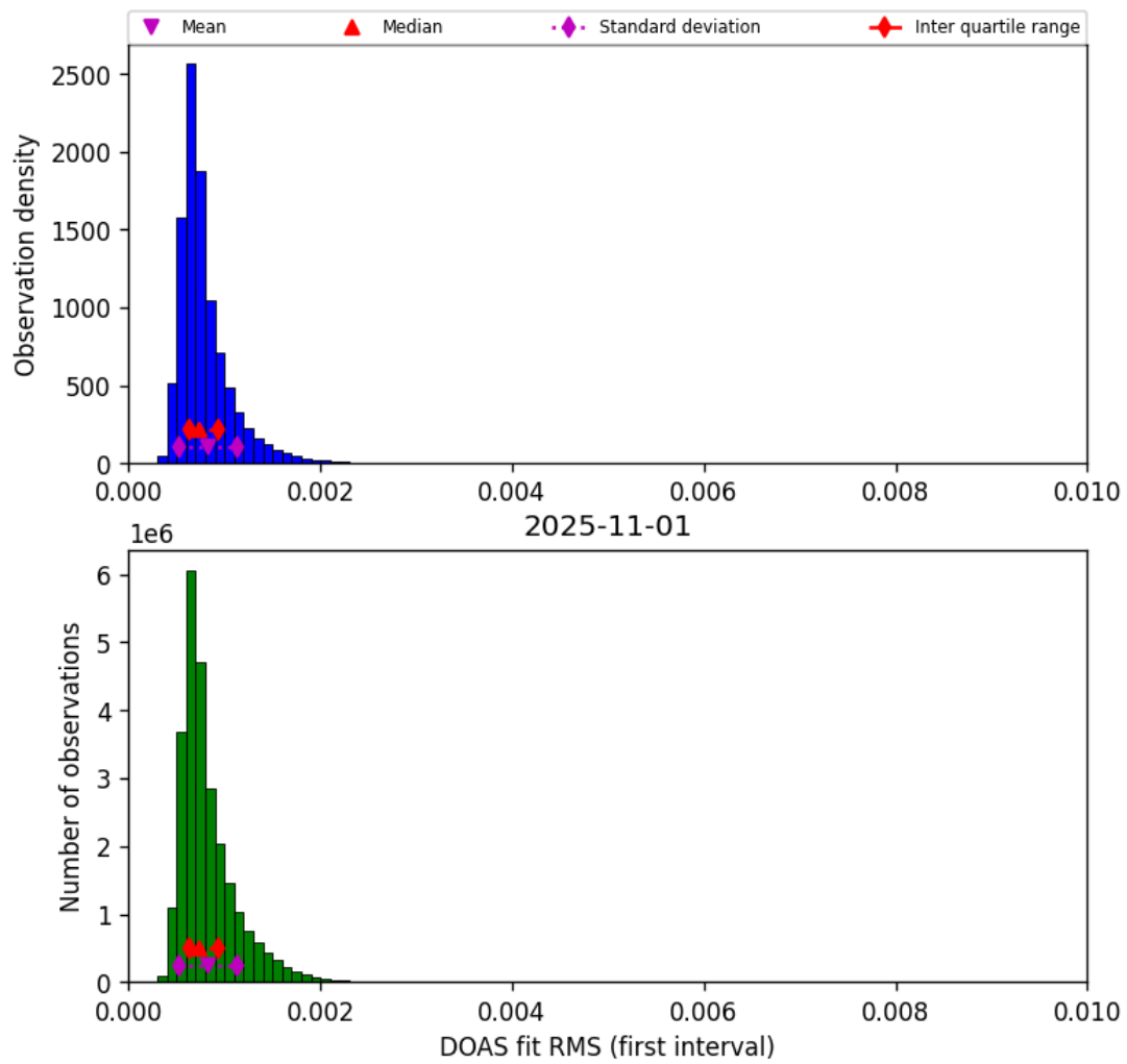
Figure 46: Histogram of “DOAS fit RMS (first interval)” for 2025-10-31 to 2025-11-02
