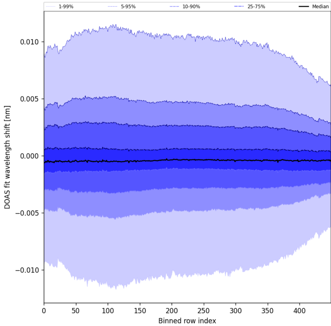
Figure 58: Along track statistics of “DOAS fit wavelength shift” for 2025-10-31 to 2025-11-02
