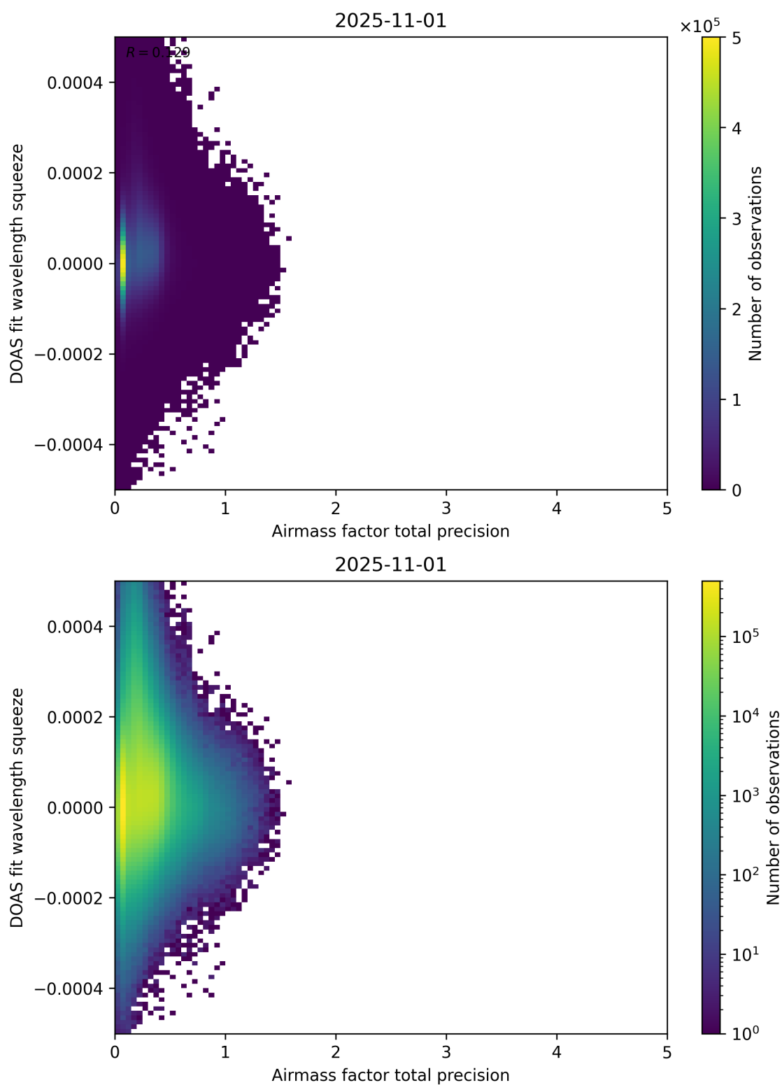
Figure 107: Scatter density plot of “Airmass factor total precision” against “DOAS fit wavelength squeeze” for 2025-10-31 to 2025-11-02.
