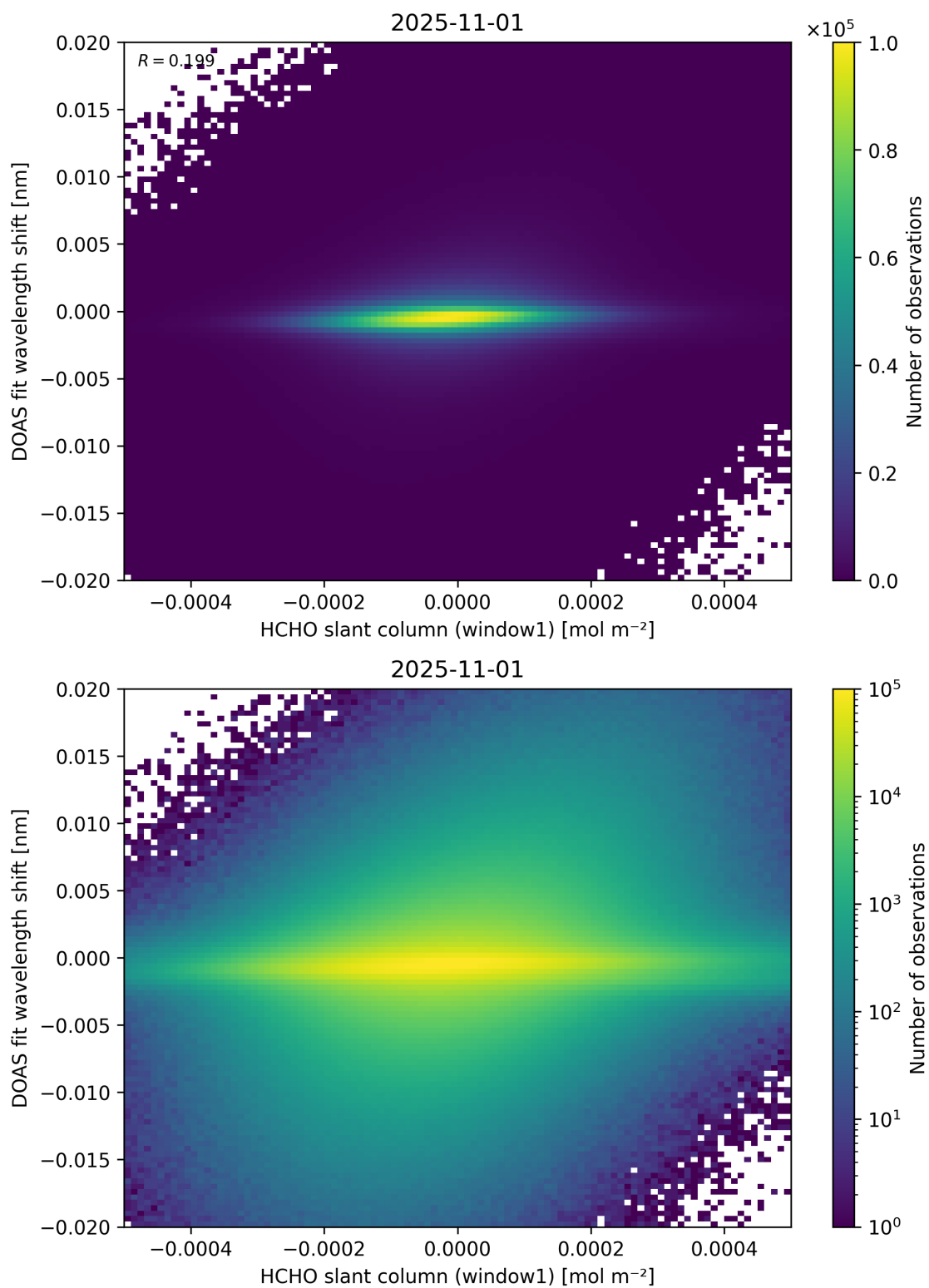
Figure 79: Scatter density plot of “HCHO slant column (window1)” against “DOAS fit wavelength shift” for 2025-10-31 to 2025-11-02.
