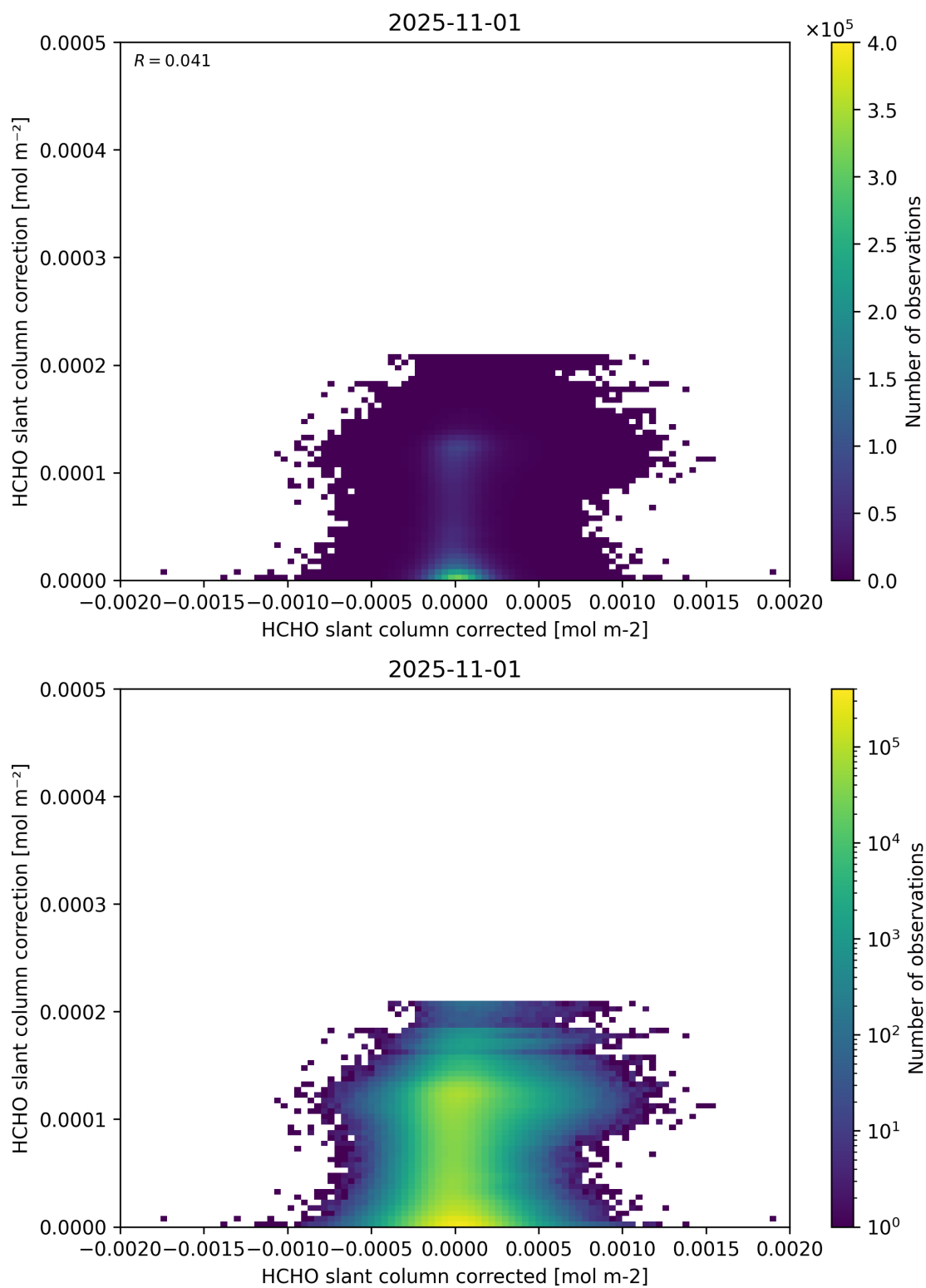
Figure 77: Scatter density plot of “HCHO slant column corrected” against “HCHO slant column correction” for 2025-10-31 to 2025-11-02.
