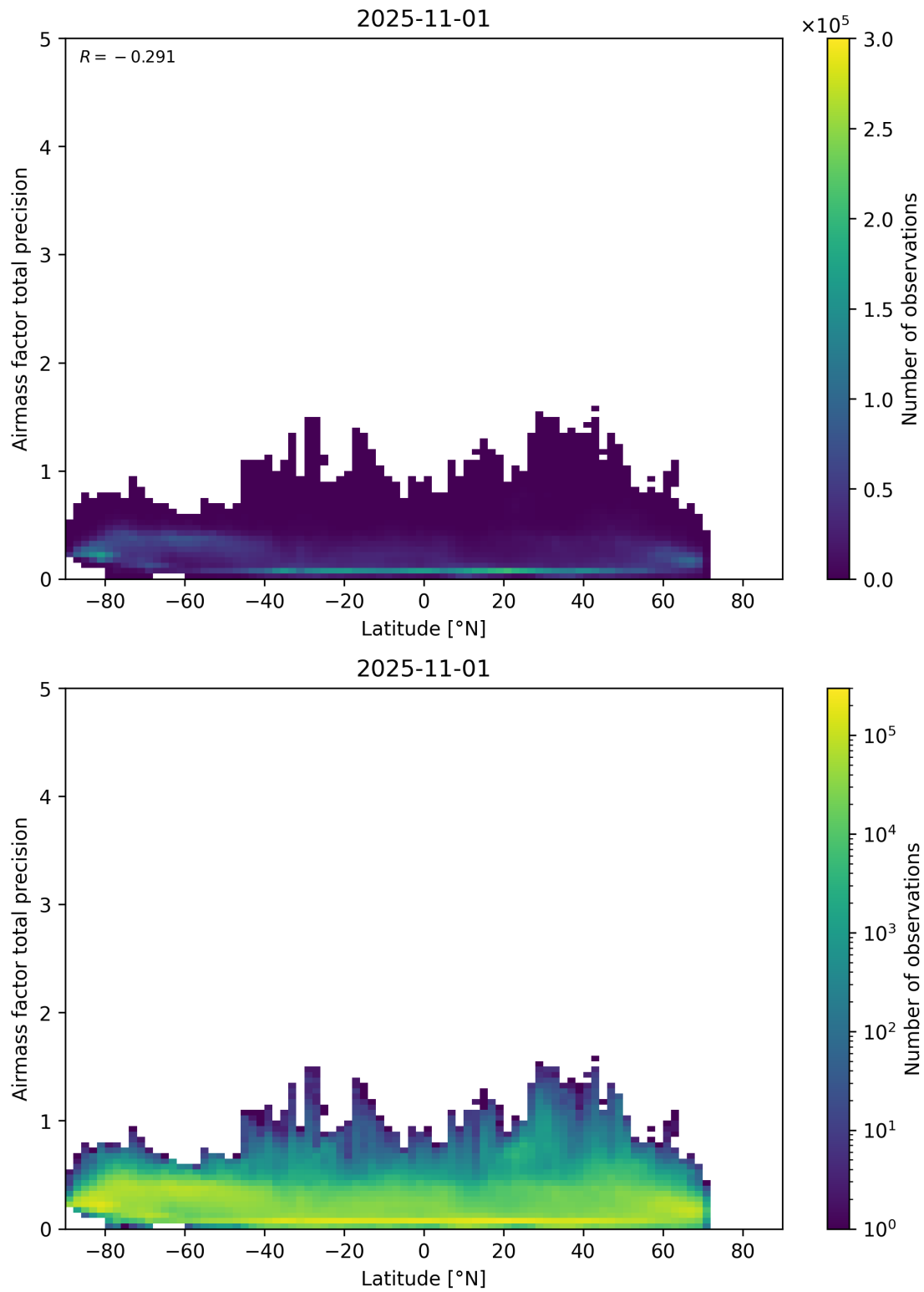
Figure 162: Scatter density plot of “Latitude” against “Airmass factor total precision” for 2025-10-31 to 2025-11-02.
