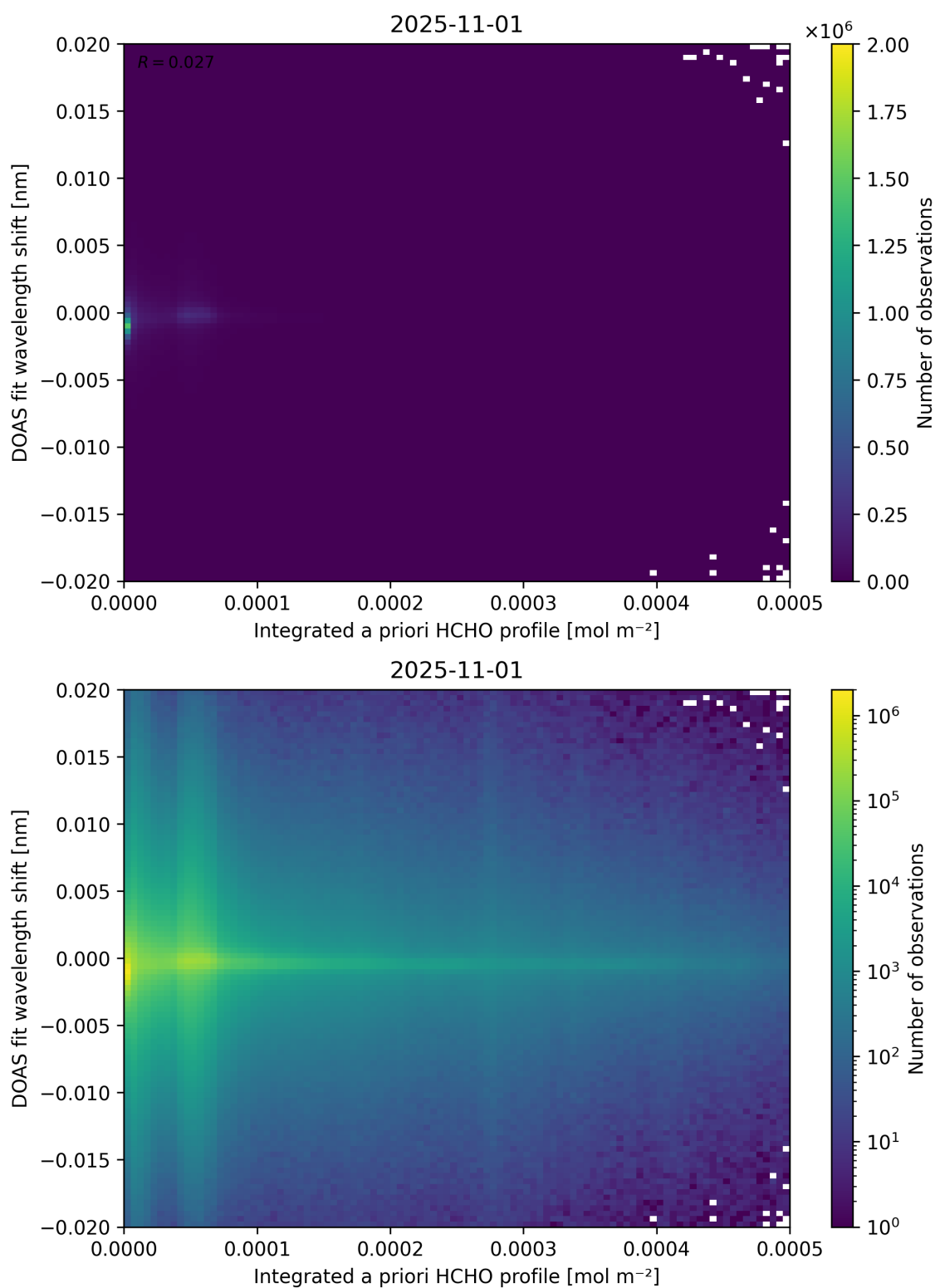
Figure 149: Scatter density plot of “Integrated a priori HCHO profile” against “DOAS fit wavelength shift” for 2025-10-31 to 2025-11-02.
