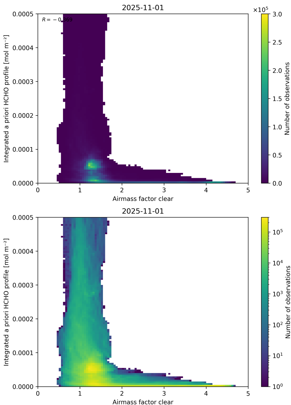
Figure 76: Scatter density plot of “Airmass factor clear” against “Integrated a priori HCHO profile” for 2025-10-31 to 2025-11-02.
