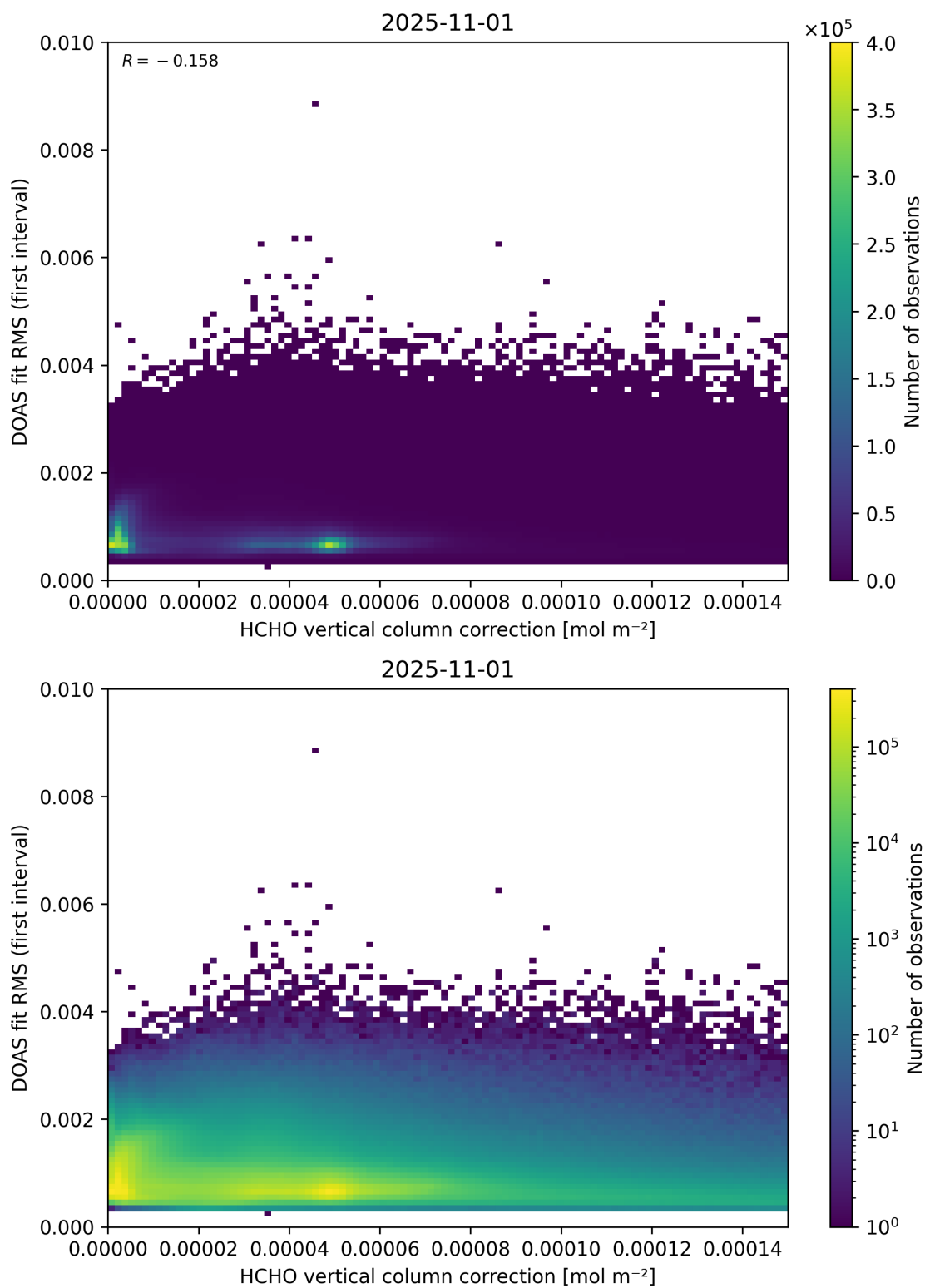
Figure 112: Scatter density plot of “HCHO vertical column correction” against “DOAS fit RMS (first interval)” for 2025-10-31 to 2025-11-02.
