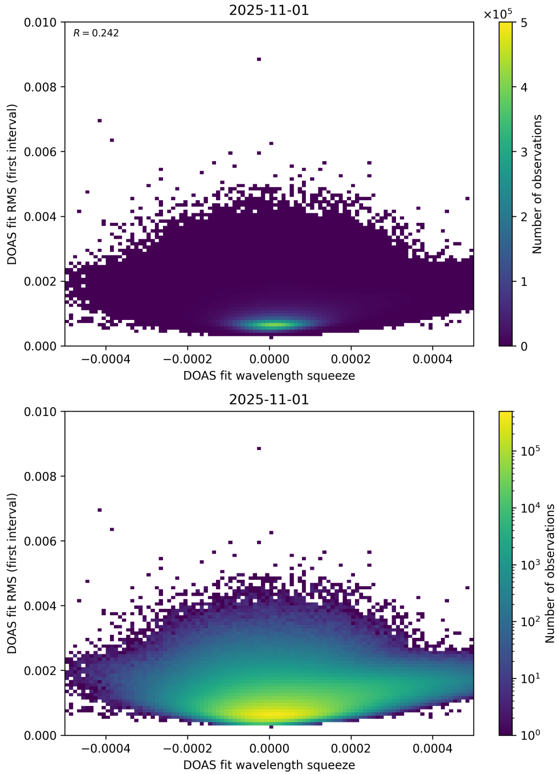
Figure 68: Scatter density plot of “DOAS fit wavelength squeeze” against “DOAS fit RMS (first interval)” for 2025-10-31 to 2025-11-02.
