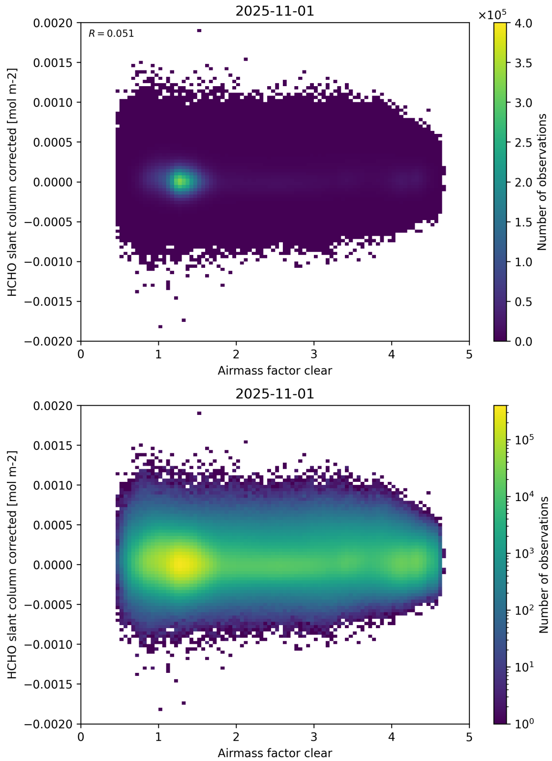
Figure 74: Scatter density plot of “Airmass factor clear” against “HCHO slant column corrected” for 2025-10-31 to 2025-11-02.
