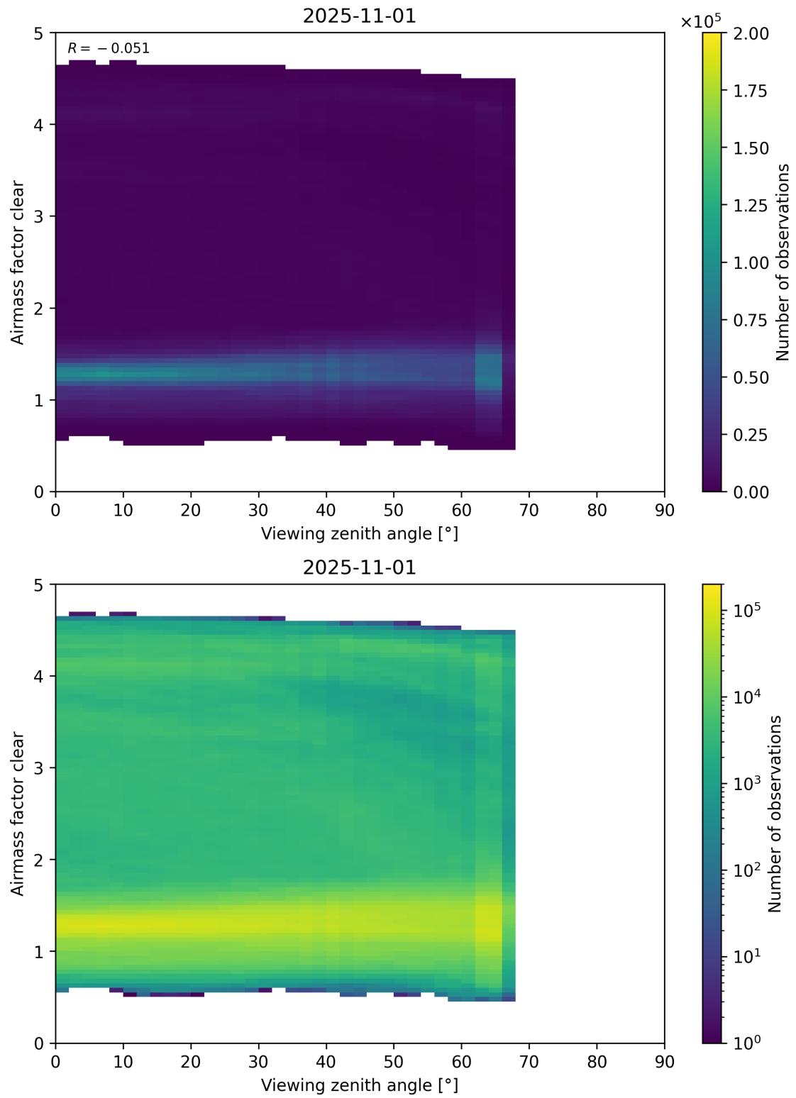
Figure 185: Scatter density plot of “Viewing zenith angle” against “Airmass factor clear” for 2025-10-31 to 2025-11-02.
