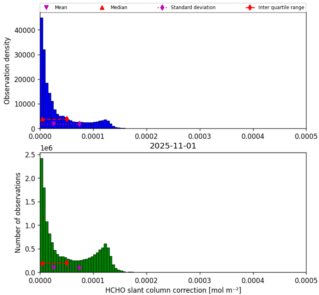
Figure 47: Histogram of “HCHO slant column correction” for 2025-10-31 to 2025-11-02
