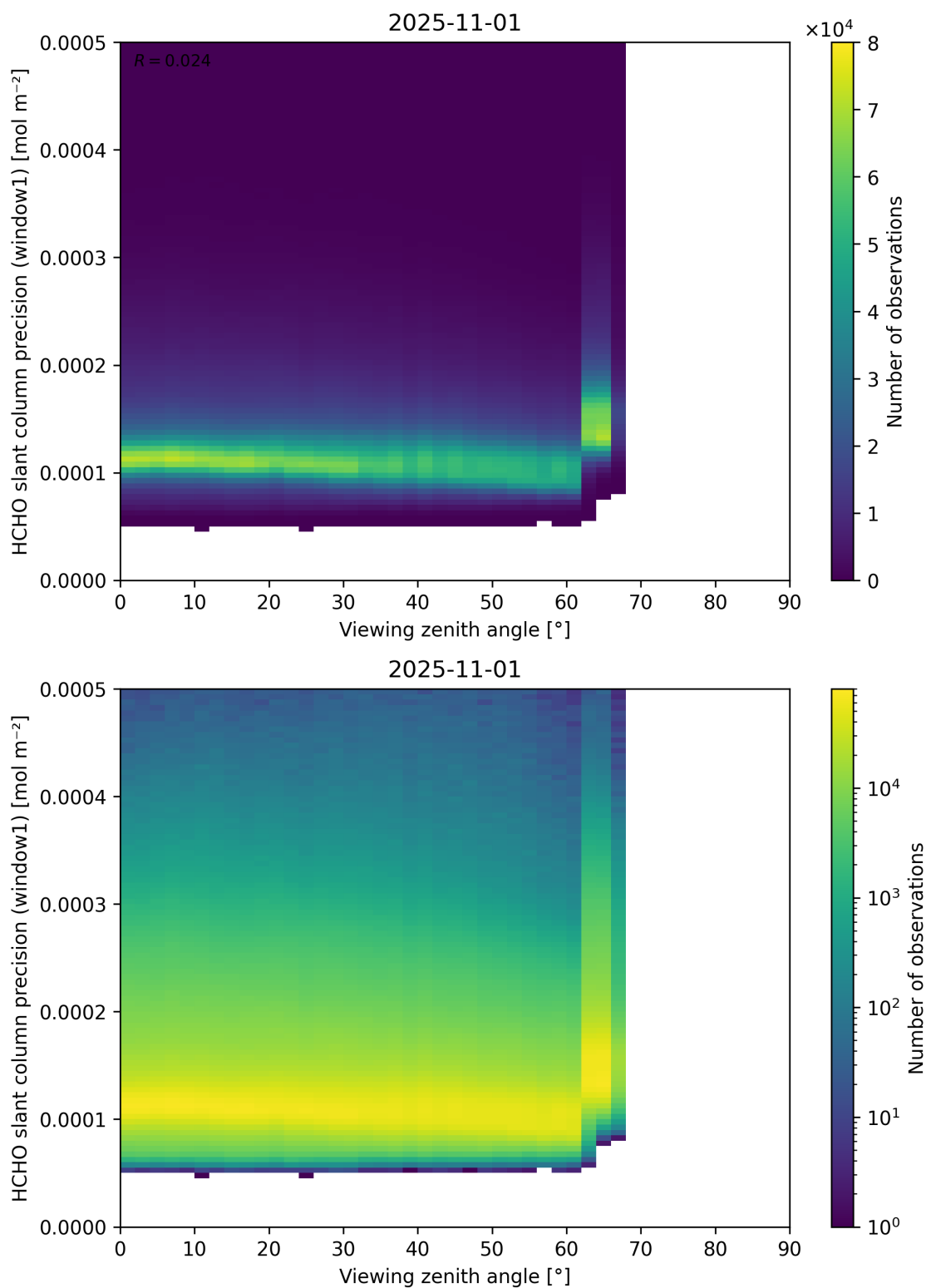
Figure 189: Scatter density plot of “Viewing zenith angle” against “HCHO slant column precision (window1)” for 2025-10-31 to 2025-11-02.
