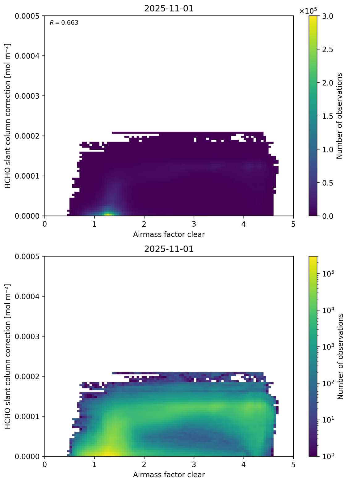
Figure 75: Scatter density plot of “Airmass factor clear” against “HCHO slant column correction” for 2025-10-31 to 2025-11-02.
