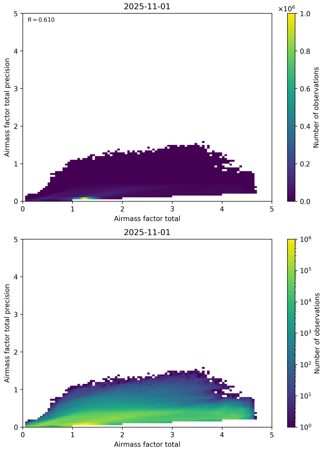
Figure 103: Scatter density plot of “Airmass factor total” against “Airmass factor total precision” for 2025-10-31 to 2025-11-02.
