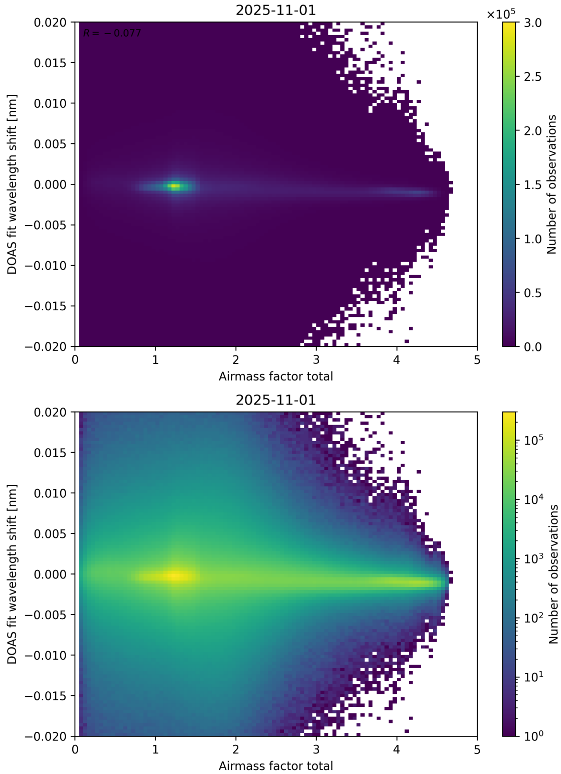
Figure 98: Scatter density plot of “Airmass factor total” against “DOAS fit wavelength shift” for 2025-10-31 to 2025-11-02.
