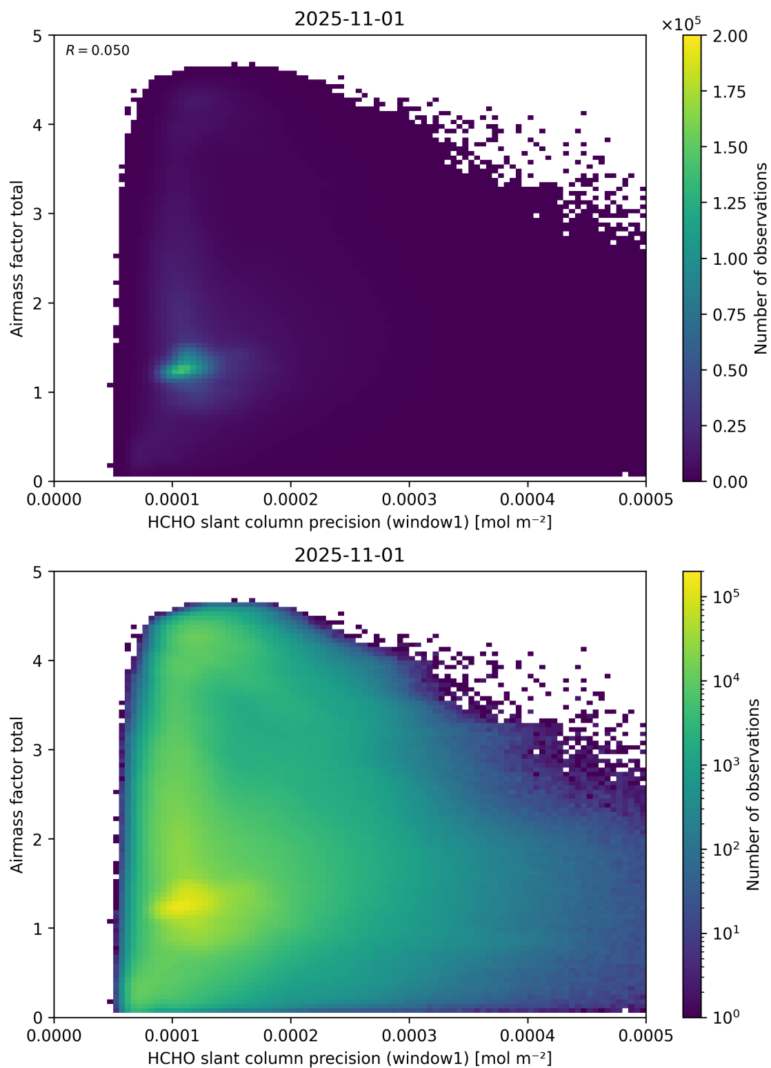
Figure 94: Scatter density plot of “HCHO slant column precision (window1)” against “Airmass factor total” for 2025-10-31 to 2025-11-02.
