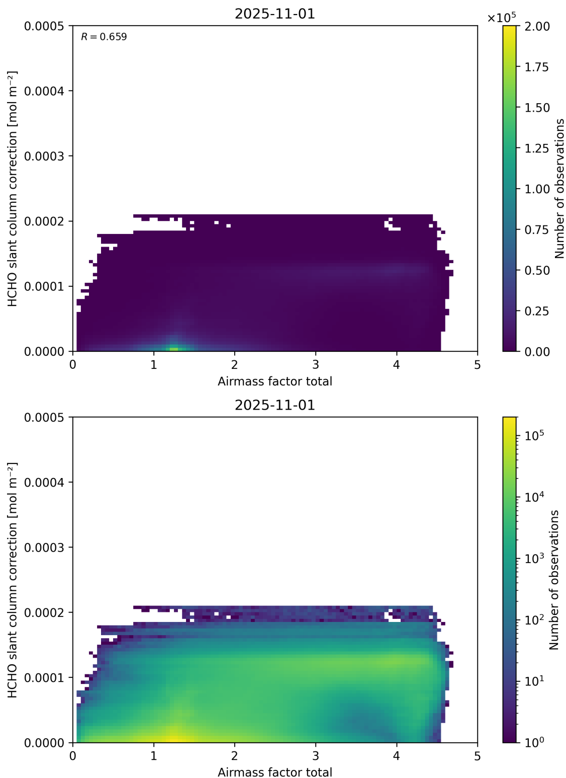
Figure 102: Scatter density plot of “Airmass factor total” against “HCHO slant column correction” for 2025-10-31 to 2025-11-02.
