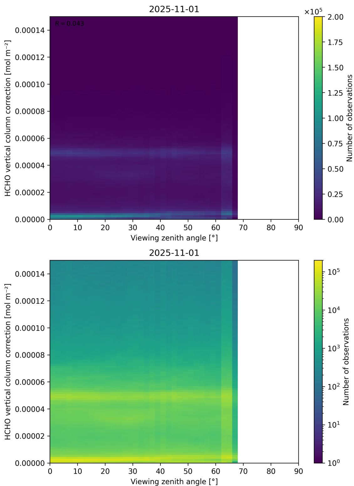
Figure 193: Scatter density plot of “Viewing zenith angle” against “HCHO vertical column correction” for 2025-10-31 to 2025-11-02.
