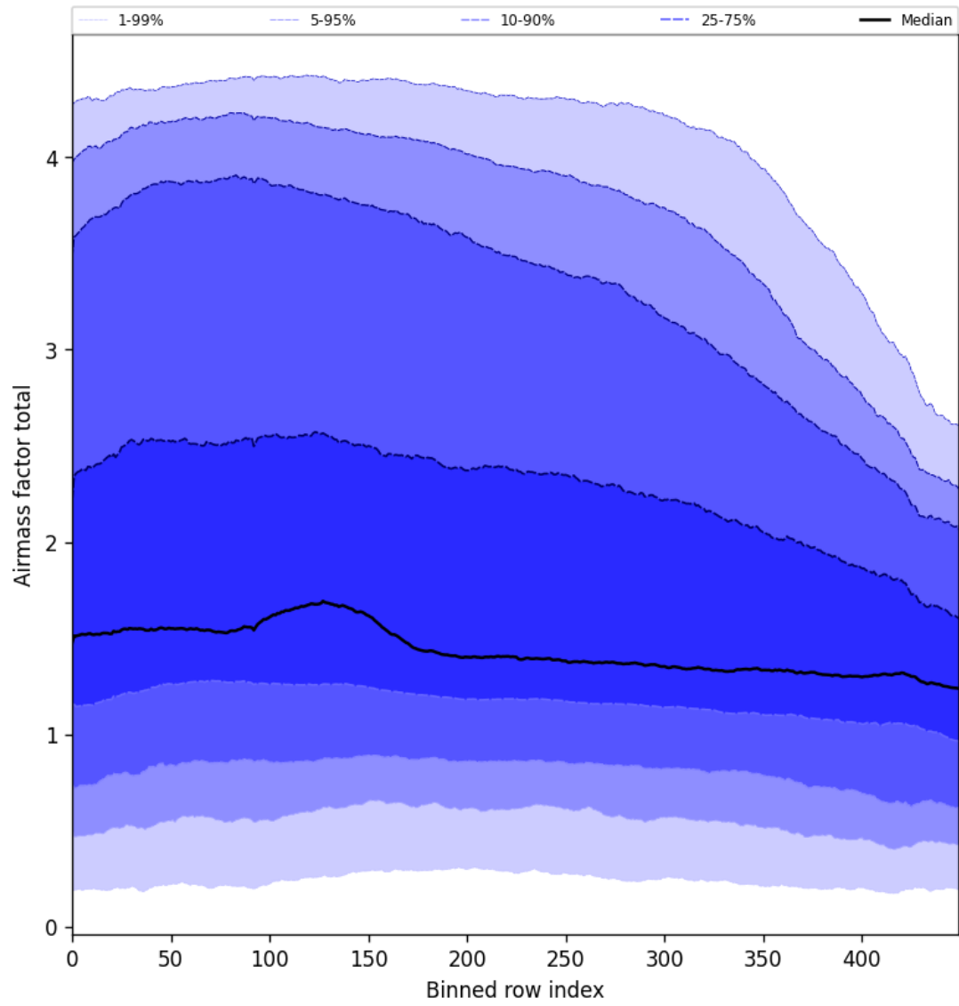
Figure 54: Along track statistics of “Airmass factor total” for 2025-10-31 to 2025-11-02
