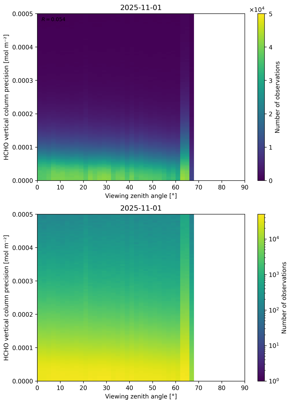
Figure 194: Scatter density plot of “Viewing zenith angle” against “HCHO vertical column precision” for 2025-10-31 to 2025-11-02.
