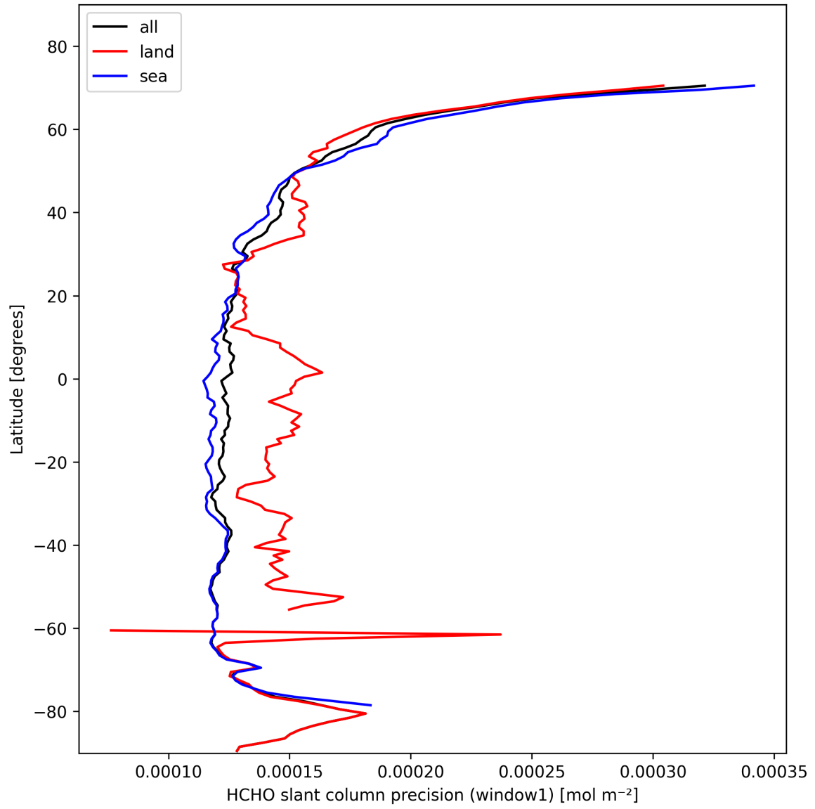
Figure 25: Zonal average of "HCHO slant column precision (window1)" for 2025-10-31 to 2025-11-02.
