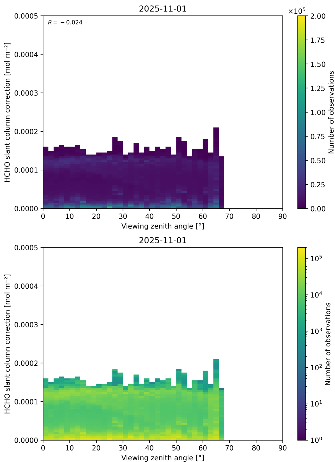
Figure 187: Scatter density plot of “Viewing zenith angle” against “HCHO slant column correction” for 2025-10-31 to 2025-11-02.
