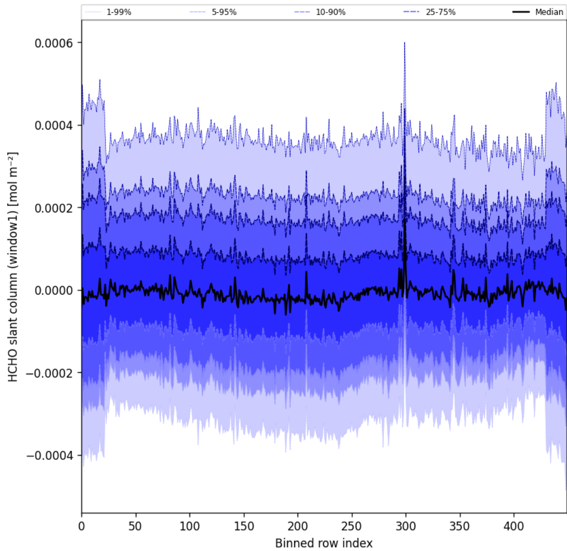
Figure 52: Along track statistics of “HCHO slant column (window1)” for 2025-10-31 to 2025-11-02
