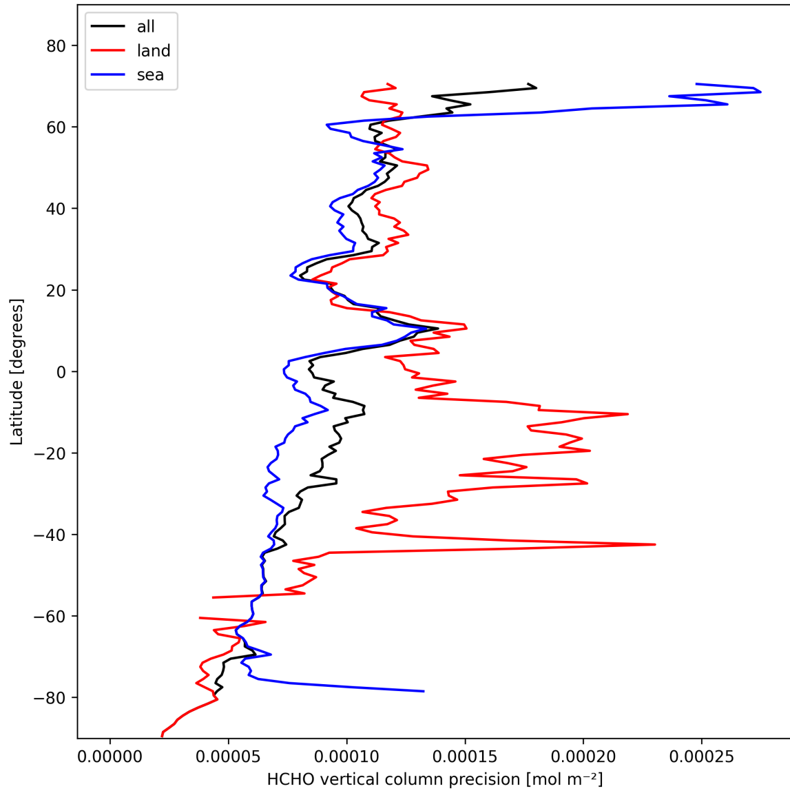
Figure 22: Zonal average of “HCHO vertical column precision” for 2025-10-31 to 2025-11-02.
