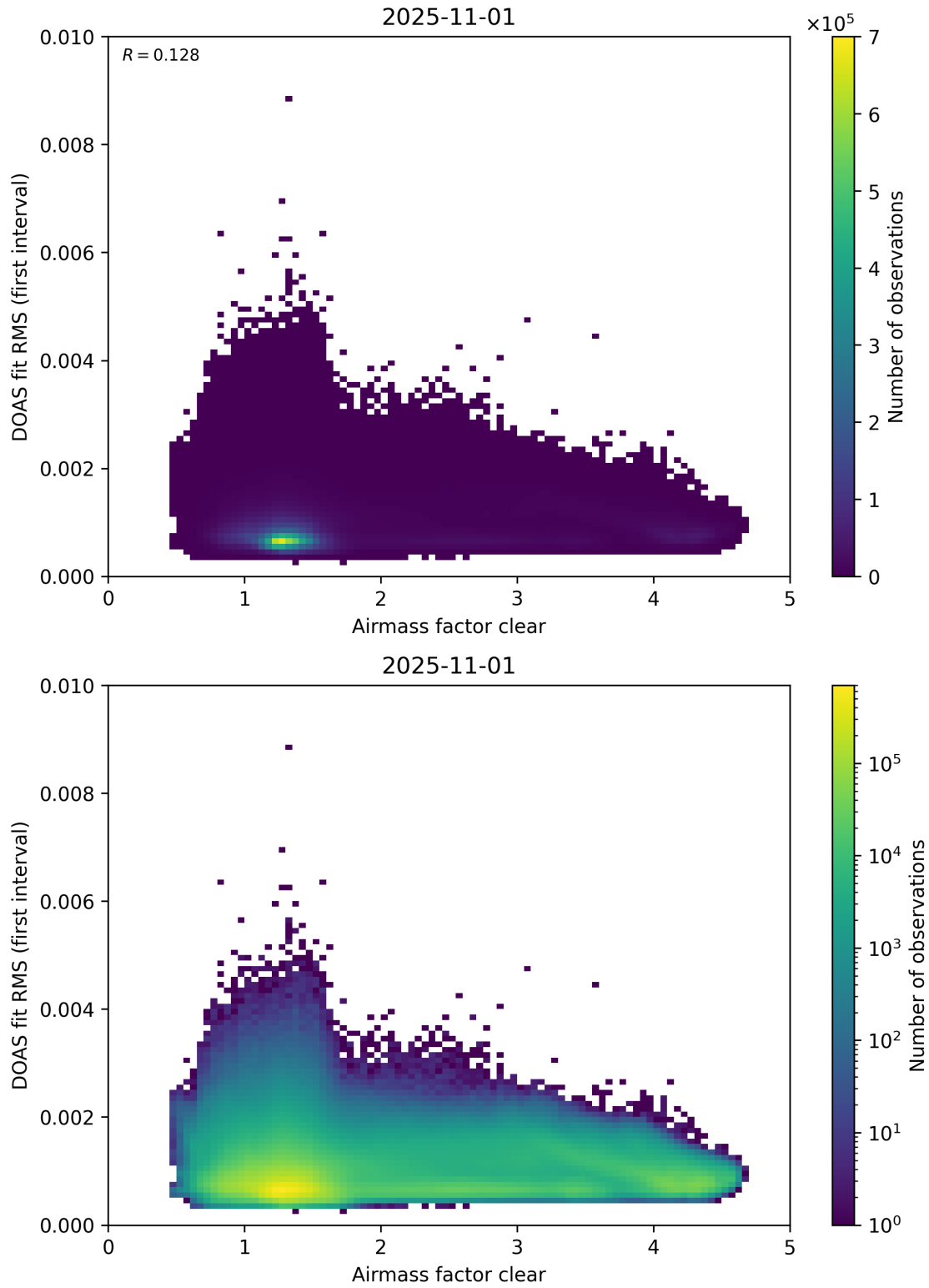
Figure 71: Scatter density plot of “Airmass factor clear” against “DOAS fit RMS (first interval)” for 2025-10-31 to 2025-11-02.
