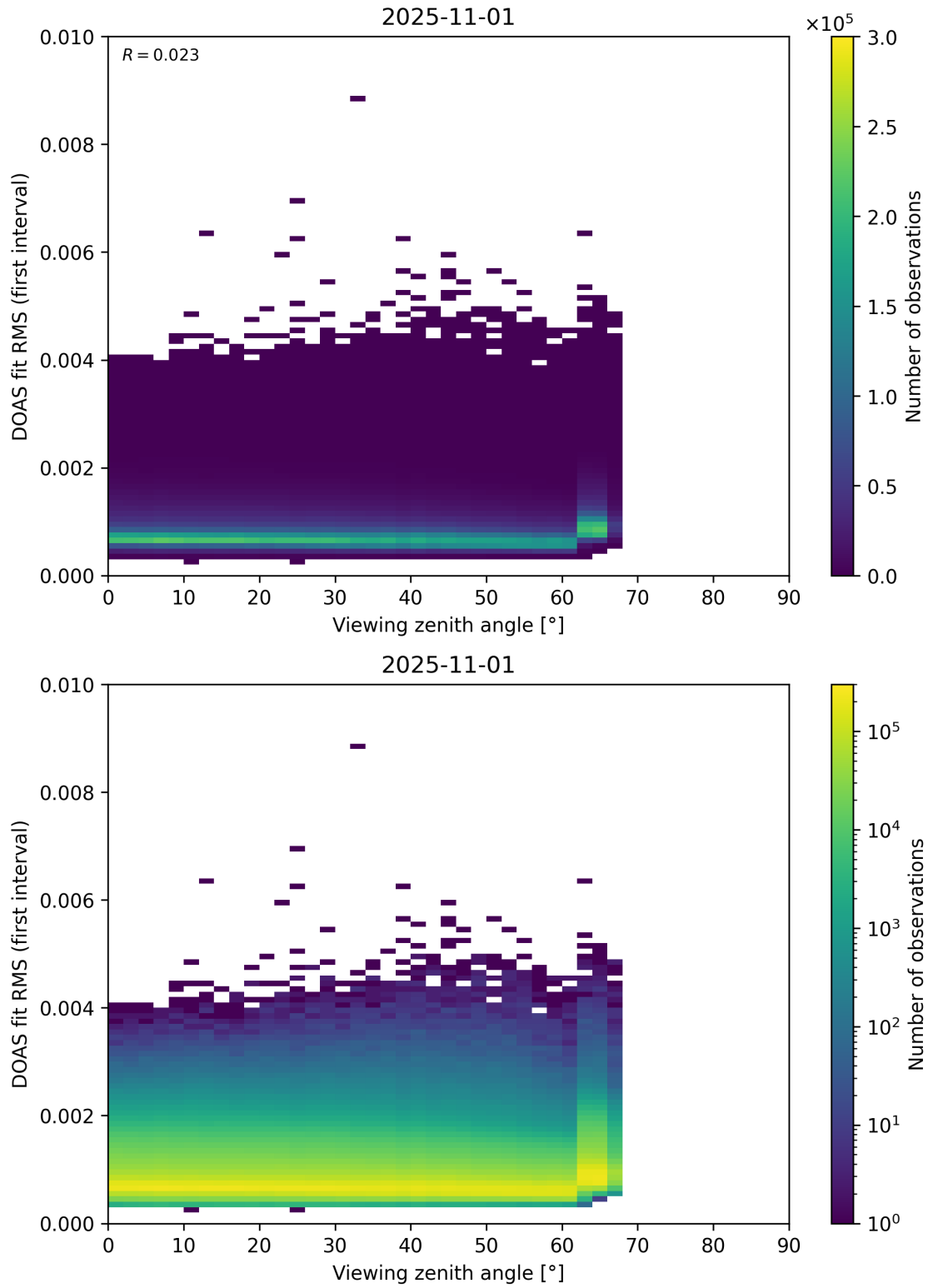
Figure 182: Scatter density plot of “Viewing zenith angle” against “DOAS fit RMS (first interval)” for 2025-10-31 to 2025-11-02.
