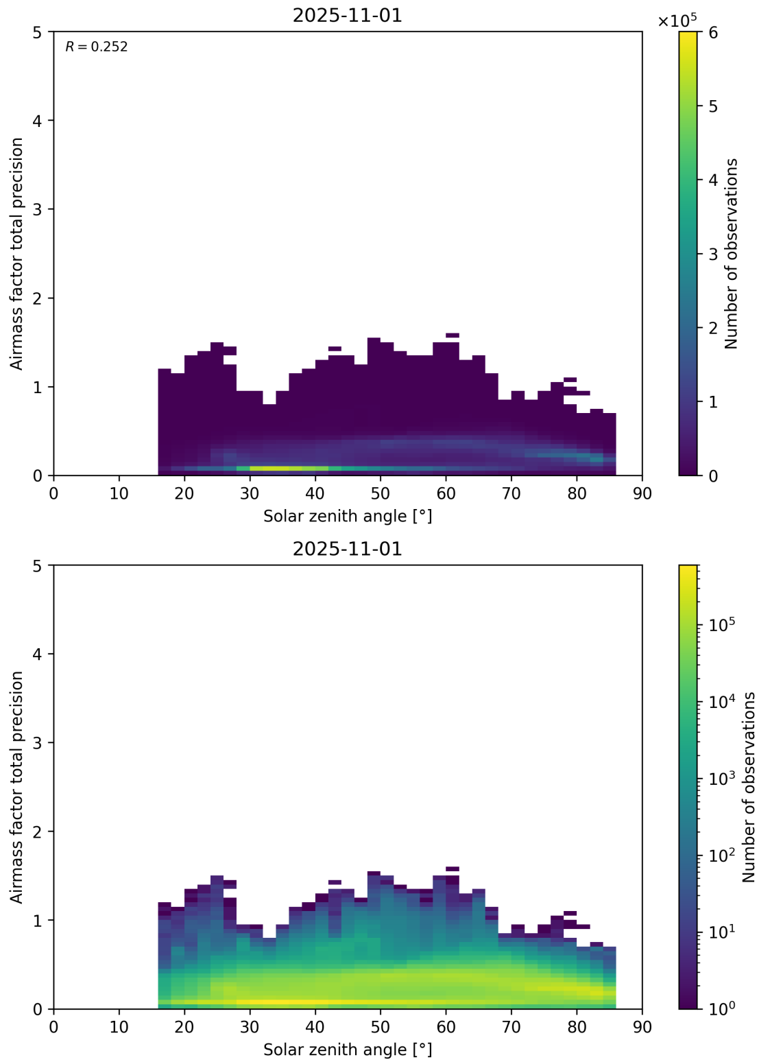
Figure 176: Scatter density plot of “Solar zenith angle” against “Airmass factor total precision” for 2025-10-31 to 2025-11-02.
