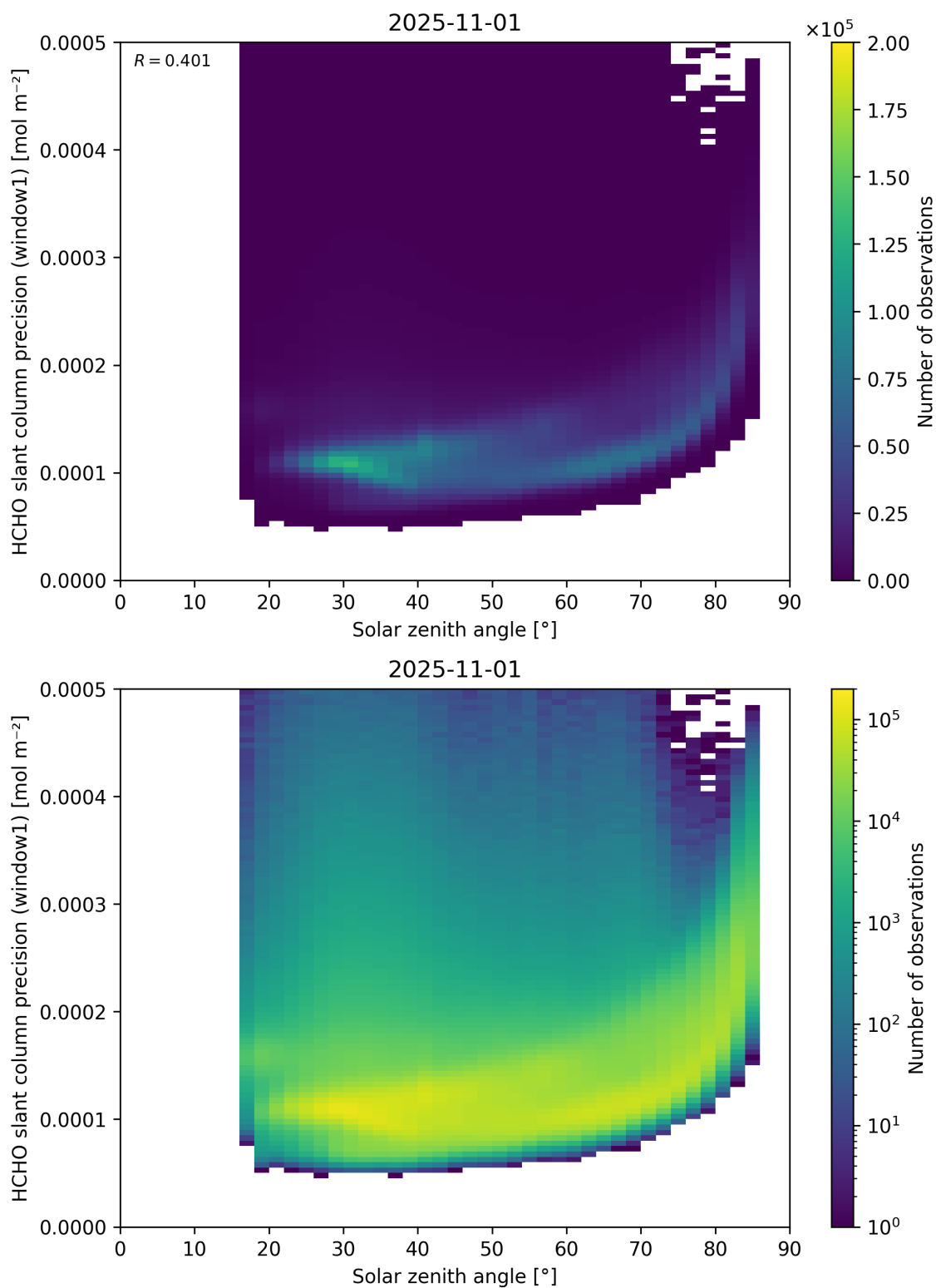
Figure 174: Scatter density plot of “Solar zenith angle” against “HCHO slant column precision (window1)” for 2025-10-31 to 2025-11-02.
