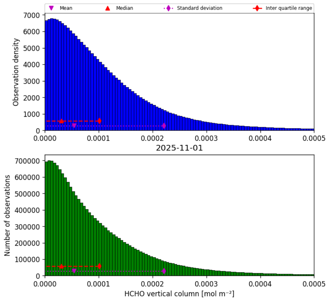
Figure 35: Histogram of “HCHO vertical column” for 2025-10-31 to 2025-11-02
