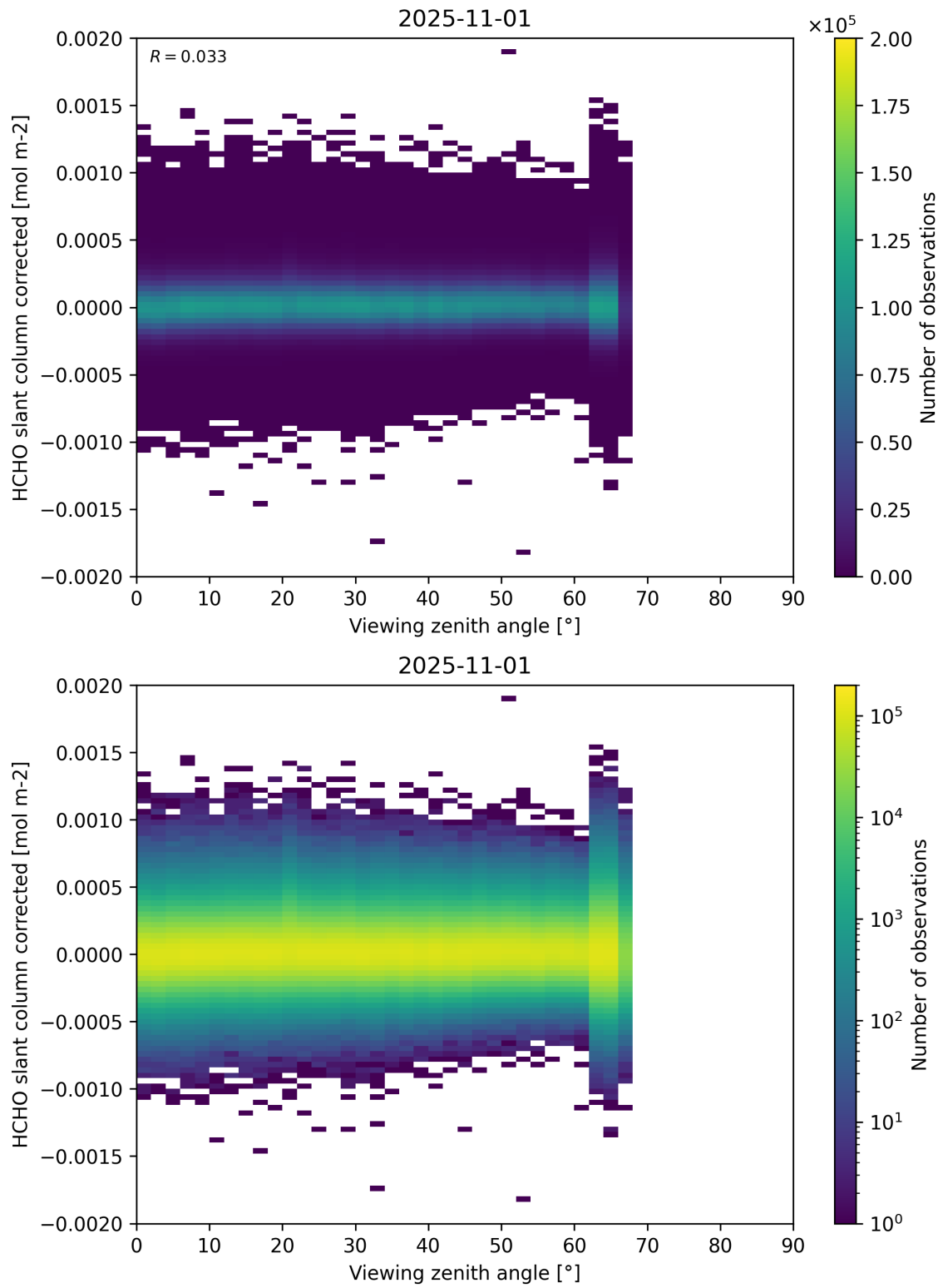
Figure 186: Scatter density plot of “Viewing zenith angle” against “HCHO slant column corrected” for 2025-10-31 to 2025-11-02.
