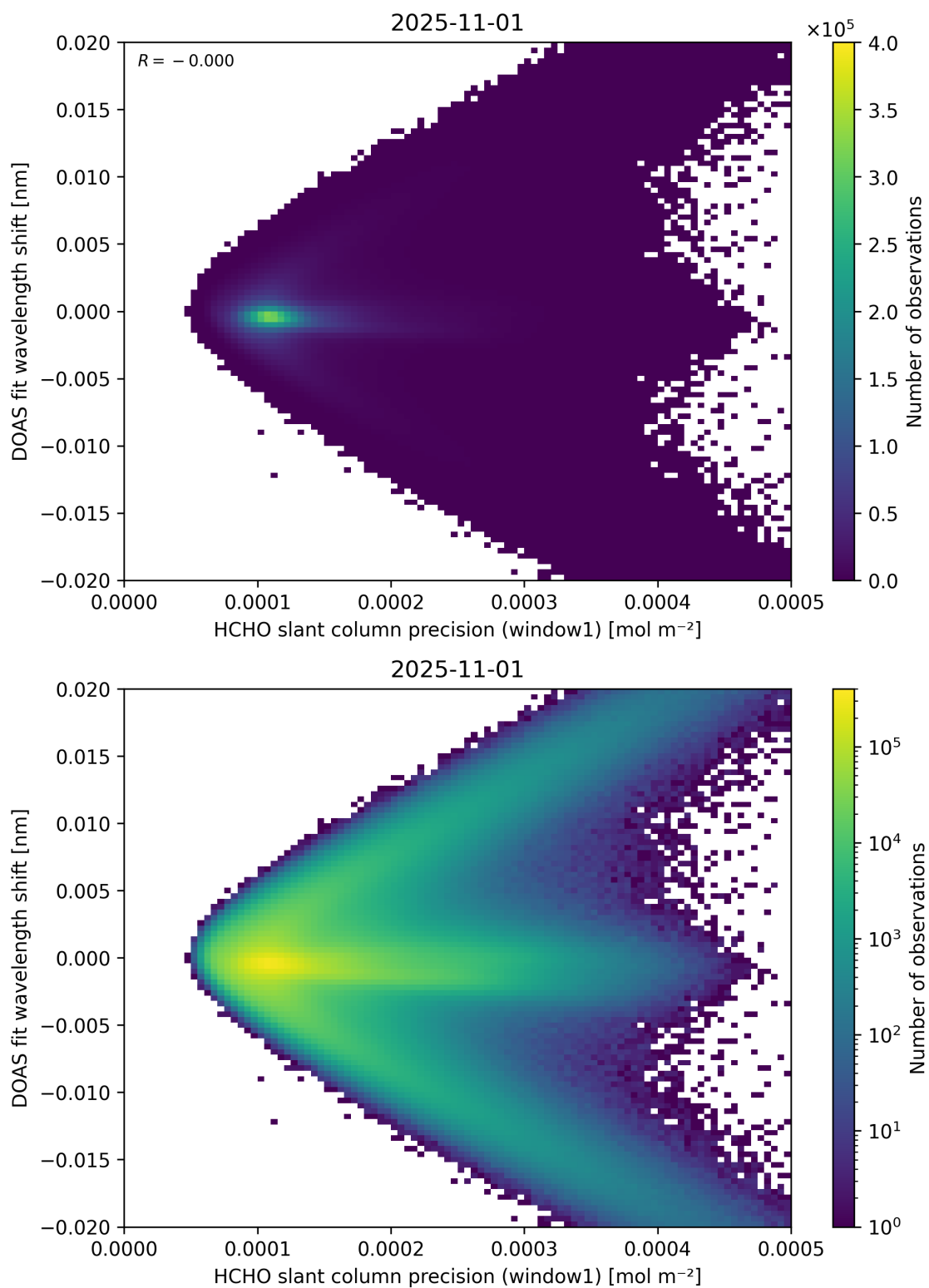
Figure 89: Scatter density plot of “HCHO slant column precision (window1)” against “DOAS fit wavelength shift” for 2025-10-31 to 2025-11-02.
