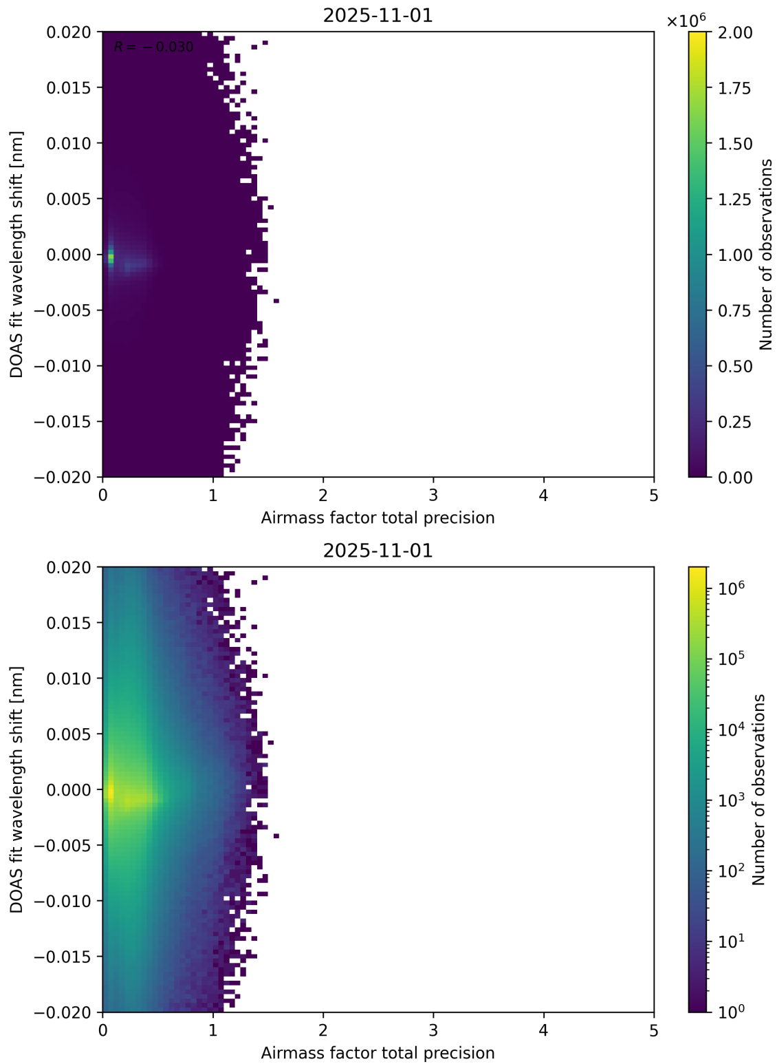
Figure 106: Scatter density plot of “Airmass factor total precision” against “DOAS fit wavelength shift” for 2025-10-31 to 2025-11-02.
