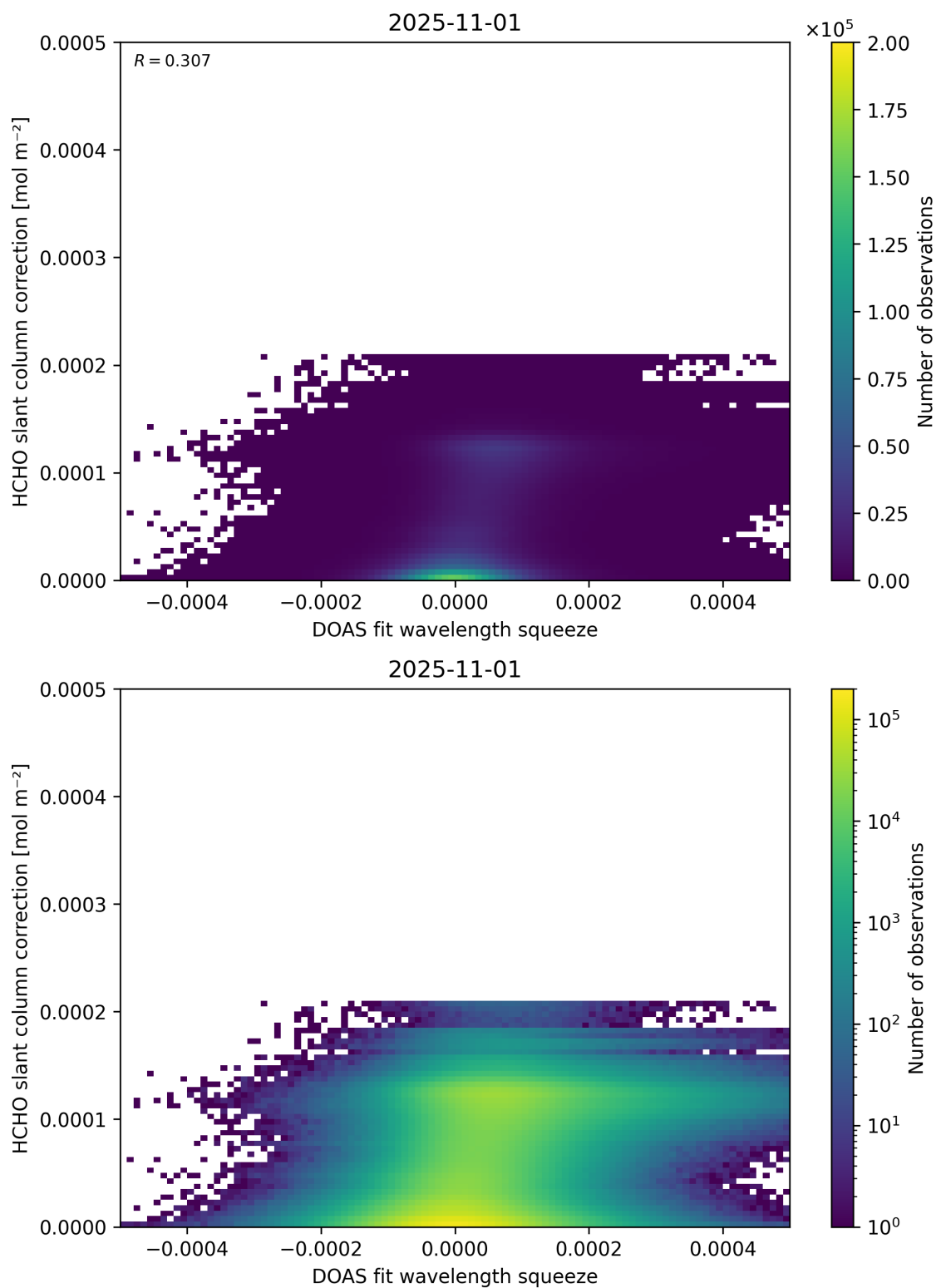
Figure 70: Scatter density plot of “DOAS fit wavelength squeeze” against “HCHO slant column correction” for 2025-10-31 to 2025-11-02.
