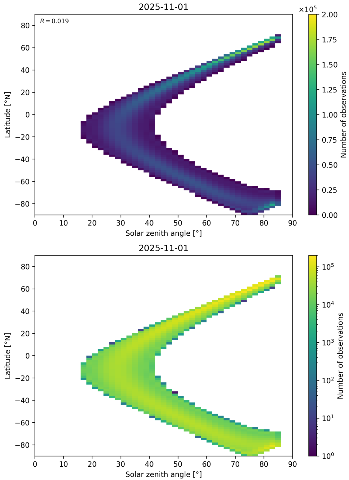
Figure 181: Scatter density plot of “Solar zenith angle” against “Latitude” for 2025-10-31 to 2025-11-02.
