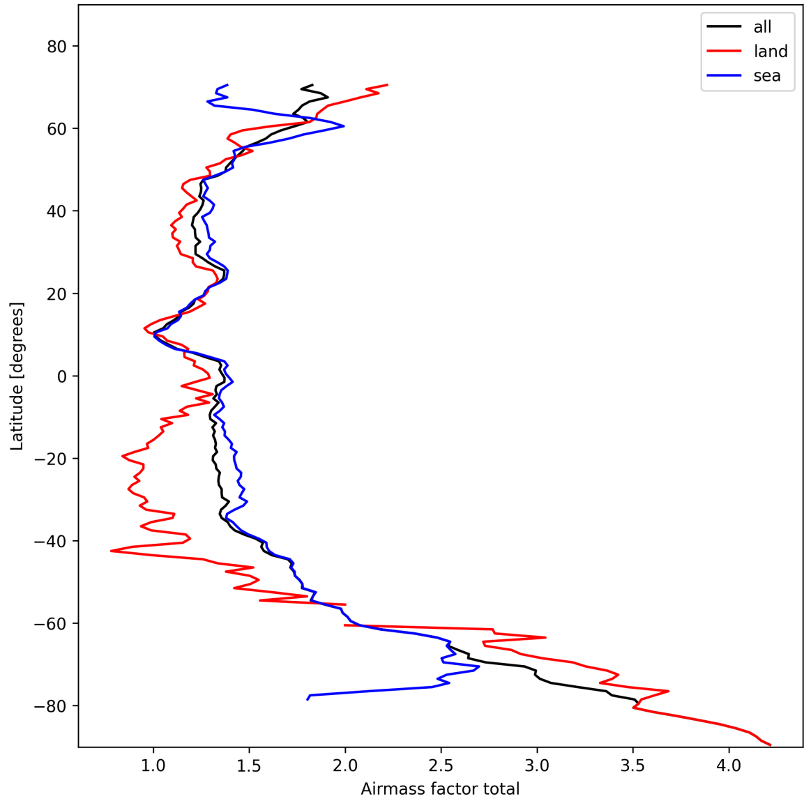
Figure 26: Zonal average of “Airmass factor total” for 2025-10-31 to 2025-11-02.
