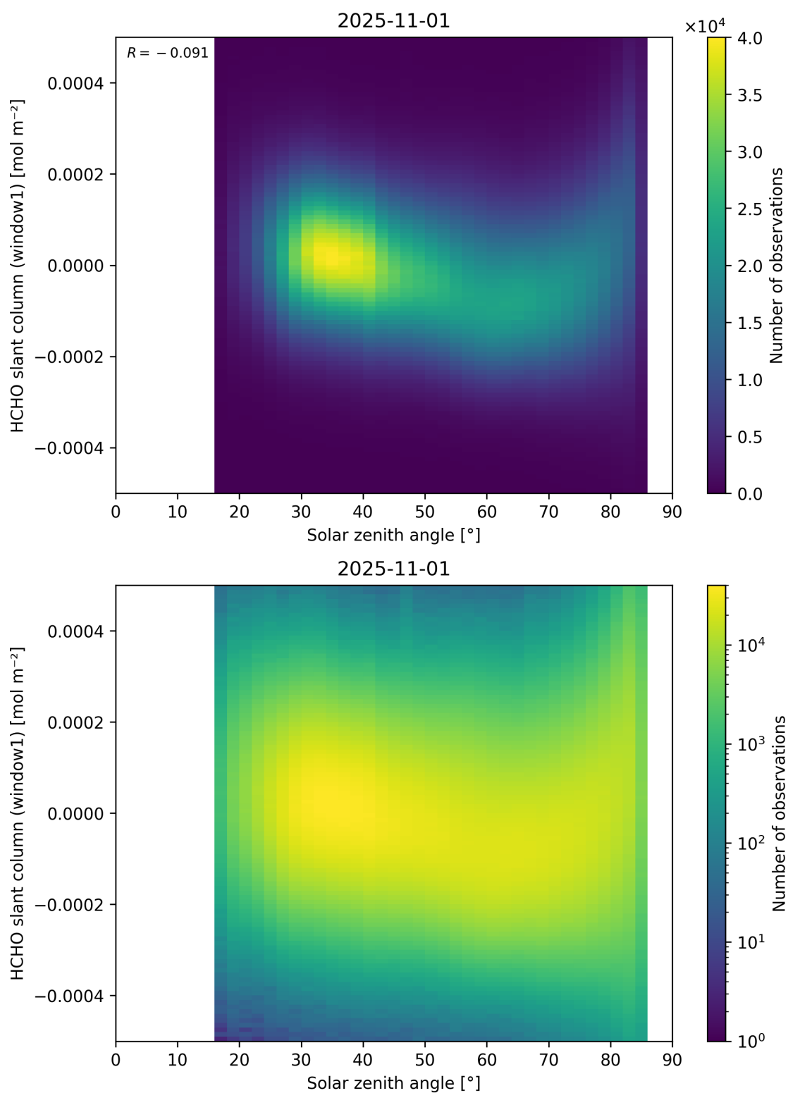
Figure 173: Scatter density plot of “Solar zenith angle” against “HCHO slant column (window1)” for 2025-10-31 to 2025-11-02.
