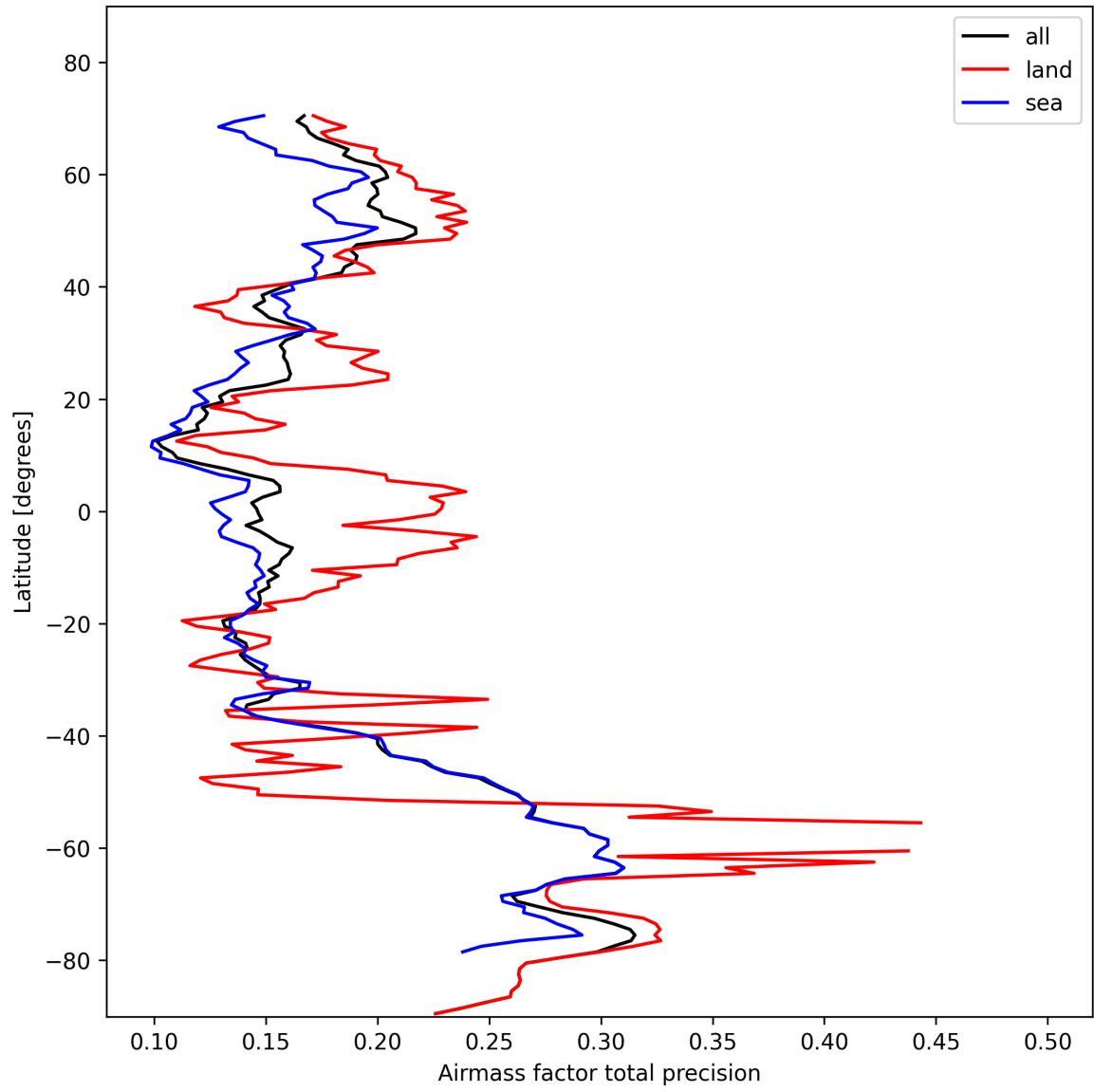
Figure 27: Zonal average of “Airmass factor total precision” for 2025-10-31 to 2025-11-02.
