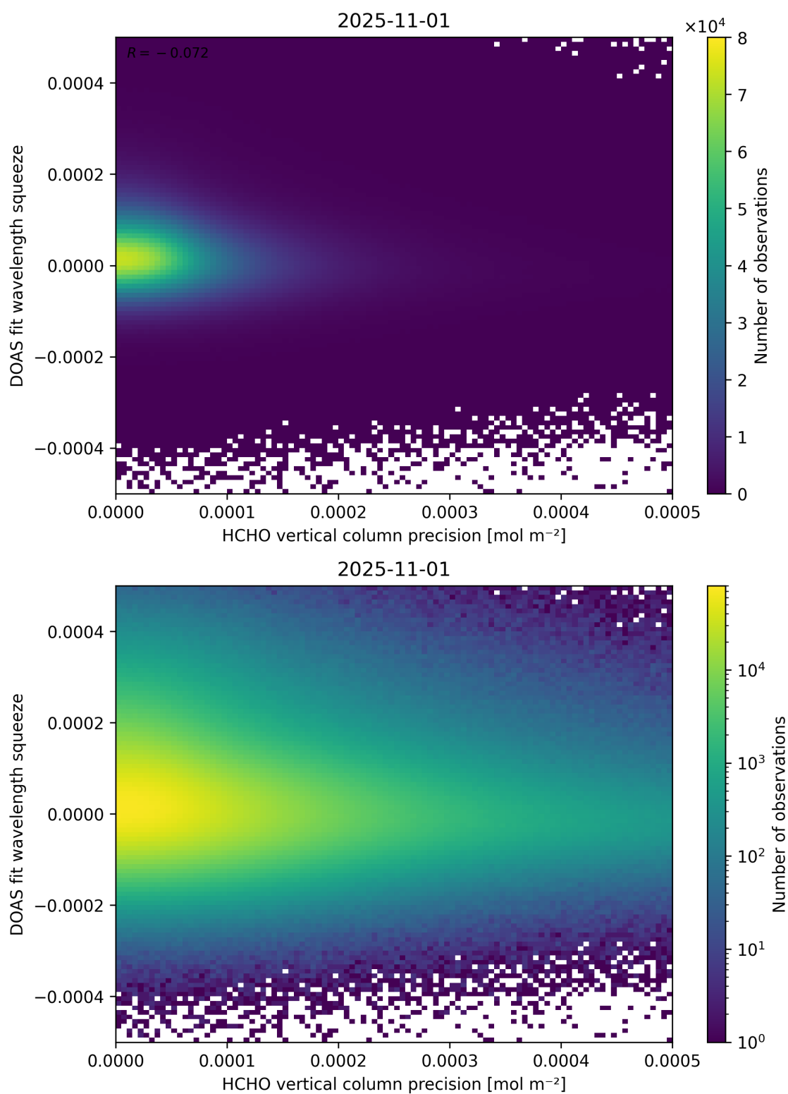
Figure 138: Scatter density plot of “HCHO vertical column precision” against “DOAS fit wavelength squeeze” for 2025-10-31 to 2025-11-02.
