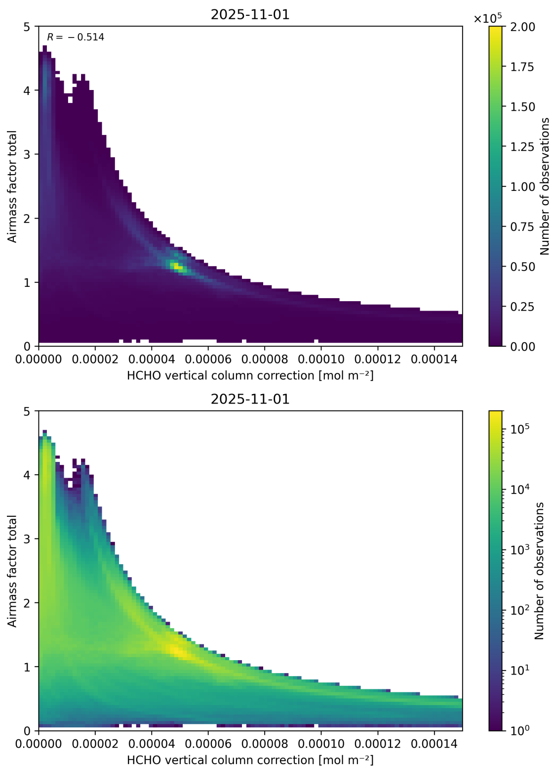
Figure 120: Scatter density plot of “HCHO vertical column correction” against “Airmass factor total” for 2025-10-31 to 2025-11-02.
