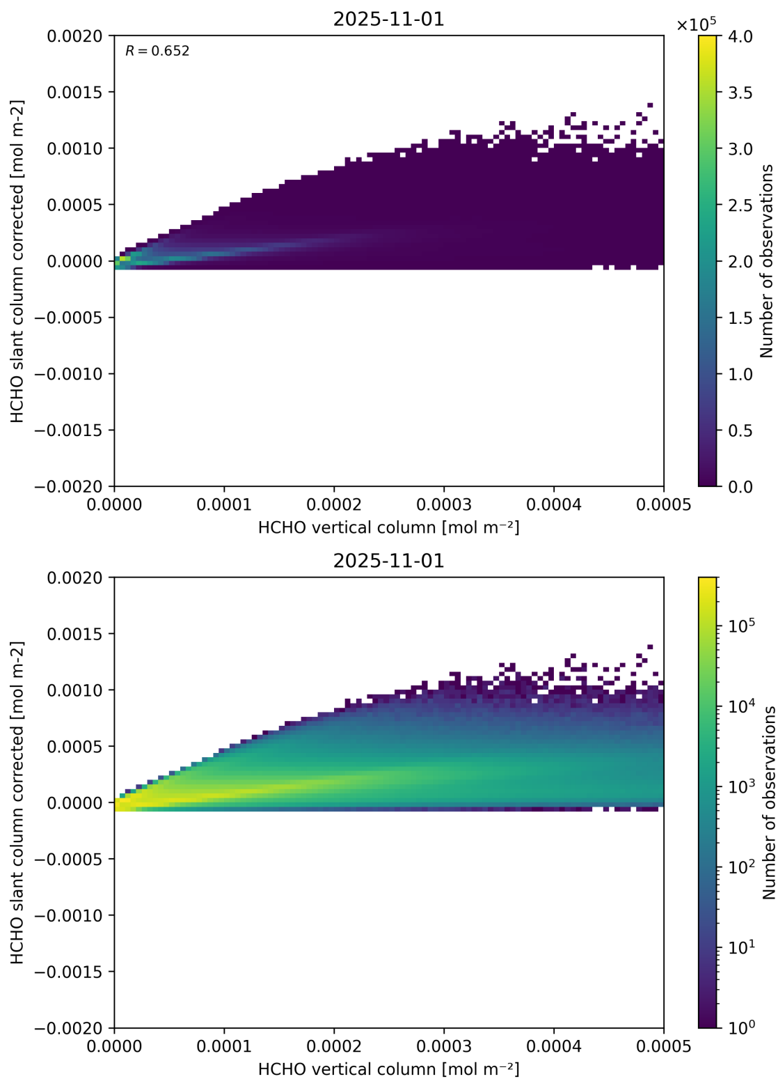
Figure 127: Scatter density plot of “HCHO vertical column” against “HCHO slant column corrected” for 2025-10-31 to 2025-11-02.
