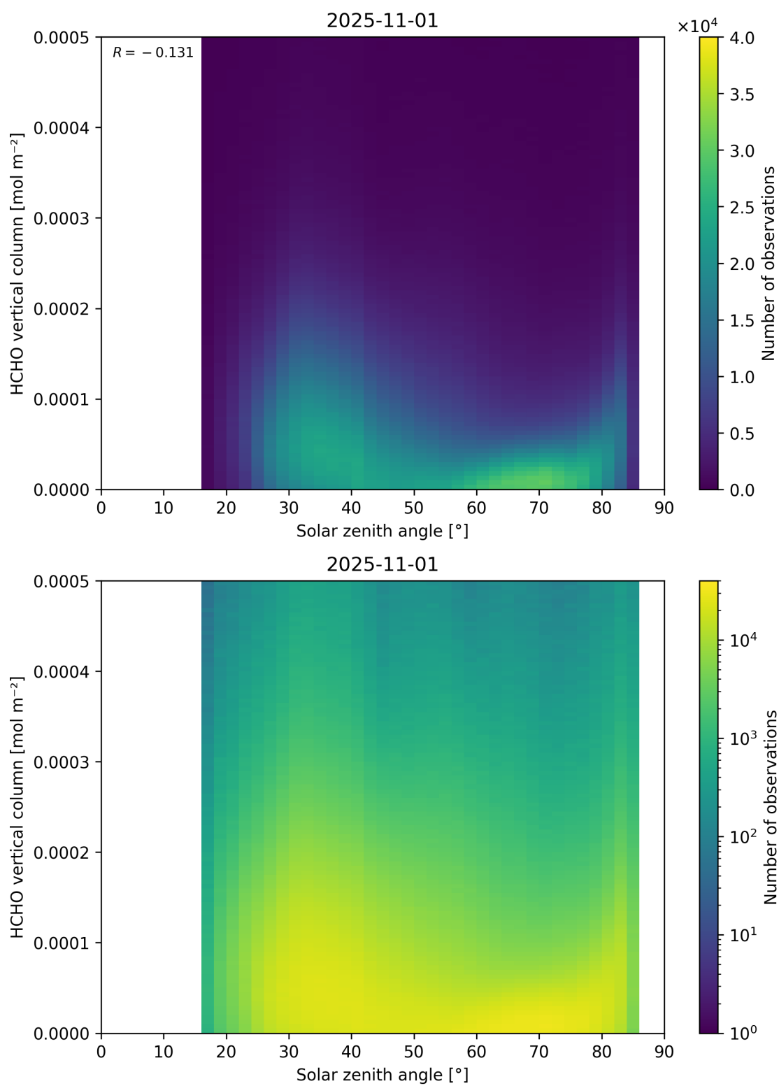
Figure 177: Scatter density plot of “Solar zenith angle” against “HCHO vertical column” for 2025-10-31 to 2025-11-02.
