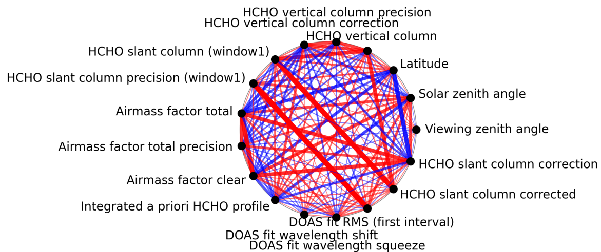
Figure 1: Map of correlation graph for 2025-10-31 to 2025-11-02.
