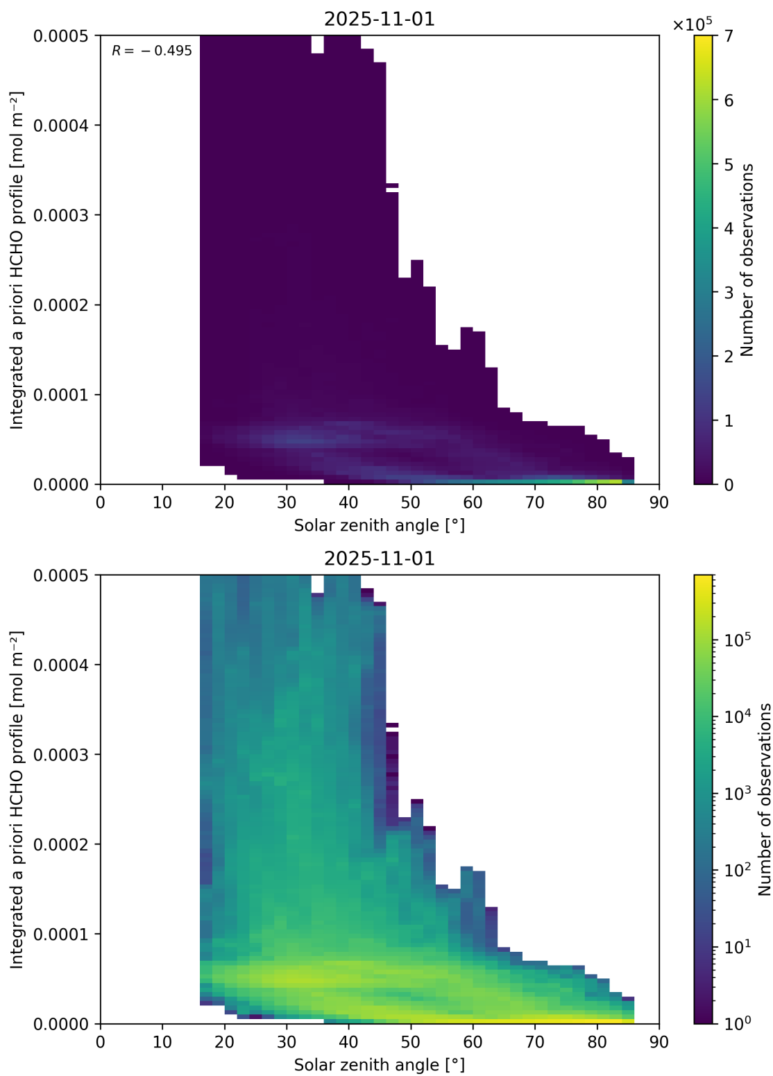
Figure 180: Scatter density plot of “Solar zenith angle” against “Integrated a priori HCHO profile” for 2025-10-31 to 2025-11-02.
