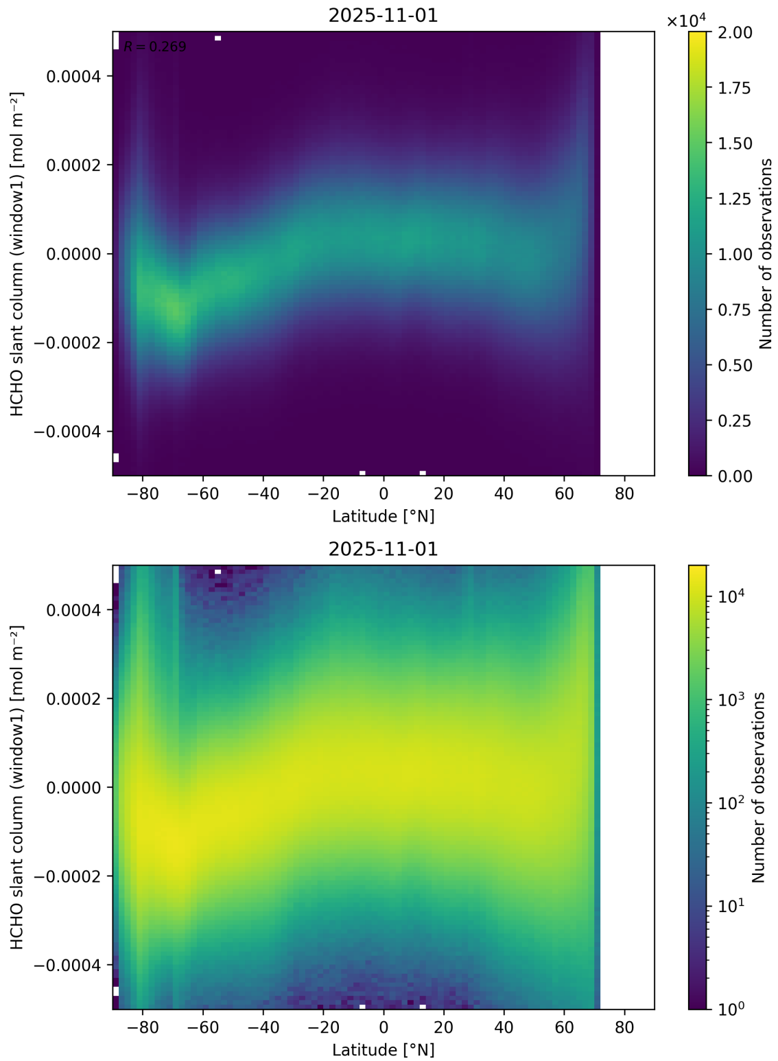
Figure 159: Scatter density plot of “Latitude” against “HCHO slant column (window1)” for 2025-10-31 to 2025-11-02.
