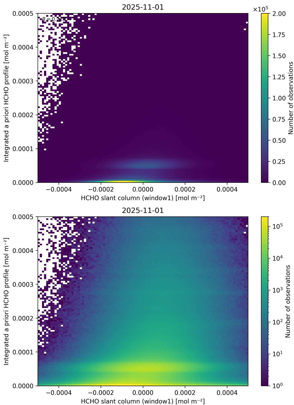
Figure 87: Scatter density plot of “HCHO slant column (window1)” against “Integrated a priori HCHO profile” for 2025-10-31 to 2025-11-02.
