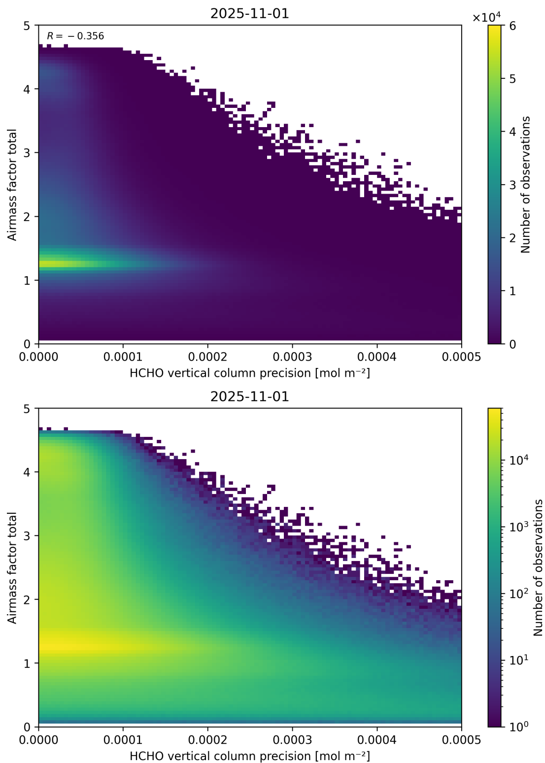
Figure 144: Scatter density plot of “HCHO vertical column precision” against “Airmass factor total” for 2025-10-31 to 2025-11-02.
