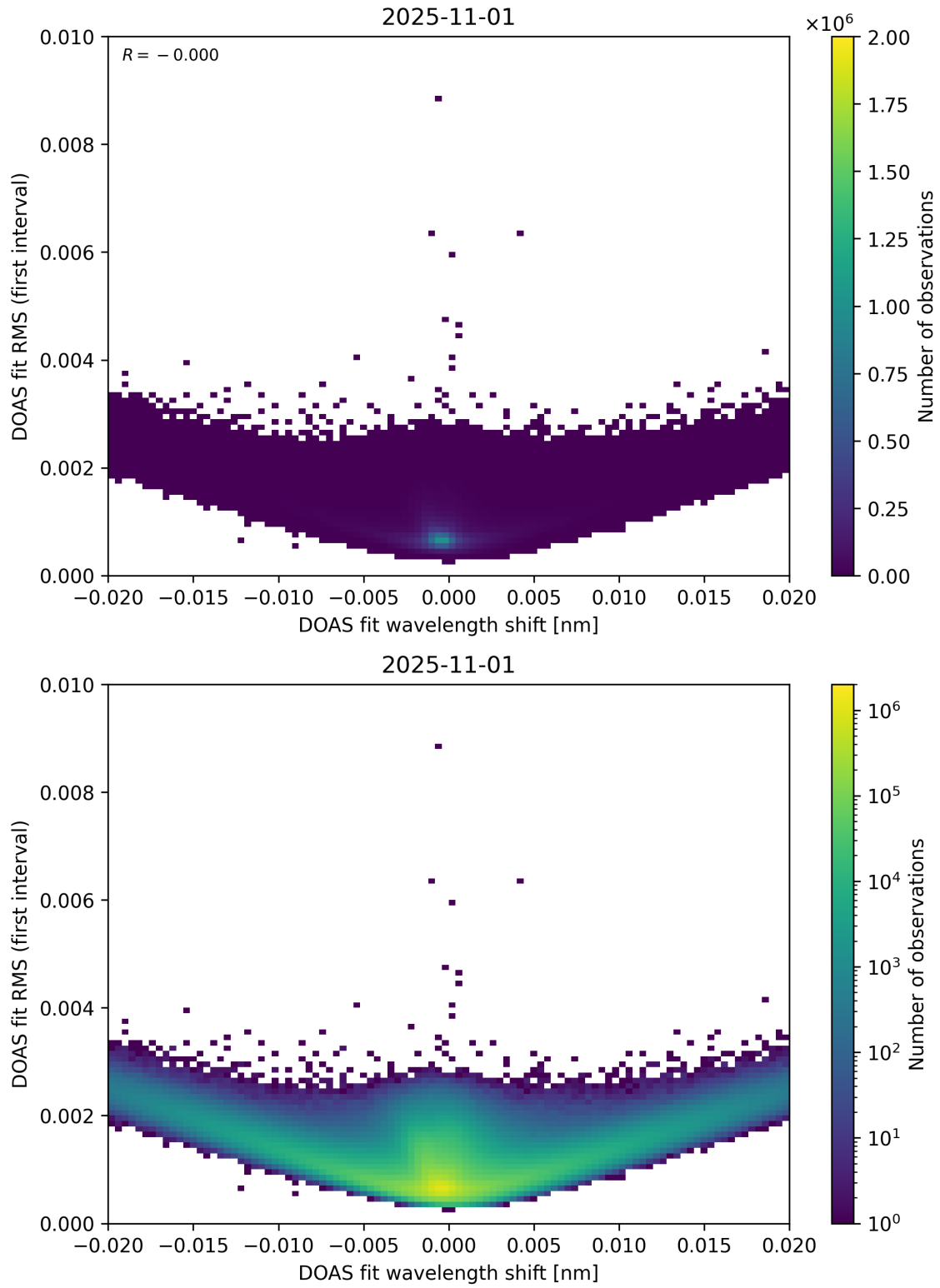
Figure 64: Scatter density plot of “DOAS fit wavelength shift” against “DOAS fit RMS (first interval)” for 2025-10-31 to 2025-11-02.
