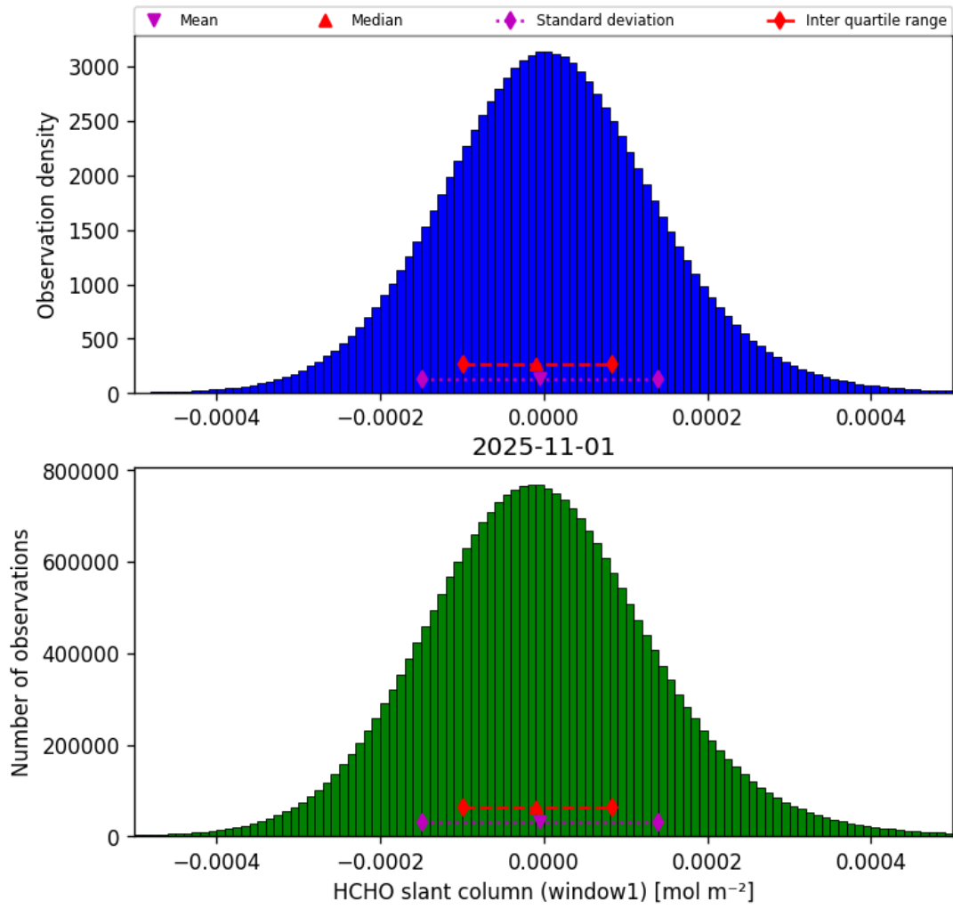
Figure 38: Histogram of “HCHO slant column (window1)” for 2025-10-31 to 2025-11-02
