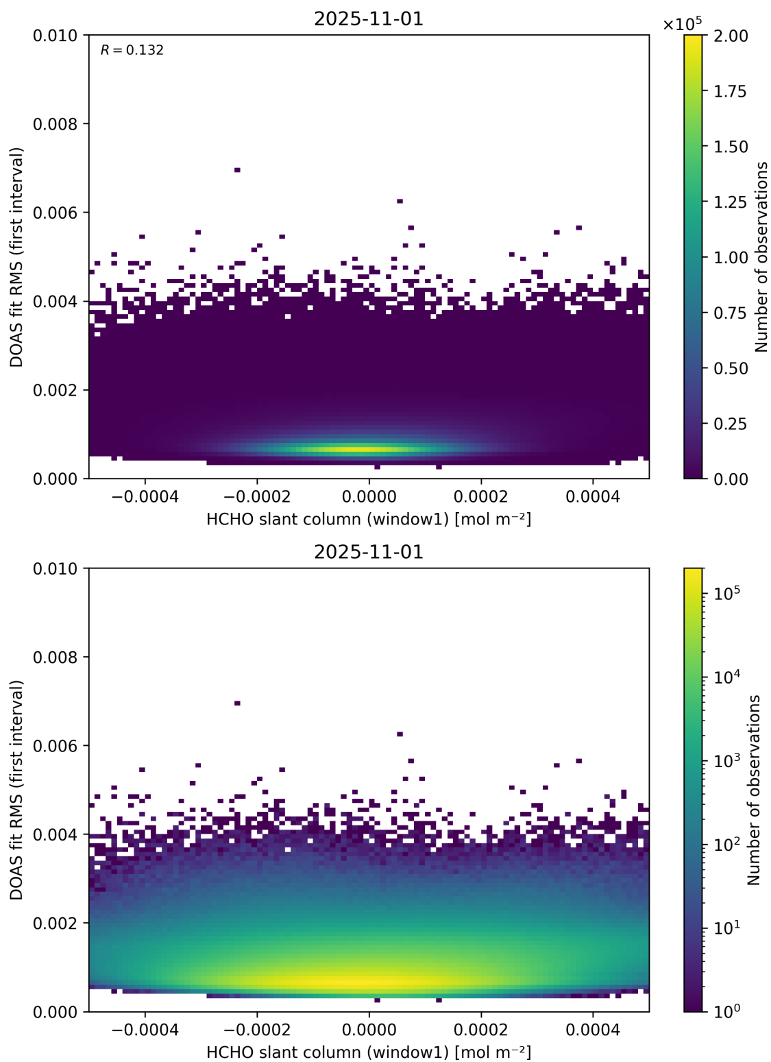
Figure 78: Scatter density plot of “HCHO slant column (window1)” against “DOAS fit RMS (first interval)” for 2025-10-31 to 2025-11-02.
