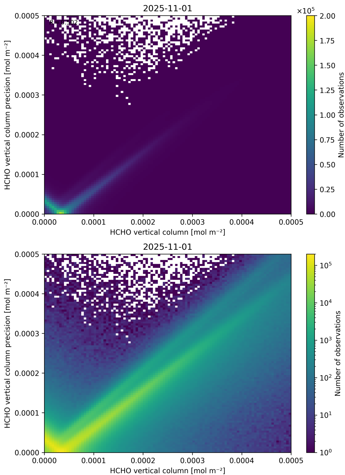
Figure 134: Scatter density plot of “HCHO vertical column” against “HCHO vertical column precision” for 2025-10-31 to 2025-11-02.
