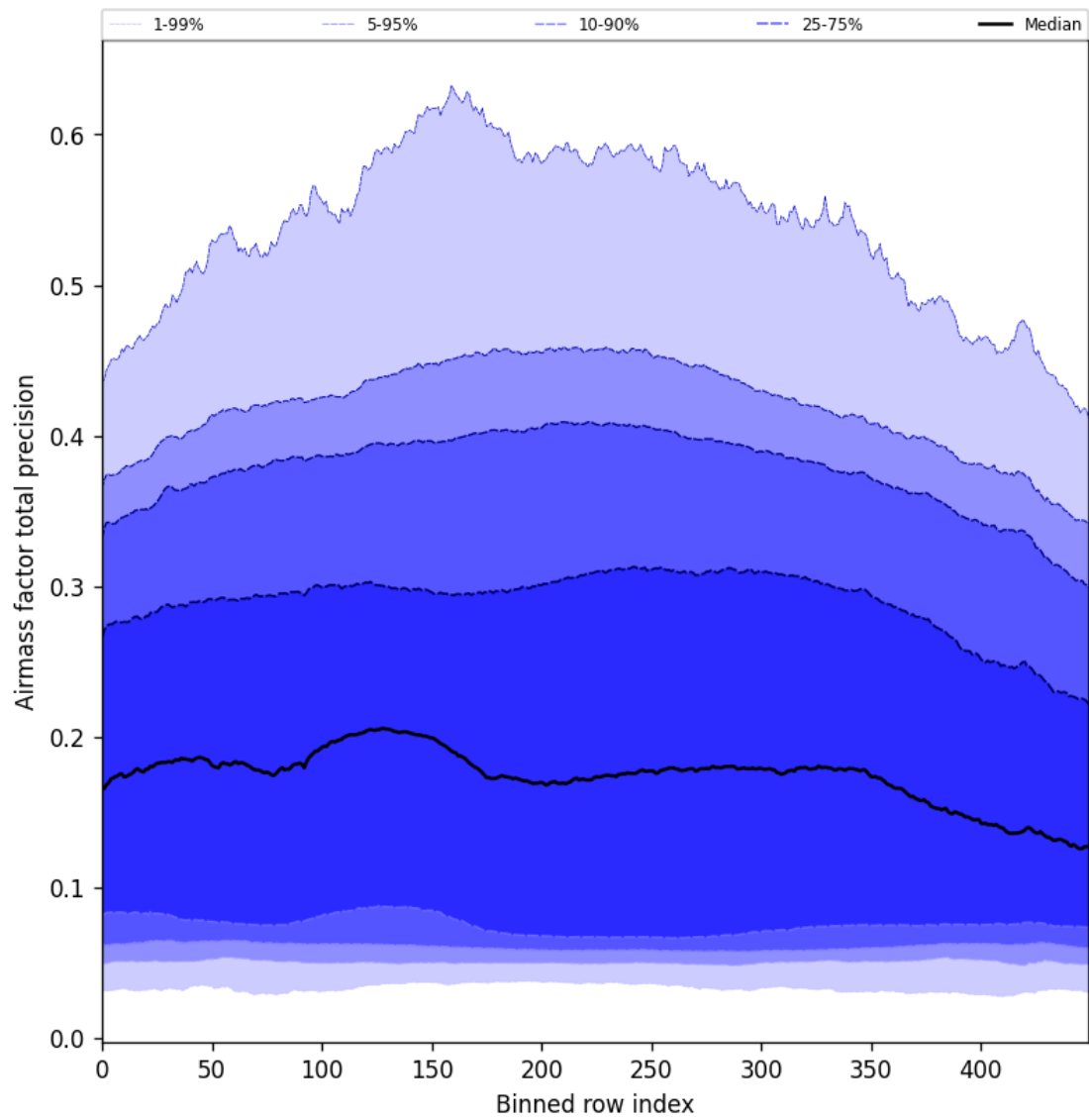
Figure 55: Along track statistics of “Airmass factor total precision” for 2025-10-31 to 2025-11-02
