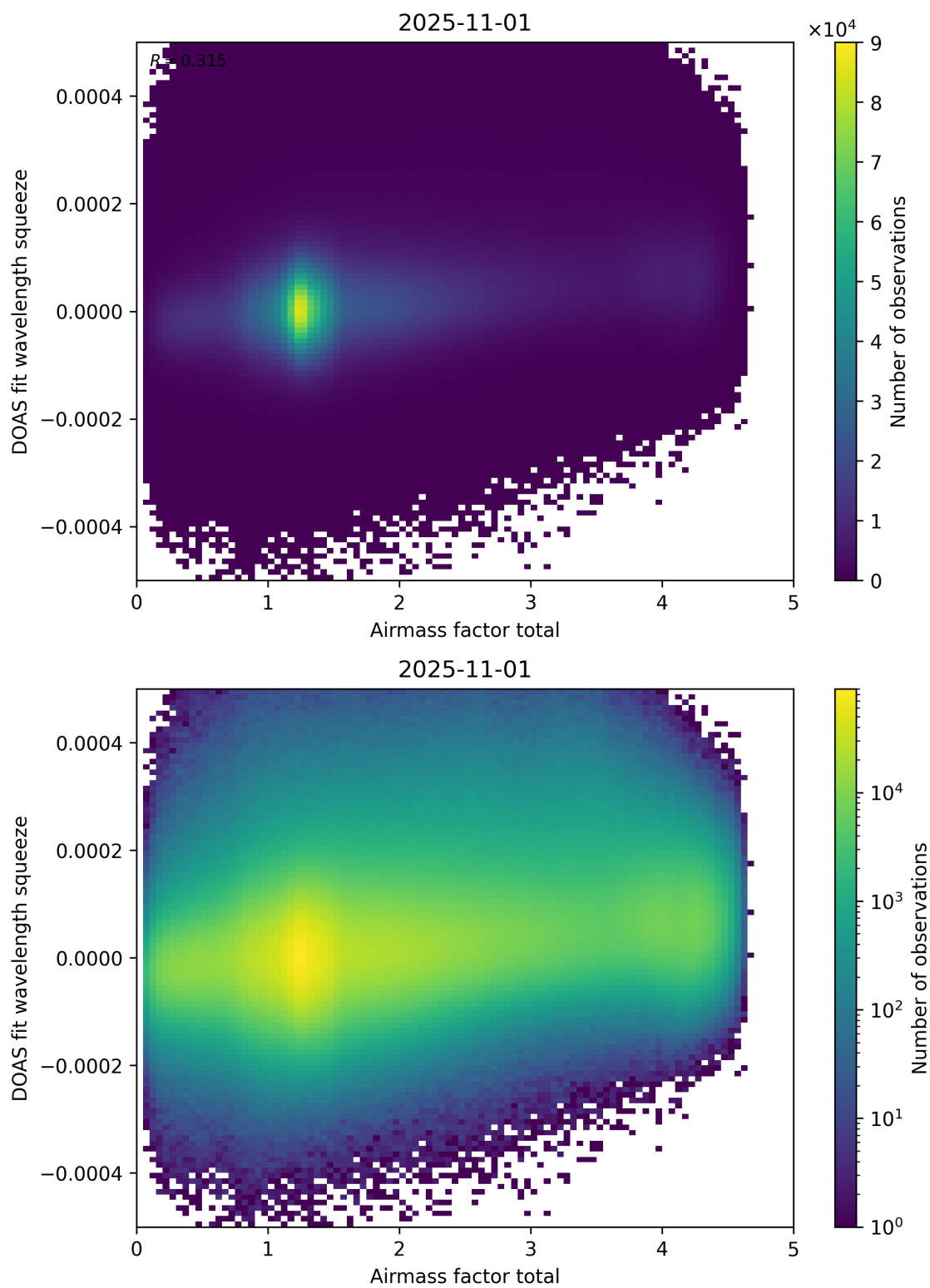
Figure 99: Scatter density plot of “Airmass factor total” against “DOAS fit wavelength squeeze” for 2025-10-31 to 2025-11-02.
