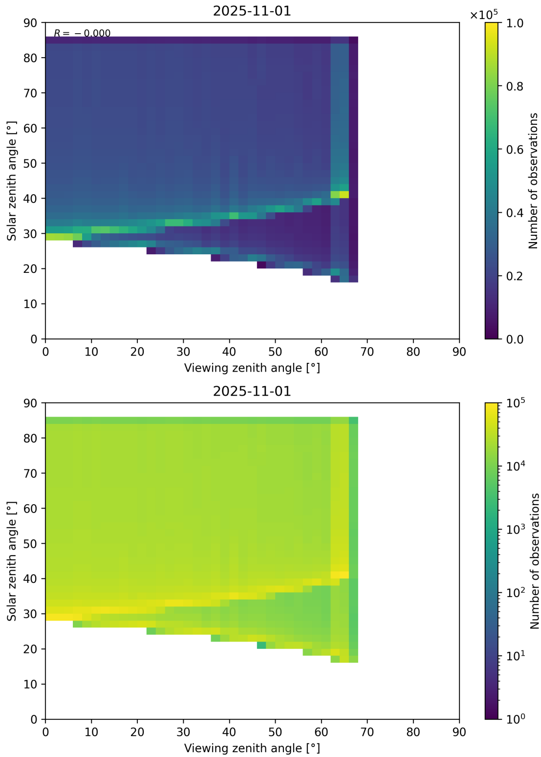
Figure 197: Scatter density plot of “Viewing zenith angle” against “Solar zenith angle” for 2025-10-31 to 2025-11-02.
