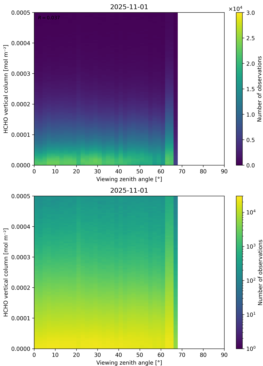
Figure 192: Scatter density plot of “Viewing zenith angle” against “HCHO vertical column” for 2025-10-31 to 2025-11-02.
