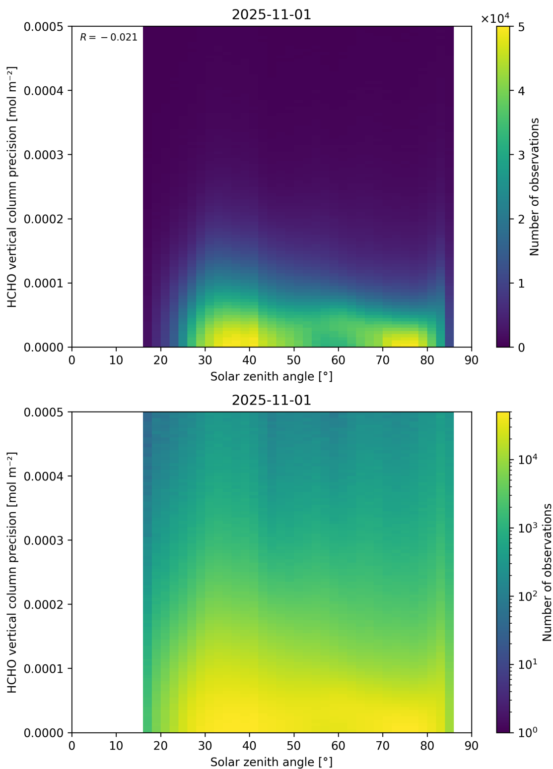
Figure 179: Scatter density plot of “Solar zenith angle” against “HCHO vertical column precision” for 2025-10-31 to 2025-11-02.
