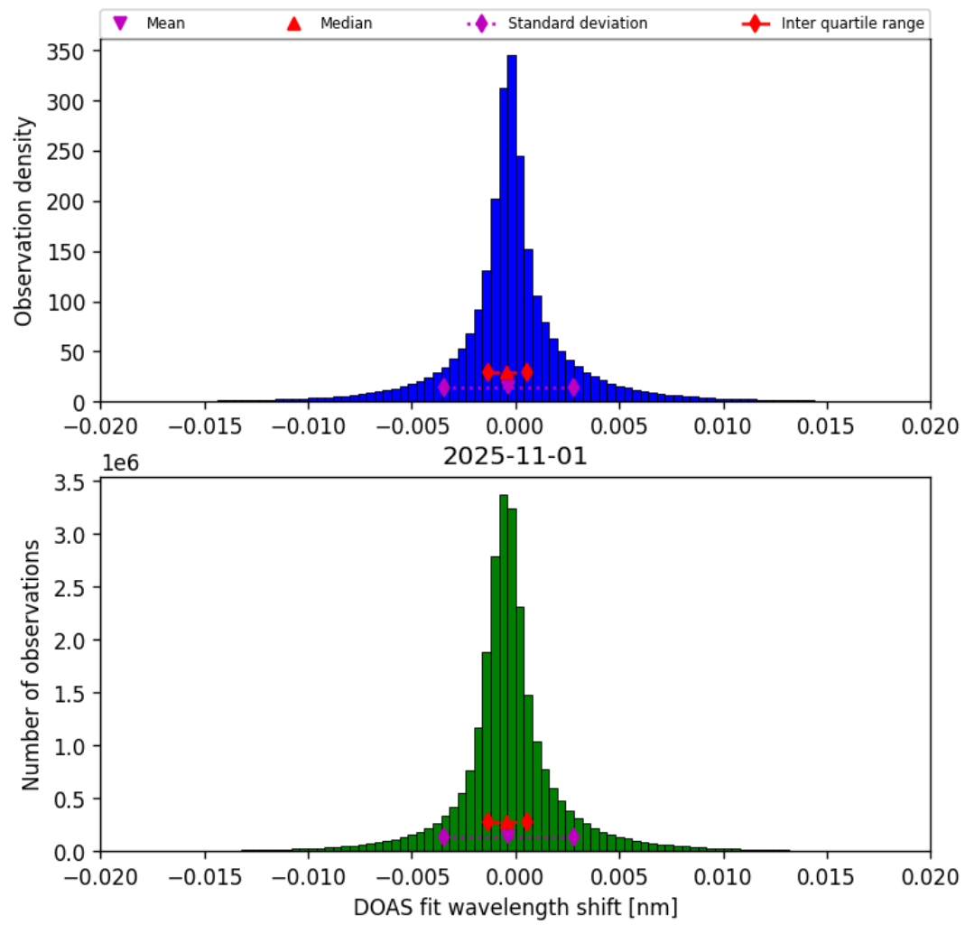
Figure 44: Histogram of “DOAS fit wavelength shift” for 2025-10-31 to 2025-11-02
