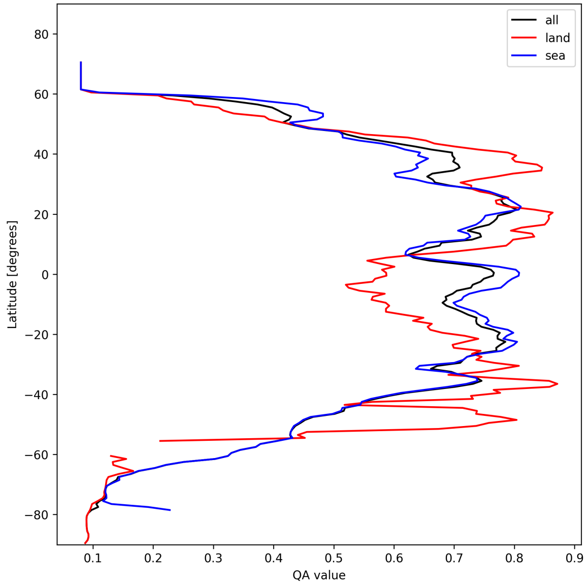
Figure 20: Zonal average of “QA value” for 2025-10-31 to 2025-11-02.
