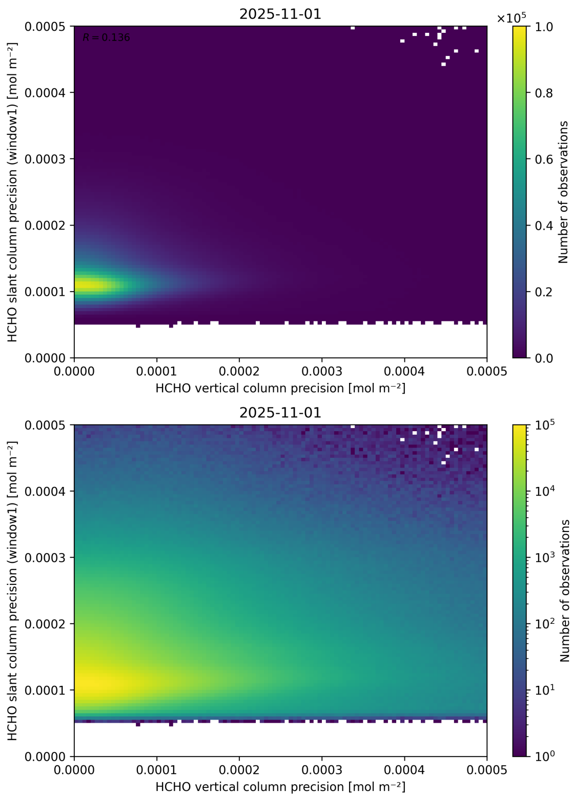
Figure 143: Scatter density plot of “HCHO vertical column precision” against “HCHO slant column precision (window1)” for 2025-10-31 to 2025-11-02.
