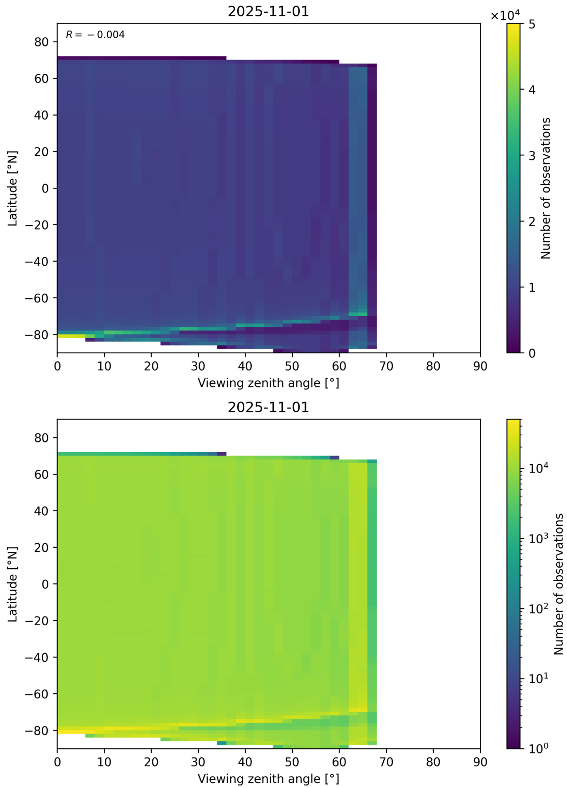
Figure 196: Scatter density plot of “Viewing zenith angle” against “Latitude” for 2025-10-31 to 2025-11-02.
