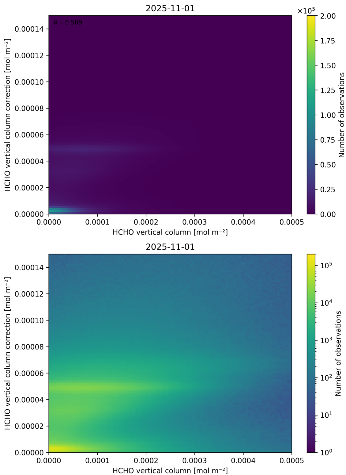
Figure 133: Scatter density plot of “HCHO vertical column” against “HCHO vertical column correction” for 2025-10-31 to 2025-11-02.
