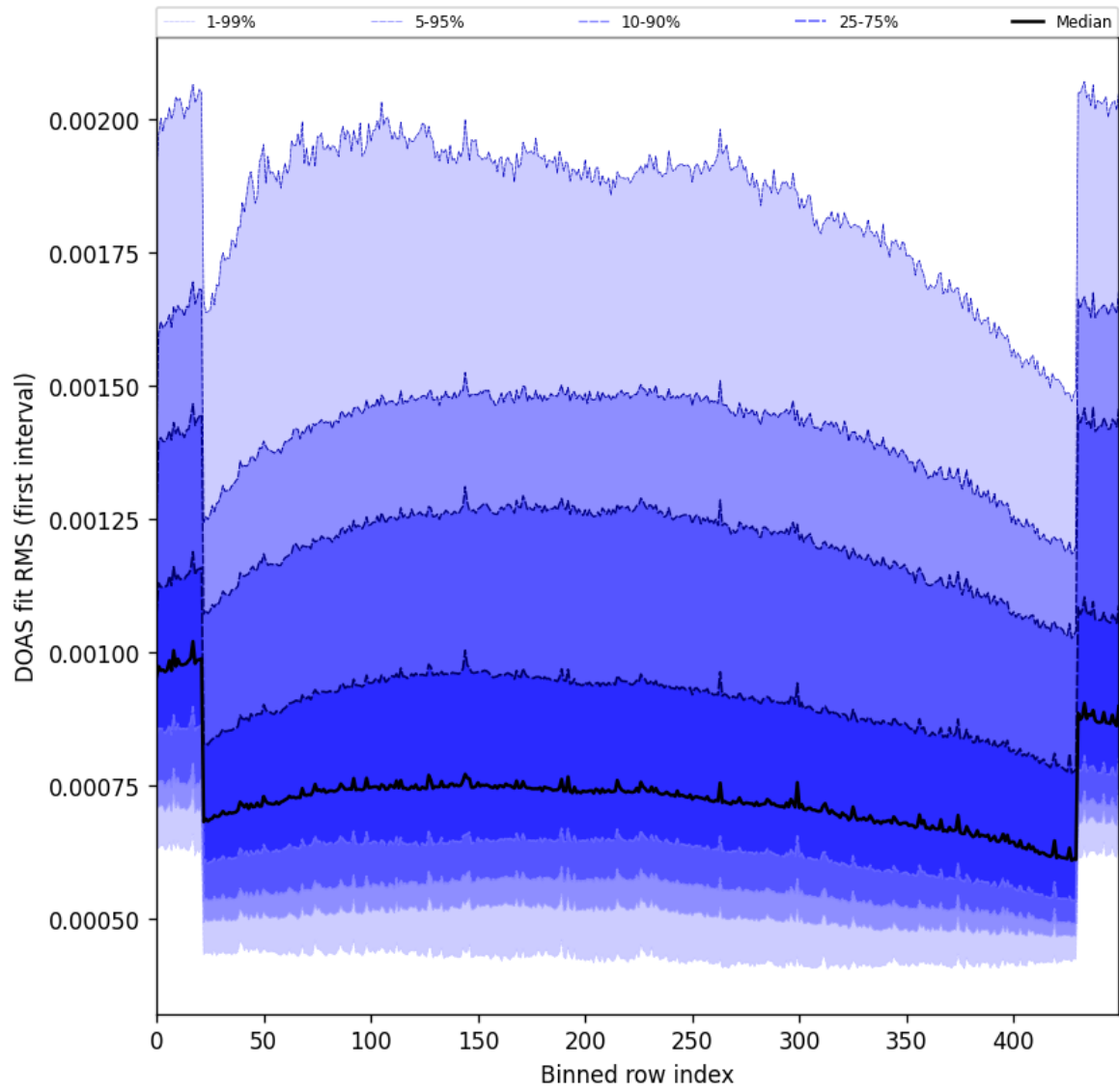
Figure 60: Along track statistics of “DOAS fit RMS (first interval)” for 2025-10-31 to 2025-11-02
