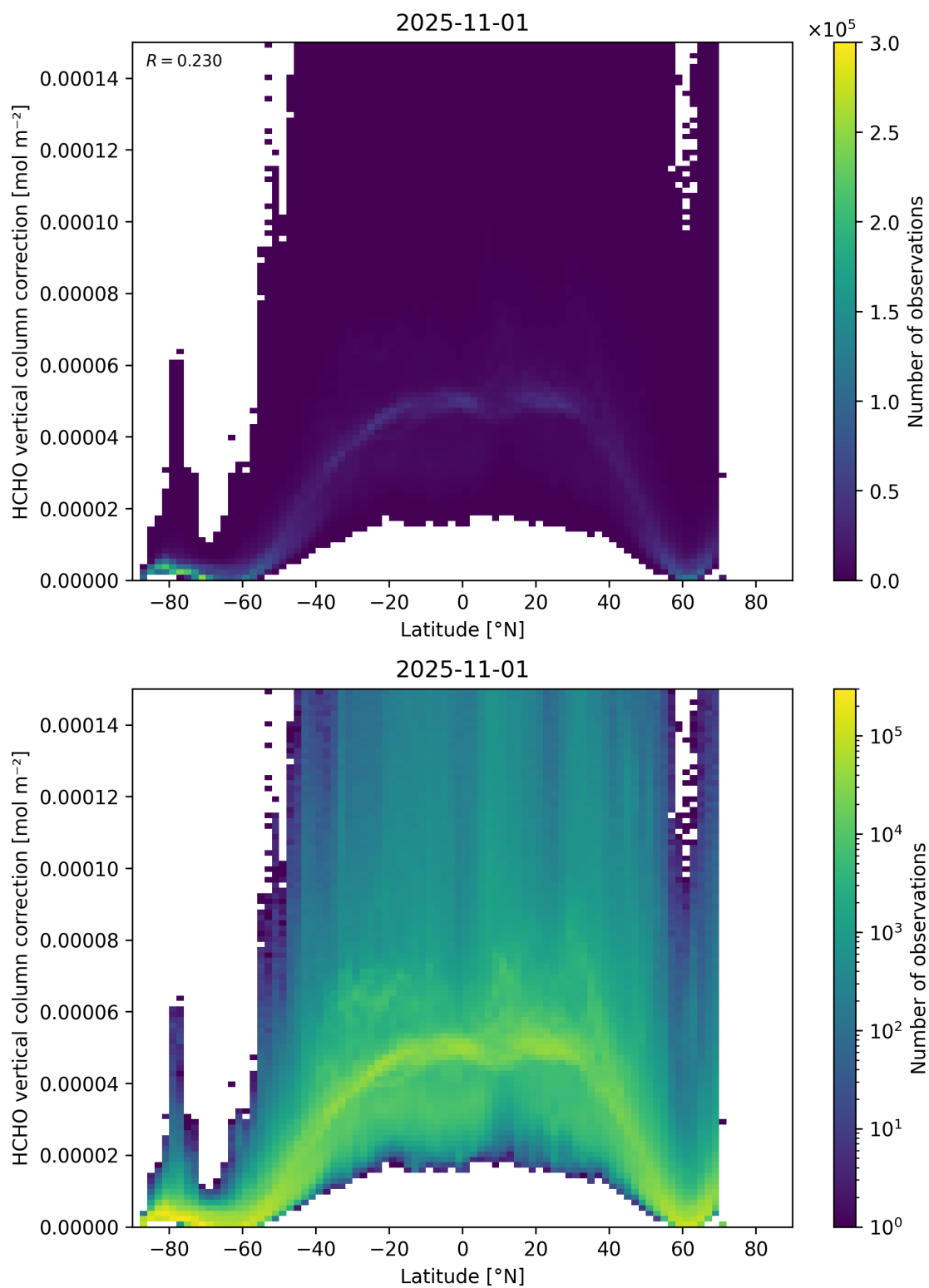
Figure 164: Scatter density plot of “Latitude” against “HCHO vertical column correction” for 2025-10-31 to 2025-11-02.
