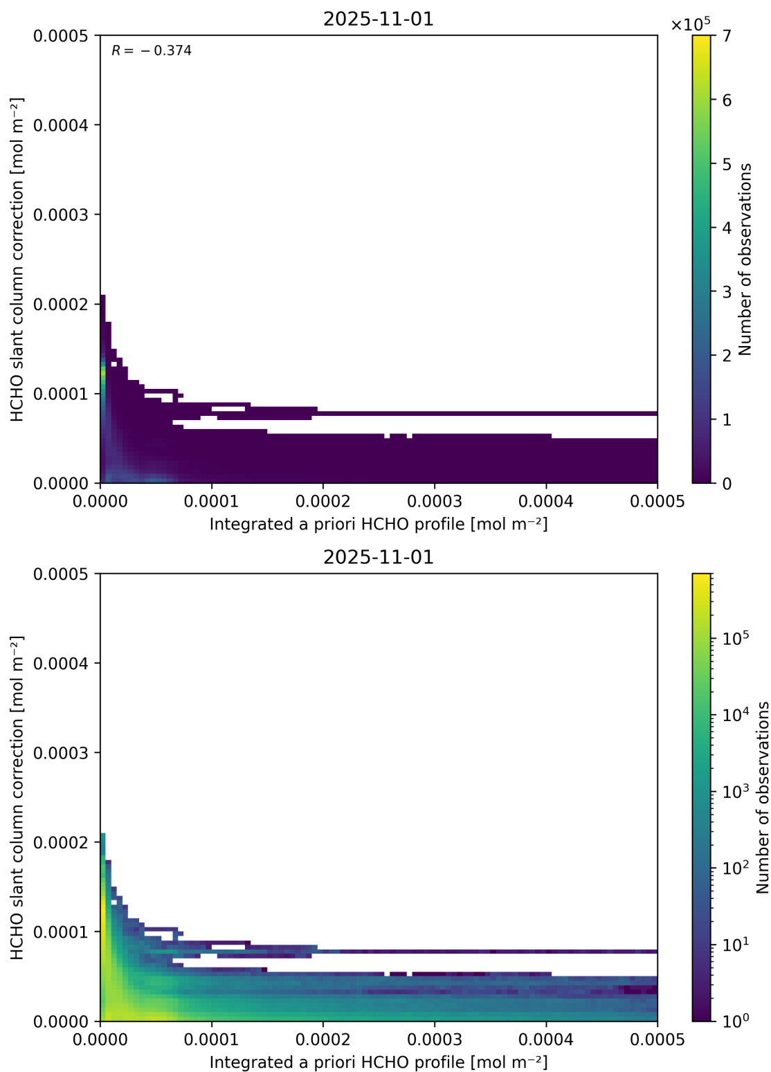
Figure 152: Scatter density plot of “Integrated a priori HCHO profile” against “HCHO slant column correction” for 2025-10-31 to 2025-11-02.
