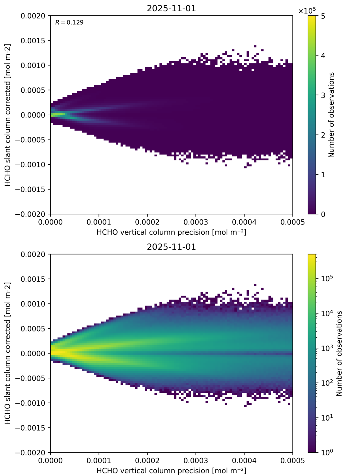
Figure 140: Scatter density plot of “HCHO vertical column precision” against “HCHO slant column corrected” for 2025-10-31 to 2025-11-02.
