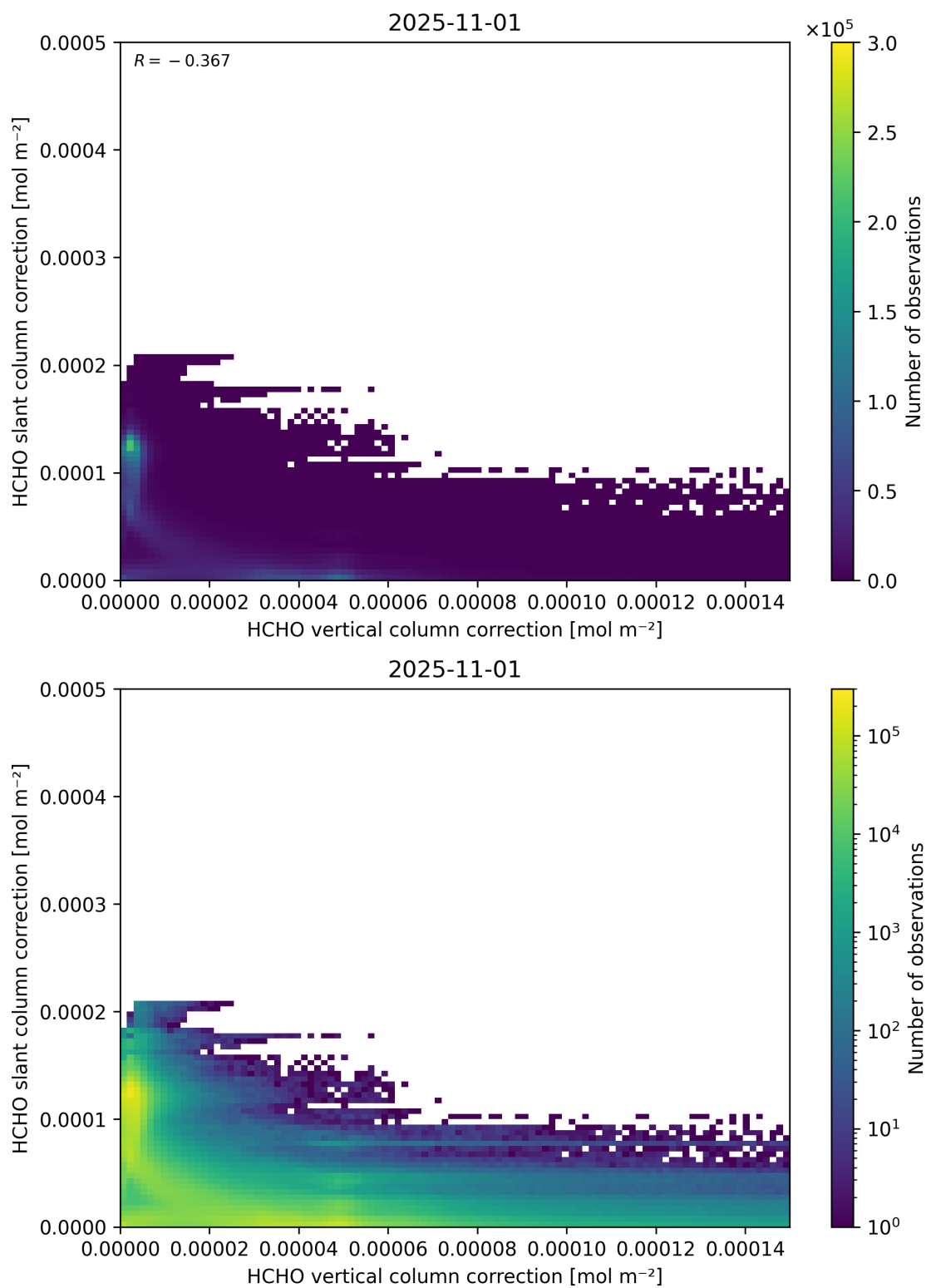
Figure 117: Scatter density plot of “HCHO vertical column correction” against “HCHO slant column correction” for 2025-10-31 to 2025-11-02.
