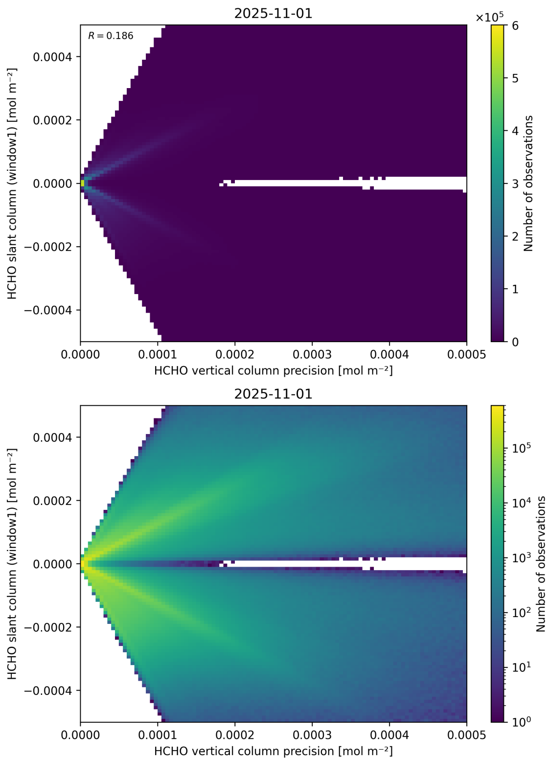
Figure 142: Scatter density plot of “HCHO vertical column precision” against “HCHO slant column (window1)” for 2025-10-31 to 2025-11-02.
