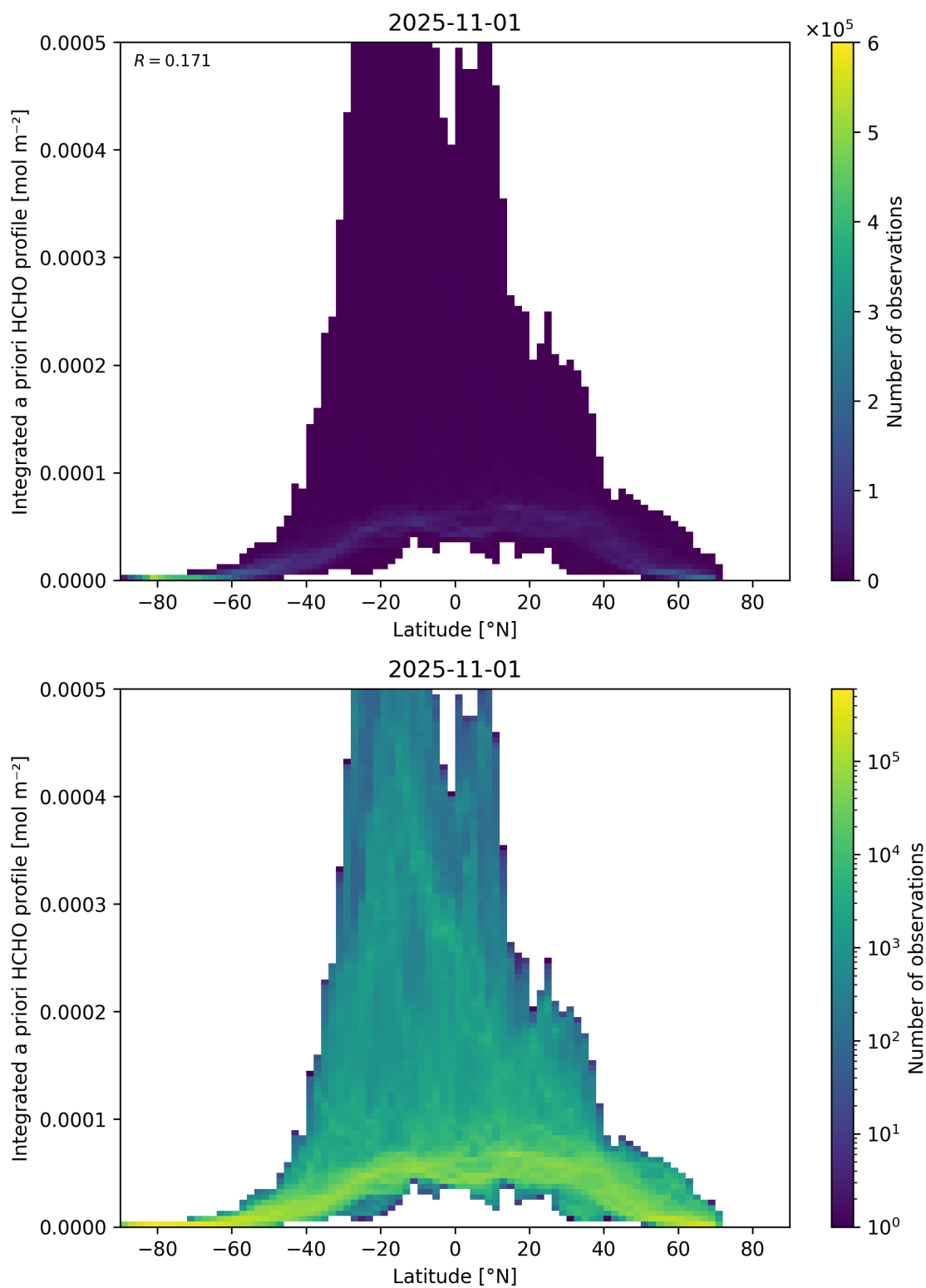
Figure 166: Scatter density plot of “Latitude” against “Integrated a priori HCHO profile” for 2025-10-31 to 2025-11-02.
