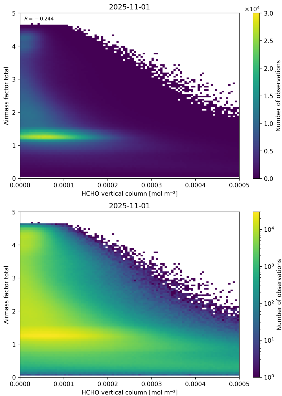
Figure 131: Scatter density plot of “HCHO vertical column” against “Airmass factor total” for 2025-10-31 to 2025-11-02.
