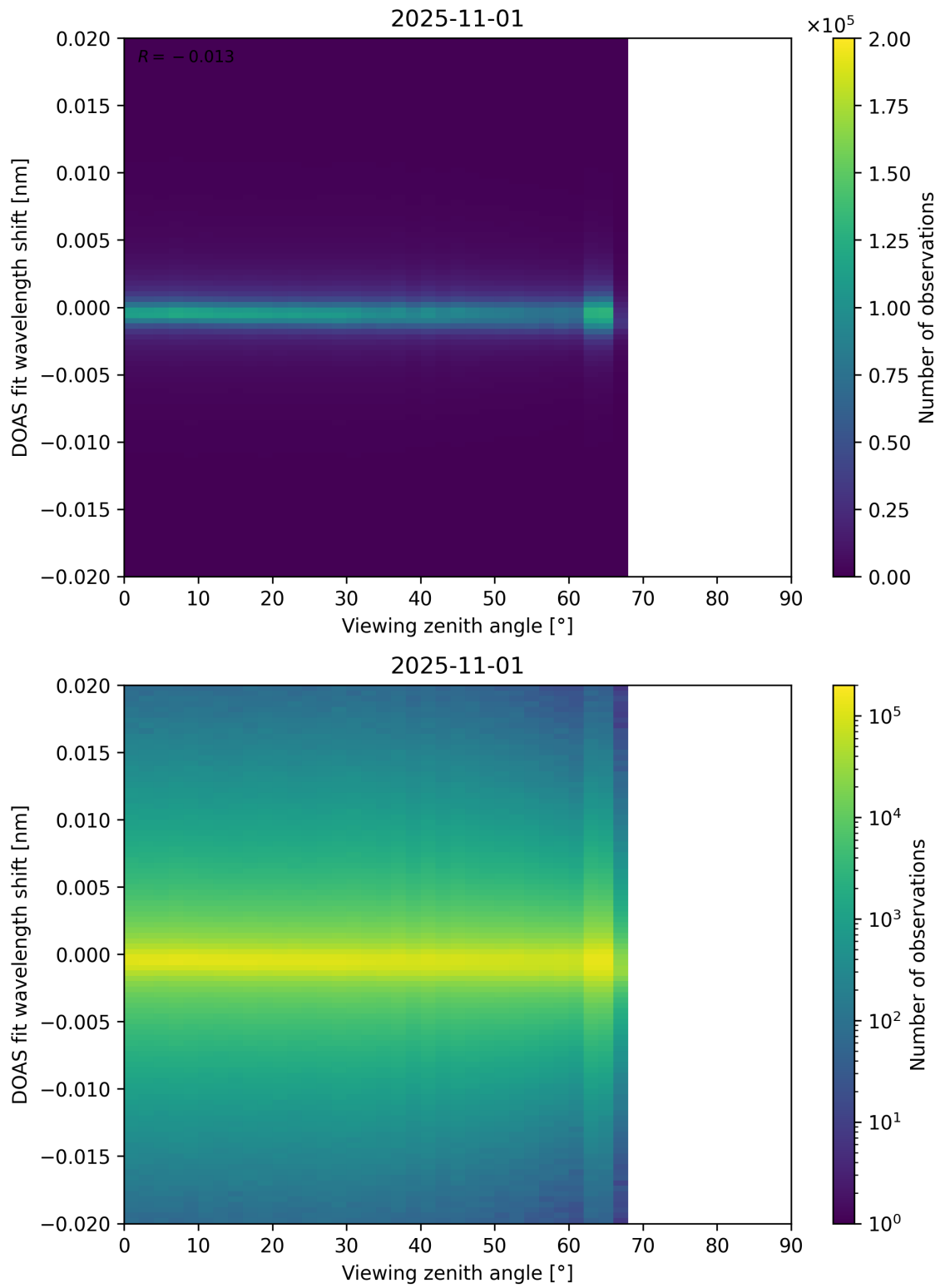
Figure 183: Scatter density plot of “Viewing zenith angle” against “DOAS fit wavelength shift” for 2025-10-31 to 2025-11-02.
