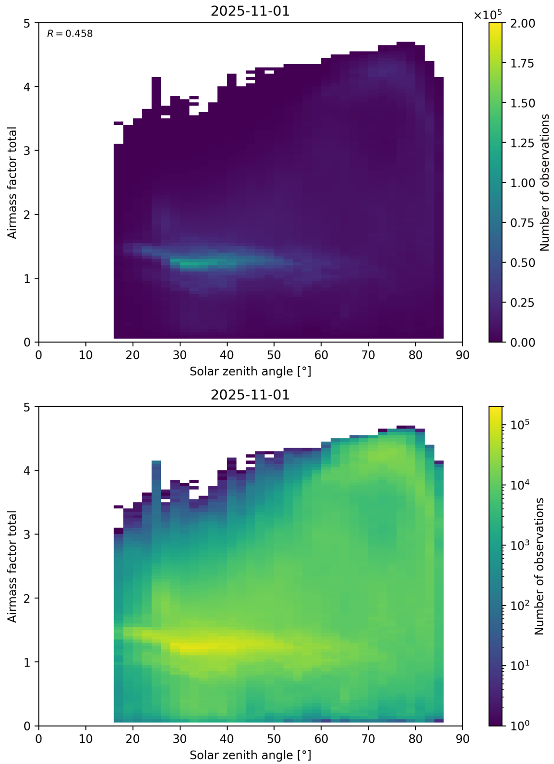
Figure 175: Scatter density plot of “Solar zenith angle” against “Airmass factor total” for 2025-10-31 to 2025-11-02.
