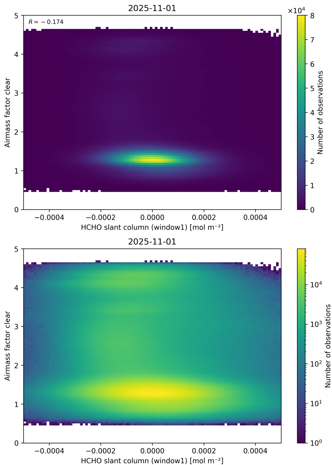
Figure 81: Scatter density plot of “HCHO slant column (window1)” against “Airmass factor clear” for 2025-10-31 to 2025-11-02.
