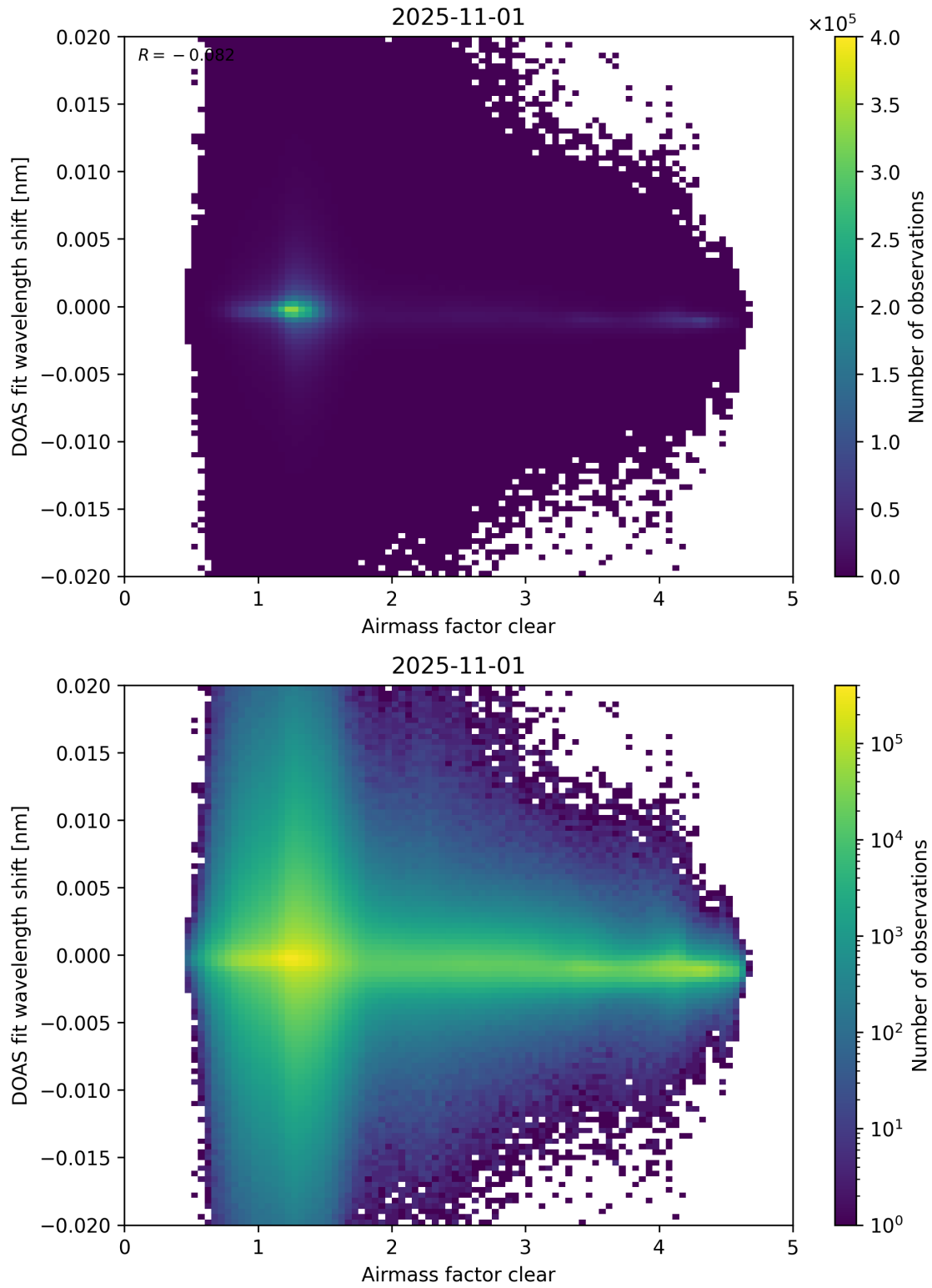
Figure 72: Scatter density plot of “Airmass factor clear” against “DOAS fit wavelength shift” for 2025-10-31 to 2025-11-02.
