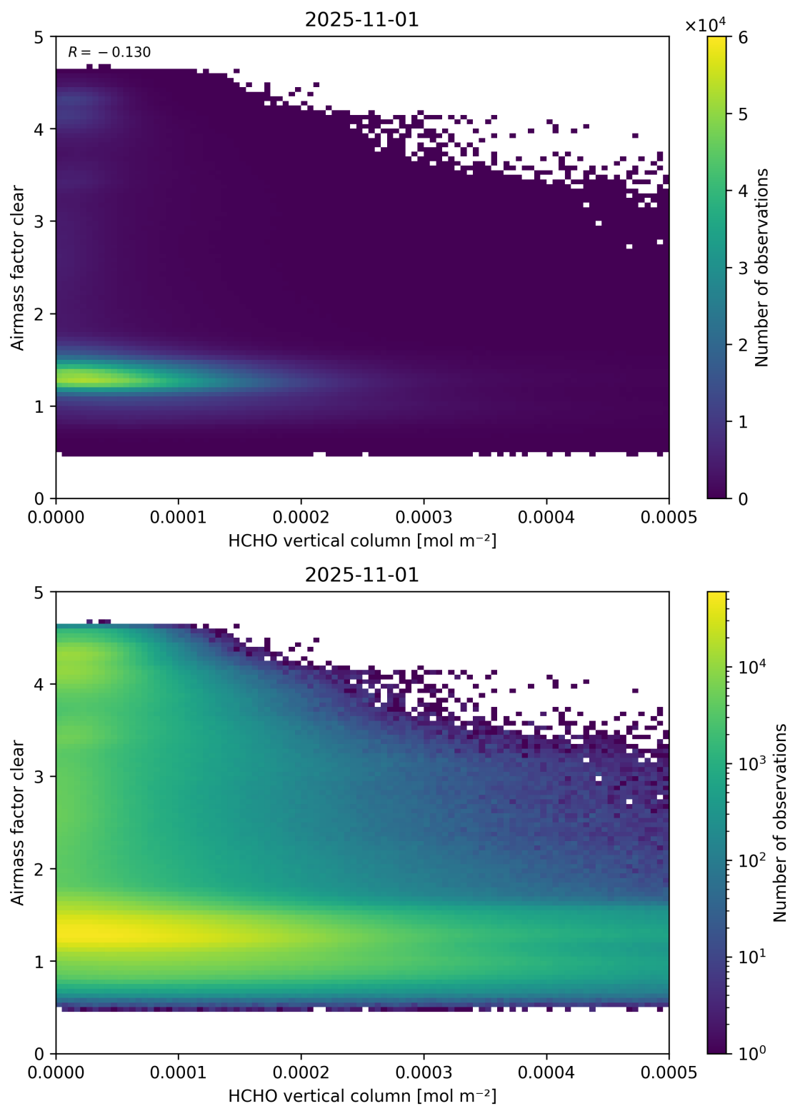
Figure 126: Scatter density plot of “HCHO vertical column” against “Airmass factor clear” for 2025-10-31 to 2025-11-02.
