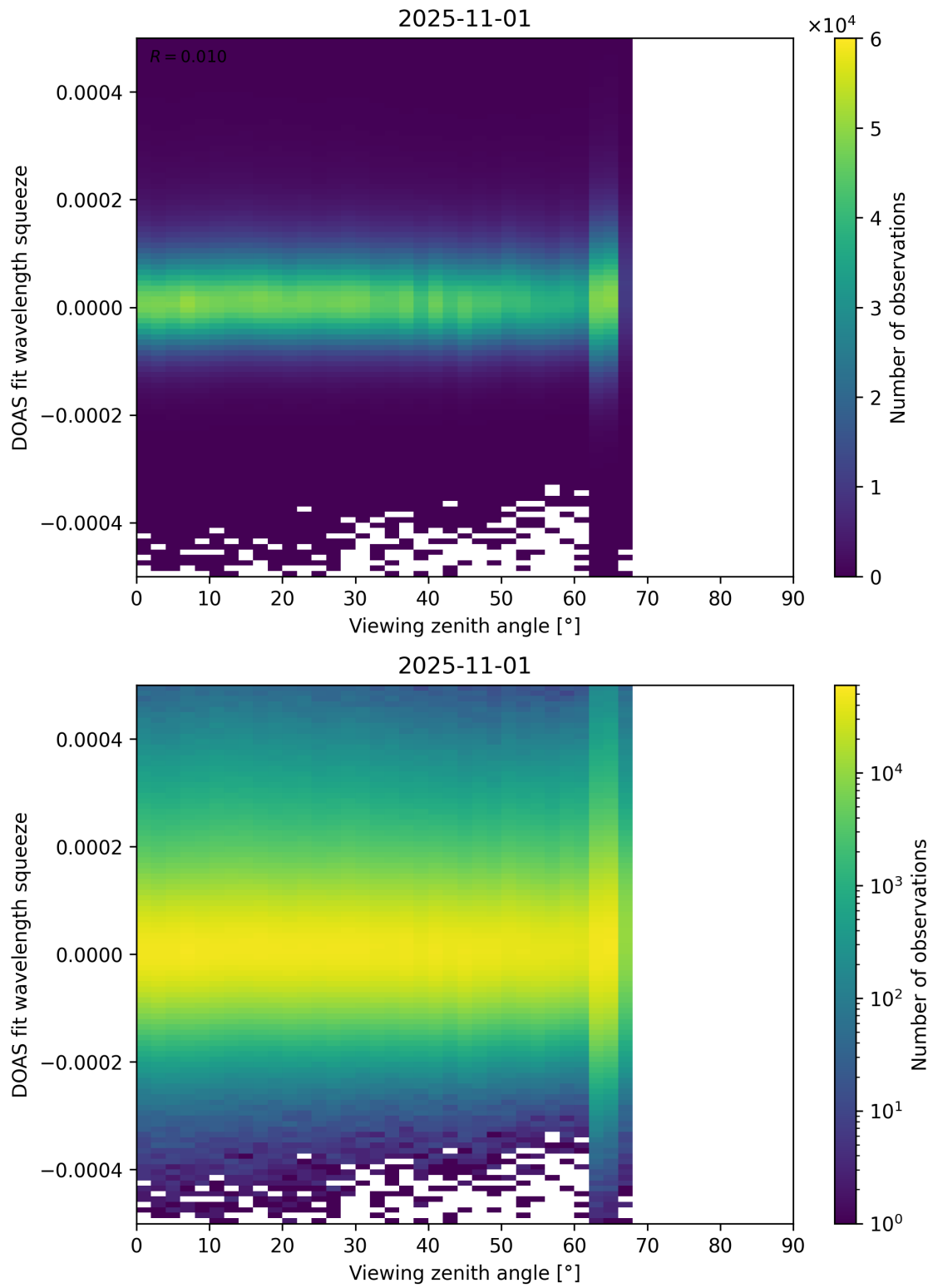
Figure 184: Scatter density plot of “Viewing zenith angle” against “DOAS fit wavelength squeeze” for 2025-10-31 to 2025-11-02.
