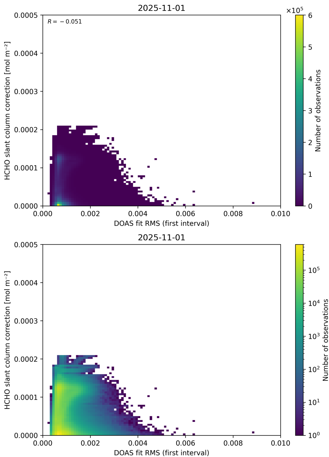
Figure 63: Scatter density plot of “DOAS fit RMS (first interval)” against “HCHO slant column correction” for 2025-10-31 to 2025-11-02.
