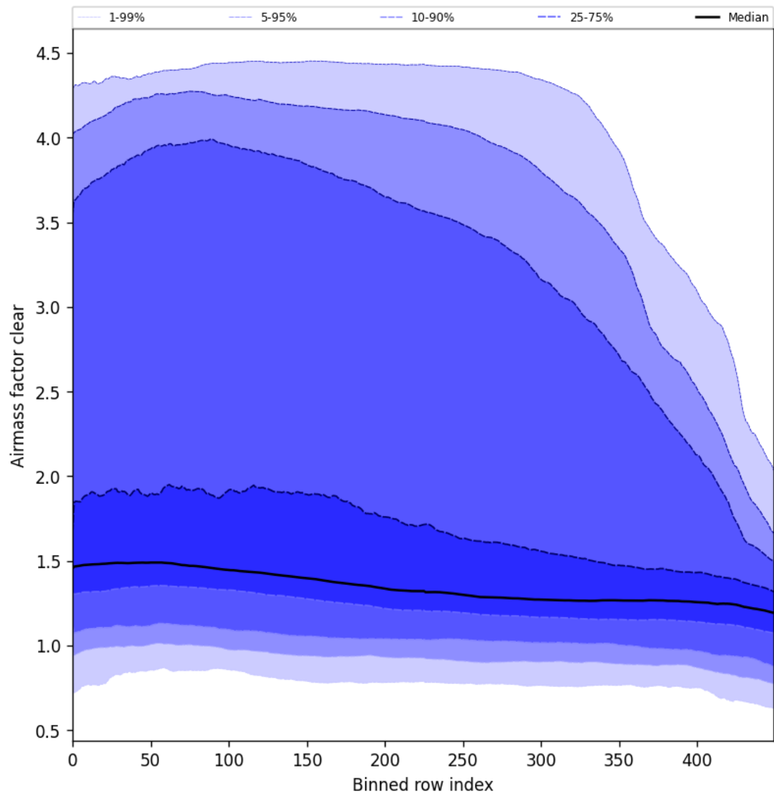
Figure 56: Along track statistics of “Air mass factor clear” for 2025-10-31 to 2025-11-02
