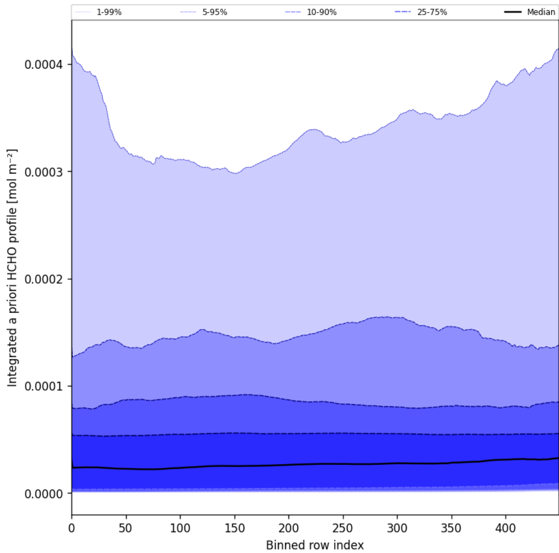
Figure 57: Along track statistics of “Integrated a priori HCHO profile” for 2025-10-31 to 2025-11-02
