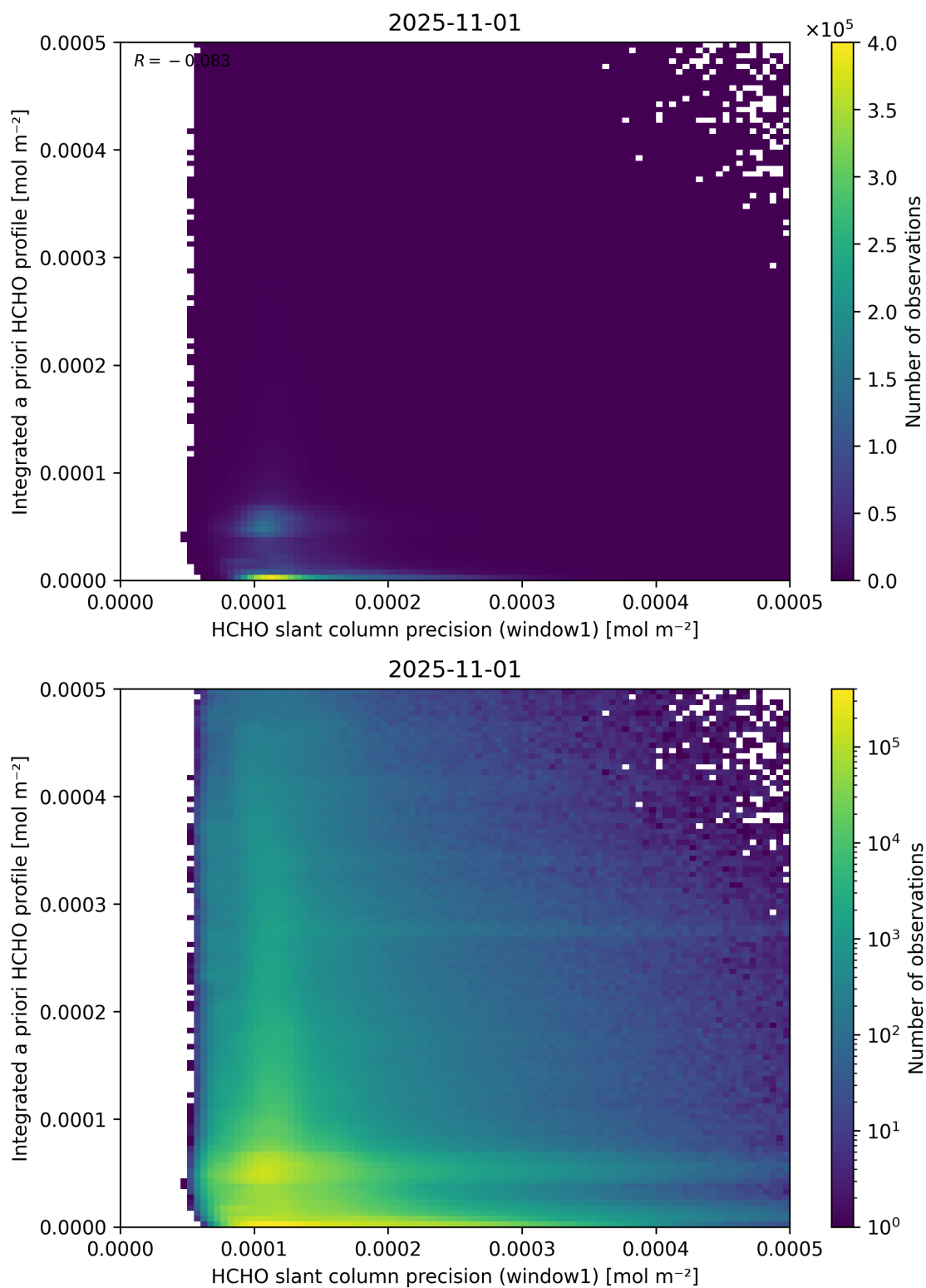
Figure 96: Scatter density plot of “HCHO slant column precision (window1)” against “Integrated a priori HCHO profile” for 2025-10-31 to 2025-11-02.
