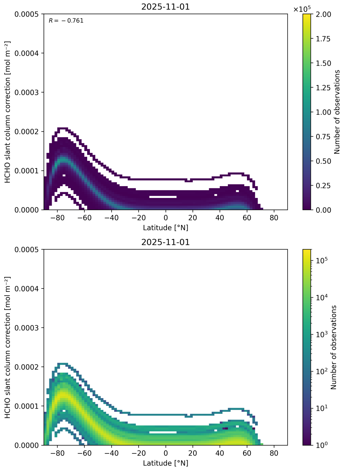
Figure 158: Scatter density plot of “Latitude” against “HCHO slant column correction” for 2025-10-31 to 2025-11-02.
