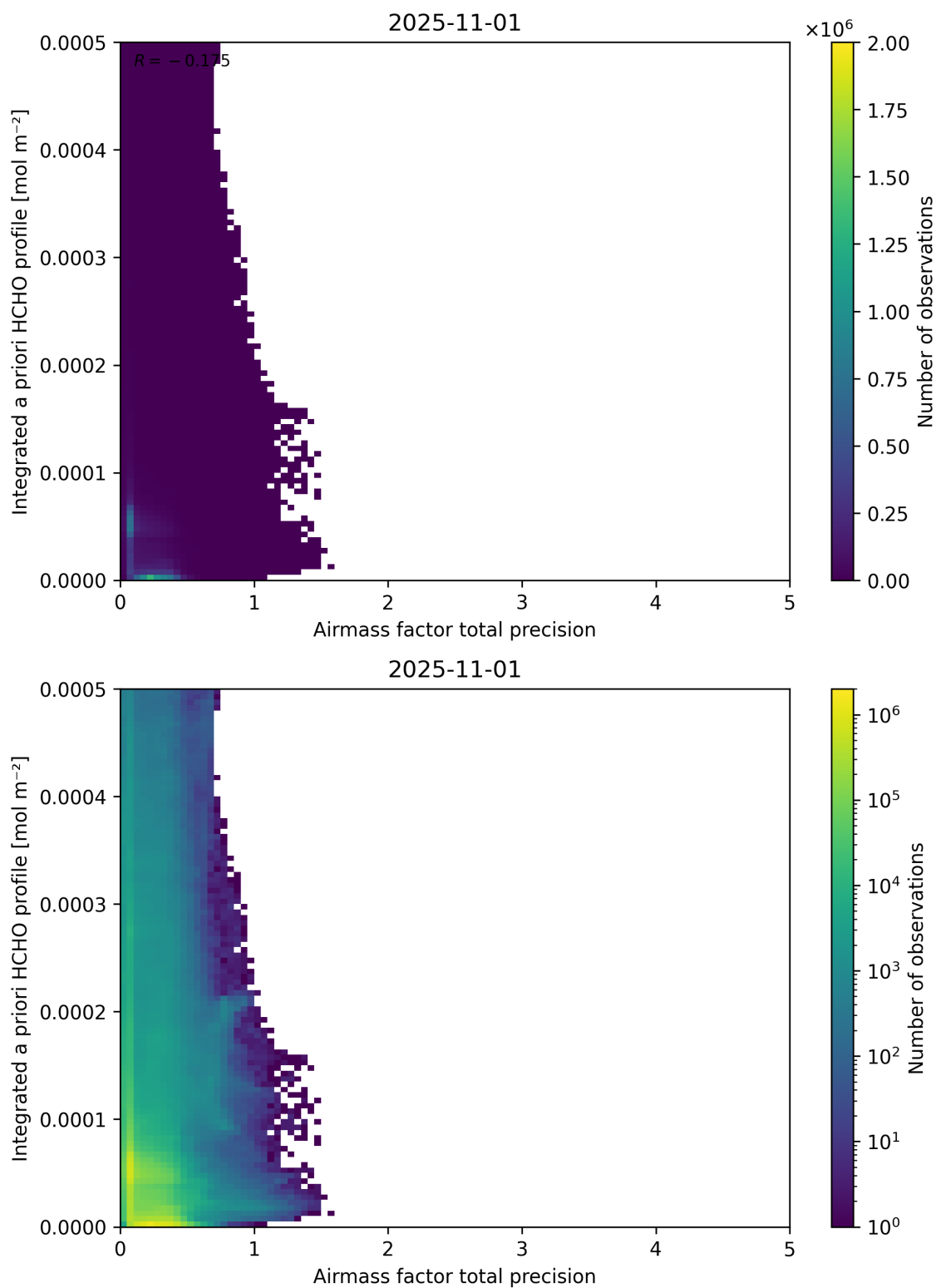
Figure 111: Scatter density plot of “Airmass factor total precision” against “Integrated a priori HCHO profile” for 2025-10-31 to 2025-11-02.
