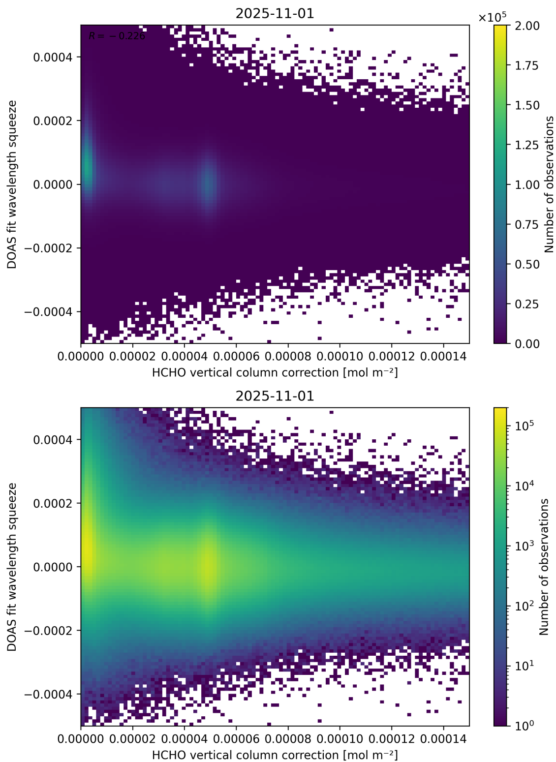
Figure 114: Scatter density plot of “HCHO vertical column correction” against “DOAS fit wavelength squeeze” for 2025-10-31 to 2025-11-02.
