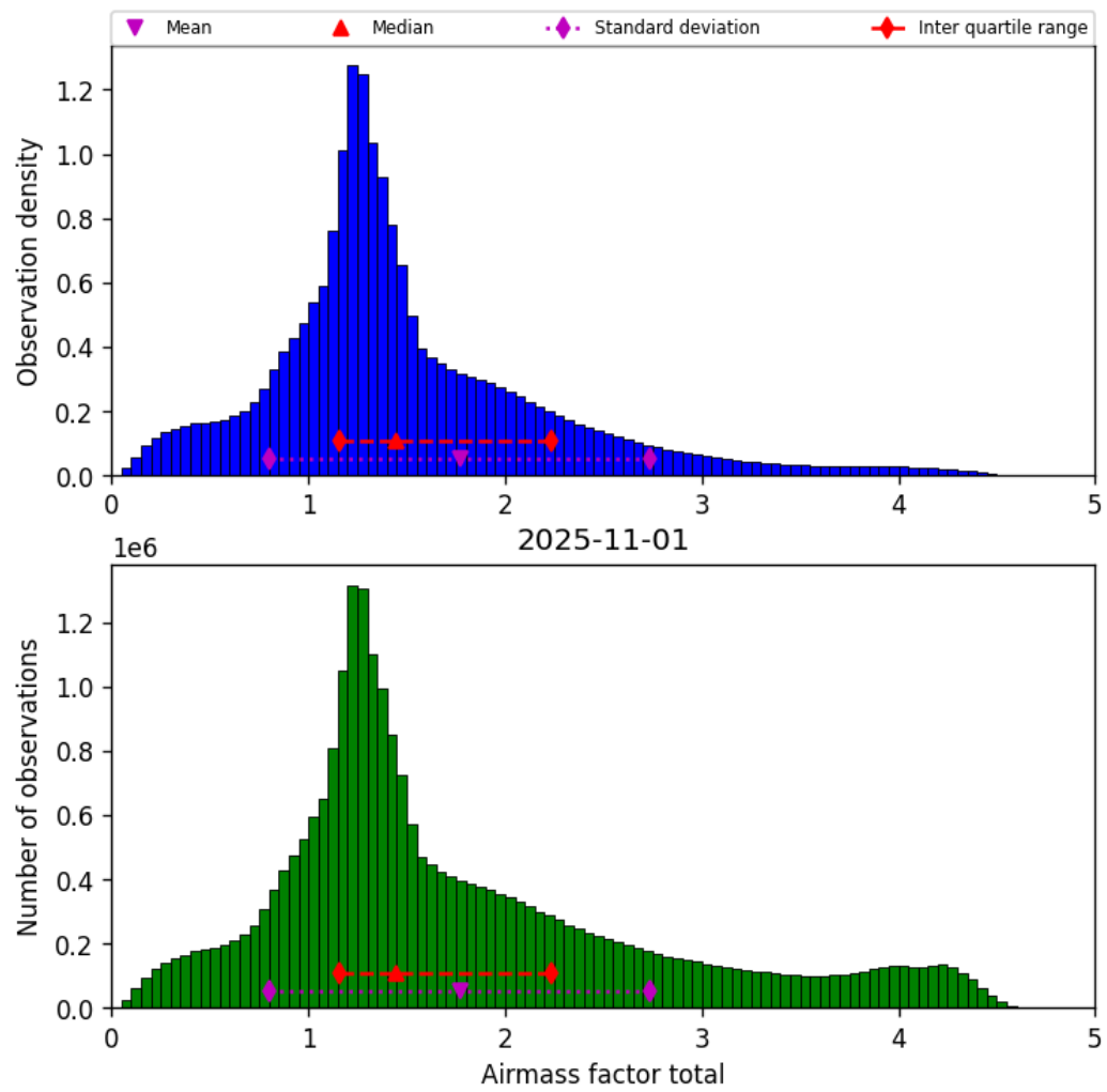
Figure 40: Histogram of “Airmass factor total” for 2025-10-31 to 2025-11-02
