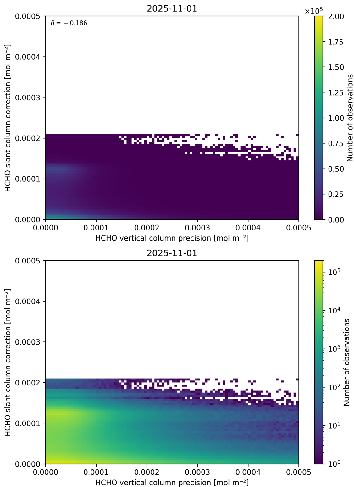
Figure 141: Scatter density plot of “HCHO vertical column precision” against “HCHO slant column correction” for 2025-10-31 to 2025-11-02.
