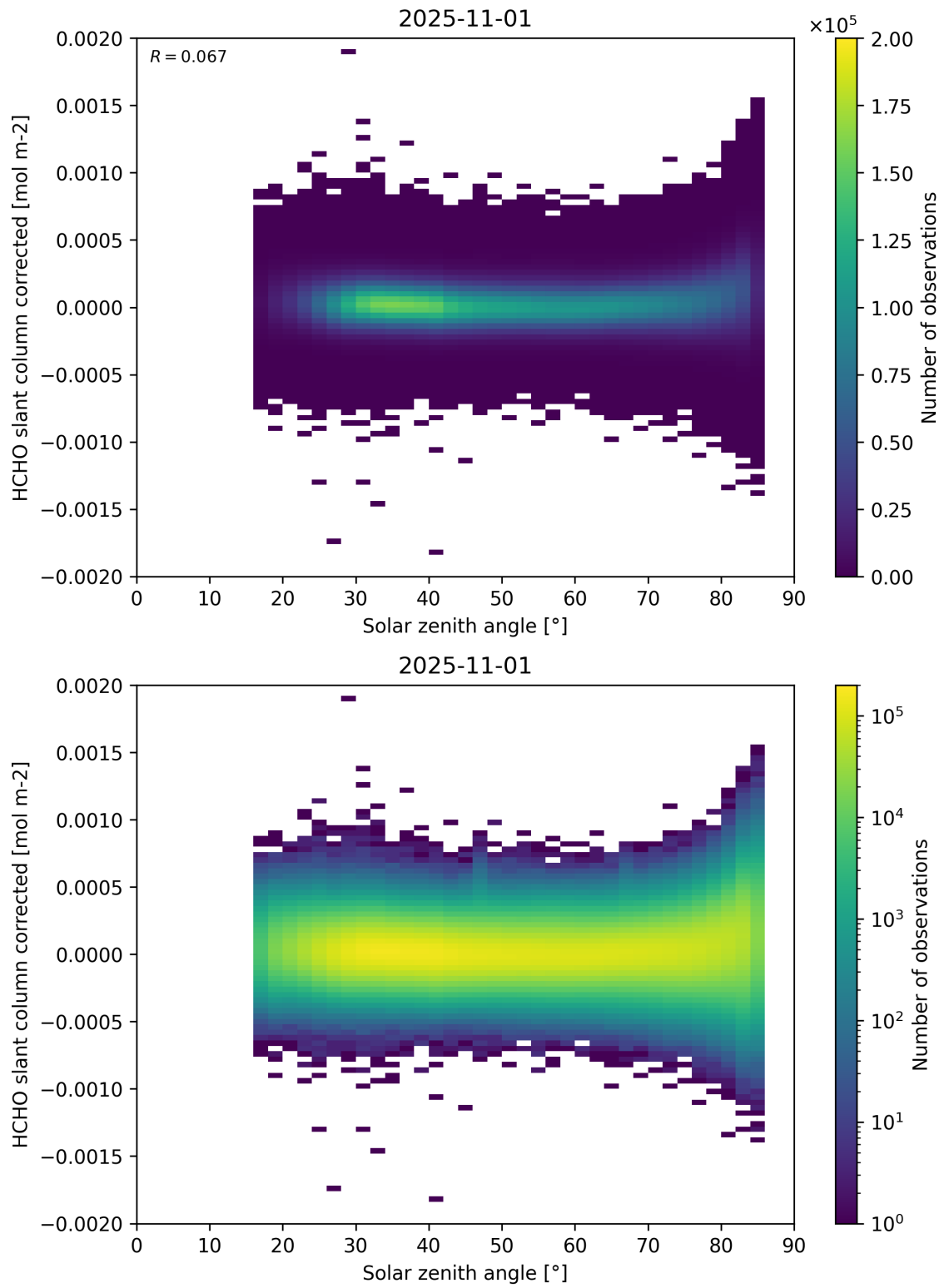
Figure 171: Scatter density plot of “Solar zenith angle” against “HCHO slant column corrected” for 2025-10-31 to 2025-11-02.
