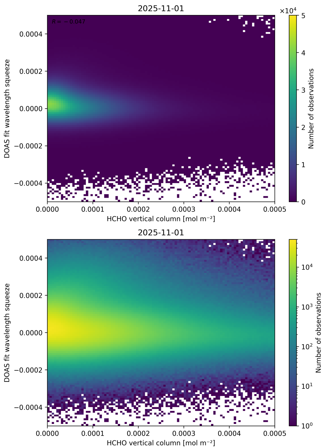
Figure 125: Scatter density plot of “HCHO vertical column” against “DOAS fit wavelength squeeze” for 2025-10-31 to 2025-11-02.
