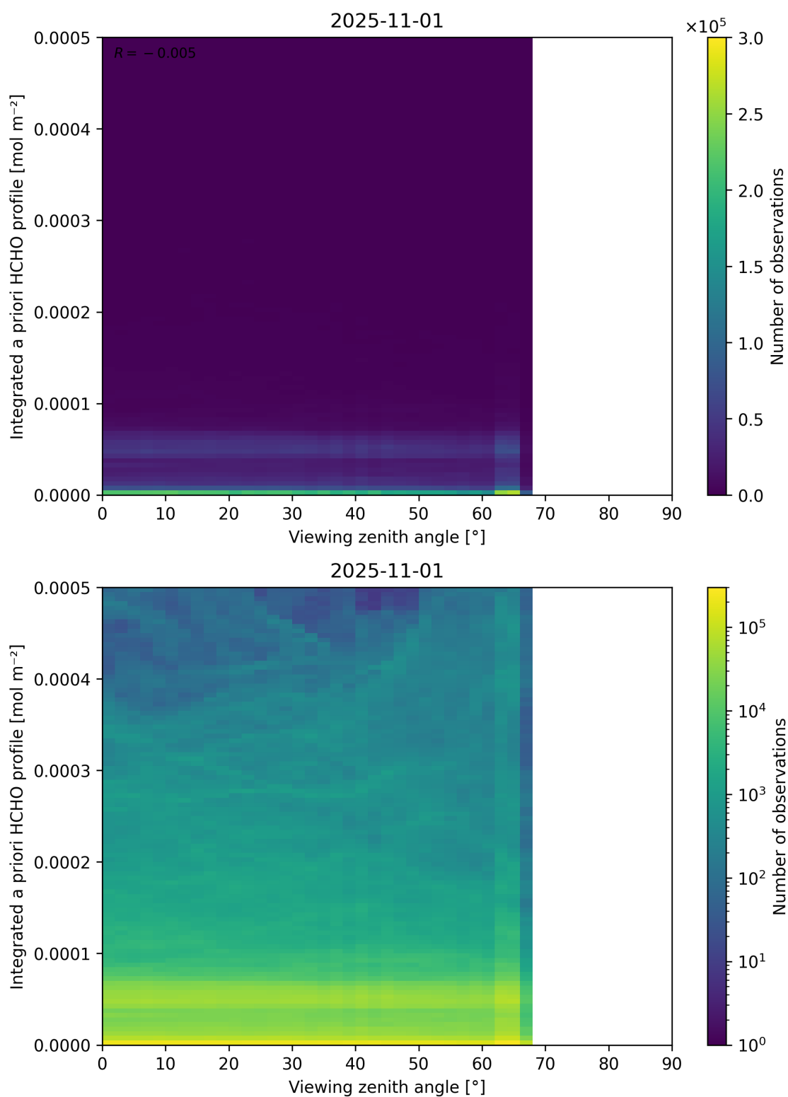
Figure 195: Scatter density plot of “Viewing zenith angle” against “Integrated a priori HCHO profile” for 2025-10-31 to 2025-11-02.
