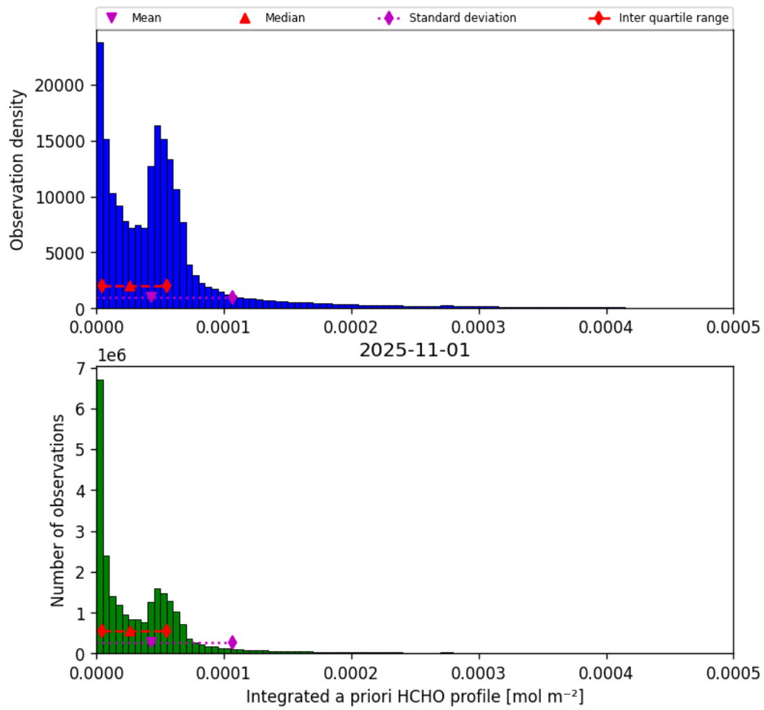
Figure 43: Histogram of “Integrated a priori HCHO profile” for 2025-10-31 to 2025-11-02
