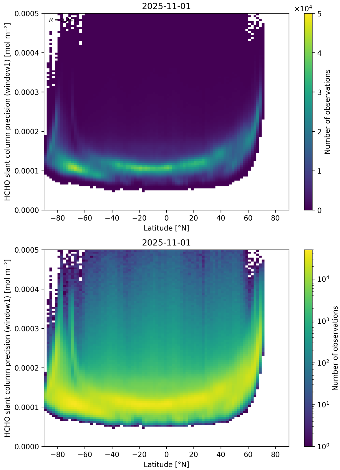
Figure 160: Scatter density plot of “Latitude” against “HCHO slant column precision (window1)” for 2025-10-31 to 2025-11-02.
