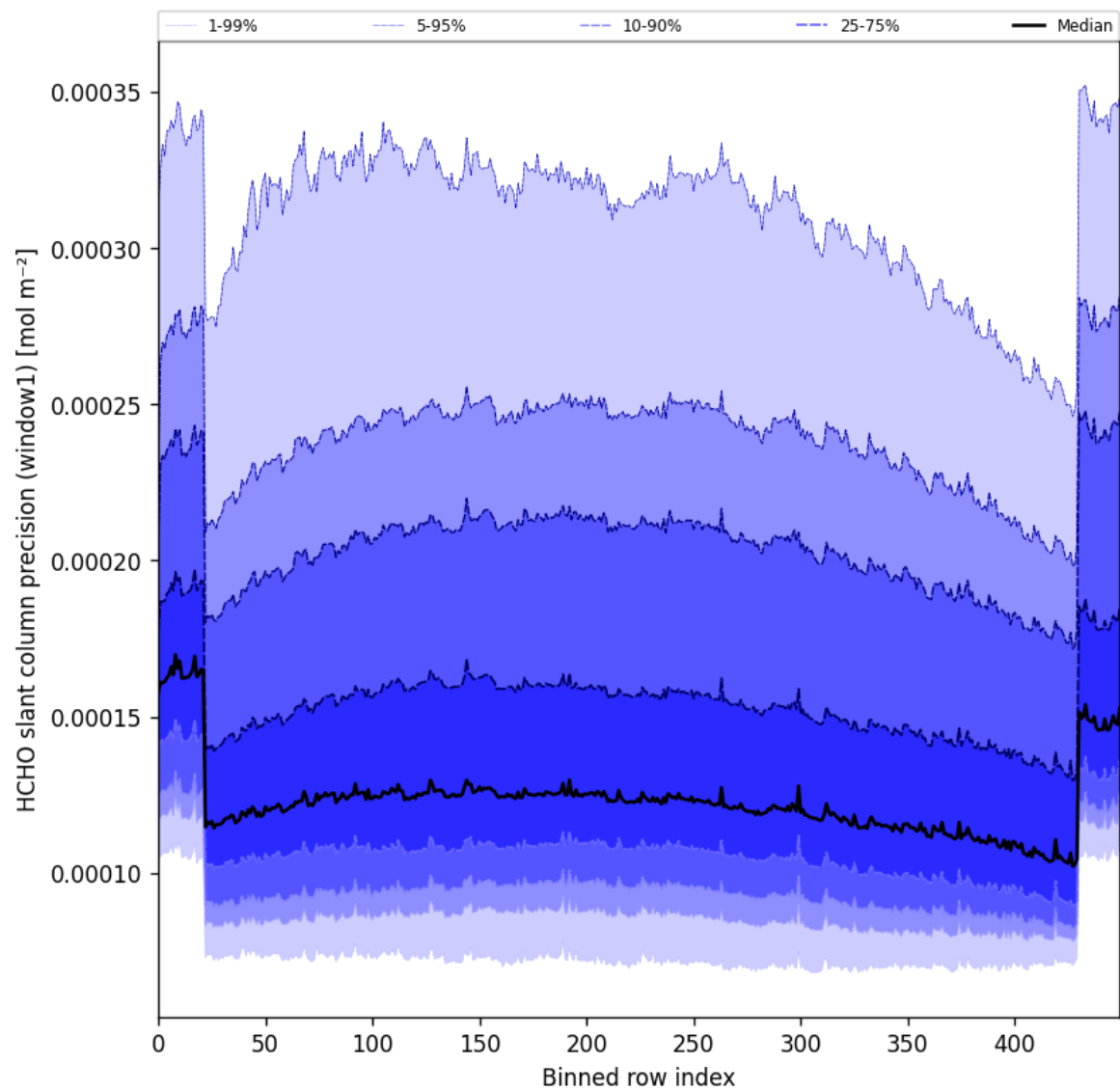
Figure 53: Along track statistics of “HCHO slant column precision (window1)” for 2025-10-31 to 2025-11-02
