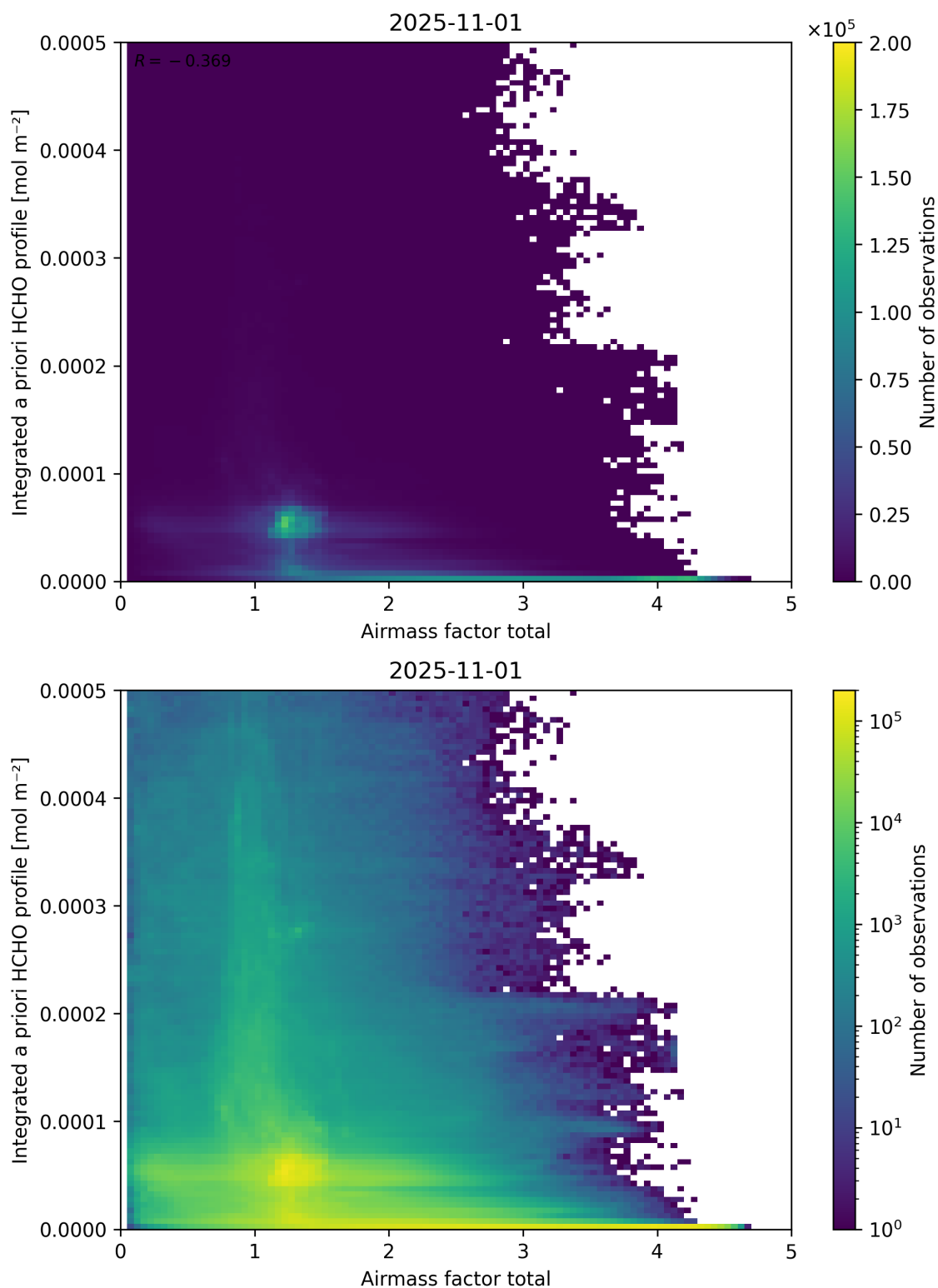
Figure 104: Scatter density plot of “Airmass factor total” against “Integrated a priori HCHO profile” for 2025-10-31 to 2025-11-02.
