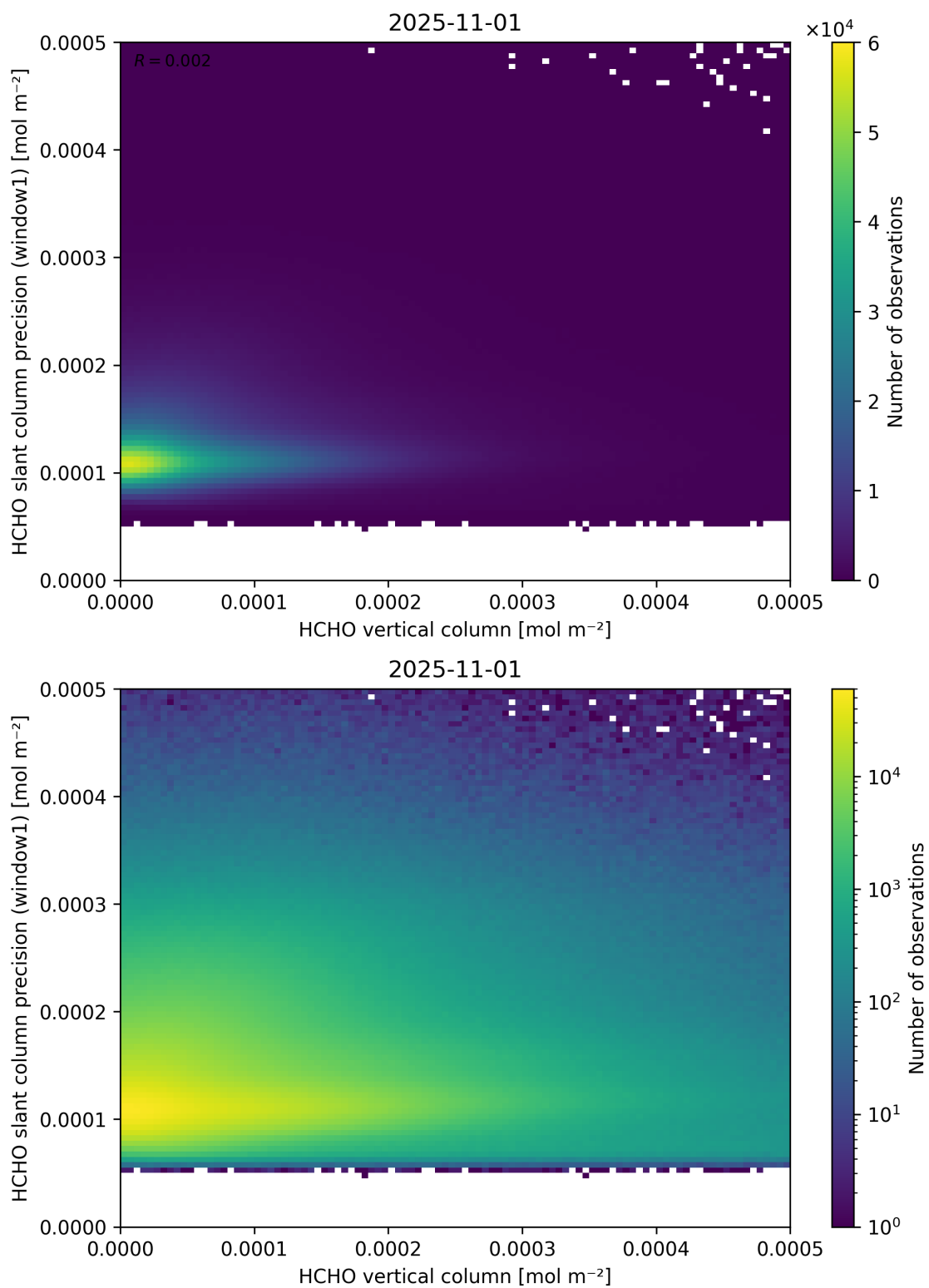
Figure 130: Scatter density plot of “HCHO vertical column” against “HCHO slant column precision (window1)” for 2025-10-31 to 2025-11-02.
