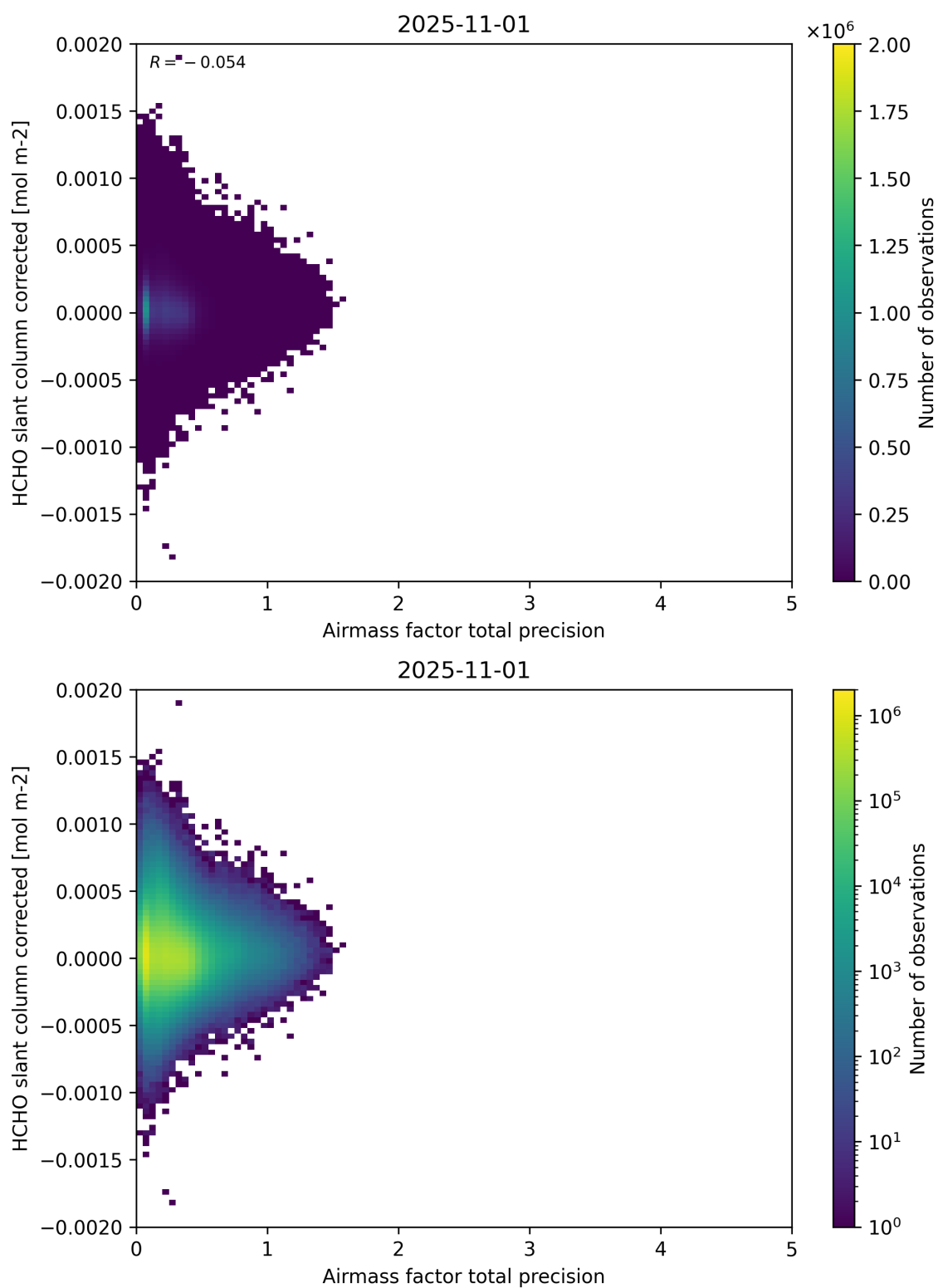
Figure 109: Scatter density plot of “Airmass factor total precision” against “HCHO slant column corrected” for 2025-10-31 to 2025-11-02.
