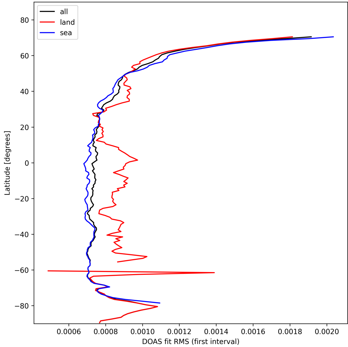
Figure 32: Zonal average of “DOAS fit RMS (first interval)” for 2025-10-31 to 2025-11-02.
