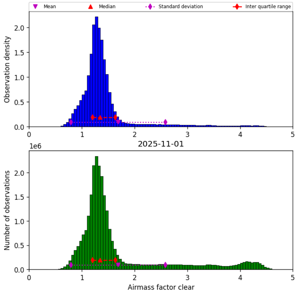
Figure 42: Histogram of “Airmass factor clear” for 2025-10-31 to 2025-11-02
