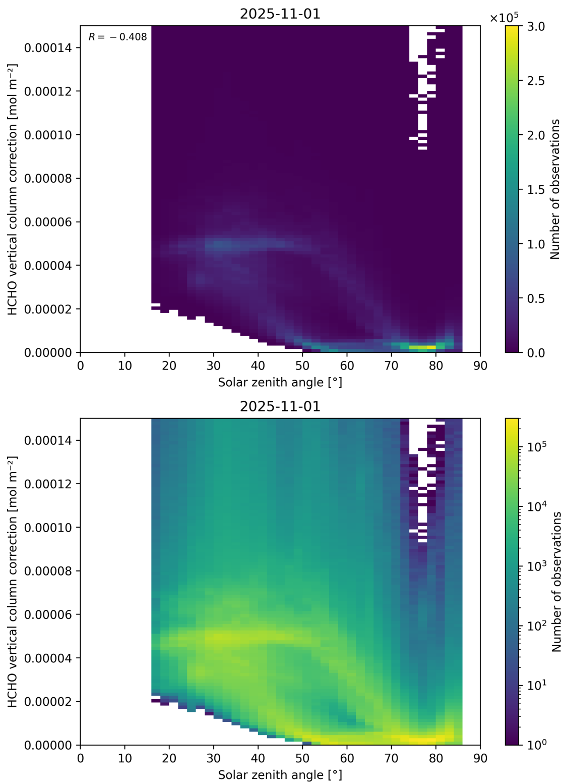
Figure 178: Scatter density plot of “Solar zenith angle” against “HCHO vertical column correction” for 2025-10-31 to 2025-11-02.
