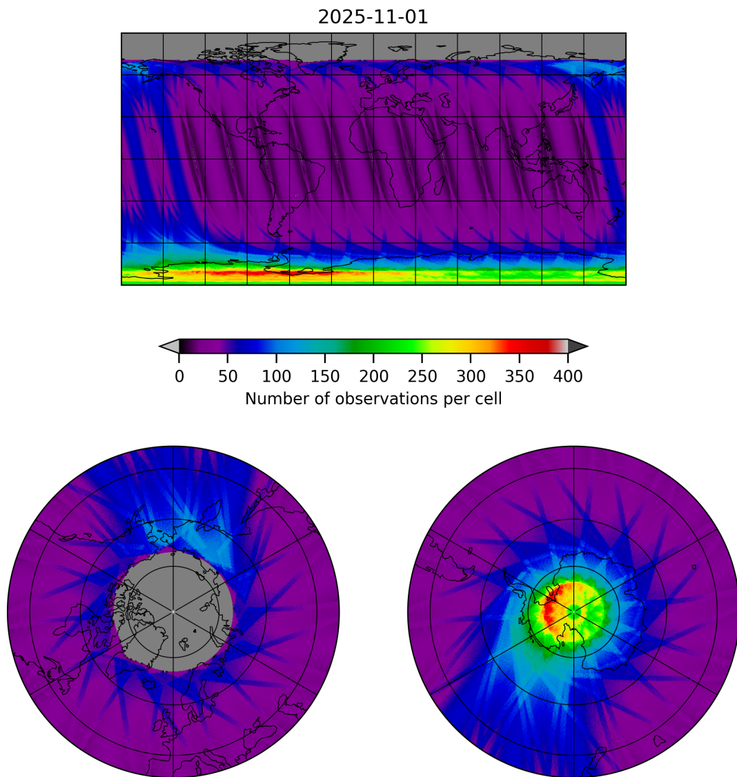
Figure 19: Map of the number of observations for 2025-10-31 to 2025-11-02
