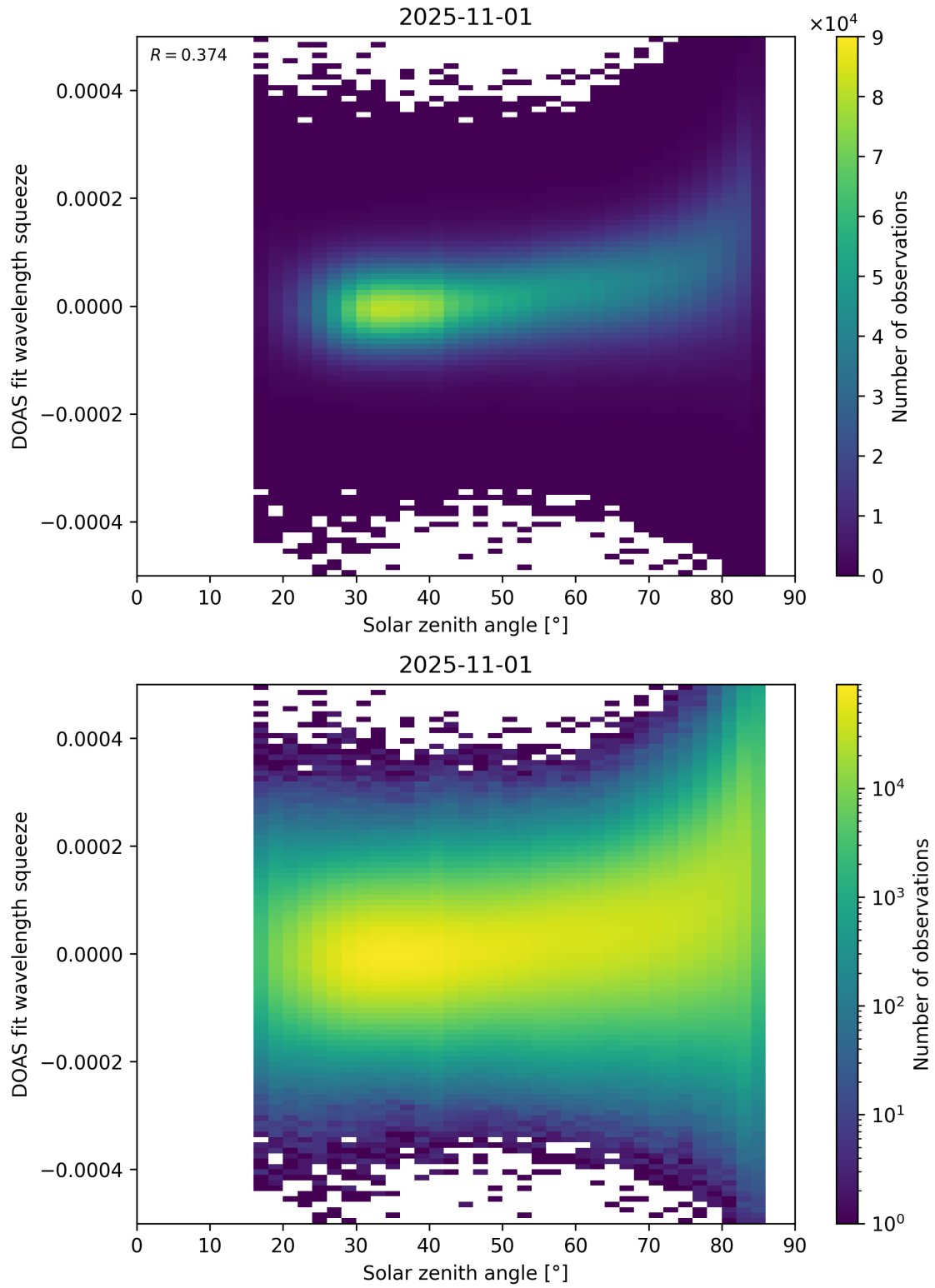
Figure 169: Scatter density plot of “Solar zenith angle” against “DOAS fit wavelength squeeze” for 2025-10-31 to 2025-11-02.
