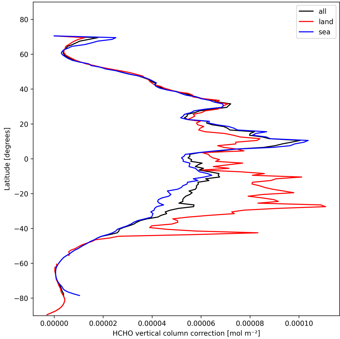
Figure 23: Zonal average of “HCHO vertical column correction” for 2025-10-31 to 2025-11-02.
