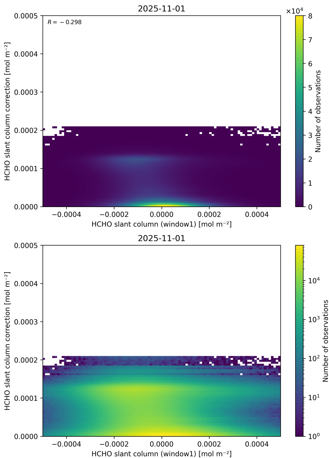
Figure 83: Scatter density plot of “HCHO slant column (window1)” against “HCHO slant column correction” for 2025-10-31 to 2025-11-02.
