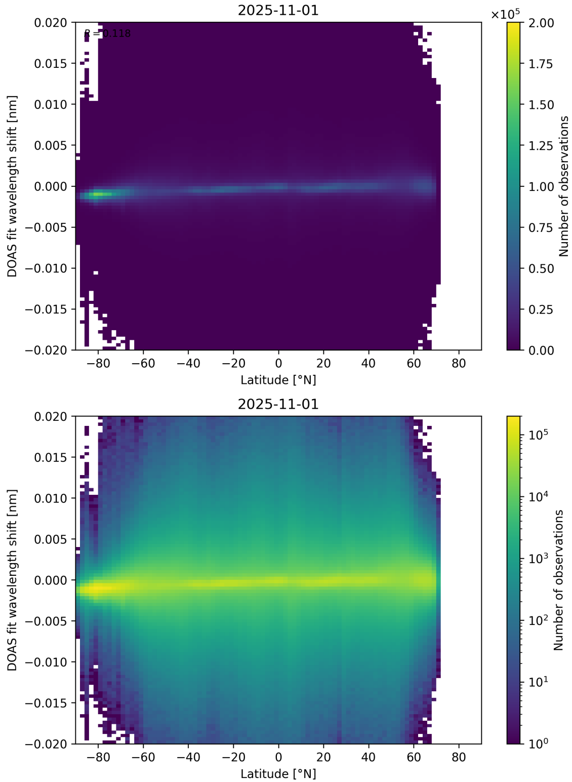
Figure 154: Scatter density plot of “Latitude” against “DOAS fit wavelength shift” for 2025-10-31 to 2025-11-02.
