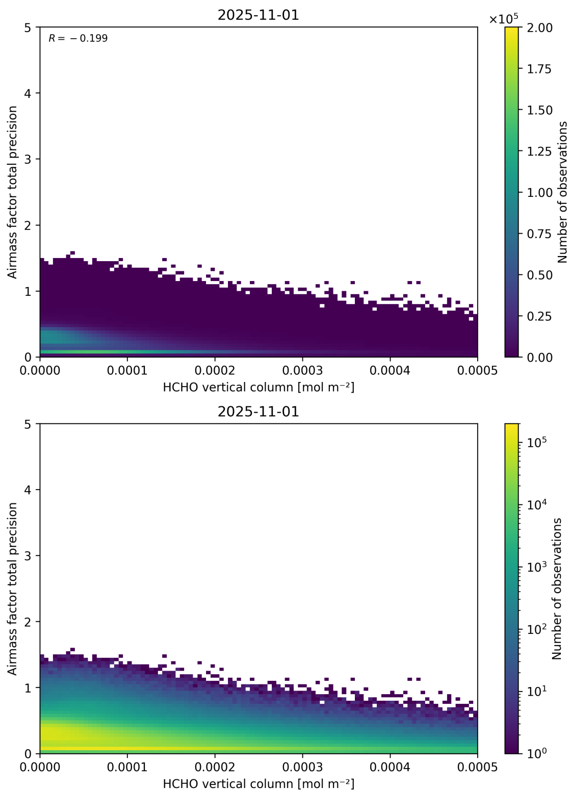
Figure 132: Scatter density plot of “HCHO vertical column” against “Airmass factor total precision” for 2025-10-31 to 2025-11-02.
