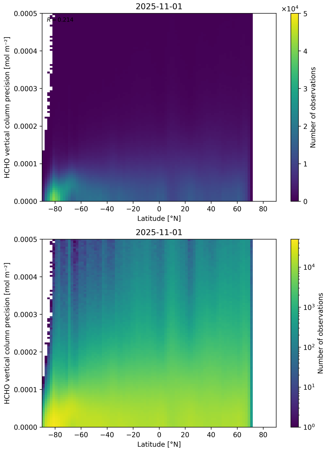
Figure 165: Scatter density plot of “Latitude” against “HCHO vertical column precision” for 2025-10-31 to 2025-11-02.
