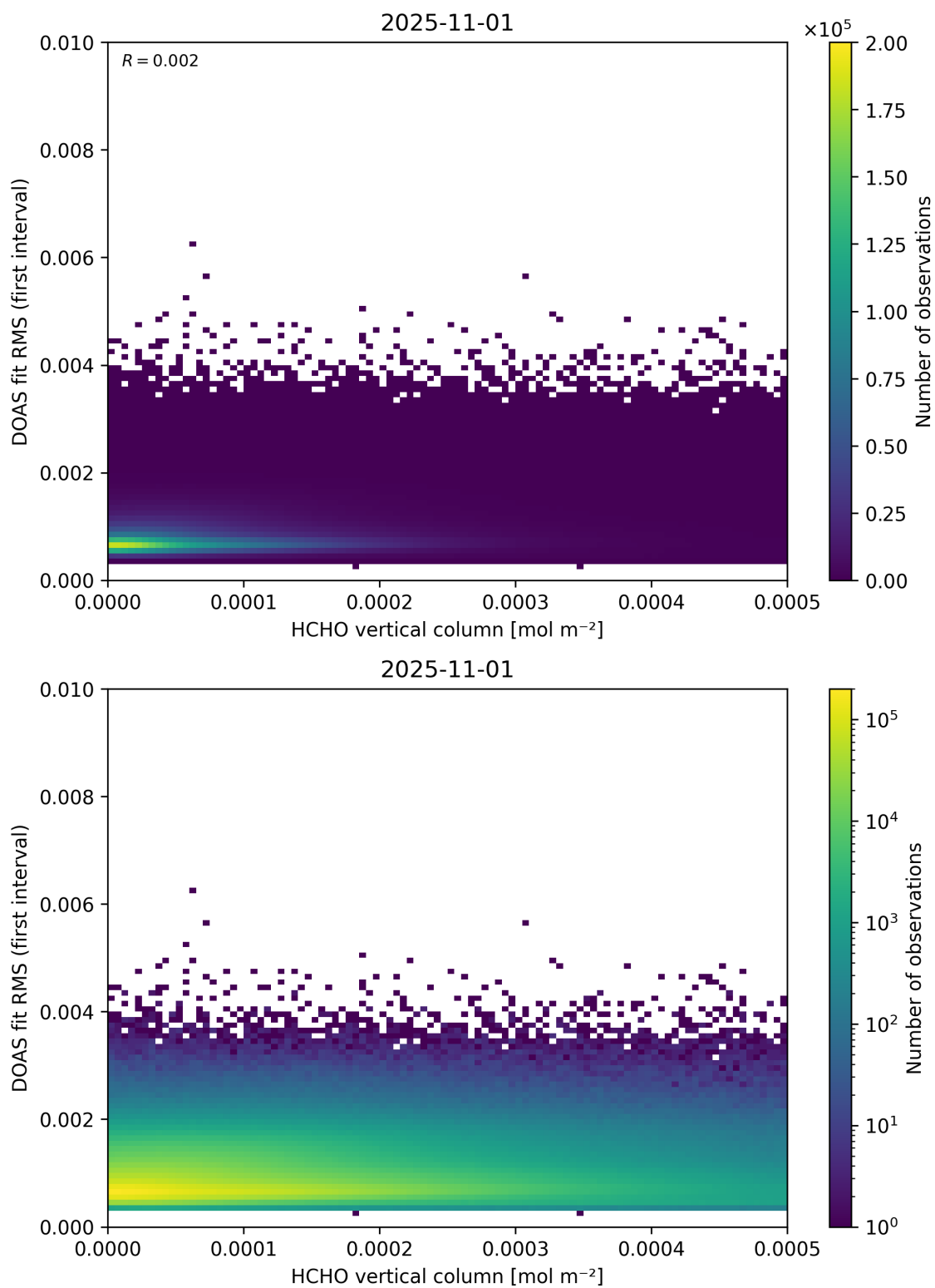
Figure 123: Scatter density plot of “HCHO vertical column” against “DOAS fit RMS (first interval)” for 2025-10-31 to 2025-11-02.
