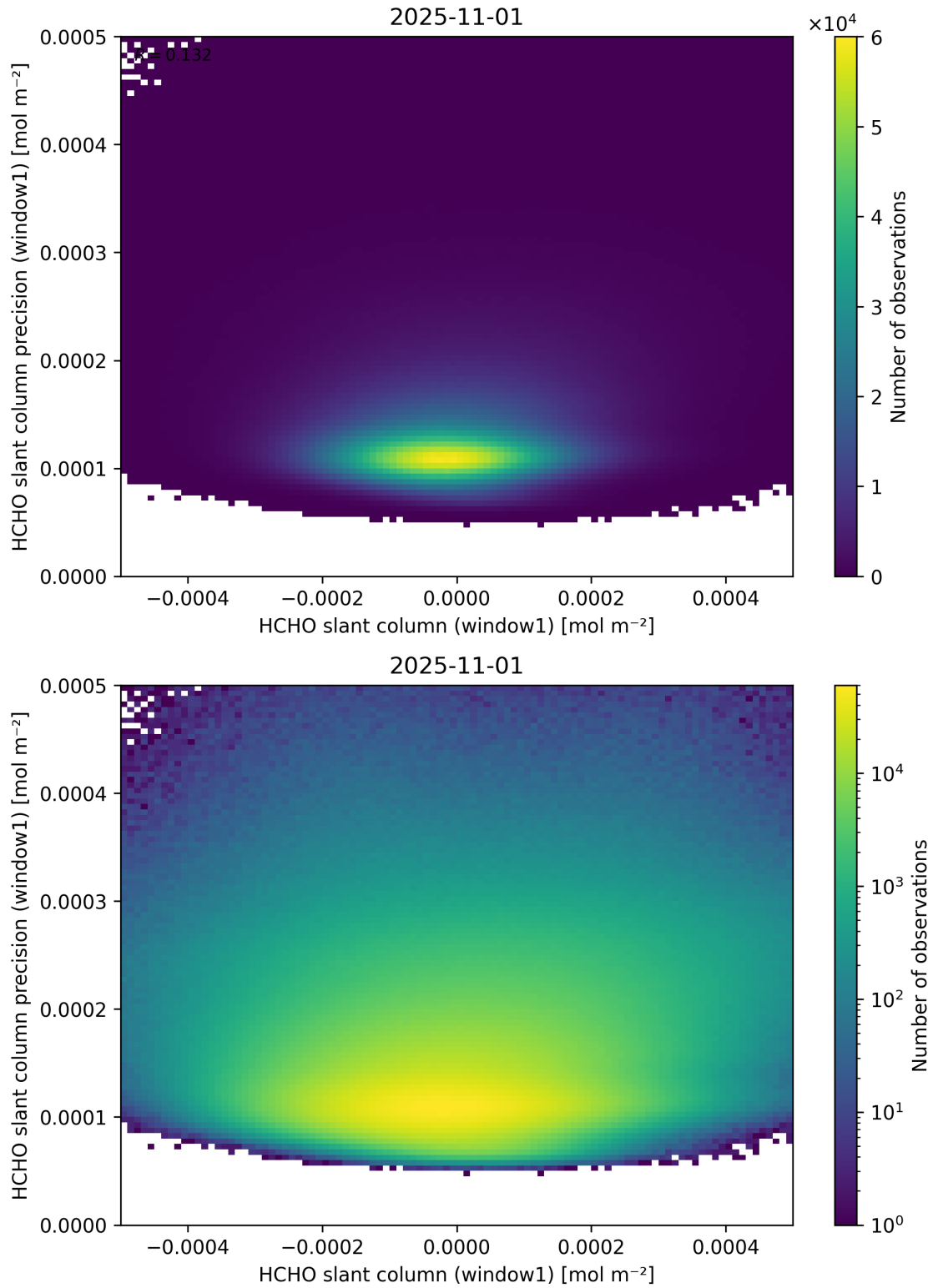
Figure 84: Scatter density plot of “HCHO slant column (window1)” against “HCHO slant column precision (window1)” for 2025-10-31 to 2025-11-02.
