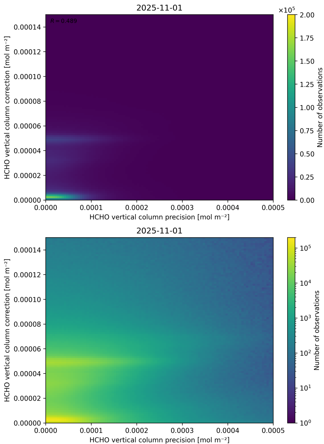
Figure 146: Scatter density plot of “HCHO vertical column precision” against “HCHO vertical column correction” for 2025-10-31 to 2025-11-02.
