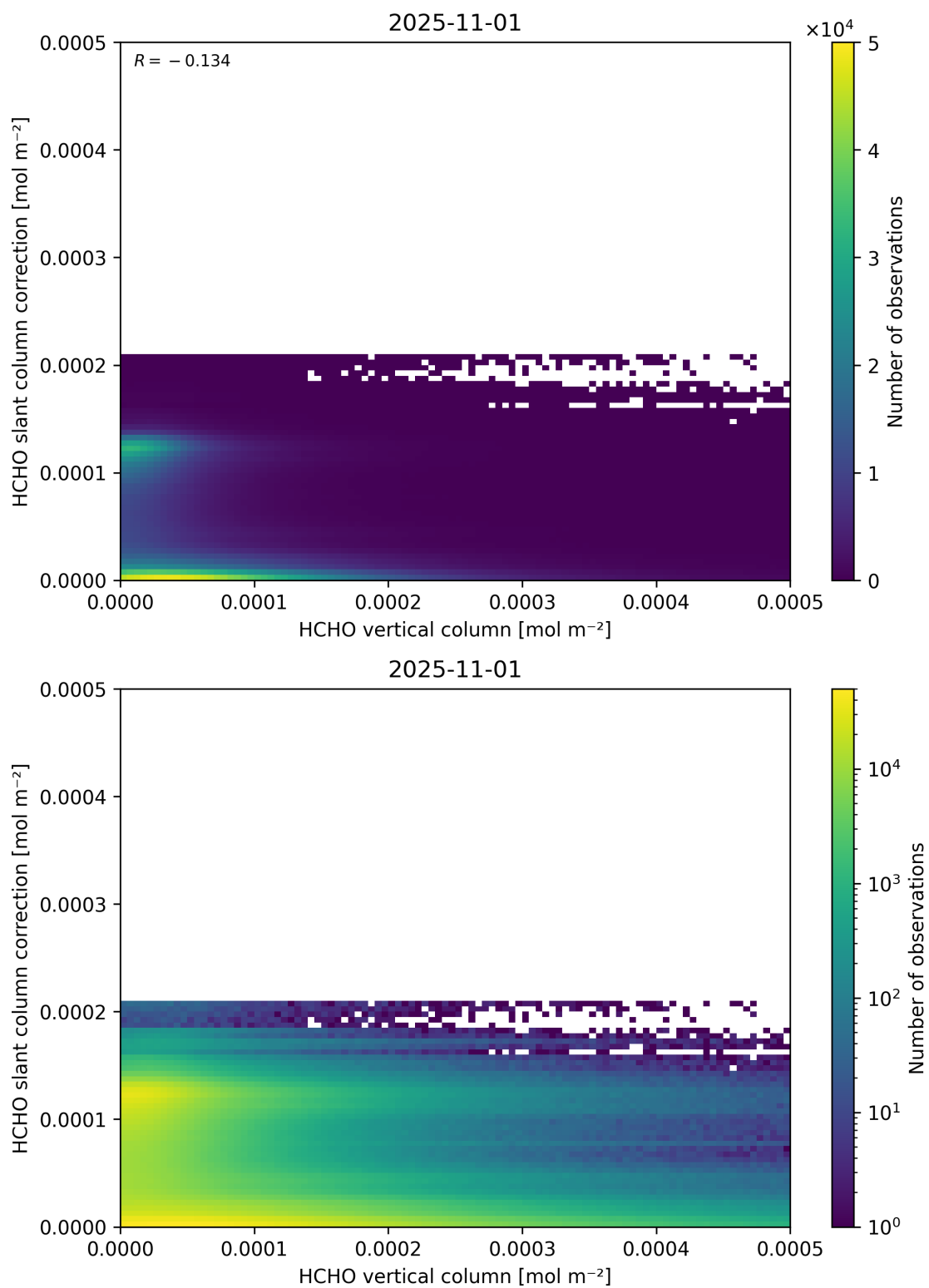
Figure 128: Scatter density plot of “HCHO vertical column” against “HCHO slant column correction” for 2025-10-31 to 2025-11-02.
