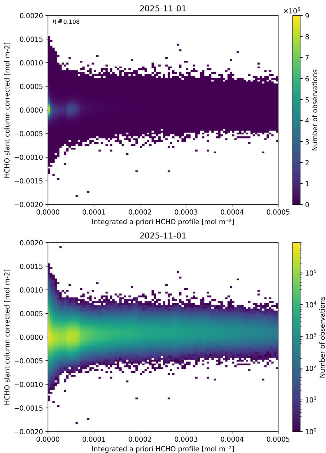
Figure 151: Scatter density plot of “Integrated a priori HCHO profile” against “HCHO slant column corrected” for 2025-10-31 to 2025-11-02.
