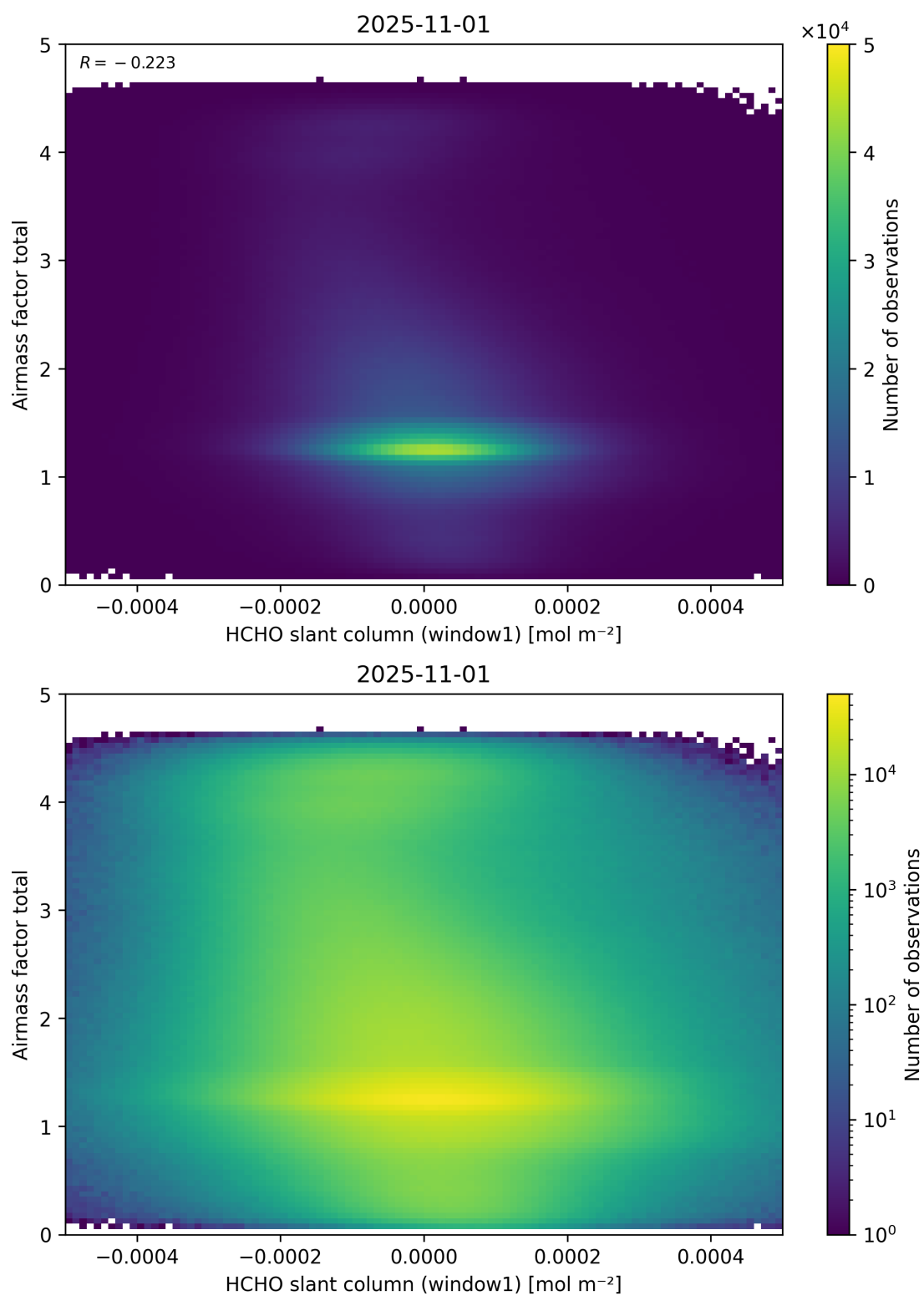
Figure 85: Scatter density plot of “HCHO slant column (window1)” against “Airmass factor total” for 2025-10-31 to 2025-11-02.
