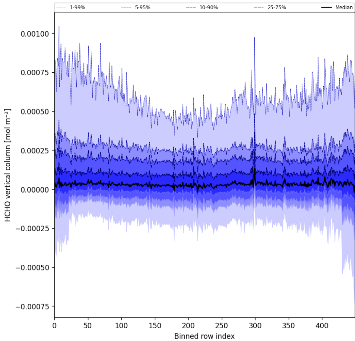
Figure 49: Along track statistics of “HCHO vertical column” for 2025-10-31 to 2025-11-02
