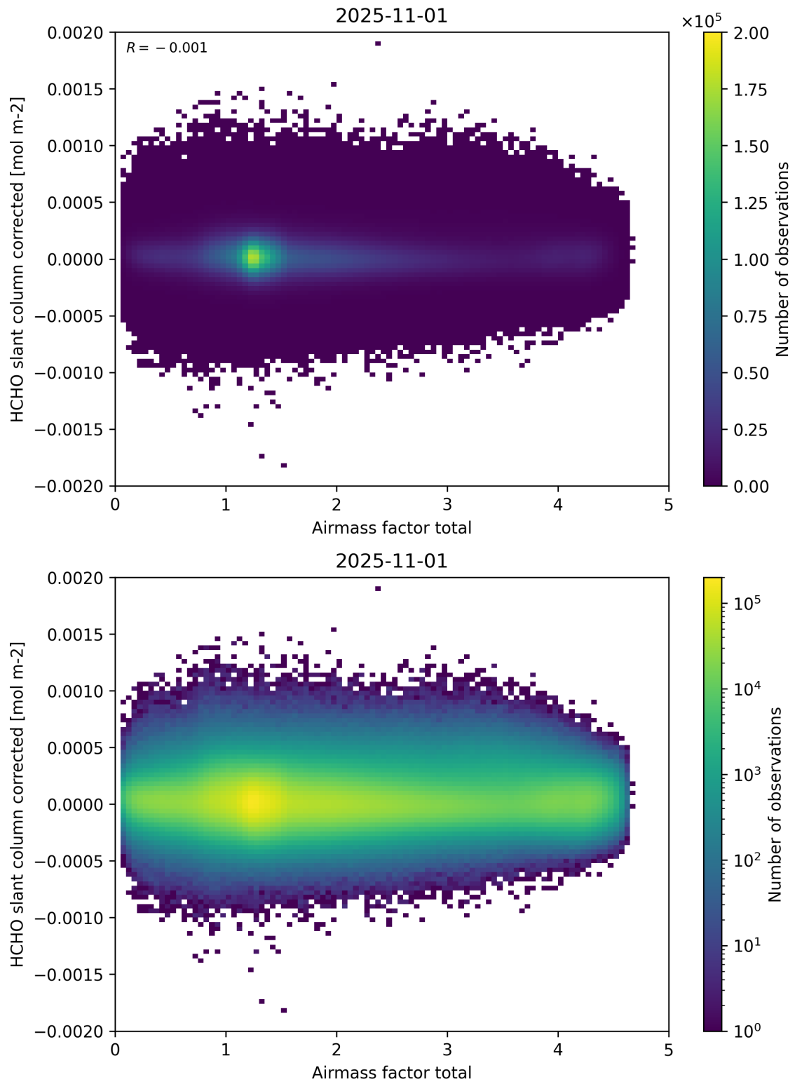
Figure 101: Scatter density plot of “Airmass factor total” against “HCHO slant column corrected” for 2025-10-31 to 2025-11-02.
