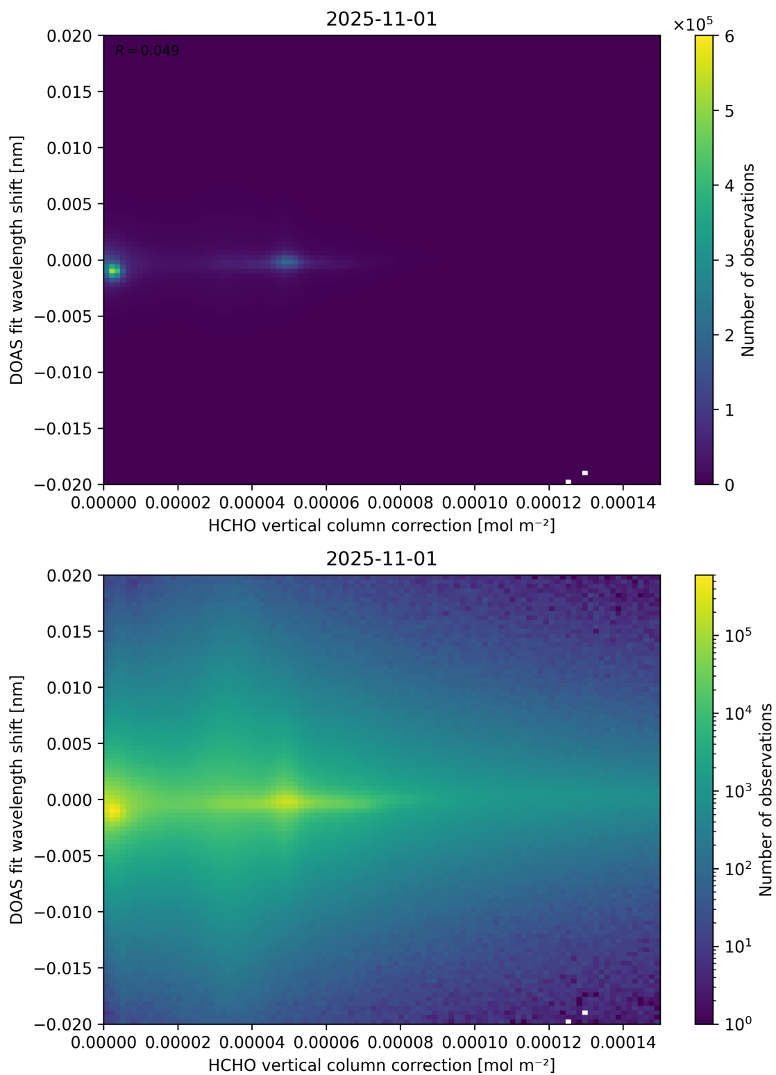
Figure 113: Scatter density plot of “HCHO vertical column correction” against “DOAS fit wavelength shift” for 2025-10-31 to 2025-11-02.
