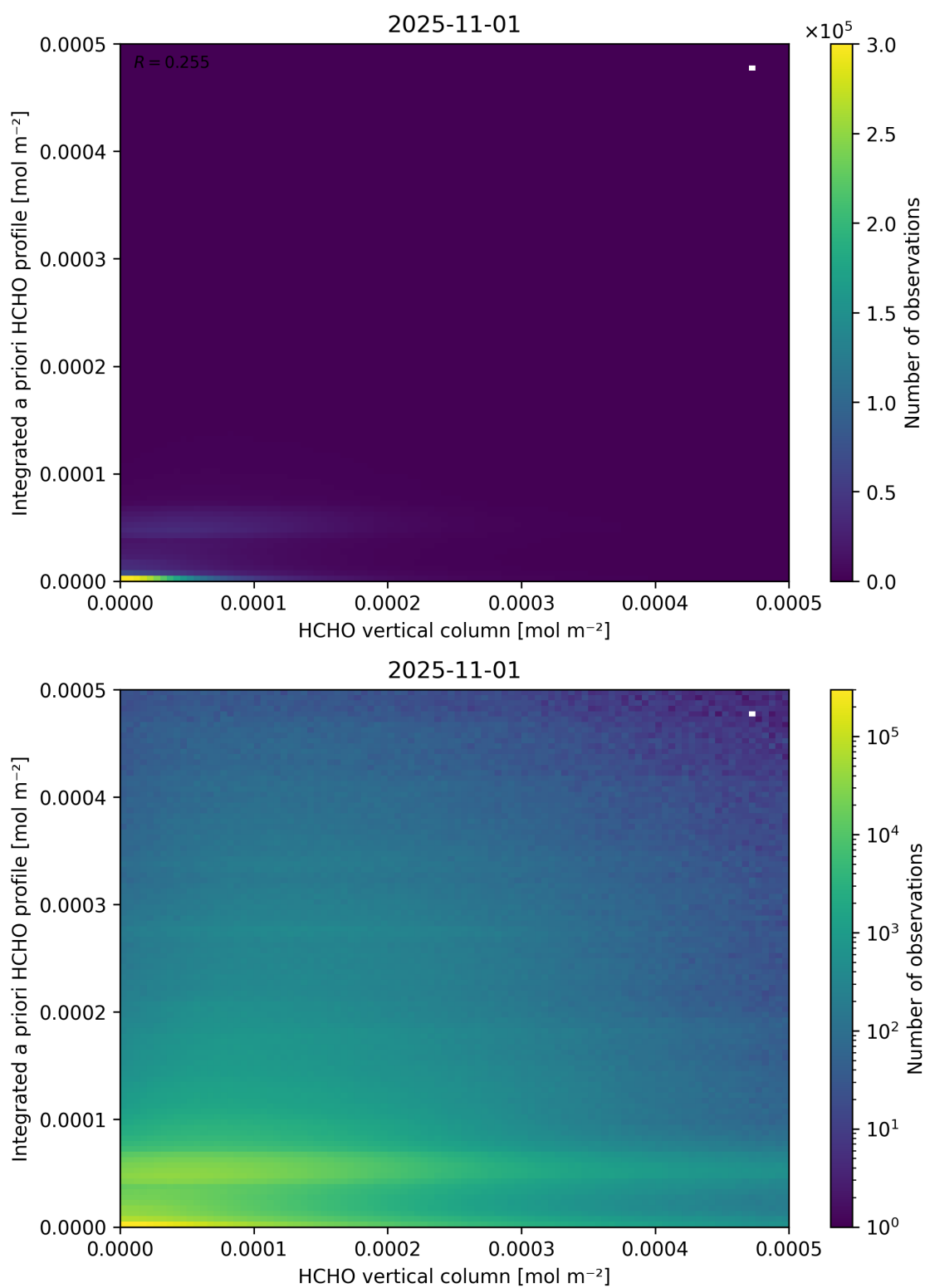
Figure 135: Scatter density plot of “HCHO vertical column” against “Integrated a priori HCHO profile” for 2025-10-31 to 2025-11-02.
