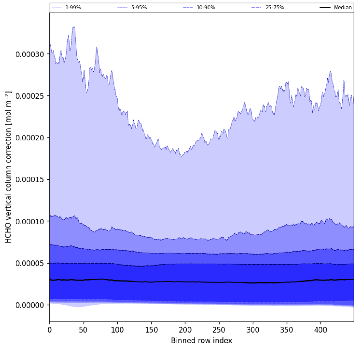
Figure 51: Along track statistics of “HCHO vertical column correction” for 2025-10-31 to 2025-11-02
