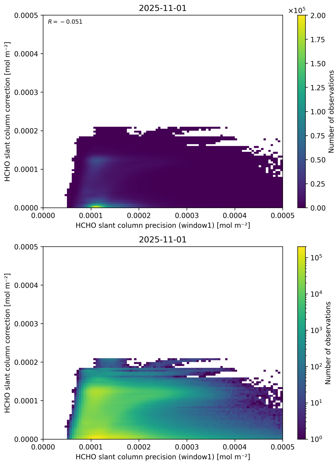
Figure 93: Scatter density plot of “HCHO slant column precision (window1)” against “HCHO slant column correction” for 2025-10-31 to 2025-11-02.
