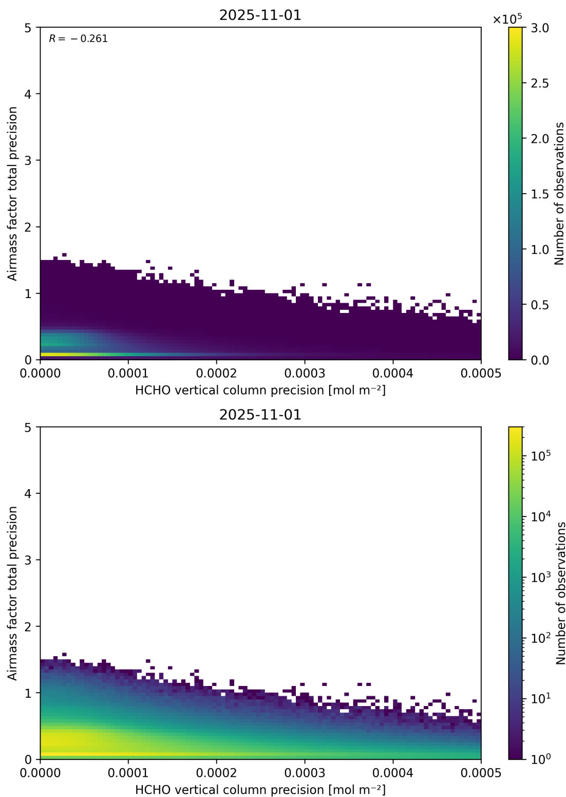
Figure 145: Scatter density plot of “HCHO vertical column precision” against “Airmass factor total precision” for 2025-10-31 to 2025-11-02.
