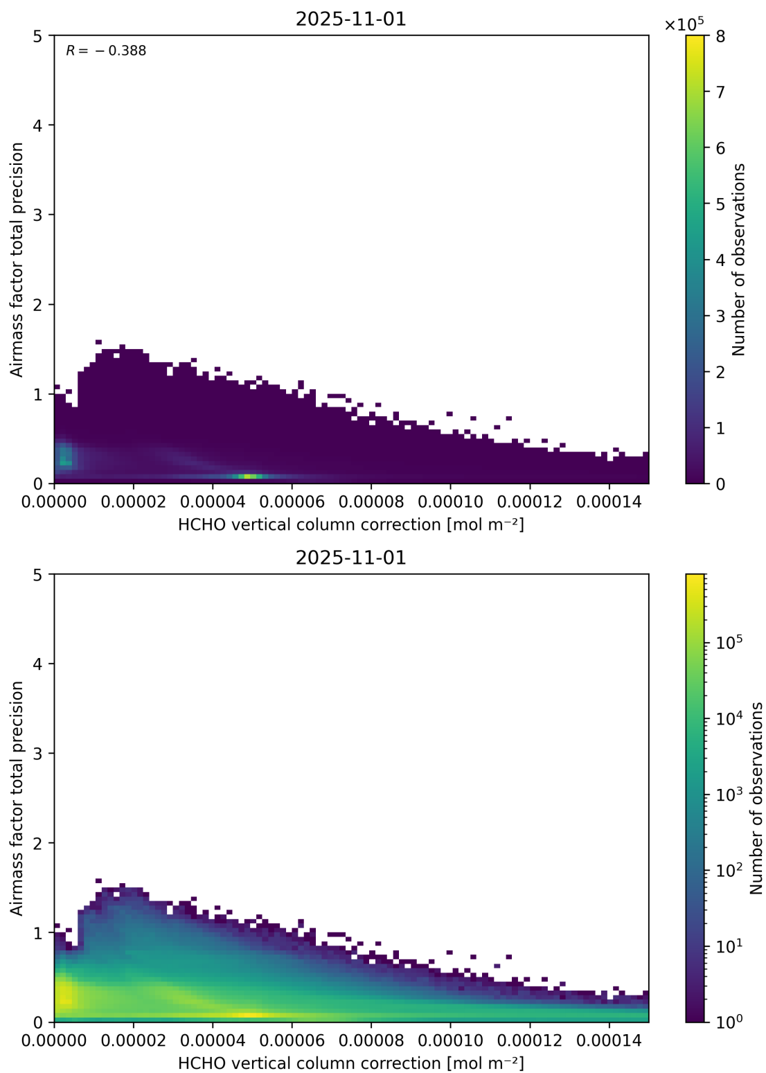
Figure 121: Scatter density plot of “HCHO vertical column correction” against “Airmass factor total precision” for 2025-10-31 to 2025-11-02.
