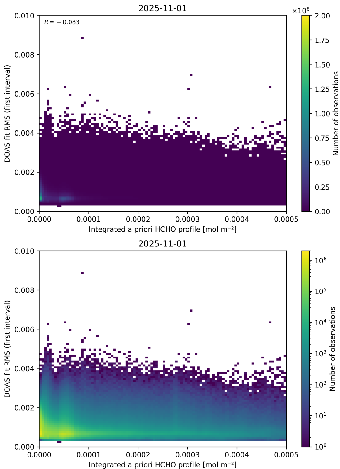
Figure 148: Scatter density plot of “Integrated a priori HCHO profile” against “DOAS fit RMS (first interval)” for 2025-10-31 to 2025-11-02.
