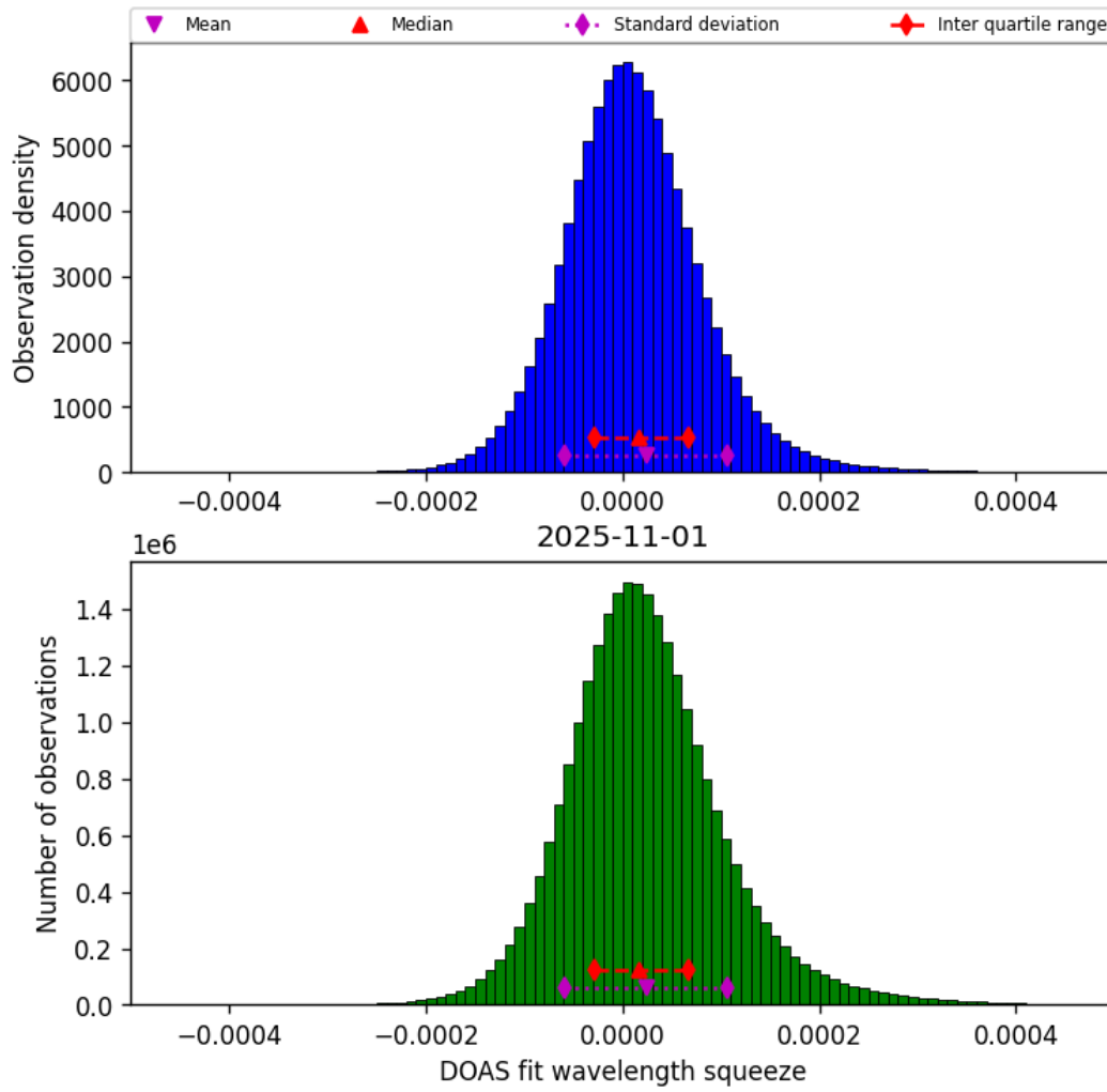
Figure 45: Histogram of “DOAS fit wavelength squeeze” for 2025-10-31 to 2025-11-02
