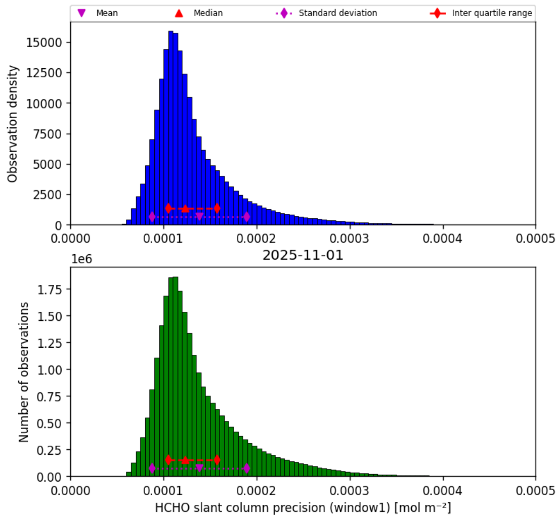
Figure 39: Histogram of “HCHO slant column precision (window1)” for 2025-10-31 to 2025-11-02
