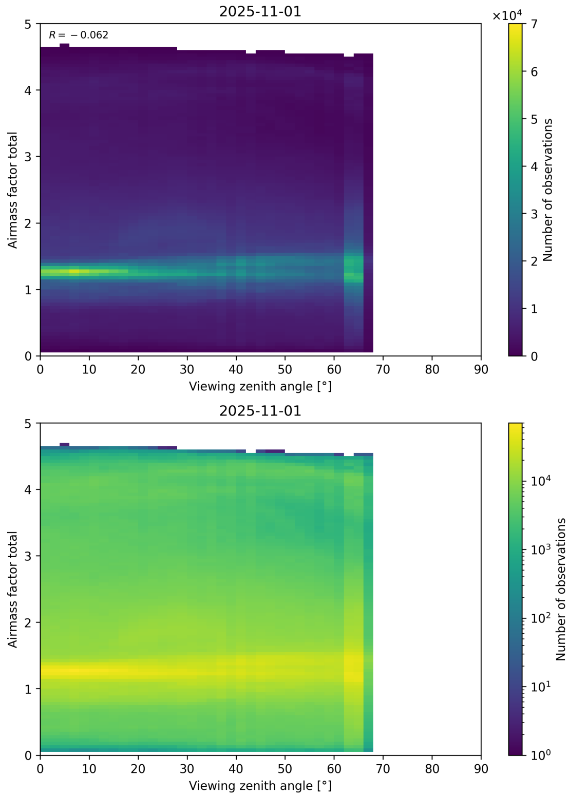
Figure 190: Scatter density plot of “Viewing zenith angle” against “Airmass factor total” for 2025-10-31 to 2025-11-02.
