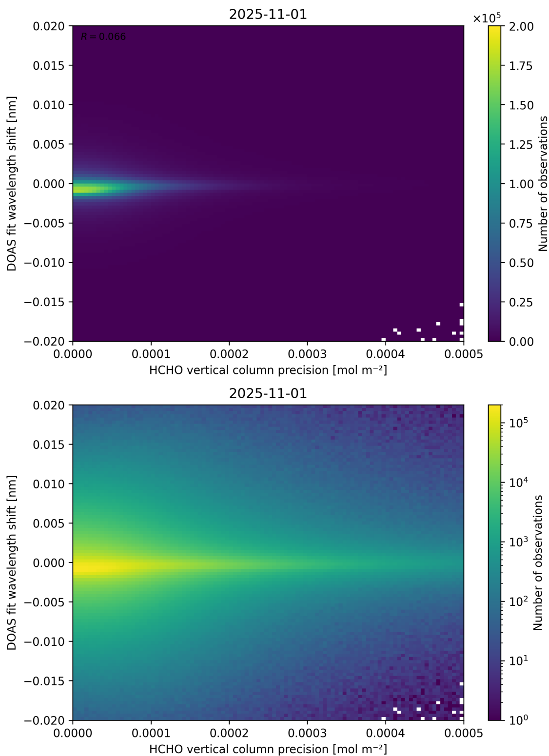
Figure 137: Scatter density plot of “HCHO vertical column precision” against “DOAS fit wavelength shift” for 2025-10-31 to 2025-11-02.
