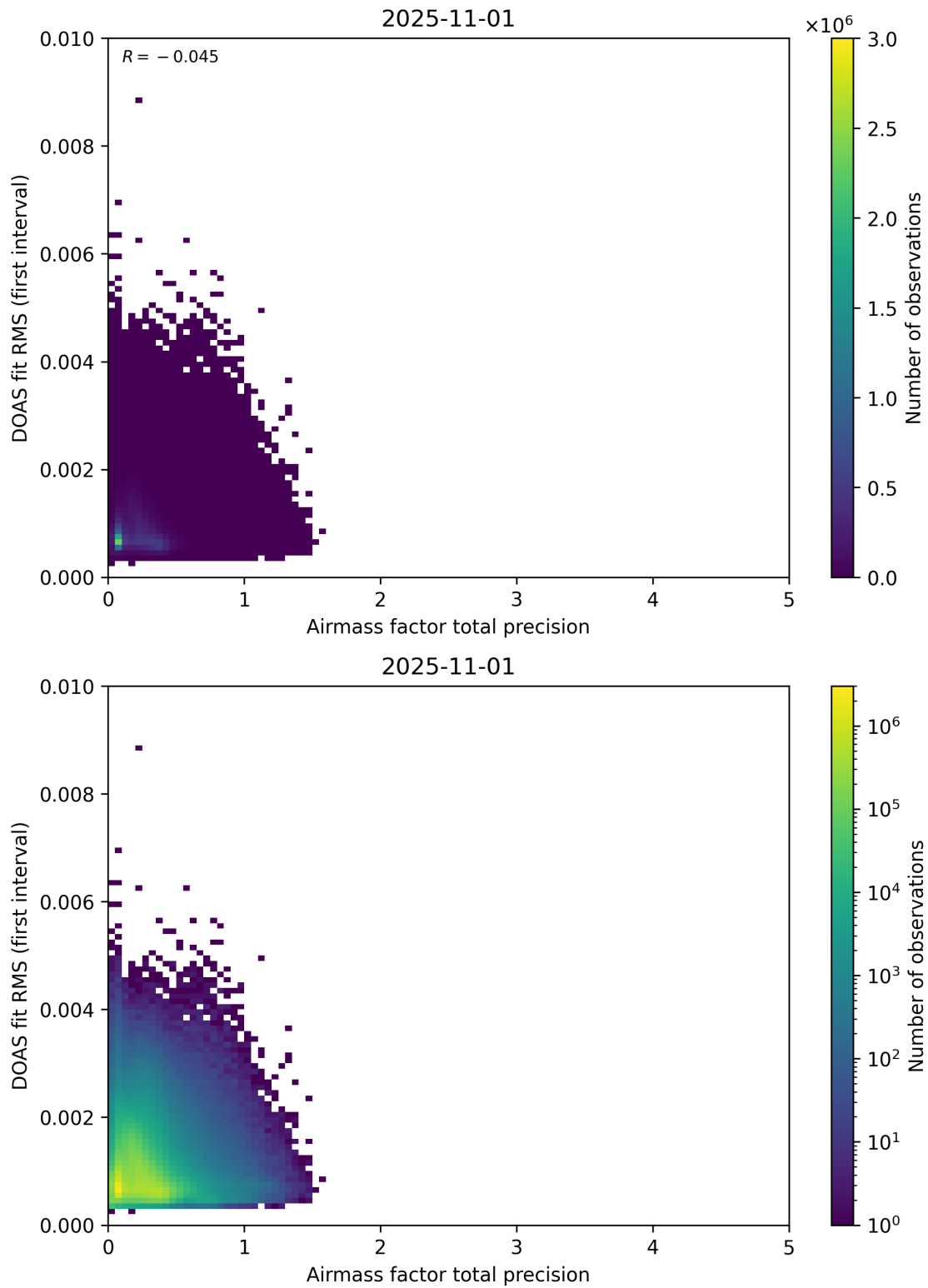
Figure 105: Scatter density plot of “Airmass factor total precision” against “DOAS fit RMS (first interval)” for 2025-10-31 to 2025-11-02.
