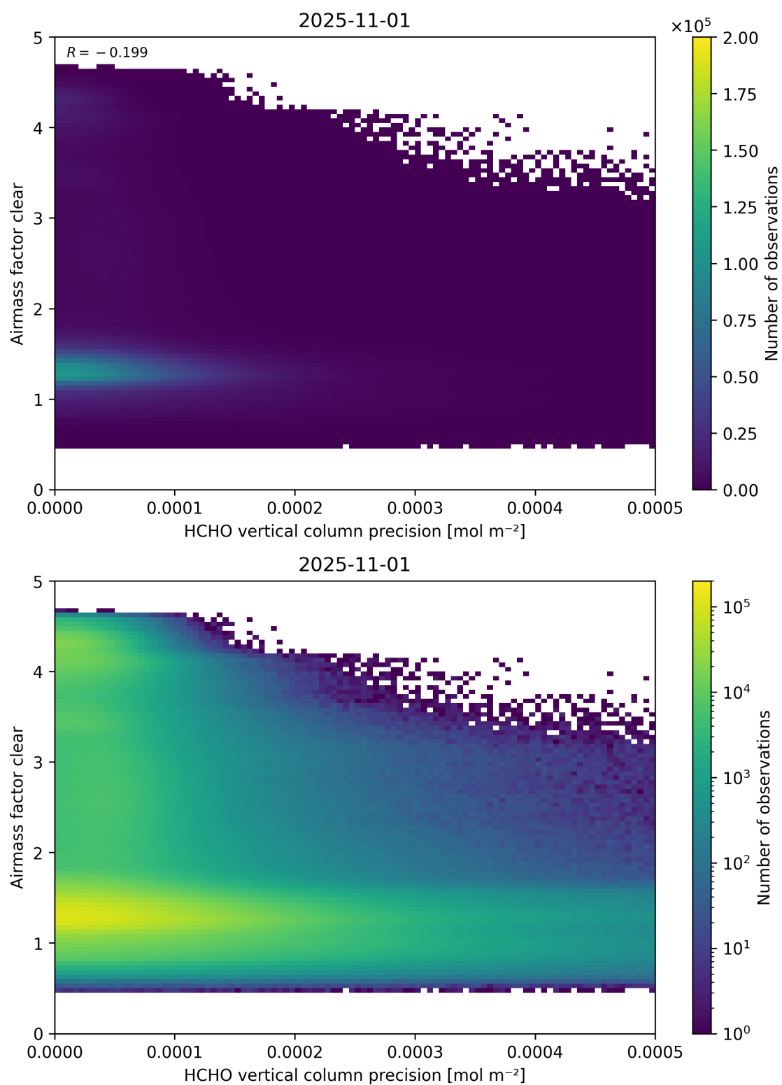
Figure 139: Scatter density plot of “HCHO vertical column precision” against “Airmass factor clear” for 2025-10-31 to 2025-11-02.
