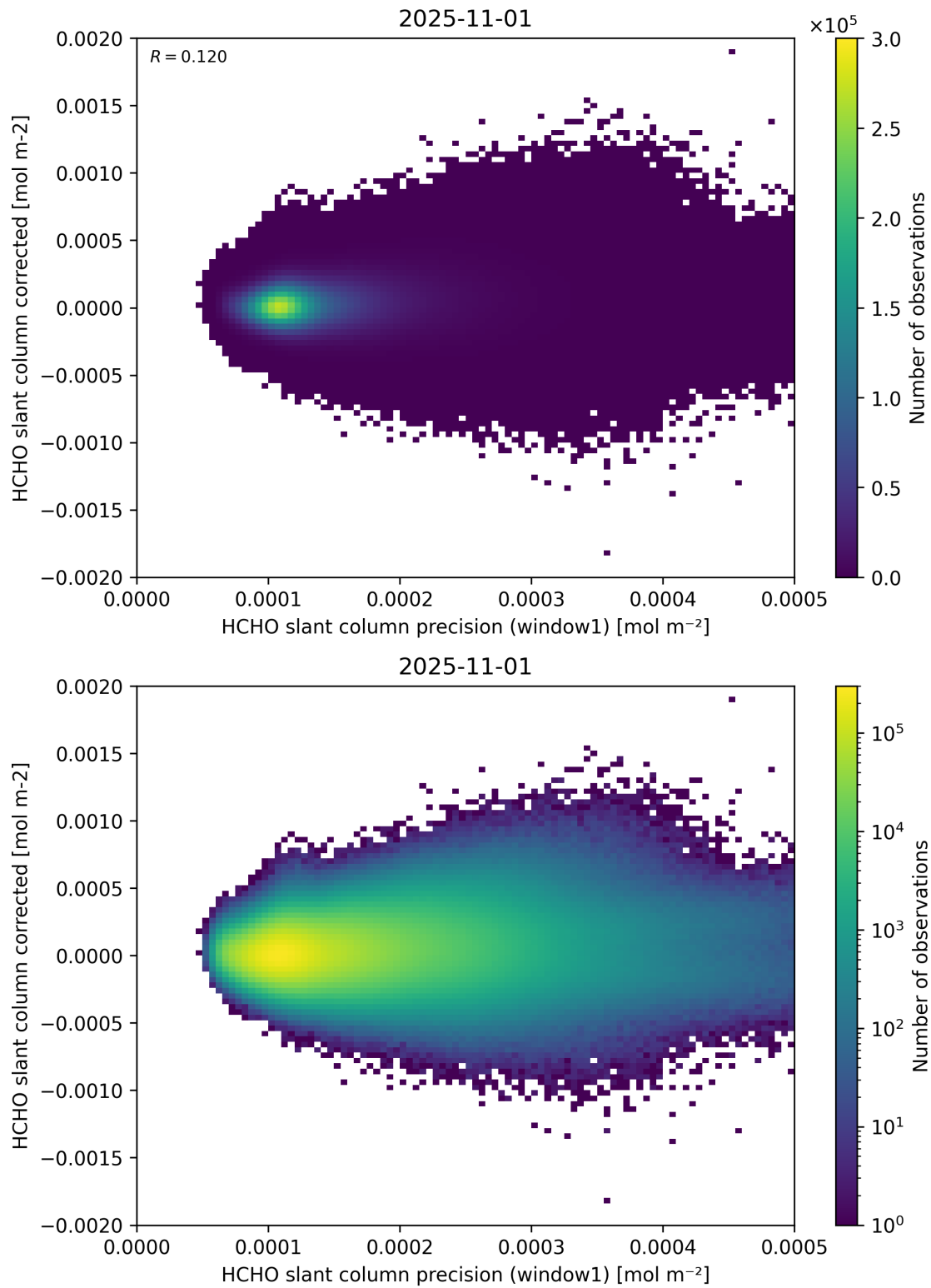
Figure 92: Scatter density plot of “HCHO slant column precision (window1)” against “HCHO slant column corrected” for 2025-10-31 to 2025-11-02.
