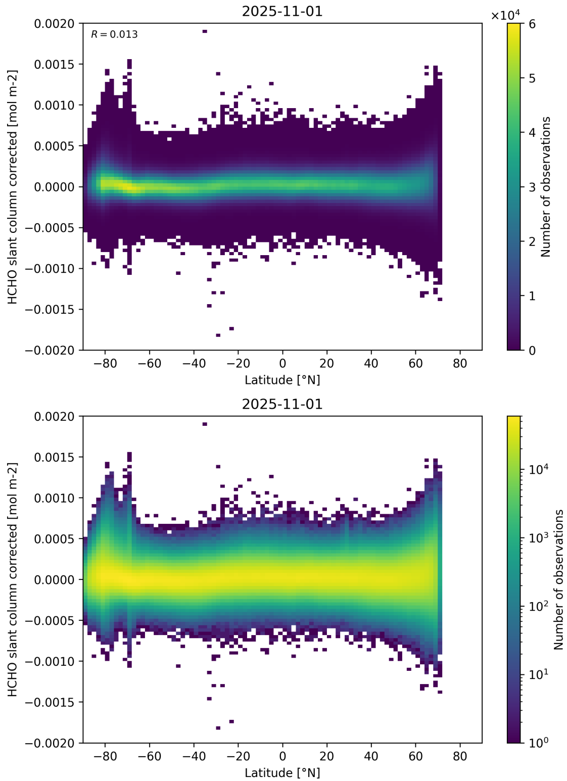
Figure 157: Scatter density plot of “Latitude” against “HCHO slant column corrected” for 2025-10-31 to 2025-11-02.
