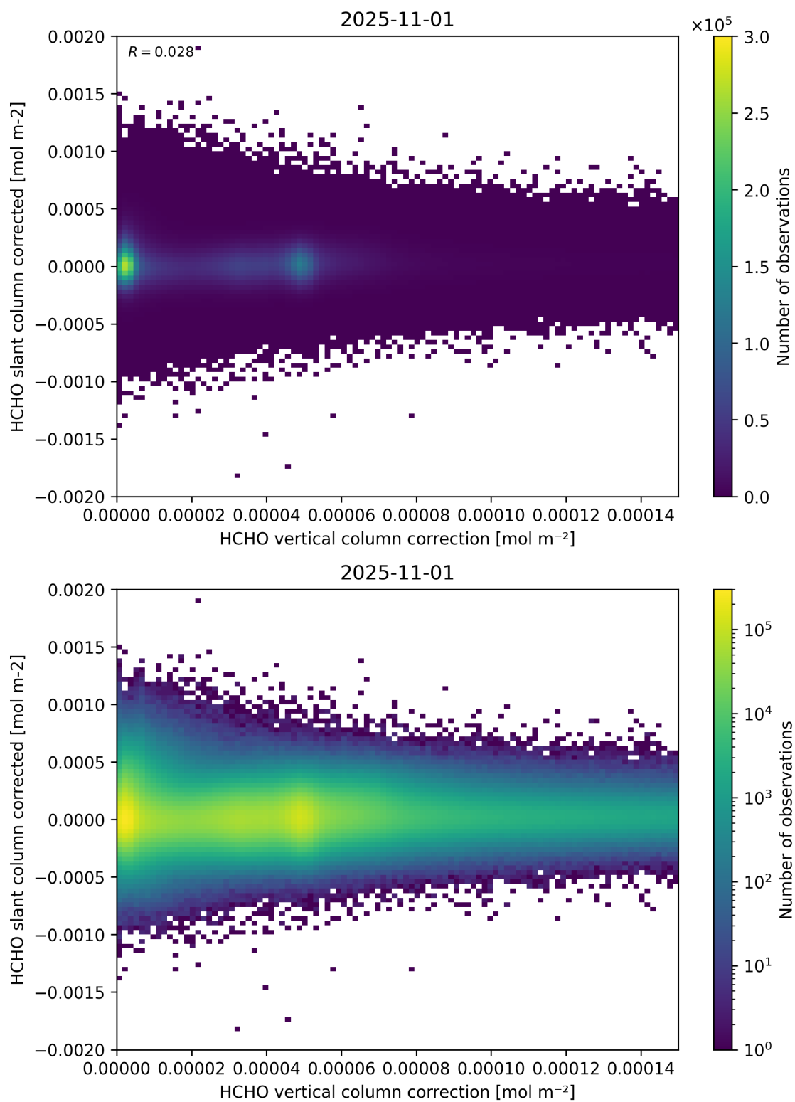
Figure 116: Scatter density plot of “HCHO vertical column correction” against “HCHO slant column corrected” for 2025-10-31 to 2025-11-02.
