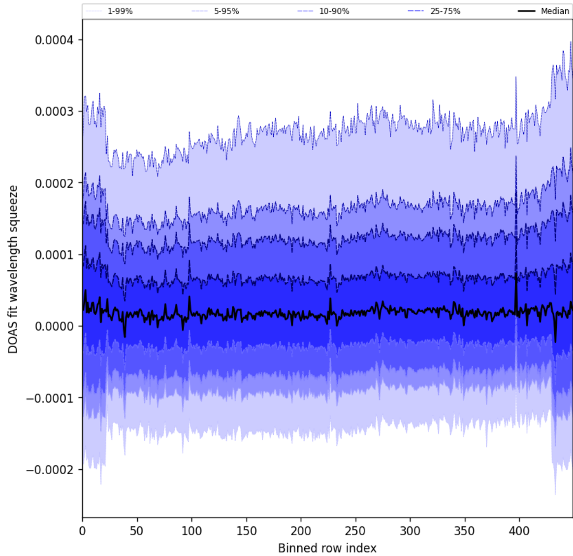
Figure 59: Along track statistics of “DOAS fit wavelength squeeze” for 2025-10-31 to 2025-11-02
