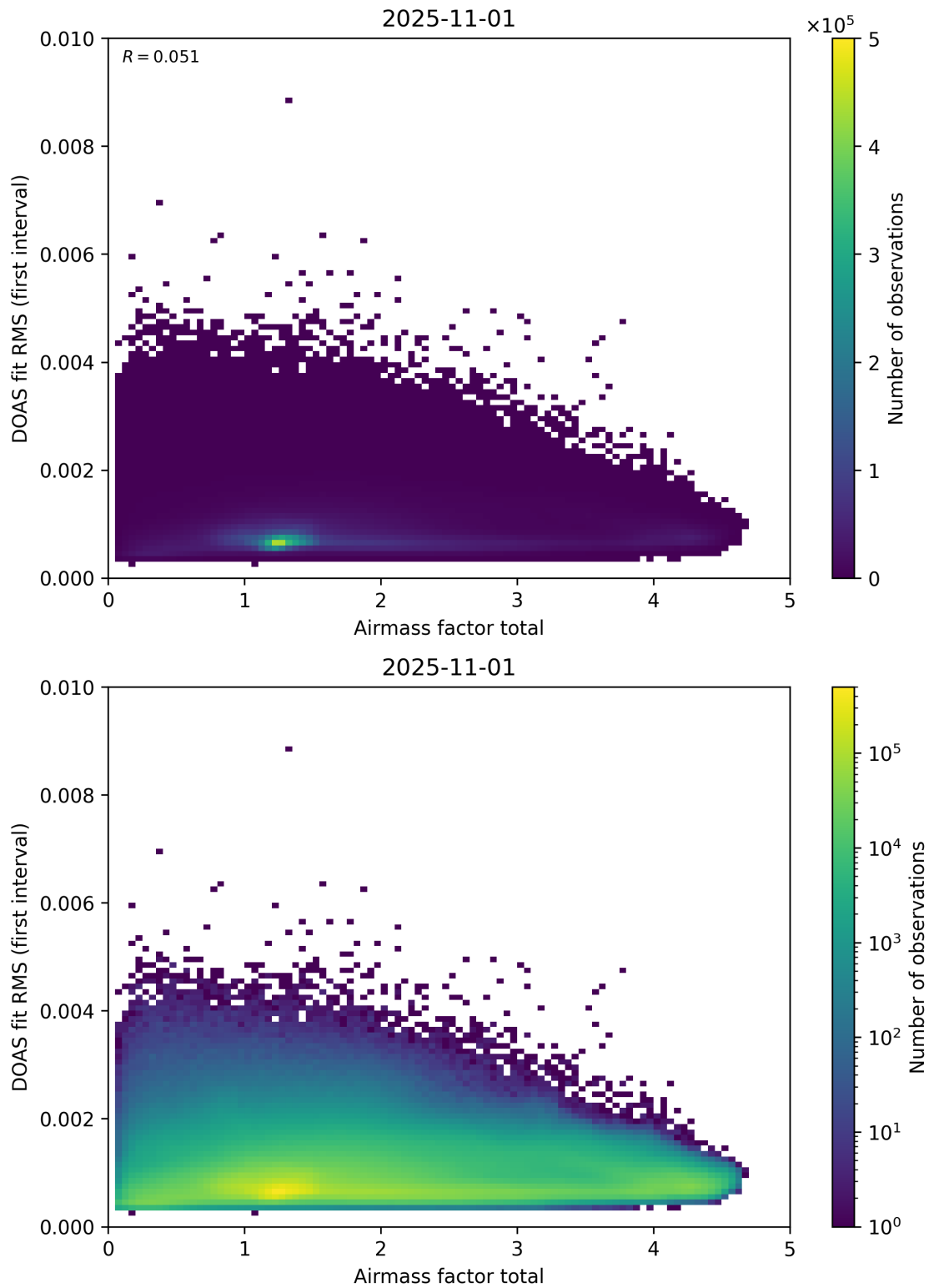
Figure 97: Scatter density plot of “Airmass factor total” against “DOAS fit RMS (first interval)” for 2025-10-31 to 2025-11-02.
