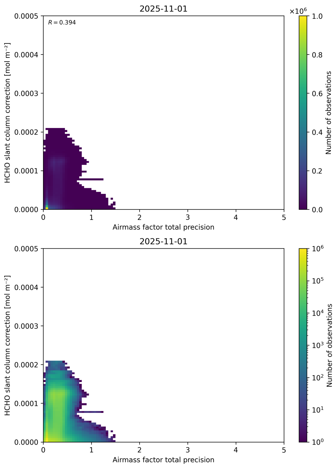
Figure 110: Scatter density plot of “Airmass factor total precision” against “HCHO slant column correction” for 2025-10-31 to 2025-11-02.
