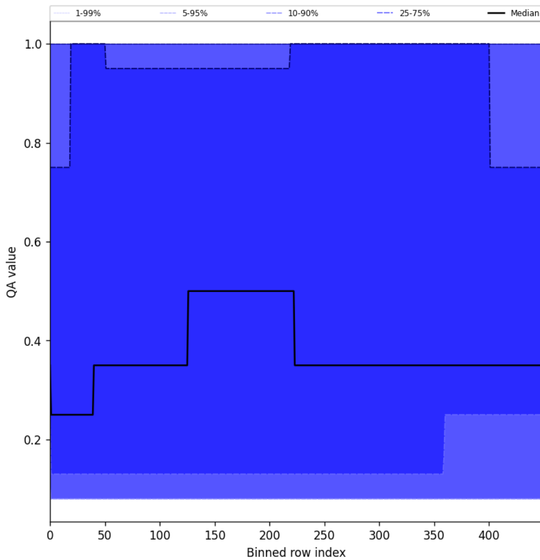
Figure 48: Along track statistics of “QA value” for 2025-10-31 to 2025-11-02
