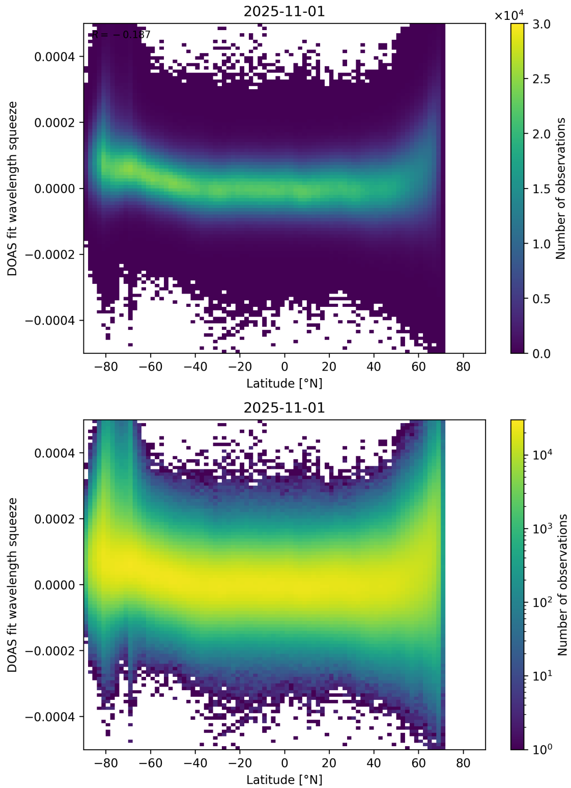
Figure 155: Scatter density plot of “Latitude” against “DOAS fit wavelength squeeze” for 2025-10-31 to 2025-11-02.
