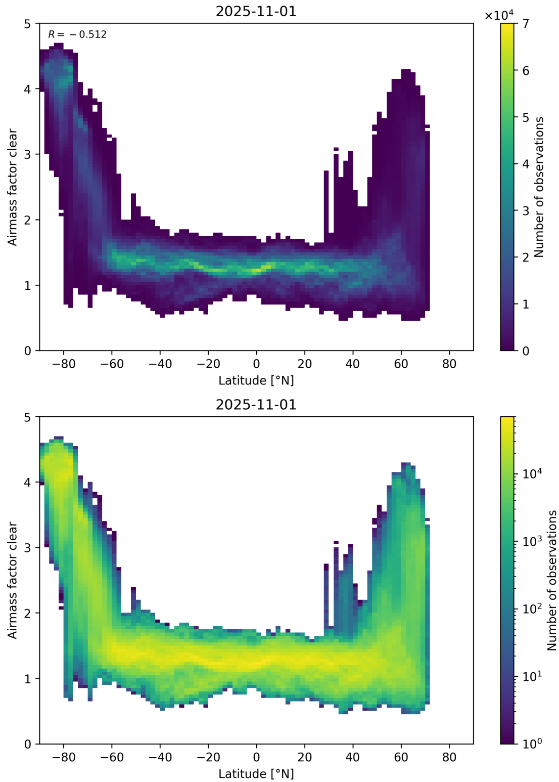
Figure 156: Scatter density plot of “Latitude” against “Airmass factor clear” for 2025-10-31 to 2025-11-02.
