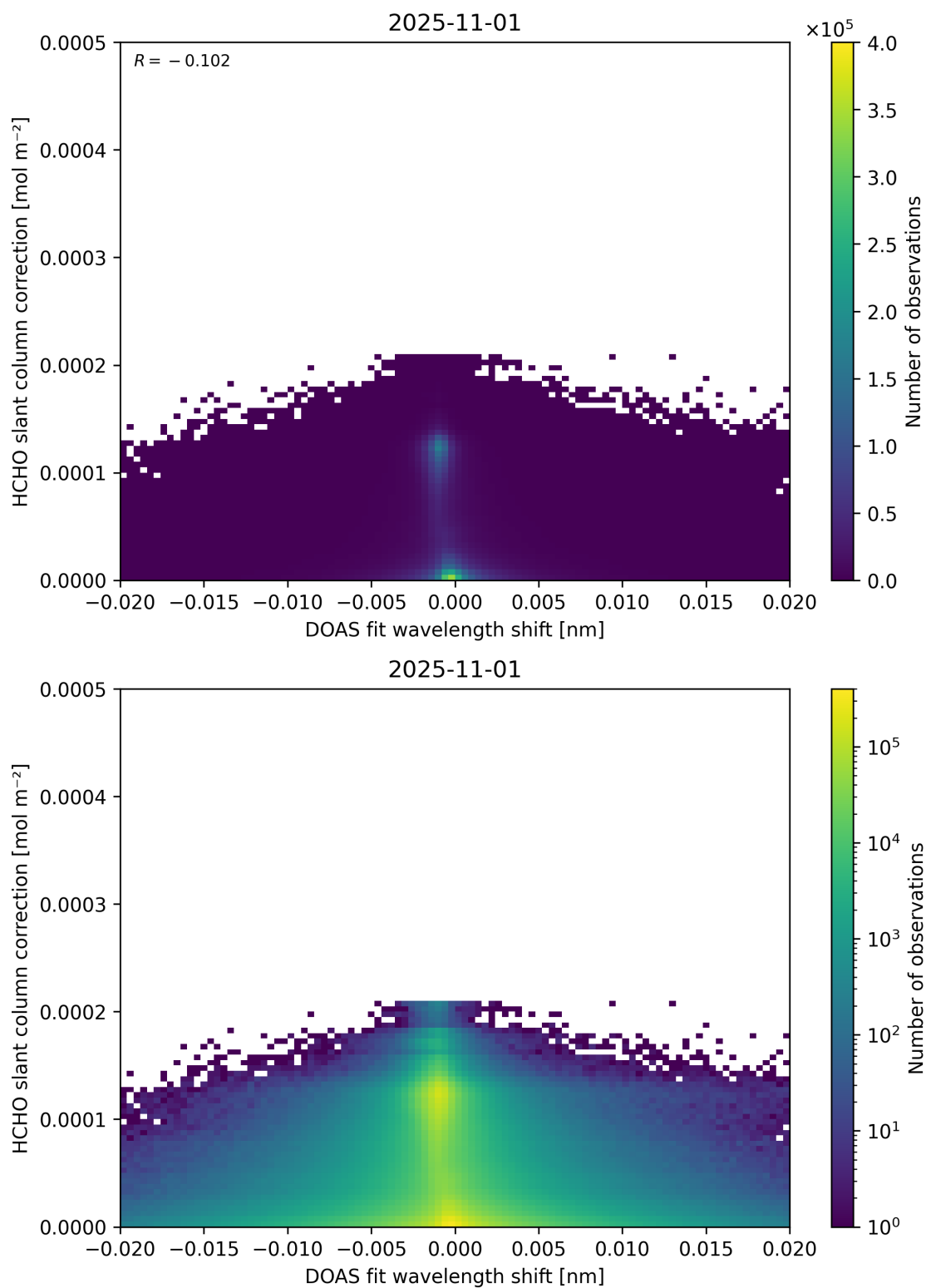
Figure 67: Scatter density plot of “DOAS fit wavelength shift” against “HCHO slant column correction” for 2025-10-31 to 2025-11-02.
