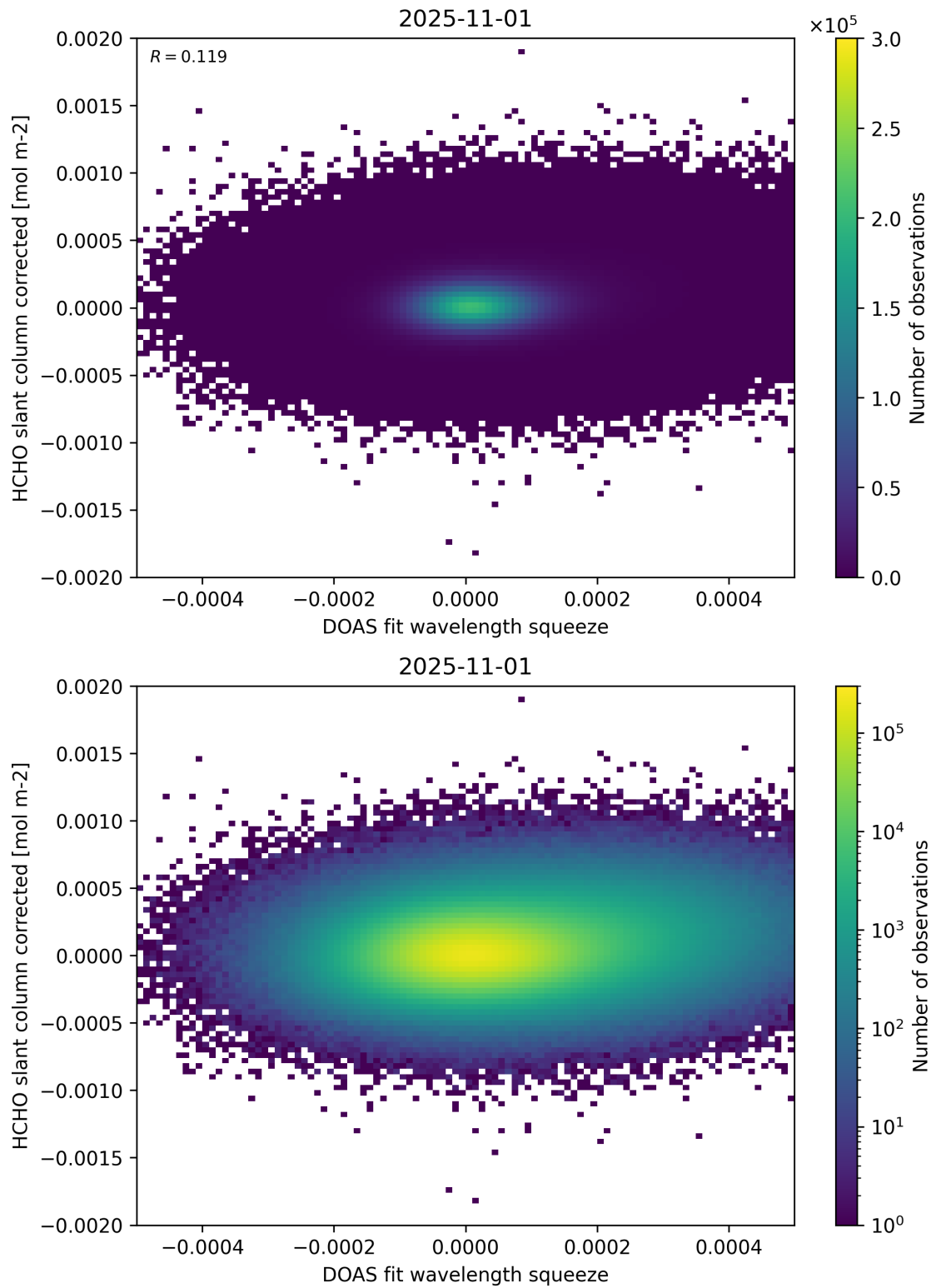
Figure 69: Scatter density plot of “DOAS fit wavelength squeeze” against “HCHO slant column corrected” for 2025-10-31 to 2025-11-02.
