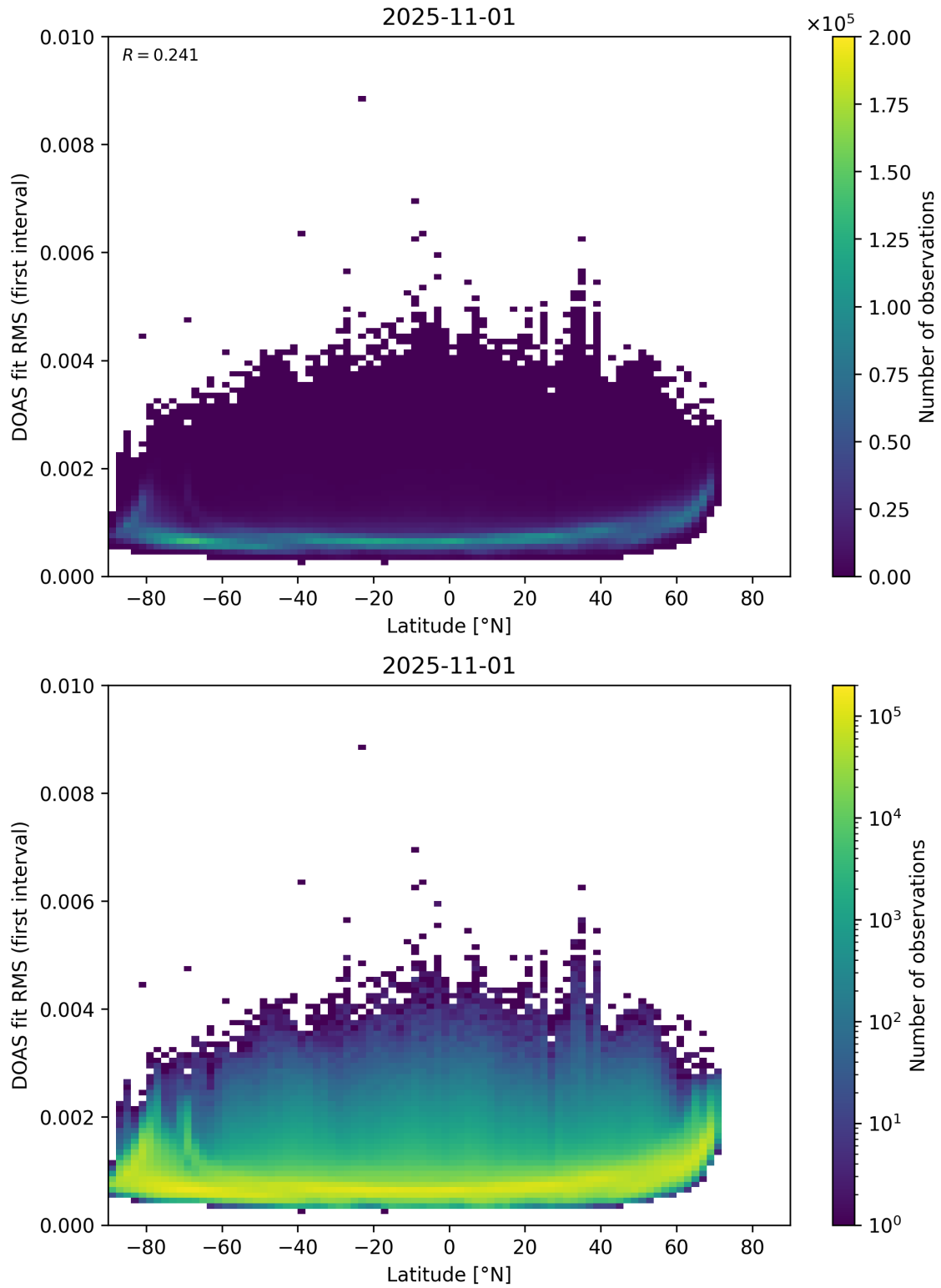
Figure 153: Scatter density plot of “Latitude” against “DOAS fit RMS (first interval)” for 2025-10-31 to 2025-11-02.
