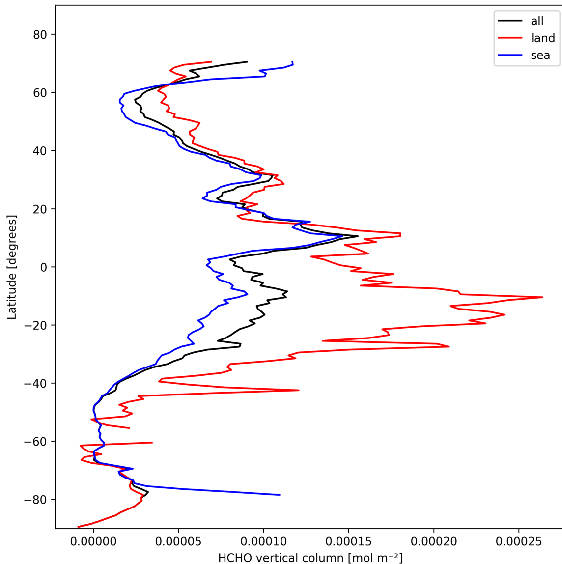
Figure 21: Zonal average of “HCHO vertical column” for 2025-10-31 to 2025-11-02.
