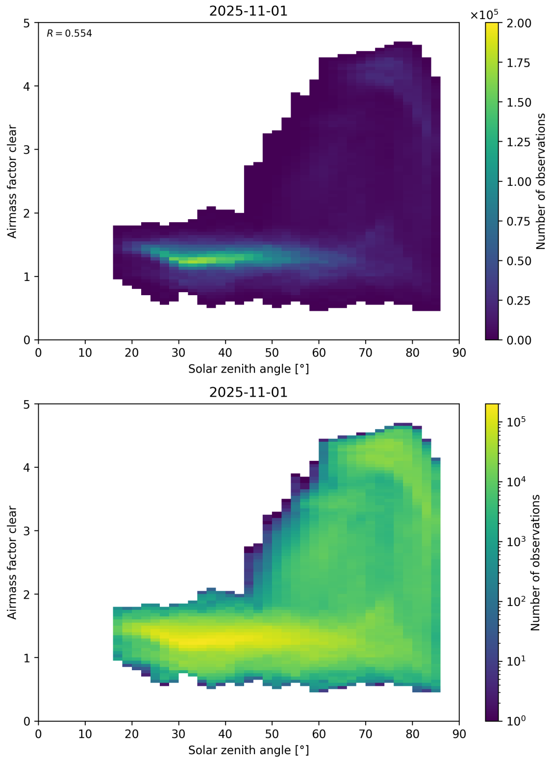
Figure 170: Scatter density plot of “Solar zenith angle” against “Airmass factor clear” for 2025-10-31 to 2025-11-02.
