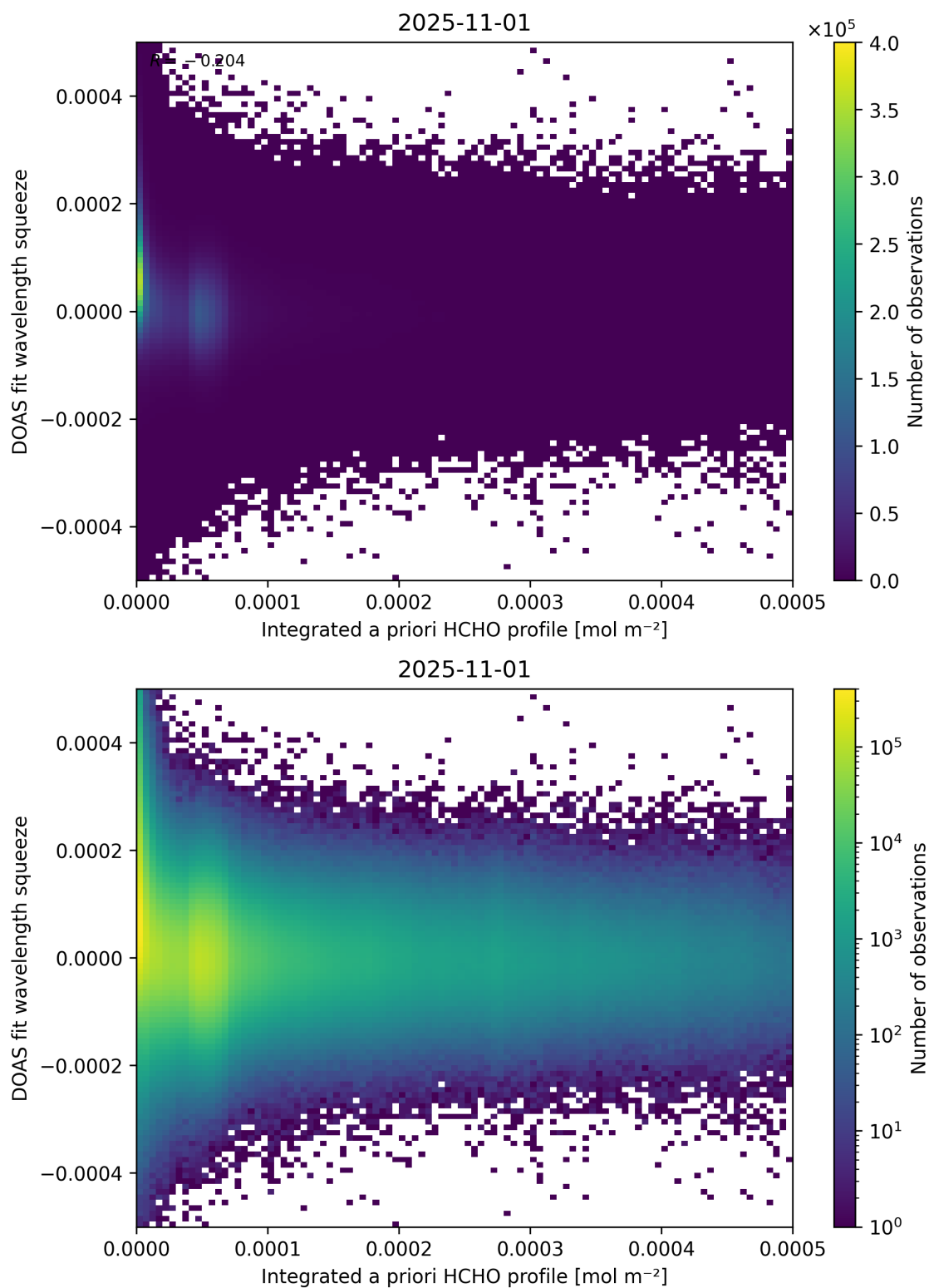
Figure 150: Scatter density plot of “Integrated a priori HCHO profile” against “DOAS fit wavelength squeeze” for 2025-10-31 to 2025-11-02.
