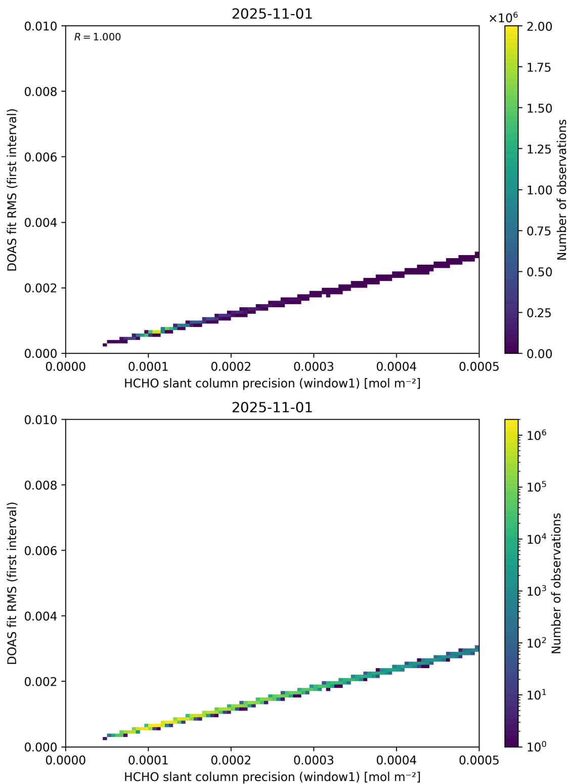
Figure 88: Scatter density plot of “HCHO slant column precision (window1)” against “DOAS fit RMS (first interval)” for 2025-10-31 to 2025-11-02.
