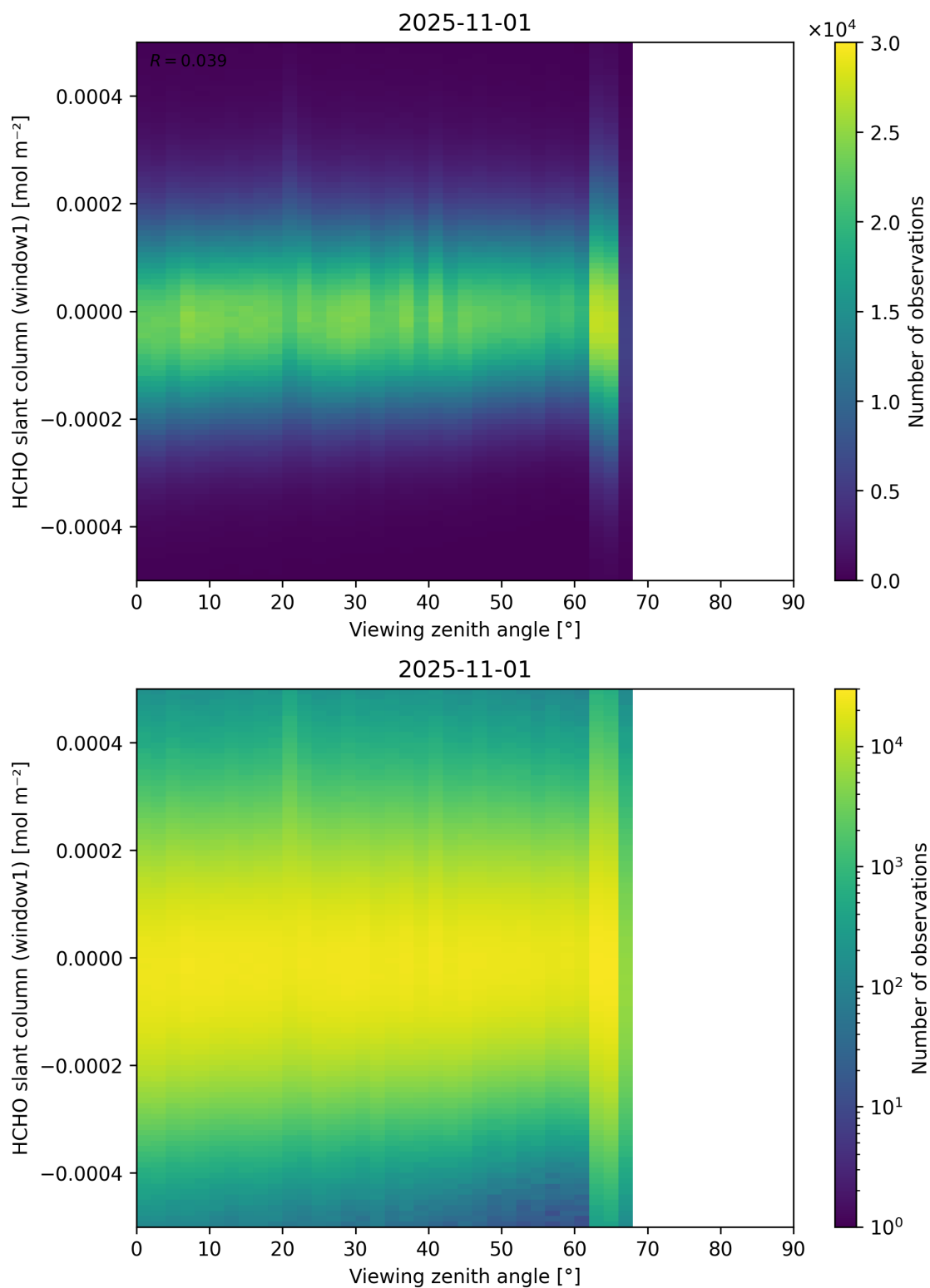
Figure 188: Scatter density plot of “Viewing zenith angle” against “HCHO slant column (window1)” for 2025-10-31 to 2025-11-02.
