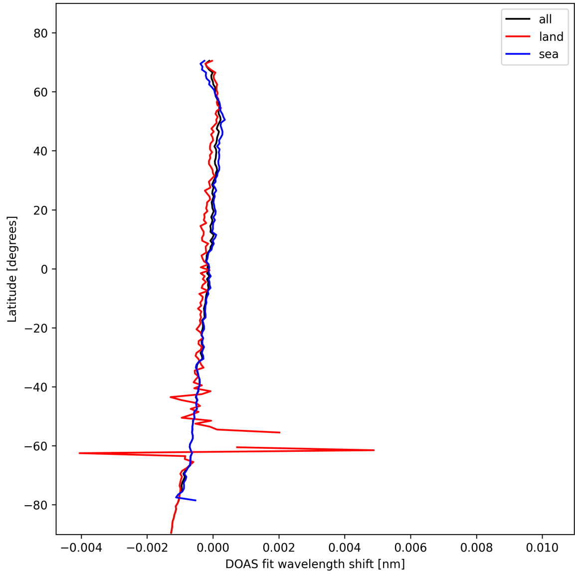
Figure 30: Zonal average of “DOAS fit wavelength shift” for 2025-10-31 to 2025-11-02.
