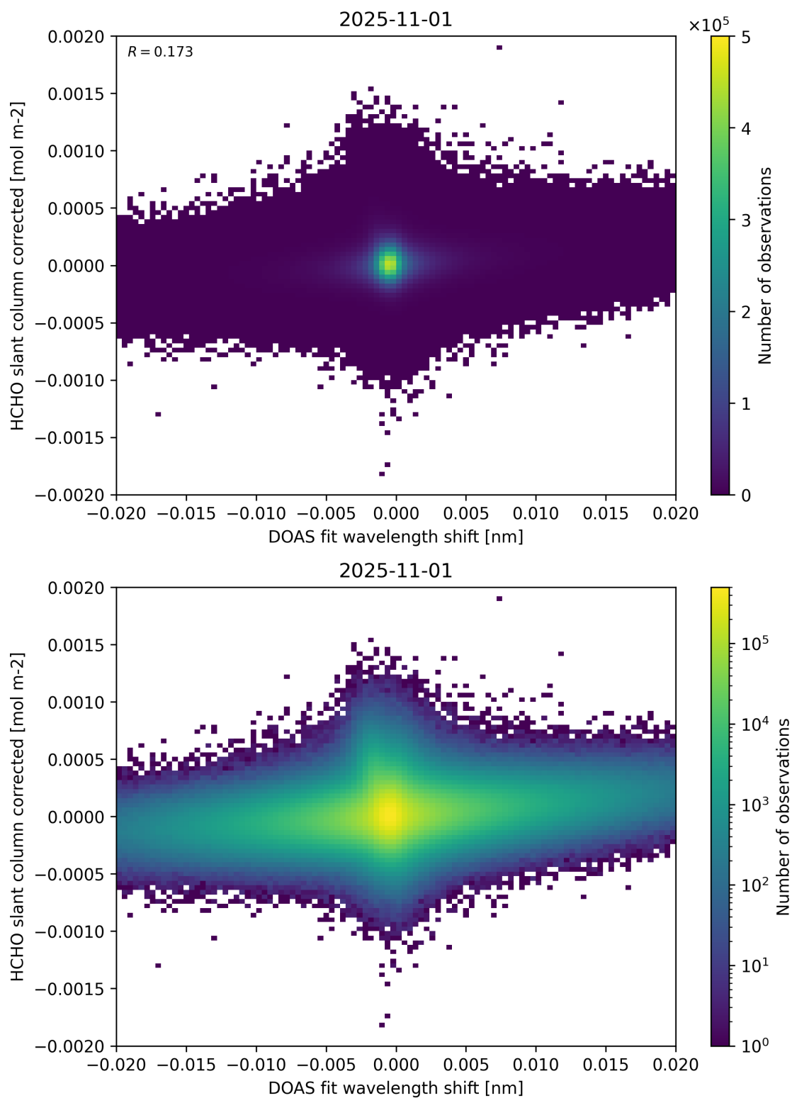
Figure 66: Scatter density plot of “DOAS fit wavelength shift” against “HCHO slant column corrected” for 2025-10-31 to 2025-11-02.
