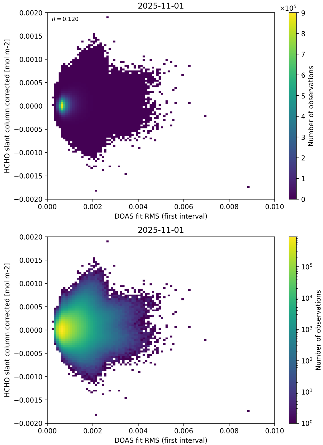
Figure 62: Scatter density plot of “DOAS fit RMS (first interval)” against “HCHO slant column corrected” for 2025-10-31 to 2025-11-02.
