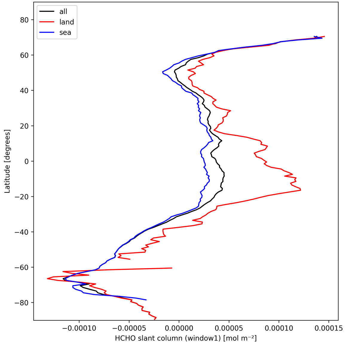
Figure 24: Zonal average of “HCHO slant column (window1)” for 2025-10-31 to 2025-11-02.
