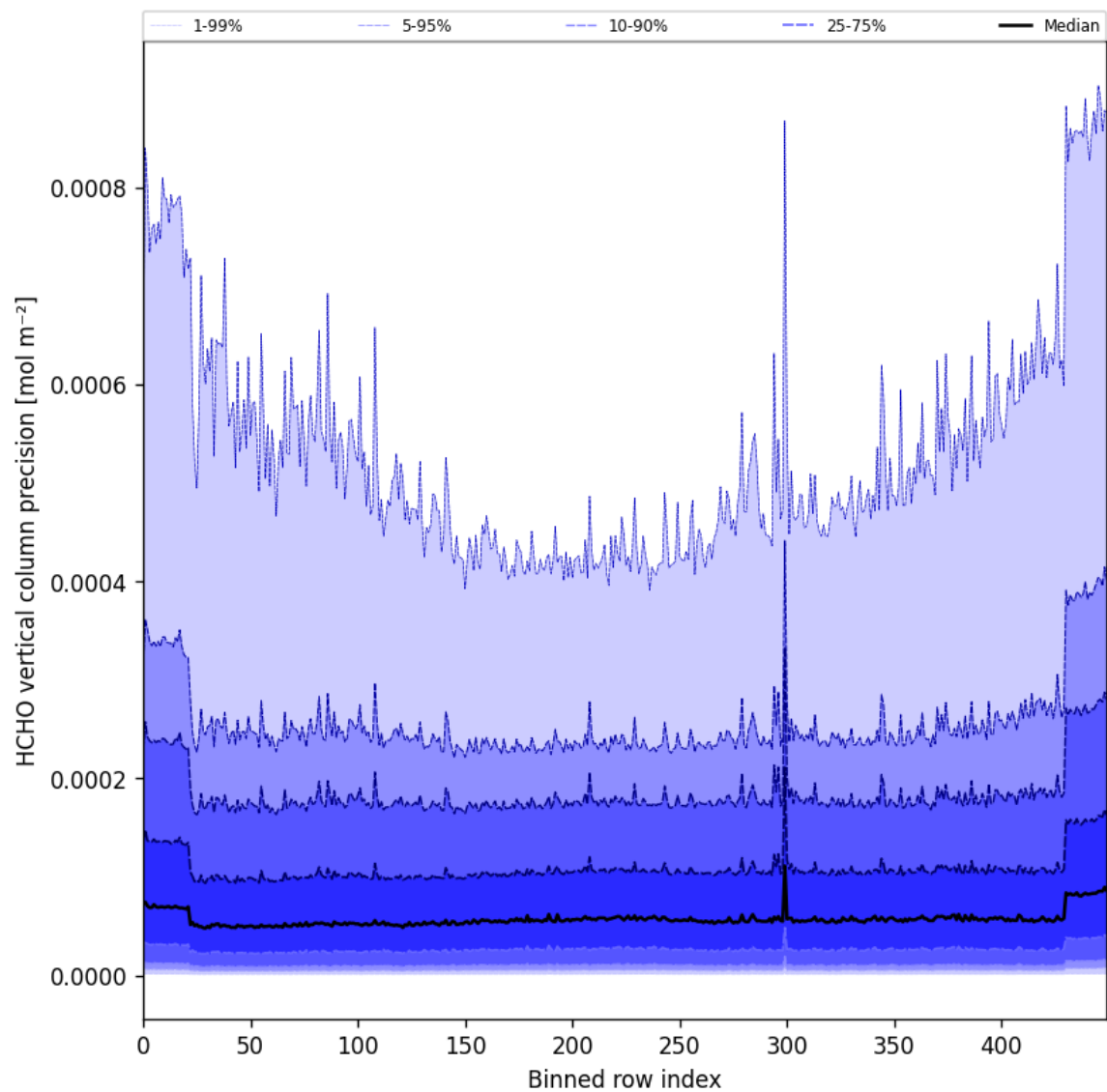
Figure 50: Along track statistics of “HCHO vertical column precision” for 2025-10-31 to 2025-11-02
