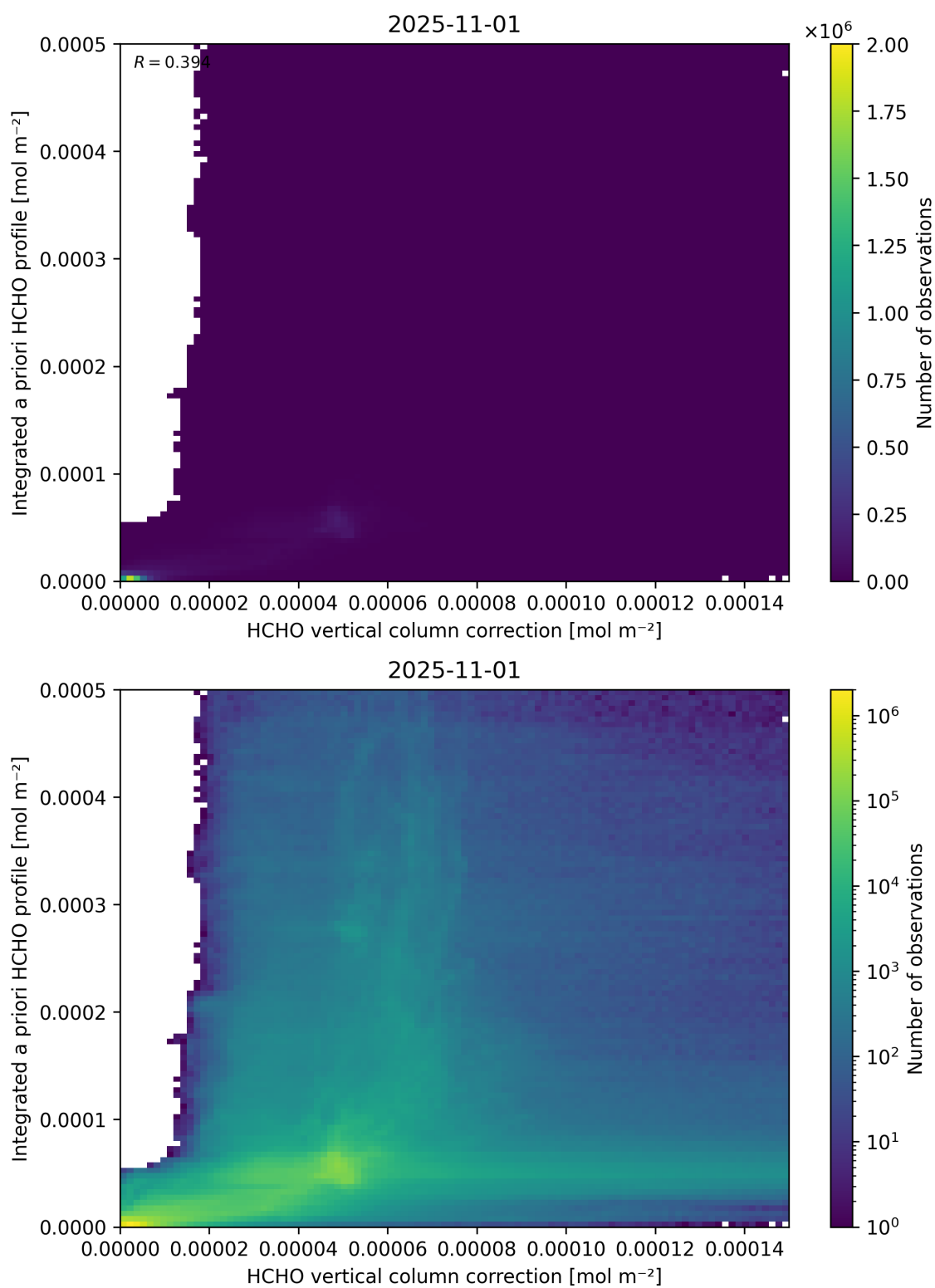
Figure 122: Scatter density plot of “HCHO vertical column correction” against “Integrated a priori HCHO profile” for 2025-10-31 to 2025-11-02.
