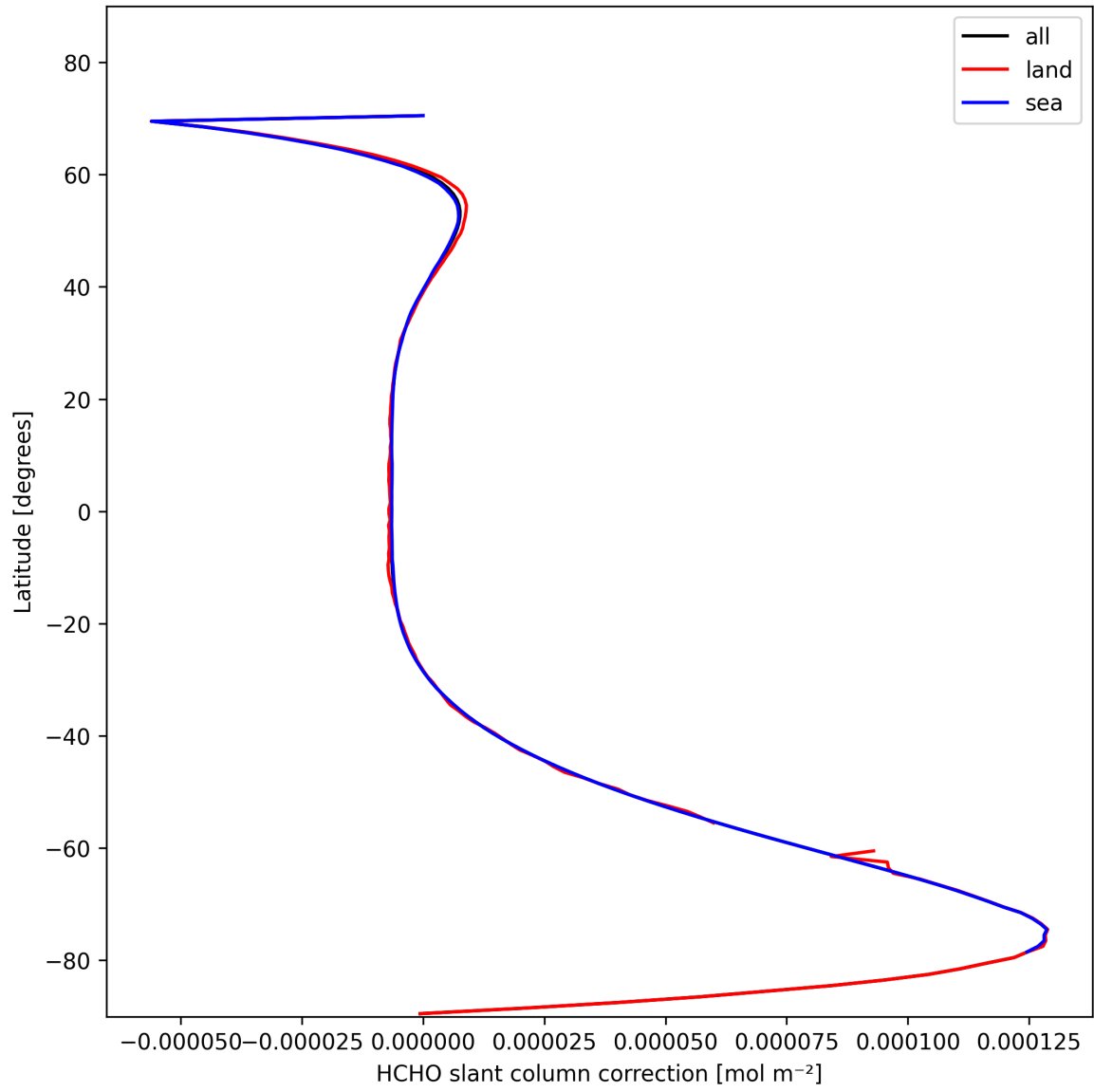
Figure 33: Zonal average of “HCHO slant column correction” for 2025-10-31 to 2025-11-02.
