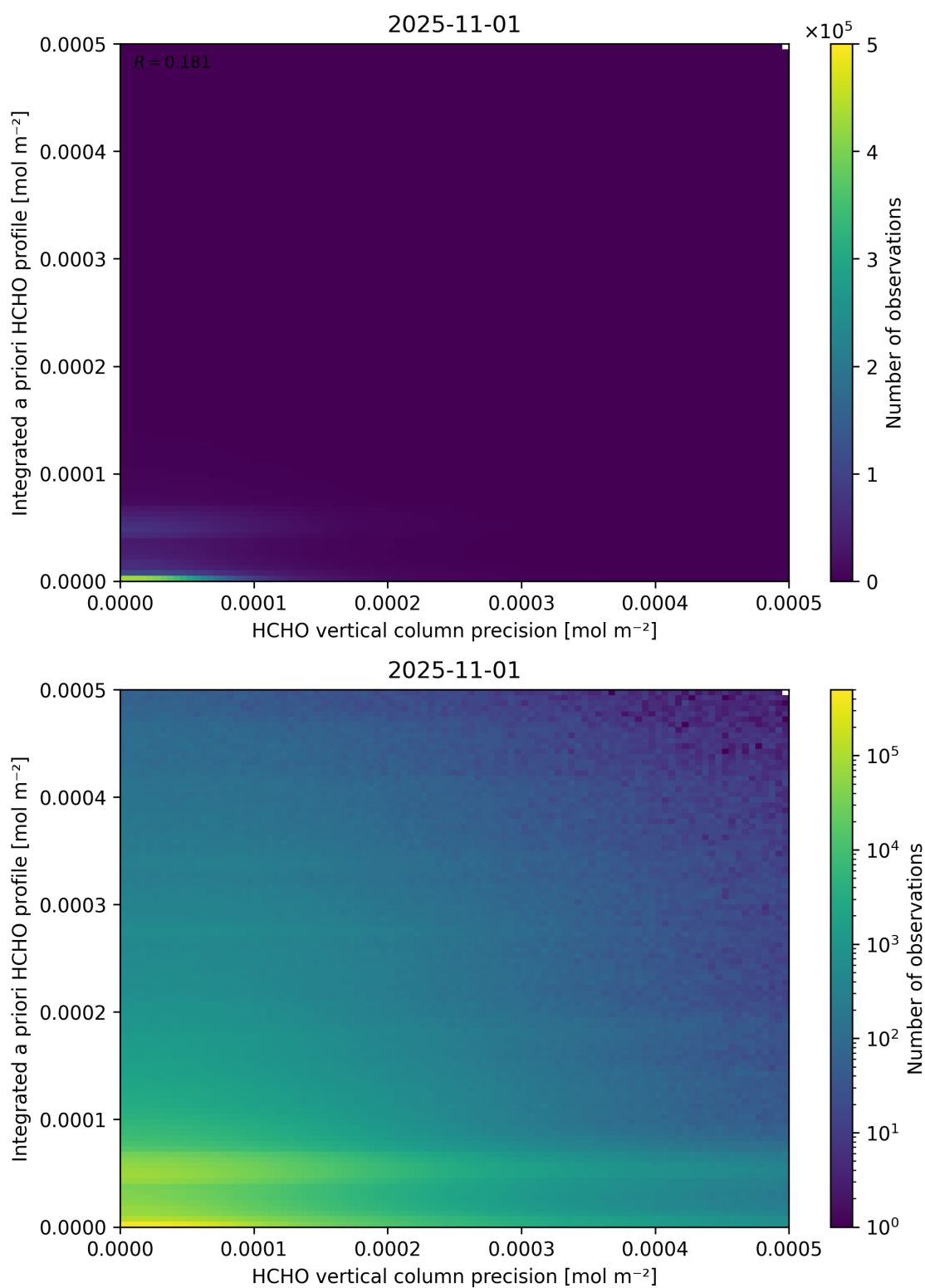
Figure 147: Scatter density plot of “HCHO vertical column precision” against “Integrated a priori HCHO profile” for 2025-10-31 to 2025-11-02.
