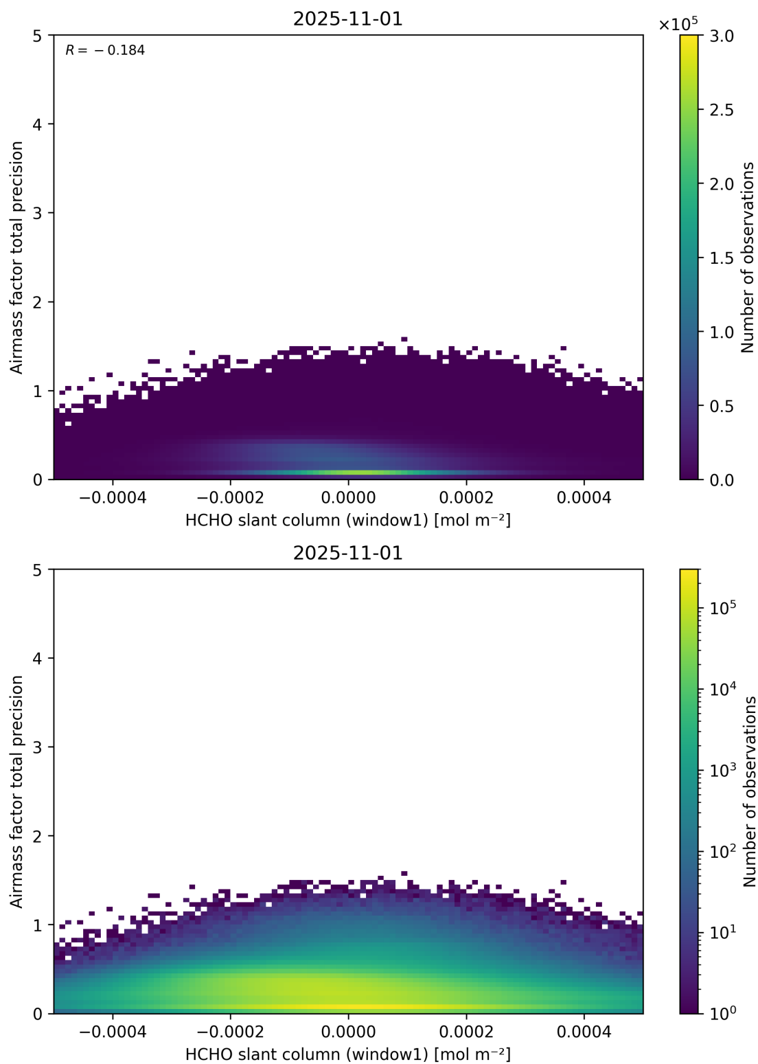
Figure 86: Scatter density plot of “HCHO slant column (window1)” against “Airmass factor total precision” for 2025-10-31 to 2025-11-02.
