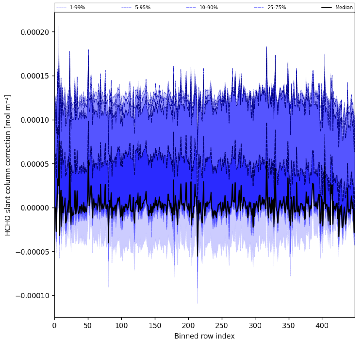
Figure 61: Along track statistics of “HCHO slant column correction” for 2025-10-31 to 2025-11-02
