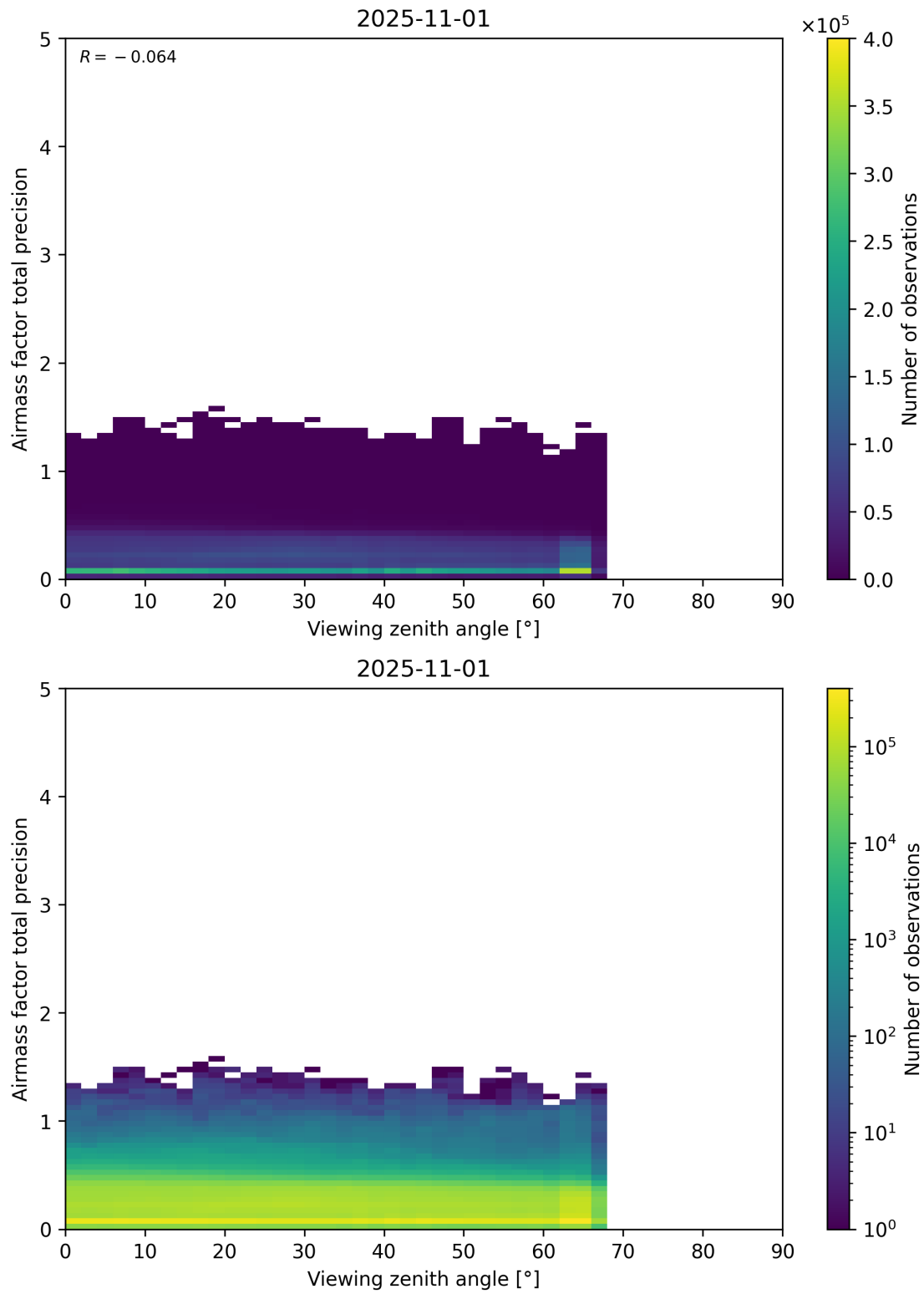
Figure 191: Scatter density plot of “Viewing zenith angle” against “Airmass factor total precision” for 2025-10-31 to 2025-11-02.
