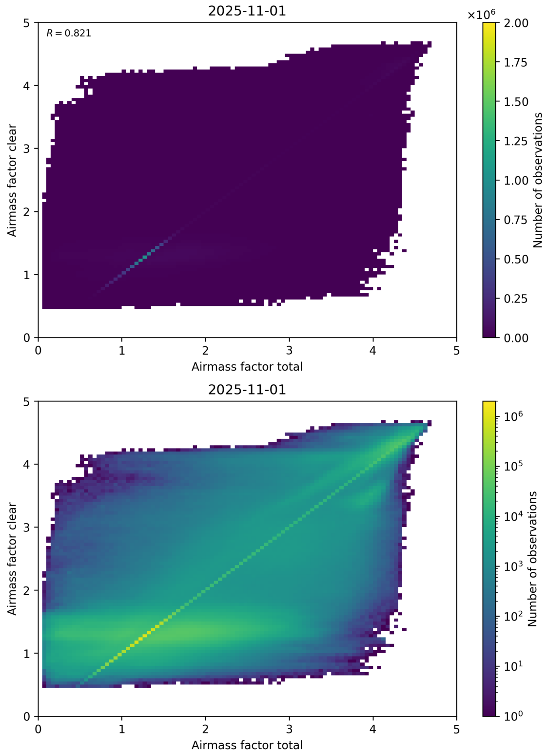
Figure 100: Scatter density plot of “Airmass factor total” against “Airmass factor clear” for 2025-10-31 to 2025-11-02.
