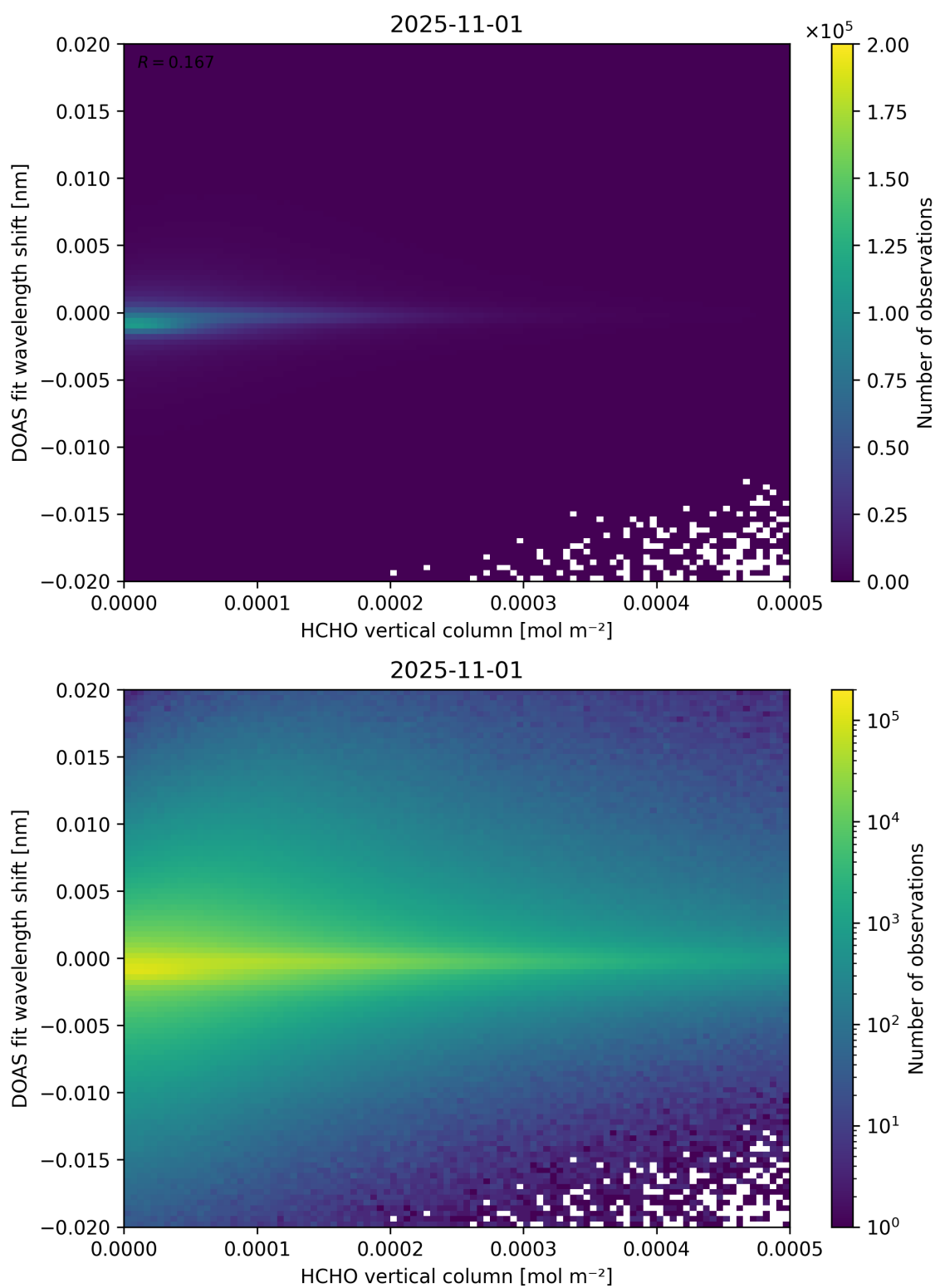
Figure 124: Scatter density plot of “HCHO vertical column” against “DOAS fit wavelength shift” for 2025-10-31 to 2025-11-02.
