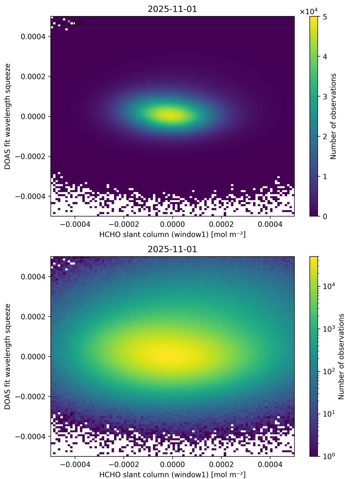
Figure 80: Scatter density plot of “HCHO slant column (window1)” against “DOAS fit wavelength squeeze” for 2025-10-31 to 2025-11-02.
