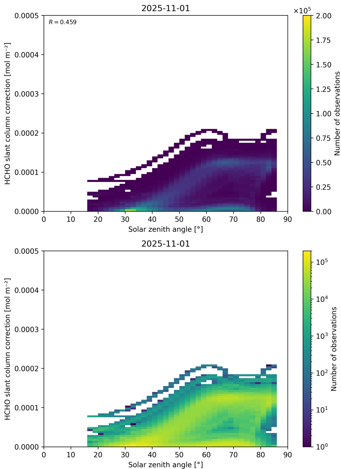
Figure 172: Scatter density plot of “Solar zenith angle” against “HCHO slant column correction” for 2025-10-31 to 2025-11-02.
