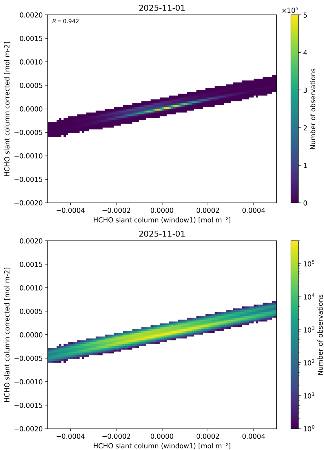
Figure 82: Scatter density plot of “HCHO slant column (window1)” against “HCHO slant column corrected” for 2025-10-31 to 2025-11-02.
