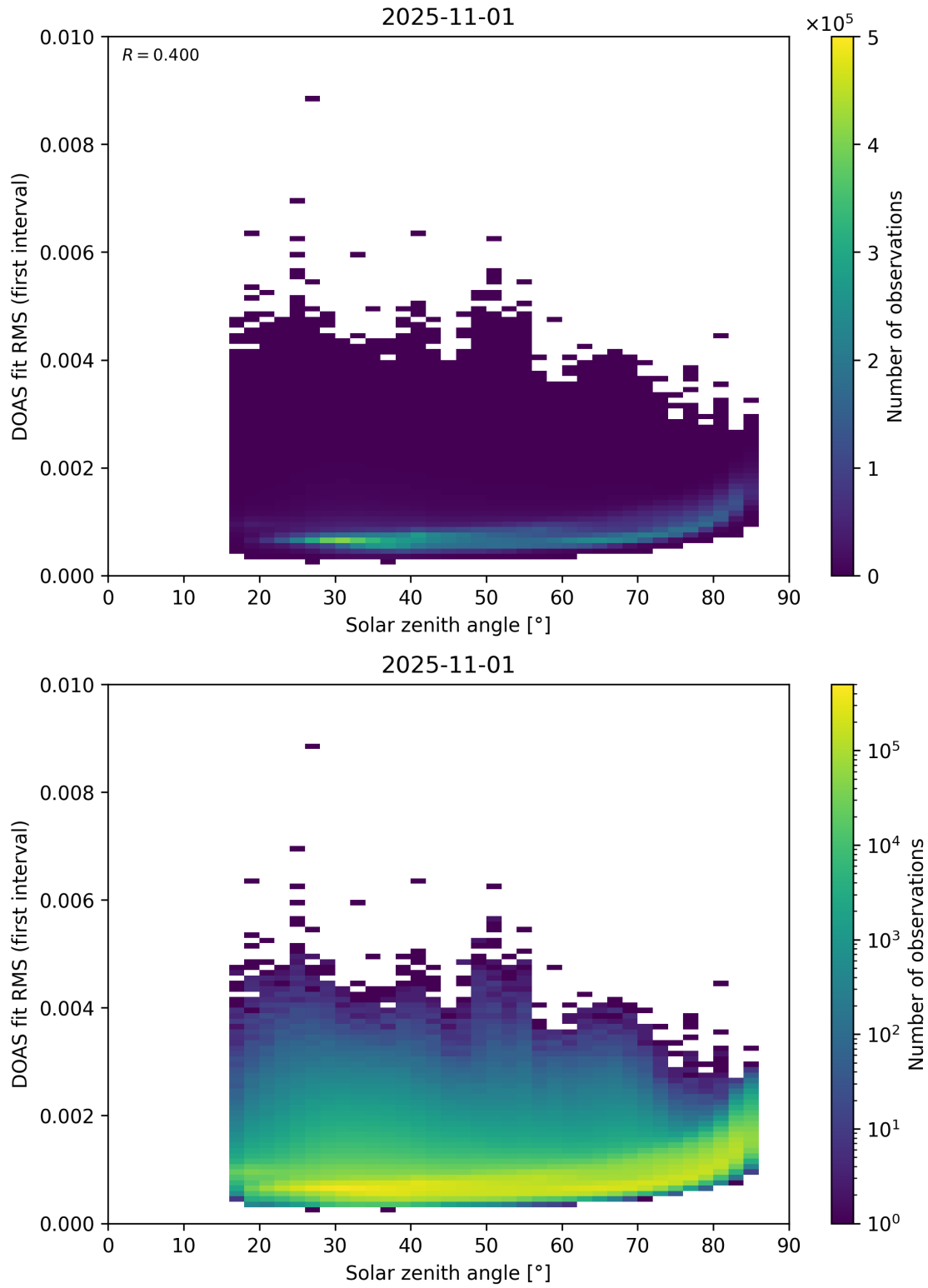
Figure 167: Scatter density plot of “Solar zenith angle” against “DOAS fit RMS (first interval)” for 2025-10-31 to 2025-11-02.
