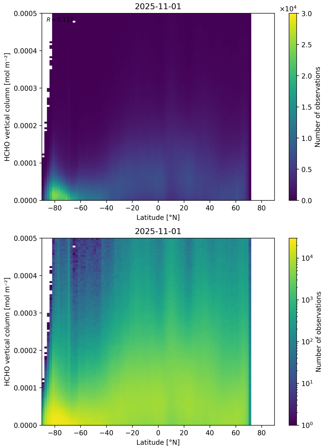
Figure 163: Scatter density plot of “Latitude” against “HCHO vertical column” for 2025-10-31 to 2025-11-02.
