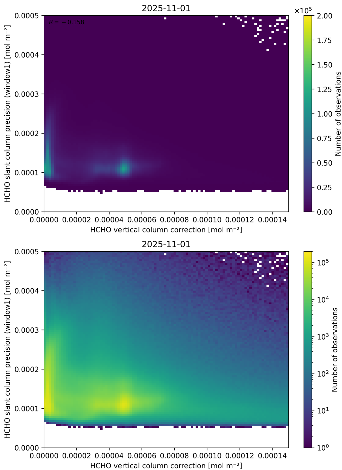
Figure 119: Scatter density plot of “HCHO vertical column correction” against “HCHO slant column precision (window1)” for 2025-10-31 to 2025-11-02.
