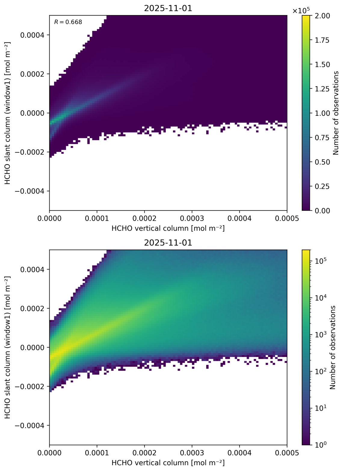
Figure 129: Scatter density plot of “HCHO vertical column” against “HCHO slant column (window1)” for 2025-10-31 to 2025-11-02.
