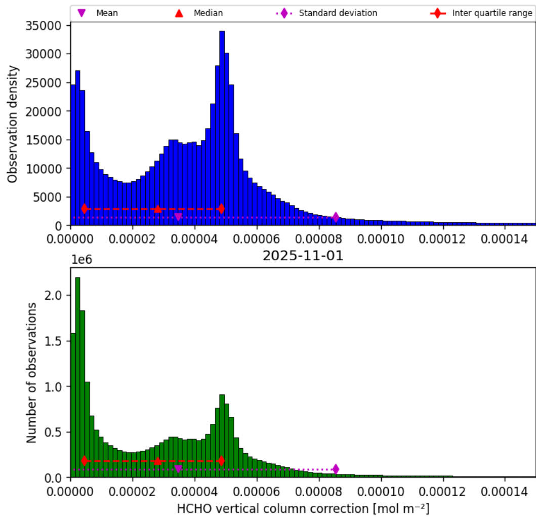
Figure 37: Histogram of “HCHO vertical column correction” for 2025-10-31 to 2025-11-02
