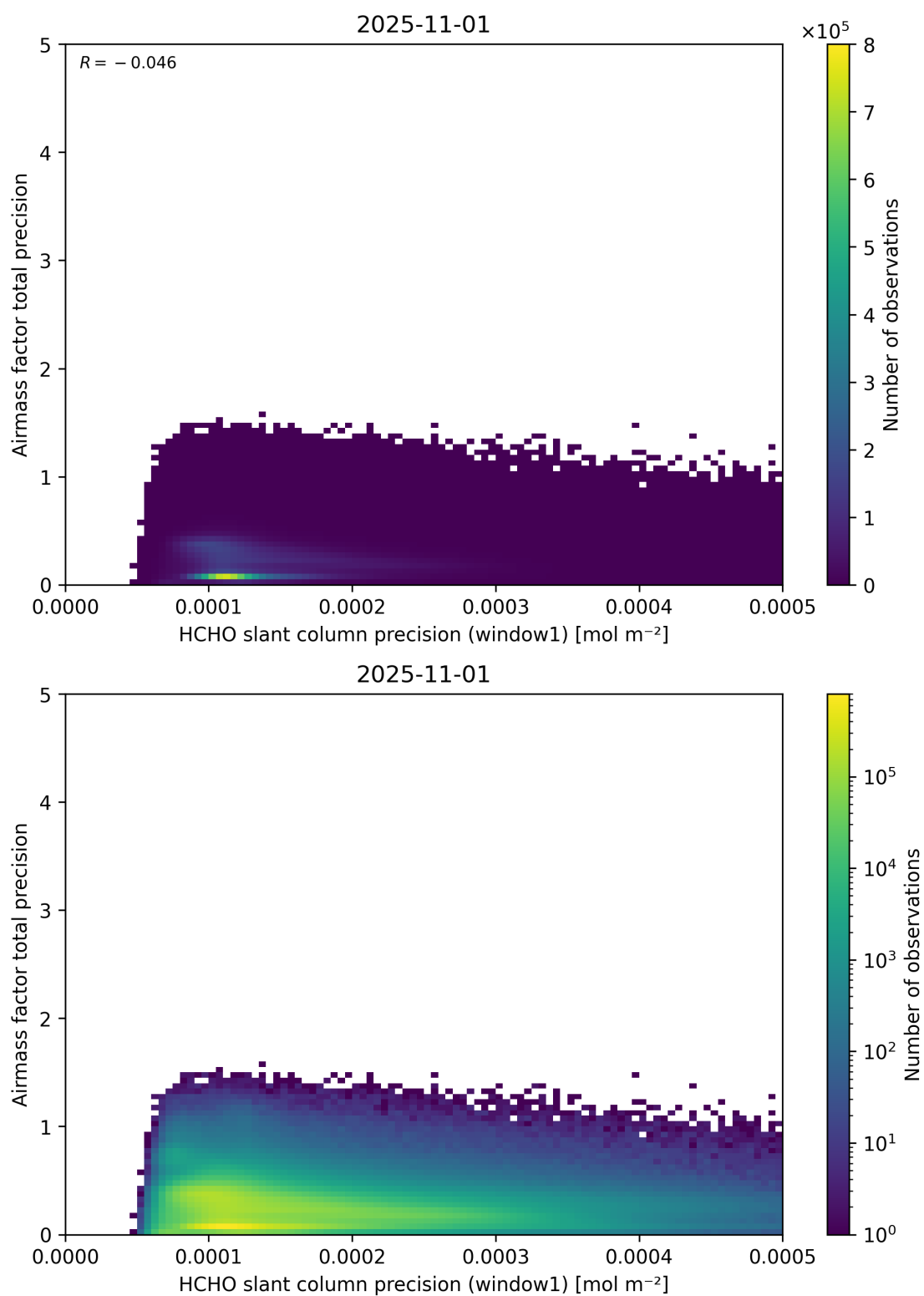
Figure 95: Scatter density plot of “HCHO slant column precision (window1)” against “Airmass factor total precision” for 2025-10-31 to 2025-11-02.
