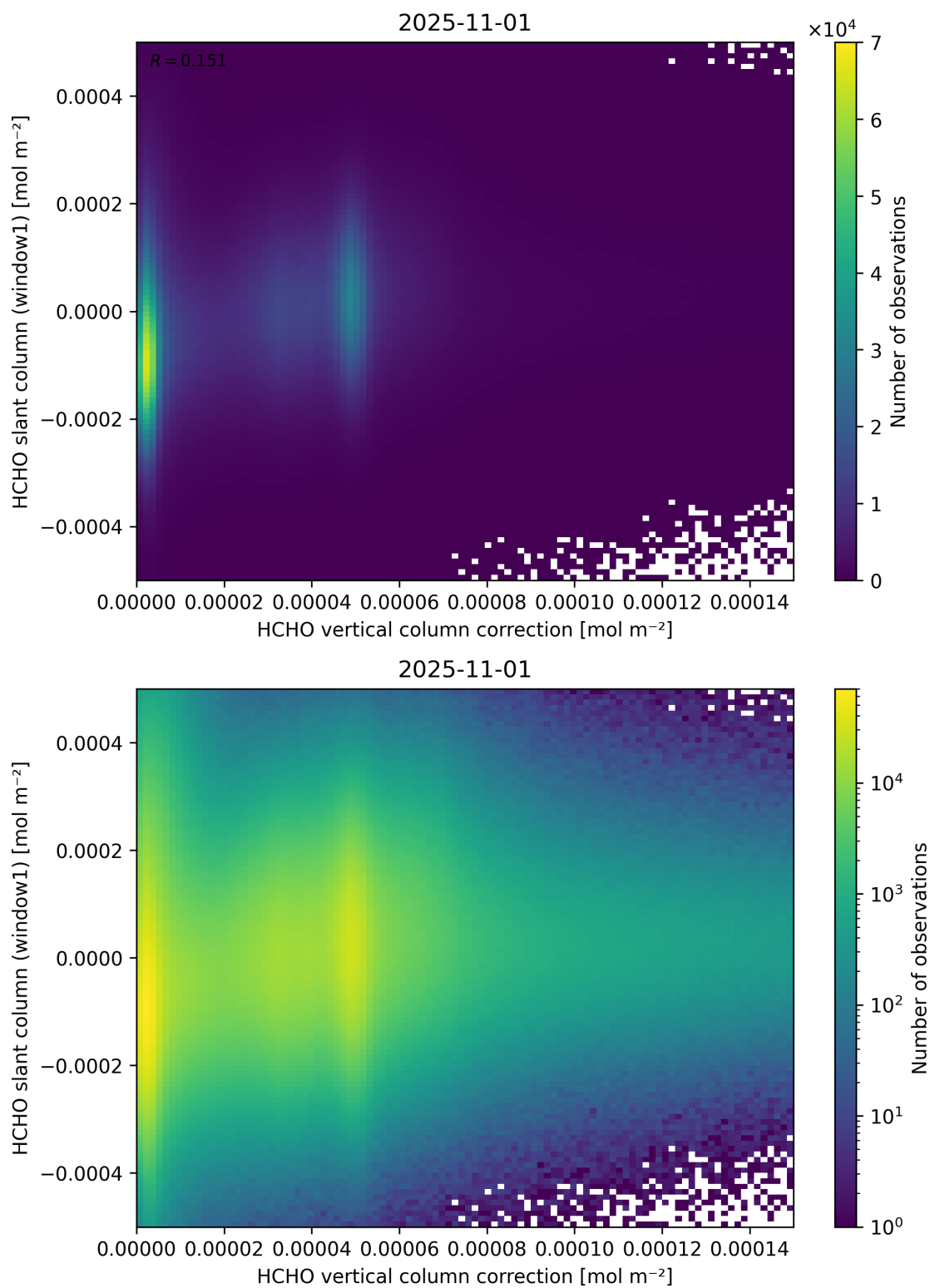
Figure 118: Scatter density plot of “HCHO vertical column correction” against “HCHO slant column (window1)” for 2025-10-31 to 2025-11-02.
