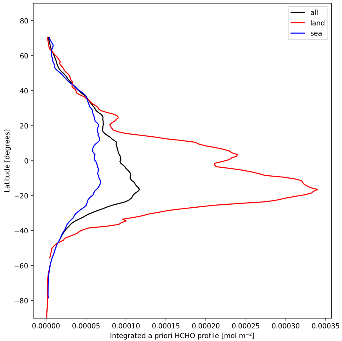
Figure 29: Zonal average of “Integrated a priori HCHO profile” for 2025-10-31 to 2025-11-02.
