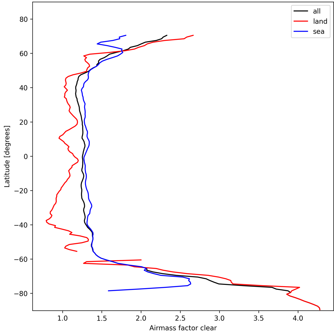
Figure 28: Zonal average of “Airmass factor clear” for 2025-10-31 to 2025-11-02.
