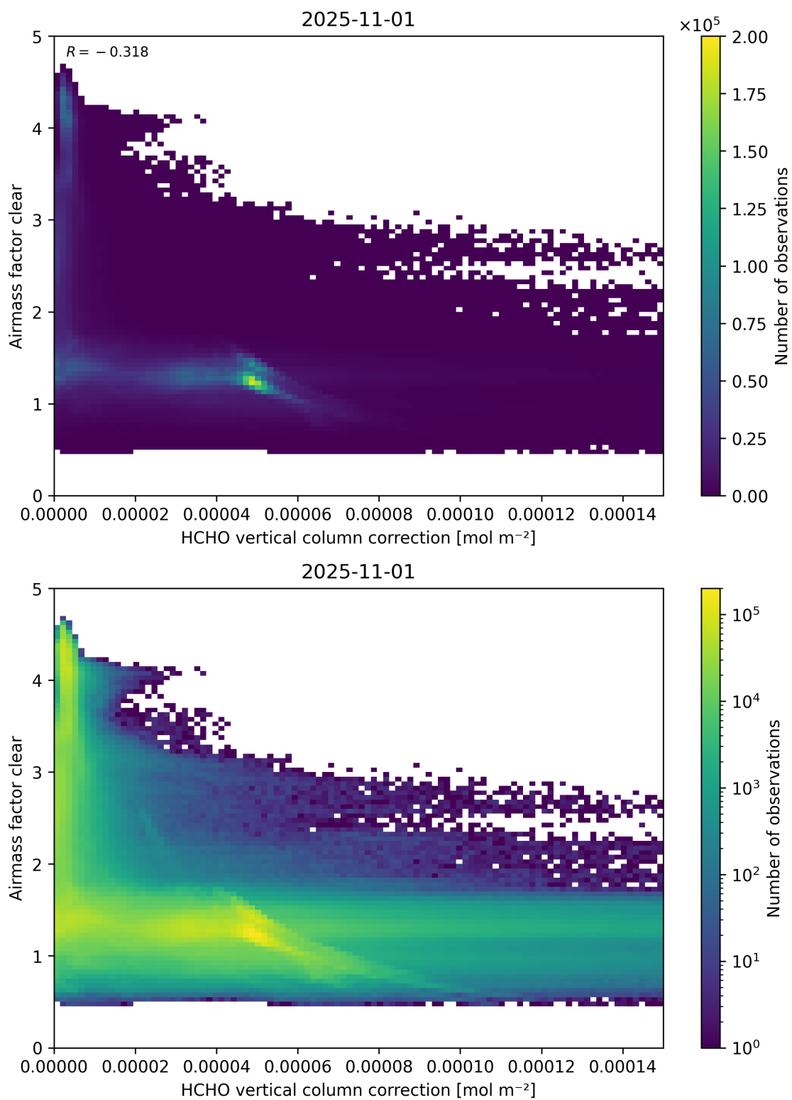
Figure 115: Scatter density plot of “HCHO vertical column correction” against “Airmass factor clear” for 2025-10-31 to 2025-11-02.
