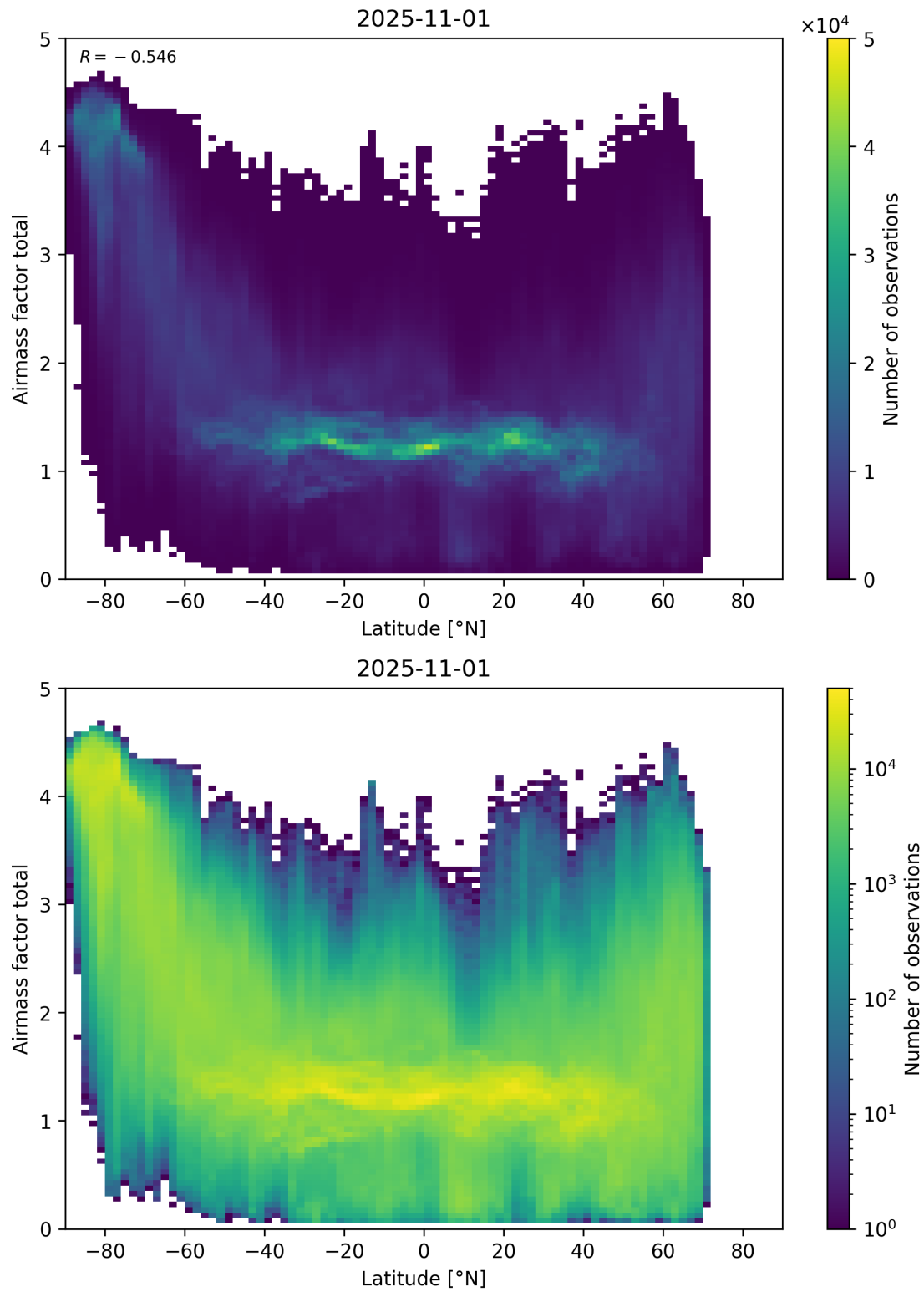
Figure 161: Scatter density plot of “Latitude” against “Airmass factor total” for 2025-10-31 to 2025-11-02.
