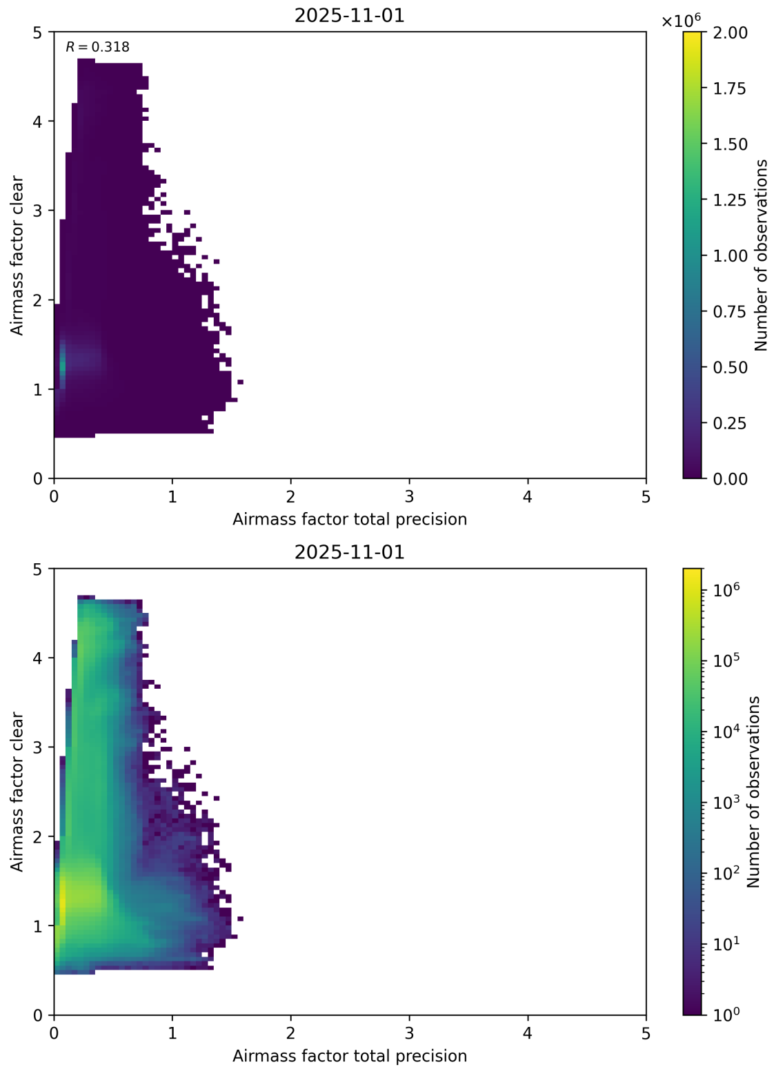
Figure 108: Scatter density plot of “Airmass factor total precision” against “Airmass factor clear” for 2025-10-31 to 2025-11-02.
