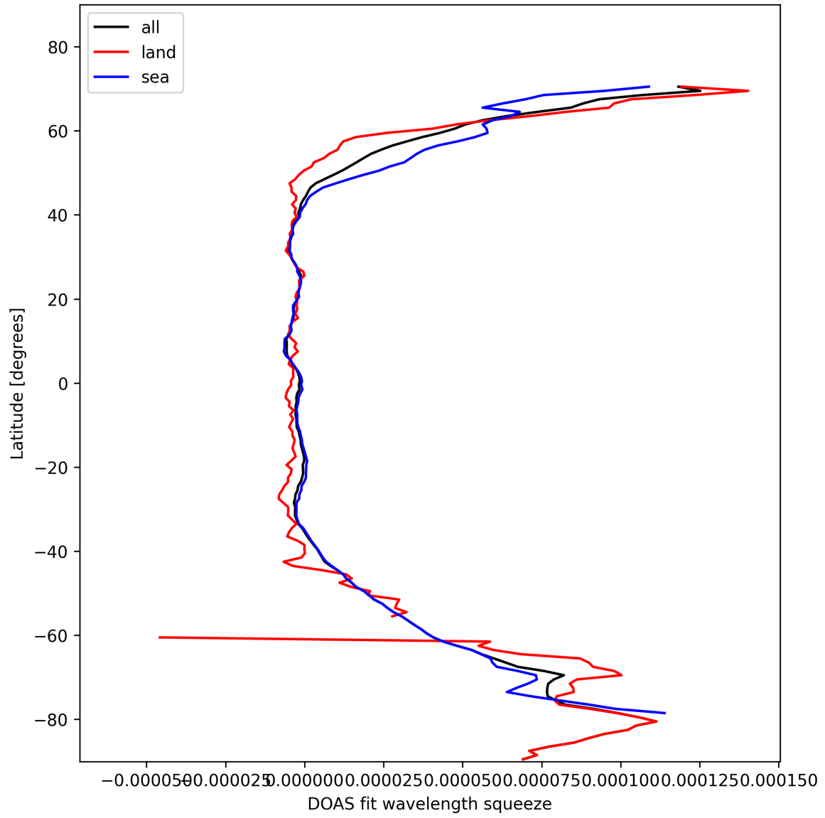
Figure 31: Zonal average of “DOAS fit wavelength squeeze” for 2025-10-31 to 2025-11-02.
