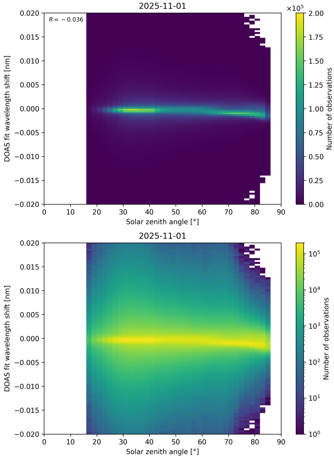
Figure 168: Scatter density plot of “Solar zenith angle” against “DOAS fit wavelength shift” for 2025-10-31 to 2025-11-02.
