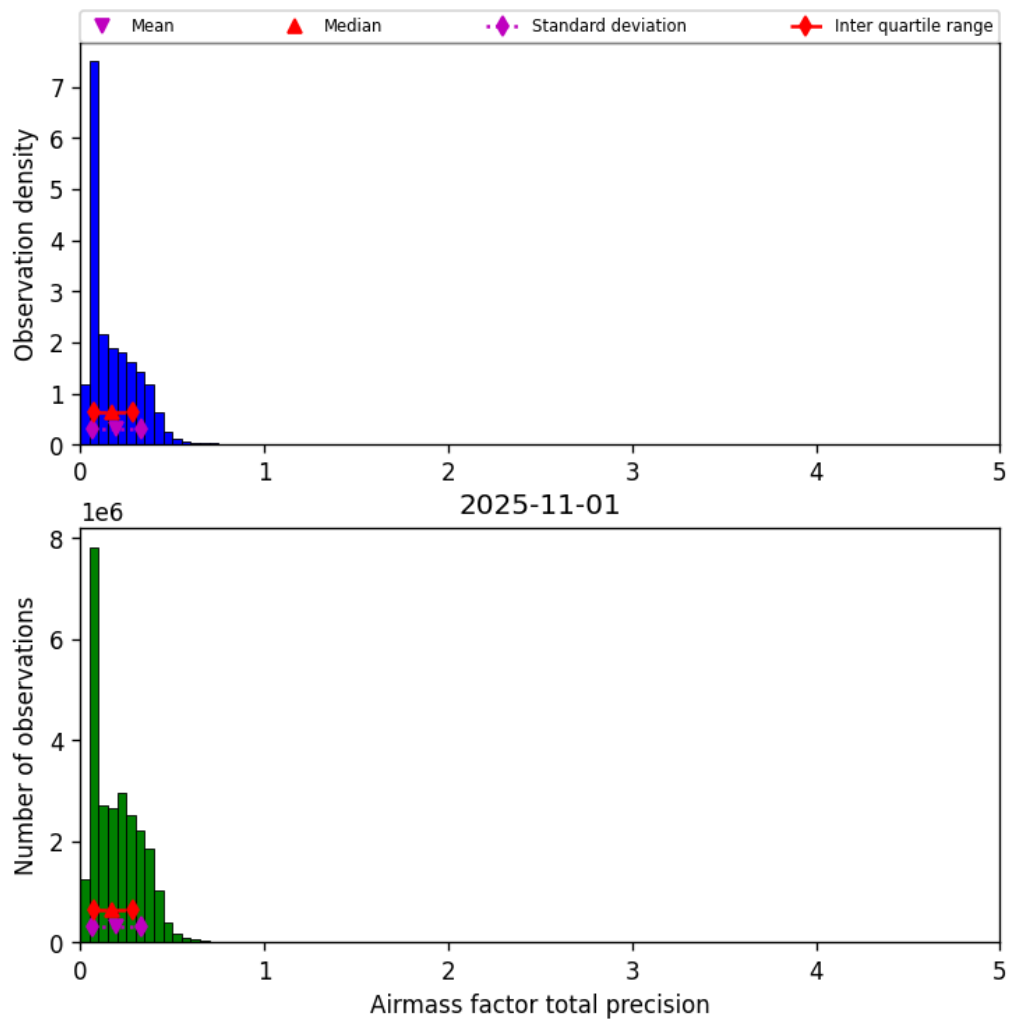
Figure 41: Histogram of “Airmass factor total precision” for 2025-10-31 to 2025-11-02
