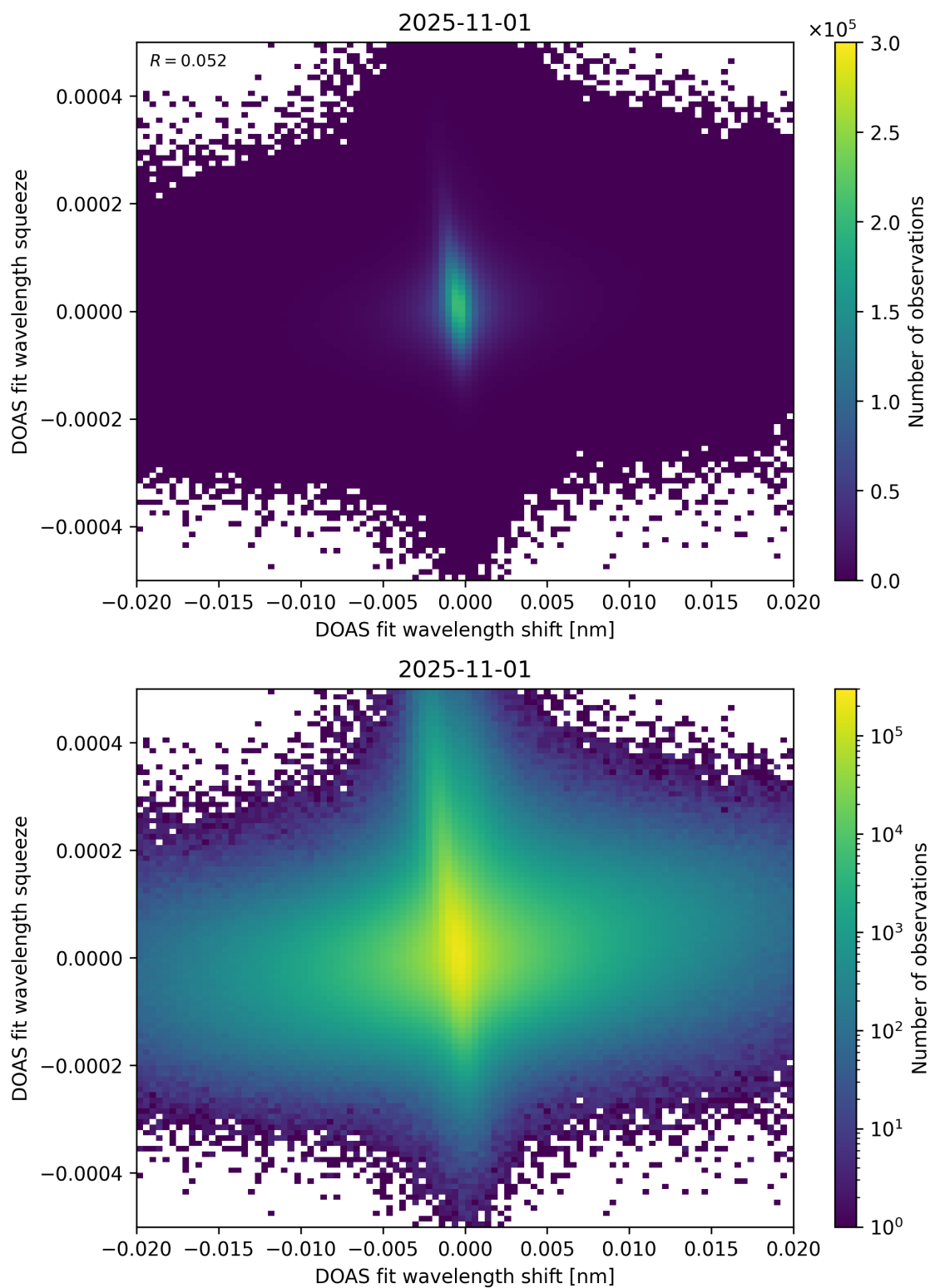
Figure 65: Scatter density plot of “DOAS fit wavelength shift” against “DOAS fit wavelength squeeze” for 2025-10-31 to 2025-11-02.
