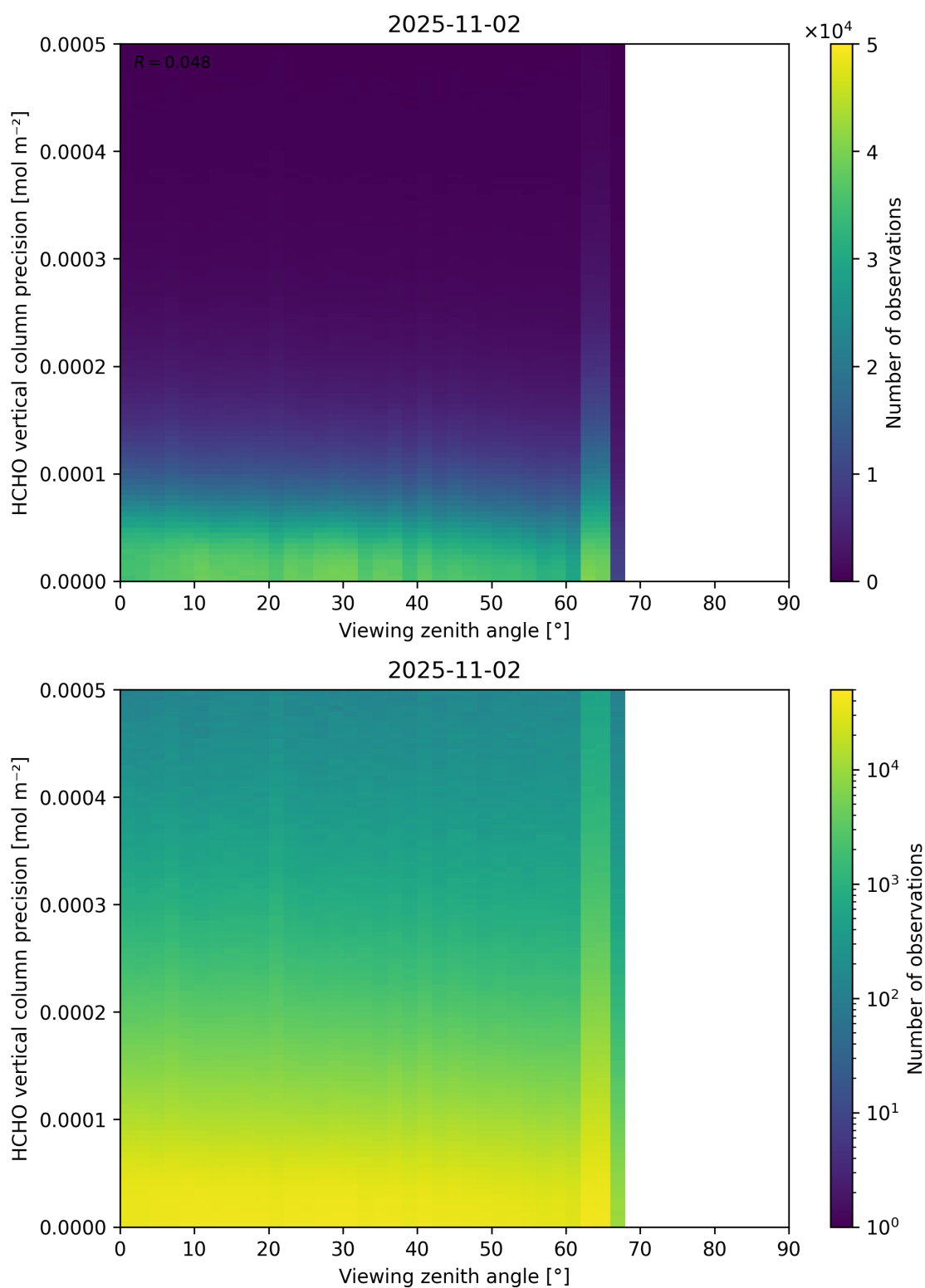
Figure 194: Scatter density plot of “Viewing zenith angle” against “HCHO vertical column precision” for 2025-11-02 to 2025-11-03.
