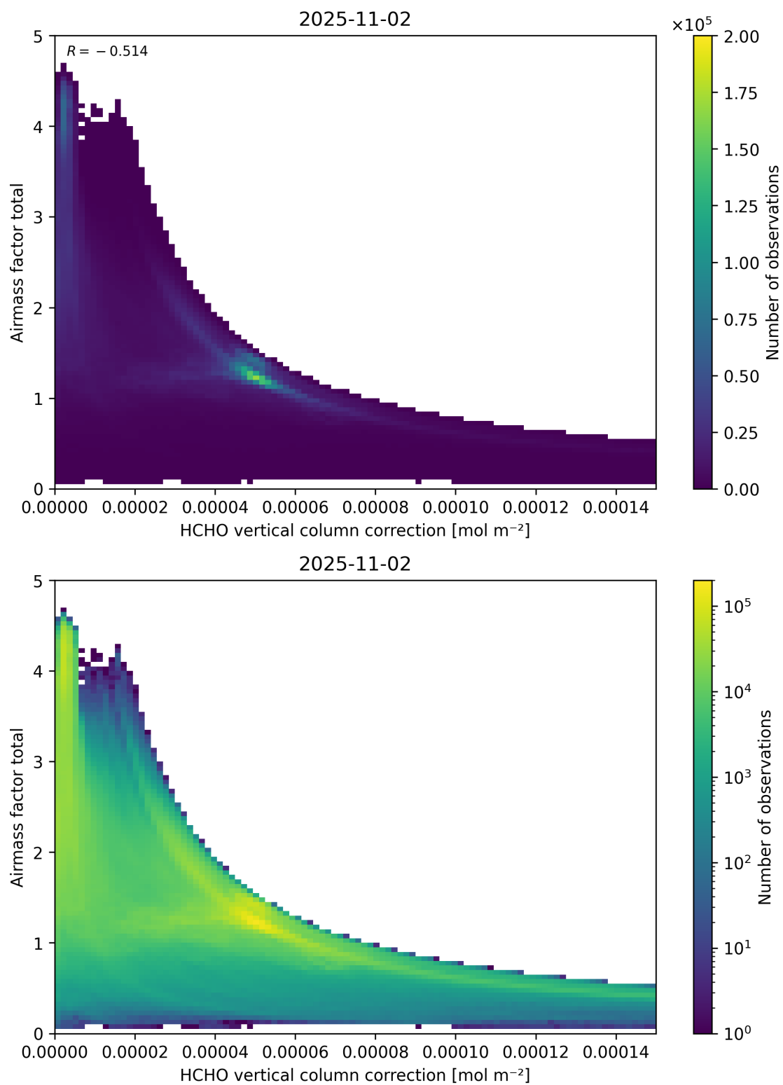
Figure 120: Scatter density plot of “HCHO vertical column correction” against “Airmass factor total” for 2025-11-02 to 2025-11-03.
