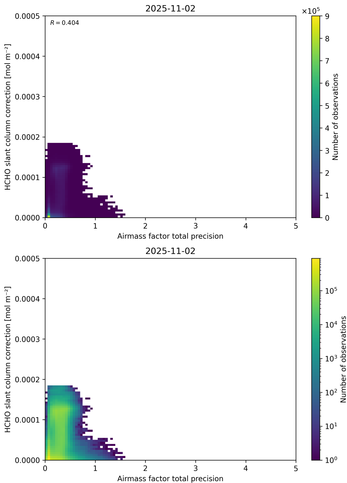
Figure 110: Scatter density plot of “Airmass factor total precision” against “HCHO slant column correction” for 2025-11-02 to 2025-11-03.
