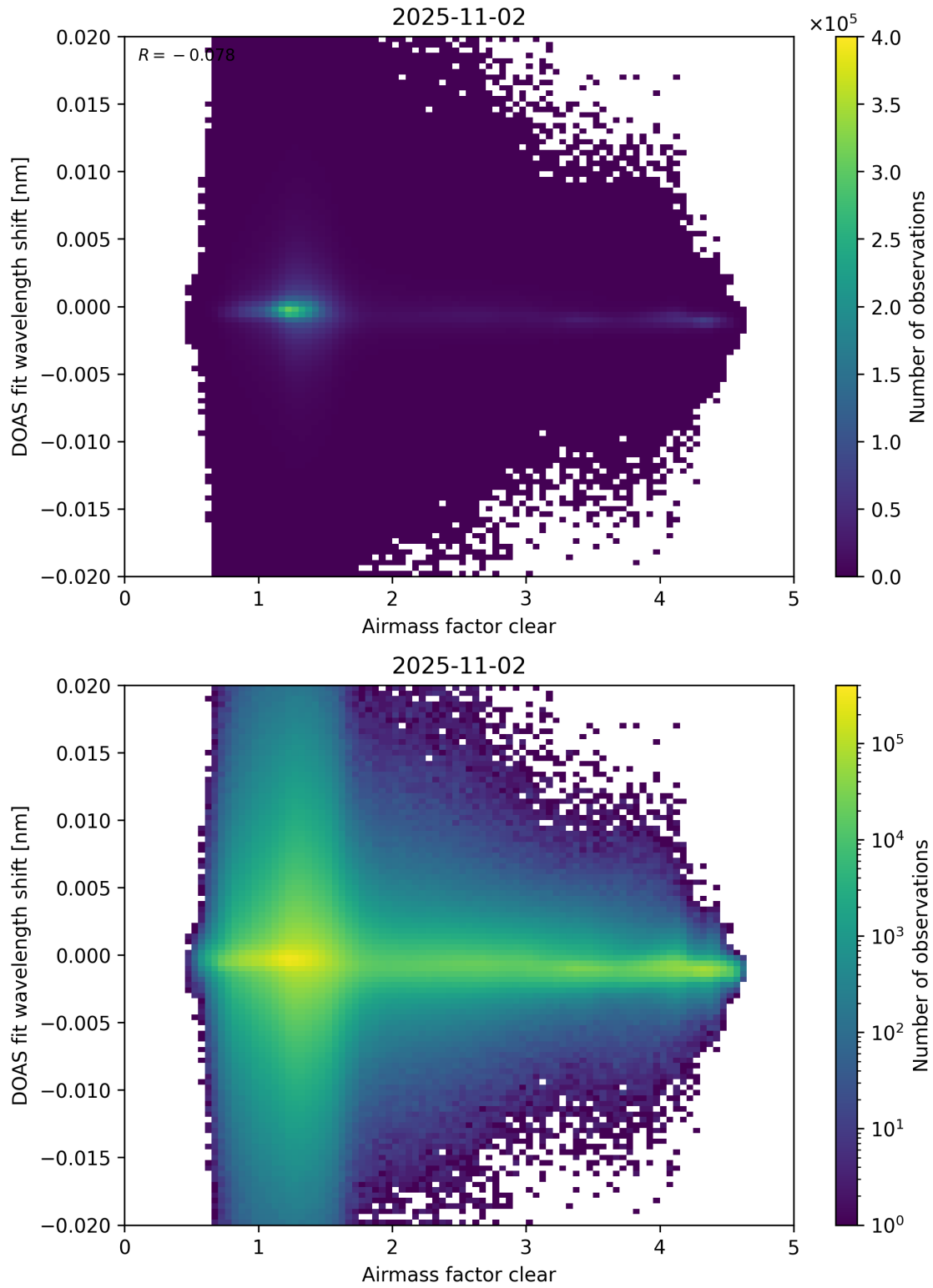
Figure 72: Scatter density plot of “Airmass factor clear” against “DOAS fit wavelength shift” for 2025-11-02 to 2025-11-03.
