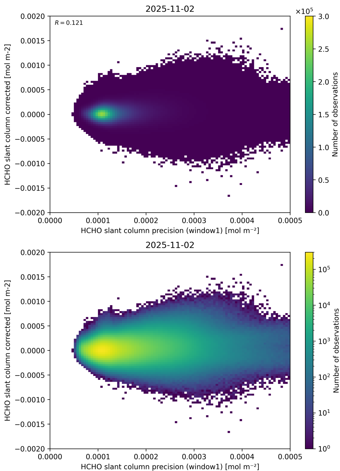
Figure 92: Scatter density plot of “HCHO slant column precision (window1)” against “HCHO slant column corrected” for 2025-11-02 to 2025-11-03.
