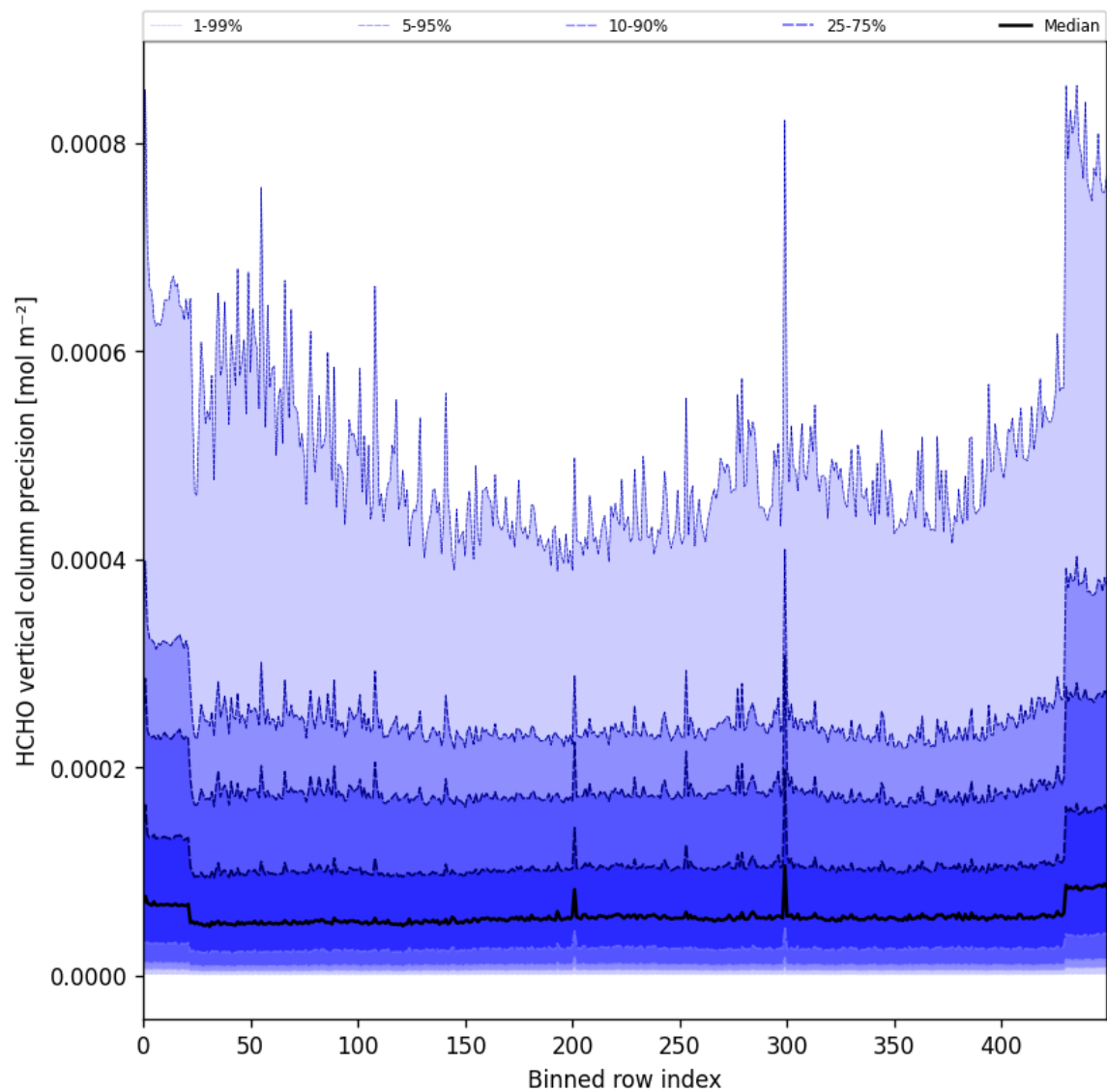
Figure 50: Along track statistics of “HCHO vertical column precision” for 2025-11-02 to 2025-11-03
