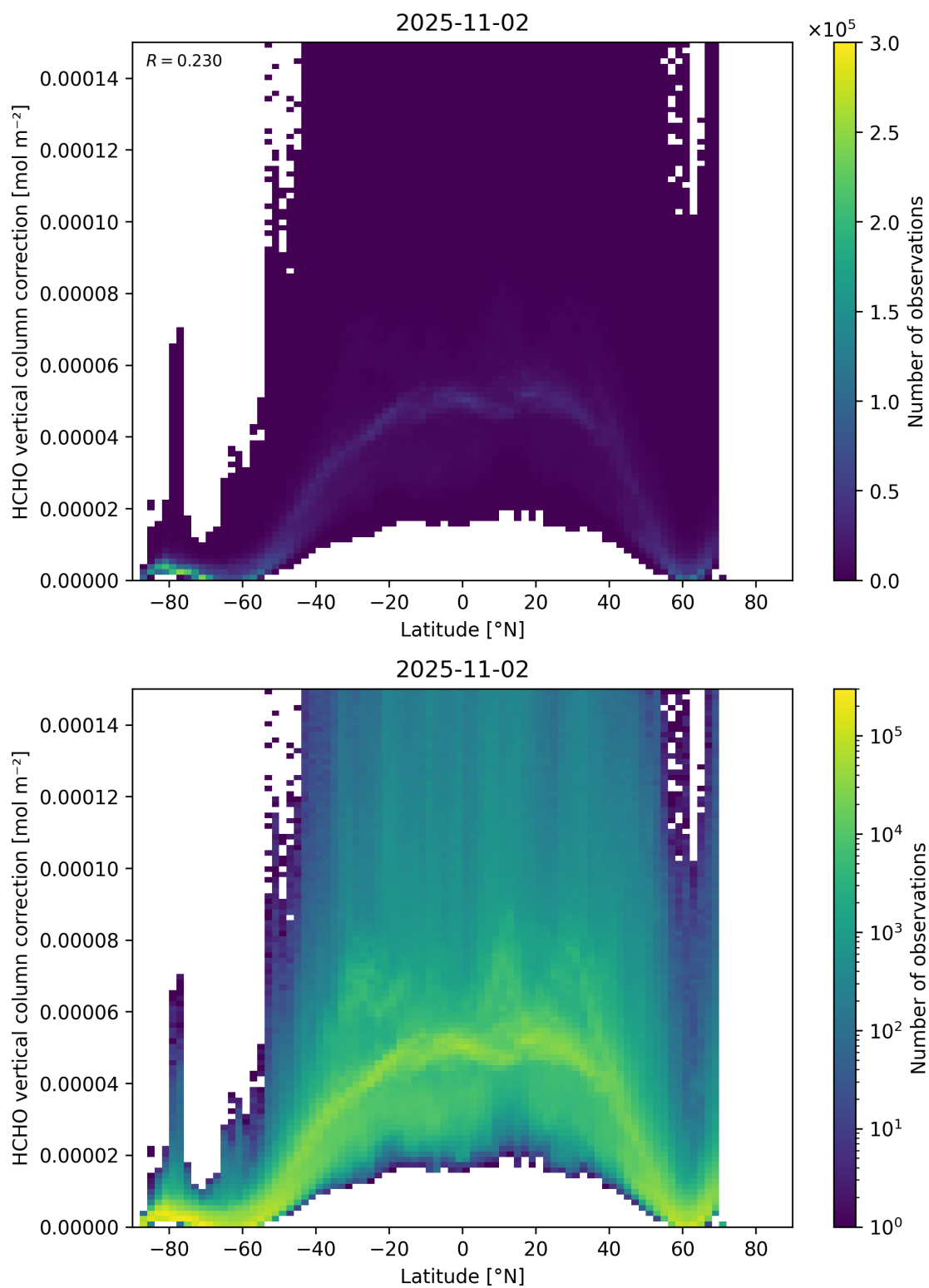
Figure 164: Scatter density plot of “Latitude” against “HCHO vertical column correction” for 2025-11-02 to 2025-11-03.
