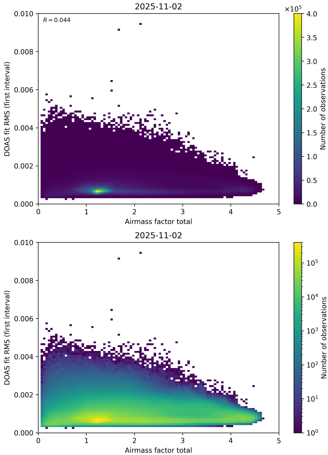
Figure 97: Scatter density plot of “Airmass factor total” against “DOAS fit RMS (first interval)” for 2025-11-02 to 2025-11-03.
