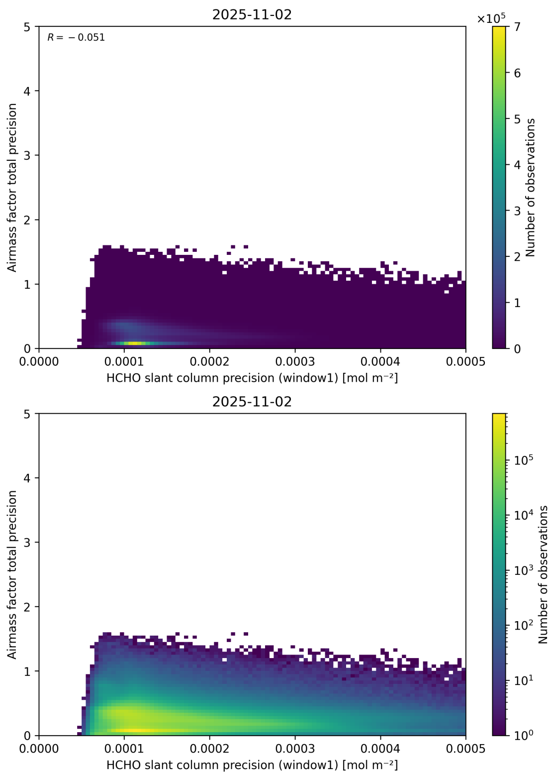
Figure 95: Scatter density plot of “HCHO slant column precision (window1)” against “Airmass factor total precision” for 2025-11-02 to 2025-11-03.
