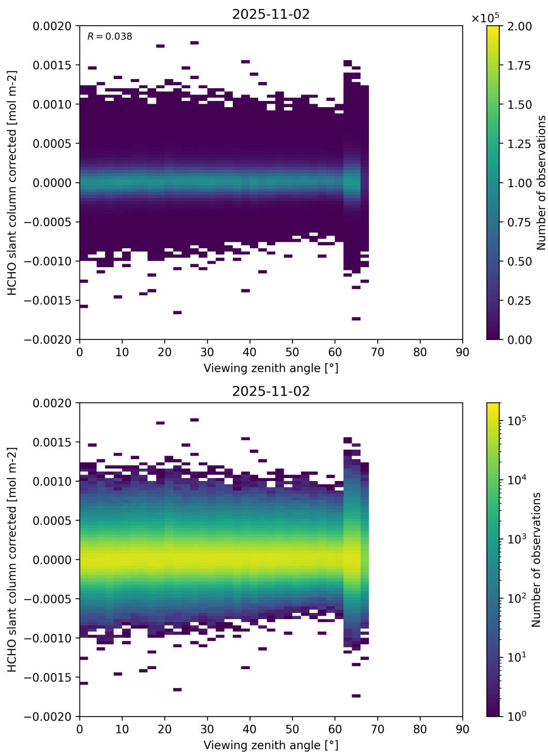
Figure 186: Scatter density plot of “Viewing zenith angle” against “HCHO slant column corrected” for 2025-11-02 to 2025-11-03.
