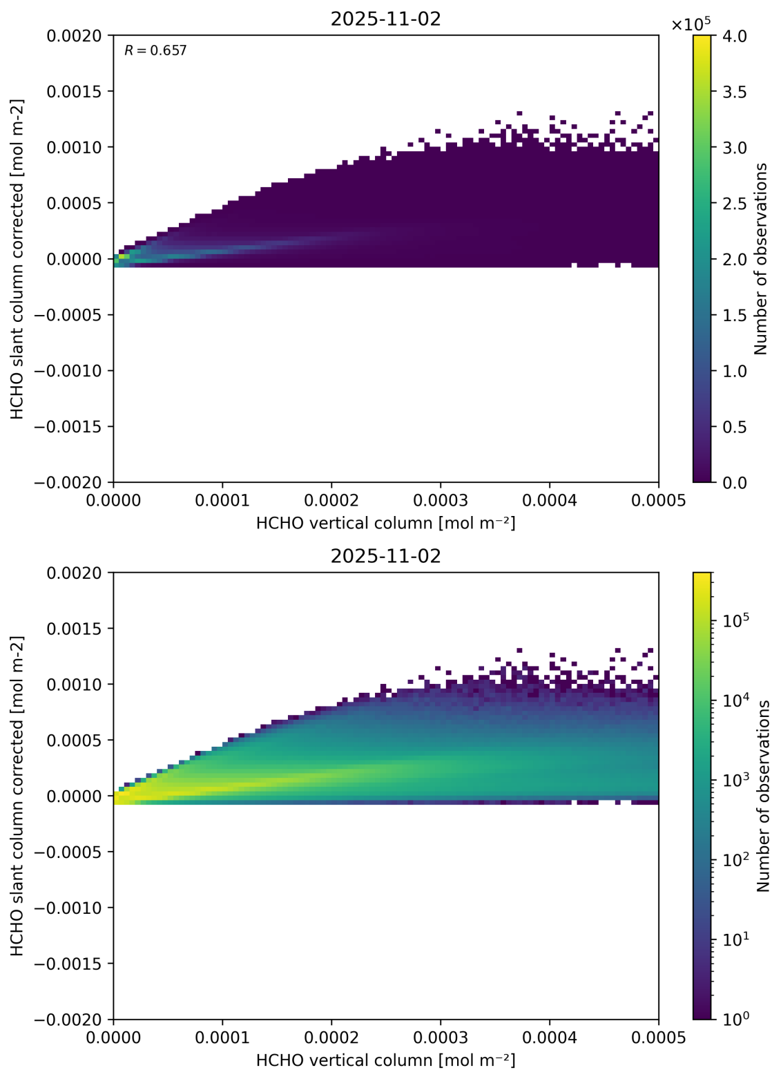
Figure 127: Scatter density plot of “HCHO vertical column” against “HCHO slant column corrected” for 2025-11-02 to 2025-11-03.
