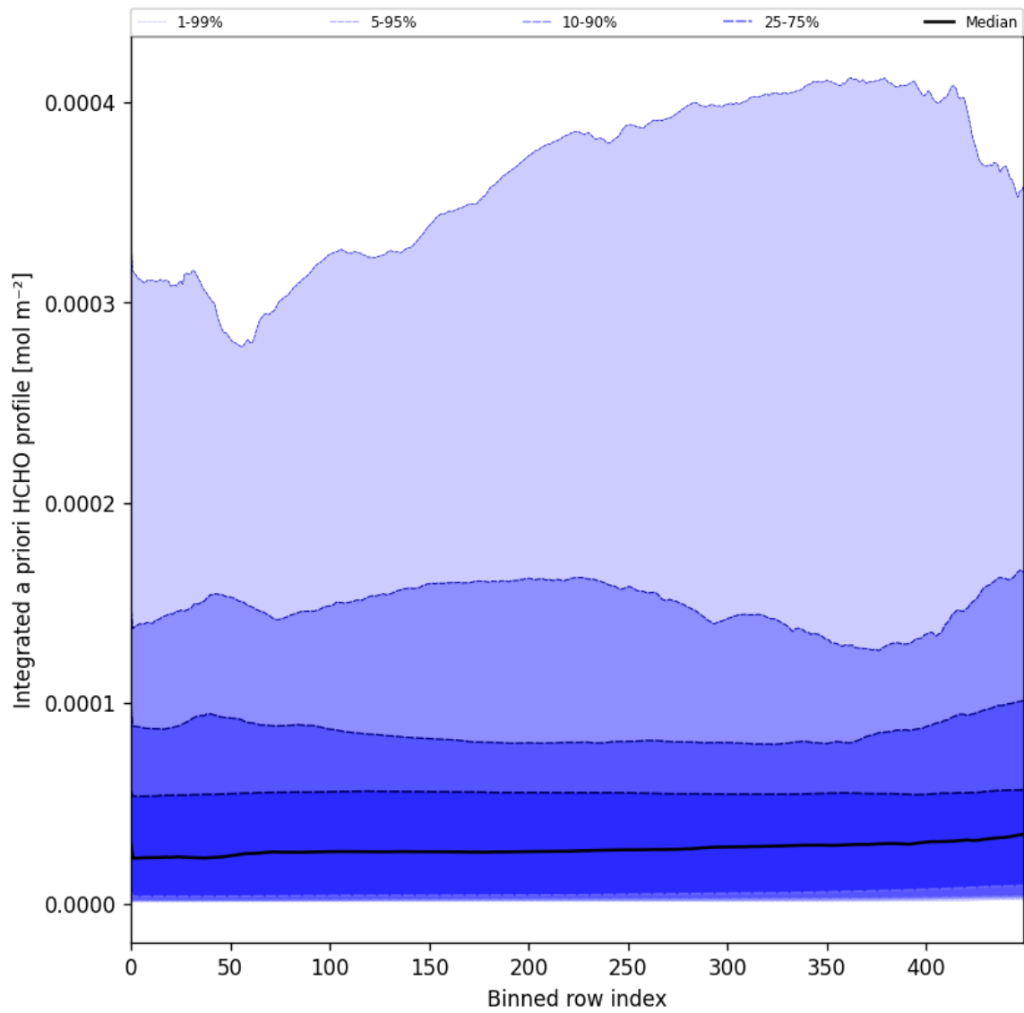
Figure 57: Along track statistics of "Integrated a priori HCHO profile" for 2025-11-02 to 2025-11-03
