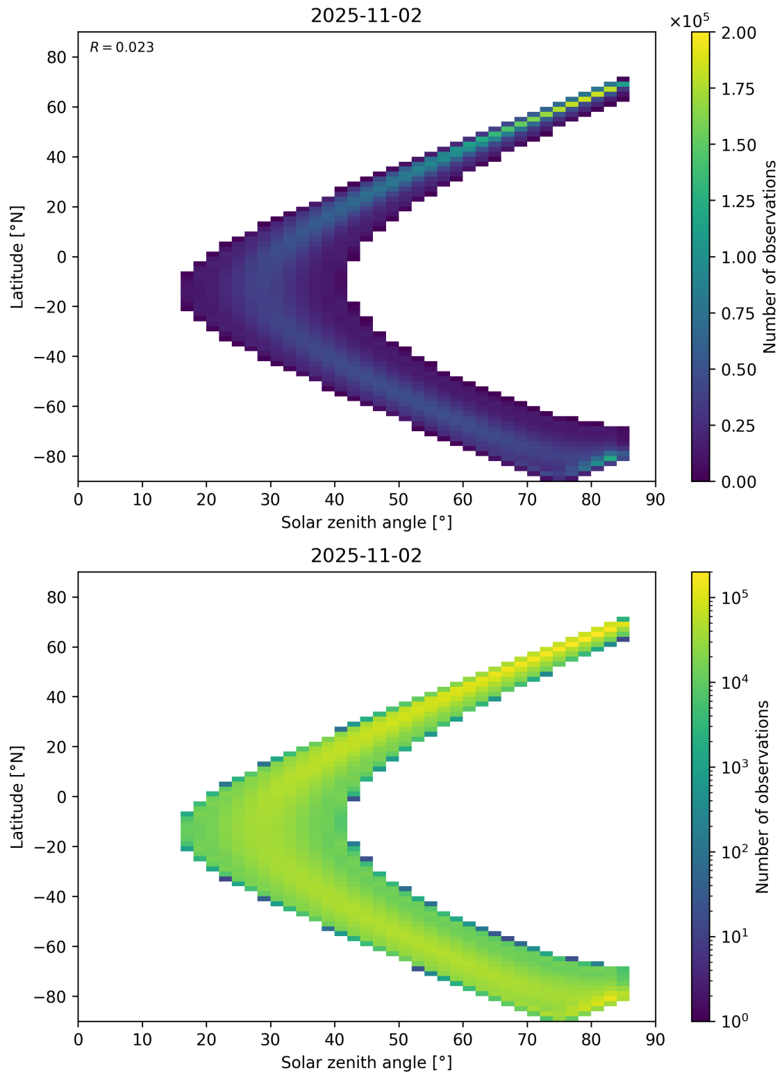
Figure 181: Scatter density plot of “Solar zenith angle” against “Latitude” for 2025-11-02 to 2025-11-03.
