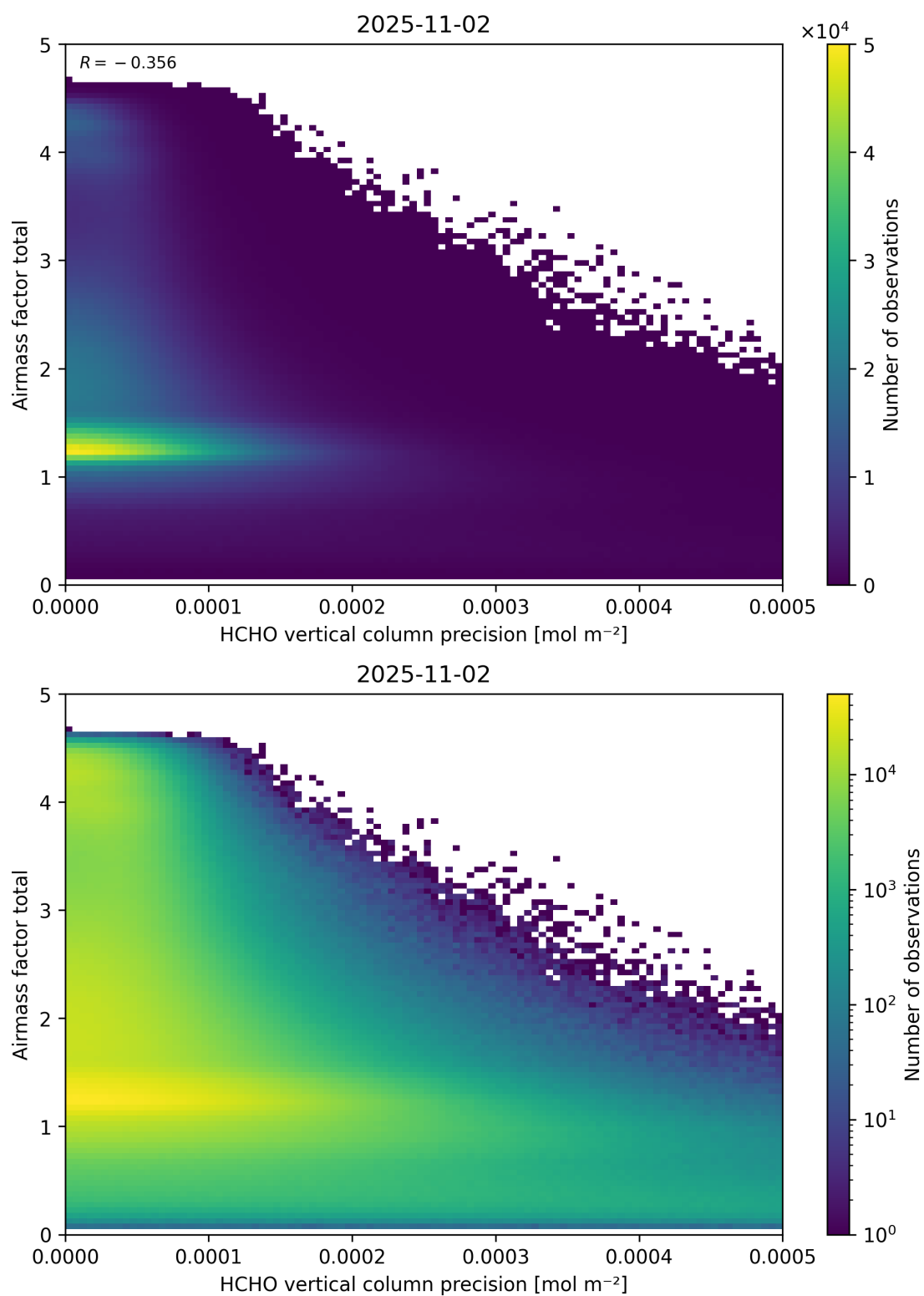
Figure 144: Scatter density plot of “HCHO vertical column precision” against “Airmass factor total” for 2025-11-02 to 2025-11-03.
