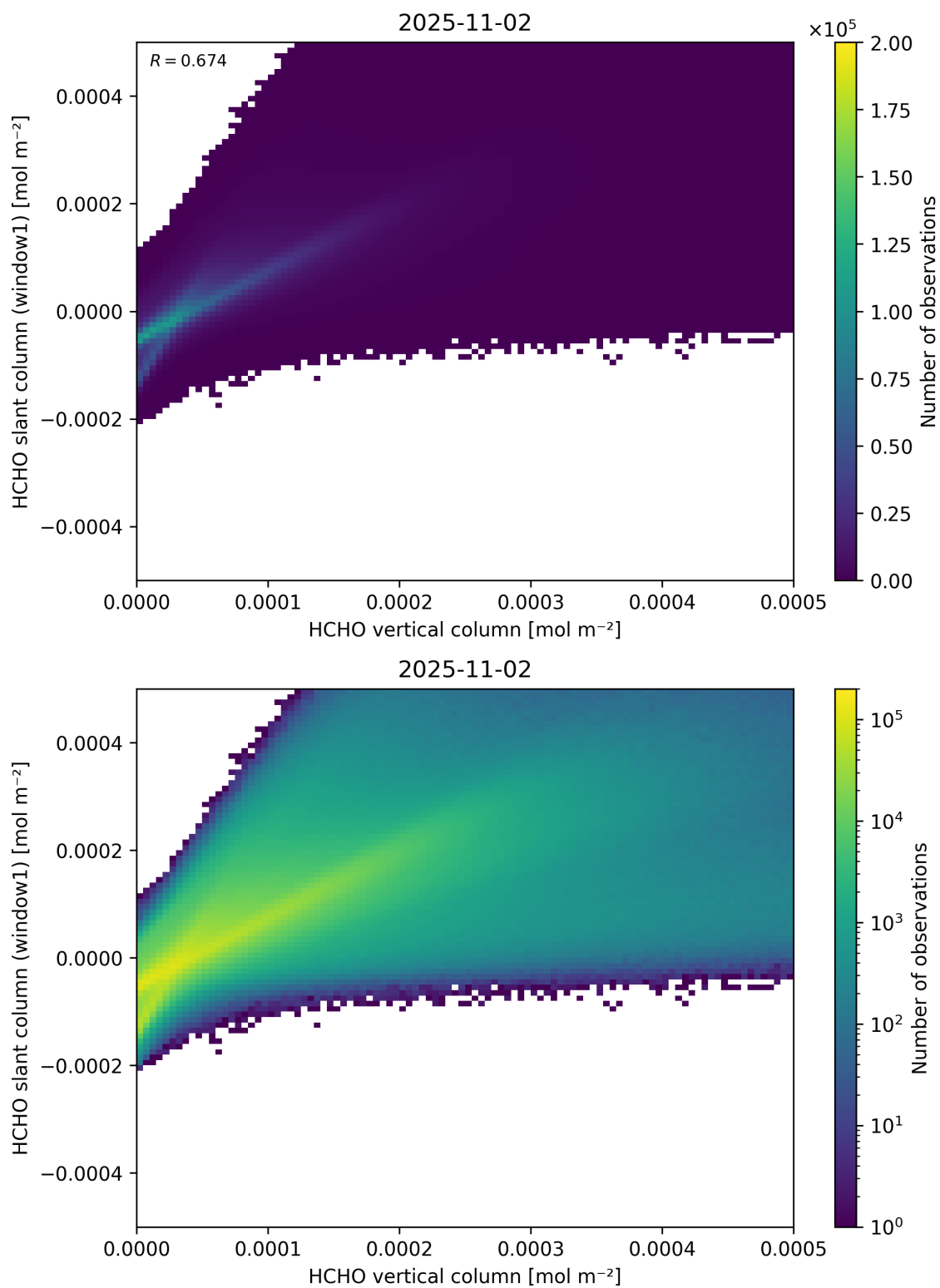
Figure 129: Scatter density plot of “HCHO vertical column” against “HCHO slant column (window1)” for 2025-11-02 to 2025-11-03.
