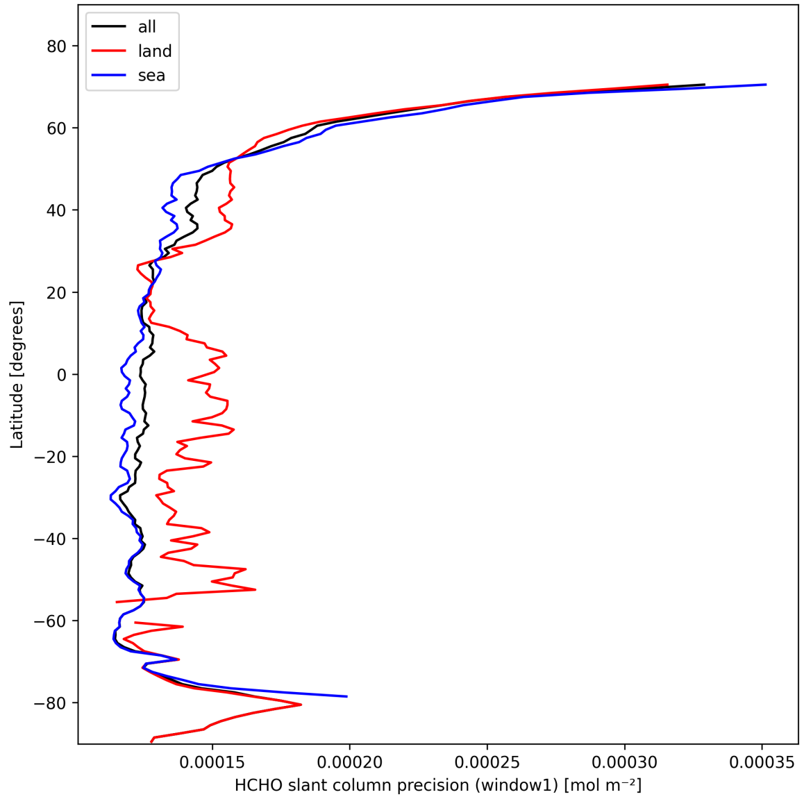
Figure 25: Zonal average of "HCHO slant column precision (window1)" for 2025-11-02 to 2025-11-03.
