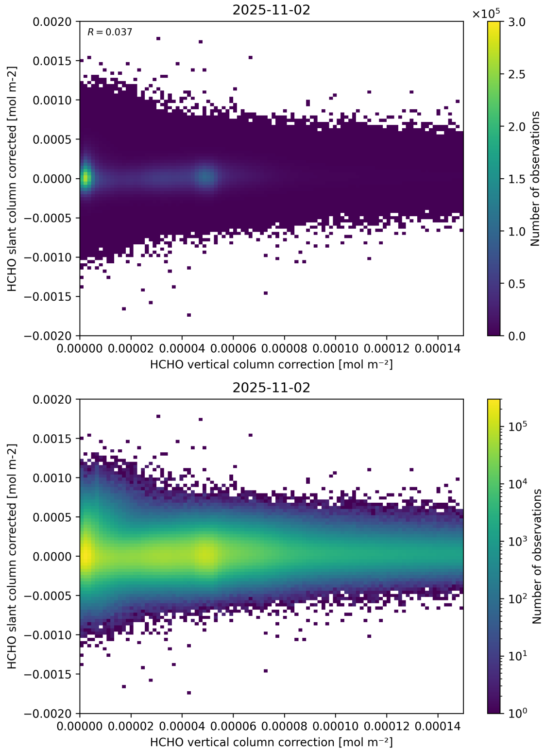
Figure 116: Scatter density plot of “HCHO vertical column correction” against “HCHO slant column corrected” for 2025-11-02 to 2025-11-03.
