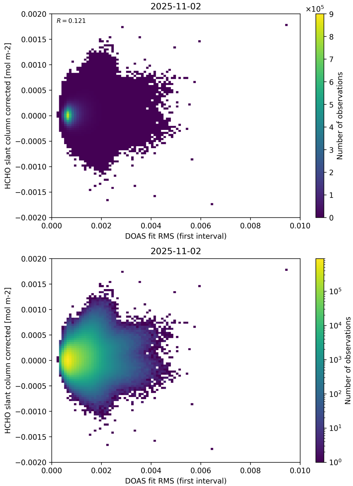
Figure 62: Scatter density plot of “DOAS fit RMS (first interval)” against “HCHO slant column corrected” for 2025-11-02 to 2025-11-03.
