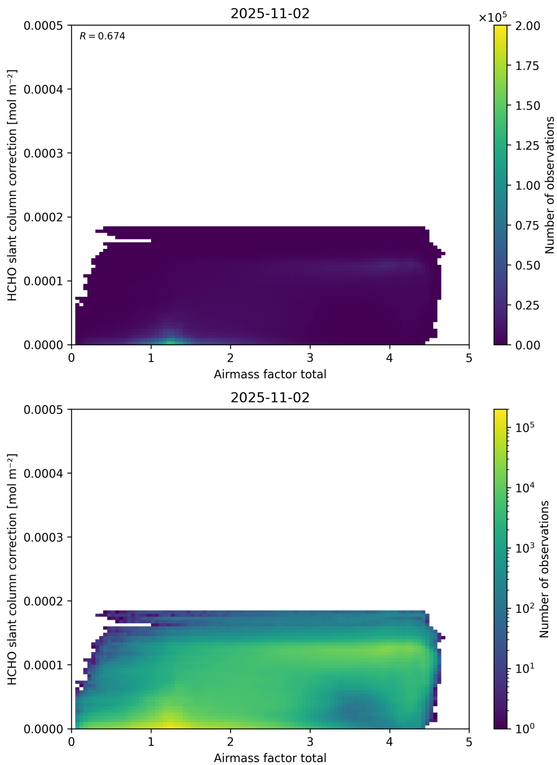
Figure 102: Scatter density plot of “Airmass factor total” against “HCHO slant column correction” for 2025-11-02 to 2025-11-03.
