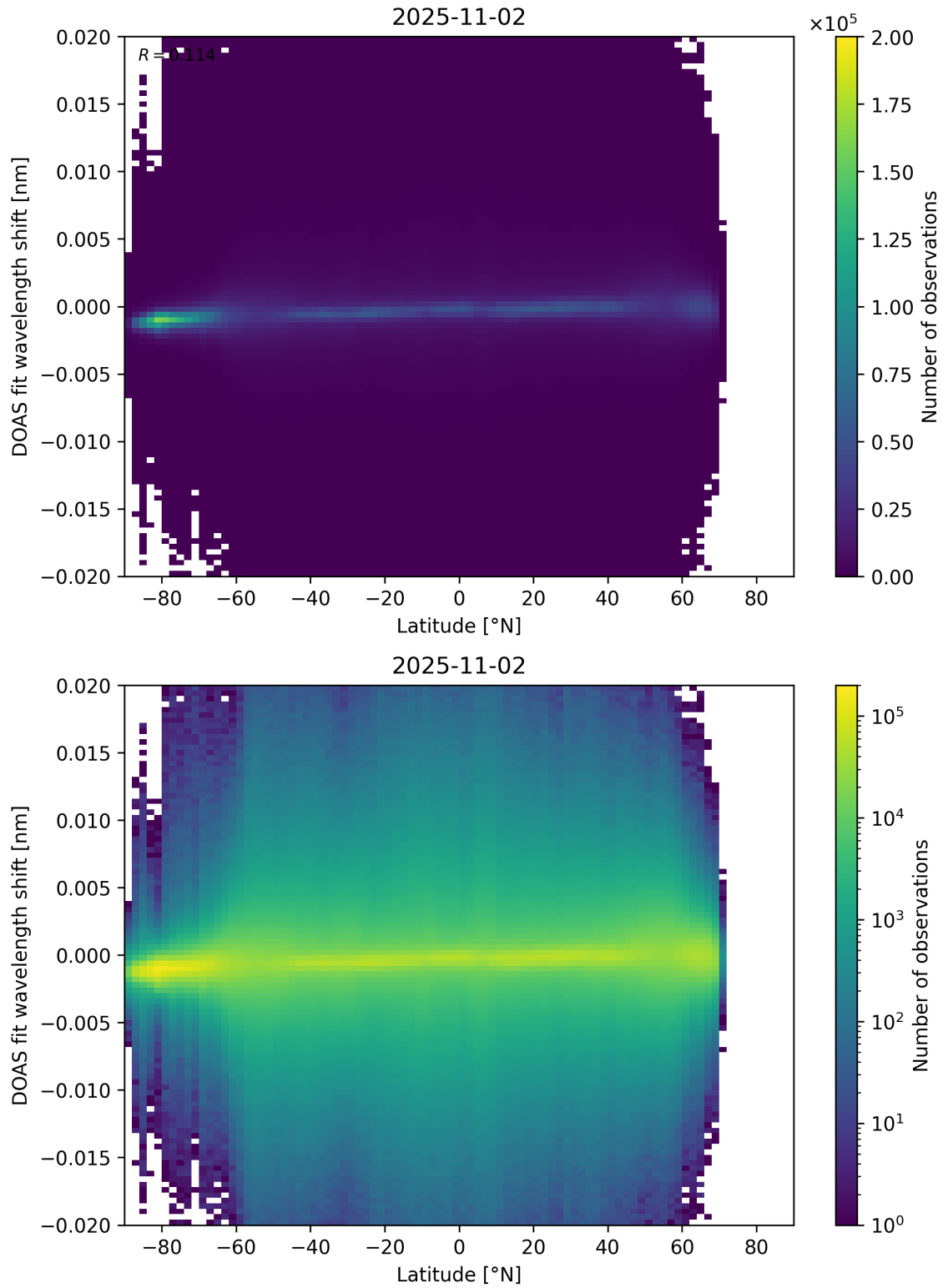
Figure 154: Scatter density plot of “Latitude” against “DOAS fit wavelength shift” for 2025-11-02 to 2025-11-03.
