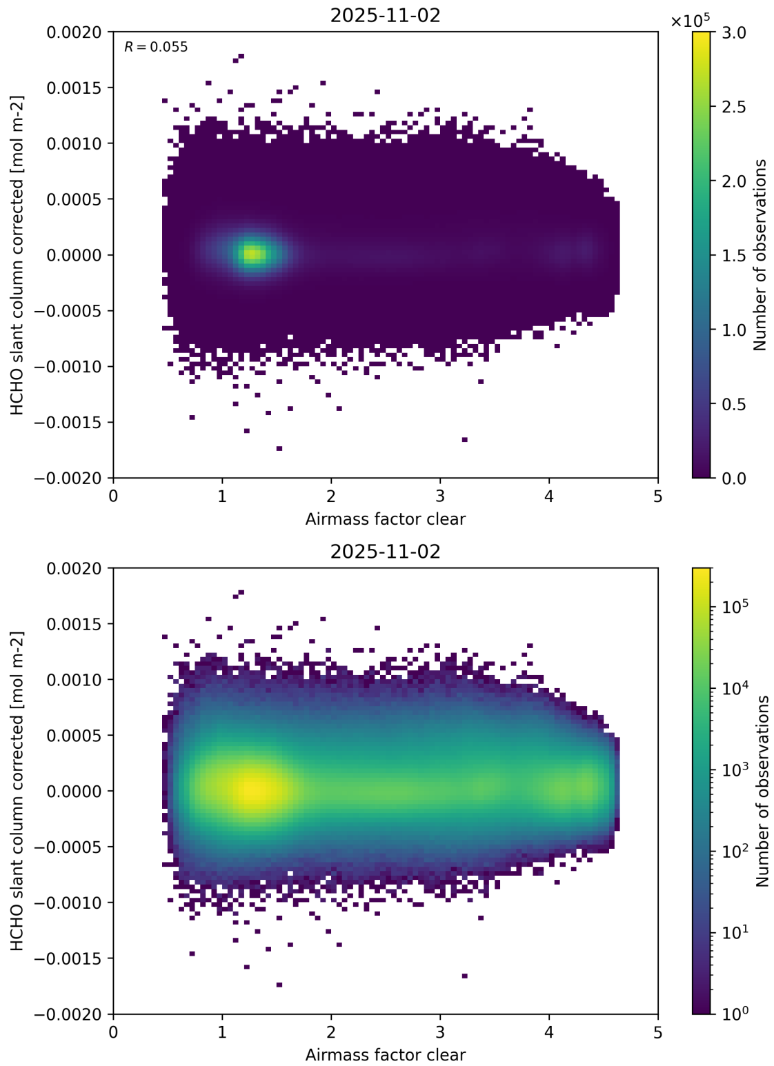
Figure 74: Scatter density plot of “Airmass factor clear” against “HCHO slant column corrected” for 2025-11-02 to 2025-11-03.
