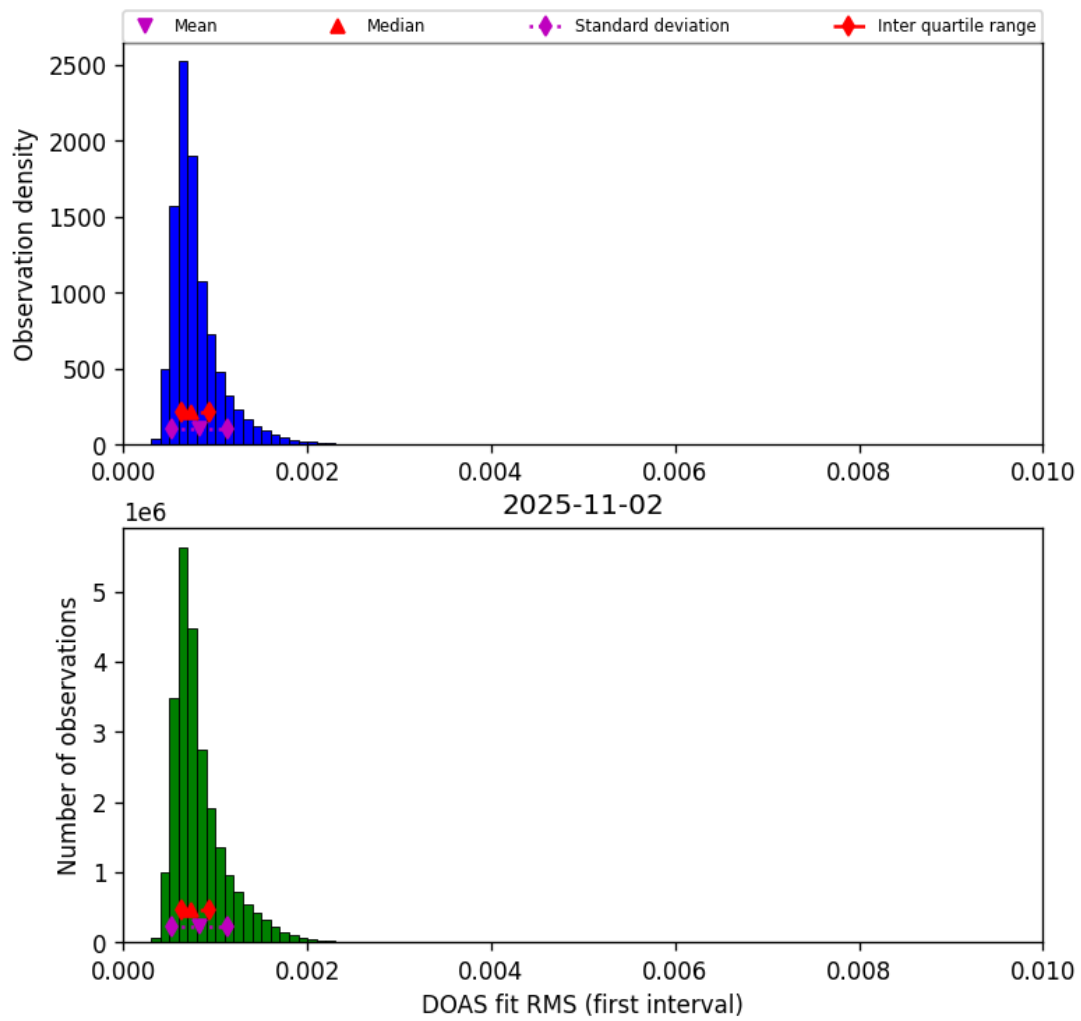
Figure 46: Histogram of “DOAS fit RMS (first interval)” for 2025-11-02 to 2025-11-03
