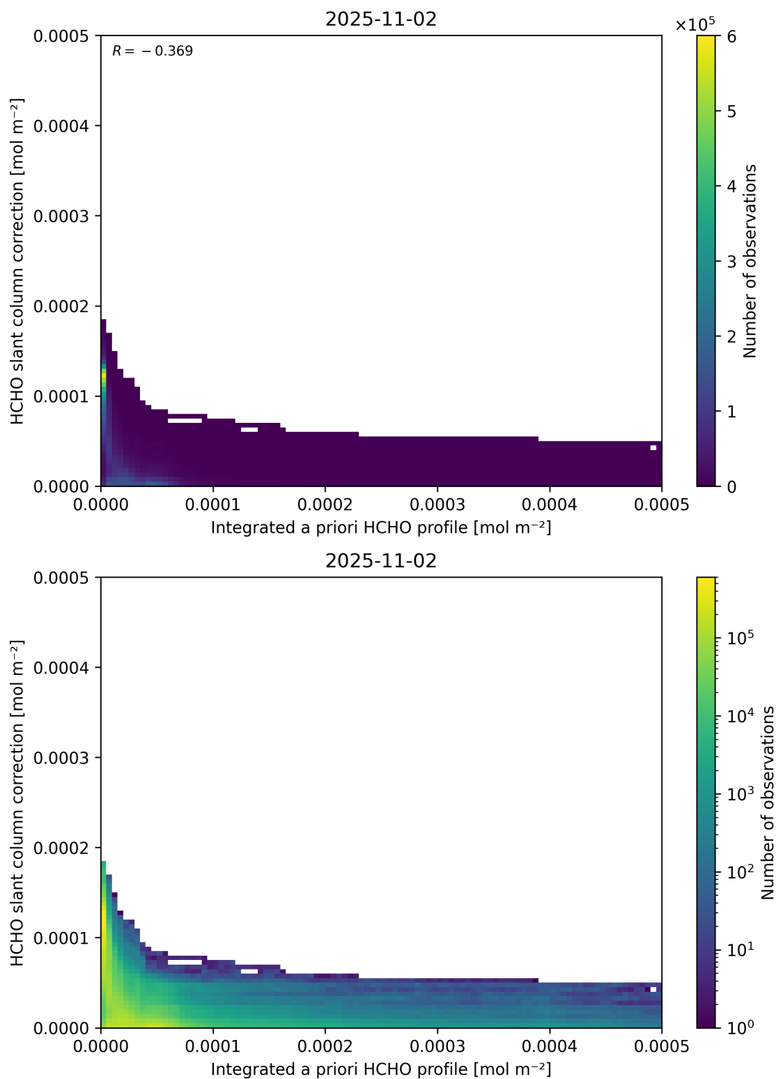
Figure 152: Scatter density plot of “Integrated a priori HCHO profile” against “HCHO slant column correction” for 2025-11-02 to 2025-11-03.
