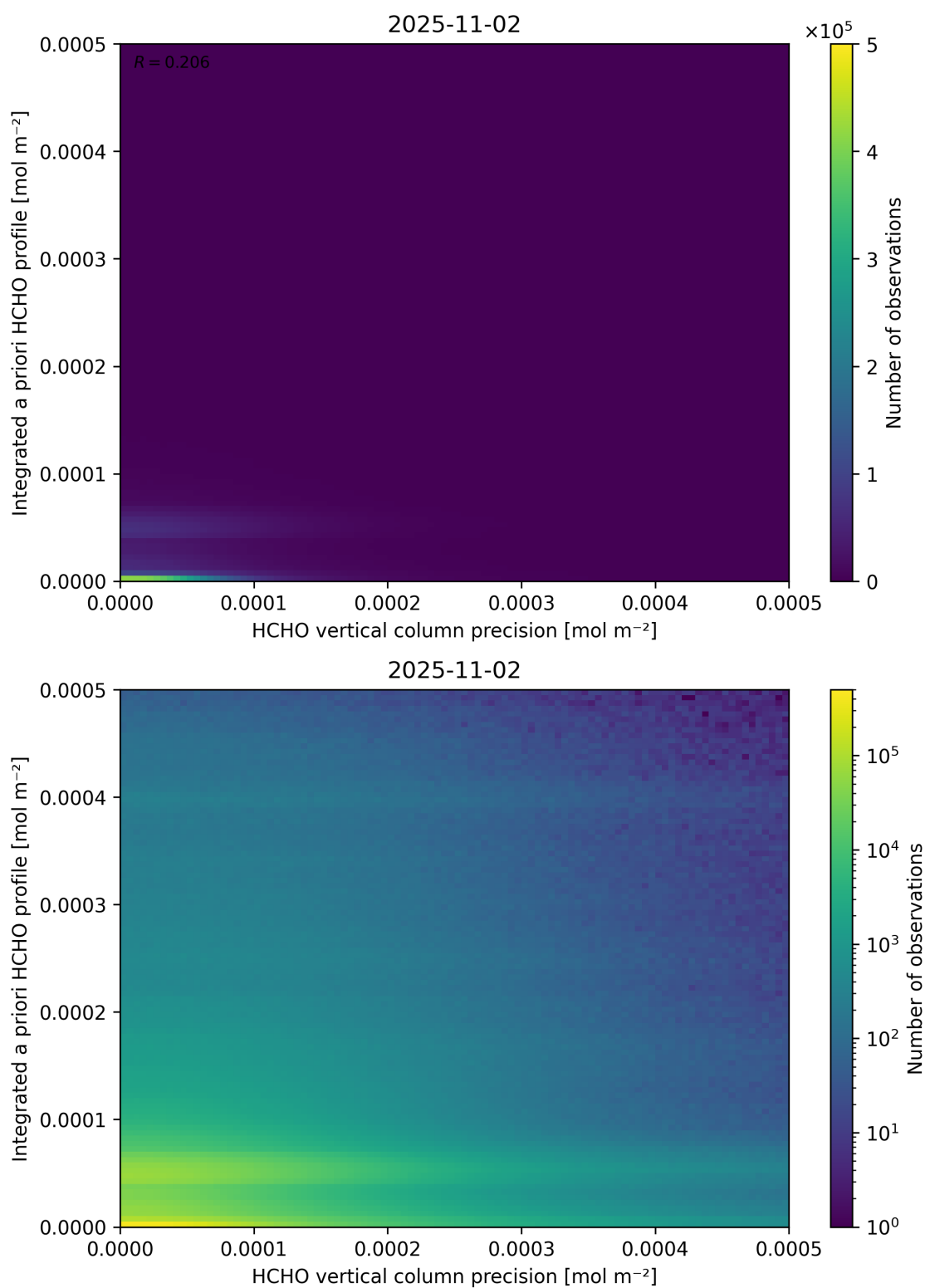
Figure 147: Scatter density plot of “HCHO vertical column precision” against “Integrated a priori HCHO profile” for 2025-11-02 to 2025-11-03.
