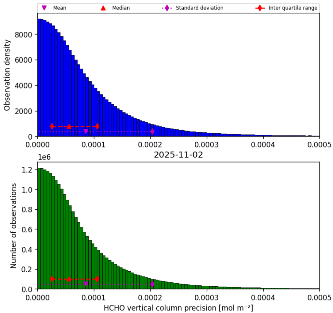
Figure 36: Histogram of “HCHO vertical column precision” for 2025-11-02 to 2025-11-03
