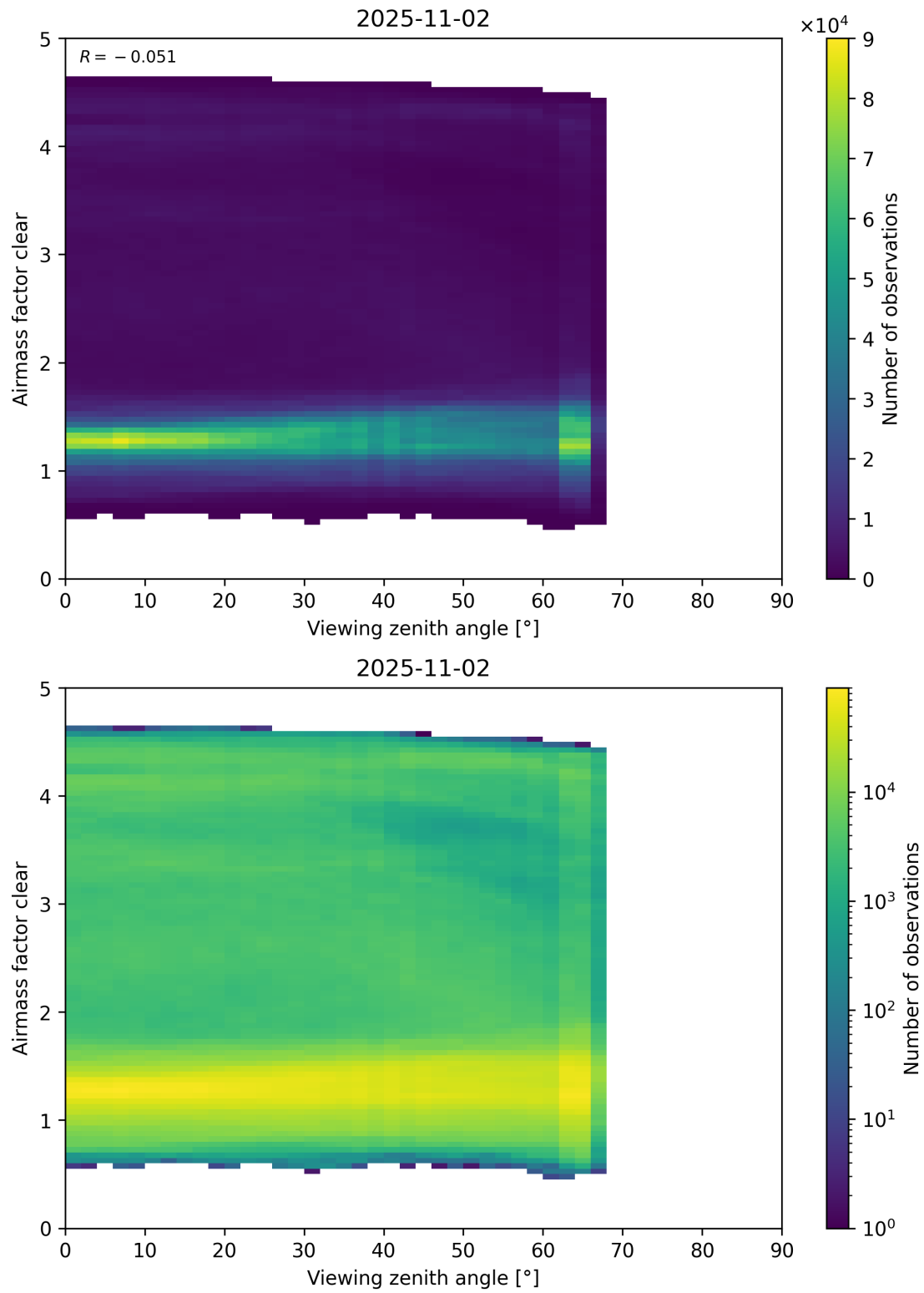
Figure 185: Scatter density plot of “Viewing zenith angle” against “Airmass factor clear” for 2025-11-02 to 2025-11-03.
