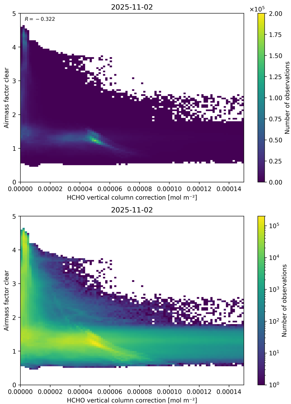
Figure 115: Scatter density plot of “HCHO vertical column correction” against “Airmass factor clear” for 2025-11-02 to 2025-11-03.
