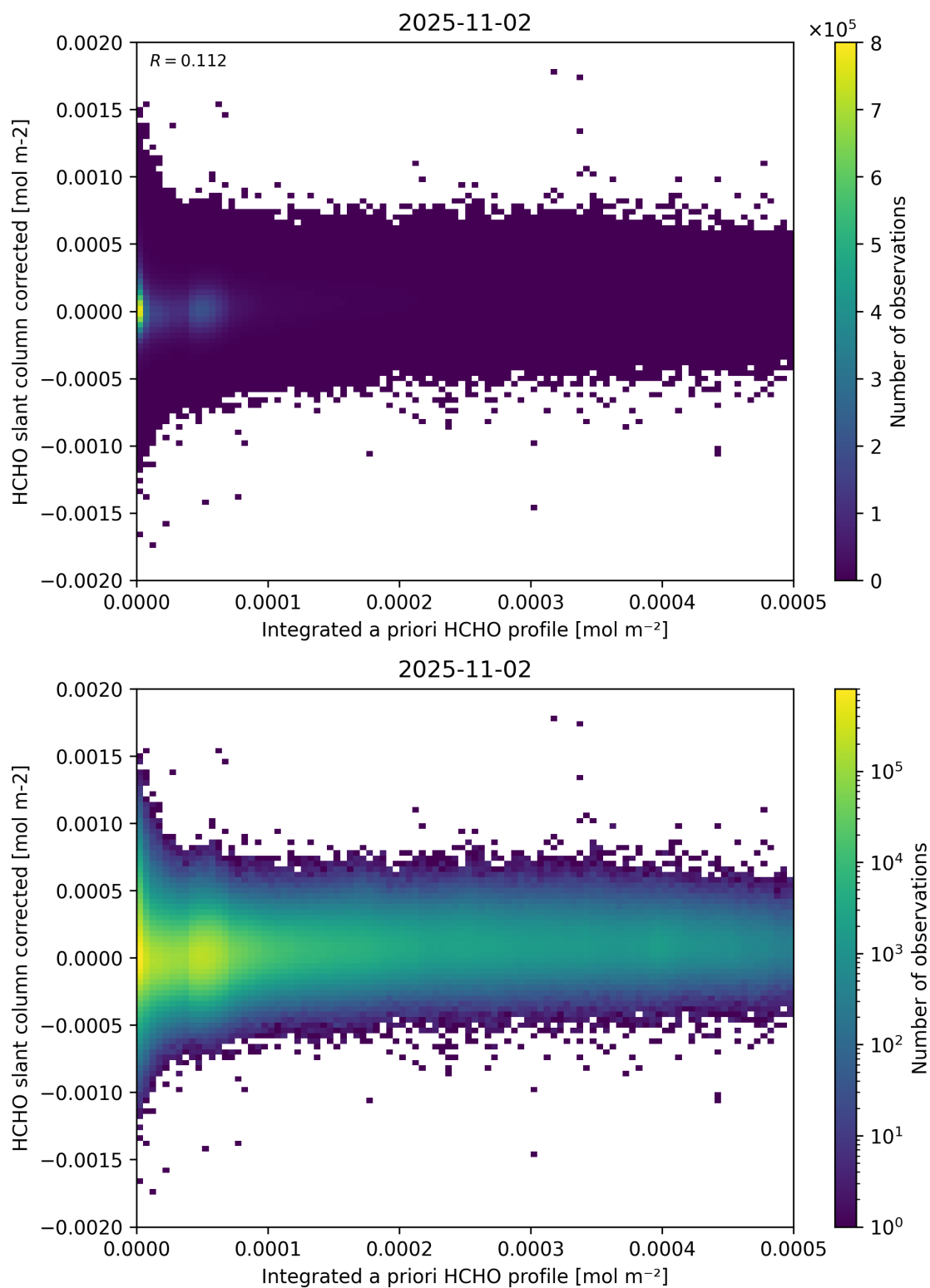
Figure 151: Scatter density plot of “Integrated a priori HCHO profile” against “HCHO slant column corrected” for 2025-11-02 to 2025-11-03.
