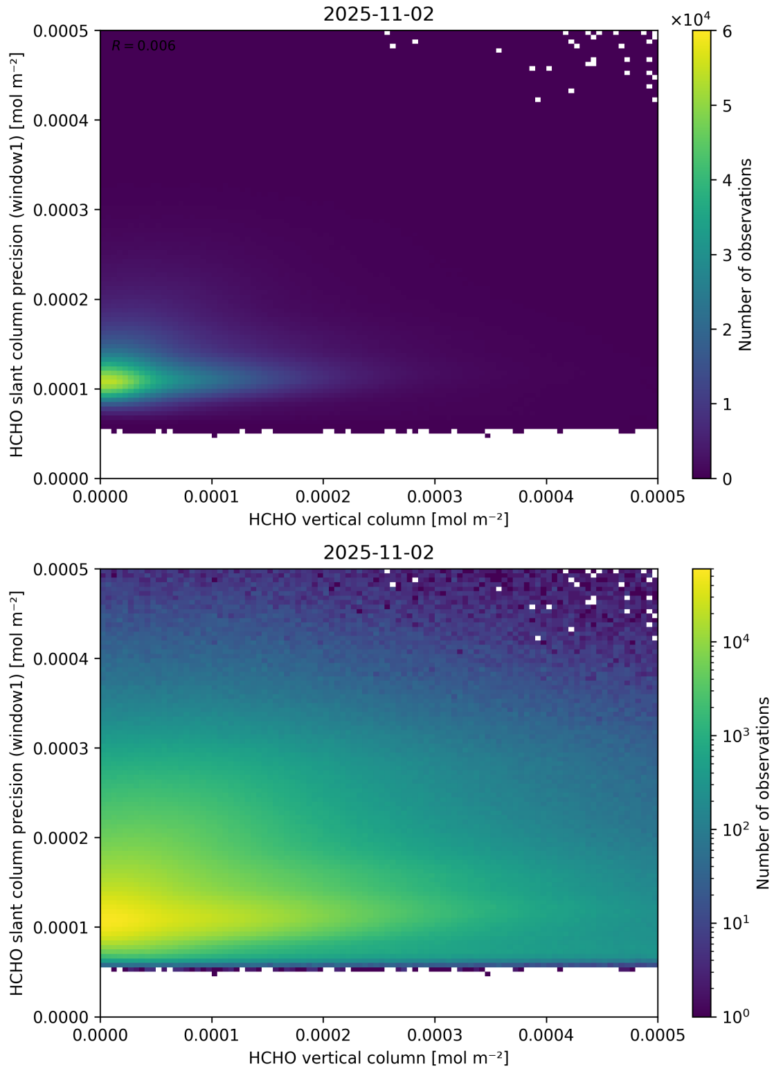
Figure 130: Scatter density plot of “HCHO vertical column” against “HCHO slant column precision (window1)” for 2025-11-02 to 2025-11-03.
