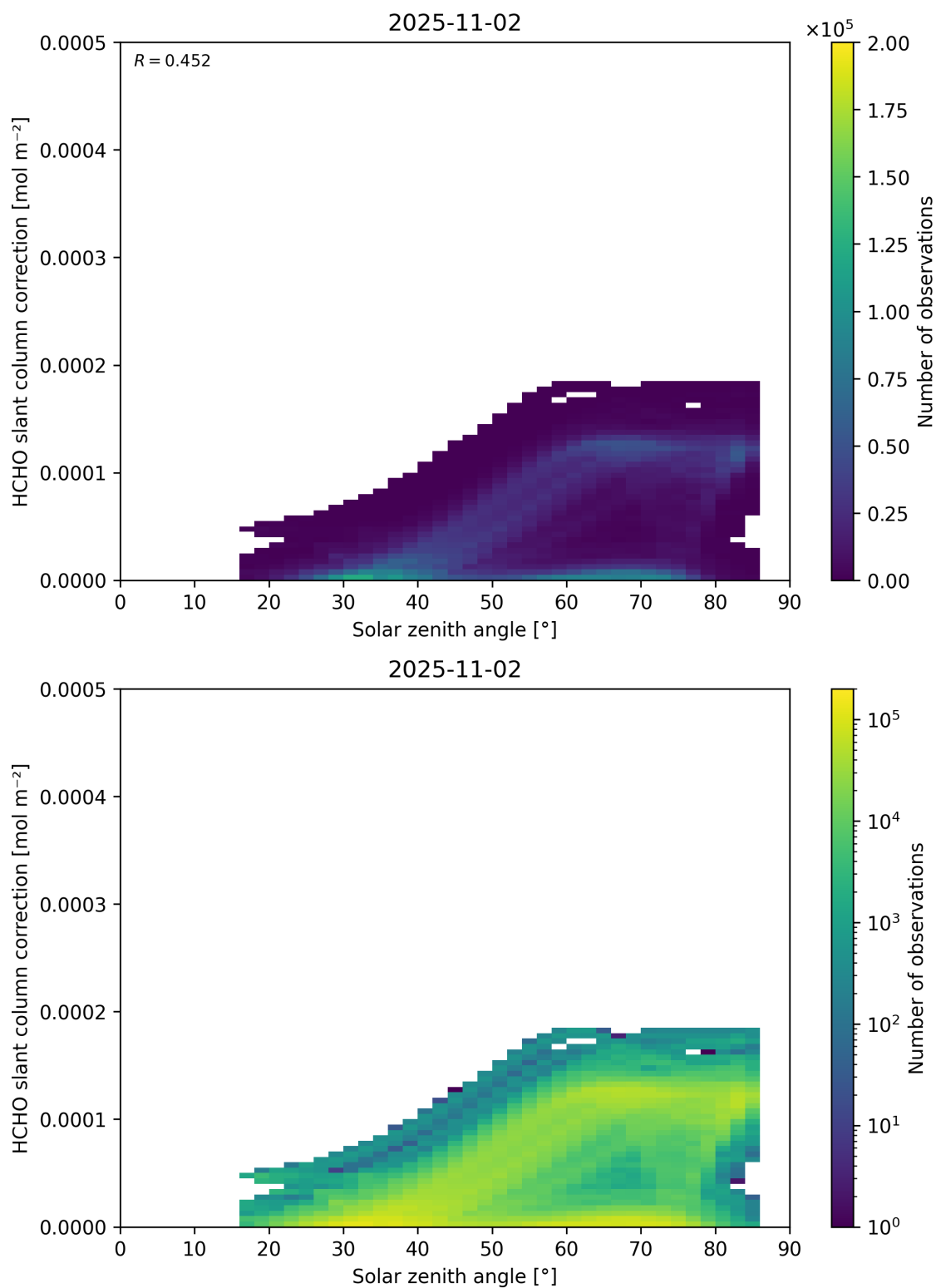
Figure 172: Scatter density plot of “Solar zenith angle” against “HCHO slant column correction” for 2025-11-02 to 2025-11-03.
