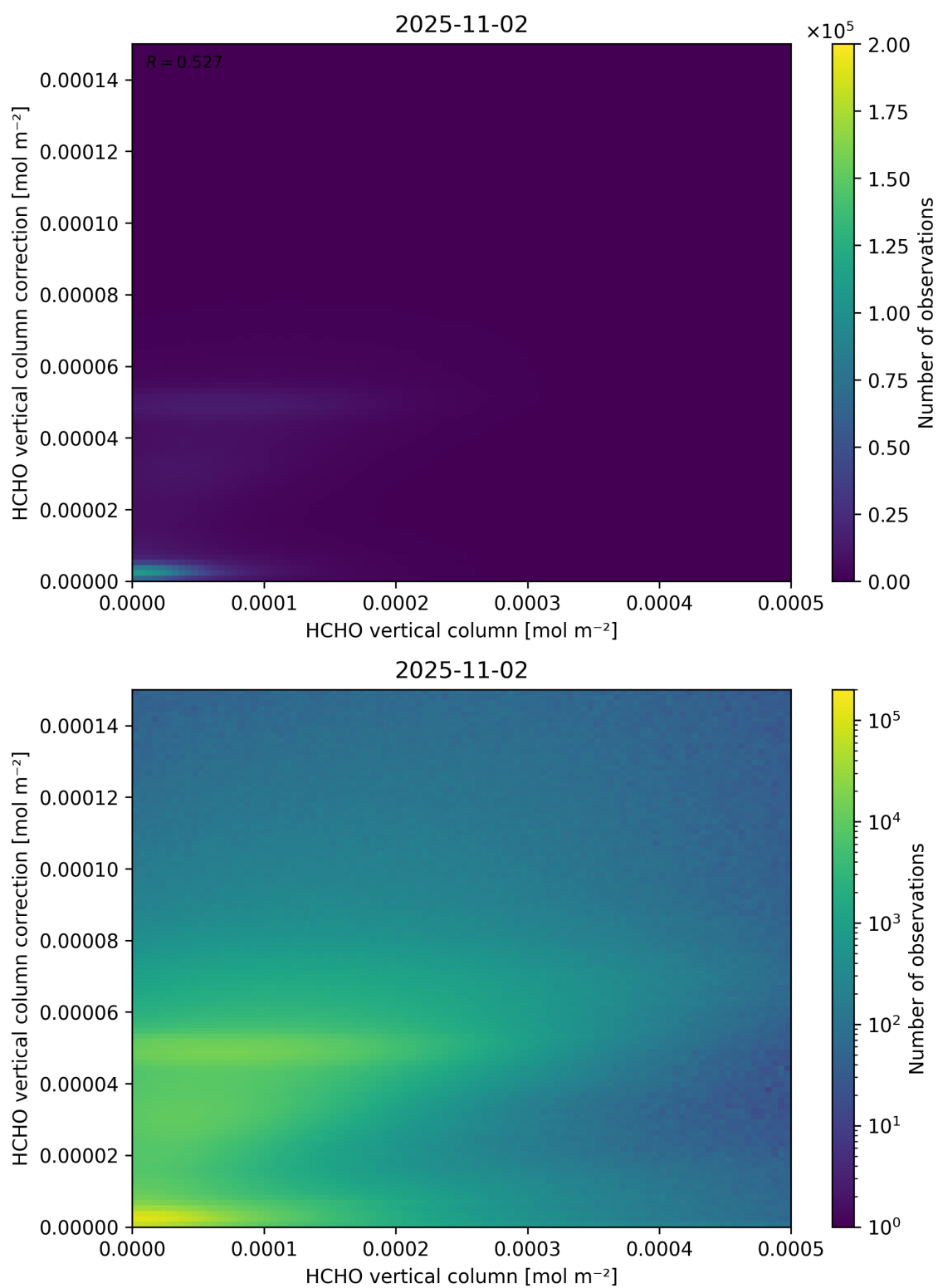
Figure 133: Scatter density plot of “HCHO vertical column” against “HCHO vertical column correction” for 2025-11-02 to 2025-11-03.
