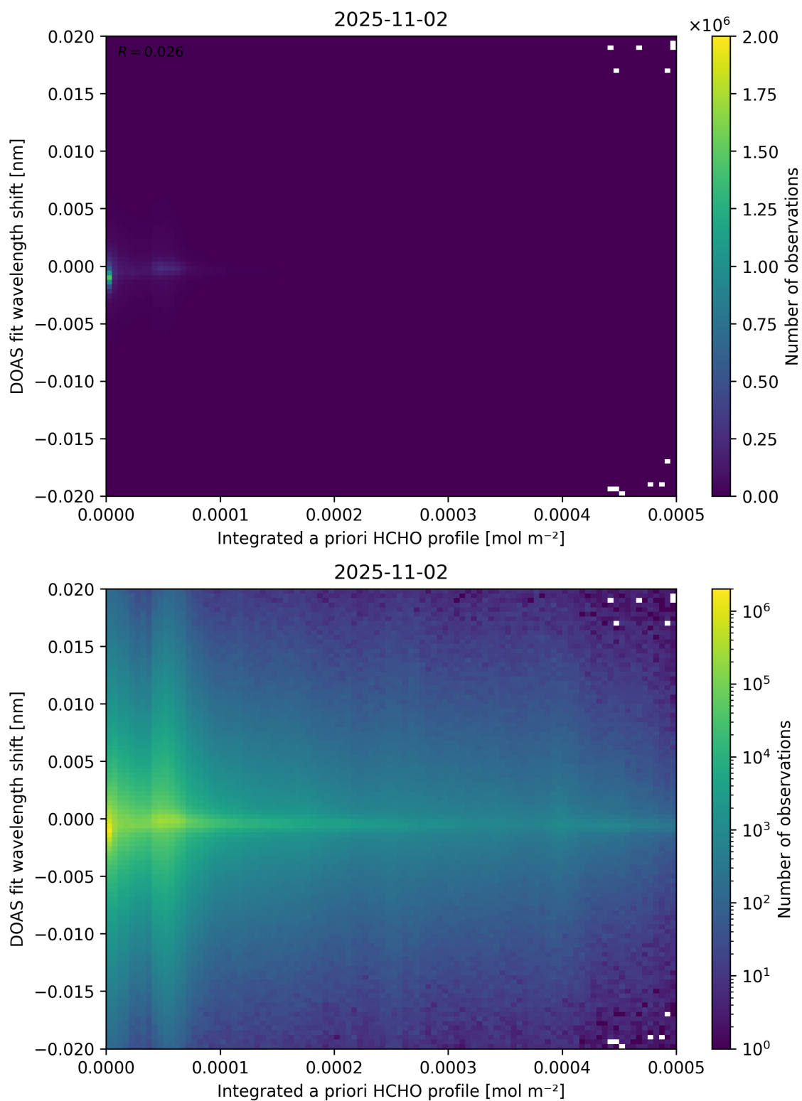
Figure 149: Scatter density plot of “Integrated a priori HCHO profile” against “DOAS fit wavelength shift” for 2025-11-02 to 2025-11-03.
