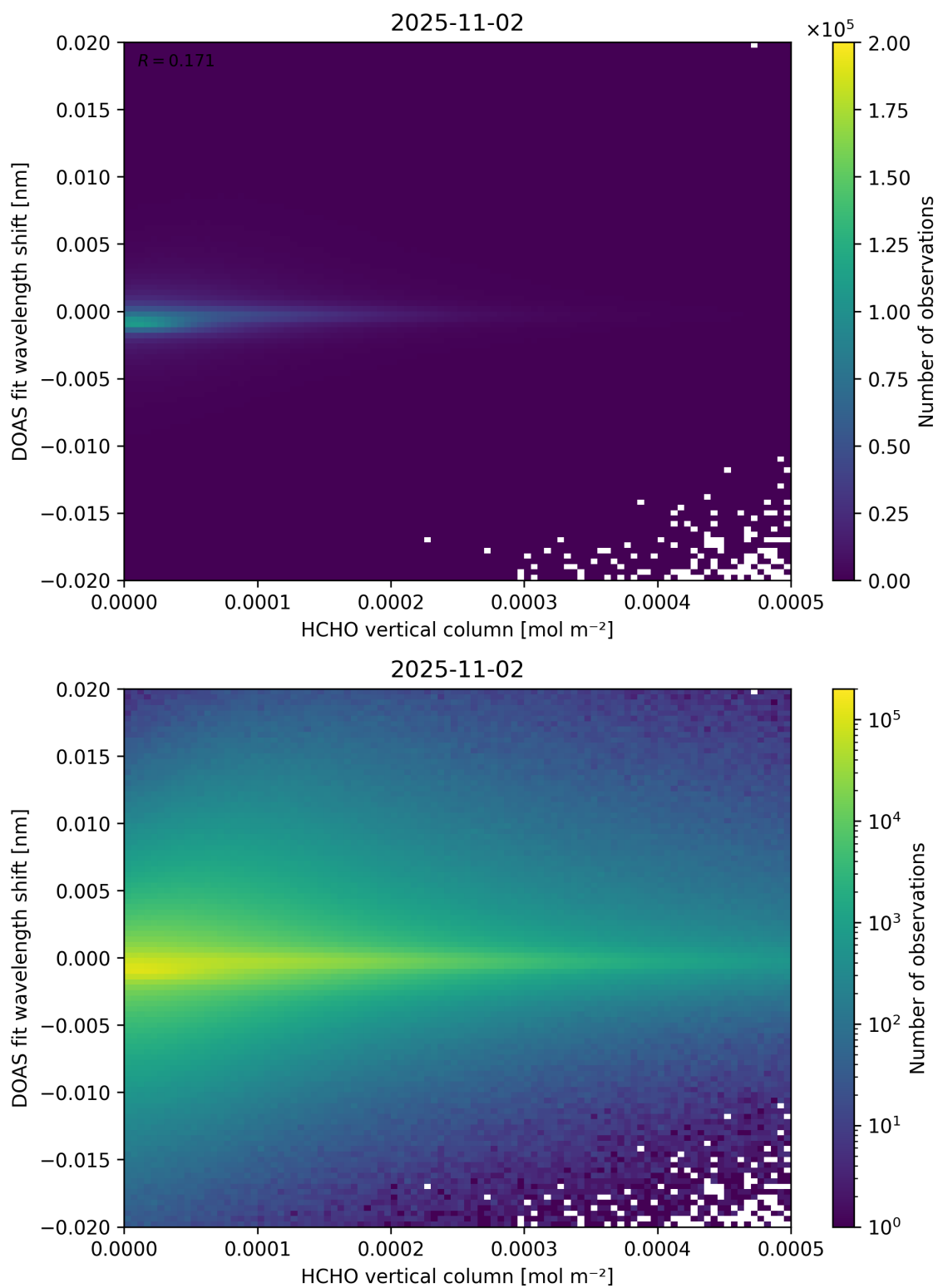
Figure 124: Scatter density plot of “HCHO vertical column” against “DOAS fit wavelength shift” for 2025-11-02 to 2025-11-03.
