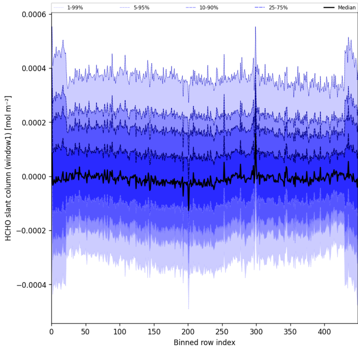
Figure 52: Along track statistics of “HCHO slant column (window1)” for 2025-11-02 to 2025-11-03
