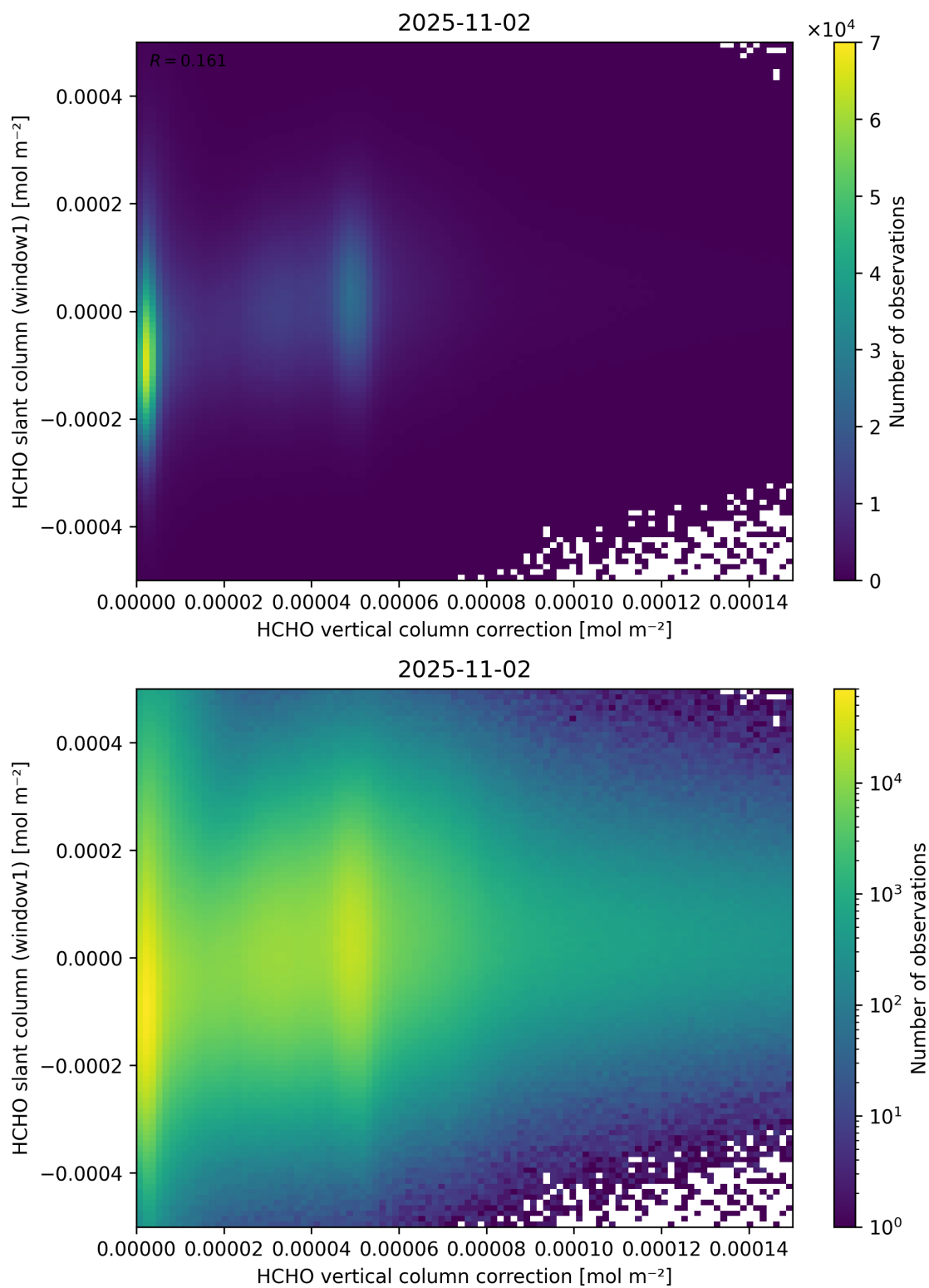
Figure 118: Scatter density plot of “HCHO vertical column correction” against “HCHO slant column (window1)” for 2025-11-02 to 2025-11-03.
