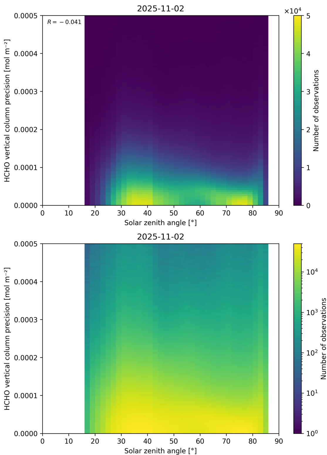
Figure 179: Scatter density plot of “Solar zenith angle” against “HCHO vertical column precision” for 2025-11-02 to 2025-11-03.
