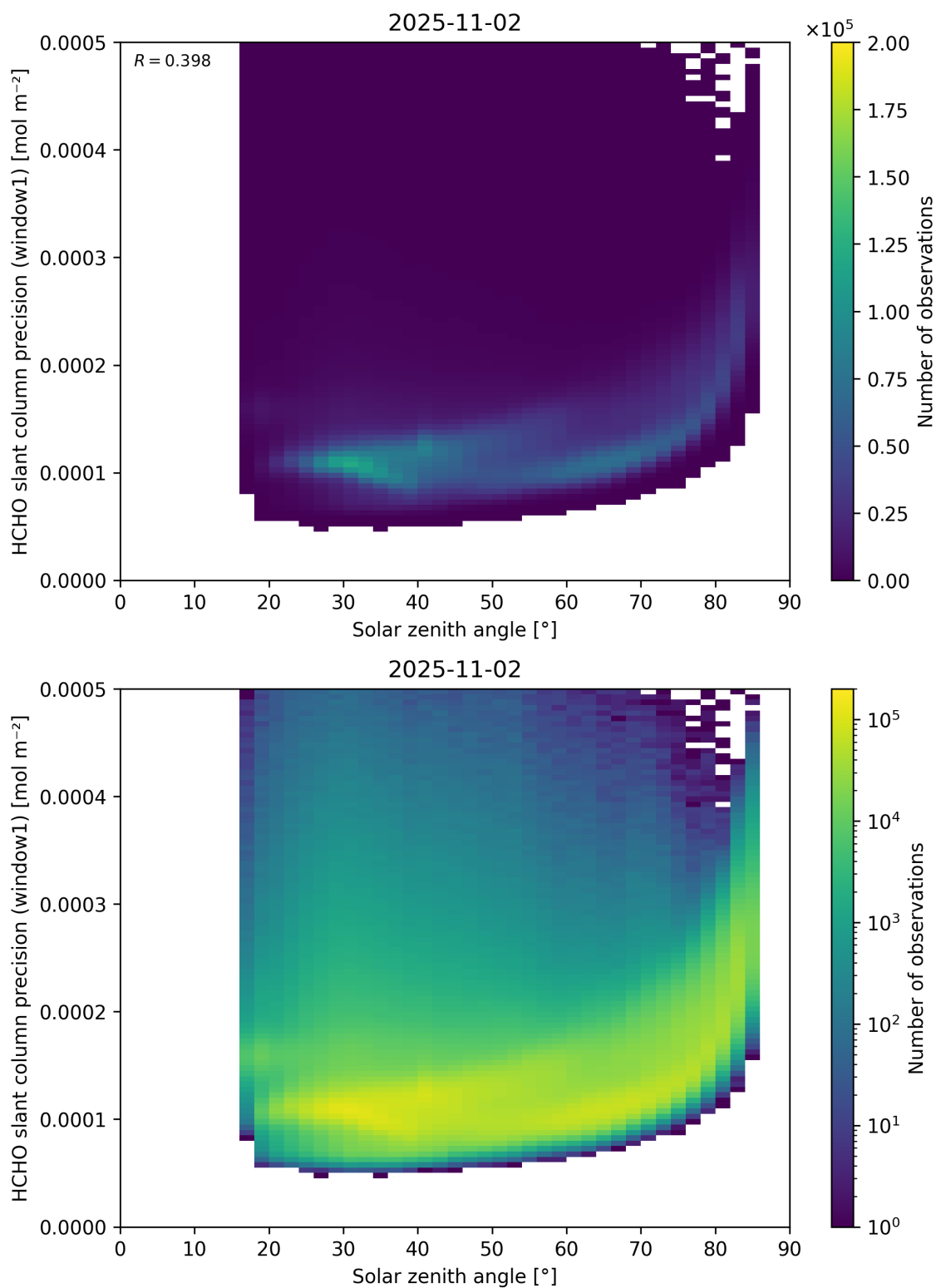
Figure 174: Scatter density plot of “Solar zenith angle” against “HCHO slant column precision (window1)” for 2025-11-02 to 2025-11-03.
