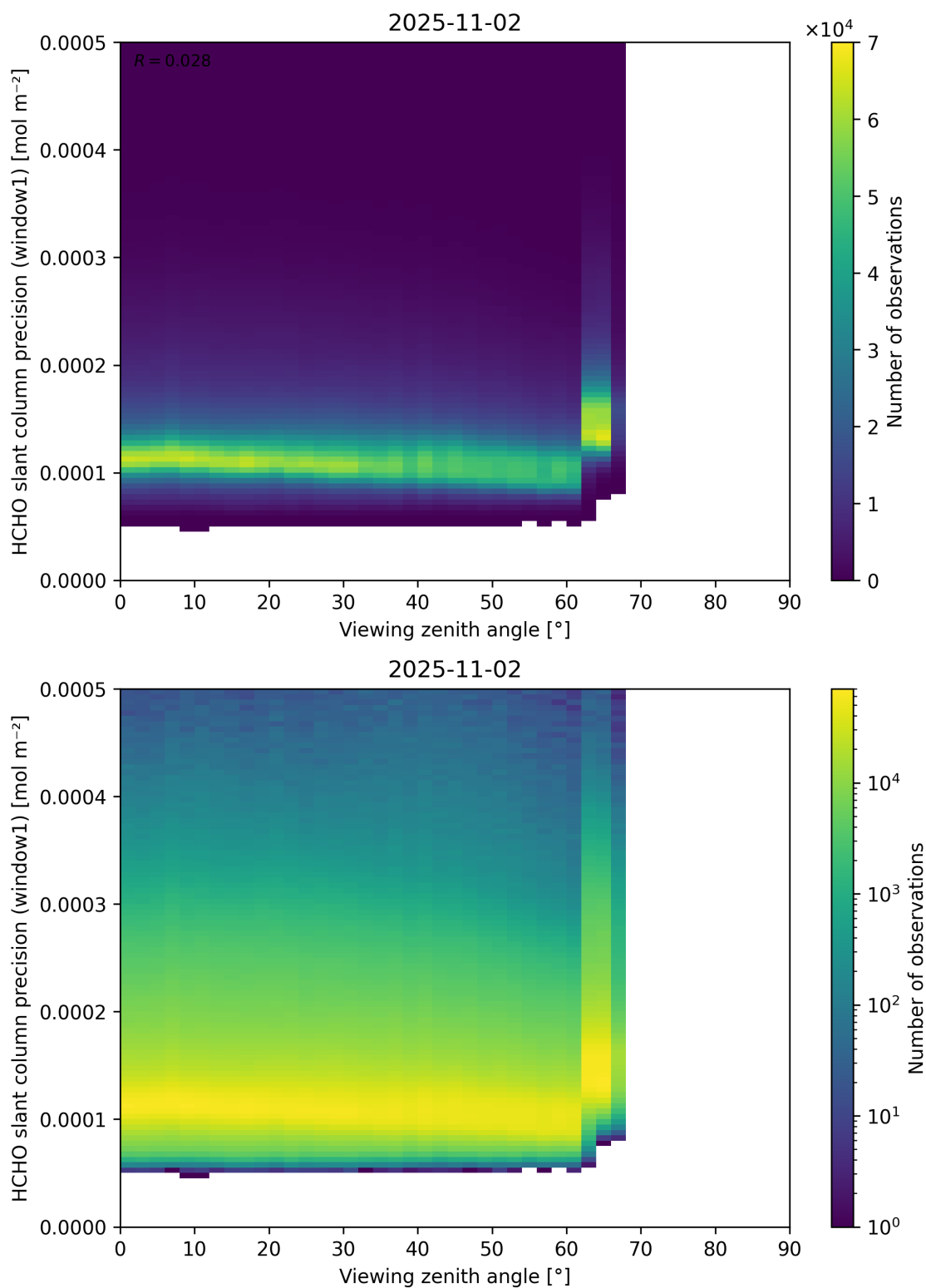
Figure 189: Scatter density plot of “Viewing zenith angle” against “HCHO slant column precision (window1)” for 2025-11-02 to 2025-11-03.
