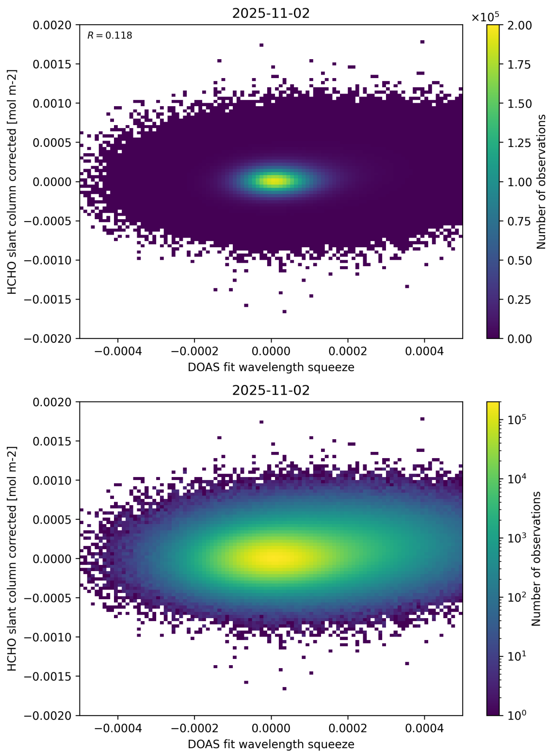
Figure 69: Scatter density plot of “DOAS fit wavelength squeeze” against “HCHO slant column corrected” for 2025-11-02 to 2025-11-03.
