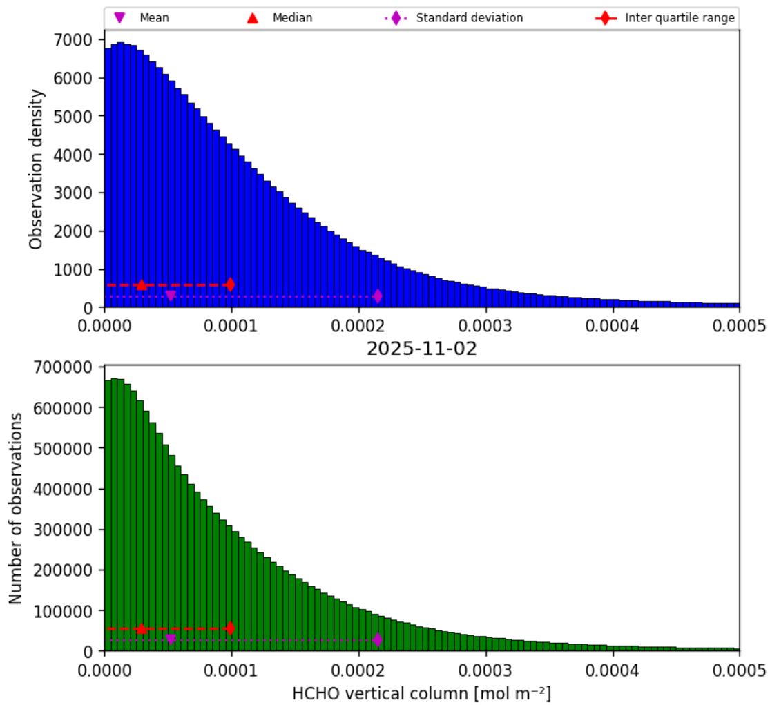
Figure 35: Histogram of “HCHO vertical column” for 2025-11-02 to 2025-11-03
