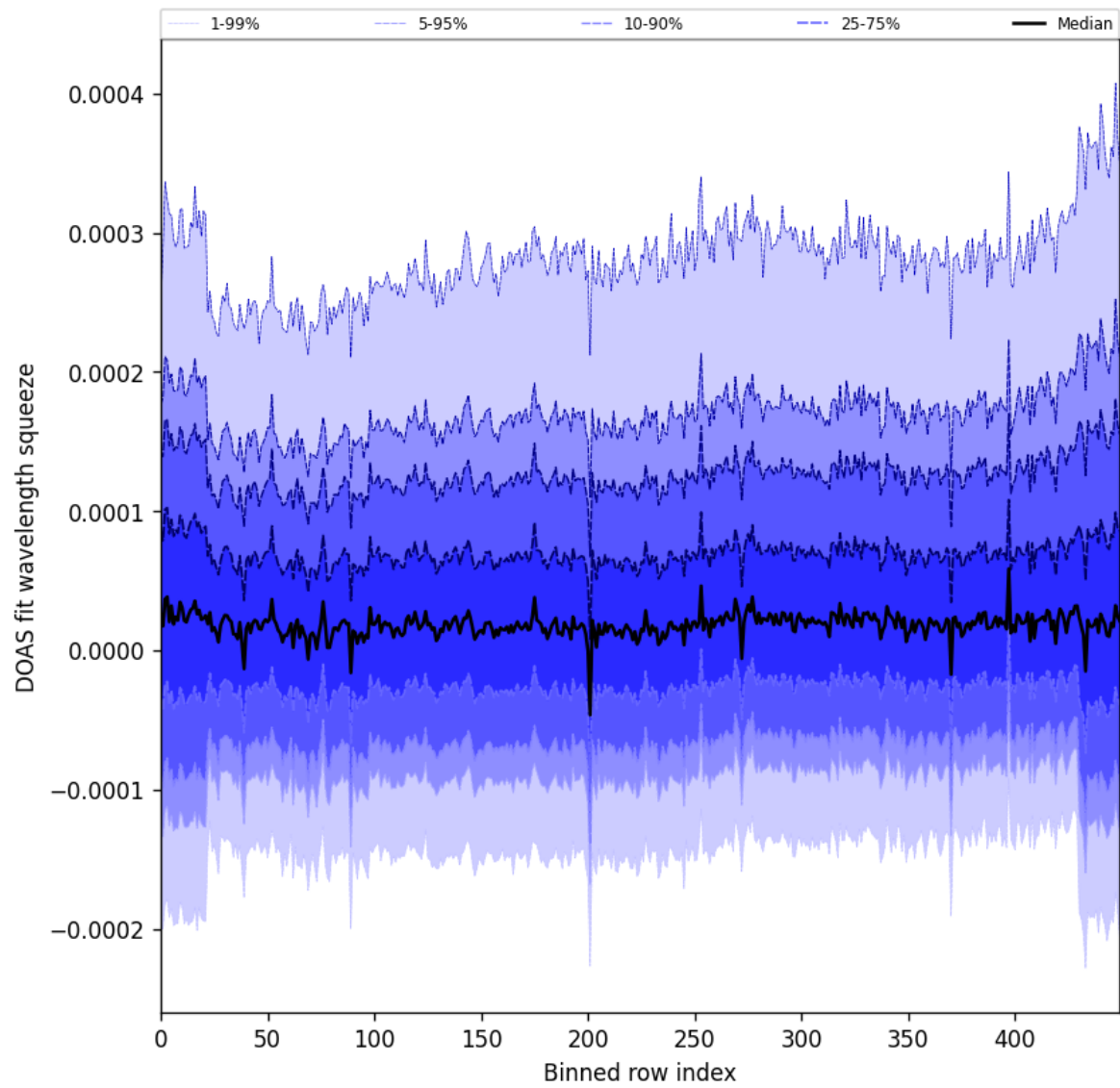
Figure 59: Along track statistics of “DOAS fit wavelength squeeze” for 2025-11-02 to 2025-11-03
