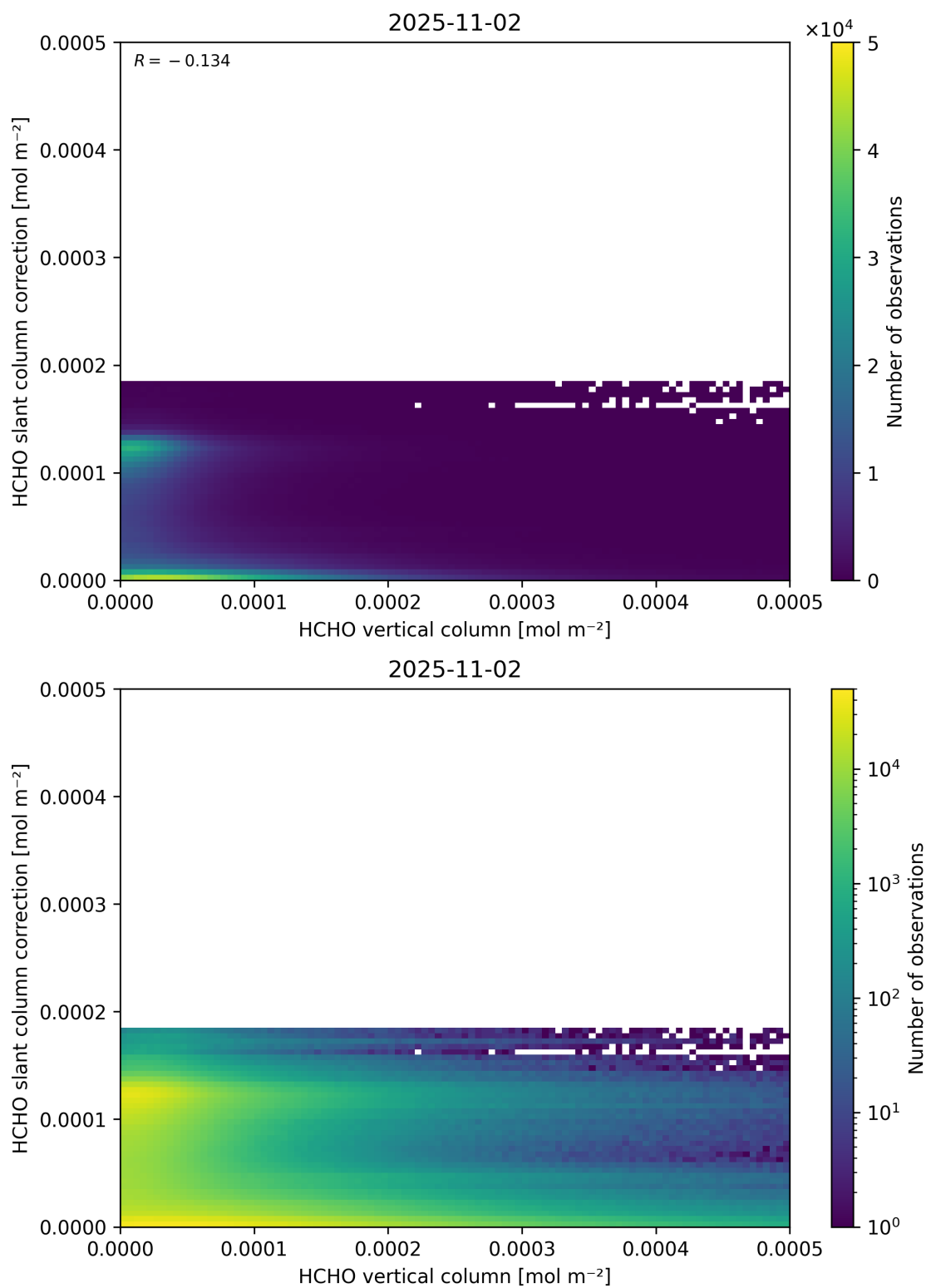
Figure 128: Scatter density plot of “HCHO vertical column” against “HCHO slant column correction” for 2025-11-02 to 2025-11-03.
