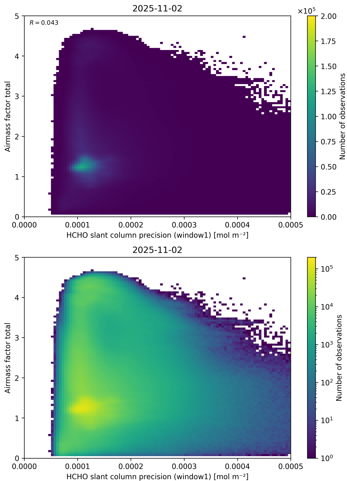
Figure 94: Scatter density plot of “HCHO slant column precision (window1)” against “Airmass factor total” for 2025-11-02 to 2025-11-03.
