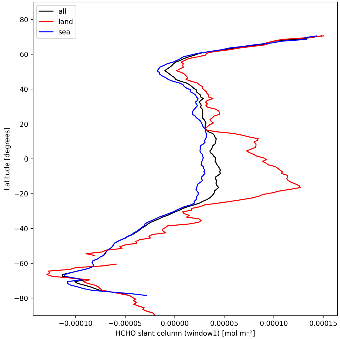
Figure 24: Zonal average of “HCHO slant column (window1)” for 2025-11-02 to 2025-11-03.
