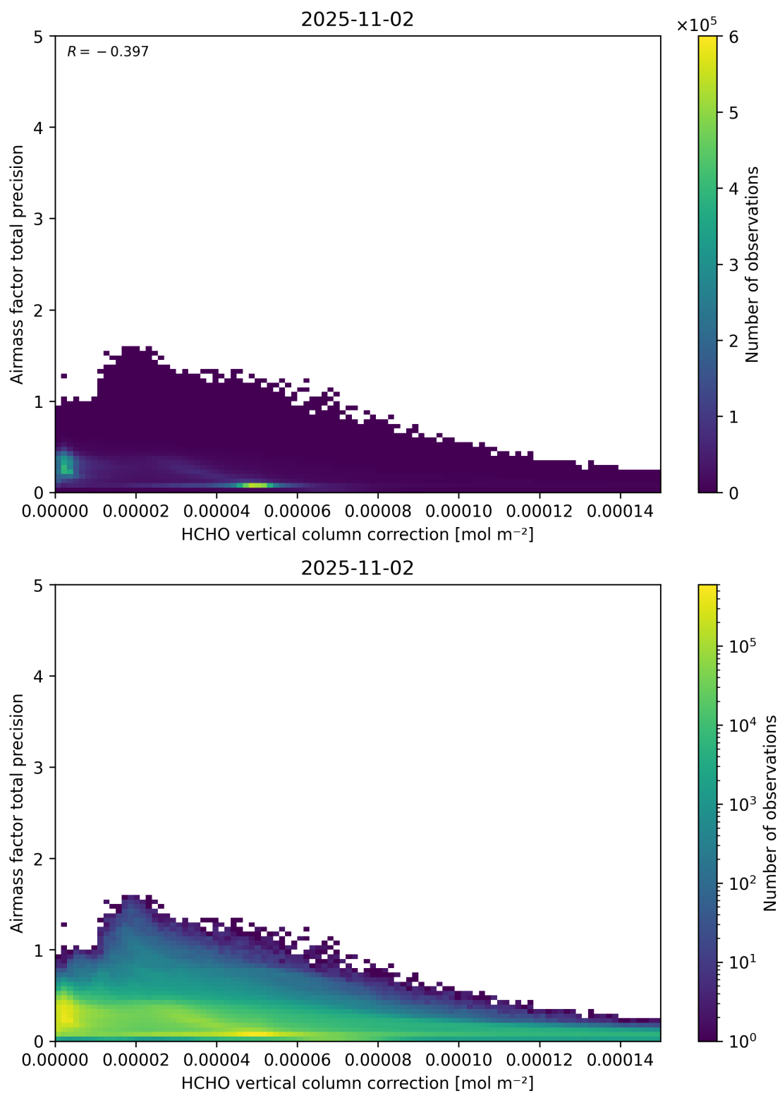
Figure 121: Scatter density plot of “HCHO vertical column correction” against “Airmass factor total precision” for 2025-11-02 to 2025-11-03.
