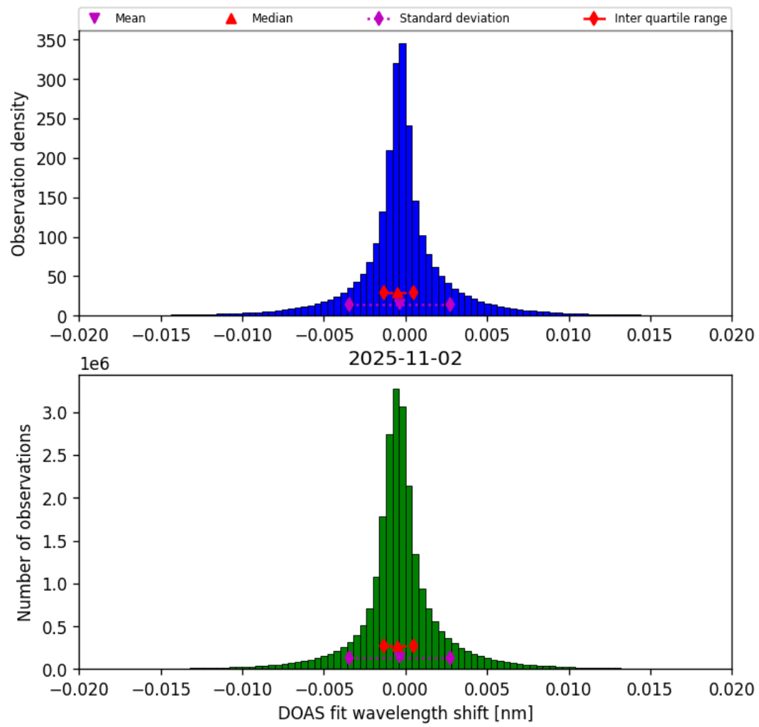
Figure 44: Histogram of “DOAS fit wavelength shift” for 2025-11-02 to 2025-11-03
