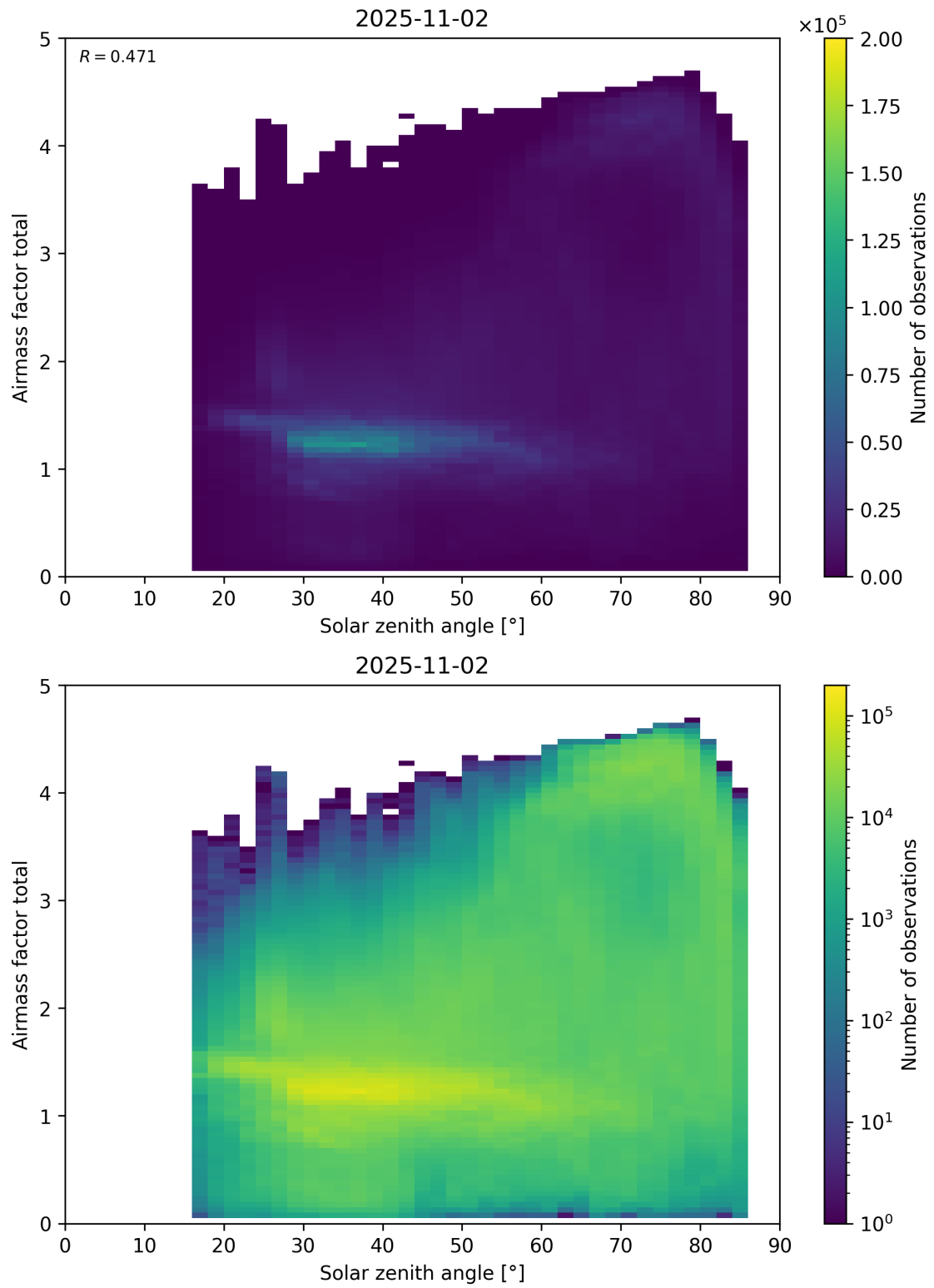
Figure 175: Scatter density plot of “Solar zenith angle” against “Airmass factor total” for 2025-11-02 to 2025-11-03.
