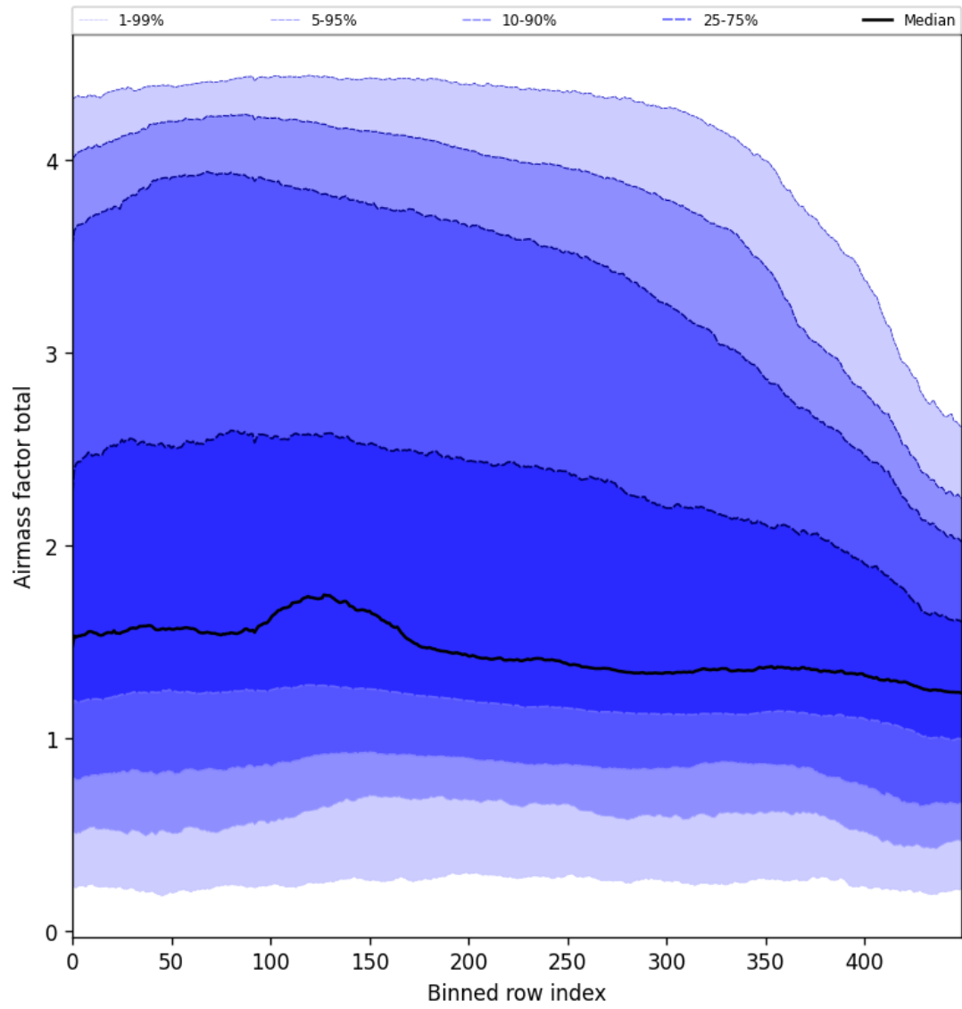
Figure 54: Along track statistics of “Airmass factor total” for 2025-11-02 to 2025-11-03
