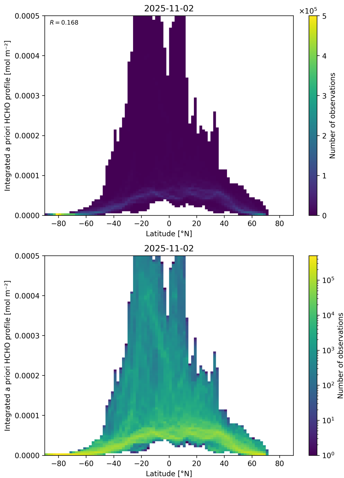
Figure 166: Scatter density plot of “Latitude” against “Integrated a priori HCHO profile” for 2025-11-02 to 2025-11-03.
