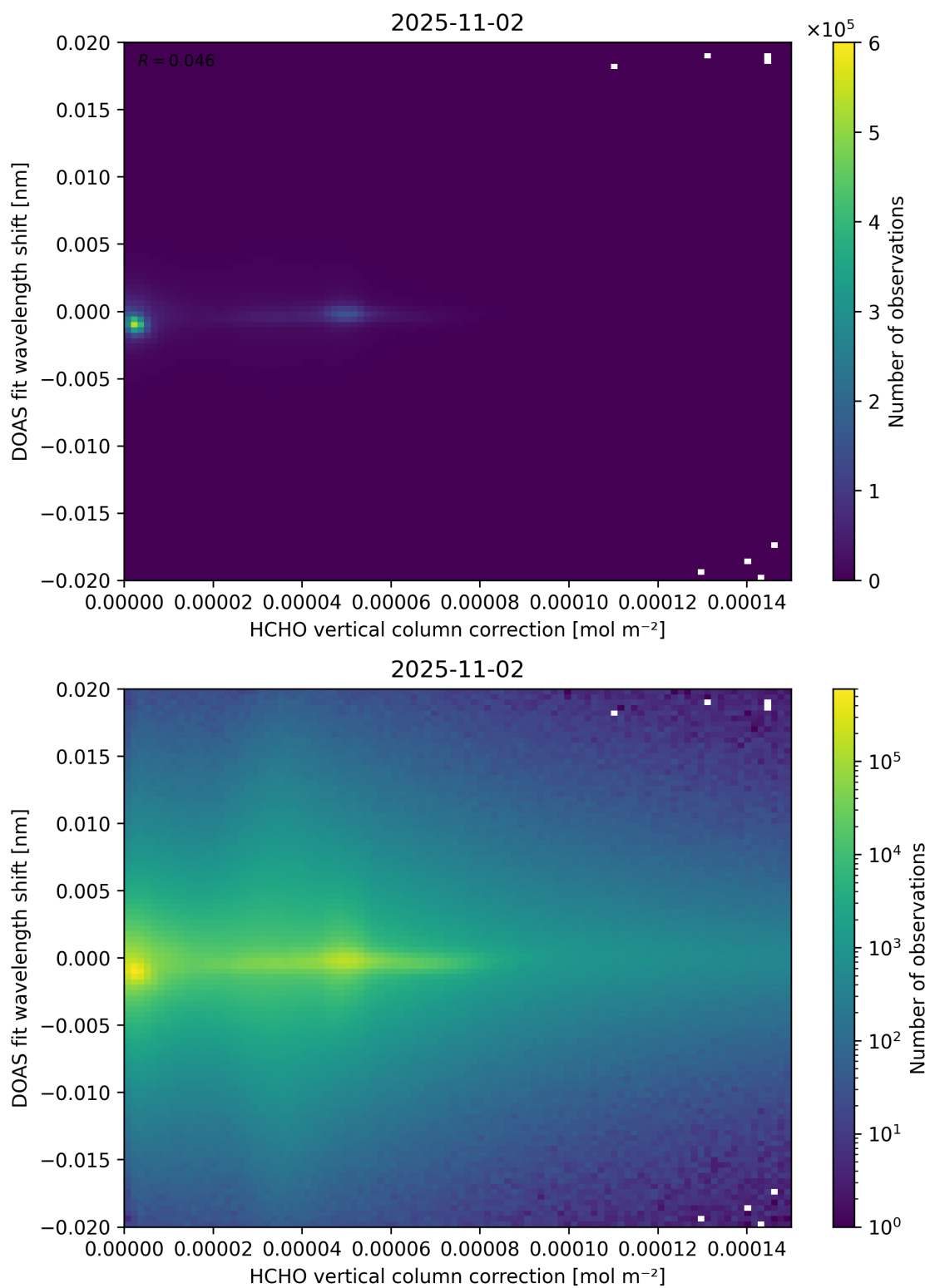
Figure 113: Scatter density plot of “HCHO vertical column correction” against “DOAS fit wavelength shift” for 2025-11-02 to 2025-11-03.
