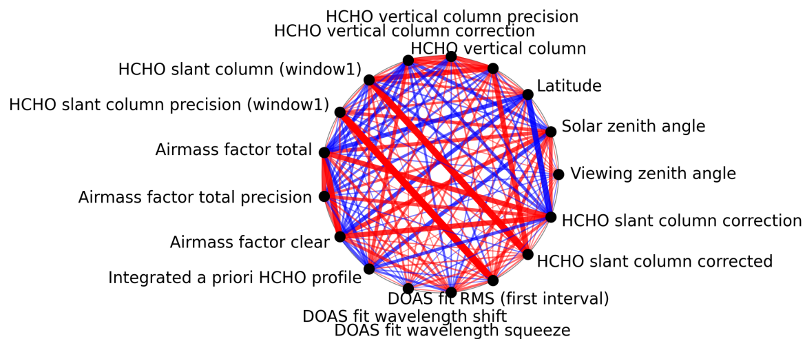
Figure 1: Map of correlation graph for 2025-11-02 to 2025-11-03.
