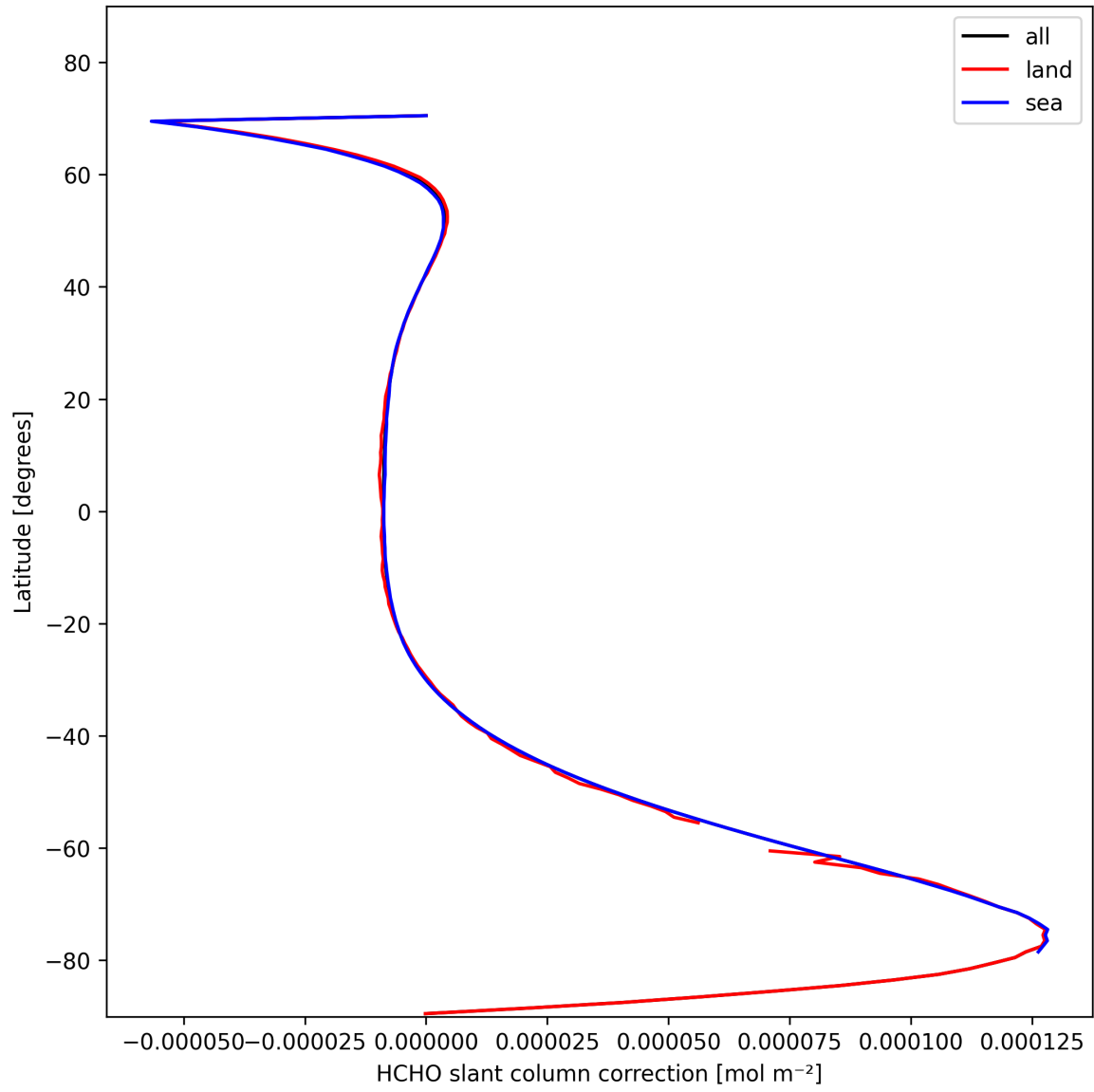
Figure 33: Zonal average of "HCHO slant column correction" for 2025-11-02 to 2025-11-03.
