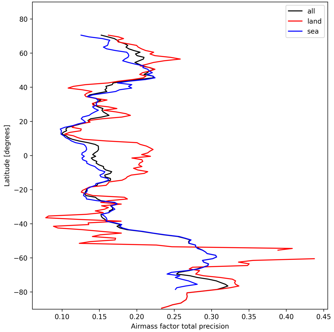
Figure 27: Zonal average of “Airmass factor total precision” for 2025-11-02 to 2025-11-03.
