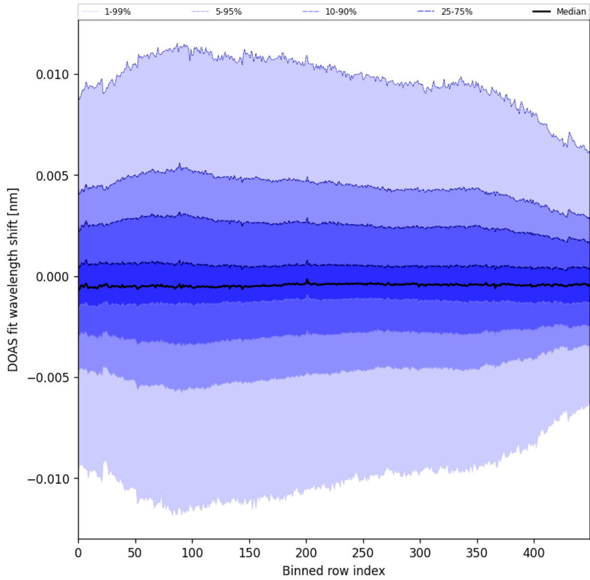
Figure 58: Along track statistics of “DOAS fit wavelength shift” for 2025-11-02 to 2025-11-03
