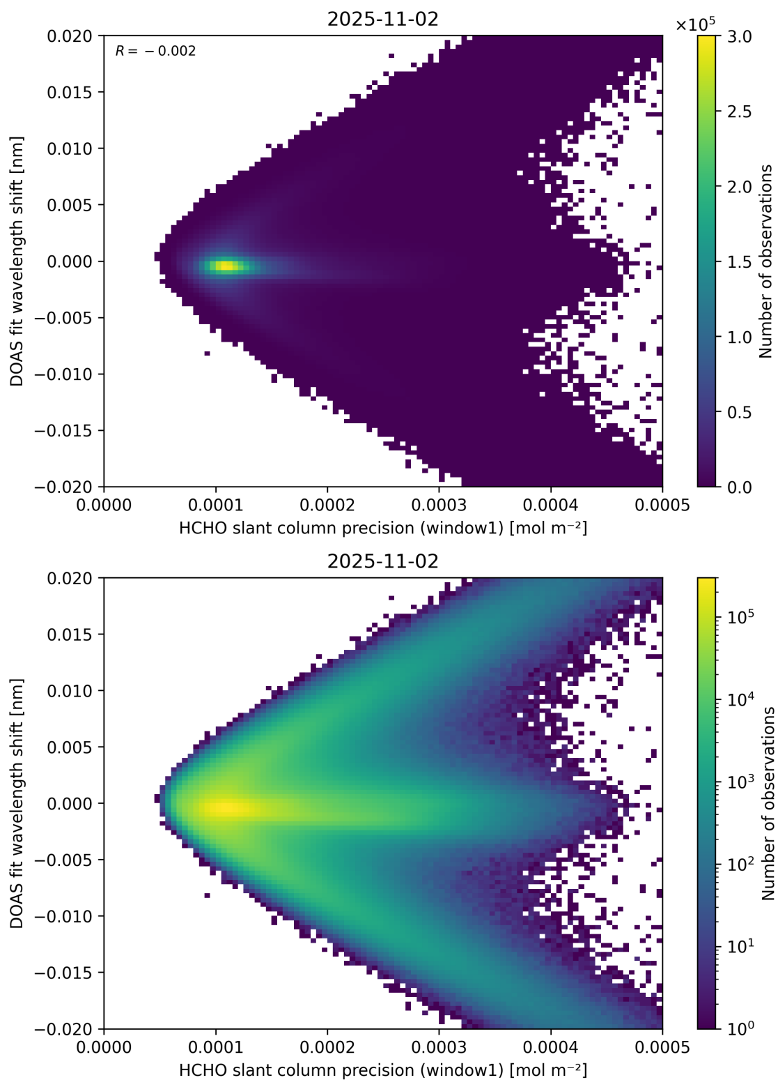
Figure 89: Scatter density plot of “HCHO slant column precision (window1)” against “DOAS fit wavelength shift” for 2025-11-02 to 2025-11-03.
