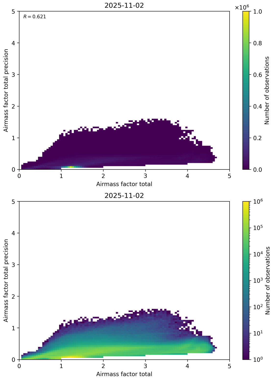
Figure 103: Scatter density plot of “Airmass factor total” against “Airmass factor total precision” for 2025-11-02 to 2025-11-03.
