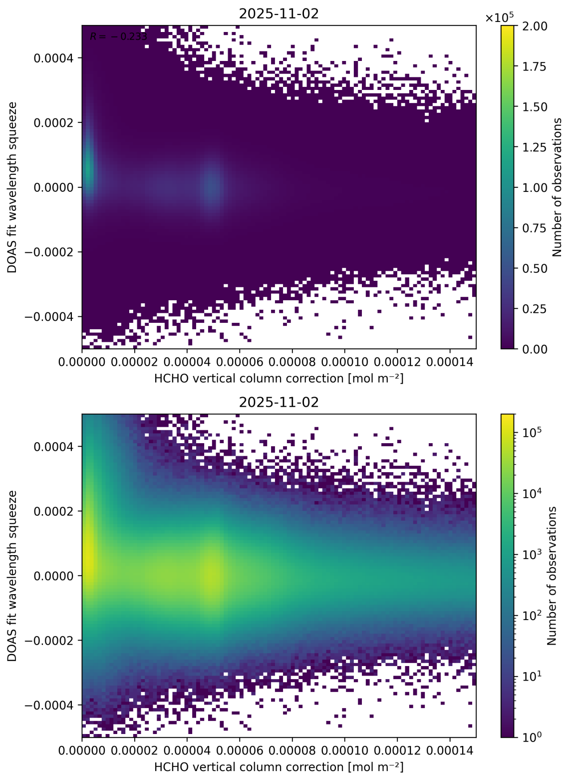
Figure 114: Scatter density plot of “HCHO vertical column correction” against “DOAS fit wavelength squeeze” for 2025-11-02 to 2025-11-03.
