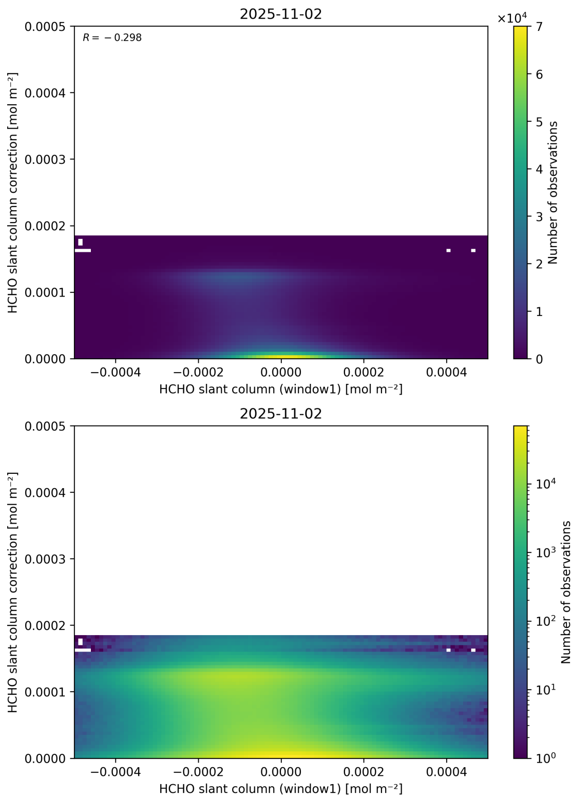
Figure 83: Scatter density plot of “HCHO slant column (window1)” against “HCHO slant column correction” for 2025-11-02 to 2025-11-03.
