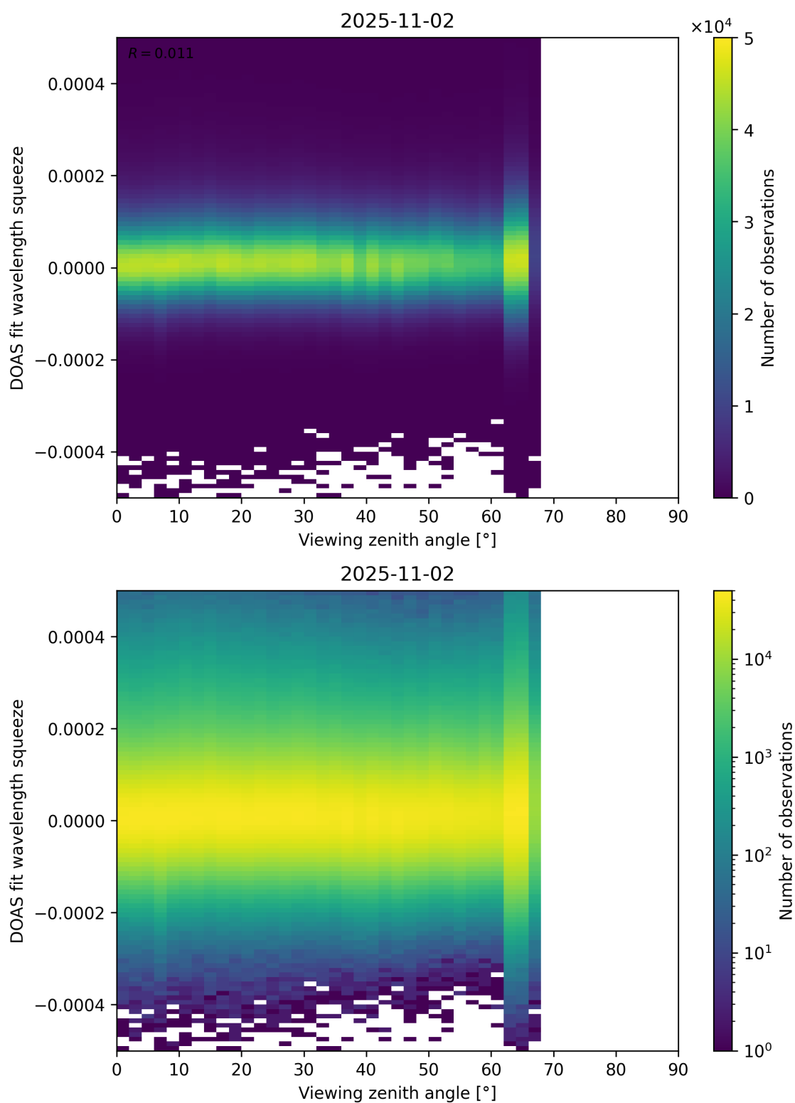
Figure 184: Scatter density plot of “Viewing zenith angle” against “DOAS fit wavelength squeeze” for 2025-11-02 to 2025-11-03.
