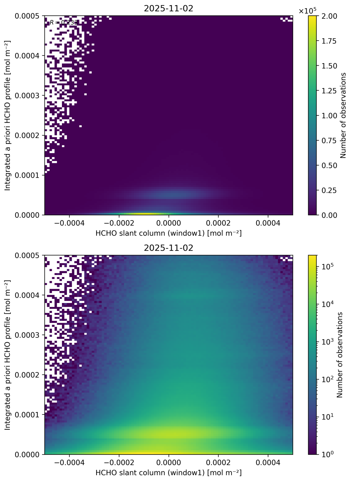
Figure 87: Scatter density plot of “HCHO slant column (window1)” against “Integrated a priori HCHO profile” for 2025-11-02 to 2025-11-03.
