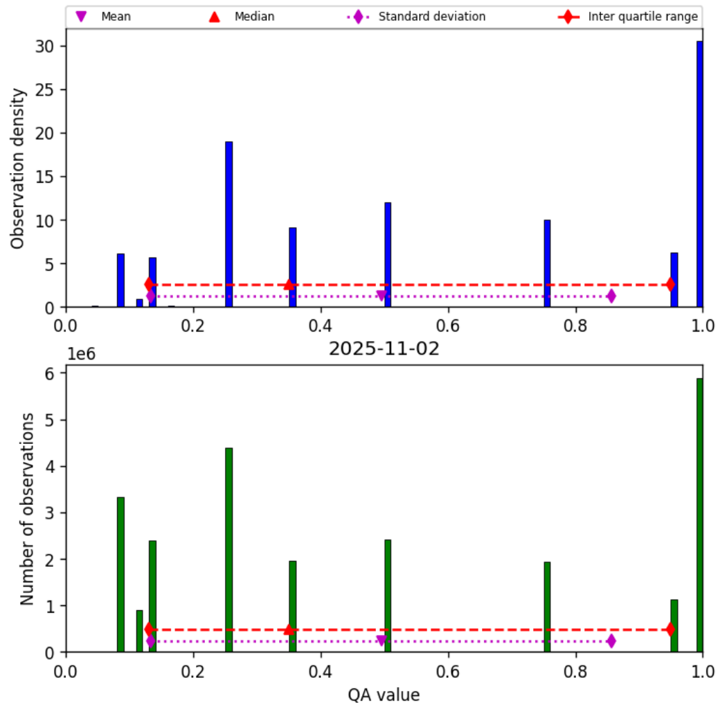
Figure 34: Histogram of “QA value” for 2025-11-02 to 2025-11-03
