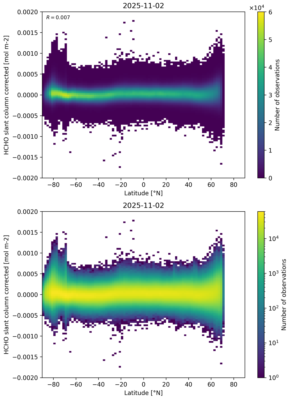
Figure 157: Scatter density plot of “Latitude” against “HCHO slant column corrected” for 2025-11-02 to 2025-11-03.
