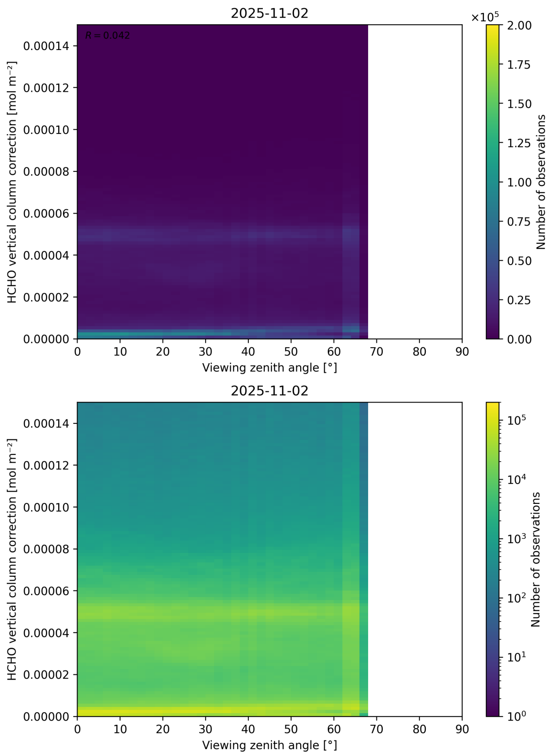
Figure 193: Scatter density plot of “Viewing zenith angle” against “HCHO vertical column correction” for 2025-11-02 to 2025-11-03.
