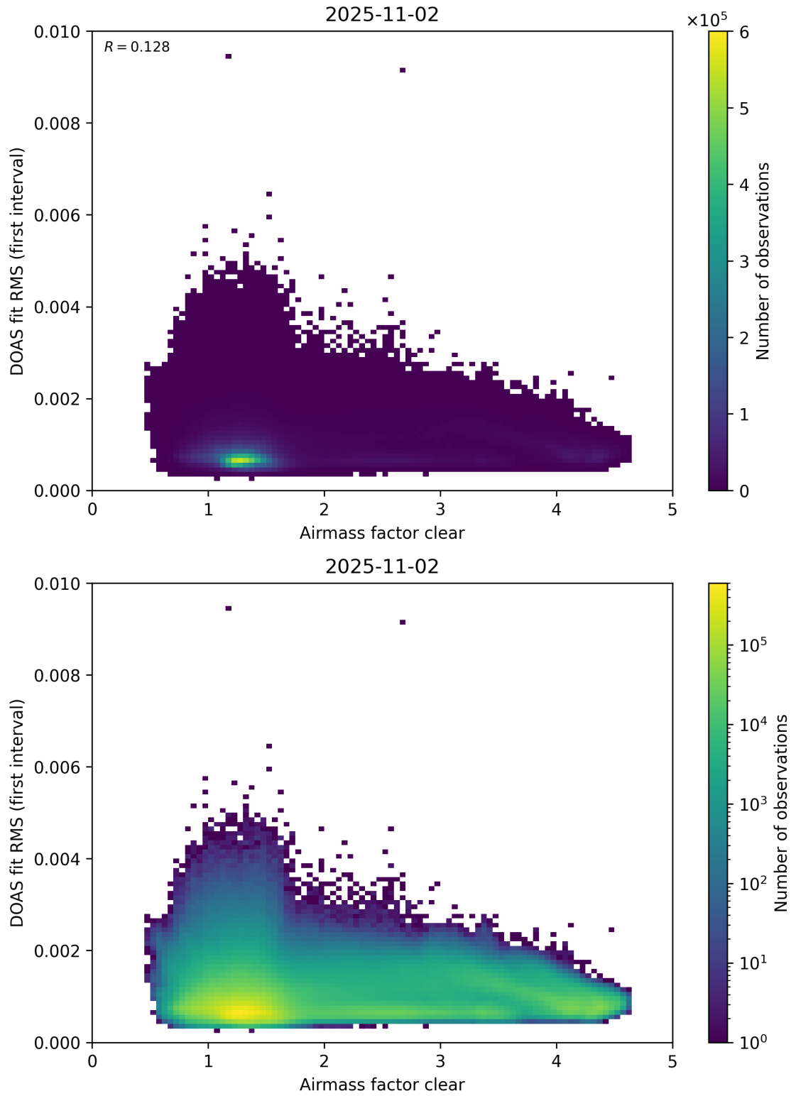
Figure 71: Scatter density plot of “Airmass factor clear” against “DOAS fit RMS (first interval)” for 2025-11-02 to 2025-11-03.
