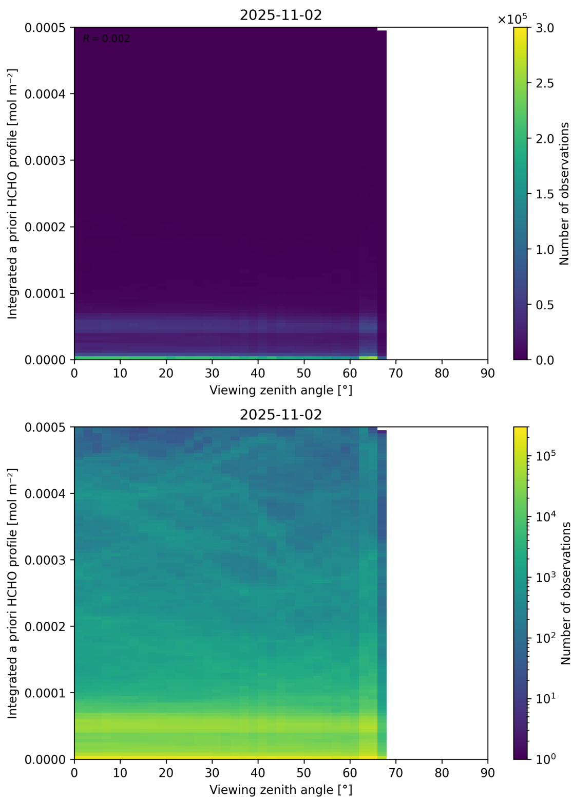
Figure 195: Scatter density plot of “Viewing zenith angle” against “Integrated a priori HCHO profile” for 2025-11-02 to 2025-11-03.
