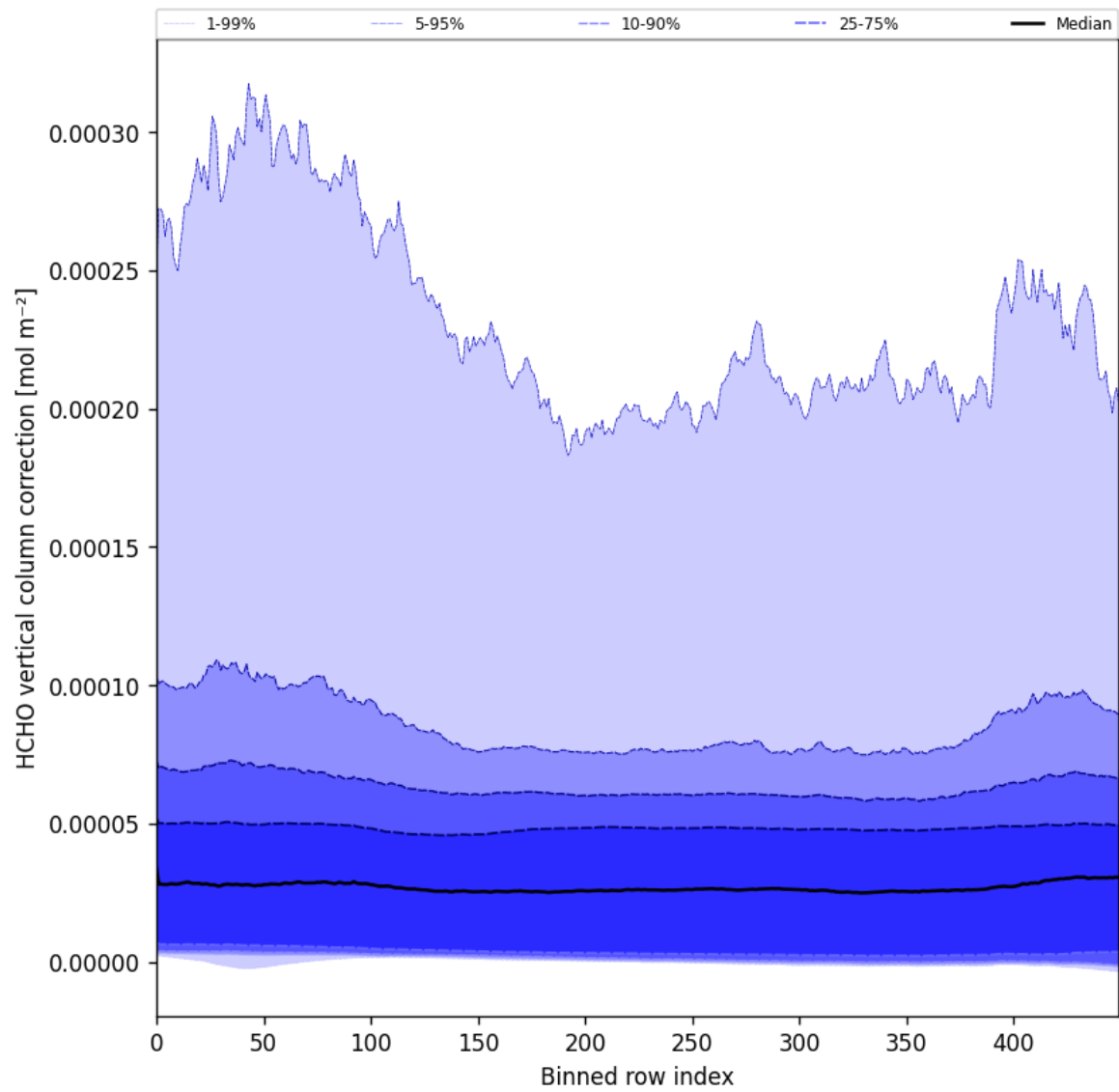
Figure 51: Along track statistics of “HCHO vertical column correction” for 2025-11-02 to 2025-11-03
