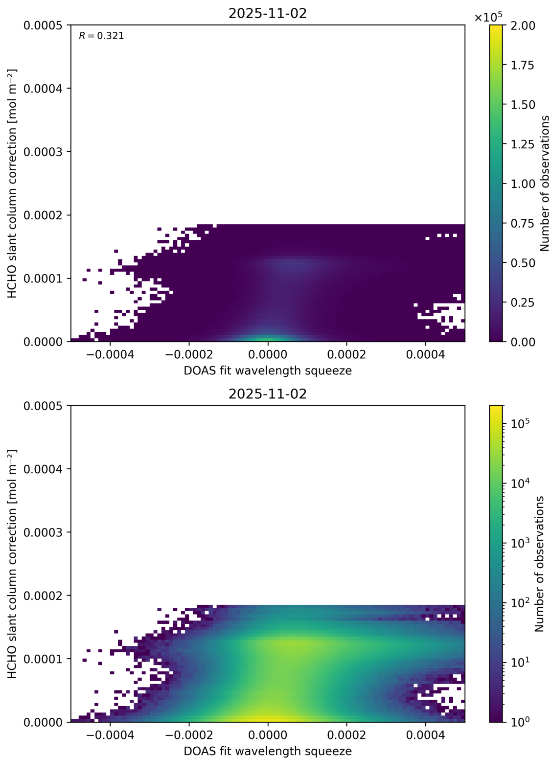
Figure 70: Scatter density plot of “DOAS fit wavelength squeeze” against “HCHO slant column correction” for 2025-11-02 to 2025-11-03.
