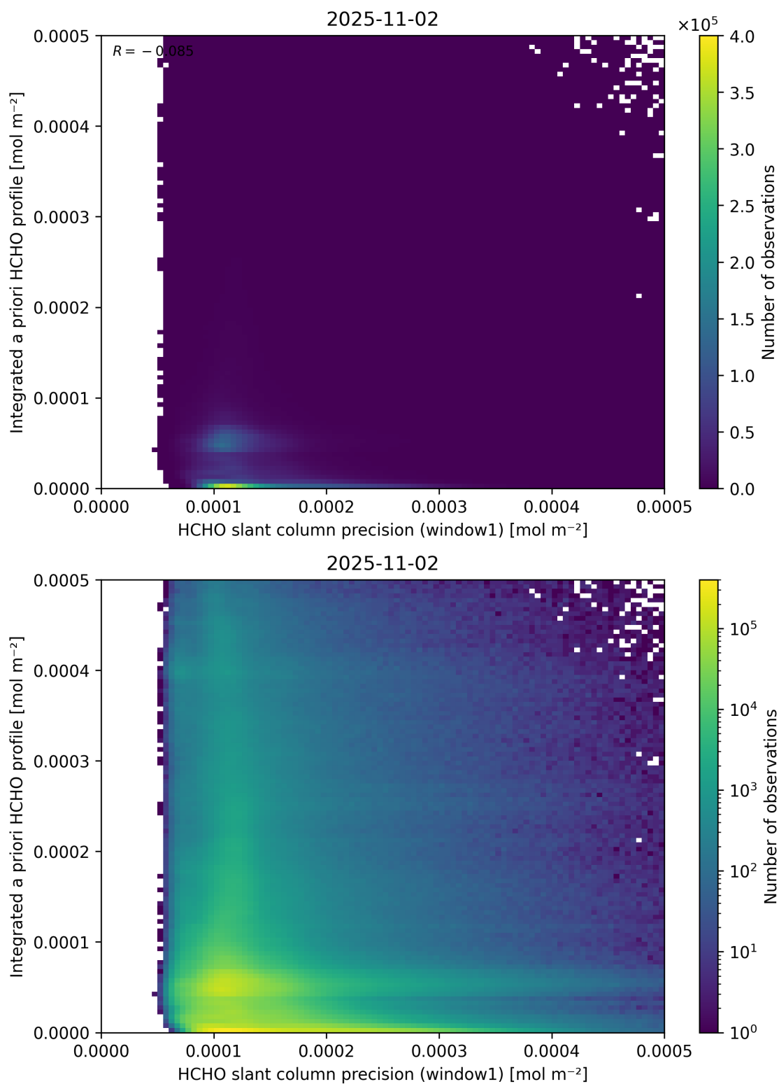
Figure 96: Scatter density plot of “HCHO slant column precision (window1)” against “Integrated a priori HCHO profile” for 2025-11-02 to 2025-11-03.
