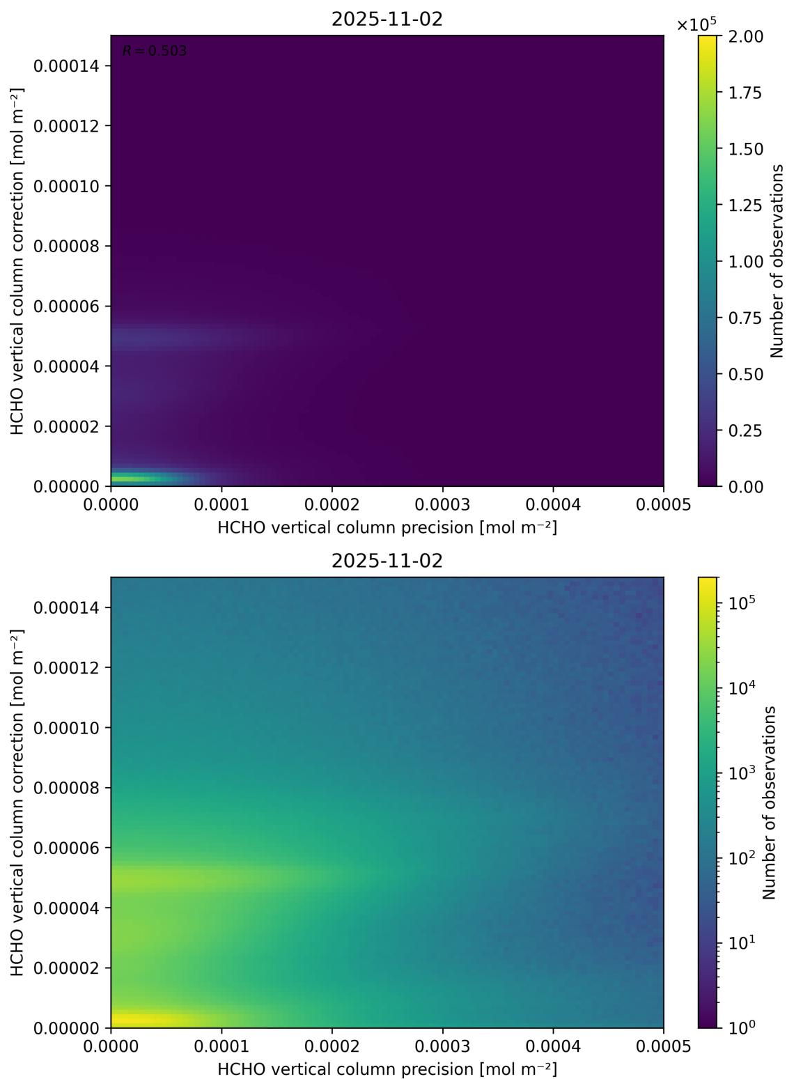
Figure 146: Scatter density plot of “HCHO vertical column precision” against “HCHO vertical column correction” for 2025-11-02 to 2025-11-03.
