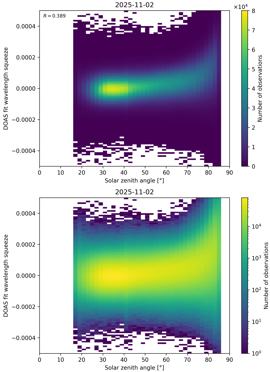
Figure 169: Scatter density plot of “Solar zenith angle” against “DOAS fit wavelength squeeze” for 2025-11-02 to 2025-11-03.
