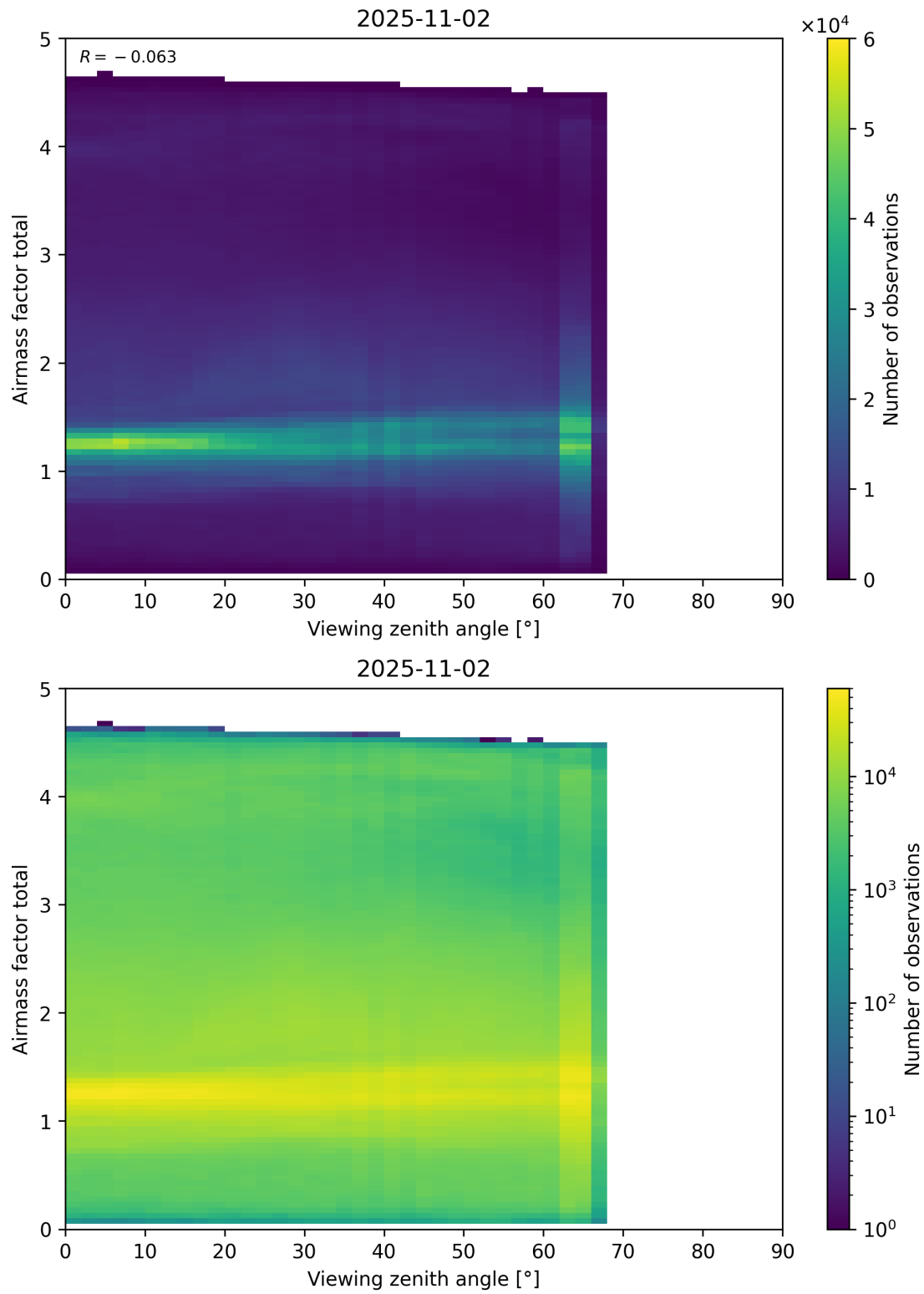
Figure 190: Scatter density plot of “Viewing zenith angle” against “Airmass factor total” for 2025-11-02 to 2025-11-03.
