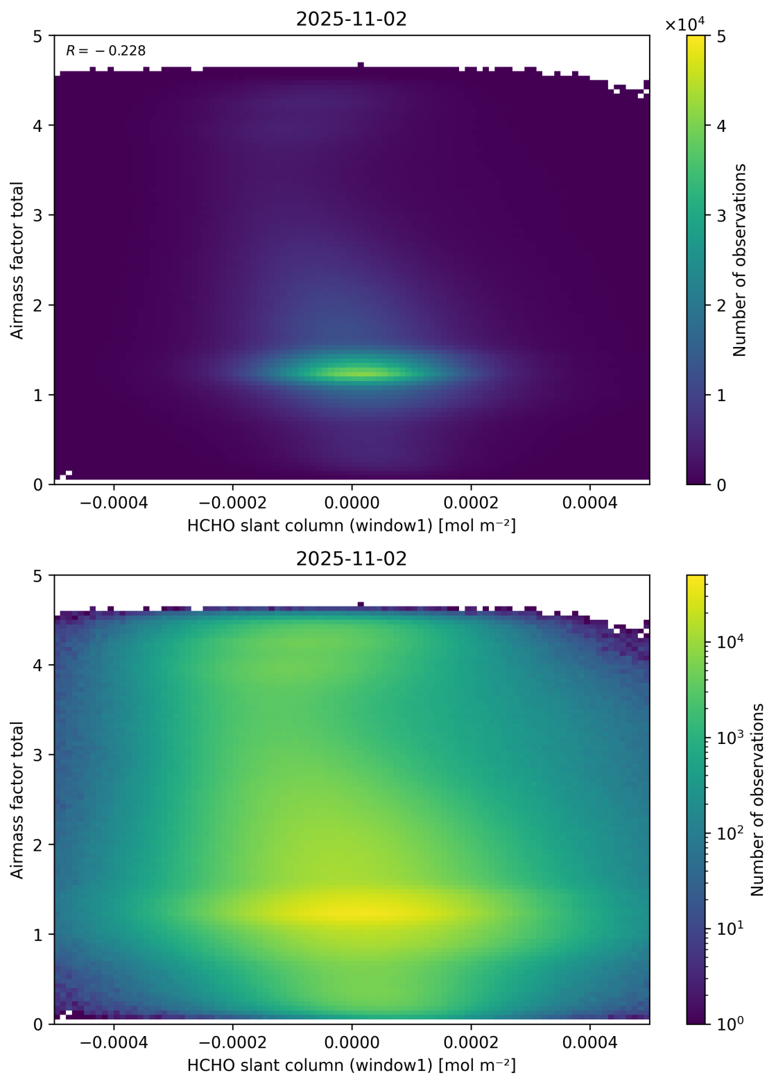
Figure 85: Scatter density plot of “HCHO slant column (window1)” against “Airmass factor total” for 2025-11-02 to 2025-11-03.
