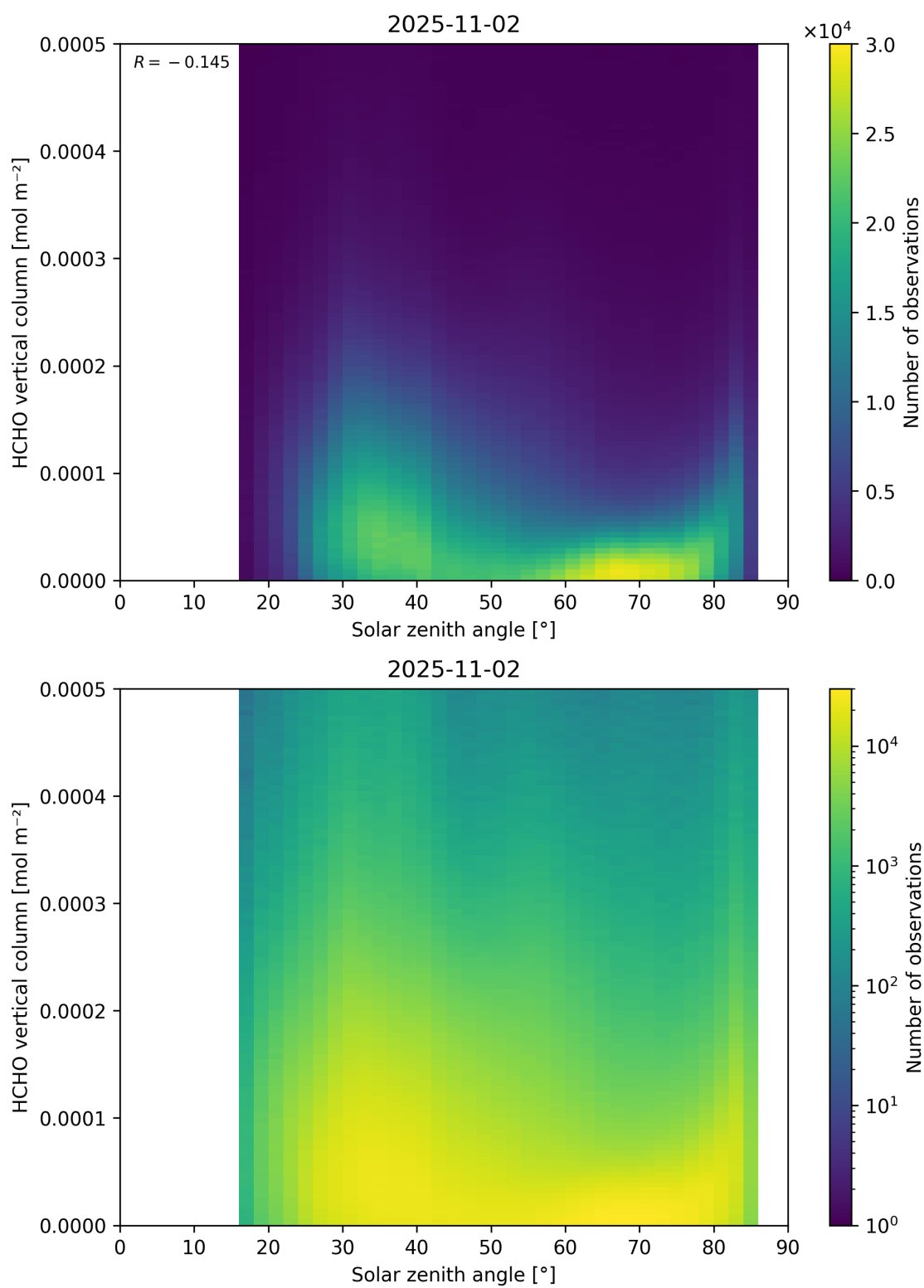
Figure 177: Scatter density plot of “Solar zenith angle” against “HCHO vertical column” for 2025-11-02 to 2025-11-03.
