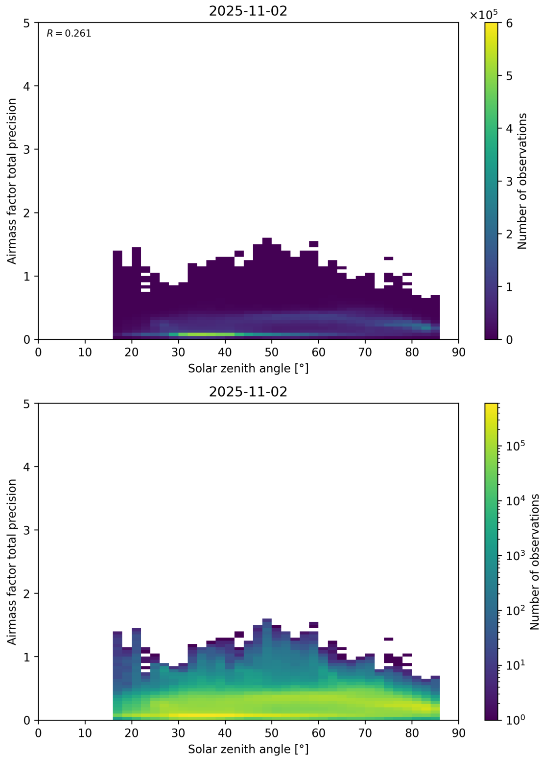
Figure 176: Scatter density plot of “Solar zenith angle” against “Airmass factor total precision” for 2025-11-02 to 2025-11-03.
