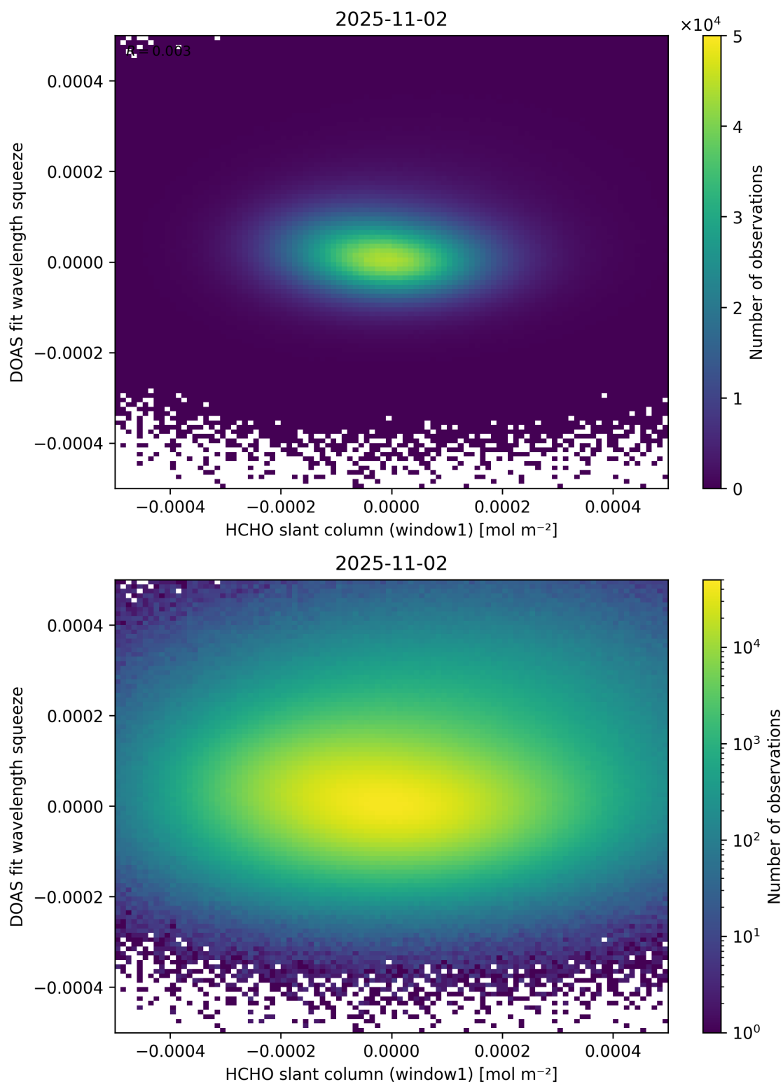
Figure 80: Scatter density plot of “HCHO slant column (window1)” against “DOAS fit wavelength squeeze” for 2025-11-02 to 2025-11-03.
