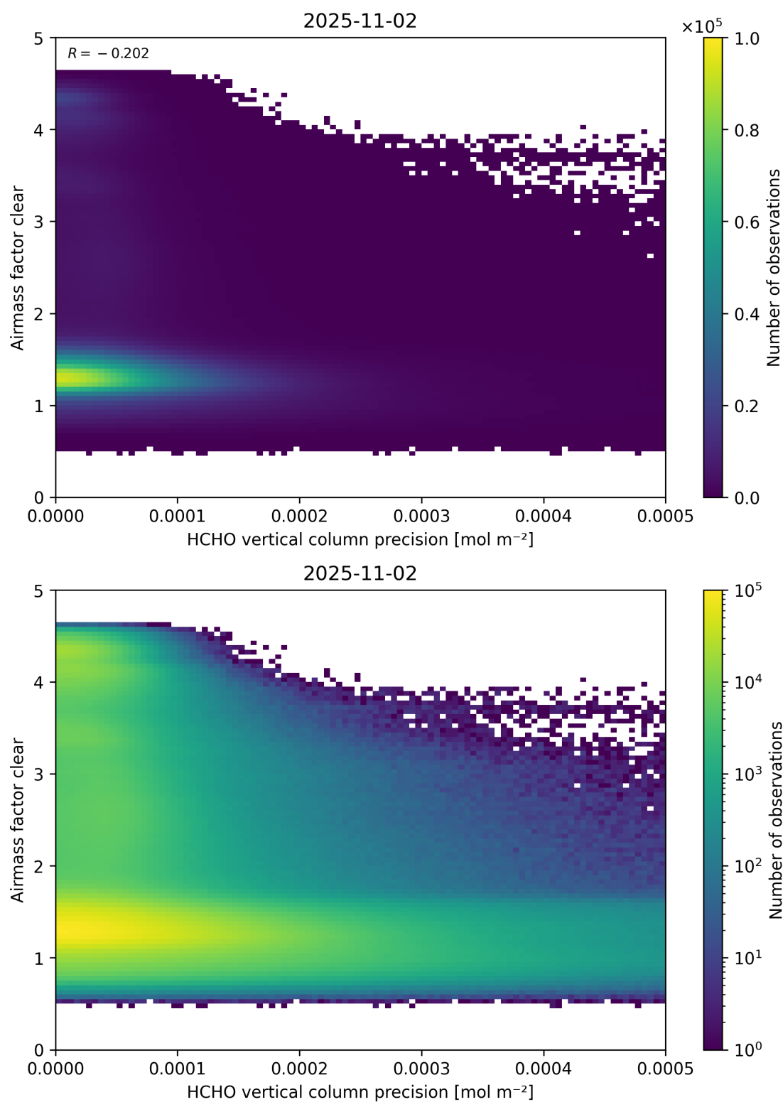
Figure 139: Scatter density plot of “HCHO vertical column precision” against “Airmass factor clear” for 2025-11-02 to 2025-11-03.
