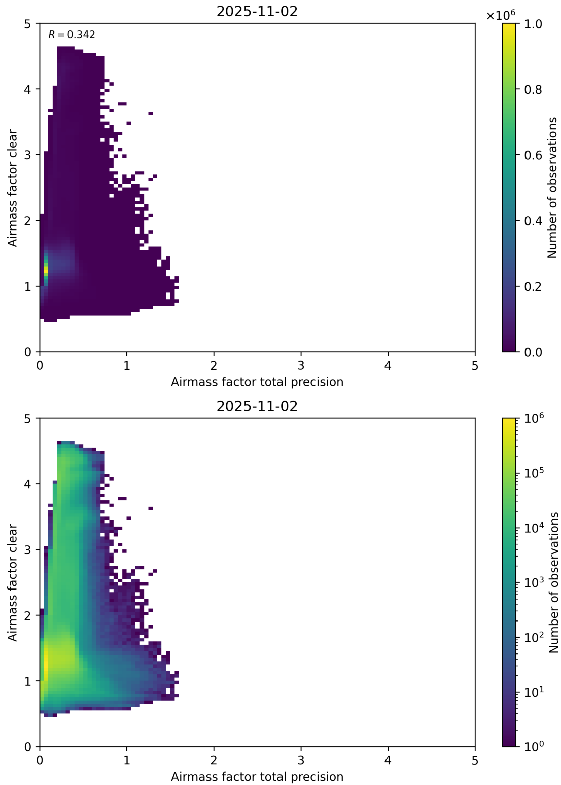
Figure 108: Scatter density plot of “Airmass factor total precision” against “Airmass factor clear” for 2025-11-02 to 2025-11-03.
