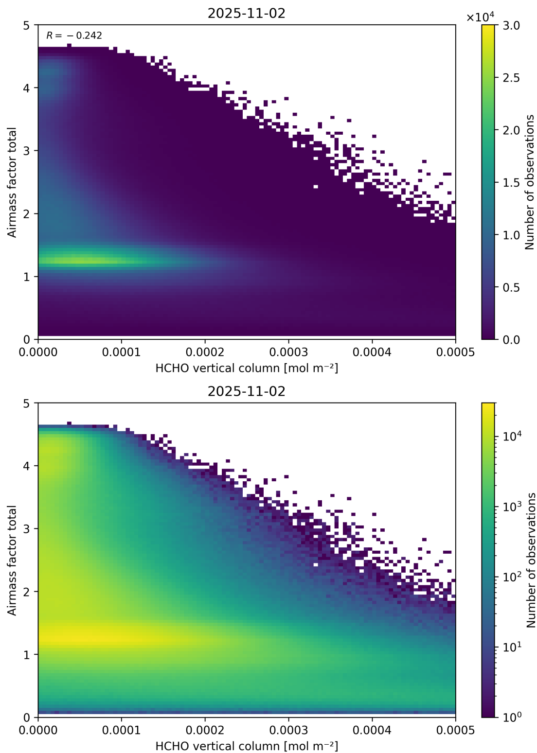
Figure 131: Scatter density plot of “HCHO vertical column” against “Airmass factor total” for 2025-11-02 to 2025-11-03.
