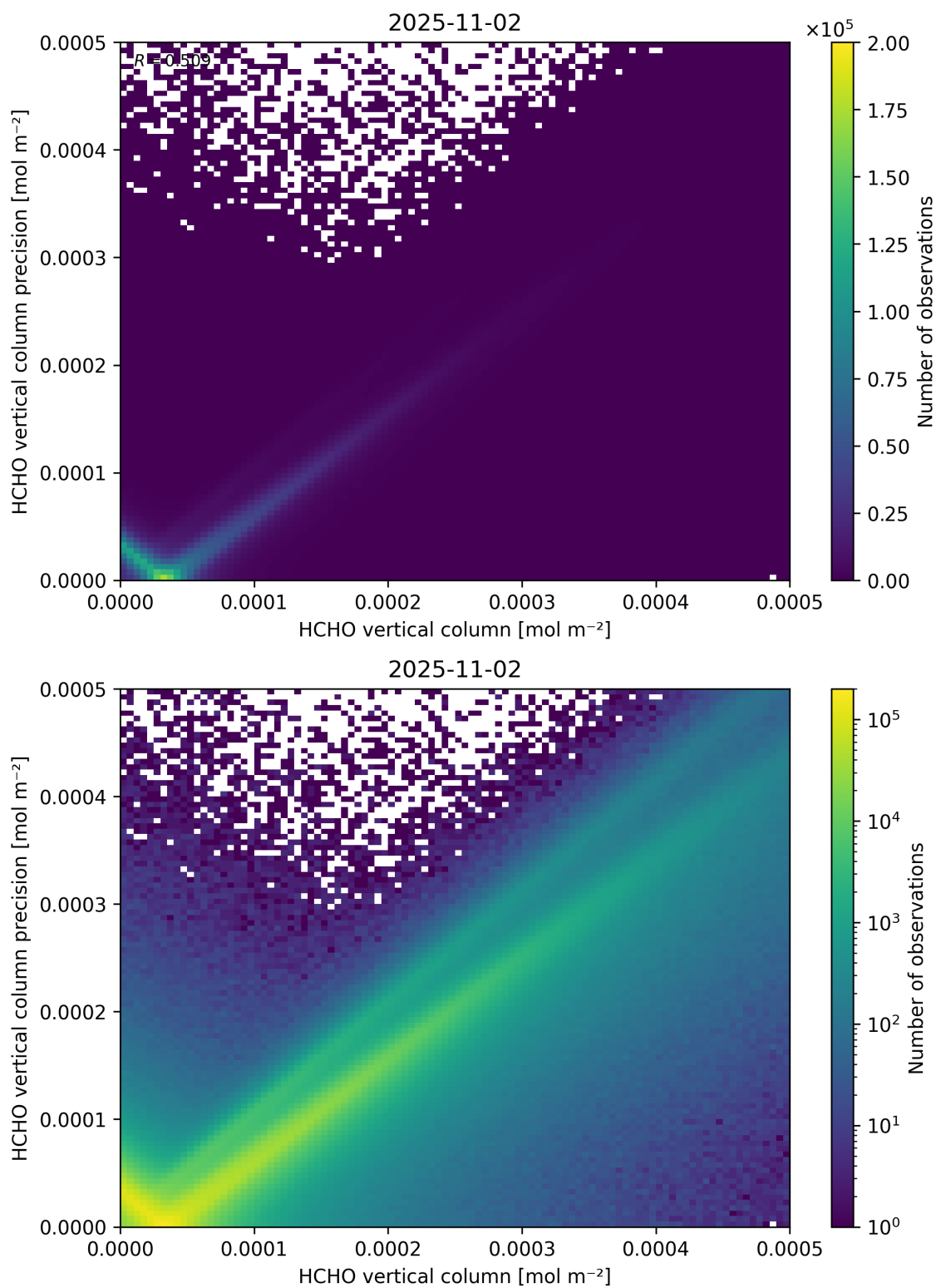
Figure 134: Scatter density plot of “HCHO vertical column” against “HCHO vertical column precision” for 2025-11-02 to 2025-11-03.
