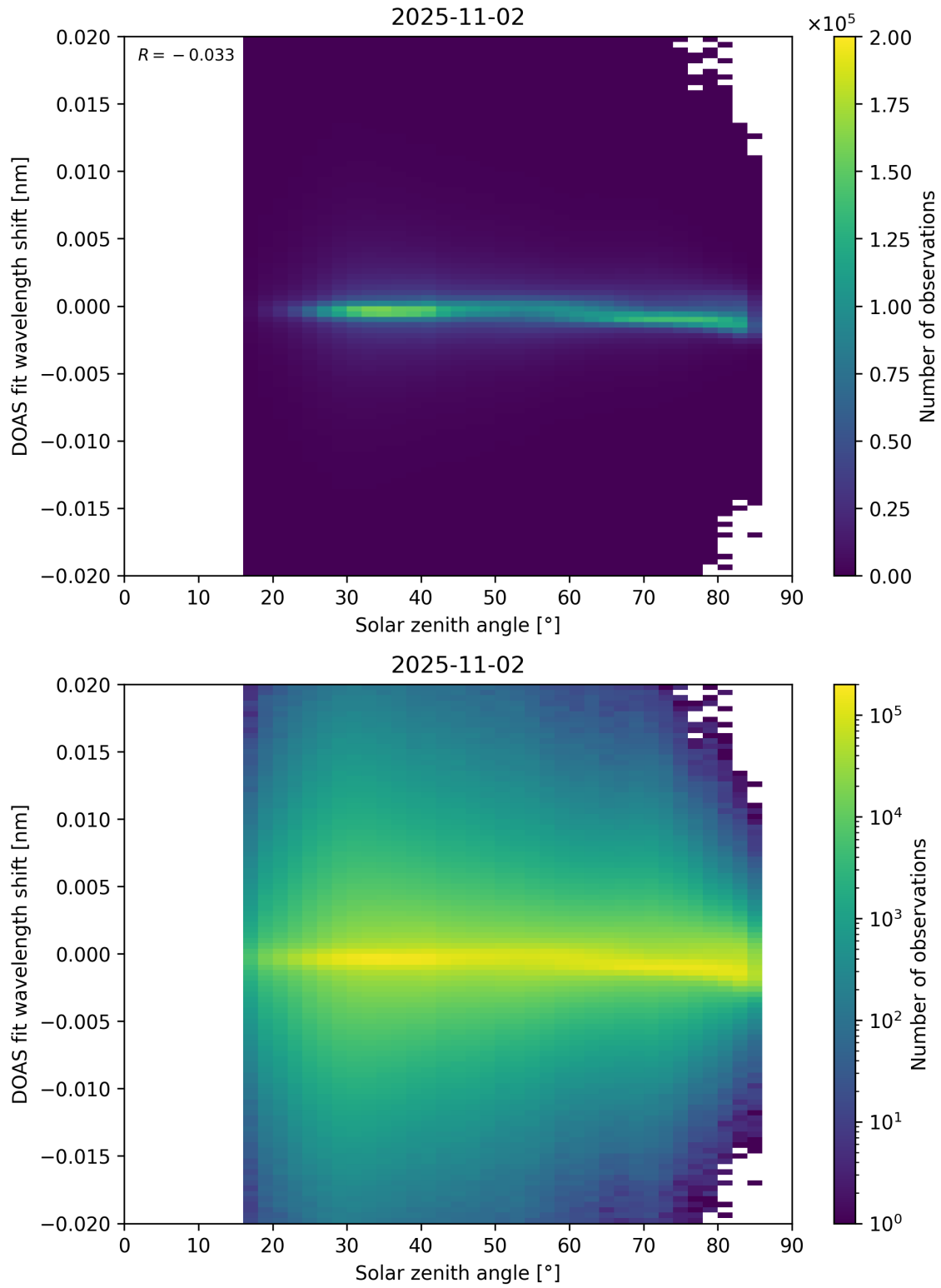
Figure 168: Scatter density plot of “Solar zenith angle” against “DOAS fit wavelength shift” for 2025-11-02 to 2025-11-03.
