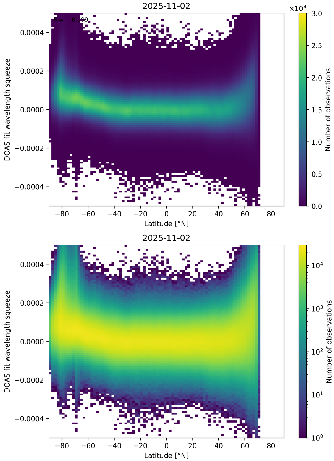
Figure 155: Scatter density plot of “Latitude” against “DOAS fit wavelength squeeze” for 2025-11-02 to 2025-11-03.
