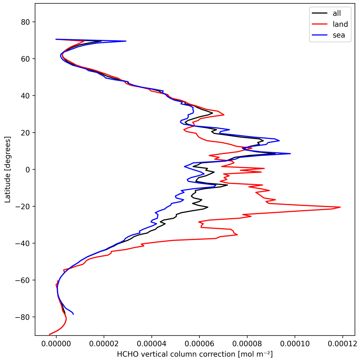
Figure 23: Zonal average of “HCHO vertical column correction” for 2025-11-02 to 2025-11-03.
