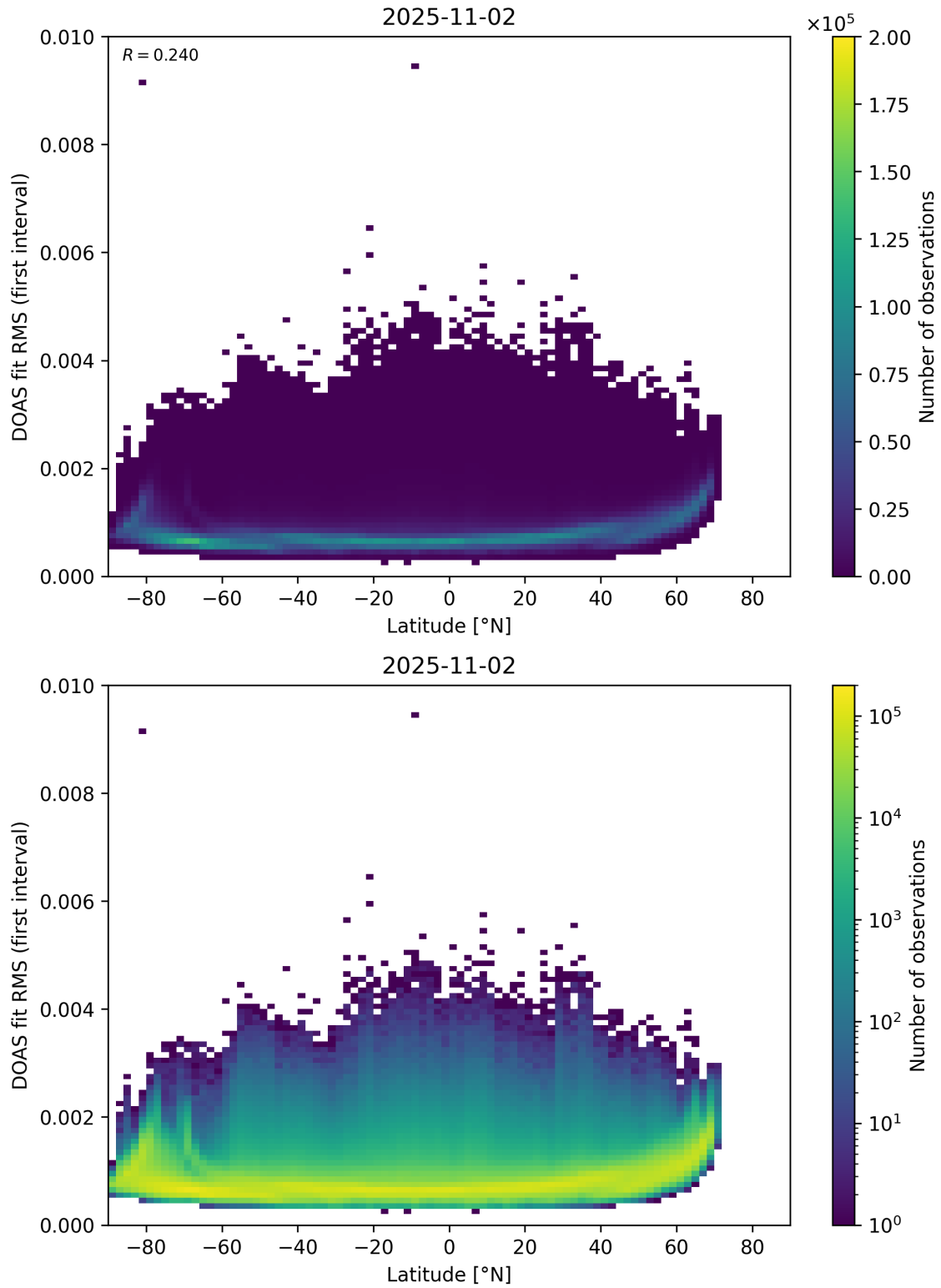
Figure 153: Scatter density plot of “Latitude” against “DOAS fit RMS (first interval)” for 2025-11-02 to 2025-11-03.
