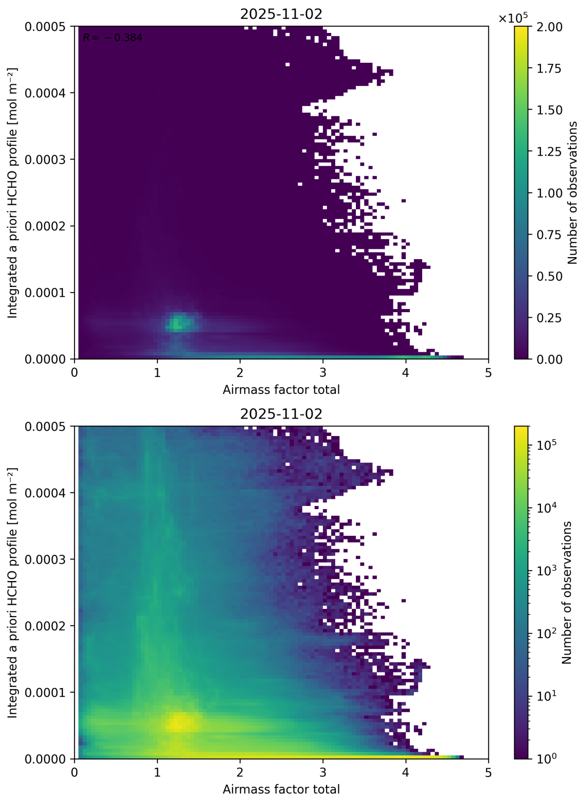
Figure 104: Scatter density plot of “Airmass factor total” against “Integrated a priori HCHO profile” for 2025-11-02 to 2025-11-03.
