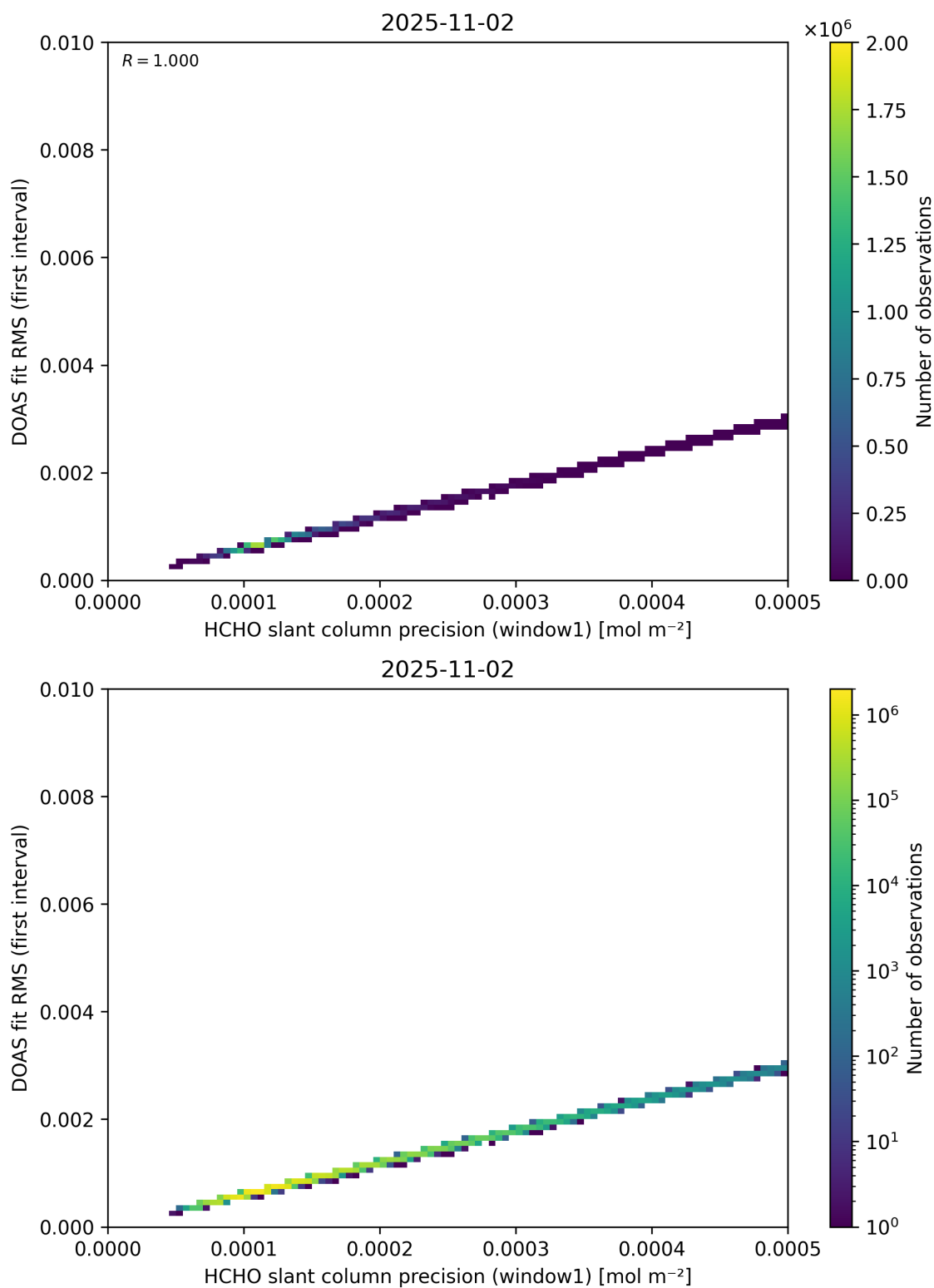
Figure 88: Scatter density plot of “HCHO slant column precision (window1)” against “DOAS fit RMS (first interval)” for 2025-11-02 to 2025-11-03.
