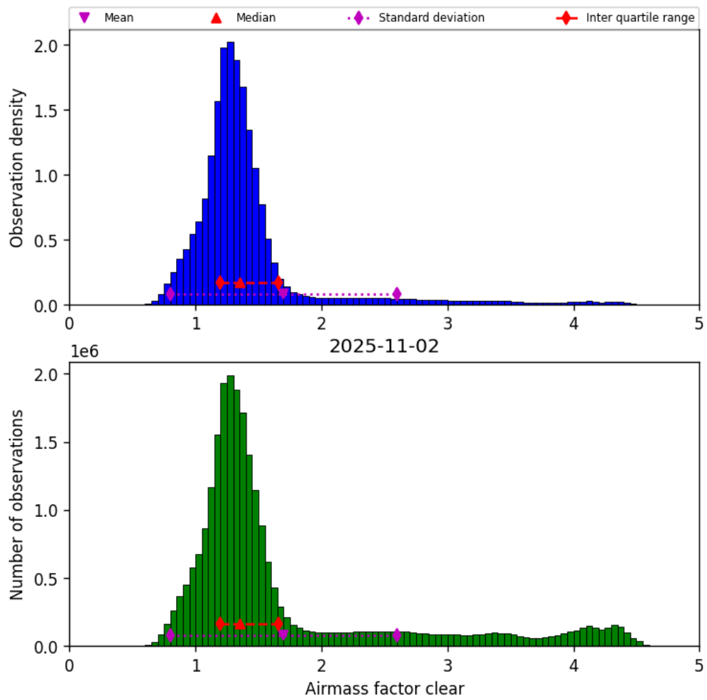
Figure 42: Histogram of “Airmass factor clear” for 2025-11-02 to 2025-11-03
