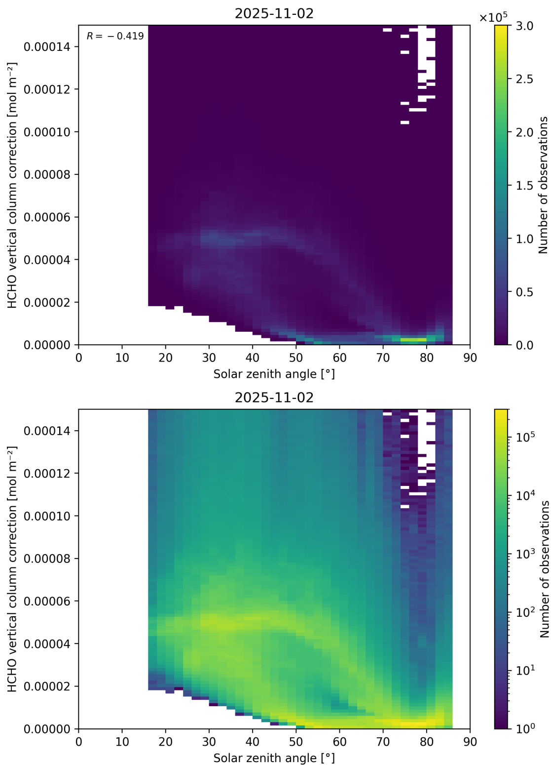
Figure 178: Scatter density plot of “Solar zenith angle” against “HCHO vertical column correction” for 2025-11-02 to 2025-11-03.
