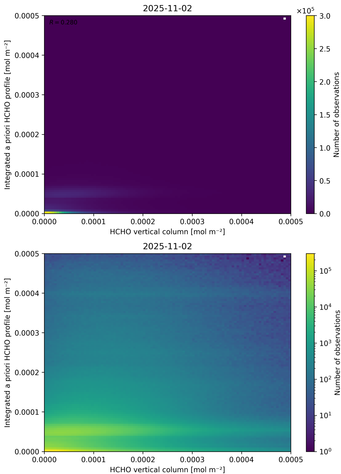
Figure 135: Scatter density plot of “HCHO vertical column” against “Integrated a priori HCHO profile” for 2025-11-02 to 2025-11-03.
