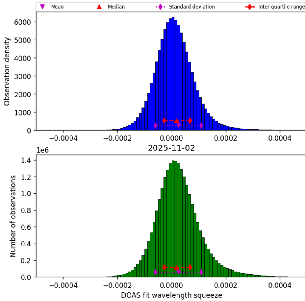
Figure 45: Histogram of “DOAS fit wavelength squeeze” for 2025-11-02 to 2025-11-03
