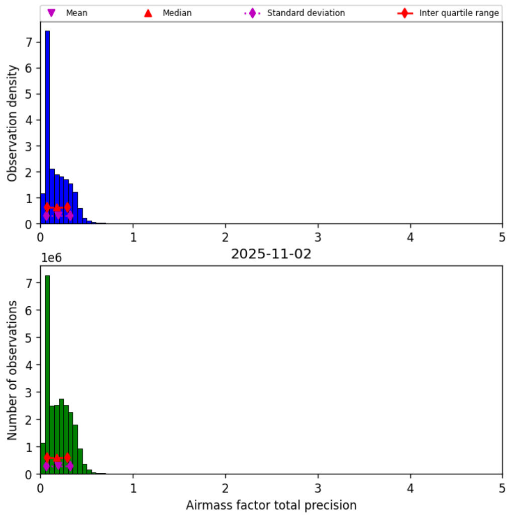
Figure 41: Histogram of “Airmass factor total precision” for 2025-11-02 to 2025-11-03
