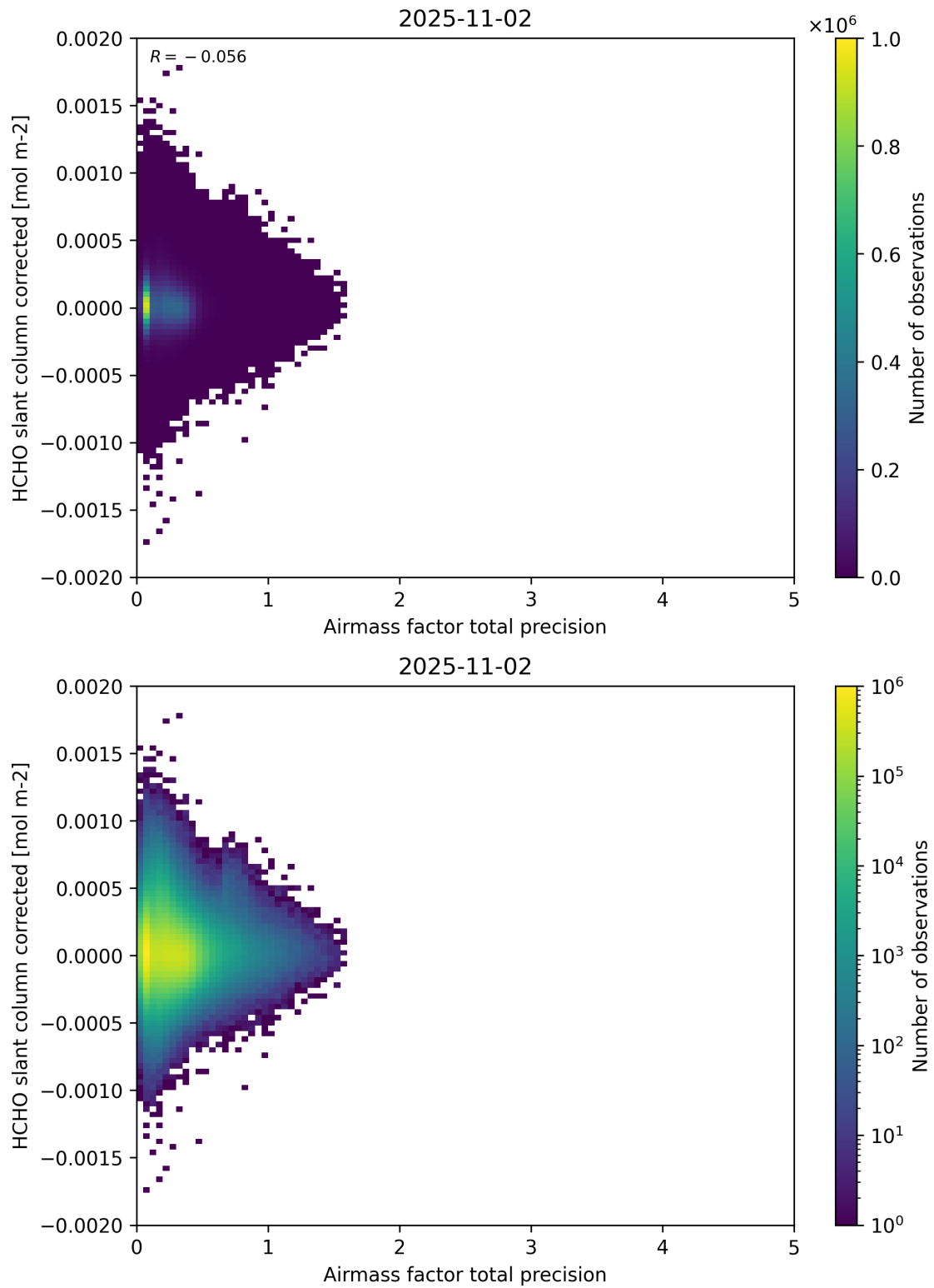
Figure 109: Scatter density plot of “Airmass factor total precision” against “HCHO slant column corrected” for 2025-11-02 to 2025-11-03.
