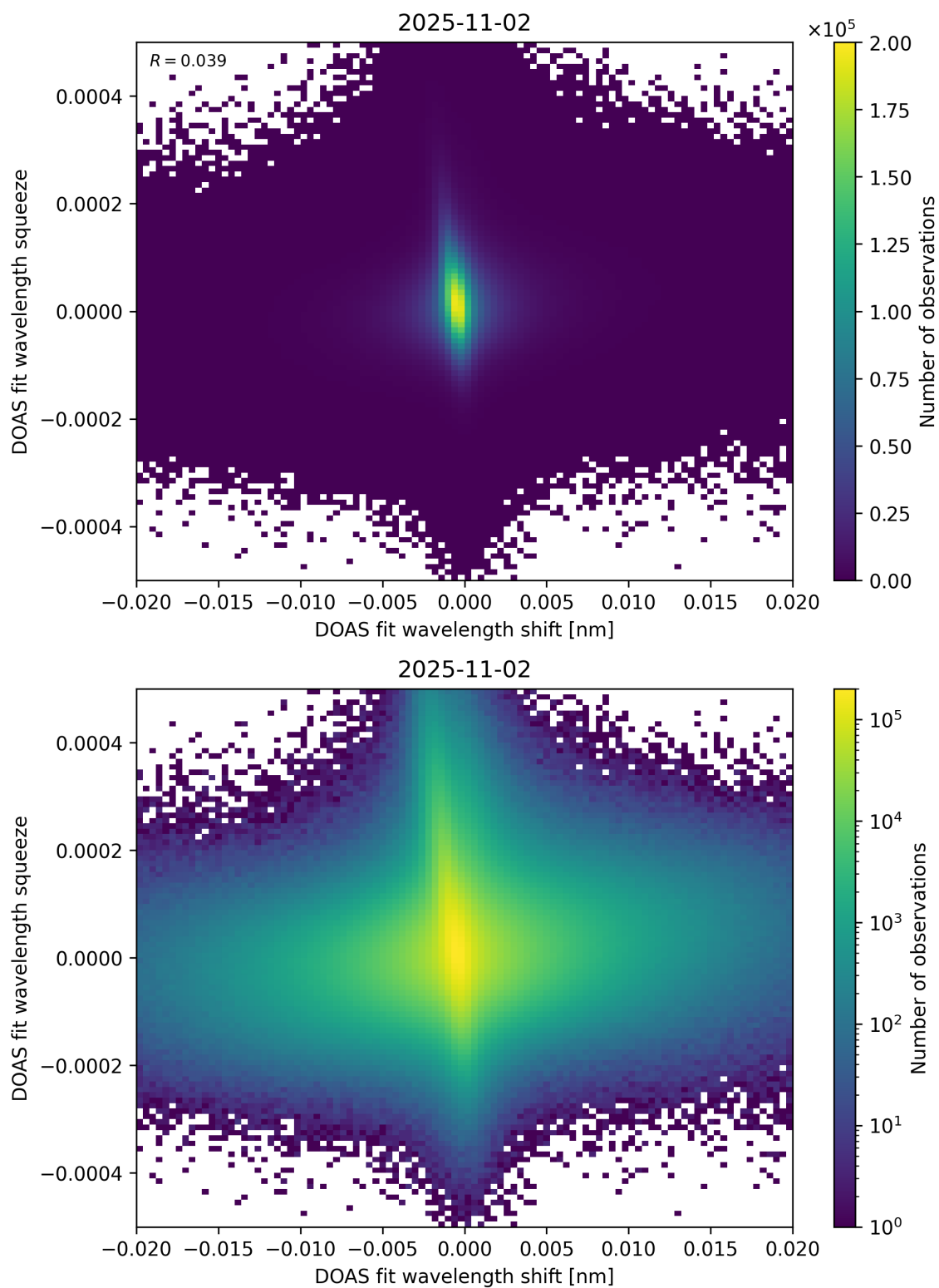
Figure 65: Scatter density plot of “DOAS fit wavelength shift” against “DOAS fit wavelength squeeze” for 2025-11-02 to 2025-11-03.
