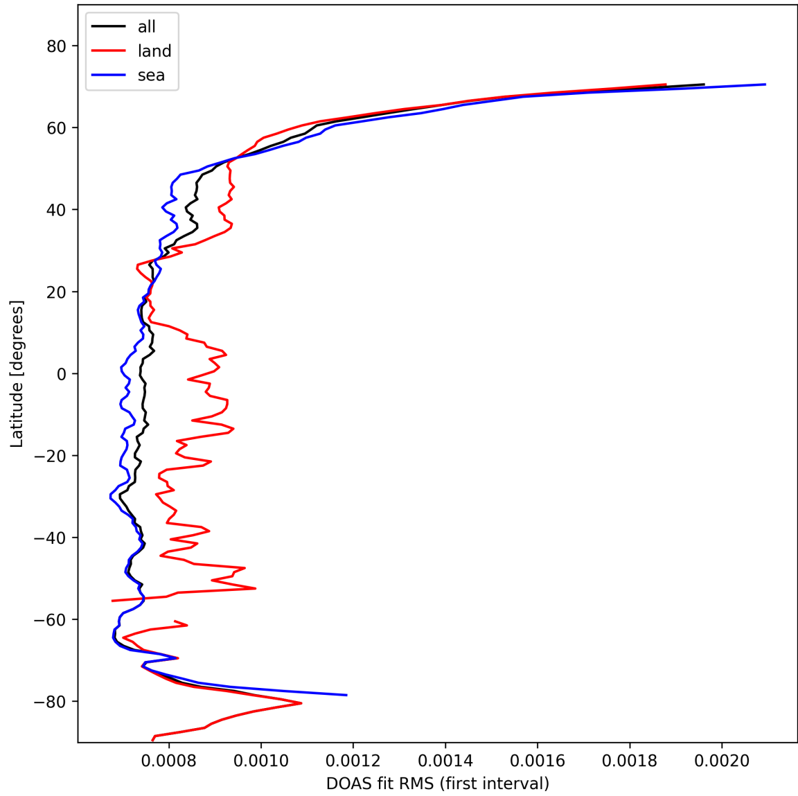
Figure 32: Zonal average of “DOAS fit RMS (first interval)” for 2025-11-02 to 2025-11-03.
