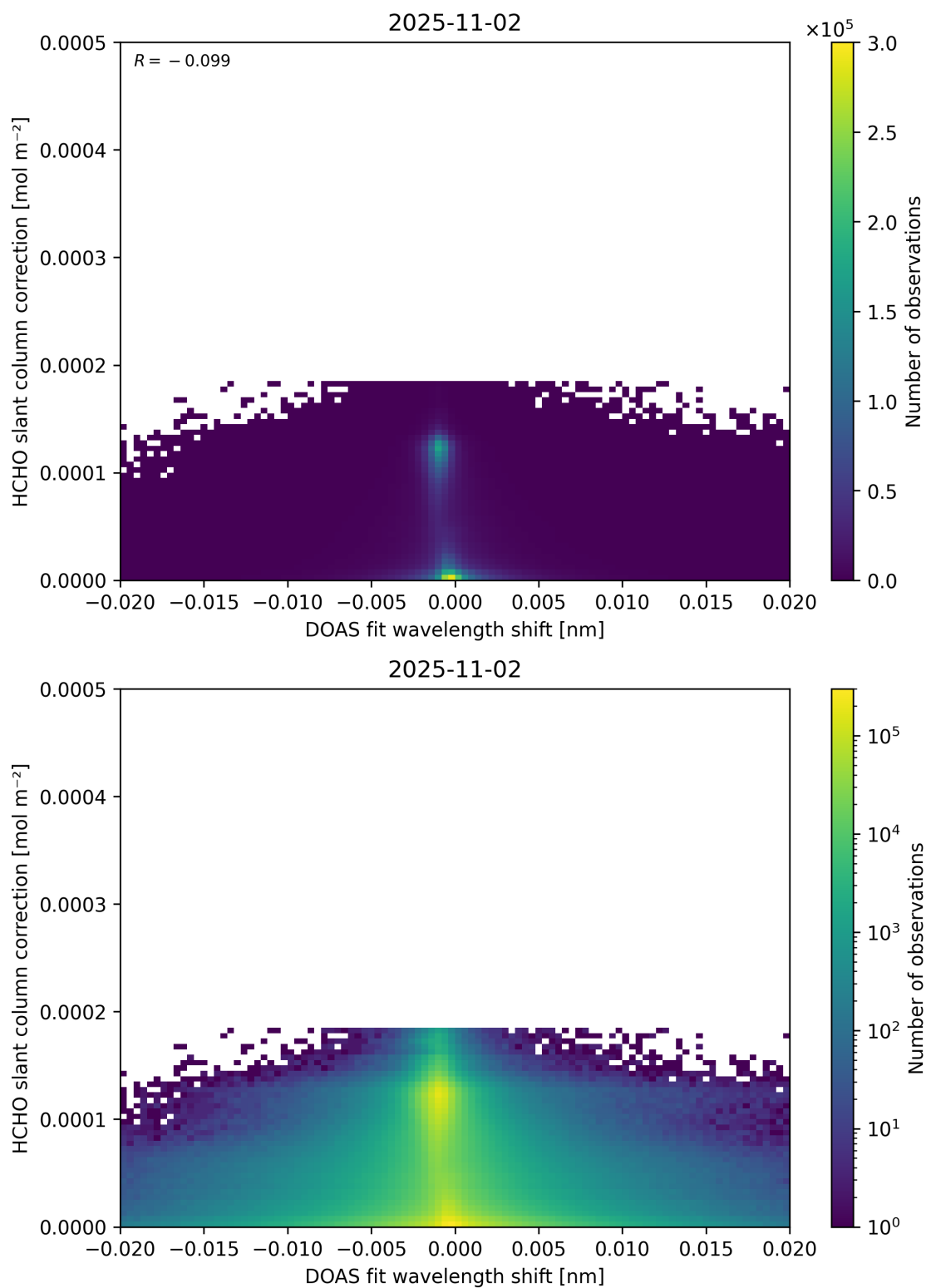
Figure 67: Scatter density plot of “DOAS fit wavelength shift” against “HCHO slant column correction” for 2025-11-02 to 2025-11-03.
