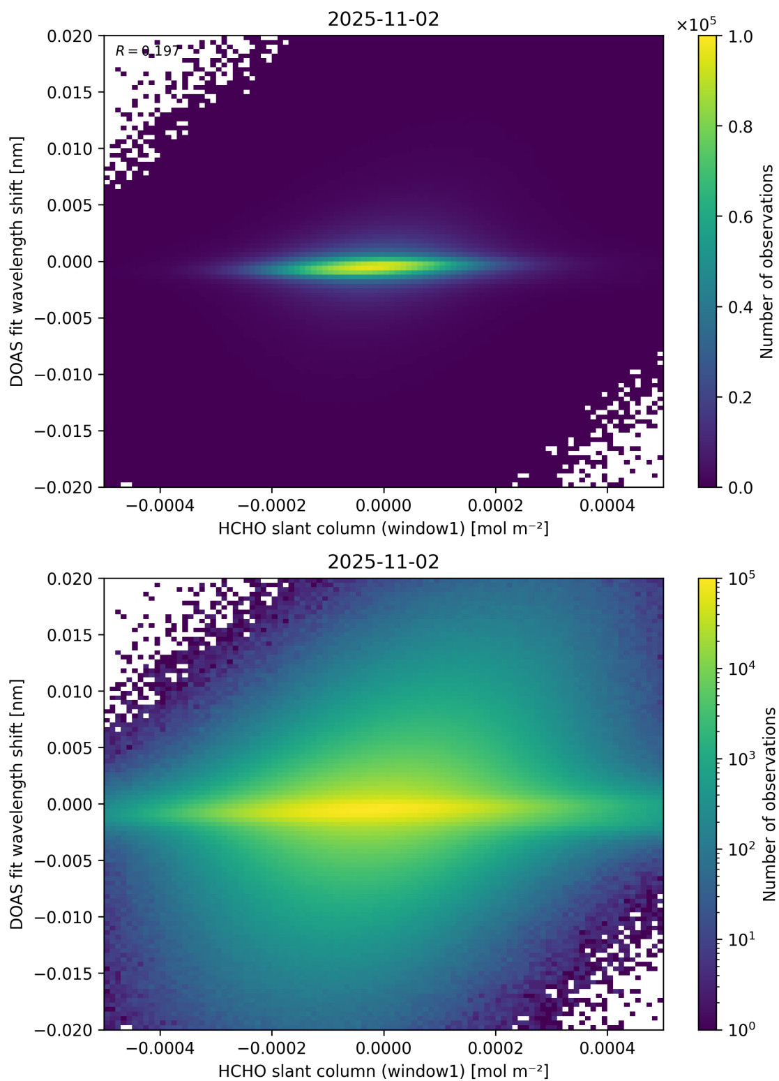
Figure 79: Scatter density plot of “HCHO slant column (window1)” against “DOAS fit wavelength shift” for 2025-11-02 to 2025-11-03.
