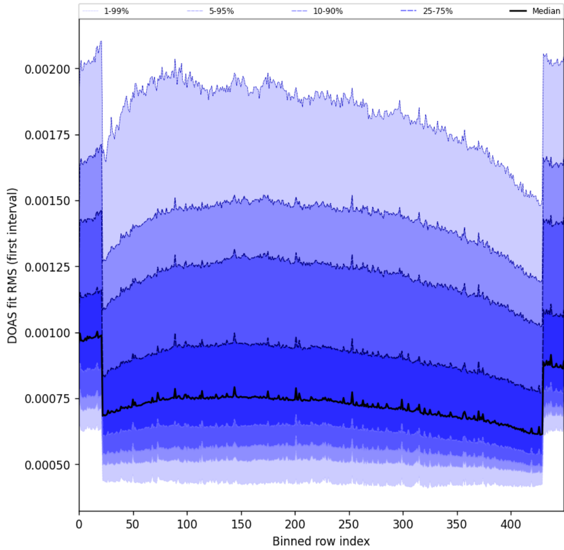
Figure 60: Along track statistics of “DOAS fit RMS (first interval)” for 2025-11-02 to 2025-11-03
