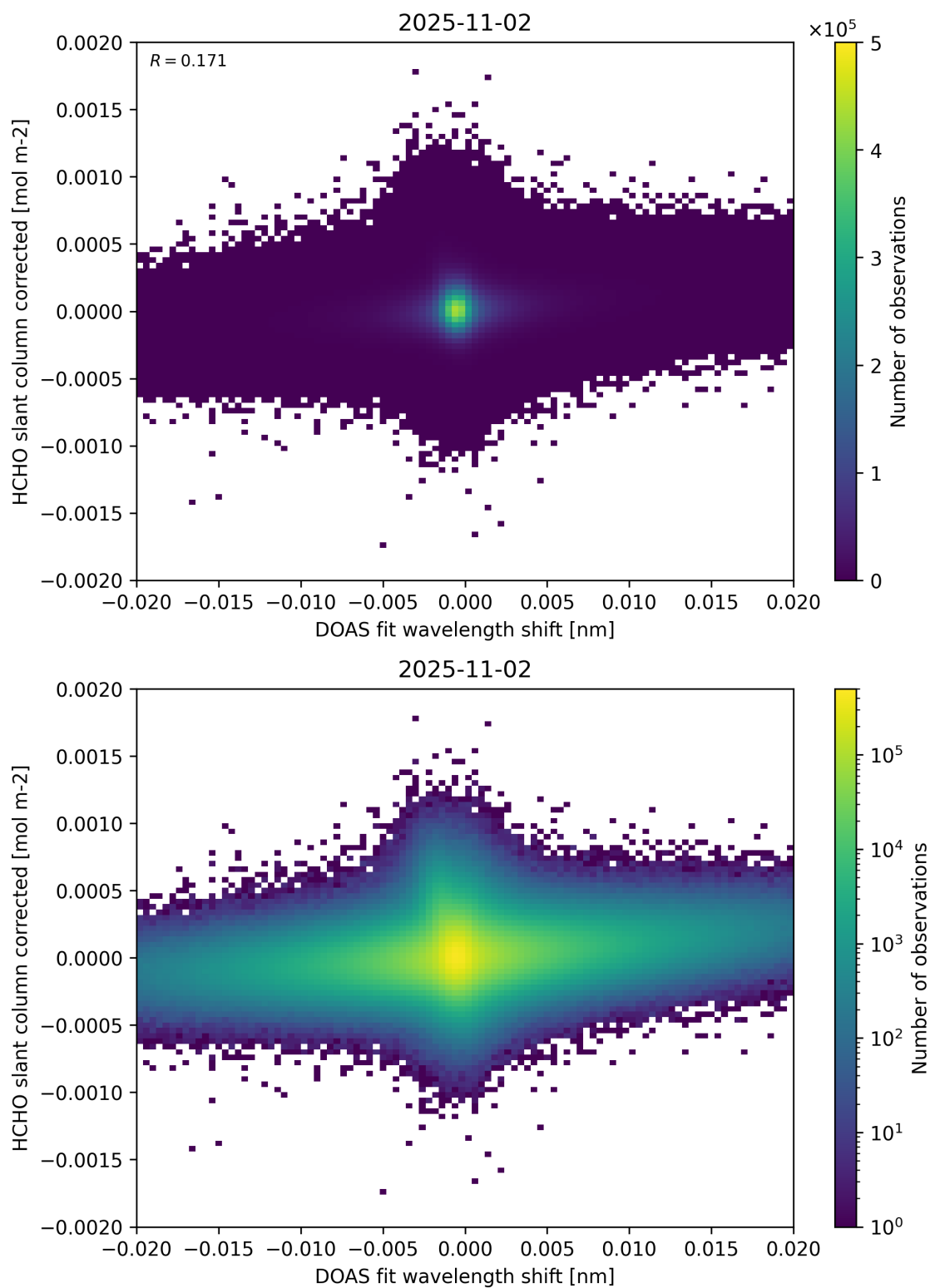
Figure 66: Scatter density plot of “DOAS fit wavelength shift” against “HCHO slant column corrected” for 2025-11-02 to 2025-11-03.
