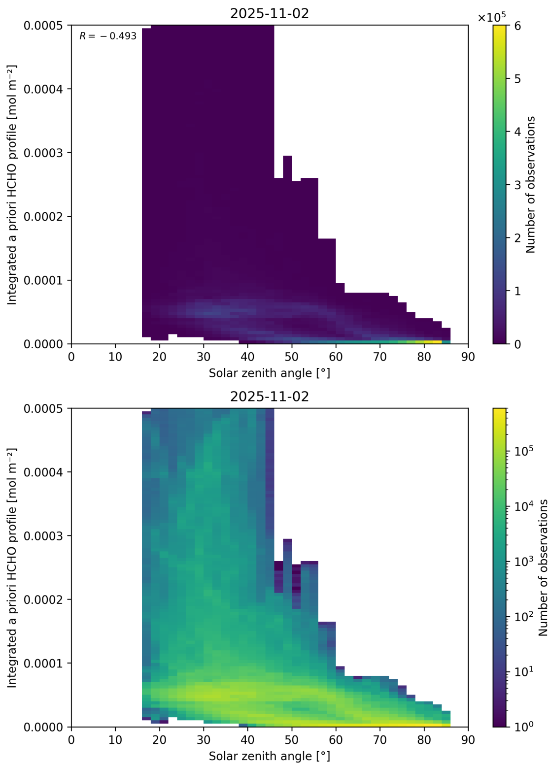
Figure 180: Scatter density plot of “Solar zenith angle” against “Integrated a priori HCHO profile” for 2025-11-02 to 2025-11-03.
