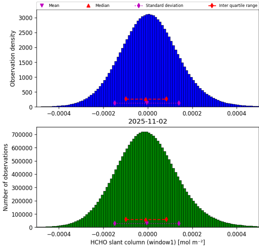
Figure 38: Histogram of “HCHO slant column (window1)” for 2025-11-02 to 2025-11-03
