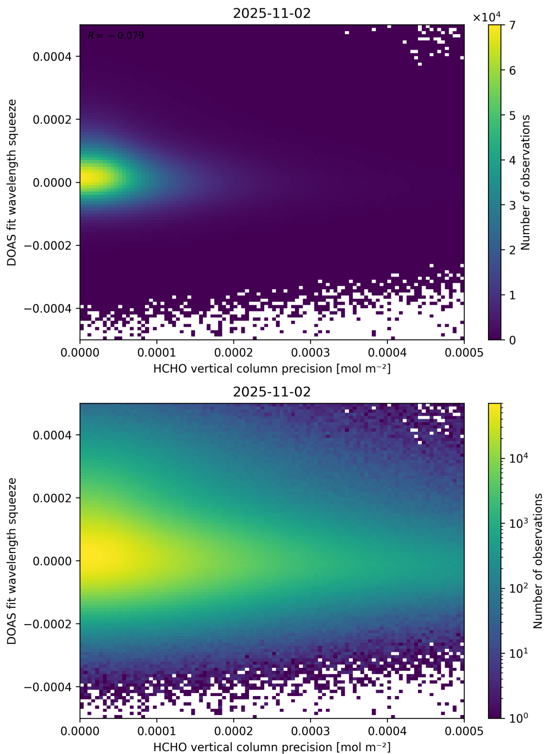
Figure 138: Scatter density plot of “HCHO vertical column precision” against “DOAS fit wavelength squeeze” for 2025-11-02 to 2025-11-03.
