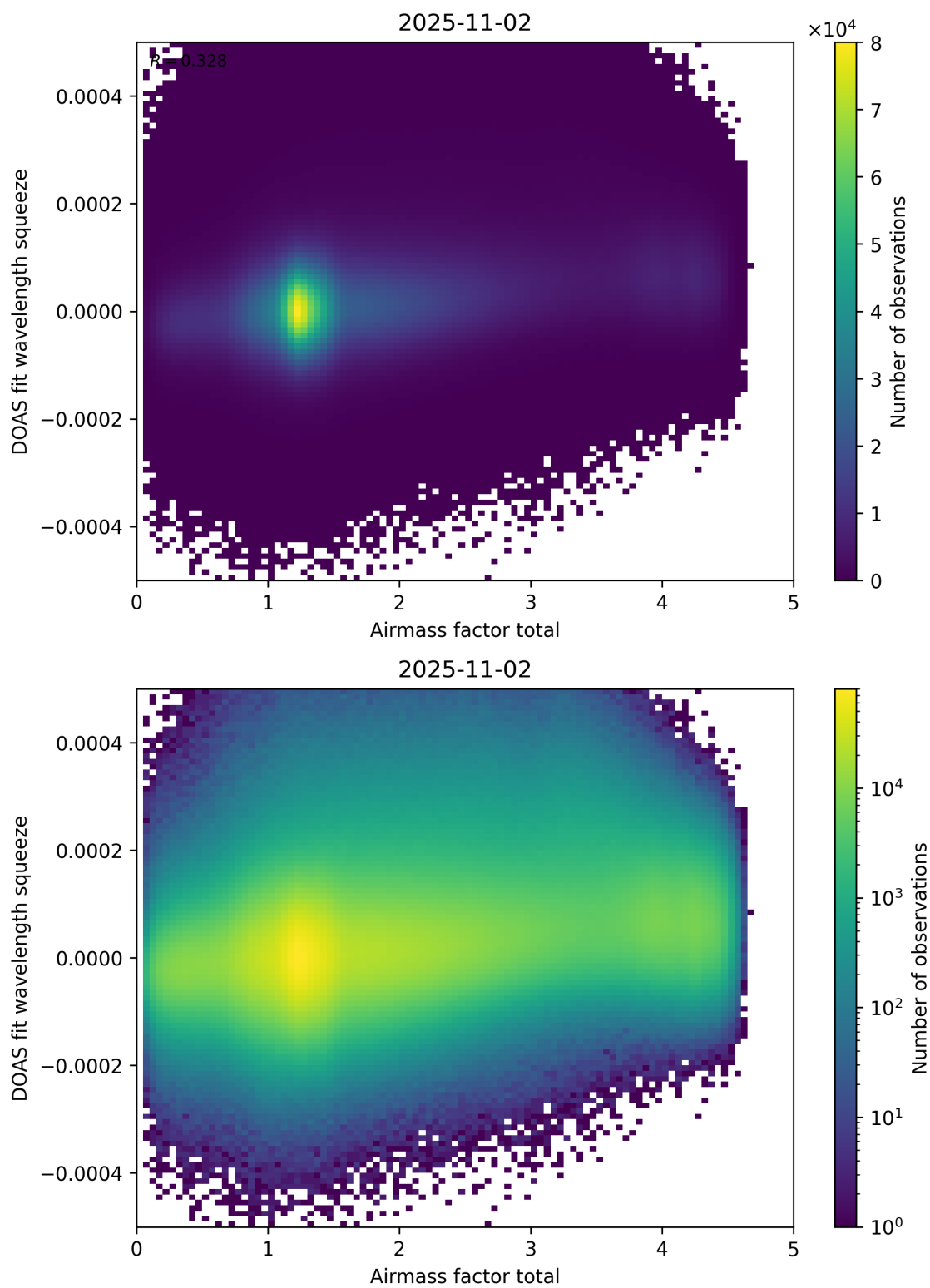
Figure 99: Scatter density plot of “Airmass factor total” against “DOAS fit wavelength squeeze” for 2025-11-02 to 2025-11-03.
