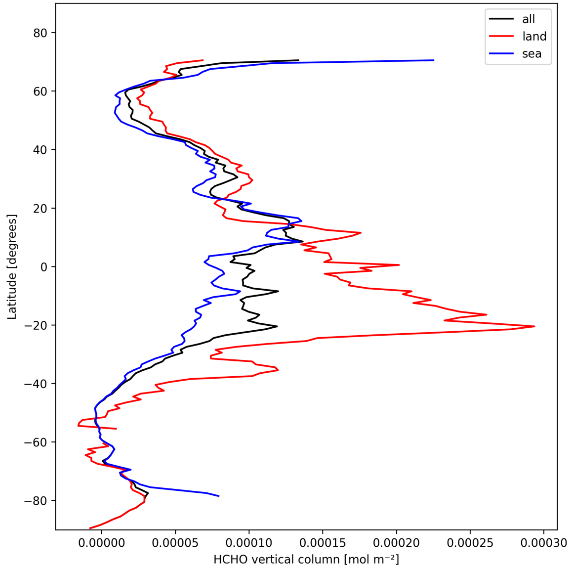
Figure 21: Zonal average of “HCHO vertical column” for 2025-11-02 to 2025-11-03.
