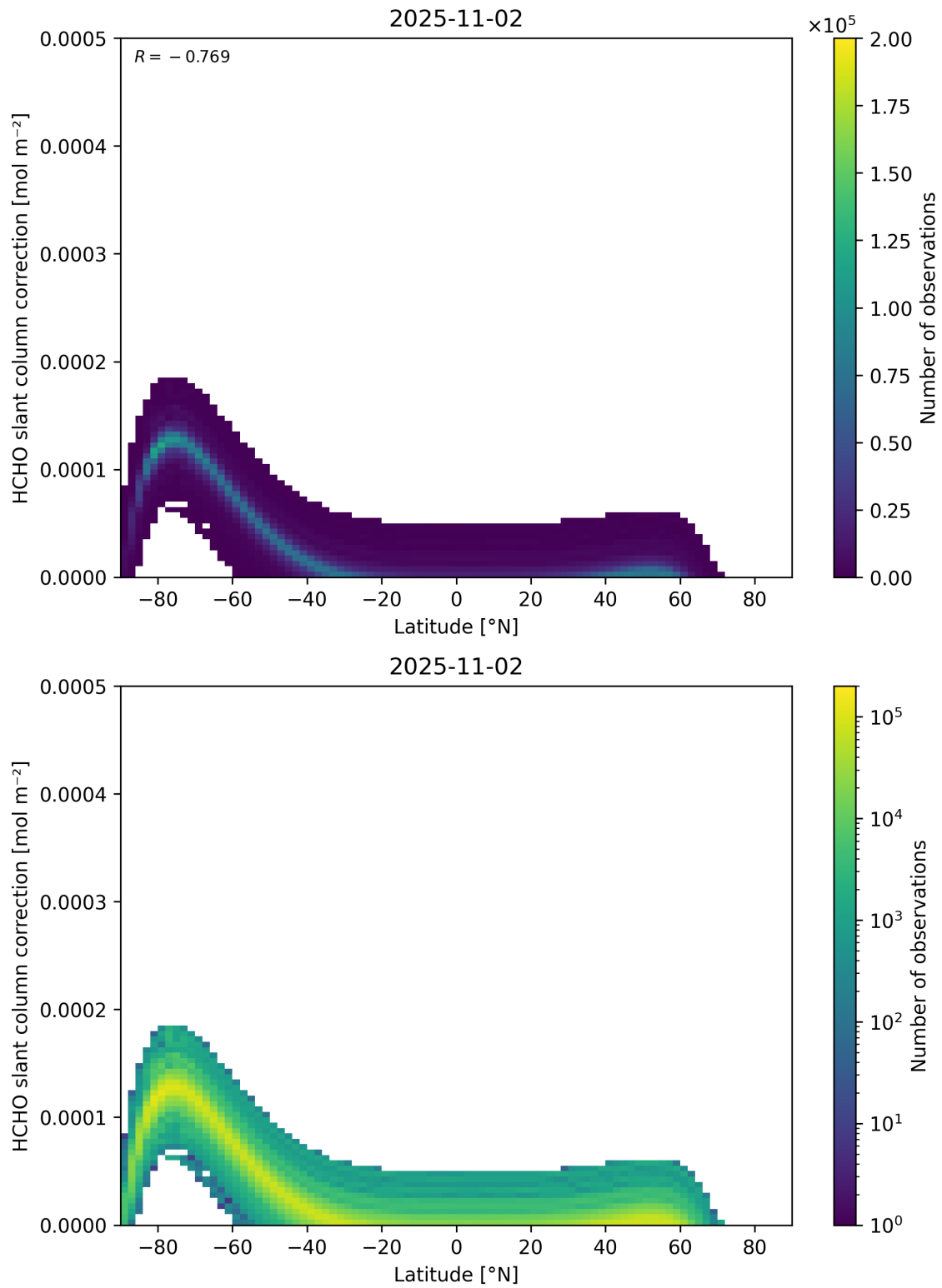
Figure 158: Scatter density plot of “Latitude” against “HCHO slant column correction” for 2025-11-02 to 2025-11-03.
