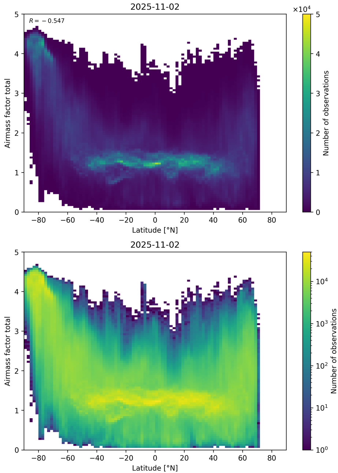
Figure 161: Scatter density plot of “Latitude” against “Airmass factor total” for 2025-11-02 to 2025-11-03.
