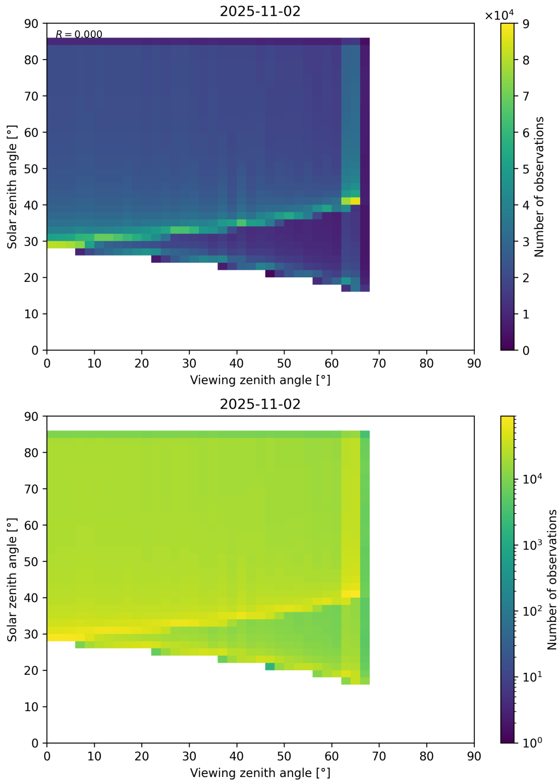
Figure 197: Scatter density plot of “Viewing zenith angle” against “Solar zenith angle” for 2025-11-02 to 2025-11-03.
