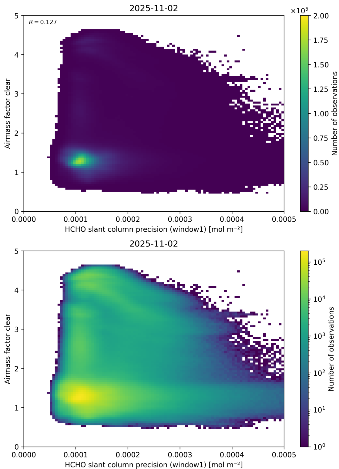
Figure 91: Scatter density plot of “HCHO slant column precision (window1)” against “Airmass factor clear” for 2025-11-02 to 2025-11-03.
