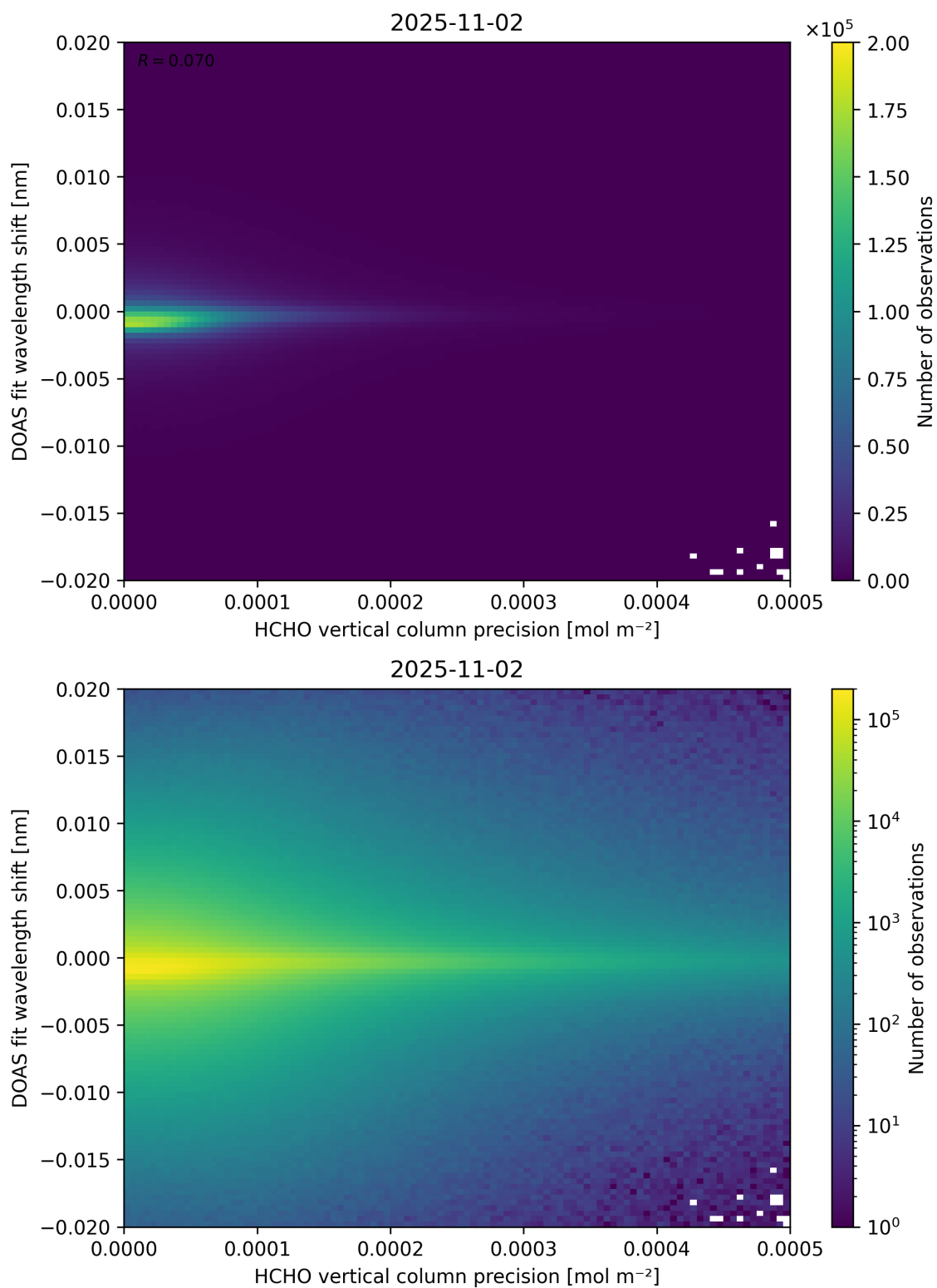
Figure 137: Scatter density plot of “HCHO vertical column precision” against “DOAS fit wavelength shift” for 2025-11-02 to 2025-11-03.
