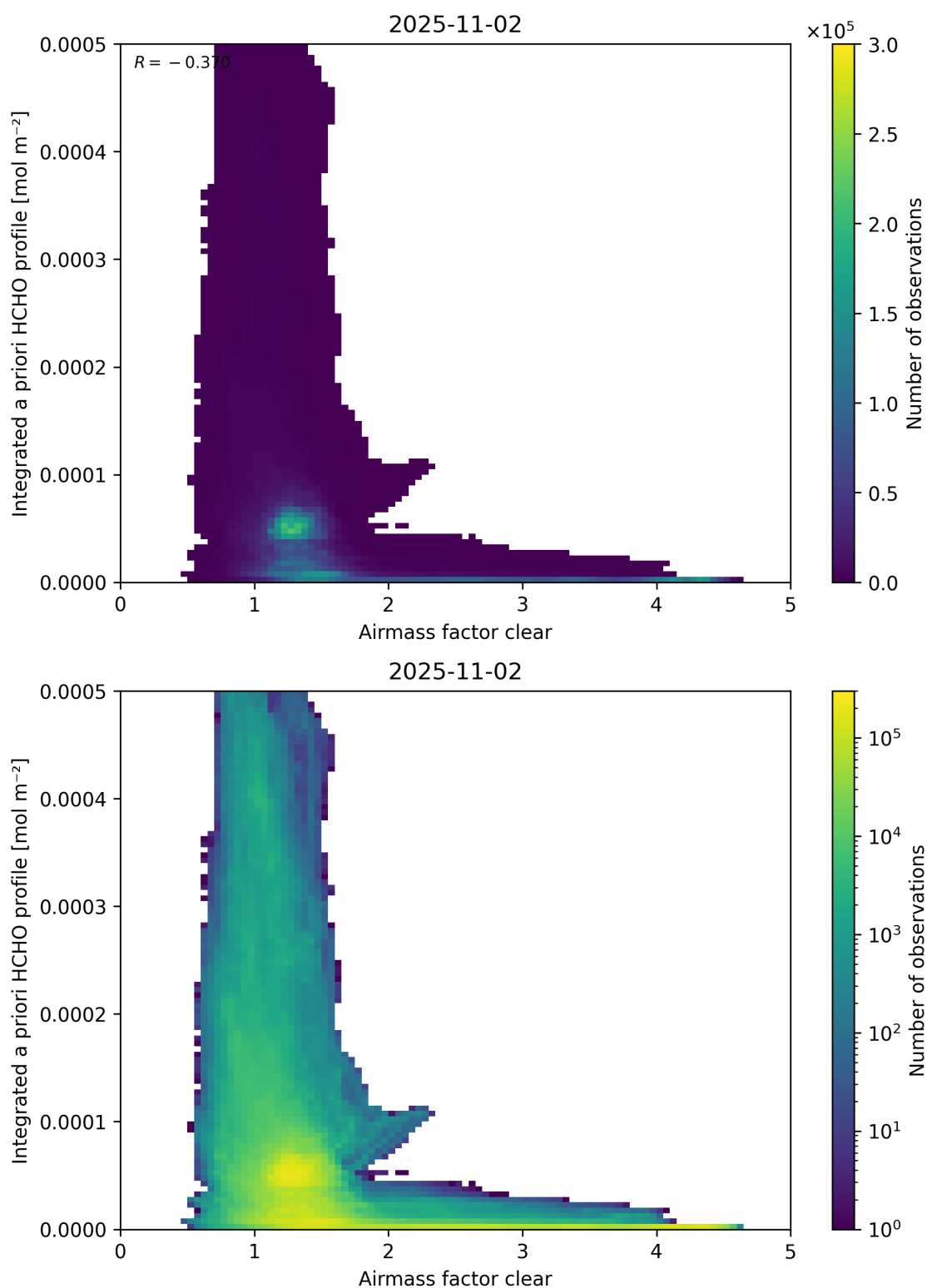
Figure 76: Scatter density plot of “Airmass factor clear” against “Integrated a priori HCHO profile” for 2025-11-02 to 2025-11-03.
