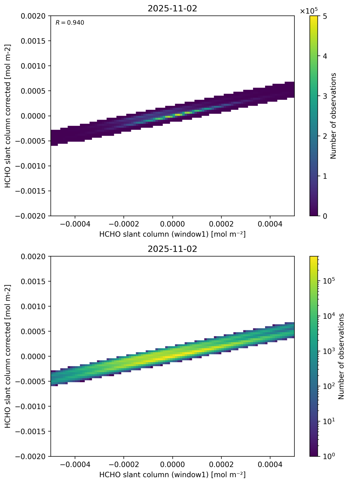
Figure 82: Scatter density plot of “HCHO slant column (window1)” against “HCHO slant column corrected” for 2025-11-02 to 2025-11-03.
