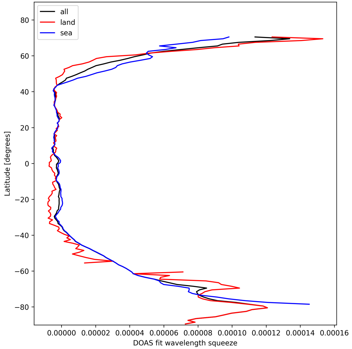
Figure 31: Zonal average of “DOAS fit wavelength squeeze” for 2025-11-02 to 2025-11-03.
