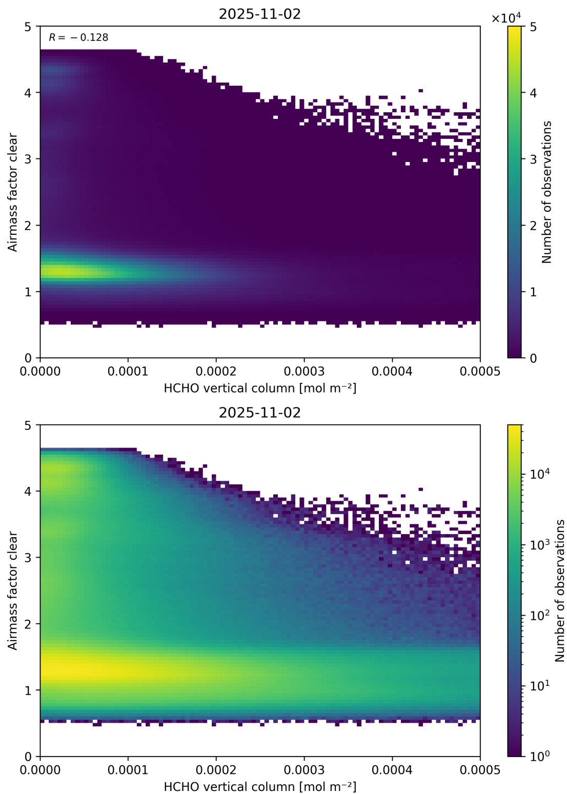
Figure 126: Scatter density plot of “HCHO vertical column” against “Airmass factor clear” for 2025-11-02 to 2025-11-03.
