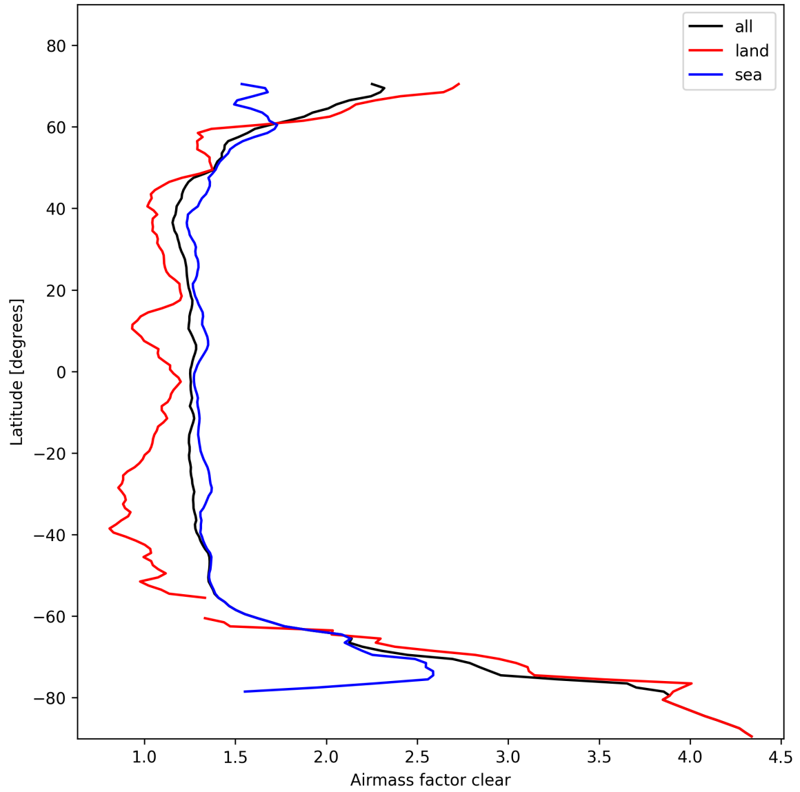
Figure 28: Zonal average of “Airmass factor clear” for 2025-11-02 to 2025-11-03.
