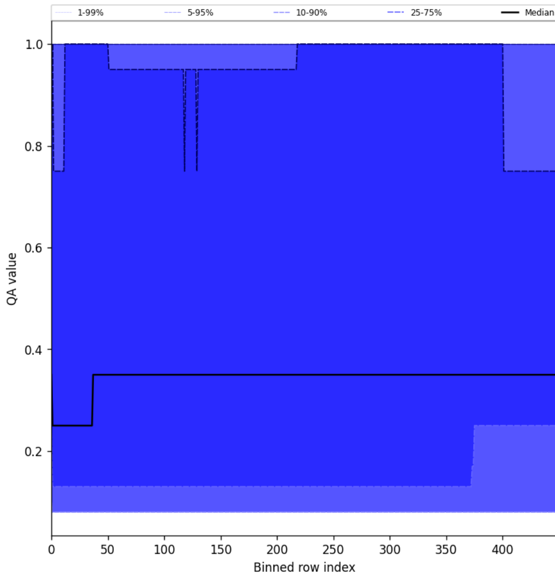
Figure 48: Along track statistics of “QA value” for 2025-11-02 to 2025-11-03
