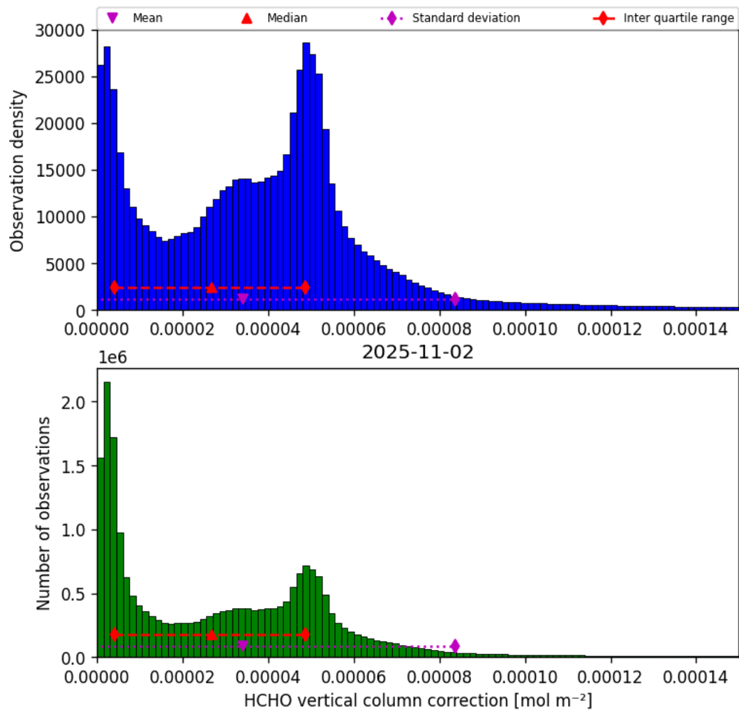
Figure 37: Histogram of “HCHO vertical column correction” for 2025-11-02 to 2025-11-03
