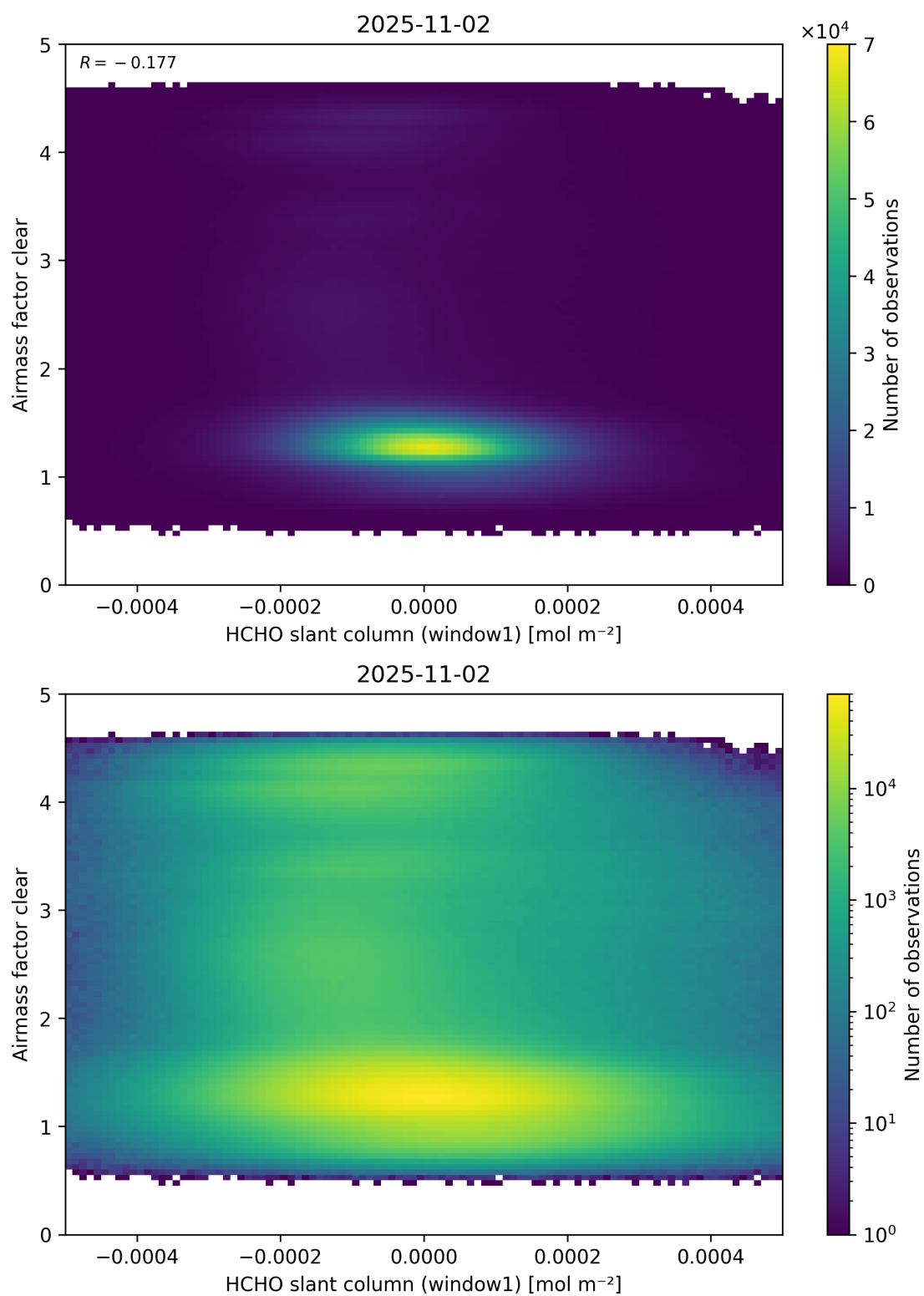
Figure 81: Scatter density plot of “HCHO slant column (window1)” against “Airmass factor clear” for 2025-11-02 to 2025-11-03.
