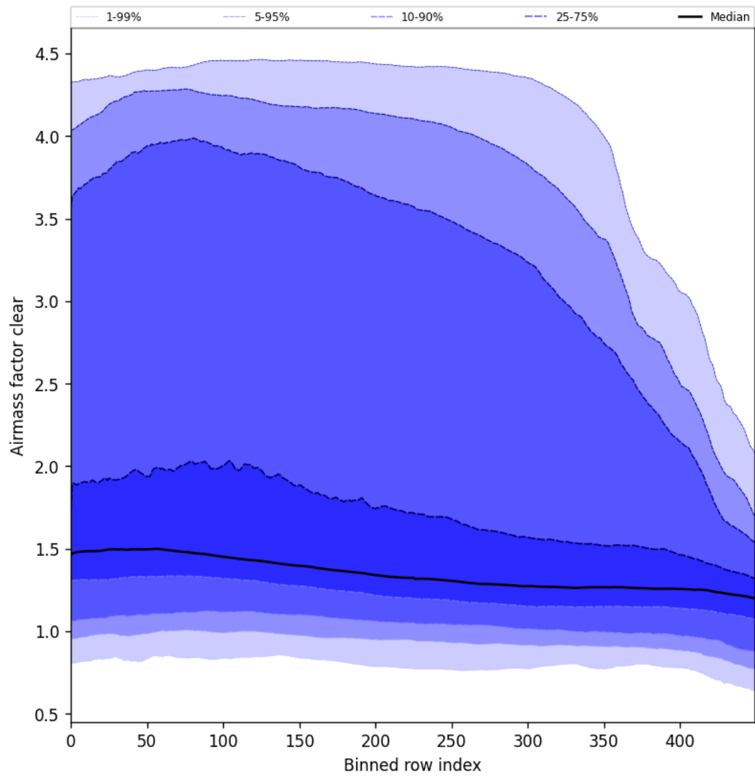
Figure 56: Along track statistics of “Airmass factor clear” for 2025-11-02 to 2025-11-03
