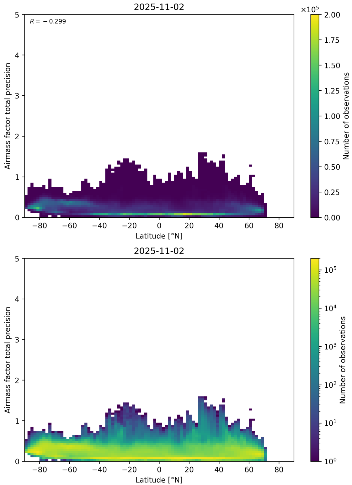
Figure 162: Scatter density plot of “Latitude” against “Airmass factor total precision” for 2025-11-02 to 2025-11-03.
