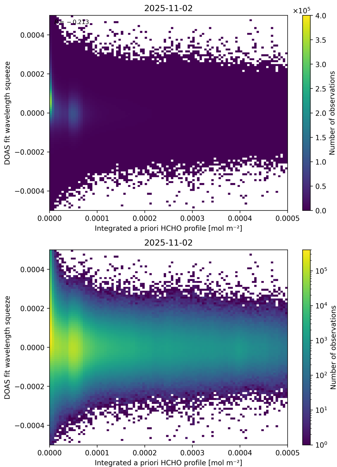
Figure 150: Scatter density plot of “Integrated a priori HCHO profile” against “DOAS fit wavelength squeeze” for 2025-11-02 to 2025-11-03.
