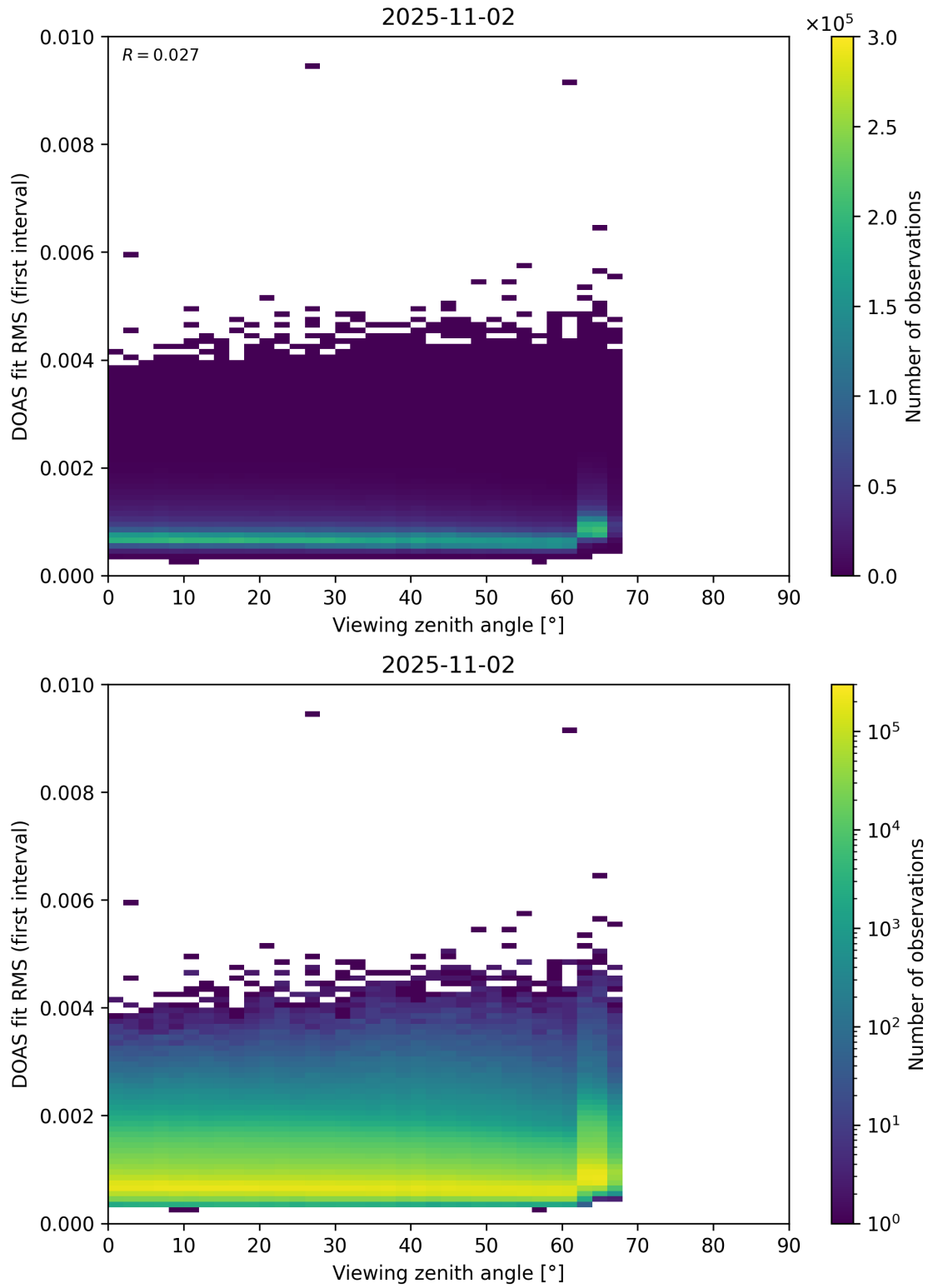
Figure 182: Scatter density plot of “Viewing zenith angle” against “DOAS fit RMS (first interval)” for 2025-11-02 to 2025-11-03.
