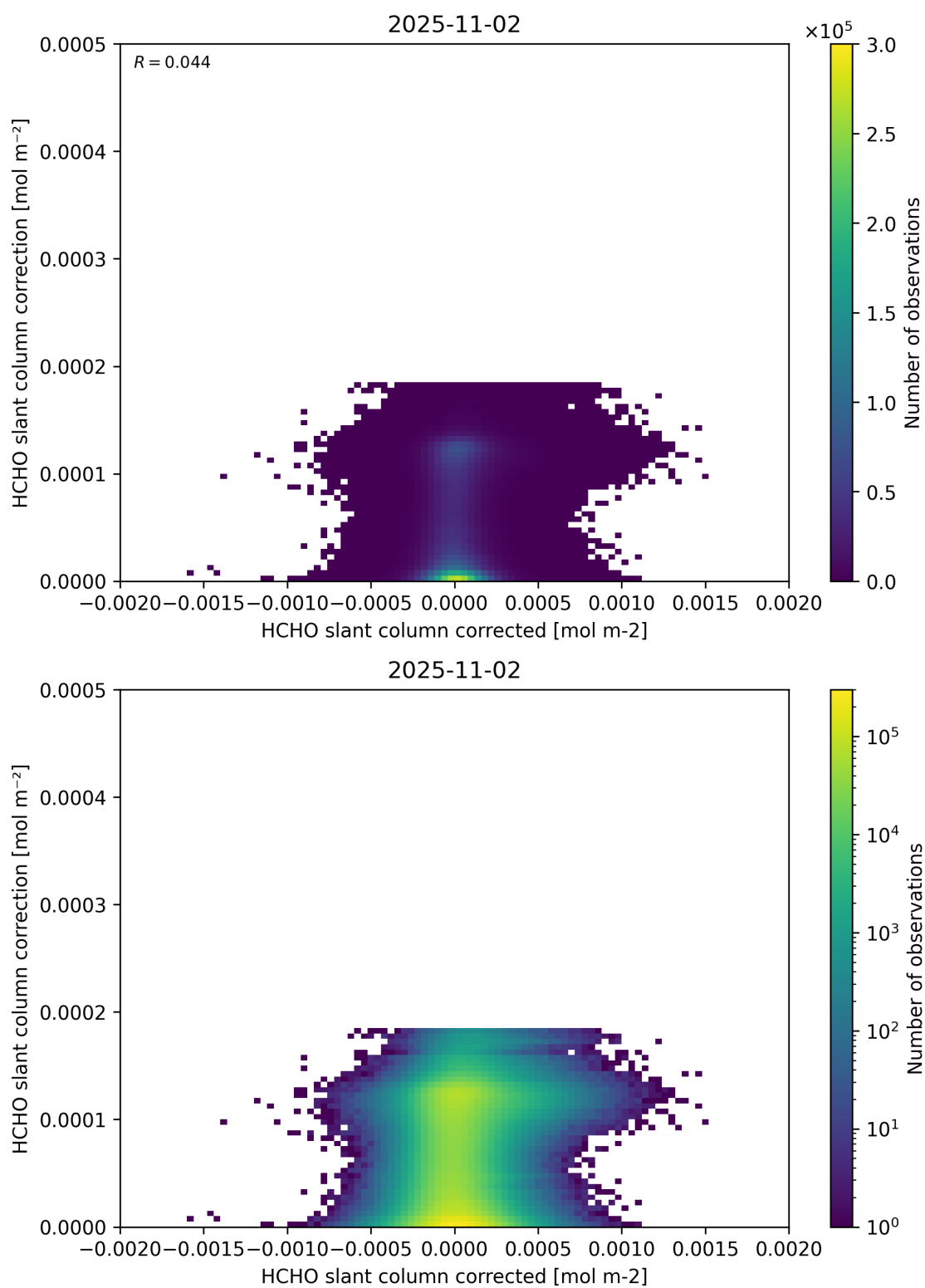
Figure 77: Scatter density plot of “HCHO slant column corrected” against “HCHO slant column correction” for 2025-11-02 to 2025-11-03.
