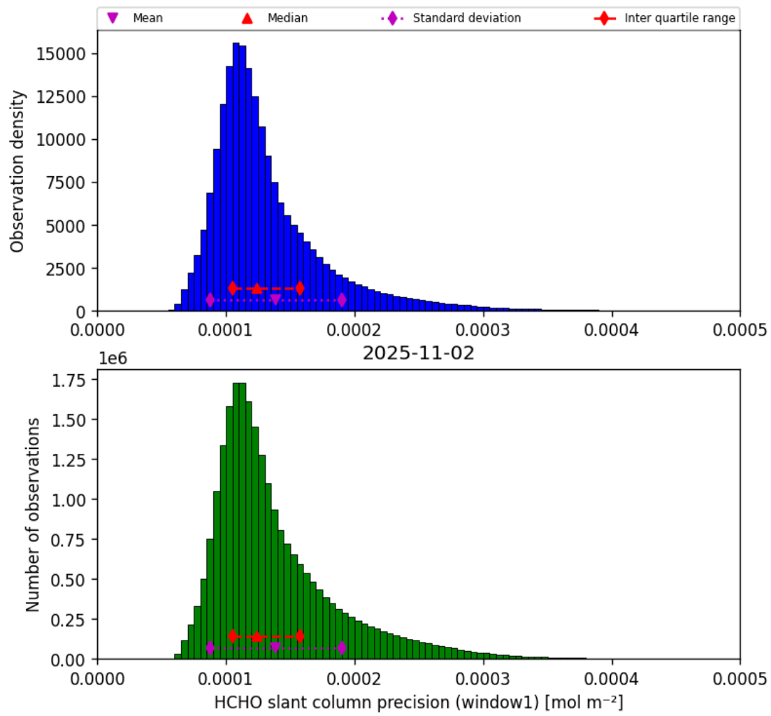
Figure 39: Histogram of “HCHO slant column precision (window1)” for 2025-11-02 to 2025-11-03
