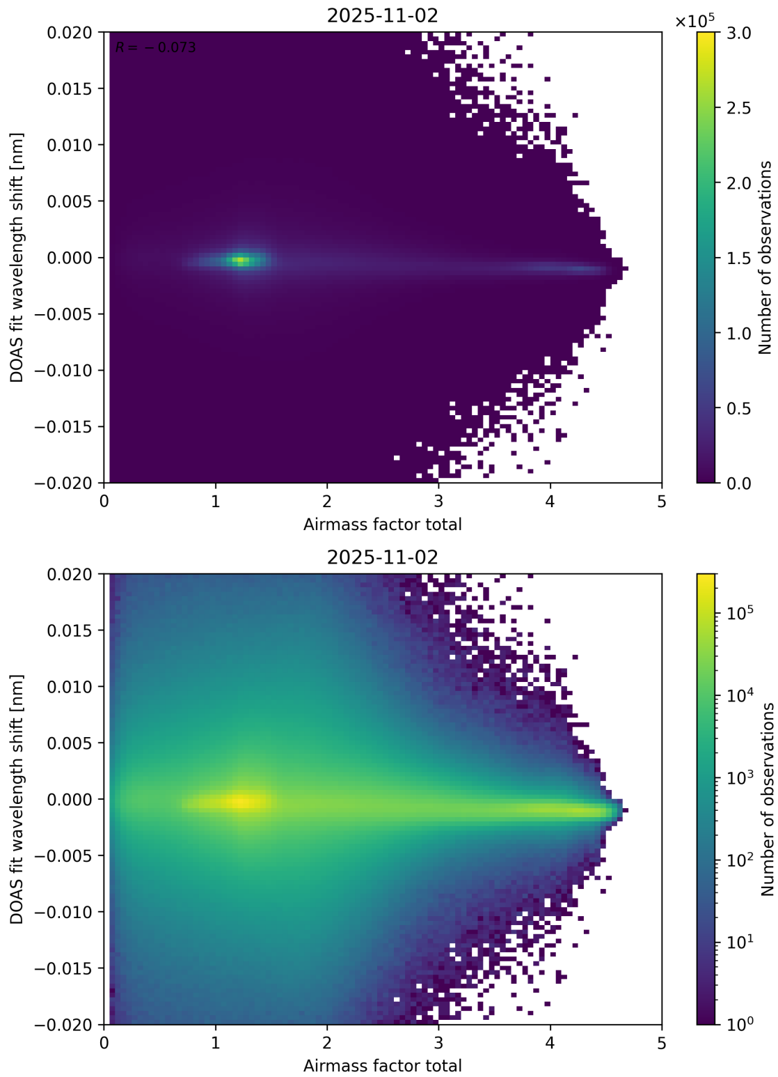
Figure 98: Scatter density plot of “Airmass factor total” against “DOAS fit wavelength shift” for 2025-11-02 to 2025-11-03.
