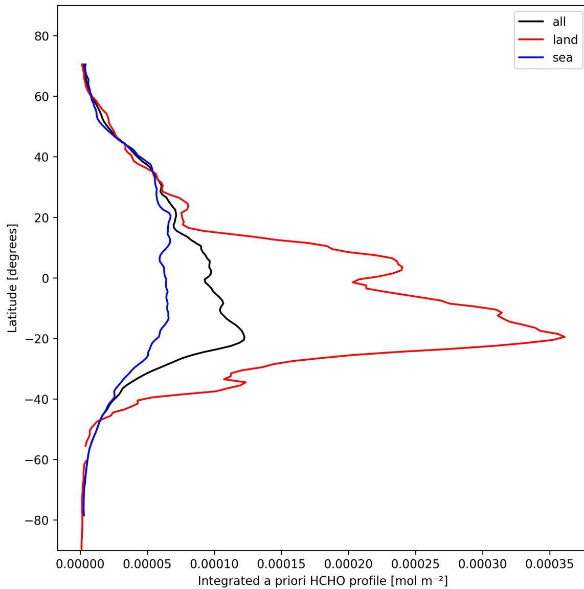
Figure 29: Zonal average of “Integrated a priori HCHO profile” for 2025-11-02 to 2025-11-03.
