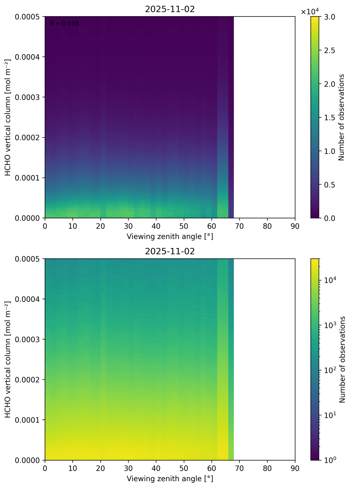
Figure 192: Scatter density plot of “Viewing zenith angle” against “HCHO vertical column” for 2025-11-02 to 2025-11-03.
