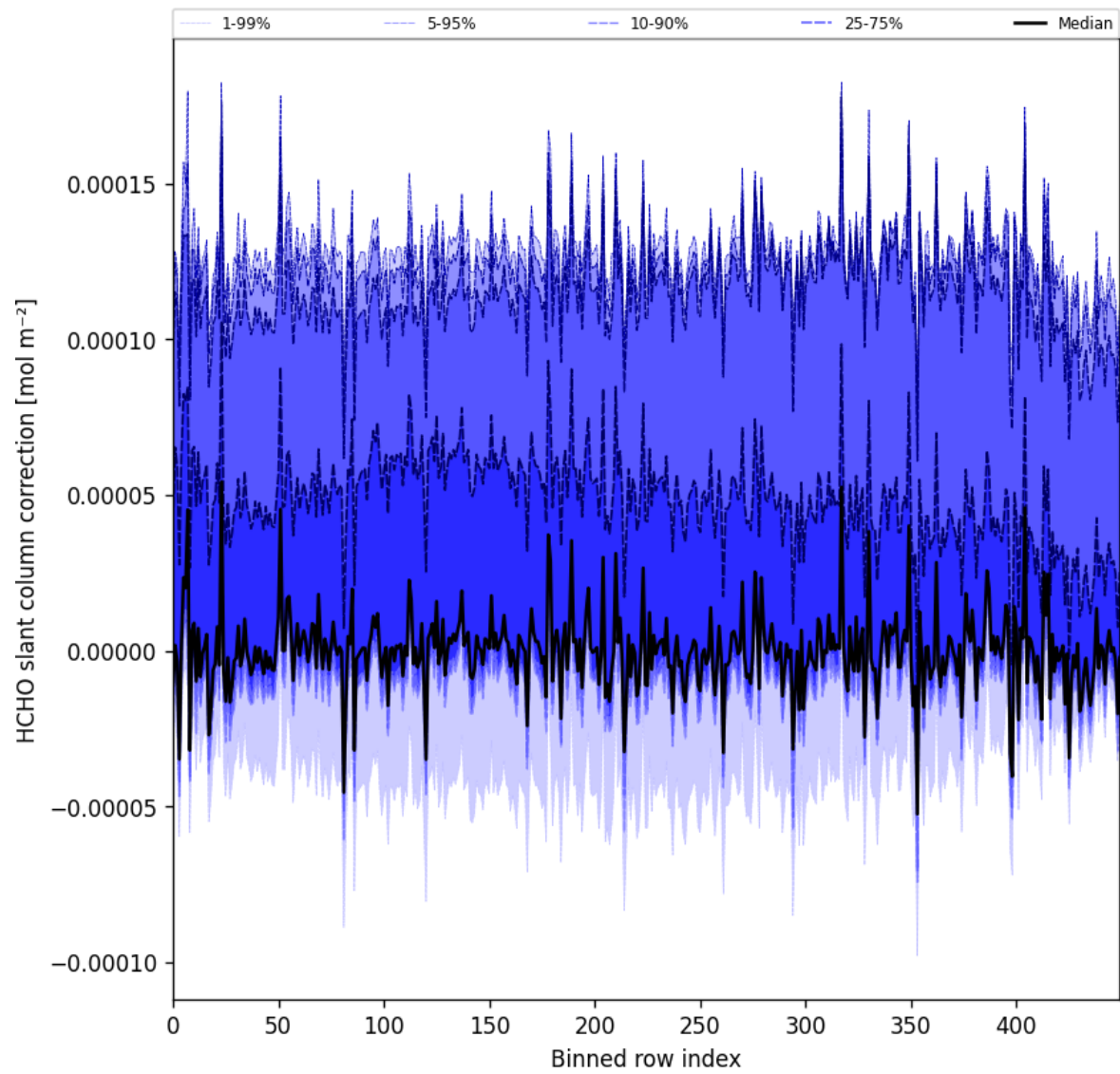
Figure 61: Along track statistics of “HCHO slant column correction” for 2025-11-02 to 2025-11-03
