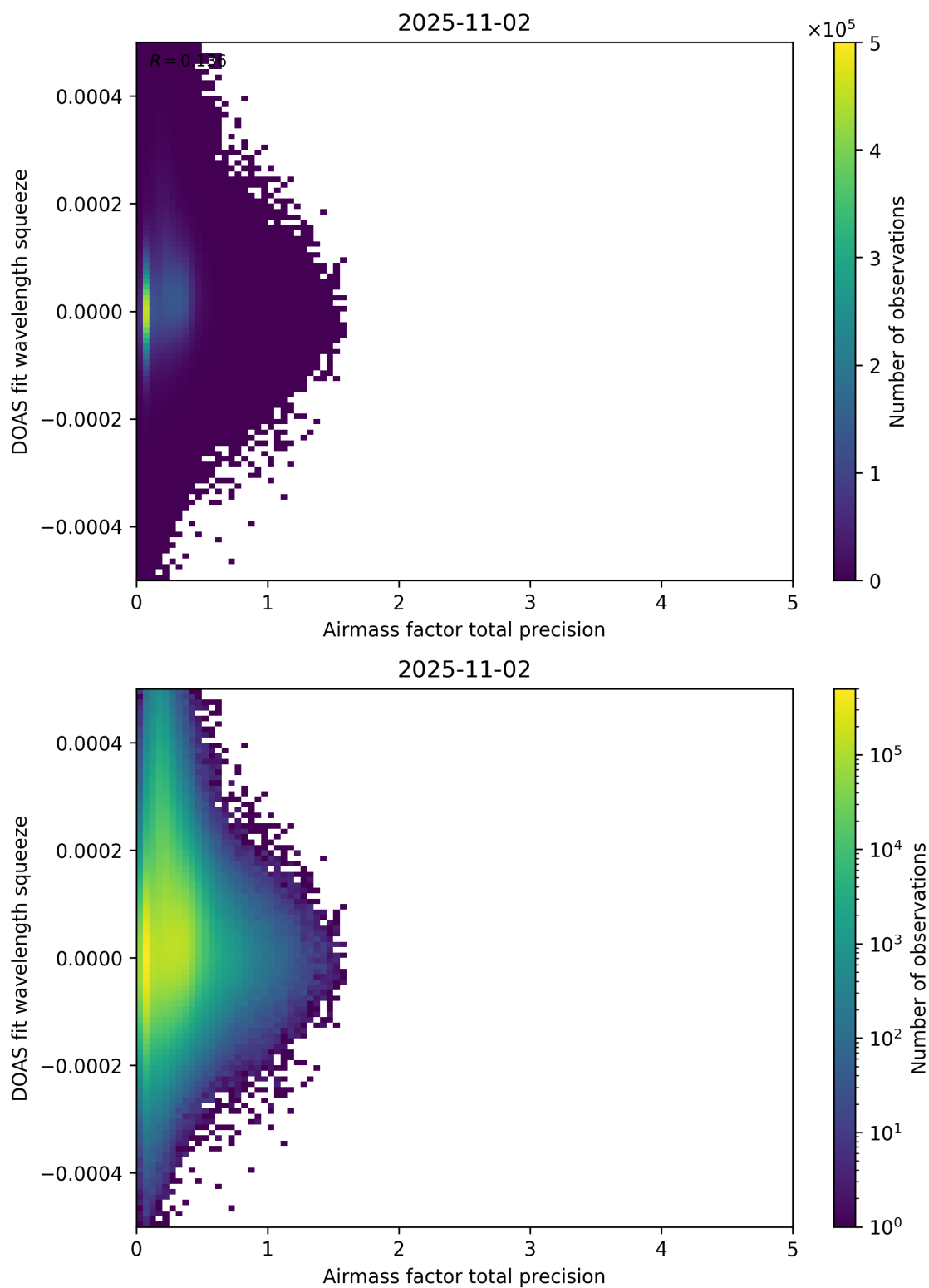
Figure 107: Scatter density plot of “Airmass factor total precision” against “DOAS fit wavelength squeeze” for 2025-11-02 to 2025-11-03.
