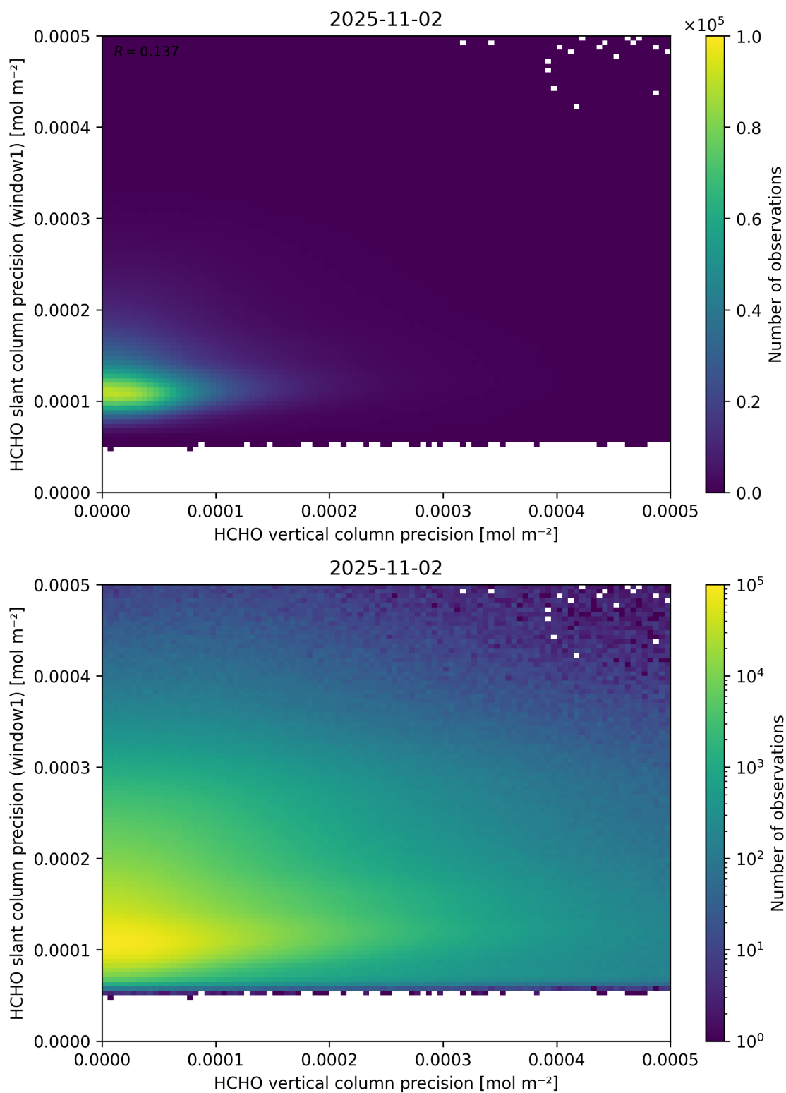
Figure 143: Scatter density plot of “HCHO vertical column precision” against “HCHO slant column precision (window1)” for 2025-11-02 to 2025-11-03.
