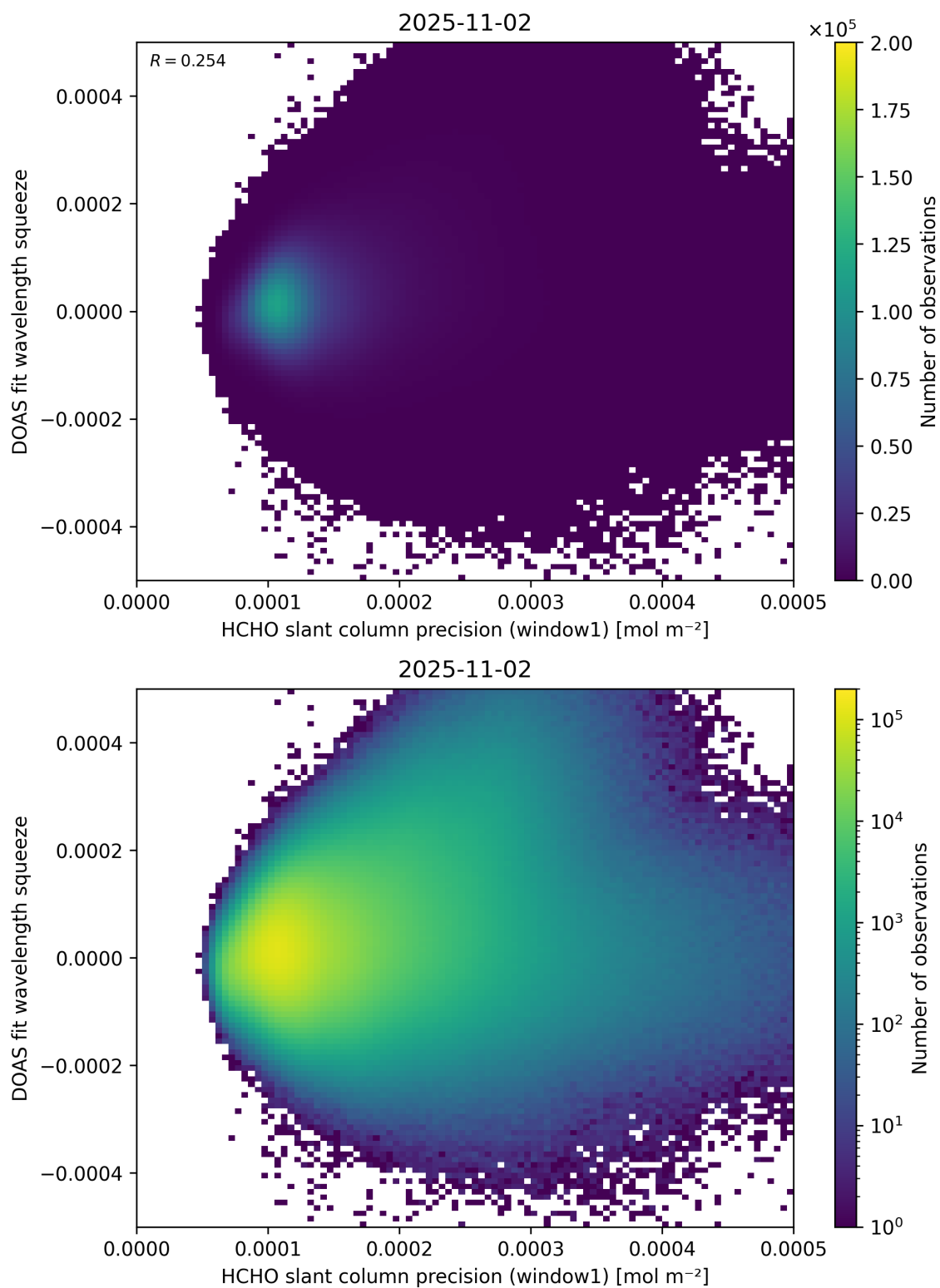
Figure 90: Scatter density plot of “HCHO slant column precision (window1)” against “DOAS fit wavelength squeeze” for 2025-11-02 to 2025-11-03.
