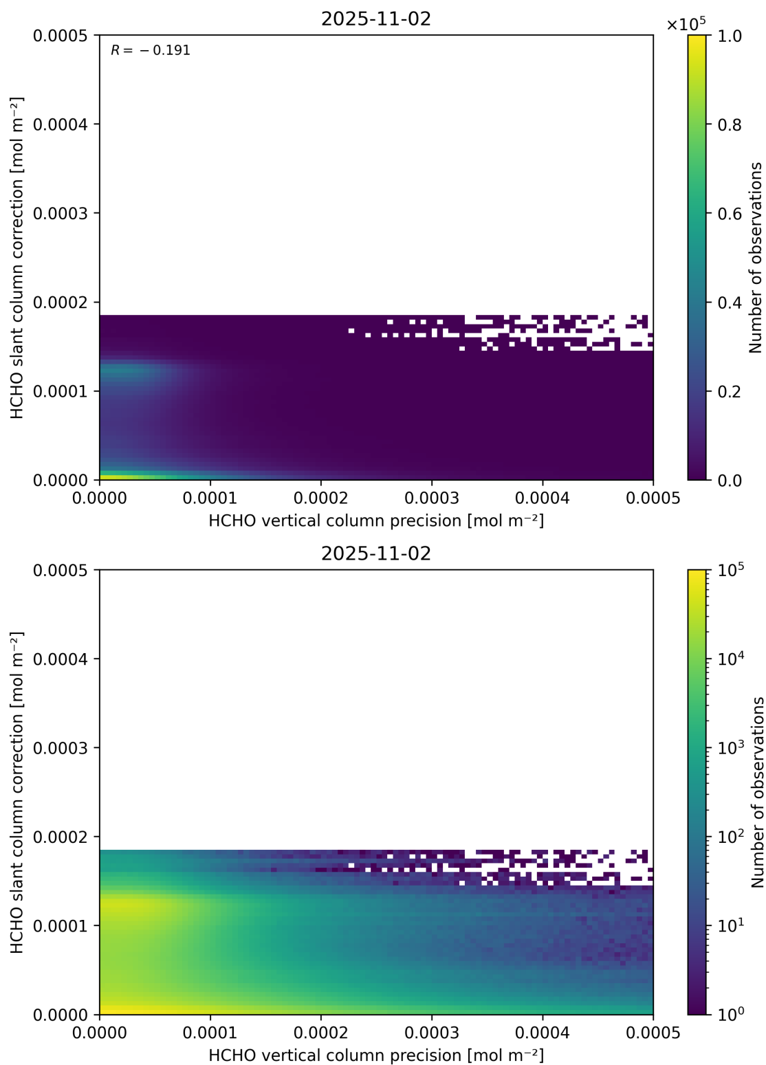
Figure 141: Scatter density plot of “HCHO vertical column precision” against “HCHO slant column correction” for 2025-11-02 to 2025-11-03.
