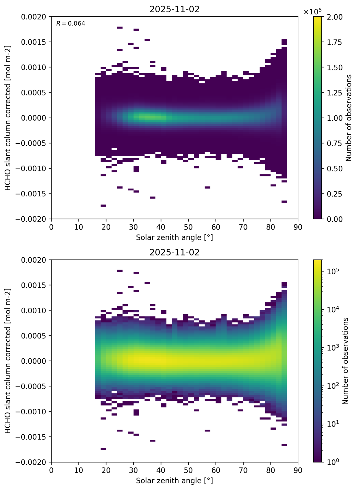
Figure 171: Scatter density plot of “Solar zenith angle” against “HCHO slant column corrected” for 2025-11-02 to 2025-11-03.
