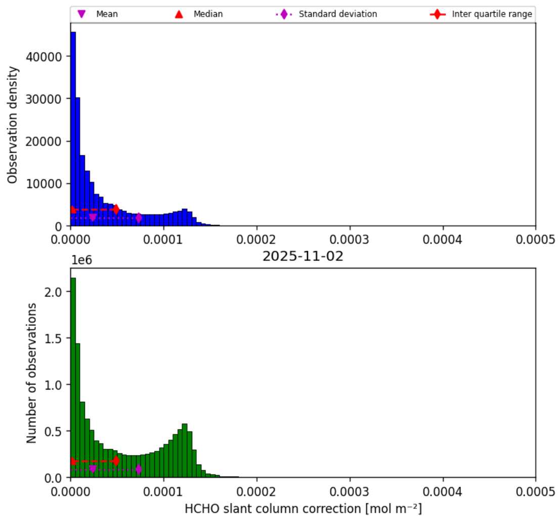
Figure 47: Histogram of “HCHO slant column correction” for 2025-11-02 to 2025-11-03
