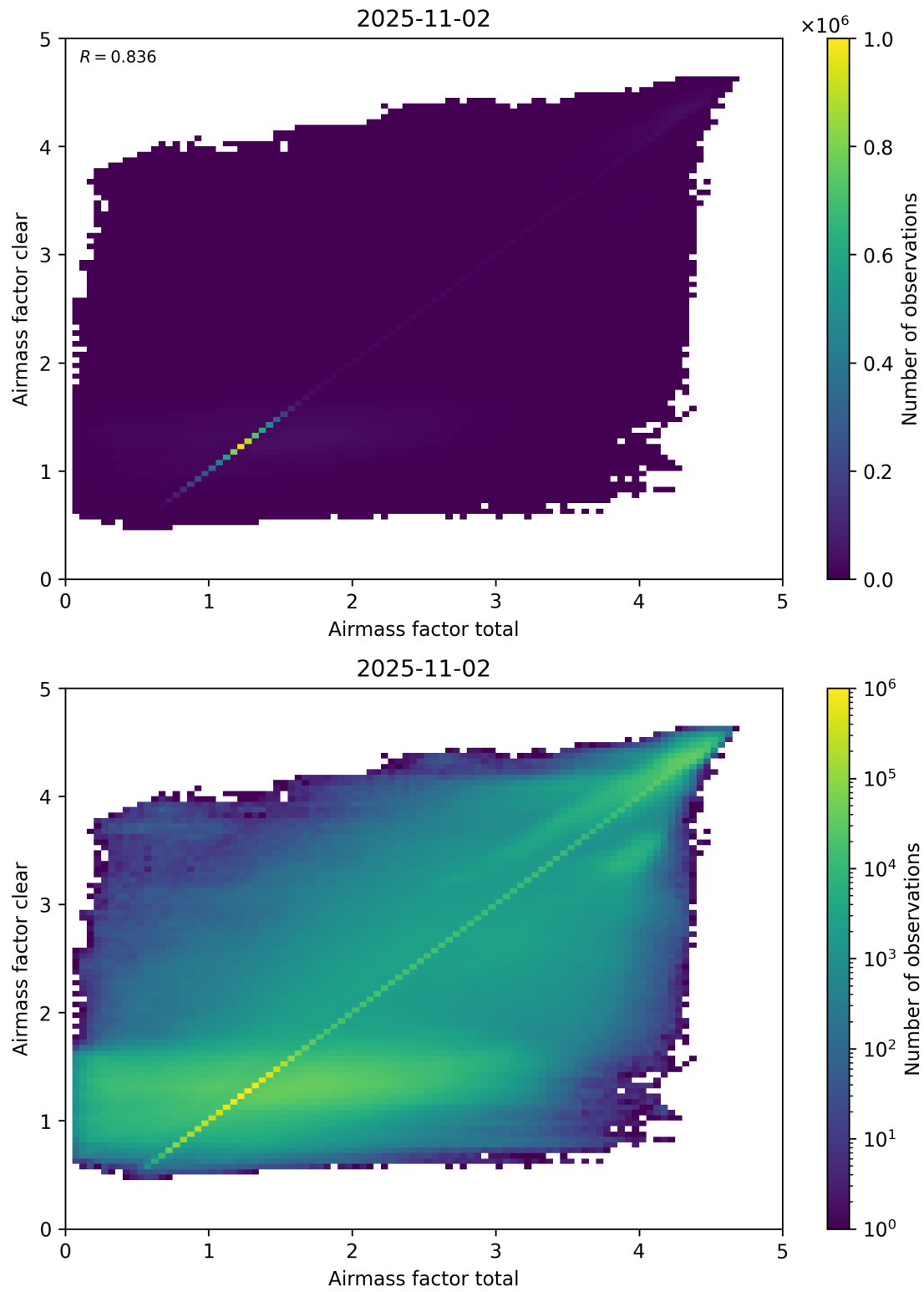
Figure 100: Scatter density plot of “Airmass factor total” against “Airmass factor clear” for 2025-11-02 to 2025-11-03.
