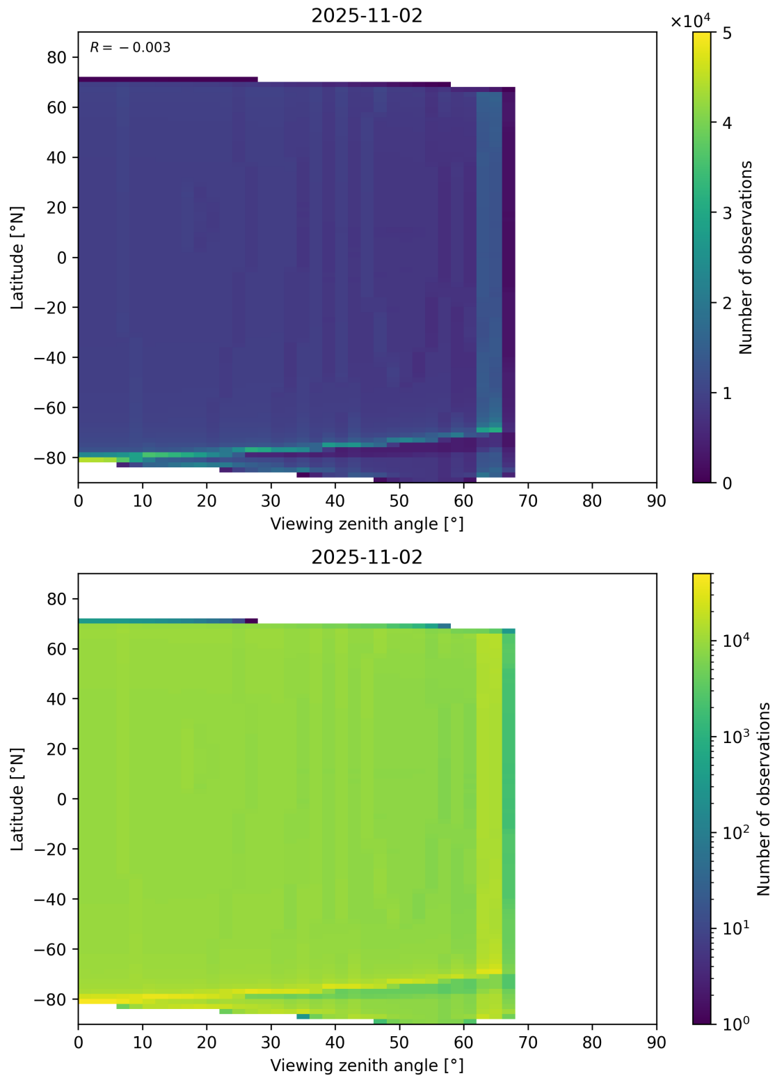
Figure 196: Scatter density plot of “Viewing zenith angle” against “Latitude” for 2025-11-02 to 2025-11-03.
