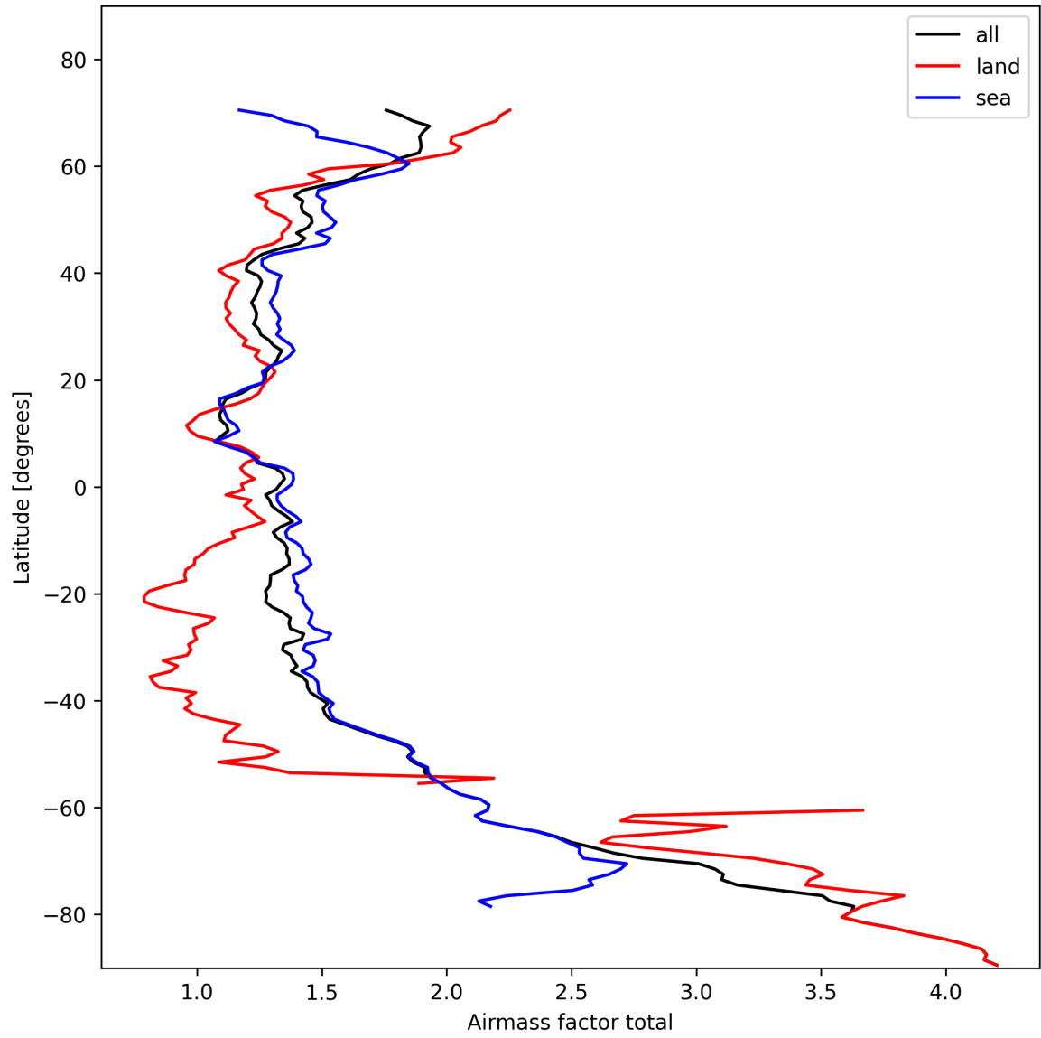
Figure 26: Zonal average of “Airmass factor total” for 2025-11-02 to 2025-11-03.
