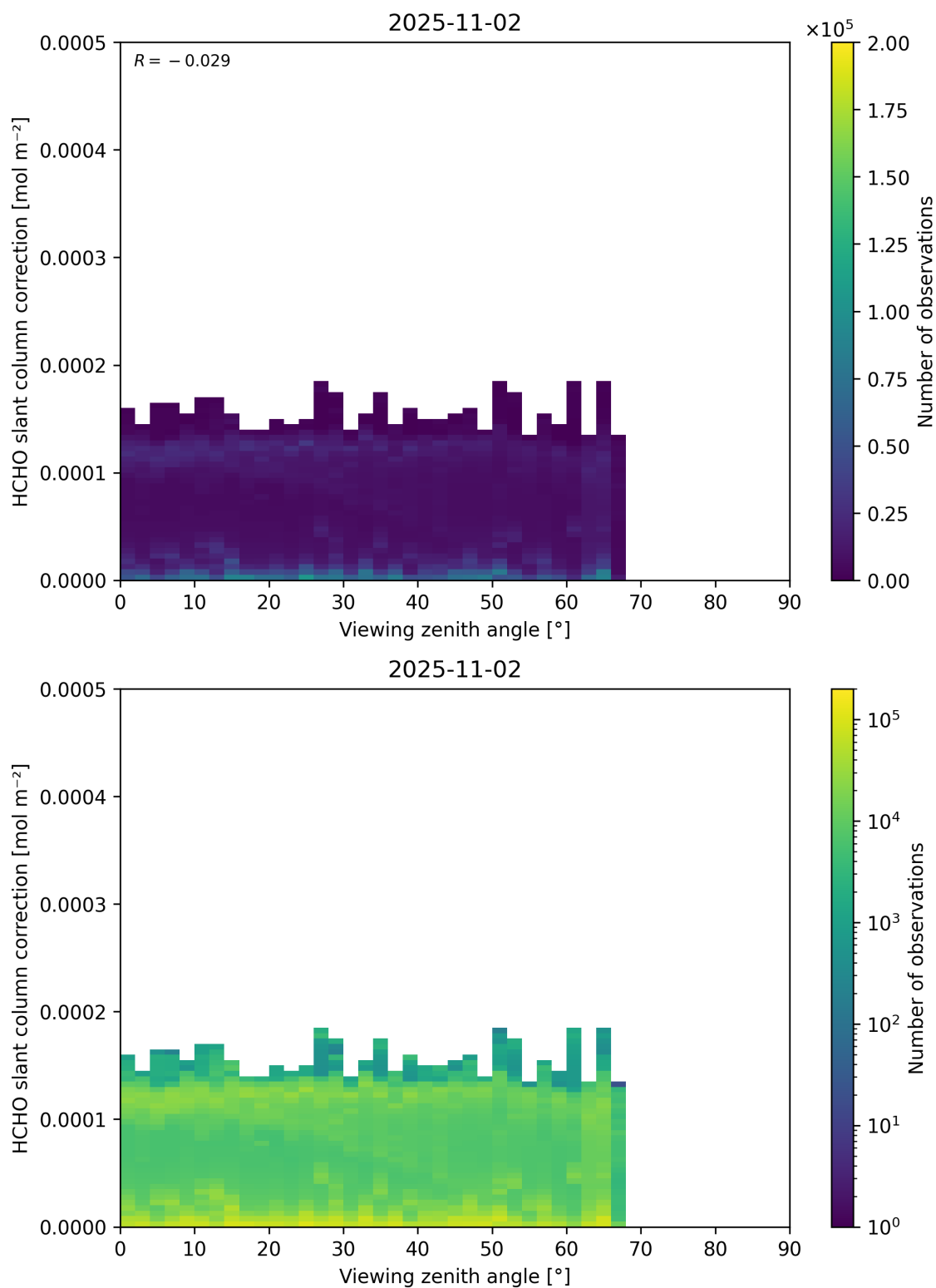
Figure 187: Scatter density plot of “Viewing zenith angle” against “HCHO slant column correction” for 2025-11-02 to 2025-11-03.
