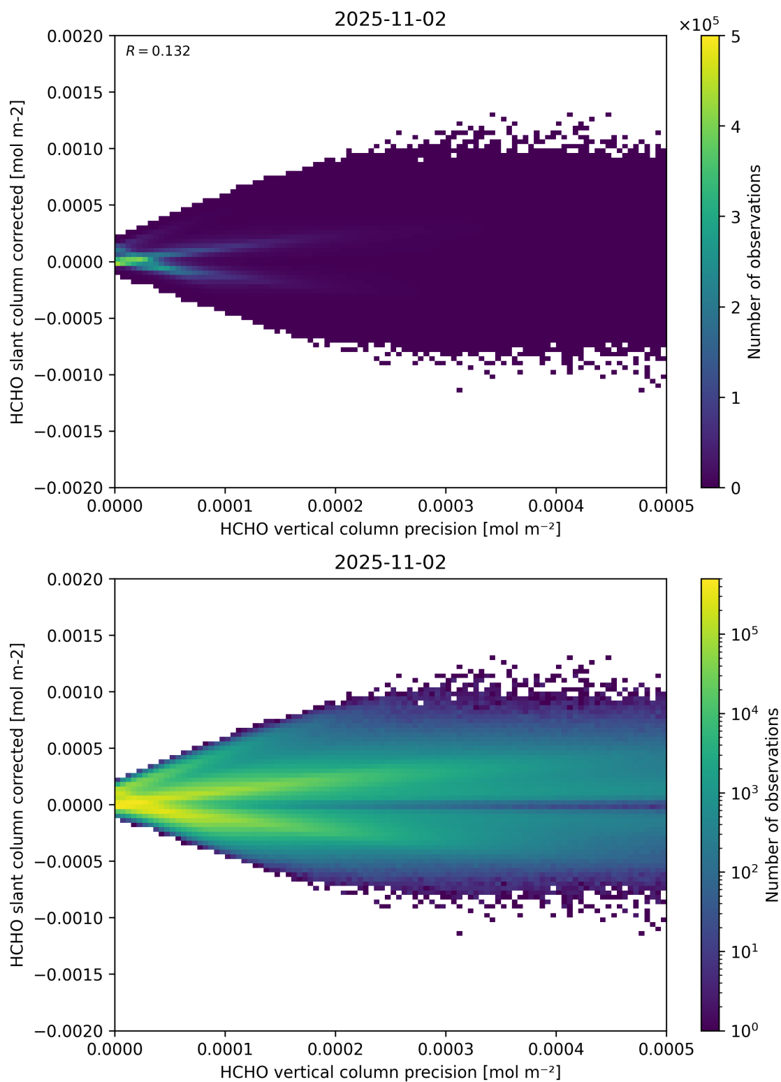
Figure 140: Scatter density plot of “HCHO vertical column precision” against “HCHO slant column corrected” for 2025-11-02 to 2025-11-03.
