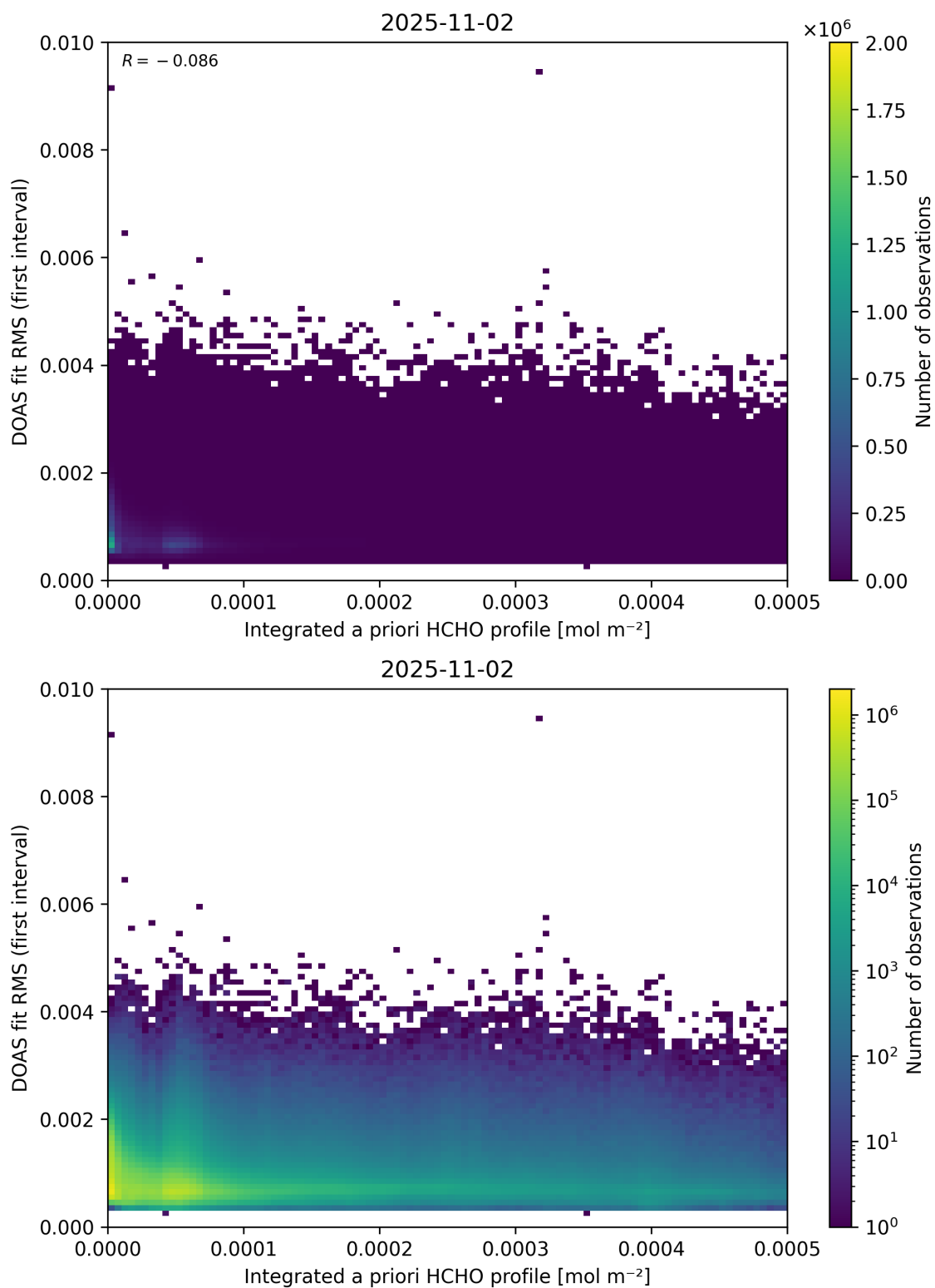
Figure 148: Scatter density plot of “Integrated a priori HCHO profile” against “DOAS fit RMS (first interval)” for 2025-11-02 to 2025-11-03.
