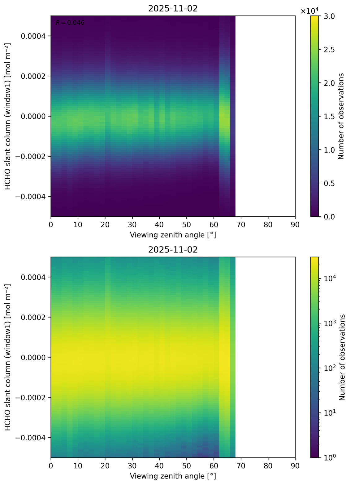
Figure 188: Scatter density plot of “Viewing zenith angle” against “HCHO slant column (window1)” for 2025-11-02 to 2025-11-03.
