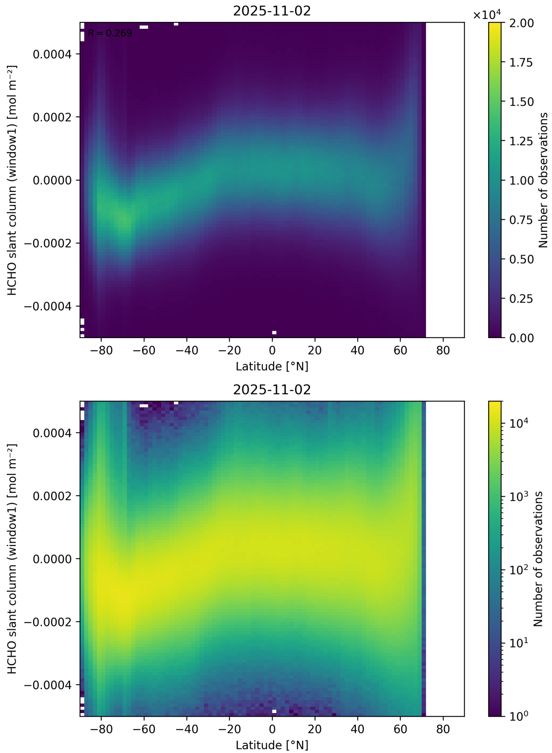
Figure 159: Scatter density plot of “Latitude” against “HCHO slant column (window1)” for 2025-11-02 to 2025-11-03.
