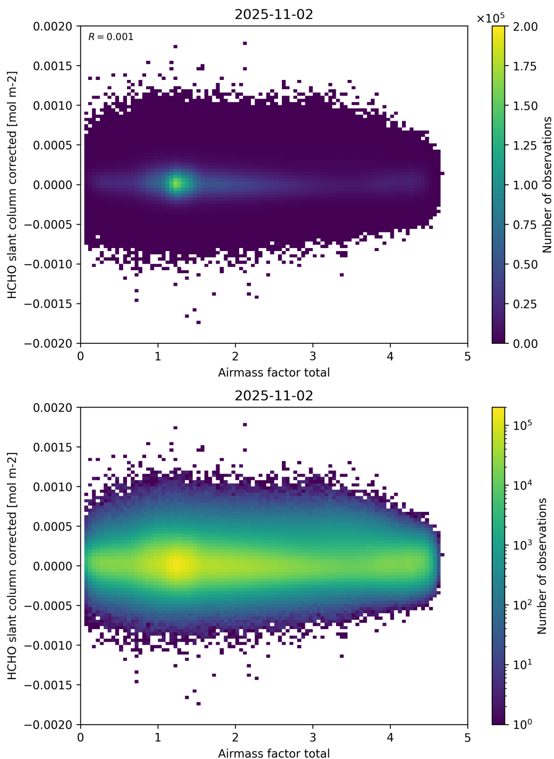
Figure 101: Scatter density plot of “Airmass factor total” against “HCHO slant column corrected” for 2025-11-02 to 2025-11-03.
