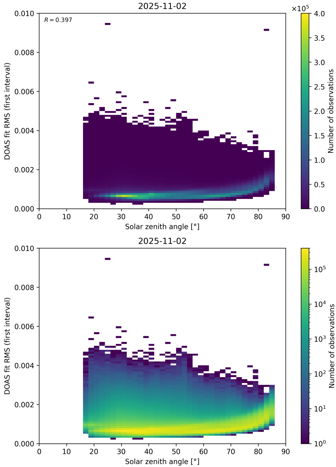
Figure 167: Scatter density plot of “Solar zenith angle” against “DOAS fit RMS (first interval)” for 2025-11-02 to 2025-11-03.
