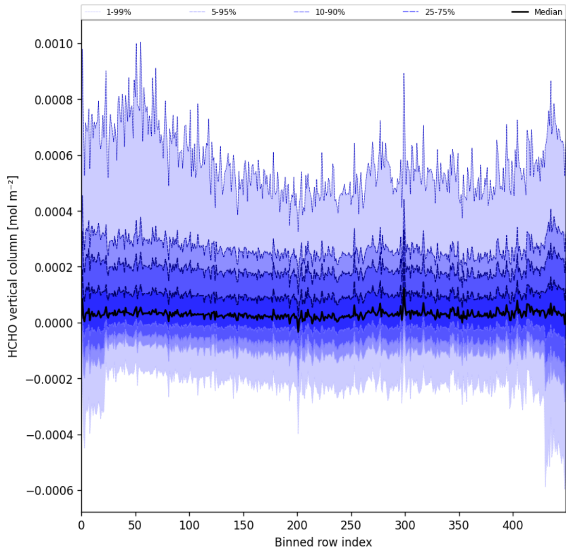
Figure 49: Along track statistics of “HCHO vertical column” for 2025-11-02 to 2025-11-03
