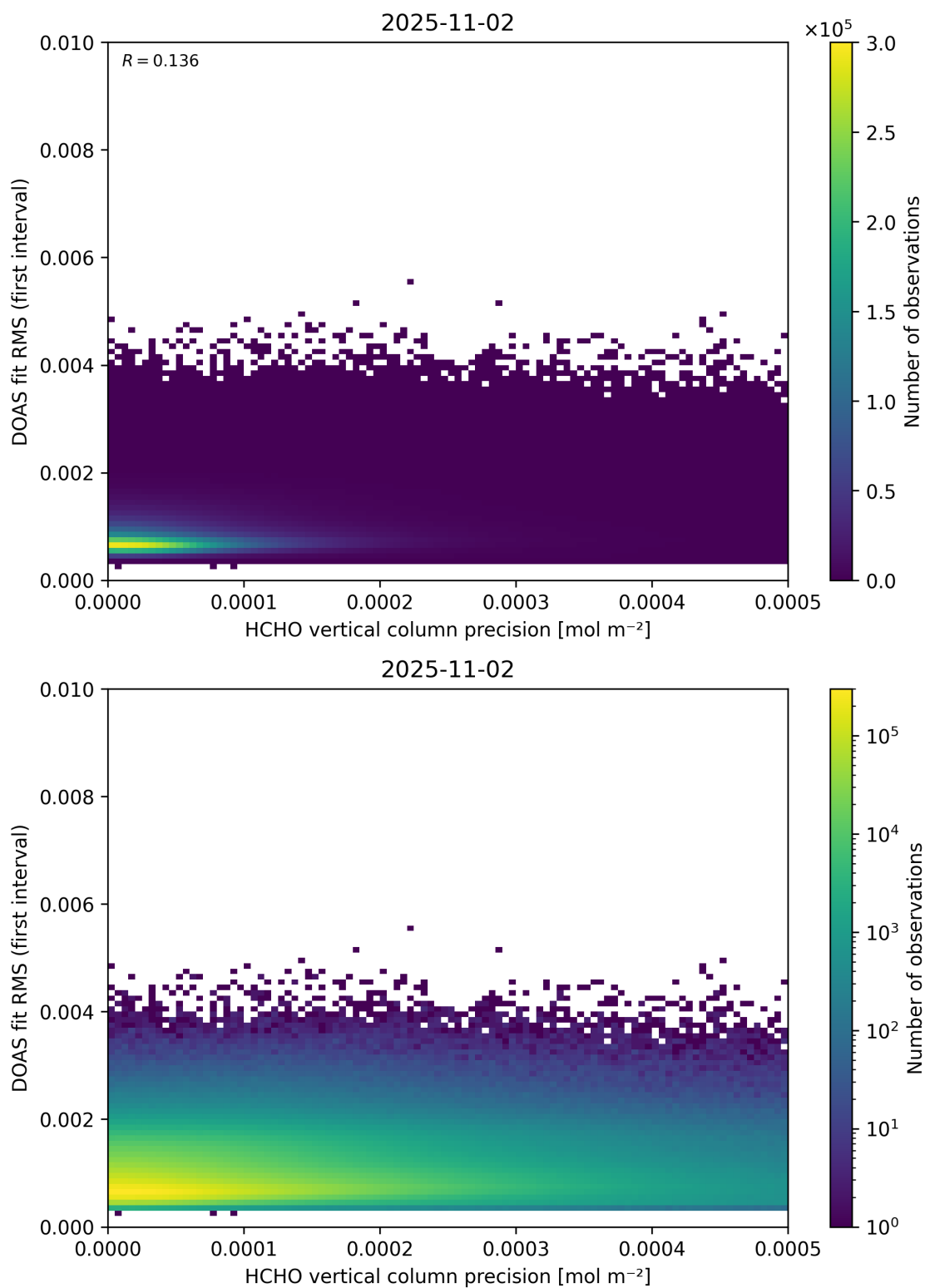
Figure 136: Scatter density plot of “HCHO vertical column precision” against “DOAS fit RMS (first interval)” for 2025-11-02 to 2025-11-03.
