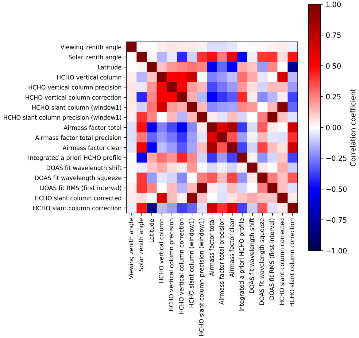
Figure 2: Map of correlation matrix for 2025-11-02 to 2025-11-03.
