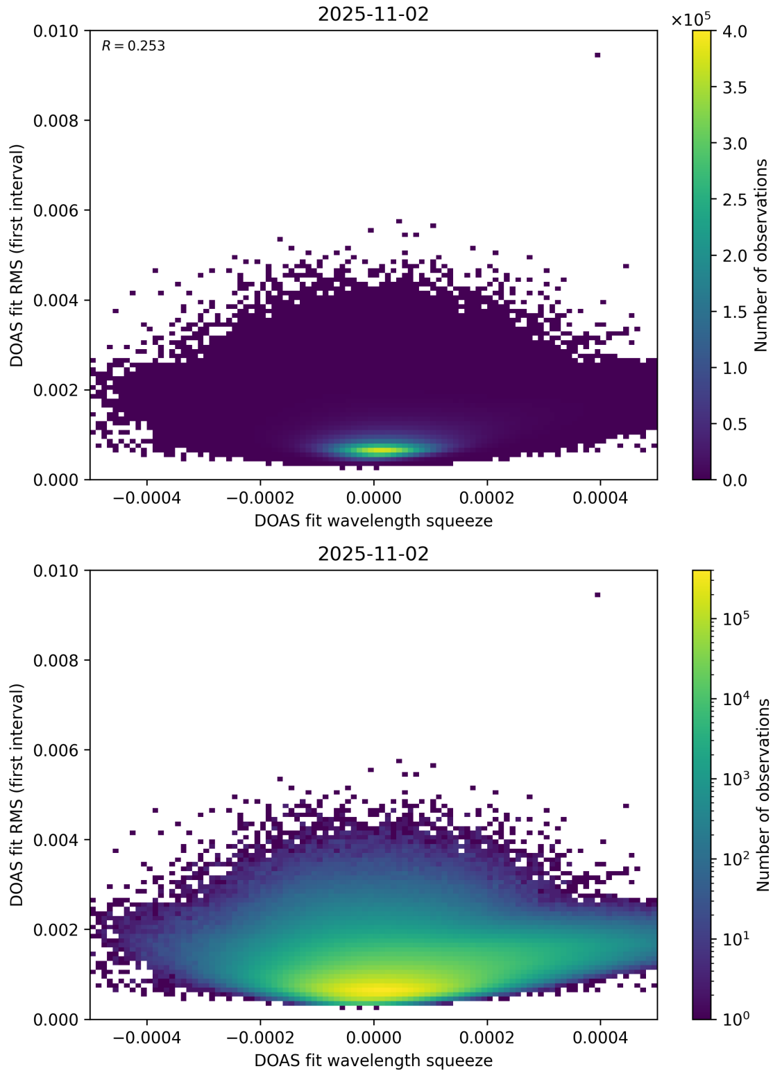
Figure 68: Scatter density plot of “DOAS fit wavelength squeeze” against “DOAS fit RMS (first interval)” for 2025-11-02 to 2025-11-03.
