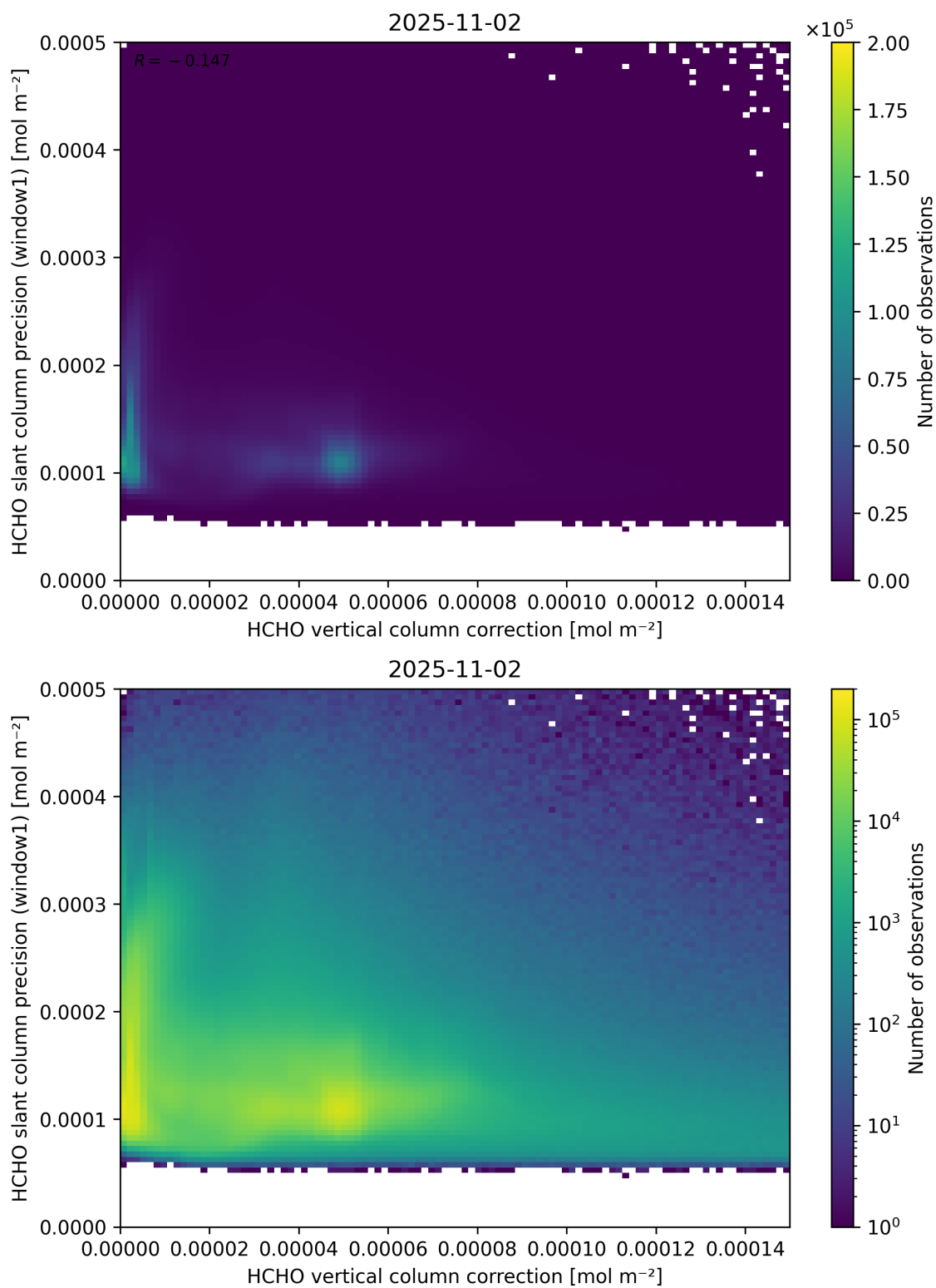
Figure 119: Scatter density plot of “HCHO vertical column correction” against “HCHO slant column precision (window1)” for 2025-11-02 to 2025-11-03.
