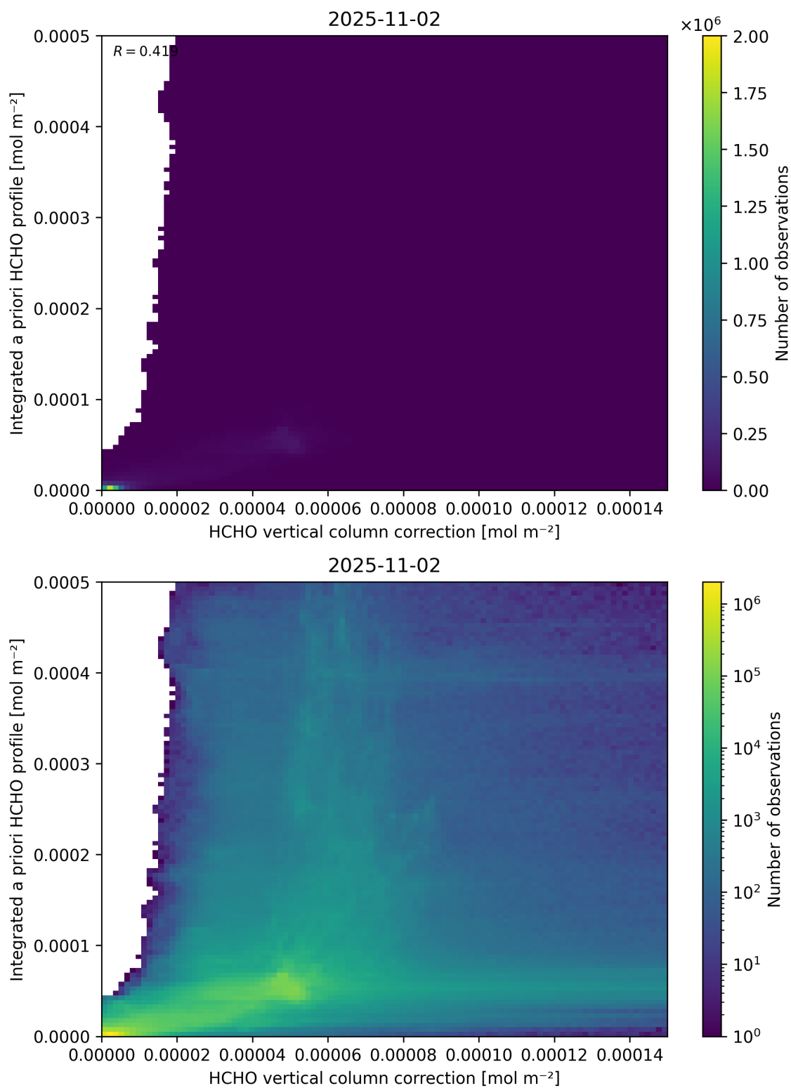
Figure 122: Scatter density plot of “HCHO vertical column correction” against “Integrated a priori HCHO profile” for 2025-11-02 to 2025-11-03.
