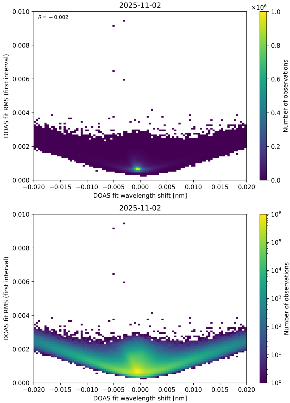
Figure 64: Scatter density plot of “DOAS fit wavelength shift” against “DOAS fit RMS (first interval)” for 2025-11-02 to 2025-11-03.
