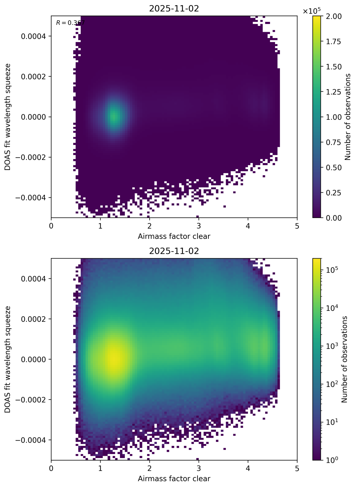
Figure 73: Scatter density plot of “Airmass factor clear” against “DOAS fit wavelength squeeze” for 2025-11-02 to 2025-11-03.
