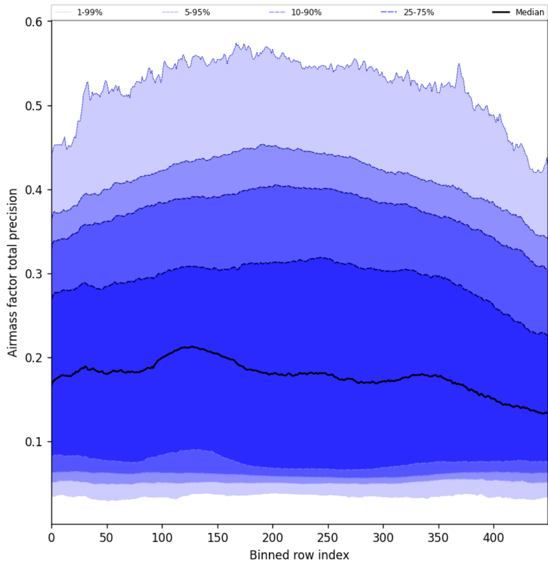
Figure 55: Along track statistics of “Airmass factor total precision” for 2025-11-02 to 2025-11-03
