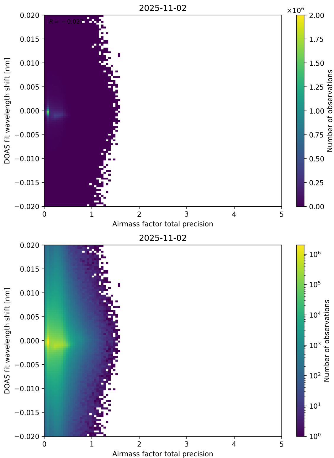
Figure 106: Scatter density plot of “Airmass factor total precision” against “DOAS fit wavelength shift” for 2025-11-02 to 2025-11-03.
