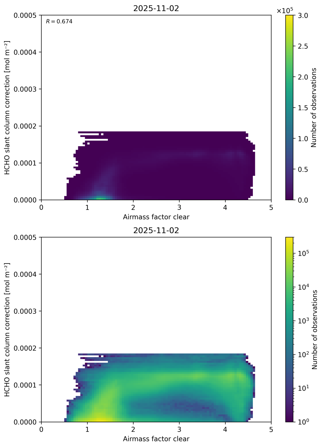
Figure 75: Scatter density plot of “Airmass factor clear” against “HCHO slant column correction” for 2025-11-02 to 2025-11-03.
