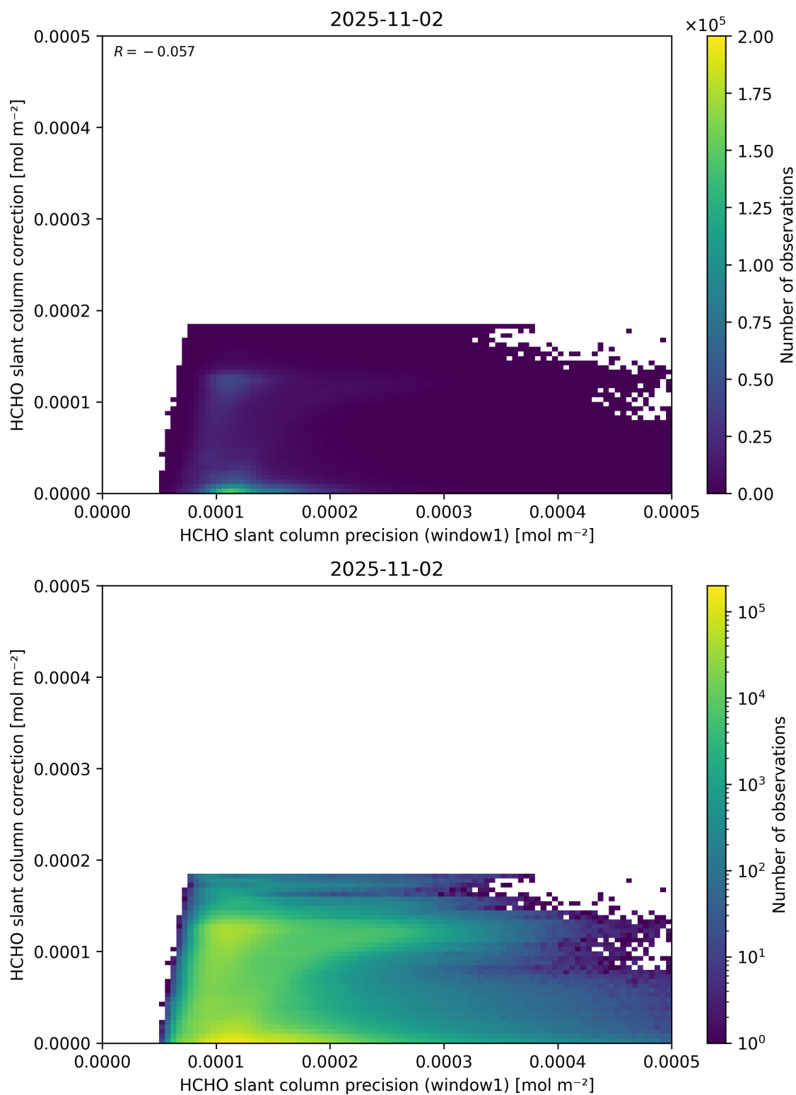
Figure 93: Scatter density plot of “HCHO slant column precision (window1)” against “HCHO slant column correction” for 2025-11-02 to 2025-11-03.
