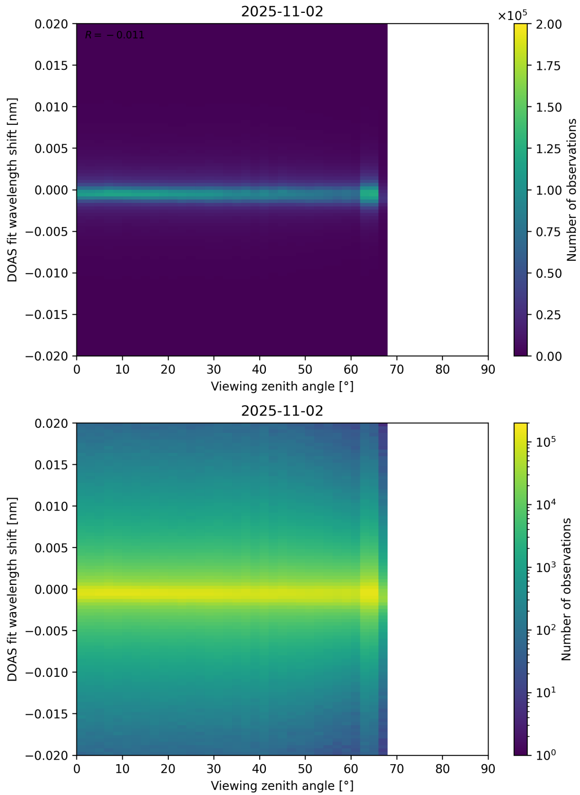
Figure 183: Scatter density plot of “Viewing zenith angle” against “DOAS fit wavelength shift” for 2025-11-02 to 2025-11-03.
