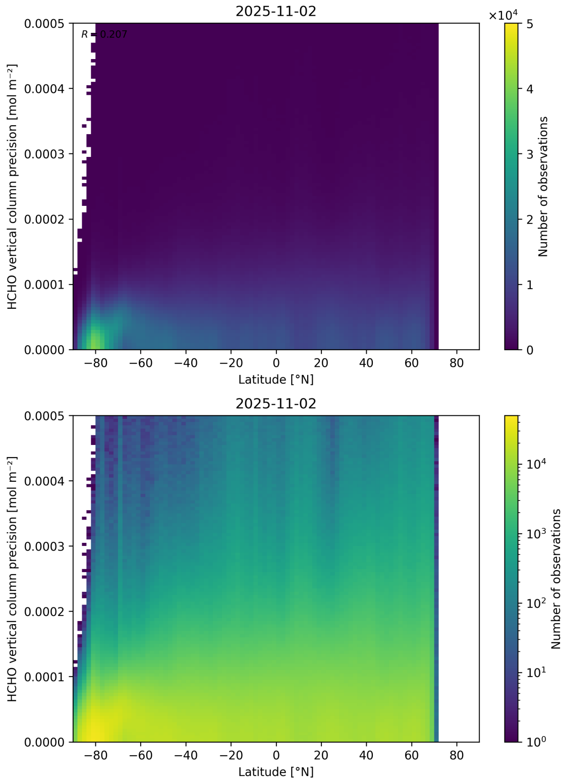
Figure 165: Scatter density plot of “Latitude” against “HCHO vertical column precision” for 2025-11-02 to 2025-11-03.
