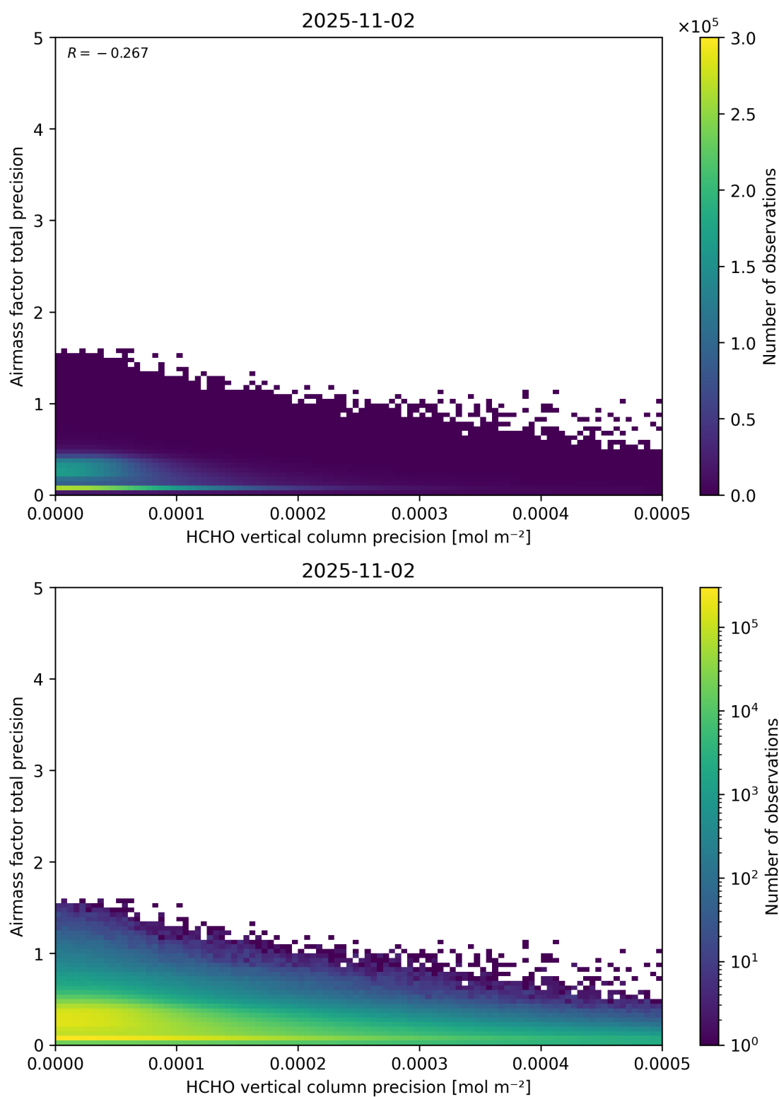
Figure 145: Scatter density plot of “HCHO vertical column precision” against “Airmass factor total precision” for 2025-11-02 to 2025-11-03.
