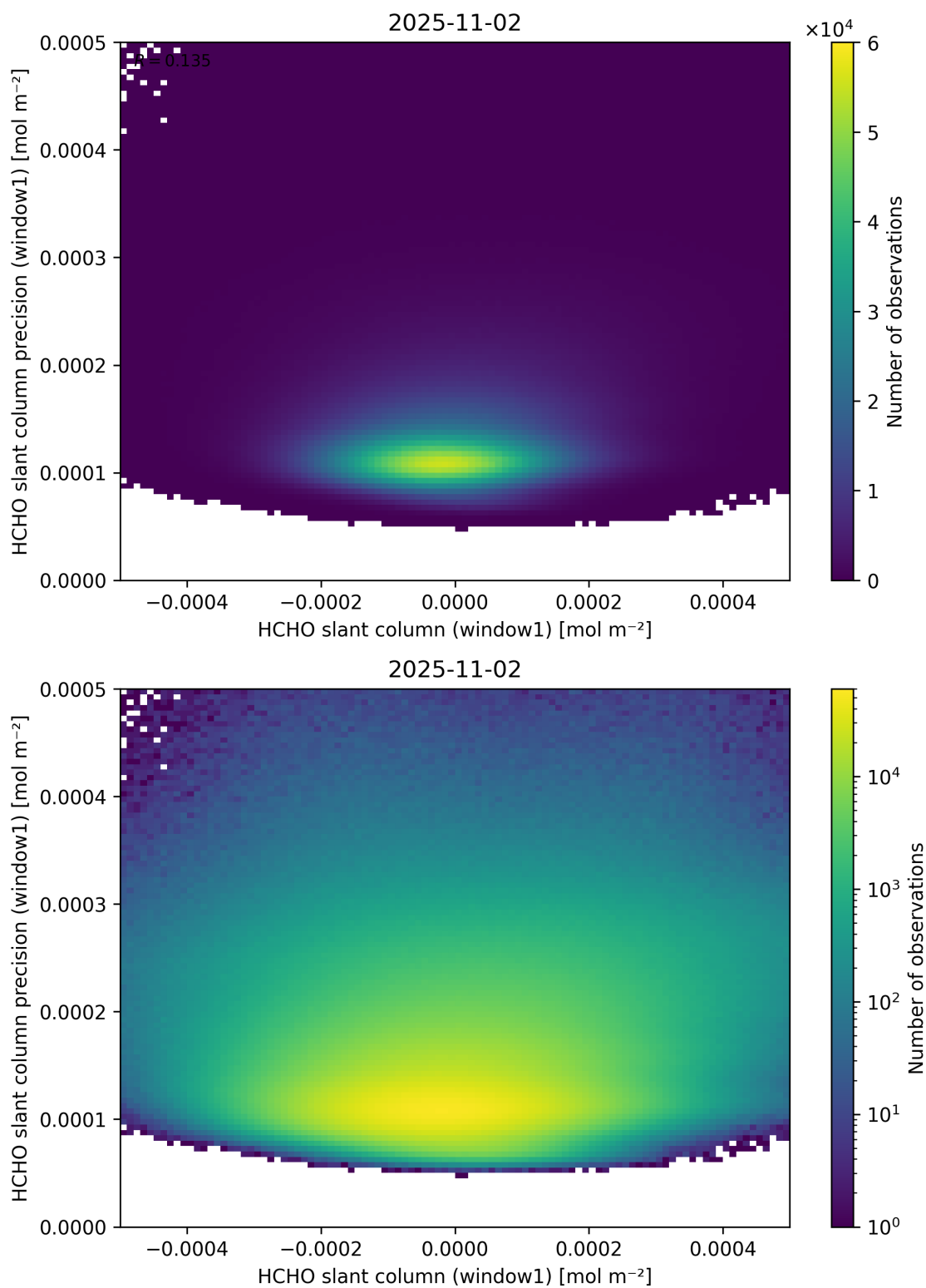
Figure 84: Scatter density plot of “HCHO slant column (window1)” against “HCHO slant column precision (window1)” for 2025-11-02 to 2025-11-03.
