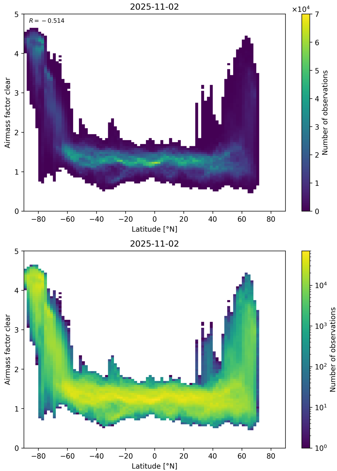
Figure 156: Scatter density plot of “Latitude” against “Airmass factor clear” for 2025-11-02 to 2025-11-03.
