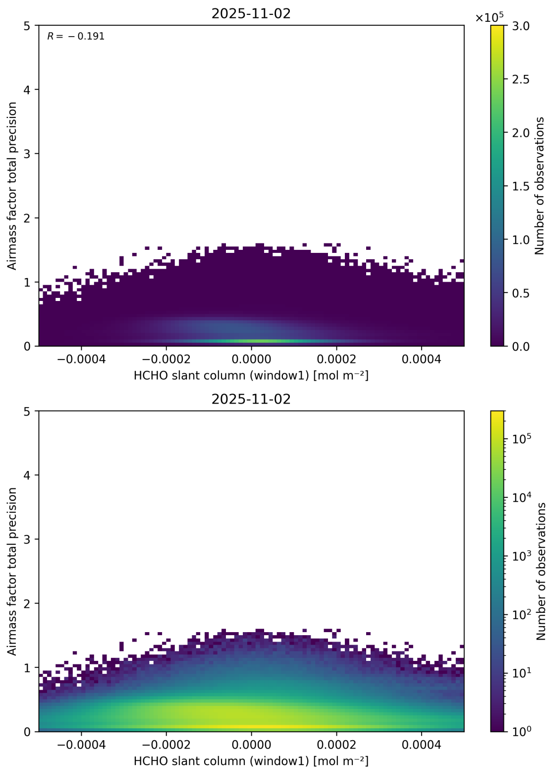
Figure 86: Scatter density plot of “HCHO slant column (window1)” against “Airmass factor total precision” for 2025-11-02 to 2025-11-03.
