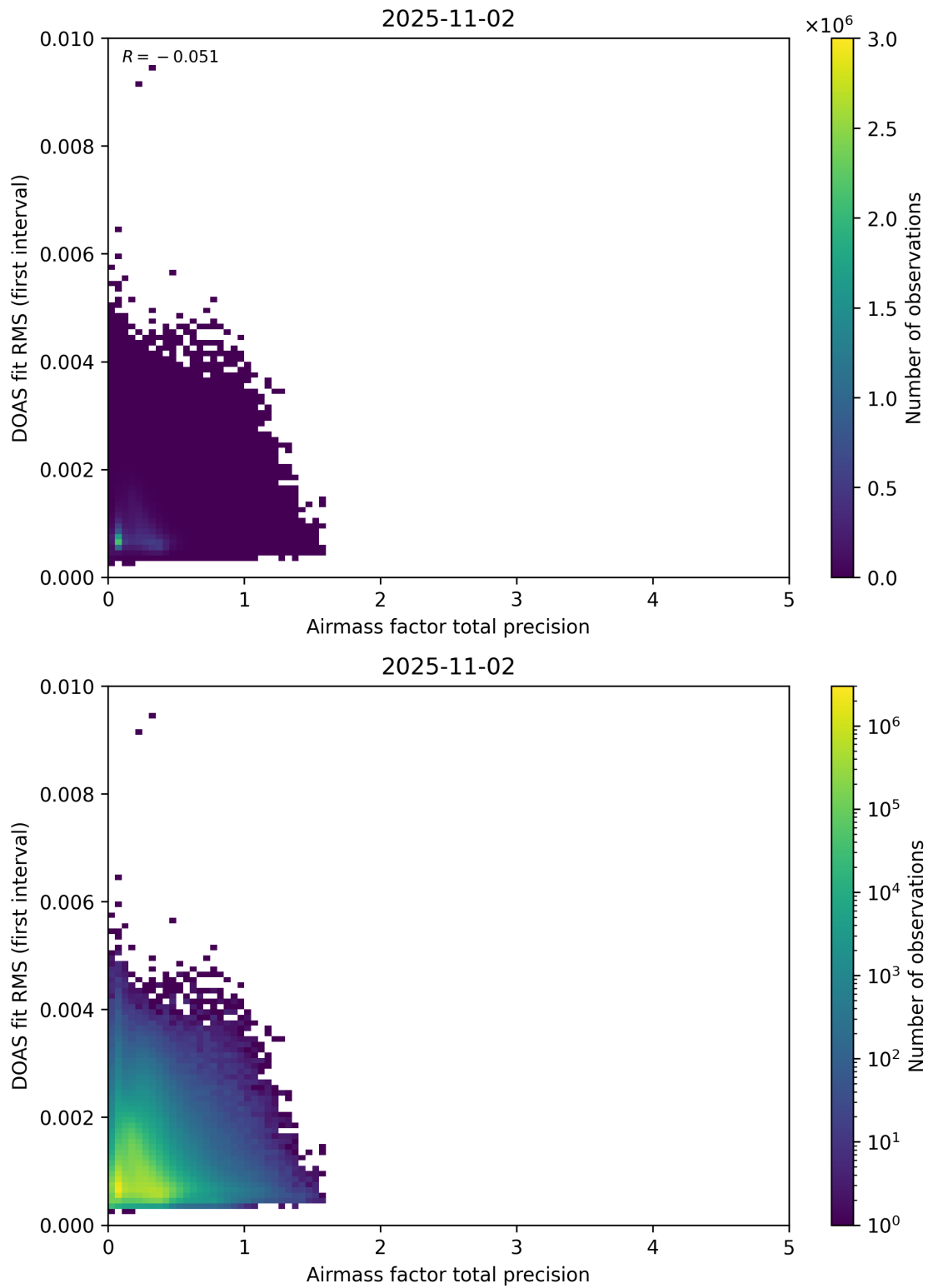
Figure 105: Scatter density plot of “Airmass factor total precision” against “DOAS fit RMS (first interval)” for 2025-11-02 to 2025-11-03.
