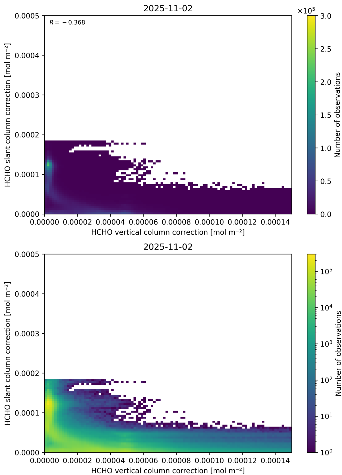
Figure 117: Scatter density plot of “HCHO vertical column correction” against “HCHO slant column correction” for 2025-11-02 to 2025-11-03.
