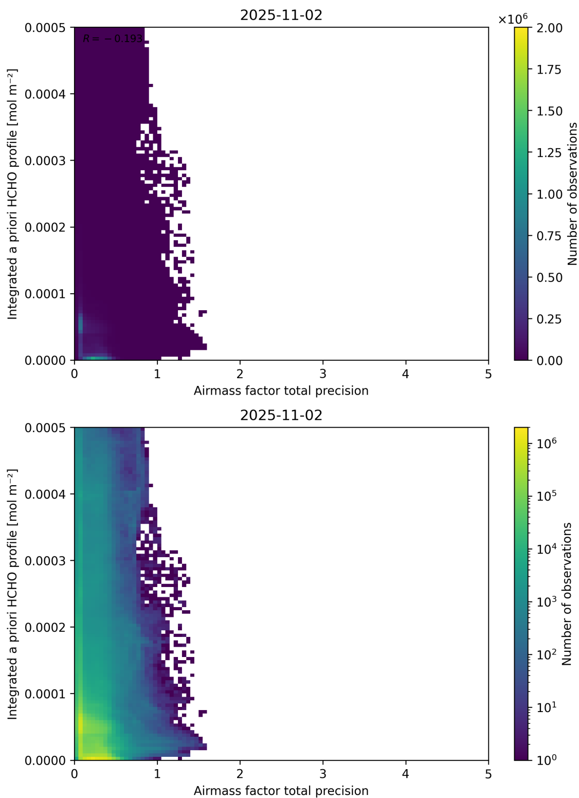
Figure 111: Scatter density plot of “Airmass factor total precision” against “Integrated a priori HCHO profile” for 2025-11-02 to 2025-11-03.
