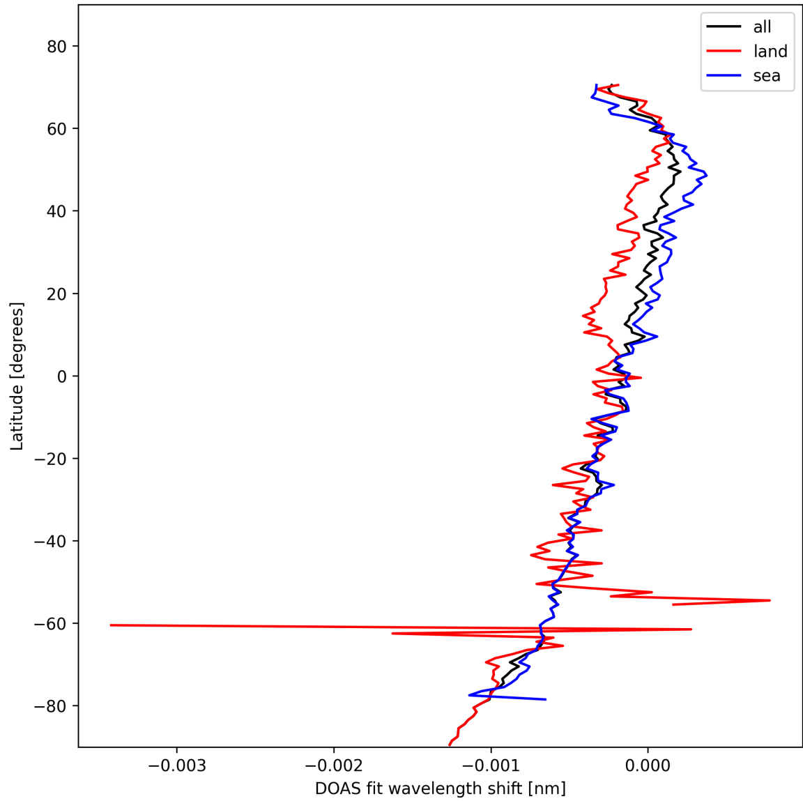
Figure 30: Zonal average of “DOAS fit wavelength shift” for 2025-11-02 to 2025-11-03.
