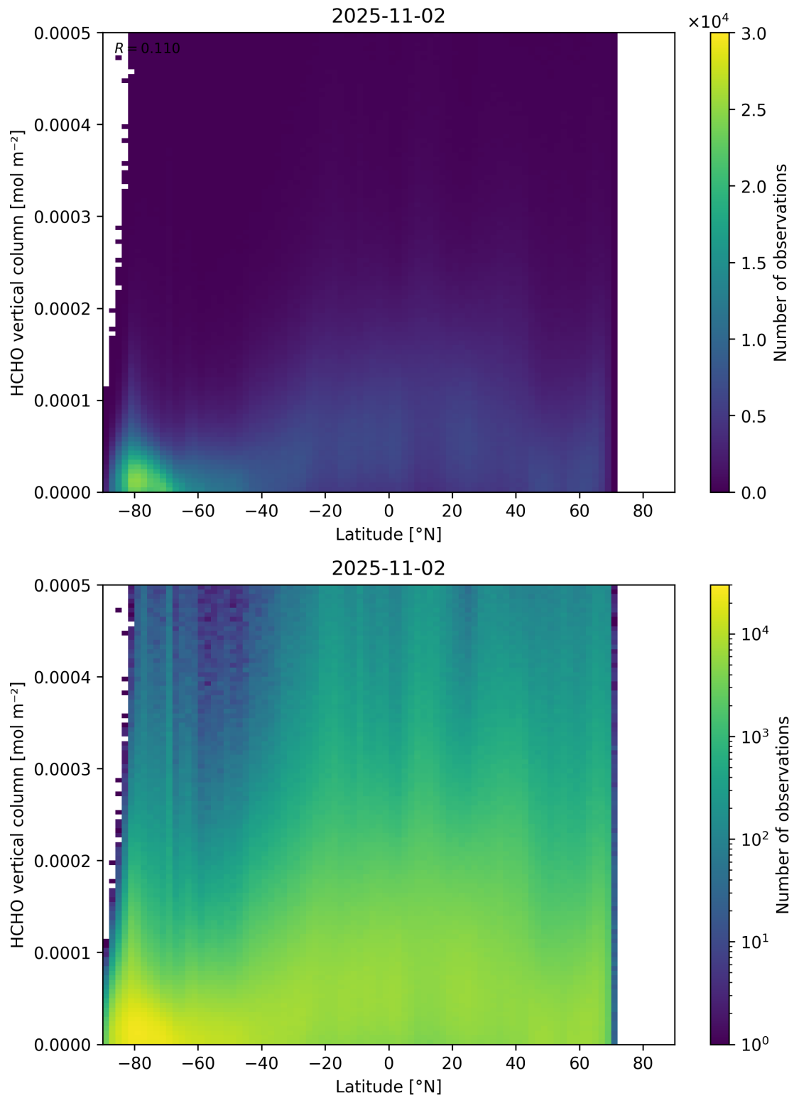
Figure 163: Scatter density plot of “Latitude” against “HCHO vertical column” for 2025-11-02 to 2025-11-03.
