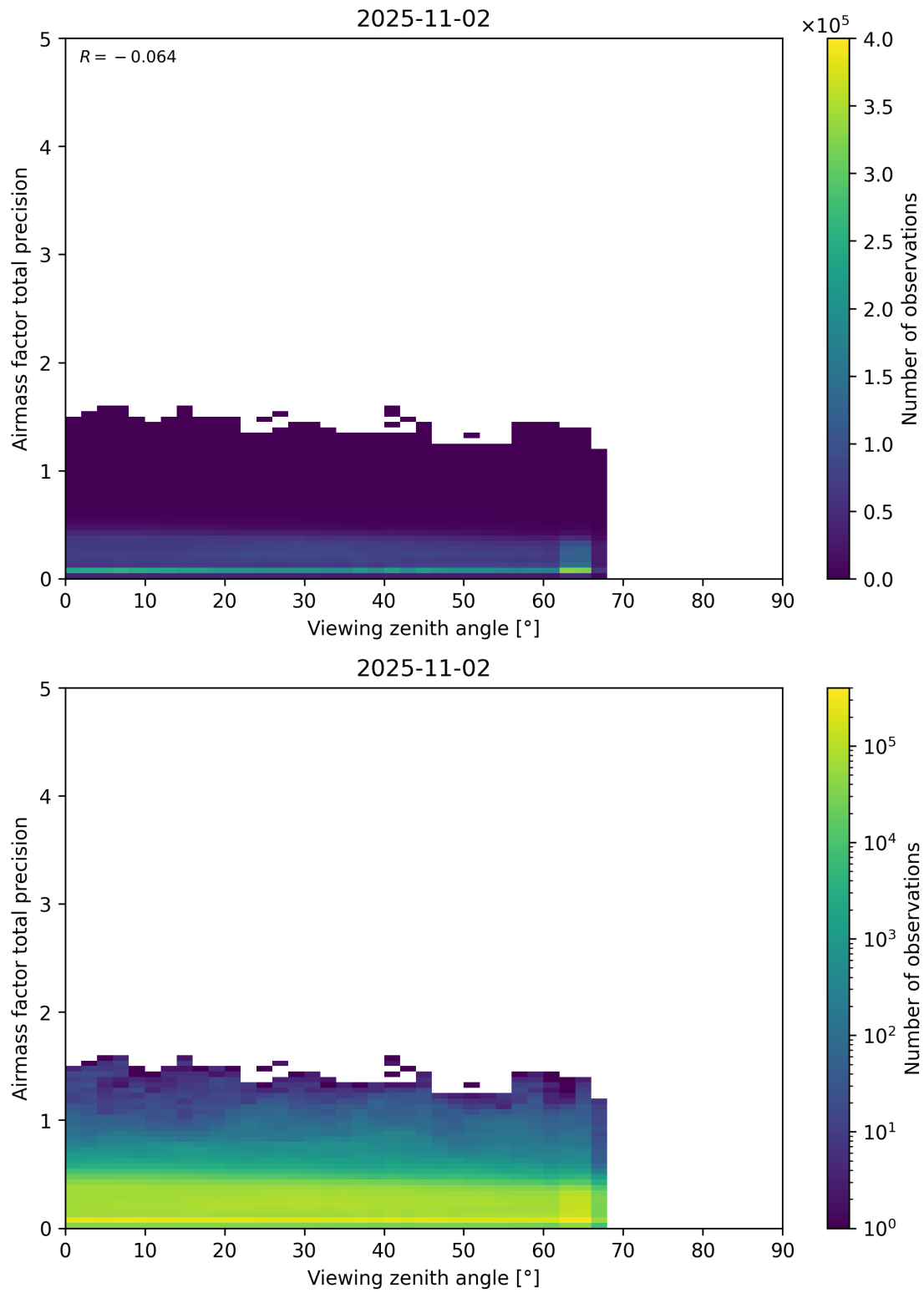
Figure 191: Scatter density plot of “Viewing zenith angle” against “Airmass factor total precision” for 2025-11-02 to 2025-11-03.
