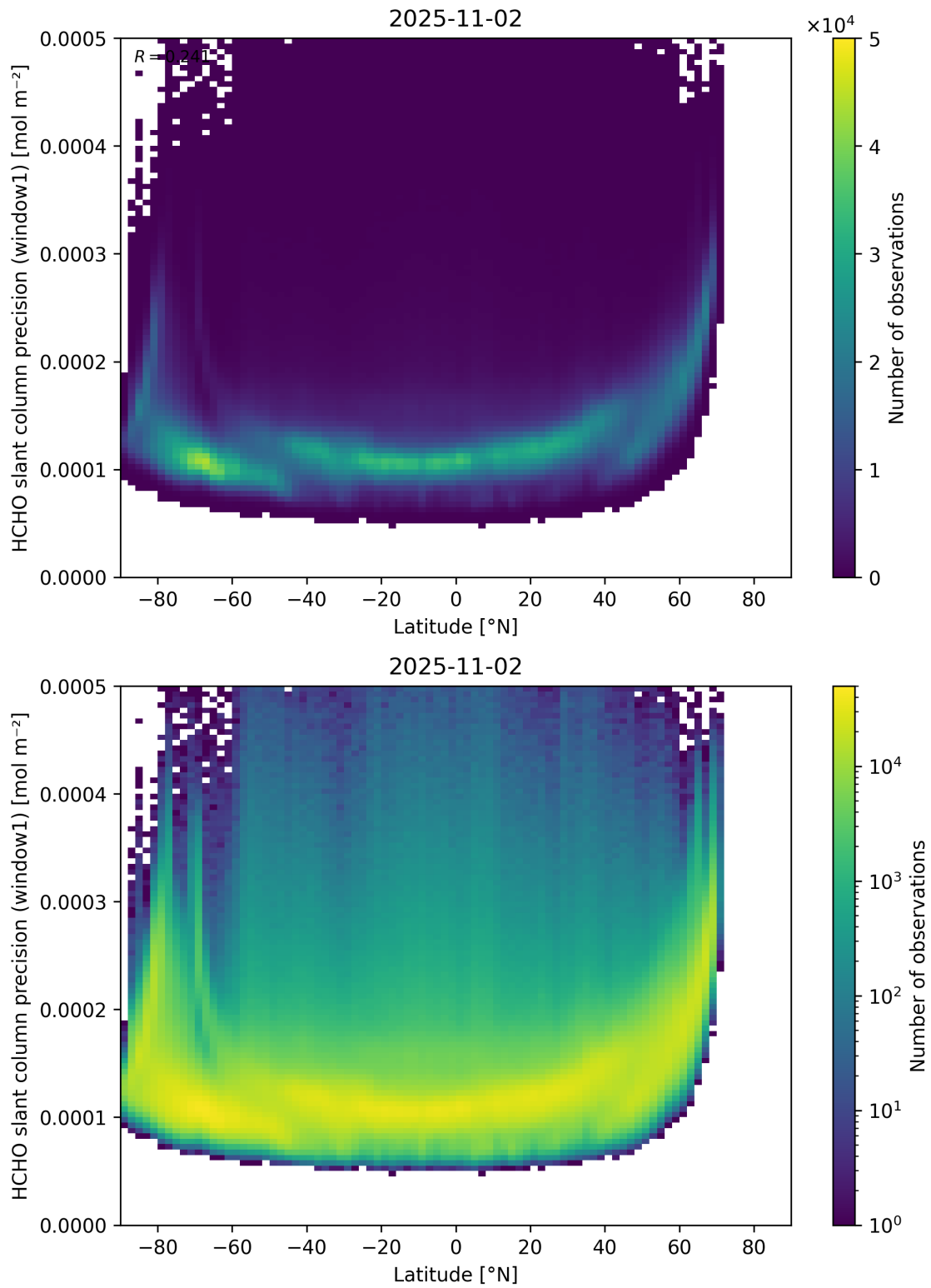
Figure 160: Scatter density plot of “Latitude” against “HCHO slant column precision (window1)” for 2025-11-02 to 2025-11-03.
