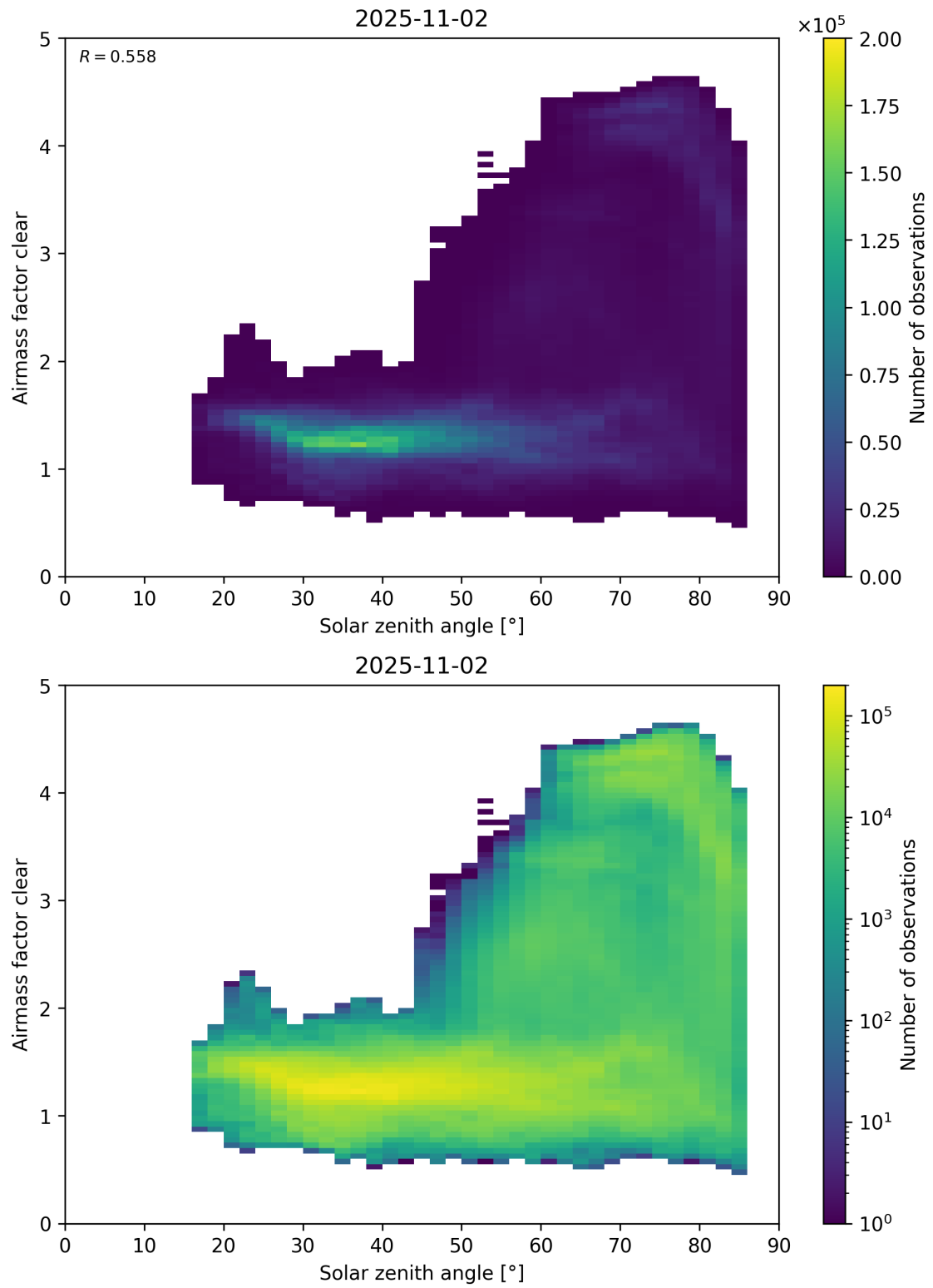
Figure 170: Scatter density plot of “Solar zenith angle” against “Airmass factor clear” for 2025-11-02 to 2025-11-03.
