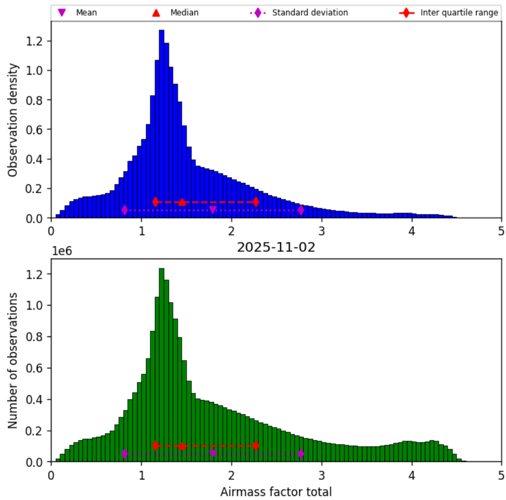
Figure 40: Histogram of “Airmass factor total” for 2025-11-02 to 2025-11-03
