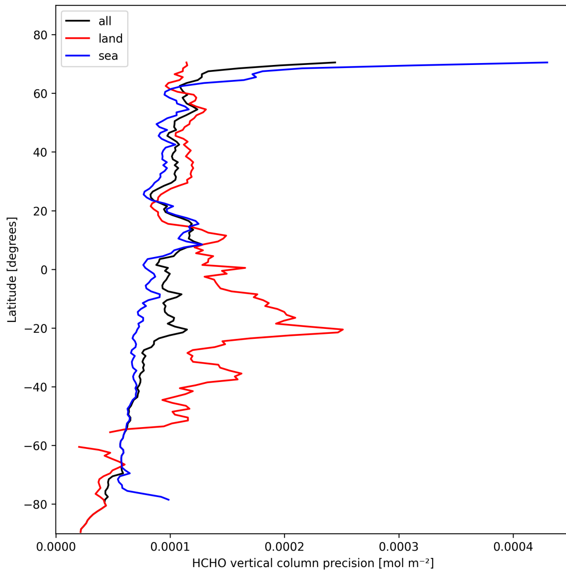
Figure 22: Zonal average of “HCHO vertical column precision” for 2025-11-02 to 2025-11-03.
