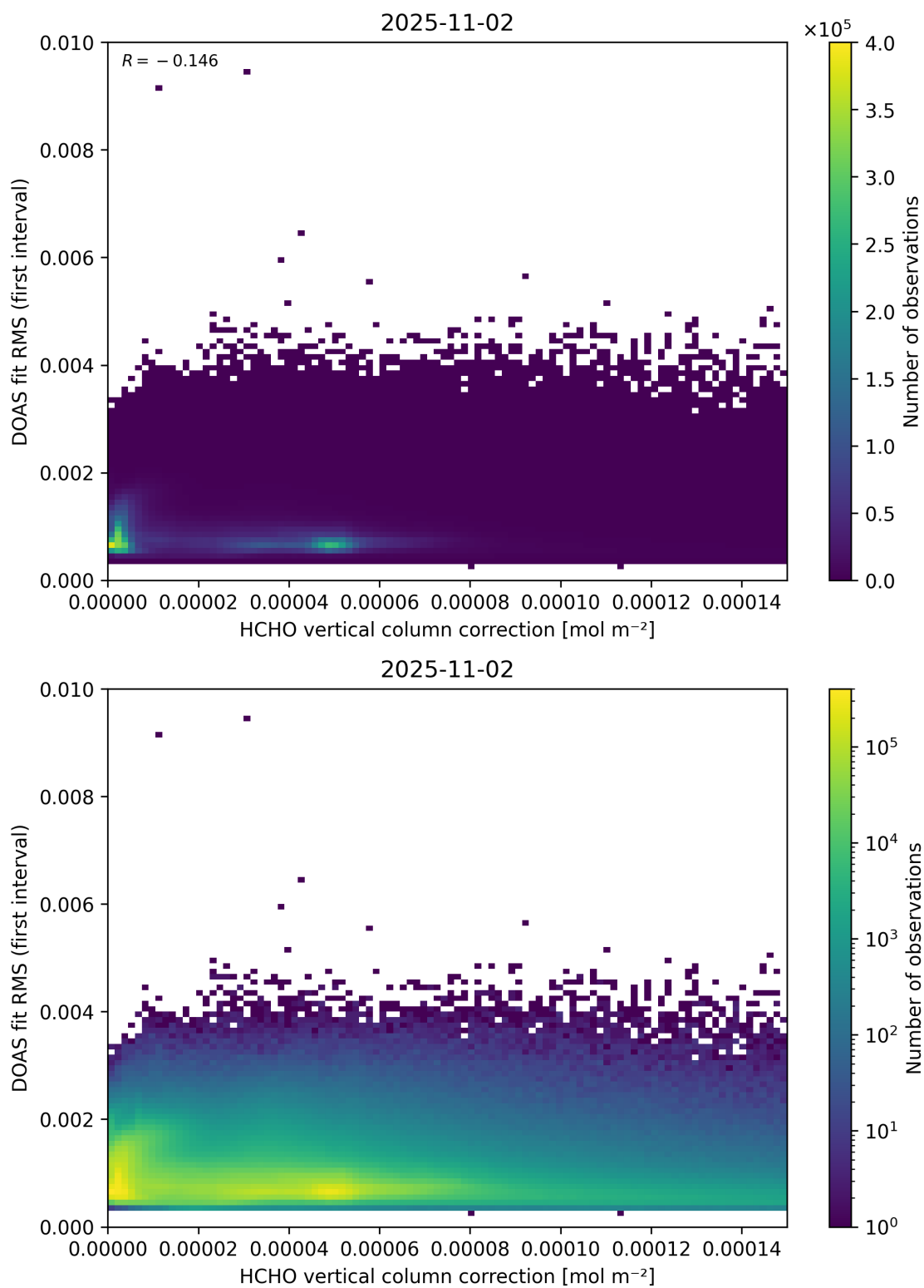
Figure 112: Scatter density plot of “HCHO vertical column correction” against “DOAS fit RMS (first interval)” for 2025-11-02 to 2025-11-03.
