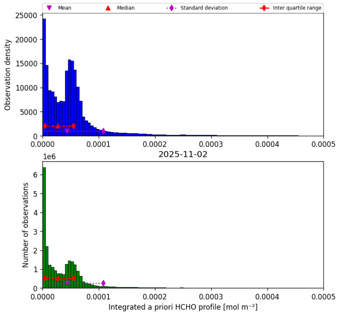
Figure 43: Histogram of “Integrated a priori HCHO profile” for 2025-11-02 to 2025-11-03
