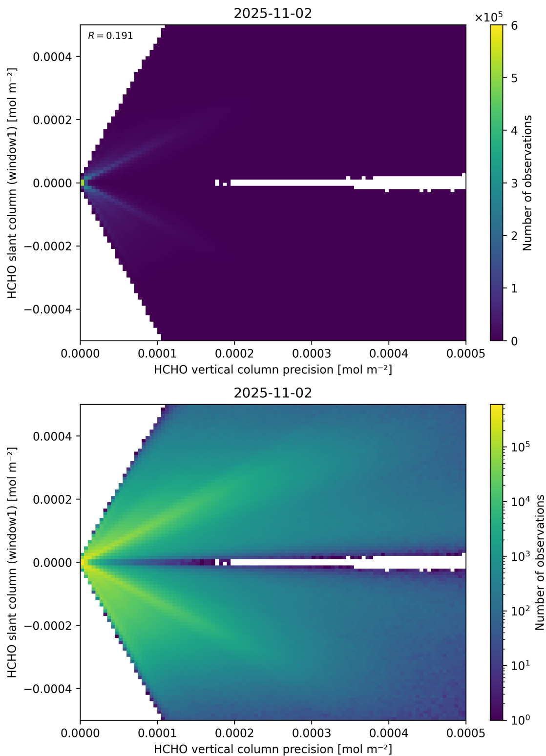
Figure 142: Scatter density plot of “HCHO vertical column precision” against “HCHO slant column (window1)” for 2025-11-02 to 2025-11-03.
