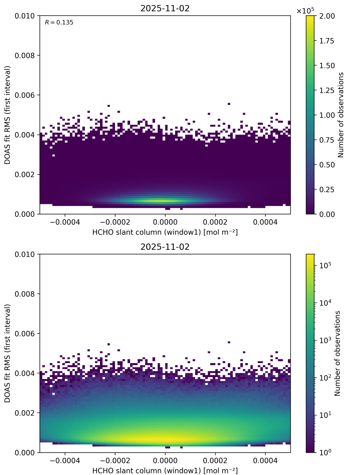
Figure 78: Scatter density plot of “HCHO slant column (window1)” against “DOAS fit RMS (first interval)” for 2025-11-02 to 2025-11-03.
