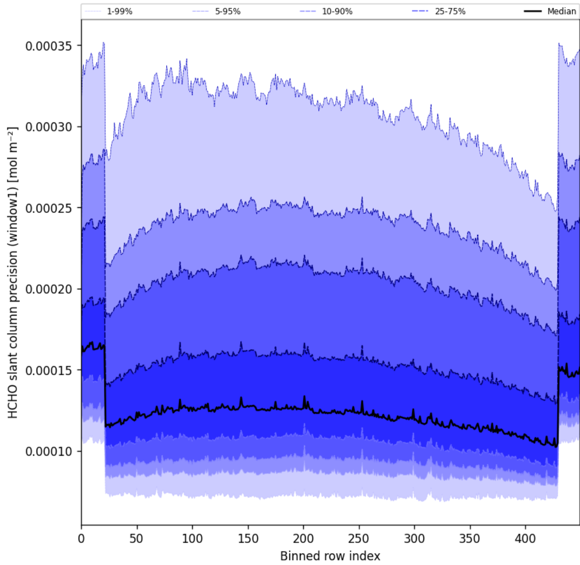
Figure 53: Along track statistics of “HCHO slant column precision (window1)” for 2025-11-02 to 2025-11-03
