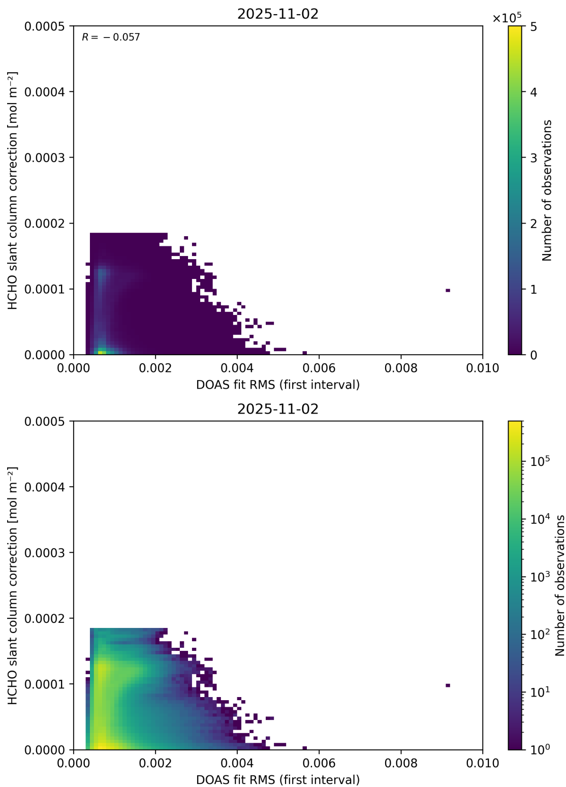
Figure 63: Scatter density plot of “DOAS fit RMS (first interval)” against “HCHO slant column correction” for 2025-11-02 to 2025-11-03.
