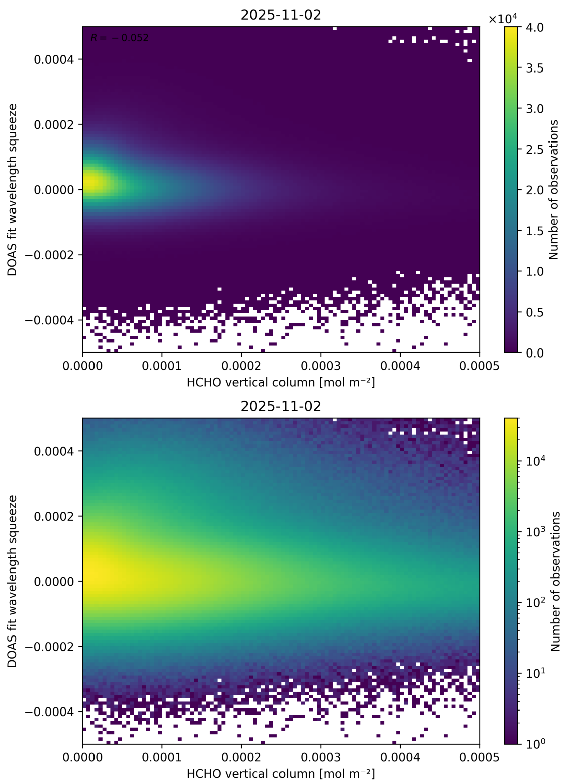
Figure 125: Scatter density plot of “HCHO vertical column” against “DOAS fit wavelength squeeze” for 2025-11-02 to 2025-11-03.
