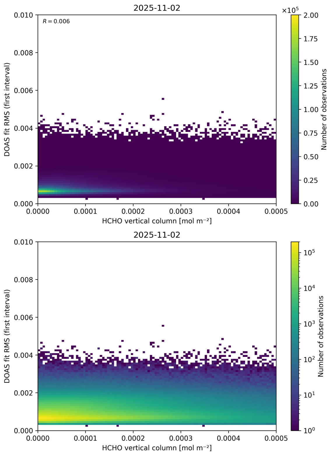
Figure 123: Scatter density plot of “HCHO vertical column” against “DOAS fit RMS (first interval)” for 2025-11-02 to 2025-11-03.
