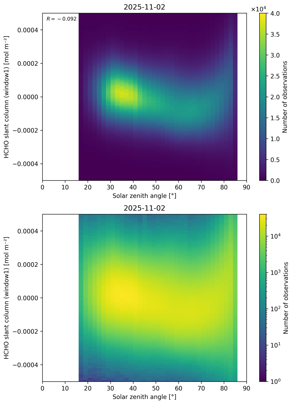
Figure 173: Scatter density plot of “Solar zenith angle” against “HCHO slant column (window1)” for 2025-11-02 to 2025-11-03.
