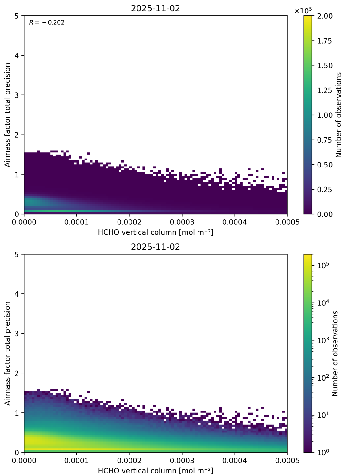
Figure 132: Scatter density plot of “HCHO vertical column” against “Airmass factor total precision” for 2025-11-02 to 2025-11-03.
