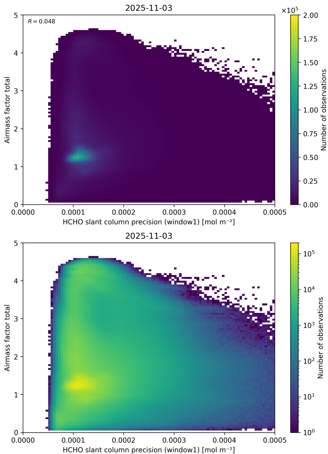
Figure 94: Scatter density plot of “HCHO slant column precision (window1)” against “Airmass factor total” for 2025-11-02 to 2025-11-04.
