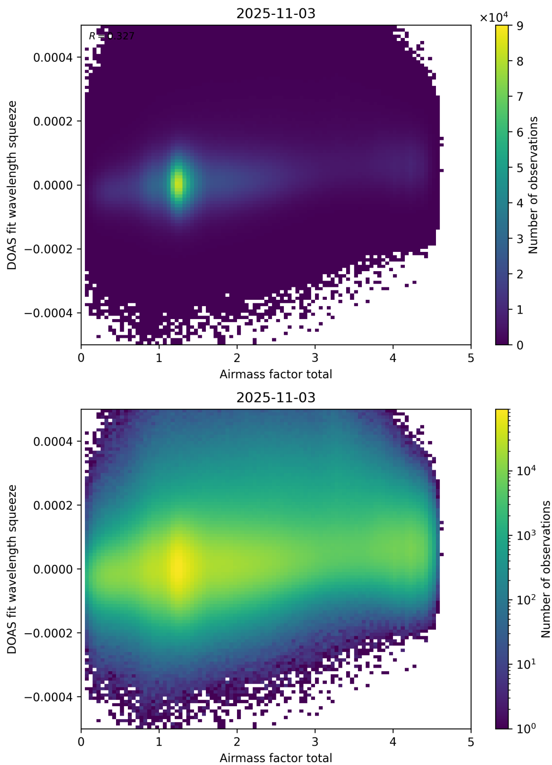
Figure 99: Scatter density plot of “Airmass factor total” against “DOAS fit wavelength squeeze” for 2025-11-02 to 2025-11-04.
