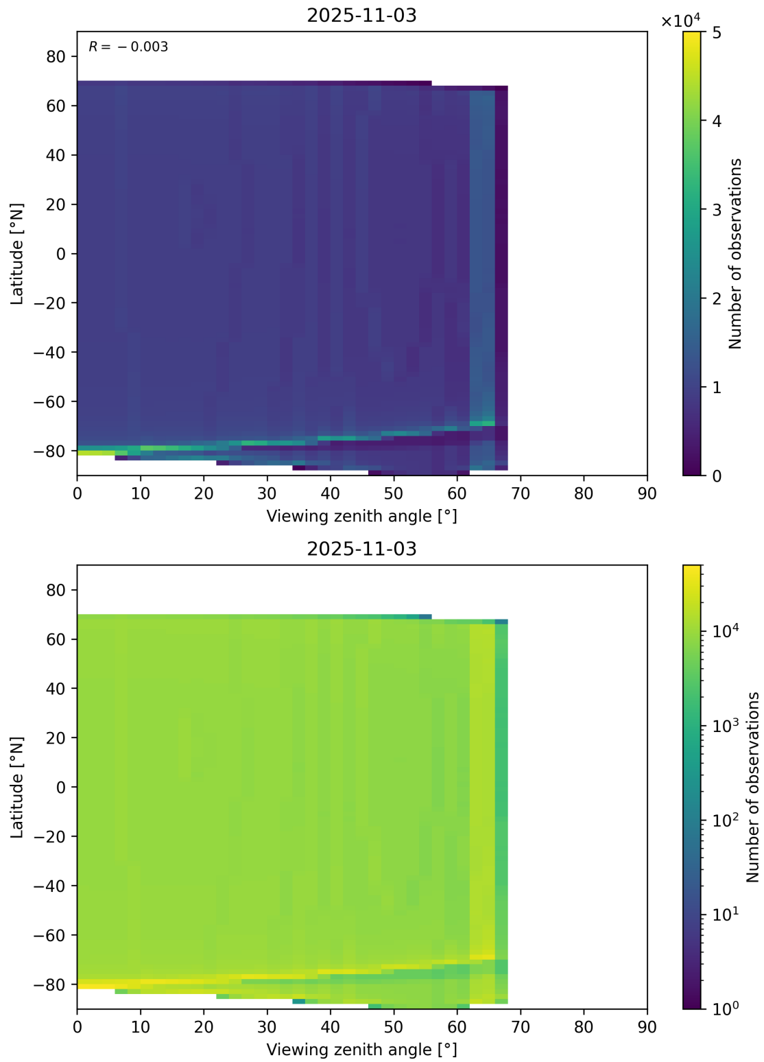
Figure 196: Scatter density plot of “Viewing zenith angle” against “Latitude” for 2025-11-02 to 2025-11-04.
