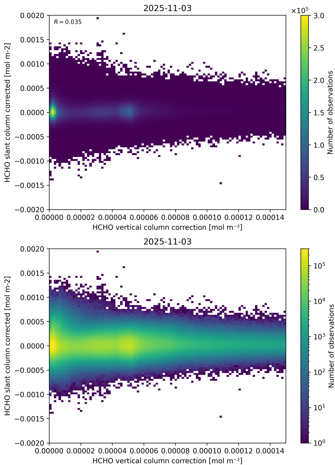
Figure 116: Scatter density plot of “HCHO vertical column correction” against “HCHO slant column corrected” for 2025-11-02 to 2025-11-04.
