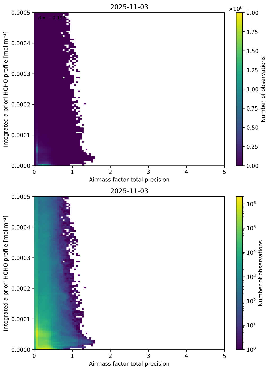
Figure 111: Scatter density plot of “Airmass factor total precision” against “Integrated a priori HCHO profile” for 2025-11-02 to 2025-11-04.
