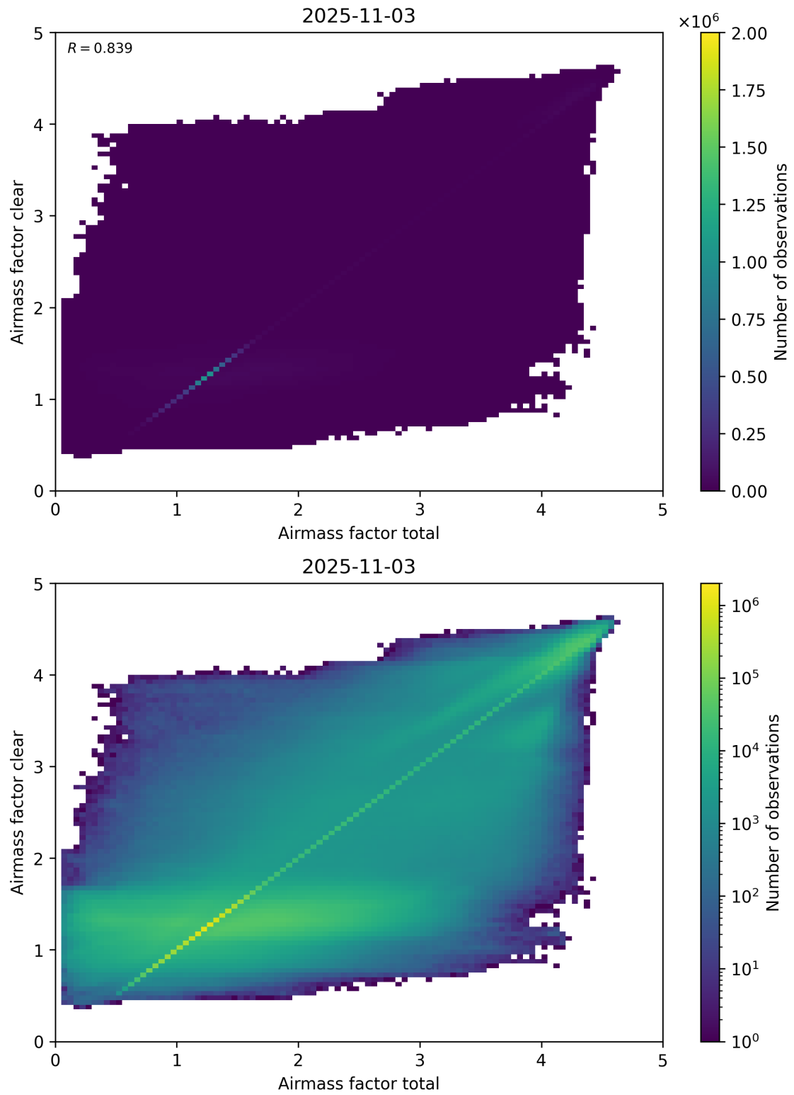
Figure 100: Scatter density plot of “Airmass factor total” against “Airmass factor clear” for 2025-11-02 to 2025-11-04.
