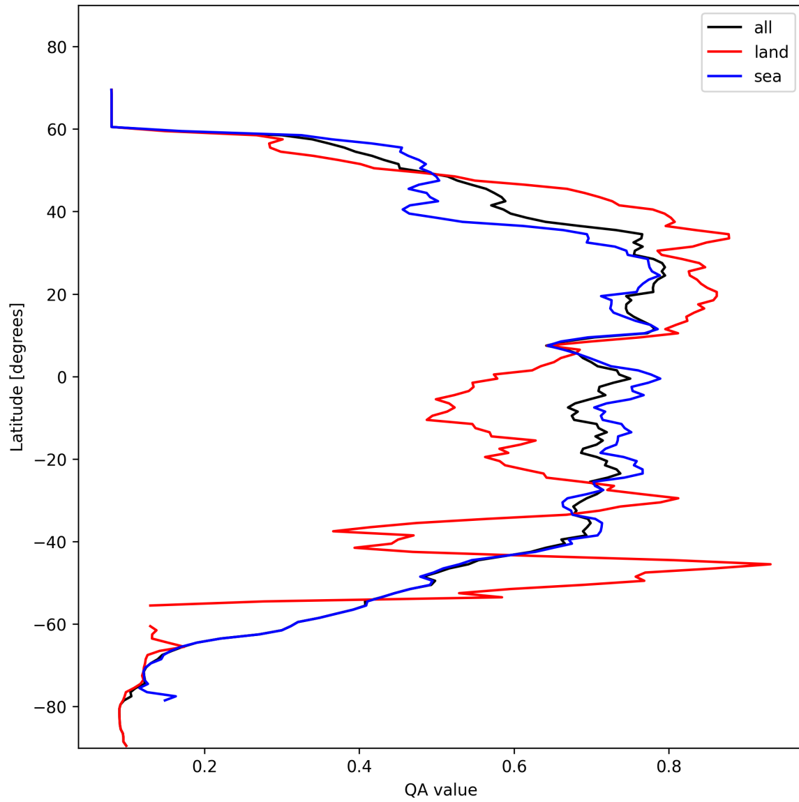
Figure 20: Zonal average of “QA value” for 2025-11-02 to 2025-11-04.
