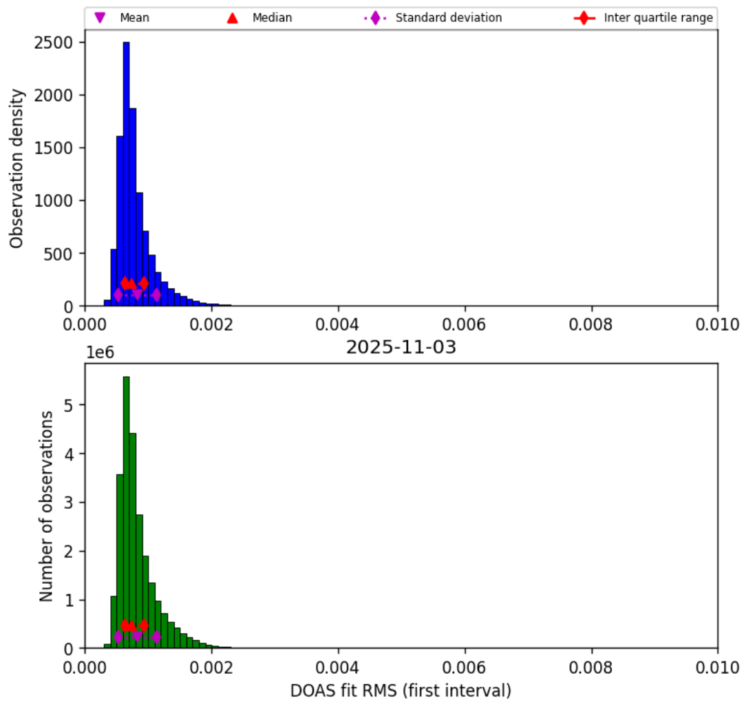
Figure 46: Histogram of “DOAS fit RMS (first interval)” for 2025-11-02 to 2025-11-04
