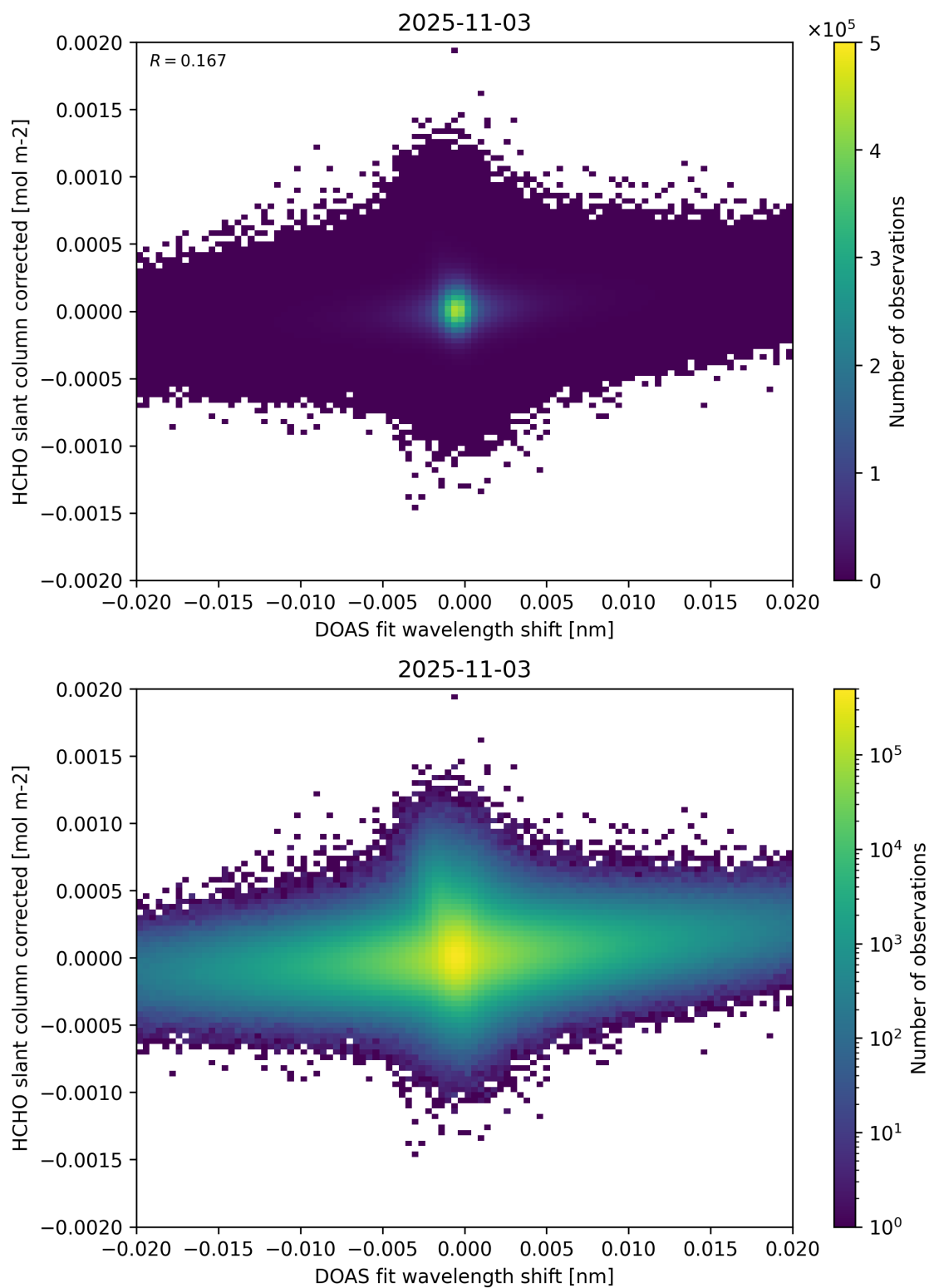
Figure 66: Scatter density plot of “DOAS fit wavelength shift” against “HCHO slant column corrected” for 2025-11-02 to 2025-11-04.
