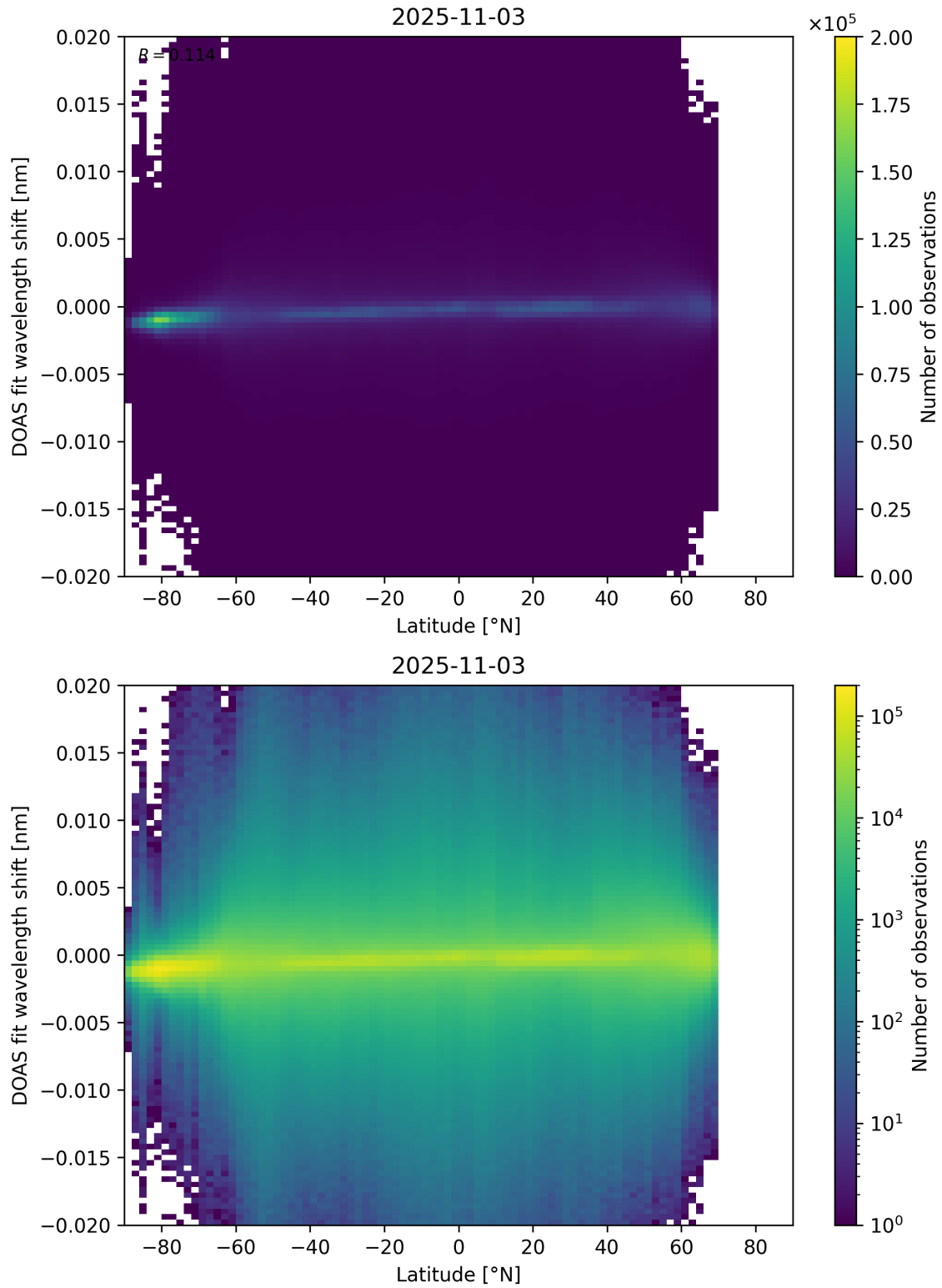
Figure 154: Scatter density plot of “Latitude” against “DOAS fit wavelength shift” for 2025-11-02 to 2025-11-04.
