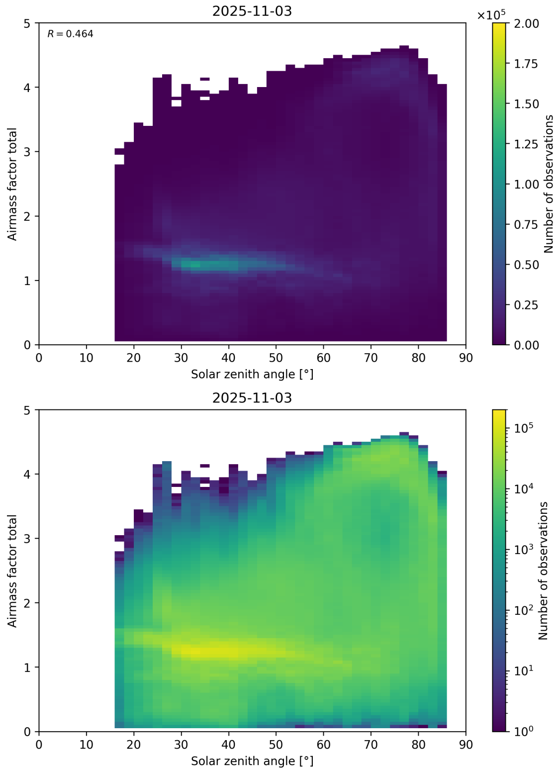
Figure 175: Scatter density plot of “Solar zenith angle” against “Airmass factor total” for 2025-11-02 to 2025-11-04.
