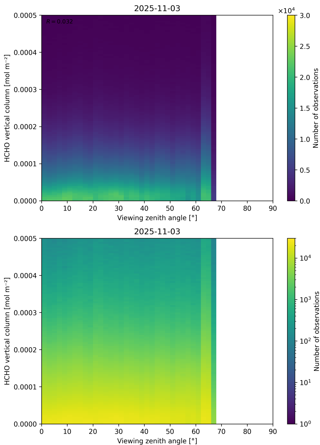
Figure 192: Scatter density plot of “Viewing zenith angle” against “HCHO vertical column” for 2025-11-02 to 2025-11-04.
