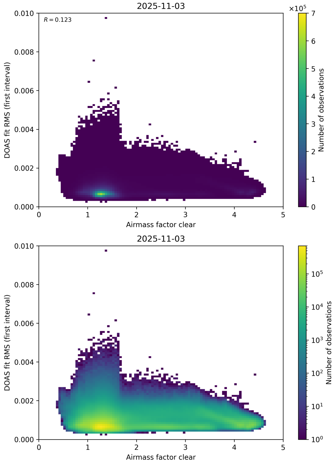
Figure 71: Scatter density plot of “Airmass factor clear” against “DOAS fit RMS (first interval)” for 2025-11-02 to 2025-11-04.
