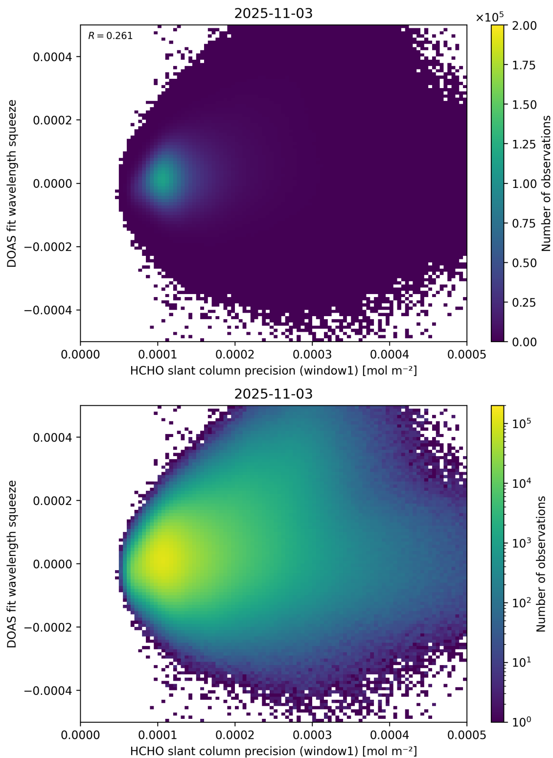
Figure 90: Scatter density plot of “HCHO slant column precision (window1)” against “DOAS fit wavelength squeeze” for 2025-11-02 to 2025-11-04.
