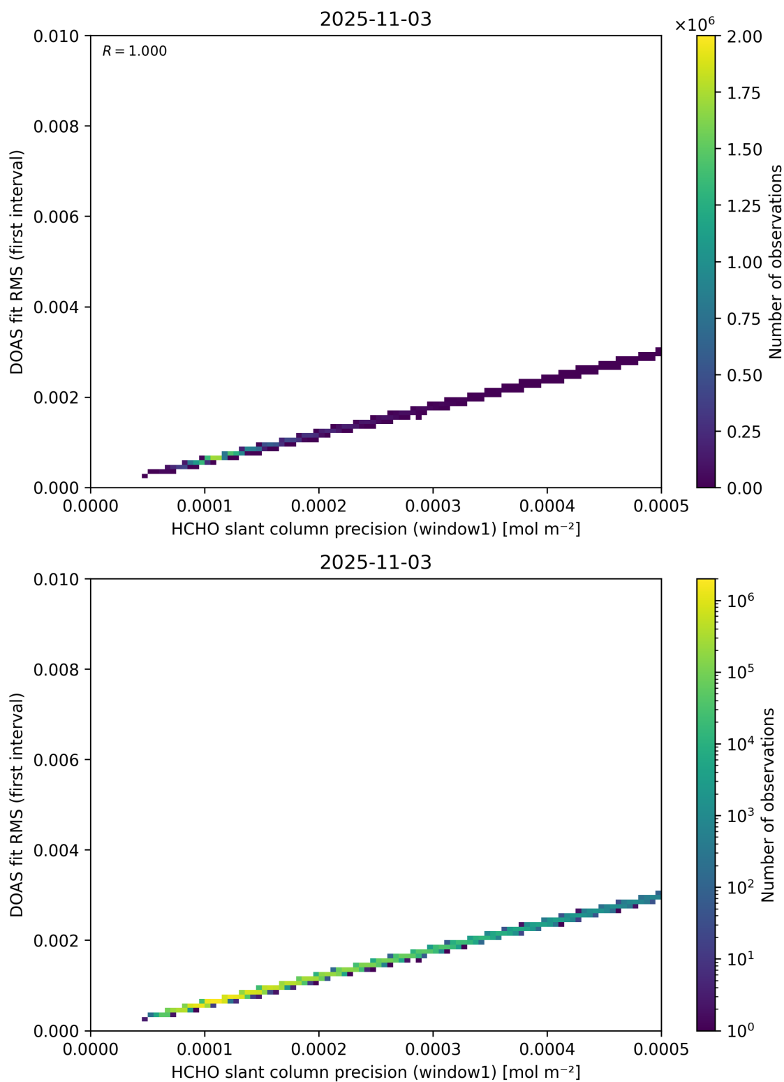
Figure 88: Scatter density plot of “HCHO slant column precision (window1)” against “DOAS fit RMS (first interval)” for 2025-11-02 to 2025-11-04.
