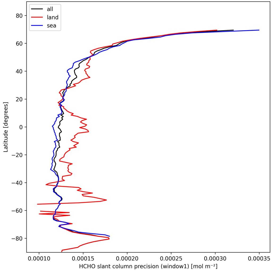
Figure 25: Zonal average of “HCHO slant column precision (window1)” for 2025-11-02 to 2025-11-04.
