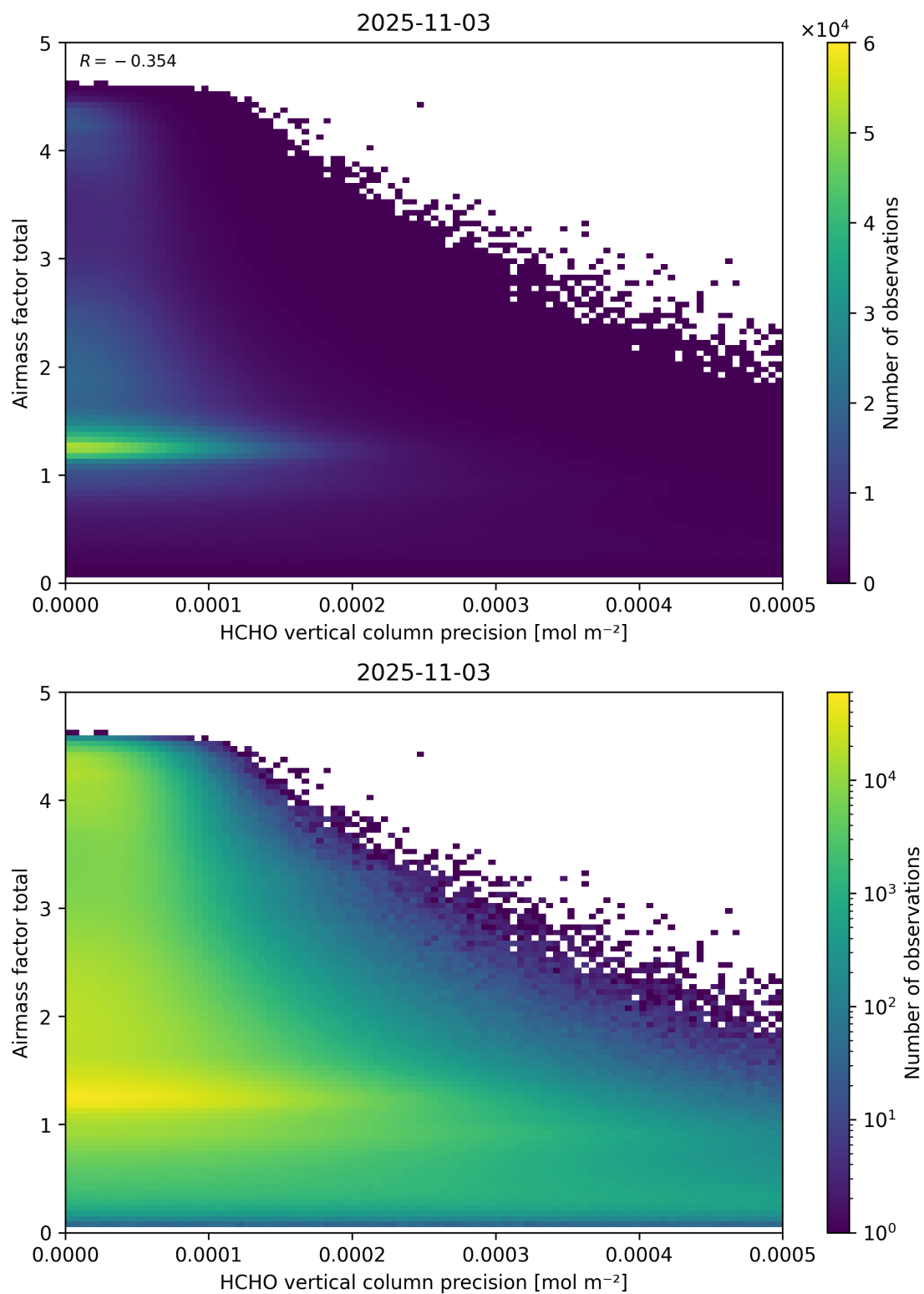
Figure 144: Scatter density plot of “HCHO vertical column precision” against “Airmass factor total” for 2025-11-02 to 2025-11-04.
