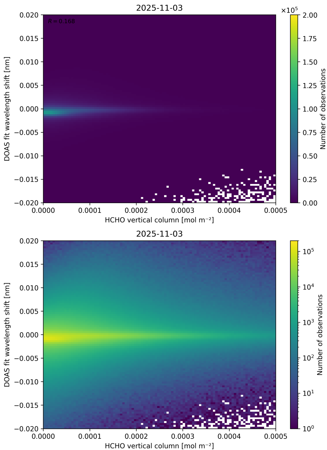
Figure 124: Scatter density plot of “HCHO vertical column” against “DOAS fit wavelength shift” for 2025-11-02 to 2025-11-04.
