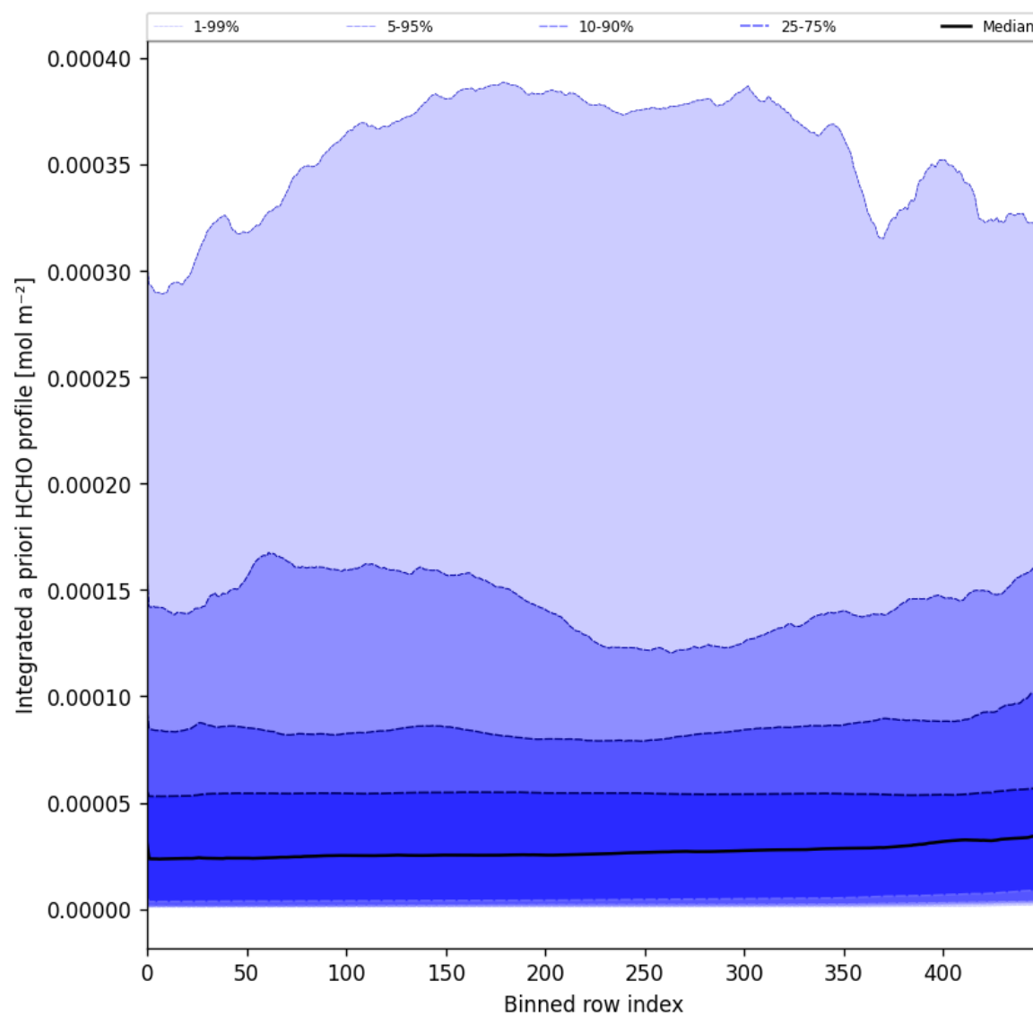
Figure 57: Along track statistics of “Integrated a priori HCHO profile” for 2025-11-02 to 2025-11-04
