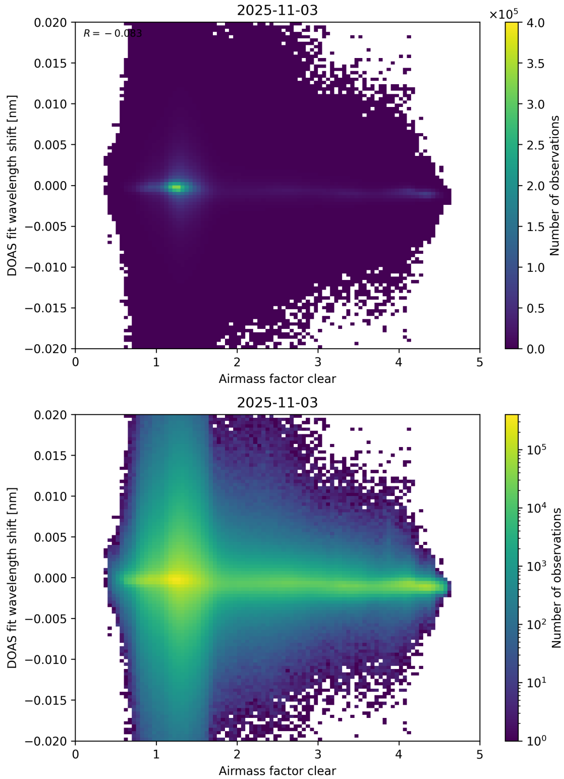
Figure 72: Scatter density plot of “Airmass factor clear” against “DOAS fit wavelength shift” for 2025-11-02 to 2025-11-04.
