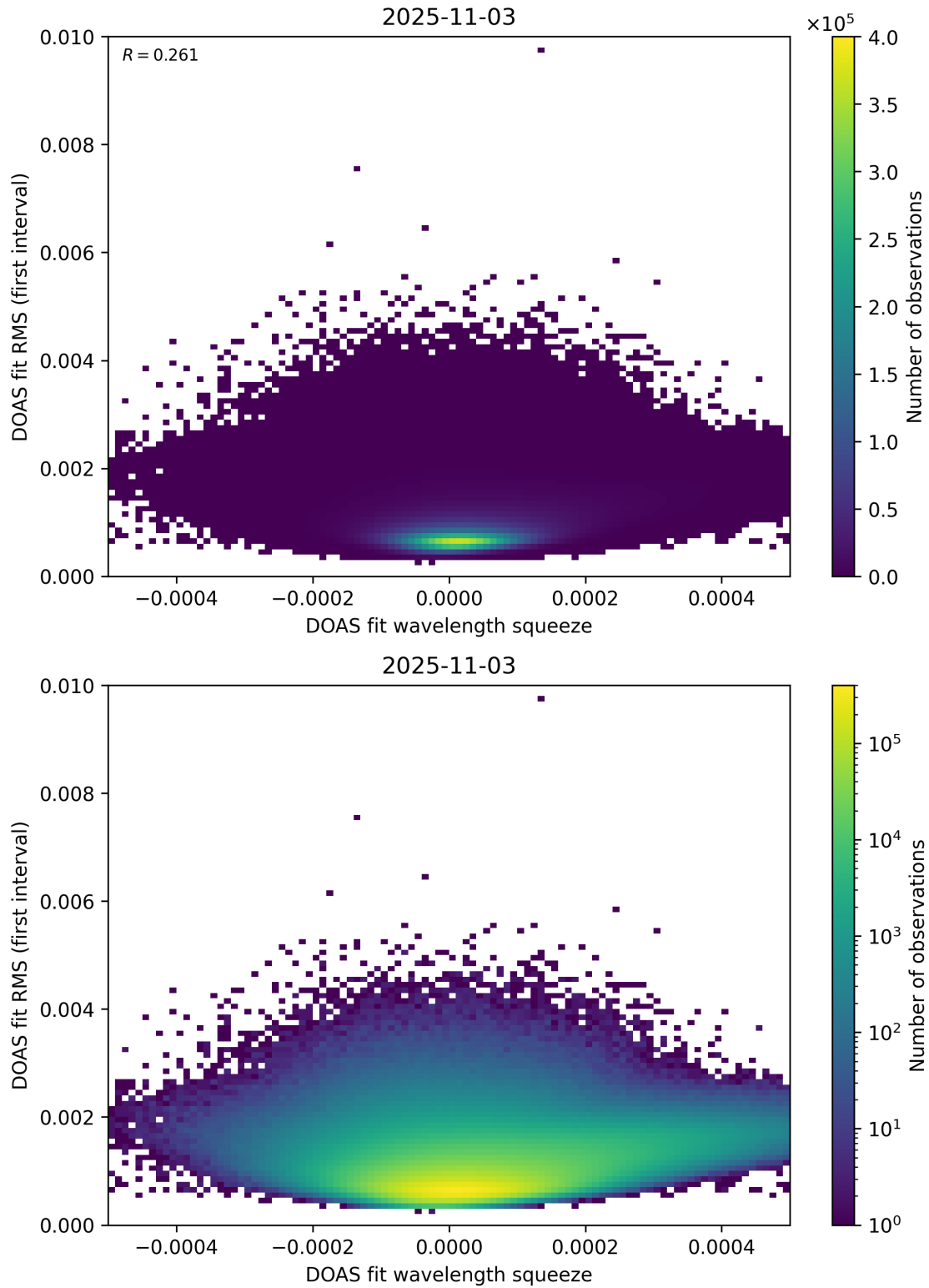
Figure 68: Scatter density plot of “DOAS fit wavelength squeeze” against “DOAS fit RMS (first interval)” for 2025-11-02 to 2025-11-04.
