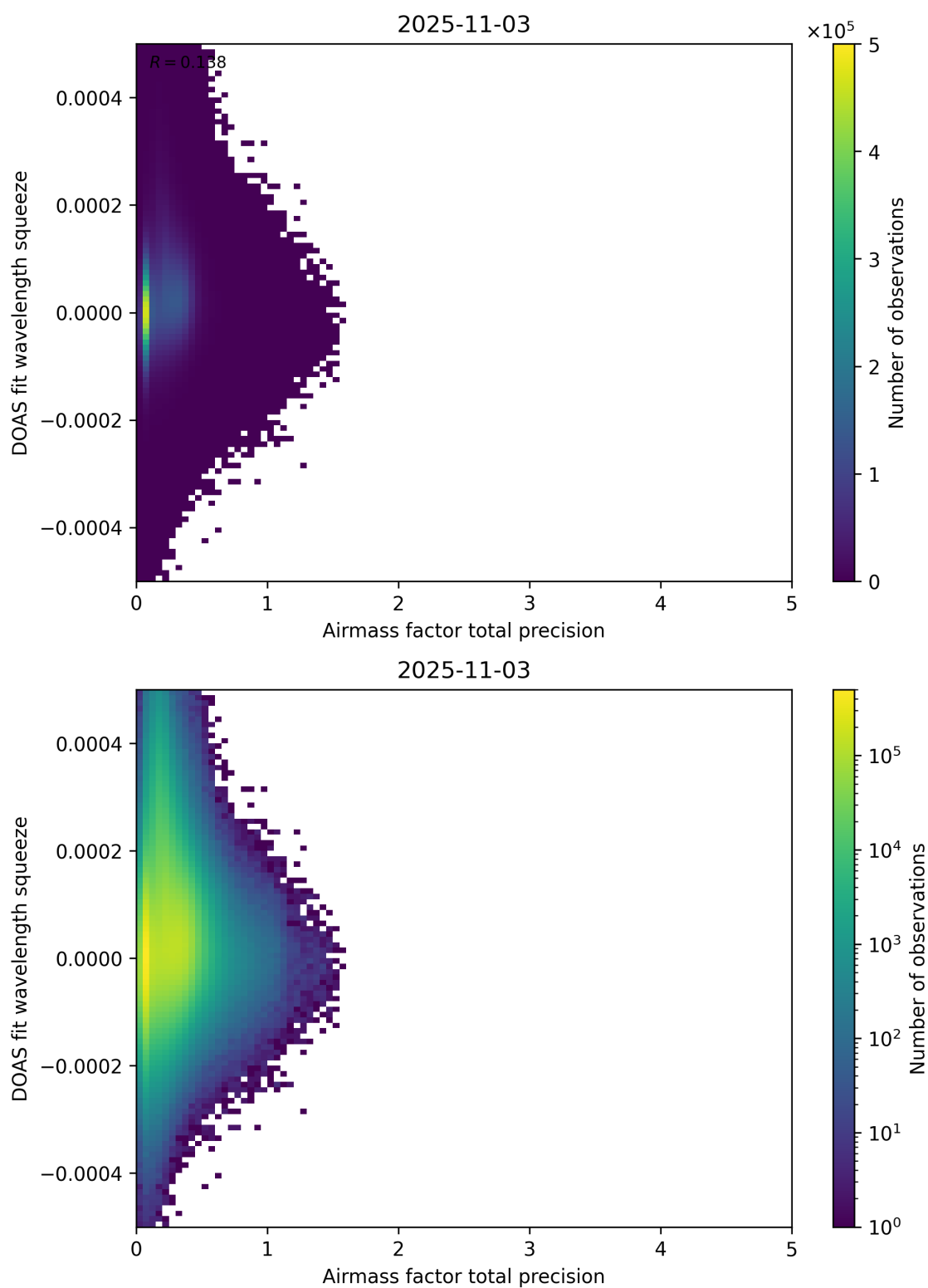
Figure 107: Scatter density plot of “Airmass factor total precision” against “DOAS fit wavelength squeeze” for 2025-11-02 to 2025-11-04.
