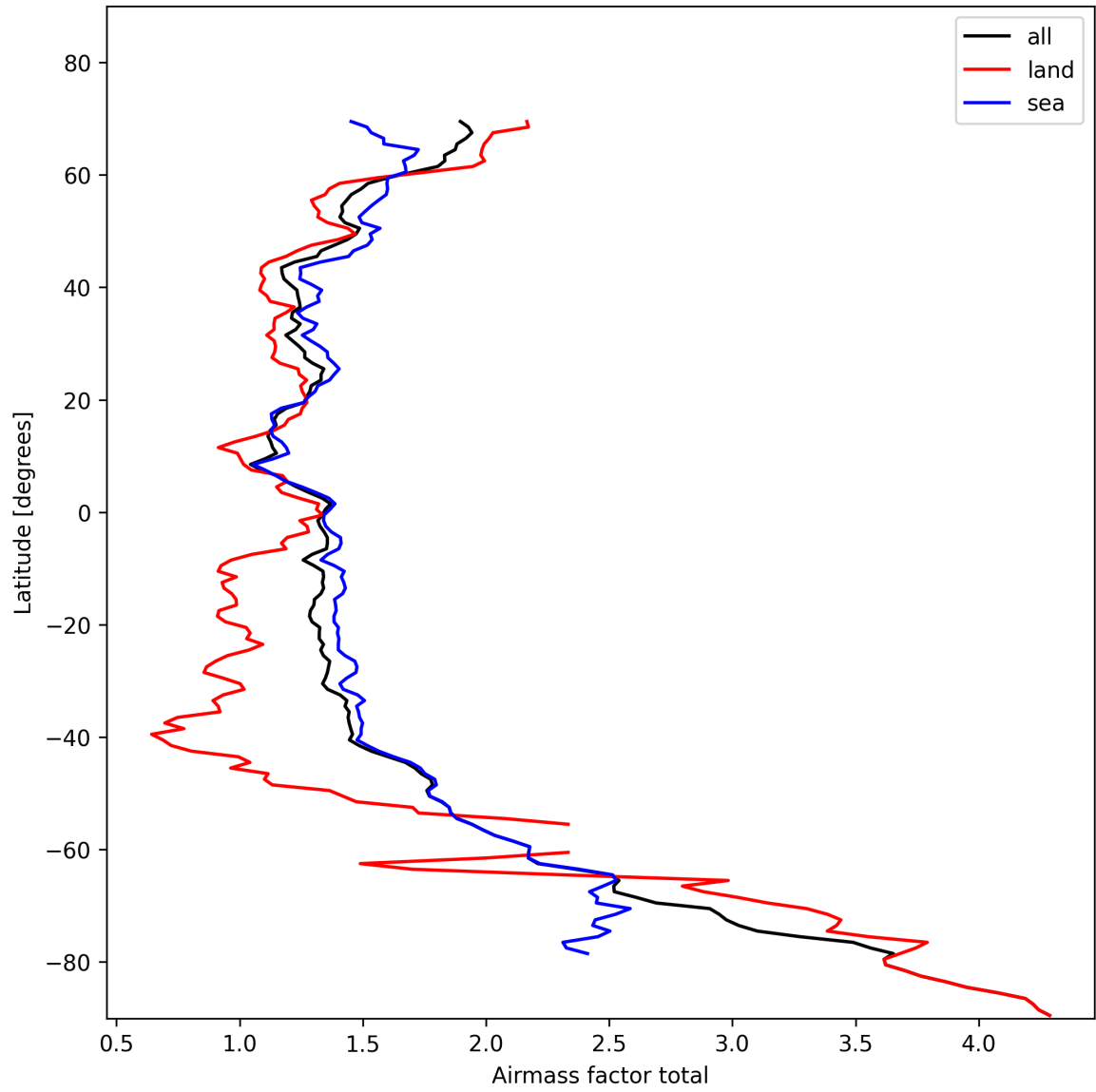
Figure 26: Zonal average of “Airmass factor total” for 2025-11-02 to 2025-11-04.
