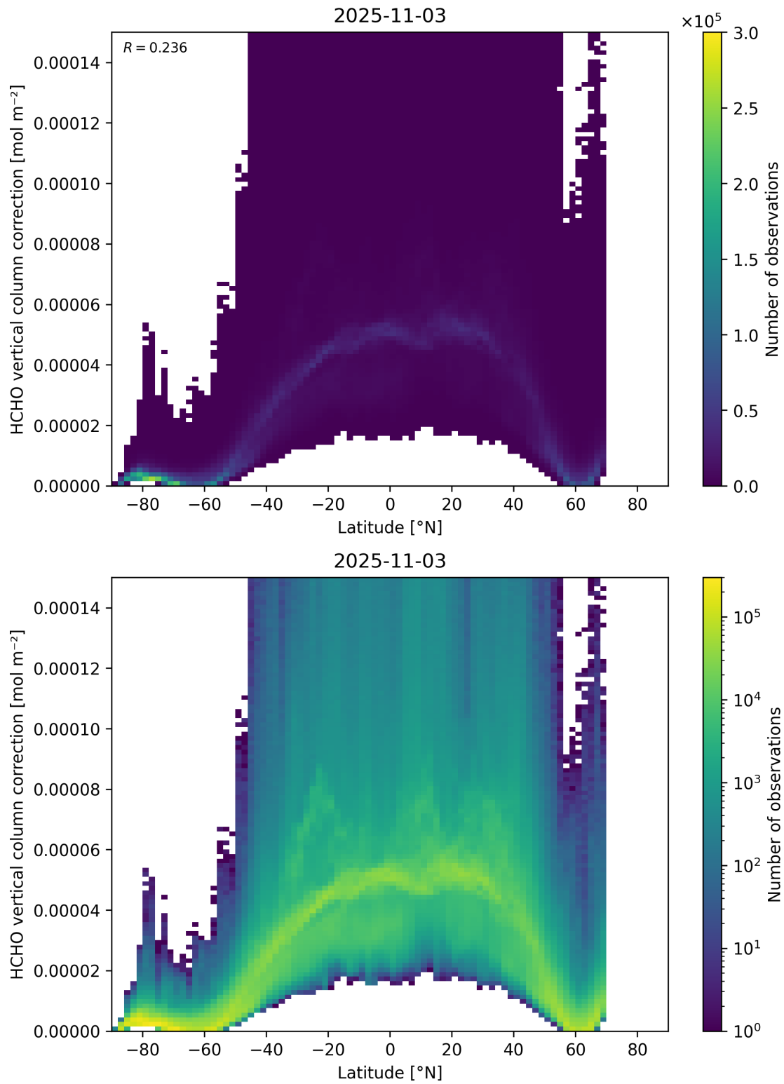
Figure 164: Scatter density plot of “Latitude” against “HCHO vertical column correction” for 2025-11-02 to 2025-11-04.
