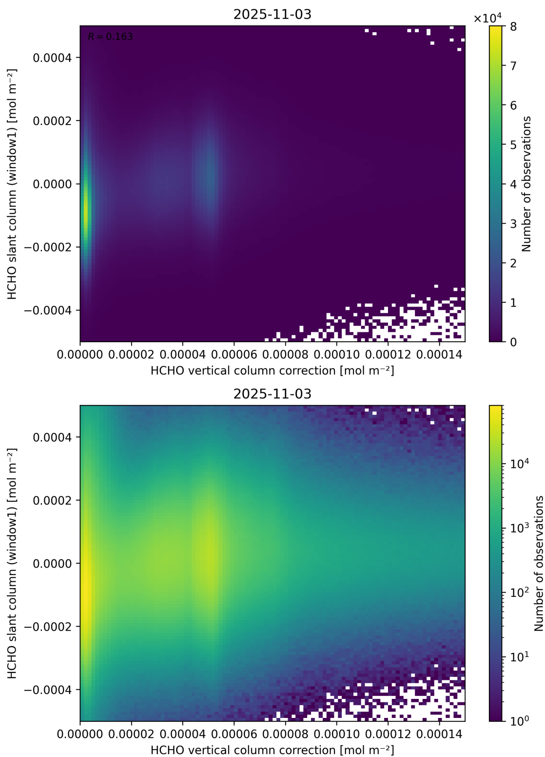
Figure 118: Scatter density plot of “HCHO vertical column correction” against “HCHO slant column (window1)” for 2025-11-02 to 2025-11-04.
