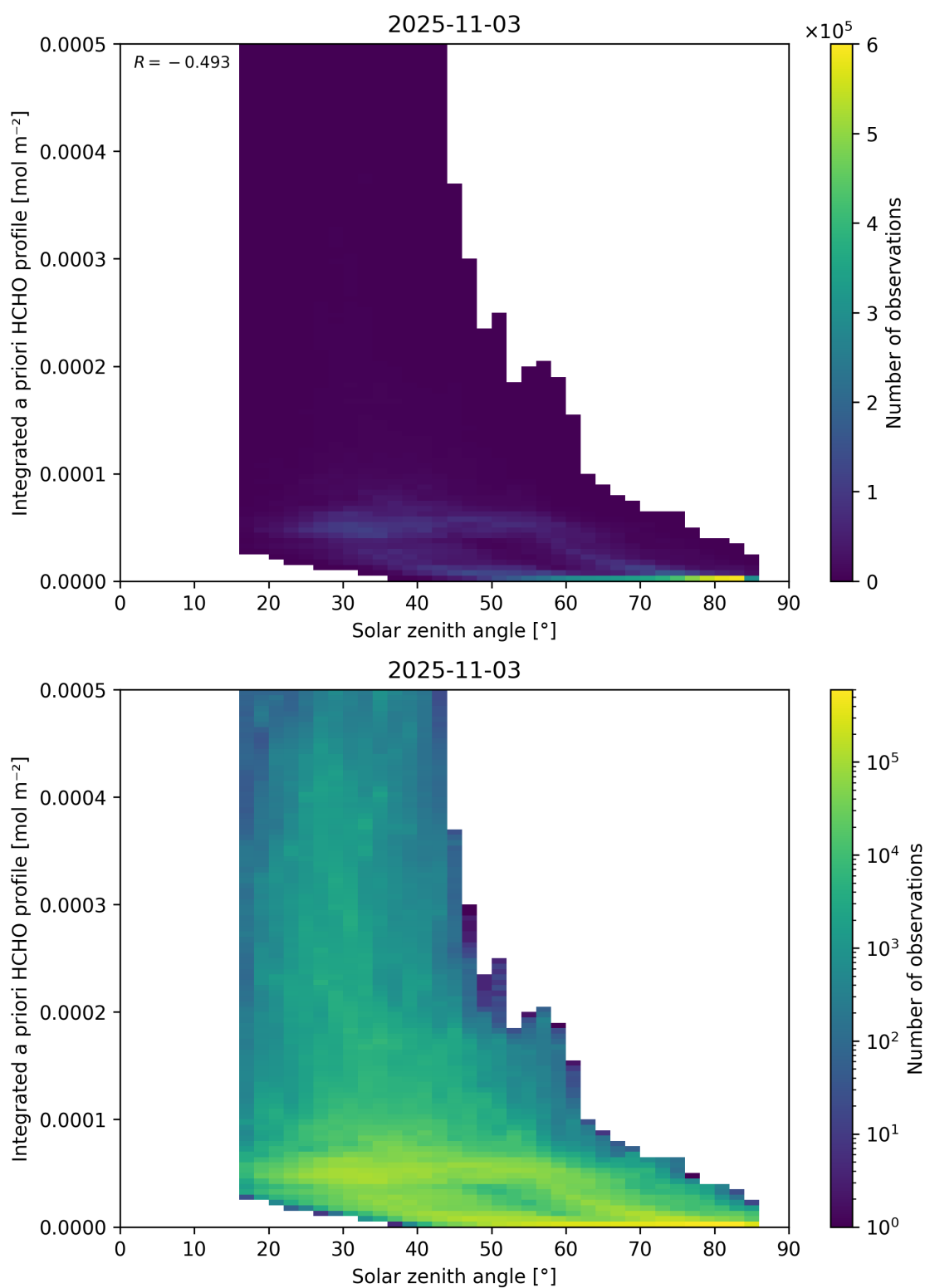
Figure 180: Scatter density plot of “Solar zenith angle” against “Integrated a priori HCHO profile” for 2025-11-02 to 2025-11-04.
