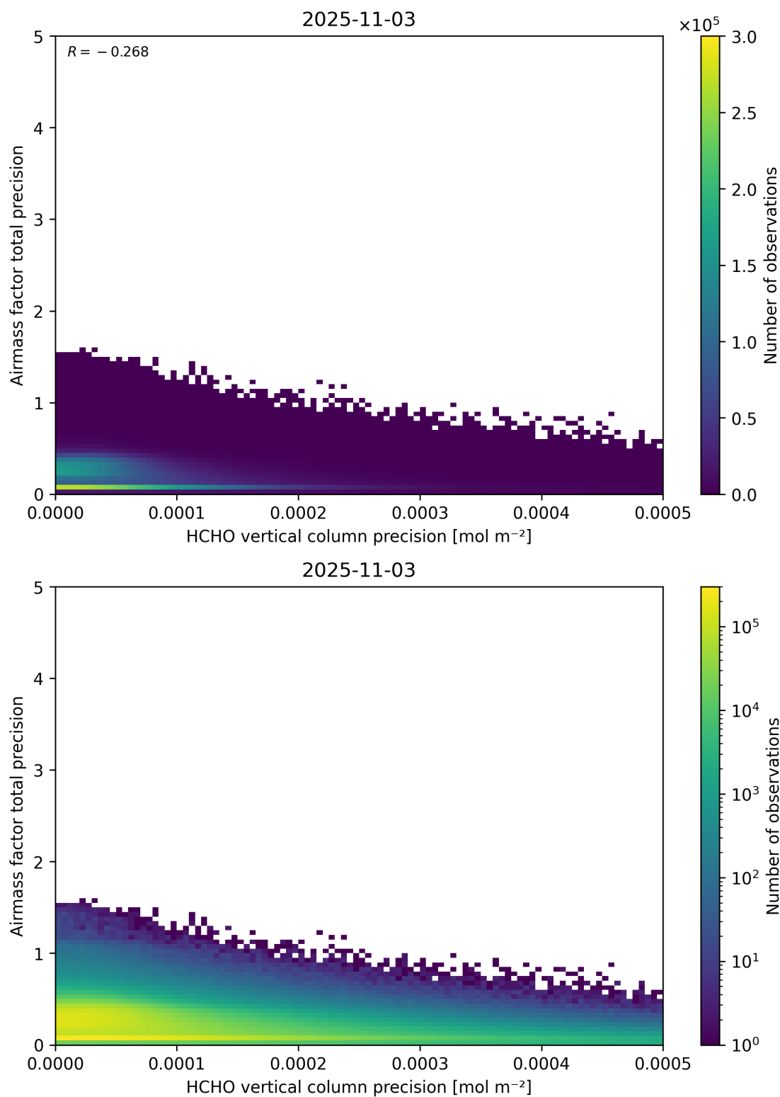
Figure 145: Scatter density plot of “HCHO vertical column precision” against “Airmass factor total precision” for 2025-11-02 to 2025-11-04.
