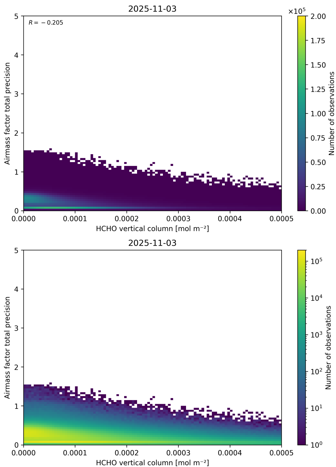
Figure 132: Scatter density plot of “HCHO vertical column” against “Airmass factor total precision” for 2025-11-02 to 2025-11-04.
