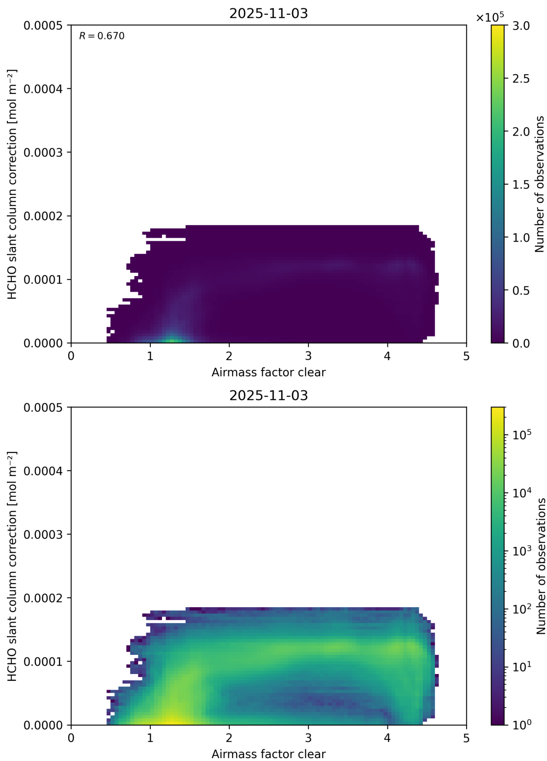
Figure 75: Scatter density plot of “Airmass factor clear” against “HCHO slant column correction” for 2025-11-02 to 2025-11-04.
