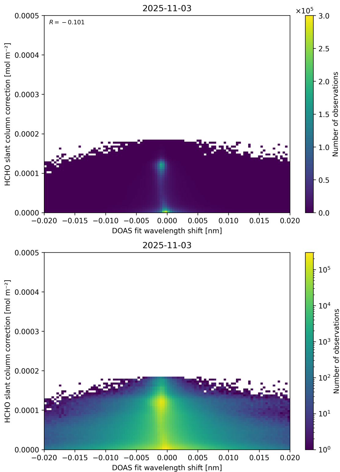
Figure 67: Scatter density plot of “DOAS fit wavelength shift” against “HCHO slant column correction” for 2025-11-02 to 2025-11-04.
