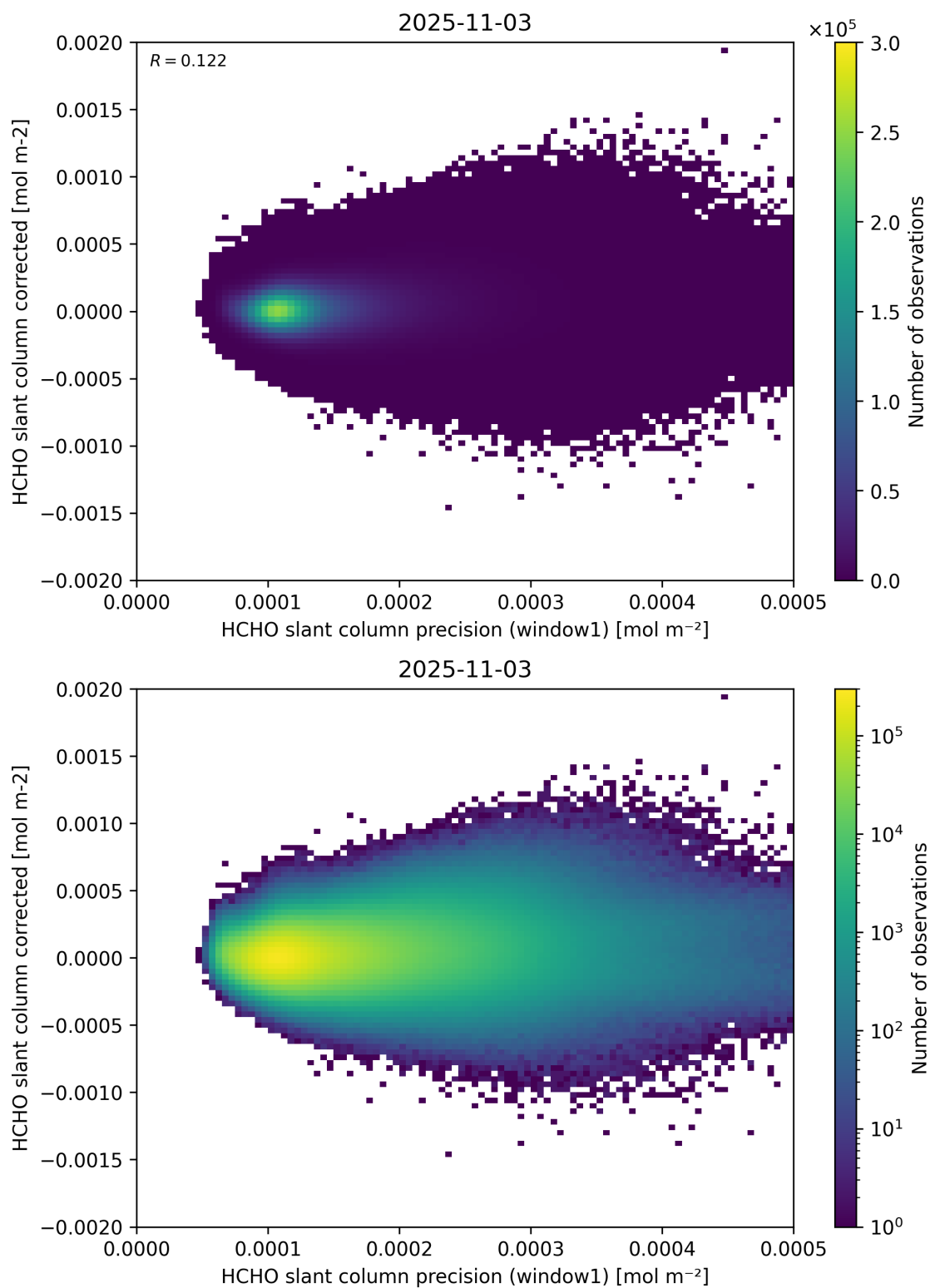
Figure 92: Scatter density plot of “HCHO slant column precision (window1)” against “HCHO slant column corrected” for 2025-11-02 to 2025-11-04.
