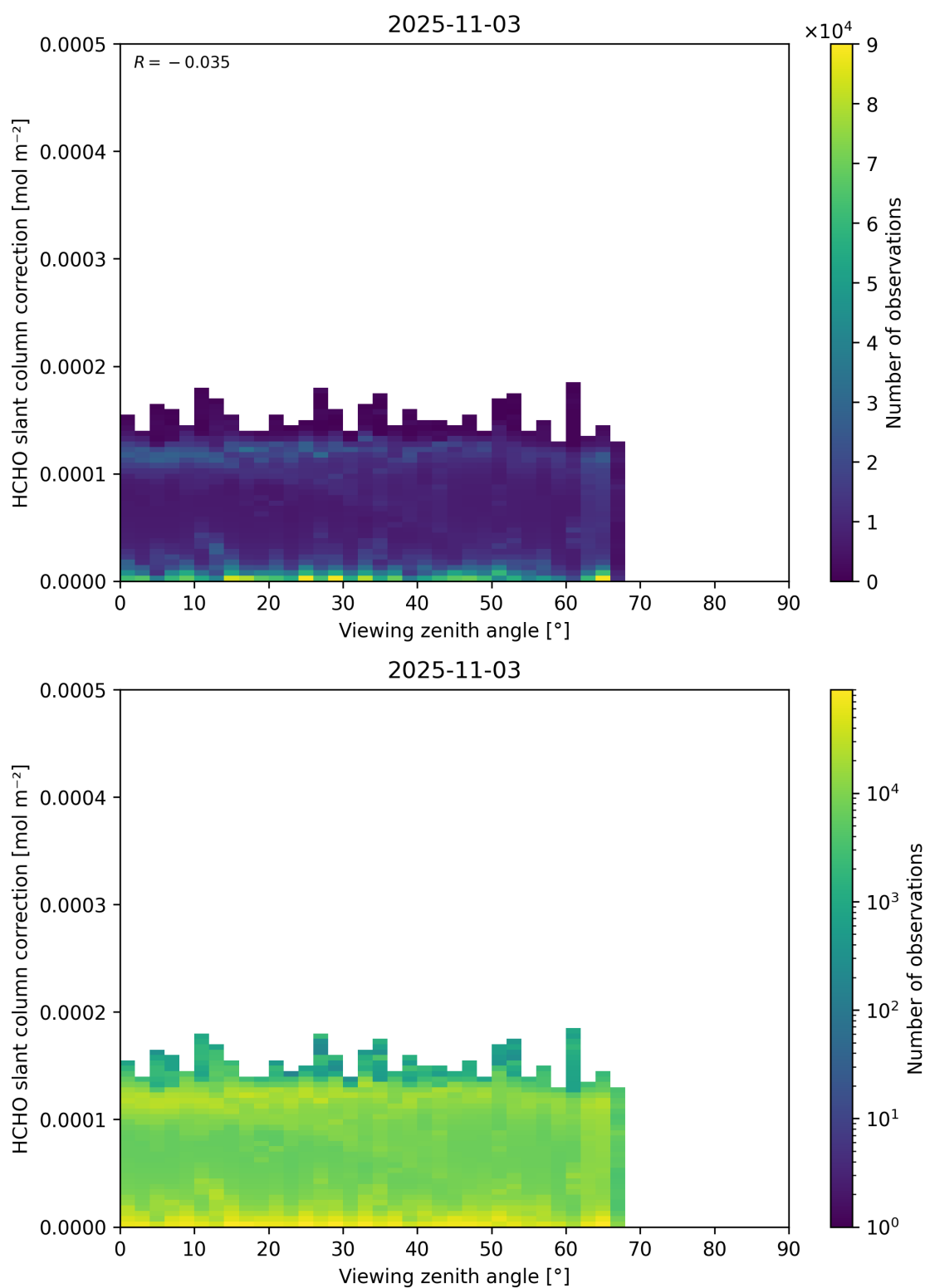
Figure 187: Scatter density plot of “Viewing zenith angle” against “HCHO slant column correction” for 2025-11-02 to 2025-11-04.
