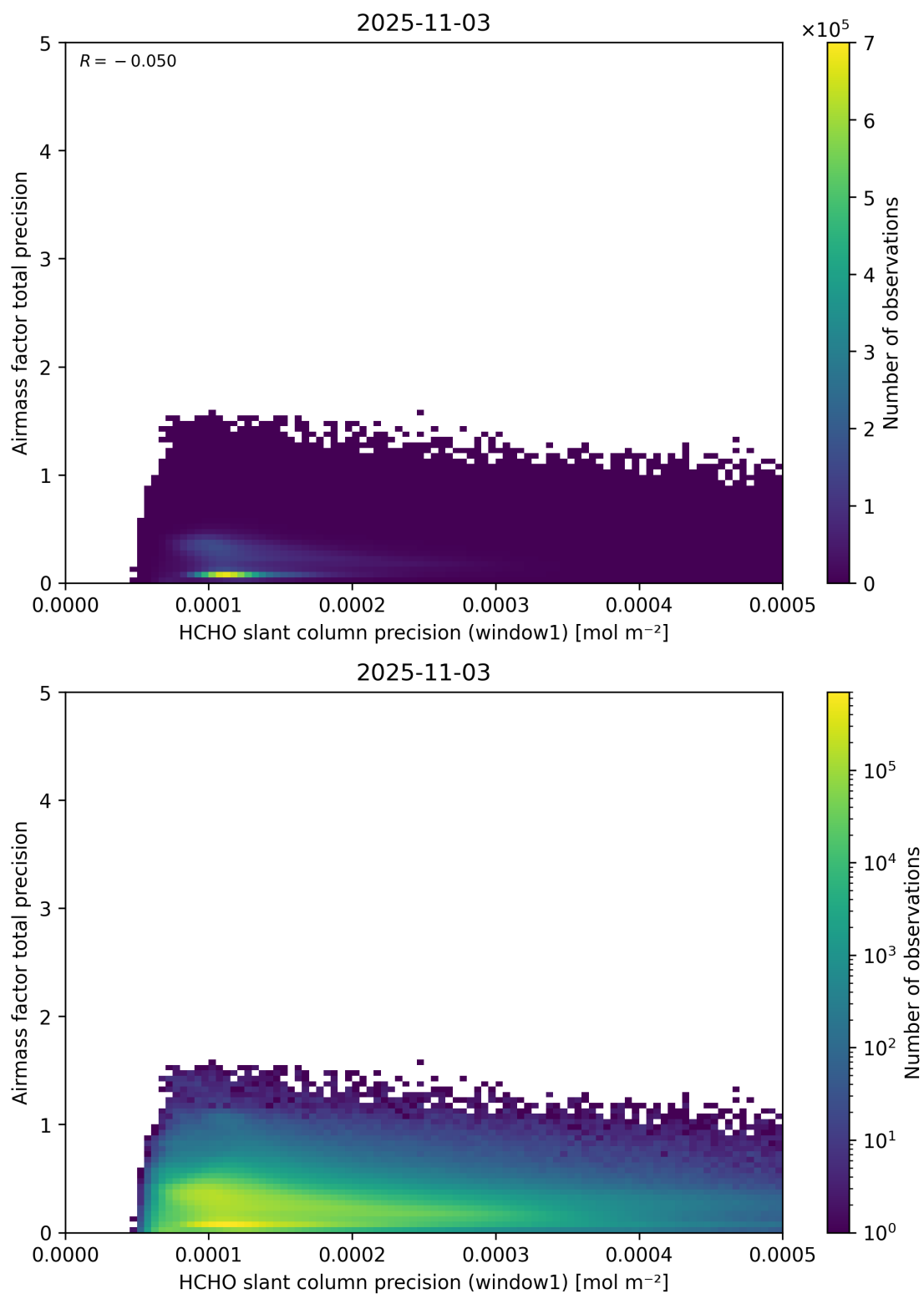
Figure 95: Scatter density plot of “HCHO slant column precision (window1)” against “Airmass factor total precision” for 2025-11-02 to 2025-11-04.
