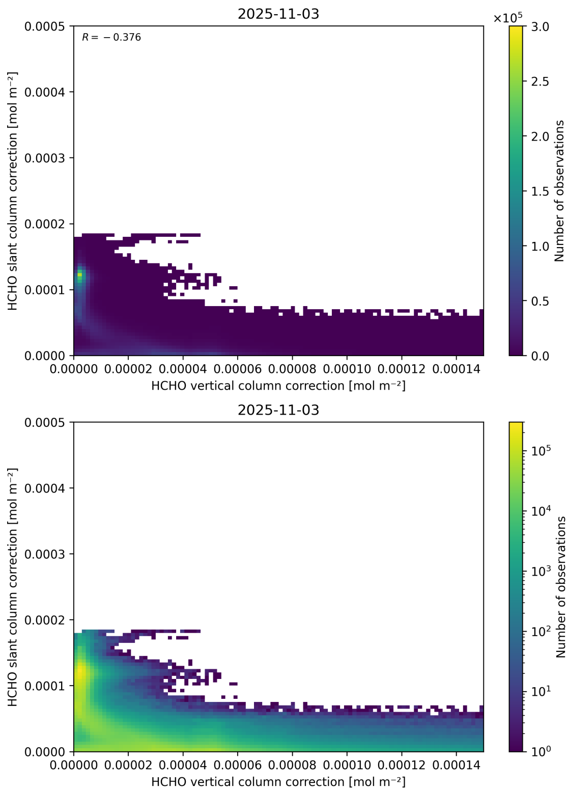
Figure 117: Scatter density plot of “HCHO vertical column correction” against “HCHO slant column correction” for 2025-11-02 to 2025-11-04.
