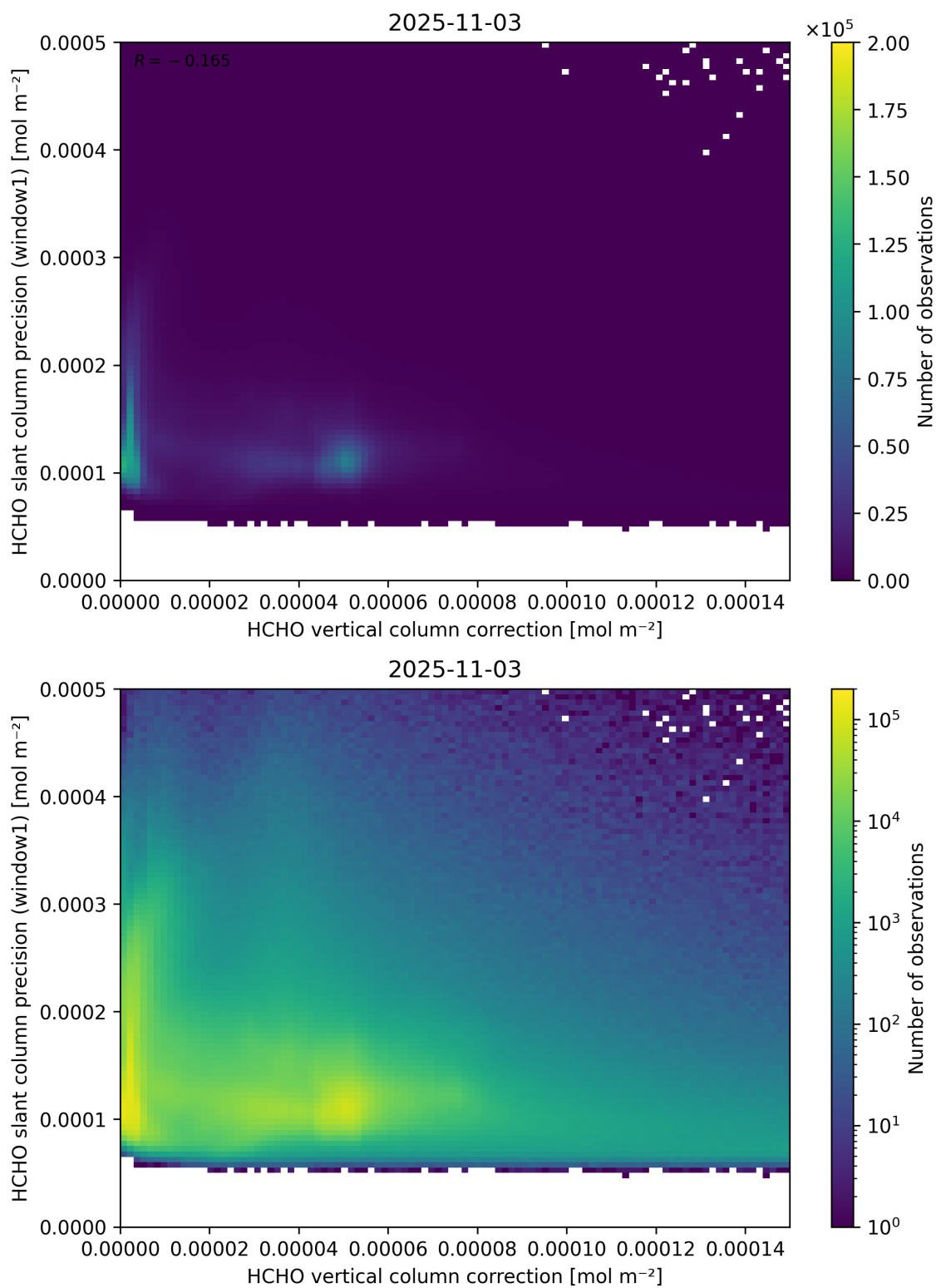
Figure 119: Scatter density plot of “HCHO vertical column correction” against “HCHO slant column precision (window1)” for 2025-11-02 to 2025-11-04.
