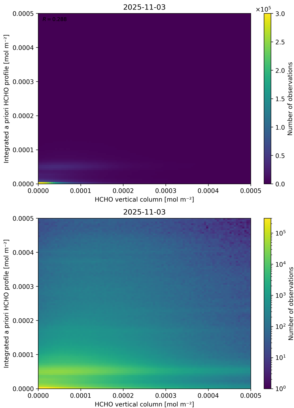
Figure 135: Scatter density plot of “HCHO vertical column” against “Integrated a priori HCHO profile” for 2025-11-02 to 2025-11-04.
