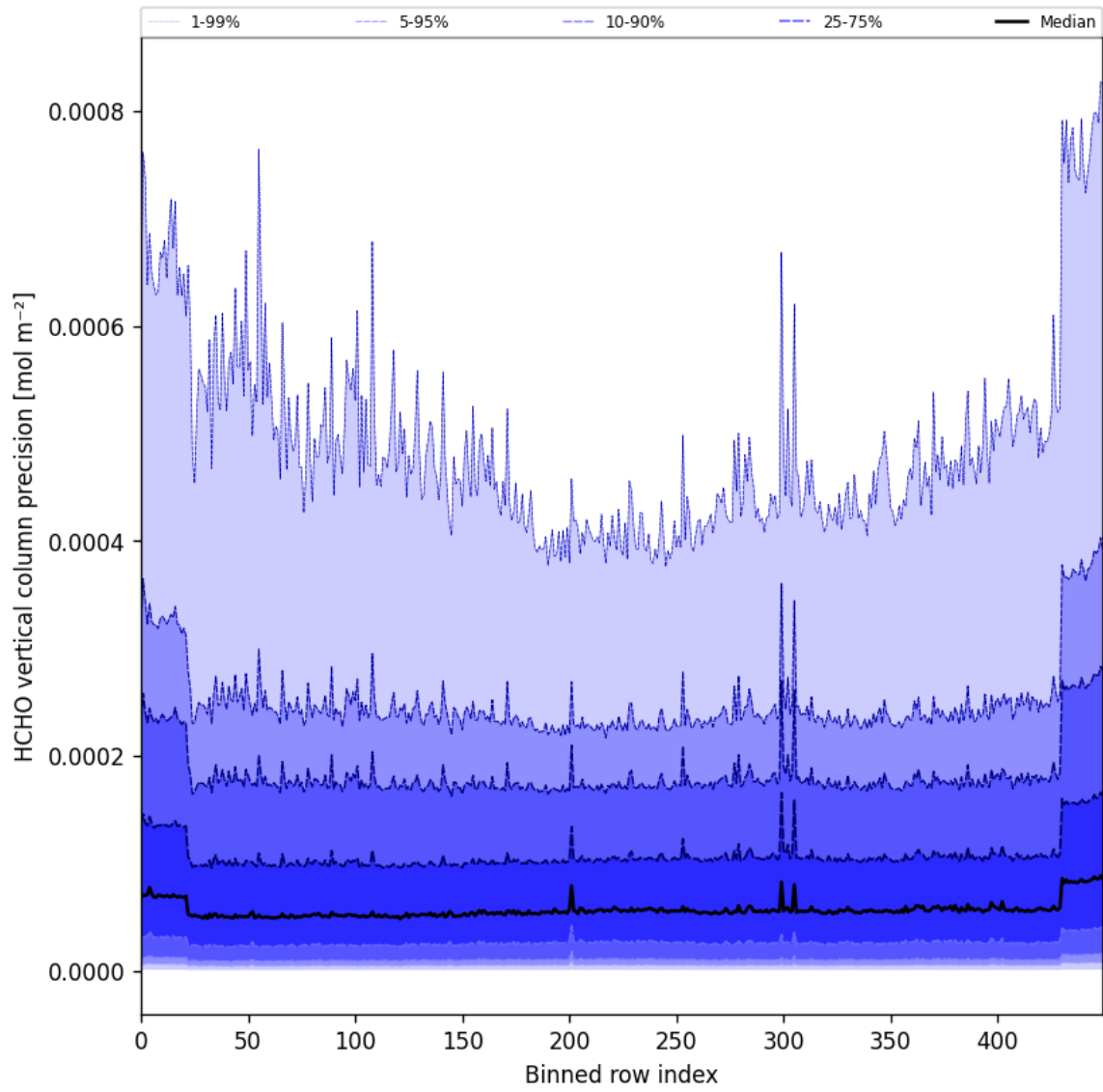
Figure 50: Along track statistics of "HCHO vertical column precision" for 2025-11-02 to 2025-11-04
