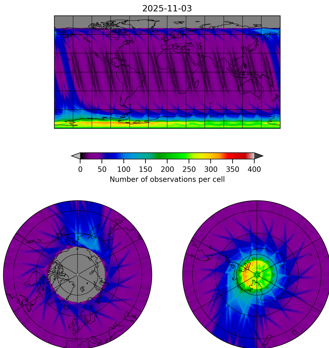
Figure 19: Map of the number of observations for 2025-11-02 to 2025-11-04
