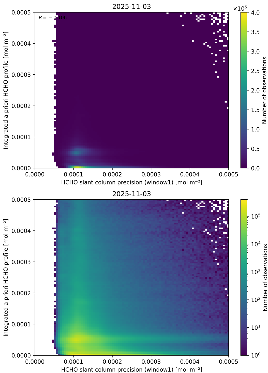
Figure 96: Scatter density plot of “HCHO slant column precision (window1)” against “Integrated a priori HCHO profile” for 2025-11-02 to 2025-11-04.
