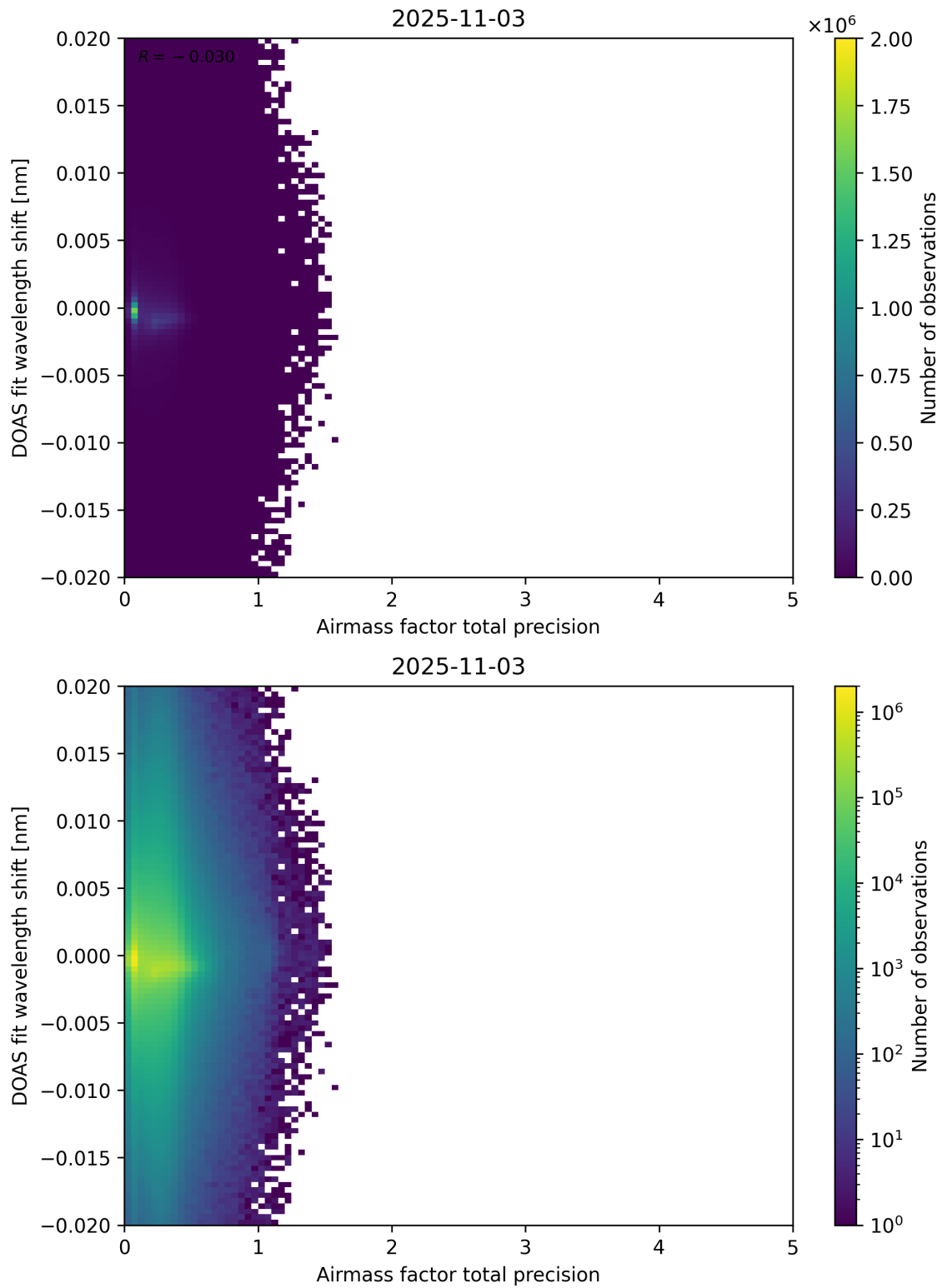
Figure 106: Scatter density plot of “Airmass factor total precision” against “DOAS fit wavelength shift” for 2025-11-02 to 2025-11-04.
