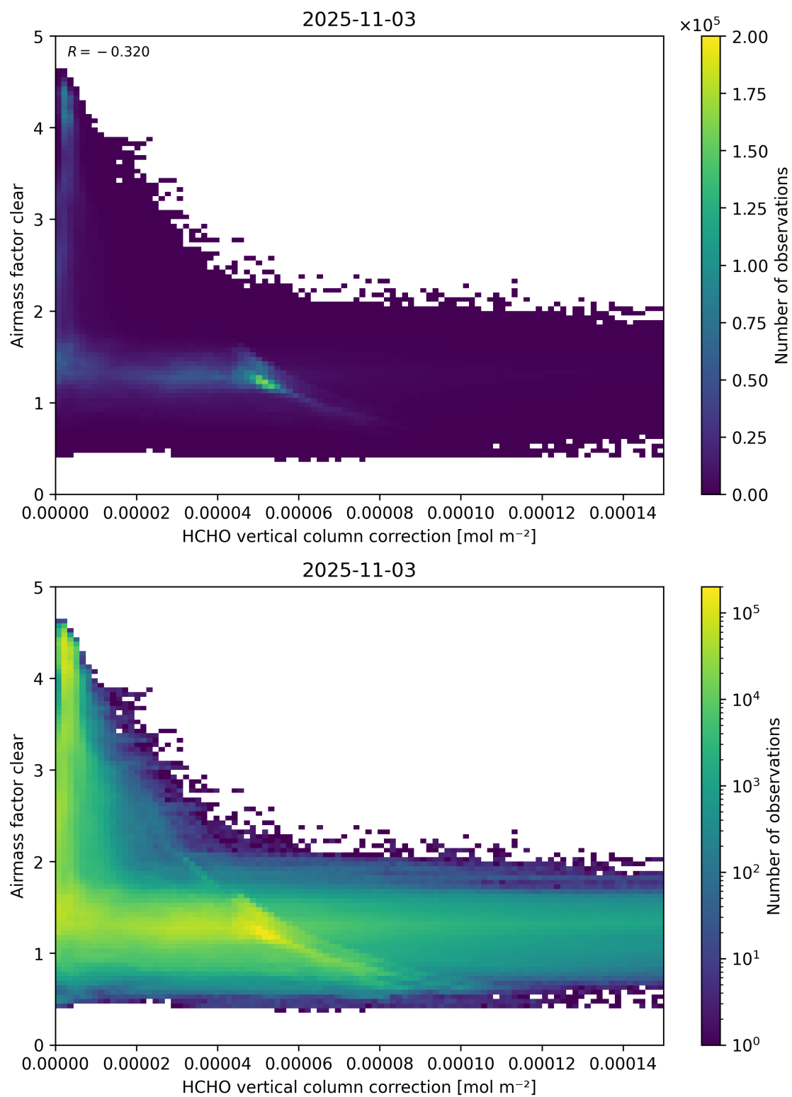
Figure 115: Scatter density plot of “HCHO vertical column correction” against “Airmass factor clear” for 2025-11-02 to 2025-11-04.
