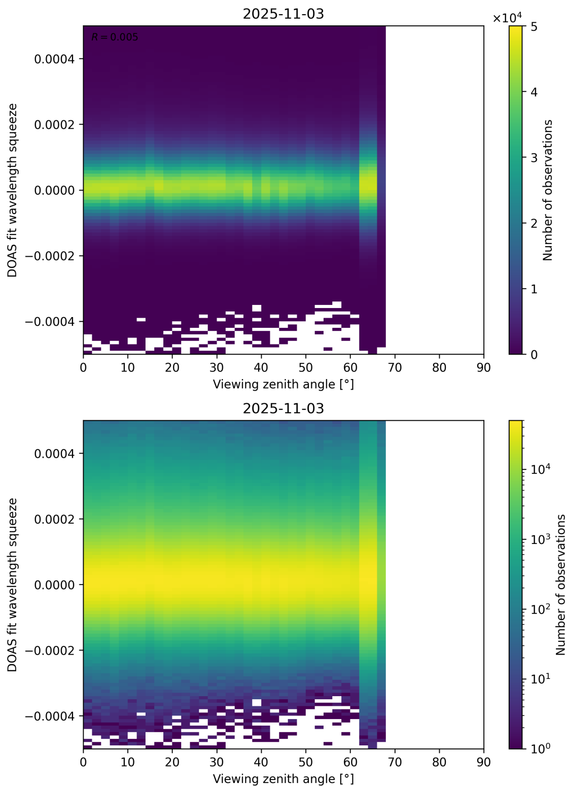
Figure 184: Scatter density plot of “Viewing zenith angle” against “DOAS fit wavelength squeeze” for 2025-11-02 to 2025-11-04.
