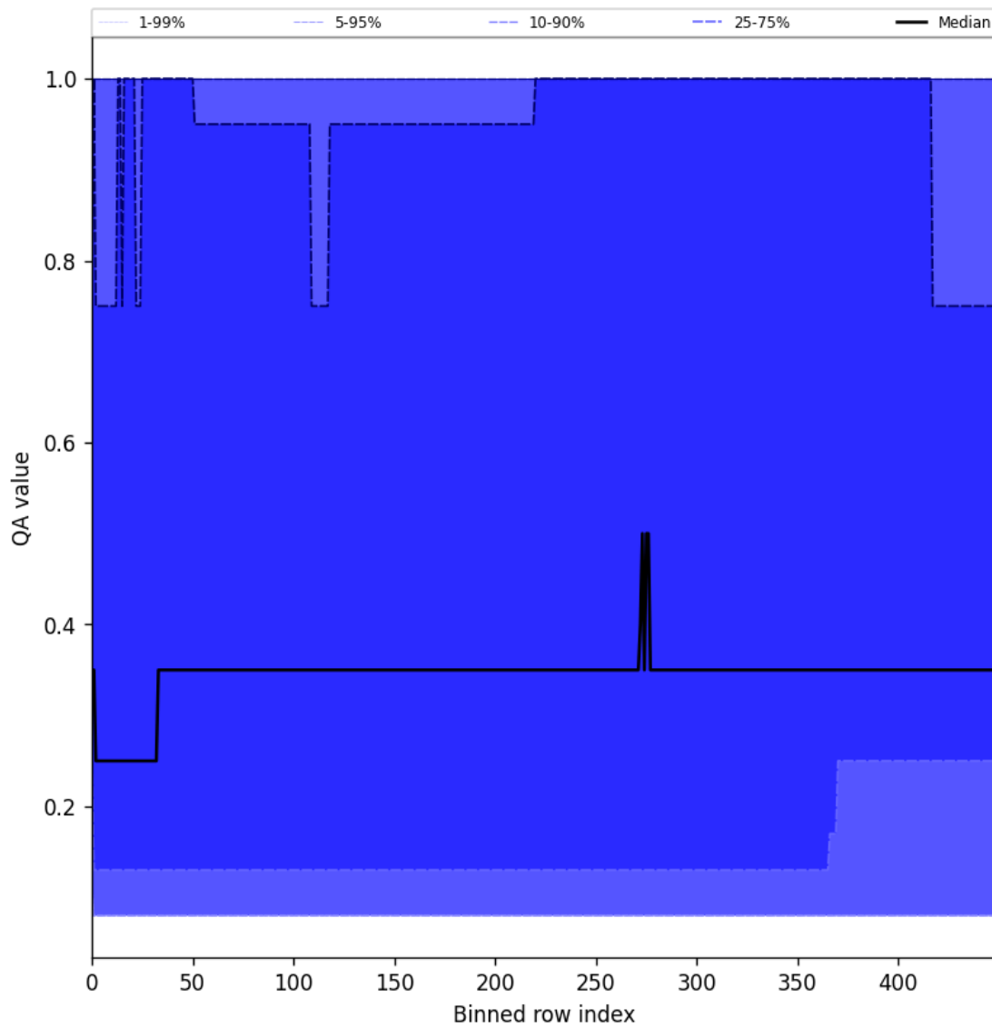
Figure 48: Along track statistics of “QA value” for 2025-11-02 to 2025-11-04
