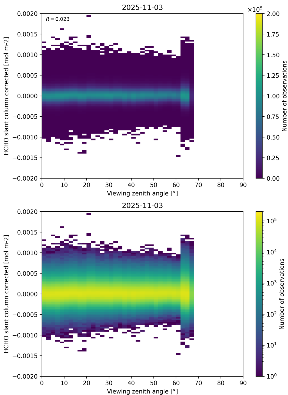
Figure 186: Scatter density plot of “Viewing zenith angle” against “HCHO slant column corrected” for 2025-11-02 to 2025-11-04.
