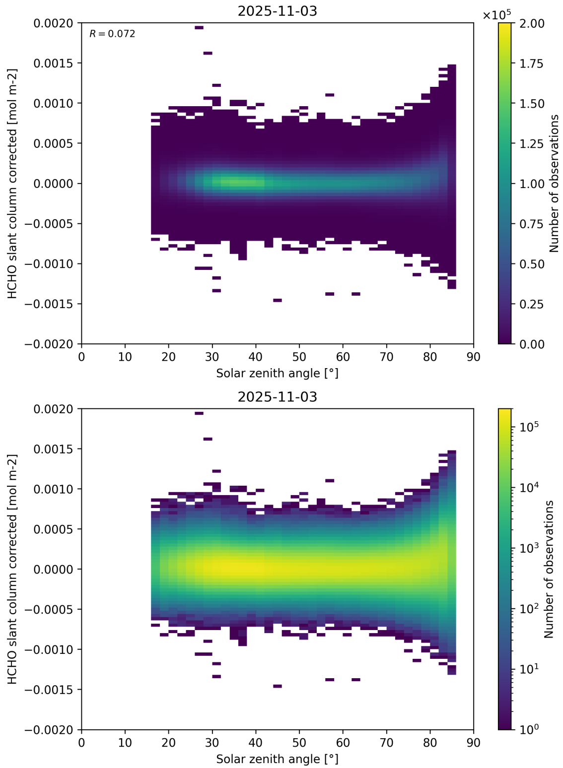
Figure 171: Scatter density plot of “Solar zenith angle” against “HCHO slant column corrected” for 2025-11-02 to 2025-11-04.
