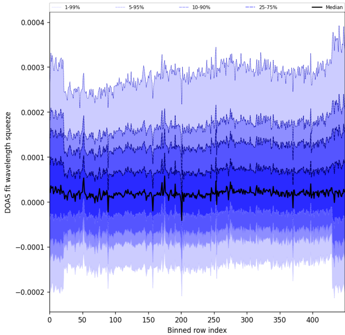
Figure 59: Along track statistics of “DOAS fit wavelength squeeze” for 2025-11-02 to 2025-11-04
