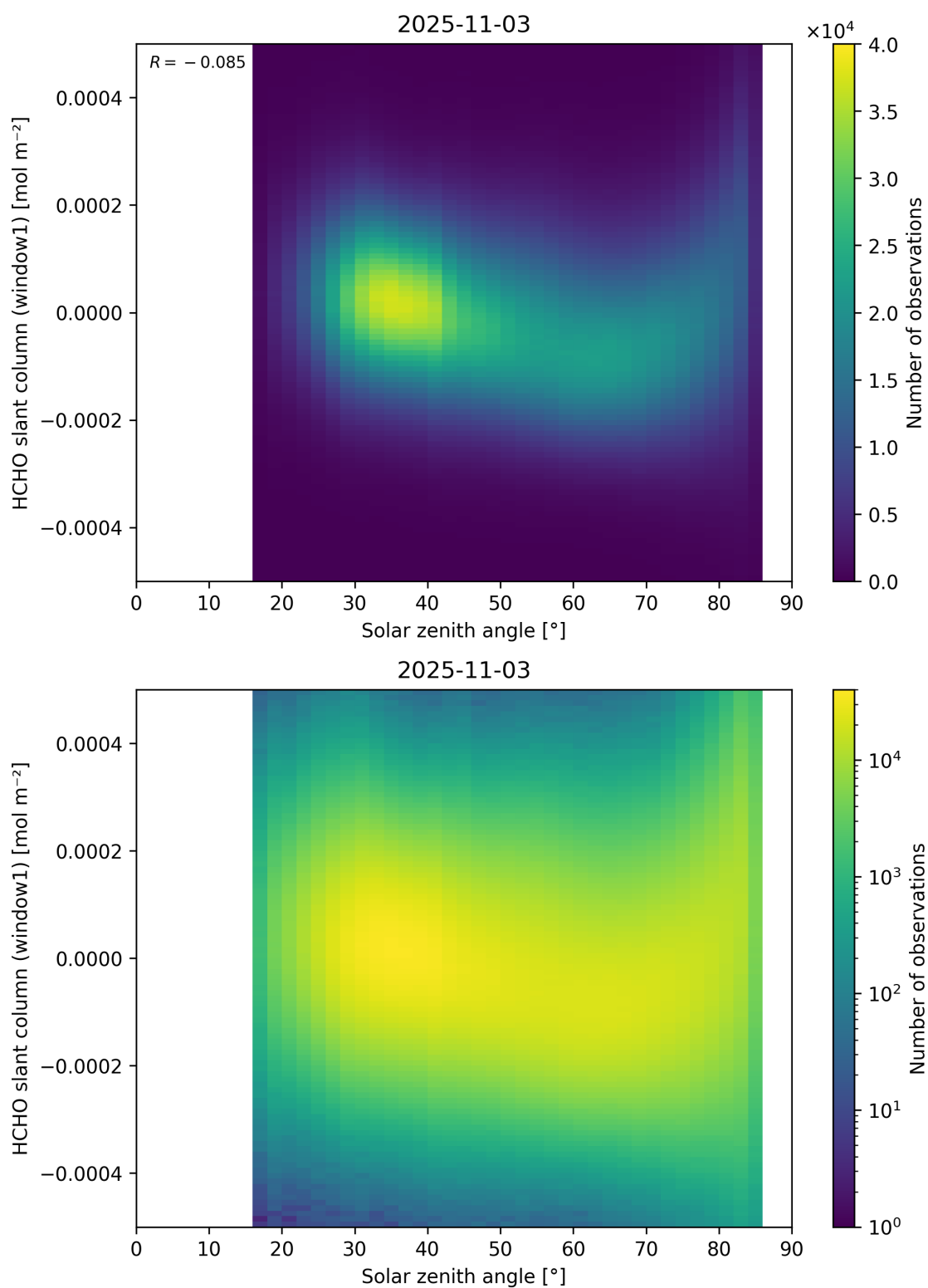
Figure 173: Scatter density plot of “Solar zenith angle” against “HCHO slant column (window1)” for 2025-11-02 to 2025-11-04.
