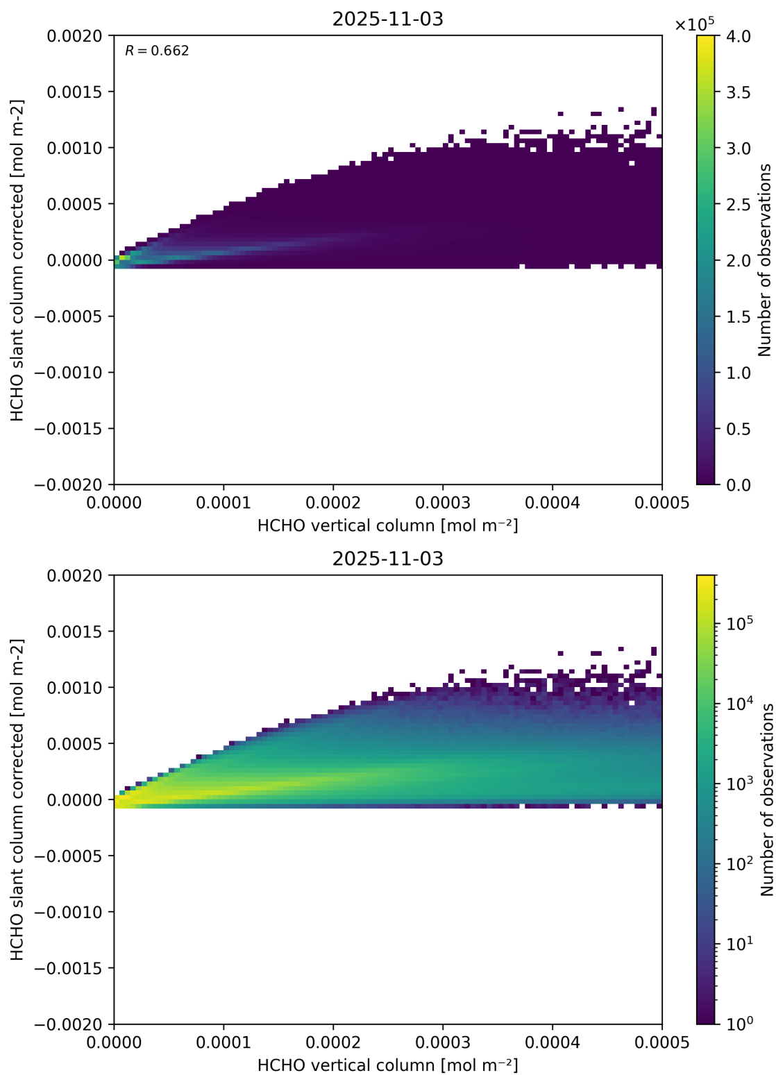
Figure 127: Scatter density plot of “HCHO vertical column” against “HCHO slant column corrected” for 2025-11-02 to 2025-11-04.
