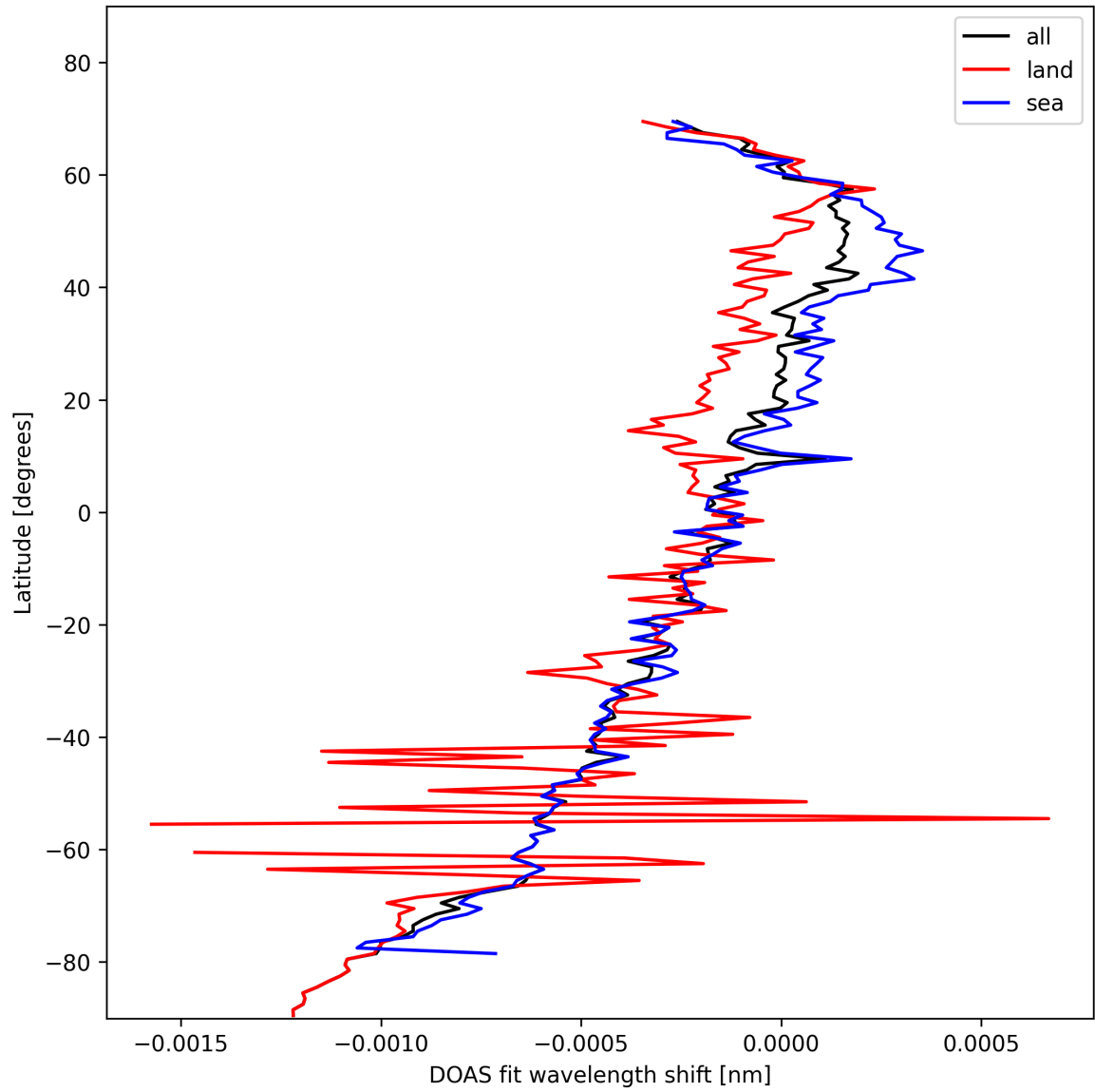
Figure 30: Zonal average of “DOAS fit wavelength shift” for 2025-11-02 to 2025-11-04.
