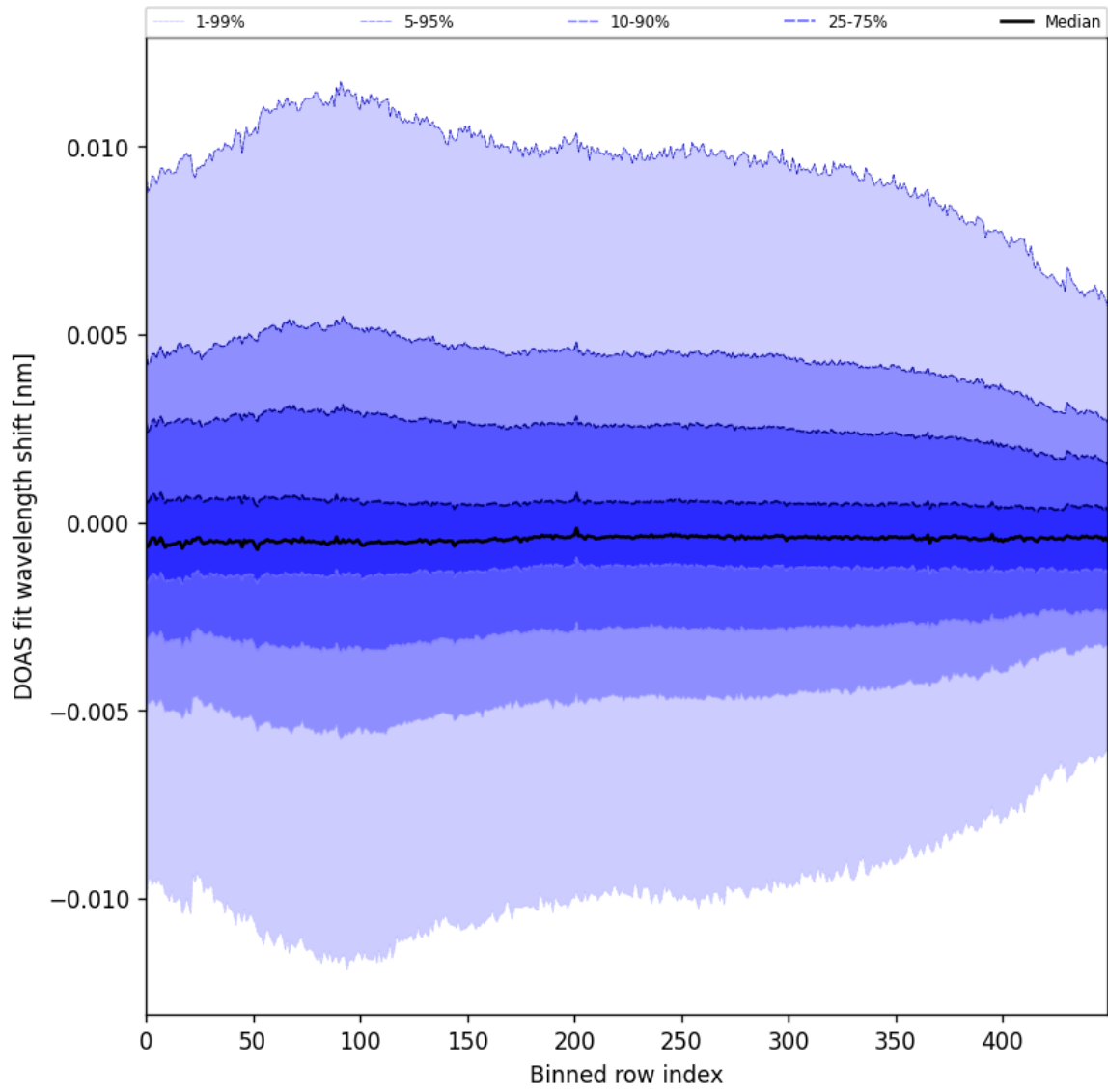
Figure 58: Along track statistics of “DOAS fit wavelength shift” for 2025-11-02 to 2025-11-04
