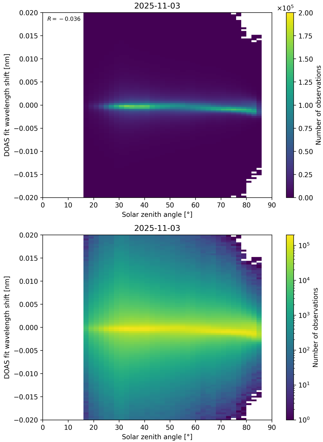
Figure 168: Scatter density plot of “Solar zenith angle” against “DOAS fit wavelength shift” for 2025-11-02 to 2025-11-04.
