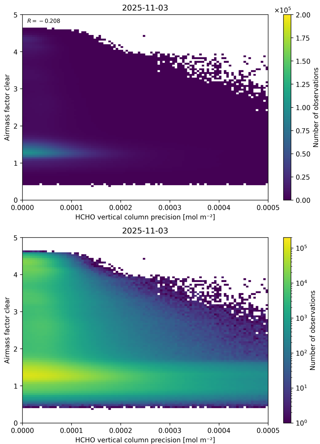
Figure 139: Scatter density plot of “HCHO vertical column precision” against “Airmass factor clear” for 2025-11-02 to 2025-11-04.
