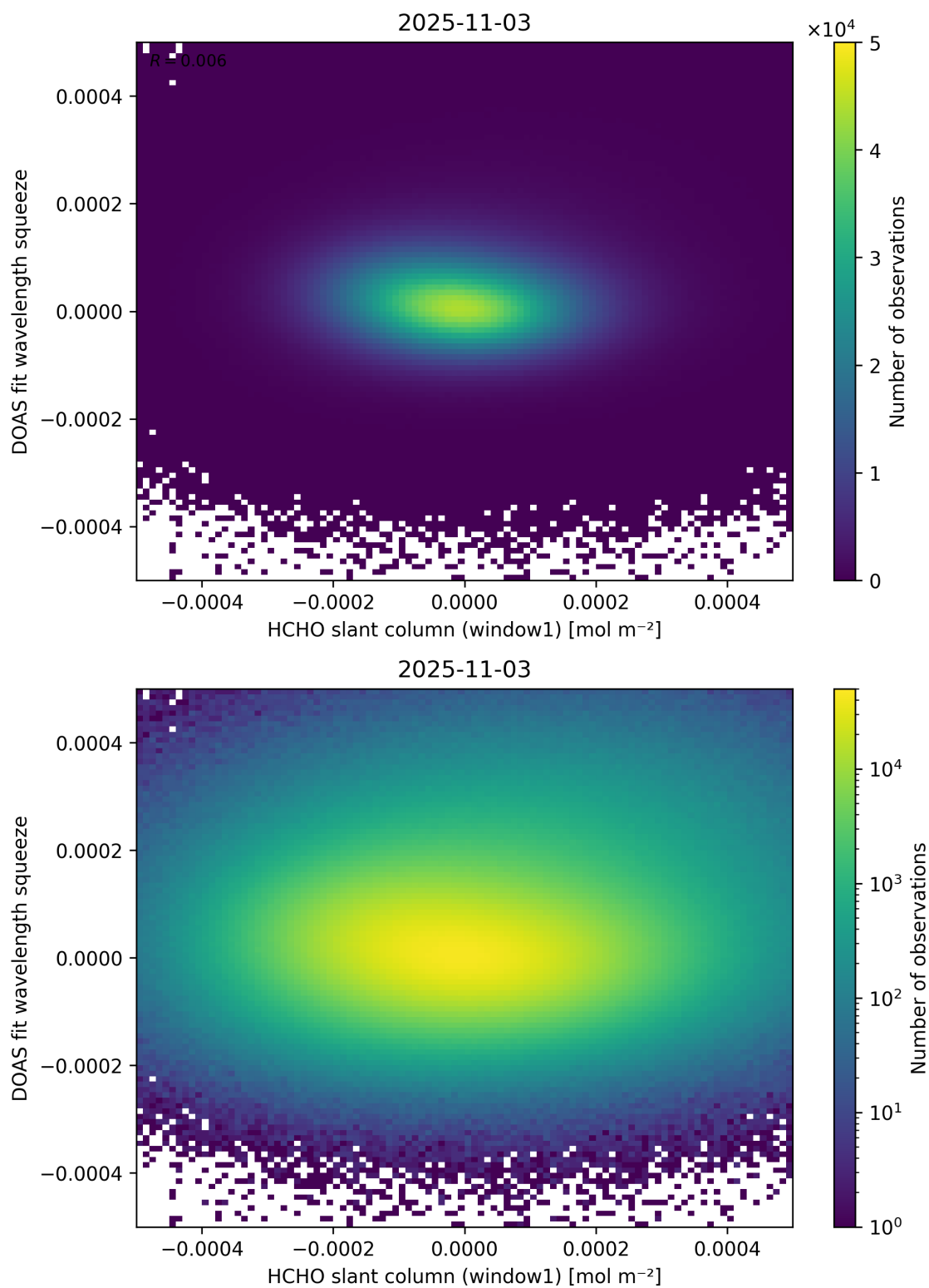
Figure 80: Scatter density plot of “HCHO slant column (window1)” against “DOAS fit wavelength squeeze” for 2025-11-02 to 2025-11-04.
