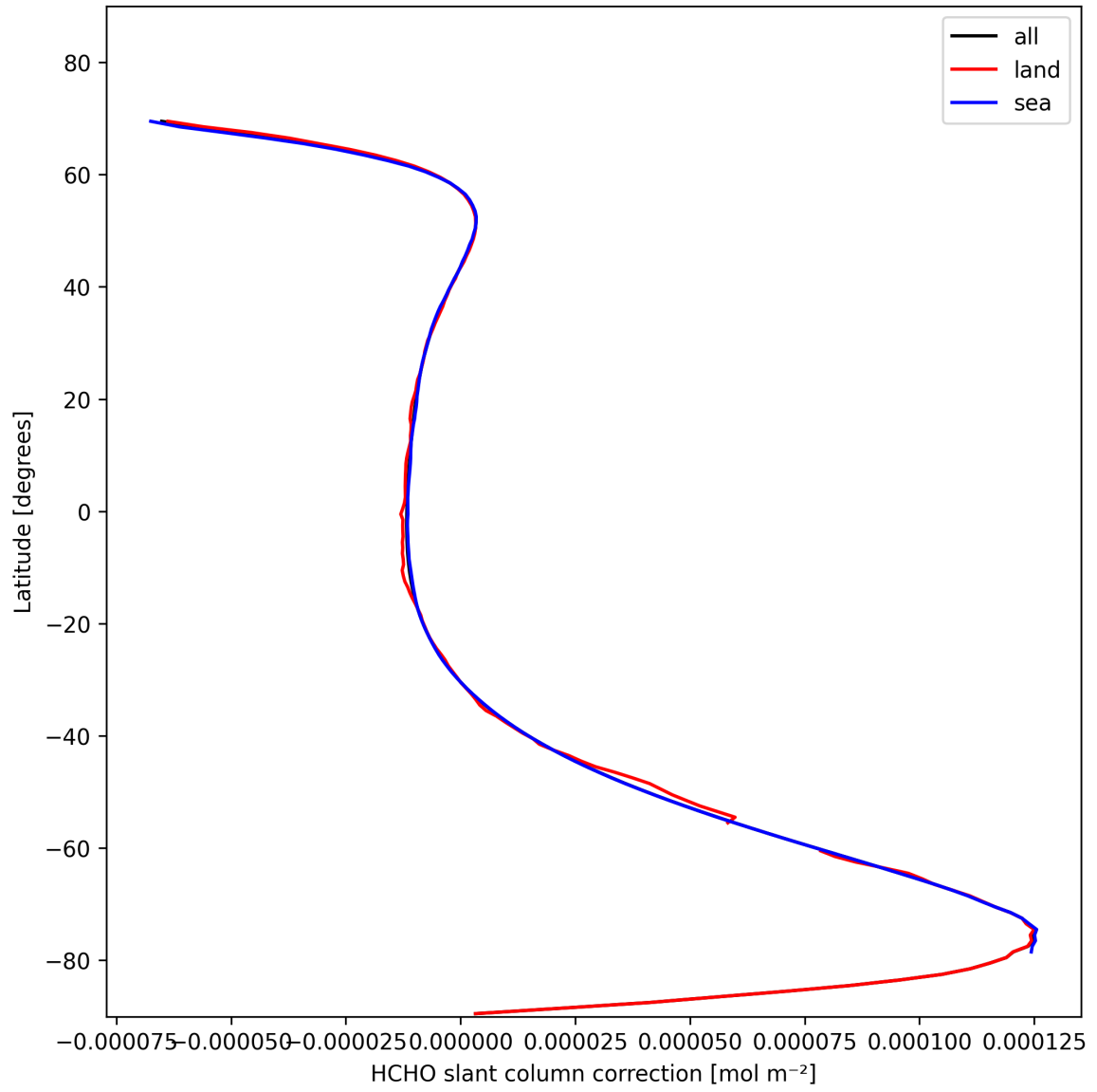
Figure 33: Zonal average of “HCHO slant column correction” for 2025-11-02 to 2025-11-04.
