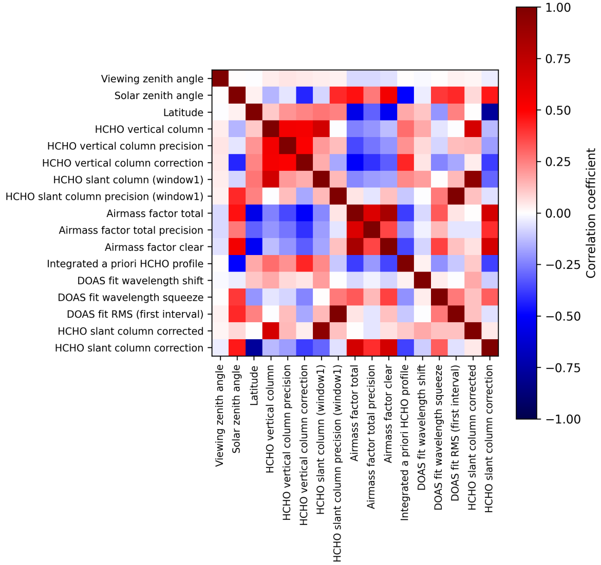
Figure 2: Map of correlation matrix for 2025-11-02 to 2025-11-04.
