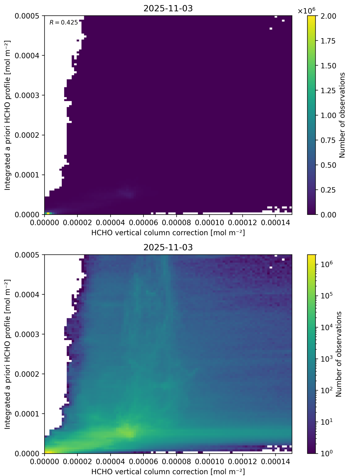
Figure 122: Scatter density plot of “HCHO vertical column correction” against “Integrated a priori HCHO profile” for 2025-11-02 to 2025-11-04.
