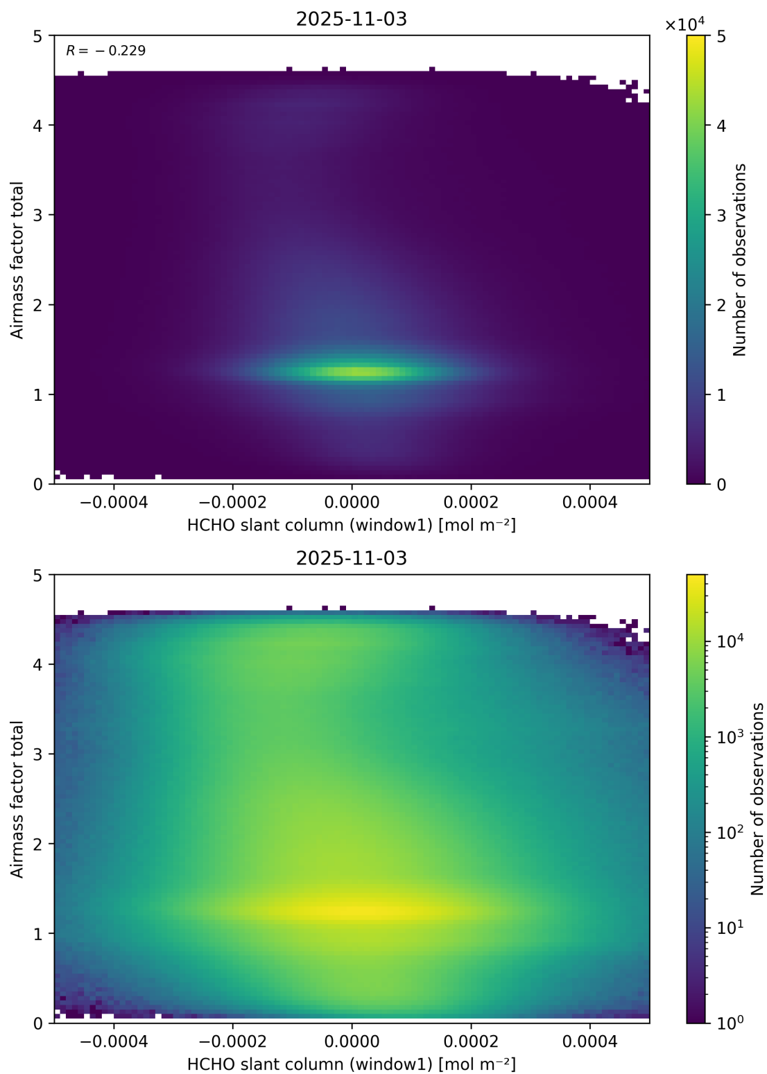
Figure 85: Scatter density plot of “HCHO slant column (window1)” against “Airmass factor total” for 2025-11-02 to 2025-11-04.
