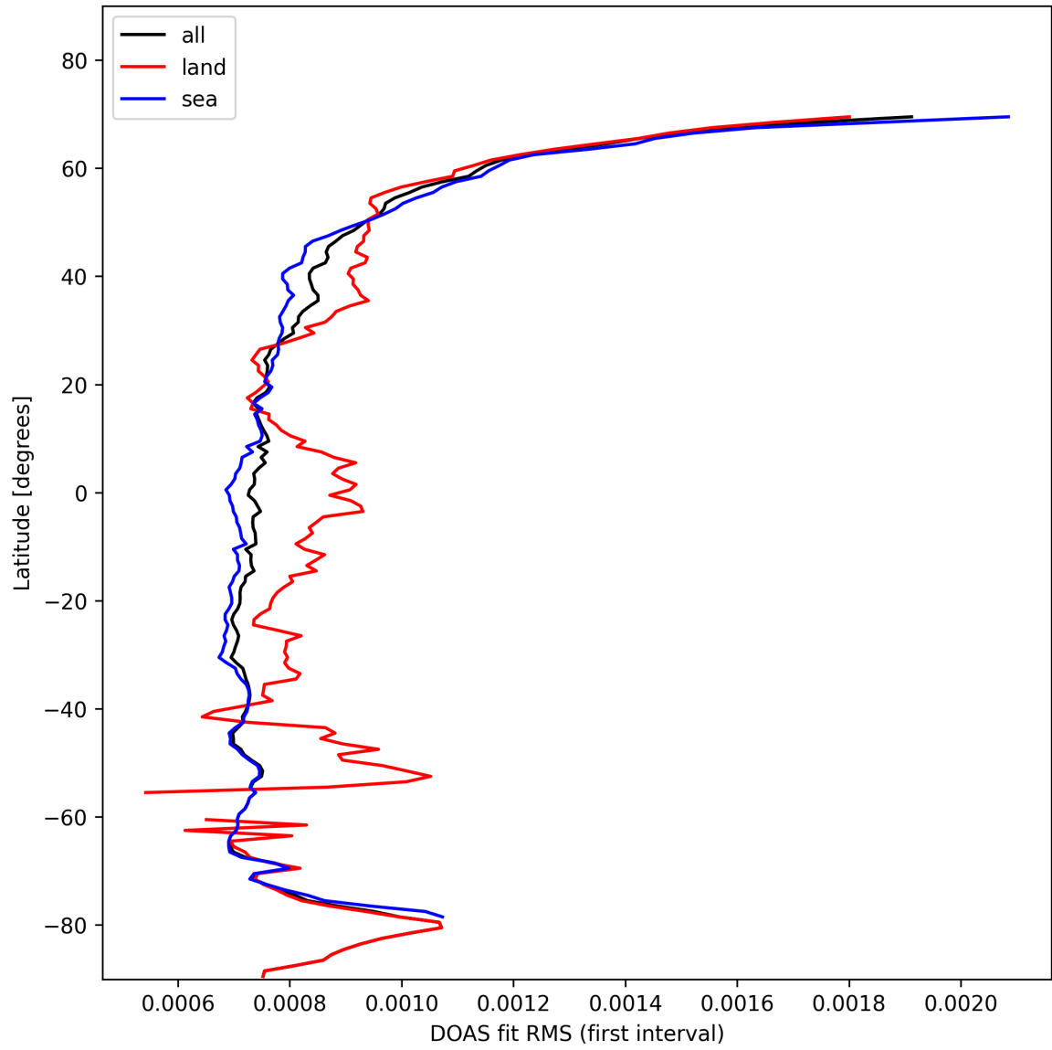
Figure 32: Zonal average of “DOAS fit RMS (first interval)” for 2025-11-02 to 2025-11-04.
