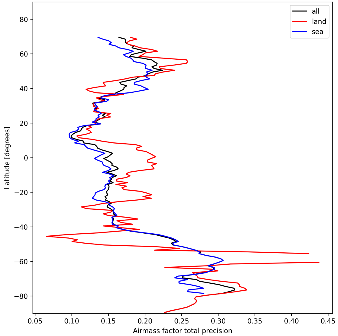
Figure 27: Zonal average of “Airmass factor total precision” for 2025-11-02 to 2025-11-04.
