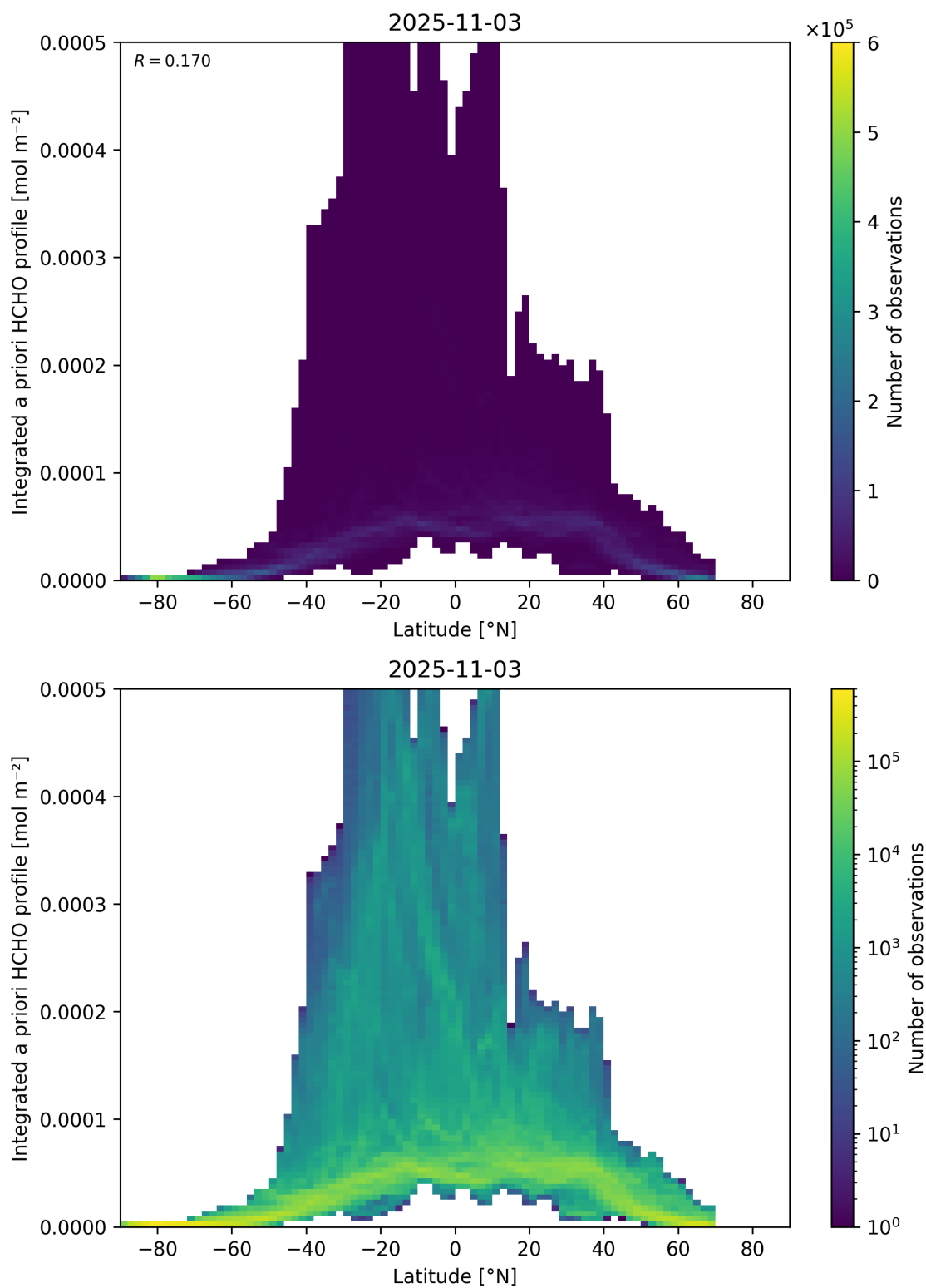
Figure 166: Scatter density plot of “Latitude” against “Integrated a priori HCHO profile” for 2025-11-02 to 2025-11-04.
