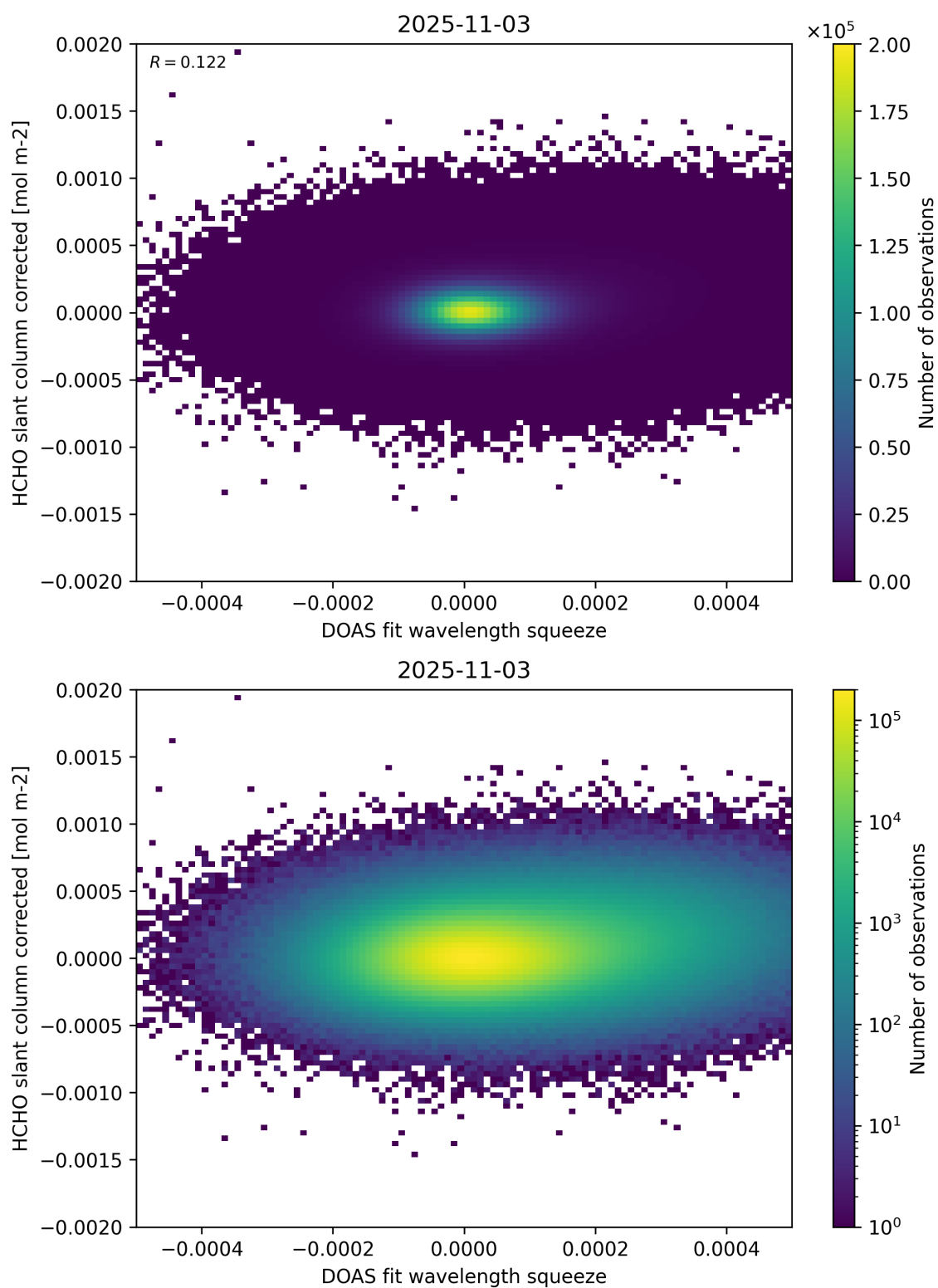
Figure 69: Scatter density plot of “DOAS fit wavelength squeeze” against “HCHO slant column corrected” for 2025-11-02 to 2025-11-04.
