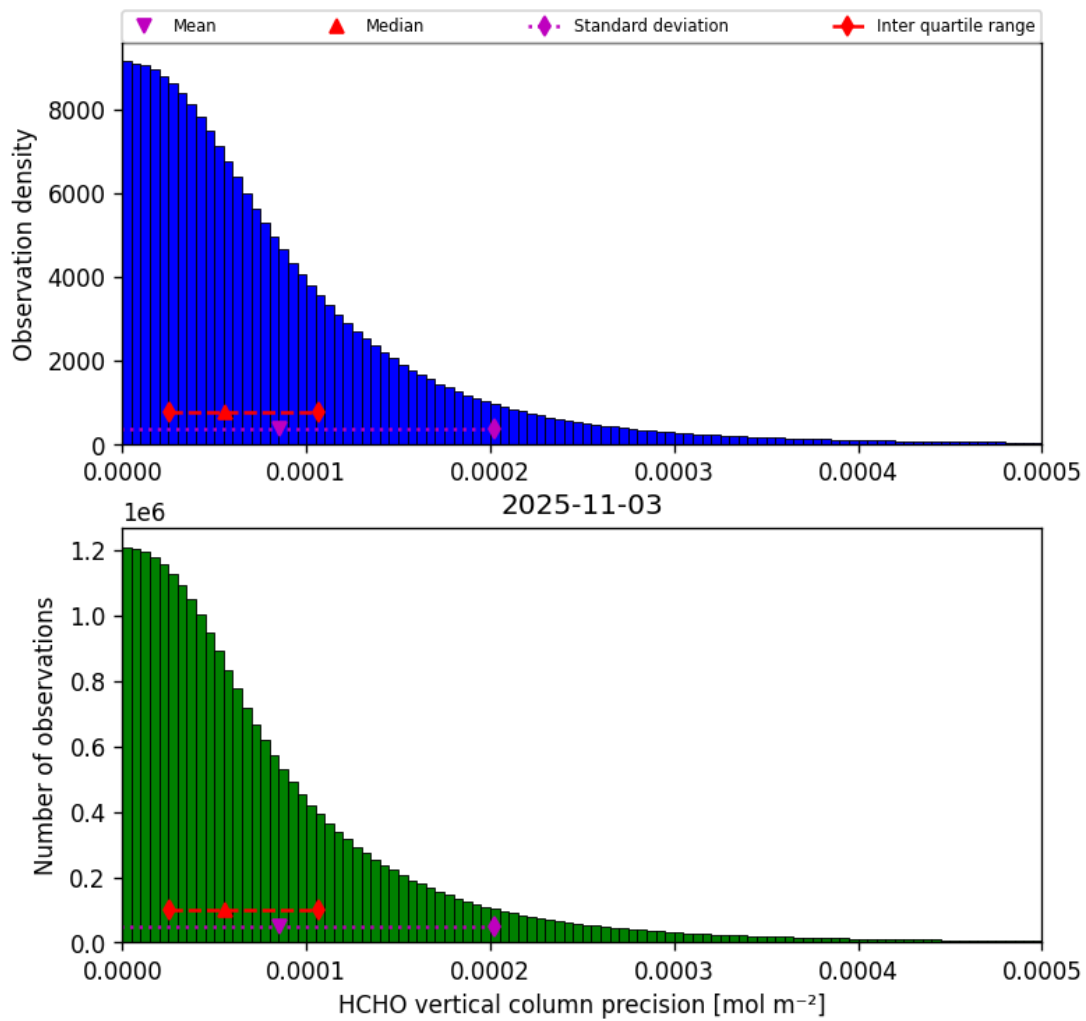
Figure 36: Histogram of “HCHO vertical column precision” for 2025-11-02 to 2025-11-04
