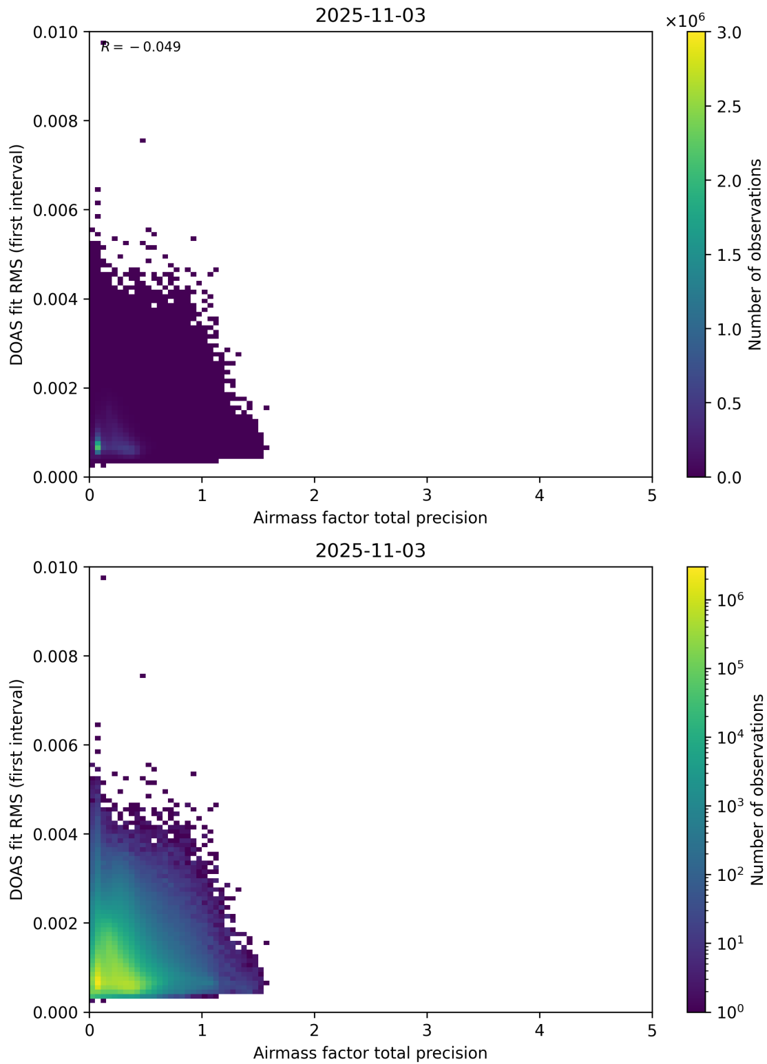
Figure 105: Scatter density plot of “Airmass factor total precision” against “DOAS fit RMS (first interval)” for 2025-11-02 to 2025-11-04.
