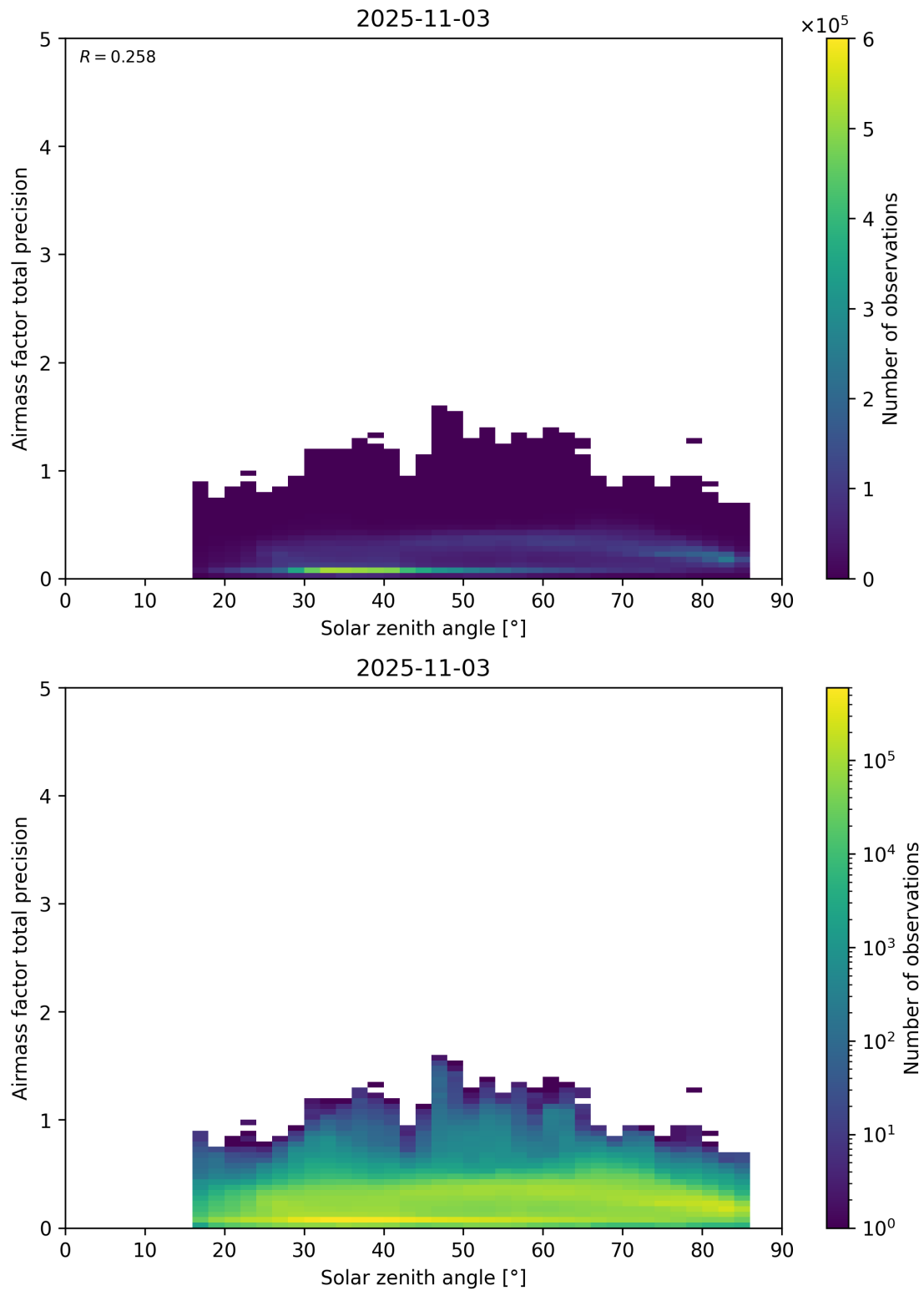
Figure 176: Scatter density plot of “Solar zenith angle” against “Airmass factor total precision” for 2025-11-02 to 2025-11-04.
