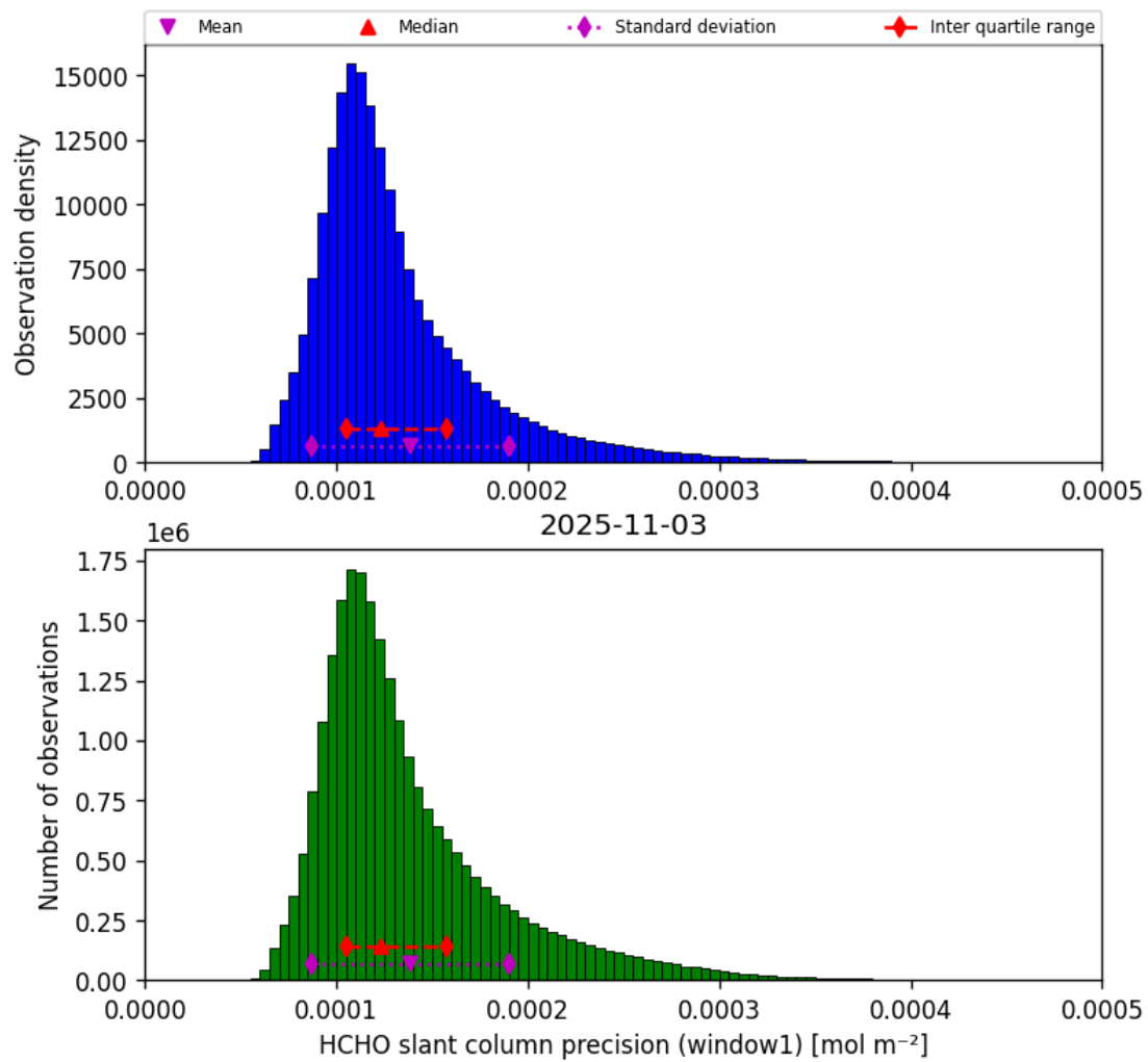
Figure 39: Histogram of “HCHO slant column precision (window1)” for 2025-11-02 to 2025-11-04
