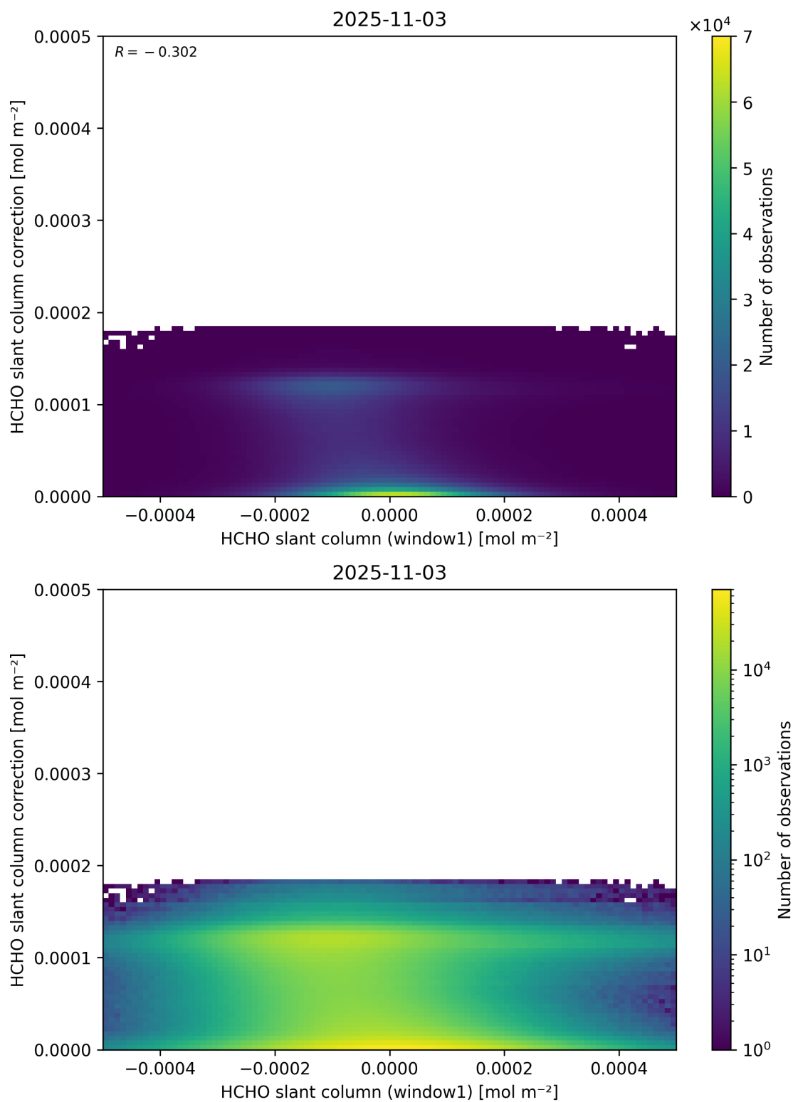
Figure 83: Scatter density plot of “HCHO slant column (window1)” against “HCHO slant column correction” for 2025-11-02 to 2025-11-04.
