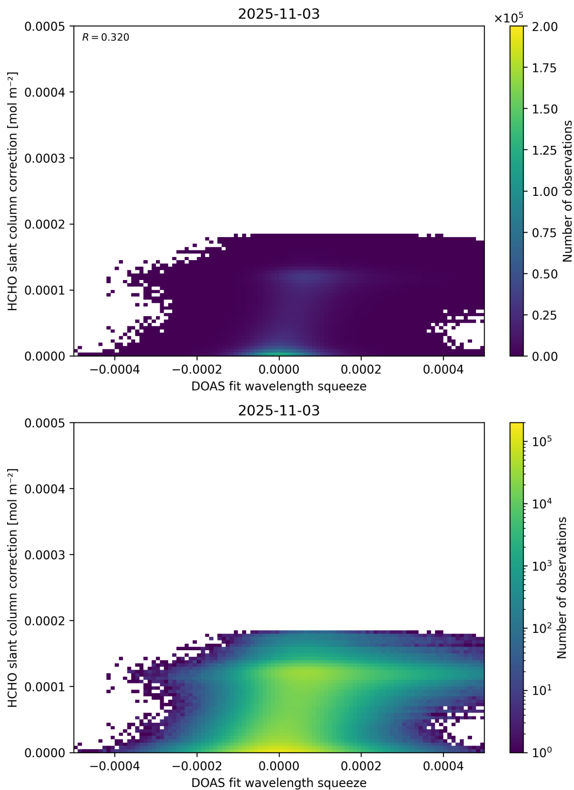
Figure 70: Scatter density plot of “DOAS fit wavelength squeeze” against “HCHO slant column correction” for 2025-11-02 to 2025-11-04.
