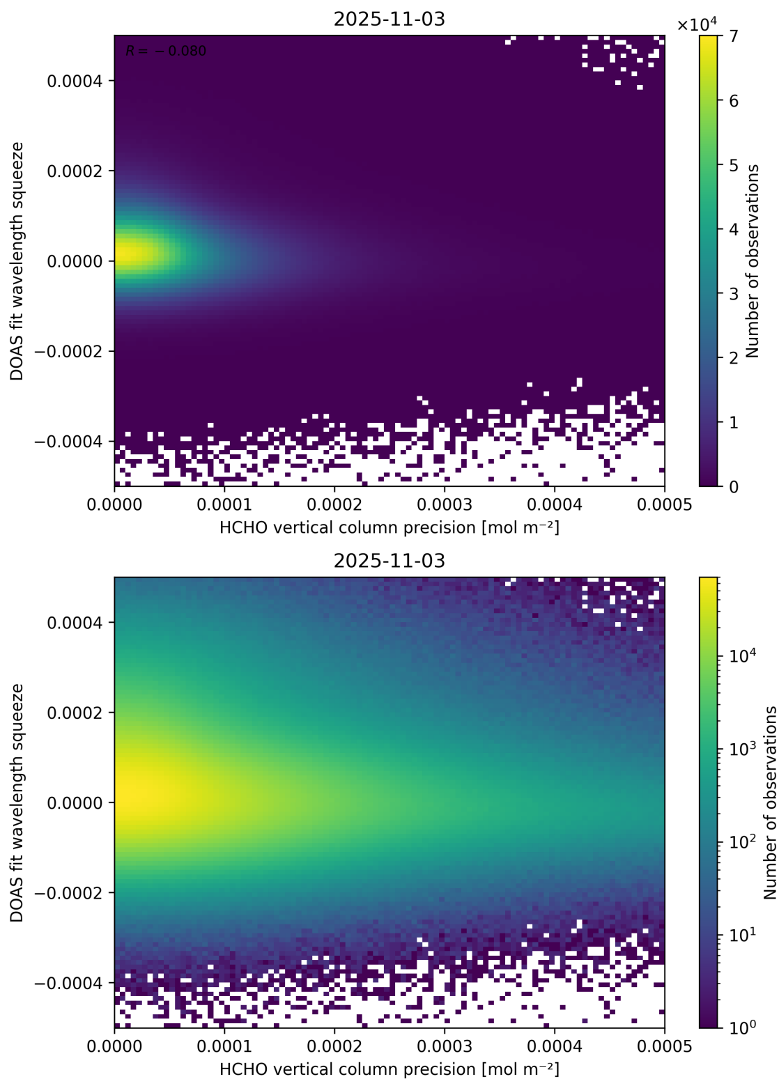
Figure 138: Scatter density plot of “HCHO vertical column precision” against “DOAS fit wavelength squeeze” for 2025-11-02 to 2025-11-04.
