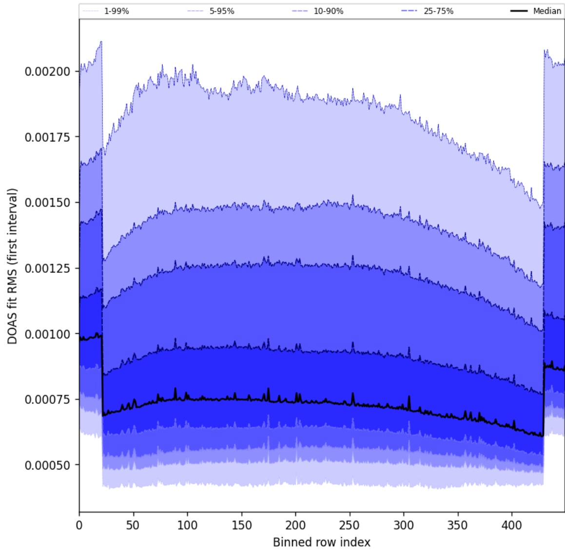
Figure 60: Along track statistics of “DOAS fit RMS (first interval)” for 2025-11-02 to 2025-11-04
