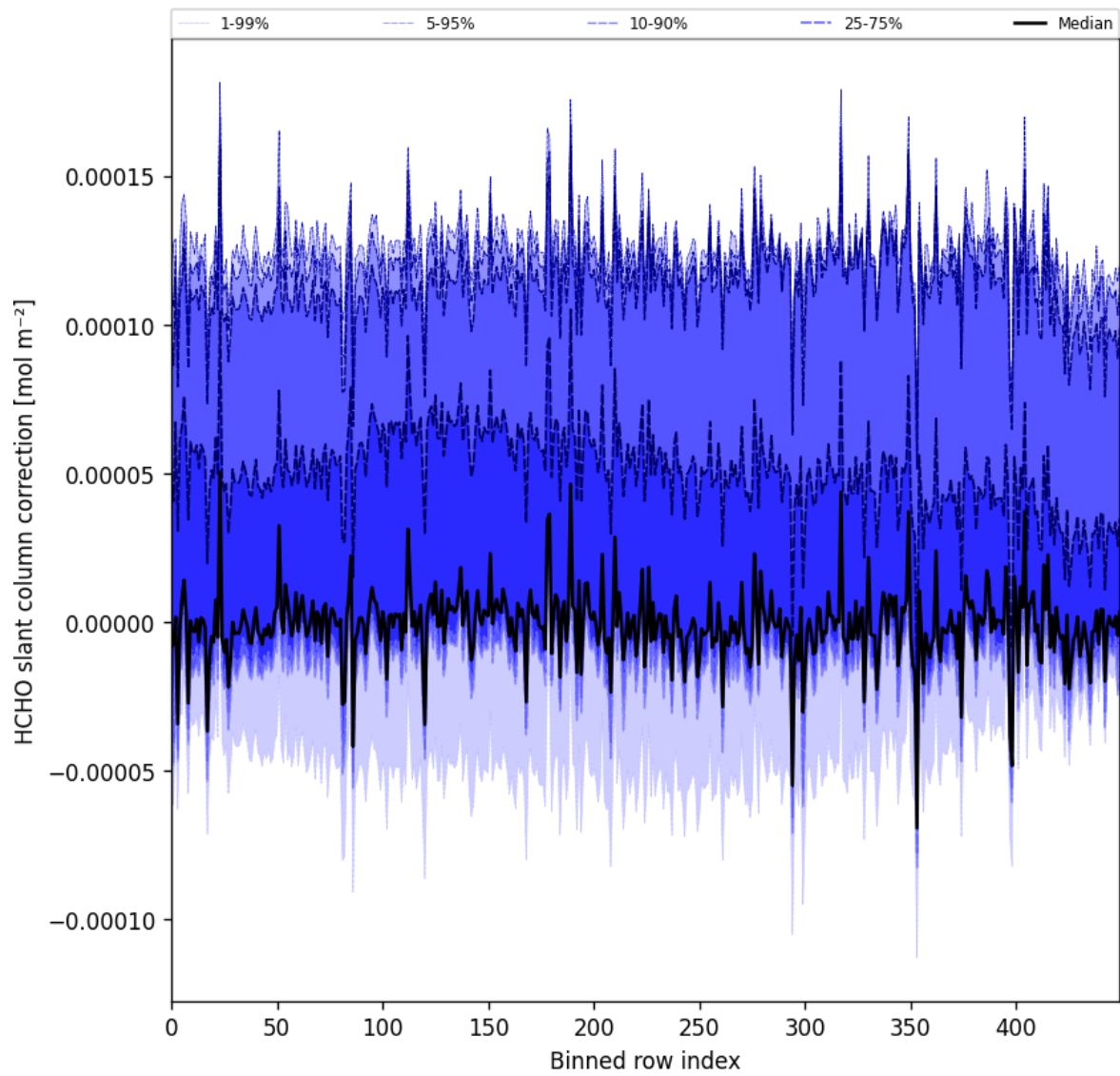
Figure 61: Along track statistics of “HCHO slant column correction” for 2025-11-02 to 2025-11-04
