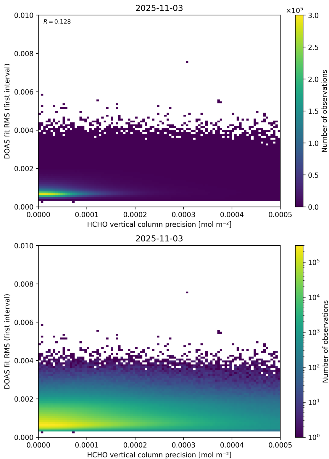
Figure 136: Scatter density plot of “HCHO vertical column precision” against “DOAS fit RMS (first interval)” for 2025-11-02 to 2025-11-04.
