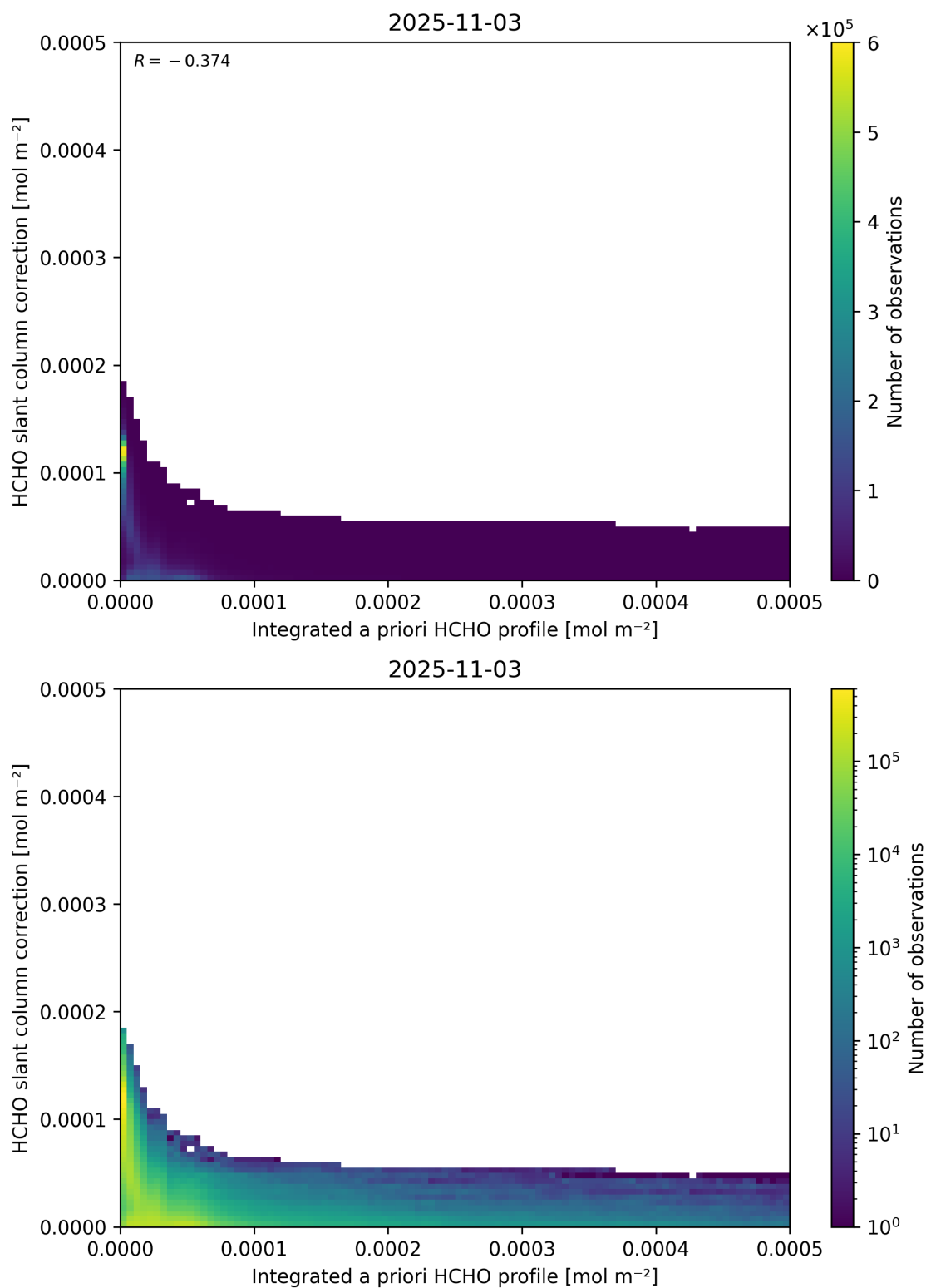
Figure 152: Scatter density plot of “Integrated a priori HCHO profile” against “HCHO slant column correction” for 2025-11-02 to 2025-11-04.
