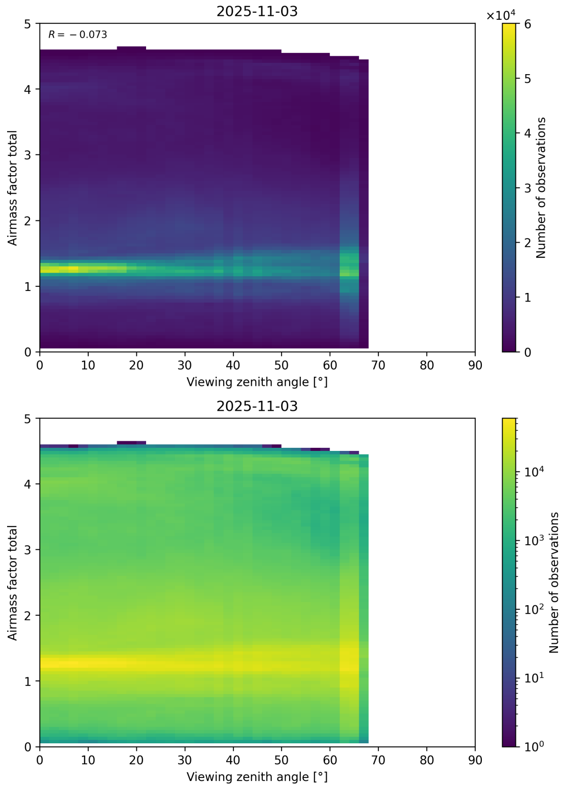
Figure 190: Scatter density plot of “Viewing zenith angle” against “Airmass factor total” for 2025-11-02 to 2025-11-04.
