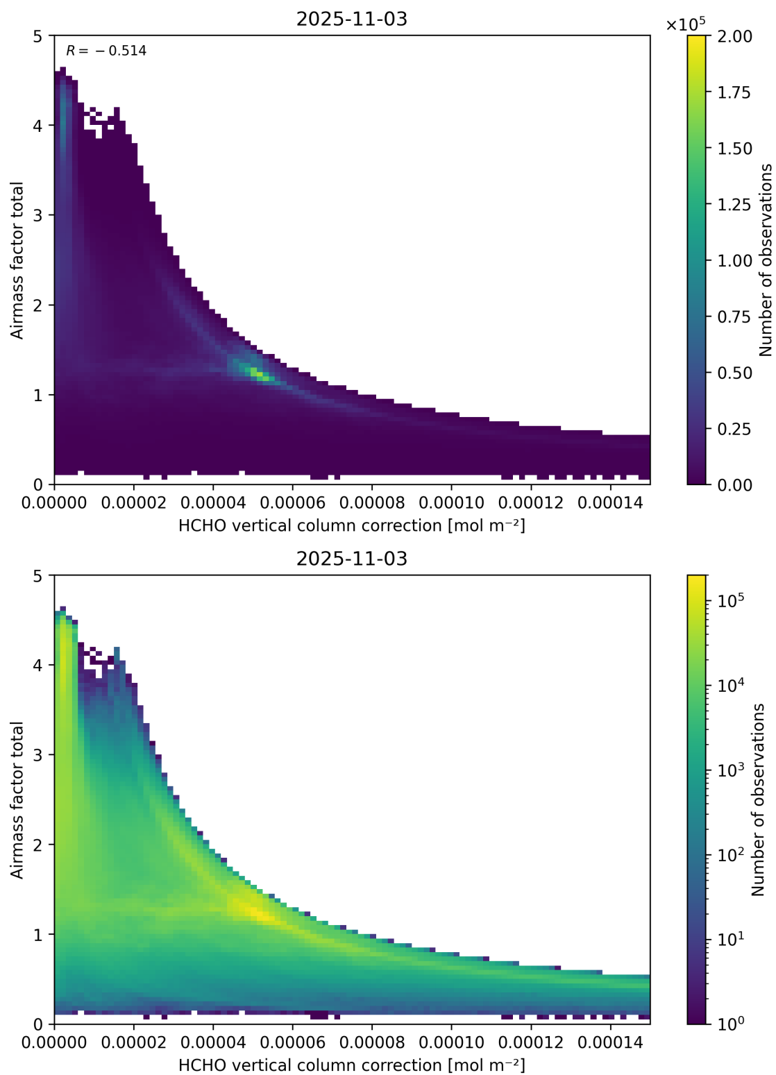
Figure 120: Scatter density plot of “HCHO vertical column correction” against “Airmass factor total” for 2025-11-02 to 2025-11-04.
