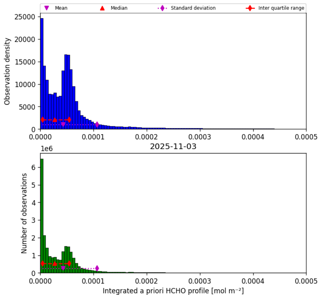
Figure 43: Histogram of “Integrated a priori HCHO profile” for 2025-11-02 to 2025-11-04
