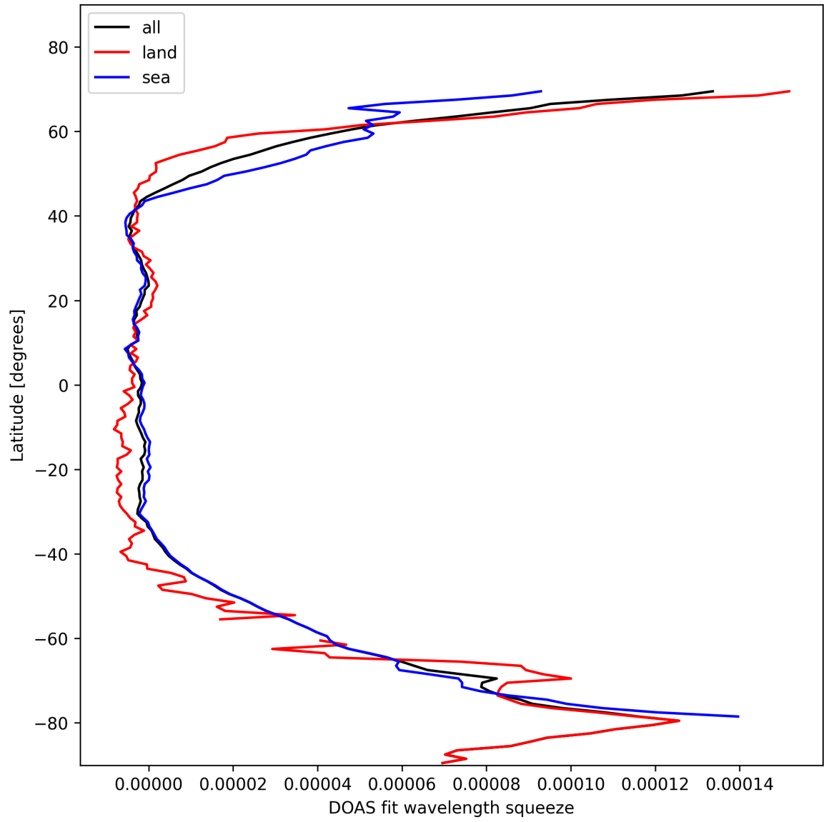
Figure 31: Zonal average of “DOAS fit wavelength squeeze” for 2025-11-02 to 2025-11-04.
