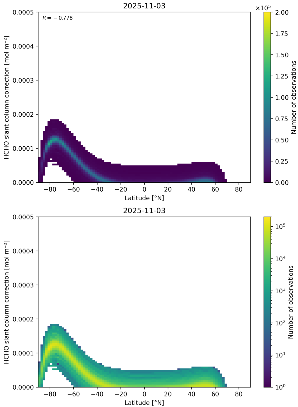
Figure 158: Scatter density plot of “Latitude” against “HCHO slant column correction” for 2025-11-02 to 2025-11-04.
