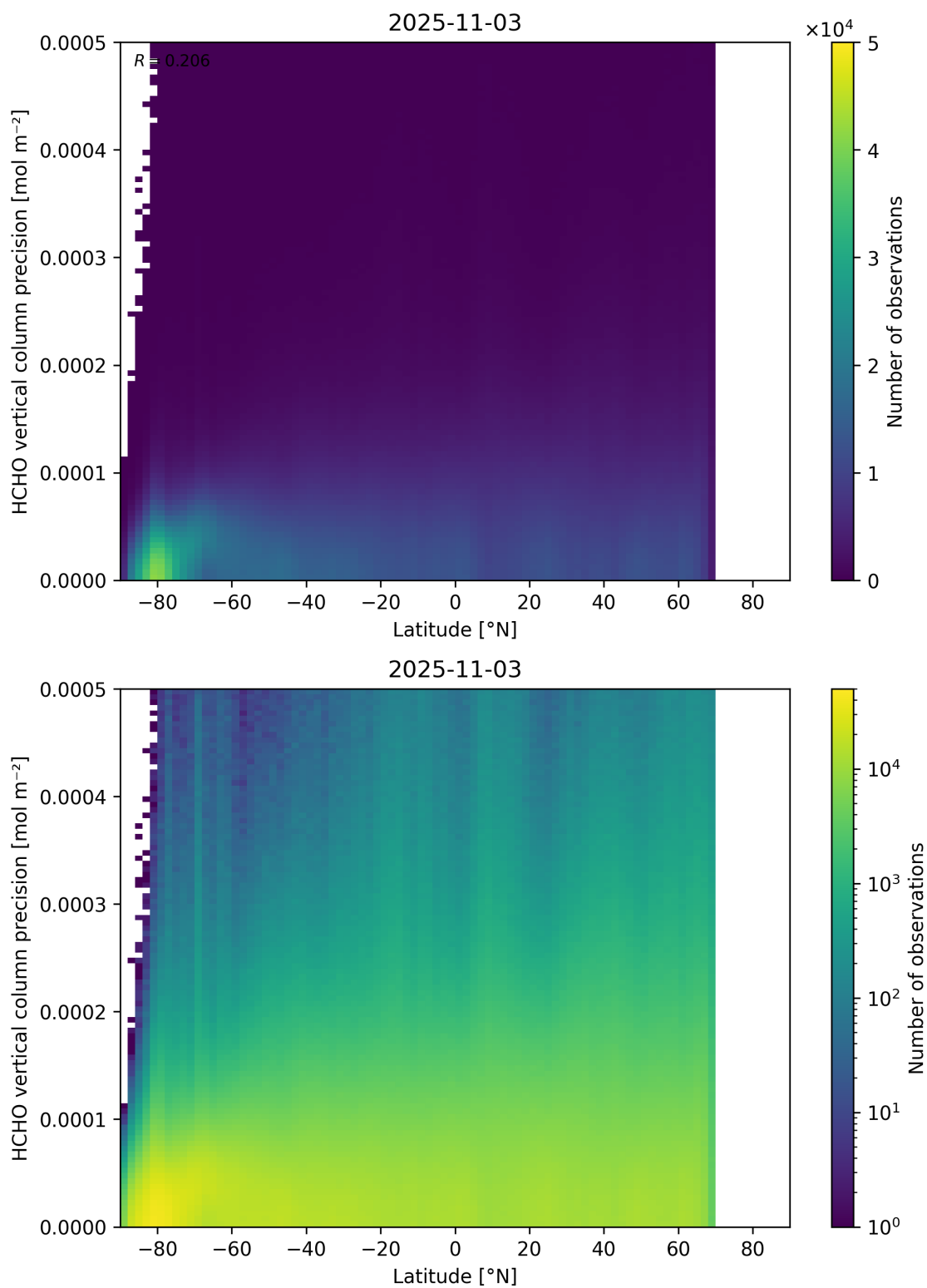
Figure 165: Scatter density plot of “Latitude” against “HCHO vertical column precision” for 2025-11-02 to 2025-11-04.
