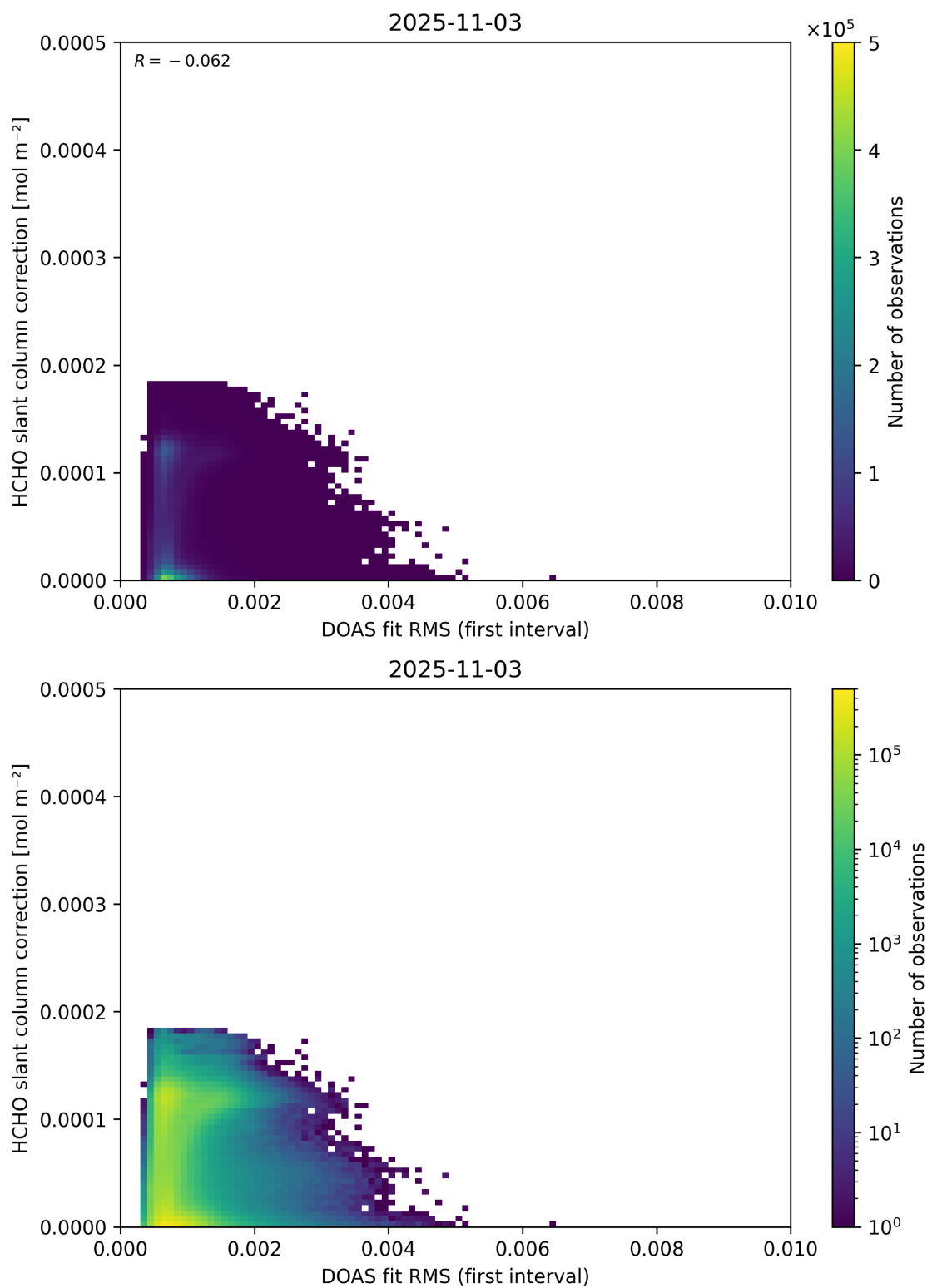
Figure 63: Scatter density plot of “DOAS fit RMS (first interval)” against “HCHO slant column correction” for 2025-11-02 to 2025-11-04.
