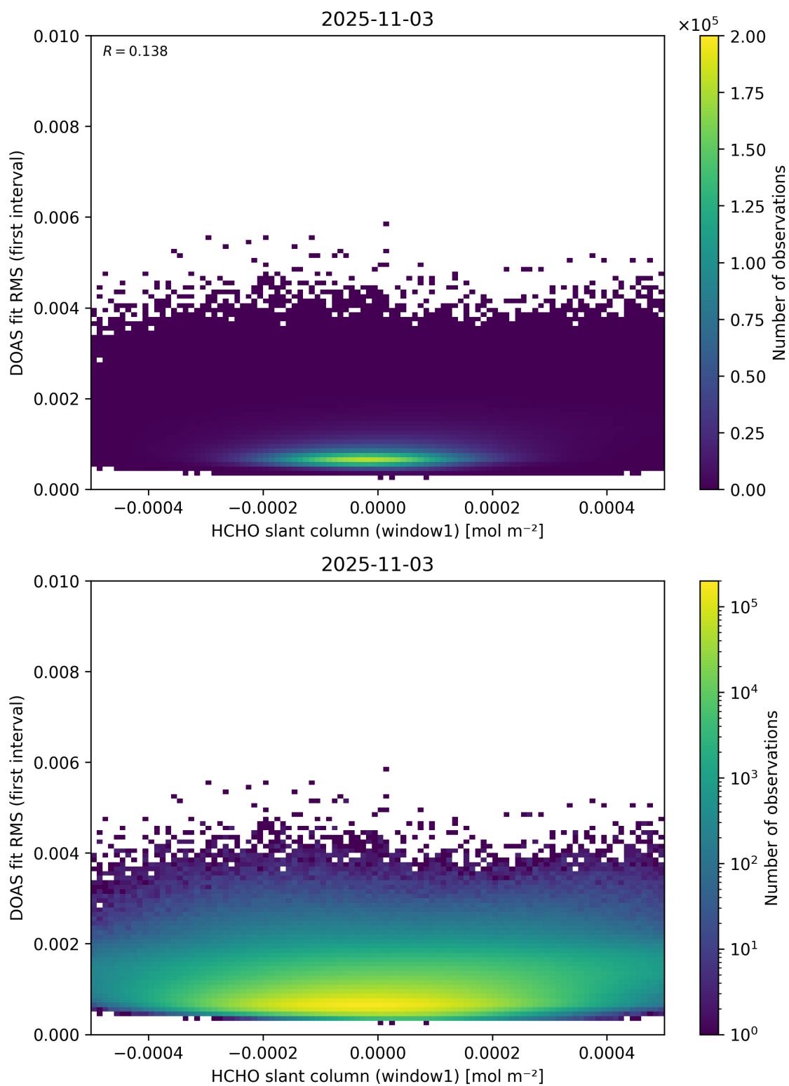
Figure 78: Scatter density plot of “HCHO slant column (window1)” against “DOAS fit RMS (first interval)” for 2025-11-02 to 2025-11-04.
