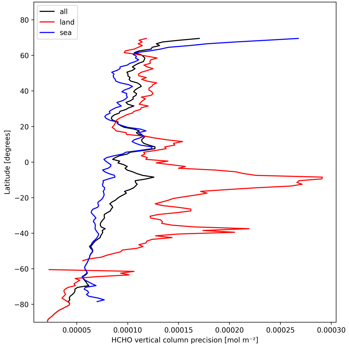
Figure 22: Zonal average of “HCHO vertical column precision” for 2025-11-02 to 2025-11-04.
