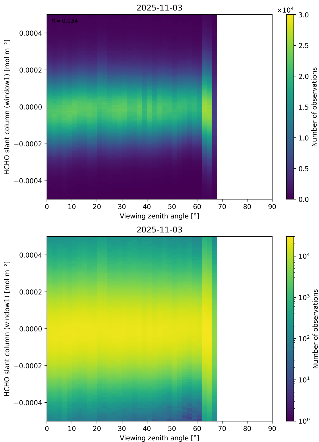
Figure 188: Scatter density plot of “Viewing zenith angle” against “HCHO slant column (window1)” for 2025-11-02 to 2025-11-04.
