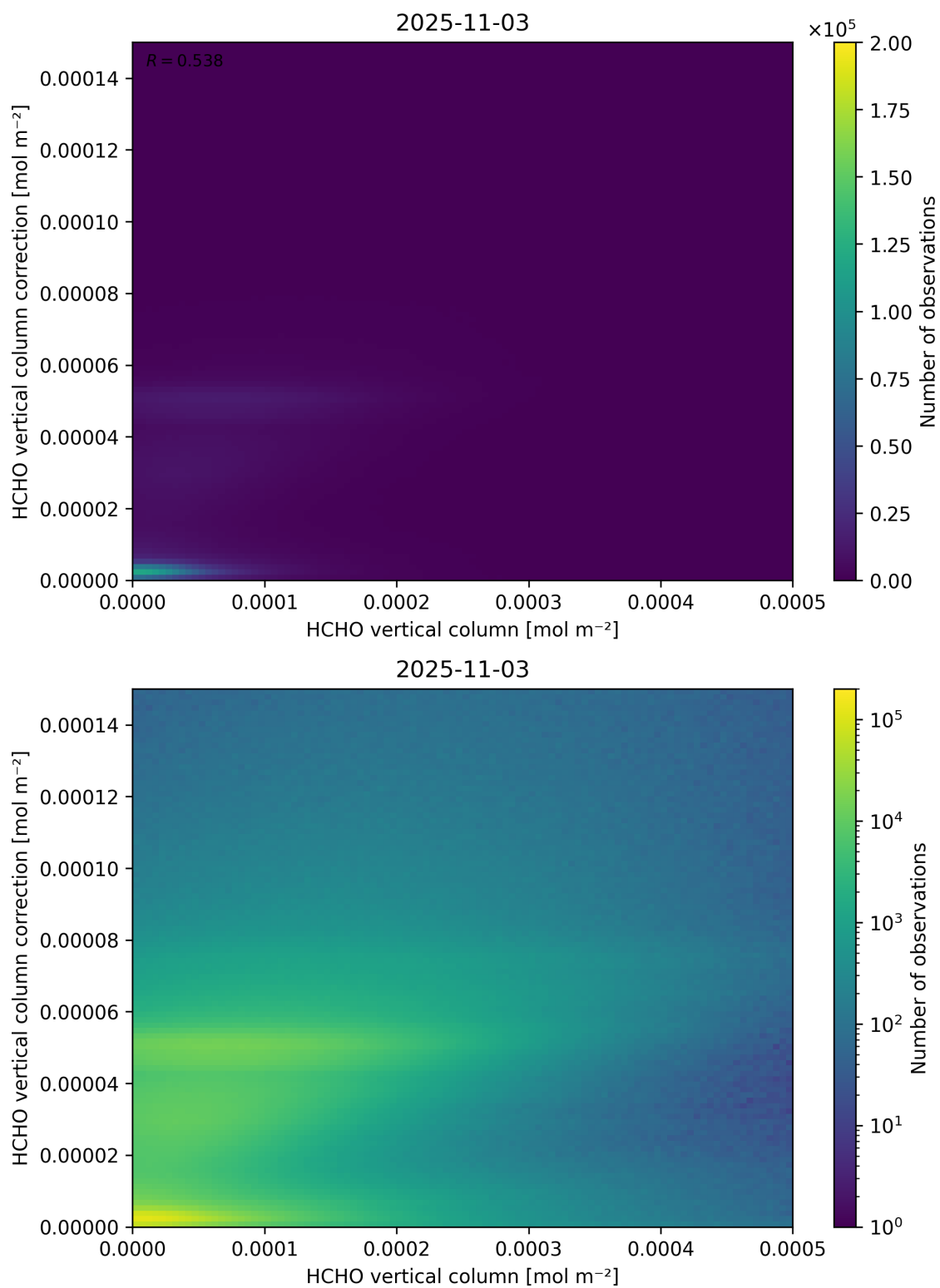
Figure 133: Scatter density plot of “HCHO vertical column” against “HCHO vertical column correction” for 2025-11-02 to 2025-11-04.
