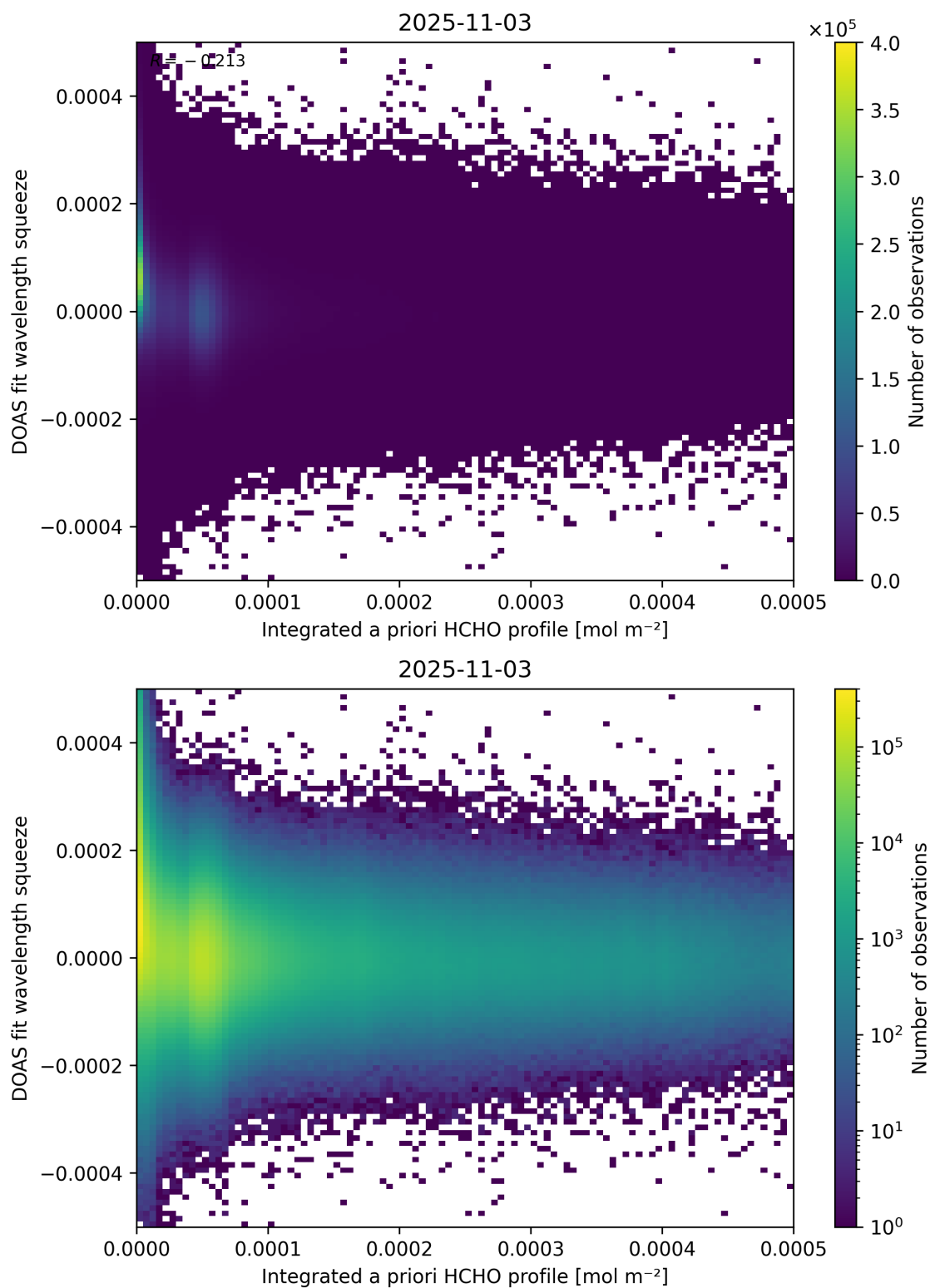
Figure 150: Scatter density plot of “Integrated a priori HCHO profile” against “DOAS fit wavelength squeeze” for 2025-11-02 to 2025-11-04.
