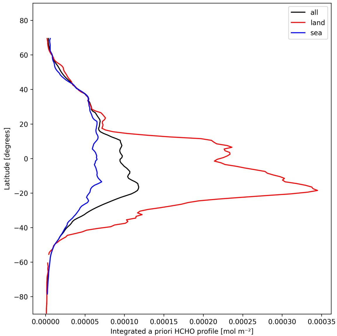
Figure 29: Zonal average of “Integrated a priori HCHO profile” for 2025-11-02 to 2025-11-04.
