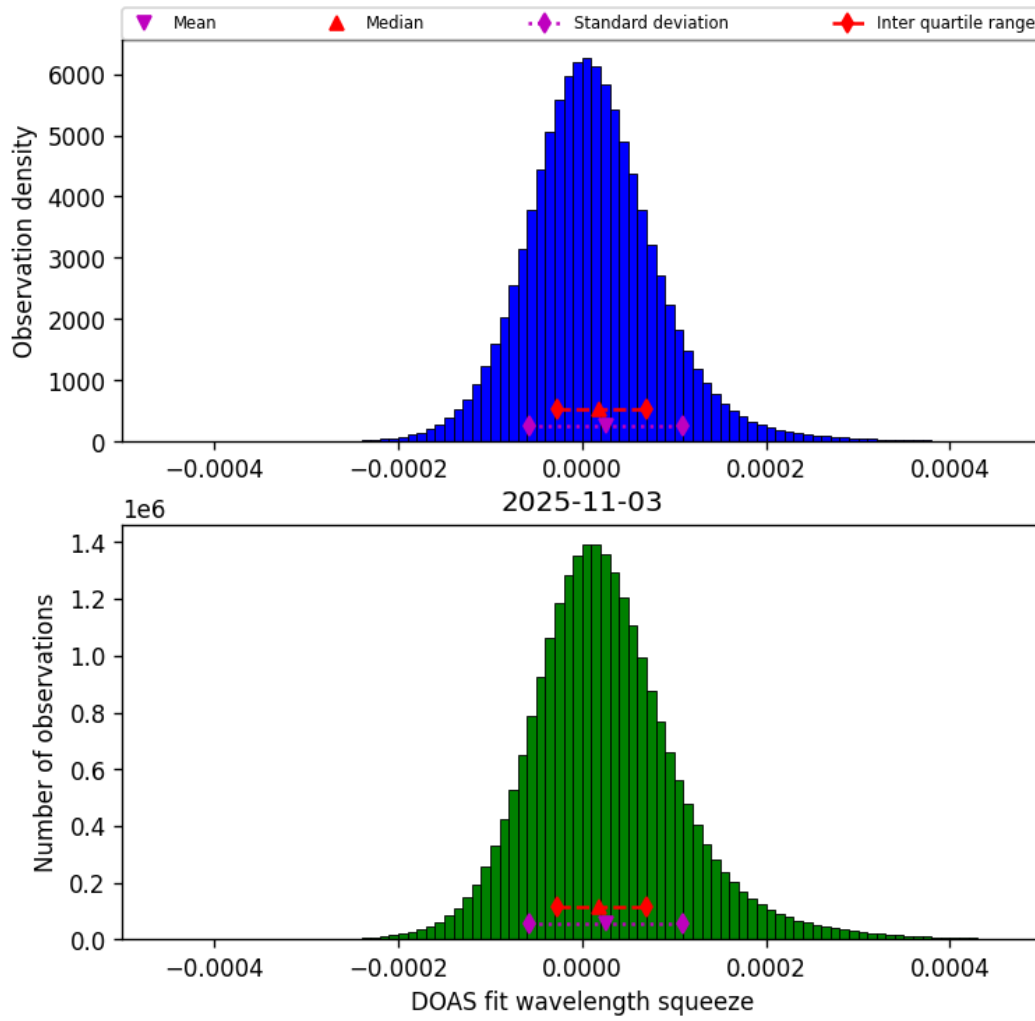
Figure 45: Histogram of “DOAS fit wavelength squeeze” for 2025-11-02 to 2025-11-04
