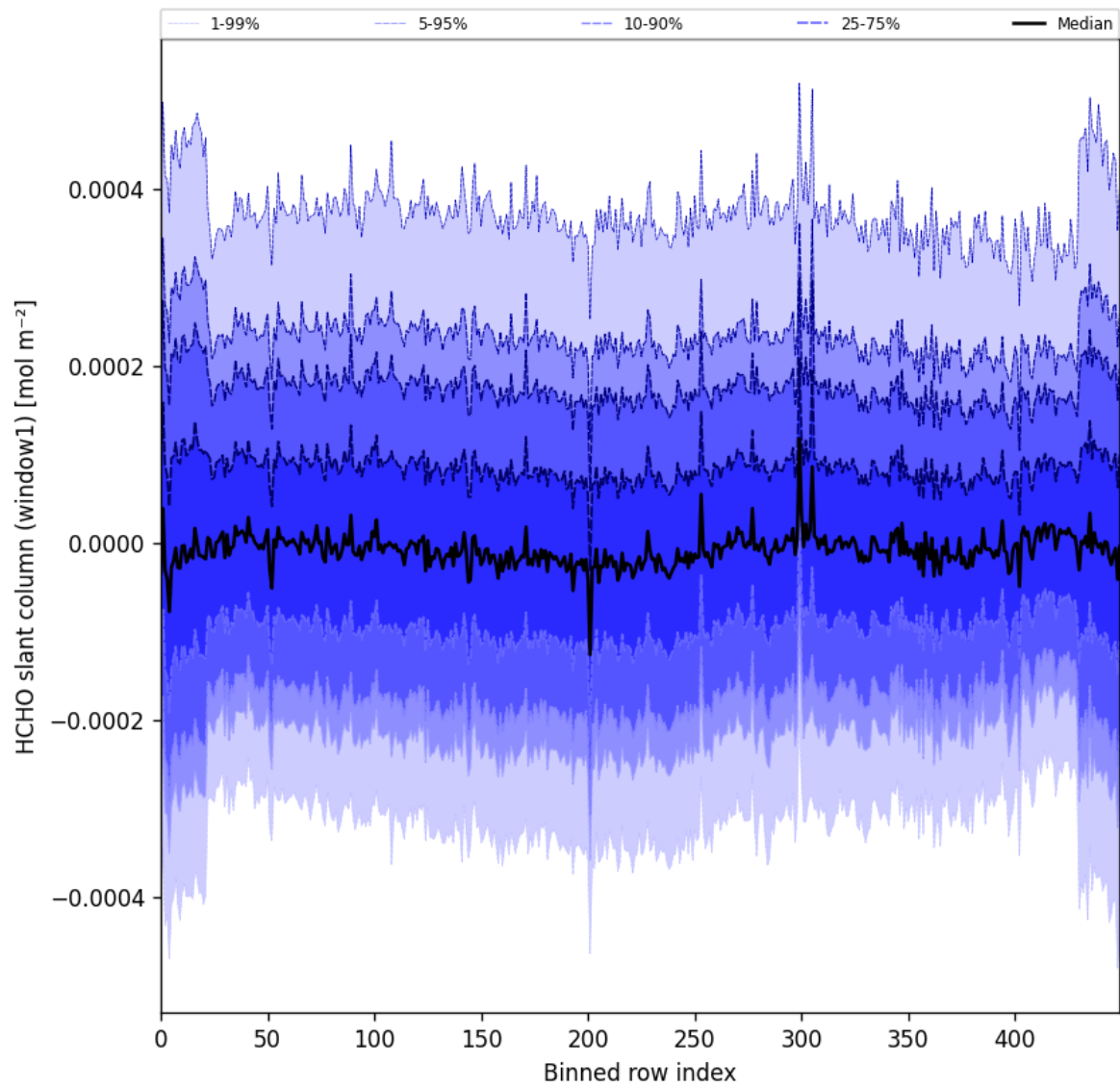
Figure 52: Along track statistics of “HCHO slant column (window1)” for 2025-11-02 to 2025-11-04
