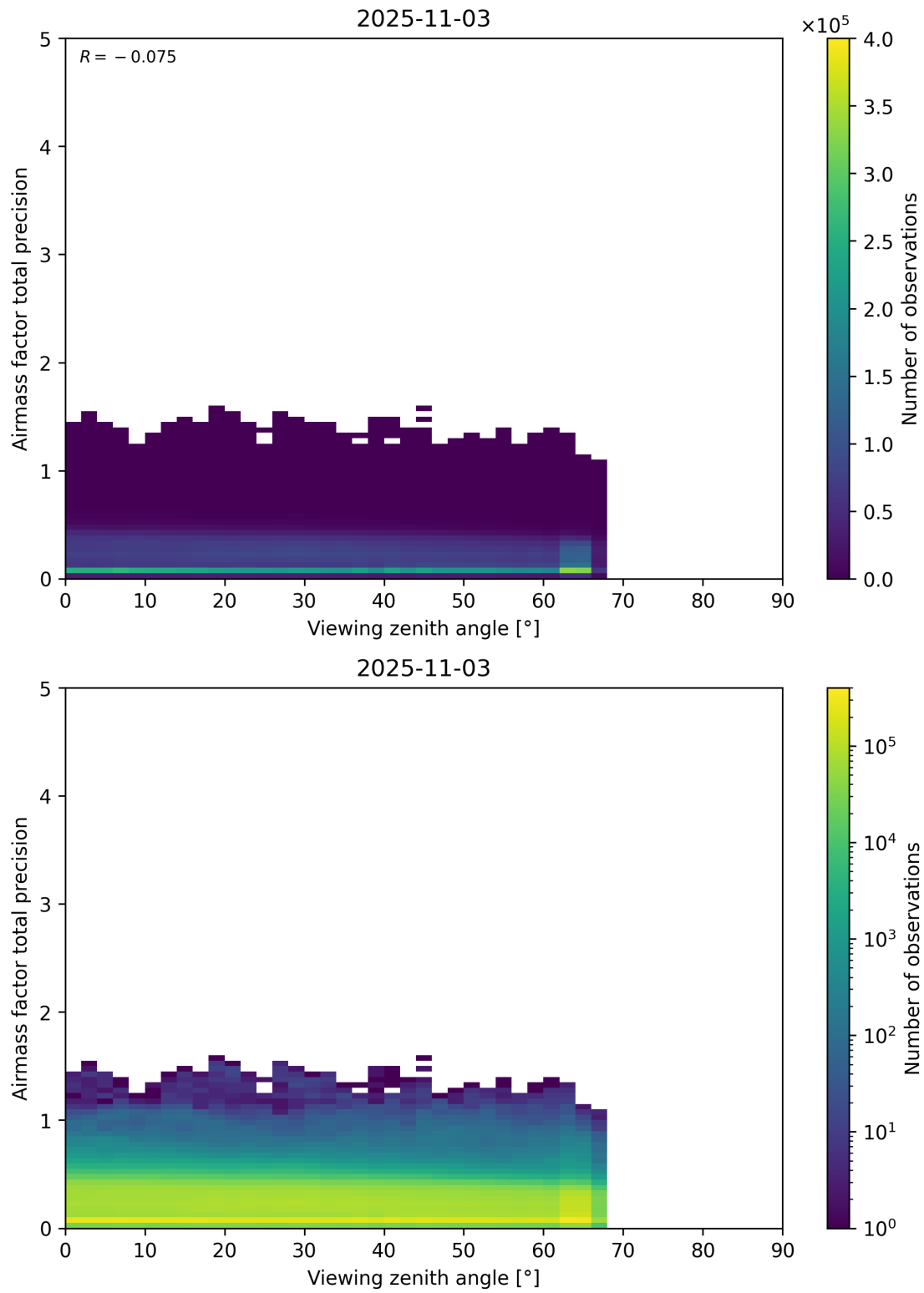
Figure 191: Scatter density plot of “Viewing zenith angle” against “Airmass factor total precision” for 2025-11-02 to 2025-11-04.
