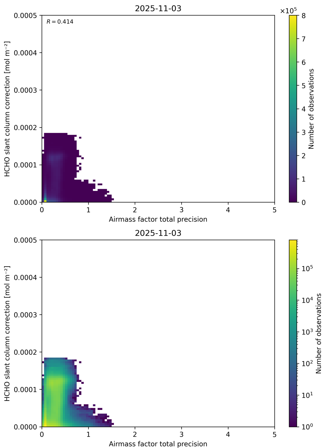
Figure 110: Scatter density plot of “Airmass factor total precision” against “HCHO slant column correction” for 2025-11-02 to 2025-11-04.
