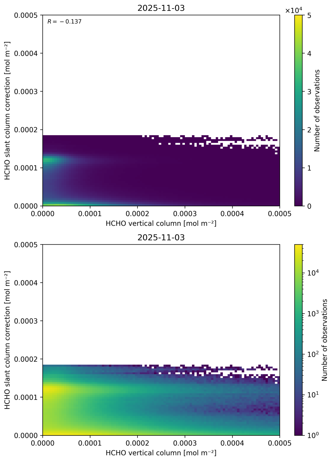
Figure 128: Scatter density plot of “HCHO vertical column” against “HCHO slant column correction” for 2025-11-02 to 2025-11-04.
