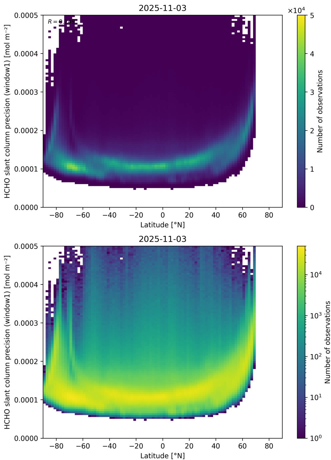
Figure 160: Scatter density plot of “Latitude” against “HCHO slant column precision (window1)” for 2025-11-02 to 2025-11-04.
