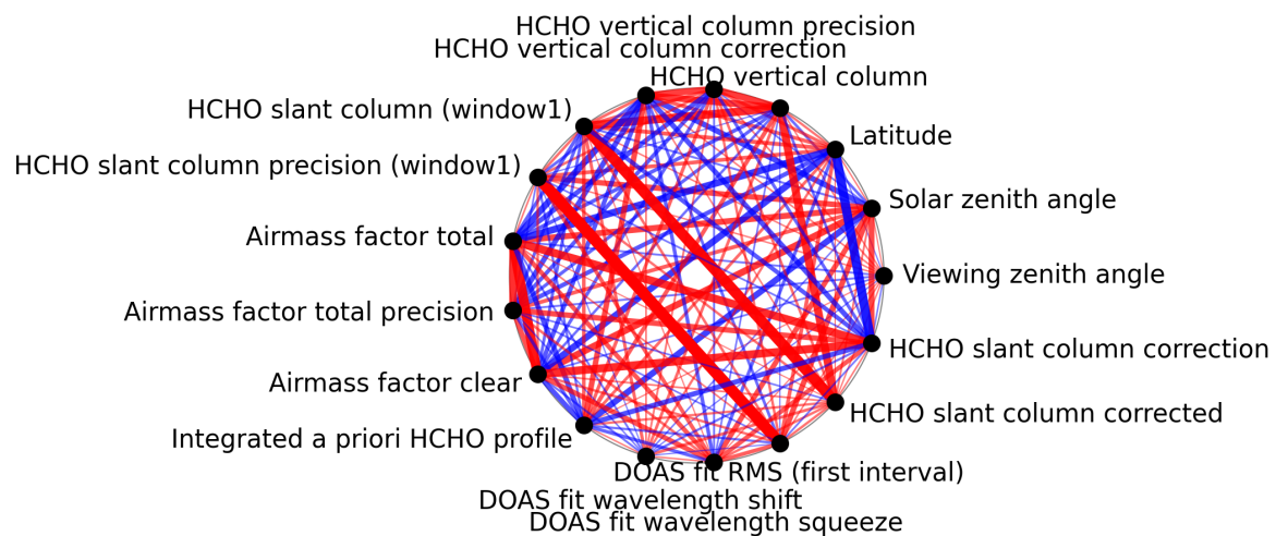
Figure 1: Map of correlation graph for 2025-11-02 to 2025-11-04.
