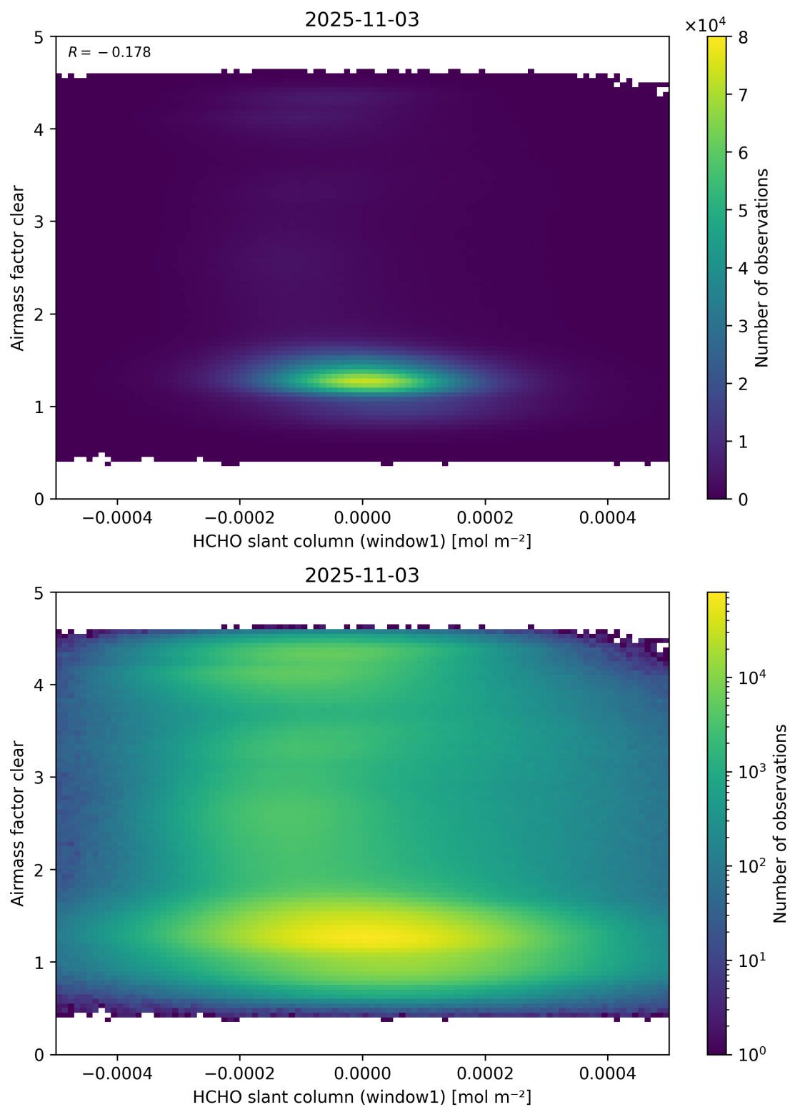
Figure 81: Scatter density plot of “HCHO slant column (window1)” against “Airmass factor clear” for 2025-11-02 to 2025-11-04.
