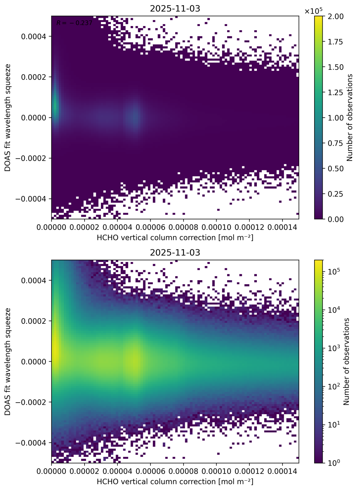
Figure 114: Scatter density plot of “HCHO vertical column correction” against “DOAS fit wavelength squeeze” for 2025-11-02 to 2025-11-04.
