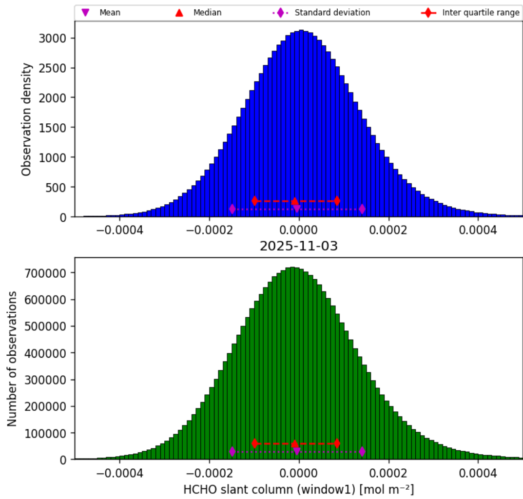
Figure 38: Histogram of “HCHO slant column (window1)” for 2025-11-02 to 2025-11-04
