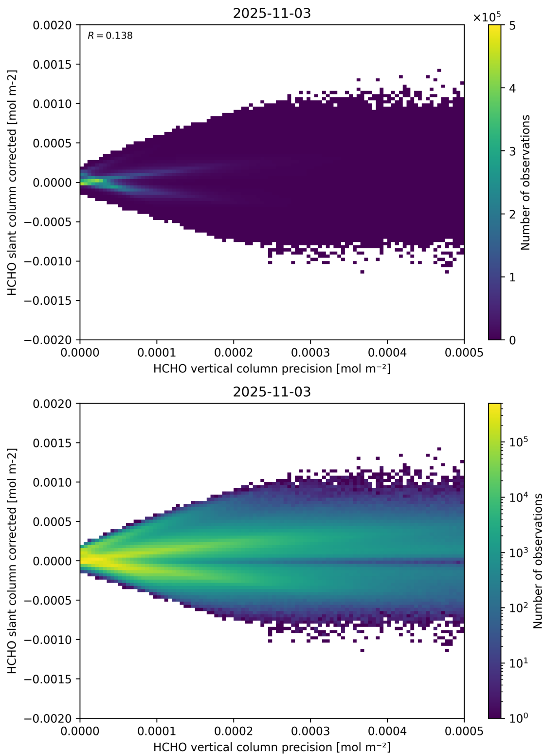
Figure 140: Scatter density plot of “HCHO vertical column precision” against “HCHO slant column corrected” for 2025-11-02 to 2025-11-04.
