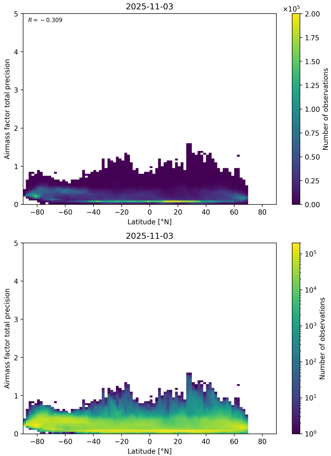
Figure 162: Scatter density plot of “Latitude” against “Airmass factor total precision” for 2025-11-02 to 2025-11-04.
