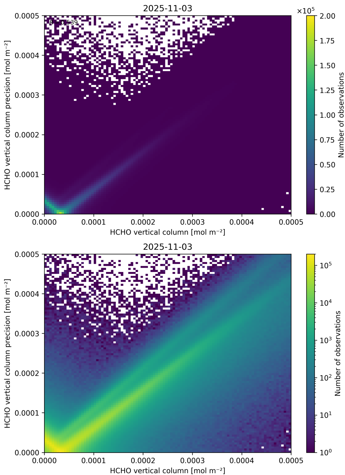
Figure 134: Scatter density plot of “HCHO vertical column” against “HCHO vertical column precision” for 2025-11-02 to 2025-11-04.
