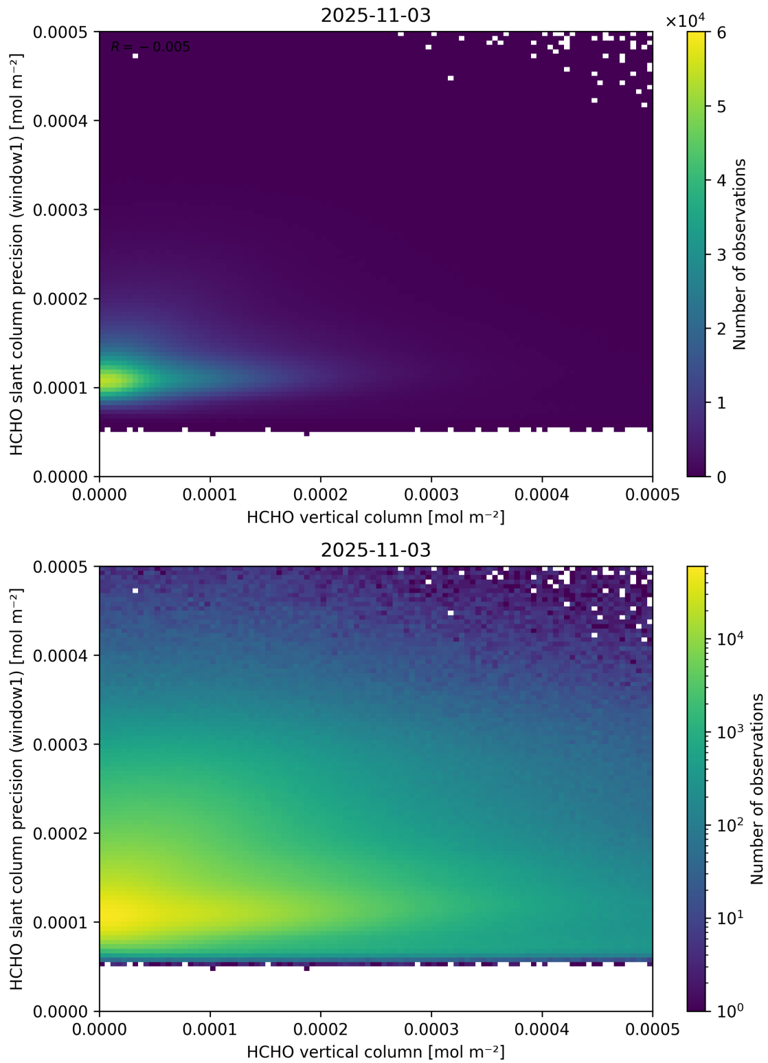
Figure 130: Scatter density plot of “HCHO vertical column” against “HCHO slant column precision (window1)” for 2025-11-02 to 2025-11-04.
