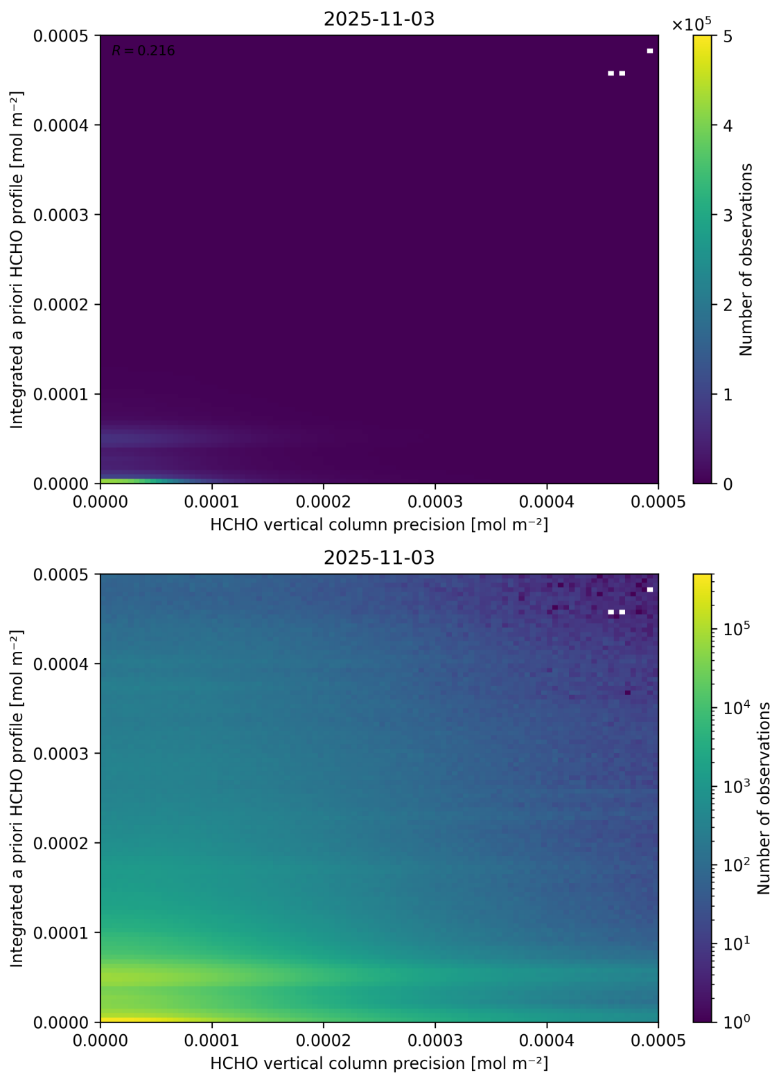
Figure 147: Scatter density plot of “HCHO vertical column precision” against “Integrated a priori HCHO profile” for 2025-11-02 to 2025-11-04.
