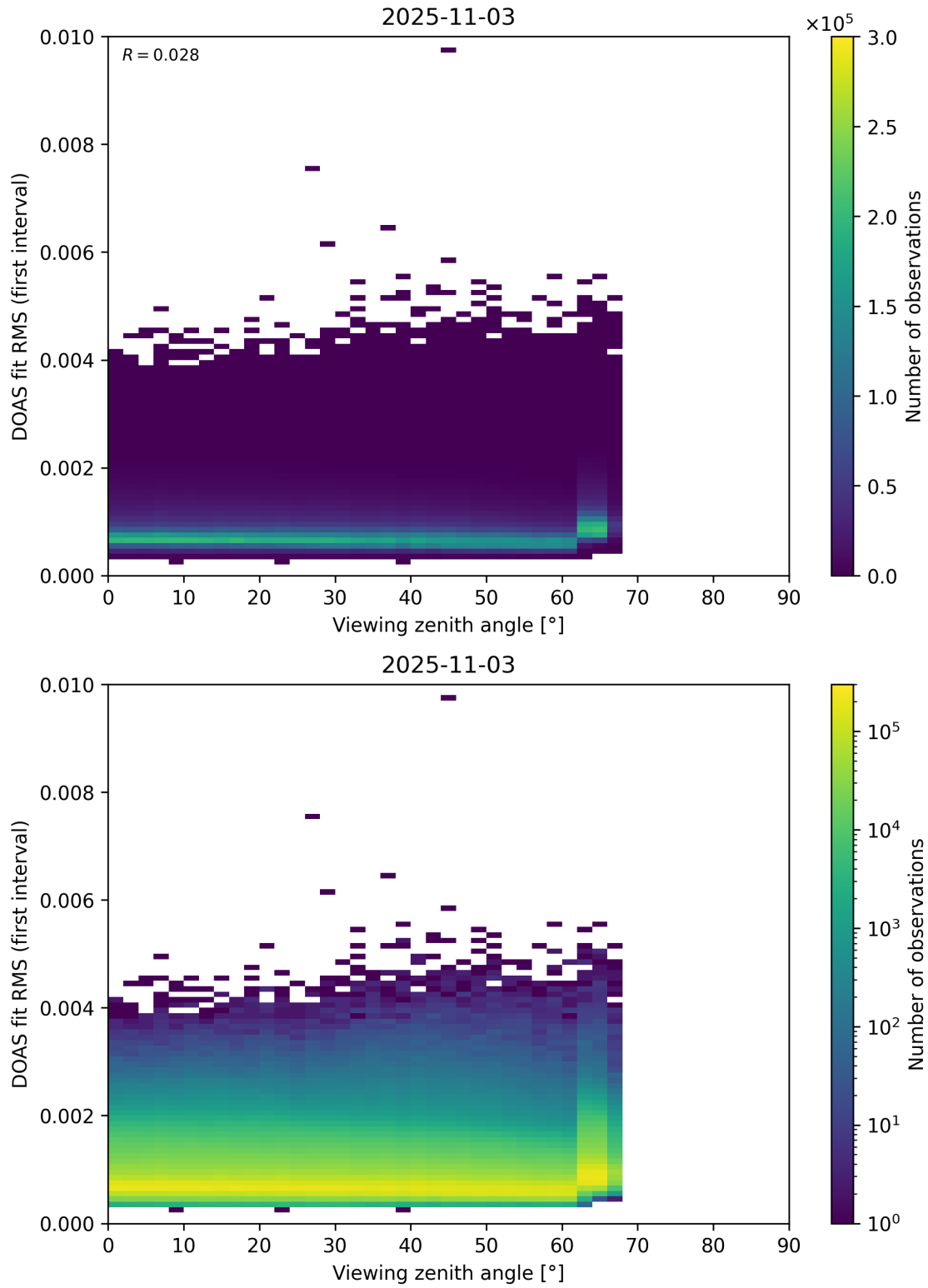
Figure 182: Scatter density plot of “Viewing zenith angle” against “DOAS fit RMS (first interval)” for 2025-11-02 to 2025-11-04.
