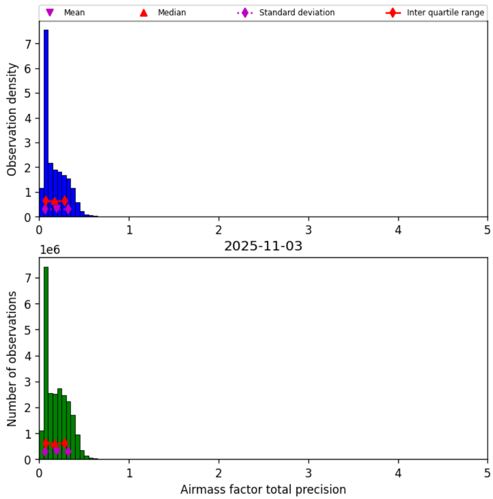
Figure 41: Histogram of “Airmass factor total precision” for 2025-11-02 to 2025-11-04
