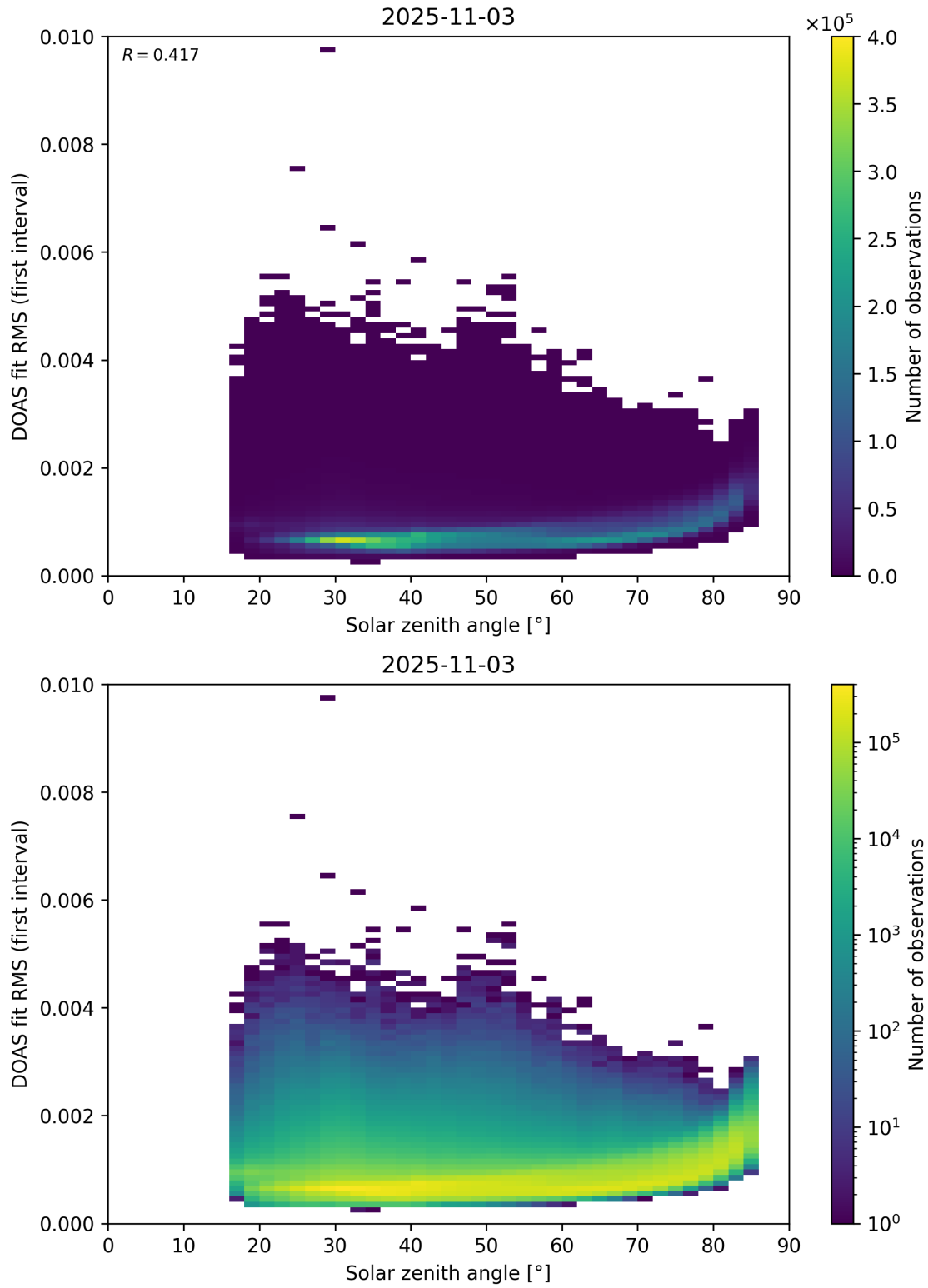
Figure 167: Scatter density plot of “Solar zenith angle” against “DOAS fit RMS (first interval)” for 2025-11-02 to 2025-11-04.
