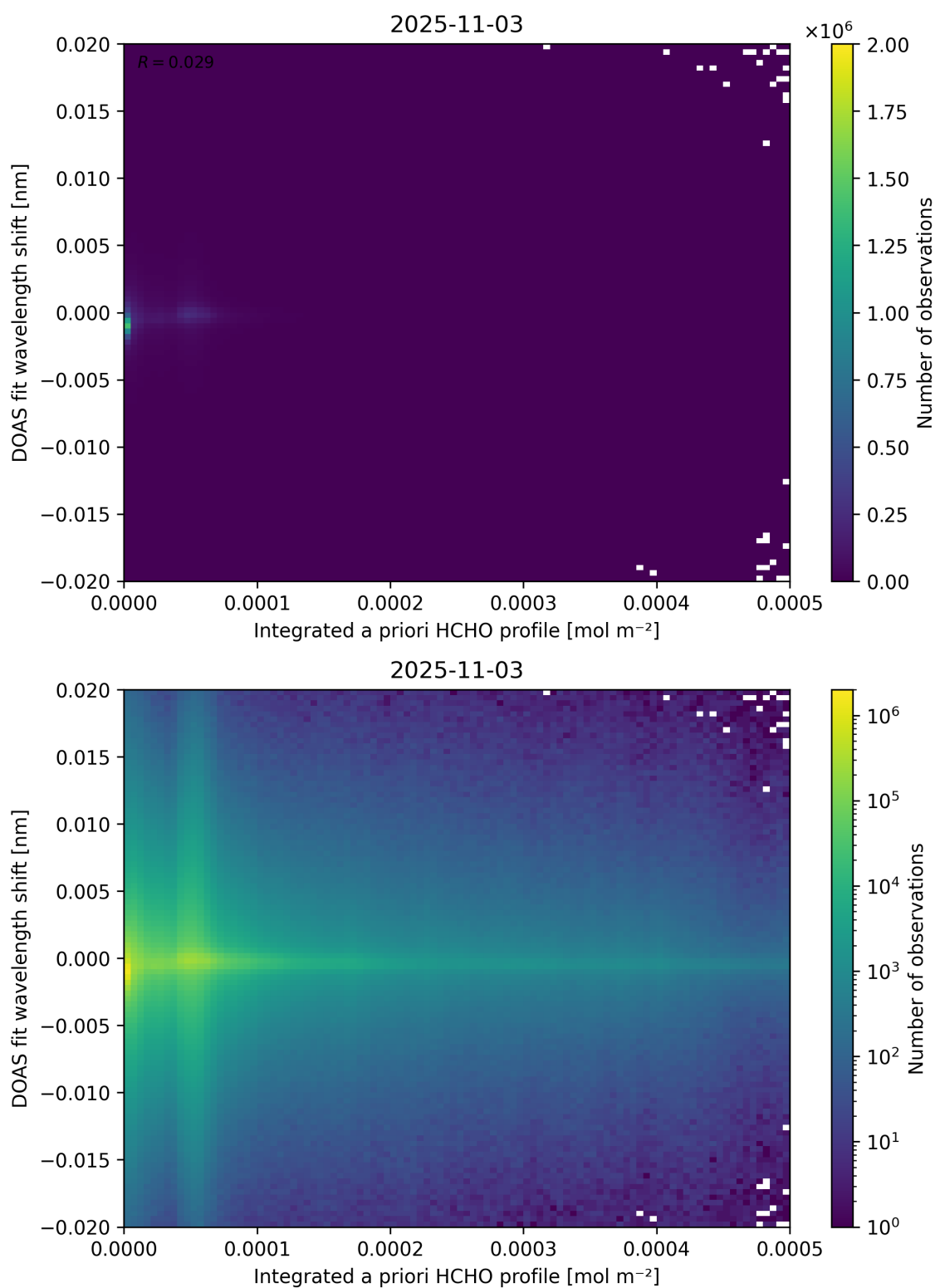
Figure 149: Scatter density plot of “Integrated a priori HCHO profile” against “DOAS fit wavelength shift” for 2025-11-02 to 2025-11-04.
