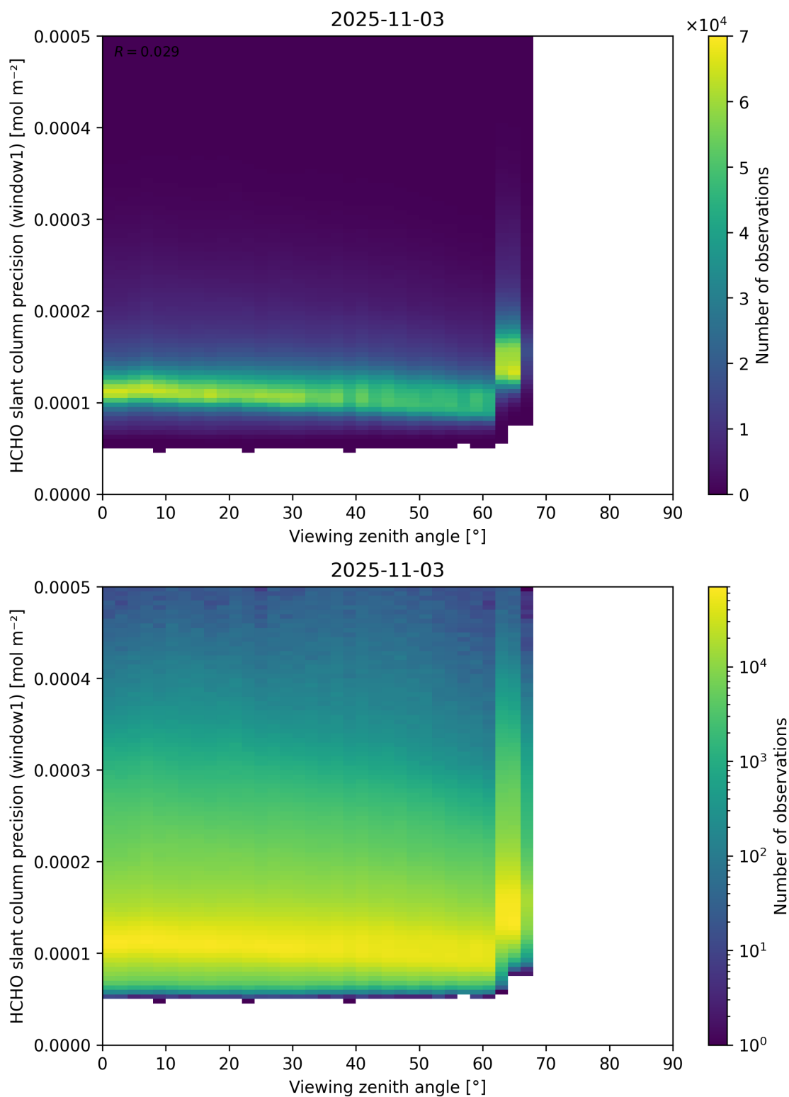
Figure 189: Scatter density plot of “Viewing zenith angle” against “HCHO slant column precision (window1)” for 2025-11-02 to 2025-11-04.
