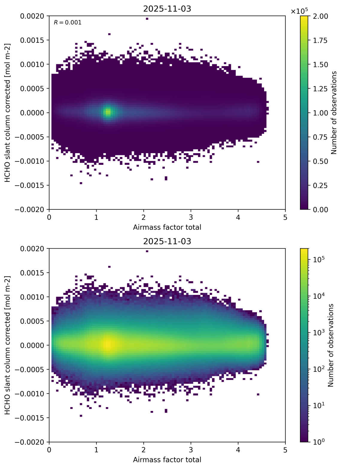
Figure 101: Scatter density plot of “Airmass factor total” against “HCHO slant column corrected” for 2025-11-02 to 2025-11-04.
