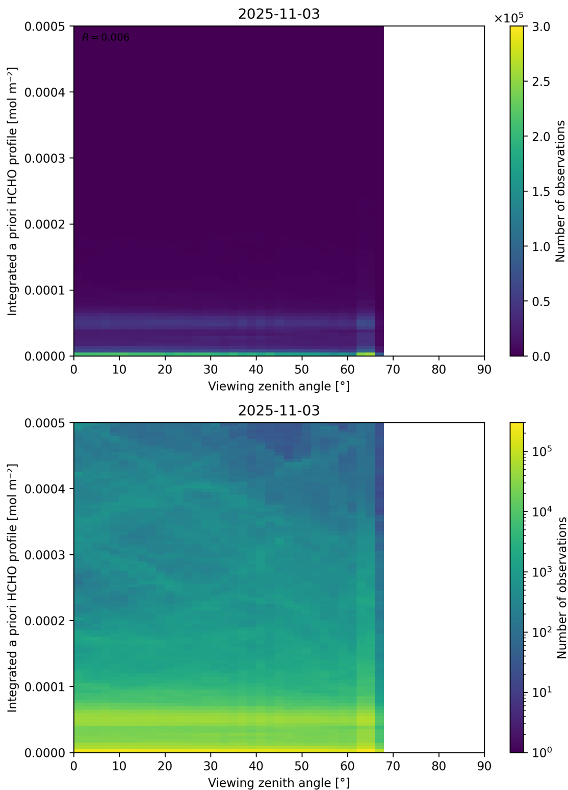
Figure 195: Scatter density plot of “Viewing zenith angle” against “Integrated a priori HCHO profile” for 2025-11-02 to 2025-11-04.
