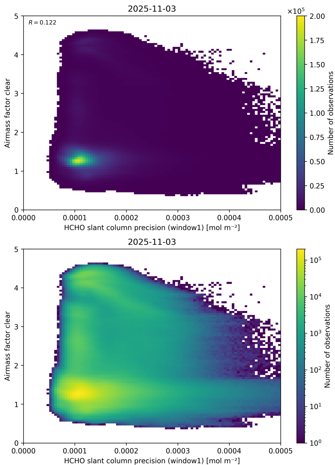
Figure 91: Scatter density plot of “HCHO slant column precision (window1)” against “Airmass factor clear” for 2025-11-02 to 2025-11-04.
