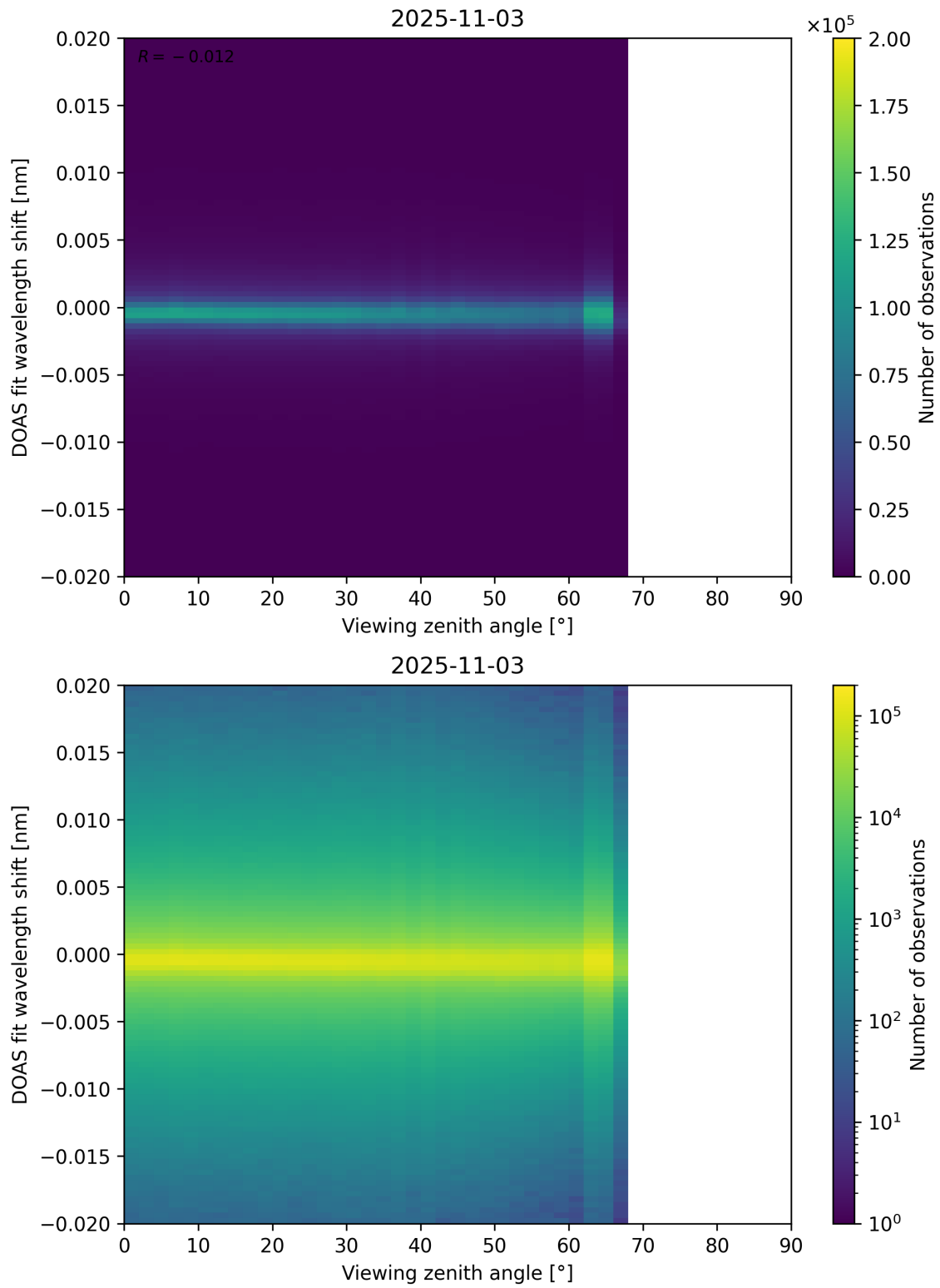
Figure 183: Scatter density plot of “Viewing zenith angle” against “DOAS fit wavelength shift” for 2025-11-02 to 2025-11-04.
