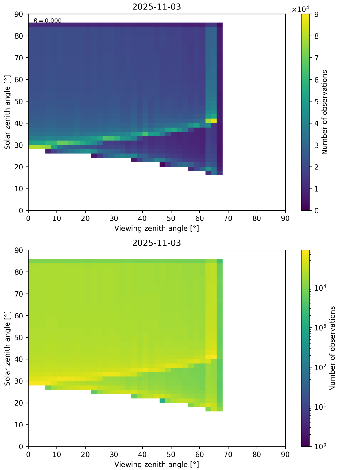
Figure 197: Scatter density plot of “Viewing zenith angle” against “Solar zenith angle” for 2025-11-02 to 2025-11-04.
