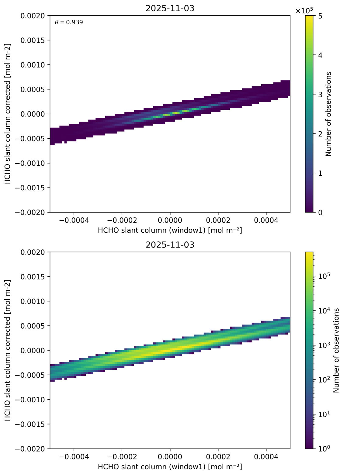
Figure 82: Scatter density plot of “HCHO slant column (window1)” against “HCHO slant column corrected” for 2025-11-02 to 2025-11-04.
