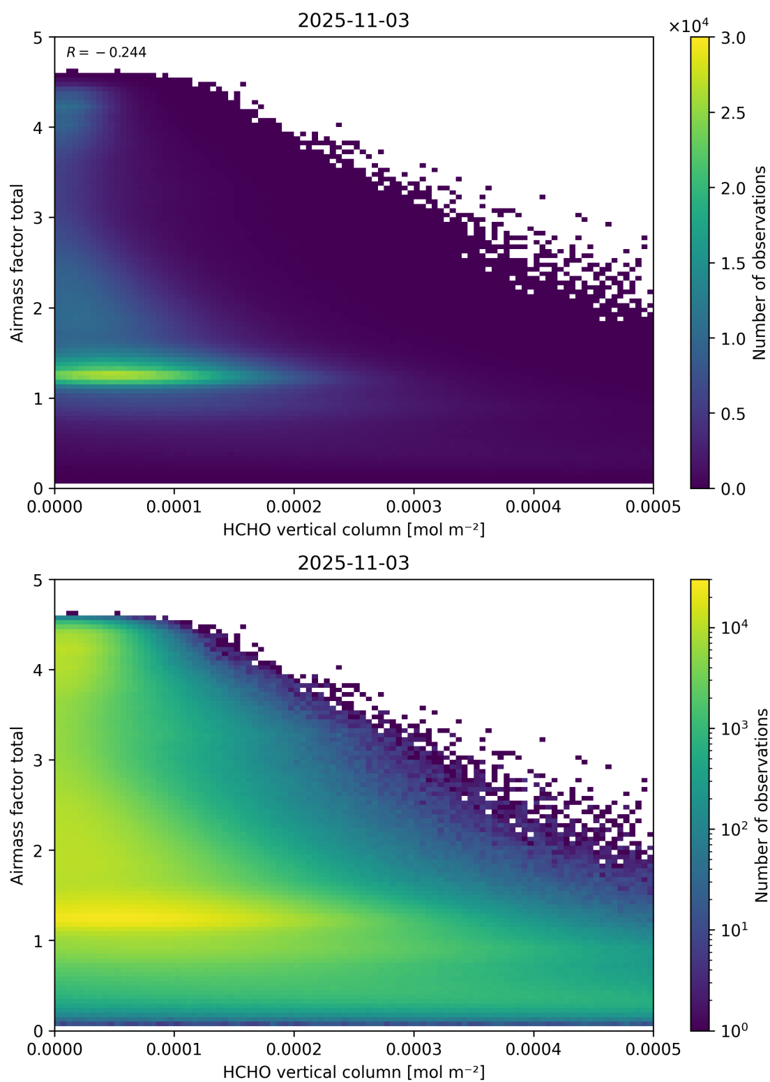
Figure 131: Scatter density plot of “HCHO vertical column” against “Airmass factor total” for 2025-11-02 to 2025-11-04.
