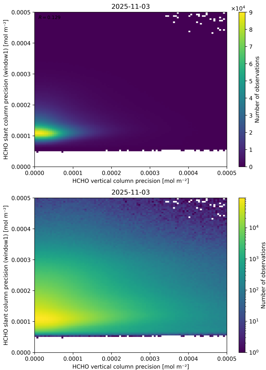
Figure 143: Scatter density plot of “HCHO vertical column precision” against “HCHO slant column precision (window1)” for 2025-11-02 to 2025-11-04.
