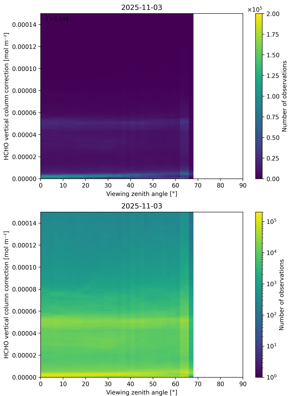
Figure 193: Scatter density plot of “Viewing zenith angle” against “HCHO vertical column correction” for 2025-11-02 to 2025-11-04.
