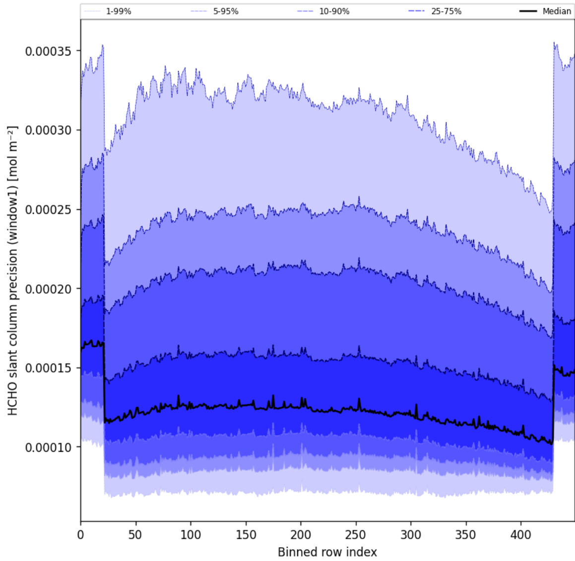
Figure 53: Along track statistics of “HCHO slant column precision (window1)” for 2025-11-02 to 2025-11-04
