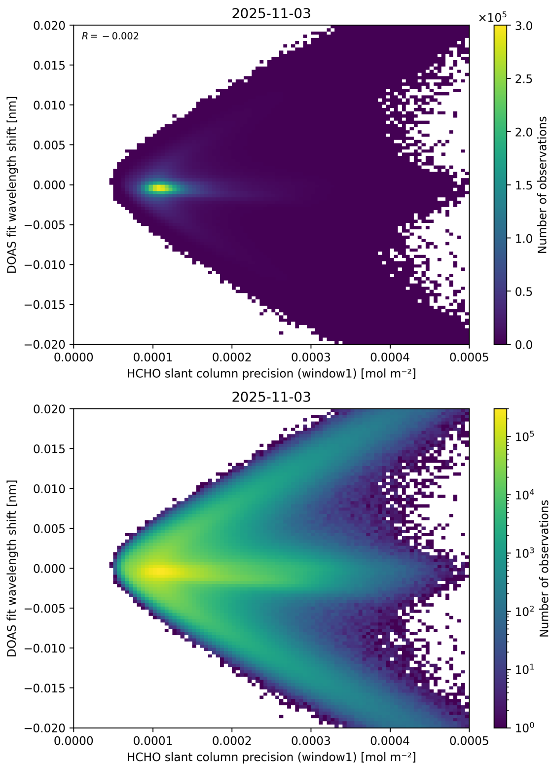
Figure 89: Scatter density plot of “HCHO slant column precision (window1)” against “DOAS fit wavelength shift” for 2025-11-02 to 2025-11-04.
