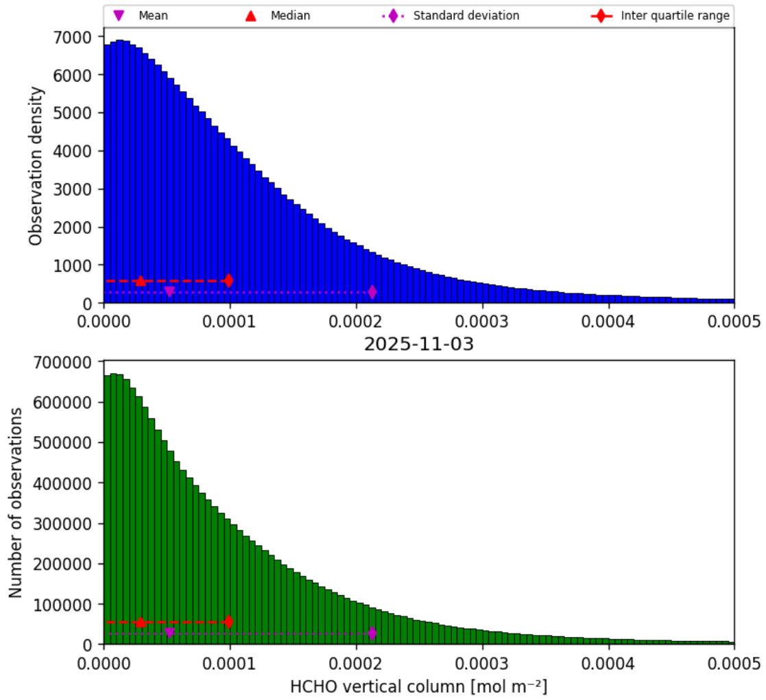
Figure 35: Histogram of “HCHO vertical column” for 2025-11-02 to 2025-11-04
