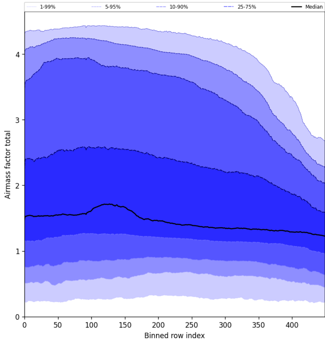
Figure 54: Along track statistics of “Airmass factor total” for 2025-11-02 to 2025-11-04
