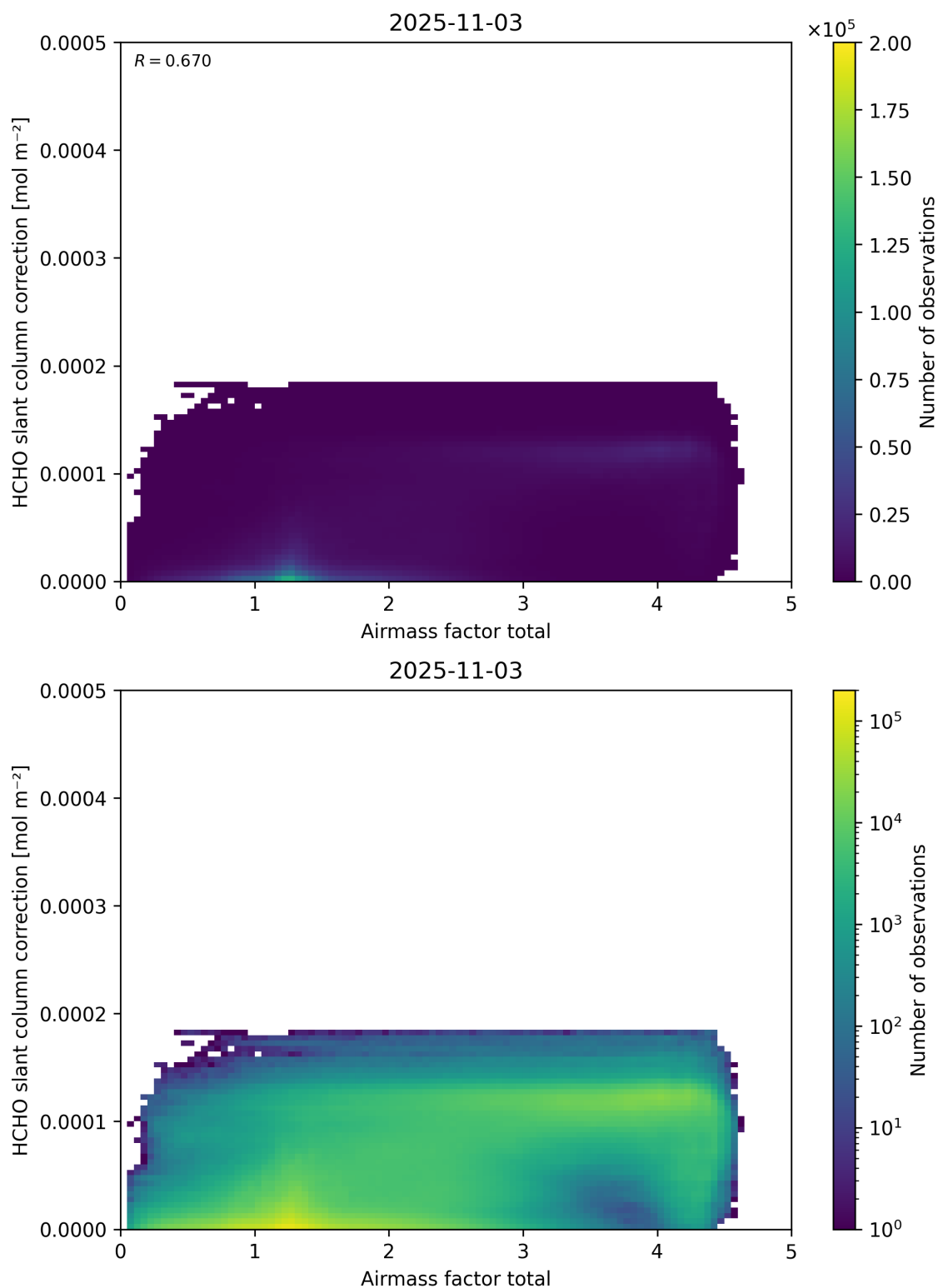
Figure 102: Scatter density plot of “Airmass factor total” against “HCHO slant column correction” for 2025-11-02 to 2025-11-04.
