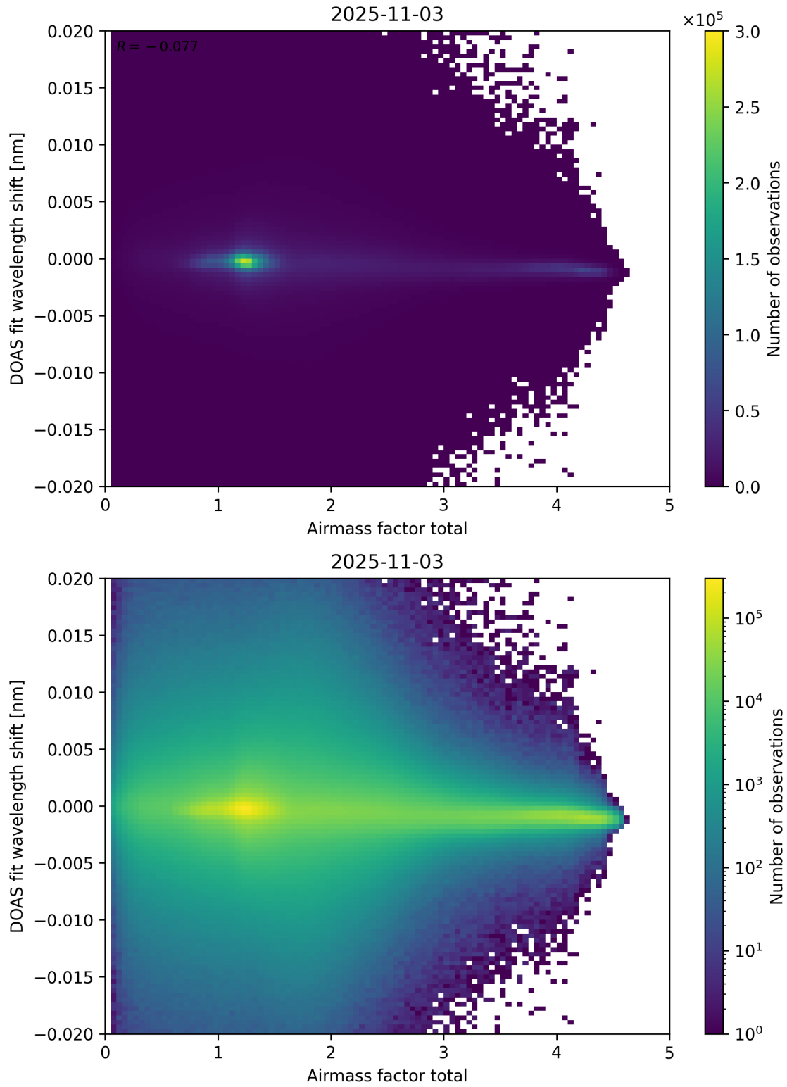
Figure 98: Scatter density plot of “Airmass factor total” against “DOAS fit wavelength shift” for 2025-11-02 to 2025-11-04.
