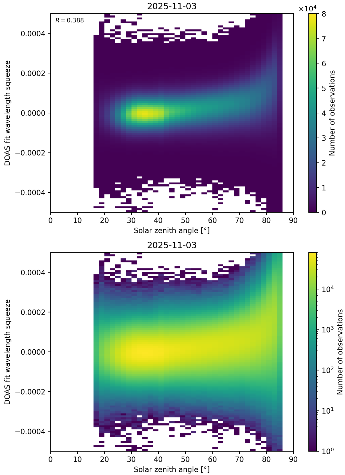
Figure 169: Scatter density plot of “Solar zenith angle” against “DOAS fit wavelength squeeze” for 2025-11-02 to 2025-11-04.
