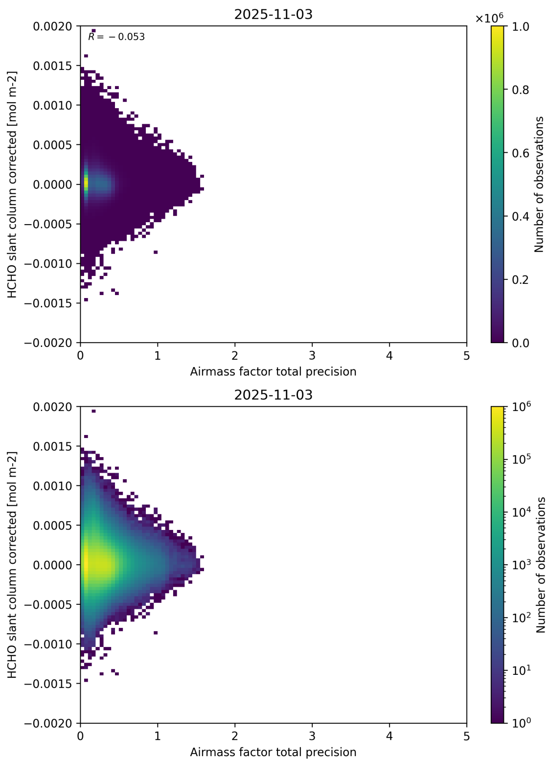
Figure 109: Scatter density plot of “Airmass factor total precision” against “HCHO slant column corrected” for 2025-11-02 to 2025-11-04.
