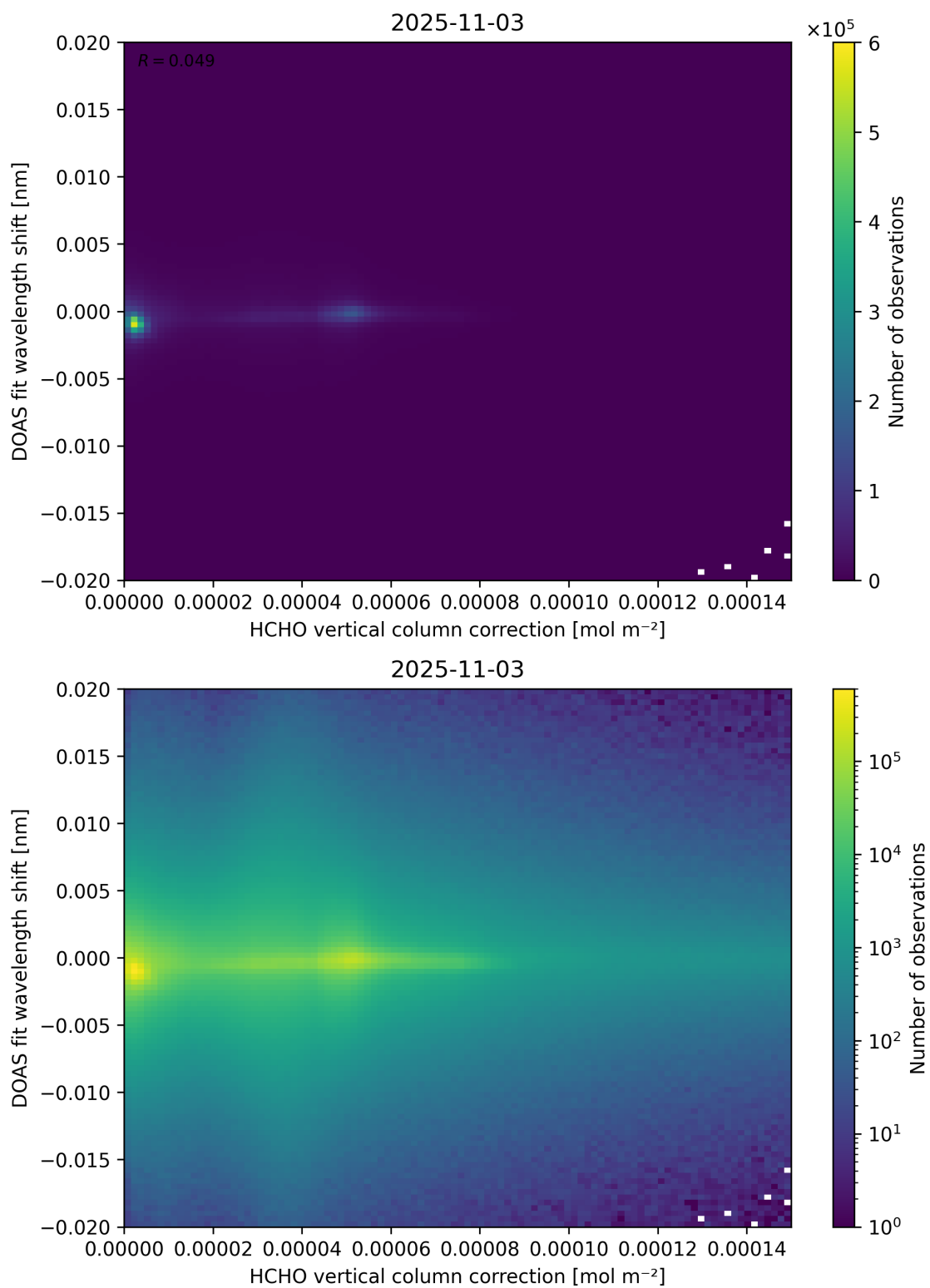
Figure 113: Scatter density plot of “HCHO vertical column correction” against “DOAS fit wavelength shift” for 2025-11-02 to 2025-11-04.
