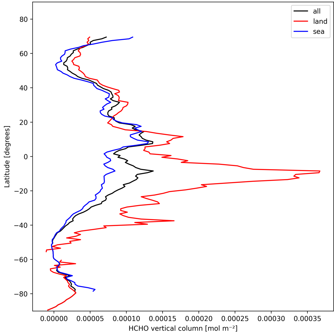
Figure 21: Zonal average of “HCHO vertical column” for 2025-11-02 to 2025-11-04.
