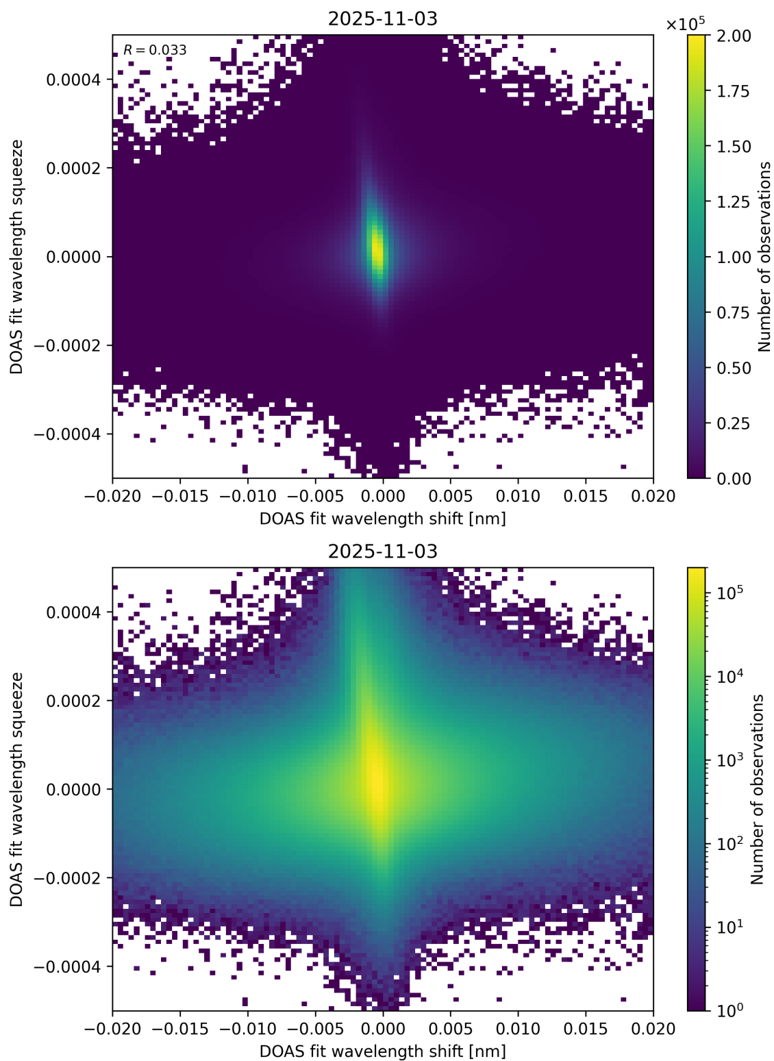
Figure 65: Scatter density plot of “DOAS fit wavelength shift” against “DOAS fit wavelength squeeze” for 2025-11-02 to 2025-11-04.
