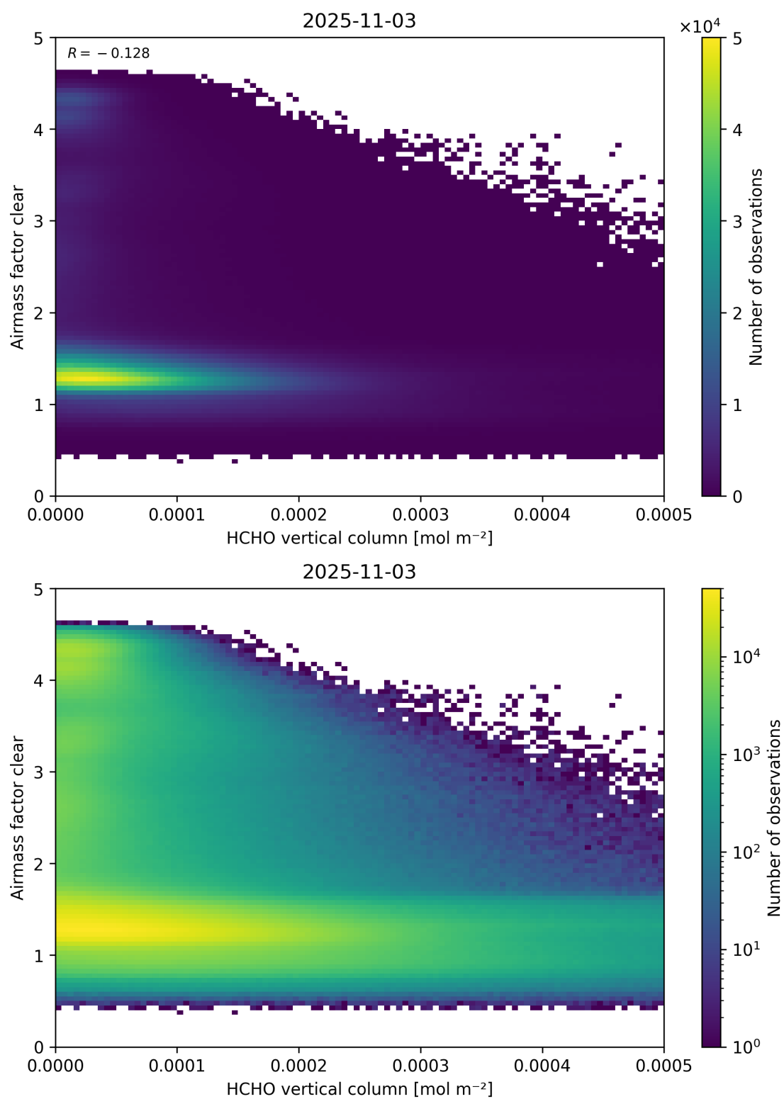
Figure 126: Scatter density plot of “HCHO vertical column” against “Airmass factor clear” for 2025-11-02 to 2025-11-04.
