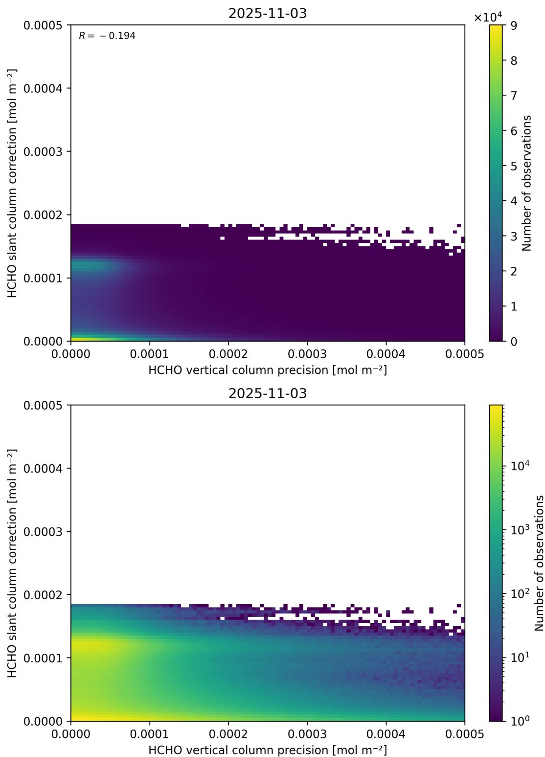
Figure 141: Scatter density plot of “HCHO vertical column precision” against “HCHO slant column correction” for 2025-11-02 to 2025-11-04.
