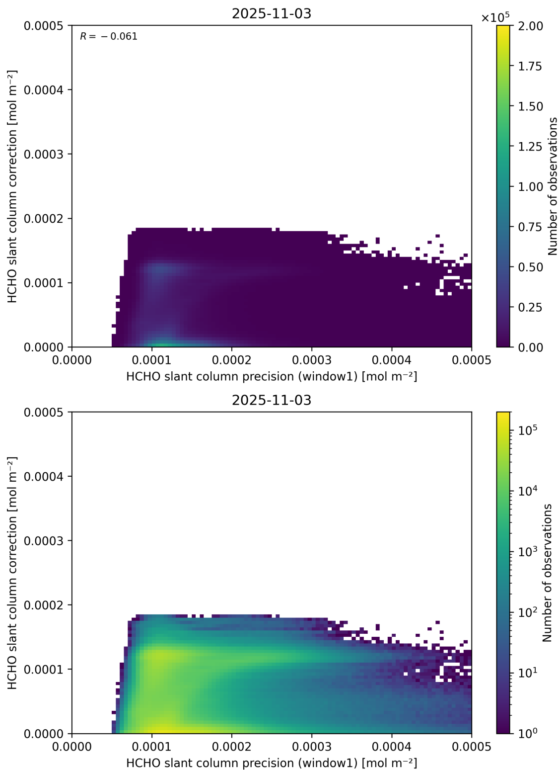
Figure 93: Scatter density plot of “HCHO slant column precision (window1)” against “HCHO slant column correction” for 2025-11-02 to 2025-11-04.
