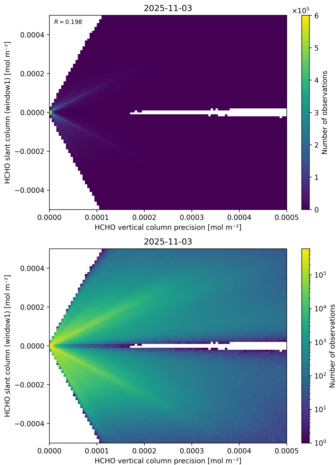
Figure 142: Scatter density plot of “HCHO vertical column precision” against “HCHO slant column (window1)” for 2025-11-02 to 2025-11-04.
