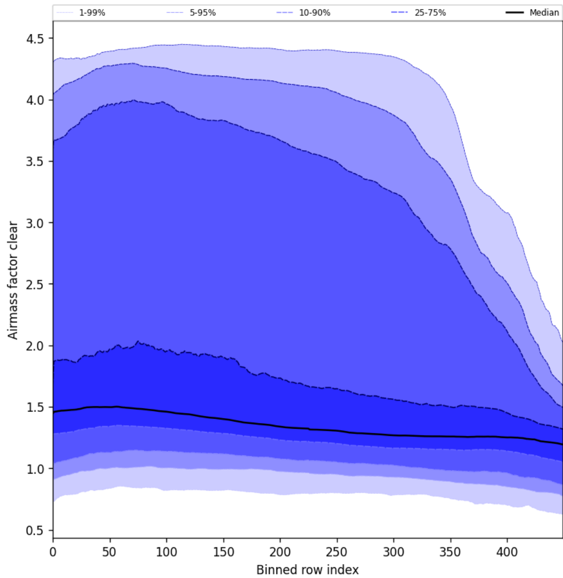
Figure 56: Along track statistics of “Airmass factor clear” for 2025-11-02 to 2025-11-04
