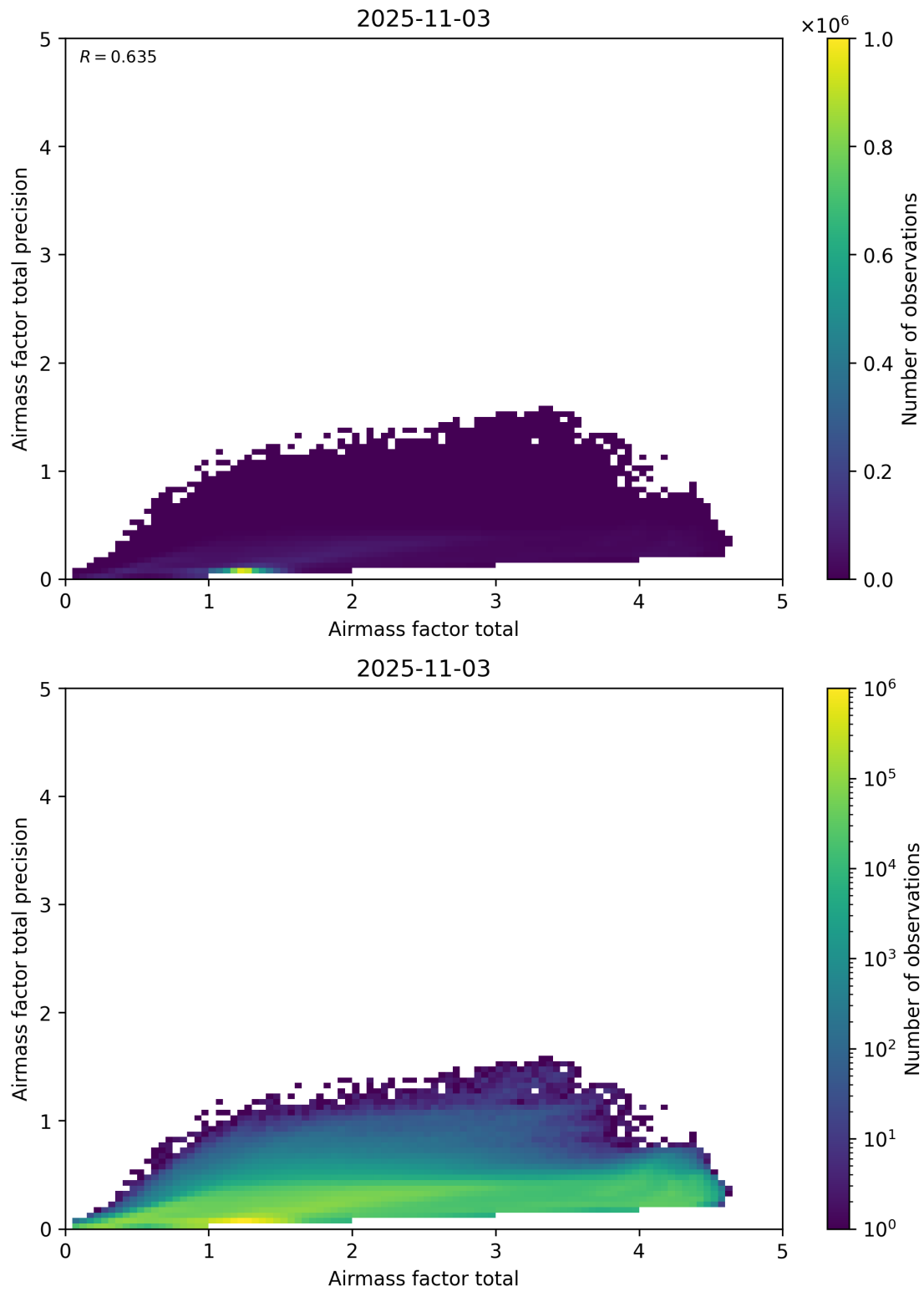
Figure 103: Scatter density plot of “Airmass factor total” against “Airmass factor total precision” for 2025-11-02 to 2025-11-04.
