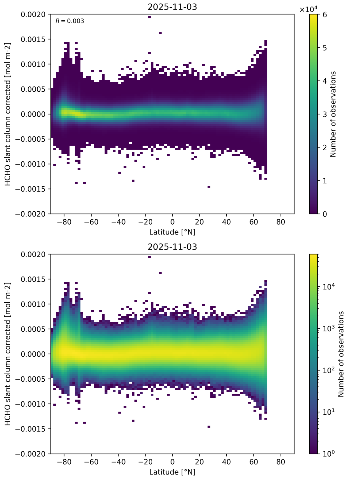
Figure 157: Scatter density plot of “Latitude” against “HCHO slant column corrected” for 2025-11-02 to 2025-11-04.
