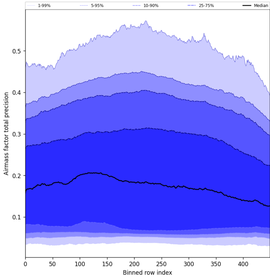
Figure 55: Along track statistics of “Airmass factor total precision” for 2025-11-02 to 2025-11-04
