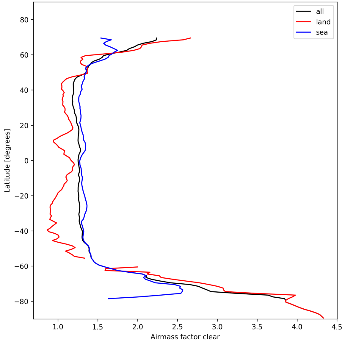
Figure 28: Zonal average of “Airmass factor clear” for 2025-11-02 to 2025-11-04.
