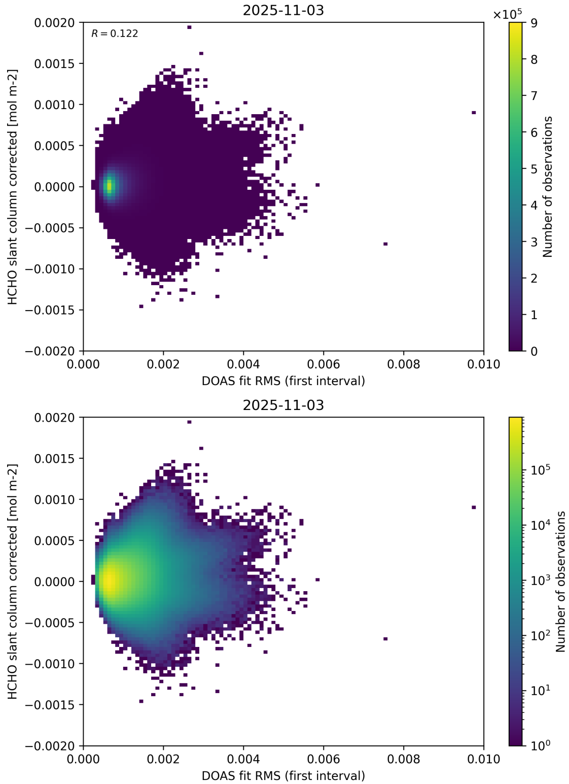
Figure 62: Scatter density plot of “DOAS fit RMS (first interval)” against “HCHO slant column corrected” for 2025-11-02 to 2025-11-04.
