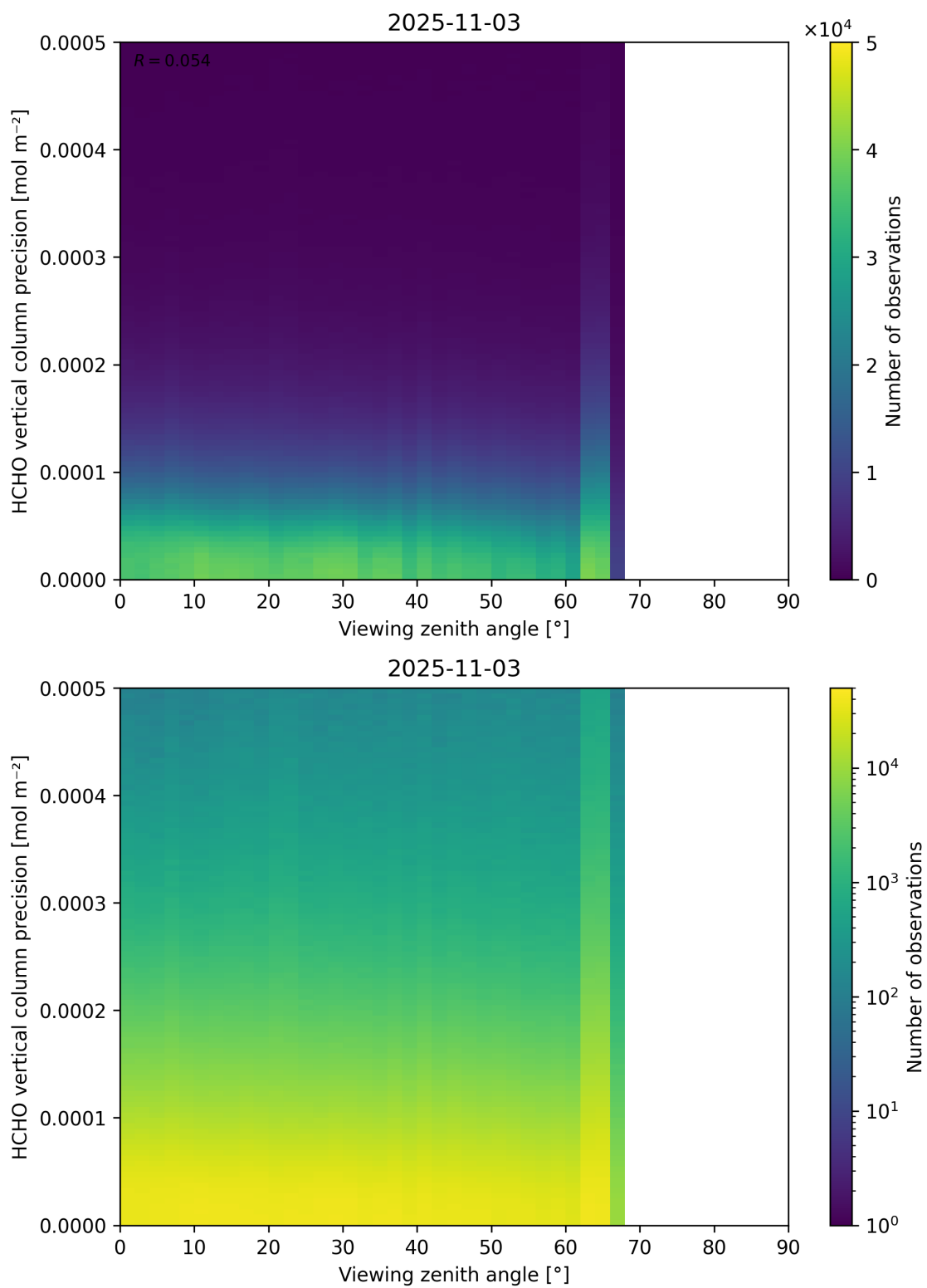
Figure 194: Scatter density plot of “Viewing zenith angle” against “HCHO vertical column precision” for 2025-11-02 to 2025-11-04.
