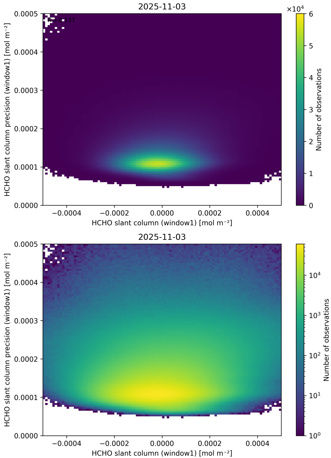
Figure 84: Scatter density plot of “HCHO slant column (window1)” against “HCHO slant column precision (window1)” for 2025-11-02 to 2025-11-04.
