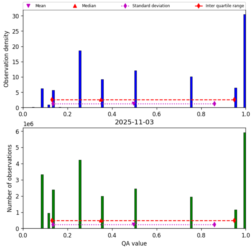
Figure 34: Histogram of “QA value” for 2025-11-02 to 2025-11-04
