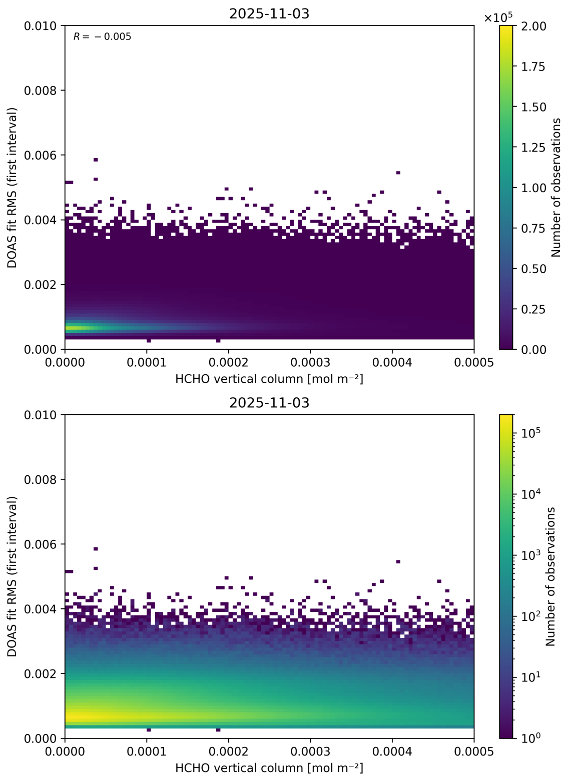
Figure 123: Scatter density plot of “HCHO vertical column” against “DOAS fit RMS (first interval)” for 2025-11-02 to 2025-11-04.
