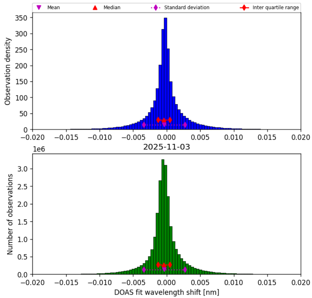
Figure 44: Histogram of “DOAS fit wavelength shift” for 2025-11-02 to 2025-11-04
