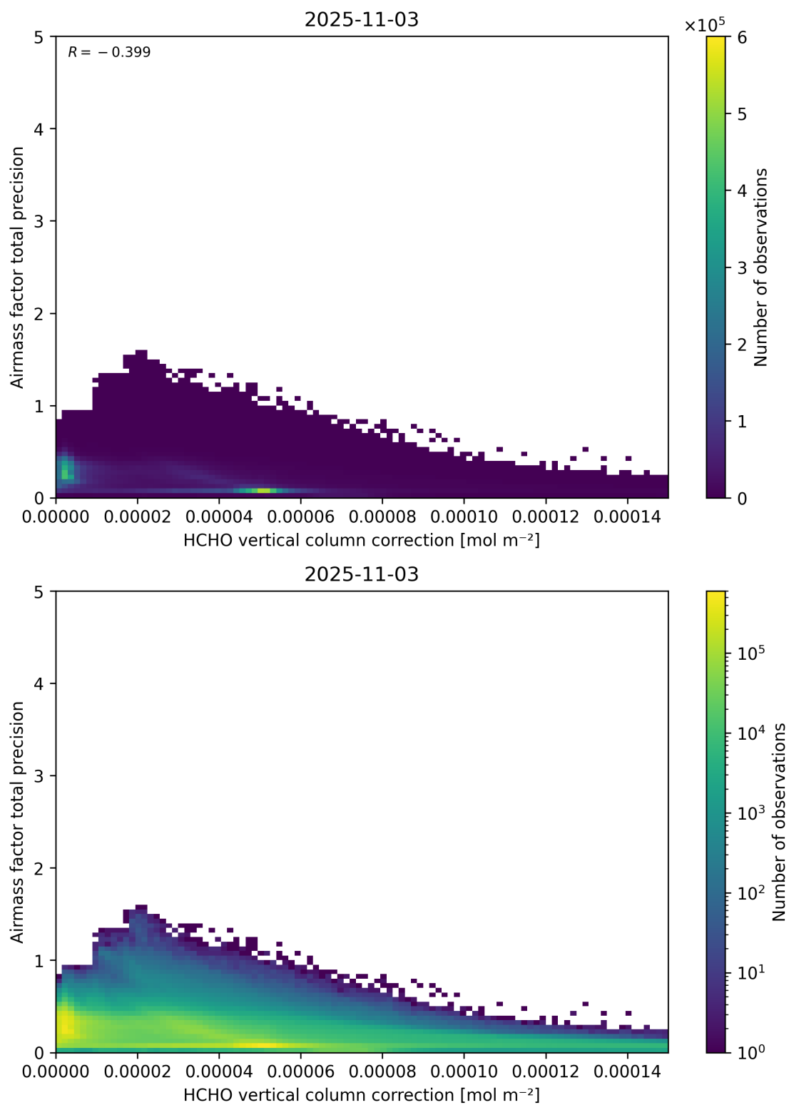
Figure 121: Scatter density plot of “HCHO vertical column correction” against “Airmass factor total precision” for 2025-11-02 to 2025-11-04.
