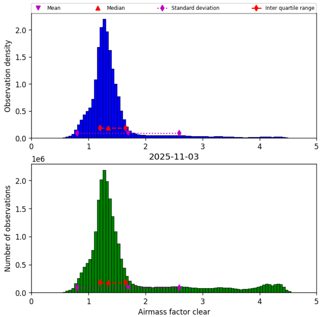
Figure 42: Histogram of “Airmass factor clear” for 2025-11-02 to 2025-11-04
