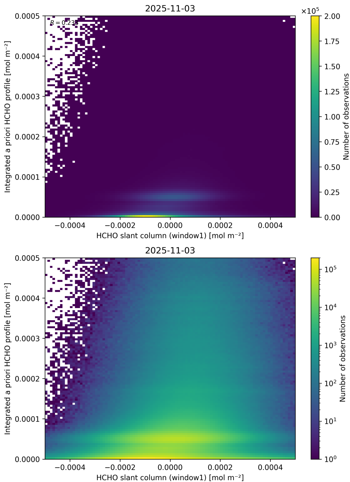
Figure 87: Scatter density plot of “HCHO slant column (window1)” against “Integrated a priori HCHO profile” for 2025-11-02 to 2025-11-04.
