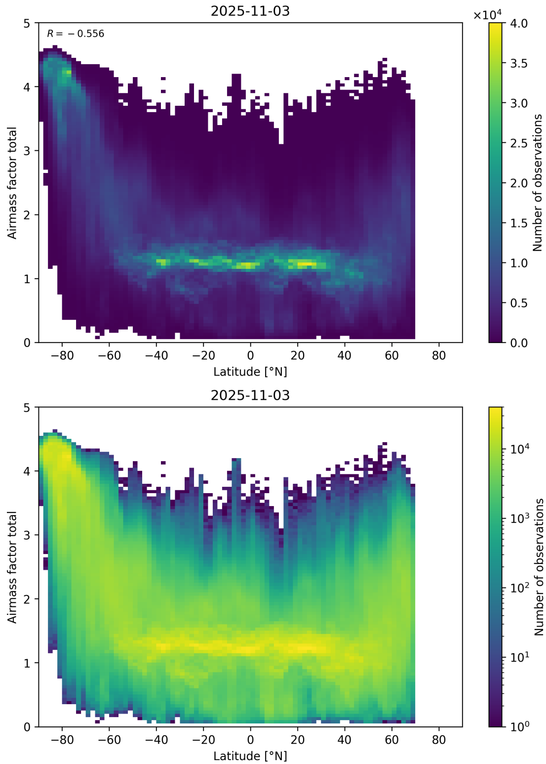
Figure 161: Scatter density plot of “Latitude” against “Airmass factor total” for 2025-11-02 to 2025-11-04.
