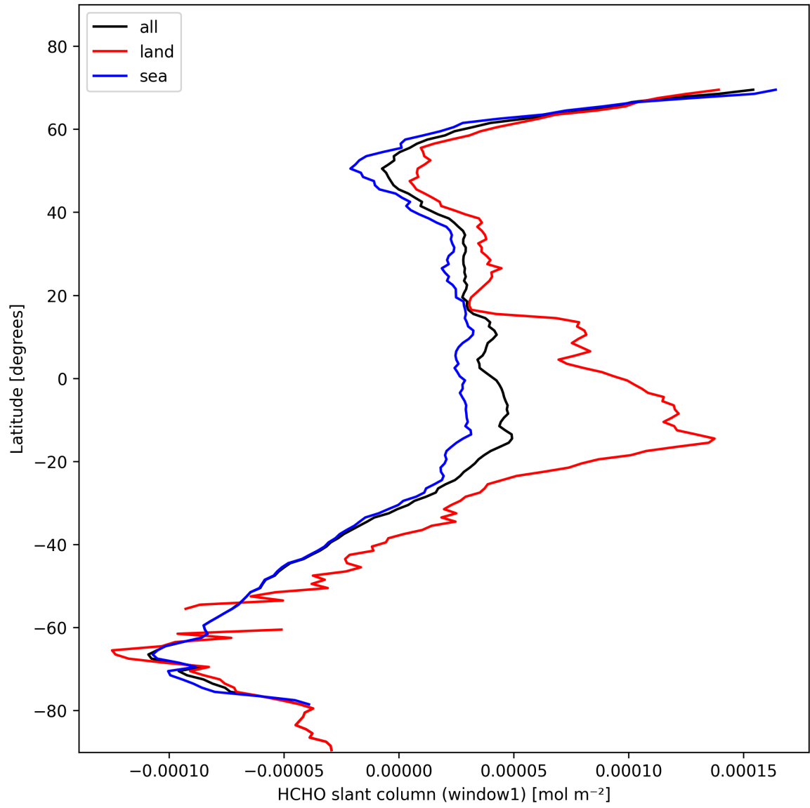
Figure 24: Zonal average of “HCHO slant column (window1)” for 2025-11-02 to 2025-11-04.
