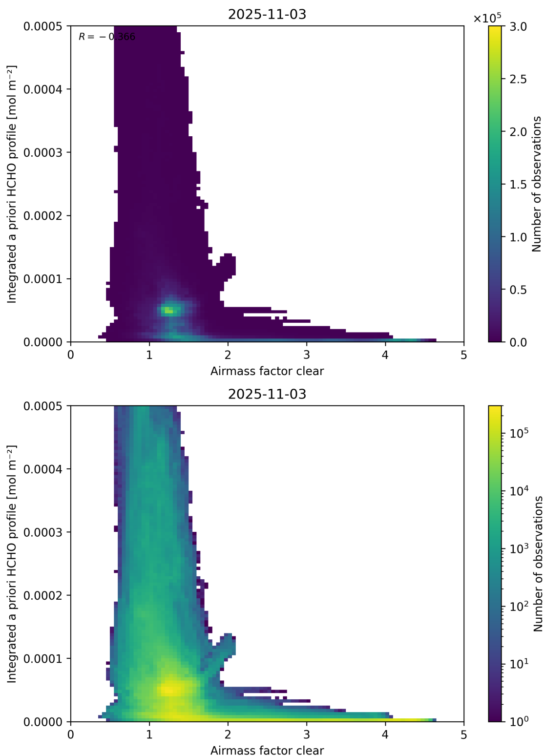
Figure 76: Scatter density plot of “Airmass factor clear” against “Integrated a priori HCHO profile” for 2025-11-02 to 2025-11-04.
