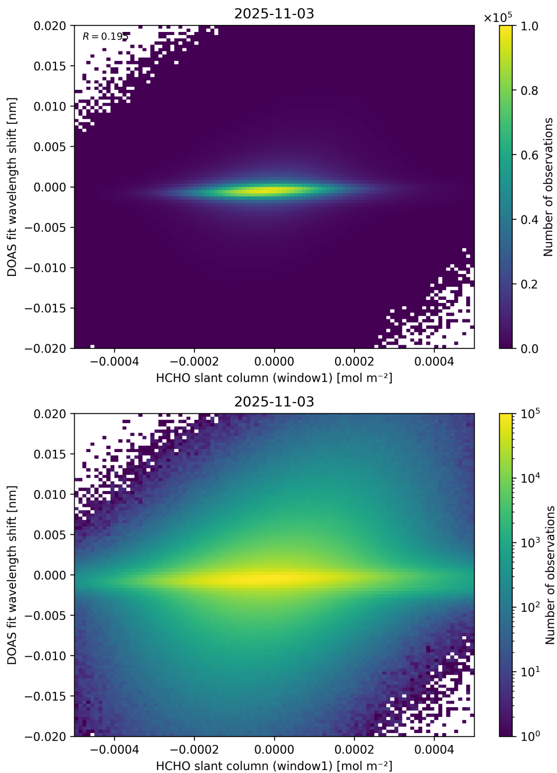
Figure 79: Scatter density plot of “HCHO slant column (window1)” against “DOAS fit wavelength shift” for 2025-11-02 to 2025-11-04.
