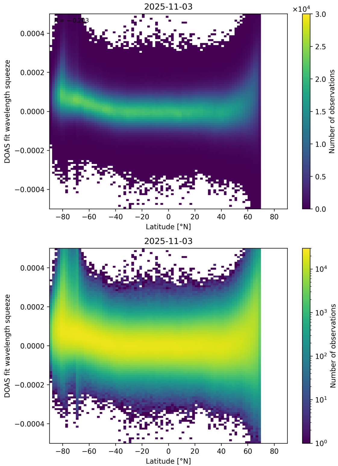
Figure 155: Scatter density plot of “Latitude” against “DOAS fit wavelength squeeze” for 2025-11-02 to 2025-11-04.
