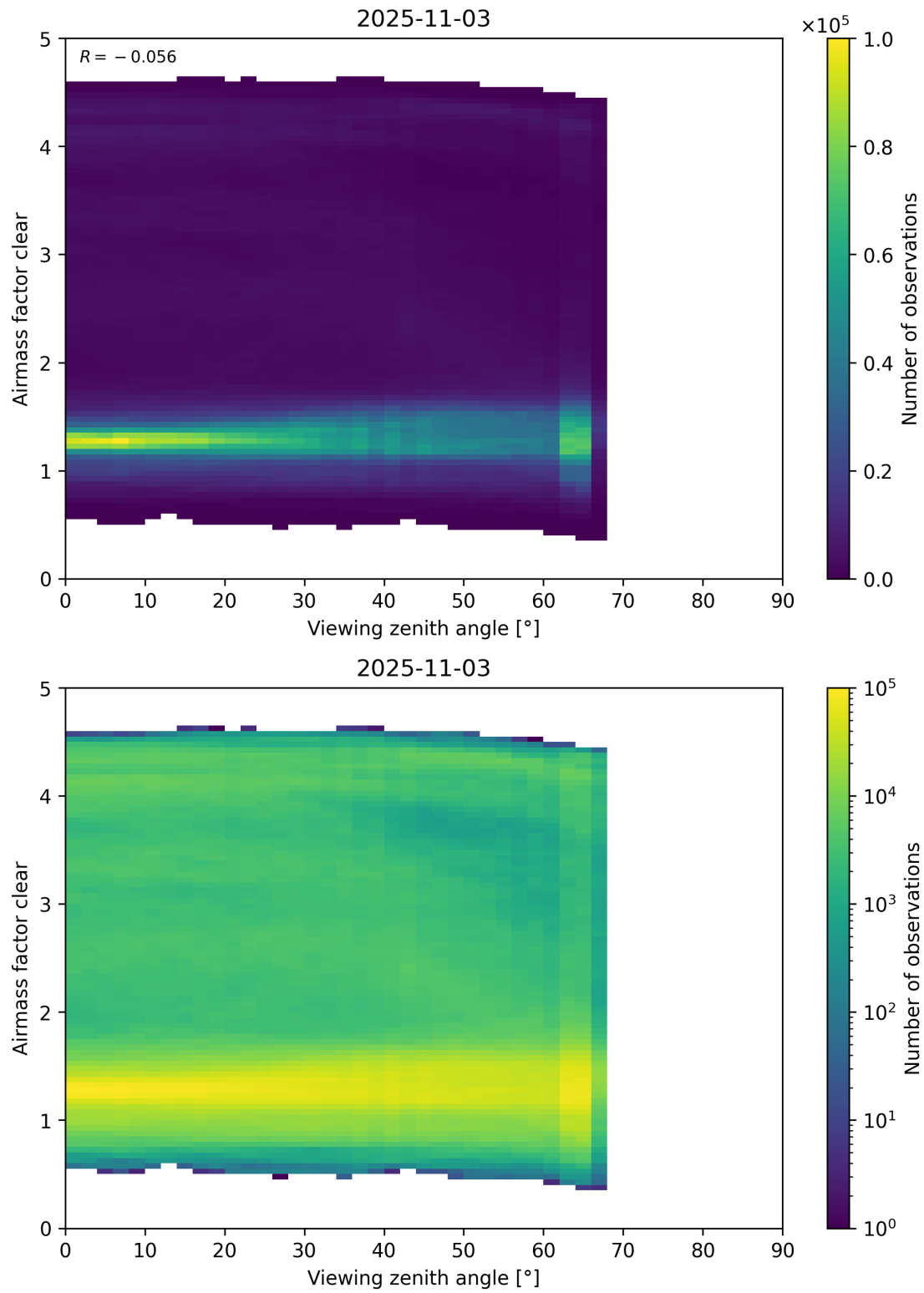
Figure 185: Scatter density plot of “Viewing zenith angle” against “Airmass factor clear” for 2025-11-02 to 2025-11-04.
