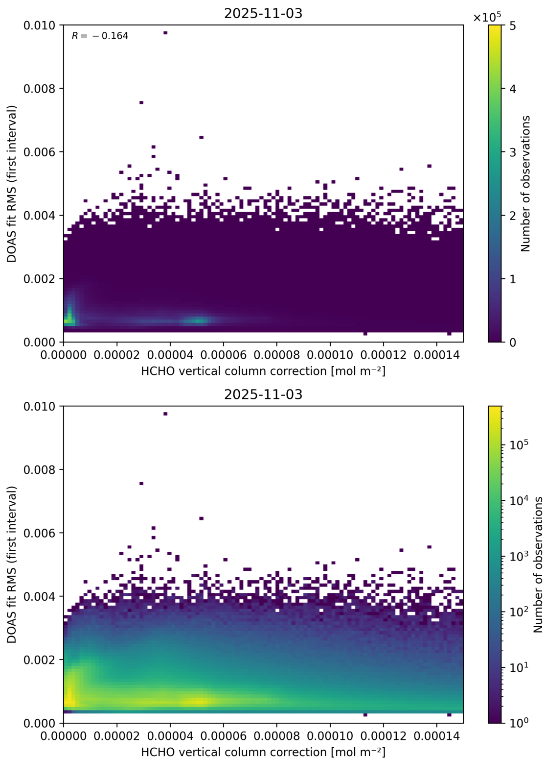
Figure 112: Scatter density plot of “HCHO vertical column correction” against “DOAS fit RMS (first interval)” for 2025-11-02 to 2025-11-04.
