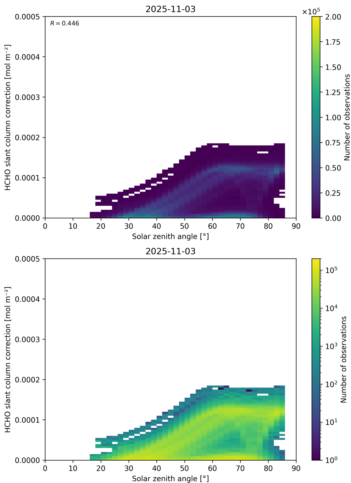
Figure 172: Scatter density plot of “Solar zenith angle” against “HCHO slant column correction” for 2025-11-02 to 2025-11-04.
