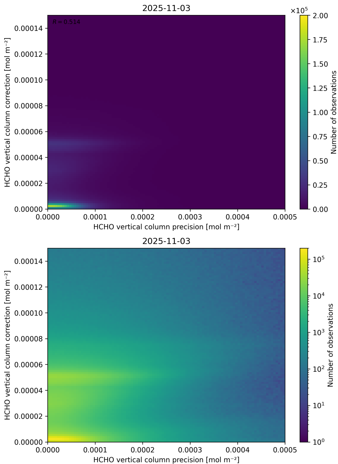
Figure 146: Scatter density plot of “HCHO vertical column precision” against “HCHO vertical column correction” for 2025-11-02 to 2025-11-04.
