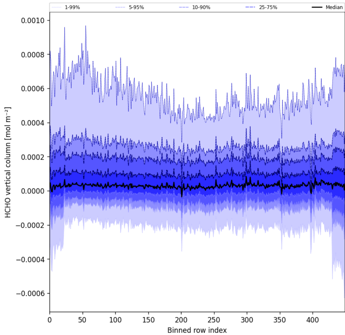
Figure 49: Along track statistics of “HCHO vertical column” for 2025-11-02 to 2025-11-04
