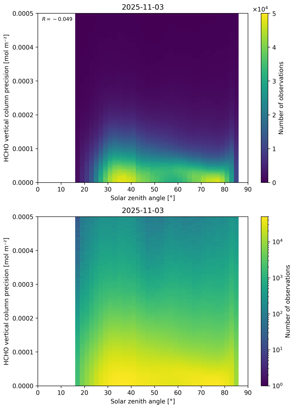
Figure 179: Scatter density plot of “Solar zenith angle” against “HCHO vertical column precision” for 2025-11-02 to 2025-11-04.
