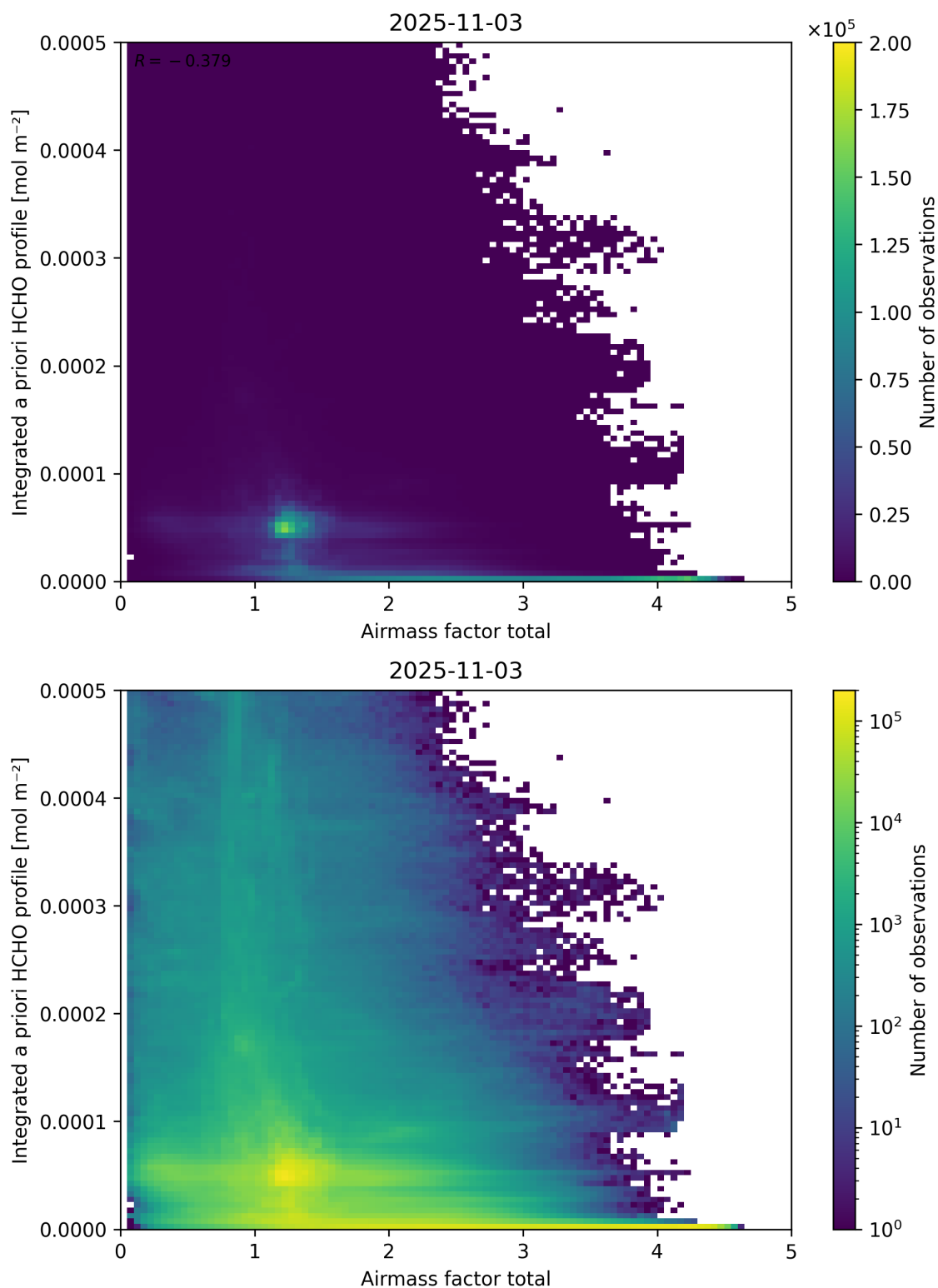
Figure 104: Scatter density plot of “Airmass factor total” against “Integrated a priori HCHO profile” for 2025-11-02 to 2025-11-04.
