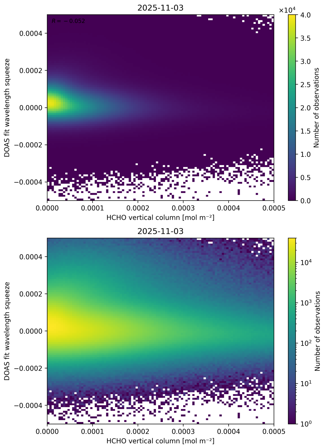
Figure 125: Scatter density plot of “HCHO vertical column” against “DOAS fit wavelength squeeze” for 2025-11-02 to 2025-11-04.
