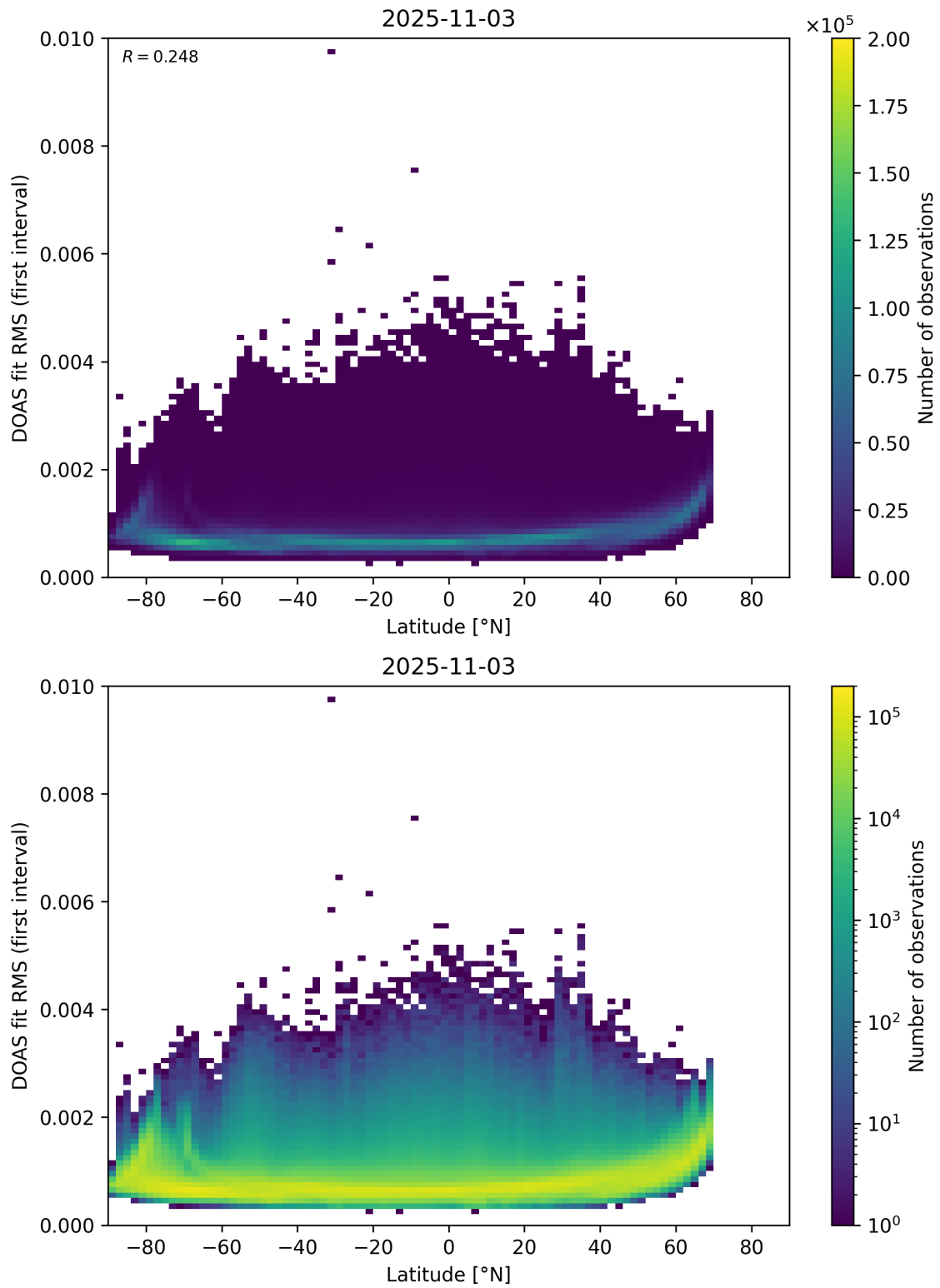
Figure 153: Scatter density plot of “Latitude” against “DOAS fit RMS (first interval)” for 2025-11-02 to 2025-11-04.
