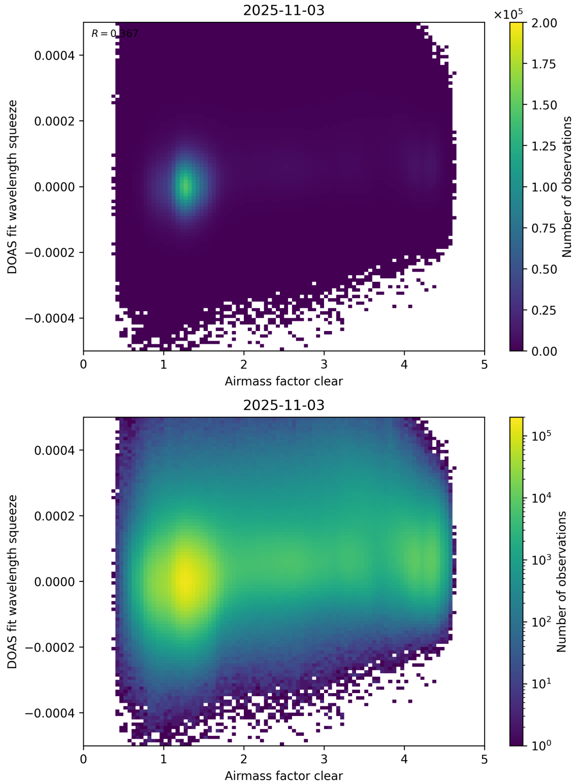
Figure 73: Scatter density plot of “Airmass factor clear” against “DOAS fit wavelength squeeze” for 2025-11-02 to 2025-11-04.
