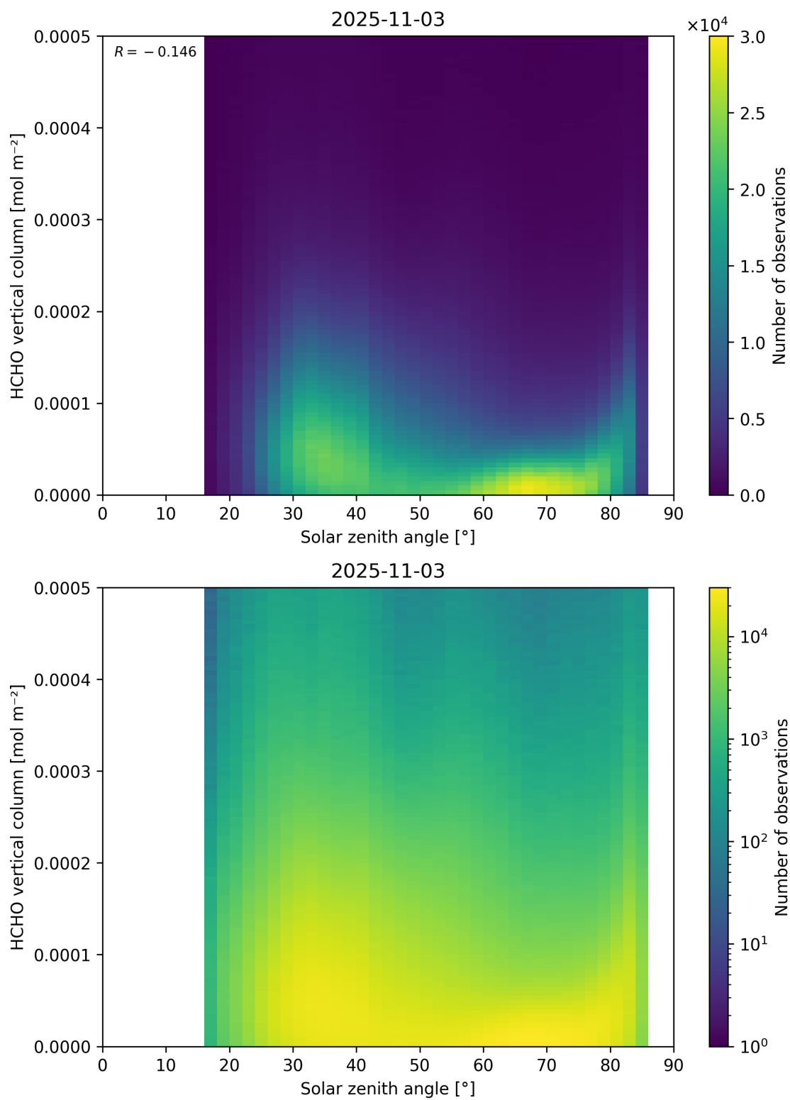
Figure 177: Scatter density plot of “Solar zenith angle” against “HCHO vertical column” for 2025-11-02 to 2025-11-04.
