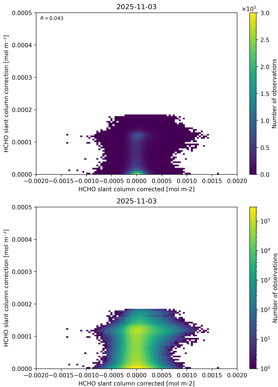
Figure 77: Scatter density plot of “HCHO slant column corrected” against “HCHO slant column correction” for 2025-11-02 to 2025-11-04.
