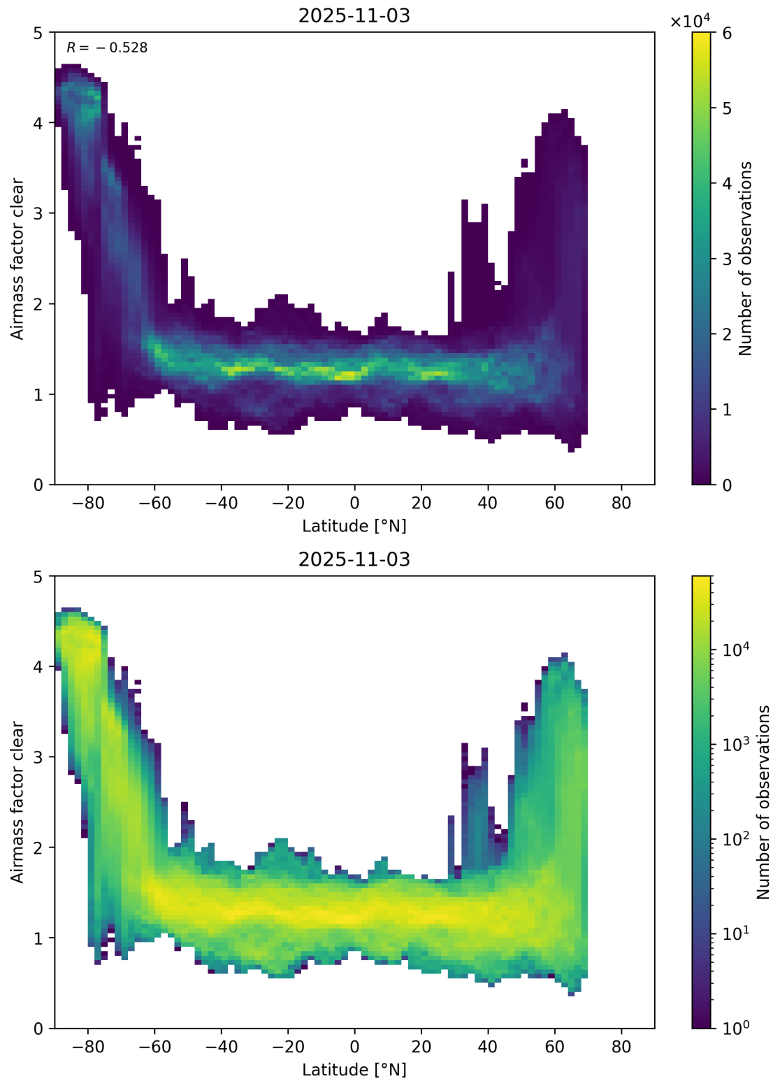
Figure 156: Scatter density plot of “Latitude” against “Airmass factor clear” for 2025-11-02 to 2025-11-04.
