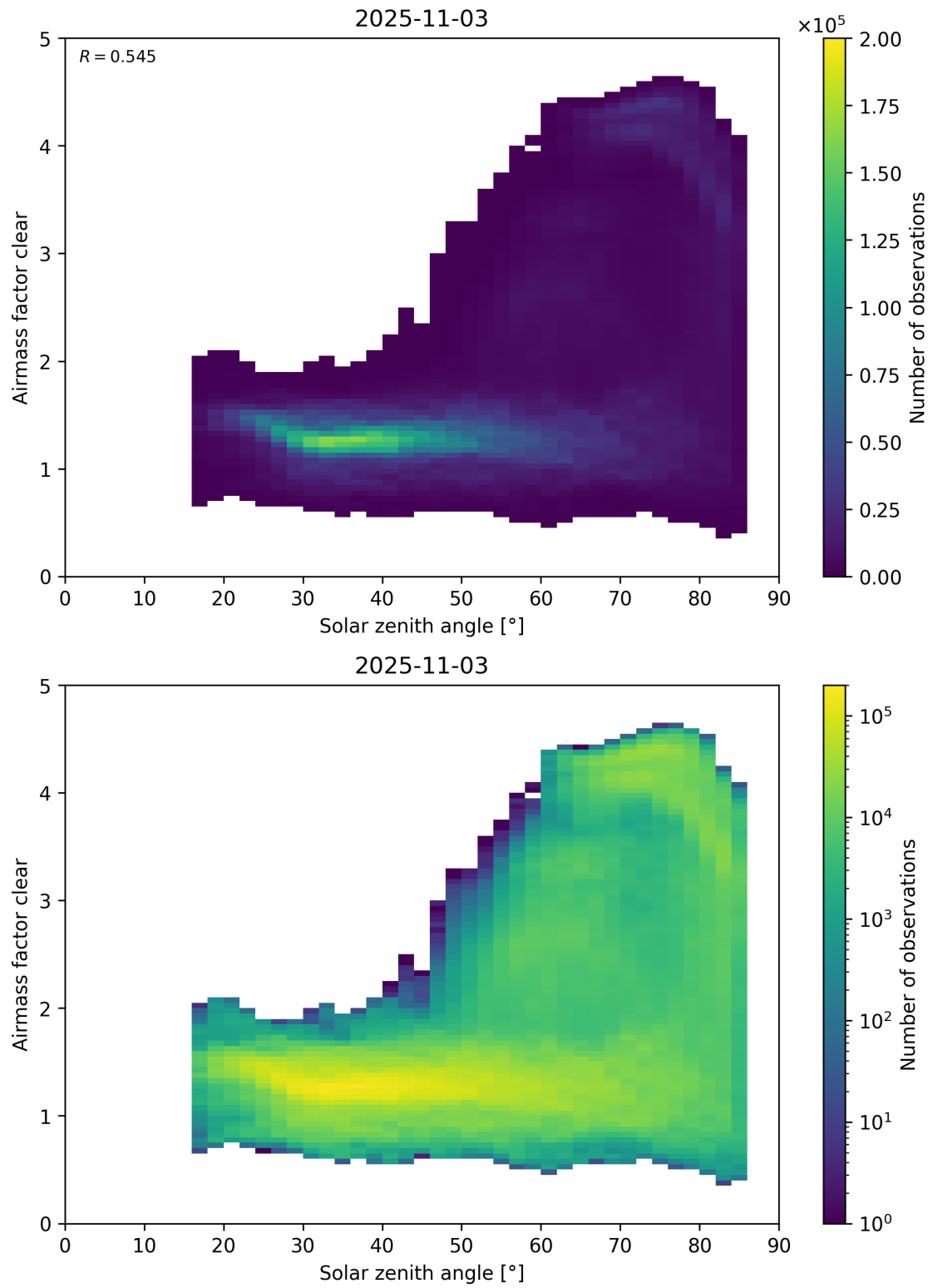
Figure 170: Scatter density plot of “Solar zenith angle” against “Airmass factor clear” for 2025-11-02 to 2025-11-04.
