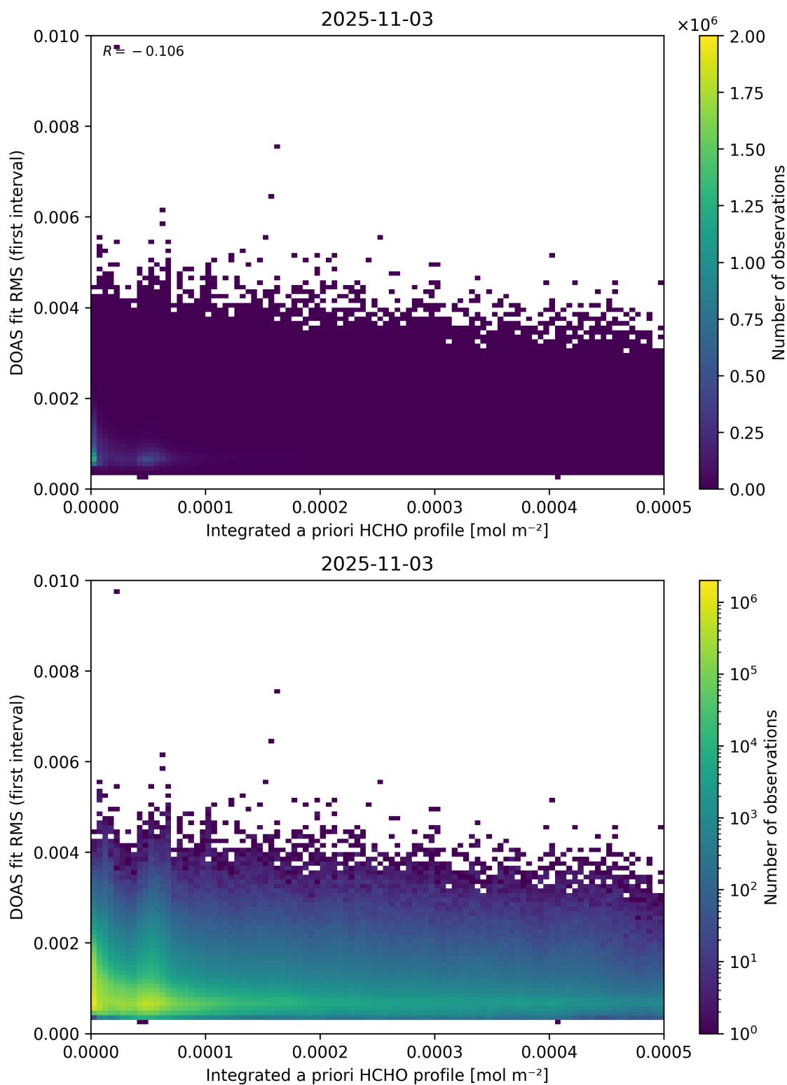
Figure 148: Scatter density plot of “Integrated a priori HCHO profile” against “DOAS fit RMS (first interval)” for 2025-11-02 to 2025-11-04.
