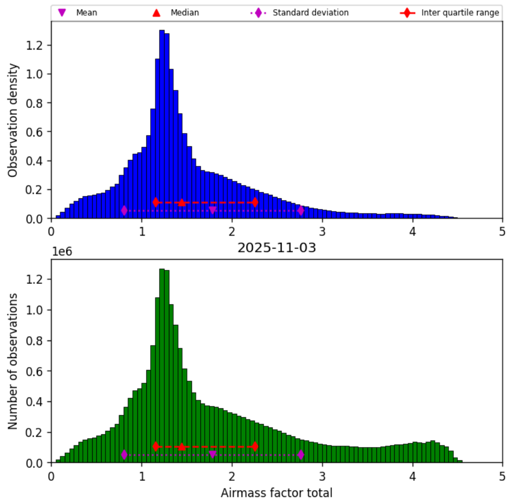
Figure 40: Histogram of “Airmass factor total” for 2025-11-02 to 2025-11-04
