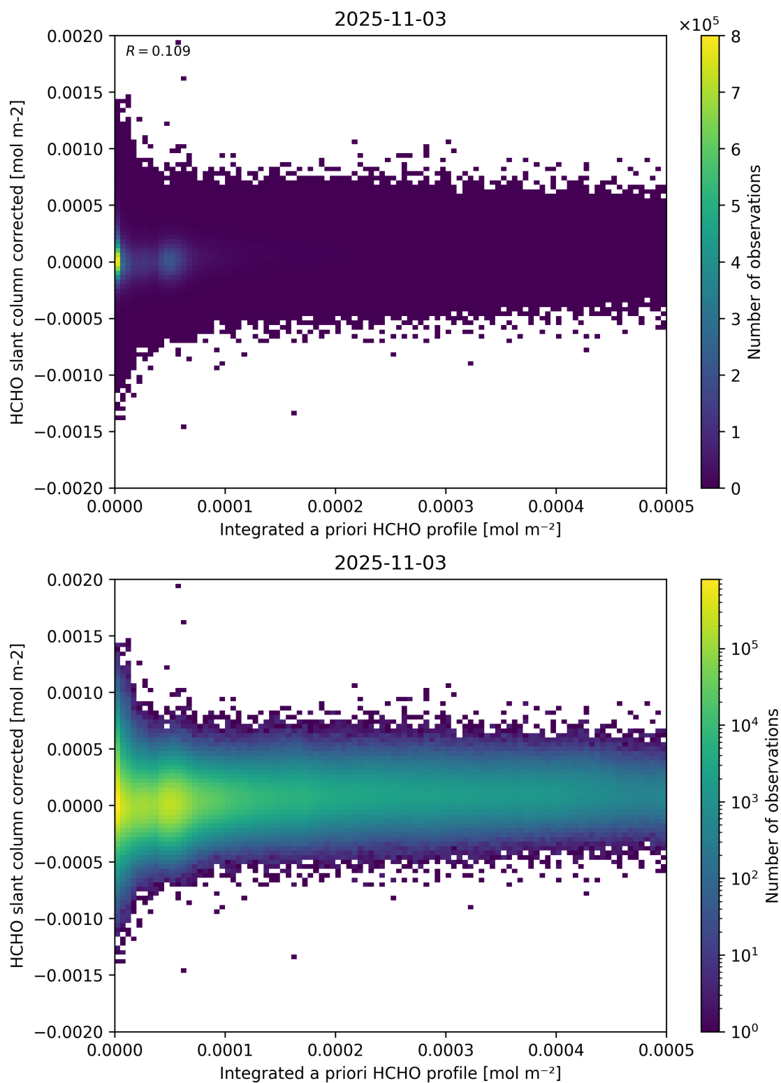
Figure 151: Scatter density plot of “Integrated a priori HCHO profile” against “HCHO slant column corrected” for 2025-11-02 to 2025-11-04.
