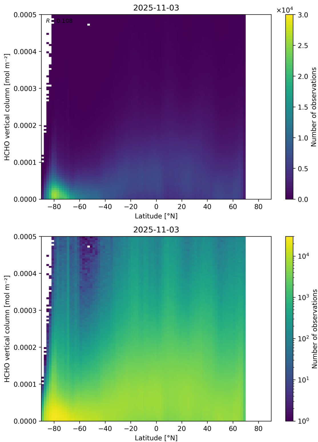
Figure 163: Scatter density plot of “Latitude” against “HCHO vertical column” for 2025-11-02 to 2025-11-04.
