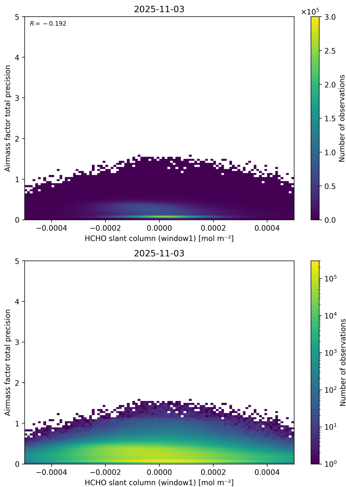
Figure 86: Scatter density plot of “HCHO slant column (window1)” against “Airmass factor total precision” for 2025-11-02 to 2025-11-04.
