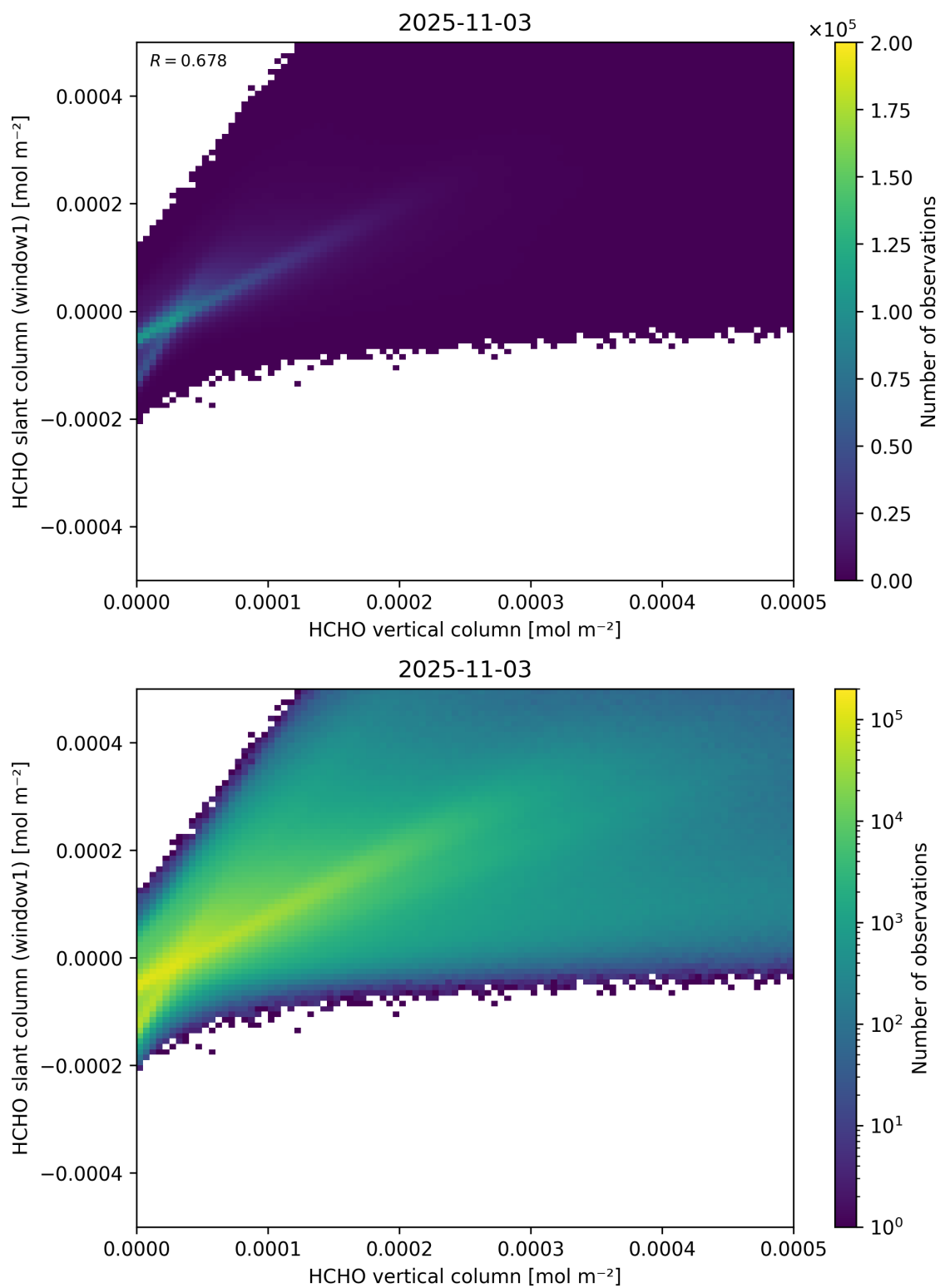
Figure 129: Scatter density plot of “HCHO vertical column” against “HCHO slant column (window1)” for 2025-11-02 to 2025-11-04.
