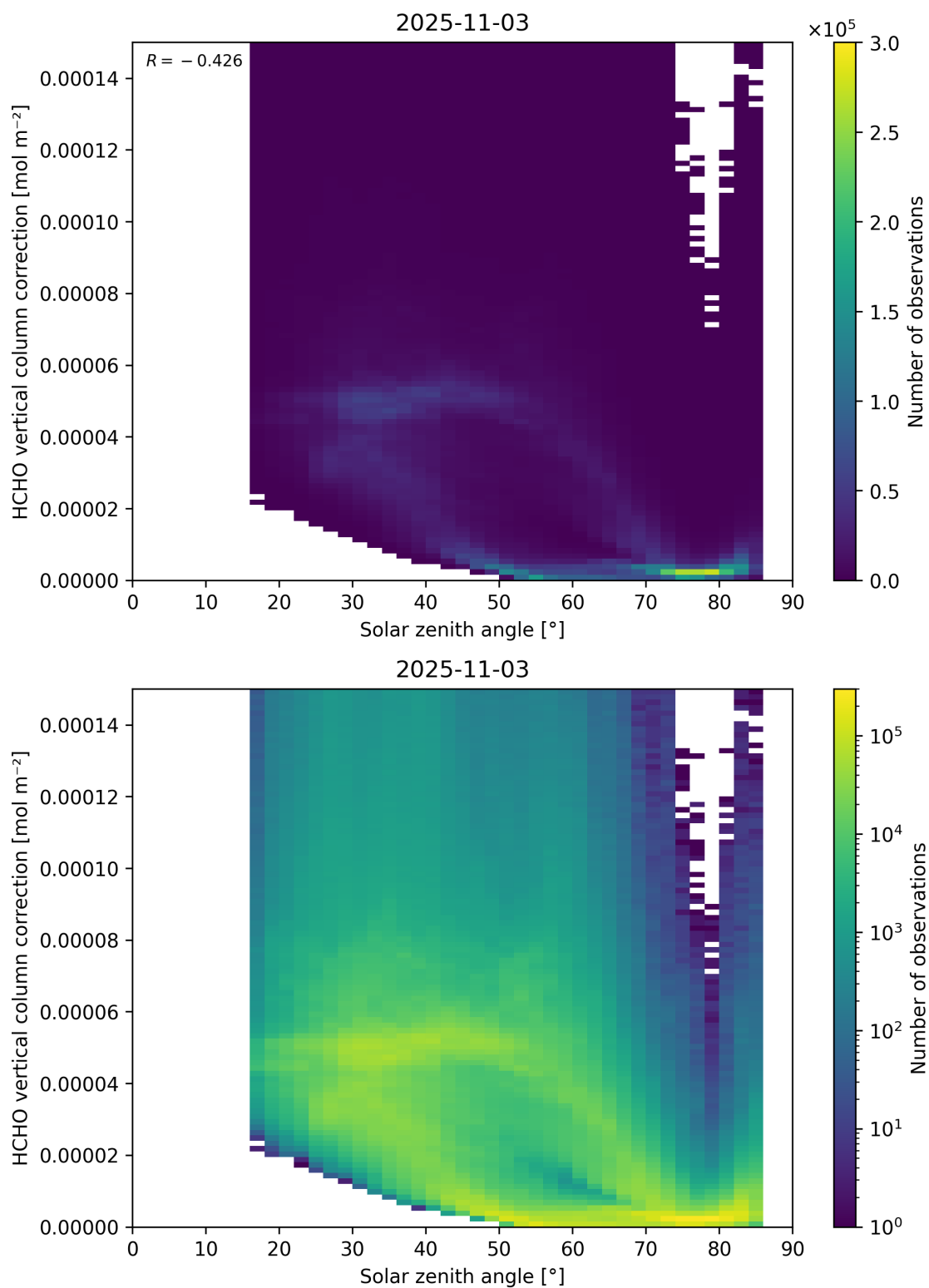
Figure 178: Scatter density plot of “Solar zenith angle” against “HCHO vertical column correction” for 2025-11-02 to 2025-11-04.
