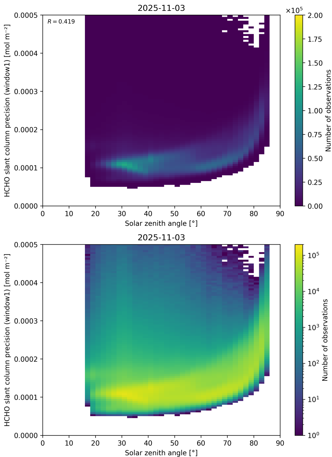
Figure 174: Scatter density plot of “Solar zenith angle” against “HCHO slant column precision (window1)” for 2025-11-02 to 2025-11-04.
