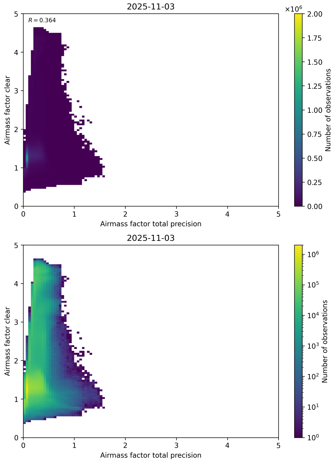
Figure 108: Scatter density plot of “Airmass factor total precision” against “Airmass factor clear” for 2025-11-02 to 2025-11-04.
