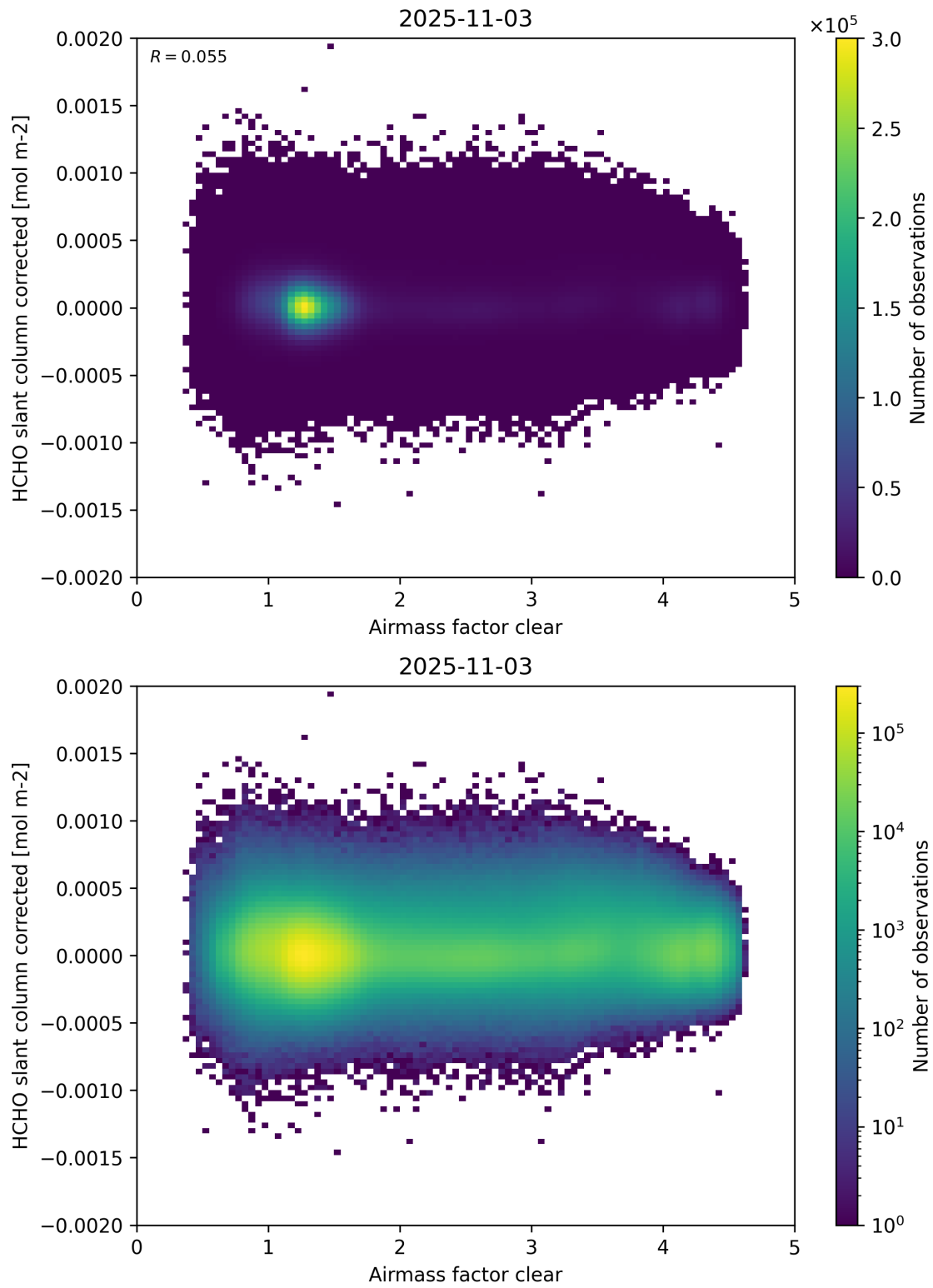
Figure 74: Scatter density plot of “Airmass factor clear” against “HCHO slant column corrected” for 2025-11-02 to 2025-11-04.
