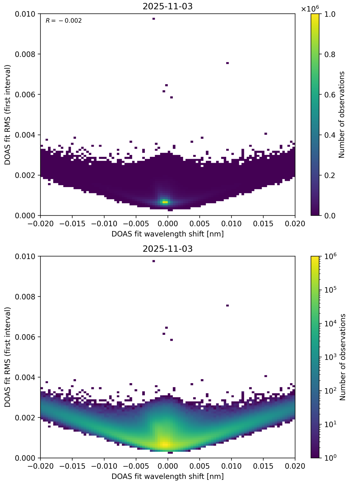
Figure 64: Scatter density plot of “DOAS fit wavelength shift” against “DOAS fit RMS (first interval)” for 2025-11-02 to 2025-11-04.
