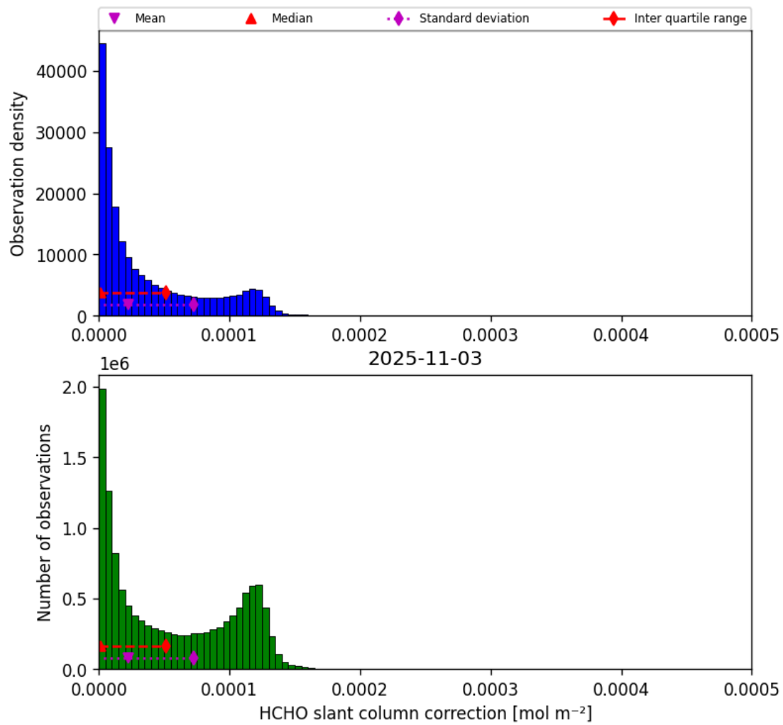
Figure 47: Histogram of “HCHO slant column correction” for 2025-11-02 to 2025-11-04
