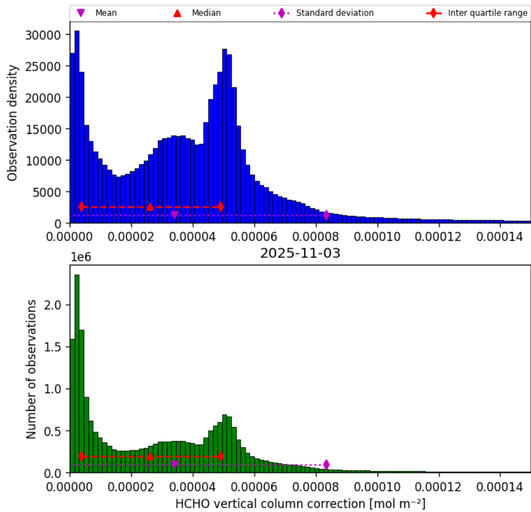
Figure 37: Histogram of “HCHO vertical column correction” for 2025-11-02 to 2025-11-04
