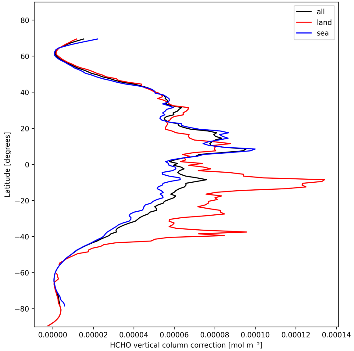
Figure 23: Zonal average of “HCHO vertical column correction” for 2025-11-02 to 2025-11-04.
