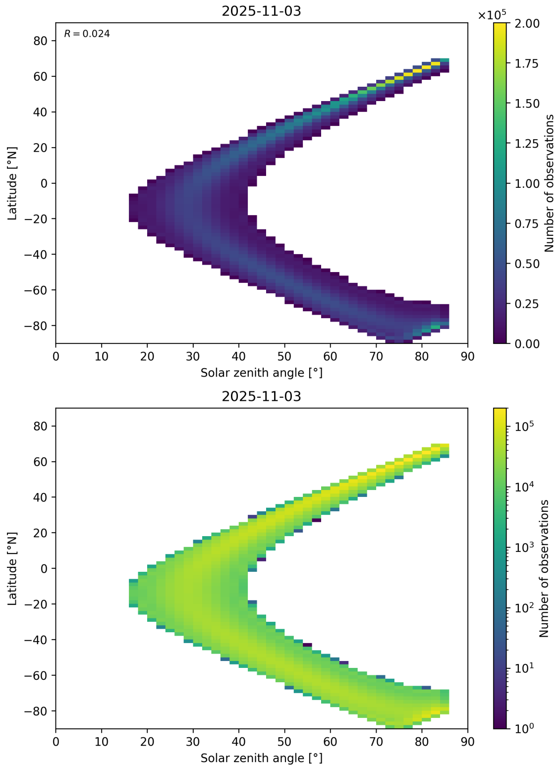
Figure 181: Scatter density plot of “Solar zenith angle” against “Latitude” for 2025-11-02 to 2025-11-04.
