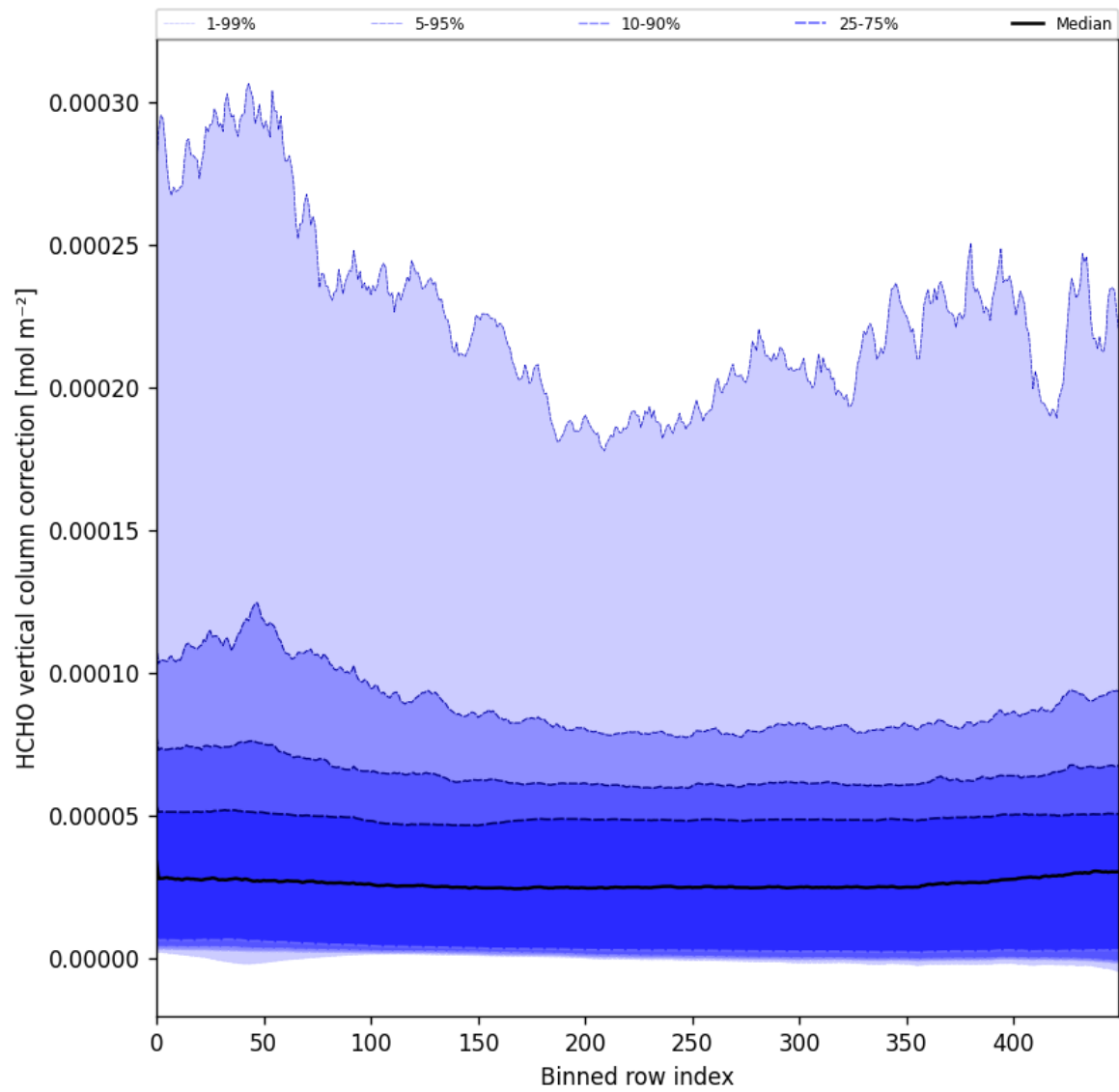
Figure 51: Along track statistics of “HCHO vertical column correction” for 2025-11-02 to 2025-11-04
