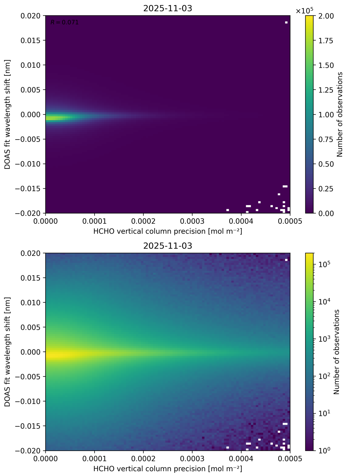
Figure 137: Scatter density plot of “HCHO vertical column precision” against “DOAS fit wavelength shift” for 2025-11-02 to 2025-11-04.
