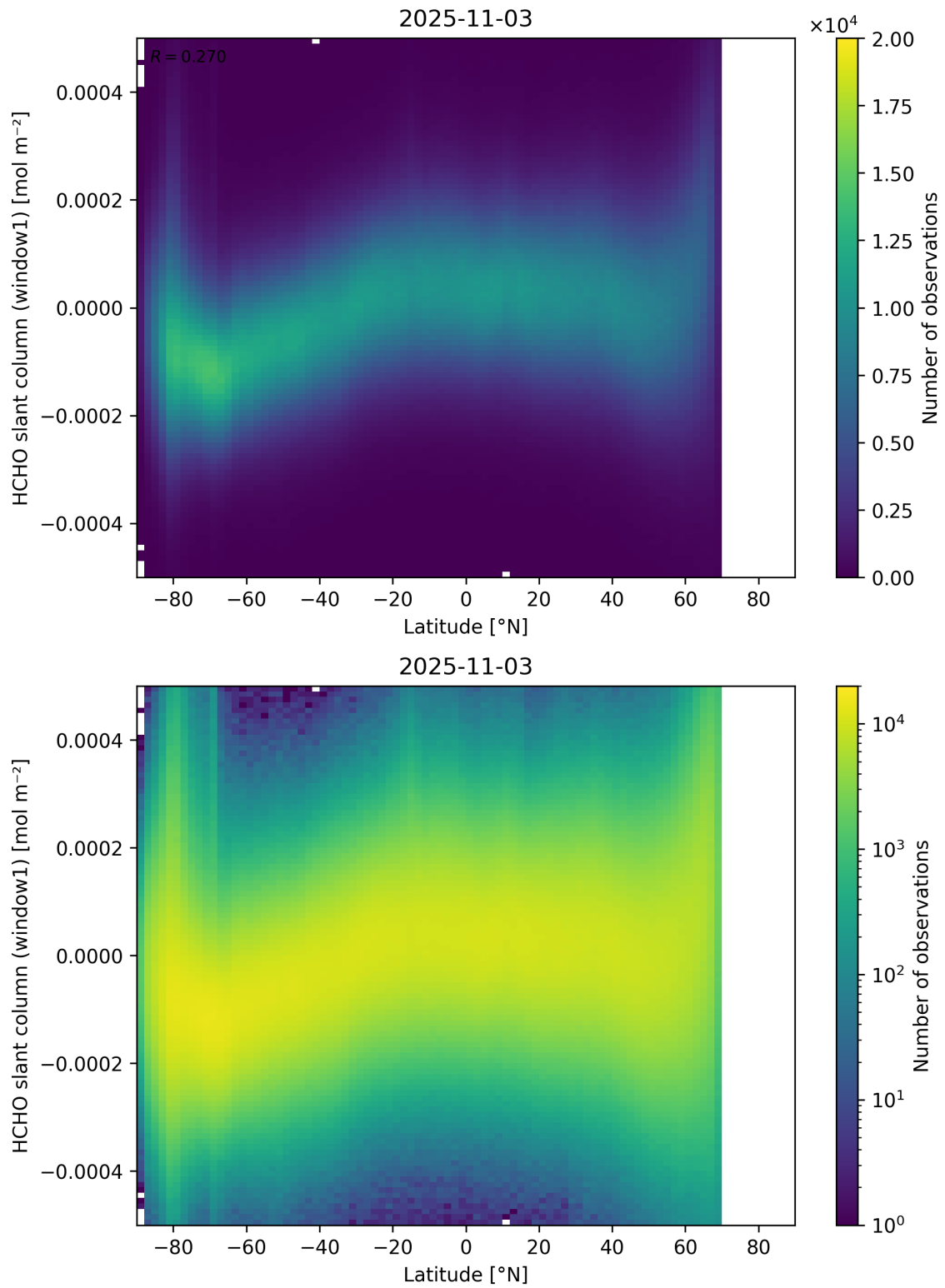
Figure 159: Scatter density plot of “Latitude” against “HCHO slant column (window1)” for 2025-11-02 to 2025-11-04.
