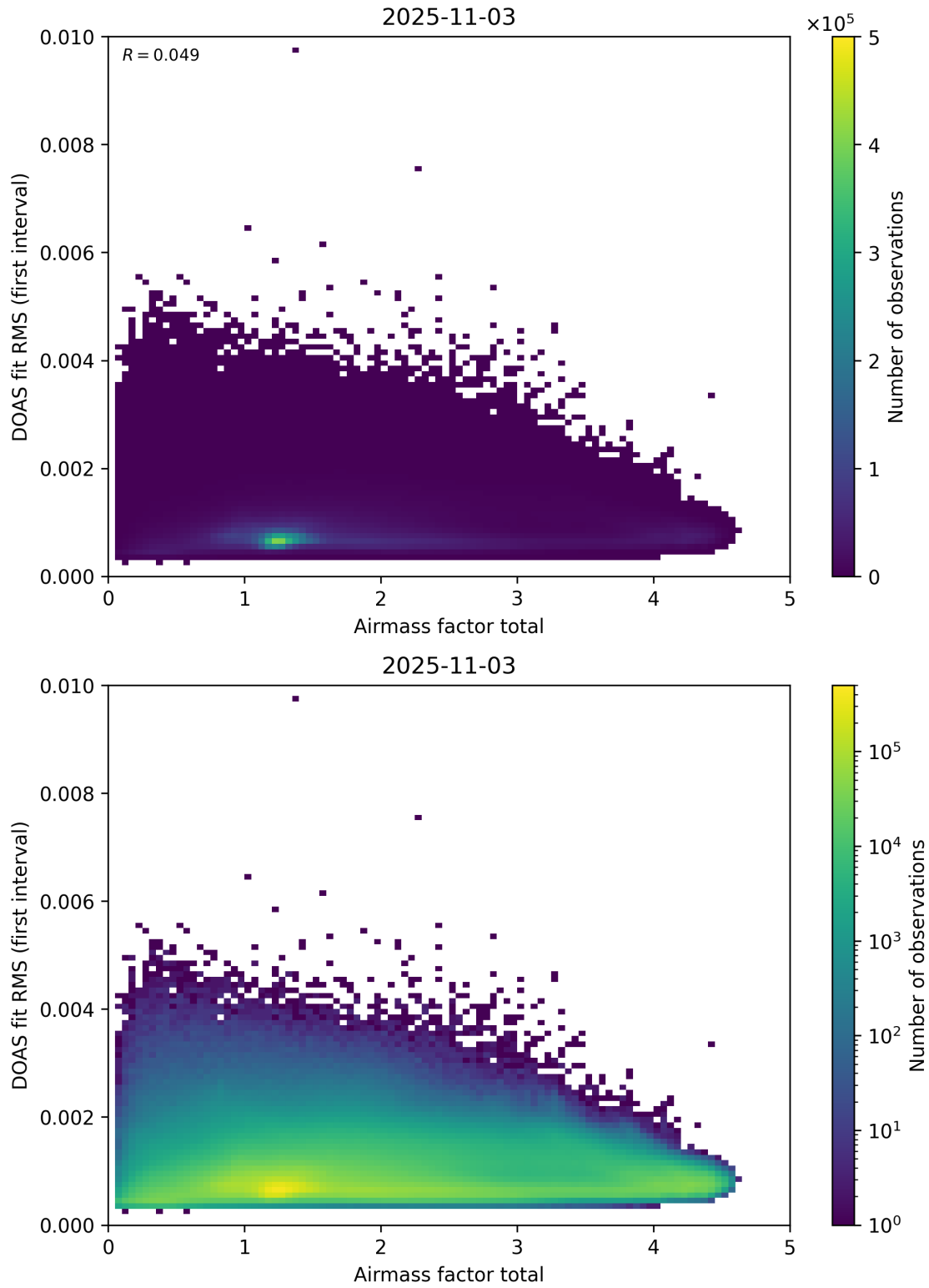
Figure 97: Scatter density plot of “Airmass factor total” against “DOAS fit RMS (first interval)” for 2025-11-02 to 2025-11-04.
