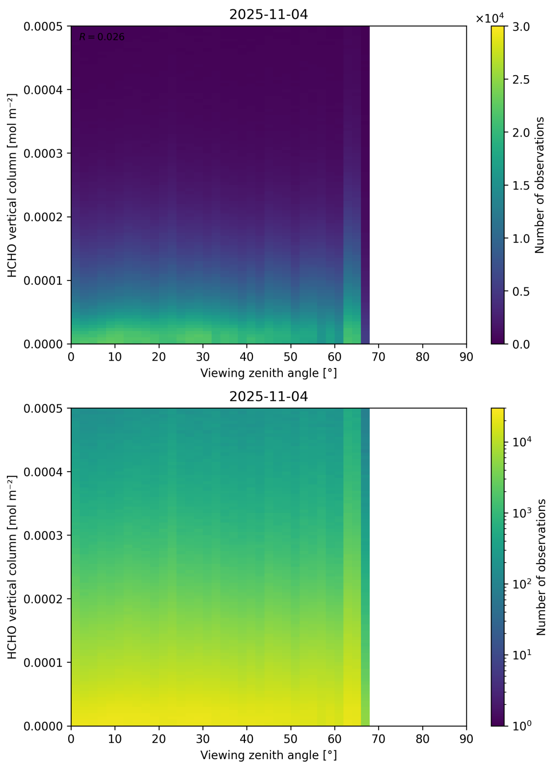
Figure 192: Scatter density plot of “Viewing zenith angle” against “HCHO vertical column” for 2025-11-03 to 2025-11-05.
