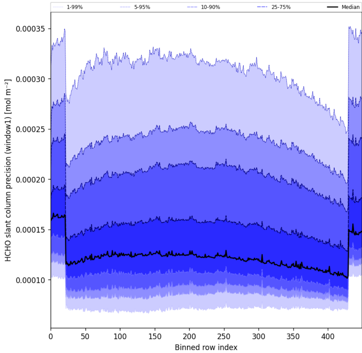
Figure 53: Along track statistics of “HCHO slant column precision (window1)” for 2025-11-03 to 2025-11-05
