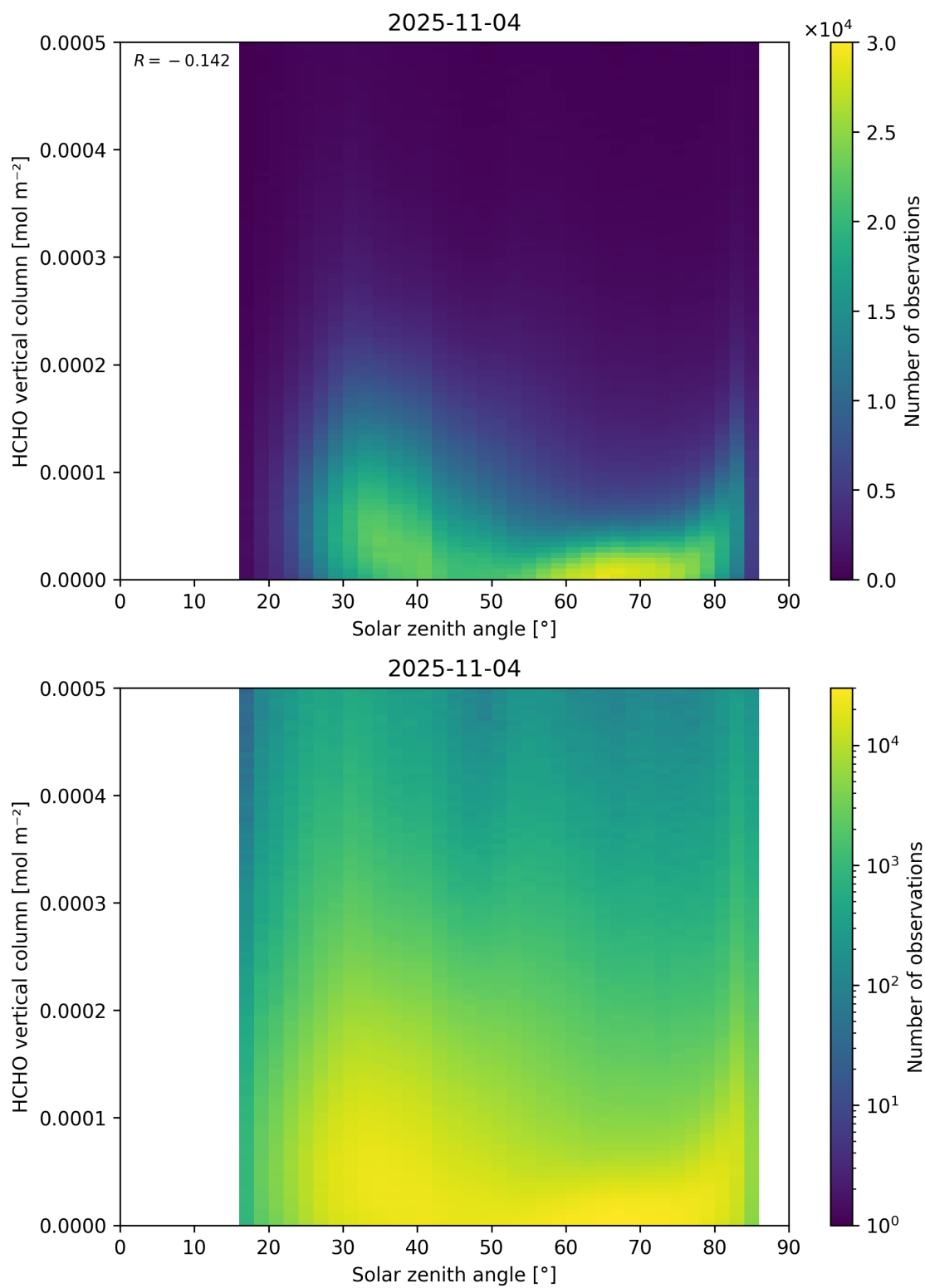
Figure 177: Scatter density plot of “Solar zenith angle” against “HCHO vertical column” for 2025-11-03 to 2025-11-05.
