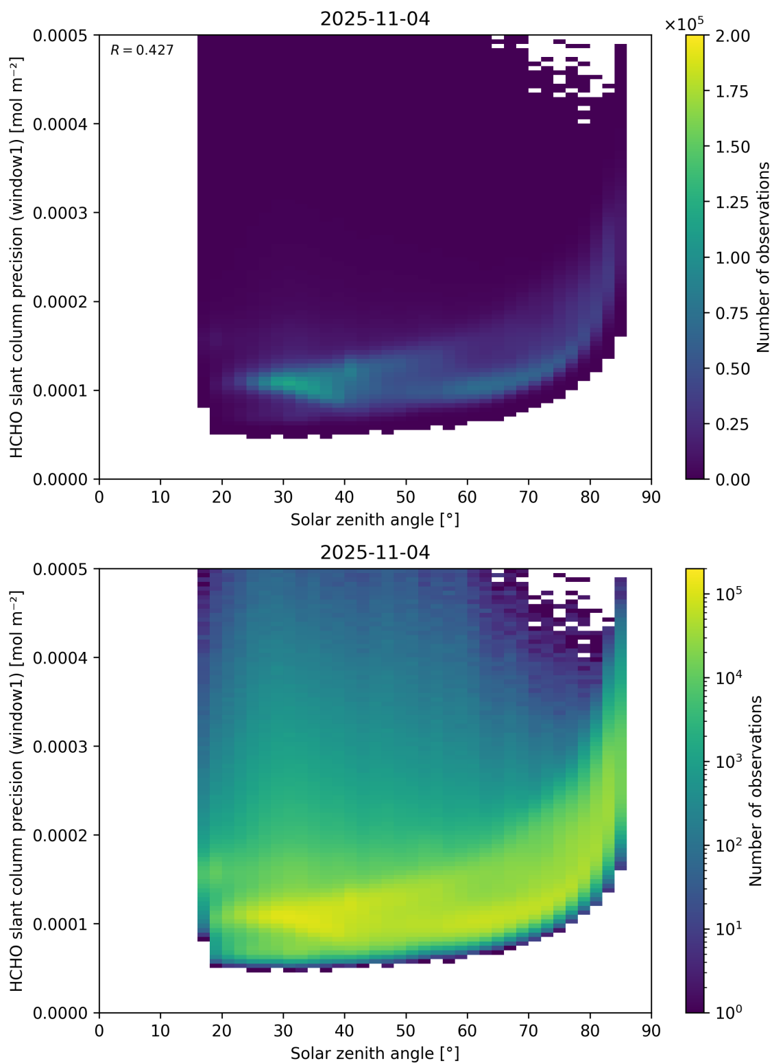
Figure 174: Scatter density plot of “Solar zenith angle” against “HCHO slant column precision (window1)” for 2025-11-03 to 2025-11-05.
