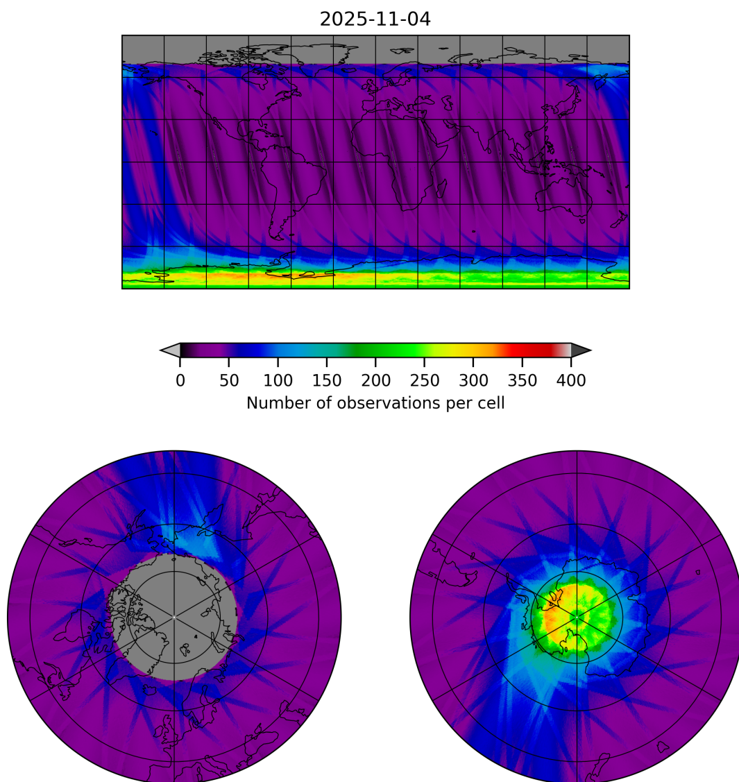
Figure 19: Map of the number of observations for 2025-11-03 to 2025-11-05
