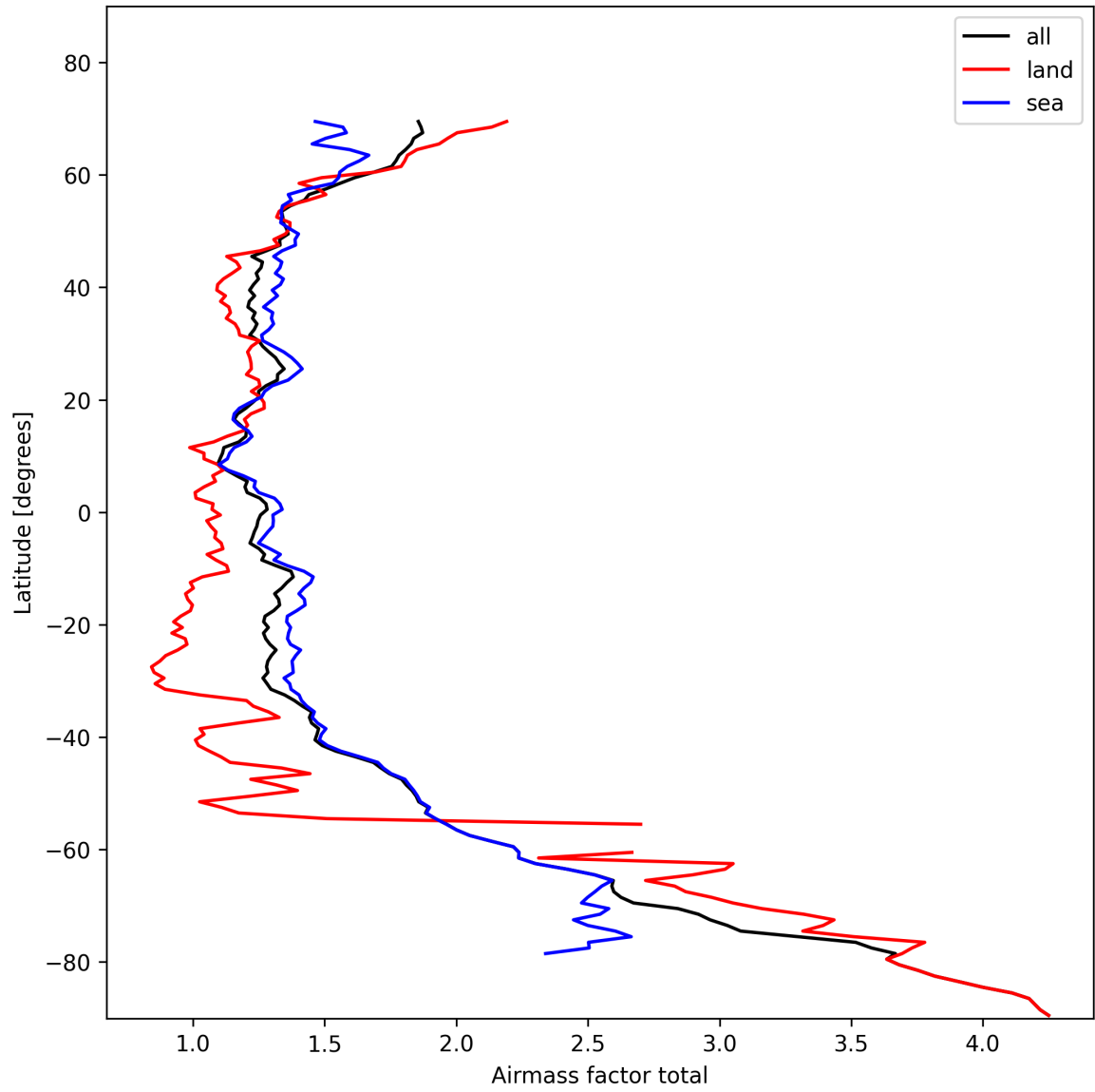
Figure 26: Zonal average of “Airmass factor total” for 2025-11-03 to 2025-11-05.
