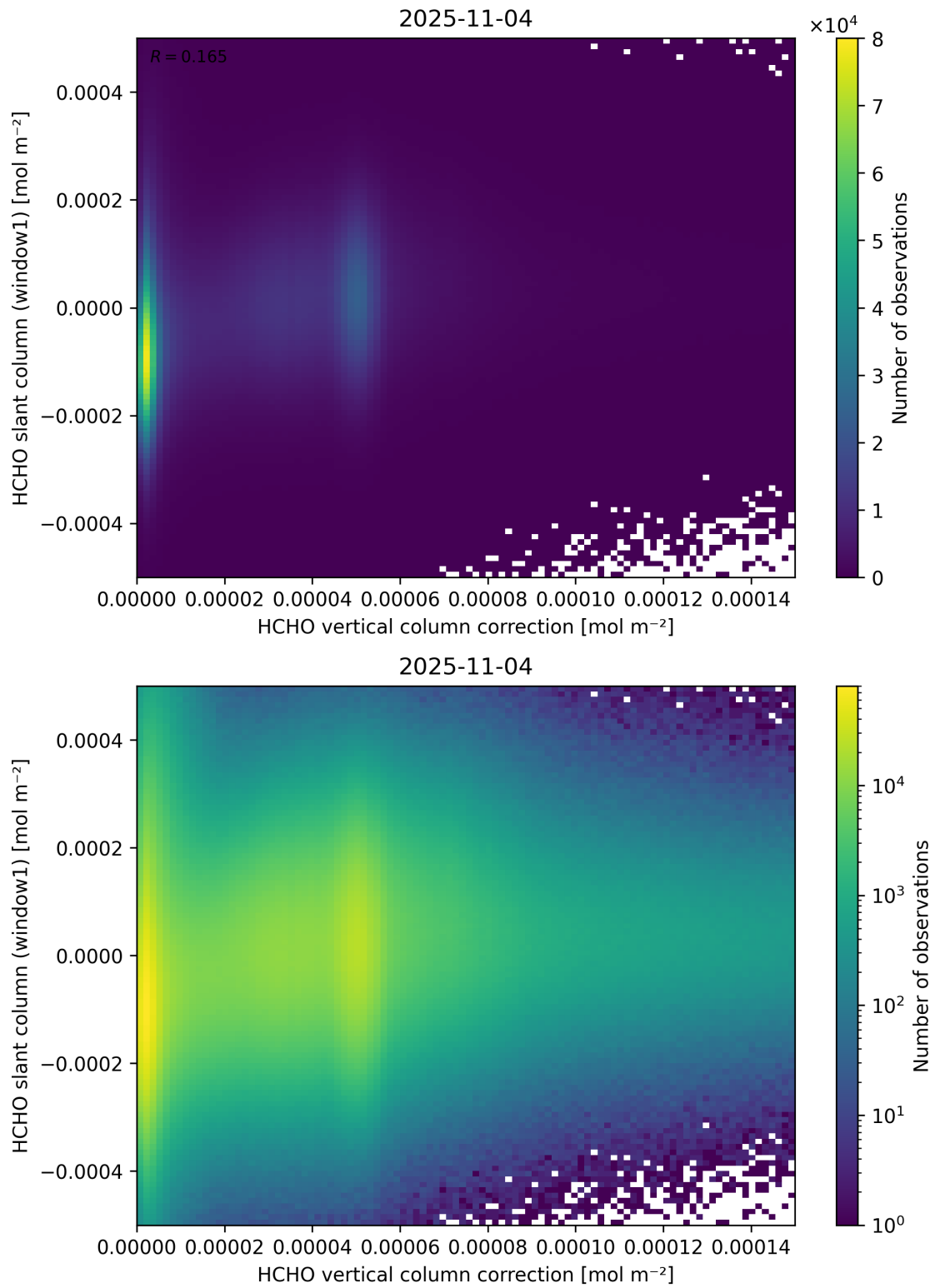
Figure 118: Scatter density plot of “HCHO vertical column correction” against “HCHO slant column (window1)” for 2025-11-03 to 2025-11-05.
