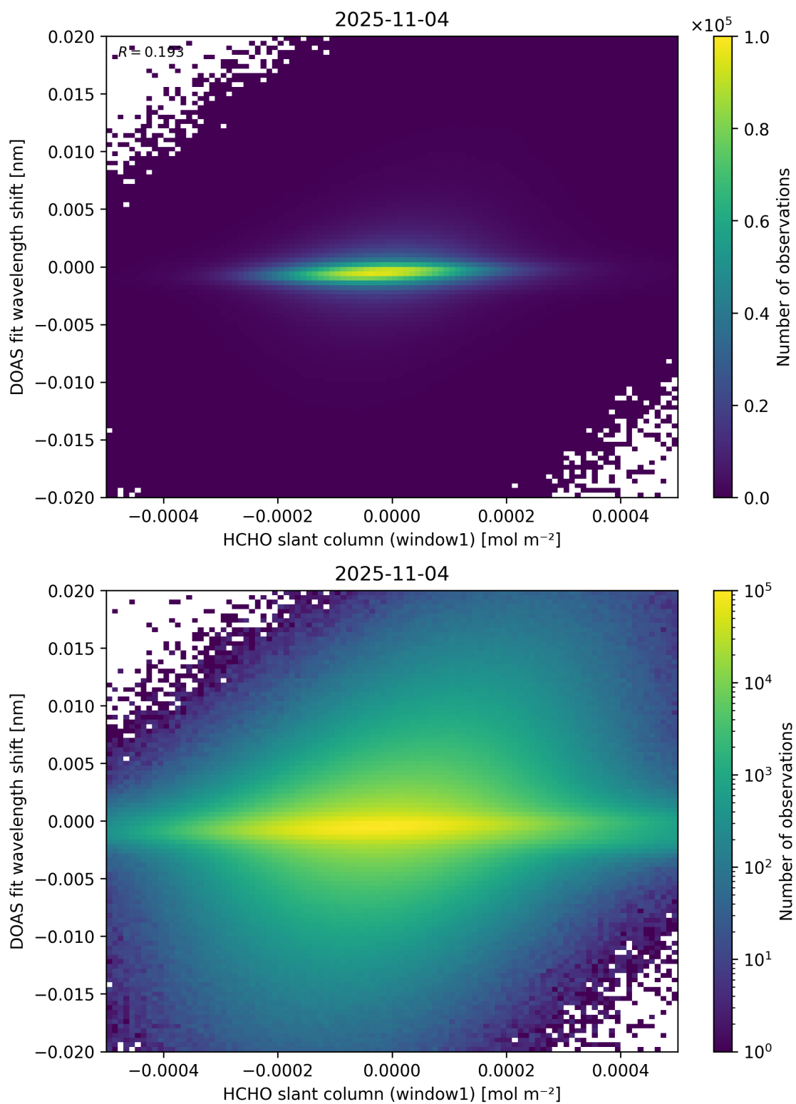
Figure 79: Scatter density plot of “HCHO slant column (window1)” against “DOAS fit wavelength shift” for 2025-11-03 to 2025-11-05.
