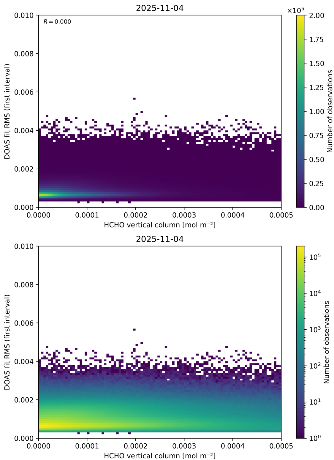
Figure 123: Scatter density plot of “HCHO vertical column” against “DOAS fit RMS (first interval)” for 2025-11-03 to 2025-11-05.
