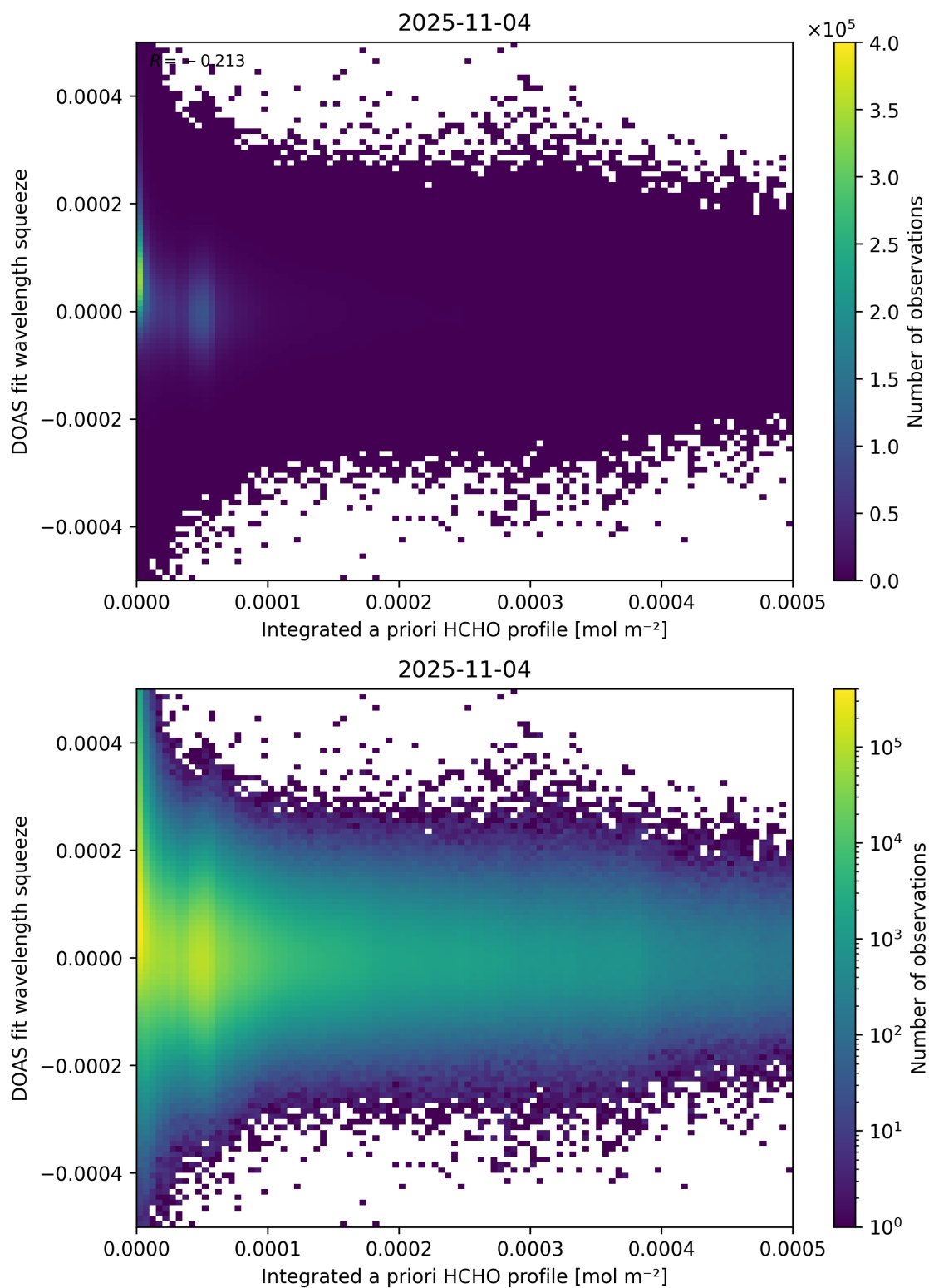
Figure 150: Scatter density plot of “Integrated a priori HCHO profile” against “DOAS fit wavelength squeeze” for 2025-11-03 to 2025-11-05.
