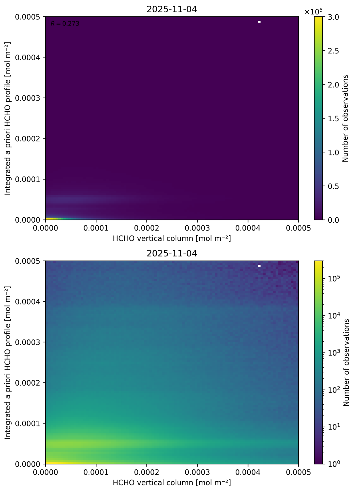
Figure 135: Scatter density plot of “HCHO vertical column” against “Integrated a priori HCHO profile” for 2025-11-03 to 2025-11-05.
