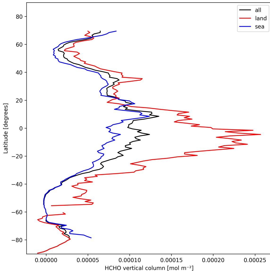
Figure 21: Zonal average of “HCHO vertical column” for 2025-11-03 to 2025-11-05.
