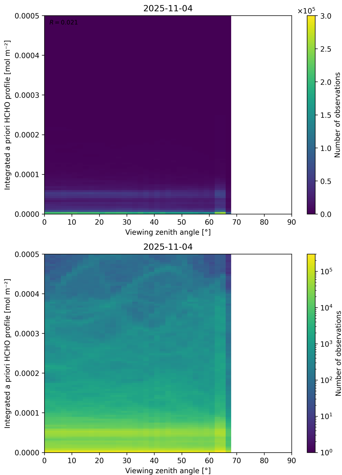
Figure 195: Scatter density plot of “Viewing zenith angle” against “Integrated a priori HCHO profile” for 2025-11-03 to 2025-11-05.
