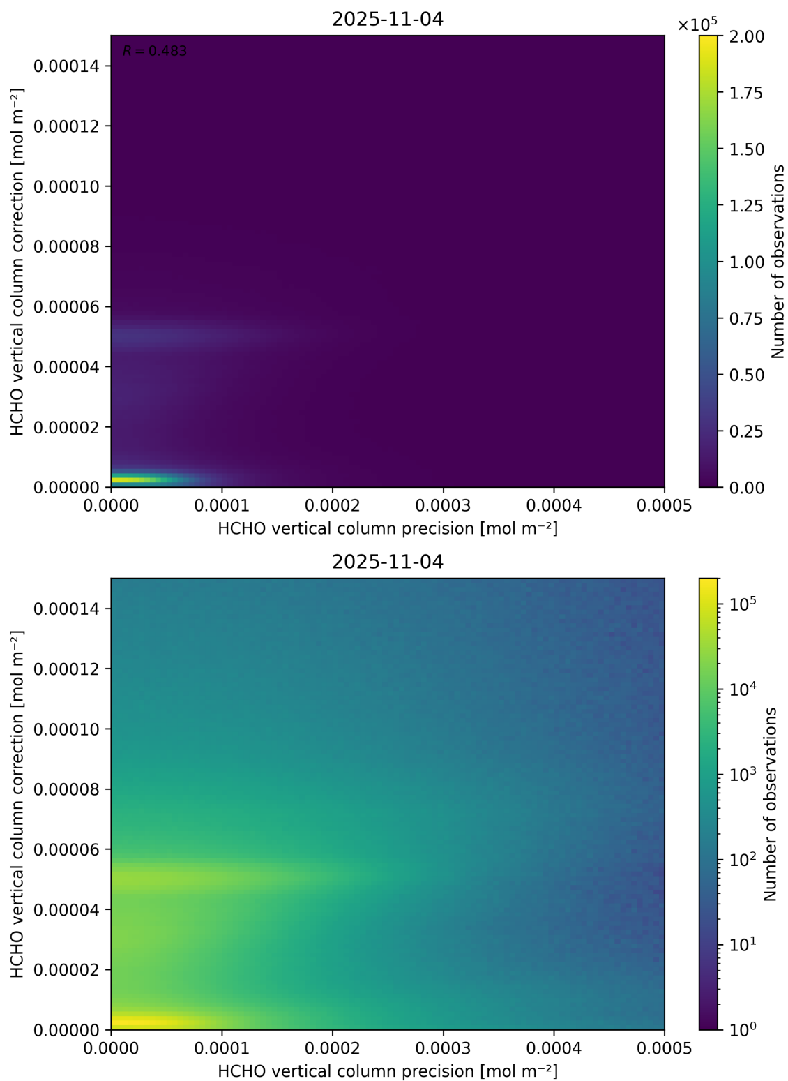
Figure 146: Scatter density plot of “HCHO vertical column precision” against “HCHO vertical column correction” for 2025-11-03 to 2025-11-05.
