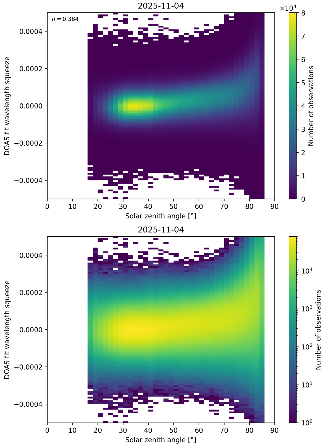
Figure 169: Scatter density plot of “Solar zenith angle” against “DOAS fit wavelength squeeze” for 2025-11-03 to 2025-11-05.
