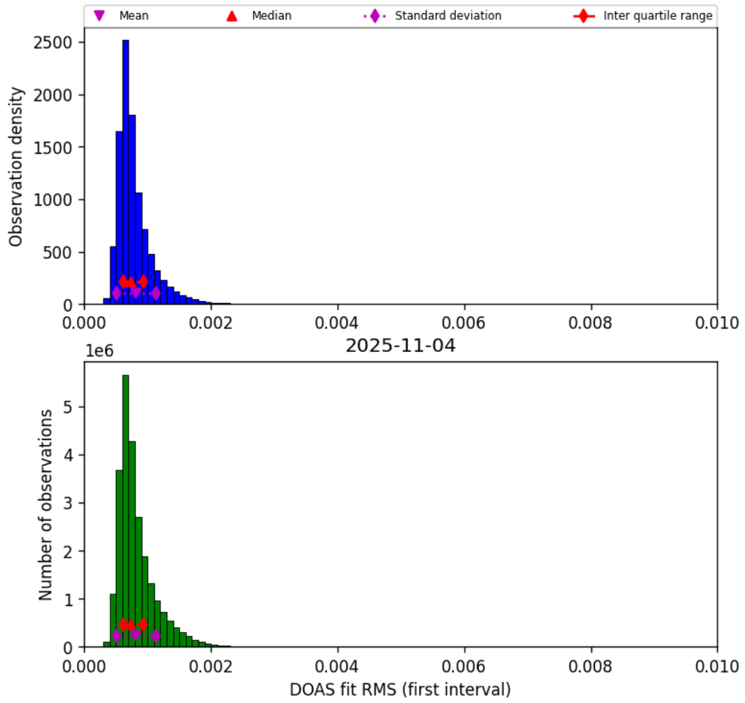
Figure 46: Histogram of “DOAS fit RMS (first interval)” for 2025-11-03 to 2025-11-05
