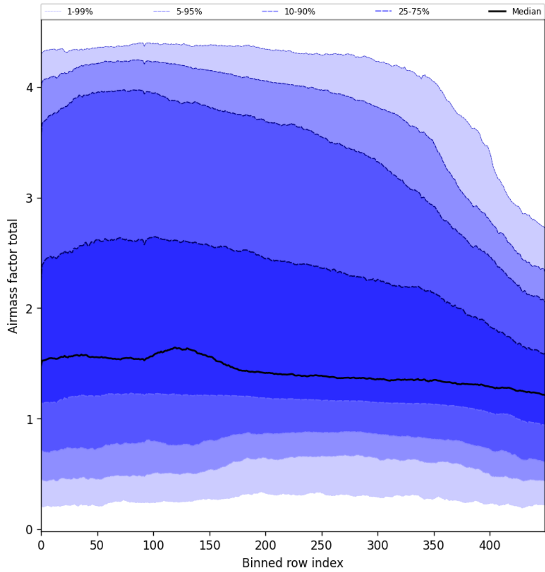
Figure 54: Along track statistics of “Airmass factor total” for 2025-11-03 to 2025-11-05
