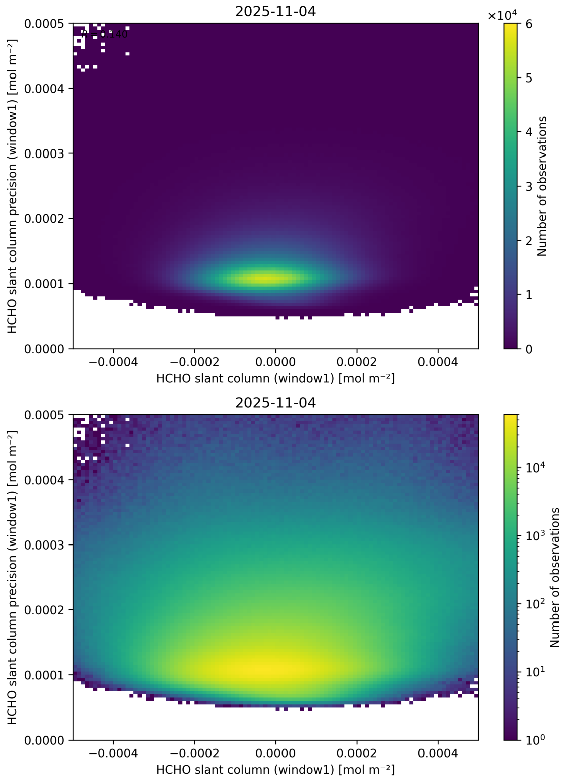
Figure 84: Scatter density plot of “HCHO slant column (window1)” against “HCHO slant column precision (window1)” for 2025-11-03 to 2025-11-05.
