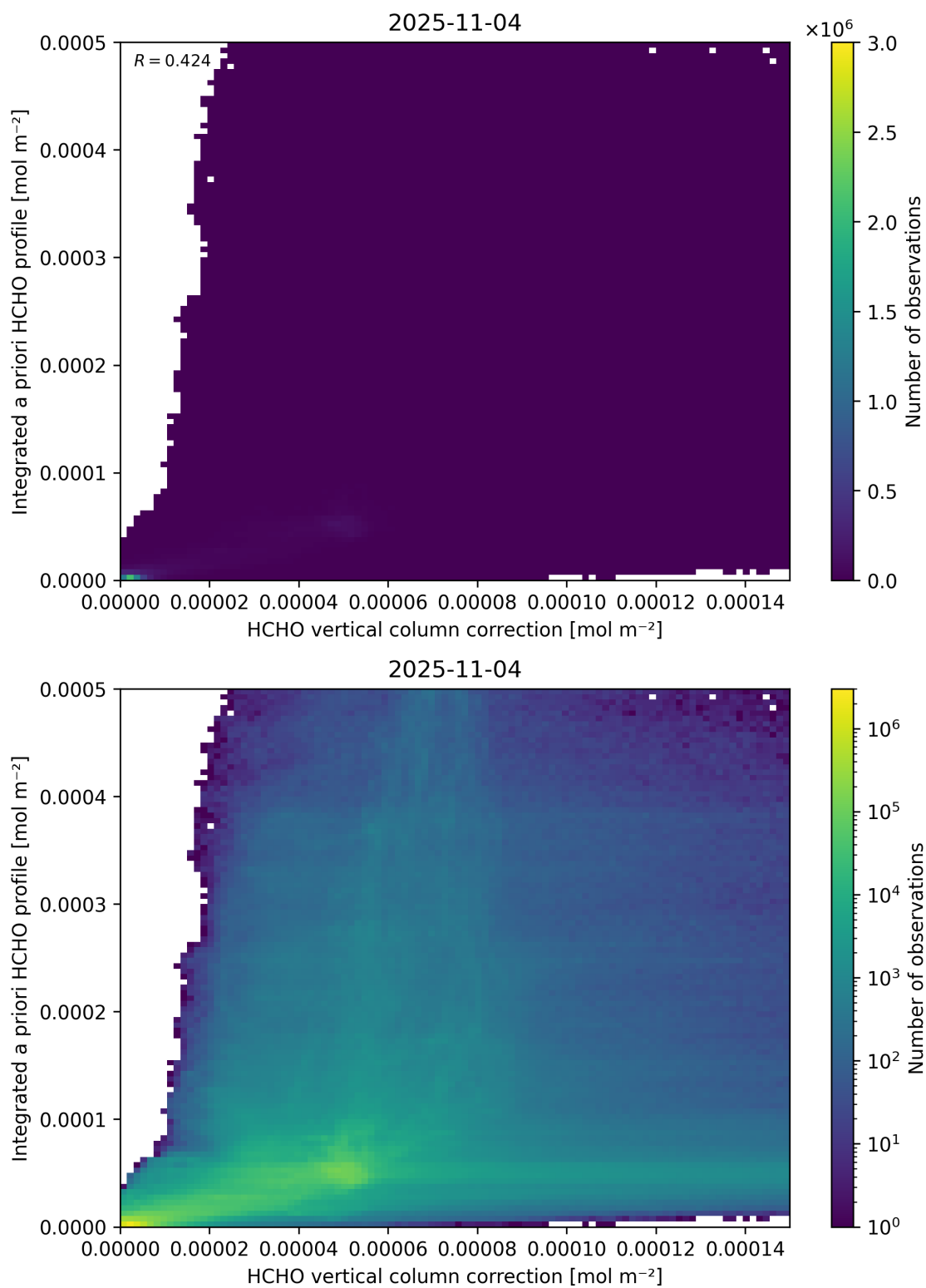
Figure 122: Scatter density plot of “HCHO vertical column correction” against “Integrated a priori HCHO profile” for 2025-11-03 to 2025-11-05.
