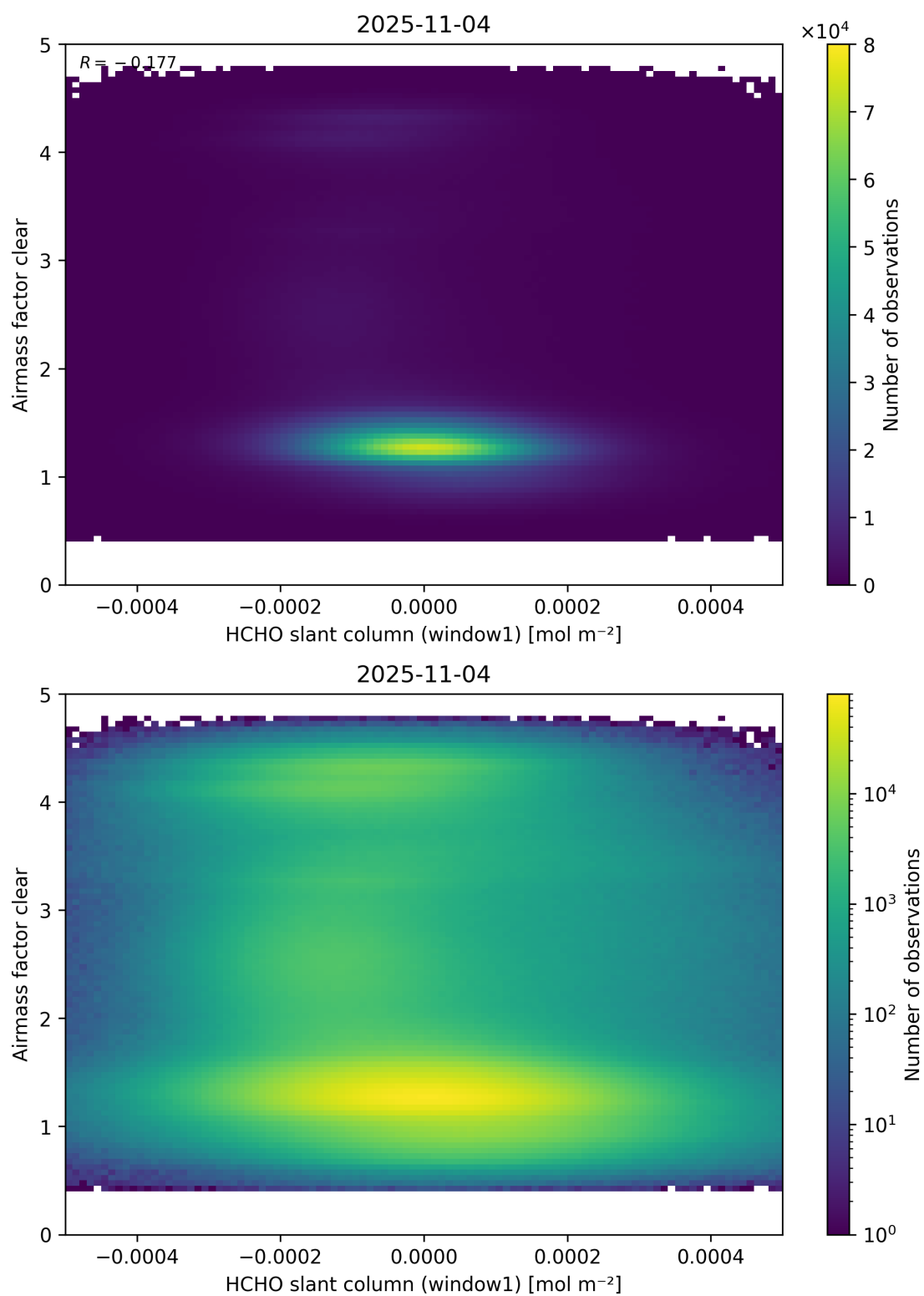
Figure 81: Scatter density plot of “HCHO slant column (window1)” against “Airmass factor clear” for 2025-11-03 to 2025-11-05.
