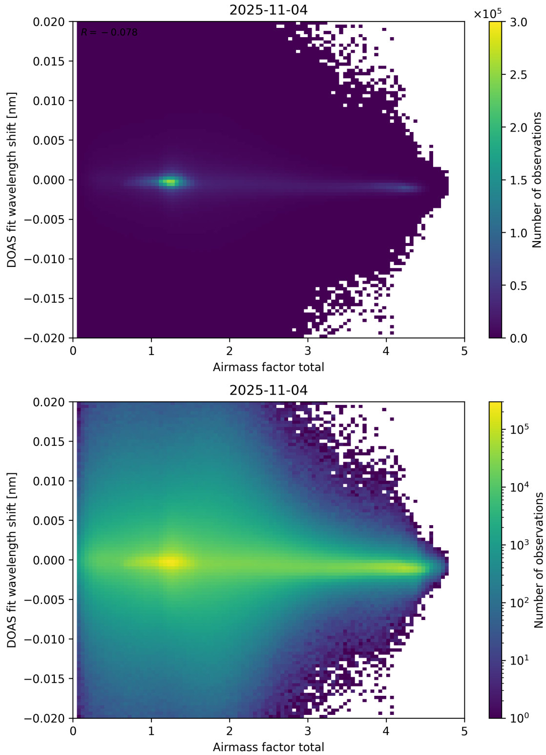
Figure 98: Scatter density plot of “Airmass factor total” against “DOAS fit wavelength shift” for 2025-11-03 to 2025-11-05.
