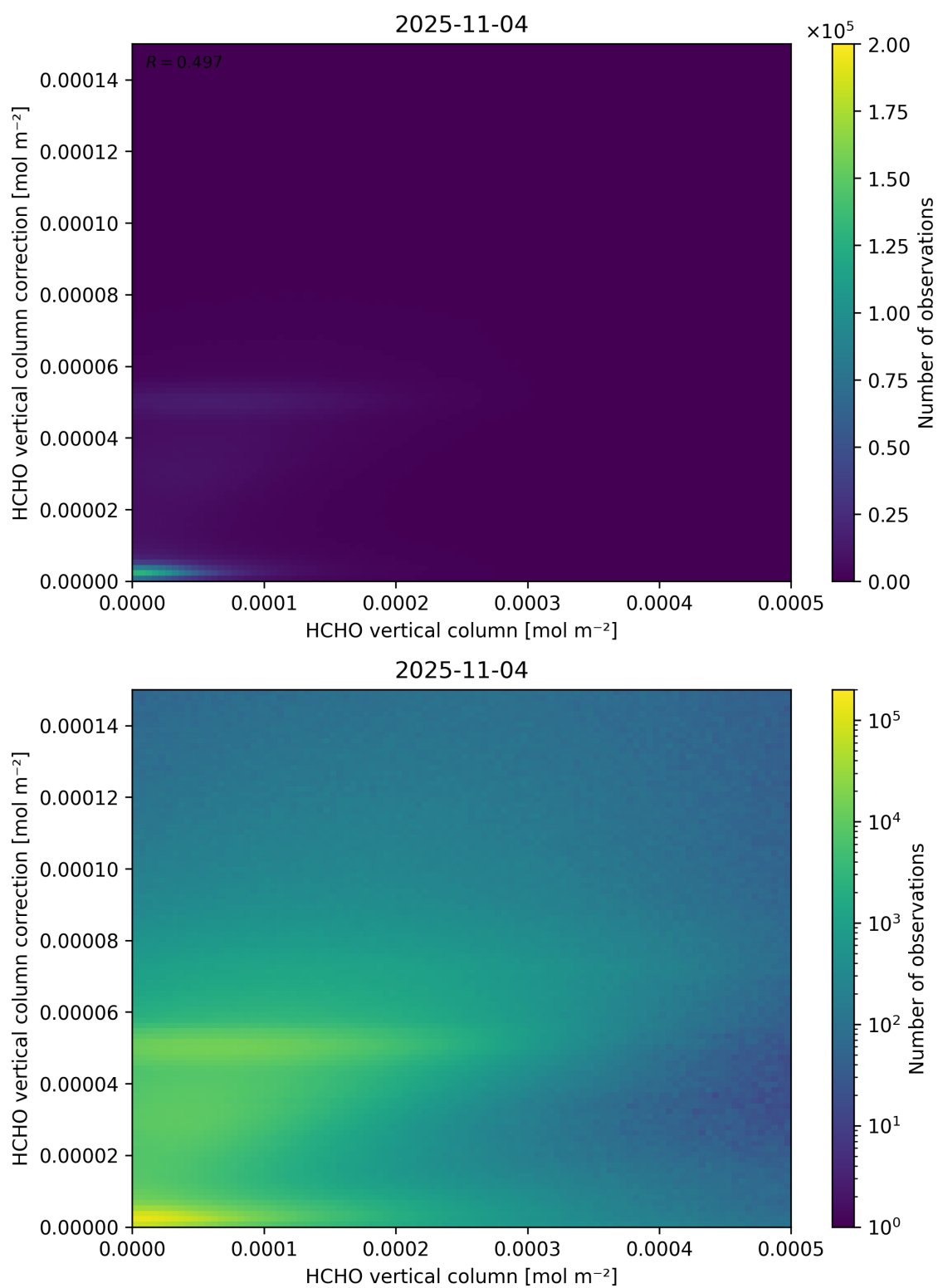
Figure 133: Scatter density plot of “HCHO vertical column” against “HCHO vertical column correction” for 2025-11-03 to 2025-11-05.
