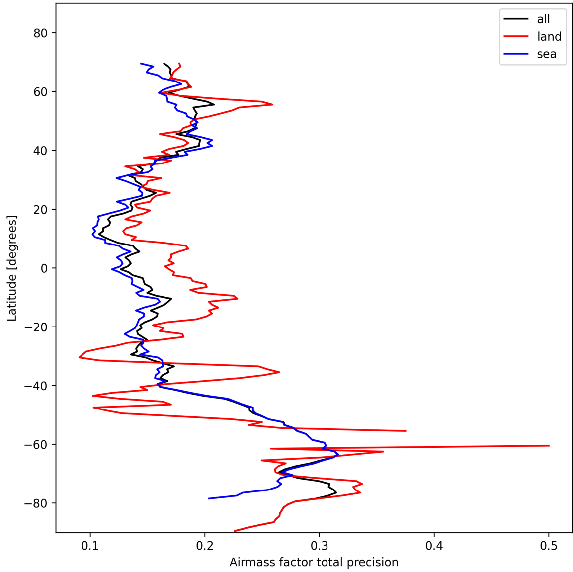
Figure 27: Zonal average of “Airmass factor total precision” for 2025-11-03 to 2025-11-05.
