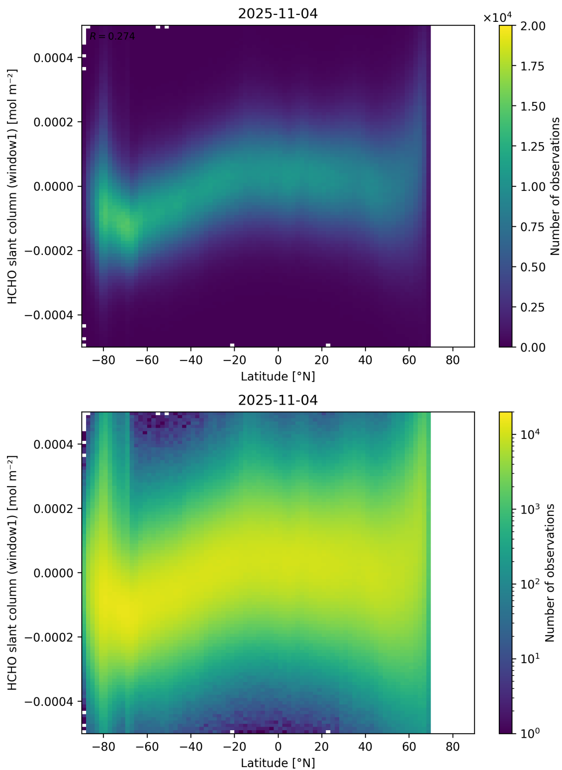
Figure 159: Scatter density plot of “Latitude” against “HCHO slant column (window1)” for 2025-11-03 to 2025-11-05.
