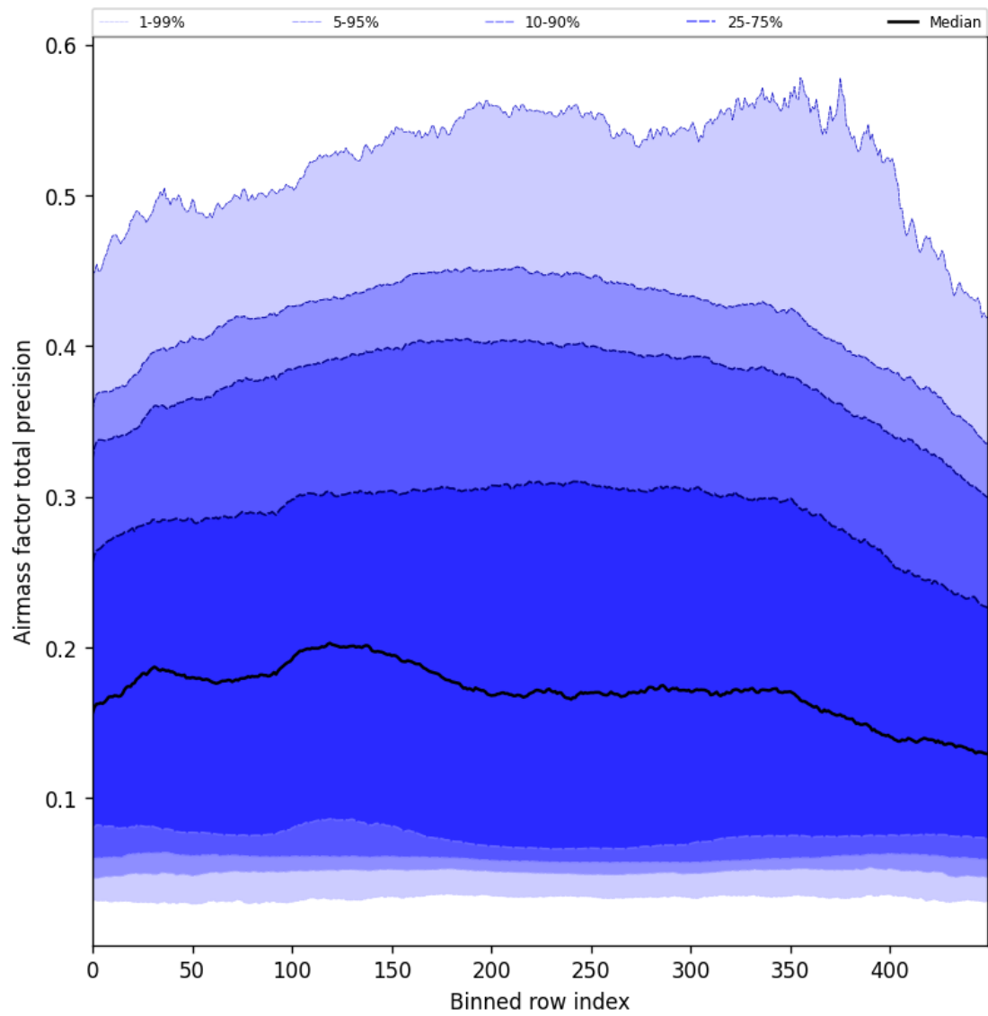
Figure 55: Along track statistics of “Airmass factor total precision” for 2025-11-03 to 2025-11-05
