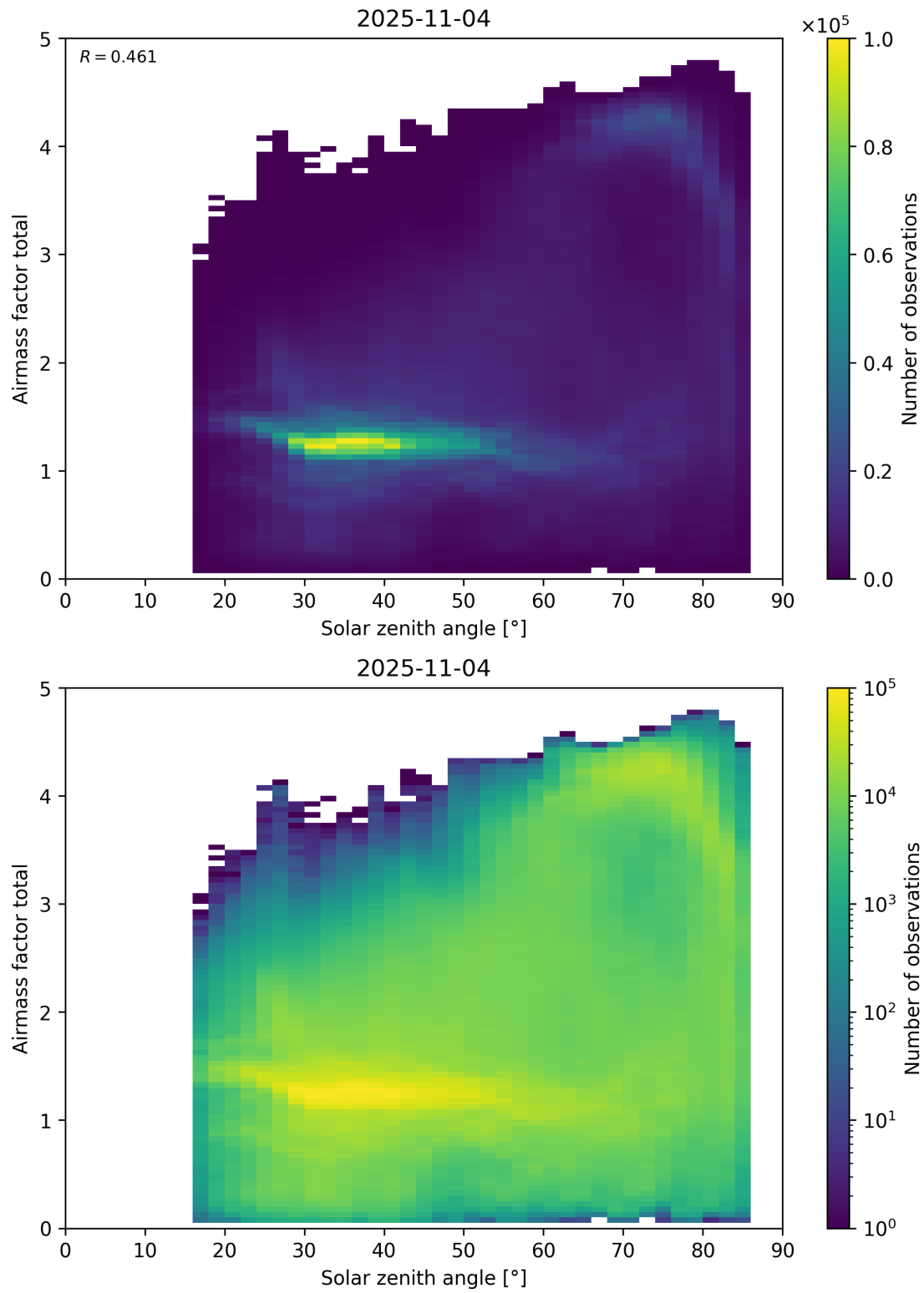
Figure 175: Scatter density plot of “Solar zenith angle” against “Airmass factor total” for 2025-11-03 to 2025-11-05.
