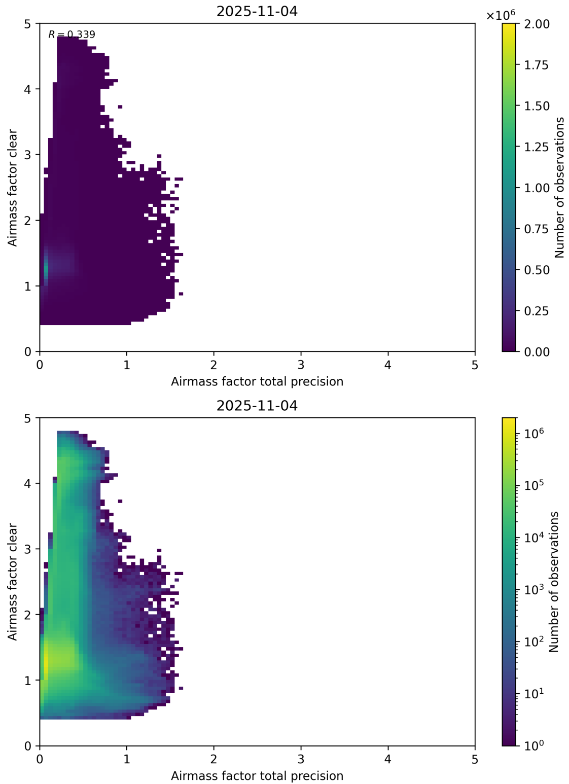
Figure 108: Scatter density plot of “Airmass factor total precision” against “Airmass factor clear” for 2025-11-03 to 2025-11-05.
