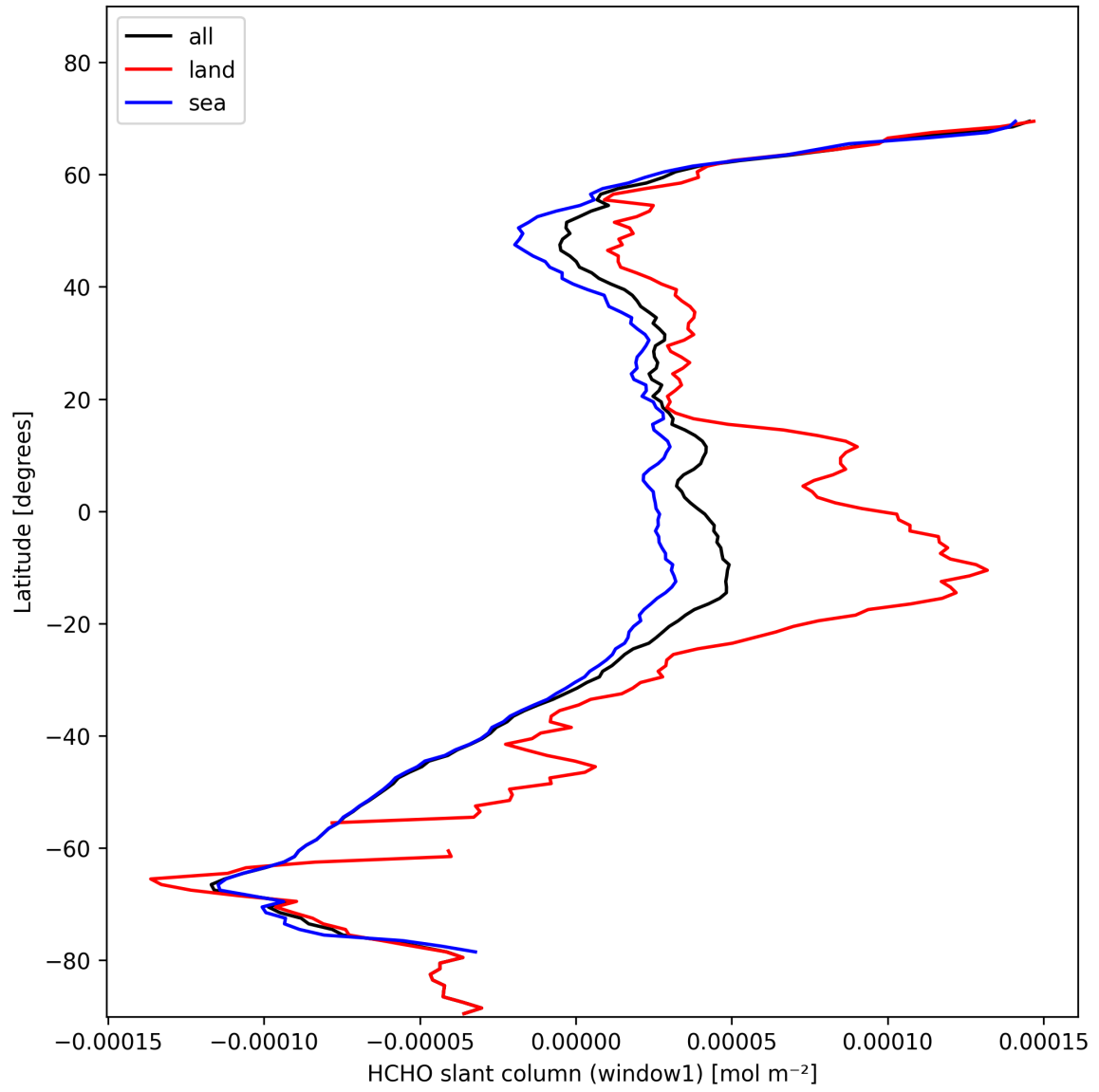
Figure 24: Zonal average of “HCHO slant column (window1)” for 2025-11-03 to 2025-11-05.
