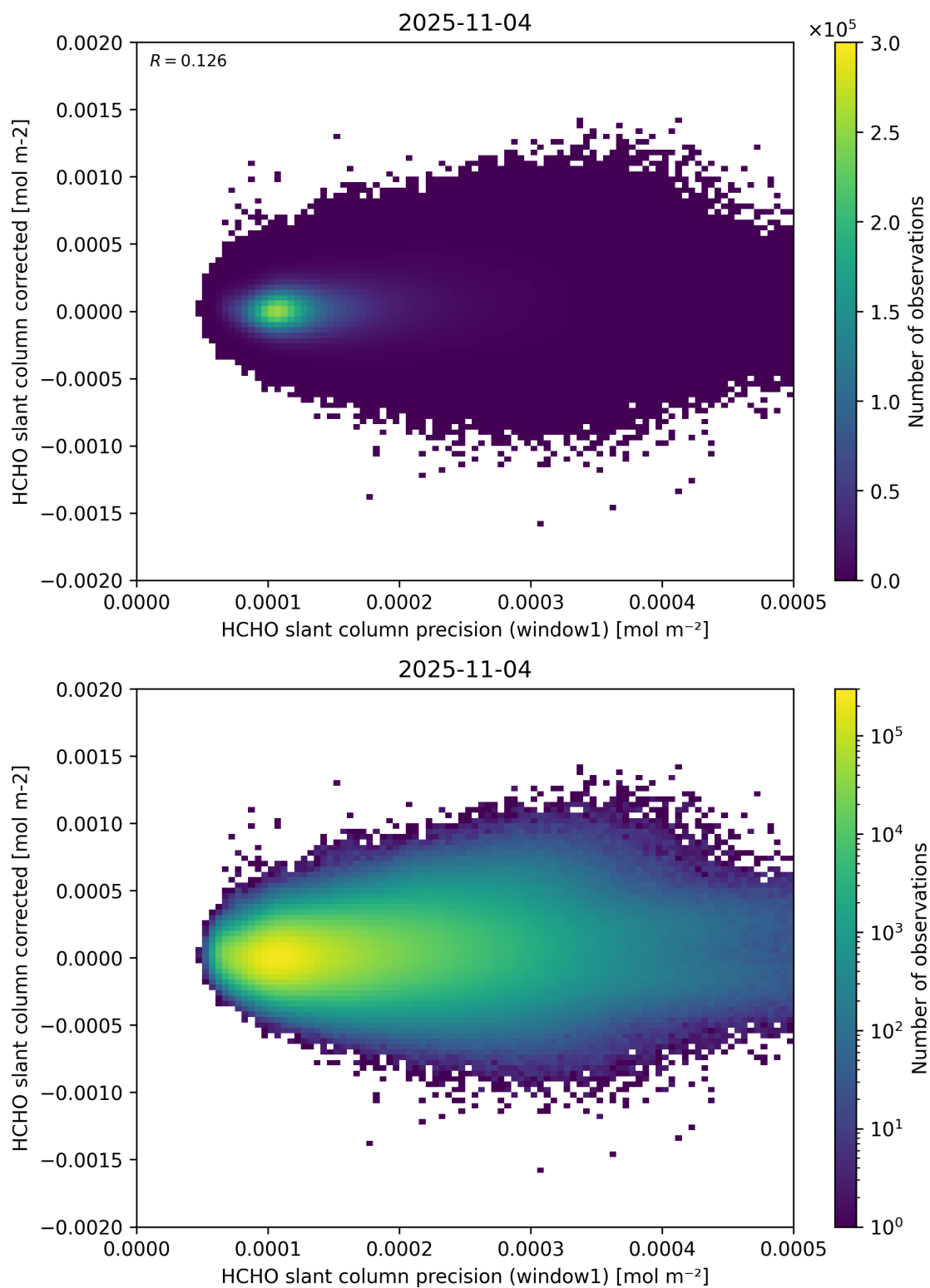
Figure 92: Scatter density plot of “HCHO slant column precision (window1)” against “HCHO slant column corrected” for 2025-11-03 to 2025-11-05.
