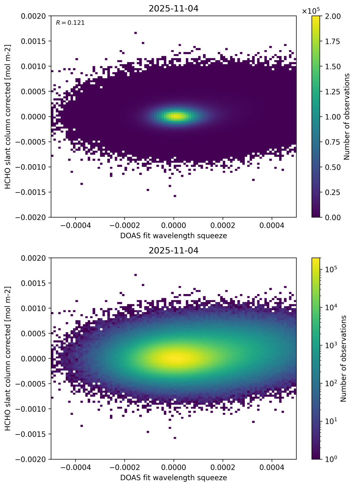
Figure 69: Scatter density plot of “DOAS fit wavelength squeeze” against “HCHO slant column corrected” for 2025-11-03 to 2025-11-05.
