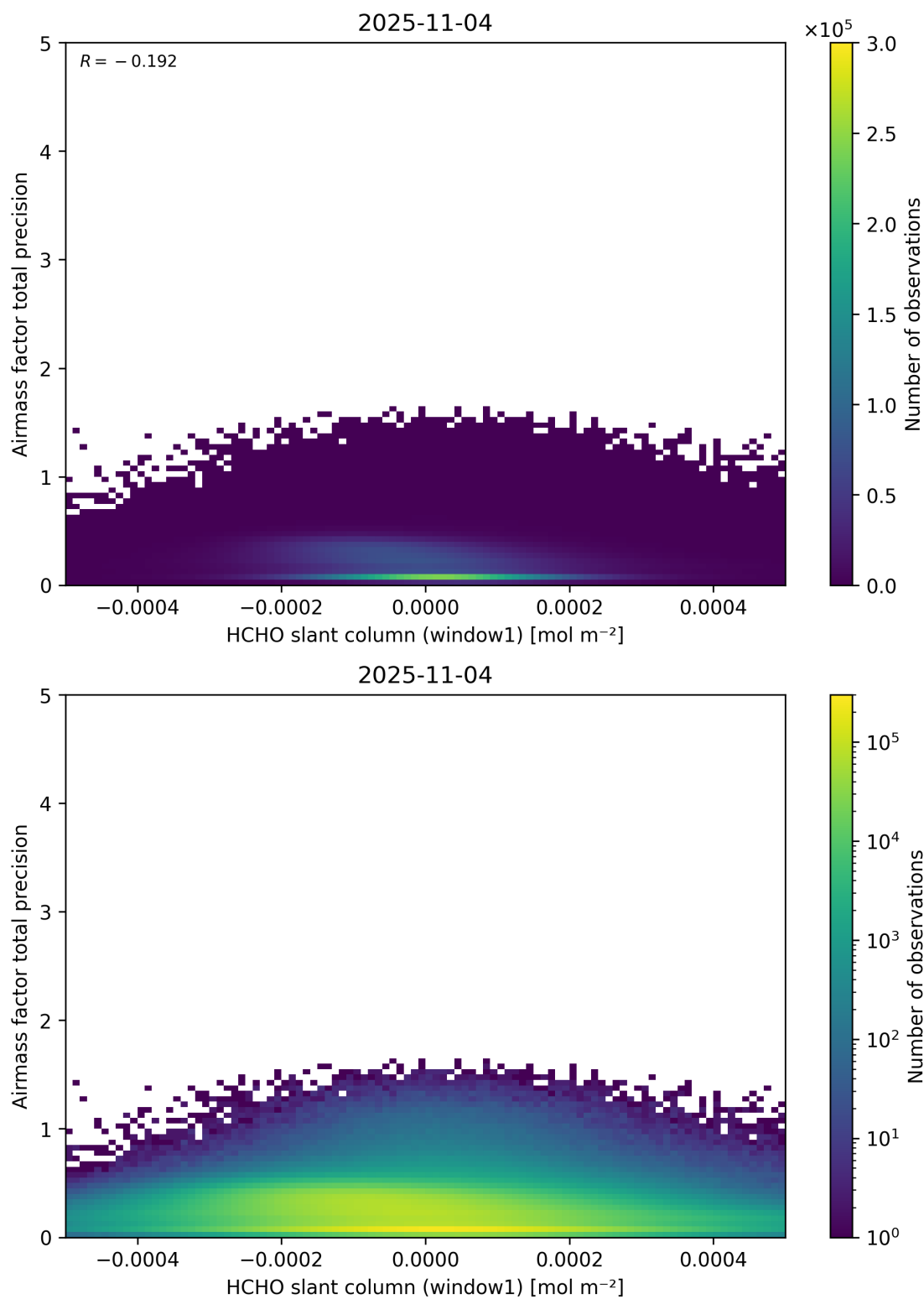
Figure 86: Scatter density plot of “HCHO slant column (window1)” against “Airmass factor total precision” for 2025-11-03 to 2025-11-05.
