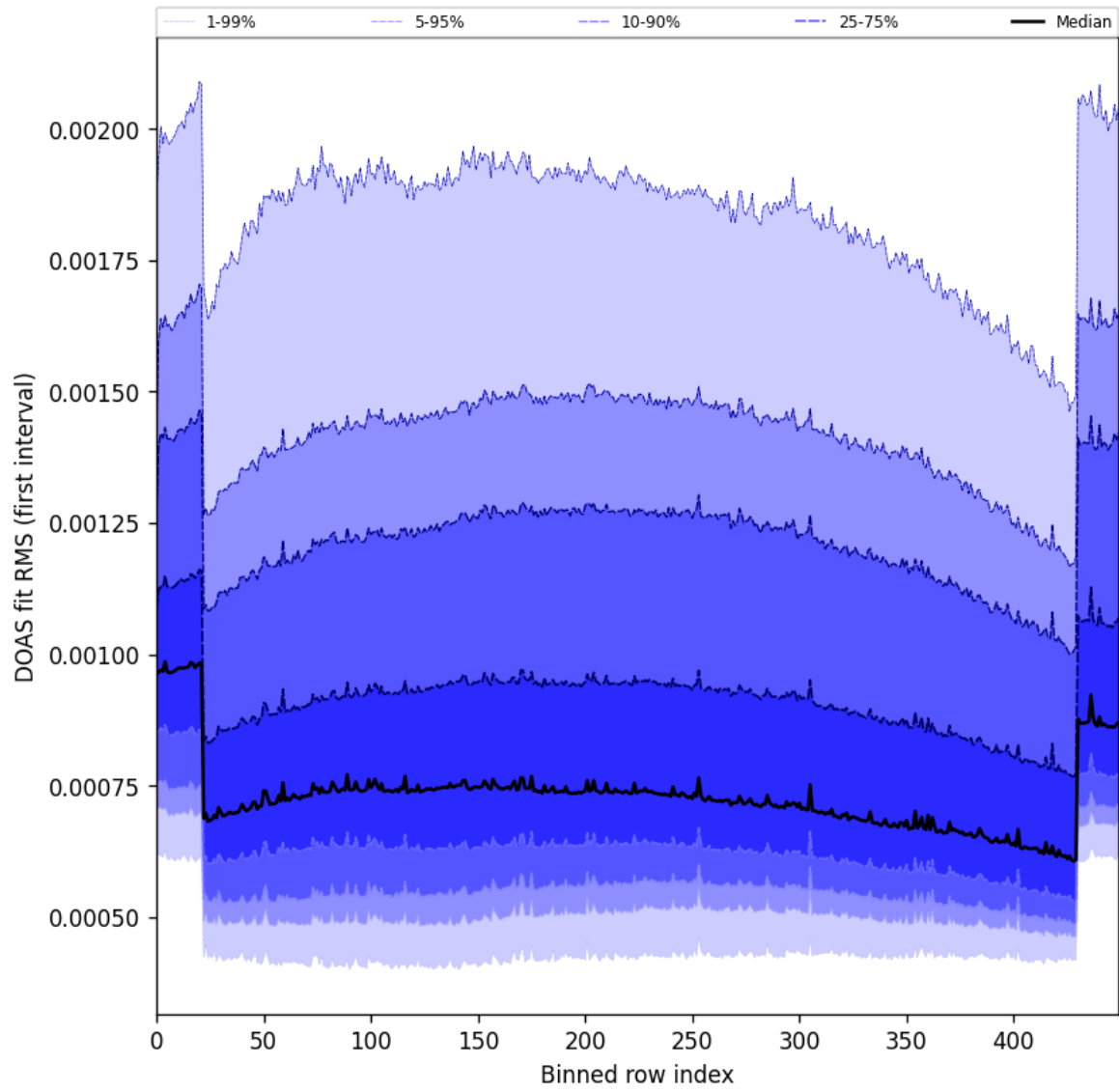
Figure 60: Along track statistics of “DOAS fit RMS (first interval)” for 2025-11-03 to 2025-11-05
