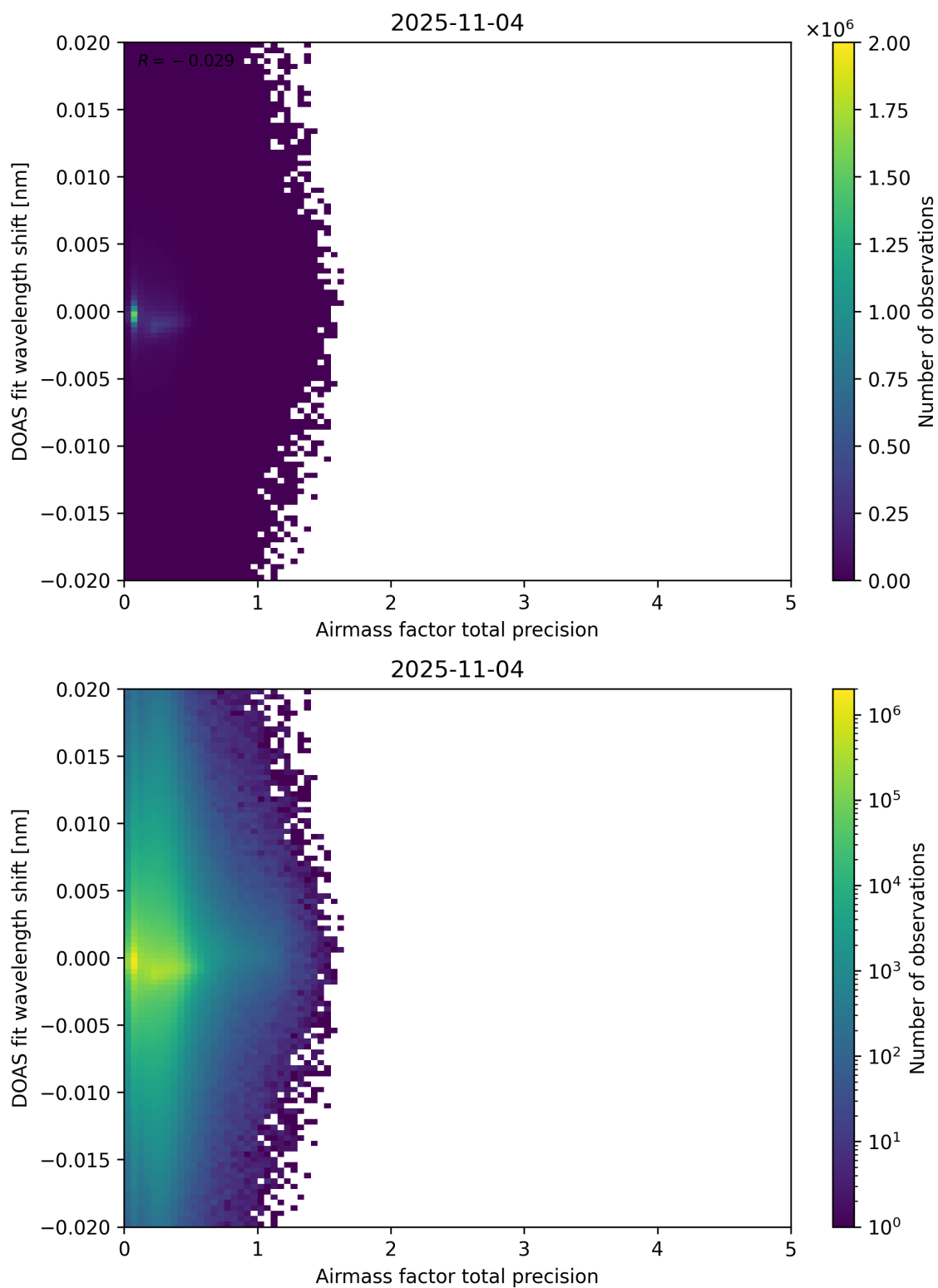
Figure 106: Scatter density plot of “Airmass factor total precision” against “DOAS fit wavelength shift” for 2025-11-03 to 2025-11-05.
