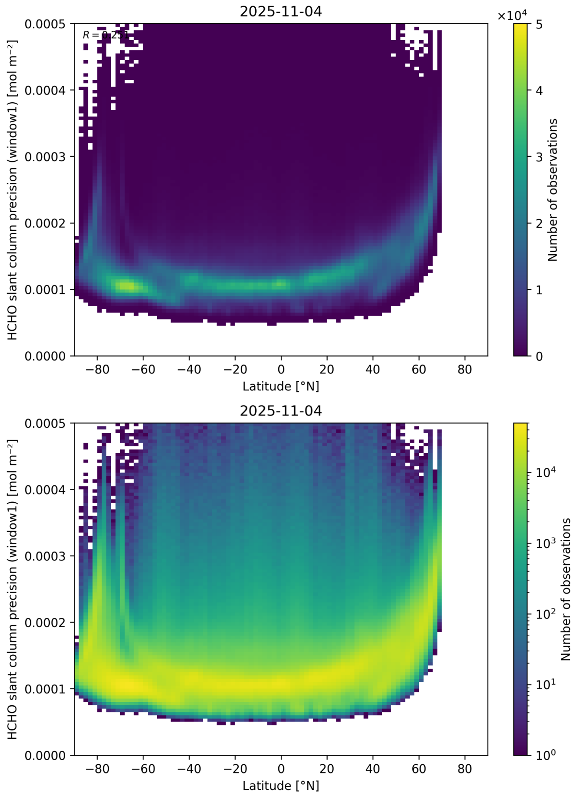
Figure 160: Scatter density plot of “Latitude” against “HCHO slant column precision (window1)” for 2025-11-03 to 2025-11-05.
