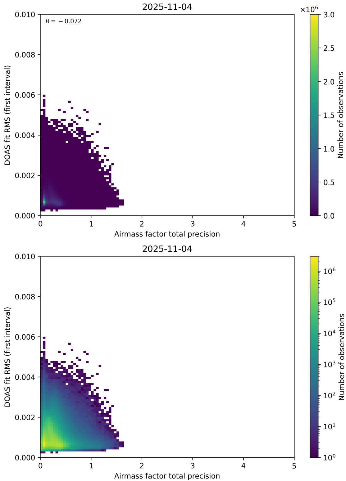
Figure 105: Scatter density plot of “Airmass factor total precision” against “DOAS fit RMS (first interval)” for 2025-11-03 to 2025-11-05.
