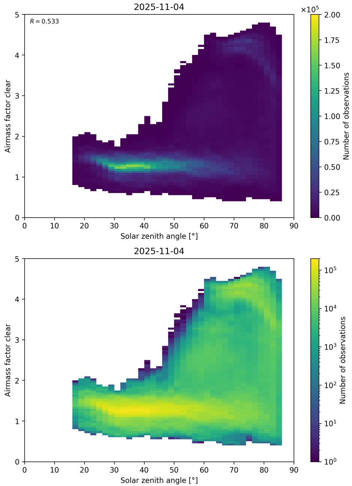
Figure 170: Scatter density plot of “Solar zenith angle” against “Airmass factor clear” for 2025-11-03 to 2025-11-05.
