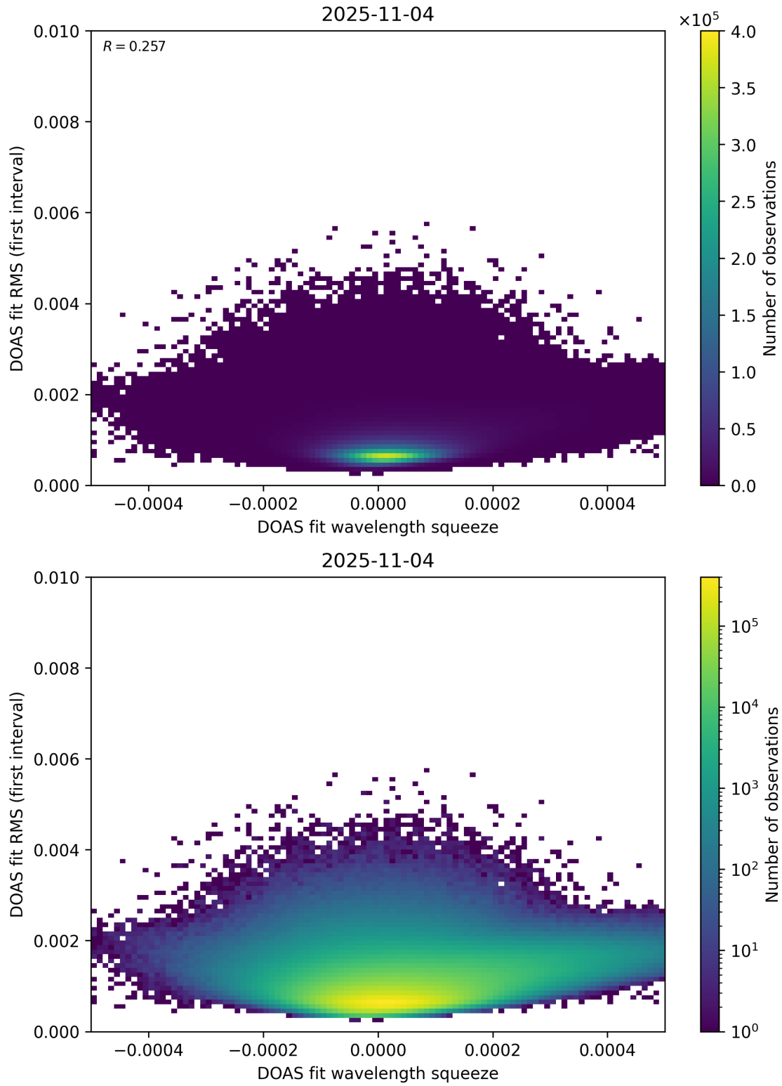
Figure 68: Scatter density plot of “DOAS fit wavelength squeeze” against “DOAS fit RMS (first interval)” for 2025-11-03 to 2025-11-05.
