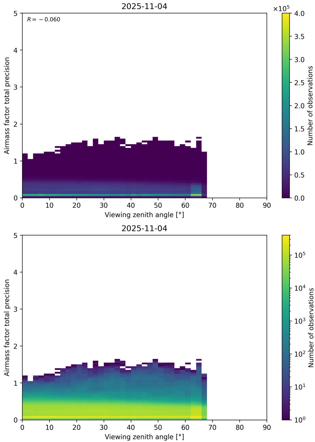
Figure 191: Scatter density plot of “Viewing zenith angle” against “Airmass factor total precision” for 2025-11-03 to 2025-11-05.
