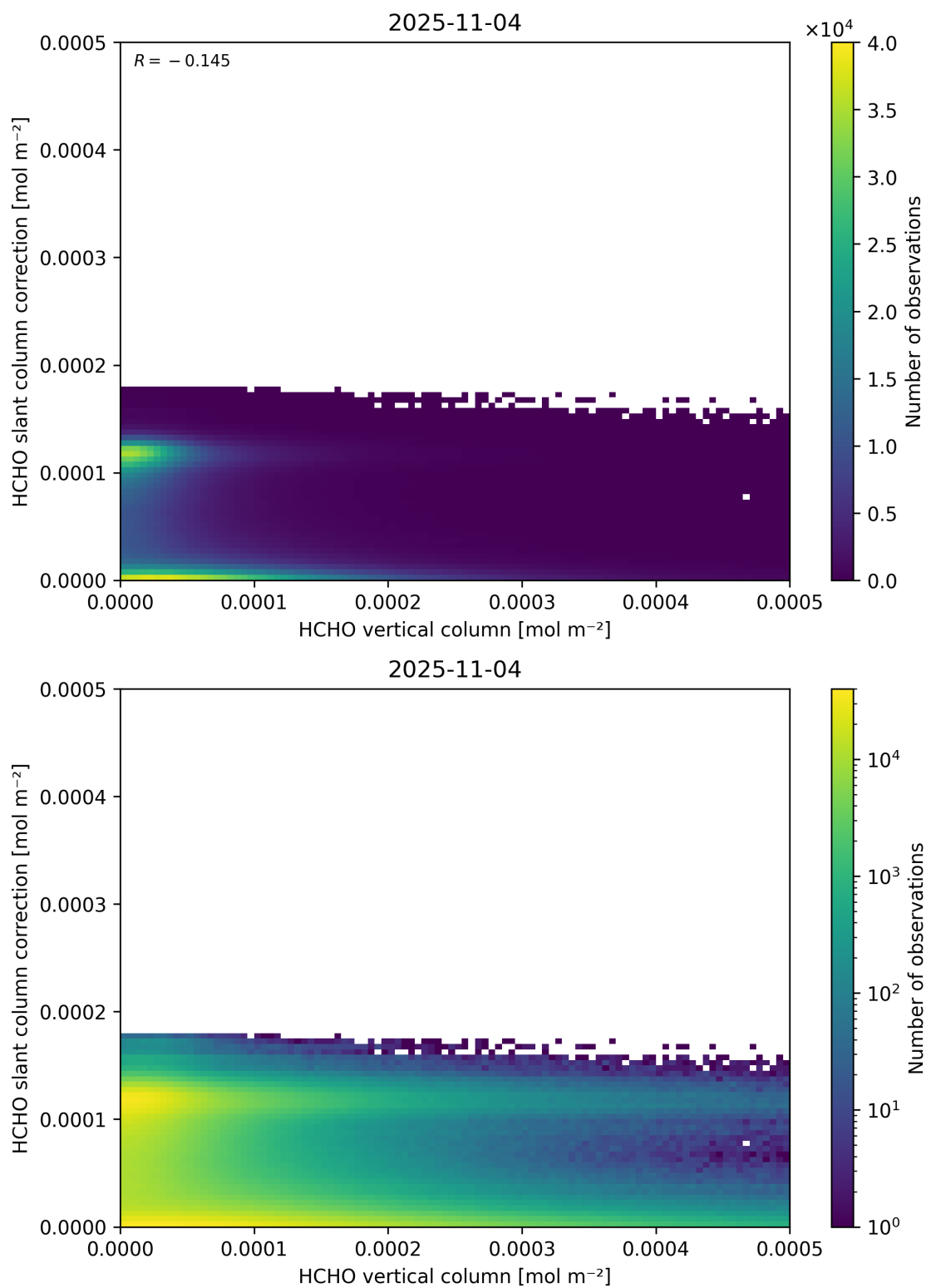
Figure 128: Scatter density plot of “HCHO vertical column” against “HCHO slant column correction” for 2025-11-03 to 2025-11-05.
