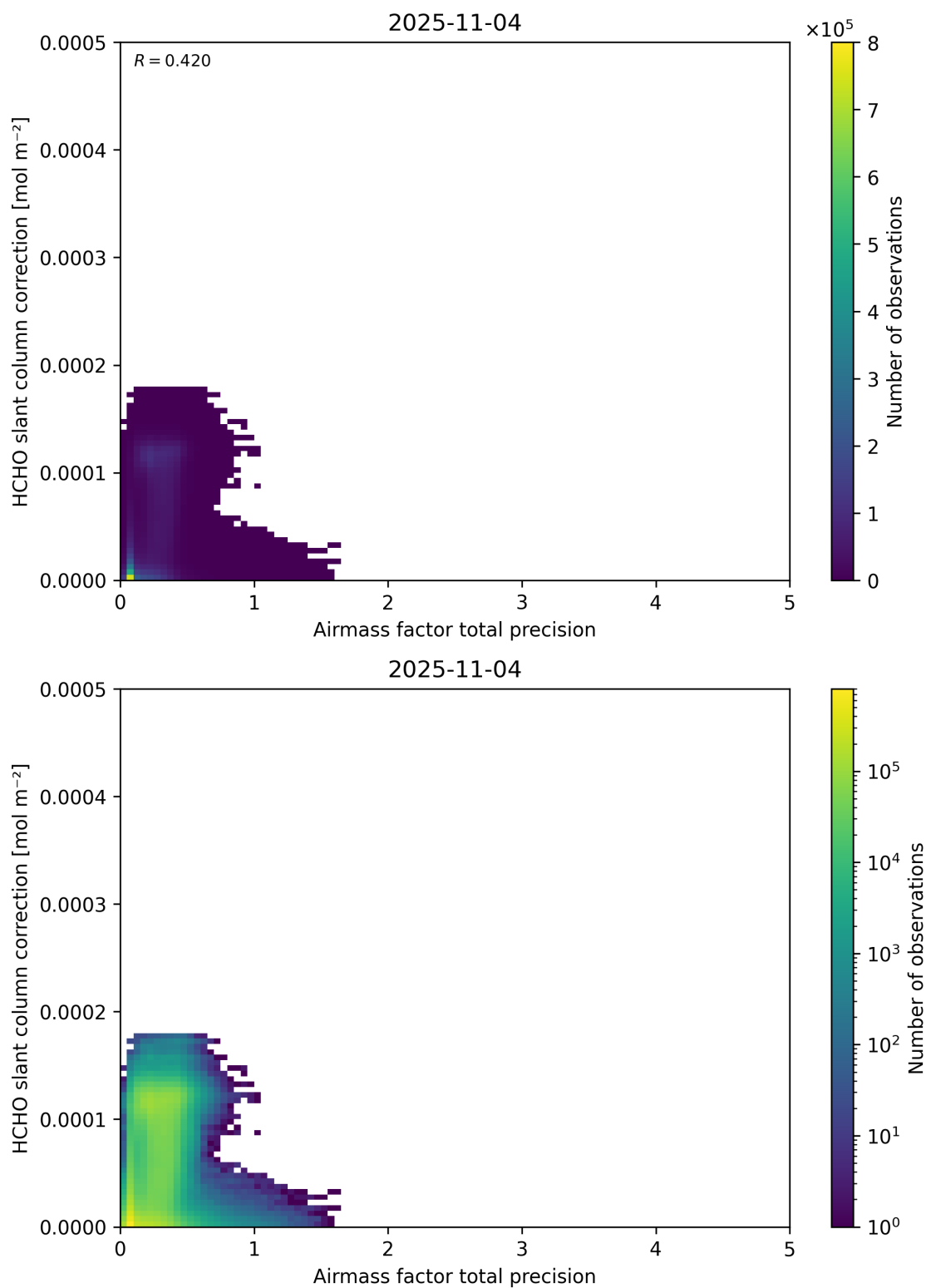
Figure 110: Scatter density plot of “Airmass factor total precision” against “HCHO slant column correction” for 2025-11-03 to 2025-11-05.
