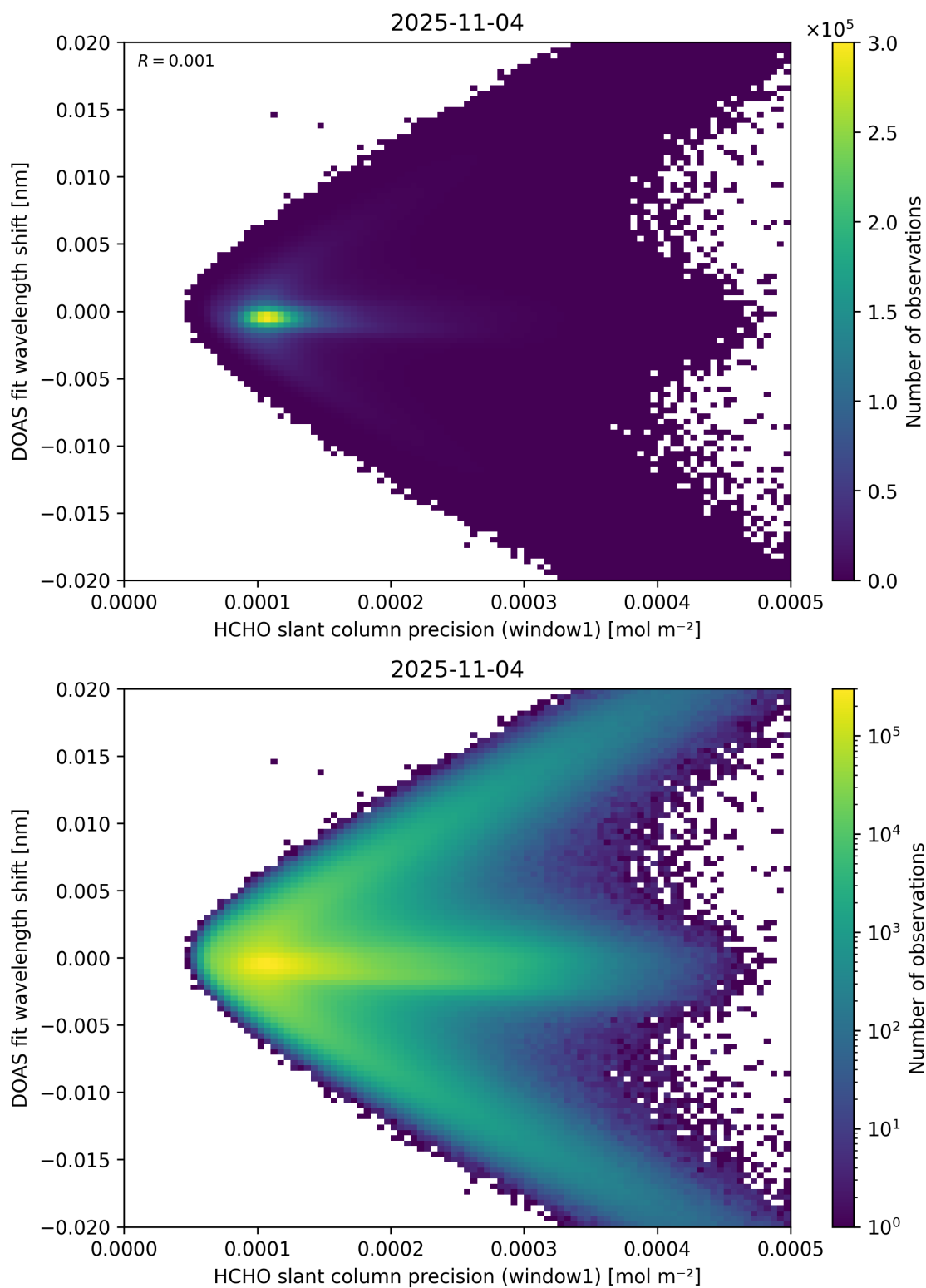
Figure 89: Scatter density plot of “HCHO slant column precision (window1)” against “DOAS fit wavelength shift” for 2025-11-03 to 2025-11-05.
