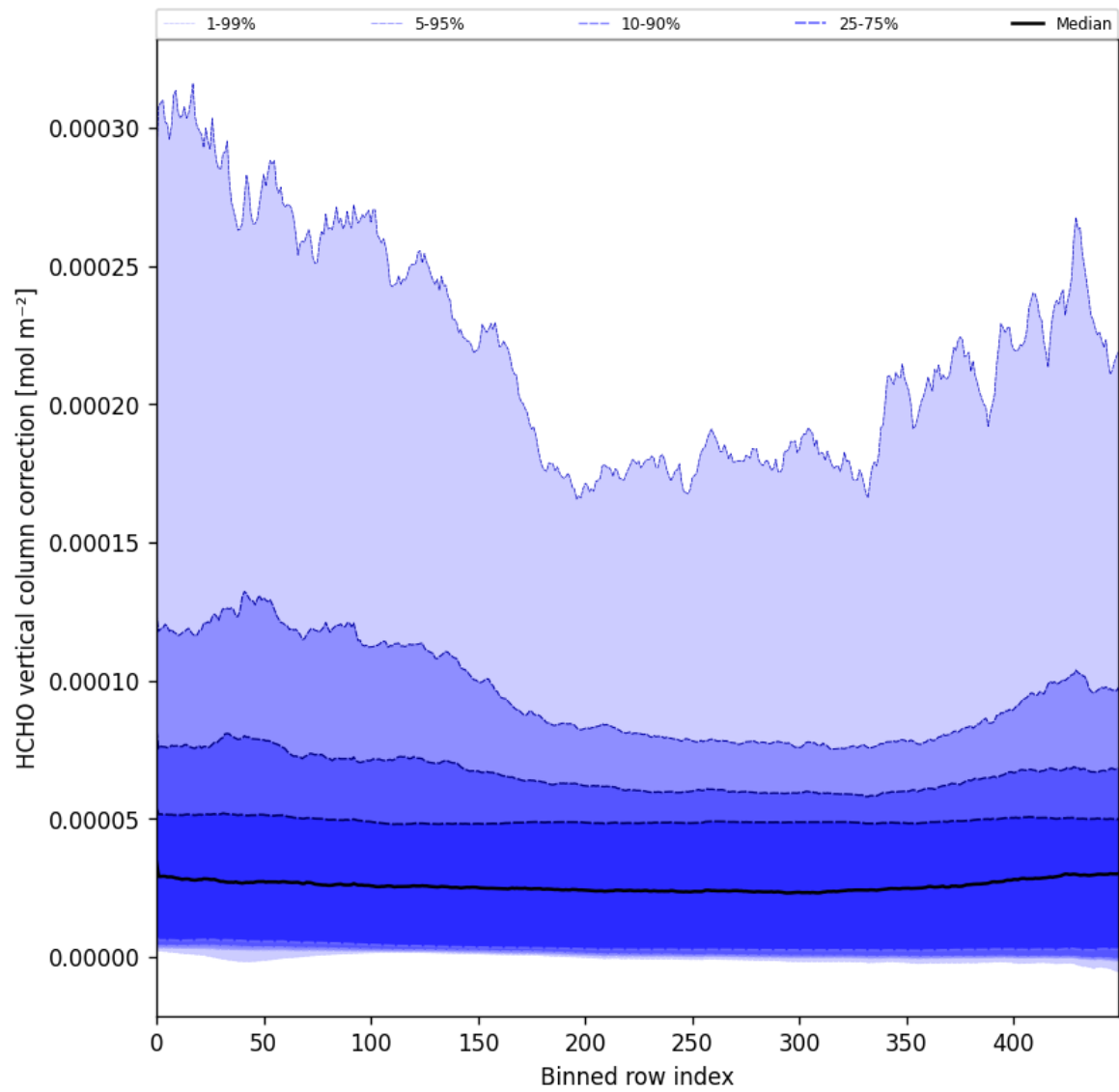
Figure 51: Along track statistics of “HCHO vertical column correction” for 2025-11-03 to 2025-11-05
