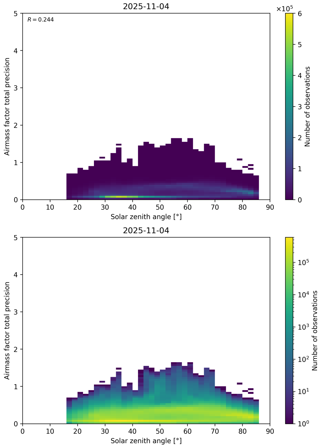
Figure 176: Scatter density plot of “Solar zenith angle” against “Airmass factor total precision” for 2025-11-03 to 2025-11-05.
