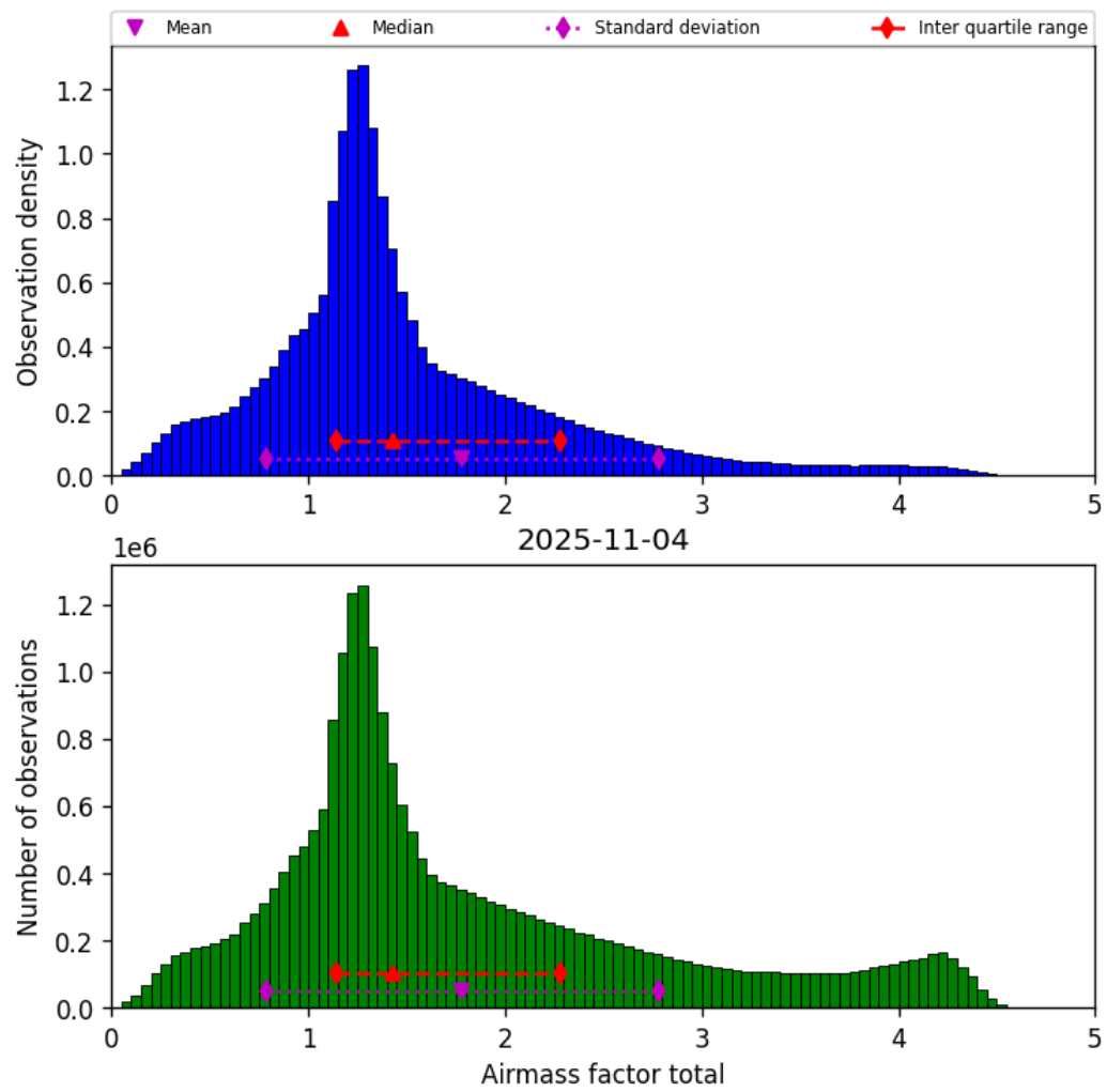
Figure 40: Histogram of “Airmass factor total” for 2025-11-03 to 2025-11-05
