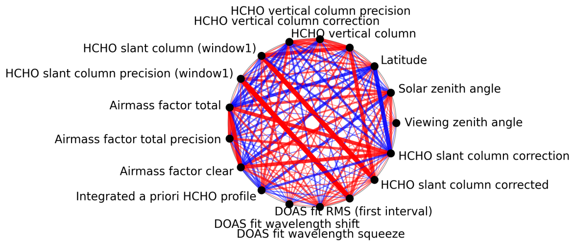
Figure 1: Map of correlation graph for 2025-11-03 to 2025-11-05.
