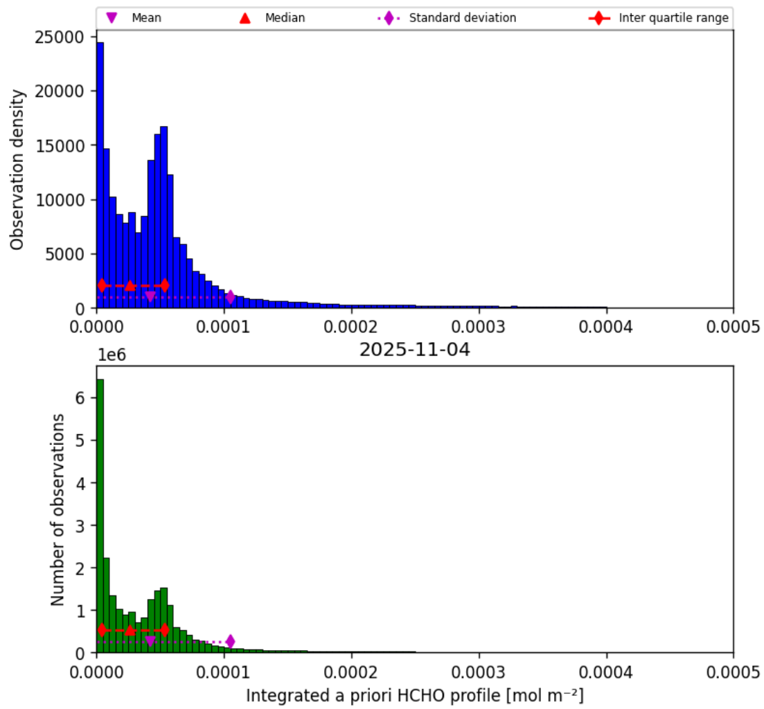
Figure 43: Histogram of “Integrated a priori HCHO profile” for 2025-11-03 to 2025-11-05
