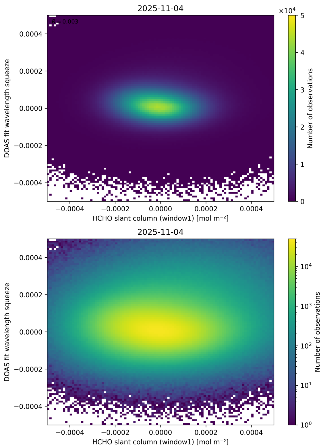
Figure 80: Scatter density plot of “HCHO slant column (window1)” against “DOAS fit wavelength squeeze” for 2025-11-03 to 2025-11-05.
