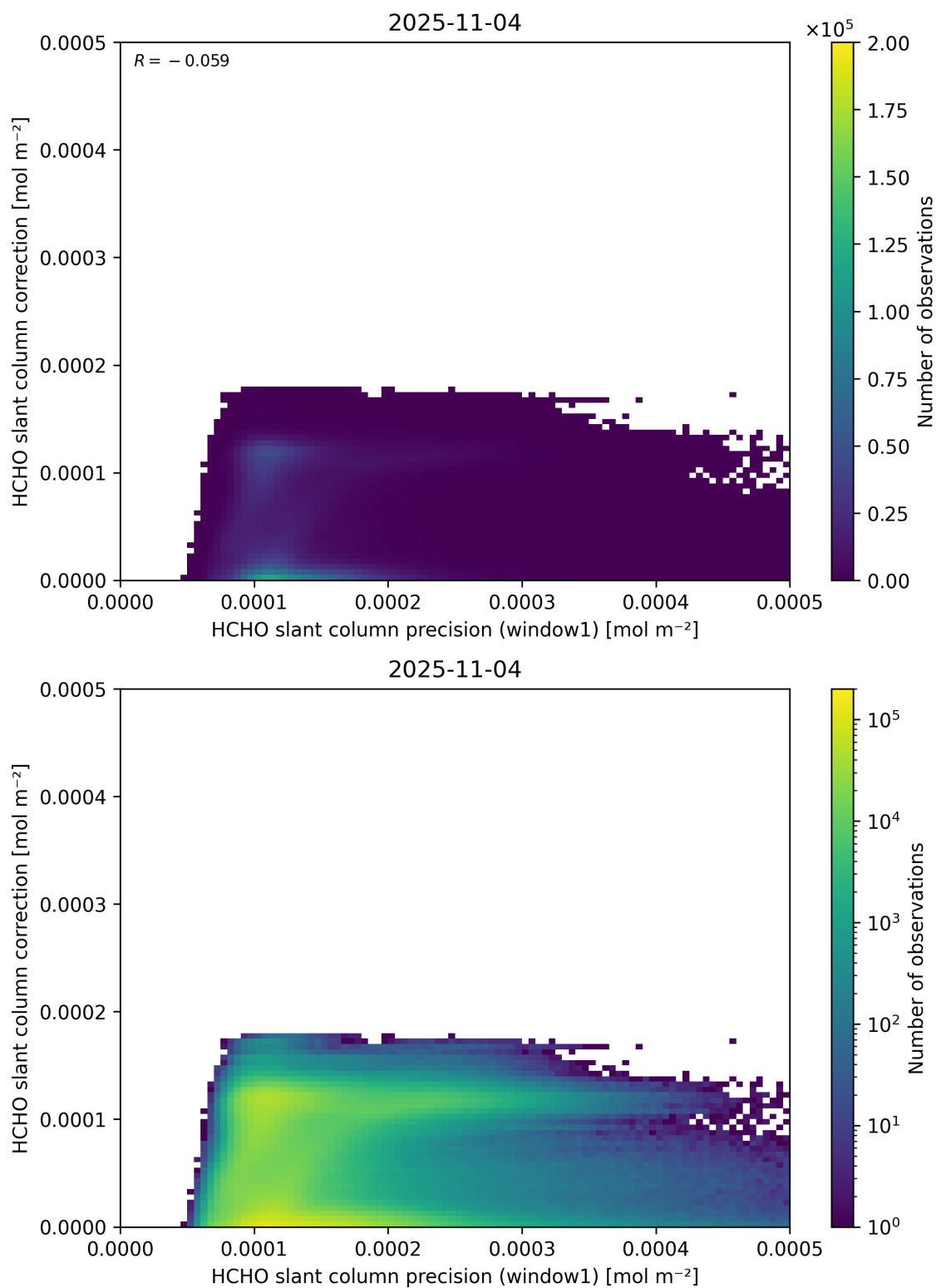
Figure 93: Scatter density plot of “HCHO slant column precision (window1)” against “HCHO slant column correction” for 2025-11-03 to 2025-11-05.
