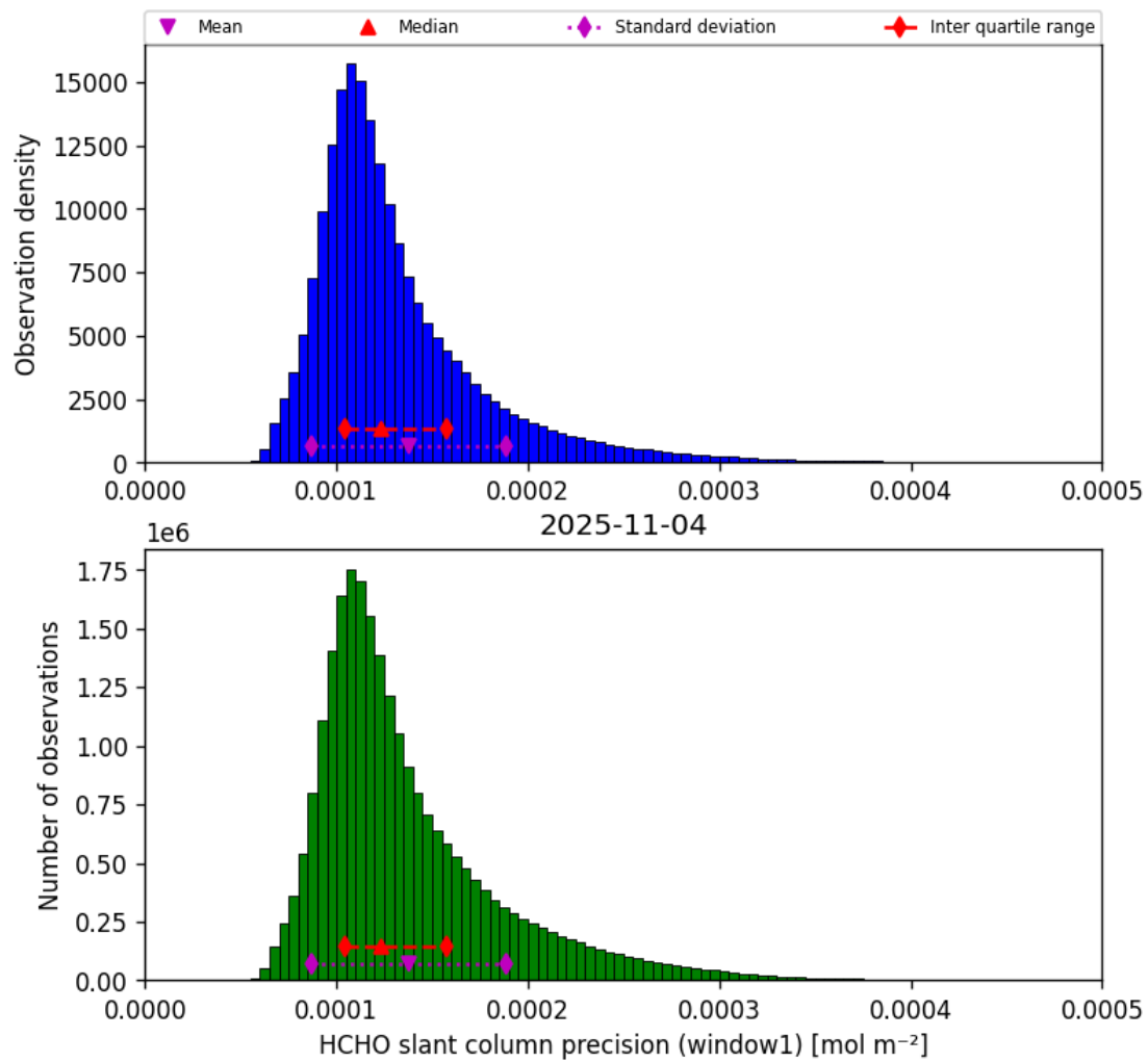
Figure 39: Histogram of “HCHO slant column precision (window1)” for 2025-11-03 to 2025-11-05
