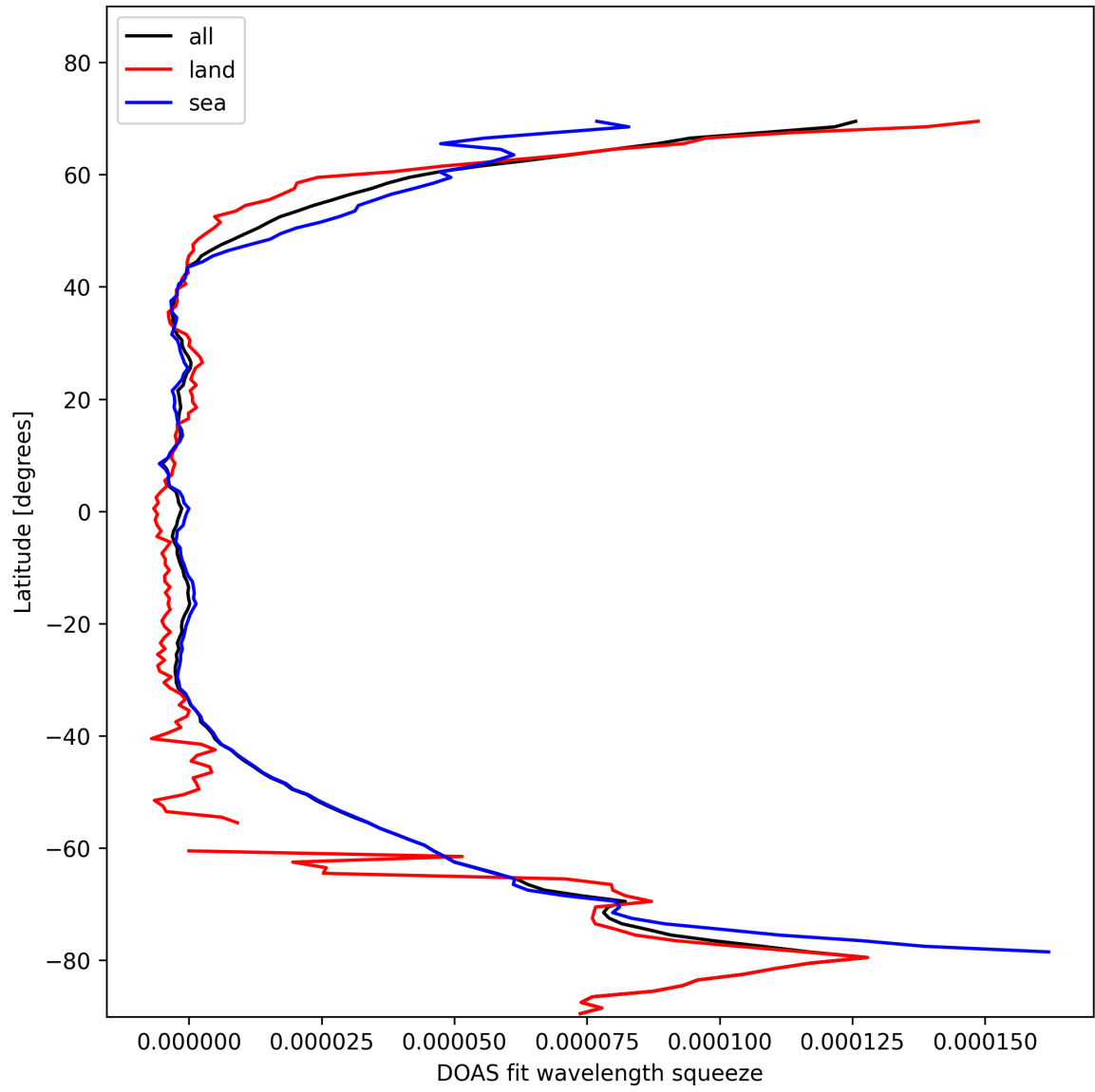
Figure 31: Zonal average of “DOAS fit wavelength squeeze” for 2025-11-03 to 2025-11-05.
