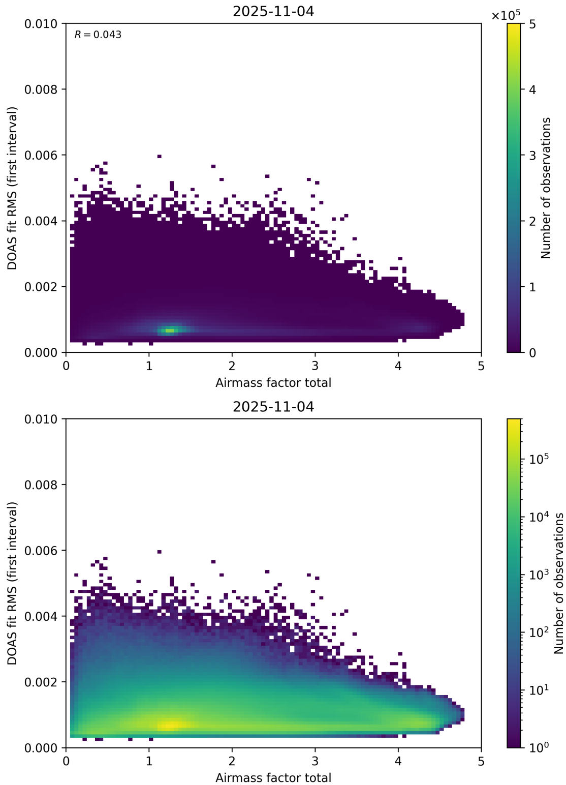
Figure 97: Scatter density plot of “Airmass factor total” against “DOAS fit RMS (first interval)” for 2025-11-03 to 2025-11-05.
