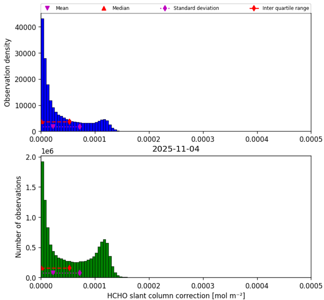
Figure 47: Histogram of “HCHO slant column correction” for 2025-11-03 to 2025-11-05
