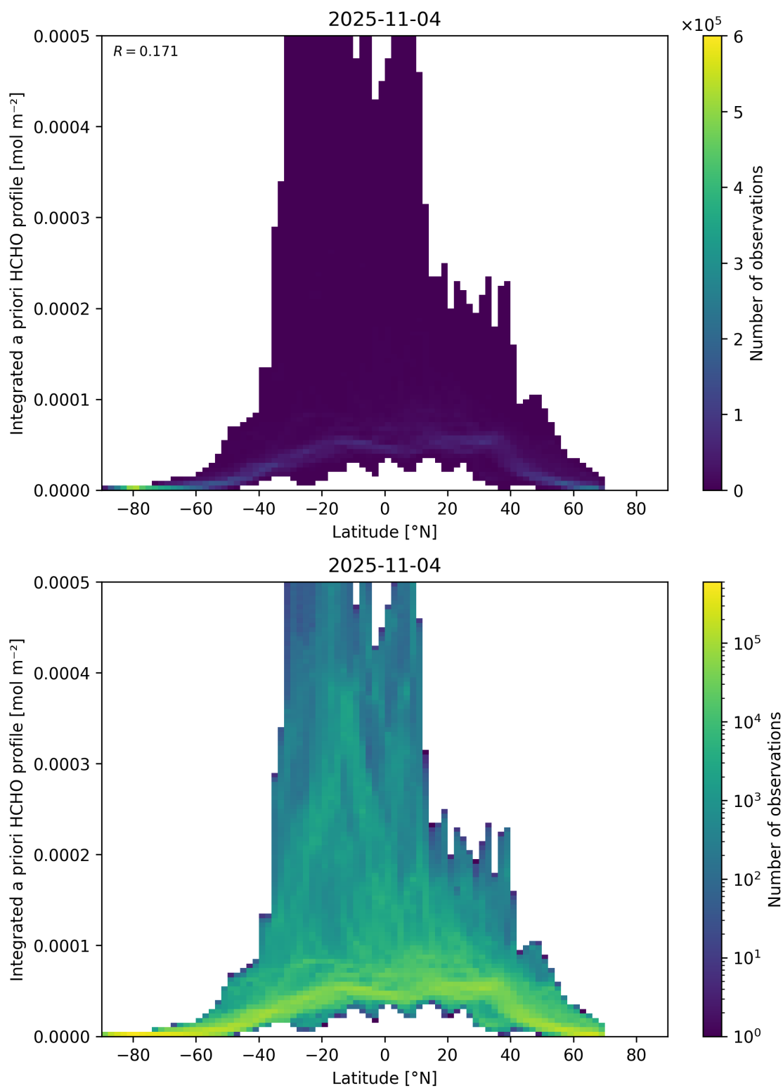
Figure 166: Scatter density plot of “Latitude” against “Integrated a priori HCHO profile” for 2025-11-03 to 2025-11-05.
