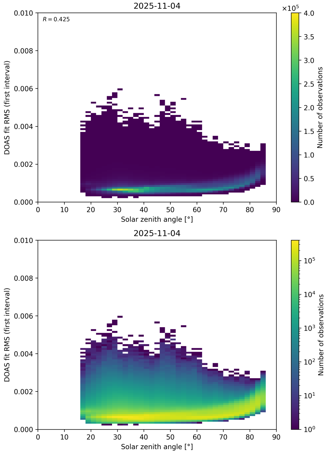
Figure 167: Scatter density plot of “Solar zenith angle” against “DOAS fit RMS (first interval)” for 2025-11-03 to 2025-11-05.
