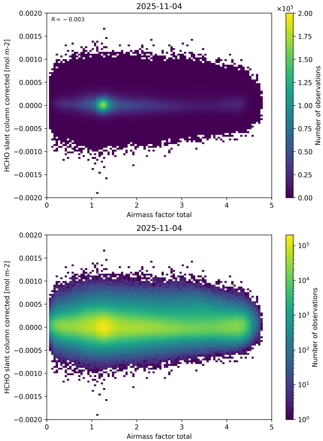
Figure 101: Scatter density plot of “Airmass factor total” against “HCHO slant column corrected” for 2025-11-03 to 2025-11-05.
