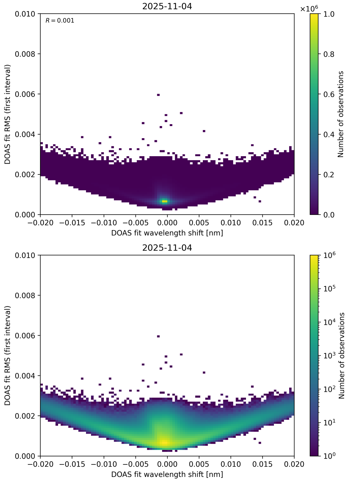
Figure 64: Scatter density plot of “DOAS fit wavelength shift” against “DOAS fit RMS (first interval)” for 2025-11-03 to 2025-11-05.
