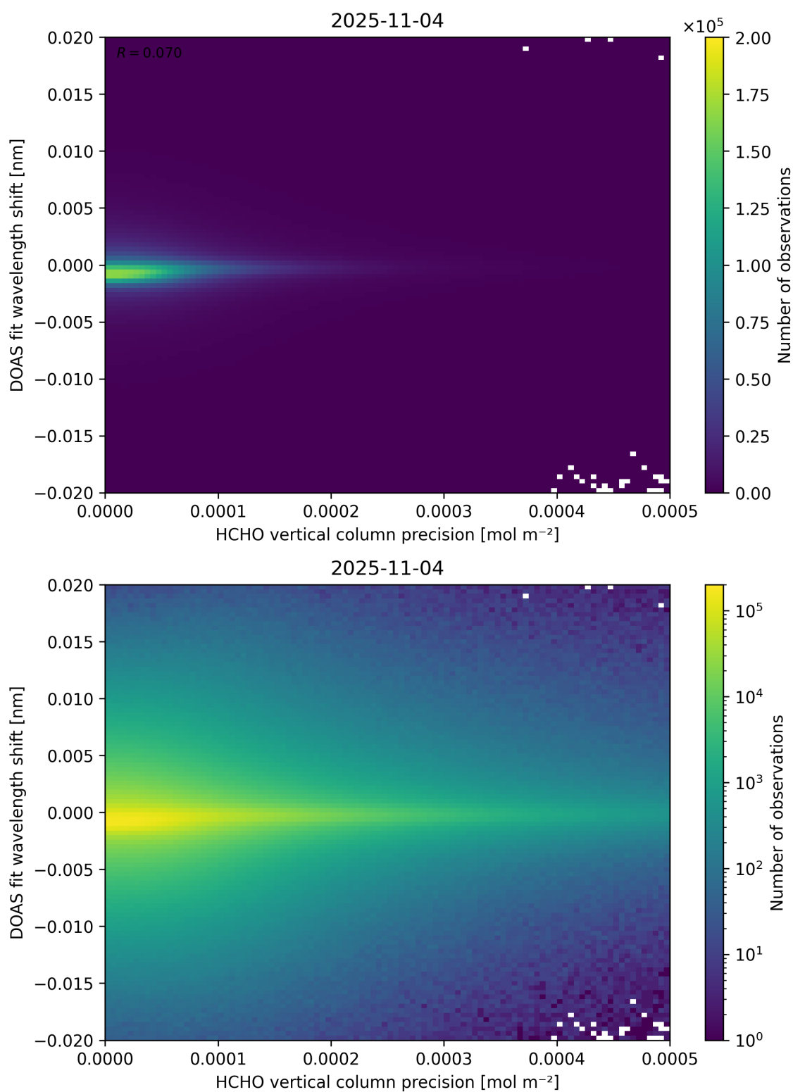
Figure 137: Scatter density plot of “HCHO vertical column precision” against “DOAS fit wavelength shift” for 2025-11-03 to 2025-11-05.
