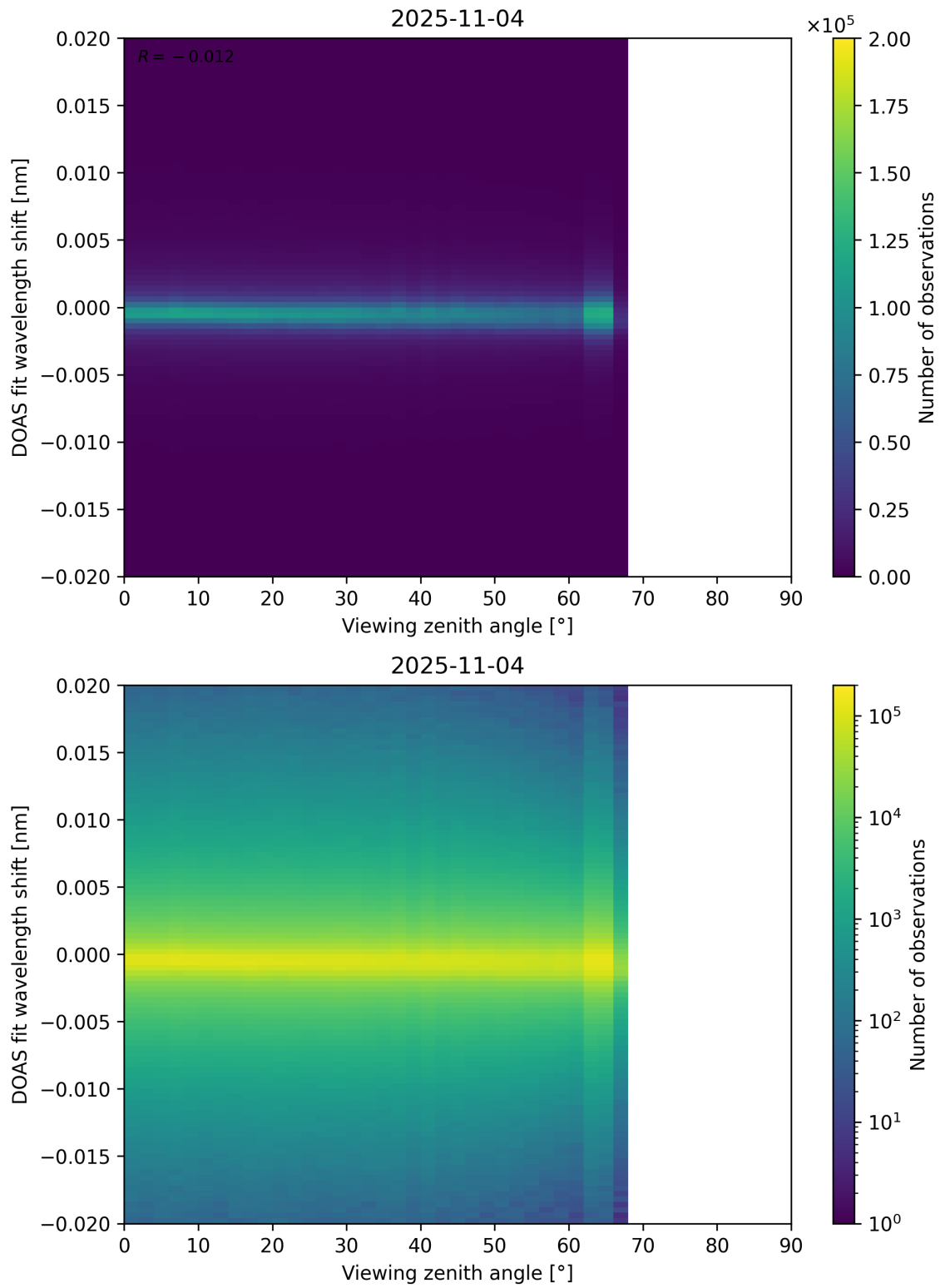
Figure 183: Scatter density plot of “Viewing zenith angle” against “DOAS fit wavelength shift” for 2025-11-03 to 2025-11-05.
