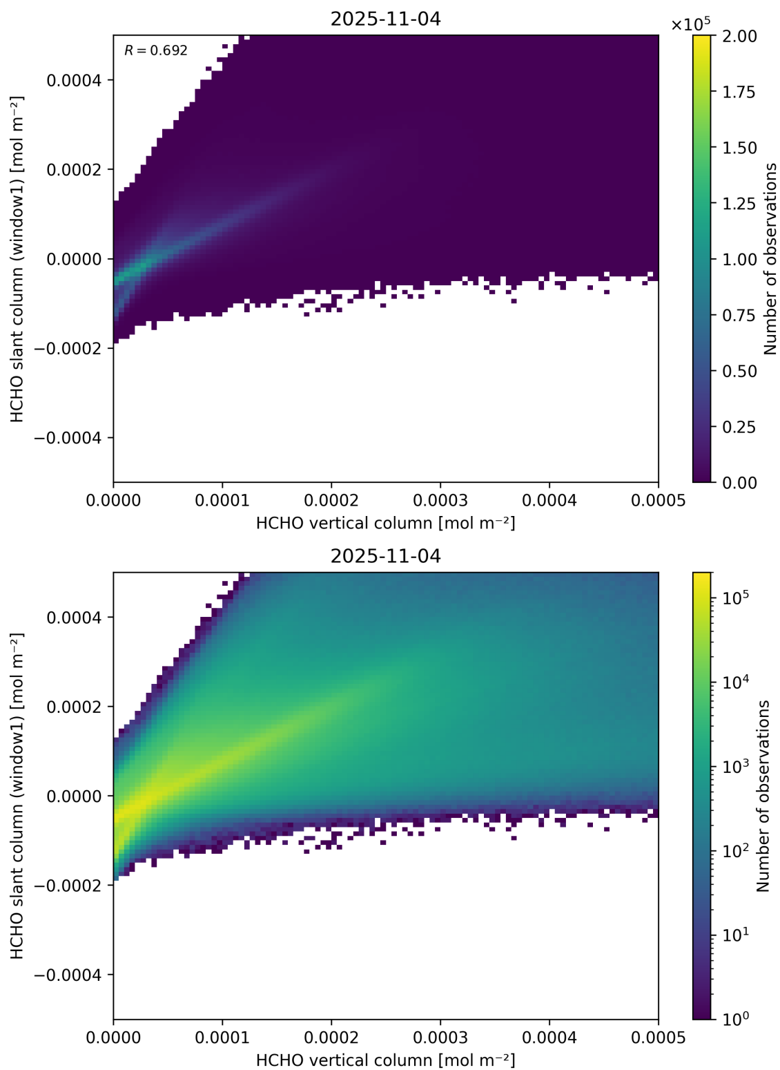
Figure 129: Scatter density plot of “HCHO vertical column” against “HCHO slant column (window1)” for 2025-11-03 to 2025-11-05.
