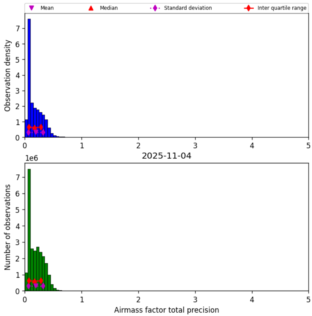
Figure 41: Histogram of “Airmass factor total precision” for 2025-11-03 to 2025-11-05
