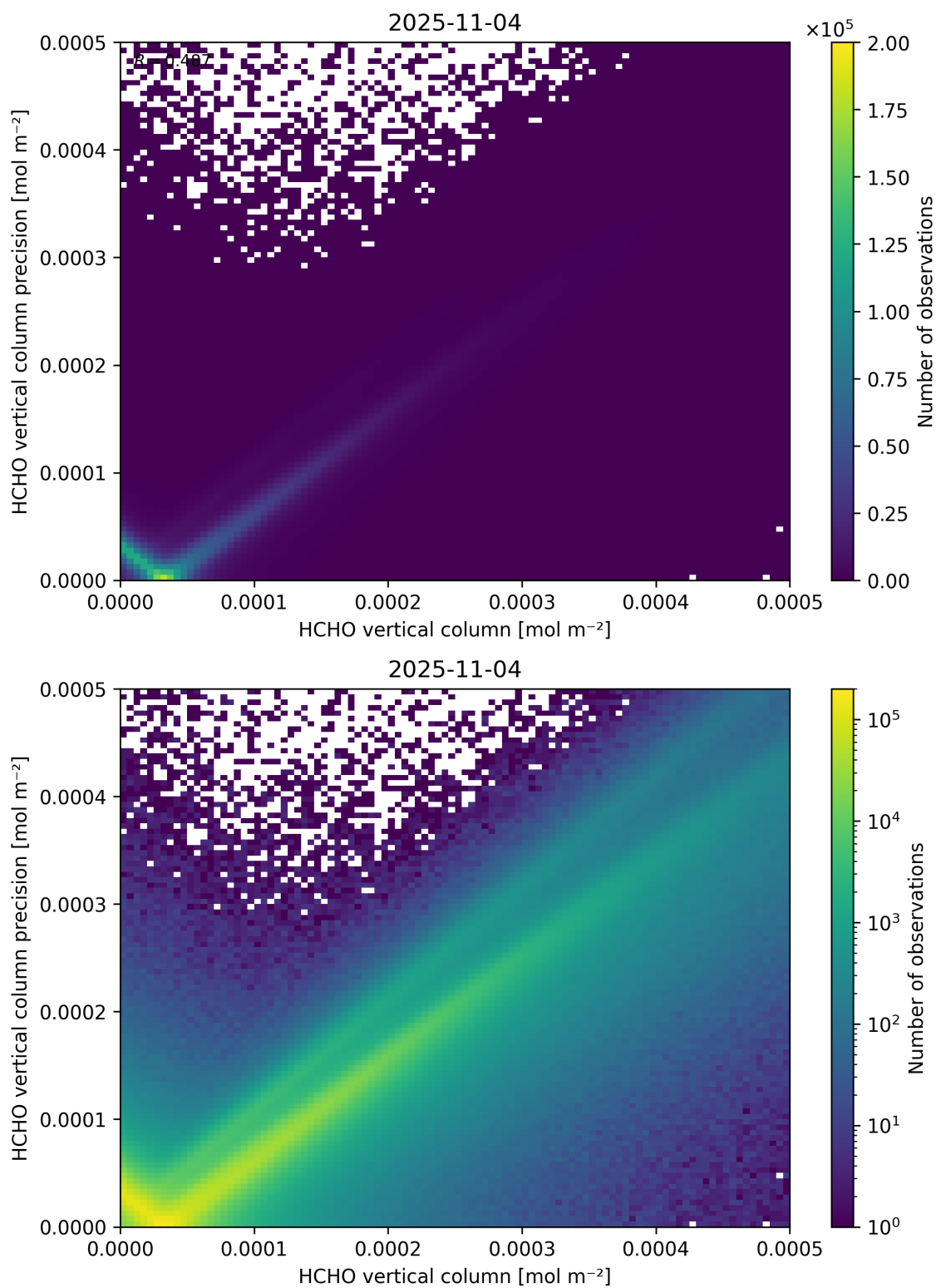
Figure 134: Scatter density plot of “HCHO vertical column” against “HCHO vertical column precision” for 2025-11-03 to 2025-11-05.
