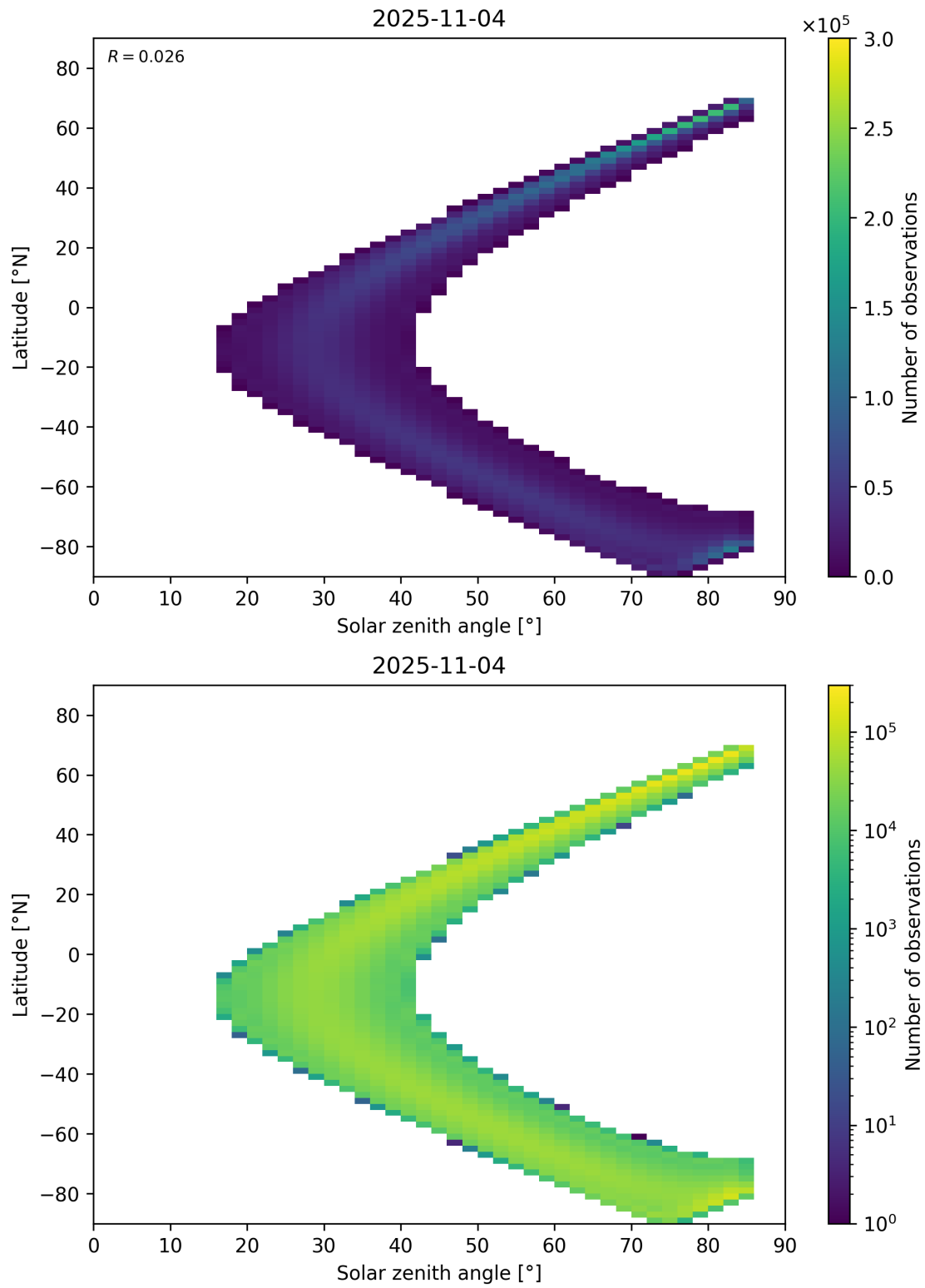
Figure 181: Scatter density plot of “Solar zenith angle” against “Latitude” for 2025-11-03 to 2025-11-05.
