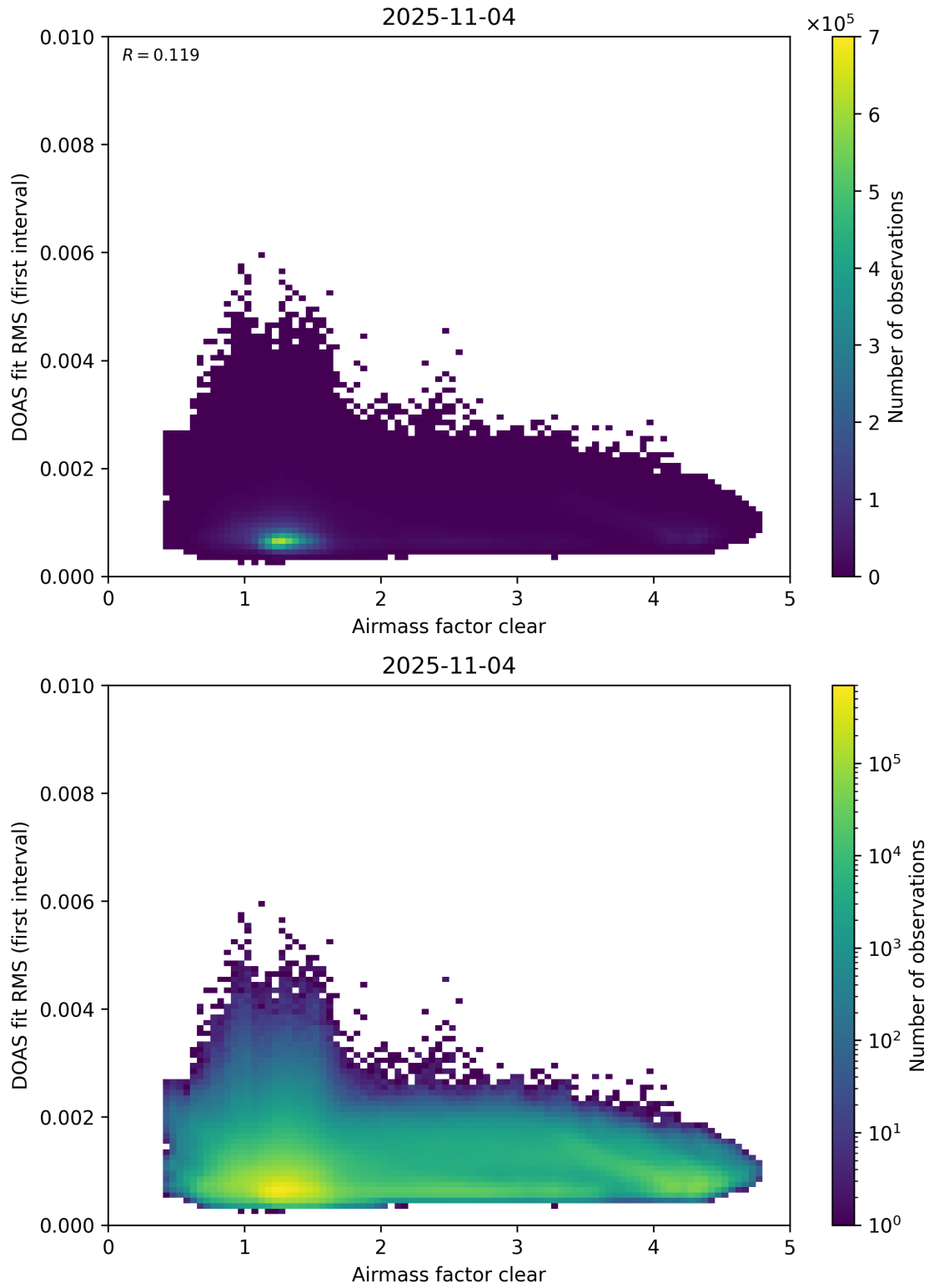
Figure 71: Scatter density plot of “Airmass factor clear” against “DOAS fit RMS (first interval)” for 2025-11-03 to 2025-11-05.
