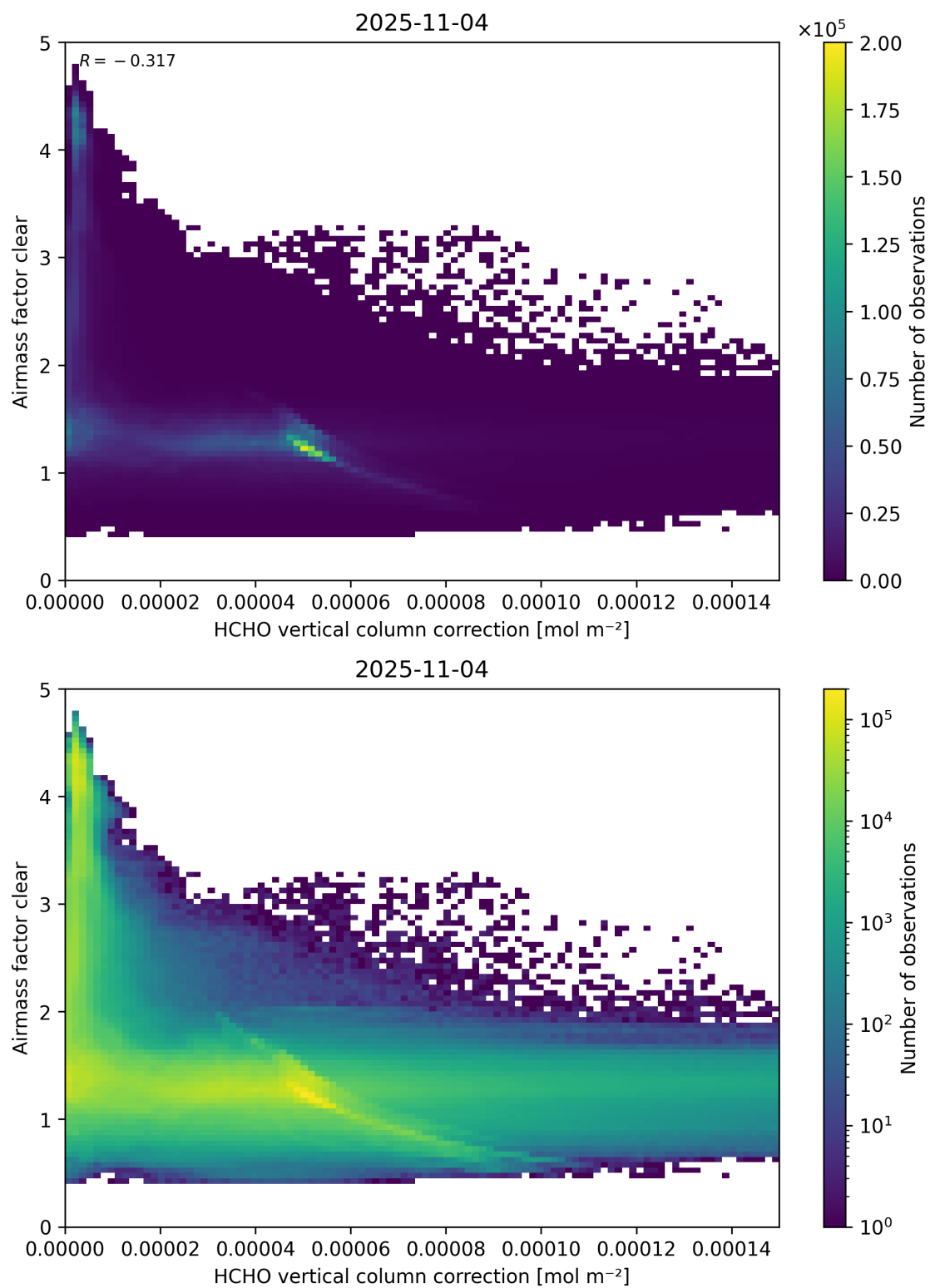
Figure 115: Scatter density plot of “HCHO vertical column correction” against “Airmass factor clear” for 2025-11-03 to 2025-11-05.
