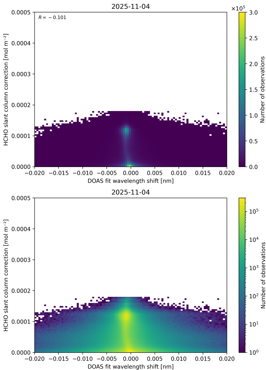
Figure 67: Scatter density plot of “DOAS fit wavelength shift” against “HCHO slant column correction” for 2025-11-03 to 2025-11-05.
