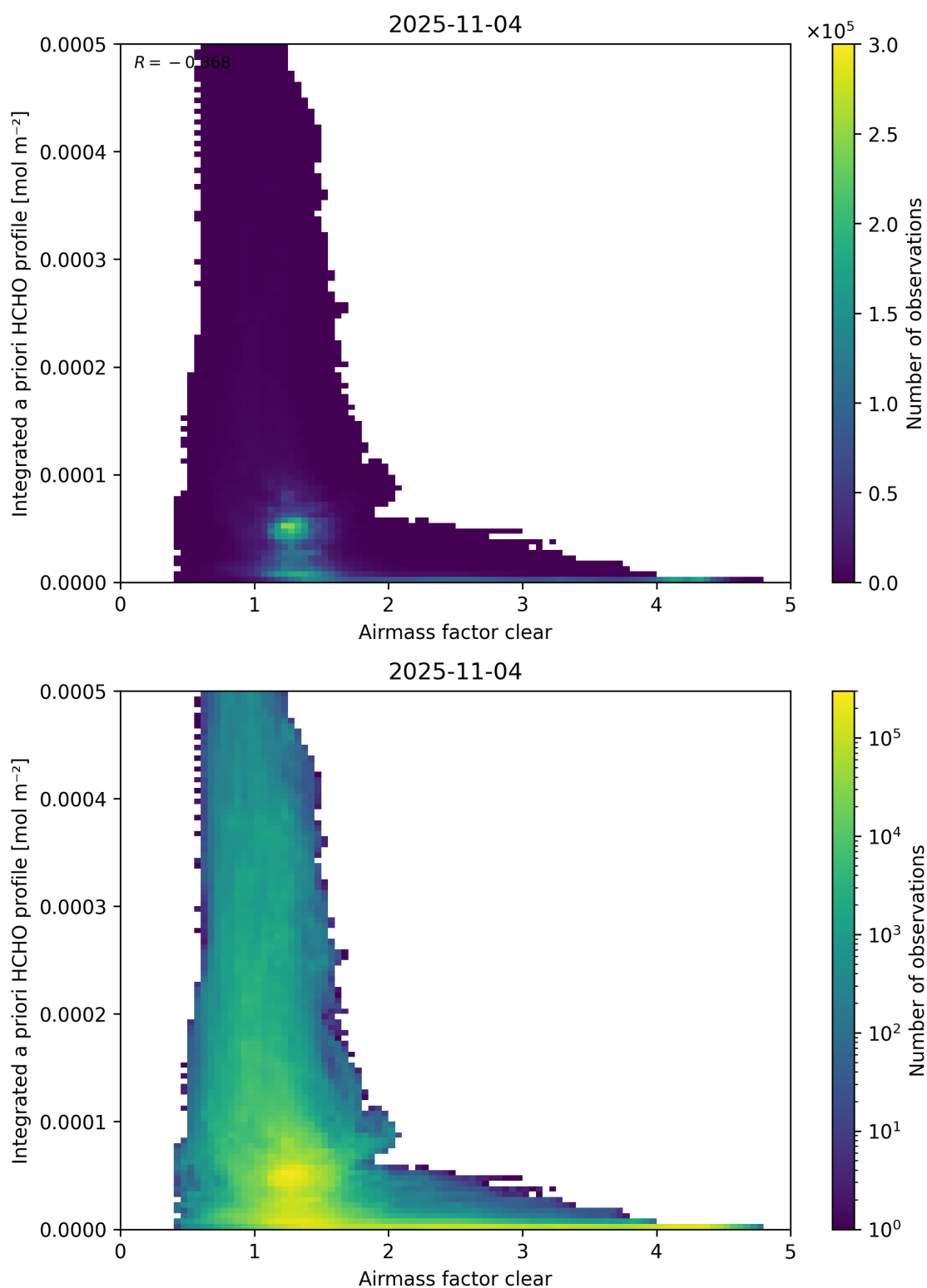
Figure 76: Scatter density plot of “Airmass factor clear” against “Integrated a priori HCHO profile” for 2025-11-03 to 2025-11-05.
