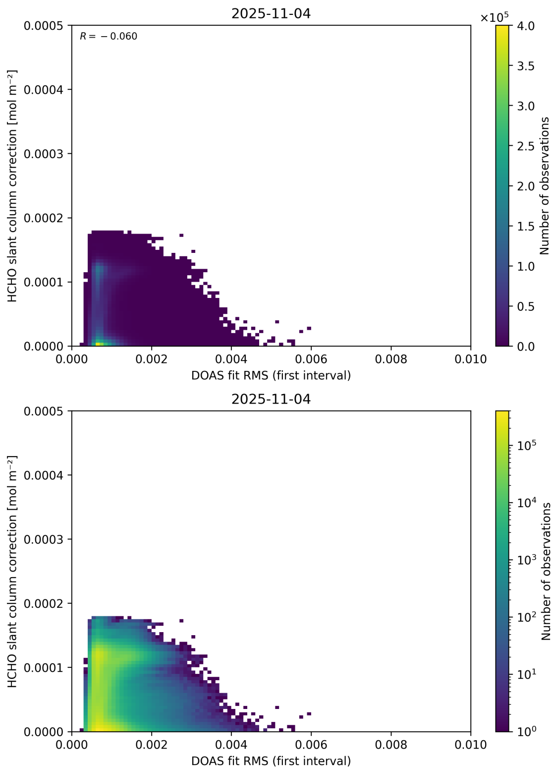
Figure 63: Scatter density plot of “DOAS fit RMS (first interval)” against “HCHO slant column correction” for 2025-11-03 to 2025-11-05.
