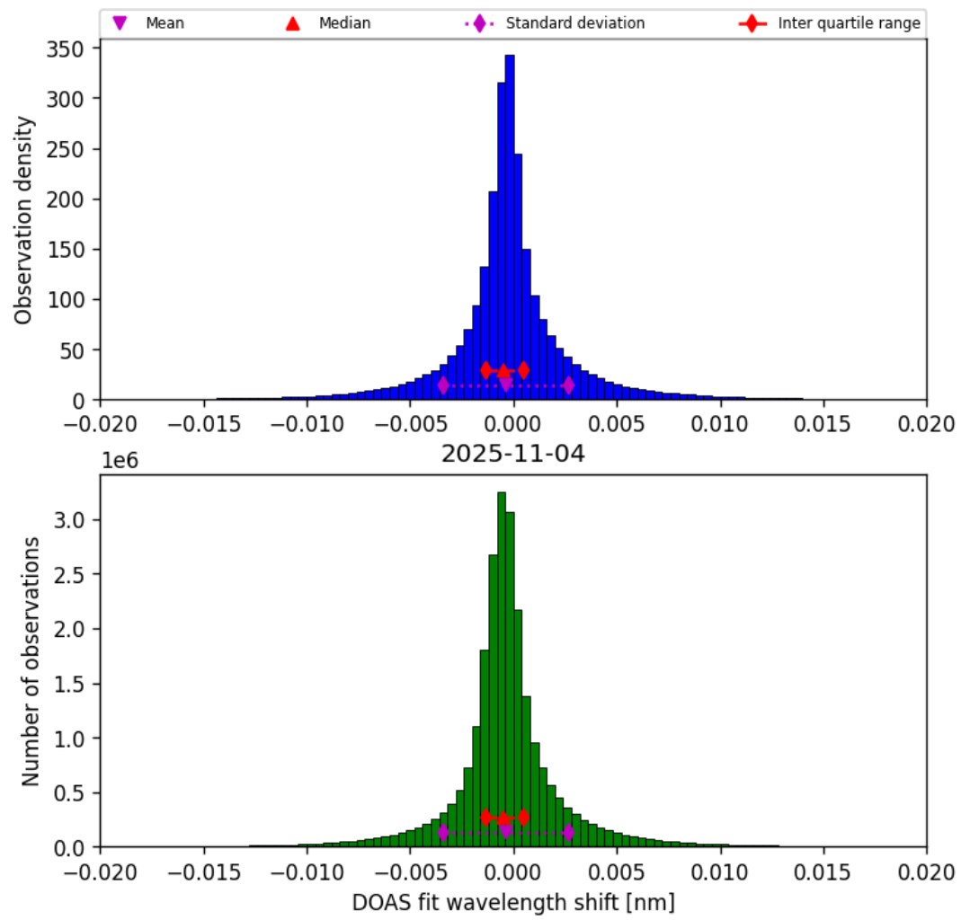
Figure 44: Histogram of “DOAS fit wavelength shift” for 2025-11-03 to 2025-11-05
