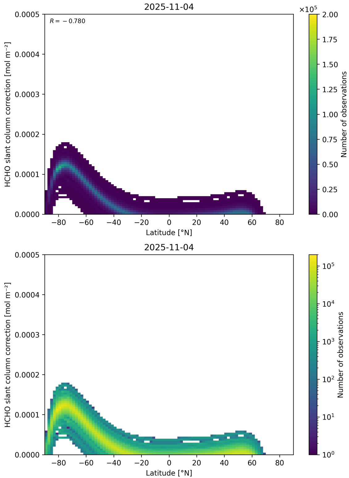
Figure 158: Scatter density plot of “Latitude” against “HCHO slant column correction” for 2025-11-03 to 2025-11-05.
