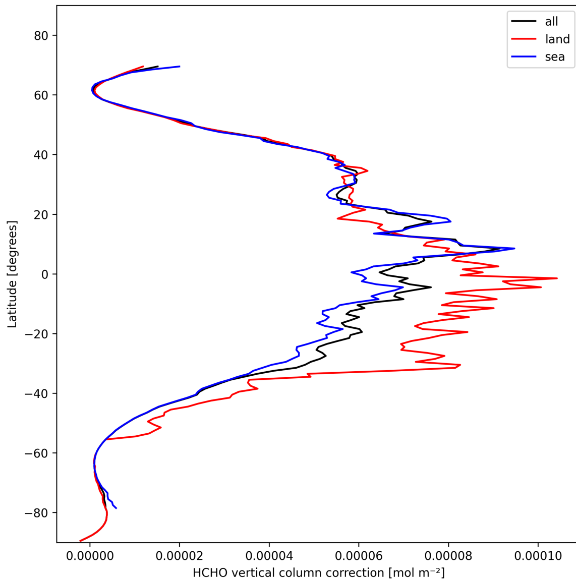
Figure 23: Zonal average of “HCHO vertical column correction” for 2025-11-03 to 2025-11-05.
