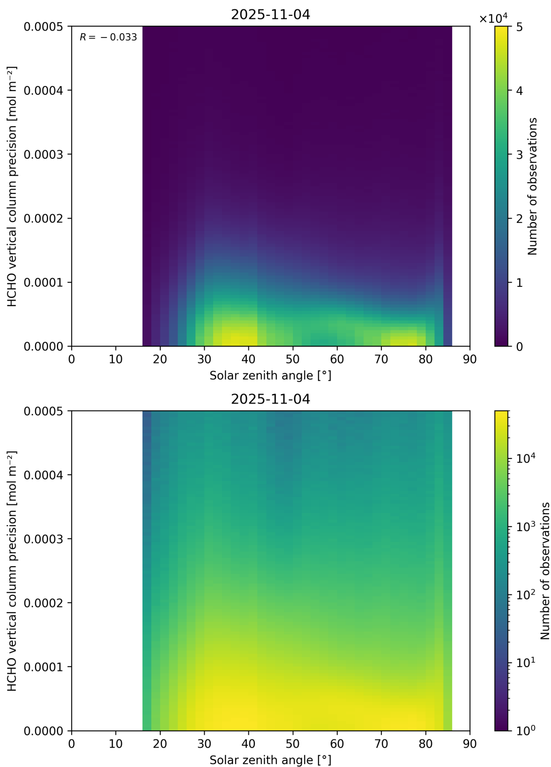
Figure 179: Scatter density plot of “Solar zenith angle” against “HCHO vertical column precision” for 2025-11-03 to 2025-11-05.
