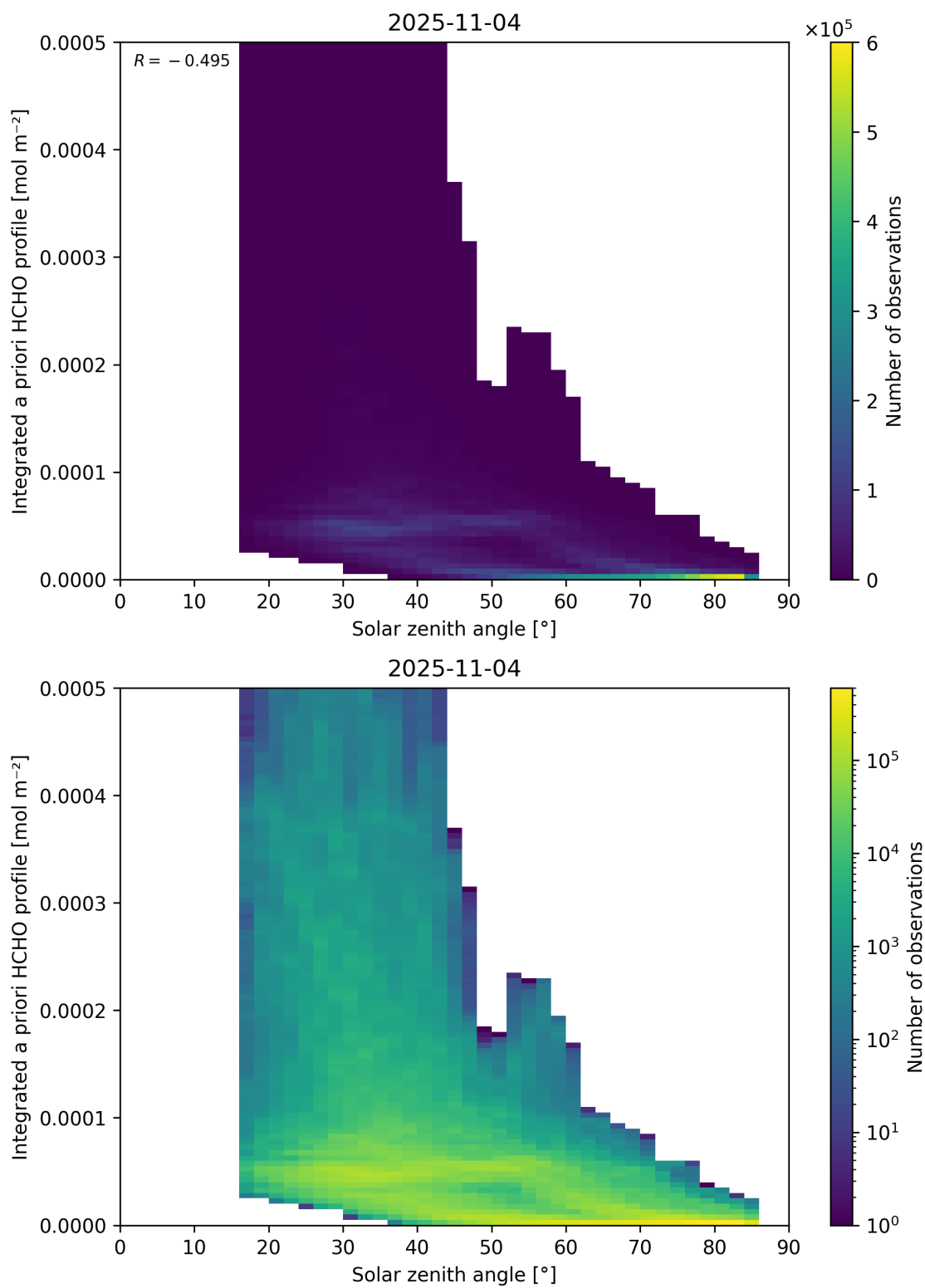
Figure 180: Scatter density plot of “Solar zenith angle” against “Integrated a priori HCHO profile” for 2025-11-03 to 2025-11-05.
