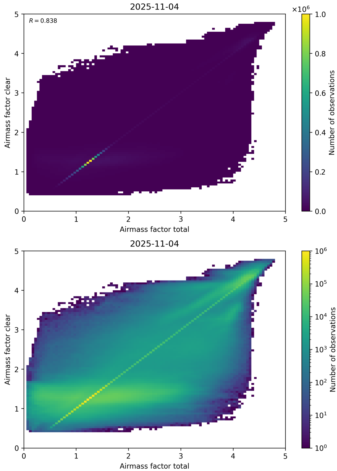
Figure 100: Scatter density plot of “Airmass factor total” against “Airmass factor clear” for 2025-11-03 to 2025-11-05.
