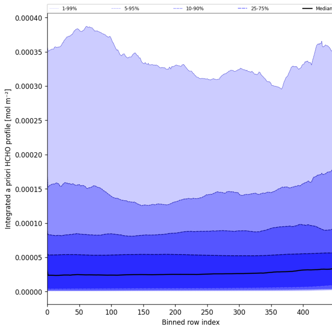
Figure 57: Along track statistics of “Integrated a priori HCHO profile” for 2025-11-03 to 2025-11-05
