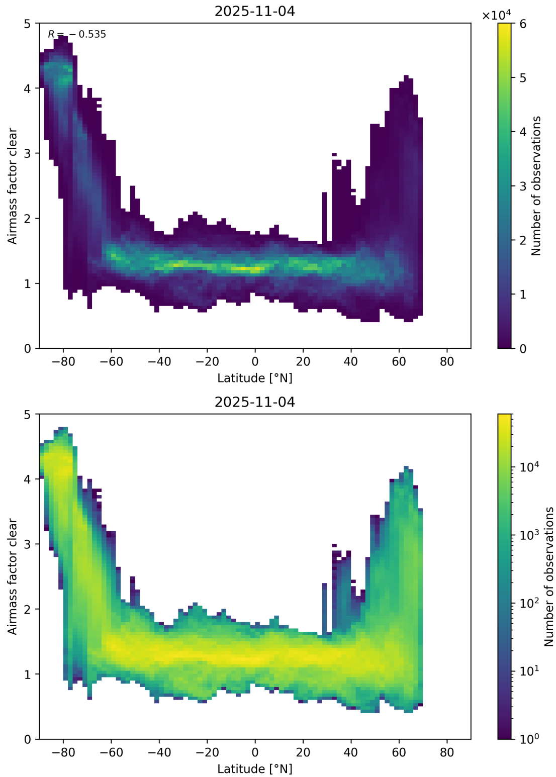
Figure 156: Scatter density plot of “Latitude” against “Airmass factor clear” for 2025-11-03 to 2025-11-05.
