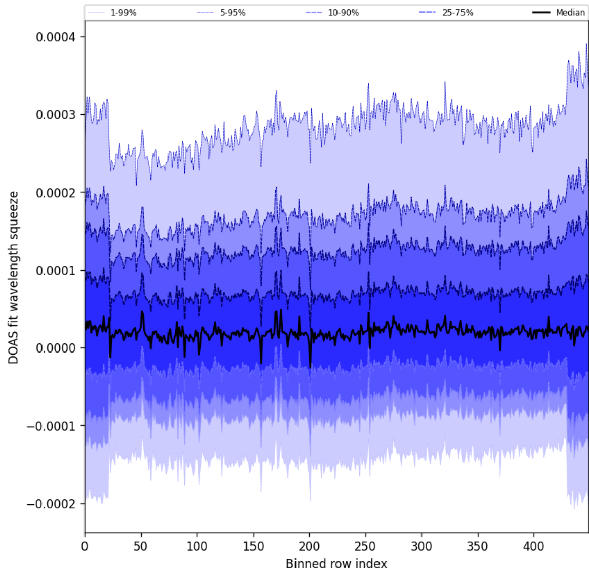
Figure 59: Along track statistics of “DOAS fit wavelength squeeze” for 2025-11-03 to 2025-11-05
