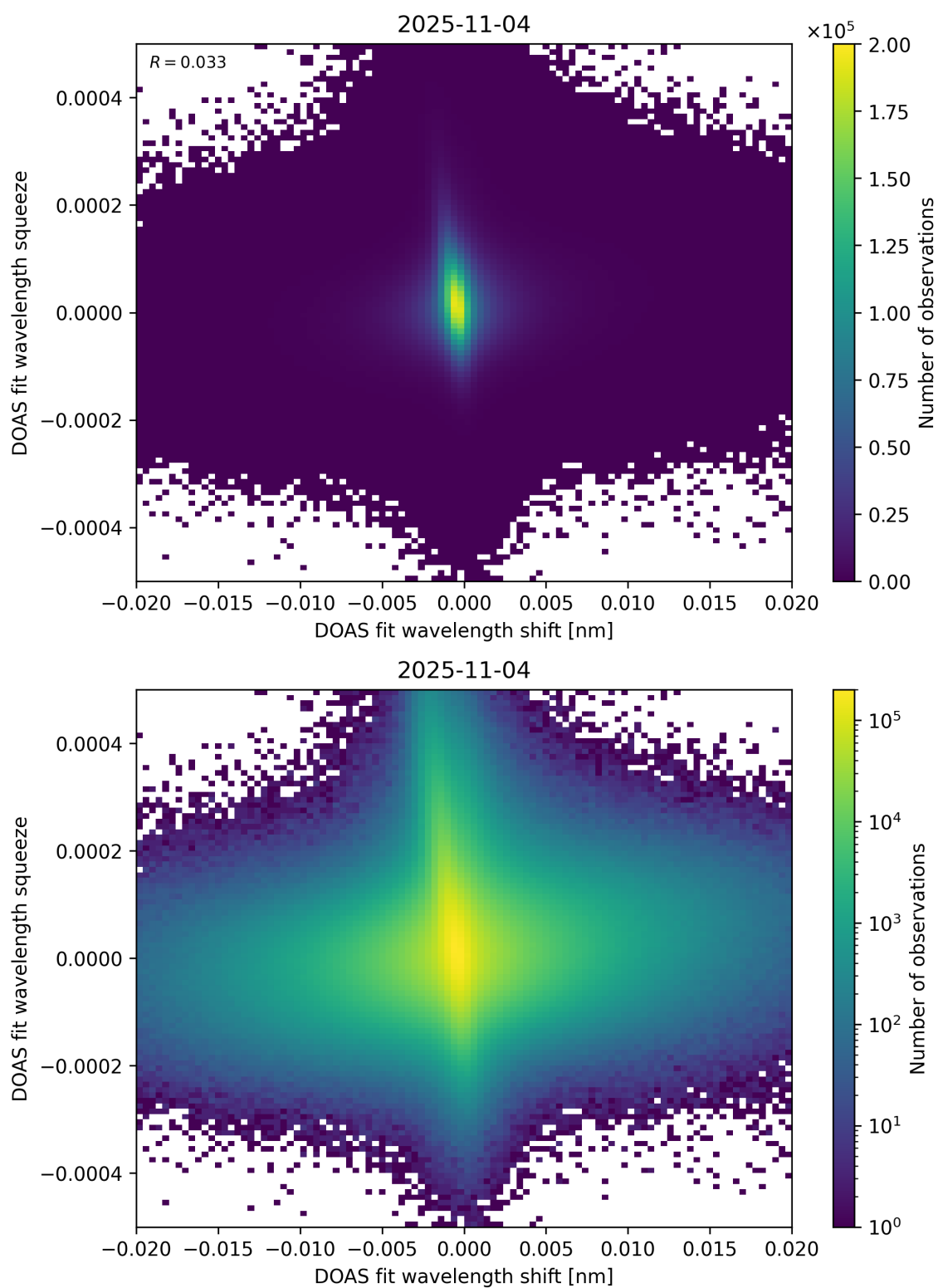
Figure 65: Scatter density plot of “DOAS fit wavelength shift” against “DOAS fit wavelength squeeze” for 2025-11-03 to 2025-11-05.
