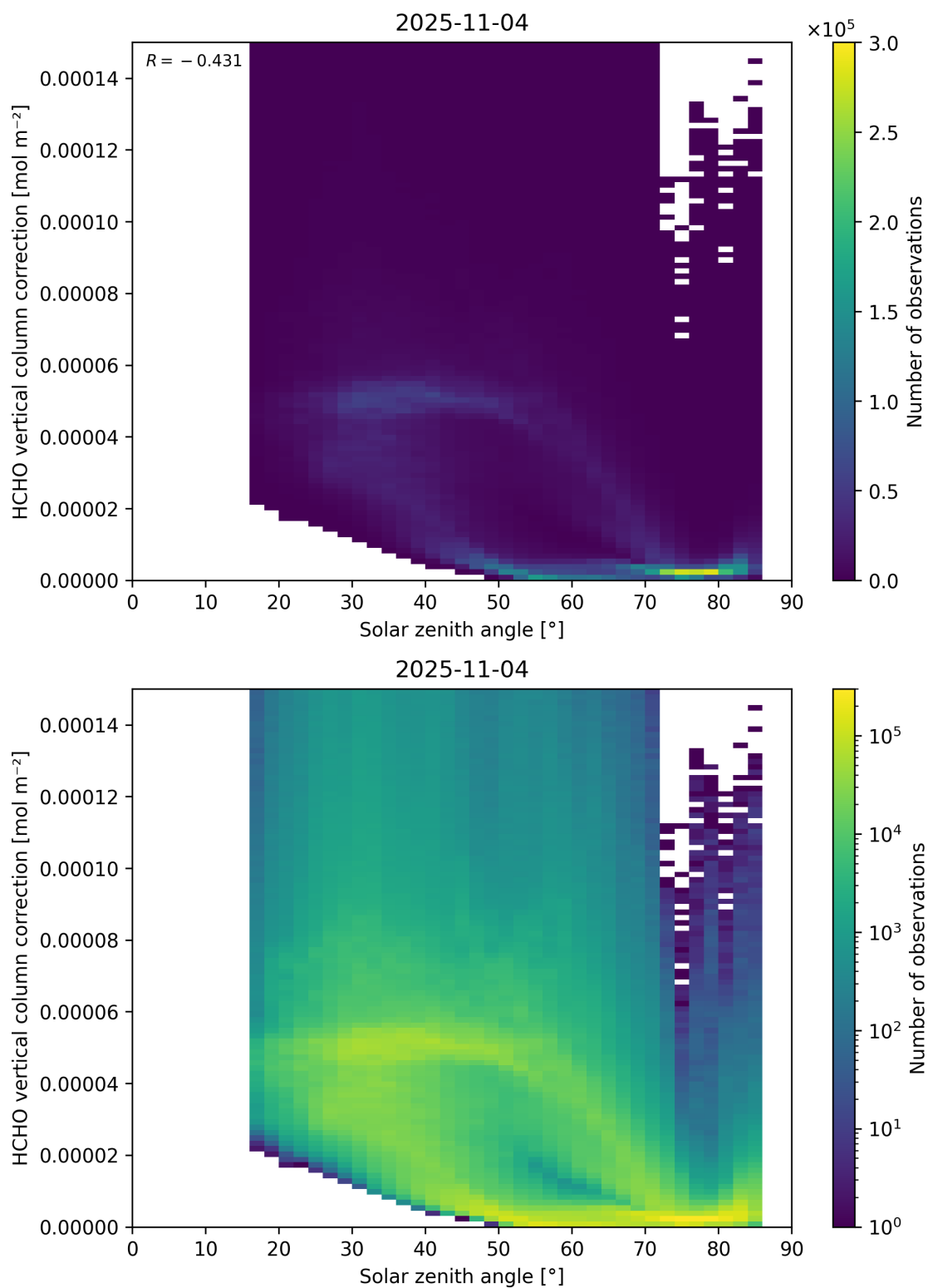
Figure 178: Scatter density plot of “Solar zenith angle” against “HCHO vertical column correction” for 2025-11-03 to 2025-11-05.
