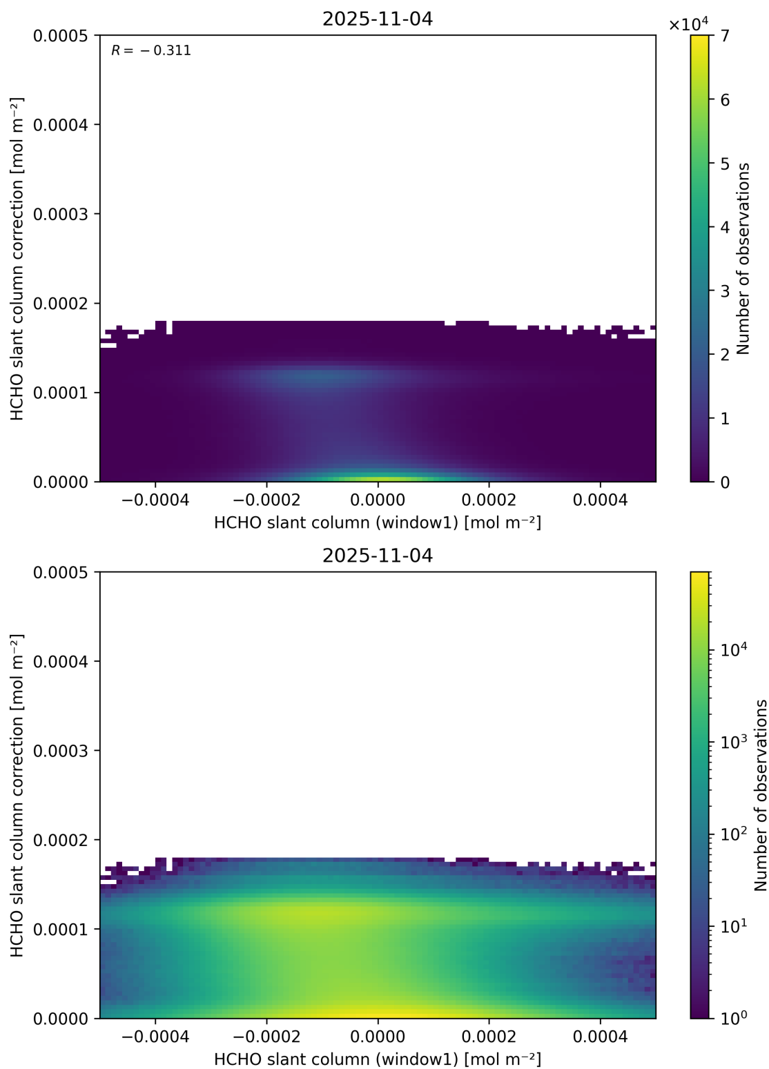
Figure 83: Scatter density plot of “HCHO slant column (window1)” against “HCHO slant column correction” for 2025-11-03 to 2025-11-05.
