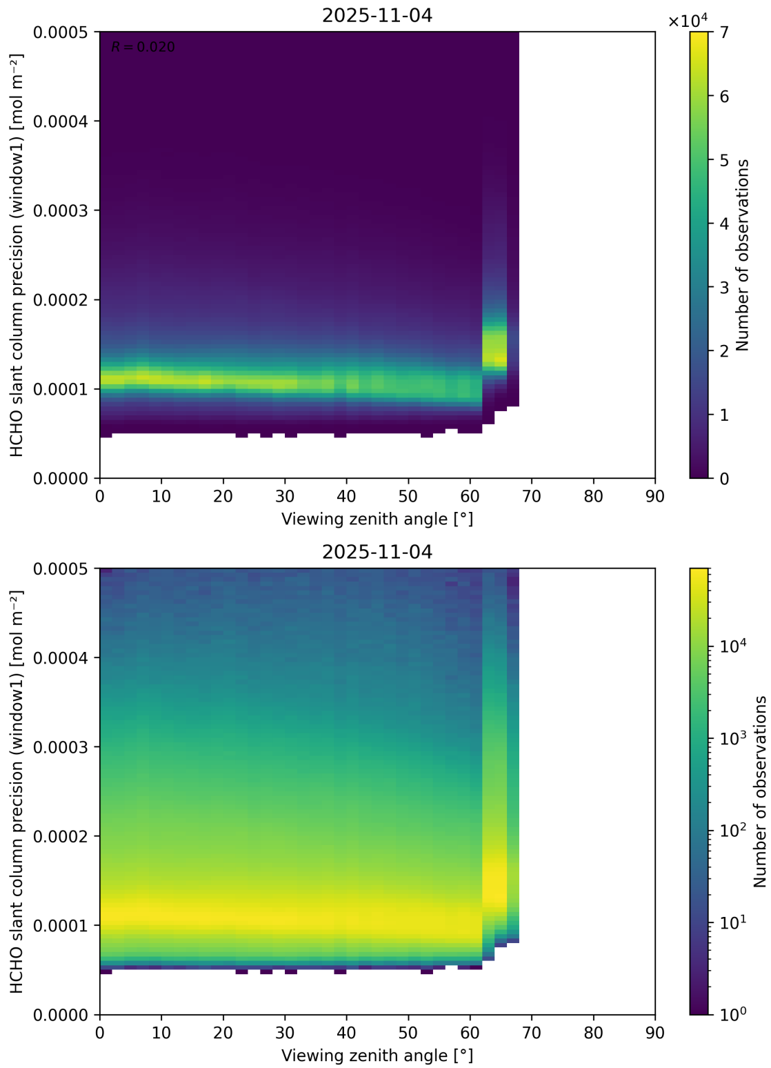
Figure 189: Scatter density plot of “Viewing zenith angle” against “HCHO slant column precision (window1)” for 2025-11-03 to 2025-11-05.
