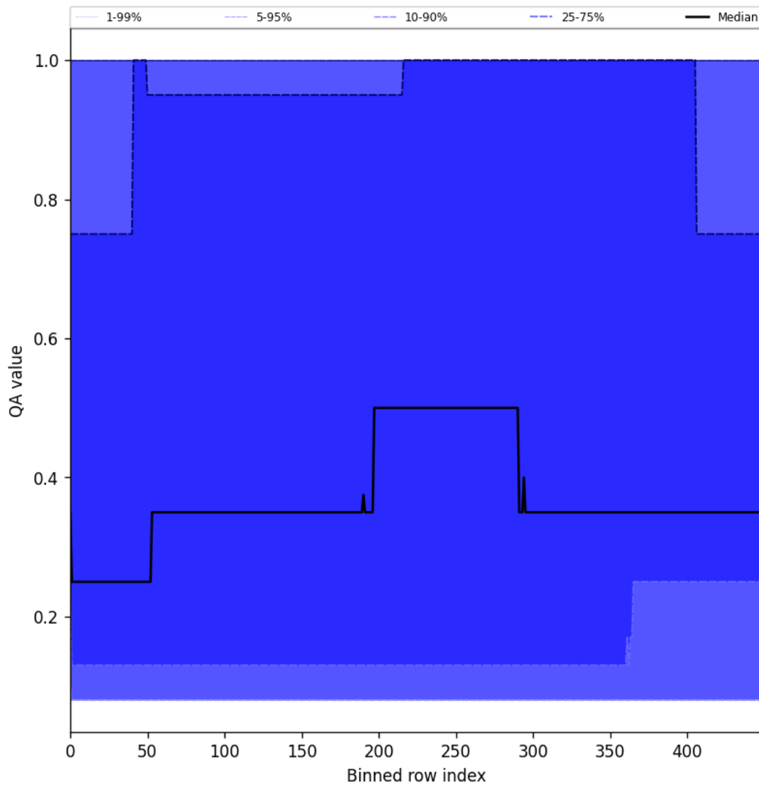
Figure 48: Along track statistics of “QA value” for 2025-11-03 to 2025-11-05
