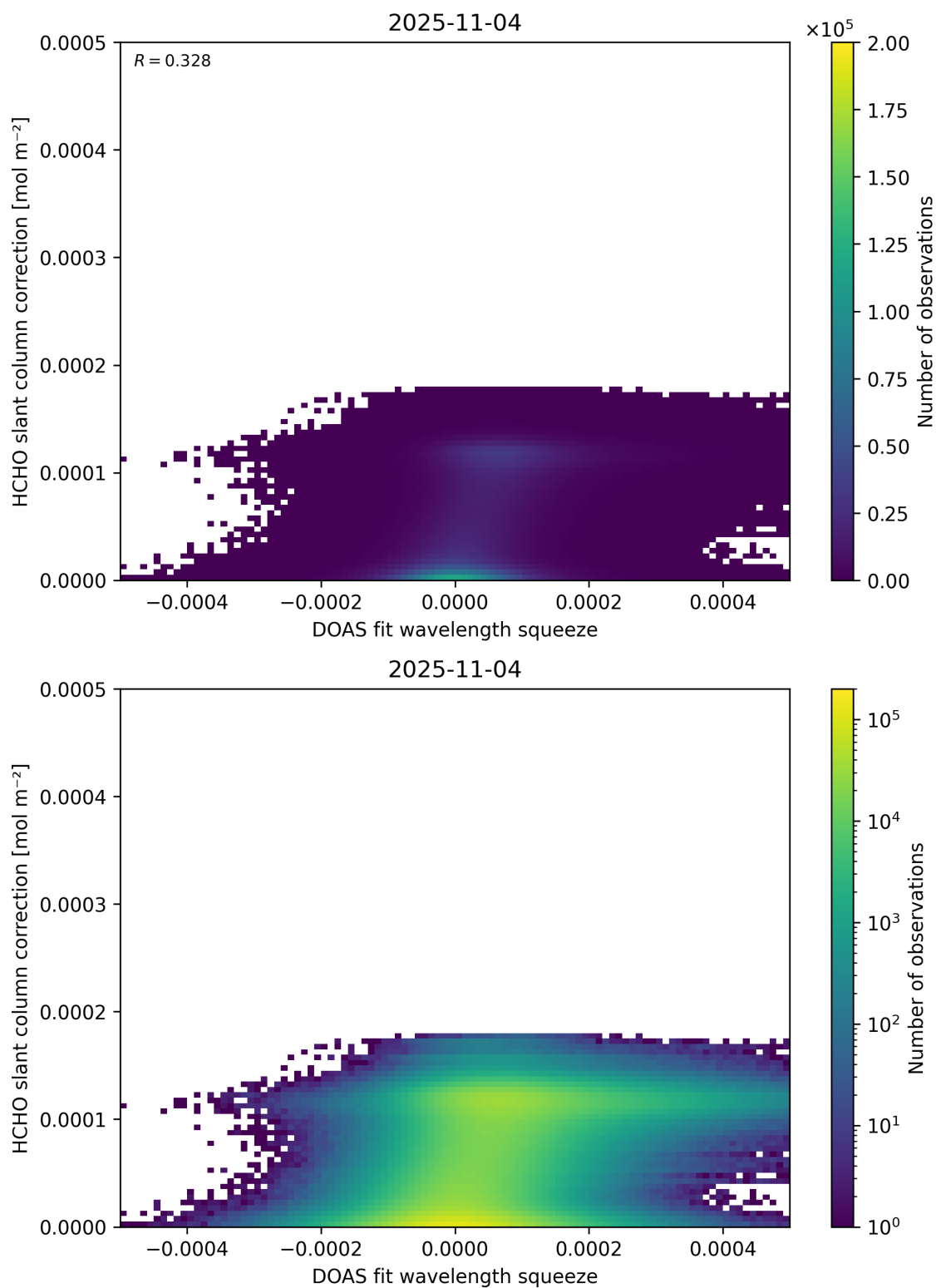
Figure 70: Scatter density plot of “DOAS fit wavelength squeeze” against “HCHO slant column correction” for 2025-11-03 to 2025-11-05.
