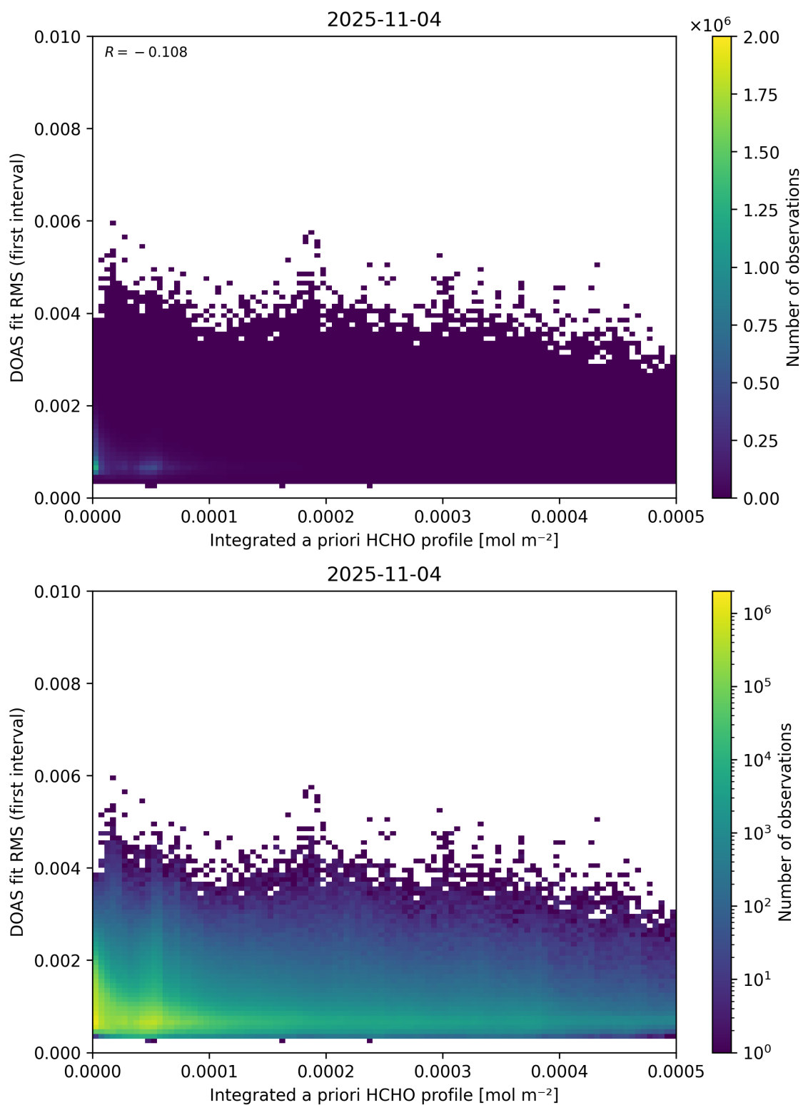
Figure 148: Scatter density plot of “Integrated a priori HCHO profile” against “DOAS fit RMS (first interval)” for 2025-11-03 to 2025-11-05.
