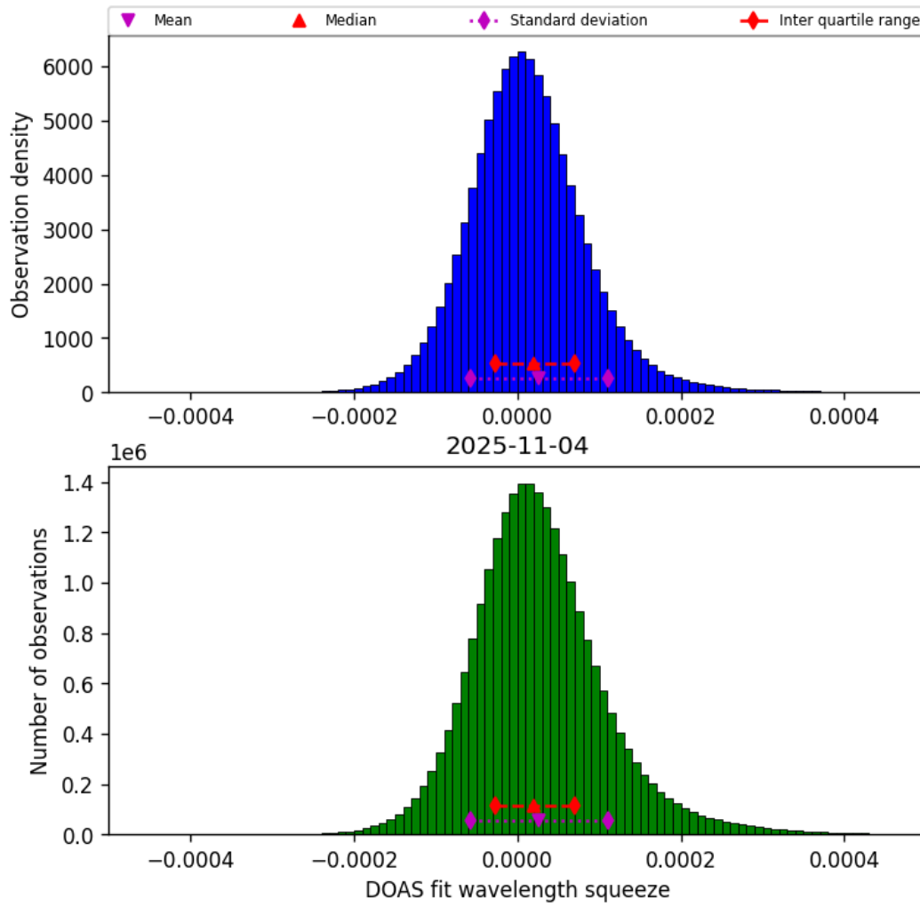
Figure 45: Histogram of “DOAS fit wavelength squeeze” for 2025-11-03 to 2025-11-05
