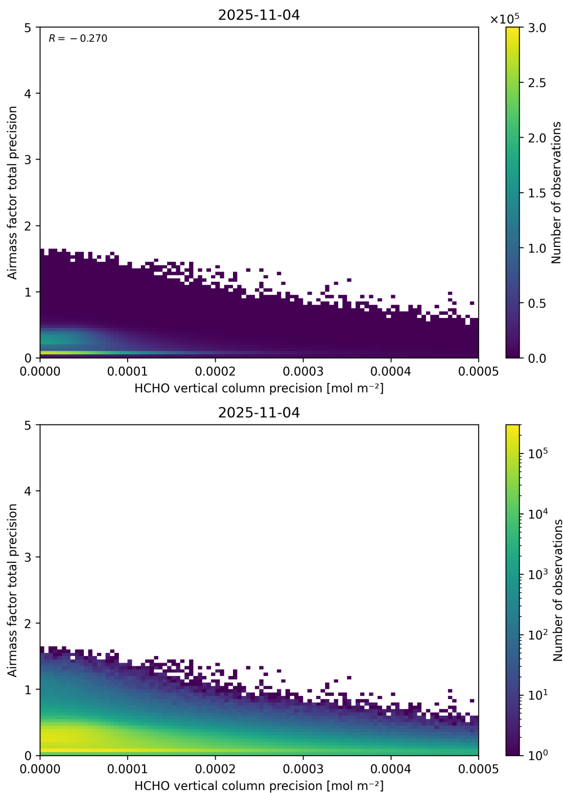
Figure 145: Scatter density plot of “HCHO vertical column precision” against “Airmass factor total precision” for 2025-11-03 to 2025-11-05.
