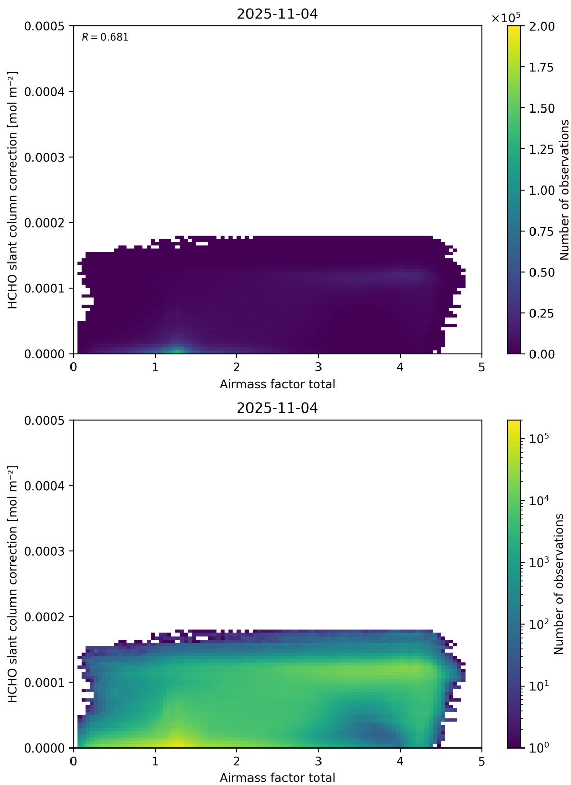
Figure 102: Scatter density plot of “Airmass factor total” against “HCHO slant column correction” for 2025-11-03 to 2025-11-05.
