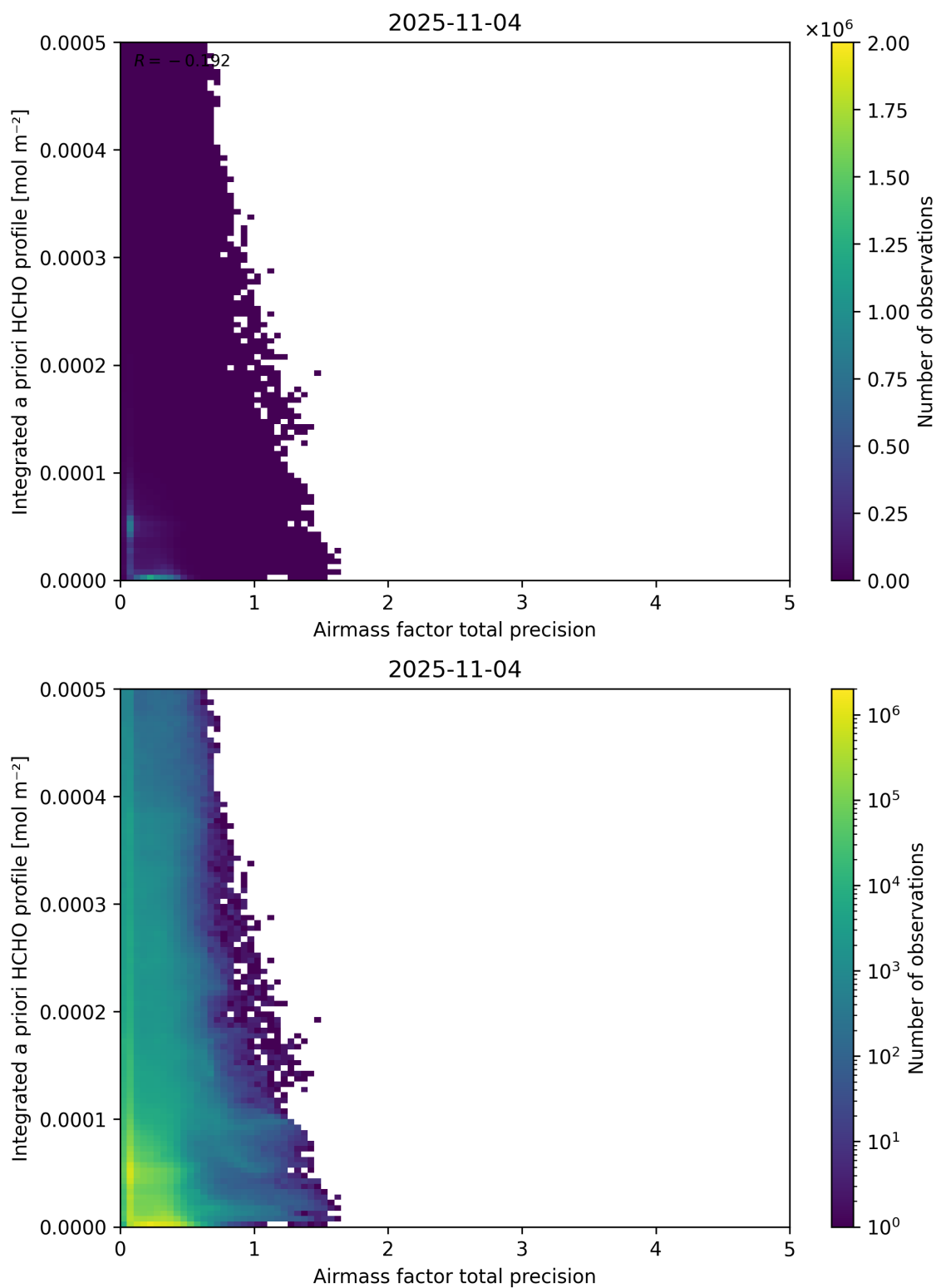
Figure 111: Scatter density plot of “Airmass factor total precision” against “Integrated a priori HCHO profile” for 2025-11-03 to 2025-11-05.
