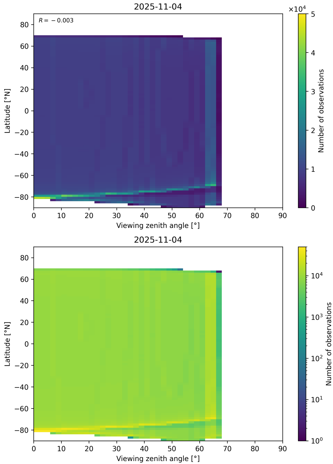
Figure 196: Scatter density plot of “Viewing zenith angle” against “Latitude” for 2025-11-03 to 2025-11-05.
