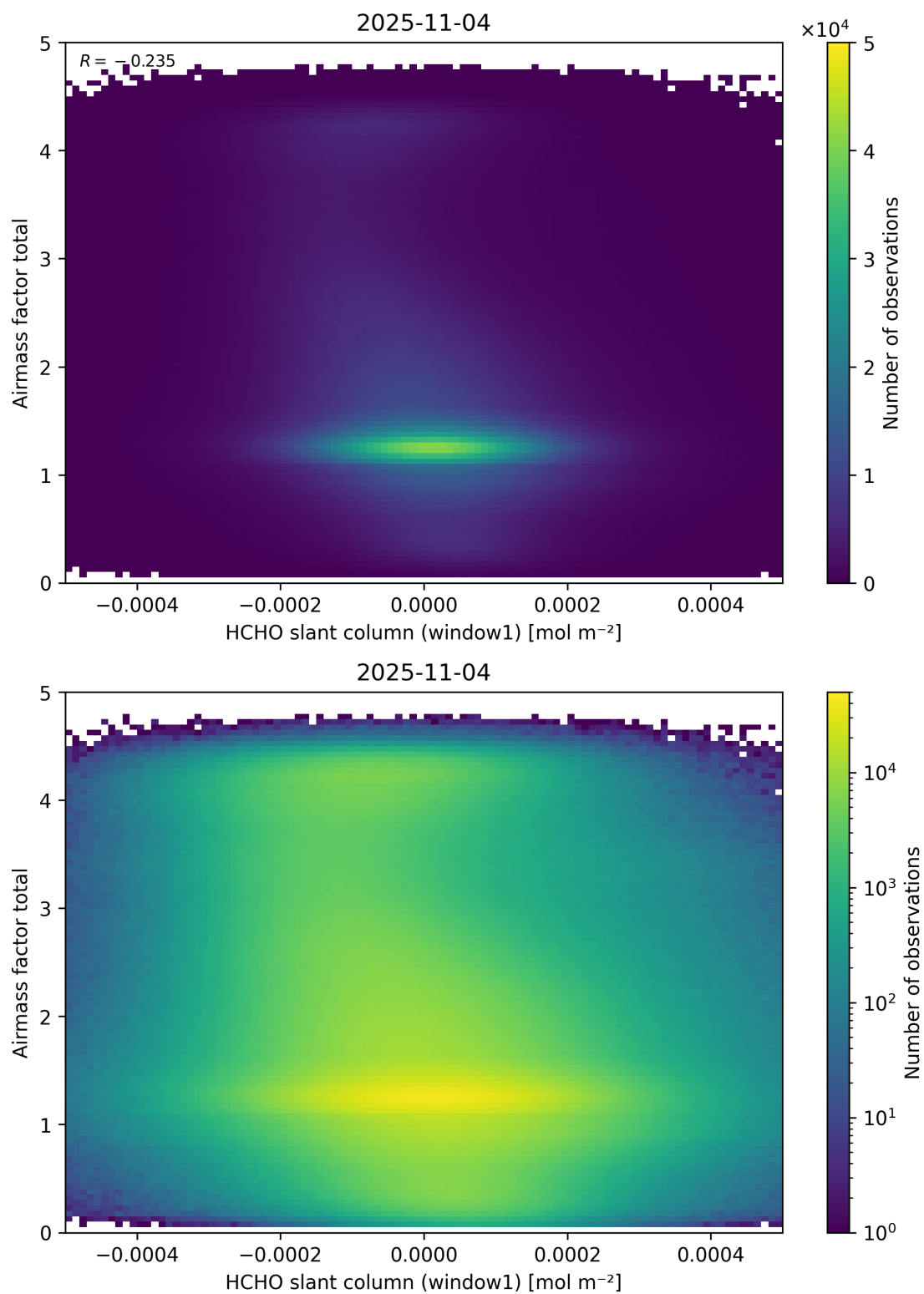
Figure 85: Scatter density plot of “HCHO slant column (window1)” against “Airmass factor total” for 2025-11-03 to 2025-11-05.
