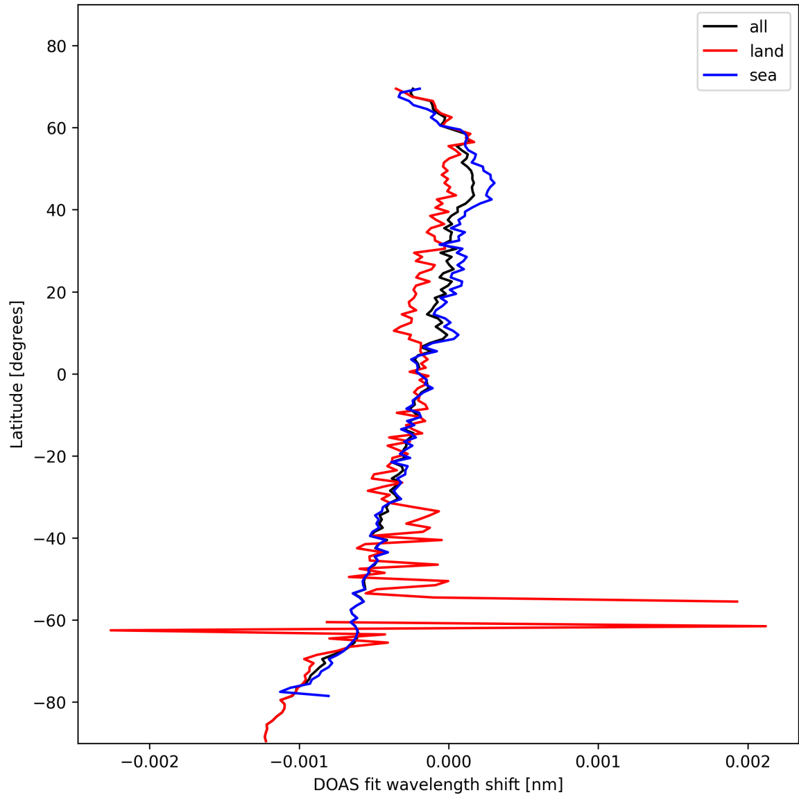
Figure 30: Zonal average of “DOAS fit wavelength shift” for 2025-11-03 to 2025-11-05.
