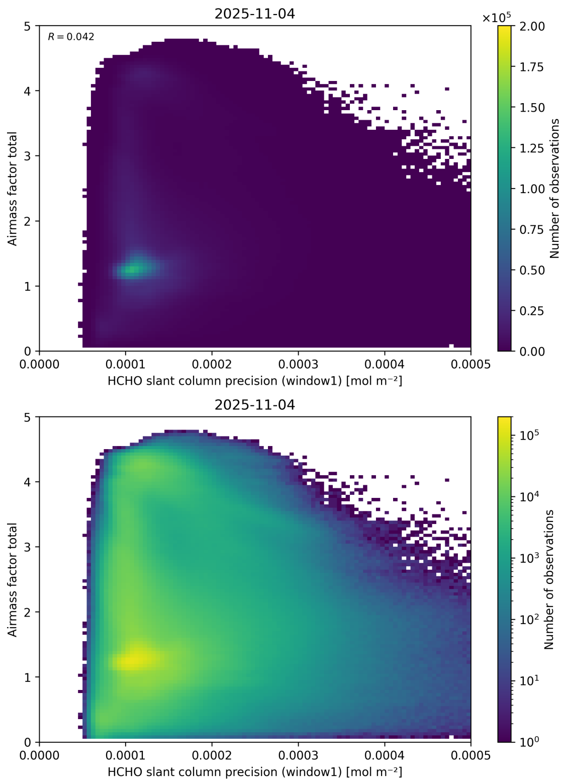
Figure 94: Scatter density plot of “HCHO slant column precision (window1)” against “Airmass factor total” for 2025-11-03 to 2025-11-05.
