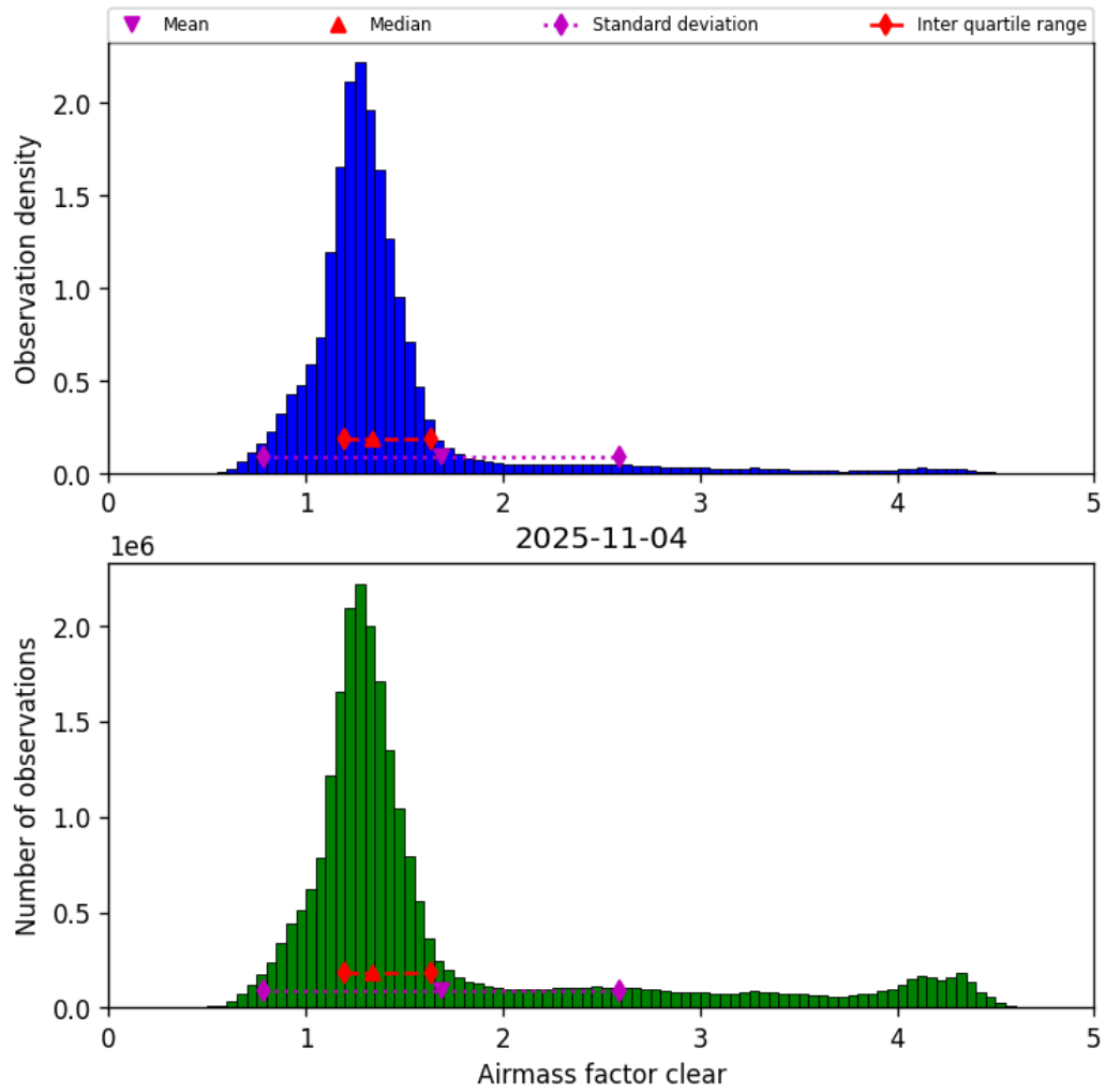
Figure 42: Histogram of “Airmass factor clear” for 2025-11-03 to 2025-11-05
