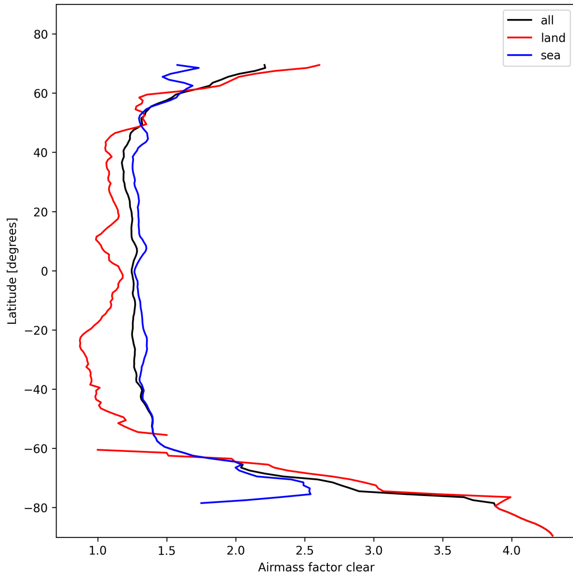
Figure 28: Zonal average of “Airmass factor clear” for 2025-11-03 to 2025-11-05.
