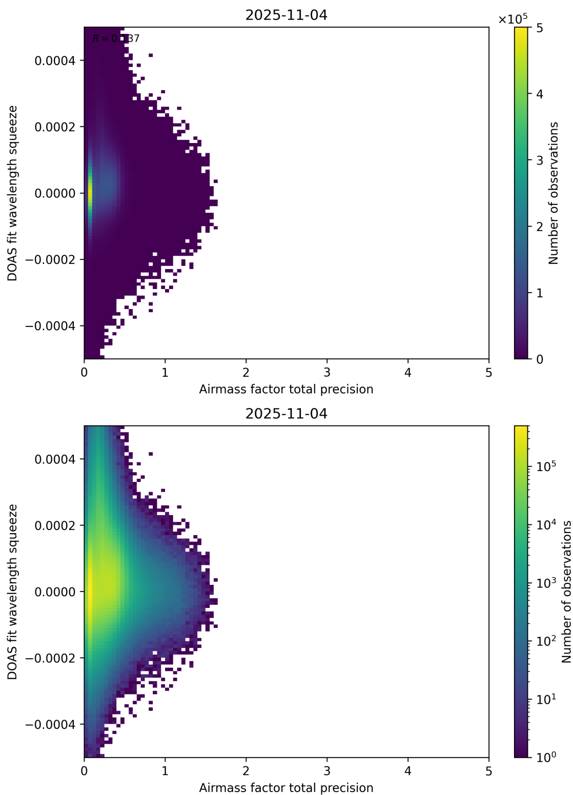
Figure 107: Scatter density plot of “Airmass factor total precision” against “DOAS fit wavelength squeeze” for 2025-11-03 to 2025-11-05.
