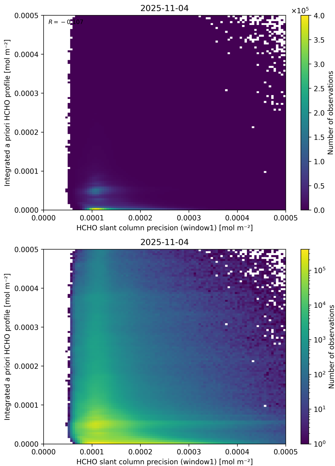
Figure 96: Scatter density plot of “HCHO slant column precision (window1)” against “Integrated a priori HCHO profile” for 2025-11-03 to 2025-11-05.
