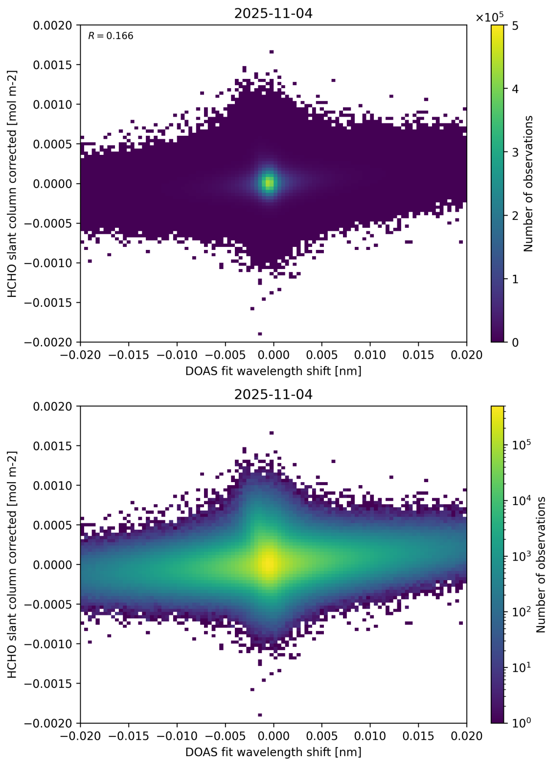
Figure 66: Scatter density plot of “DOAS fit wavelength shift” against “HCHO slant column corrected” for 2025-11-03 to 2025-11-05.
