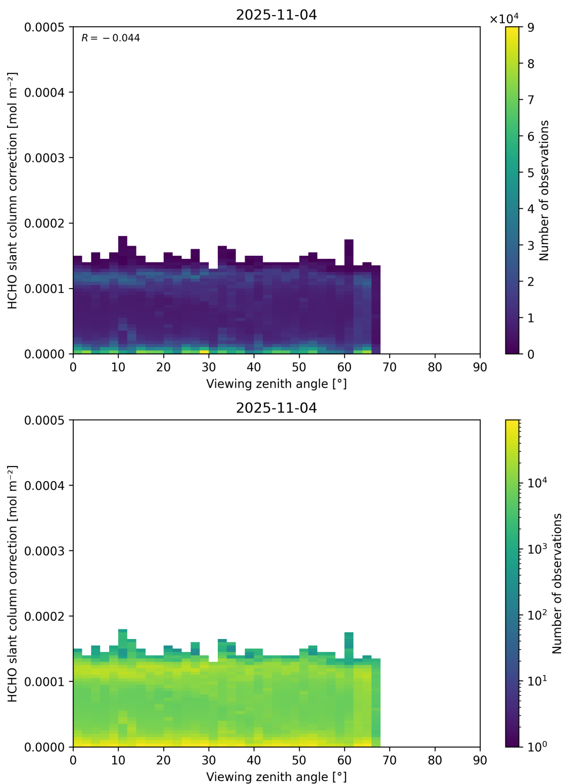
Figure 187: Scatter density plot of “Viewing zenith angle” against “HCHO slant column correction” for 2025-11-03 to 2025-11-05.
