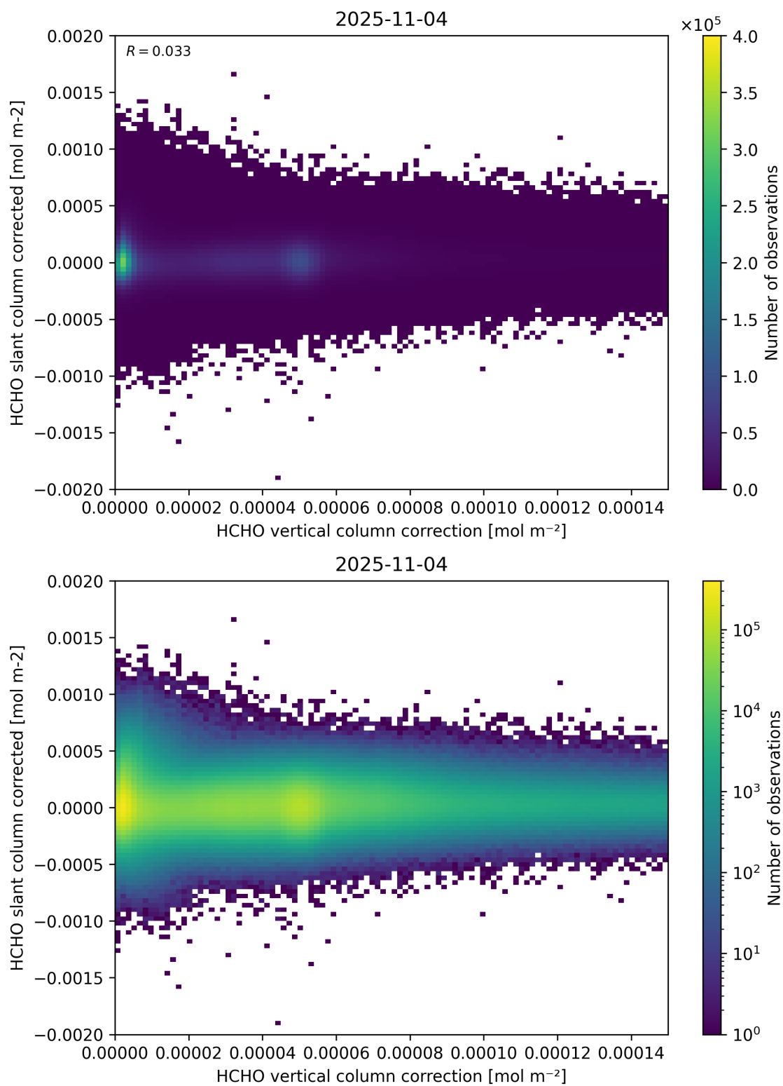
Figure 116: Scatter density plot of “HCHO vertical column correction” against “HCHO slant column corrected” for 2025-11-03 to 2025-11-05.
