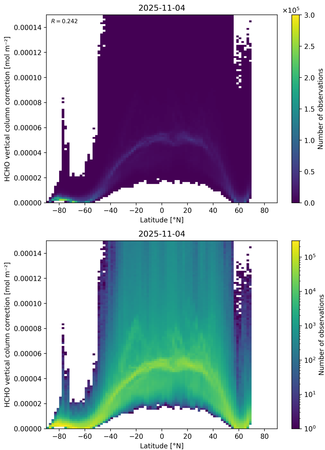
Figure 164: Scatter density plot of “Latitude” against “HCHO vertical column correction” for 2025-11-03 to 2025-11-05.
