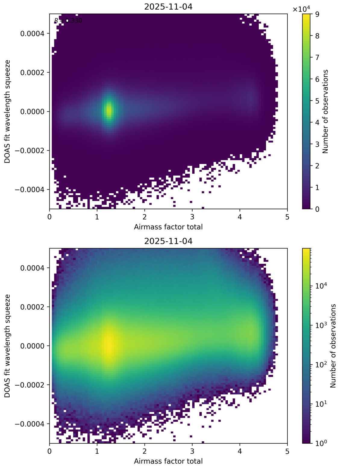
Figure 99: Scatter density plot of “Airmass factor total” against “DOAS fit wavelength squeeze” for 2025-11-03 to 2025-11-05.
