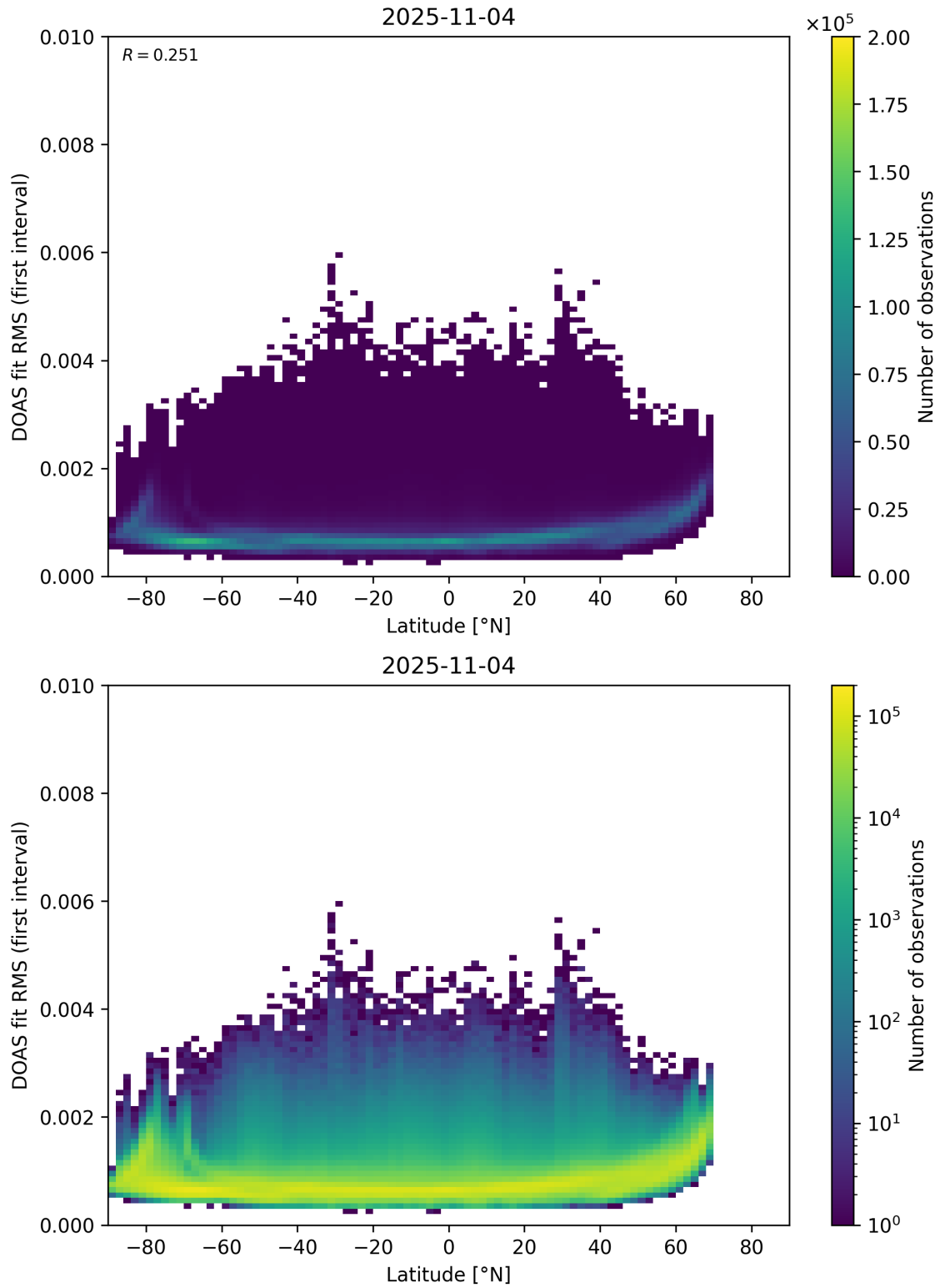
Figure 153: Scatter density plot of “Latitude” against “DOAS fit RMS (first interval)” for 2025-11-03 to 2025-11-05.
