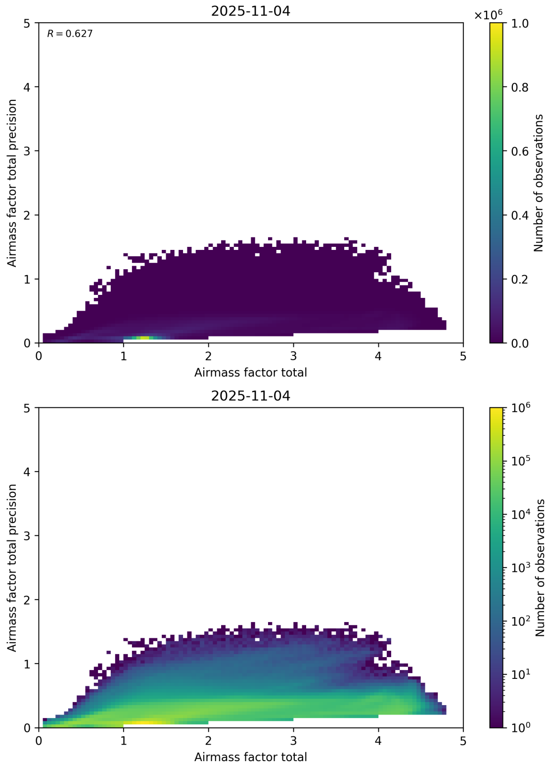
Figure 103: Scatter density plot of “Airmass factor total” against “Airmass factor total precision” for 2025-11-03 to 2025-11-05.
