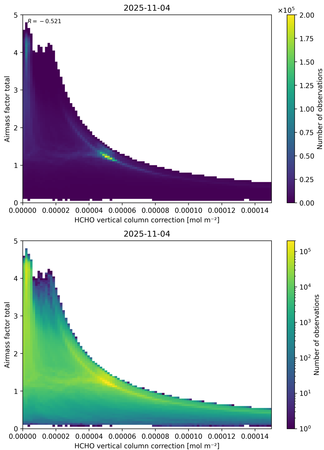
Figure 120: Scatter density plot of “HCHO vertical column correction” against “Airmass factor total” for 2025-11-03 to 2025-11-05.
