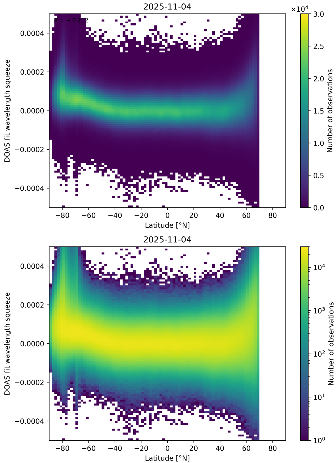
Figure 155: Scatter density plot of “Latitude” against “DOAS fit wavelength squeeze” for 2025-11-03 to 2025-11-05.
