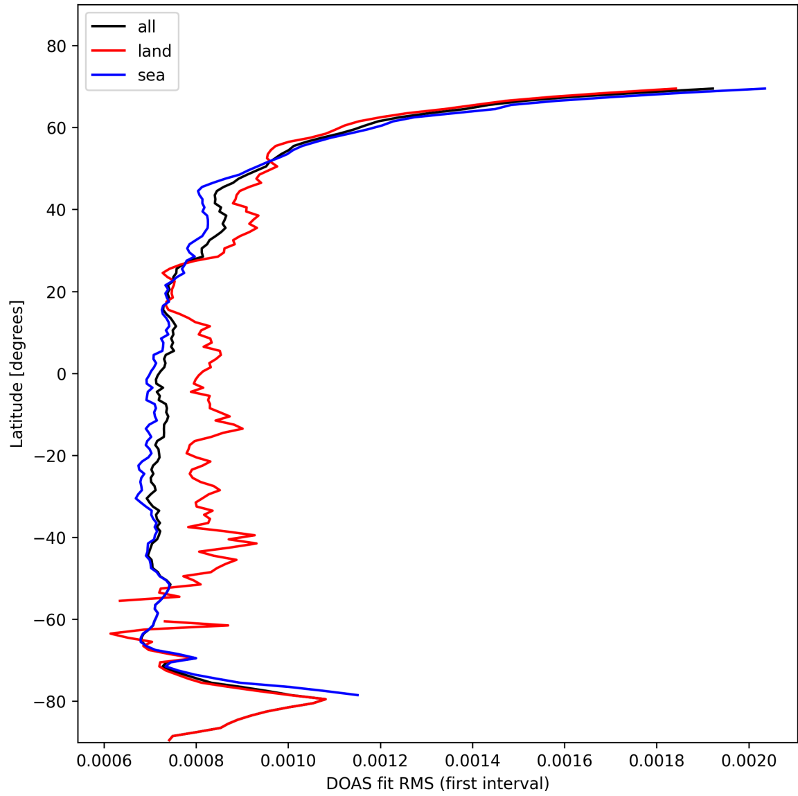
Figure 32: Zonal average of “DOAS fit RMS (first interval)” for 2025-11-03 to 2025-11-05.
