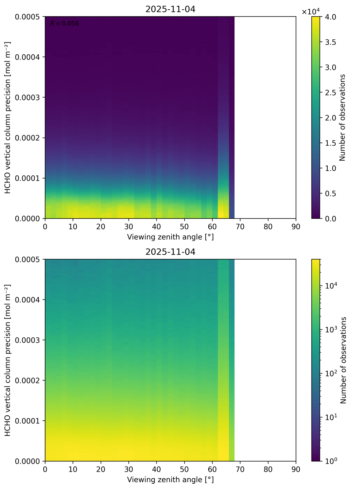
Figure 194: Scatter density plot of “Viewing zenith angle” against “HCHO vertical column precision” for 2025-11-03 to 2025-11-05.
