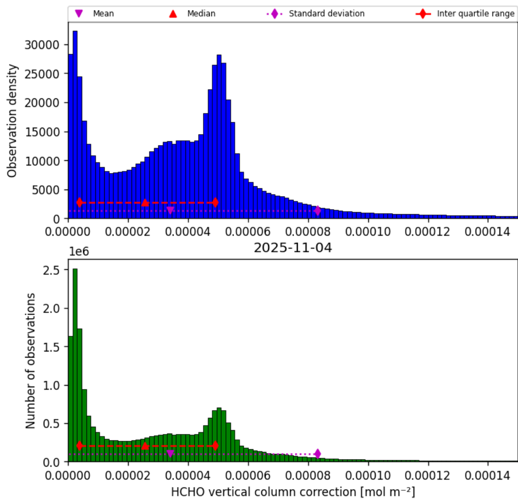
Figure 37: Histogram of “HCHO vertical column correction” for 2025-11-03 to 2025-11-05
