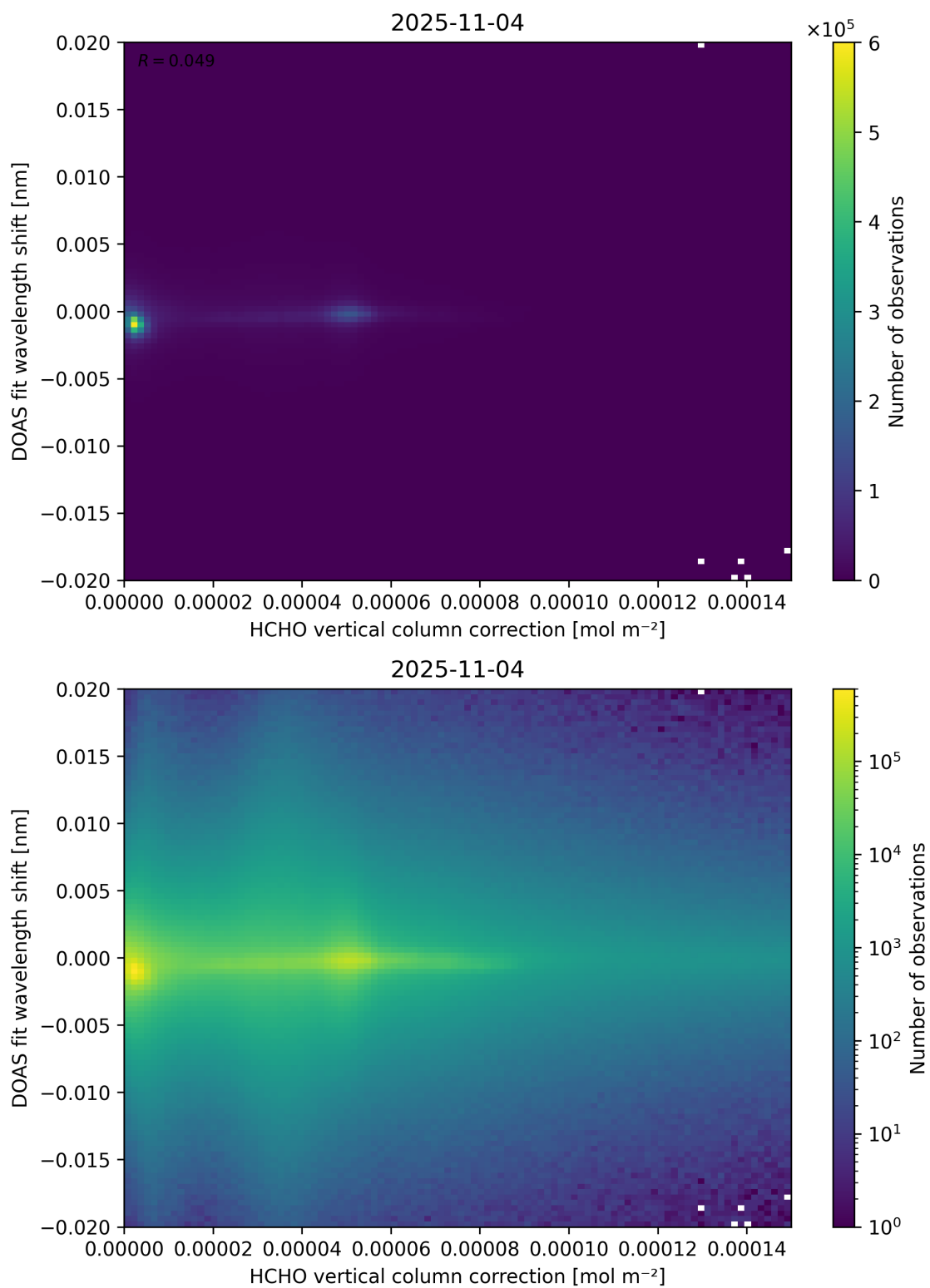
Figure 113: Scatter density plot of “HCHO vertical column correction” against “DOAS fit wavelength shift” for 2025-11-03 to 2025-11-05.
