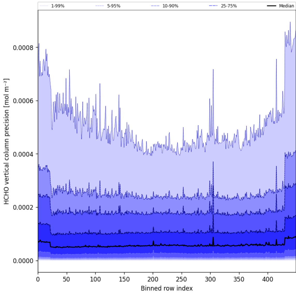
Figure 50: Along track statistics of “HCHO vertical column precision” for 2025-11-03 to 2025-11-05
