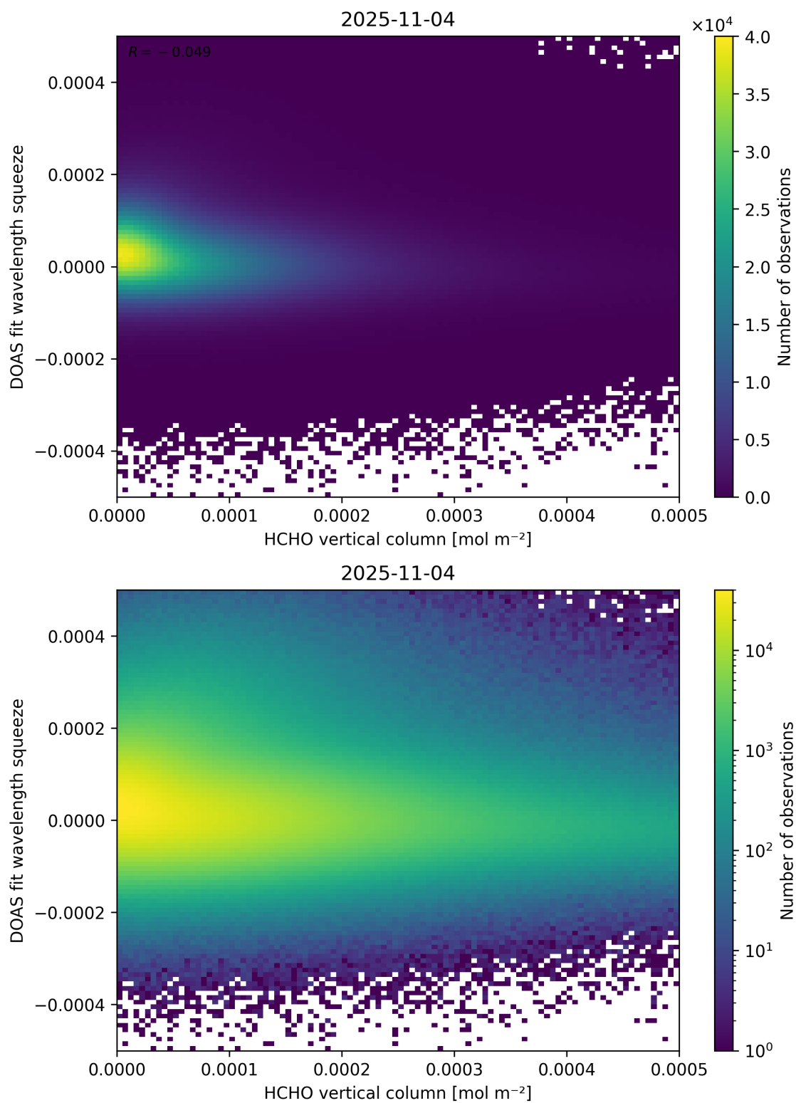
Figure 125: Scatter density plot of “HCHO vertical column” against “DOAS fit wavelength squeeze” for 2025-11-03 to 2025-11-05.
