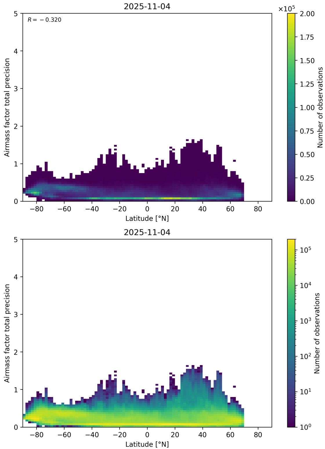
Figure 162: Scatter density plot of “Latitude” against “Airmass factor total precision” for 2025-11-03 to 2025-11-05.
