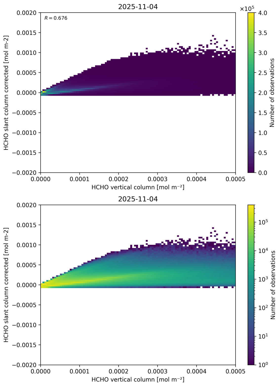
Figure 127: Scatter density plot of “HCHO vertical column” against “HCHO slant column corrected” for 2025-11-03 to 2025-11-05.
