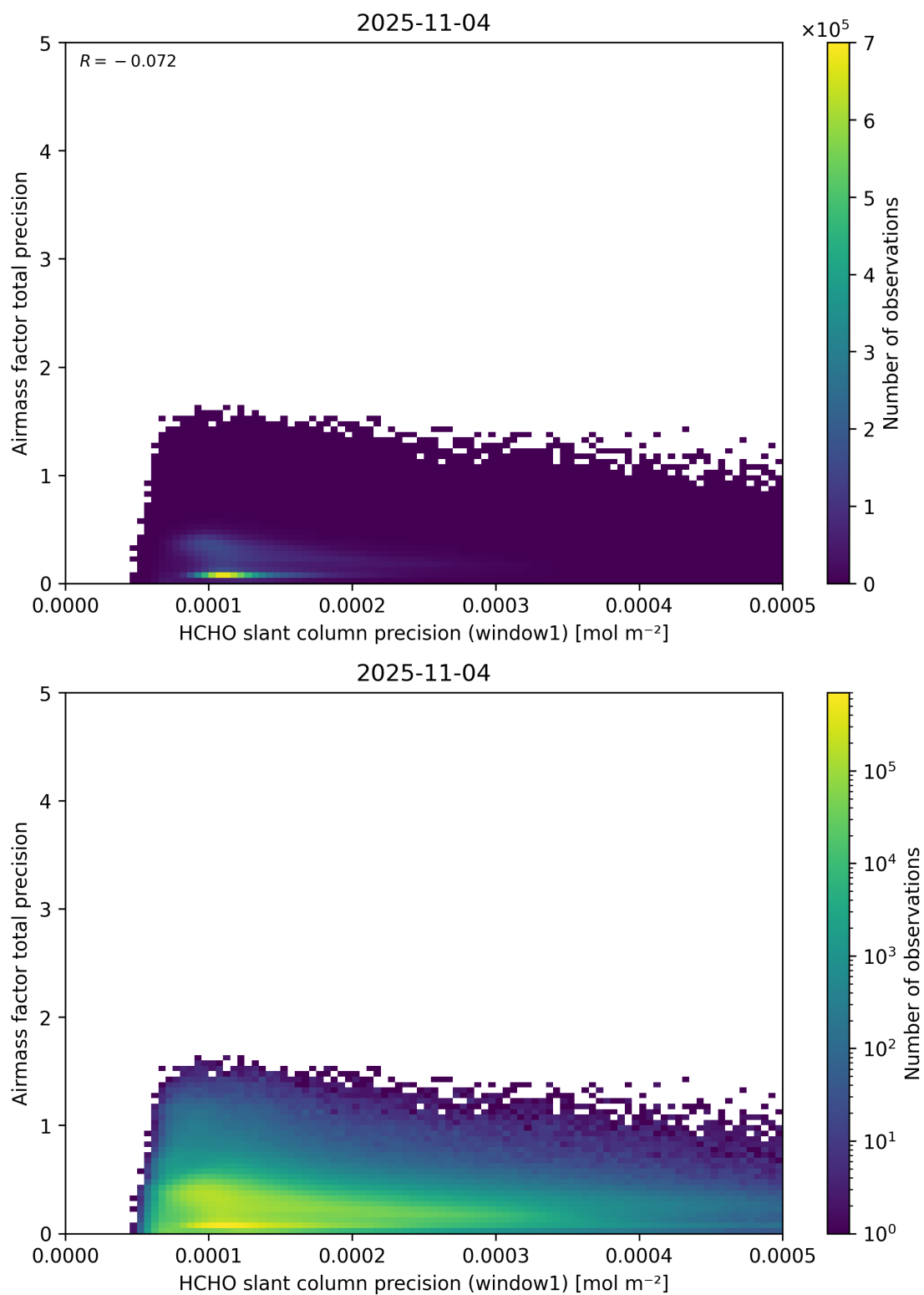
Figure 95: Scatter density plot of “HCHO slant column precision (window1)” against “Airmass factor total precision” for 2025-11-03 to 2025-11-05.
