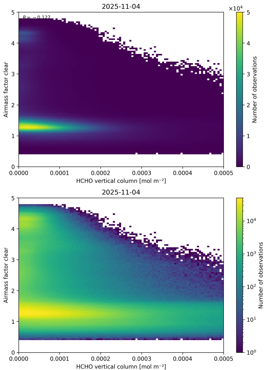
Figure 126: Scatter density plot of “HCHO vertical column” against “Airmass factor clear” for 2025-11-03 to 2025-11-05.
