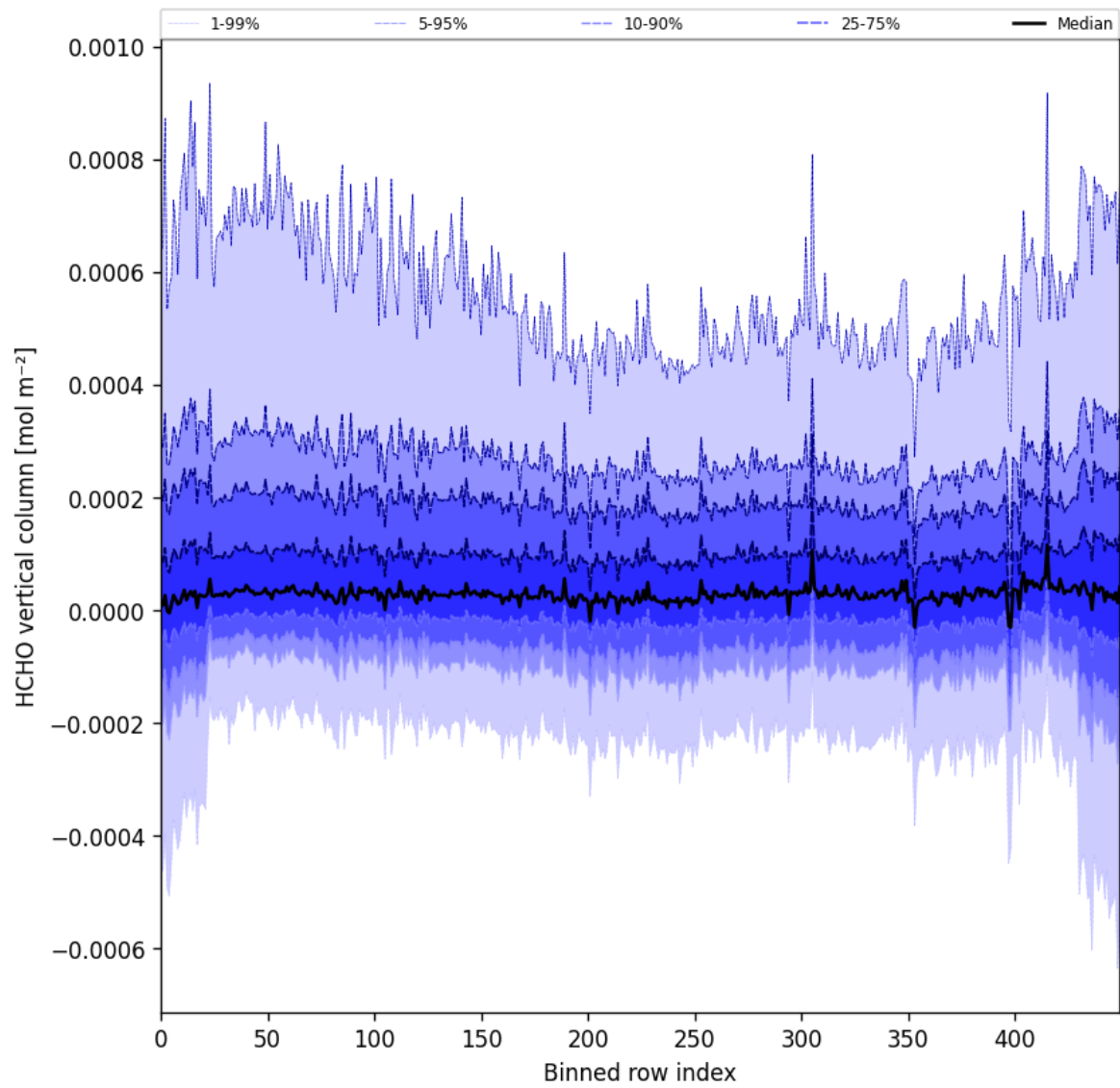
Figure 49: Along track statistics of “HCHO vertical column” for 2025-11-03 to 2025-11-05
