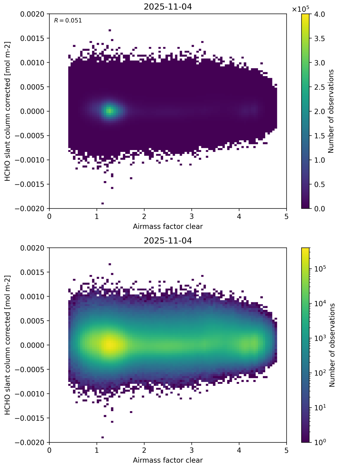
Figure 74: Scatter density plot of “Airmass factor clear” against “HCHO slant column corrected” for 2025-11-03 to 2025-11-05.
