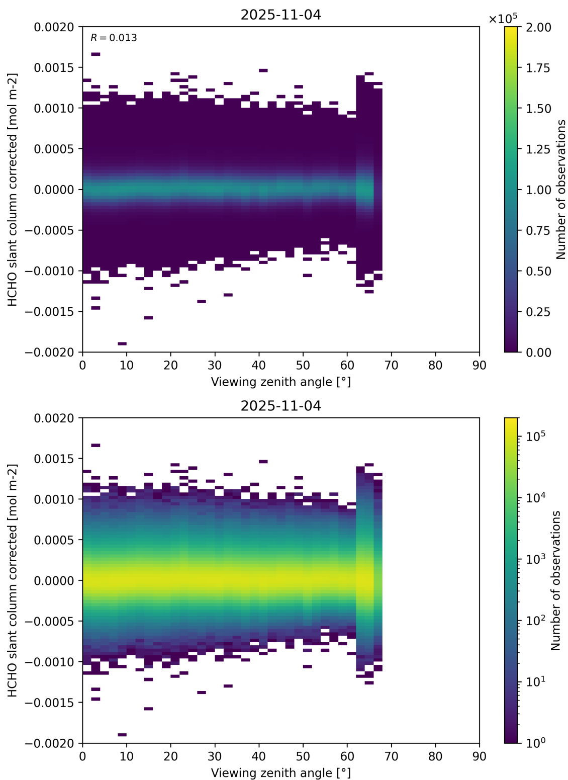
Figure 186: Scatter density plot of “Viewing zenith angle” against “HCHO slant column corrected” for 2025-11-03 to 2025-11-05.
