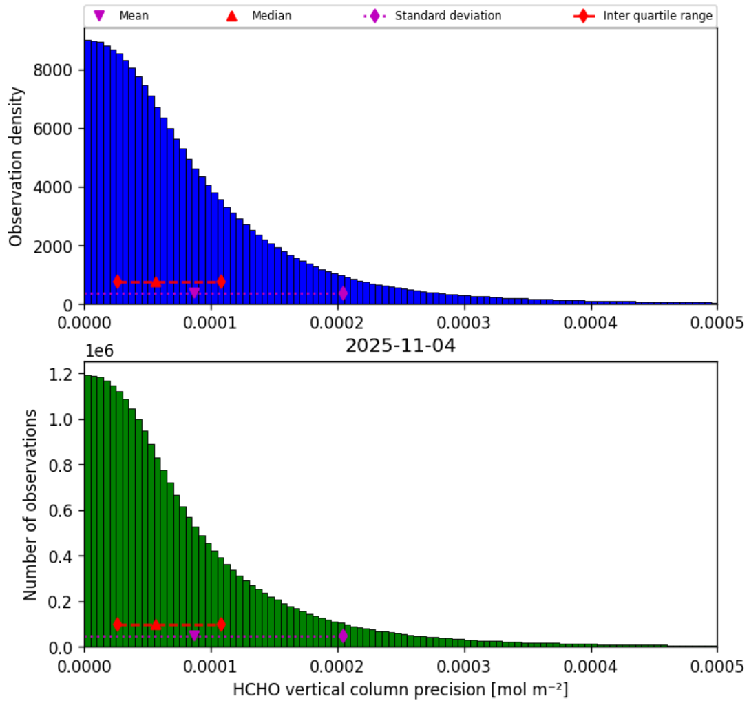
Figure 36: Histogram of “HCHO vertical column precision” for 2025-11-03 to 2025-11-05
