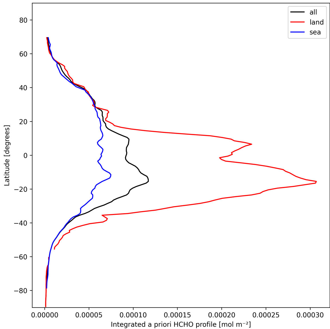
Figure 29: Zonal average of “Integrated a priori HCHO profile” for 2025-11-03 to 2025-11-05.
