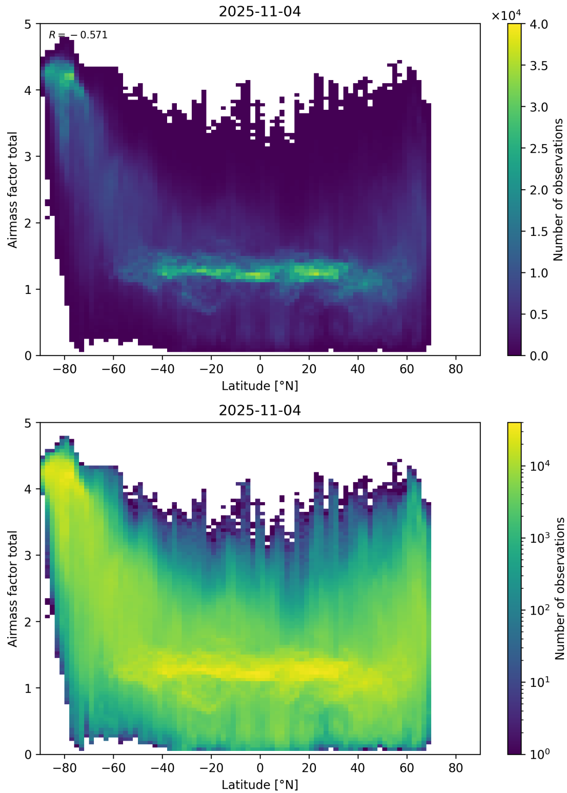
Figure 161: Scatter density plot of “Latitude” against “Airmass factor total” for 2025-11-03 to 2025-11-05.
