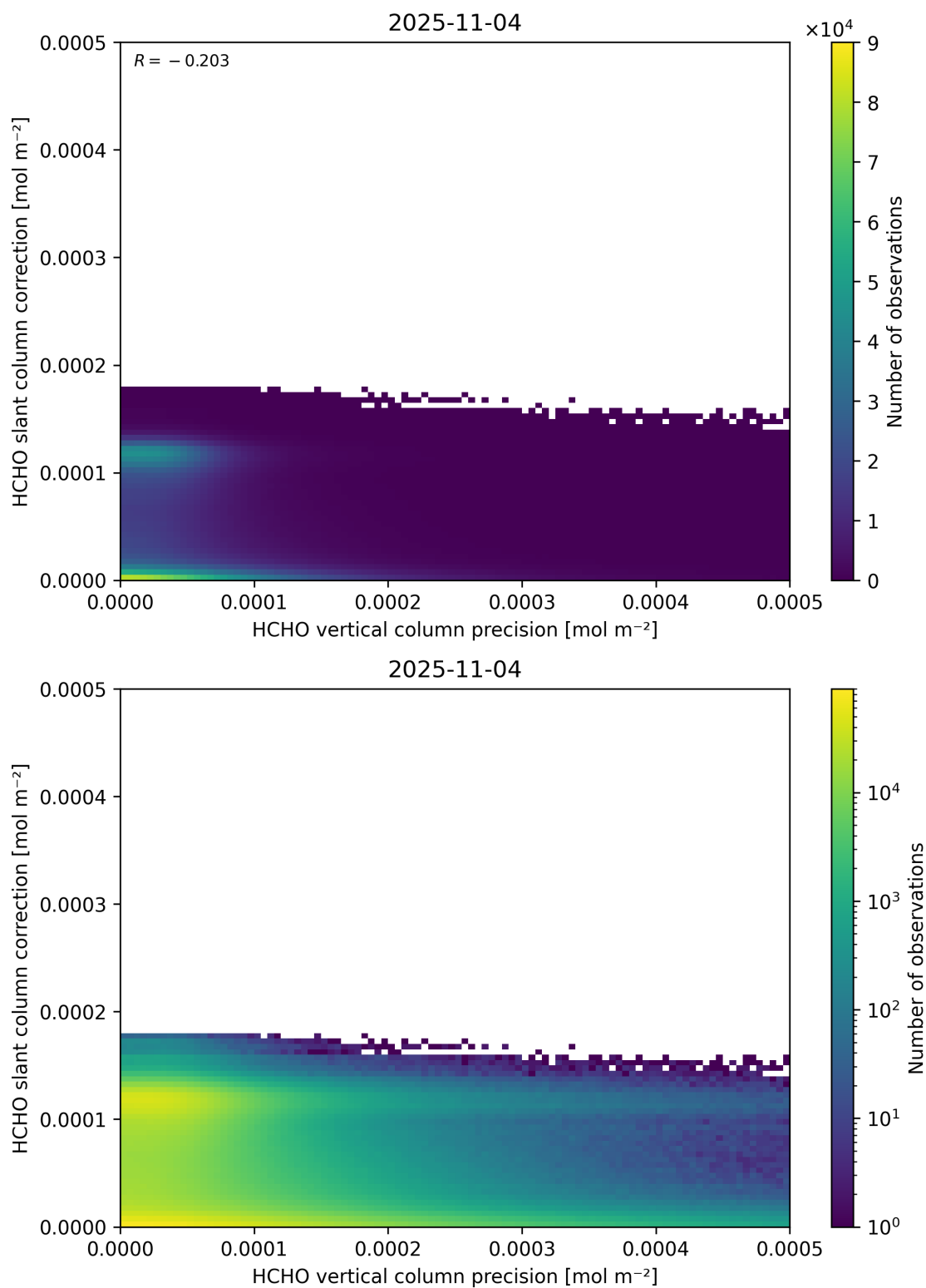
Figure 141: Scatter density plot of “HCHO vertical column precision” against “HCHO slant column correction” for 2025-11-03 to 2025-11-05.
