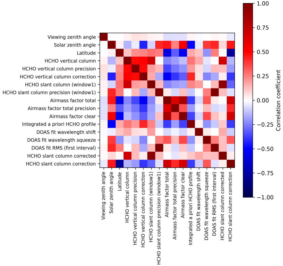
Figure 2: Map of correlation matrix for 2025-11-03 to 2025-11-05.
