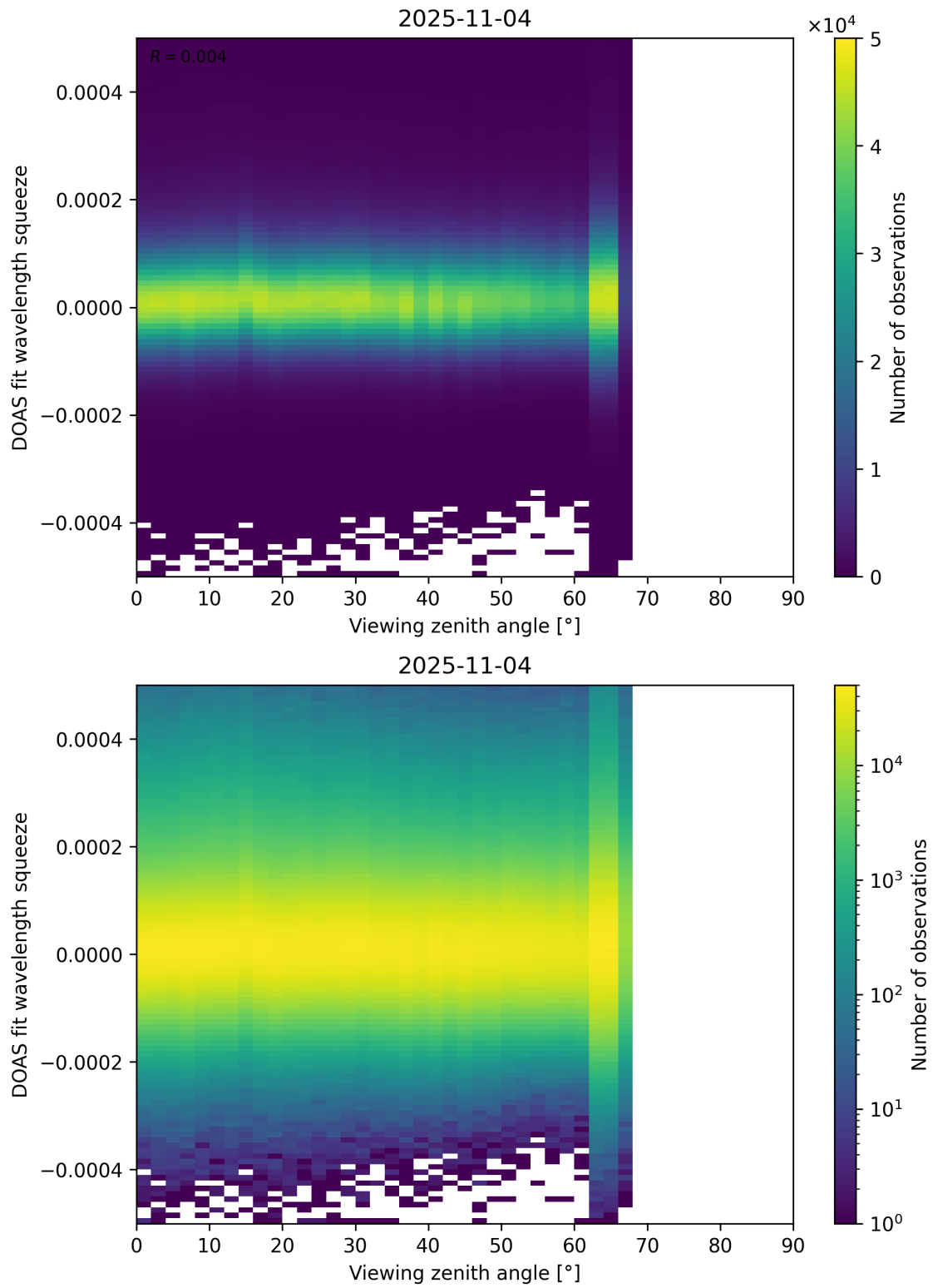
Figure 184: Scatter density plot of “Viewing zenith angle” against “DOAS fit wavelength squeeze” for 2025-11-03 to 2025-11-05.
