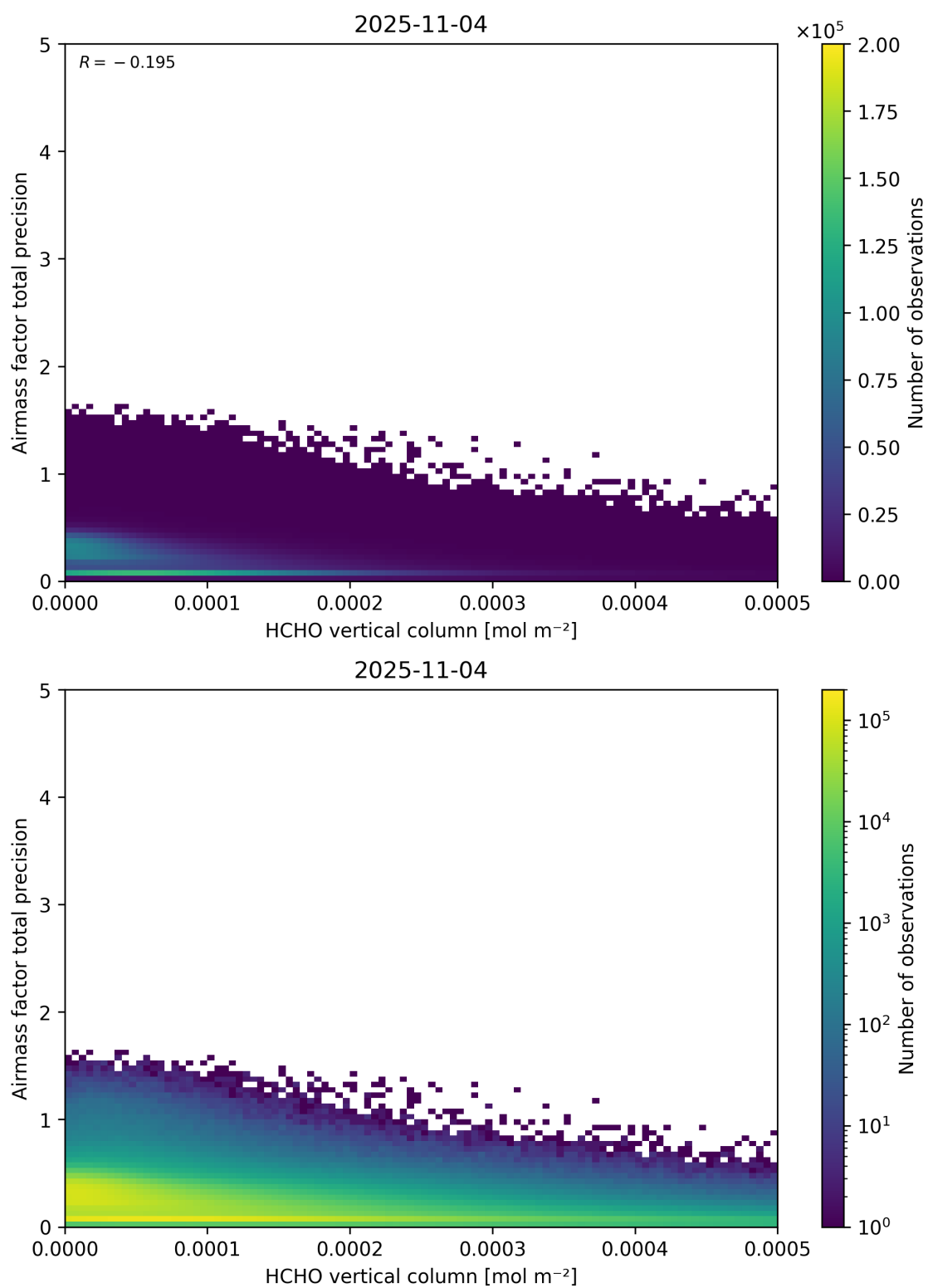
Figure 132: Scatter density plot of “HCHO vertical column” against “Airmass factor total precision” for 2025-11-03 to 2025-11-05.
