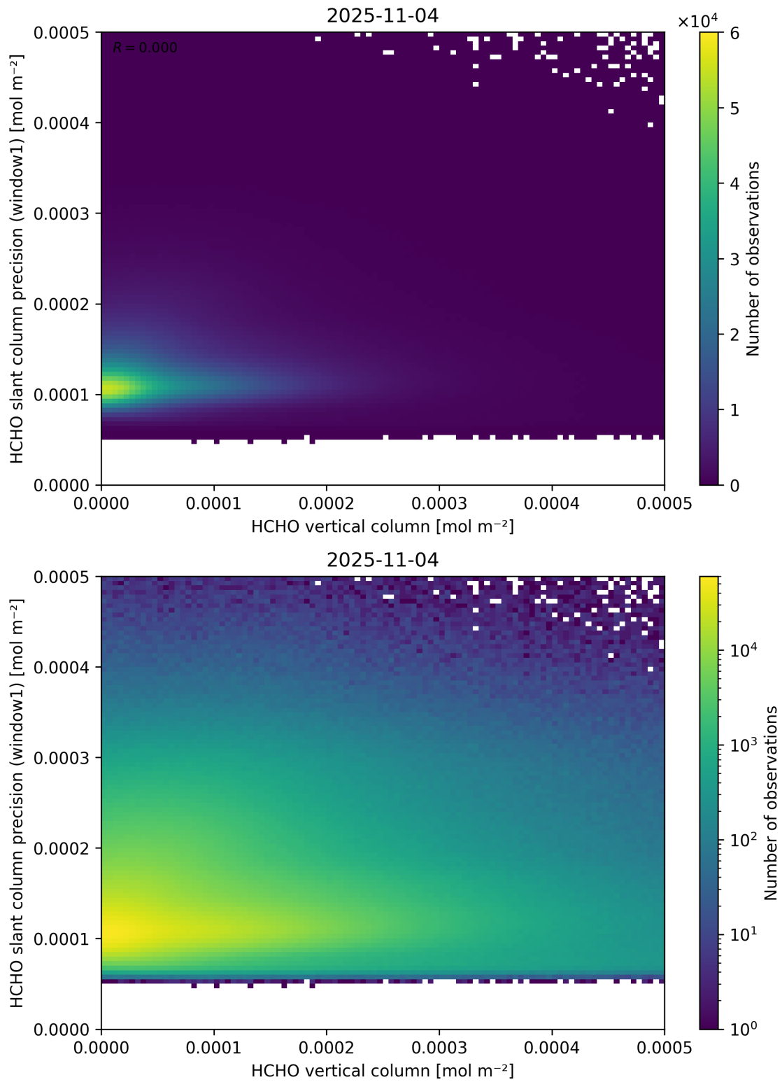
Figure 130: Scatter density plot of “HCHO vertical column” against “HCHO slant column precision (window1)” for 2025-11-03 to 2025-11-05.
