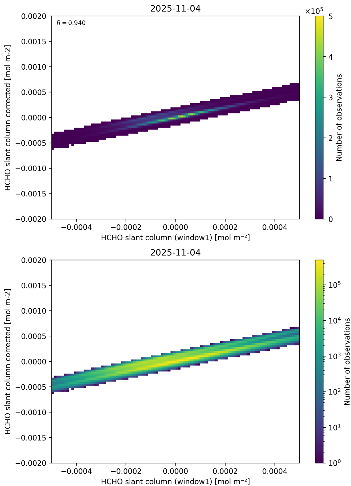
Figure 82: Scatter density plot of “HCHO slant column (window1)” against “HCHO slant column corrected” for 2025-11-03 to 2025-11-05.
