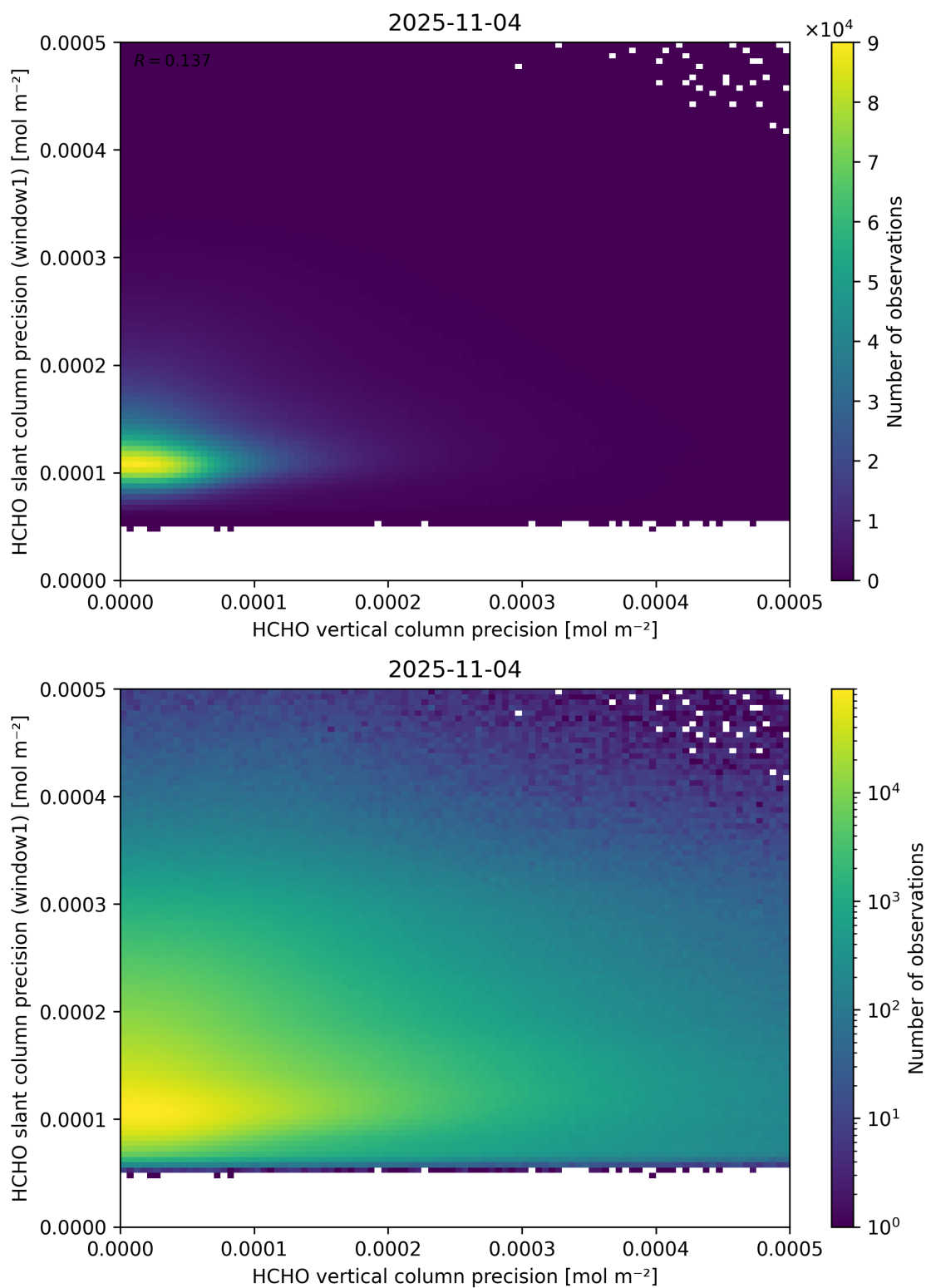
Figure 143: Scatter density plot of “HCHO vertical column precision” against “HCHO slant column precision (window1)” for 2025-11-03 to 2025-11-05.
