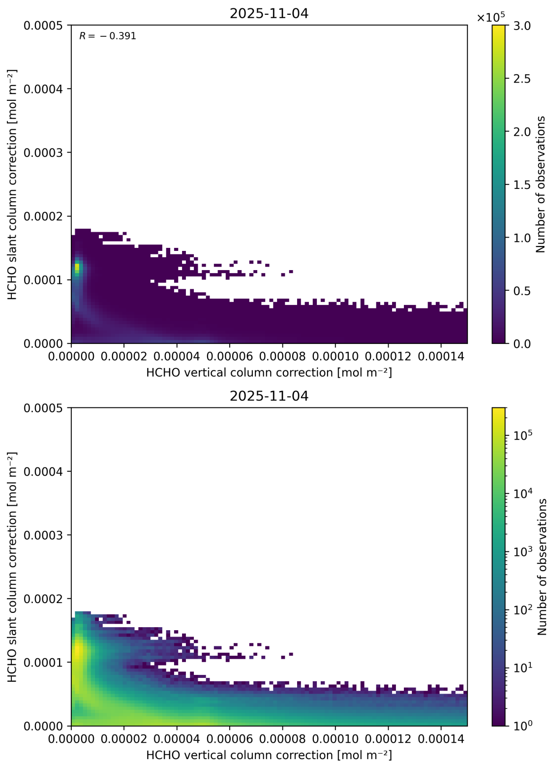
Figure 117: Scatter density plot of “HCHO vertical column correction” against “HCHO slant column correction” for 2025-11-03 to 2025-11-05.
