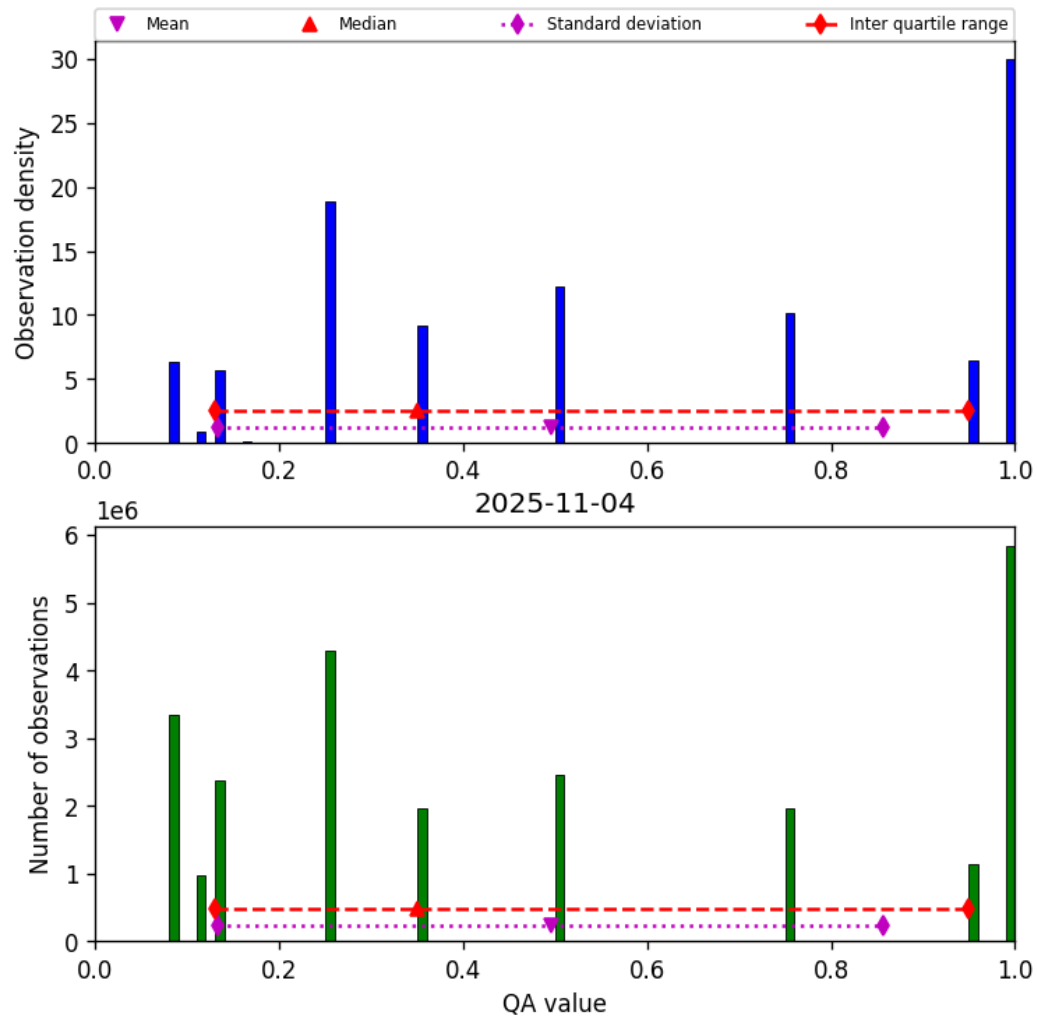
Figure 34: Histogram of “QA value” for 2025-11-03 to 2025-11-05
