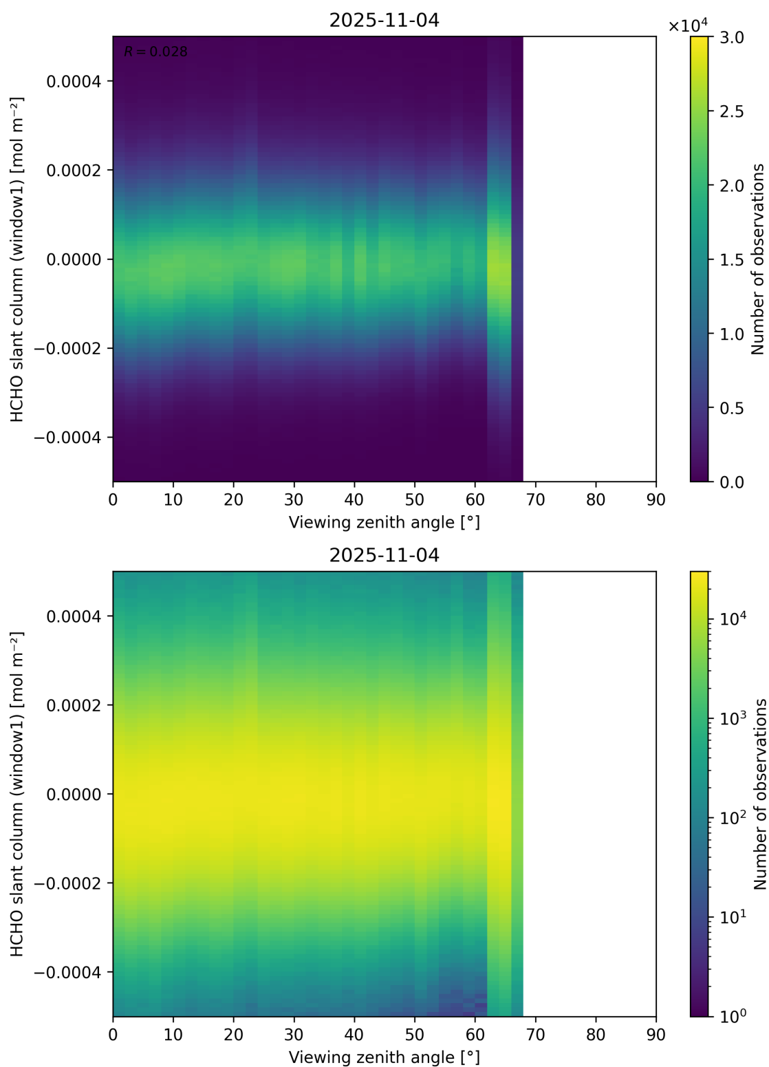
Figure 188: Scatter density plot of “Viewing zenith angle” against “HCHO slant column (window1)” for 2025-11-03 to 2025-11-05.
