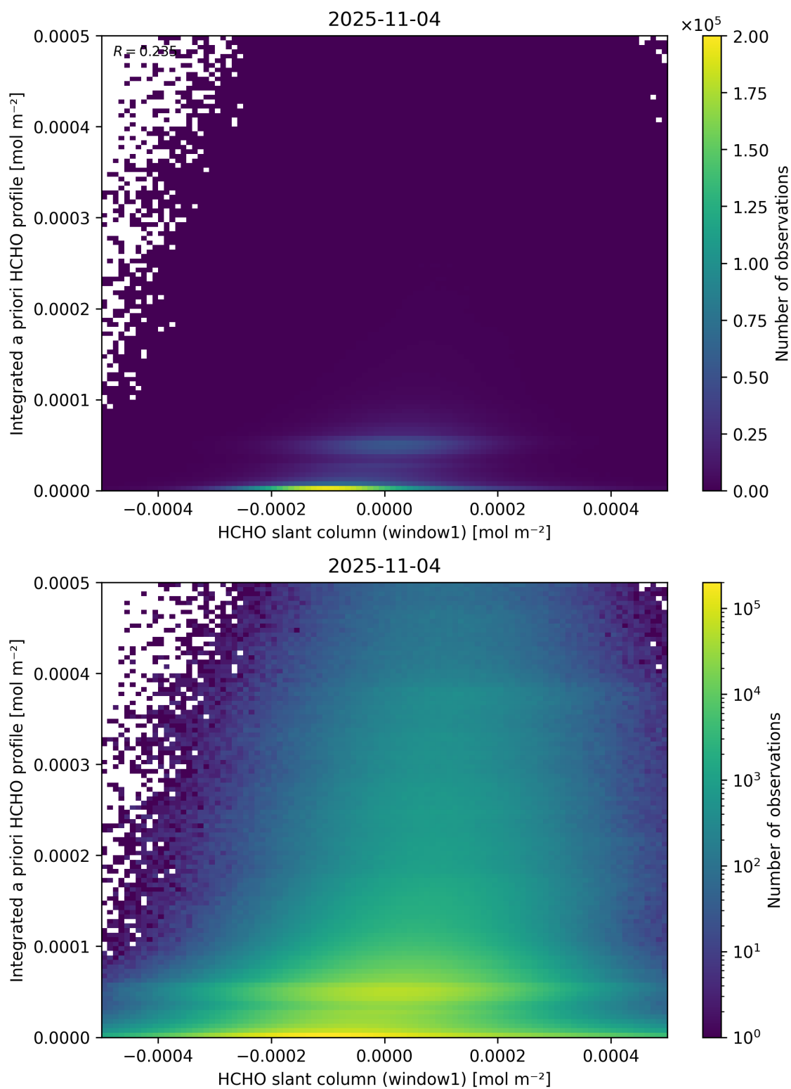
Figure 87: Scatter density plot of “HCHO slant column (window1)” against “Integrated a priori HCHO profile” for 2025-11-03 to 2025-11-05.
