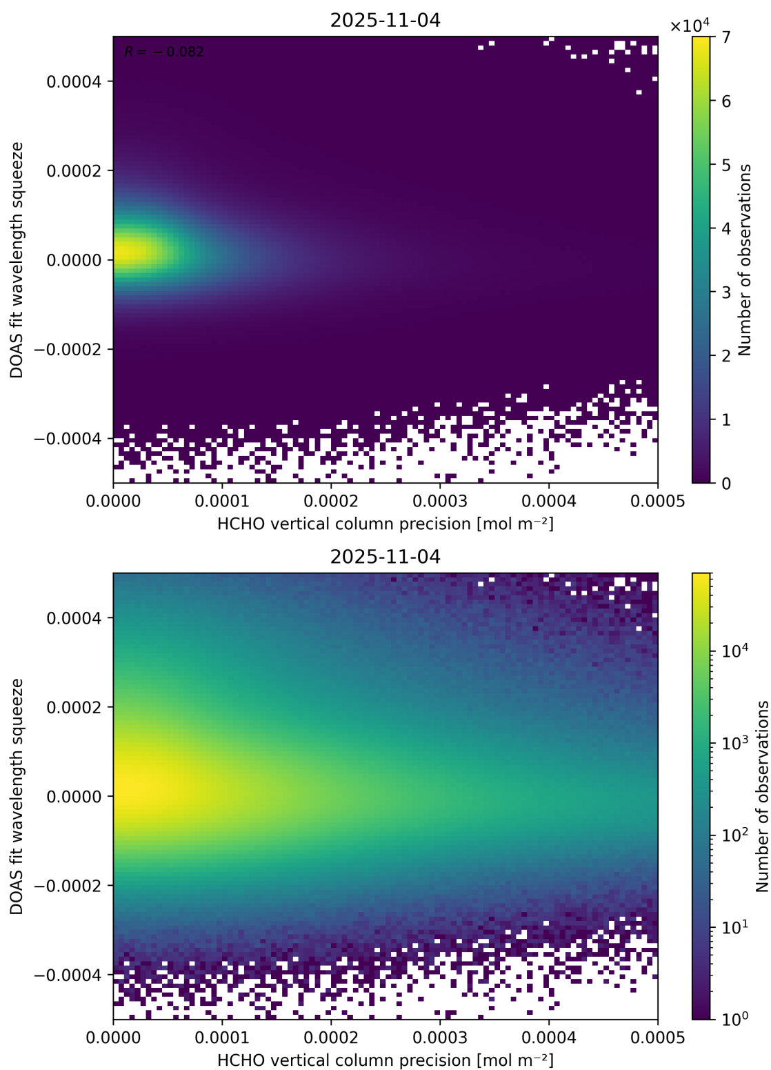
Figure 138: Scatter density plot of “HCHO vertical column precision” against “DOAS fit wavelength squeeze” for 2025-11-03 to 2025-11-05.
