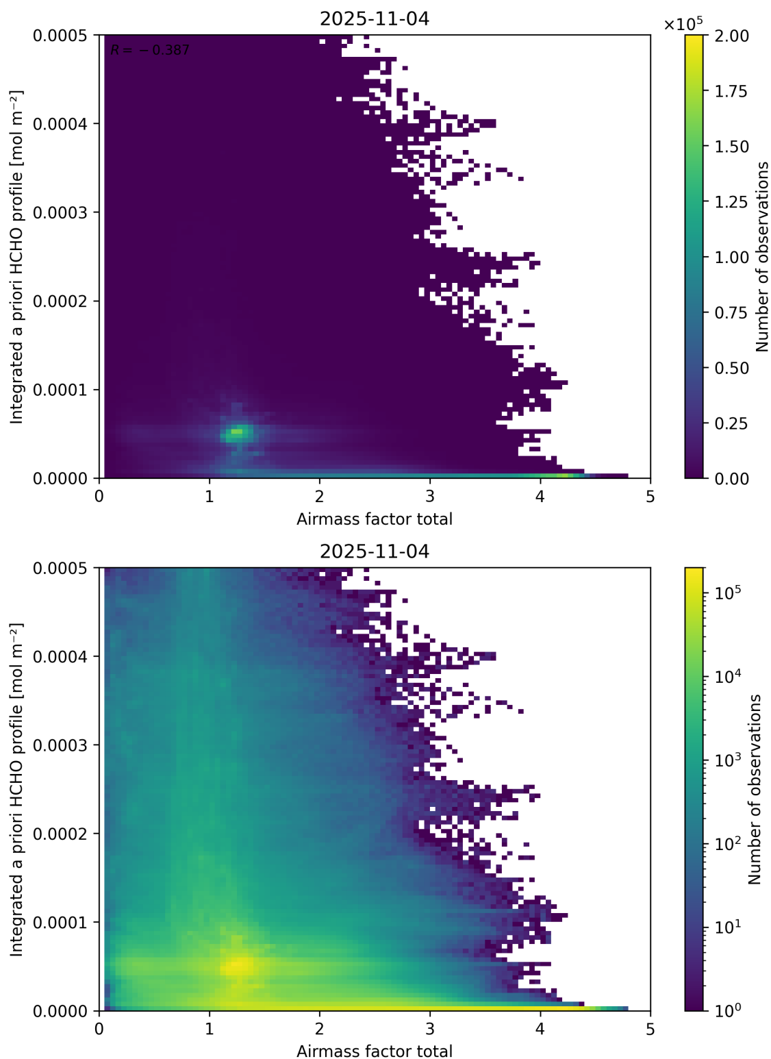
Figure 104: Scatter density plot of “Airmass factor total” against “Integrated a priori HCHO profile” for 2025-11-03 to 2025-11-05.
