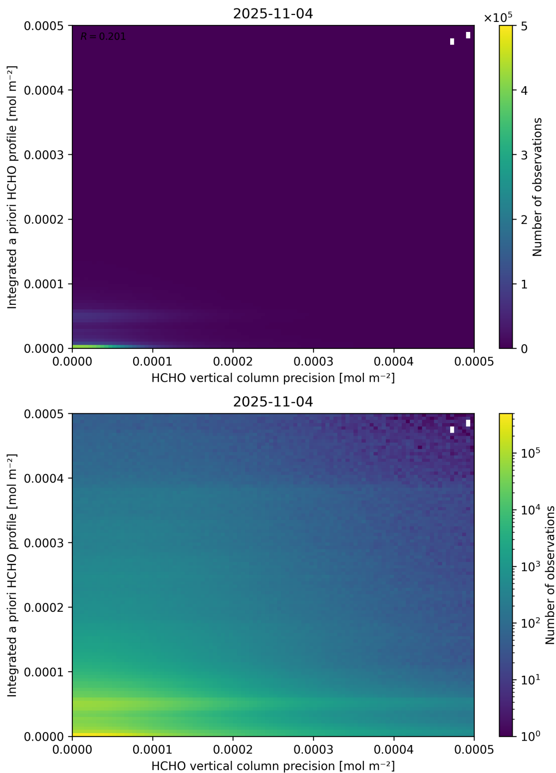
Figure 147: Scatter density plot of “HCHO vertical column precision” against “Integrated a priori HCHO profile” for 2025-11-03 to 2025-11-05.
