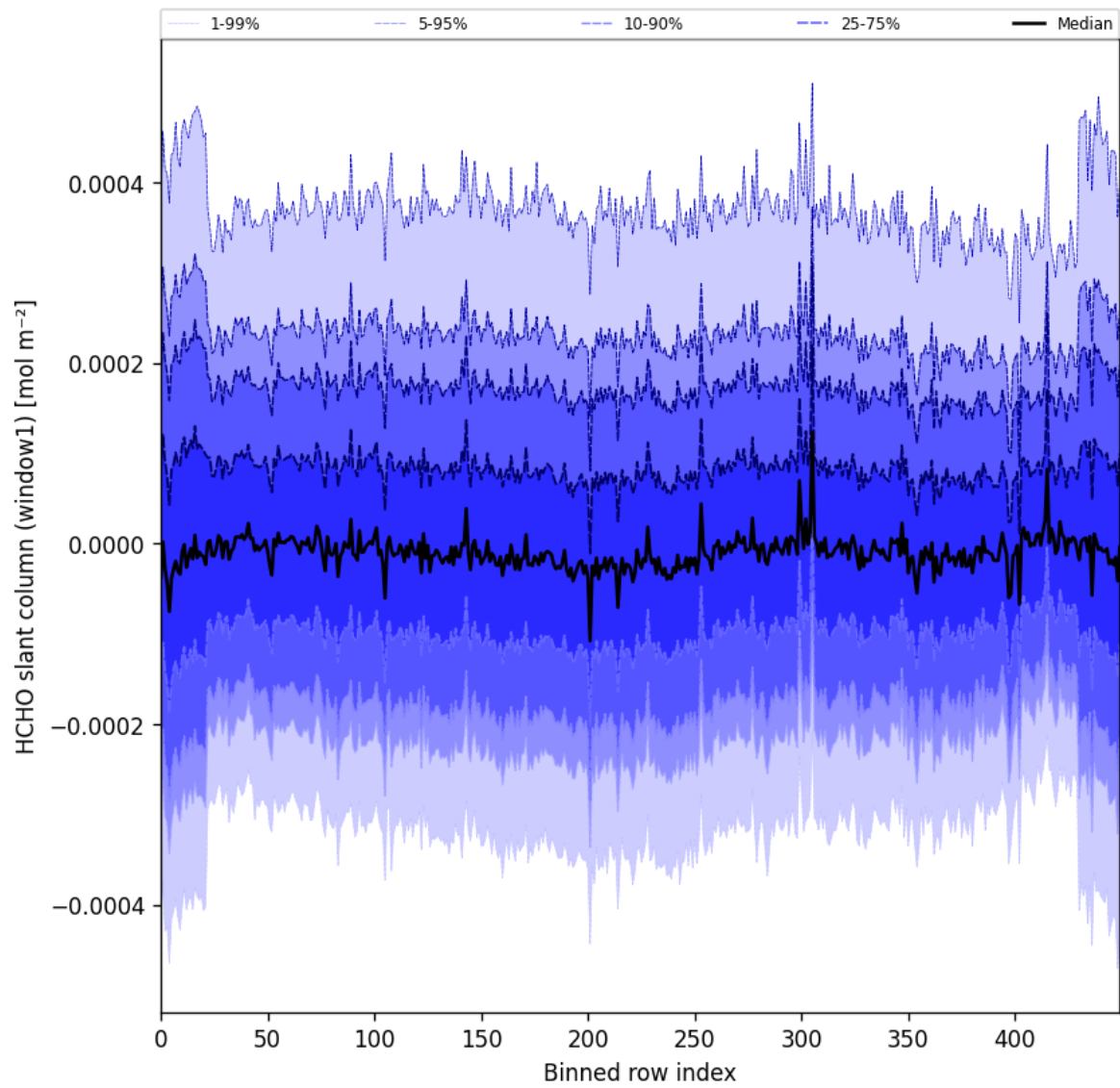
Figure 52: Along track statistics of “HCHO slant column (window1)” for 2025-11-03 to 2025-11-05
