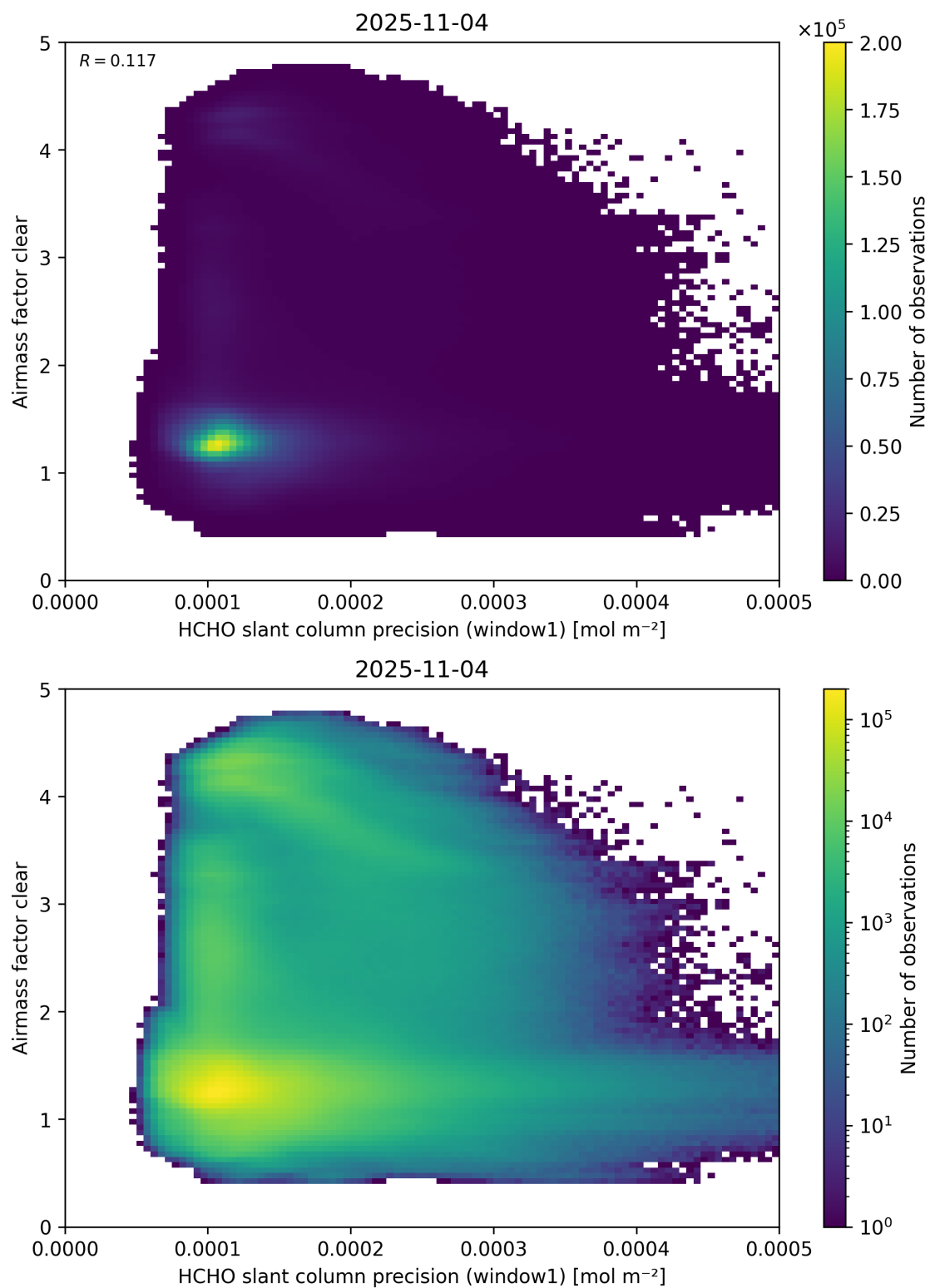
Figure 91: Scatter density plot of “HCHO slant column precision (window1)” against “Airmass factor clear” for 2025-11-03 to 2025-11-05.
