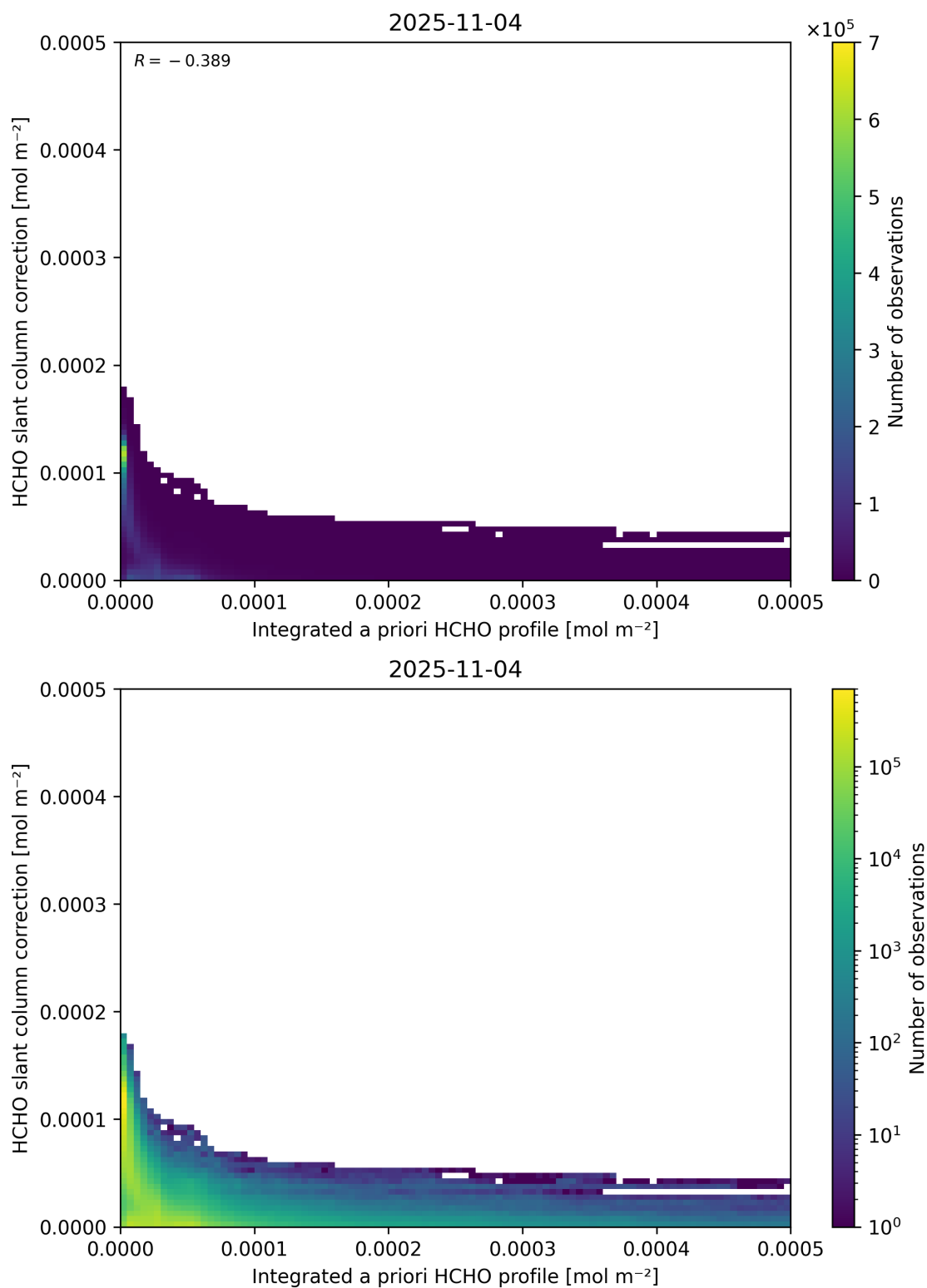
Figure 152: Scatter density plot of “Integrated a priori HCHO profile” against “HCHO slant column correction” for 2025-11-03 to 2025-11-05.
