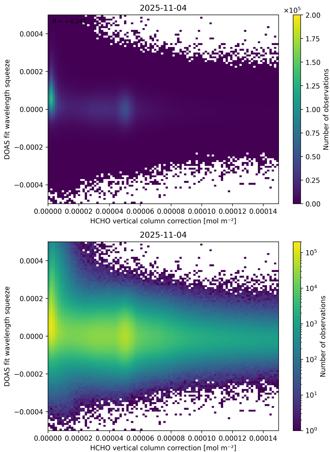
Figure 114: Scatter density plot of “HCHO vertical column correction” against “DOAS fit wavelength squeeze” for 2025-11-03 to 2025-11-05.
