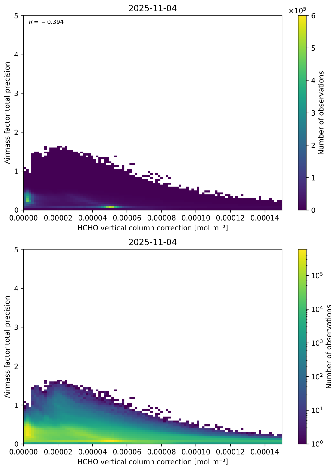
Figure 121: Scatter density plot of “HCHO vertical column correction” against “Airmass factor total precision” for 2025-11-03 to 2025-11-05.
