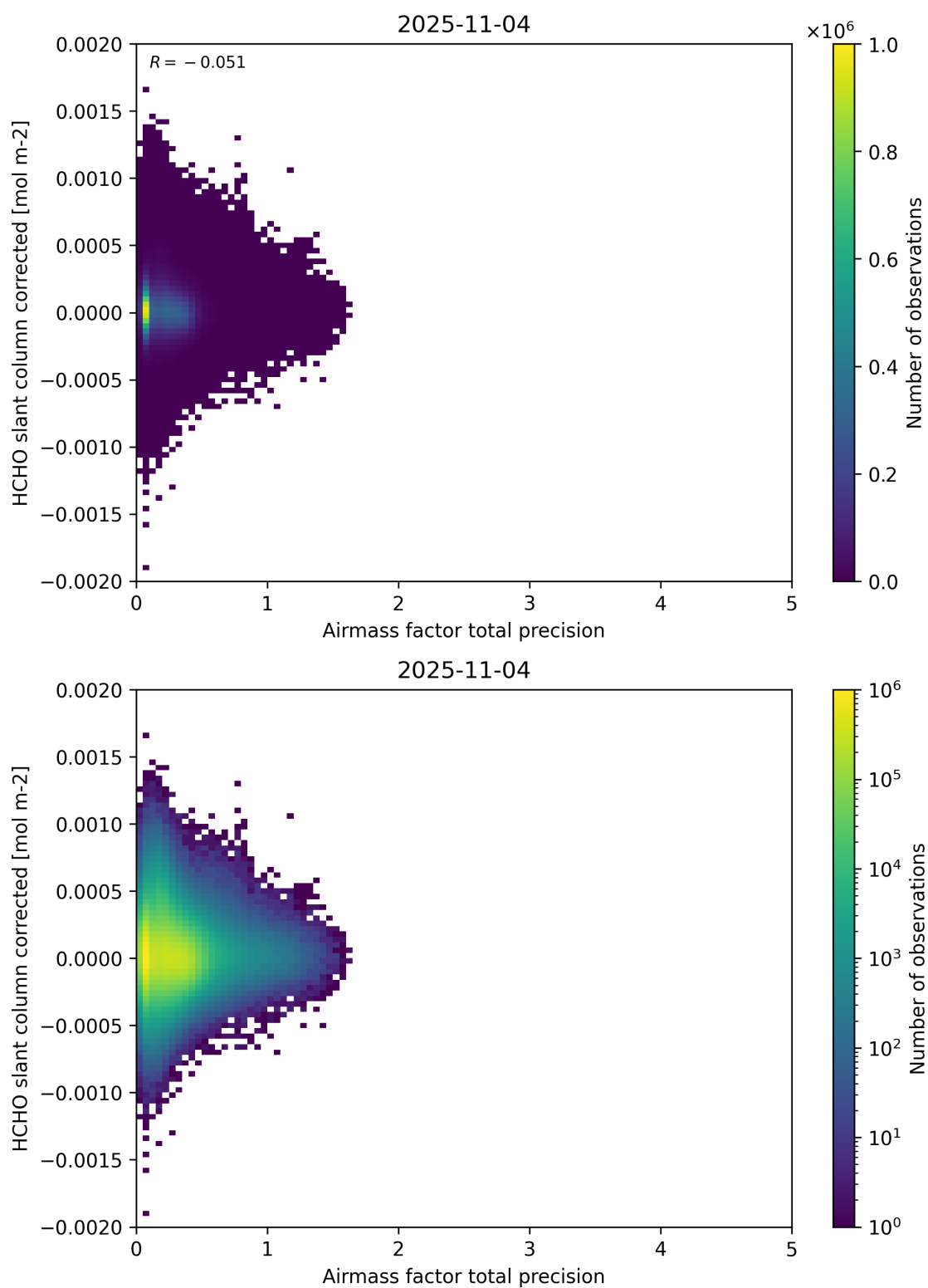
Figure 109: Scatter density plot of “Airmass factor total precision” against “HCHO slant column corrected” for 2025-11-03 to 2025-11-05.
