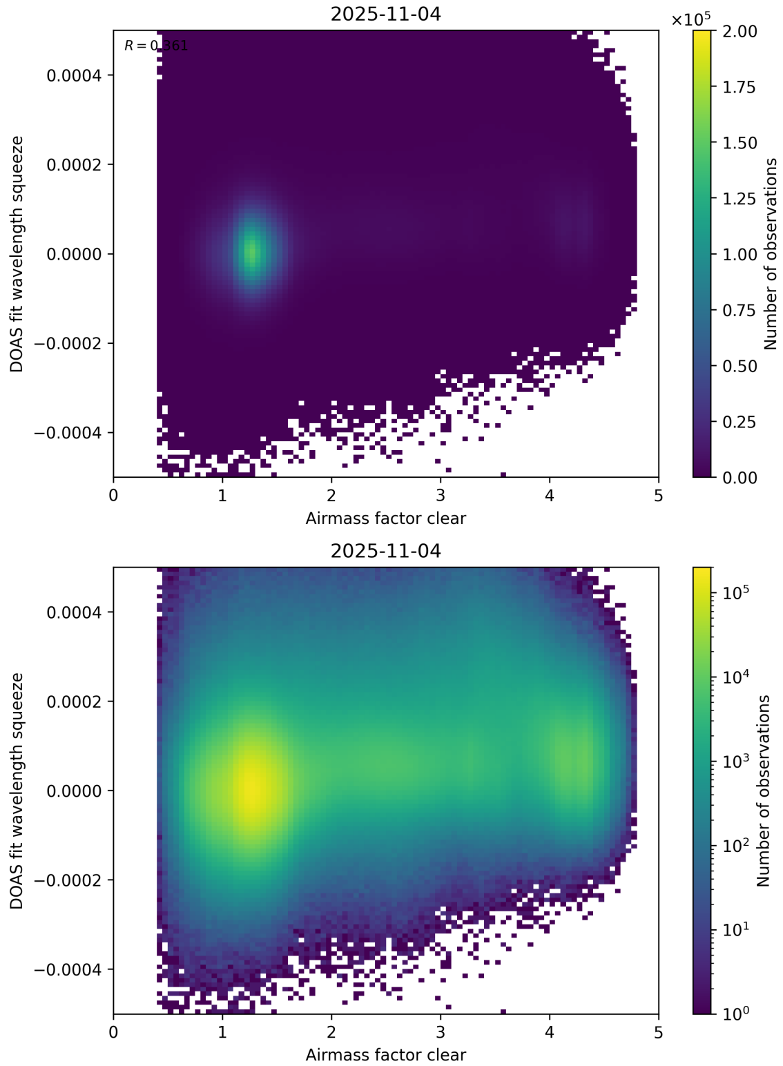
Figure 73: Scatter density plot of “Airmass factor clear” against “DOAS fit wavelength squeeze” for 2025-11-03 to 2025-11-05.
