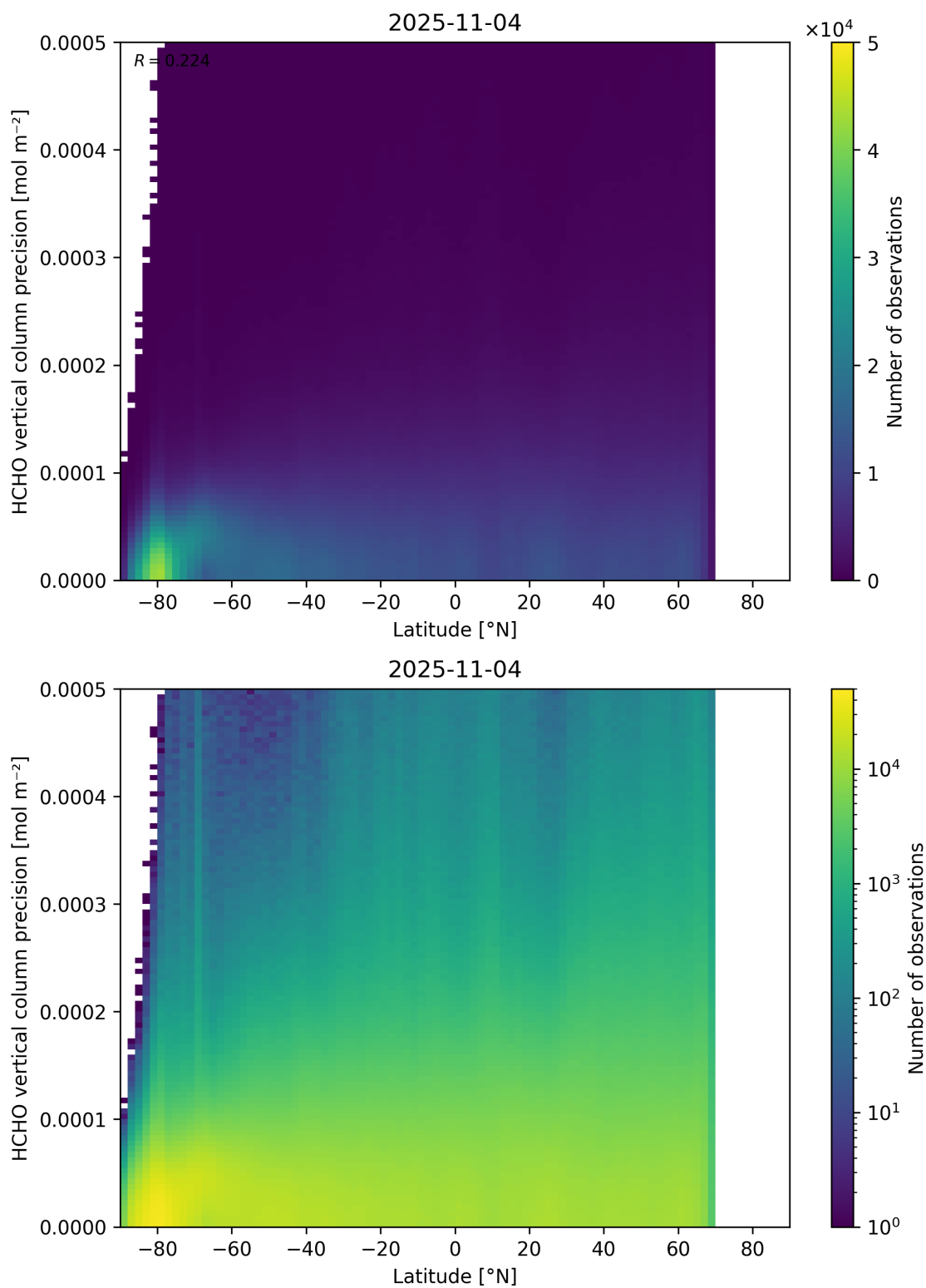
Figure 165: Scatter density plot of “Latitude” against “HCHO vertical column precision” for 2025-11-03 to 2025-11-05.
