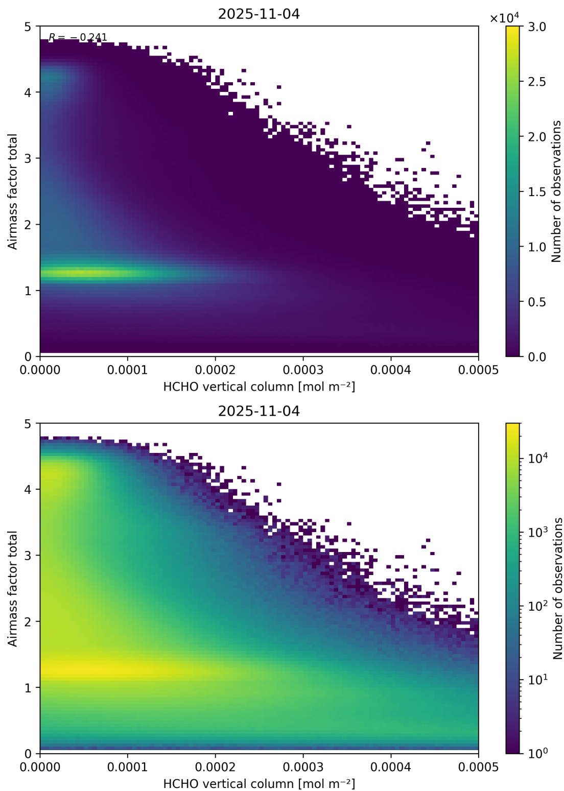
Figure 131: Scatter density plot of “HCHO vertical column” against “Airmass factor total” for 2025-11-03 to 2025-11-05.
