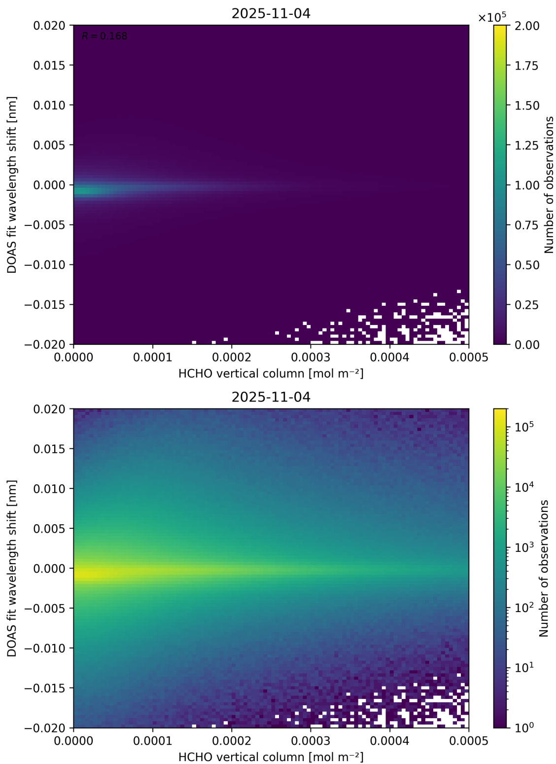
Figure 124: Scatter density plot of “HCHO vertical column” against “DOAS fit wavelength shift” for 2025-11-03 to 2025-11-05.
