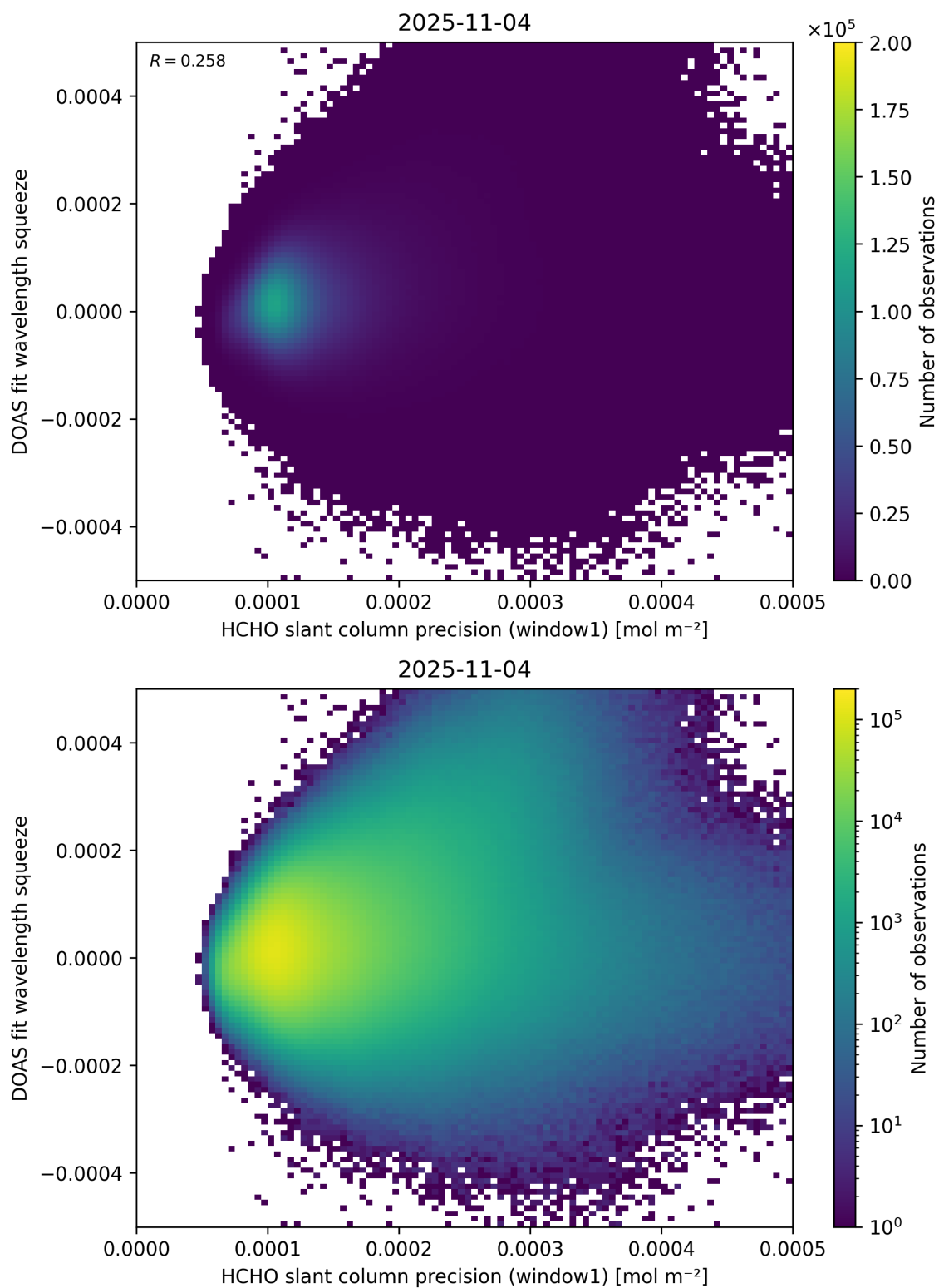
Figure 90: Scatter density plot of “HCHO slant column precision (window1)” against “DOAS fit wavelength squeeze” for 2025-11-03 to 2025-11-05.
