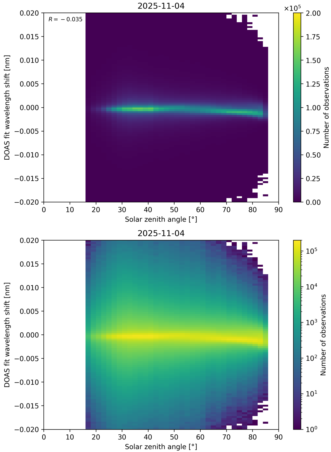
Figure 168: Scatter density plot of “Solar zenith angle” against “DOAS fit wavelength shift” for 2025-11-03 to 2025-11-05.
