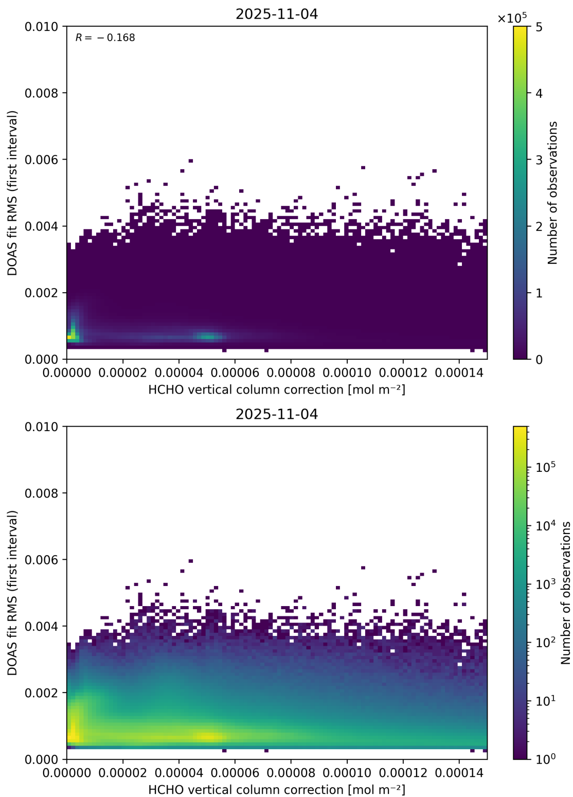
Figure 112: Scatter density plot of “HCHO vertical column correction” against “DOAS fit RMS (first interval)” for 2025-11-03 to 2025-11-05.
