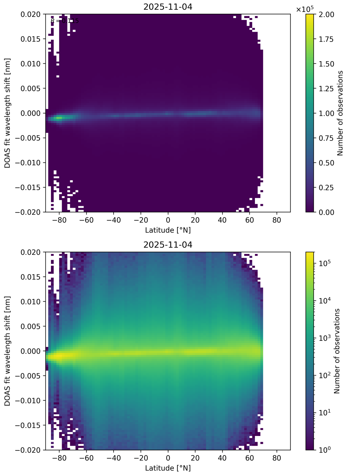
Figure 154: Scatter density plot of “Latitude” against “DOAS fit wavelength shift” for 2025-11-03 to 2025-11-05.
