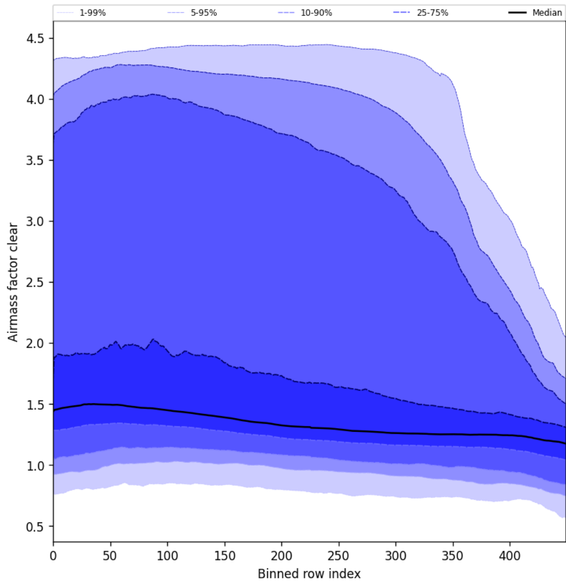
Figure 56: Along track statistics of “Air mass factor clear” for 2025-11-03 to 2025-11-05
