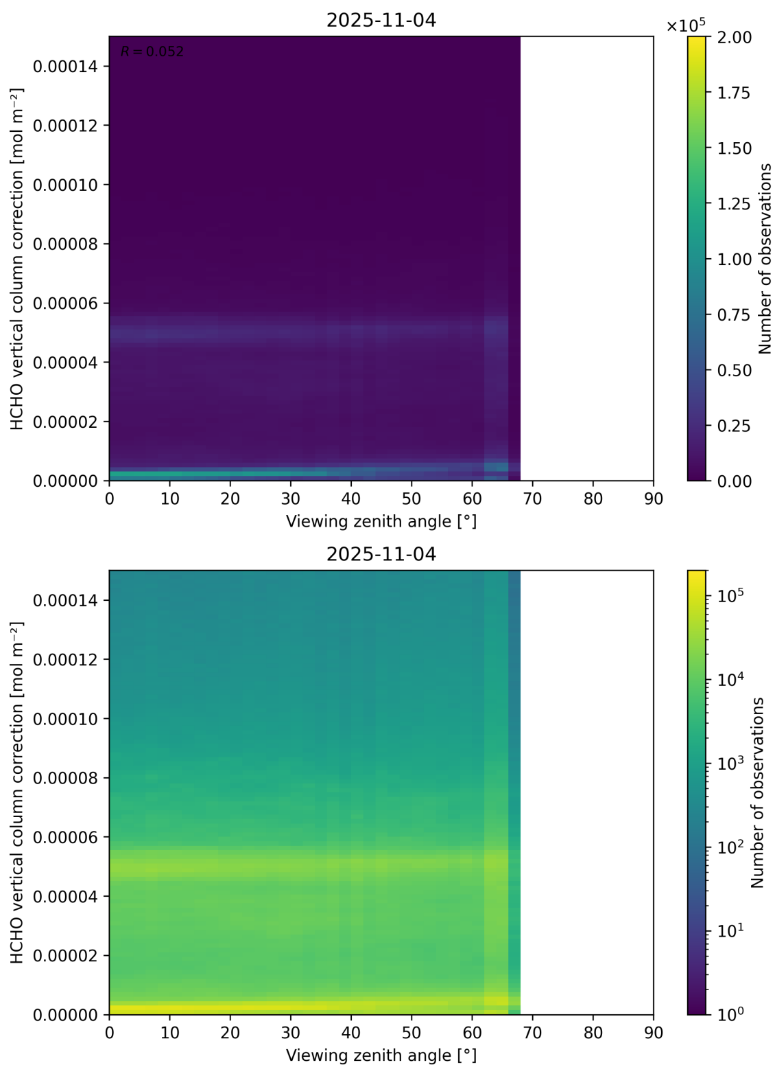
Figure 193: Scatter density plot of “Viewing zenith angle” against “HCHO vertical column correction” for 2025-11-03 to 2025-11-05.
