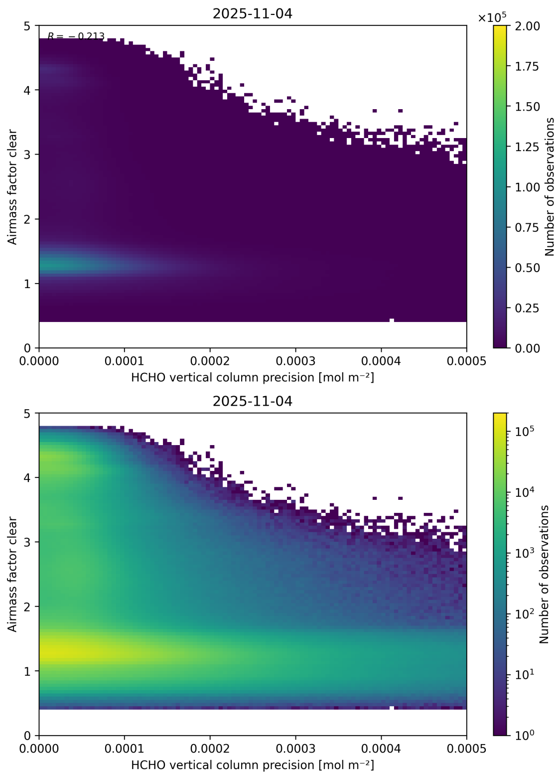
Figure 139: Scatter density plot of “HCHO vertical column precision” against “Airmass factor clear” for 2025-11-03 to 2025-11-05.
