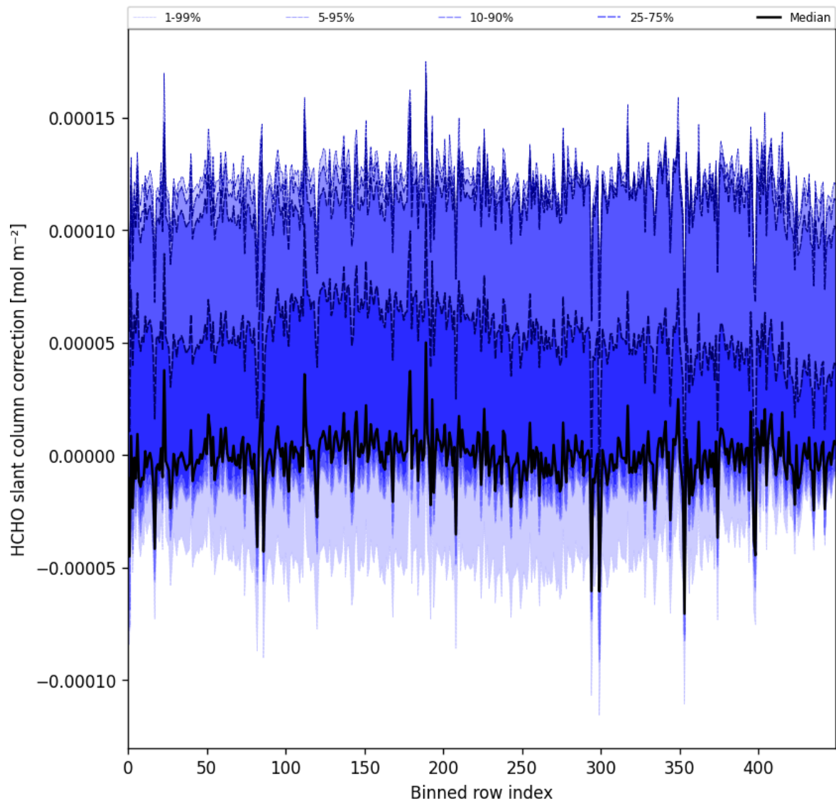
Figure 61: Along track statistics of “HCHO slant column correction” for 2025-11-03 to 2025-11-05
