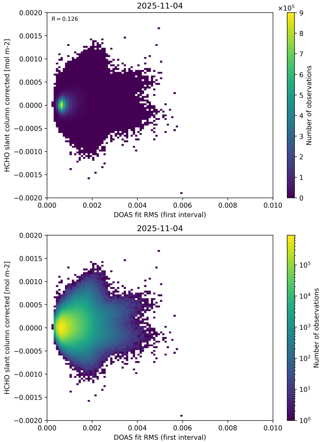
Figure 62: Scatter density plot of “DOAS fit RMS (first interval)” against “HCHO slant column corrected” for 2025-11-03 to 2025-11-05.
