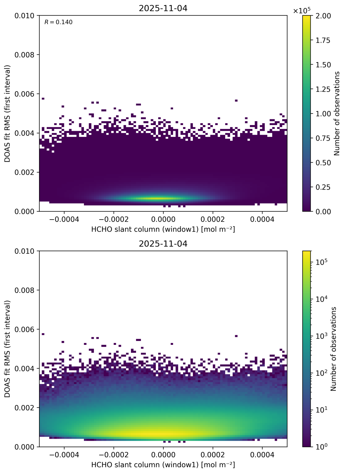
Figure 78: Scatter density plot of “HCHO slant column (window1)” against “DOAS fit RMS (first interval)” for 2025-11-03 to 2025-11-05.
