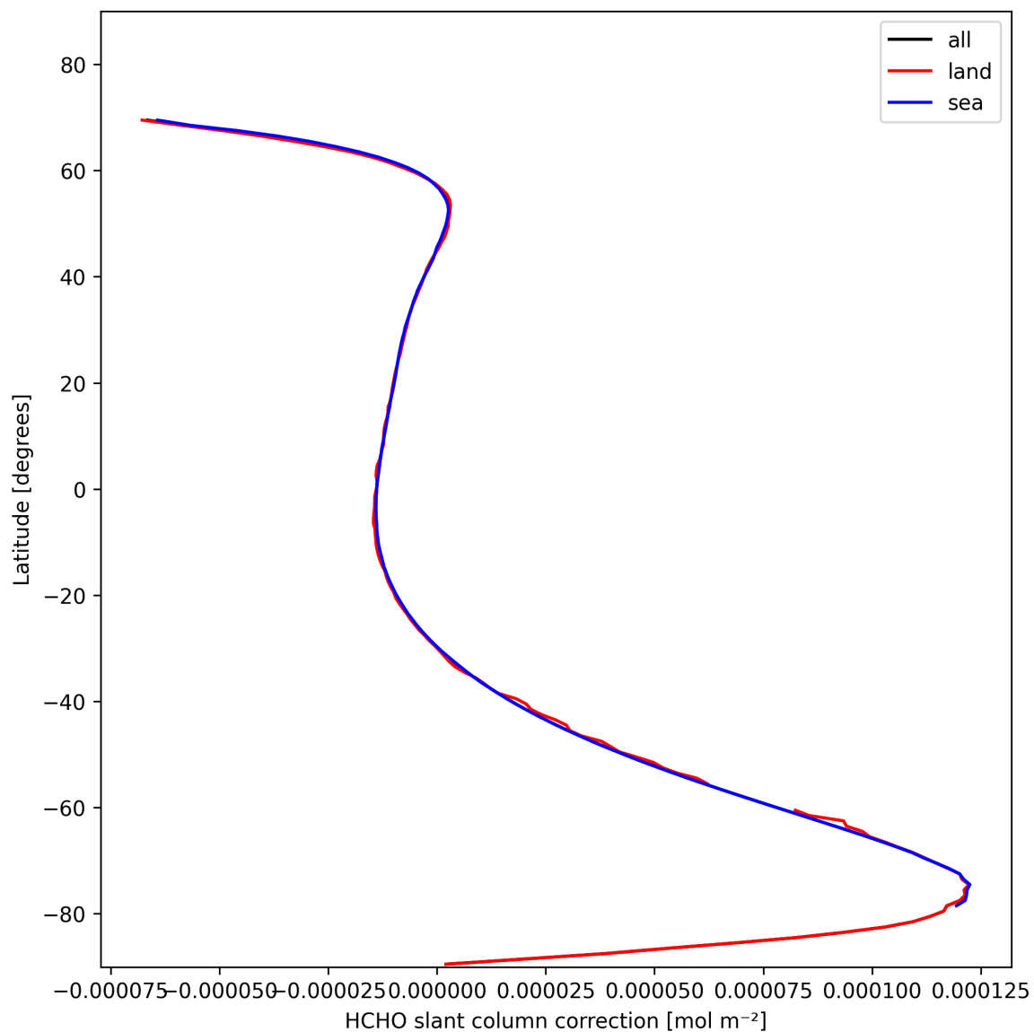
Figure 33: Zonal average of “HCHO slant column correction” for 2025-11-03 to 2025-11-05.
