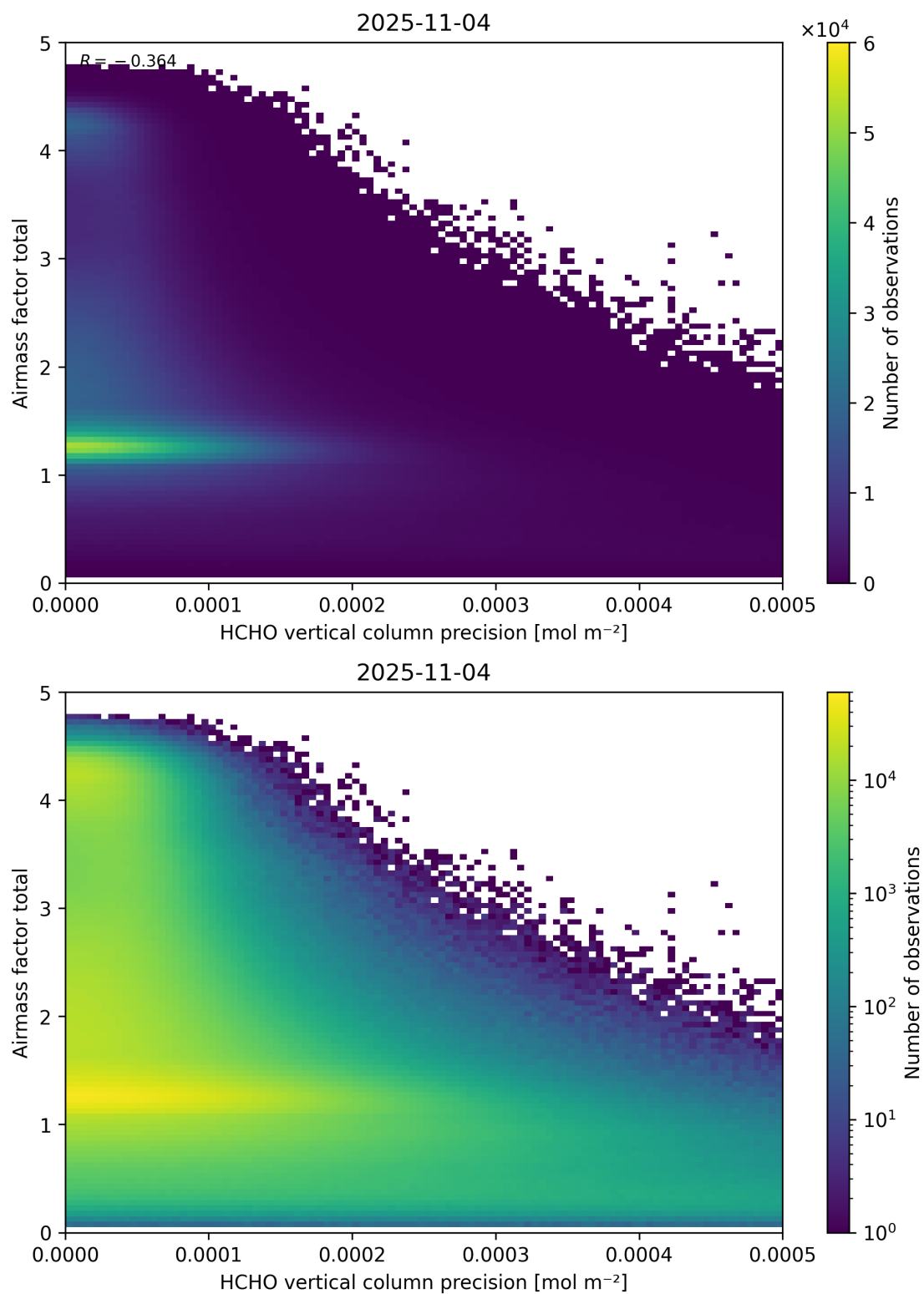
Figure 144: Scatter density plot of “HCHO vertical column precision” against “Airmass factor total” for 2025-11-03 to 2025-11-05.
