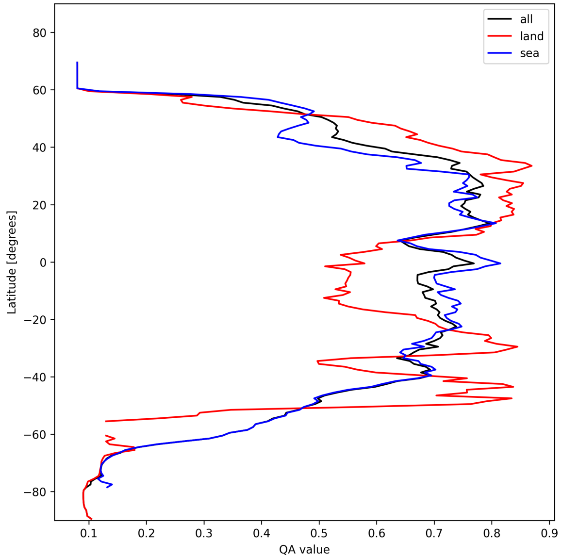
Figure 20: Zonal average of “QA value” for 2025-11-03 to 2025-11-05.
