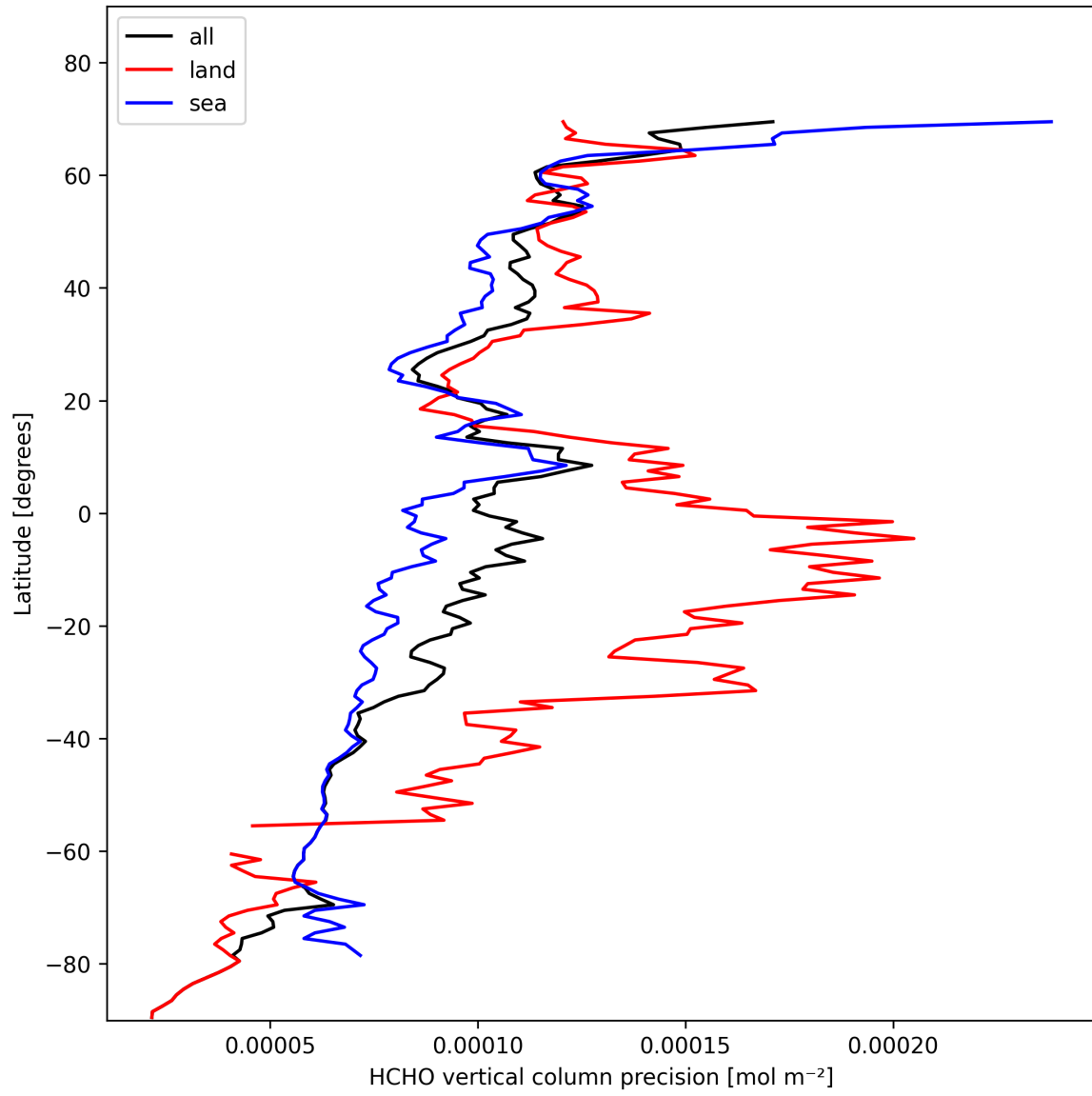
Figure 22: Zonal average of "HCHO vertical column precision" for 2025-11-03 to 2025-11-05.
