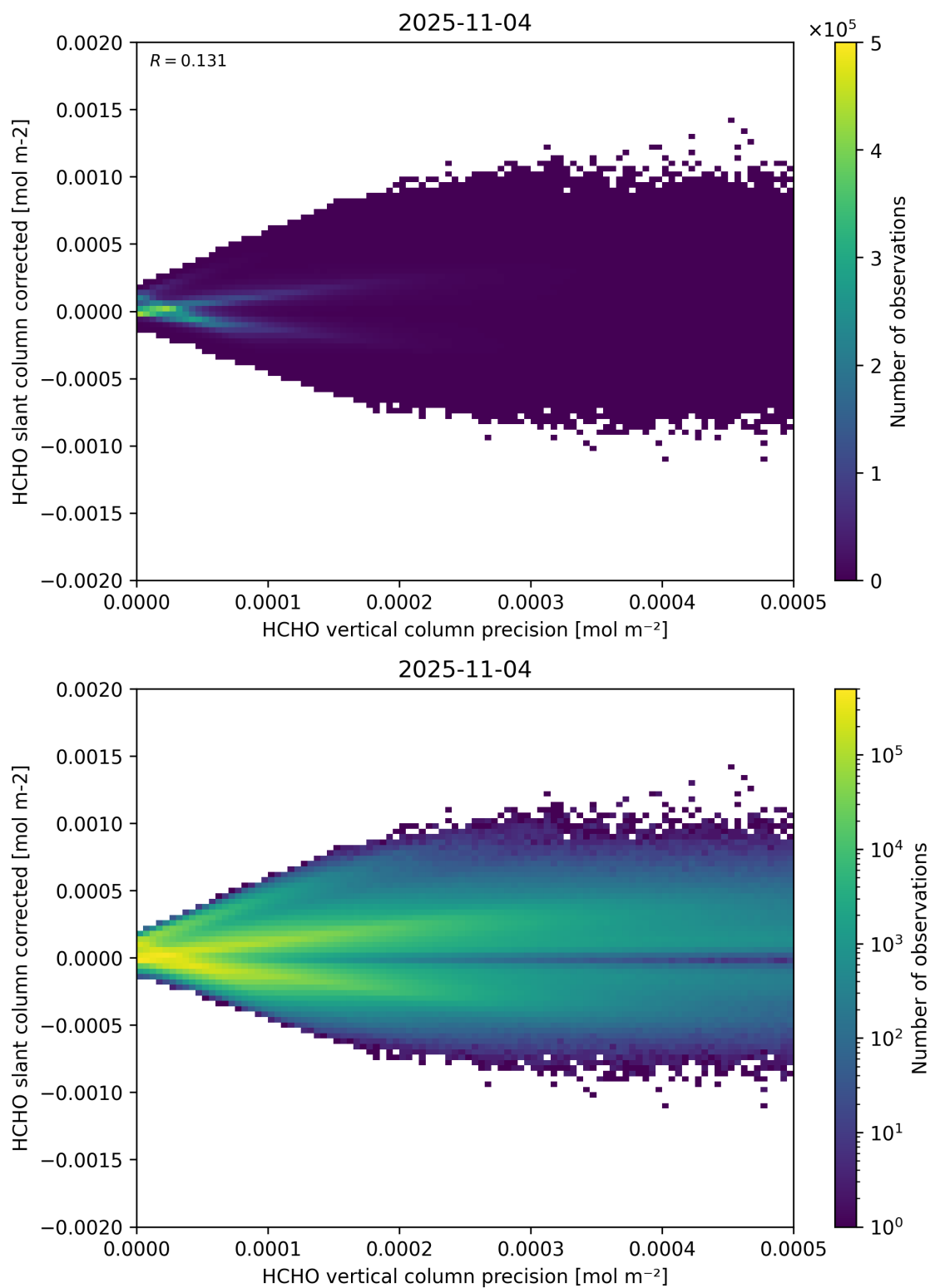
Figure 140: Scatter density plot of “HCHO vertical column precision” against “HCHO slant column corrected” for 2025-11-03 to 2025-11-05.
