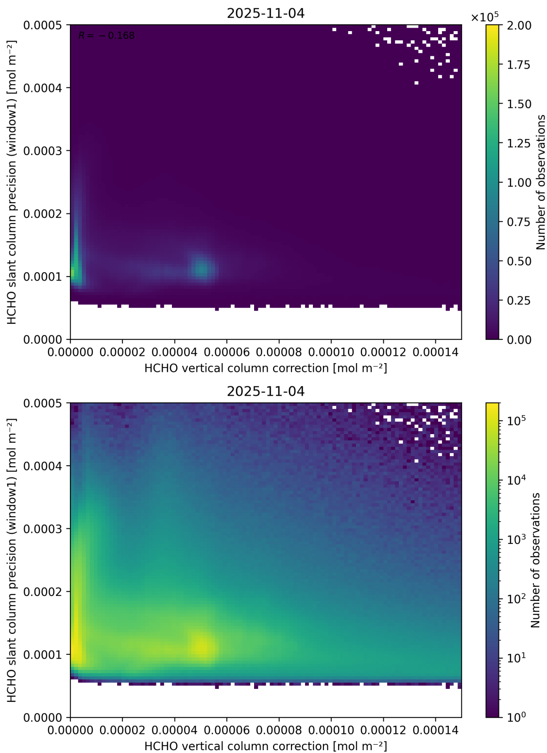
Figure 119: Scatter density plot of “HCHO vertical column correction” against “HCHO slant column precision (window1)” for 2025-11-03 to 2025-11-05.
