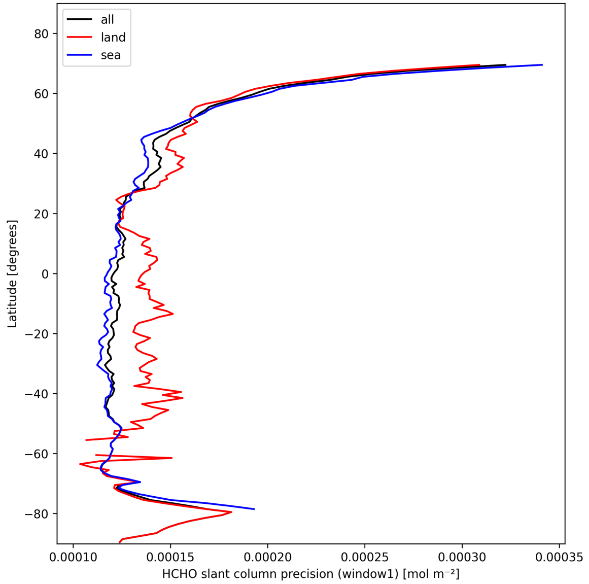
Figure 25: Zonal average of “HCHO slant column precision (window1)” for 2025-11-03 to 2025-11-05.
