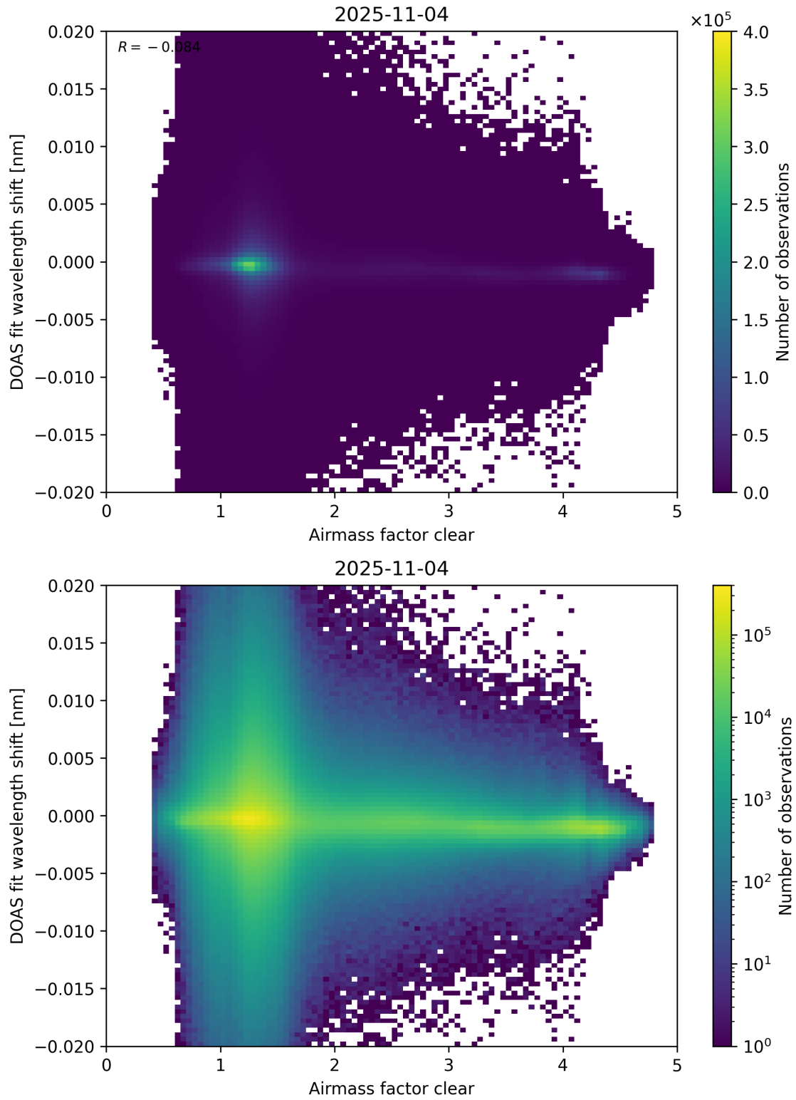
Figure 72: Scatter density plot of “Airmass factor clear” against “DOAS fit wavelength shift” for 2025-11-03 to 2025-11-05.
