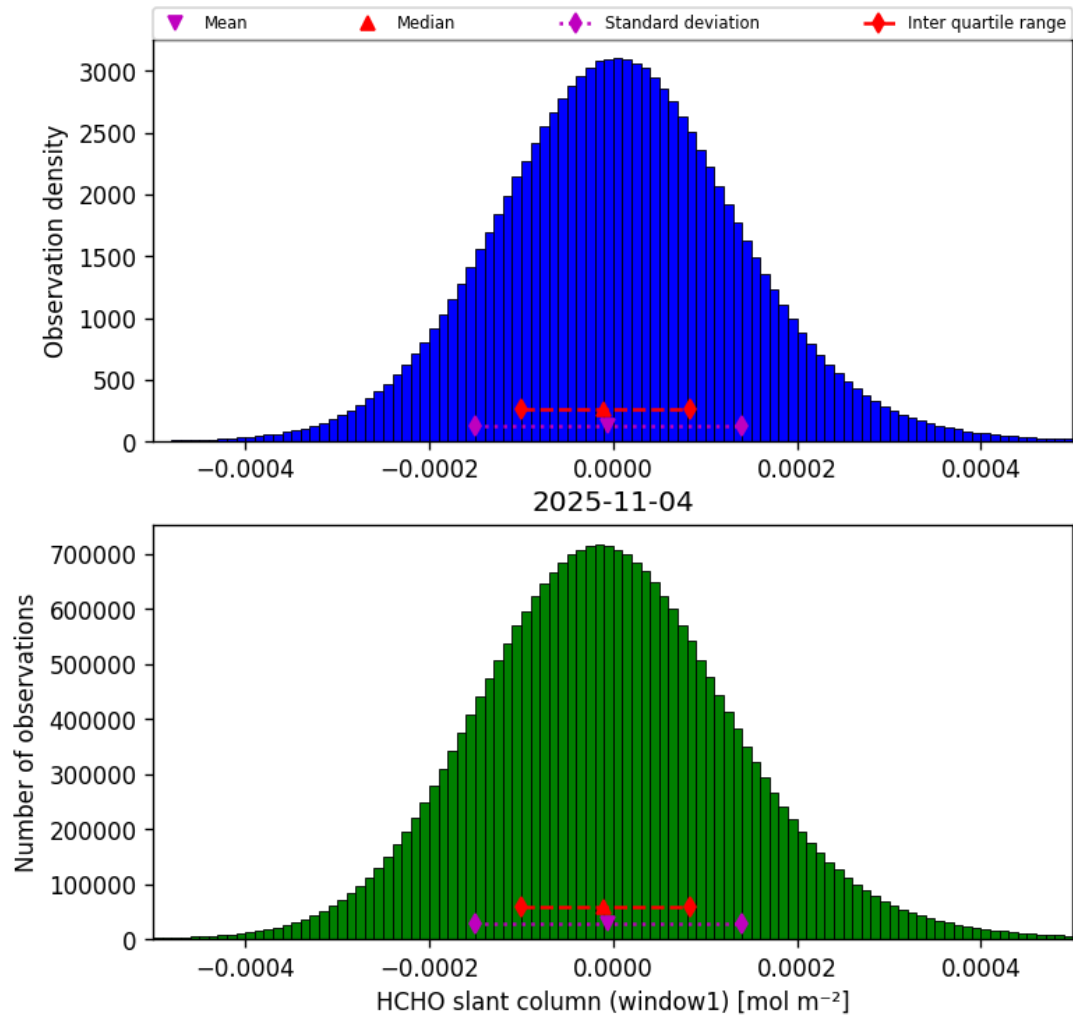
Figure 38: Histogram of “HCHO slant column (window1)” for 2025-11-03 to 2025-11-05
