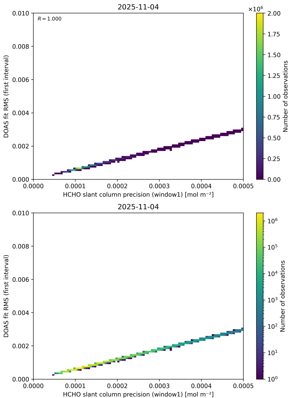
Figure 88: Scatter density plot of “HCHO slant column precision (window1)” against “DOAS fit RMS (first interval)” for 2025-11-03 to 2025-11-05.
