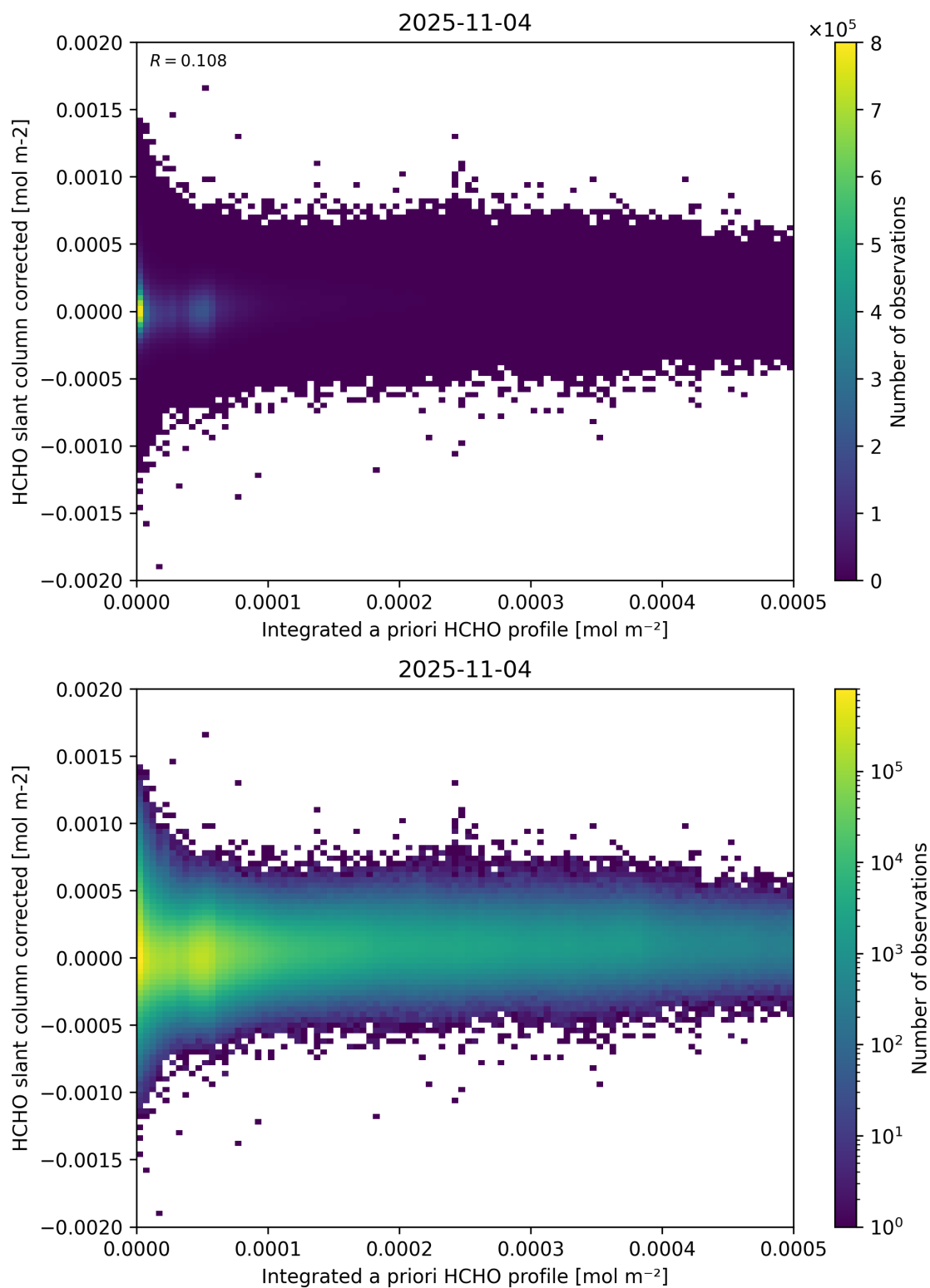
Figure 151: Scatter density plot of “Integrated a priori HCHO profile” against “HCHO slant column corrected” for 2025-11-03 to 2025-11-05.
