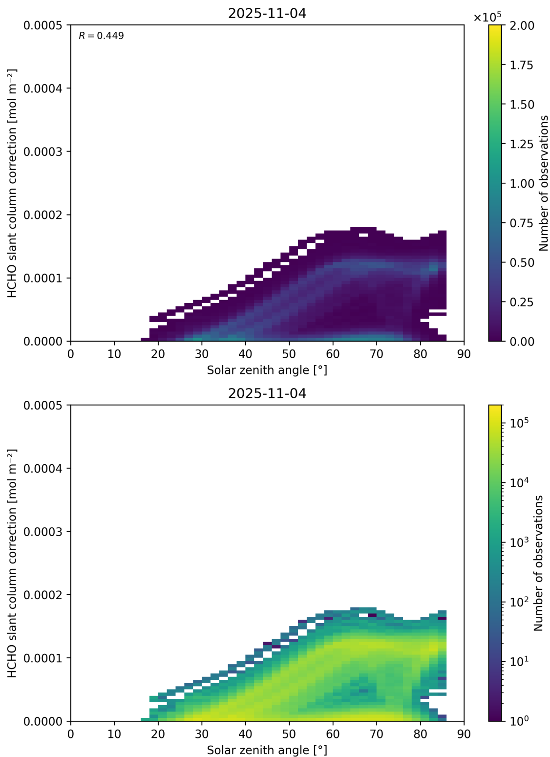
Figure 172: Scatter density plot of “Solar zenith angle” against “HCHO slant column correction” for 2025-11-03 to 2025-11-05.
