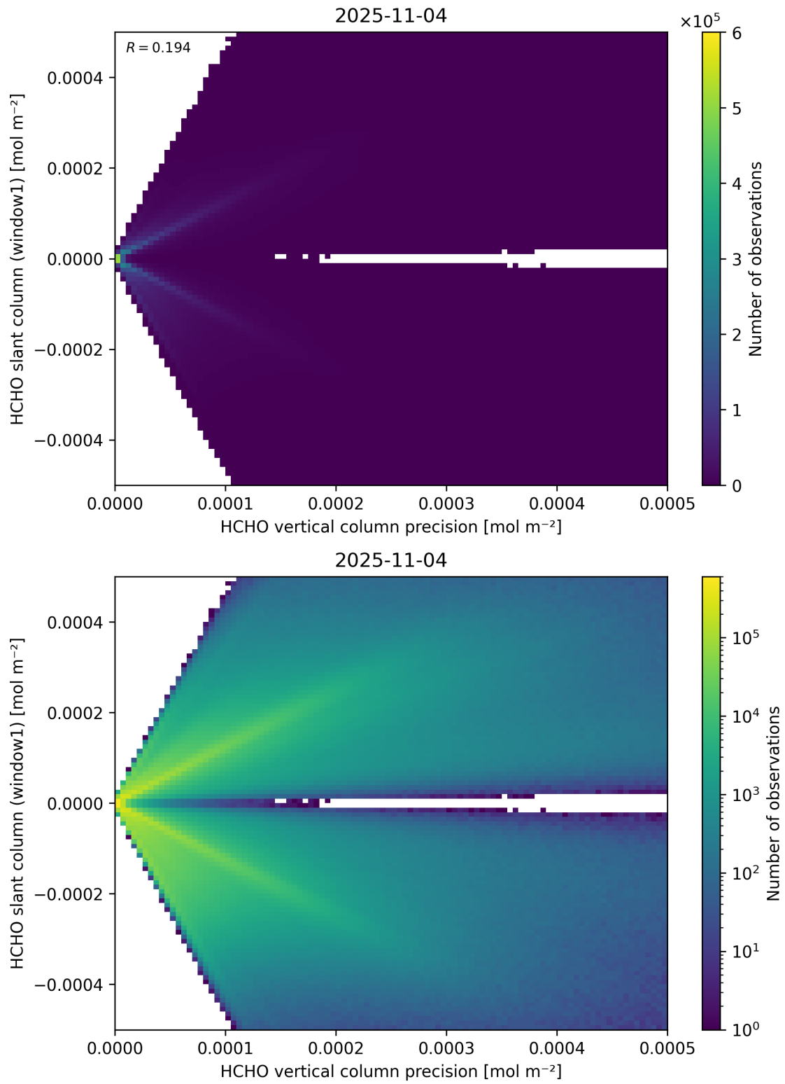
Figure 142: Scatter density plot of “HCHO vertical column precision” against “HCHO slant column (window1)” for 2025-11-03 to 2025-11-05.
