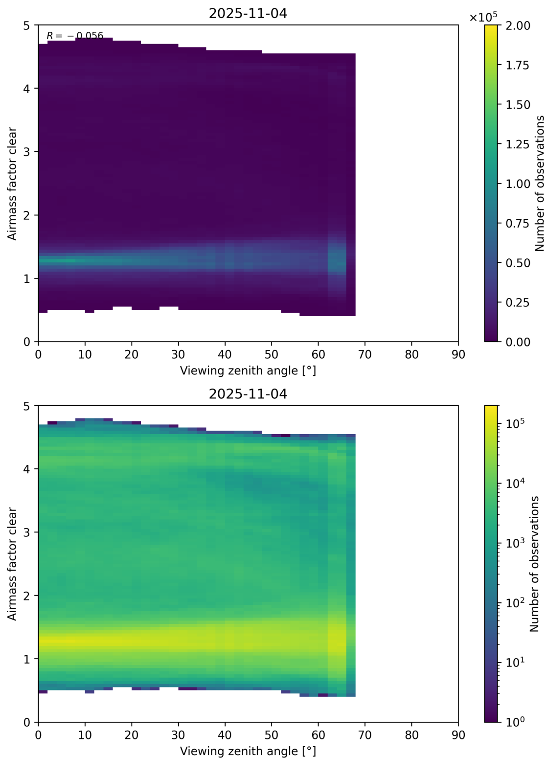
Figure 185: Scatter density plot of “Viewing zenith angle” against “Airmass factor clear” for 2025-11-03 to 2025-11-05.
