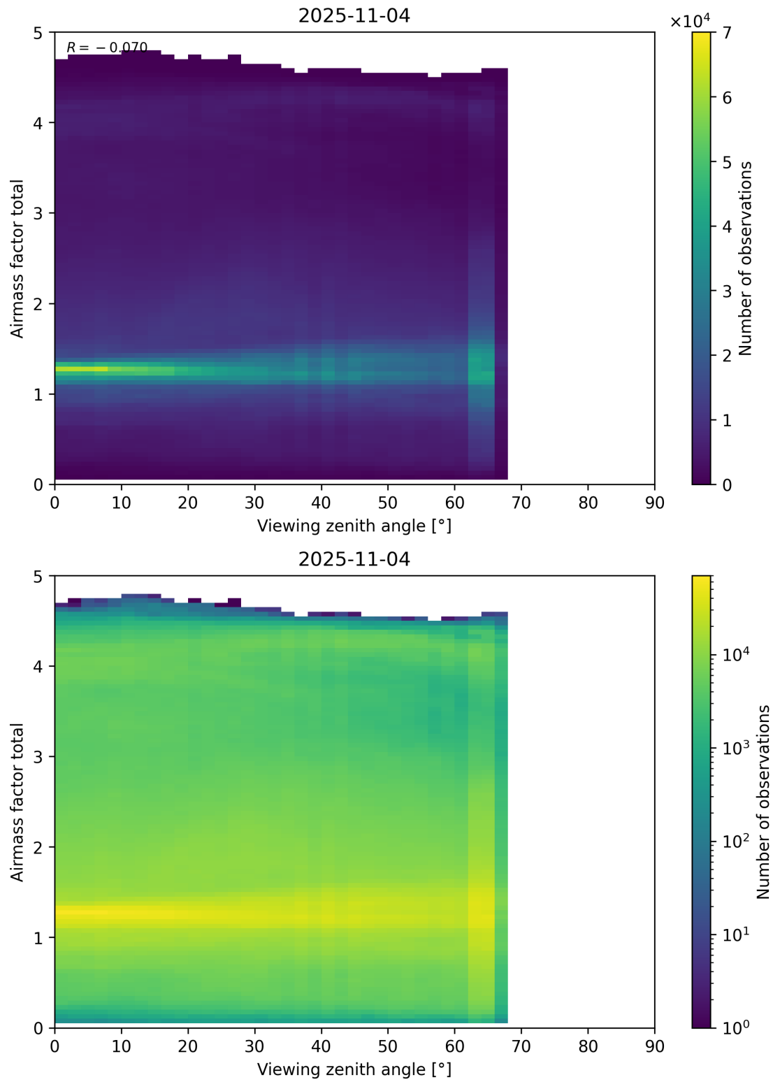
Figure 190: Scatter density plot of “Viewing zenith angle” against “Airmass factor total” for 2025-11-03 to 2025-11-05.
