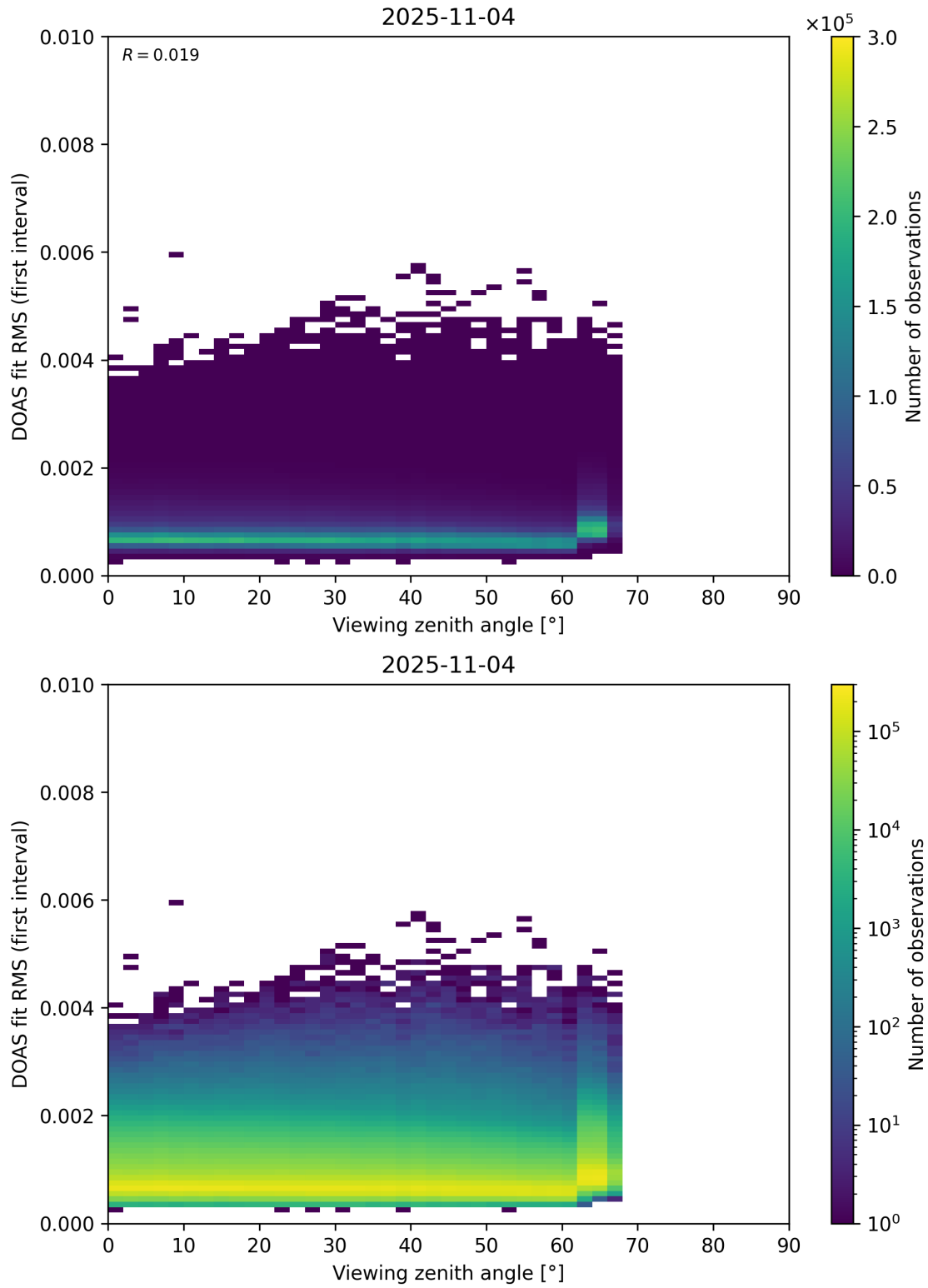
Figure 182: Scatter density plot of “Viewing zenith angle” against “DOAS fit RMS (first interval)” for 2025-11-03 to 2025-11-05.
