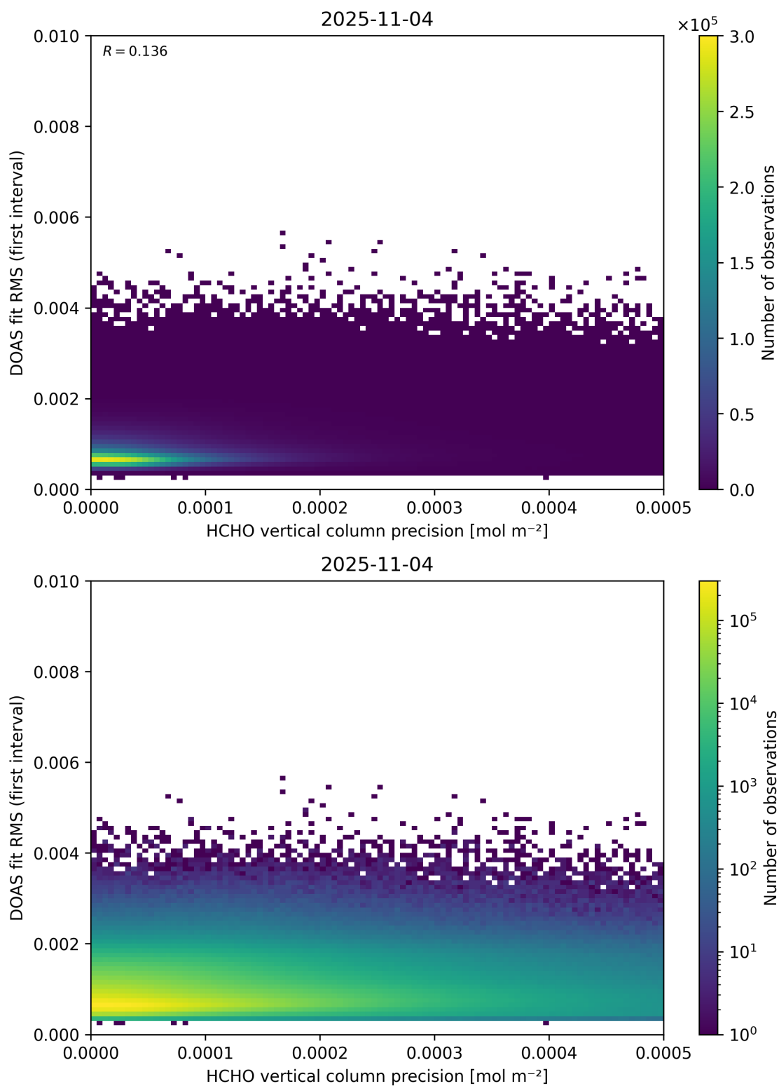
Figure 136: Scatter density plot of “HCHO vertical column precision” against “DOAS fit RMS (first interval)” for 2025-11-03 to 2025-11-05.
