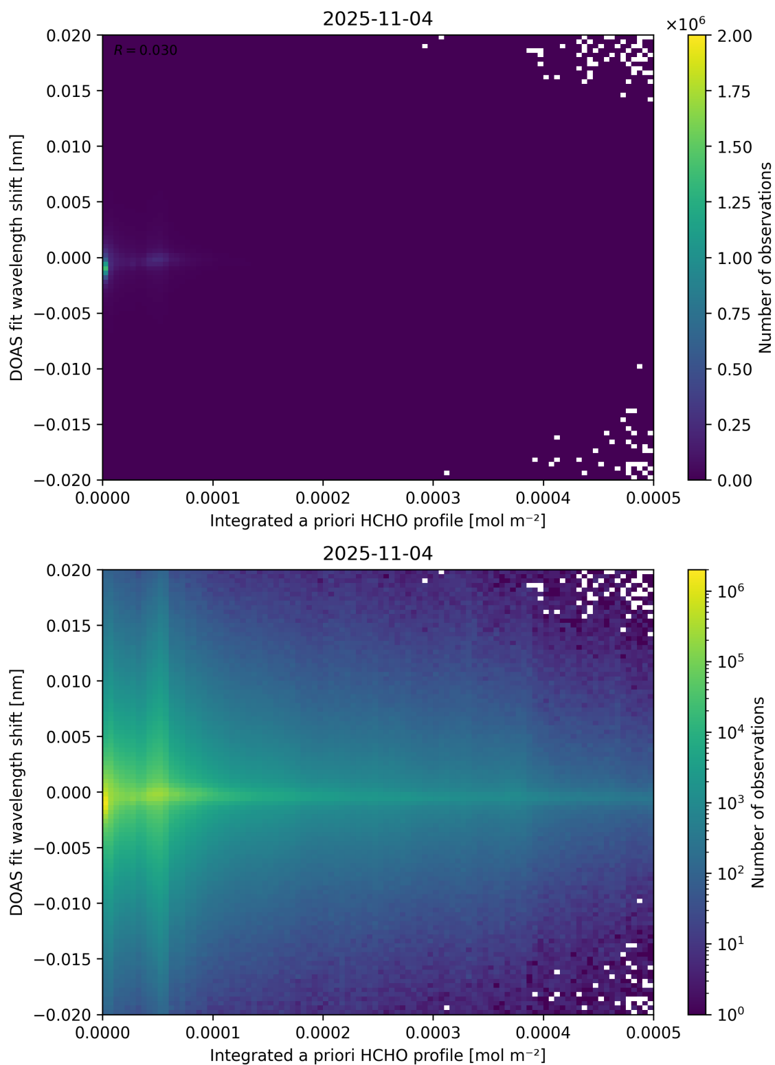
Figure 149: Scatter density plot of “Integrated a priori HCHO profile” against “DOAS fit wavelength shift” for 2025-11-03 to 2025-11-05.
