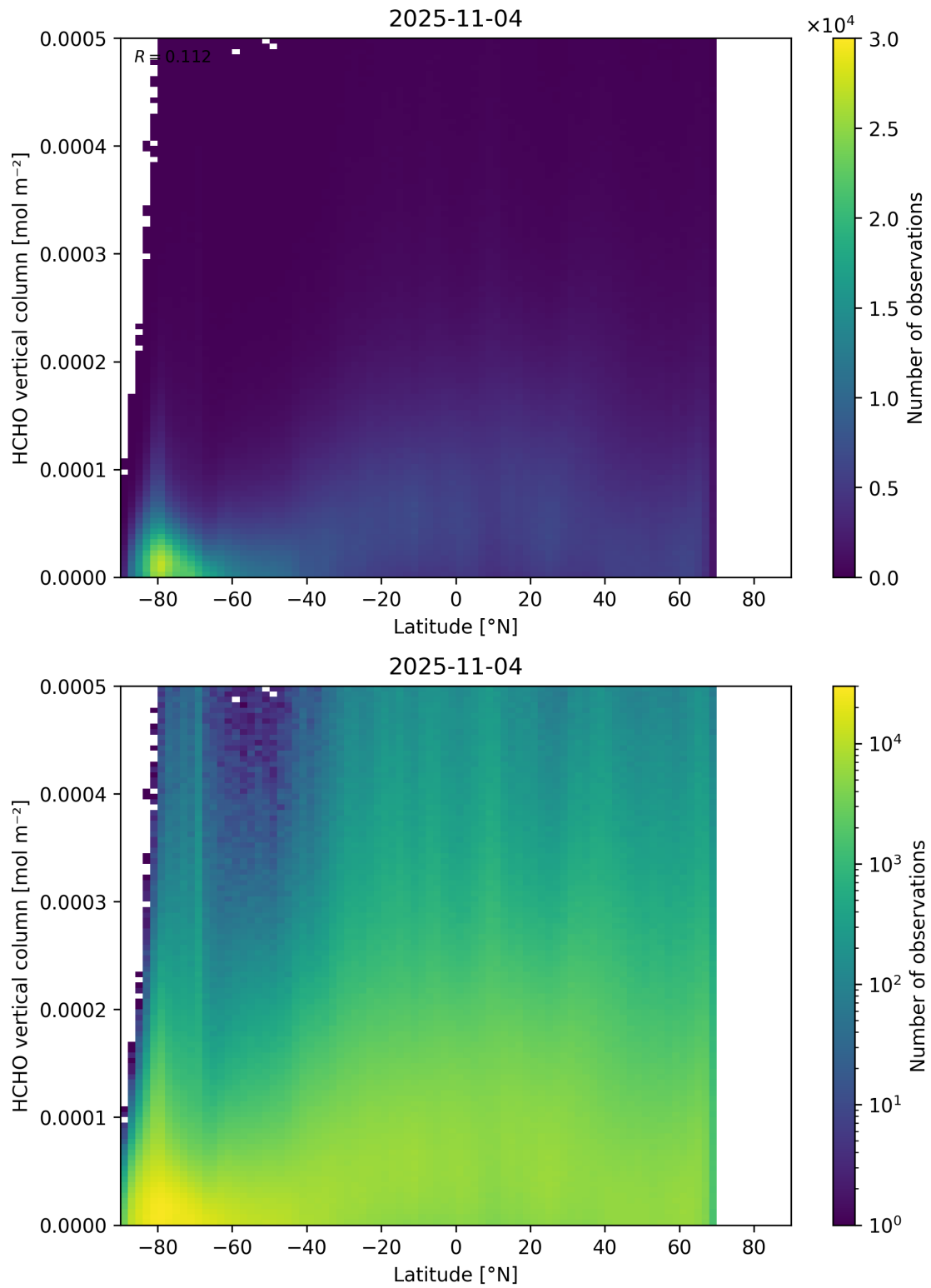
Figure 163: Scatter density plot of “Latitude” against “HCHO vertical column” for 2025-11-03 to 2025-11-05.
