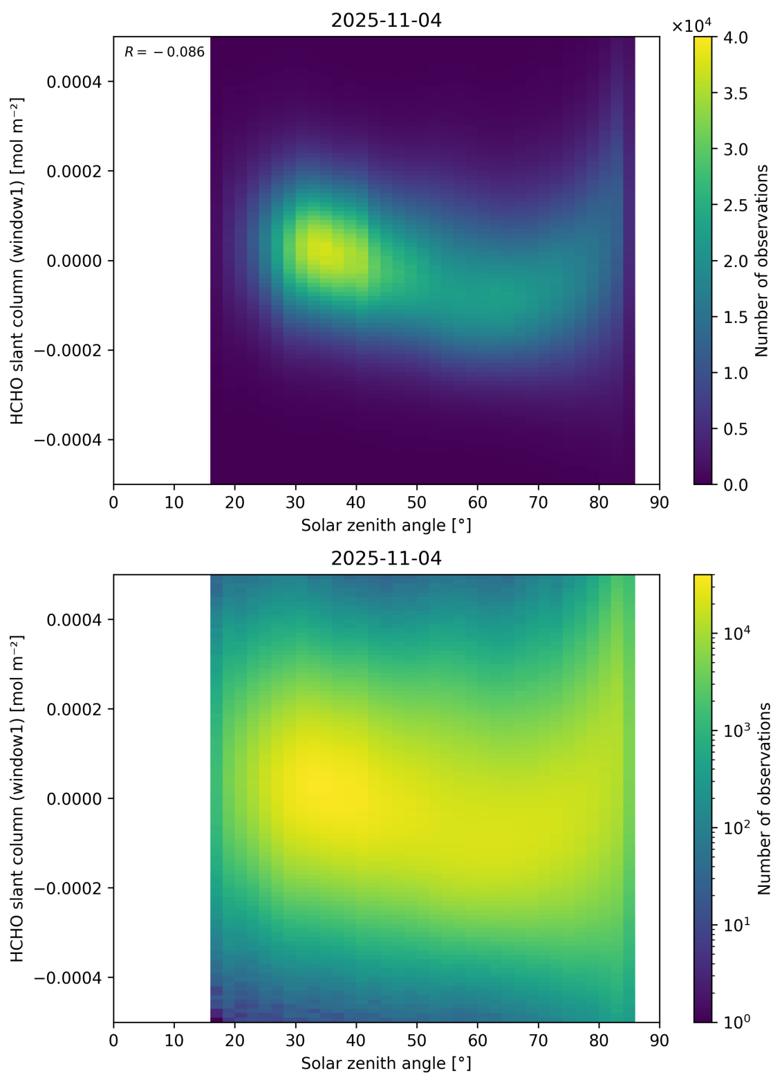
Figure 173: Scatter density plot of “Solar zenith angle” against “HCHO slant column (window1)” for 2025-11-03 to 2025-11-05.
