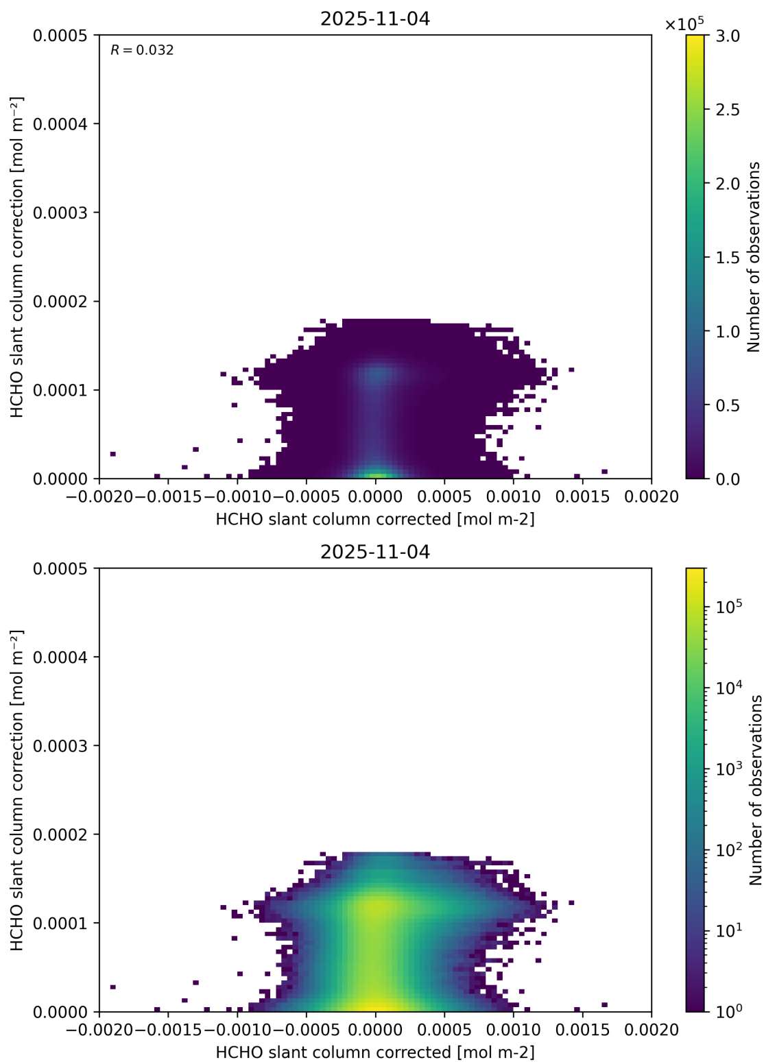
Figure 77: Scatter density plot of “HCHO slant column corrected” against “HCHO slant column correction” for 2025-11-03 to 2025-11-05.
