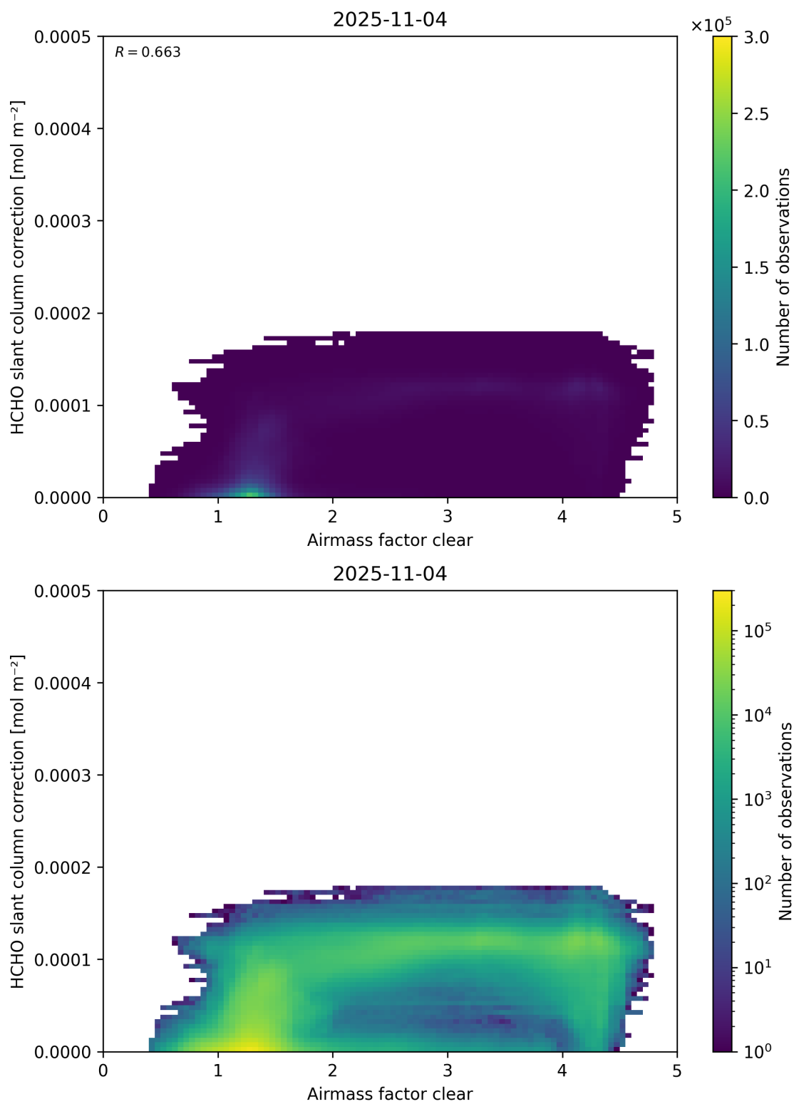
Figure 75: Scatter density plot of “Airmass factor clear” against “HCHO slant column correction” for 2025-11-03 to 2025-11-05.
