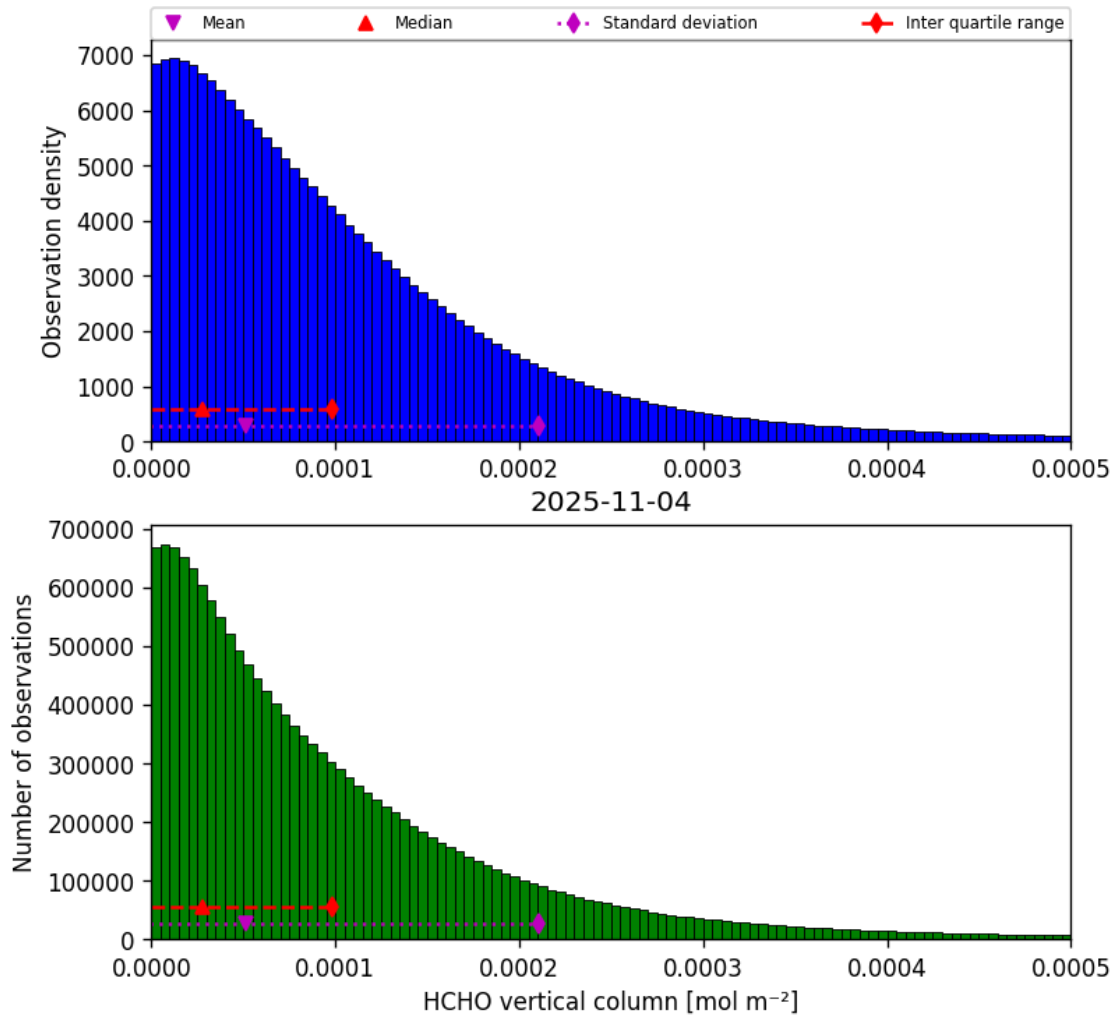
Figure 35: Histogram of “HCHO vertical column” for 2025-11-03 to 2025-11-05
