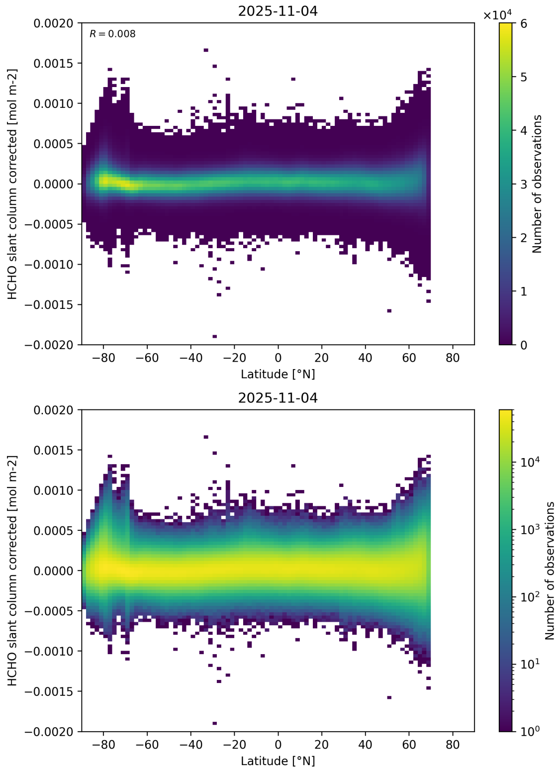
Figure 157: Scatter density plot of “Latitude” against “HCHO slant column corrected” for 2025-11-03 to 2025-11-05.
