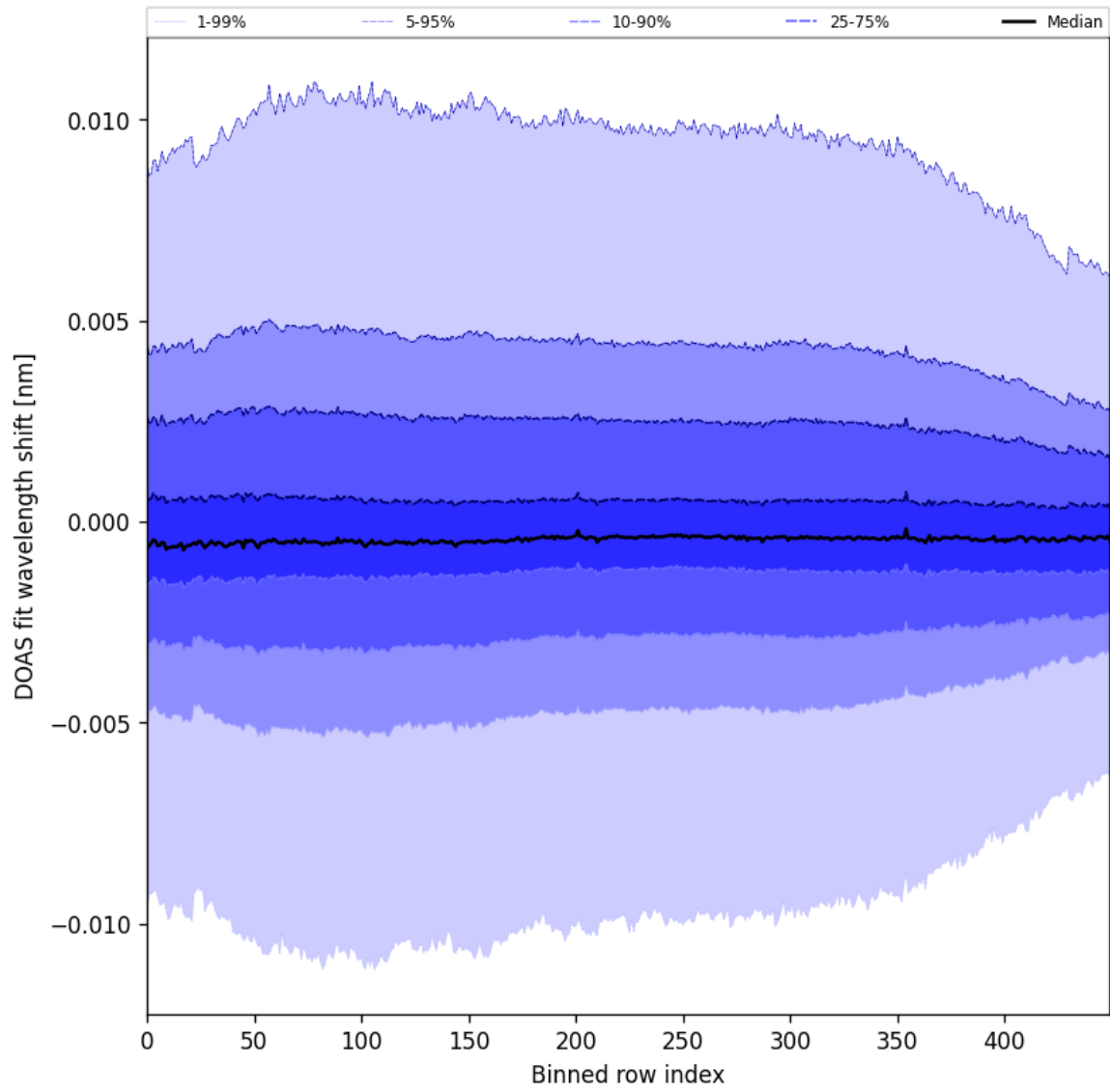
Figure 58: Along track statistics of “DOAS fit wavelength shift” for 2025-11-03 to 2025-11-05
