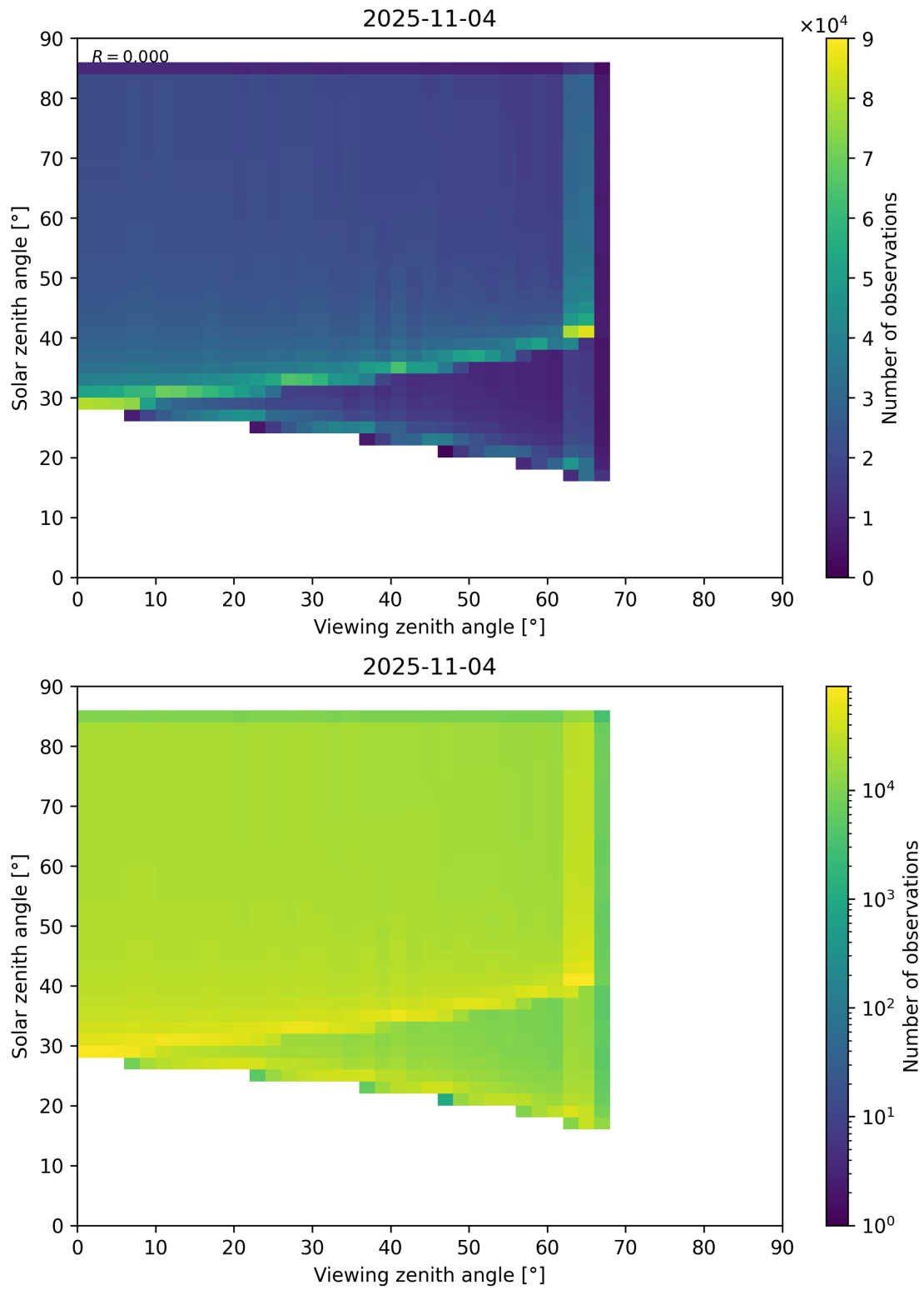
Figure 197: Scatter density plot of “Viewing zenith angle” against “Solar zenith angle” for 2025-11-03 to 2025-11-05.
