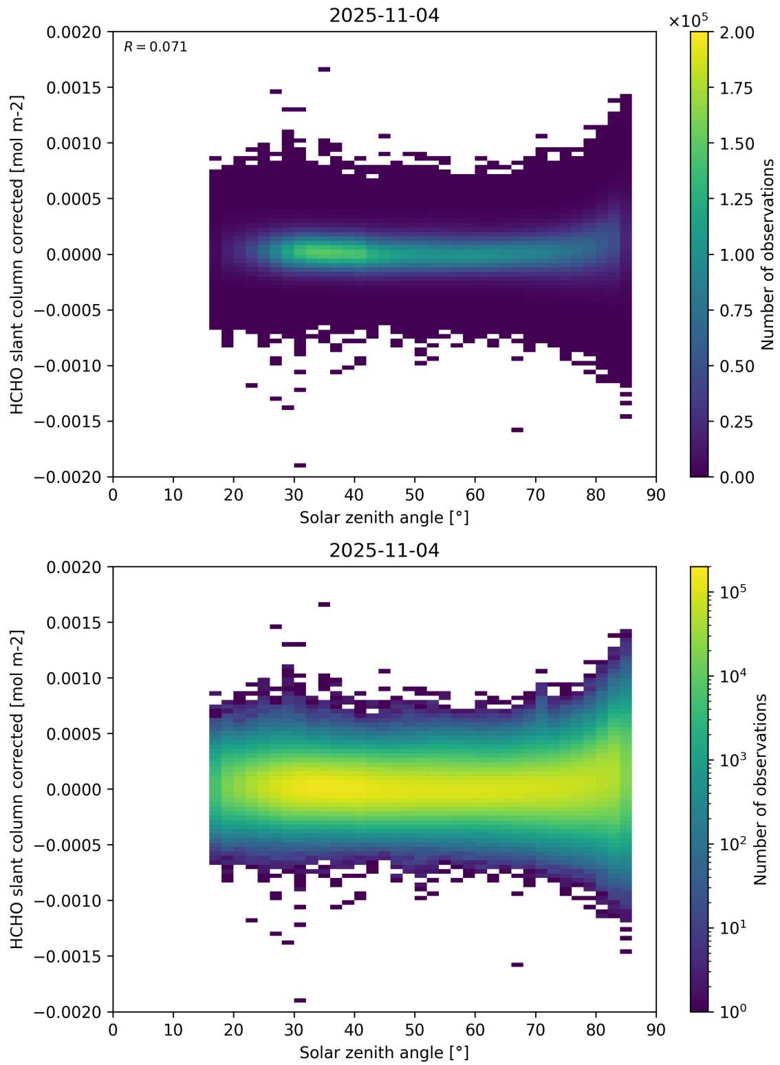
Figure 171: Scatter density plot of “Solar zenith angle” against “HCHO slant column corrected” for 2025-11-03 to 2025-11-05.
