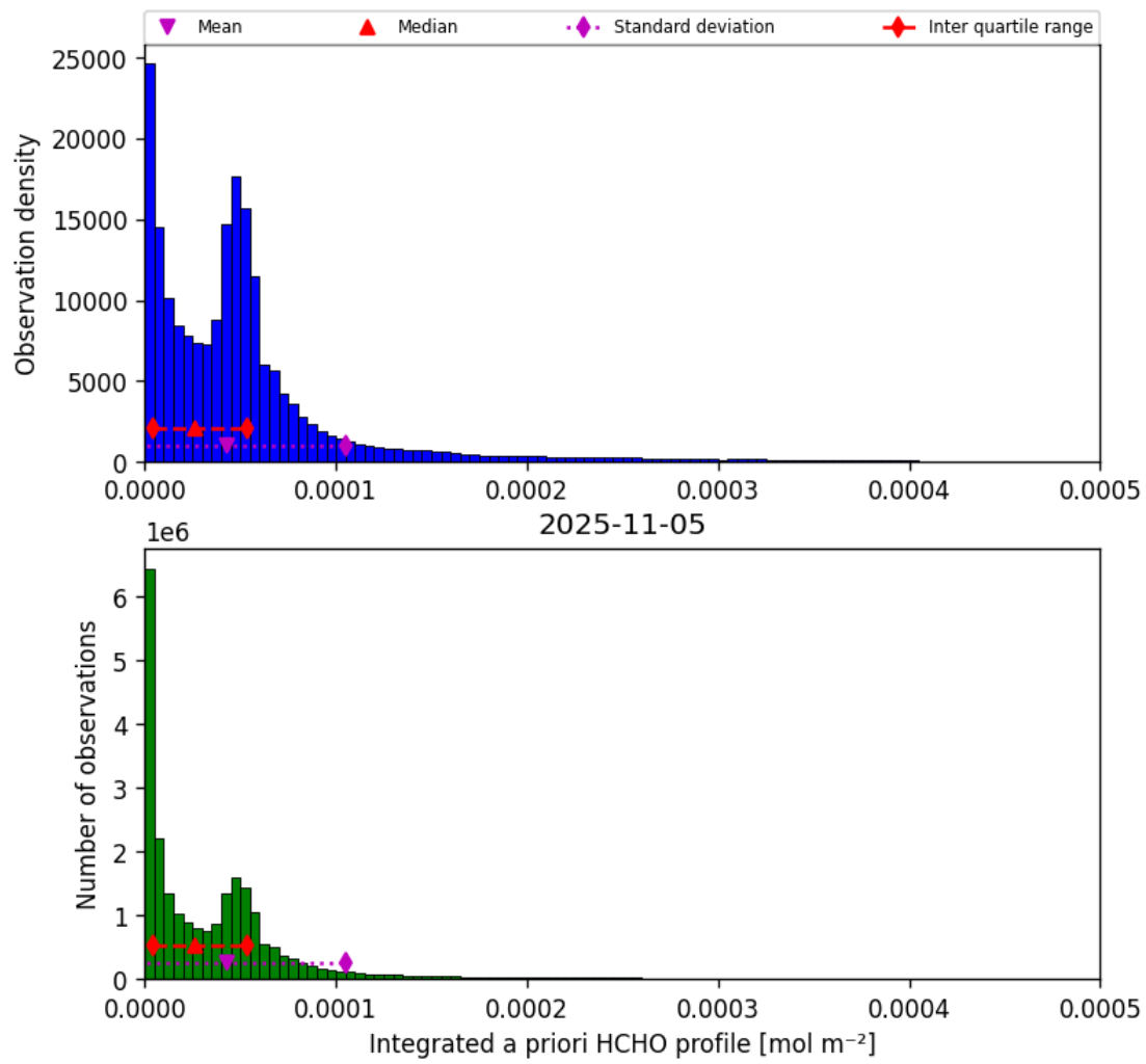
Figure 43: Histogram of “Integrated a priori HCHO profile” for 2025-11-04 to 2025-11-06
