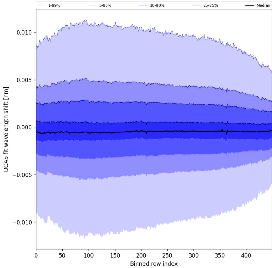
Figure 58: Along track statistics of “DOAS fit wavelength shift” for 2025-11-04 to 2025-11-06
