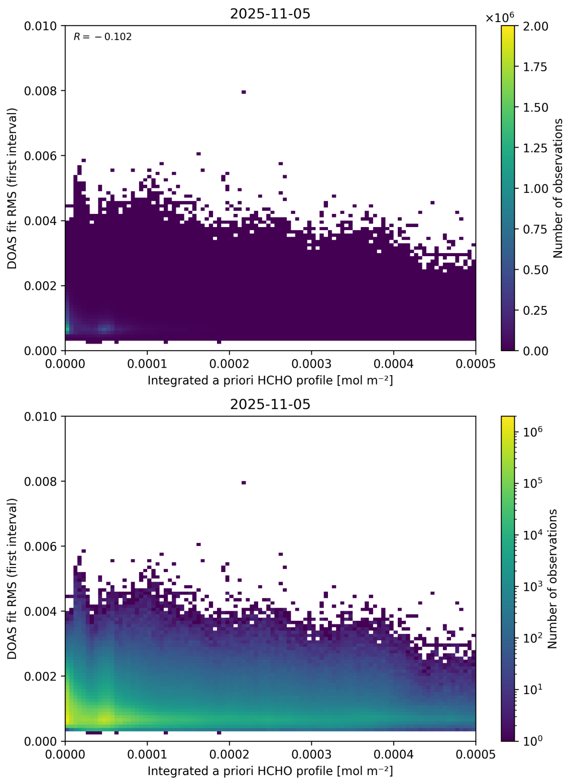
Figure 148: Scatter density plot of “Integrated a priori HCHO profile” against “DOAS fit RMS (first interval)” for 2025-11-04 to 2025-11-06.
