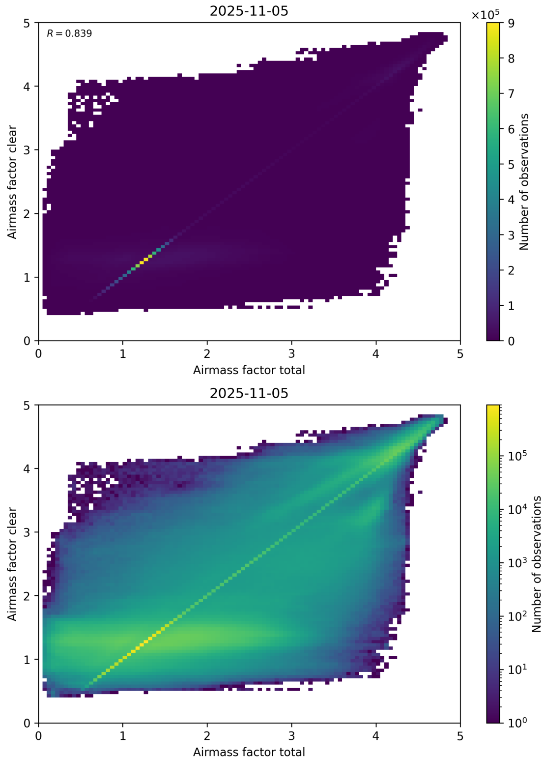
Figure 100: Scatter density plot of “Airmass factor total” against “Airmass factor clear” for 2025-11-04 to 2025-11-06.
