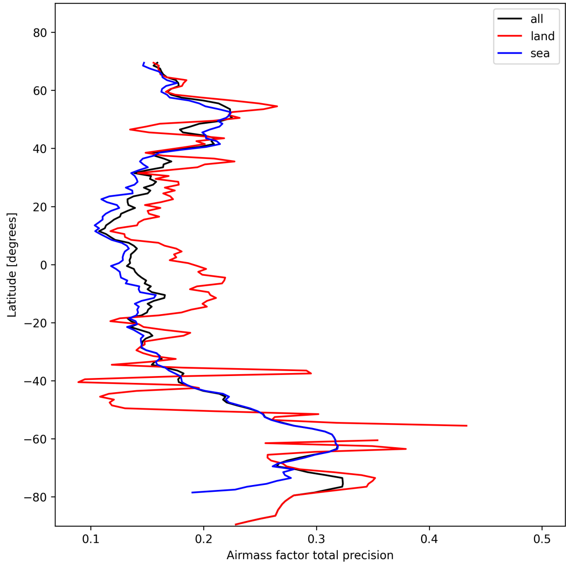
Figure 27: Zonal average of “Airmass factor total precision” for 2025-11-04 to 2025-11-06.
