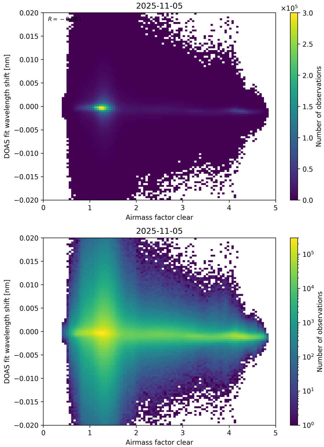
Figure 72: Scatter density plot of “Airmass factor clear” against “DOAS fit wavelength shift” for 2025-11-04 to 2025-11-06.
