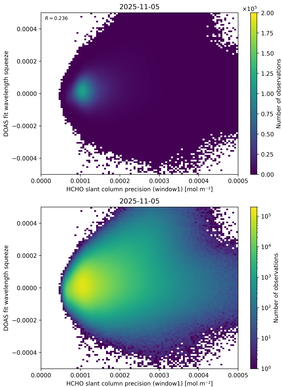
Figure 90: Scatter density plot of “HCHO slant column precision (window1)” against “DOAS fit wavelength squeeze” for 2025-11-04 to 2025-11-06.
