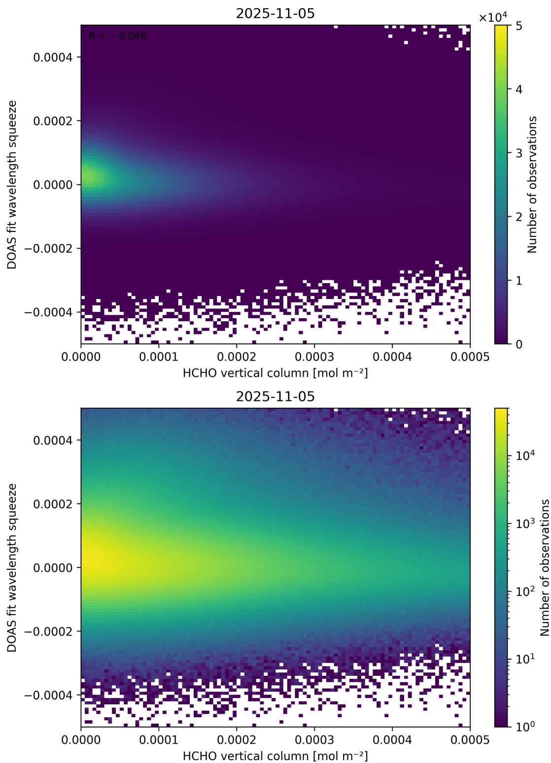
Figure 125: Scatter density plot of “HCHO vertical column” against “DOAS fit wavelength squeeze” for 2025-11-04 to 2025-11-06.
