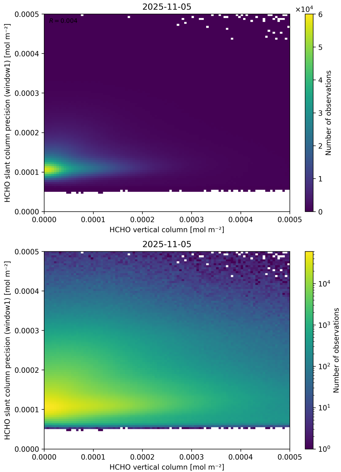
Figure 130: Scatter density plot of “HCHO vertical column” against “HCHO slant column precision (window1)” for 2025-11-04 to 2025-11-06.
