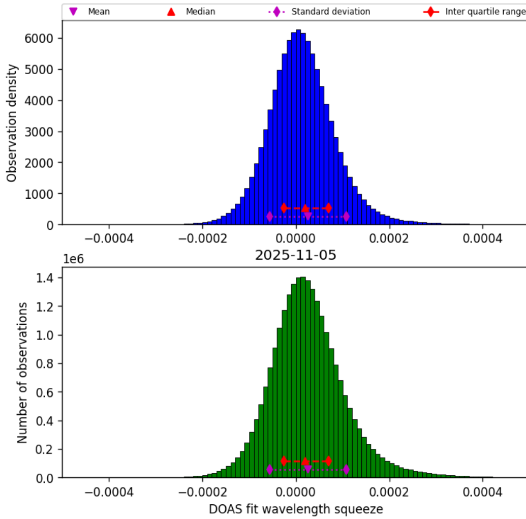
Figure 45: Histogram of “DOAS fit wavelength squeeze” for 2025-11-04 to 2025-11-06
