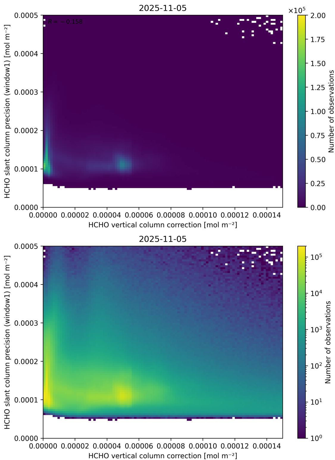
Figure 119: Scatter density plot of “HCHO vertical column correction” against “HCHO slant column precision (window1)” for 2025-11-04 to 2025-11-06.
