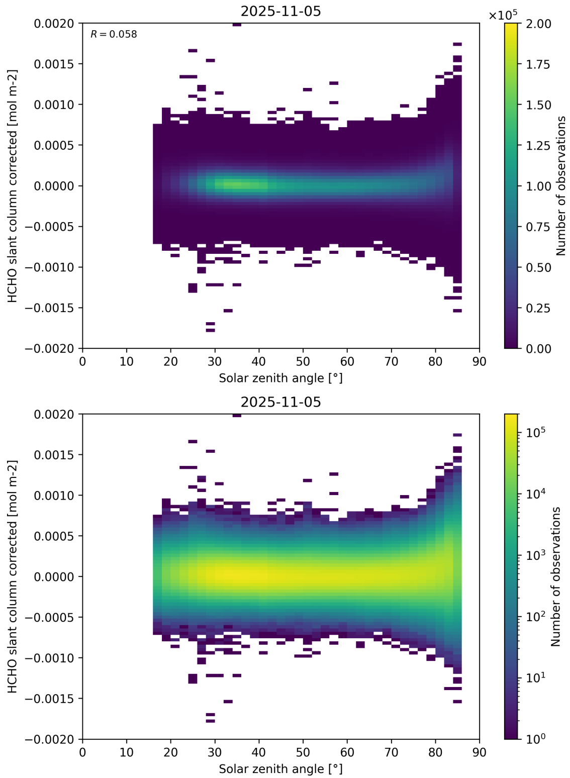
Figure 171: Scatter density plot of “Solar zenith angle” against “HCHO slant column corrected” for 2025-11-04 to 2025-11-06.
