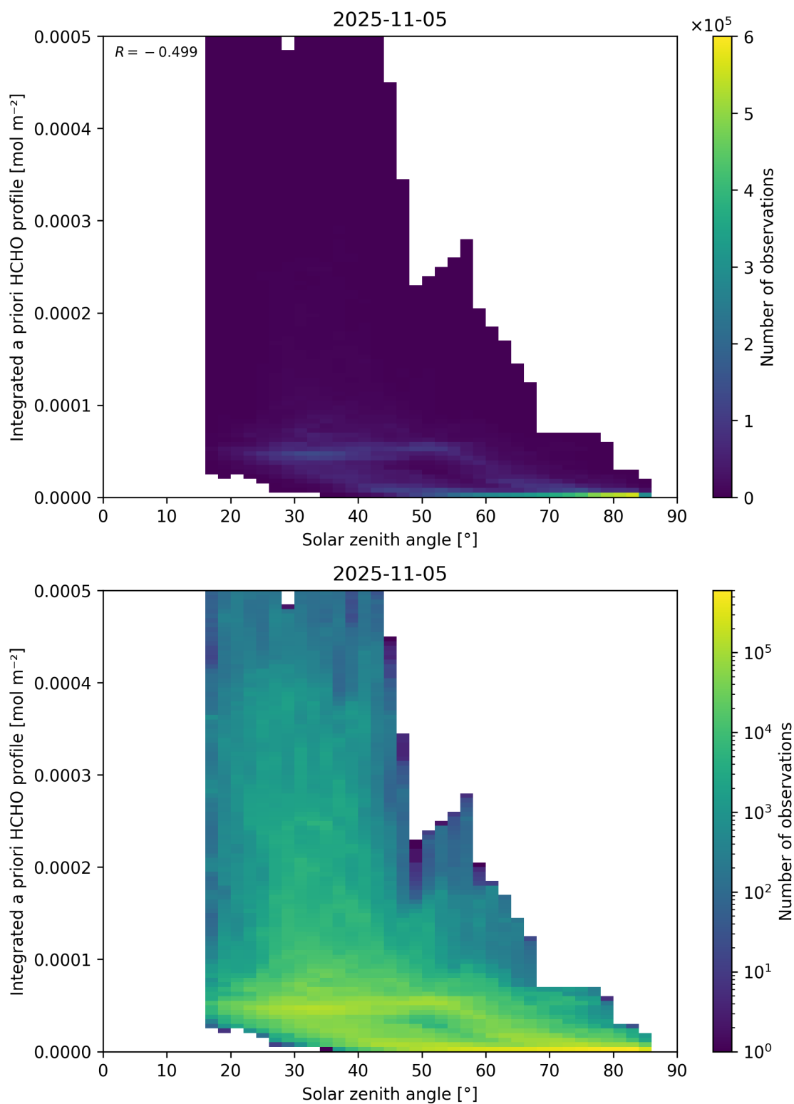
Figure 180: Scatter density plot of “Solar zenith angle” against “Integrated a priori HCHO profile” for 2025-11-04 to 2025-11-06.
