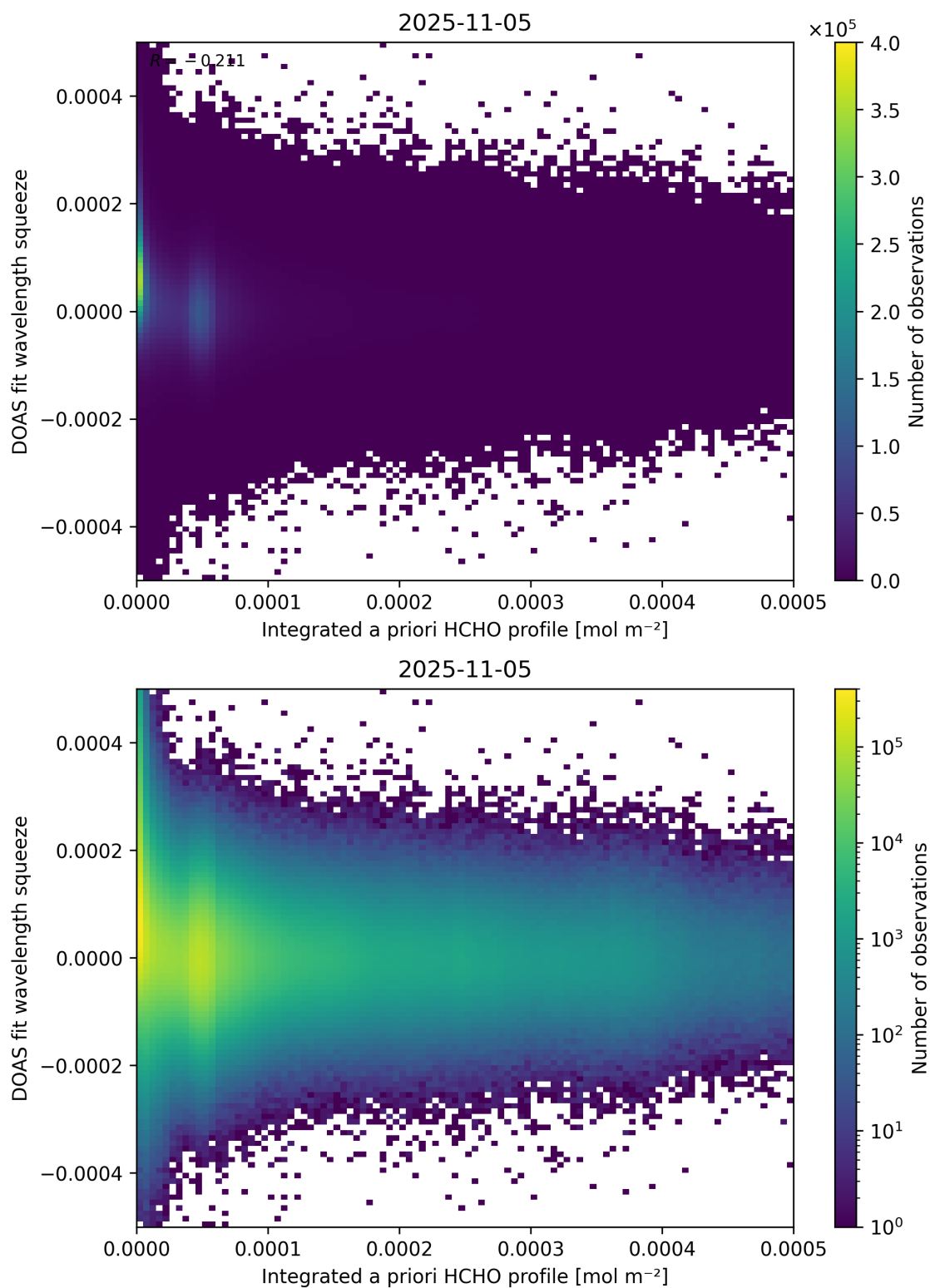
Figure 150: Scatter density plot of “Integrated a priori HCHO profile” against “DOAS fit wavelength squeeze” for 2025-11-04 to 2025-11-06.
