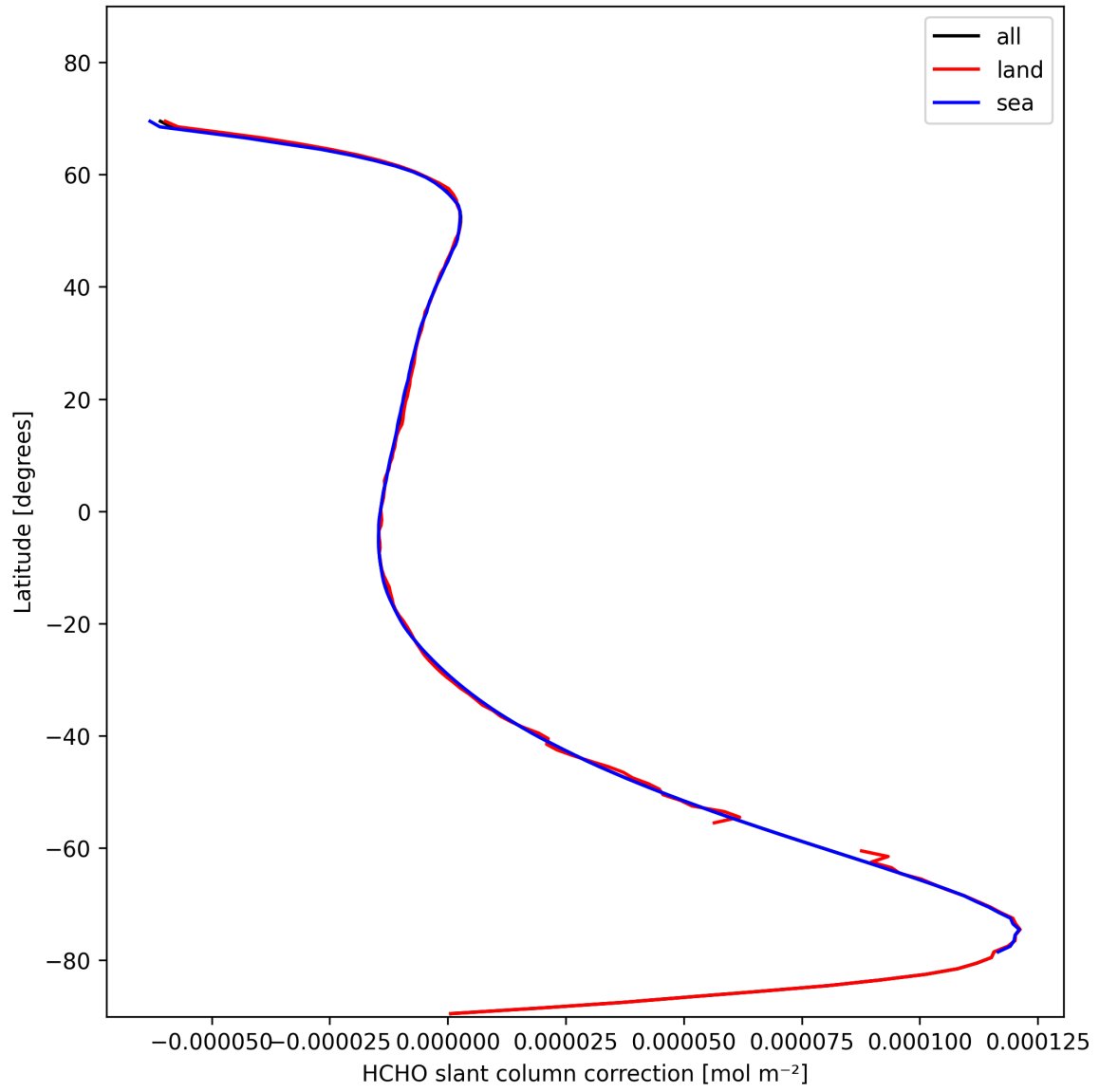
Figure 33: Zonal average of “HCHO slant column correction” for 2025-11-04 to 2025-11-06.
