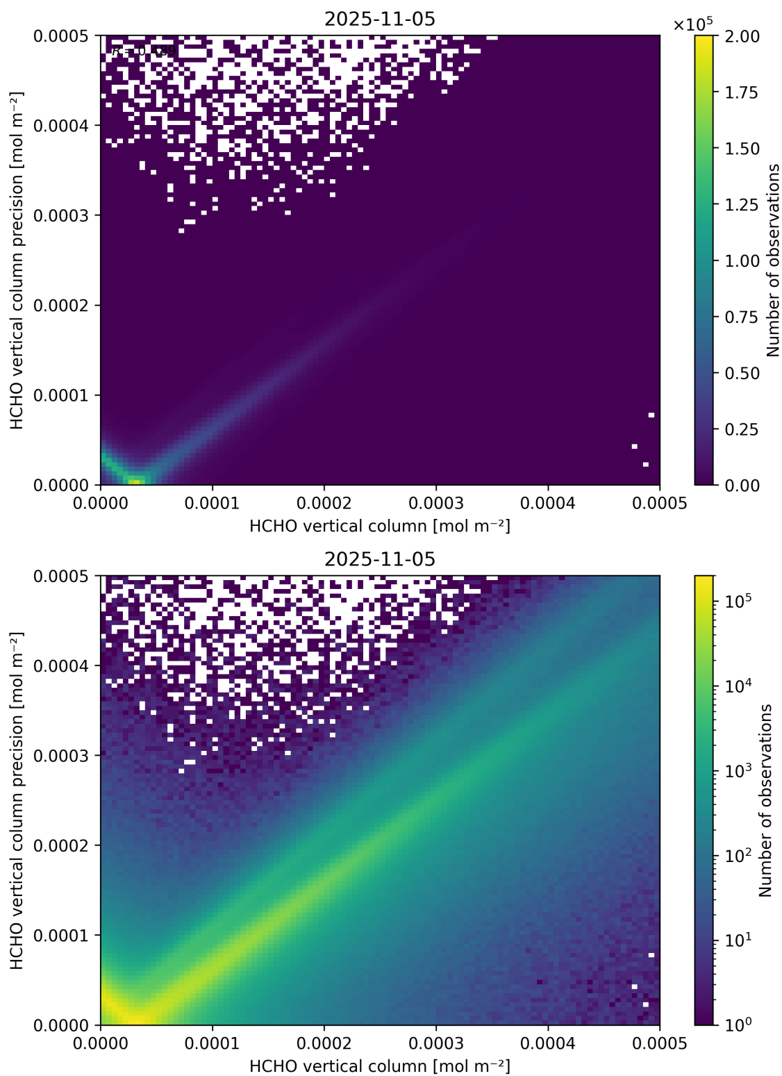
Figure 134: Scatter density plot of “HCHO vertical column” against “HCHO vertical column precision” for 2025-11-04 to 2025-11-06.
