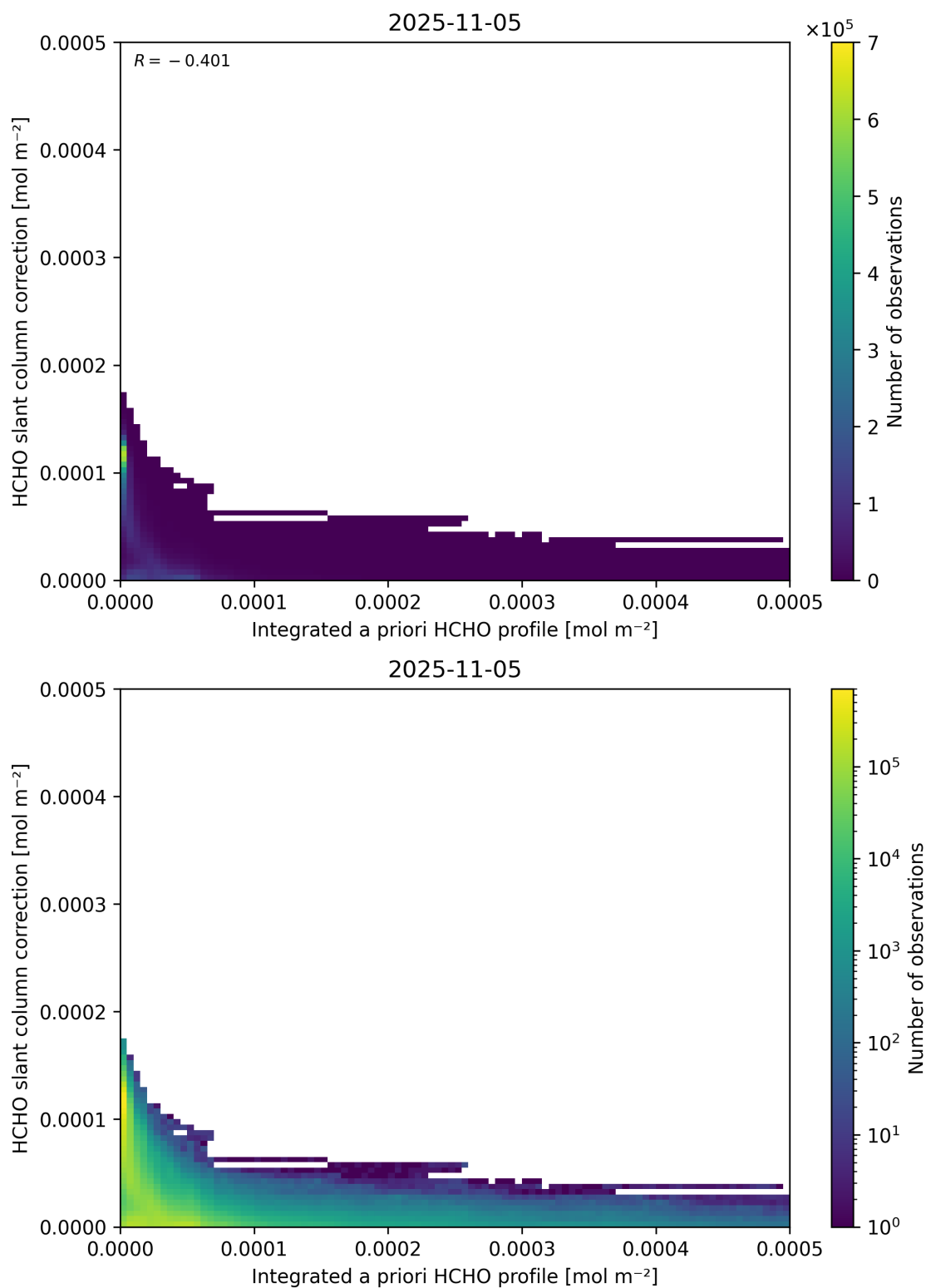
Figure 152: Scatter density plot of “Integrated a priori HCHO profile” against “HCHO slant column correction” for 2025-11-04 to 2025-11-06.
