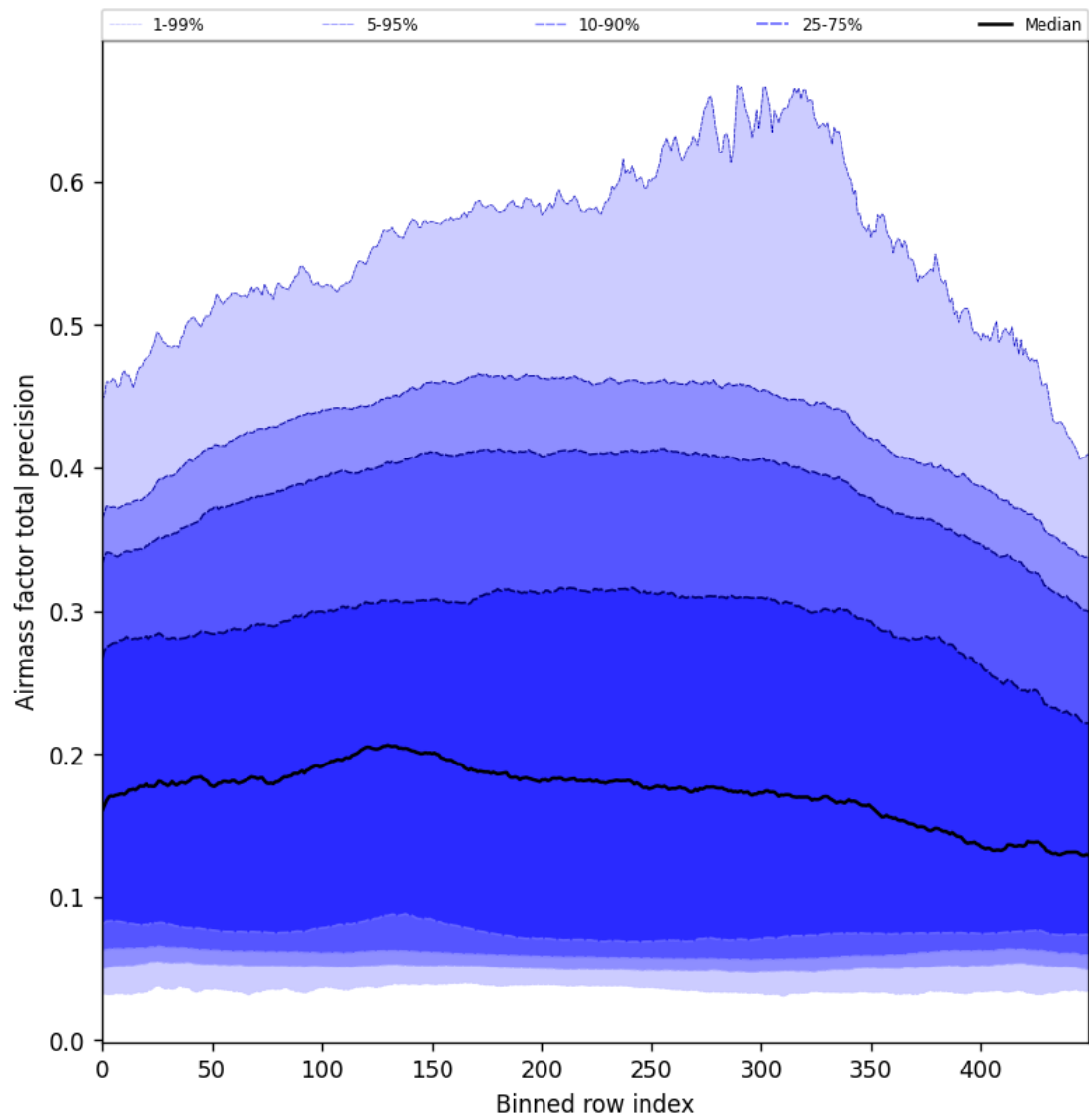
Figure 55: Along track statistics of “Airmass factor total precision” for 2025-11-04 to 2025-11-06
