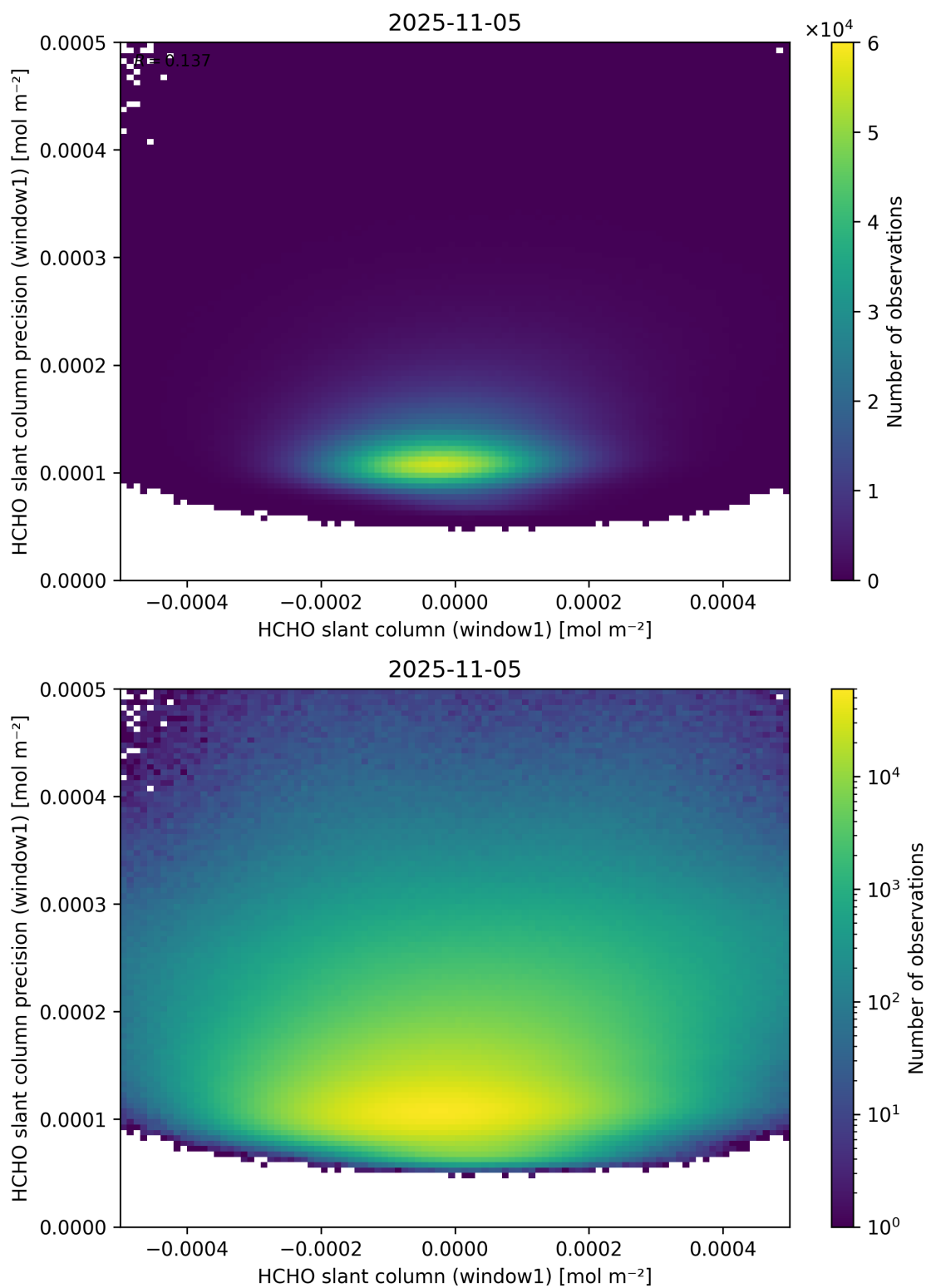
Figure 84: Scatter density plot of “HCHO slant column (window1)” against “HCHO slant column precision (window1)” for 2025-11-04 to 2025-11-06.
