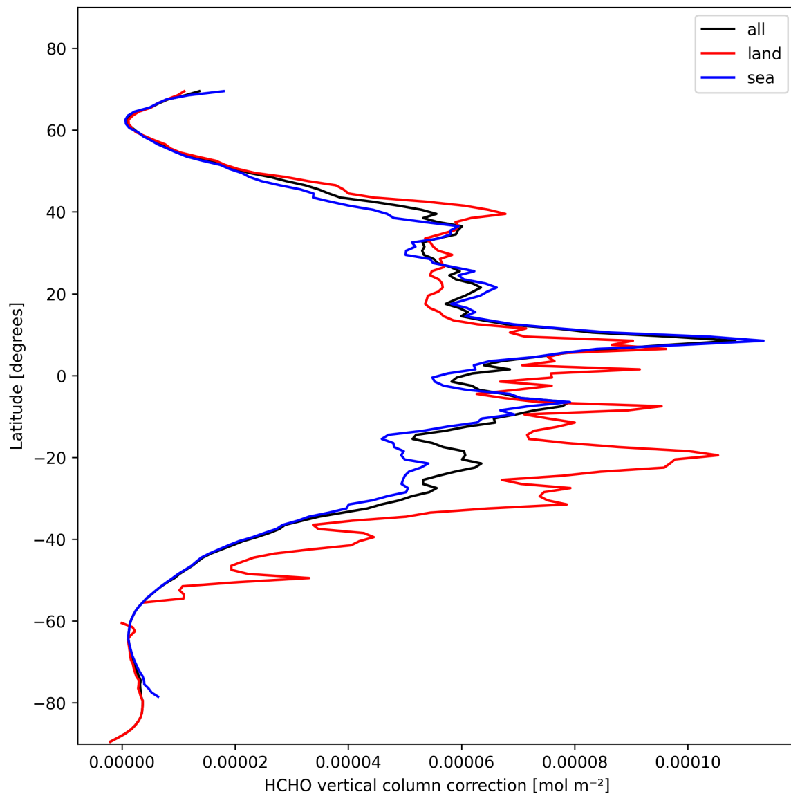
Figure 23: Zonal average of “HCHO vertical column correction” for 2025-11-04 to 2025-11-06.
