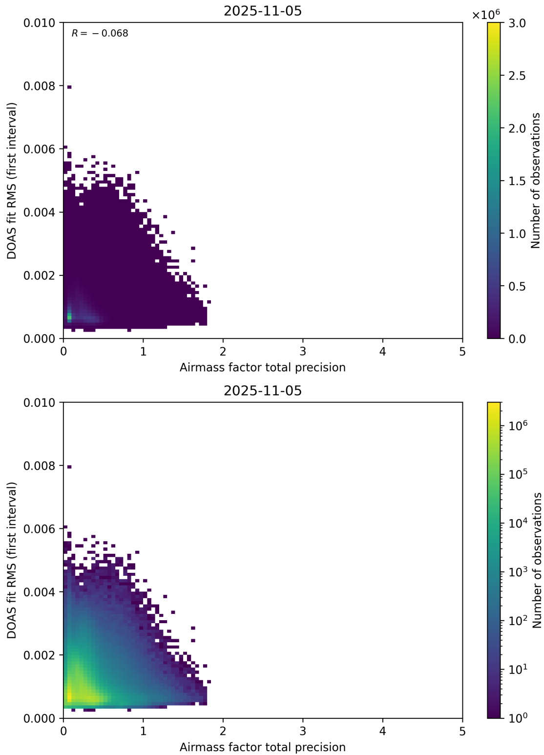
Figure 105: Scatter density plot of “Airmass factor total precision” against “DOAS fit RMS (first interval)” for 2025-11-04 to 2025-11-06.
