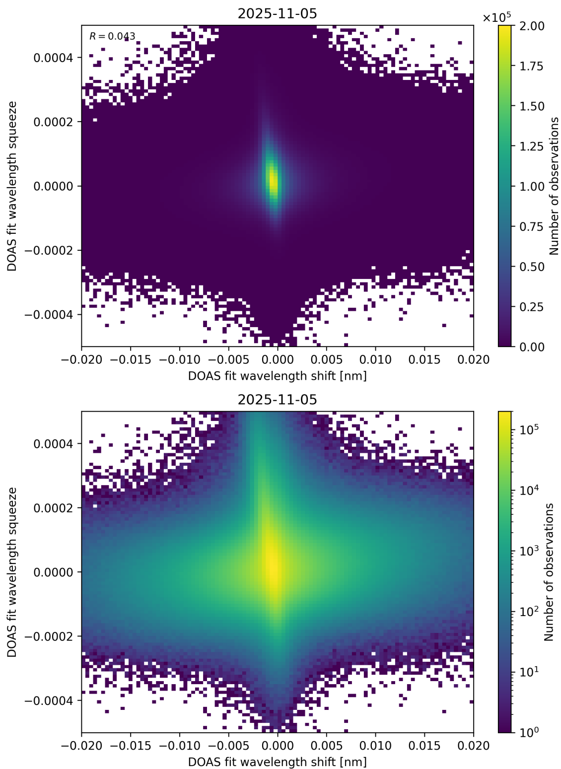
Figure 65: Scatter density plot of “DOAS fit wavelength shift” against “DOAS fit wavelength squeeze” for 2025-11-04 to 2025-11-06.
