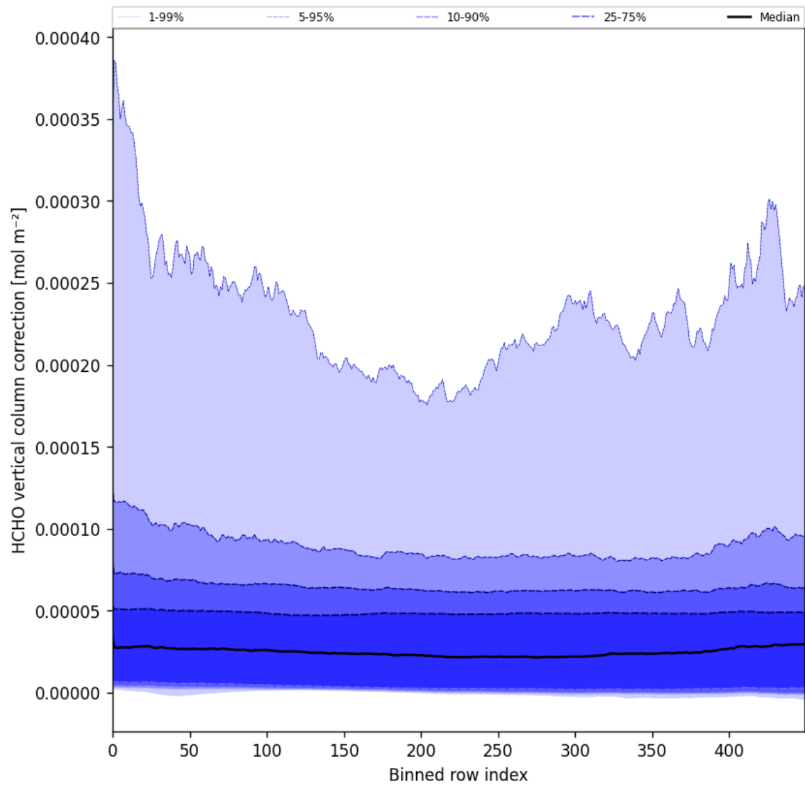
Figure 51: Along track statistics of “HCHO vertical column correction” for 2025-11-04 to 2025-11-06
