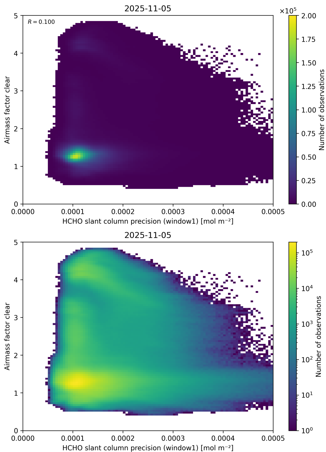
Figure 91: Scatter density plot of “HCHO slant column precision (window1)” against “Airmass factor clear” for 2025-11-04 to 2025-11-06.
