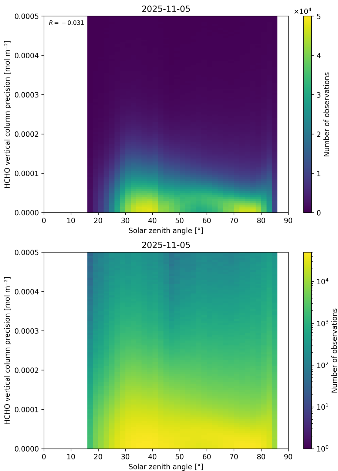
Figure 179: Scatter density plot of “Solar zenith angle” against “HCHO vertical column precision” for 2025-11-04 to 2025-11-06.
