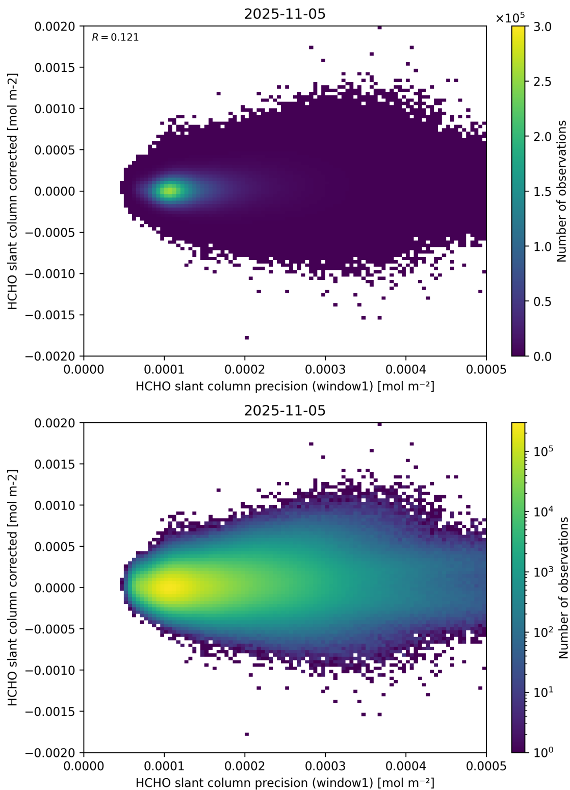
Figure 92: Scatter density plot of “HCHO slant column precision (window1)” against “HCHO slant column corrected” for 2025-11-04 to 2025-11-06.
