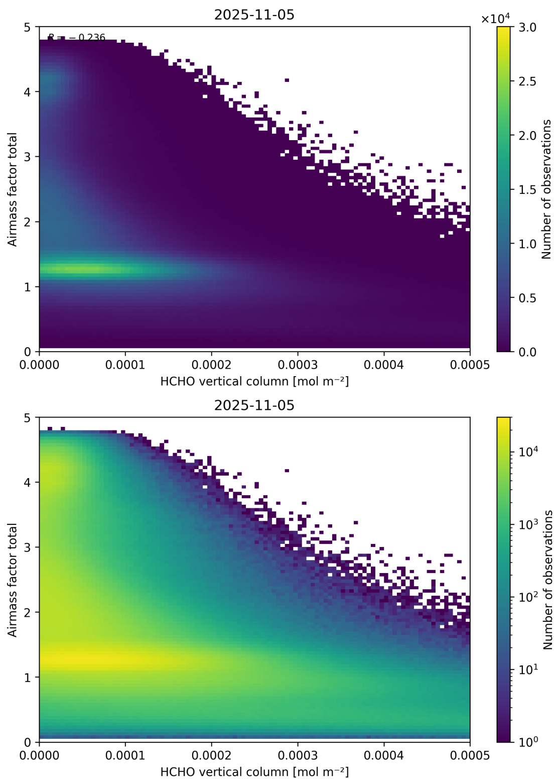
Figure 131: Scatter density plot of “HCHO vertical column” against “Airmass factor total” for 2025-11-04 to 2025-11-06.
