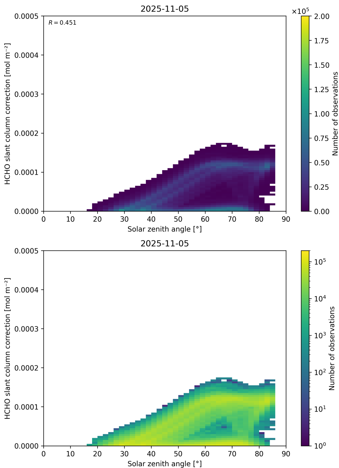
Figure 172: Scatter density plot of “Solar zenith angle” against “HCHO slant column correction” for 2025-11-04 to 2025-11-06.
