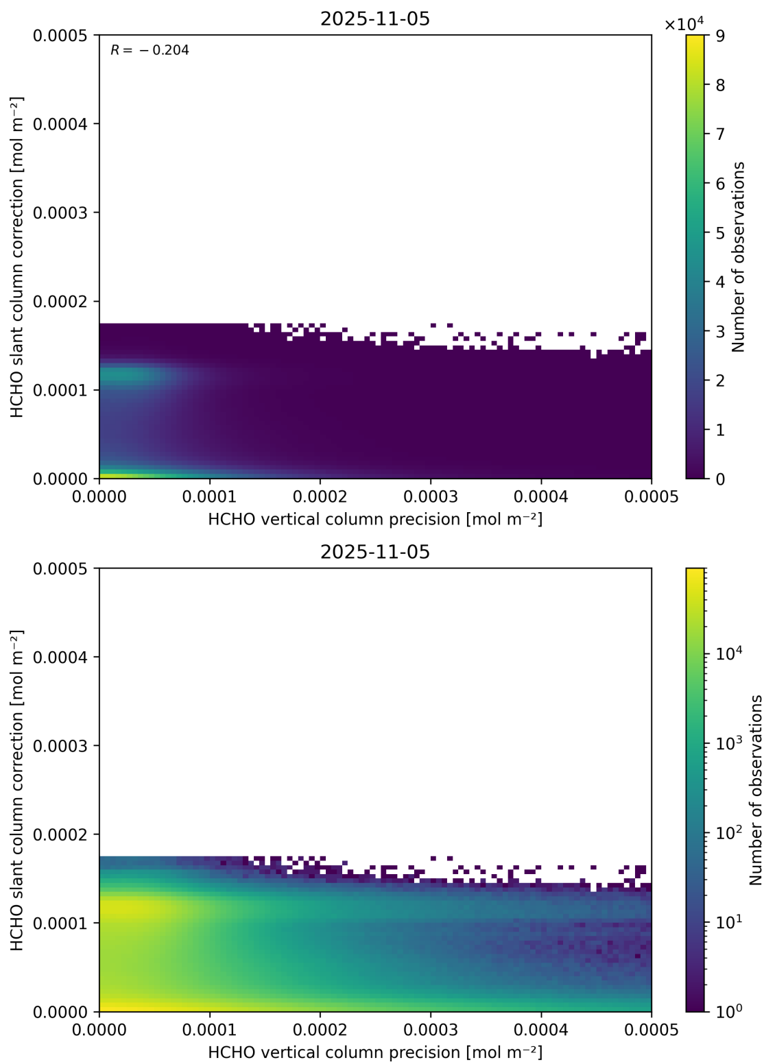
Figure 141: Scatter density plot of “HCHO vertical column precision” against “HCHO slant column correction” for 2025-11-04 to 2025-11-06.
