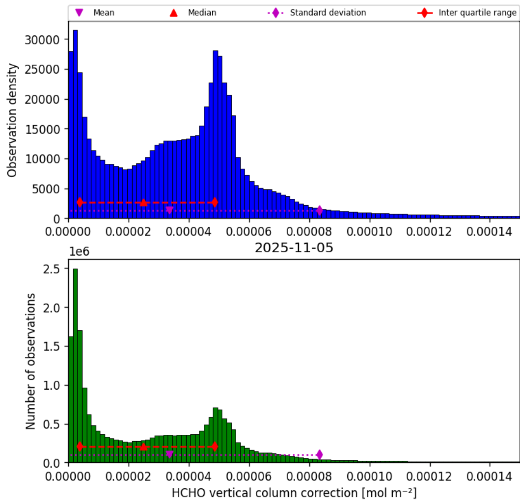
Figure 37: Histogram of “HCHO vertical column correction” for 2025-11-04 to 2025-11-06
