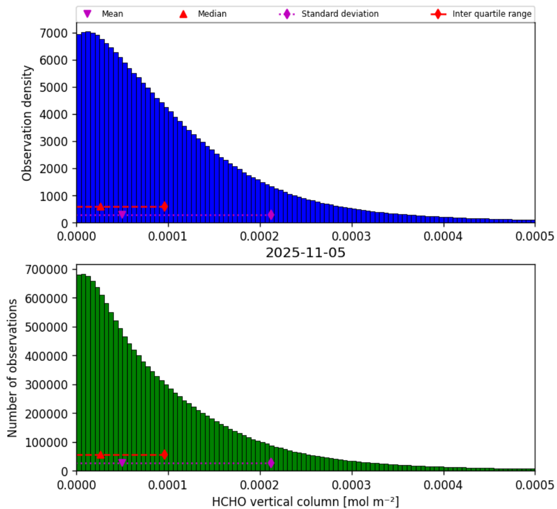
Figure 35: Histogram of “HCHO vertical column” for 2025-11-04 to 2025-11-06
