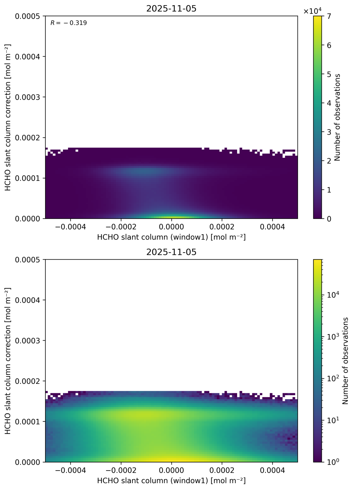
Figure 83: Scatter density plot of “HCHO slant column (window1)” against “HCHO slant column correction” for 2025-11-04 to 2025-11-06.
