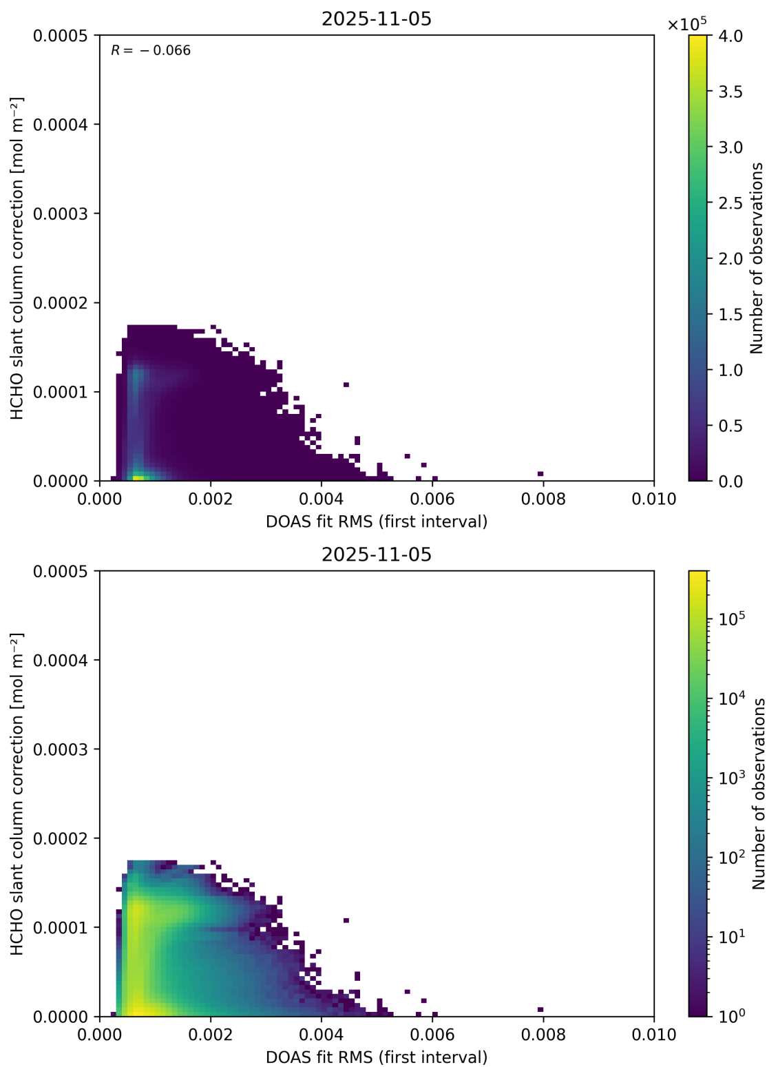
Figure 63: Scatter density plot of “DOAS fit RMS (first interval)” against “HCHO slant column correction” for 2025-11-04 to 2025-11-06.
