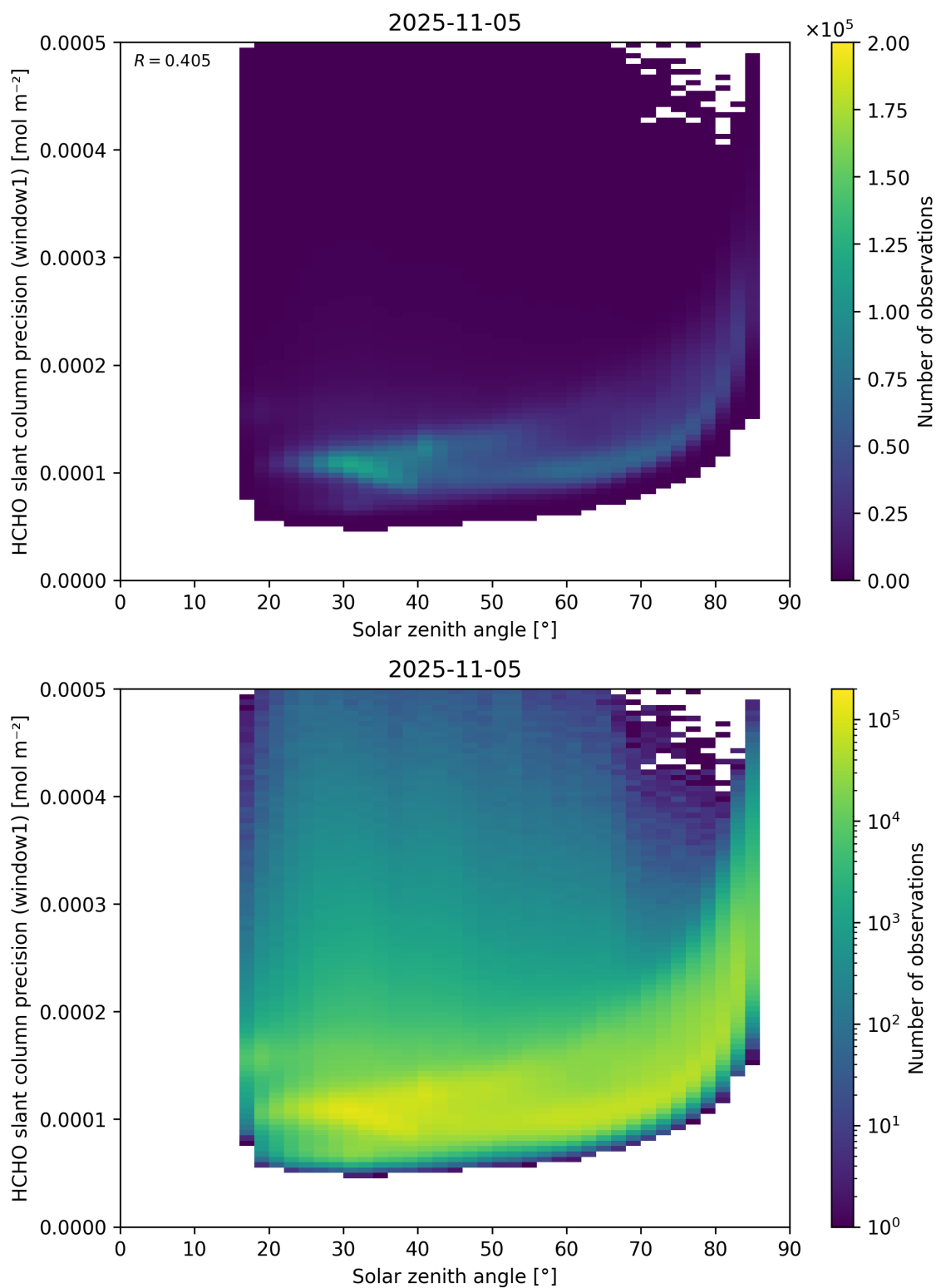
Figure 174: Scatter density plot of “Solar zenith angle” against “HCHO slant column precision (window1)” for 2025-11-04 to 2025-11-06.
