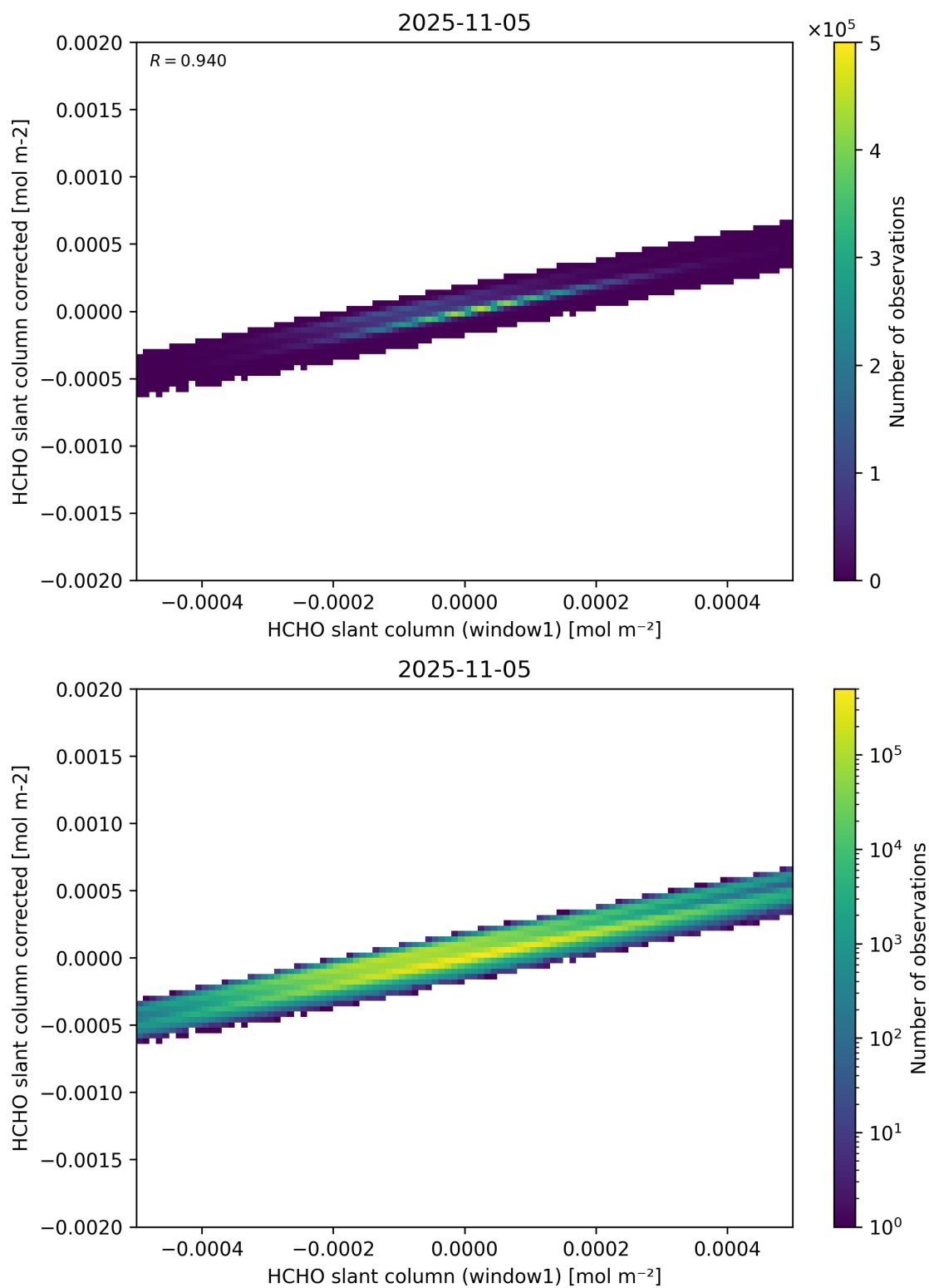
Figure 82: Scatter density plot of “HCHO slant column (window1)” against “HCHO slant column corrected” for 2025-11-04 to 2025-11-06.
