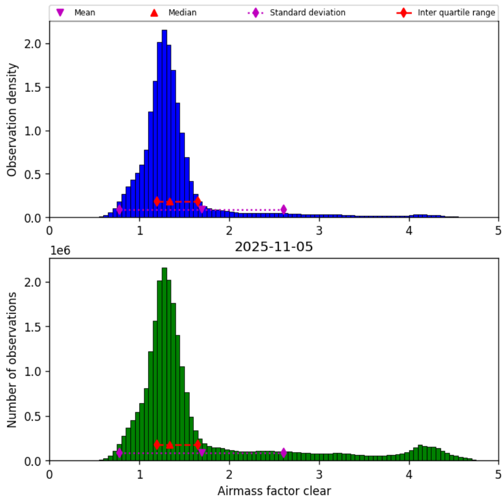
Figure 42: Histogram of “Airmass factor clear” for 2025-11-04 to 2025-11-06
