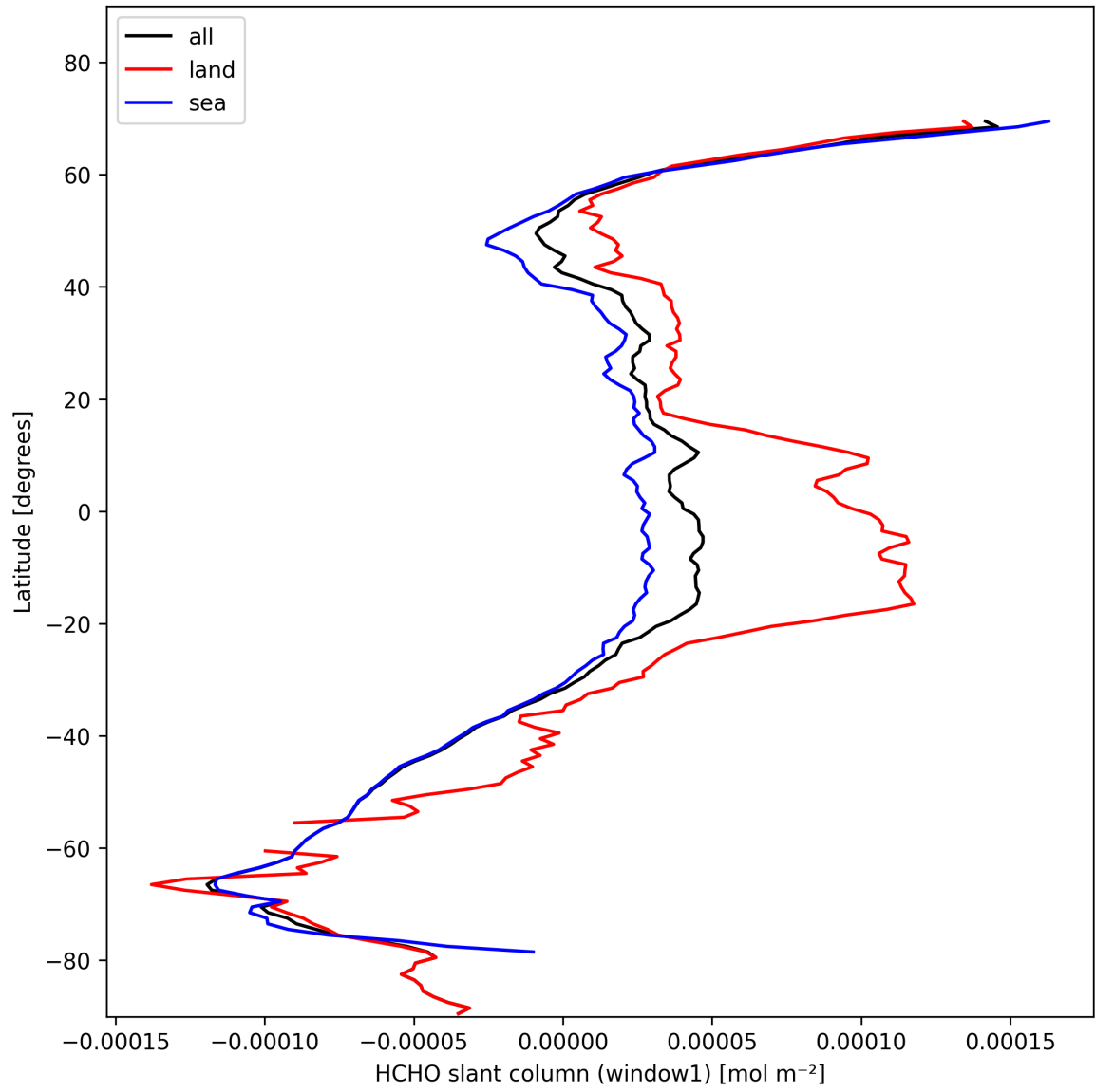
Figure 24: Zonal average of “HCHO slant column (window1)” for 2025-11-04 to 2025-11-06.
