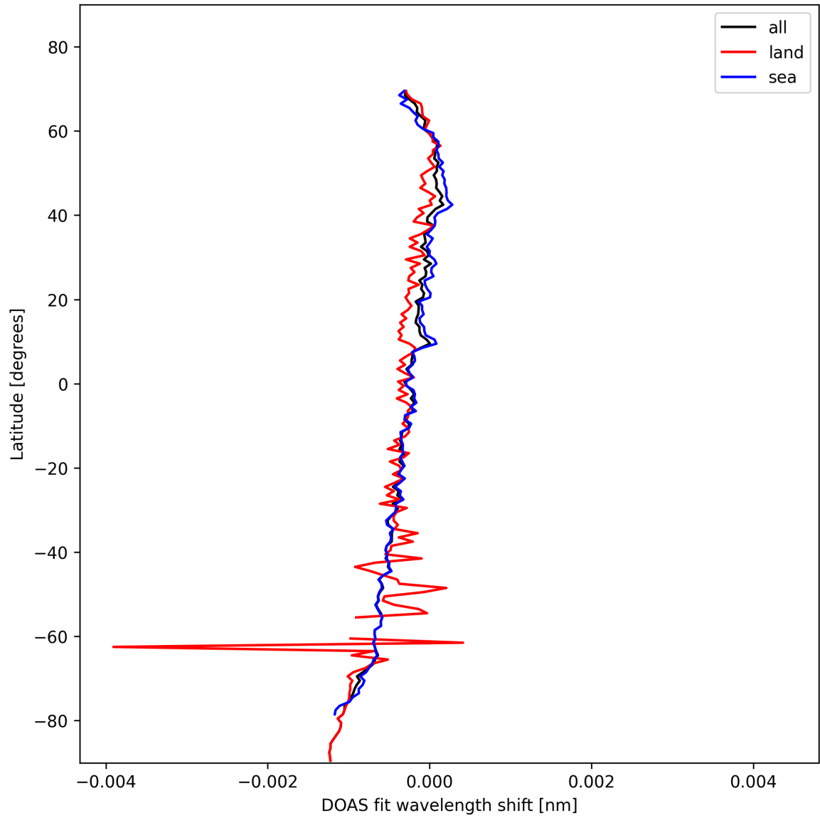
Figure 30: Zonal average of “DOAS fit wavelength shift” for 2025-11-04 to 2025-11-06.
