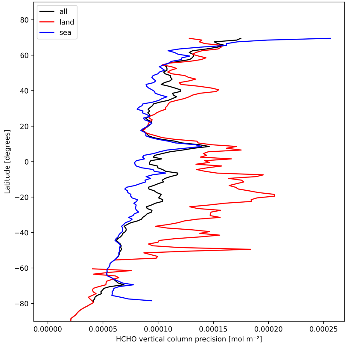
Figure 22: Zonal average of “HCHO vertical column precision” for 2025-11-04 to 2025-11-06.
