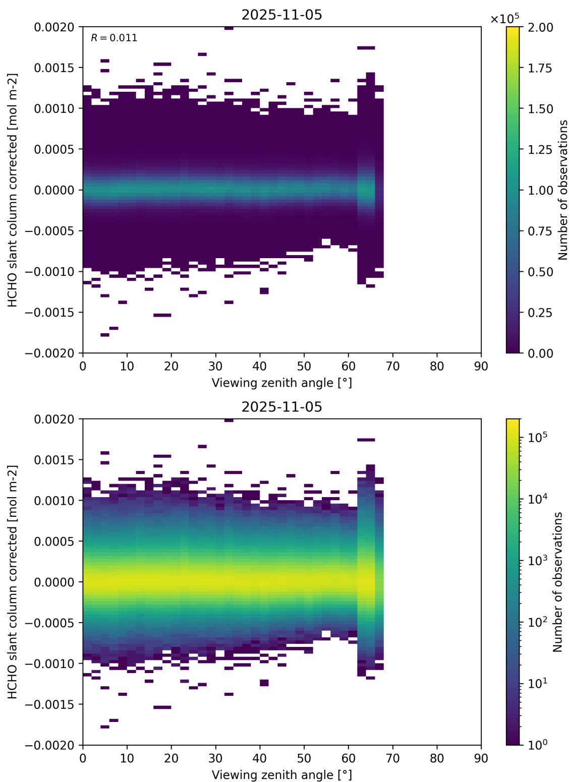
Figure 186: Scatter density plot of “Viewing zenith angle” against “HCHO slant column corrected” for 2025-11-04 to 2025-11-06.
