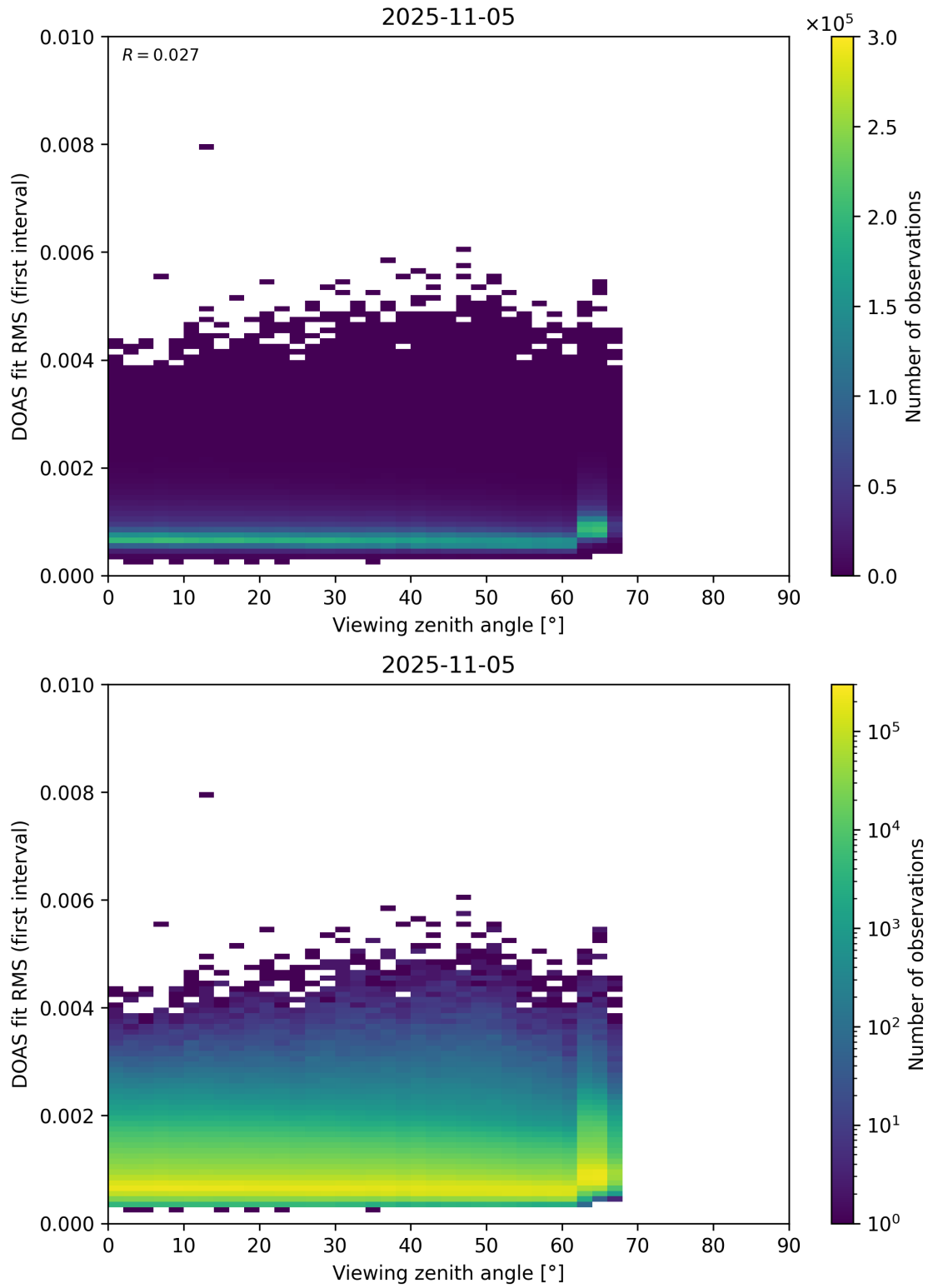
Figure 182: Scatter density plot of “Viewing zenith angle” against “DOAS fit RMS (first interval)” for 2025-11-04 to 2025-11-06.
