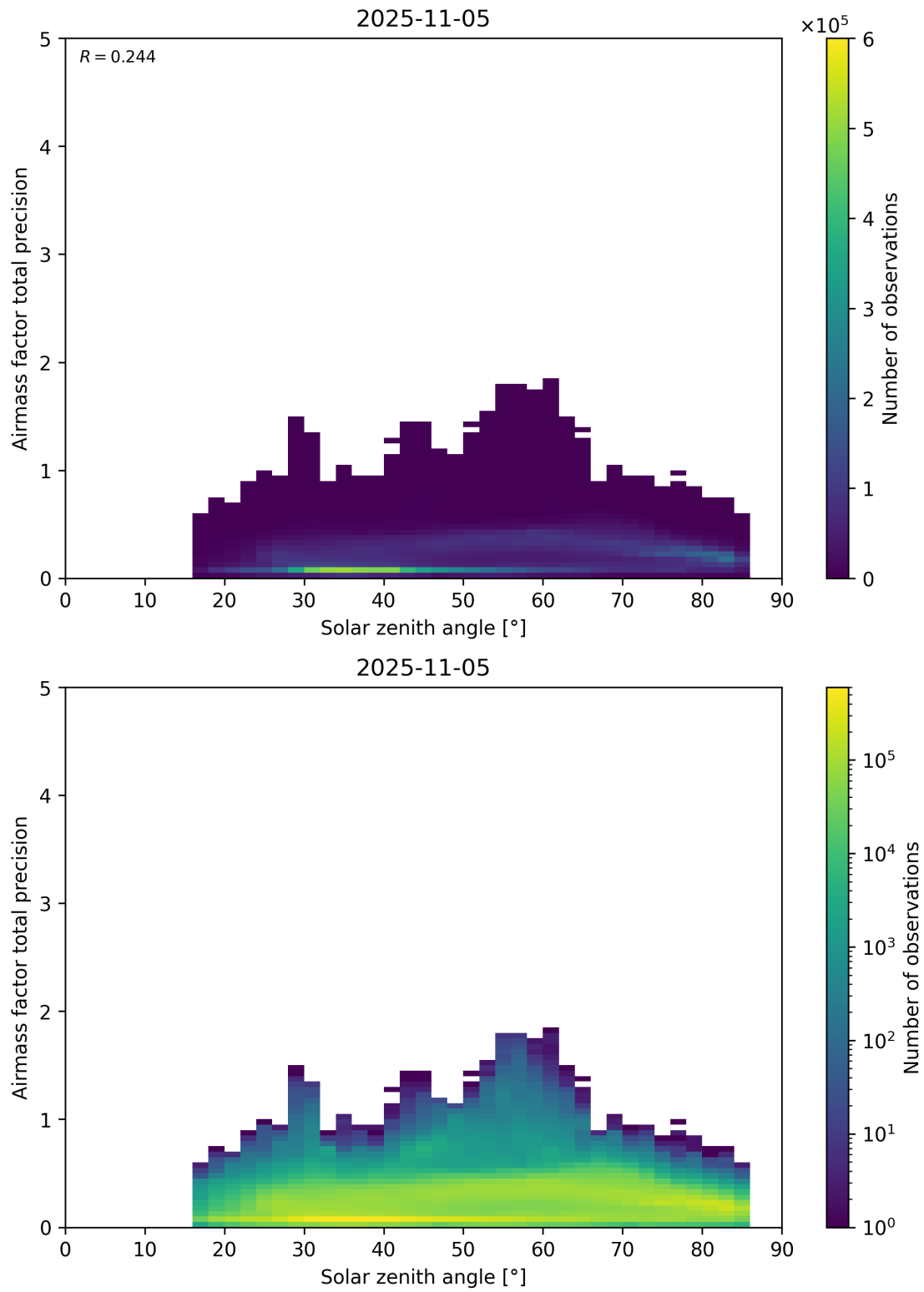
Figure 176: Scatter density plot of “Solar zenith angle” against “Airmass factor total precision” for 2025-11-04 to 2025-11-06.
