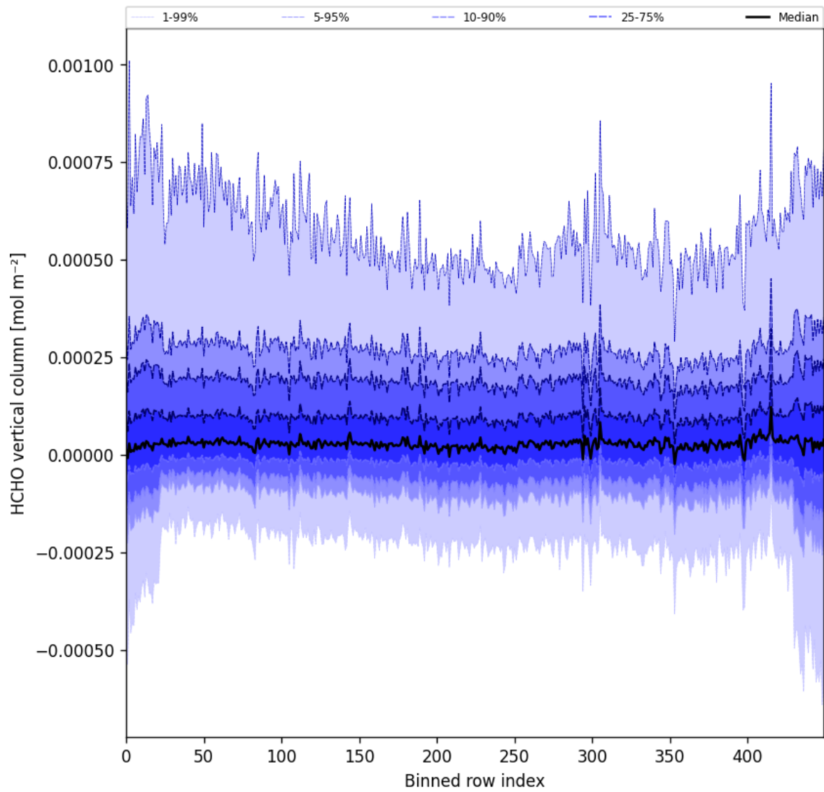
Figure 49: Along track statistics of “HCHO vertical column” for 2025-11-04 to 2025-11-06
