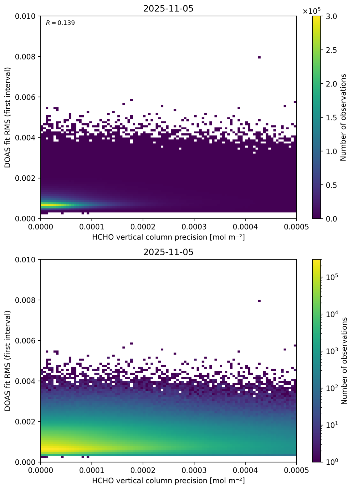
Figure 136: Scatter density plot of “HCHO vertical column precision” against “DOAS fit RMS (first interval)” for 2025-11-04 to 2025-11-06.
