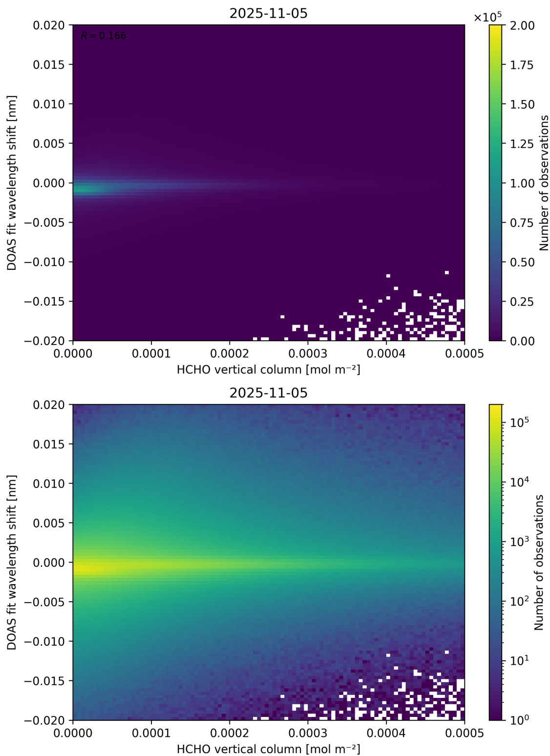
Figure 124: Scatter density plot of “HCHO vertical column” against “DOAS fit wavelength shift” for 2025-11-04 to 2025-11-06.
