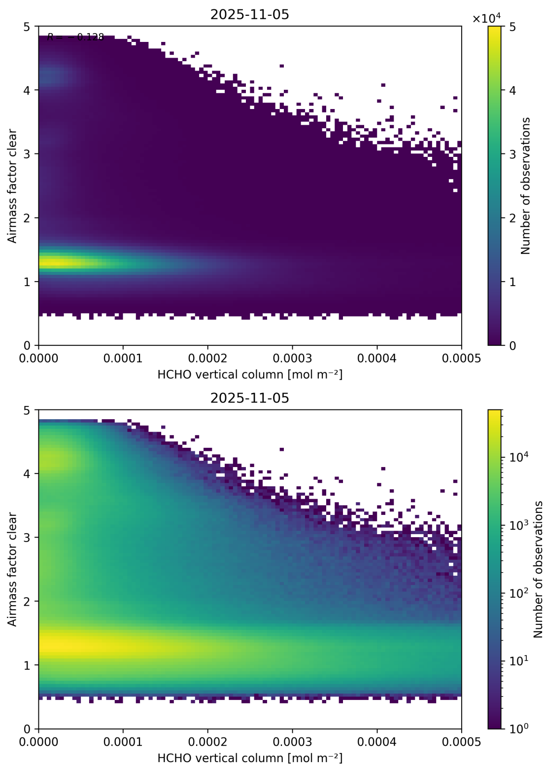
Figure 126: Scatter density plot of “HCHO vertical column” against “Airmass factor clear” for 2025-11-04 to 2025-11-06.
