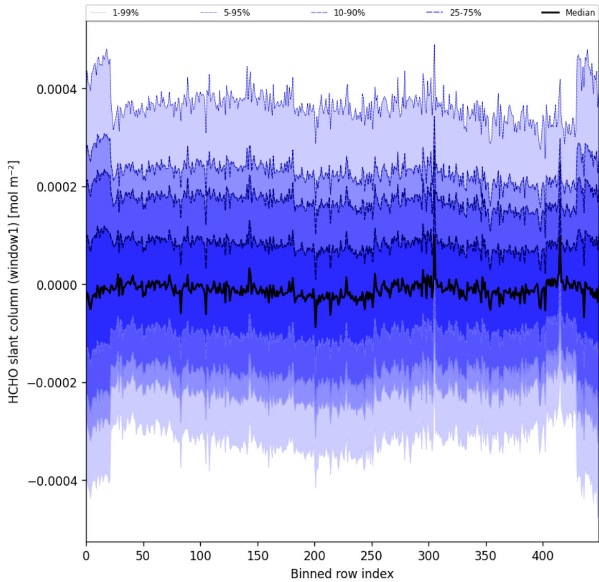
Figure 52: Along track statistics of “HCHO slant column (window1)” for 2025-11-04 to 2025-11-06
