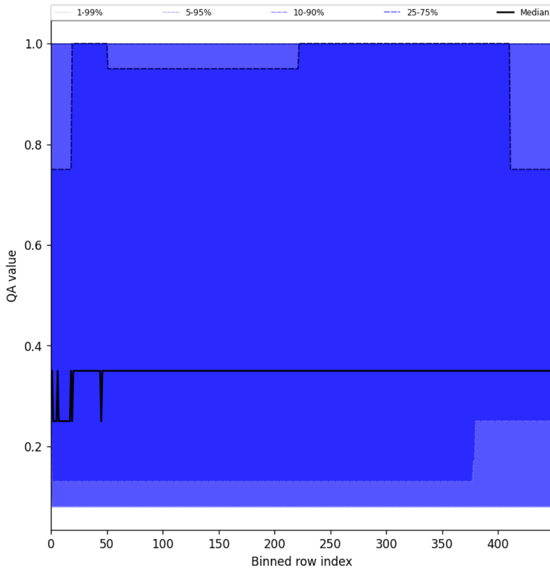
Figure 48: Along track statistics of “QA value” for 2025-11-04 to 2025-11-06
