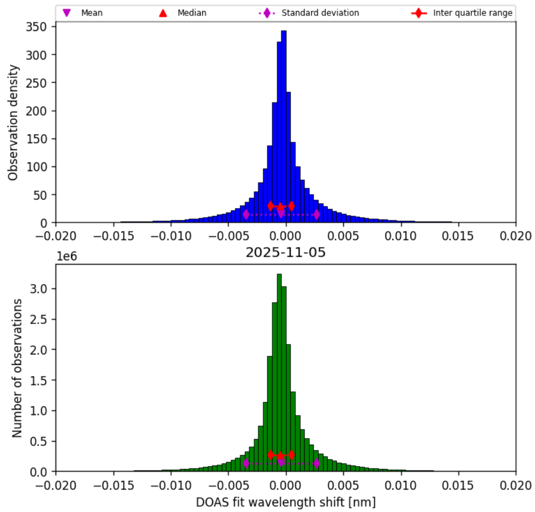
Figure 44: Histogram of “DOAS fit wavelength shift” for 2025-11-04 to 2025-11-06
