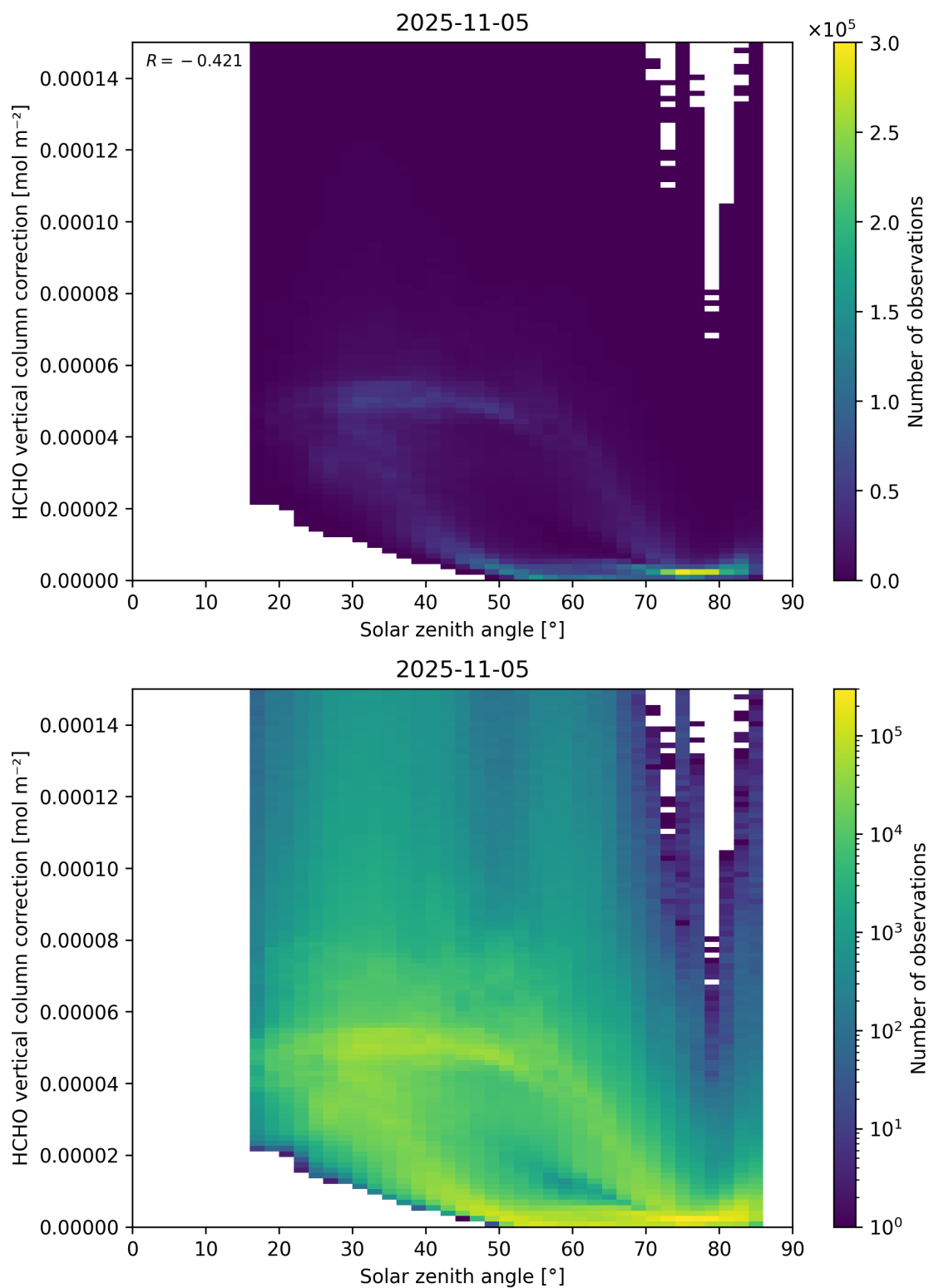
Figure 178: Scatter density plot of “Solar zenith angle” against “HCHO vertical column correction” for 2025-11-04 to 2025-11-06.
