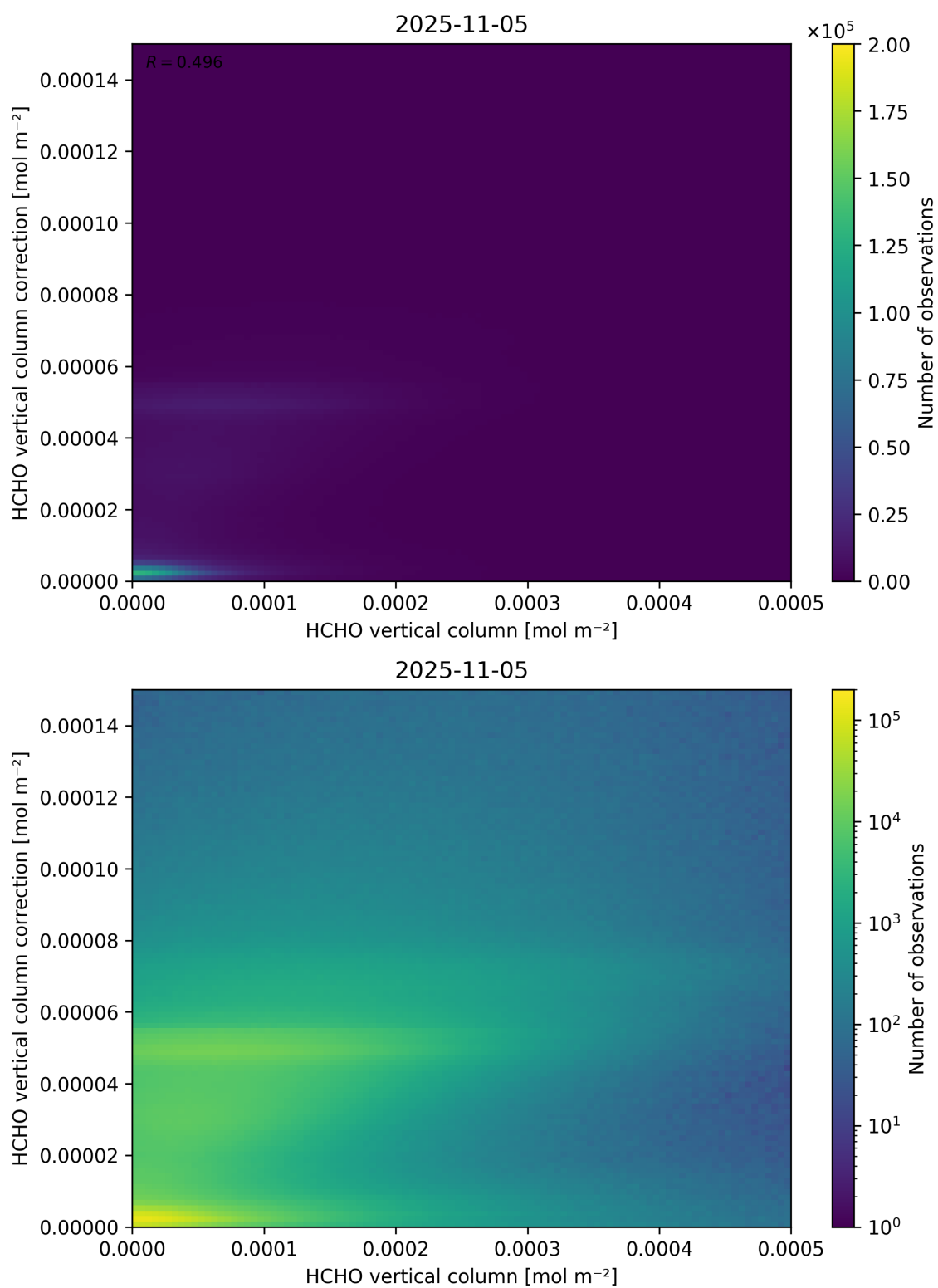
Figure 133: Scatter density plot of “HCHO vertical column” against “HCHO vertical column correction” for 2025-11-04 to 2025-11-06.
