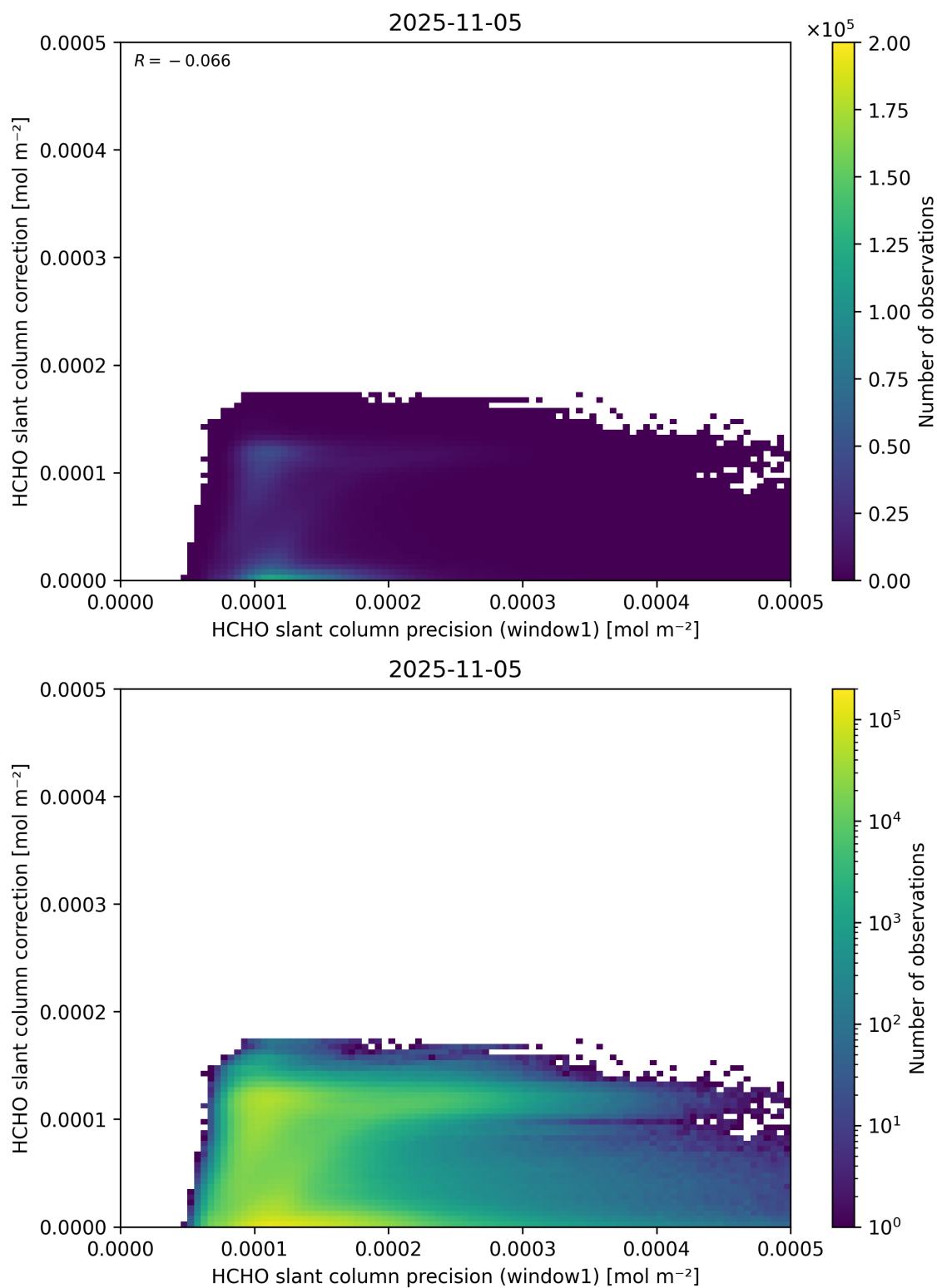
Figure 93: Scatter density plot of “HCHO slant column precision (window1)” against “HCHO slant column correction” for 2025-11-04 to 2025-11-06.
