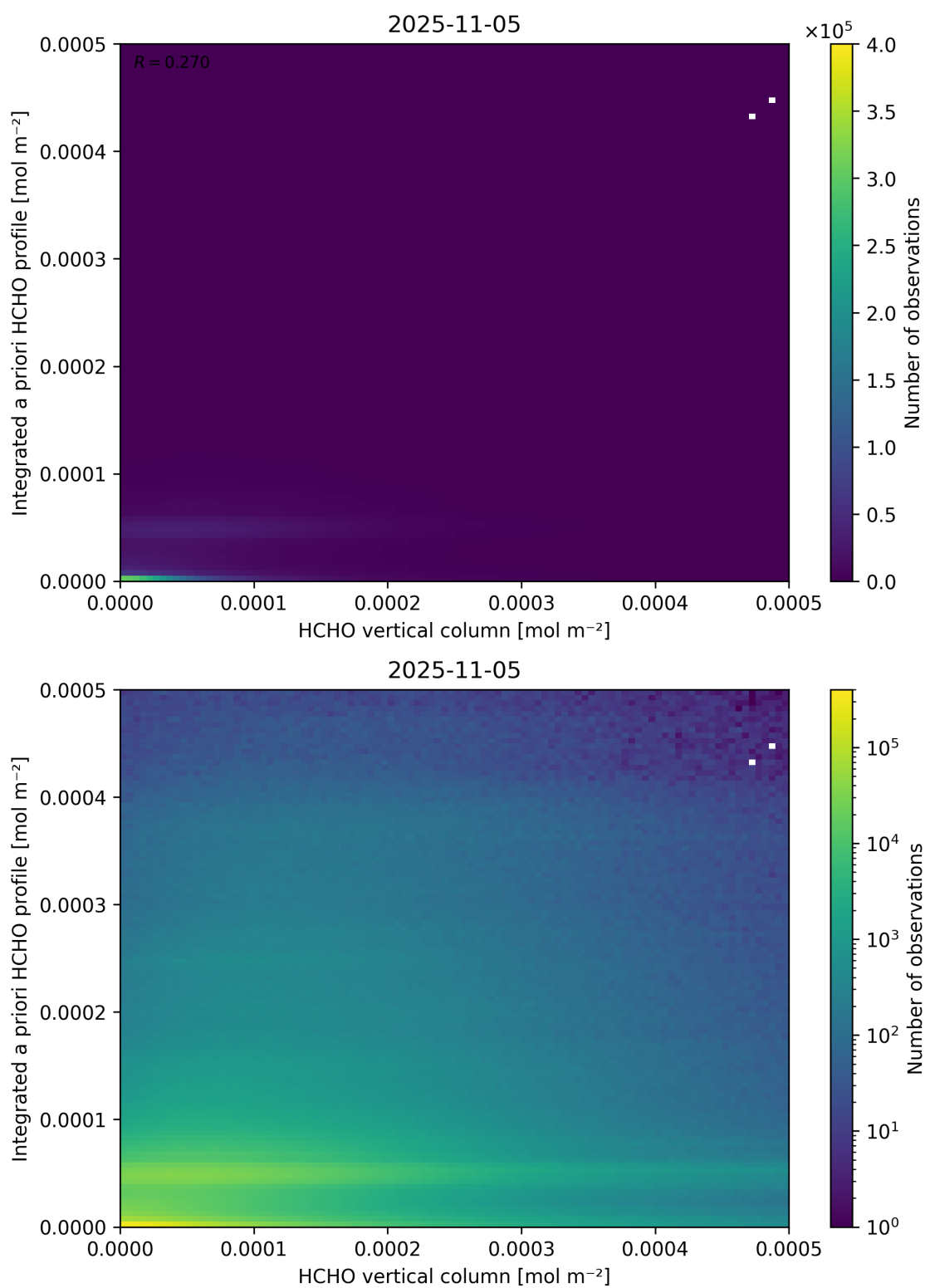
Figure 135: Scatter density plot of “HCHO vertical column” against “Integrated a priori HCHO profile” for 2025-11-04 to 2025-11-06.
