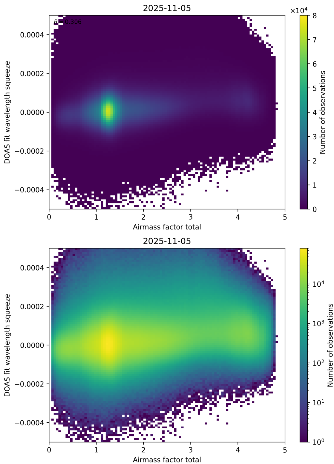
Figure 99: Scatter density plot of “Airmass factor total” against “DOAS fit wavelength squeeze” for 2025-11-04 to 2025-11-06.
