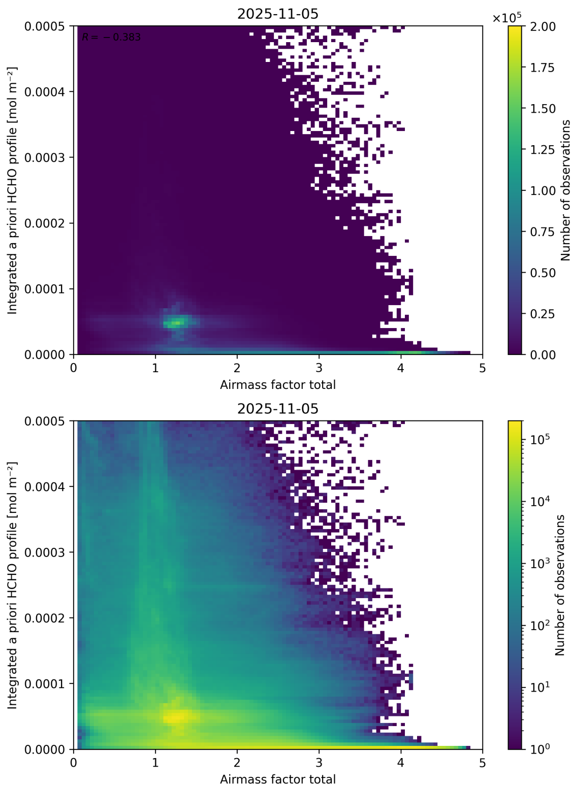
Figure 104: Scatter density plot of “Airmass factor total” against “Integrated a priori HCHO profile” for 2025-11-04 to 2025-11-06.
