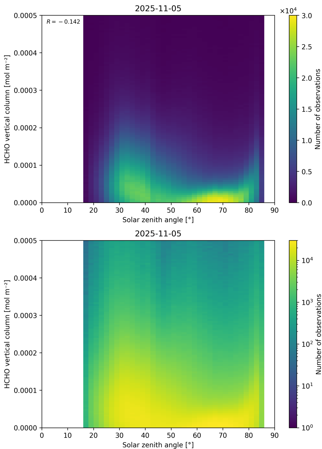
Figure 177: Scatter density plot of “Solar zenith angle” against “HCHO vertical column” for 2025-11-04 to 2025-11-06.
