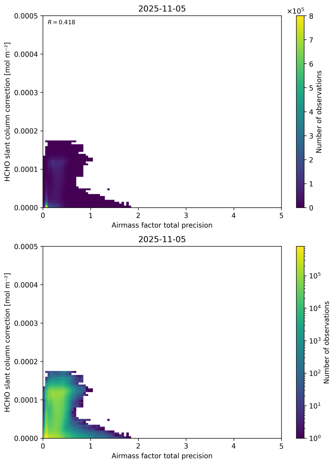
Figure 110: Scatter density plot of “Airmass factor total precision” against “HCHO slant column correction” for 2025-11-04 to 2025-11-06.
