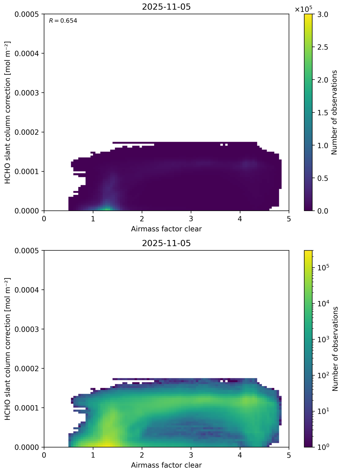
Figure 75: Scatter density plot of “Airmass factor clear” against “HCHO slant column correction” for 2025-11-04 to 2025-11-06.
