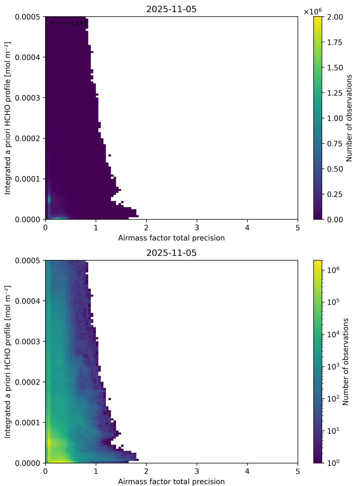
Figure 111: Scatter density plot of “Airmass factor total precision” against “Integrated a priori HCHO profile” for 2025-11-04 to 2025-11-06.
