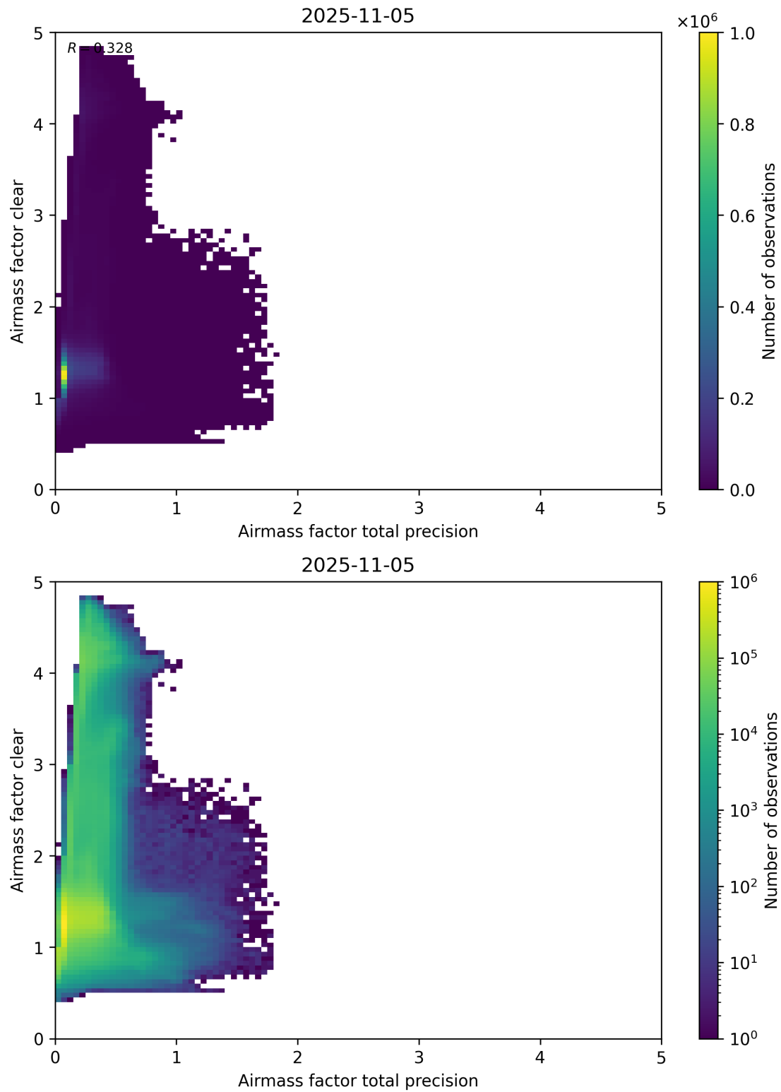
Figure 108: Scatter density plot of “Airmass factor total precision” against “Airmass factor clear” for 2025-11-04 to 2025-11-06.
