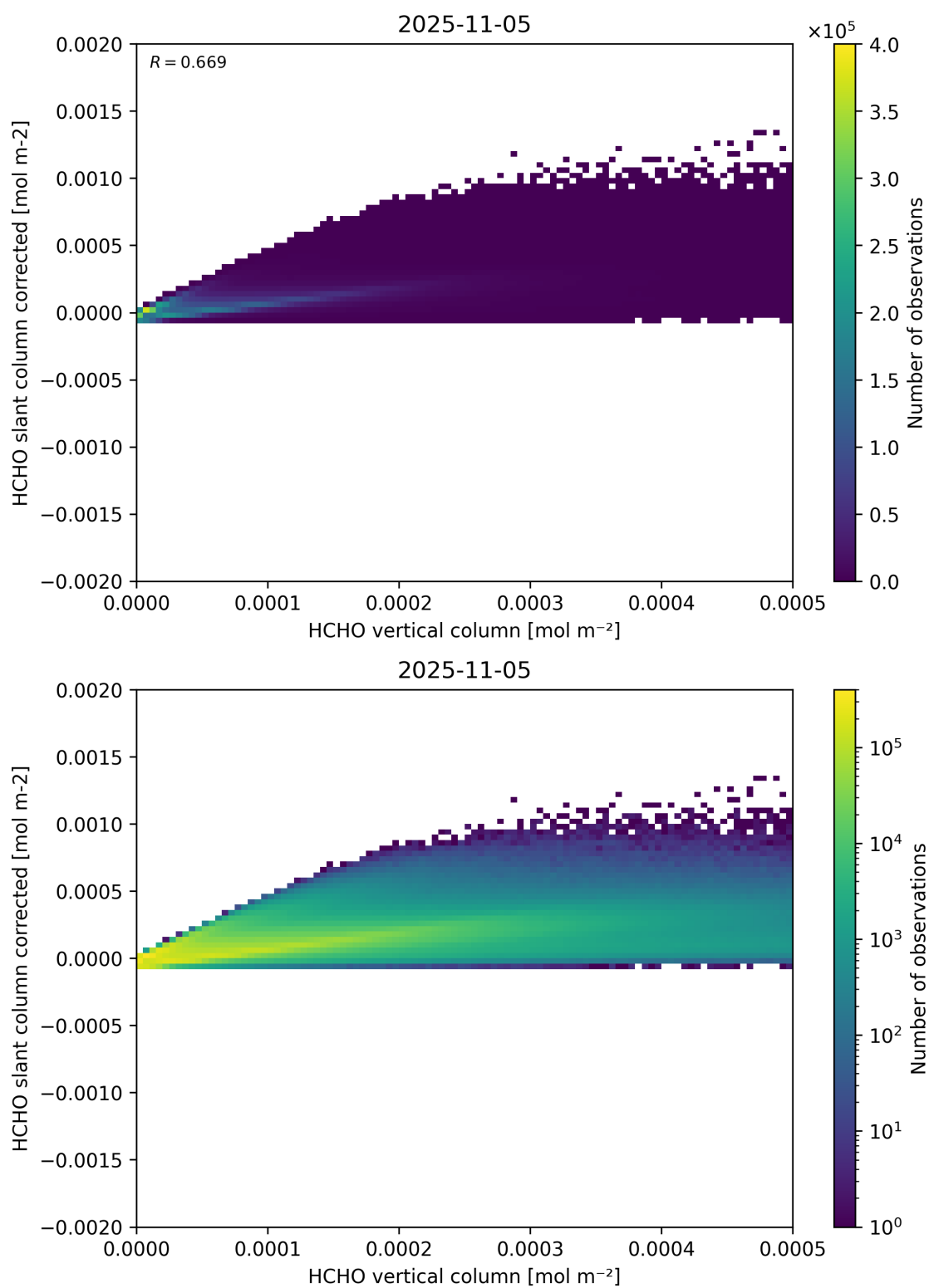
Figure 127: Scatter density plot of “HCHO vertical column” against “HCHO slant column corrected” for 2025-11-04 to 2025-11-06.
