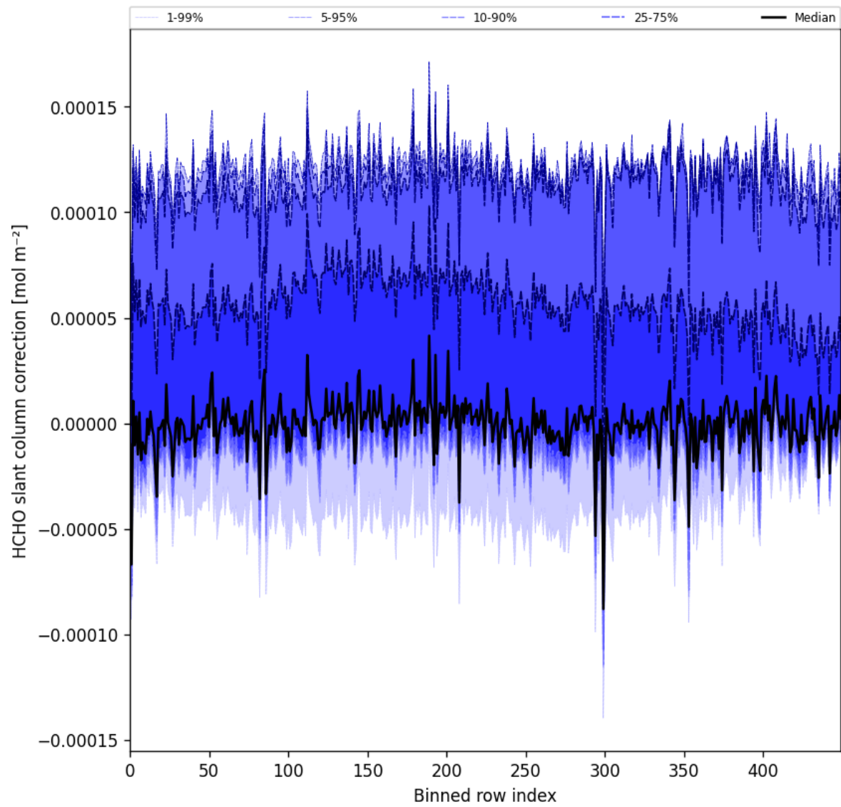
Figure 61: Along track statistics of “HCHO slant column correction” for 2025-11-04 to 2025-11-06
