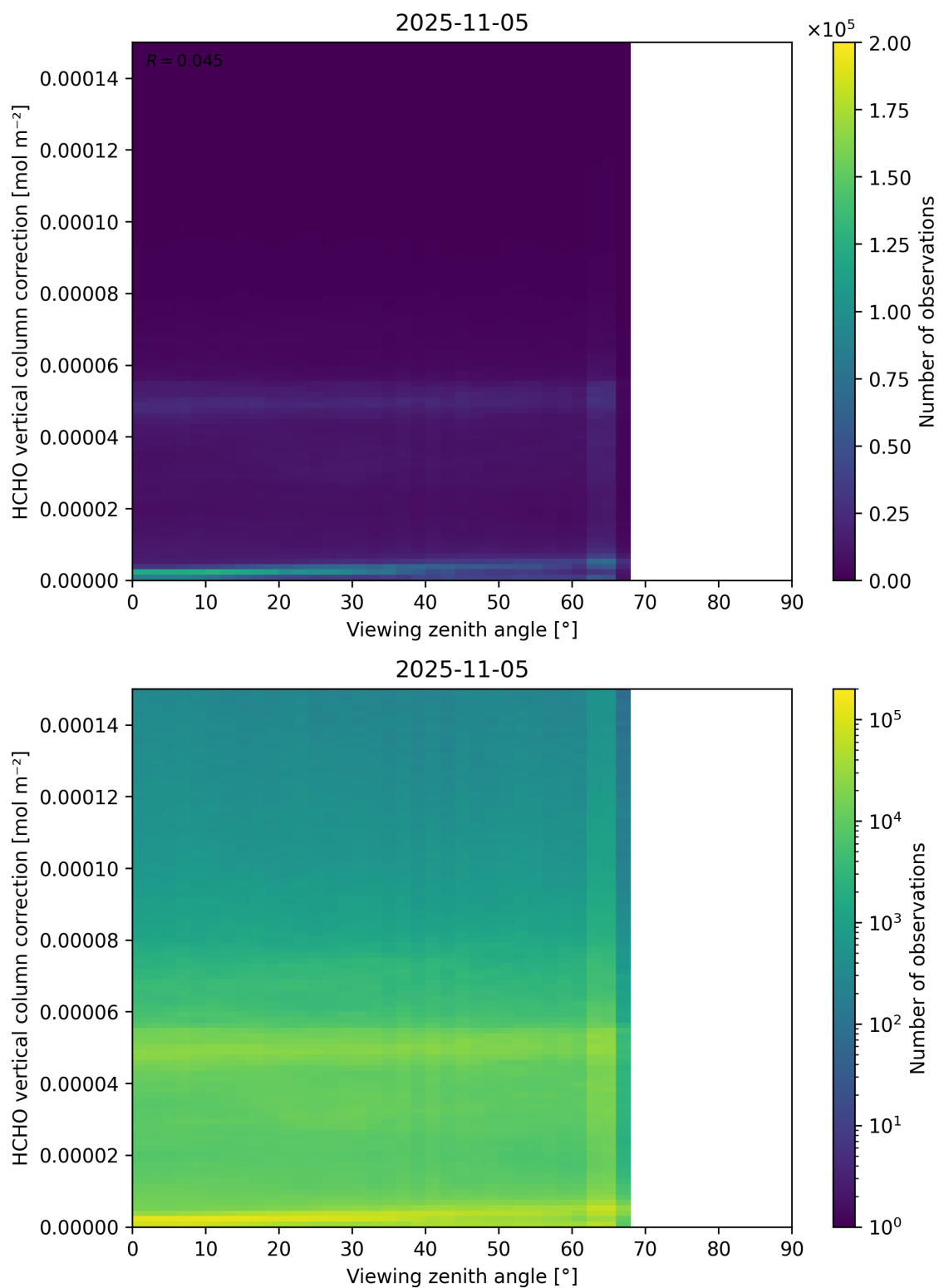
Figure 193: Scatter density plot of “Viewing zenith angle” against “HCHO vertical column correction” for 2025-11-04 to 2025-11-06.
