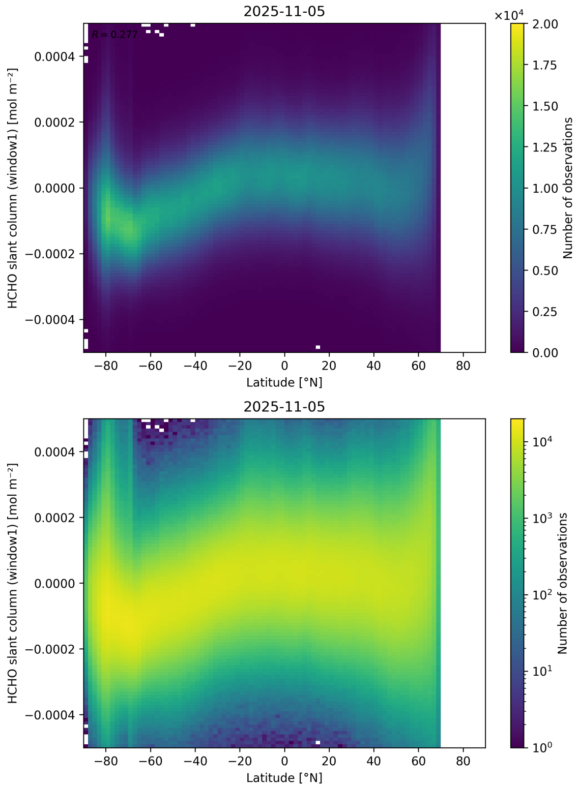
Figure 159: Scatter density plot of “Latitude” against “HCHO slant column (window1)” for 2025-11-04 to 2025-11-06.
