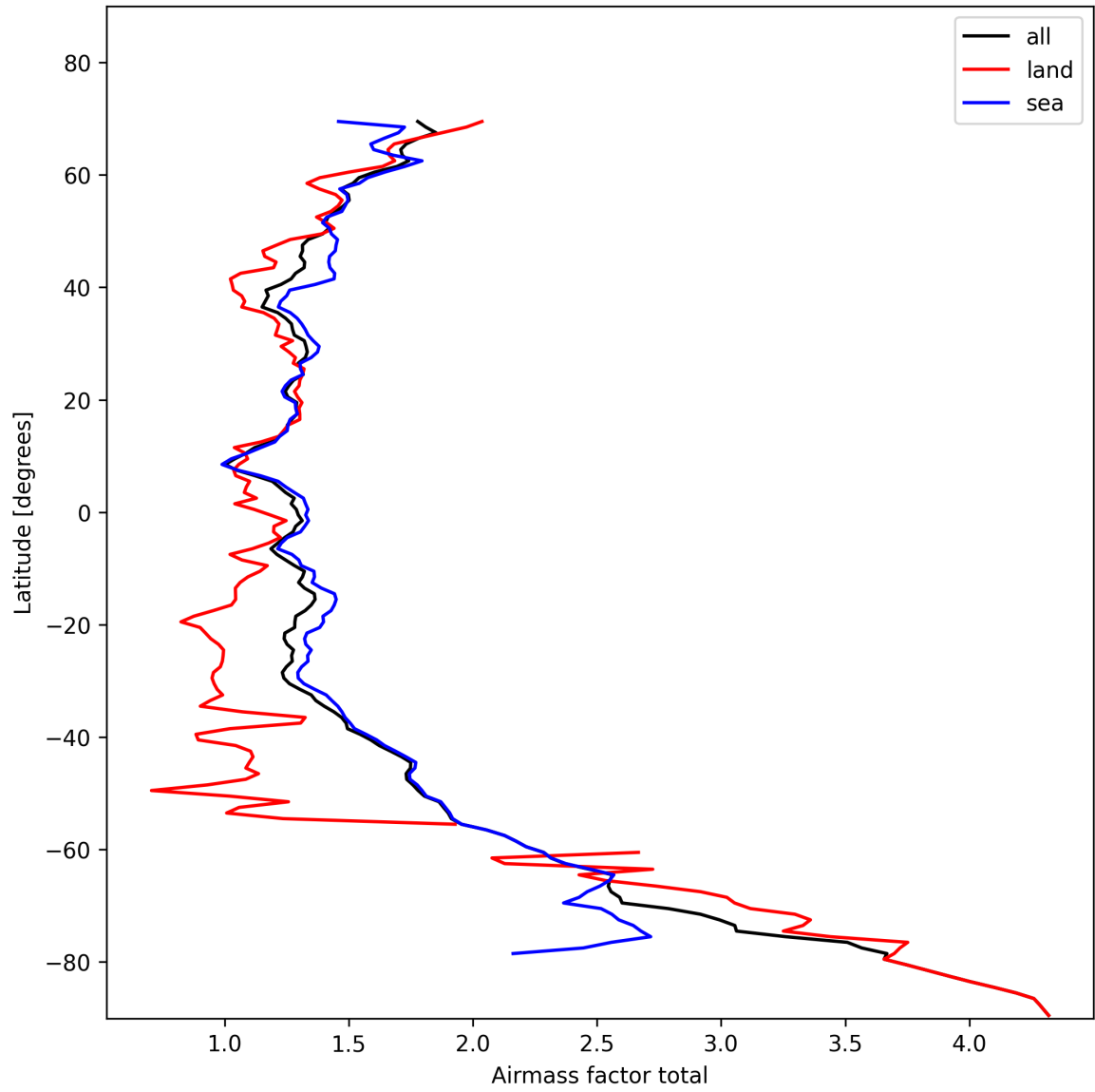
Figure 26: Zonal average of “Airmass factor total” for 2025-11-04 to 2025-11-06.
