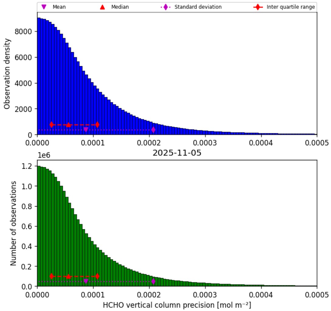
Figure 36: Histogram of “HCHO vertical column precision” for 2025-11-04 to 2025-11-06
