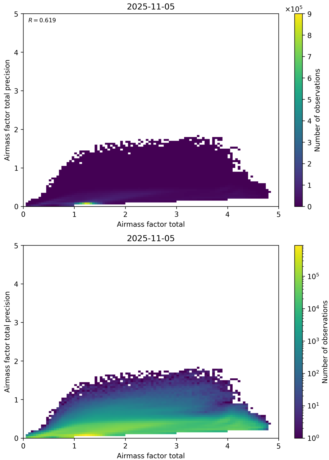
Figure 103: Scatter density plot of “Airmass factor total” against “Airmass factor total precision” for 2025-11-04 to 2025-11-06.
