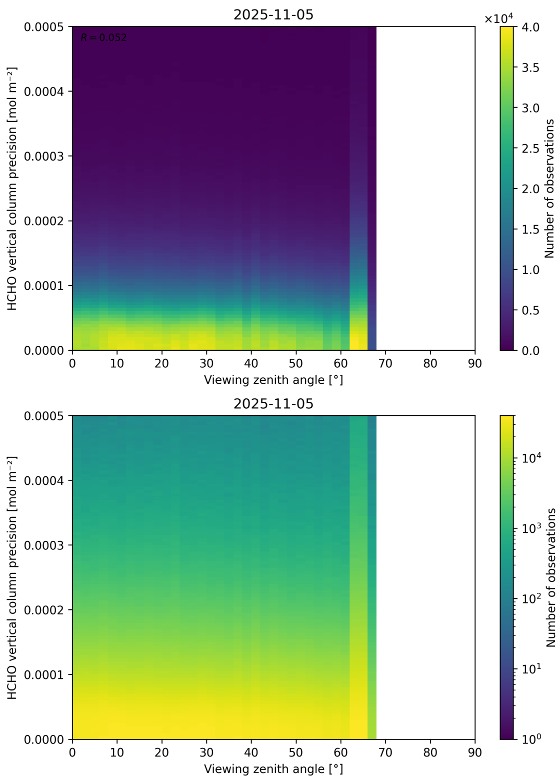
Figure 194: Scatter density plot of “Viewing zenith angle” against “HCHO vertical column precision” for 2025-11-04 to 2025-11-06.
