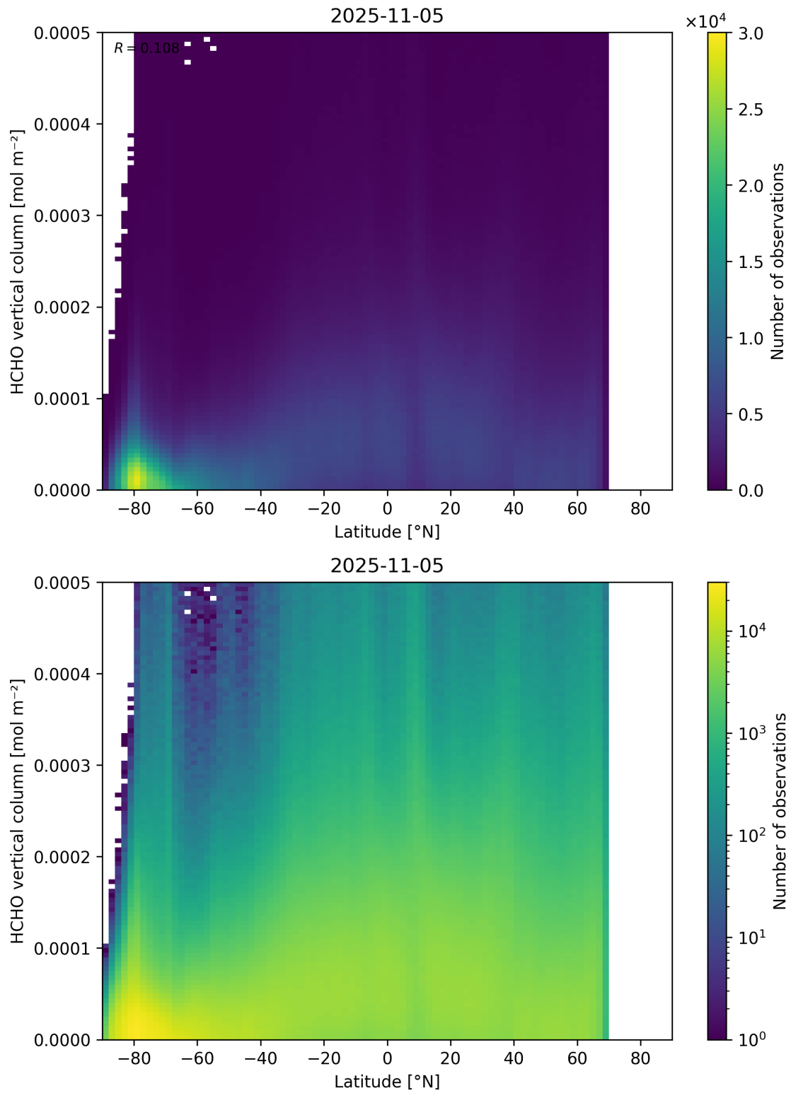
Figure 163: Scatter density plot of “Latitude” against “HCHO vertical column” for 2025-11-04 to 2025-11-06.
