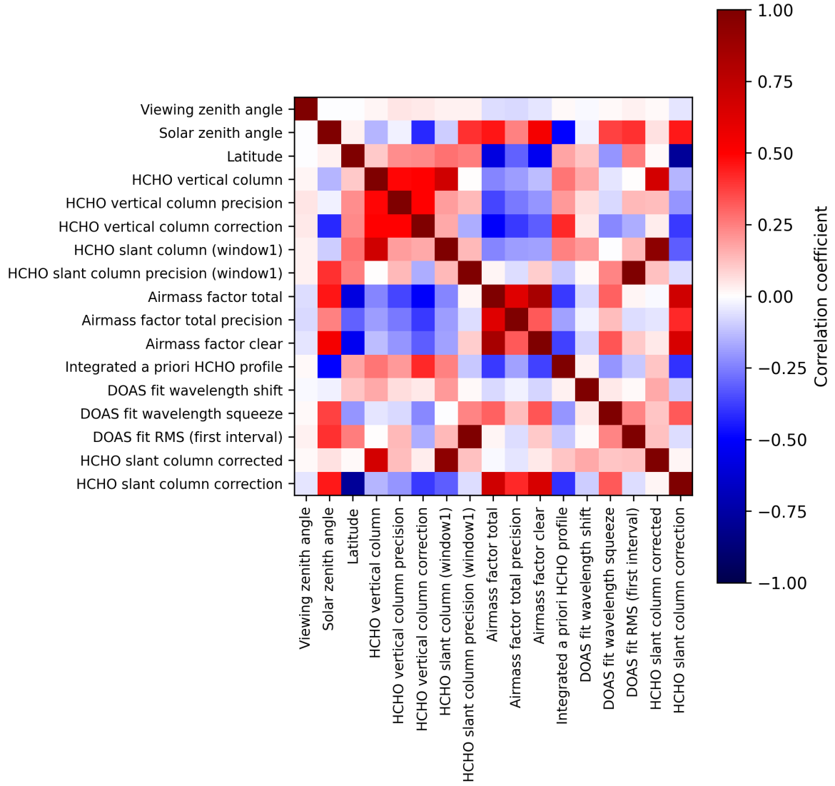
Figure 2: Map of correlation matrix for 2025-11-04 to 2025-11-06.
