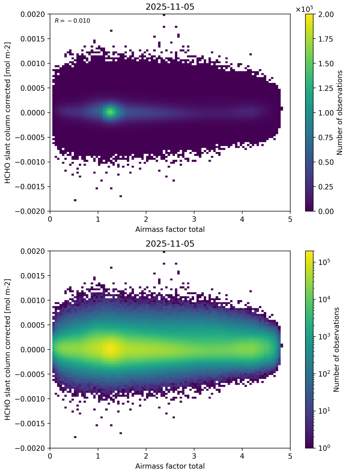
Figure 101: Scatter density plot of “Airmass factor total” against “HCHO slant column corrected” for 2025-11-04 to 2025-11-06.
