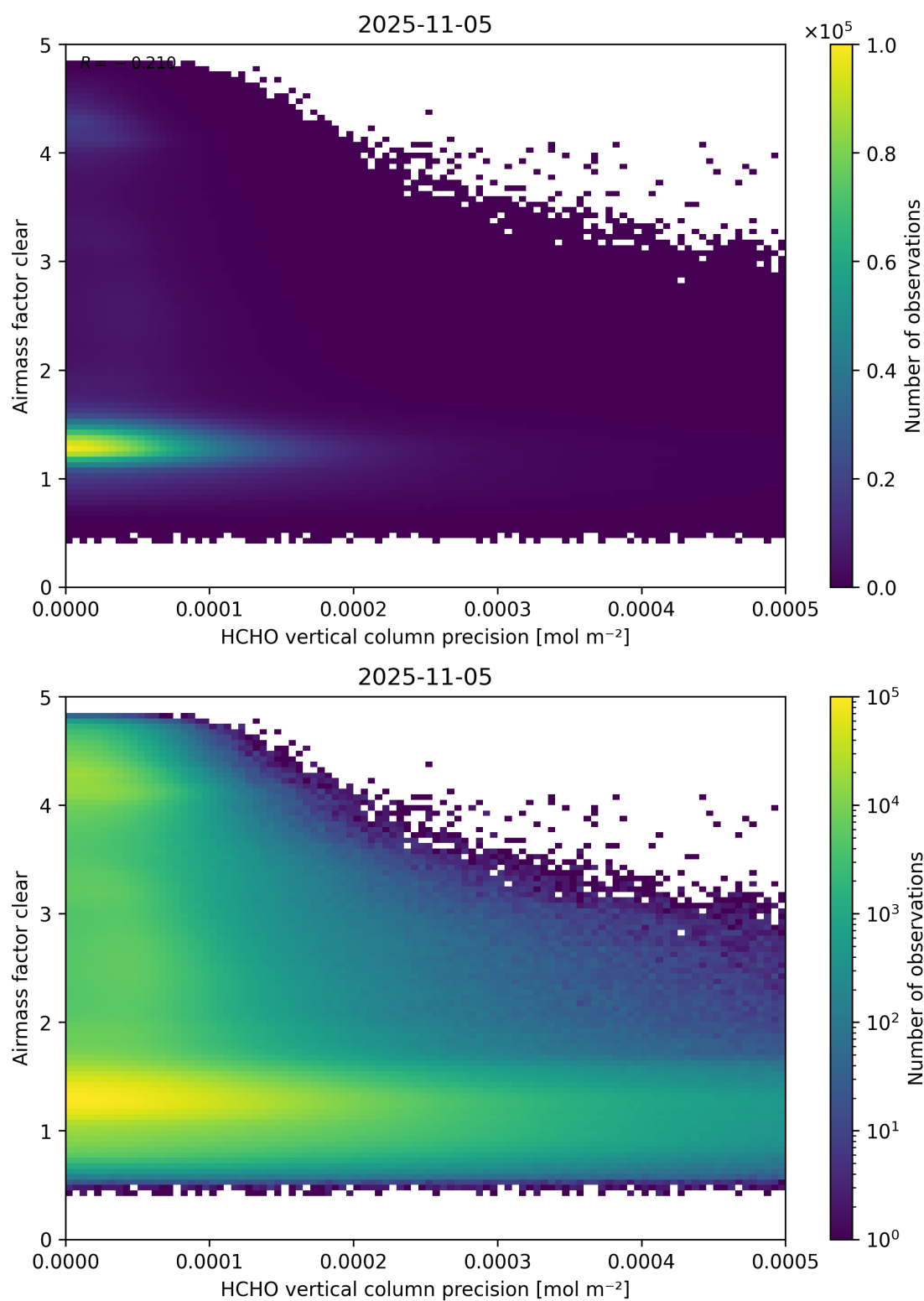
Figure 139: Scatter density plot of “HCHO vertical column precision” against “Airmass factor clear” for 2025-11-04 to 2025-11-06.
