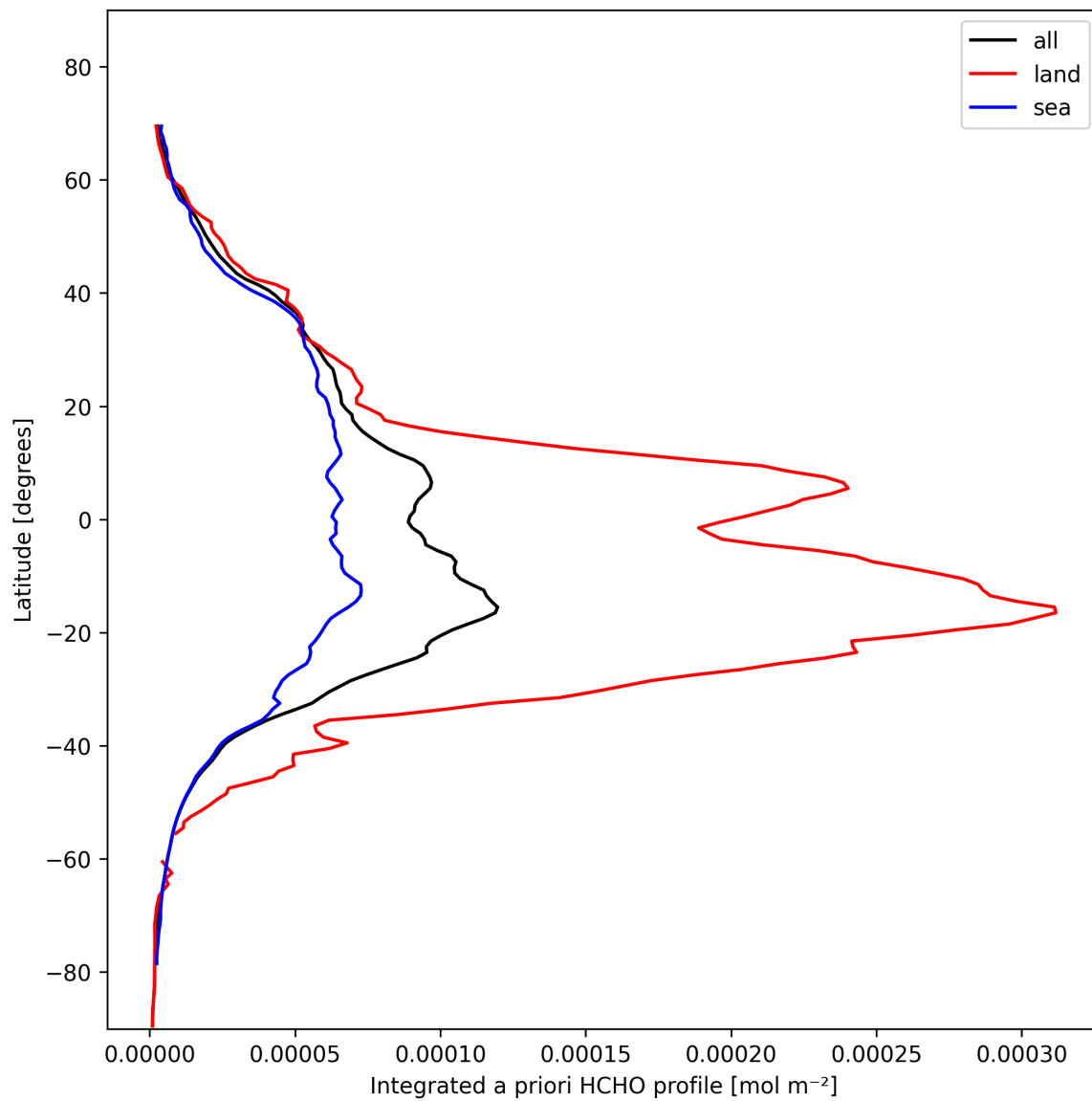
Figure 29: Zonal average of “Integrated a priori HCHO profile” for 2025-11-04 to 2025-11-06.
