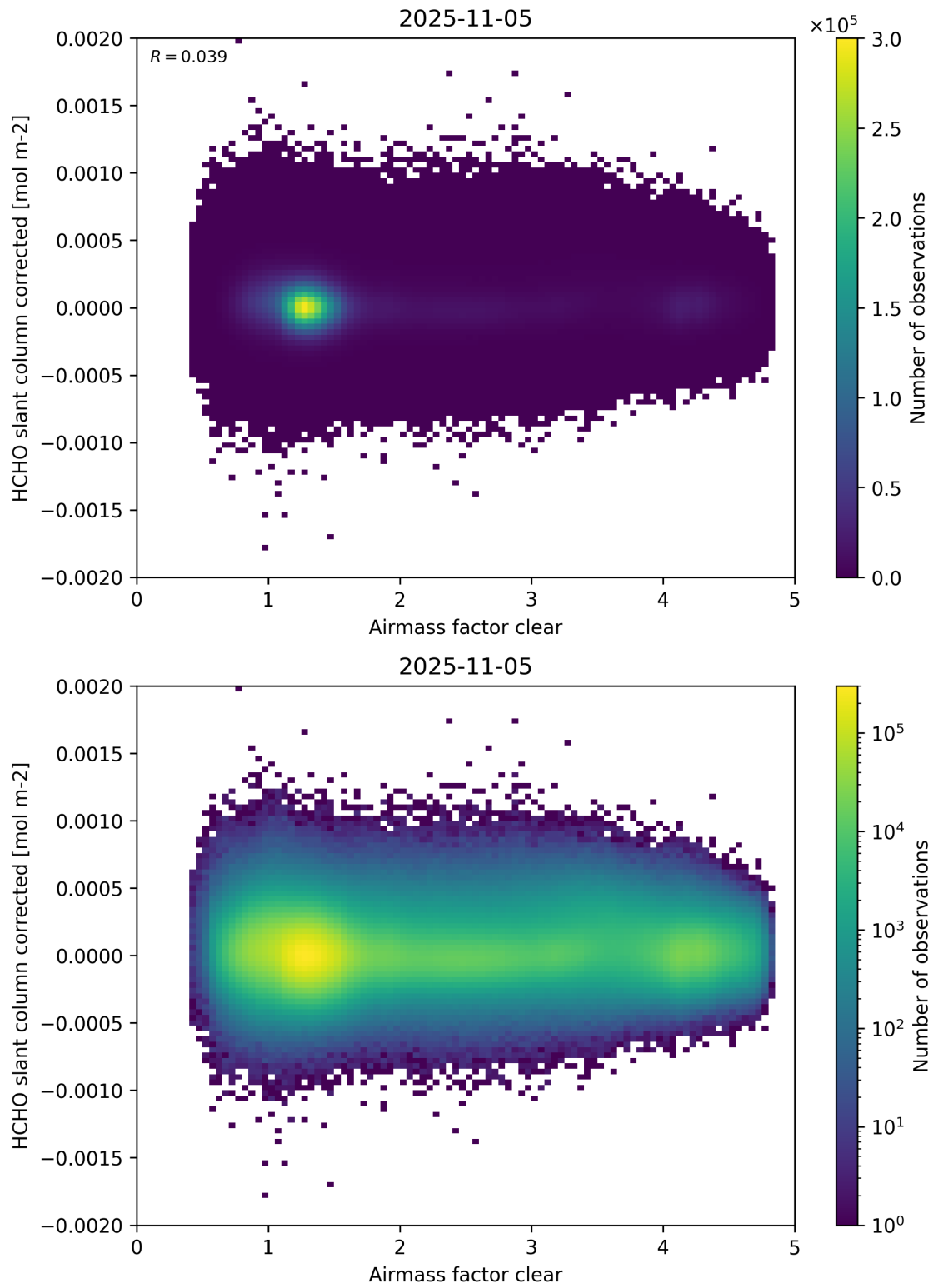
Figure 74: Scatter density plot of “Airmass factor clear” against “HCHO slant column corrected” for 2025-11-04 to 2025-11-06.
