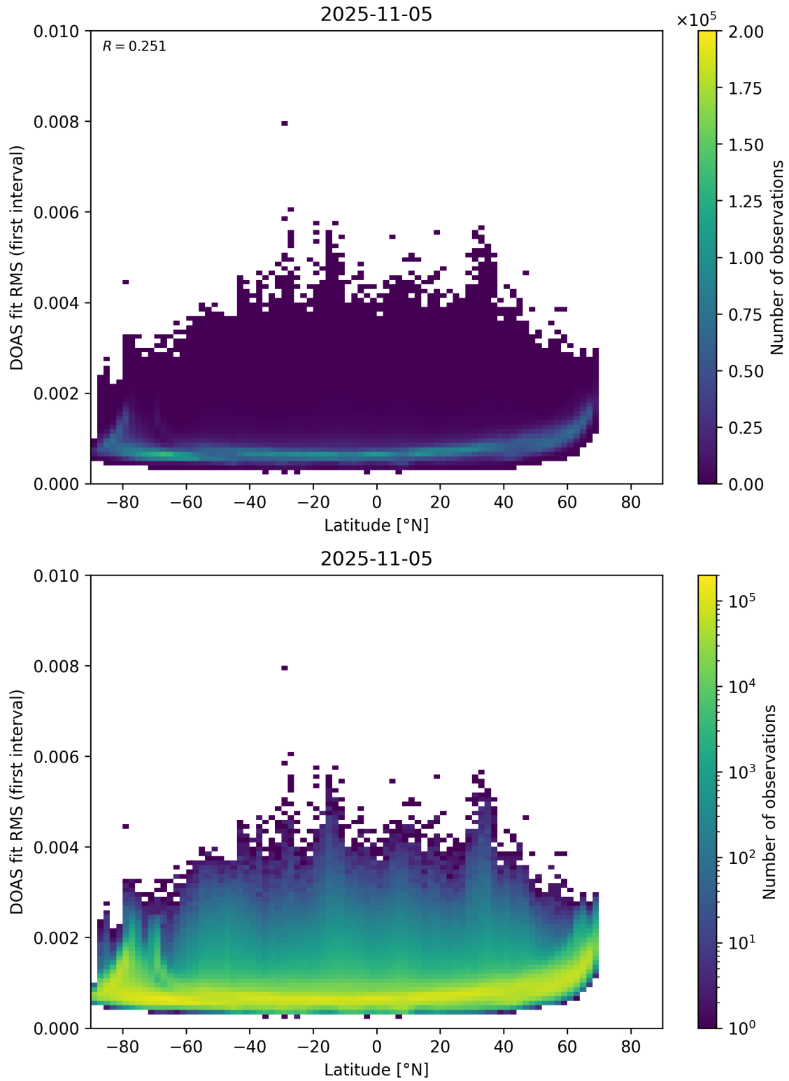
Figure 153: Scatter density plot of “Latitude” against “DOAS fit RMS (first interval)” for 2025-11-04 to 2025-11-06.
