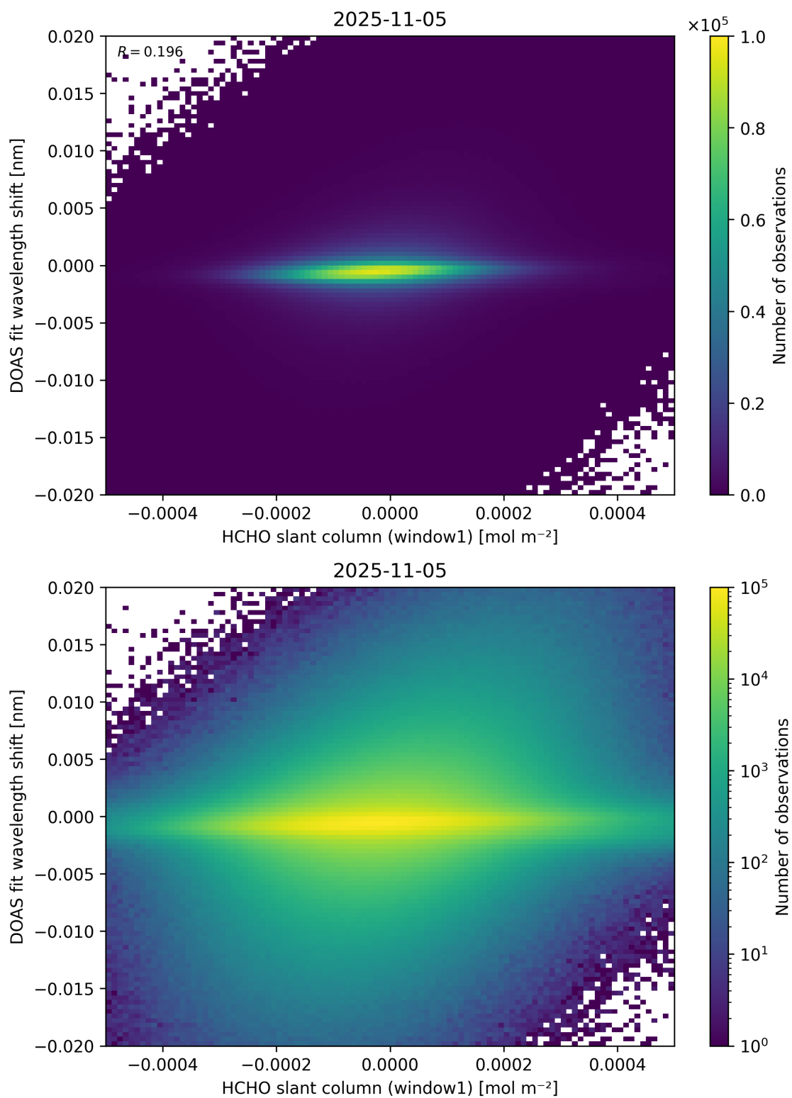
Figure 79: Scatter density plot of “HCHO slant column (window1)” against “DOAS fit wavelength shift” for 2025-11-04 to 2025-11-06.
