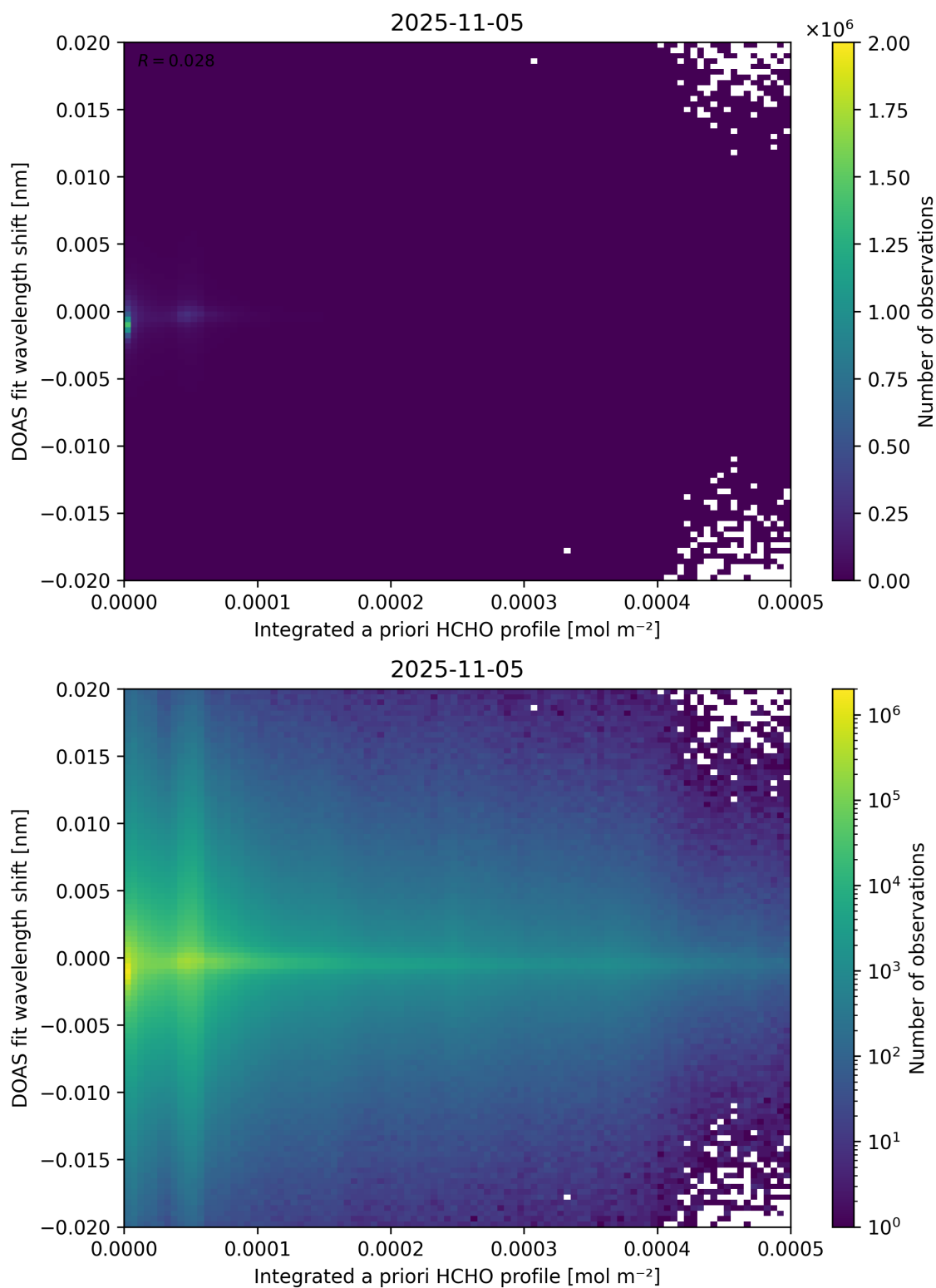
Figure 149: Scatter density plot of “Integrated a priori HCHO profile” against “DOAS fit wavelength shift” for 2025-11-04 to 2025-11-06.
