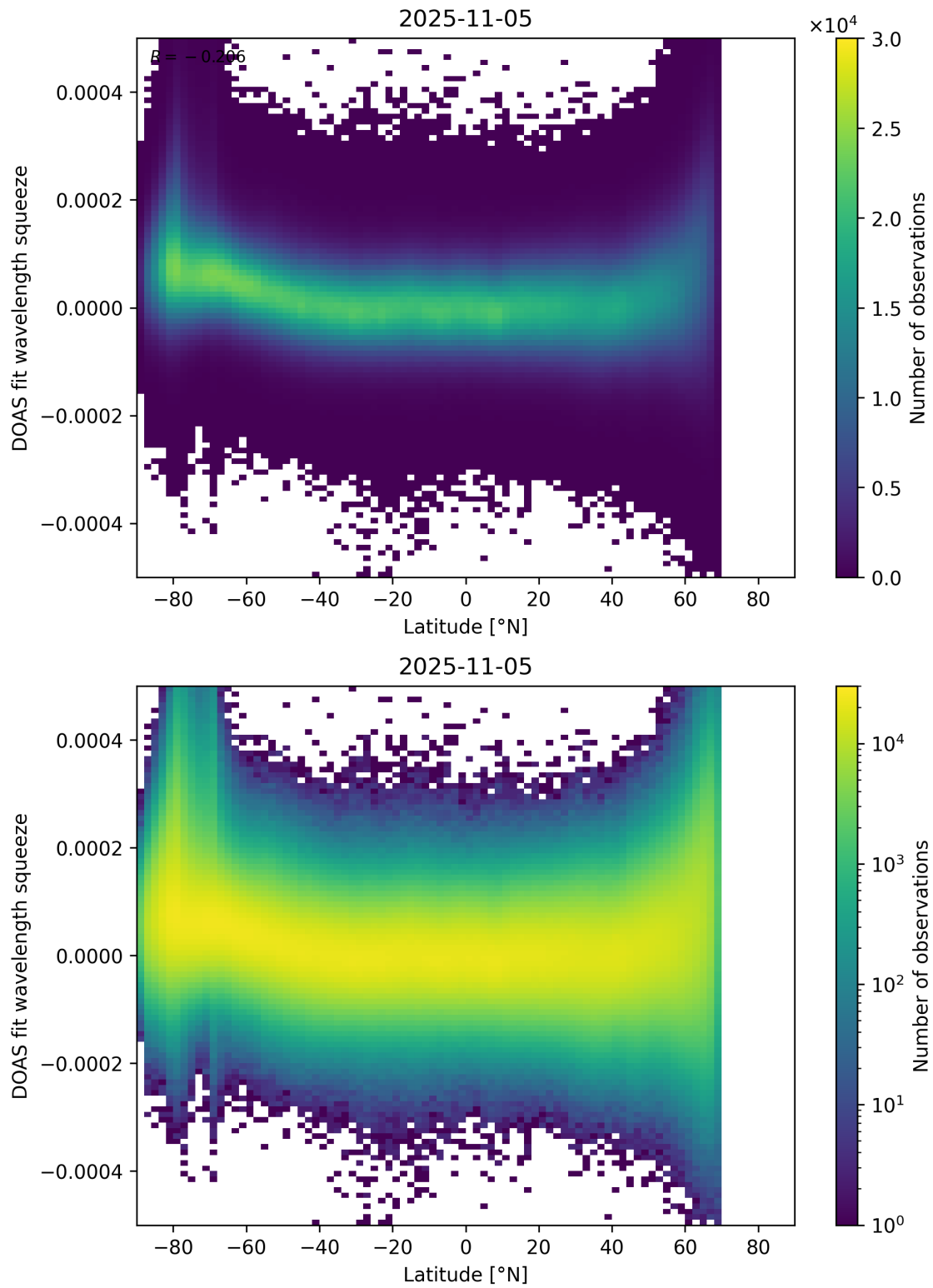
Figure 155: Scatter density plot of “Latitude” against “DOAS fit wavelength squeeze” for 2025-11-04 to 2025-11-06.
