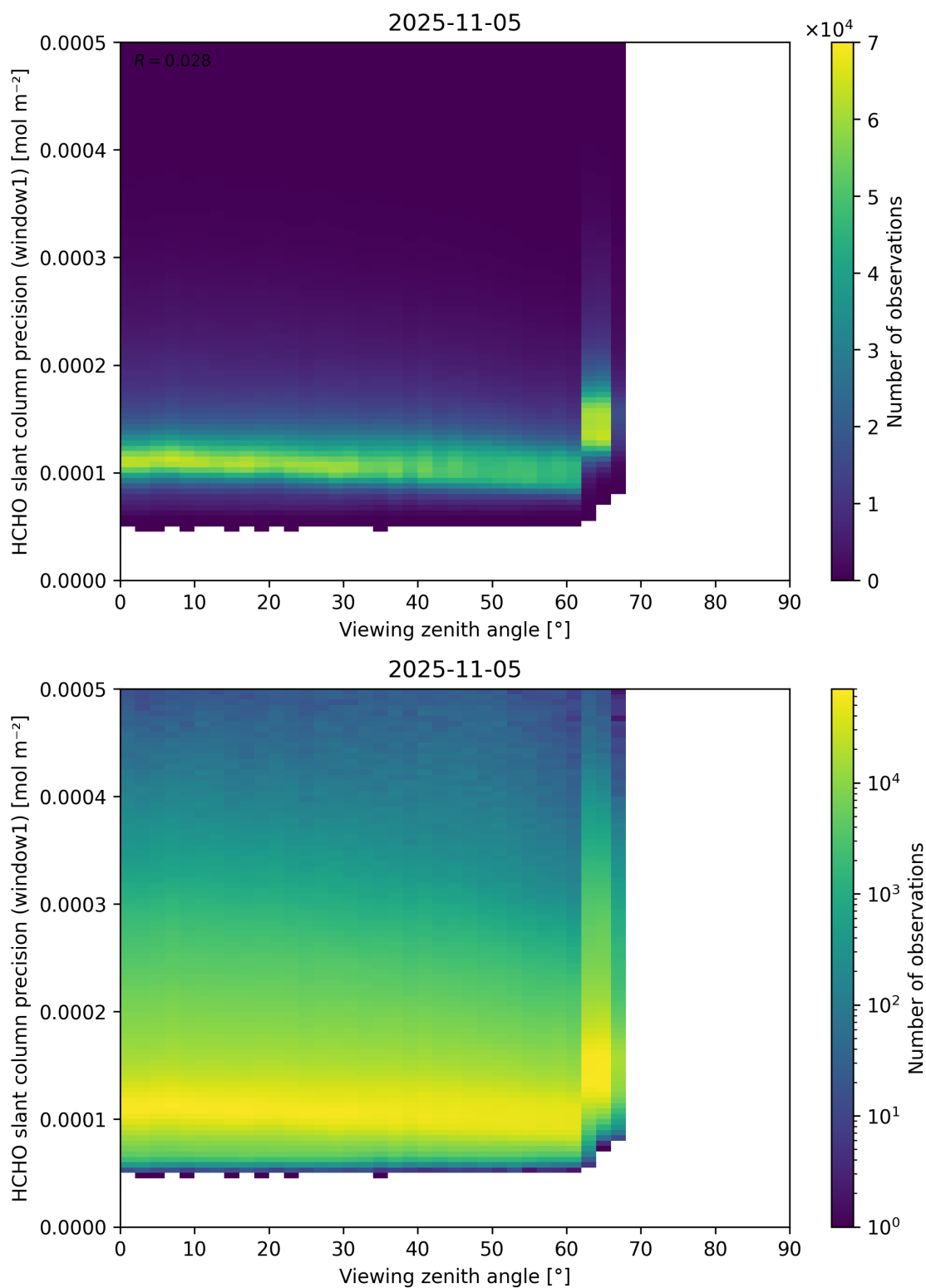
Figure 189: Scatter density plot of “Viewing zenith angle” against “HCHO slant column precision (window1)” for 2025-11-04 to 2025-11-06.
