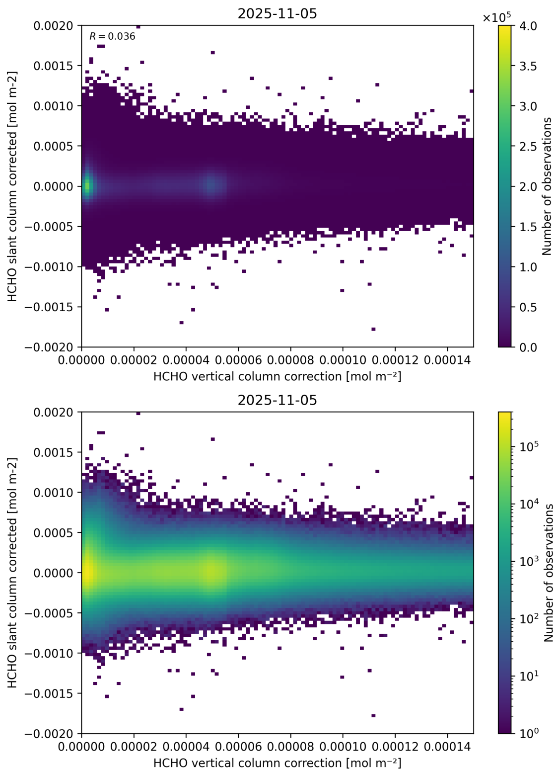
Figure 116: Scatter density plot of “HCHO vertical column correction” against “HCHO slant column corrected” for 2025-11-04 to 2025-11-06.
