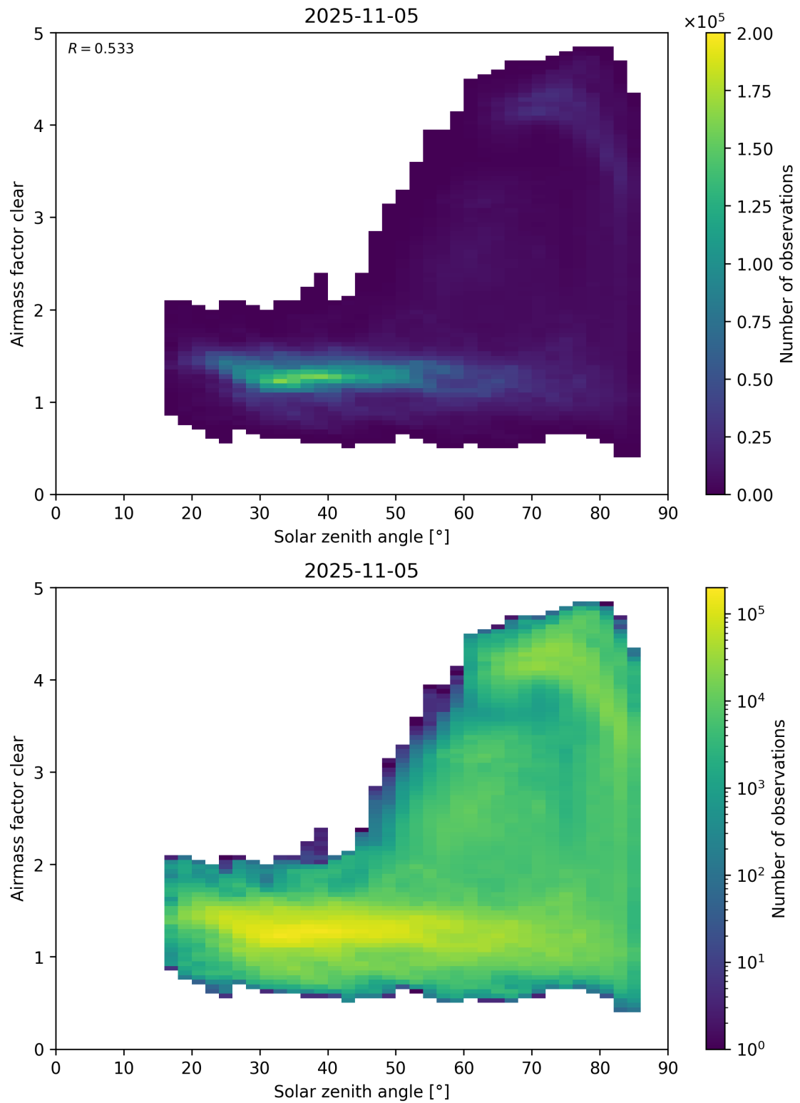
Figure 170: Scatter density plot of “Solar zenith angle” against “Airmass factor clear” for 2025-11-04 to 2025-11-06.
