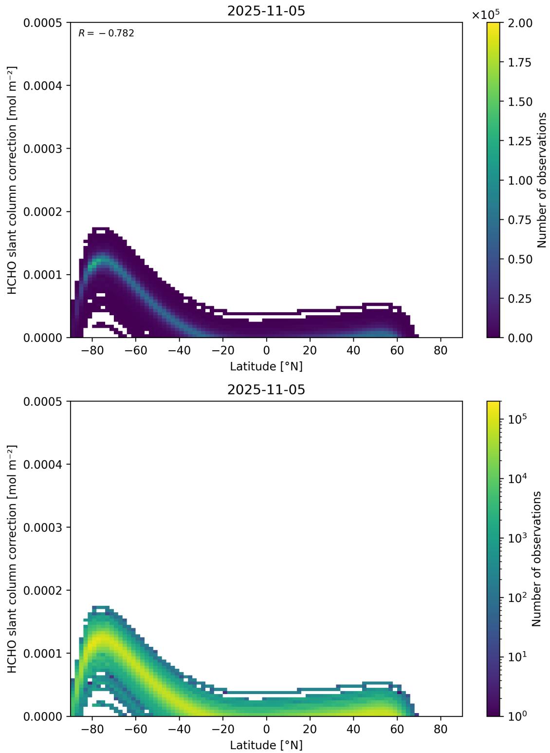
Figure 158: Scatter density plot of “Latitude” against “HCHO slant column correction” for 2025-11-04 to 2025-11-06.
