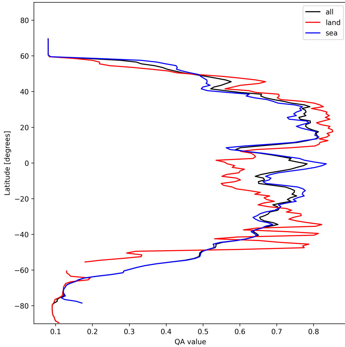
Figure 20: Zonal average of “QA value” for 2025-11-04 to 2025-11-06.
