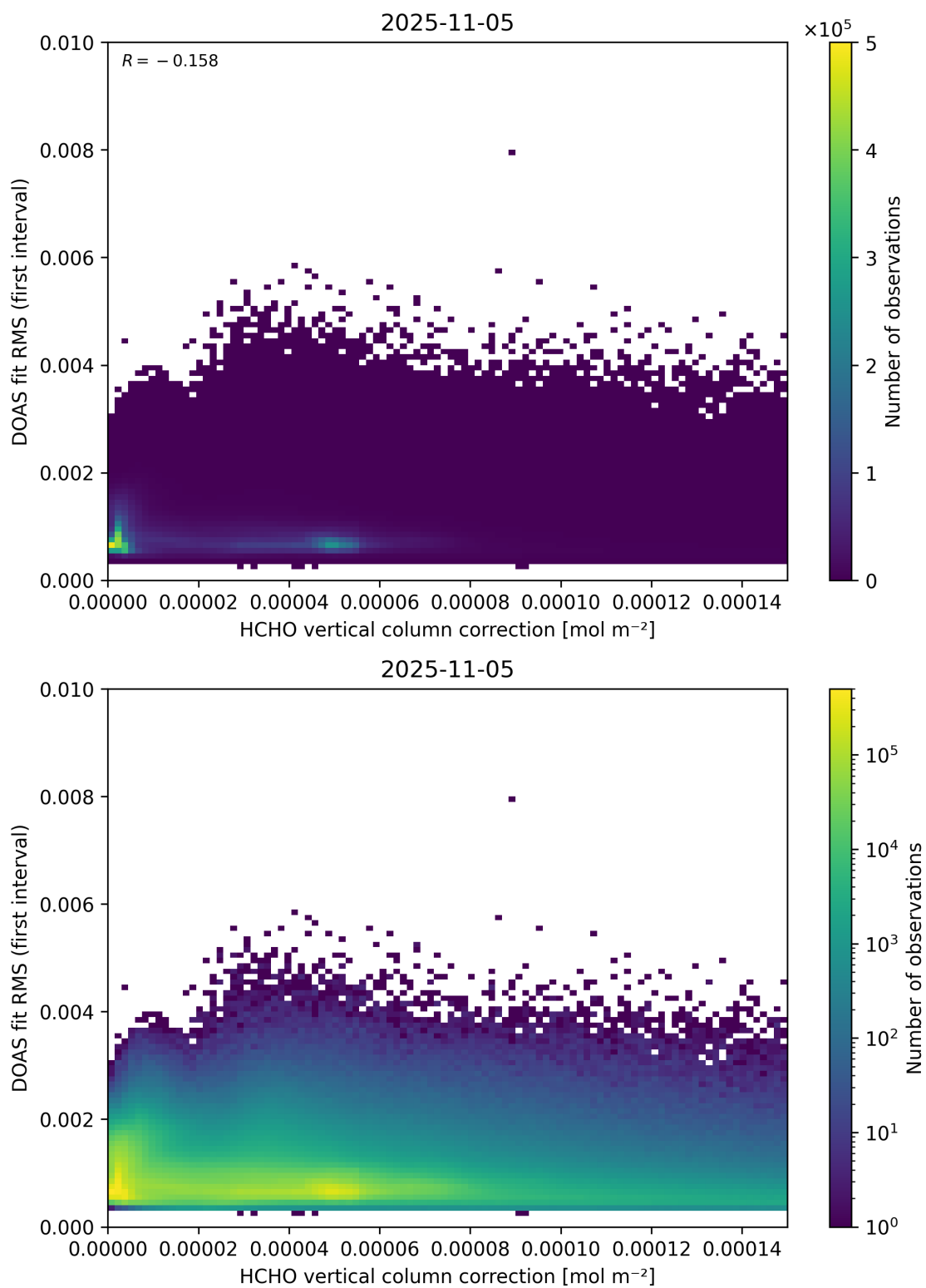
Figure 112: Scatter density plot of “HCHO vertical column correction” against “DOAS fit RMS (first interval)” for 2025-11-04 to 2025-11-06.
