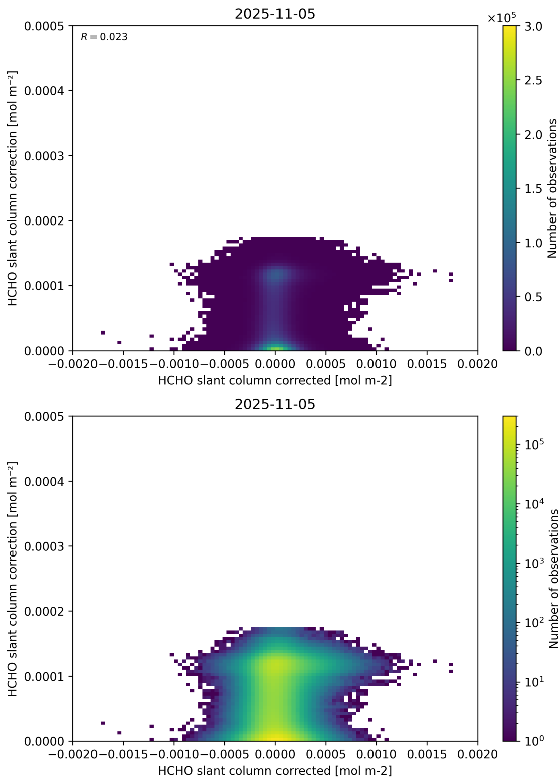
Figure 77: Scatter density plot of “HCHO slant column corrected” against “HCHO slant column correction” for 2025-11-04 to 2025-11-06.
