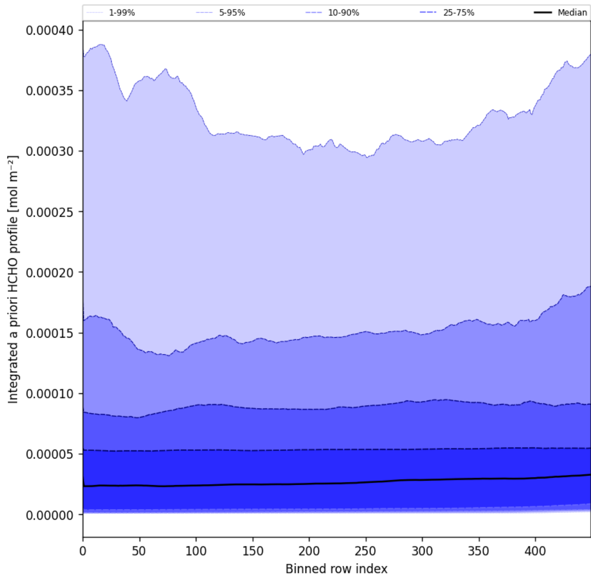
Figure 57: Along track statistics of "Integrated a priori HCHO profile" for 2025-11-04 to 2025-11-06
