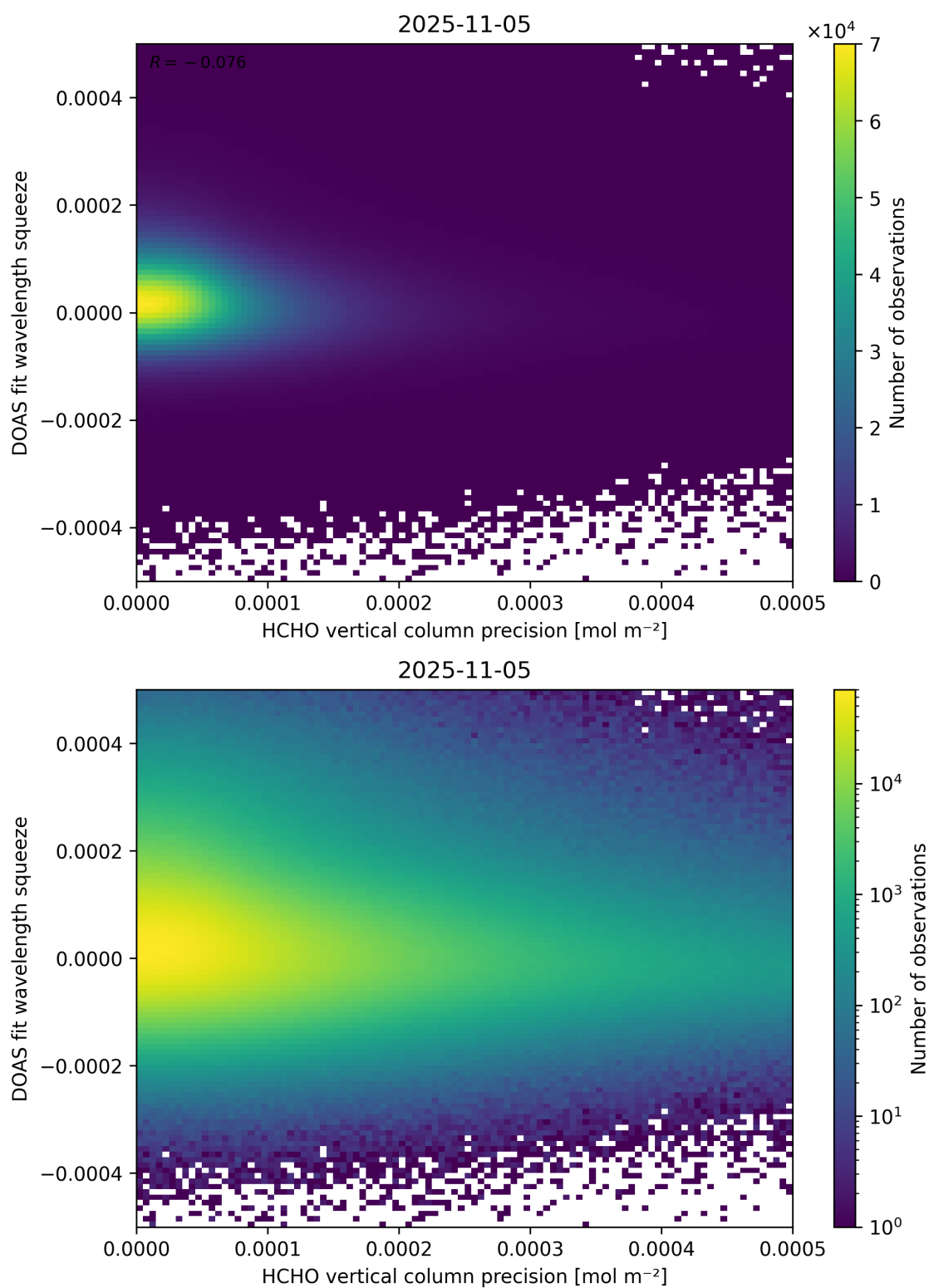
Figure 138: Scatter density plot of “HCHO vertical column precision” against “DOAS fit wavelength squeeze” for 2025-11-04 to 2025-11-06.
