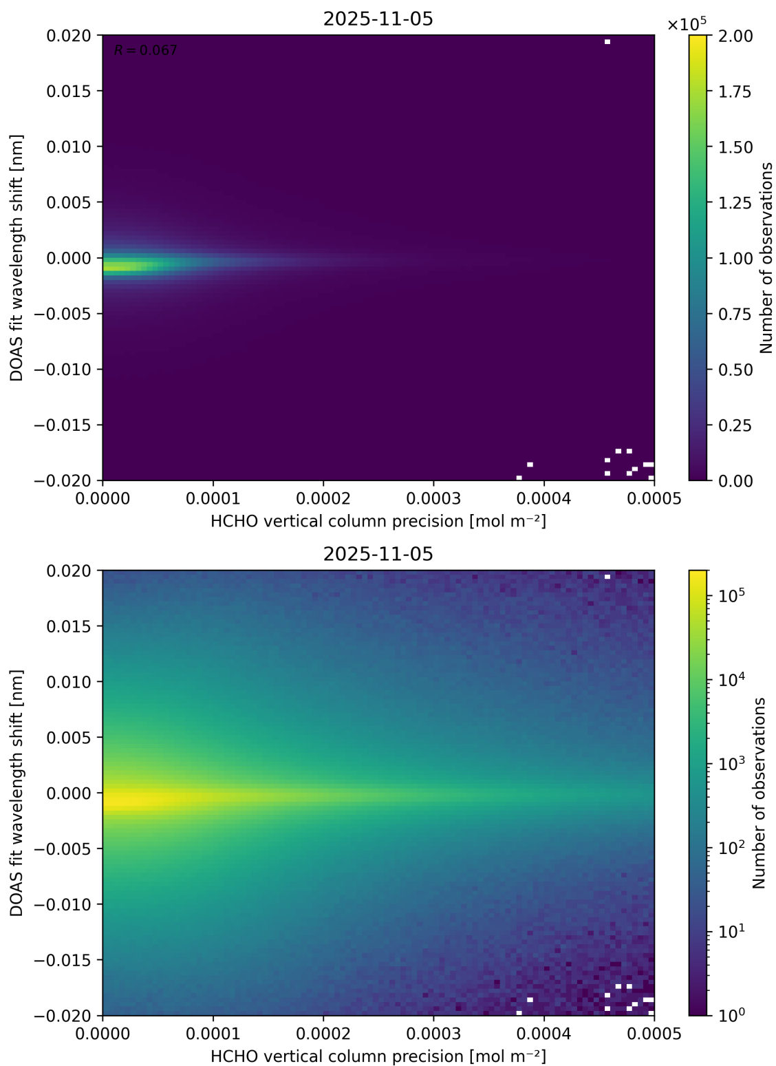
Figure 137: Scatter density plot of “HCHO vertical column precision” against “DOAS fit wavelength shift” for 2025-11-04 to 2025-11-06.
