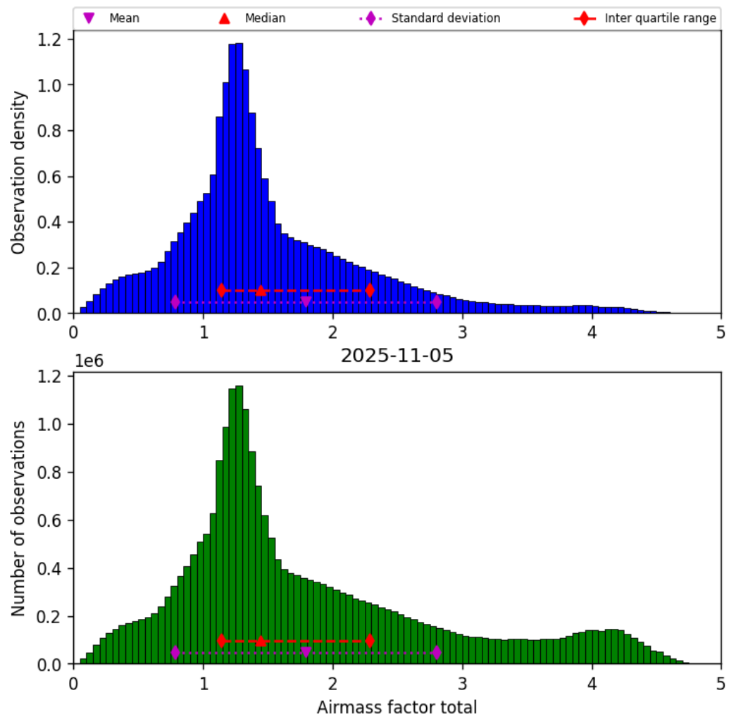
Figure 40: Histogram of “Airmass factor total” for 2025-11-04 to 2025-11-06
