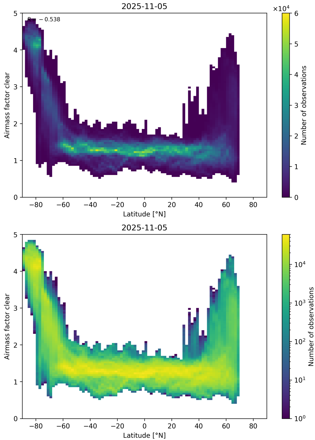
Figure 156: Scatter density plot of “Latitude” against “Airmass factor clear” for 2025-11-04 to 2025-11-06.
