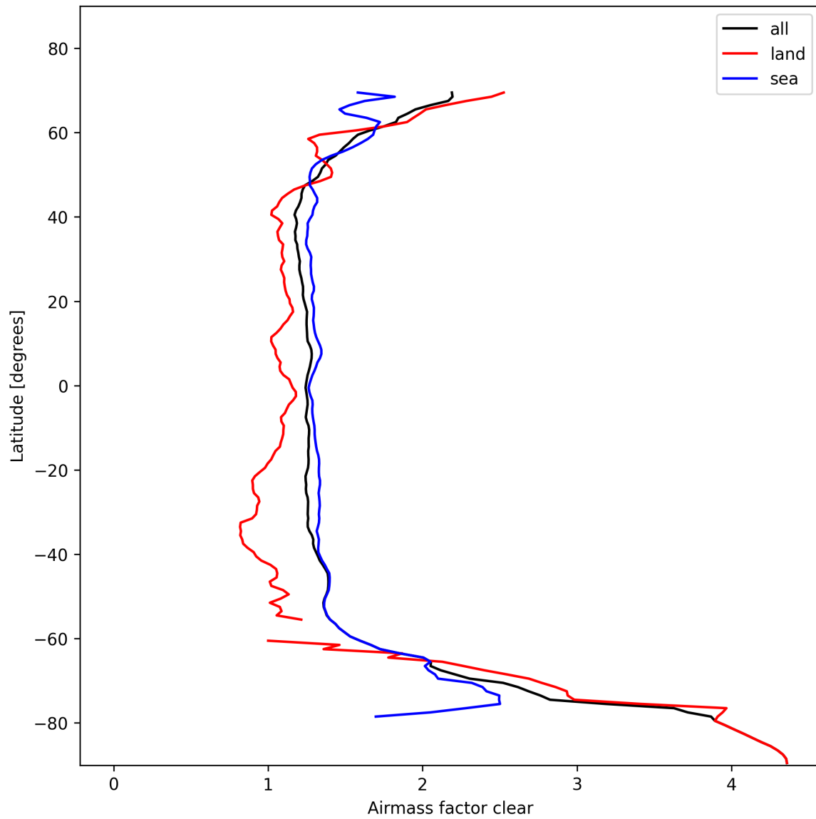
Figure 28: Zonal average of “Airmass factor clear” for 2025-11-04 to 2025-11-06.
