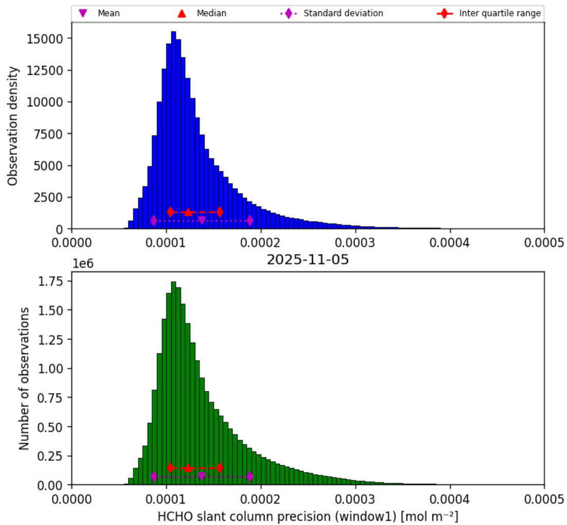
Figure 39: Histogram of “HCHO slant column precision (window1)” for 2025-11-04 to 2025-11-06
