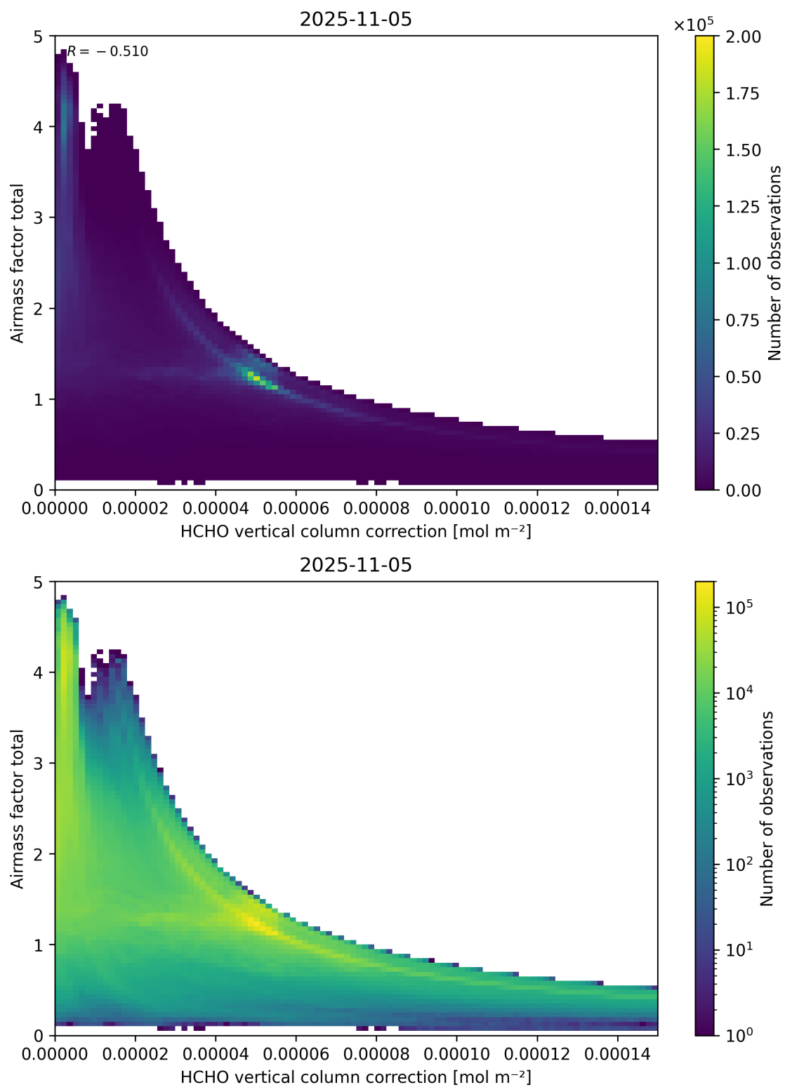
Figure 120: Scatter density plot of “HCHO vertical column correction” against “Airmass factor total” for 2025-11-04 to 2025-11-06.
