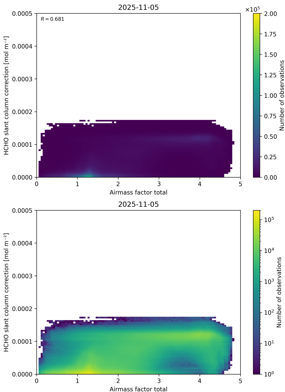
Figure 102: Scatter density plot of “Airmass factor total” against “HCHO slant column correction” for 2025-11-04 to 2025-11-06.
