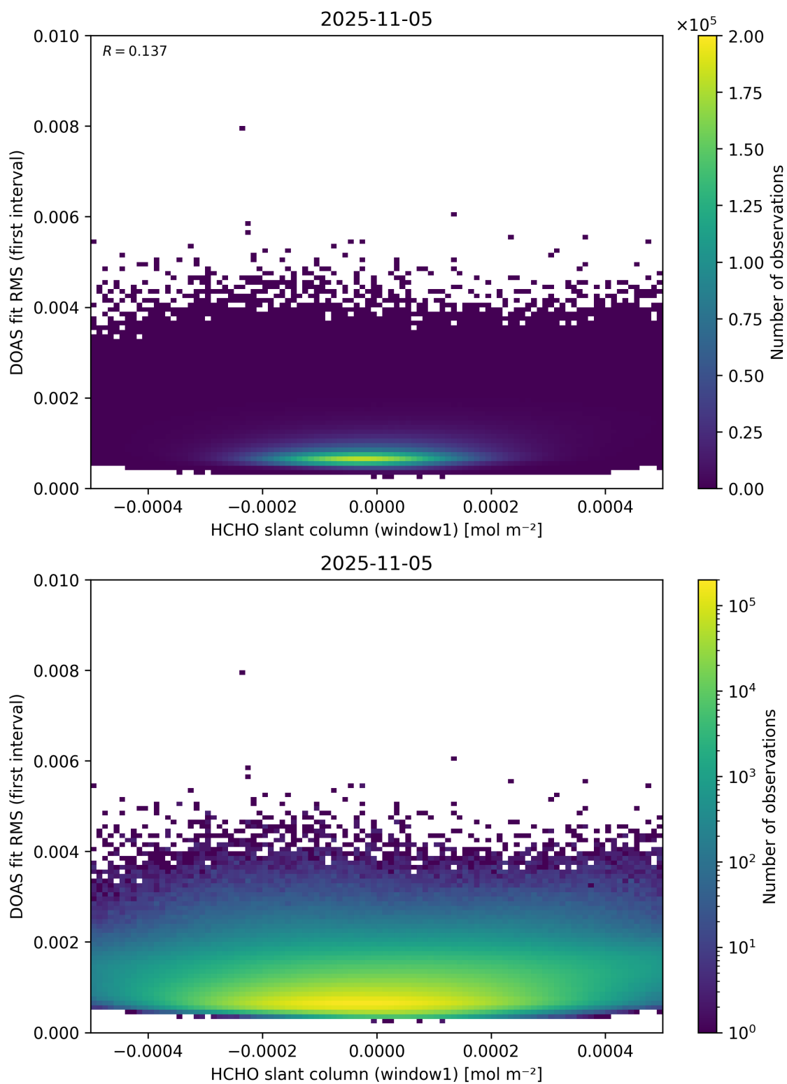
Figure 78: Scatter density plot of “HCHO slant column (window1)” against “DOAS fit RMS (first interval)” for 2025-11-04 to 2025-11-06.
