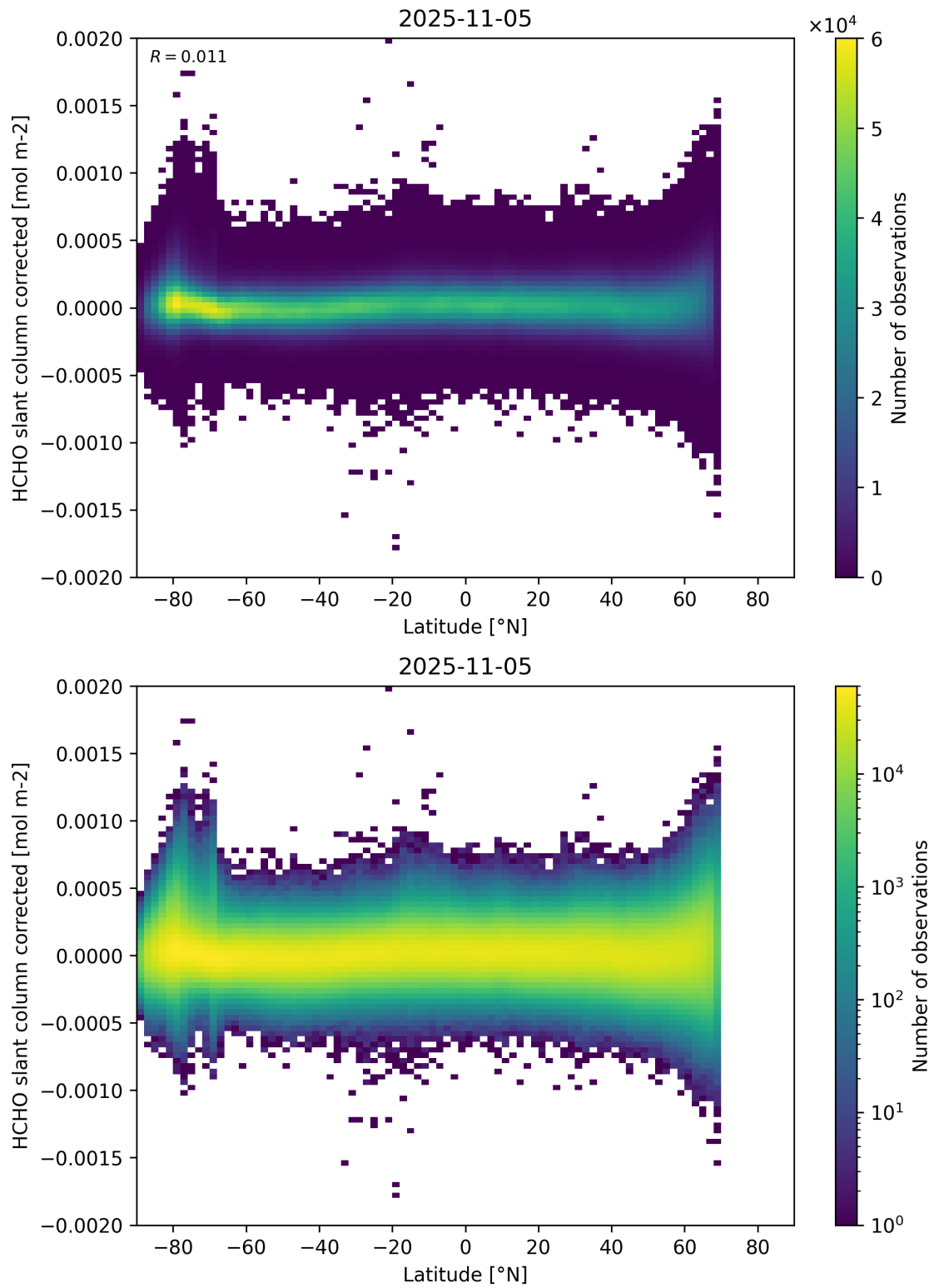
Figure 157: Scatter density plot of “Latitude” against “HCHO slant column corrected” for 2025-11-04 to 2025-11-06.
