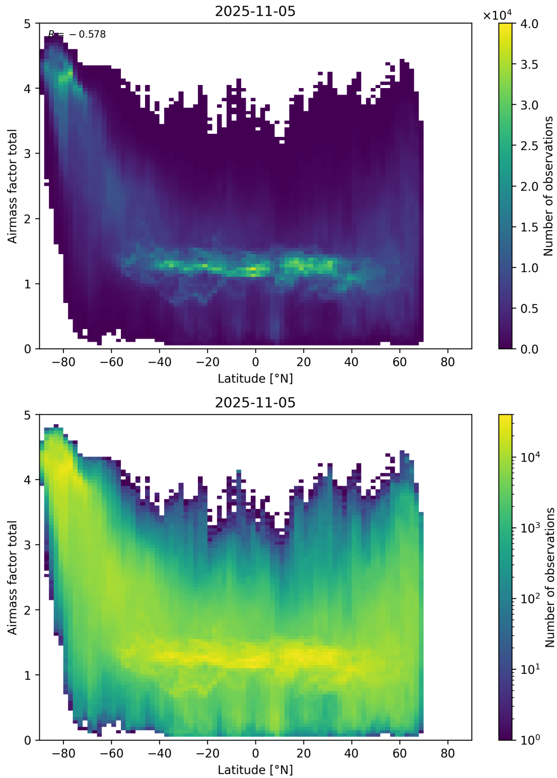
Figure 161: Scatter density plot of “Latitude” against “Airmass factor total” for 2025-11-04 to 2025-11-06.
