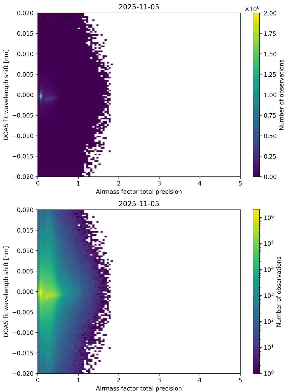
Figure 106: Scatter density plot of “Airmass factor total precision” against “DOAS fit wavelength shift” for 2025-11-04 to 2025-11-06.
