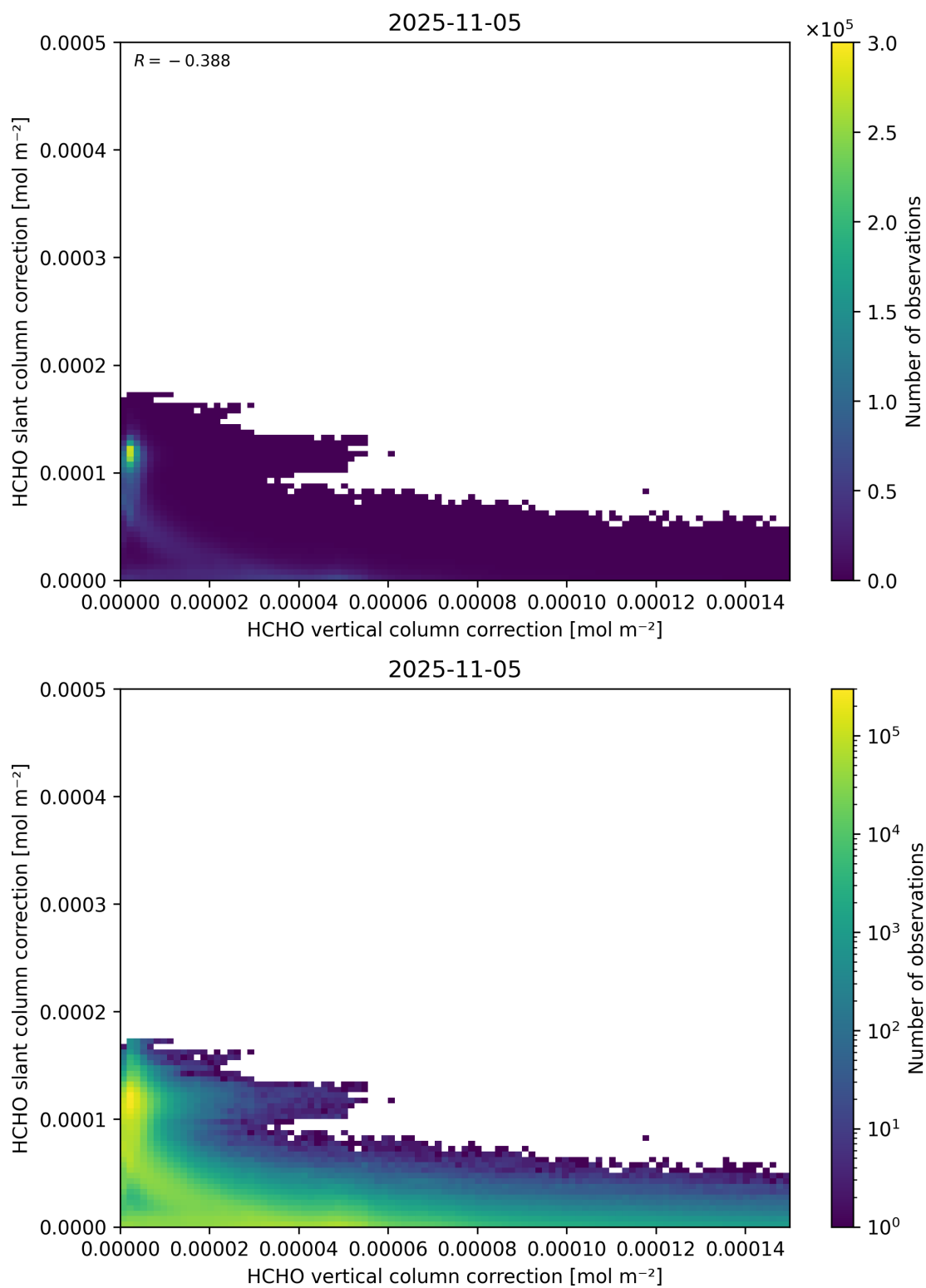
Figure 117: Scatter density plot of “HCHO vertical column correction” against “HCHO slant column correction” for 2025-11-04 to 2025-11-06.
