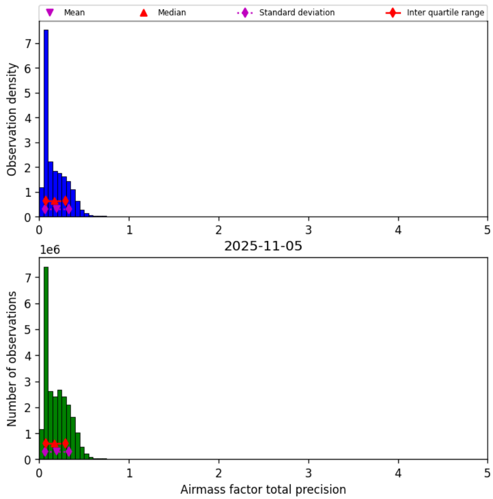
Figure 41: Histogram of “Airmass factor total precision” for 2025-11-04 to 2025-11-06
