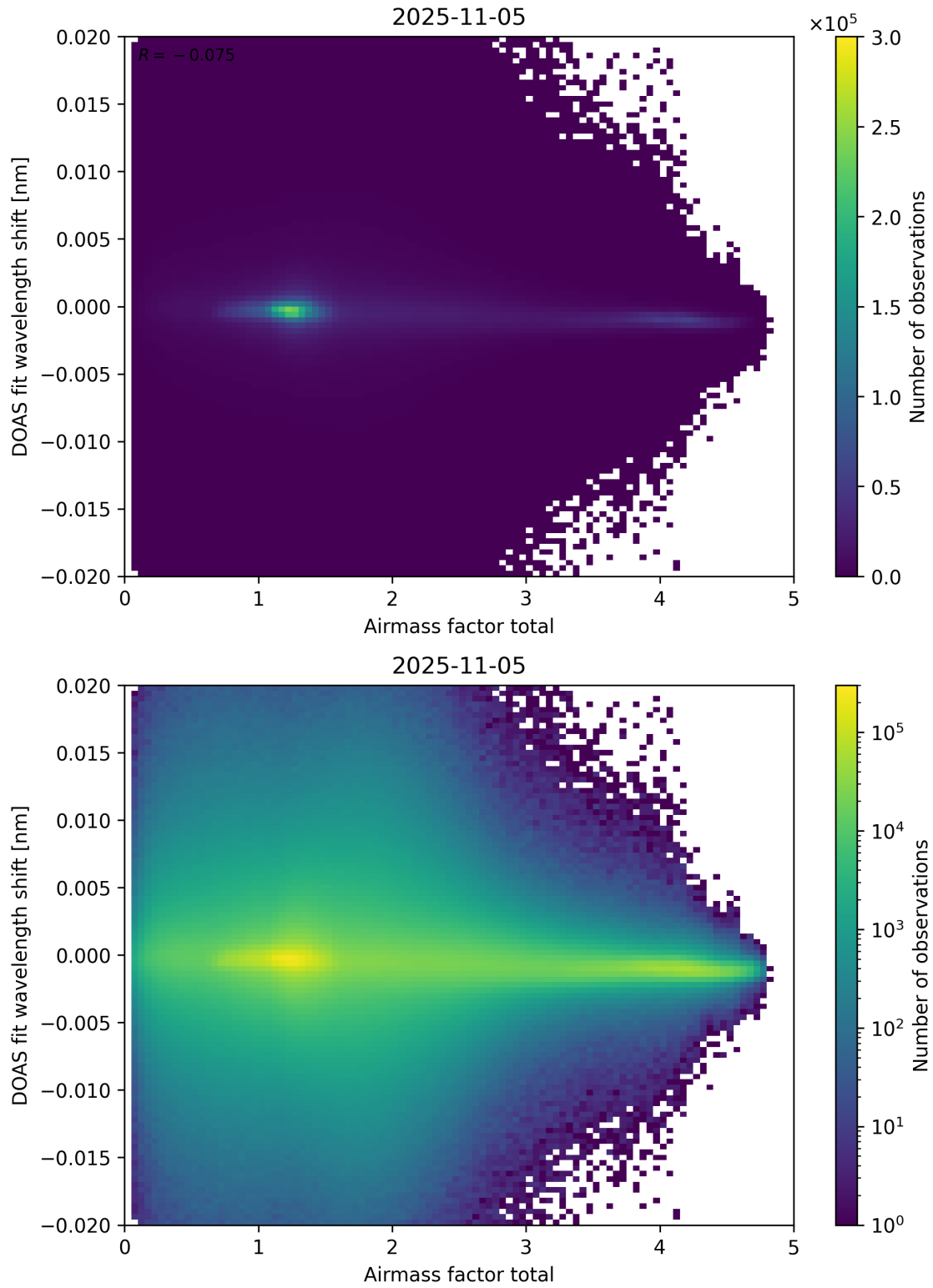
Figure 98: Scatter density plot of “Airmass factor total” against “DOAS fit wavelength shift” for 2025-11-04 to 2025-11-06.
