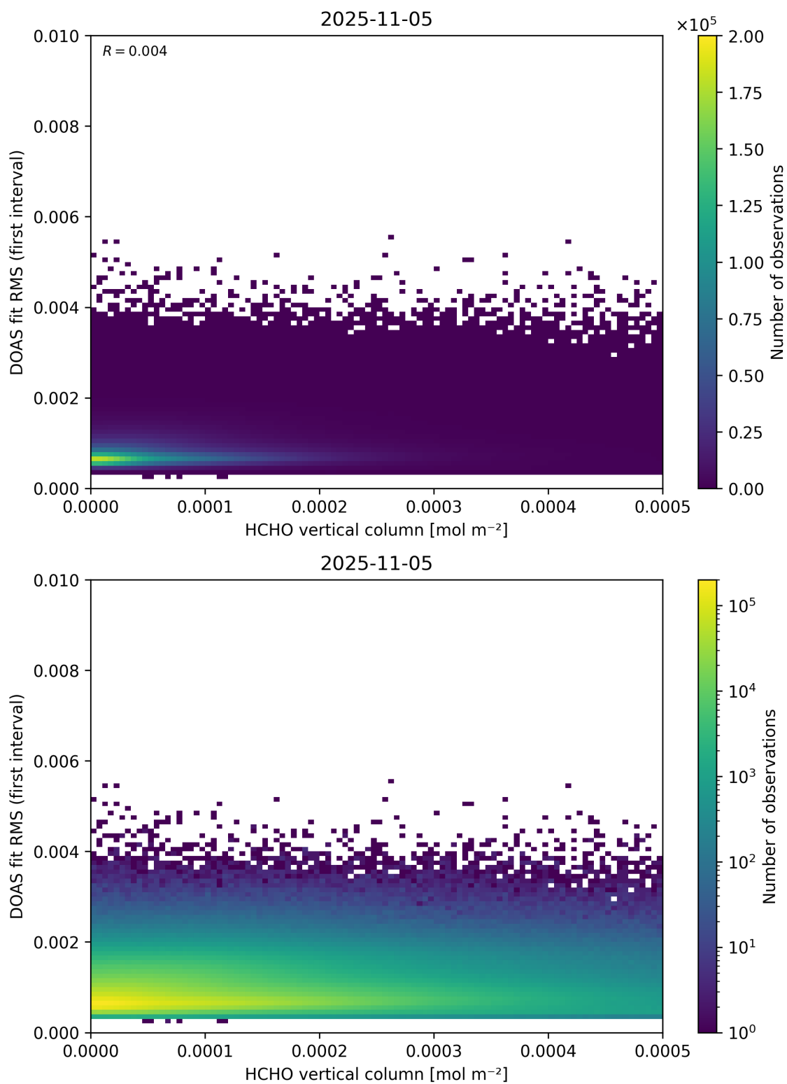
Figure 123: Scatter density plot of “HCHO vertical column” against “DOAS fit RMS (first interval)” for 2025-11-04 to 2025-11-06.
