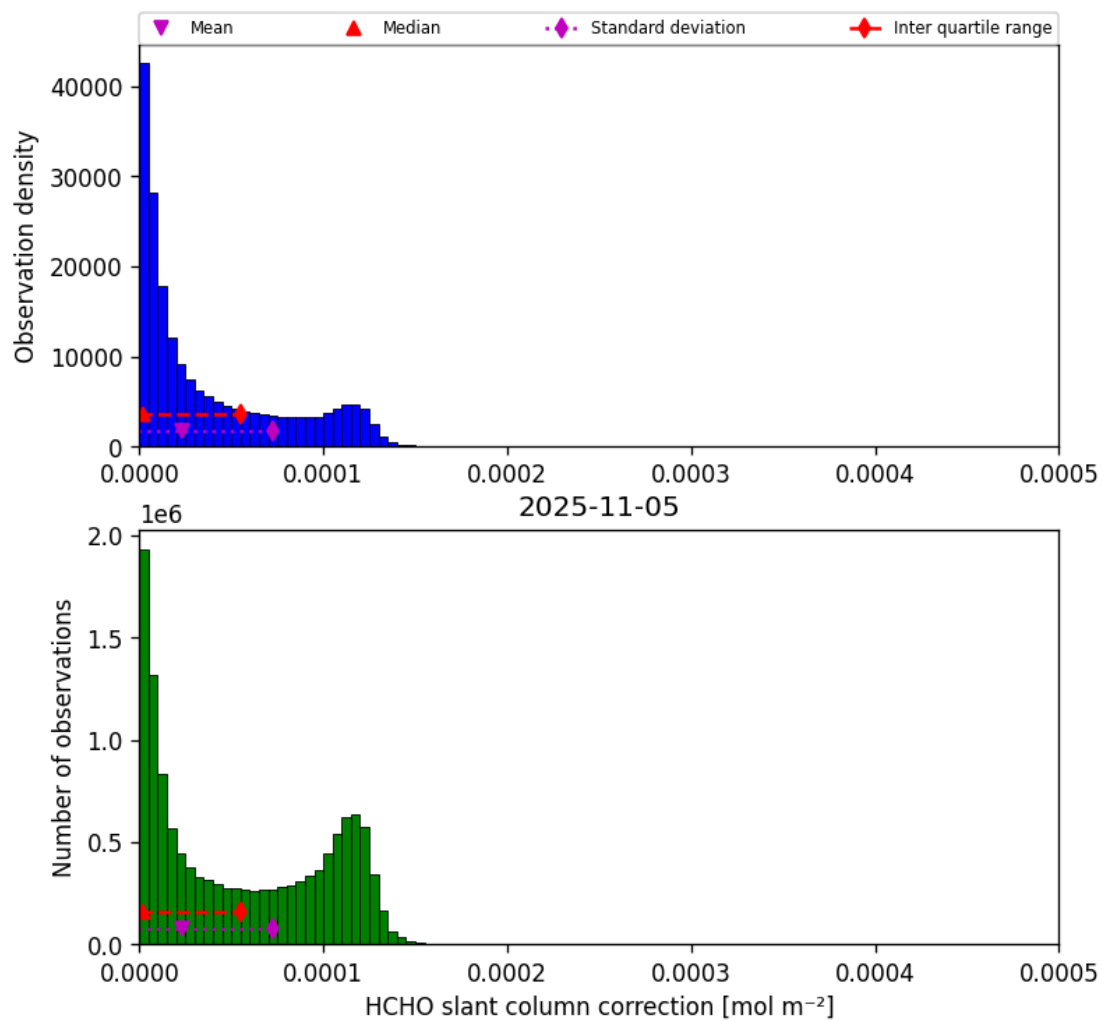
Figure 47: Histogram of “HCHO slant column correction” for 2025-11-04 to 2025-11-06
