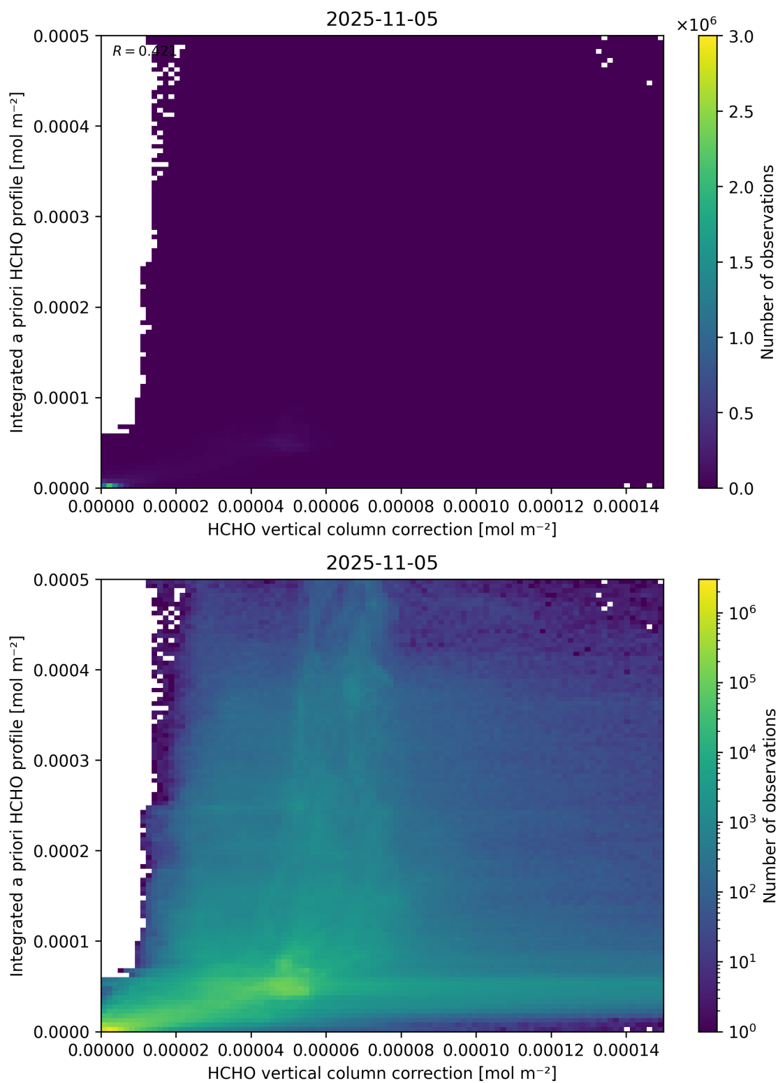
Figure 122: Scatter density plot of “HCHO vertical column correction” against “Integrated a priori HCHO profile” for 2025-11-04 to 2025-11-06.
