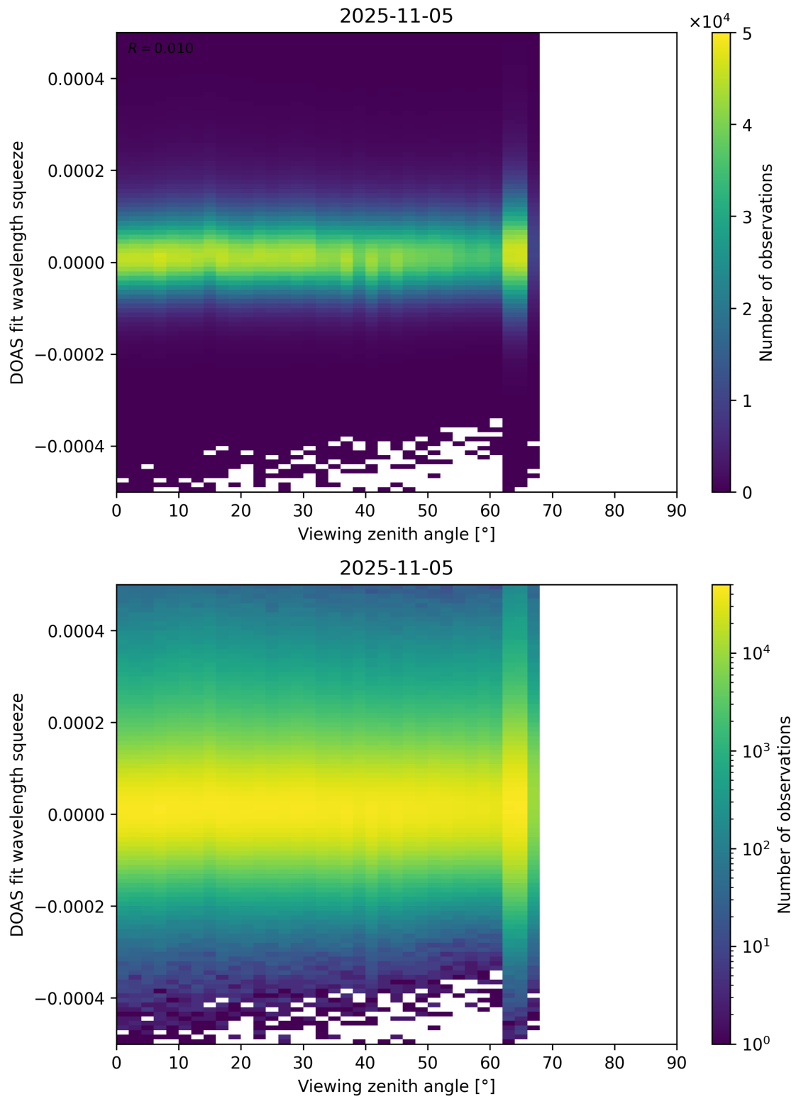
Figure 184: Scatter density plot of “Viewing zenith angle” against “DOAS fit wavelength squeeze” for 2025-11-04 to 2025-11-06.
