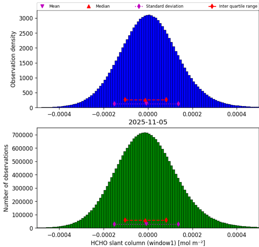
Figure 38: Histogram of “HCHO slant column (window1)” for 2025-11-04 to 2025-11-06
