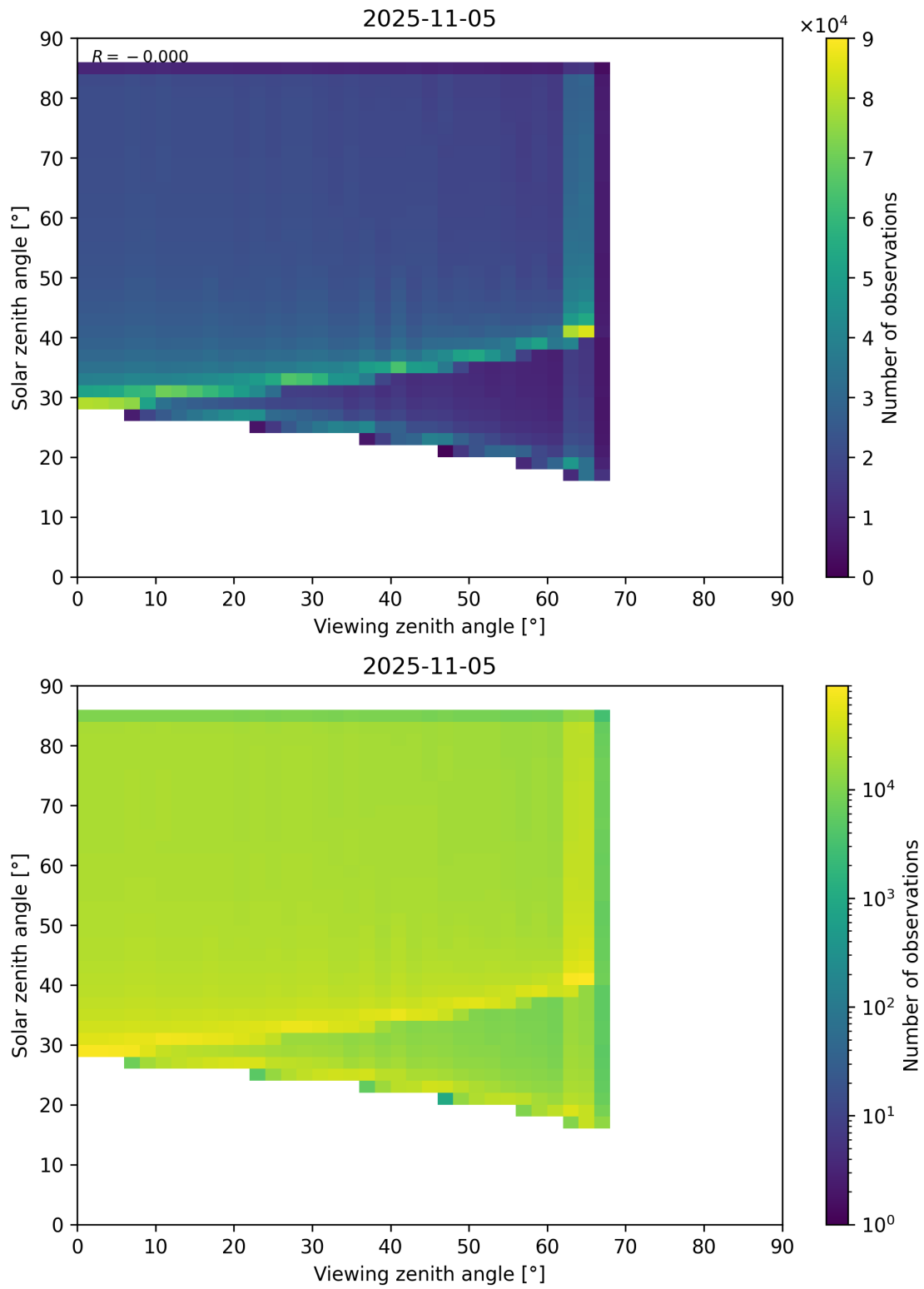
Figure 197: Scatter density plot of “Viewing zenith angle” against “Solar zenith angle” for 2025-11-04 to 2025-11-06.
