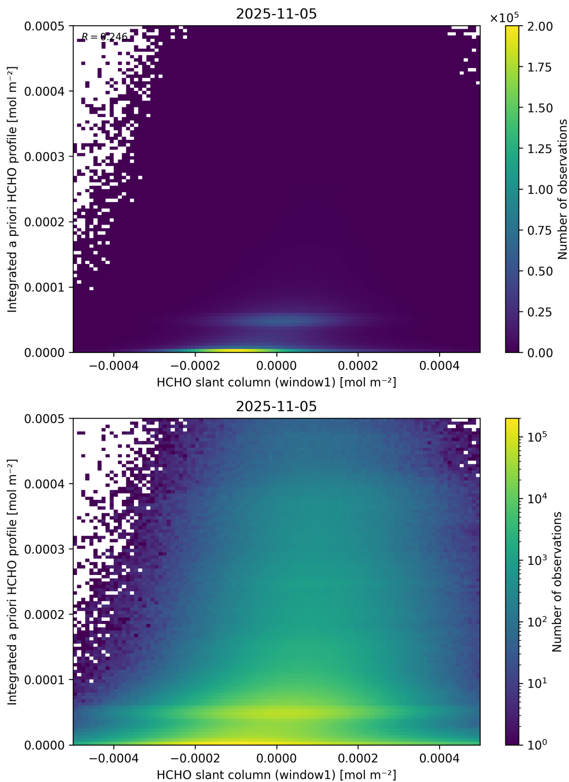
Figure 87: Scatter density plot of “HCHO slant column (window1)” against “Integrated a priori HCHO profile” for 2025-11-04 to 2025-11-06.
