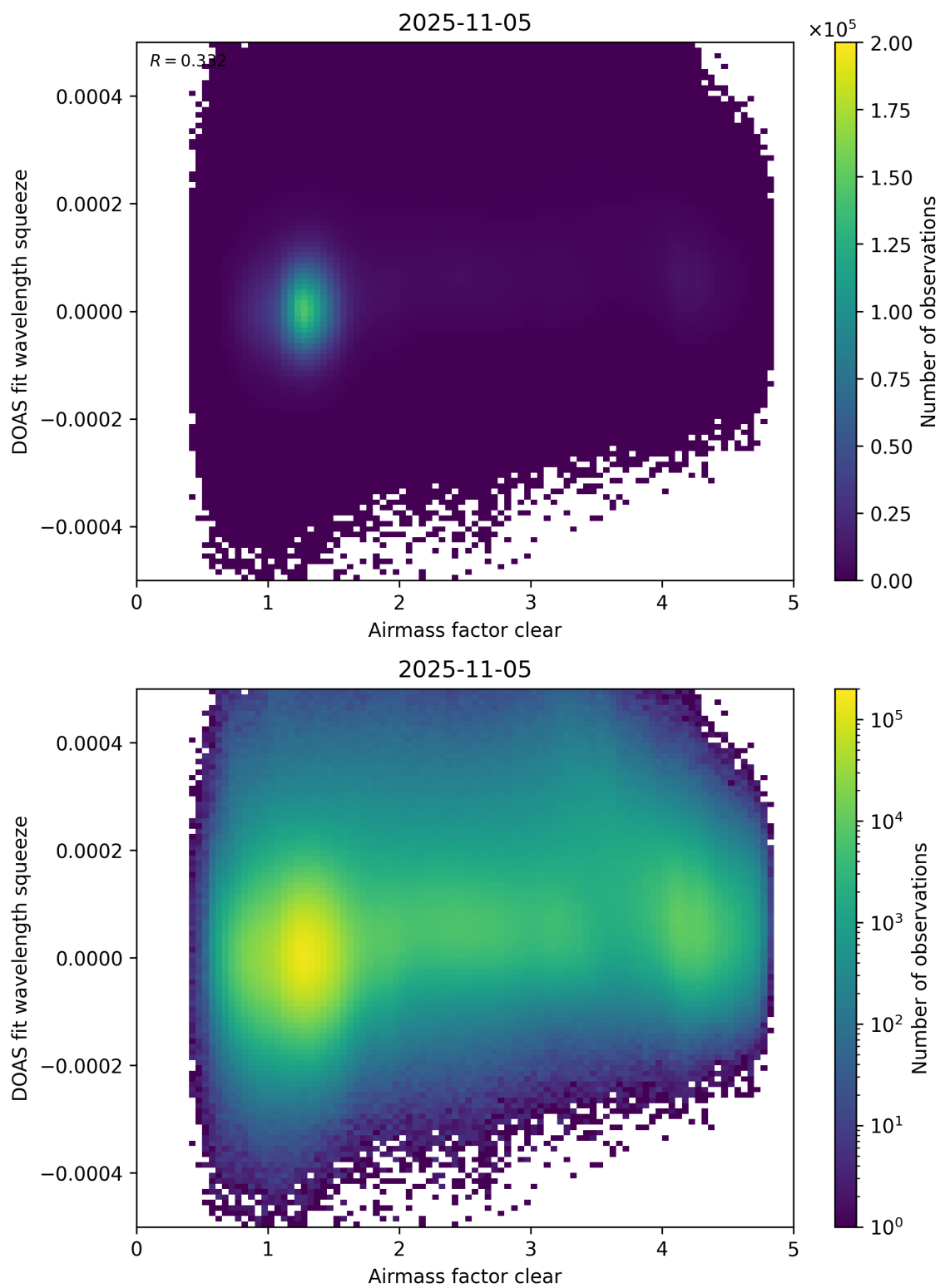
Figure 73: Scatter density plot of “Airmass factor clear” against “DOAS fit wavelength squeeze” for 2025-11-04 to 2025-11-06.
