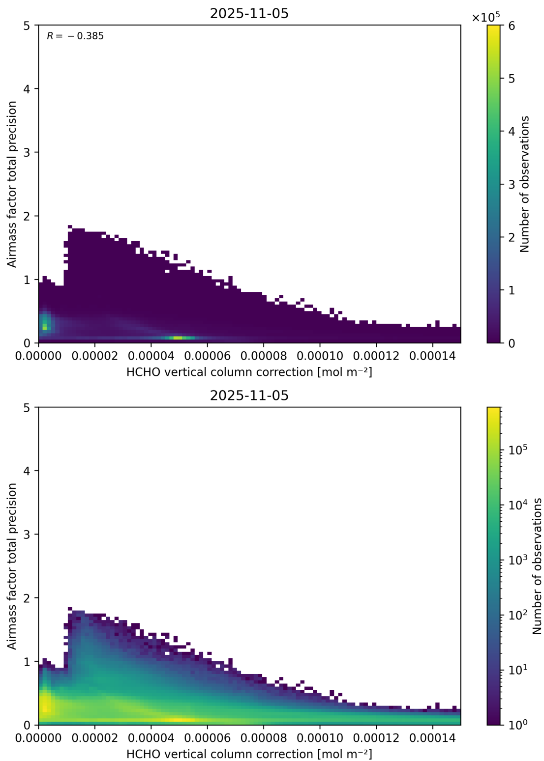
Figure 121: Scatter density plot of “HCHO vertical column correction” against “Airmass factor total precision” for 2025-11-04 to 2025-11-06.
