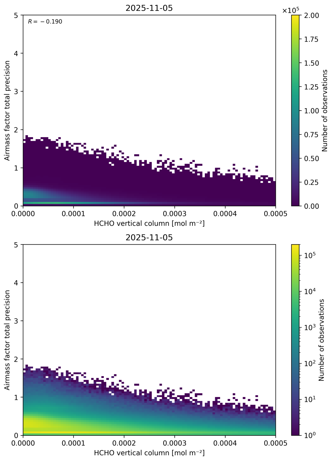
Figure 132: Scatter density plot of “HCHO vertical column” against “Airmass factor total precision” for 2025-11-04 to 2025-11-06.
