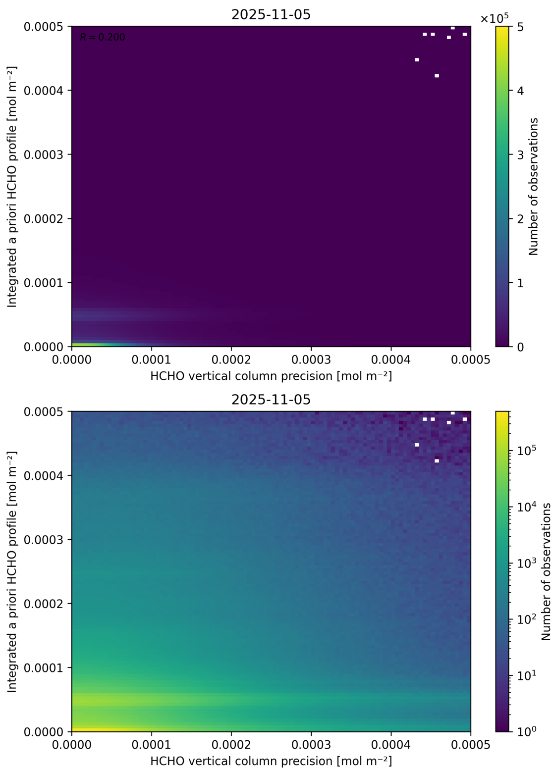
Figure 147: Scatter density plot of “HCHO vertical column precision” against “Integrated a priori HCHO profile” for 2025-11-04 to 2025-11-06.
