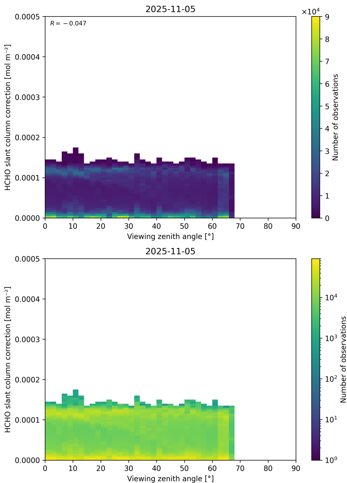
Figure 187: Scatter density plot of “Viewing zenith angle” against “HCHO slant column correction” for 2025-11-04 to 2025-11-06.
