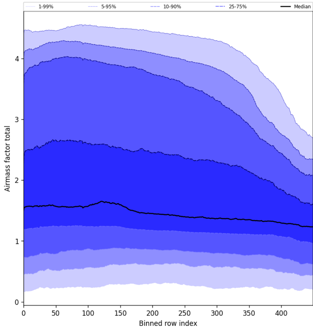
Figure 54: Along track statistics of “Airmass factor total” for 2025-11-04 to 2025-11-06
