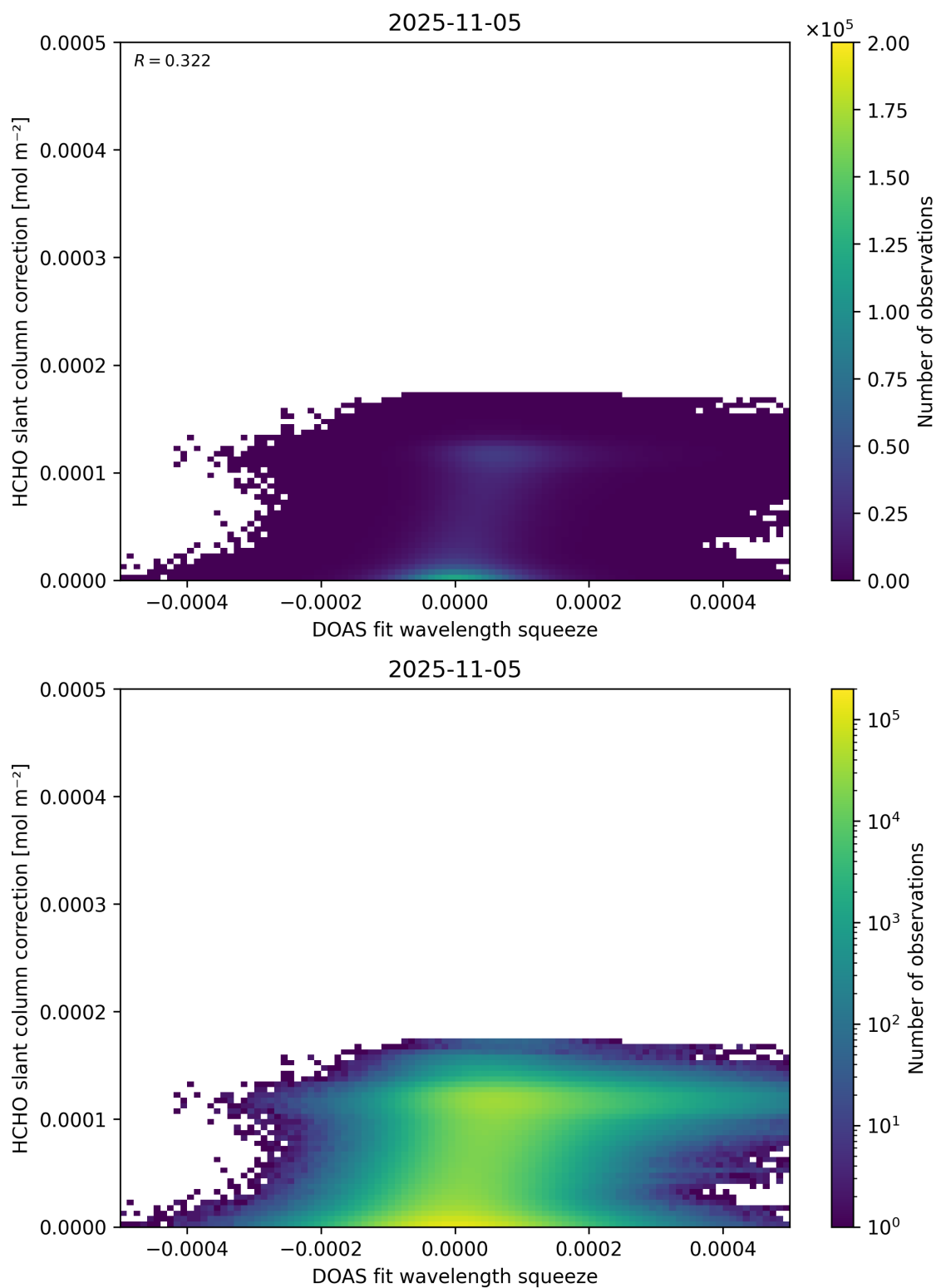
Figure 70: Scatter density plot of “DOAS fit wavelength squeeze” against “HCHO slant column correction” for 2025-11-04 to 2025-11-06.
