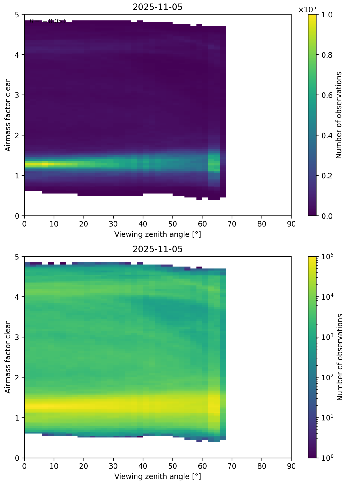
Figure 185: Scatter density plot of “Viewing zenith angle” against “Airmass factor clear” for 2025-11-04 to 2025-11-06.
