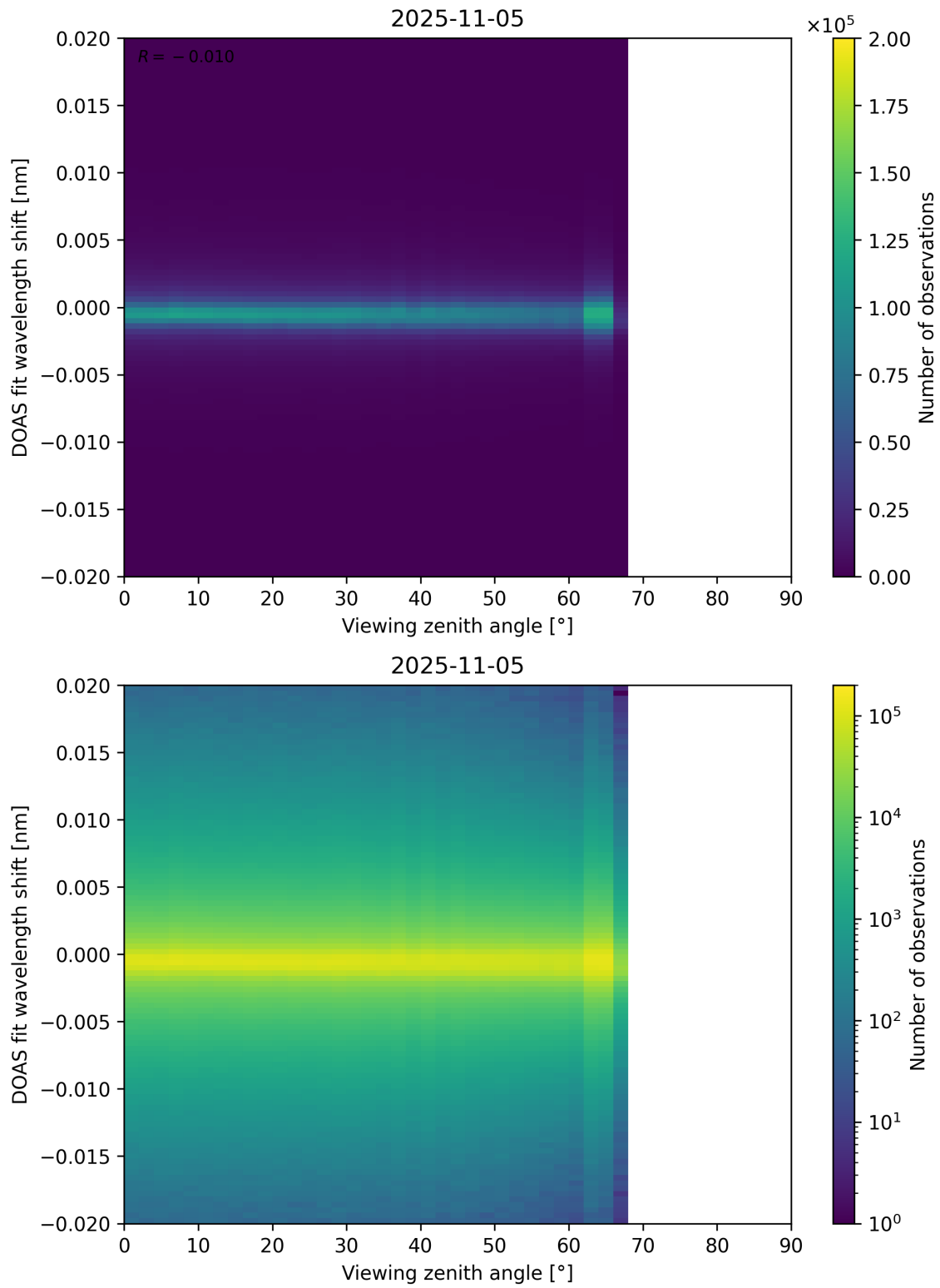
Figure 183: Scatter density plot of “Viewing zenith angle” against “DOAS fit wavelength shift” for 2025-11-04 to 2025-11-06.
