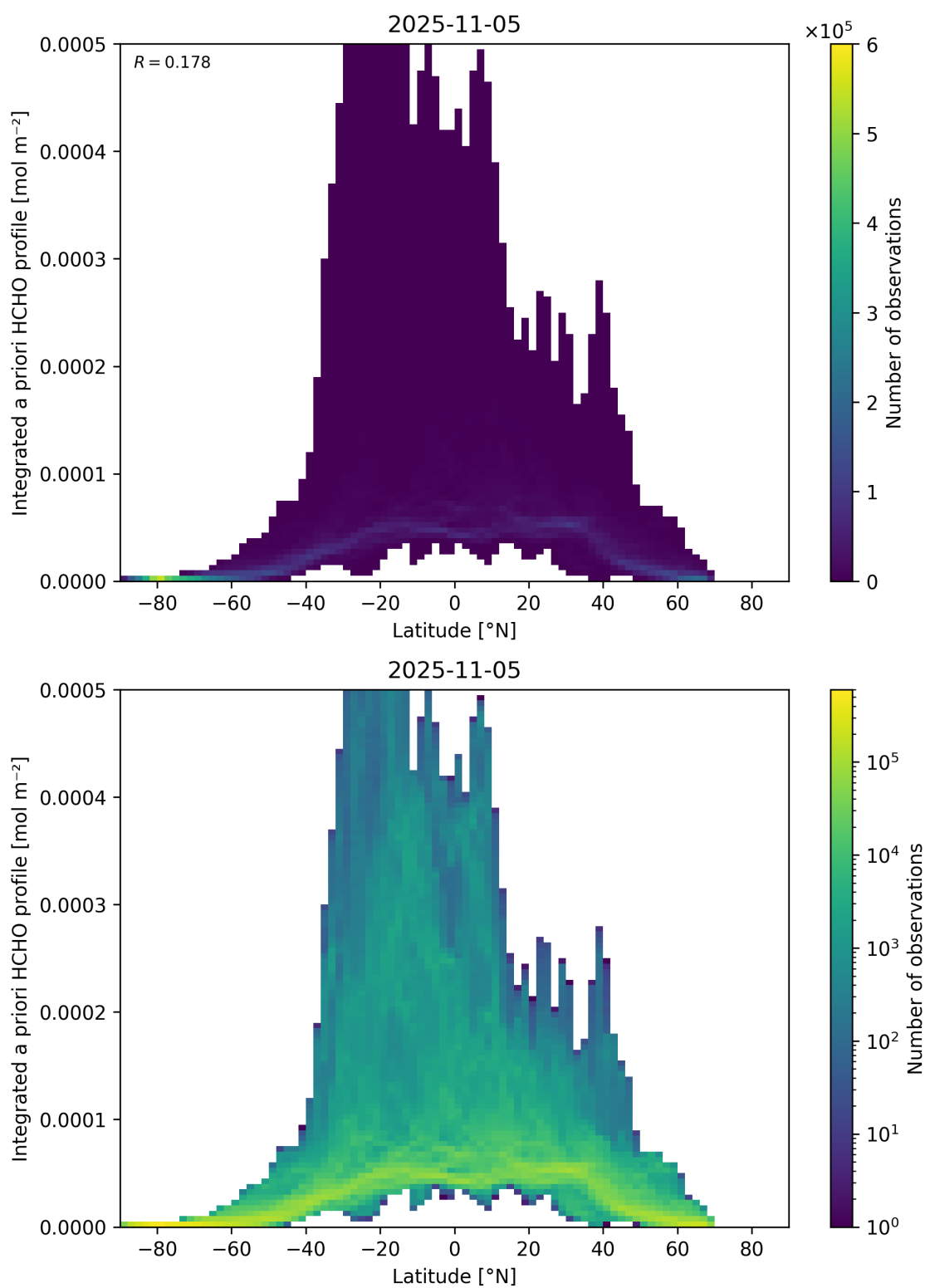
Figure 166: Scatter density plot of “Latitude” against “Integrated a priori HCHO profile” for 2025-11-04 to 2025-11-06.
