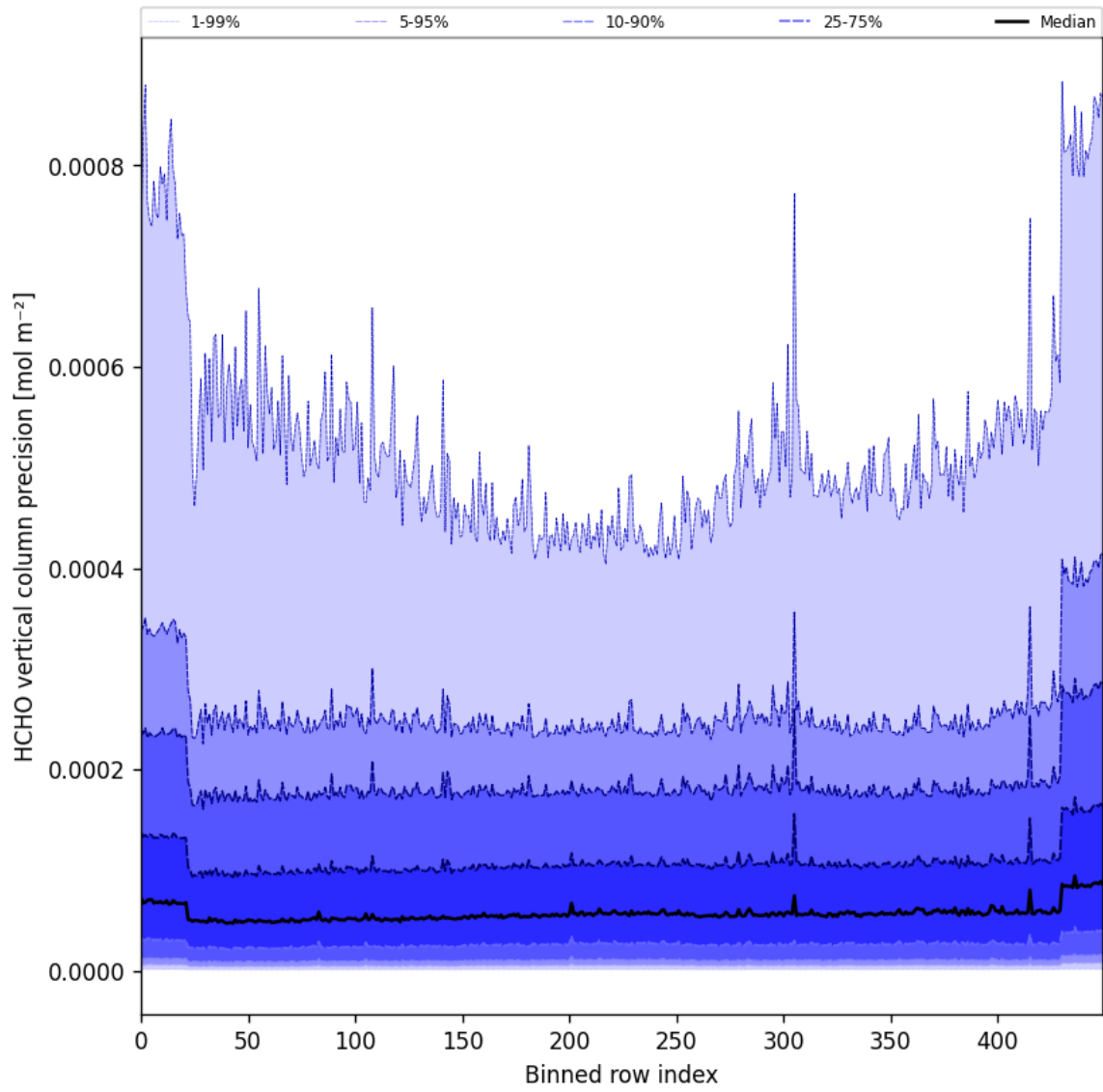
Figure 50: Along track statistics of “HCHO vertical column precision” for 2025-11-04 to 2025-11-06
