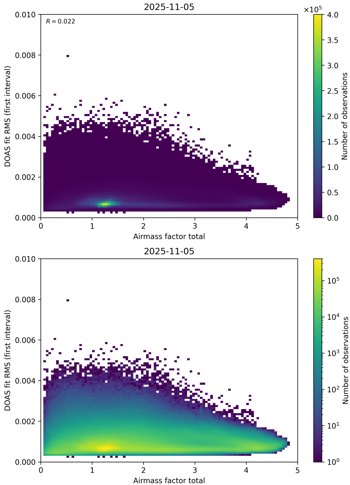
Figure 97: Scatter density plot of “Airmass factor total” against “DOAS fit RMS (first interval)” for 2025-11-04 to 2025-11-06.
