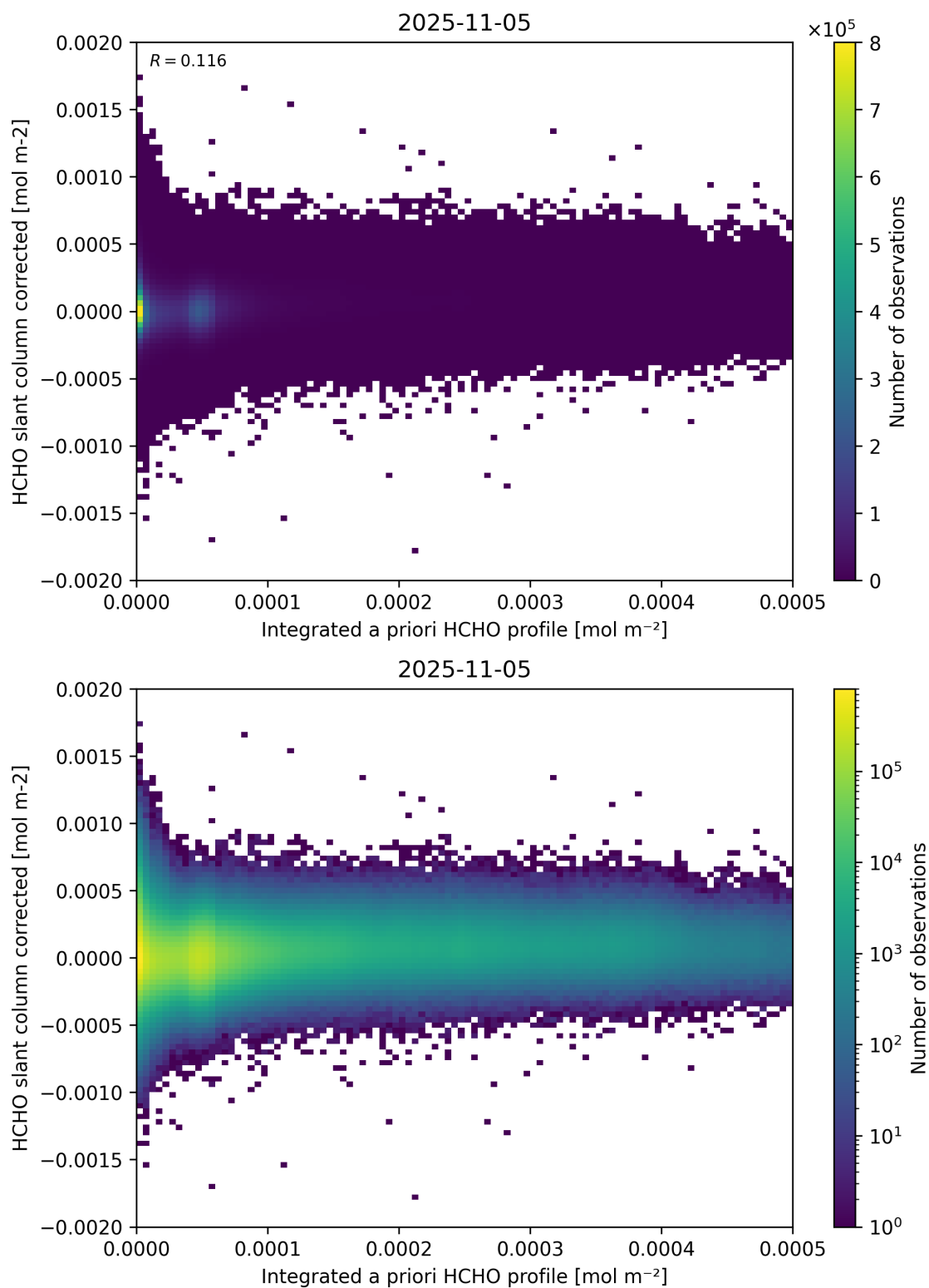
Figure 151: Scatter density plot of “Integrated a priori HCHO profile” against “HCHO slant column corrected” for 2025-11-04 to 2025-11-06.
