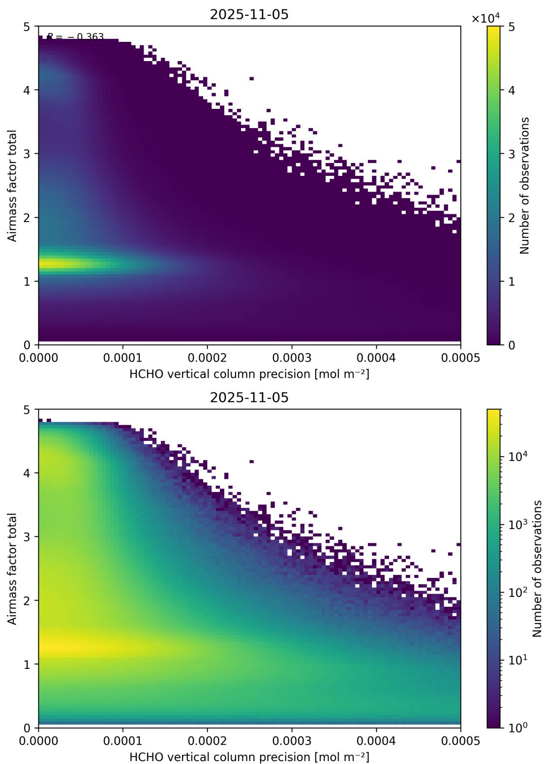
Figure 144: Scatter density plot of “HCHO vertical column precision” against “Airmass factor total” for 2025-11-04 to 2025-11-06.
