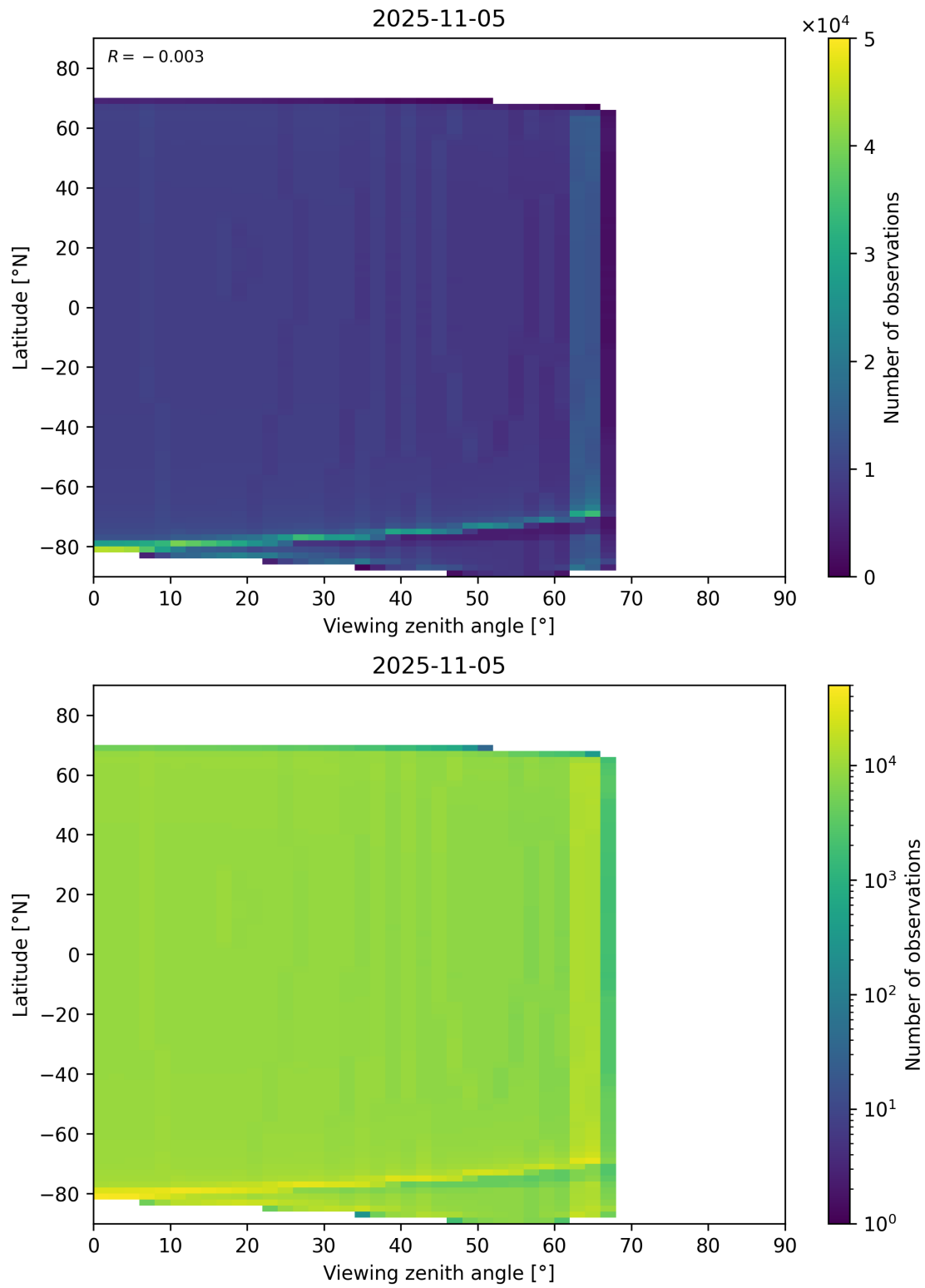
Figure 196: Scatter density plot of “Viewing zenith angle” against “Latitude” for 2025-11-04 to 2025-11-06.
