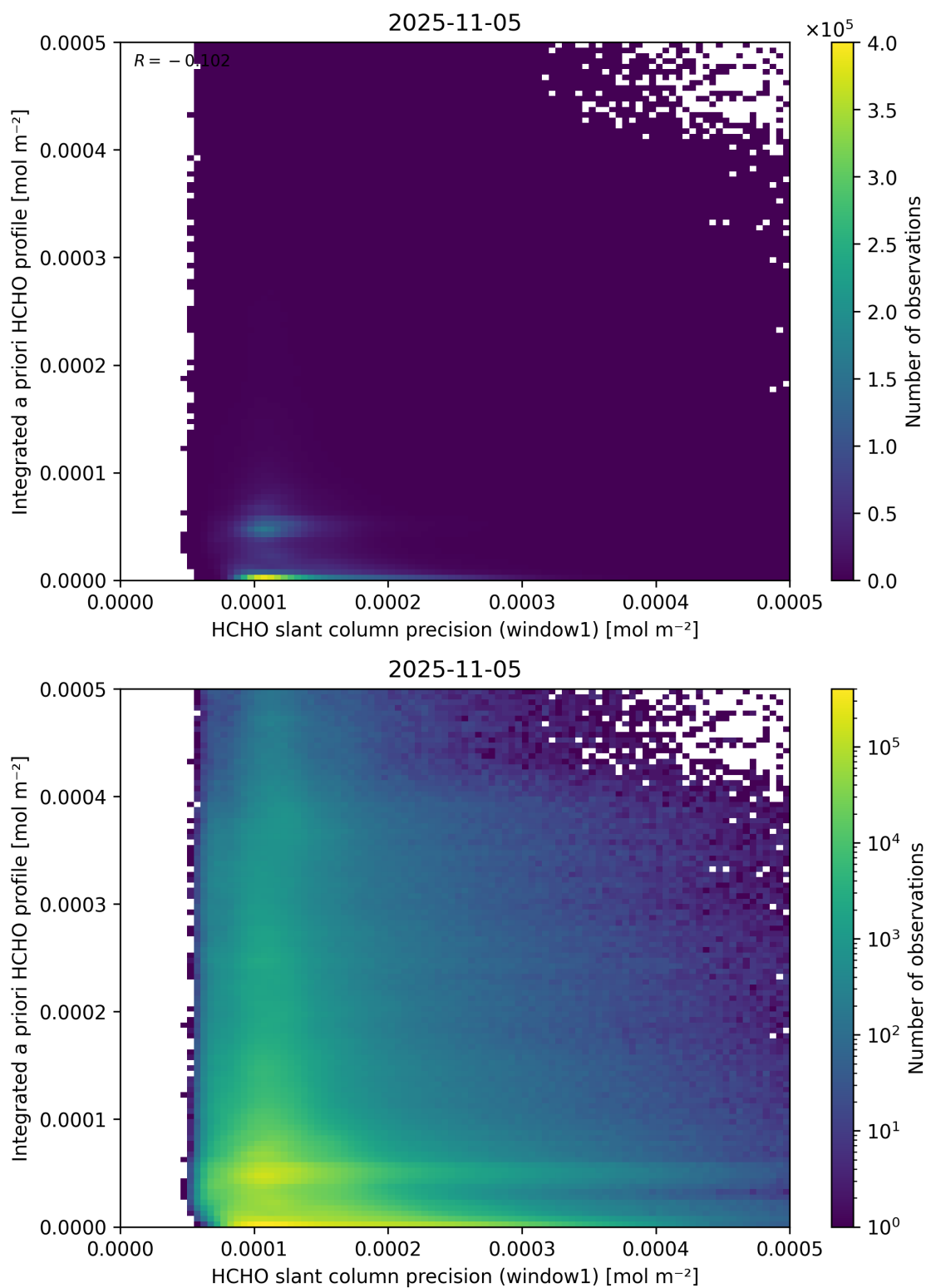
Figure 96: Scatter density plot of “HCHO slant column precision (window1)” against “Integrated a priori HCHO profile” for 2025-11-04 to 2025-11-06.
