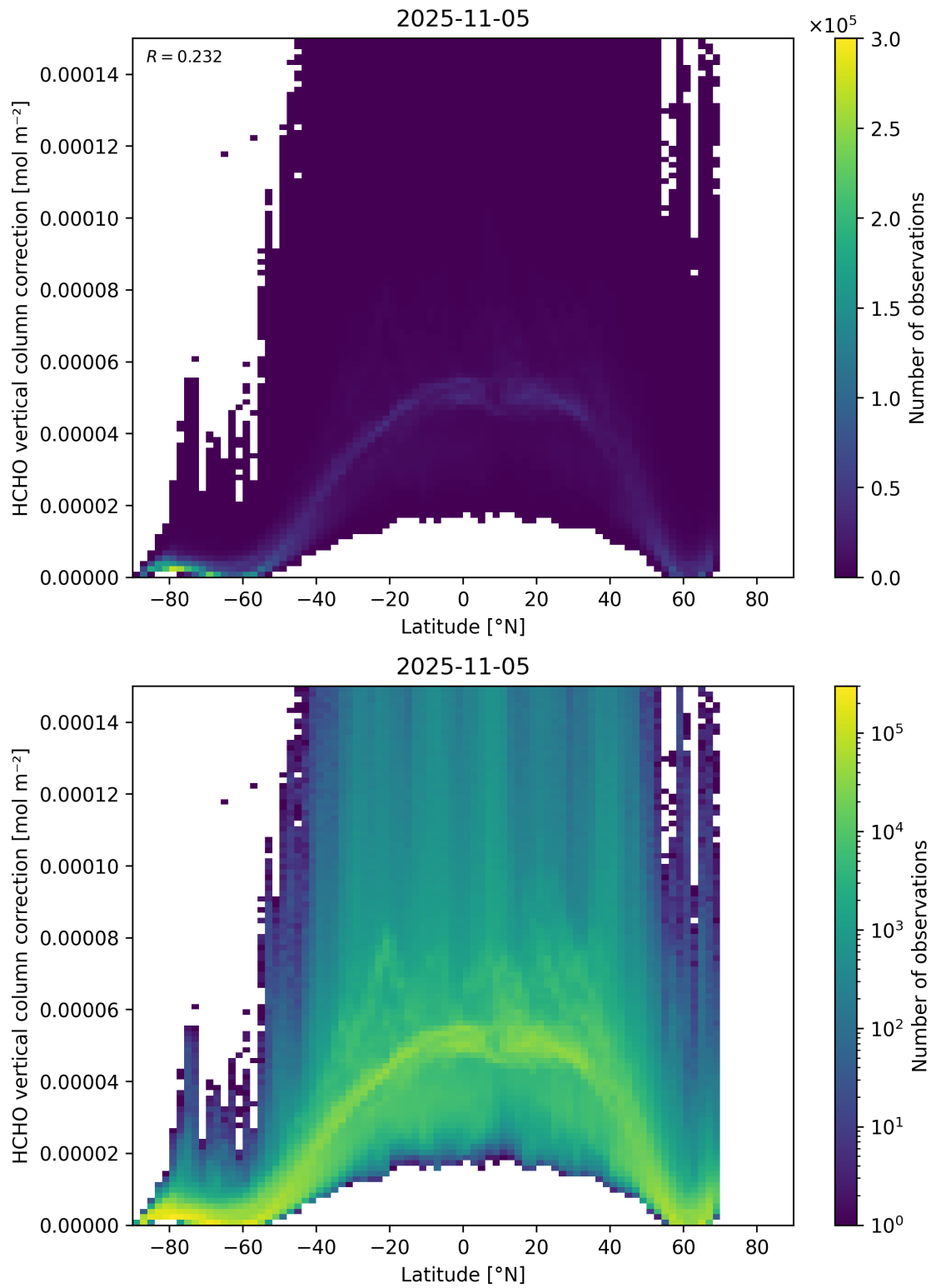
Figure 164: Scatter density plot of “Latitude” against “HCHO vertical column correction” for 2025-11-04 to 2025-11-06.
