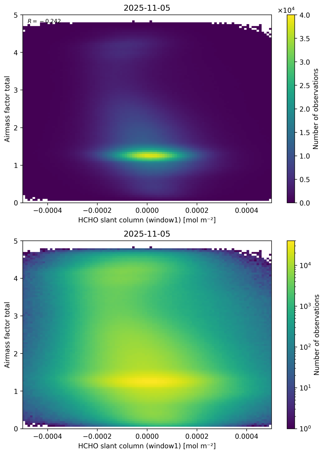
Figure 85: Scatter density plot of “HCHO slant column (window1)” against “Airmass factor total” for 2025-11-04 to 2025-11-06.
