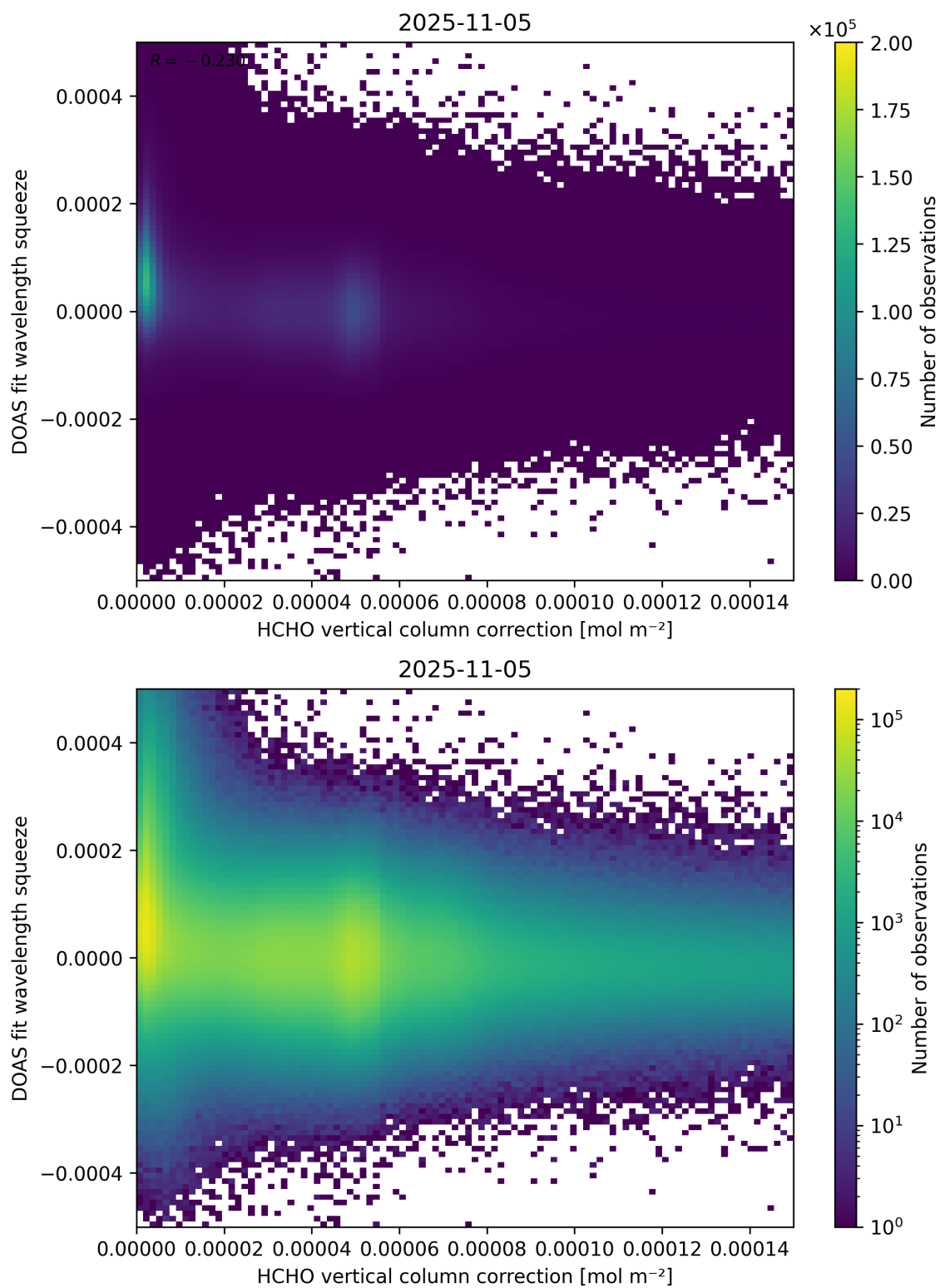
Figure 114: Scatter density plot of “HCHO vertical column correction” against “DOAS fit wavelength squeeze” for 2025-11-04 to 2025-11-06.
