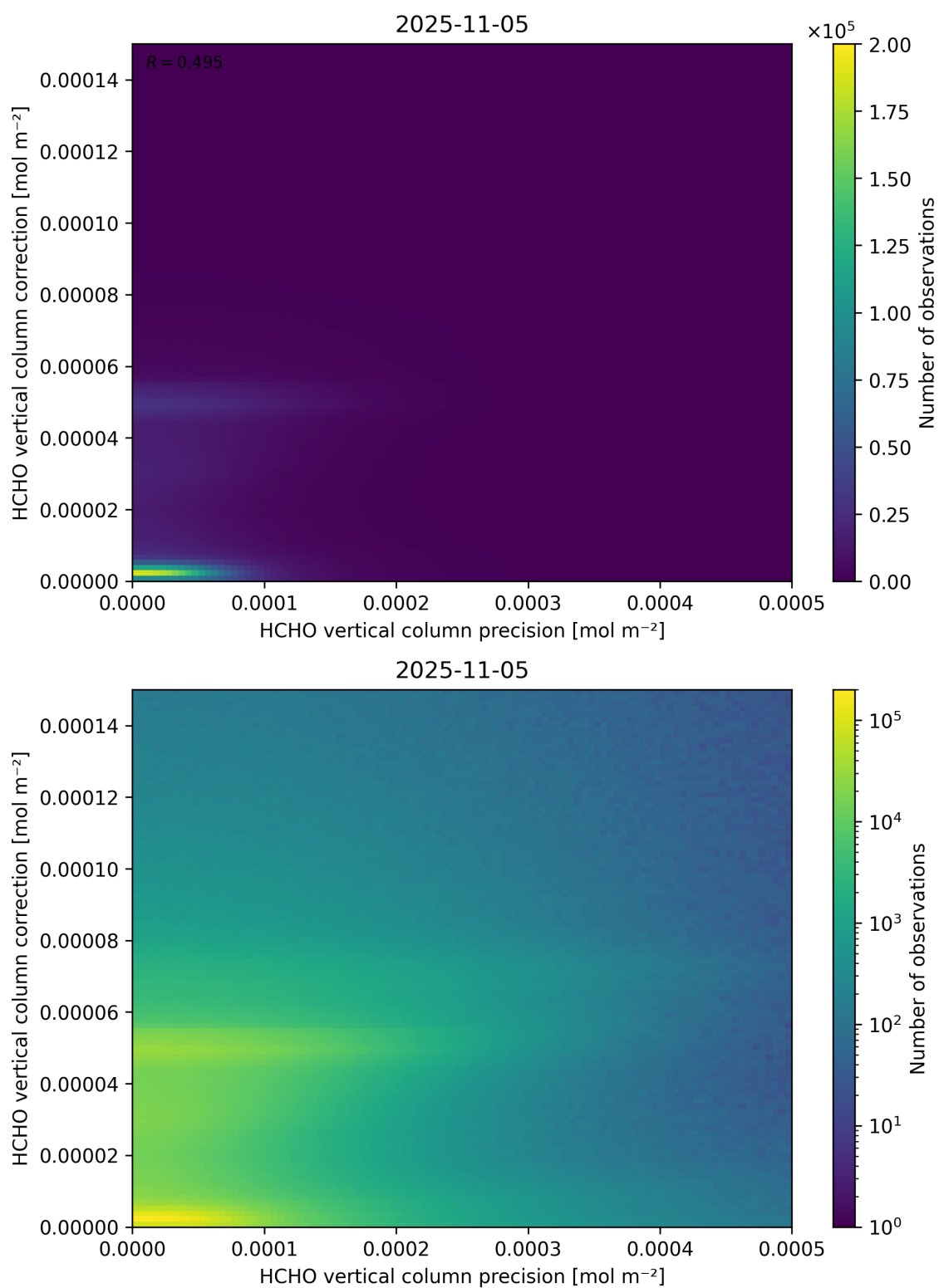
Figure 146: Scatter density plot of “HCHO vertical column precision” against “HCHO vertical column correction” for 2025-11-04 to 2025-11-06.
