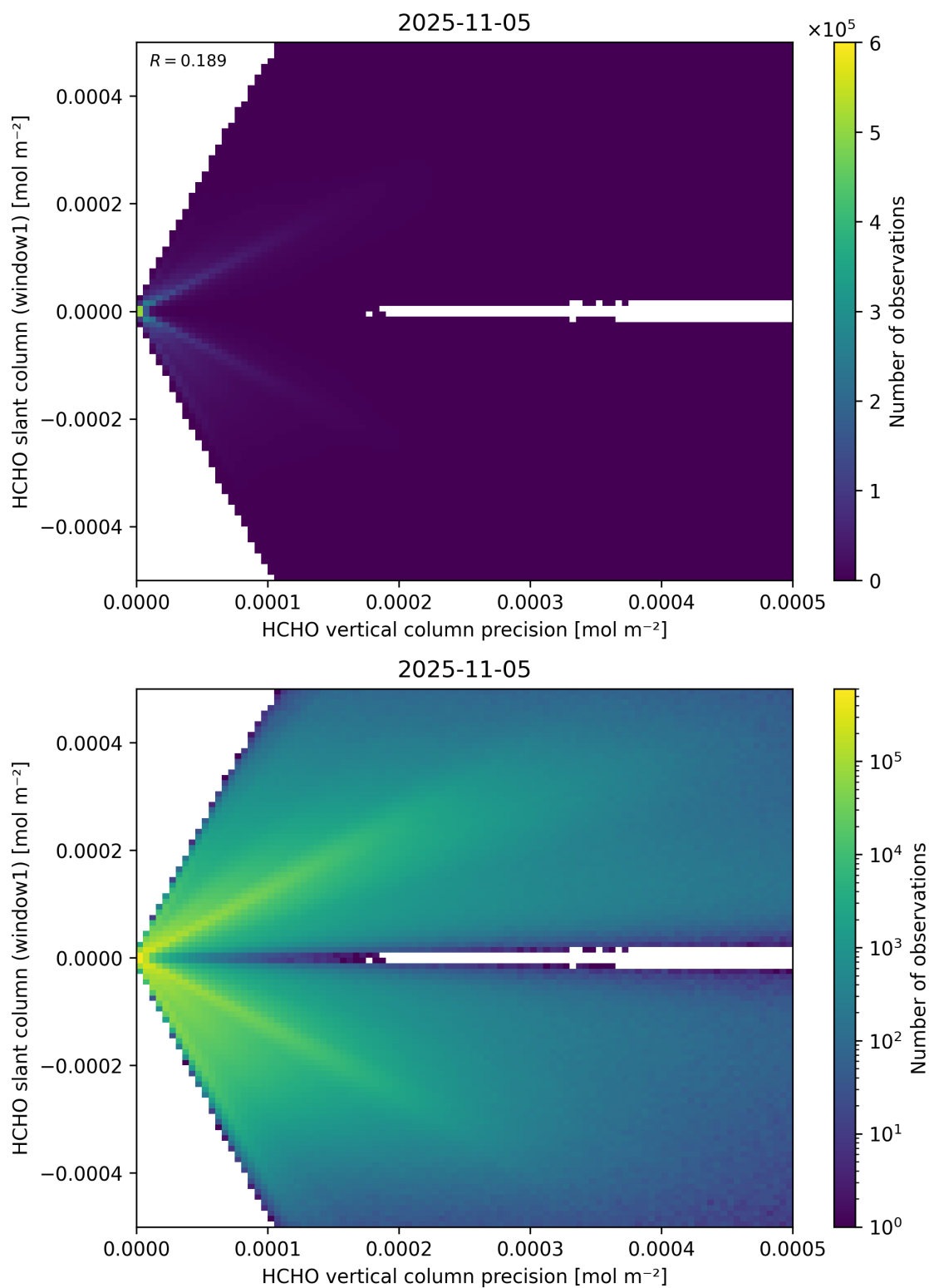
Figure 142: Scatter density plot of “HCHO vertical column precision” against “HCHO slant column (window1)” for 2025-11-04 to 2025-11-06.
