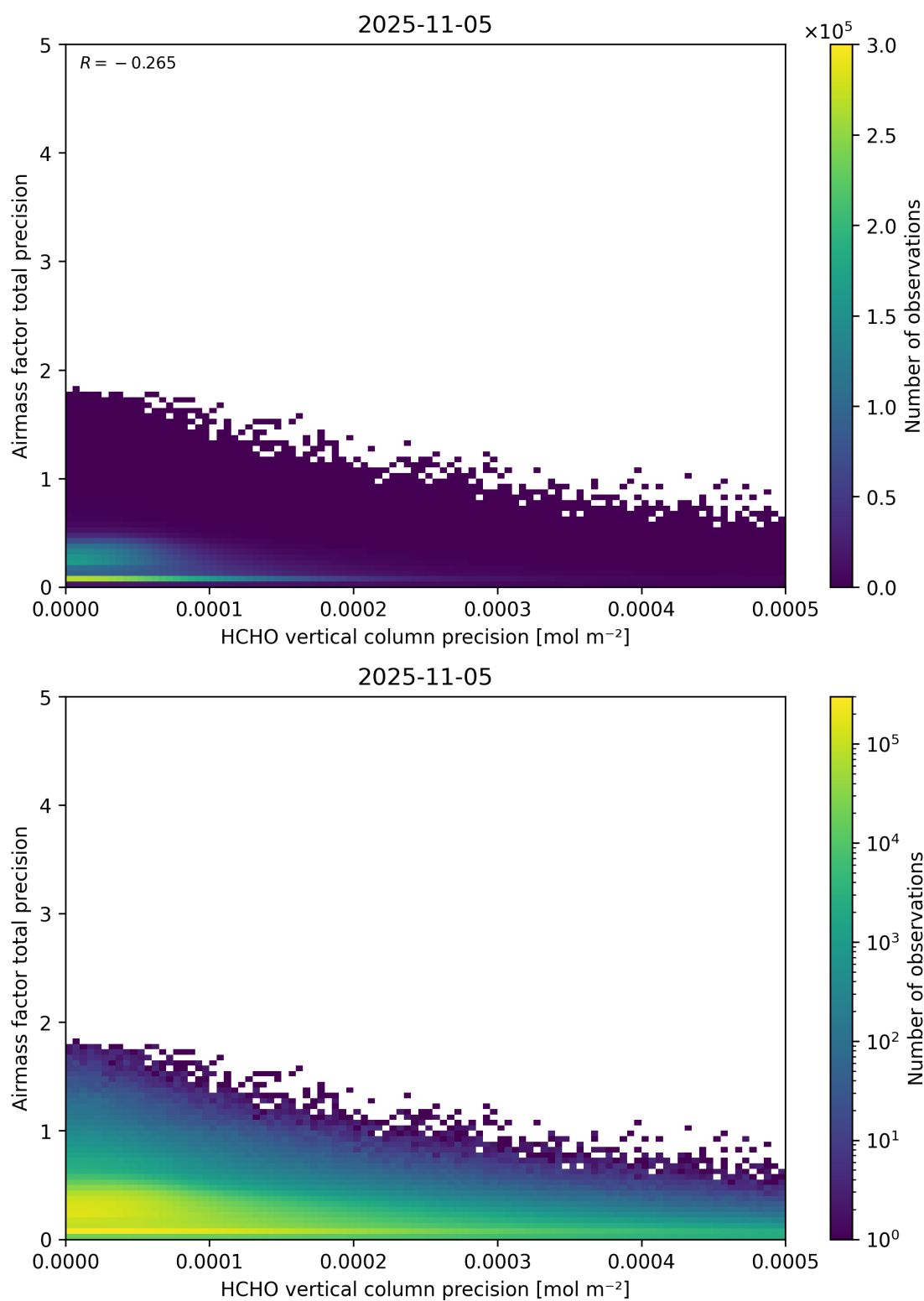
Figure 145: Scatter density plot of “HCHO vertical column precision” against “Airmass factor total precision” for 2025-11-04 to 2025-11-06.
