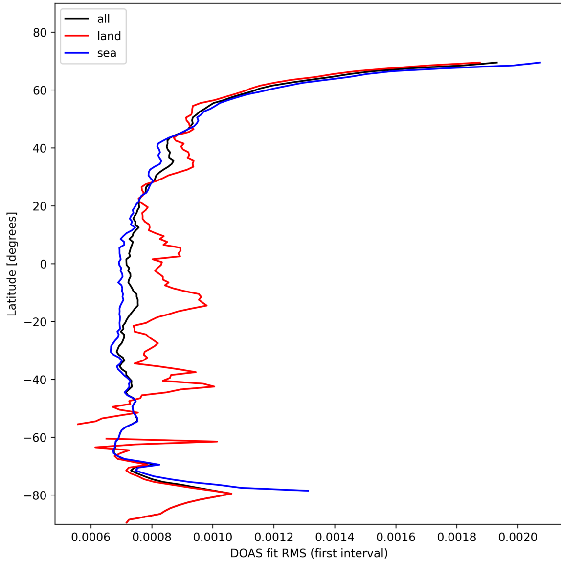
Figure 32: Zonal average of “DOAS fit RMS (first interval)” for 2025-11-04 to 2025-11-06.
