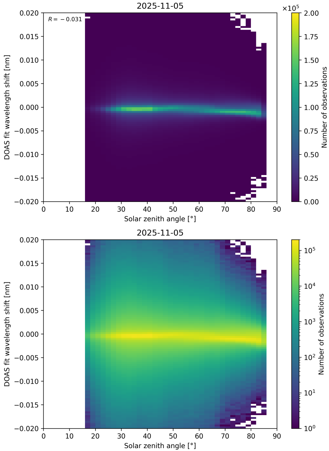
Figure 168: Scatter density plot of “Solar zenith angle” against “DOAS fit wavelength shift” for 2025-11-04 to 2025-11-06.
