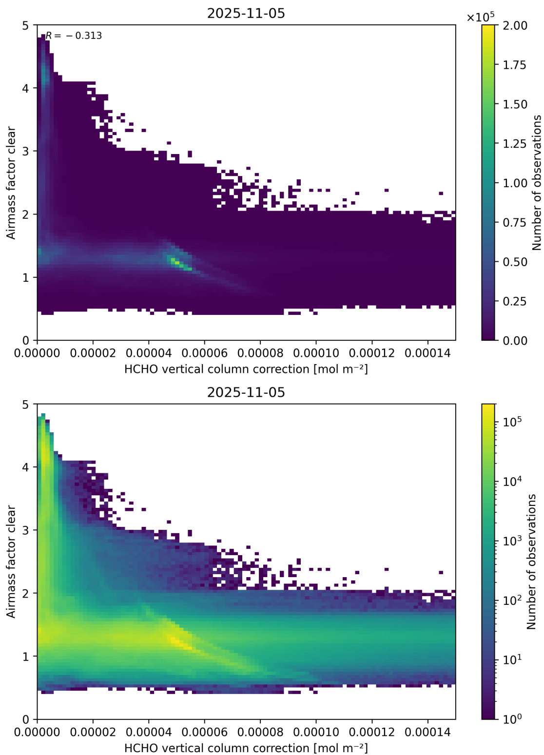
Figure 115: Scatter density plot of “HCHO vertical column correction” against “Airmass factor clear” for 2025-11-04 to 2025-11-06.
