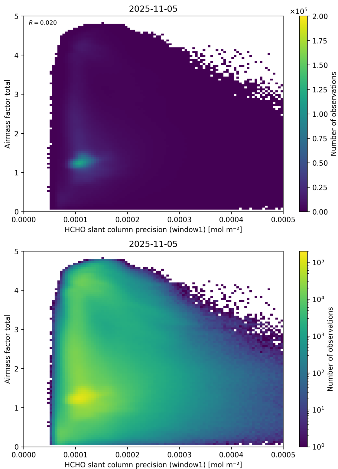
Figure 94: Scatter density plot of “HCHO slant column precision (window1)” against “Airmass factor total” for 2025-11-04 to 2025-11-06.
