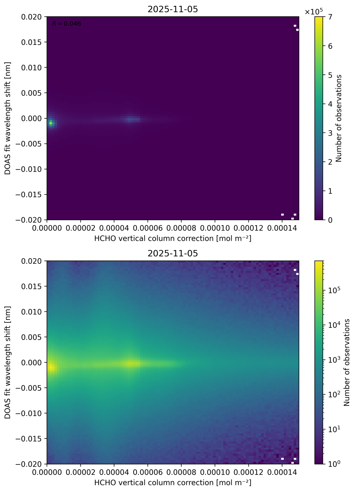
Figure 113: Scatter density plot of “HCHO vertical column correction” against “DOAS fit wavelength shift” for 2025-11-04 to 2025-11-06.
