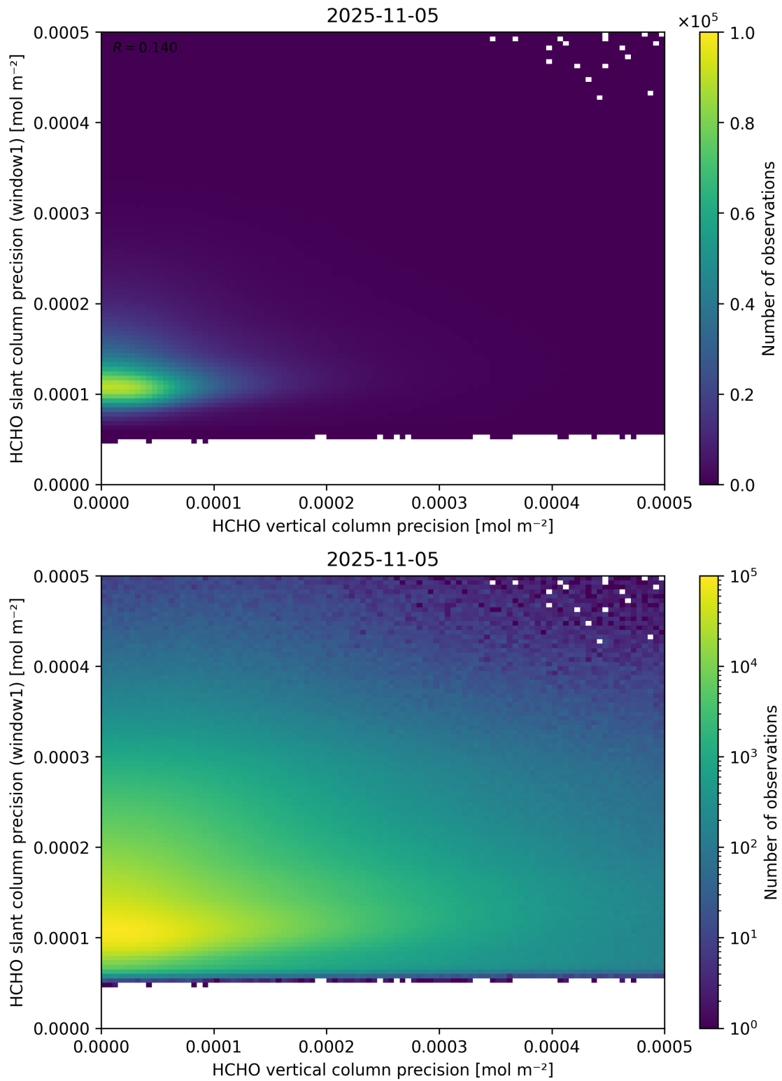
Figure 143: Scatter density plot of “HCHO vertical column precision” against “HCHO slant column precision (window1)” for 2025-11-04 to 2025-11-06.
