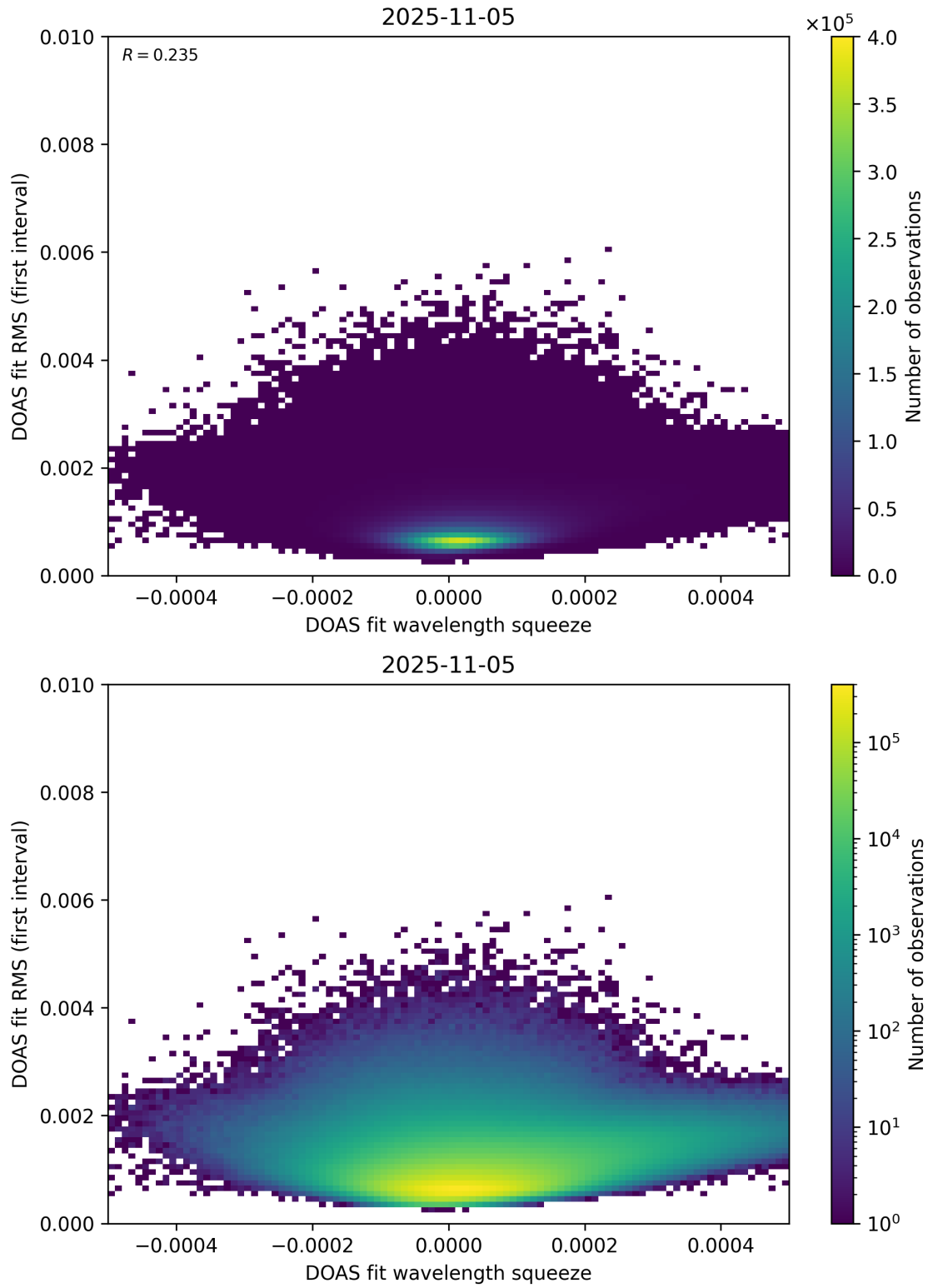
Figure 68: Scatter density plot of “DOAS fit wavelength squeeze” against “DOAS fit RMS (first interval)” for 2025-11-04 to 2025-11-06.
