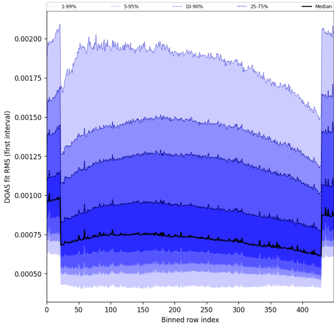
Figure 60: Along track statistics of “DOAS fit RMS (first interval)” for 2025-11-04 to 2025-11-06
