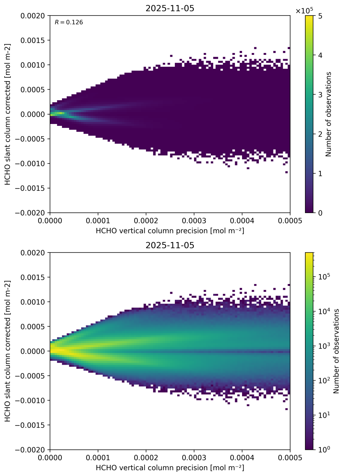
Figure 140: Scatter density plot of “HCHO vertical column precision” against “HCHO slant column corrected” for 2025-11-04 to 2025-11-06.
