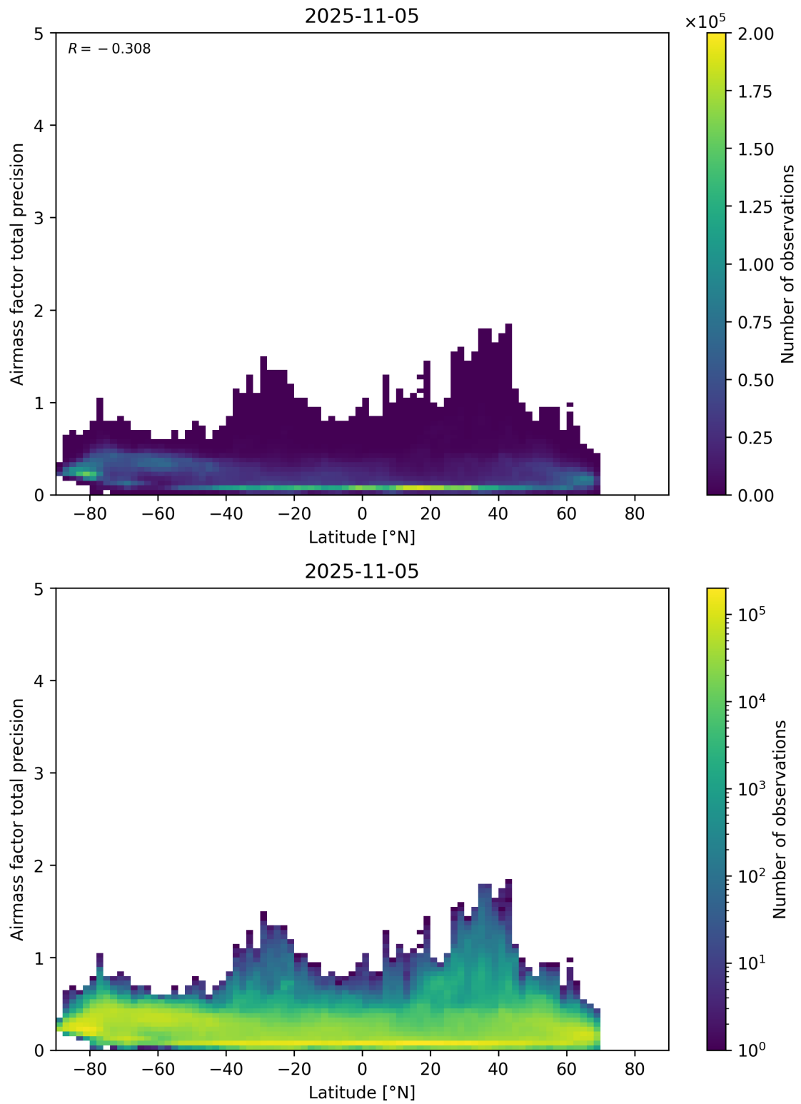
Figure 162: Scatter density plot of “Latitude” against “Airmass factor total precision” for 2025-11-04 to 2025-11-06.
