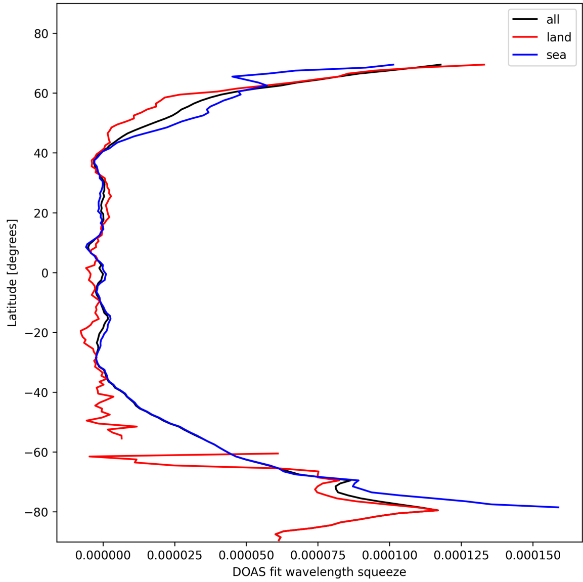
Figure 31: Zonal average of “DOAS fit wavelength squeeze” for 2025-11-04 to 2025-11-06.
