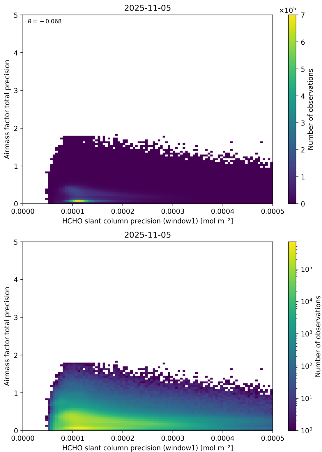
Figure 95: Scatter density plot of “HCHO slant column precision (window1)” against “Airmass factor total precision” for 2025-11-04 to 2025-11-06.
