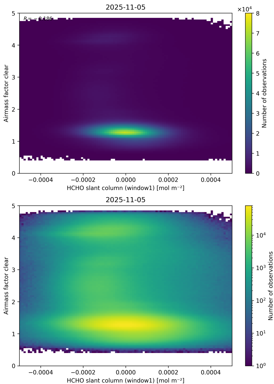
Figure 81: Scatter density plot of “HCHO slant column (window1)” against “Airmass factor clear” for 2025-11-04 to 2025-11-06.
