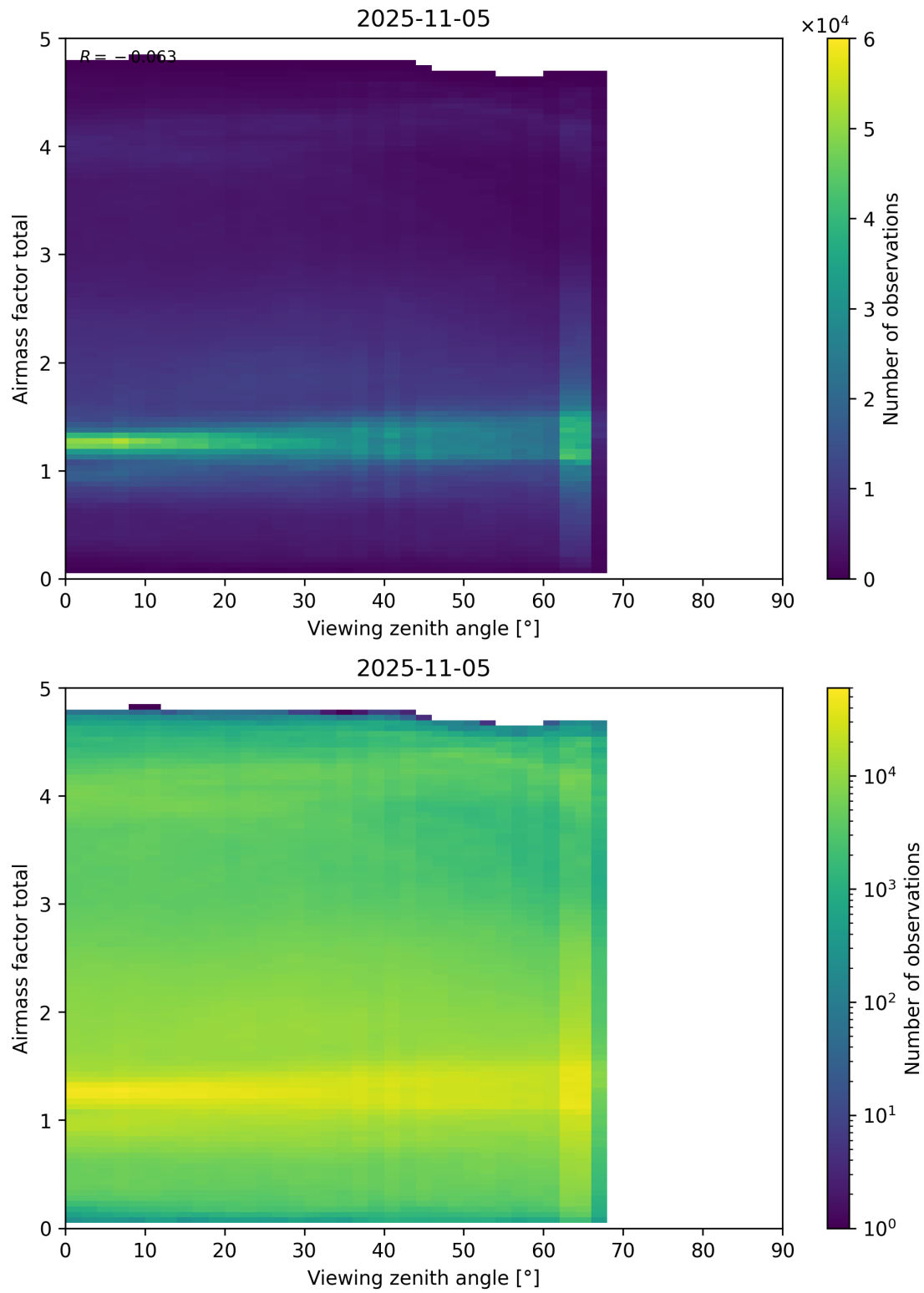
Figure 190: Scatter density plot of “Viewing zenith angle” against “Airmass factor total” for 2025-11-04 to 2025-11-06.
