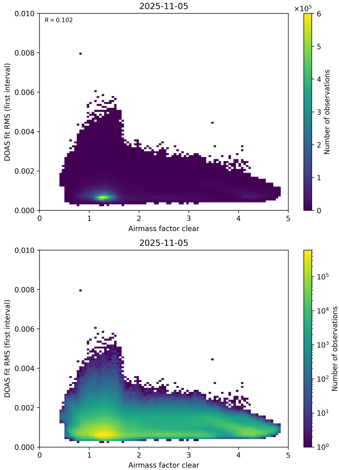
Figure 71: Scatter density plot of “Airmass factor clear” against “DOAS fit RMS (first interval)” for 2025-11-04 to 2025-11-06.
