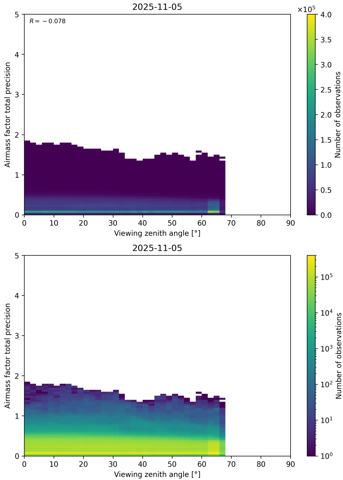
Figure 191: Scatter density plot of “Viewing zenith angle” against “Airmass factor total precision” for 2025-11-04 to 2025-11-06.
