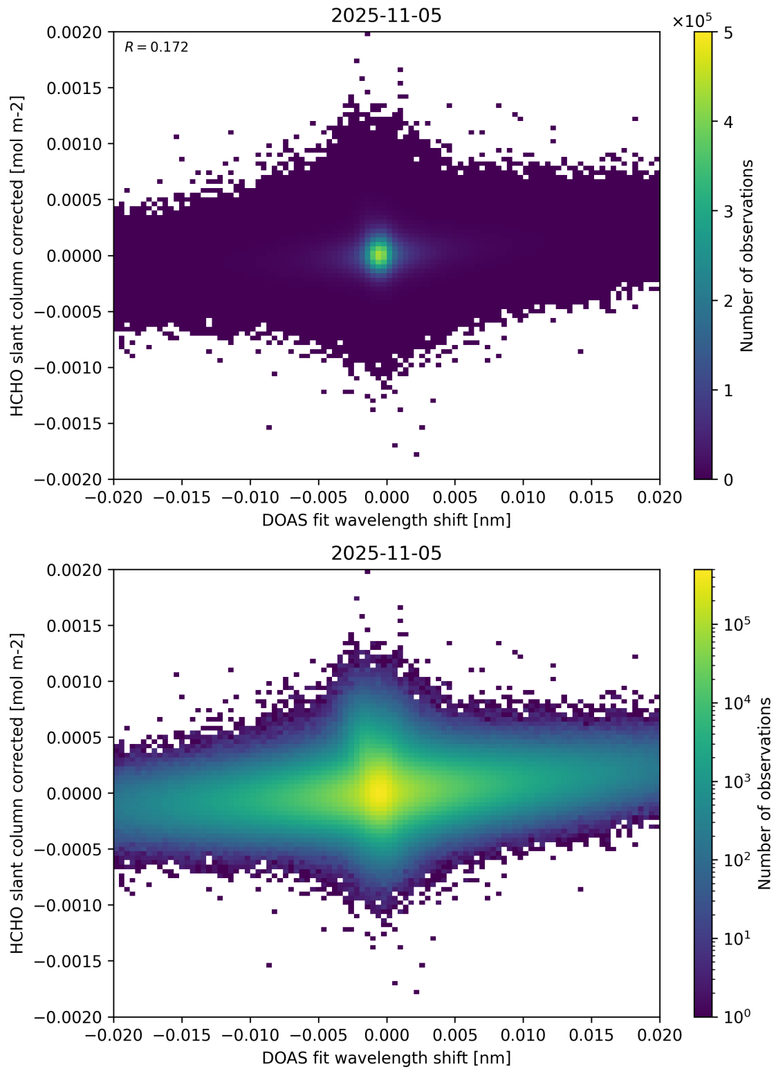
Figure 66: Scatter density plot of “DOAS fit wavelength shift” against “HCHO slant column corrected” for 2025-11-04 to 2025-11-06.
