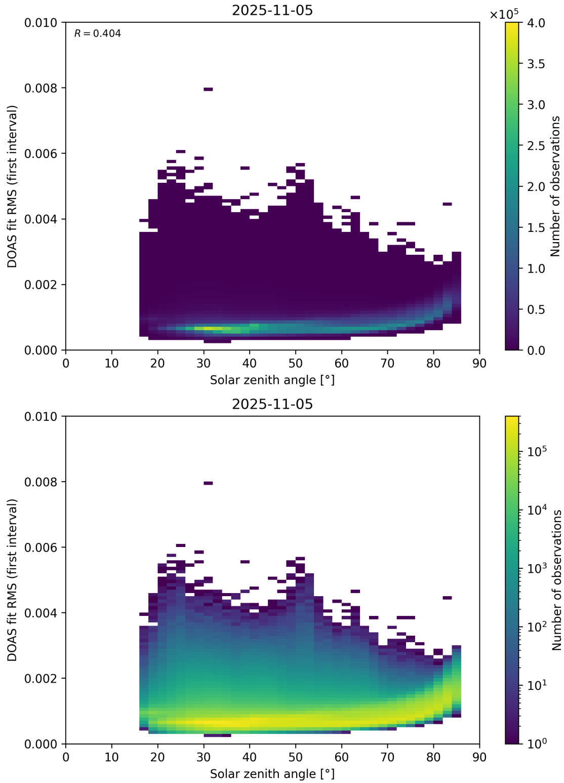
Figure 167: Scatter density plot of “Solar zenith angle” against “DOAS fit RMS (first interval)” for 2025-11-04 to 2025-11-06.
