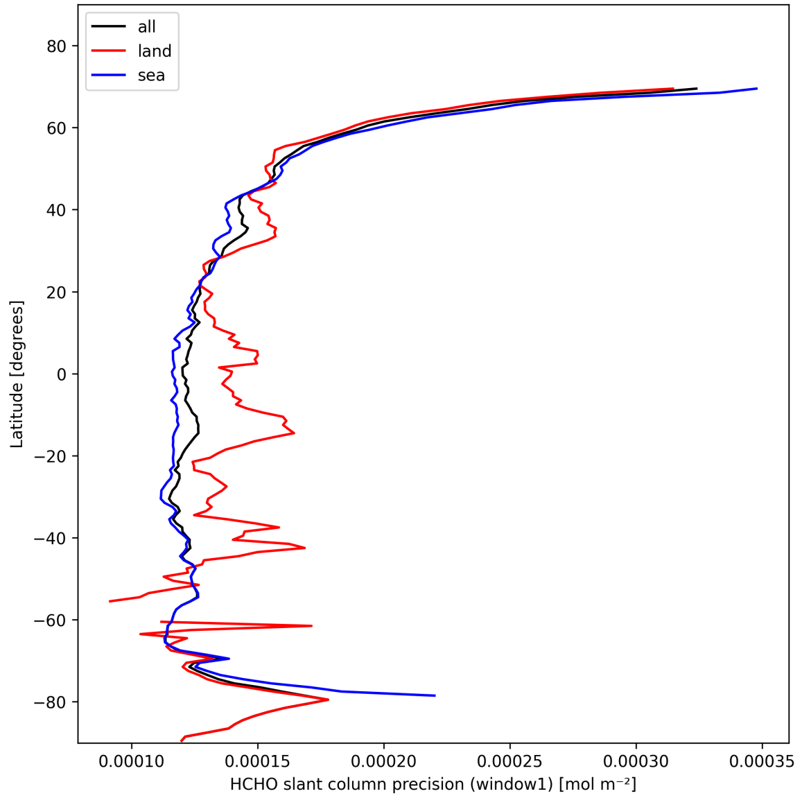
Figure 25: Zonal average of “HCHO slant column precision (window1)” for 2025-11-04 to 2025-11-06.
