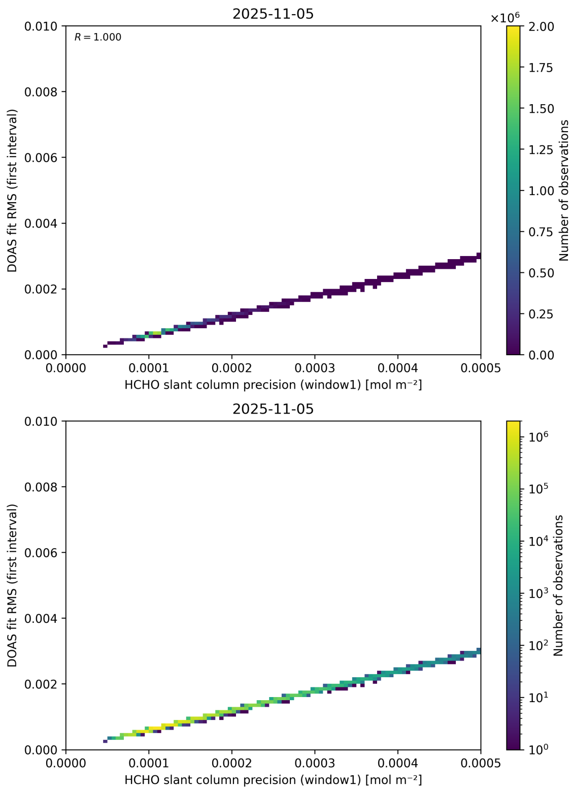
Figure 88: Scatter density plot of “HCHO slant column precision (window1)” against “DOAS fit RMS (first interval)” for 2025-11-04 to 2025-11-06.
