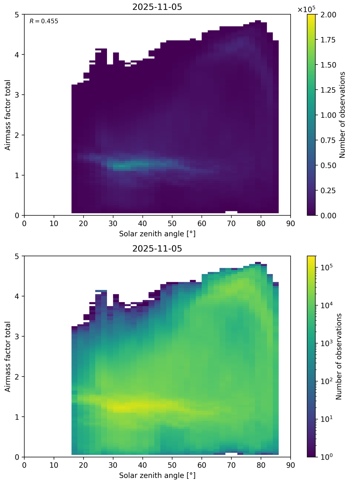
Figure 175: Scatter density plot of “Solar zenith angle” against “Airmass factor total” for 2025-11-04 to 2025-11-06.
