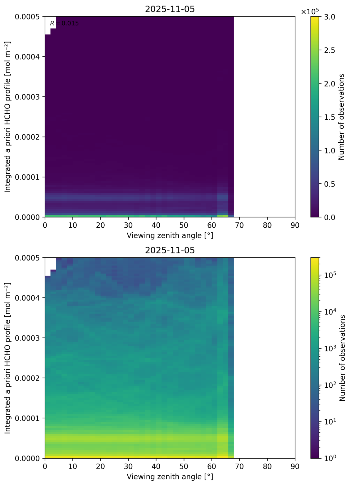
Figure 195: Scatter density plot of “Viewing zenith angle” against “Integrated a priori HCHO profile” for 2025-11-04 to 2025-11-06.
