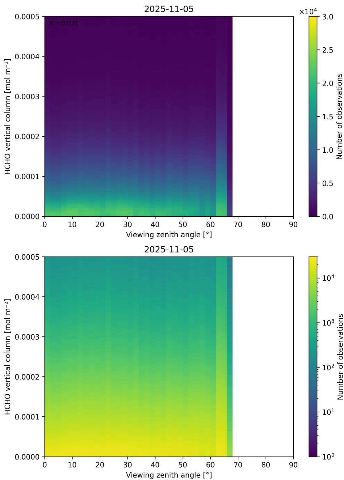
Figure 192: Scatter density plot of “Viewing zenith angle” against “HCHO vertical column” for 2025-11-04 to 2025-11-06.
