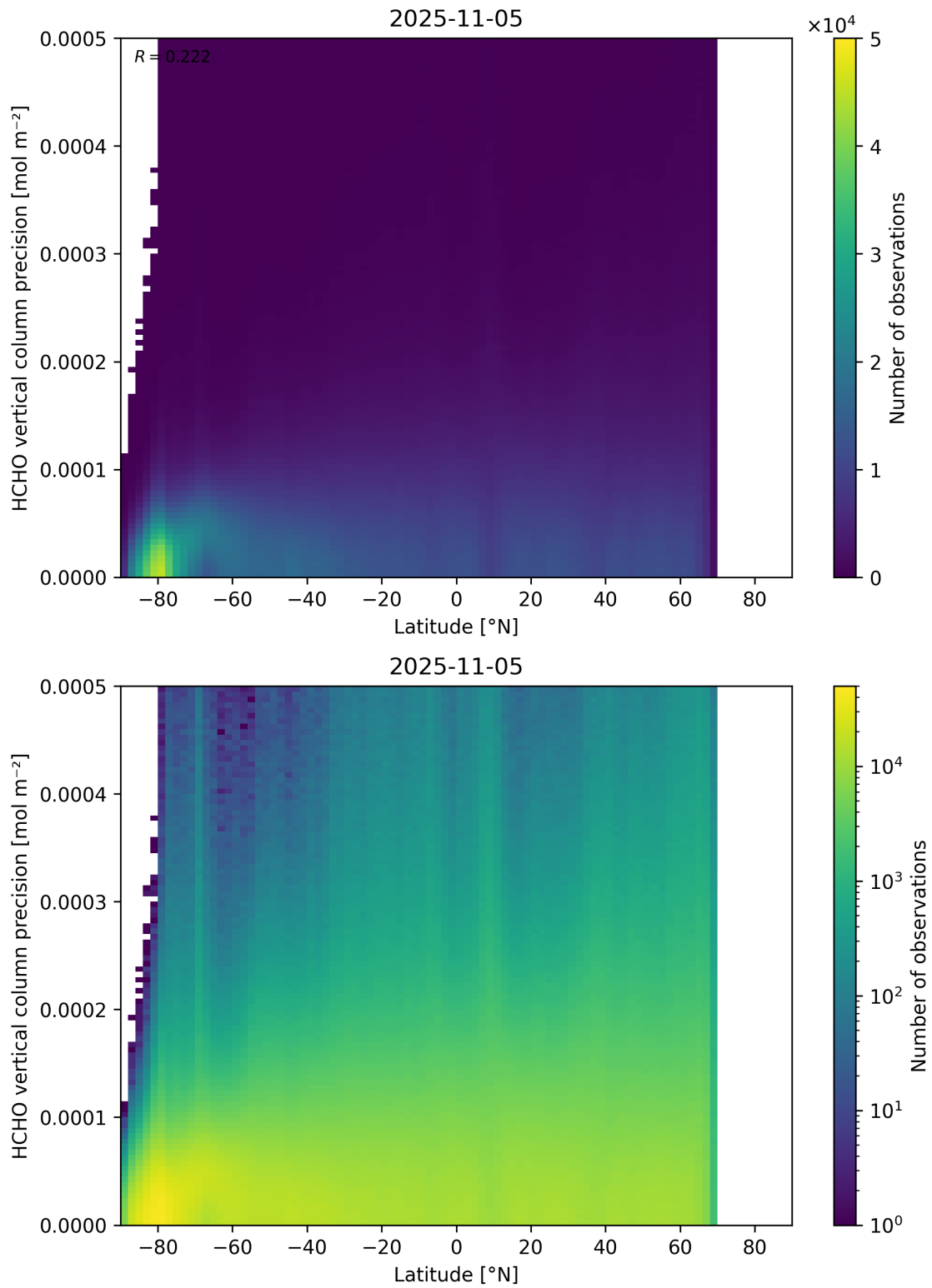
Figure 165: Scatter density plot of “Latitude” against “HCHO vertical column precision” for 2025-11-04 to 2025-11-06.
