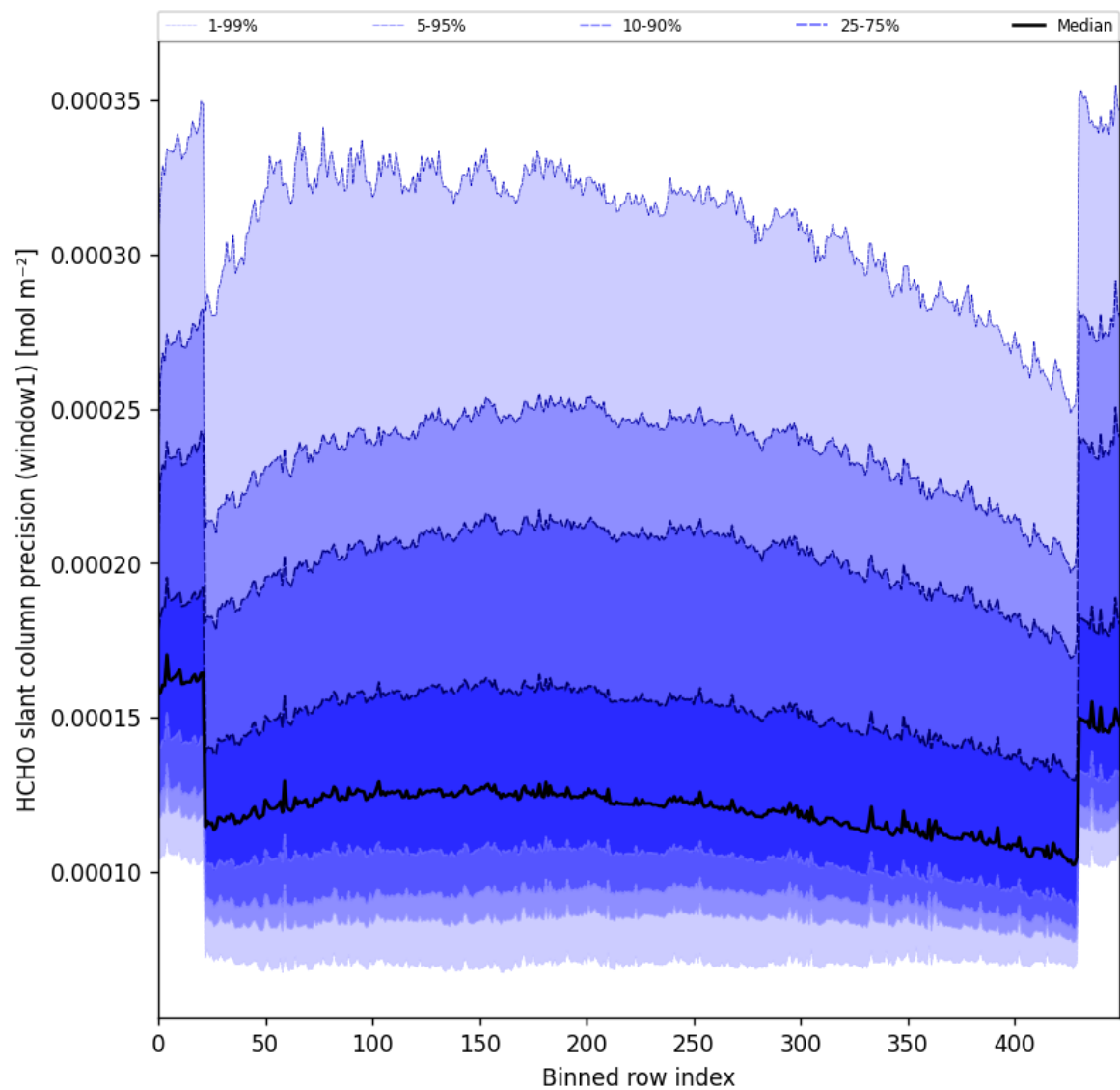
Figure 53: Along track statistics of “HCHO slant column precision (window1)” for 2025-11-04 to 2025-11-06
