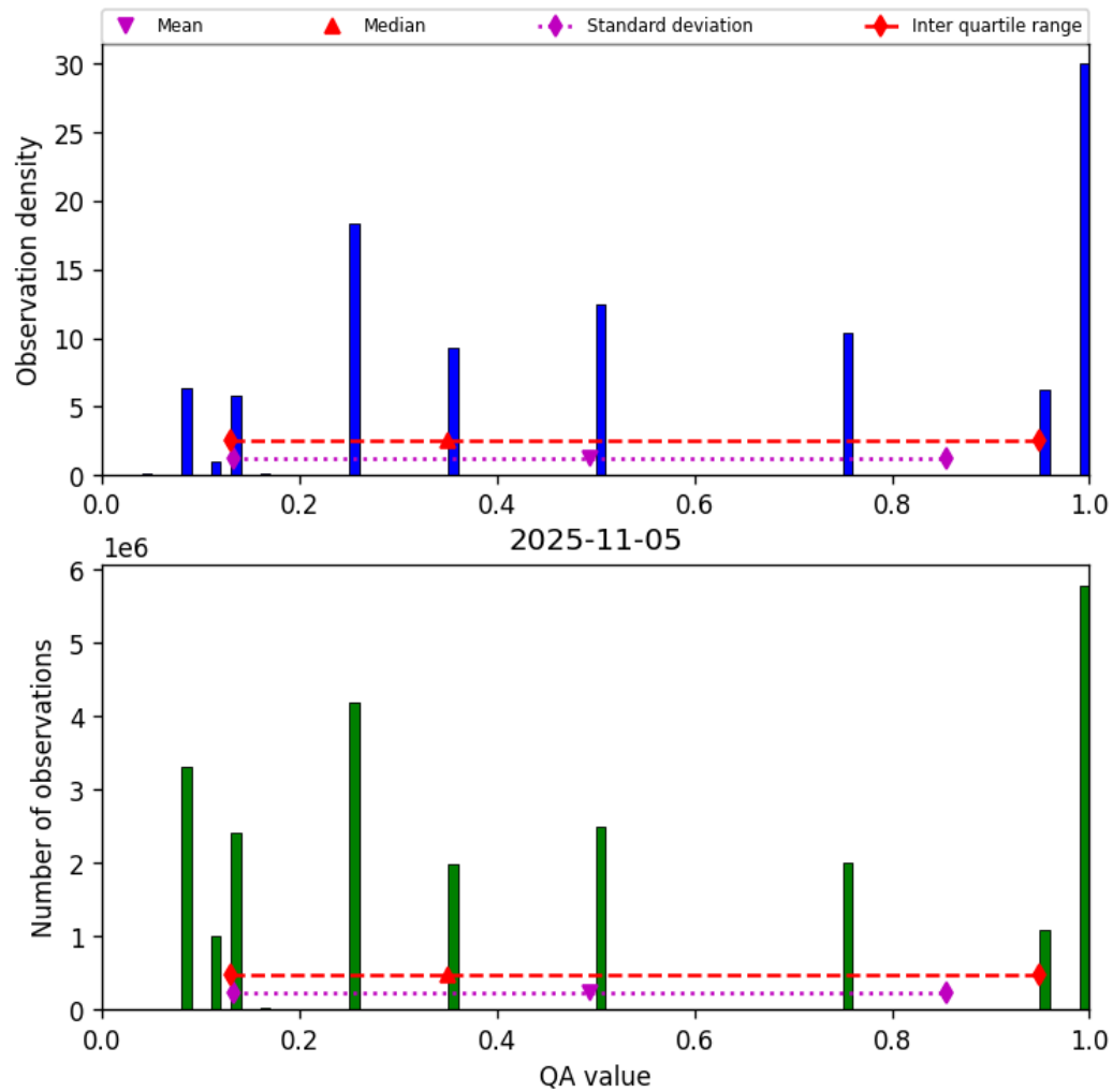
Figure 34: Histogram of “QA value” for 2025-11-04 to 2025-11-06
