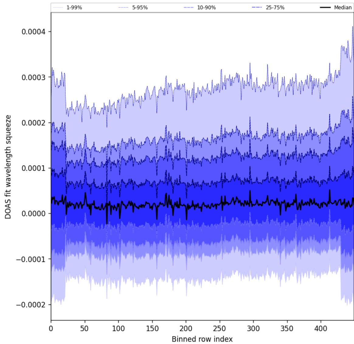
Figure 59: Along track statistics of “DOAS fit wavelength squeeze” for 2025-11-04 to 2025-11-06
