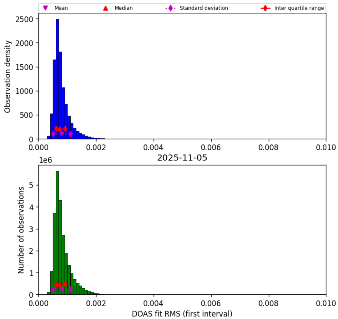
Figure 46: Histogram of “DOAS fit RMS (first interval)” for 2025-11-04 to 2025-11-06
