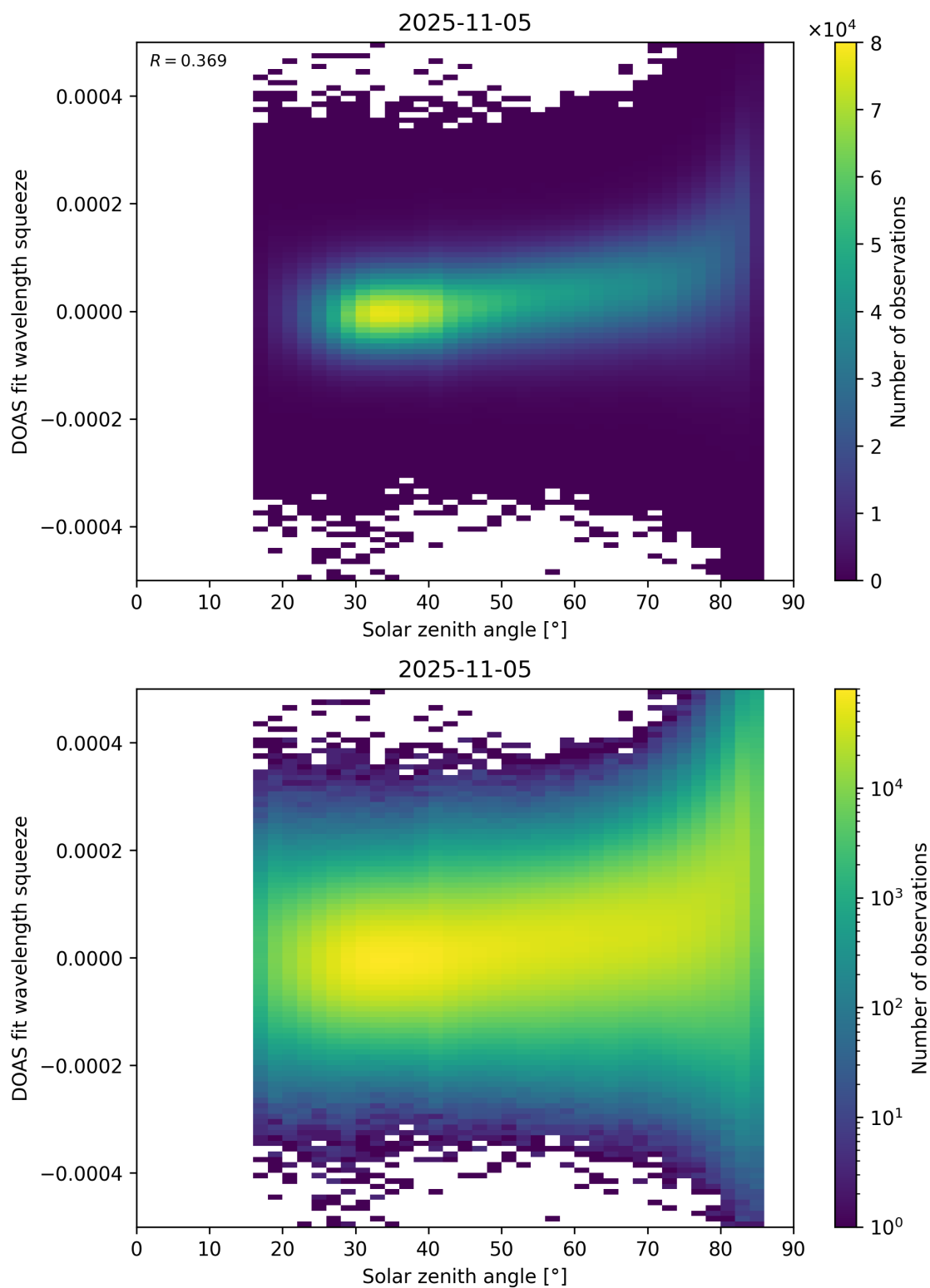
Figure 169: Scatter density plot of “Solar zenith angle” against “DOAS fit wavelength squeeze” for 2025-11-04 to 2025-11-06.
