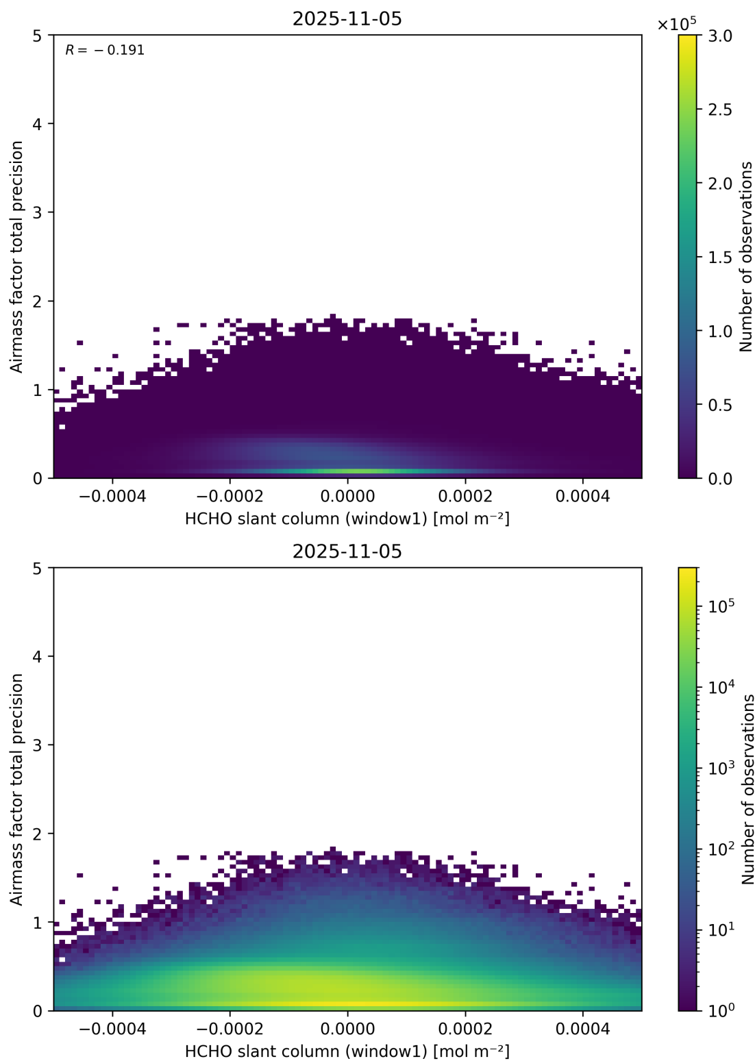
Figure 86: Scatter density plot of “HCHO slant column (window1)” against “Airmass factor total precision” for 2025-11-04 to 2025-11-06.
