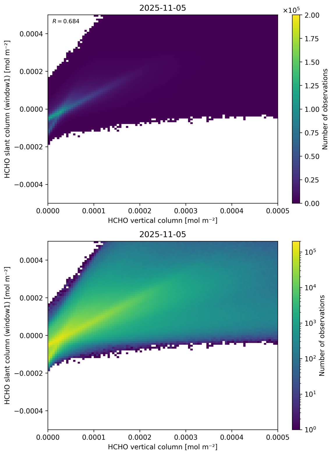
Figure 129: Scatter density plot of “HCHO vertical column” against “HCHO slant column (window1)” for 2025-11-04 to 2025-11-06.
