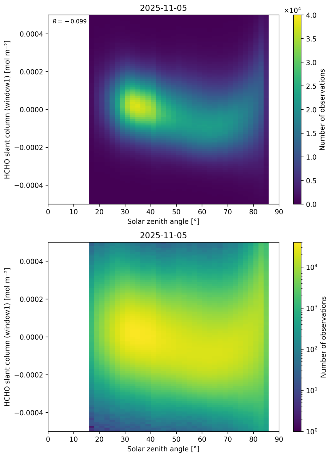
Figure 173: Scatter density plot of “Solar zenith angle” against “HCHO slant column (window1)” for 2025-11-04 to 2025-11-06.
