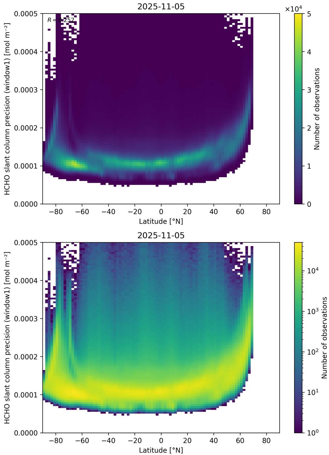
Figure 160: Scatter density plot of “Latitude” against “HCHO slant column precision (window1)” for 2025-11-04 to 2025-11-06.
