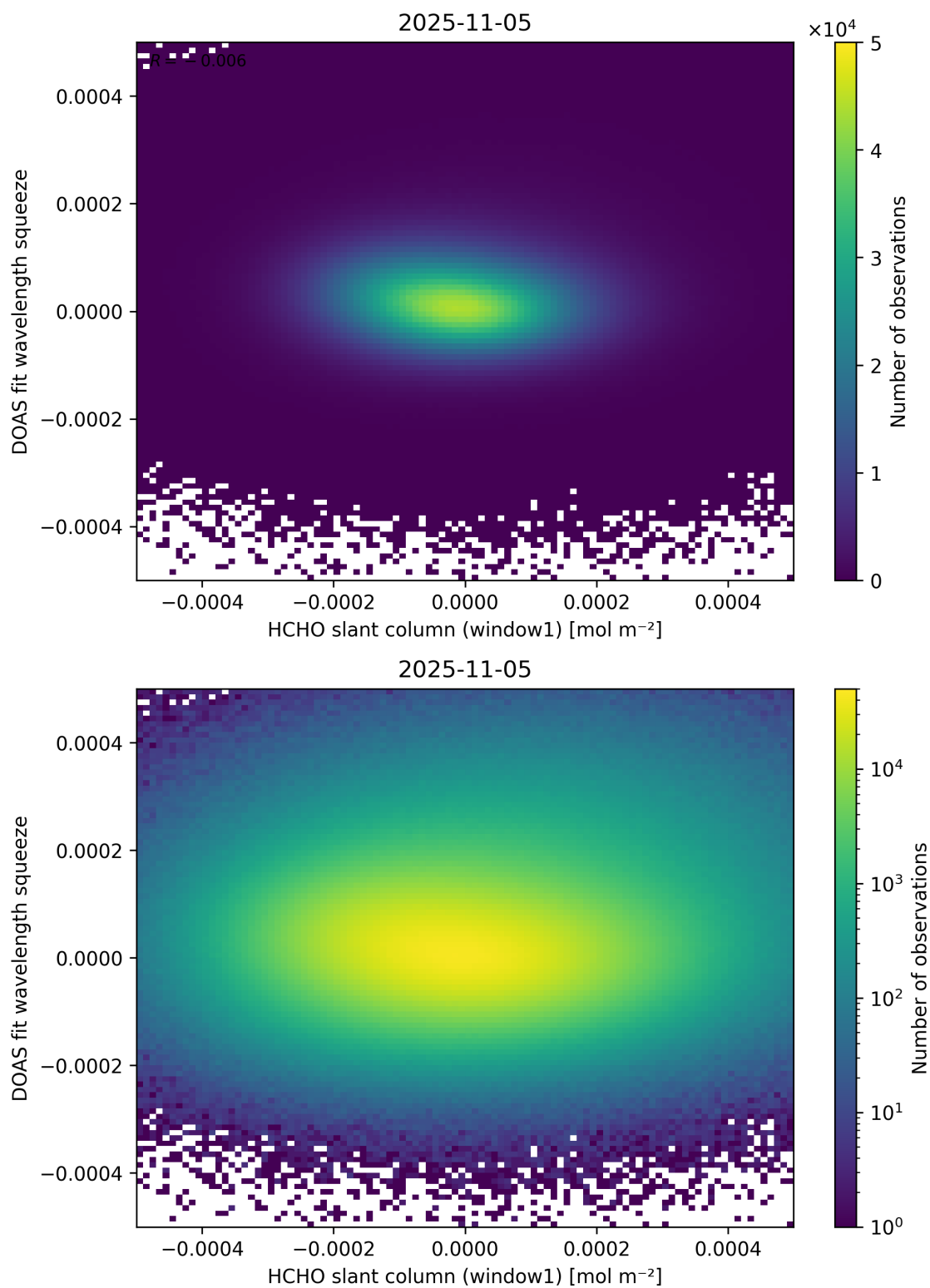
Figure 80: Scatter density plot of “HCHO slant column (window1)” against “DOAS fit wavelength squeeze” for 2025-11-04 to 2025-11-06.
