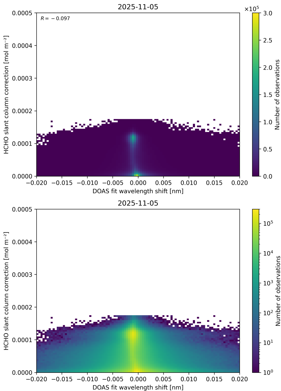
Figure 67: Scatter density plot of “DOAS fit wavelength shift” against “HCHO slant column correction” for 2025-11-04 to 2025-11-06.
