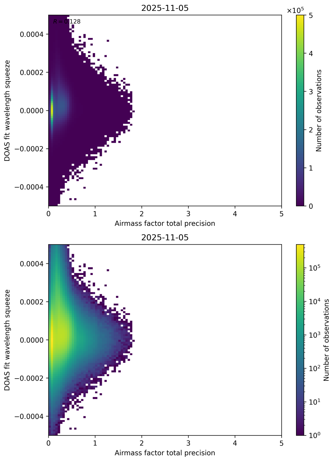
Figure 107: Scatter density plot of “Airmass factor total precision” against “DOAS fit wavelength squeeze” for 2025-11-04 to 2025-11-06.
