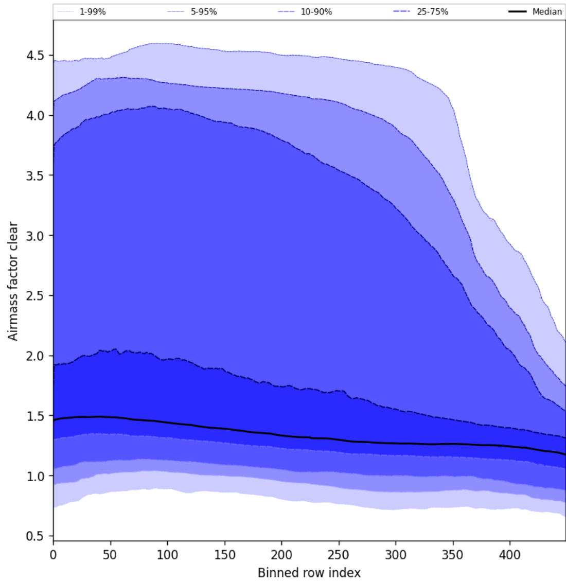
Figure 56: Along track statistics of “Airmass factor clear” for 2025-11-04 to 2025-11-06
