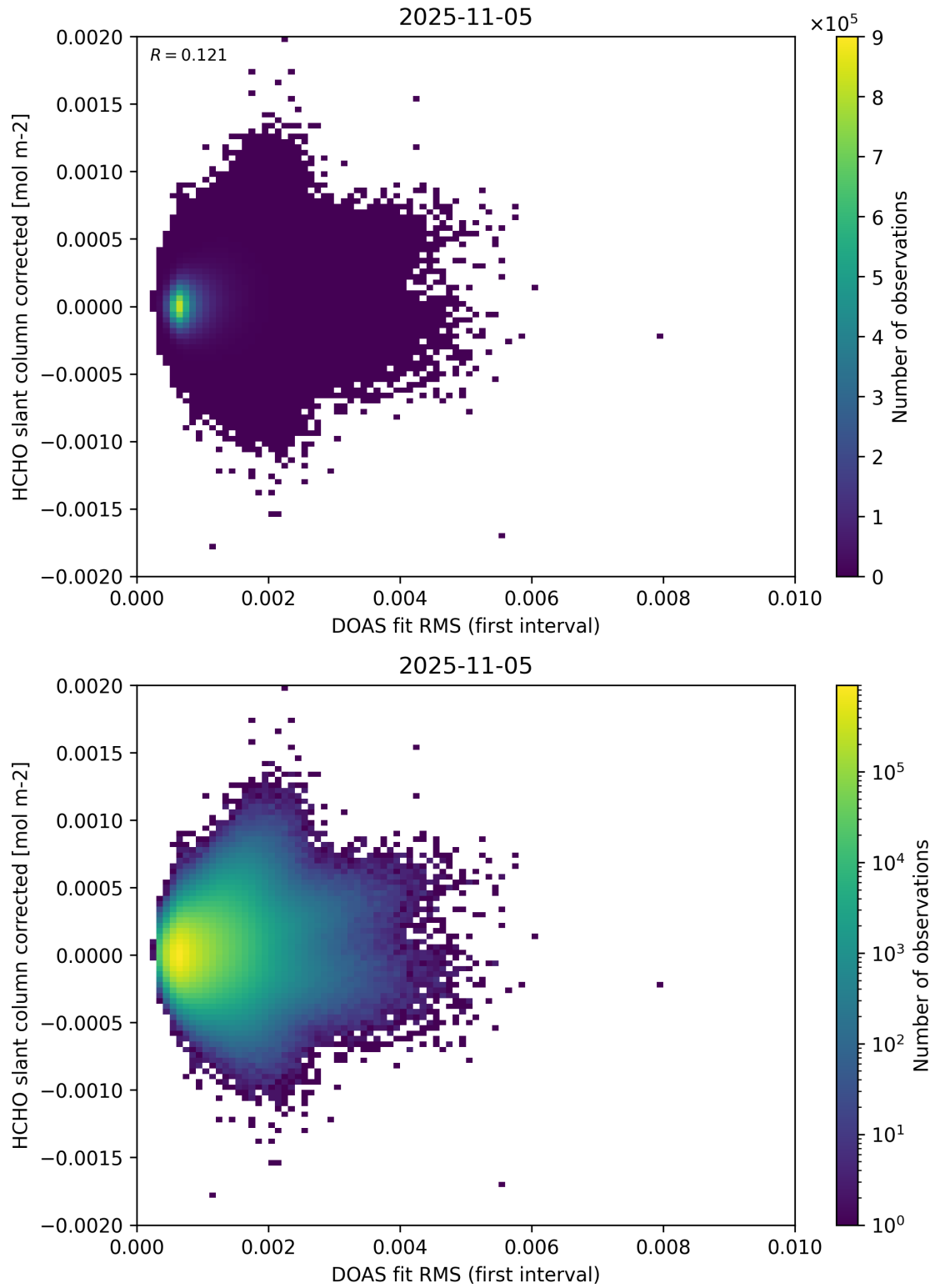
Figure 62: Scatter density plot of “DOAS fit RMS (first interval)” against “HCHO slant column corrected” for 2025-11-04 to 2025-11-06.
