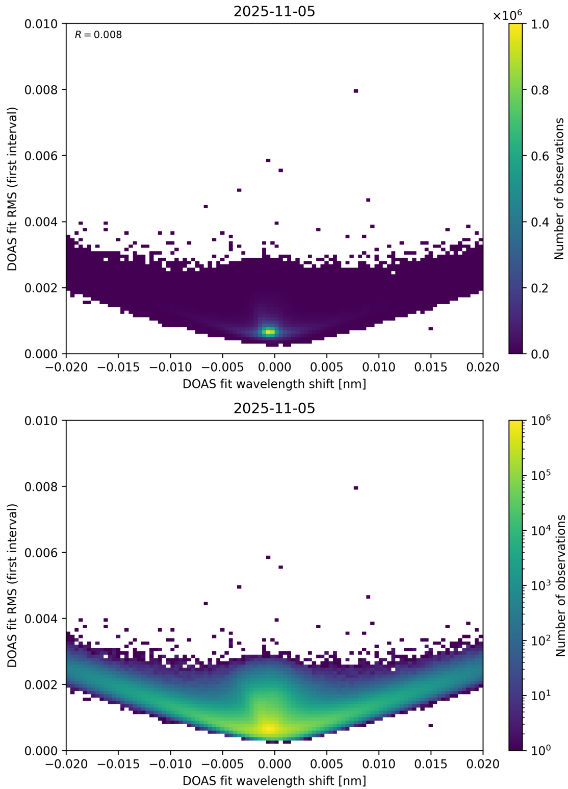
Figure 64: Scatter density plot of “DOAS fit wavelength shift” against “DOAS fit RMS (first interval)” for 2025-11-04 to 2025-11-06.
