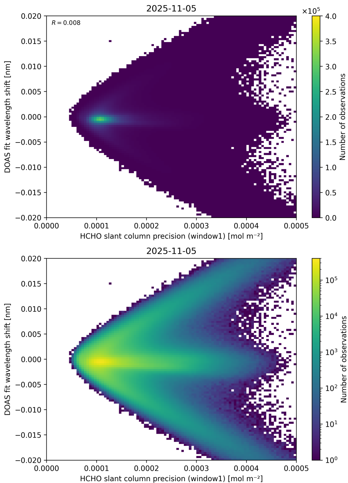
Figure 89: Scatter density plot of “HCHO slant column precision (window1)” against “DOAS fit wavelength shift” for 2025-11-04 to 2025-11-06.
