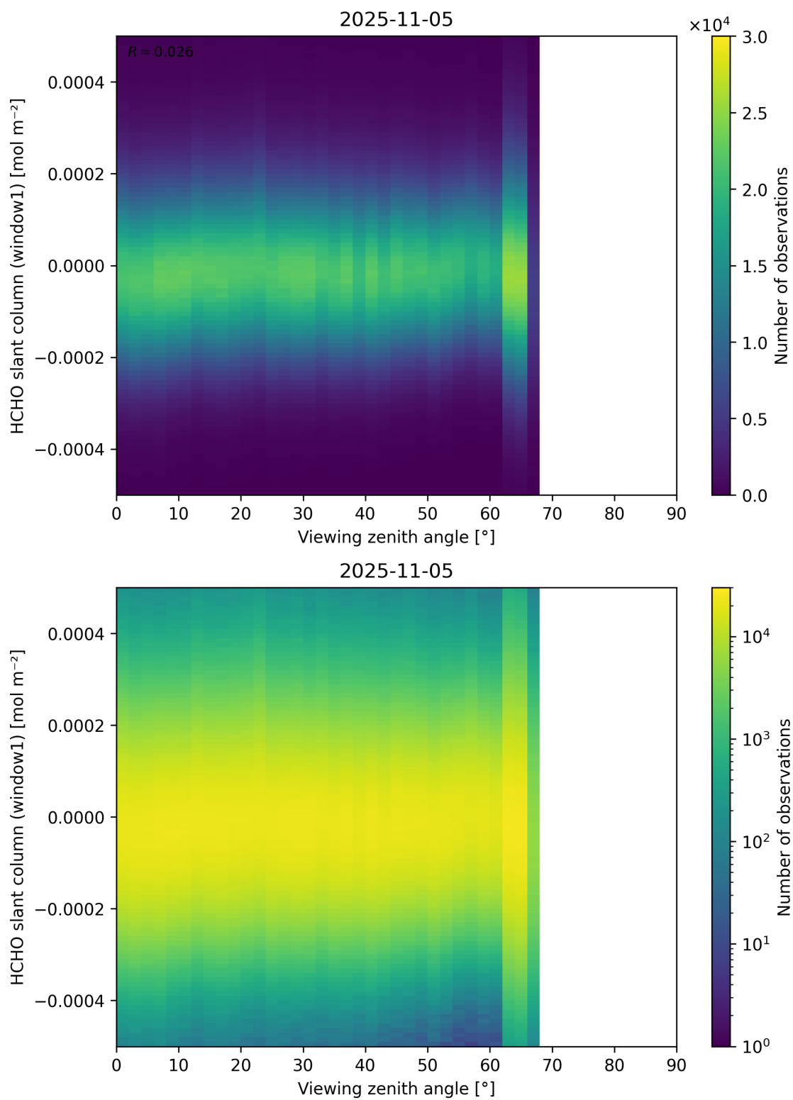
Figure 188: Scatter density plot of “Viewing zenith angle” against “HCHO slant column (window1)” for 2025-11-04 to 2025-11-06.
