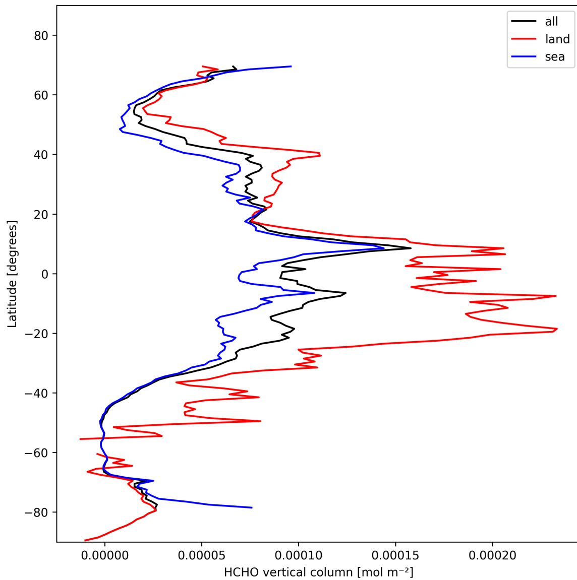
Figure 21: Zonal average of “HCHO vertical column” for 2025-11-04 to 2025-11-06.
