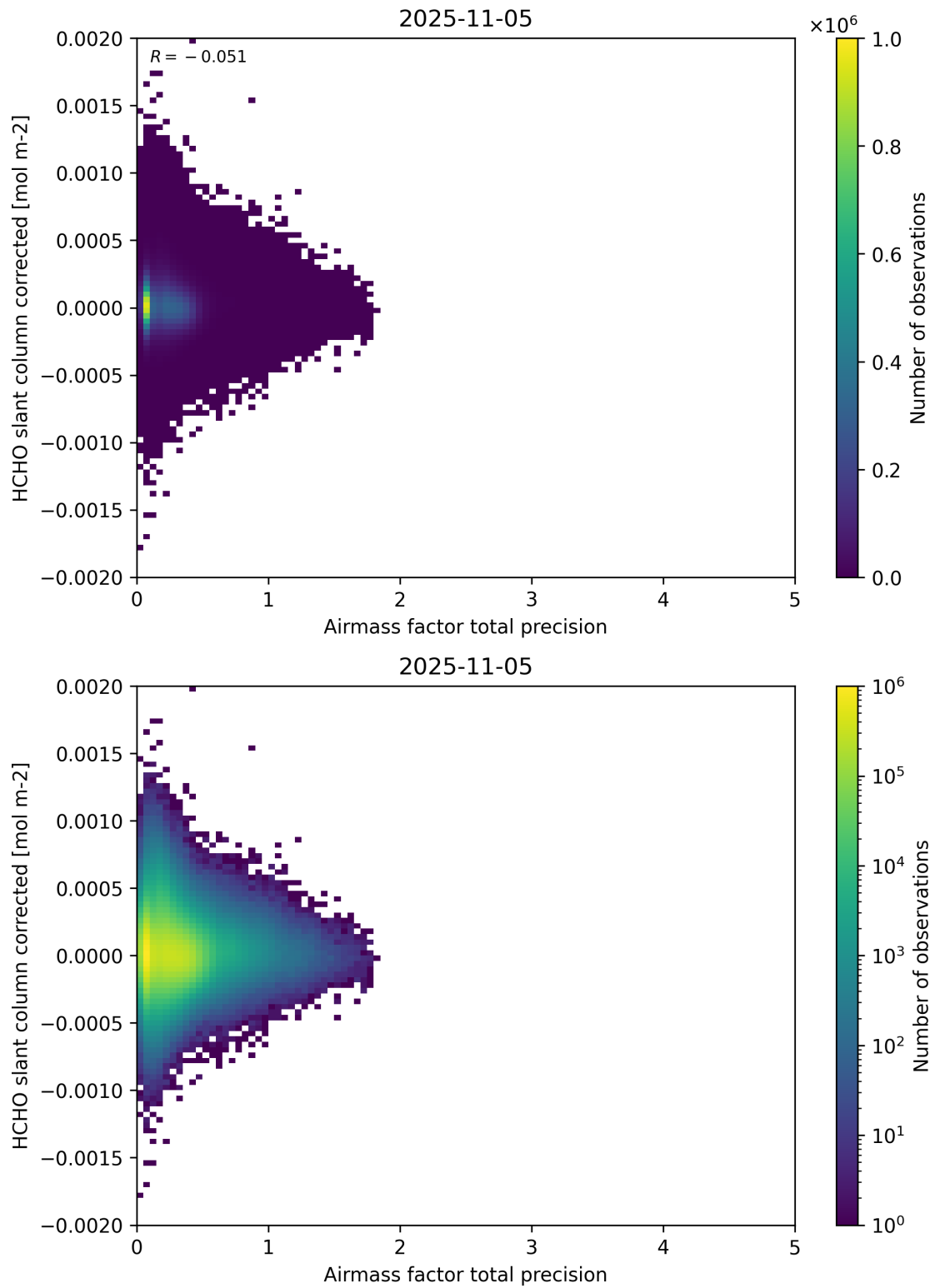
Figure 109: Scatter density plot of “Airmass factor total precision” against “HCHO slant column corrected” for 2025-11-04 to 2025-11-06.
