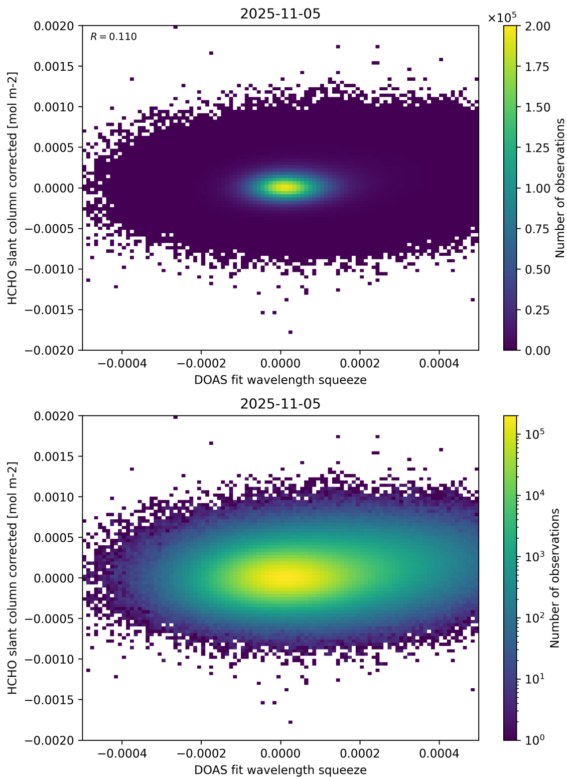
Figure 69: Scatter density plot of “DOAS fit wavelength squeeze” against “HCHO slant column corrected” for 2025-11-04 to 2025-11-06.
