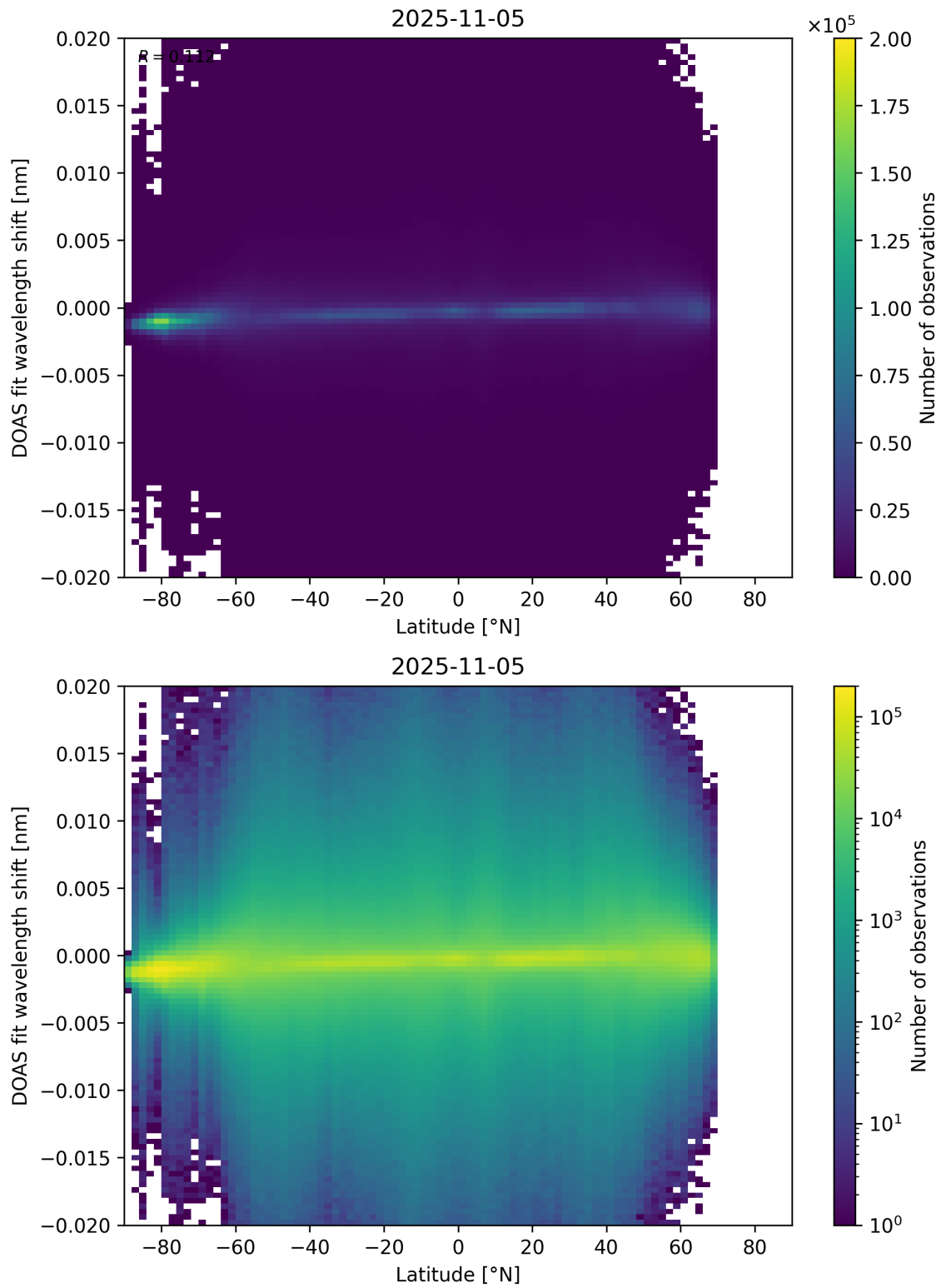
Figure 154: Scatter density plot of “Latitude” against “DOAS fit wavelength shift” for 2025-11-04 to 2025-11-06.
