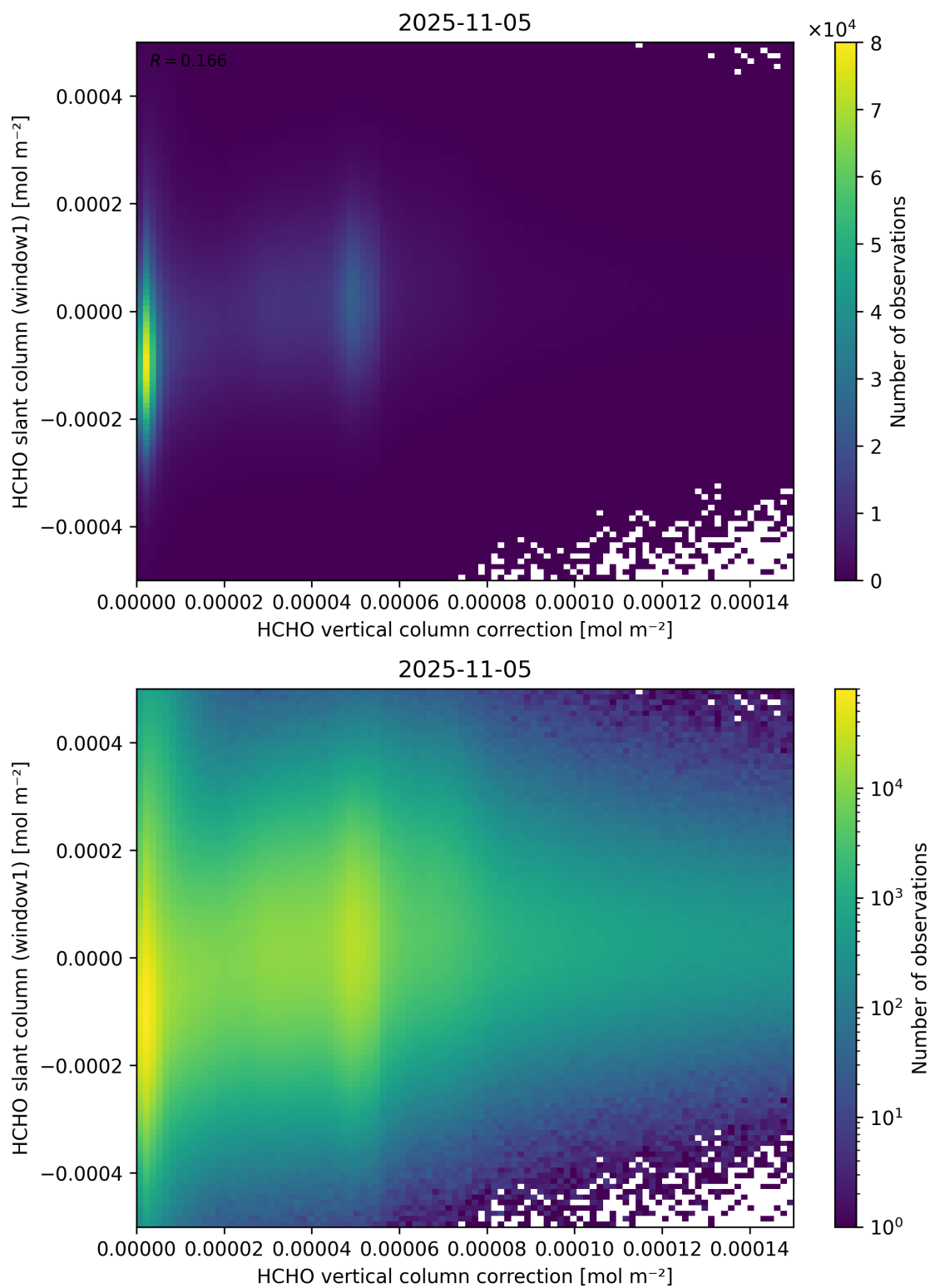
Figure 118: Scatter density plot of “HCHO vertical column correction” against “HCHO slant column (window1)” for 2025-11-04 to 2025-11-06.
