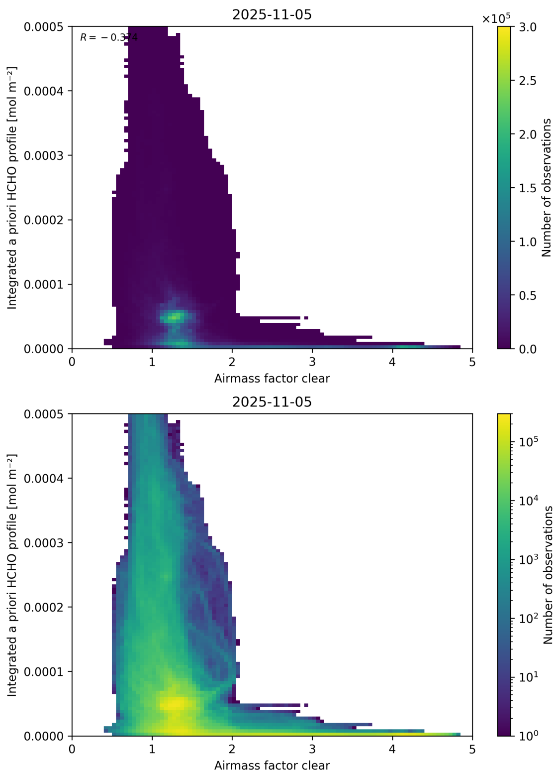
Figure 76: Scatter density plot of “Airmass factor clear” against “Integrated a priori HCHO profile” for 2025-11-04 to 2025-11-06.
