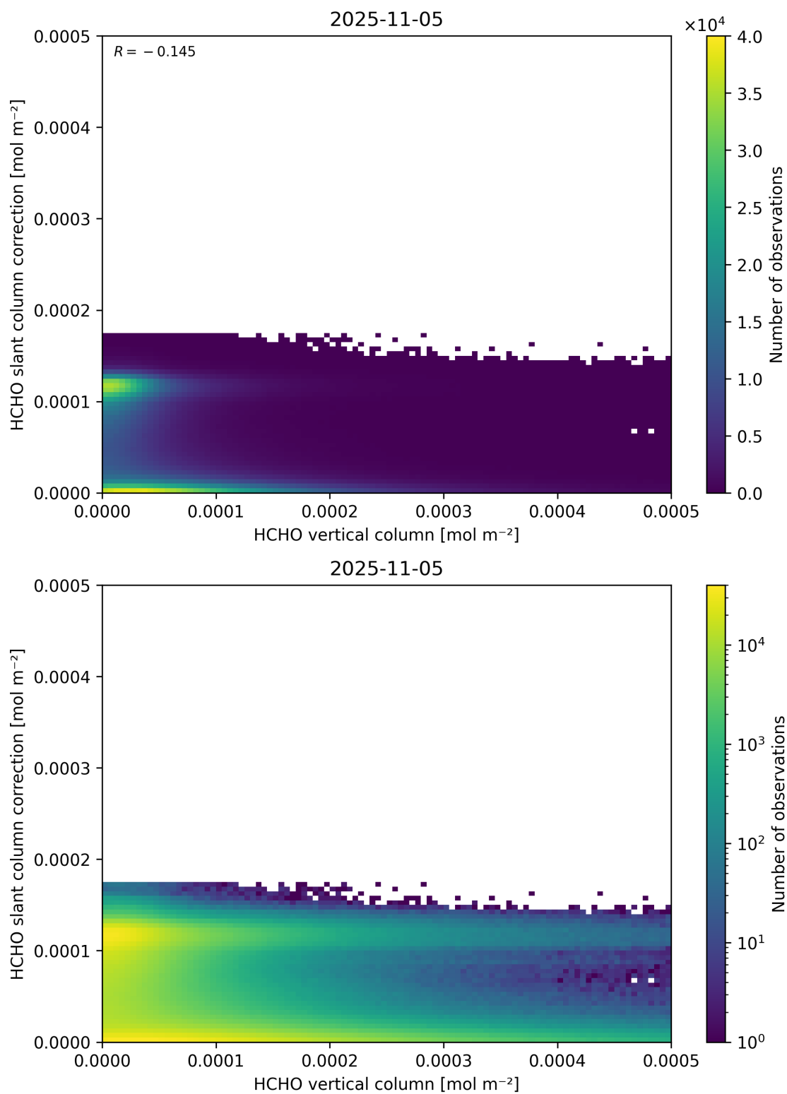
Figure 128: Scatter density plot of “HCHO vertical column” against “HCHO slant column correction” for 2025-11-04 to 2025-11-06.
