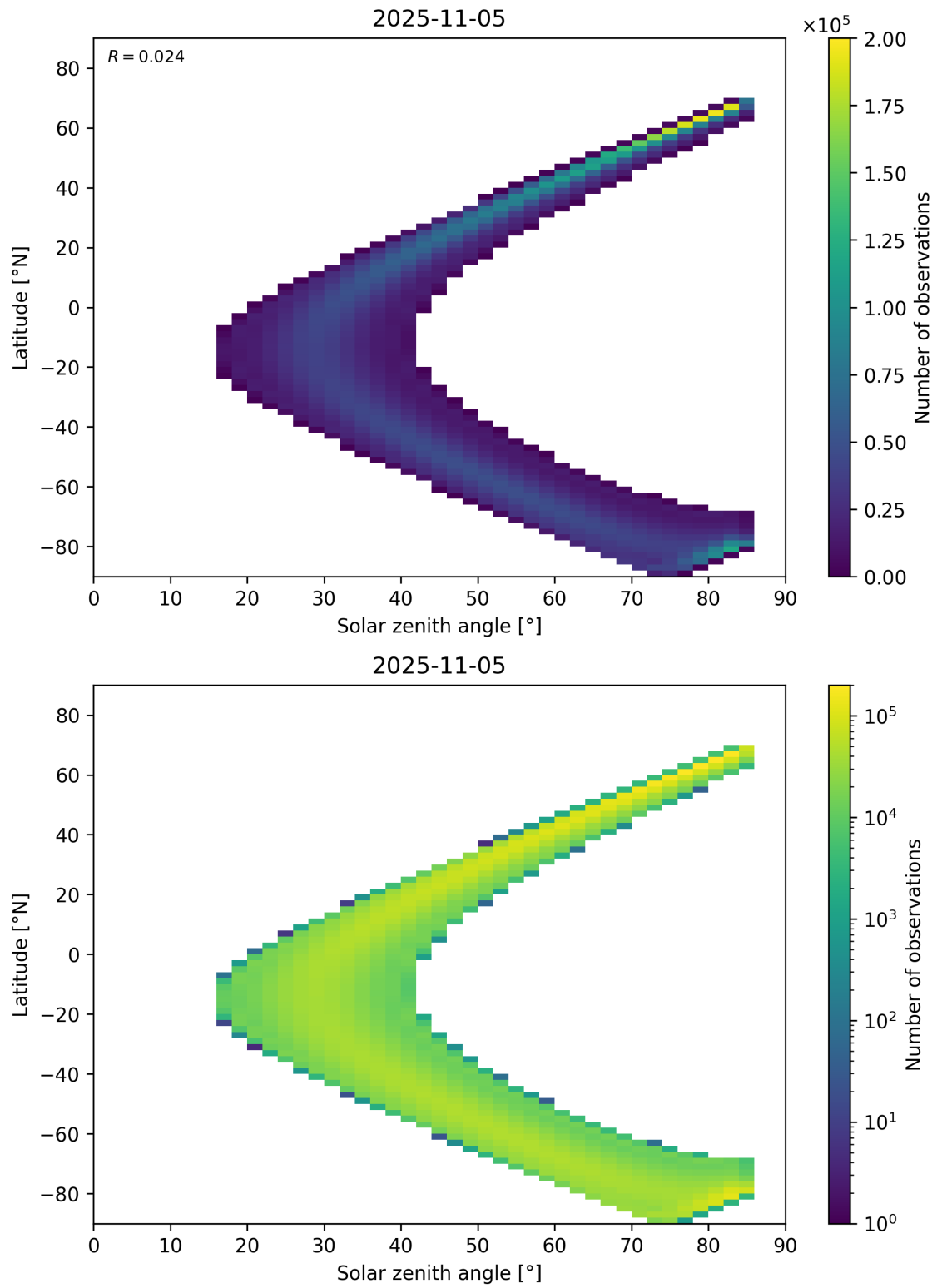
Figure 181: Scatter density plot of “Solar zenith angle” against “Latitude” for 2025-11-04 to 2025-11-06.
