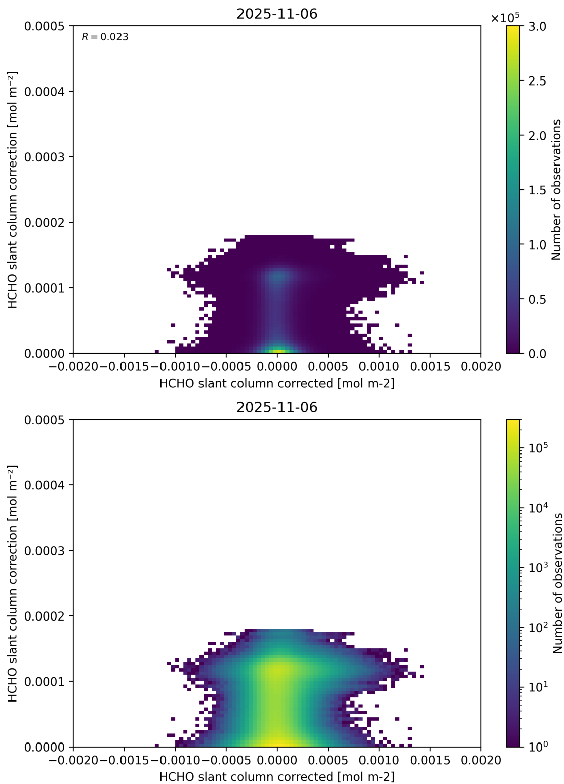
Figure 77: Scatter density plot of “HCHO slant column corrected” against “HCHO slant column correction” for 2025-11-05 to 2025-11-07.
