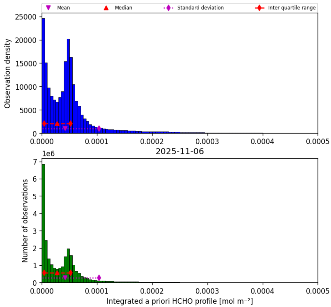
Figure 43: Histogram of “Integrated a priori HCHO profile” for 2025-11-05 to 2025-11-07
