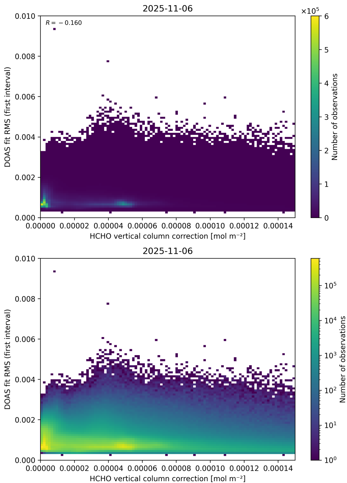
Figure 112: Scatter density plot of “HCHO vertical column correction” against “DOAS fit RMS (first interval)” for 2025-11-05 to 2025-11-07.
