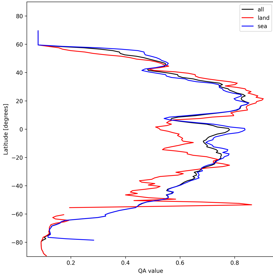
Figure 20: Zonal average of “QA value” for 2025-11-05 to 2025-11-07.
