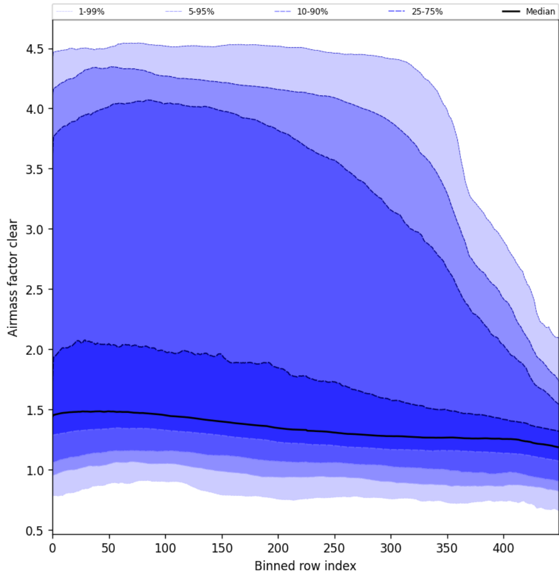
Figure 56: Along track statistics of “Airmass factor clear” for 2025-11-05 to 2025-11-07
