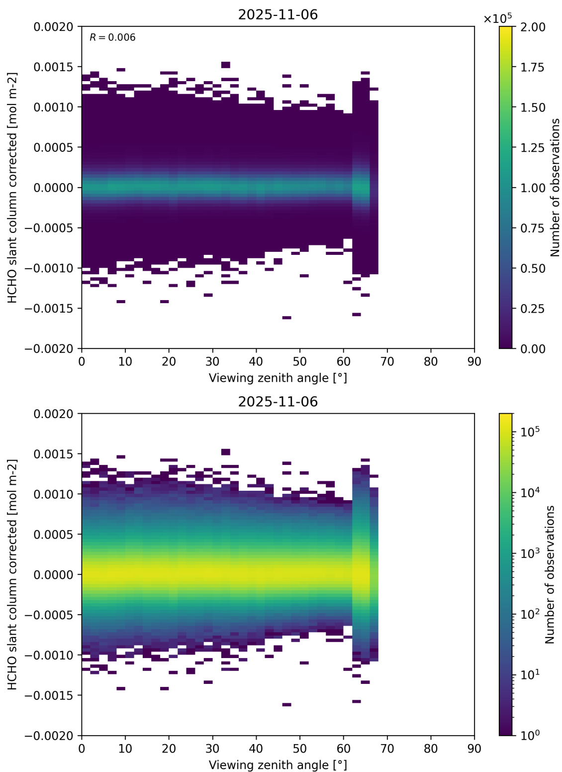
Figure 186: Scatter density plot of “Viewing zenith angle” against “HCHO slant column corrected” for 2025-11-05 to 2025-11-07.
