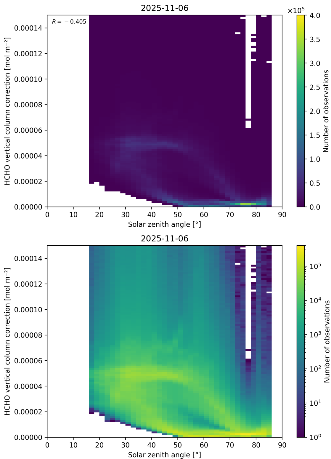
Figure 178: Scatter density plot of “Solar zenith angle” against “HCHO vertical column correction” for 2025-11-05 to 2025-11-07.
