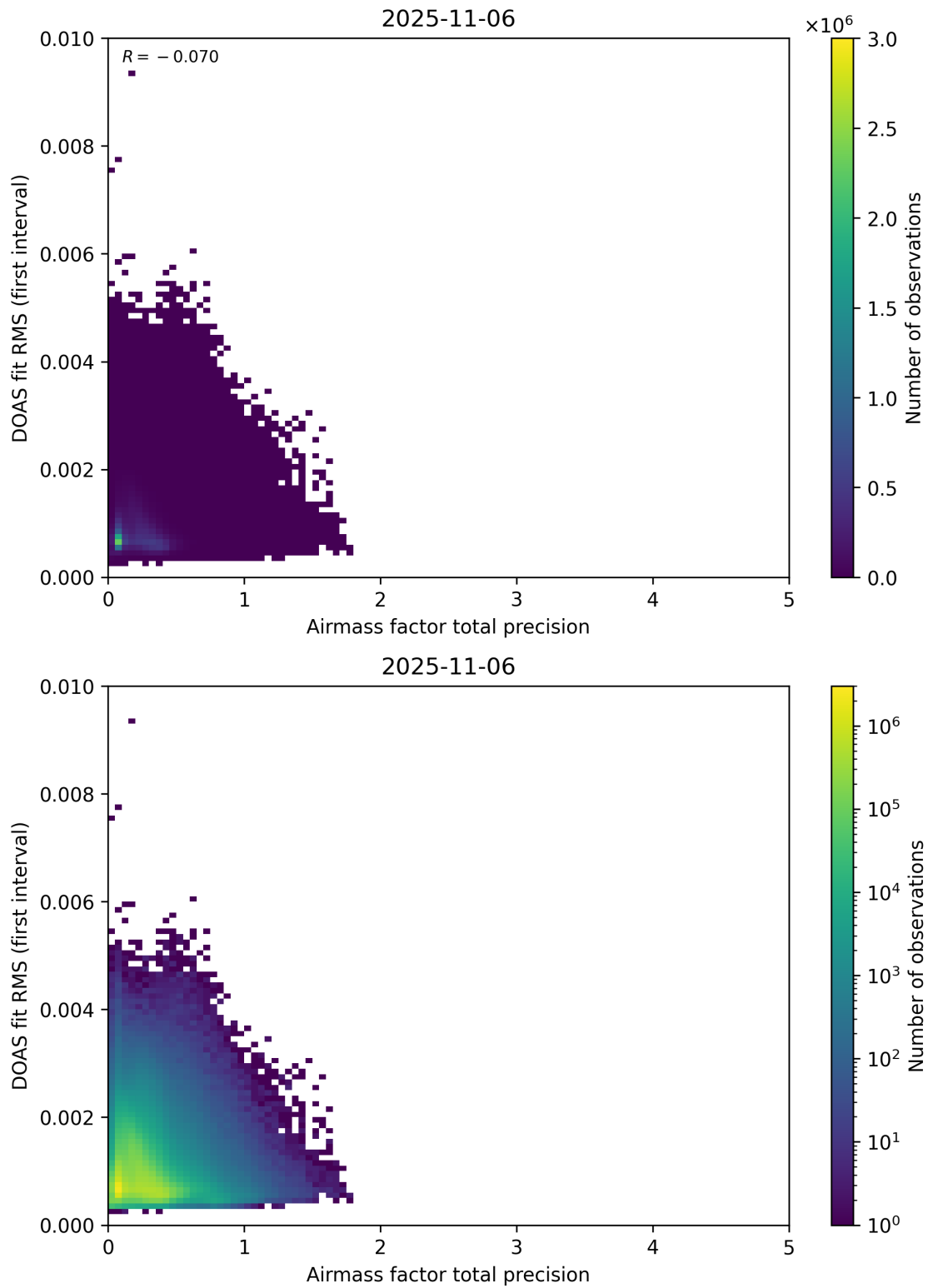
Figure 105: Scatter density plot of “Airmass factor total precision” against “DOAS fit RMS (first interval)” for 2025-11-05 to 2025-11-07.
