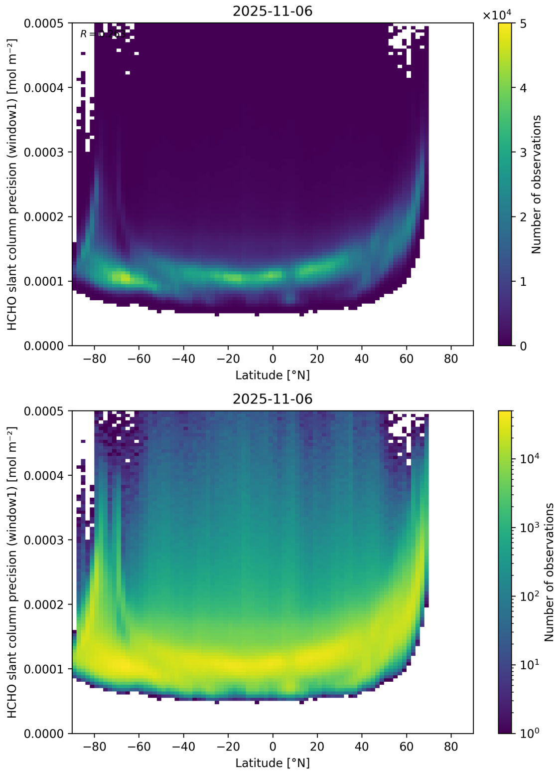
Figure 160: Scatter density plot of “Latitude” against “HCHO slant column precision (window1)” for 2025-11-05 to 2025-11-07.
