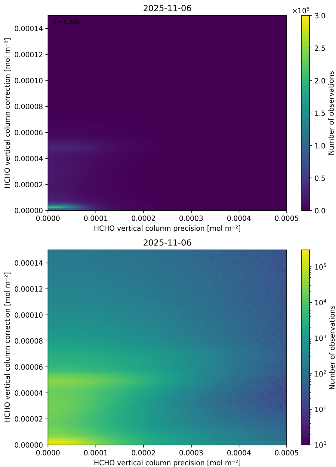
Figure 146: Scatter density plot of “HCHO vertical column precision” against “HCHO vertical column correction” for 2025-11-05 to 2025-11-07.
