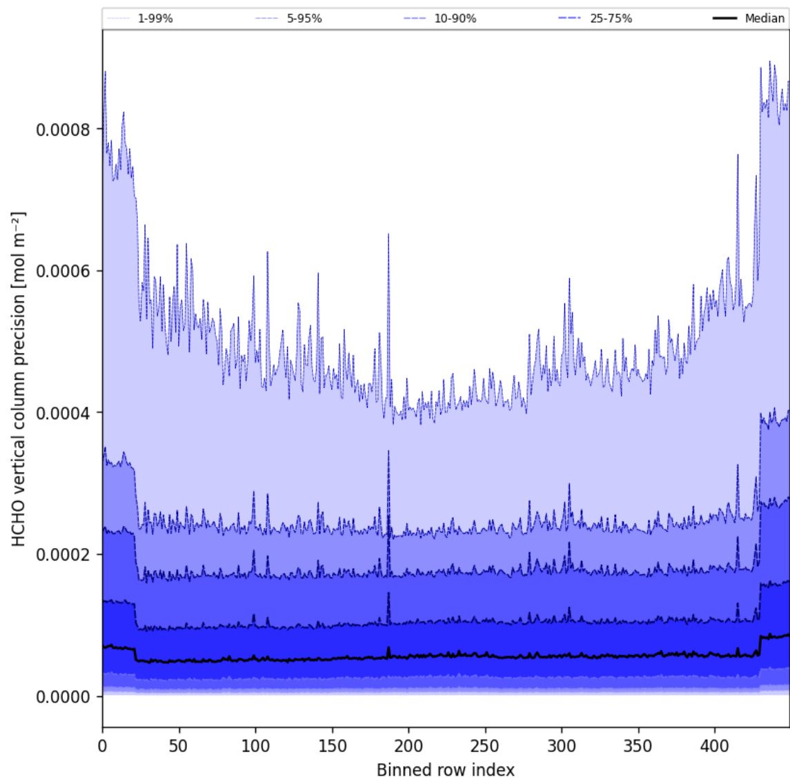
Figure 50: Along track statistics of “HCHO vertical column precision” for 2025-11-05 to 2025-11-07
