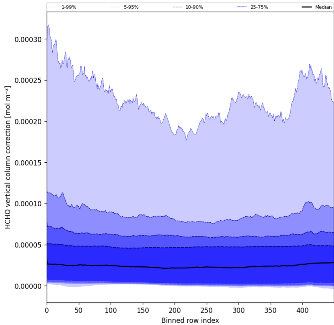
Figure 51: Along track statistics of “HCHO vertical column correction” for 2025-11-05 to 2025-11-07
