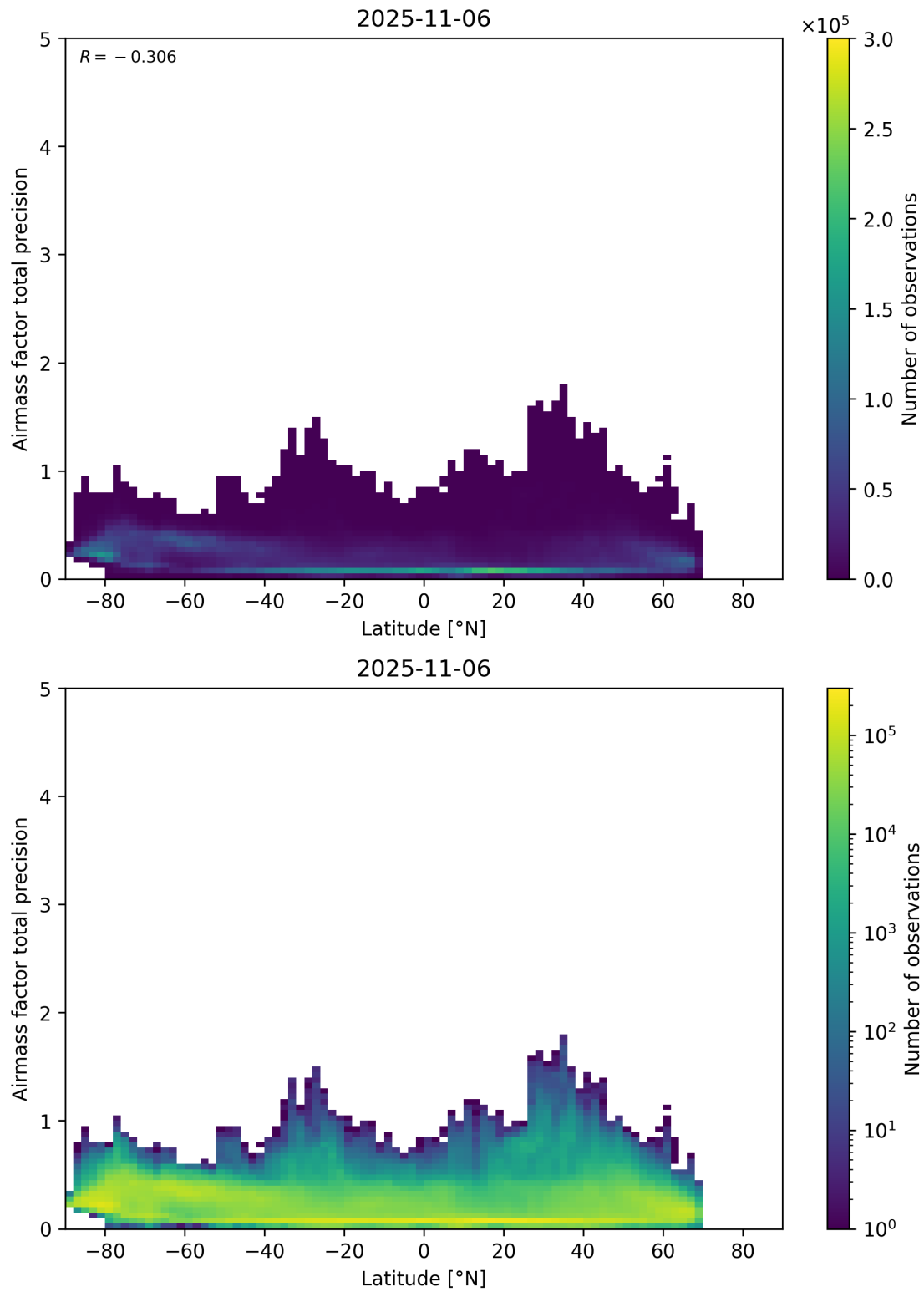
Figure 162: Scatter density plot of “Latitude” against “Airmass factor total precision” for 2025-11-05 to 2025-11-07.
