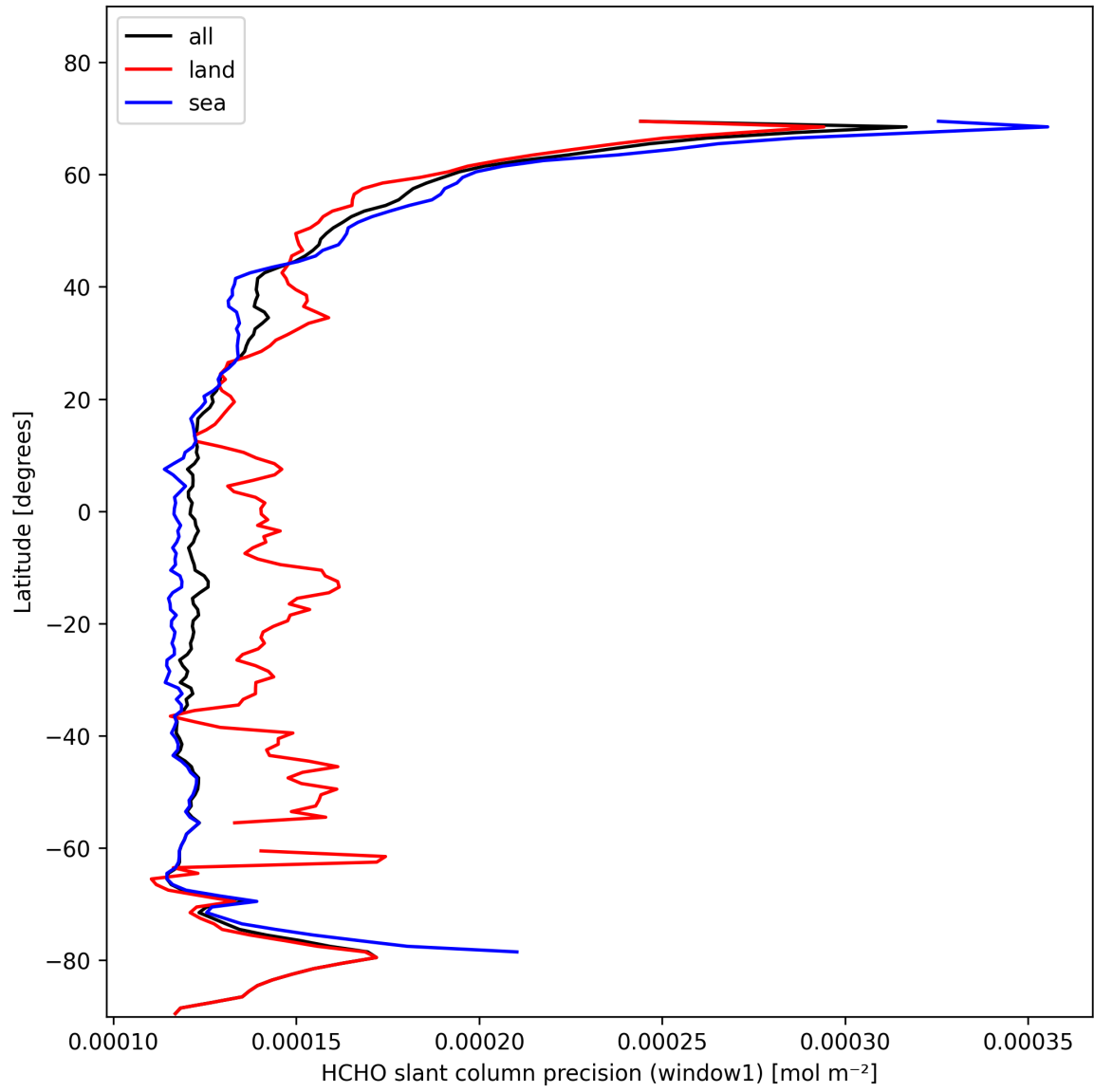
Figure 25: Zonal average of “HCHO slant column precision (window1)” for 2025-11-05 to 2025-11-07.
