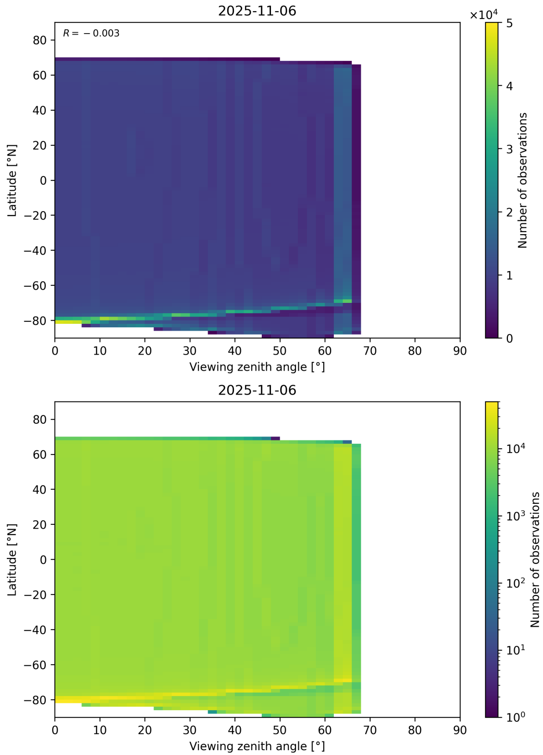
Figure 196: Scatter density plot of “Viewing zenith angle” against “Latitude” for 2025-11-05 to 2025-11-07.
