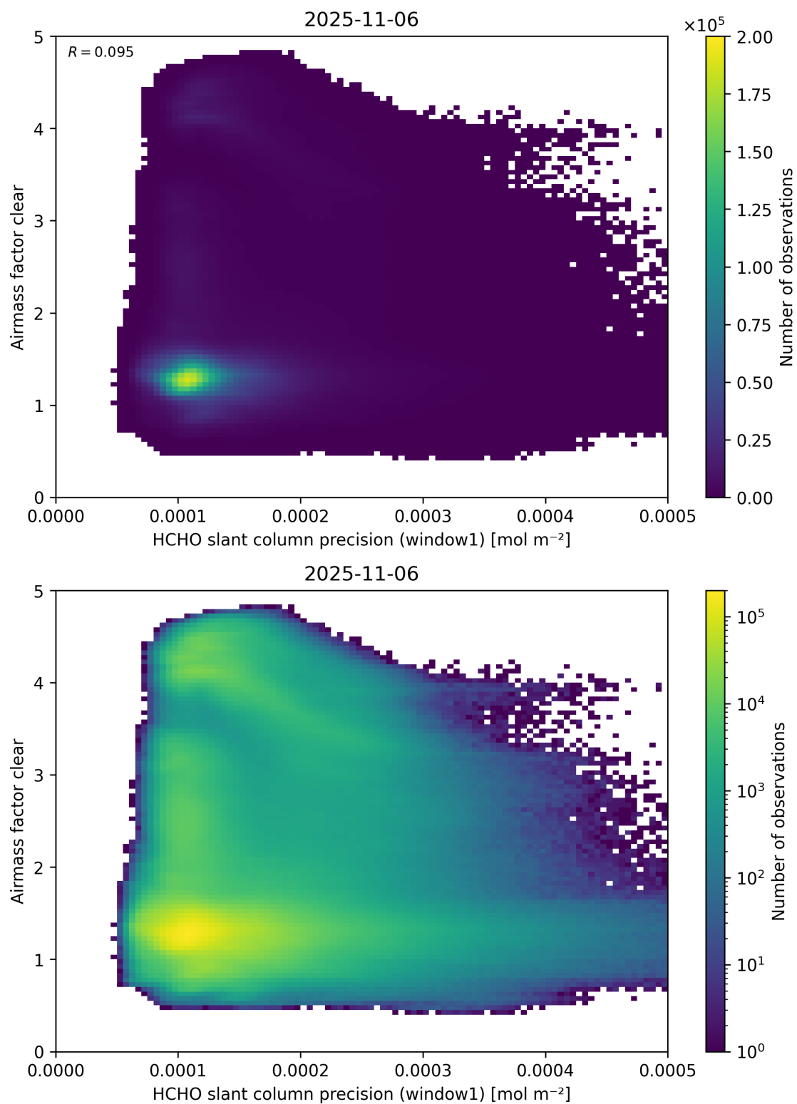
Figure 91: Scatter density plot of “HCHO slant column precision (window1)” against “Airmass factor clear” for 2025-11-05 to 2025-11-07.
