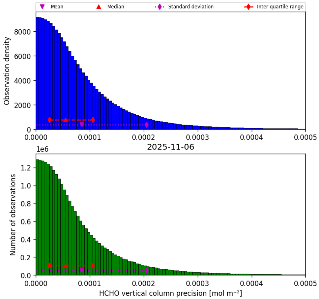
Figure 36: Histogram of “HCHO vertical column precision” for 2025-11-05 to 2025-11-07
