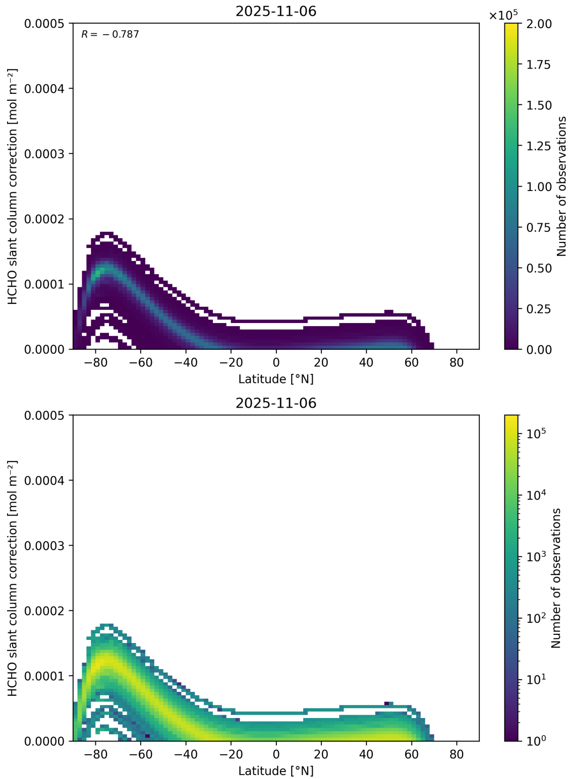
Figure 158: Scatter density plot of “Latitude” against “HCHO slant column correction” for 2025-11-05 to 2025-11-07.
