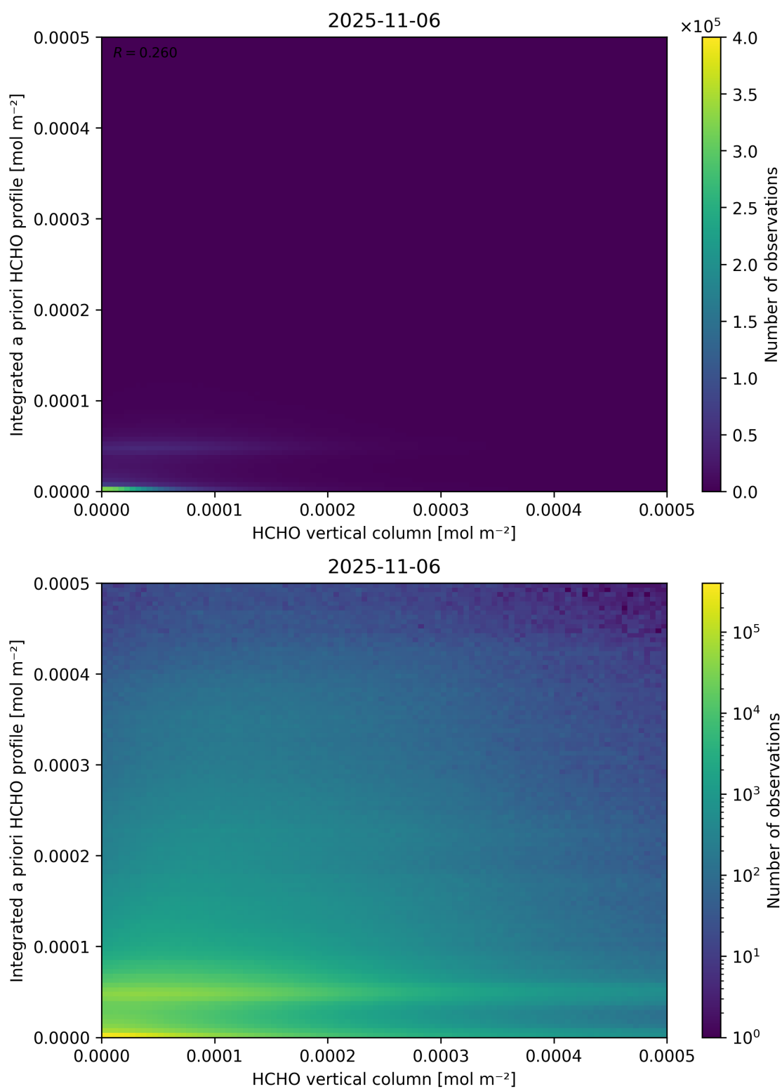
Figure 135: Scatter density plot of “HCHO vertical column” against “Integrated a priori HCHO profile” for 2025-11-05 to 2025-11-07.
