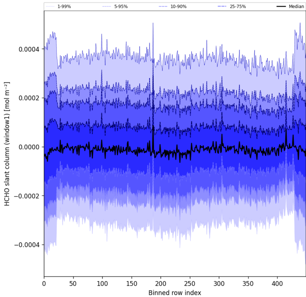
Figure 52: Along track statistics of “HCHO slant column (window1)” for 2025-11-05 to 2025-11-07
