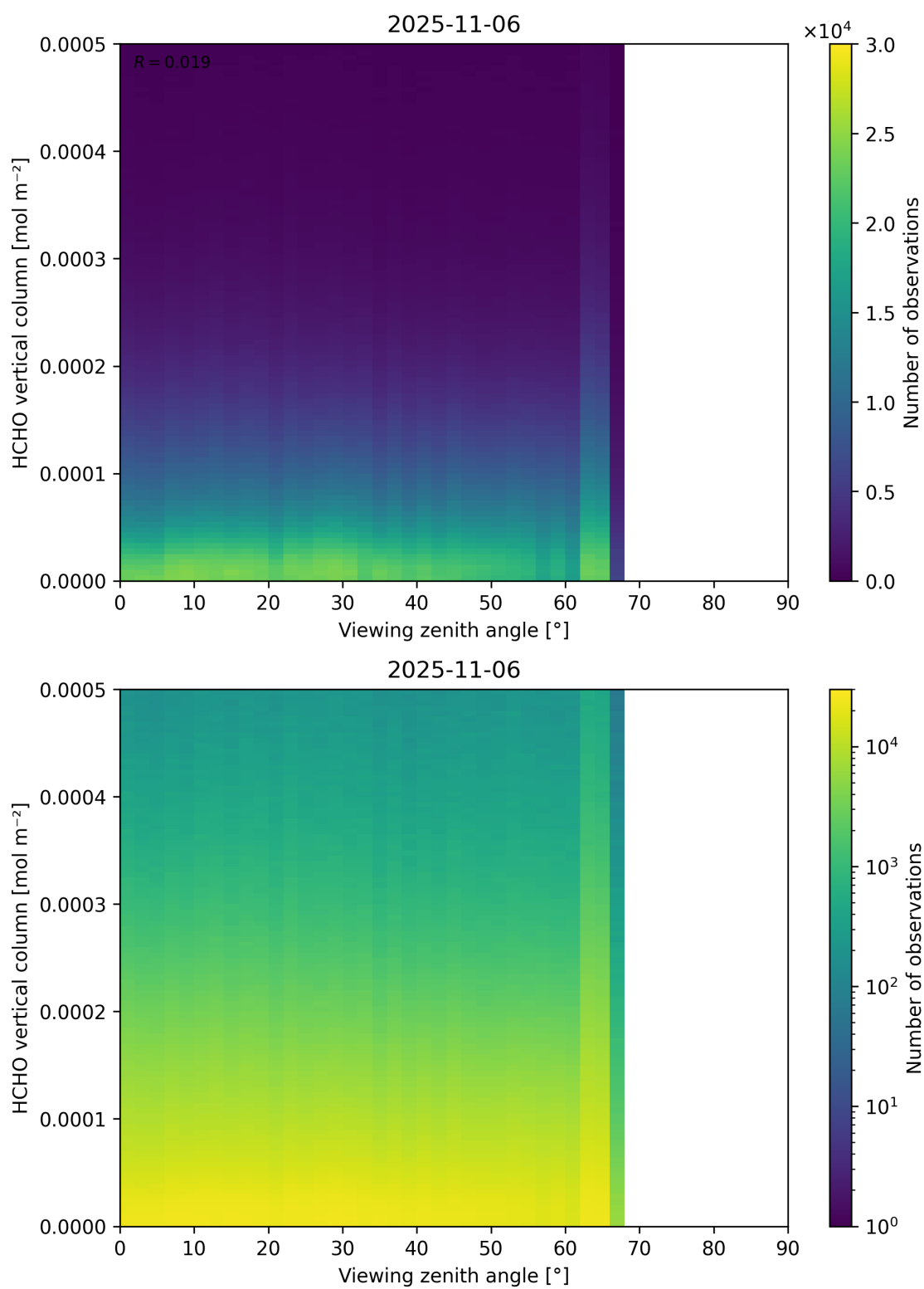
Figure 192: Scatter density plot of “Viewing zenith angle” against “HCHO vertical column” for 2025-11-05 to 2025-11-07.
