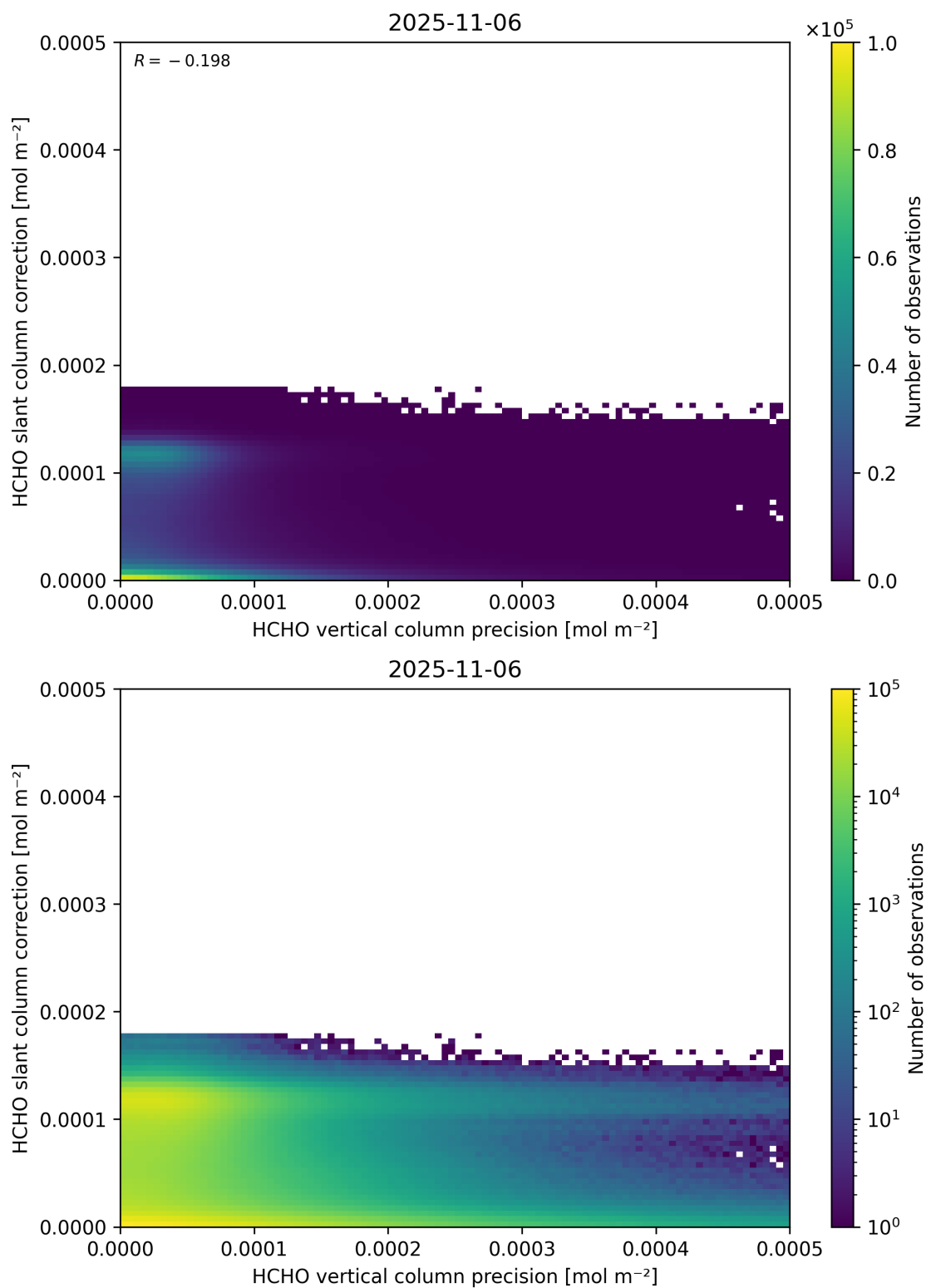
Figure 141: Scatter density plot of “HCHO vertical column precision” against “HCHO slant column correction” for 2025-11-05 to 2025-11-07.
