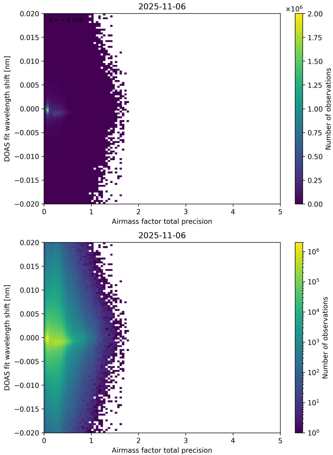
Figure 106: Scatter density plot of “Airmass factor total precision” against “DOAS fit wavelength shift” for 2025-11-05 to 2025-11-07.
