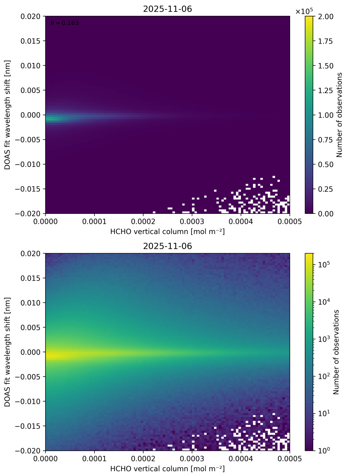
Figure 124: Scatter density plot of “HCHO vertical column” against “DOAS fit wavelength shift” for 2025-11-05 to 2025-11-07.
