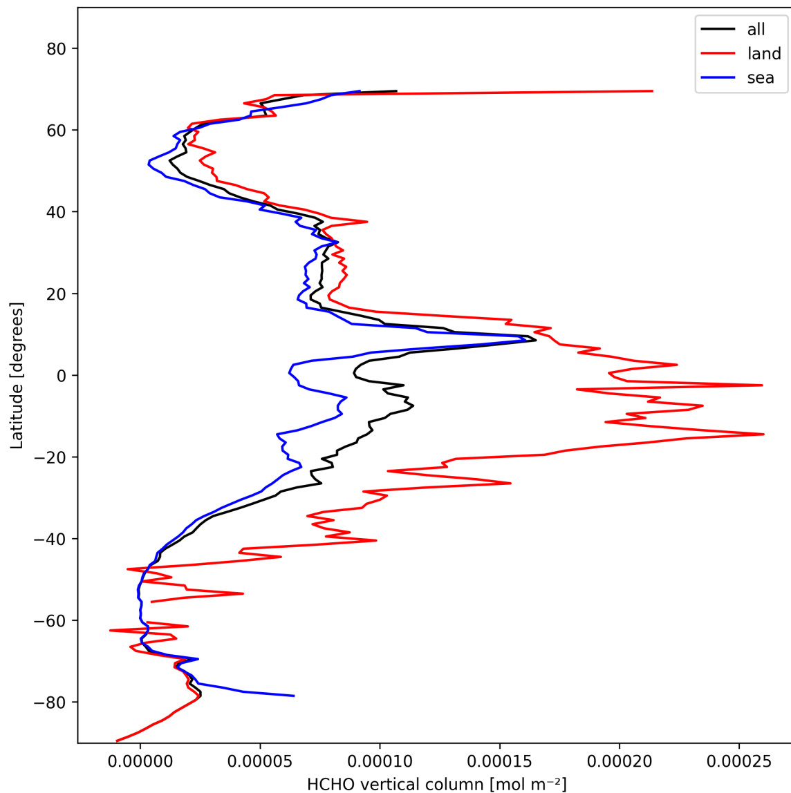
Figure 21: Zonal average of “HCHO vertical column” for 2025-11-05 to 2025-11-07.
