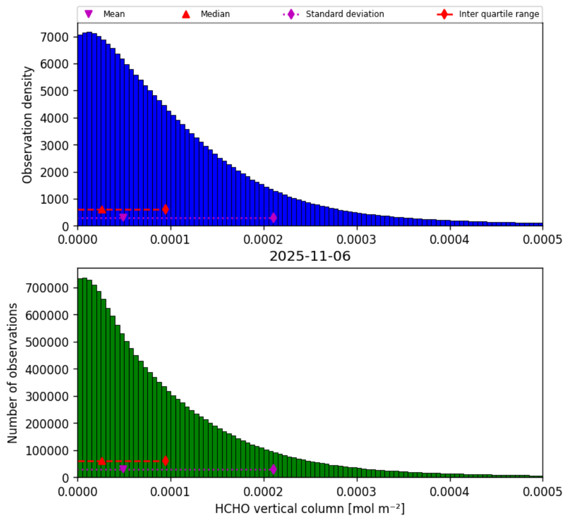
Figure 35: Histogram of “HCHO vertical column” for 2025-11-05 to 2025-11-07
