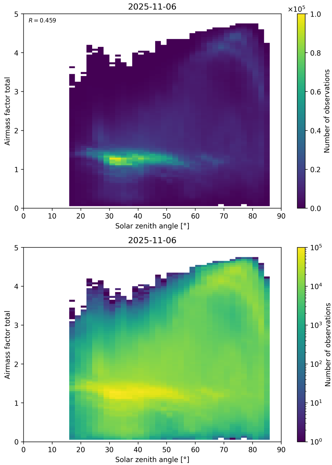
Figure 175: Scatter density plot of “Solar zenith angle” against “Airmass factor total” for 2025-11-05 to 2025-11-07.
