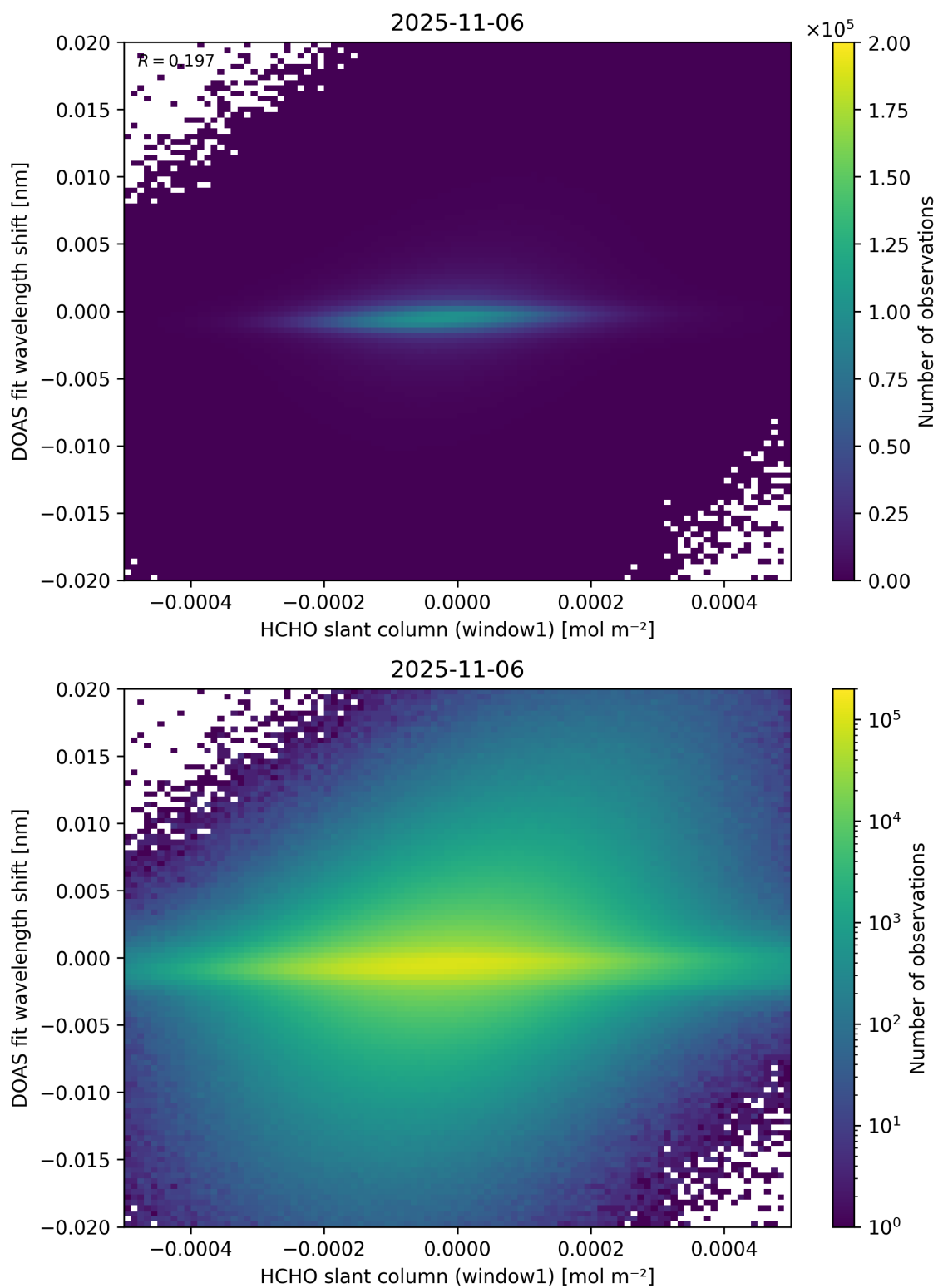
Figure 79: Scatter density plot of “HCHO slant column (window1)” against “DOAS fit wavelength shift” for 2025-11-05 to 2025-11-07.
