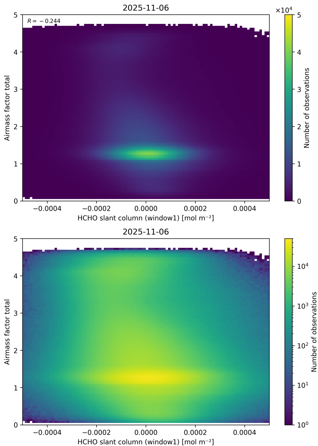
Figure 85: Scatter density plot of “HCHO slant column (window1)” against “Airmass factor total” for 2025-11-05 to 2025-11-07.
