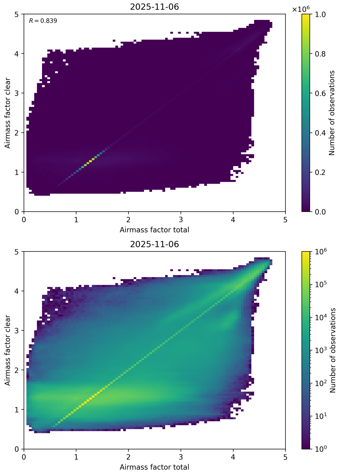
Figure 100: Scatter density plot of “Airmass factor total” against “Airmass factor clear” for 2025-11-05 to 2025-11-07.
