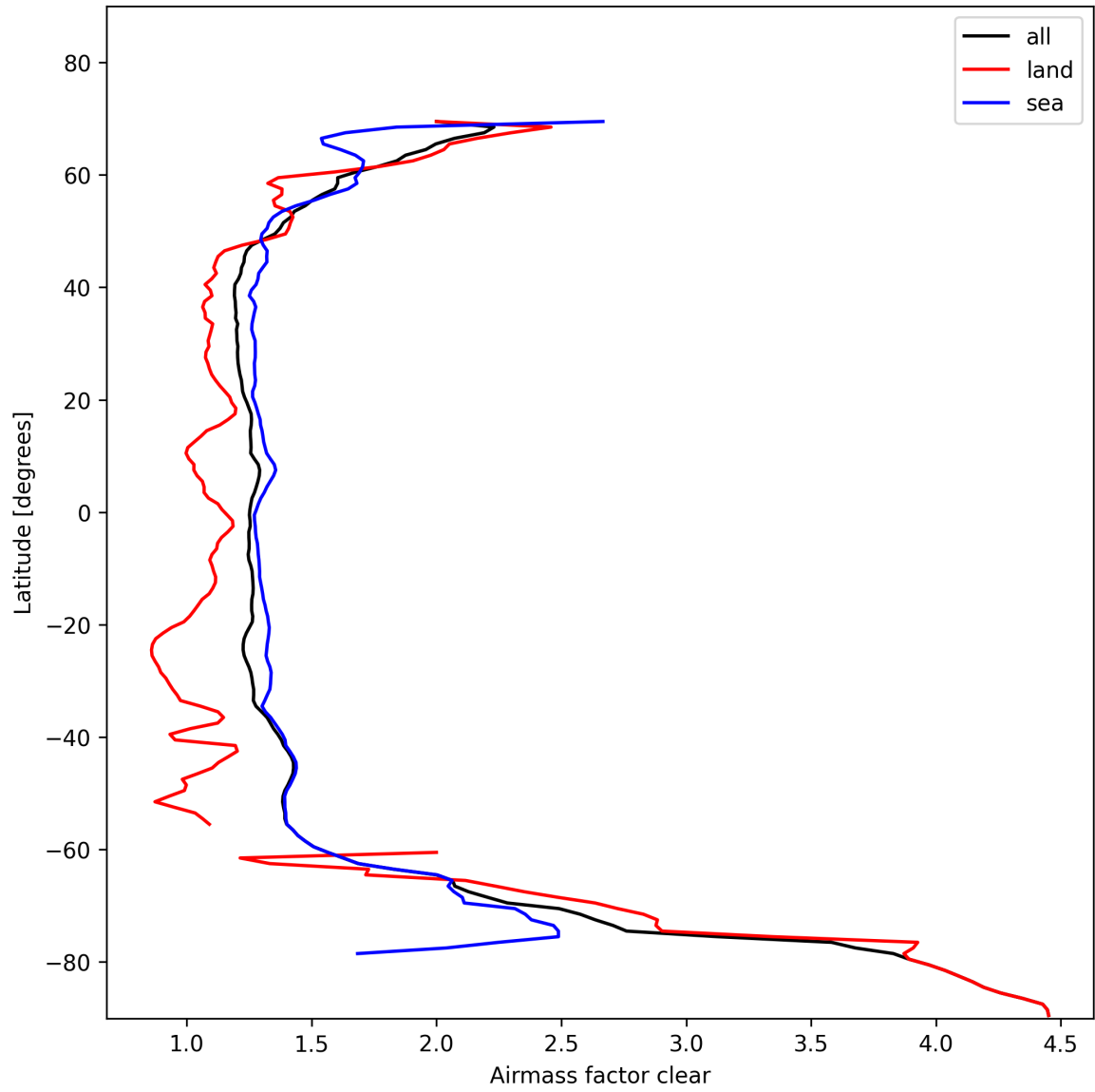
Figure 28: Zonal average of “Airmass factor clear” for 2025-11-05 to 2025-11-07.
