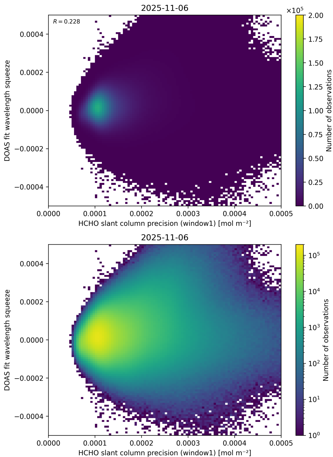
Figure 90: Scatter density plot of “HCHO slant column precision (window1)” against “DOAS fit wavelength squeeze” for 2025-11-05 to 2025-11-07.
