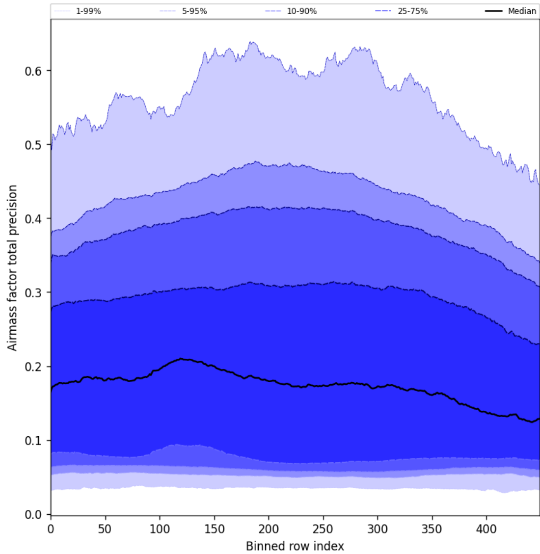
Figure 55: Along track statistics of “Airmass factor total precision” for 2025-11-05 to 2025-11-07
