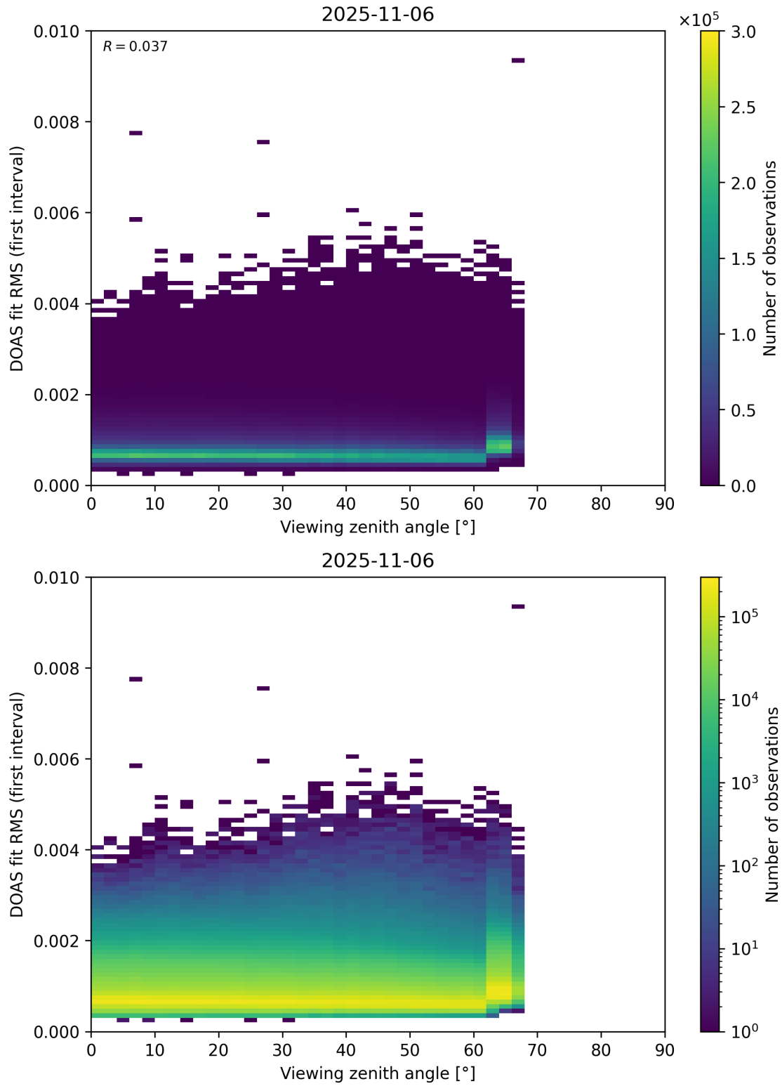
Figure 182: Scatter density plot of “Viewing zenith angle” against “DOAS fit RMS (first interval)” for 2025-11-05 to 2025-11-07.
