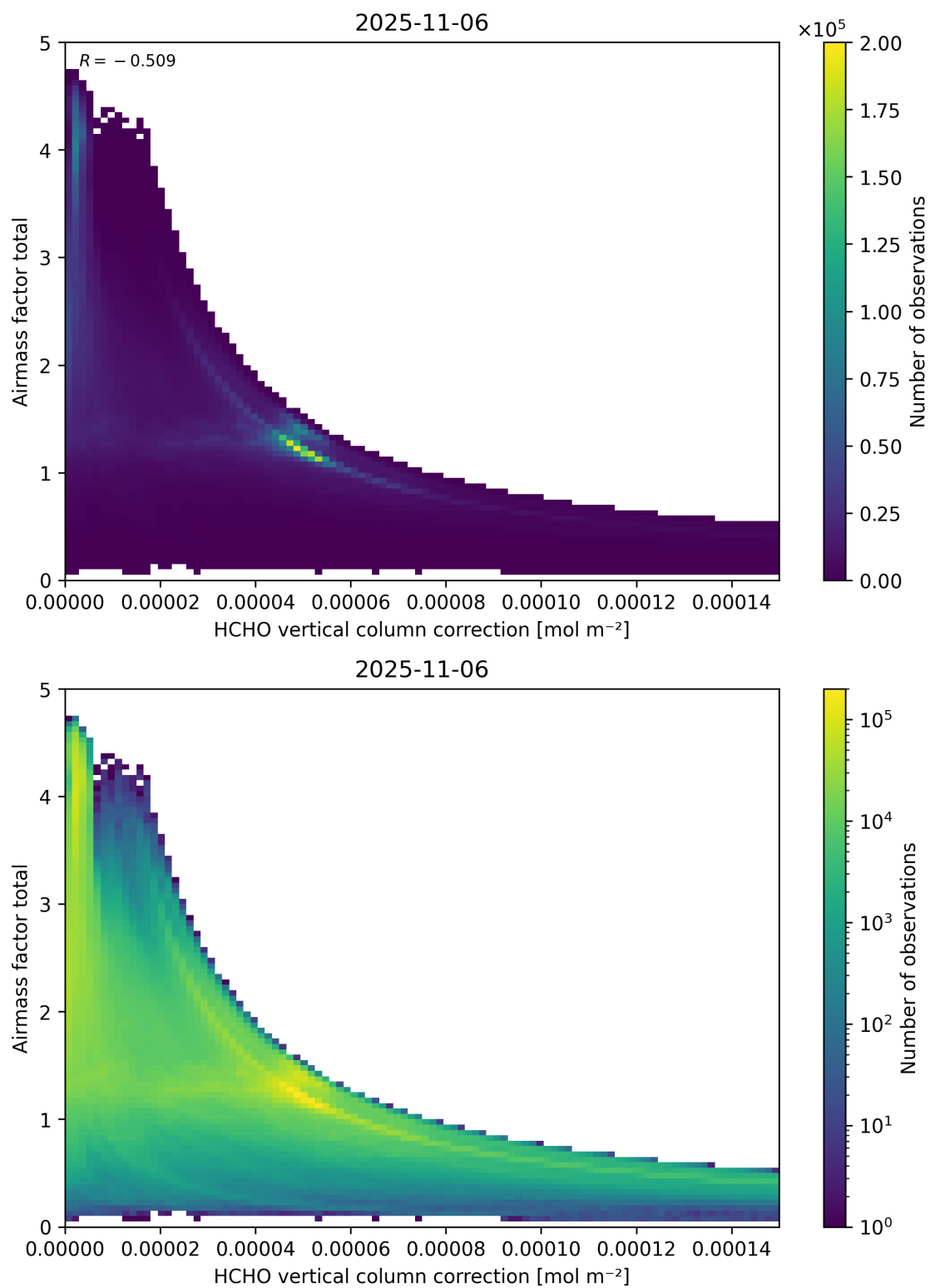
Figure 120: Scatter density plot of “HCHO vertical column correction” against “Airmass factor total” for 2025-11-05 to 2025-11-07.
