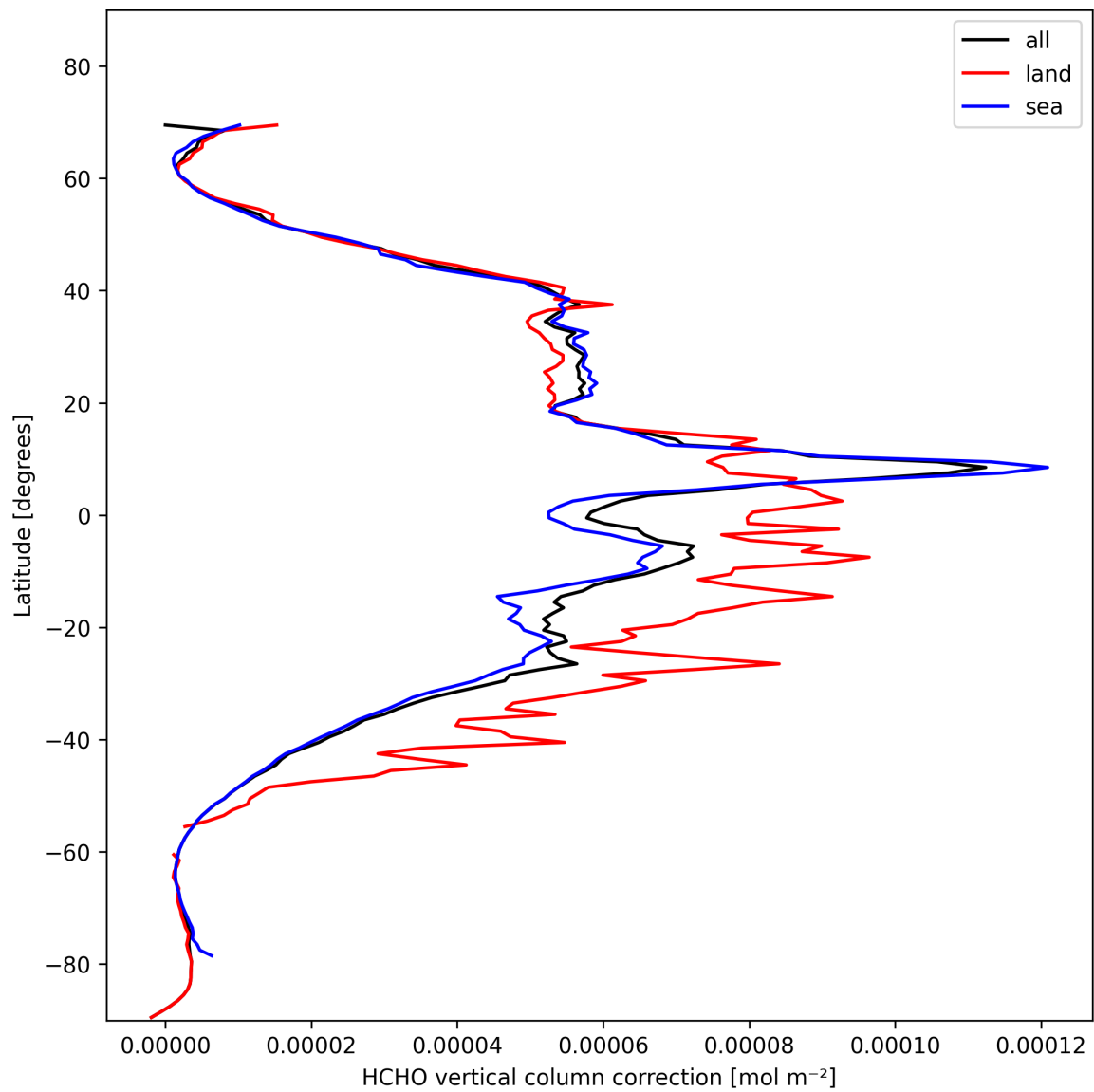
Figure 23: Zonal average of “HCHO vertical column correction” for 2025-11-05 to 2025-11-07.
