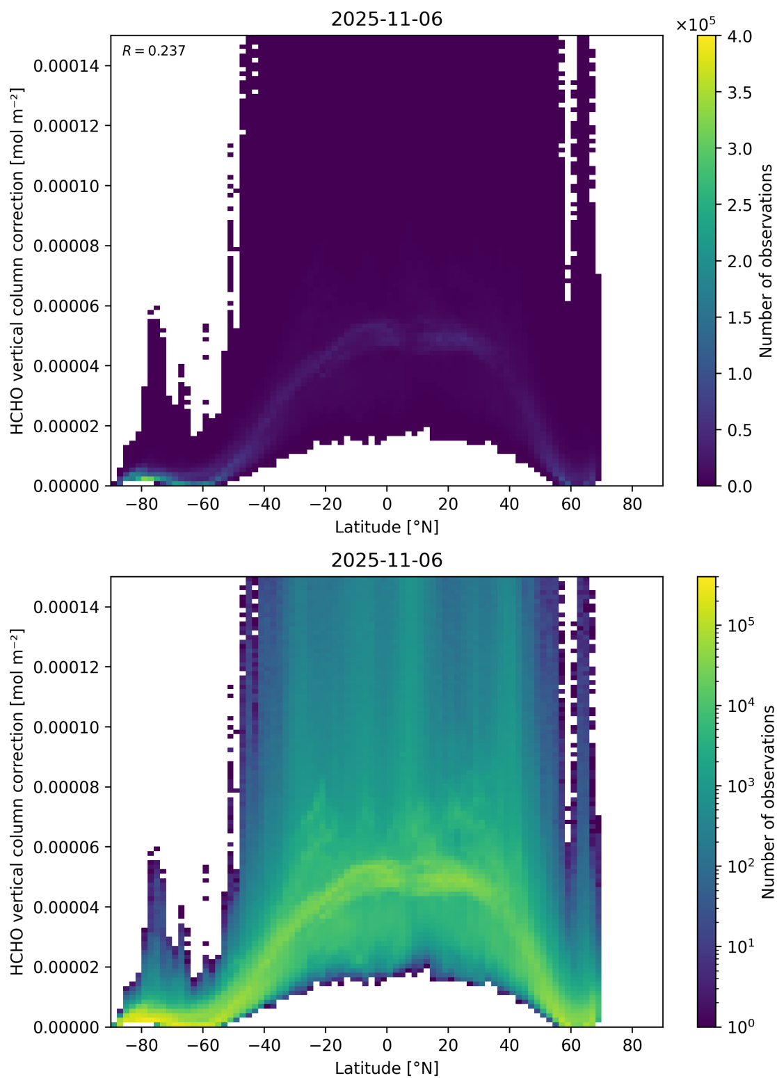
Figure 164: Scatter density plot of “Latitude” against “HCHO vertical column correction” for 2025-11-05 to 2025-11-07.
