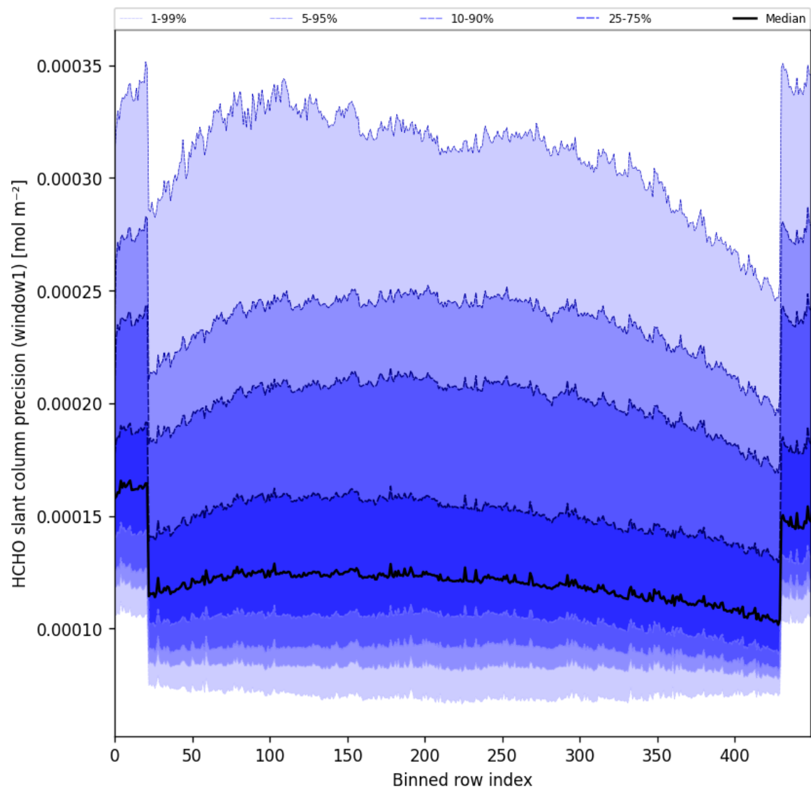
Figure 53: Along track statistics of “HCHO slant column precision (window1)” for 2025-11-05 to 2025-11-07
