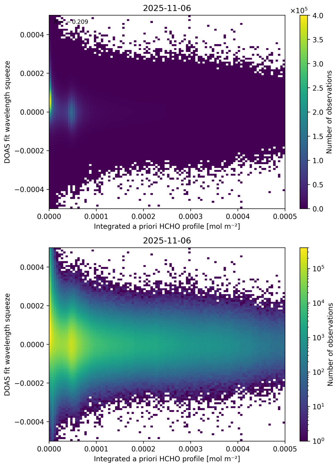
Figure 150: Scatter density plot of “Integrated a priori HCHO profile” against “DOAS fit wavelength squeeze” for 2025-11-05 to 2025-11-07.
