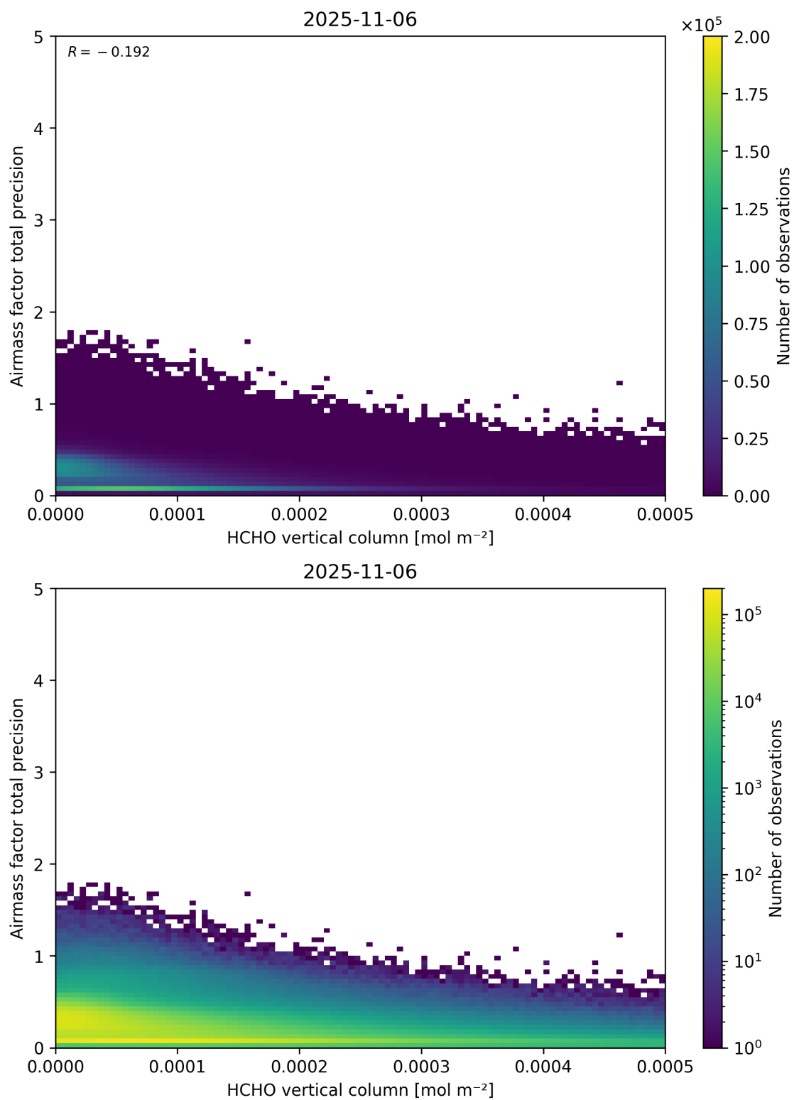
Figure 132: Scatter density plot of “HCHO vertical column” against “Airmass factor total precision” for 2025-11-05 to 2025-11-07.
