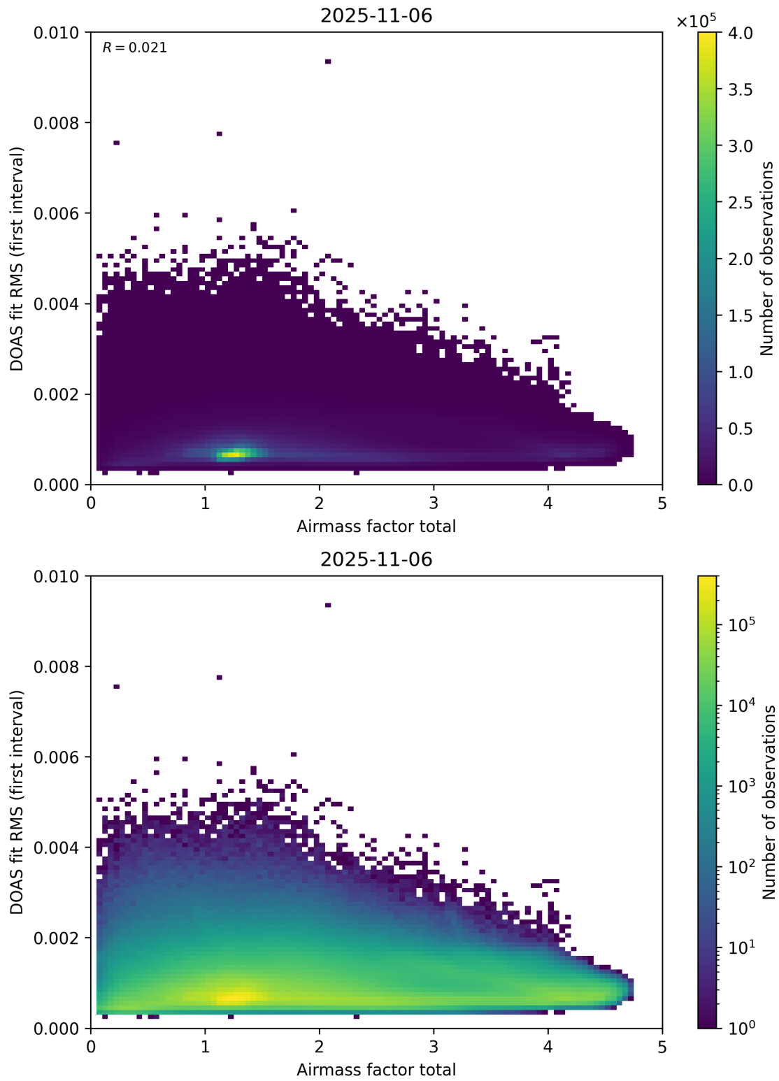
Figure 97: Scatter density plot of “Airmass factor total” against “DOAS fit RMS (first interval)” for 2025-11-05 to 2025-11-07.
