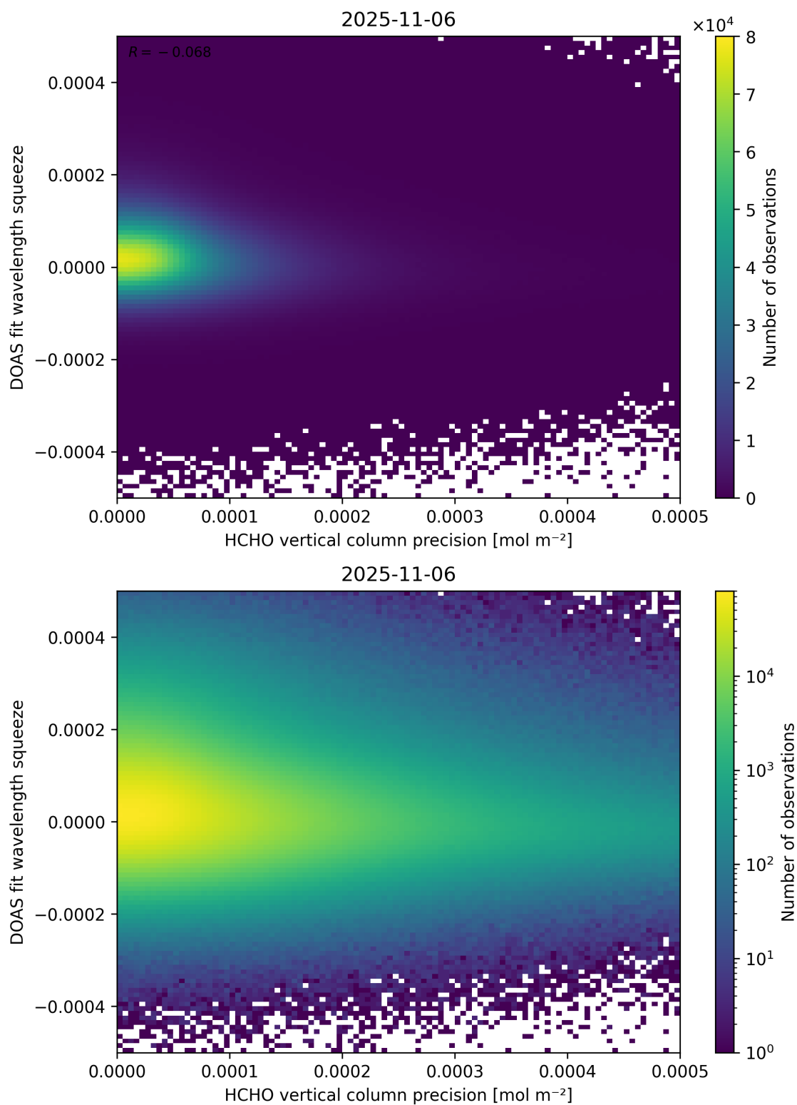
Figure 138: Scatter density plot of “HCHO vertical column precision” against “DOAS fit wavelength squeeze” for 2025-11-05 to 2025-11-07.
