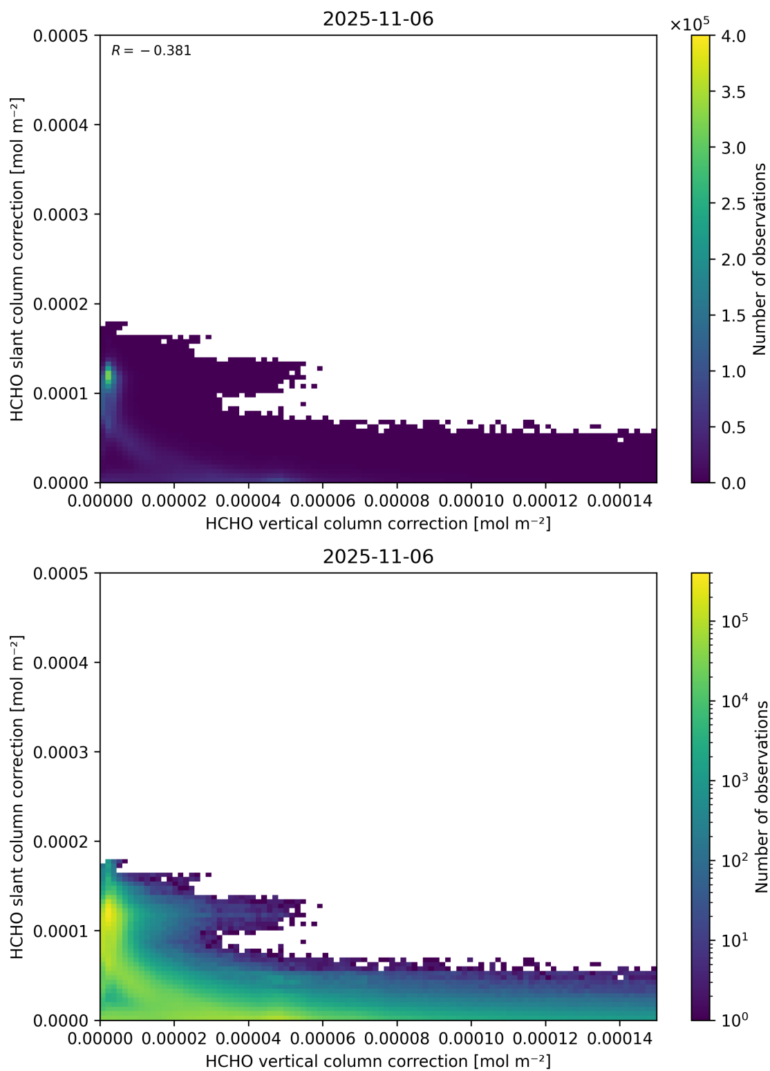
Figure 117: Scatter density plot of “HCHO vertical column correction” against “HCHO slant column correction” for 2025-11-05 to 2025-11-07.
