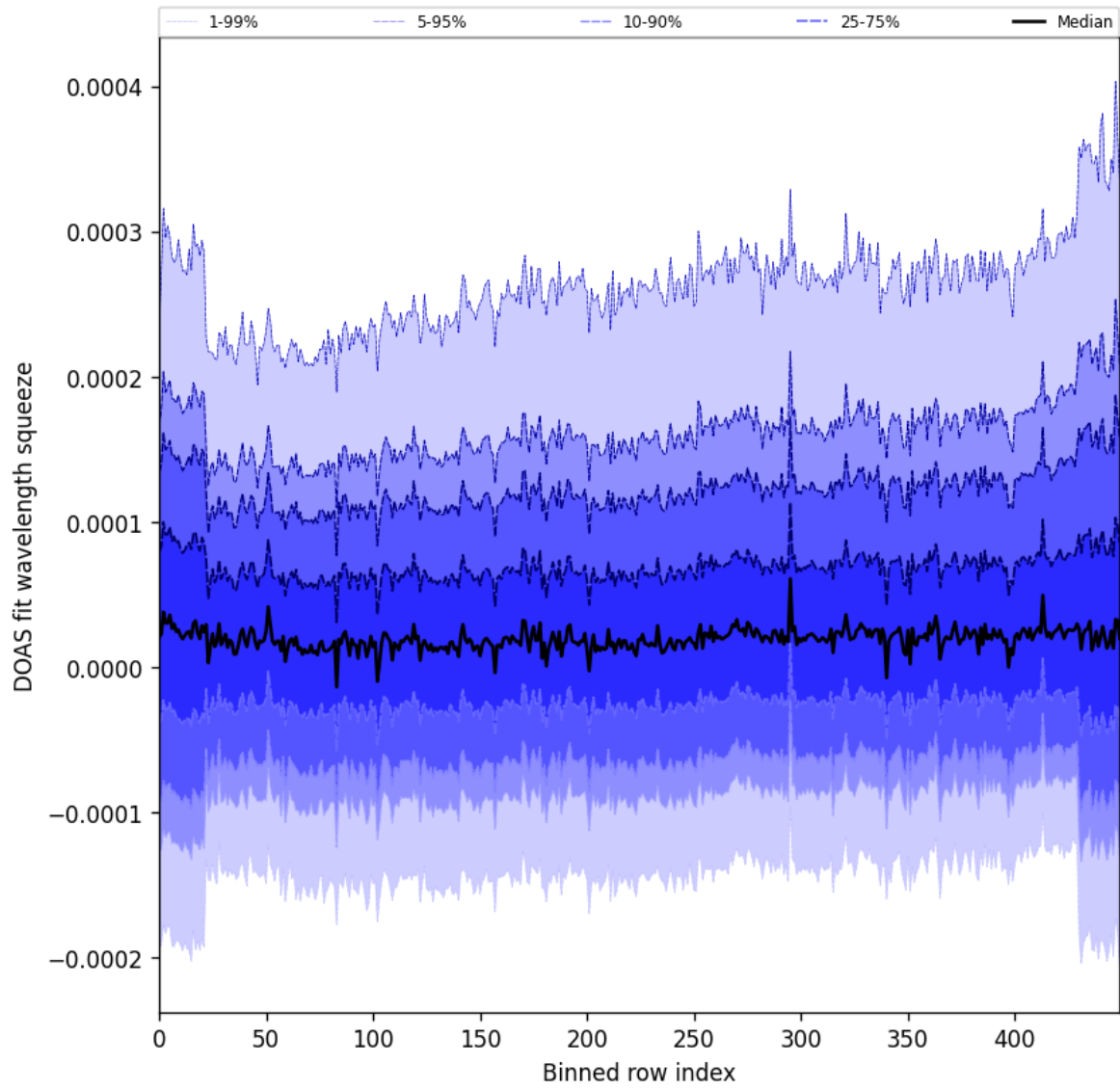
Figure 59: Along track statistics of “DOAS fit wavelength squeeze” for 2025-11-05 to 2025-11-07
