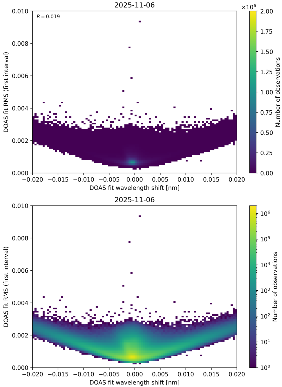
Figure 64: Scatter density plot of “DOAS fit wavelength shift” against “DOAS fit RMS (first interval)” for 2025-11-05 to 2025-11-07.
