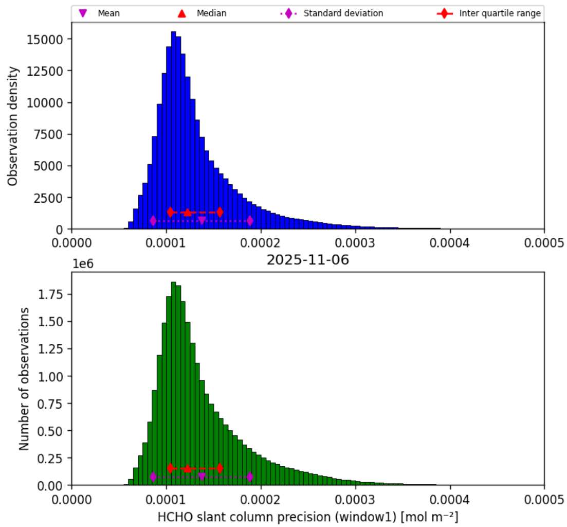
Figure 39: Histogram of “HCHO slant column precision (window1)” for 2025-11-05 to 2025-11-07
