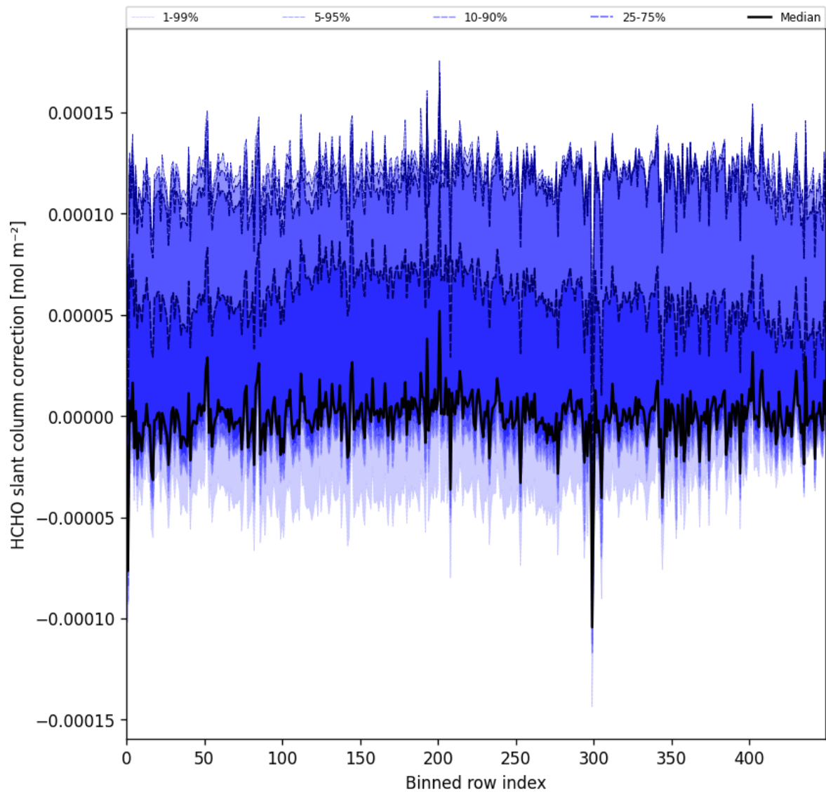
Figure 61: Along track statistics of “HCHO slant column correction” for 2025-11-05 to 2025-11-07
