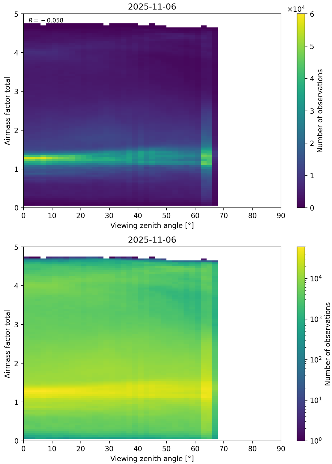
Figure 190: Scatter density plot of “Viewing zenith angle” against “Airmass factor total” for 2025-11-05 to 2025-11-07.
