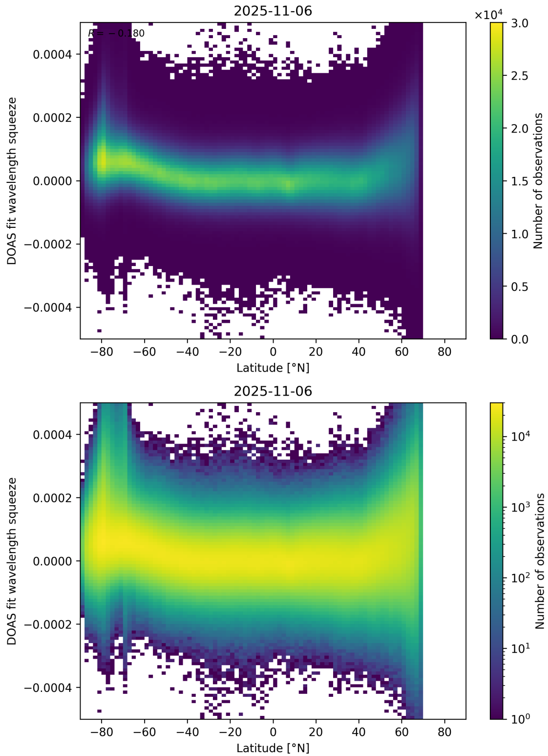
Figure 155: Scatter density plot of “Latitude” against “DOAS fit wavelength squeeze” for 2025-11-05 to 2025-11-07.
