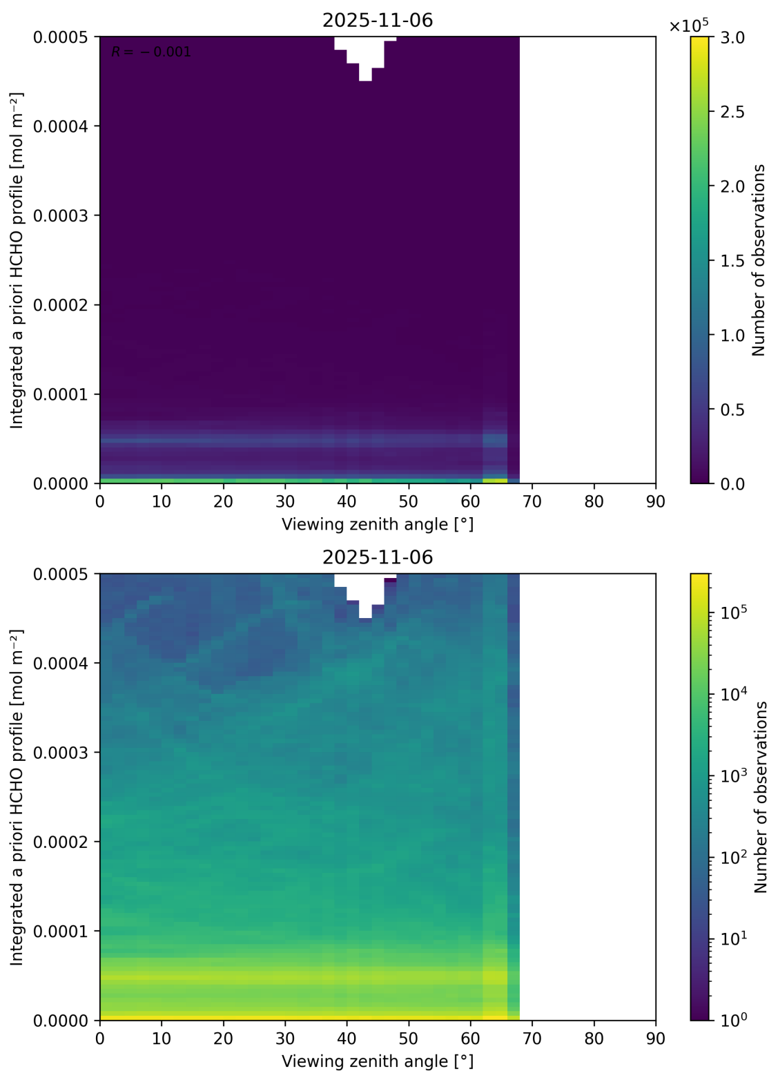
Figure 195: Scatter density plot of “Viewing zenith angle” against “Integrated a priori HCHO profile” for 2025-11-05 to 2025-11-07.
