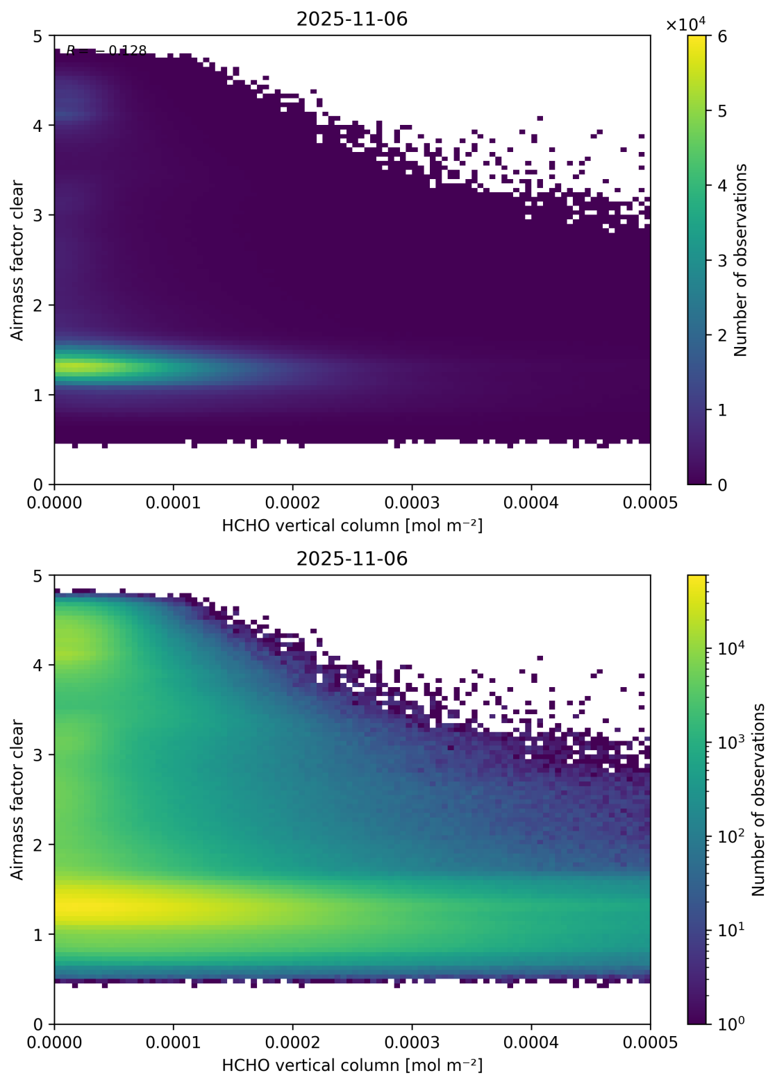
Figure 126: Scatter density plot of “HCHO vertical column” against “Airmass factor clear” for 2025-11-05 to 2025-11-07.
