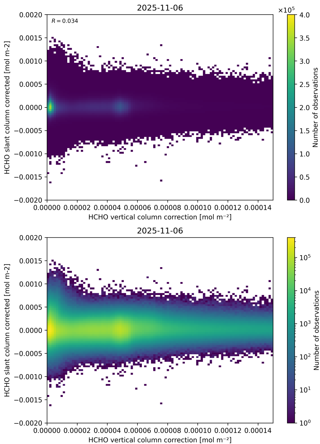
Figure 116: Scatter density plot of “HCHO vertical column correction” against “HCHO slant column corrected” for 2025-11-05 to 2025-11-07.
