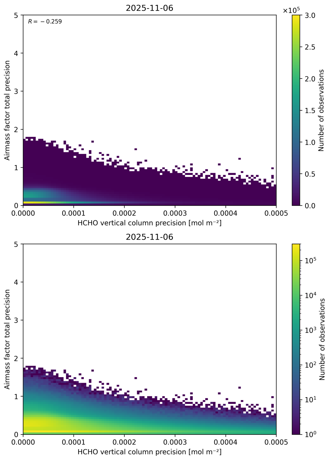
Figure 145: Scatter density plot of “HCHO vertical column precision” against “Airmass factor total precision” for 2025-11-05 to 2025-11-07.
