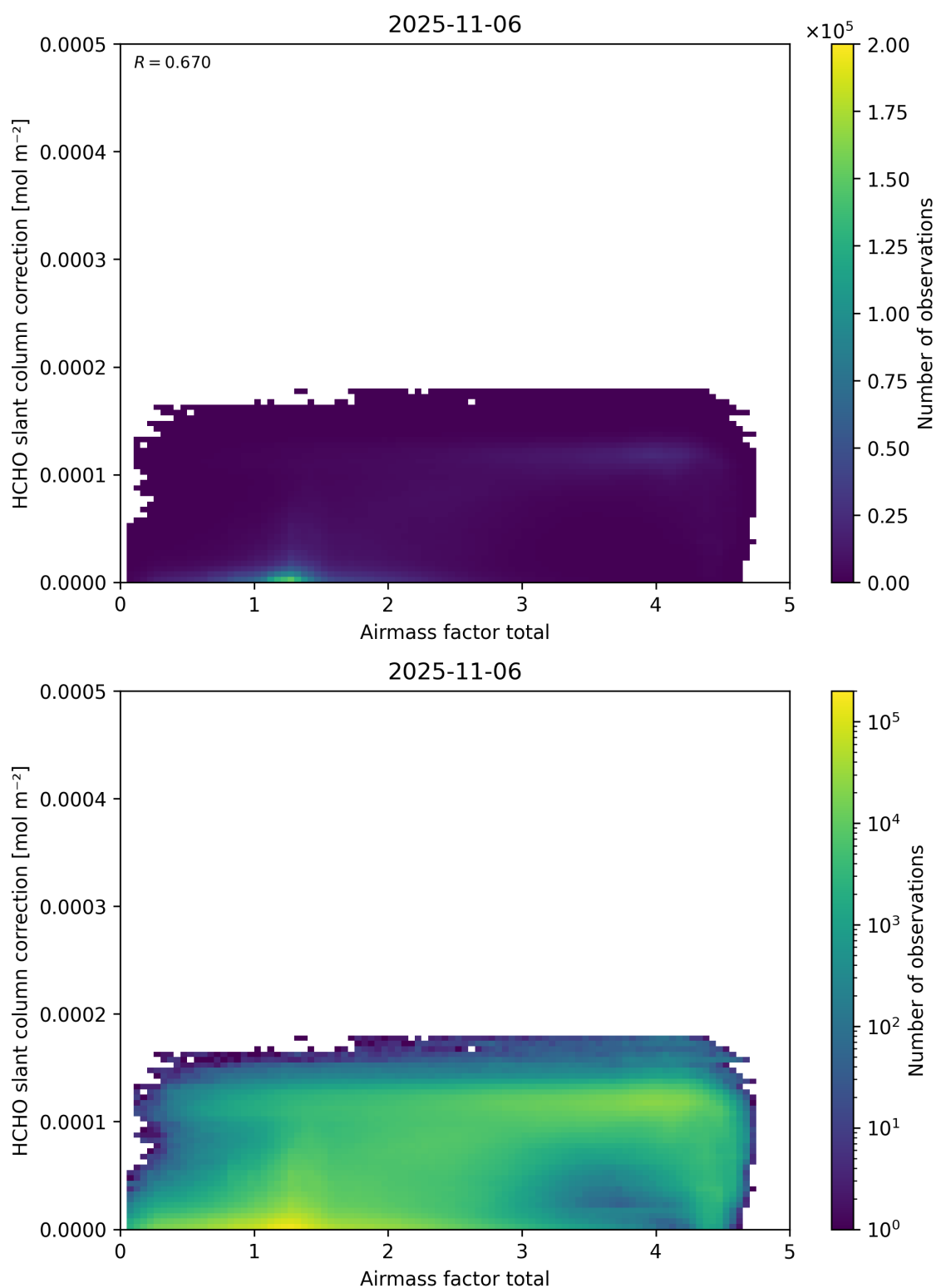
Figure 102: Scatter density plot of “Airmass factor total” against “HCHO slant column correction” for 2025-11-05 to 2025-11-07.
