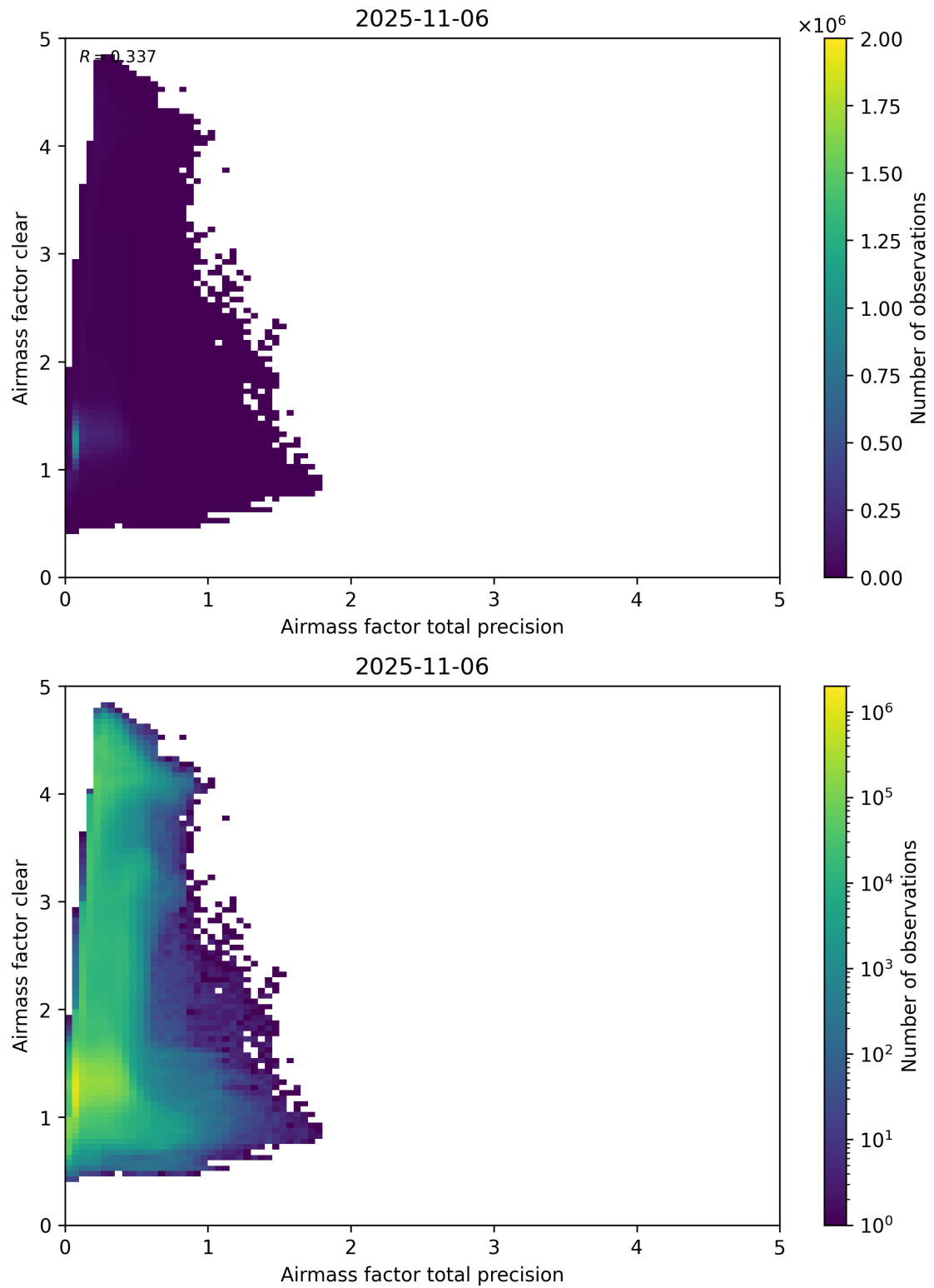
Figure 108: Scatter density plot of “Airmass factor total precision” against “Airmass factor clear” for 2025-11-05 to 2025-11-07.
