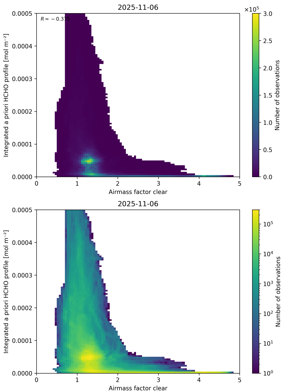
Figure 76: Scatter density plot of “Airmass factor clear” against “Integrated a priori HCHO profile” for 2025-11-05 to 2025-11-07.
