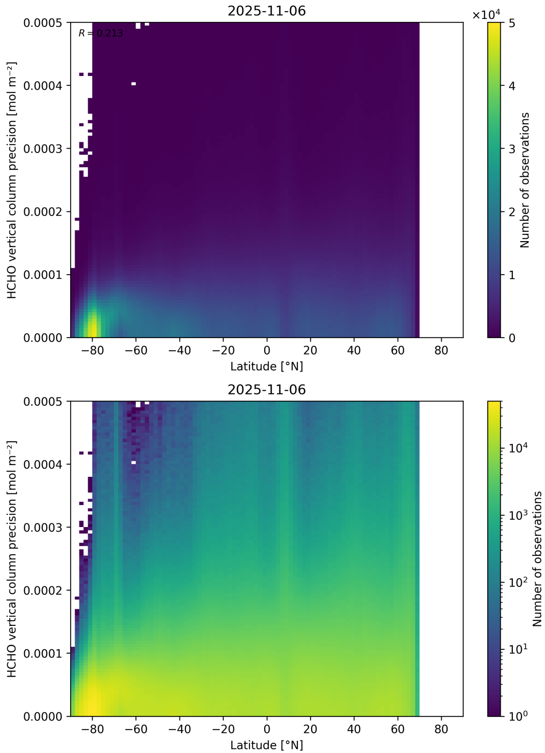
Figure 165: Scatter density plot of “Latitude” against “HCHO vertical column precision” for 2025-11-05 to 2025-11-07.
