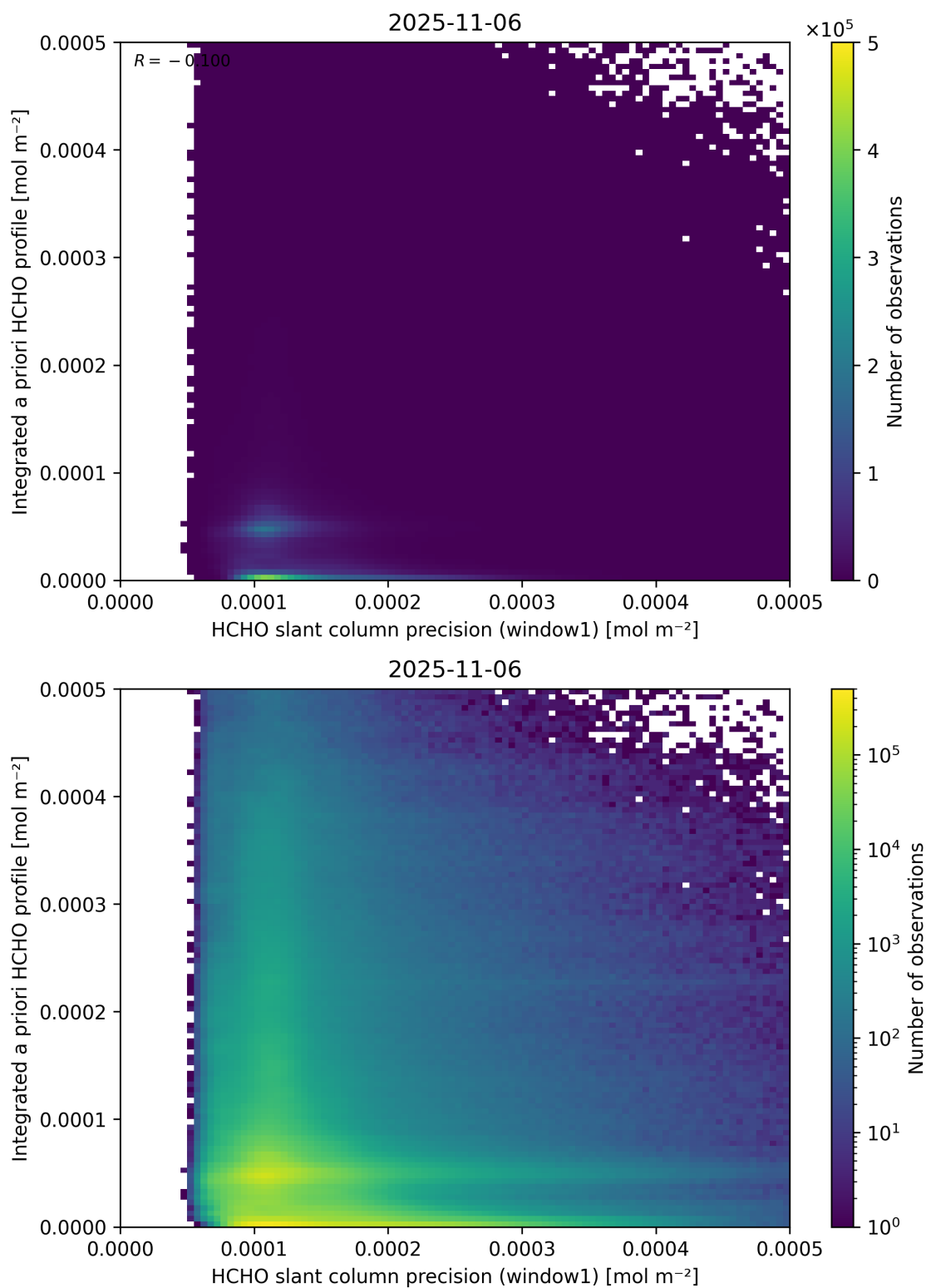
Figure 96: Scatter density plot of “HCHO slant column precision (window1)” against “Integrated a priori HCHO profile” for 2025-11-05 to 2025-11-07.
