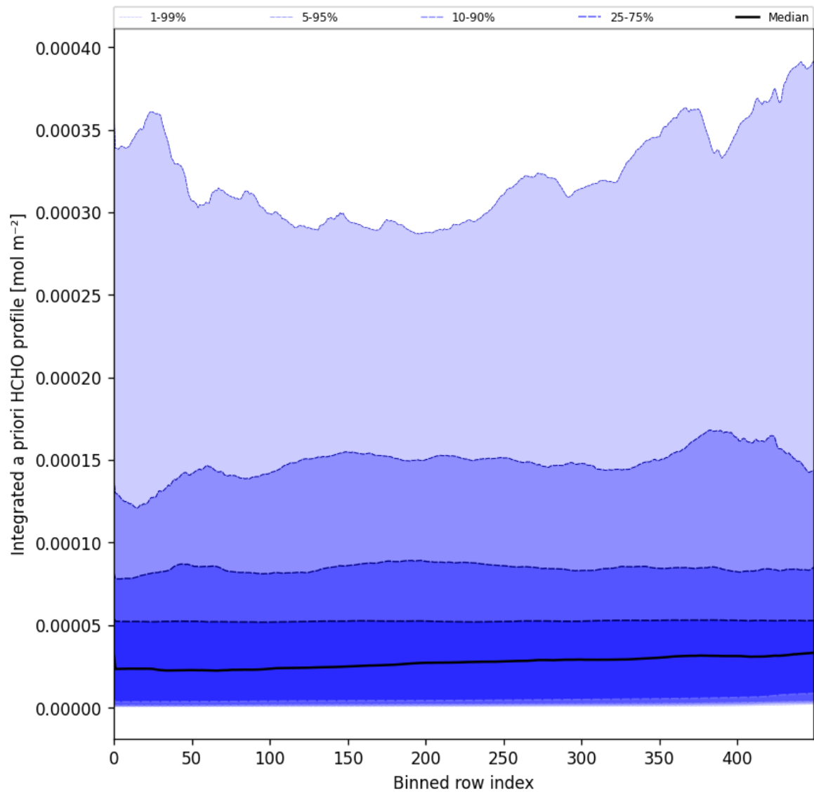
Figure 57: Along track statistics of “Integrated a priori HCHO profile” for 2025-11-05 to 2025-11-07
