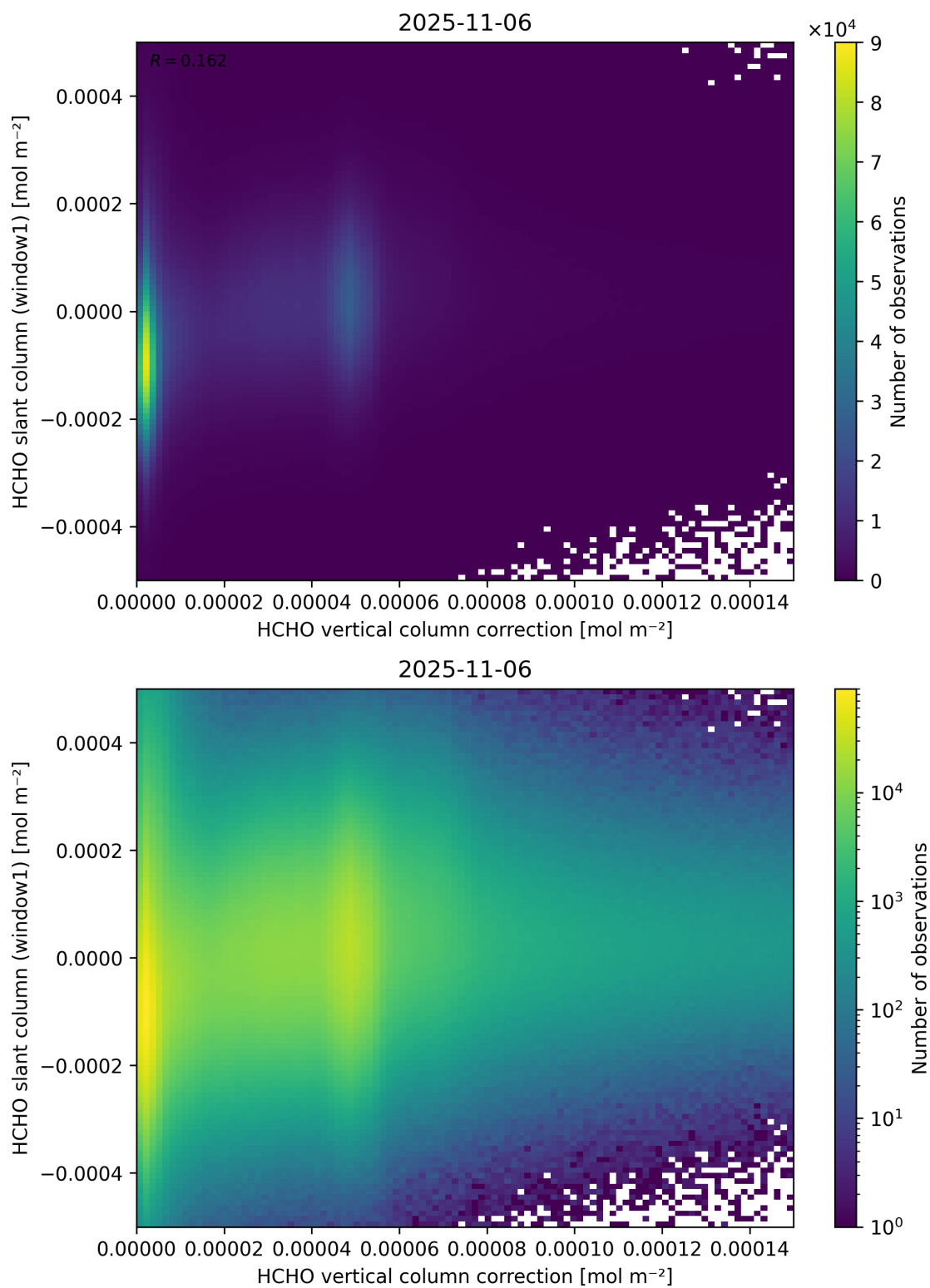
Figure 118: Scatter density plot of “HCHO vertical column correction” against “HCHO slant column (window1)” for 2025-11-05 to 2025-11-07.
