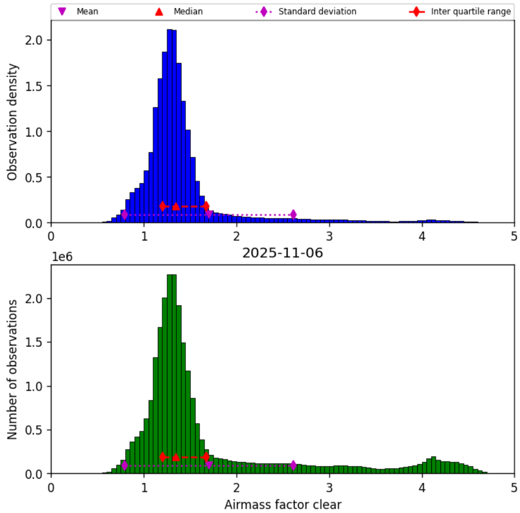
Figure 42: Histogram of “Airmass factor clear” for 2025-11-05 to 2025-11-07
