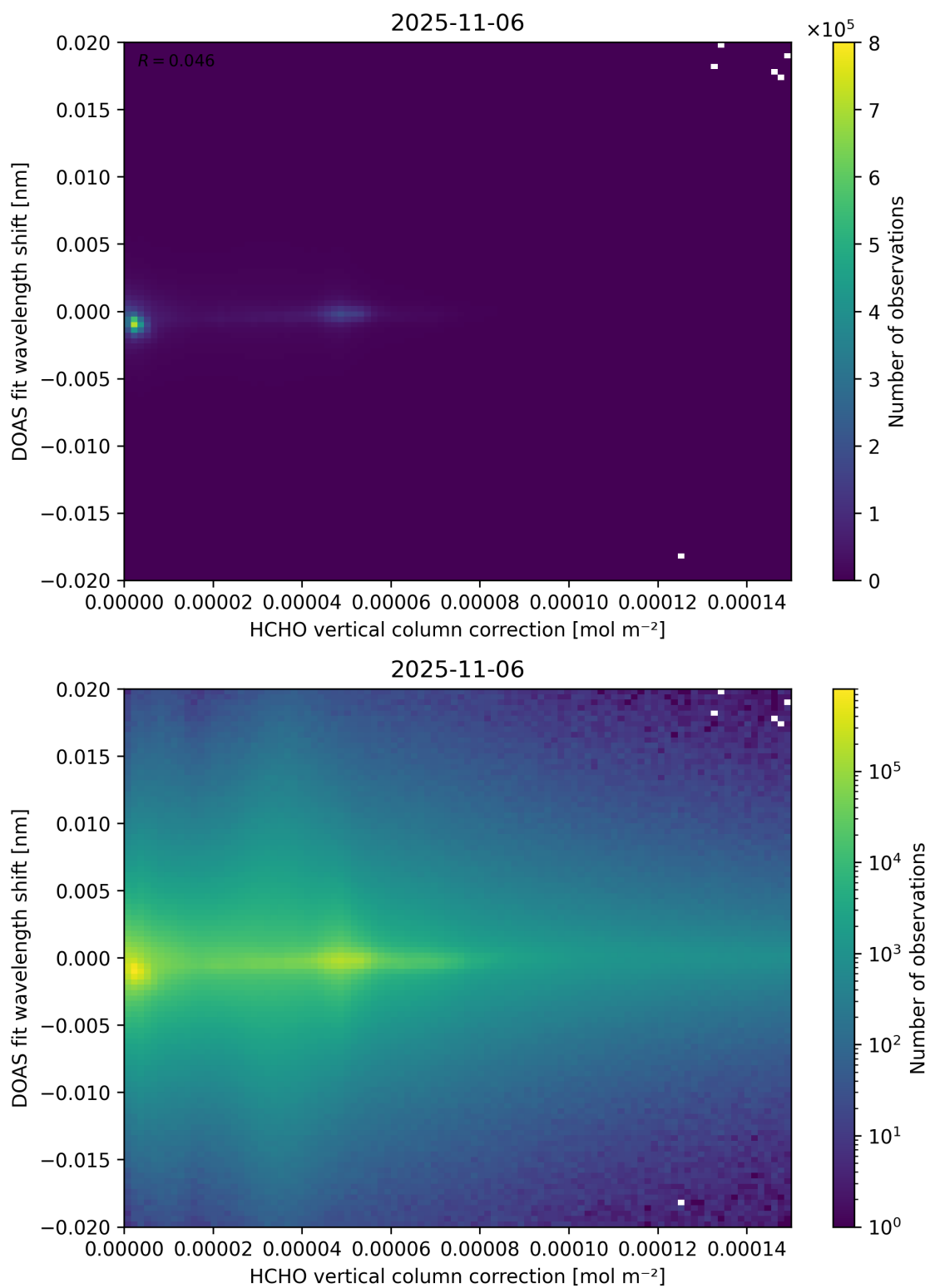
Figure 113: Scatter density plot of “HCHO vertical column correction” against “DOAS fit wavelength shift” for 2025-11-05 to 2025-11-07.
