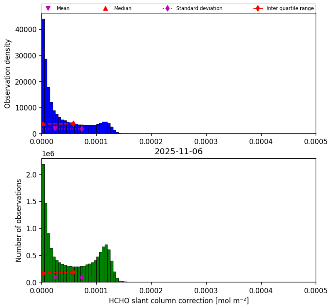
Figure 47: Histogram of “HCHO slant column correction” for 2025-11-05 to 2025-11-07
