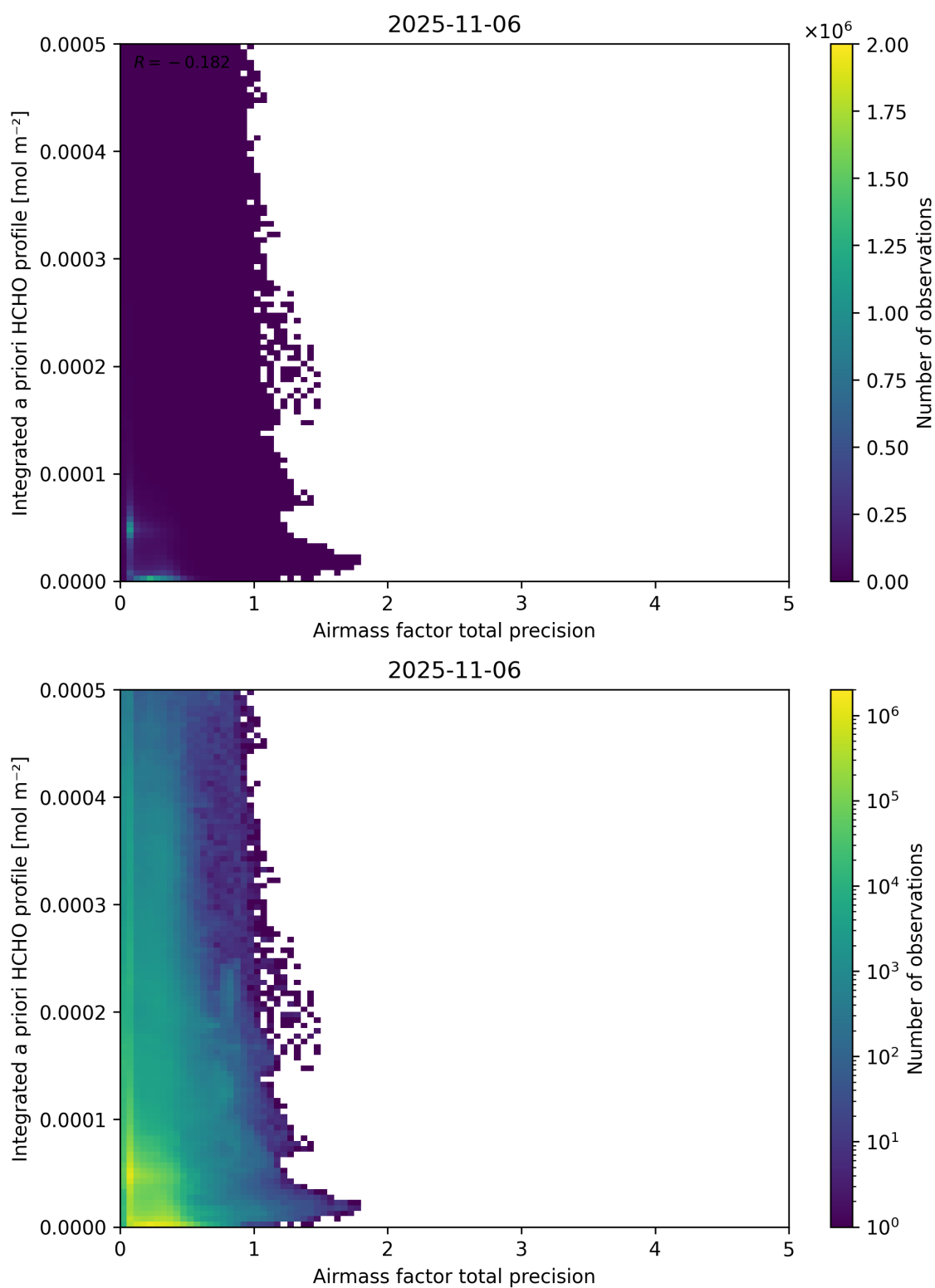
Figure 111: Scatter density plot of “Airmass factor total precision” against “Integrated a priori HCHO profile” for 2025-11-05 to 2025-11-07.
