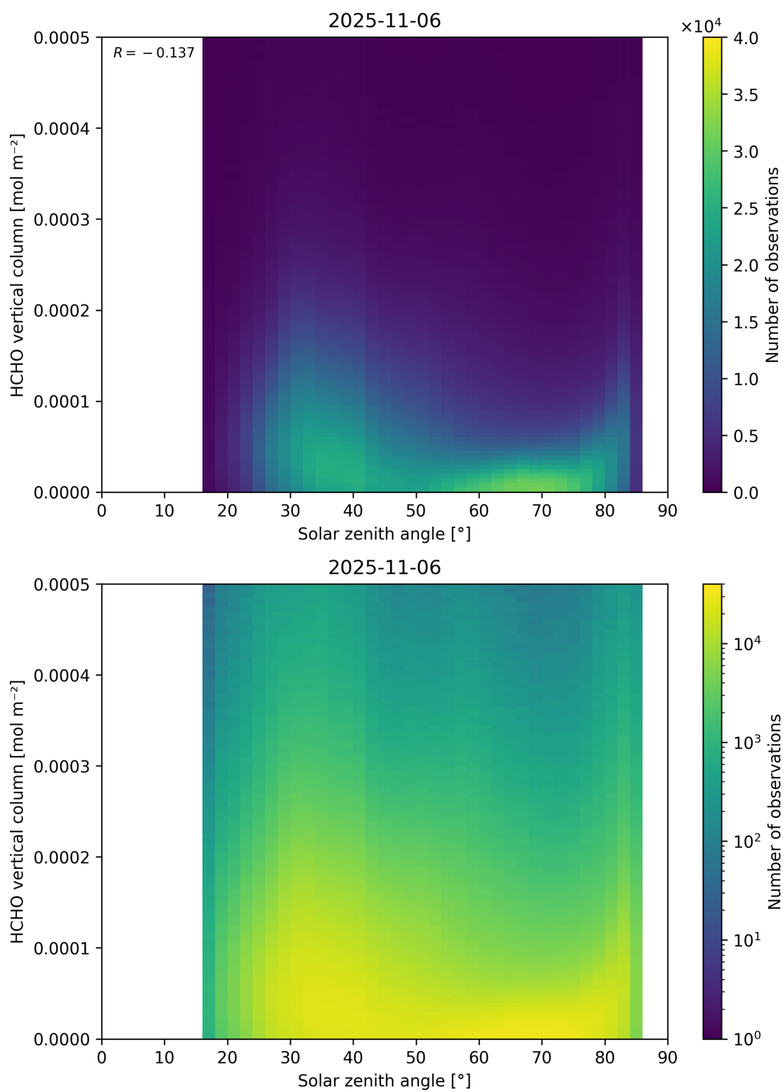
Figure 177: Scatter density plot of “Solar zenith angle” against “HCHO vertical column” for 2025-11-05 to 2025-11-07.
