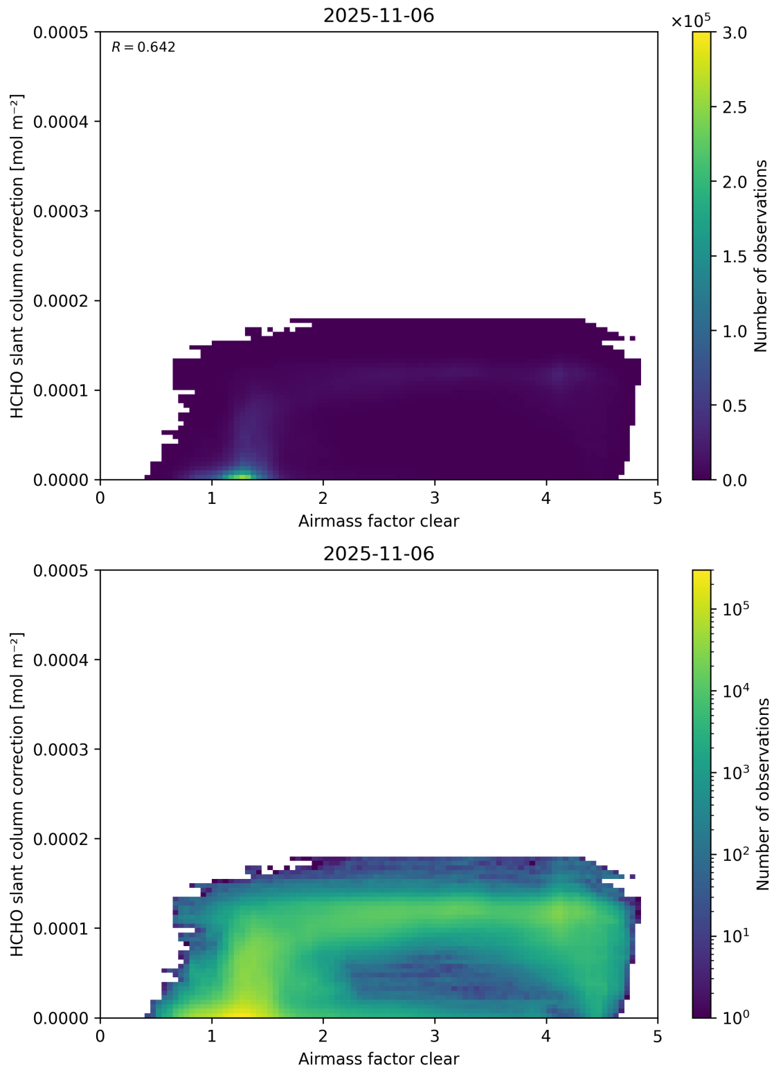
Figure 75: Scatter density plot of “Airmass factor clear” against “HCHO slant column correction” for 2025-11-05 to 2025-11-07.
