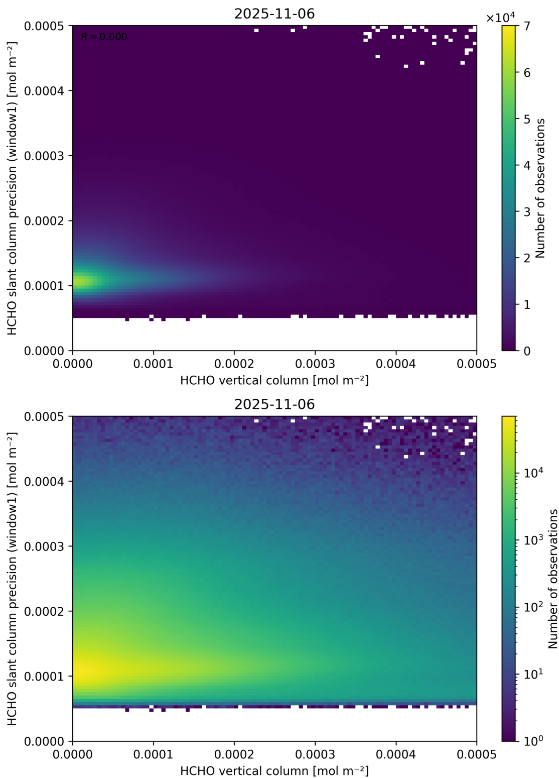
Figure 130: Scatter density plot of “HCHO vertical column” against “HCHO slant column precision (window1)” for 2025-11-05 to 2025-11-07.
