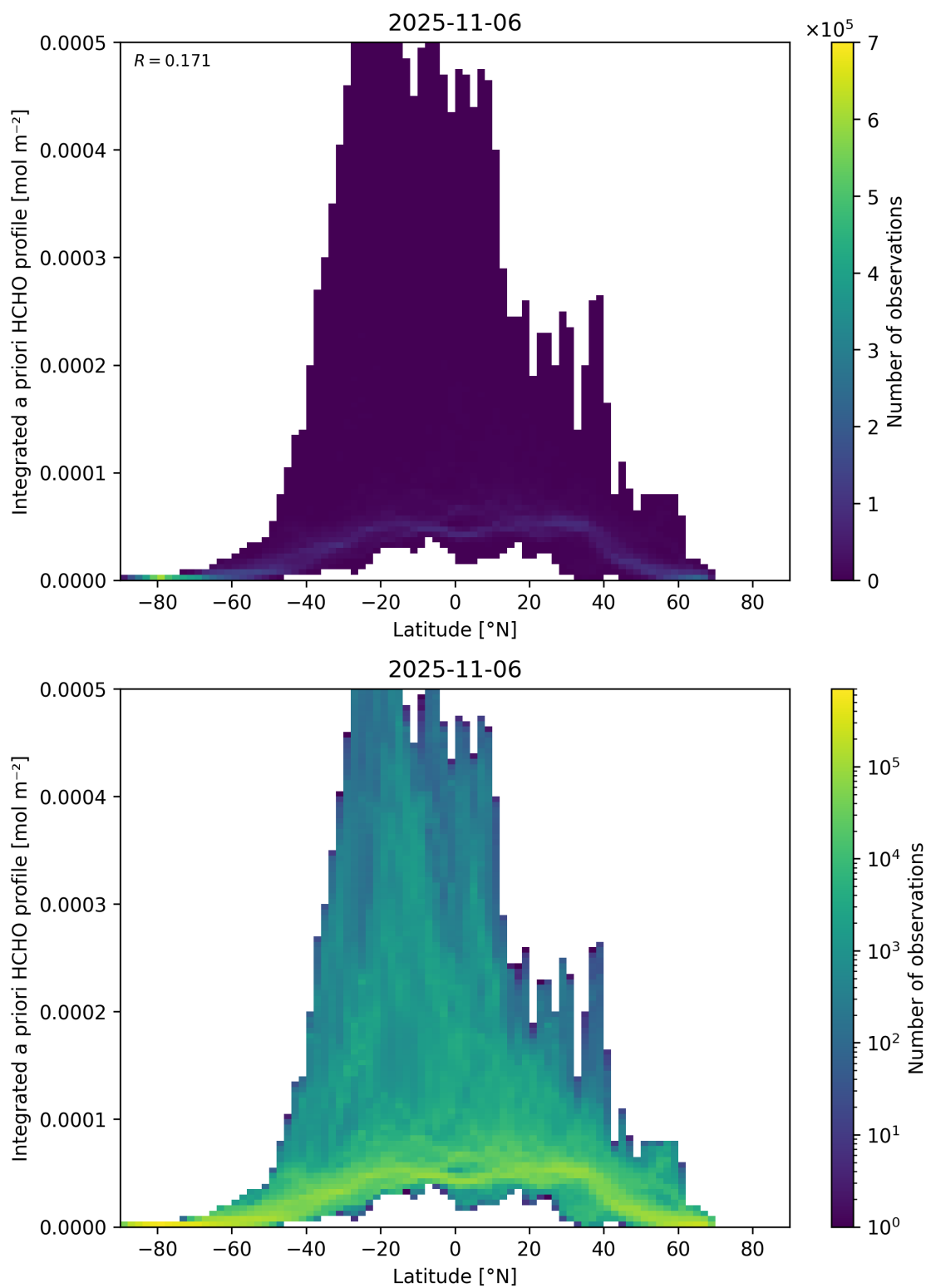
Figure 166: Scatter density plot of “Latitude” against “Integrated a priori HCHO profile” for 2025-11-05 to 2025-11-07.
