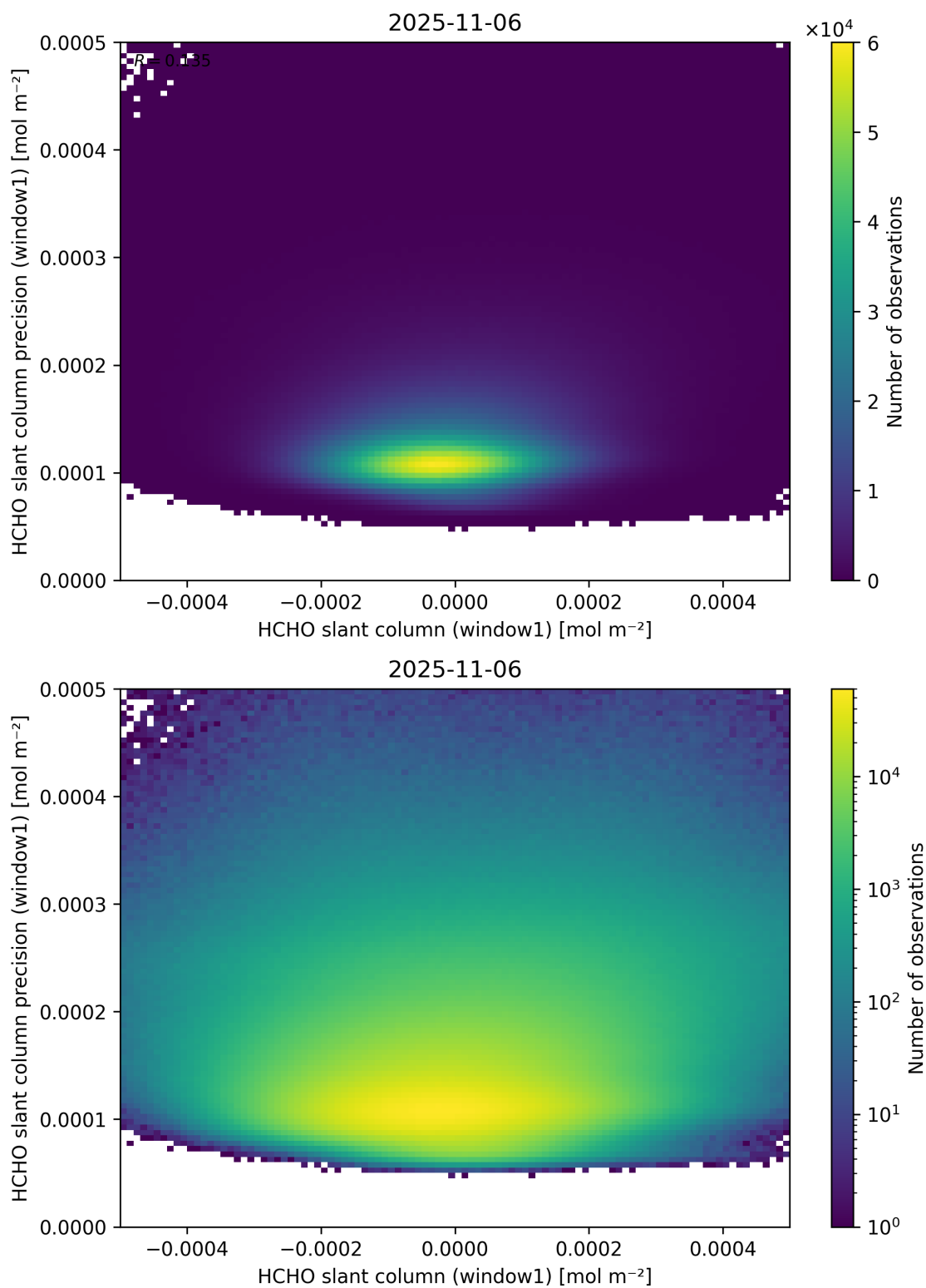
Figure 84: Scatter density plot of “HCHO slant column (window1)” against “HCHO slant column precision (window1)” for 2025-11-05 to 2025-11-07.
