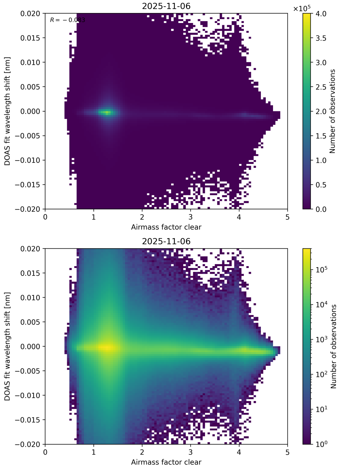
Figure 72: Scatter density plot of “Airmass factor clear” against “DOAS fit wavelength shift” for 2025-11-05 to 2025-11-07.
