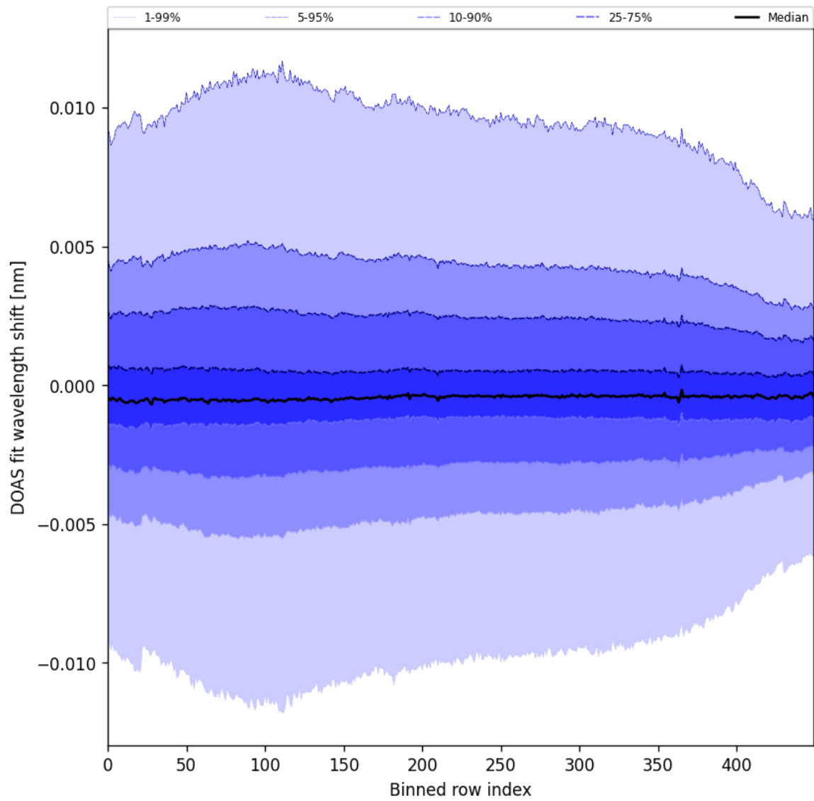
Figure 58: Along track statistics of “DOAS fit wavelength shift” for 2025-11-05 to 2025-11-07
