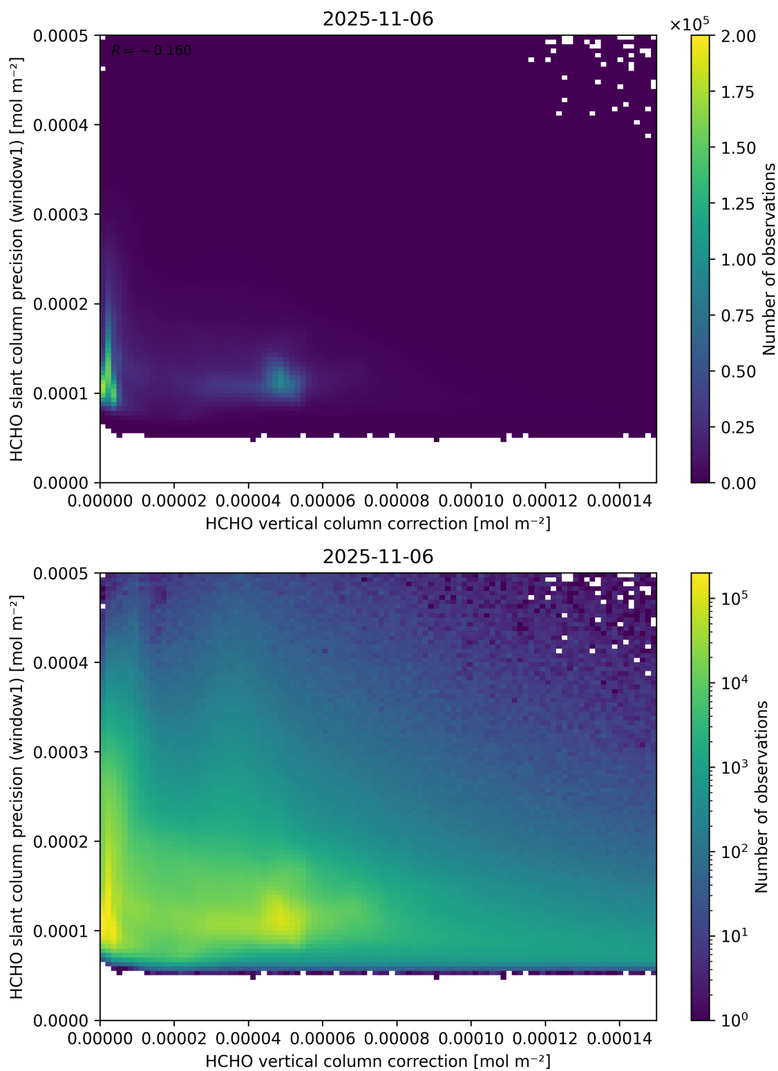
Figure 119: Scatter density plot of “HCHO vertical column correction” against “HCHO slant column precision (window1)” for 2025-11-05 to 2025-11-07.
