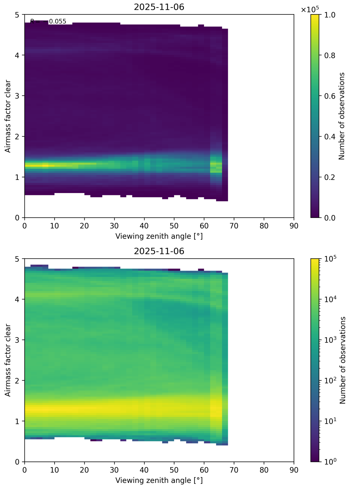
Figure 185: Scatter density plot of “Viewing zenith angle” against “Airmass factor clear” for 2025-11-05 to 2025-11-07.
