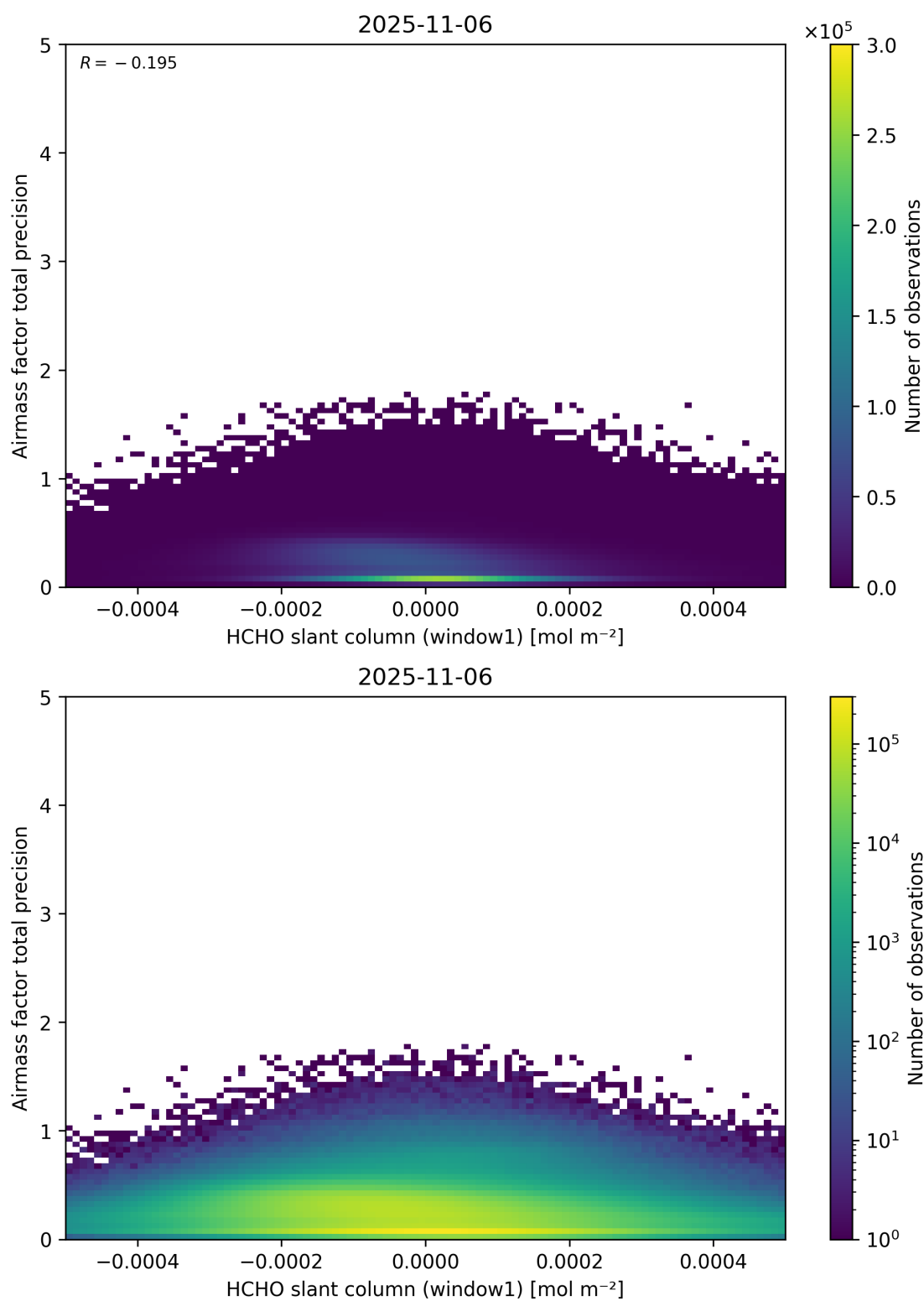
Figure 86: Scatter density plot of “HCHO slant column (window1)” against “Airmass factor total precision” for 2025-11-05 to 2025-11-07.
