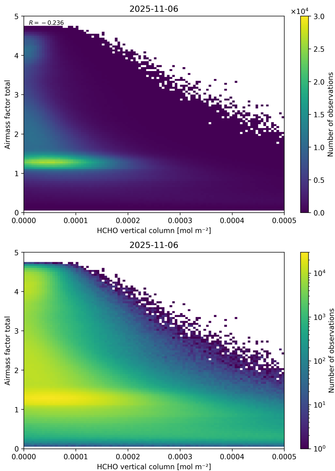
Figure 131: Scatter density plot of “HCHO vertical column” against “Airmass factor total” for 2025-11-05 to 2025-11-07.
