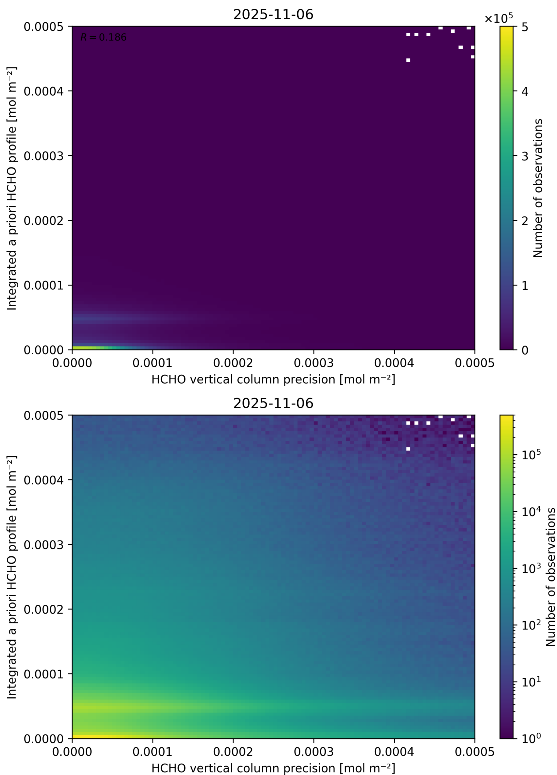
Figure 147: Scatter density plot of “HCHO vertical column precision” against “Integrated a priori HCHO profile” for 2025-11-05 to 2025-11-07.
