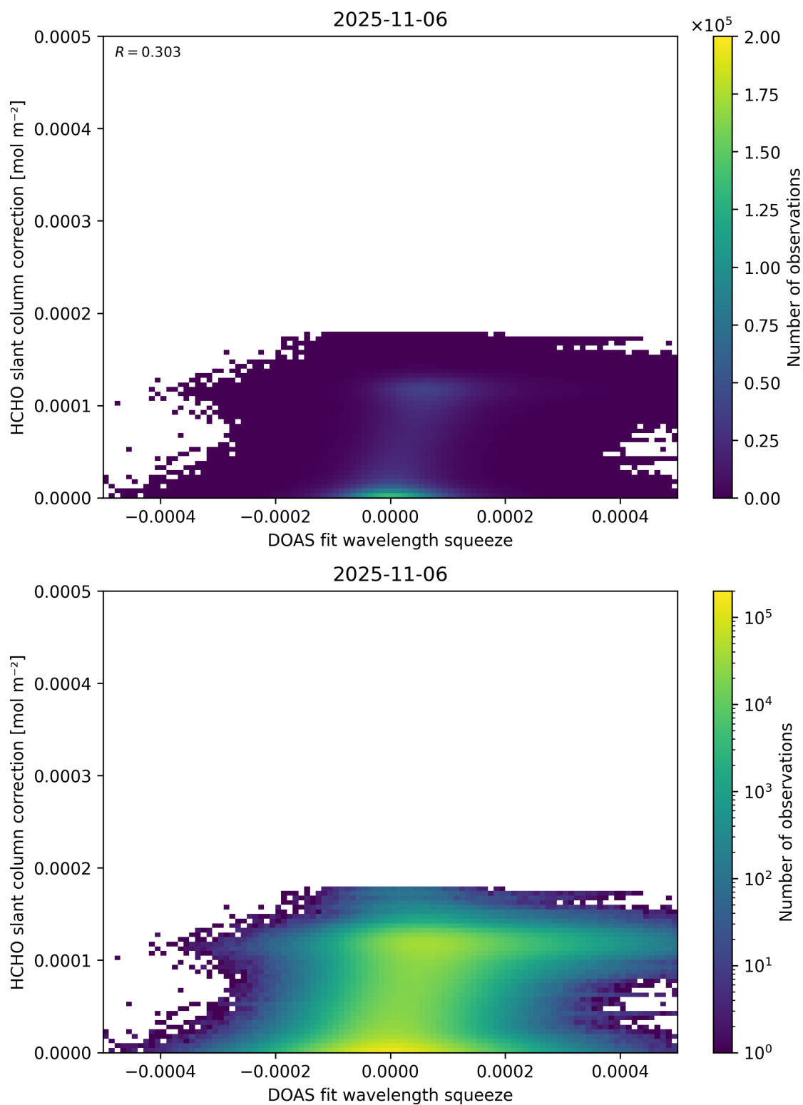
Figure 70: Scatter density plot of “DOAS fit wavelength squeeze” against “HCHO slant column correction” for 2025-11-05 to 2025-11-07.
