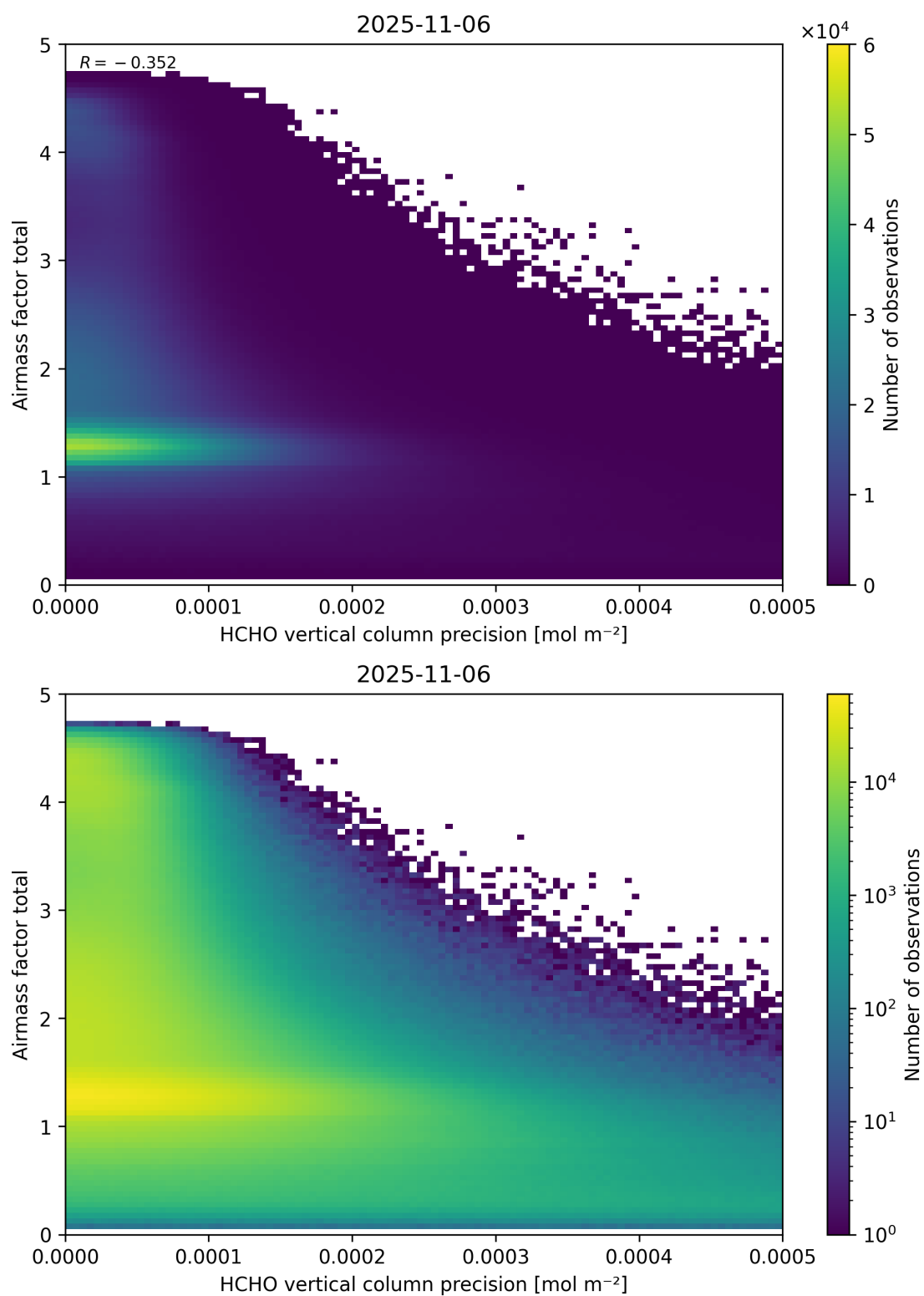
Figure 144: Scatter density plot of “HCHO vertical column precision” against “Airmass factor total” for 2025-11-05 to 2025-11-07.
