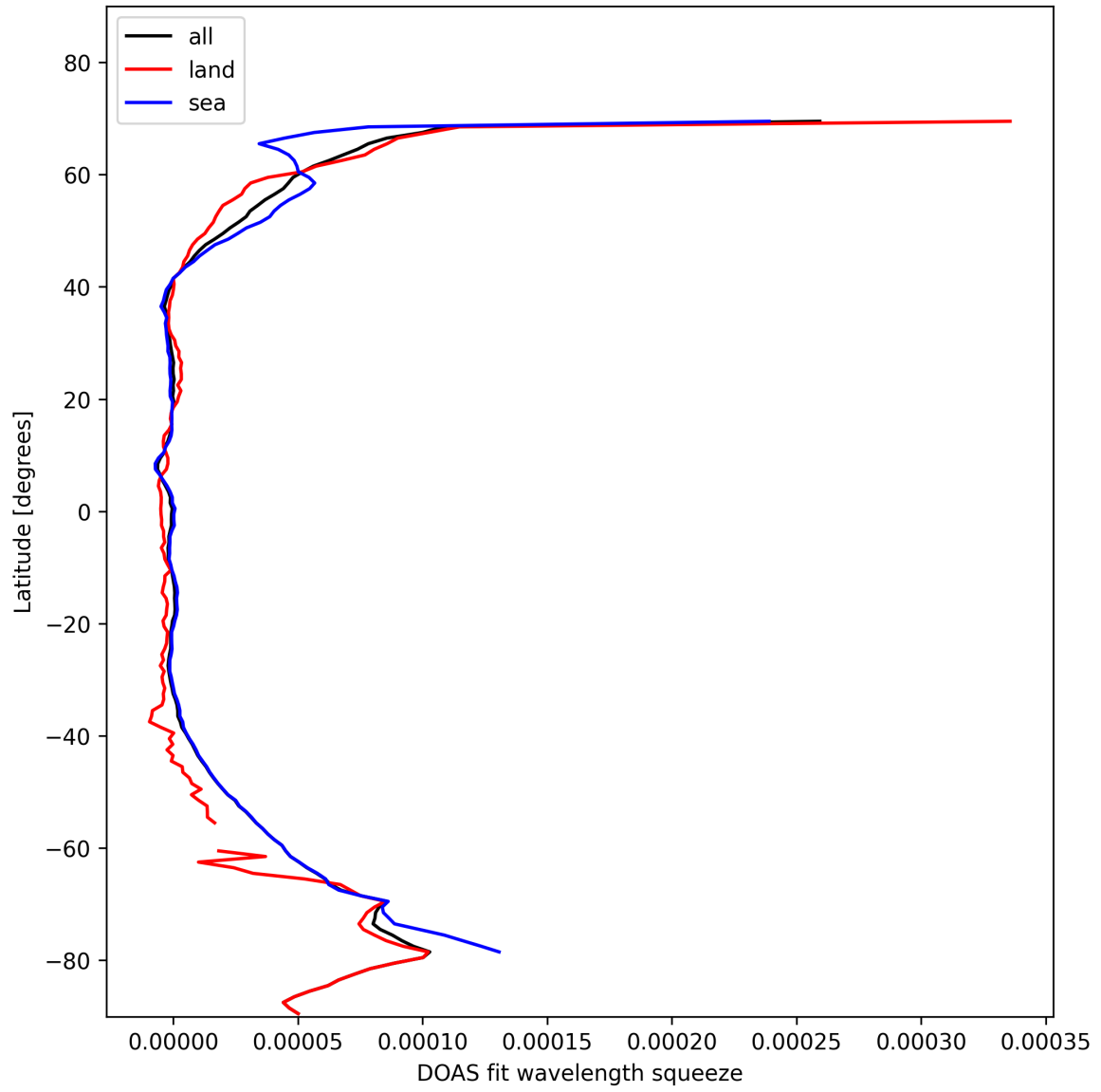
Figure 31: Zonal average of “DOAS fit wavelength squeeze” for 2025-11-05 to 2025-11-07.
