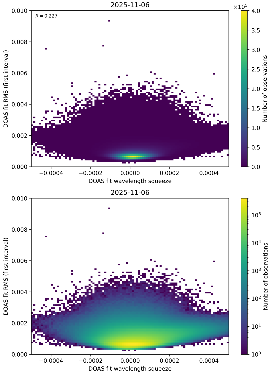
Figure 68: Scatter density plot of “DOAS fit wavelength squeeze” against “DOAS fit RMS (first interval)” for 2025-11-05 to 2025-11-07.
