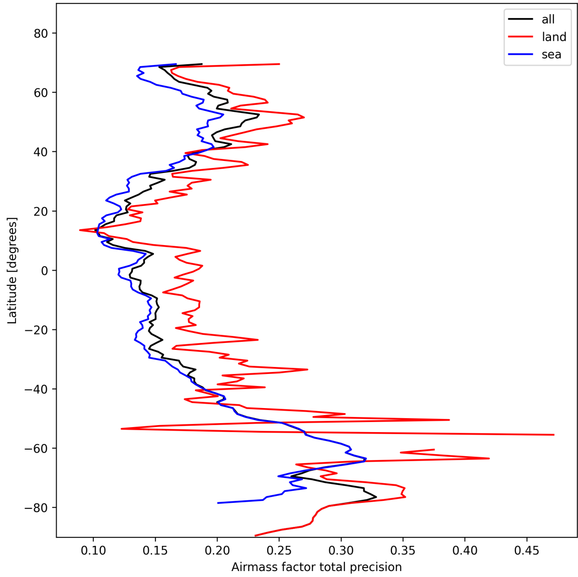
Figure 27: Zonal average of “Airmass factor total precision” for 2025-11-05 to 2025-11-07.
