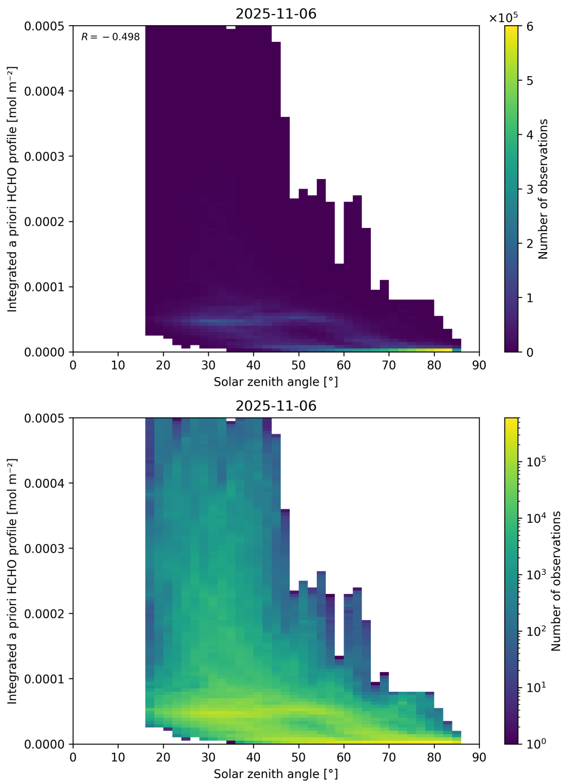
Figure 180: Scatter density plot of “Solar zenith angle” against “Integrated a priori HCHO profile” for 2025-11-05 to 2025-11-07.
