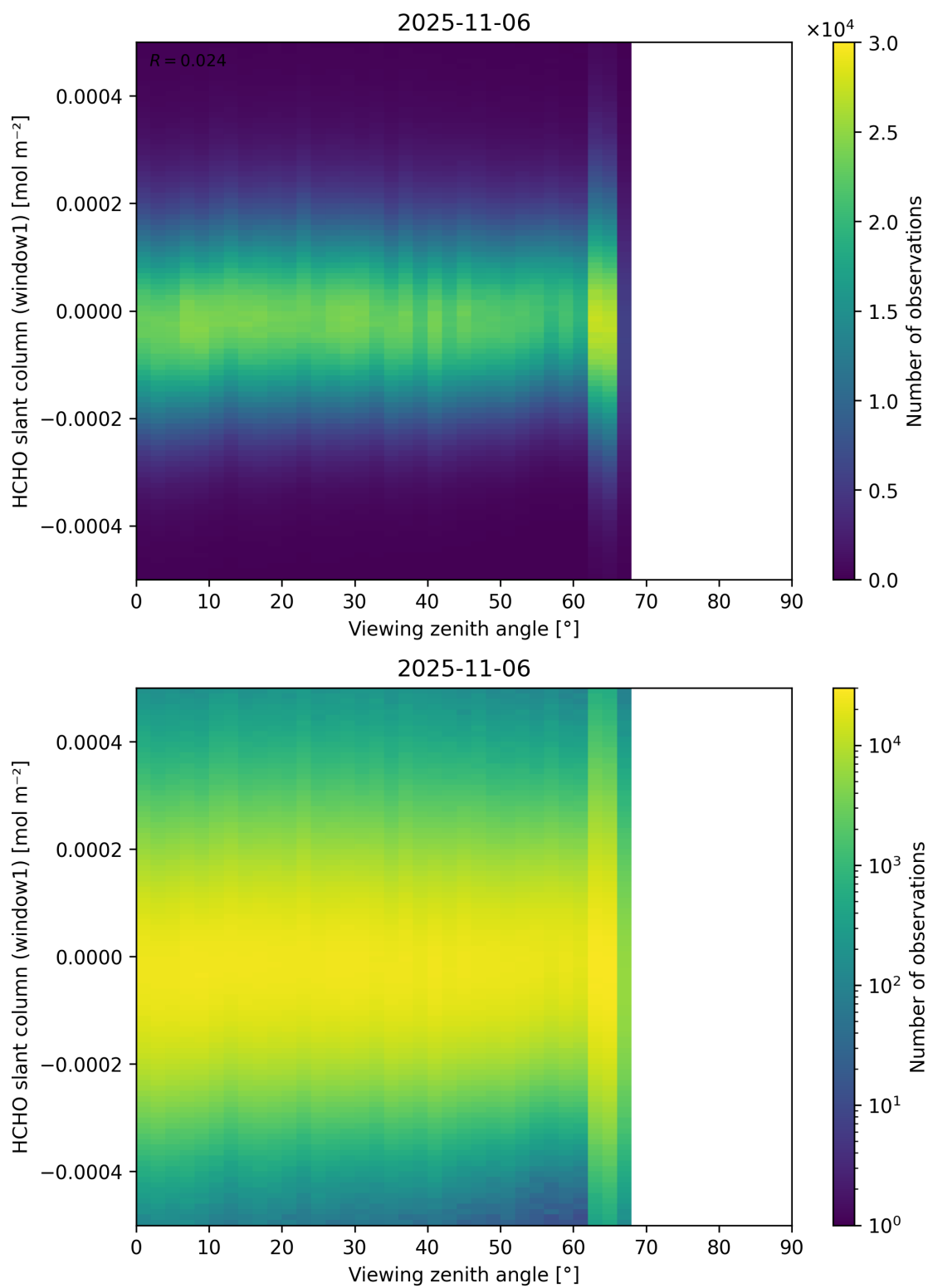
Figure 188: Scatter density plot of “Viewing zenith angle” against “HCHO slant column (window1)” for 2025-11-05 to 2025-11-07.
