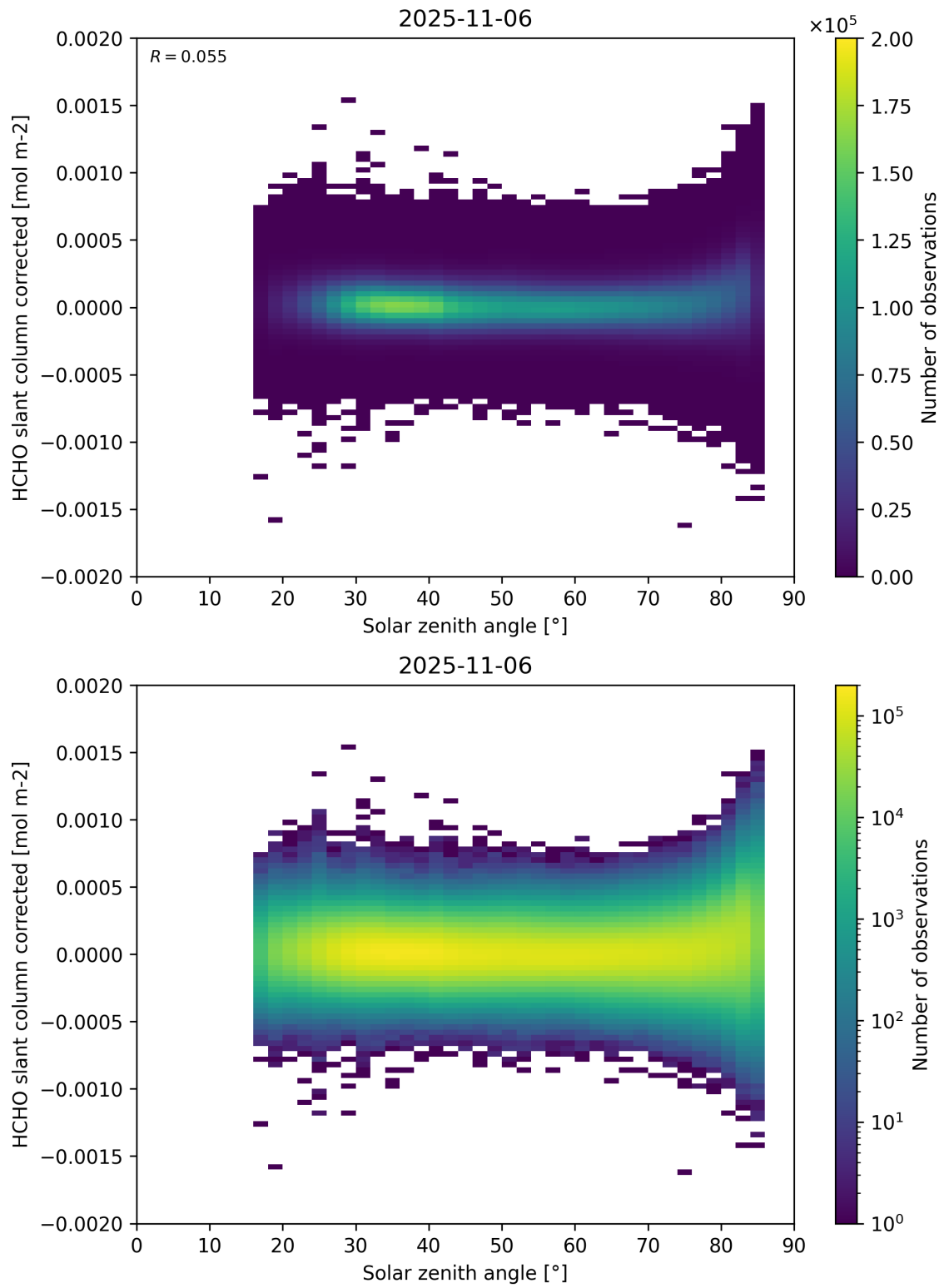
Figure 171: Scatter density plot of “Solar zenith angle” against “HCHO slant column corrected” for 2025-11-05 to 2025-11-07.
