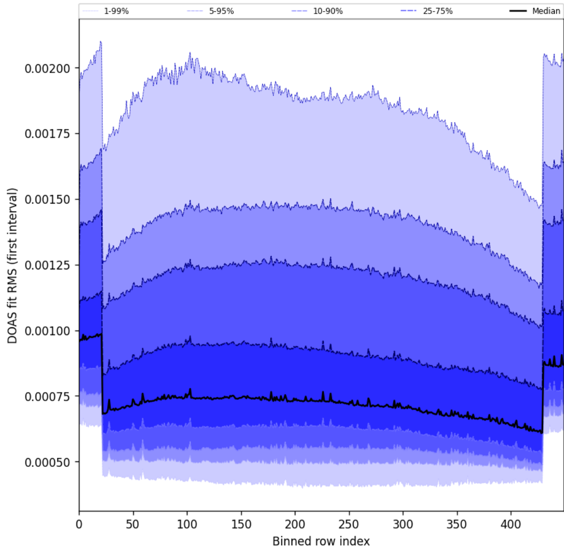
Figure 60: Along track statistics of “DOAS fit RMS (first interval)” for 2025-11-05 to 2025-11-07
