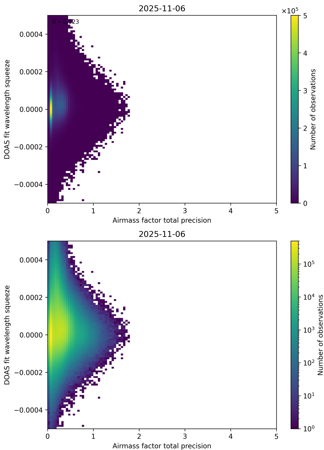
Figure 107: Scatter density plot of “Airmass factor total precision” against “DOAS fit wavelength squeeze” for 2025-11-05 to 2025-11-07.
