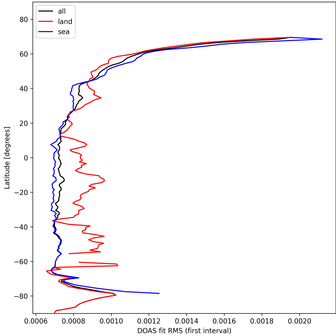
Figure 32: Zonal average of “DOAS fit RMS (first interval)” for 2025-11-05 to 2025-11-07.
