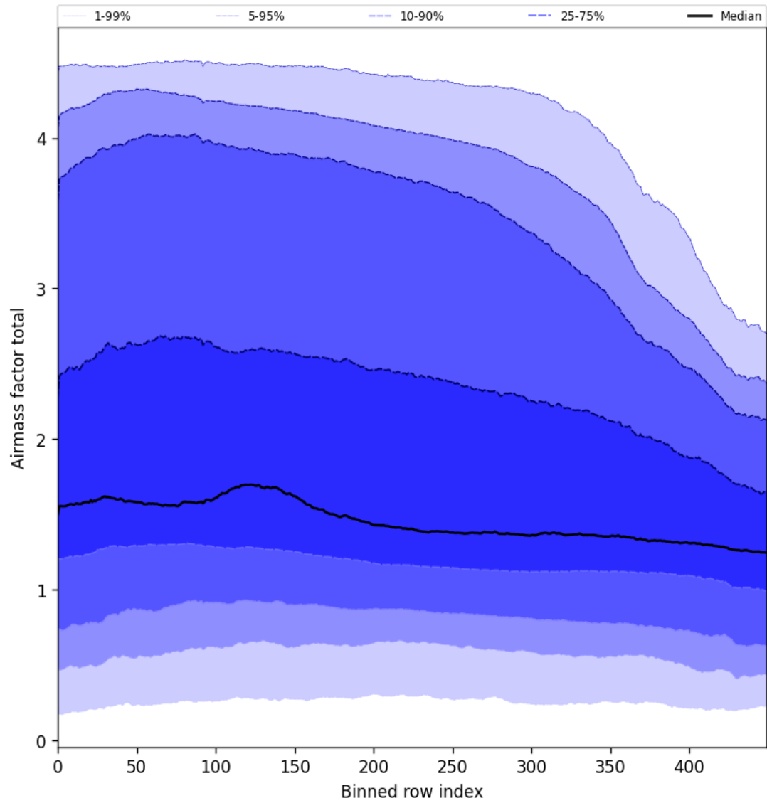
Figure 54: Along track statistics of “Airmass factor total” for 2025-11-05 to 2025-11-07
