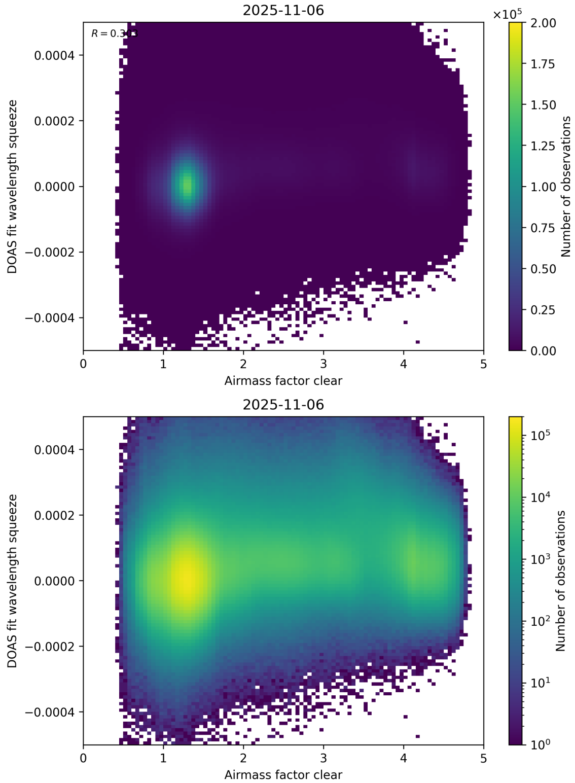
Figure 73: Scatter density plot of “Airmass factor clear” against “DOAS fit wavelength squeeze” for 2025-11-05 to 2025-11-07.
