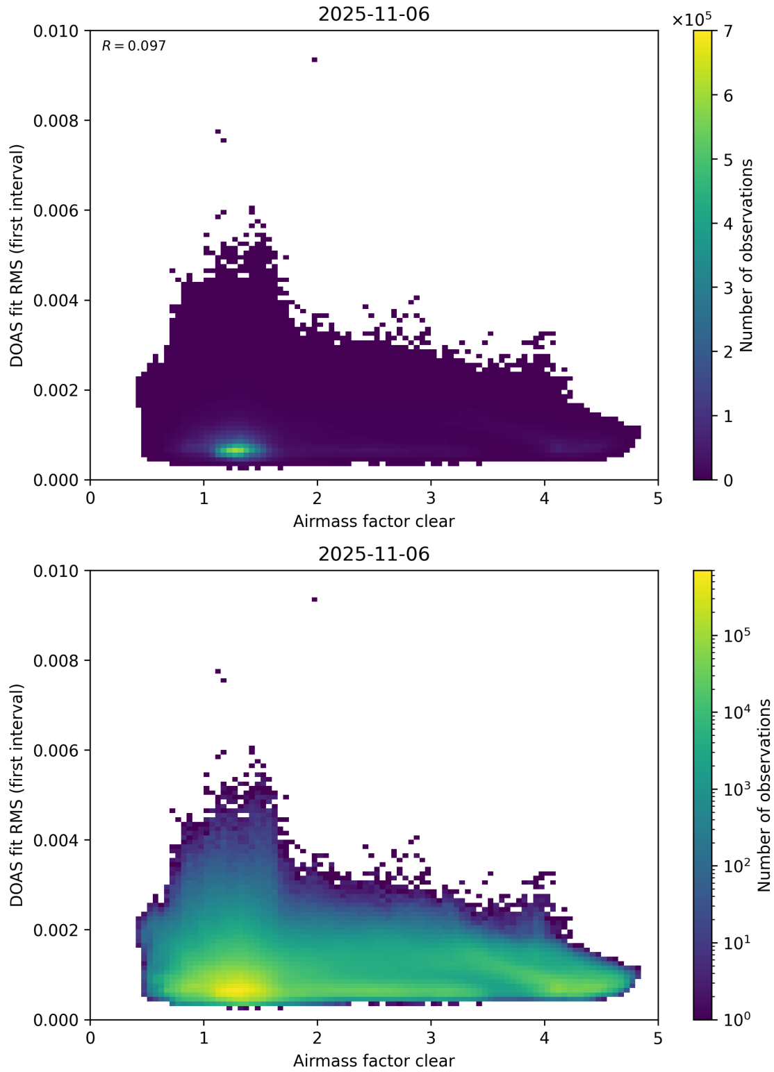
Figure 71: Scatter density plot of “Airmass factor clear” against “DOAS fit RMS (first interval)” for 2025-11-05 to 2025-11-07.
