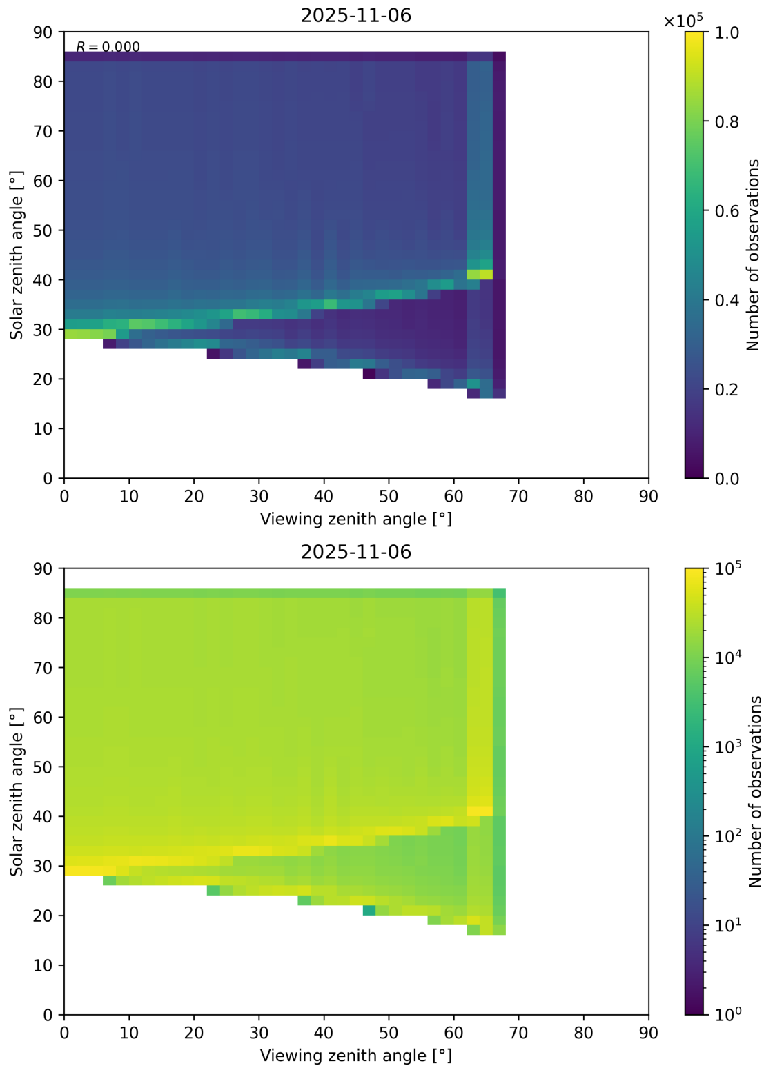
Figure 197: Scatter density plot of “Viewing zenith angle” against “Solar zenith angle” for 2025-11-05 to 2025-11-07.
