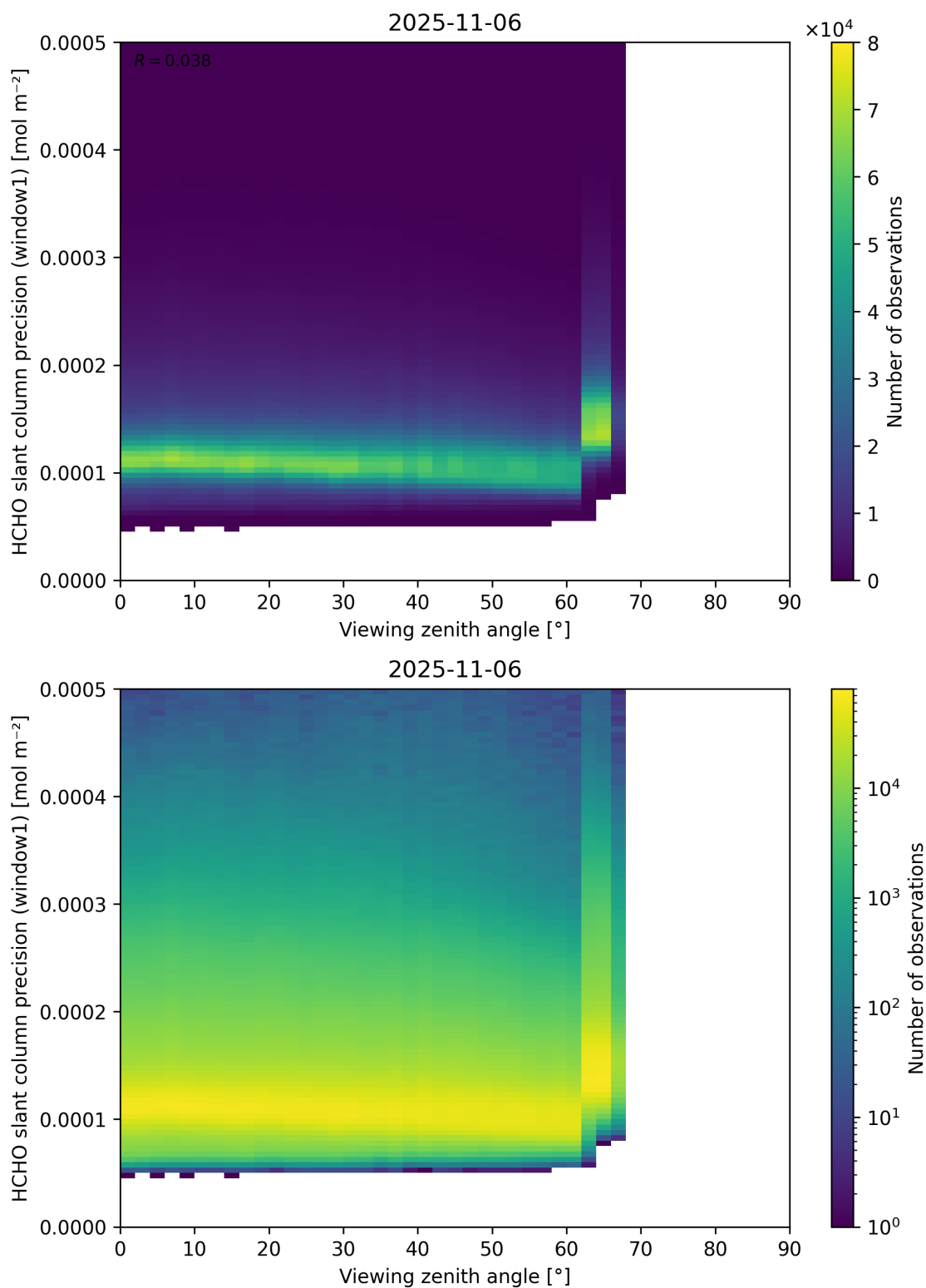
Figure 189: Scatter density plot of “Viewing zenith angle” against “HCHO slant column precision (window1)” for 2025-11-05 to 2025-11-07.
