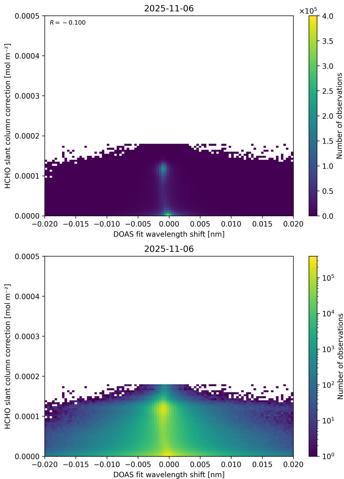
Figure 67: Scatter density plot of “DOAS fit wavelength shift” against “HCHO slant column correction” for 2025-11-05 to 2025-11-07.
