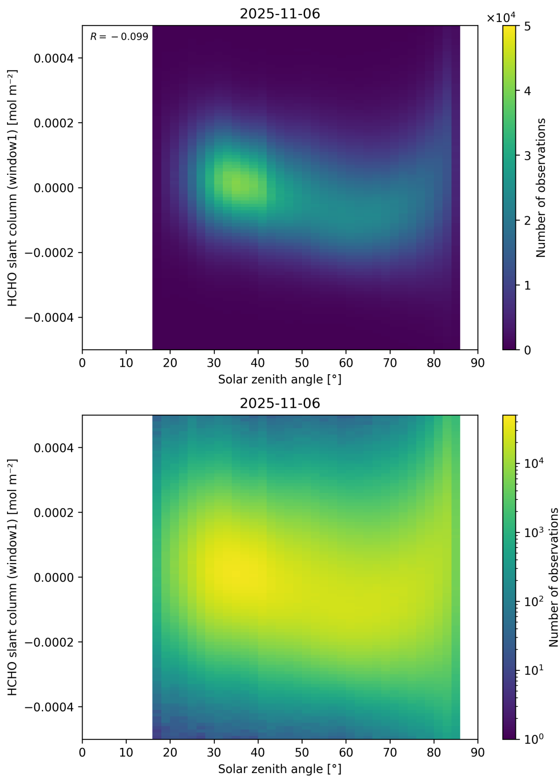
Figure 173: Scatter density plot of “Solar zenith angle” against “HCHO slant column (window1)” for 2025-11-05 to 2025-11-07.
