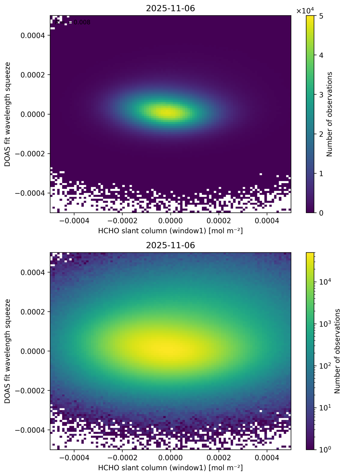
Figure 80: Scatter density plot of “HCHO slant column (window1)” against “DOAS fit wavelength squeeze” for 2025-11-05 to 2025-11-07.
