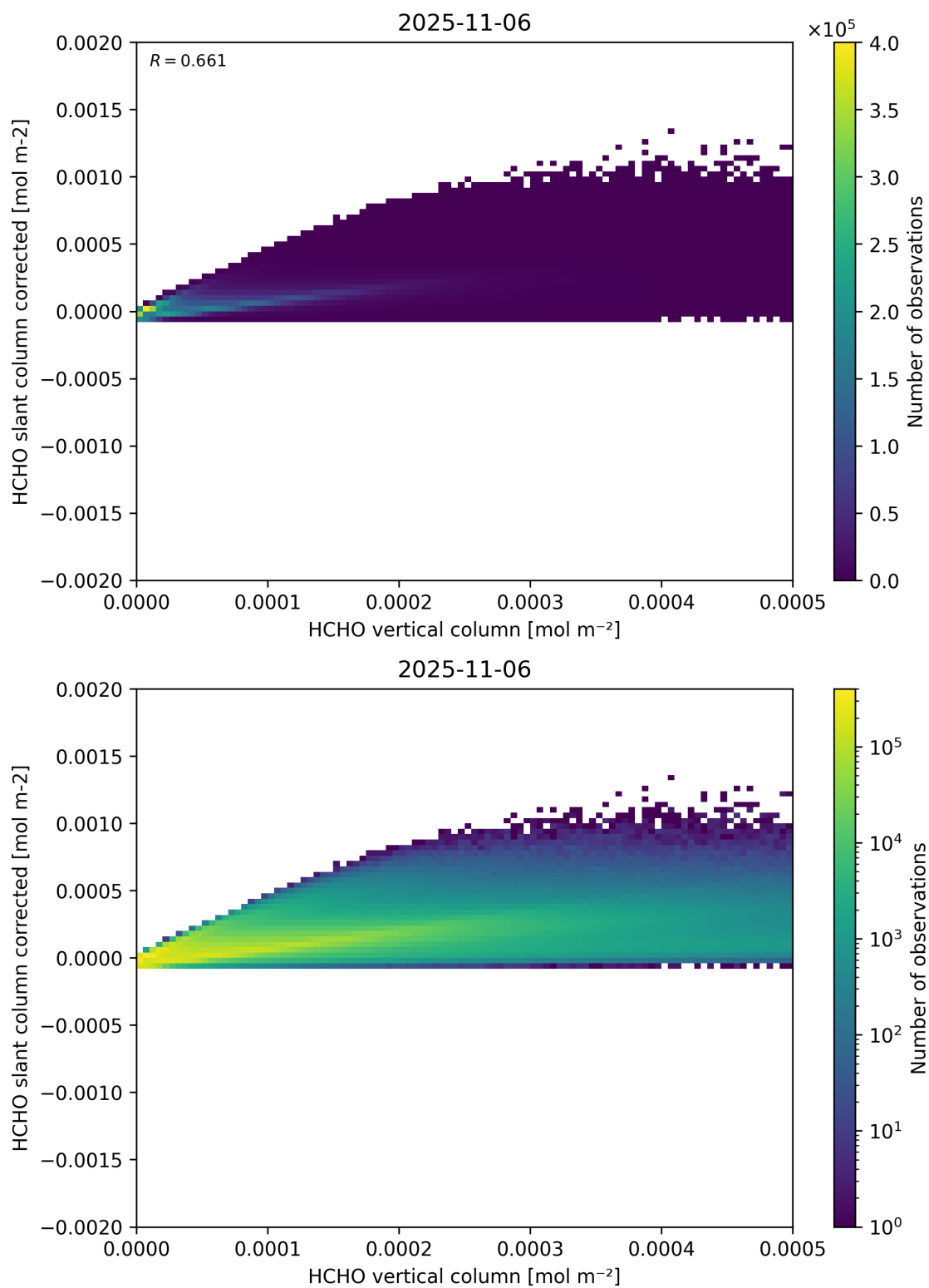
Figure 127: Scatter density plot of “HCHO vertical column” against “HCHO slant column corrected” for 2025-11-05 to 2025-11-07.
