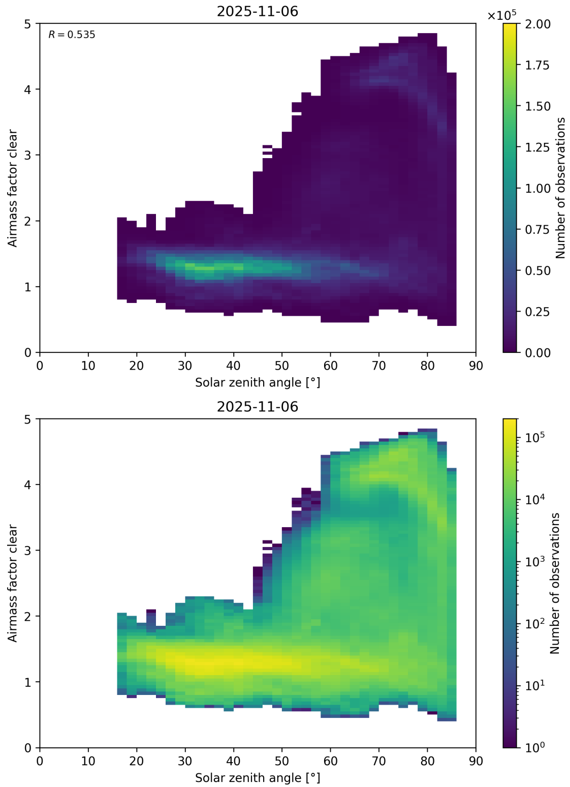
Figure 170: Scatter density plot of “Solar zenith angle” against “Airmass factor clear” for 2025-11-05 to 2025-11-07.
