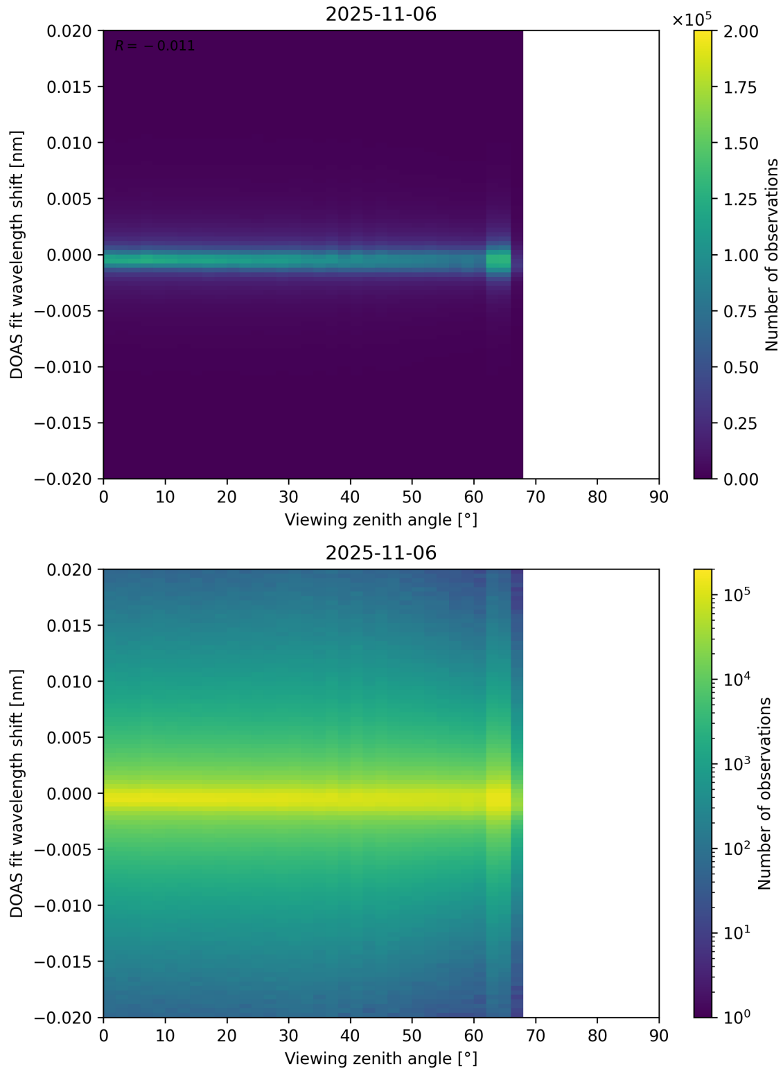
Figure 183: Scatter density plot of “Viewing zenith angle” against “DOAS fit wavelength shift” for 2025-11-05 to 2025-11-07.
