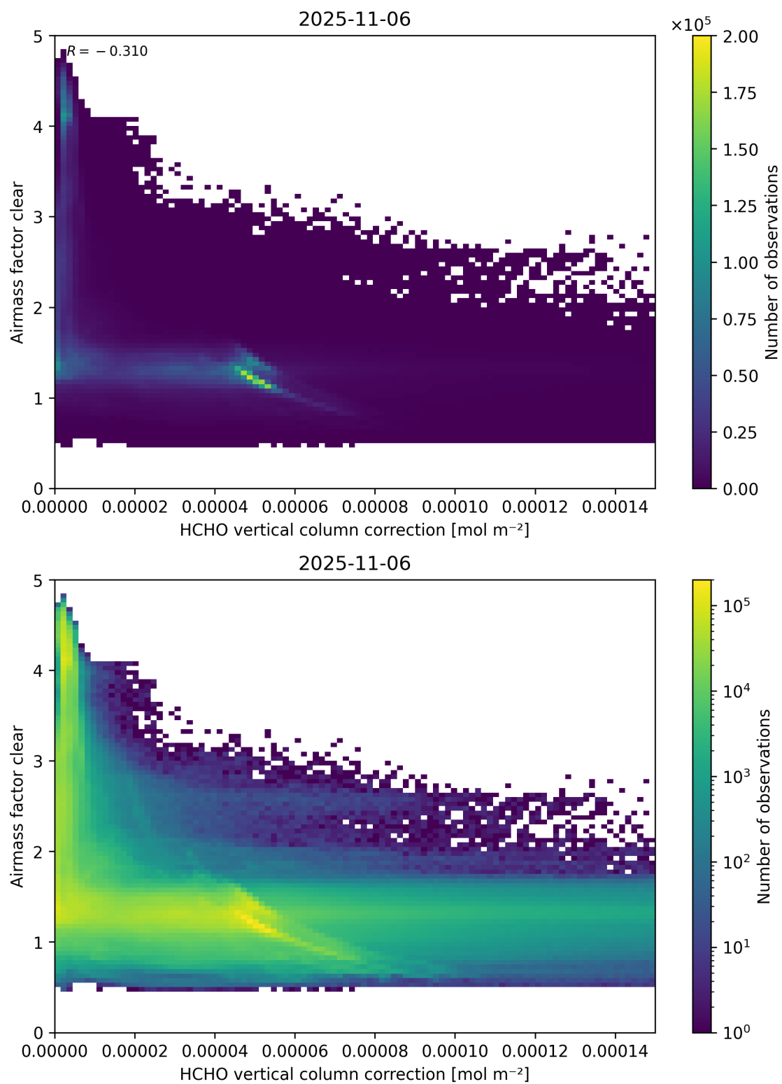
Figure 115: Scatter density plot of “HCHO vertical column correction” against “Airmass factor clear” for 2025-11-05 to 2025-11-07.
