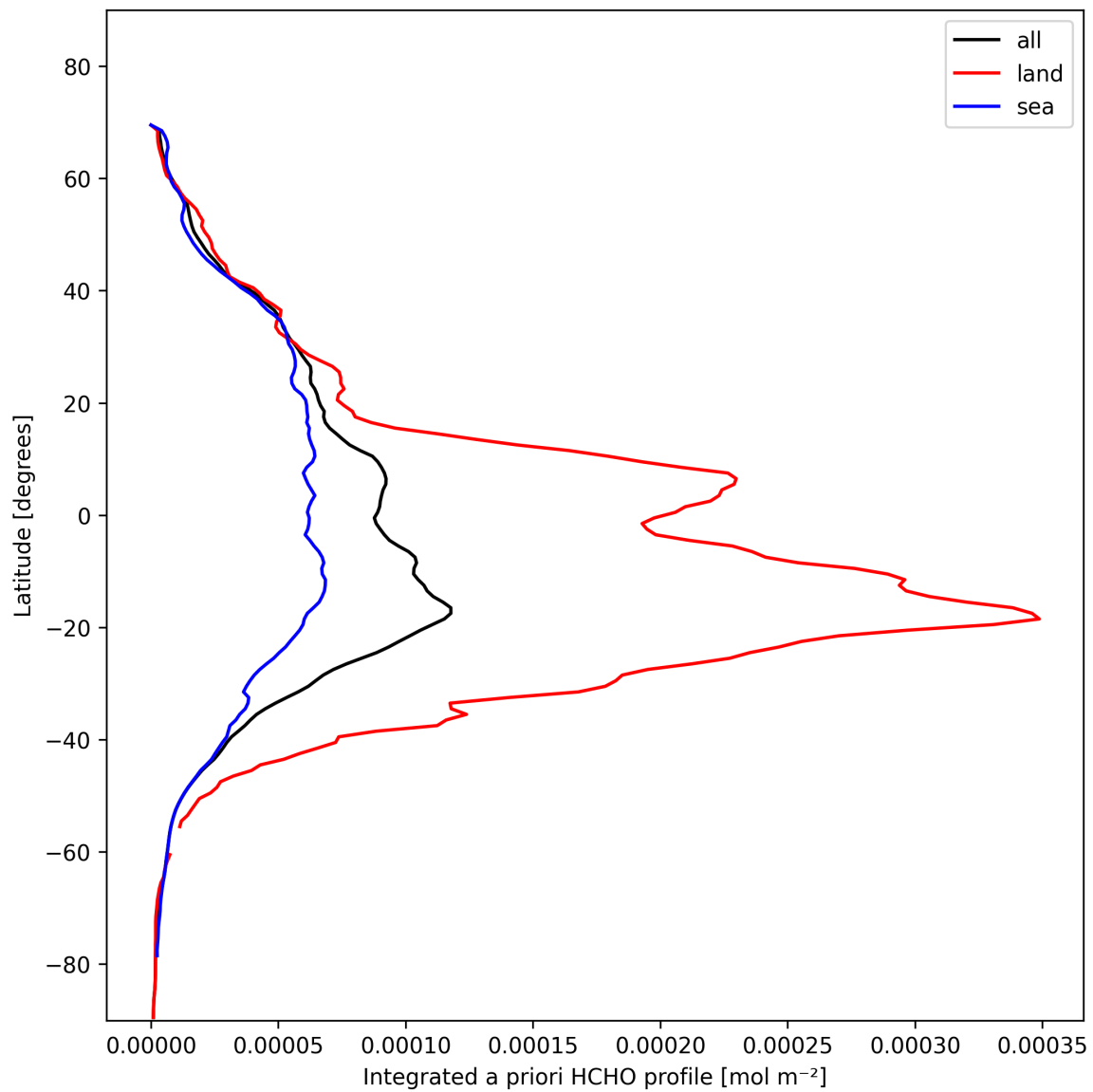
Figure 29: Zonal average of “Integrated a priori HCHO profile” for 2025-11-05 to 2025-11-07.
