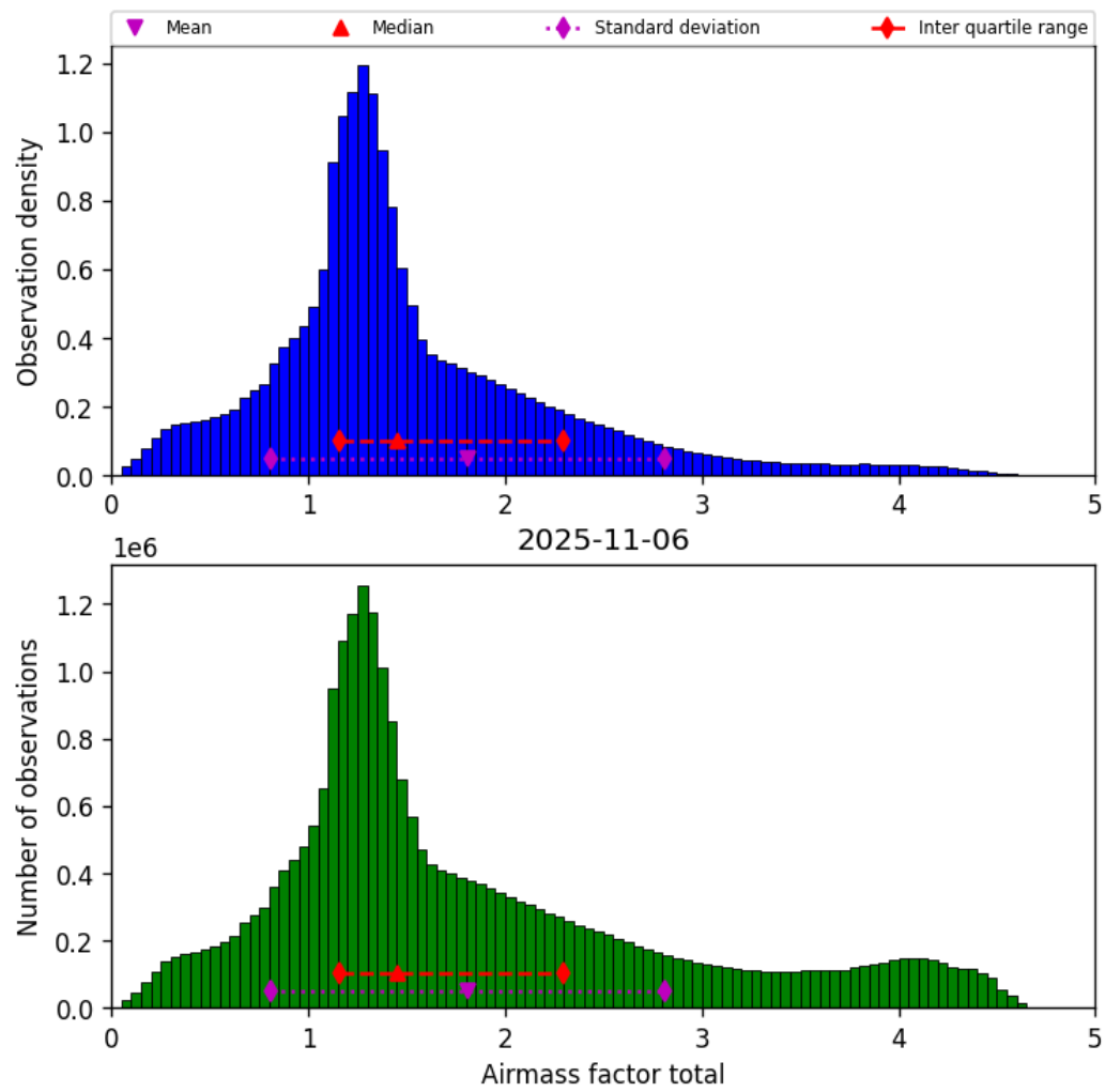
Figure 40: Histogram of “Airmass factor total” for 2025-11-05 to 2025-11-07
