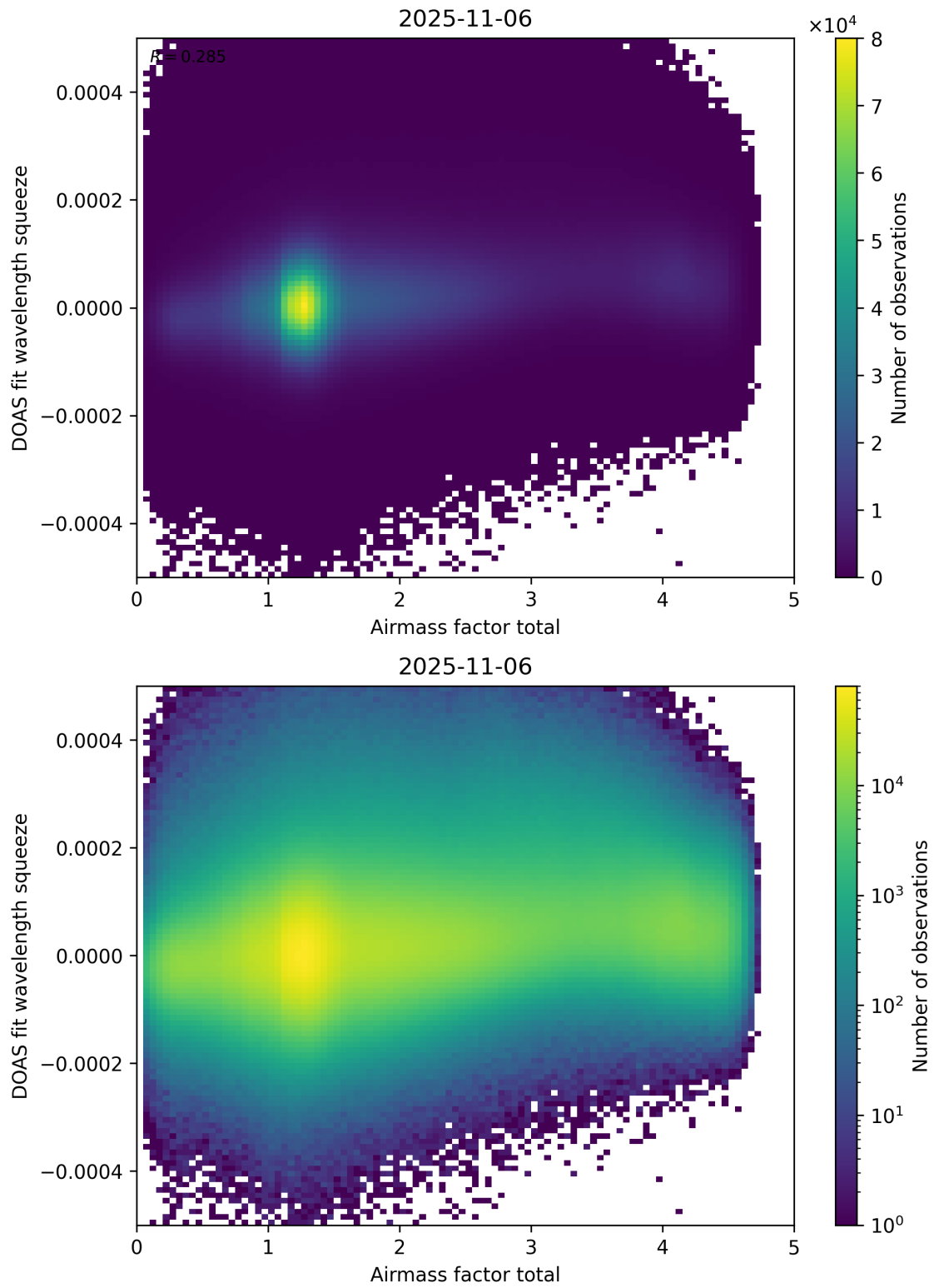
Figure 99: Scatter density plot of “Airmass factor total” against “DOAS fit wavelength squeeze” for 2025-11-05 to 2025-11-07.
