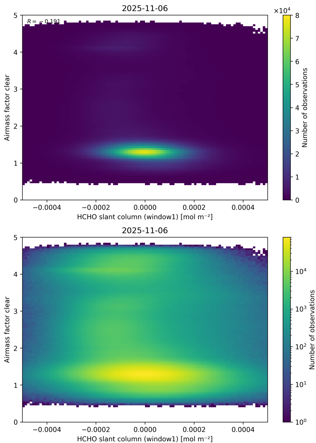
Figure 81: Scatter density plot of “HCHO slant column (window1)” against “Airmass factor clear” for 2025-11-05 to 2025-11-07.
