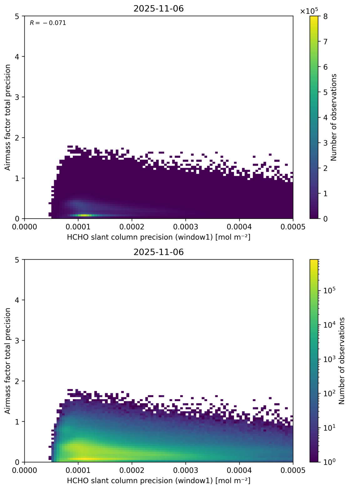
Figure 95: Scatter density plot of “HCHO slant column precision (window1)” against “Airmass factor total precision” for 2025-11-05 to 2025-11-07.
