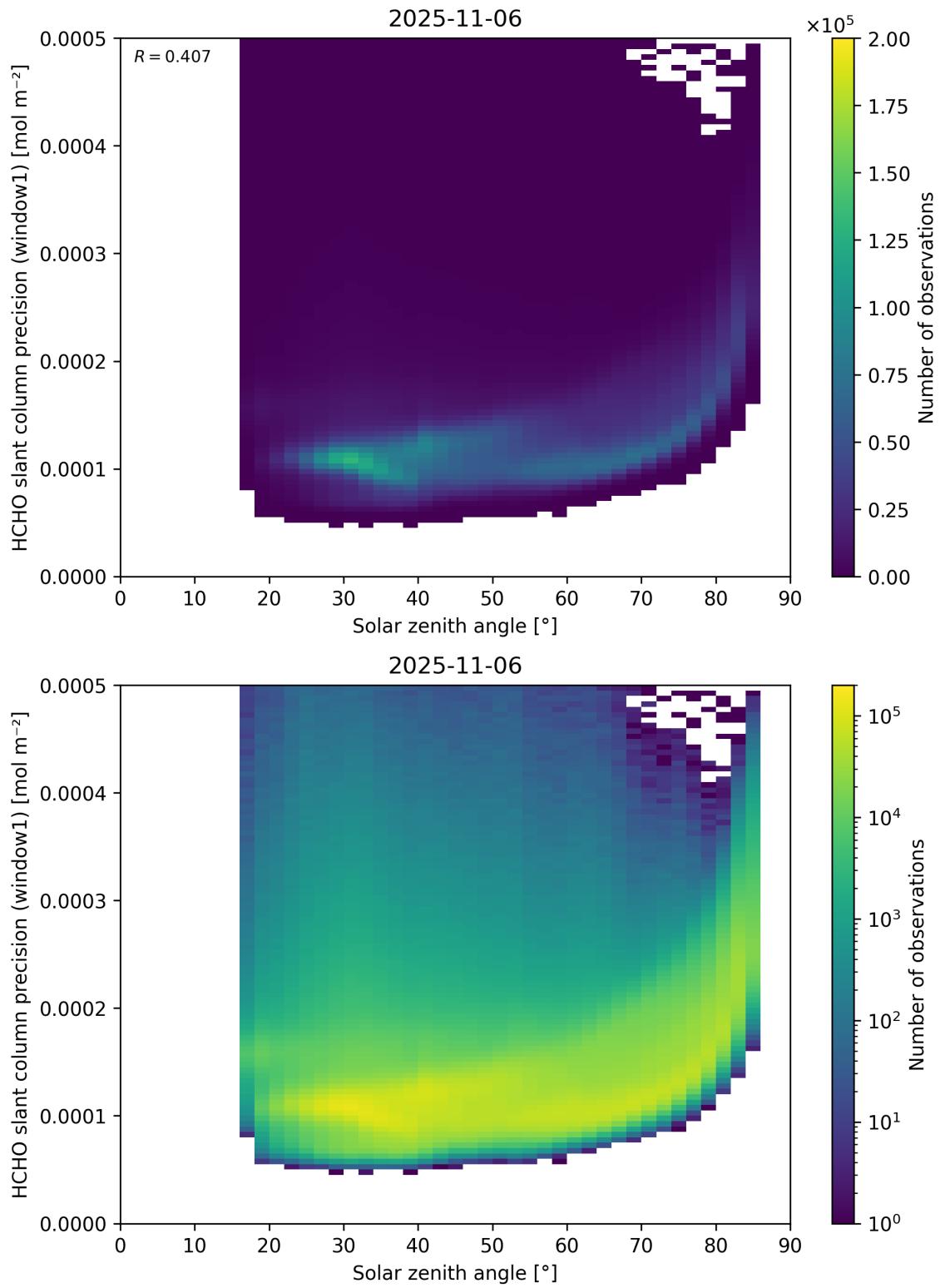
Figure 174: Scatter density plot of “Solar zenith angle” against “HCHO slant column precision (window1)” for 2025-11-05 to 2025-11-07.
