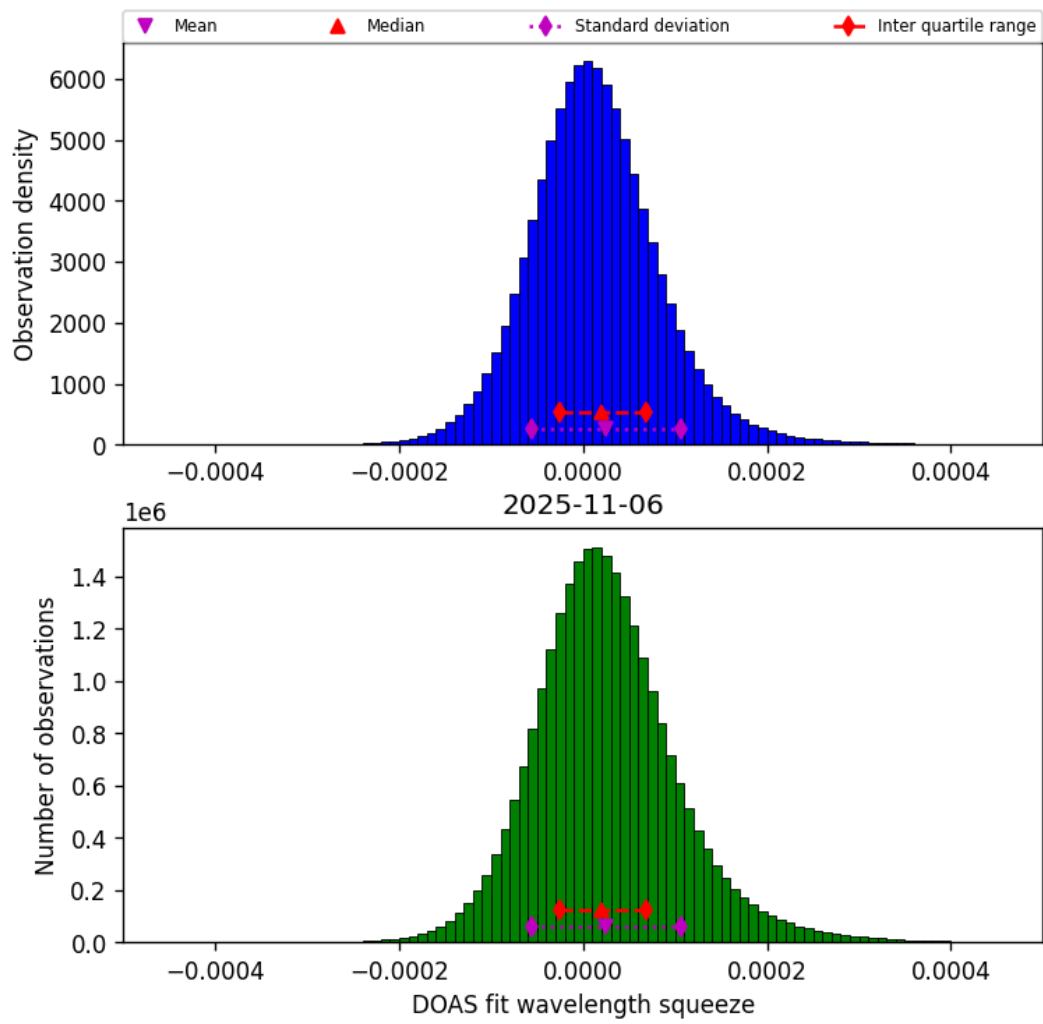
Figure 45: Histogram of “DOAS fit wavelength squeeze” for 2025-11-05 to 2025-11-07
