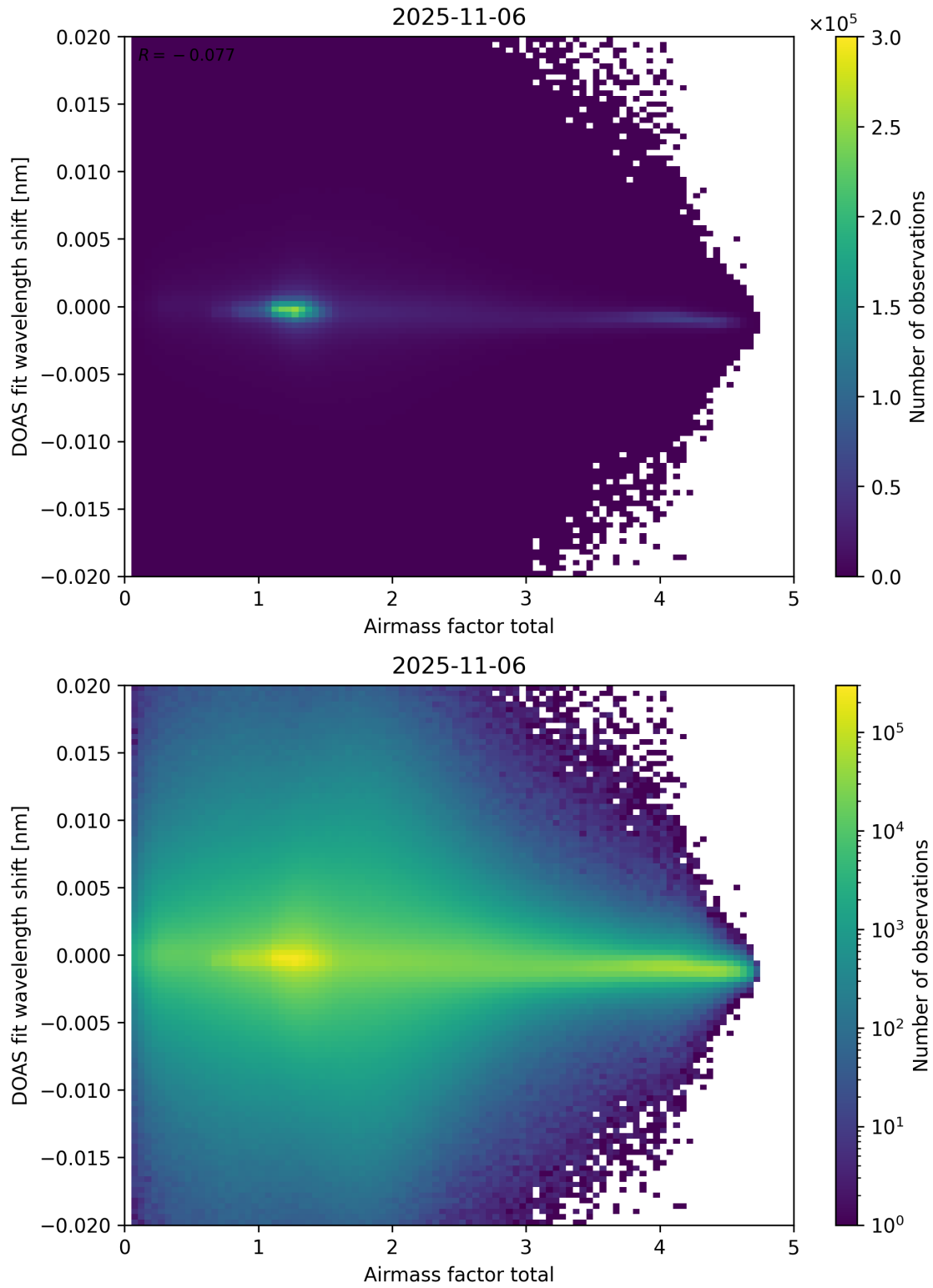
Figure 98: Scatter density plot of “Airmass factor total” against “DOAS fit wavelength shift” for 2025-11-05 to 2025-11-07.
