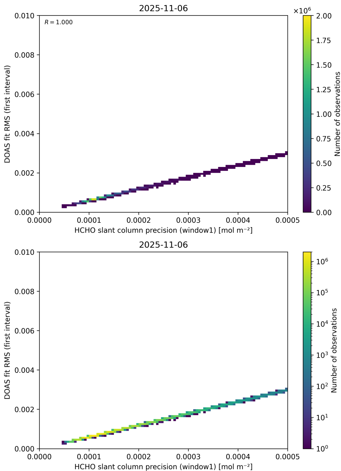
Figure 88: Scatter density plot of “HCHO slant column precision (window1)” against “DOAS fit RMS (first interval)” for 2025-11-05 to 2025-11-07.
