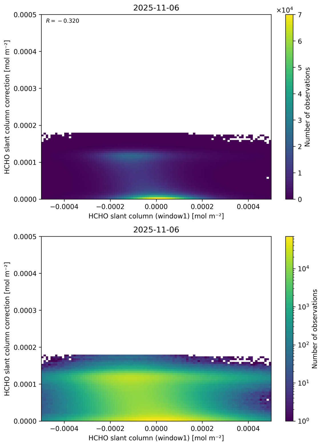
Figure 83: Scatter density plot of “HCHO slant column (window1)” against “HCHO slant column correction” for 2025-11-05 to 2025-11-07.
