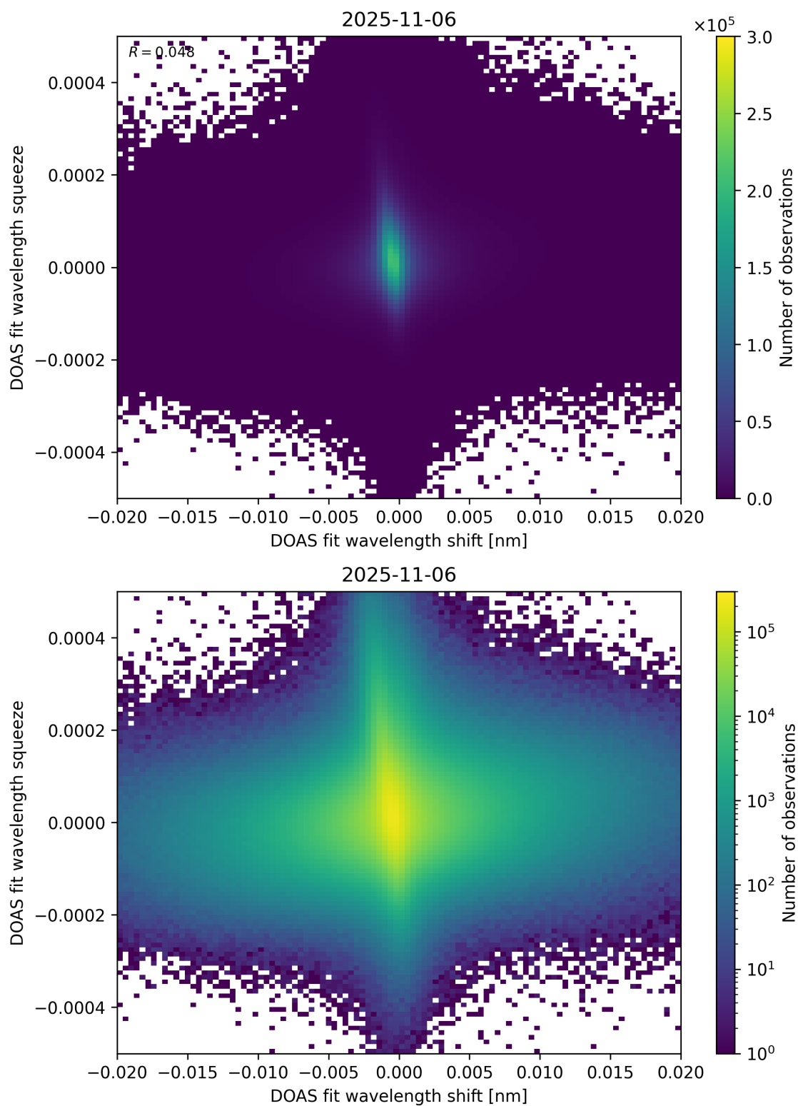
Figure 65: Scatter density plot of “DOAS fit wavelength shift” against “DOAS fit wavelength squeeze” for 2025-11-05 to 2025-11-07.
