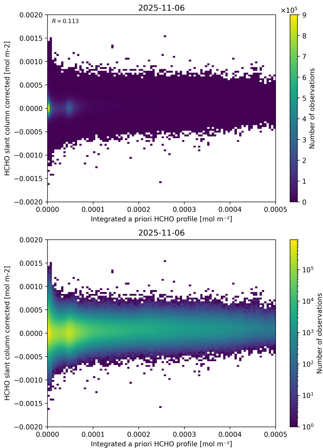
Figure 151: Scatter density plot of “Integrated a priori HCHO profile” against “HCHO slant column corrected” for 2025-11-05 to 2025-11-07.
