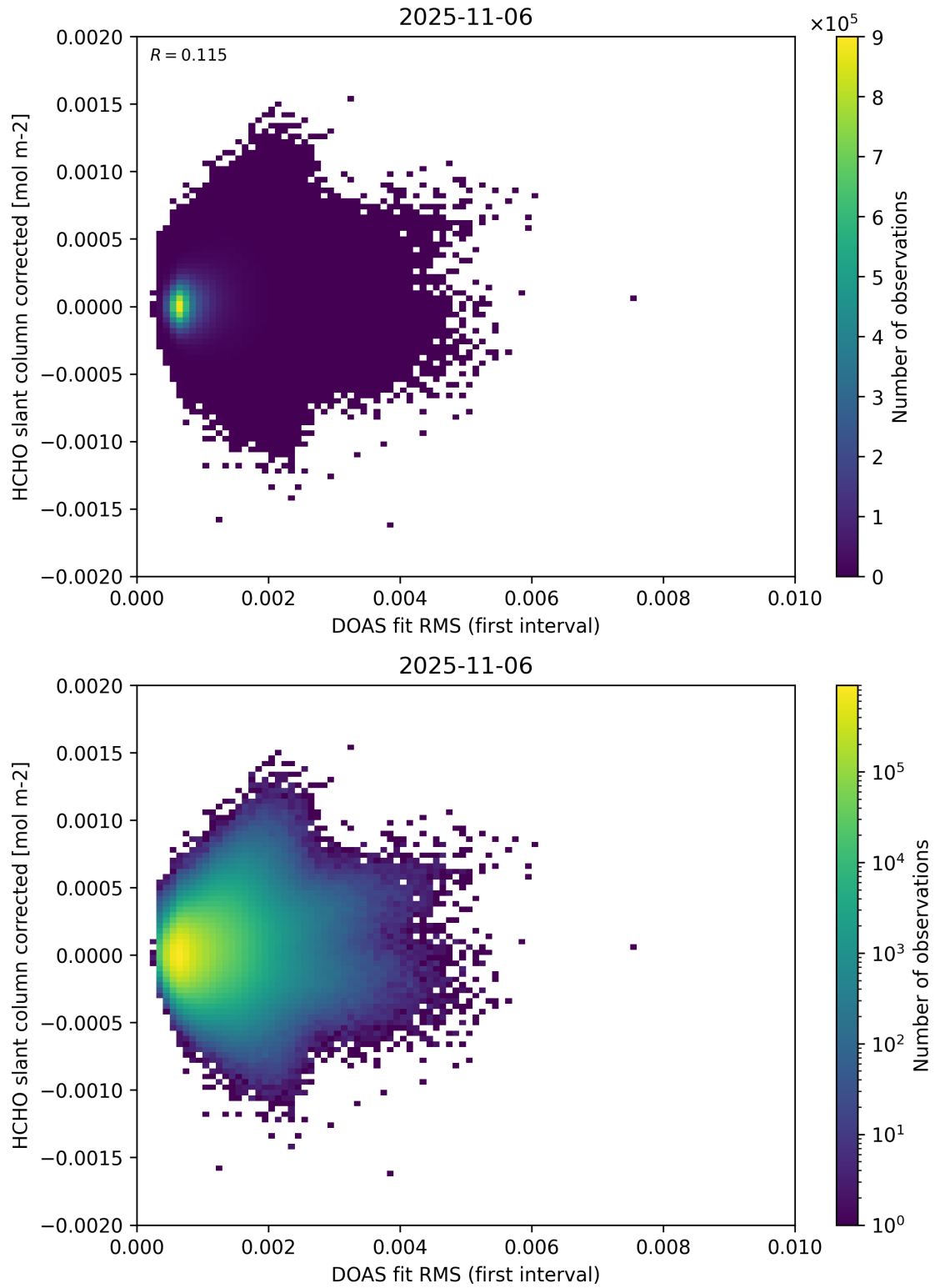
Figure 62: Scatter density plot of “DOAS fit RMS (first interval)” against “HCHO slant column corrected” for 2025-11-05 to 2025-11-07.
