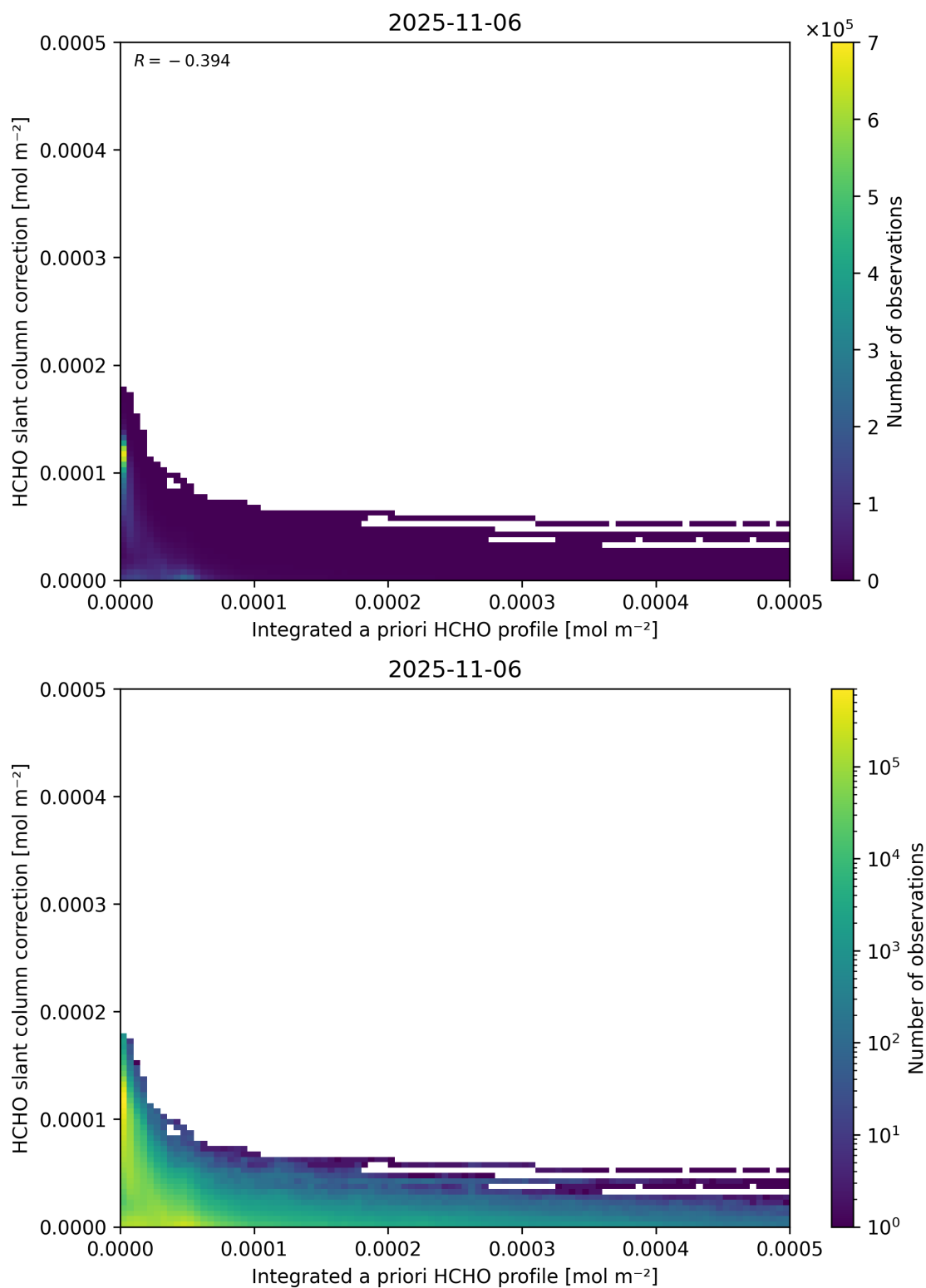
Figure 152: Scatter density plot of “Integrated a priori HCHO profile” against “HCHO slant column correction” for 2025-11-05 to 2025-11-07.
