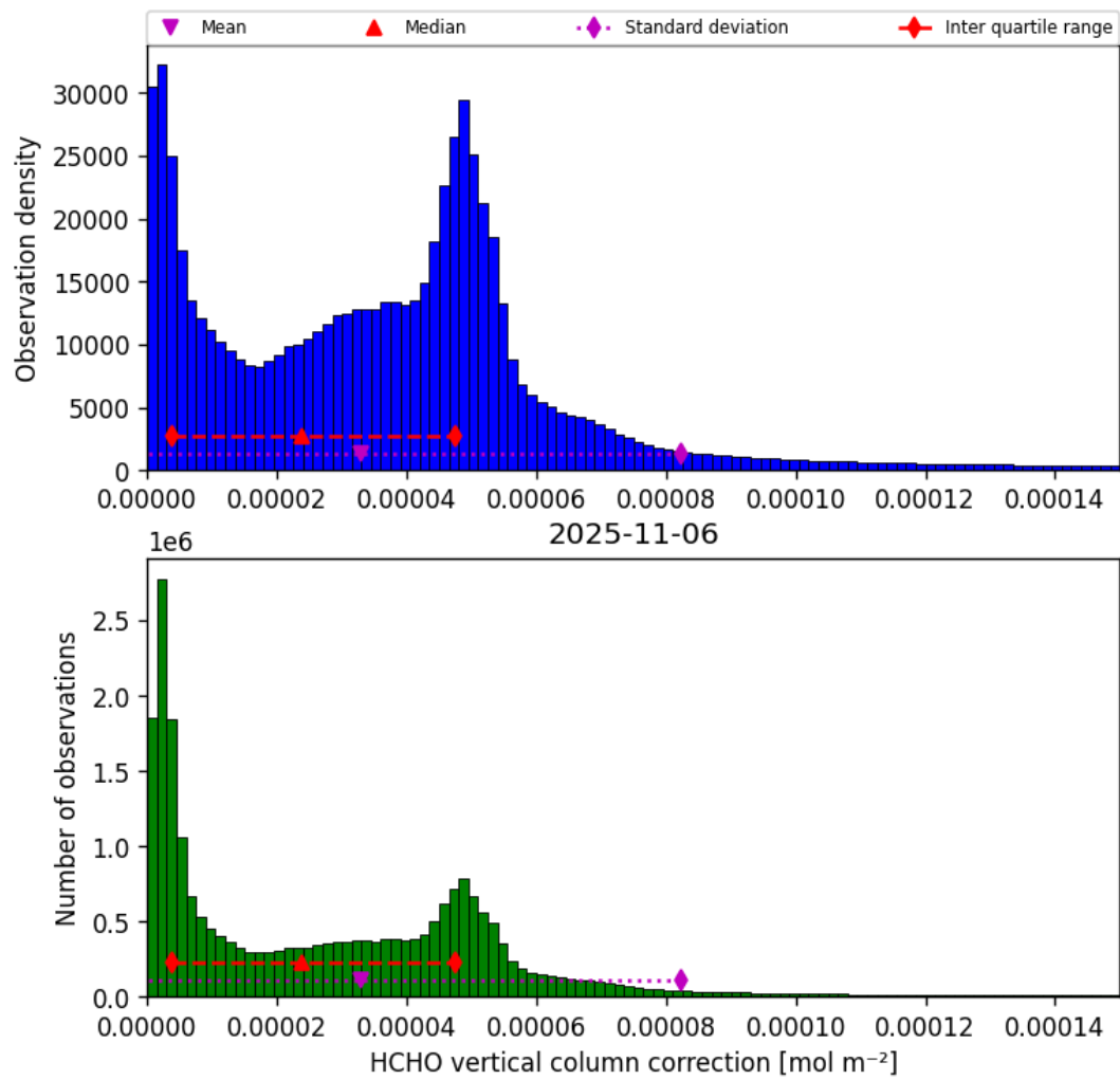
Figure 37: Histogram of “HCHO vertical column correction” for 2025-11-05 to 2025-11-07
