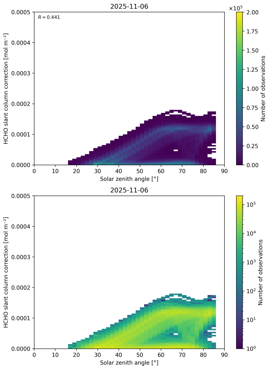
Figure 172: Scatter density plot of “Solar zenith angle” against “HCHO slant column correction” for 2025-11-05 to 2025-11-07.
