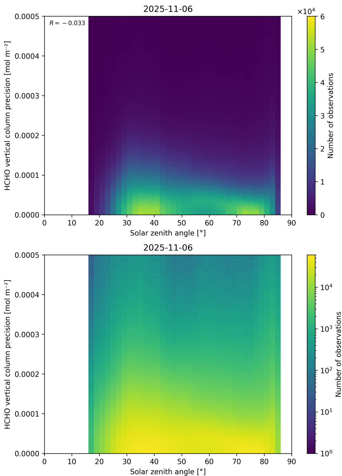
Figure 179: Scatter density plot of “Solar zenith angle” against “HCHO vertical column precision” for 2025-11-05 to 2025-11-07.
