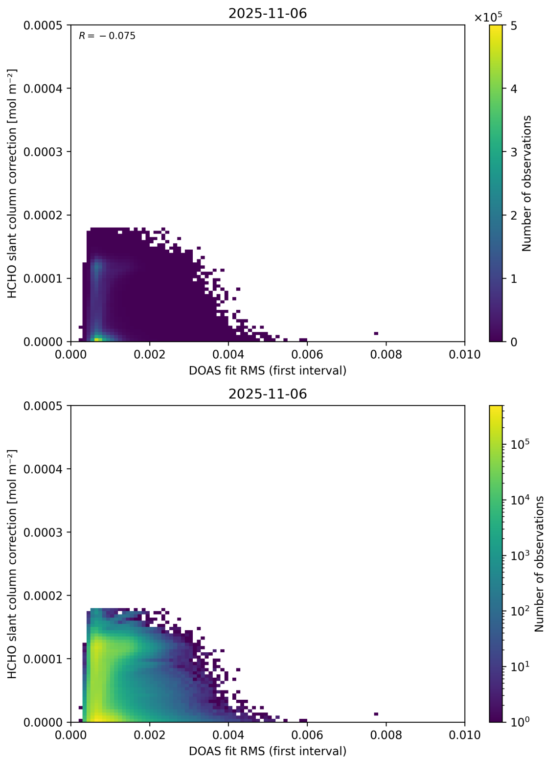
Figure 63: Scatter density plot of “DOAS fit RMS (first interval)” against “HCHO slant column correction” for 2025-11-05 to 2025-11-07.
