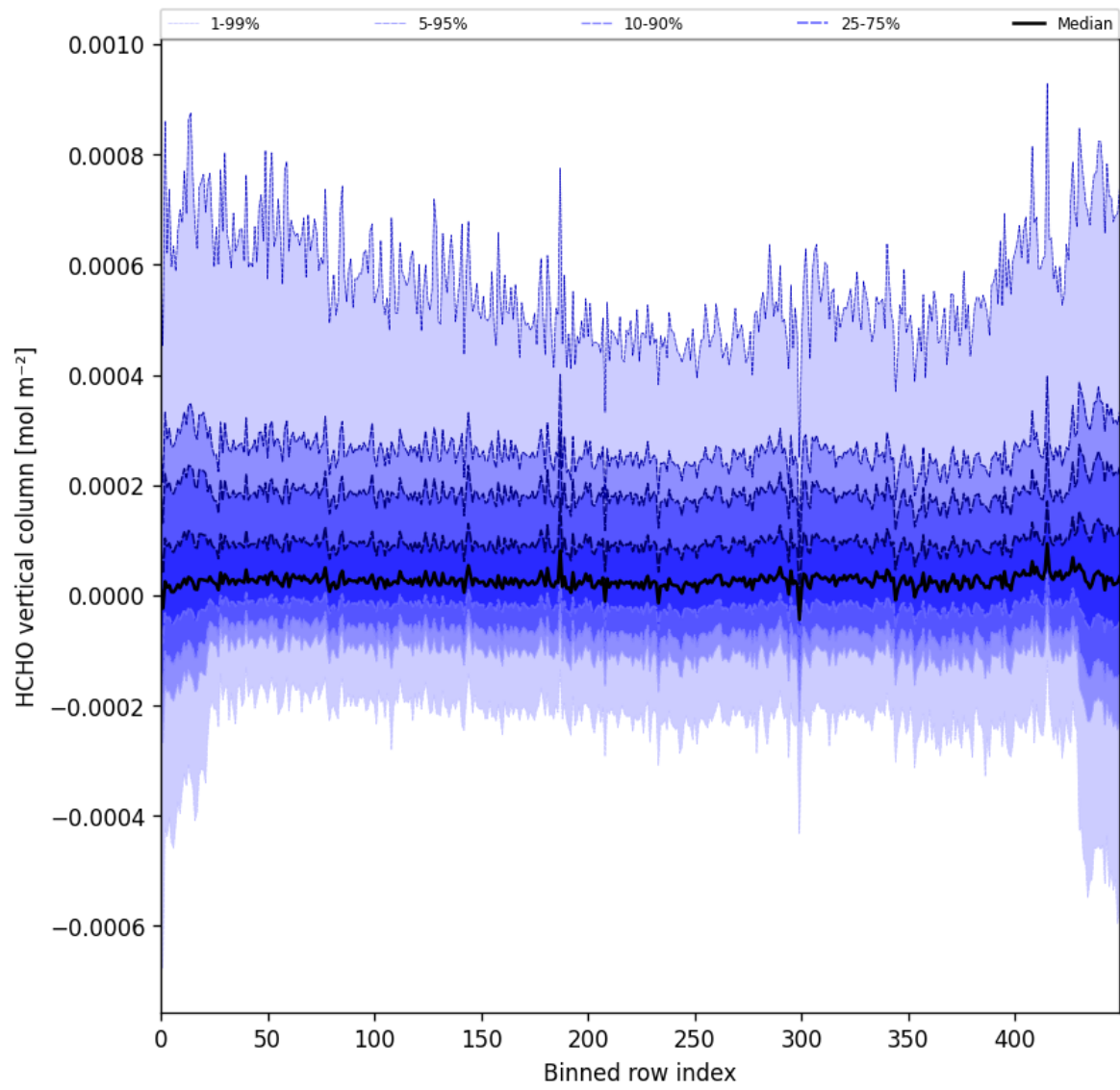
Figure 49: Along track statistics of “HCHO vertical column” for 2025-11-05 to 2025-11-07
