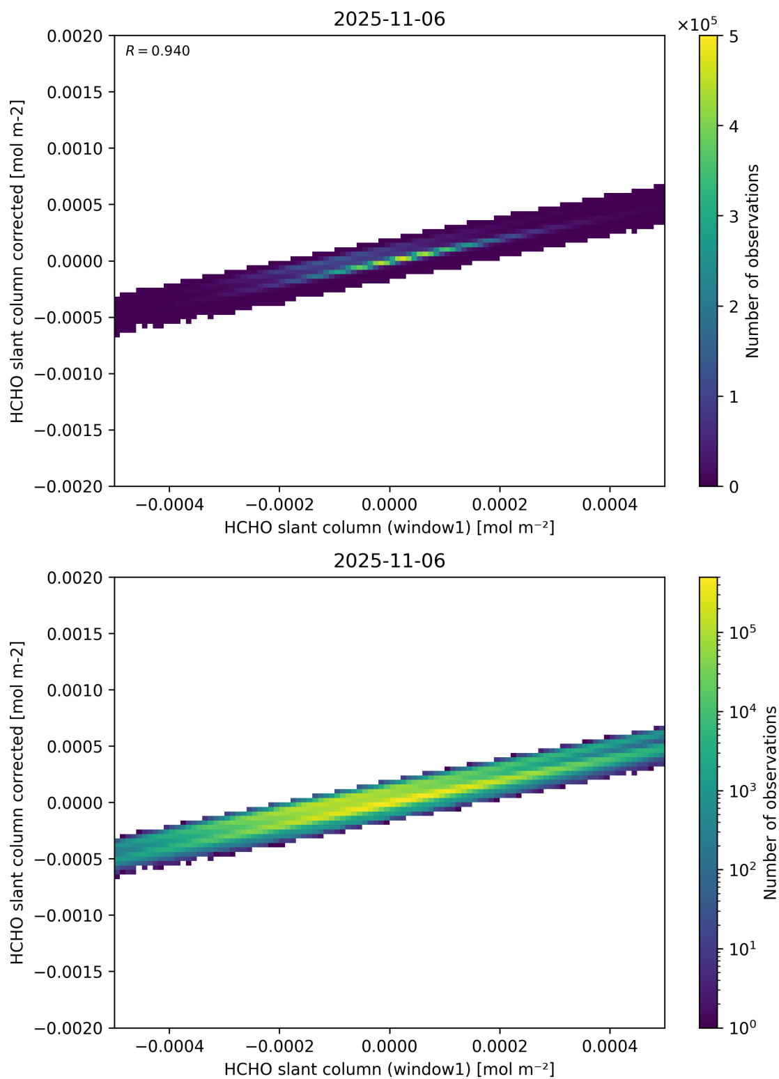
Figure 82: Scatter density plot of “HCHO slant column (window1)” against “HCHO slant column corrected” for 2025-11-05 to 2025-11-07.
