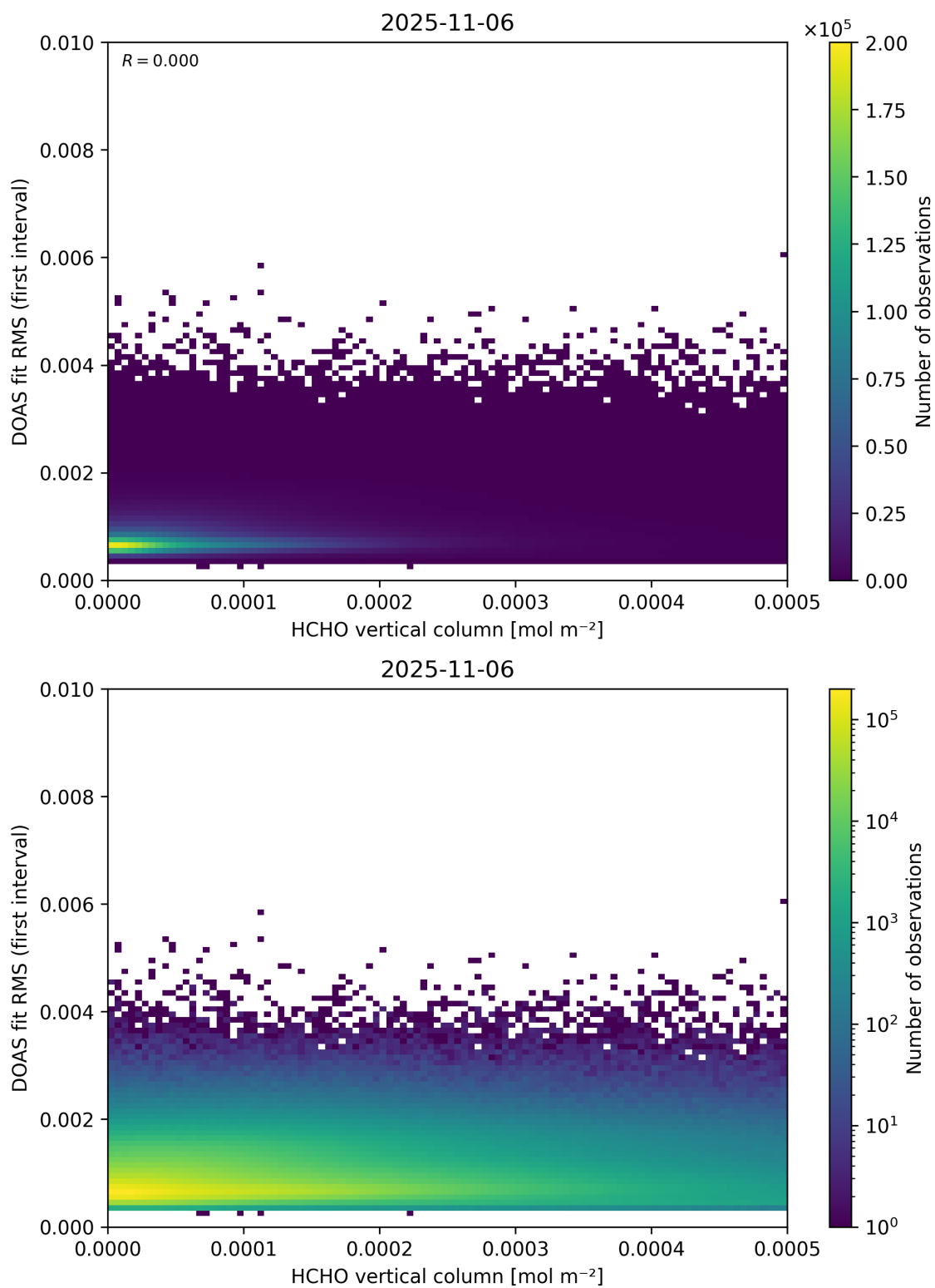
Figure 123: Scatter density plot of “HCHO vertical column” against “DOAS fit RMS (first interval)” for 2025-11-05 to 2025-11-07.
