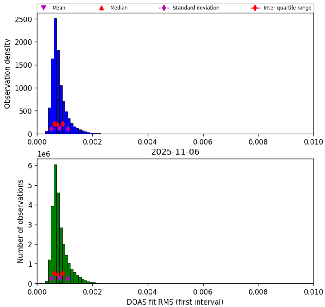
Figure 46: Histogram of “DOAS fit RMS (first interval)” for 2025-11-05 to 2025-11-07
