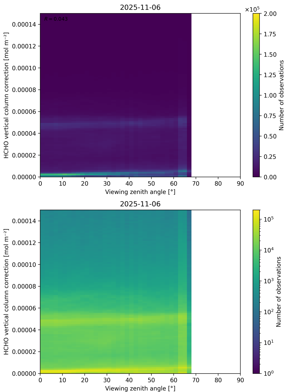
Figure 193: Scatter density plot of “Viewing zenith angle” against “HCHO vertical column correction” for 2025-11-05 to 2025-11-07.
