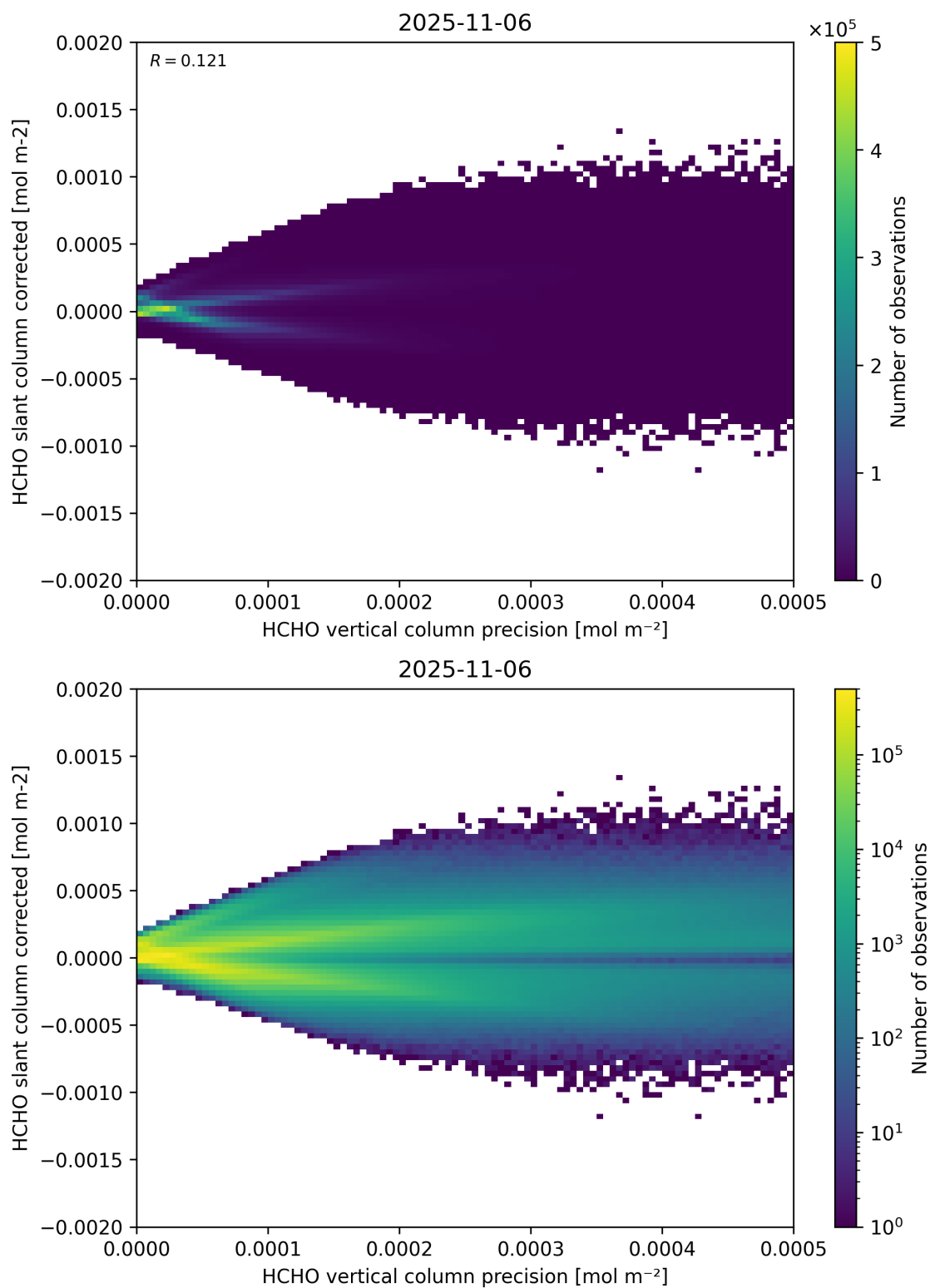
Figure 140: Scatter density plot of “HCHO vertical column precision” against “HCHO slant column corrected” for 2025-11-05 to 2025-11-07.
