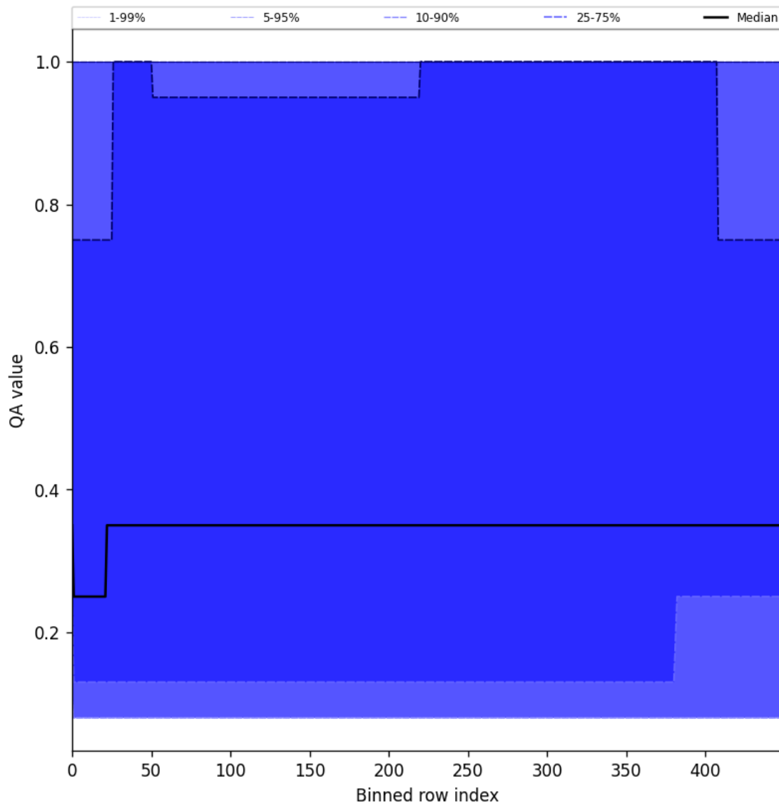
Figure 48: Along track statistics of “QA value” for 2025-11-05 to 2025-11-07
