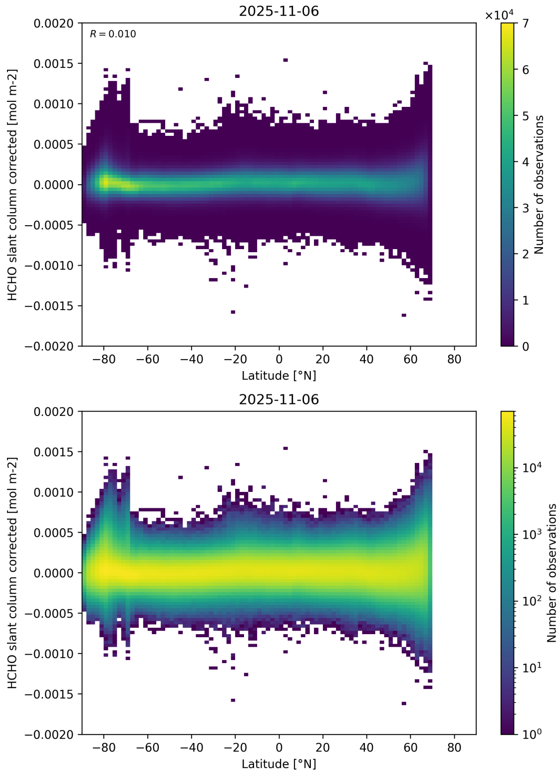
Figure 157: Scatter density plot of “Latitude” against “HCHO slant column corrected” for 2025-11-05 to 2025-11-07.
