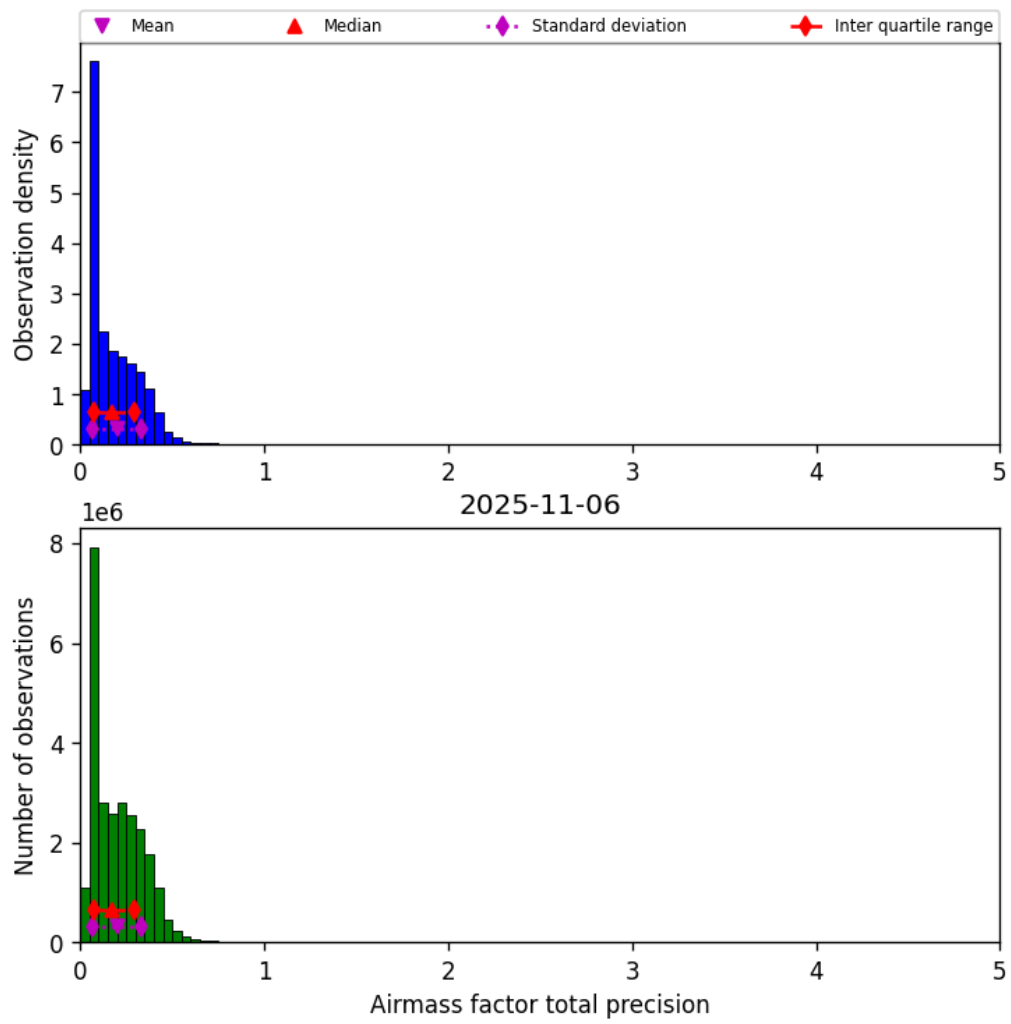
Figure 41: Histogram of “Airmass factor total precision” for 2025-11-05 to 2025-11-07
