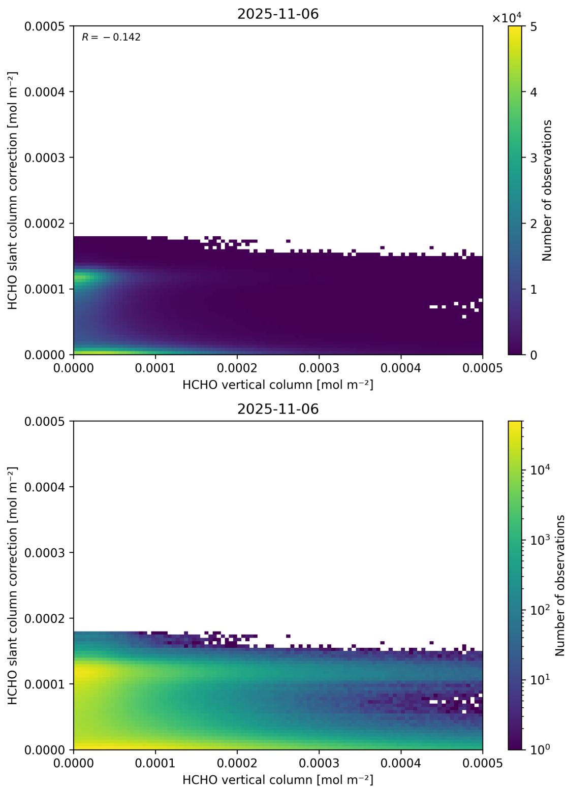
Figure 128: Scatter density plot of “HCHO vertical column” against “HCHO slant column correction” for 2025-11-05 to 2025-11-07.
