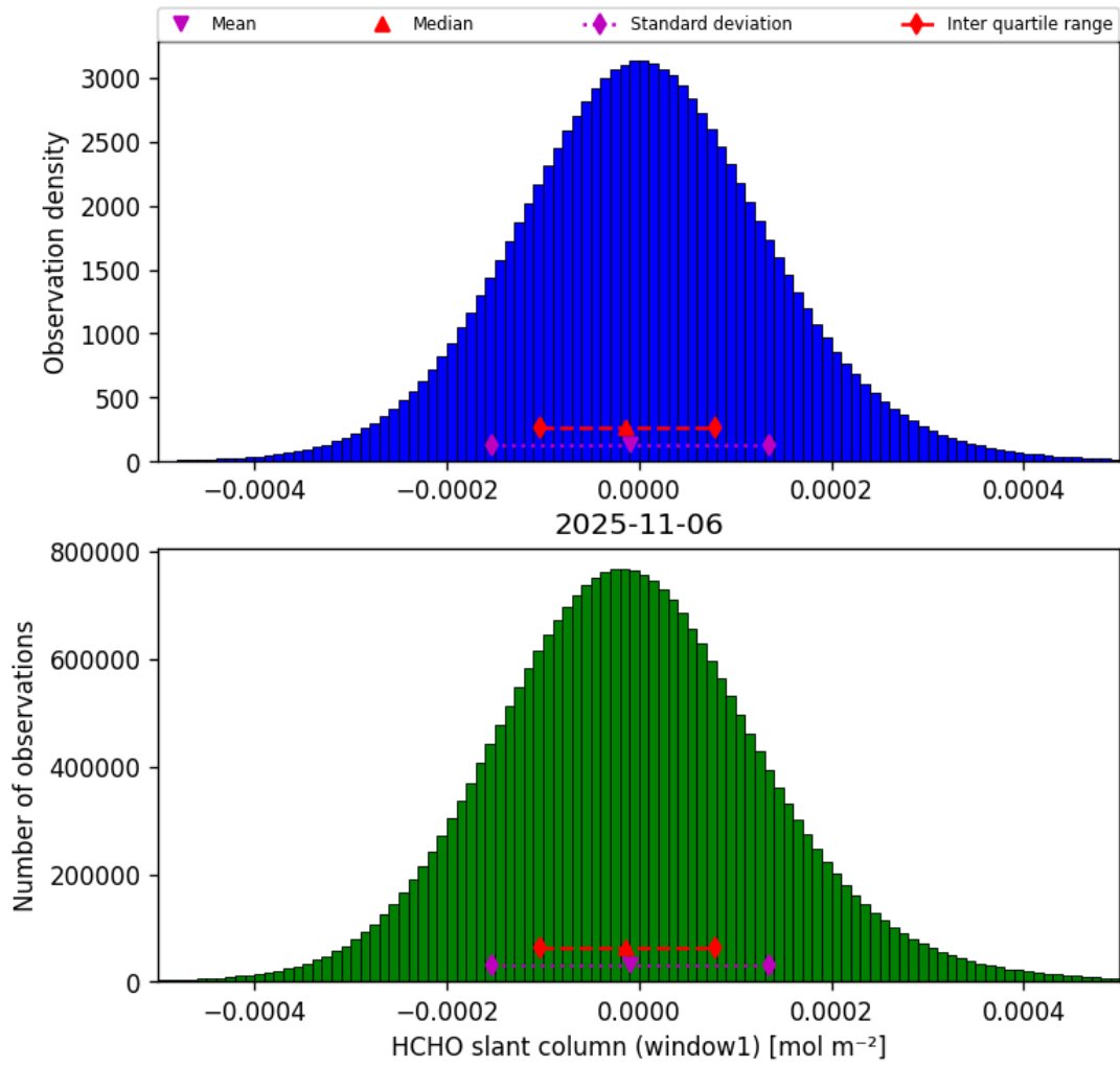
Figure 38: Histogram of “HCHO slant column (window1)” for 2025-11-05 to 2025-11-07
