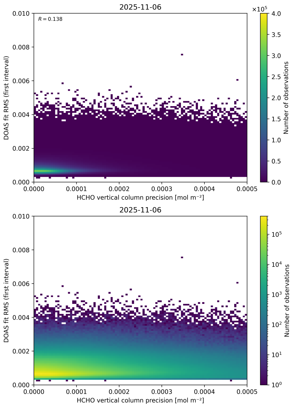
Figure 136: Scatter density plot of “HCHO vertical column precision” against “DOAS fit RMS (first interval)” for 2025-11-05 to 2025-11-07.
