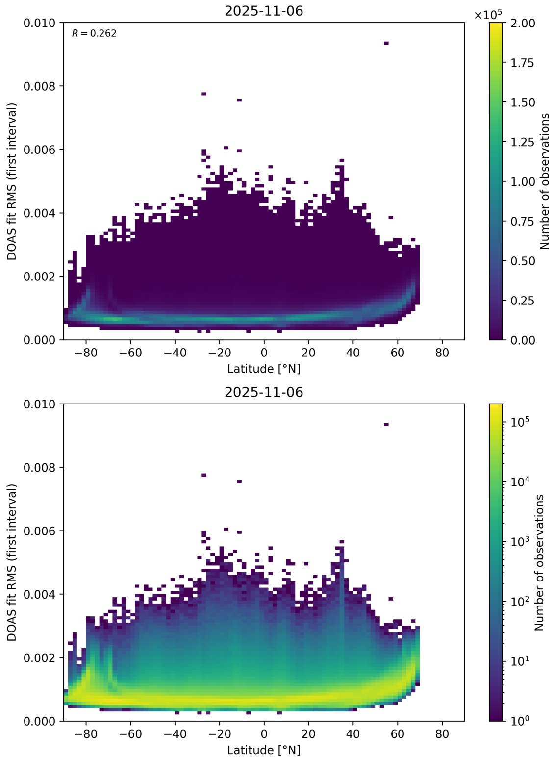
Figure 153: Scatter density plot of “Latitude” against “DOAS fit RMS (first interval)” for 2025-11-05 to 2025-11-07.
