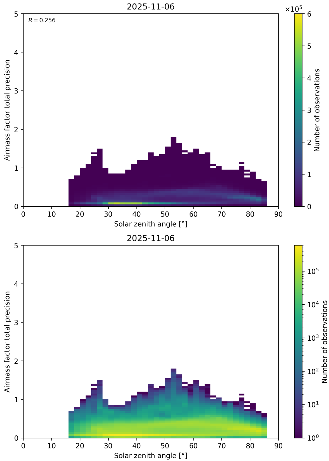
Figure 176: Scatter density plot of “Solar zenith angle” against “Airmass factor total precision” for 2025-11-05 to 2025-11-07.
