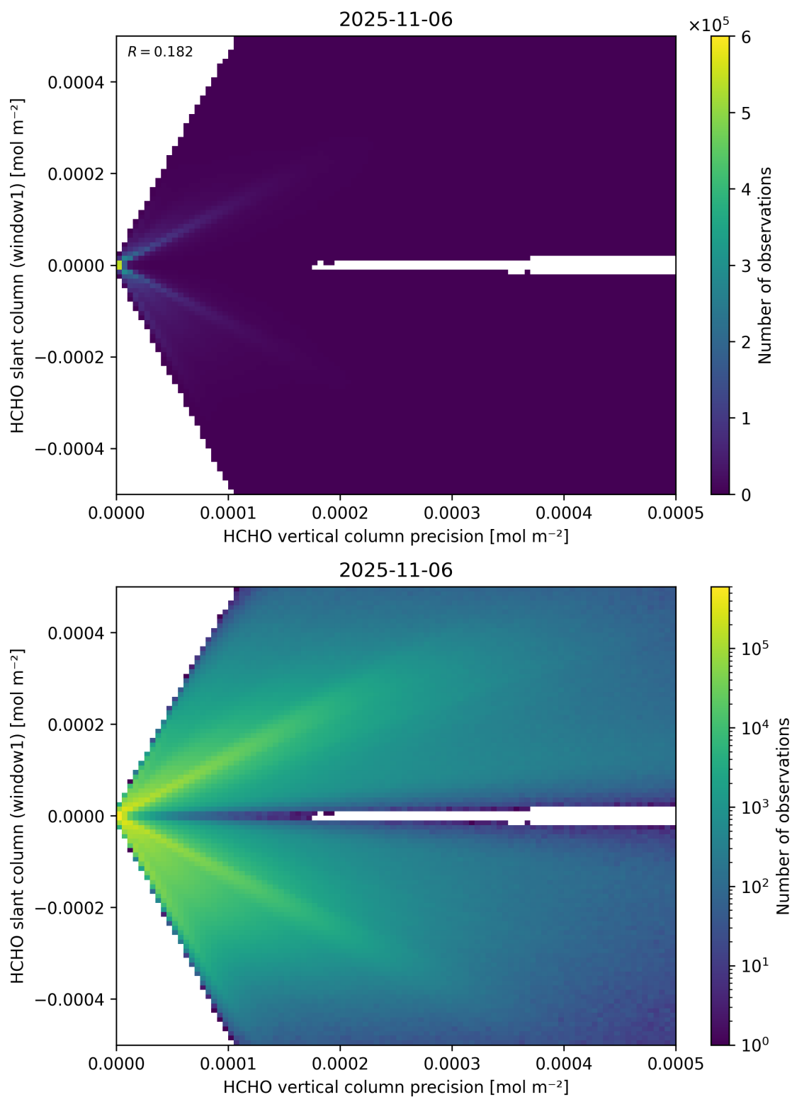
Figure 142: Scatter density plot of “HCHO vertical column precision” against “HCHO slant column (window1)” for 2025-11-05 to 2025-11-07.
