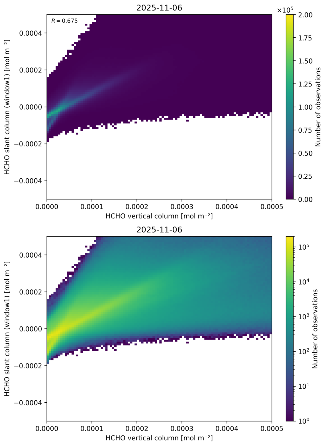
Figure 129: Scatter density plot of “HCHO vertical column” against “HCHO slant column (window1)” for 2025-11-05 to 2025-11-07.
