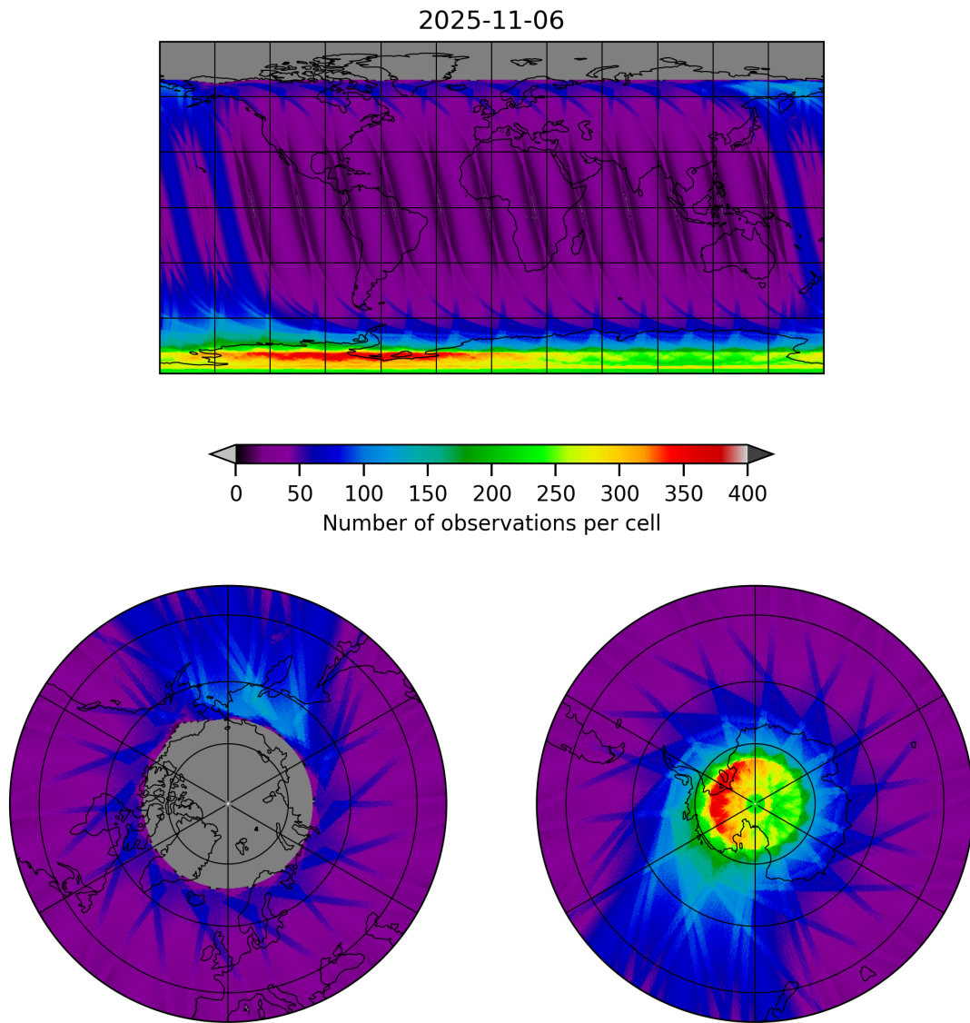
Figure 19: Map of the number of observations for 2025-11-05 to 2025-11-07
