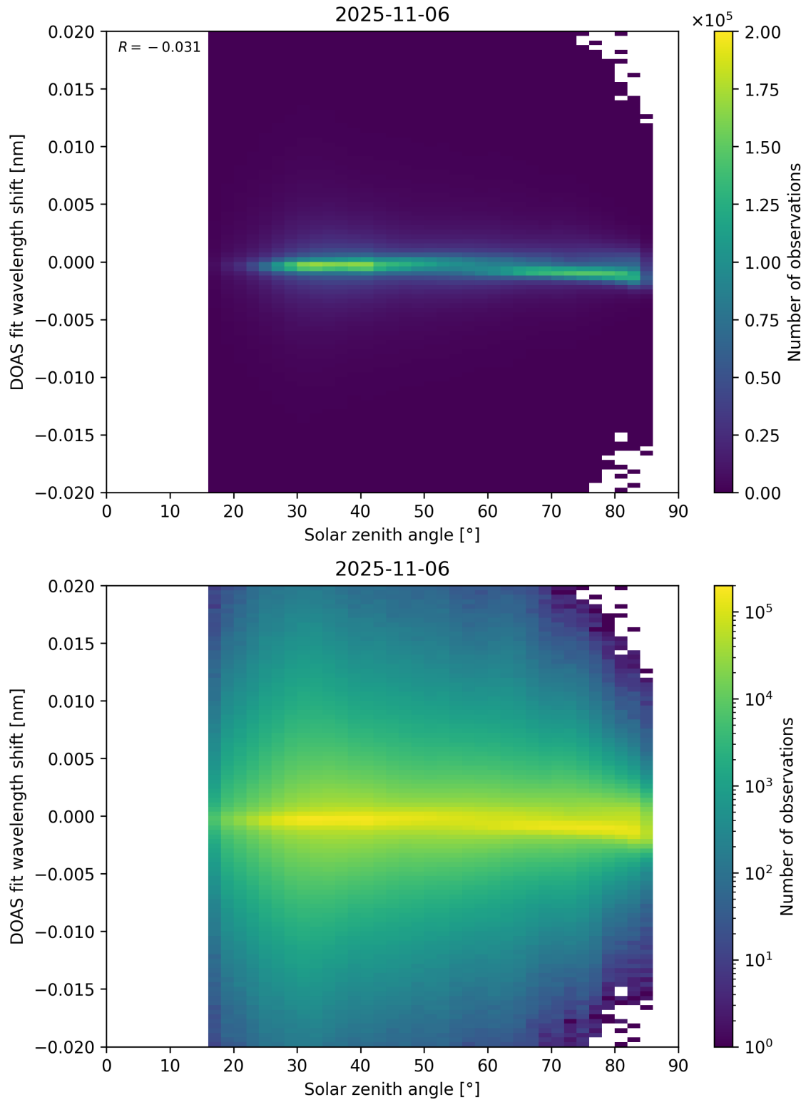
Figure 168: Scatter density plot of “Solar zenith angle” against “DOAS fit wavelength shift” for 2025-11-05 to 2025-11-07.
