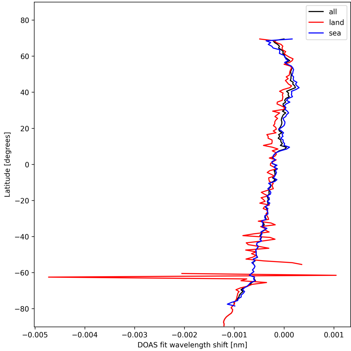
Figure 30: Zonal average of “DOAS fit wavelength shift” for 2025-11-05 to 2025-11-07.
