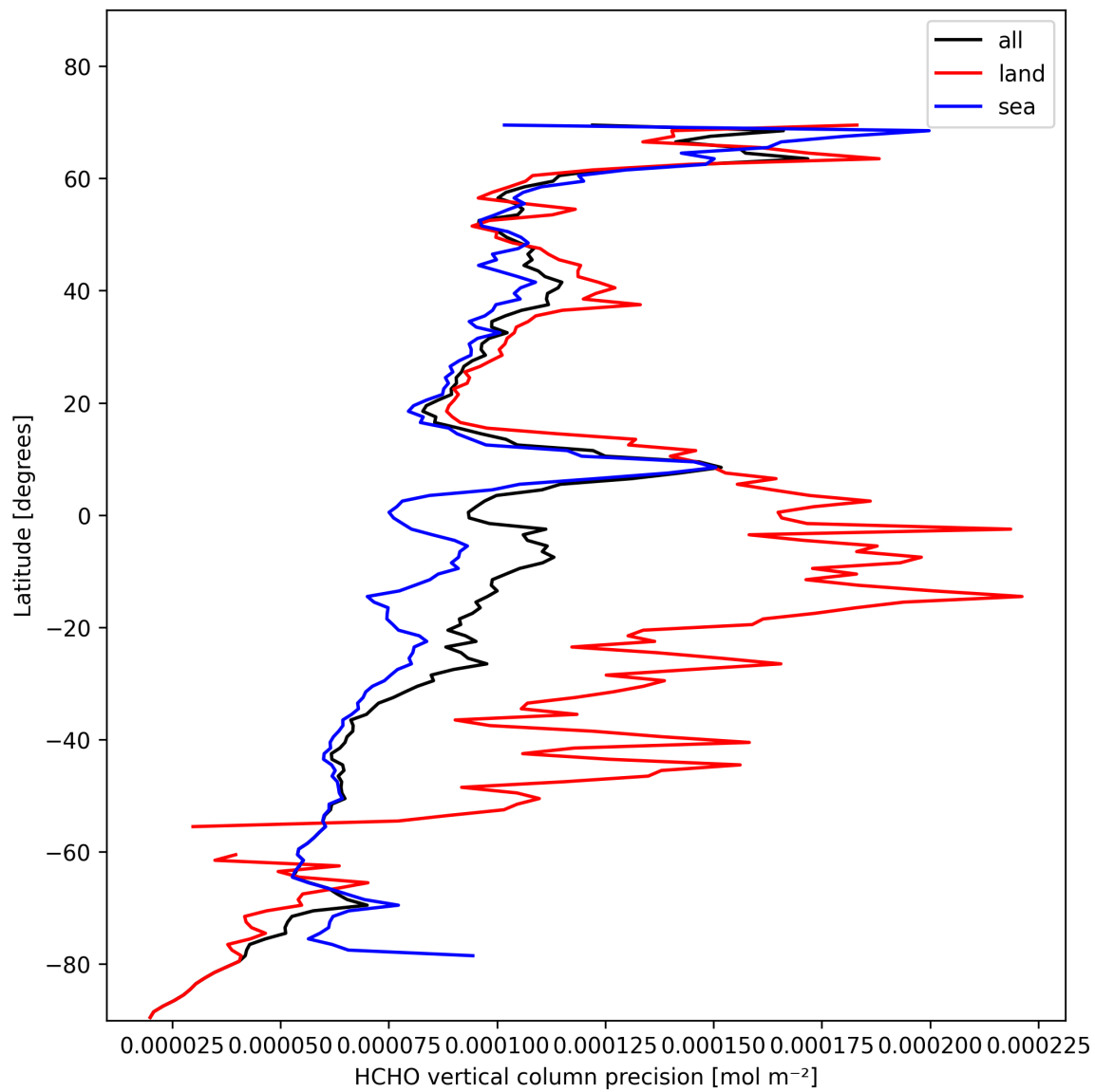
Figure 22: Zonal average of “HCHO vertical column precision” for 2025-11-05 to 2025-11-07.
