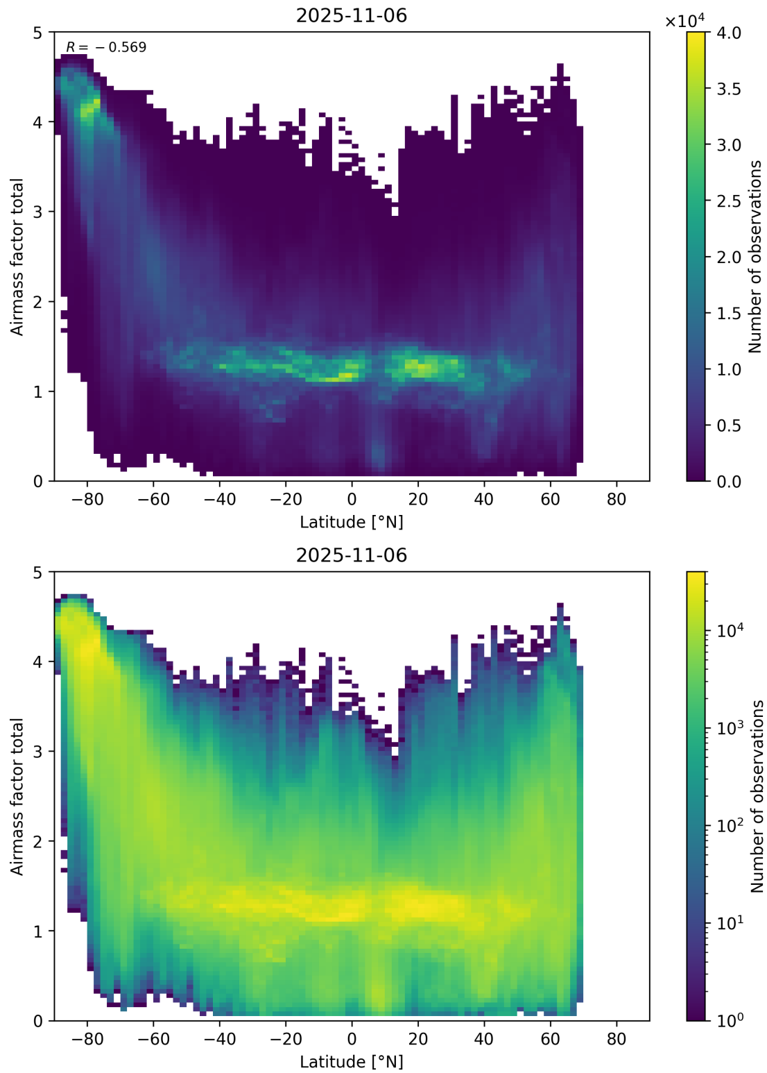
Figure 161: Scatter density plot of “Latitude” against “Airmass factor total” for 2025-11-05 to 2025-11-07.
