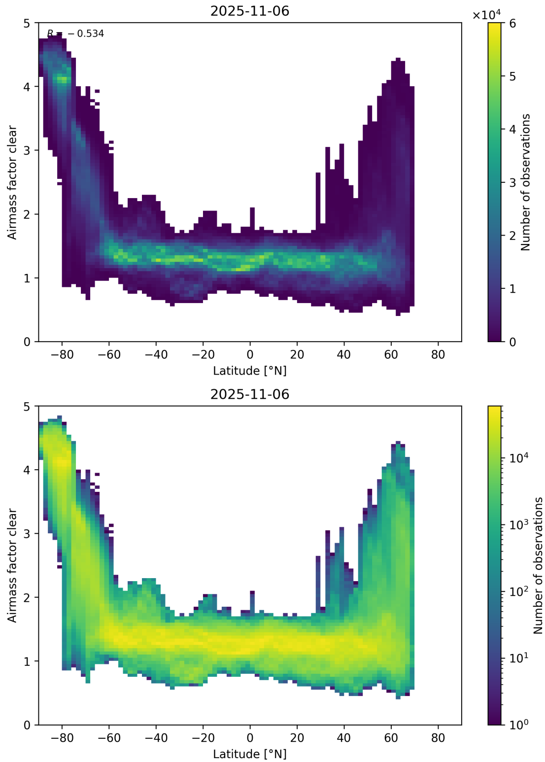
Figure 156: Scatter density plot of “Latitude” against “Airmass factor clear” for 2025-11-05 to 2025-11-07.
