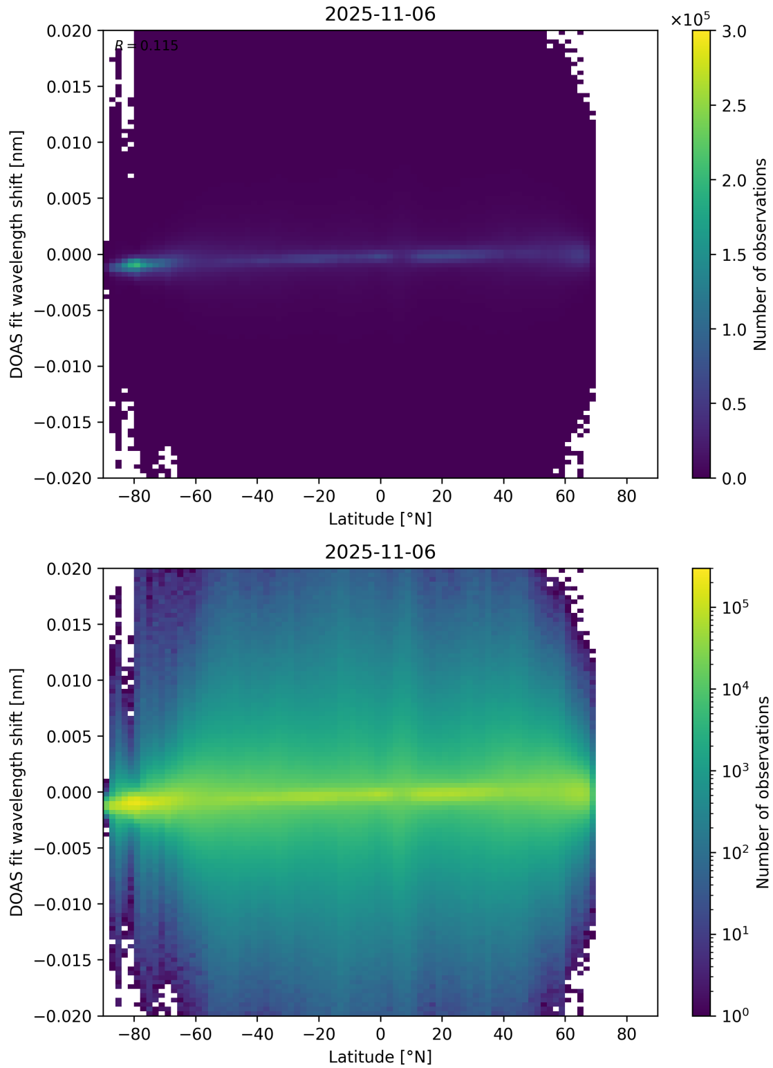
Figure 154: Scatter density plot of “Latitude” against “DOAS fit wavelength shift” for 2025-11-05 to 2025-11-07.
