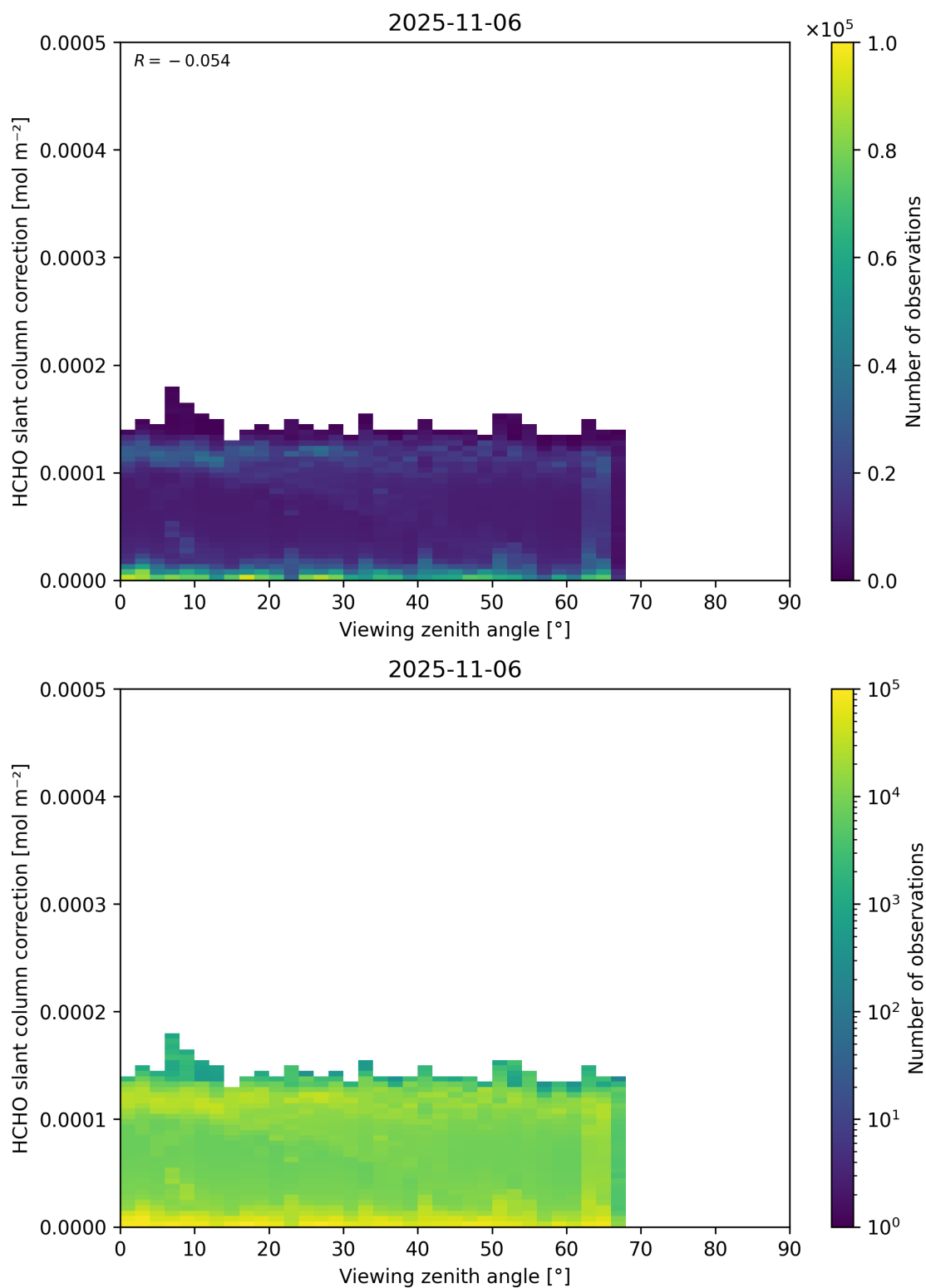
Figure 187: Scatter density plot of “Viewing zenith angle” against “HCHO slant column correction” for 2025-11-05 to 2025-11-07.
