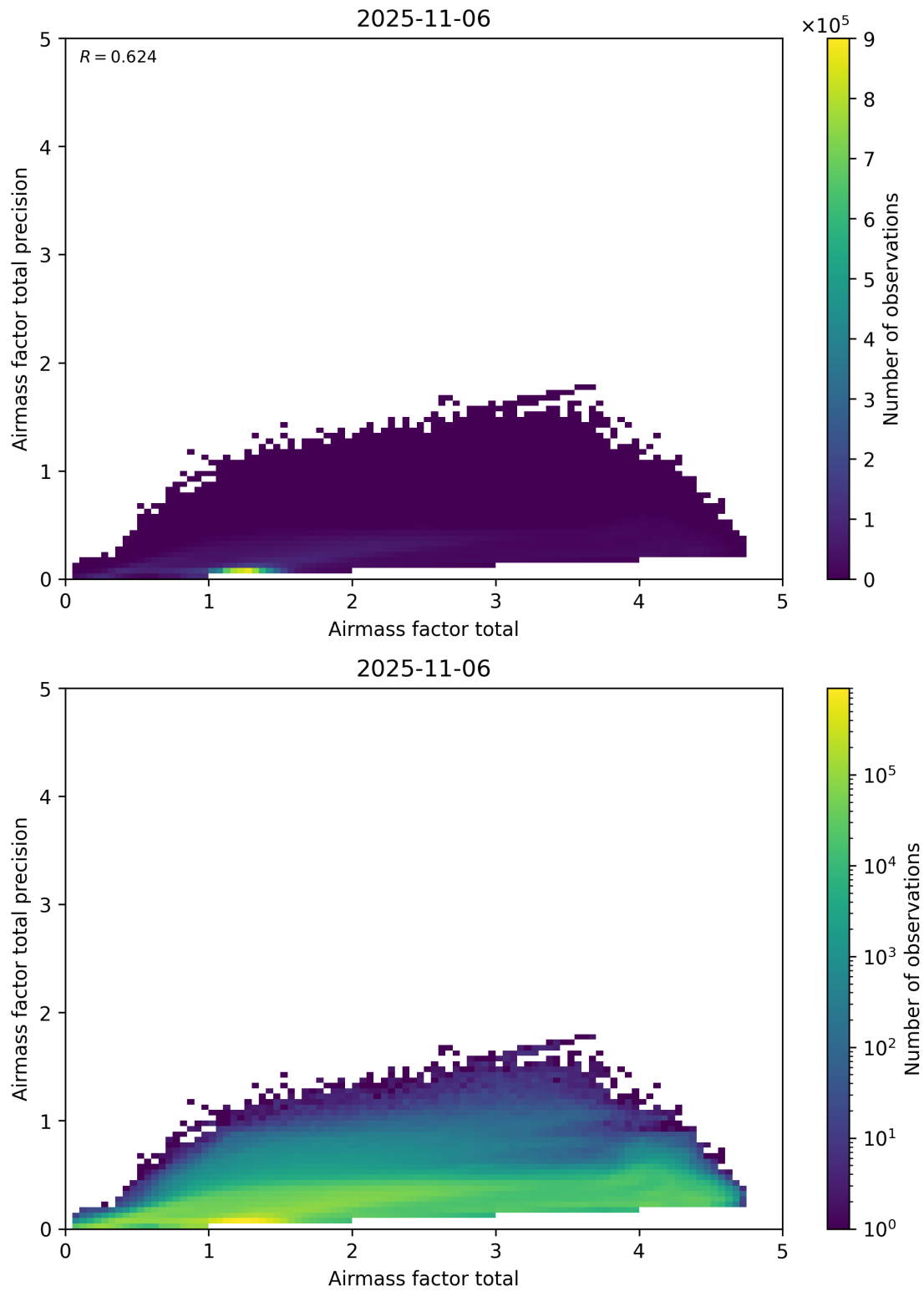
Figure 103: Scatter density plot of “Airmass factor total” against “Airmass factor total precision” for 2025-11-05 to 2025-11-07.
