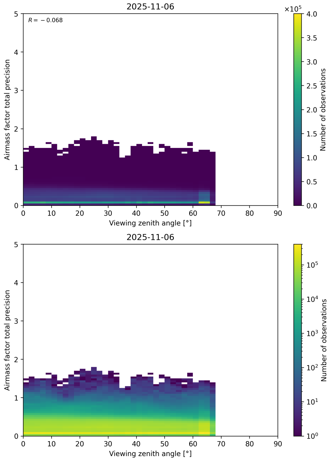
Figure 191: Scatter density plot of “Viewing zenith angle” against “Airmass factor total precision” for 2025-11-05 to 2025-11-07.
