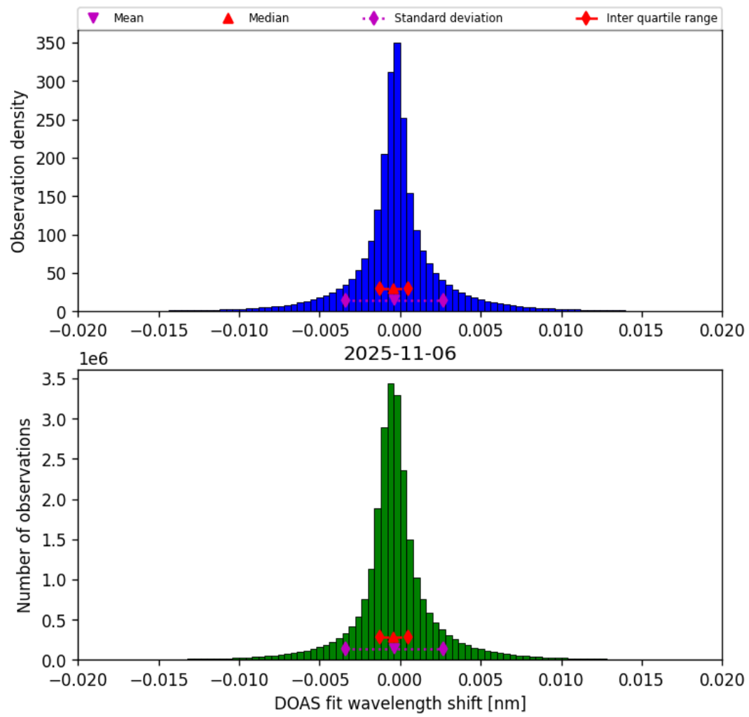
Figure 44: Histogram of “DOAS fit wavelength shift” for 2025-11-05 to 2025-11-07
