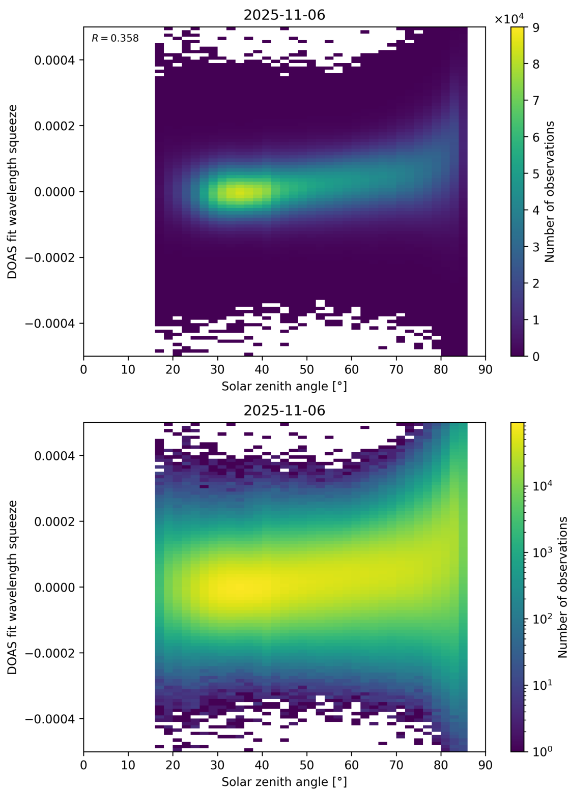
Figure 169: Scatter density plot of “Solar zenith angle” against “DOAS fit wavelength squeeze” for 2025-11-05 to 2025-11-07.
