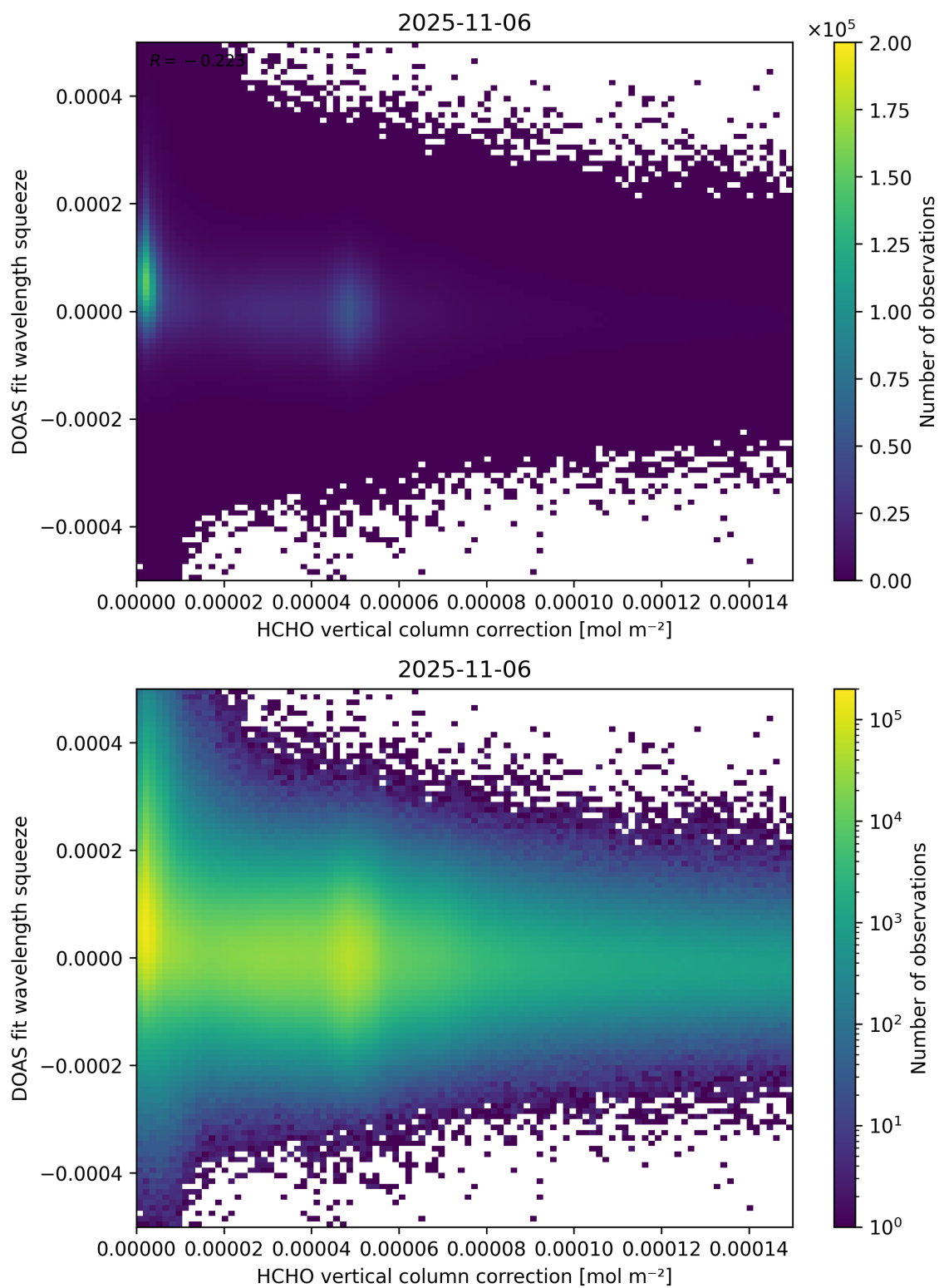
Figure 114: Scatter density plot of “HCHO vertical column correction” against “DOAS fit wavelength squeeze” for 2025-11-05 to 2025-11-07.
