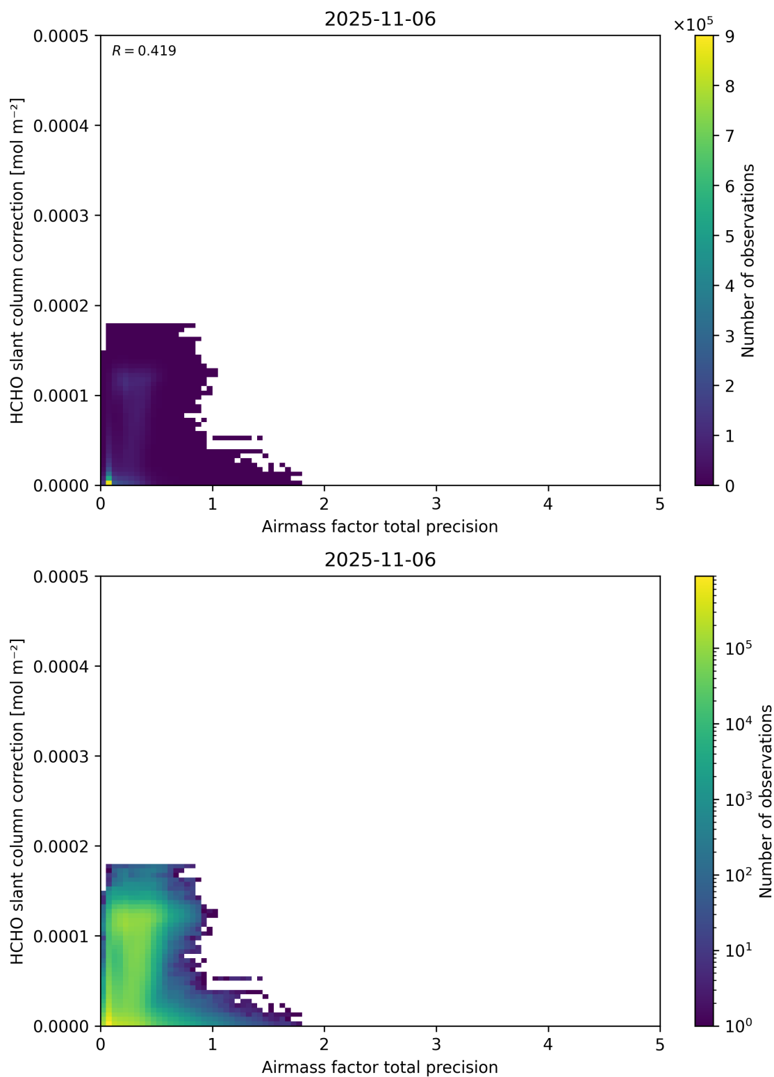
Figure 110: Scatter density plot of “Airmass factor total precision” against “HCHO slant column correction” for 2025-11-05 to 2025-11-07.
