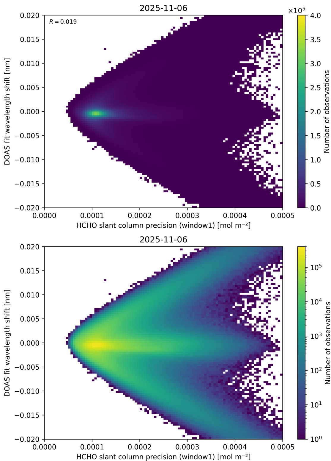
Figure 89: Scatter density plot of “HCHO slant column precision (window1)” against “DOAS fit wavelength shift” for 2025-11-05 to 2025-11-07.
