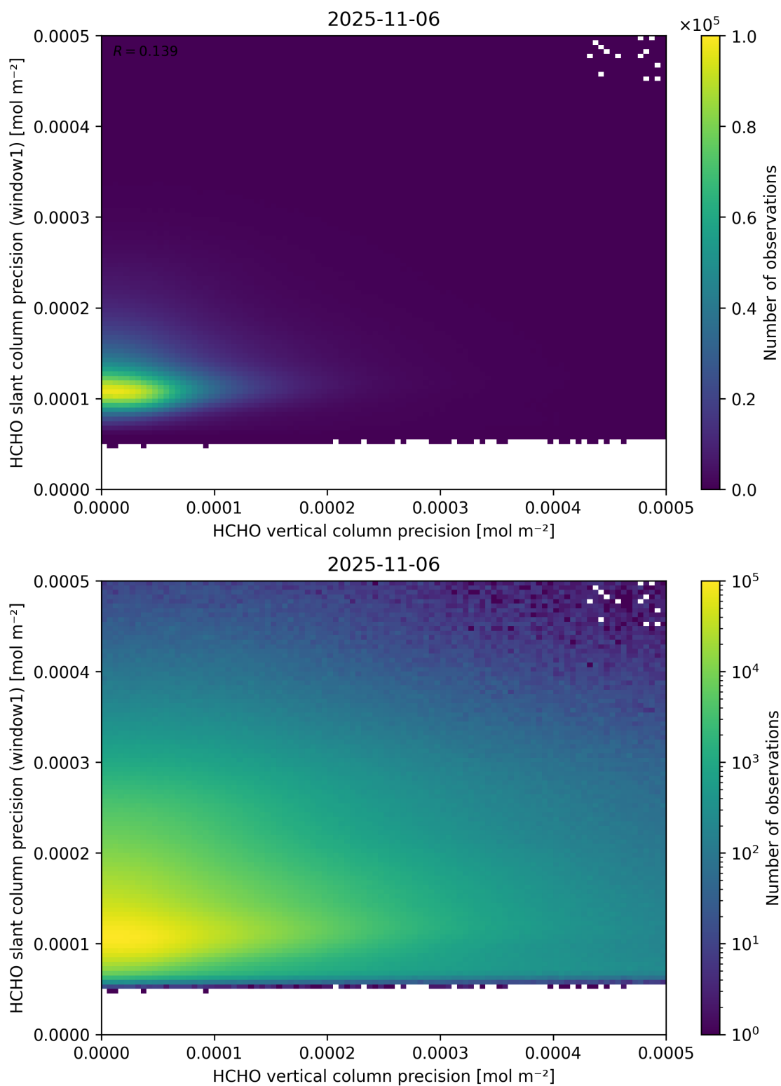
Figure 143: Scatter density plot of “HCHO vertical column precision” against “HCHO slant column precision (window1)” for 2025-11-05 to 2025-11-07.
