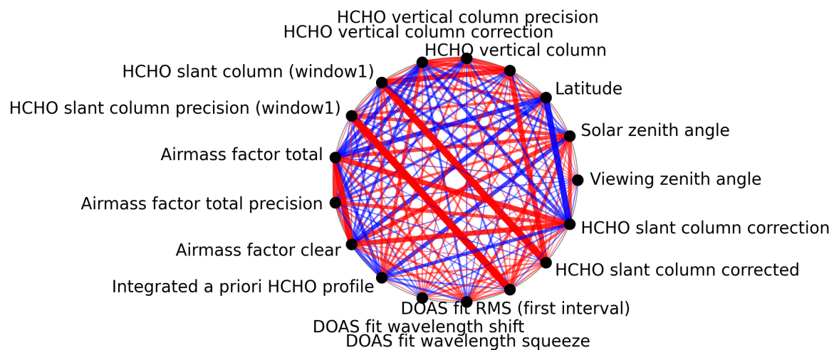
Figure 1: Map of correlation graph for 2025-11-05 to 2025-11-07.
