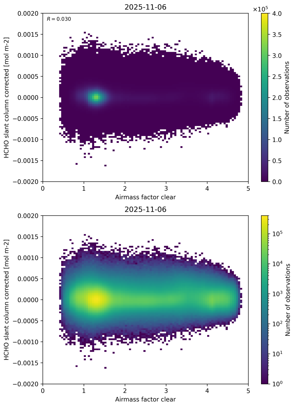
Figure 74: Scatter density plot of “Airmass factor clear” against “HCHO slant column corrected” for 2025-11-05 to 2025-11-07.
