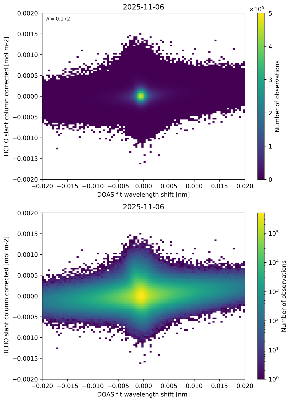
Figure 66: Scatter density plot of “DOAS fit wavelength shift” against “HCHO slant column corrected” for 2025-11-05 to 2025-11-07.
