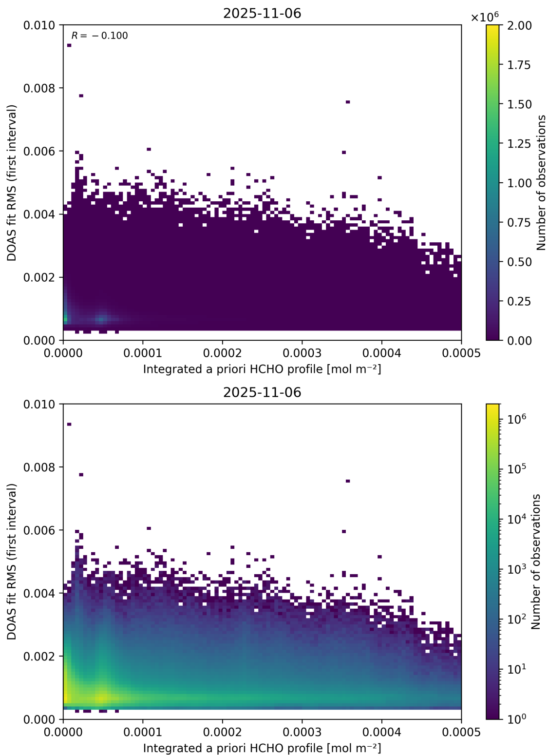
Figure 148: Scatter density plot of “Integrated a priori HCHO profile” against “DOAS fit RMS (first interval)” for 2025-11-05 to 2025-11-07.
