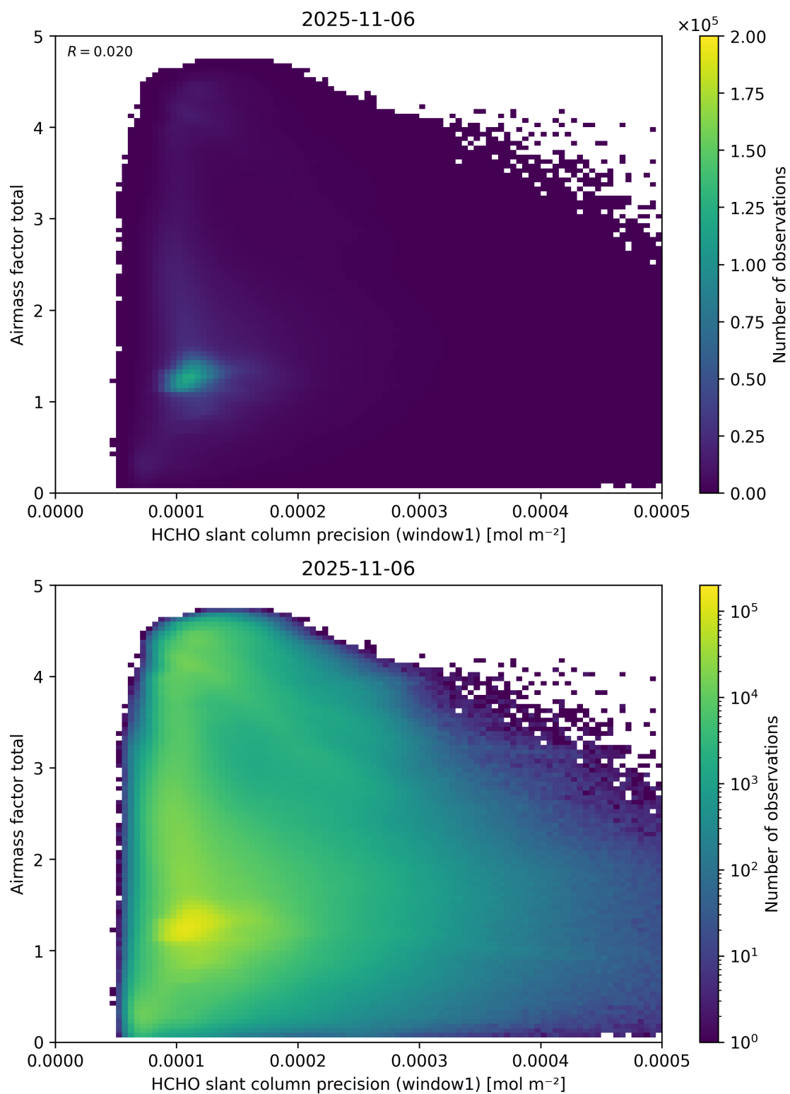
Figure 94: Scatter density plot of “HCHO slant column precision (window1)” against “Airmass factor total” for 2025-11-05 to 2025-11-07.
