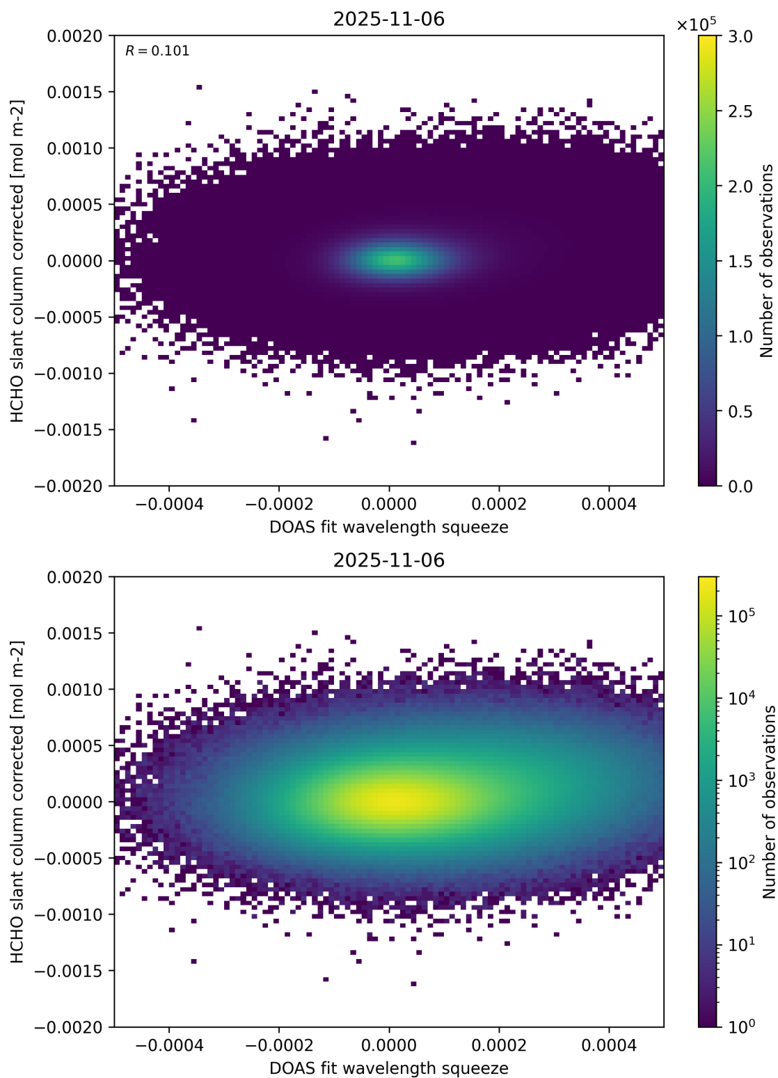
Figure 69: Scatter density plot of “DOAS fit wavelength squeeze” against “HCHO slant column corrected” for 2025-11-05 to 2025-11-07.
