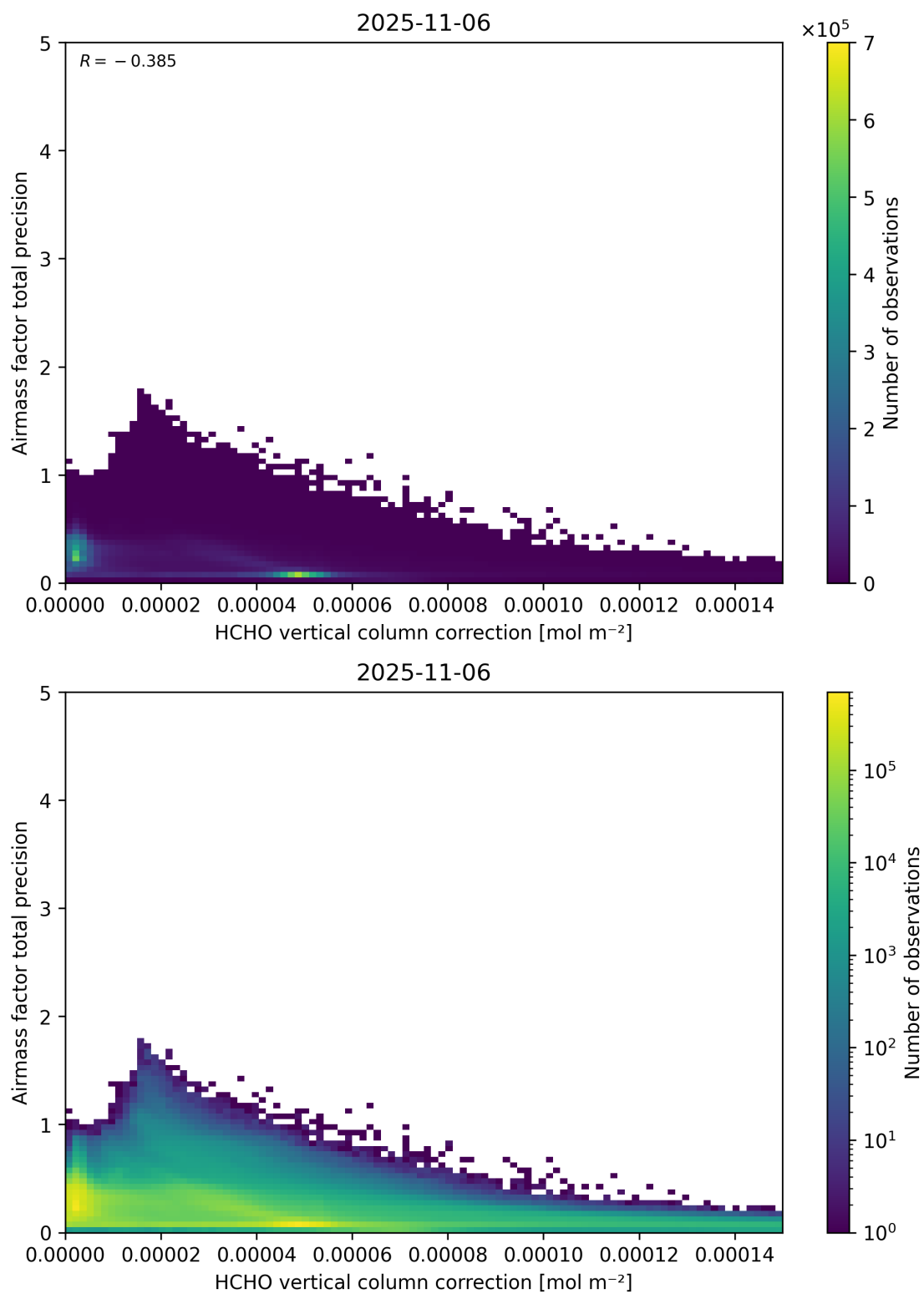
Figure 121: Scatter density plot of “HCHO vertical column correction” against “Airmass factor total precision” for 2025-11-05 to 2025-11-07.
