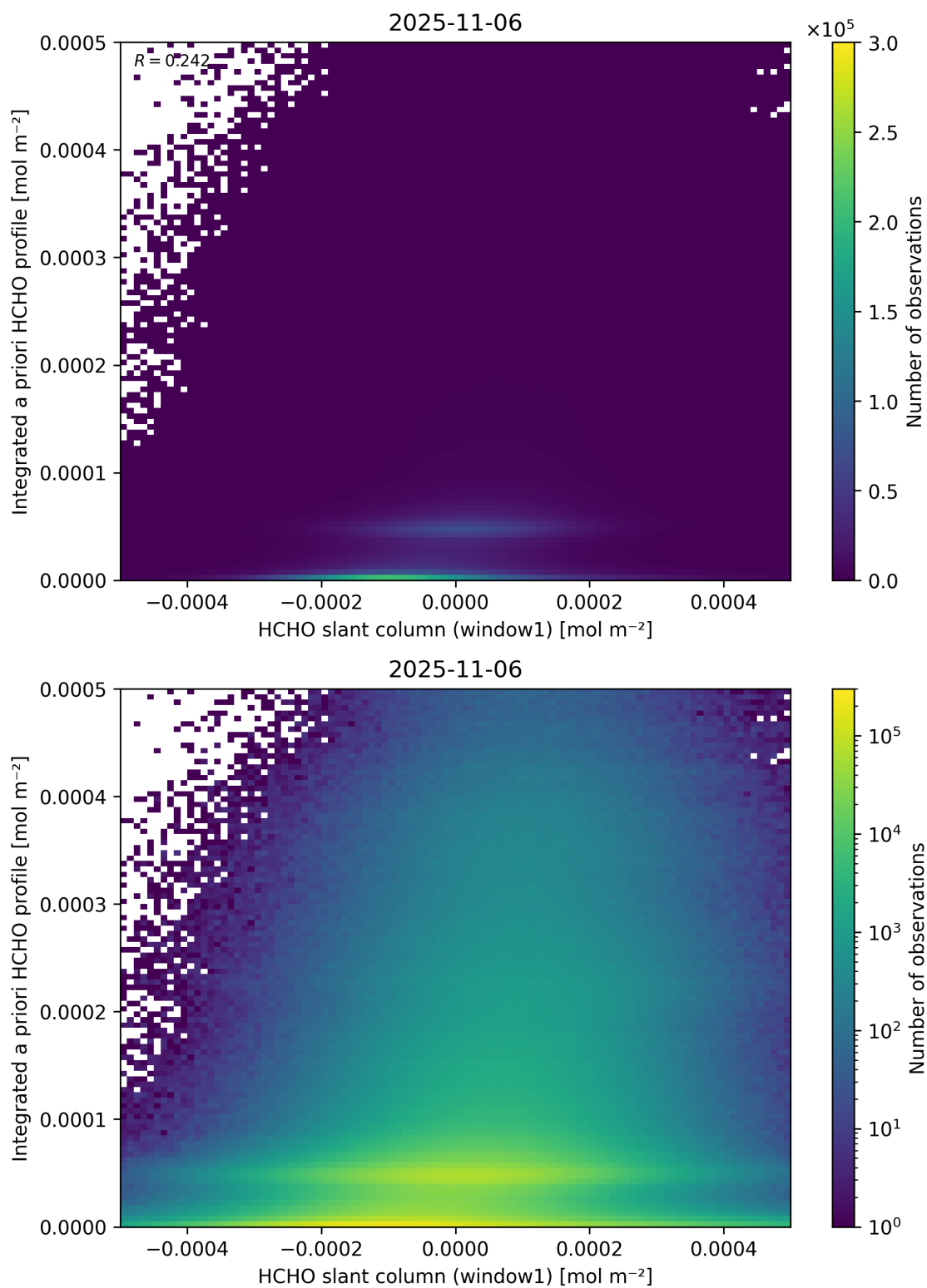
Figure 87: Scatter density plot of “HCHO slant column (window1)” against “Integrated a priori HCHO profile” for 2025-11-05 to 2025-11-07.
