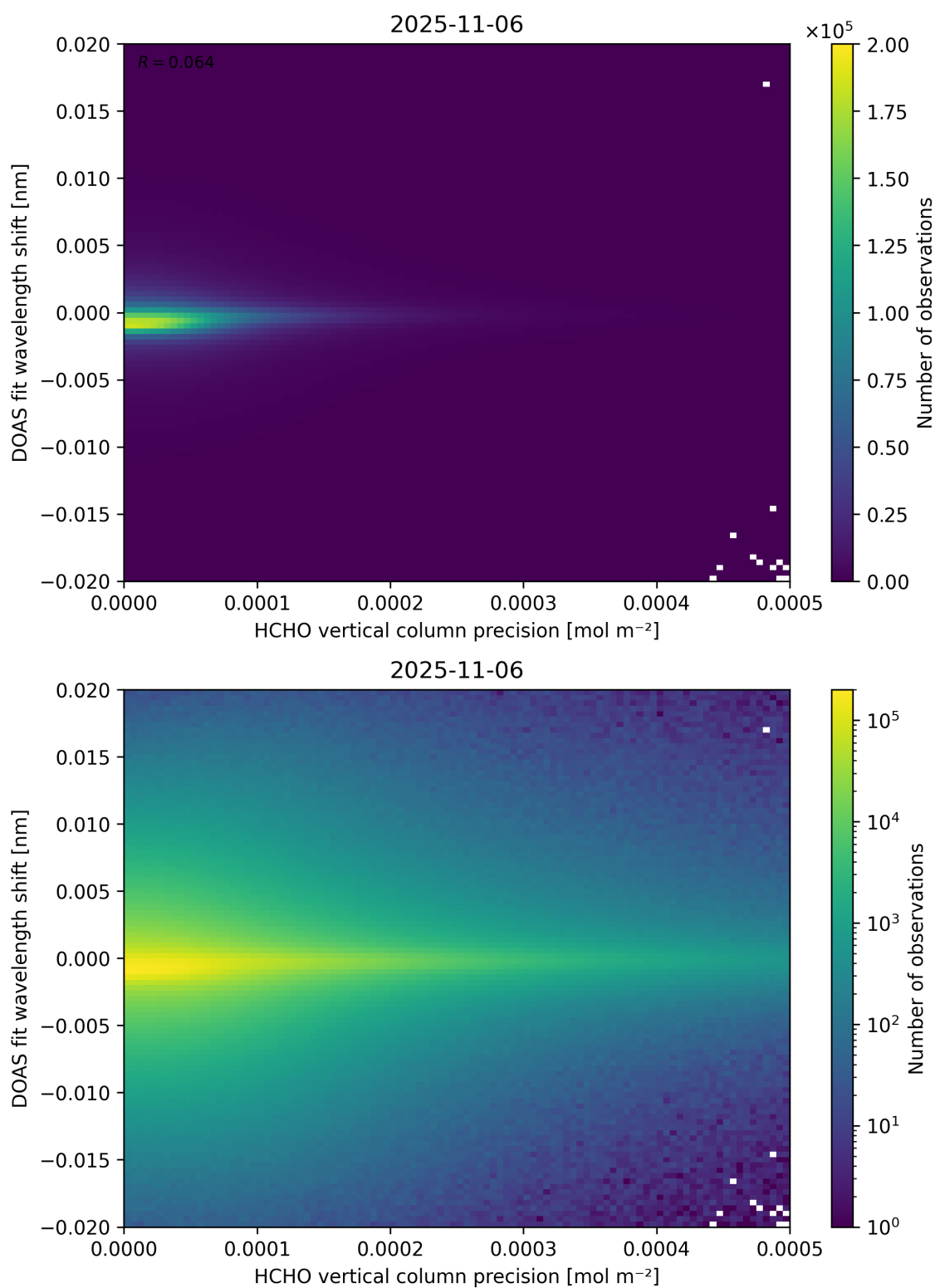
Figure 137: Scatter density plot of “HCHO vertical column precision” against “DOAS fit wavelength shift” for 2025-11-05 to 2025-11-07.
