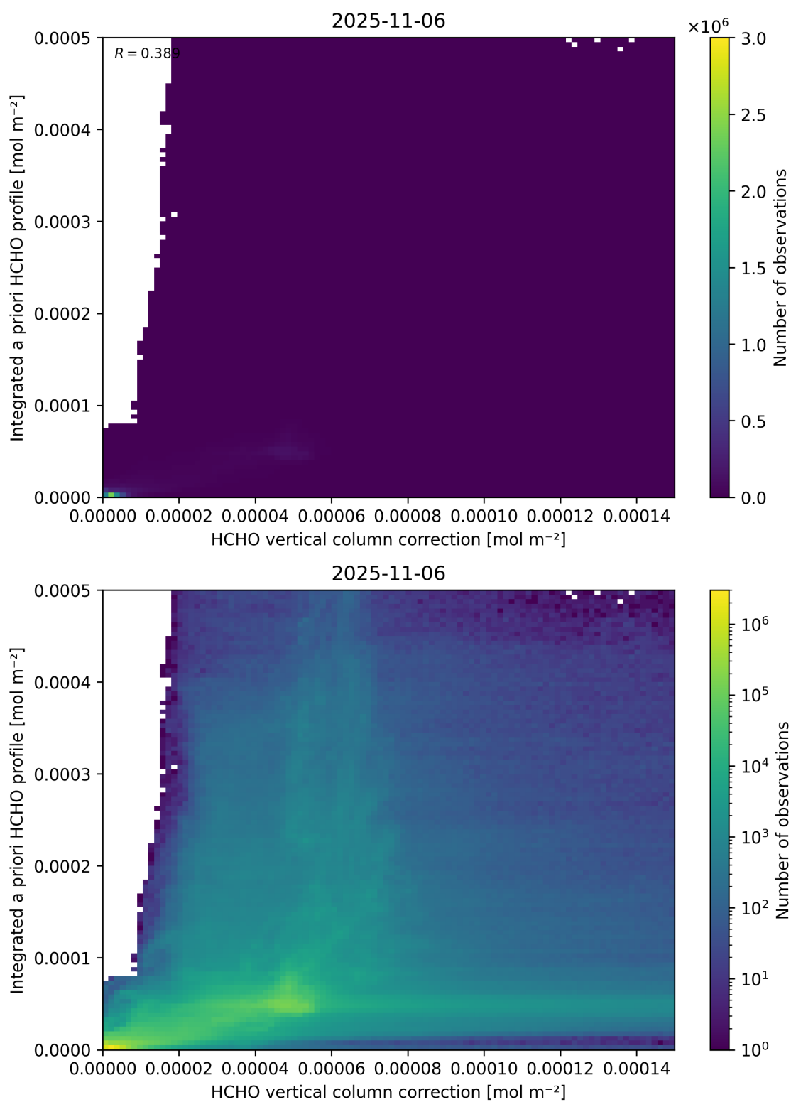
Figure 122: Scatter density plot of “HCHO vertical column correction” against “Integrated a priori HCHO profile” for 2025-11-05 to 2025-11-07.
