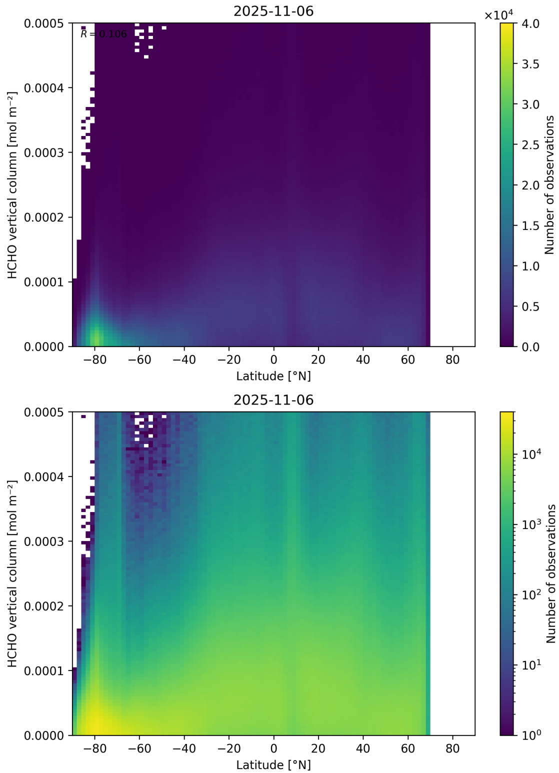
Figure 163: Scatter density plot of “Latitude” against “HCHO vertical column” for 2025-11-05 to 2025-11-07.
