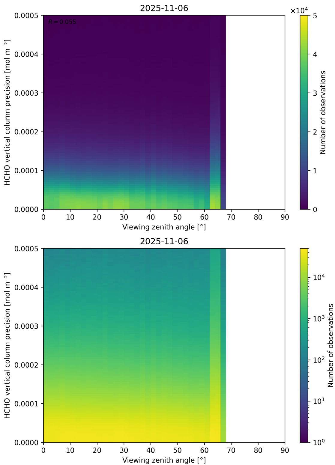
Figure 194: Scatter density plot of “Viewing zenith angle” against “HCHO vertical column precision” for 2025-11-05 to 2025-11-07.
