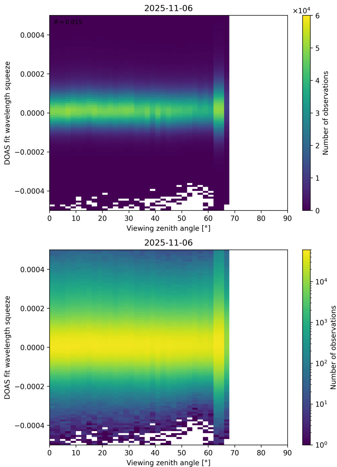
Figure 184: Scatter density plot of “Viewing zenith angle” against “DOAS fit wavelength squeeze” for 2025-11-05 to 2025-11-07.
