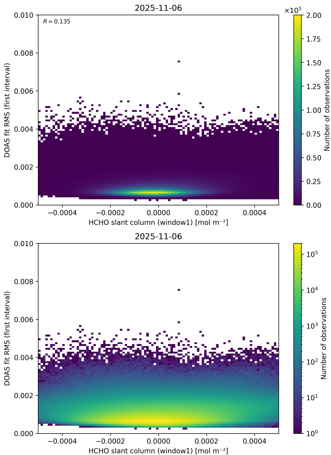
Figure 78: Scatter density plot of “HCHO slant column (window1)” against “DOAS fit RMS (first interval)” for 2025-11-05 to 2025-11-07.
