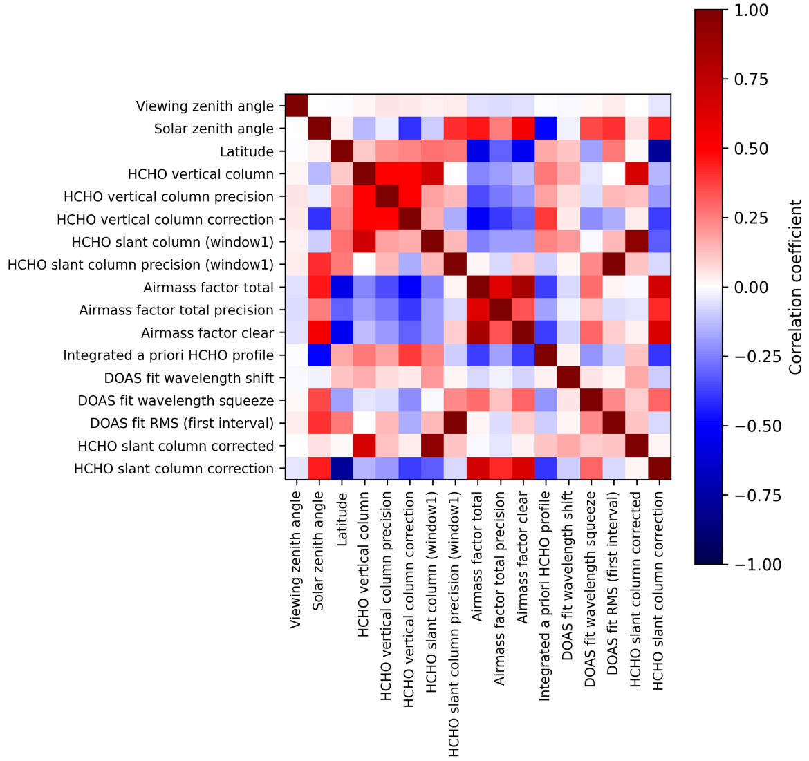
Figure 2: Map of correlation matrix for 2025-11-05 to 2025-11-07.
