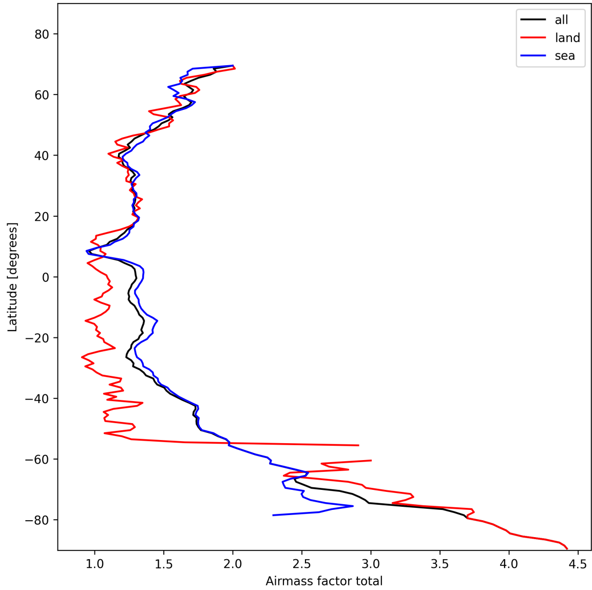
Figure 26: Zonal average of “Airmass factor total” for 2025-11-05 to 2025-11-07.
