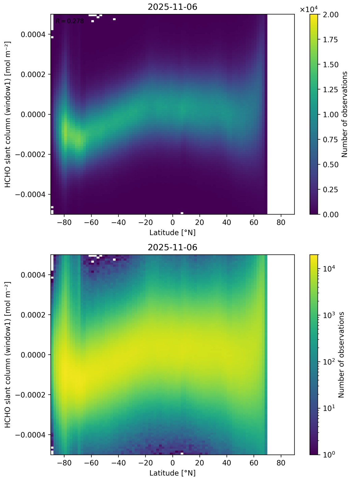
Figure 159: Scatter density plot of “Latitude” against “HCHO slant column (window1)” for 2025-11-05 to 2025-11-07.
