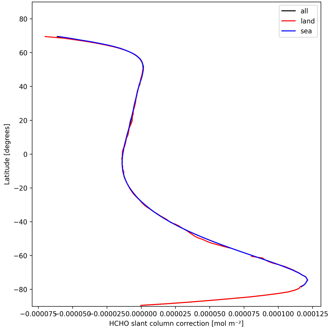
Figure 33: Zonal average of “HCHO slant column correction” for 2025-11-05 to 2025-11-07.
