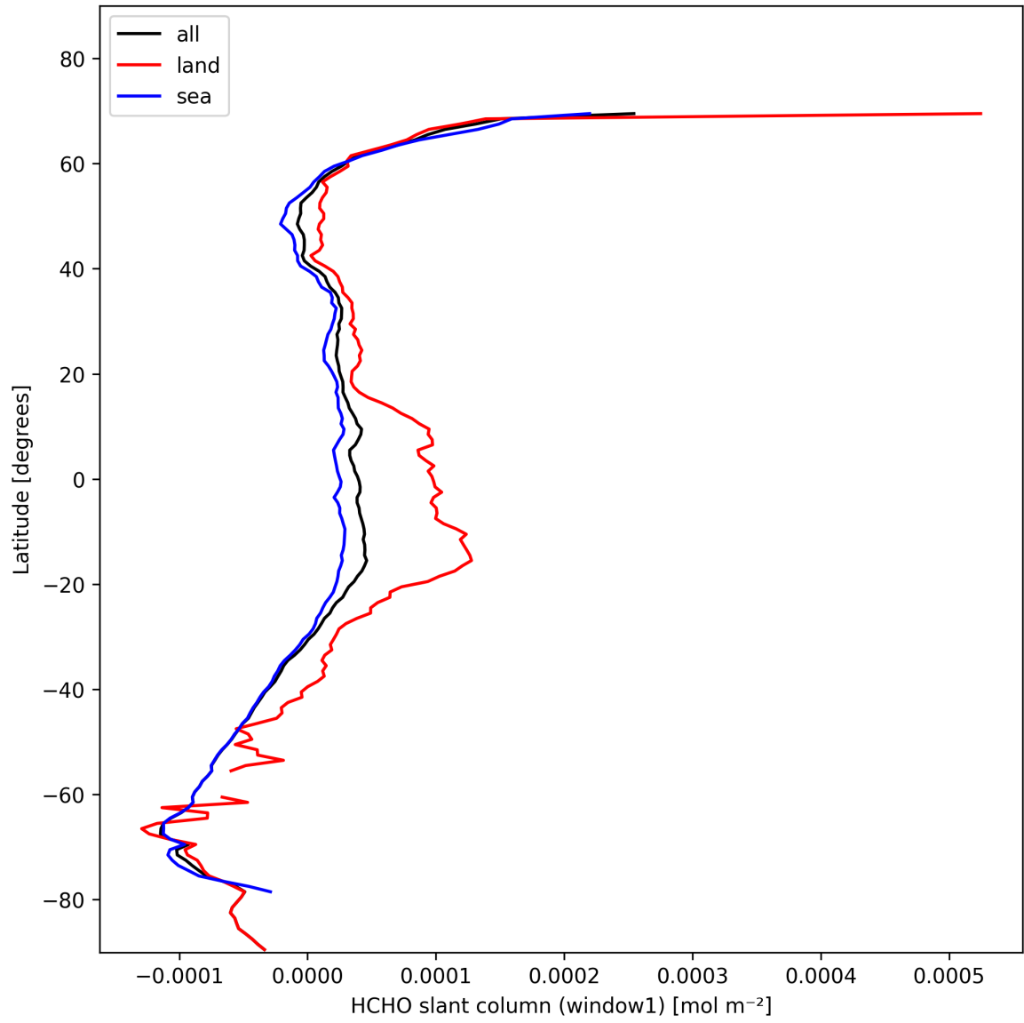
Figure 24: Zonal average of “HCHO slant column (window1)” for 2025-11-05 to 2025-11-07.
