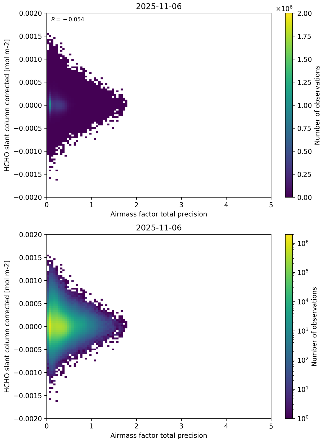
Figure 109: Scatter density plot of “Airmass factor total precision” against “HCHO slant column corrected” for 2025-11-05 to 2025-11-07.
