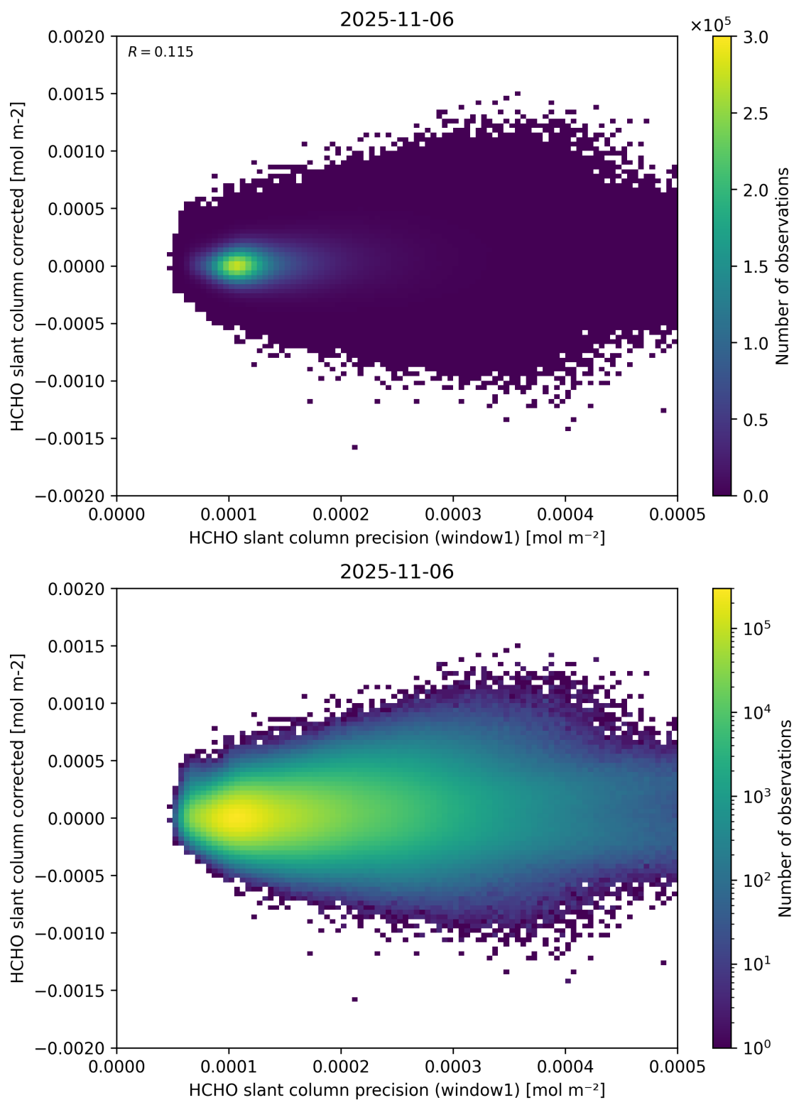
Figure 92: Scatter density plot of “HCHO slant column precision (window1)” against “HCHO slant column corrected” for 2025-11-05 to 2025-11-07.
