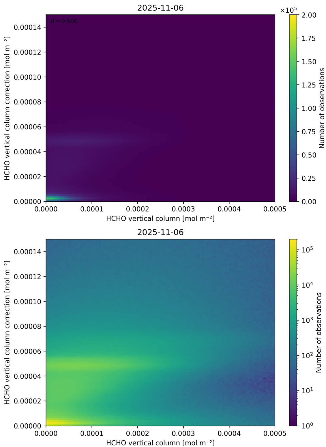
Figure 133: Scatter density plot of “HCHO vertical column” against “HCHO vertical column correction” for 2025-11-05 to 2025-11-07.
