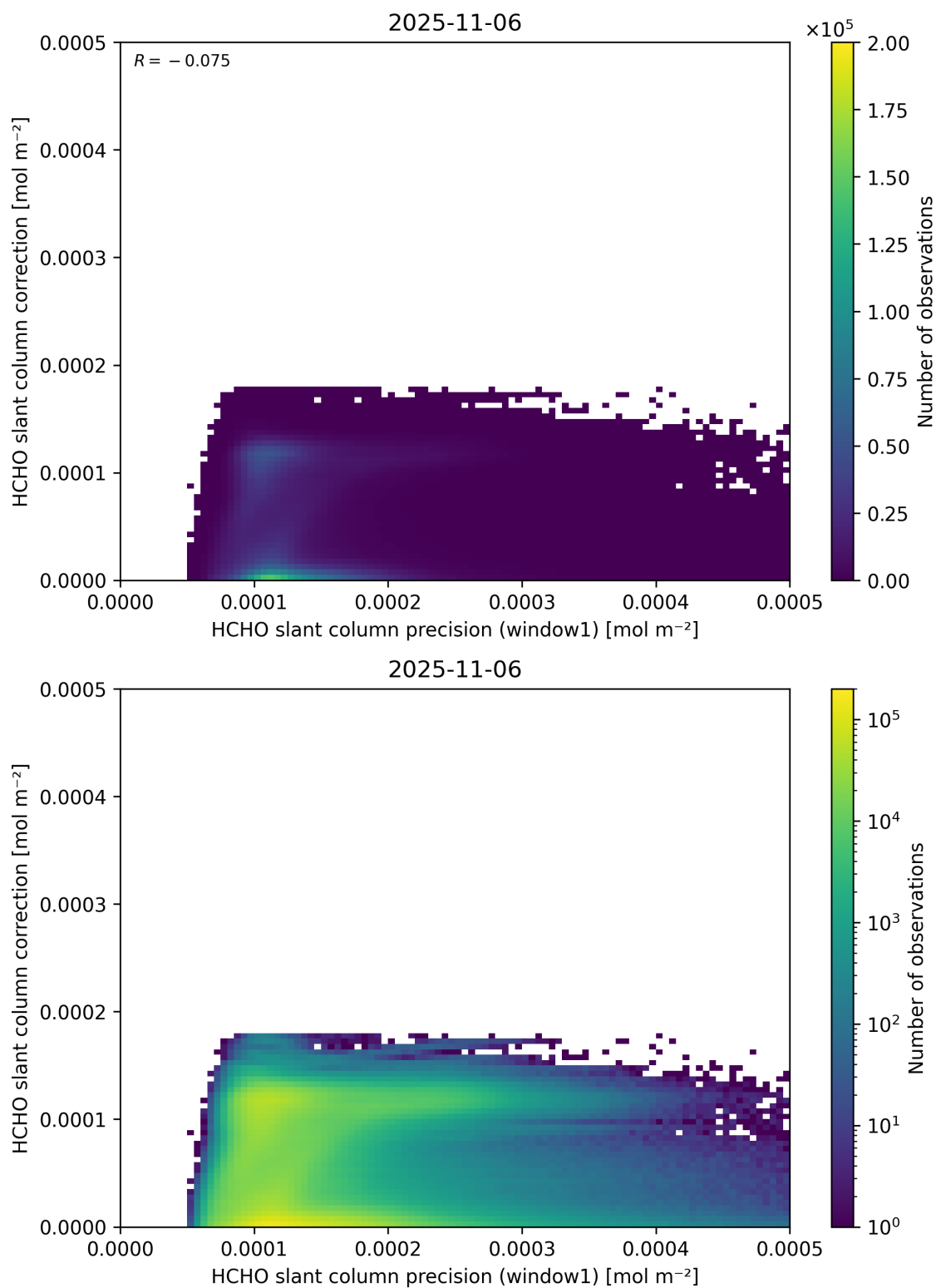
Figure 93: Scatter density plot of “HCHO slant column precision (window1)” against “HCHO slant column correction” for 2025-11-05 to 2025-11-07.
