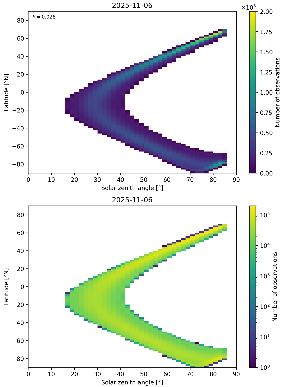
Figure 181: Scatter density plot of “Solar zenith angle” against “Latitude” for 2025-11-05 to 2025-11-07.
