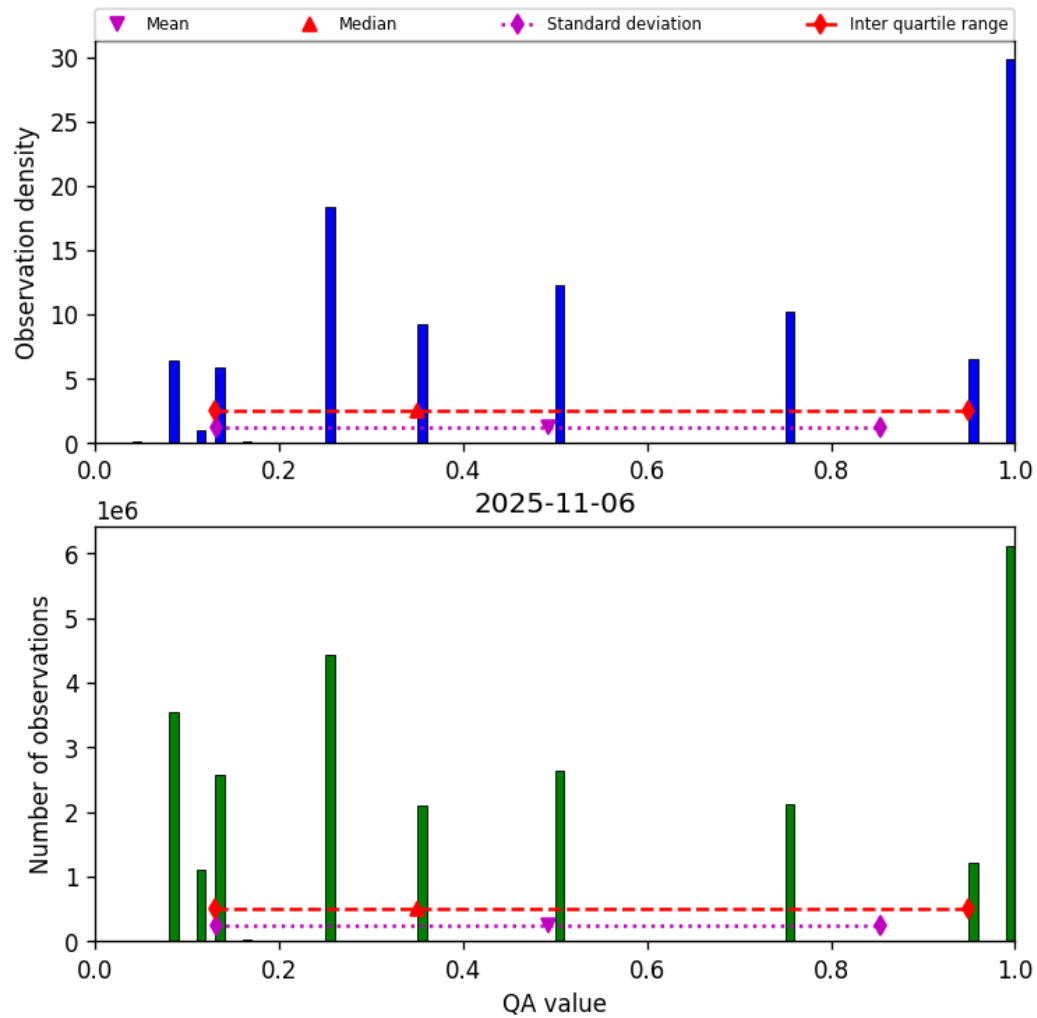
Figure 34: Histogram of “QA value” for 2025-11-05 to 2025-11-07
