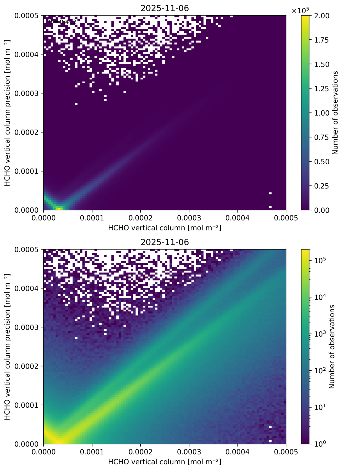
Figure 134: Scatter density plot of “HCHO vertical column” against “HCHO vertical column precision” for 2025-11-05 to 2025-11-07.
