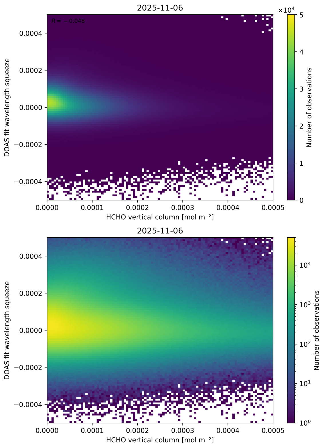
Figure 125: Scatter density plot of “HCHO vertical column” against “DOAS fit wavelength squeeze” for 2025-11-05 to 2025-11-07.
