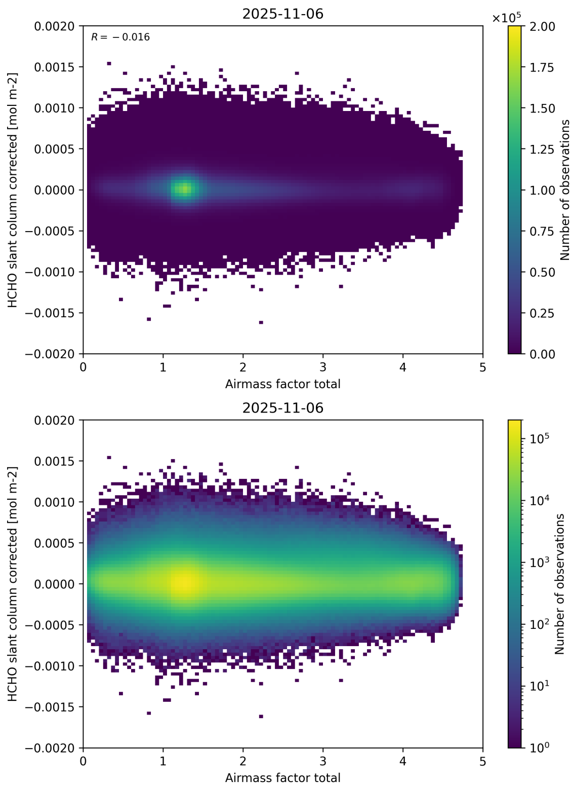
Figure 101: Scatter density plot of “Airmass factor total” against “HCHO slant column corrected” for 2025-11-05 to 2025-11-07.
