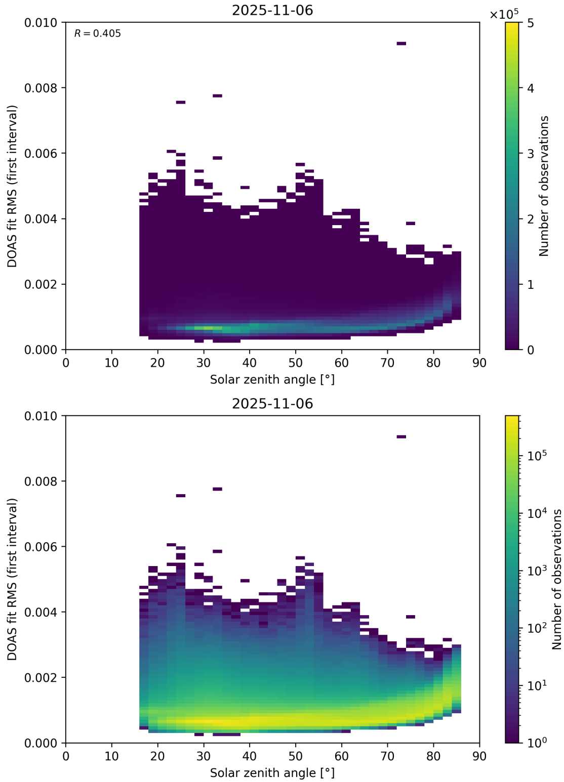
Figure 167: Scatter density plot of “Solar zenith angle” against “DOAS fit RMS (first interval)” for 2025-11-05 to 2025-11-07.
