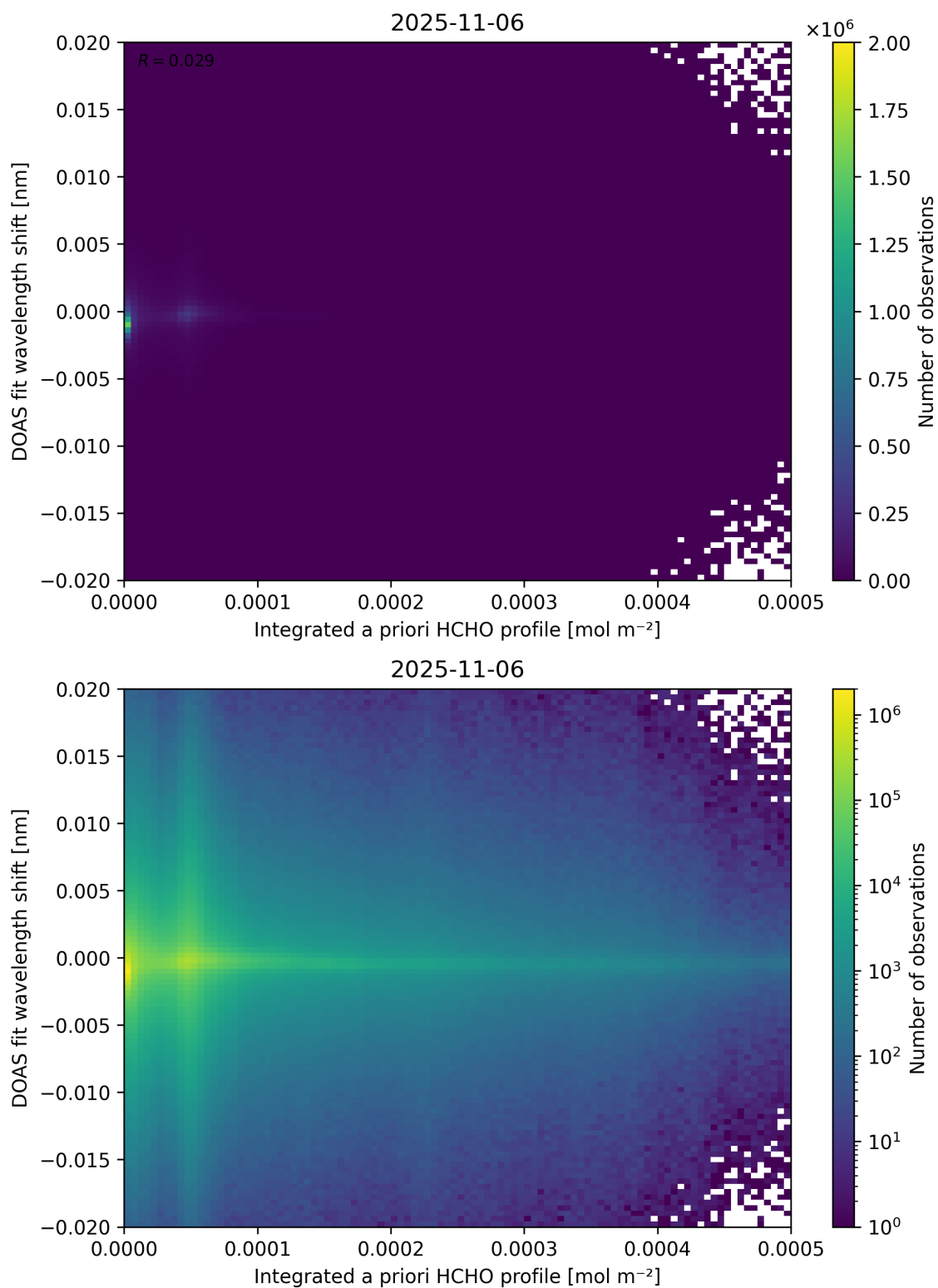
Figure 149: Scatter density plot of “Integrated a priori HCHO profile” against “DOAS fit wavelength shift” for 2025-11-05 to 2025-11-07.
