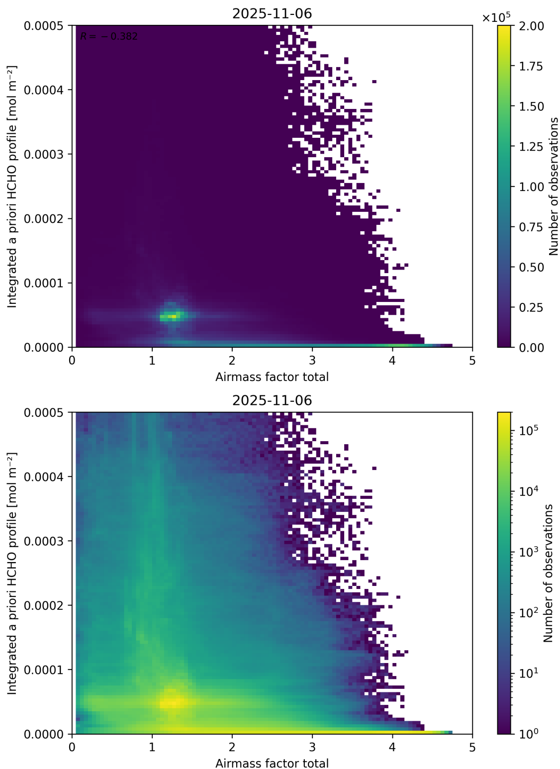
Figure 104: Scatter density plot of “Airmass factor total” against “Integrated a priori HCHO profile” for 2025-11-05 to 2025-11-07.
