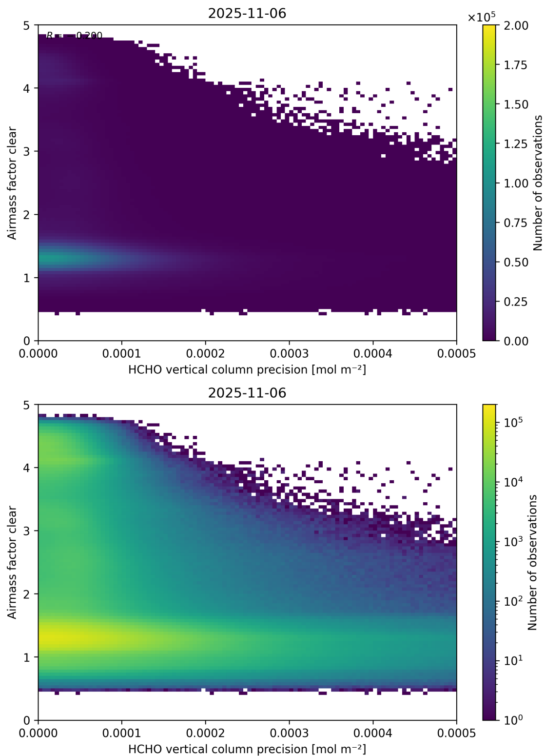
Figure 139: Scatter density plot of “HCHO vertical column precision” against “Airmass factor clear” for 2025-11-05 to 2025-11-07.
