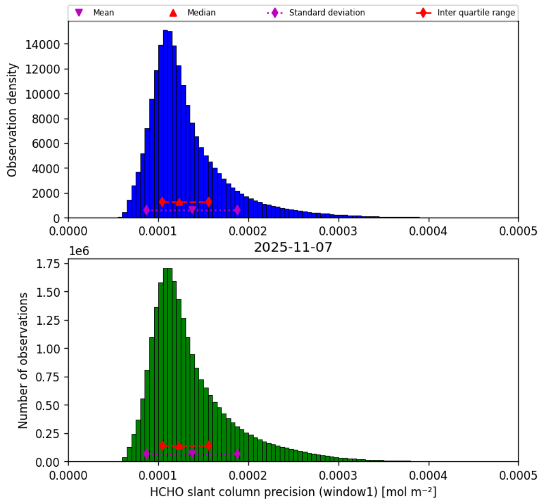
Figure 39: Histogram of “HCHO slant column precision (window1)” for 2025-11-07 to 2025-11-08
