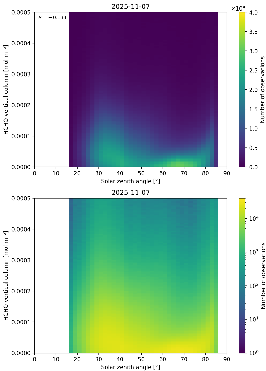
Figure 177: Scatter density plot of “Solar zenith angle” against “HCHO vertical column” for 2025-11-07 to 2025-11-08.
