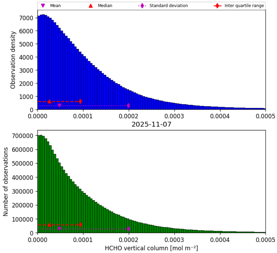
Figure 35: Histogram of “HCHO vertical column” for 2025-11-07 to 2025-11-08
