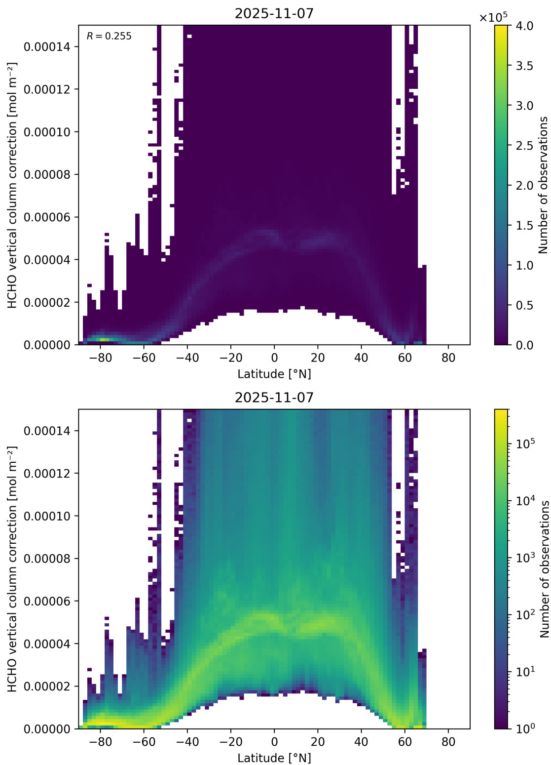
Figure 164: Scatter density plot of “Latitude” against “HCHO vertical column correction” for 2025-11-07 to 2025-11-08.
