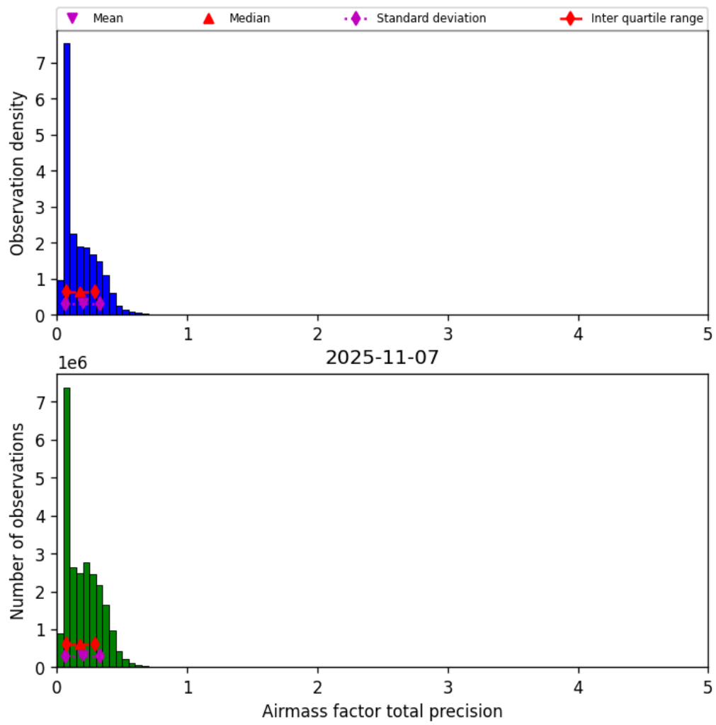
Figure 41: Histogram of “Airmass factor total precision” for 2025-11-07 to 2025-11-08
