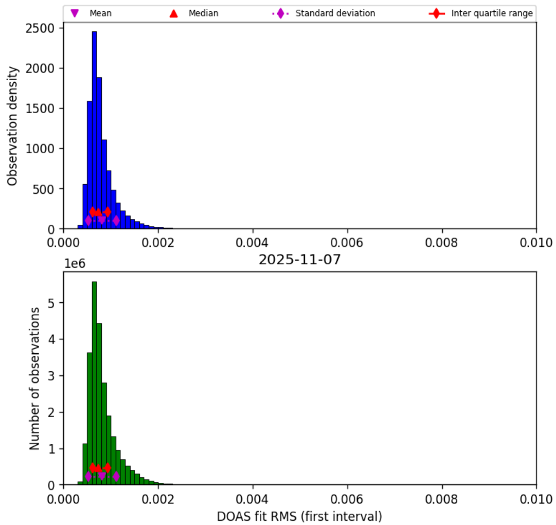
Figure 46: Histogram of “DOAS fit RMS (first interval)” for 2025-11-07 to 2025-11-08
