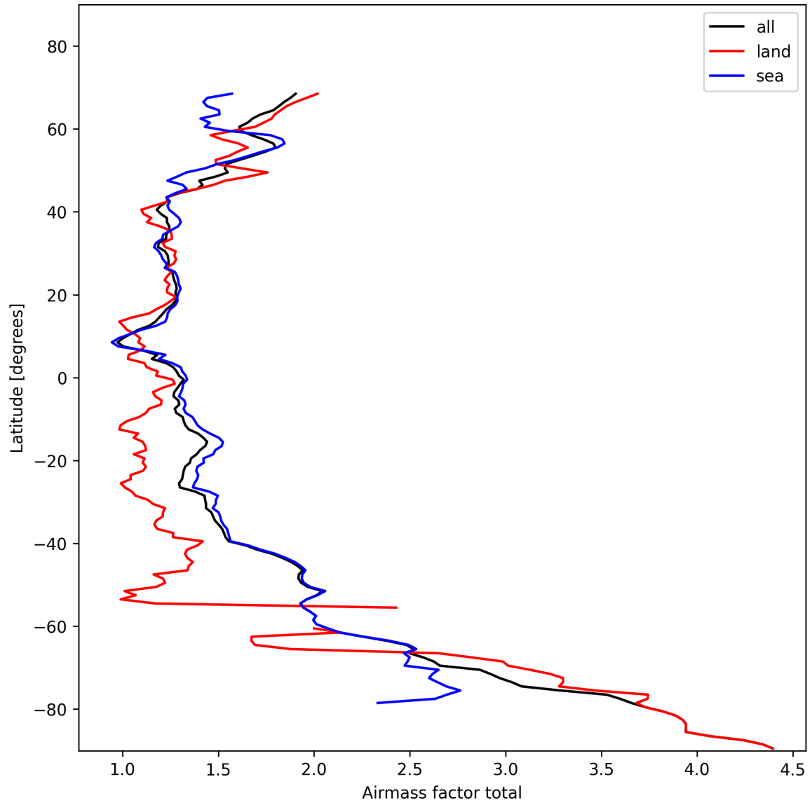
Figure 26: Zonal average of “Airmass factor total” for 2025-11-07 to 2025-11-08.
