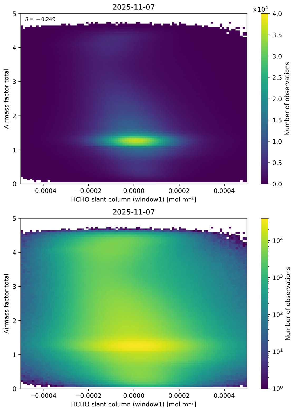
Figure 85: Scatter density plot of “HCHO slant column (window1)” against “Airmass factor total” for 2025-11-07 to 2025-11-08.
