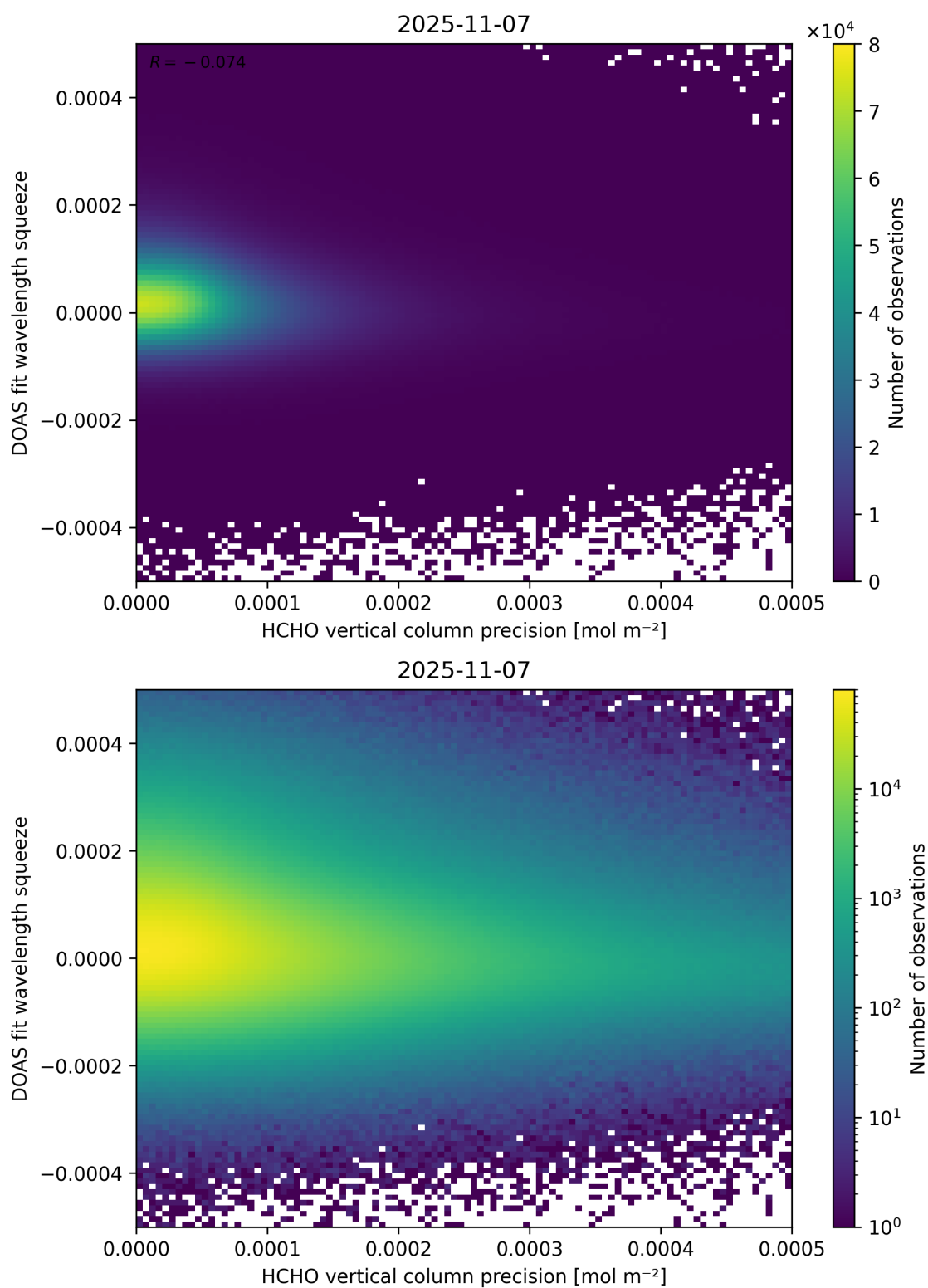
Figure 138: Scatter density plot of “HCHO vertical column precision” against “DOAS fit wavelength squeeze” for 2025-11-07 to 2025-11-08.
