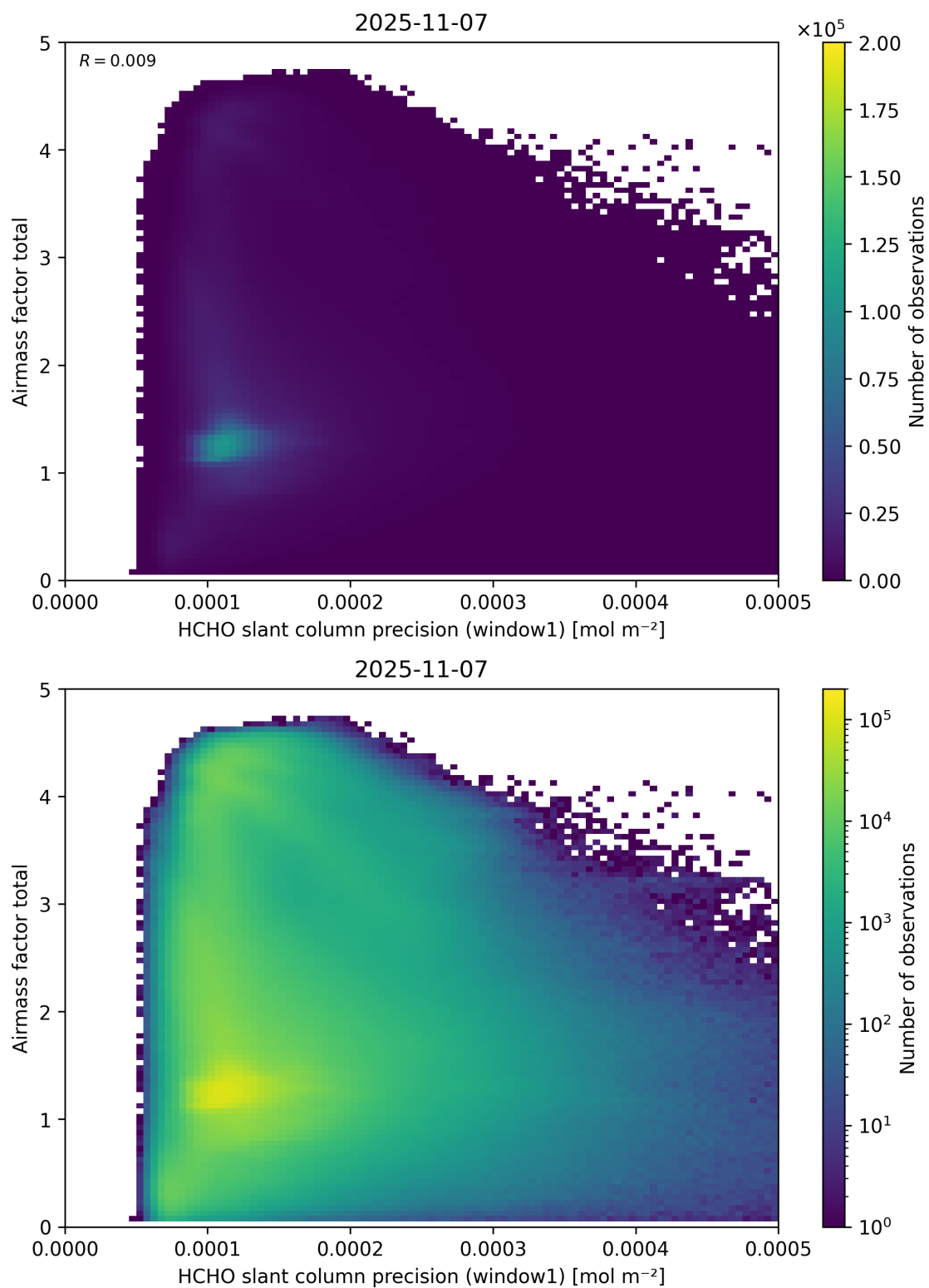
Figure 94: Scatter density plot of “HCHO slant column precision (window1)” against “Airmass factor total” for 2025-11-07 to 2025-11-08.
