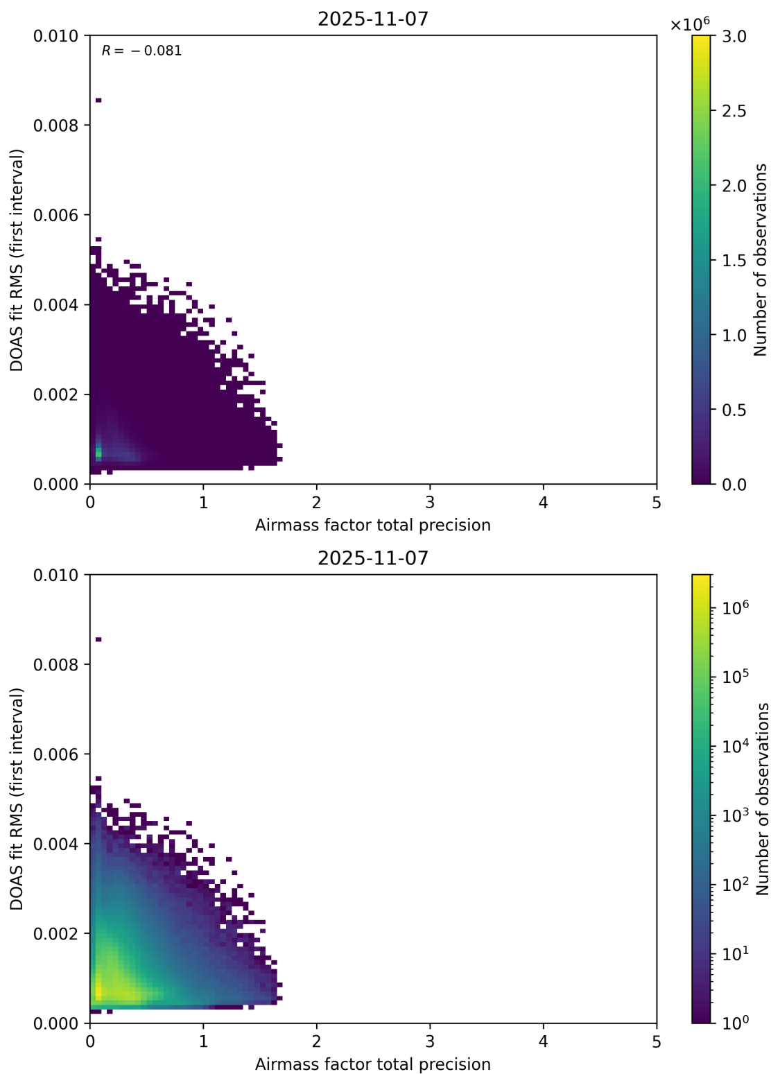
Figure 105: Scatter density plot of “Airmass factor total precision” against “DOAS fit RMS (first interval)” for 2025-11-07 to 2025-11-08.
