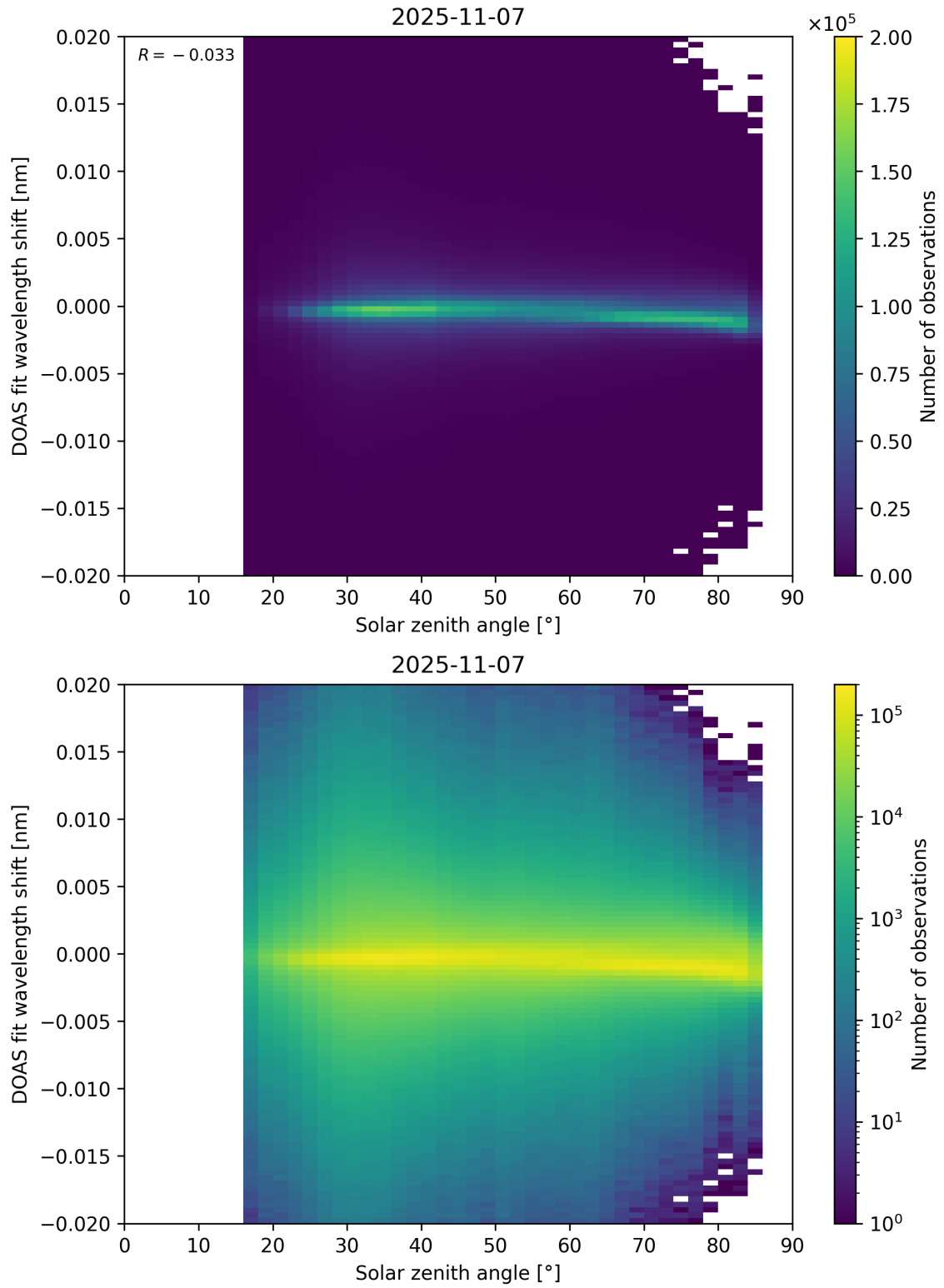
Figure 168: Scatter density plot of “Solar zenith angle” against “DOAS fit wavelength shift” for 2025-11-07 to 2025-11-08.
