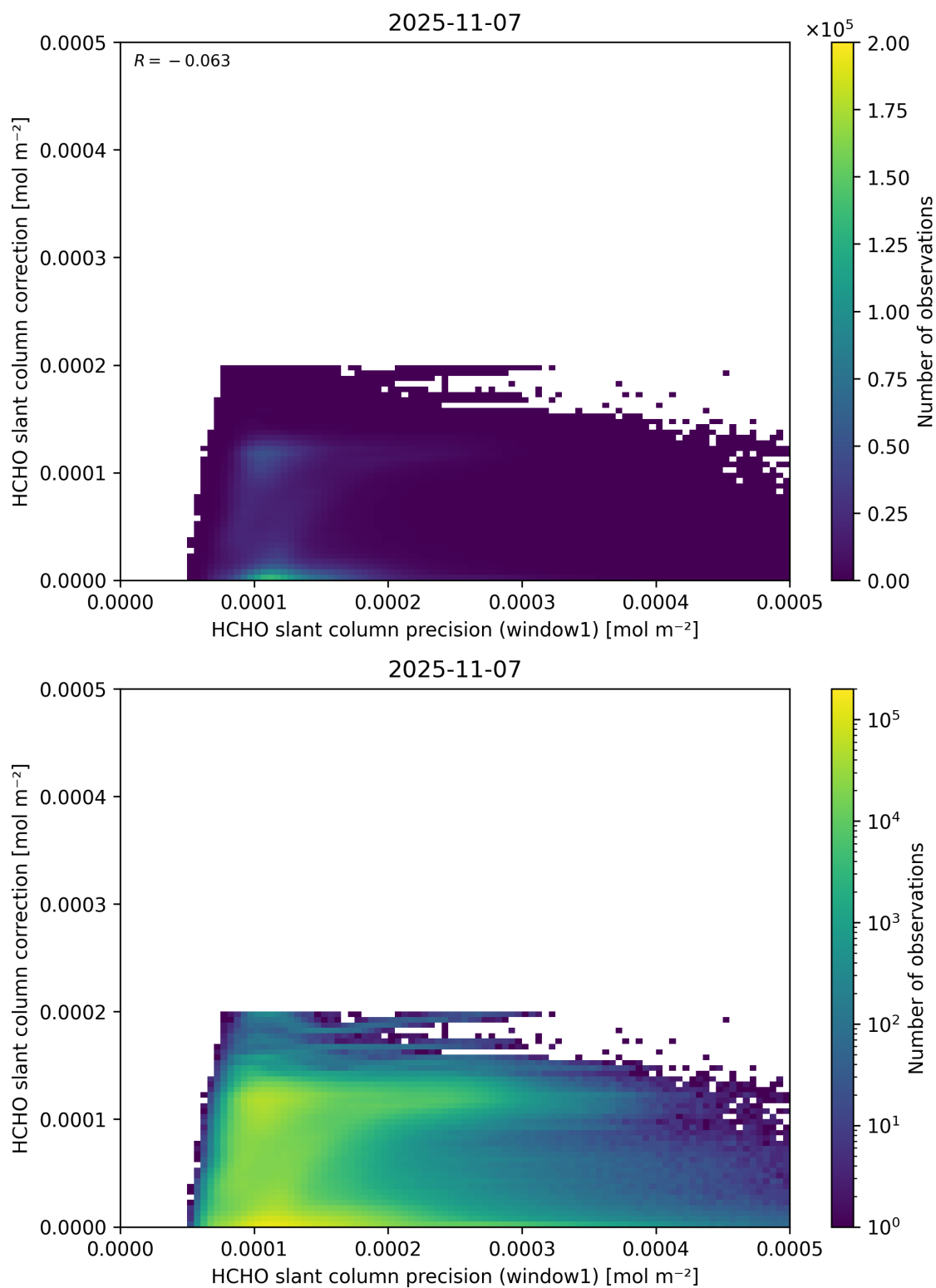
Figure 93: Scatter density plot of “HCHO slant column precision (window1)” against “HCHO slant column correction” for 2025-11-07 to 2025-11-08.
