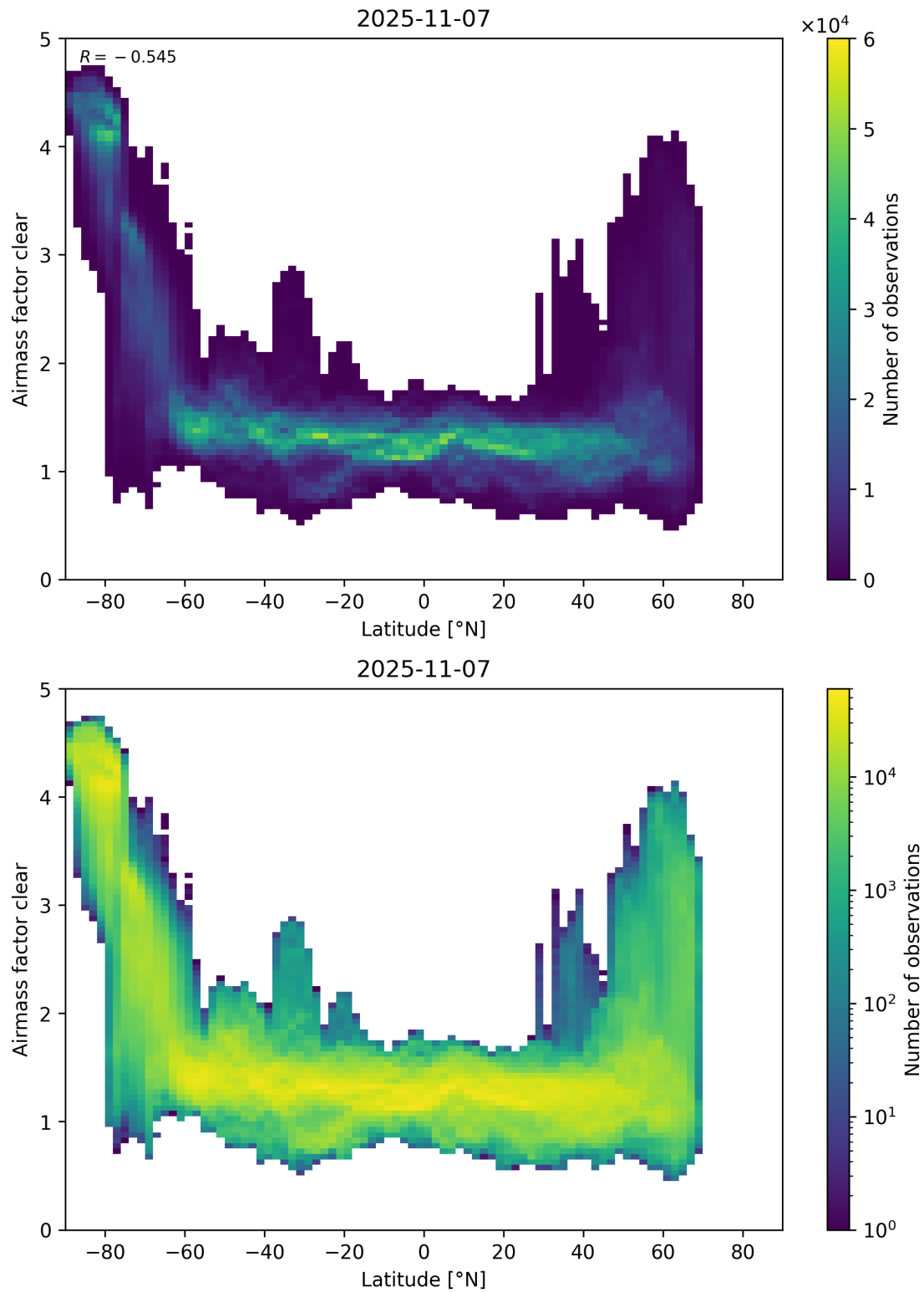
Figure 156: Scatter density plot of “Latitude” against “Airmass factor clear” for 2025-11-07 to 2025-11-08.
