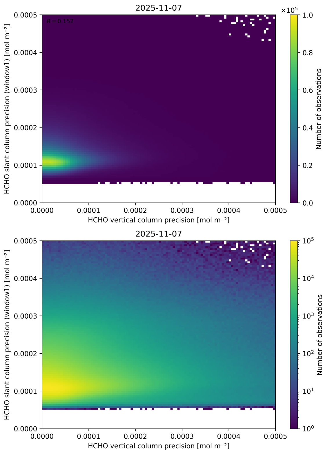
Figure 143: Scatter density plot of “HCHO vertical column precision” against “HCHO slant column precision (window1)” for 2025-11-07 to 2025-11-08.
