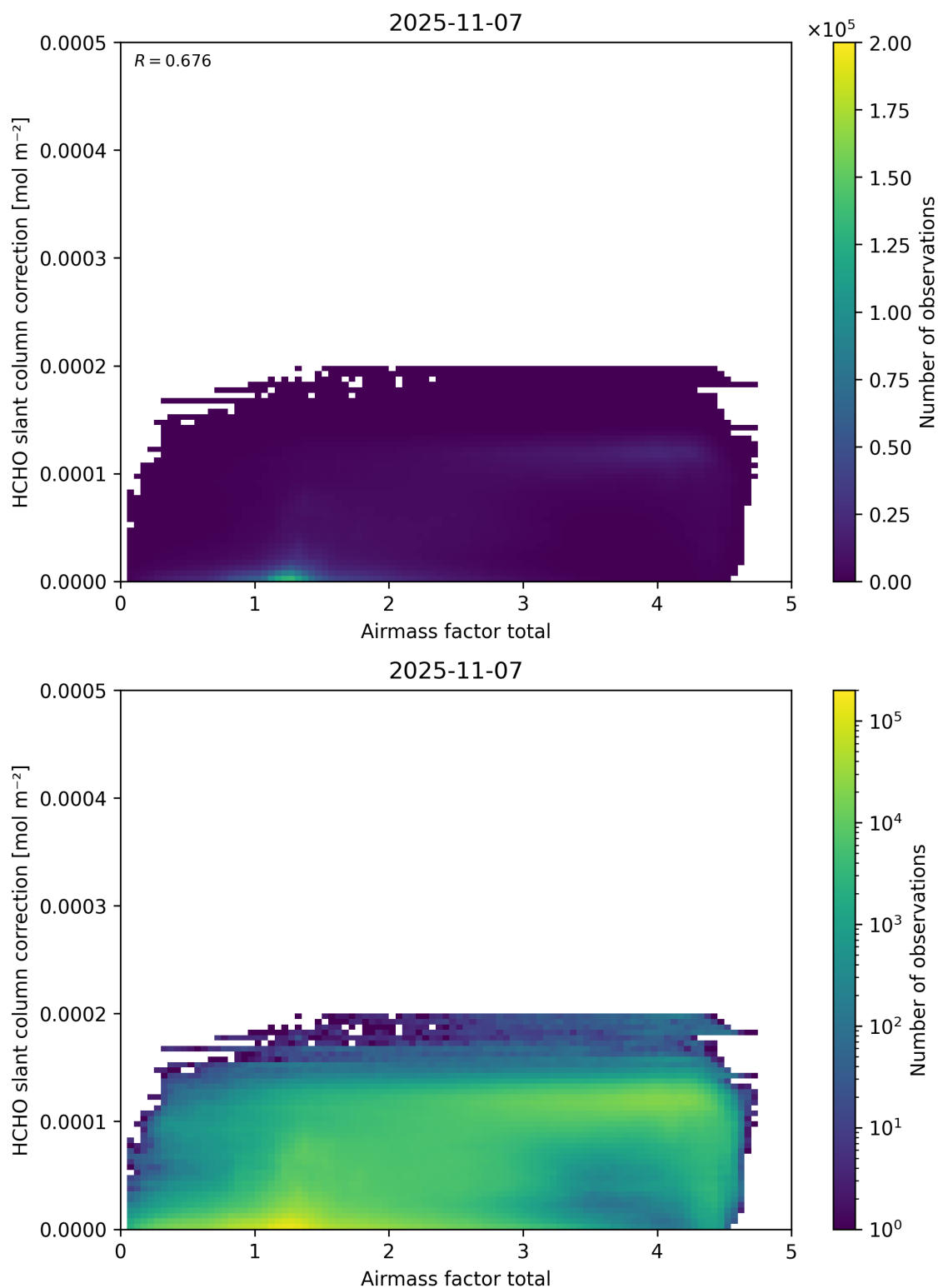
Figure 102: Scatter density plot of “Airmass factor total” against “HCHO slant column correction” for 2025-11-07 to 2025-11-08.
