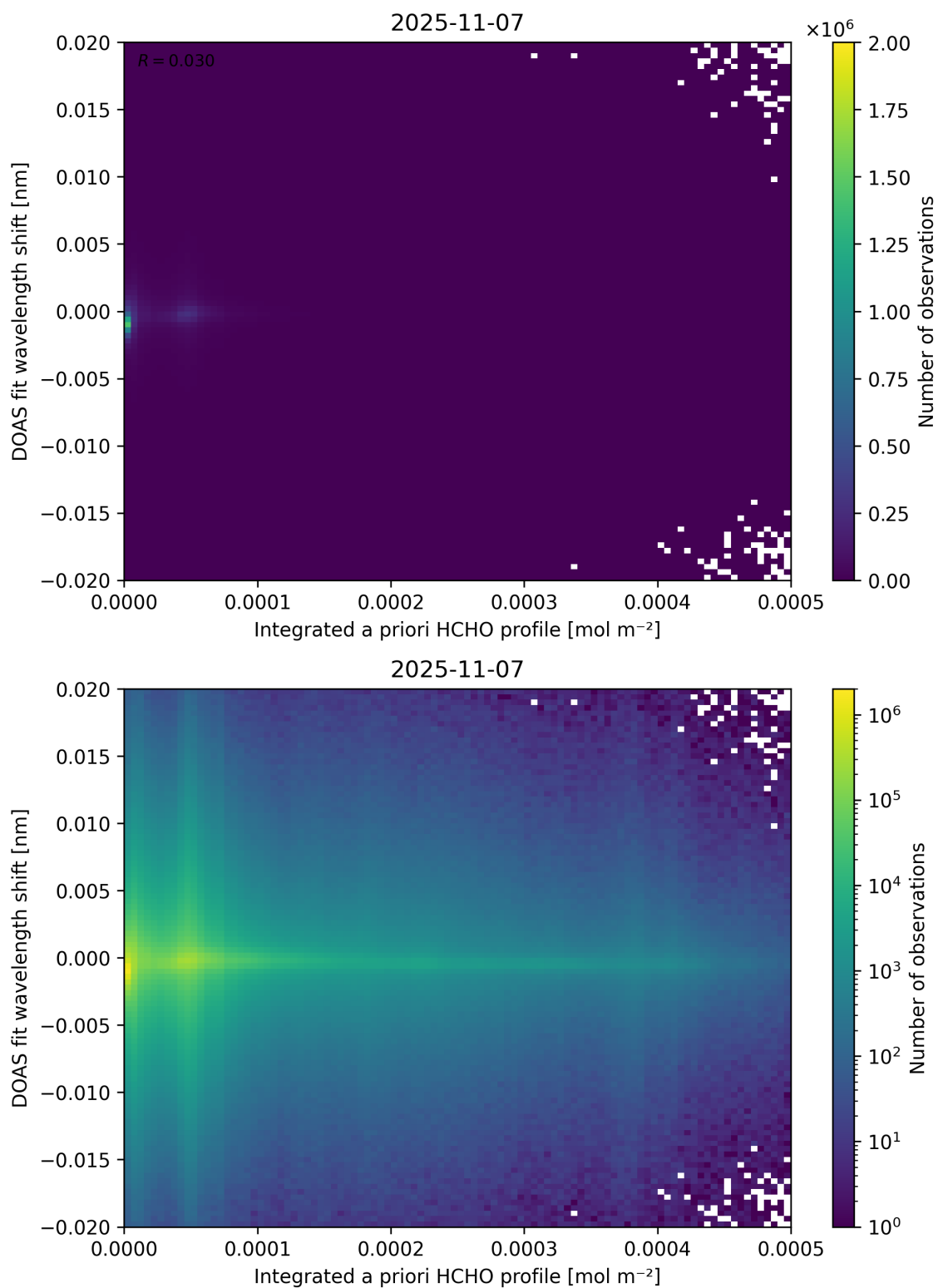
Figure 149: Scatter density plot of “Integrated a priori HCHO profile” against “DOAS fit wavelength shift” for 2025-11-07 to 2025-11-08.
