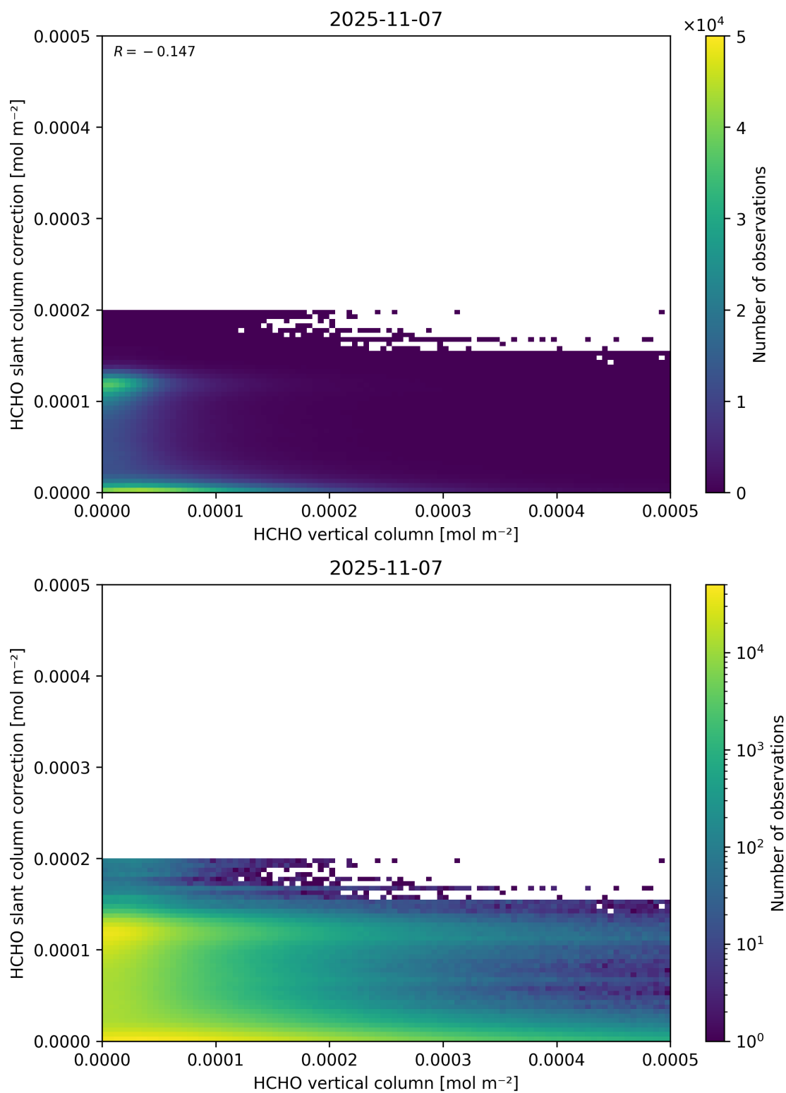
Figure 128: Scatter density plot of “HCHO vertical column” against “HCHO slant column correction” for 2025-11-07 to 2025-11-08.
