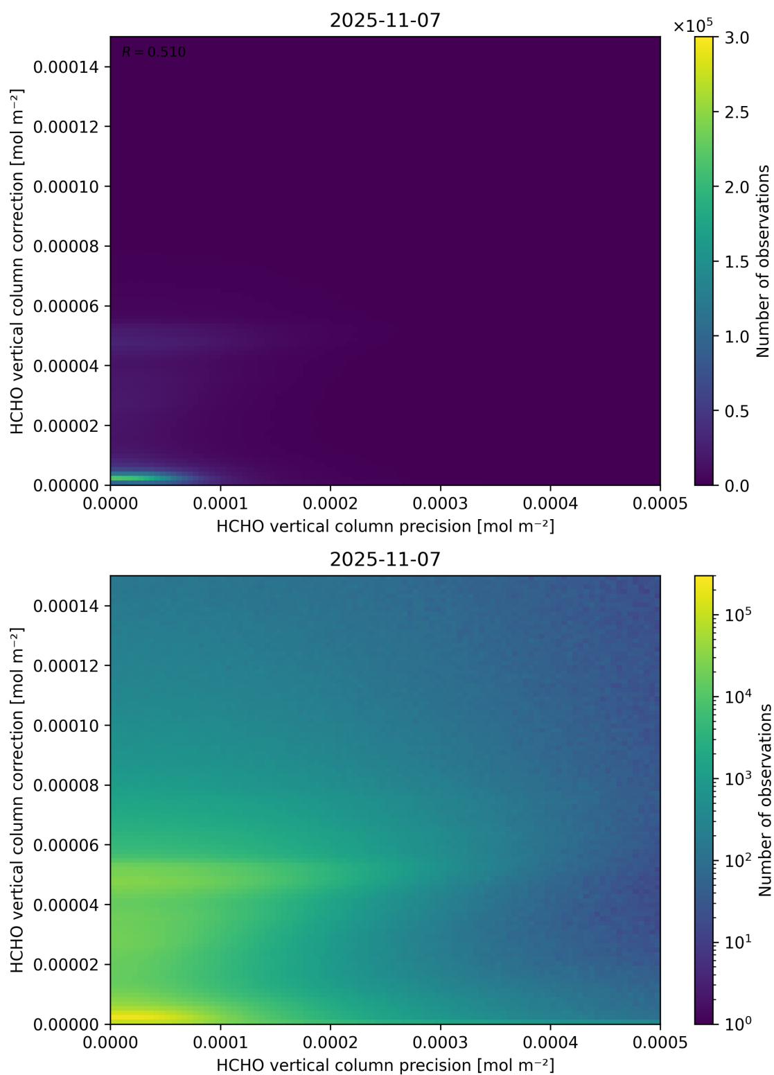
Figure 146: Scatter density plot of “HCHO vertical column precision” against “HCHO vertical column correction” for 2025-11-07 to 2025-11-08.
