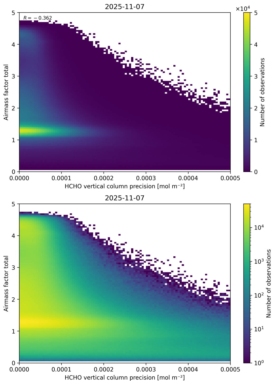
Figure 144: Scatter density plot of “HCHO vertical column precision” against “Airmass factor total” for 2025-11-07 to 2025-11-08.
