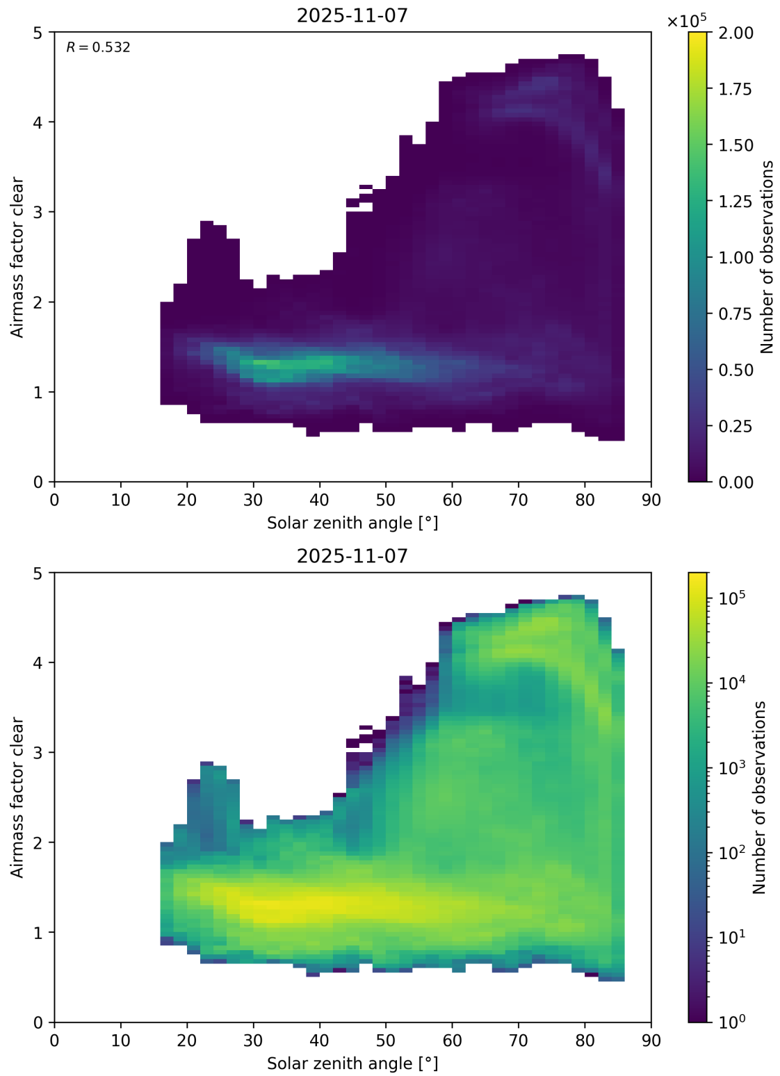
Figure 170: Scatter density plot of “Solar zenith angle” against “Airmass factor clear” for 2025-11-07 to 2025-11-08.
