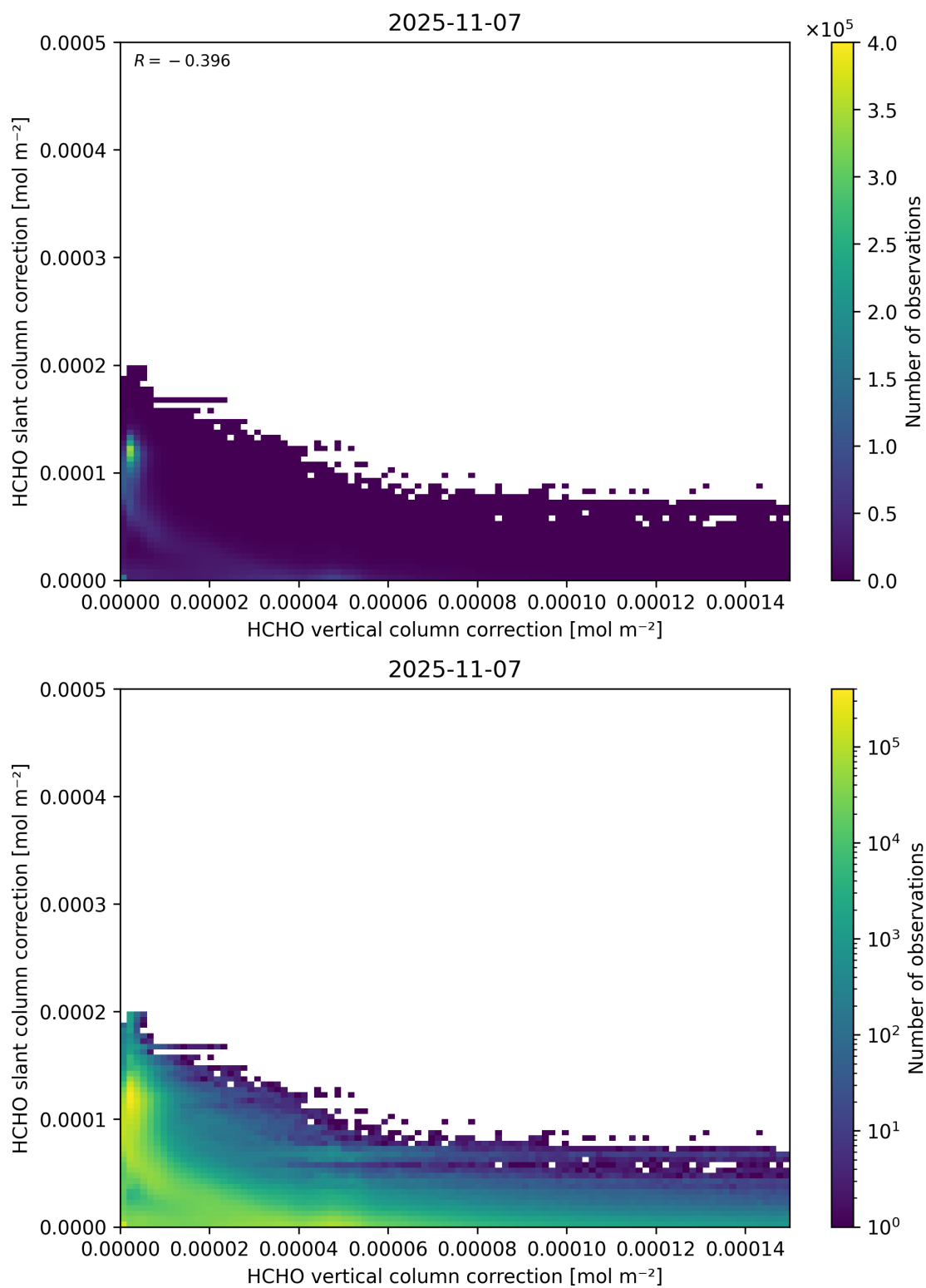
Figure 117: Scatter density plot of “HCHO vertical column correction” against “HCHO slant column correction” for 2025-11-07 to 2025-11-08.
