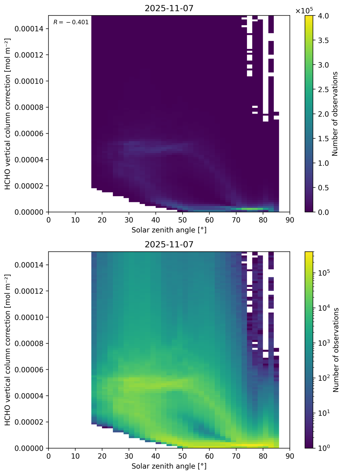
Figure 178: Scatter density plot of “Solar zenith angle” against “HCHO vertical column correction” for 2025-11-07 to 2025-11-08.
