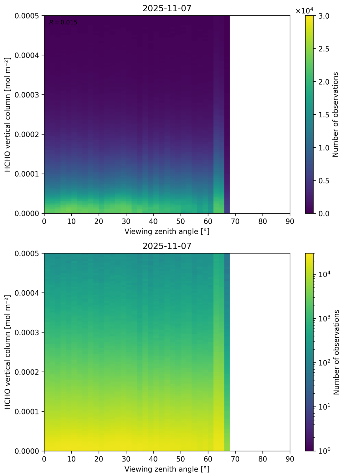
Figure 192: Scatter density plot of “Viewing zenith angle” against “HCHO vertical column” for 2025-11-07 to 2025-11-08.
