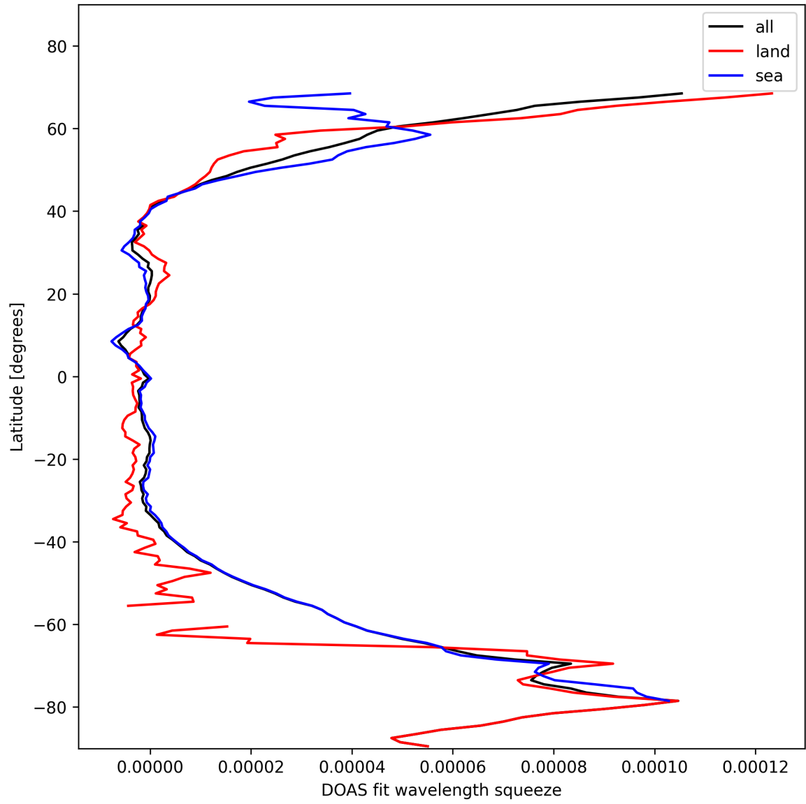
Figure 31: Zonal average of “DOAS fit wavelength squeeze” for 2025-11-07 to 2025-11-08.
