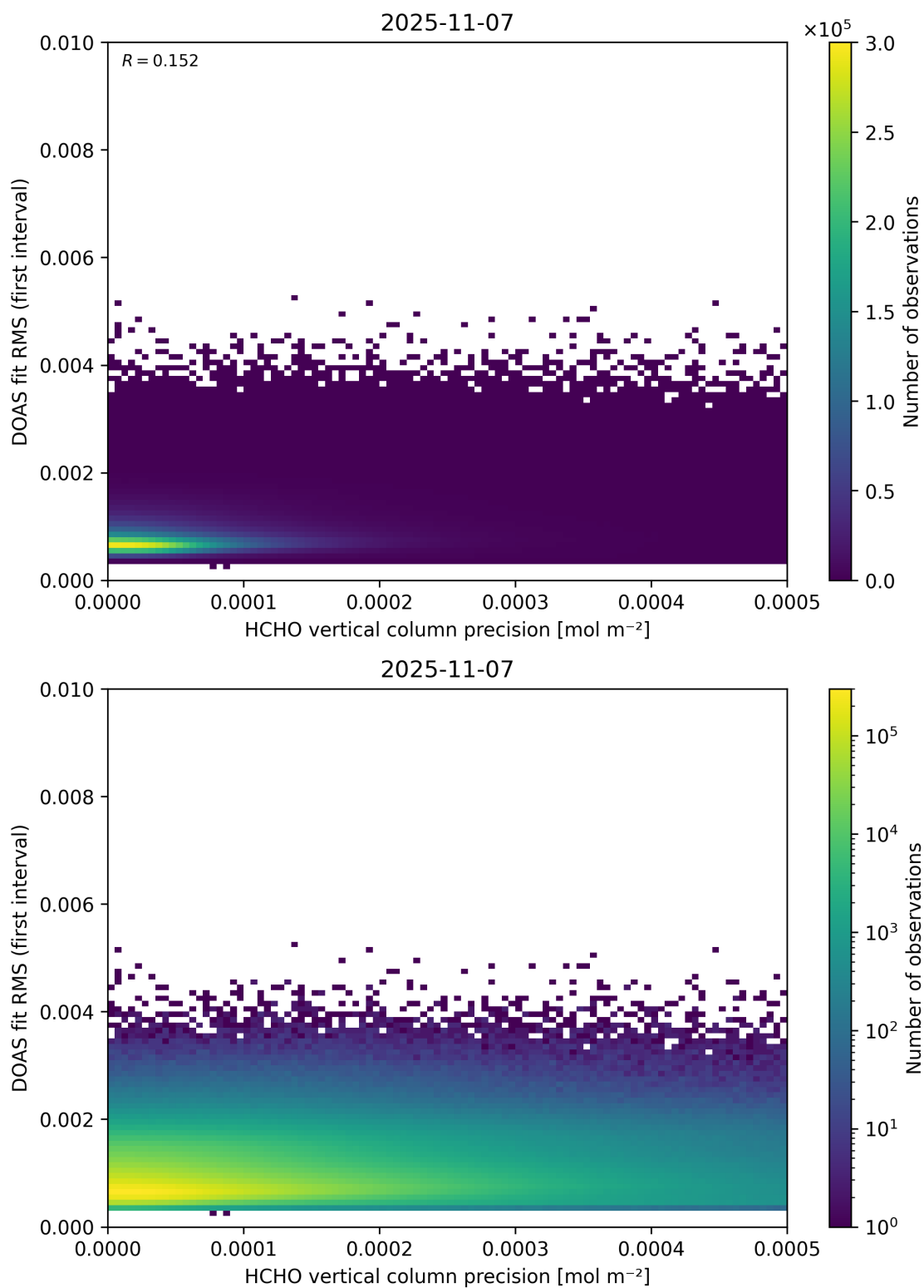
Figure 136: Scatter density plot of “HCHO vertical column precision” against “DOAS fit RMS (first interval)” for 2025-11-07 to 2025-11-08.
