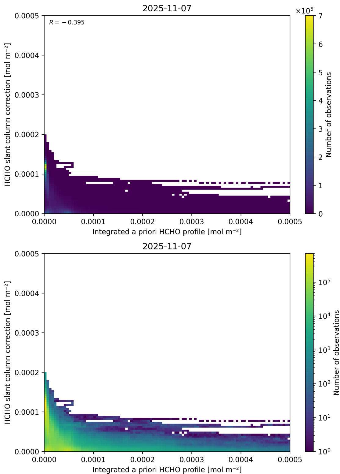
Figure 152: Scatter density plot of “Integrated a priori HCHO profile” against “HCHO slant column correction” for 2025-11-07 to 2025-11-08.
