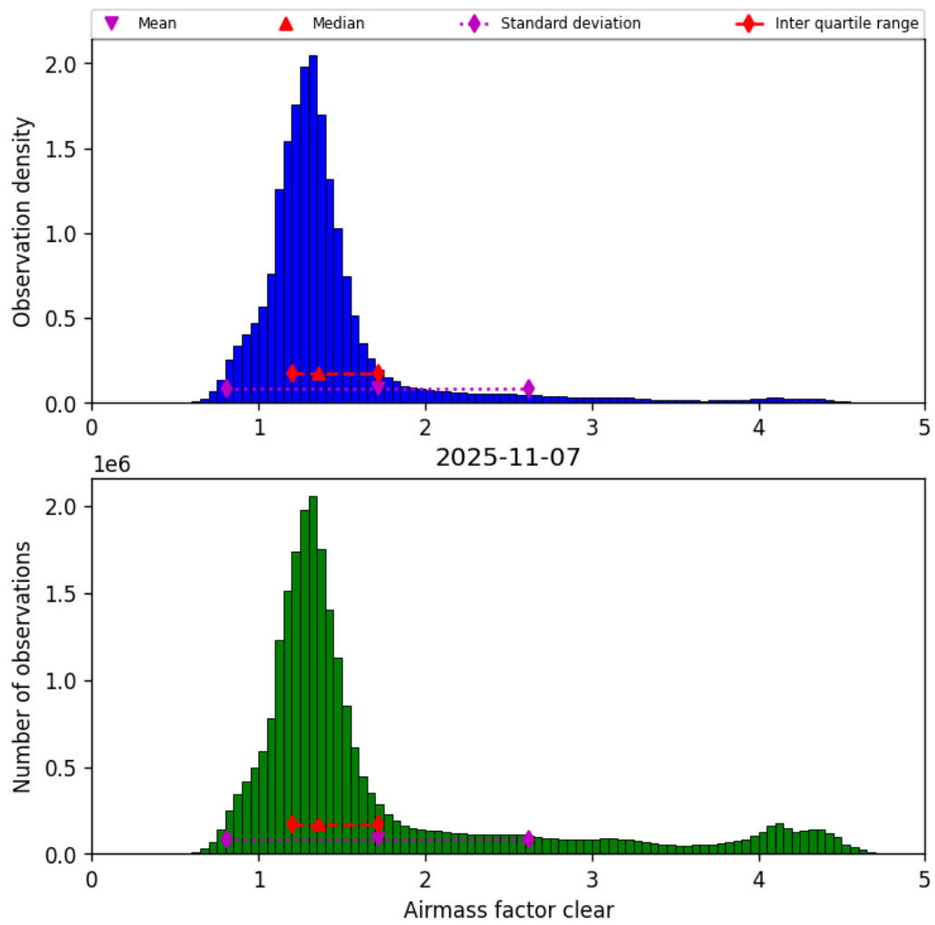
Figure 42: Histogram of “Airmass factor clear” for 2025-11-07 to 2025-11-08
