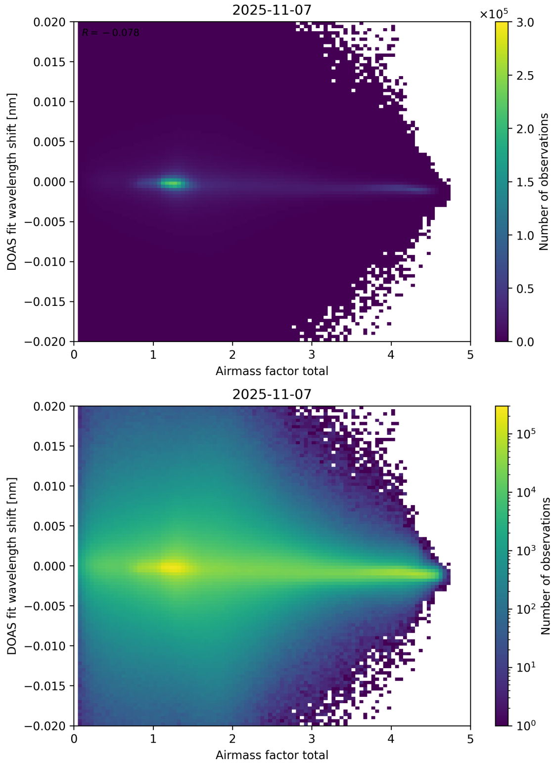
Figure 98: Scatter density plot of “Airmass factor total” against “DOAS fit wavelength shift” for 2025-11-07 to 2025-11-08.
