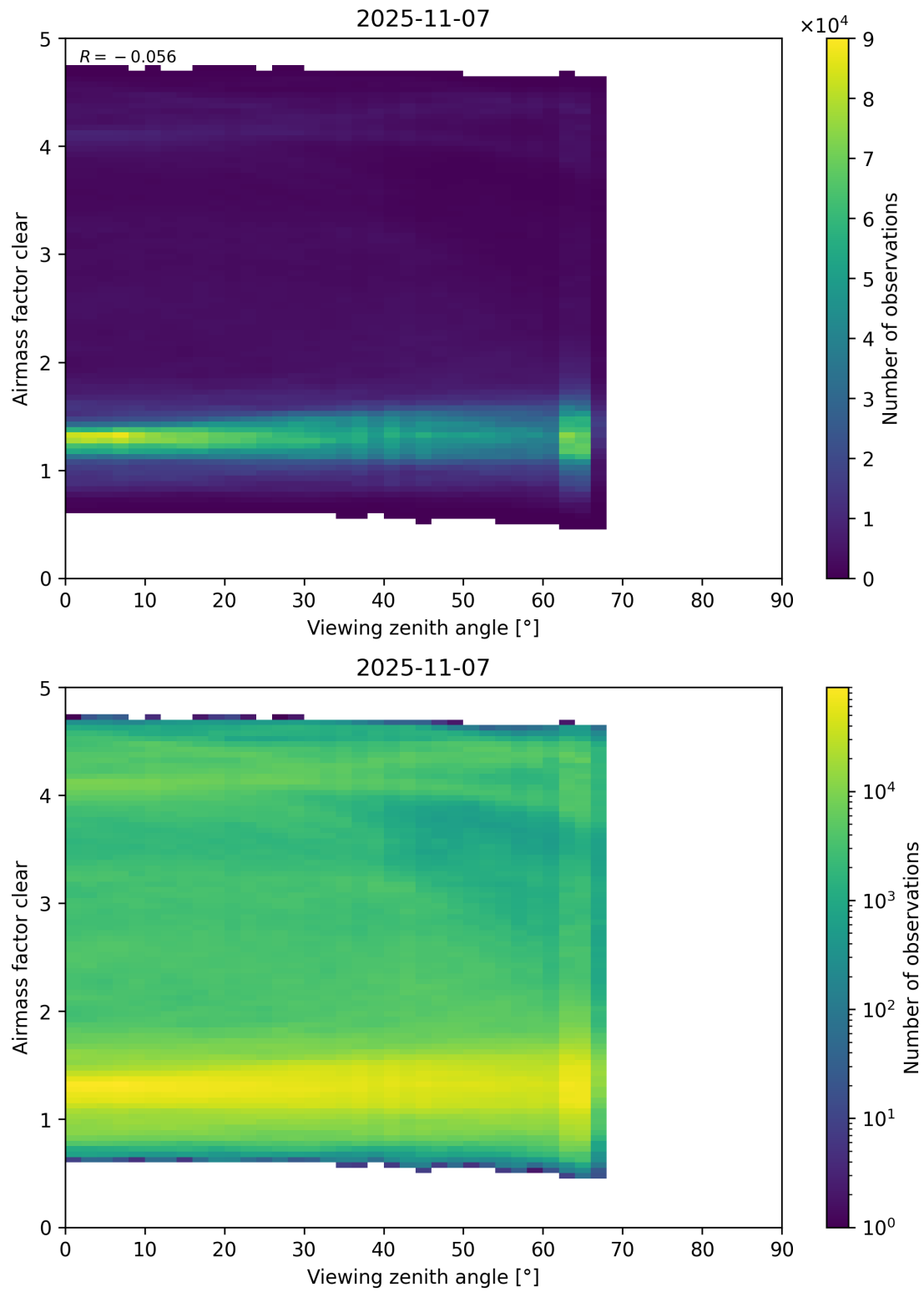
Figure 185: Scatter density plot of “Viewing zenith angle” against “Airmass factor clear” for 2025-11-07 to 2025-11-08.
