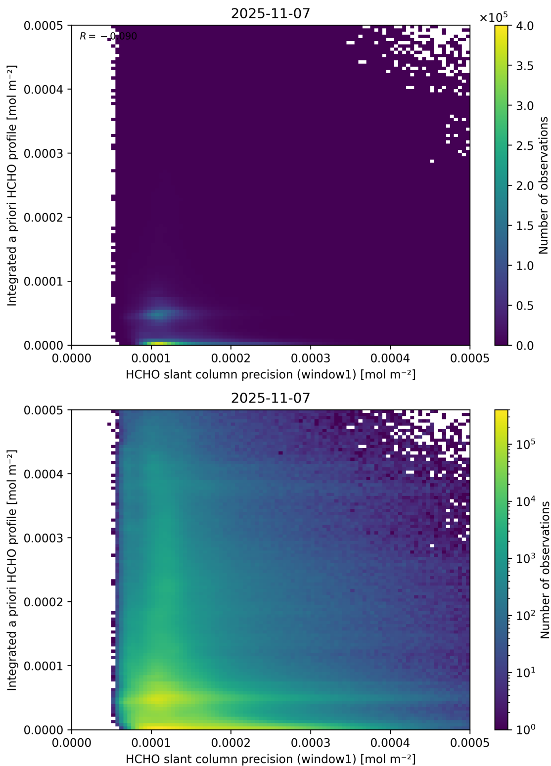
Figure 96: Scatter density plot of “HCHO slant column precision (window1)” against “Integrated a priori HCHO profile” for 2025-11-07 to 2025-11-08.
