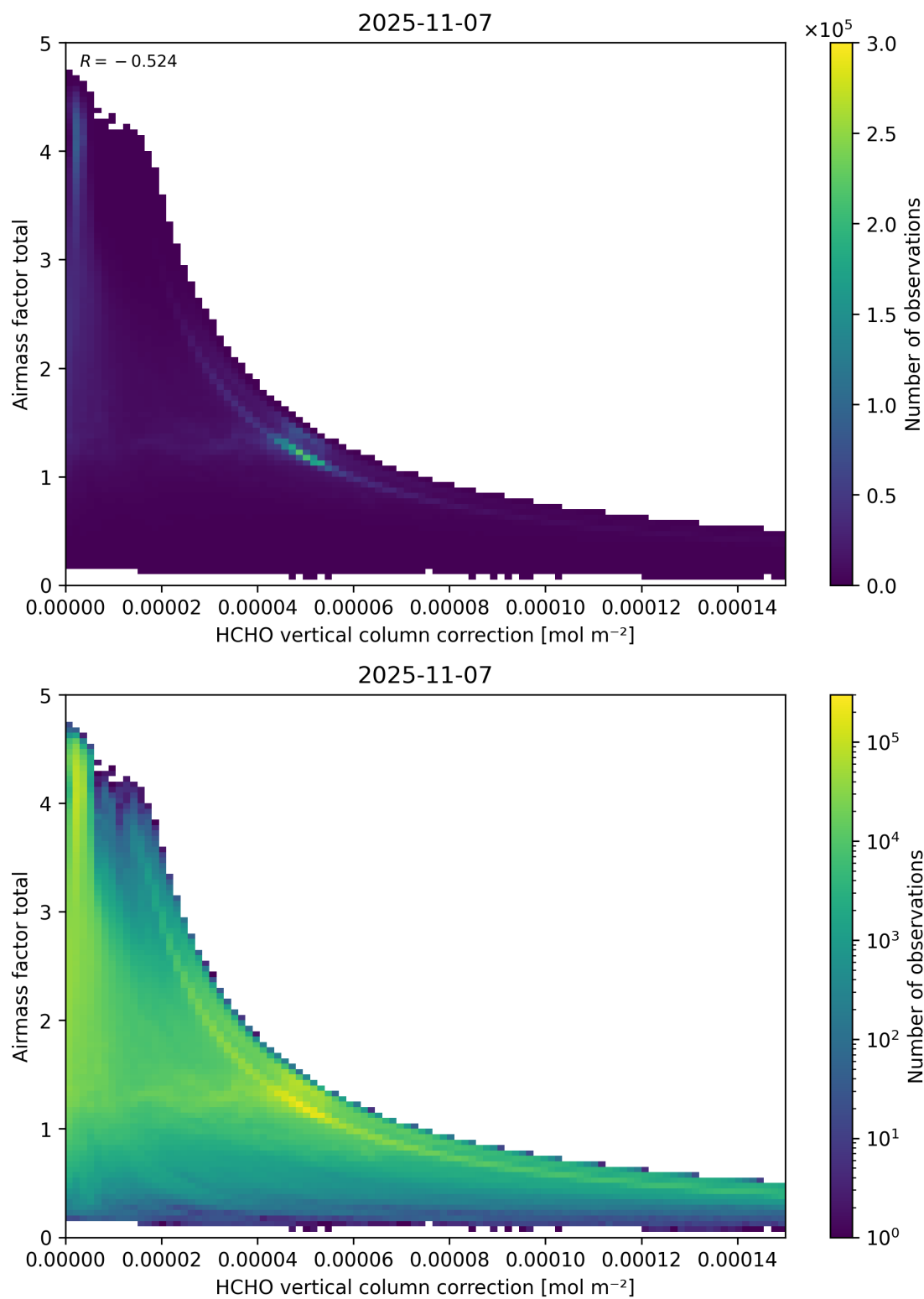
Figure 120: Scatter density plot of “HCHO vertical column correction” against “Airmass factor total” for 2025-11-07 to 2025-11-08.
