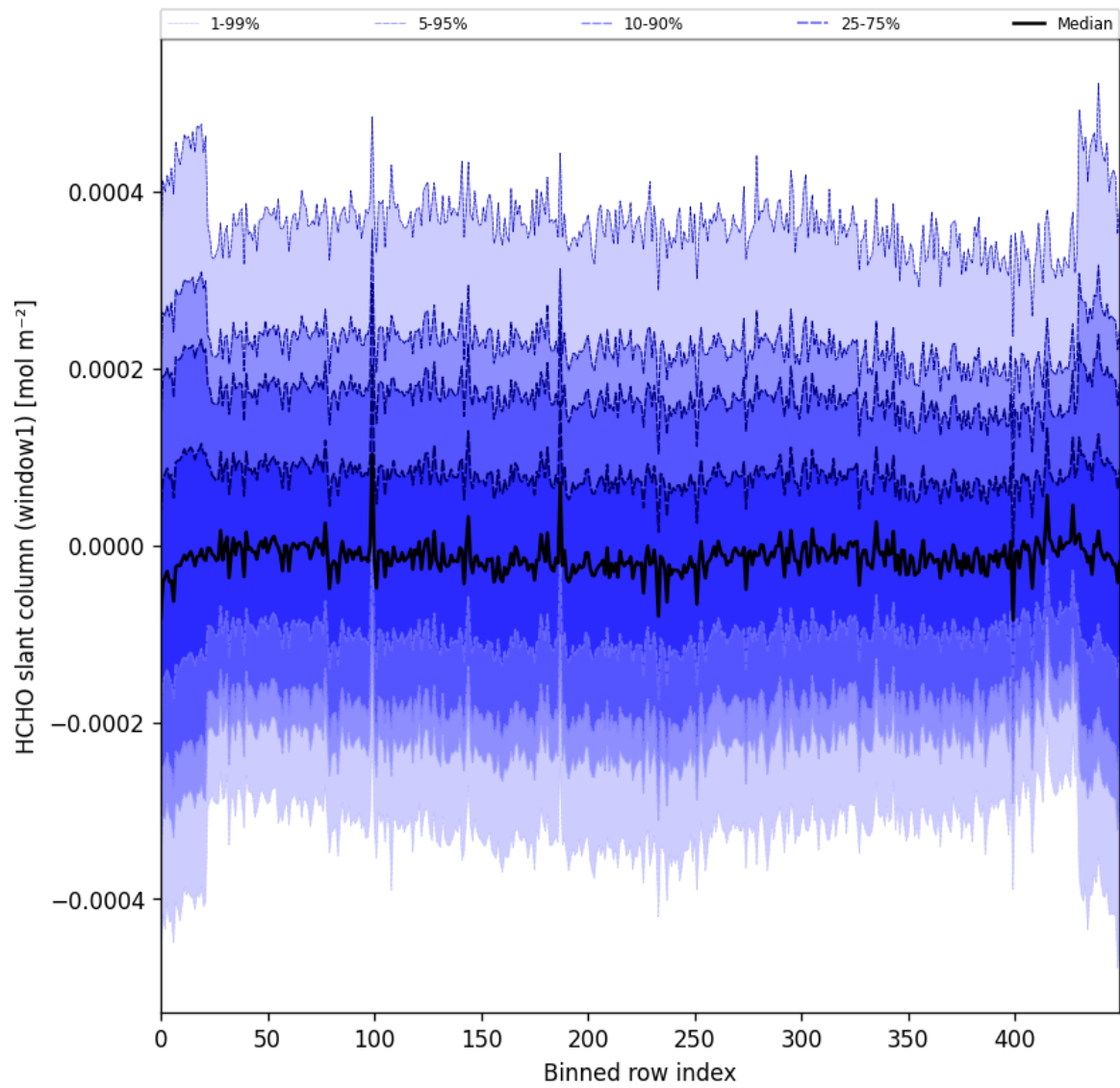
Figure 52: Along track statistics of “HCHO slant column (window1)” for 2025-11-07 to 2025-11-08
