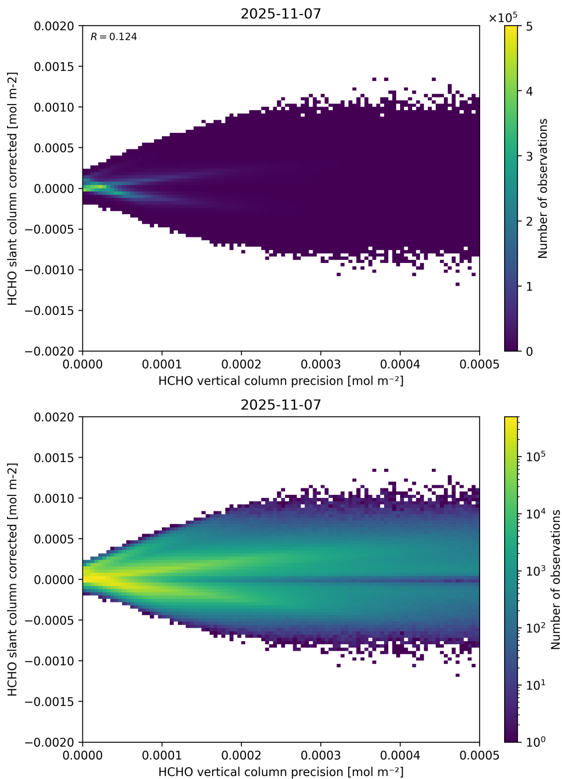
Figure 140: Scatter density plot of “HCHO vertical column precision” against “HCHO slant column corrected” for 2025-11-07 to 2025-11-08.
