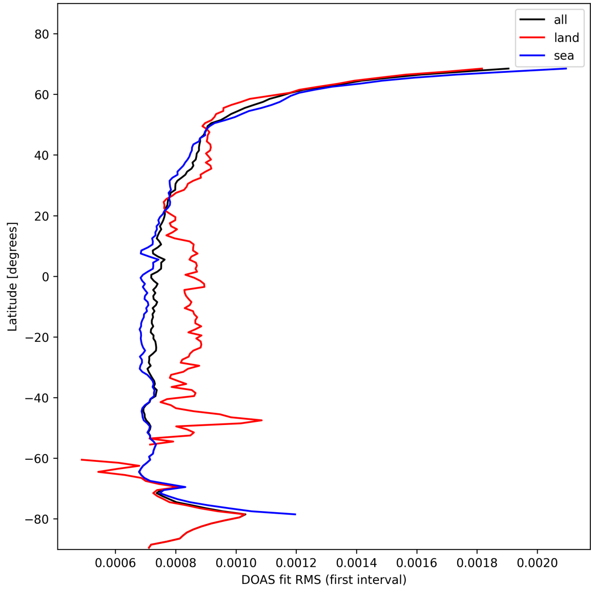
Figure 32: Zonal average of “DOAS fit RMS (first interval)” for 2025-11-07 to 2025-11-08.
