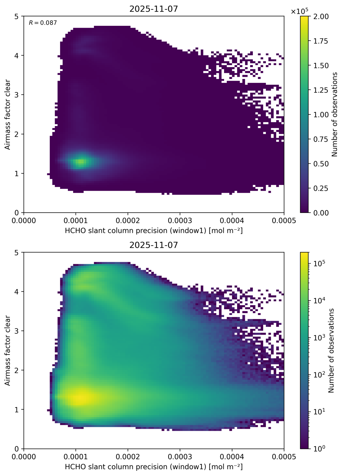
Figure 91: Scatter density plot of “HCHO slant column precision (window1)” against “Airmass factor clear” for 2025-11-07 to 2025-11-08.
