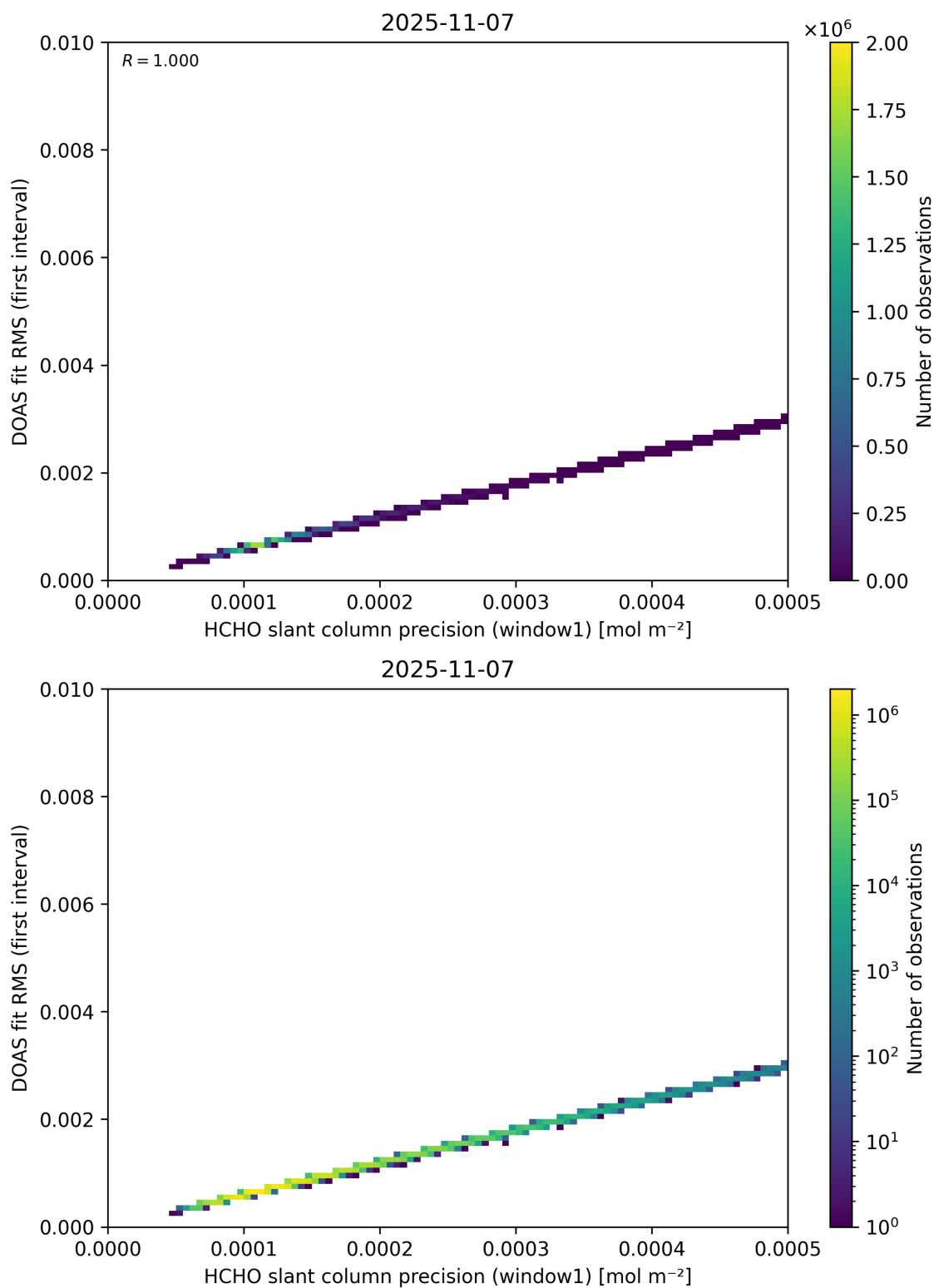
Figure 88: Scatter density plot of “HCHO slant column precision (window1)” against “DOAS fit RMS (first interval)” for 2025-11-07 to 2025-11-08.
