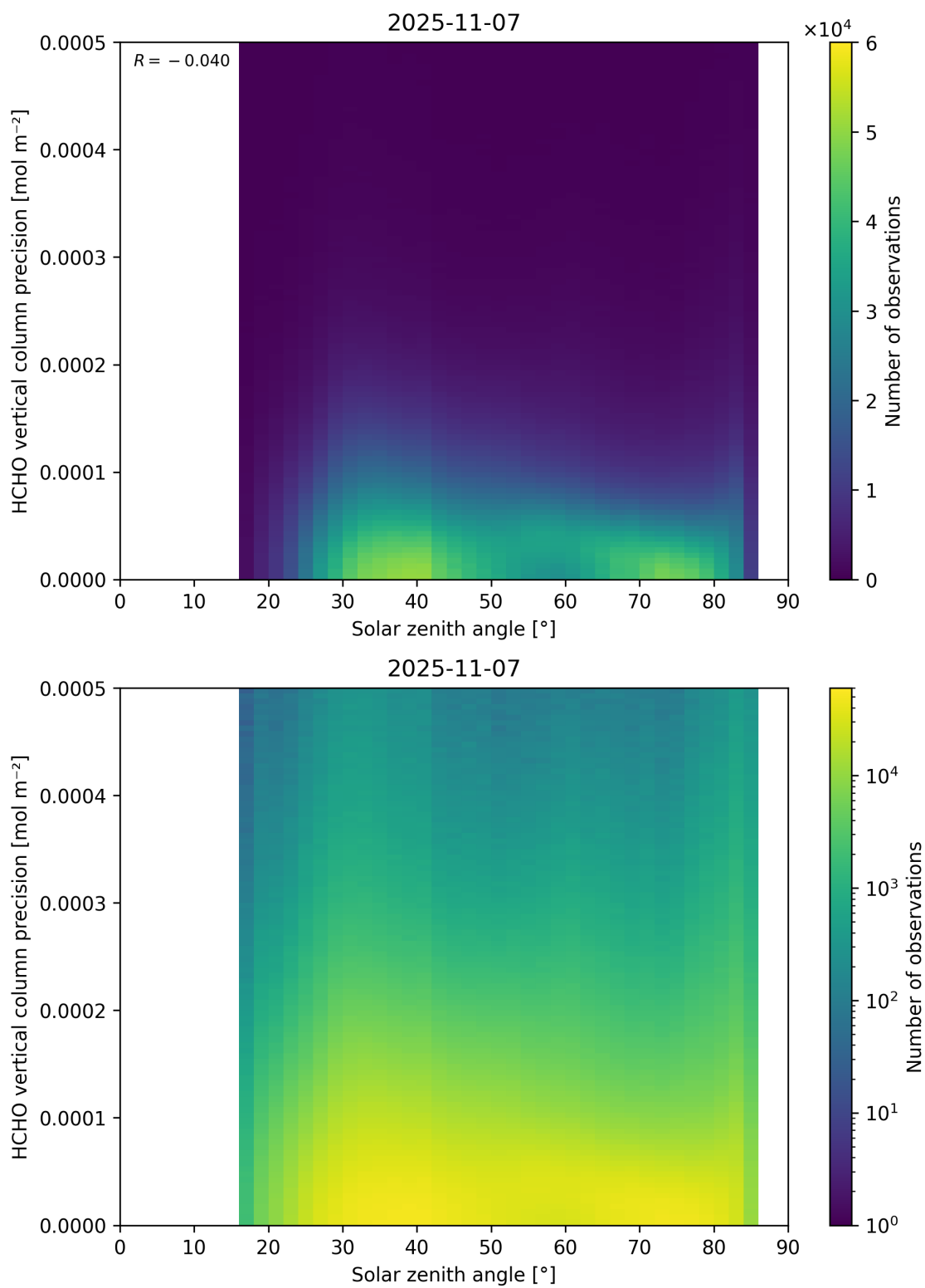
Figure 179: Scatter density plot of “Solar zenith angle” against “HCHO vertical column precision” for 2025-11-07 to 2025-11-08.
