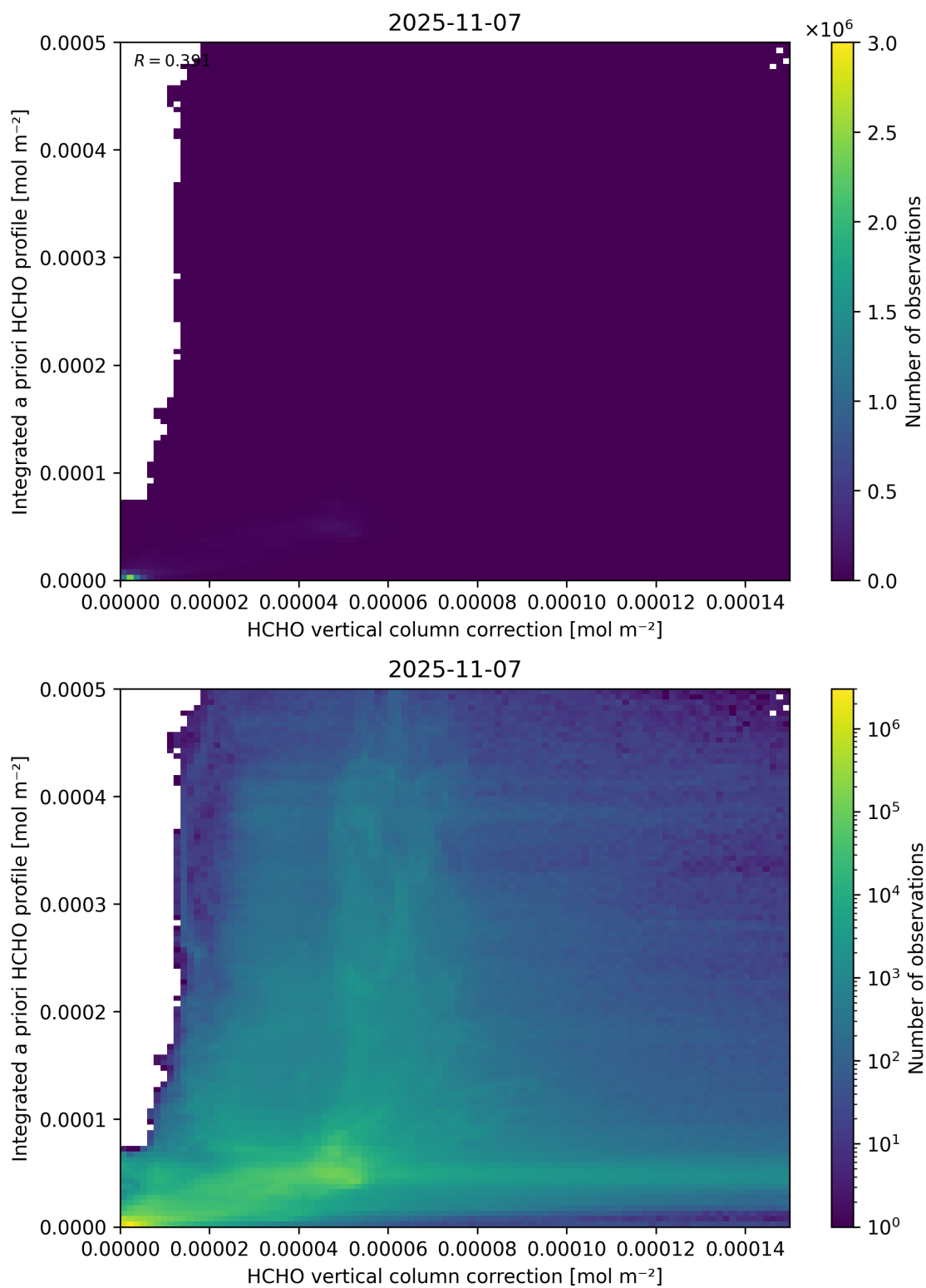
Figure 122: Scatter density plot of “HCHO vertical column correction” against “Integrated a priori HCHO profile” for 2025-11-07 to 2025-11-08.
