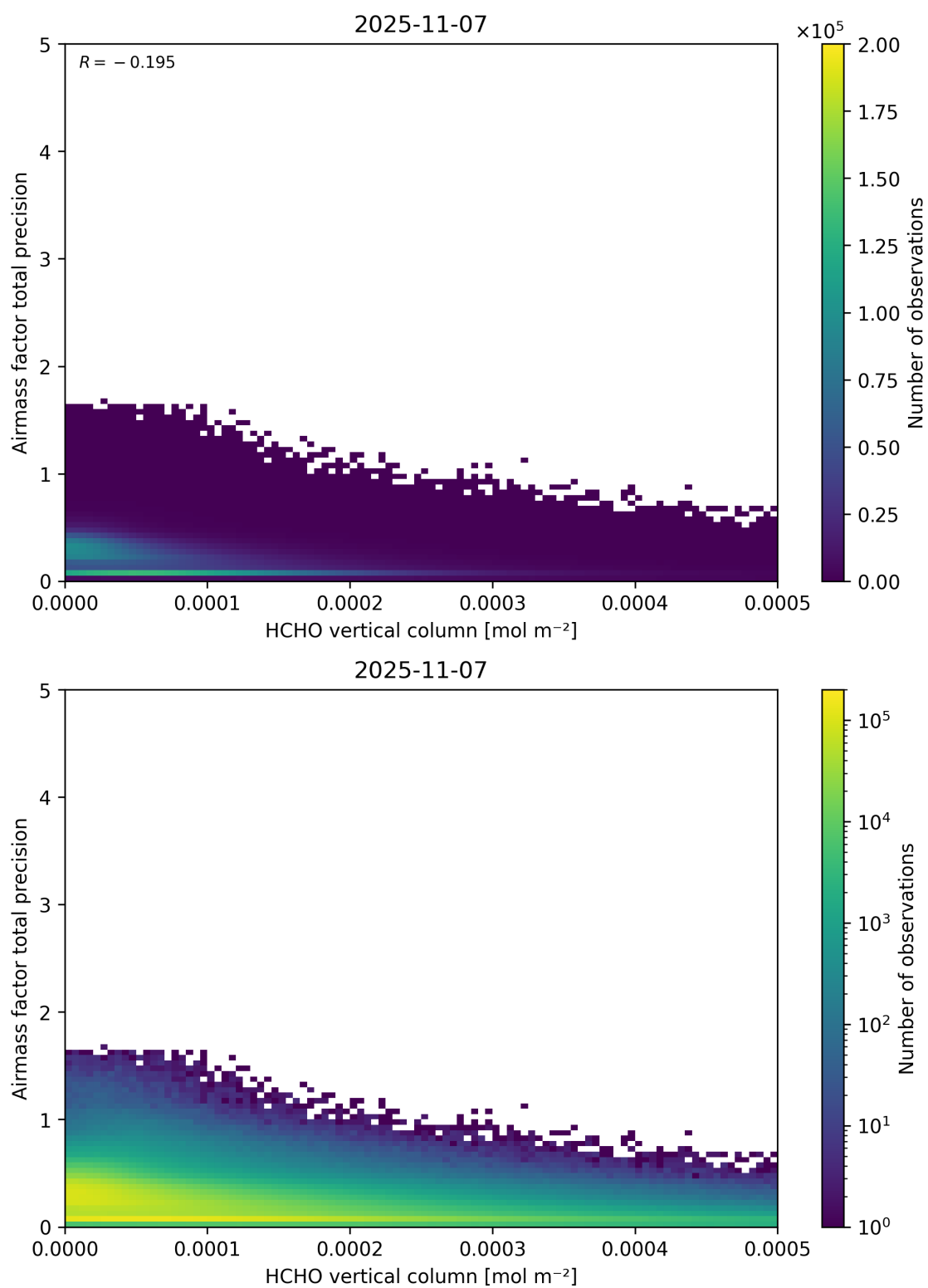
Figure 132: Scatter density plot of “HCHO vertical column” against “Airmass factor total precision” for 2025-11-07 to 2025-11-08.
