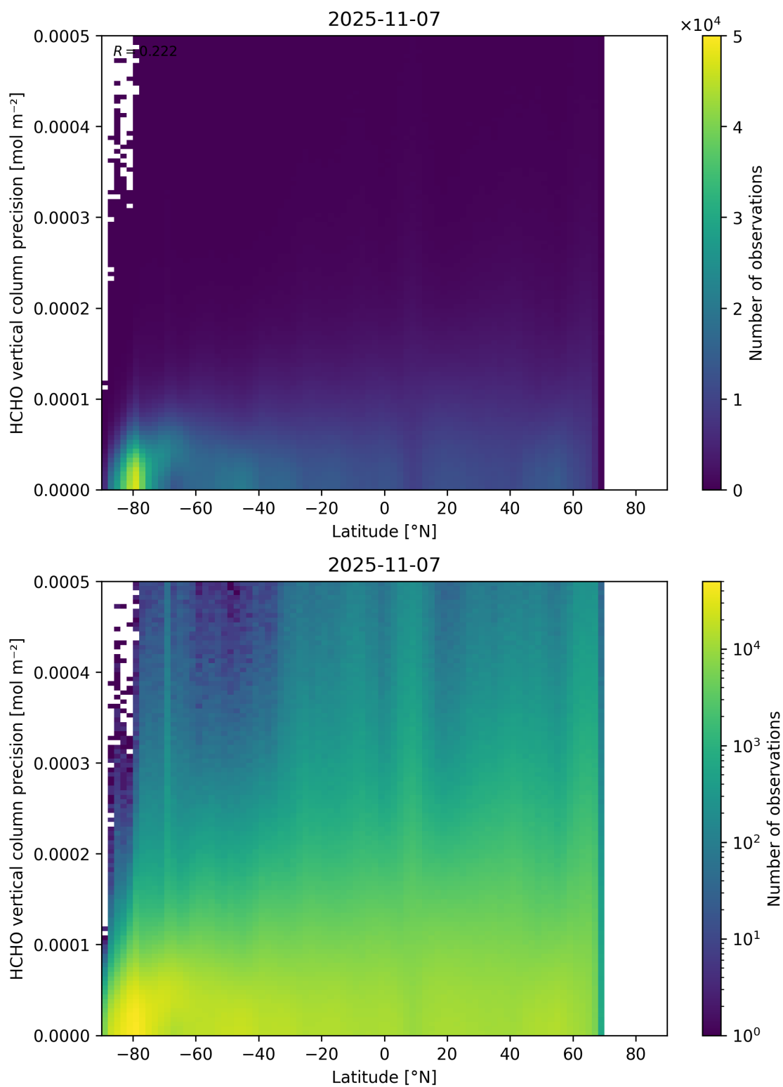
Figure 165: Scatter density plot of “Latitude” against “HCHO vertical column precision” for 2025-11-07 to 2025-11-08.
