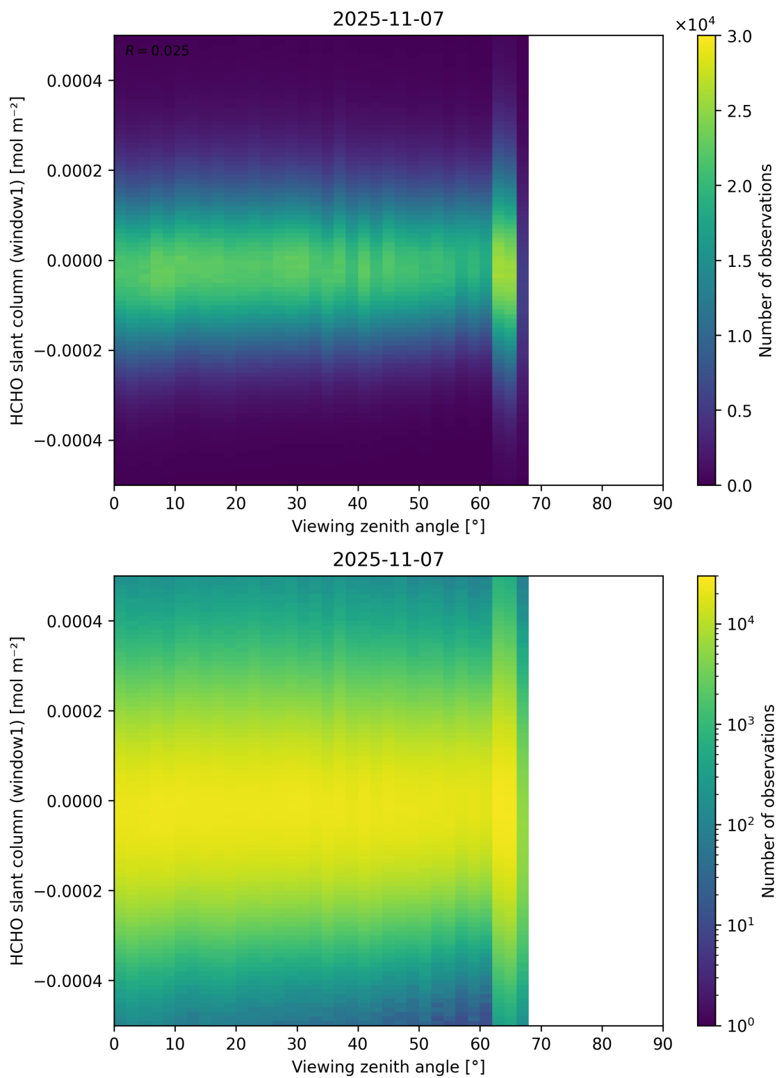
Figure 188: Scatter density plot of “Viewing zenith angle” against “HCHO slant column (window1)” for 2025-11-07 to 2025-11-08.
