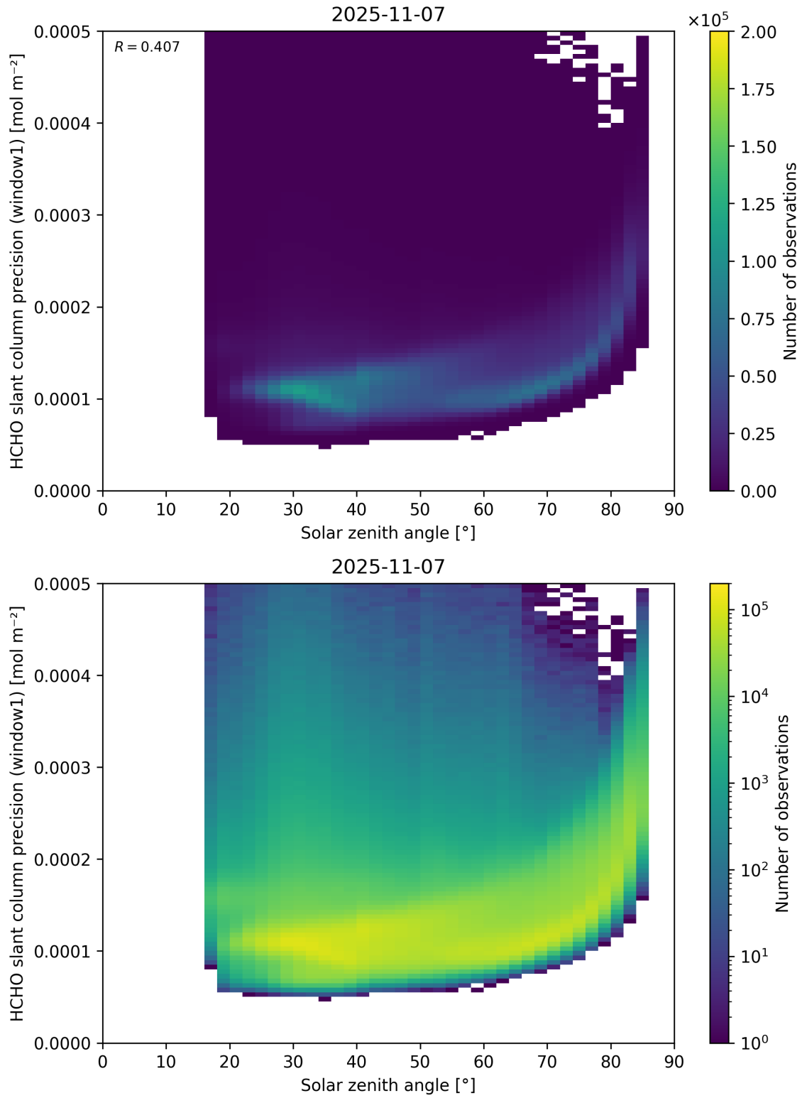
Figure 174: Scatter density plot of “Solar zenith angle” against “HCHO slant column precision (window1)” for 2025-11-07 to 2025-11-08.
