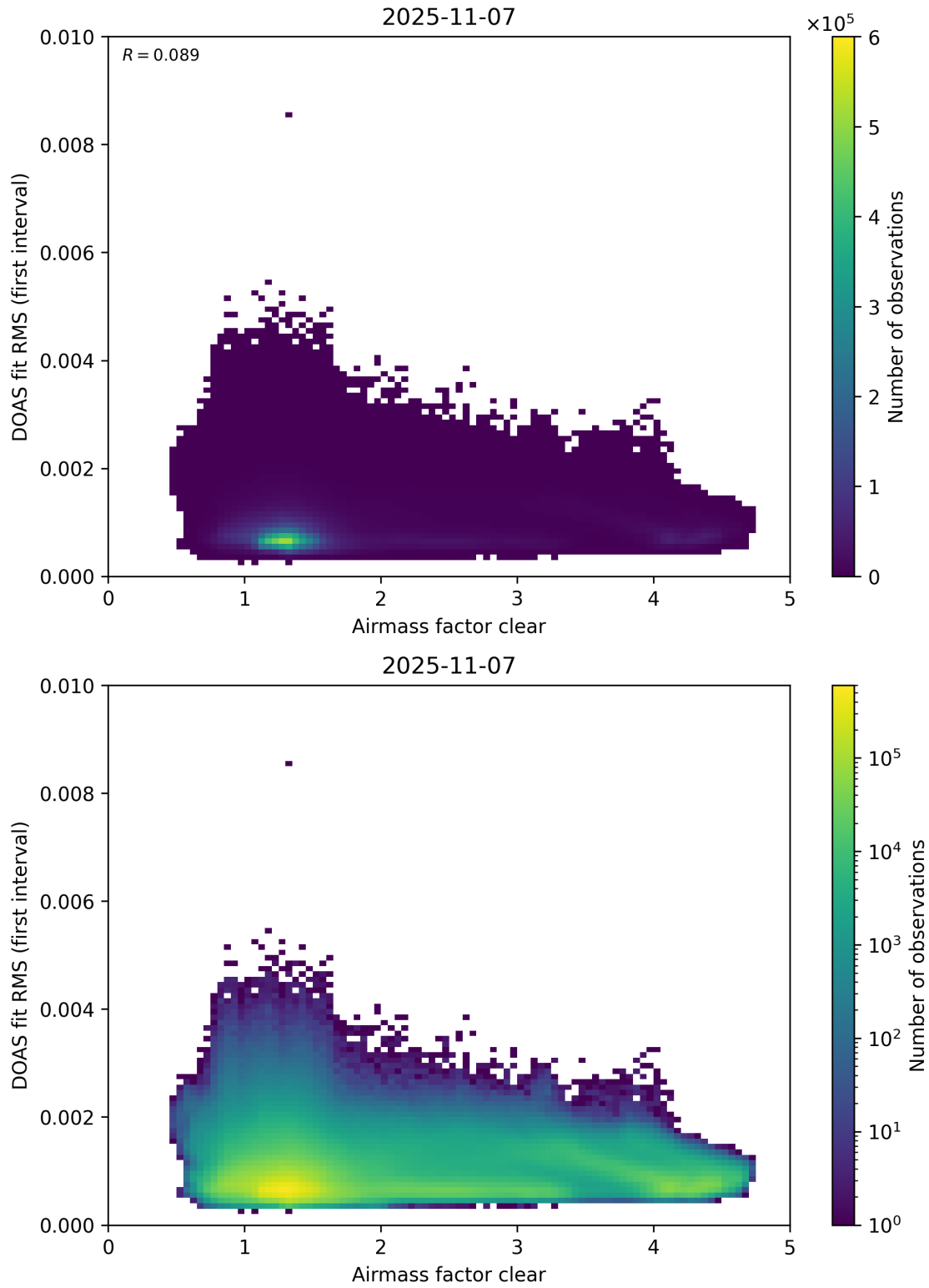
Figure 71: Scatter density plot of “Airmass factor clear” against “DOAS fit RMS (first interval)” for 2025-11-07 to 2025-11-08.
