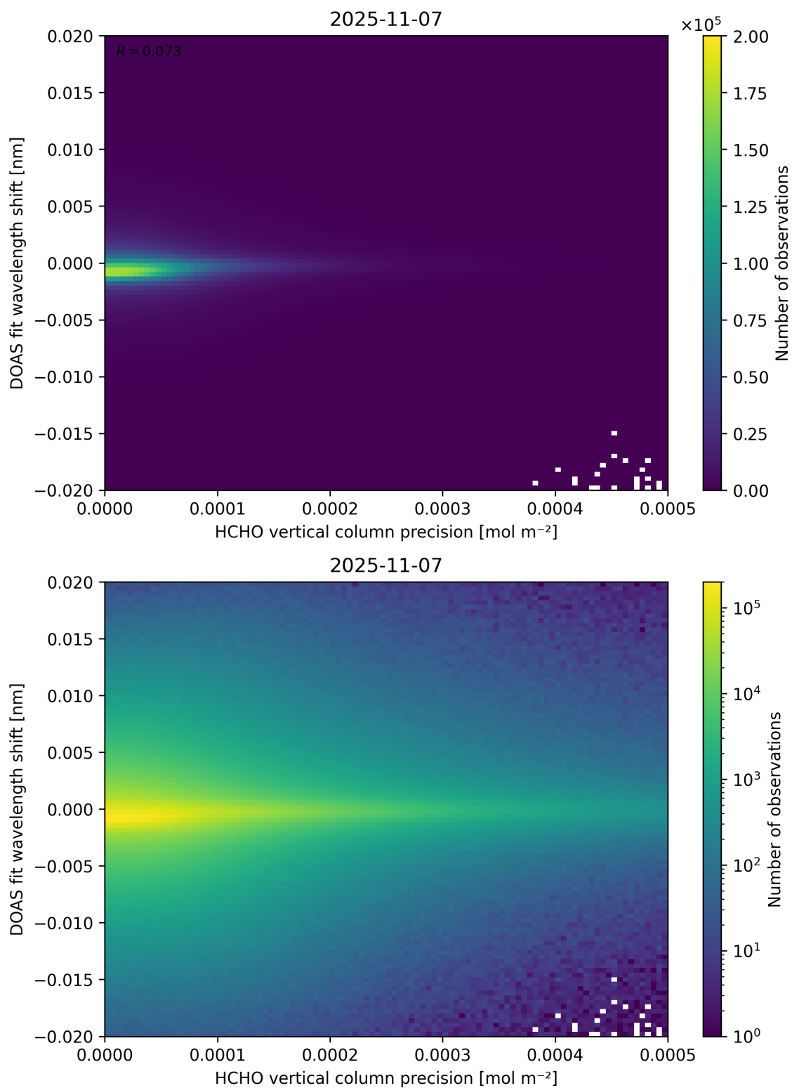
Figure 137: Scatter density plot of “HCHO vertical column precision” against “DOAS fit wavelength shift” for 2025-11-07 to 2025-11-08.
