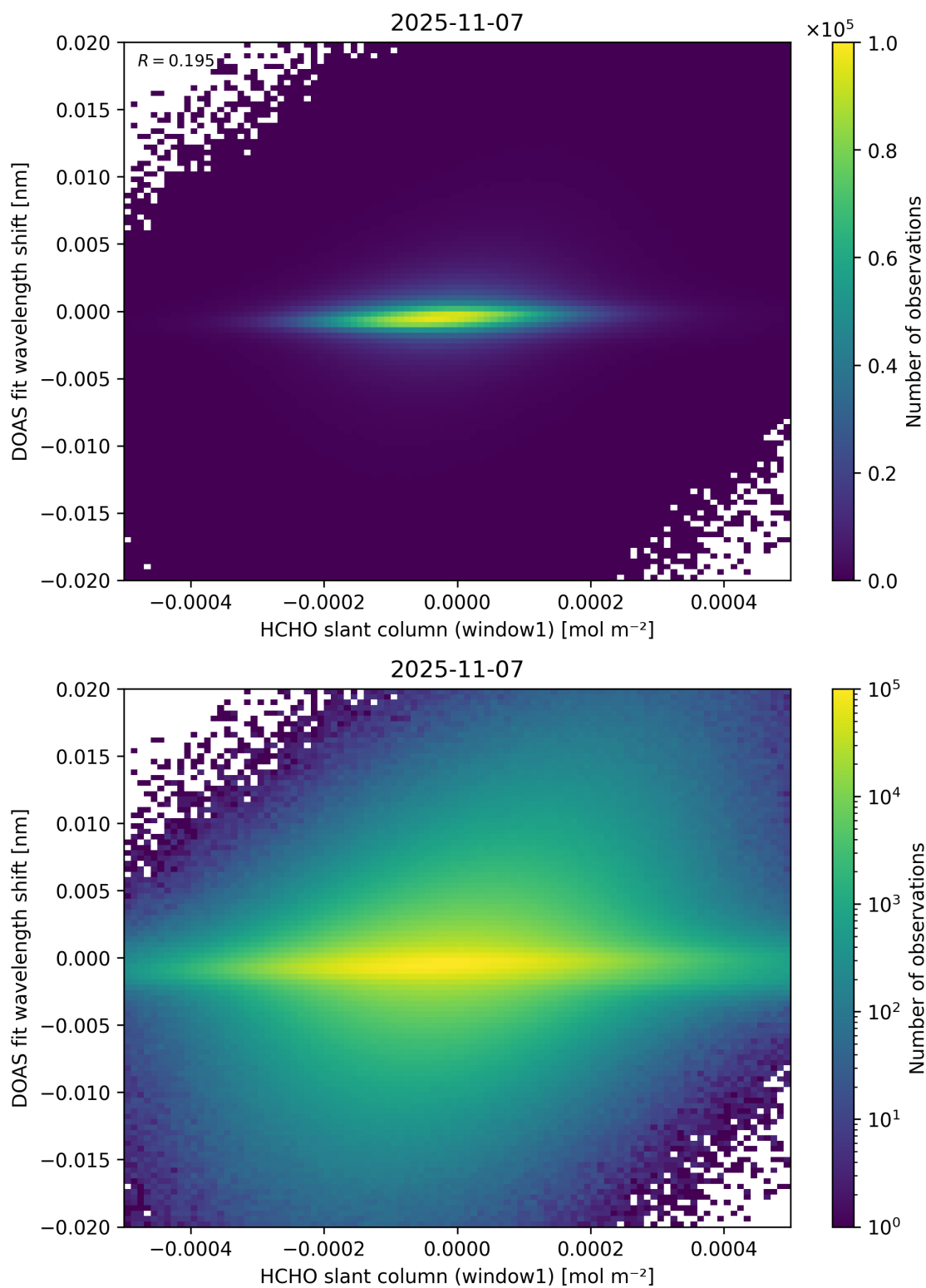
Figure 79: Scatter density plot of “HCHO slant column (window1)” against “DOAS fit wavelength shift” for 2025-11-07 to 2025-11-08.
