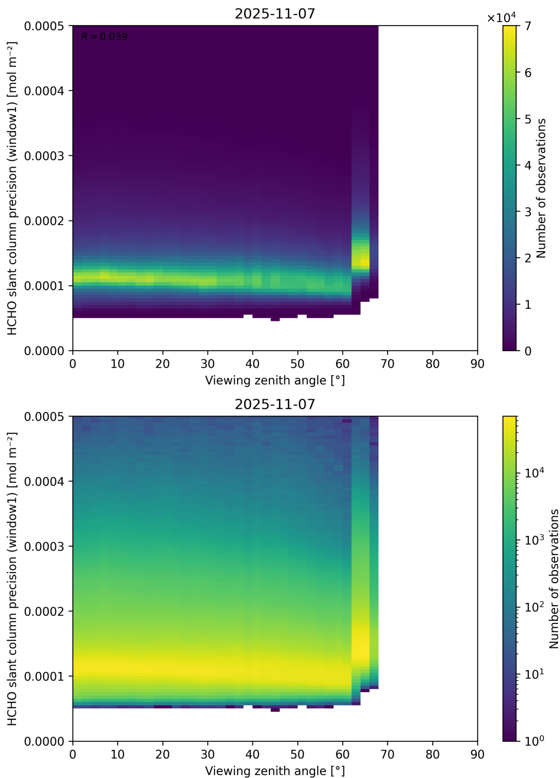
Figure 189: Scatter density plot of “Viewing zenith angle” against “HCHO slant column precision (window1)” for 2025-11-07 to 2025-11-08.
