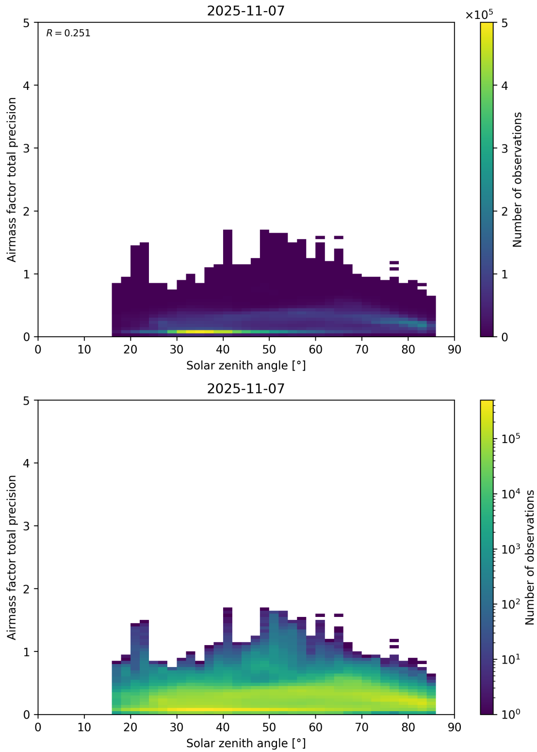
Figure 176: Scatter density plot of “Solar zenith angle” against “Airmass factor total precision” for 2025-11-07 to 2025-11-08.
