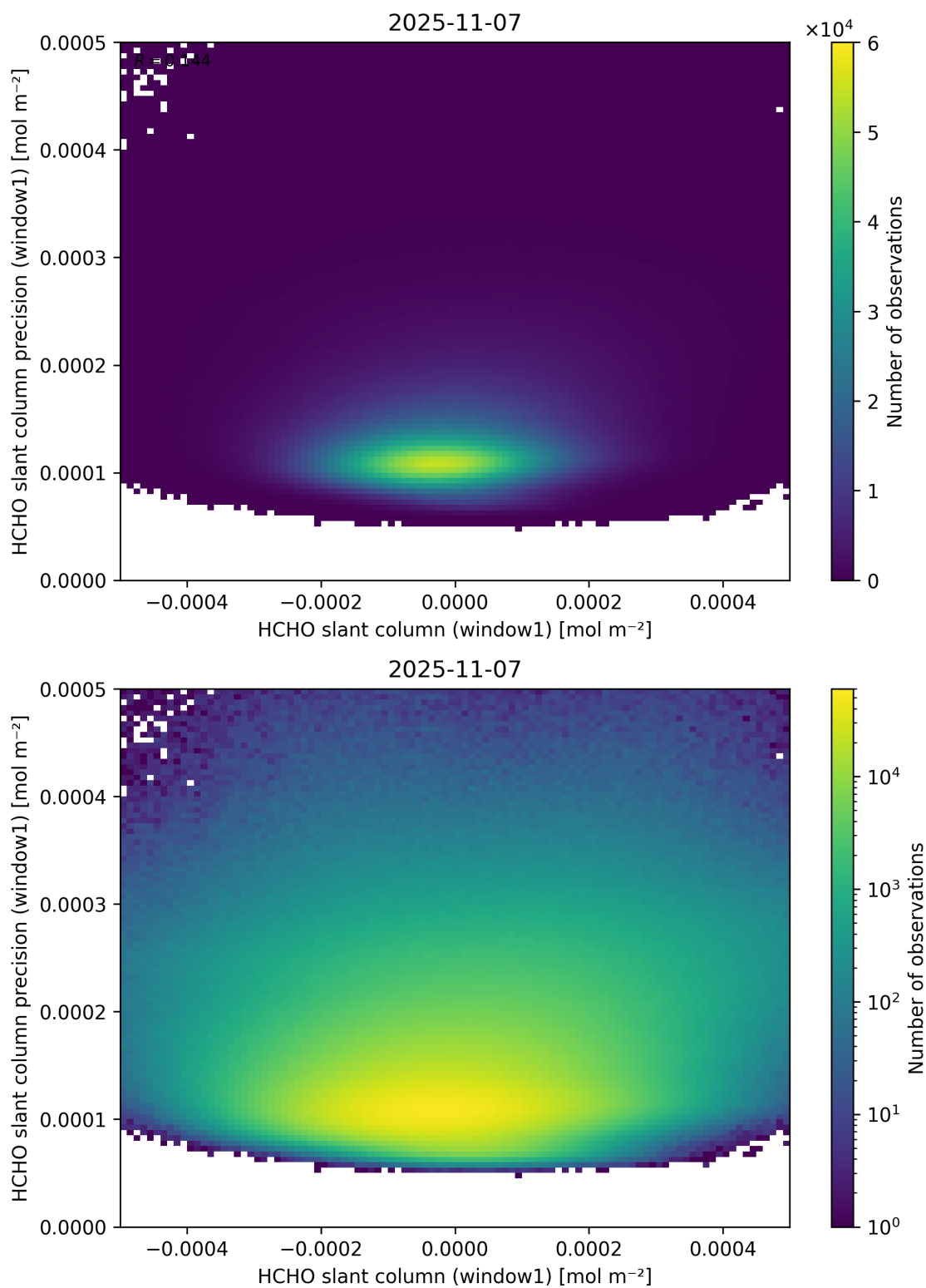
Figure 84: Scatter density plot of “HCHO slant column (window1)” against “HCHO slant column precision (window1)” for 2025-11-07 to 2025-11-08.
