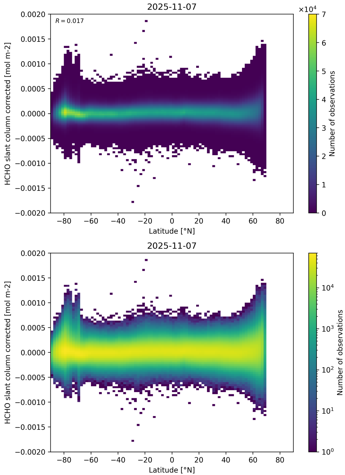
Figure 157: Scatter density plot of “Latitude” against “HCHO slant column corrected” for 2025-11-07 to 2025-11-08.
