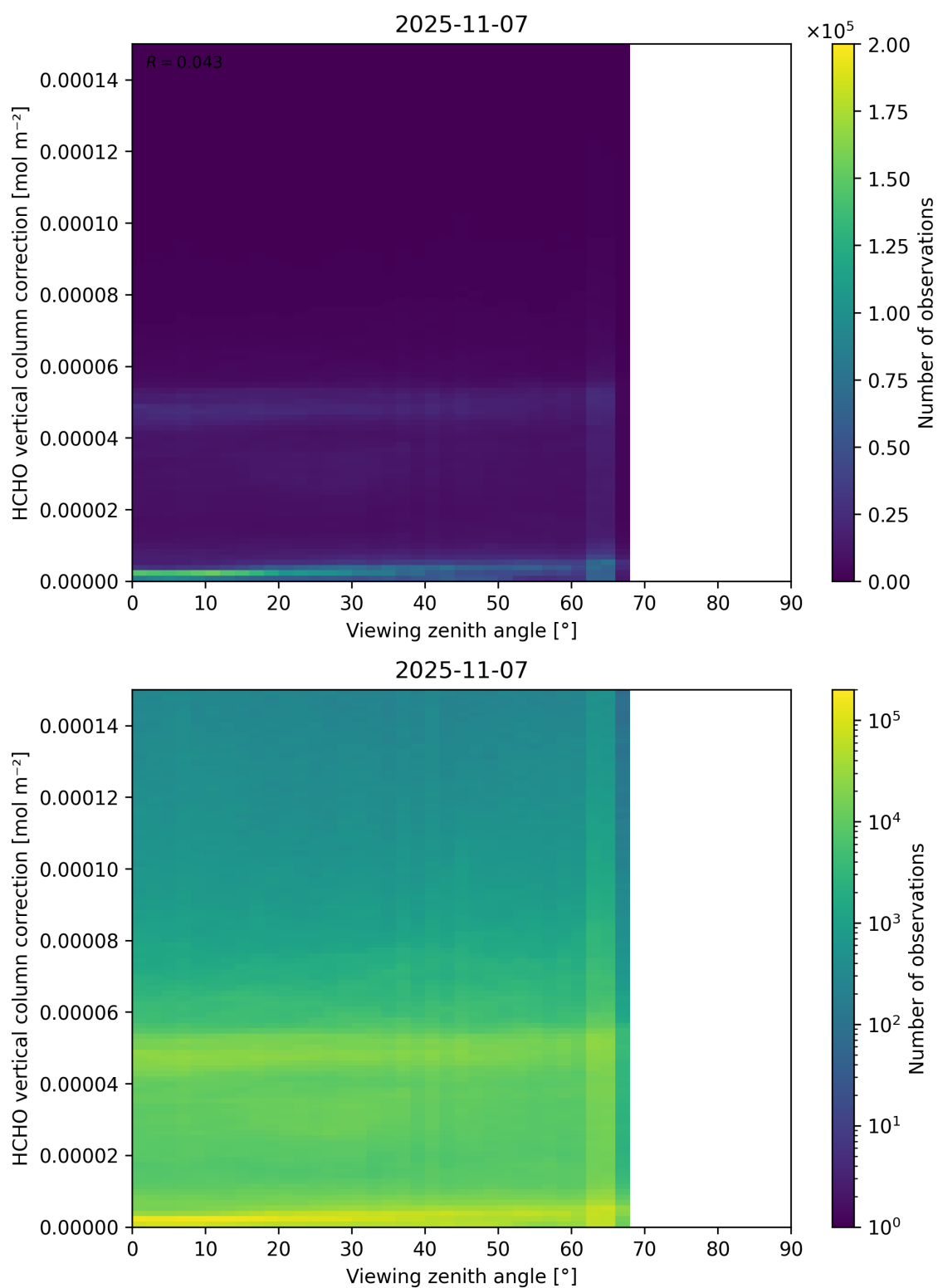
Figure 193: Scatter density plot of “Viewing zenith angle” against “HCHO vertical column correction” for 2025-11-07 to 2025-11-08.
