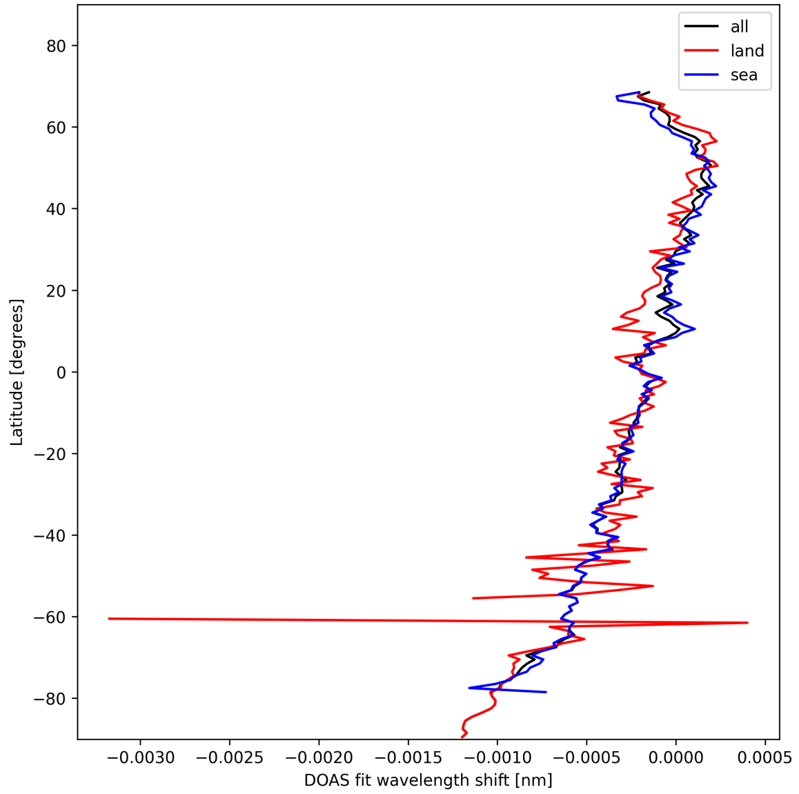
Figure 30: Zonal average of “DOAS fit wavelength shift” for 2025-11-07 to 2025-11-08.
