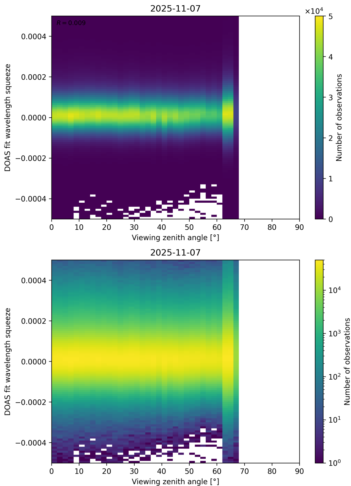
Figure 184: Scatter density plot of “Viewing zenith angle” against “DOAS fit wavelength squeeze” for 2025-11-07 to 2025-11-08.
