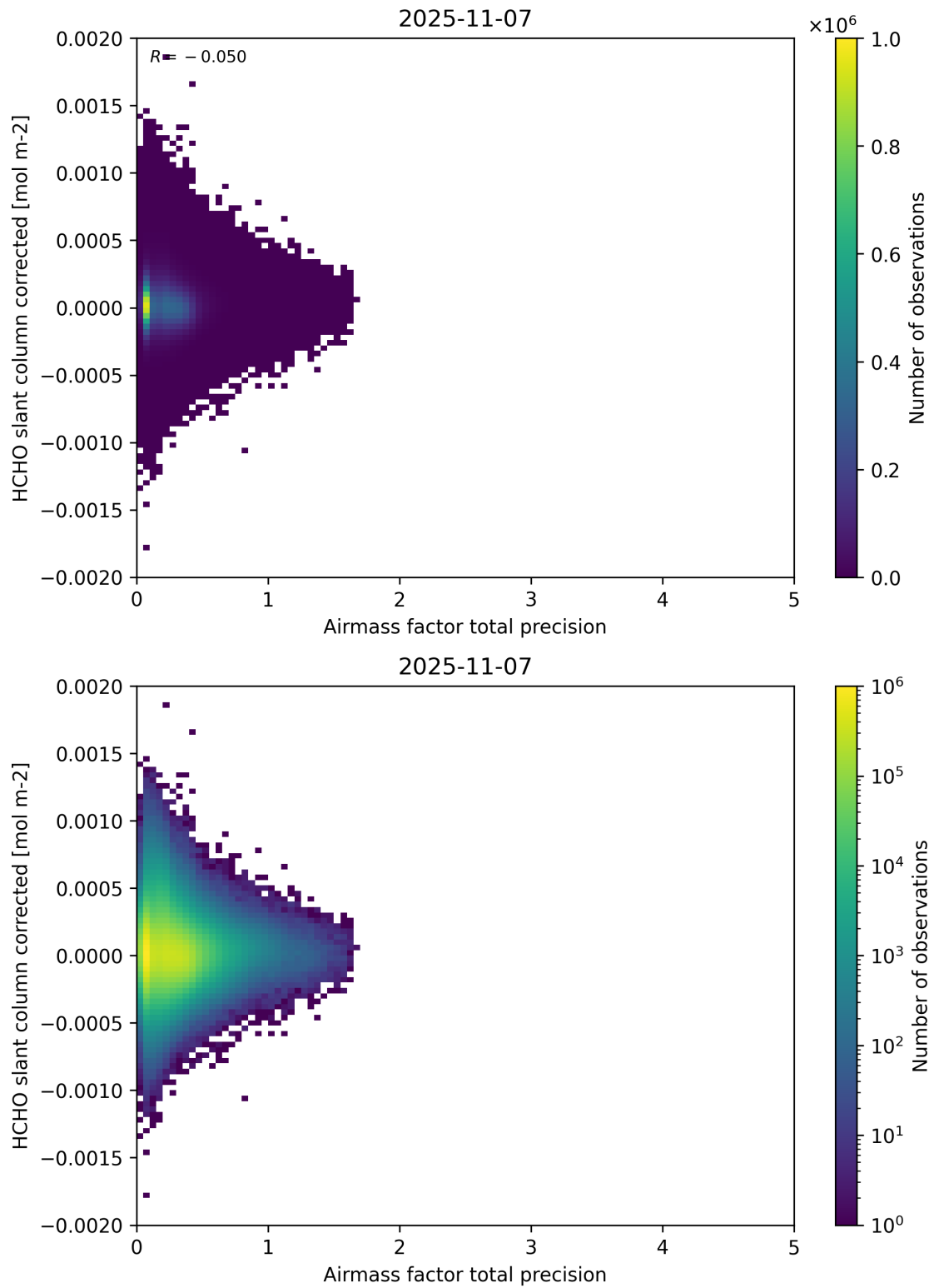
Figure 109: Scatter density plot of “Airmass factor total precision” against “HCHO slant column corrected” for 2025-11-07 to 2025-11-08.
