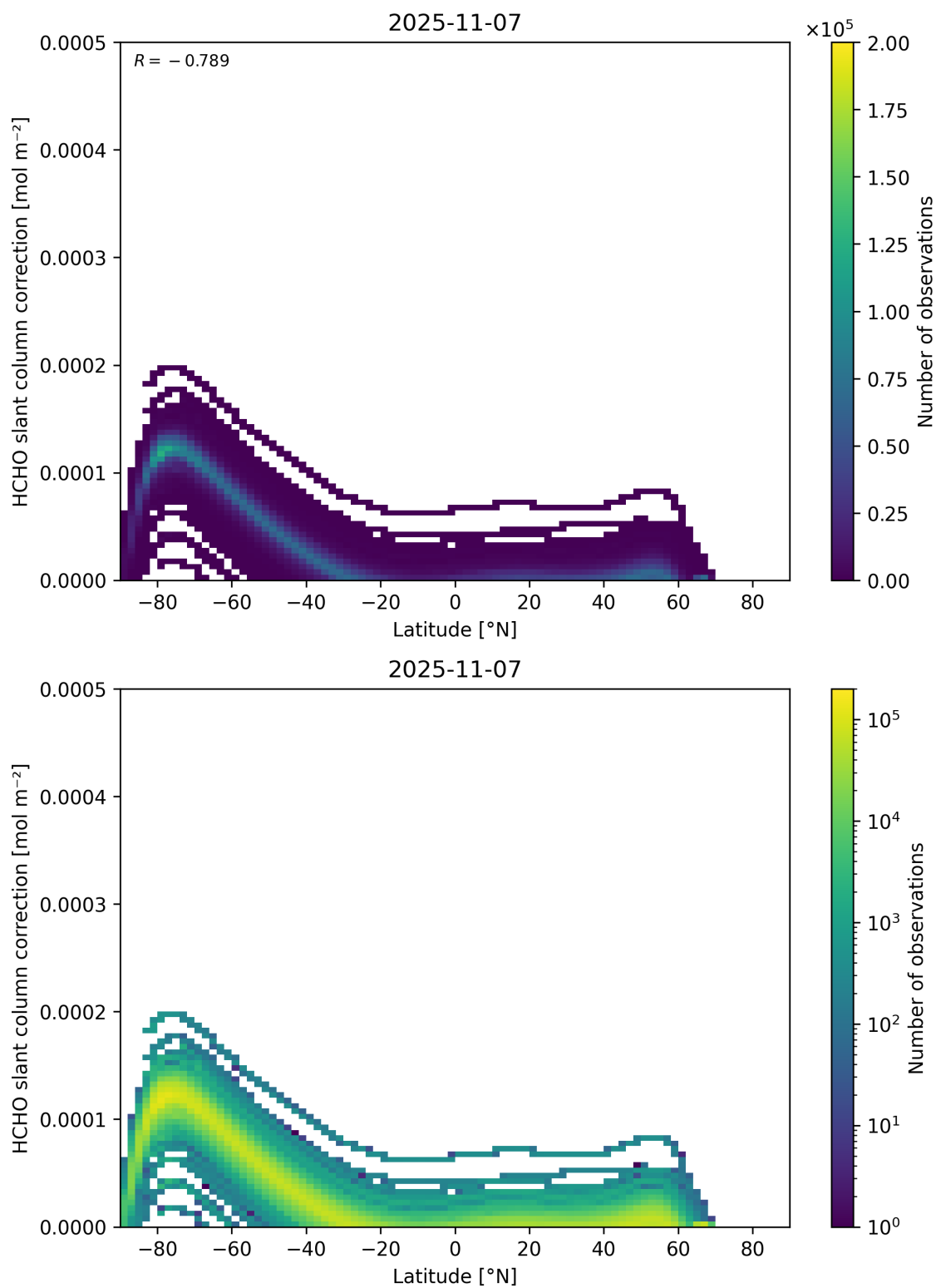
Figure 158: Scatter density plot of “Latitude” against “HCHO slant column correction” for 2025-11-07 to 2025-11-08.
