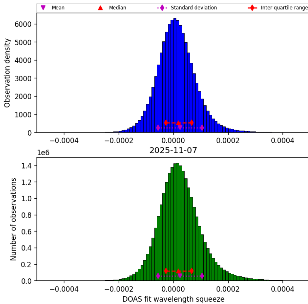
Figure 45: Histogram of “DOAS fit wavelength squeeze” for 2025-11-07 to 2025-11-08
