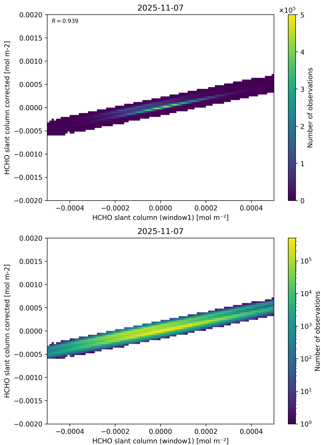
Figure 82: Scatter density plot of “HCHO slant column (window1)” against “HCHO slant column corrected” for 2025-11-07 to 2025-11-08.
