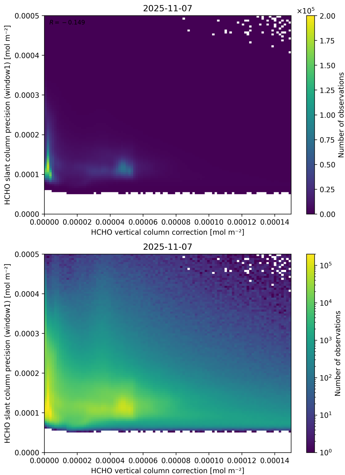
Figure 119: Scatter density plot of “HCHO vertical column correction” against “HCHO slant column precision (window1)” for 2025-11-07 to 2025-11-08.
