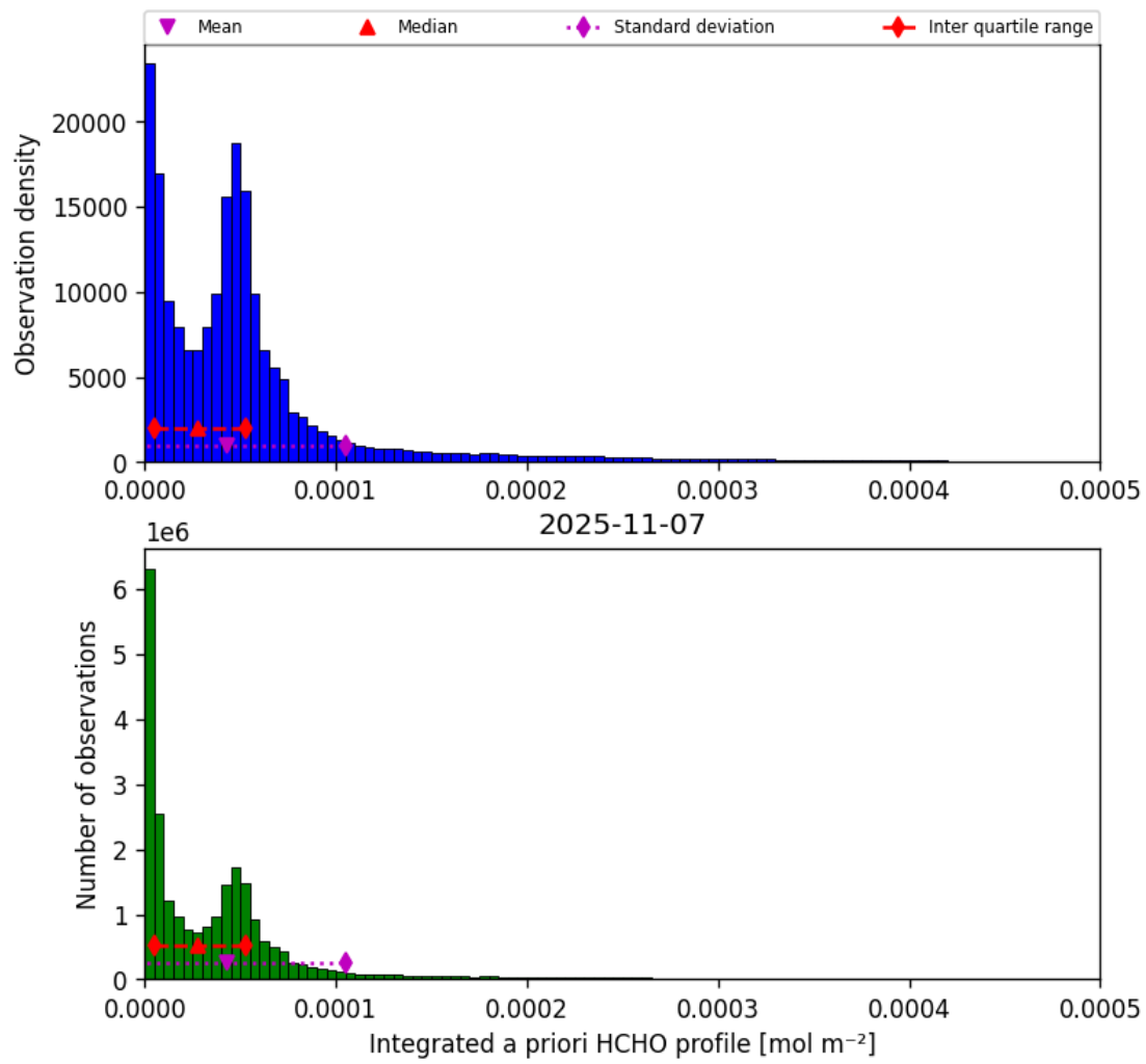
Figure 43: Histogram of “Integrated a priori HCHO profile” for 2025-11-07 to 2025-11-08
