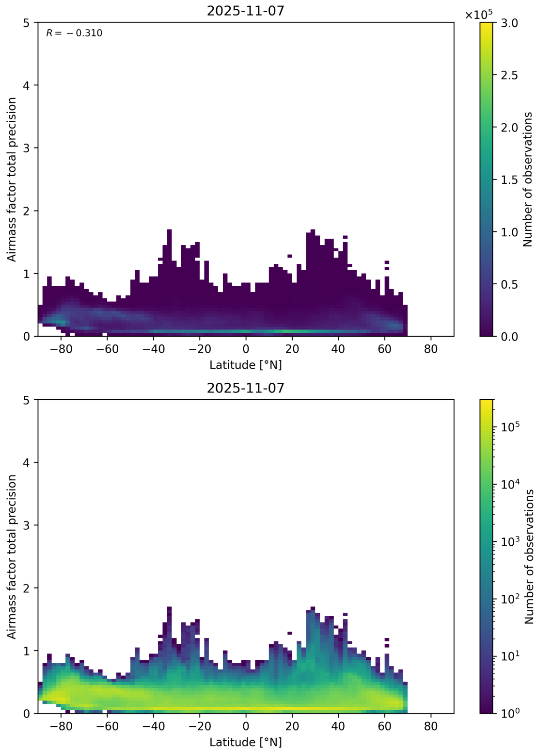
Figure 162: Scatter density plot of “Latitude” against “Airmass factor total precision” for 2025-11-07 to 2025-11-08.
