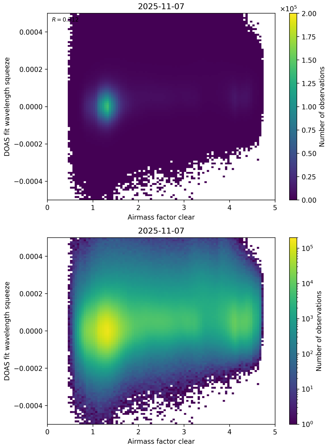
Figure 73: Scatter density plot of “Airmass factor clear” against “DOAS fit wavelength squeeze” for 2025-11-07 to 2025-11-08.
