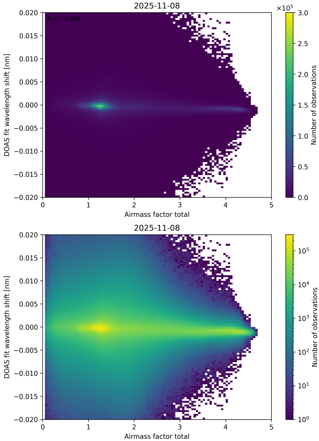
Figure 98: Scatter density plot of “Airmass factor total” against “DOAS fit wavelength shift” for 2025-11-07 to 2025-11-09.
