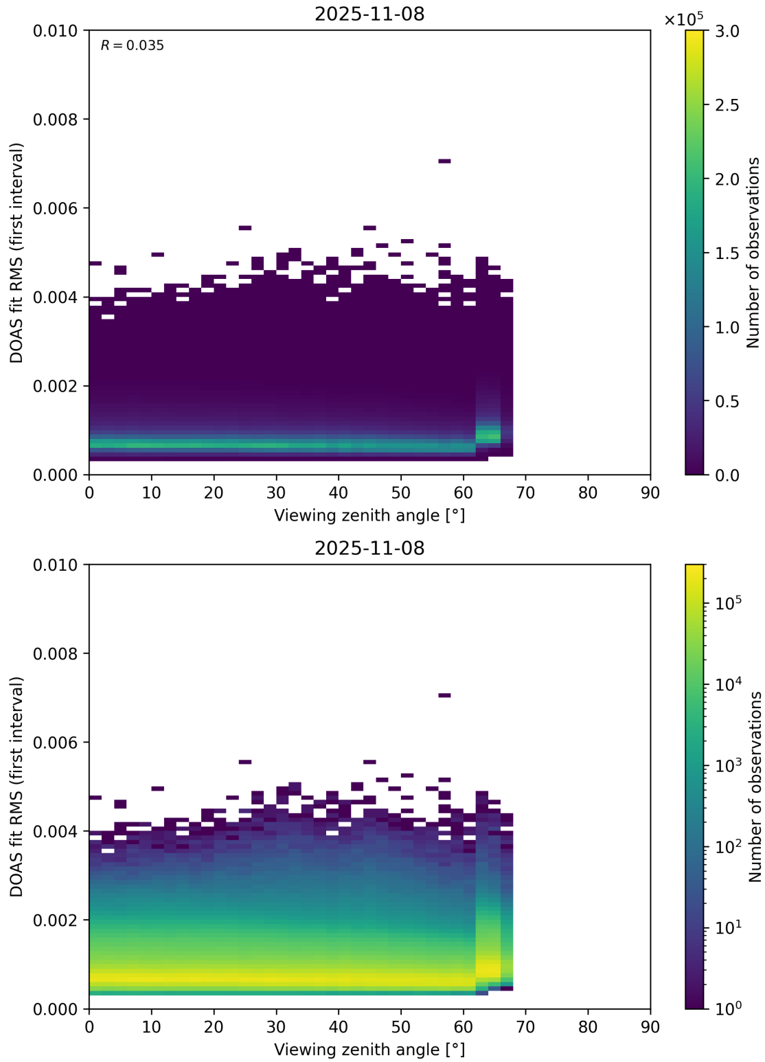
Figure 182: Scatter density plot of “Viewing zenith angle” against “DOAS fit RMS (first interval)” for 2025-11-07 to 2025-11-09.
