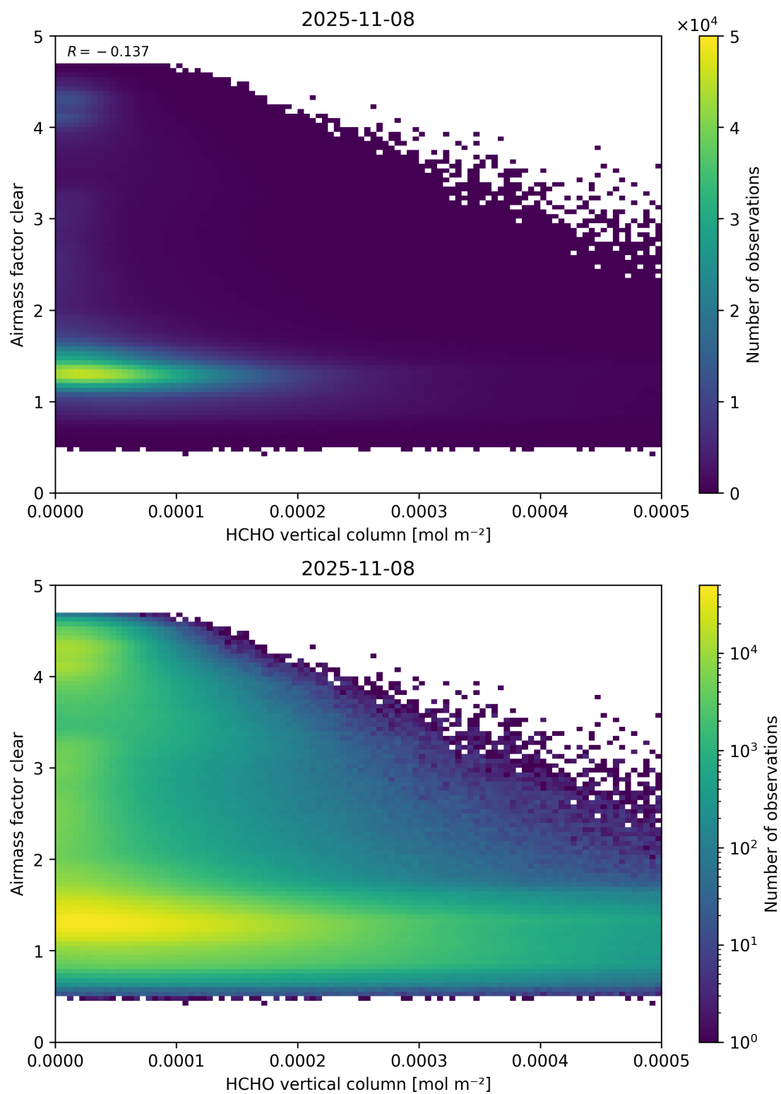
Figure 126: Scatter density plot of “HCHO vertical column” against “Airmass factor clear” for 2025-11-07 to 2025-11-09.
