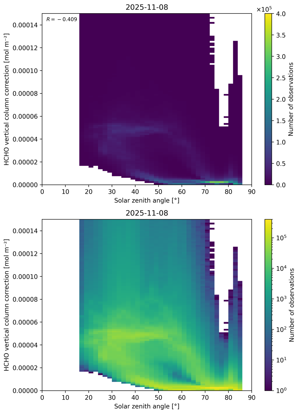
Figure 178: Scatter density plot of “Solar zenith angle” against “HCHO vertical column correction” for 2025-11-07 to 2025-11-09.
