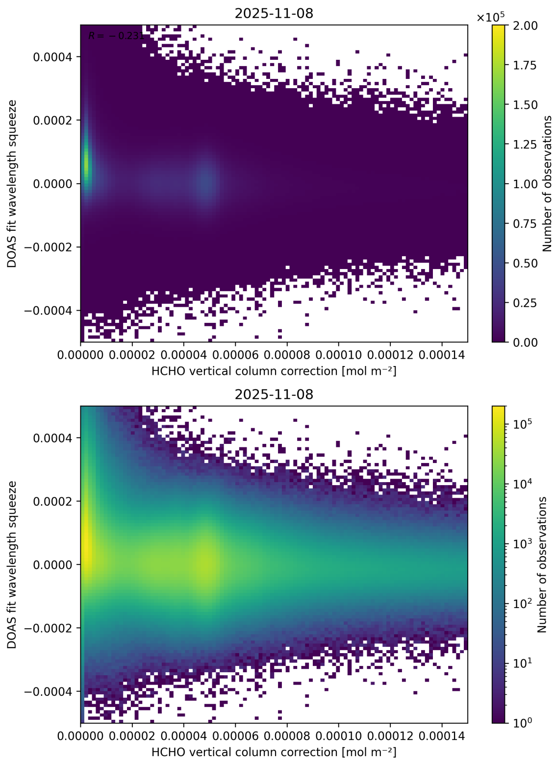
Figure 114: Scatter density plot of “HCHO vertical column correction” against “DOAS fit wavelength squeeze” for 2025-11-07 to 2025-11-09.
