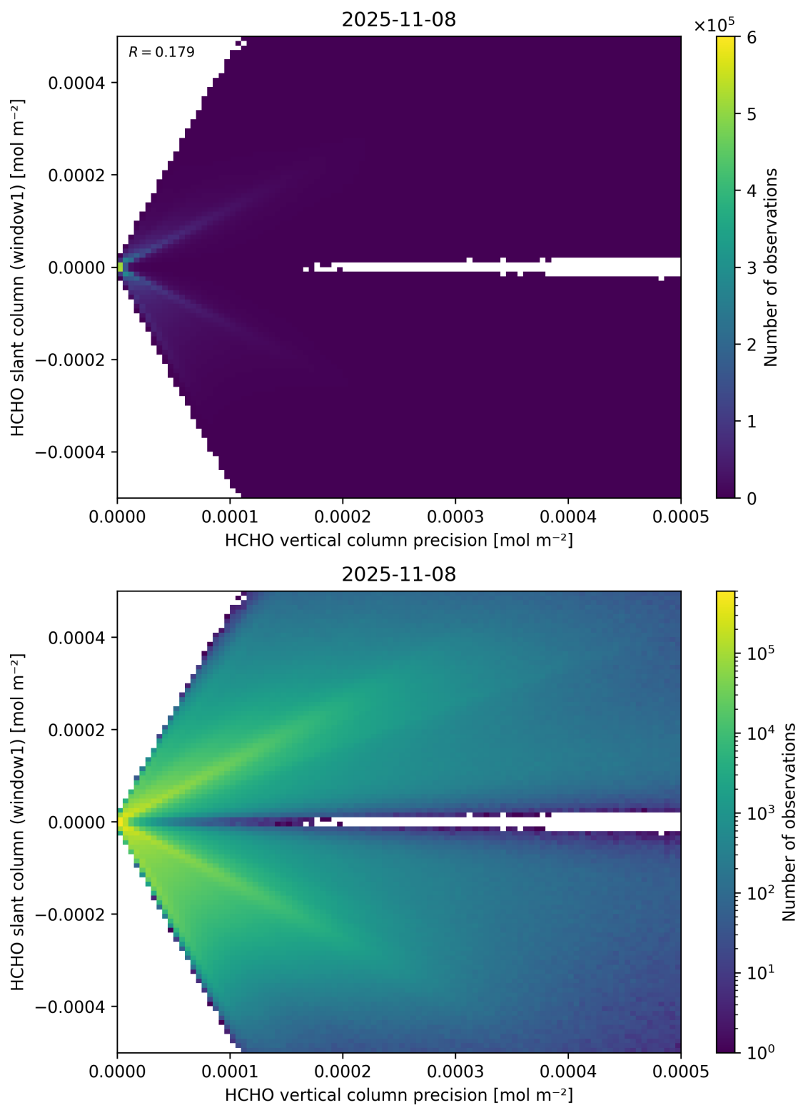
Figure 142: Scatter density plot of “HCHO vertical column precision” against “HCHO slant column (window1)” for 2025-11-07 to 2025-11-09.
