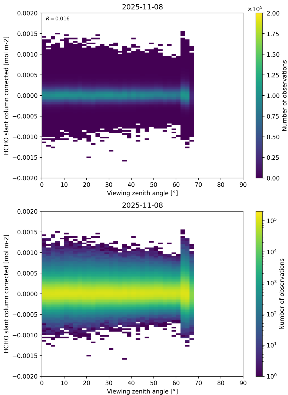
Figure 186: Scatter density plot of “Viewing zenith angle” against “HCHO slant column corrected” for 2025-11-07 to 2025-11-09.
