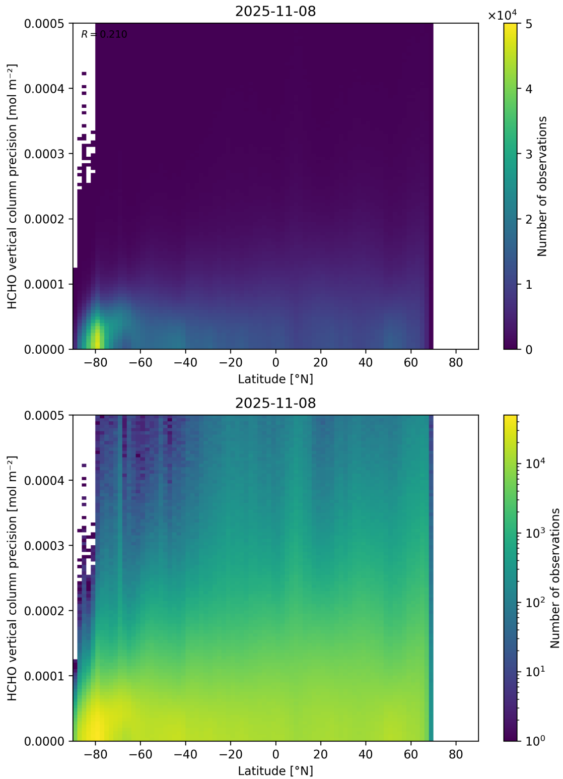
Figure 165: Scatter density plot of “Latitude” against “HCHO vertical column precision” for 2025-11-07 to 2025-11-09.
