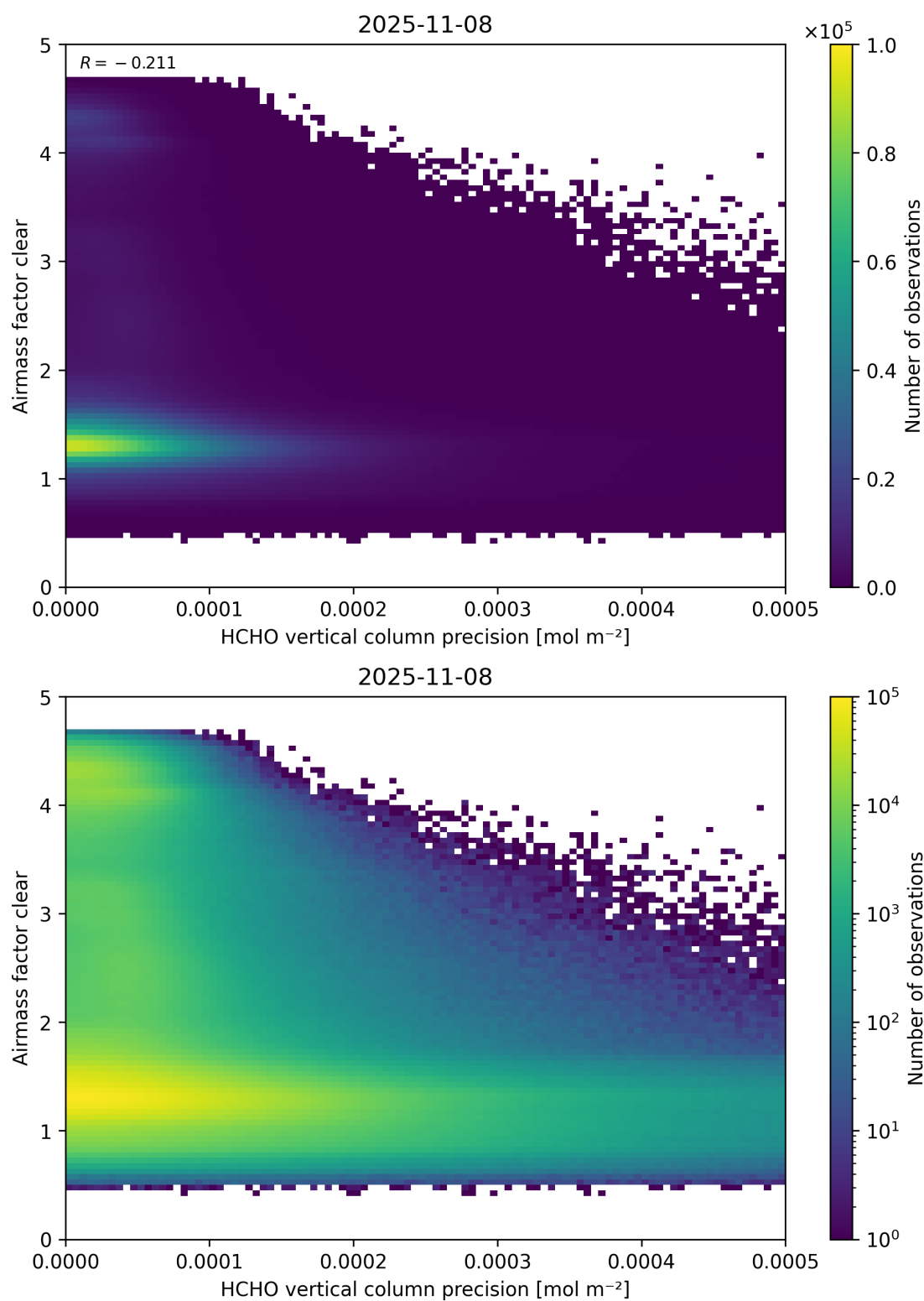
Figure 139: Scatter density plot of “HCHO vertical column precision” against “Airmass factor clear” for 2025-11-07 to 2025-11-09.
