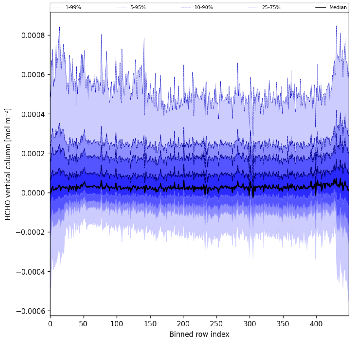
Figure 49: Along track statistics of “HCHO vertical column” for 2025-11-07 to 2025-11-09
