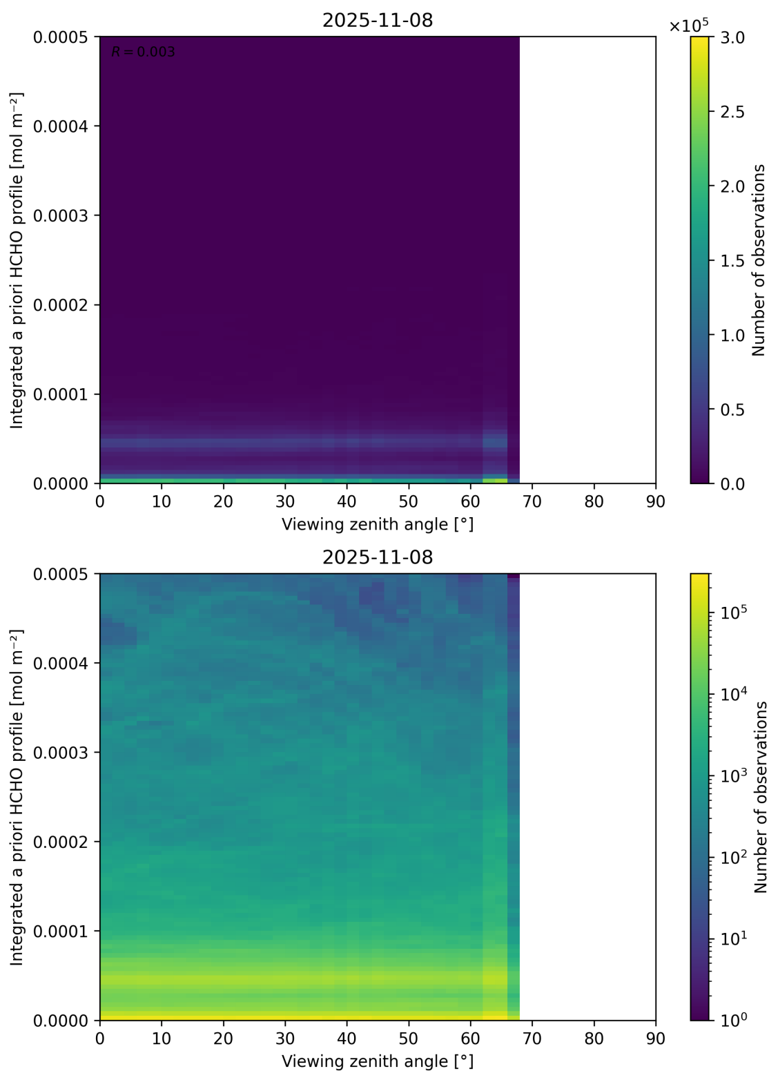
Figure 195: Scatter density plot of “Viewing zenith angle” against “Integrated a priori HCHO profile” for 2025-11-07 to 2025-11-09.
