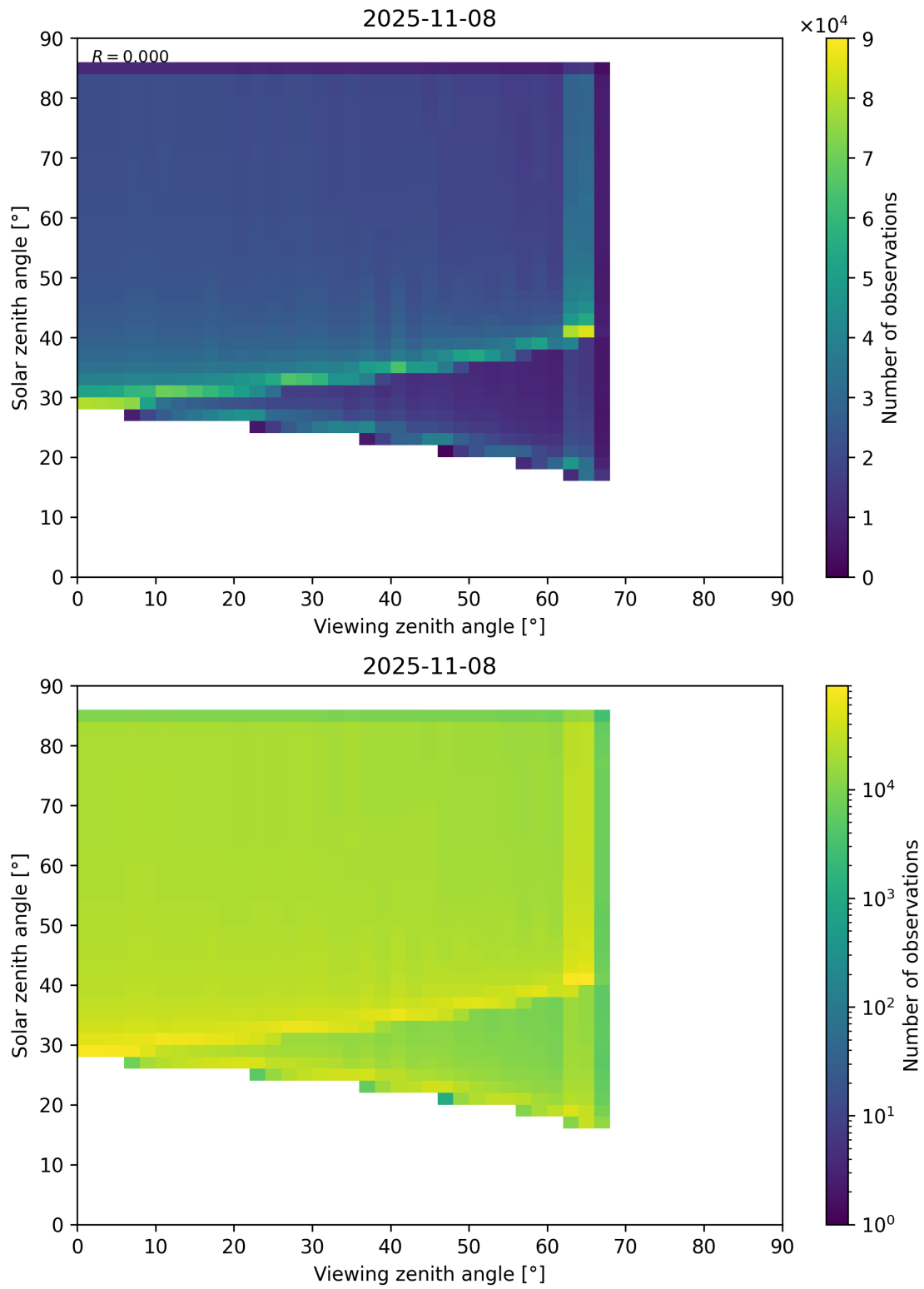
Figure 197: Scatter density plot of “Viewing zenith angle” against “Solar zenith angle” for 2025-11-07 to 2025-11-09.
