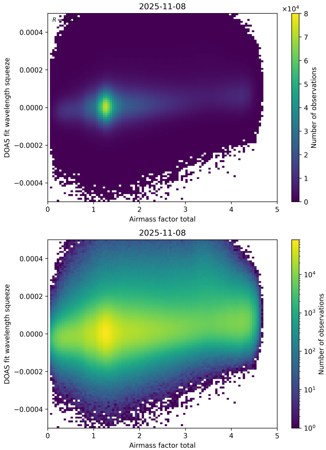
Figure 99: Scatter density plot of “Airmass factor total” against “DOAS fit wavelength squeeze” for 2025-11-07 to 2025-11-09.
