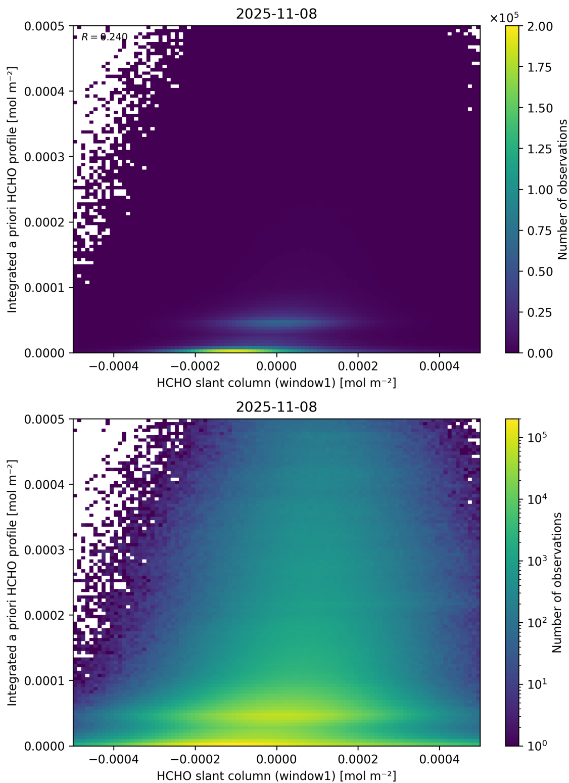
Figure 87: Scatter density plot of “HCHO slant column (window1)” against “Integrated a priori HCHO profile” for 2025-11-07 to 2025-11-09.
