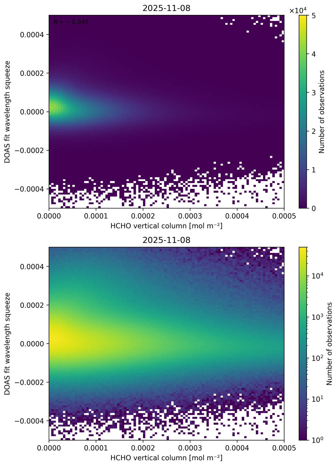
Figure 125: Scatter density plot of “HCHO vertical column” against “DOAS fit wavelength squeeze” for 2025-11-07 to 2025-11-09.
