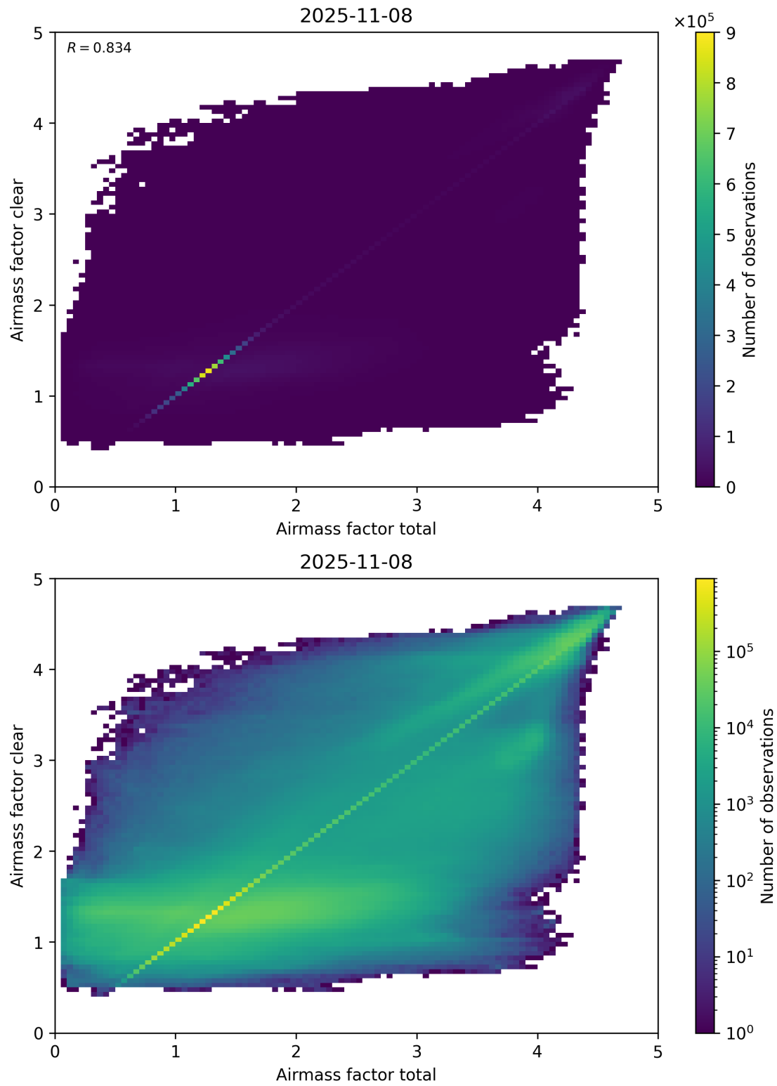
Figure 100: Scatter density plot of “Airmass factor total” against “Airmass factor clear” for 2025-11-07 to 2025-11-09.
