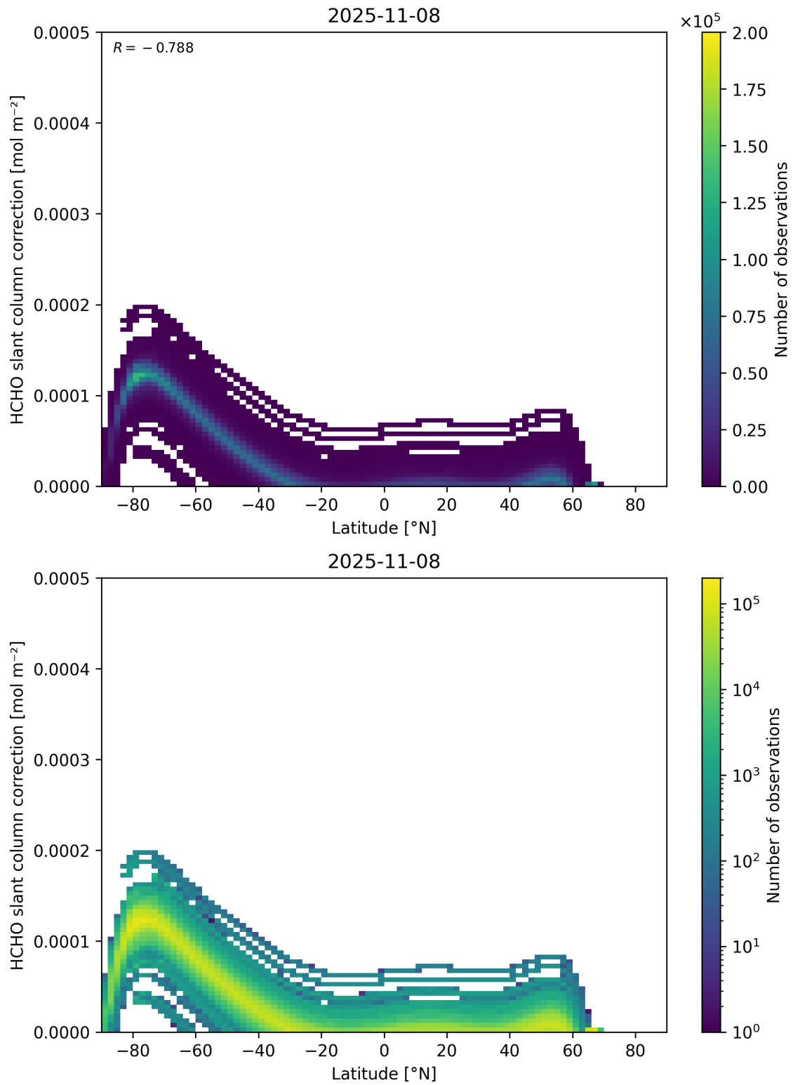
Figure 158: Scatter density plot of “Latitude” against “HCHO slant column correction” for 2025-11-07 to 2025-11-09.
