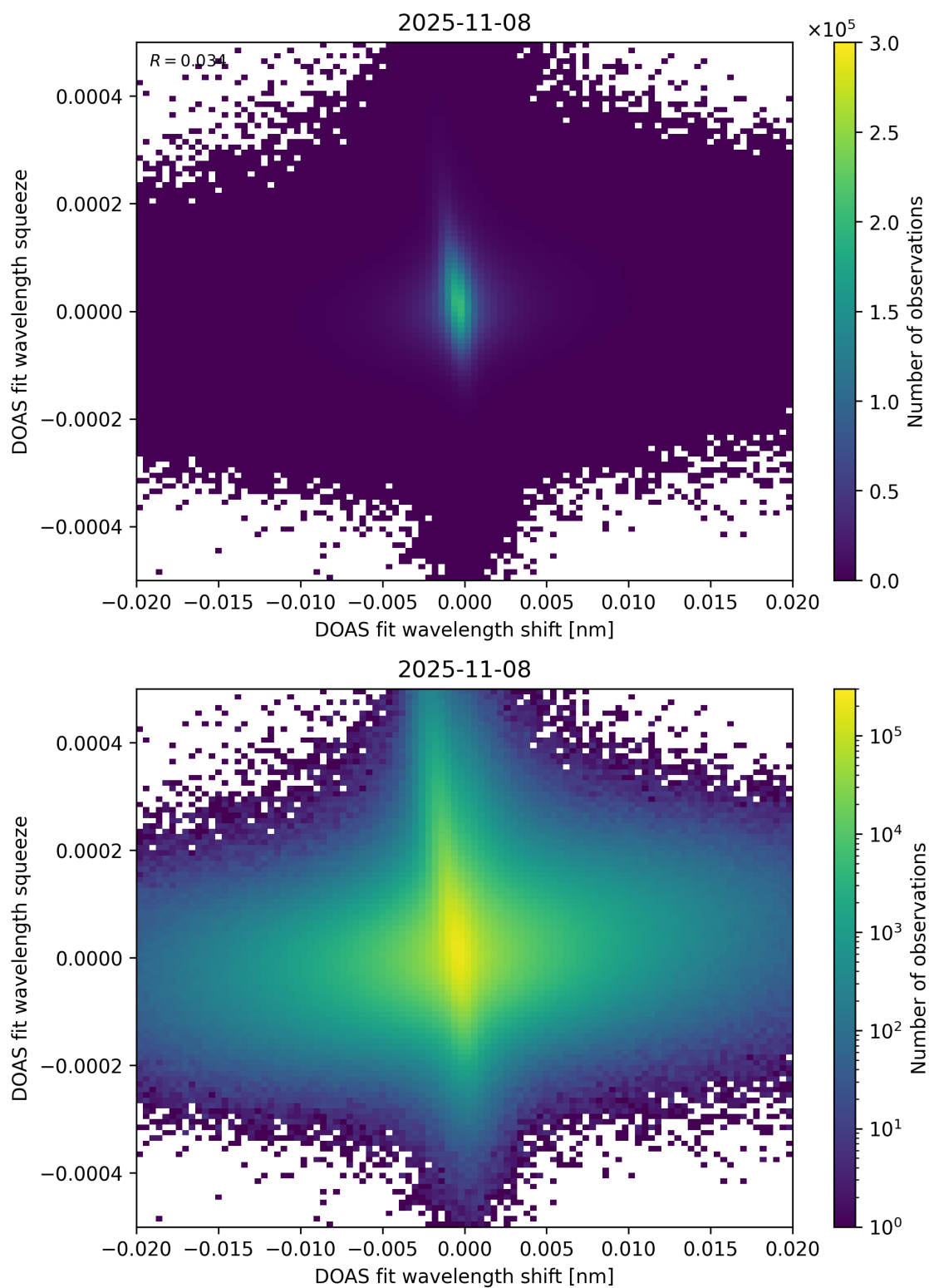
Figure 65: Scatter density plot of “DOAS fit wavelength shift” against “DOAS fit wavelength squeeze” for 2025-11-07 to 2025-11-09.
