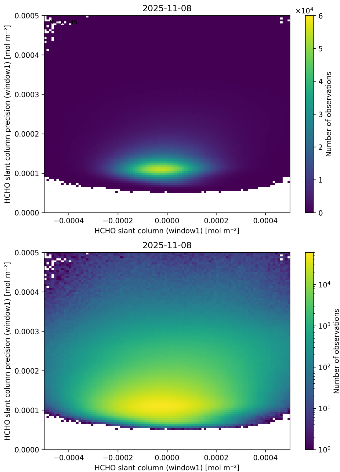
Figure 84: Scatter density plot of “HCHO slant column (window1)” against “HCHO slant column precision (window1)” for 2025-11-07 to 2025-11-09.
