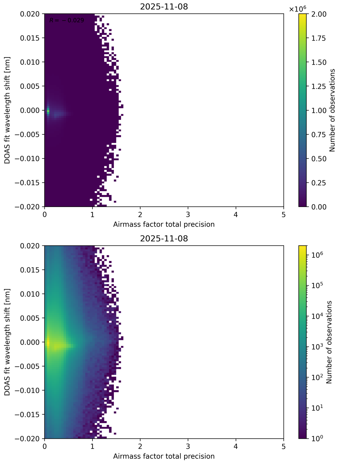
Figure 106: Scatter density plot of “Airmass factor total precision” against “DOAS fit wavelength shift” for 2025-11-07 to 2025-11-09.
