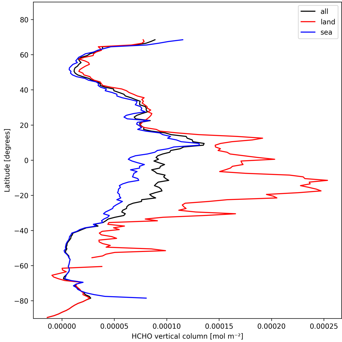
Figure 21: Zonal average of “HCHO vertical column” for 2025-11-07 to 2025-11-09.
