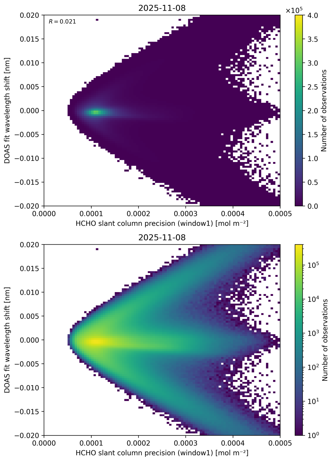
Figure 89: Scatter density plot of “HCHO slant column precision (window1)” against “DOAS fit wavelength shift” for 2025-11-07 to 2025-11-09.
