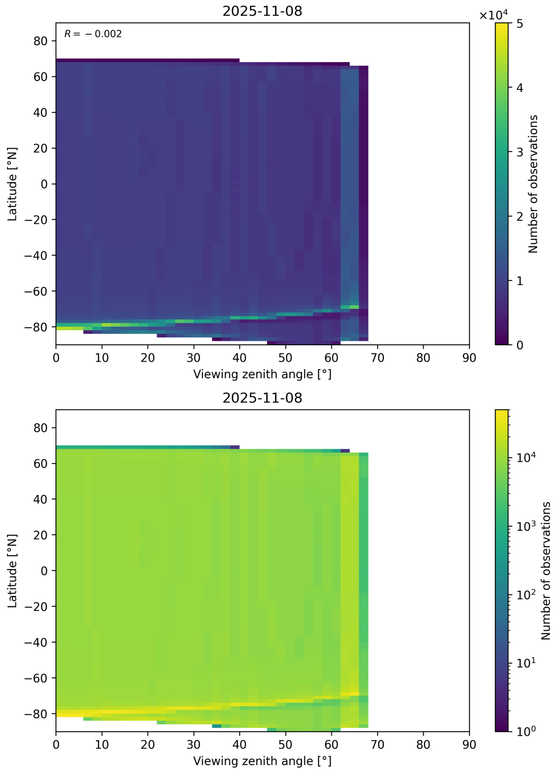
Figure 196: Scatter density plot of “Viewing zenith angle” against “Latitude” for 2025-11-07 to 2025-11-09.
