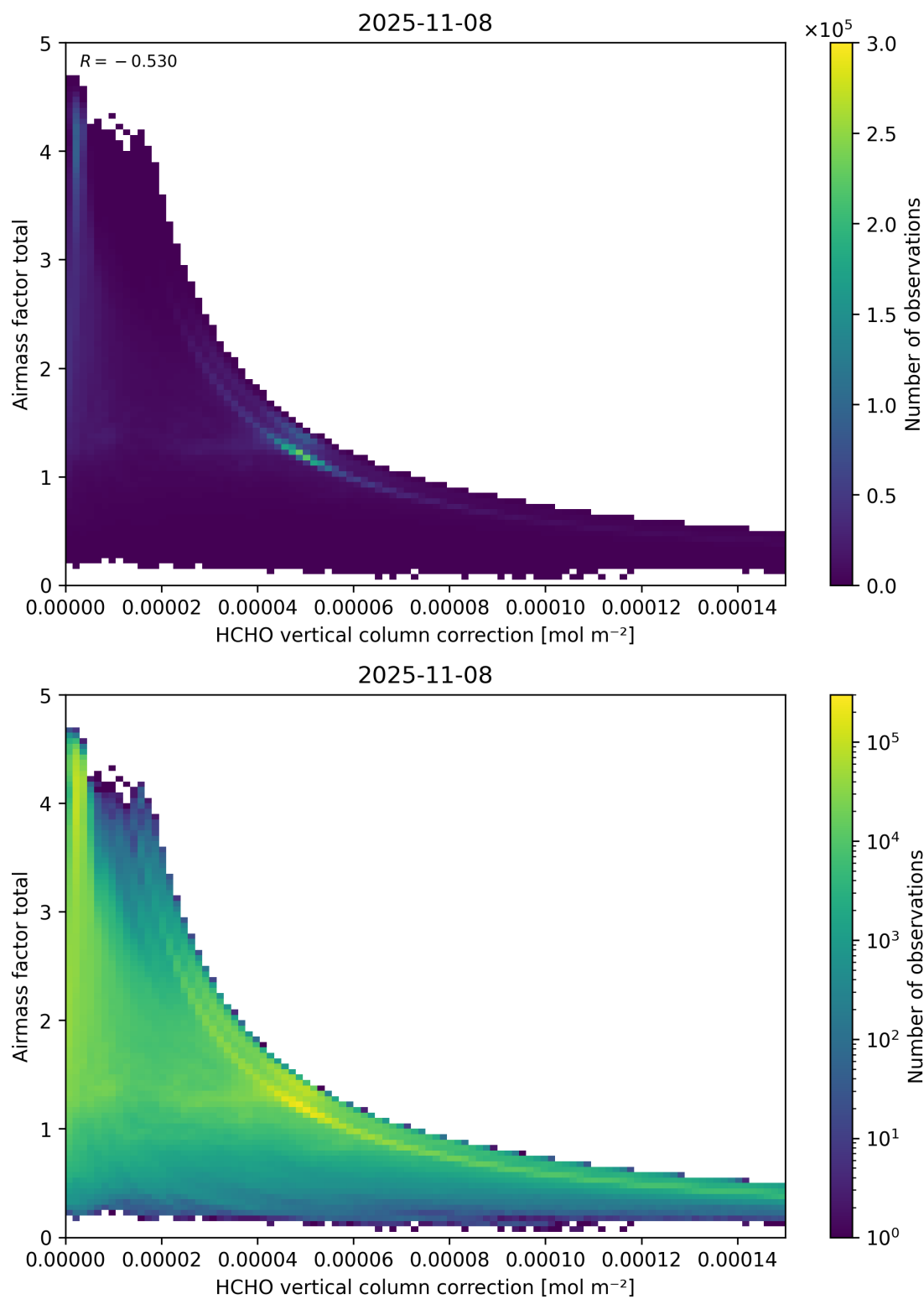
Figure 120: Scatter density plot of “HCHO vertical column correction” against “Airmass factor total” for 2025-11-07 to 2025-11-09.
