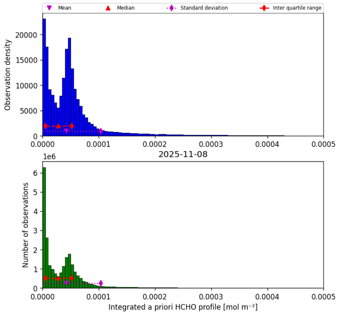
Figure 43: Histogram of “Integrated a priori HCHO profile” for 2025-11-07 to 2025-11-09
