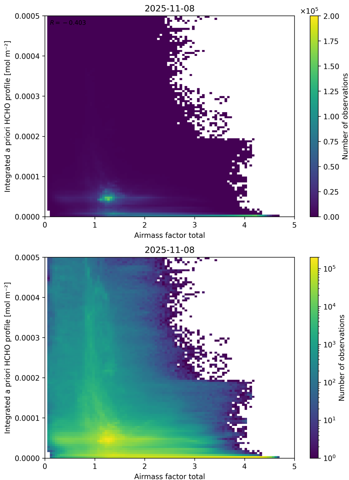
Figure 104: Scatter density plot of “Airmass factor total” against “Integrated a priori HCHO profile” for 2025-11-07 to 2025-11-09.
