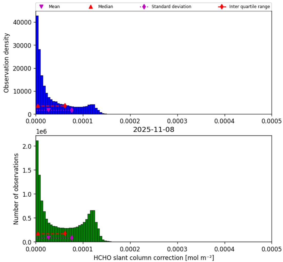
Figure 47: Histogram of “HCHO slant column correction” for 2025-11-07 to 2025-11-09
