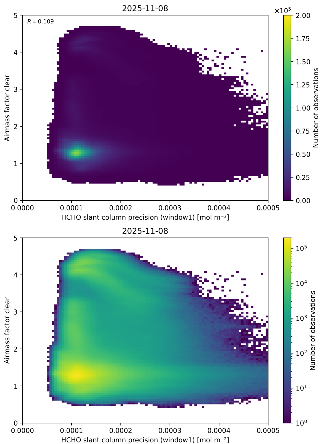
Figure 91: Scatter density plot of “HCHO slant column precision (window1)” against “Airmass factor clear” for 2025-11-07 to 2025-11-09.
