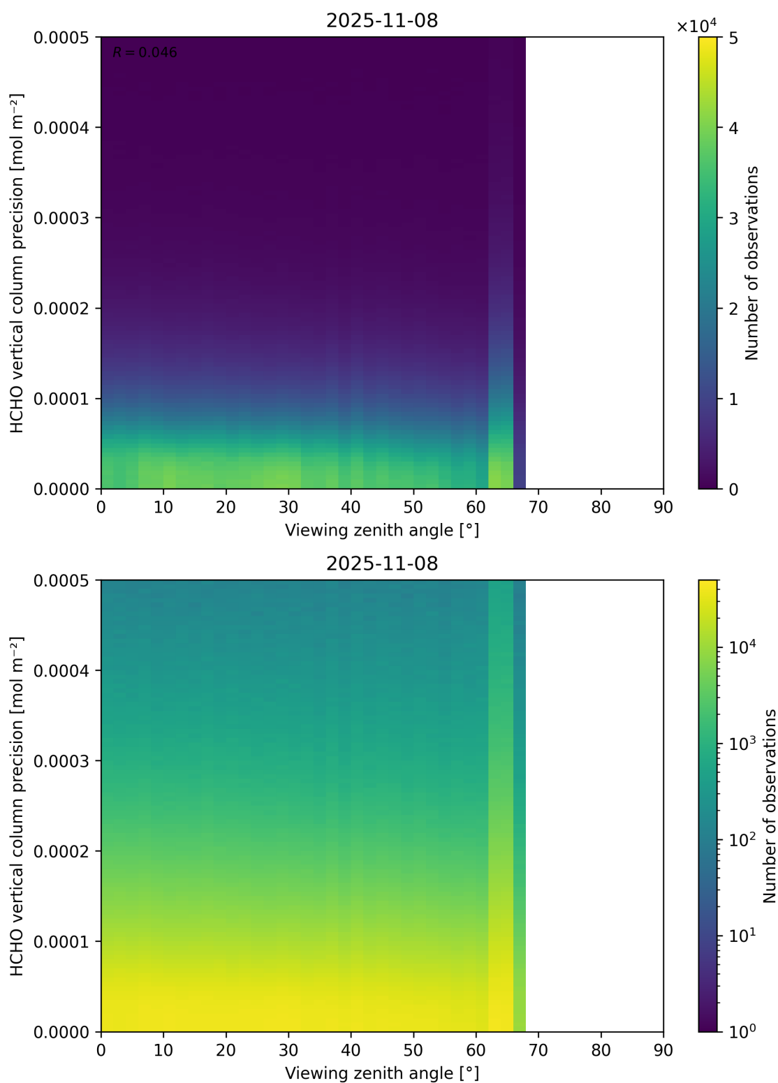
Figure 194: Scatter density plot of “Viewing zenith angle” against “HCHO vertical column precision” for 2025-11-07 to 2025-11-09.
