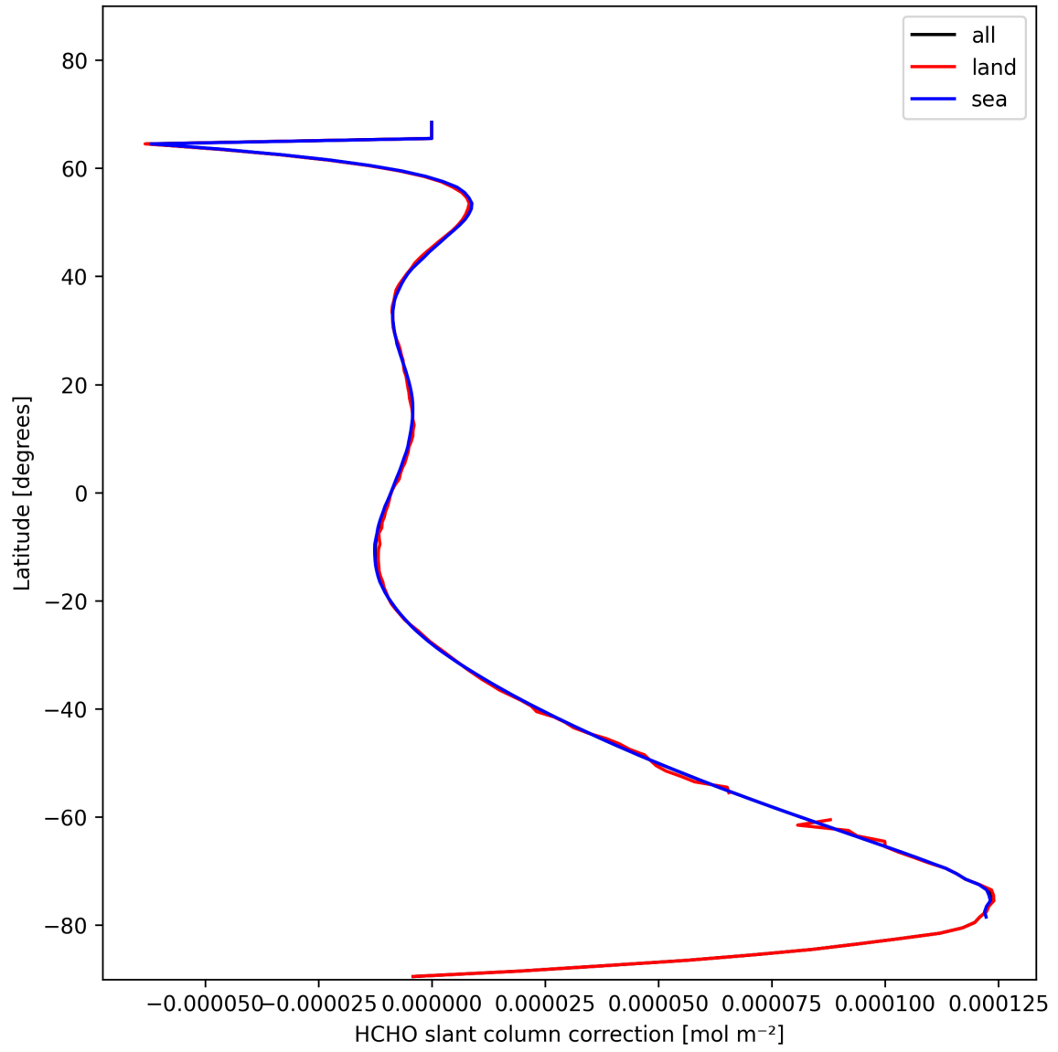
Figure 33: Zonal average of “HCHO slant column correction” for 2025-11-07 to 2025-11-09.
