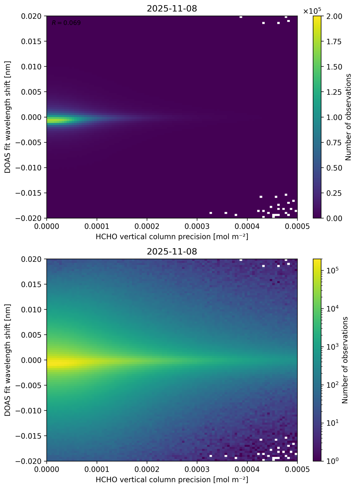
Figure 137: Scatter density plot of “HCHO vertical column precision” against “DOAS fit wavelength shift” for 2025-11-07 to 2025-11-09.
