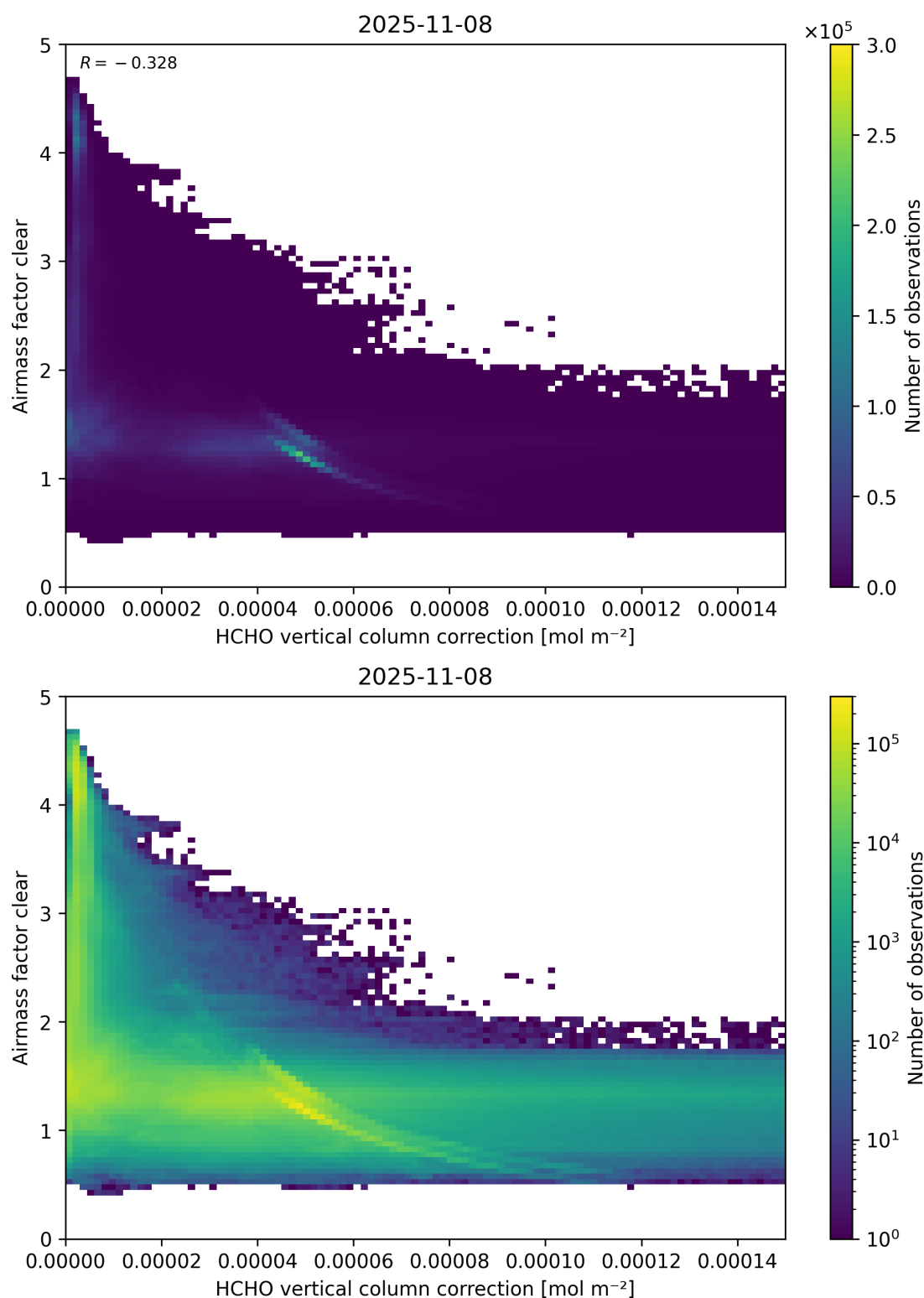
Figure 115: Scatter density plot of “HCHO vertical column correction” against “Airmass factor clear” for 2025-11-07 to 2025-11-09.
