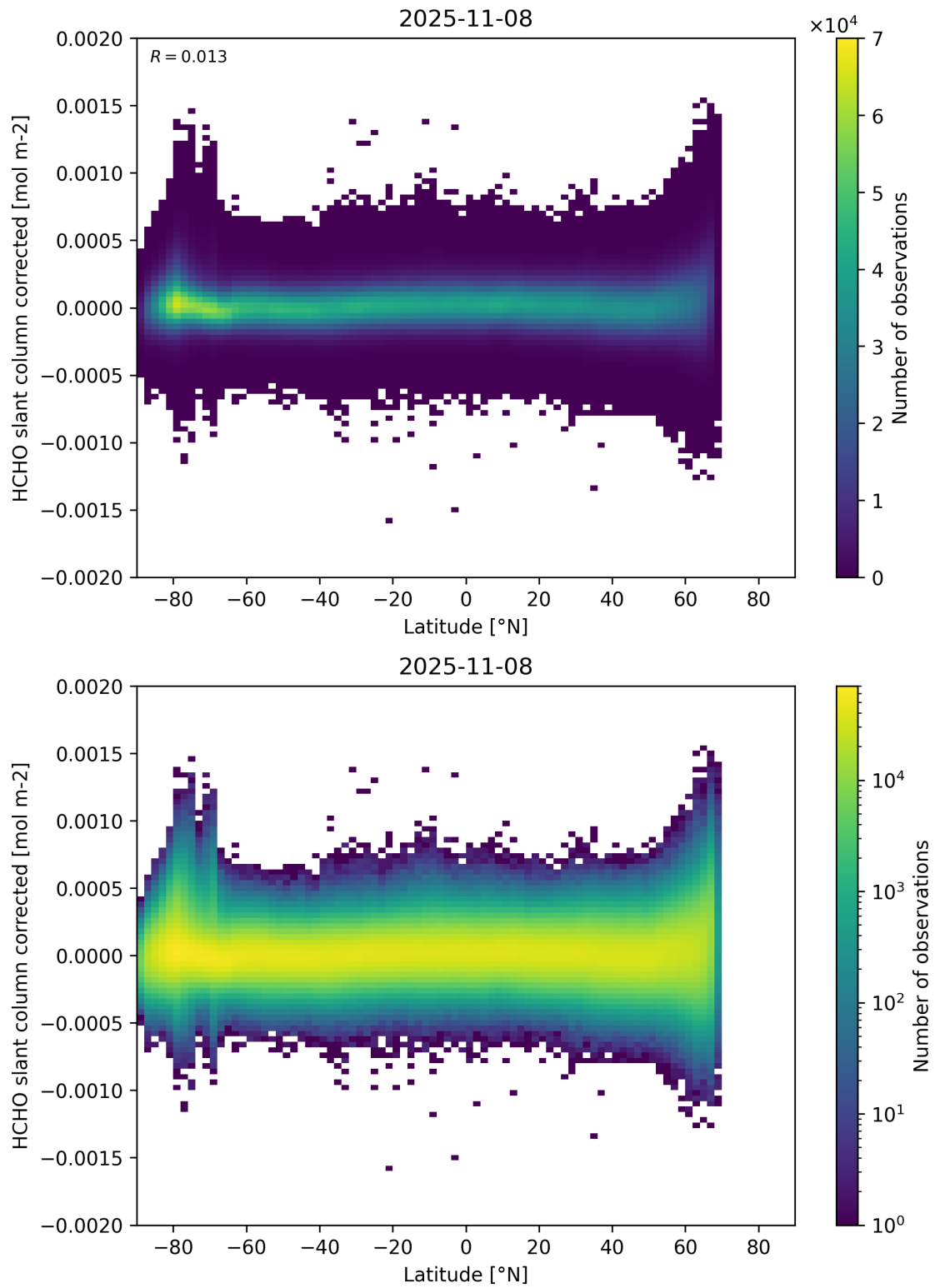
Figure 157: Scatter density plot of “Latitude” against “HCHO slant column corrected” for 2025-11-07 to 2025-11-09.
