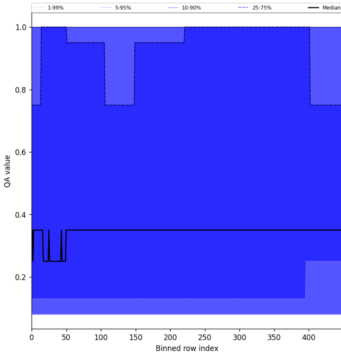
Figure 48: Along track statistics of “QA value” for 2025-11-07 to 2025-11-09
