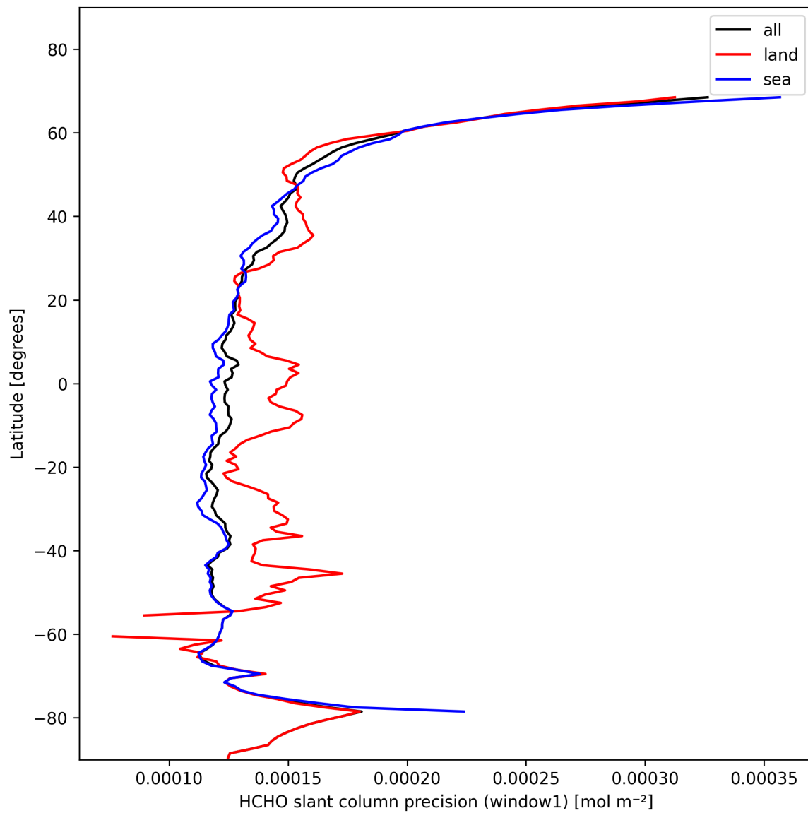
Figure 25: Zonal average of “HCHO slant column precision (window1)” for 2025-11-07 to 2025-11-09.
