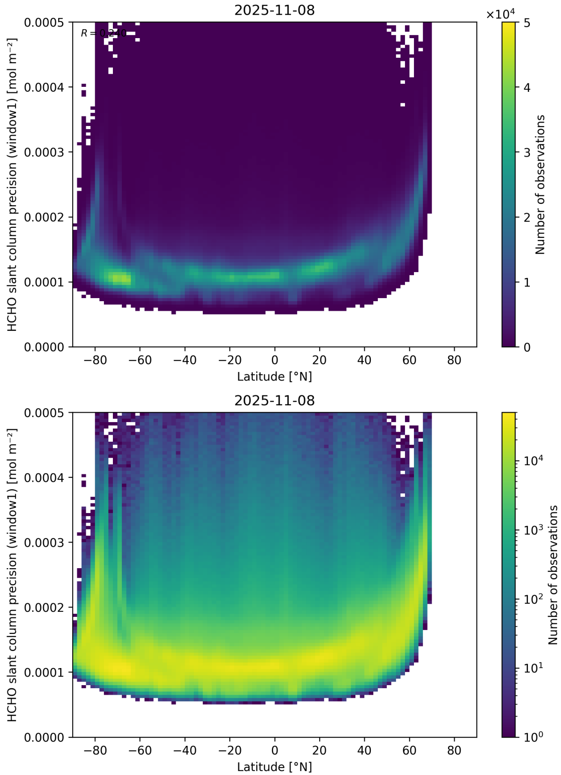
Figure 160: Scatter density plot of “Latitude” against “HCHO slant column precision (window1)” for 2025-11-07 to 2025-11-09.
