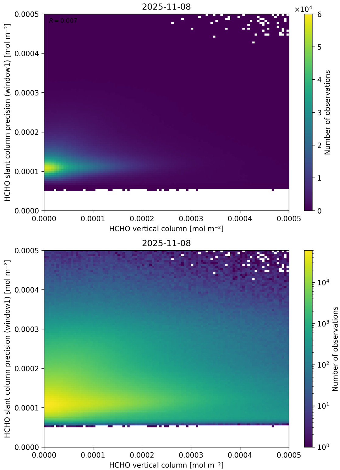
Figure 130: Scatter density plot of “HCHO vertical column” against “HCHO slant column precision (window1)” for 2025-11-07 to 2025-11-09.
