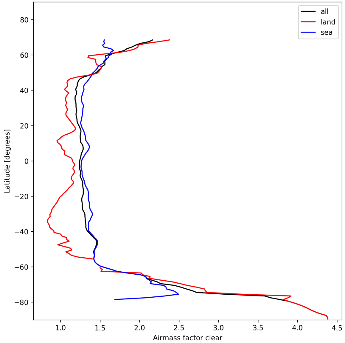
Figure 28: Zonal average of “Airmass factor clear” for 2025-11-07 to 2025-11-09.
