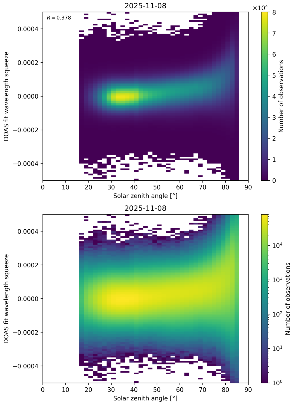
Figure 169: Scatter density plot of “Solar zenith angle” against “DOAS fit wavelength squeeze” for 2025-11-07 to 2025-11-09.
