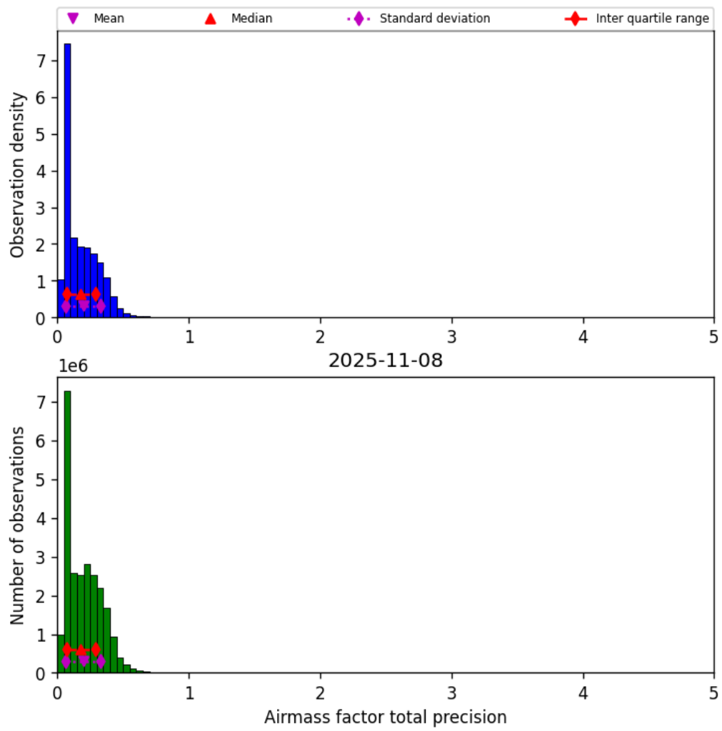
Figure 41: Histogram of “Airmass factor total precision” for 2025-11-07 to 2025-11-09
