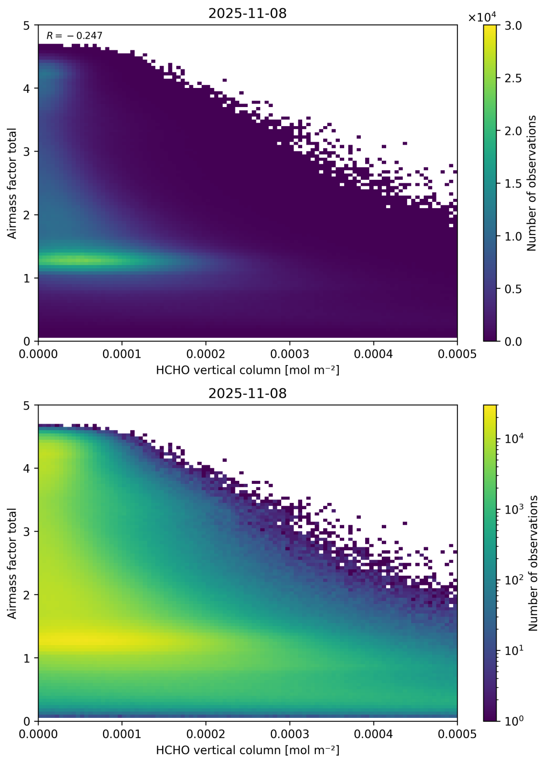
Figure 131: Scatter density plot of “HCHO vertical column” against “Airmass factor total” for 2025-11-07 to 2025-11-09.
