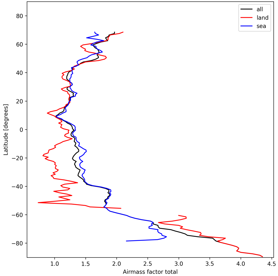
Figure 26: Zonal average of “Airmass factor total” for 2025-11-07 to 2025-11-09.
