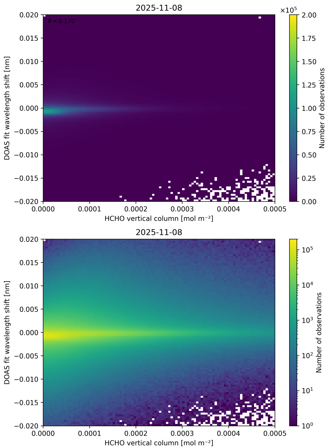
Figure 124: Scatter density plot of “HCHO vertical column” against “DOAS fit wavelength shift” for 2025-11-07 to 2025-11-09.
