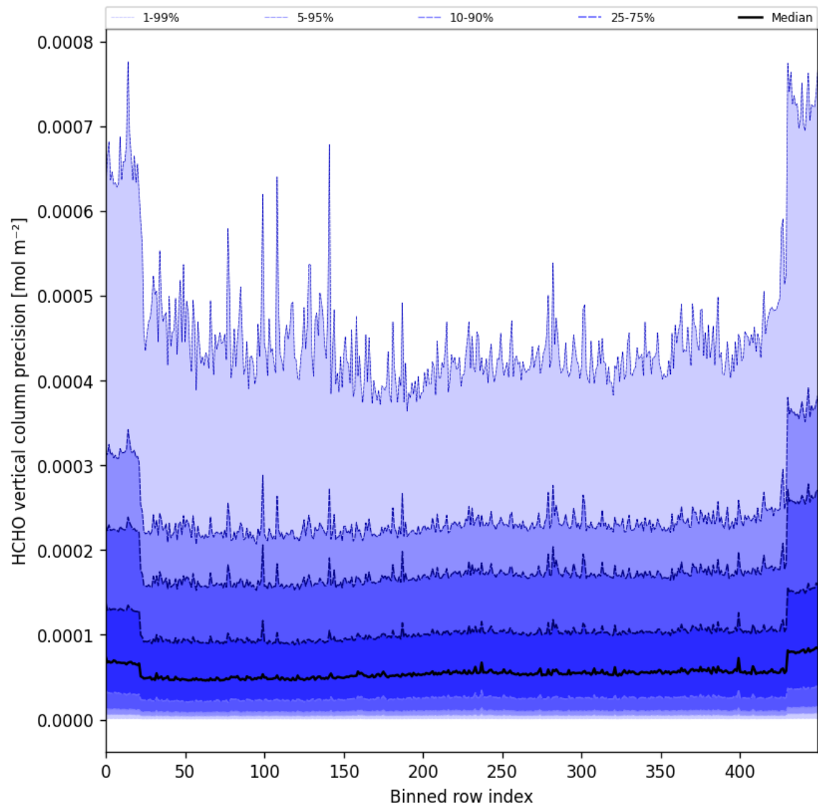
Figure 50: Along track statistics of "HCHO vertical column precision" for 2025-11-07 to 2025-11-09
