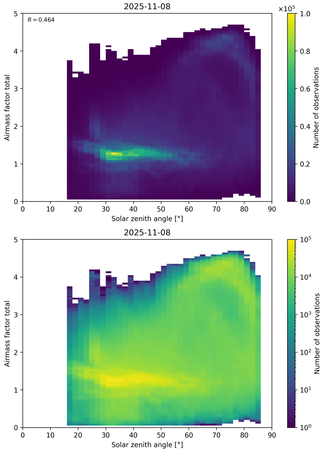
Figure 175: Scatter density plot of “Solar zenith angle” against “Airmass factor total” for 2025-11-07 to 2025-11-09.
