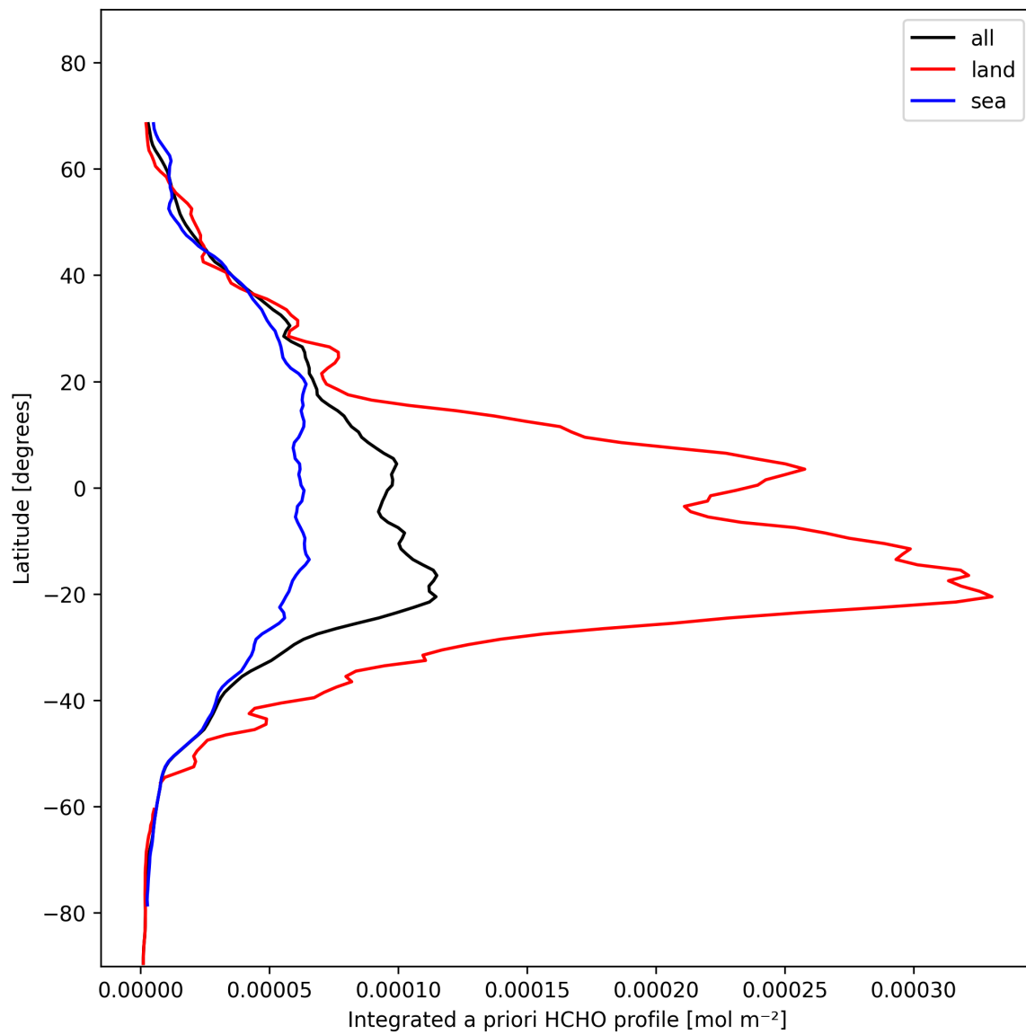
Figure 29: Zonal average of “Integrated a priori HCHO profile” for 2025-11-07 to 2025-11-09.
