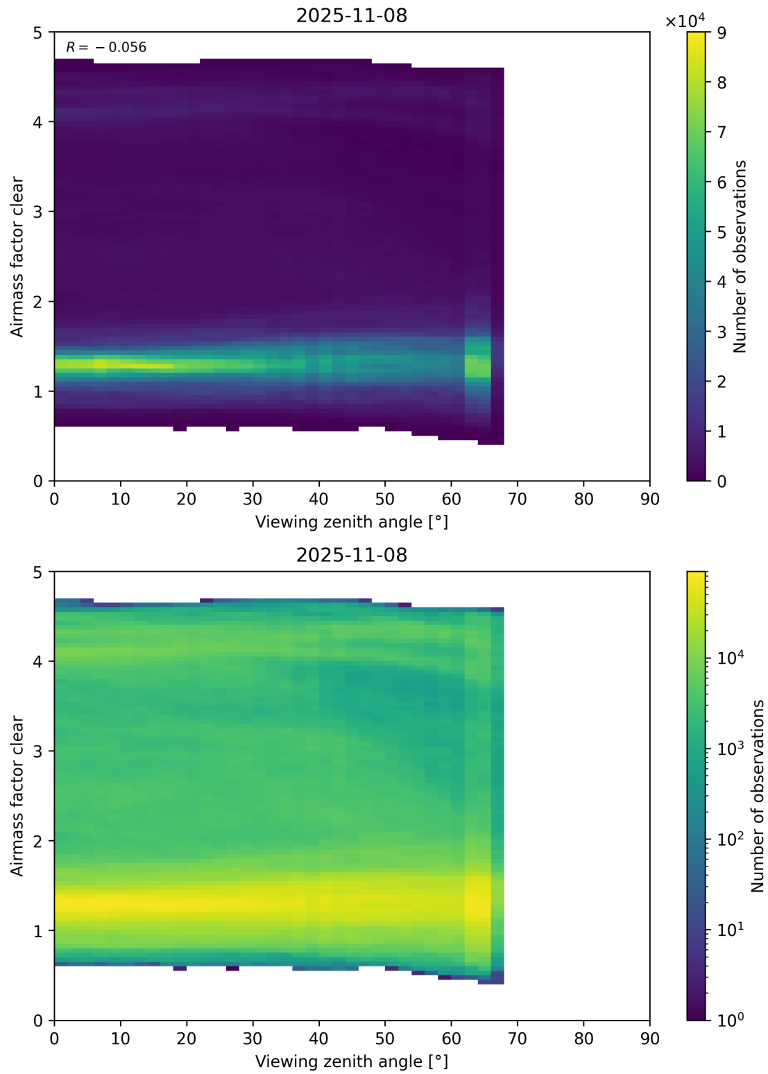
Figure 185: Scatter density plot of “Viewing zenith angle” against “Airmass factor clear” for 2025-11-07 to 2025-11-09.
