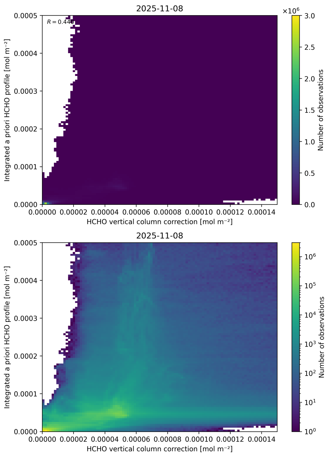
Figure 122: Scatter density plot of “HCHO vertical column correction” against “Integrated a priori HCHO profile” for 2025-11-07 to 2025-11-09.
