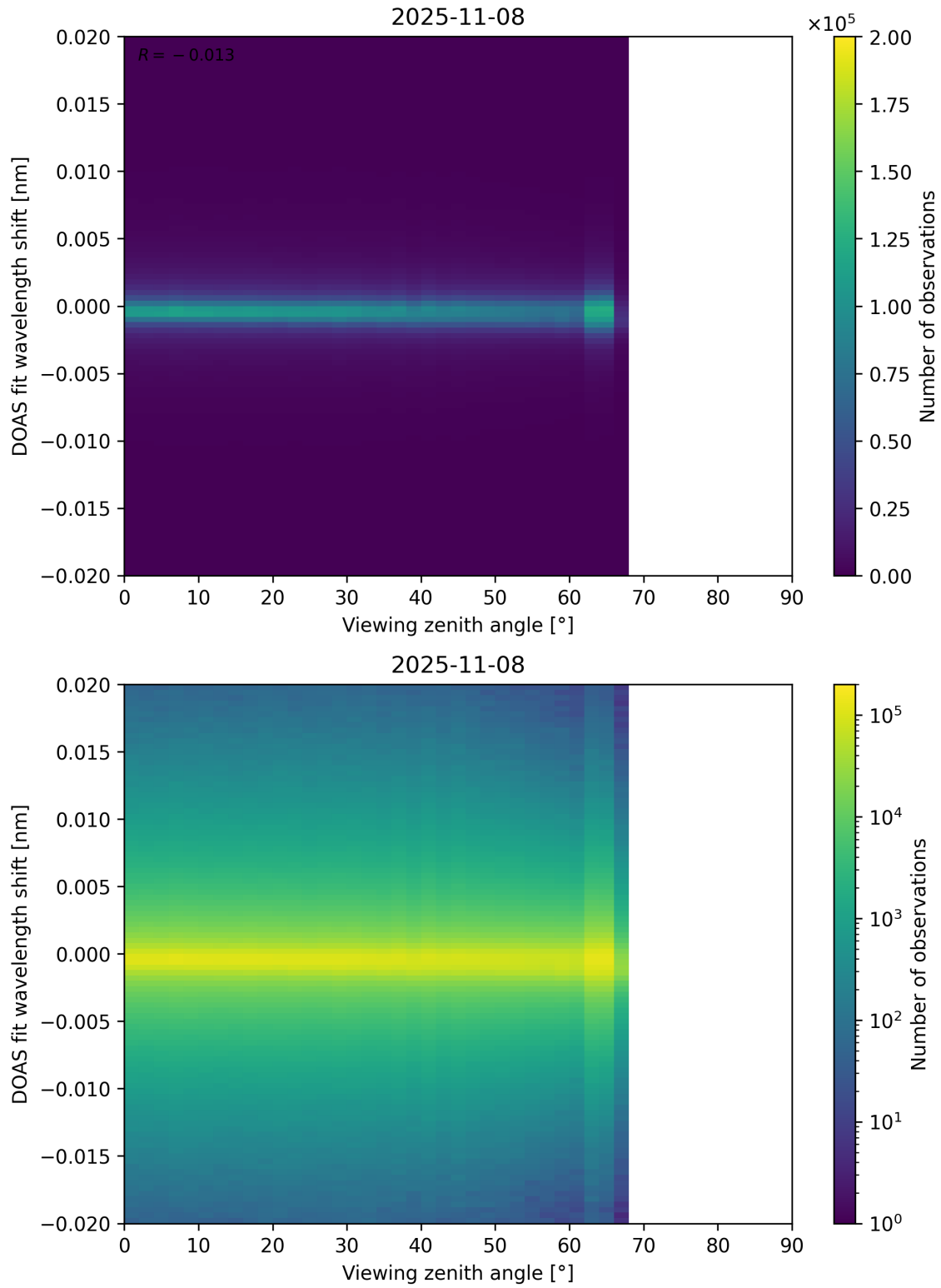
Figure 183: Scatter density plot of “Viewing zenith angle” against “DOAS fit wavelength shift” for 2025-11-07 to 2025-11-09.
