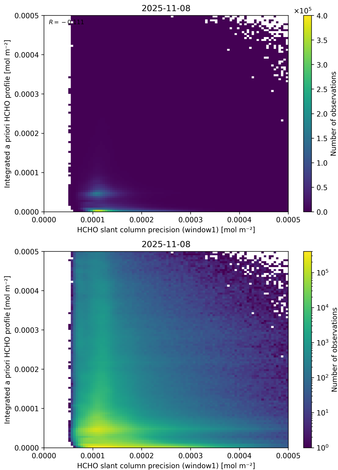
Figure 96: Scatter density plot of “HCHO slant column precision (window1)” against “Integrated a priori HCHO profile” for 2025-11-07 to 2025-11-09.
