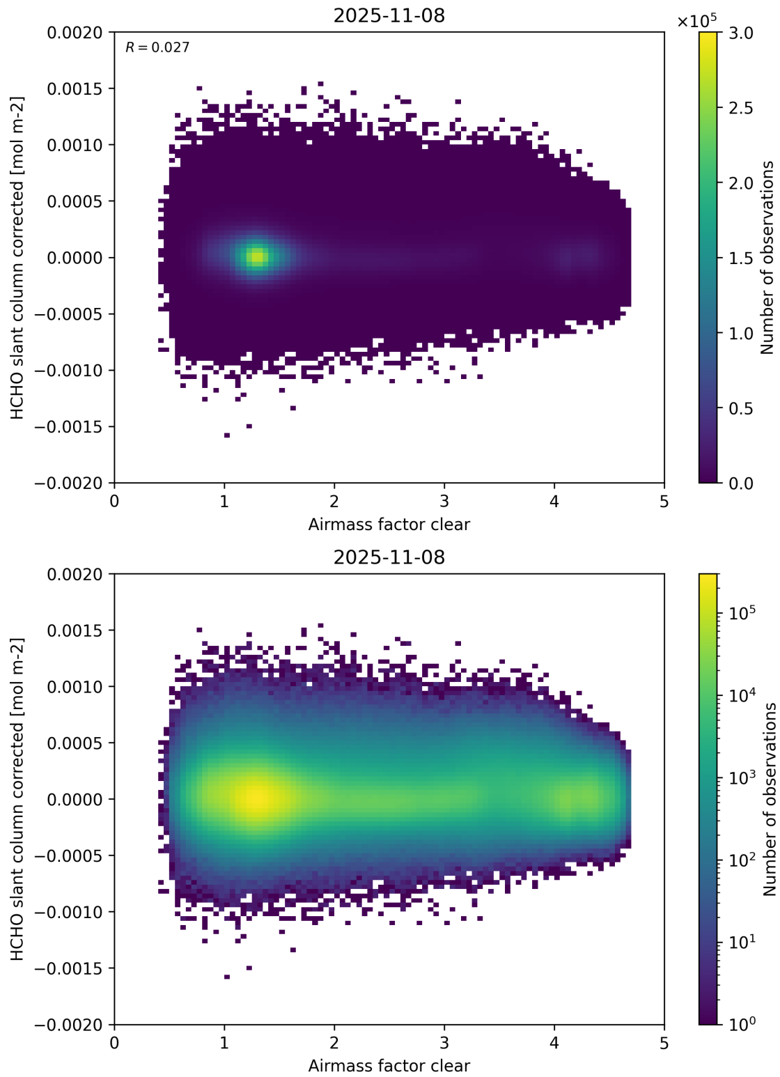
Figure 74: Scatter density plot of “Airmass factor clear” against “HCHO slant column corrected” for 2025-11-07 to 2025-11-09.
