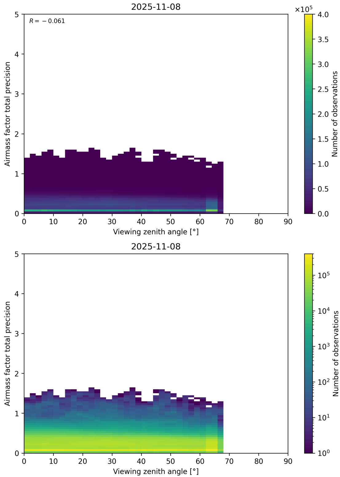
Figure 191: Scatter density plot of “Viewing zenith angle” against “Airmass factor total precision” for 2025-11-07 to 2025-11-09.
