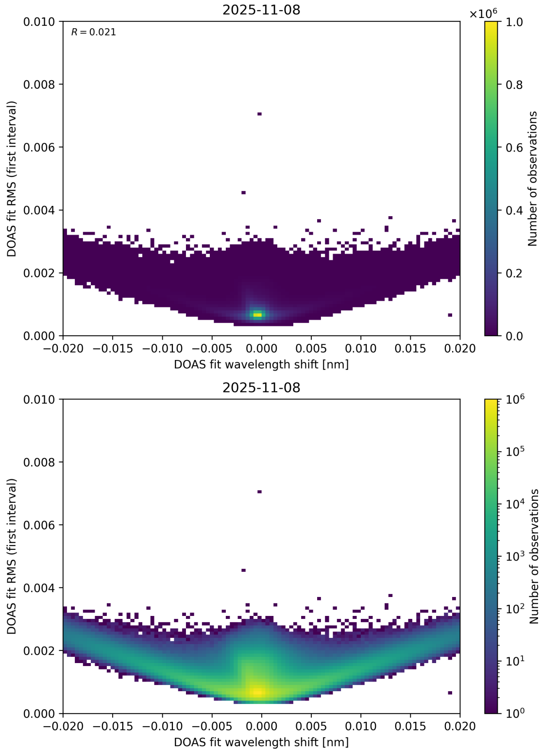
Figure 64: Scatter density plot of “DOAS fit wavelength shift” against “DOAS fit RMS (first interval)” for 2025-11-07 to 2025-11-09.
