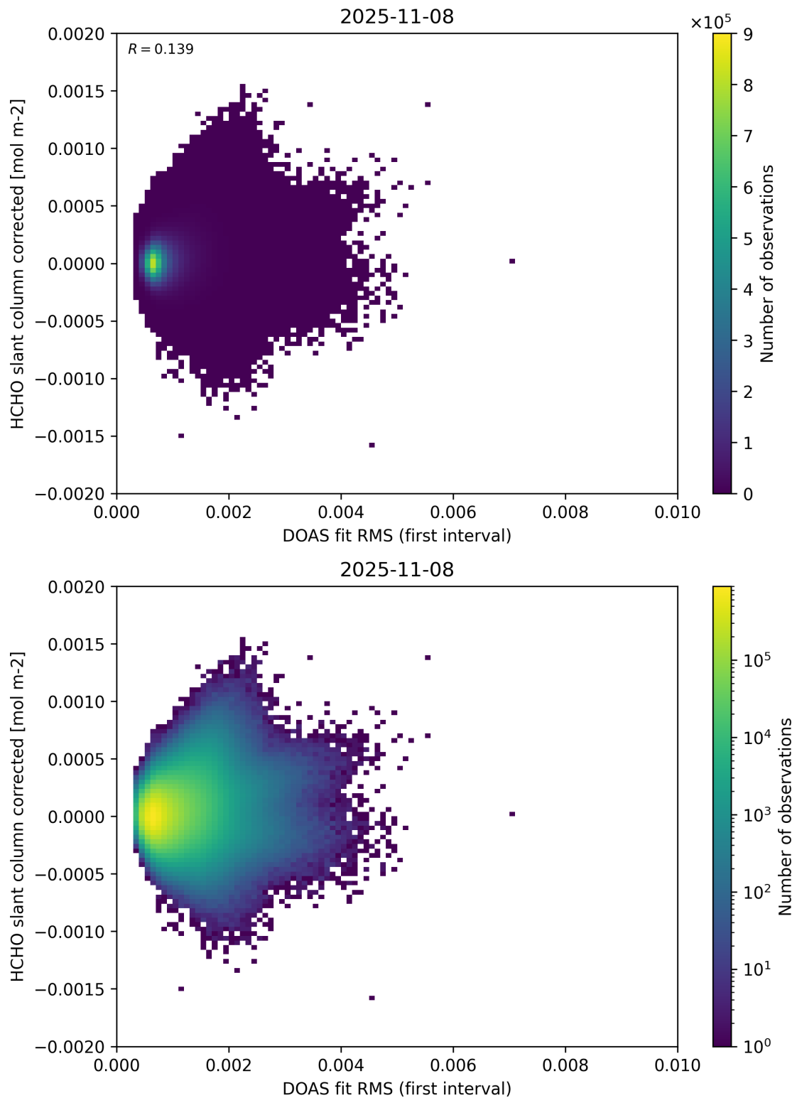
Figure 62: Scatter density plot of “DOAS fit RMS (first interval)” against “HCHO slant column corrected” for 2025-11-07 to 2025-11-09.
