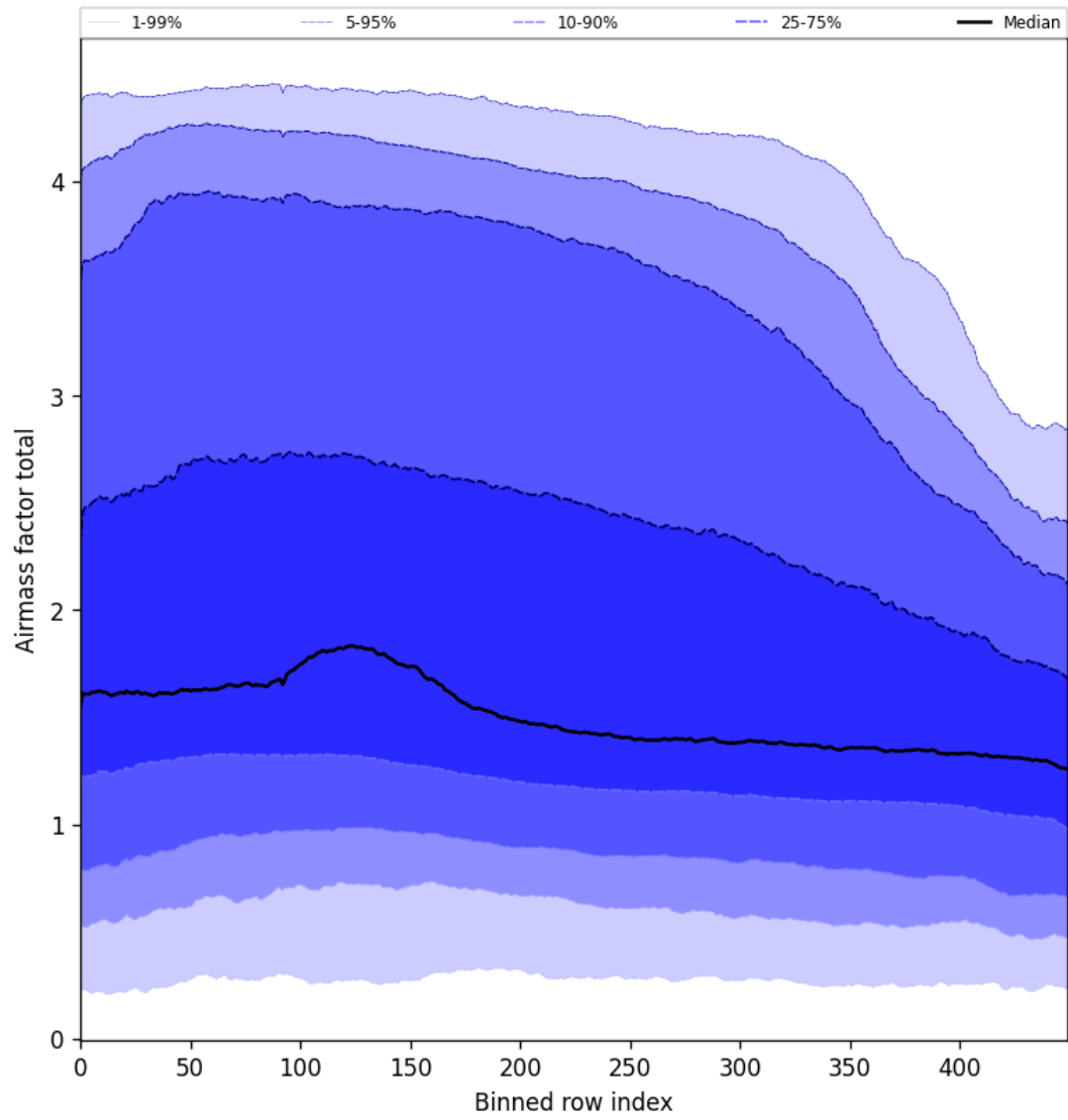
Figure 54: Along track statistics of “Airmass factor total” for 2025-11-07 to 2025-11-09
