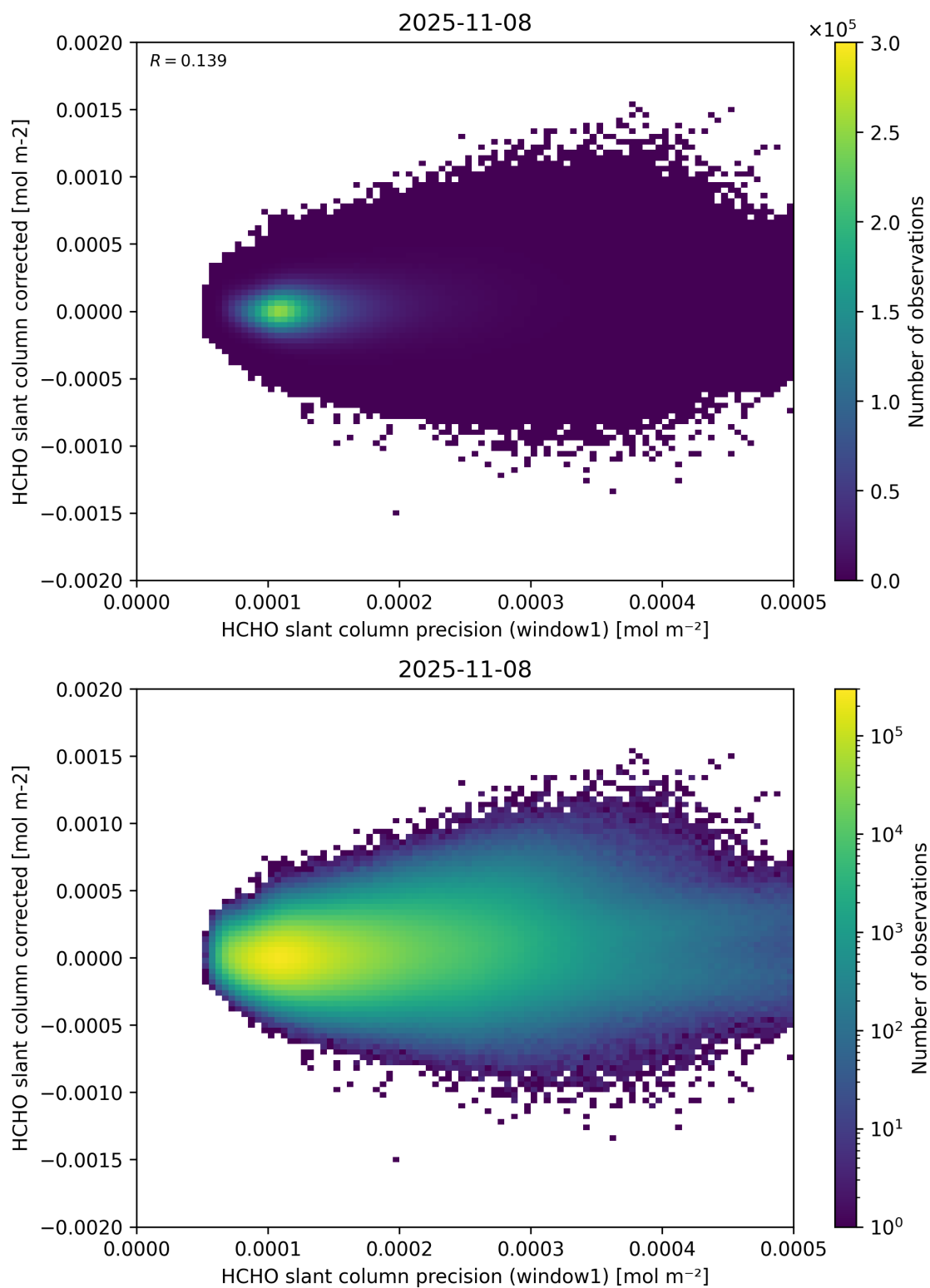
Figure 92: Scatter density plot of “HCHO slant column precision (window1)” against “HCHO slant column corrected” for 2025-11-07 to 2025-11-09.
