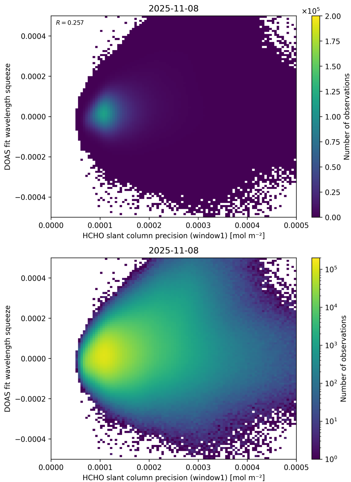
Figure 90: Scatter density plot of “HCHO slant column precision (window1)” against “DOAS fit wavelength squeeze” for 2025-11-07 to 2025-11-09.
