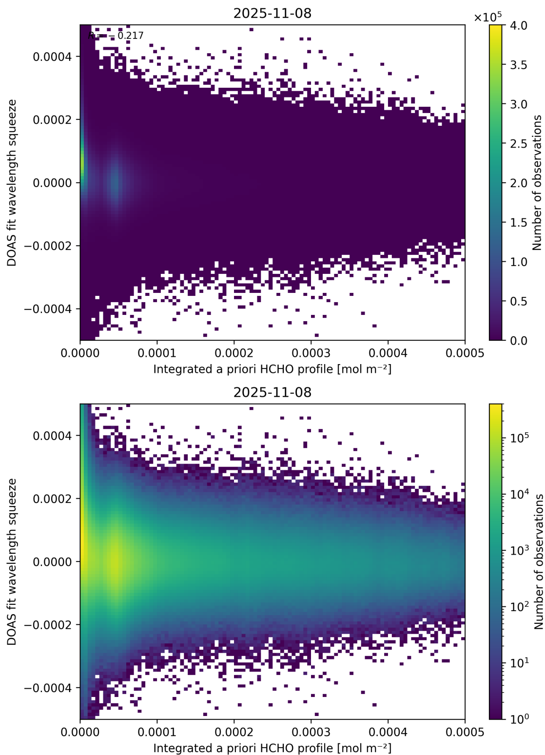
Figure 150: Scatter density plot of “Integrated a priori HCHO profile” against “DOAS fit wavelength squeeze” for 2025-11-07 to 2025-11-09.
