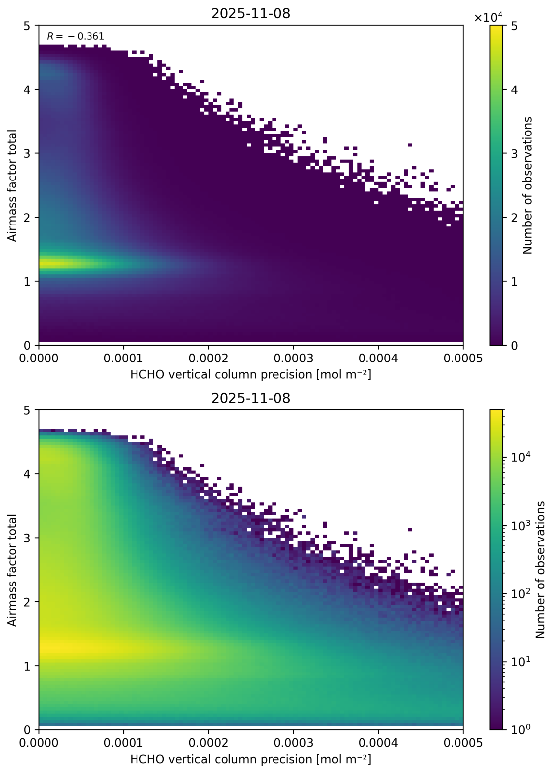
Figure 144: Scatter density plot of “HCHO vertical column precision” against “Airmass factor total” for 2025-11-07 to 2025-11-09.
