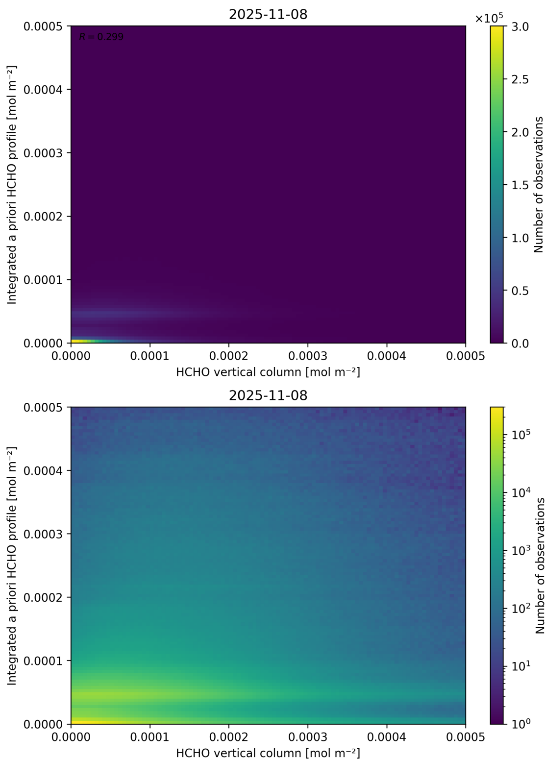
Figure 135: Scatter density plot of “HCHO vertical column” against “Integrated a priori HCHO profile” for 2025-11-07 to 2025-11-09.
