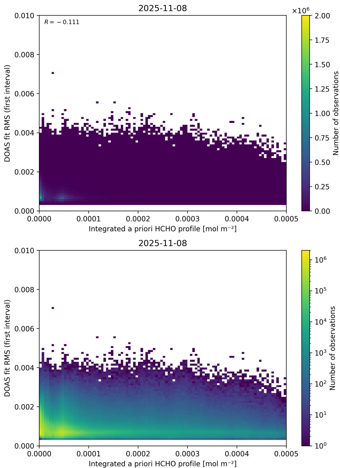
Figure 148: Scatter density plot of “Integrated a priori HCHO profile” against “DOAS fit RMS (first interval)” for 2025-11-07 to 2025-11-09.
