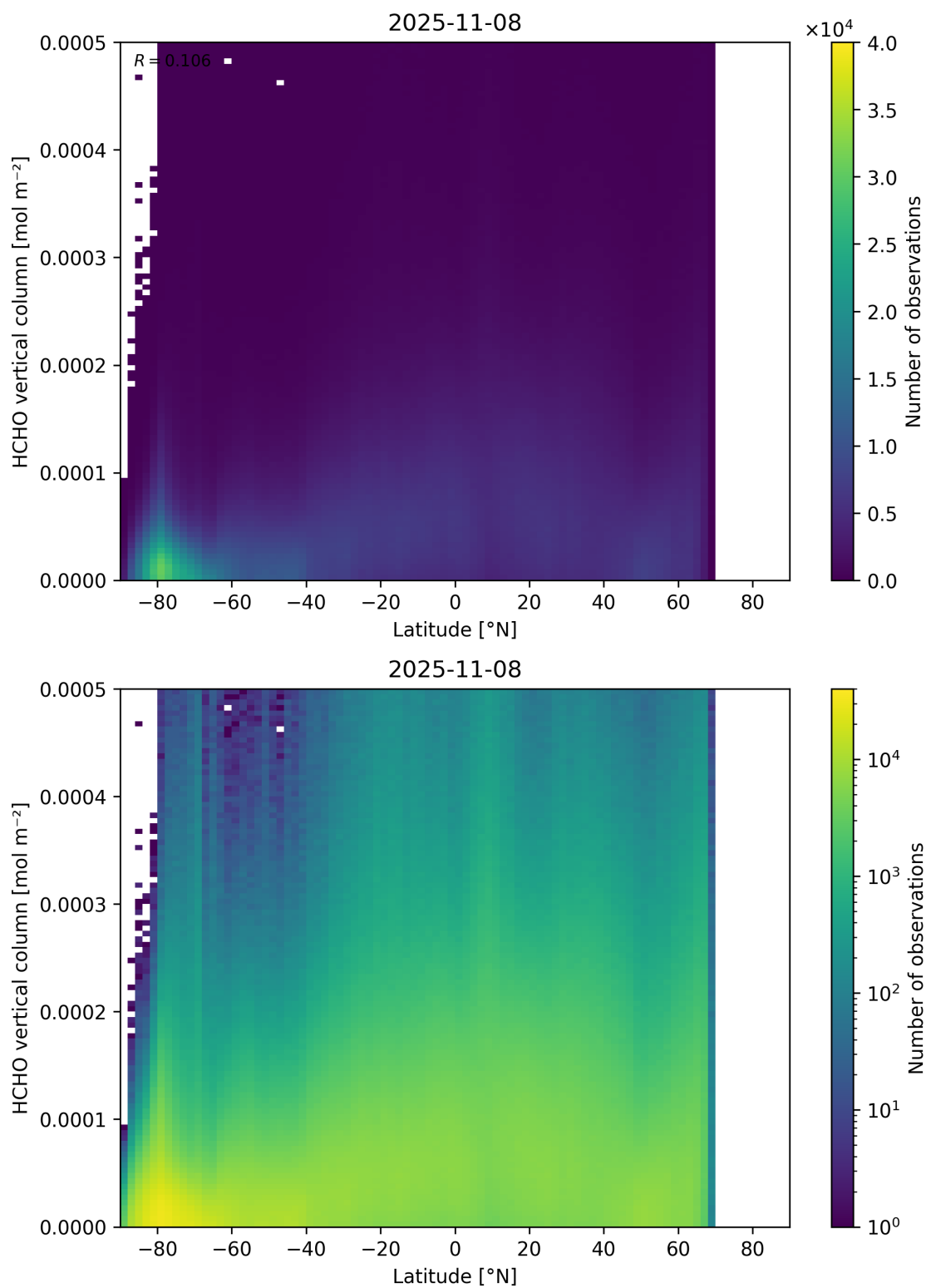
Figure 163: Scatter density plot of “Latitude” against “HCHO vertical column” for 2025-11-07 to 2025-11-09.
