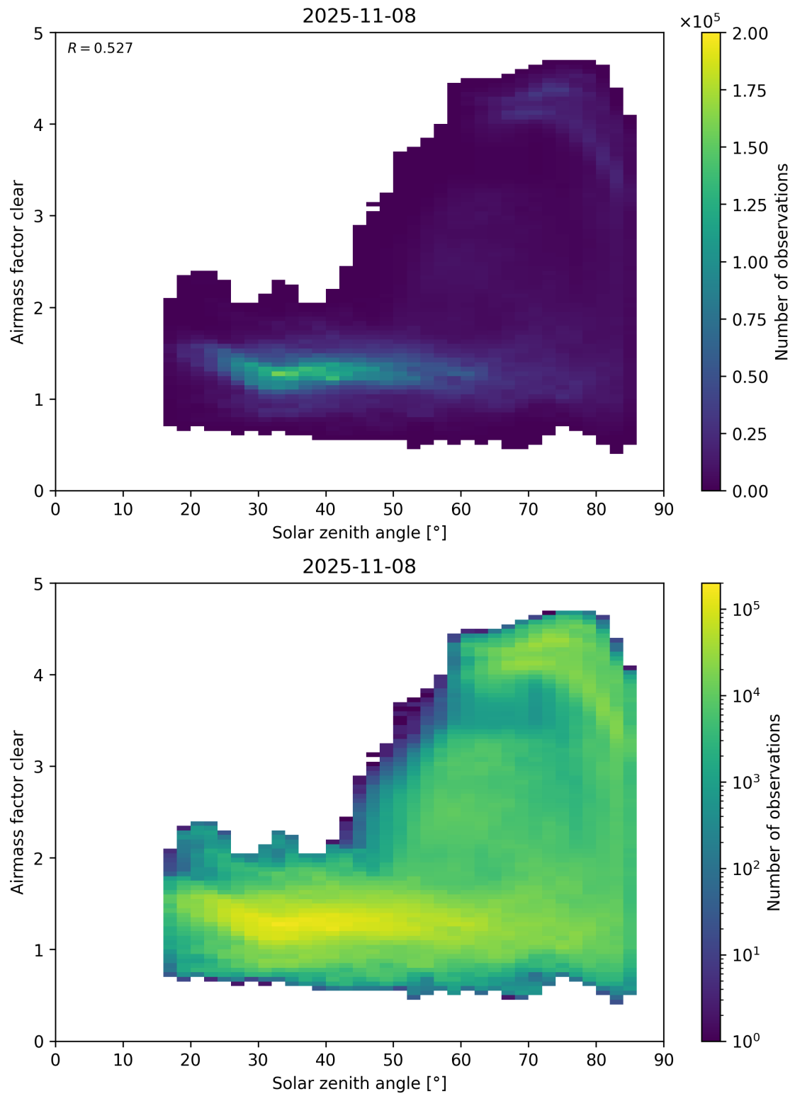
Figure 170: Scatter density plot of “Solar zenith angle” against “Airmass factor clear” for 2025-11-07 to 2025-11-09.
