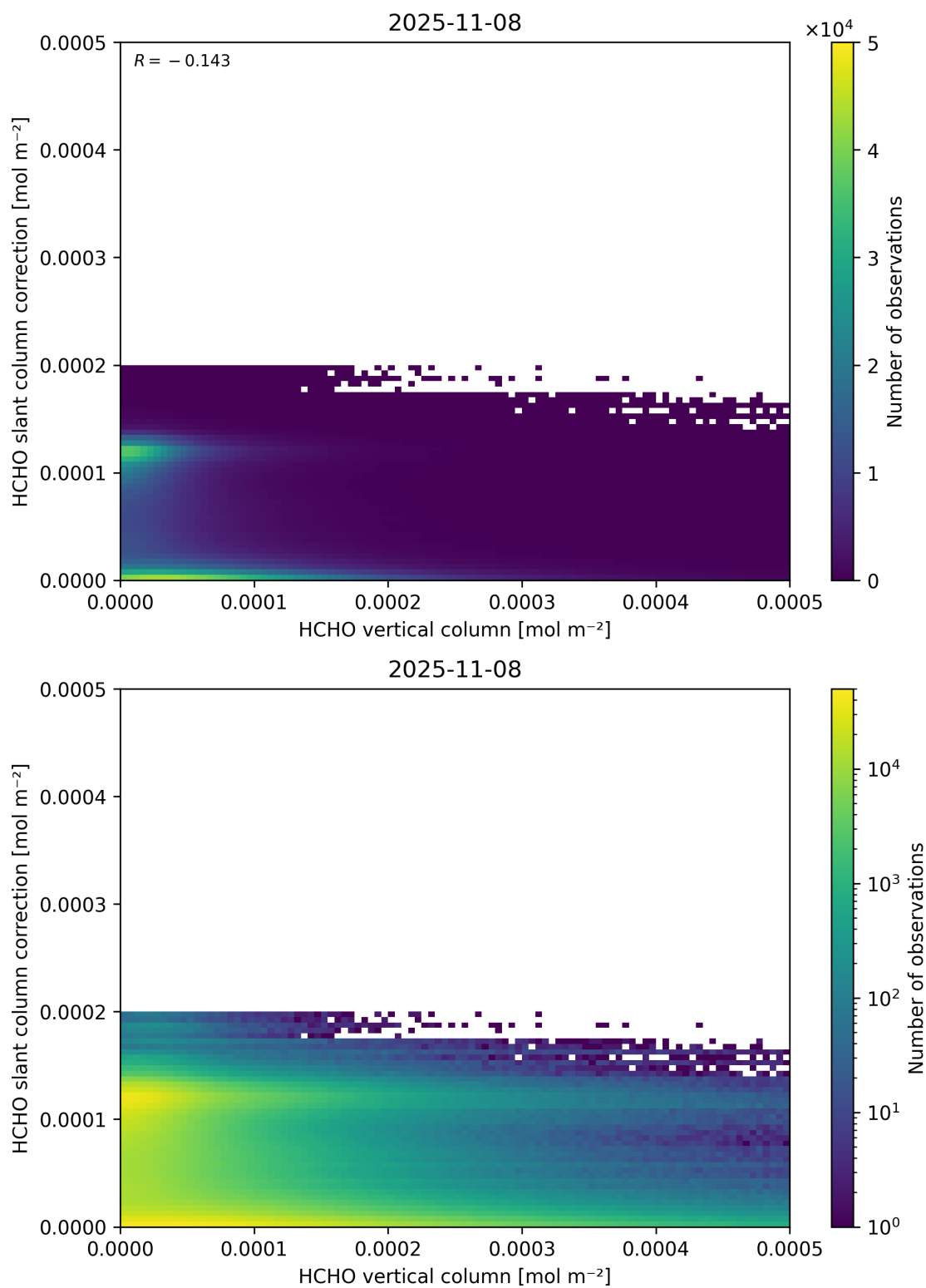
Figure 128: Scatter density plot of “HCHO vertical column” against “HCHO slant column correction” for 2025-11-07 to 2025-11-09.
