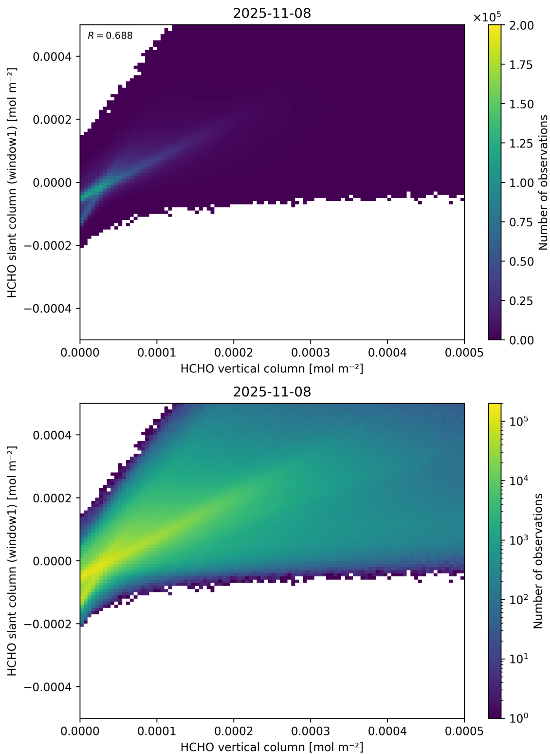
Figure 129: Scatter density plot of “HCHO vertical column” against “HCHO slant column (window1)” for 2025-11-07 to 2025-11-09.
