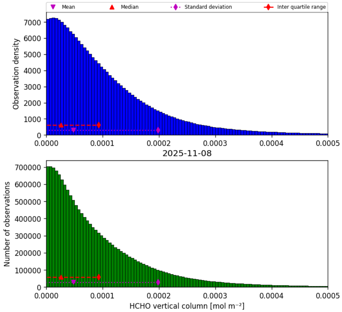
Figure 35: Histogram of “HCHO vertical column” for 2025-11-07 to 2025-11-09
