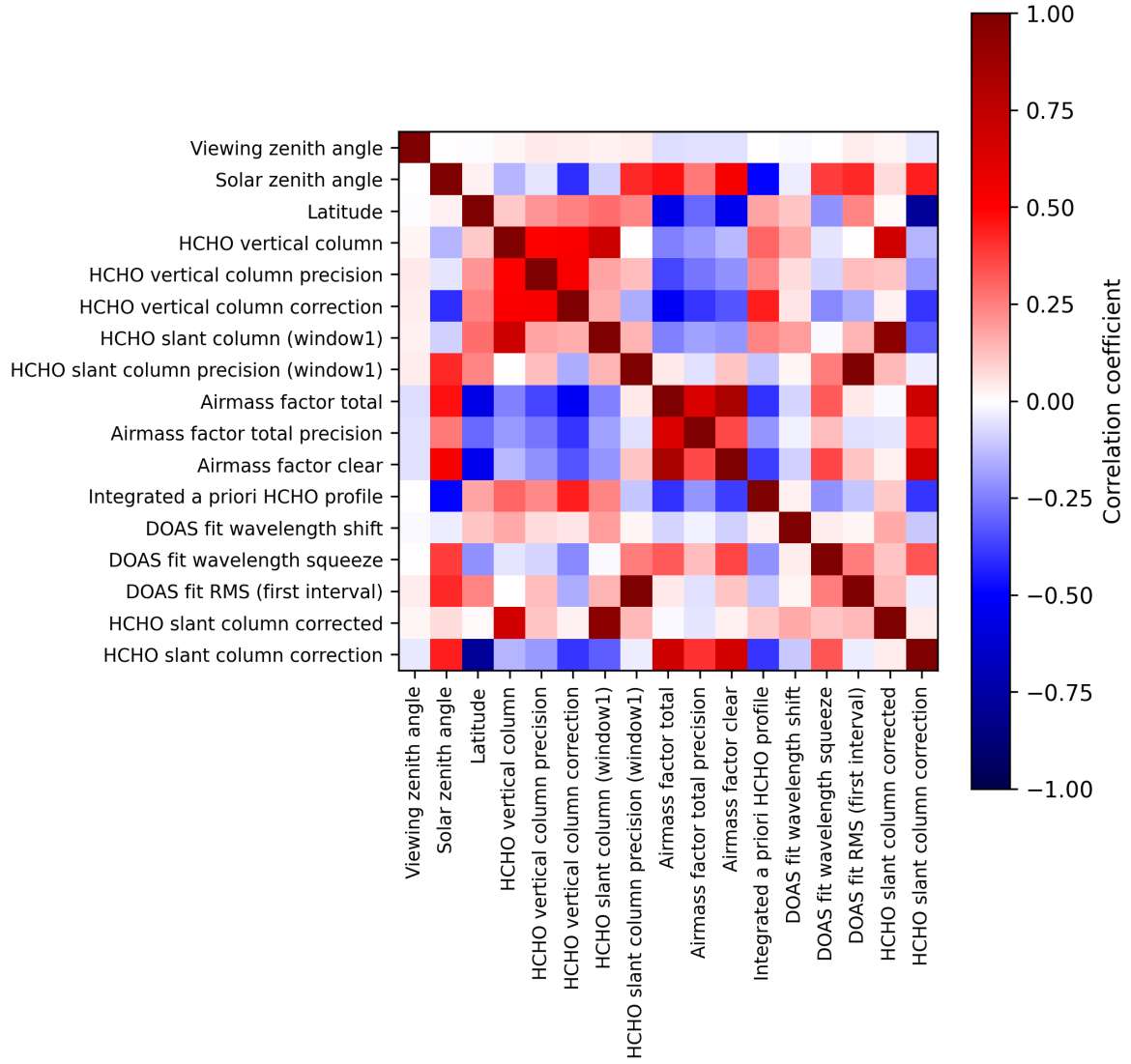
Figure 2: Map of correlation matrix for 2025-11-07 to 2025-11-09.
