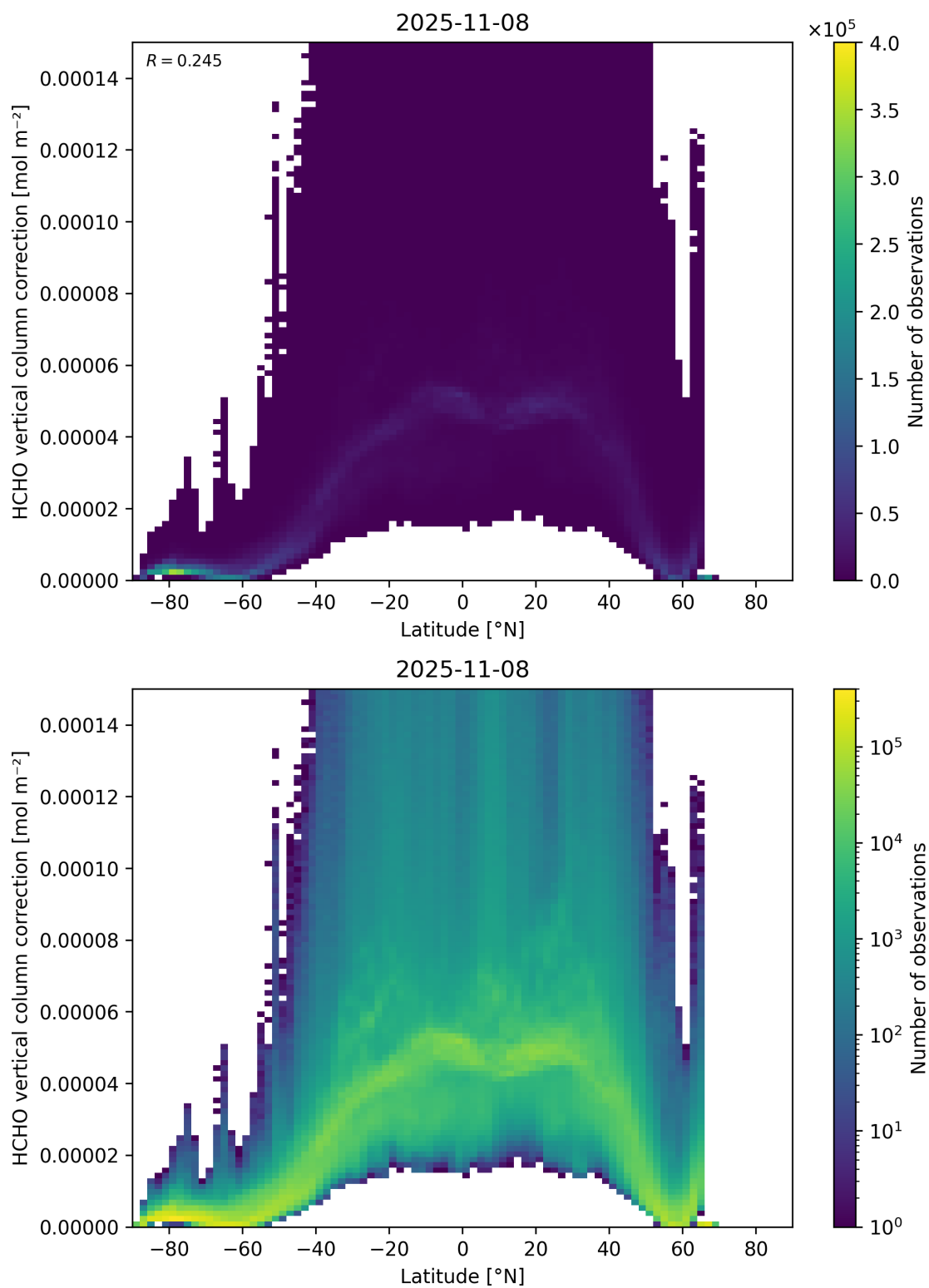
Figure 164: Scatter density plot of “Latitude” against “HCHO vertical column correction” for 2025-11-07 to 2025-11-09.
