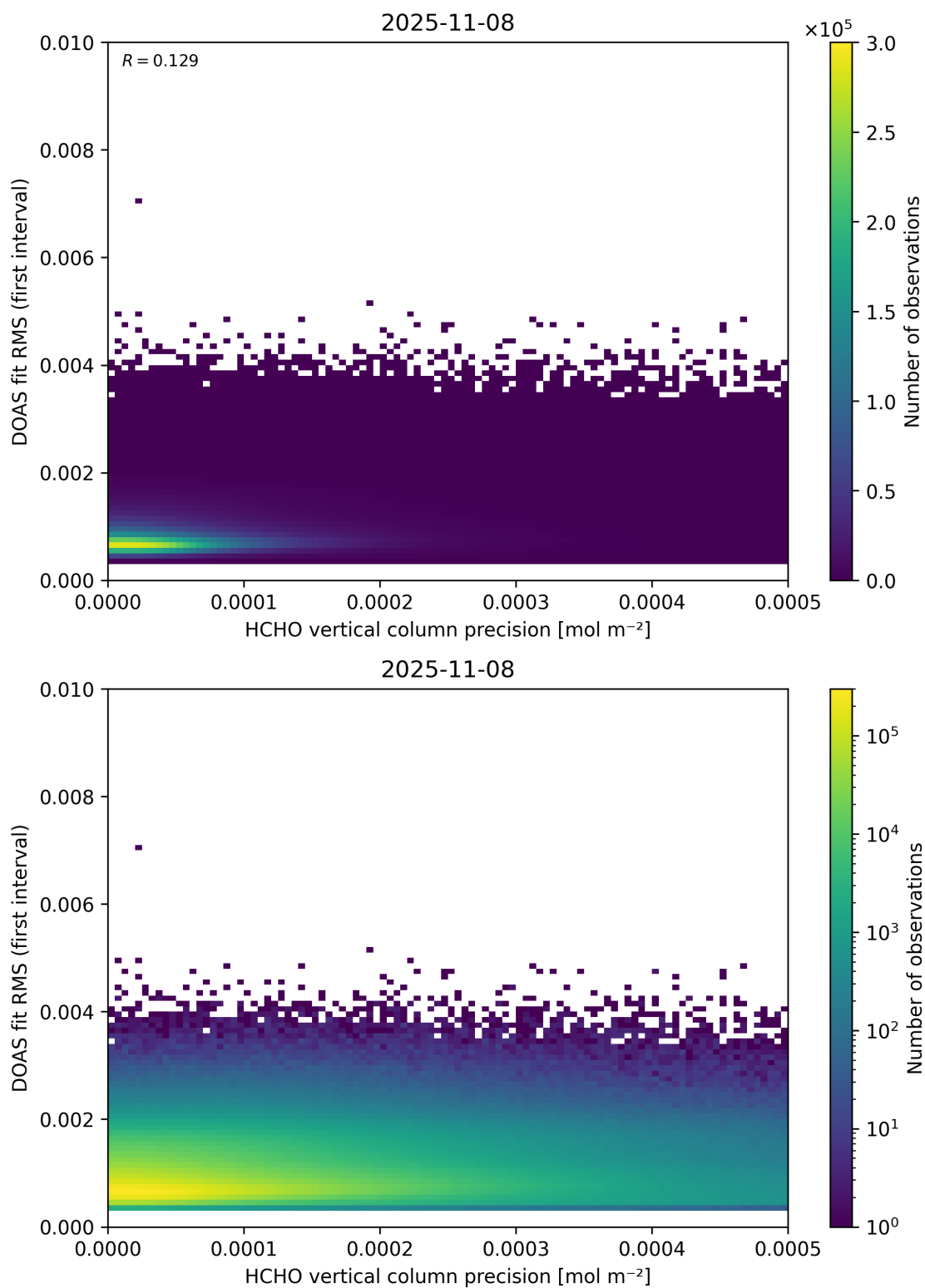
Figure 136: Scatter density plot of “HCHO vertical column precision” against “DOAS fit RMS (first interval)” for 2025-11-07 to 2025-11-09.
