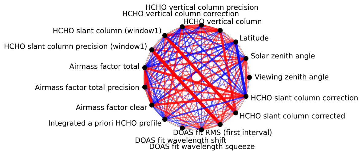
Figure 1: Map of correlation graph for 2025-11-07 to 2025-11-09.
