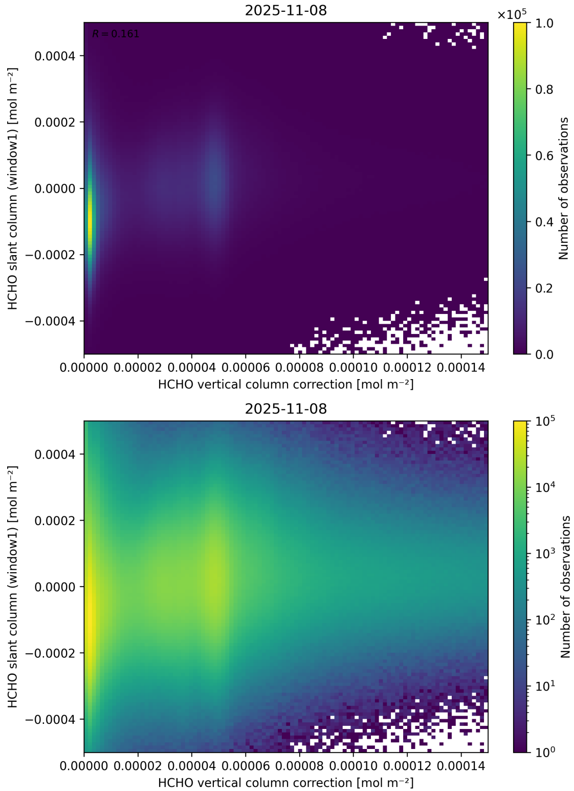
Figure 118: Scatter density plot of “HCHO vertical column correction” against “HCHO slant column (window1)” for 2025-11-07 to 2025-11-09.
