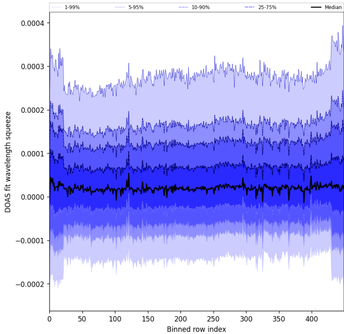
Figure 59: Along track statistics of “DOAS fit wavelength squeeze” for 2025-11-07 to 2025-11-09
