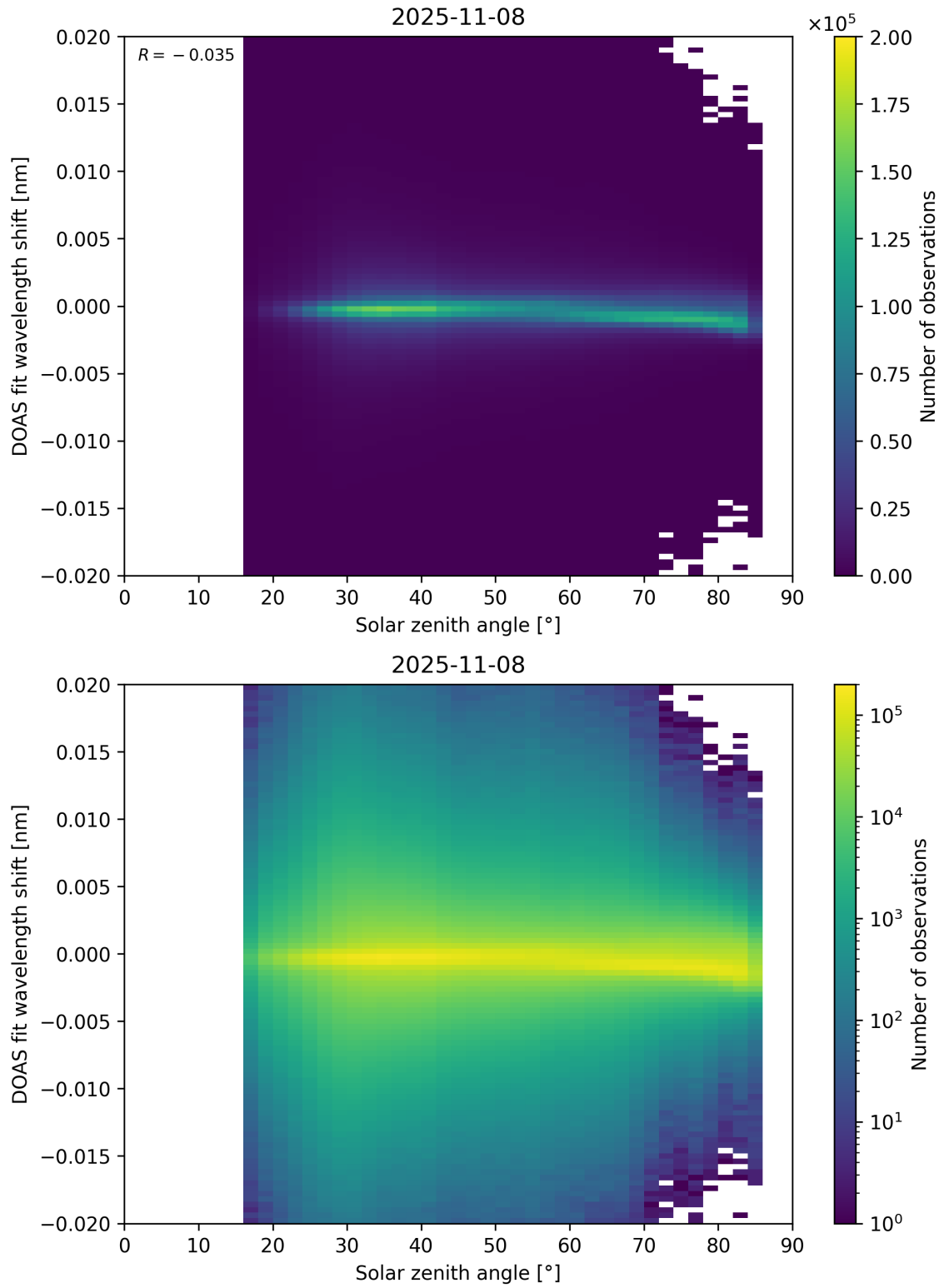
Figure 168: Scatter density plot of “Solar zenith angle” against “DOAS fit wavelength shift” for 2025-11-07 to 2025-11-09.
