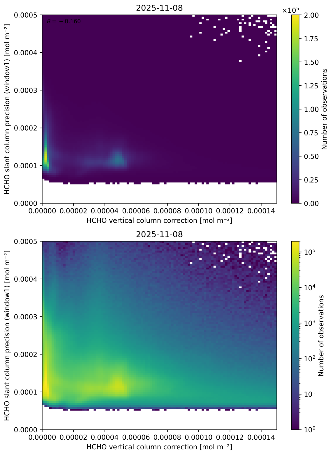
Figure 119: Scatter density plot of “HCHO vertical column correction” against “HCHO slant column precision (window1)” for 2025-11-07 to 2025-11-09.
