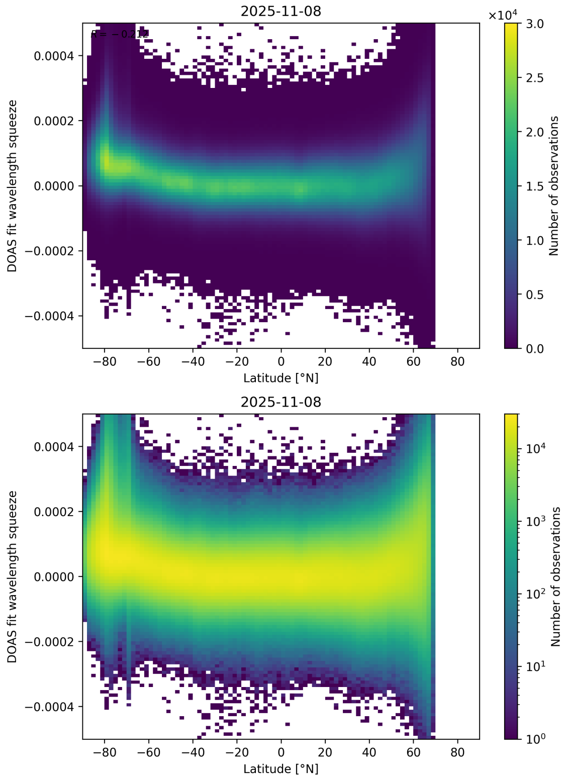
Figure 155: Scatter density plot of “Latitude” against “DOAS fit wavelength squeeze” for 2025-11-07 to 2025-11-09.
