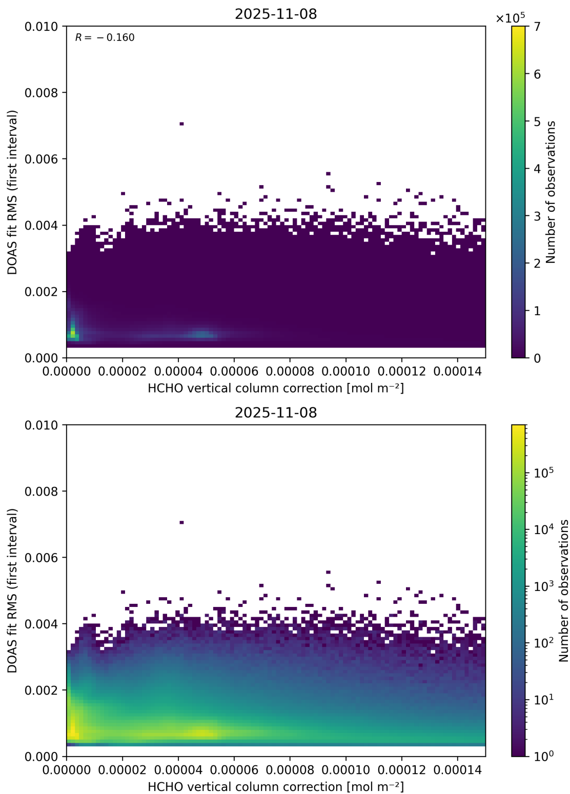
Figure 112: Scatter density plot of “HCHO vertical column correction” against “DOAS fit RMS (first interval)” for 2025-11-07 to 2025-11-09.
