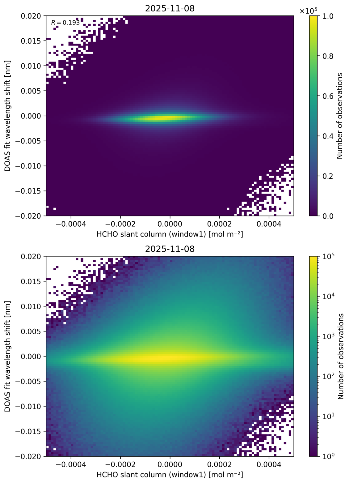
Figure 79: Scatter density plot of “HCHO slant column (window1)” against “DOAS fit wavelength shift” for 2025-11-07 to 2025-11-09.
