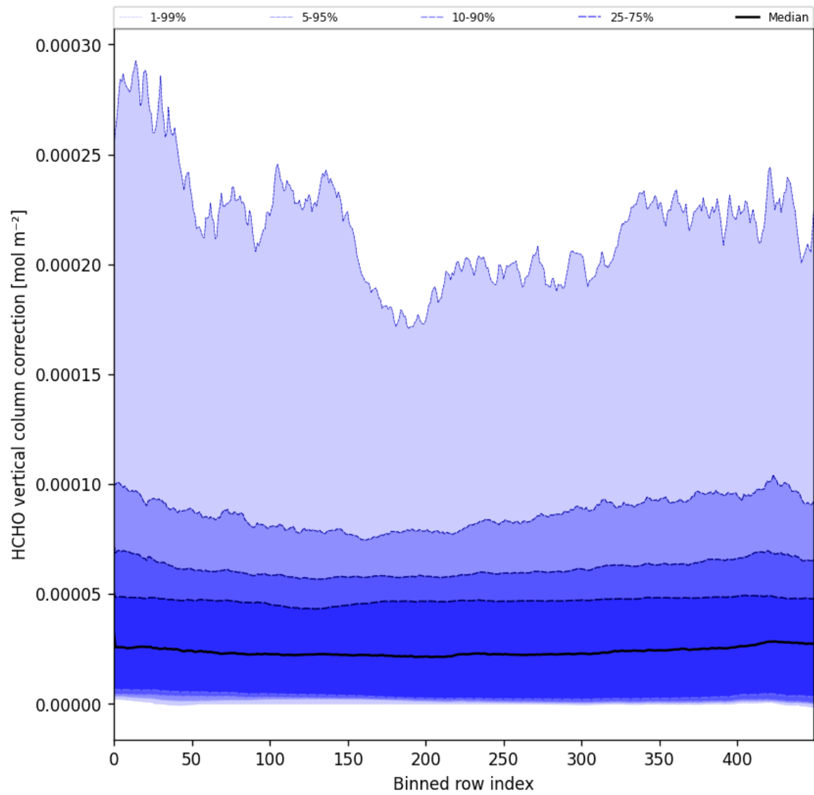
Figure 51: Along track statistics of “HCHO vertical column correction” for 2025-11-07 to 2025-11-09
