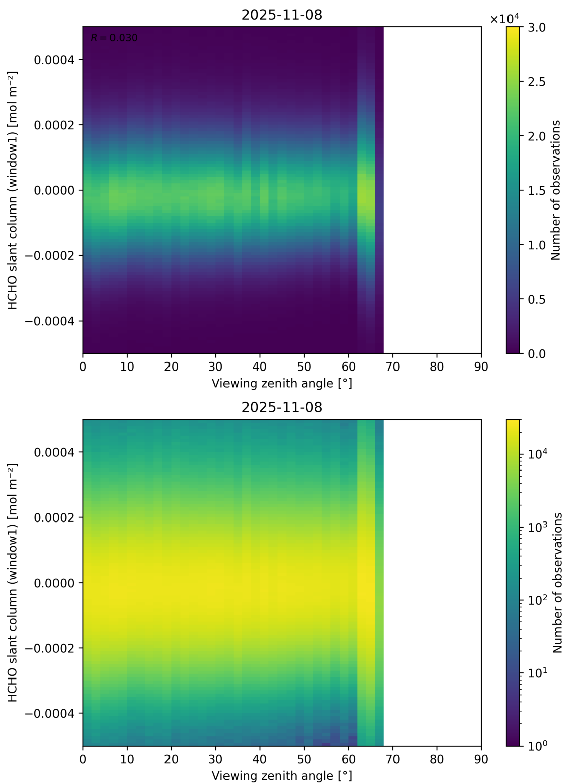
Figure 188: Scatter density plot of “Viewing zenith angle” against “HCHO slant column (window1)” for 2025-11-07 to 2025-11-09.
