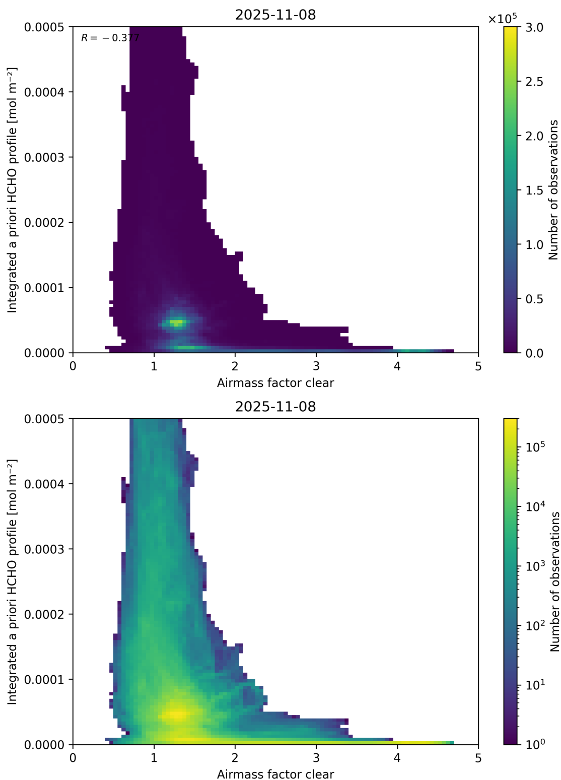
Figure 76: Scatter density plot of “Airmass factor clear” against “Integrated a priori HCHO profile” for 2025-11-07 to 2025-11-09.
