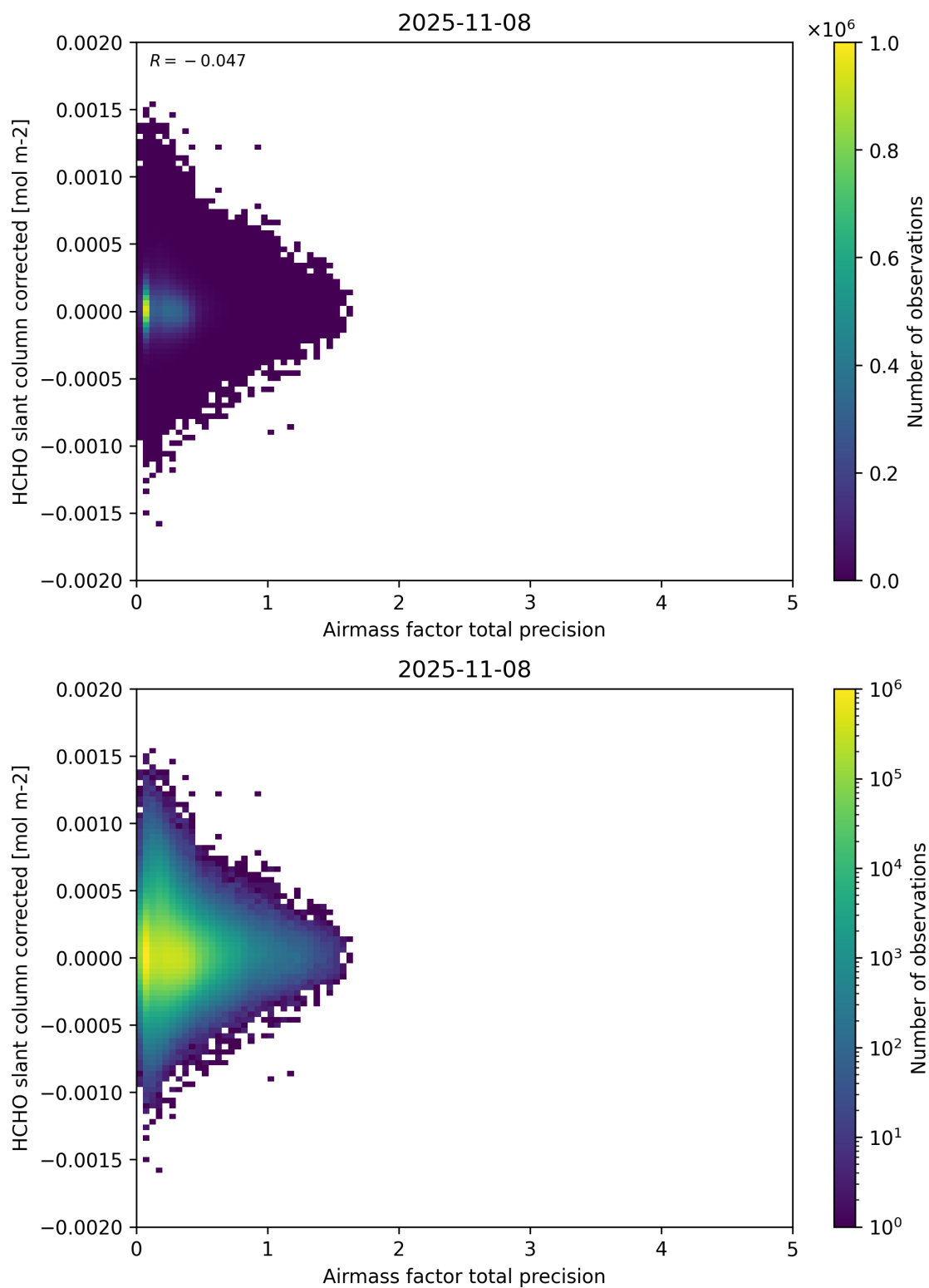
Figure 109: Scatter density plot of “Airmass factor total precision” against “HCHO slant column corrected” for 2025-11-07 to 2025-11-09.
