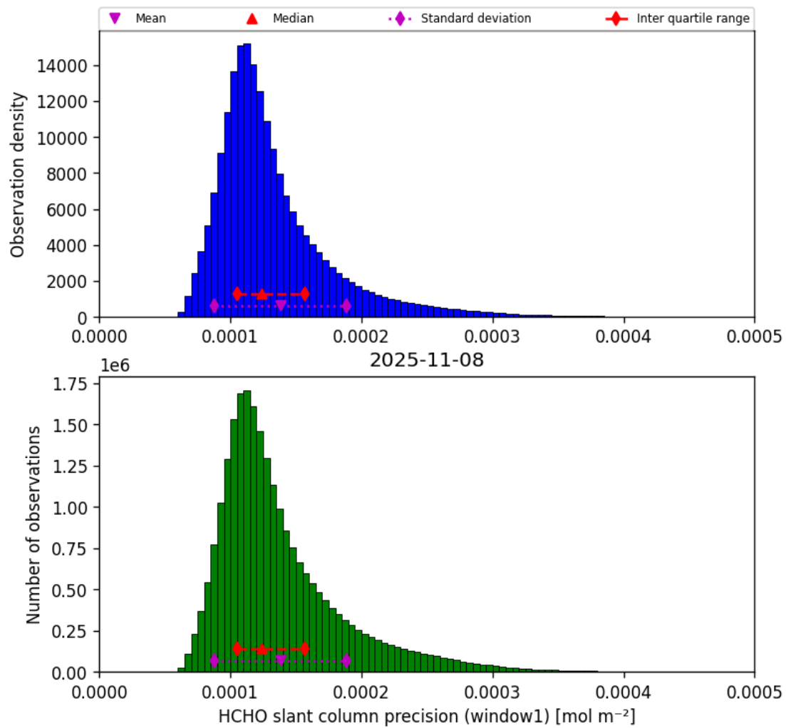
Figure 39: Histogram of “HCHO slant column precision (window1)” for 2025-11-07 to 2025-11-09
