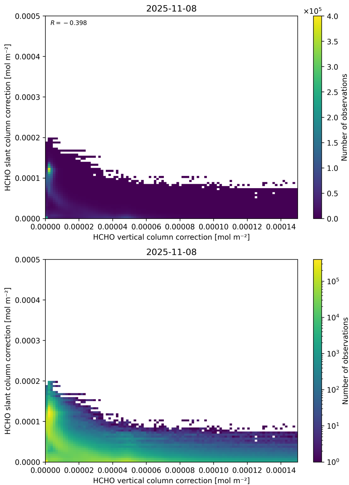
Figure 117: Scatter density plot of “HCHO vertical column correction” against “HCHO slant column correction” for 2025-11-07 to 2025-11-09.
