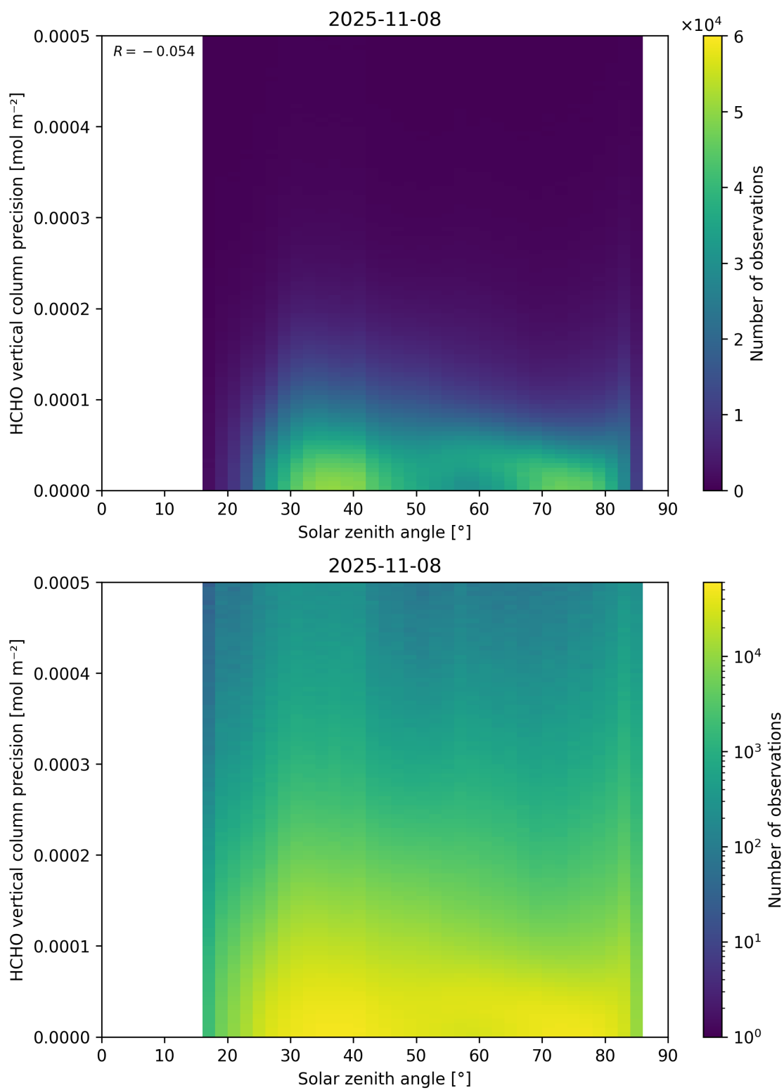
Figure 179: Scatter density plot of “Solar zenith angle” against “HCHO vertical column precision” for 2025-11-07 to 2025-11-09.
