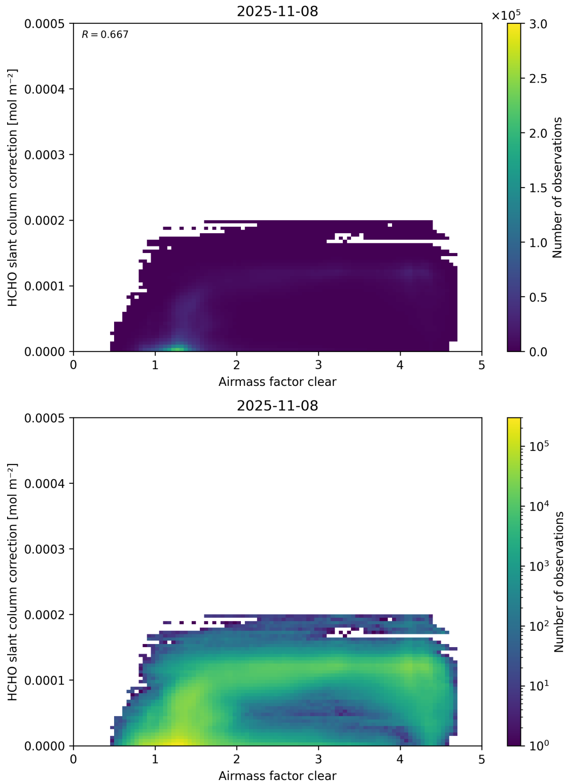
Figure 75: Scatter density plot of “Airmass factor clear” against “HCHO slant column correction” for 2025-11-07 to 2025-11-09.
