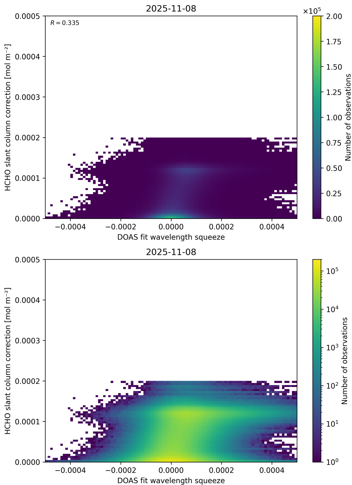
Figure 70: Scatter density plot of “DOAS fit wavelength squeeze” against “HCHO slant column correction” for 2025-11-07 to 2025-11-09.
