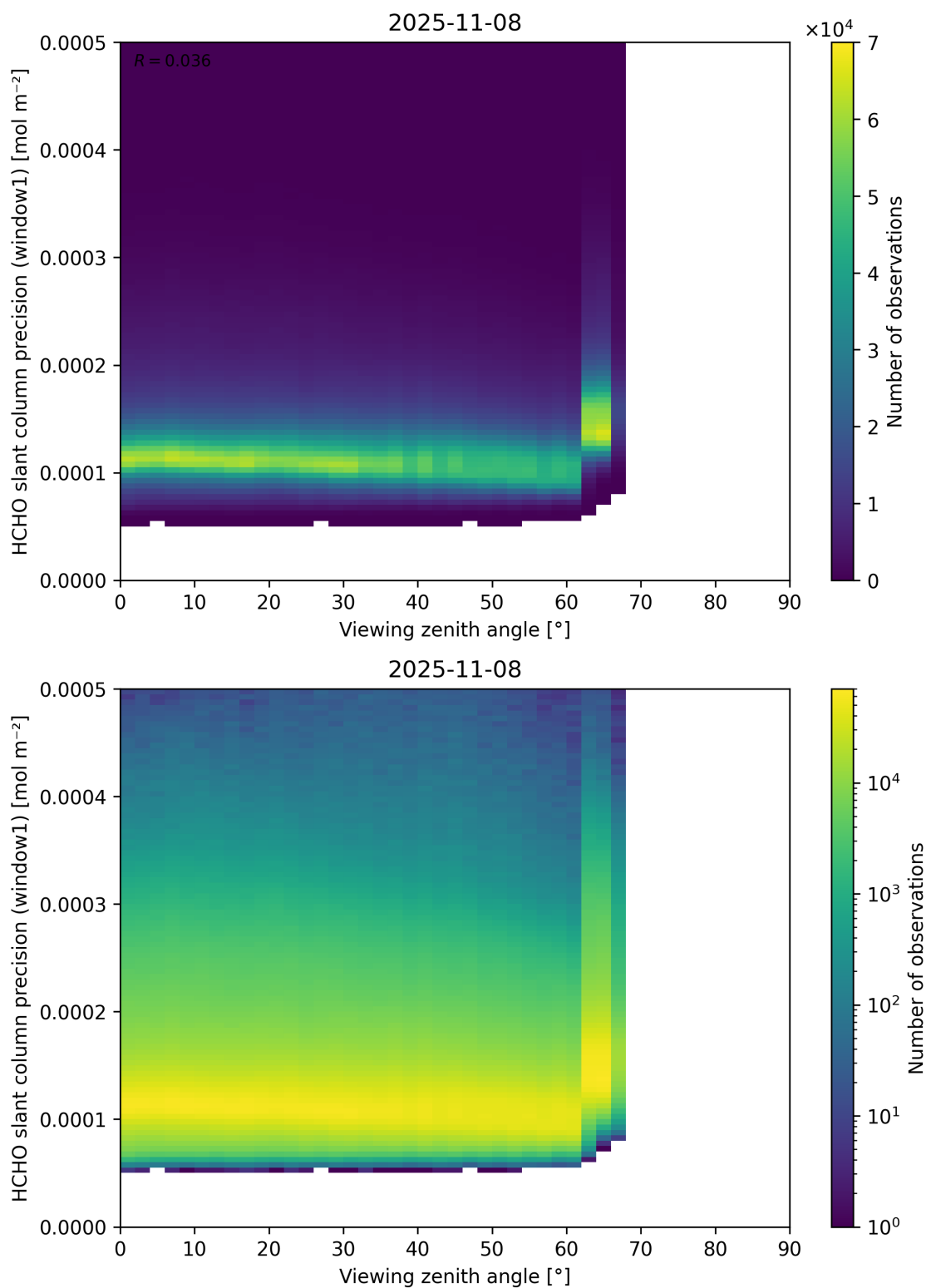
Figure 189: Scatter density plot of “Viewing zenith angle” against “HCHO slant column precision (window1)” for 2025-11-07 to 2025-11-09.
