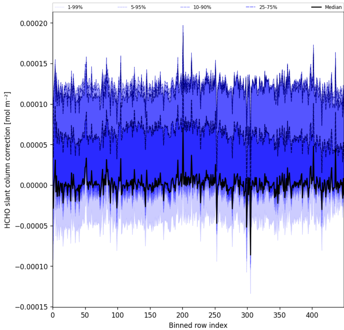
Figure 61: Along track statistics of “HCHO slant column correction” for 2025-11-07 to 2025-11-09
