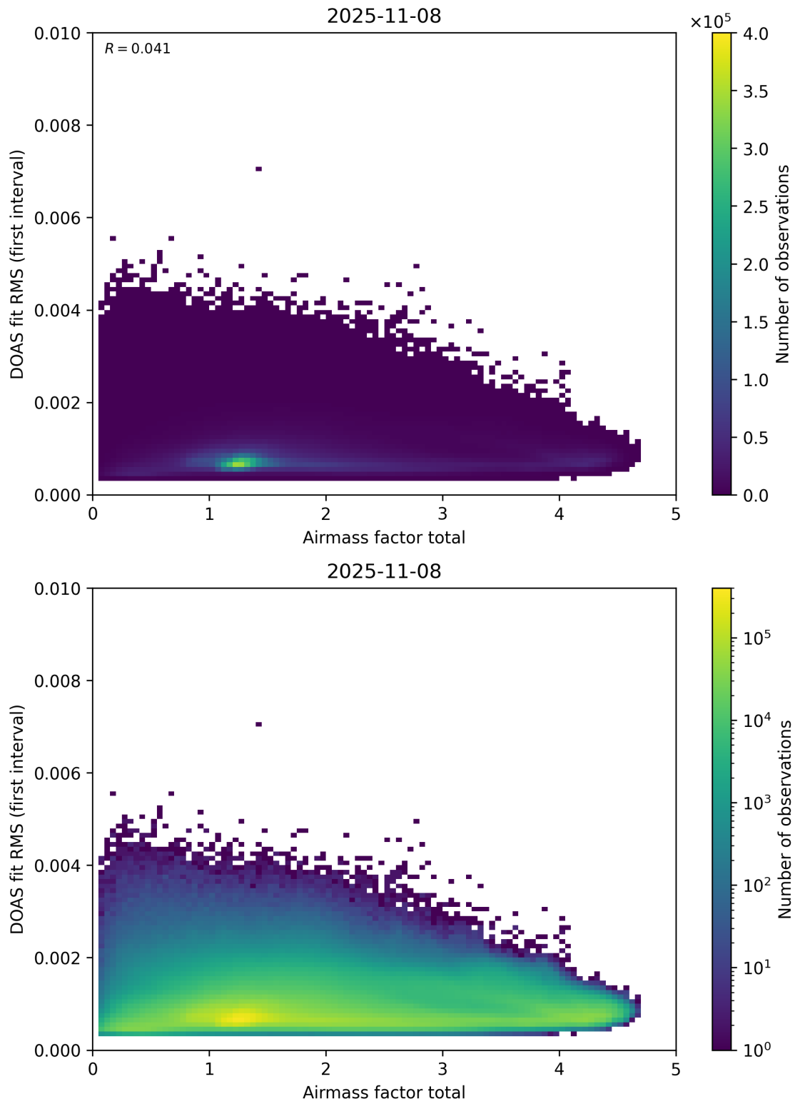
Figure 97: Scatter density plot of “Airmass factor total” against “DOAS fit RMS (first interval)” for 2025-11-07 to 2025-11-09.
