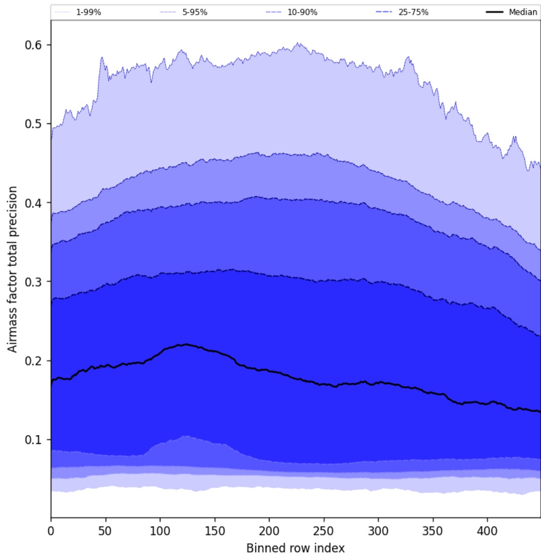
Figure 55: Along track statistics of “Airmass factor total precision” for 2025-11-07 to 2025-11-09
