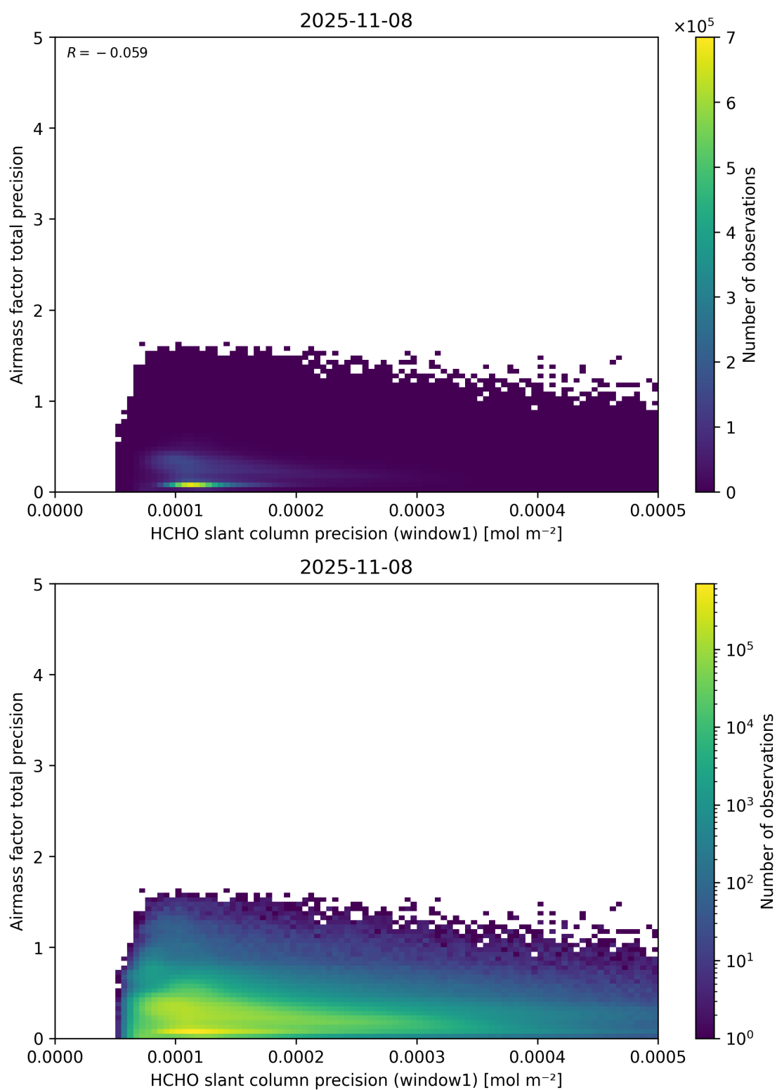
Figure 95: Scatter density plot of “HCHO slant column precision (window1)” against “Airmass factor total precision” for 2025-11-07 to 2025-11-09.
