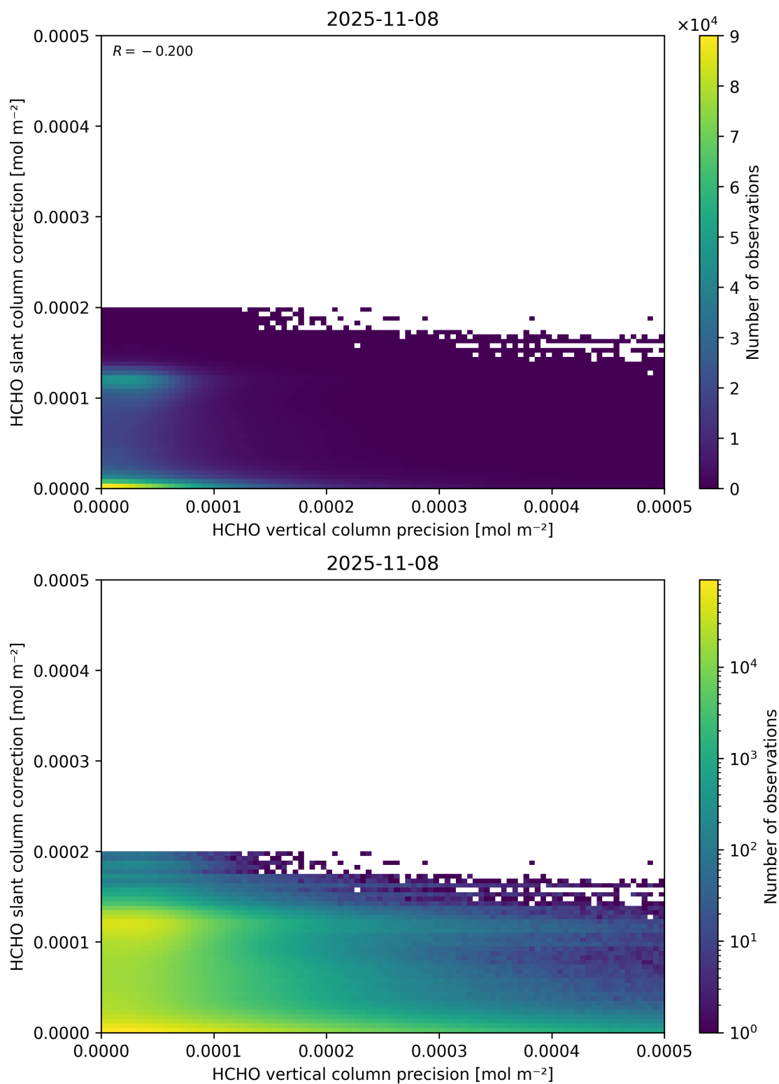
Figure 141: Scatter density plot of “HCHO vertical column precision” against “HCHO slant column correction” for 2025-11-07 to 2025-11-09.
