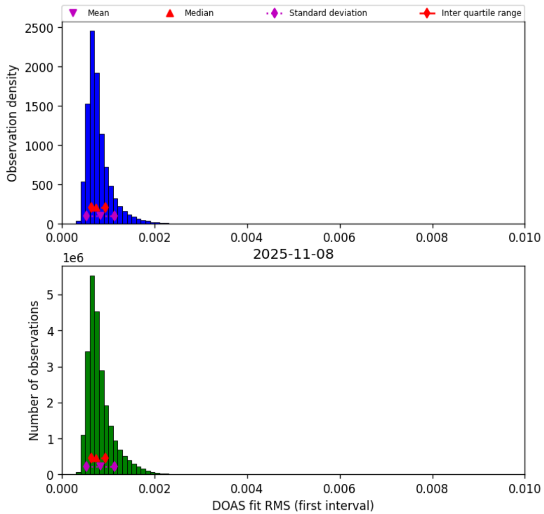
Figure 46: Histogram of “DOAS fit RMS (first interval)” for 2025-11-07 to 2025-11-09
