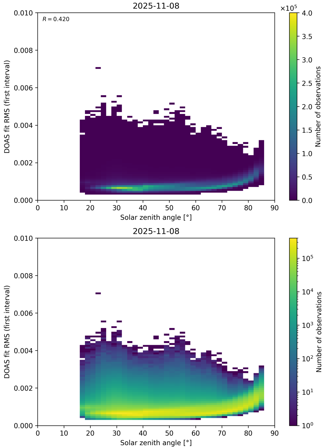
Figure 167: Scatter density plot of “Solar zenith angle” against “DOAS fit RMS (first interval)” for 2025-11-07 to 2025-11-09.
