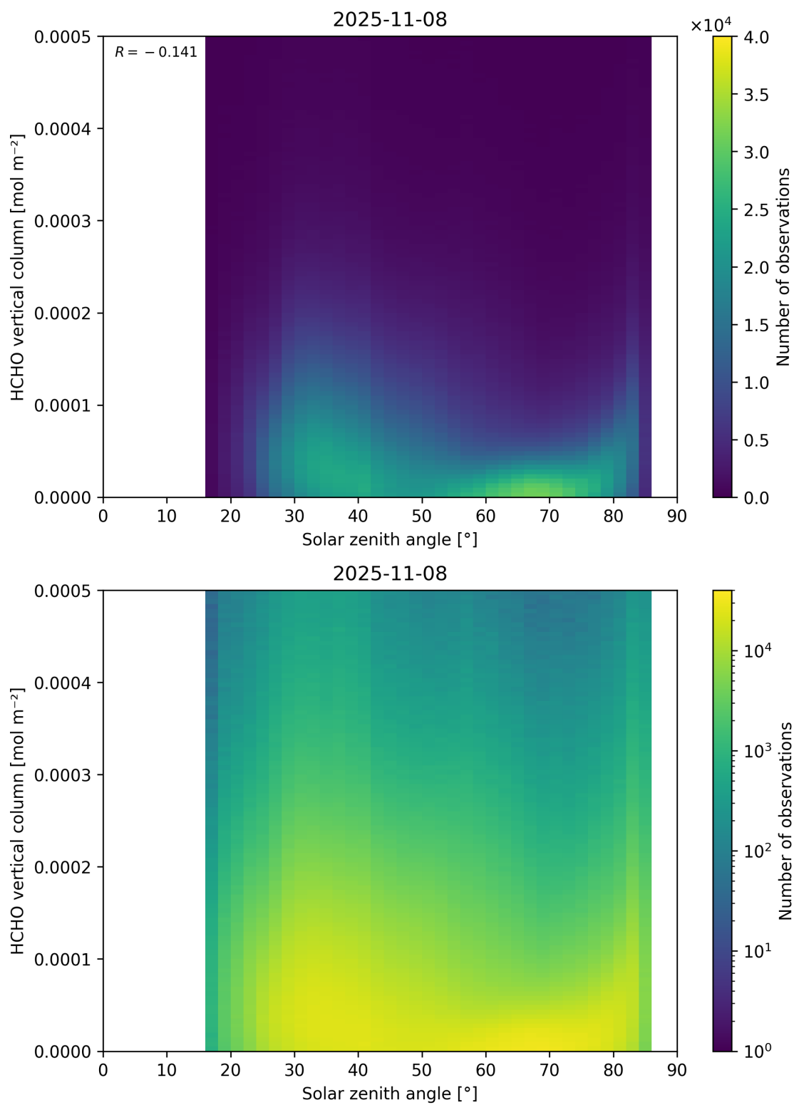
Figure 177: Scatter density plot of “Solar zenith angle” against “HCHO vertical column” for 2025-11-07 to 2025-11-09.
