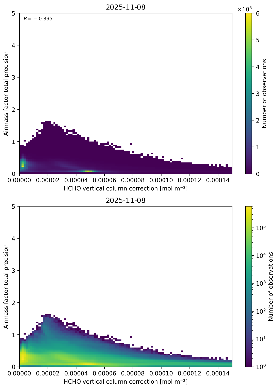
Figure 121: Scatter density plot of “HCHO vertical column correction” against “Airmass factor total precision” for 2025-11-07 to 2025-11-09.
