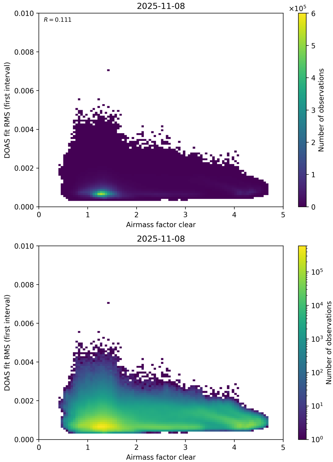
Figure 71: Scatter density plot of “Airmass factor clear” against “DOAS fit RMS (first interval)” for 2025-11-07 to 2025-11-09.
