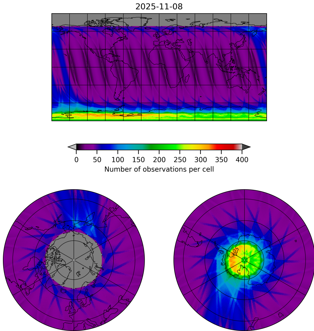
Figure 19: Map of the number of observations for 2025-11-07 to 2025-11-09
