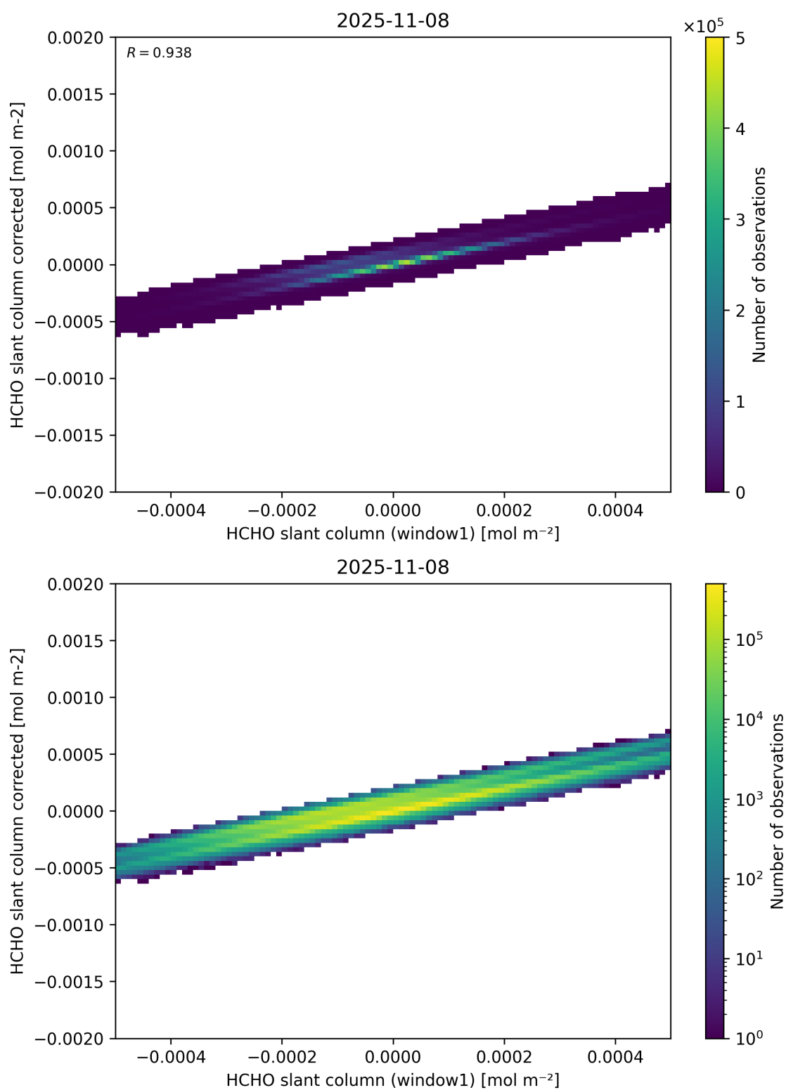
Figure 82: Scatter density plot of “HCHO slant column (window1)” against “HCHO slant column corrected” for 2025-11-07 to 2025-11-09.
