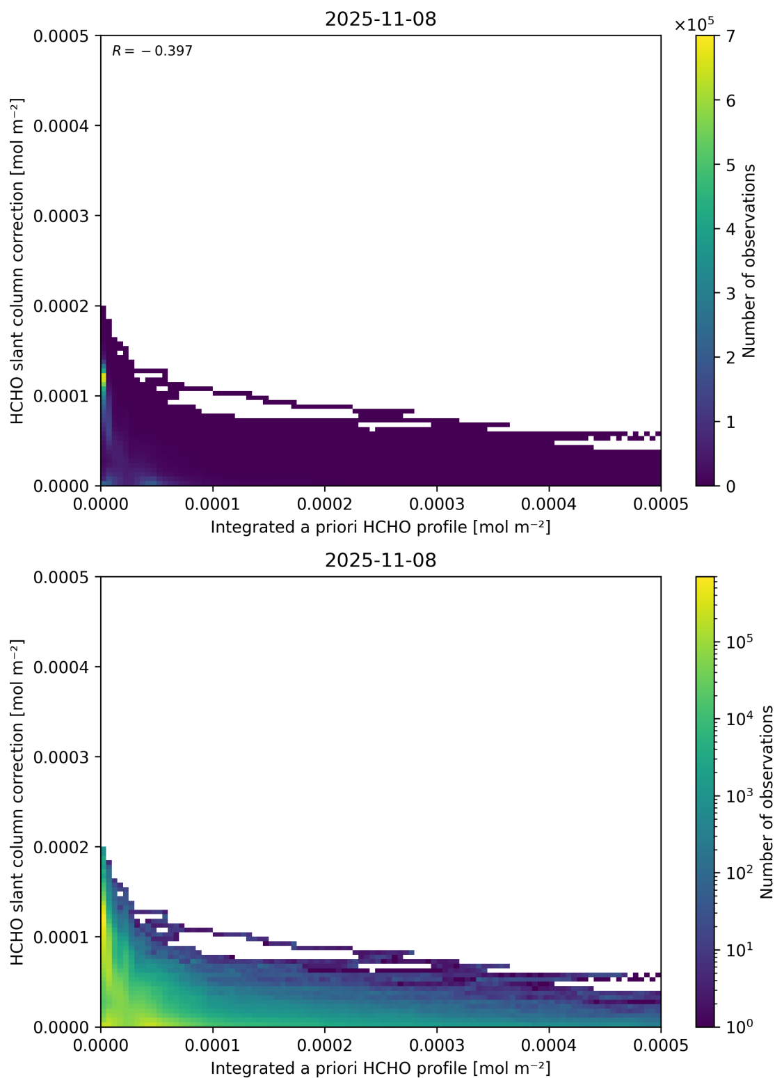
Figure 152: Scatter density plot of “Integrated a priori HCHO profile” against “HCHO slant column correction” for 2025-11-07 to 2025-11-09.
