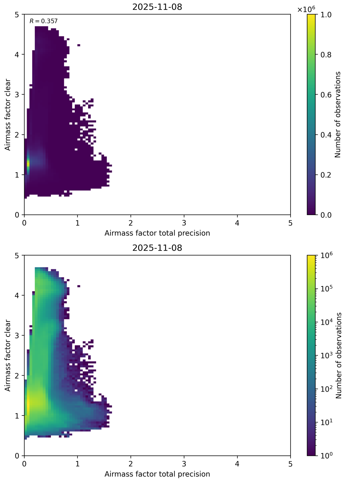
Figure 108: Scatter density plot of “Airmass factor total precision” against “Airmass factor clear” for 2025-11-07 to 2025-11-09.
