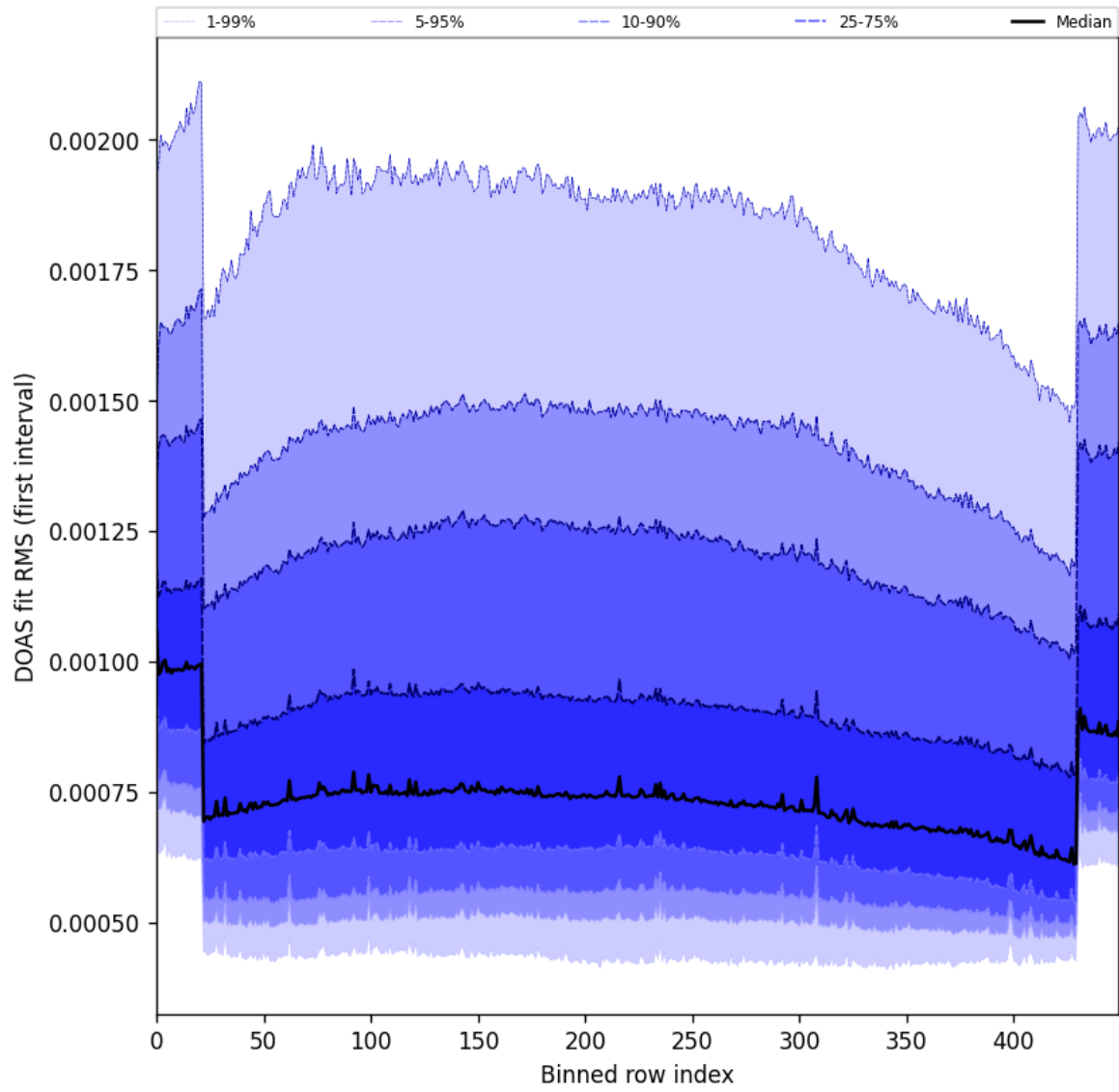
Figure 60: Along track statistics of “DOAS fit RMS (first interval)” for 2025-11-07 to 2025-11-09
