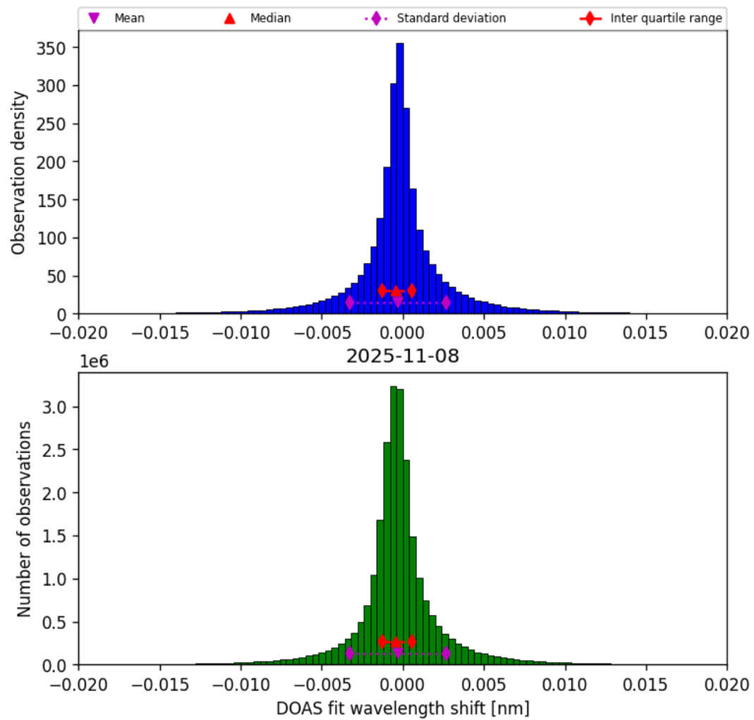
Figure 44: Histogram of “DOAS fit wavelength shift” for 2025-11-07 to 2025-11-09
