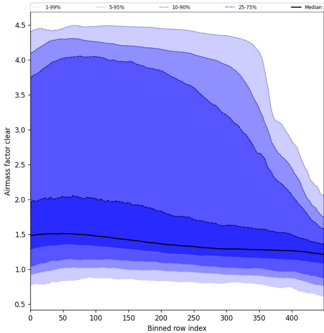
Figure 56: Along track statistics of “Air mass factor clear” for 2025-11-07 to 2025-11-09
