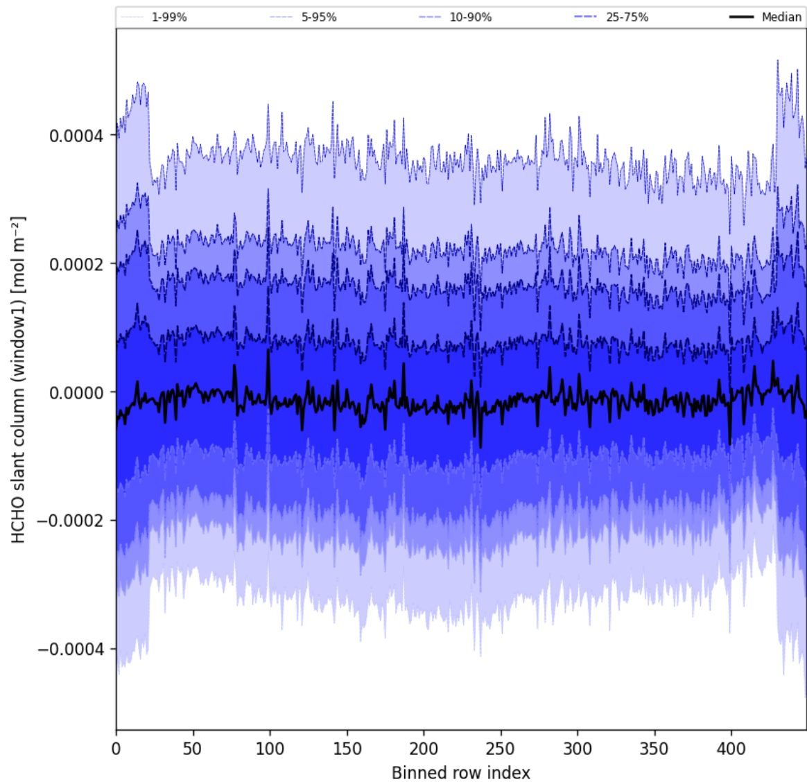
Figure 52: Along track statistics of “HCHO slant column (window1)” for 2025-11-07 to 2025-11-09
