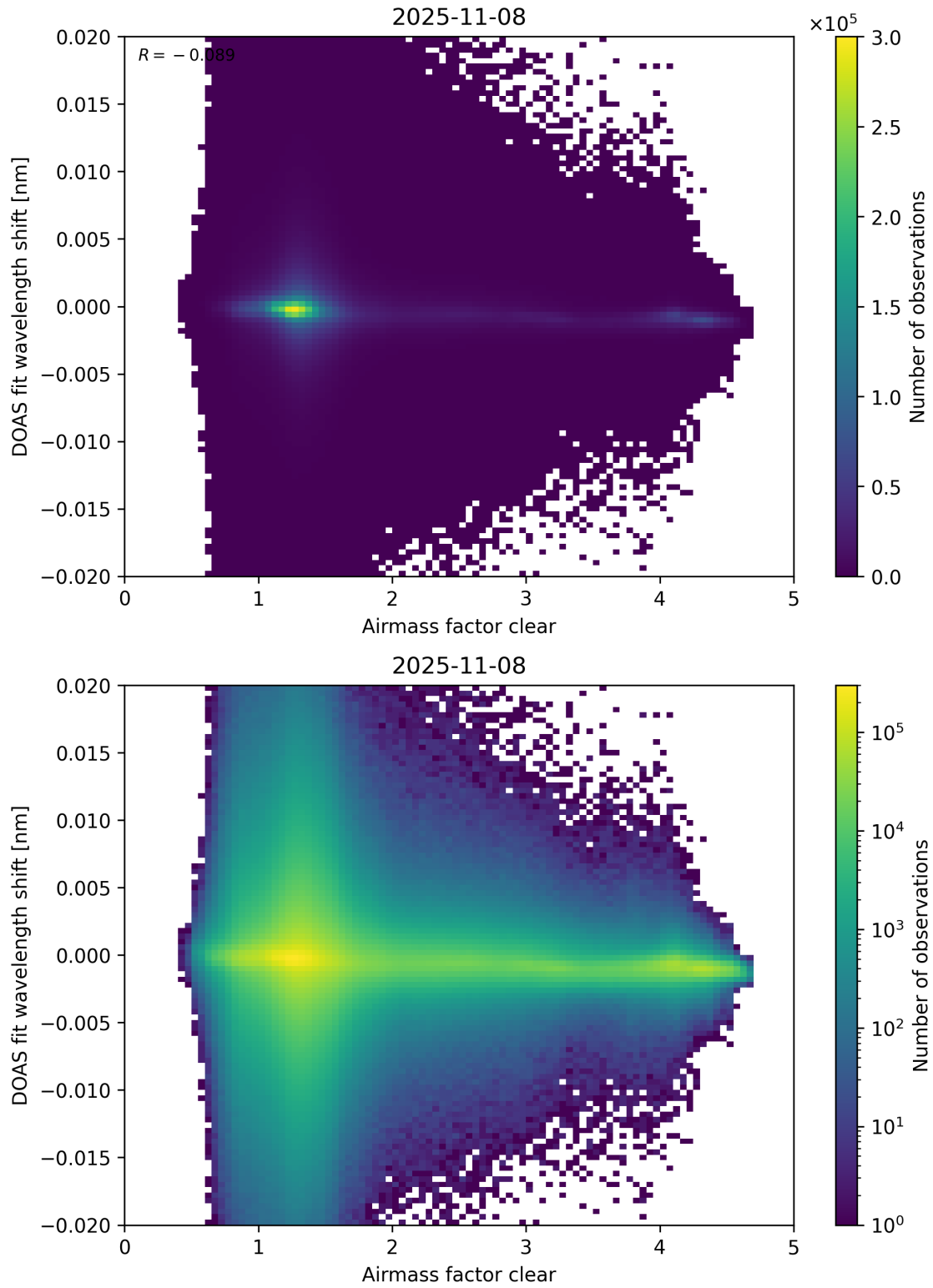
Figure 72: Scatter density plot of “Airmass factor clear” against “DOAS fit wavelength shift” for 2025-11-07 to 2025-11-09.
