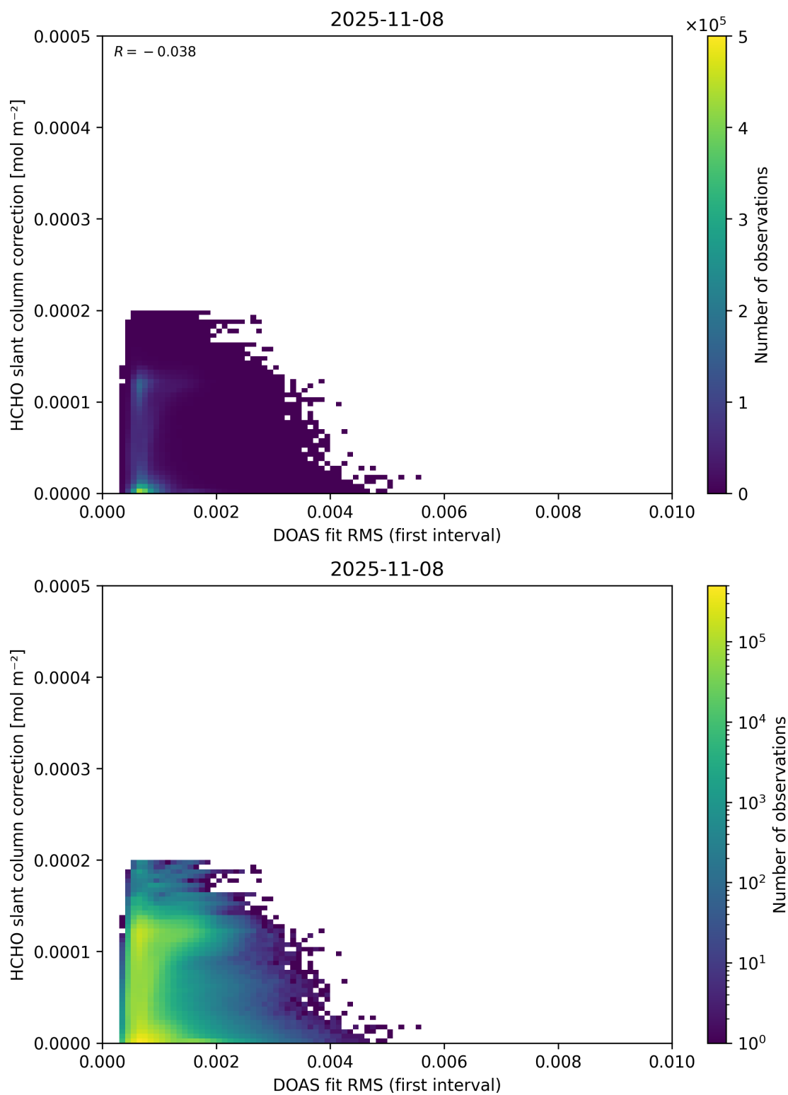
Figure 63: Scatter density plot of “DOAS fit RMS (first interval)” against “HCHO slant column correction” for 2025-11-07 to 2025-11-09.
