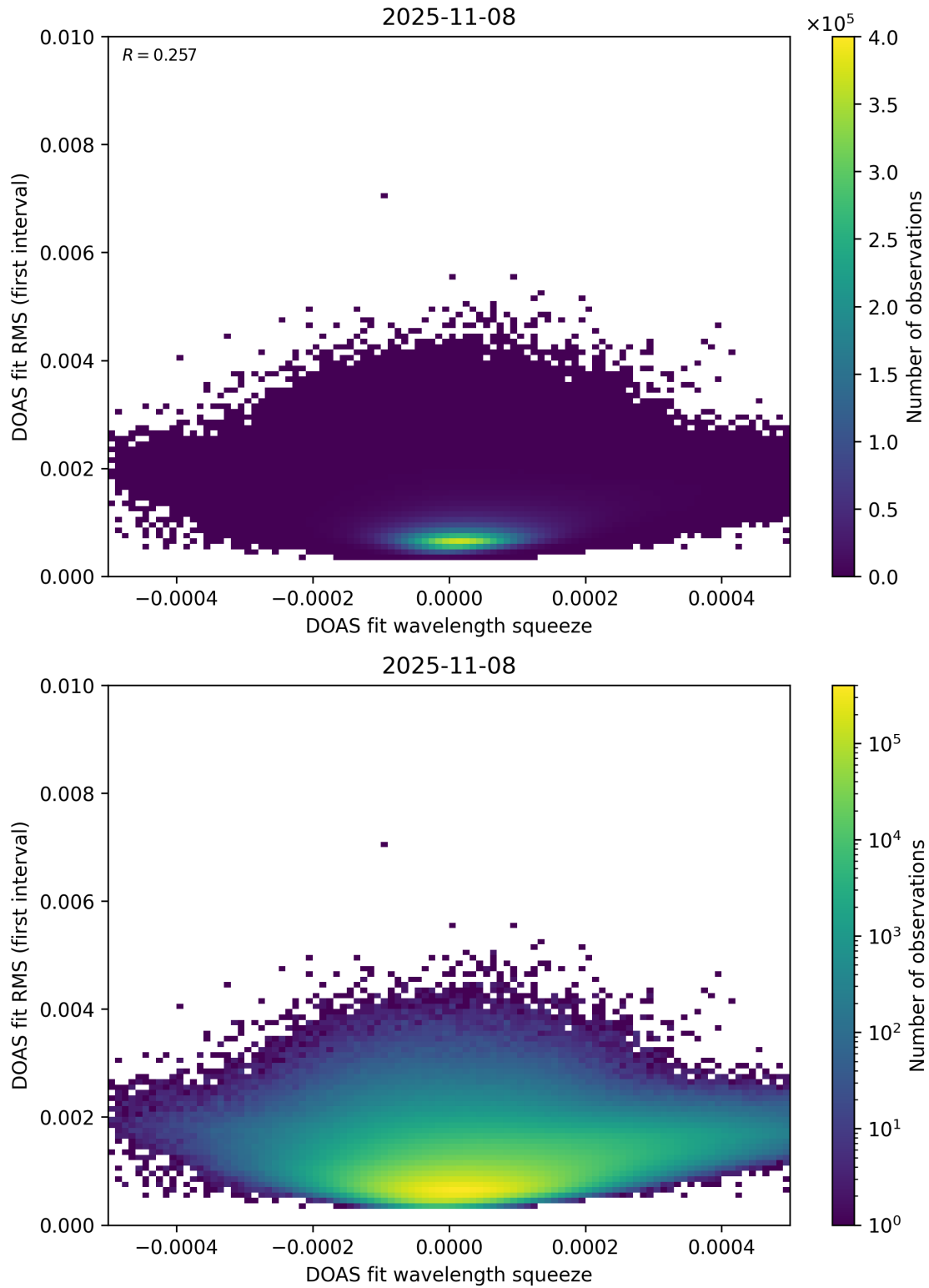
Figure 68: Scatter density plot of “DOAS fit wavelength squeeze” against “DOAS fit RMS (first interval)” for 2025-11-07 to 2025-11-09.
