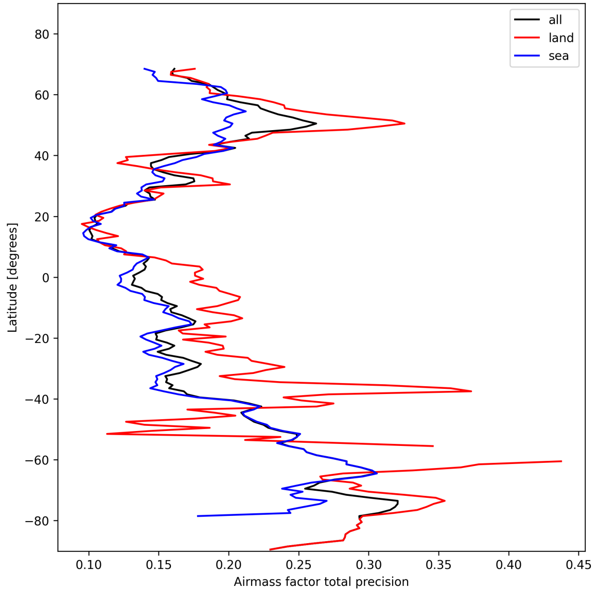
Figure 27: Zonal average of “Airmass factor total precision” for 2025-11-07 to 2025-11-09.
