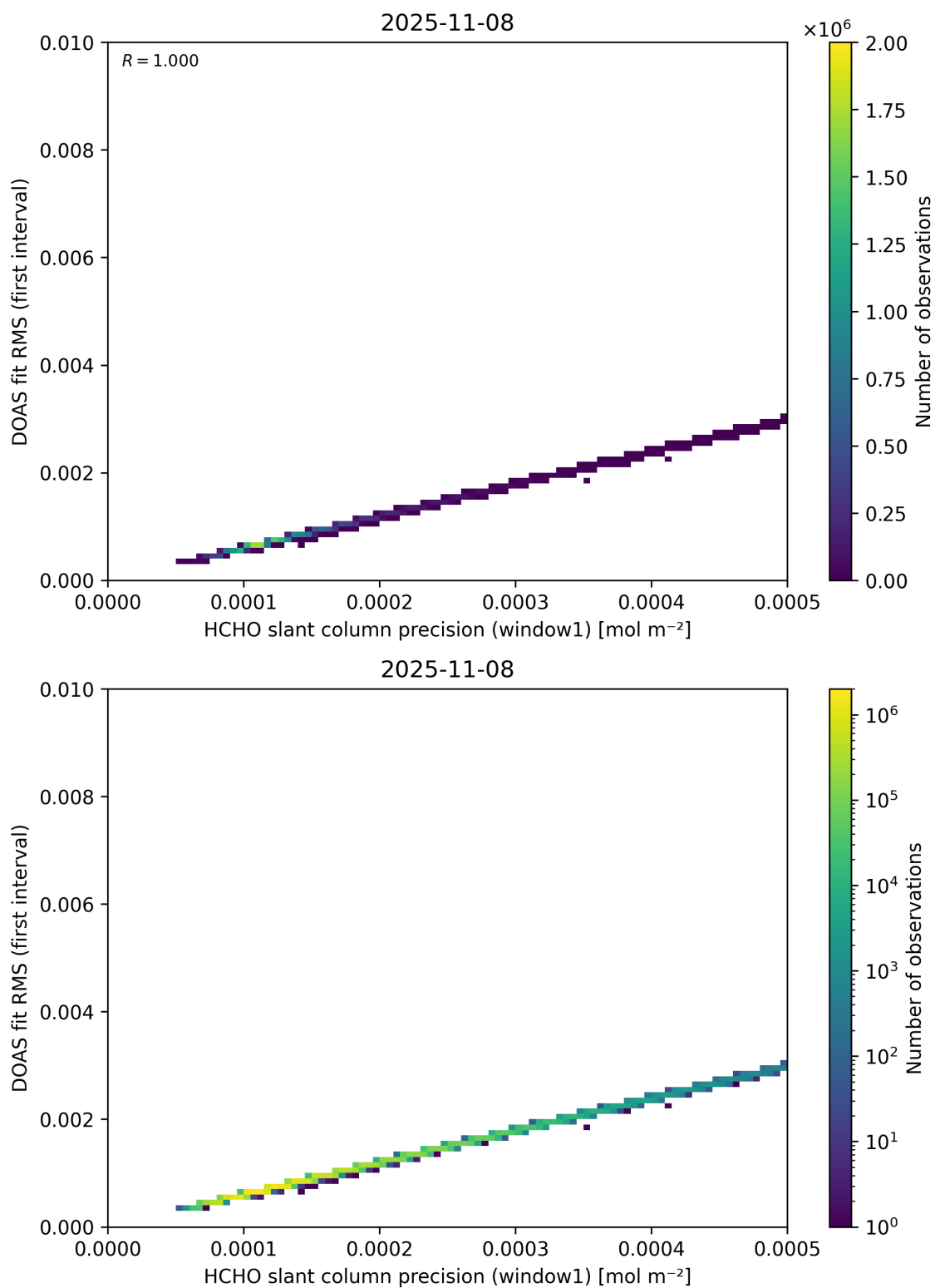
Figure 88: Scatter density plot of “HCHO slant column precision (window1)” against “DOAS fit RMS (first interval)” for 2025-11-07 to 2025-11-09.
