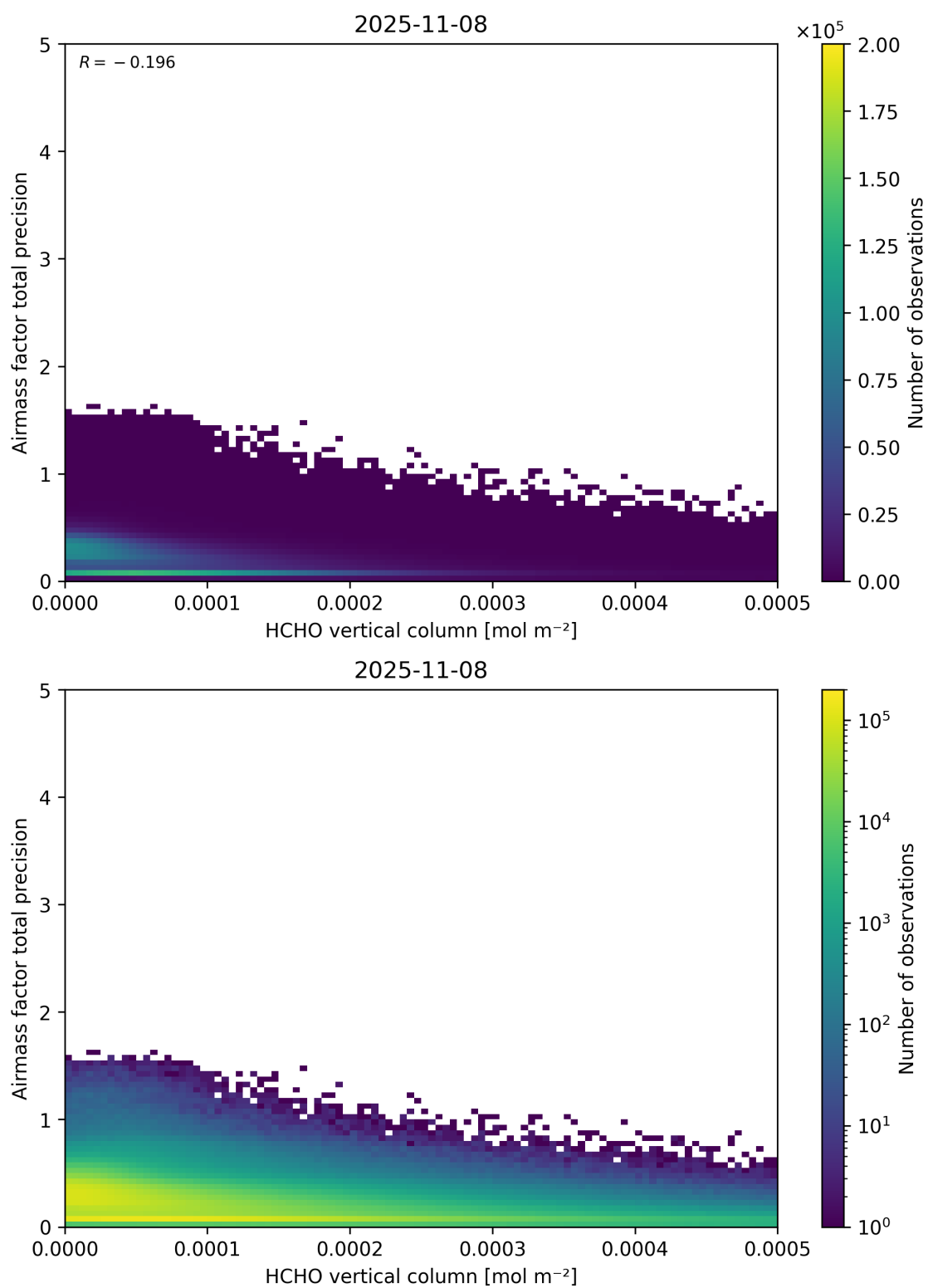
Figure 132: Scatter density plot of “HCHO vertical column” against “Airmass factor total precision” for 2025-11-07 to 2025-11-09.
