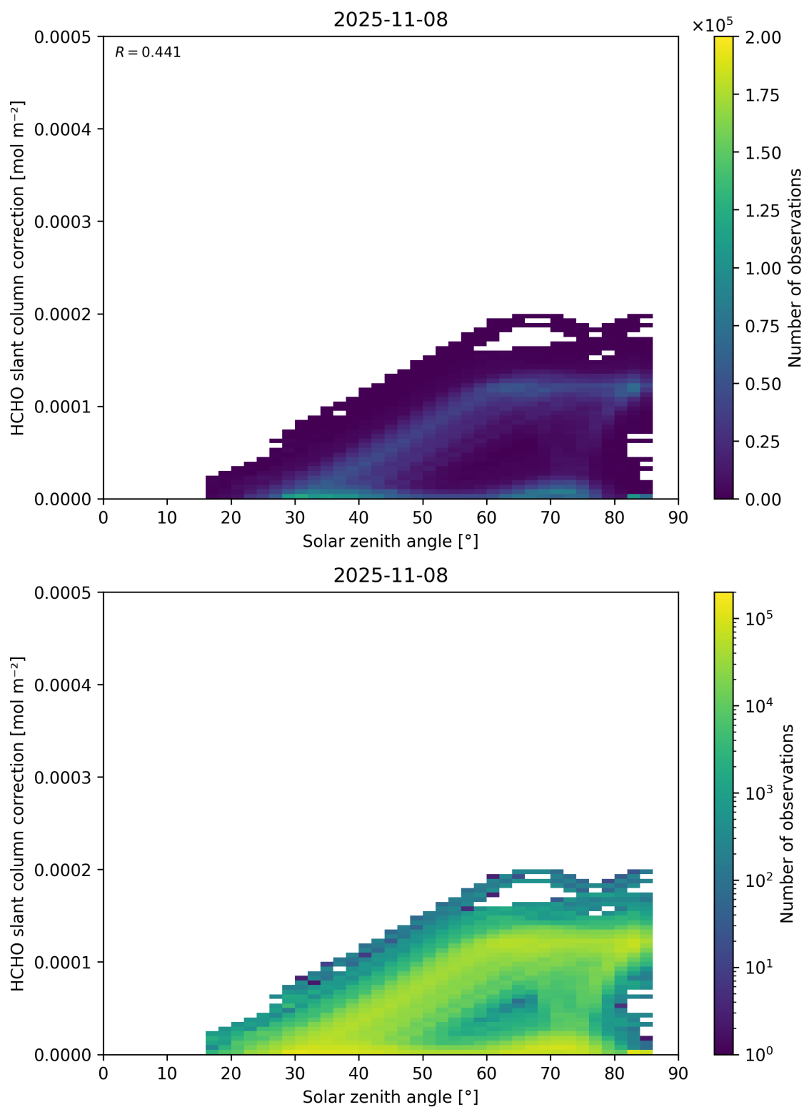
Figure 172: Scatter density plot of “Solar zenith angle” against “HCHO slant column correction” for 2025-11-07 to 2025-11-09.
