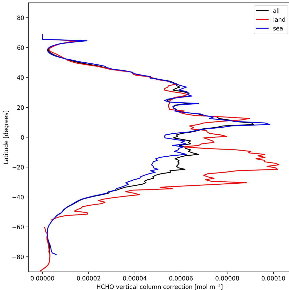
Figure 23: Zonal average of “HCHO vertical column correction” for 2025-11-07 to 2025-11-09.
