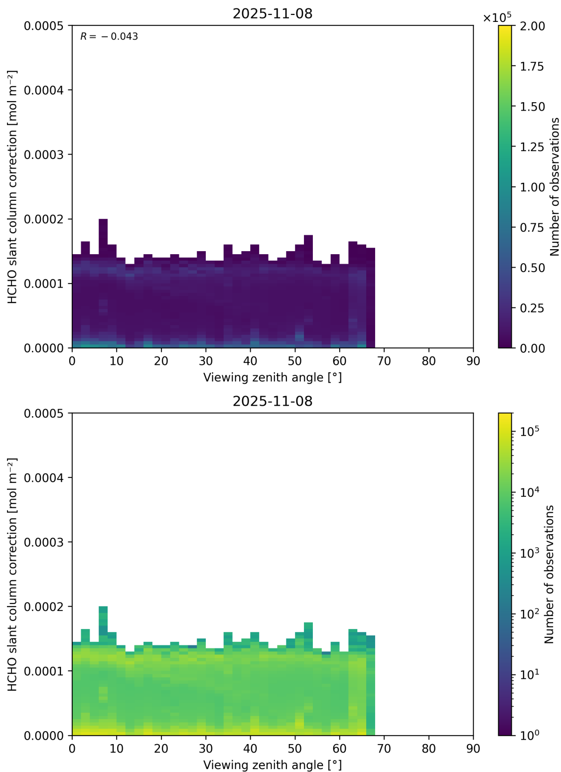
Figure 187: Scatter density plot of “Viewing zenith angle” against “HCHO slant column correction” for 2025-11-07 to 2025-11-09.
