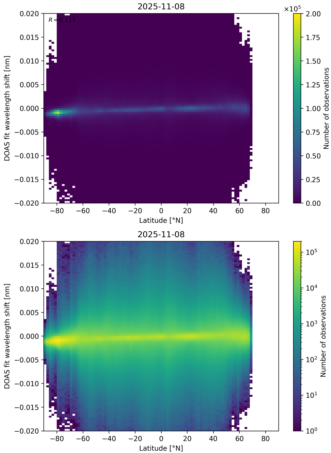
Figure 154: Scatter density plot of “Latitude” against “DOAS fit wavelength shift” for 2025-11-07 to 2025-11-09.
