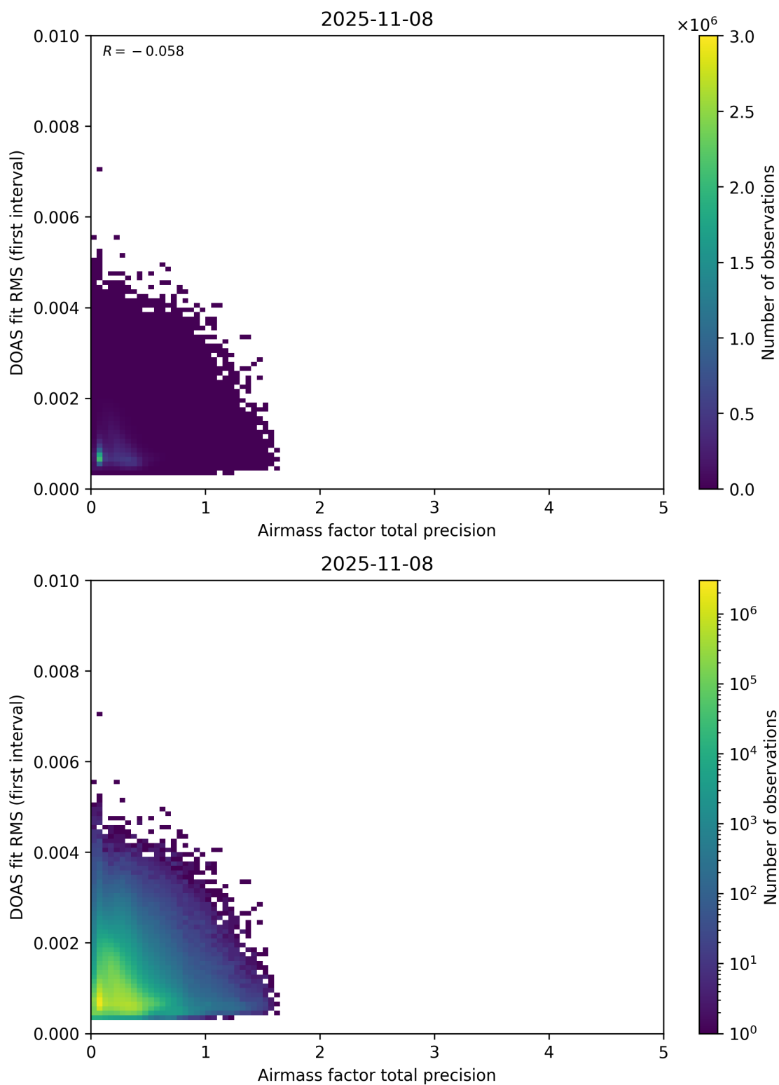
Figure 105: Scatter density plot of “Airmass factor total precision” against “DOAS fit RMS (first interval)” for 2025-11-07 to 2025-11-09.
