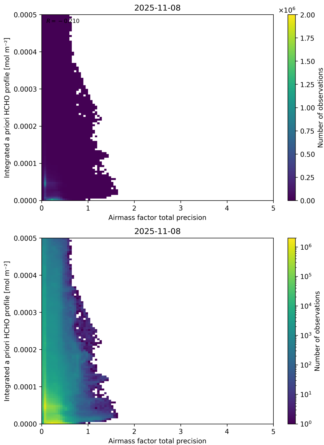
Figure 111: Scatter density plot of “Airmass factor total precision” against “Integrated a priori HCHO profile” for 2025-11-07 to 2025-11-09.
