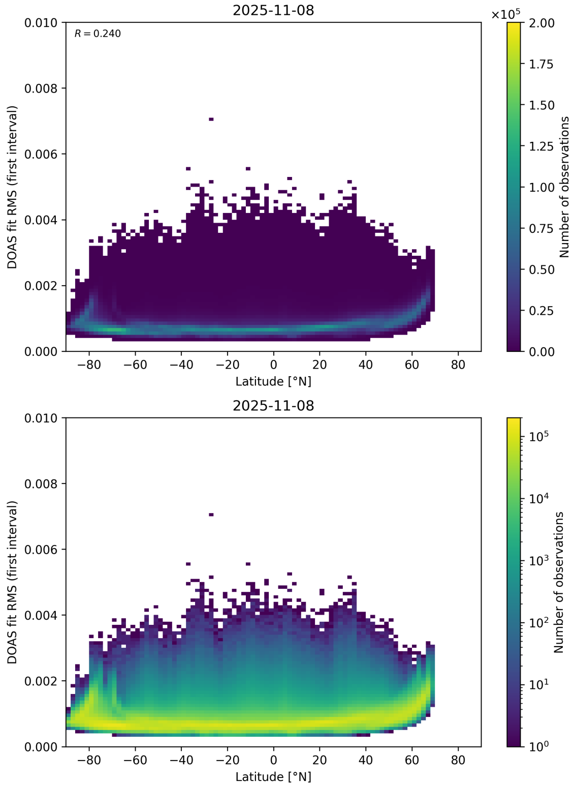
Figure 153: Scatter density plot of “Latitude” against “DOAS fit RMS (first interval)” for 2025-11-07 to 2025-11-09.
