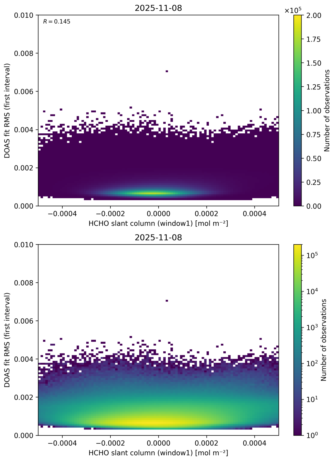
Figure 78: Scatter density plot of “HCHO slant column (window1)” against “DOAS fit RMS (first interval)” for 2025-11-07 to 2025-11-09.
