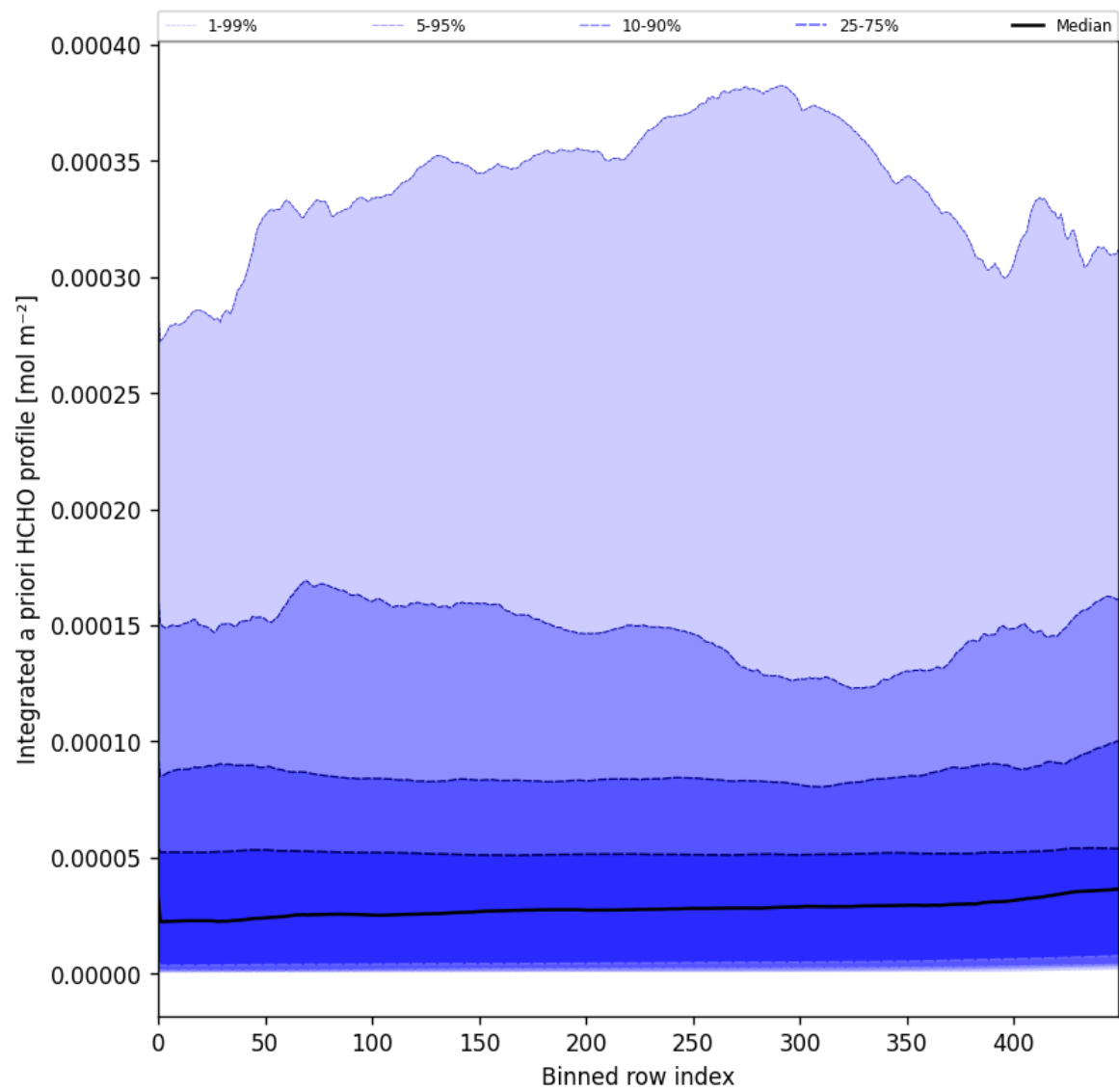
Figure 57: Along track statistics of “Integrated a priori HCHO profile” for 2025-11-07 to 2025-11-09
