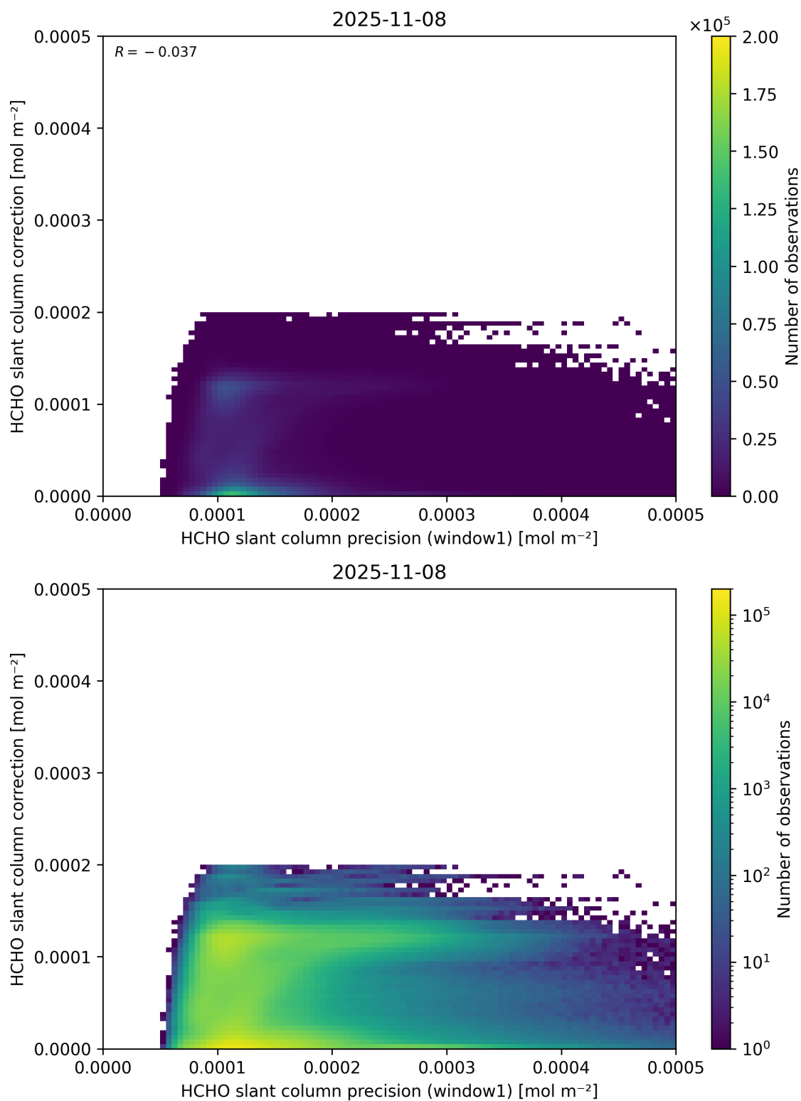
Figure 93: Scatter density plot of “HCHO slant column precision (window1)” against “HCHO slant column correction” for 2025-11-07 to 2025-11-09.
