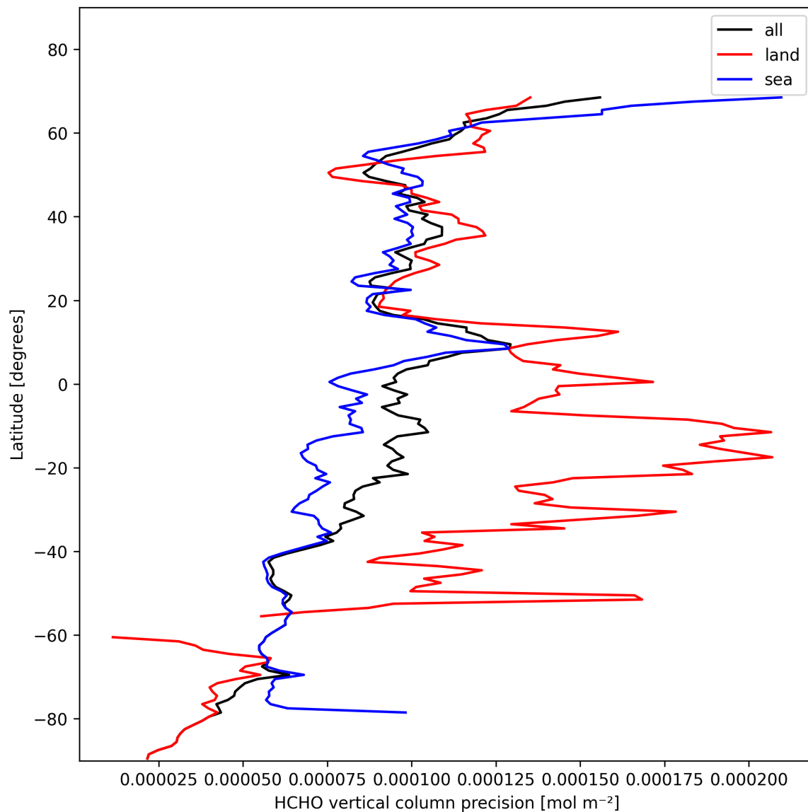
Figure 22: Zonal average of “HCHO vertical column precision” for 2025-11-07 to 2025-11-09.
