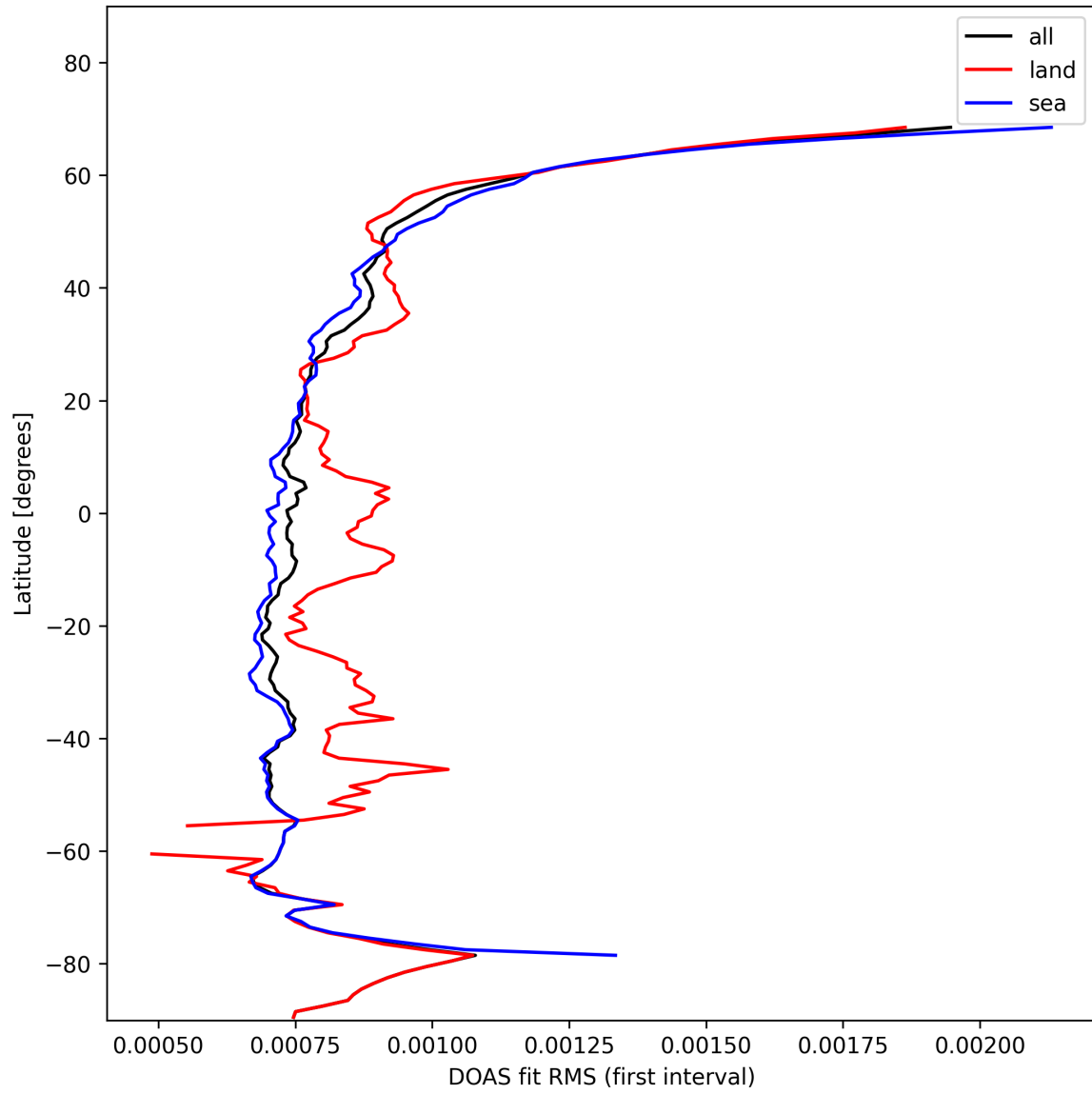
Figure 32: Zonal average of “DOAS fit RMS (first interval)” for 2025-11-07 to 2025-11-09.
