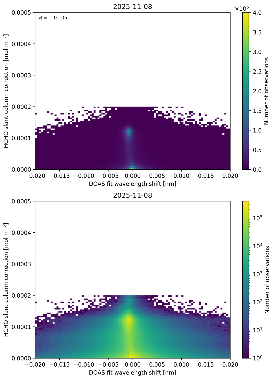
Figure 67: Scatter density plot of “DOAS fit wavelength shift” against “HCHO slant column correction” for 2025-11-07 to 2025-11-09.
