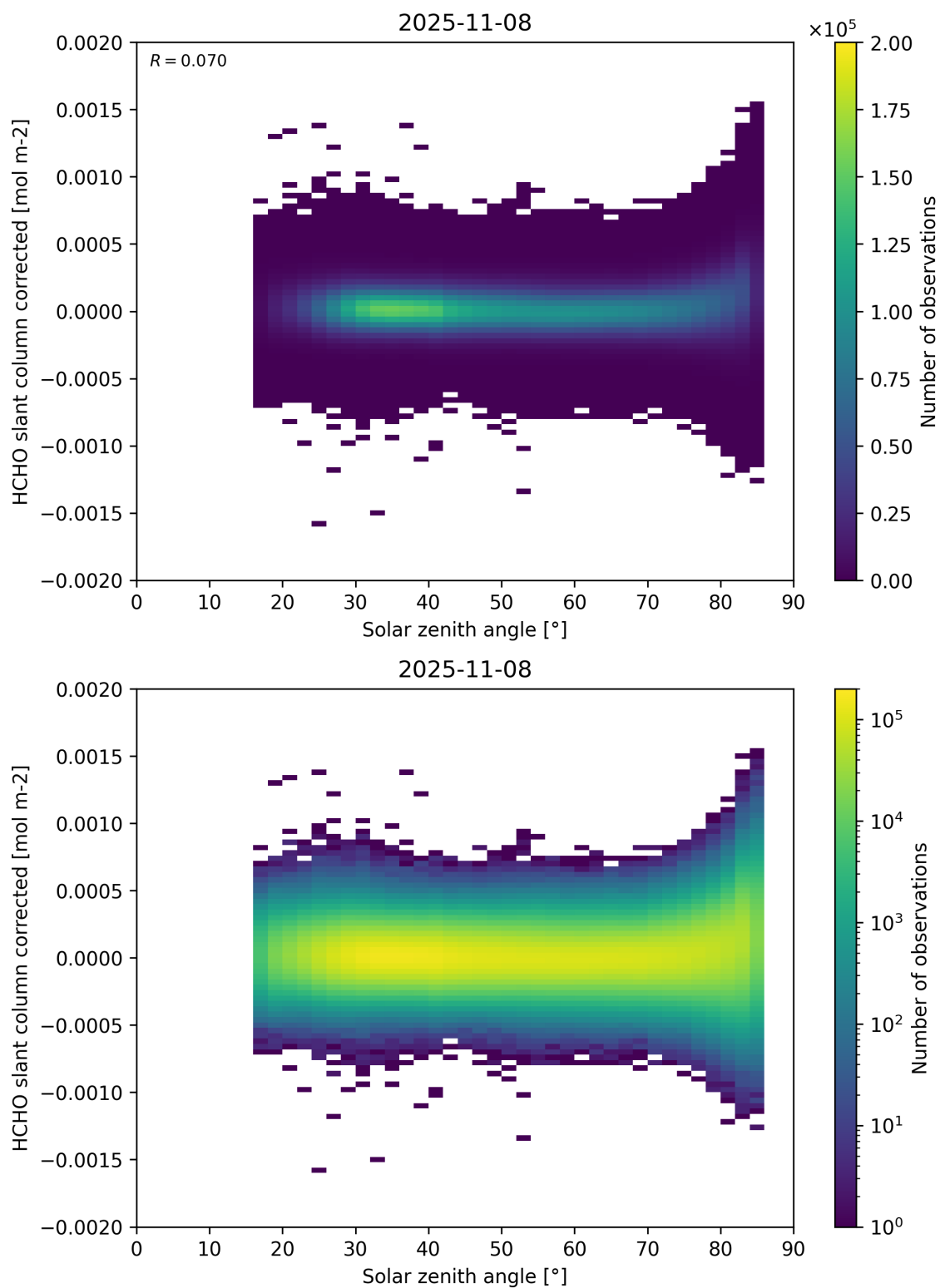
Figure 171: Scatter density plot of “Solar zenith angle” against “HCHO slant column corrected” for 2025-11-07 to 2025-11-09.
