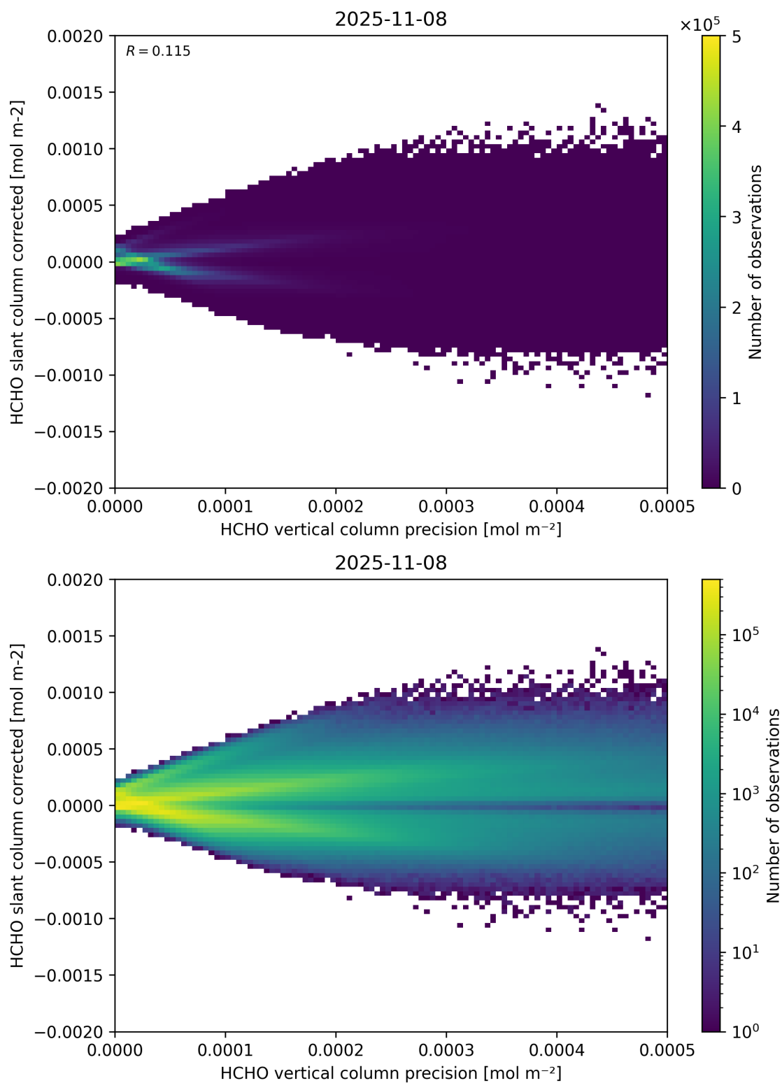
Figure 140: Scatter density plot of “HCHO vertical column precision” against “HCHO slant column corrected” for 2025-11-07 to 2025-11-09.
