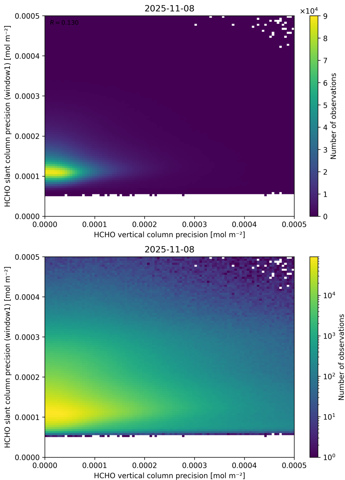
Figure 143: Scatter density plot of “HCHO vertical column precision” against “HCHO slant column precision (window1)” for 2025-11-07 to 2025-11-09.
