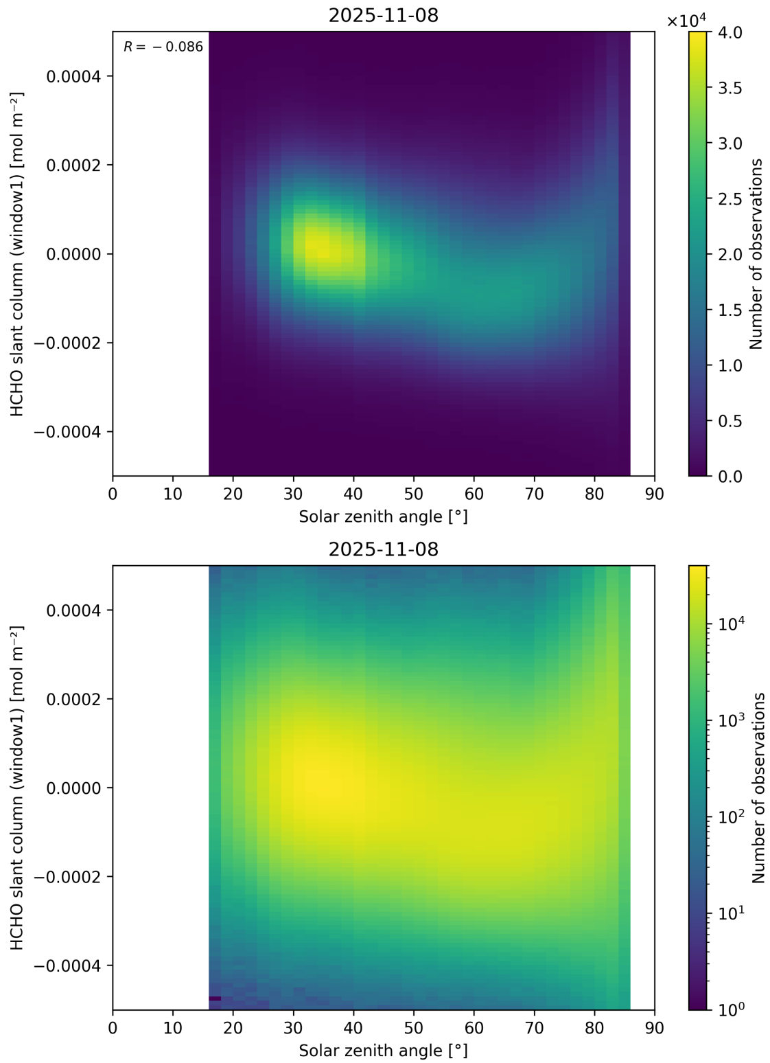
Figure 173: Scatter density plot of “Solar zenith angle” against “HCHO slant column (window1)” for 2025-11-07 to 2025-11-09.
