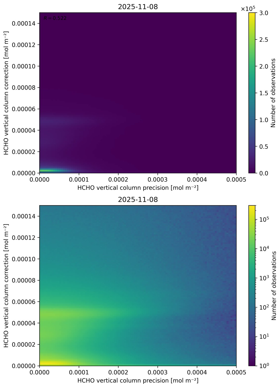
Figure 146: Scatter density plot of “HCHO vertical column precision” against “HCHO vertical column correction” for 2025-11-07 to 2025-11-09.
