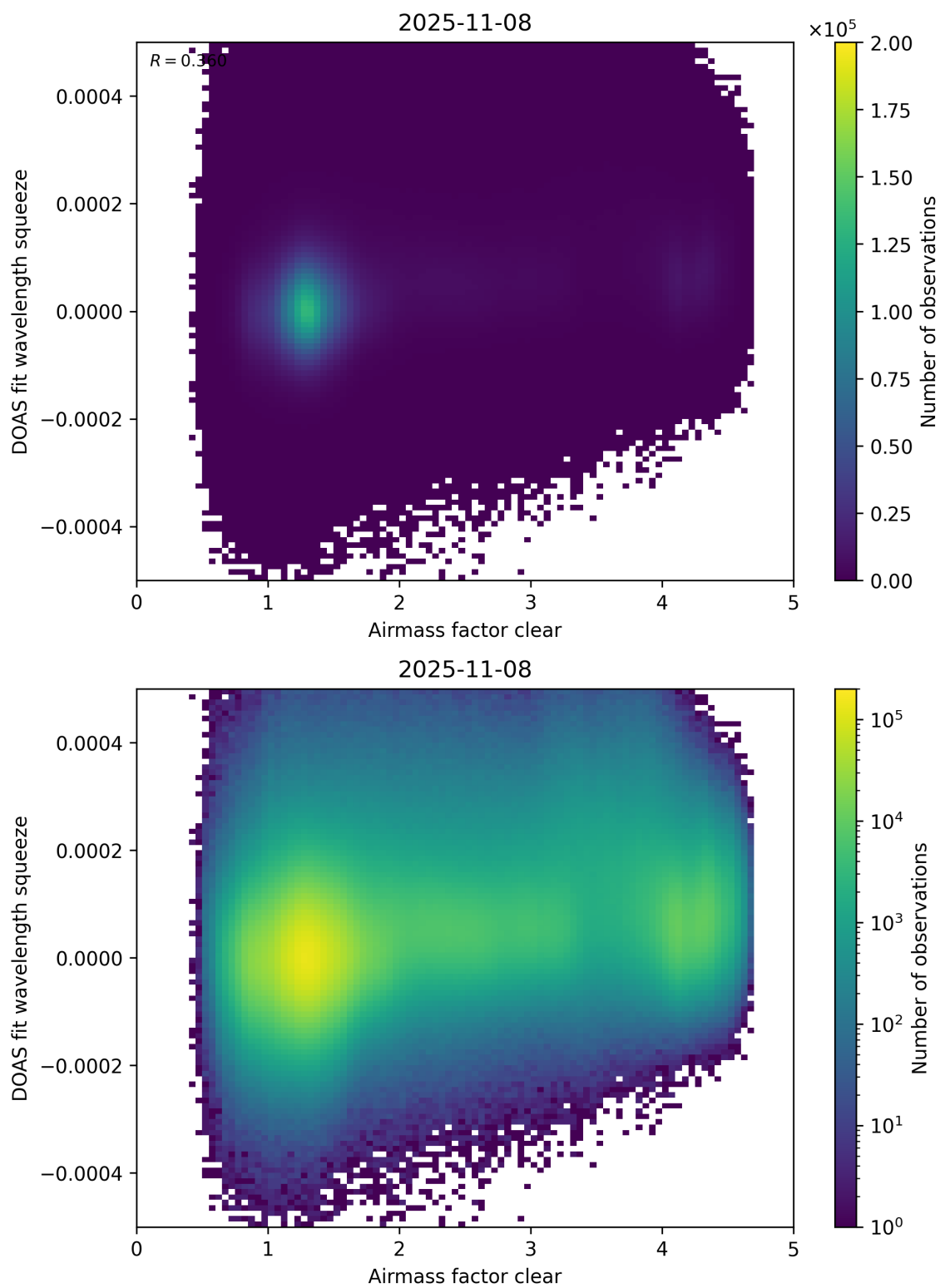
Figure 73: Scatter density plot of “Airmass factor clear” against “DOAS fit wavelength squeeze” for 2025-11-07 to 2025-11-09.
