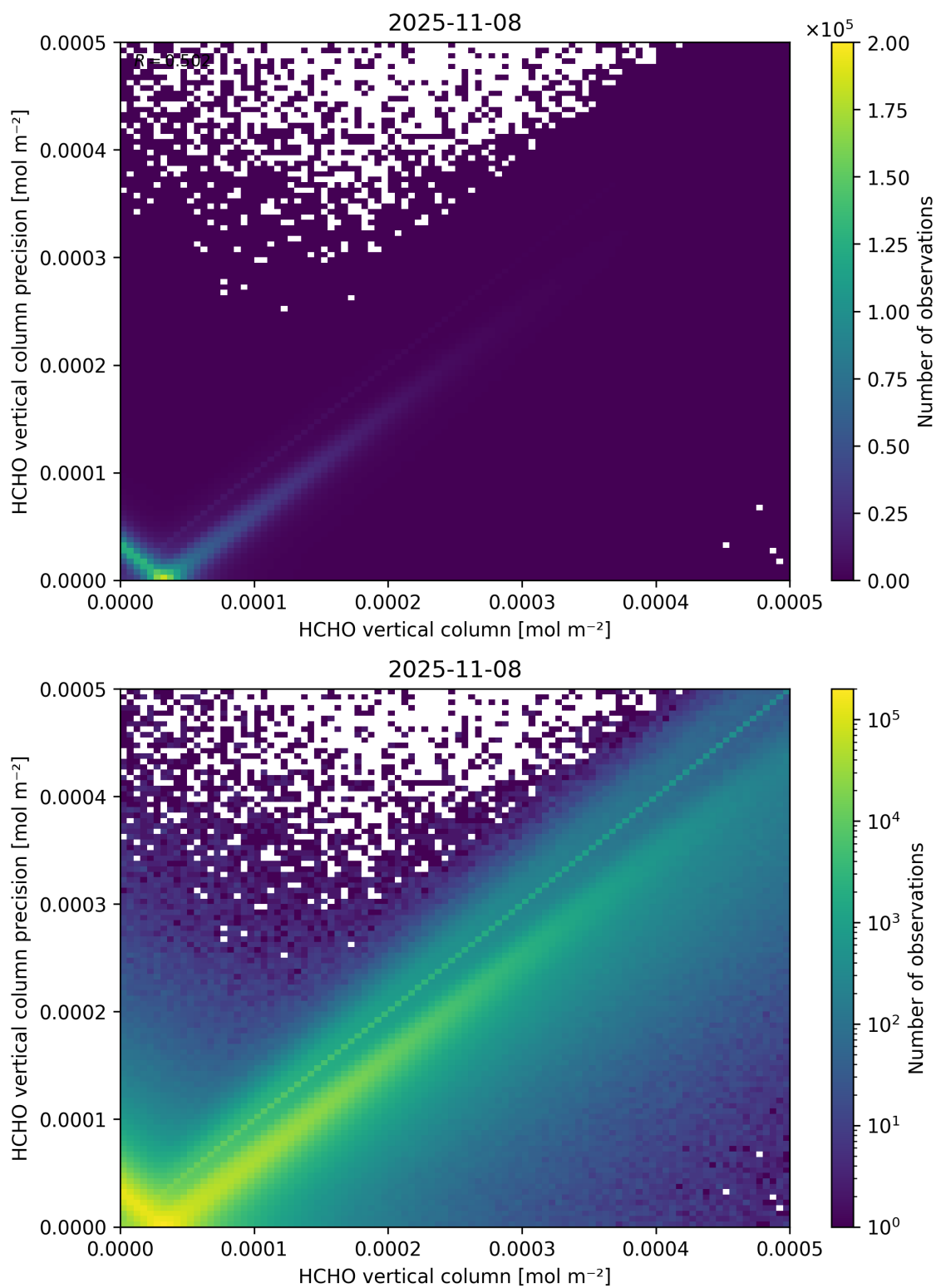
Figure 134: Scatter density plot of “HCHO vertical column” against “HCHO vertical column precision” for 2025-11-07 to 2025-11-09.
