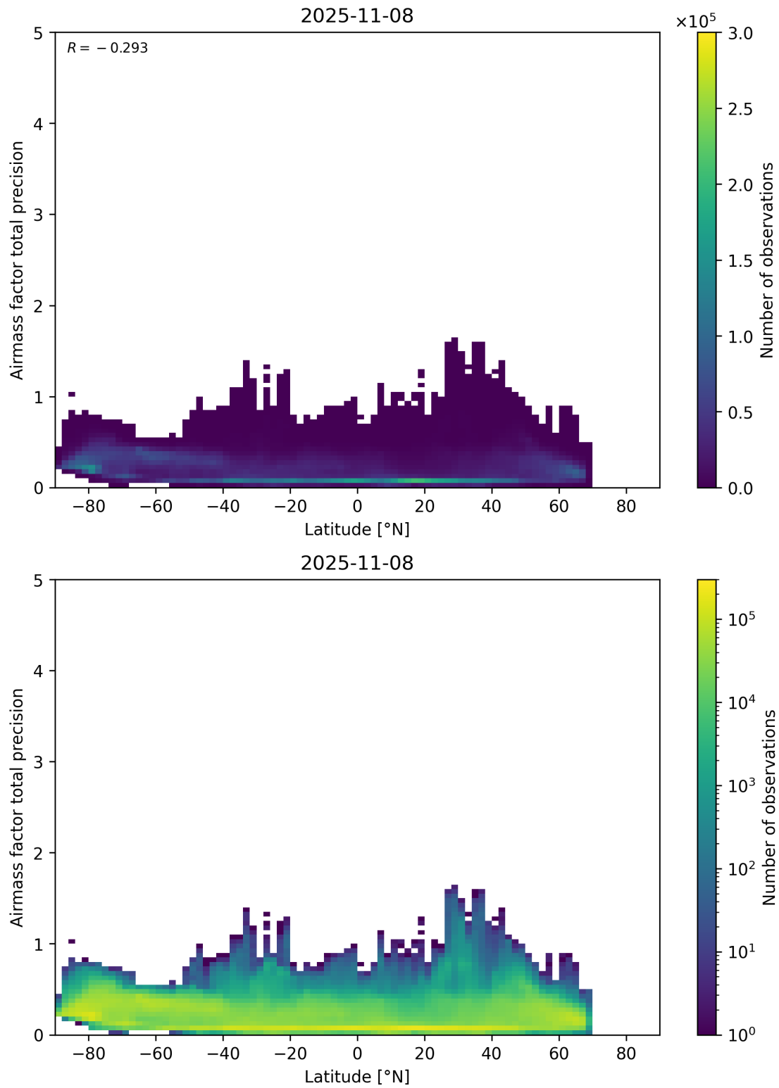
Figure 162: Scatter density plot of “Latitude” against “Airmass factor total precision” for 2025-11-07 to 2025-11-09.
