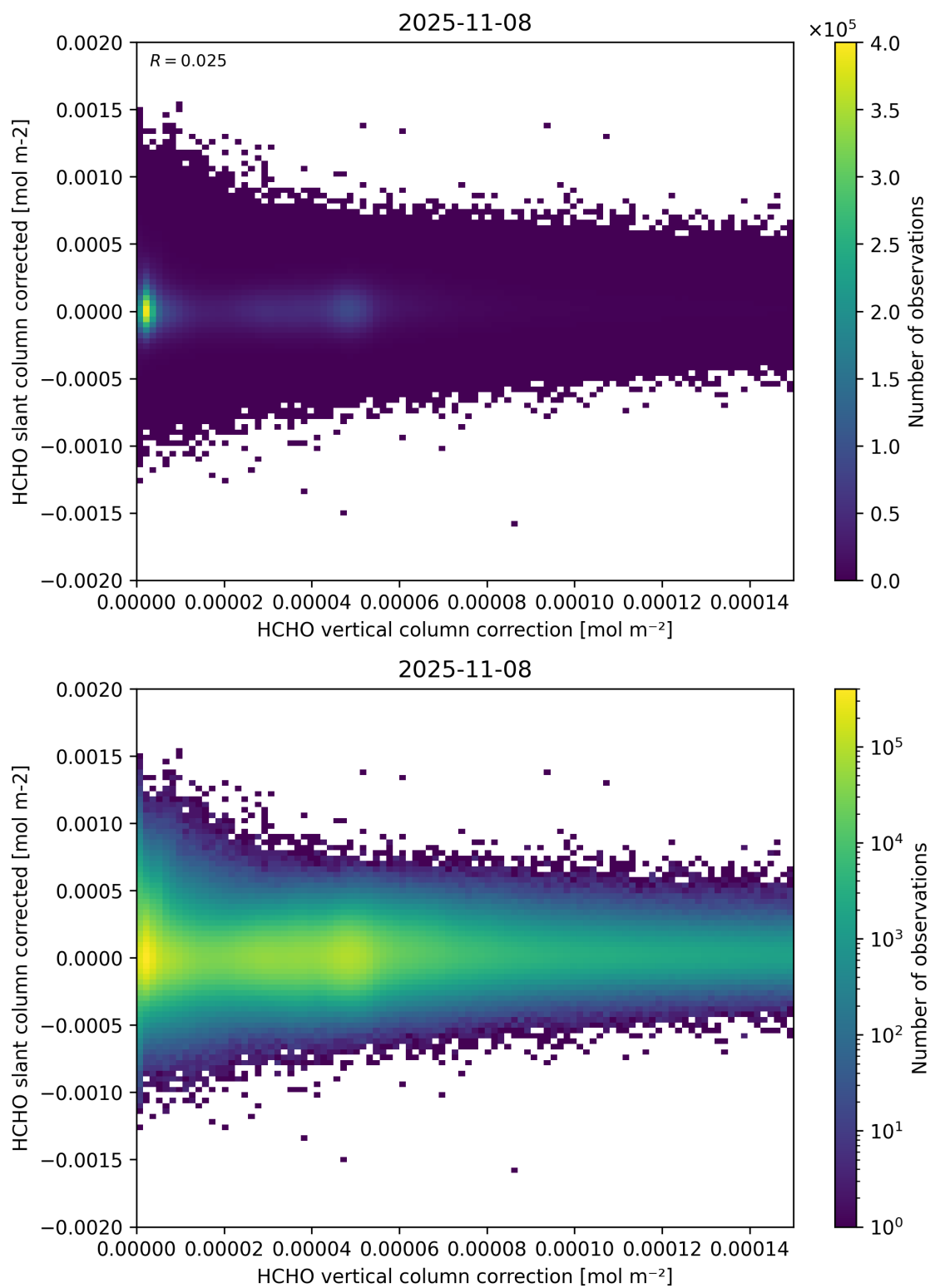
Figure 116: Scatter density plot of “HCHO vertical column correction” against “HCHO slant column corrected” for 2025-11-07 to 2025-11-09.
