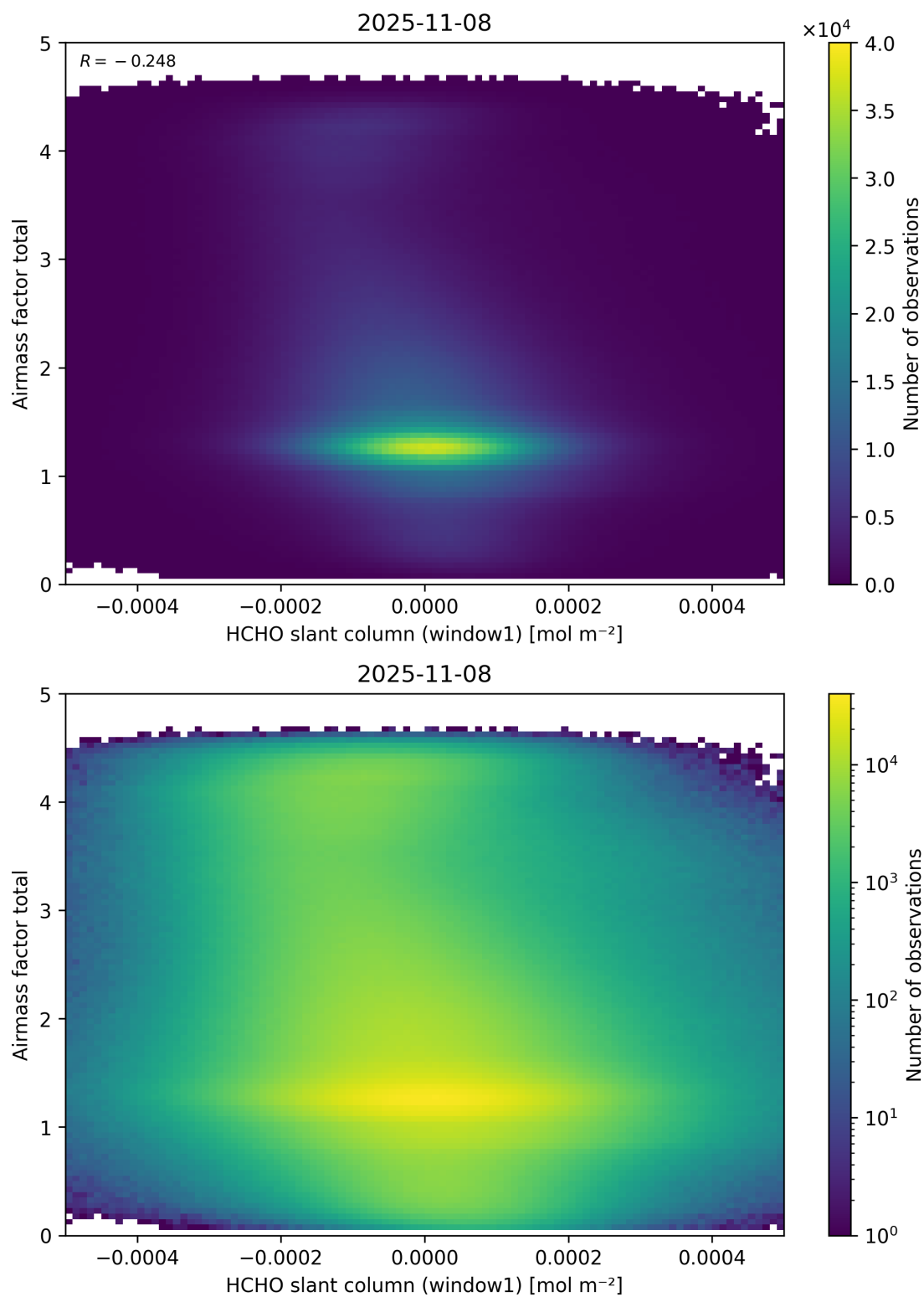
Figure 85: Scatter density plot of “HCHO slant column (window1)” against “Airmass factor total” for 2025-11-07 to 2025-11-09.
