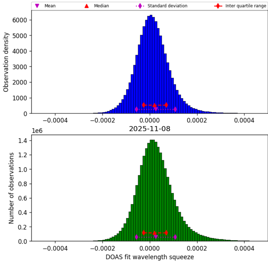
Figure 45: Histogram of “DOAS fit wavelength squeeze” for 2025-11-07 to 2025-11-09
