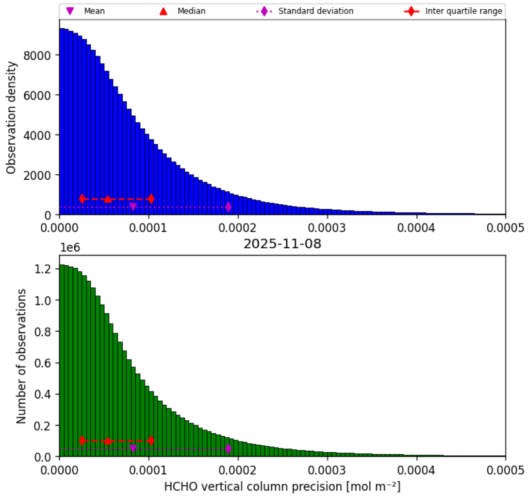
Figure 36: Histogram of “HCHO vertical column precision” for 2025-11-07 to 2025-11-09
