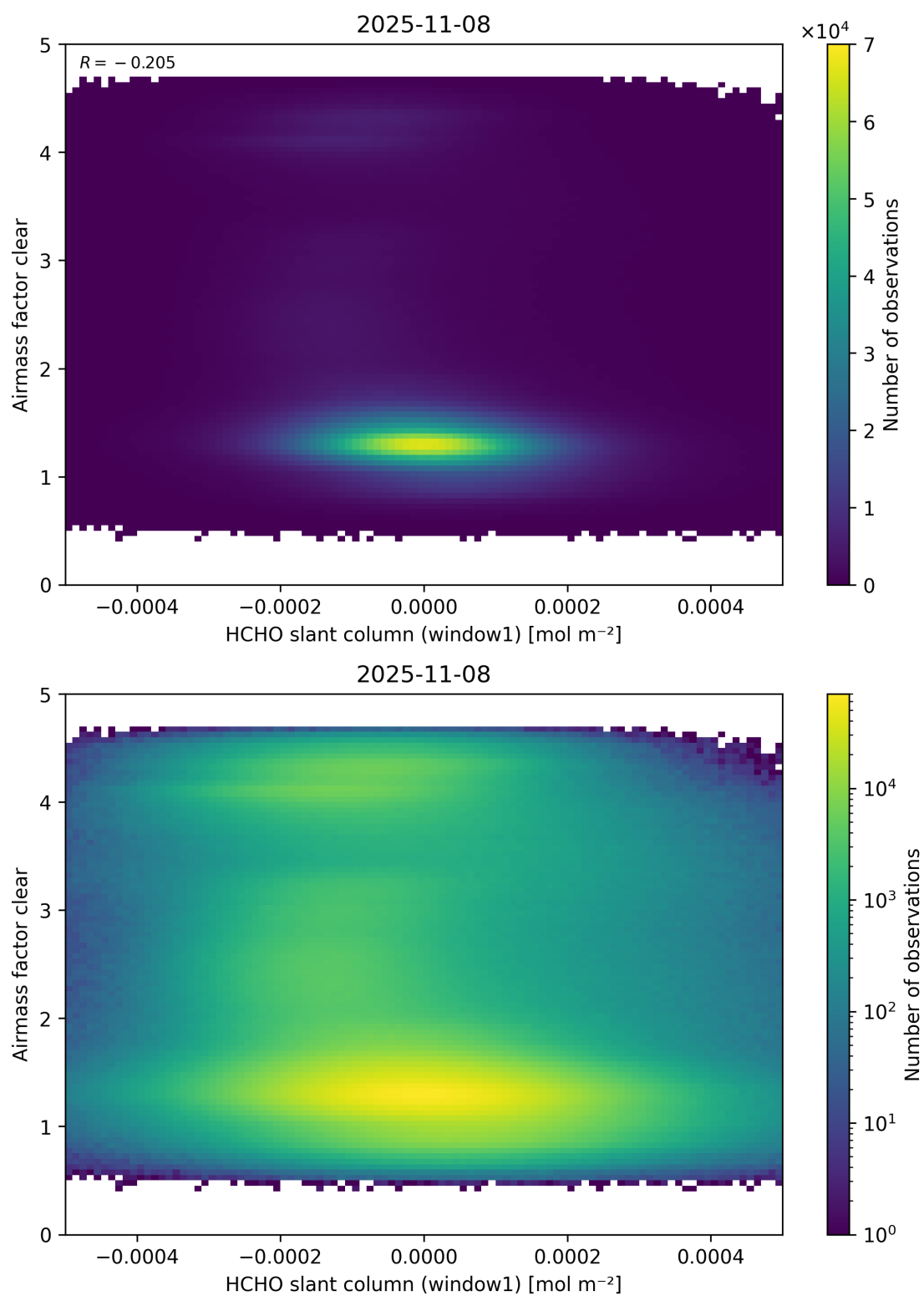
Figure 81: Scatter density plot of “HCHO slant column (window1)” against “Airmass factor clear” for 2025-11-07 to 2025-11-09.
