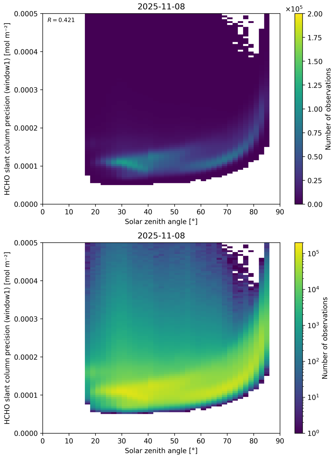
Figure 174: Scatter density plot of “Solar zenith angle” against “HCHO slant column precision (window1)” for 2025-11-07 to 2025-11-09.
