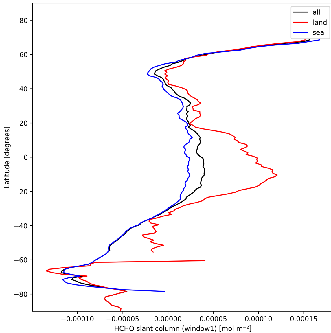
Figure 24: Zonal average of “HCHO slant column (window1)” for 2025-11-07 to 2025-11-09.
