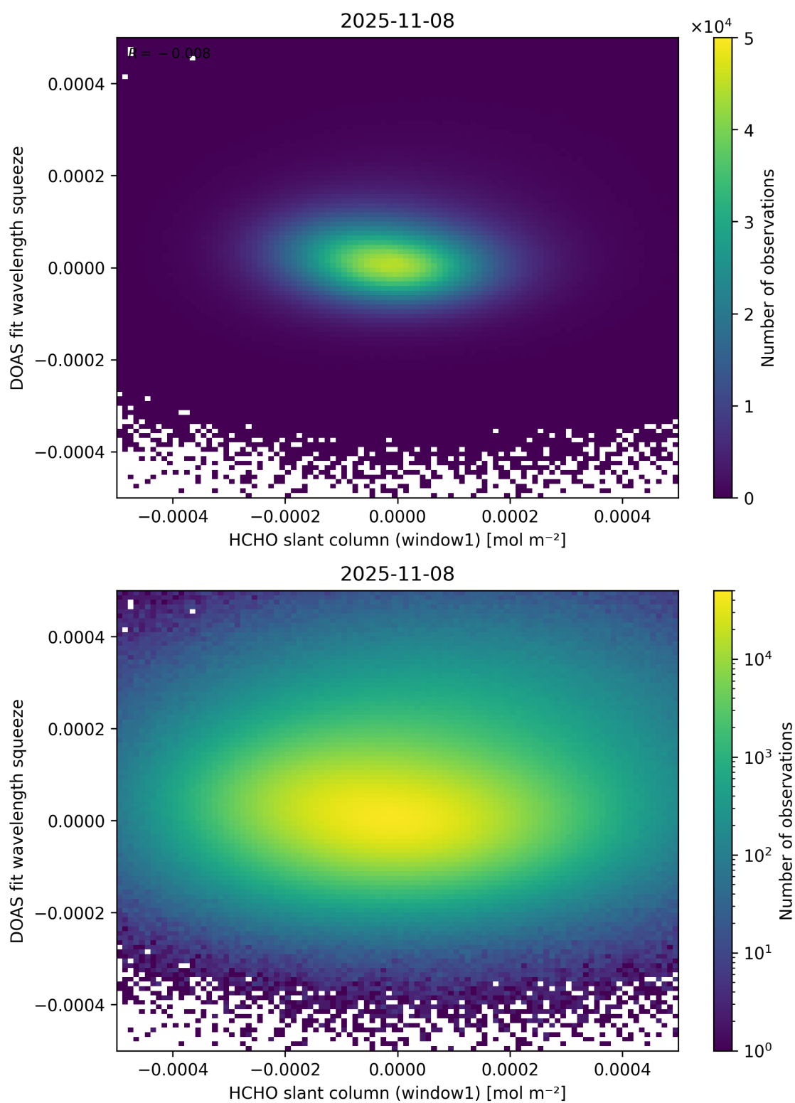
Figure 80: Scatter density plot of “HCHO slant column (window1)” against “DOAS fit wavelength squeeze” for 2025-11-07 to 2025-11-09.
