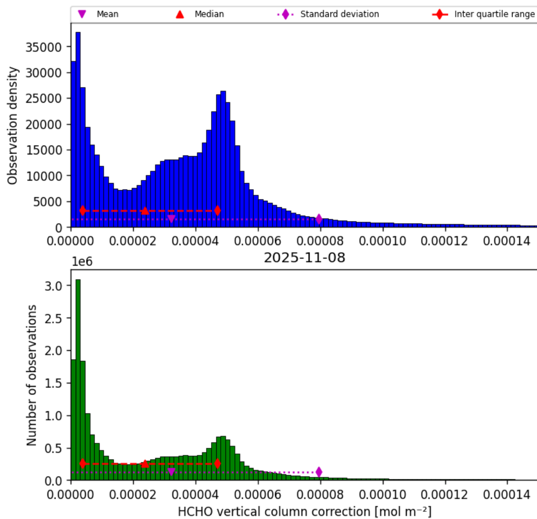
Figure 37: Histogram of “HCHO vertical column correction” for 2025-11-07 to 2025-11-09
