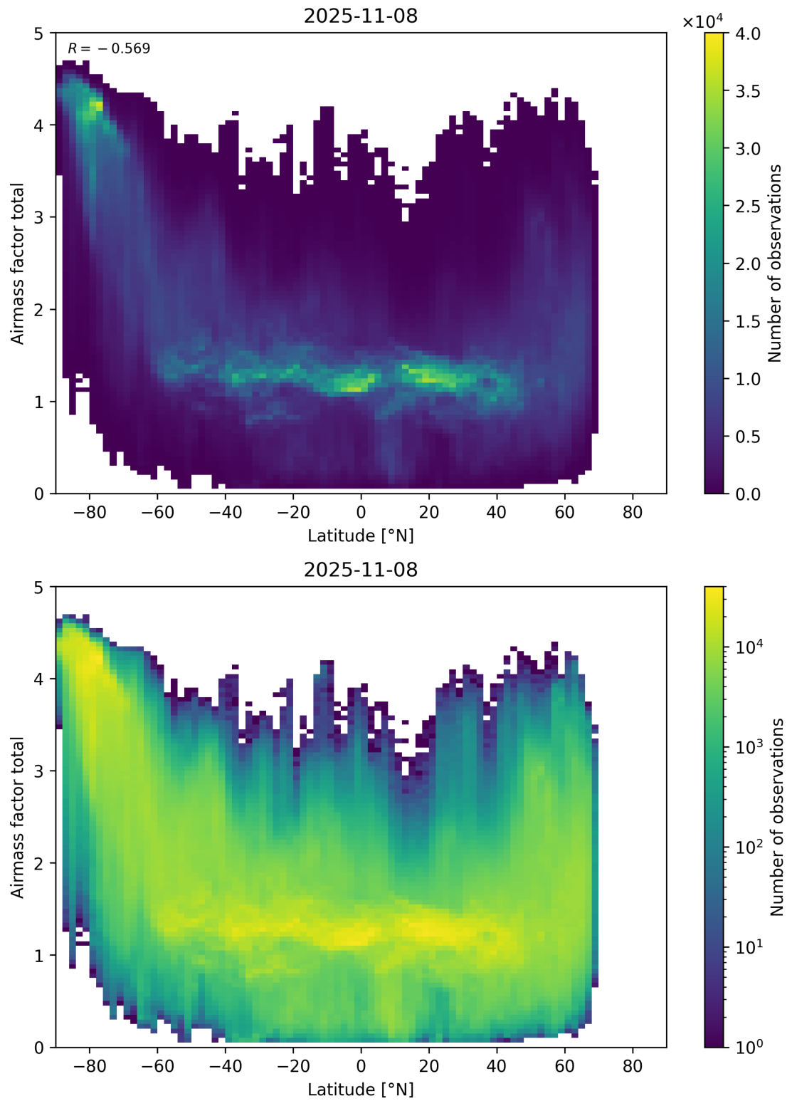
Figure 161: Scatter density plot of “Latitude” against “Airmass factor total” for 2025-11-07 to 2025-11-09.
