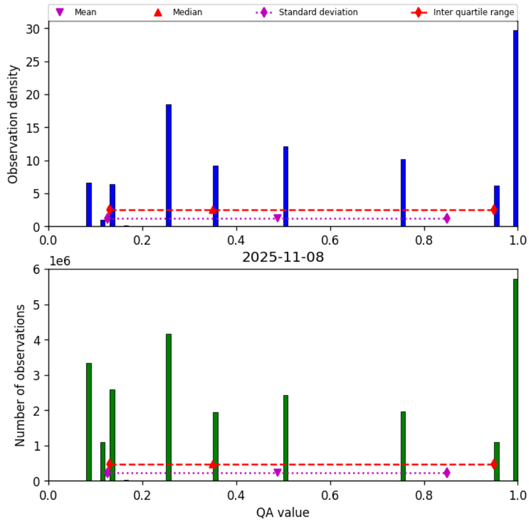
Figure 34: Histogram of “QA value” for 2025-11-07 to 2025-11-09
