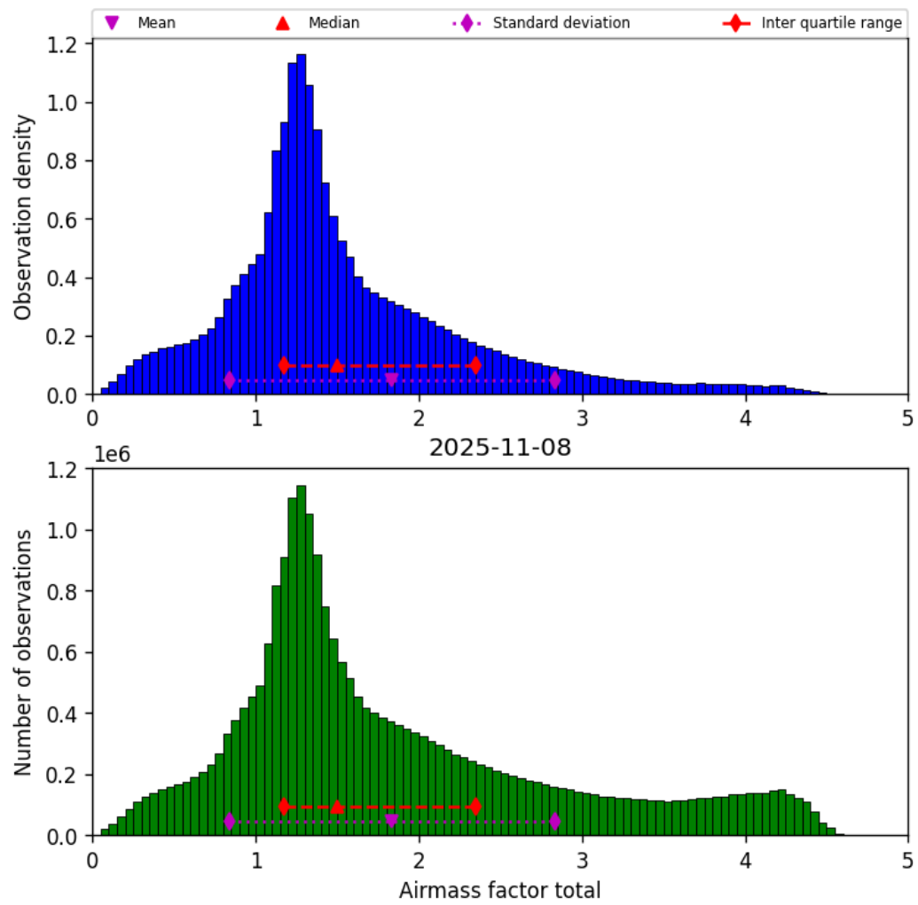
Figure 40: Histogram of “Airmass factor total” for 2025-11-07 to 2025-11-09
