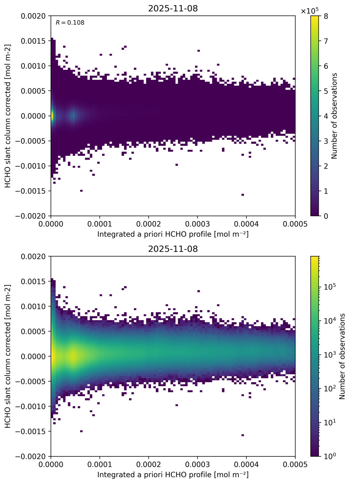
Figure 151: Scatter density plot of “Integrated a priori HCHO profile” against “HCHO slant column corrected” for 2025-11-07 to 2025-11-09.
