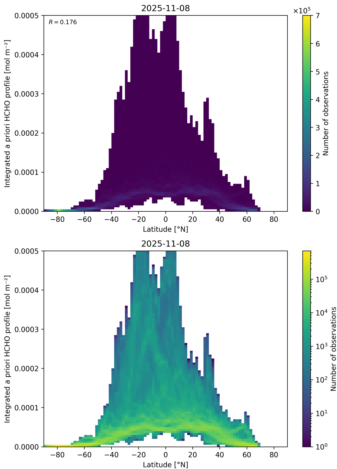
Figure 166: Scatter density plot of “Latitude” against “Integrated a priori HCHO profile” for 2025-11-07 to 2025-11-09.
