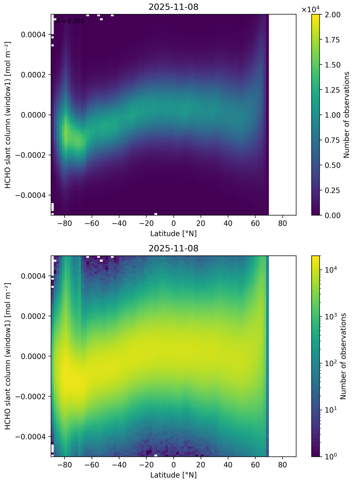
Figure 159: Scatter density plot of “Latitude” against “HCHO slant column (window1)” for 2025-11-07 to 2025-11-09.
