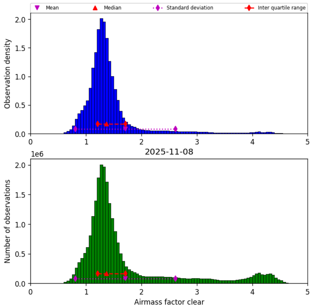
Figure 42: Histogram of “Airmass factor clear” for 2025-11-07 to 2025-11-09
