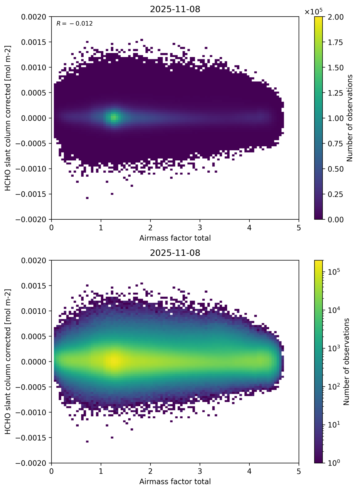
Figure 101: Scatter density plot of “Airmass factor total” against “HCHO slant column corrected” for 2025-11-07 to 2025-11-09.
