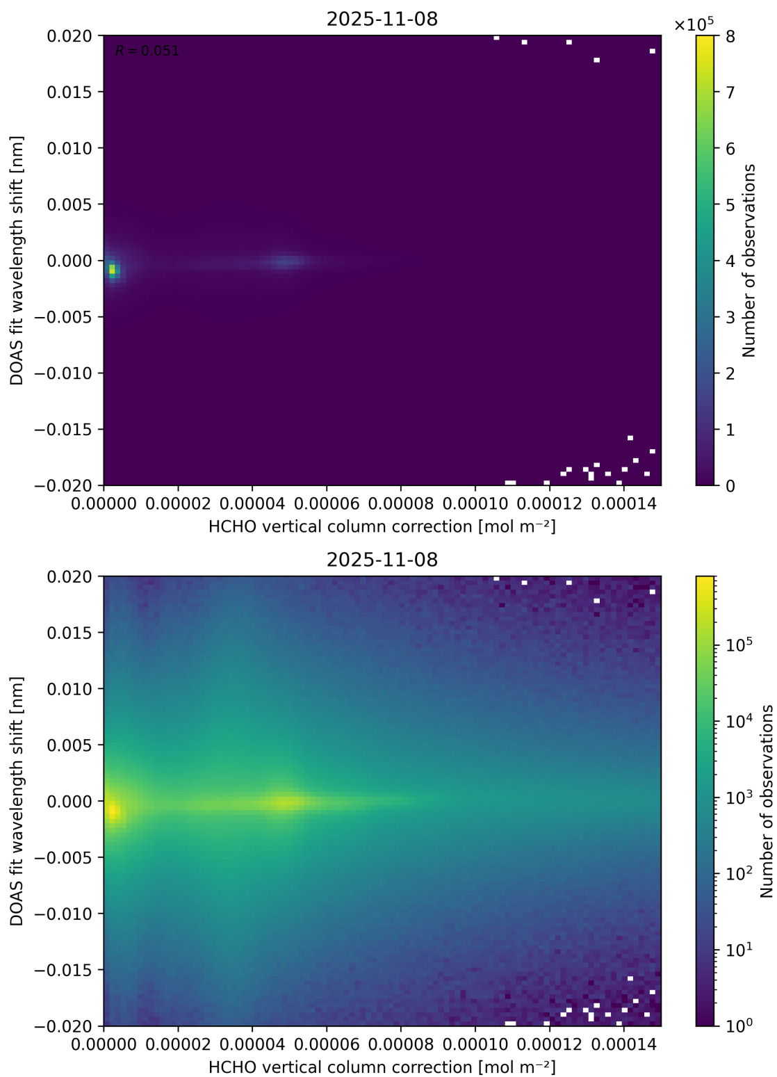
Figure 113: Scatter density plot of “HCHO vertical column correction” against “DOAS fit wavelength shift” for 2025-11-07 to 2025-11-09.
