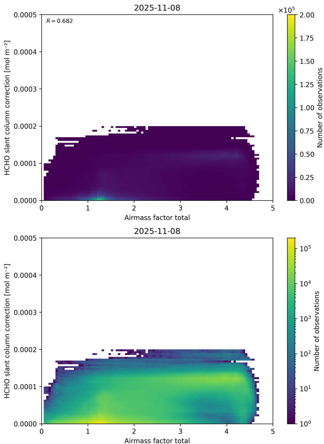
Figure 102: Scatter density plot of “Airmass factor total” against “HCHO slant column correction” for 2025-11-07 to 2025-11-09.
