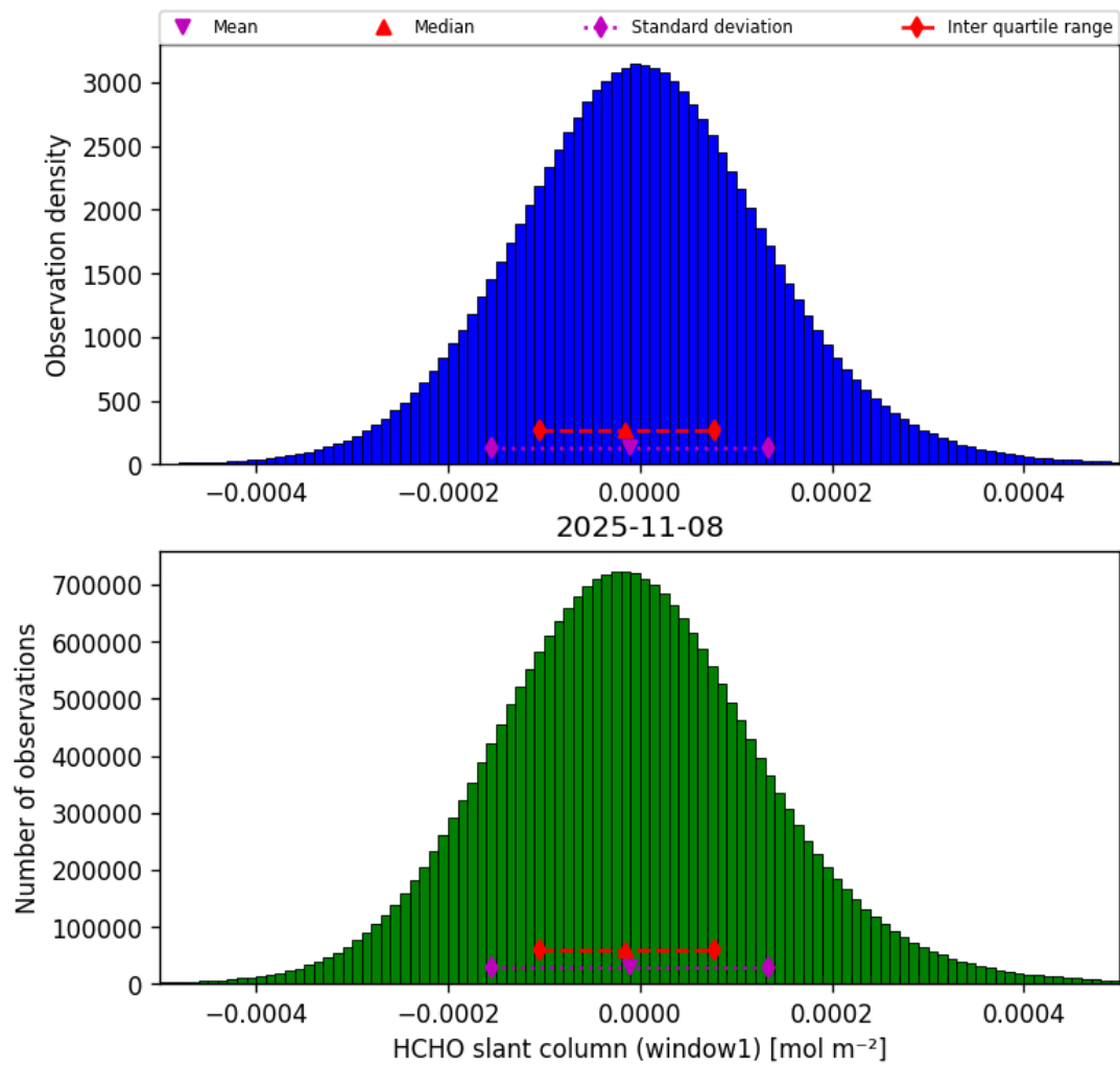
Figure 38: Histogram of “HCHO slant column (window1)” for 2025-11-07 to 2025-11-09
