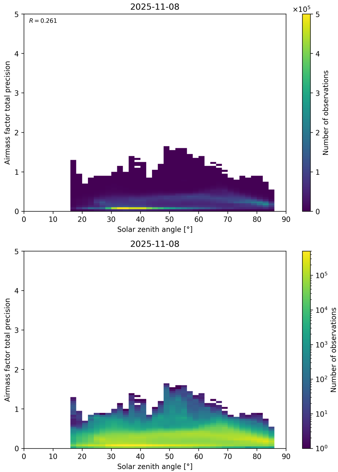
Figure 176: Scatter density plot of “Solar zenith angle” against “Airmass factor total precision” for 2025-11-07 to 2025-11-09.
