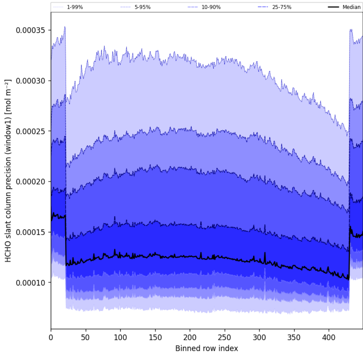
Figure 53: Along track statistics of “HCHO slant column precision (window1)” for 2025-11-07 to 2025-11-09
