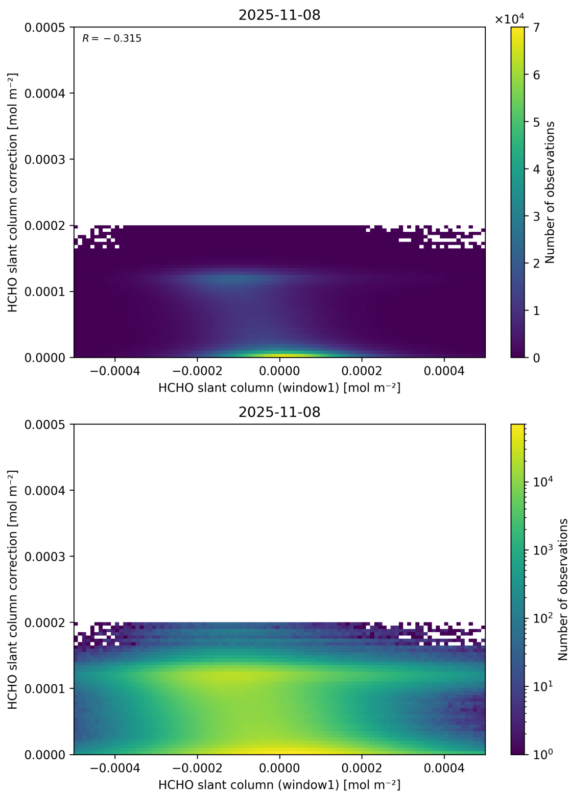
Figure 83: Scatter density plot of “HCHO slant column (window1)” against “HCHO slant column correction” for 2025-11-07 to 2025-11-09.
