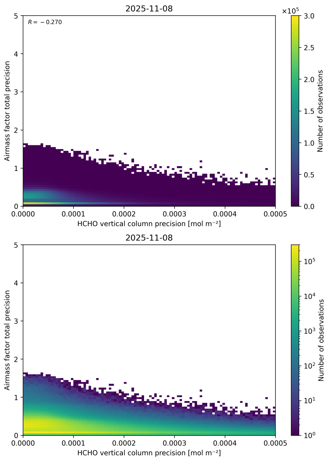
Figure 145: Scatter density plot of “HCHO vertical column precision” against “Airmass factor total precision” for 2025-11-07 to 2025-11-09.
