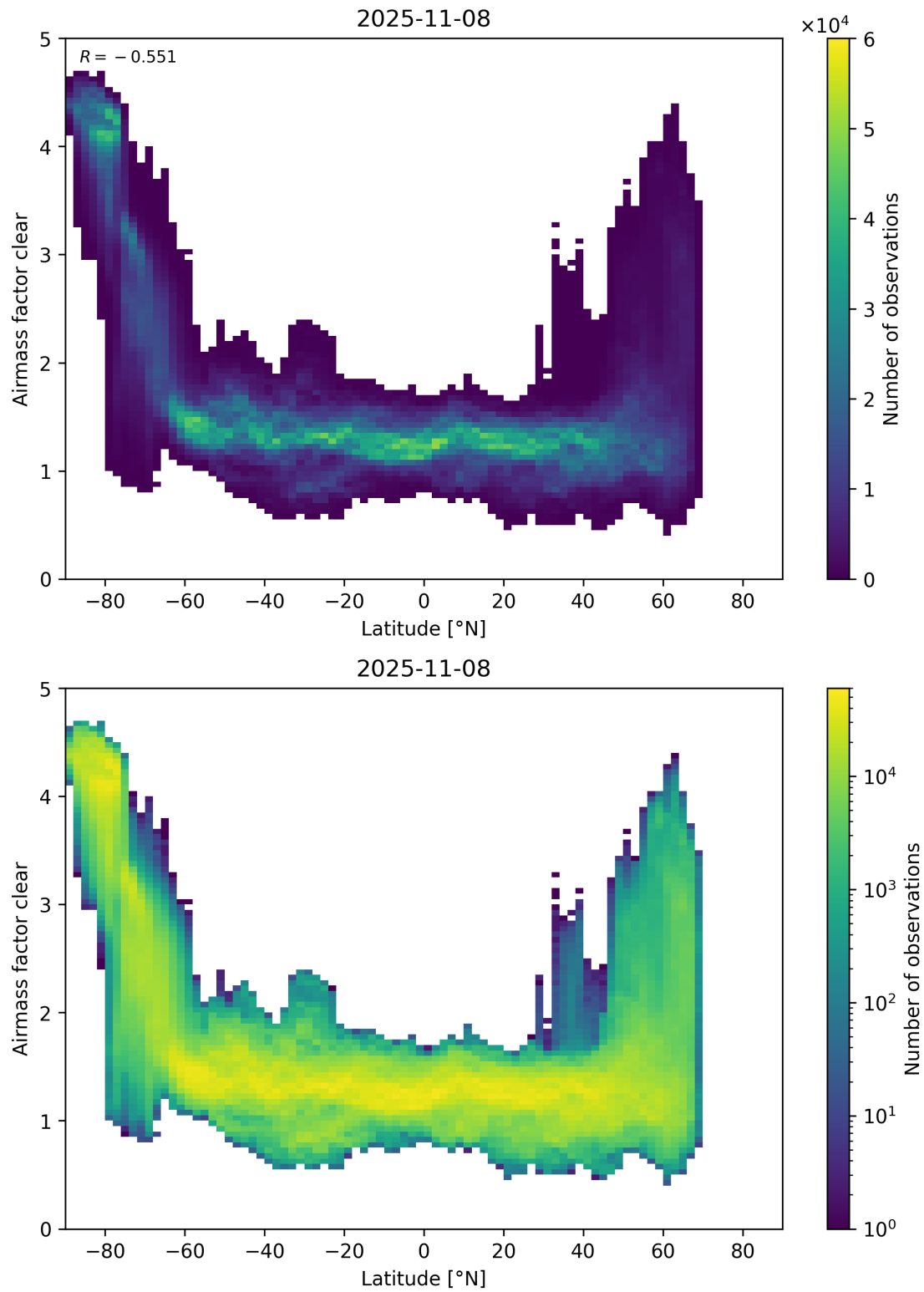
Figure 156: Scatter density plot of “Latitude” against “Airmass factor clear” for 2025-11-07 to 2025-11-09.
