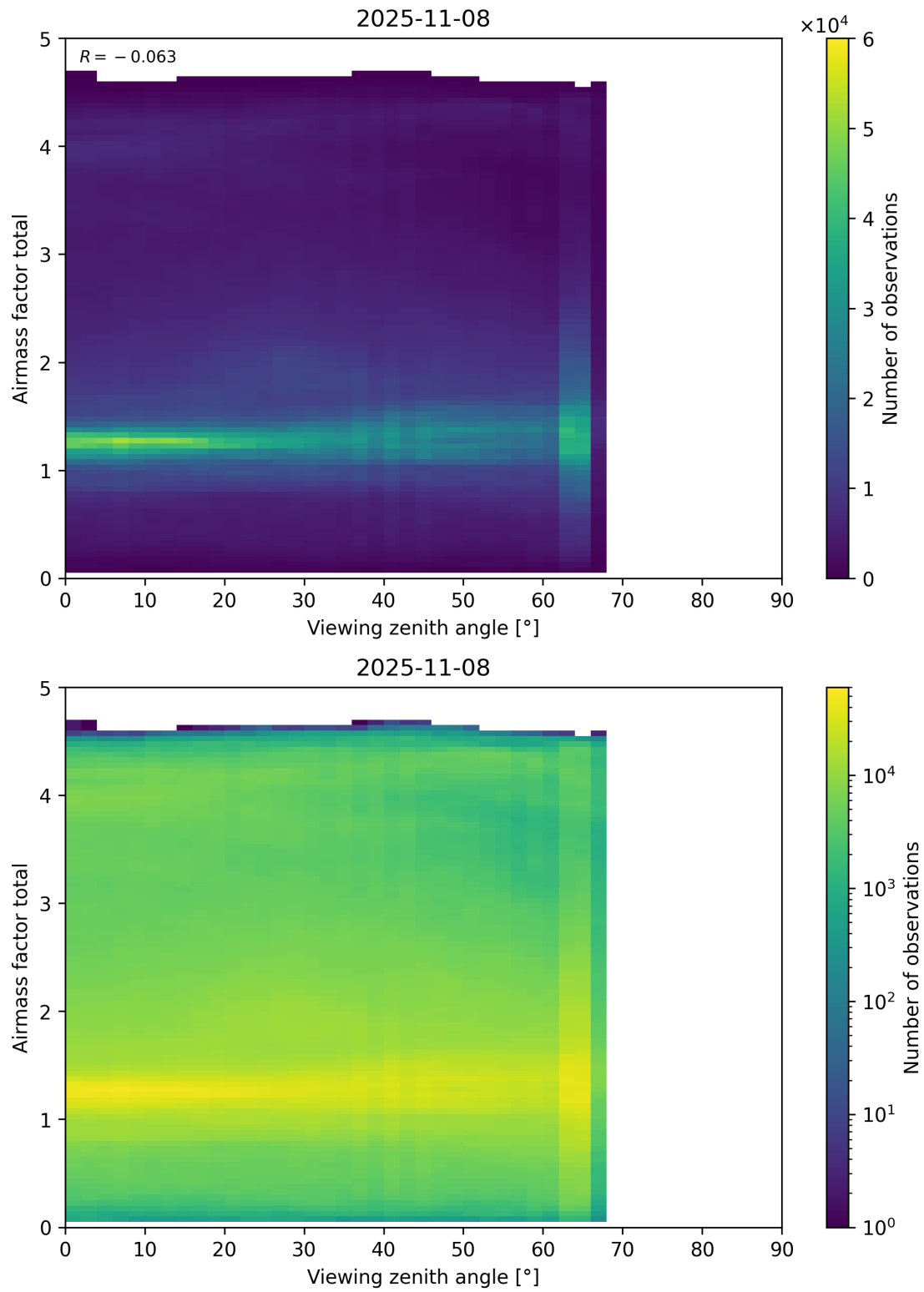
Figure 190: Scatter density plot of “Viewing zenith angle” against “Airmass factor total” for 2025-11-07 to 2025-11-09.
