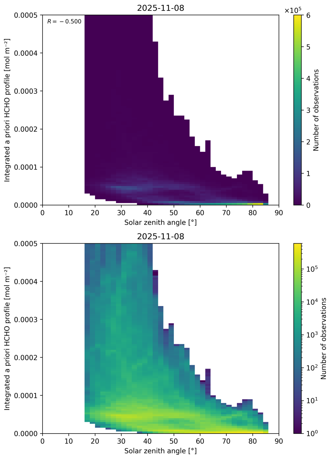
Figure 180: Scatter density plot of “Solar zenith angle” against “Integrated a priori HCHO profile” for 2025-11-07 to 2025-11-09.
