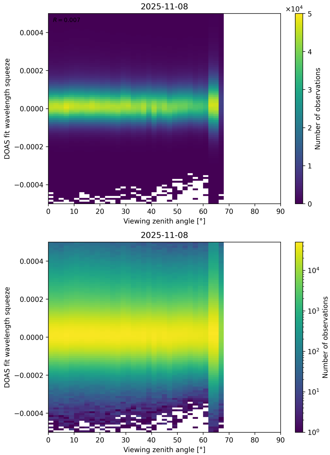
Figure 184: Scatter density plot of “Viewing zenith angle” against “DOAS fit wavelength squeeze” for 2025-11-07 to 2025-11-09.
