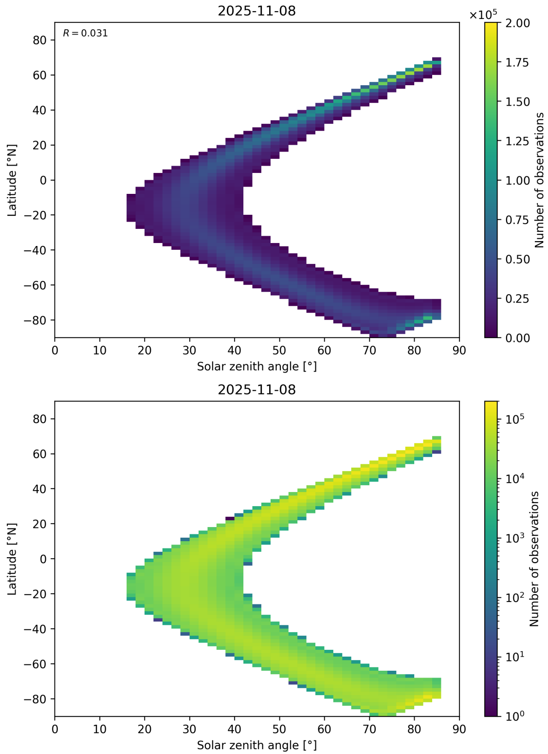
Figure 181: Scatter density plot of “Solar zenith angle” against “Latitude” for 2025-11-07 to 2025-11-09.
