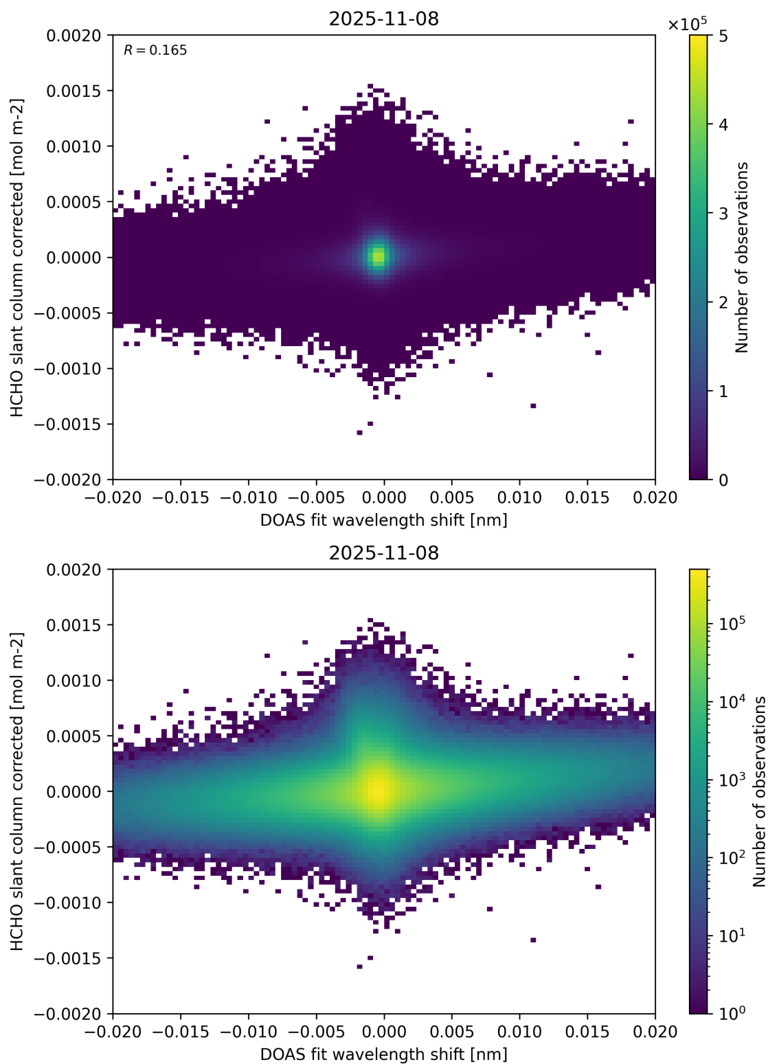
Figure 66: Scatter density plot of “DOAS fit wavelength shift” against “HCHO slant column corrected” for 2025-11-07 to 2025-11-09.
