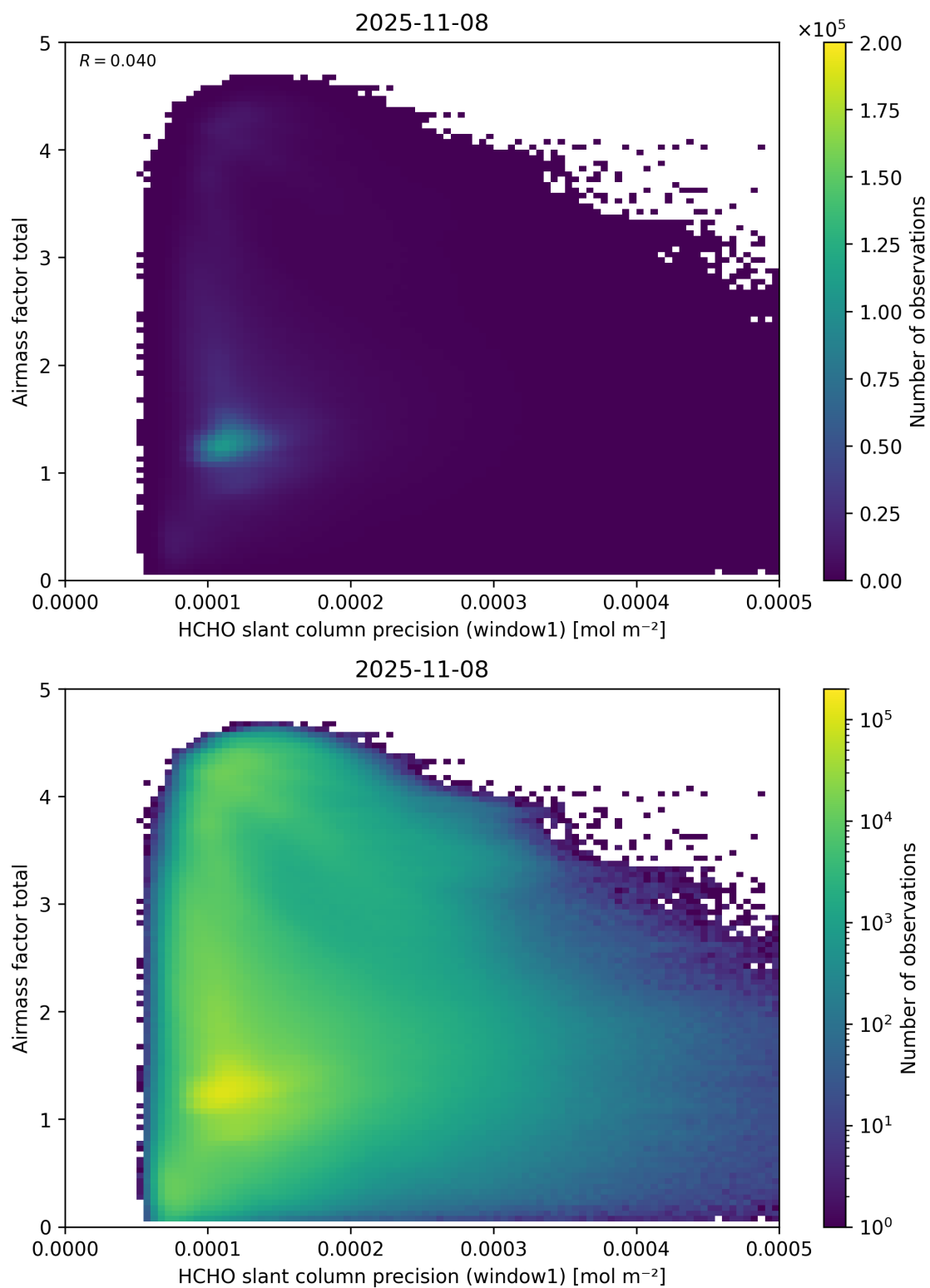
Figure 94: Scatter density plot of “HCHO slant column precision (window1)” against “Airmass factor total” for 2025-11-07 to 2025-11-09.
