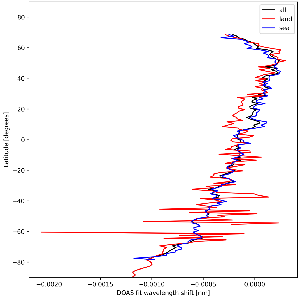
Figure 30: Zonal average of “DOAS fit wavelength shift” for 2025-11-07 to 2025-11-09.
