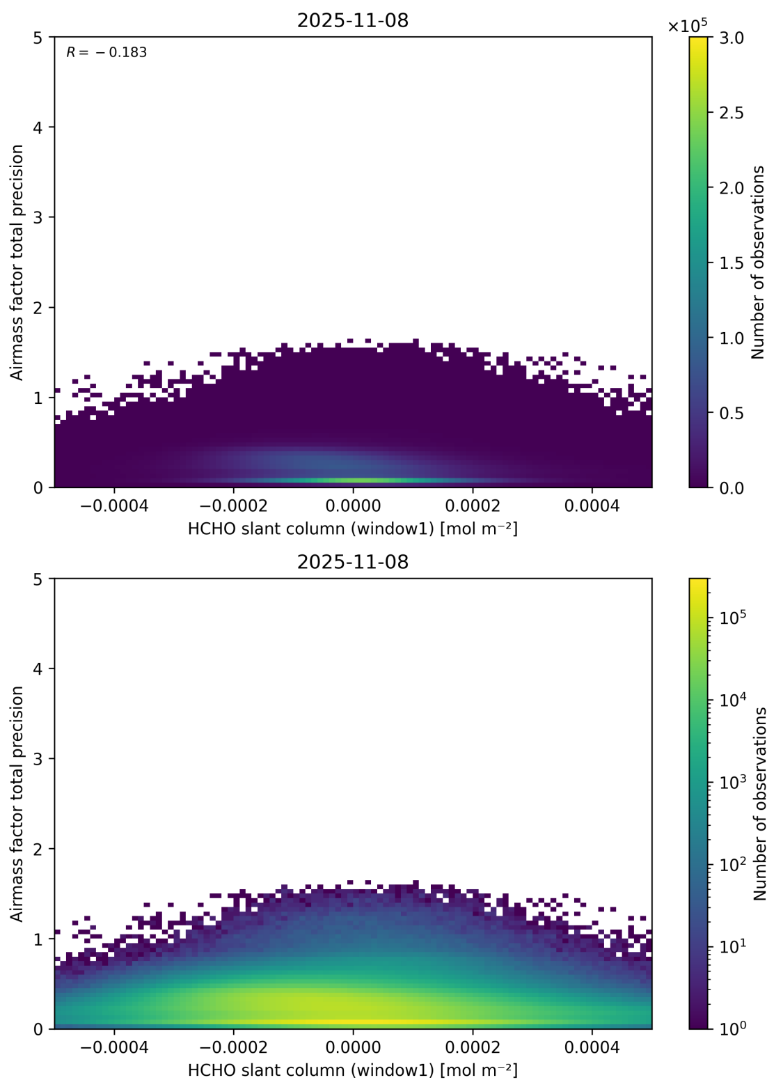
Figure 86: Scatter density plot of “HCHO slant column (window1)” against “Airmass factor total precision” for 2025-11-07 to 2025-11-09.
