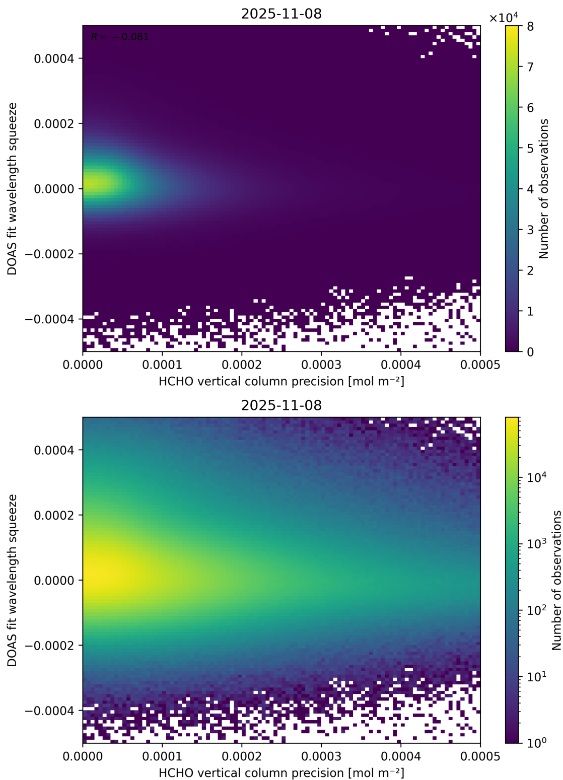
Figure 138: Scatter density plot of “HCHO vertical column precision” against “DOAS fit wavelength squeeze” for 2025-11-07 to 2025-11-09.
