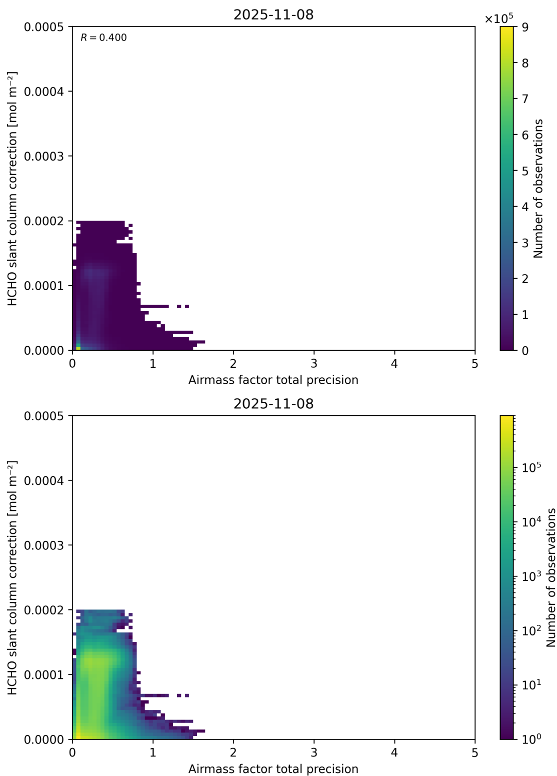
Figure 110: Scatter density plot of “Airmass factor total precision” against “HCHO slant column correction” for 2025-11-07 to 2025-11-09.
