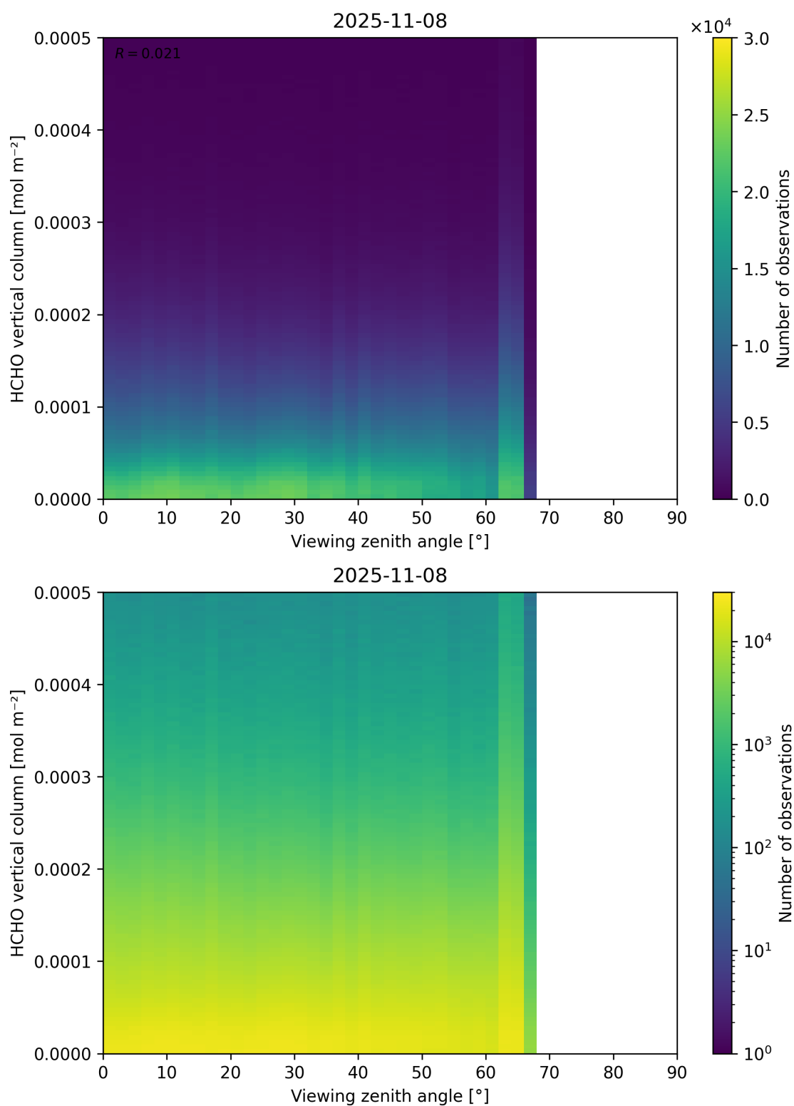
Figure 192: Scatter density plot of “Viewing zenith angle” against “HCHO vertical column” for 2025-11-07 to 2025-11-09.
