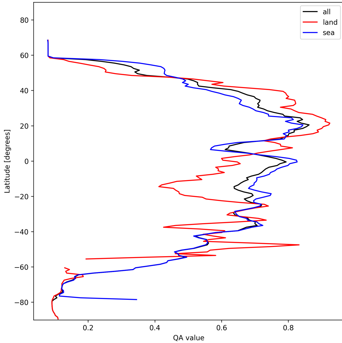
Figure 20: Zonal average of “QA value” for 2025-11-07 to 2025-11-09.
