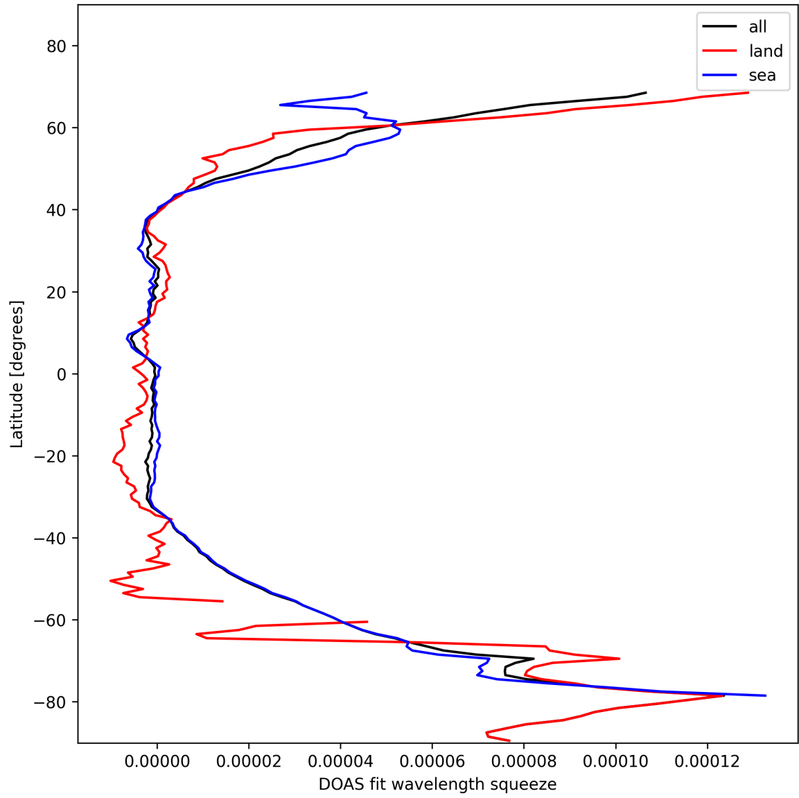
Figure 31: Zonal average of “DOAS fit wavelength squeeze” for 2025-11-07 to 2025-11-09.
