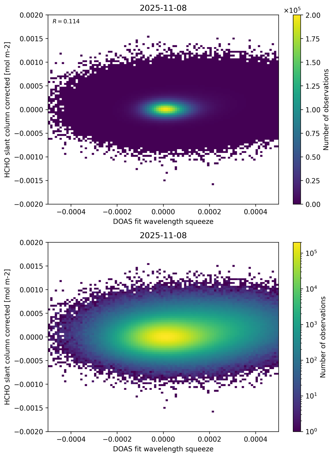
Figure 69: Scatter density plot of “DOAS fit wavelength squeeze” against “HCHO slant column corrected” for 2025-11-07 to 2025-11-09.
