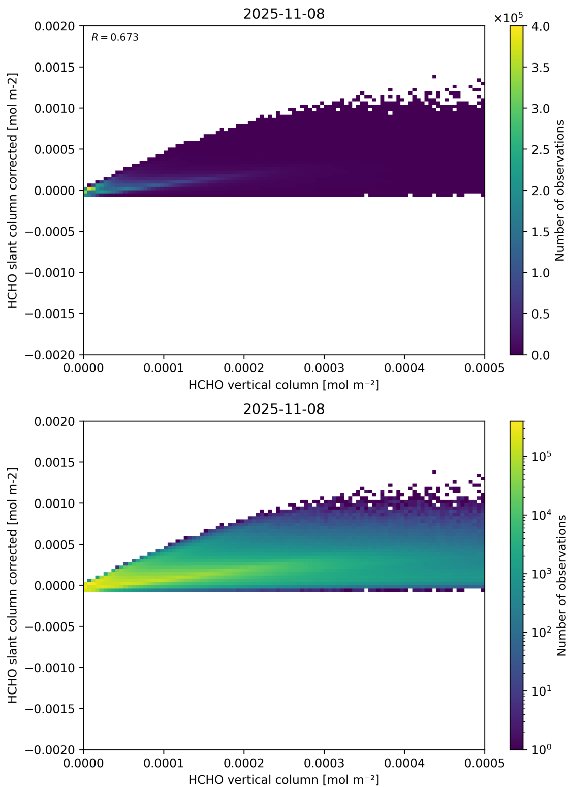
Figure 127: Scatter density plot of “HCHO vertical column” against “HCHO slant column corrected” for 2025-11-07 to 2025-11-09.
