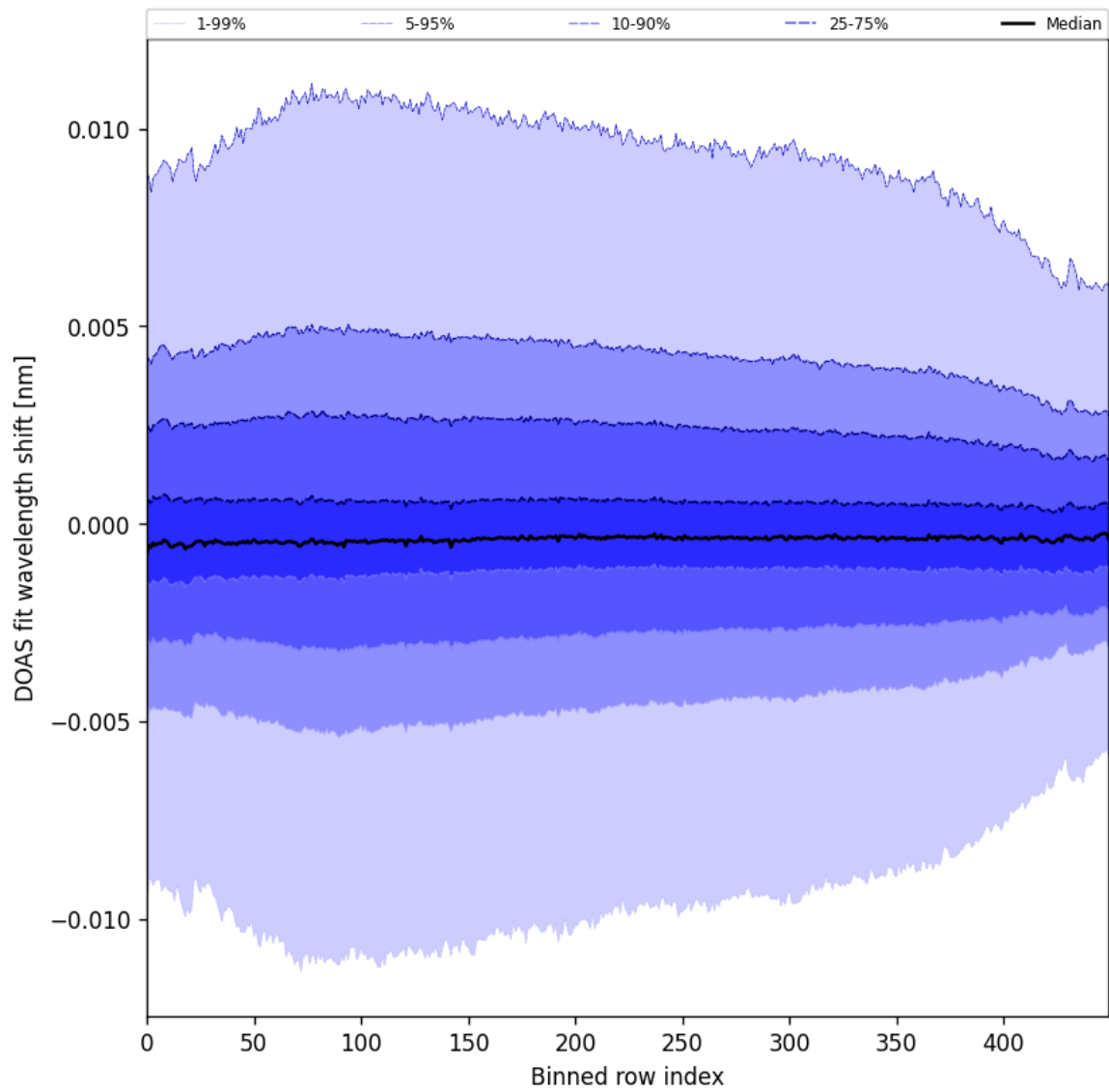
Figure 58: Along track statistics of “DOAS fit wavelength shift” for 2025-11-07 to 2025-11-09
