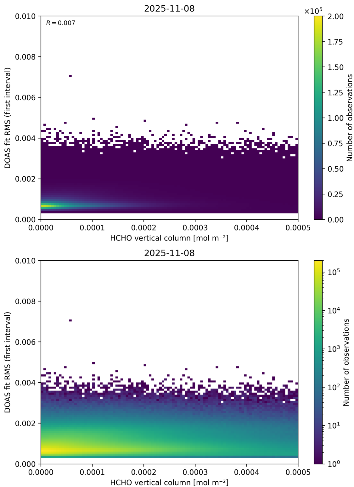
Figure 123: Scatter density plot of “HCHO vertical column” against “DOAS fit RMS (first interval)” for 2025-11-07 to 2025-11-09.
