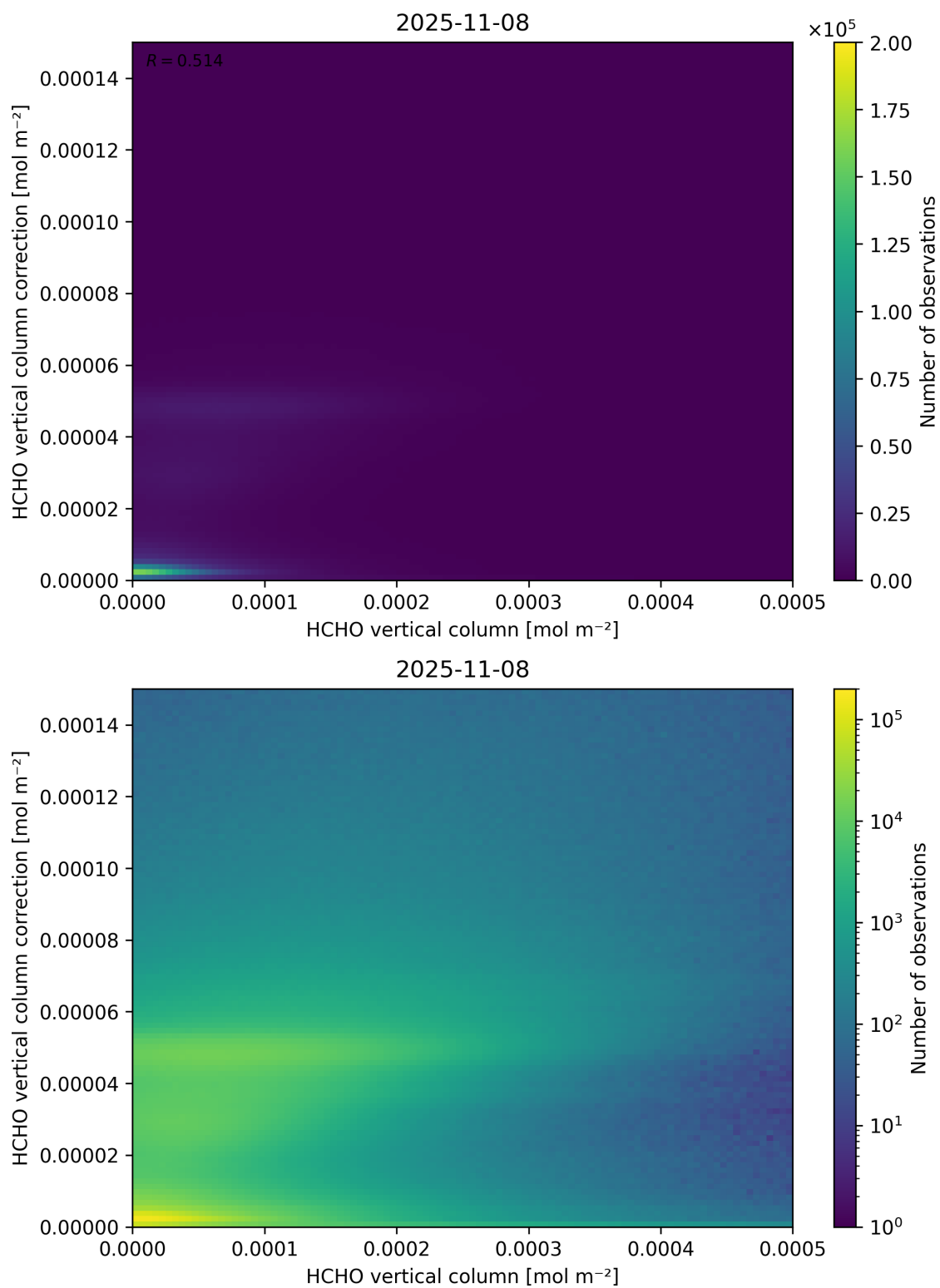
Figure 133: Scatter density plot of “HCHO vertical column” against “HCHO vertical column correction” for 2025-11-07 to 2025-11-09.
