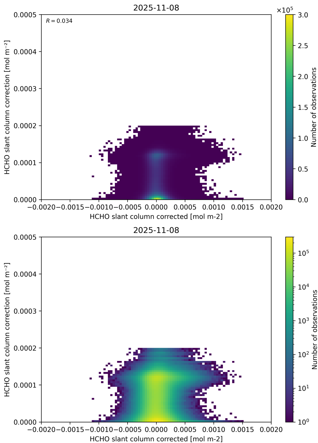
Figure 77: Scatter density plot of “HCHO slant column corrected” against “HCHO slant column correction” for 2025-11-07 to 2025-11-09.
