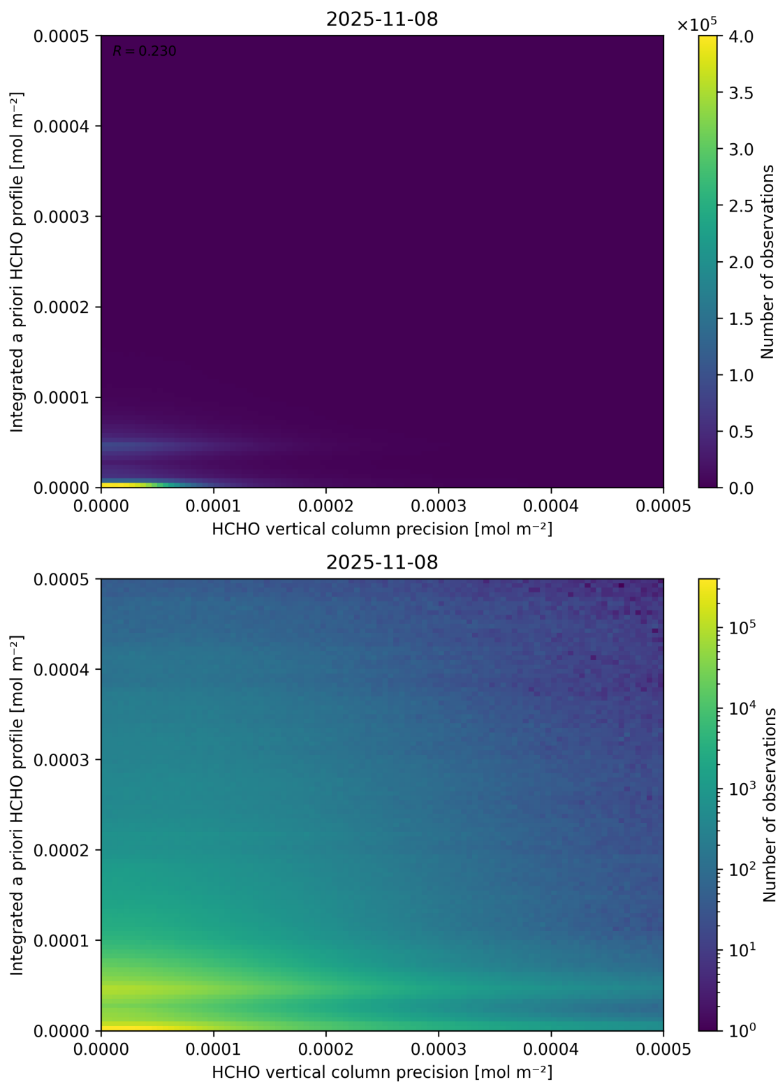
Figure 147: Scatter density plot of “HCHO vertical column precision” against “Integrated a priori HCHO profile” for 2025-11-07 to 2025-11-09.
