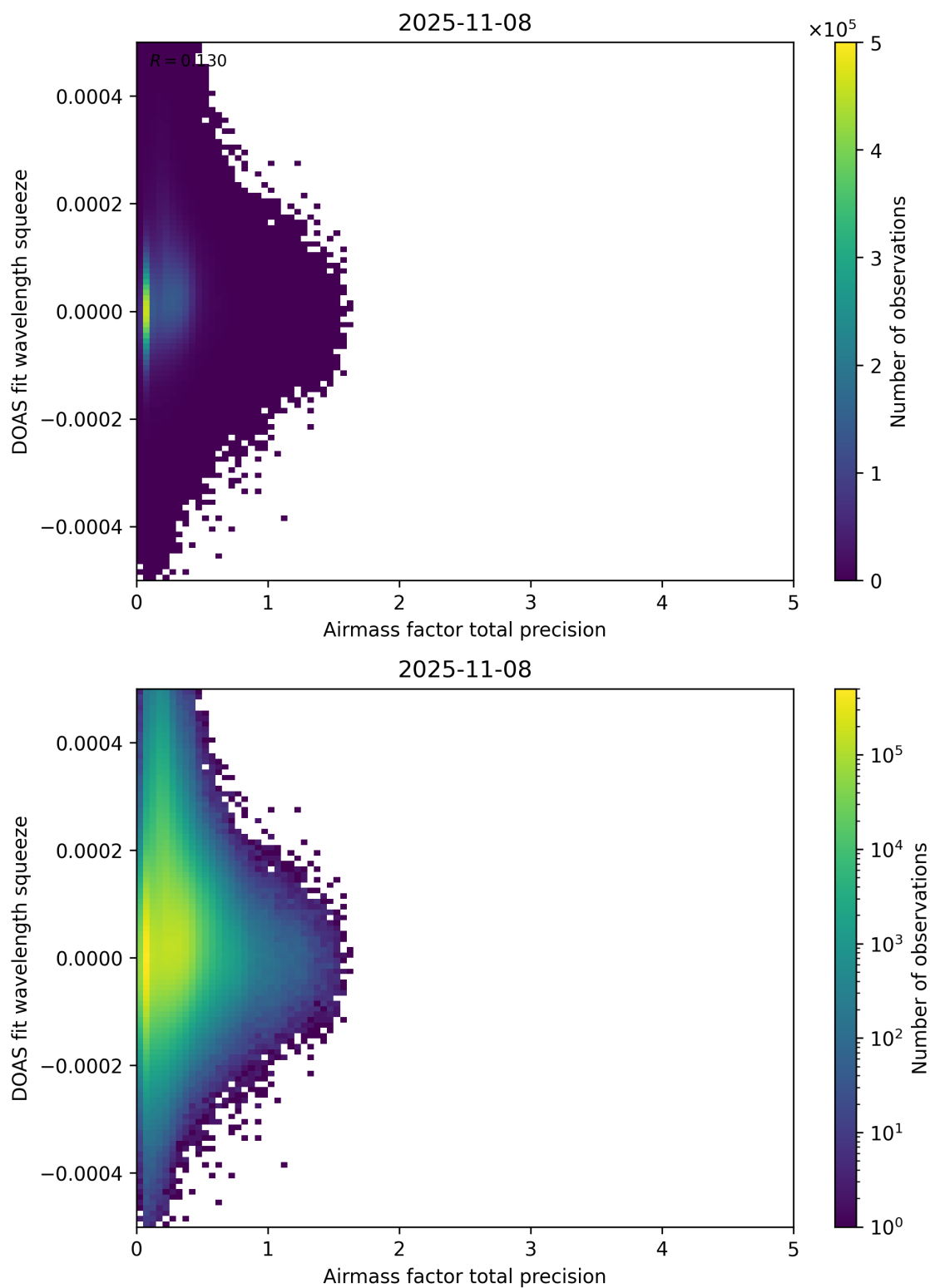
Figure 107: Scatter density plot of “Airmass factor total precision” against “DOAS fit wavelength squeeze” for 2025-11-07 to 2025-11-09.
