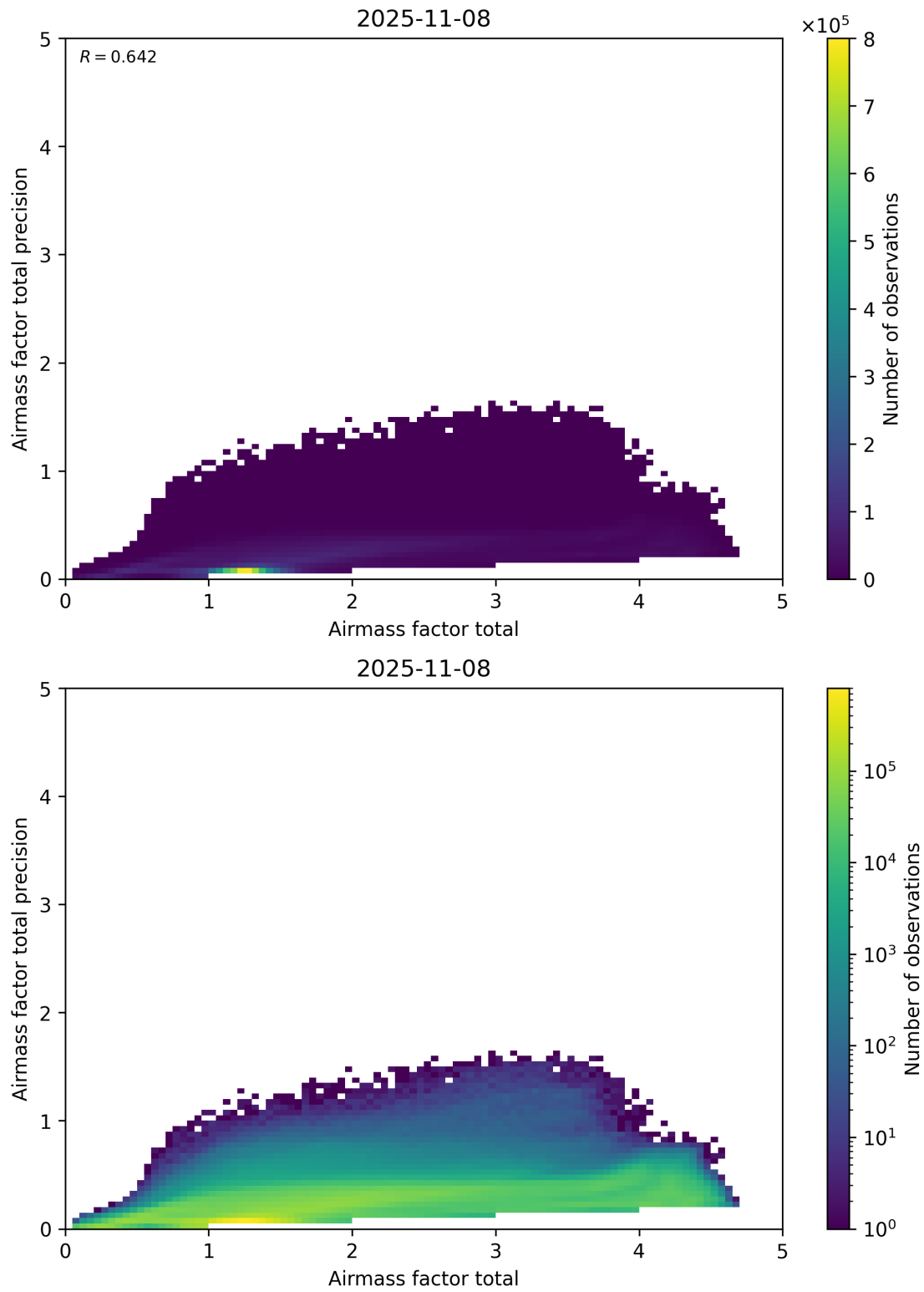
Figure 103: Scatter density plot of “Airmass factor total” against “Airmass factor total precision” for 2025-11-07 to 2025-11-09.
