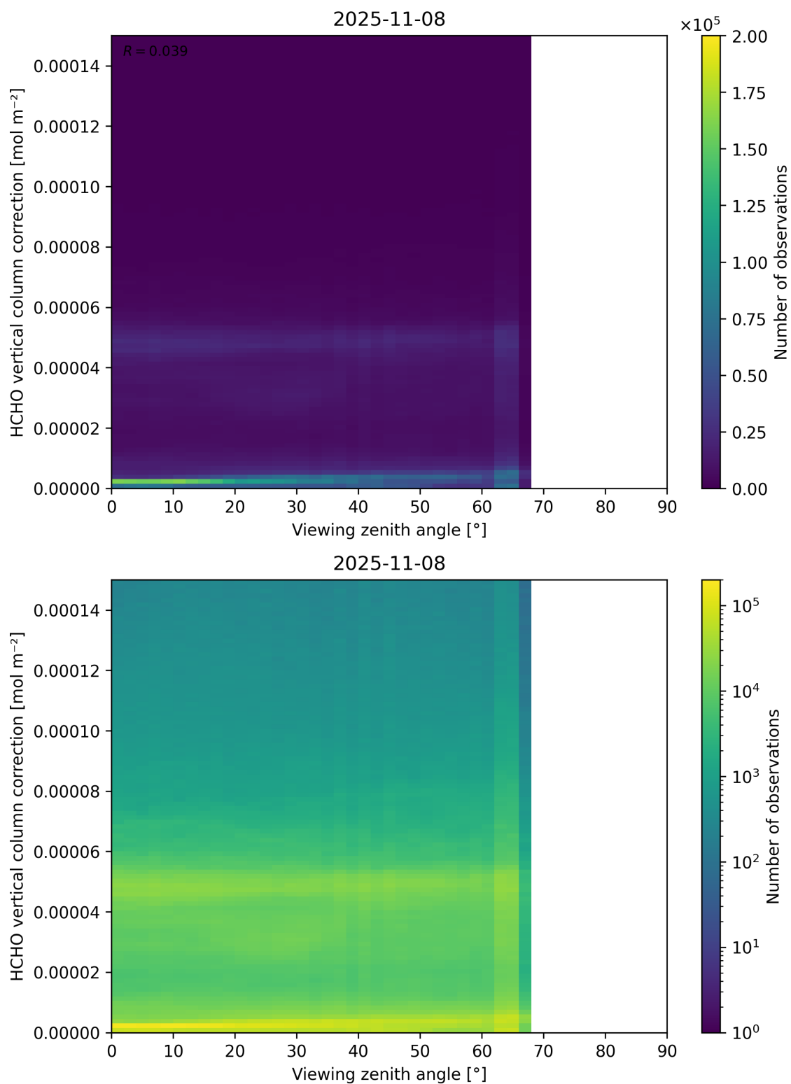
Figure 193: Scatter density plot of “Viewing zenith angle” against “HCHO vertical column correction” for 2025-11-07 to 2025-11-09.
