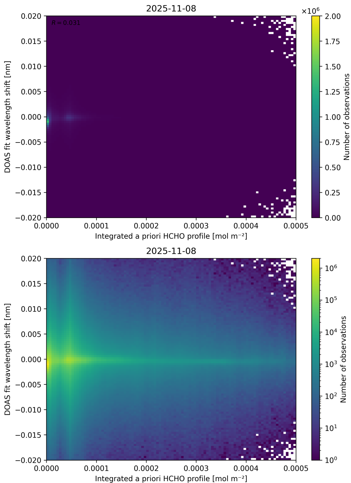
Figure 149: Scatter density plot of “Integrated a priori HCHO profile” against “DOAS fit wavelength shift” for 2025-11-07 to 2025-11-09.
