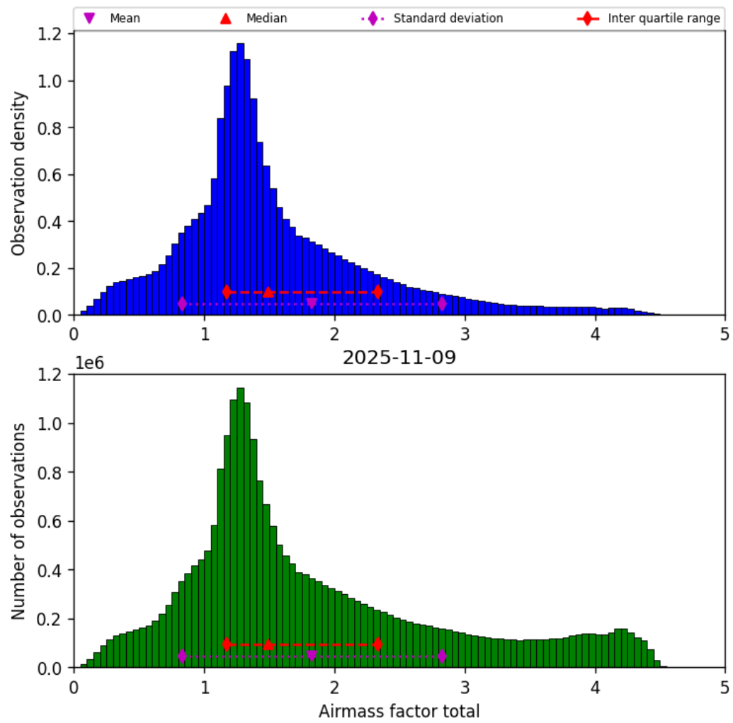
Figure 40: Histogram of “Airmass factor total” for 2025-11-08 to 2025-11-10
