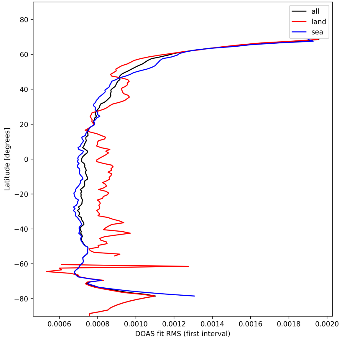
Figure 32: Zonal average of “DOAS fit RMS (first interval)” for 2025-11-08 to 2025-11-10.
