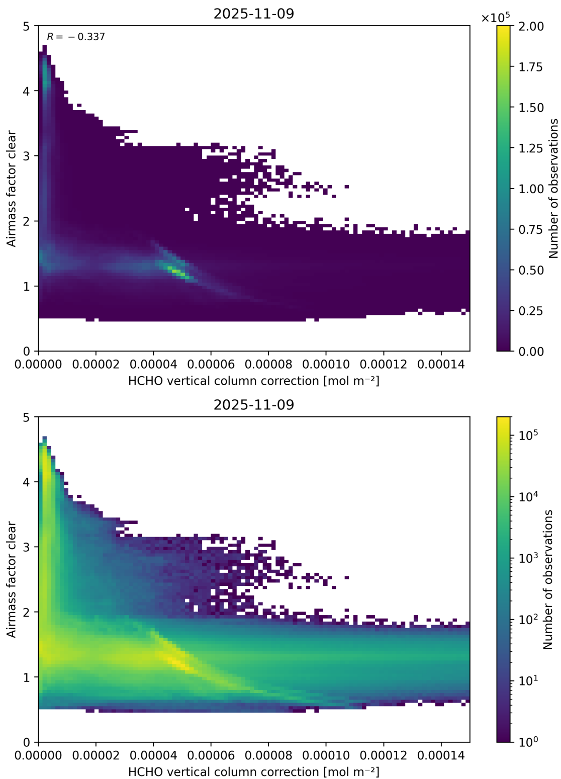
Figure 115: Scatter density plot of “HCHO vertical column correction” against “Airmass factor clear” for 2025-11-08 to 2025-11-10.
