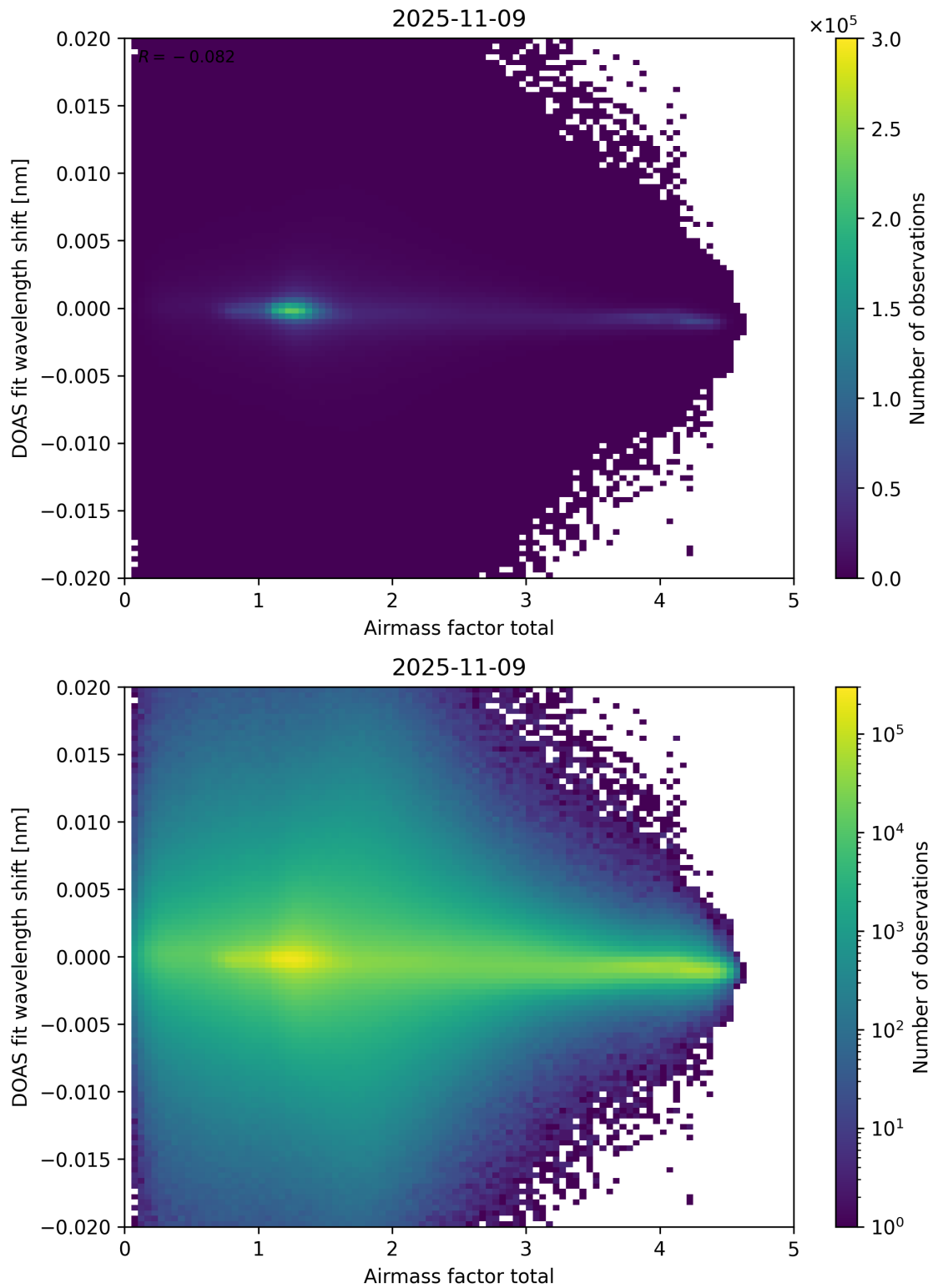
Figure 98: Scatter density plot of “Airmass factor total” against “DOAS fit wavelength shift” for 2025-11-08 to 2025-11-10.
