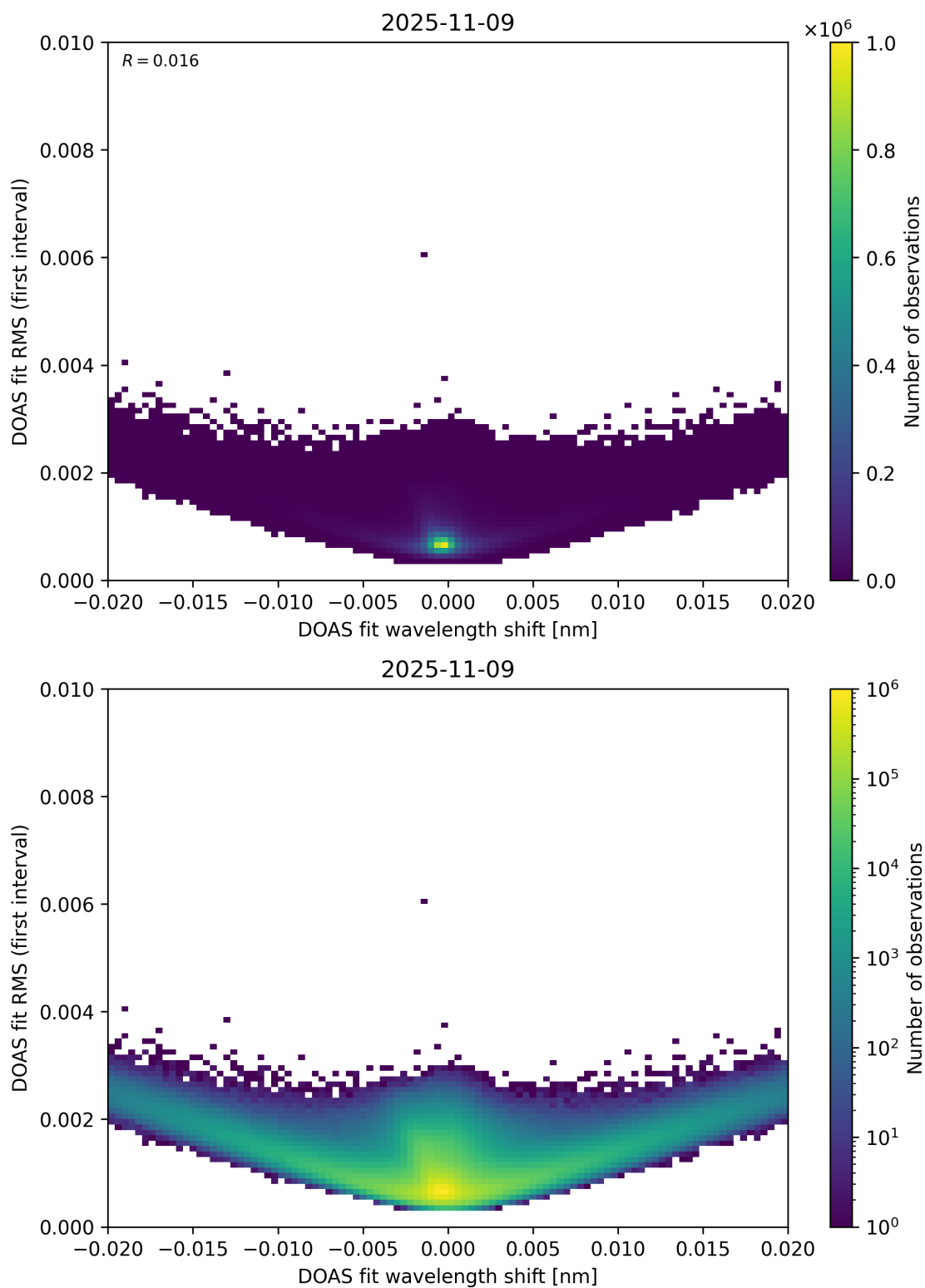
Figure 64: Scatter density plot of “DOAS fit wavelength shift” against “DOAS fit RMS (first interval)” for 2025-11-08 to 2025-11-10.
