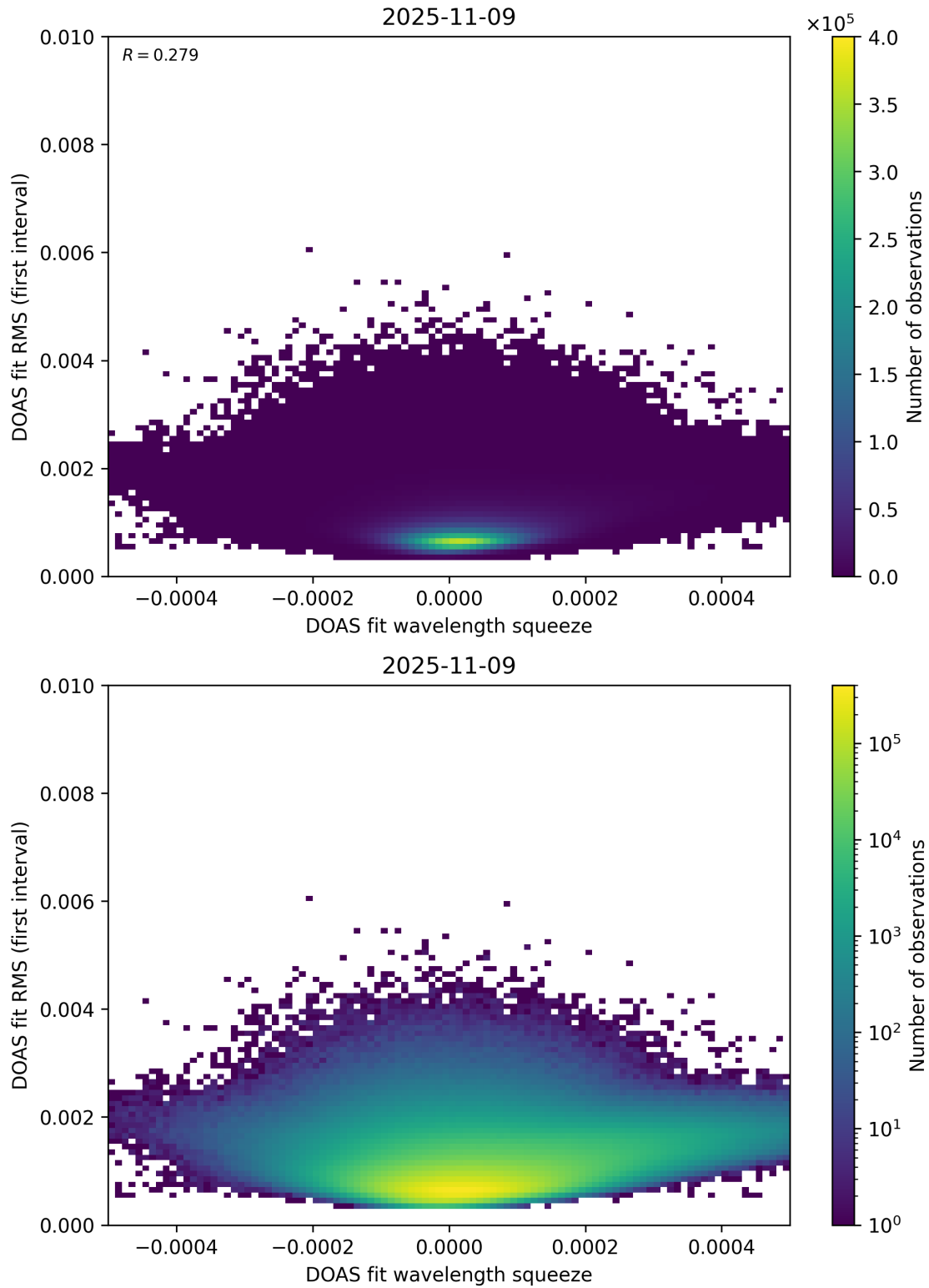
Figure 68: Scatter density plot of “DOAS fit wavelength squeeze” against “DOAS fit RMS (first interval)” for 2025-11-08 to 2025-11-10.
