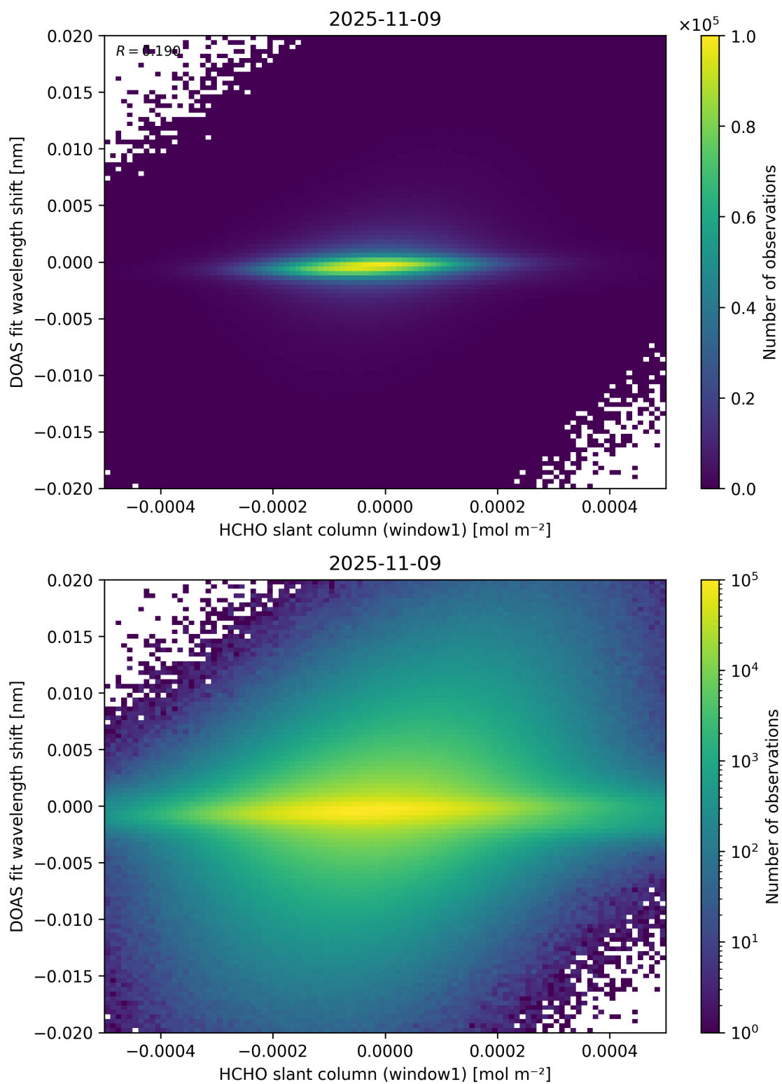
Figure 79: Scatter density plot of “HCHO slant column (window1)” against “DOAS fit wavelength shift” for 2025-11-08 to 2025-11-10.
