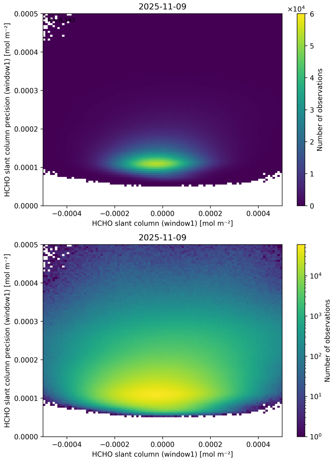
Figure 84: Scatter density plot of “HCHO slant column (window1)” against “HCHO slant column precision (window1)” for 2025-11-08 to 2025-11-10.
