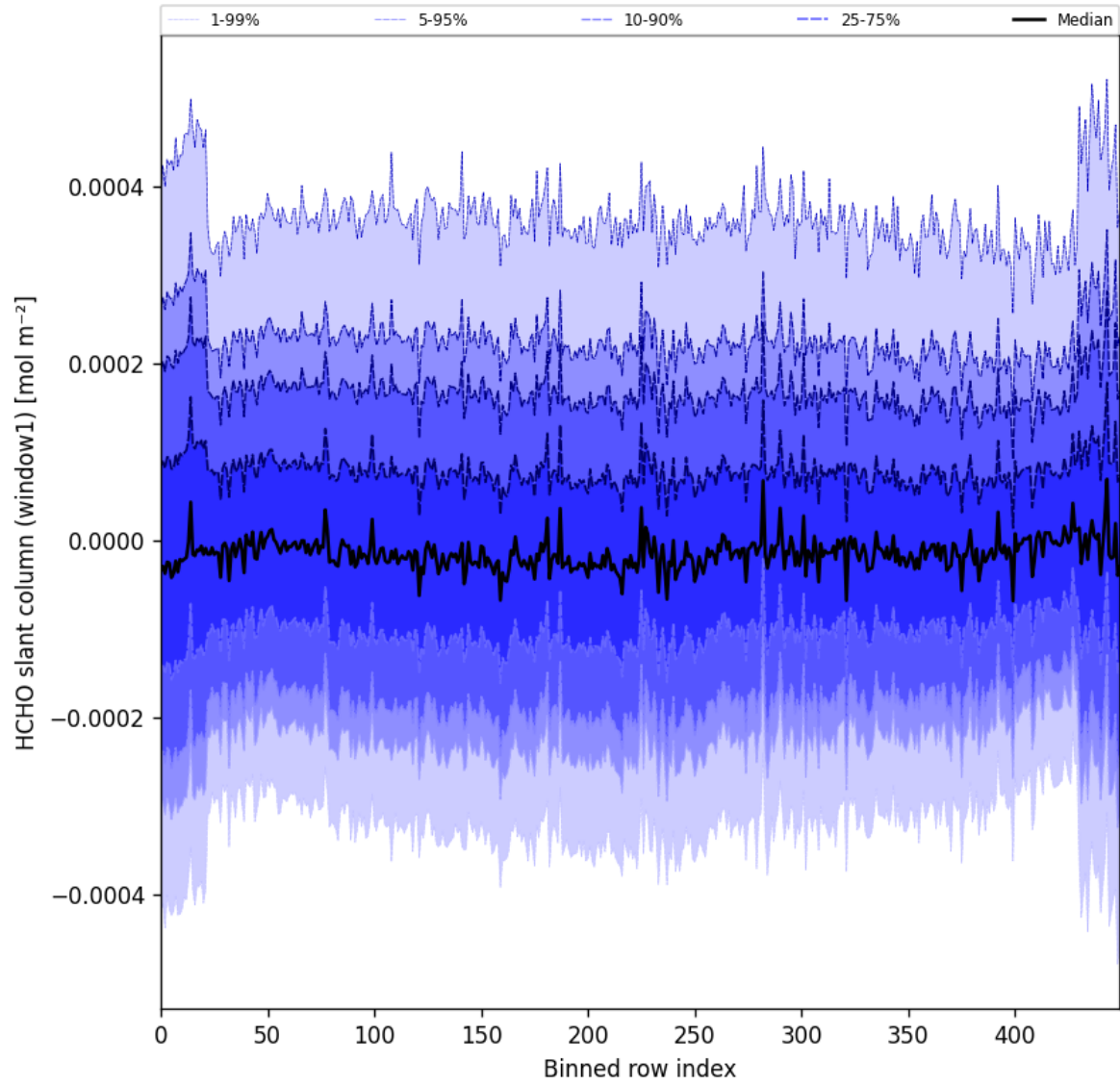
Figure 52: Along track statistics of “HCHO slant column (window1)” for 2025-11-08 to 2025-11-10
