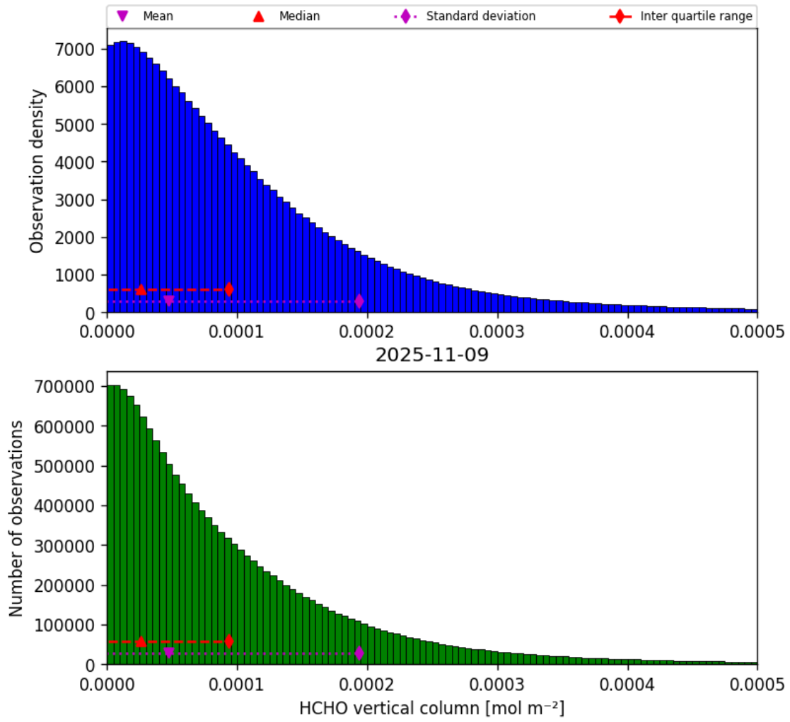
Figure 35: Histogram of “HCHO vertical column” for 2025-11-08 to 2025-11-10
