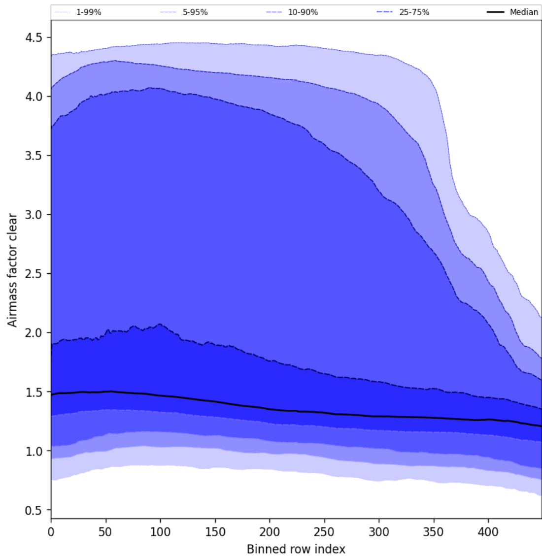
Figure 56: Along track statistics of “Air mass factor clear” for 2025-11-08 to 2025-11-10
