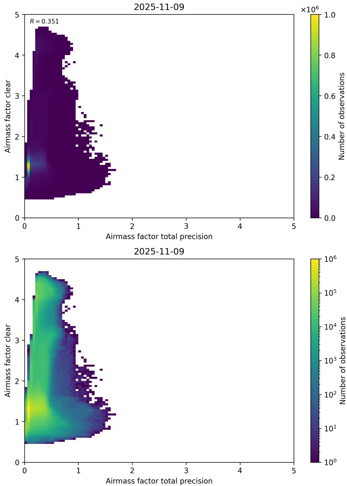
Figure 108: Scatter density plot of “Airmass factor total precision” against “Airmass factor clear” for 2025-11-08 to 2025-11-10.
