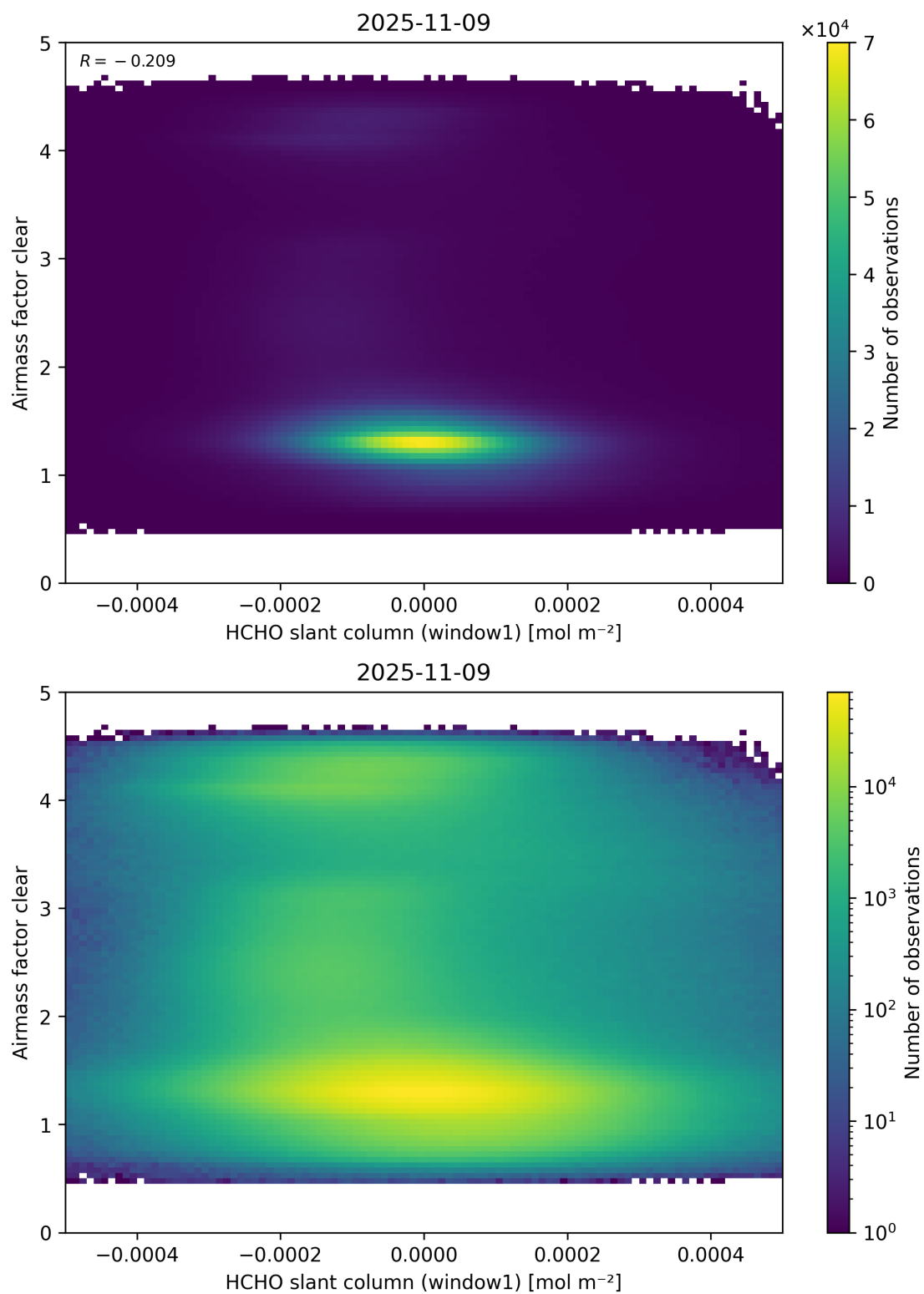
Figure 81: Scatter density plot of “HCHO slant column (window1)” against “Airmass factor clear” for 2025-11-08 to 2025-11-10.
