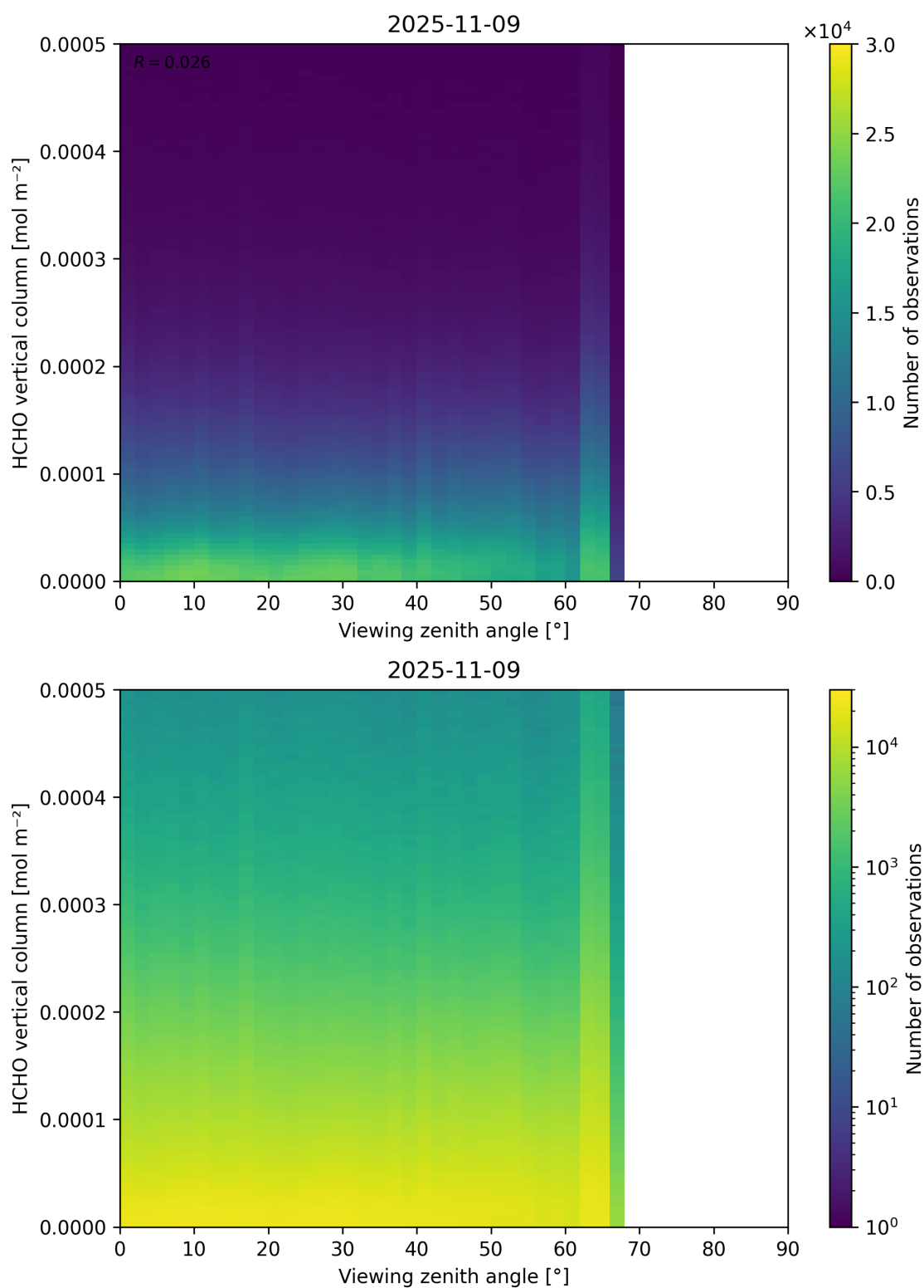
Figure 192: Scatter density plot of “Viewing zenith angle” against “HCHO vertical column” for 2025-11-08 to 2025-11-10.
