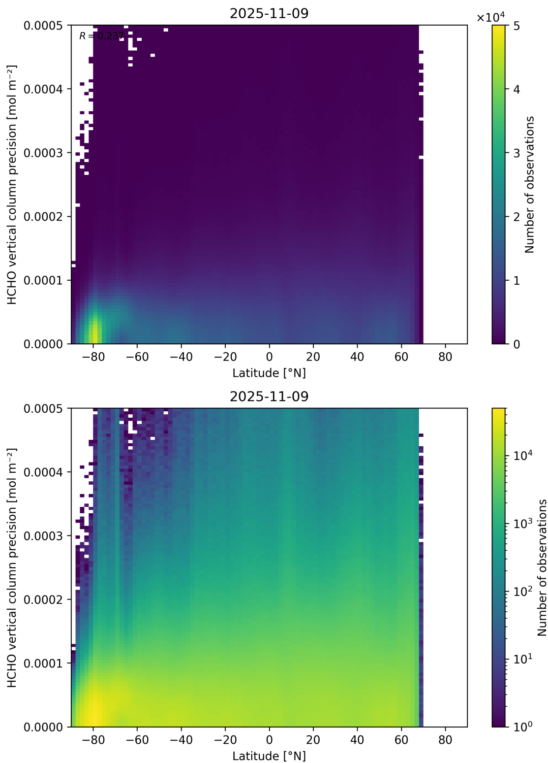
Figure 165: Scatter density plot of “Latitude” against “HCHO vertical column precision” for 2025-11-08 to 2025-11-10.
