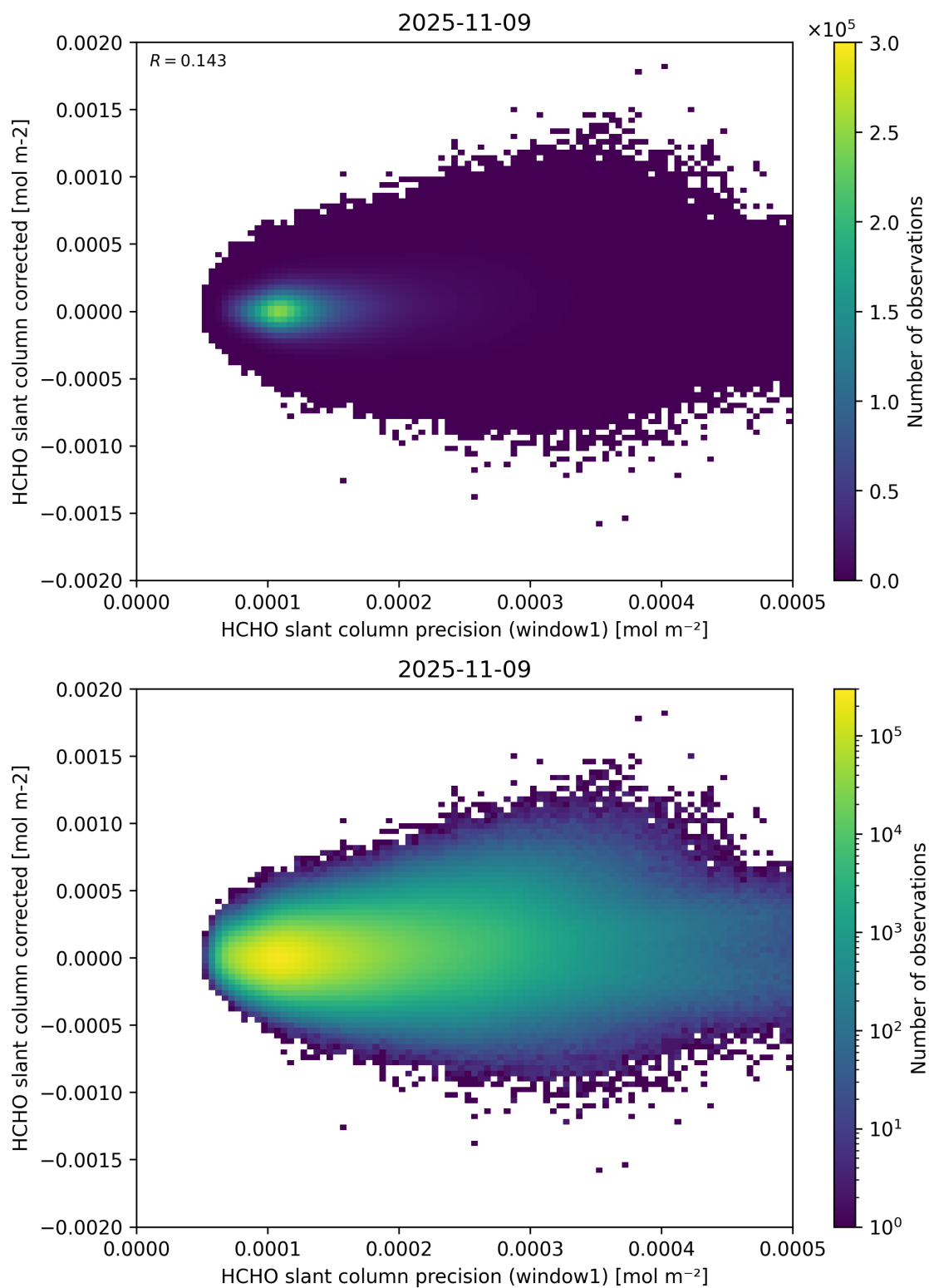
Figure 92: Scatter density plot of “HCHO slant column precision (window1)” against “HCHO slant column corrected” for 2025-11-08 to 2025-11-10.
