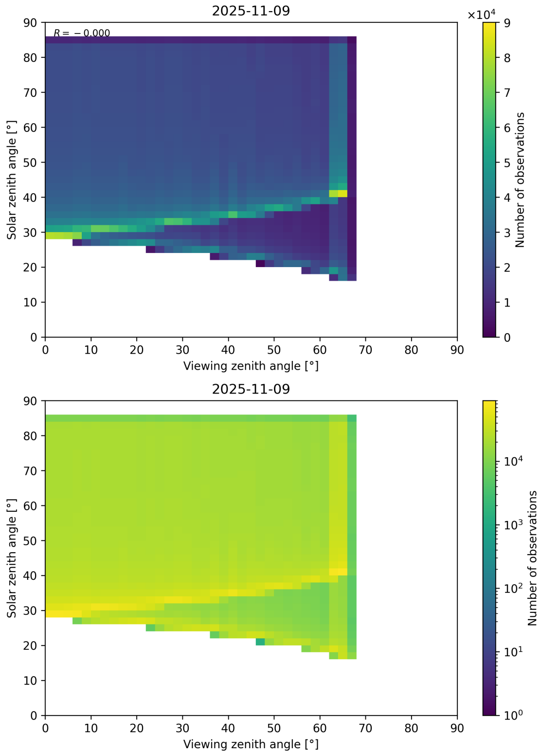
Figure 197: Scatter density plot of “Viewing zenith angle” against “Solar zenith angle” for 2025-11-08 to 2025-11-10.
