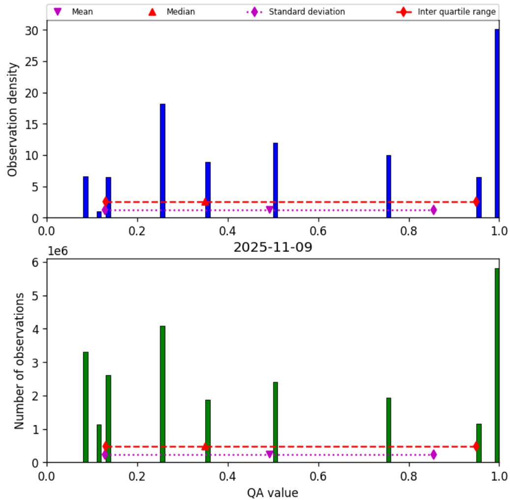
Figure 34: Histogram of “QA value” for 2025-11-08 to 2025-11-10
