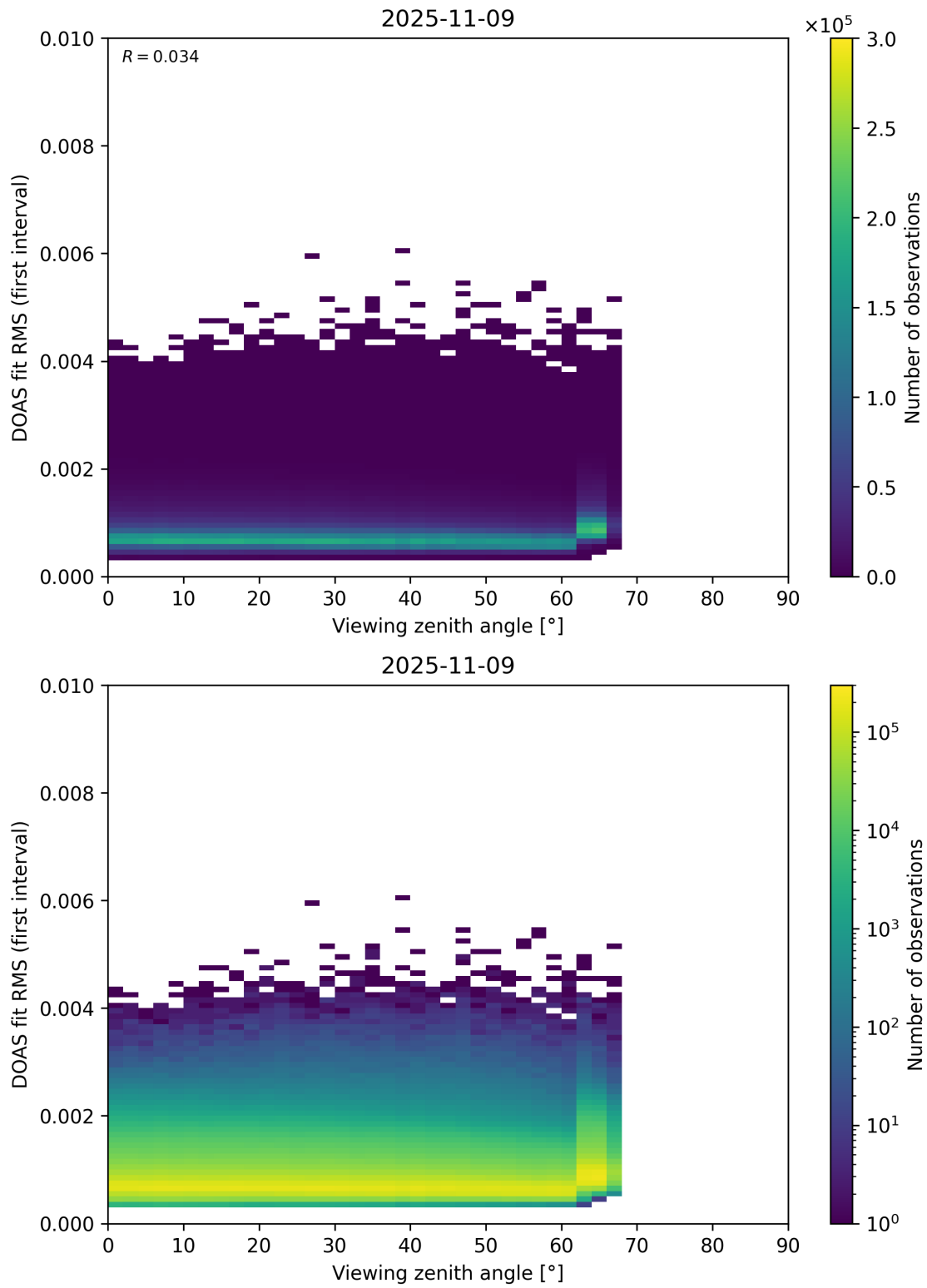
Figure 182: Scatter density plot of “Viewing zenith angle” against “DOAS fit RMS (first interval)” for 2025-11-08 to 2025-11-10.
