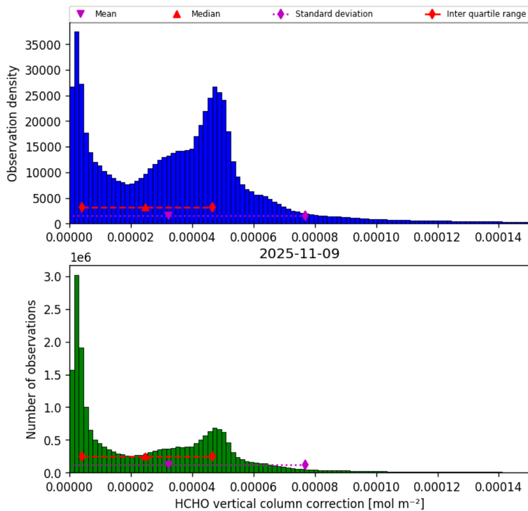
Figure 37: Histogram of “HCHO vertical column correction” for 2025-11-08 to 2025-11-10
