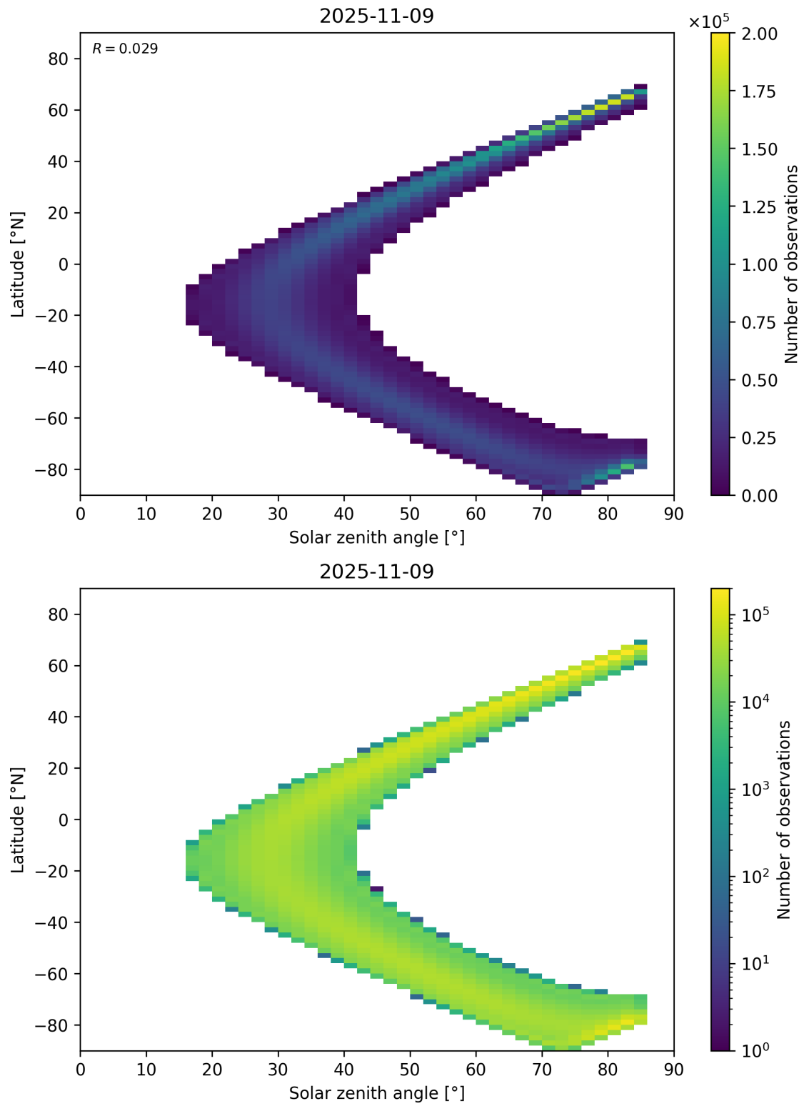
Figure 181: Scatter density plot of “Solar zenith angle” against “Latitude” for 2025-11-08 to 2025-11-10.
