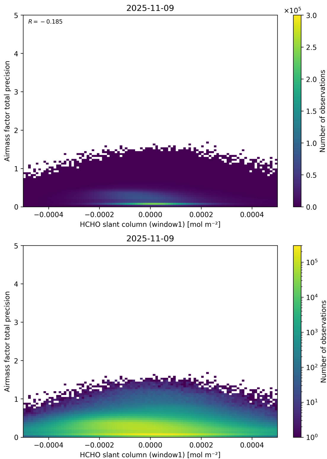
Figure 86: Scatter density plot of “HCHO slant column (window1)” against “Airmass factor total precision” for 2025-11-08 to 2025-11-10.
