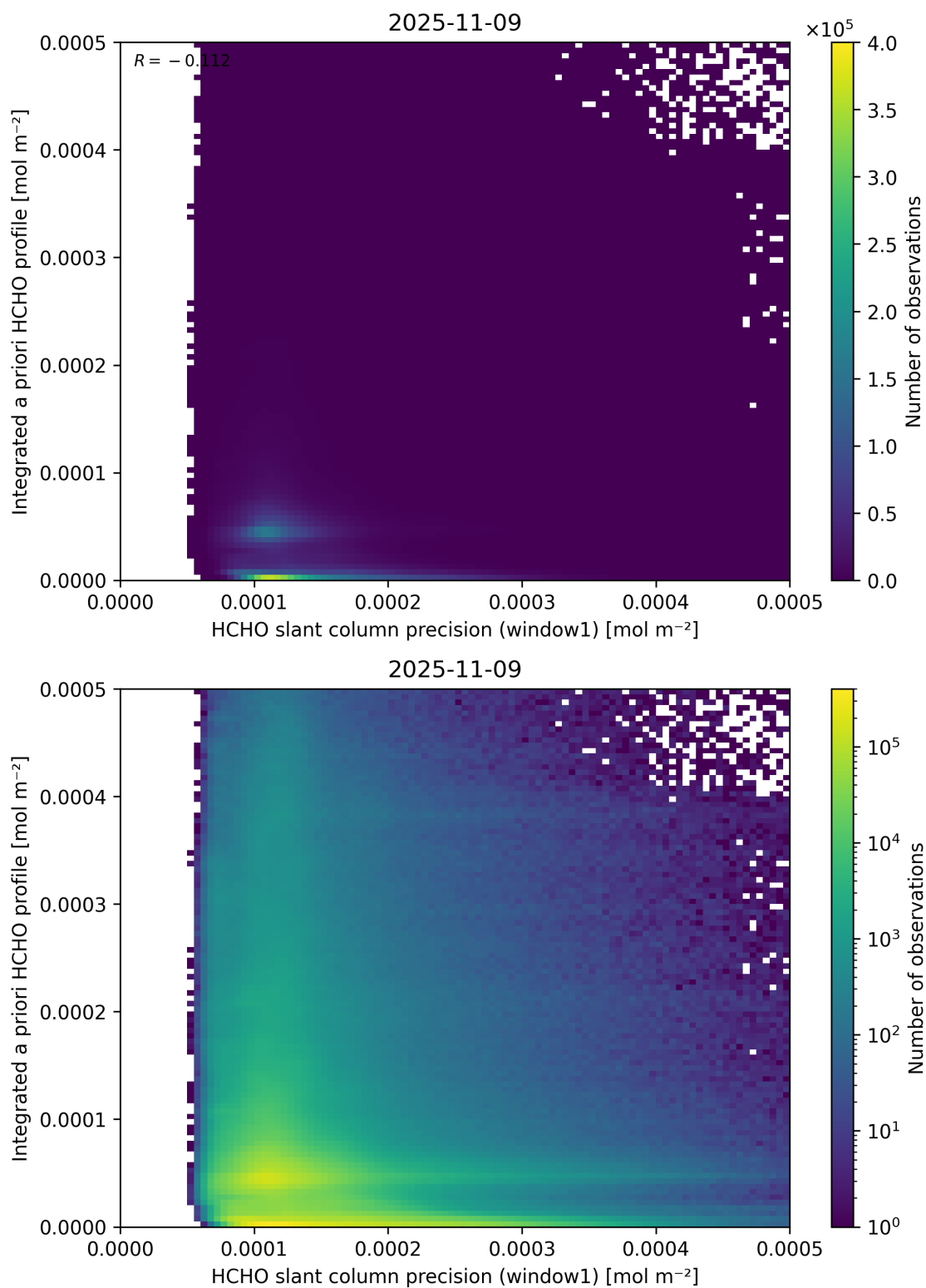
Figure 96: Scatter density plot of “HCHO slant column precision (window1)” against “Integrated a priori HCHO profile” for 2025-11-08 to 2025-11-10.
