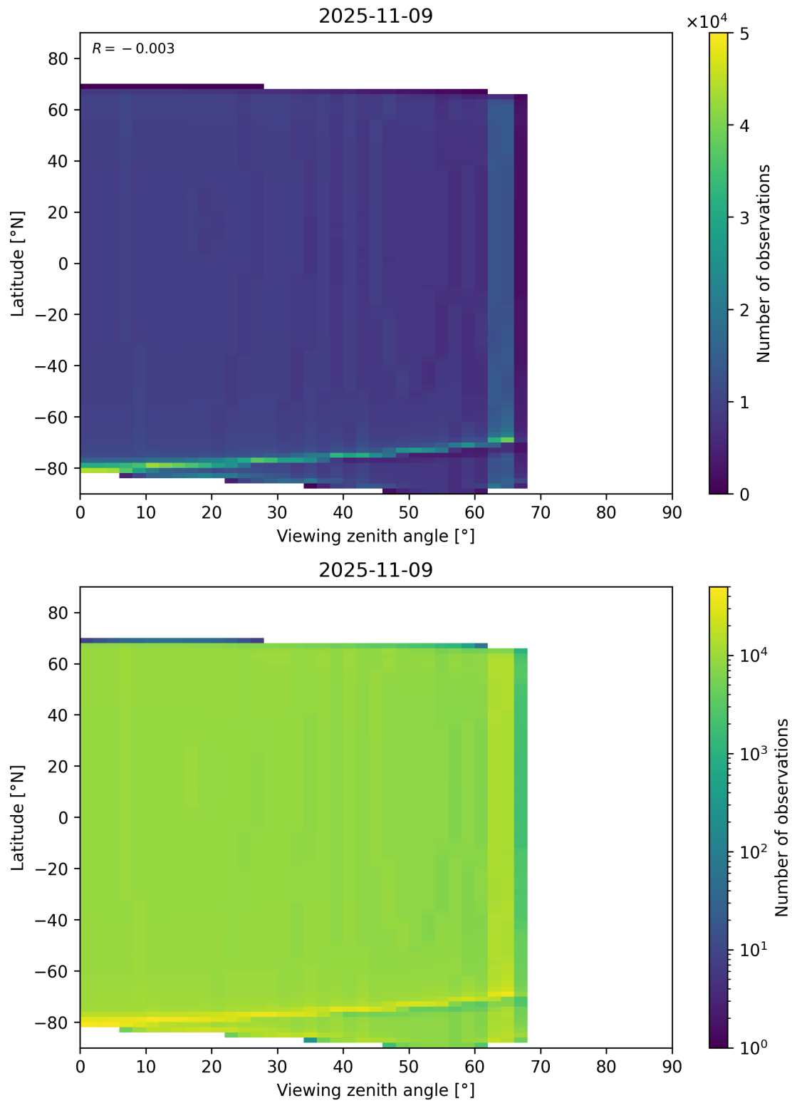
Figure 196: Scatter density plot of “Viewing zenith angle” against “Latitude” for 2025-11-08 to 2025-11-10.
