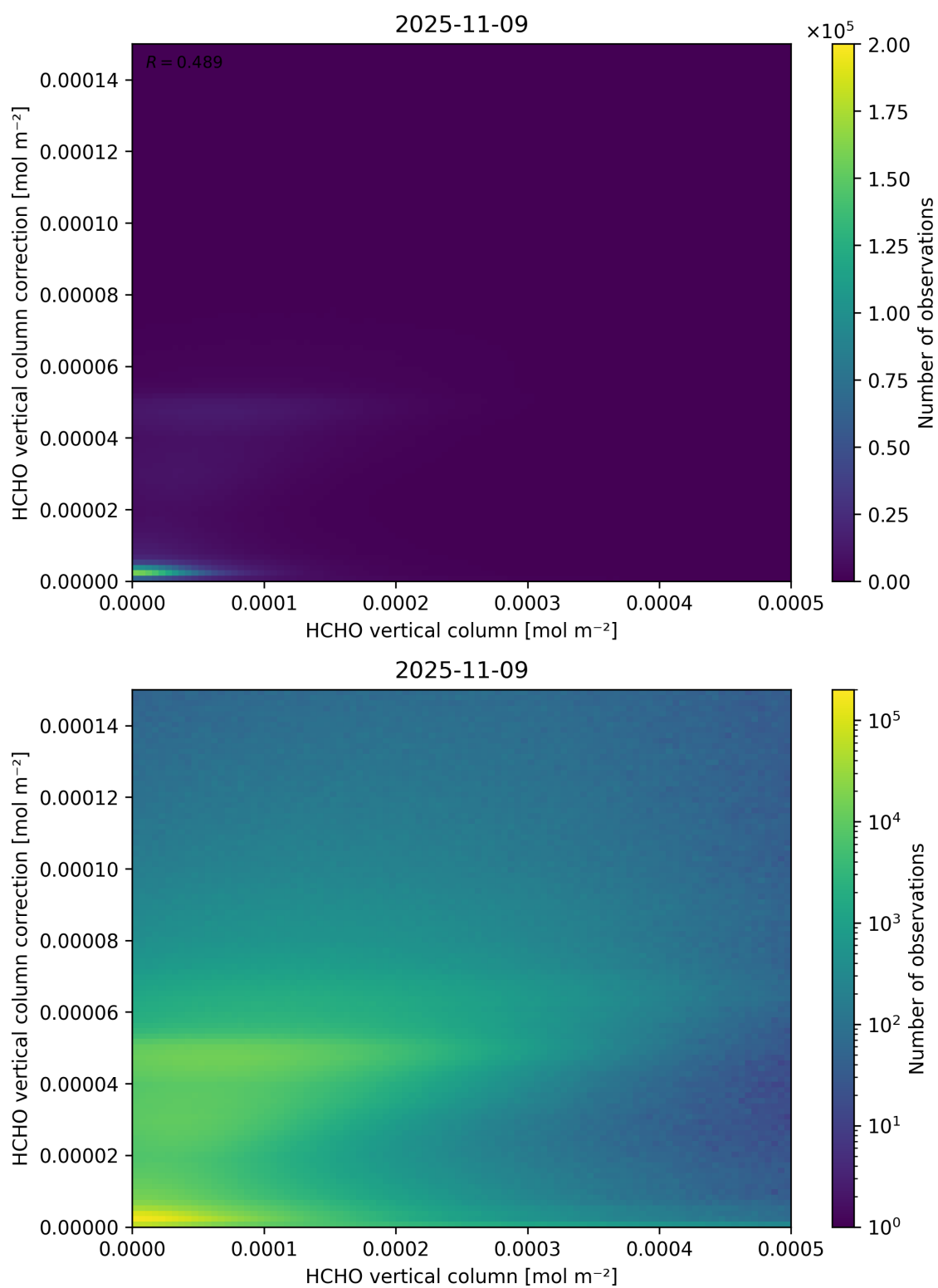
Figure 133: Scatter density plot of “HCHO vertical column” against “HCHO vertical column correction” for 2025-11-08 to 2025-11-10.
