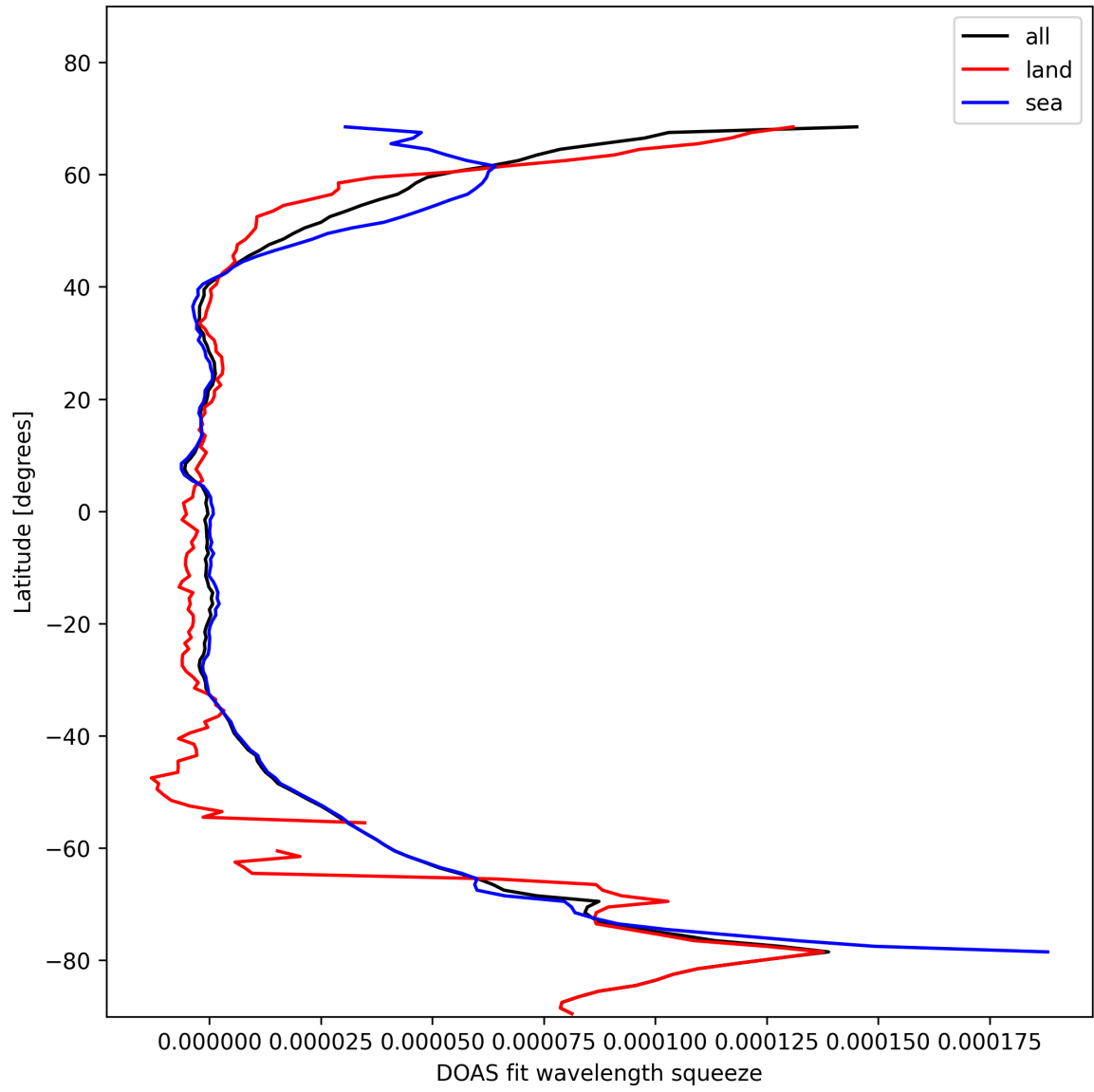
Figure 31: Zonal average of “DOAS fit wavelength squeeze” for 2025-11-08 to 2025-11-10.
