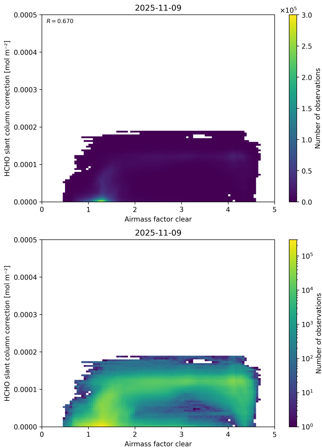
Figure 75: Scatter density plot of “Airmass factor clear” against “HCHO slant column correction” for 2025-11-08 to 2025-11-10.
