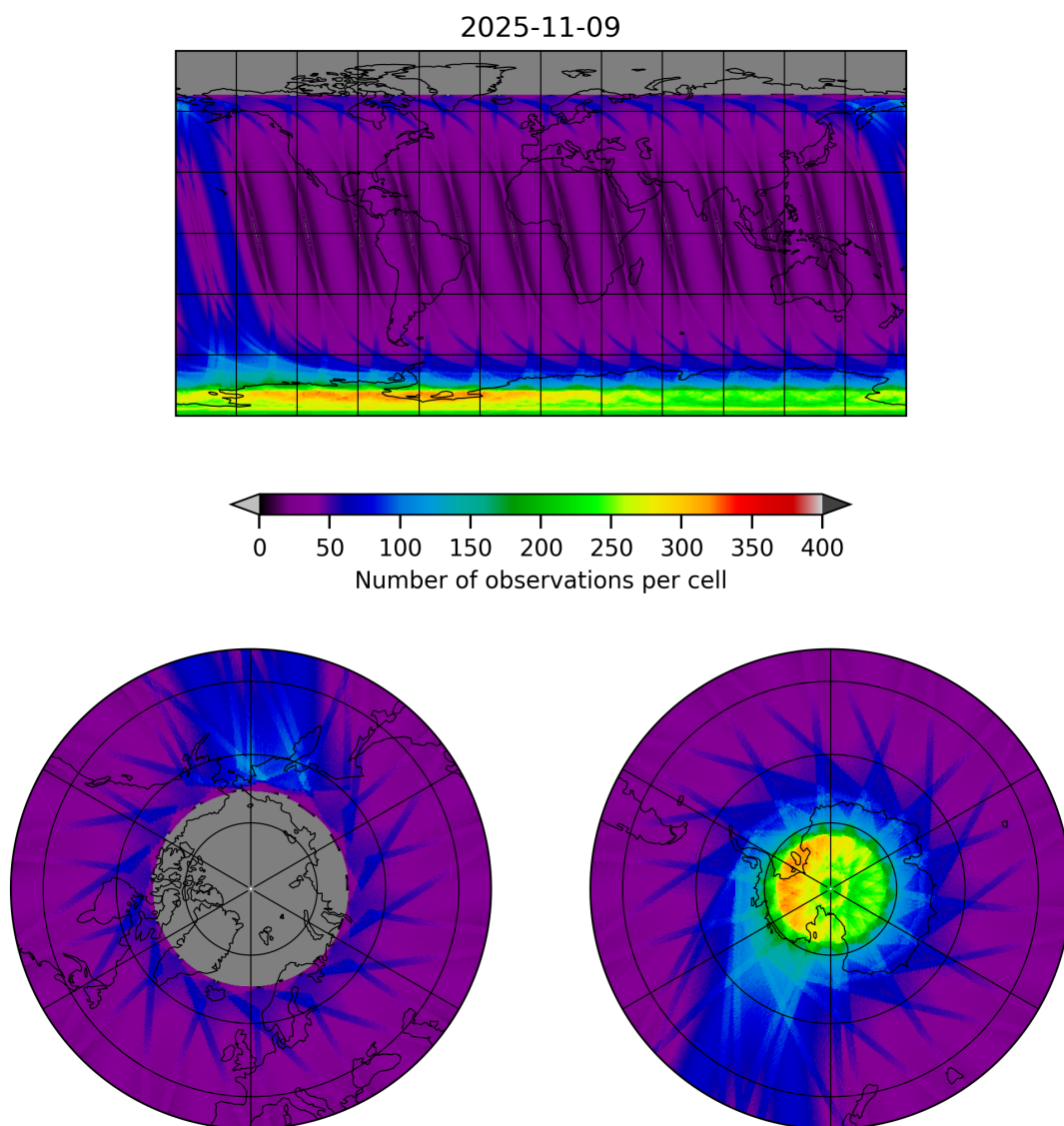
Figure 19: Map of the number of observations for 2025-11-08 to 2025-11-10
