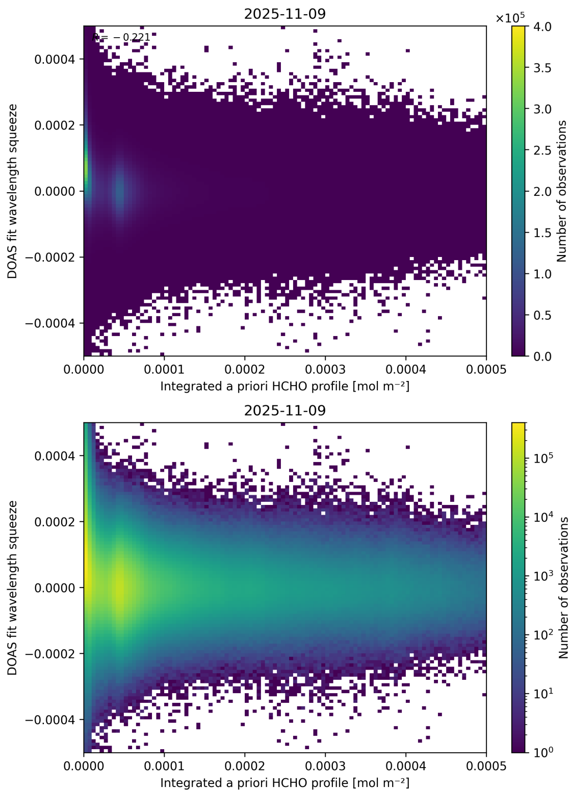
Figure 150: Scatter density plot of “Integrated a priori HCHO profile” against “DOAS fit wavelength squeeze” for 2025-11-08 to 2025-11-10.
