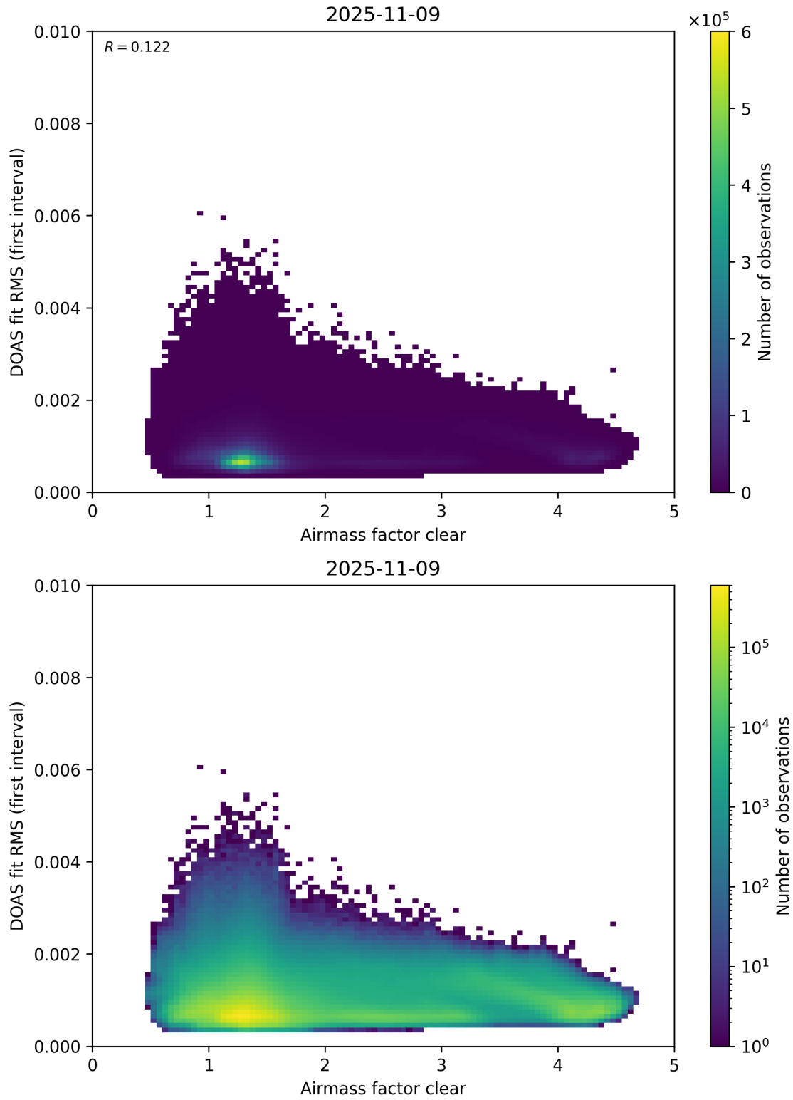
Figure 71: Scatter density plot of “Airmass factor clear” against “DOAS fit RMS (first interval)” for 2025-11-08 to 2025-11-10.
