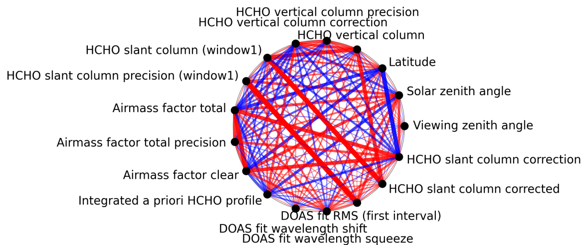
Figure 1: Map of correlation graph for 2025-11-08 to 2025-11-10.
