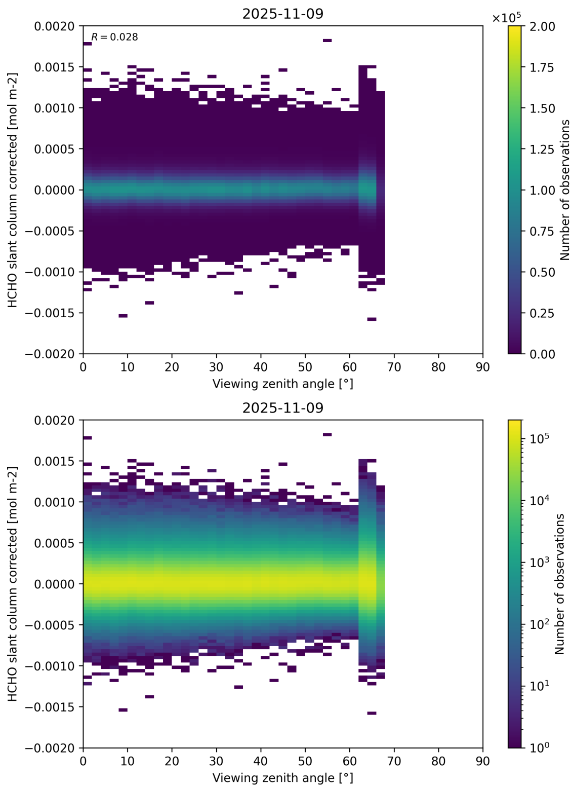
Figure 186: Scatter density plot of “Viewing zenith angle” against “HCHO slant column corrected” for 2025-11-08 to 2025-11-10.
