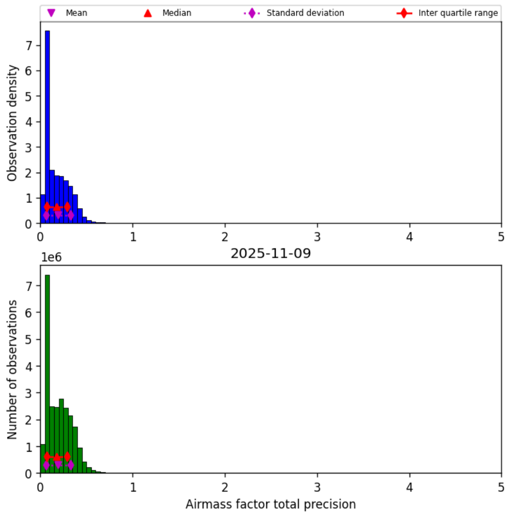
Figure 41: Histogram of “Airmass factor total precision” for 2025-11-08 to 2025-11-10
