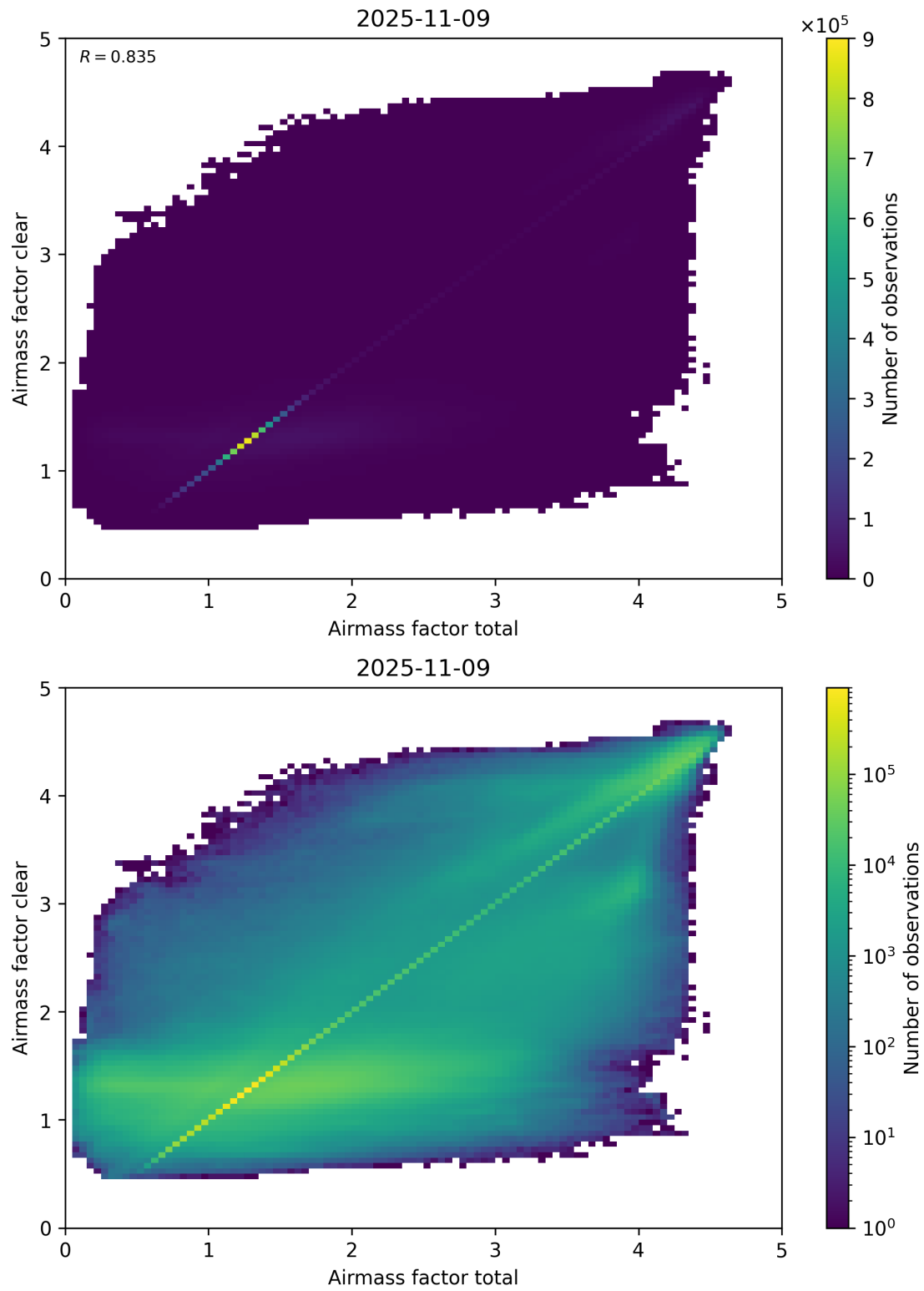
Figure 100: Scatter density plot of “Airmass factor total” against “Airmass factor clear” for 2025-11-08 to 2025-11-10.
