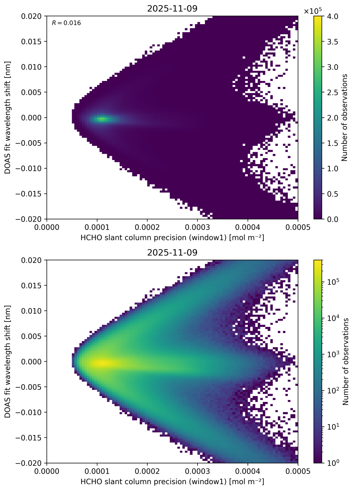
Figure 89: Scatter density plot of “HCHO slant column precision (window1)” against “DOAS fit wavelength shift” for 2025-11-08 to 2025-11-10.
