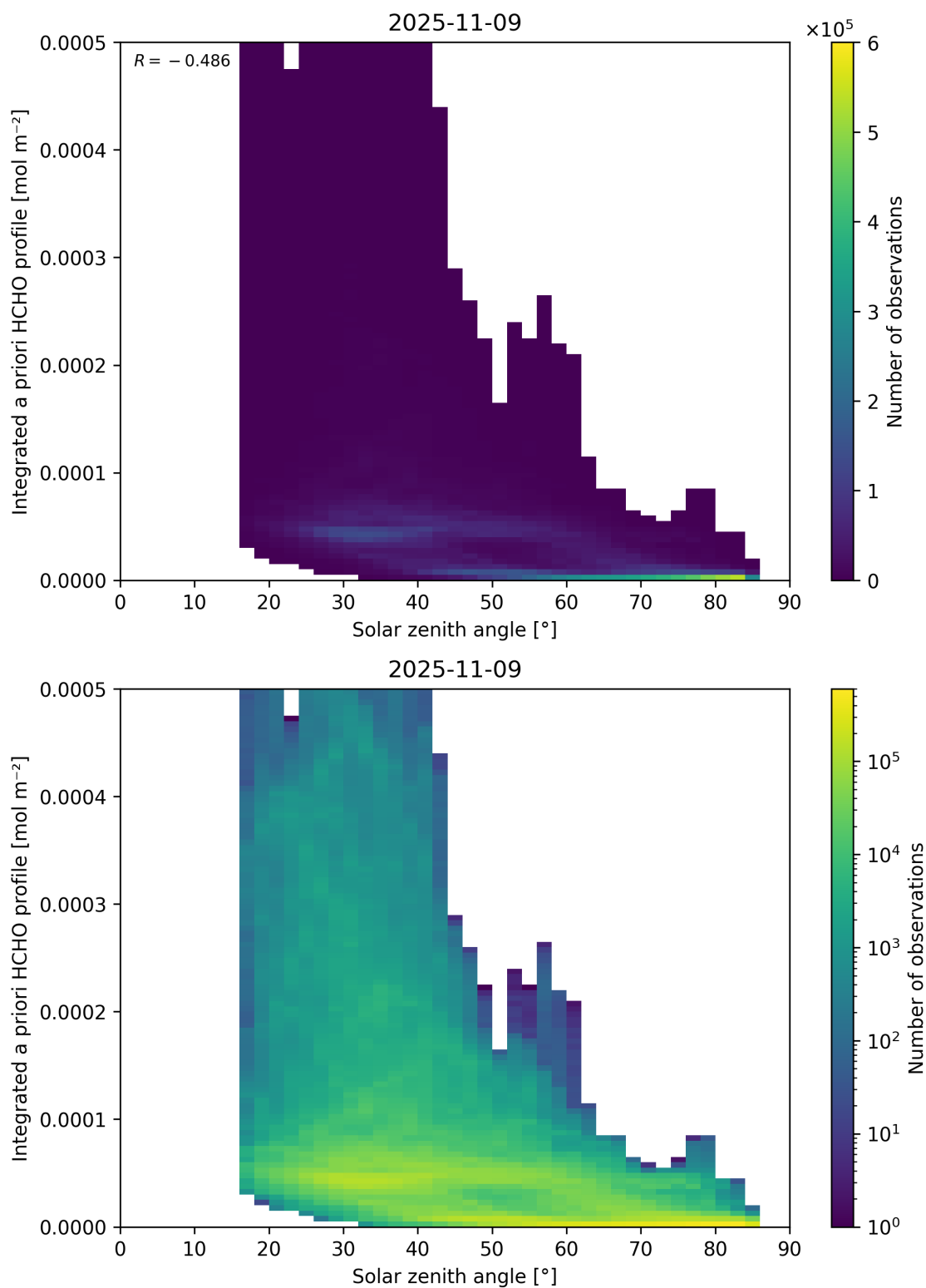
Figure 180: Scatter density plot of “Solar zenith angle” against “Integrated a priori HCHO profile” for 2025-11-08 to 2025-11-10.
