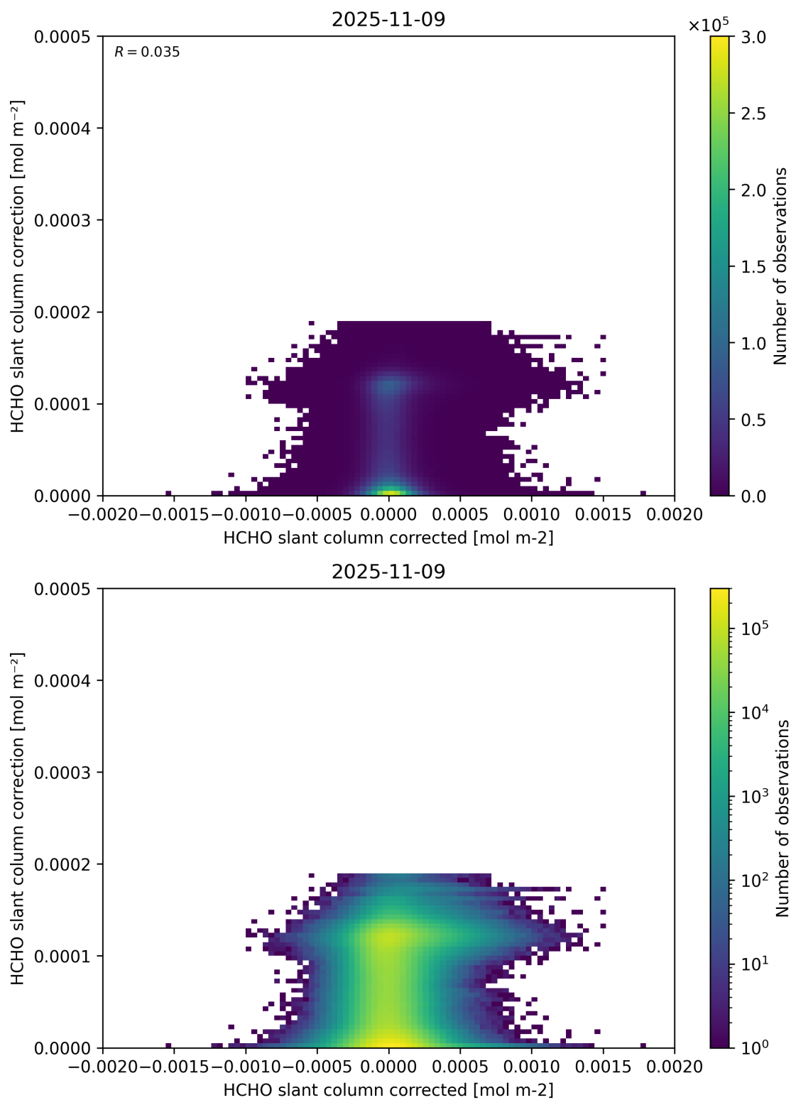
Figure 77: Scatter density plot of “HCHO slant column corrected” against “HCHO slant column correction” for 2025-11-08 to 2025-11-10.
