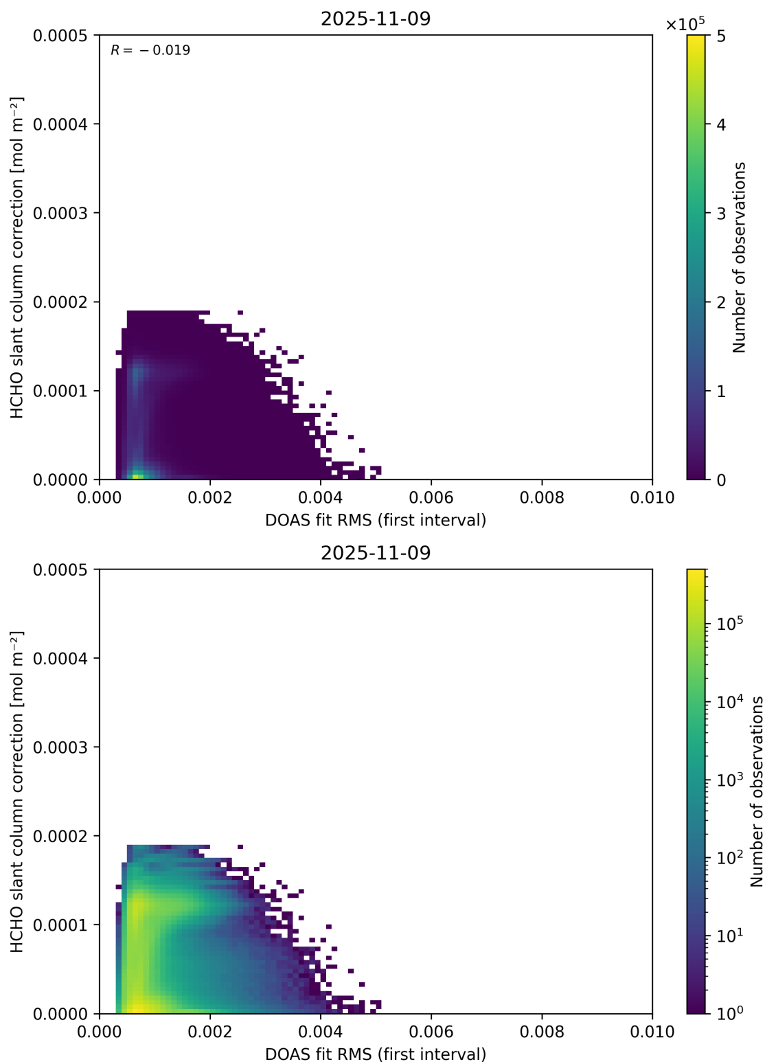
Figure 63: Scatter density plot of “DOAS fit RMS (first interval)” against “HCHO slant column correction” for 2025-11-08 to 2025-11-10.
