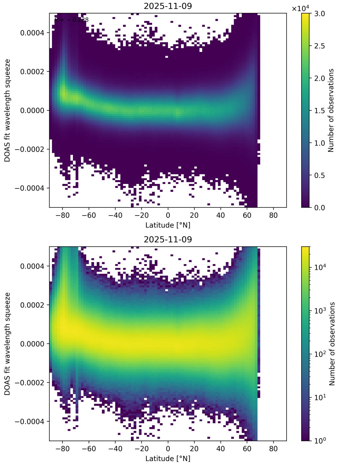
Figure 155: Scatter density plot of “Latitude” against “DOAS fit wavelength squeeze” for 2025-11-08 to 2025-11-10.
