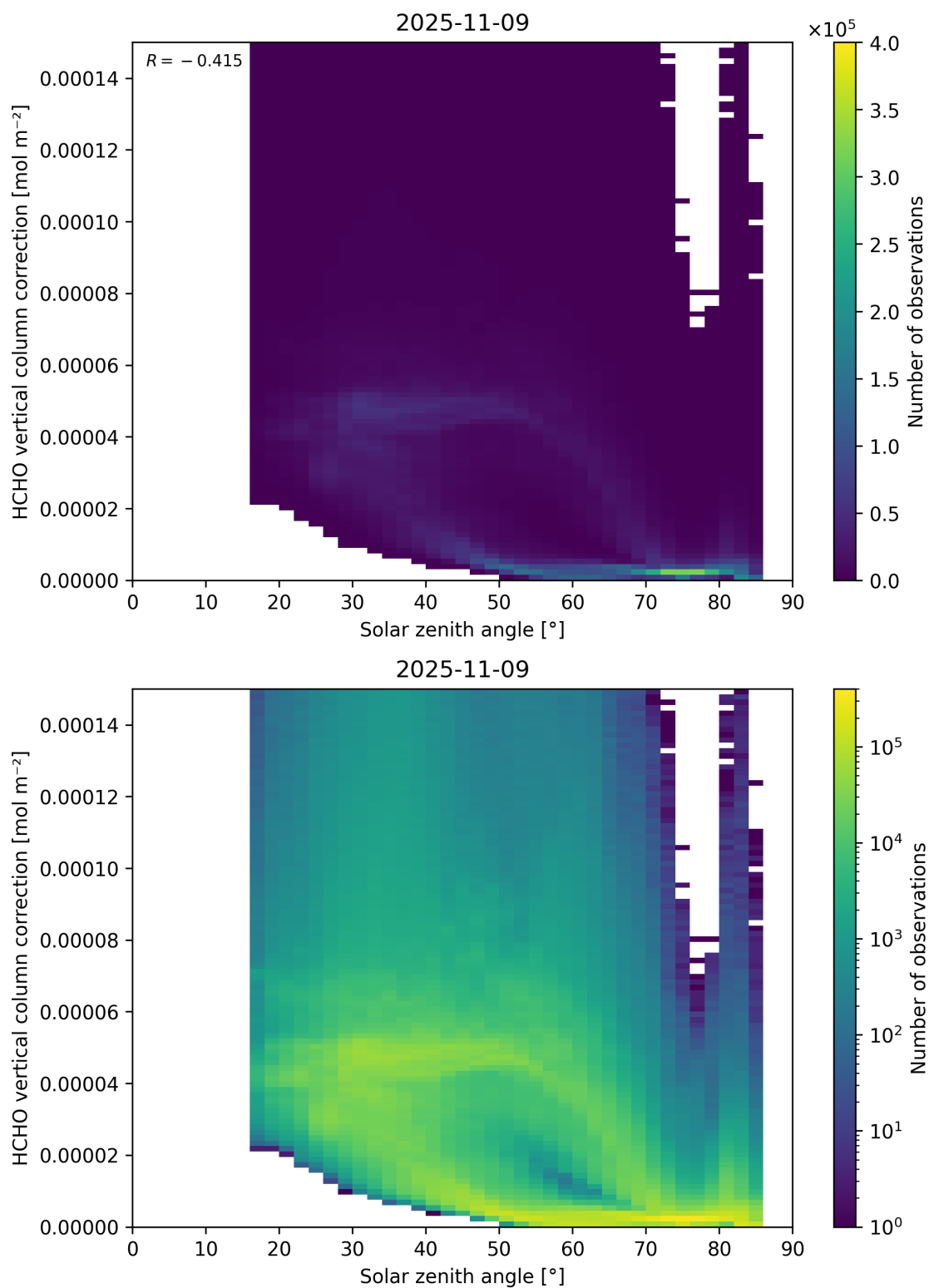
Figure 178: Scatter density plot of “Solar zenith angle” against “HCHO vertical column correction” for 2025-11-08 to 2025-11-10.
