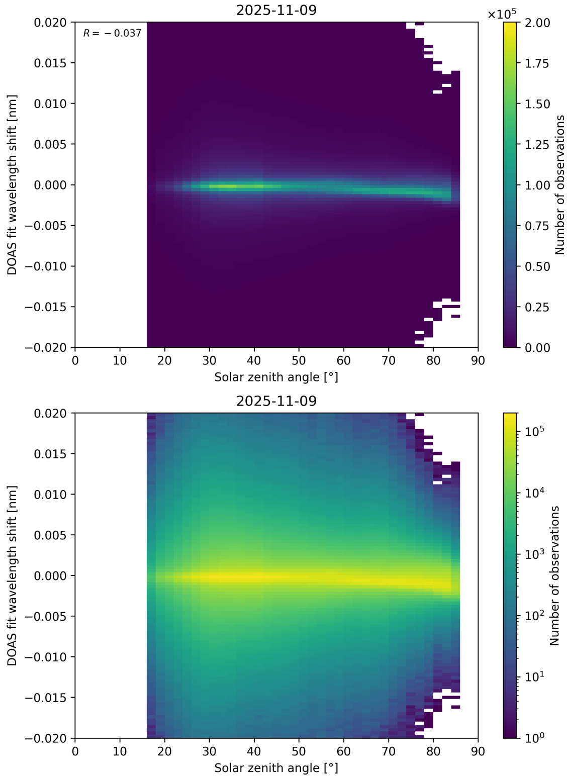
Figure 168: Scatter density plot of “Solar zenith angle” against “DOAS fit wavelength shift” for 2025-11-08 to 2025-11-10.
