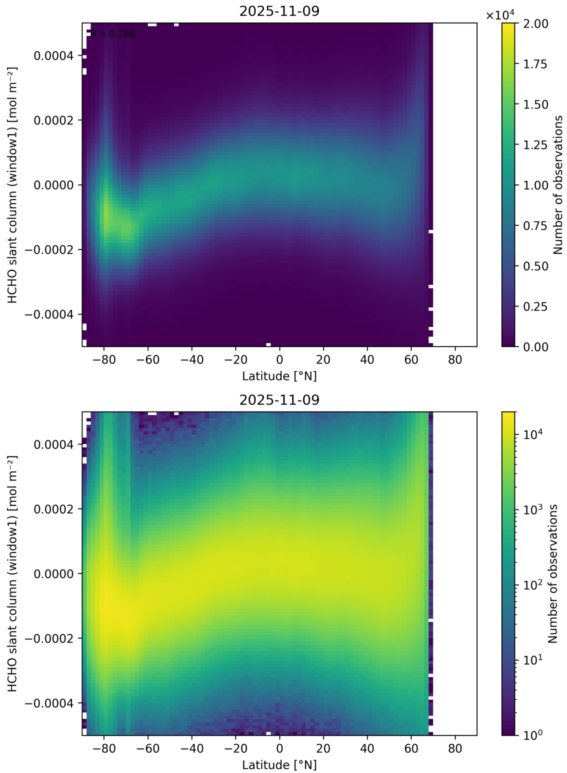
Figure 159: Scatter density plot of “Latitude” against “HCHO slant column (window1)” for 2025-11-08 to 2025-11-10.
