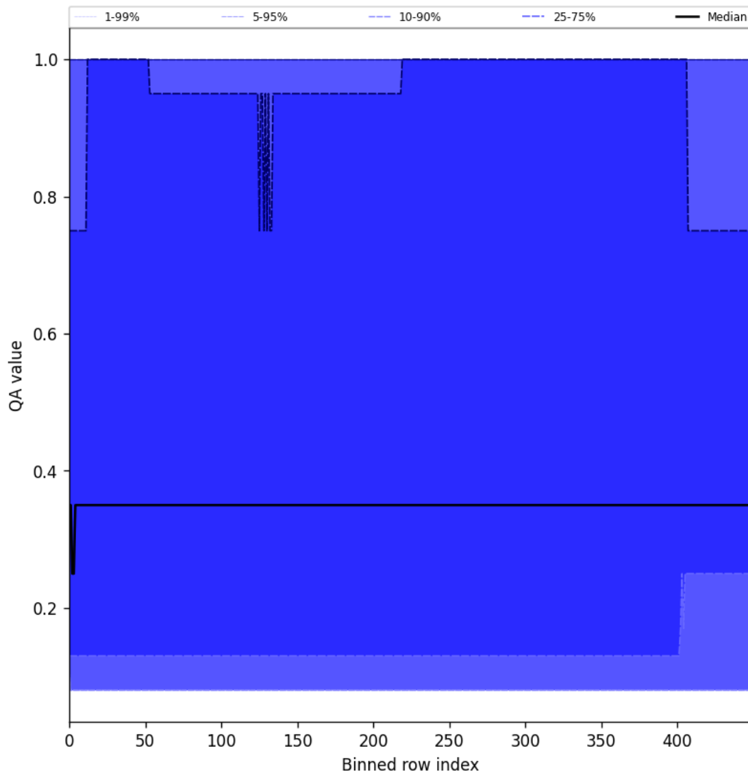
Figure 48: Along track statistics of “QA value” for 2025-11-08 to 2025-11-10
