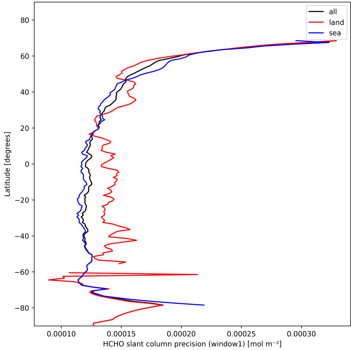
Figure 25: Zonal average of "HCHO slant column precision (window1)" for 2025-11-08 to 2025-11-10.
