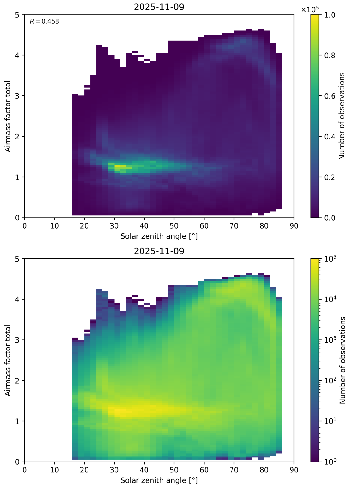
Figure 175: Scatter density plot of “Solar zenith angle” against “Airmass factor total” for 2025-11-08 to 2025-11-10.
