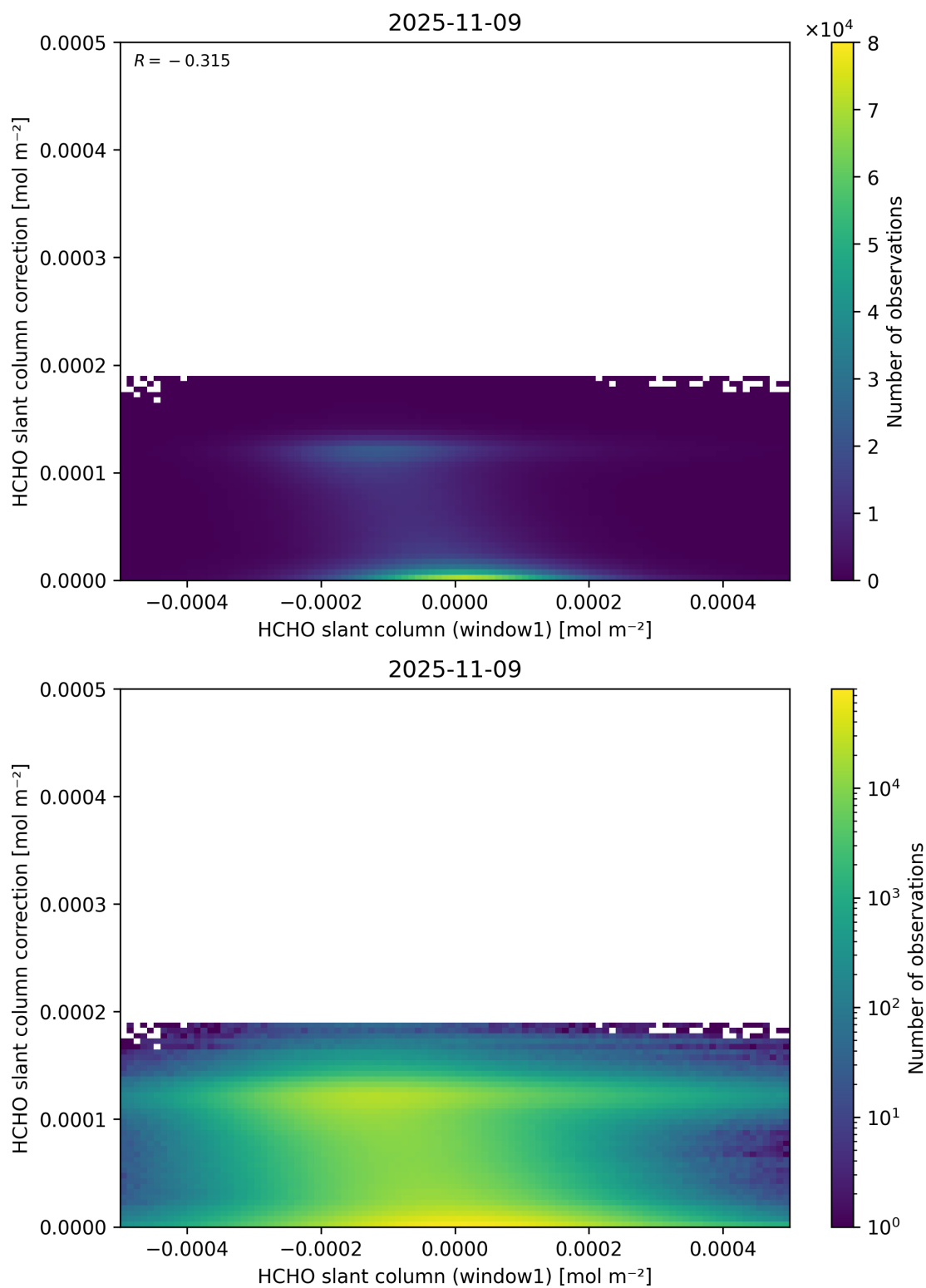
Figure 83: Scatter density plot of “HCHO slant column (window1)” against “HCHO slant column correction” for 2025-11-08 to 2025-11-10.
