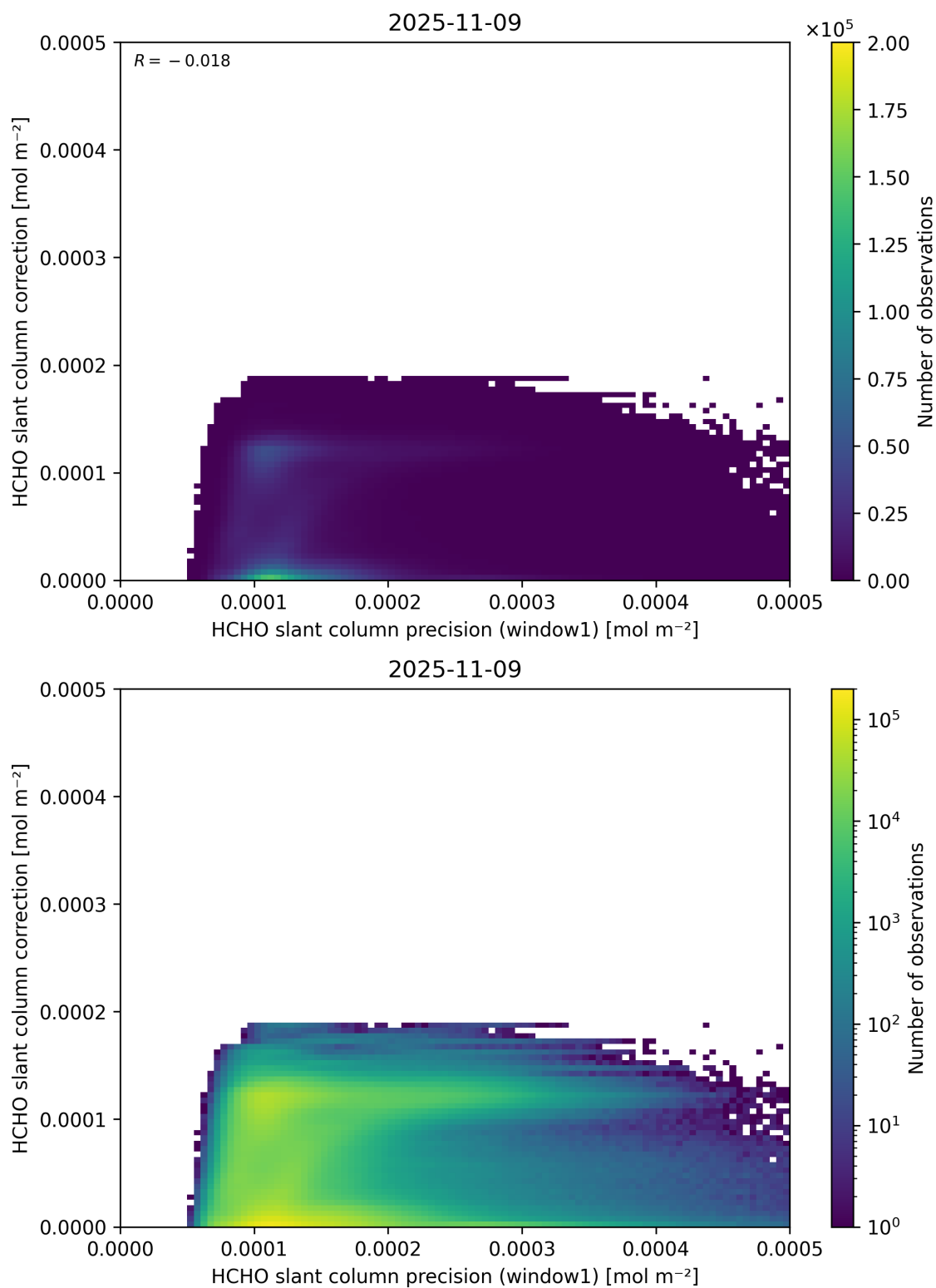
Figure 93: Scatter density plot of “HCHO slant column precision (window1)” against “HCHO slant column correction” for 2025-11-08 to 2025-11-10.
