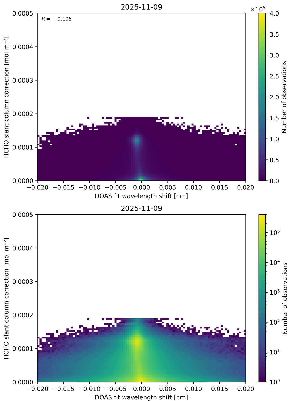
Figure 67: Scatter density plot of “DOAS fit wavelength shift” against “HCHO slant column correction” for 2025-11-08 to 2025-11-10.
