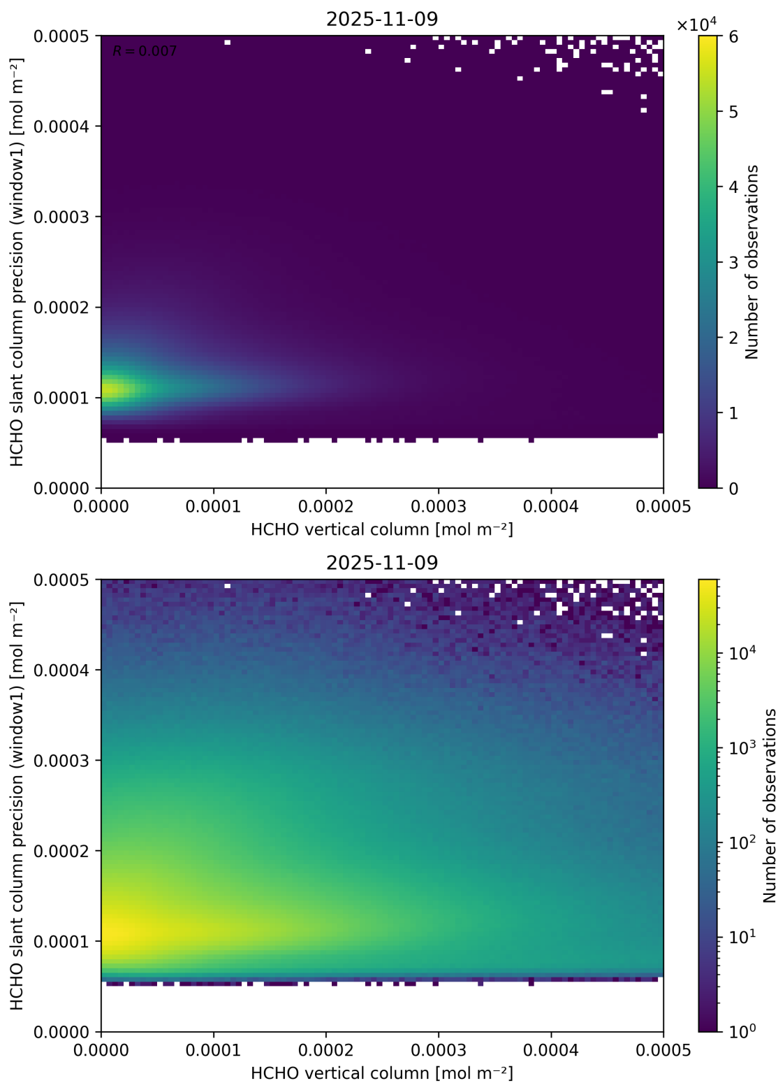
Figure 130: Scatter density plot of “HCHO vertical column” against “HCHO slant column precision (window1)” for 2025-11-08 to 2025-11-10.
