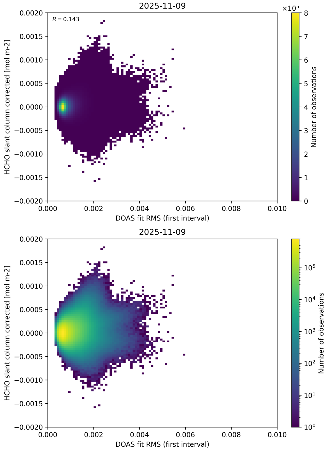
Figure 62: Scatter density plot of “DOAS fit RMS (first interval)” against “HCHO slant column corrected” for 2025-11-08 to 2025-11-10.
