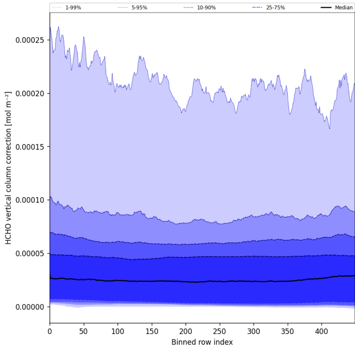
Figure 51: Along track statistics of “HCHO vertical column correction” for 2025-11-08 to 2025-11-10
