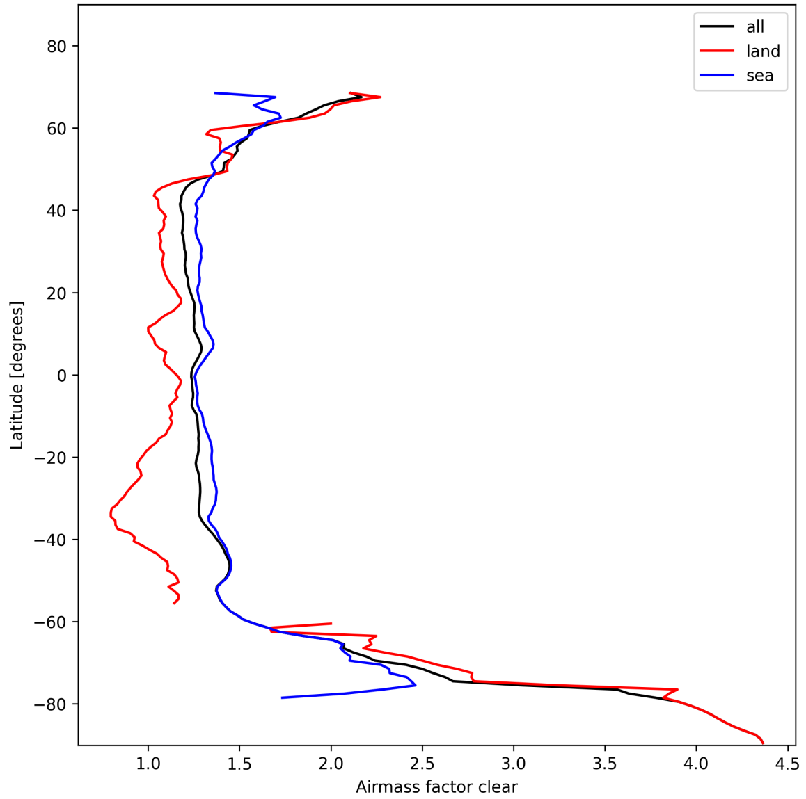
Figure 28: Zonal average of “Airmass factor clear” for 2025-11-08 to 2025-11-10.
