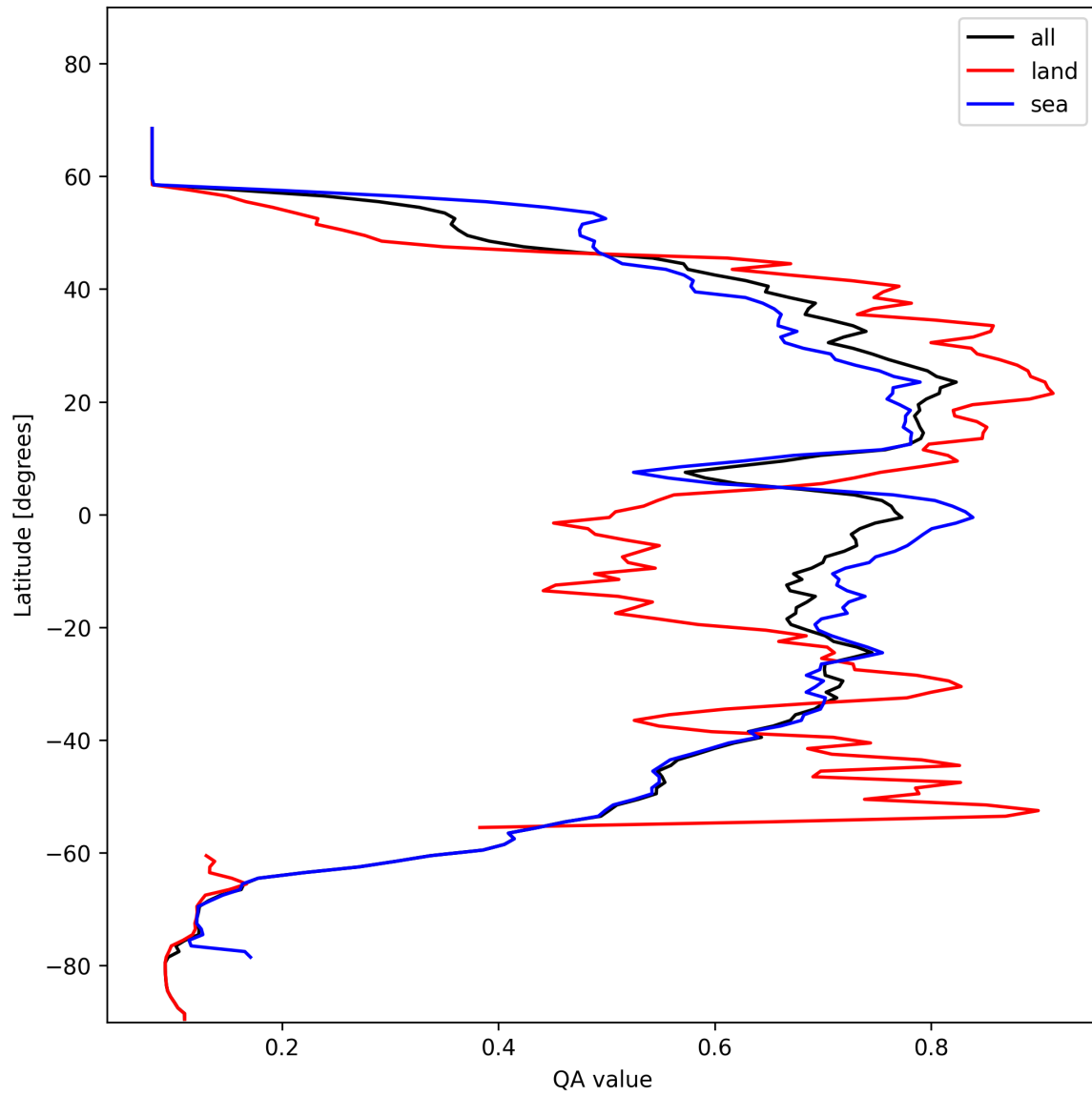
Figure 20: Zonal average of “QA value” for 2025-11-08 to 2025-11-10.
