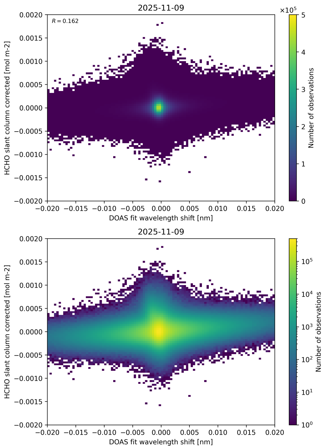
Figure 66: Scatter density plot of “DOAS fit wavelength shift” against “HCHO slant column corrected” for 2025-11-08 to 2025-11-10.
