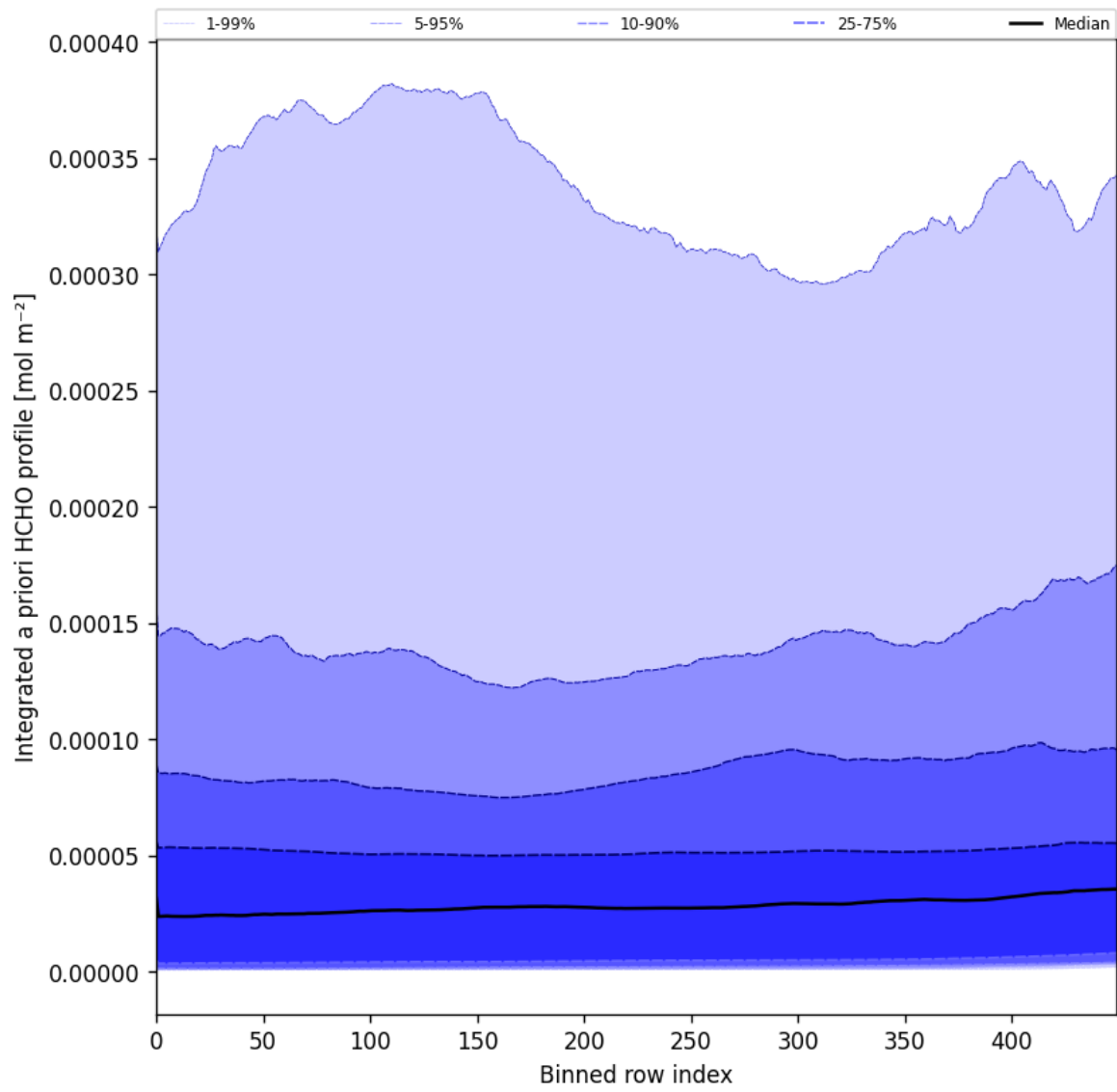
Figure 57: Along track statistics of “Integrated a priori HCHO profile” for 2025-11-08 to 2025-11-10
