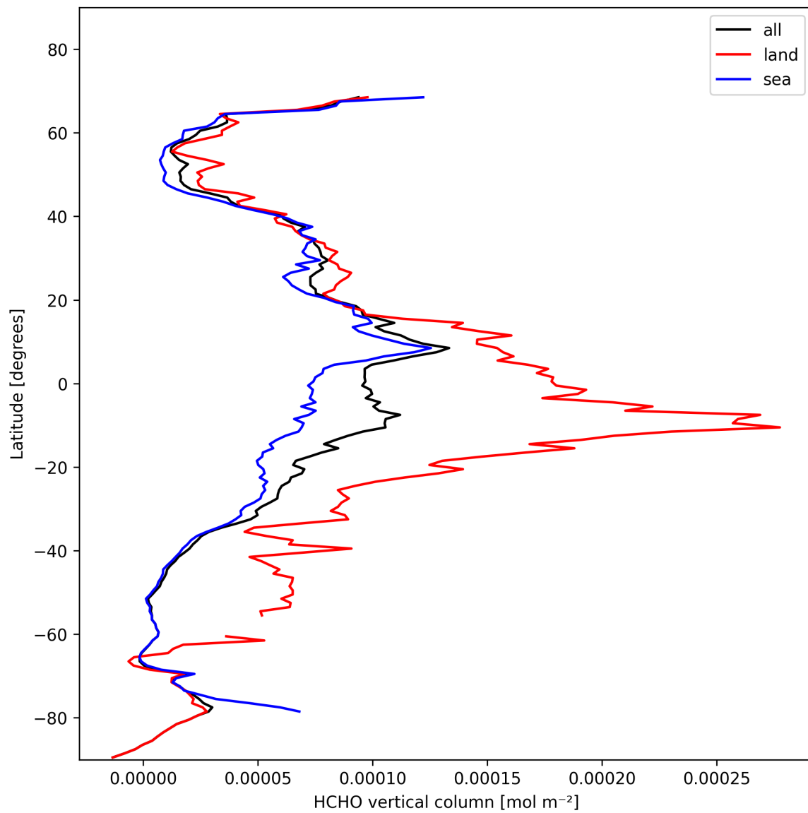
Figure 21: Zonal average of “HCHO vertical column” for 2025-11-08 to 2025-11-10.
