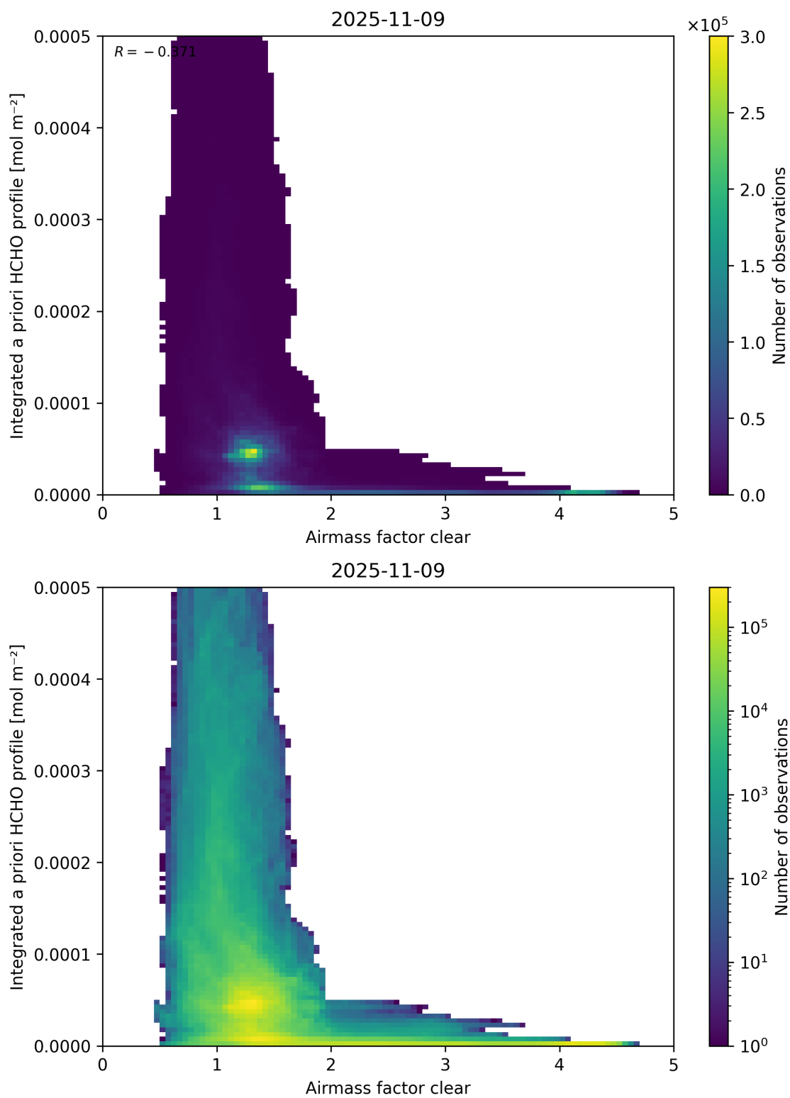
Figure 76: Scatter density plot of “Airmass factor clear” against “Integrated a priori HCHO profile” for 2025-11-08 to 2025-11-10.
