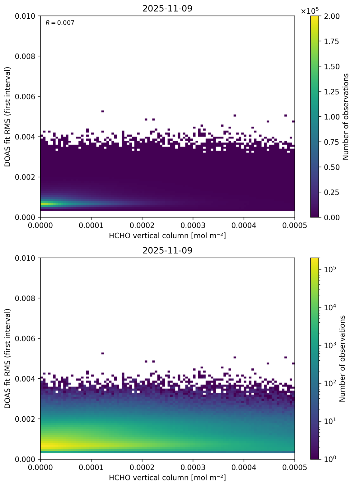
Figure 123: Scatter density plot of “HCHO vertical column” against “DOAS fit RMS (first interval)” for 2025-11-08 to 2025-11-10.
