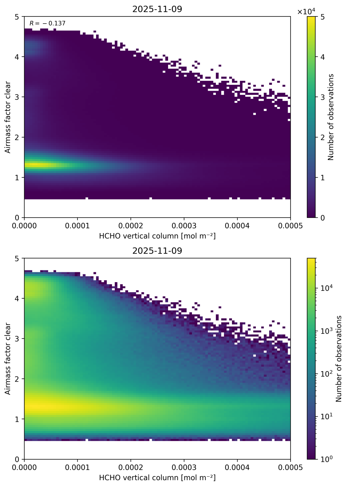
Figure 126: Scatter density plot of “HCHO vertical column” against “Airmass factor clear” for 2025-11-08 to 2025-11-10.
