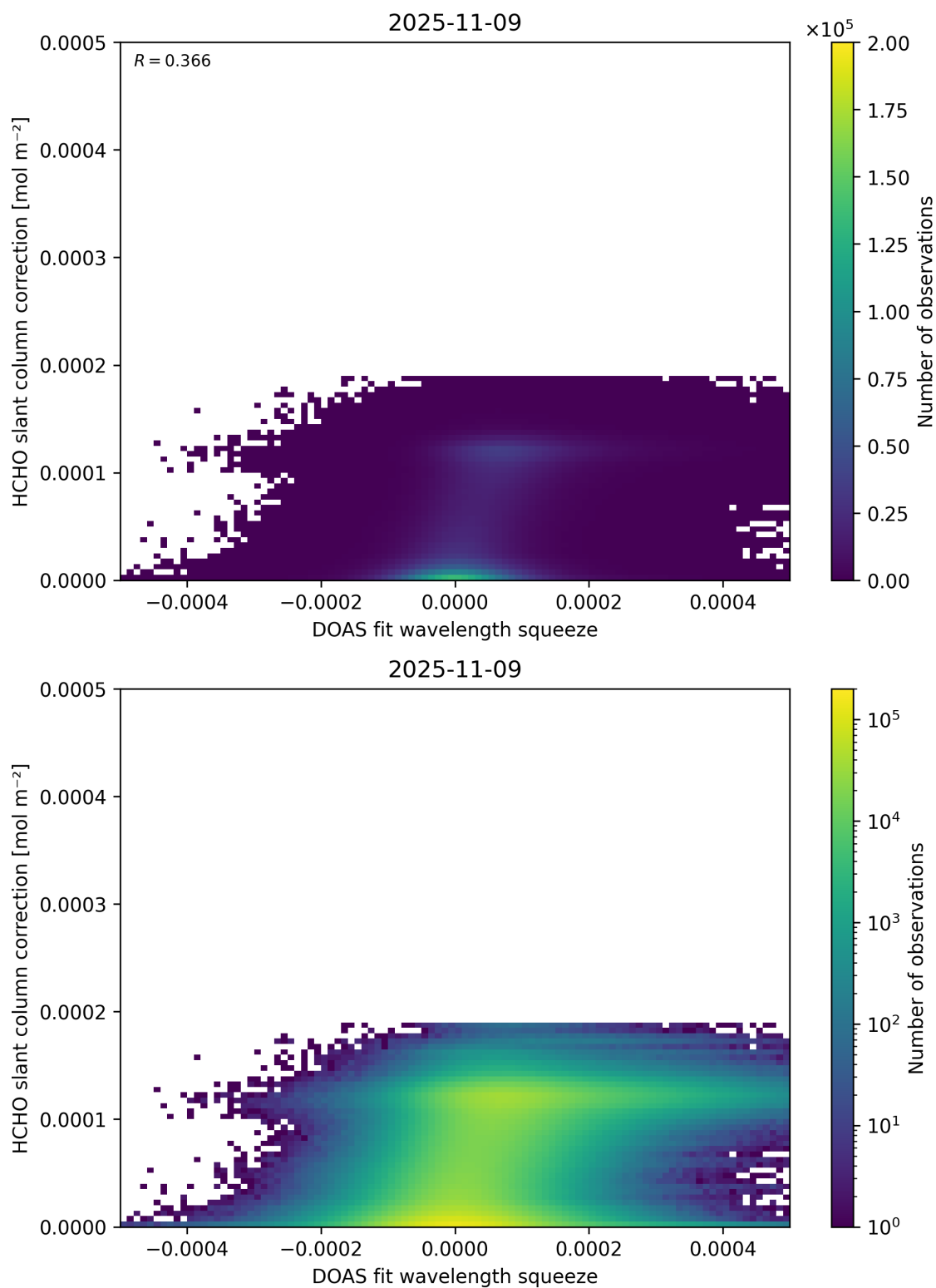
Figure 70: Scatter density plot of “DOAS fit wavelength squeeze” against “HCHO slant column correction” for 2025-11-08 to 2025-11-10.
