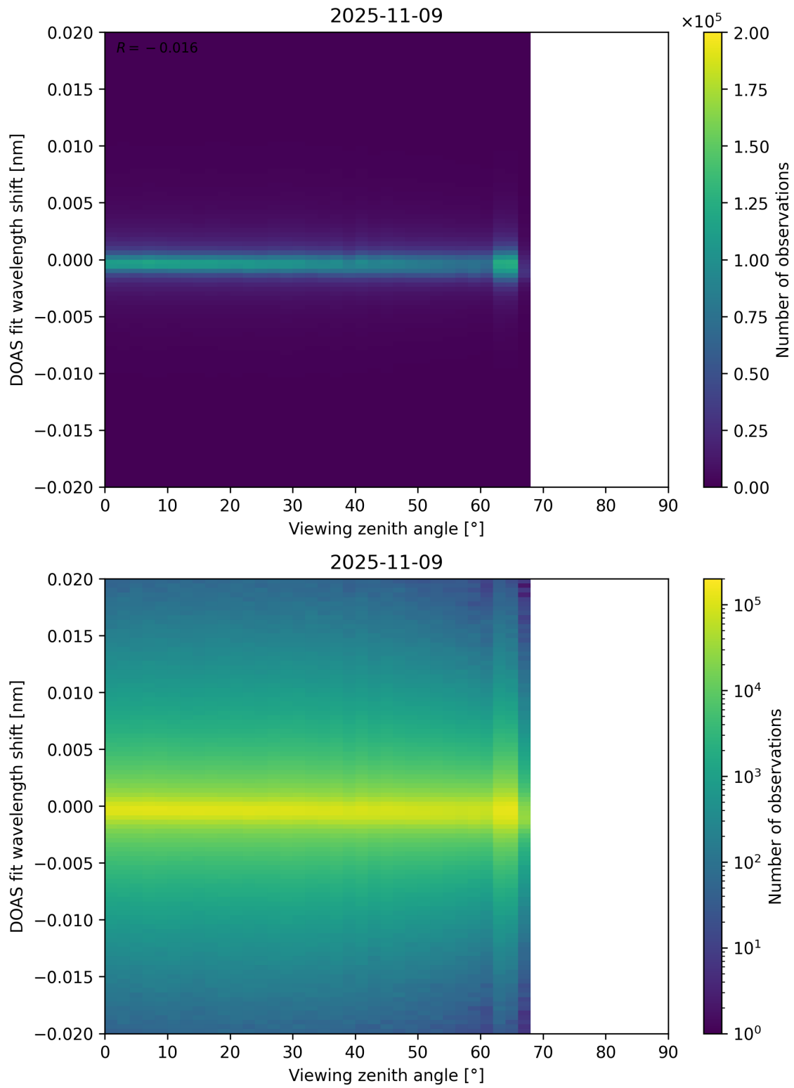
Figure 183: Scatter density plot of “Viewing zenith angle” against “DOAS fit wavelength shift” for 2025-11-08 to 2025-11-10.
