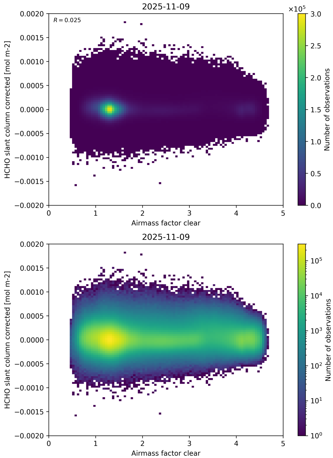
Figure 74: Scatter density plot of “Airmass factor clear” against “HCHO slant column corrected” for 2025-11-08 to 2025-11-10.
