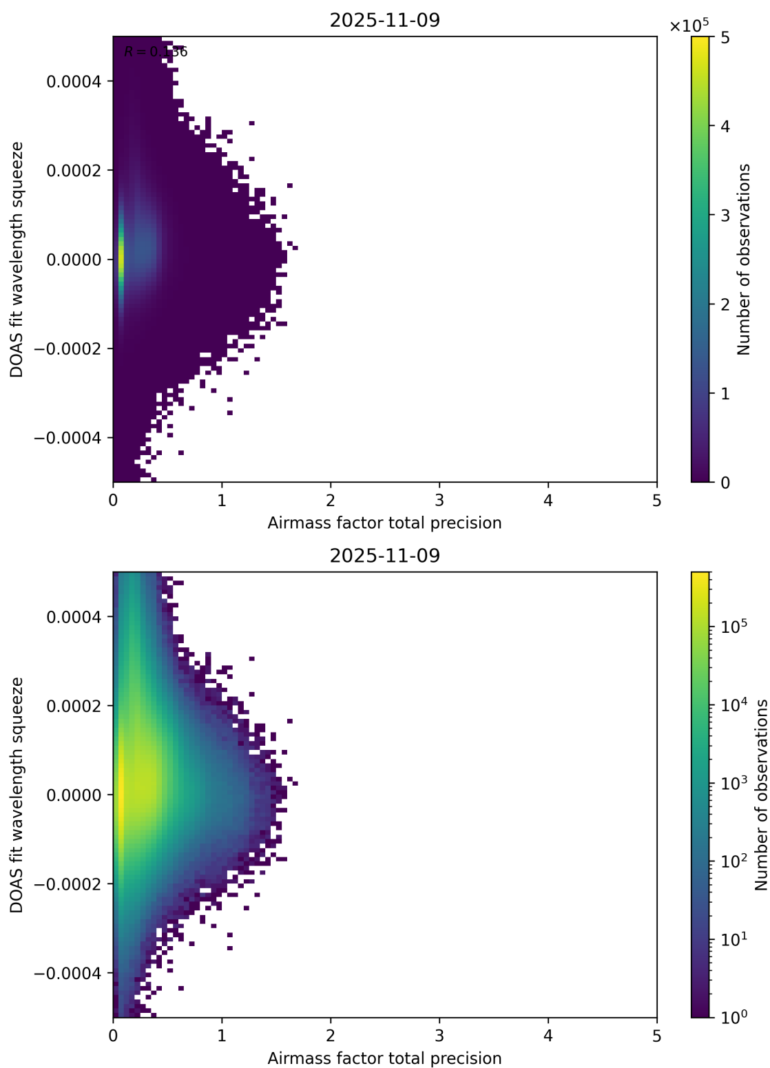
Figure 107: Scatter density plot of “Airmass factor total precision” against “DOAS fit wavelength squeeze” for 2025-11-08 to 2025-11-10.
