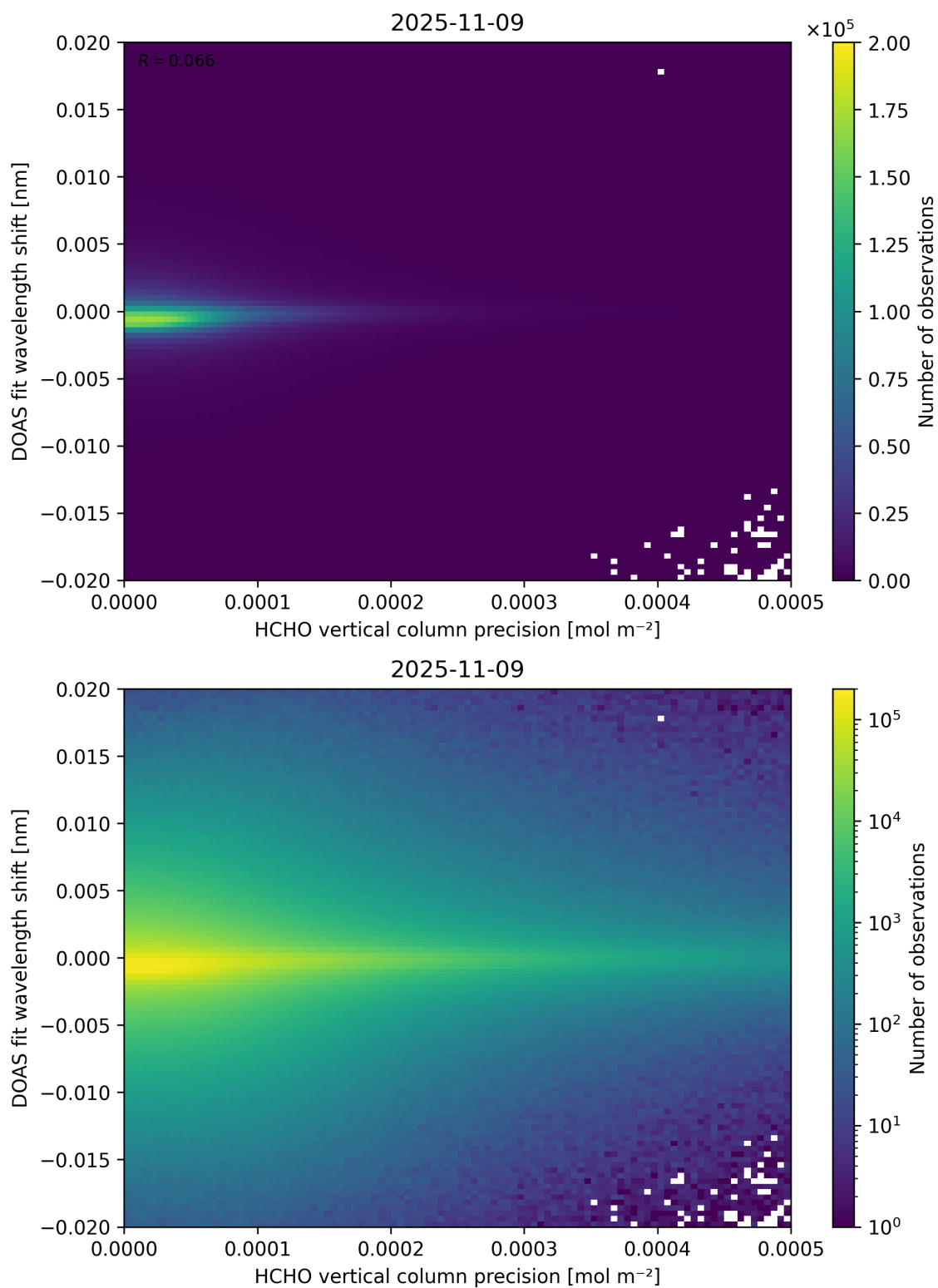
Figure 137: Scatter density plot of “HCHO vertical column precision” against “DOAS fit wavelength shift” for 2025-11-08 to 2025-11-10.
