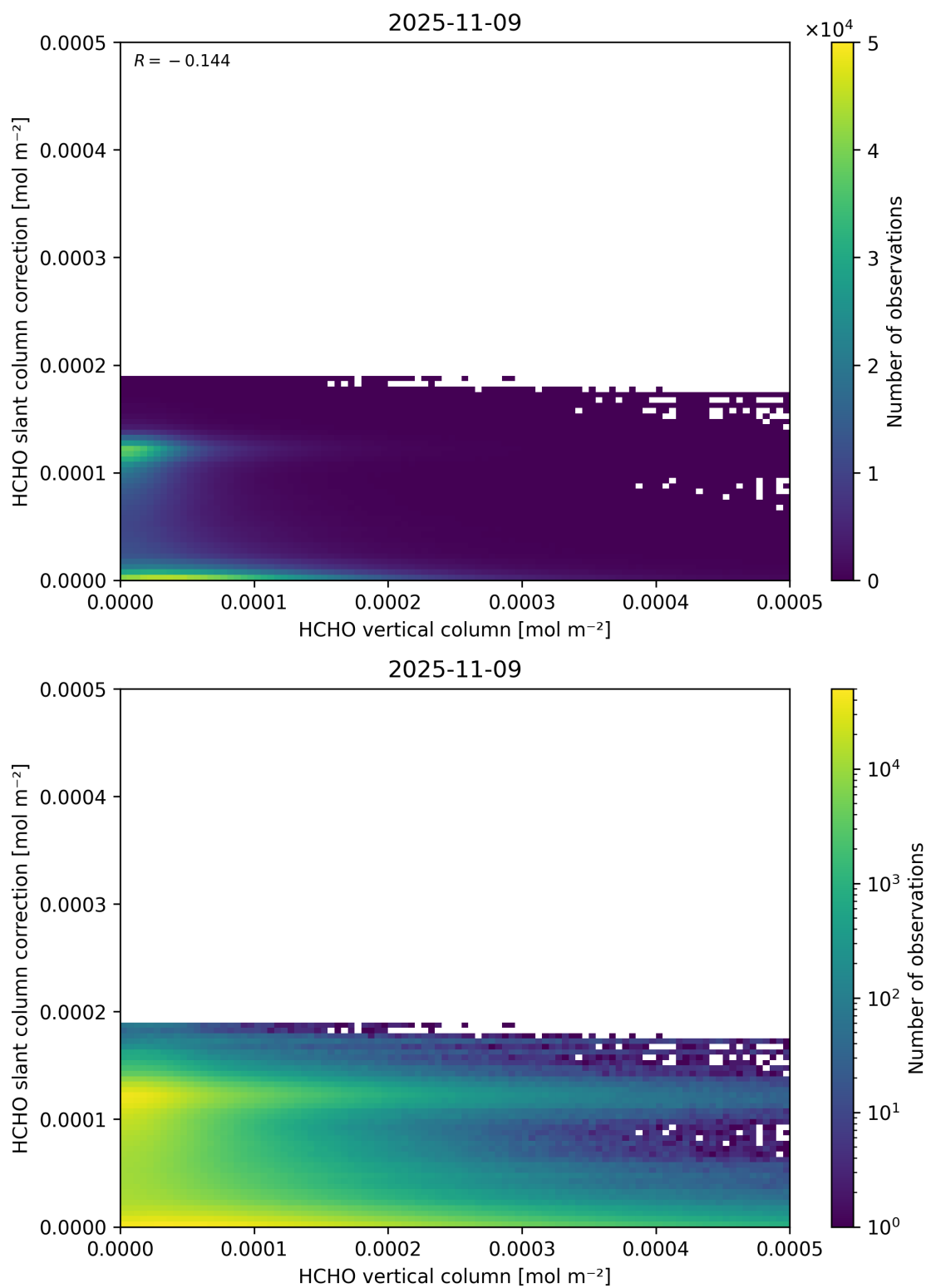
Figure 128: Scatter density plot of “HCHO vertical column” against “HCHO slant column correction” for 2025-11-08 to 2025-11-10.
