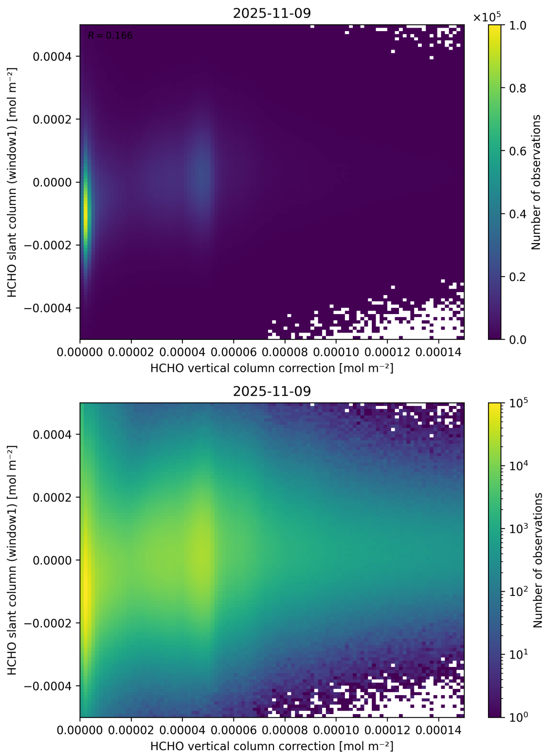
Figure 118: Scatter density plot of “HCHO vertical column correction” against “HCHO slant column (window1)” for 2025-11-08 to 2025-11-10.
