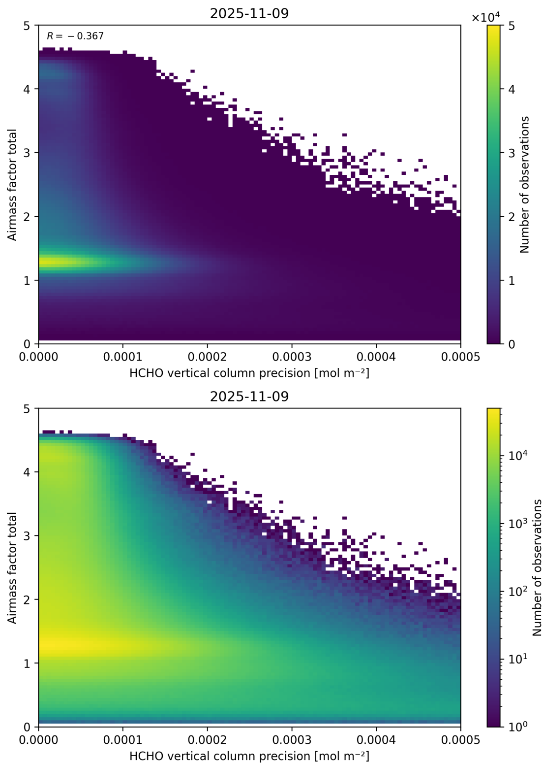
Figure 144: Scatter density plot of “HCHO vertical column precision” against “Airmass factor total” for 2025-11-08 to 2025-11-10.
