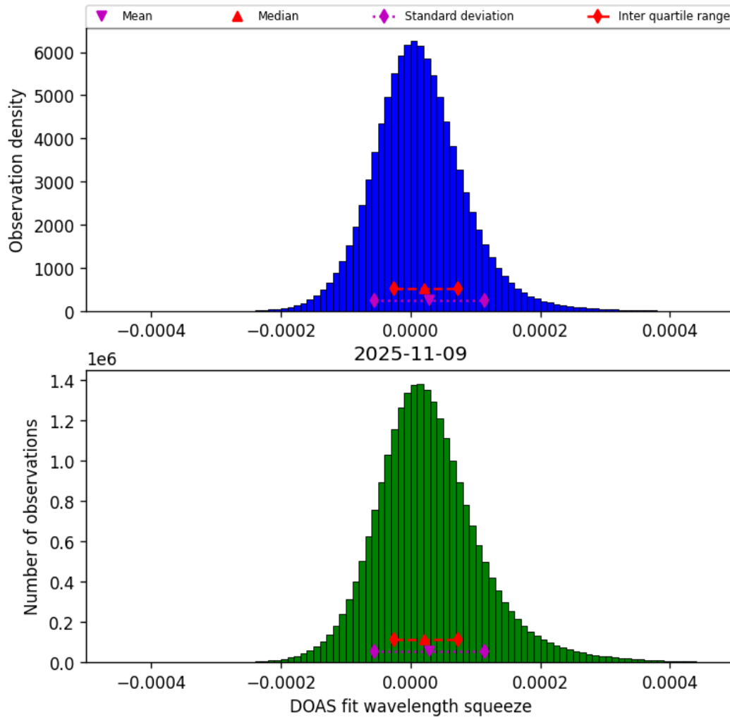
Figure 45: Histogram of “DOAS fit wavelength squeeze” for 2025-11-08 to 2025-11-10
