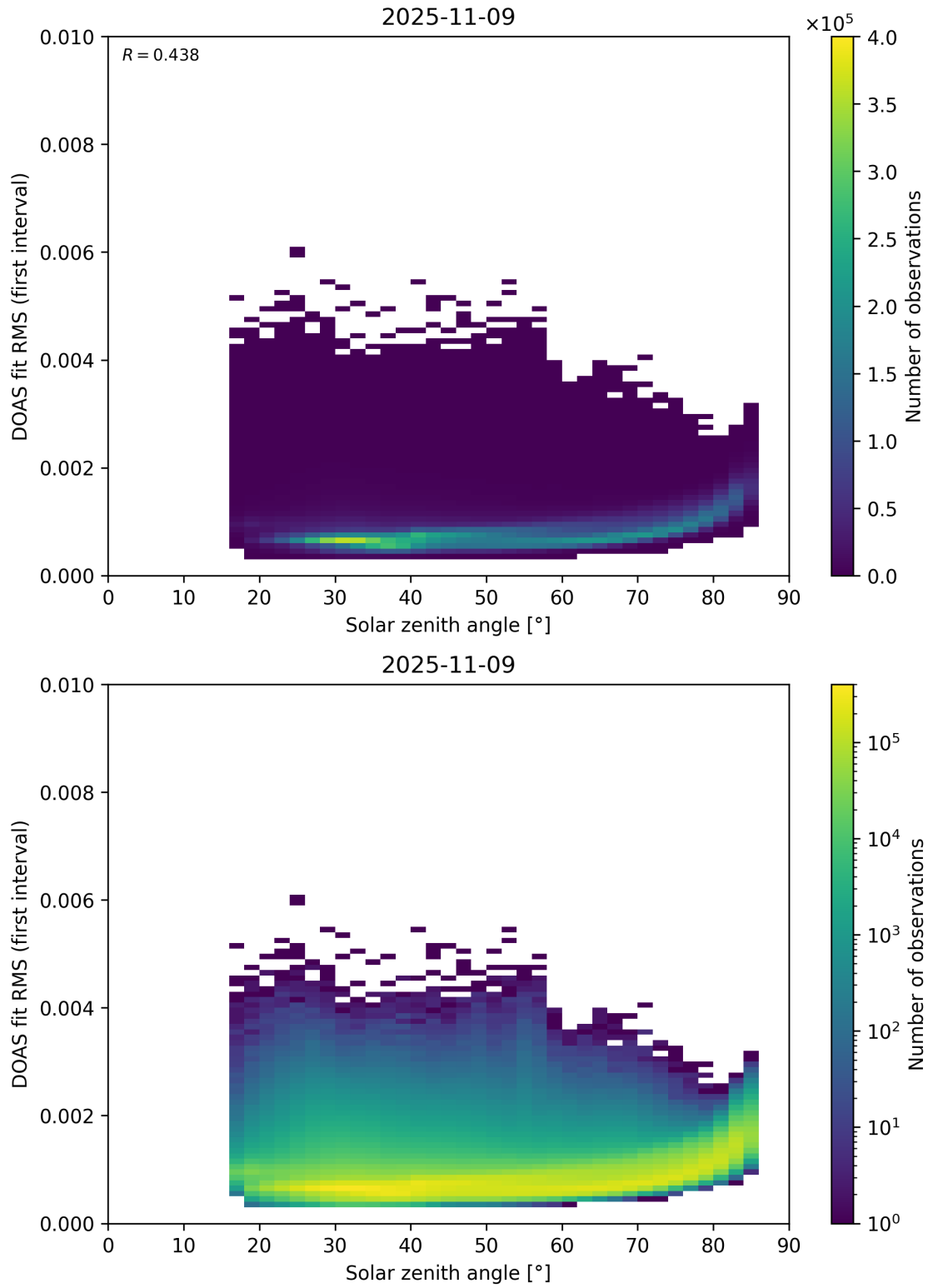
Figure 167: Scatter density plot of “Solar zenith angle” against “DOAS fit RMS (first interval)” for 2025-11-08 to 2025-11-10.
