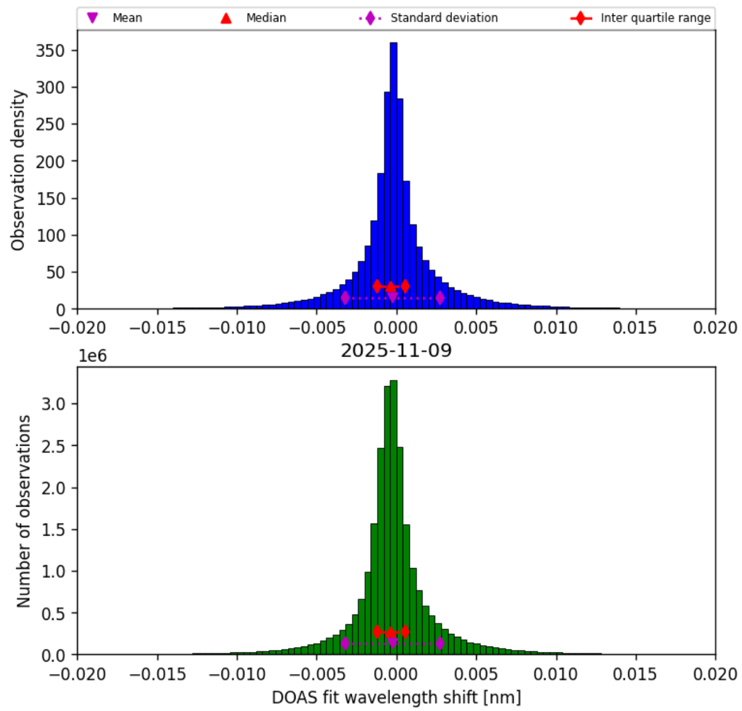
Figure 44: Histogram of “DOAS fit wavelength shift” for 2025-11-08 to 2025-11-10
