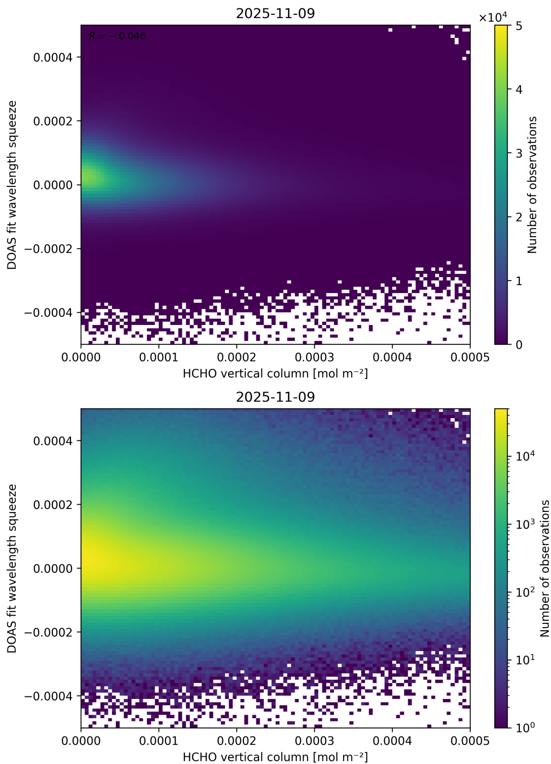
Figure 125: Scatter density plot of “HCHO vertical column” against “DOAS fit wavelength squeeze” for 2025-11-08 to 2025-11-10.
