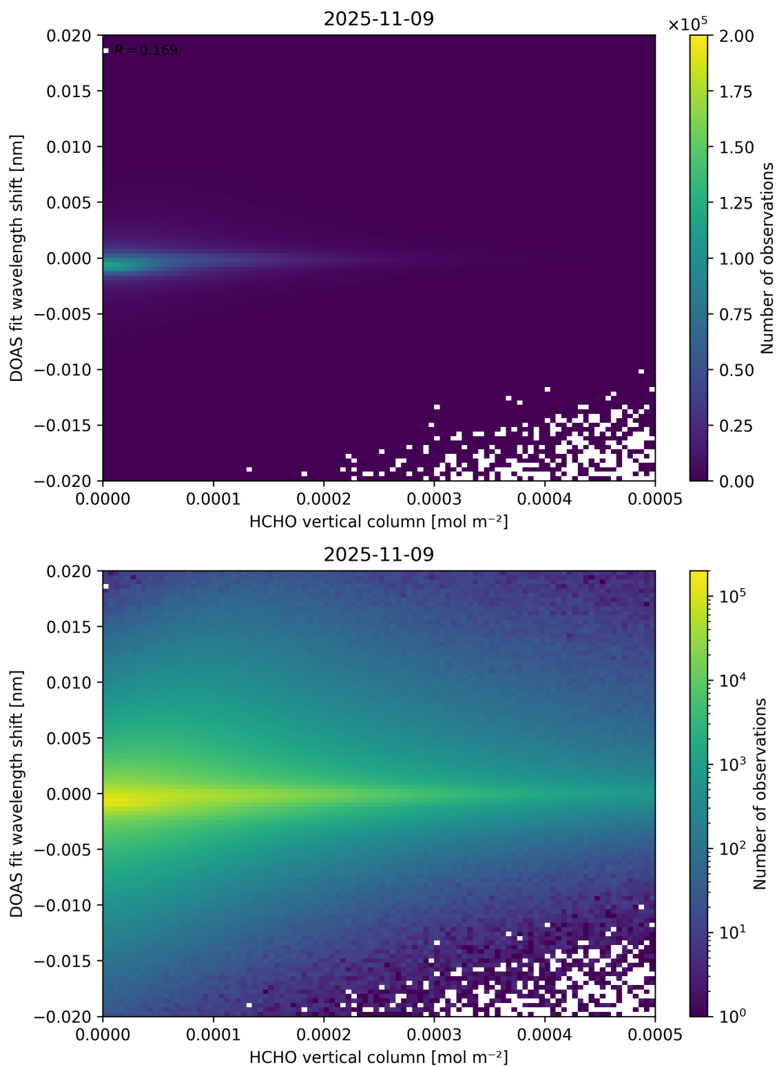
Figure 124: Scatter density plot of “HCHO vertical column” against “DOAS fit wavelength shift” for 2025-11-08 to 2025-11-10.
