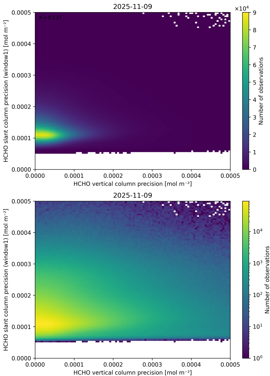
Figure 143: Scatter density plot of “HCHO vertical column precision” against “HCHO slant column precision (window1)” for 2025-11-08 to 2025-11-10.
