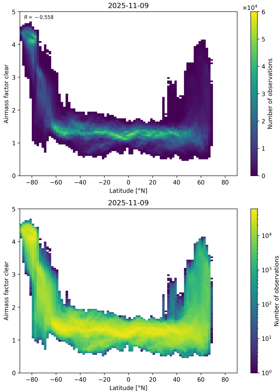
Figure 156: Scatter density plot of “Latitude” against “Airmass factor clear” for 2025-11-08 to 2025-11-10.
