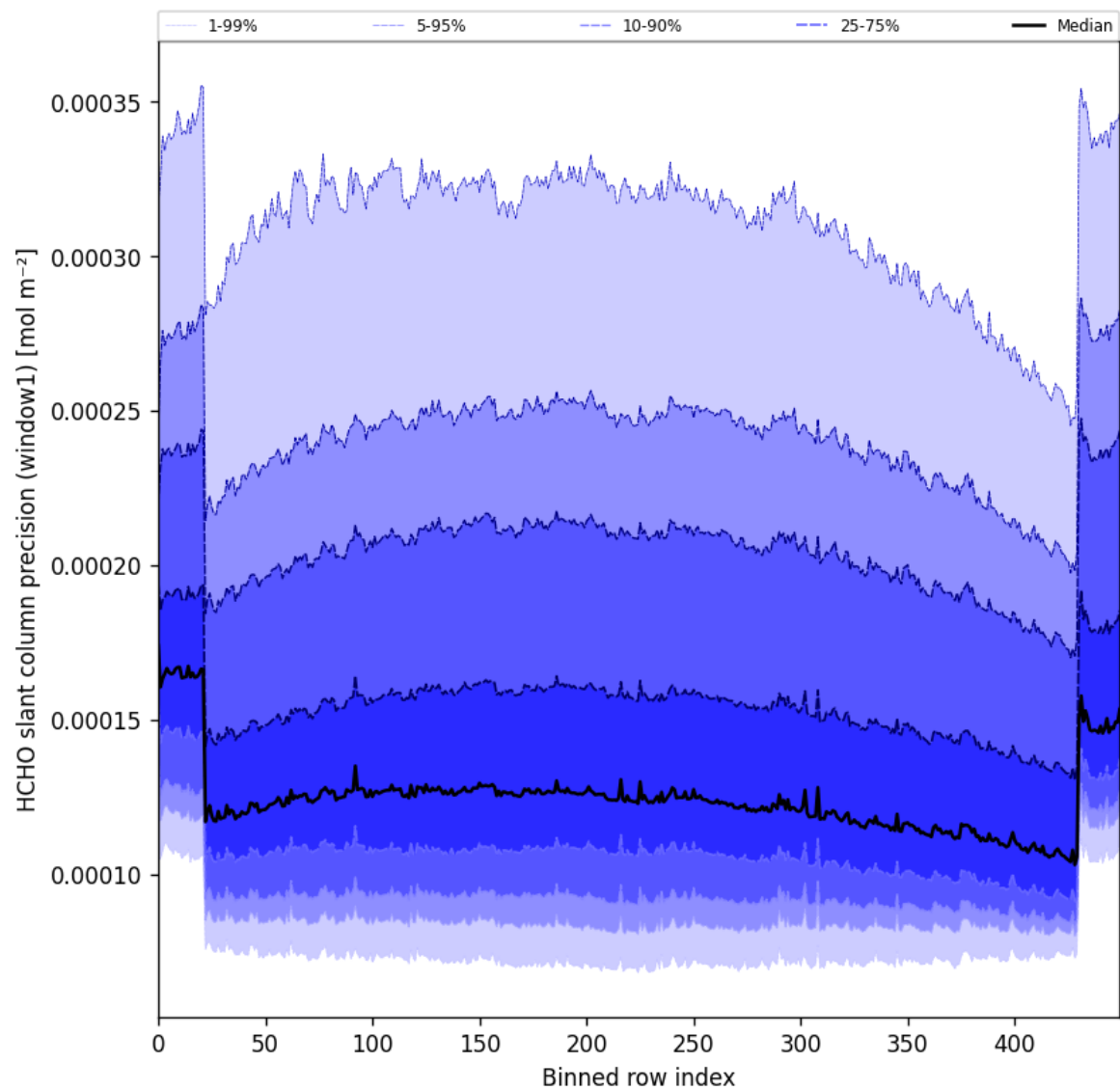
Figure 53: Along track statistics of “HCHO slant column precision (window1)” for 2025-11-08 to 2025-11-10
