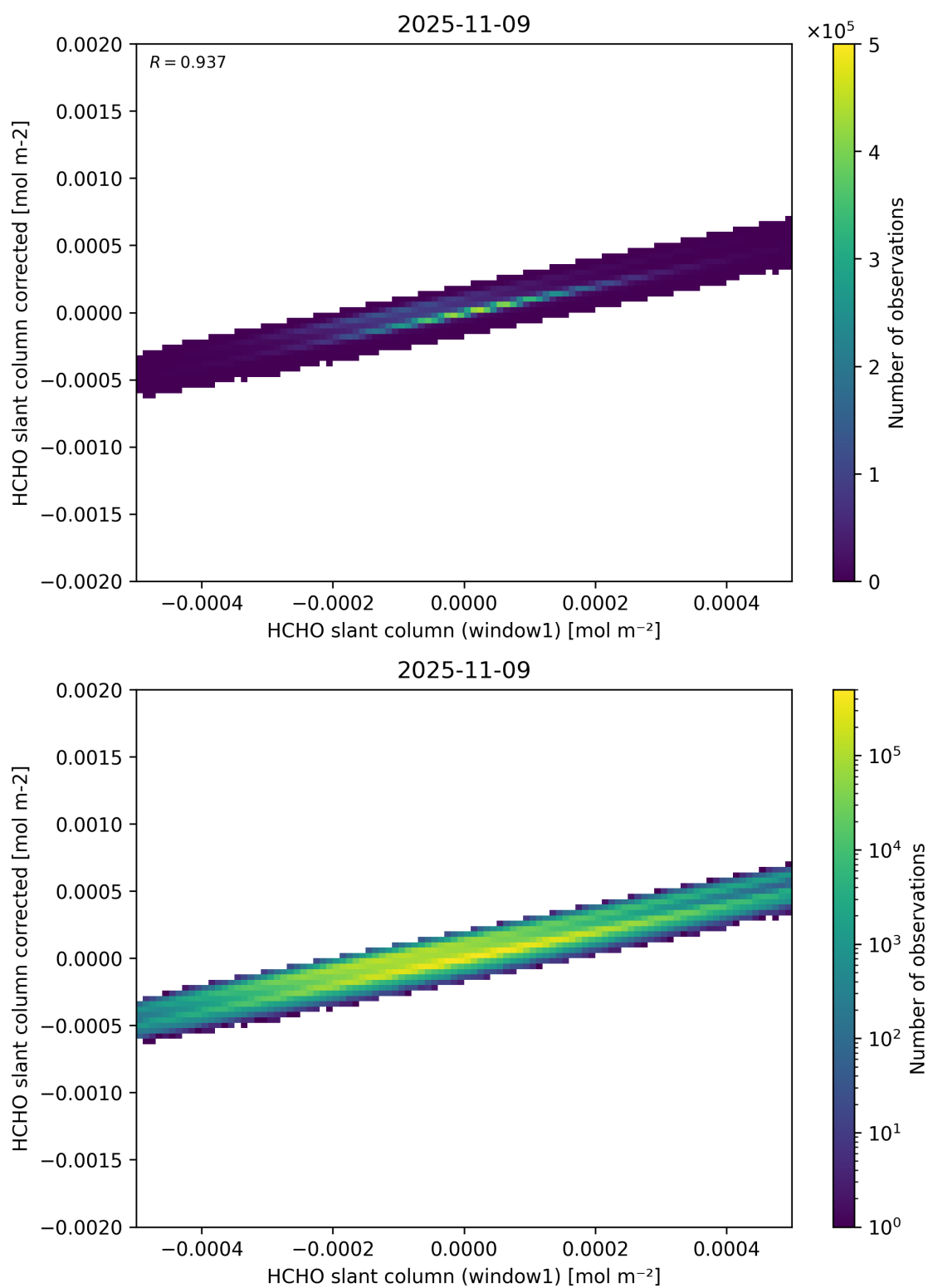
Figure 82: Scatter density plot of “HCHO slant column (window1)” against “HCHO slant column corrected” for 2025-11-08 to 2025-11-10.
