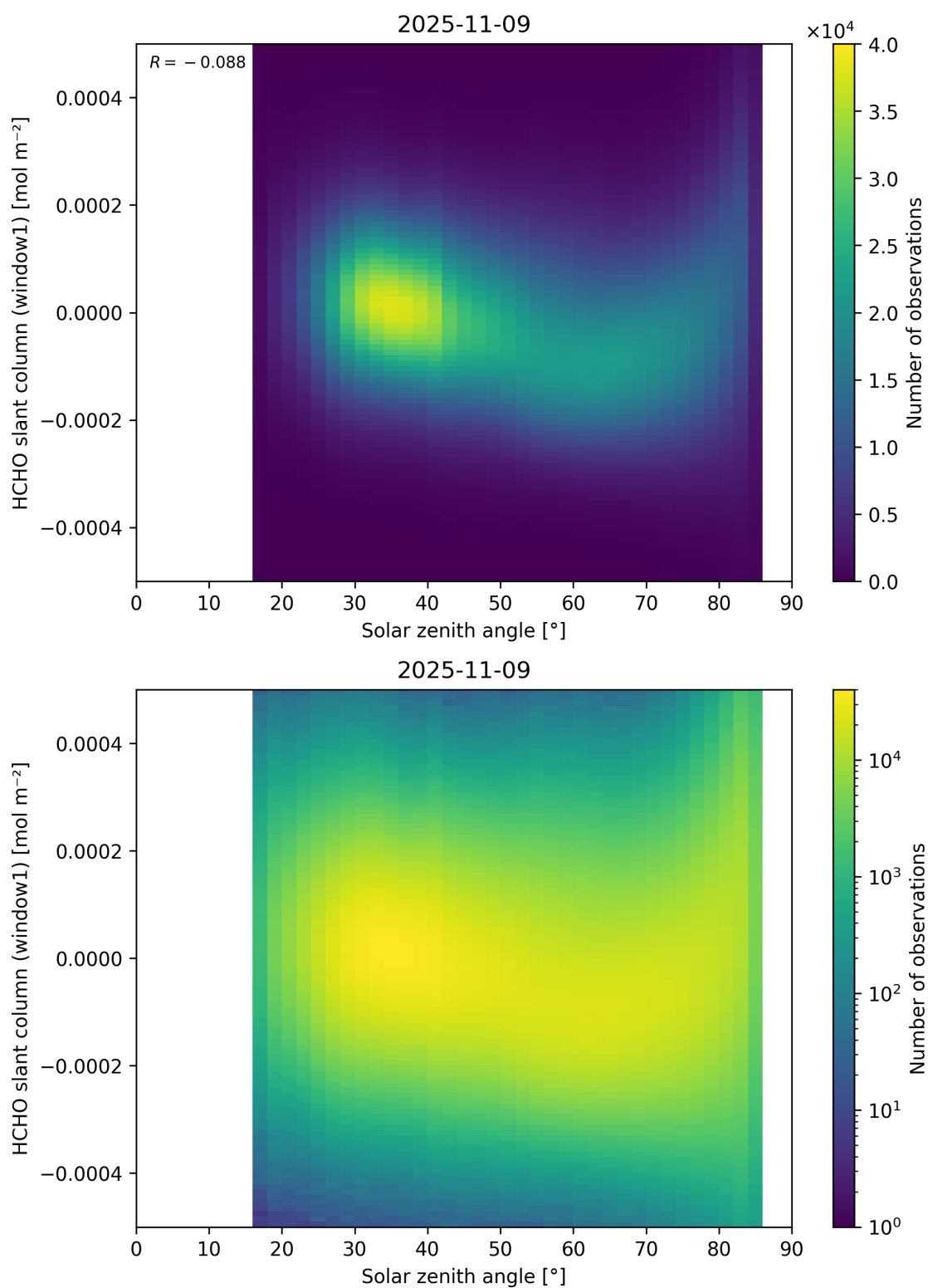
Figure 173: Scatter density plot of “Solar zenith angle” against “HCHO slant column (window1)” for 2025-11-08 to 2025-11-10.
