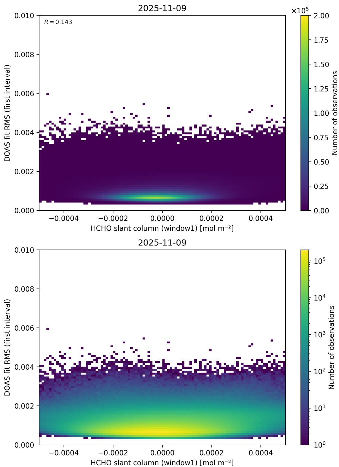
Figure 78: Scatter density plot of “HCHO slant column (window1)” against “DOAS fit RMS (first interval)” for 2025-11-08 to 2025-11-10.
