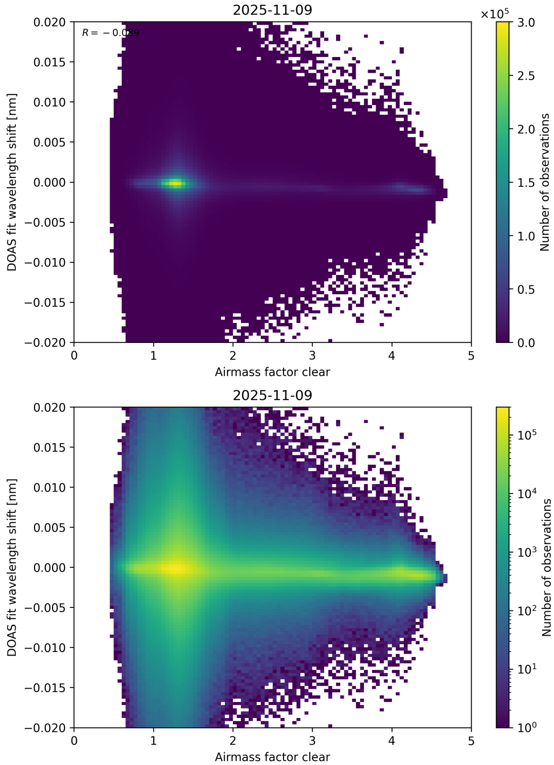
Figure 72: Scatter density plot of “Airmass factor clear” against “DOAS fit wavelength shift” for 2025-11-08 to 2025-11-10.
