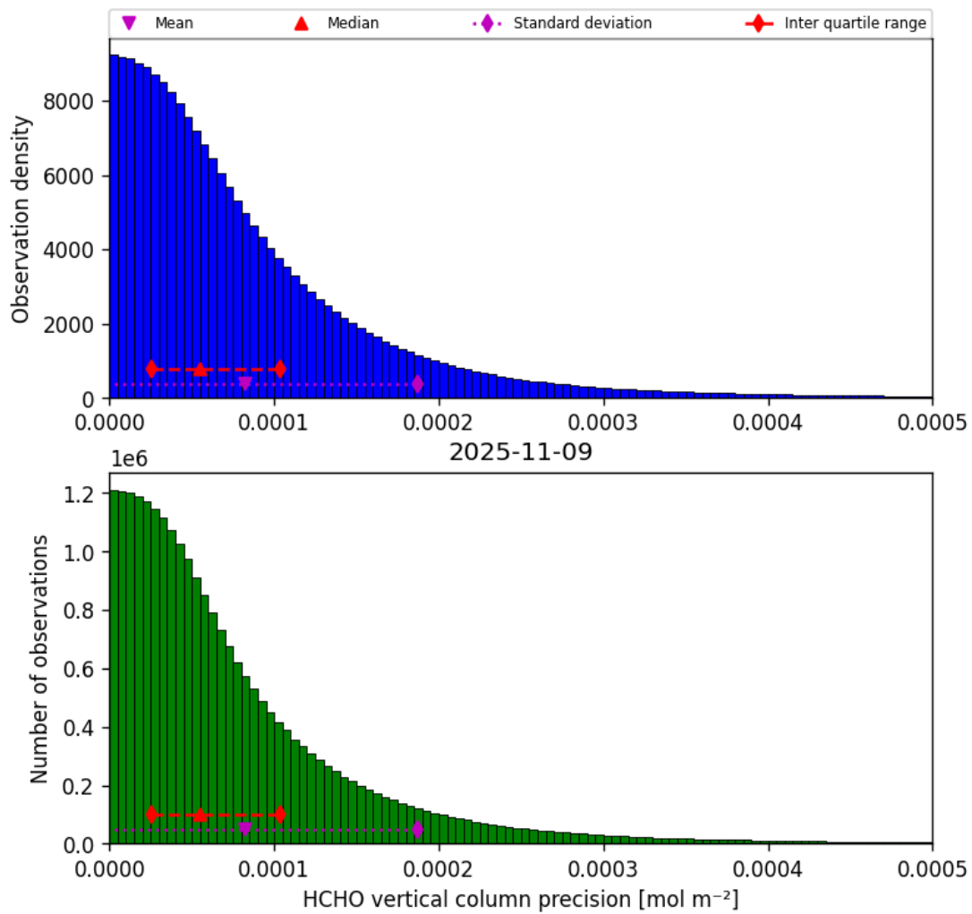
Figure 36: Histogram of “HCHO vertical column precision” for 2025-11-08 to 2025-11-10
