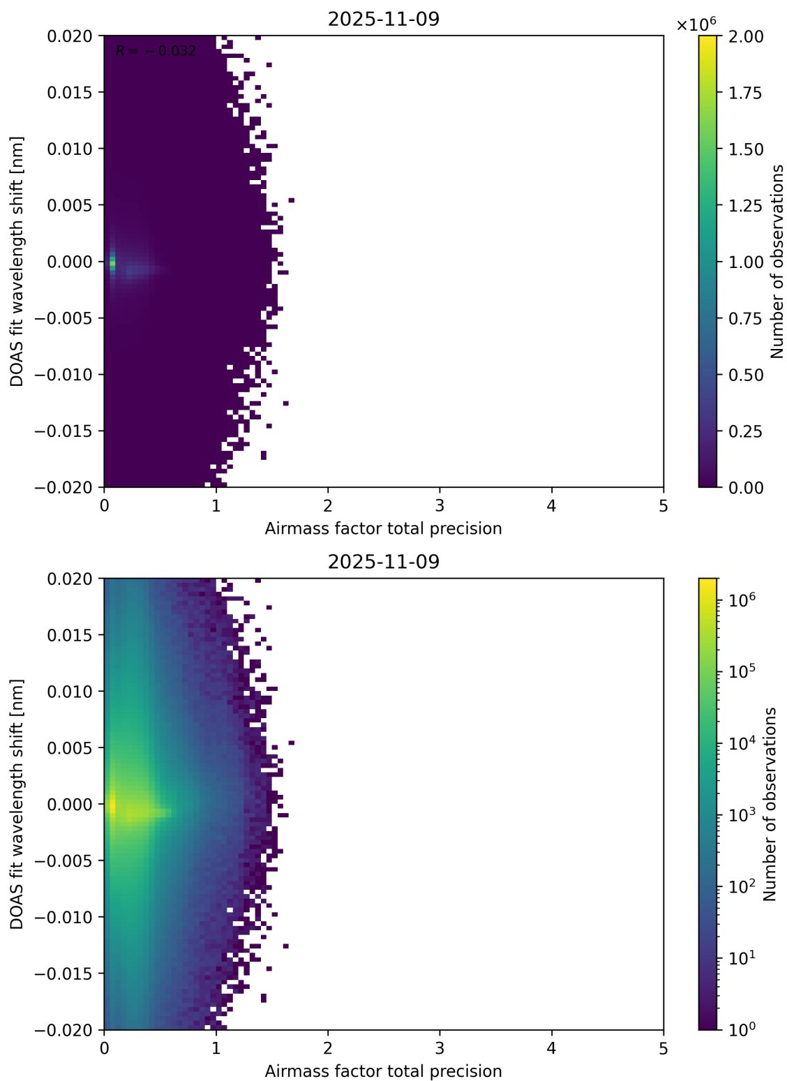
Figure 106: Scatter density plot of “Airmass factor total precision” against “DOAS fit wavelength shift” for 2025-11-08 to 2025-11-10.
