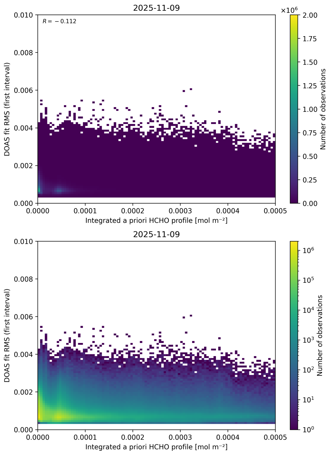
Figure 148: Scatter density plot of “Integrated a priori HCHO profile” against “DOAS fit RMS (first interval)” for 2025-11-08 to 2025-11-10.
