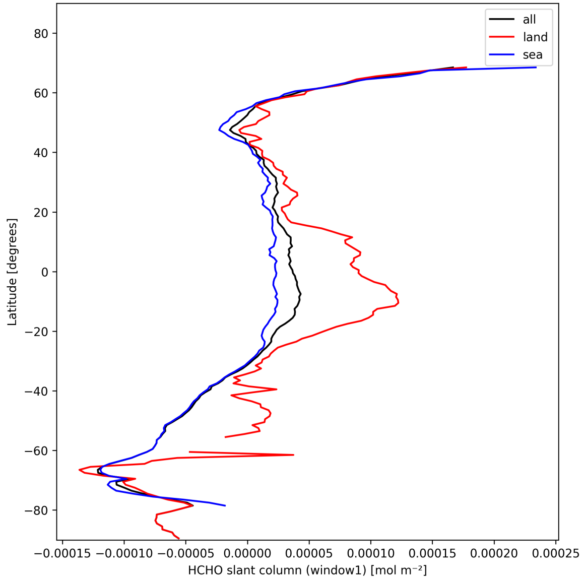
Figure 24: Zonal average of “HCHO slant column (window1)” for 2025-11-08 to 2025-11-10.
