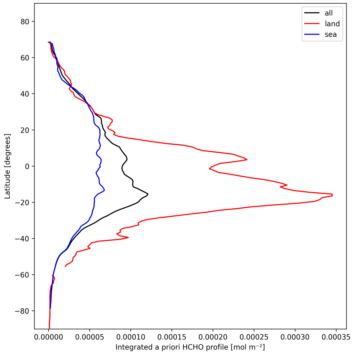
Figure 29: Zonal average of “Integrated a priori HCHO profile” for 2025-11-08 to 2025-11-10.
