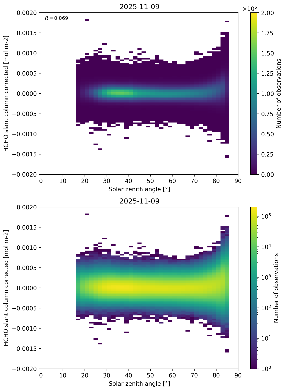
Figure 171: Scatter density plot of “Solar zenith angle” against “HCHO slant column corrected” for 2025-11-08 to 2025-11-10.
