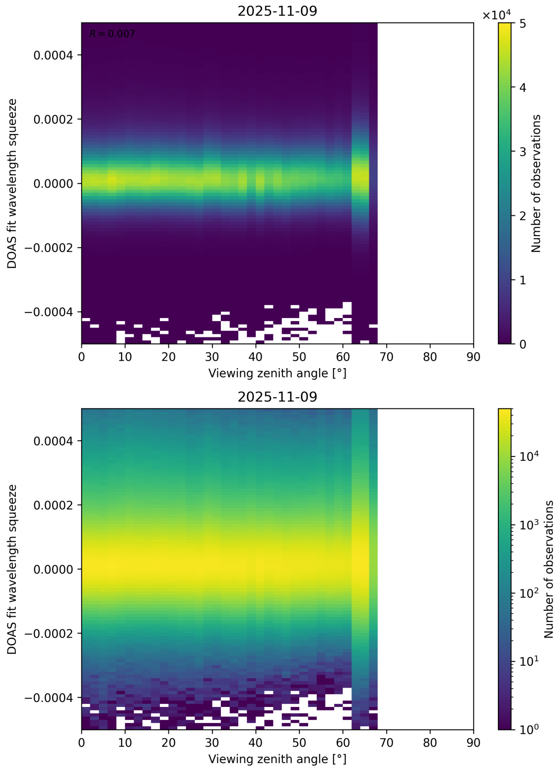
Figure 184: Scatter density plot of “Viewing zenith angle” against “DOAS fit wavelength squeeze” for 2025-11-08 to 2025-11-10.
