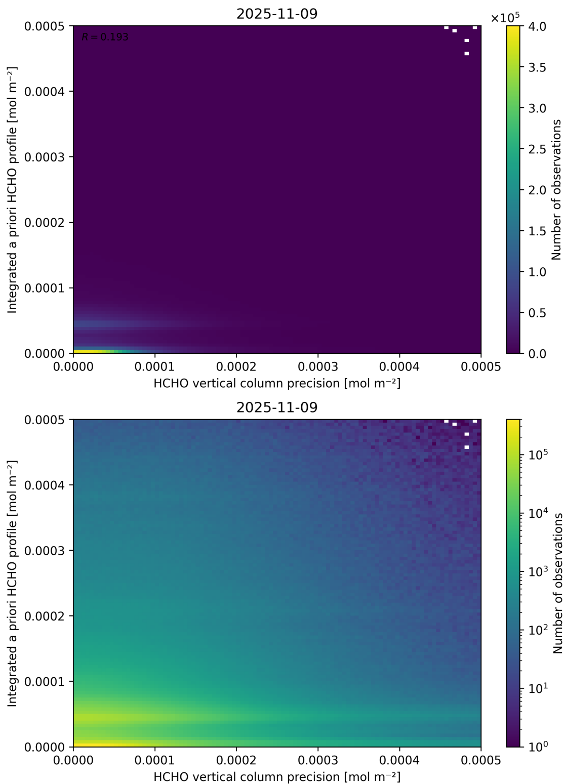
Figure 147: Scatter density plot of “HCHO vertical column precision” against “Integrated a priori HCHO profile” for 2025-11-08 to 2025-11-10.
