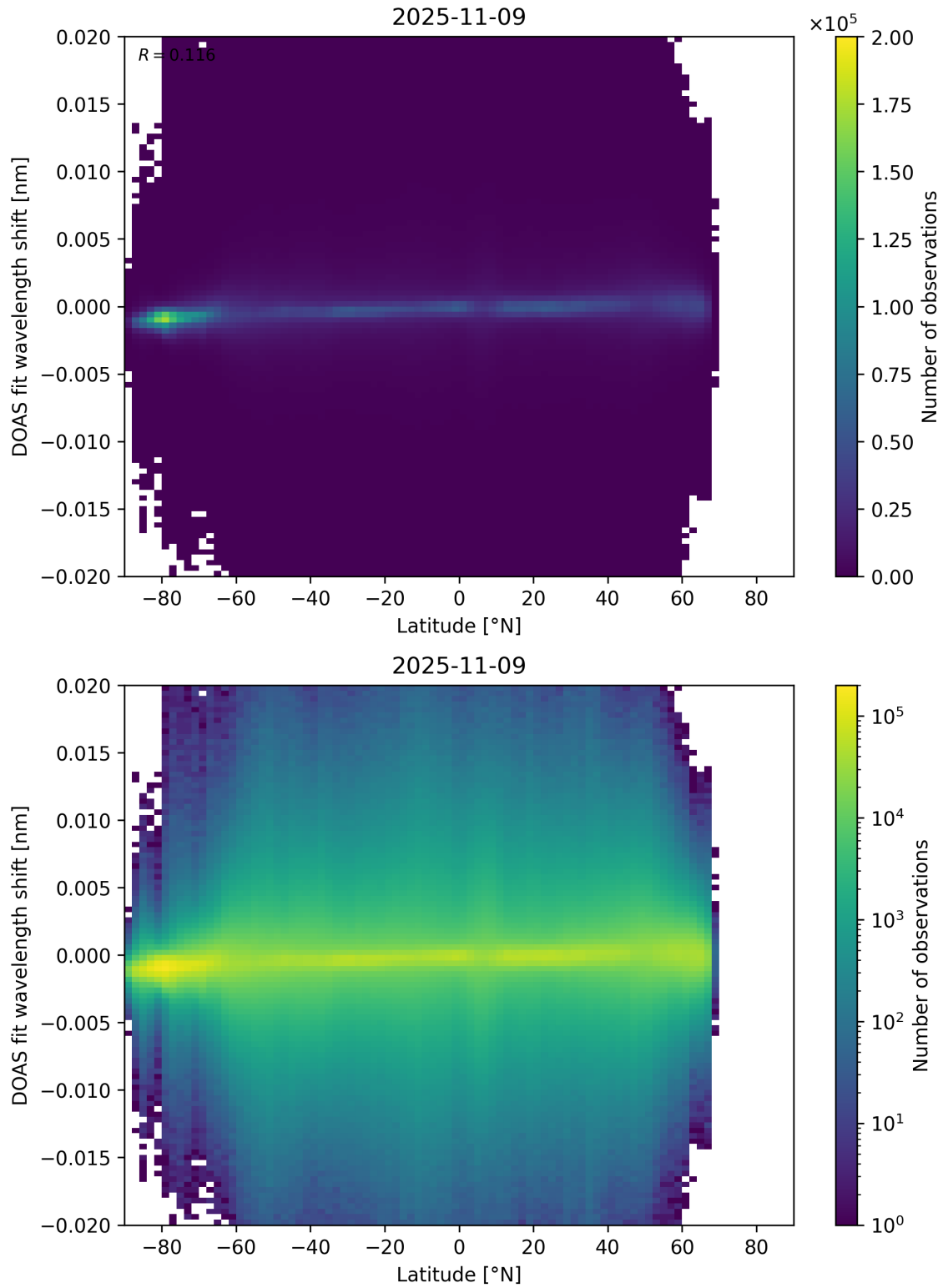
Figure 154: Scatter density plot of “Latitude” against “DOAS fit wavelength shift” for 2025-11-08 to 2025-11-10.
