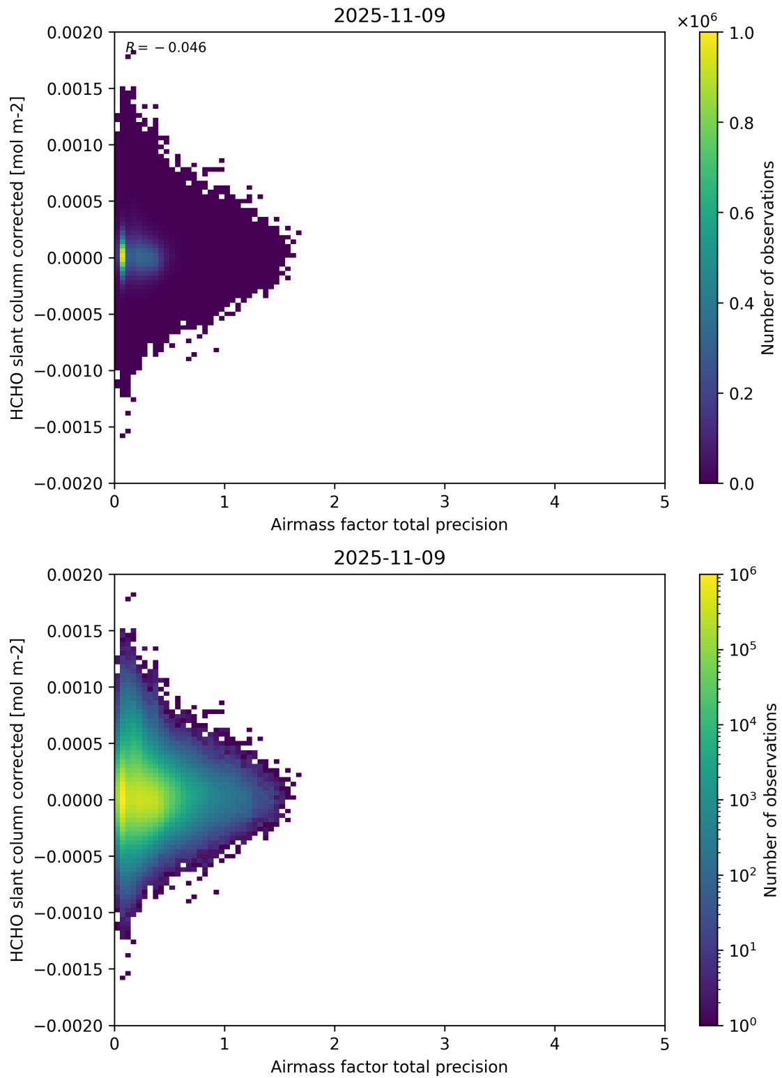
Figure 109: Scatter density plot of “Airmass factor total precision” against “HCHO slant column corrected” for 2025-11-08 to 2025-11-10.
