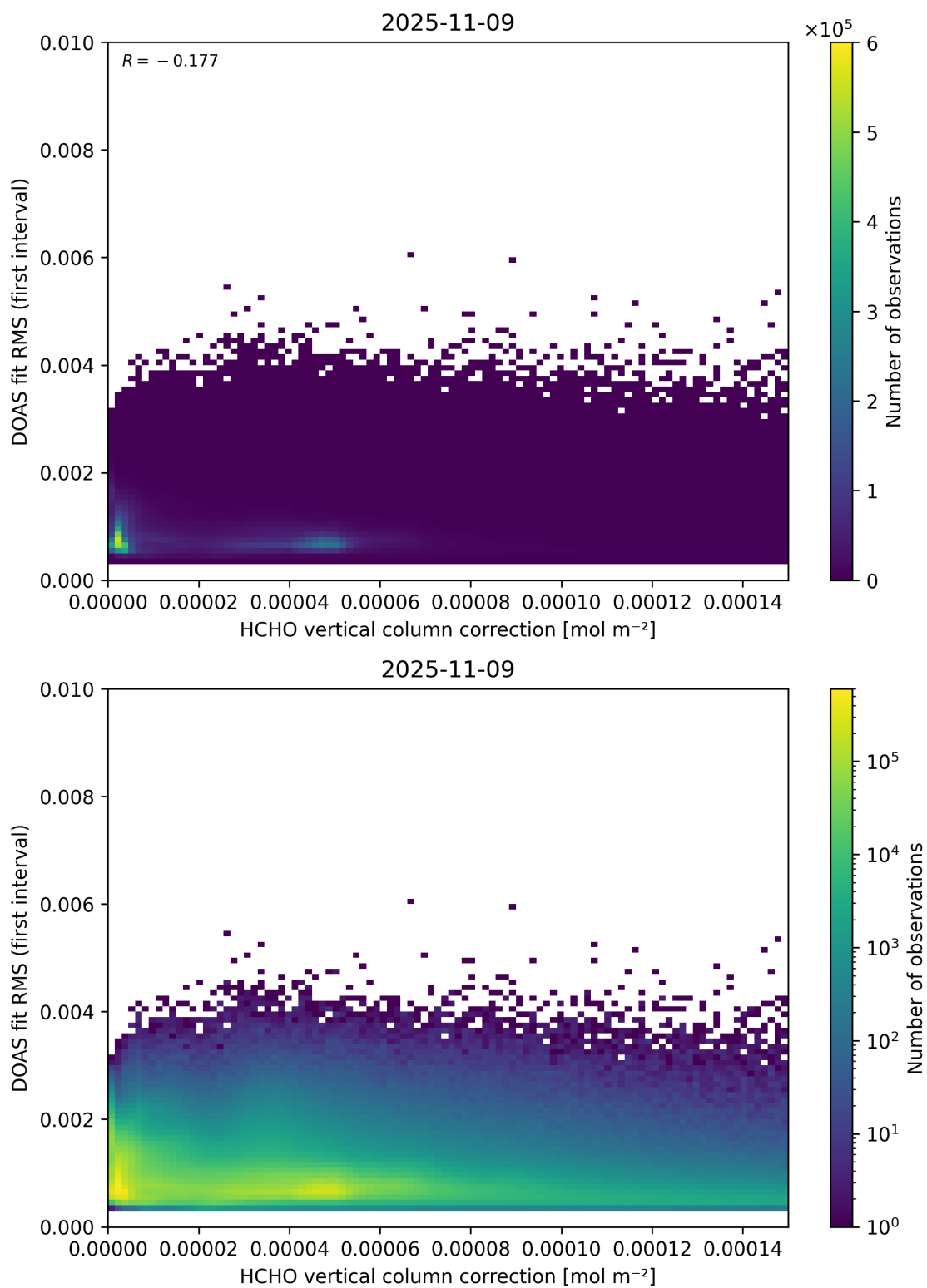
Figure 112: Scatter density plot of “HCHO vertical column correction” against “DOAS fit RMS (first interval)” for 2025-11-08 to 2025-11-10.
