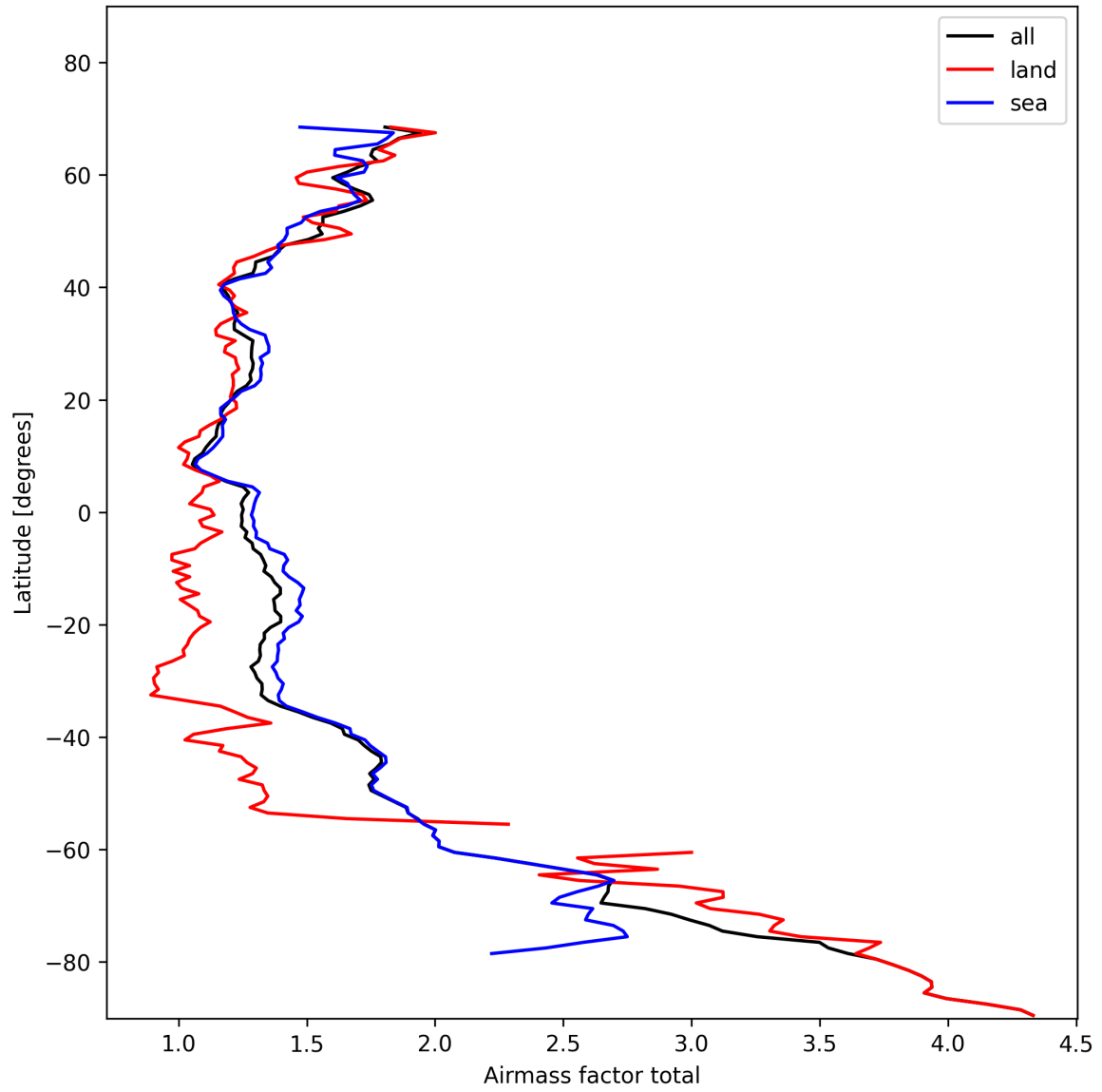
Figure 26: Zonal average of “Airmass factor total” for 2025-11-08 to 2025-11-10.
