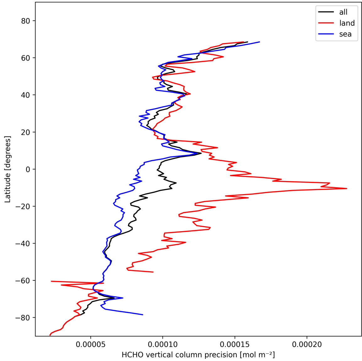
Figure 22: Zonal average of “HCHO vertical column precision” for 2025-11-08 to 2025-11-10.
