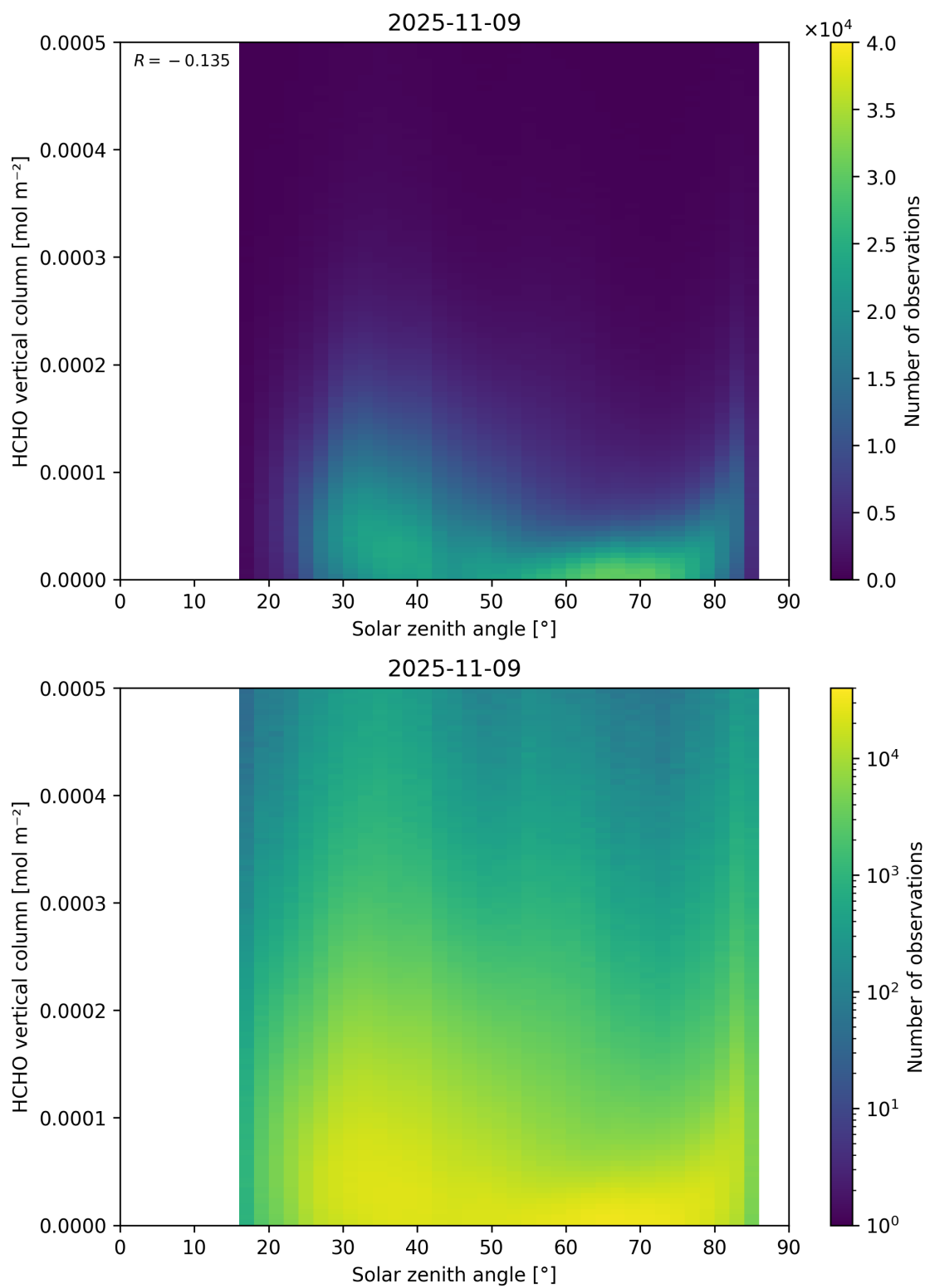
Figure 177: Scatter density plot of “Solar zenith angle” against “HCHO vertical column” for 2025-11-08 to 2025-11-10.
