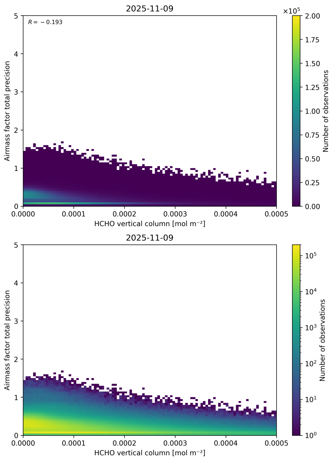
Figure 132: Scatter density plot of “HCHO vertical column” against “Airmass factor total precision” for 2025-11-08 to 2025-11-10.
