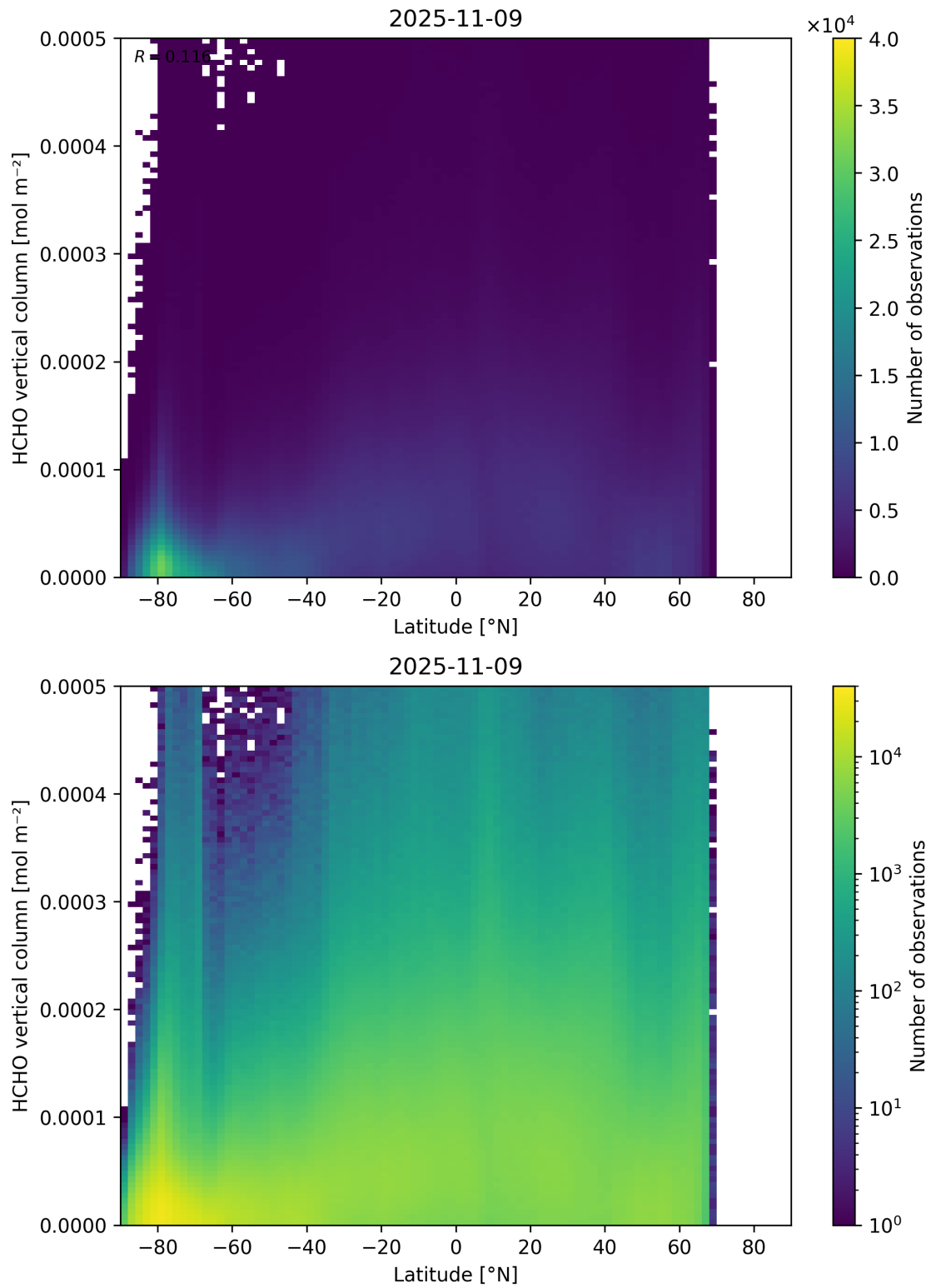
Figure 163: Scatter density plot of “Latitude” against “HCHO vertical column” for 2025-11-08 to 2025-11-10.
