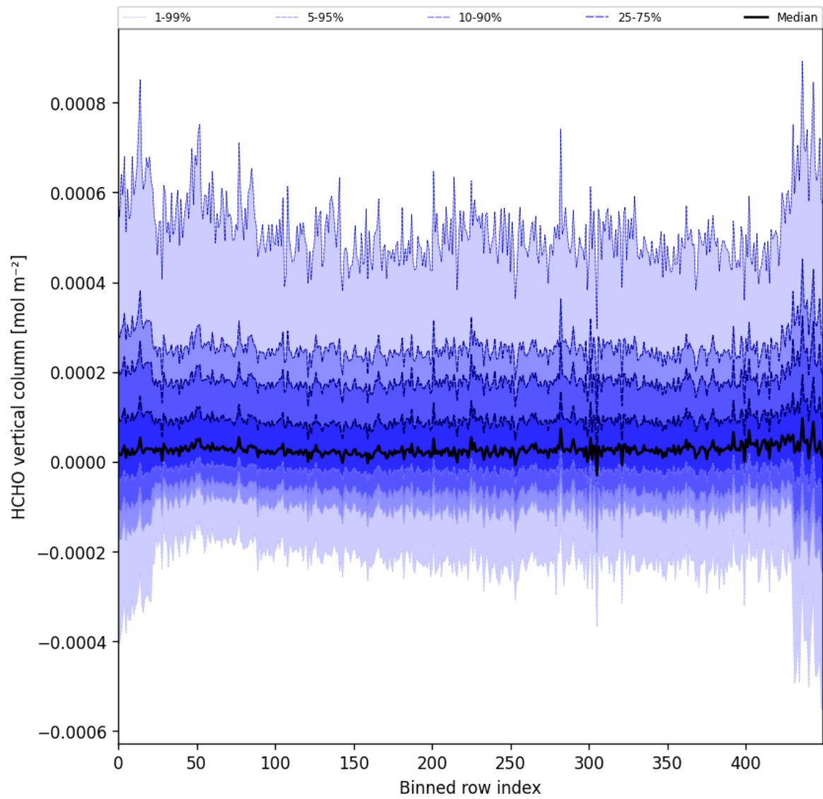
Figure 49: Along track statistics of “HCHO vertical column” for 2025-11-08 to 2025-11-10
