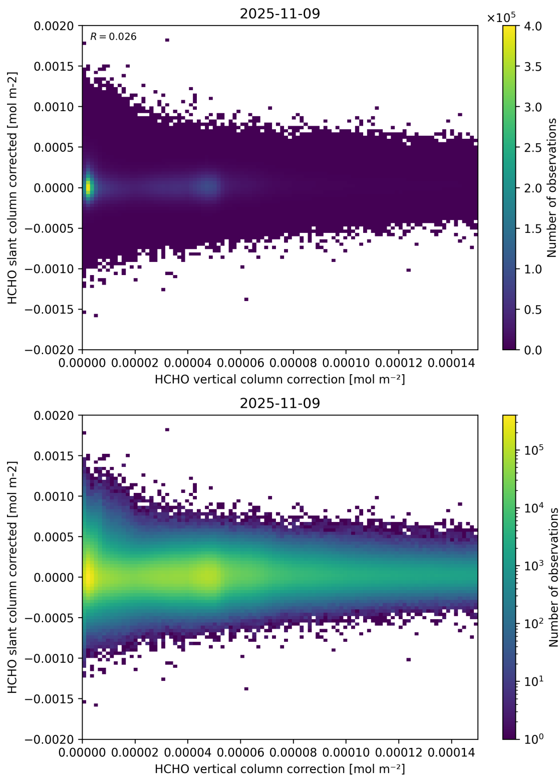
Figure 116: Scatter density plot of “HCHO vertical column correction” against “HCHO slant column corrected” for 2025-11-08 to 2025-11-10.
