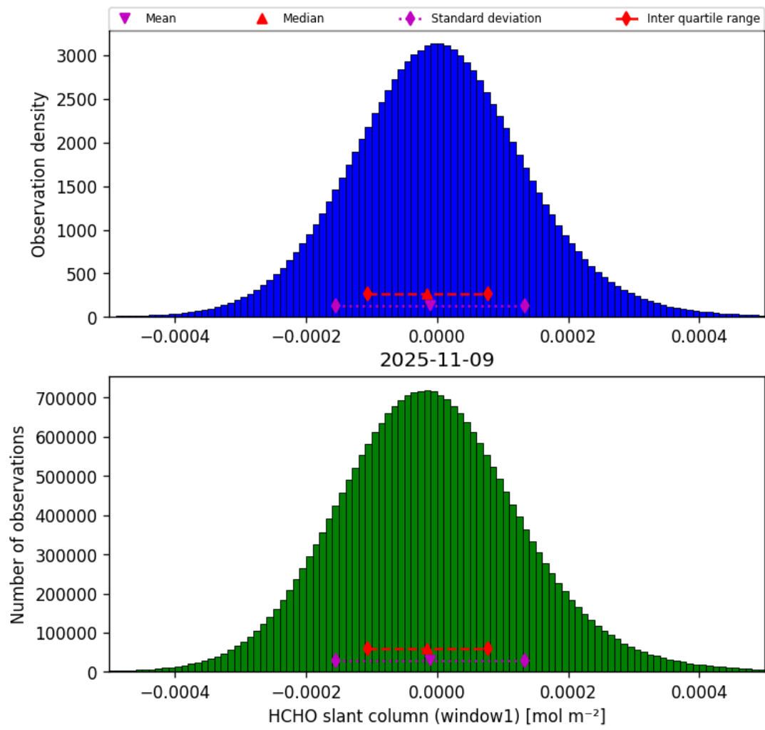
Figure 38: Histogram of “HCHO slant column (window1)” for 2025-11-08 to 2025-11-10
