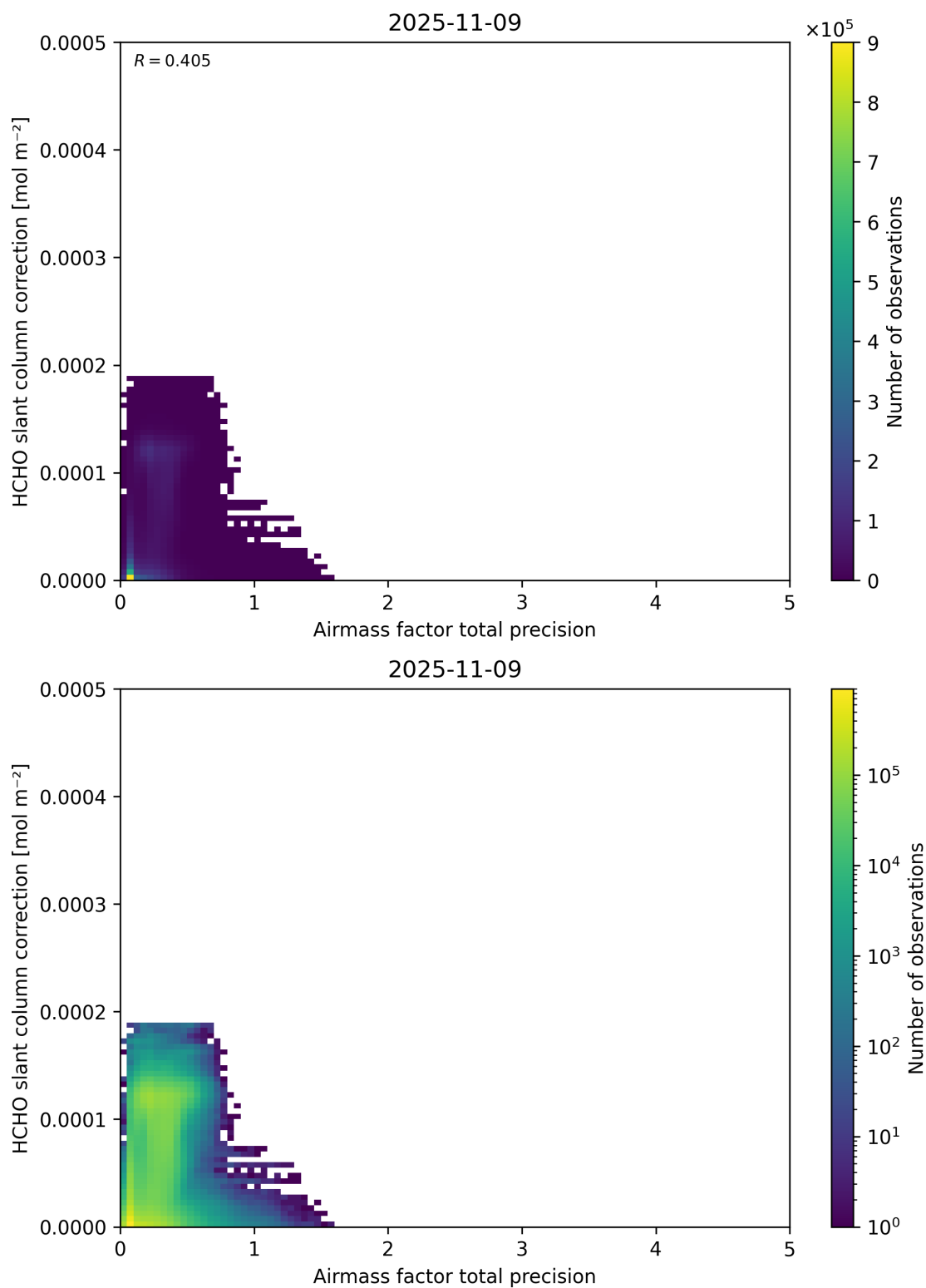
Figure 110: Scatter density plot of “Airmass factor total precision” against “HCHO slant column correction” for 2025-11-08 to 2025-11-10.
