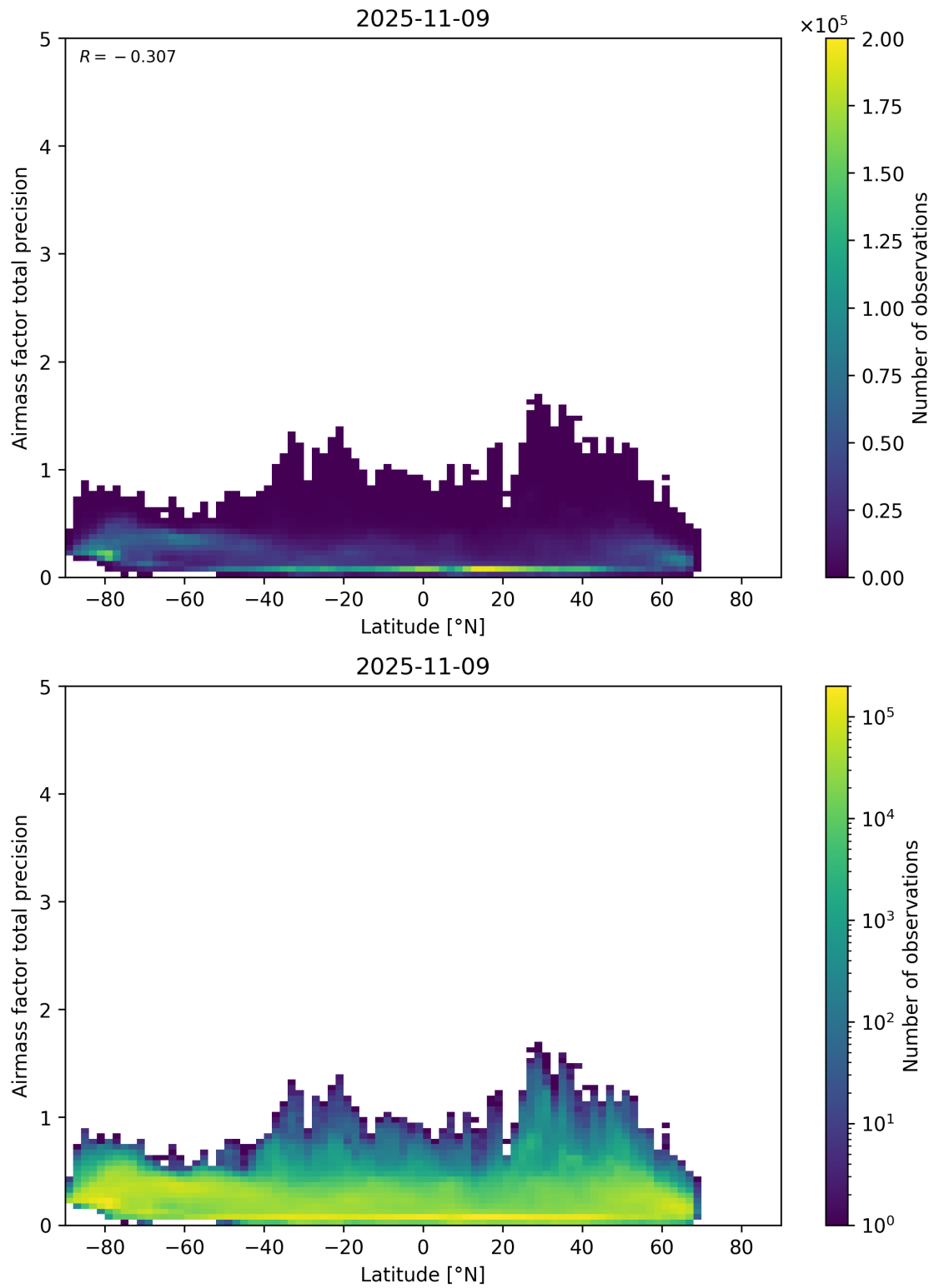
Figure 162: Scatter density plot of “Latitude” against “Airmass factor total precision” for 2025-11-08 to 2025-11-10.
