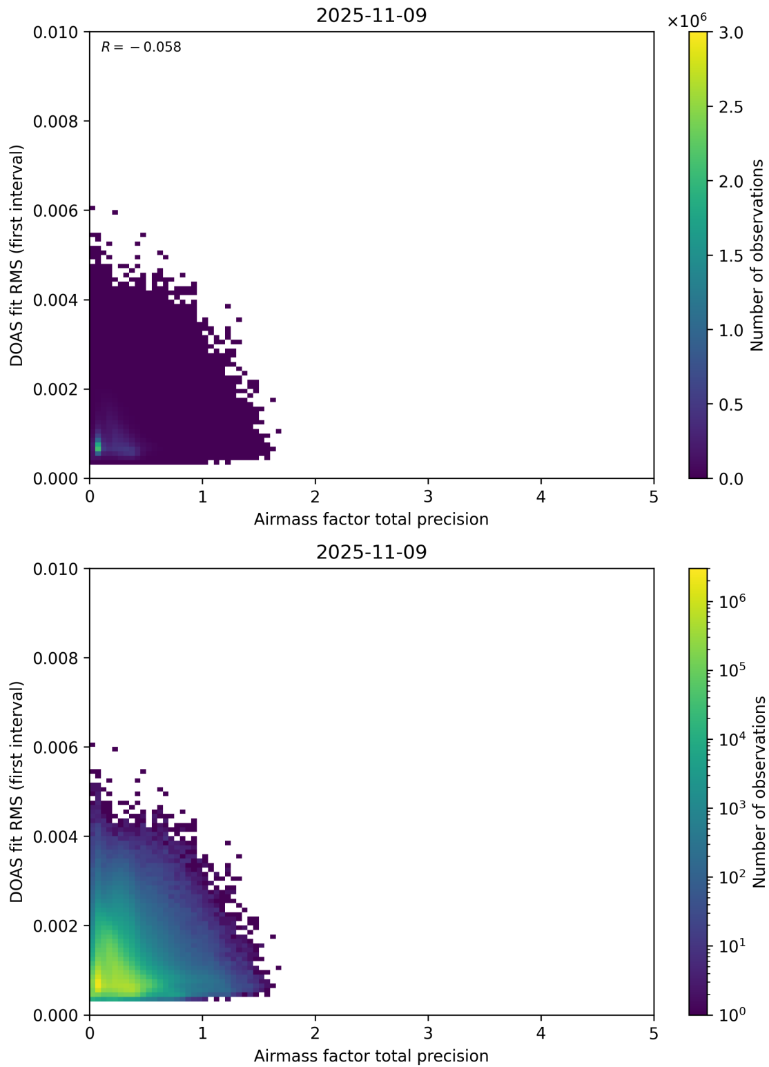
Figure 105: Scatter density plot of “Airmass factor total precision” against “DOAS fit RMS (first interval)” for 2025-11-08 to 2025-11-10.
