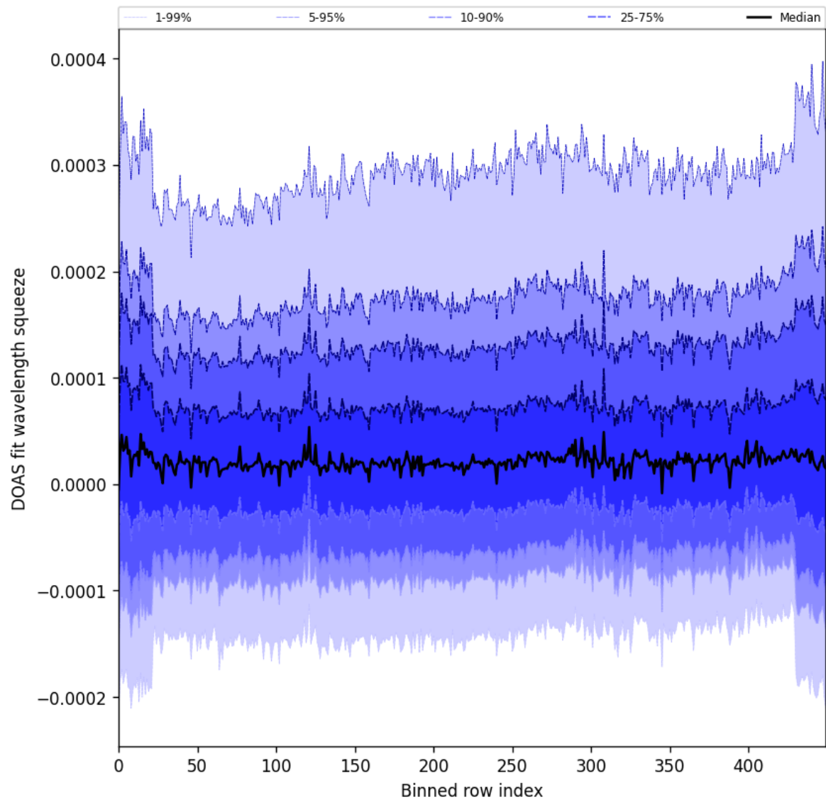
Figure 59: Along track statistics of “DOAS fit wavelength squeeze” for 2025-11-08 to 2025-11-10
