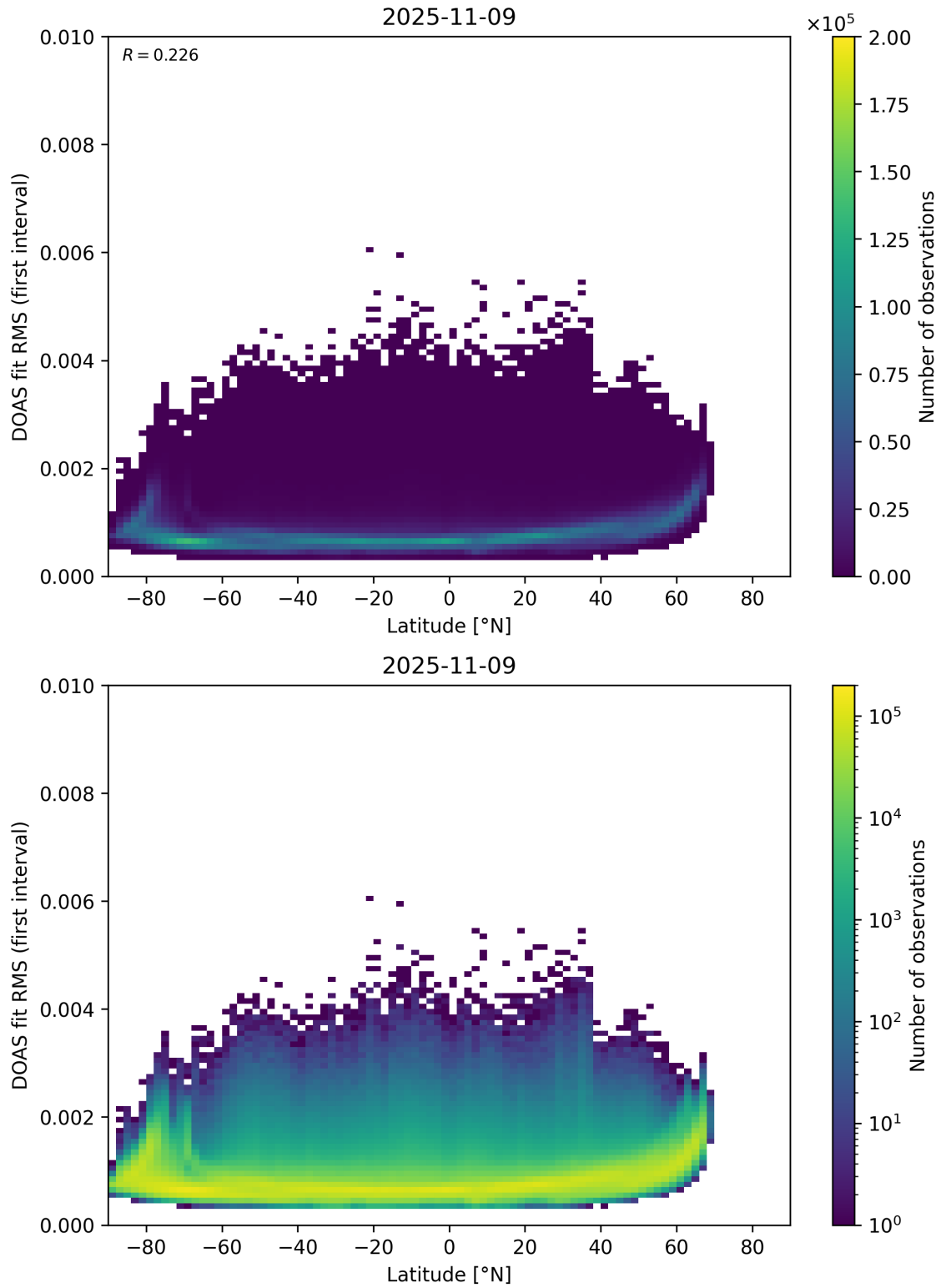
Figure 153: Scatter density plot of “Latitude” against “DOAS fit RMS (first interval)” for 2025-11-08 to 2025-11-10.
