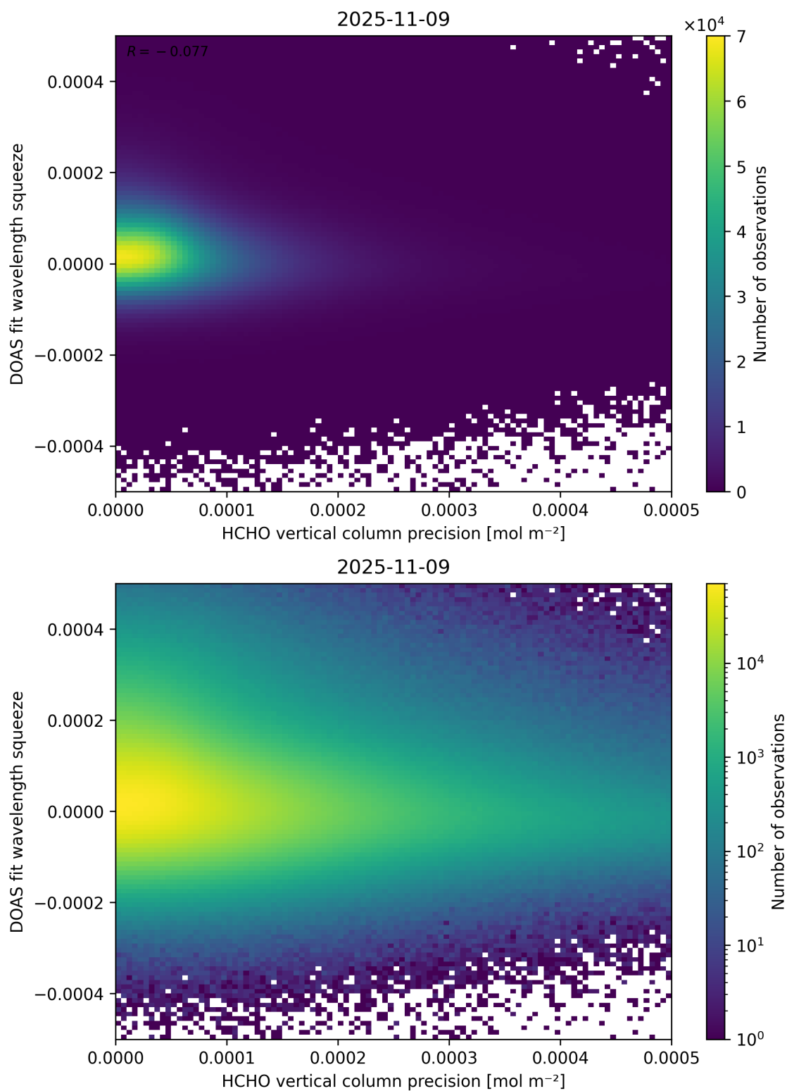
Figure 138: Scatter density plot of “HCHO vertical column precision” against “DOAS fit wavelength squeeze” for 2025-11-08 to 2025-11-10.
