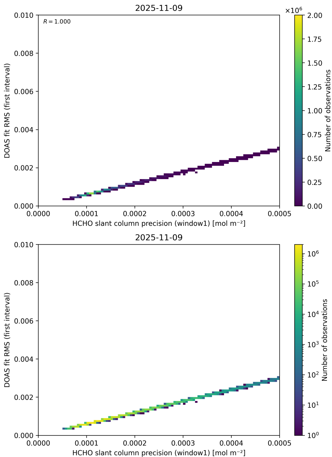
Figure 88: Scatter density plot of “HCHO slant column precision (window1)” against “DOAS fit RMS (first interval)” for 2025-11-08 to 2025-11-10.
