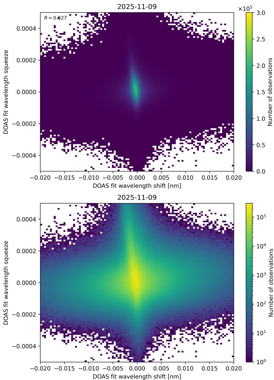
Figure 65: Scatter density plot of “DOAS fit wavelength shift” against “DOAS fit wavelength squeeze” for 2025-11-08 to 2025-11-10.
