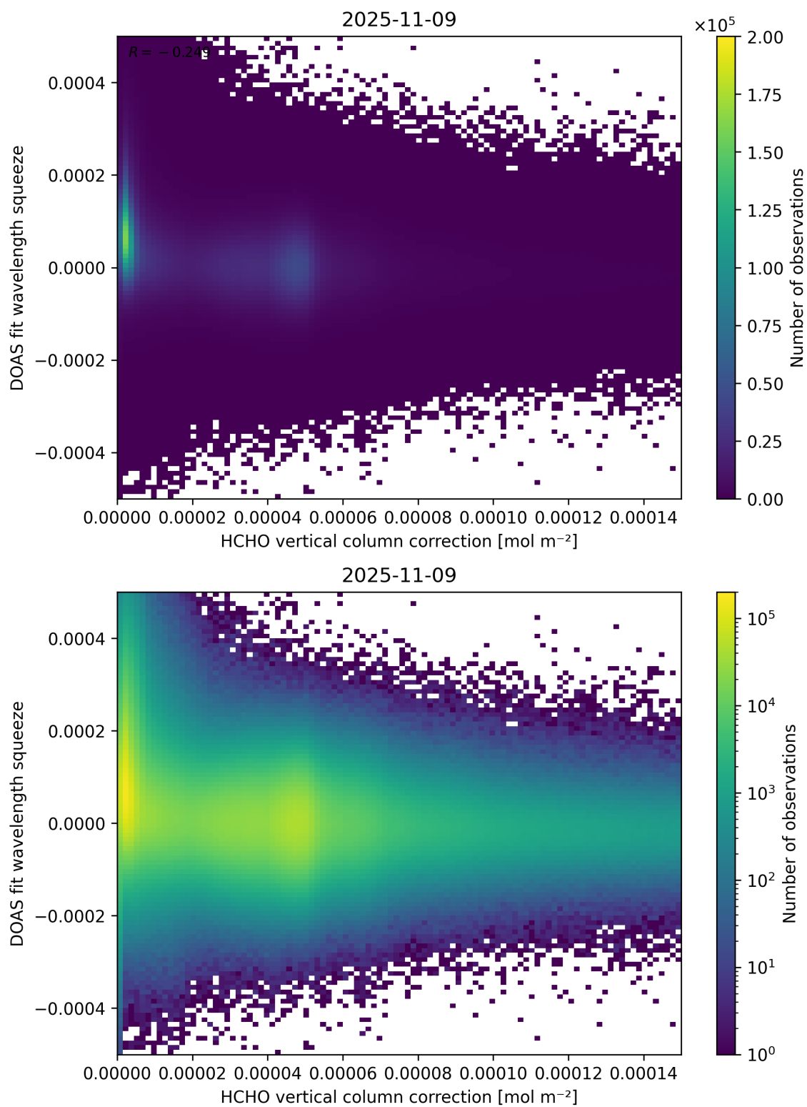
Figure 114: Scatter density plot of “HCHO vertical column correction” against “DOAS fit wavelength squeeze” for 2025-11-08 to 2025-11-10.
