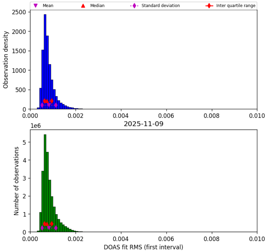
Figure 46: Histogram of “DOAS fit RMS (first interval)” for 2025-11-08 to 2025-11-10
