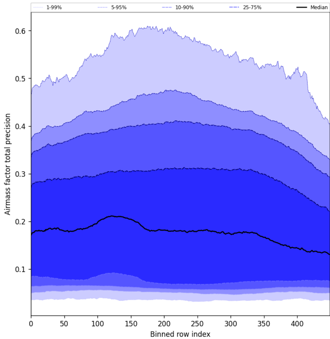
Figure 55: Along track statistics of “Airmass factor total precision” for 2025-11-08 to 2025-11-10
