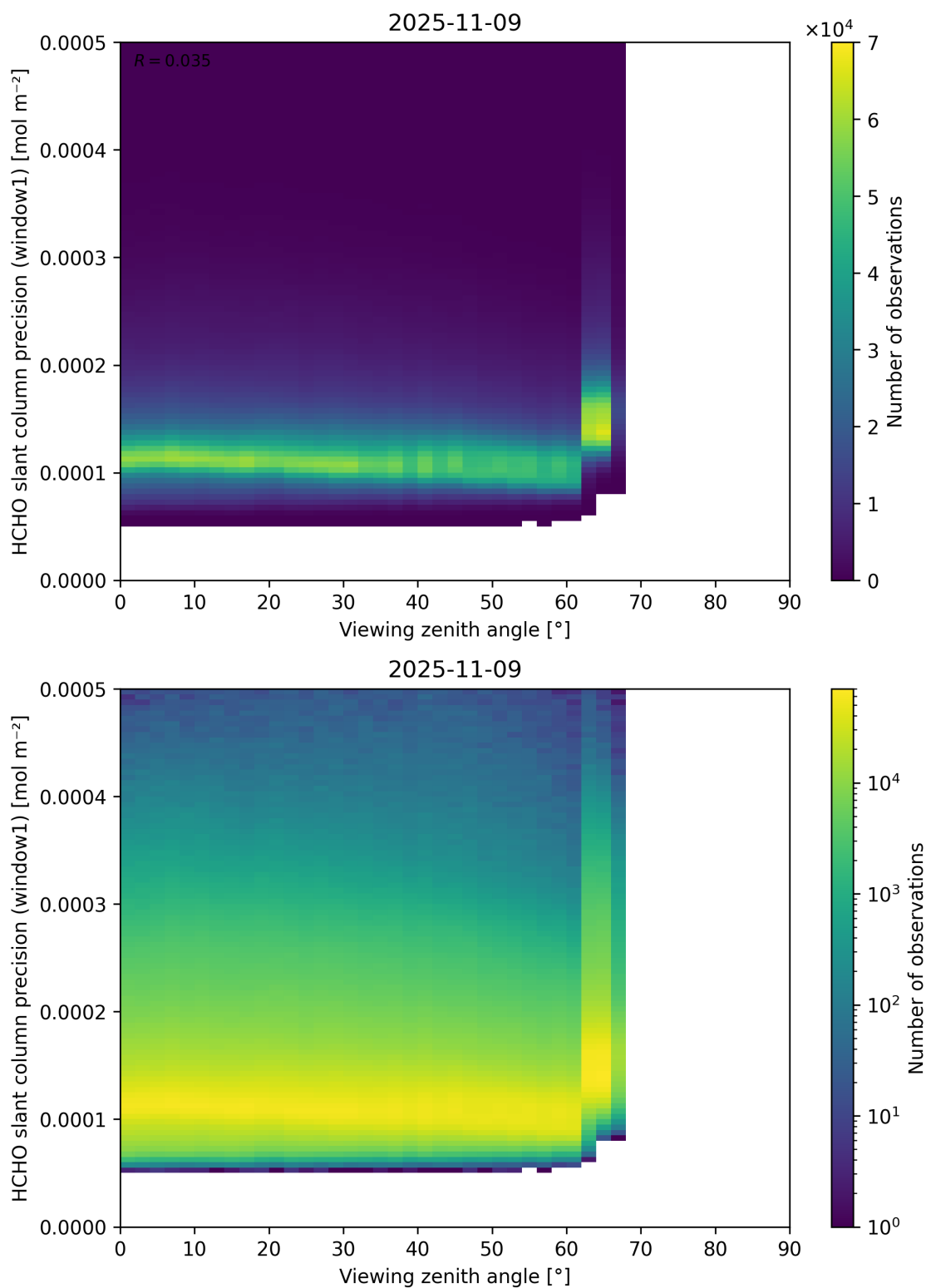
Figure 189: Scatter density plot of “Viewing zenith angle” against “HCHO slant column precision (window1)” for 2025-11-08 to 2025-11-10.
