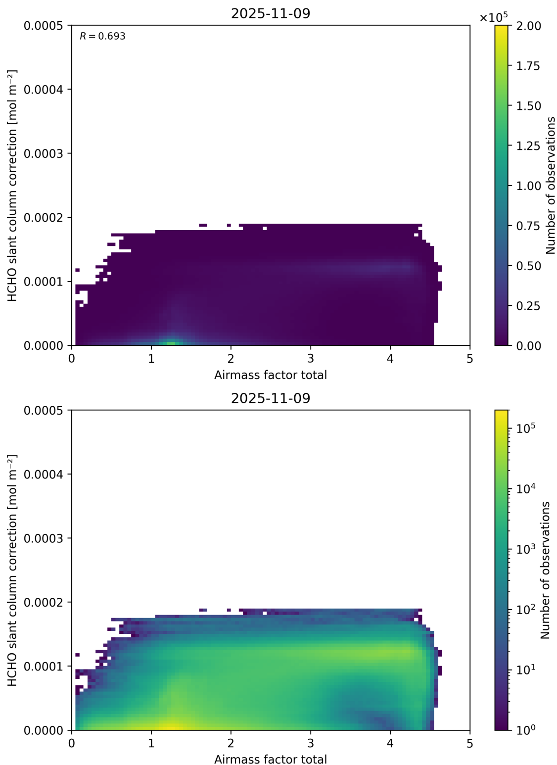
Figure 102: Scatter density plot of “Airmass factor total” against “HCHO slant column correction” for 2025-11-08 to 2025-11-10.
