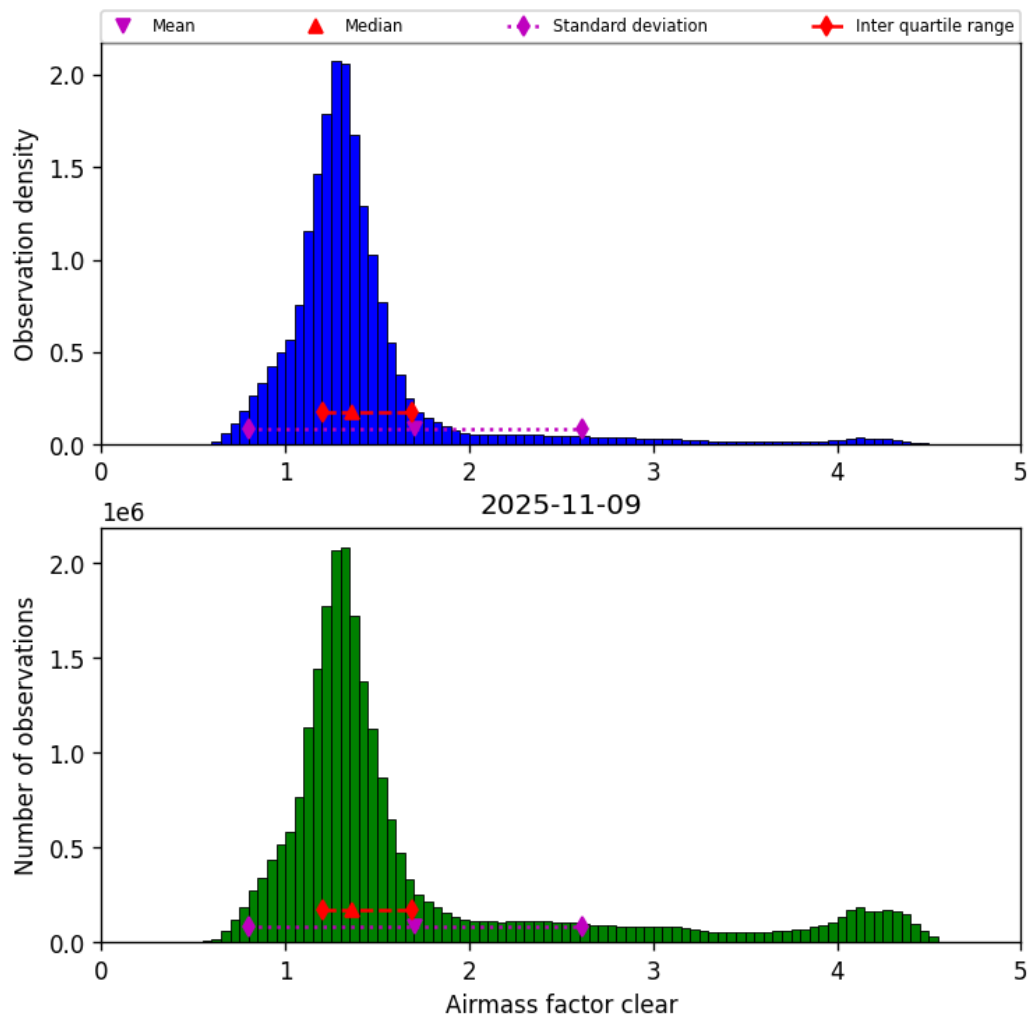
Figure 42: Histogram of “Airmass factor clear” for 2025-11-08 to 2025-11-10
