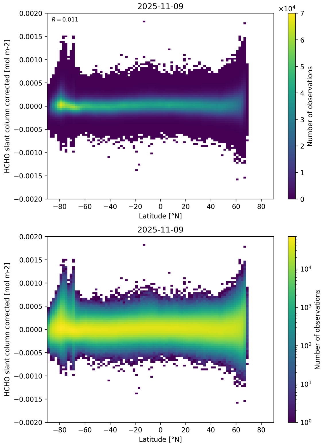
Figure 157: Scatter density plot of “Latitude” against “HCHO slant column corrected” for 2025-11-08 to 2025-11-10.
