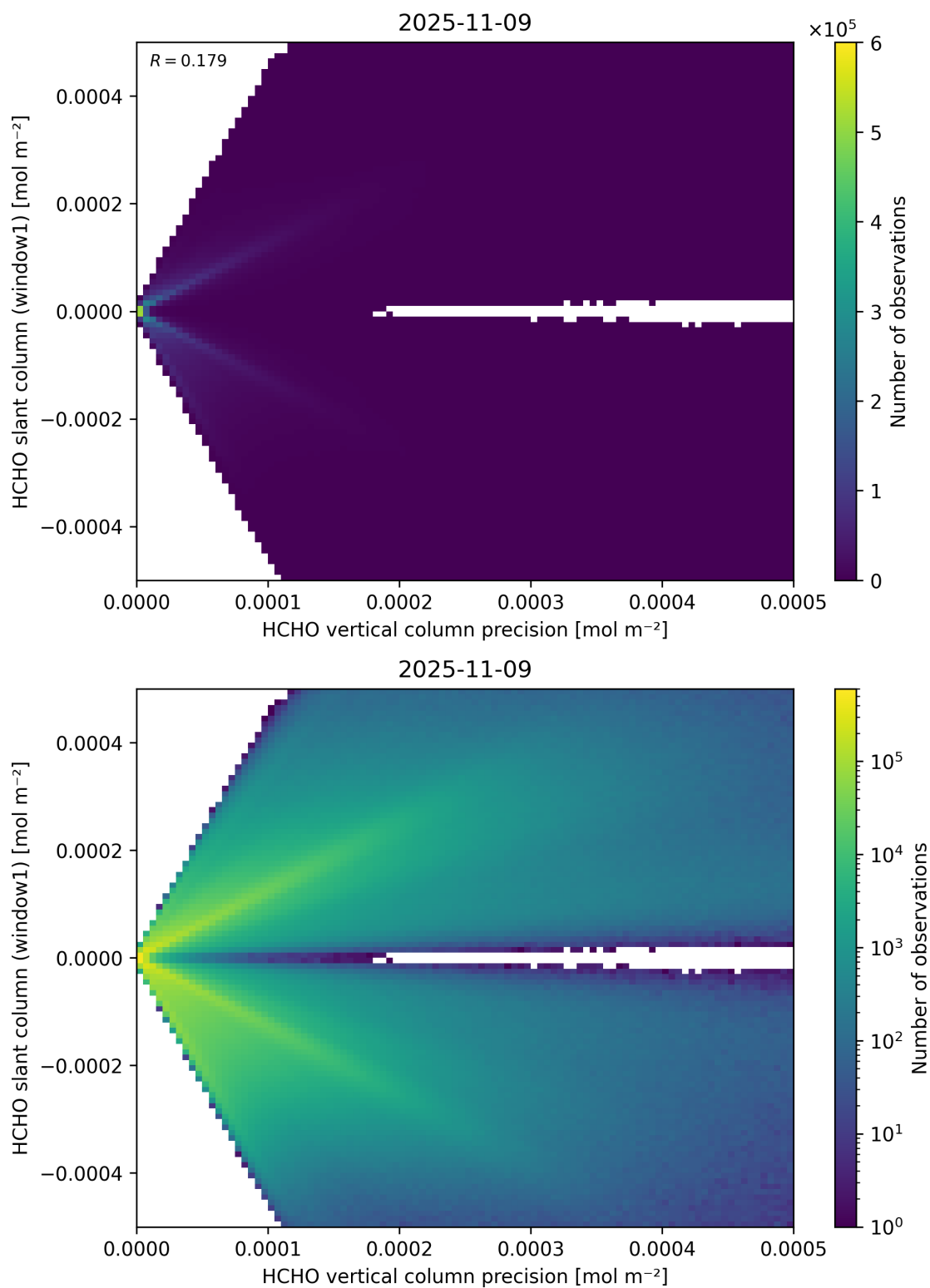
Figure 142: Scatter density plot of “HCHO vertical column precision” against “HCHO slant column (window1)” for 2025-11-08 to 2025-11-10.
