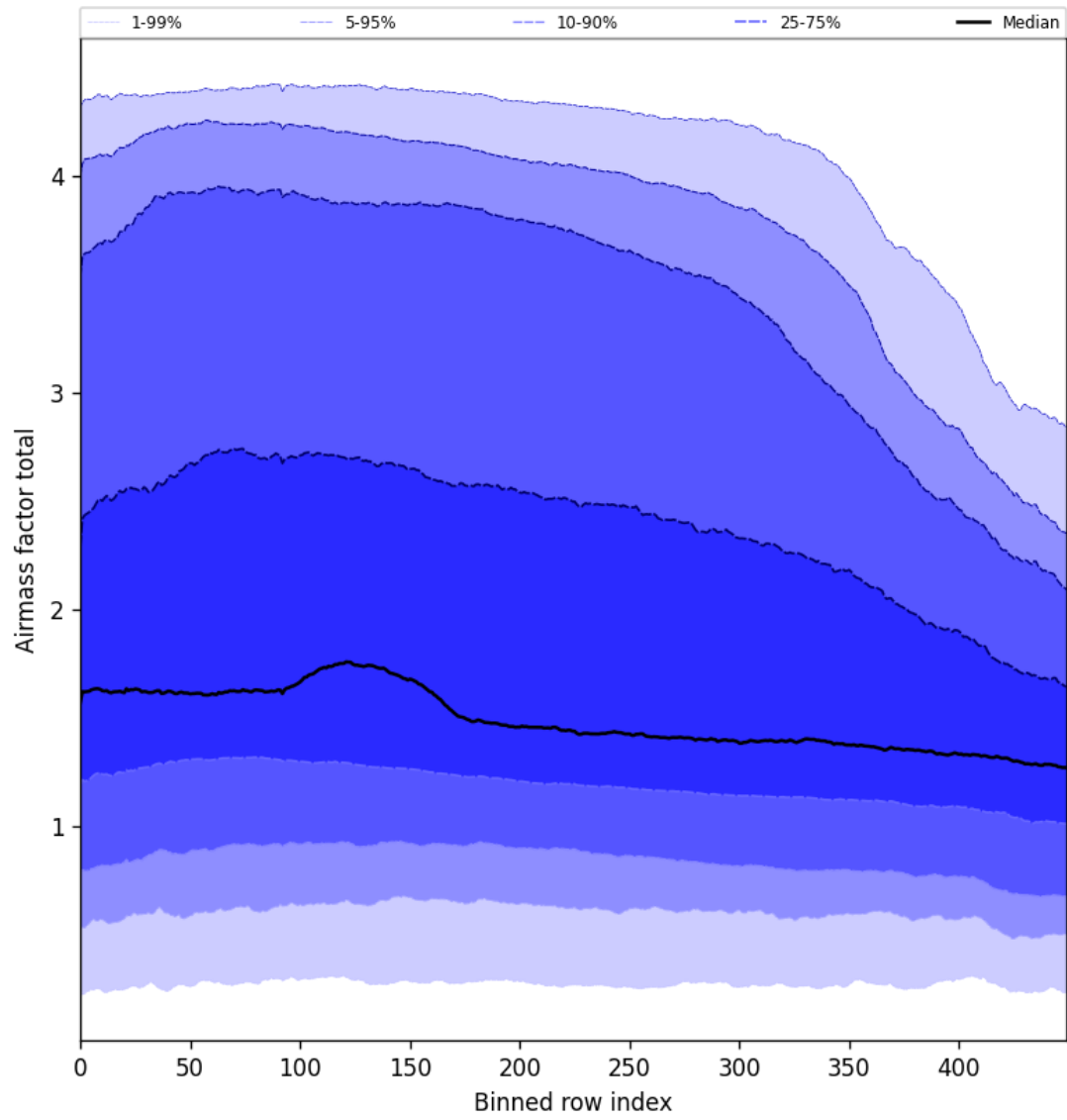
Figure 54: Along track statistics of “Airmass factor total” for 2025-11-08 to 2025-11-10
