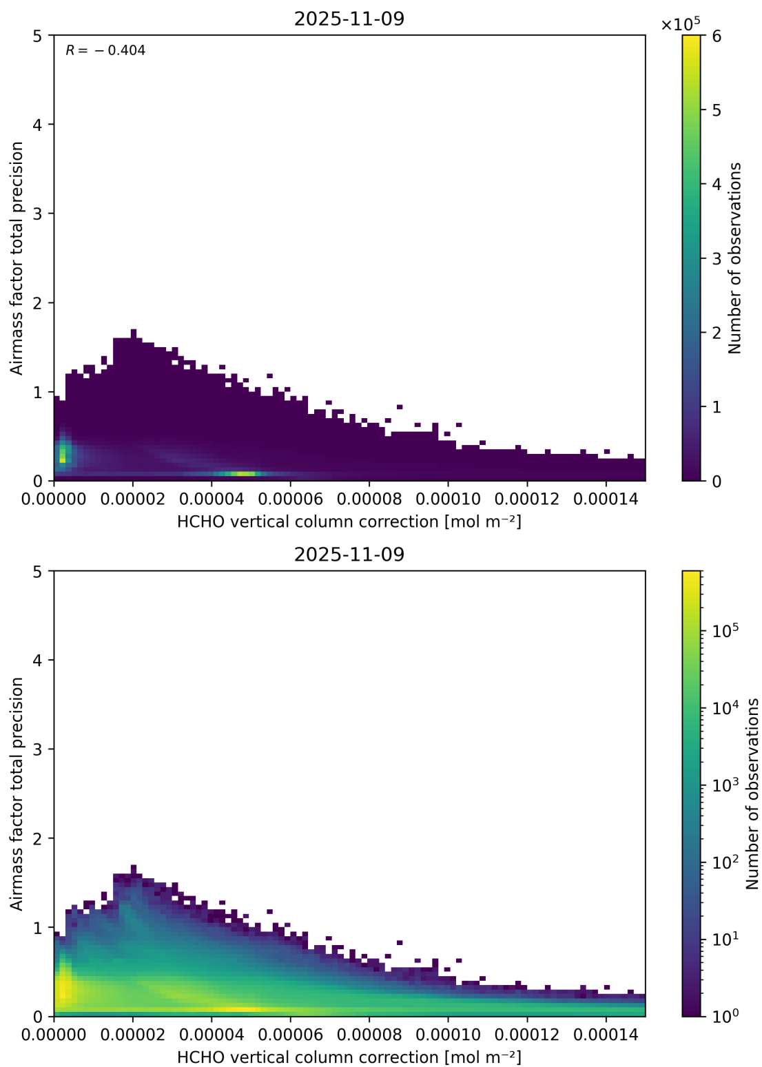
Figure 121: Scatter density plot of “HCHO vertical column correction” against “Airmass factor total precision” for 2025-11-08 to 2025-11-10.
