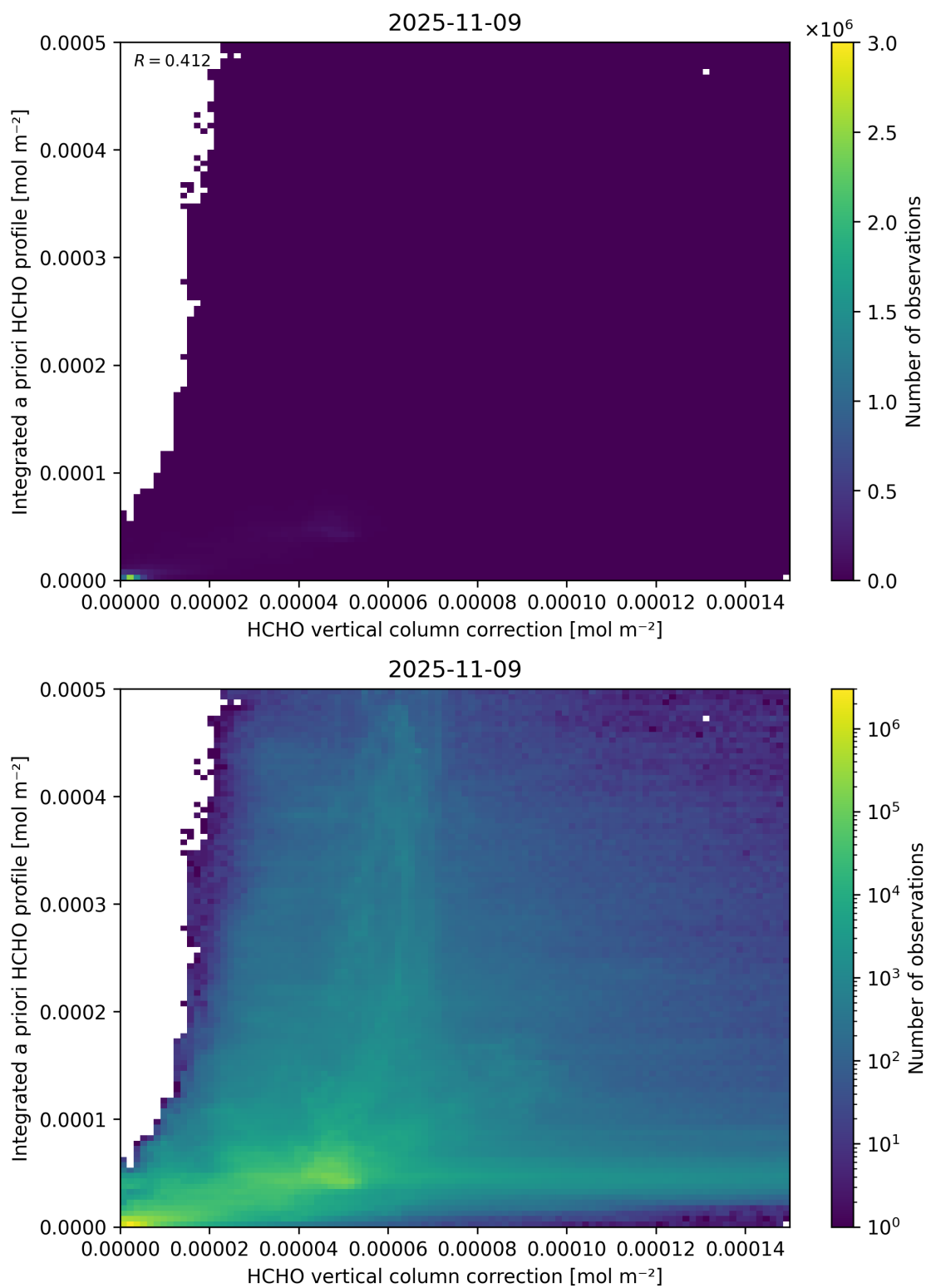
Figure 122: Scatter density plot of “HCHO vertical column correction” against “Integrated a priori HCHO profile” for 2025-11-08 to 2025-11-10.
