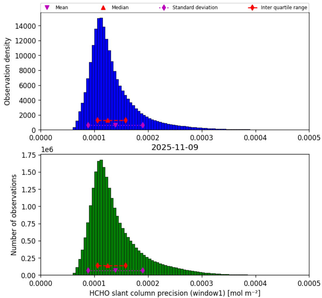
Figure 39: Histogram of “HCHO slant column precision (window1)” for 2025-11-08 to 2025-11-10
