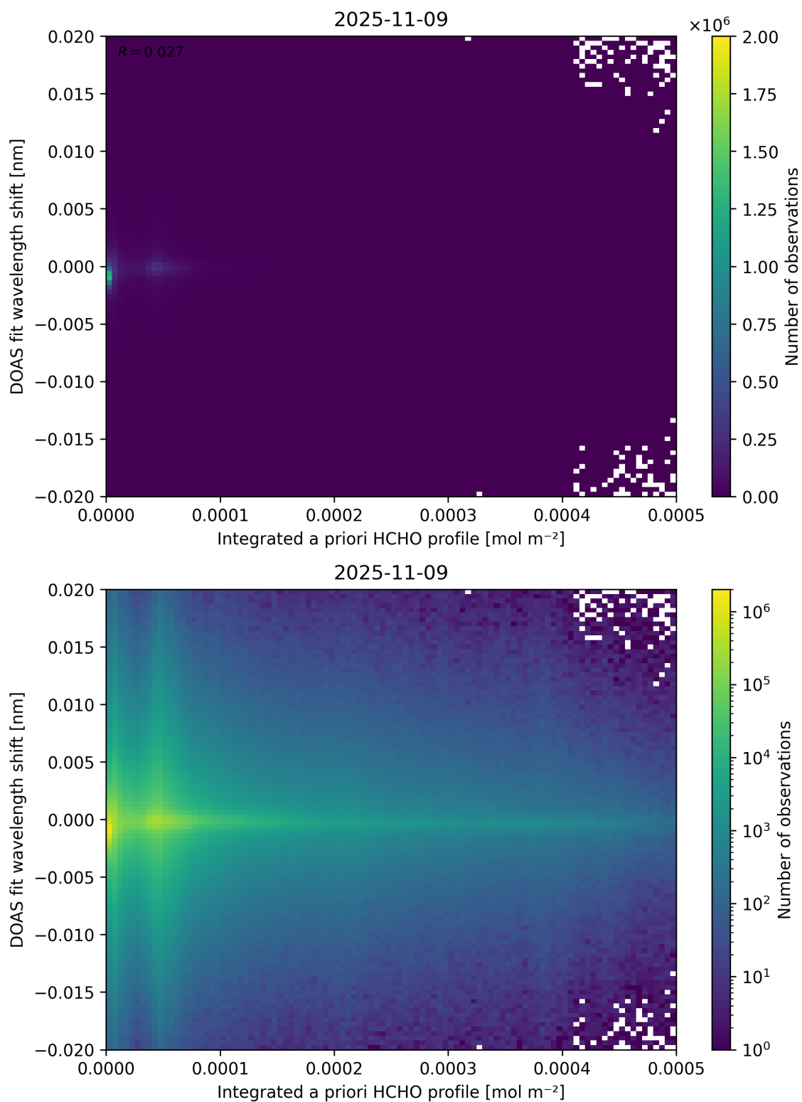
Figure 149: Scatter density plot of “Integrated a priori HCHO profile” against “DOAS fit wavelength shift” for 2025-11-08 to 2025-11-10.
