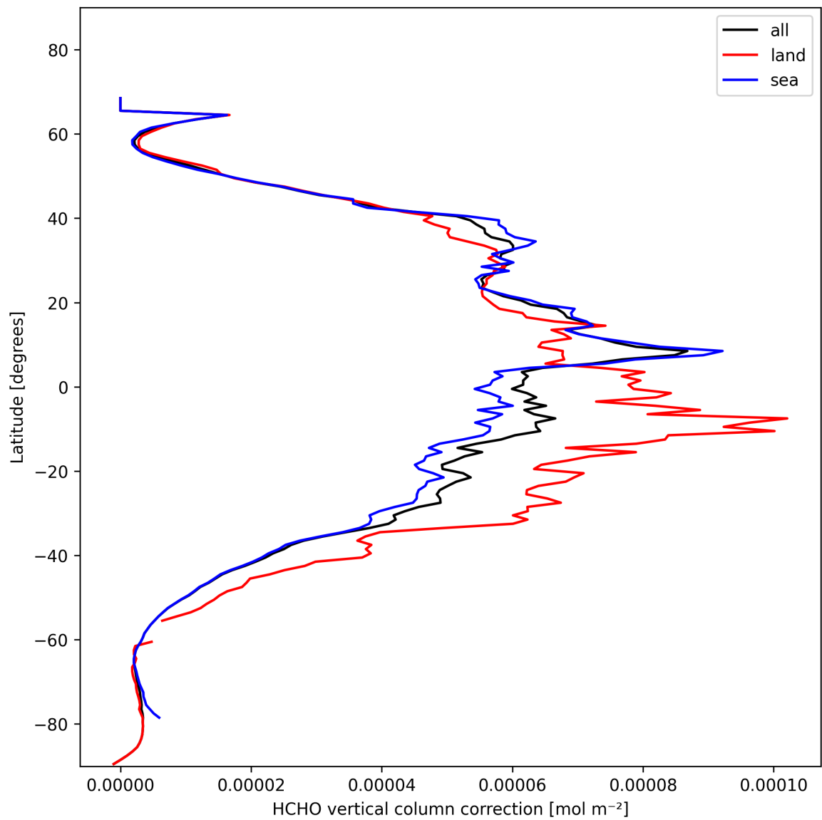
Figure 23: Zonal average of “HCHO vertical column correction” for 2025-11-08 to 2025-11-10.
