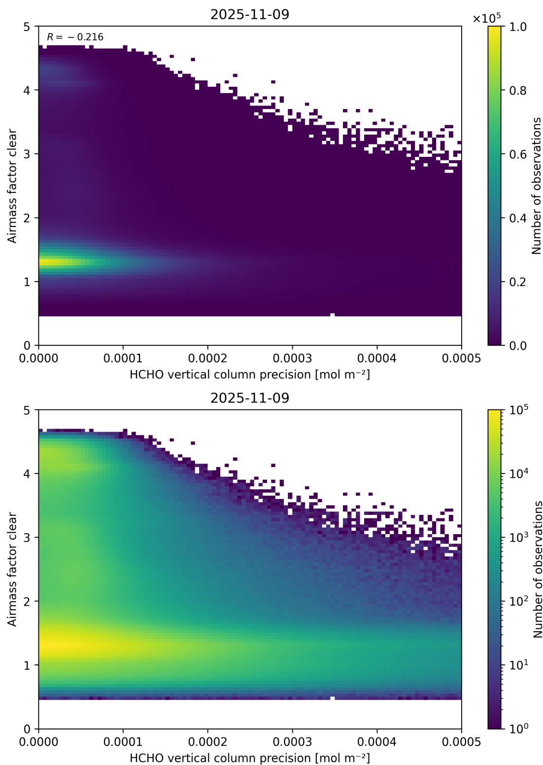
Figure 139: Scatter density plot of “HCHO vertical column precision” against “Airmass factor clear” for 2025-11-08 to 2025-11-10.
