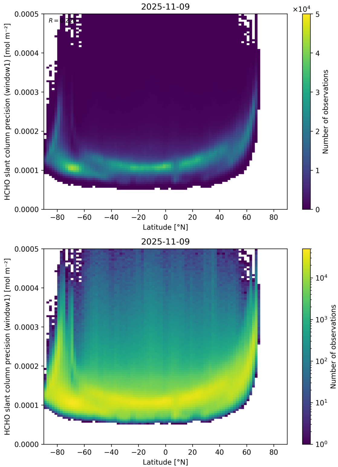
Figure 160: Scatter density plot of “Latitude” against “HCHO slant column precision (window1)” for 2025-11-08 to 2025-11-10.
