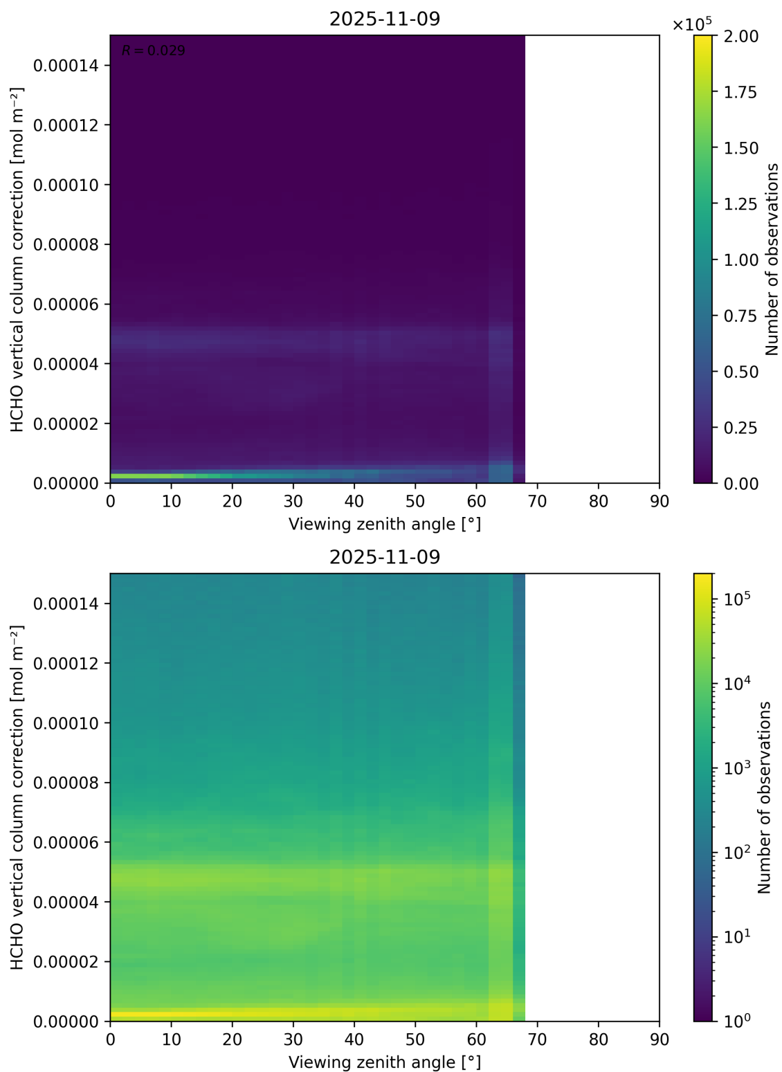
Figure 193: Scatter density plot of “Viewing zenith angle” against “HCHO vertical column correction” for 2025-11-08 to 2025-11-10.
