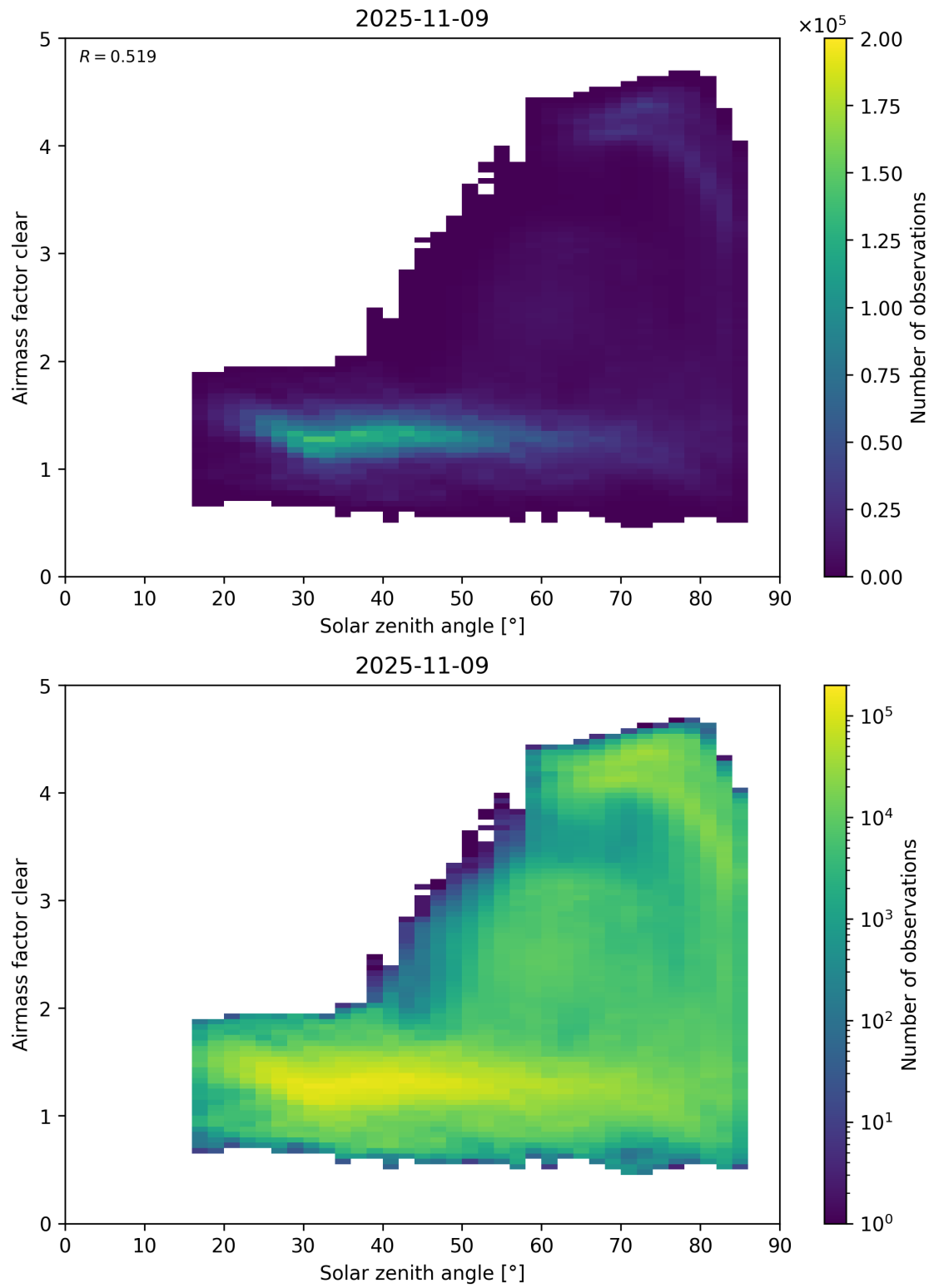
Figure 170: Scatter density plot of “Solar zenith angle” against “Airmass factor clear” for 2025-11-08 to 2025-11-10.
