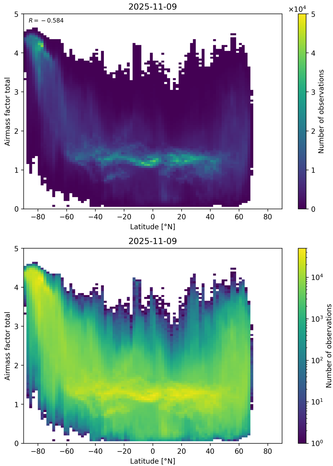
Figure 161: Scatter density plot of “Latitude” against “Airmass factor total” for 2025-11-08 to 2025-11-10.
