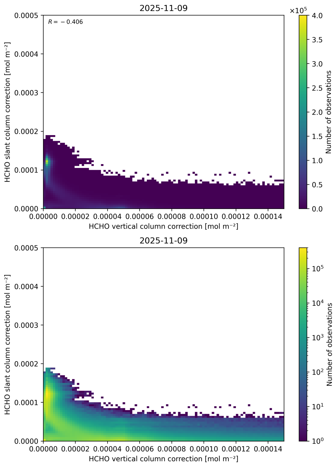
Figure 117: Scatter density plot of “HCHO vertical column correction” against “HCHO slant column correction” for 2025-11-08 to 2025-11-10.
