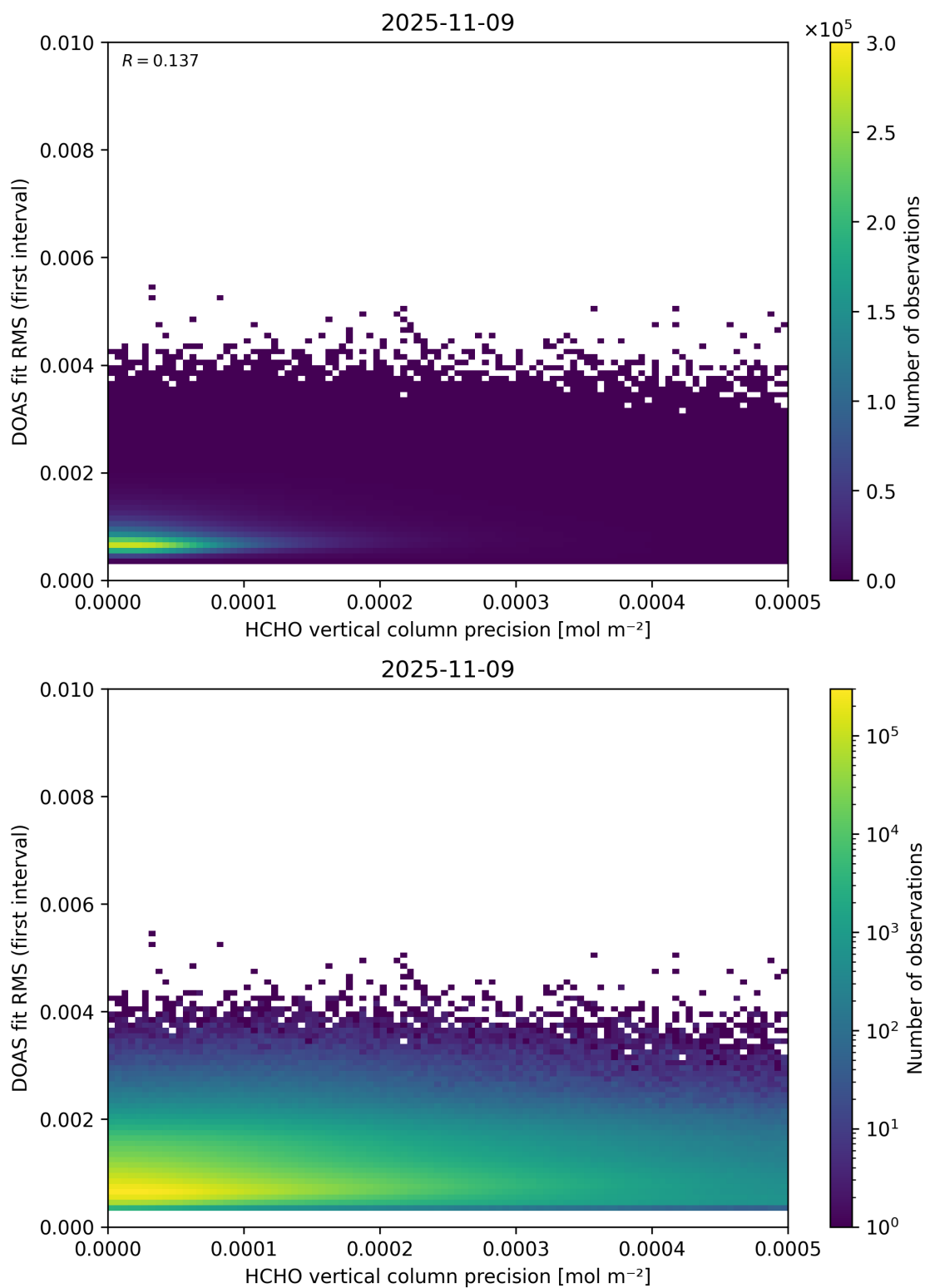
Figure 136: Scatter density plot of “HCHO vertical column precision” against “DOAS fit RMS (first interval)” for 2025-11-08 to 2025-11-10.
