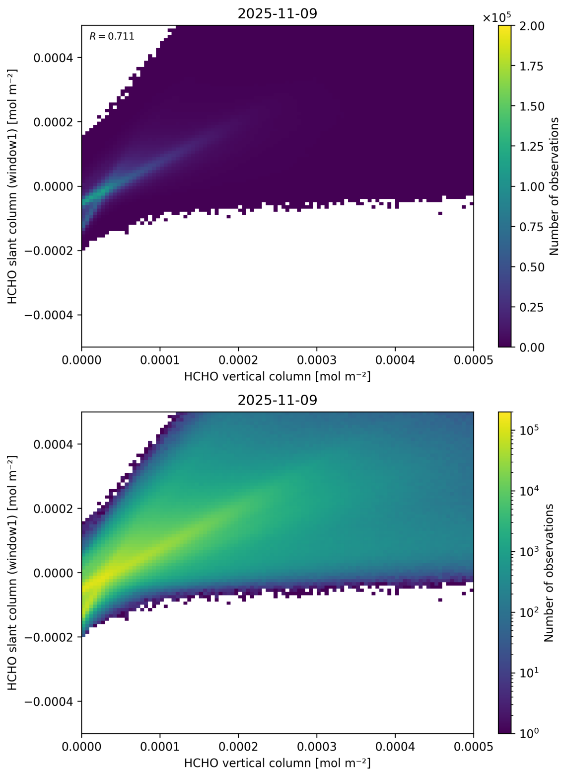
Figure 129: Scatter density plot of “HCHO vertical column” against “HCHO slant column (window1)” for 2025-11-08 to 2025-11-10.
