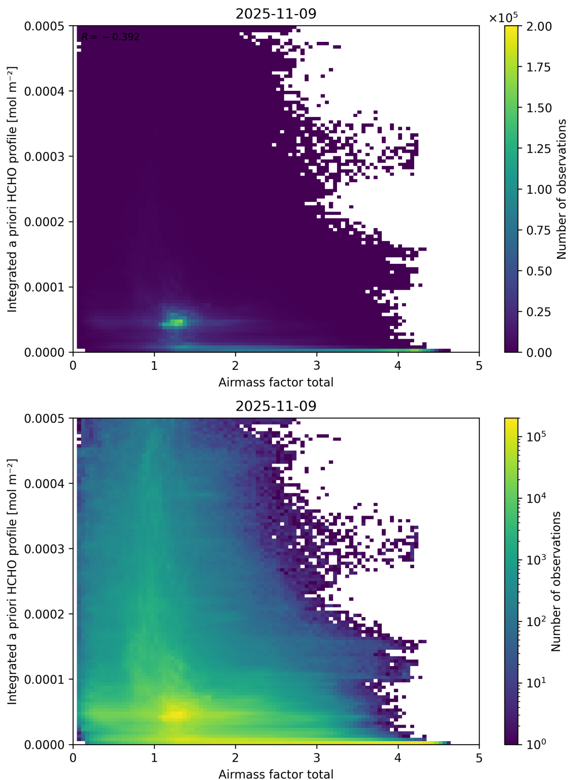
Figure 104: Scatter density plot of “Airmass factor total” against “Integrated a priori HCHO profile” for 2025-11-08 to 2025-11-10.
