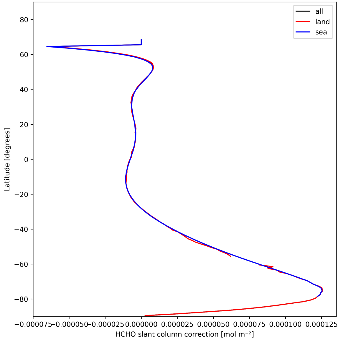
Figure 33: Zonal average of “HCHO slant column correction” for 2025-11-08 to 2025-11-10.
