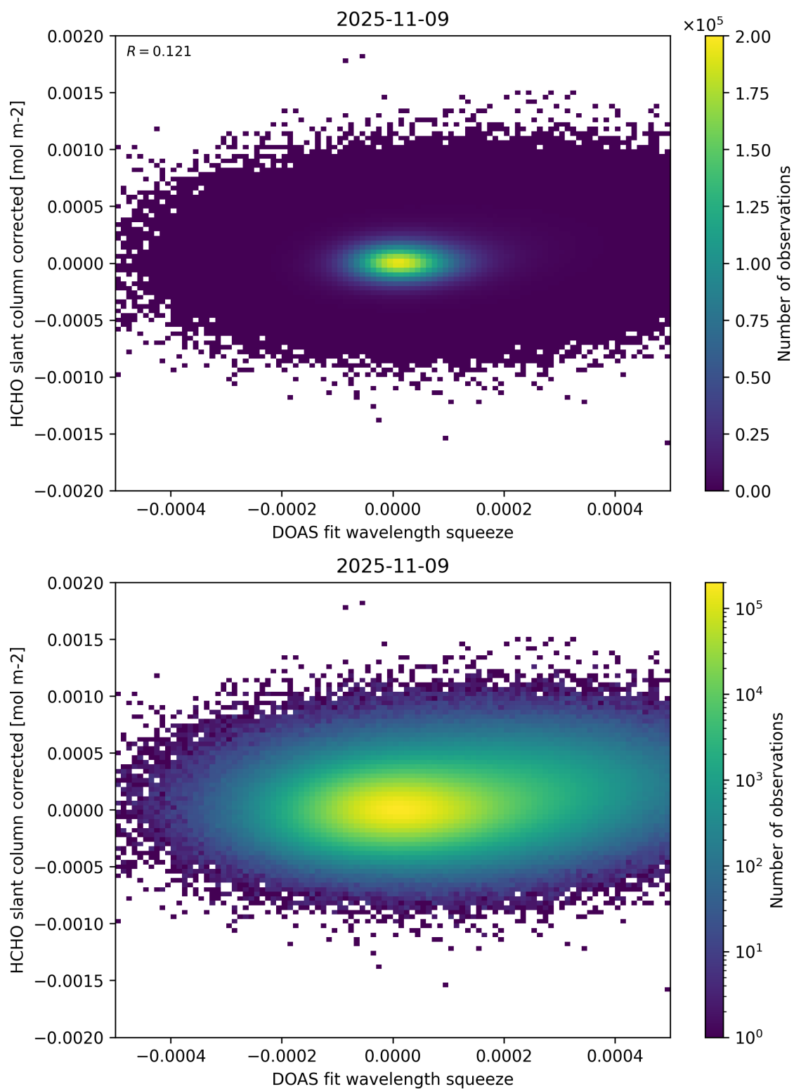
Figure 69: Scatter density plot of “DOAS fit wavelength squeeze” against “HCHO slant column corrected” for 2025-11-08 to 2025-11-10.
