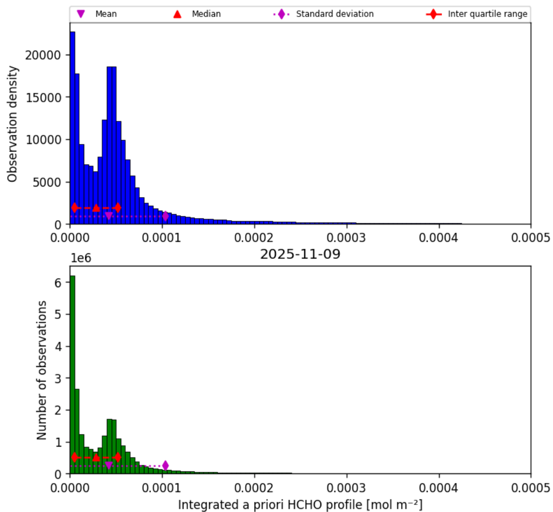
Figure 43: Histogram of “Integrated a priori HCHO profile” for 2025-11-08 to 2025-11-10
