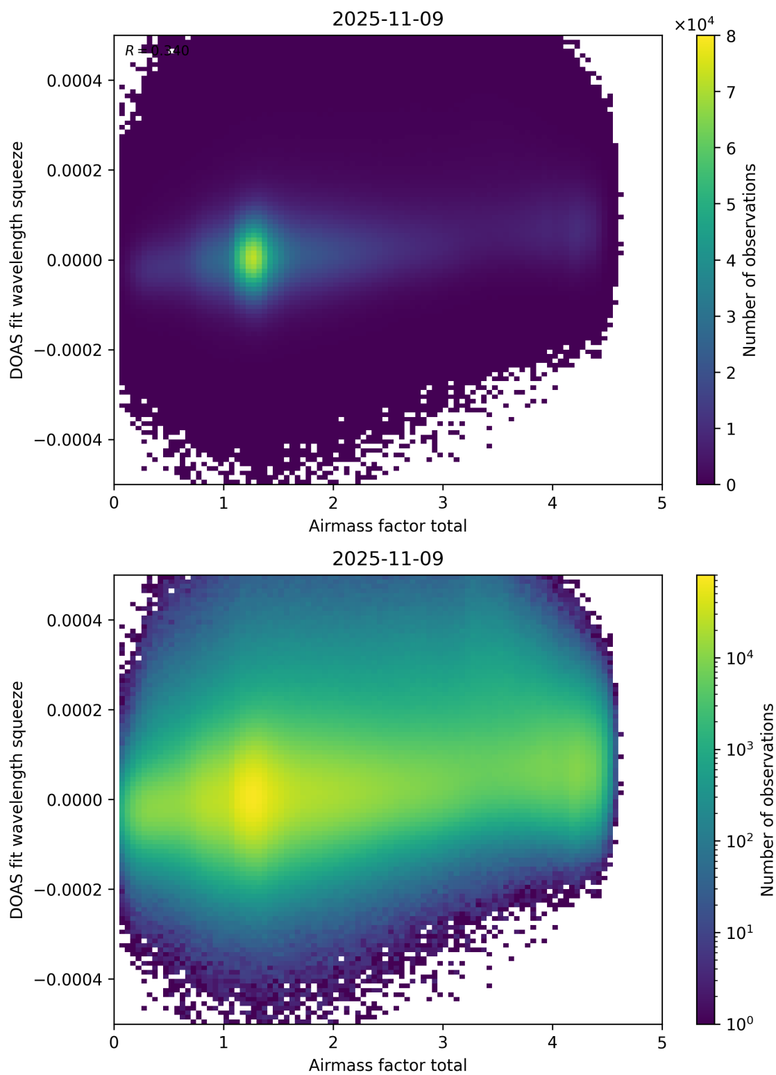
Figure 99: Scatter density plot of “Airmass factor total” against “DOAS fit wavelength squeeze” for 2025-11-08 to 2025-11-10.
