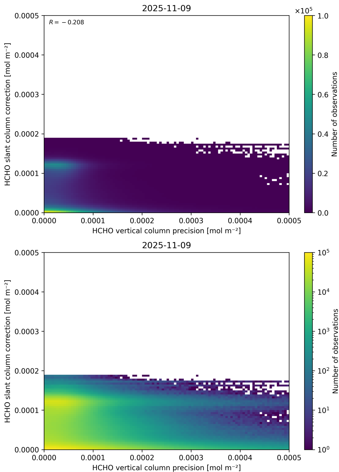
Figure 141: Scatter density plot of “HCHO vertical column precision” against “HCHO slant column correction” for 2025-11-08 to 2025-11-10.
