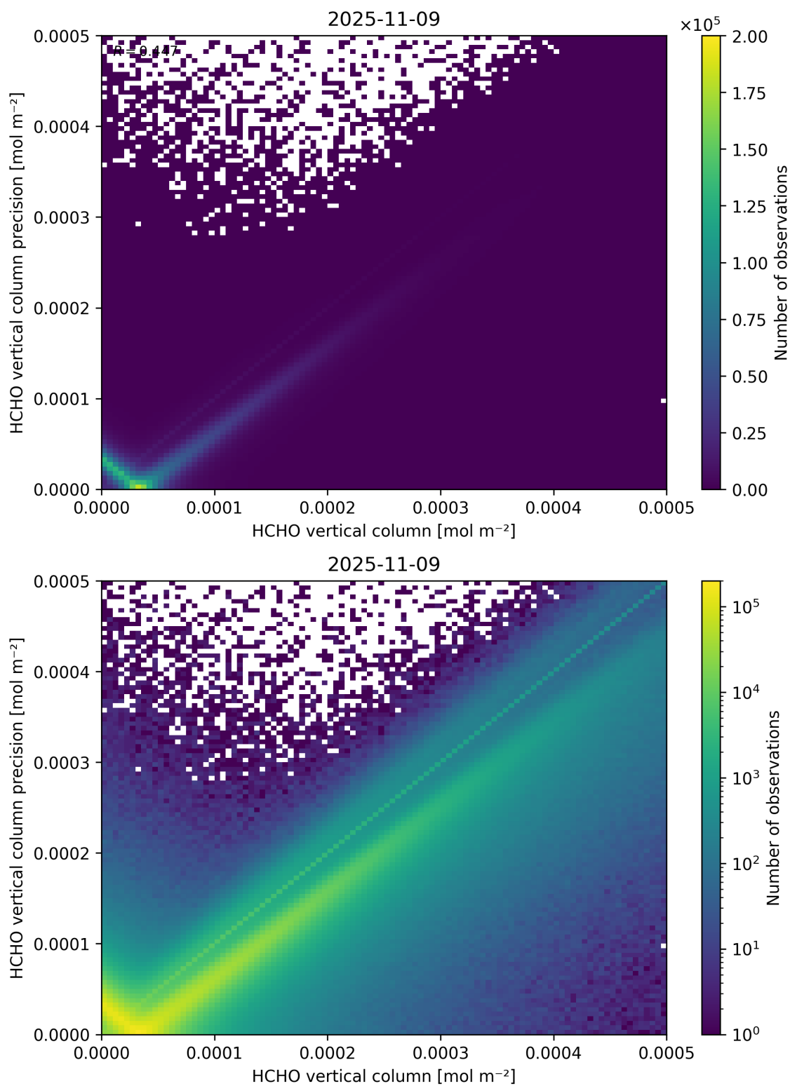
Figure 134: Scatter density plot of “HCHO vertical column” against “HCHO vertical column precision” for 2025-11-08 to 2025-11-10.
