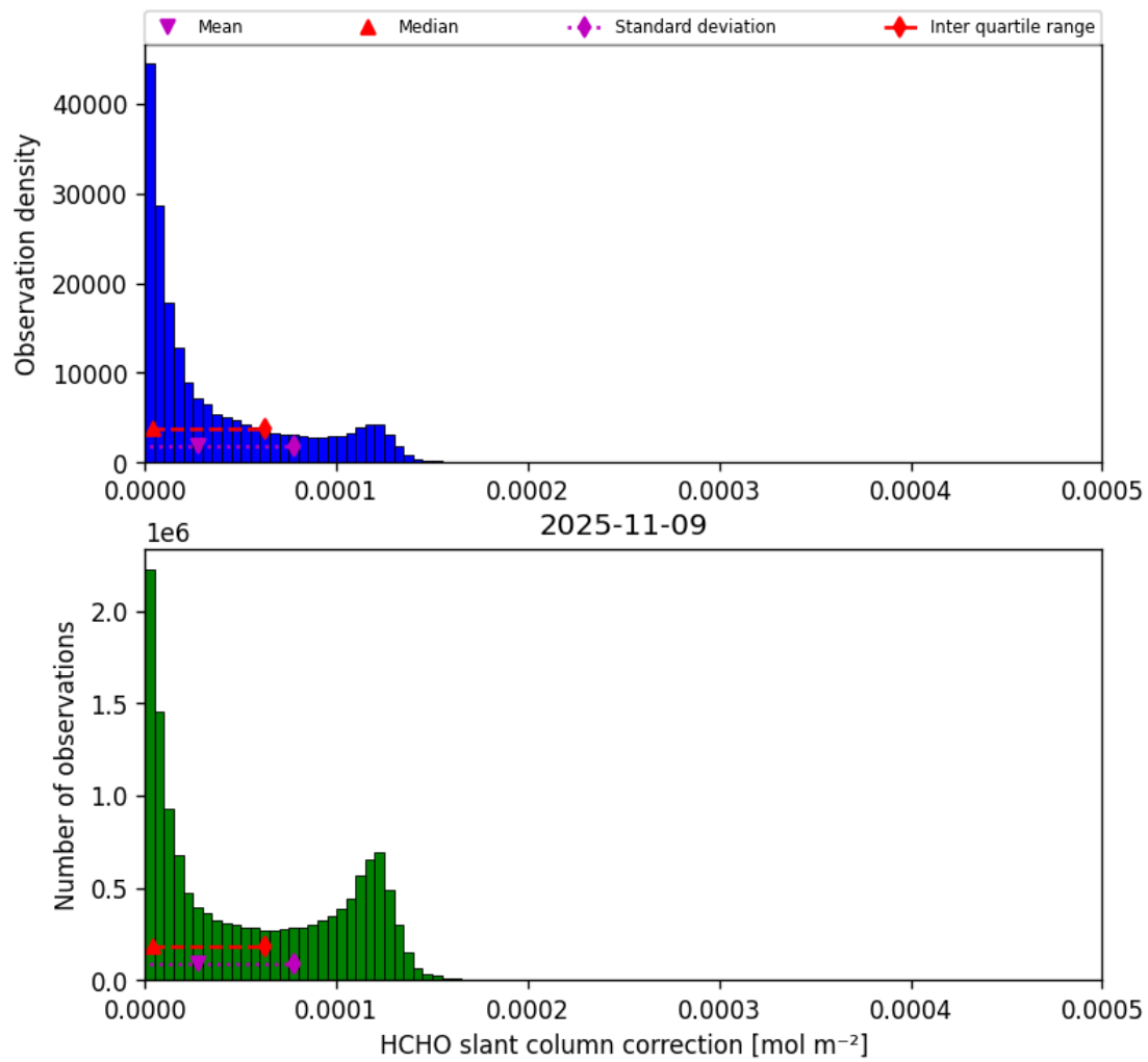
Figure 47: Histogram of “HCHO slant column correction” for 2025-11-08 to 2025-11-10
