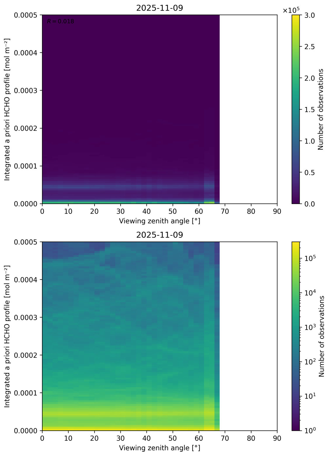
Figure 195: Scatter density plot of “Viewing zenith angle” against “Integrated a priori HCHO profile” for 2025-11-08 to 2025-11-10.
