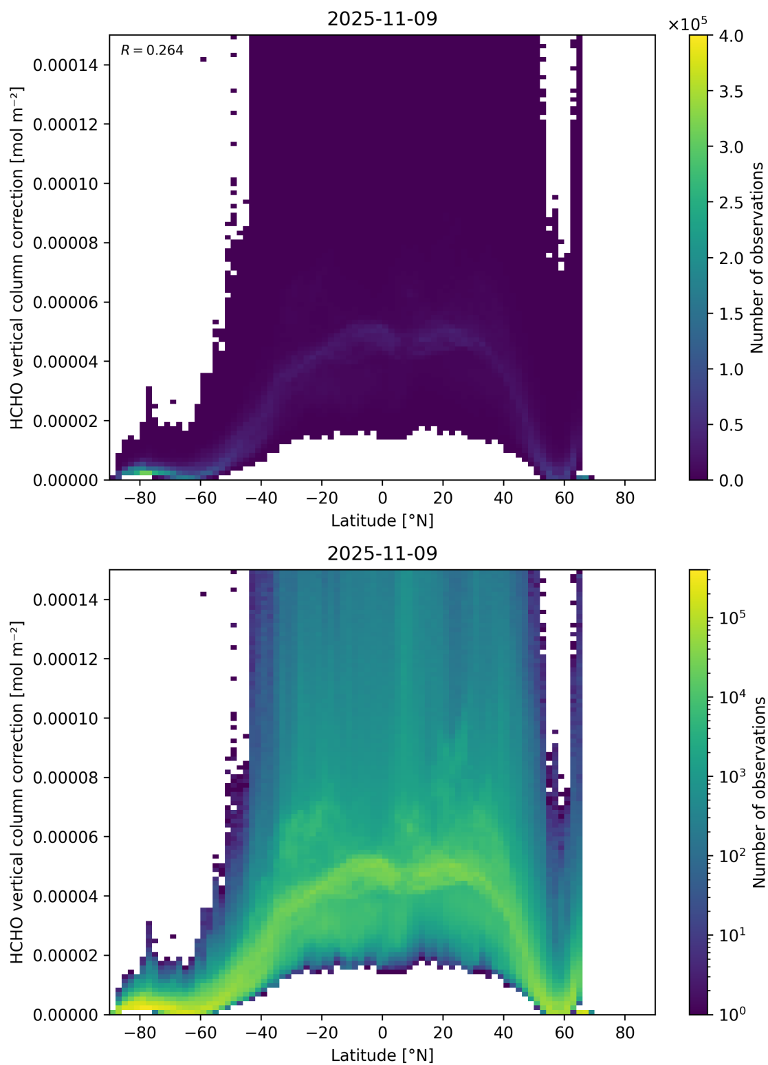
Figure 164: Scatter density plot of “Latitude” against “HCHO vertical column correction” for 2025-11-08 to 2025-11-10.
