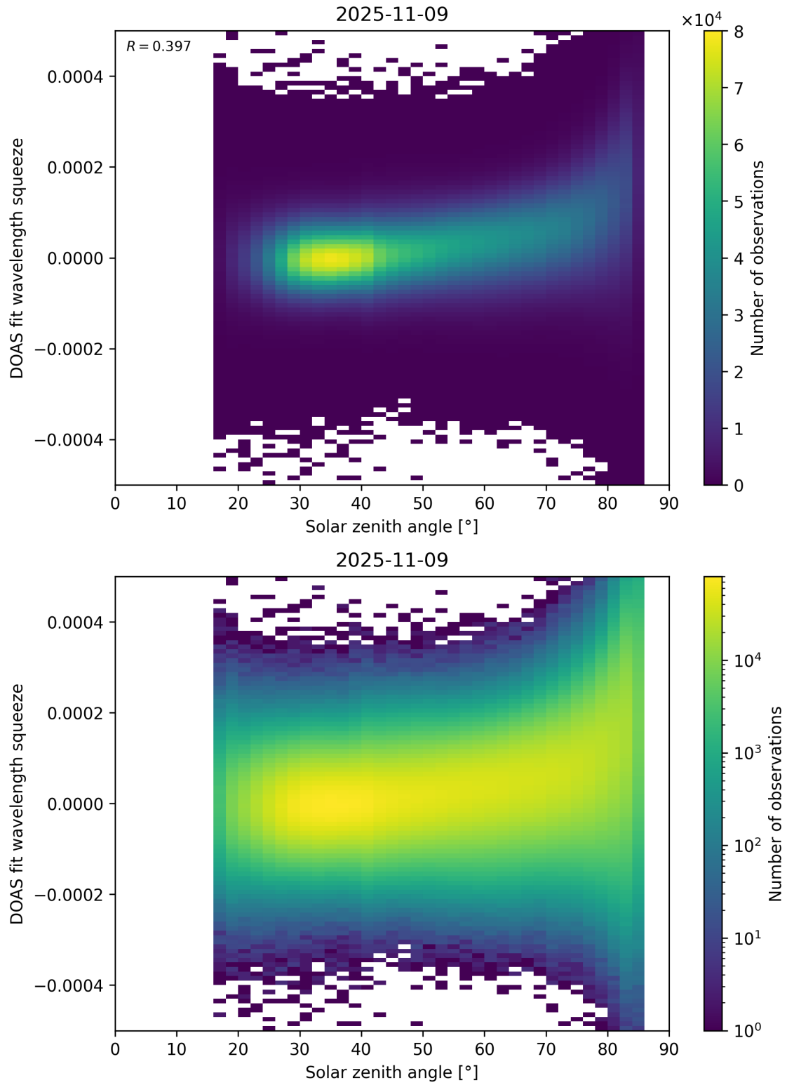
Figure 169: Scatter density plot of “Solar zenith angle” against “DOAS fit wavelength squeeze” for 2025-11-08 to 2025-11-10.
