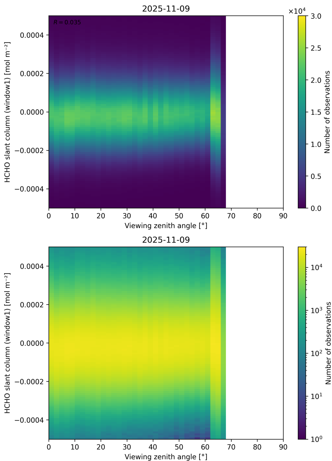
Figure 188: Scatter density plot of “Viewing zenith angle” against “HCHO slant column (window1)” for 2025-11-08 to 2025-11-10.
