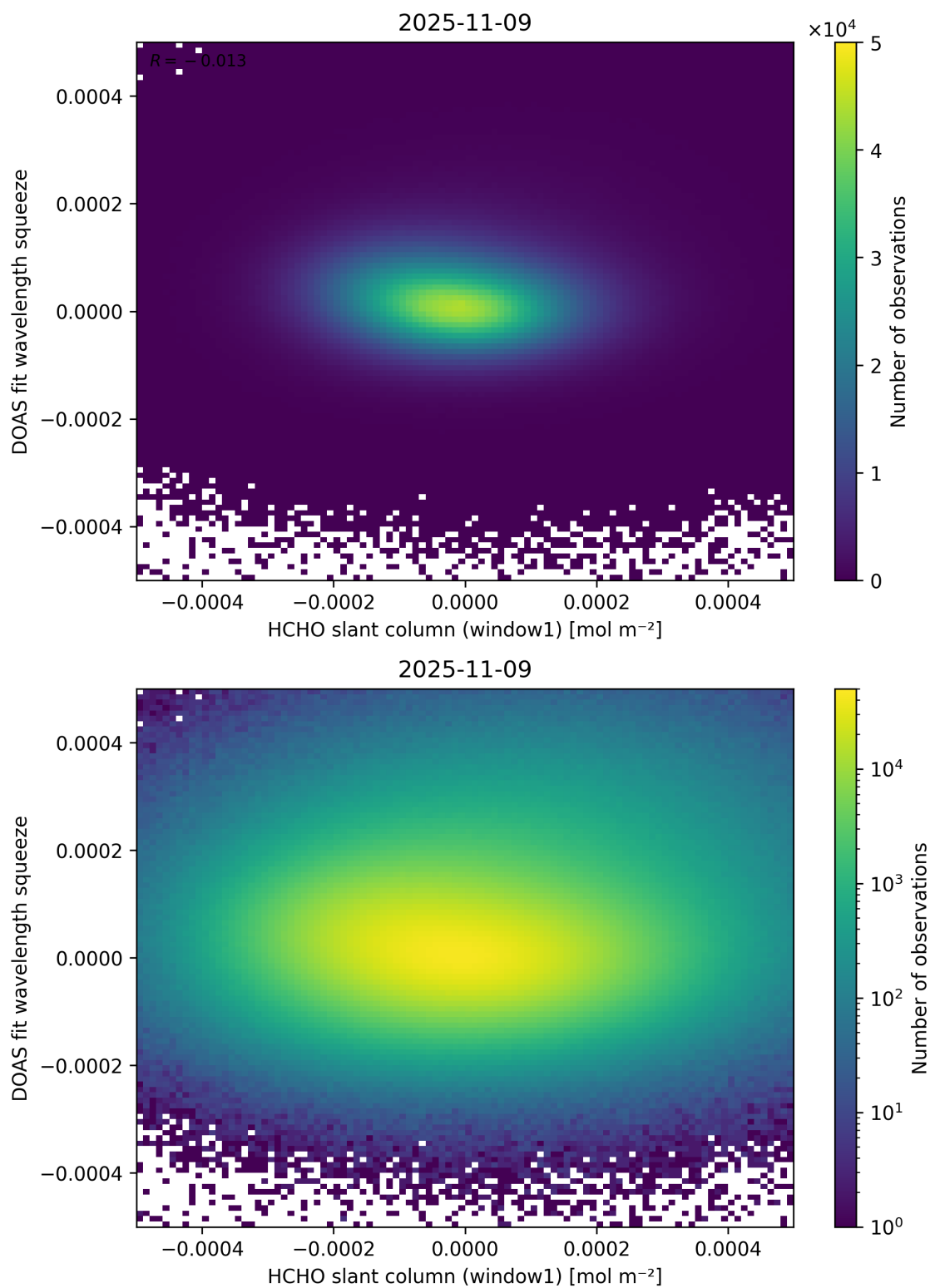
Figure 80: Scatter density plot of “HCHO slant column (window1)” against “DOAS fit wavelength squeeze” for 2025-11-08 to 2025-11-10.
