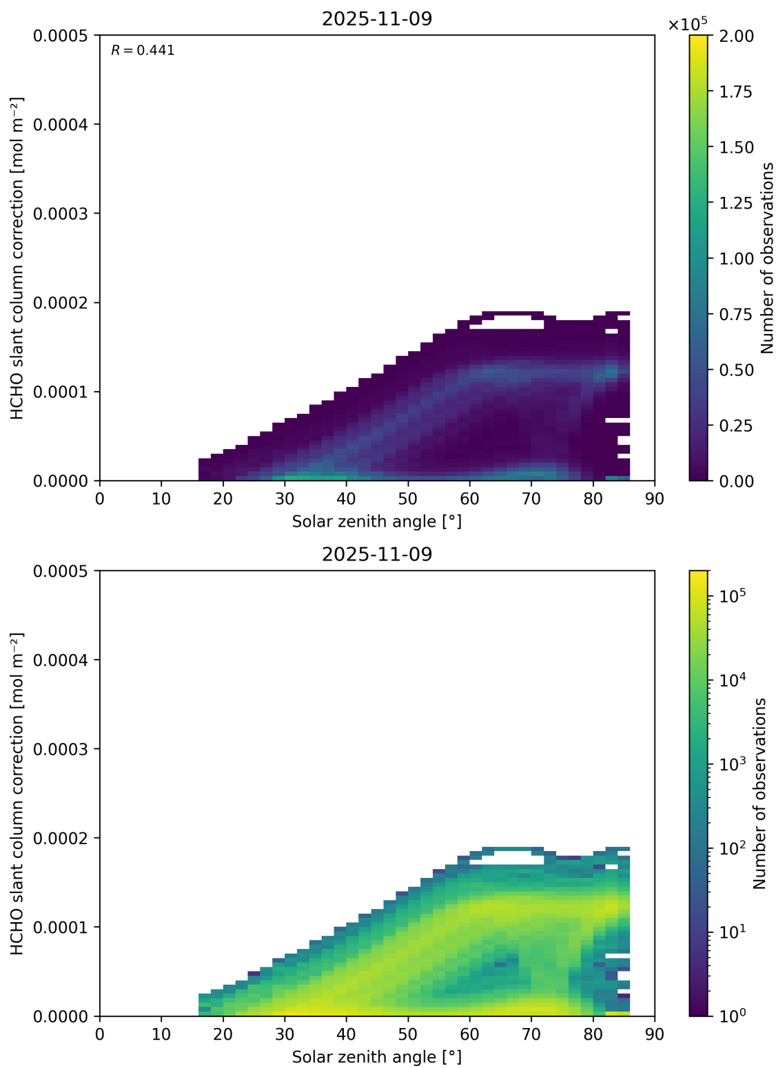
Figure 172: Scatter density plot of “Solar zenith angle” against “HCHO slant column correction” for 2025-11-08 to 2025-11-10.
