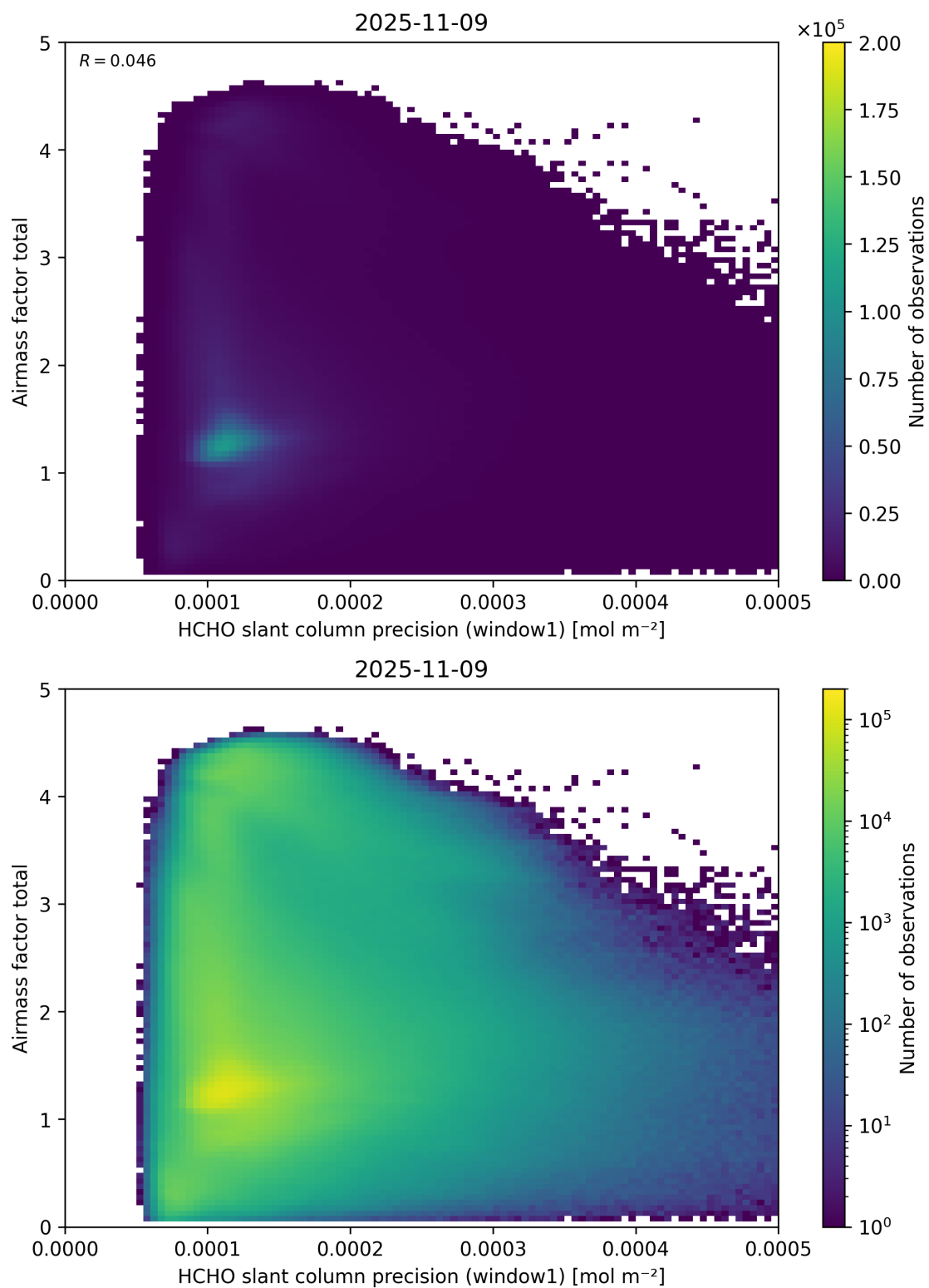
Figure 94: Scatter density plot of “HCHO slant column precision (window1)” against “Airmass factor total” for 2025-11-08 to 2025-11-10.
