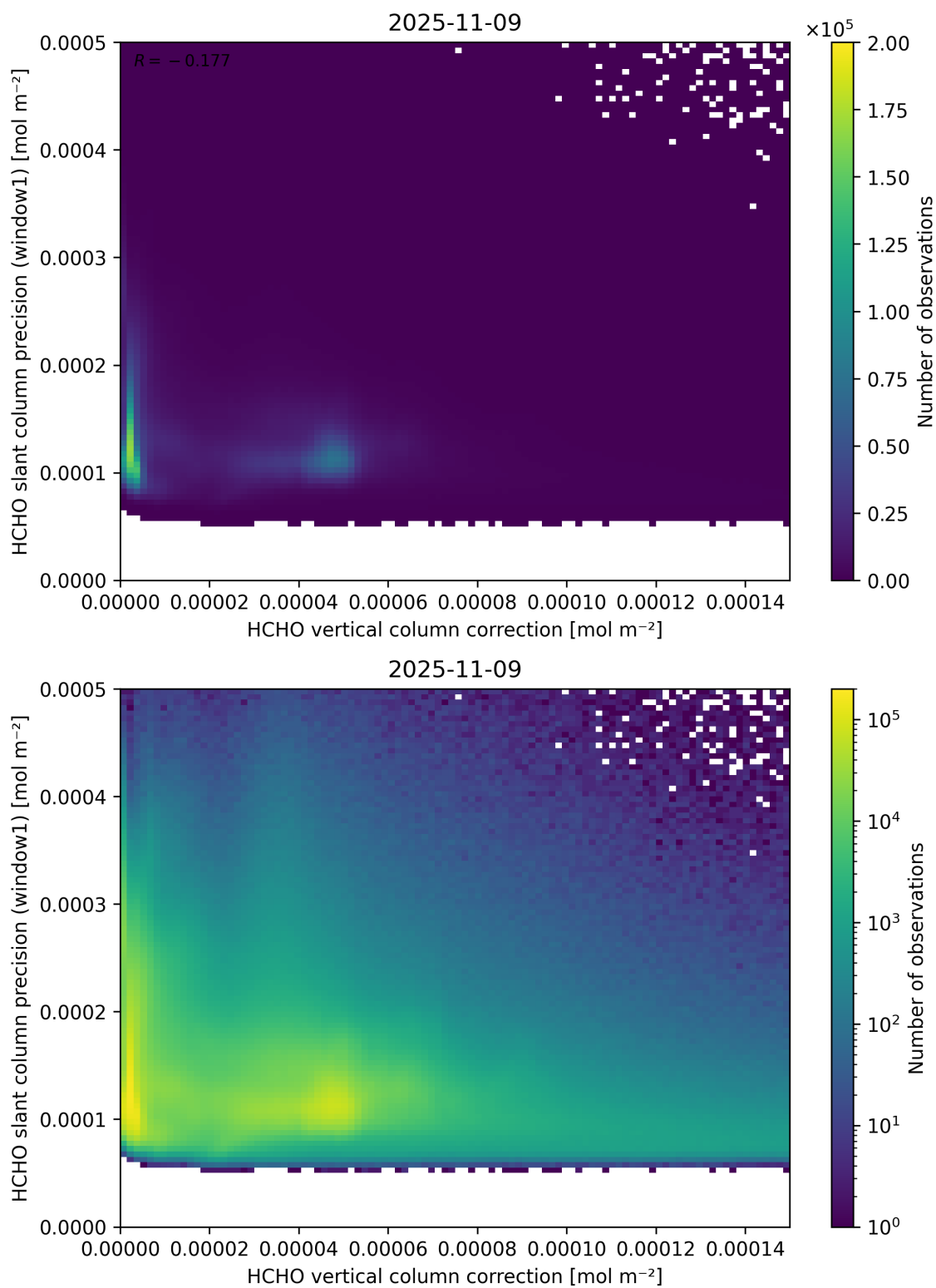
Figure 119: Scatter density plot of “HCHO vertical column correction” against “HCHO slant column precision (window1)” for 2025-11-08 to 2025-11-10.
