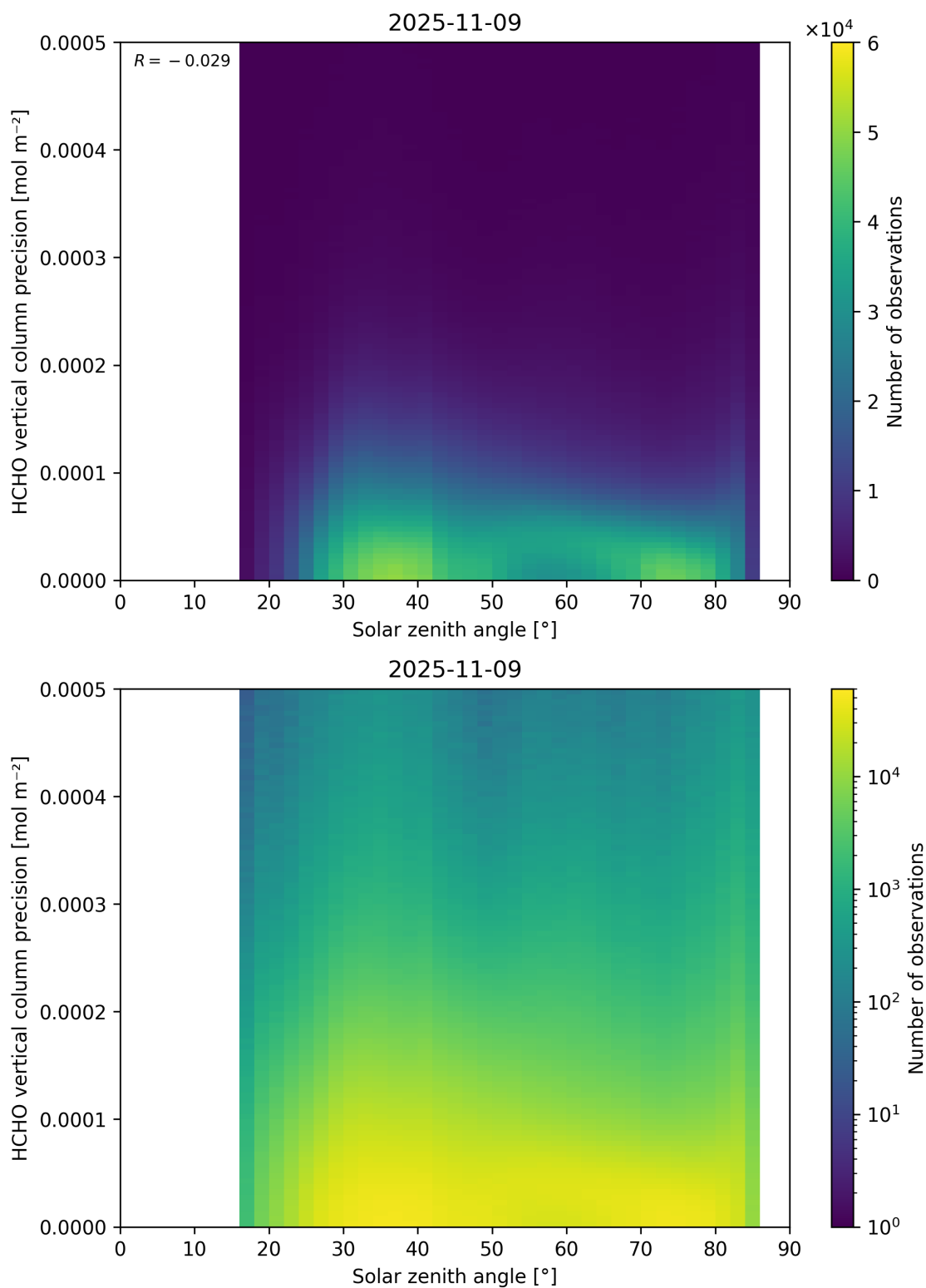
Figure 179: Scatter density plot of “Solar zenith angle” against “HCHO vertical column precision” for 2025-11-08 to 2025-11-10.
