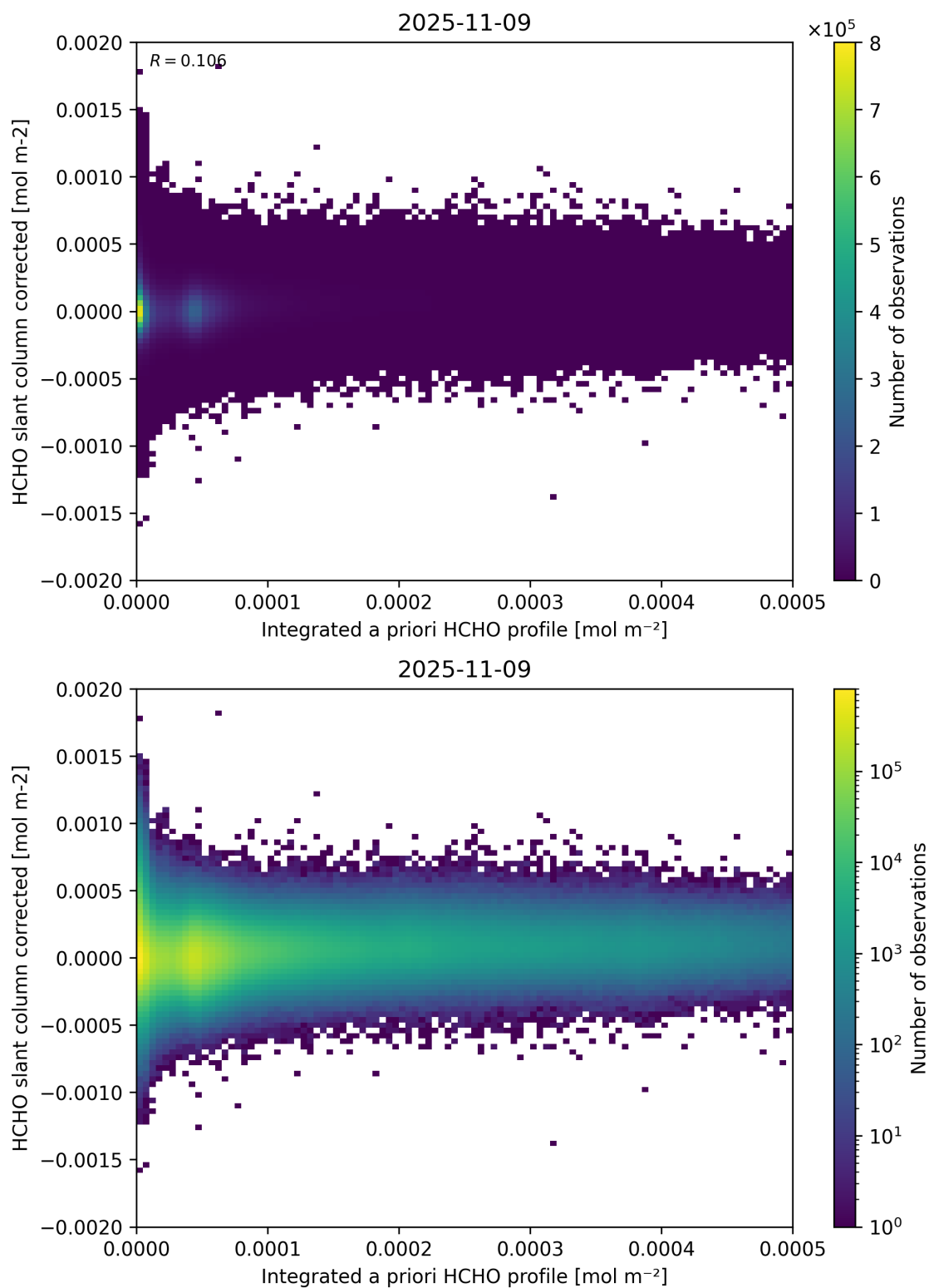
Figure 151: Scatter density plot of “Integrated a priori HCHO profile” against “HCHO slant column corrected” for 2025-11-08 to 2025-11-10.
