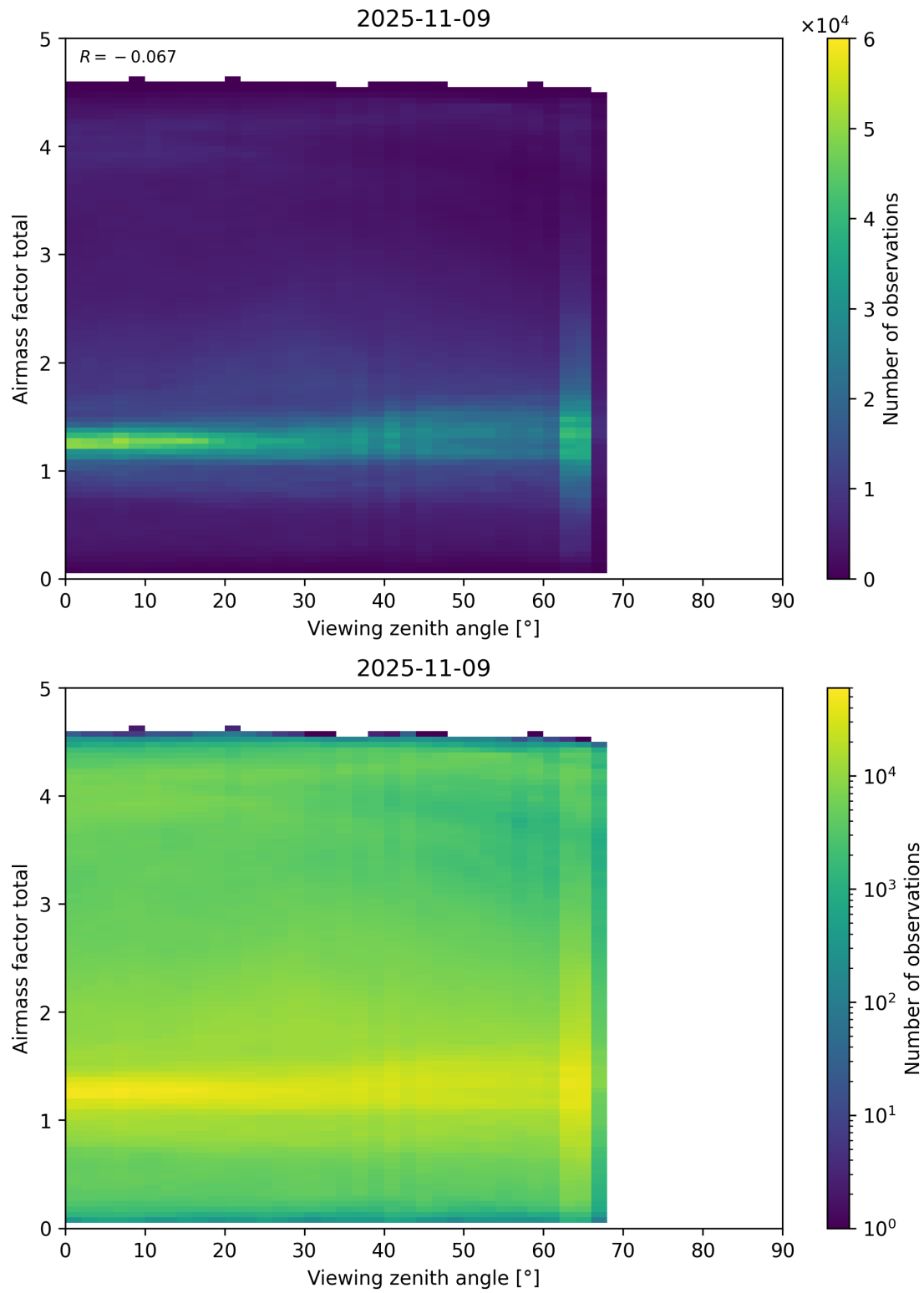
Figure 190: Scatter density plot of “Viewing zenith angle” against “Airmass factor total” for 2025-11-08 to 2025-11-10.
