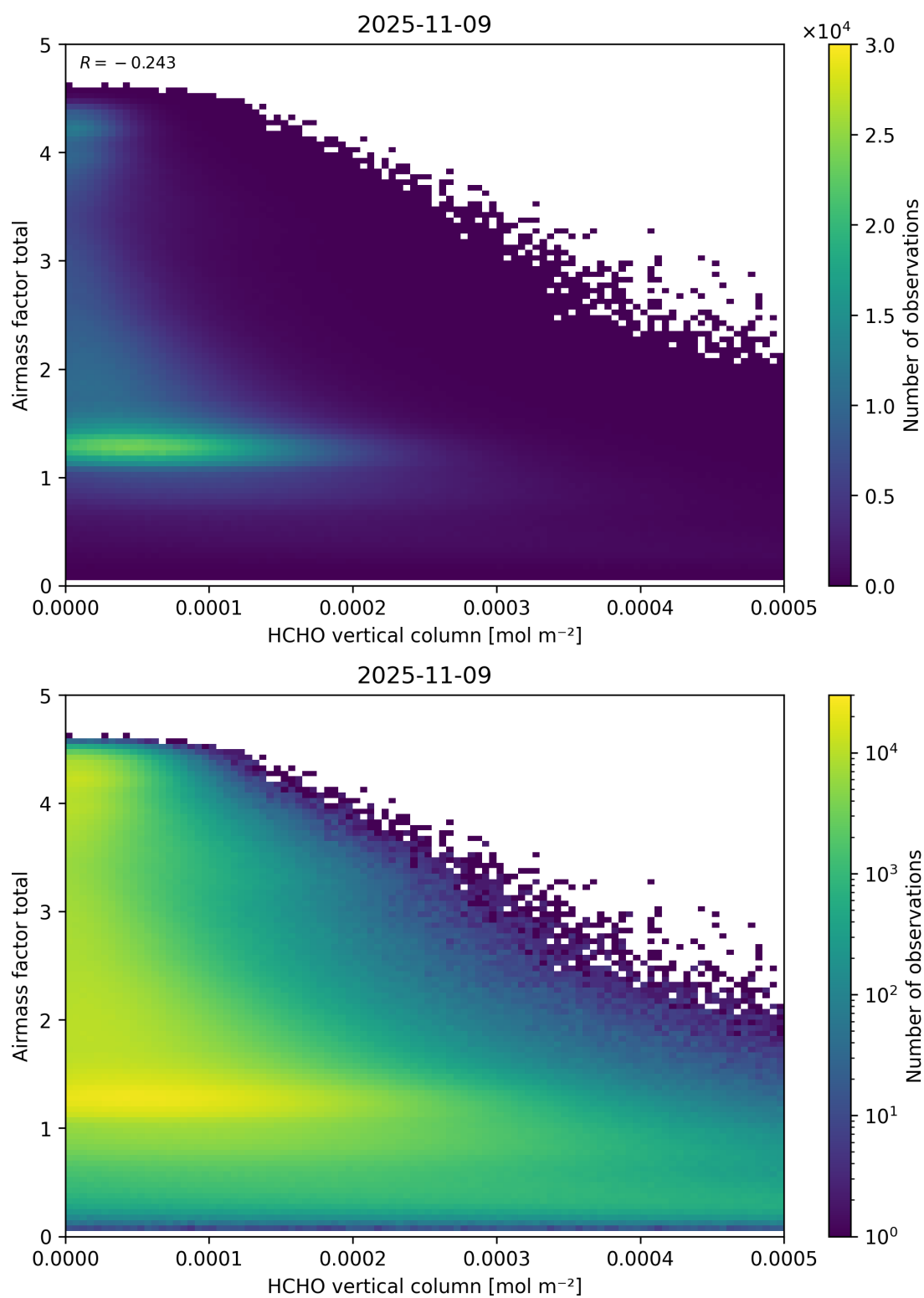
Figure 131: Scatter density plot of “HCHO vertical column” against “Airmass factor total” for 2025-11-08 to 2025-11-10.
