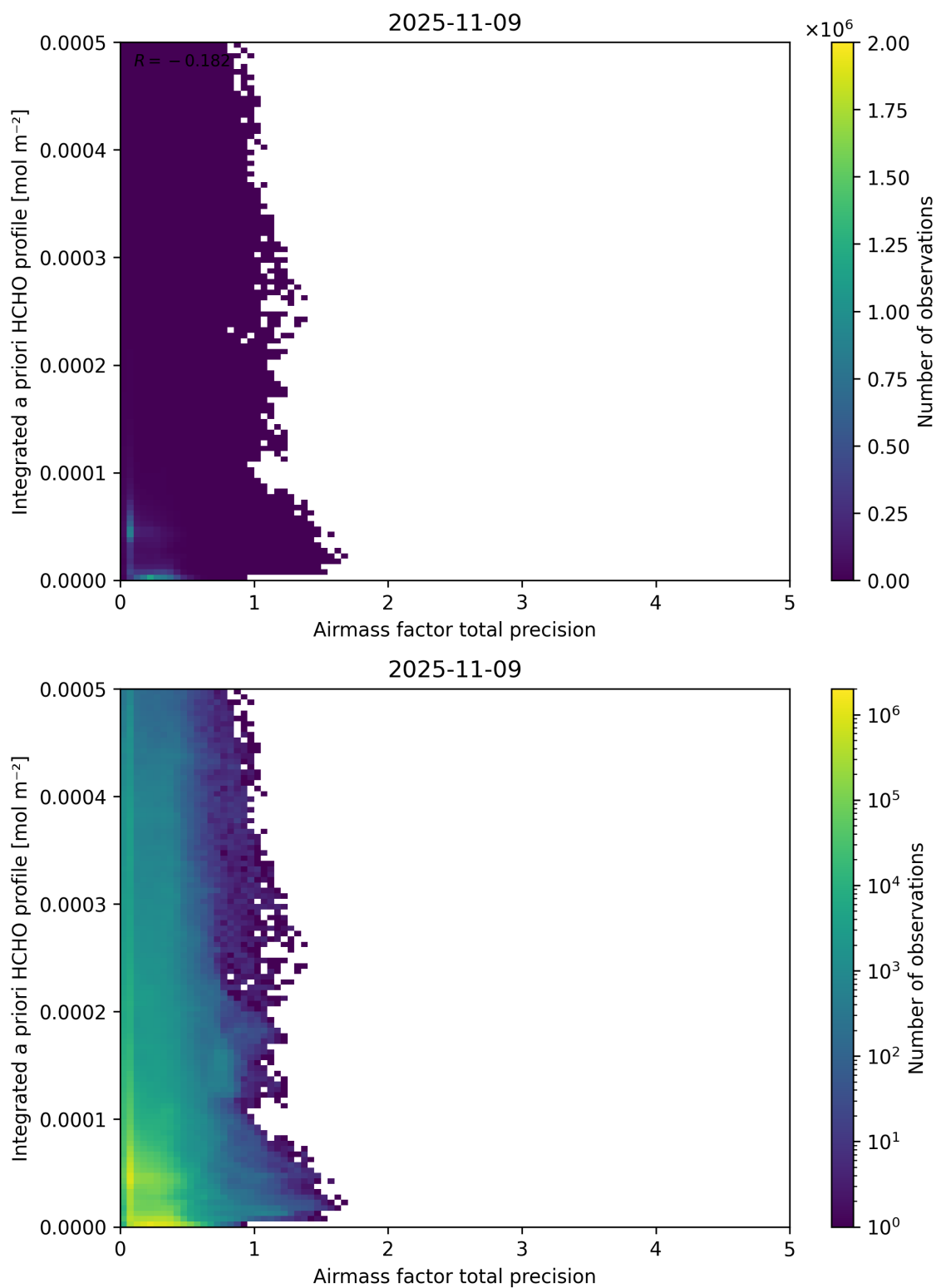
Figure 111: Scatter density plot of “Airmass factor total precision” against “Integrated a priori HCHO profile” for 2025-11-08 to 2025-11-10.
