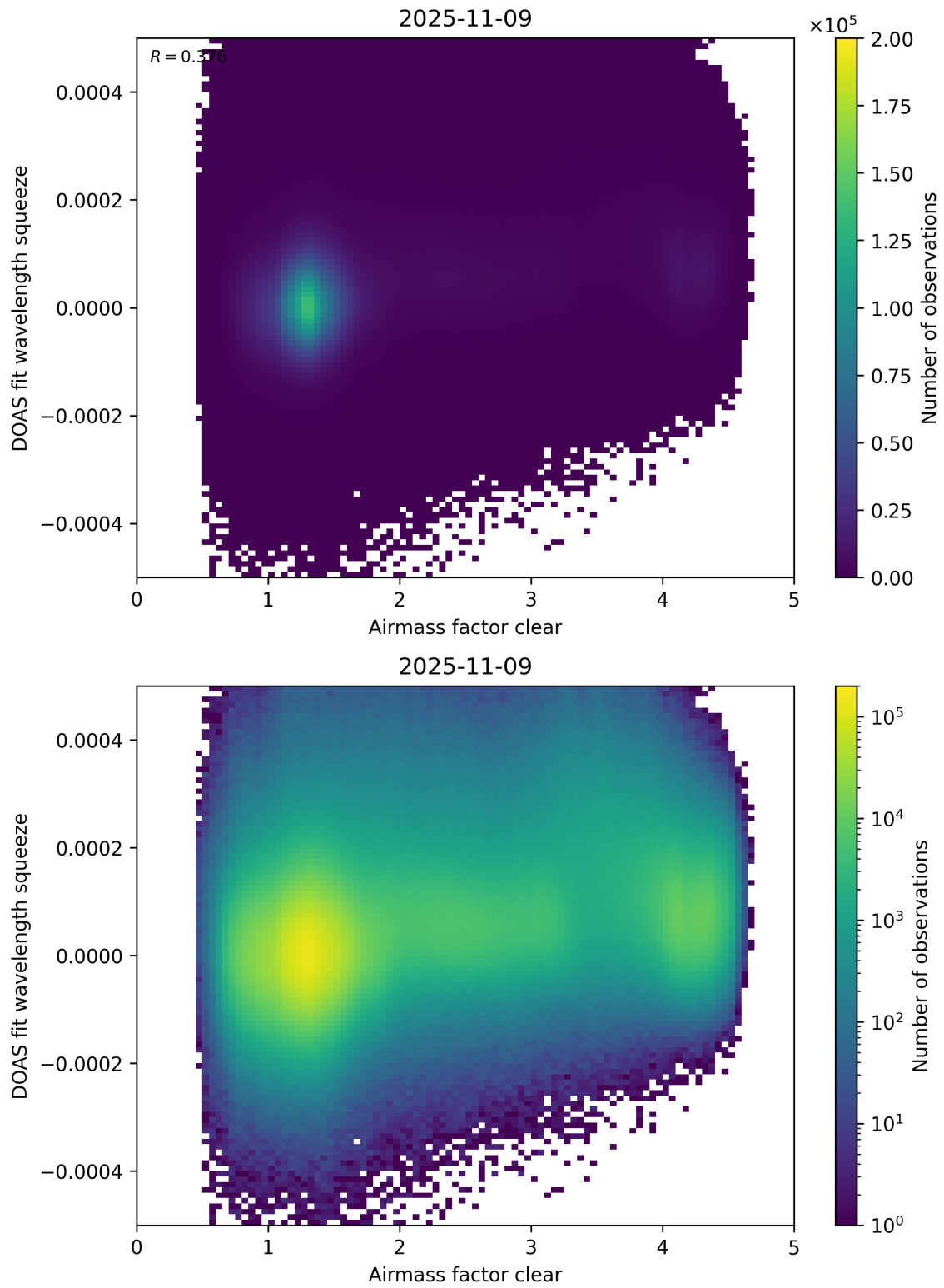
Figure 73: Scatter density plot of “Airmass factor clear” against “DOAS fit wavelength squeeze” for 2025-11-08 to 2025-11-10.
