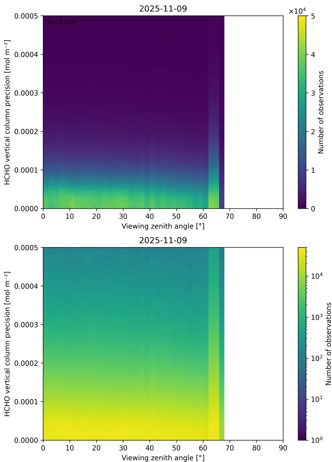
Figure 194: Scatter density plot of “Viewing zenith angle” against “HCHO vertical column precision” for 2025-11-08 to 2025-11-10.
