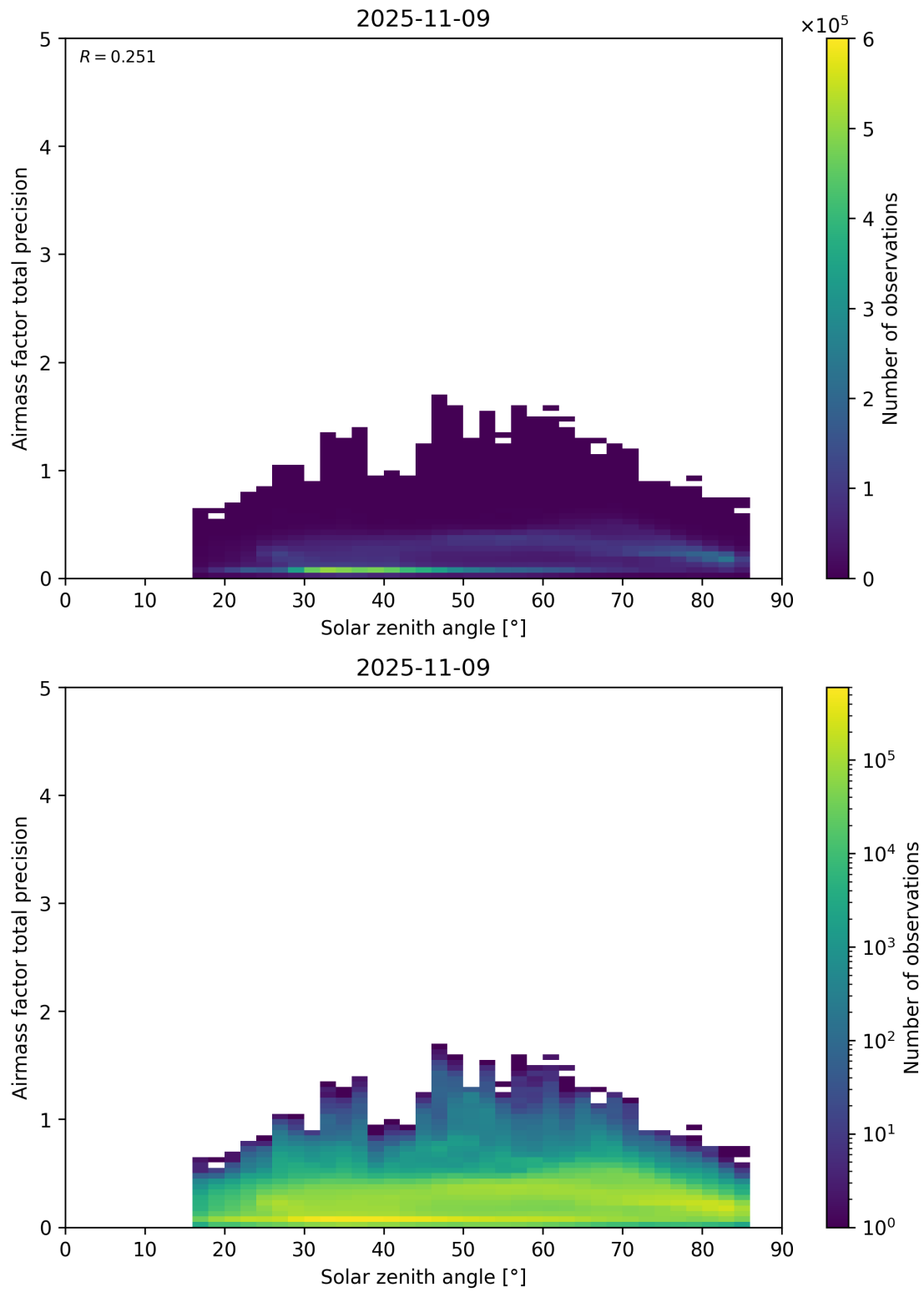
Figure 176: Scatter density plot of “Solar zenith angle” against “Airmass factor total precision” for 2025-11-08 to 2025-11-10.
