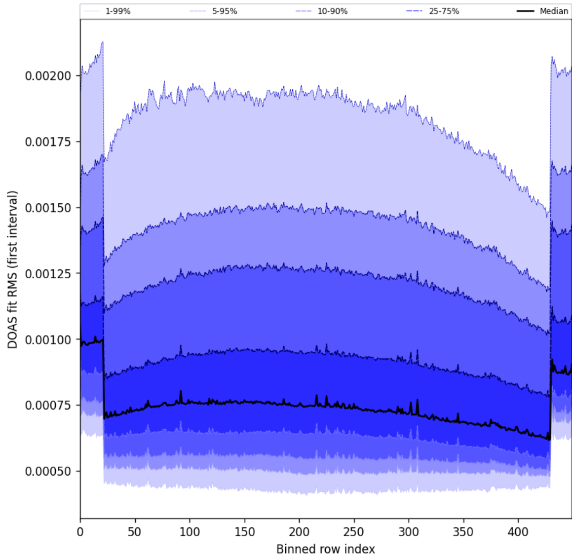
Figure 60: Along track statistics of “DOAS fit RMS (first interval)” for 2025-11-08 to 2025-11-10
