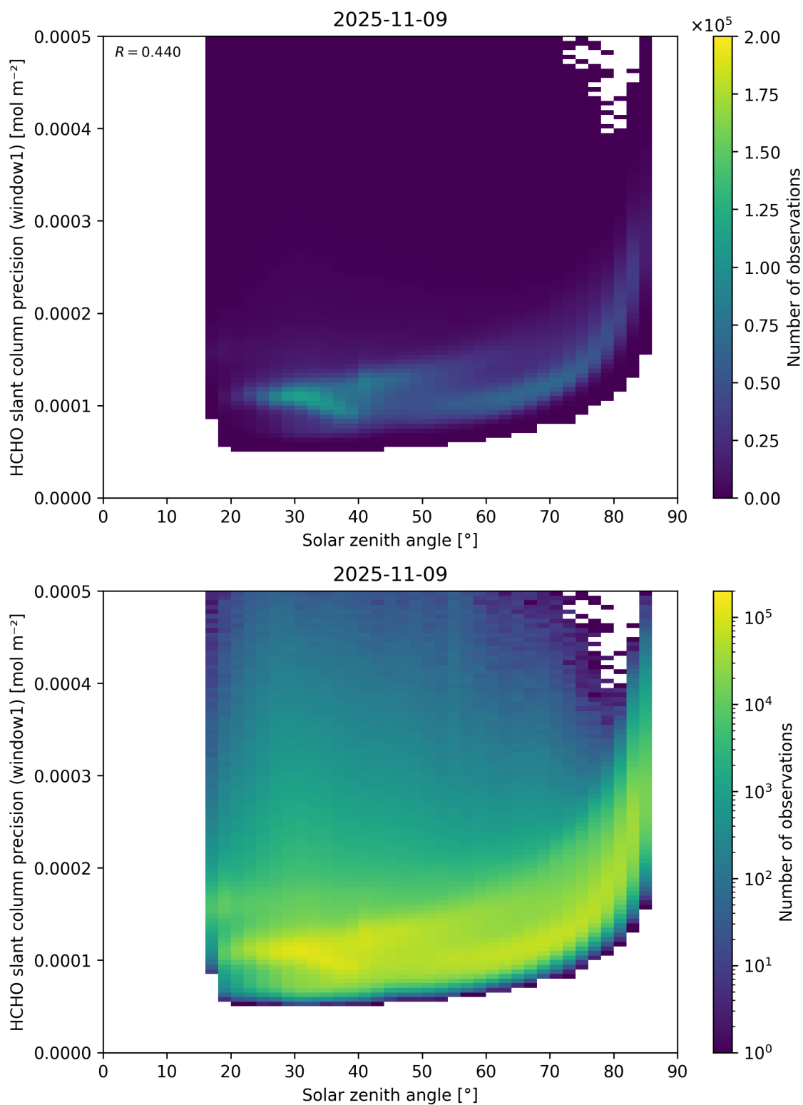
Figure 174: Scatter density plot of “Solar zenith angle” against “HCHO slant column precision (window1)” for 2025-11-08 to 2025-11-10.
