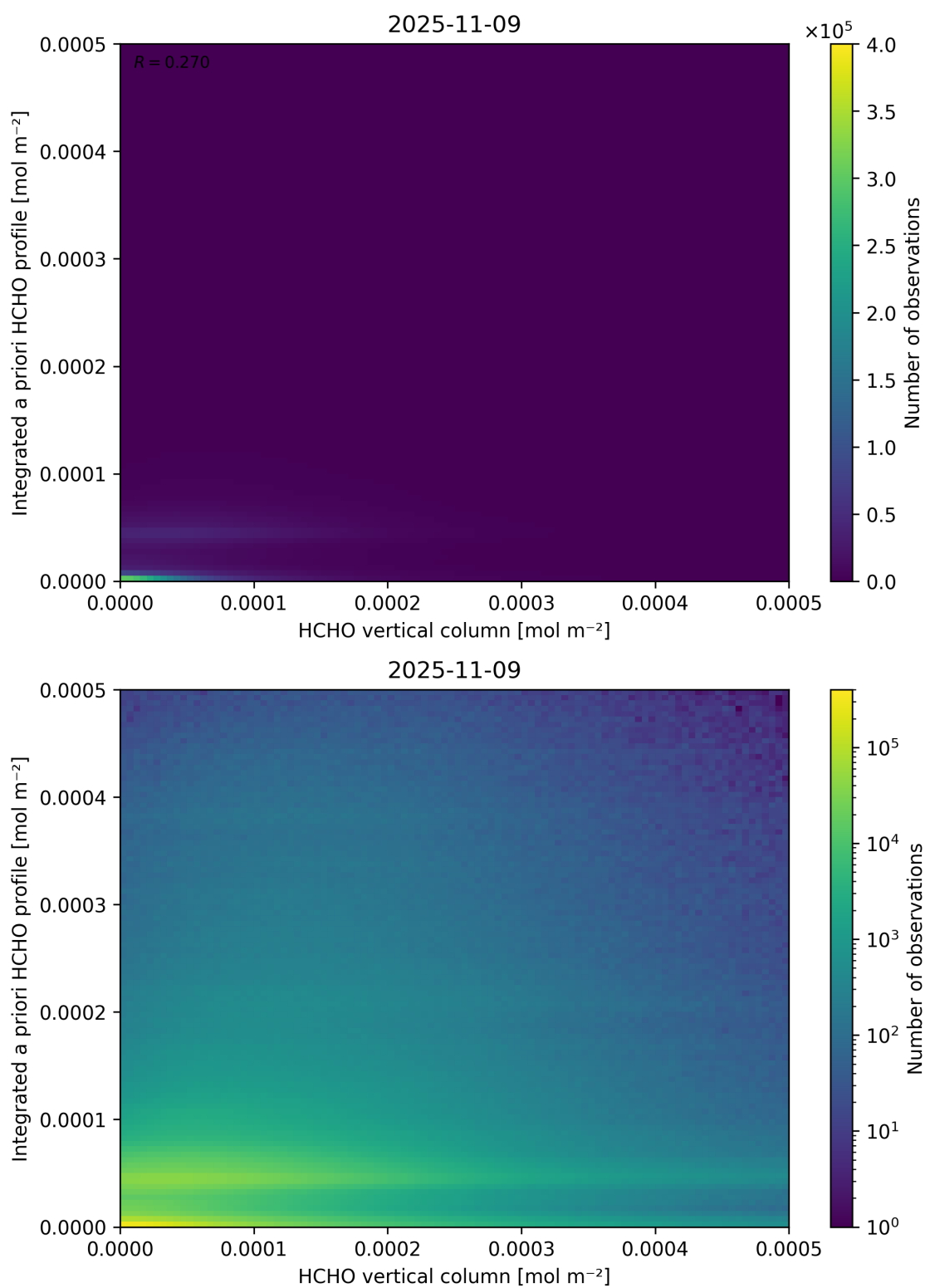
Figure 135: Scatter density plot of “HCHO vertical column” against “Integrated a priori HCHO profile” for 2025-11-08 to 2025-11-10.
