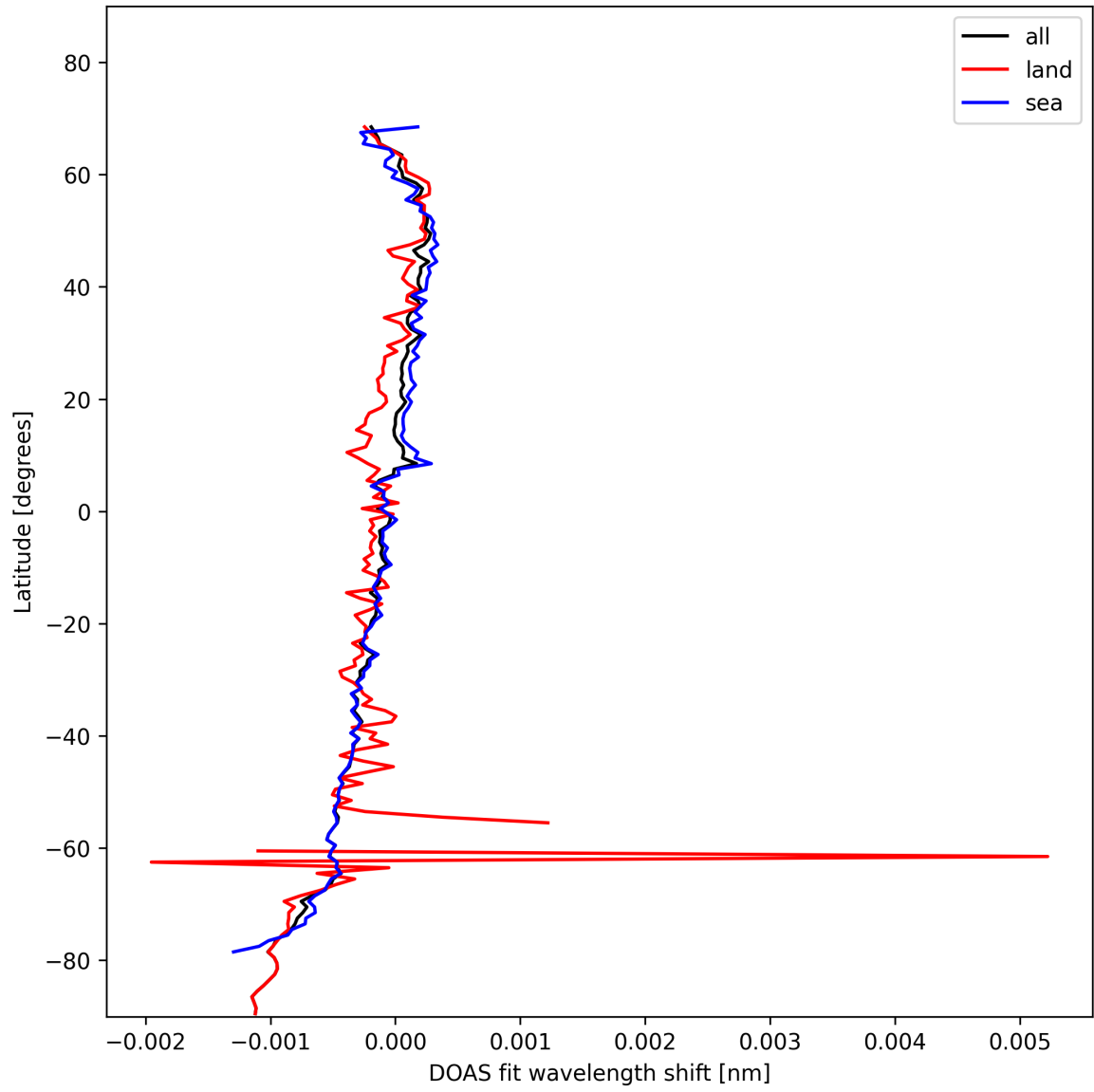
Figure 30: Zonal average of “DOAS fit wavelength shift” for 2025-11-08 to 2025-11-10.
