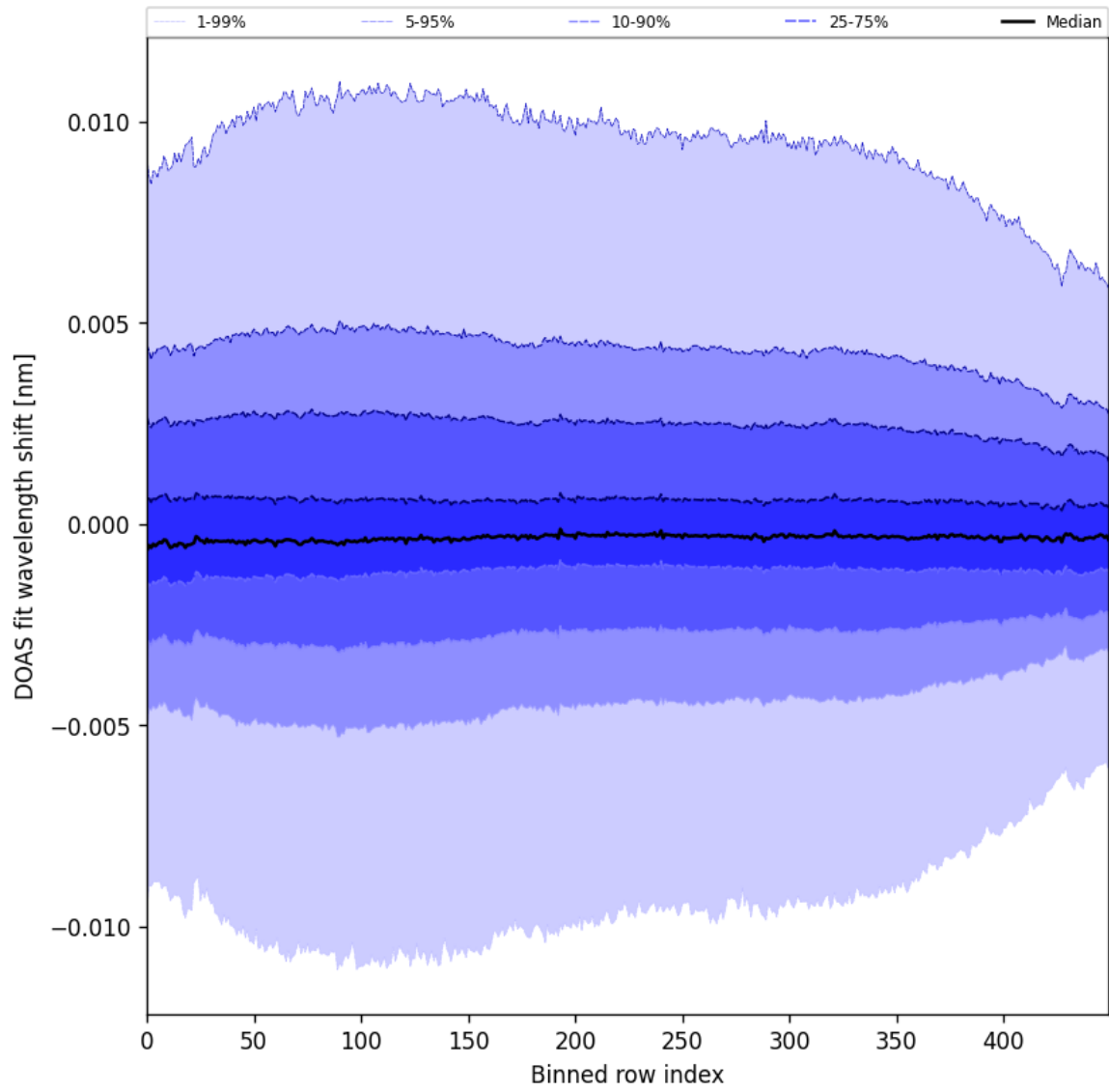
Figure 58: Along track statistics of “DOAS fit wavelength shift” for 2025-11-08 to 2025-11-10
