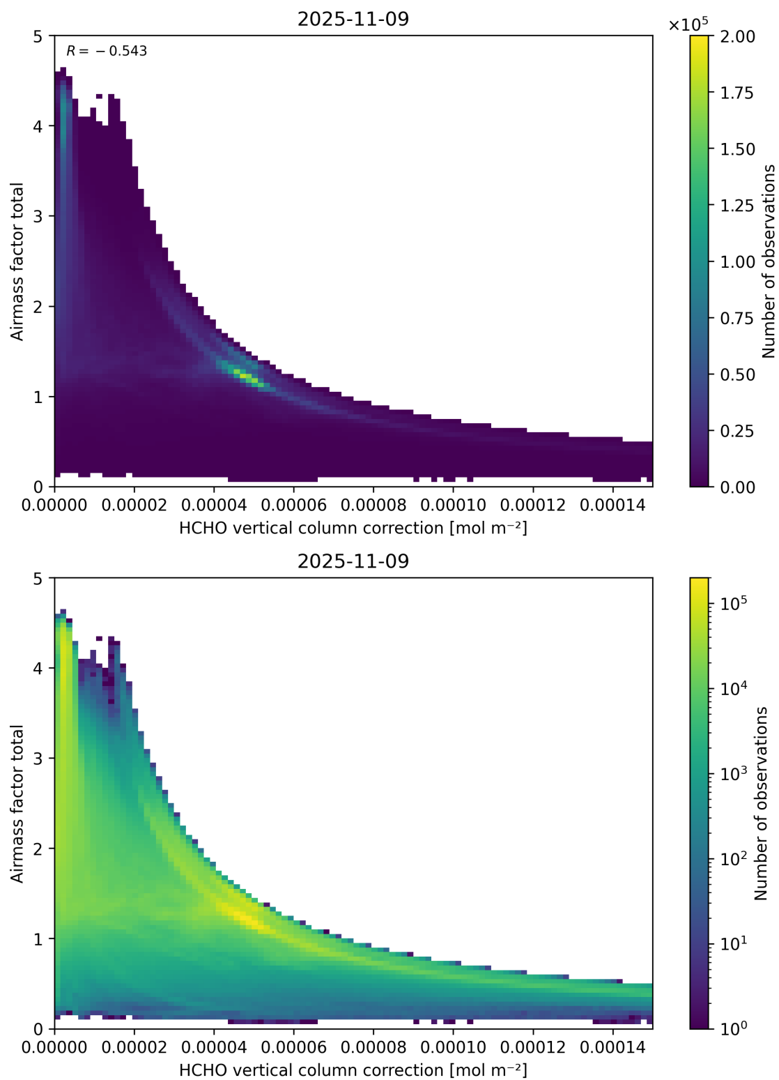
Figure 120: Scatter density plot of “HCHO vertical column correction” against “Airmass factor total” for 2025-11-08 to 2025-11-10.
