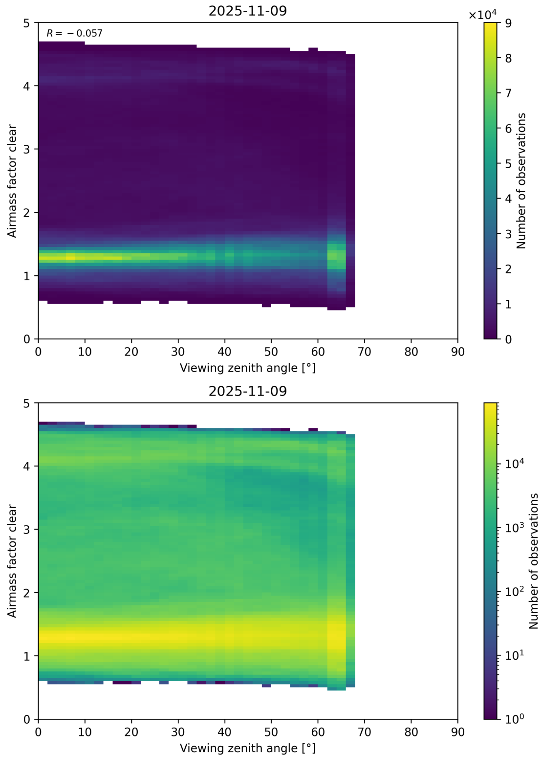
Figure 185: Scatter density plot of “Viewing zenith angle” against “Airmass factor clear” for 2025-11-08 to 2025-11-10.
