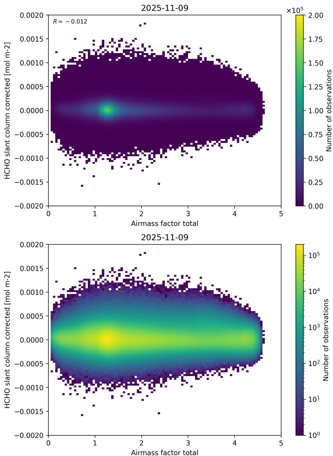
Figure 101: Scatter density plot of “Airmass factor total” against “HCHO slant column corrected” for 2025-11-08 to 2025-11-10.
