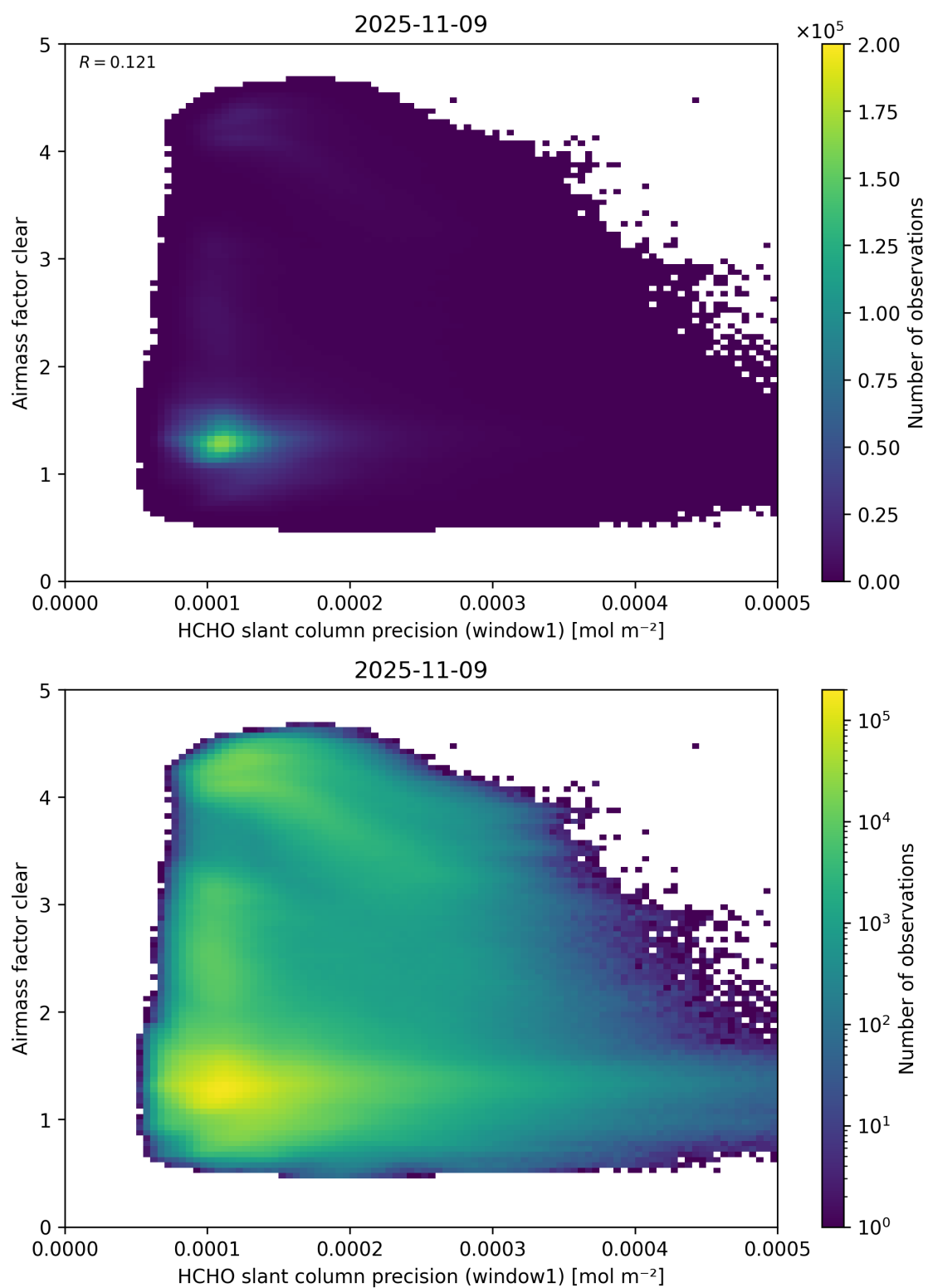
Figure 91: Scatter density plot of “HCHO slant column precision (window1)” against “Airmass factor clear” for 2025-11-08 to 2025-11-10.
