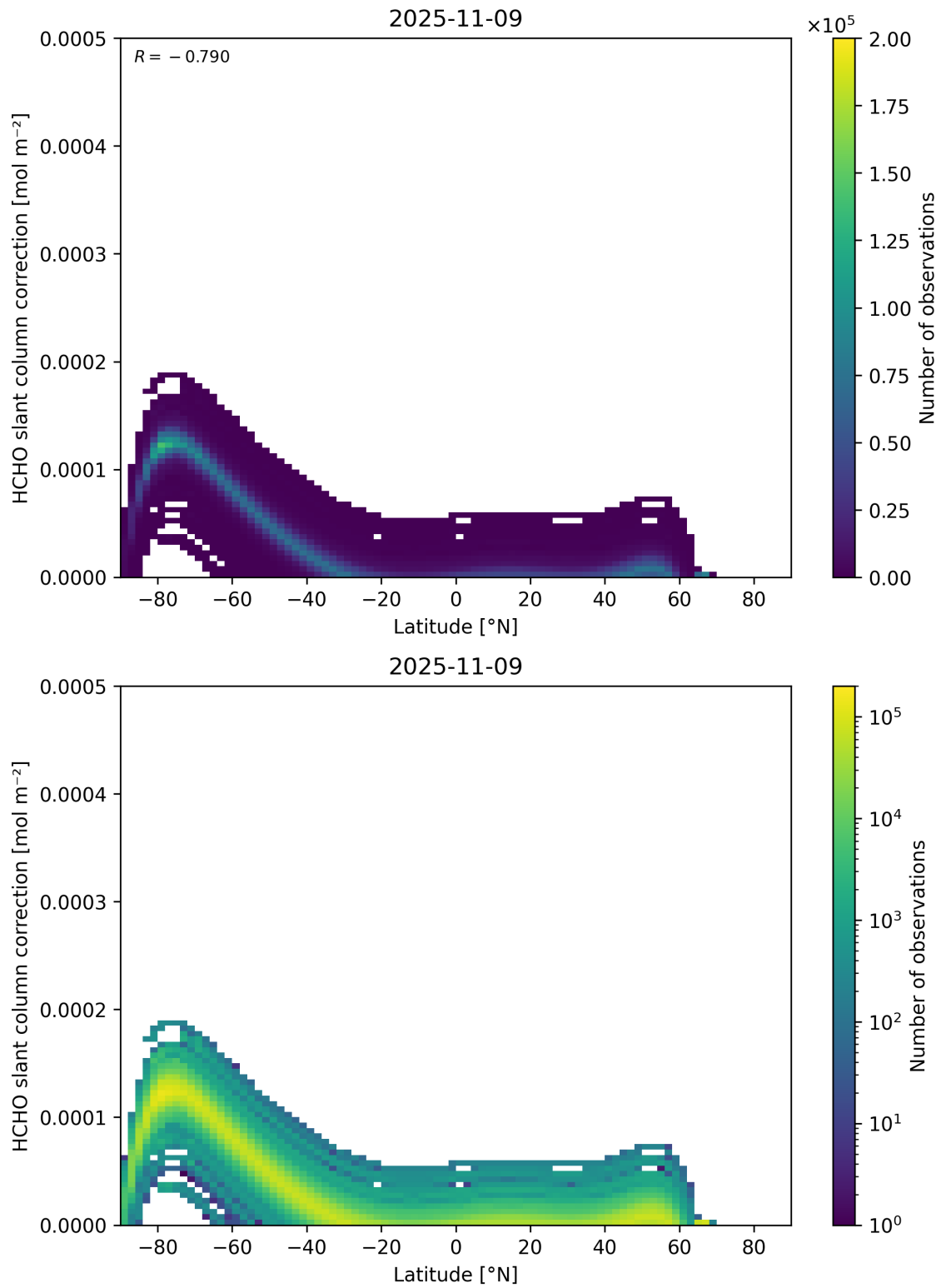
Figure 158: Scatter density plot of “Latitude” against “HCHO slant column correction” for 2025-11-08 to 2025-11-10.
