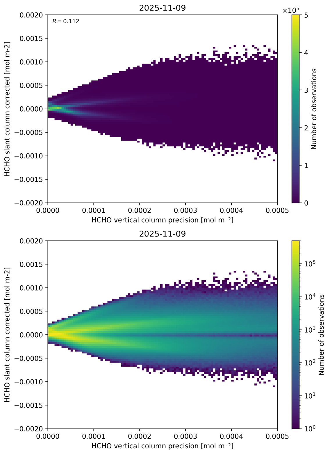
Figure 140: Scatter density plot of “HCHO vertical column precision” against “HCHO slant column corrected” for 2025-11-08 to 2025-11-10.
