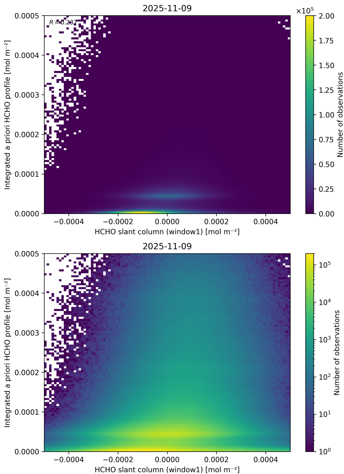
Figure 87: Scatter density plot of “HCHO slant column (window1)” against “Integrated a priori HCHO profile” for 2025-11-08 to 2025-11-10.
