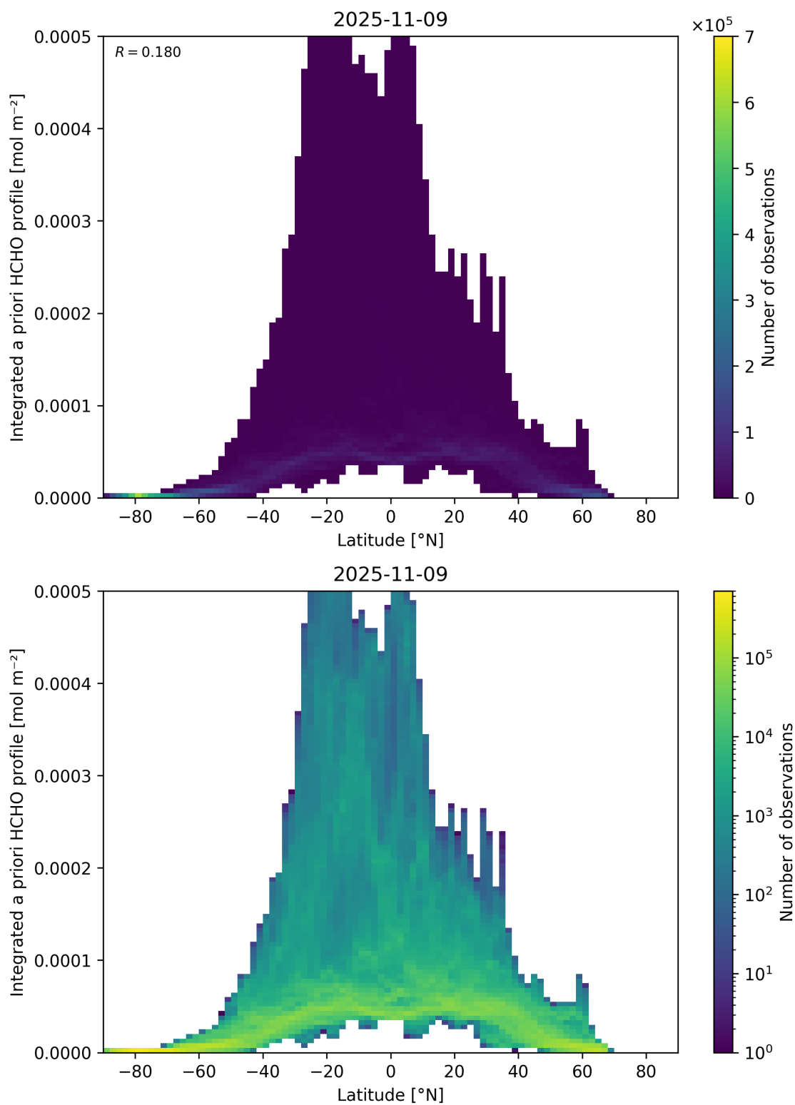
Figure 166: Scatter density plot of “Latitude” against “Integrated a priori HCHO profile” for 2025-11-08 to 2025-11-10.
