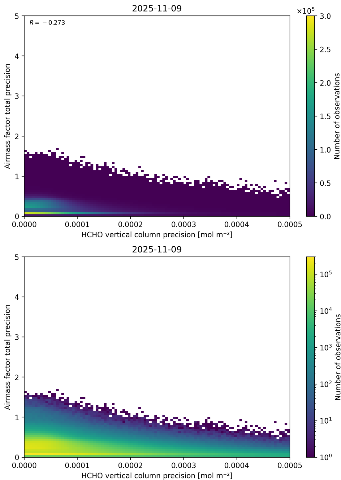
Figure 145: Scatter density plot of “HCHO vertical column precision” against “Airmass factor total precision” for 2025-11-08 to 2025-11-10.
