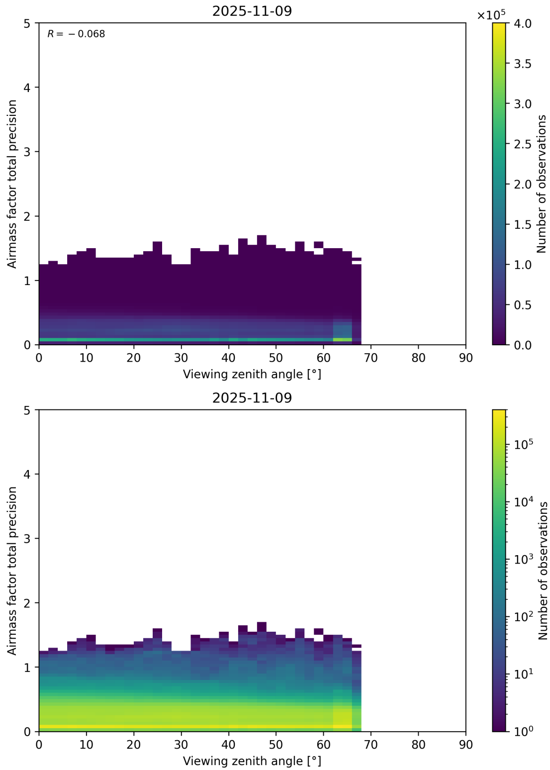
Figure 191: Scatter density plot of “Viewing zenith angle” against “Airmass factor total precision” for 2025-11-08 to 2025-11-10.
