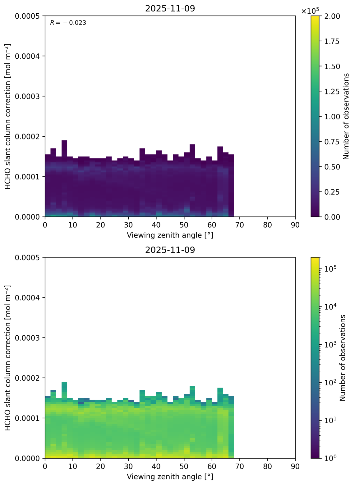
Figure 187: Scatter density plot of “Viewing zenith angle” against “HCHO slant column correction” for 2025-11-08 to 2025-11-10.
