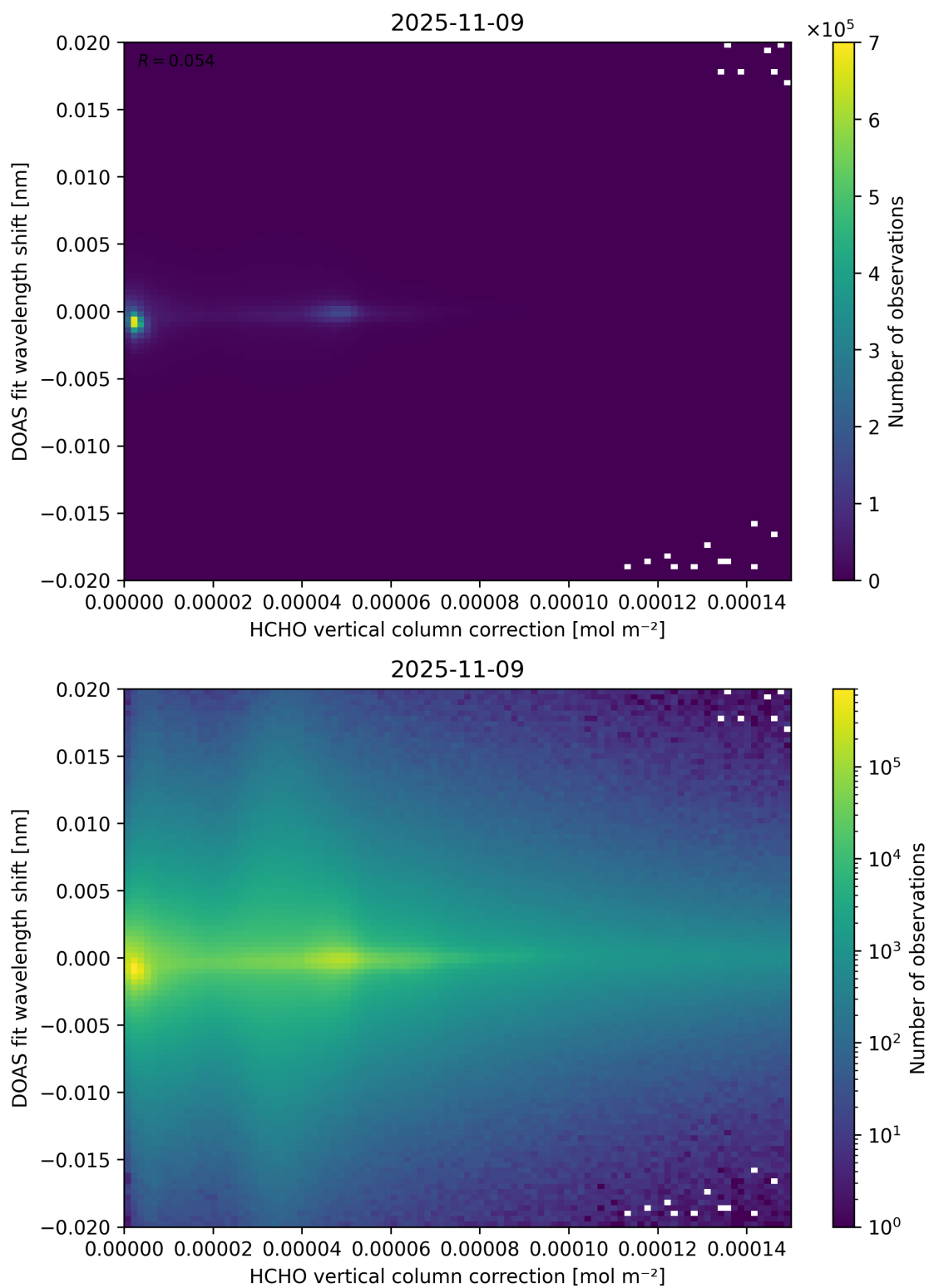
Figure 113: Scatter density plot of “HCHO vertical column correction” against “DOAS fit wavelength shift” for 2025-11-08 to 2025-11-10.
