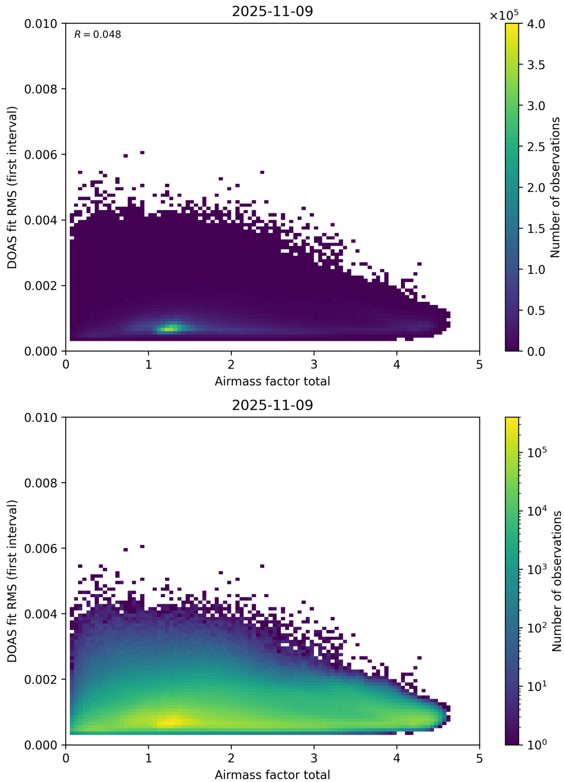
Figure 97: Scatter density plot of “Airmass factor total” against “DOAS fit RMS (first interval)” for 2025-11-08 to 2025-11-10.
