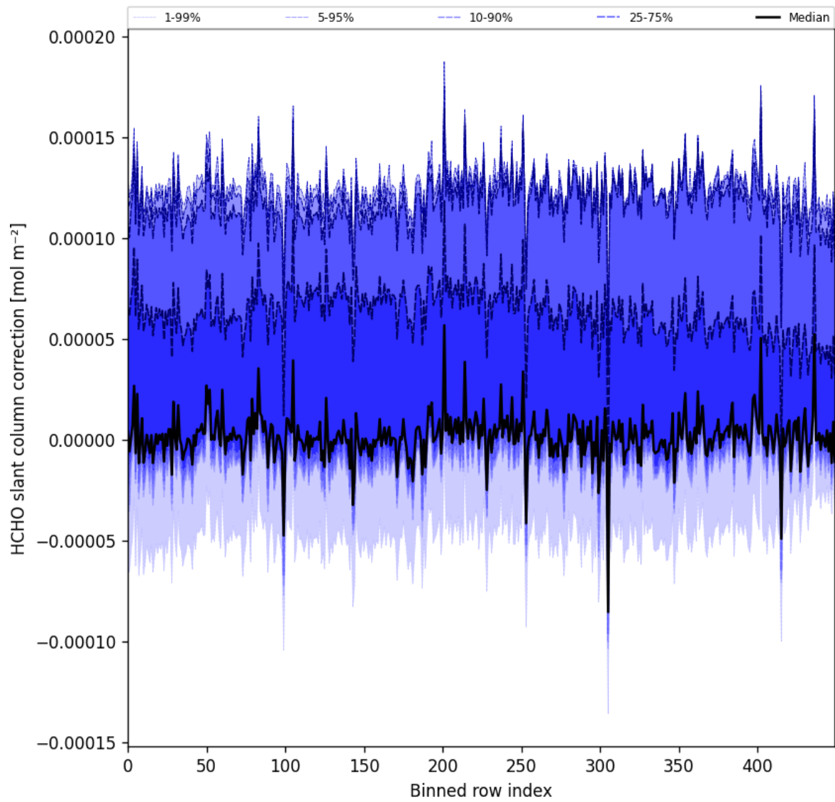
Figure 61: Along track statistics of “HCHO slant column correction” for 2025-11-08 to 2025-11-10
