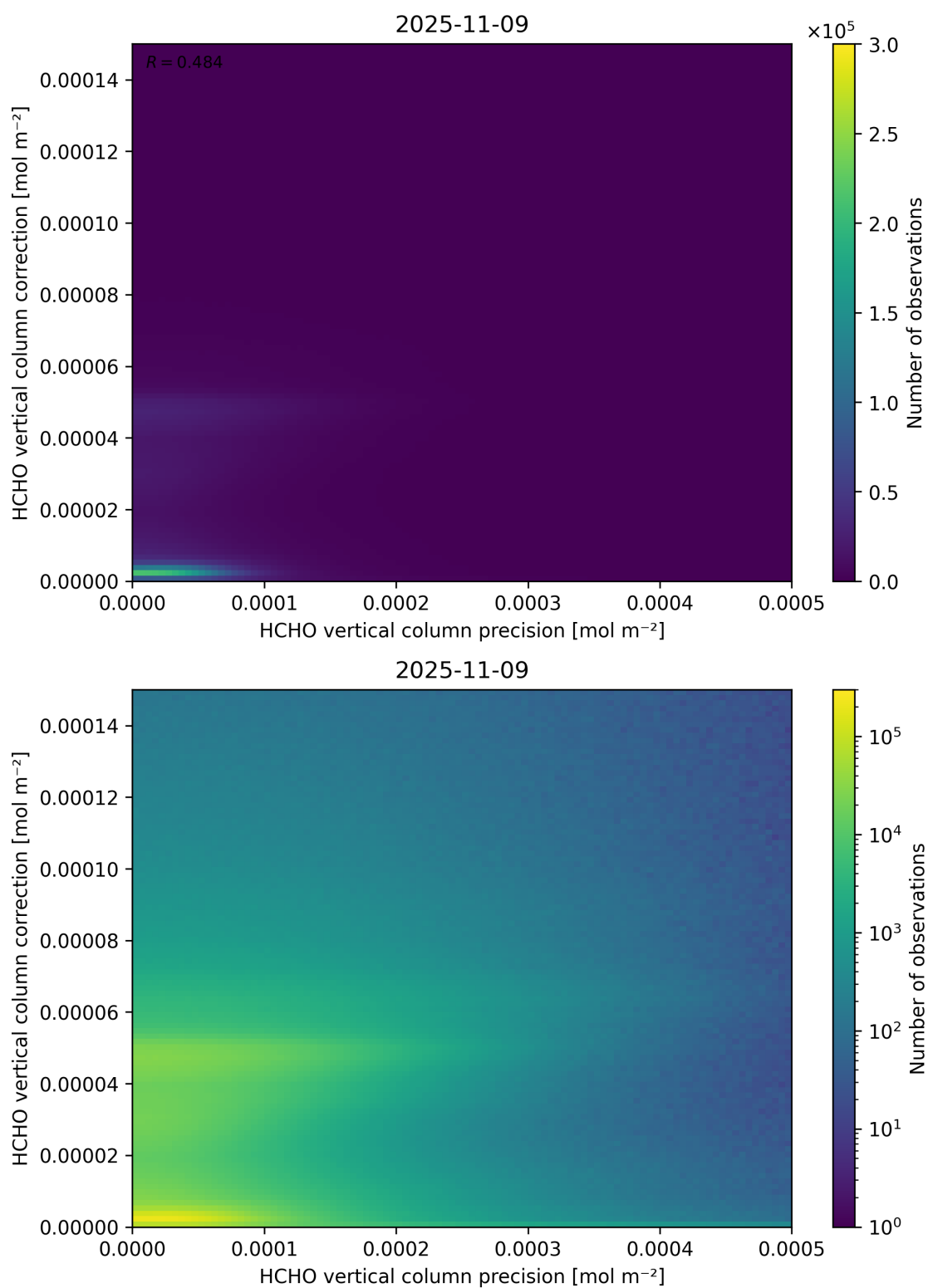
Figure 146: Scatter density plot of “HCHO vertical column precision” against “HCHO vertical column correction” for 2025-11-08 to 2025-11-10.
