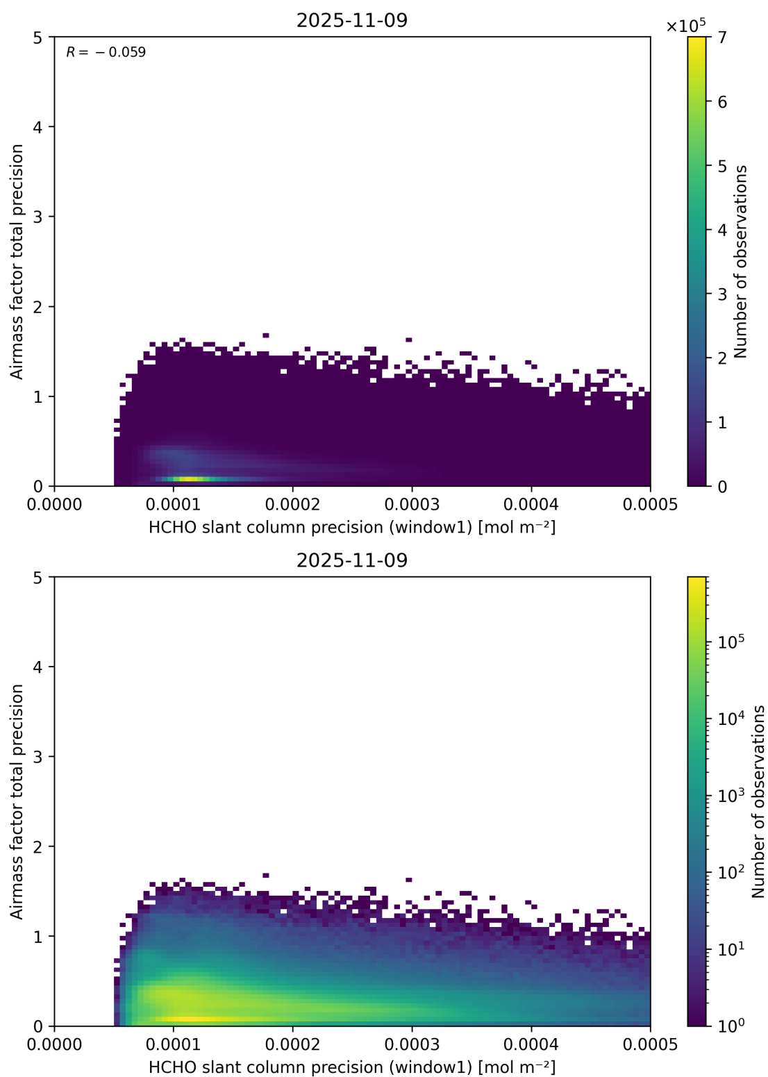
Figure 95: Scatter density plot of “HCHO slant column precision (window1)” against “Airmass factor total precision” for 2025-11-08 to 2025-11-10.
