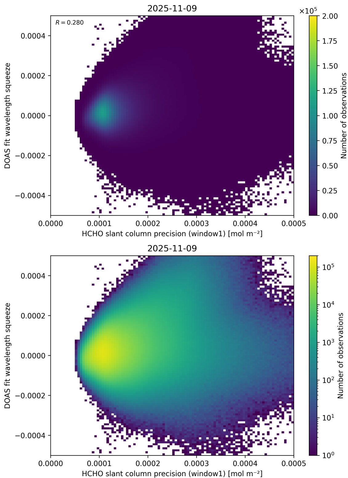
Figure 90: Scatter density plot of “HCHO slant column precision (window1)” against “DOAS fit wavelength squeeze” for 2025-11-08 to 2025-11-10.
