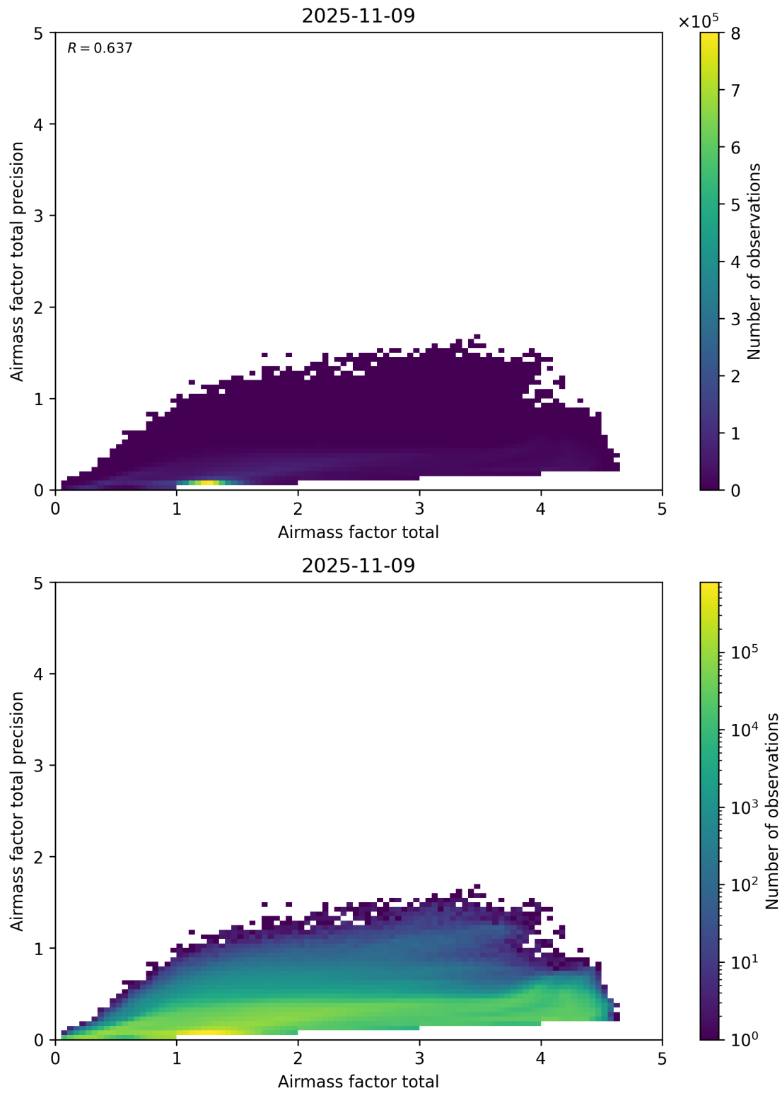
Figure 103: Scatter density plot of “Airmass factor total” against “Airmass factor total precision” for 2025-11-08 to 2025-11-10.
