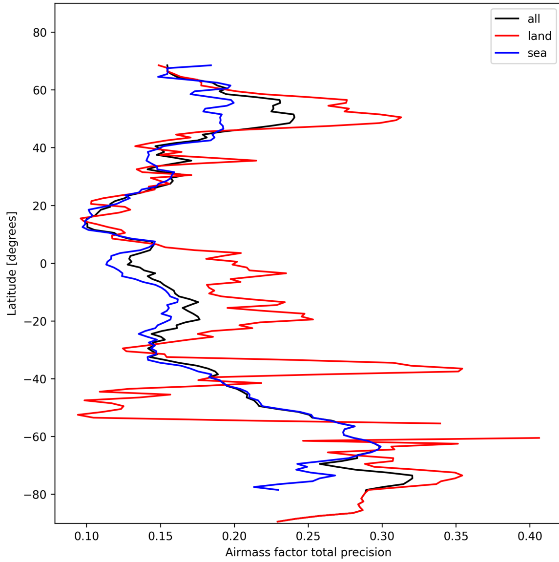
Figure 27: Zonal average of “Airmass factor total precision” for 2025-11-08 to 2025-11-10.
