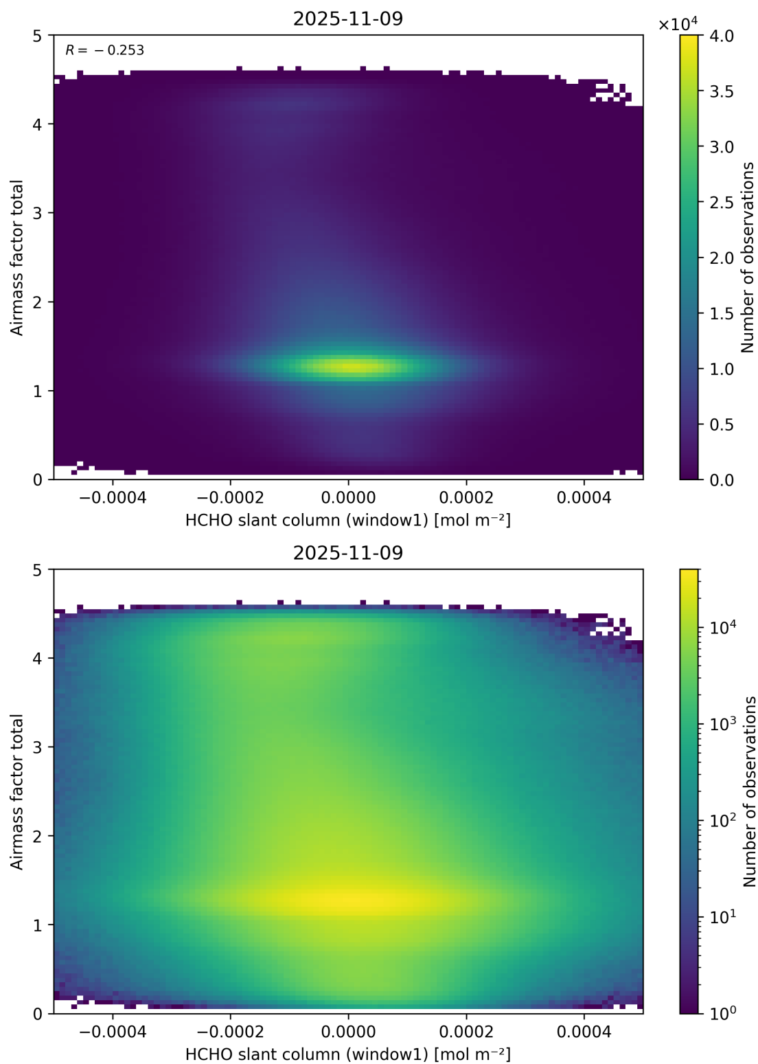
Figure 85: Scatter density plot of “HCHO slant column (window1)” against “Airmass factor total” for 2025-11-08 to 2025-11-10.
