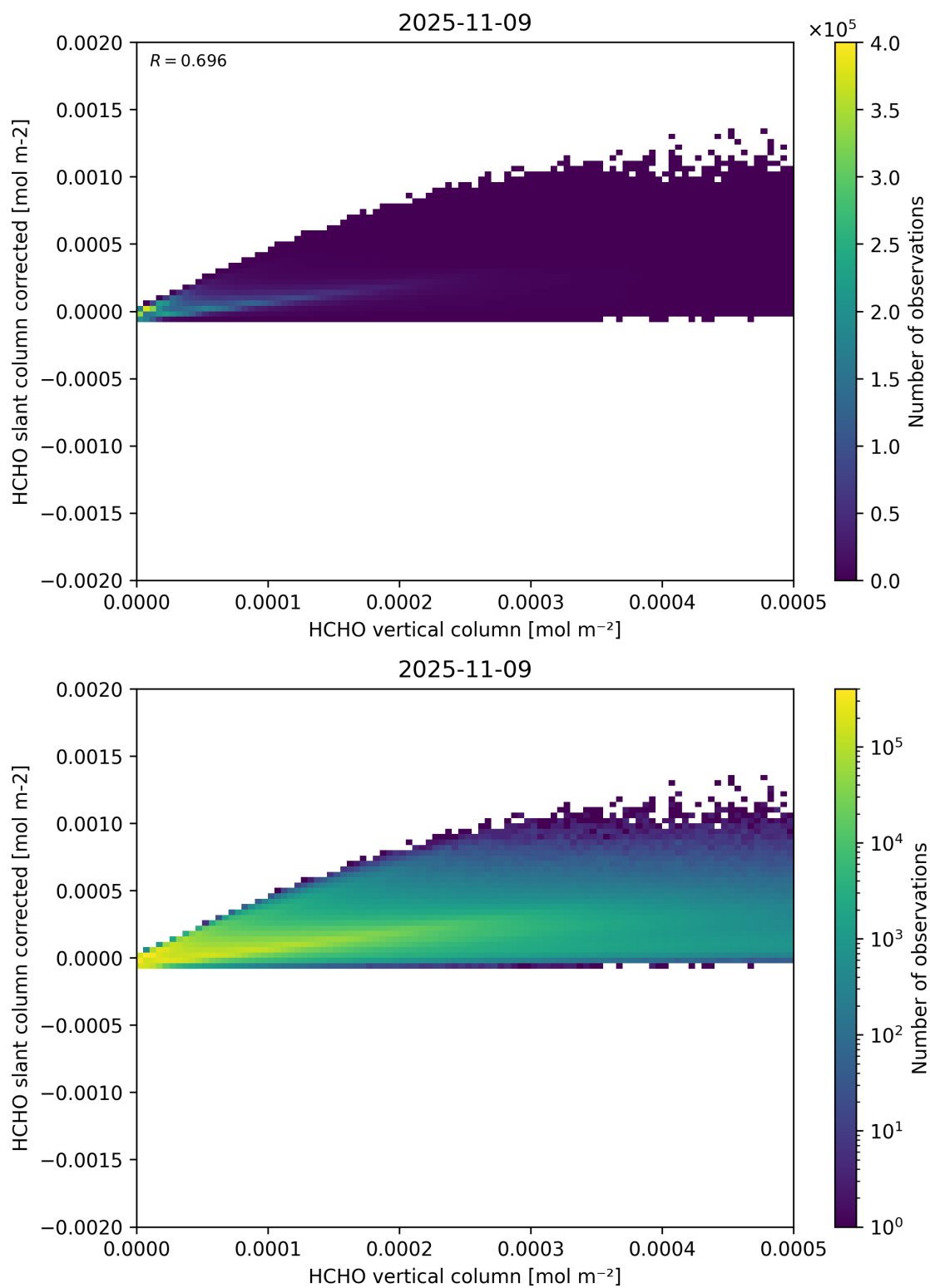
Figure 127: Scatter density plot of “HCHO vertical column” against “HCHO slant column corrected” for 2025-11-08 to 2025-11-10.
