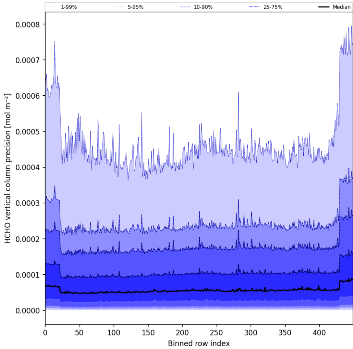
Figure 50: Along track statistics of "HCHO vertical column precision" for 2025-11-08 to 2025-11-10
