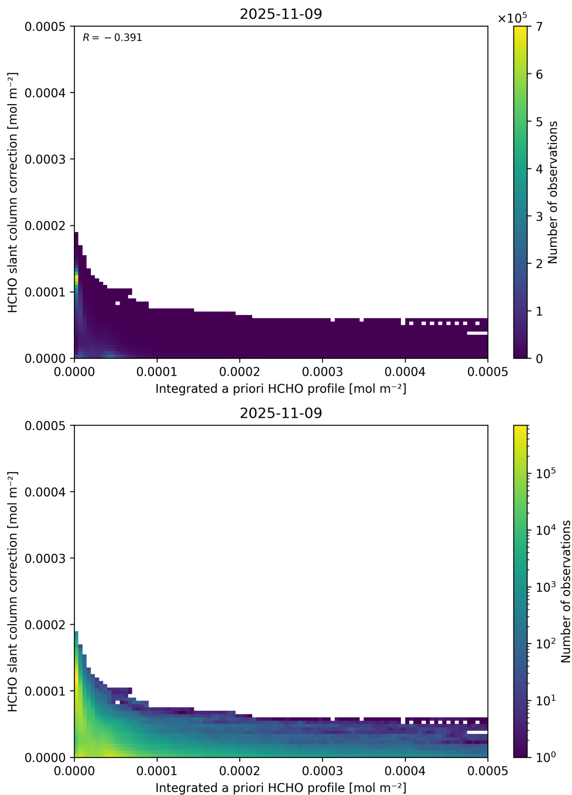
Figure 152: Scatter density plot of “Integrated a priori HCHO profile” against “HCHO slant column correction” for 2025-11-08 to 2025-11-10.
