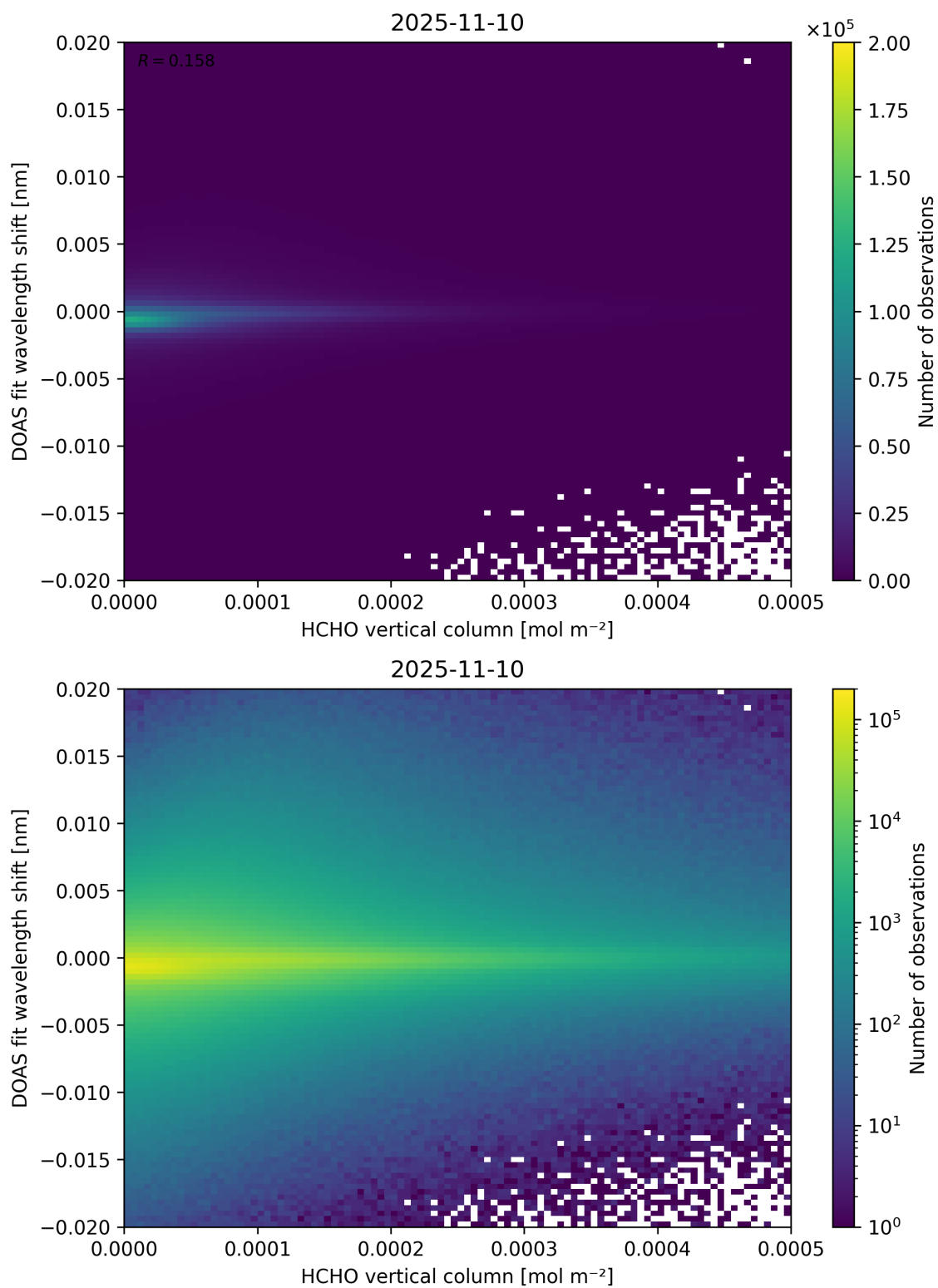
Figure 124: Scatter density plot of “HCHO vertical column” against “DOAS fit wavelength shift” for 2025-11-09 to 2025-11-11.
