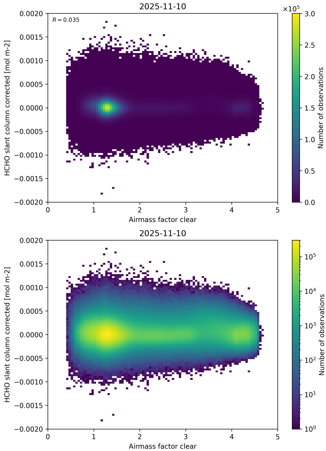
Figure 74: Scatter density plot of “Airmass factor clear” against “HCHO slant column corrected” for 2025-11-09 to 2025-11-11.
