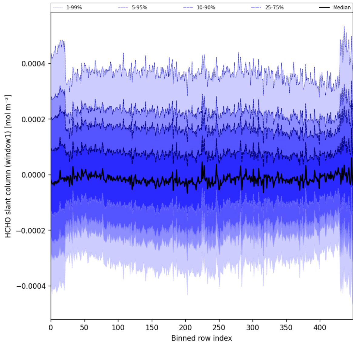
Figure 52: Along track statistics of “HCHO slant column (window1)” for 2025-11-09 to 2025-11-11
