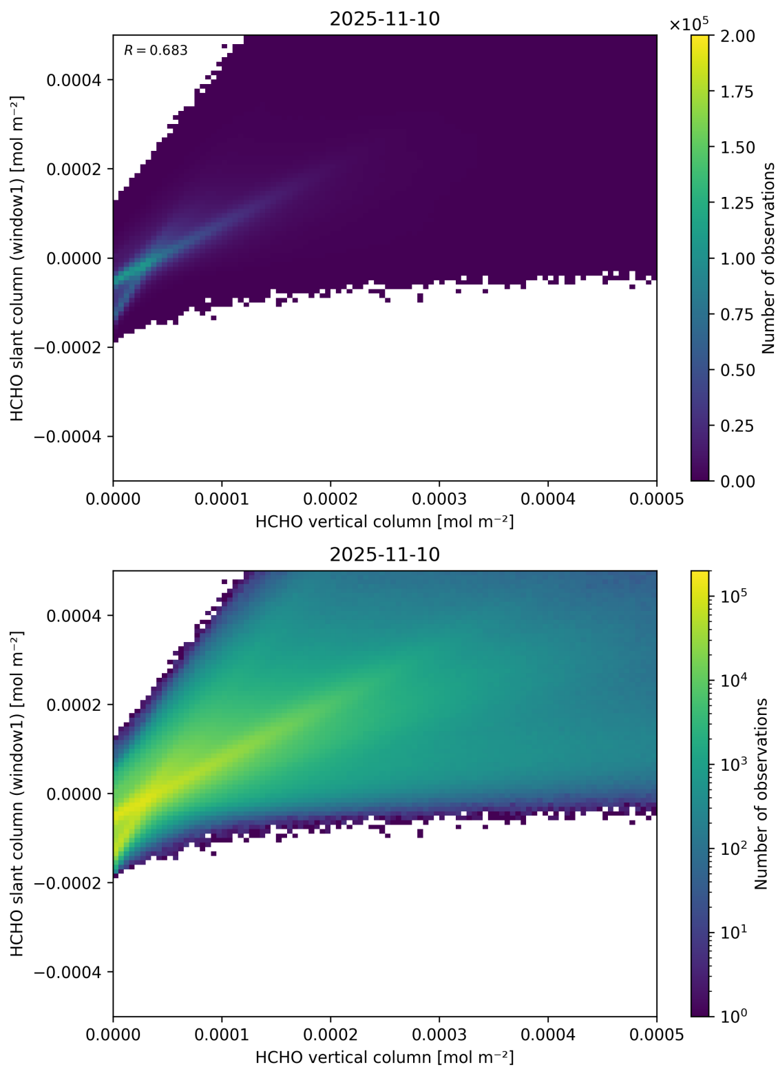
Figure 129: Scatter density plot of “HCHO vertical column” against “HCHO slant column (window1)” for 2025-11-09 to 2025-11-11.
