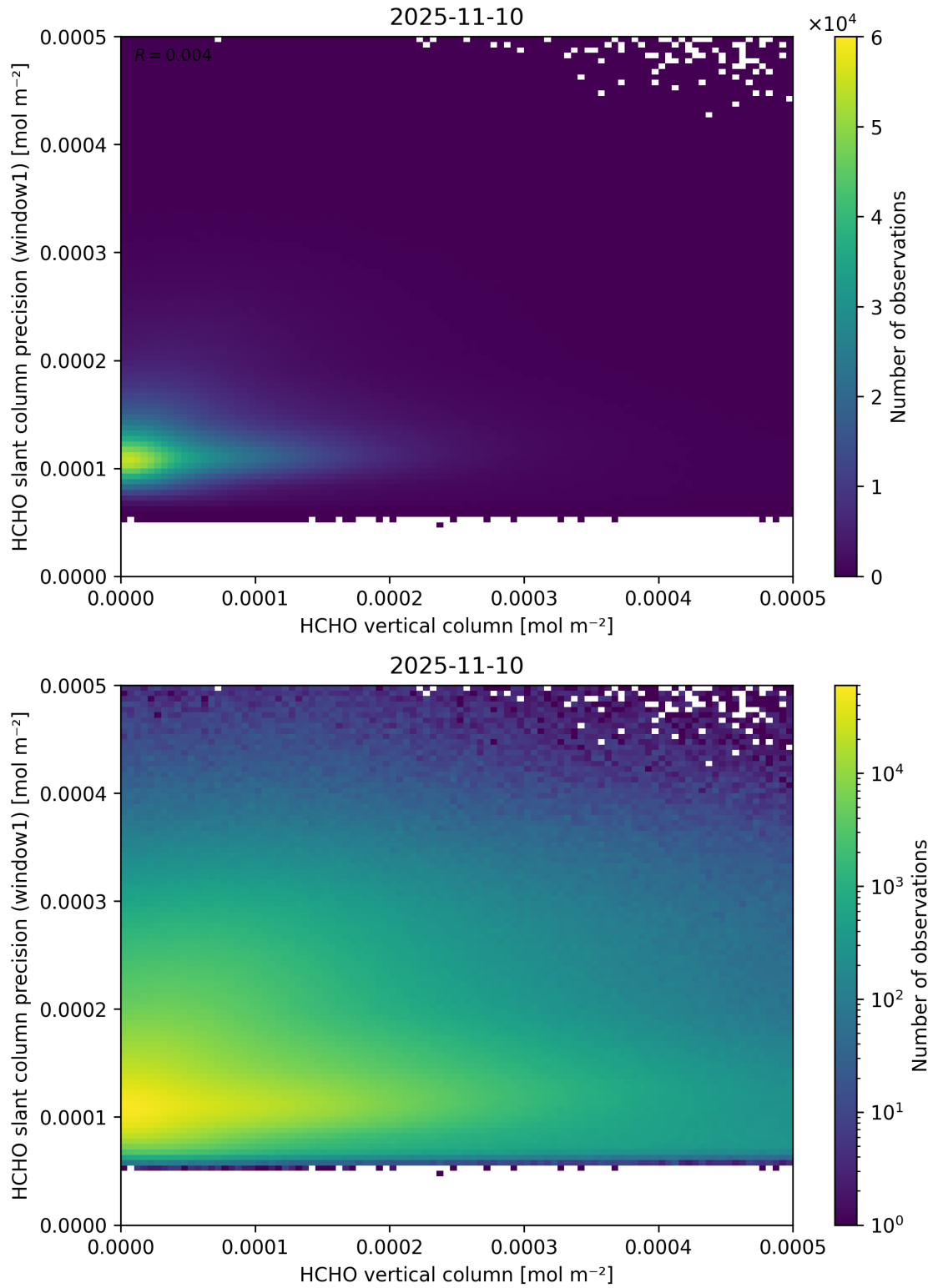
Figure 130: Scatter density plot of “HCHO vertical column” against “HCHO slant column precision (window1)” for 2025-11-09 to 2025-11-11.
