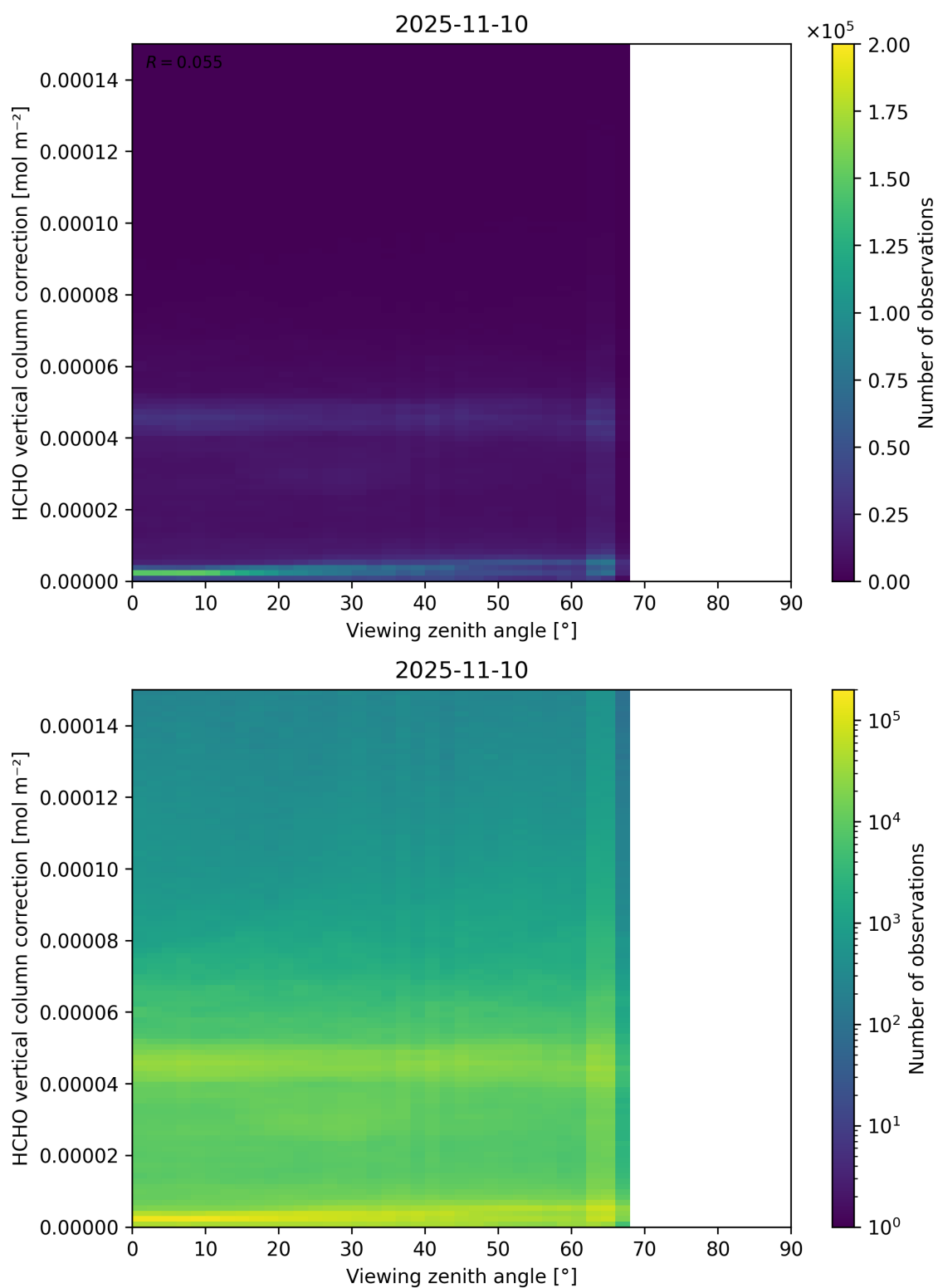
Figure 193: Scatter density plot of “Viewing zenith angle” against “HCHO vertical column correction” for 2025-11-09 to 2025-11-11.
