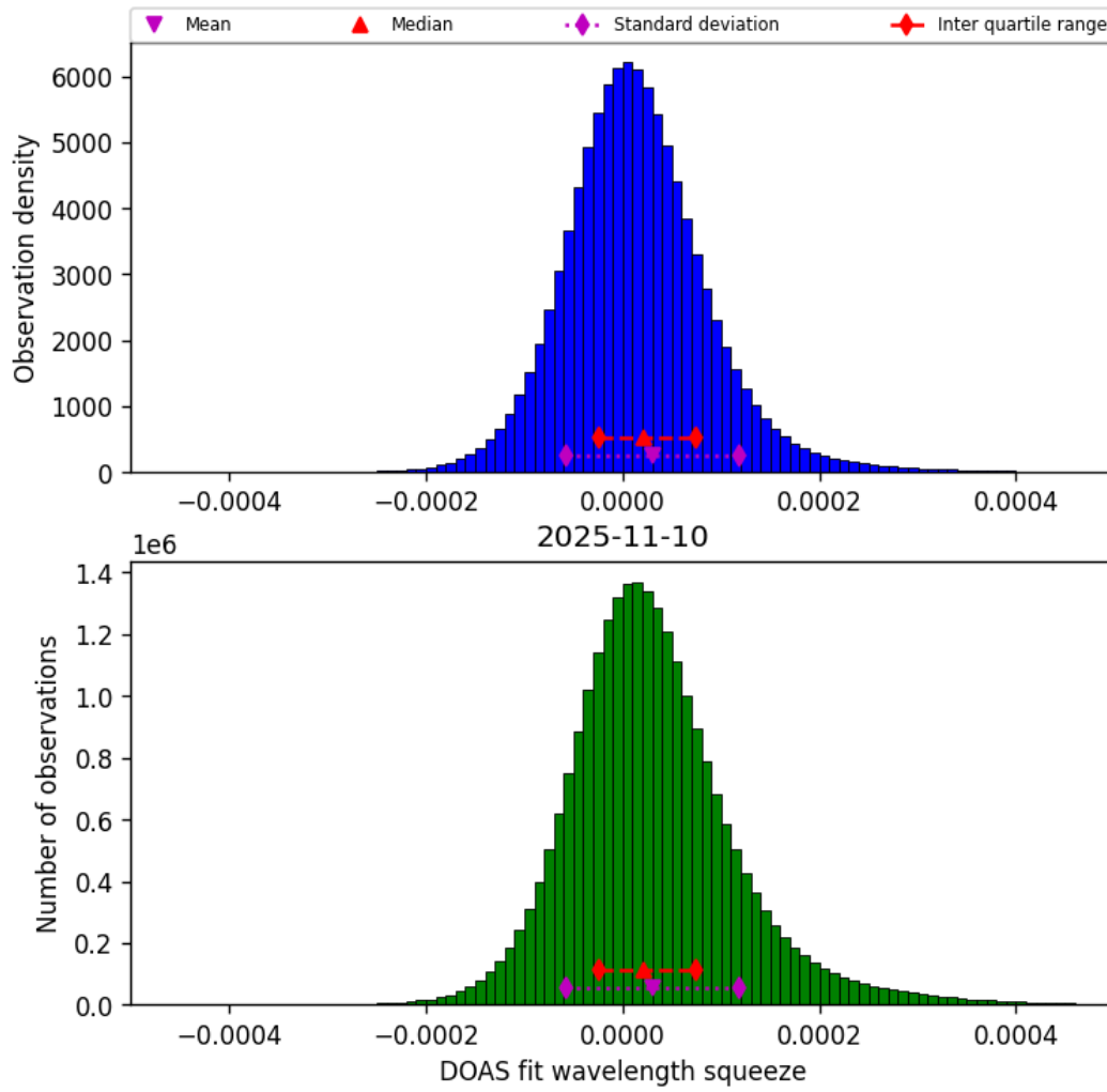
Figure 45: Histogram of “DOAS fit wavelength squeeze” for 2025-11-09 to 2025-11-11
