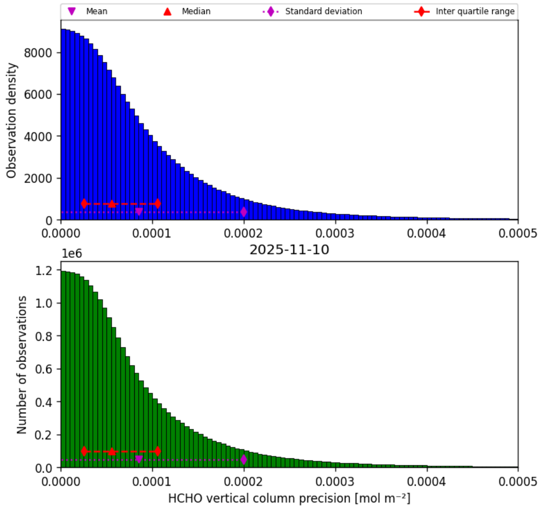
Figure 36: Histogram of “HCHO vertical column precision” for 2025-11-09 to 2025-11-11
