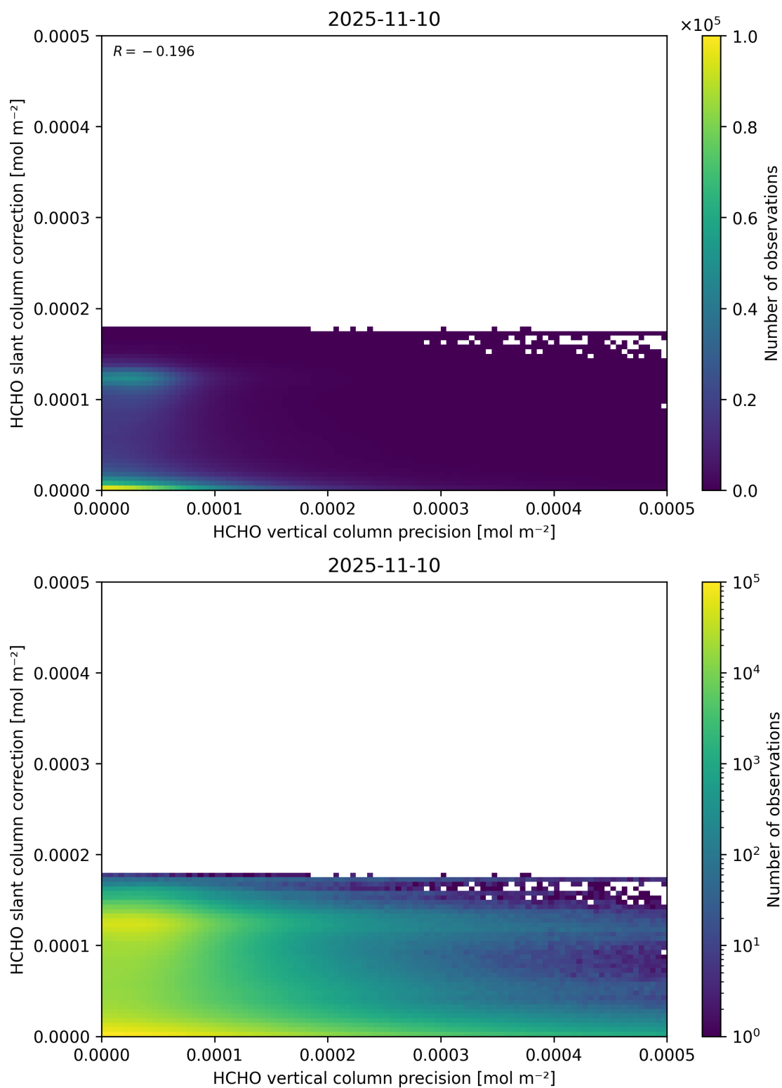
Figure 141: Scatter density plot of “HCHO vertical column precision” against “HCHO slant column correction” for 2025-11-09 to 2025-11-11.
