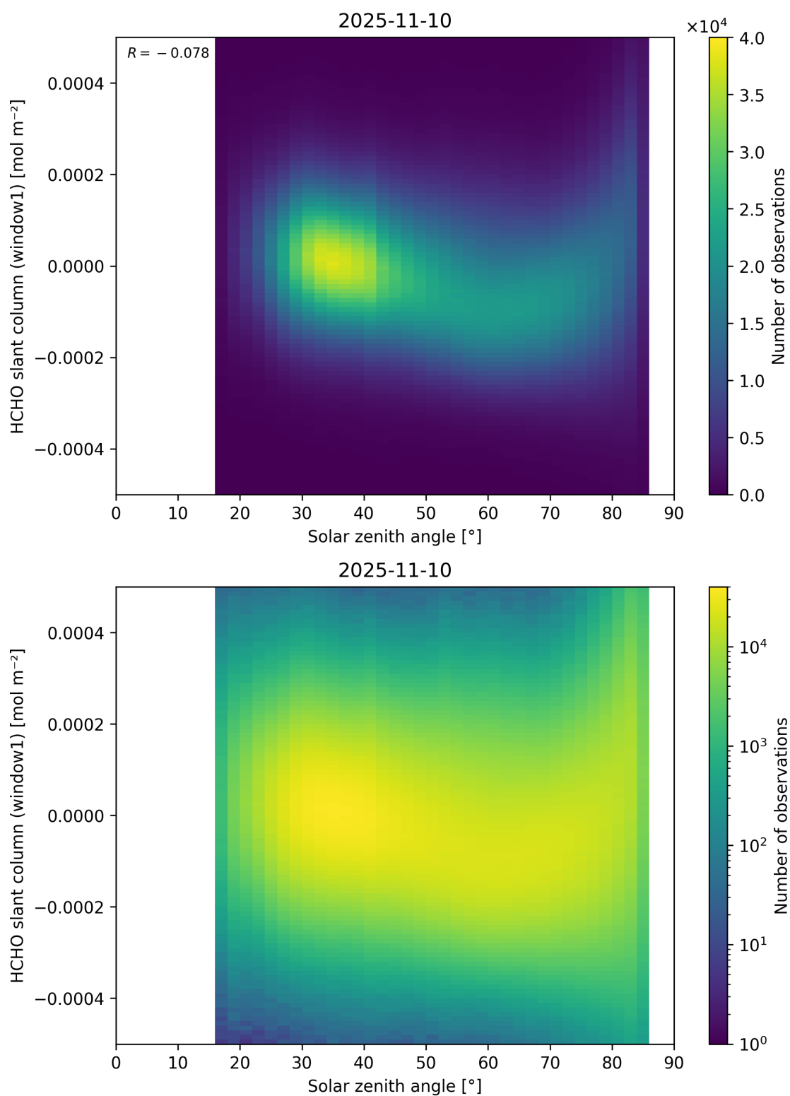
Figure 173: Scatter density plot of “Solar zenith angle” against “HCHO slant column (window1)” for 2025-11-09 to 2025-11-11.
