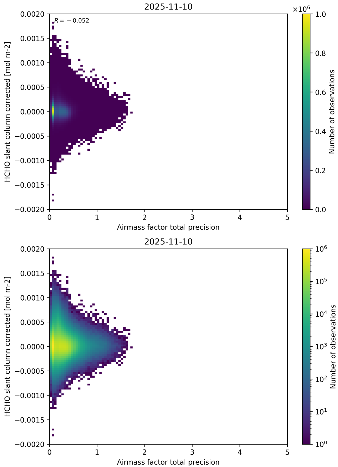
Figure 109: Scatter density plot of “Airmass factor total precision” against “HCHO slant column corrected” for 2025-11-09 to 2025-11-11.
