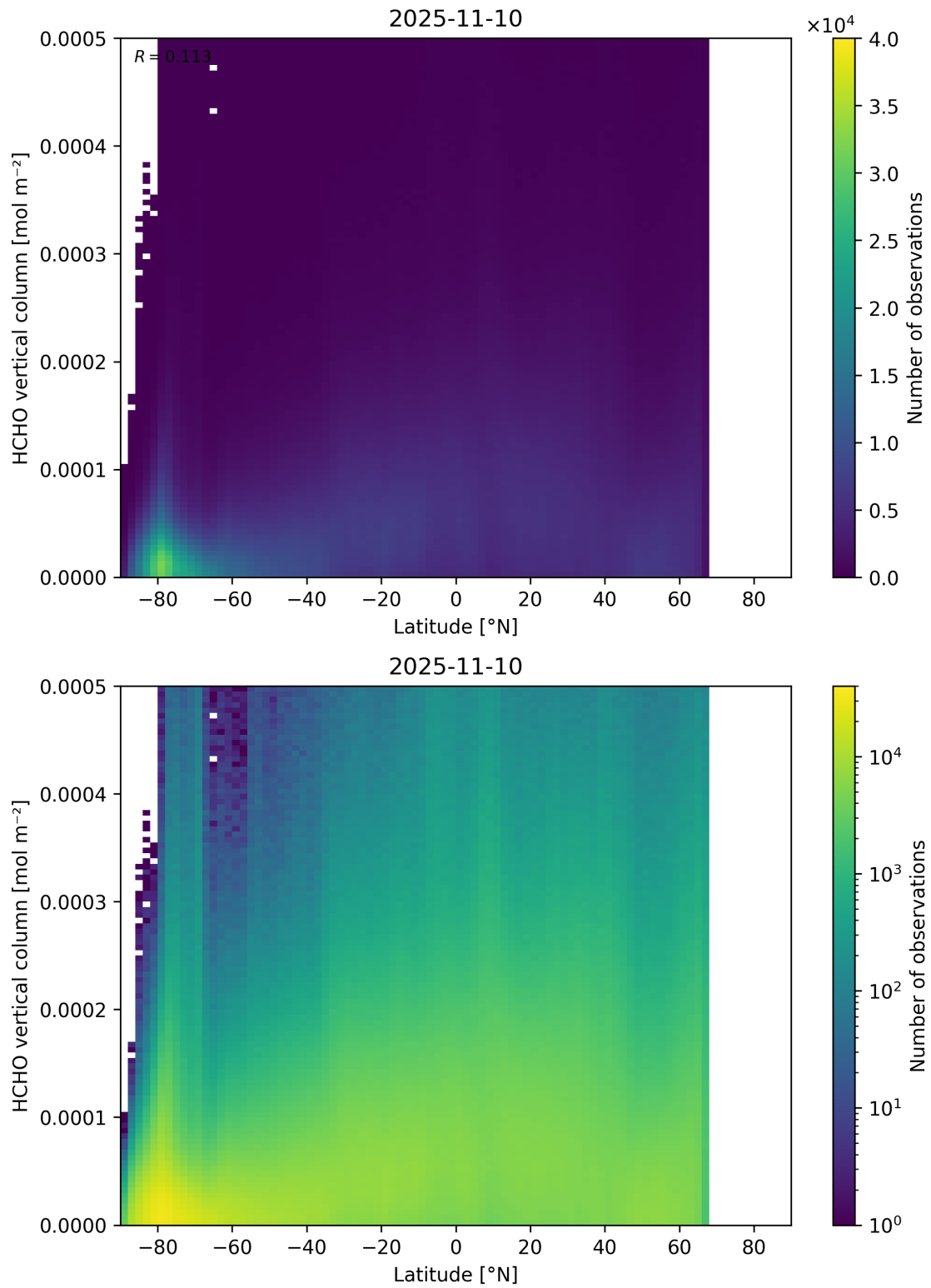
Figure 163: Scatter density plot of “Latitude” against “HCHO vertical column” for 2025-11-09 to 2025-11-11.
