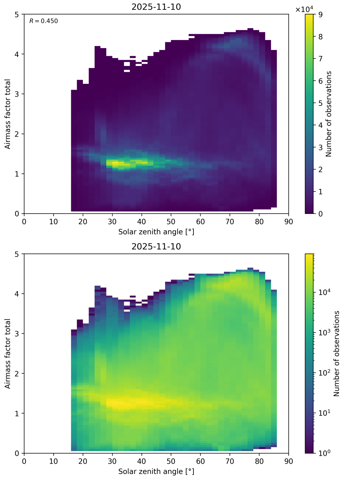
Figure 175: Scatter density plot of “Solar zenith angle” against “Airmass factor total” for 2025-11-09 to 2025-11-11.
