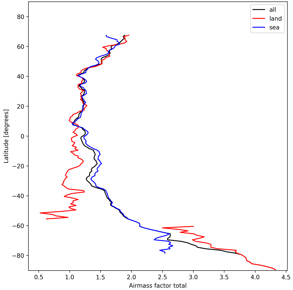
Figure 26: Zonal average of “Airmass factor total” for 2025-11-09 to 2025-11-11.
