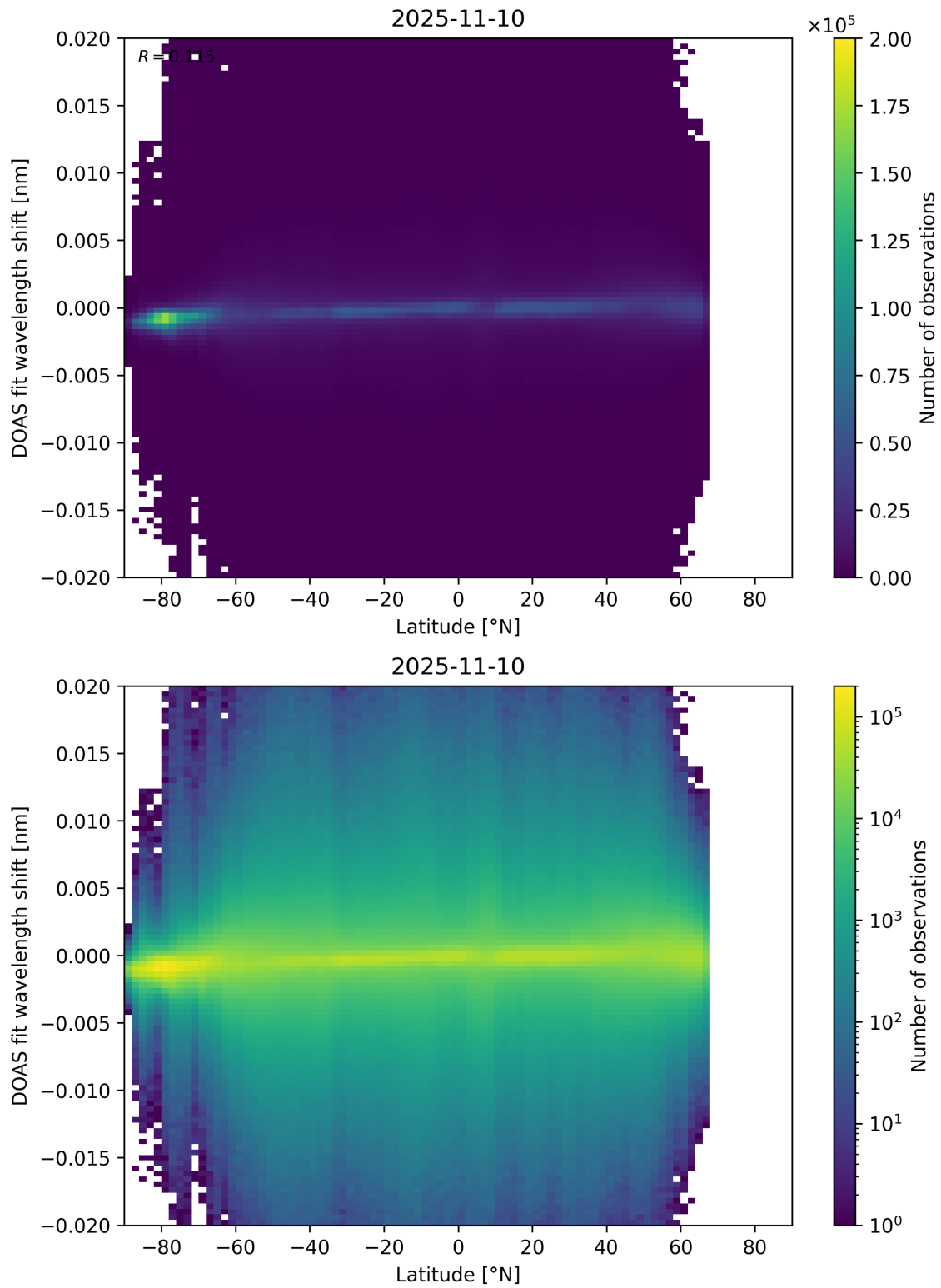
Figure 154: Scatter density plot of “Latitude” against “DOAS fit wavelength shift” for 2025-11-09 to 2025-11-11.
