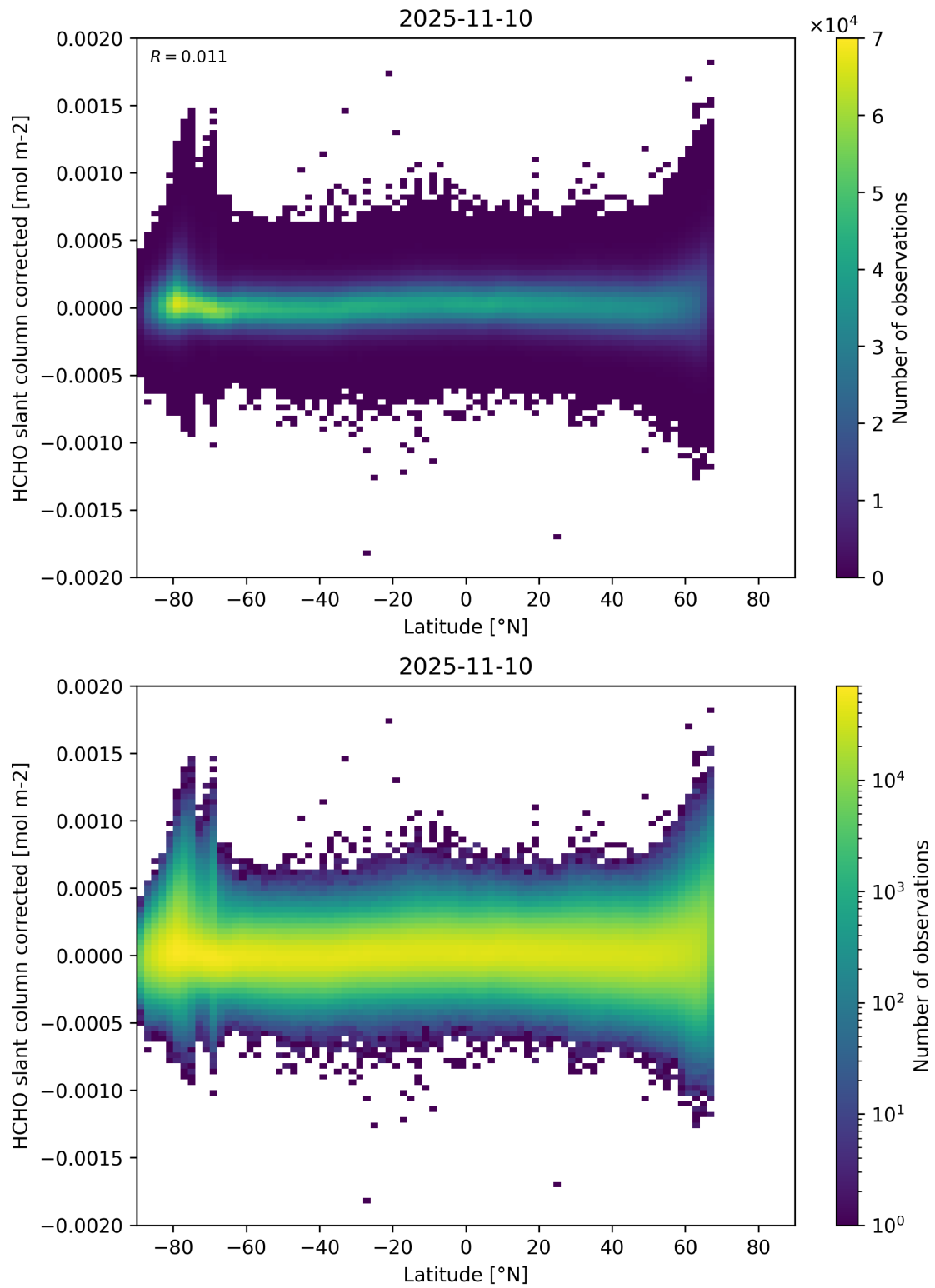
Figure 157: Scatter density plot of “Latitude” against “HCHO slant column corrected” for 2025-11-09 to 2025-11-11.
