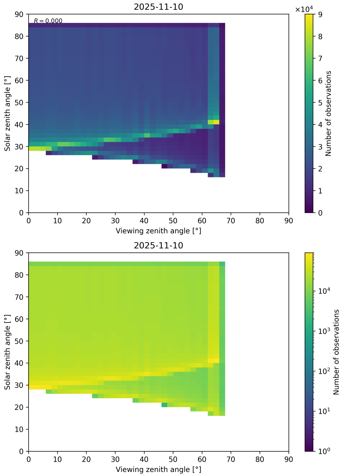
Figure 197: Scatter density plot of “Viewing zenith angle” against “Solar zenith angle” for 2025-11-09 to 2025-11-11.
