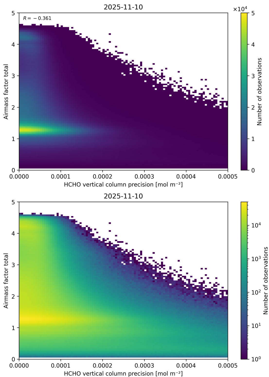
Figure 144: Scatter density plot of “HCHO vertical column precision” against “Airmass factor total” for 2025-11-09 to 2025-11-11.
