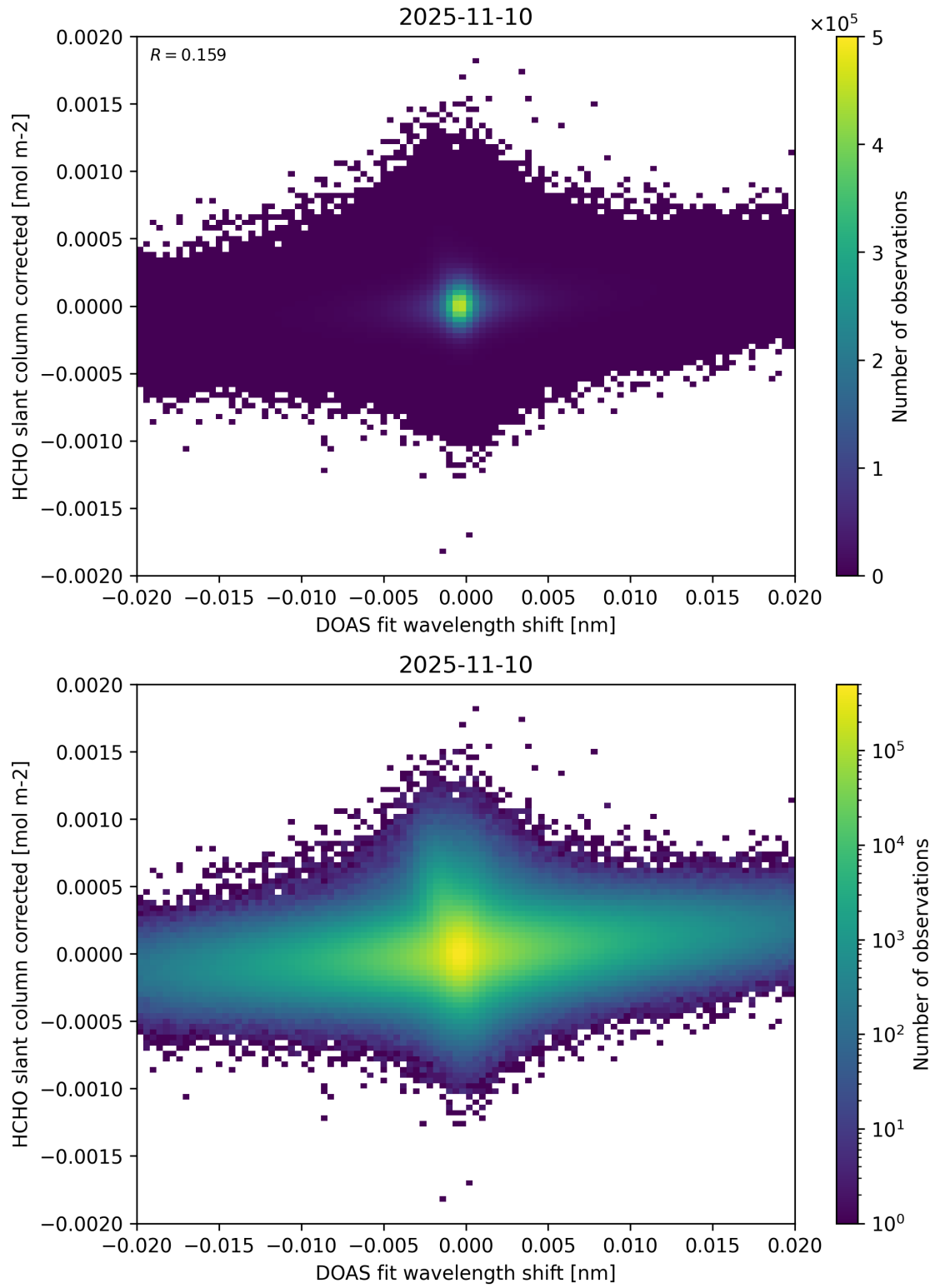
Figure 66: Scatter density plot of “DOAS fit wavelength shift” against “HCHO slant column corrected” for 2025-11-09 to 2025-11-11.
