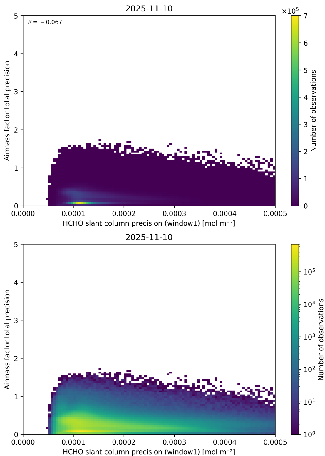
Figure 95: Scatter density plot of “HCHO slant column precision (window1)” against “Airmass factor total precision” for 2025-11-09 to 2025-11-11.
