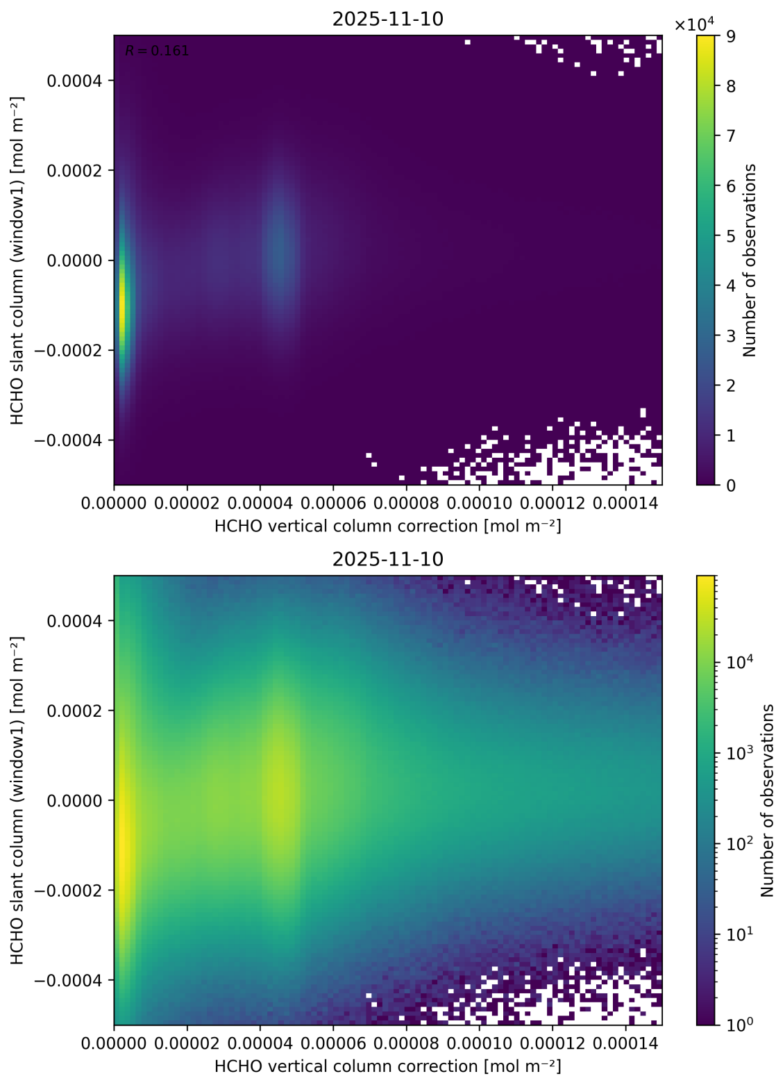
Figure 118: Scatter density plot of “HCHO vertical column correction” against “HCHO slant column (window1)” for 2025-11-09 to 2025-11-11.
