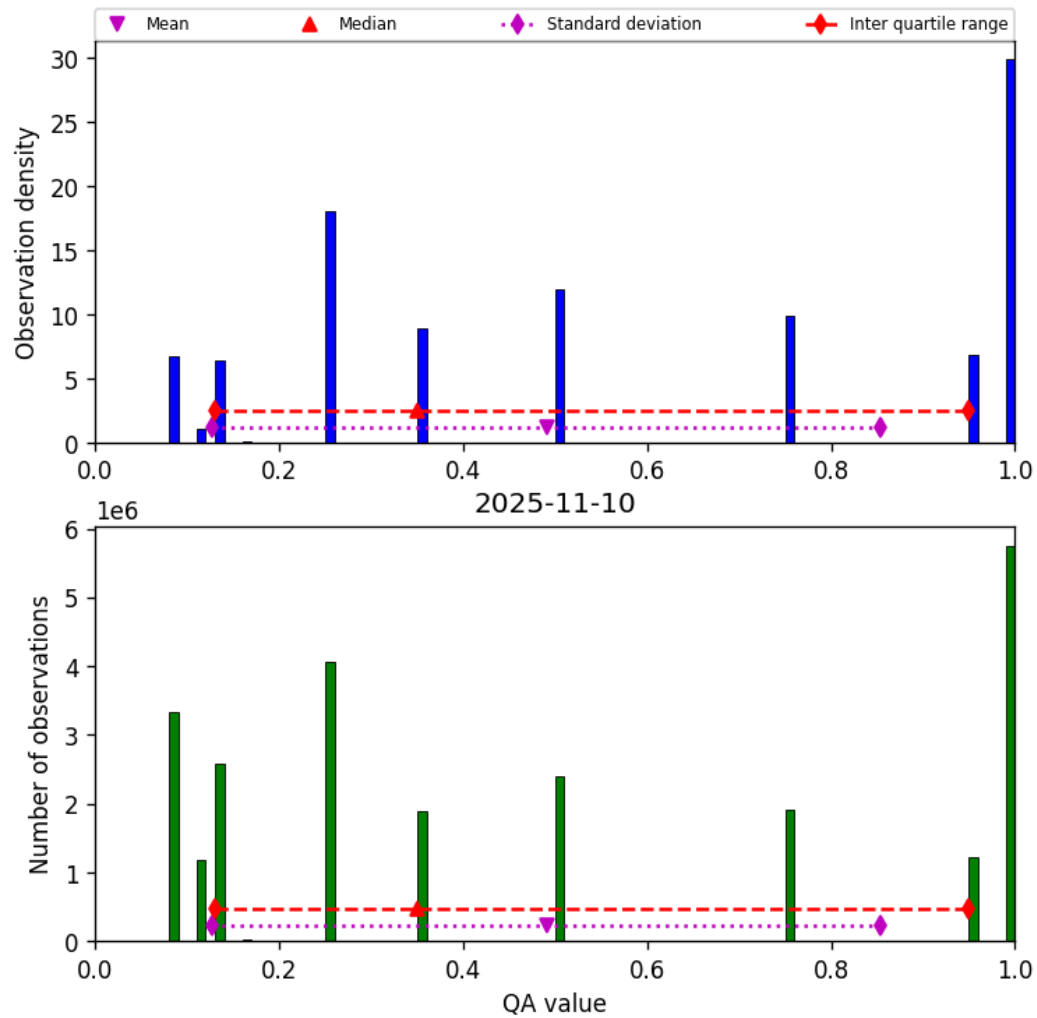
Figure 34: Histogram of “QA value” for 2025-11-09 to 2025-11-11
