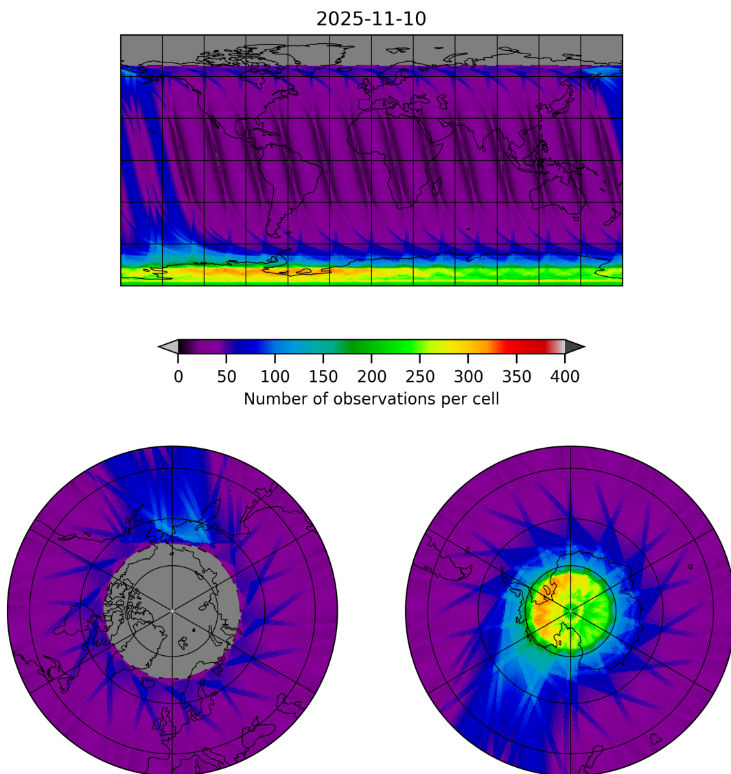
Figure 19: Map of the number of observations for 2025-11-09 to 2025-11-11
