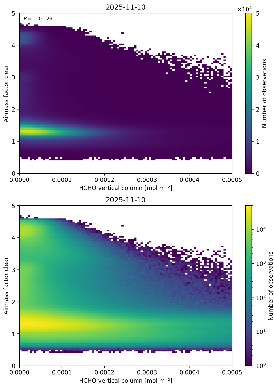
Figure 126: Scatter density plot of “HCHO vertical column” against “Airmass factor clear” for 2025-11-09 to 2025-11-11.
