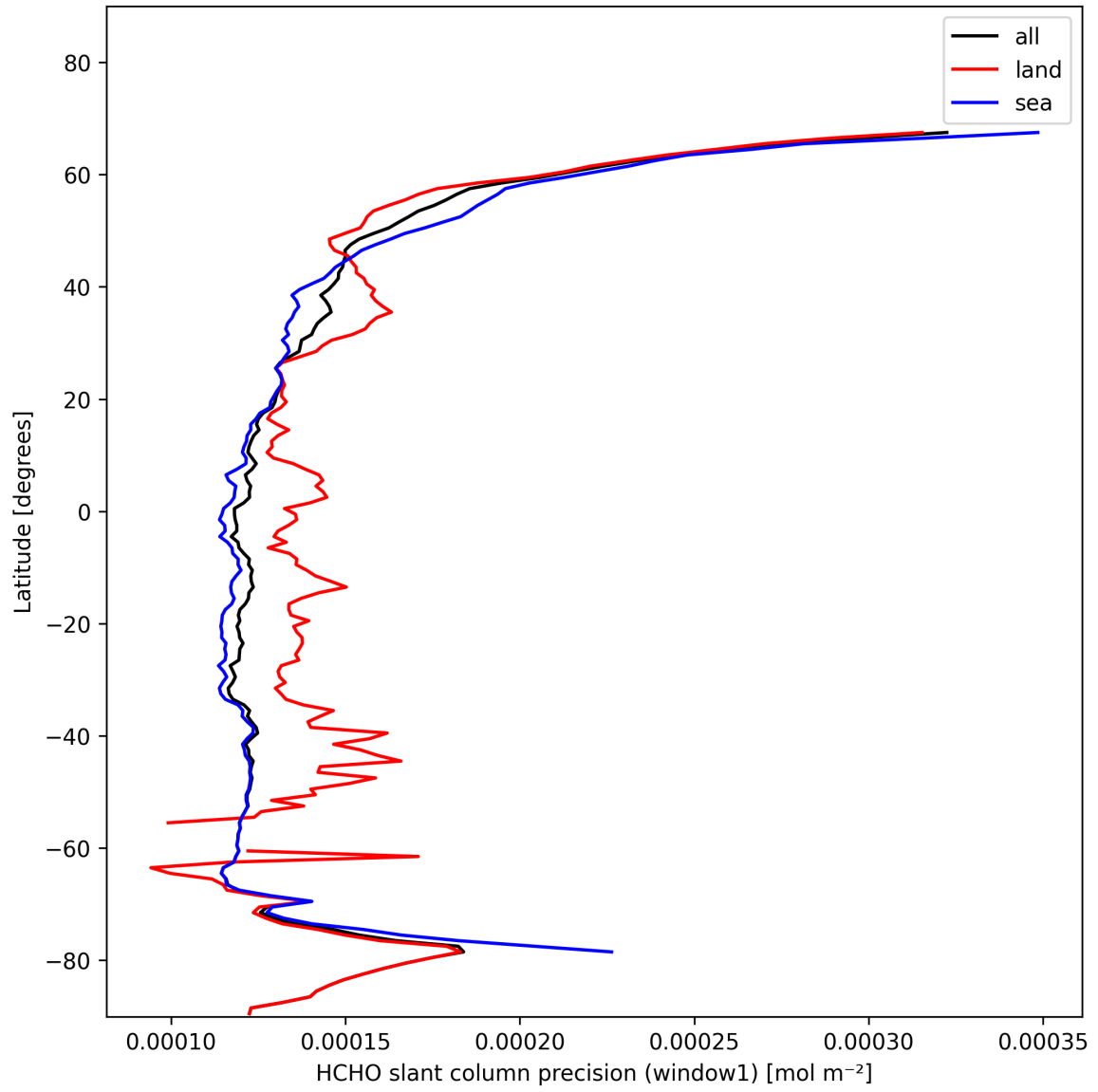
Figure 25: Zonal average of “HCHO slant column precision (window1)” for 2025-11-09 to 2025-11-11.
