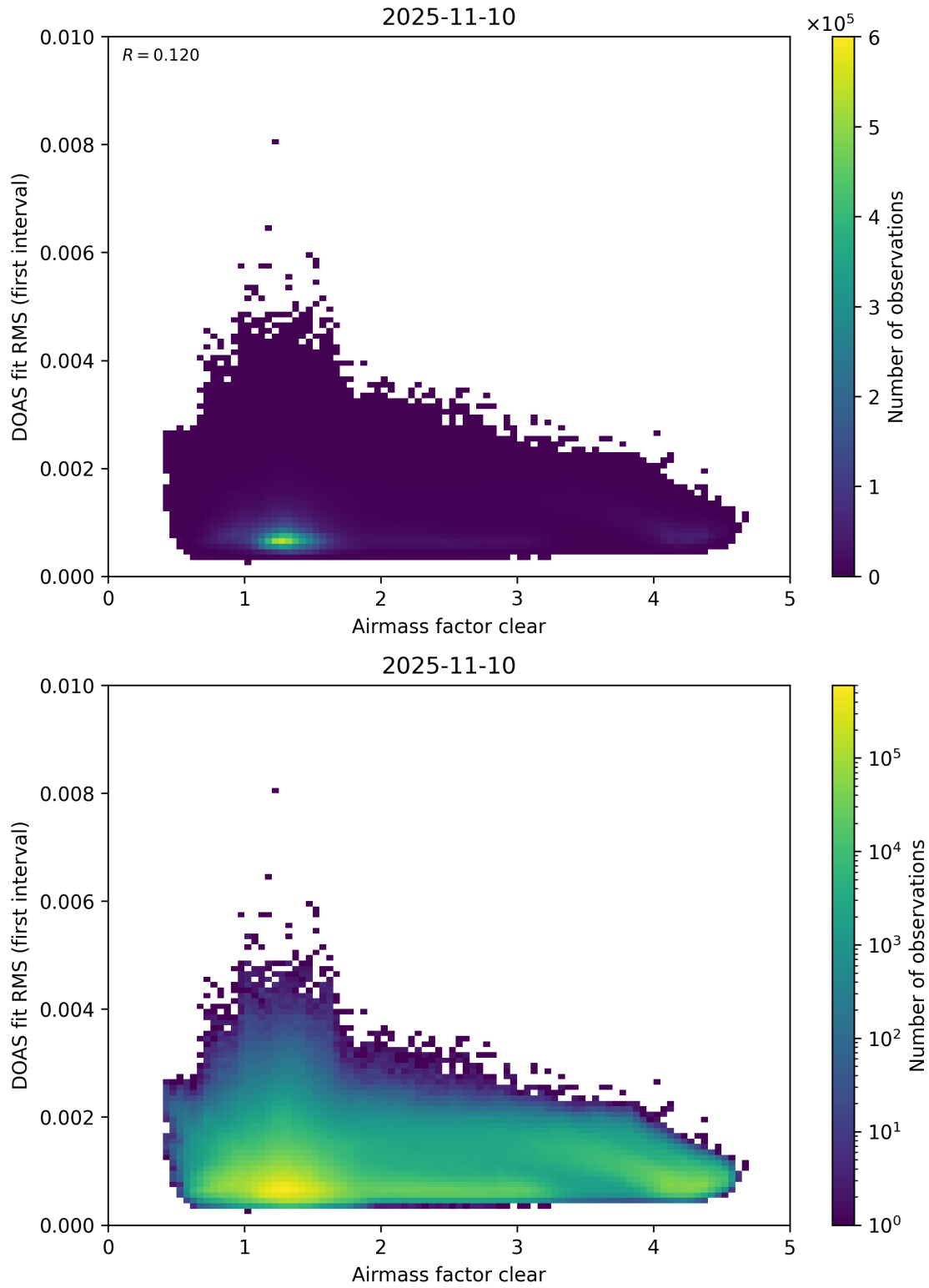
Figure 71: Scatter density plot of “Airmass factor clear” against “DOAS fit RMS (first interval)” for 2025-11-09 to 2025-11-11.
