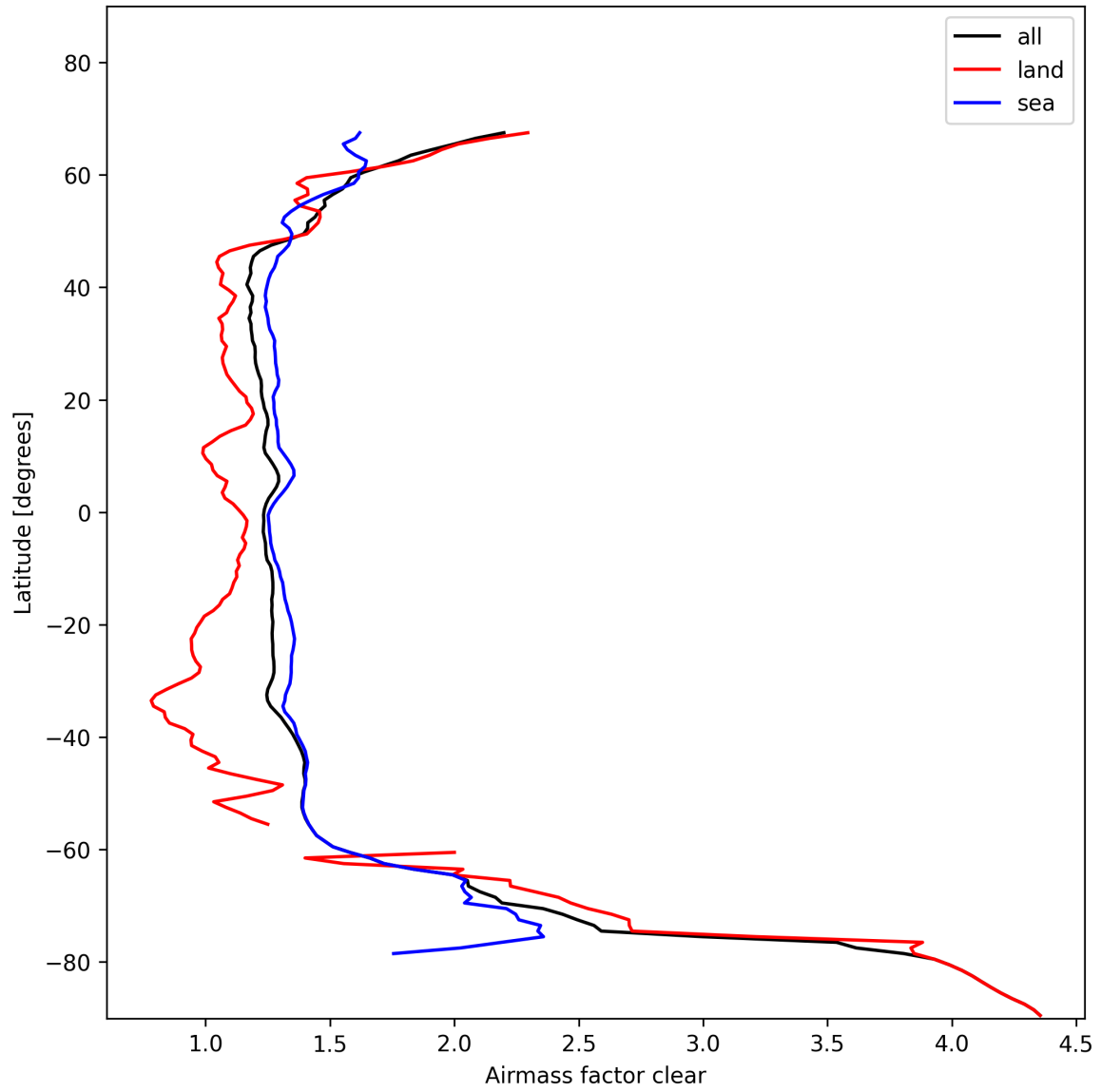
Figure 28: Zonal average of “Airmass factor clear” for 2025-11-09 to 2025-11-11.
