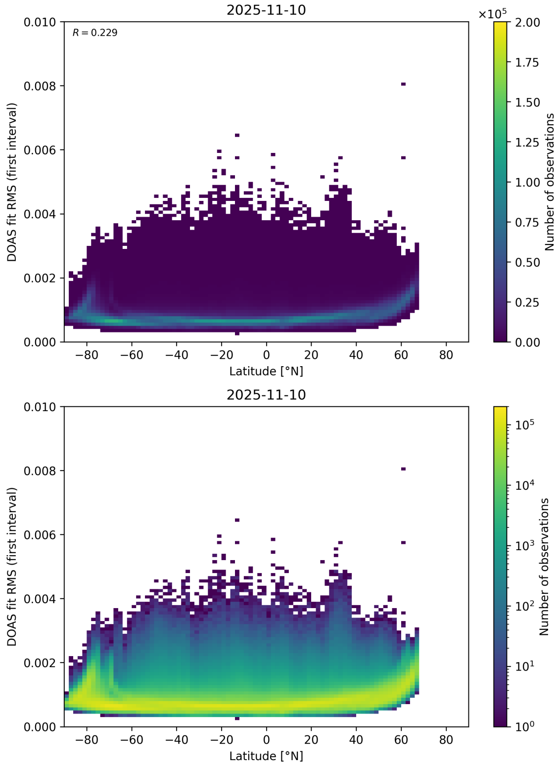
Figure 153: Scatter density plot of “Latitude” against “DOAS fit RMS (first interval)” for 2025-11-09 to 2025-11-11.
