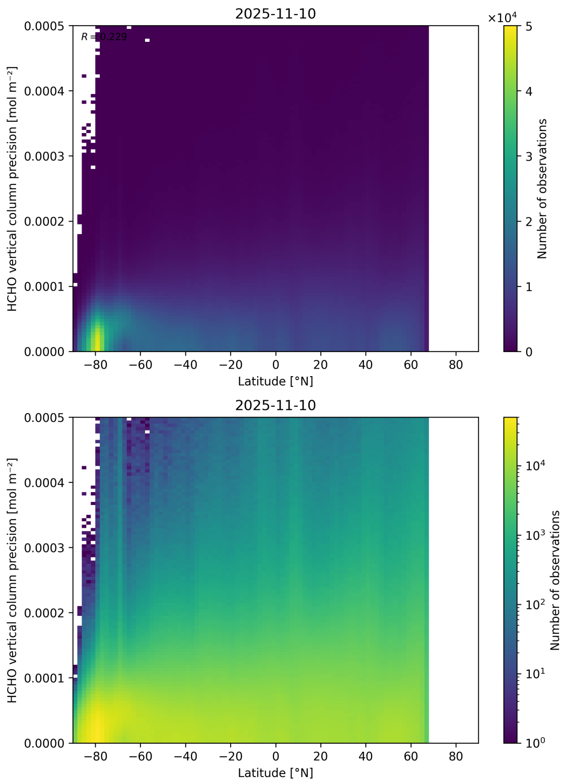
Figure 165: Scatter density plot of “Latitude” against “HCHO vertical column precision” for 2025-11-09 to 2025-11-11.
