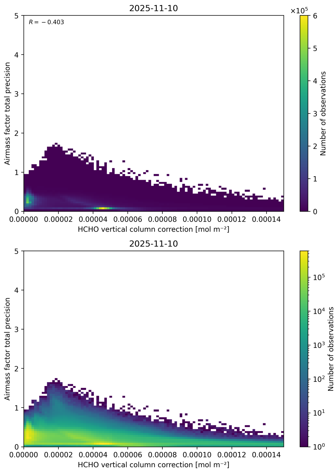
Figure 121: Scatter density plot of “HCHO vertical column correction” against “Airmass factor total precision” for 2025-11-09 to 2025-11-11.
