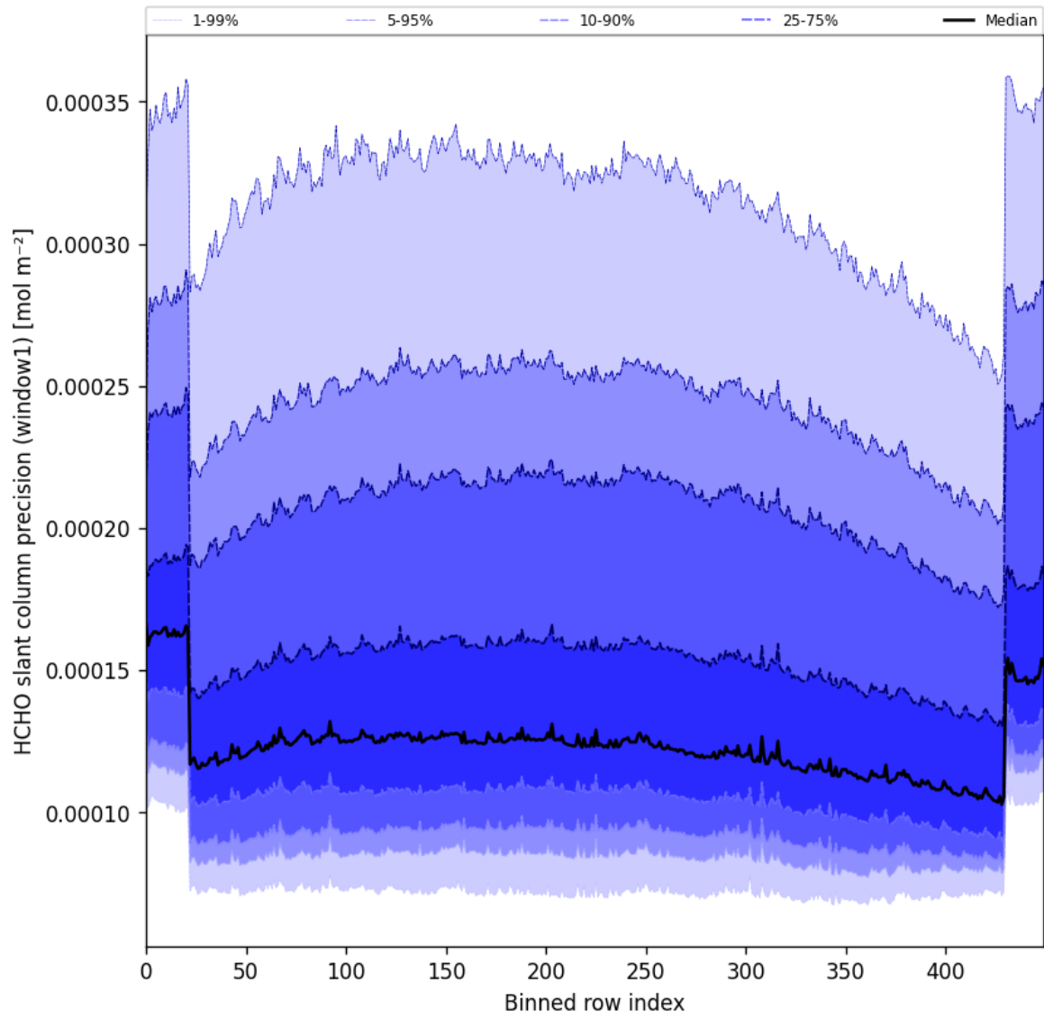
Figure 53: Along track statistics of “HCHO slant column precision (window1)” for 2025-11-09 to 2025-11-11
