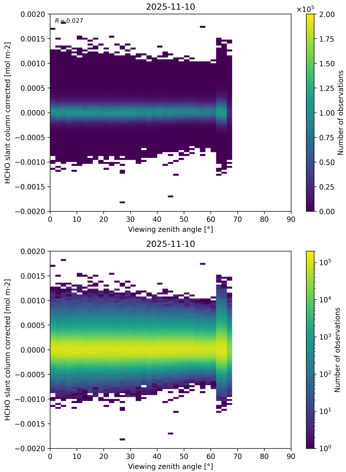
Figure 186: Scatter density plot of “Viewing zenith angle” against “HCHO slant column corrected” for 2025-11-09 to 2025-11-11.
