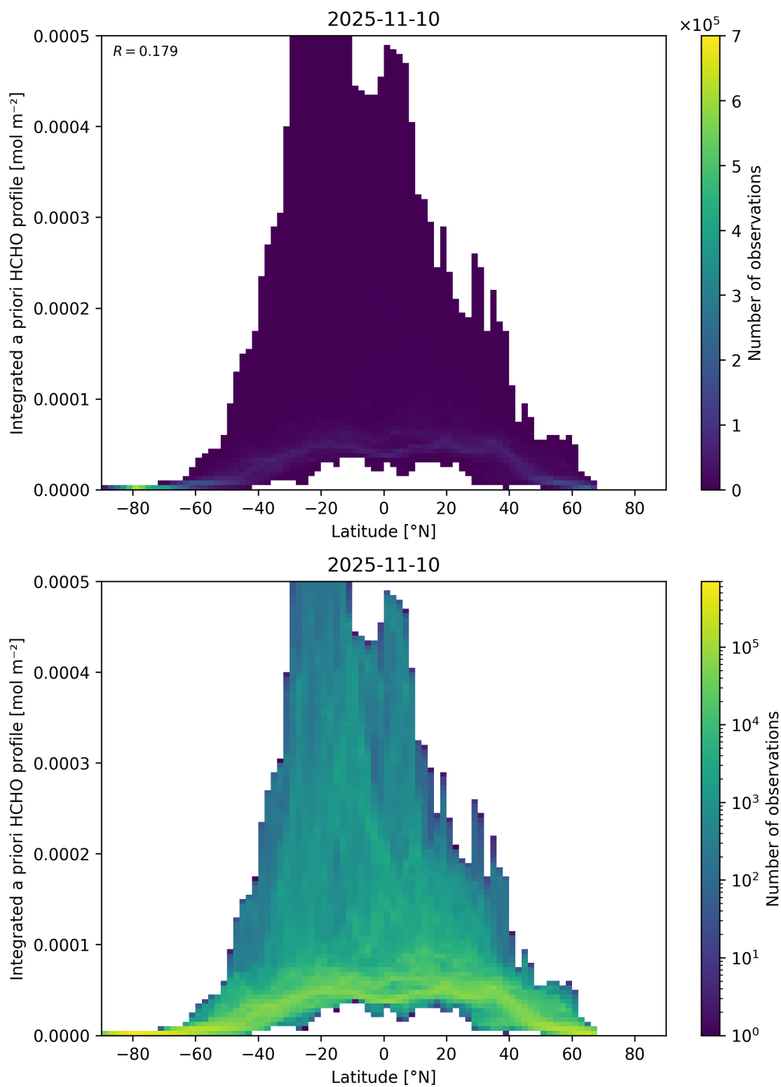
Figure 166: Scatter density plot of “Latitude” against “Integrated a priori HCHO profile” for 2025-11-09 to 2025-11-11.
