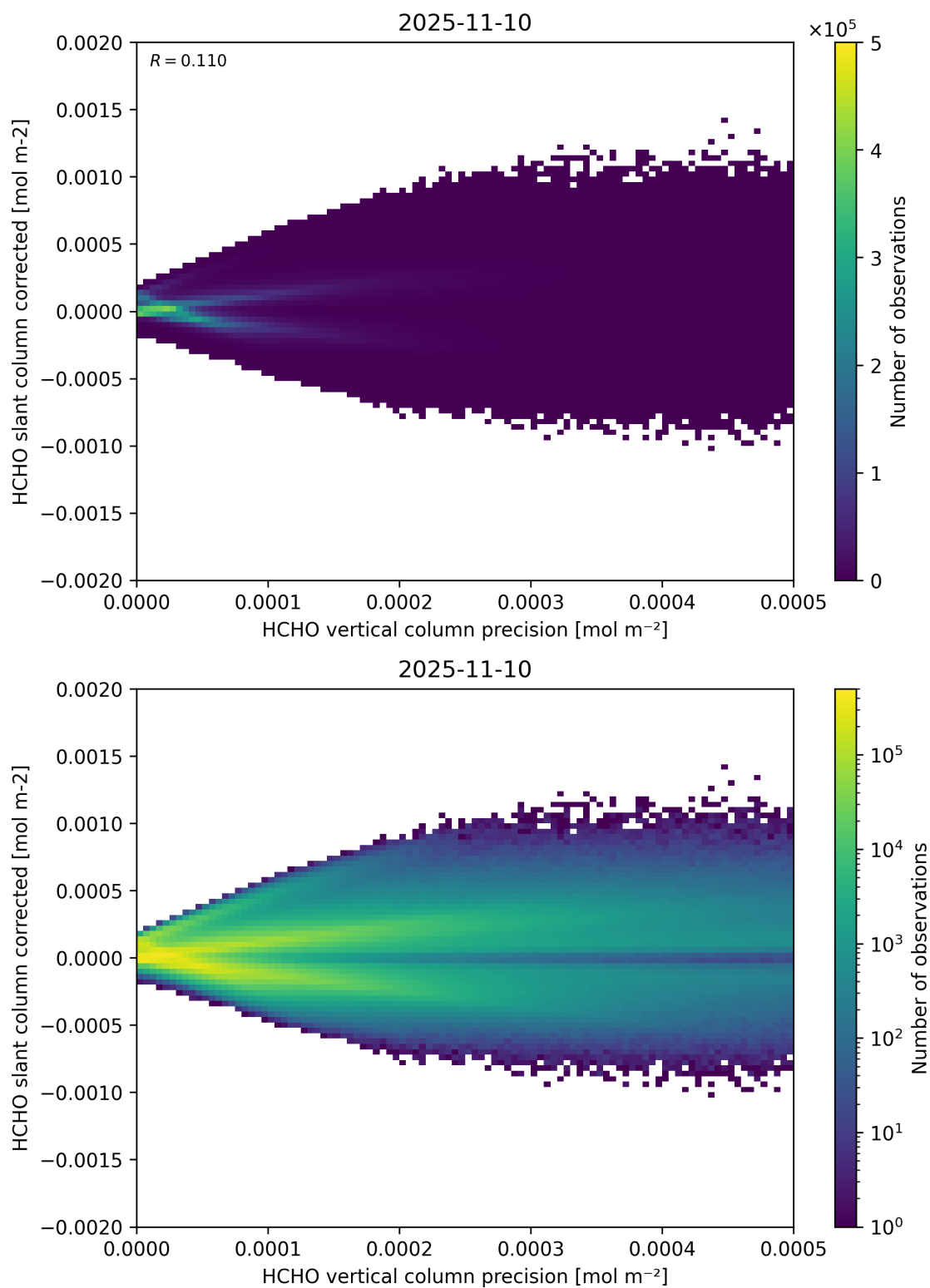
Figure 140: Scatter density plot of “HCHO vertical column precision” against “HCHO slant column corrected” for 2025-11-09 to 2025-11-11.
