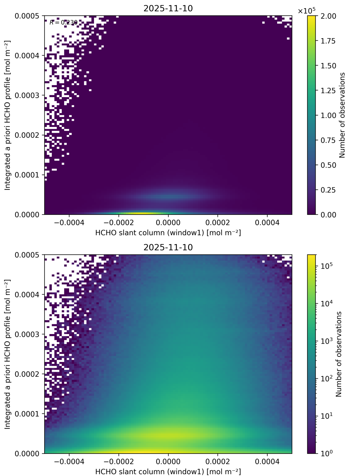
Figure 87: Scatter density plot of “HCHO slant column (window1)” against “Integrated a priori HCHO profile” for 2025-11-09 to 2025-11-11.
