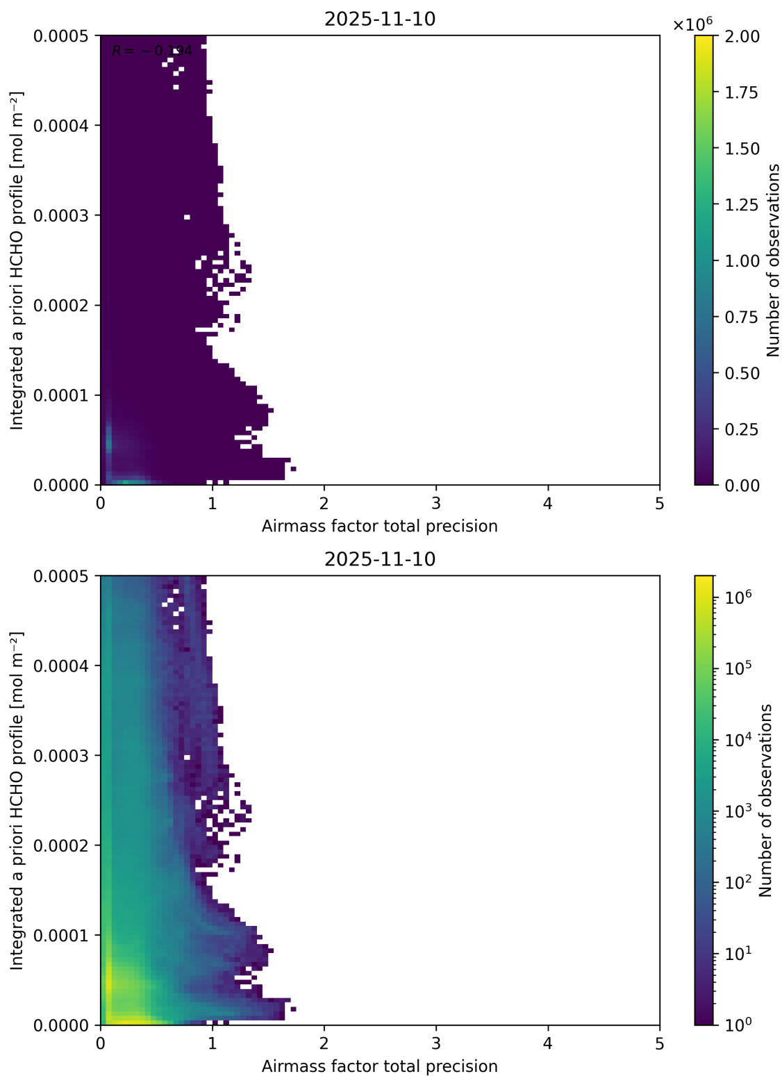
Figure 111: Scatter density plot of “Airmass factor total precision” against “Integrated a priori HCHO profile” for 2025-11-09 to 2025-11-11.
