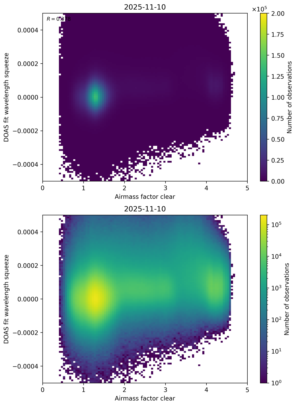
Figure 73: Scatter density plot of “Airmass factor clear” against “DOAS fit wavelength squeeze” for 2025-11-09 to 2025-11-11.
