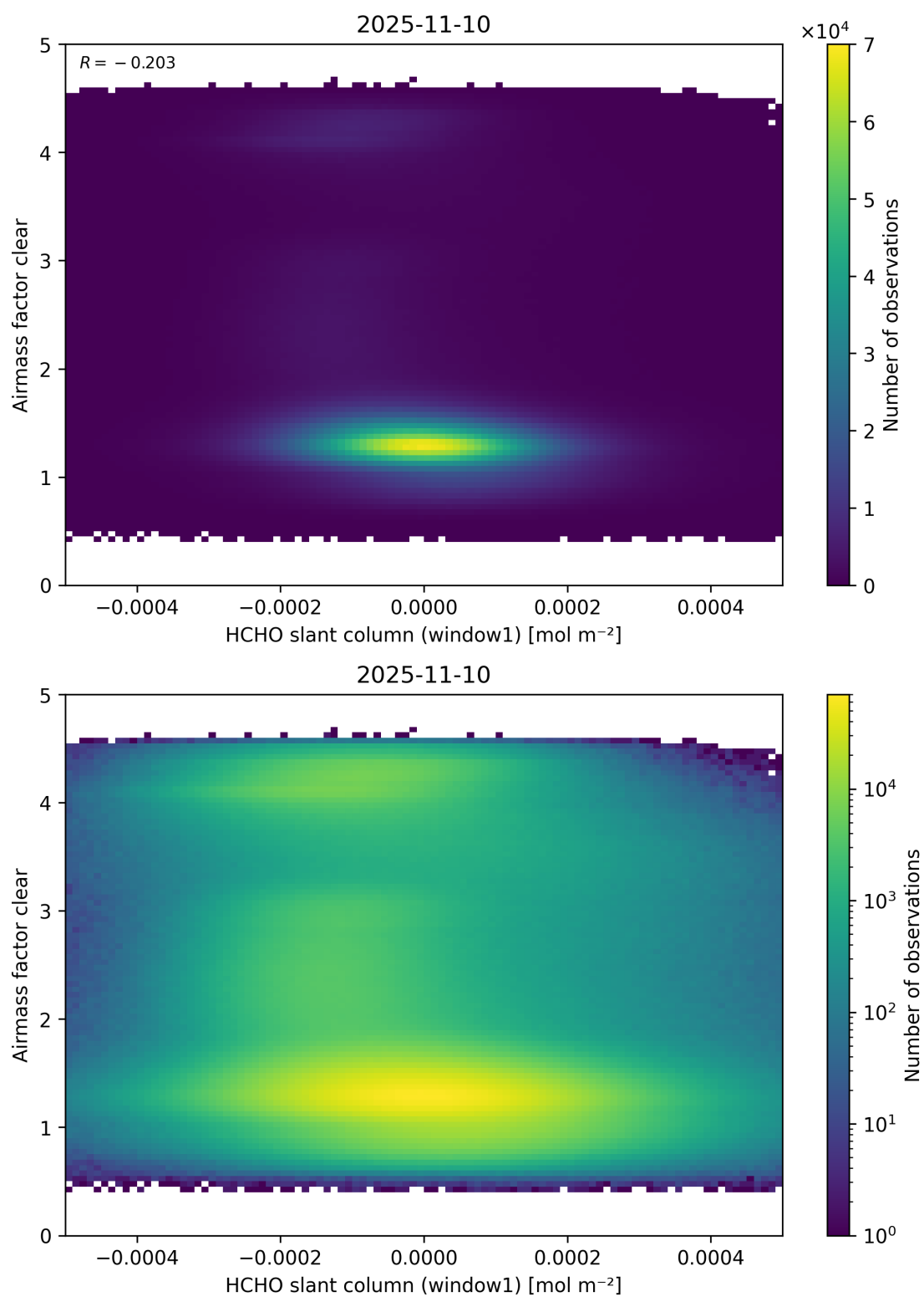
Figure 81: Scatter density plot of “HCHO slant column (window1)” against “Airmass factor clear” for 2025-11-09 to 2025-11-11.
