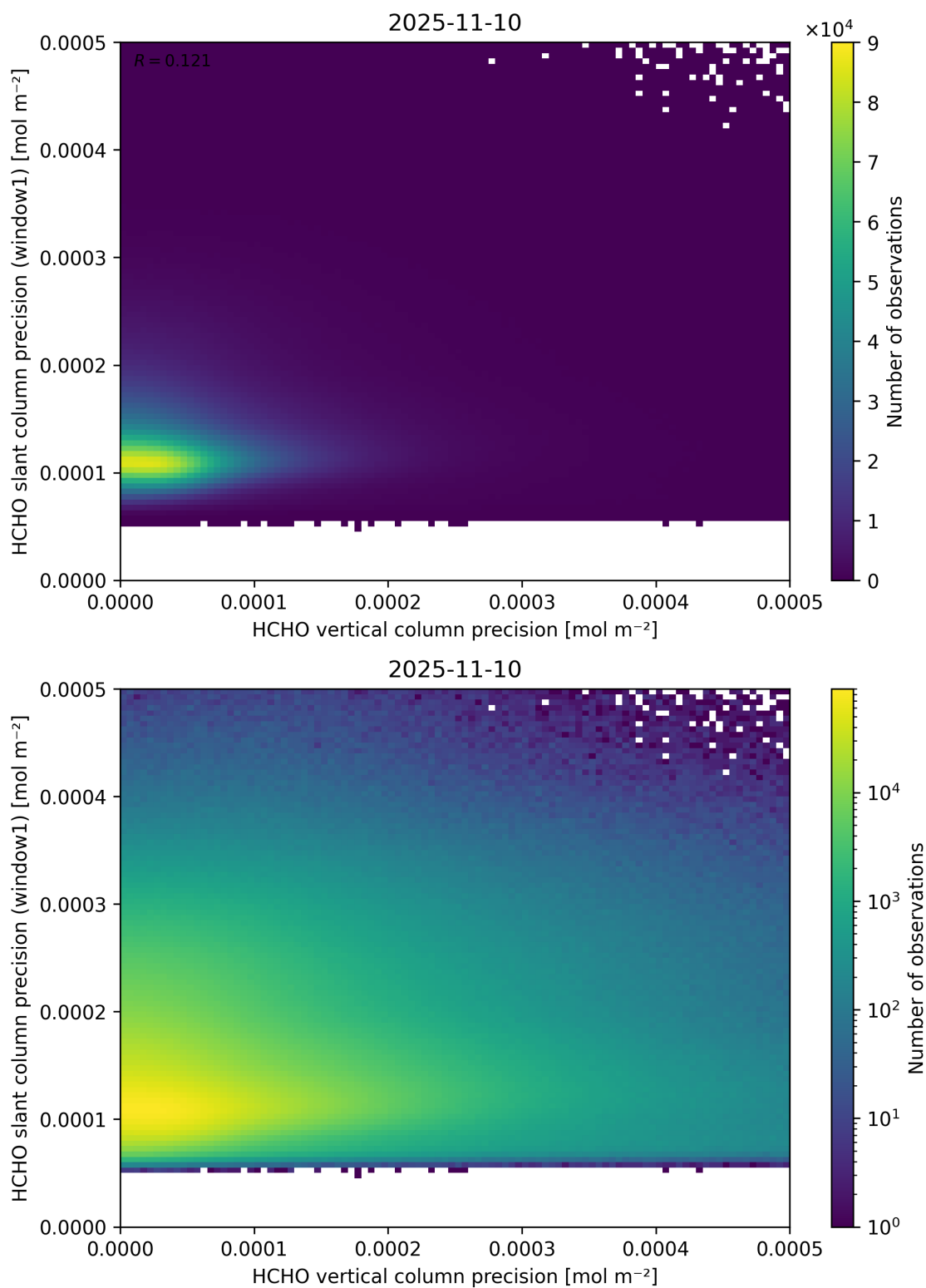
Figure 143: Scatter density plot of “HCHO vertical column precision” against “HCHO slant column precision (window1)” for 2025-11-09 to 2025-11-11.
