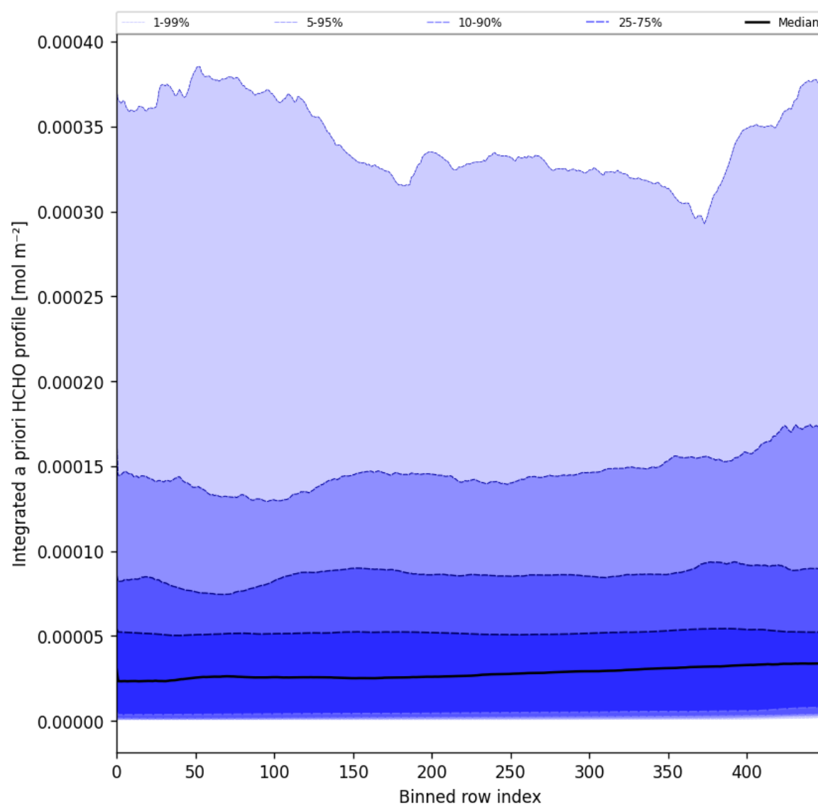
Figure 57: Along track statistics of “Integrated a priori HCHO profile” for 2025-11-09 to 2025-11-11
