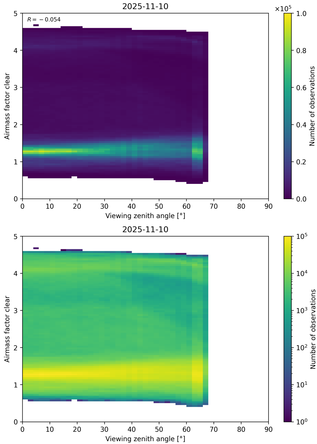
Figure 185: Scatter density plot of “Viewing zenith angle” against “Airmass factor clear” for 2025-11-09 to 2025-11-11.
