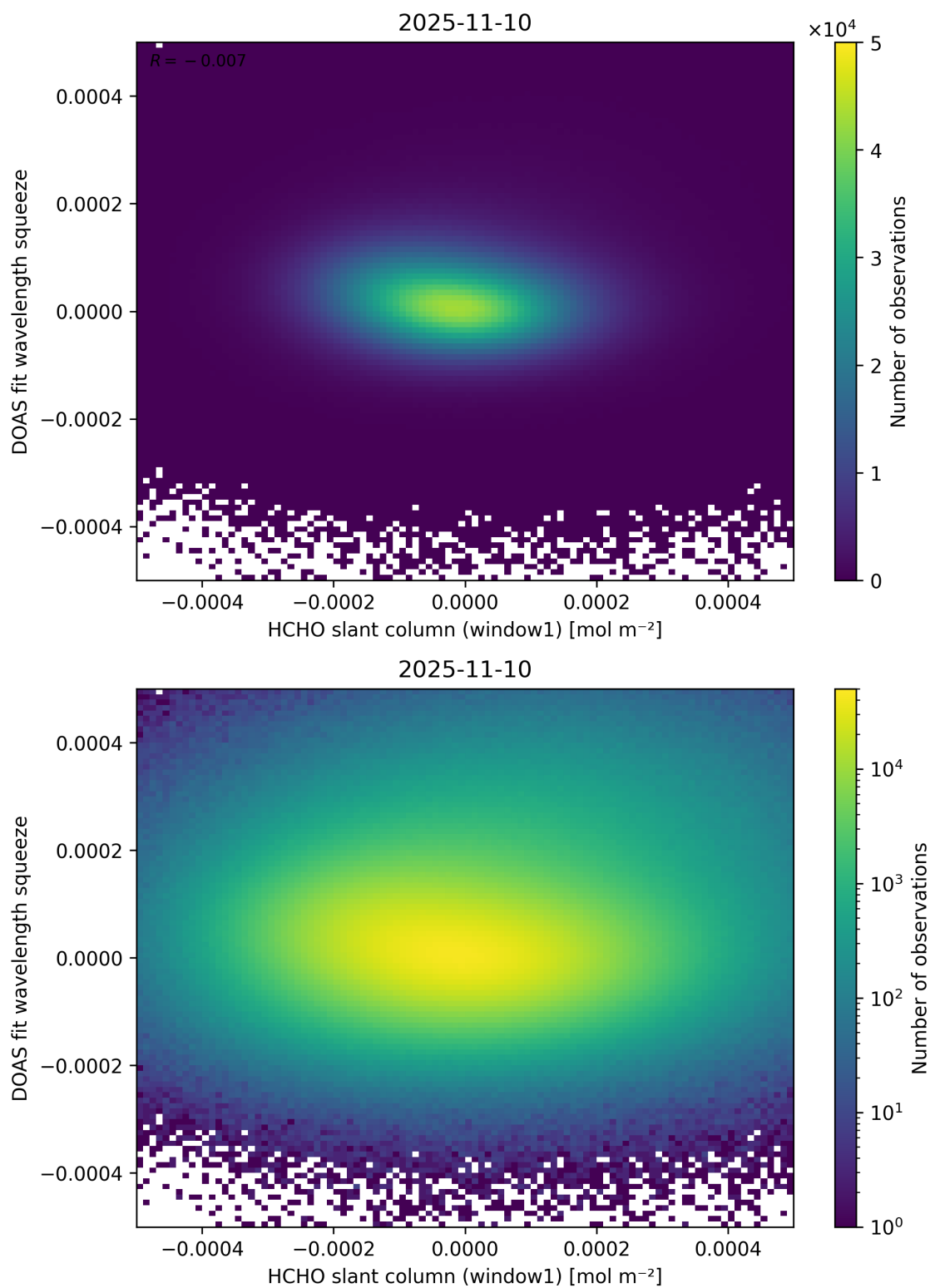
Figure 80: Scatter density plot of “HCHO slant column (window1)” against “DOAS fit wavelength squeeze” for 2025-11-09 to 2025-11-11.
