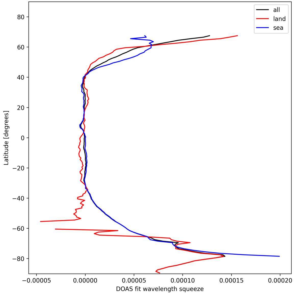
Figure 31: Zonal average of “DOAS fit wavelength squeeze” for 2025-11-09 to 2025-11-11.
