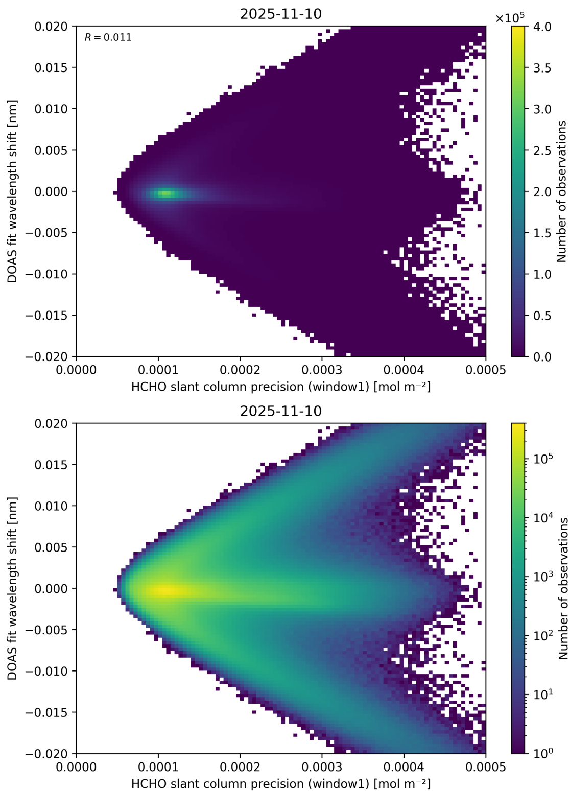
Figure 89: Scatter density plot of “HCHO slant column precision (window1)” against “DOAS fit wavelength shift” for 2025-11-09 to 2025-11-11.
