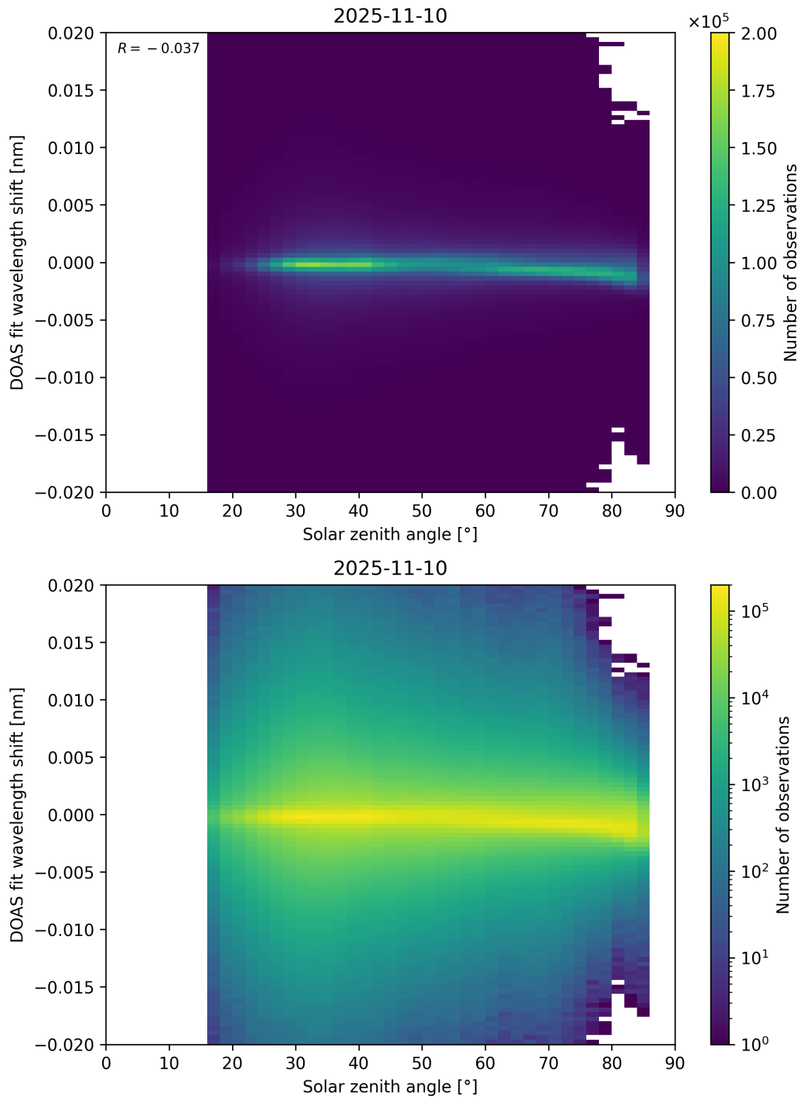
Figure 168: Scatter density plot of “Solar zenith angle” against “DOAS fit wavelength shift” for 2025-11-09 to 2025-11-11.
