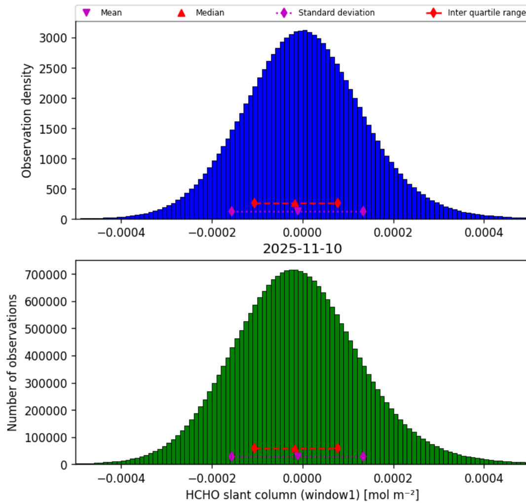
Figure 38: Histogram of “HCHO slant column (window1)” for 2025-11-09 to 2025-11-11
