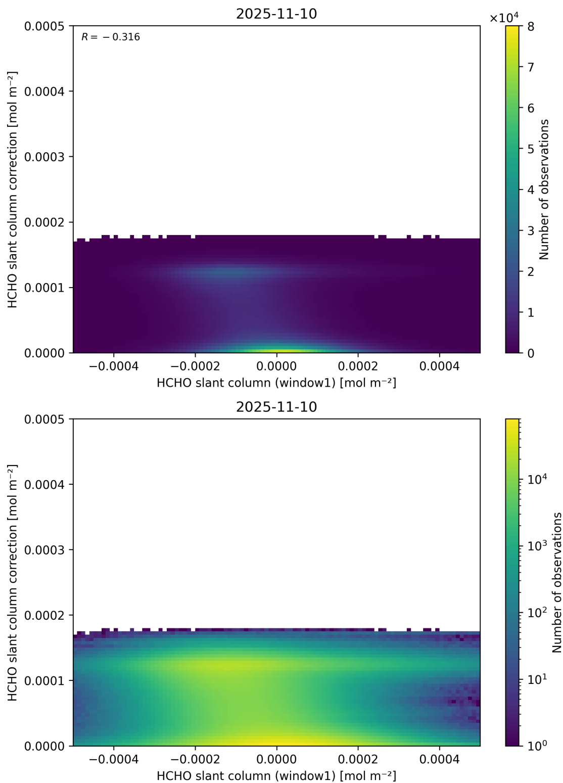
Figure 83: Scatter density plot of “HCHO slant column (window1)” against “HCHO slant column correction” for 2025-11-09 to 2025-11-11.
