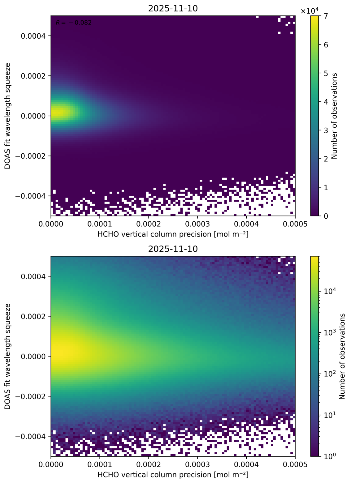
Figure 138: Scatter density plot of “HCHO vertical column precision” against “DOAS fit wavelength squeeze” for 2025-11-09 to 2025-11-11.
