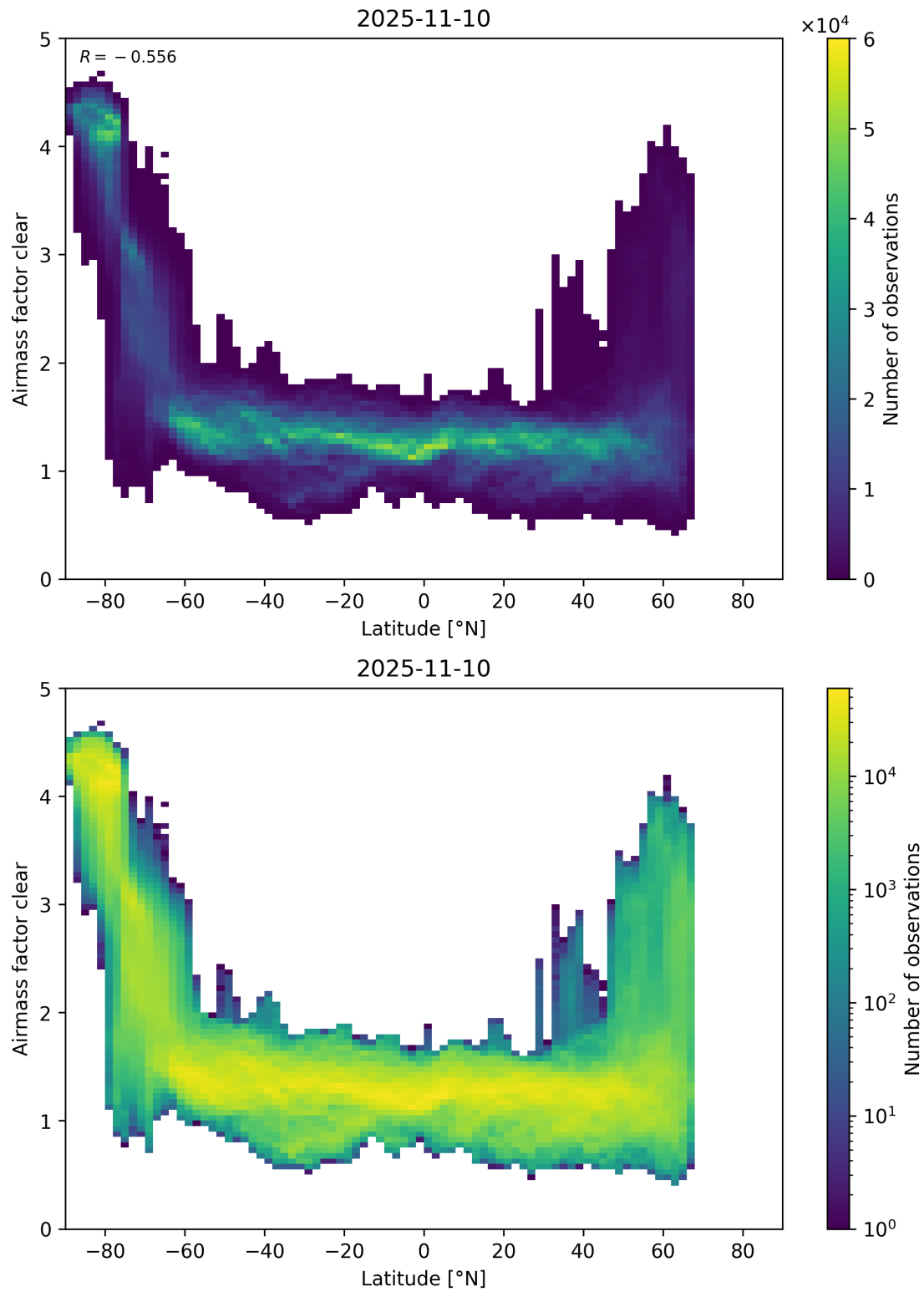
Figure 156: Scatter density plot of “Latitude” against “Airmass factor clear” for 2025-11-09 to 2025-11-11.
