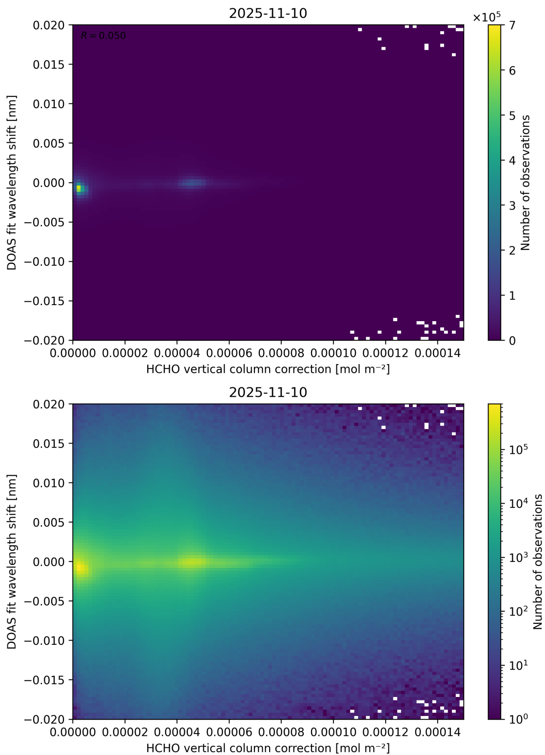
Figure 113: Scatter density plot of “HCHO vertical column correction” against “DOAS fit wavelength shift” for 2025-11-09 to 2025-11-11.
