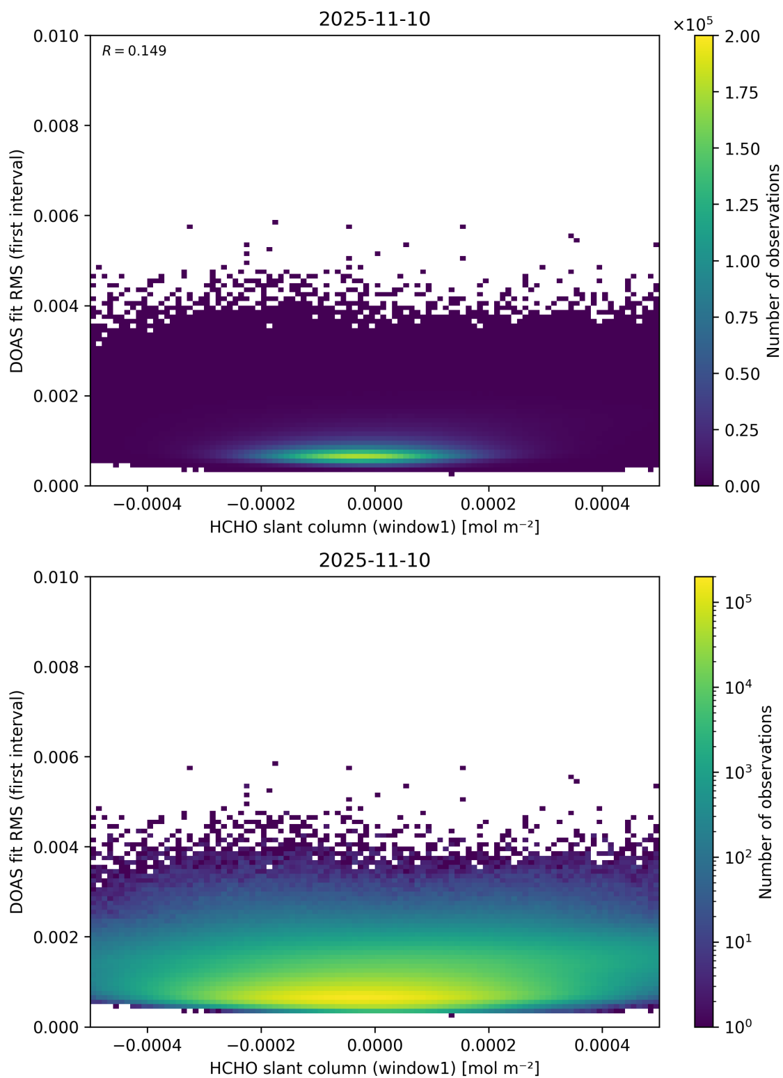
Figure 78: Scatter density plot of “HCHO slant column (window1)” against “DOAS fit RMS (first interval)” for 2025-11-09 to 2025-11-11.
