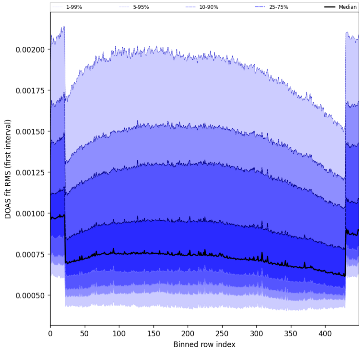
Figure 60: Along track statistics of “DOAS fit RMS (first interval)” for 2025-11-09 to 2025-11-11
