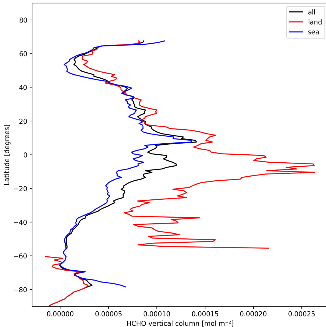
Figure 21: Zonal average of “HCHO vertical column” for 2025-11-09 to 2025-11-11.
