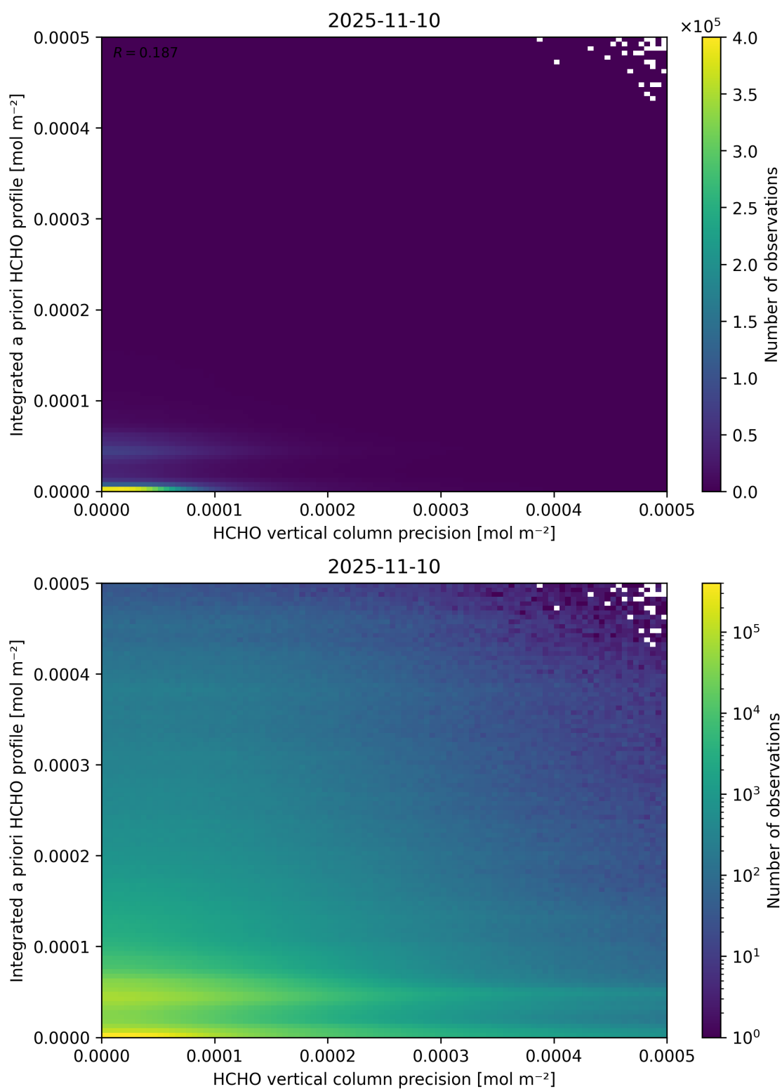
Figure 147: Scatter density plot of “HCHO vertical column precision” against “Integrated a priori HCHO profile” for 2025-11-09 to 2025-11-11.
