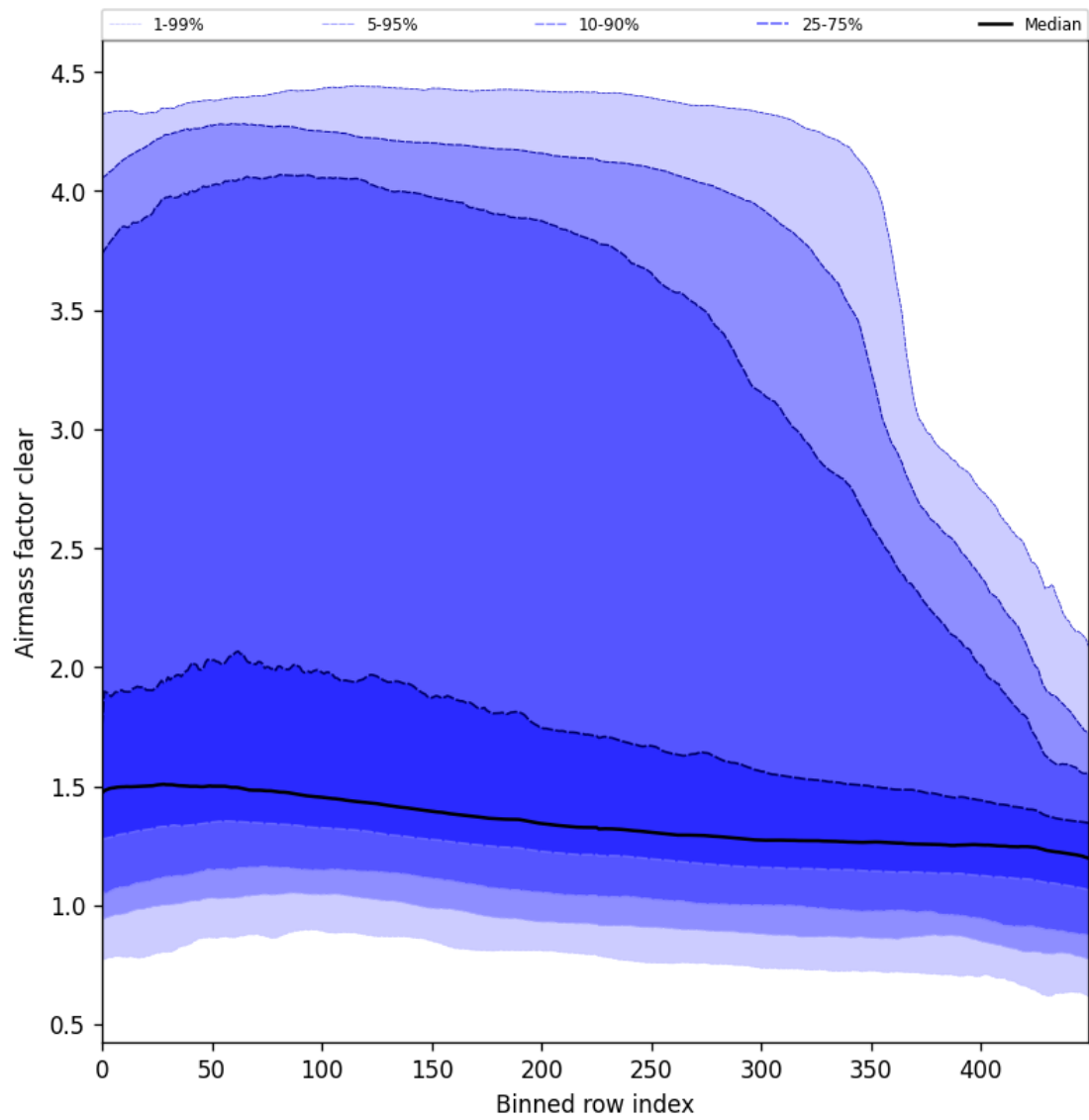
Figure 56: Along track statistics of “Airmass factor clear” for 2025-11-09 to 2025-11-11
