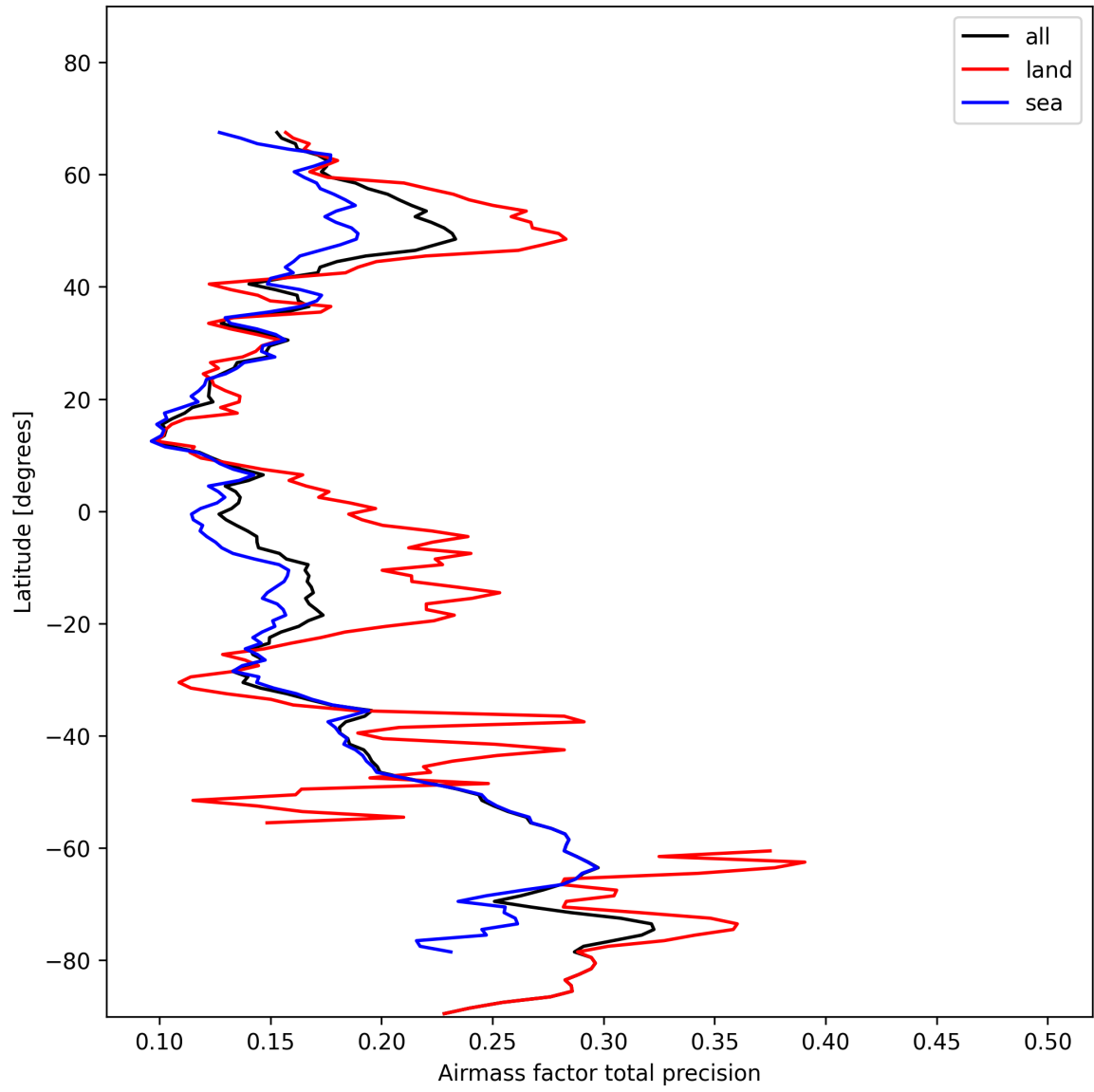
Figure 27: Zonal average of “Airmass factor total precision” for 2025-11-09 to 2025-11-11.
