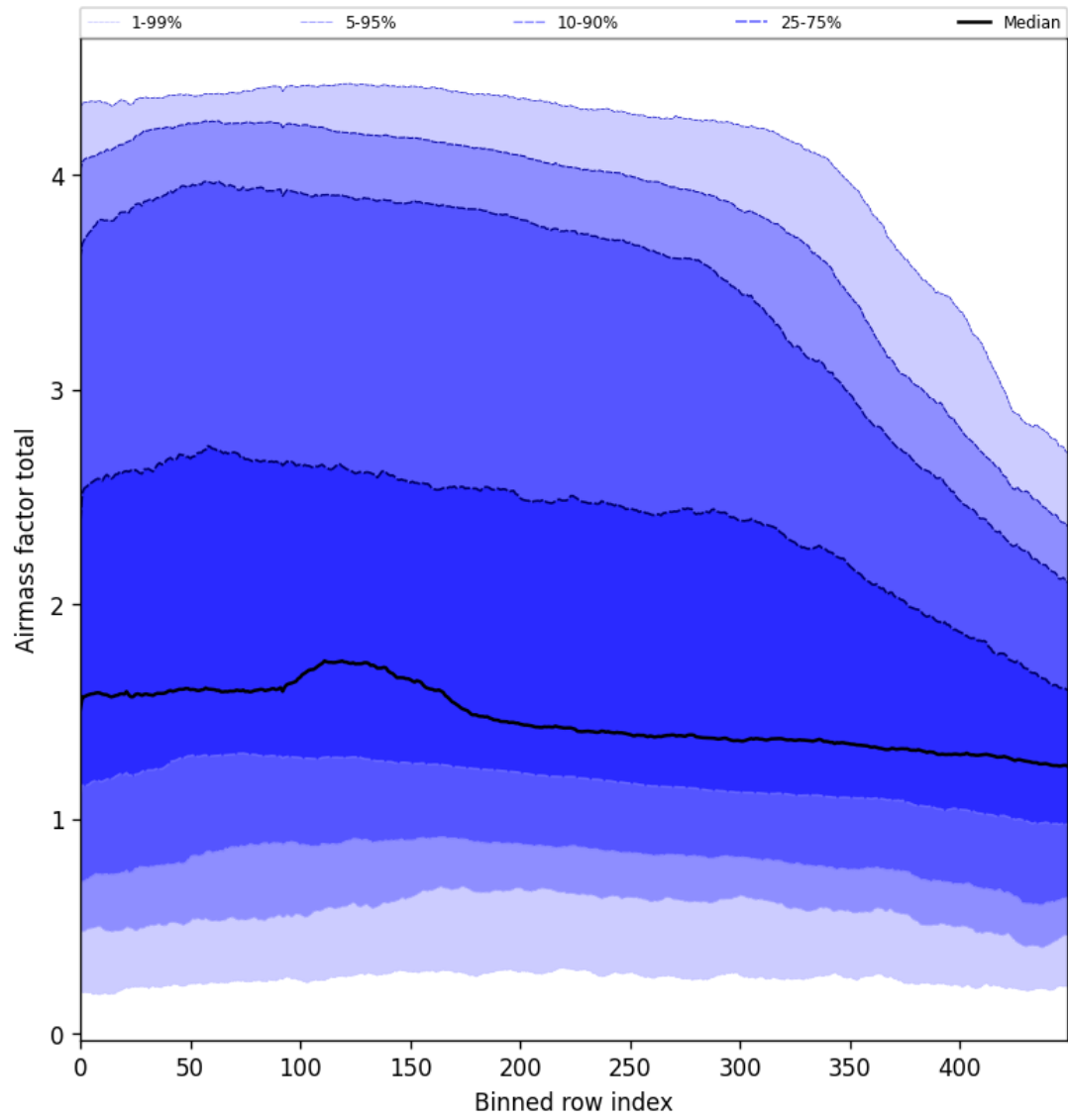
Figure 54: Along track statistics of “Airmass factor total” for 2025-11-09 to 2025-11-11
