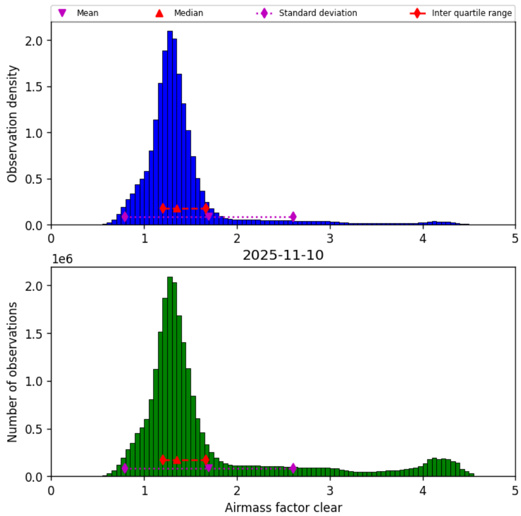
Figure 42: Histogram of “Airmass factor clear” for 2025-11-09 to 2025-11-11
