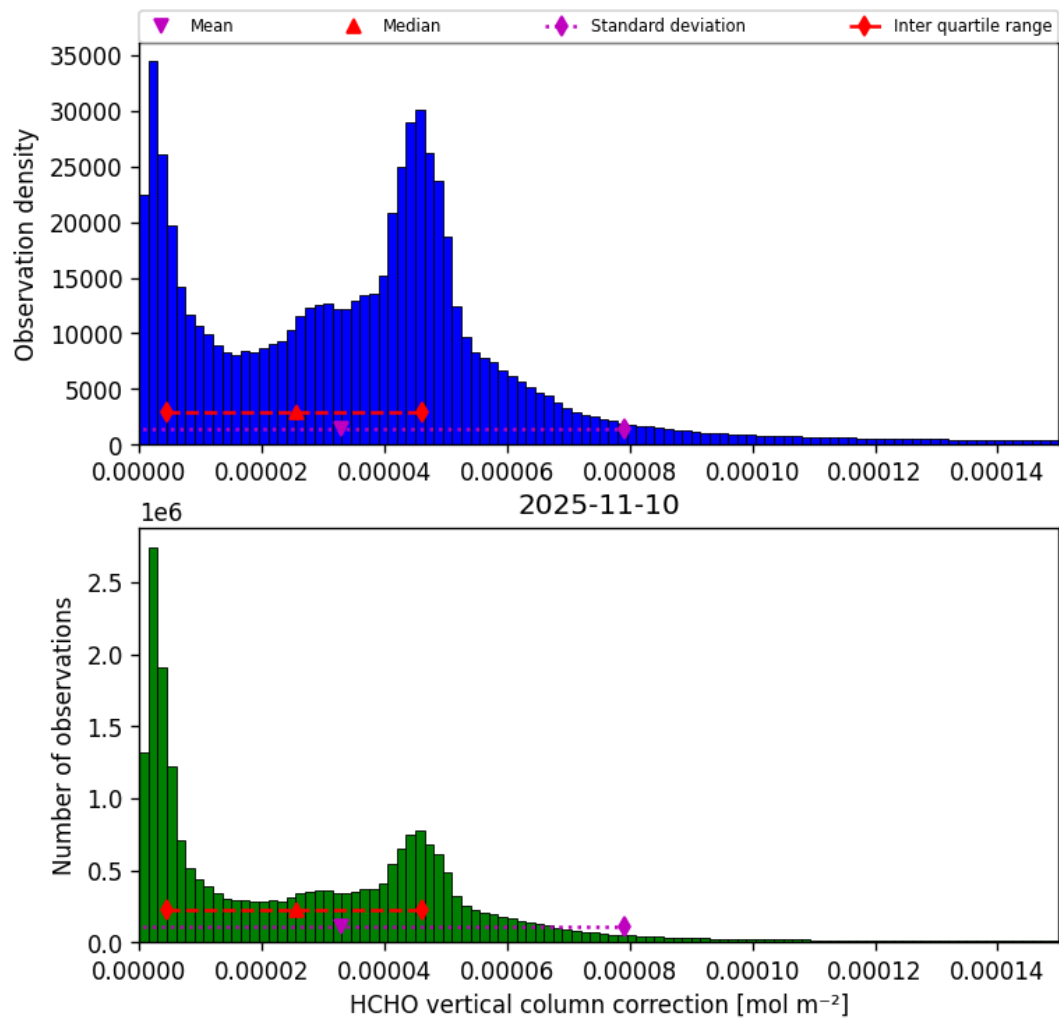
Figure 37: Histogram of “HCHO vertical column correction” for 2025-11-09 to 2025-11-11
