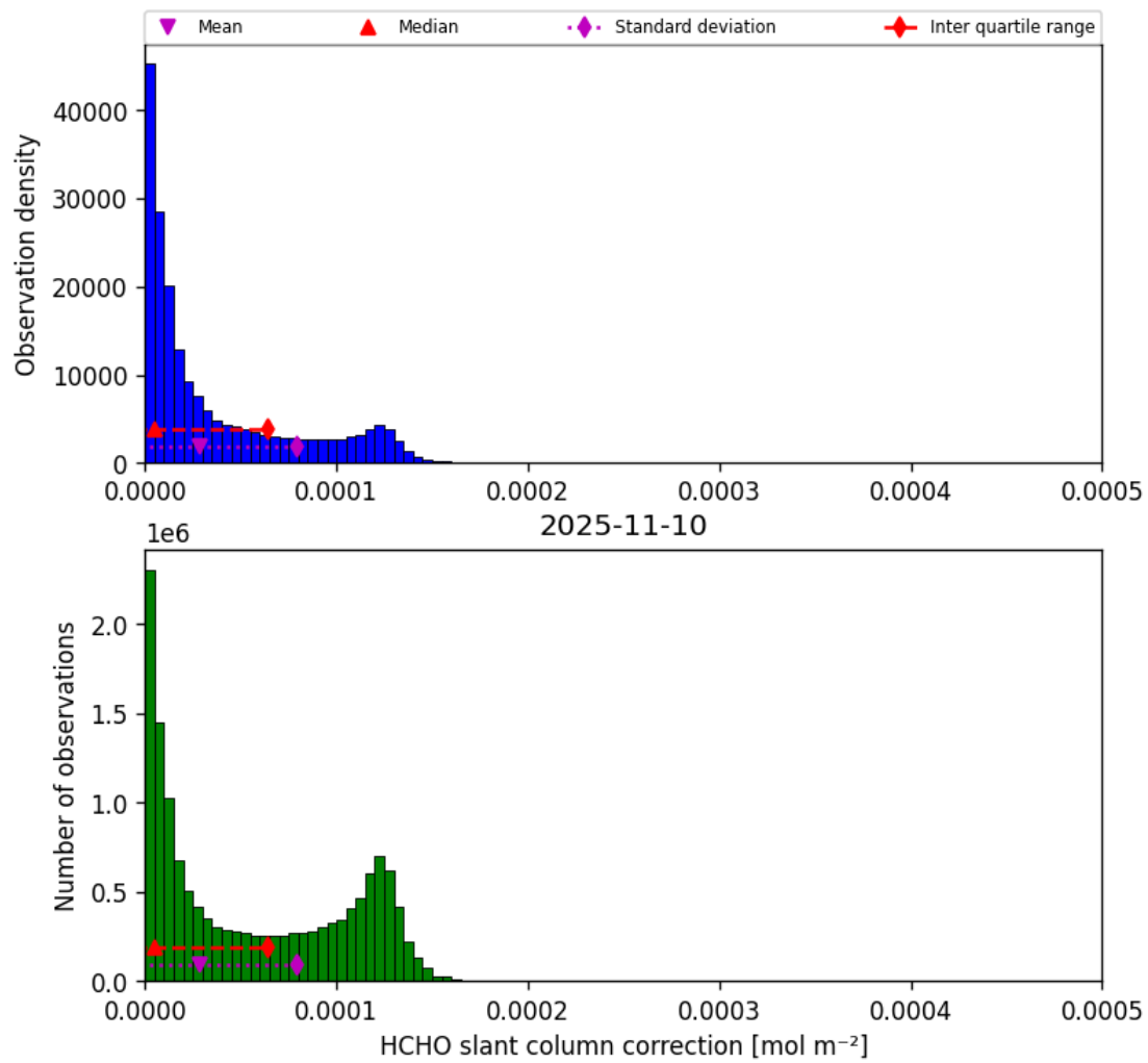
Figure 47: Histogram of “HCHO slant column correction” for 2025-11-09 to 2025-11-11
