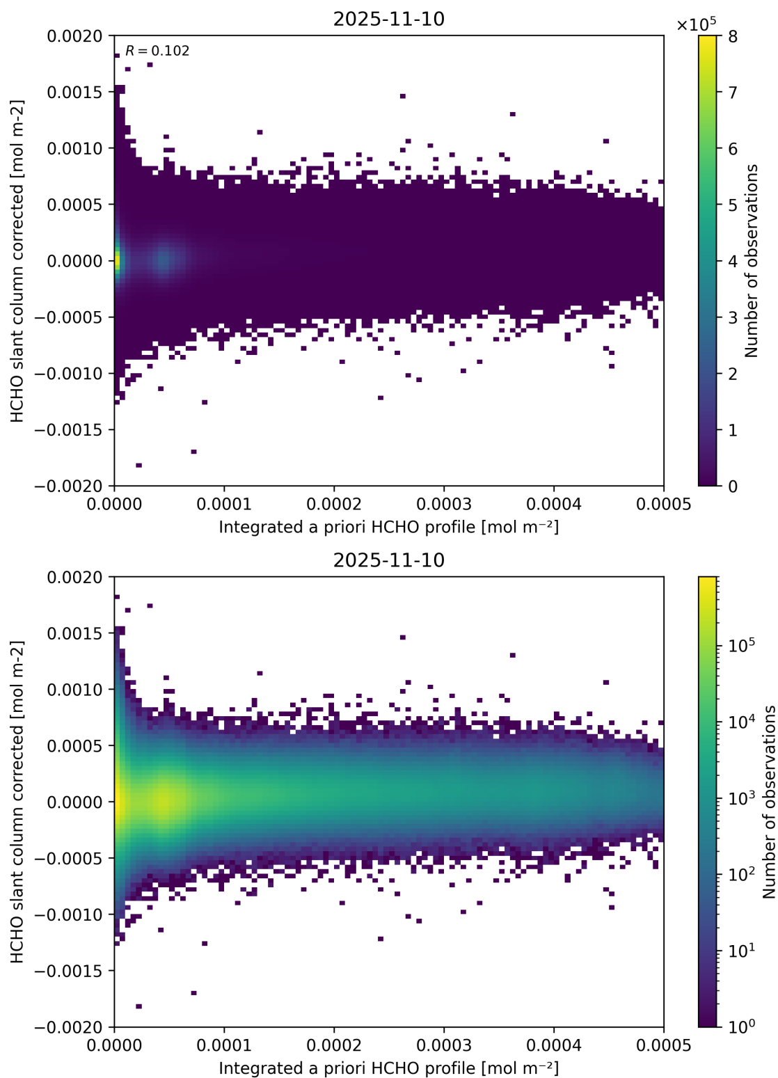
Figure 151: Scatter density plot of “Integrated a priori HCHO profile” against “HCHO slant column corrected” for 2025-11-09 to 2025-11-11.
