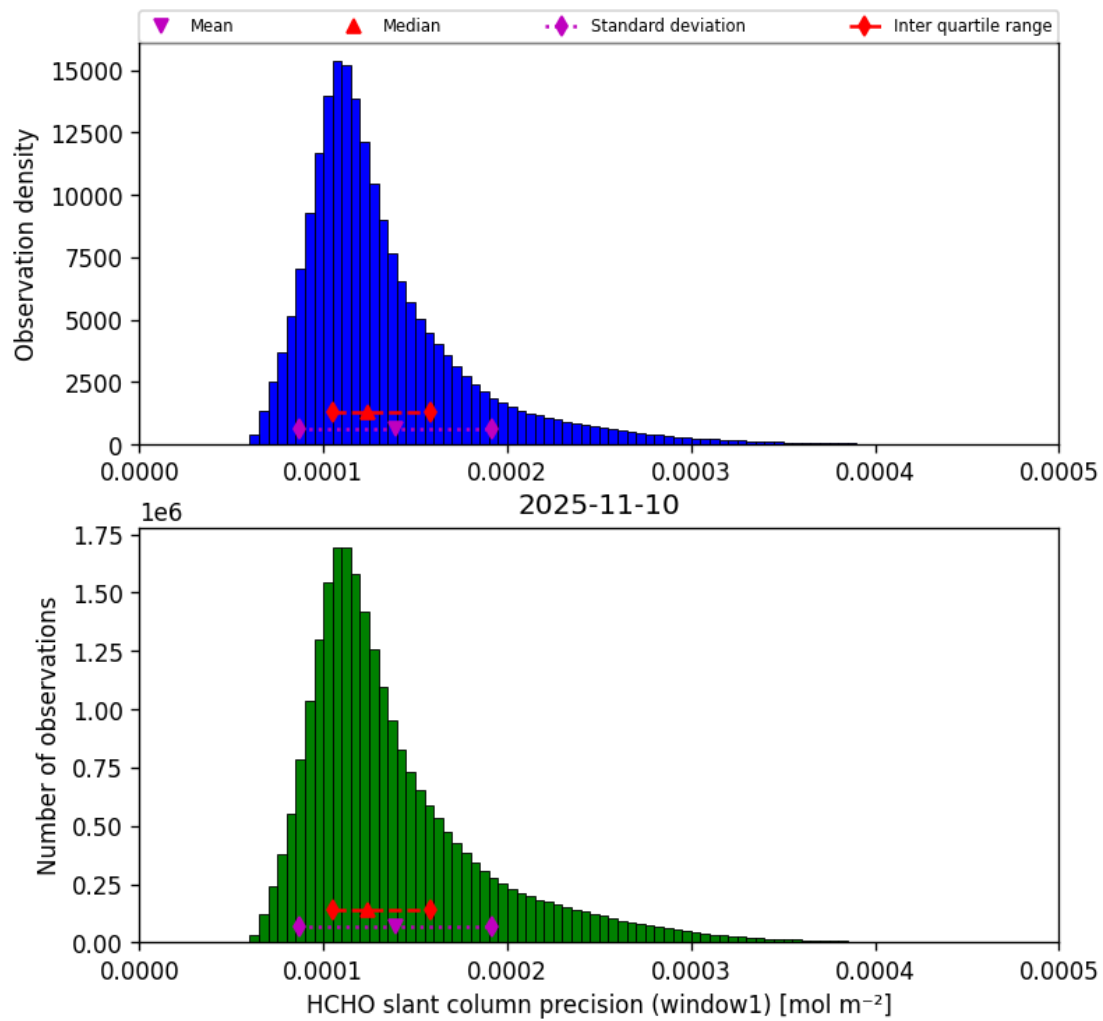
Figure 39: Histogram of “HCHO slant column precision (window1)” for 2025-11-09 to 2025-11-11
