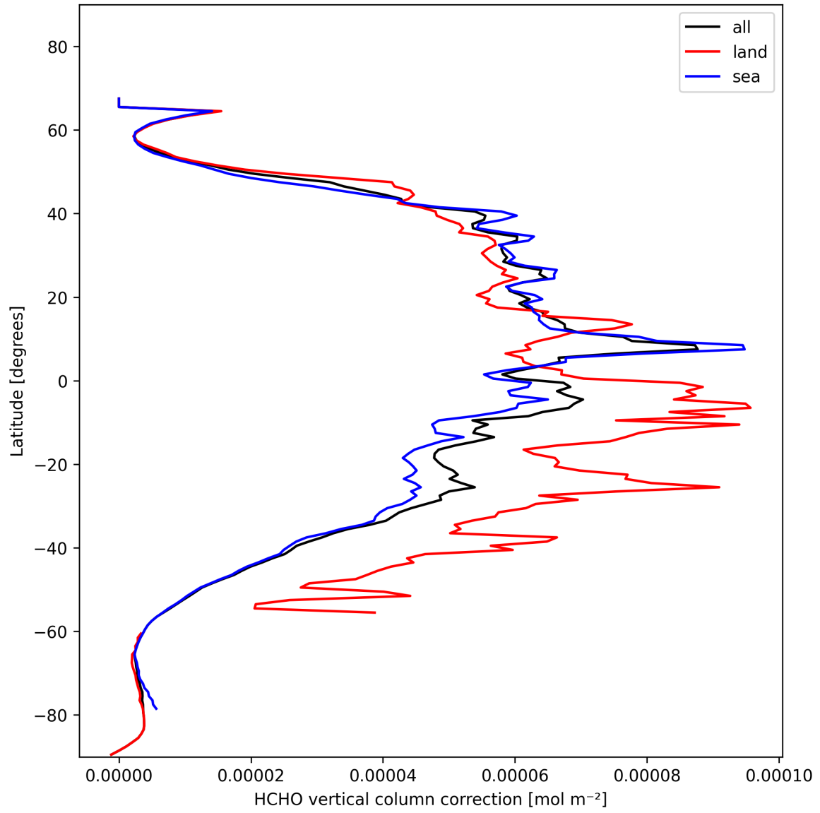
Figure 23: Zonal average of “HCHO vertical column correction” for 2025-11-09 to 2025-11-11.
