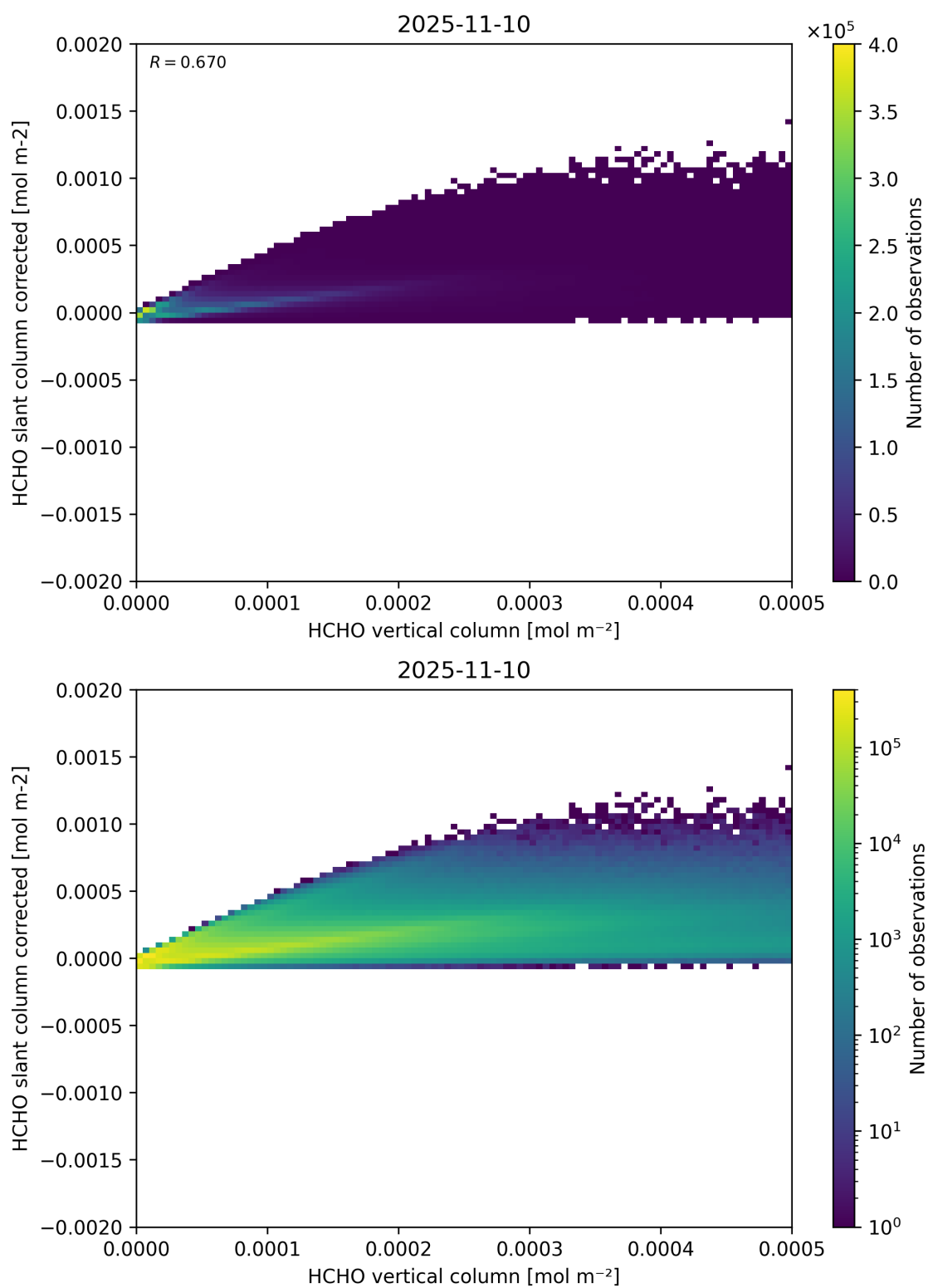
Figure 127: Scatter density plot of “HCHO vertical column” against “HCHO slant column corrected” for 2025-11-09 to 2025-11-11.
