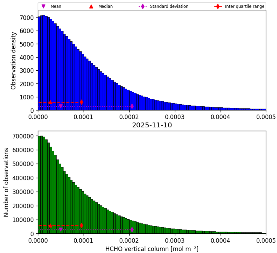
Figure 35: Histogram of “HCHO vertical column” for 2025-11-09 to 2025-11-11
