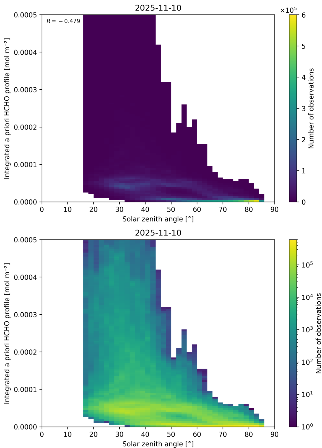
Figure 180: Scatter density plot of “Solar zenith angle” against “Integrated a priori HCHO profile” for 2025-11-09 to 2025-11-11.
