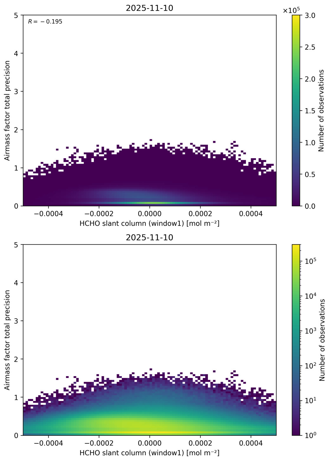
Figure 86: Scatter density plot of “HCHO slant column (window1)” against “Airmass factor total precision” for 2025-11-09 to 2025-11-11.
