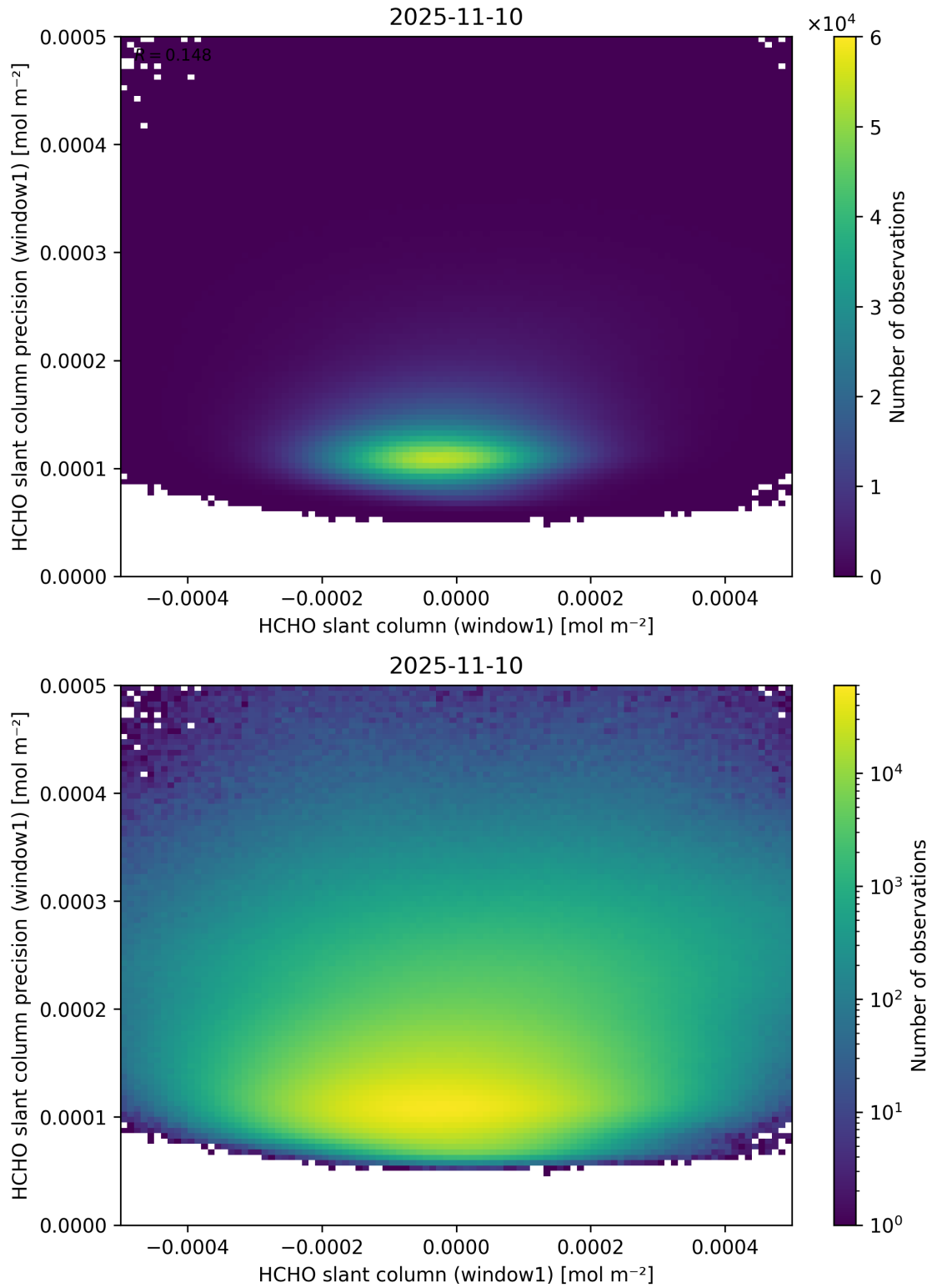
Figure 84: Scatter density plot of “HCHO slant column (window1)” against “HCHO slant column precision (window1)” for 2025-11-09 to 2025-11-11.
