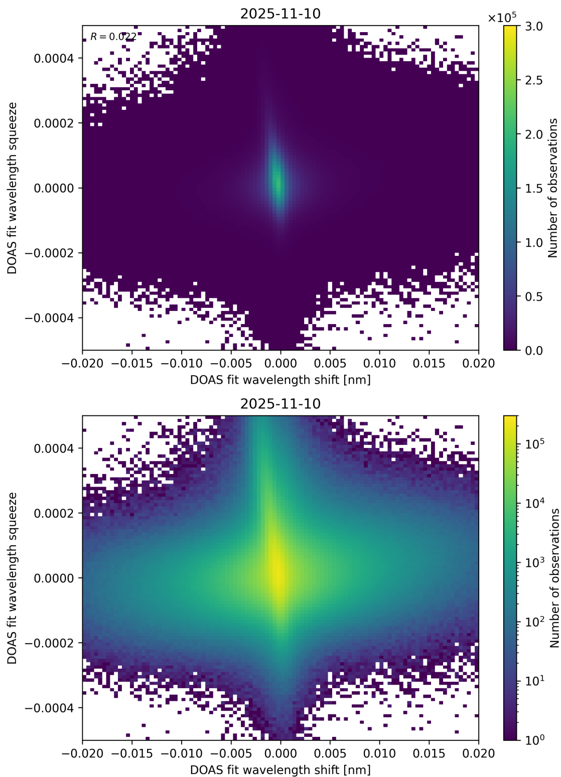
Figure 65: Scatter density plot of “DOAS fit wavelength shift” against “DOAS fit wavelength squeeze” for 2025-11-09 to 2025-11-11.
