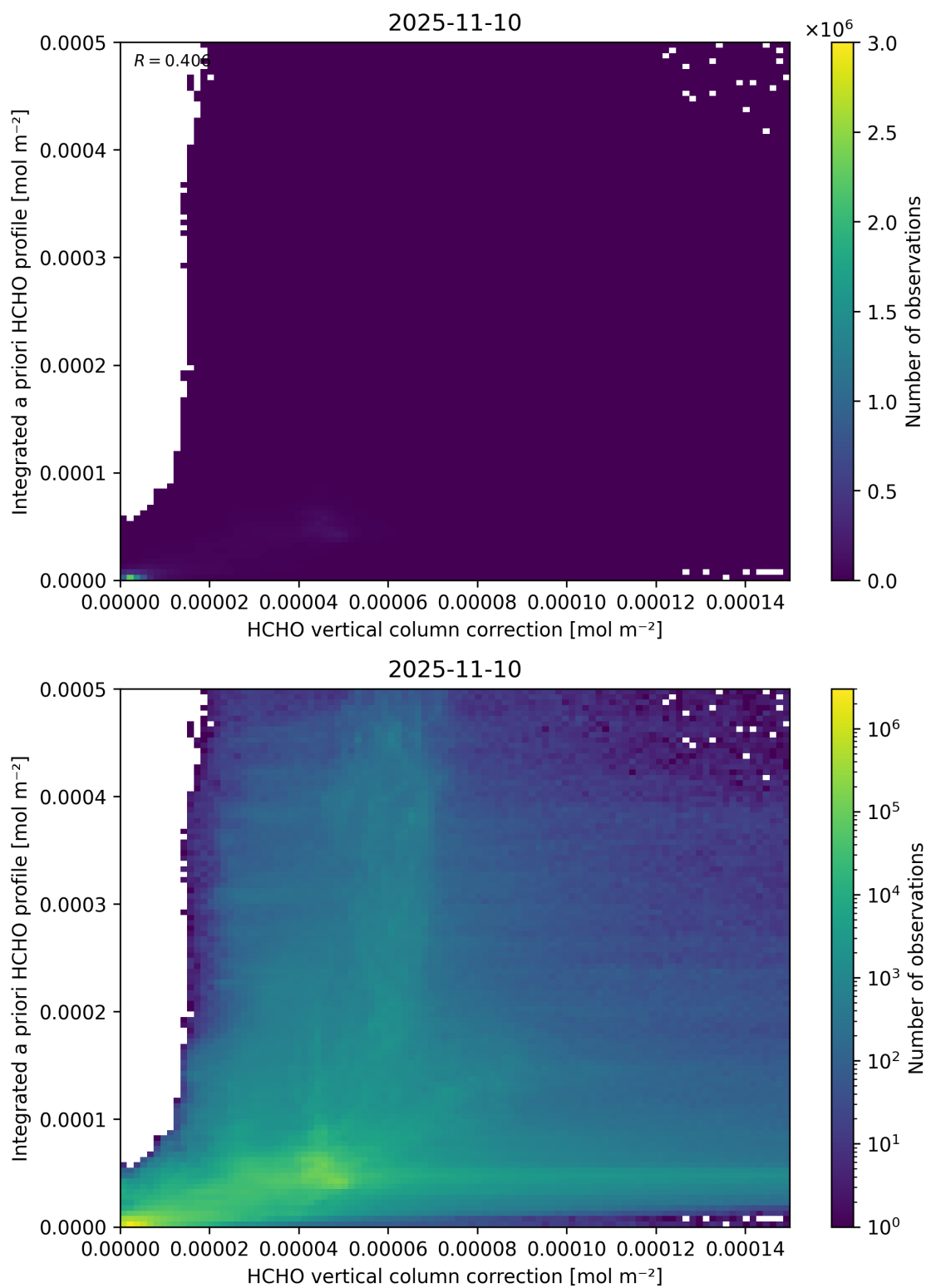
Figure 122: Scatter density plot of “HCHO vertical column correction” against “Integrated a priori HCHO profile” for 2025-11-09 to 2025-11-11.
