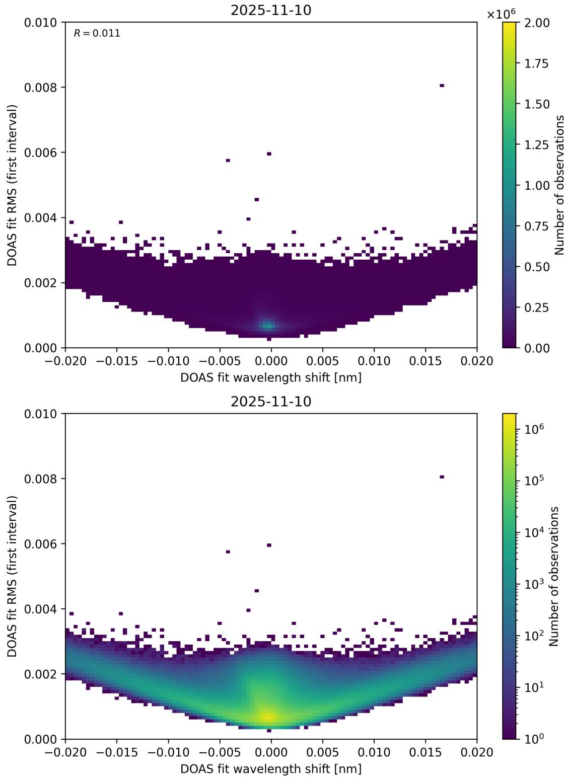
Figure 64: Scatter density plot of “DOAS fit wavelength shift” against “DOAS fit RMS (first interval)” for 2025-11-09 to 2025-11-11.
