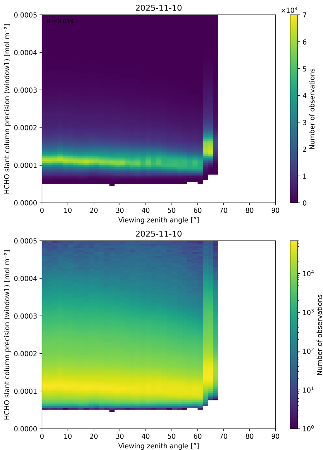
Figure 189: Scatter density plot of “Viewing zenith angle” against “HCHO slant column precision (window1)” for 2025-11-09 to 2025-11-11.
