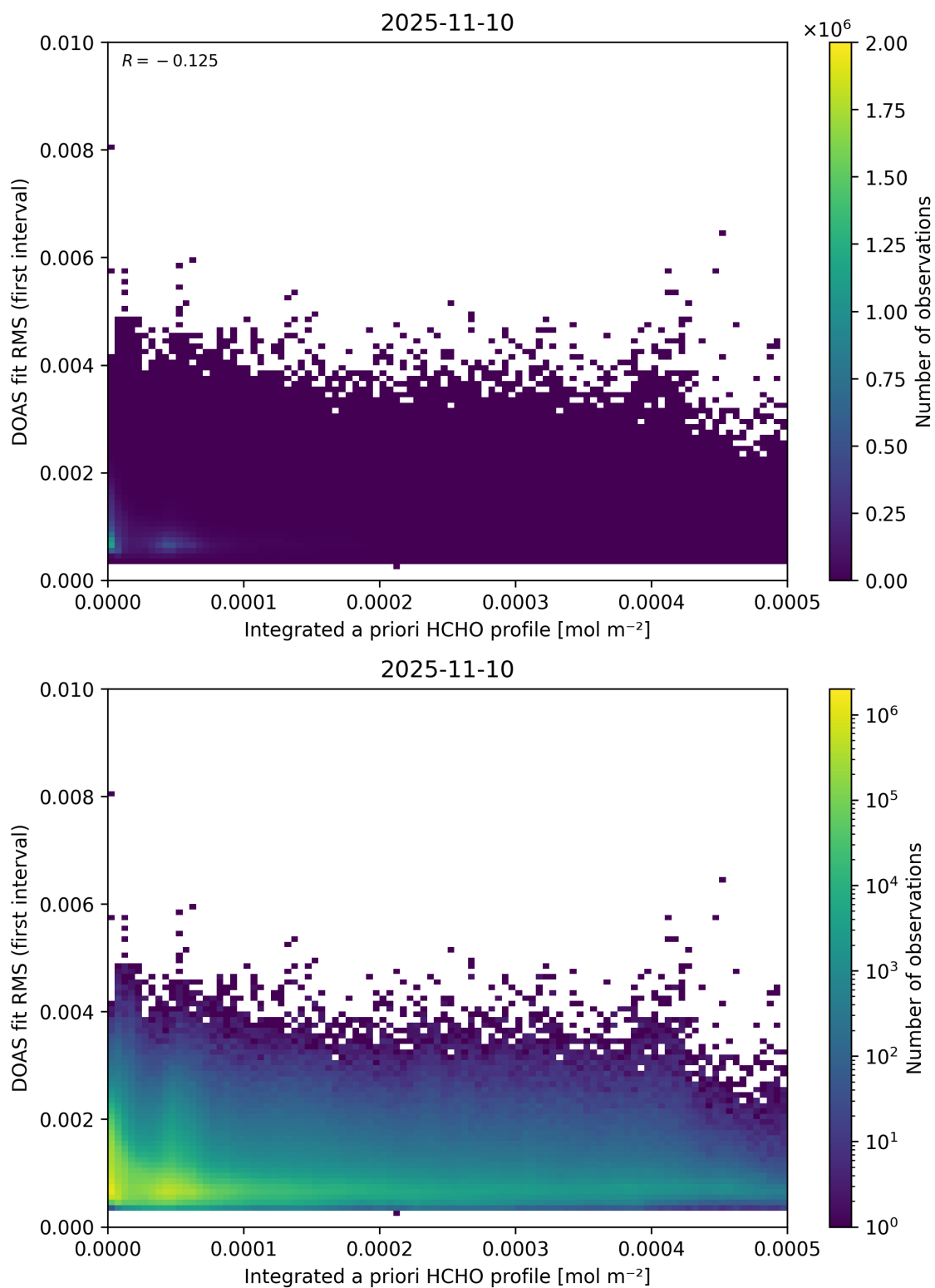
Figure 148: Scatter density plot of “Integrated a priori HCHO profile” against “DOAS fit RMS (first interval)” for 2025-11-09 to 2025-11-11.
