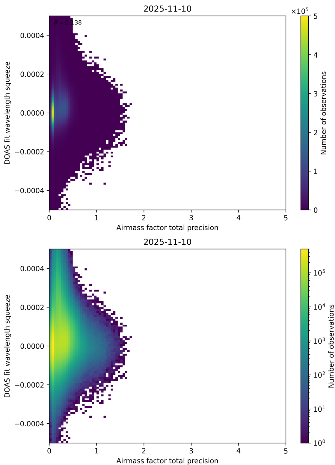
Figure 107: Scatter density plot of “Airmass factor total precision” against “DOAS fit wavelength squeeze” for 2025-11-09 to 2025-11-11.
