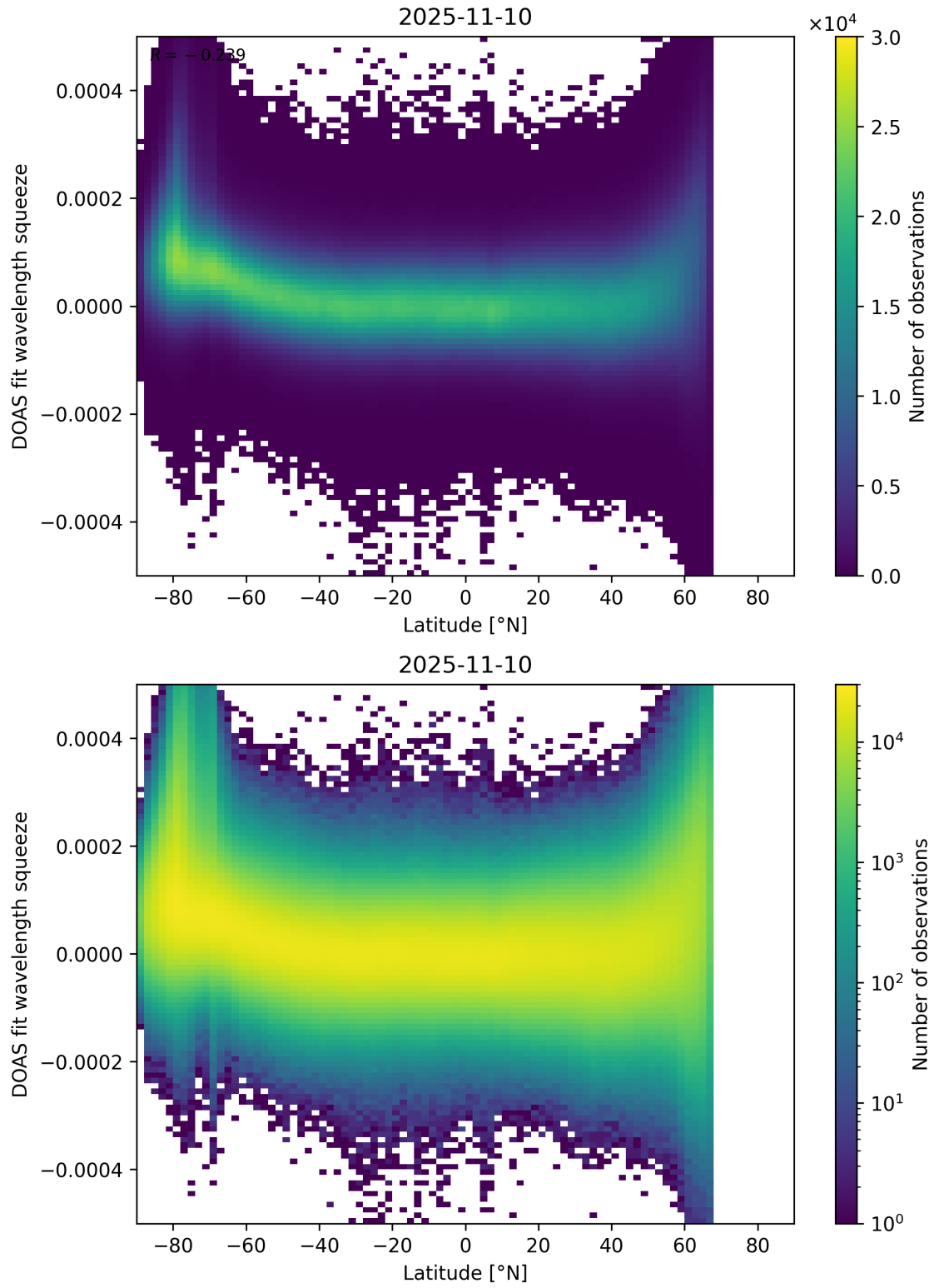
Figure 155: Scatter density plot of “Latitude” against “DOAS fit wavelength squeeze” for 2025-11-09 to 2025-11-11.
