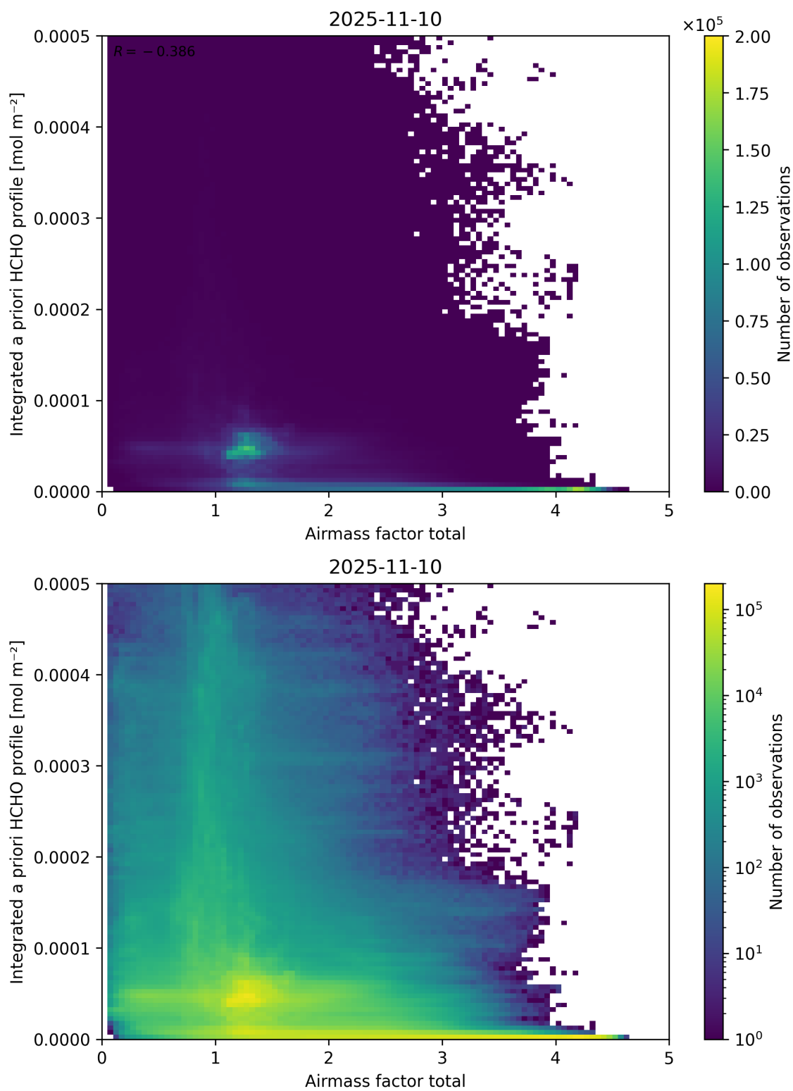
Figure 104: Scatter density plot of “Airmass factor total” against “Integrated a priori HCHO profile” for 2025-11-09 to 2025-11-11.
