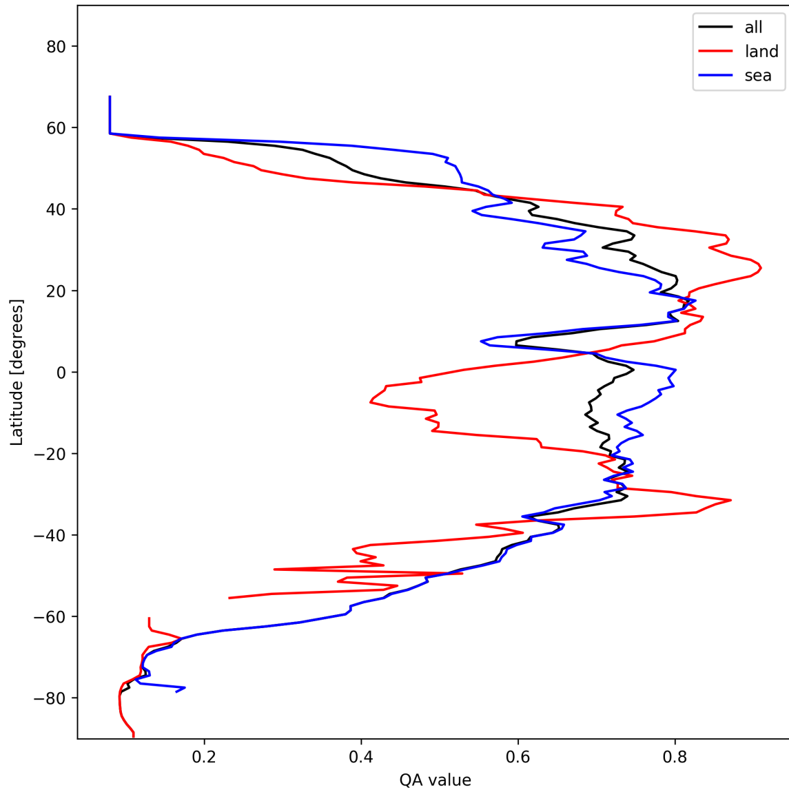
Figure 20: Zonal average of “QA value” for 2025-11-09 to 2025-11-11.
