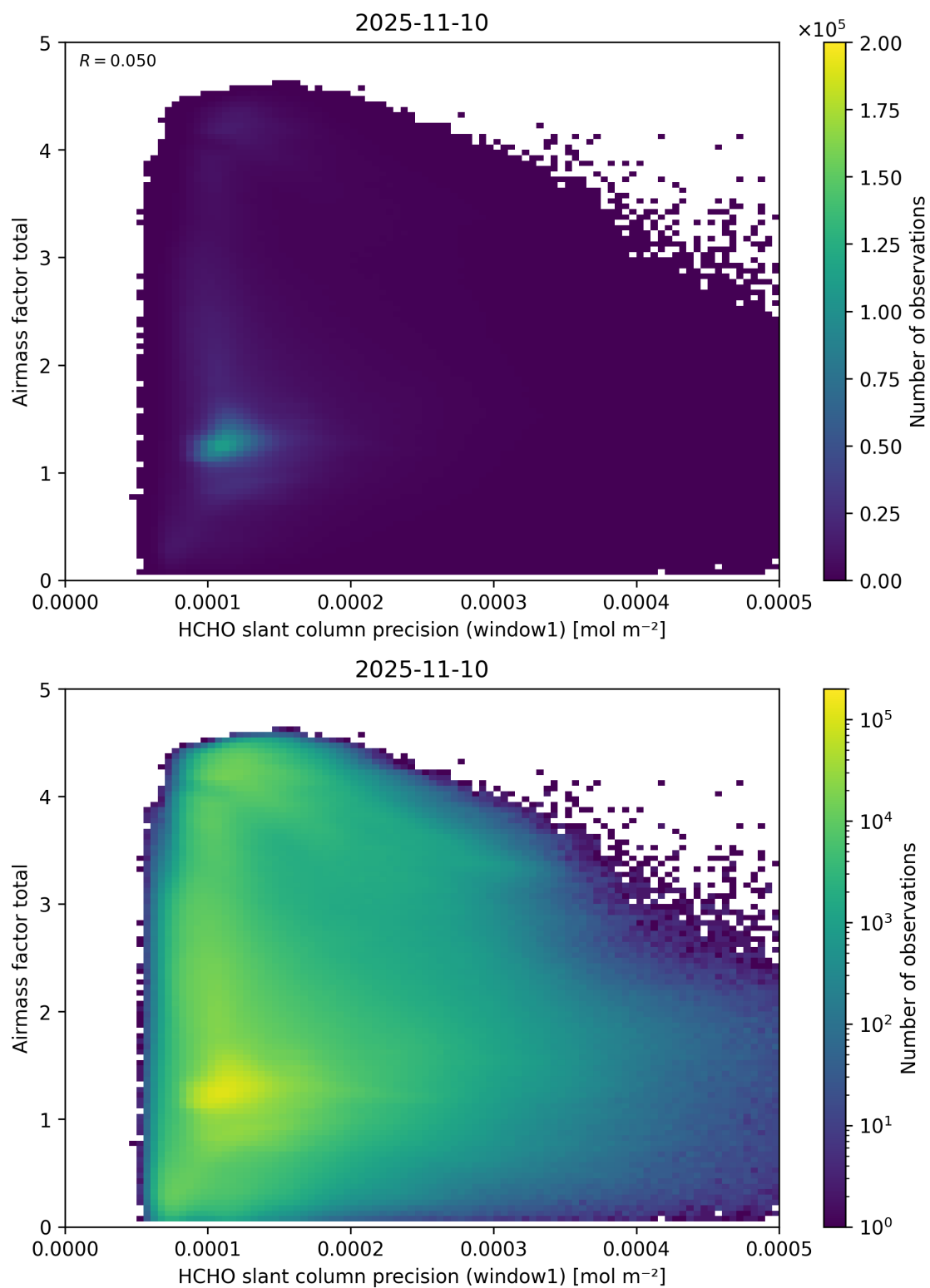
Figure 94: Scatter density plot of “HCHO slant column precision (window1)” against “Airmass factor total” for 2025-11-09 to 2025-11-11.
