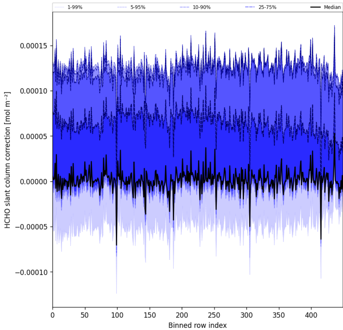
Figure 61: Along track statistics of “HCHO slant column correction” for 2025-11-09 to 2025-11-11
