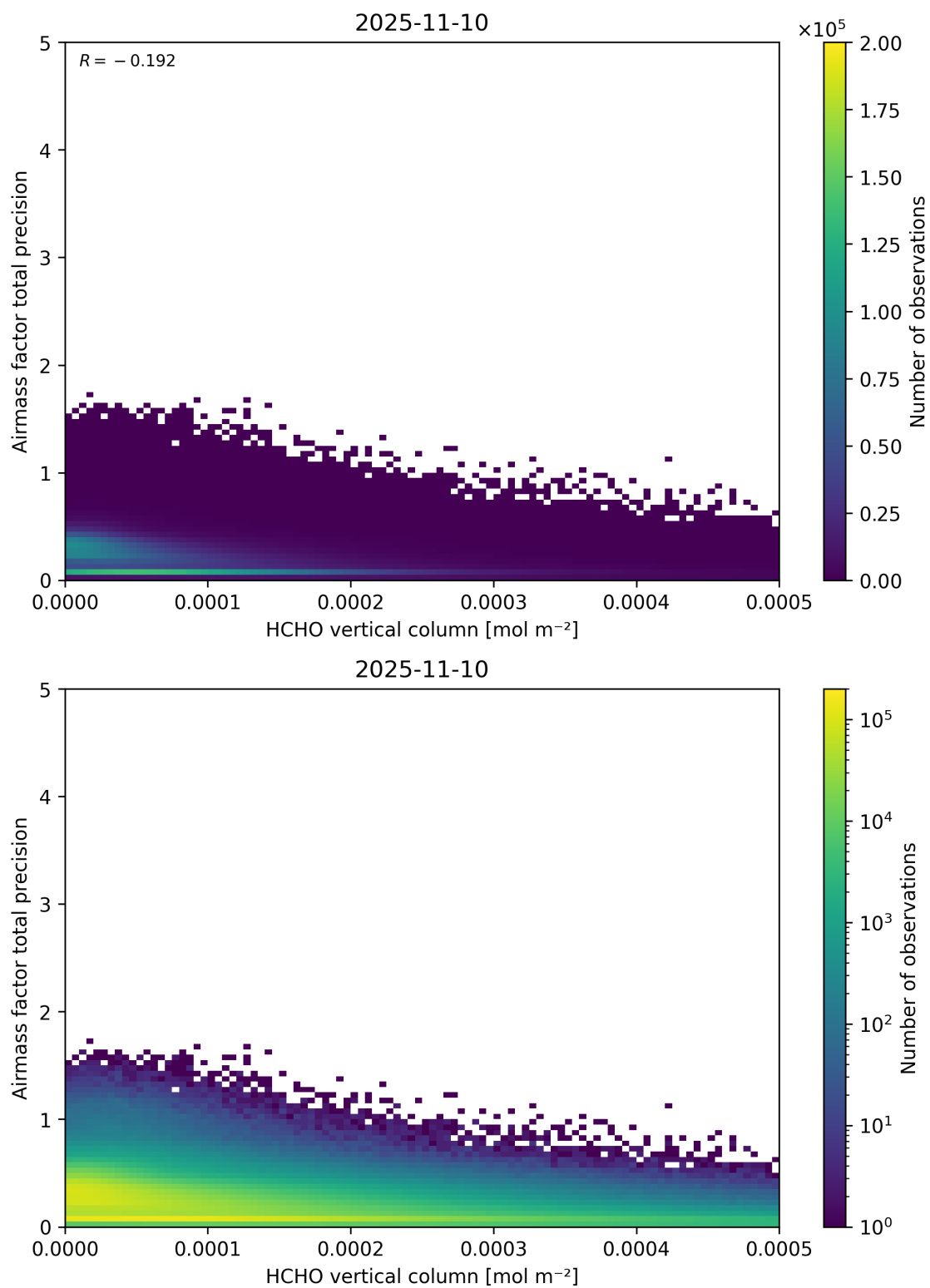
Figure 132: Scatter density plot of “HCHO vertical column” against “Airmass factor total precision” for 2025-11-09 to 2025-11-11.
