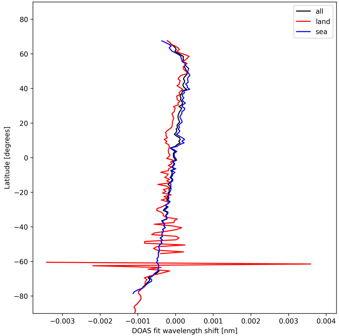
Figure 30: Zonal average of “DOAS fit wavelength shift” for 2025-11-09 to 2025-11-11.
