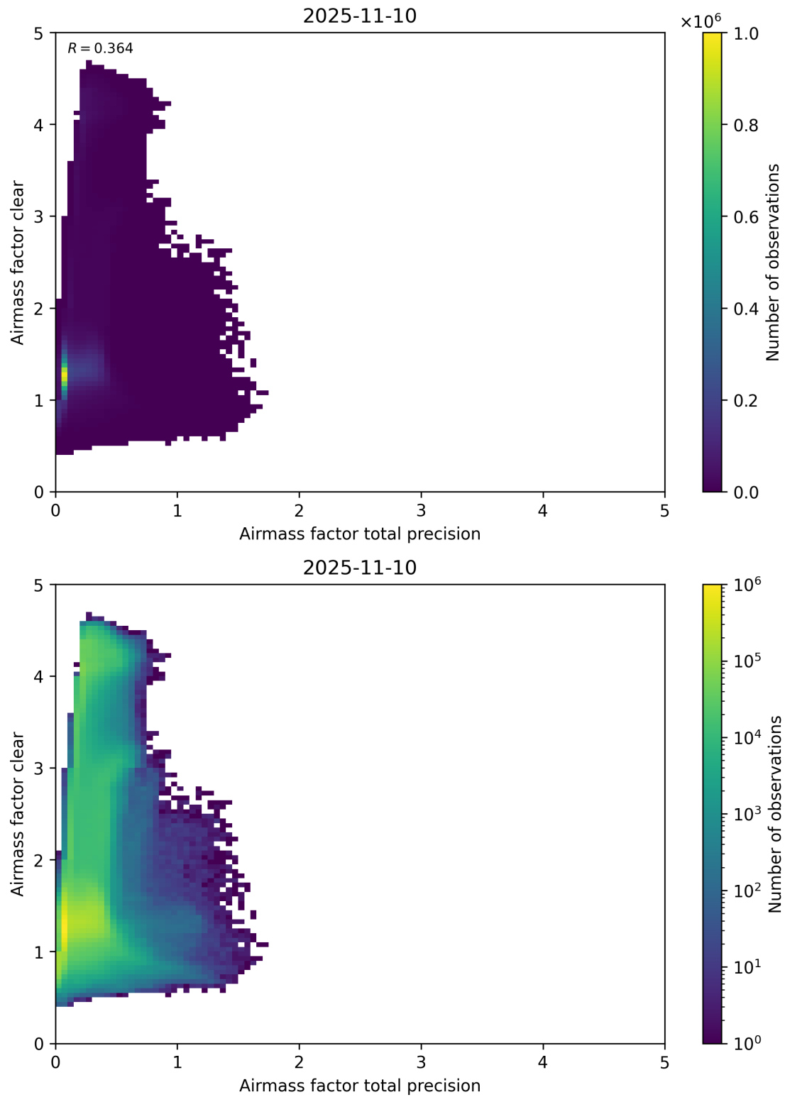
Figure 108: Scatter density plot of “Airmass factor total precision” against “Airmass factor clear” for 2025-11-09 to 2025-11-11.
