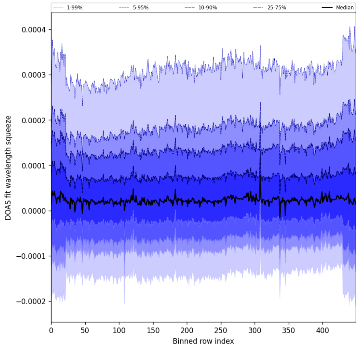
Figure 59: Along track statistics of “DOAS fit wavelength squeeze” for 2025-11-09 to 2025-11-11
