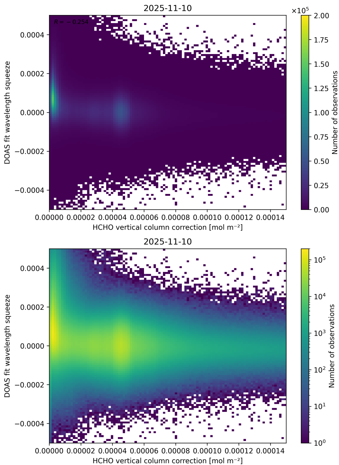
Figure 114: Scatter density plot of “HCHO vertical column correction” against “DOAS fit wavelength squeeze” for 2025-11-09 to 2025-11-11.
