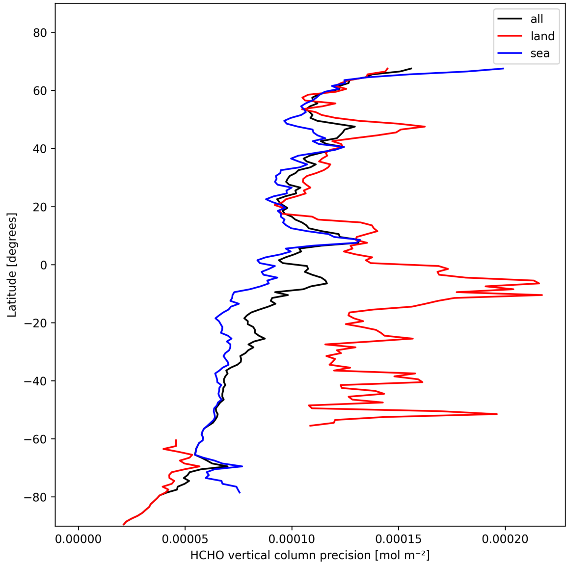
Figure 22: Zonal average of “HCHO vertical column precision” for 2025-11-09 to 2025-11-11.
