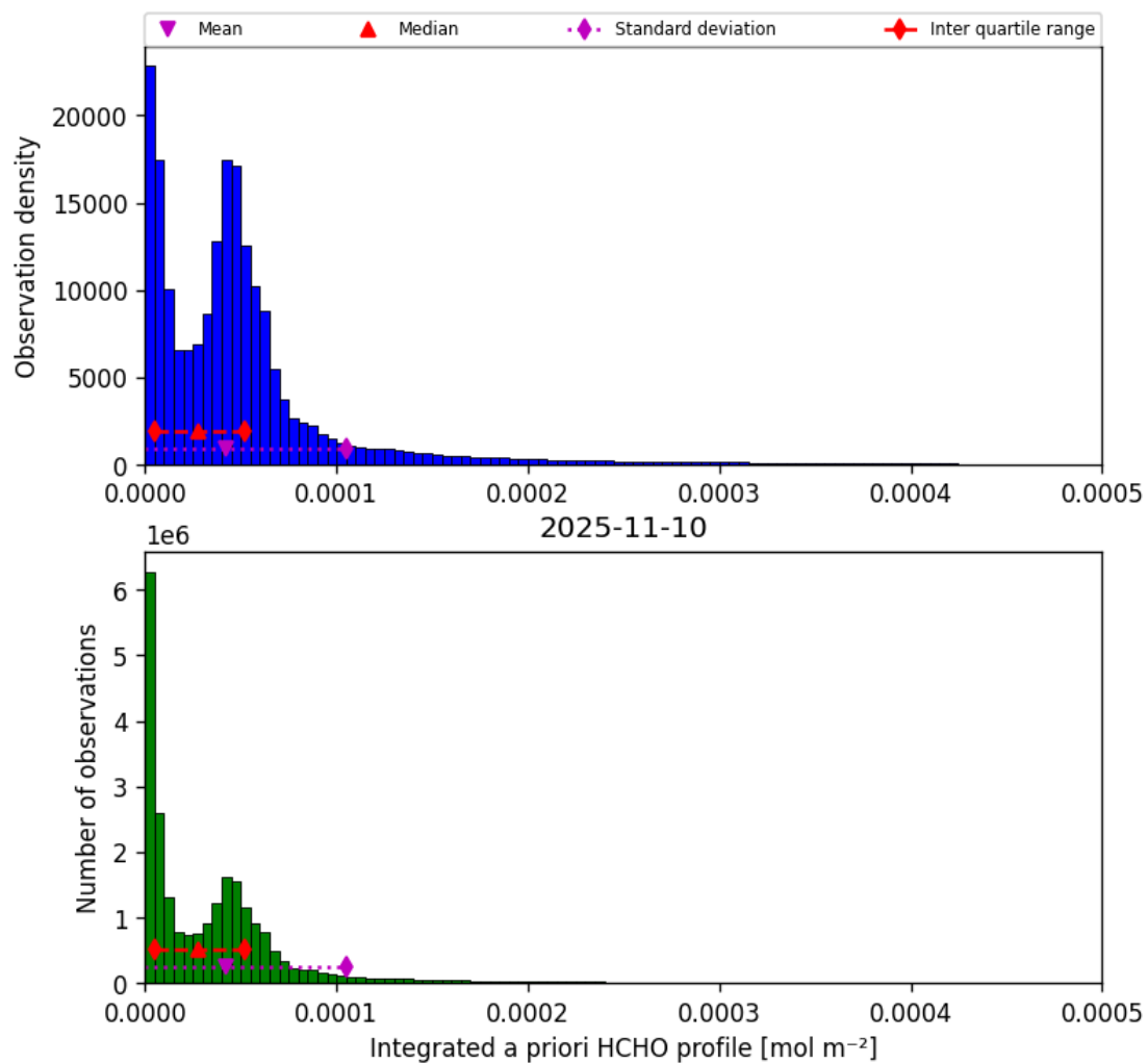
Figure 43: Histogram of “Integrated a priori HCHO profile” for 2025-11-09 to 2025-11-11
