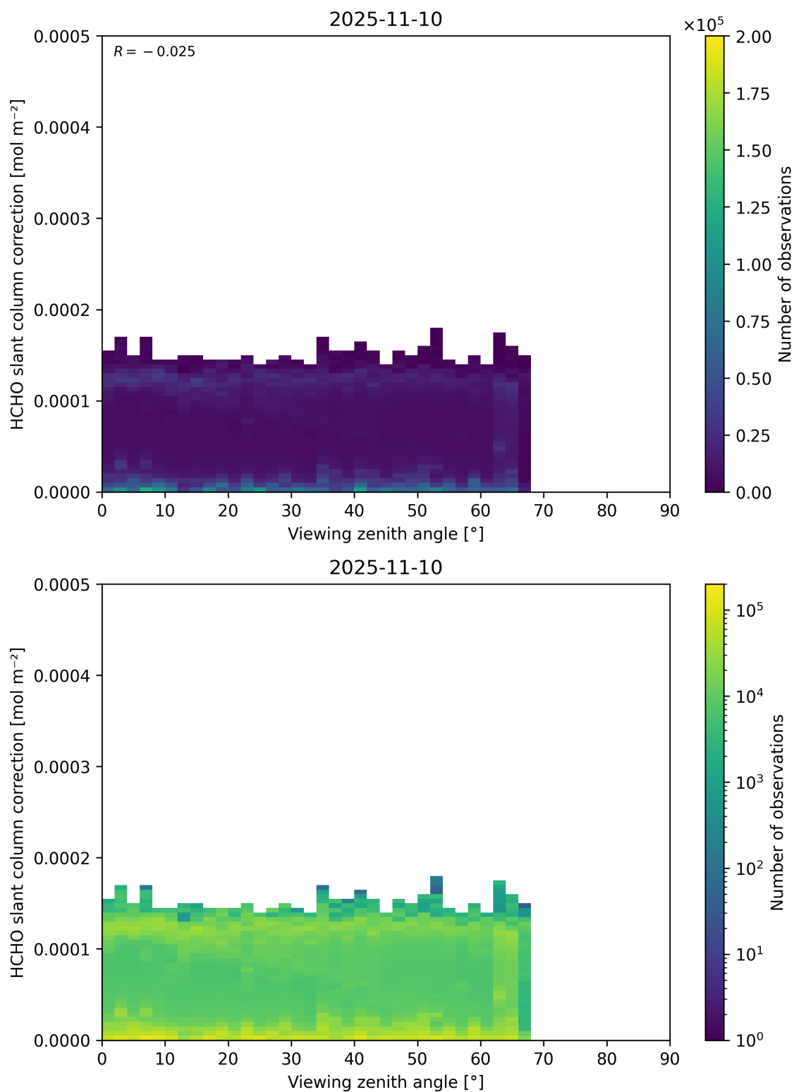
Figure 187: Scatter density plot of “Viewing zenith angle” against “HCHO slant column correction” for 2025-11-09 to 2025-11-11.
