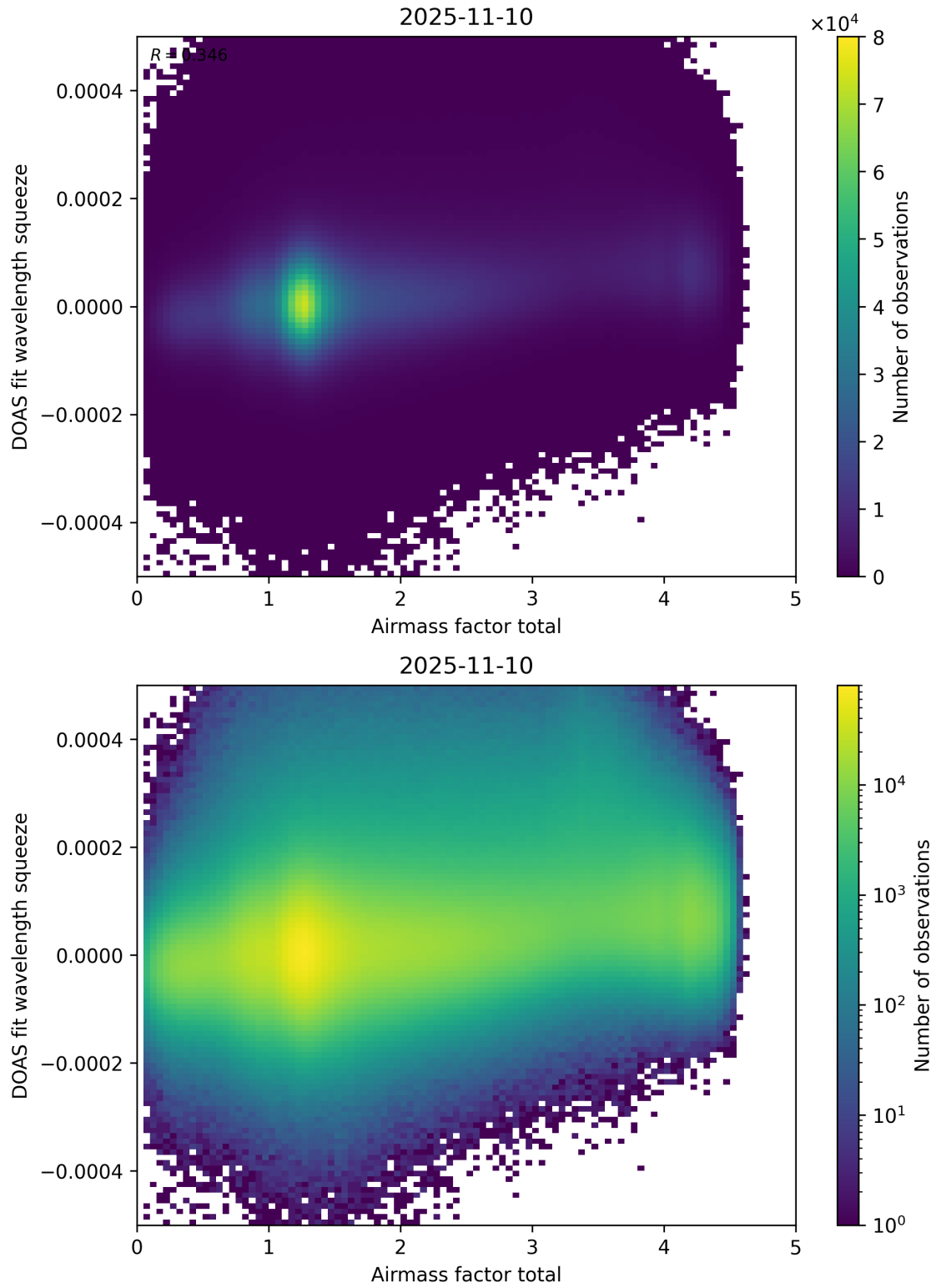
Figure 99: Scatter density plot of “Airmass factor total” against “DOAS fit wavelength squeeze” for 2025-11-09 to 2025-11-11.
