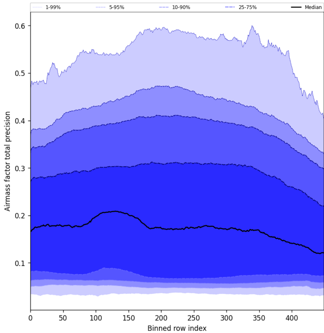
Figure 55: Along track statistics of “Airmass factor total precision” for 2025-11-09 to 2025-11-11
