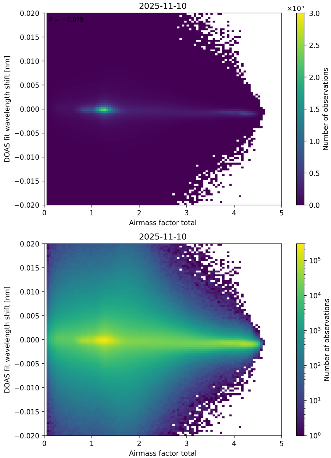
Figure 98: Scatter density plot of “Airmass factor total” against “DOAS fit wavelength shift” for 2025-11-09 to 2025-11-11.
