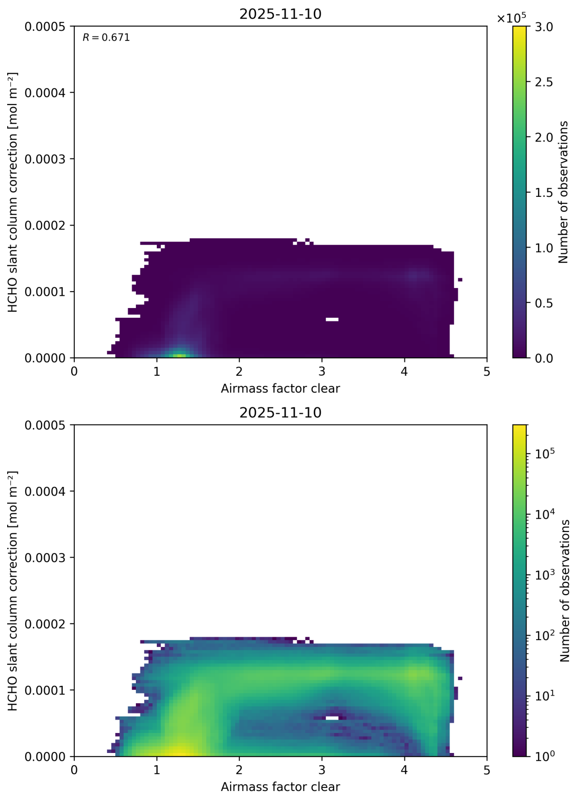
Figure 75: Scatter density plot of “Airmass factor clear” against “HCHO slant column correction” for 2025-11-09 to 2025-11-11.
