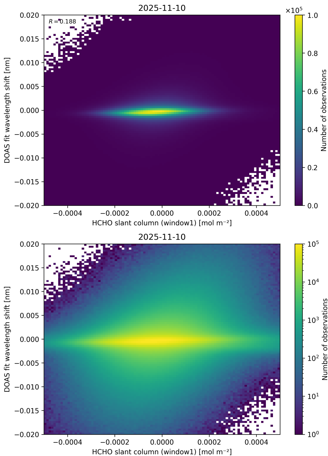
Figure 79: Scatter density plot of “HCHO slant column (window1)” against “DOAS fit wavelength shift” for 2025-11-09 to 2025-11-11.
