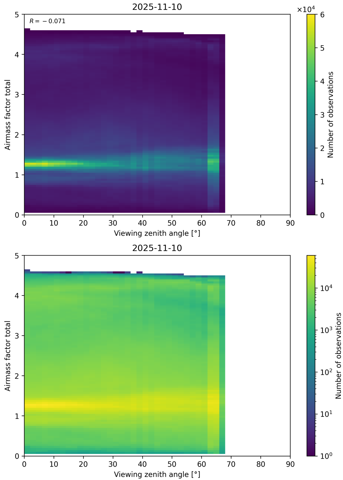
Figure 190: Scatter density plot of “Viewing zenith angle” against “Airmass factor total” for 2025-11-09 to 2025-11-11.
