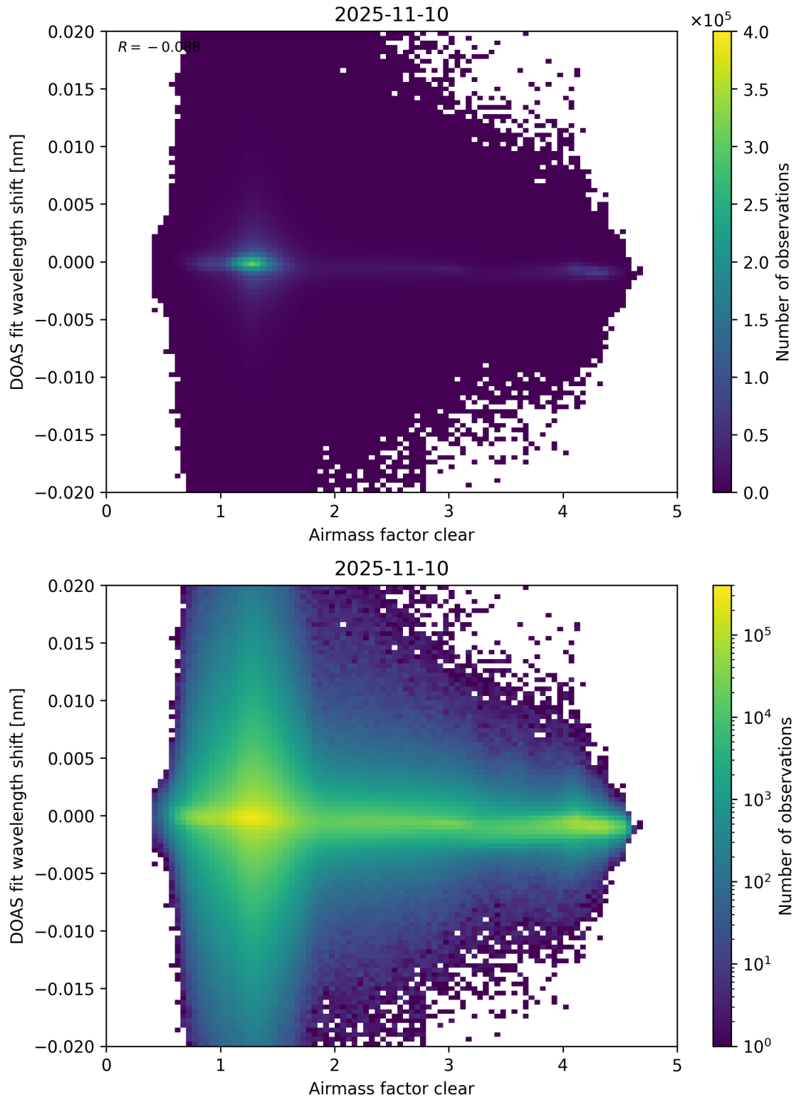
Figure 72: Scatter density plot of “Airmass factor clear” against “DOAS fit wavelength shift” for 2025-11-09 to 2025-11-11.
