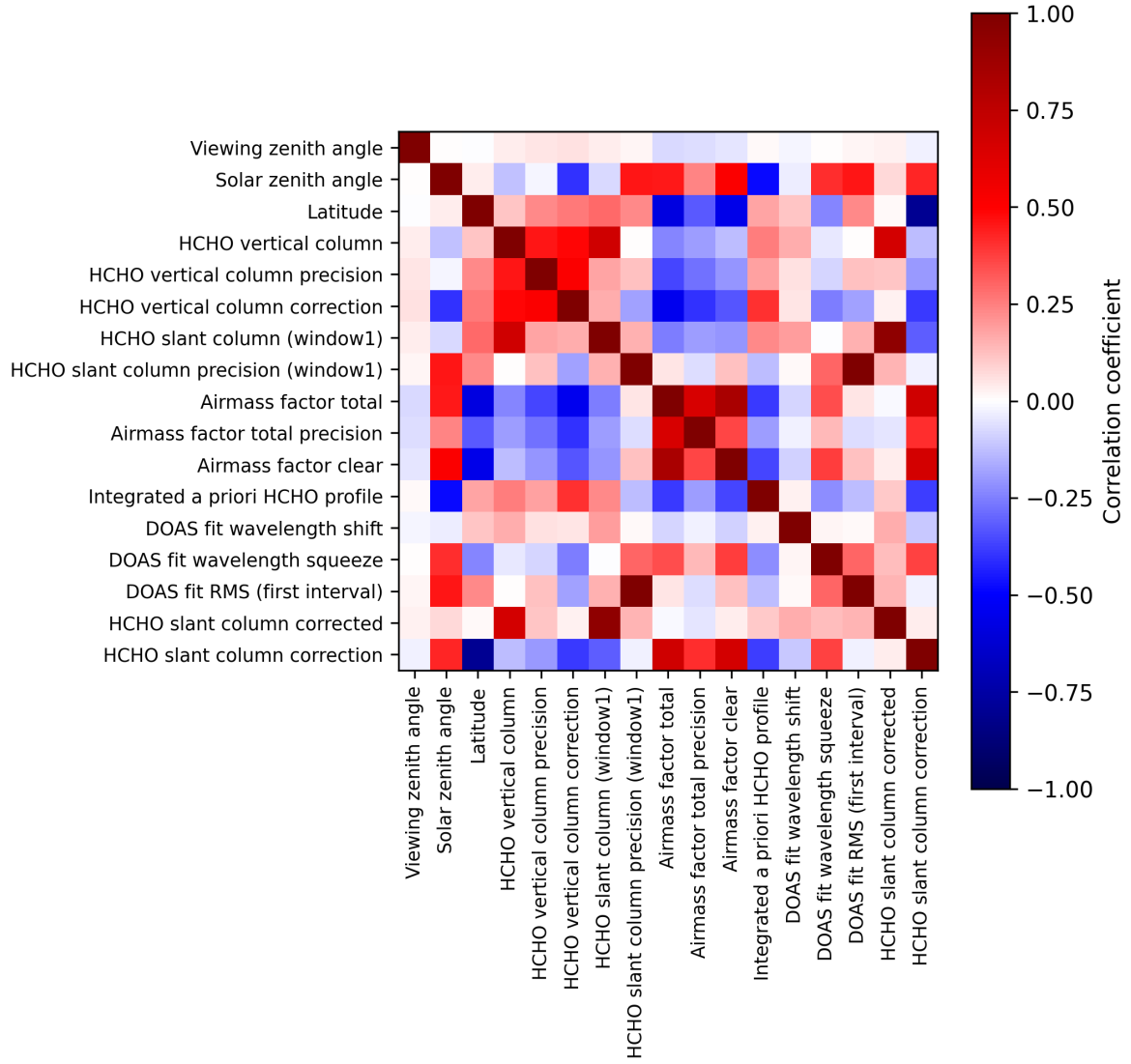
Figure 2: Map of correlation matrix for 2025-11-09 to 2025-11-11.
