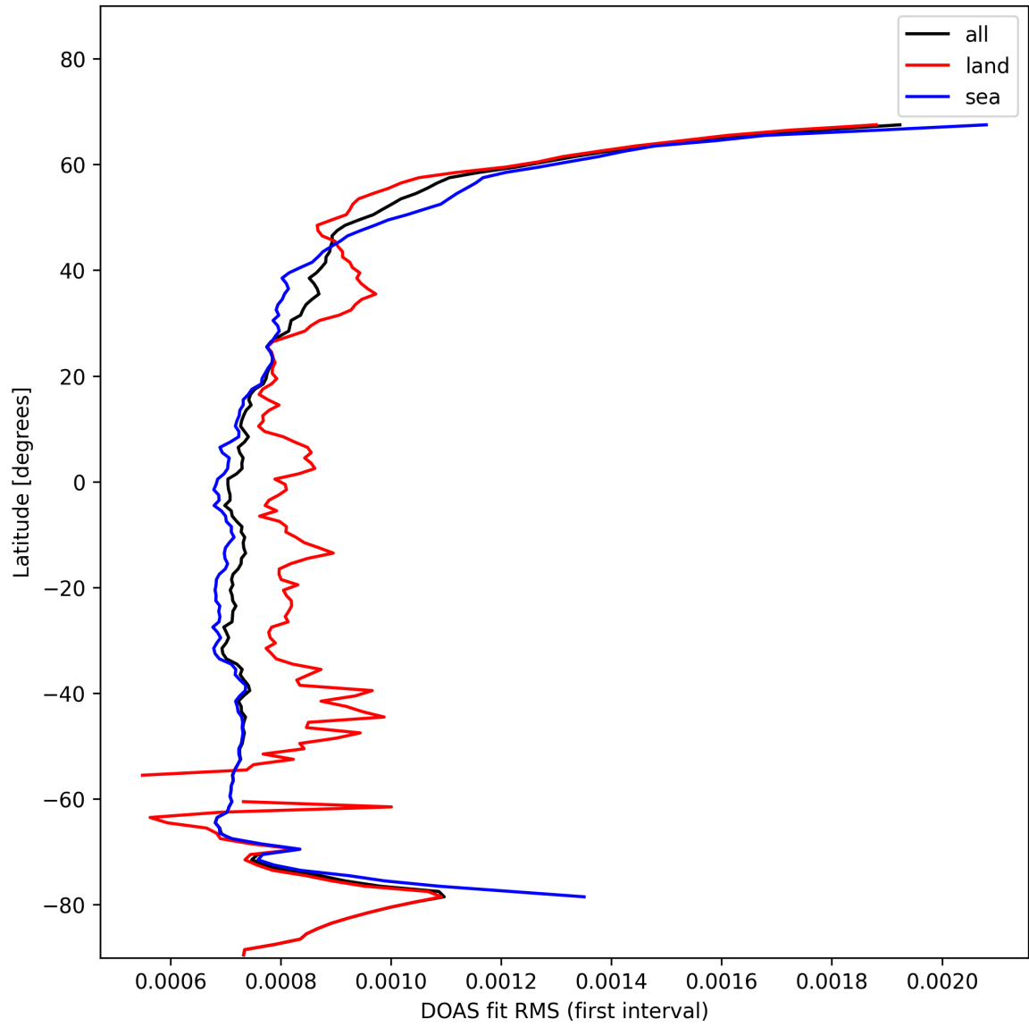
Figure 32: Zonal average of “DOAS fit RMS (first interval)” for 2025-11-09 to 2025-11-11.
