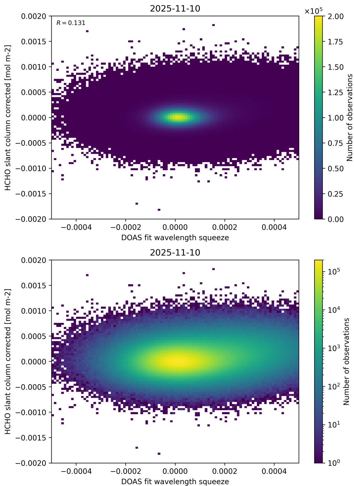
Figure 69: Scatter density plot of “DOAS fit wavelength squeeze” against “HCHO slant column corrected” for 2025-11-09 to 2025-11-11.
