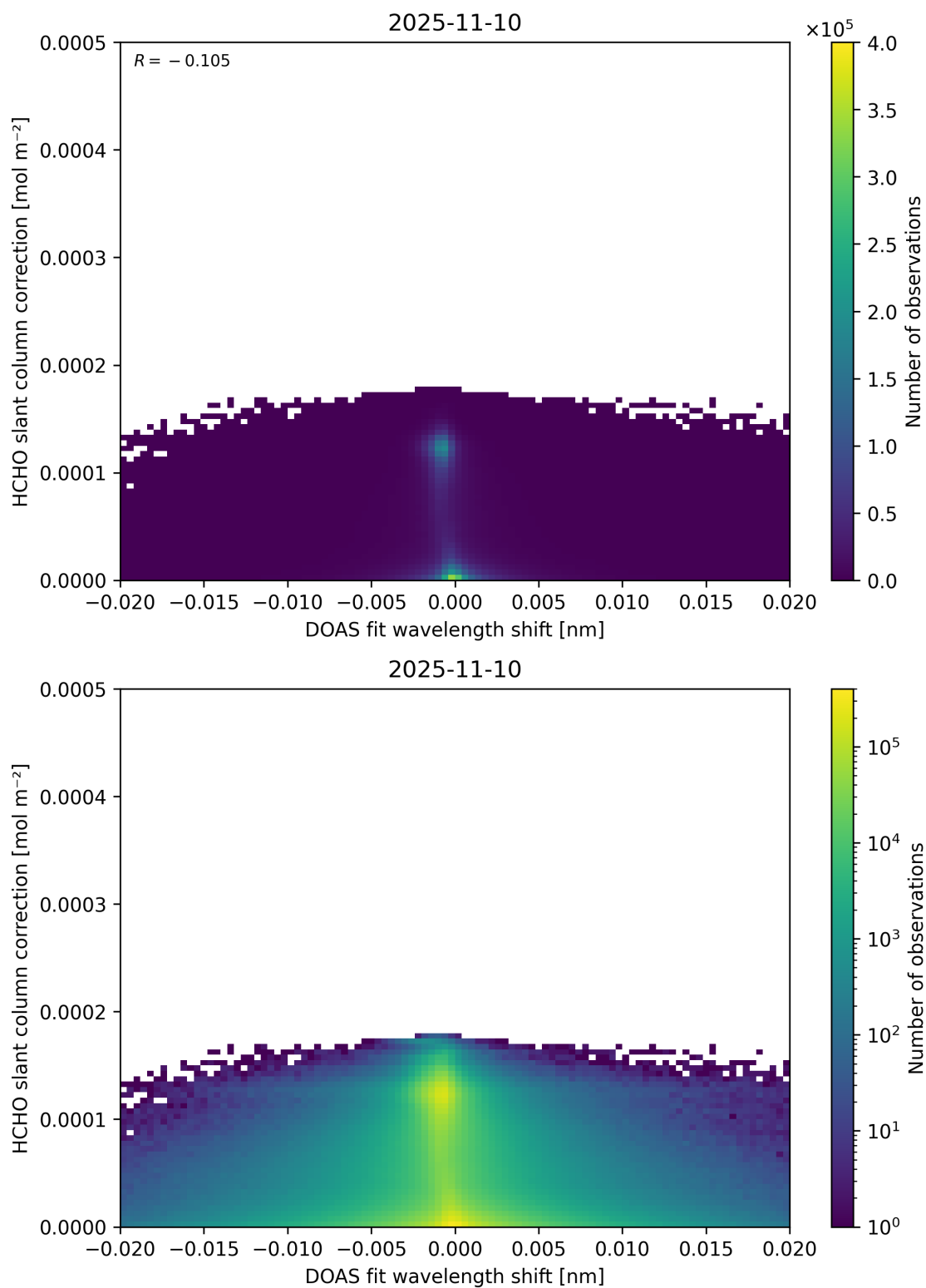
Figure 67: Scatter density plot of “DOAS fit wavelength shift” against “HCHO slant column correction” for 2025-11-09 to 2025-11-11.
