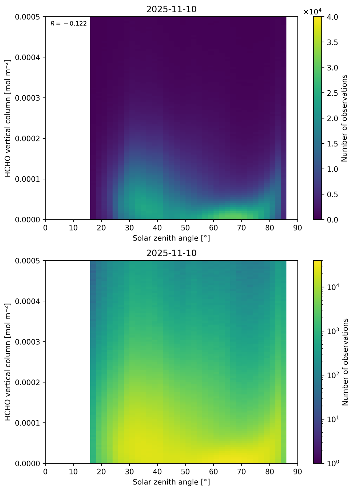
Figure 177: Scatter density plot of “Solar zenith angle” against “HCHO vertical column” for 2025-11-09 to 2025-11-11.
