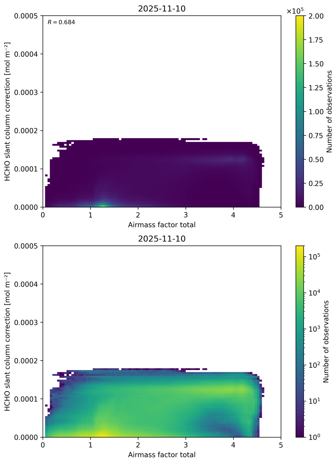
Figure 102: Scatter density plot of “Airmass factor total” against “HCHO slant column correction” for 2025-11-09 to 2025-11-11.
