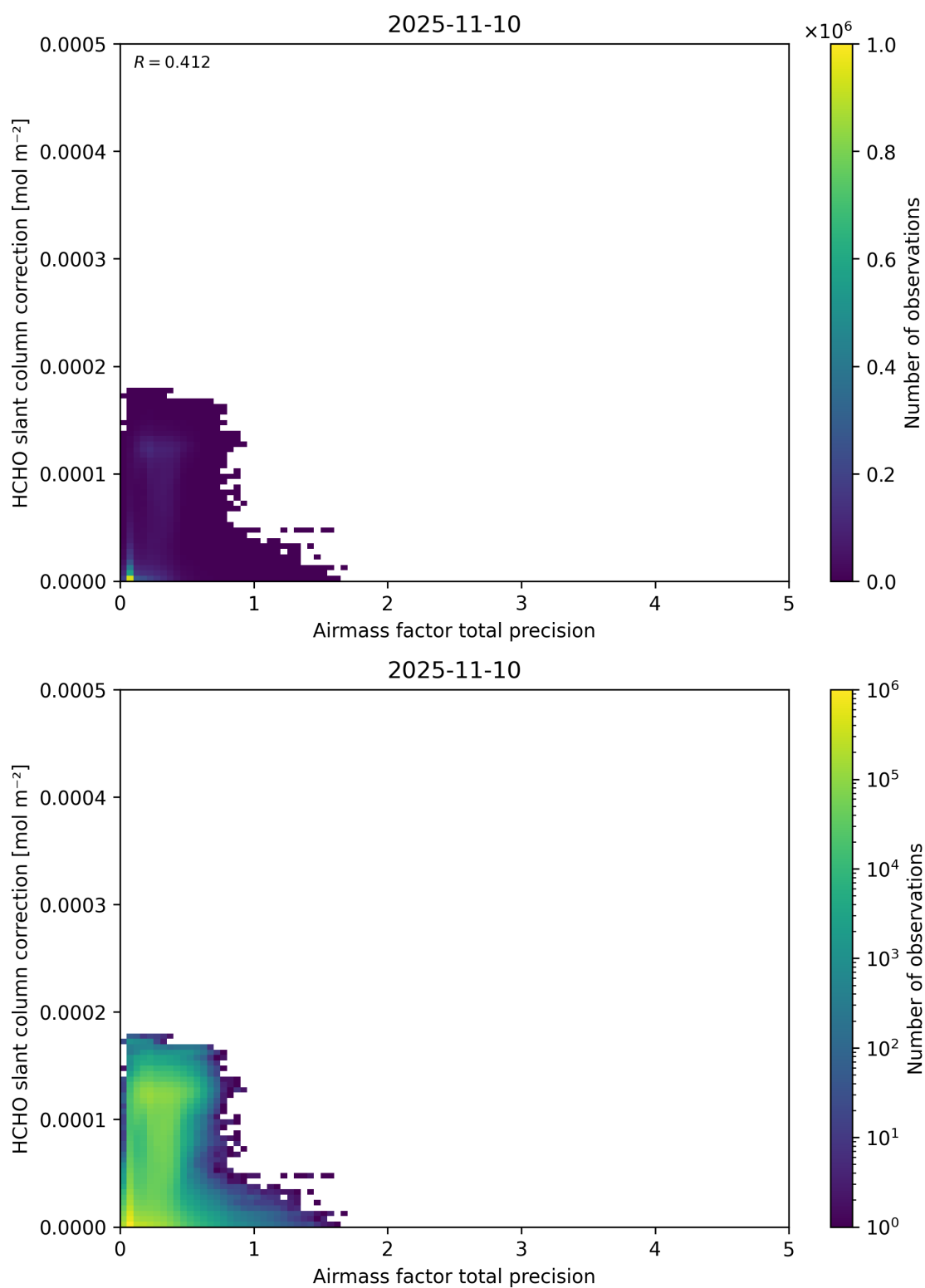
Figure 110: Scatter density plot of “Airmass factor total precision” against “HCHO slant column correction” for 2025-11-09 to 2025-11-11.
