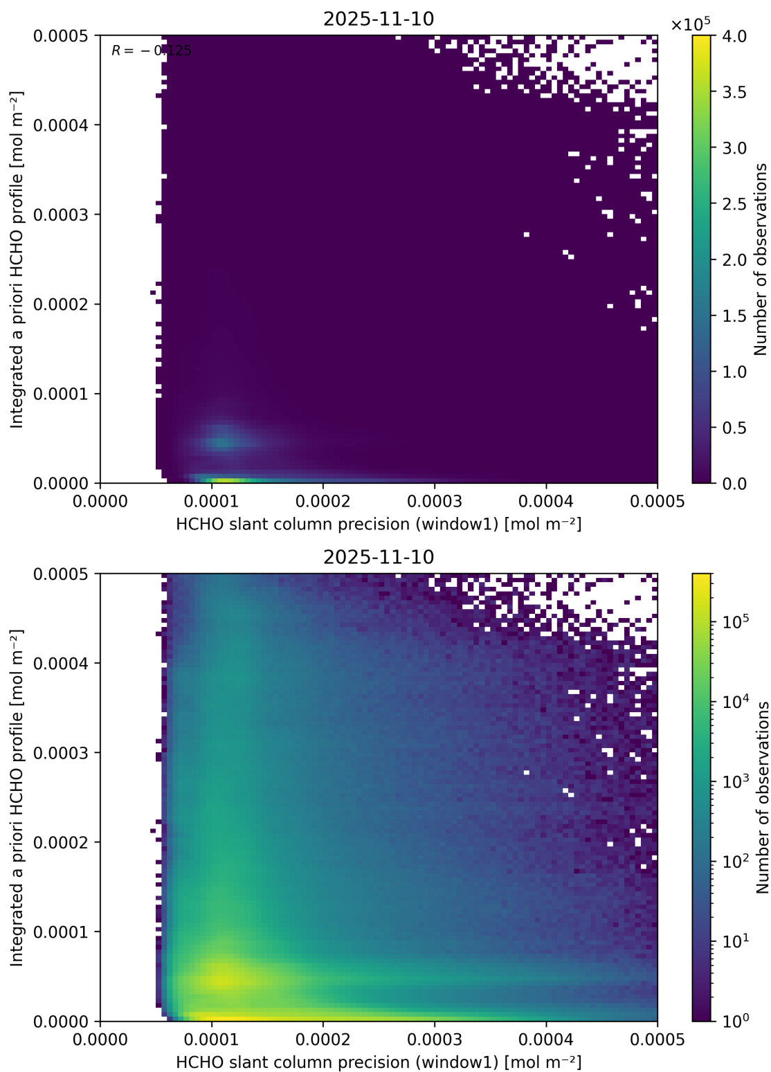
Figure 96: Scatter density plot of “HCHO slant column precision (window1)” against “Integrated a priori HCHO profile” for 2025-11-09 to 2025-11-11.
