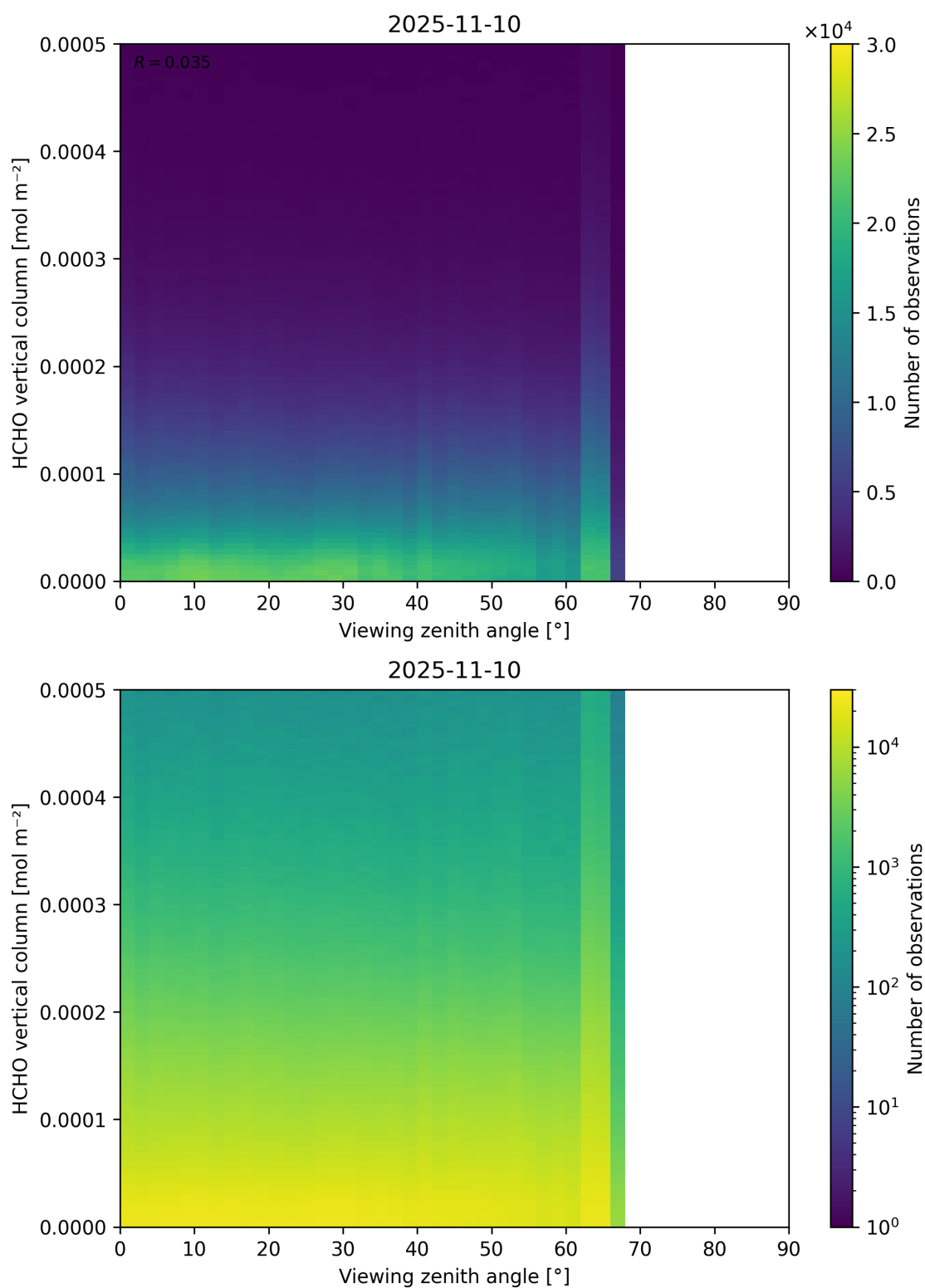
Figure 192: Scatter density plot of “Viewing zenith angle” against “HCHO vertical column” for 2025-11-09 to 2025-11-11.
