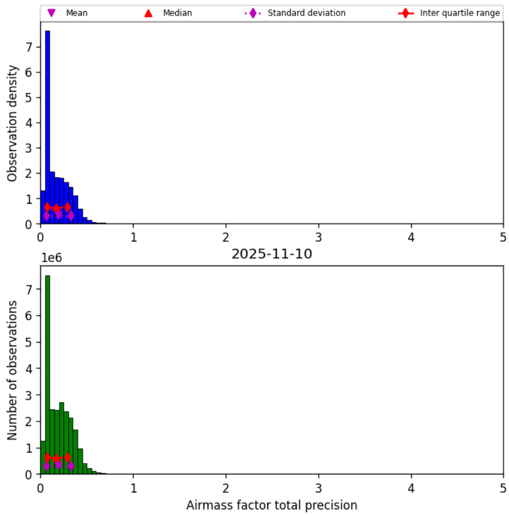
Figure 41: Histogram of “Airmass factor total precision” for 2025-11-09 to 2025-11-11
