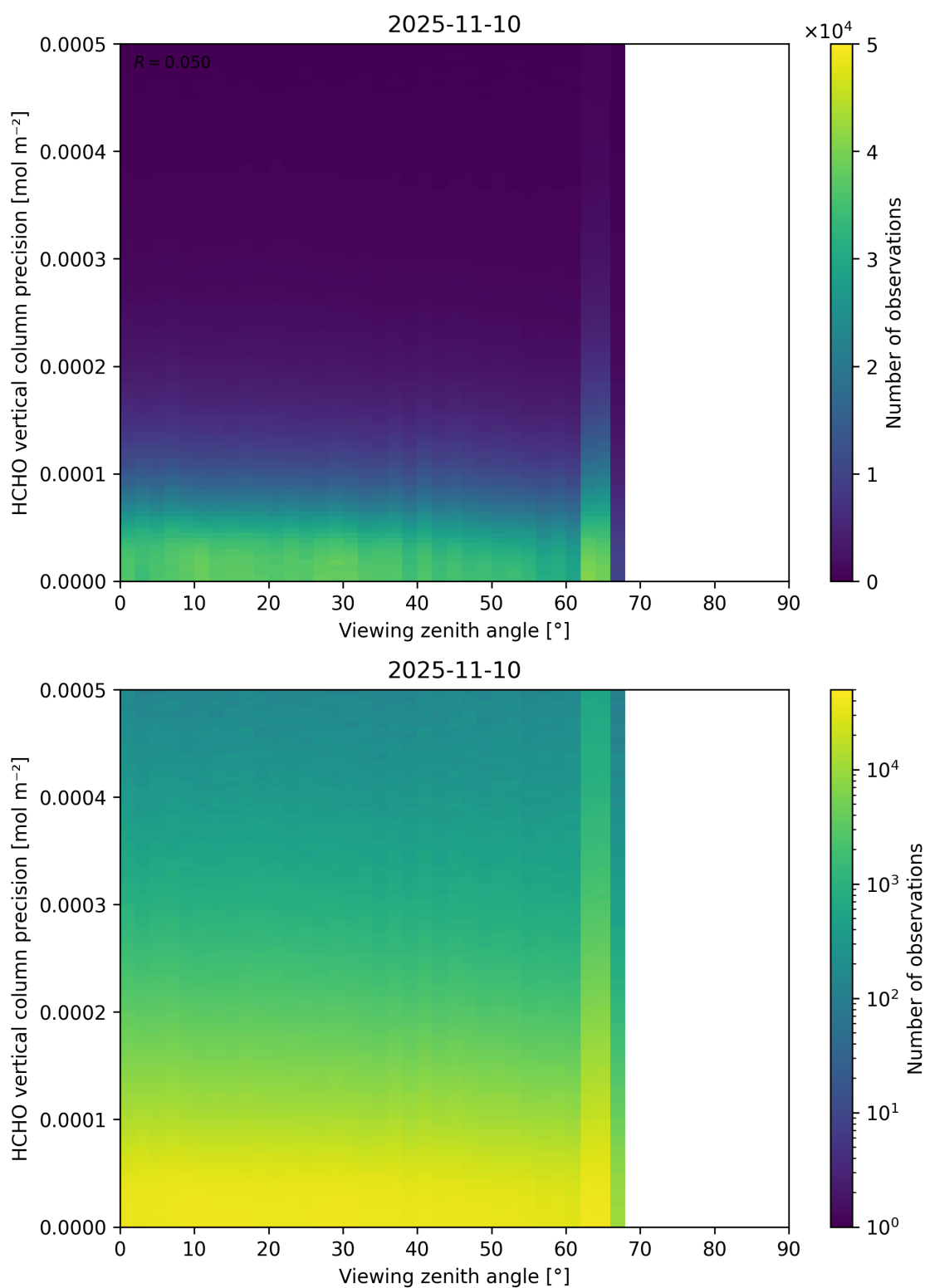
Figure 194: Scatter density plot of “Viewing zenith angle” against “HCHO vertical column precision” for 2025-11-09 to 2025-11-11.
