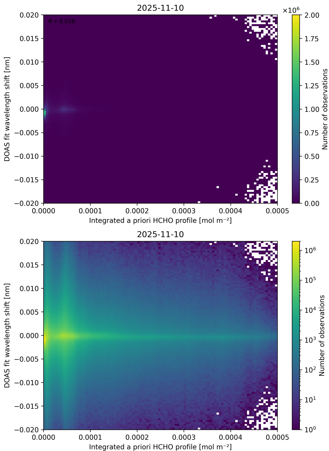
Figure 149: Scatter density plot of “Integrated a priori HCHO profile” against “DOAS fit wavelength shift” for 2025-11-09 to 2025-11-11.
