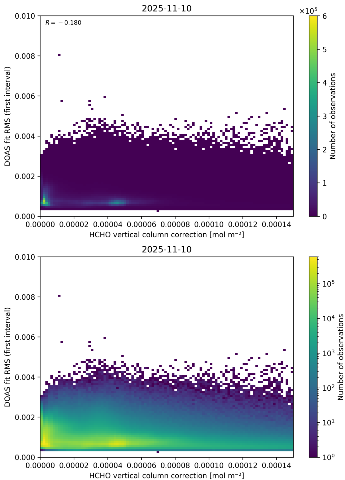
Figure 112: Scatter density plot of “HCHO vertical column correction” against “DOAS fit RMS (first interval)” for 2025-11-09 to 2025-11-11.
