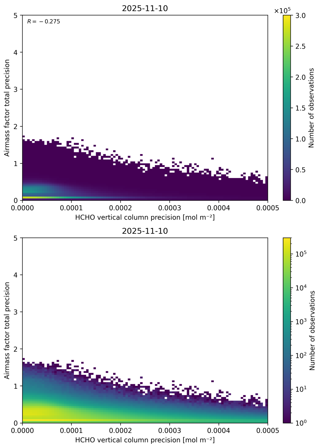
Figure 145: Scatter density plot of “HCHO vertical column precision” against “Airmass factor total precision” for 2025-11-09 to 2025-11-11.
