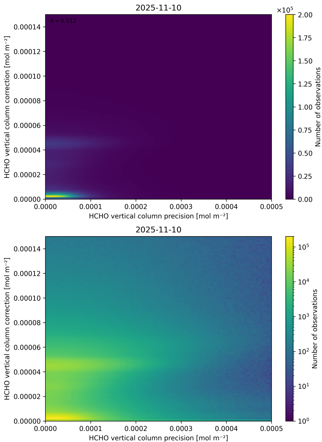
Figure 146: Scatter density plot of “HCHO vertical column precision” against “HCHO vertical column correction” for 2025-11-09 to 2025-11-11.
