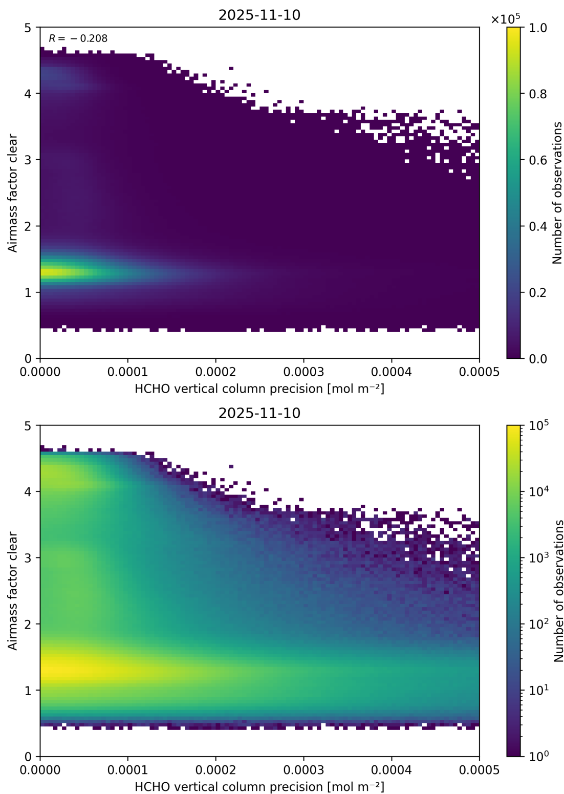
Figure 139: Scatter density plot of “HCHO vertical column precision” against “Airmass factor clear” for 2025-11-09 to 2025-11-11.
