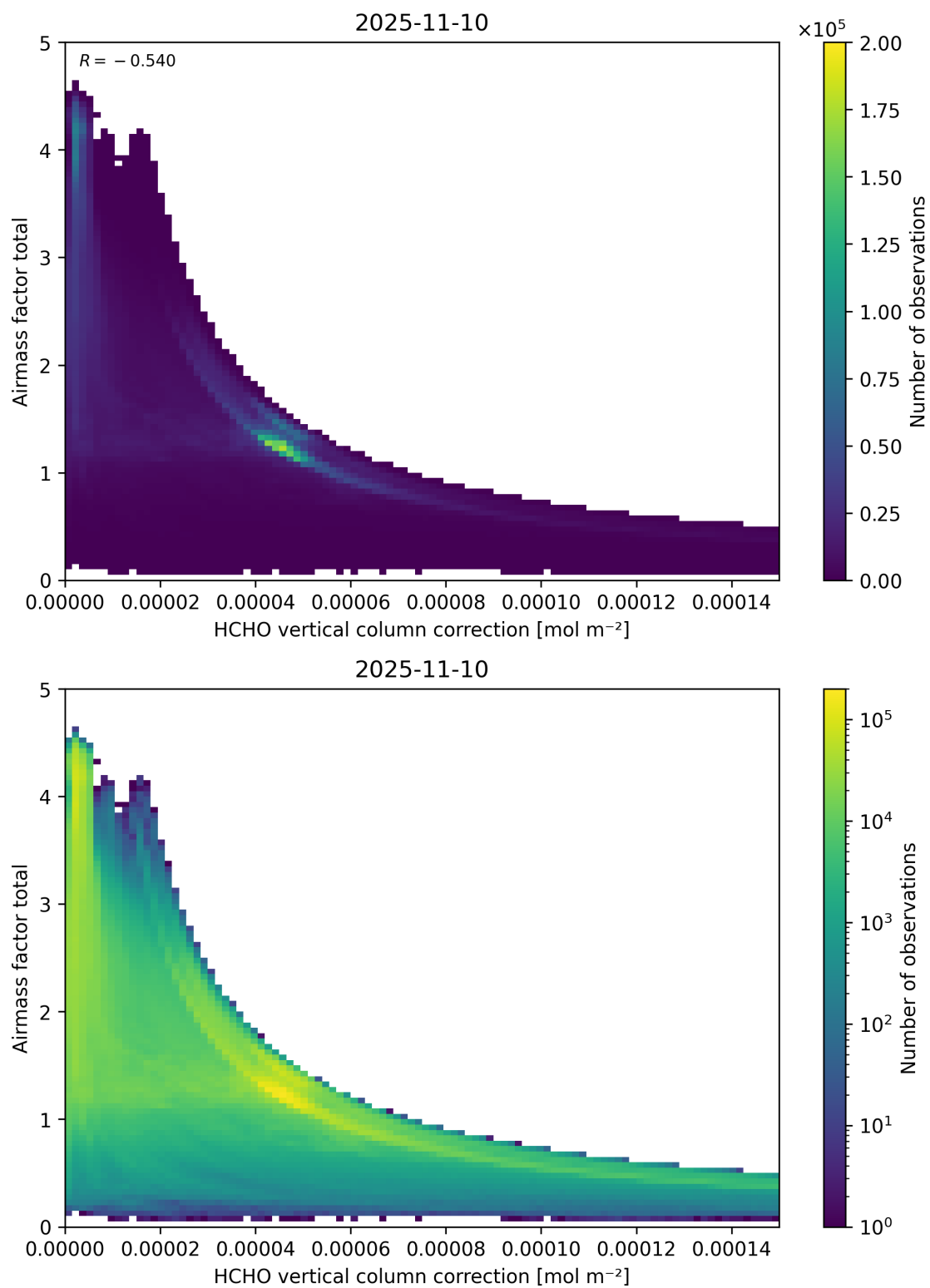
Figure 120: Scatter density plot of “HCHO vertical column correction” against “Airmass factor total” for 2025-11-09 to 2025-11-11.
