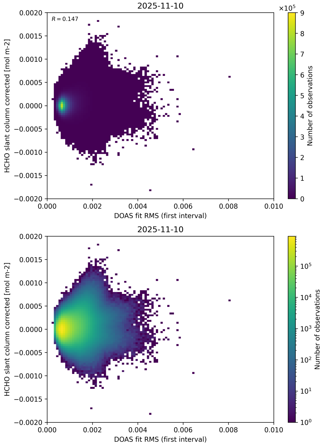
Figure 62: Scatter density plot of “DOAS fit RMS (first interval)” against “HCHO slant column corrected” for 2025-11-09 to 2025-11-11.
