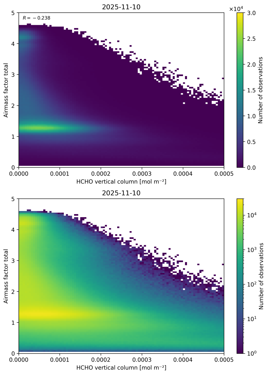
Figure 131: Scatter density plot of “HCHO vertical column” against “Airmass factor total” for 2025-11-09 to 2025-11-11.
