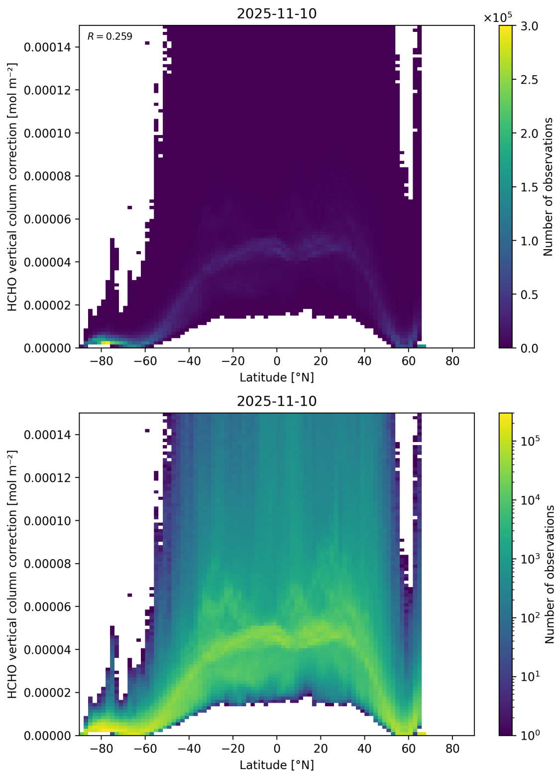
Figure 164: Scatter density plot of “Latitude” against “HCHO vertical column correction” for 2025-11-09 to 2025-11-11.
