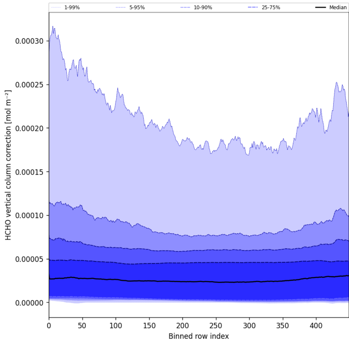
Figure 51: Along track statistics of “HCHO vertical column correction” for 2025-11-09 to 2025-11-11
