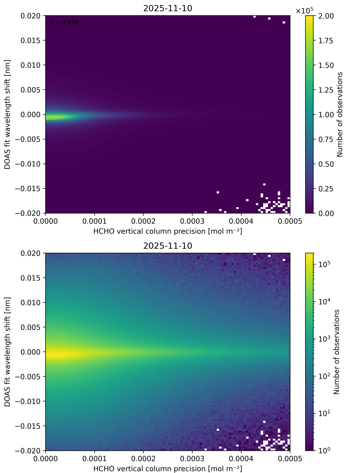
Figure 137: Scatter density plot of “HCHO vertical column precision” against “DOAS fit wavelength shift” for 2025-11-09 to 2025-11-11.
