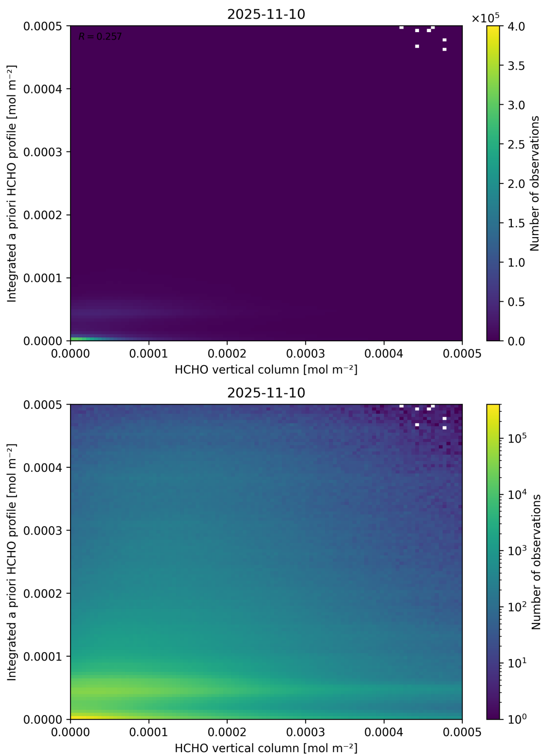
Figure 135: Scatter density plot of “HCHO vertical column” against “Integrated a priori HCHO profile” for 2025-11-09 to 2025-11-11.
