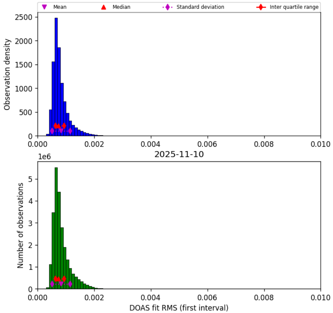
Figure 46: Histogram of “DOAS fit RMS (first interval)” for 2025-11-09 to 2025-11-11
