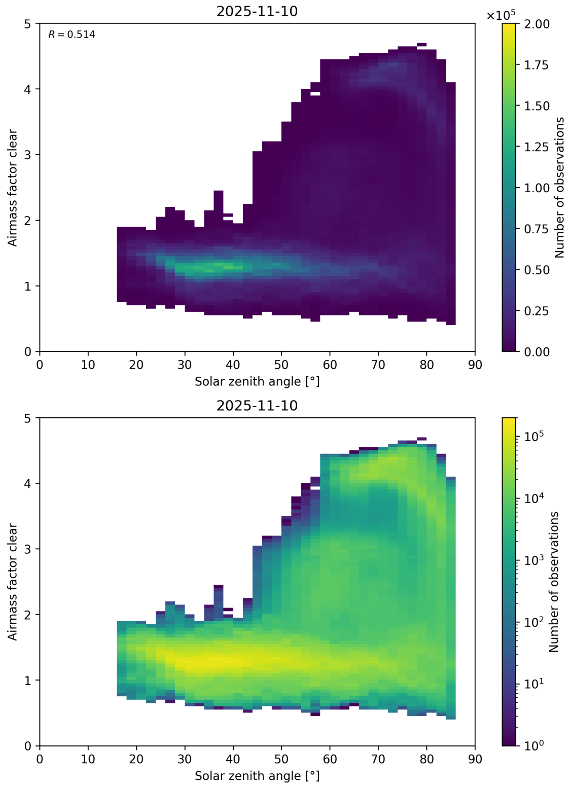
Figure 170: Scatter density plot of “Solar zenith angle” against “Airmass factor clear” for 2025-11-09 to 2025-11-11.
