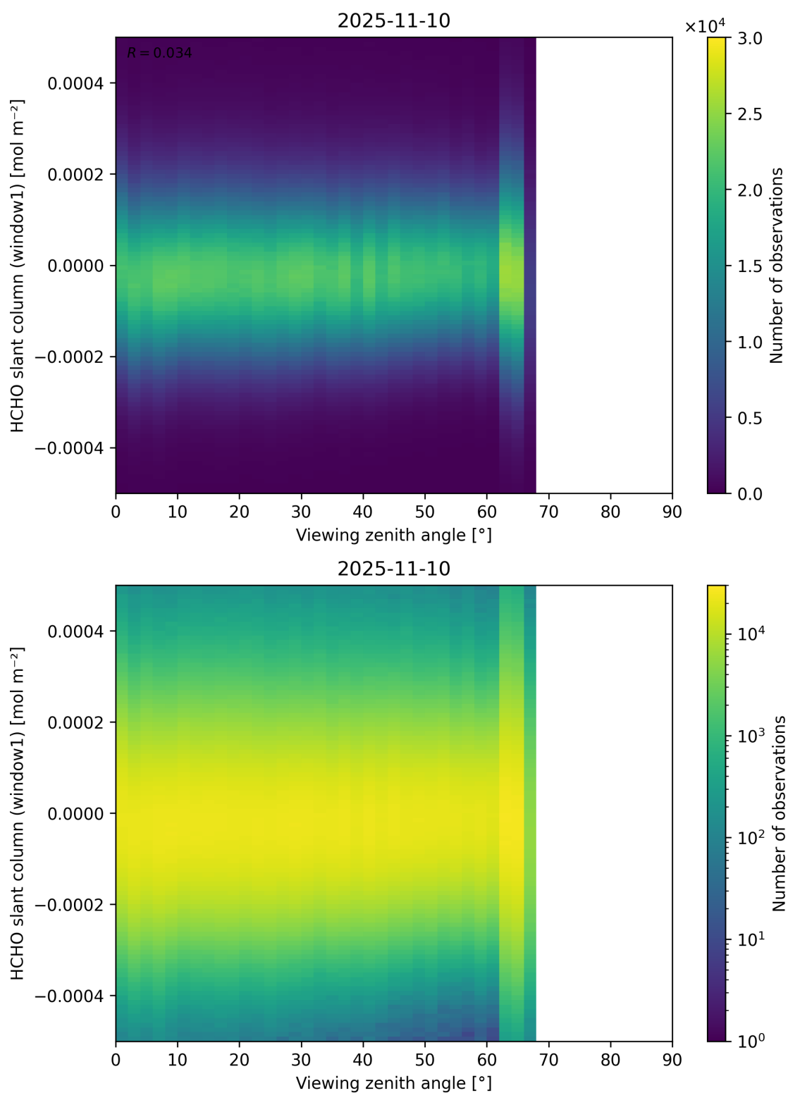
Figure 188: Scatter density plot of “Viewing zenith angle” against “HCHO slant column (window1)” for 2025-11-09 to 2025-11-11.
