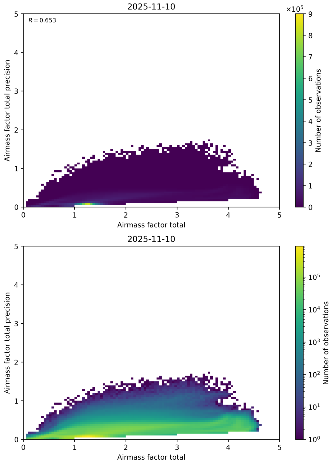
Figure 103: Scatter density plot of “Airmass factor total” against “Airmass factor total precision” for 2025-11-09 to 2025-11-11.
