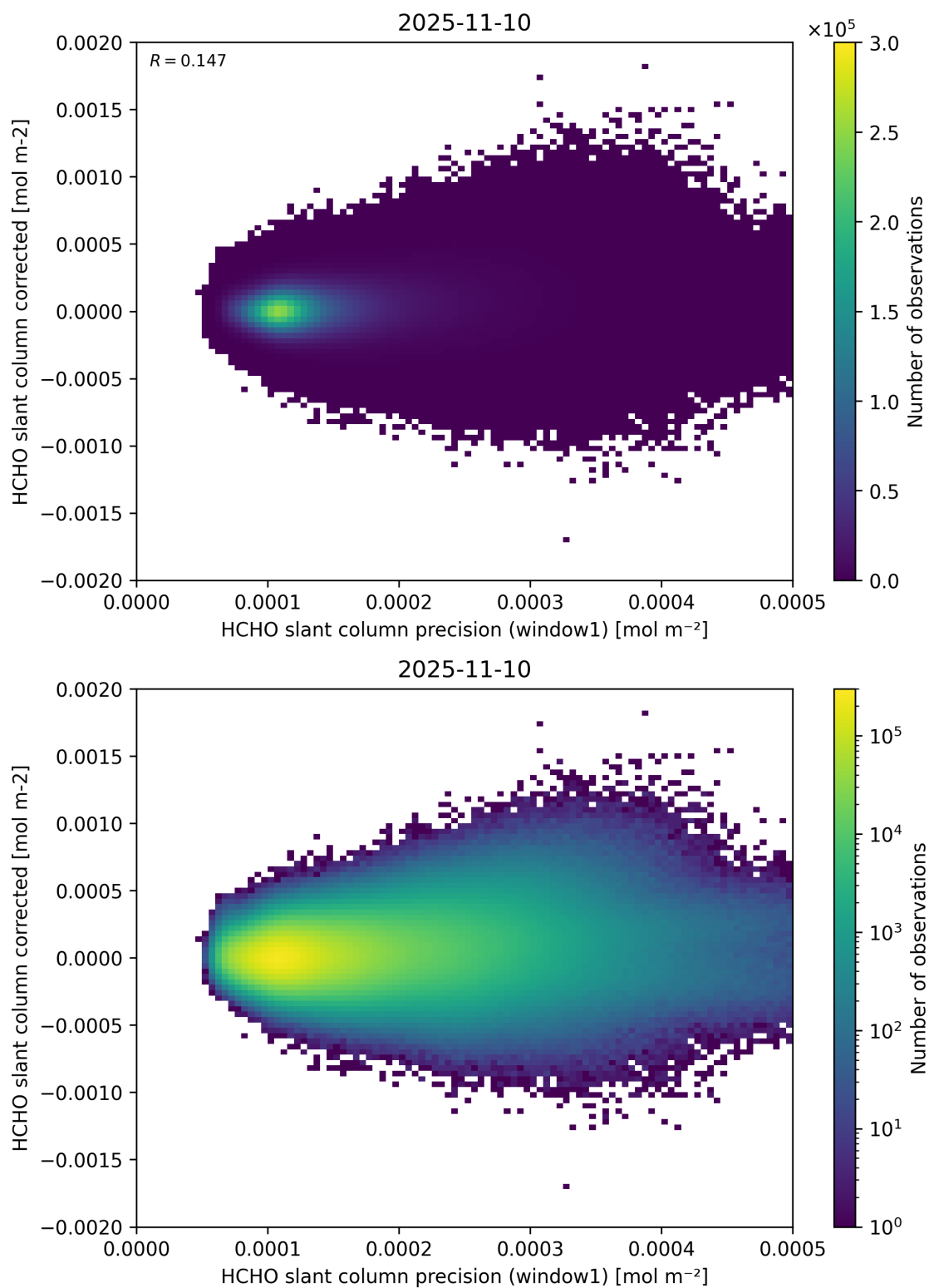
Figure 92: Scatter density plot of “HCHO slant column precision (window1)” against “HCHO slant column corrected” for 2025-11-09 to 2025-11-11.
