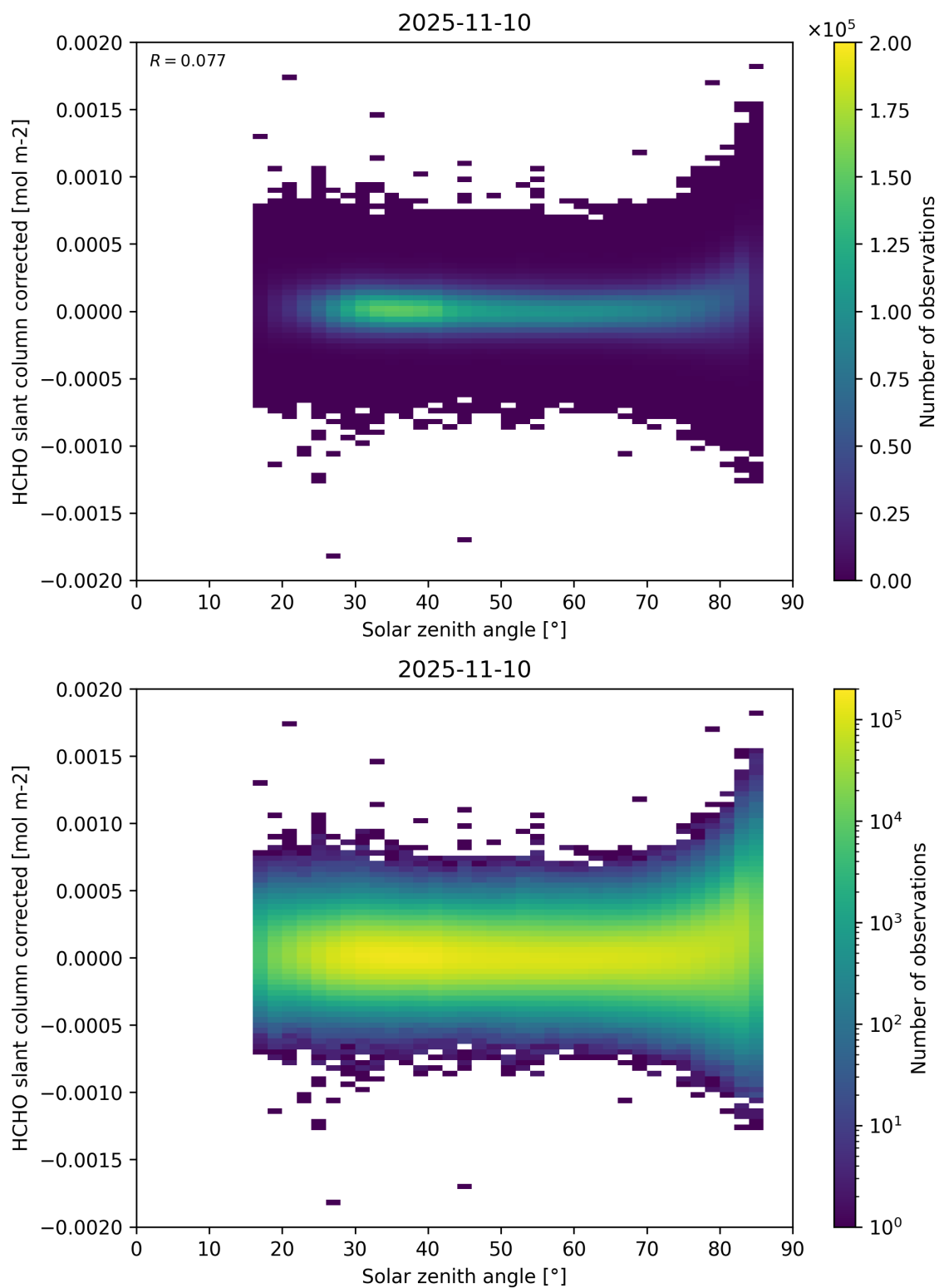
Figure 171: Scatter density plot of “Solar zenith angle” against “HCHO slant column corrected” for 2025-11-09 to 2025-11-11.
