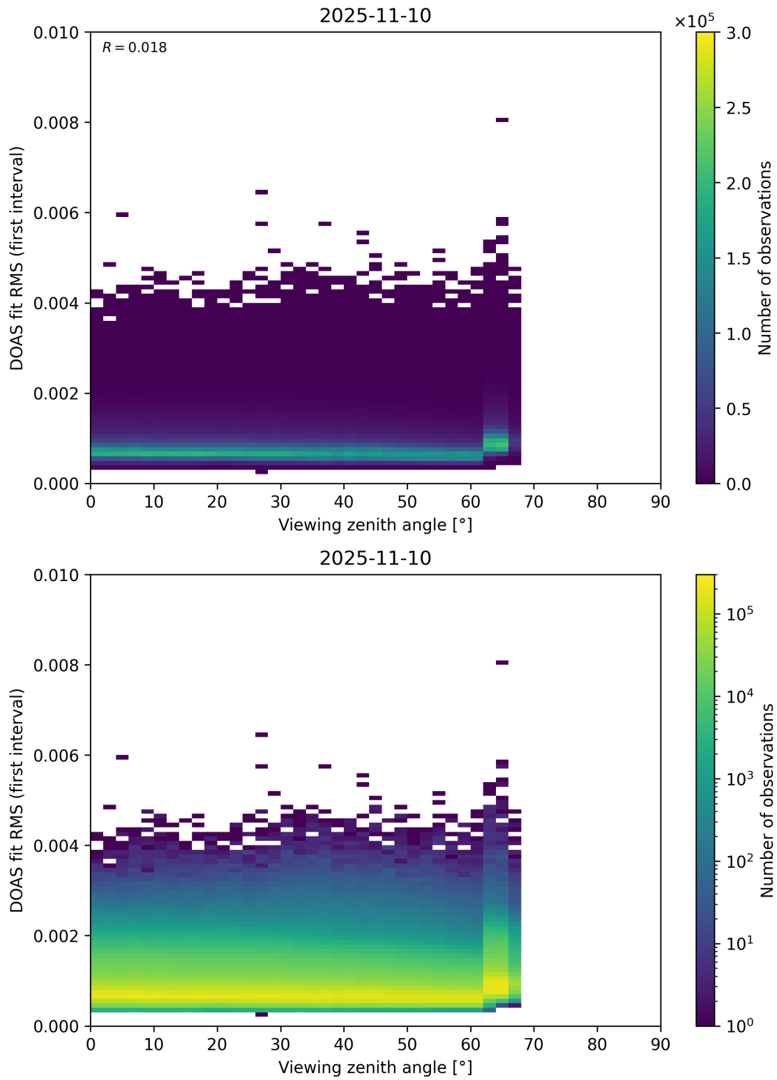
Figure 182: Scatter density plot of “Viewing zenith angle” against “DOAS fit RMS (first interval)” for 2025-11-09 to 2025-11-11.
