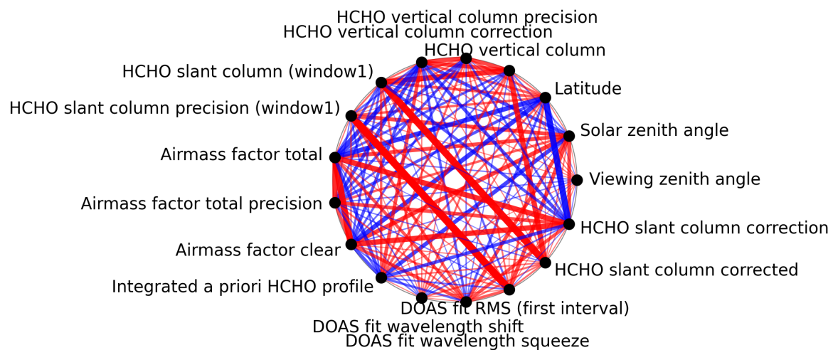
Figure 1: Map of correlation graph for 2025-11-09 to 2025-11-11.
