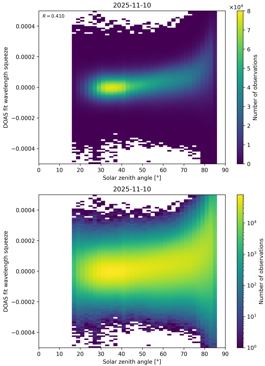
Figure 169: Scatter density plot of “Solar zenith angle” against “DOAS fit wavelength squeeze” for 2025-11-09 to 2025-11-11.
