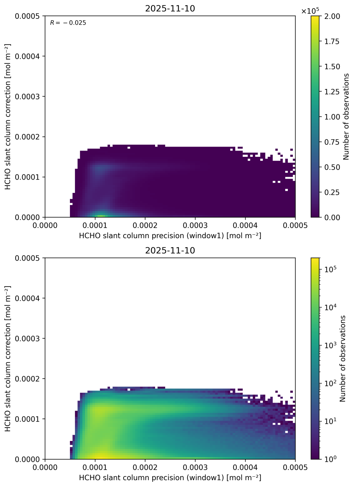
Figure 93: Scatter density plot of “HCHO slant column precision (window1)” against “HCHO slant column correction” for 2025-11-09 to 2025-11-11.
