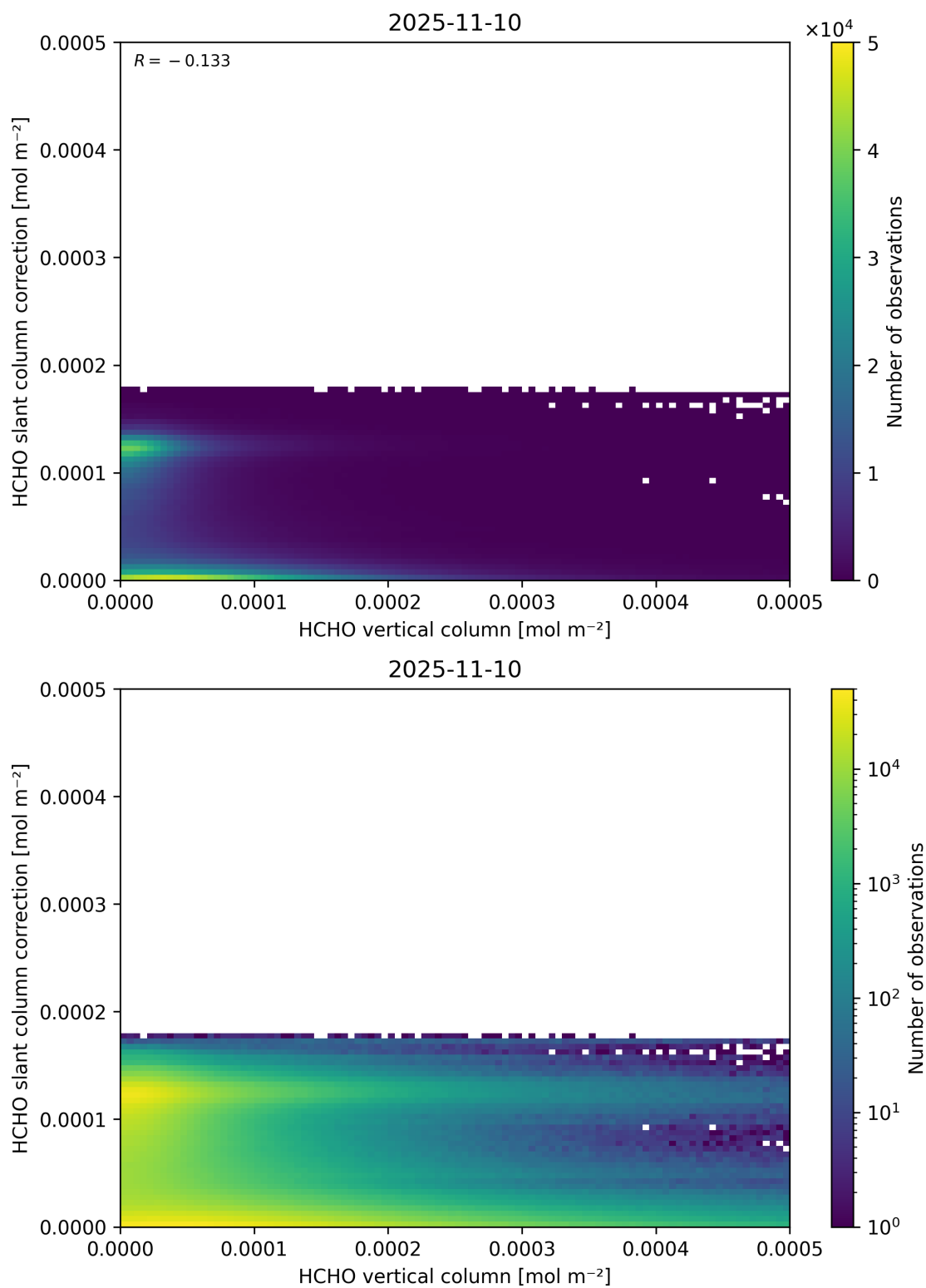
Figure 128: Scatter density plot of “HCHO vertical column” against “HCHO slant column correction” for 2025-11-09 to 2025-11-11.
