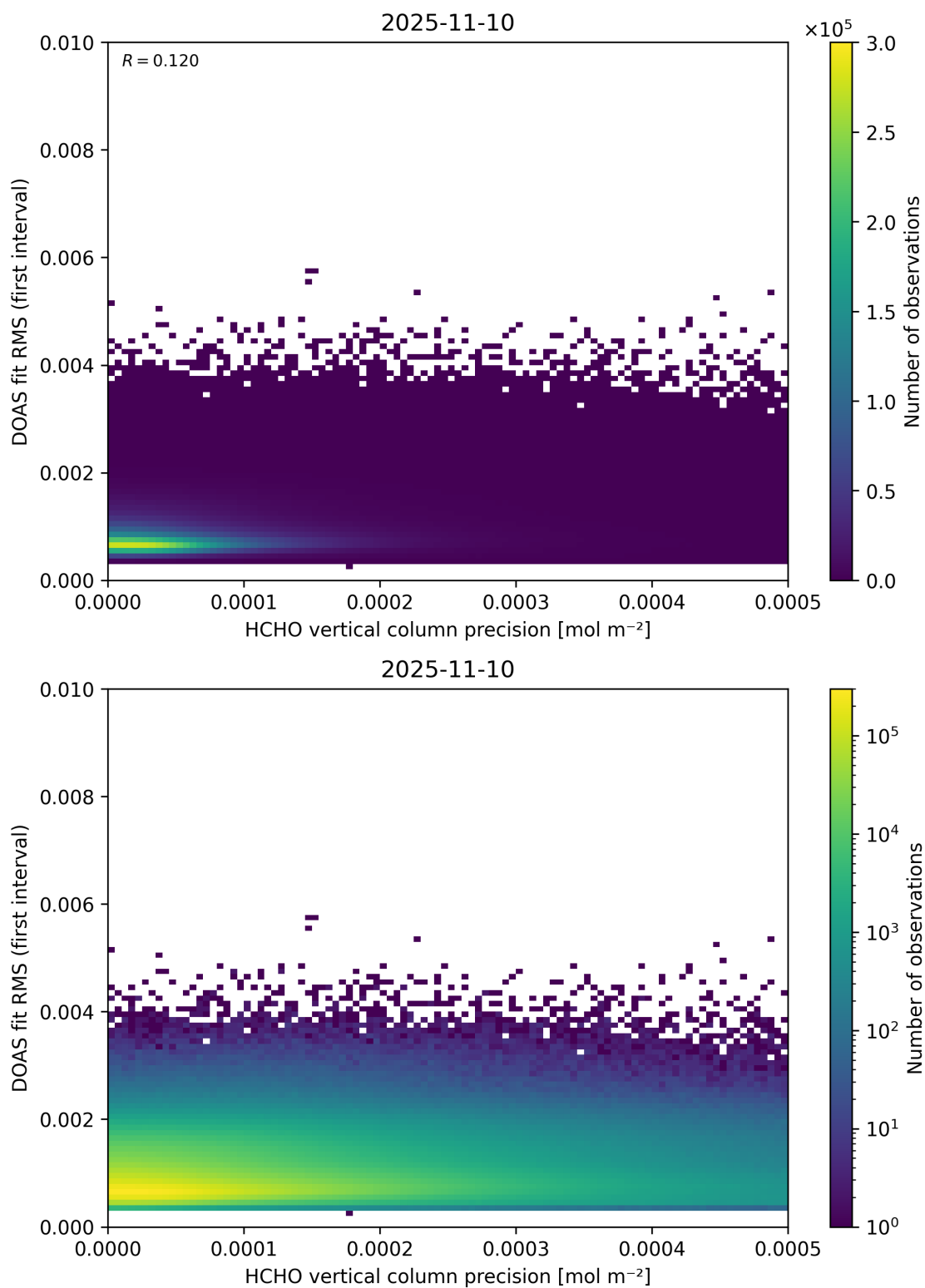
Figure 136: Scatter density plot of “HCHO vertical column precision” against “DOAS fit RMS (first interval)” for 2025-11-09 to 2025-11-11.
