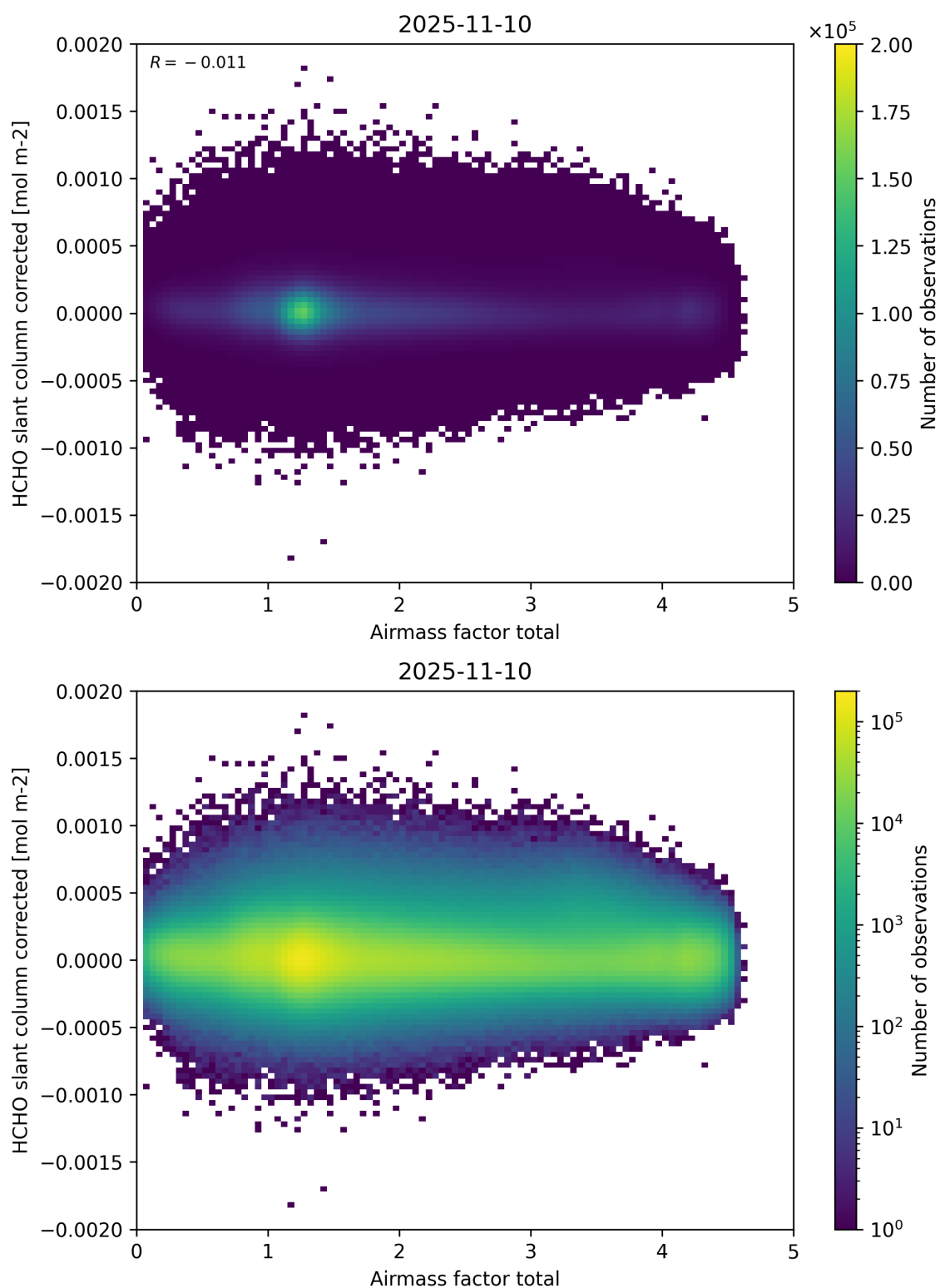
Figure 101: Scatter density plot of “Airmass factor total” against “HCHO slant column corrected” for 2025-11-09 to 2025-11-11.
