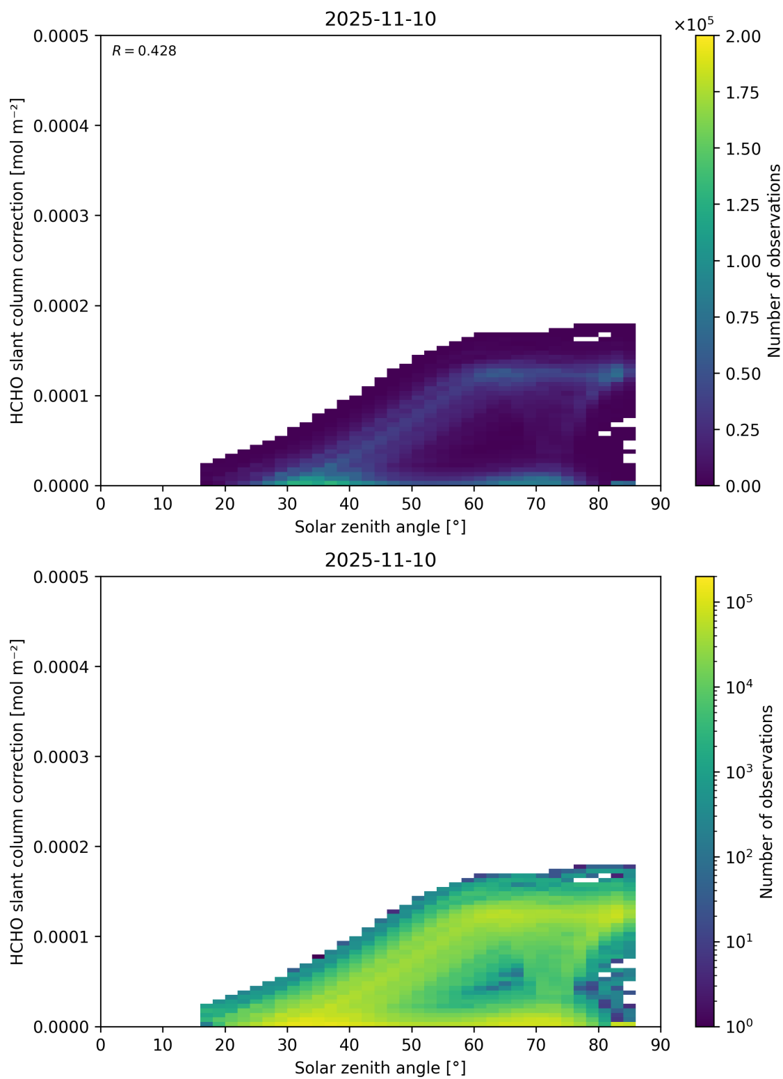
Figure 172: Scatter density plot of “Solar zenith angle” against “HCHO slant column correction” for 2025-11-09 to 2025-11-11.
