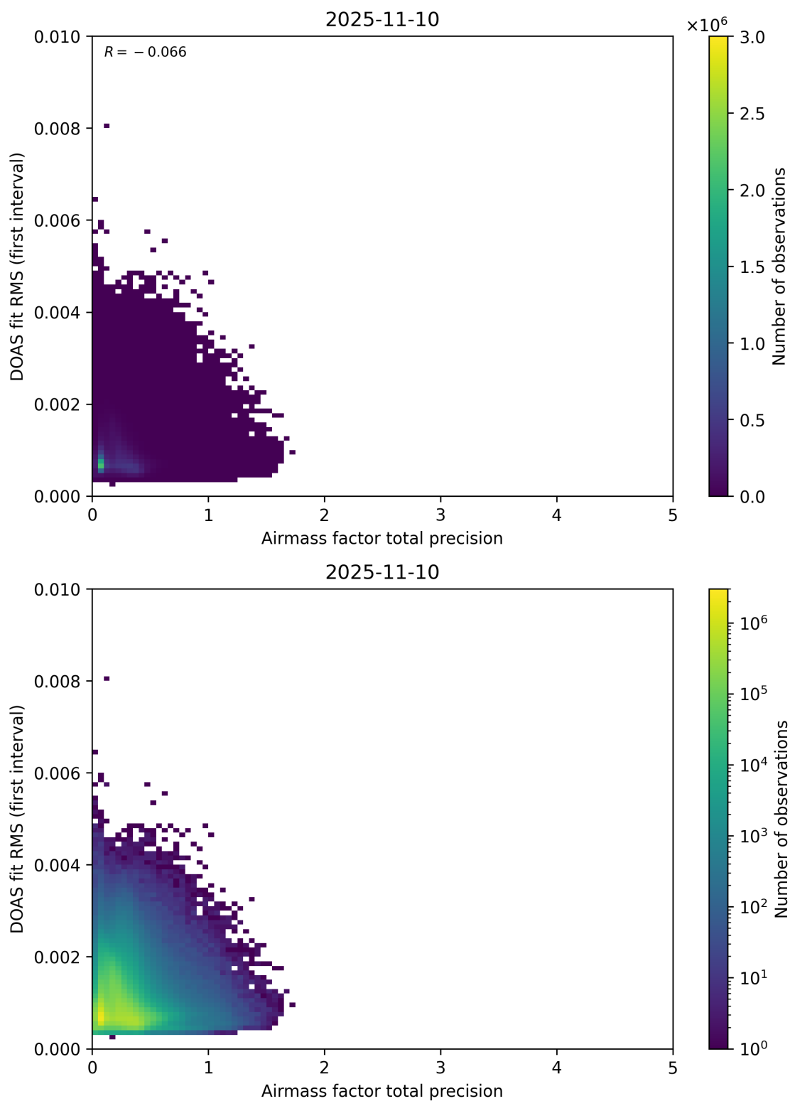
Figure 105: Scatter density plot of “Airmass factor total precision” against “DOAS fit RMS (first interval)” for 2025-11-09 to 2025-11-11.
