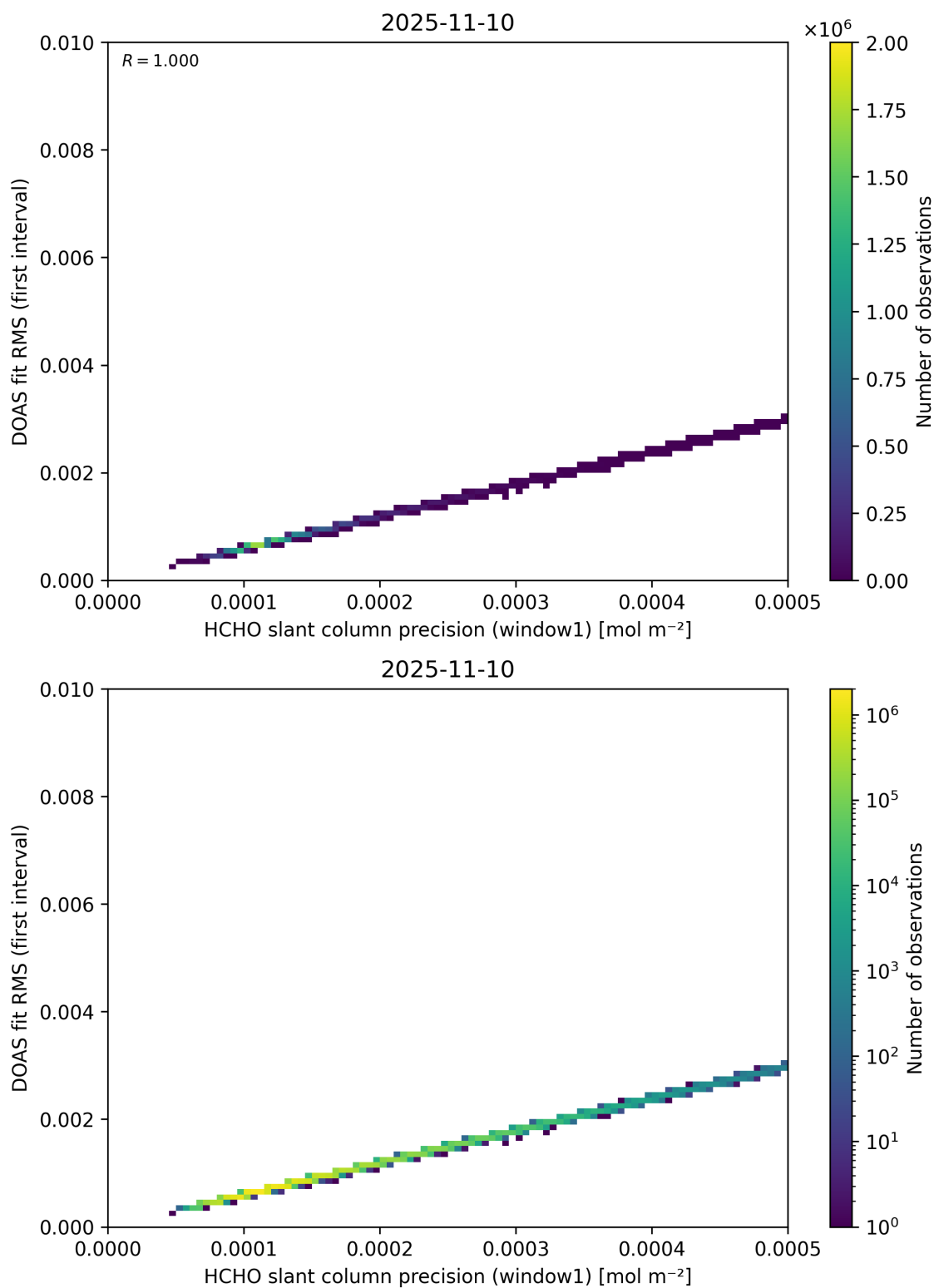
Figure 88: Scatter density plot of “HCHO slant column precision (window1)” against “DOAS fit RMS (first interval)” for 2025-11-09 to 2025-11-11.
