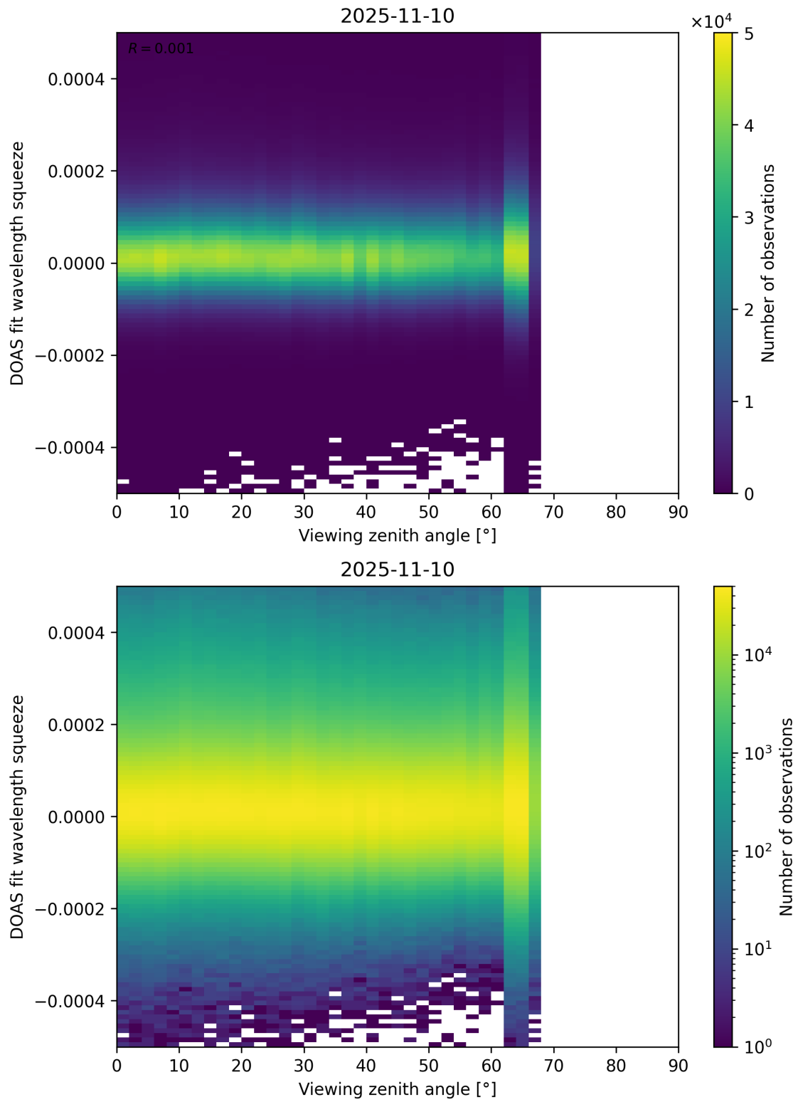
Figure 184: Scatter density plot of “Viewing zenith angle” against “DOAS fit wavelength squeeze” for 2025-11-09 to 2025-11-11.
