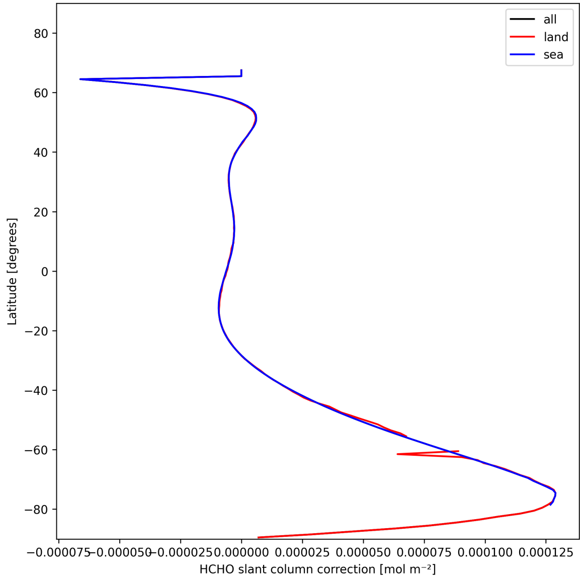
Figure 33: Zonal average of “HCHO slant column correction” for 2025-11-09 to 2025-11-11.
