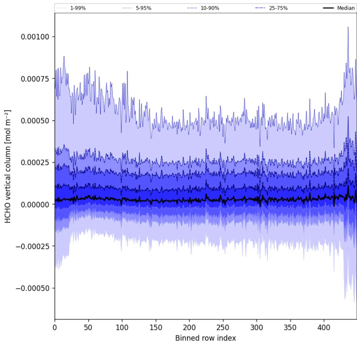
Figure 49: Along track statistics of “HCHO vertical column” for 2025-11-09 to 2025-11-11
