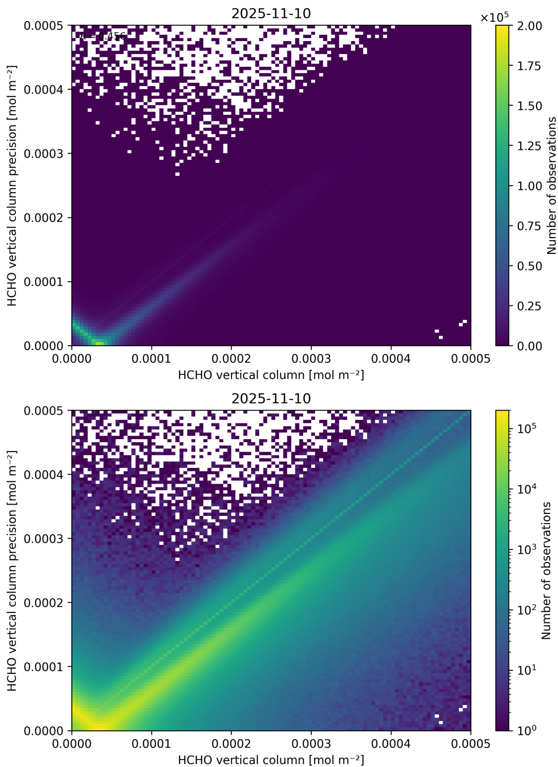
Figure 134: Scatter density plot of “HCHO vertical column” against “HCHO vertical column precision” for 2025-11-09 to 2025-11-11.
