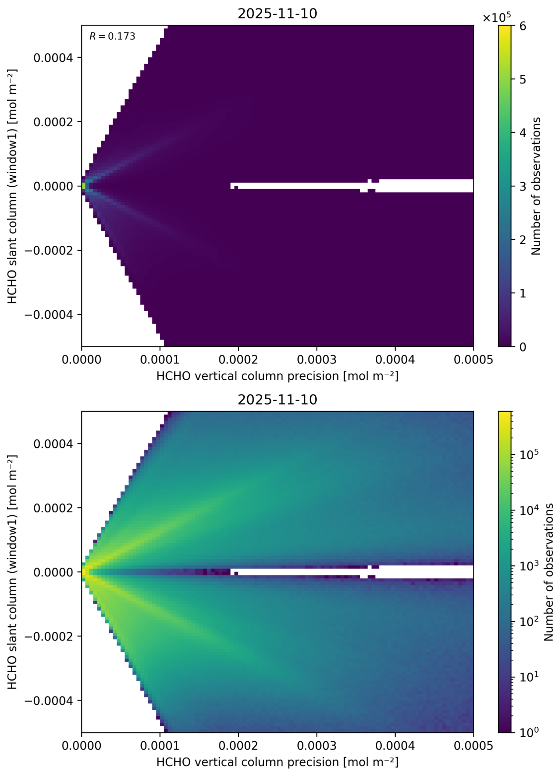
Figure 142: Scatter density plot of “HCHO vertical column precision” against “HCHO slant column (window1)” for 2025-11-09 to 2025-11-11.
