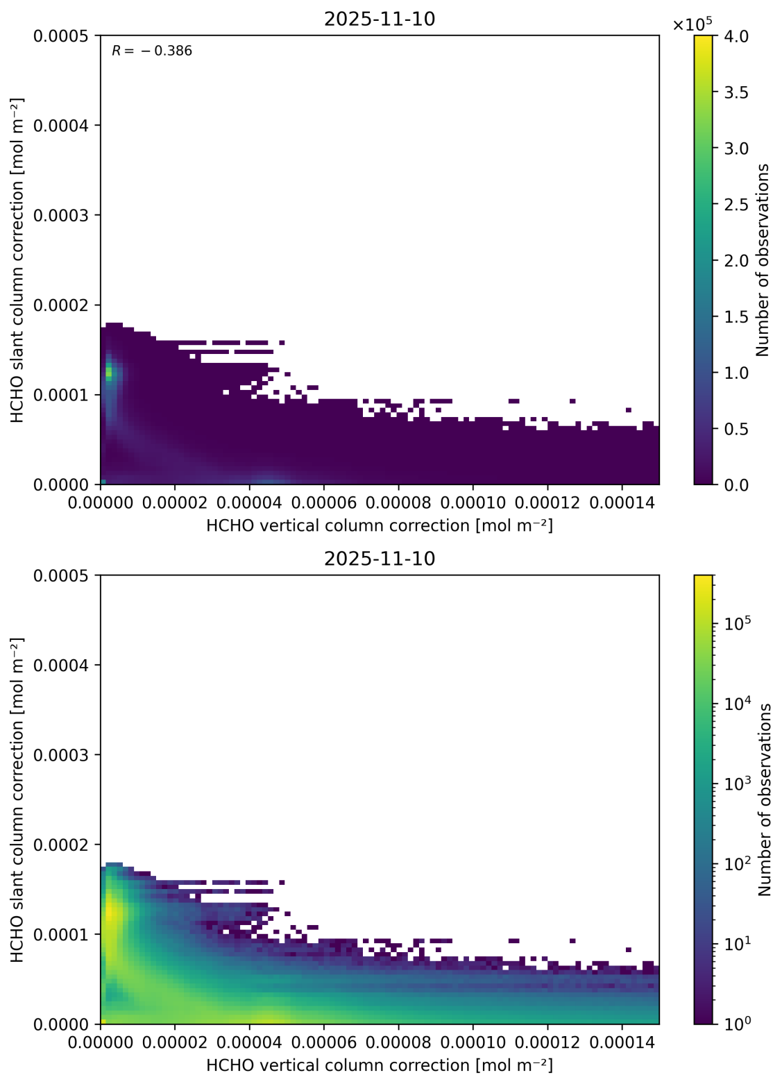
Figure 117: Scatter density plot of “HCHO vertical column correction” against “HCHO slant column correction” for 2025-11-09 to 2025-11-11.
