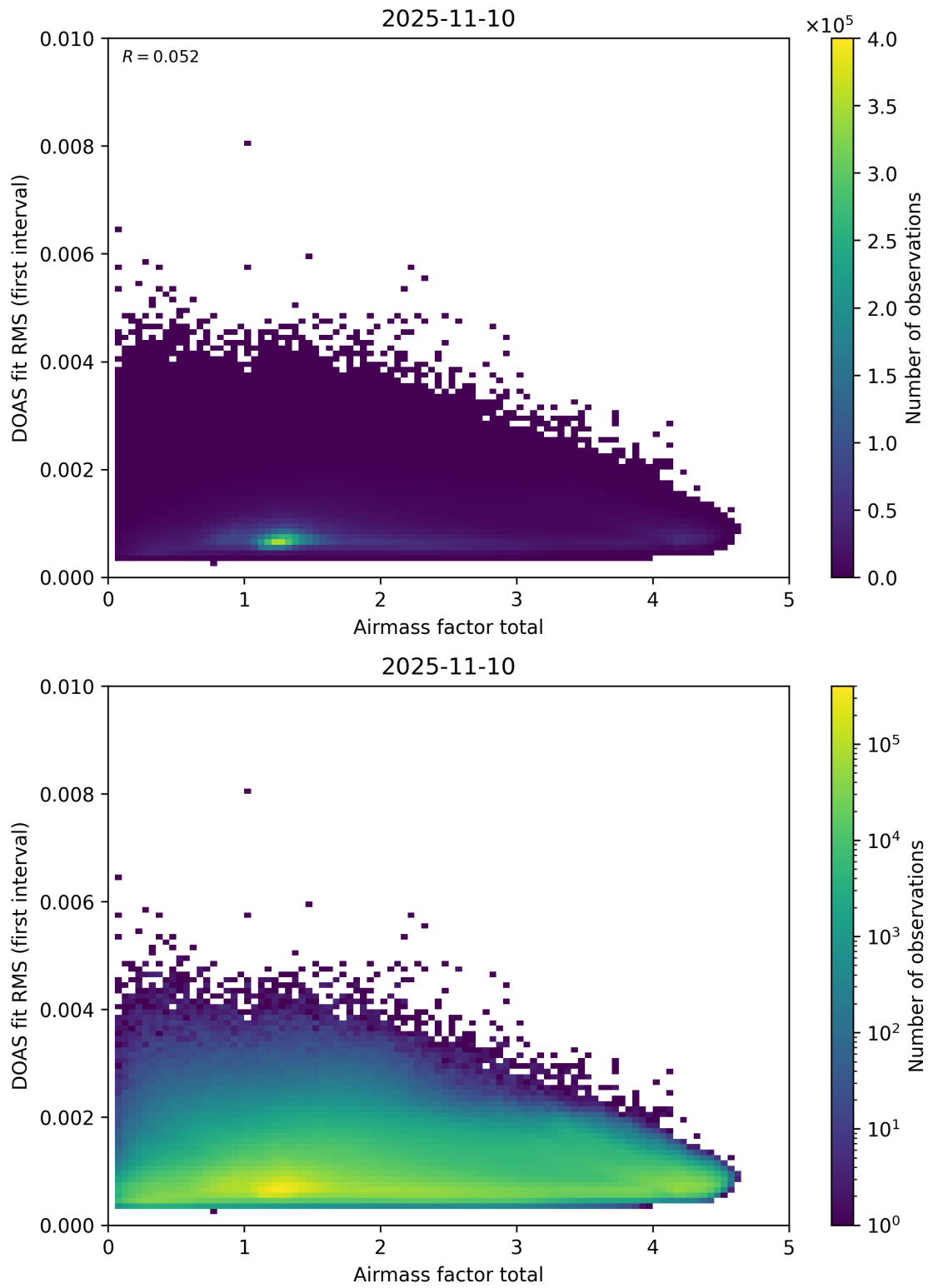
Figure 97: Scatter density plot of “Airmass factor total” against “DOAS fit RMS (first interval)” for 2025-11-09 to 2025-11-11.
