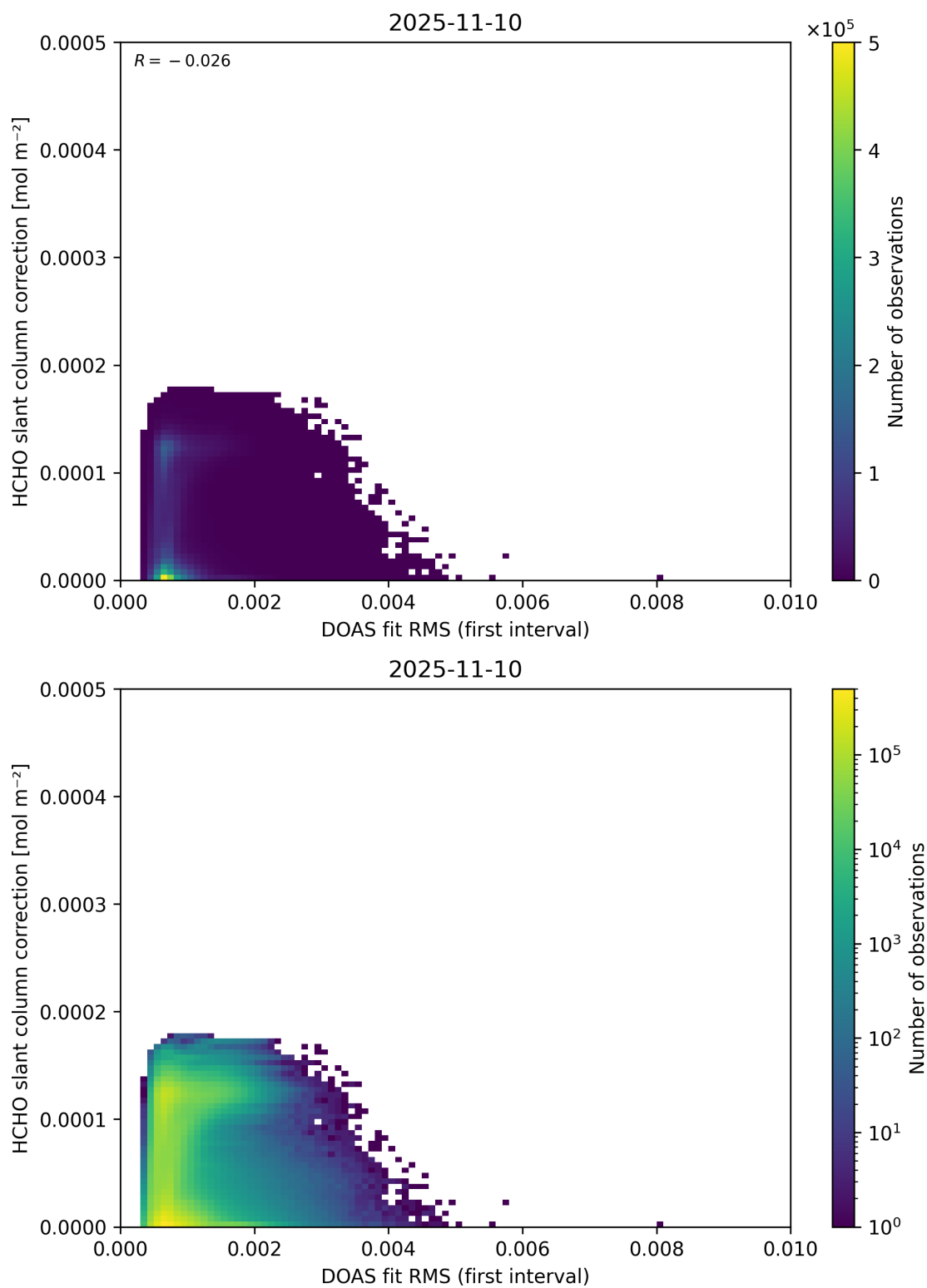
Figure 63: Scatter density plot of “DOAS fit RMS (first interval)” against “HCHO slant column correction” for 2025-11-09 to 2025-11-11.
