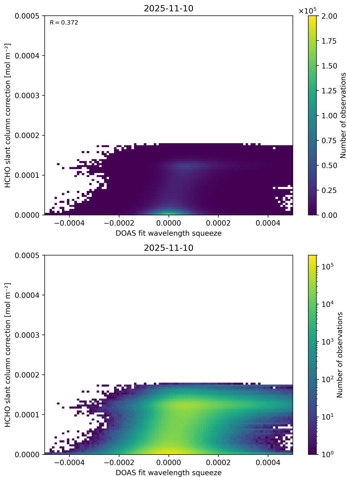
Figure 70: Scatter density plot of “DOAS fit wavelength squeeze” against “HCHO slant column correction” for 2025-11-09 to 2025-11-11.
