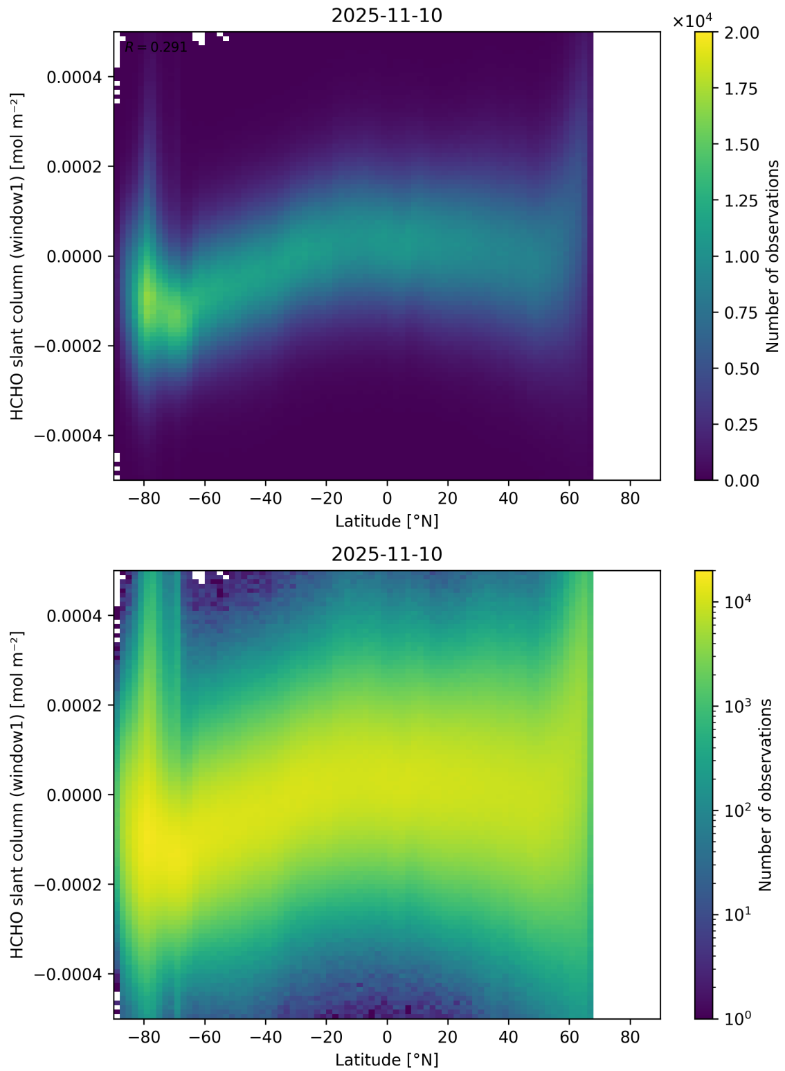
Figure 159: Scatter density plot of “Latitude” against “HCHO slant column (window1)” for 2025-11-09 to 2025-11-11.
