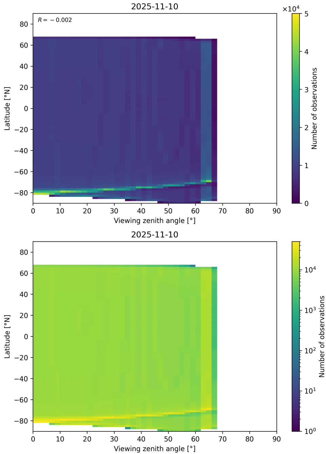
Figure 196: Scatter density plot of “Viewing zenith angle” against “Latitude” for 2025-11-09 to 2025-11-11.
