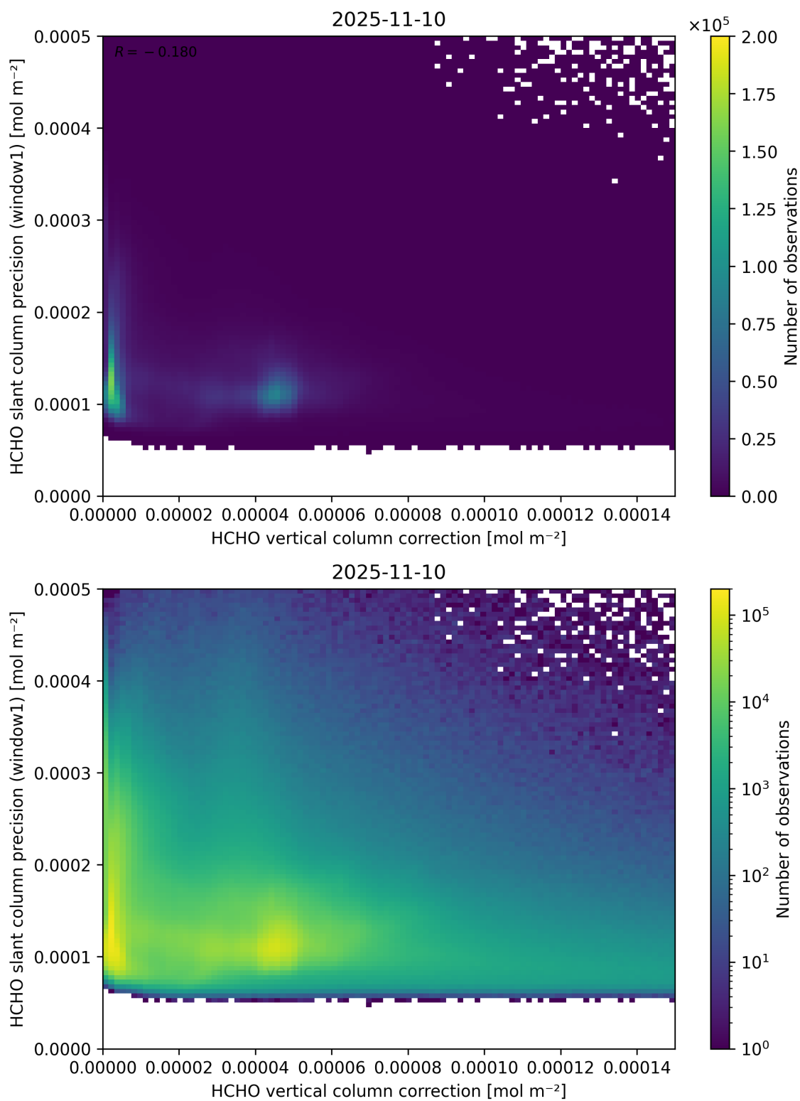
Figure 119: Scatter density plot of “HCHO vertical column correction” against “HCHO slant column precision (window1)” for 2025-11-09 to 2025-11-11.
