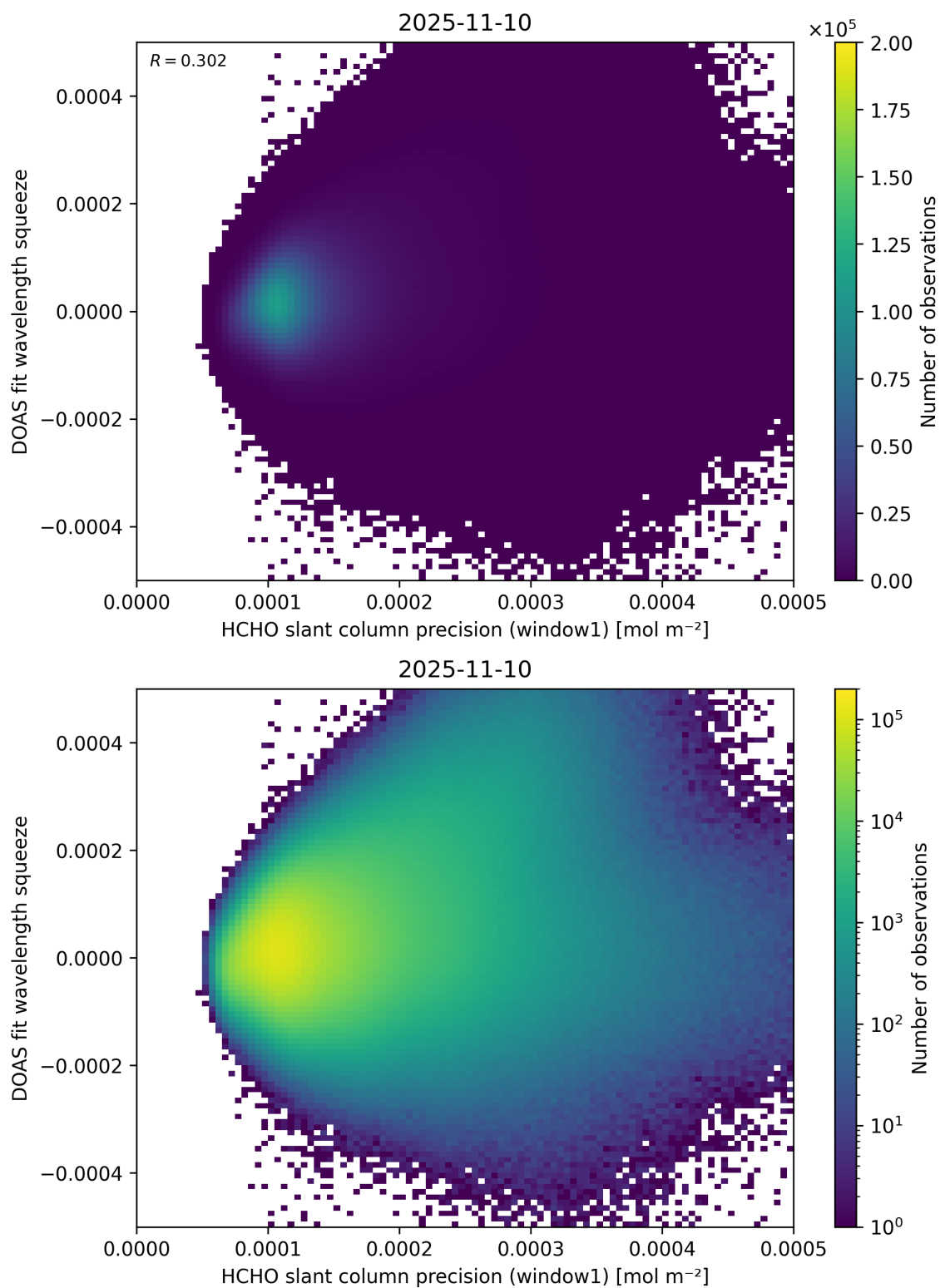
Figure 90: Scatter density plot of “HCHO slant column precision (window1)” against “DOAS fit wavelength squeeze” for 2025-11-09 to 2025-11-11.
