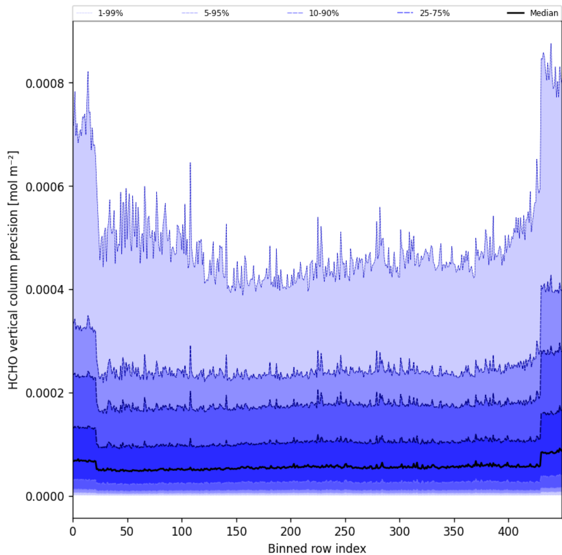
Figure 50: Along track statistics of "HCHO vertical column precision" for 2025-11-09 to 2025-11-11
