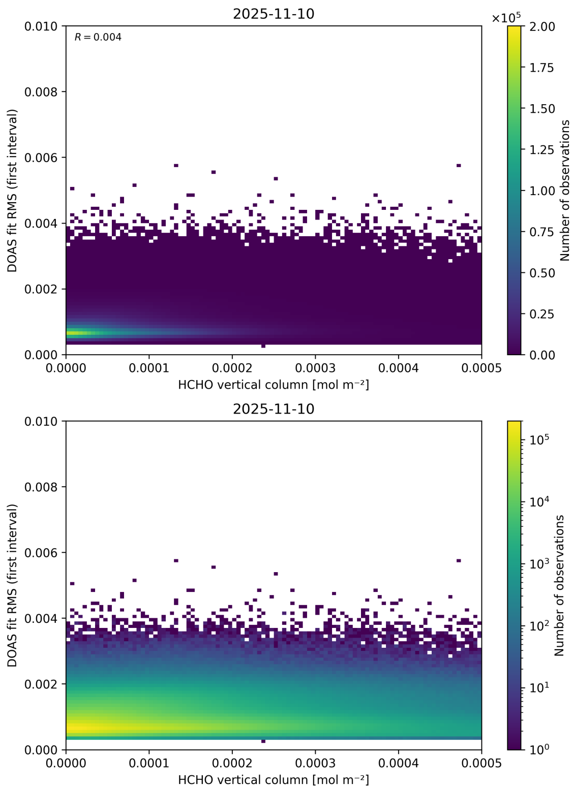
Figure 123: Scatter density plot of “HCHO vertical column” against “DOAS fit RMS (first interval)” for 2025-11-09 to 2025-11-11.
