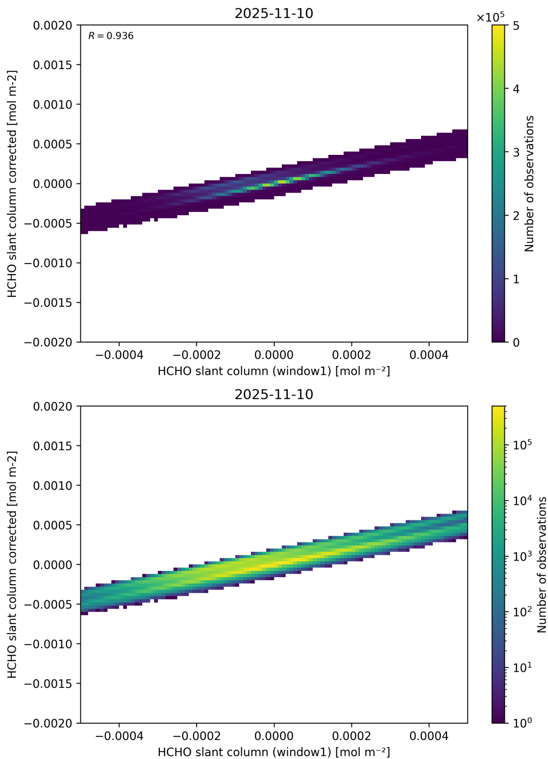
Figure 82: Scatter density plot of “HCHO slant column (window1)” against “HCHO slant column corrected” for 2025-11-09 to 2025-11-11.
