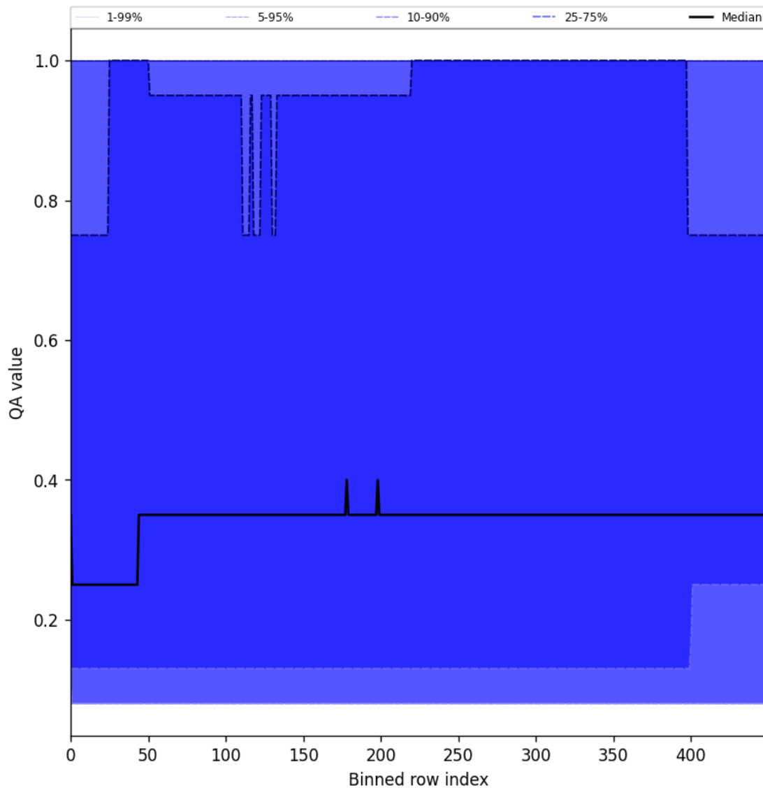
Figure 48: Along track statistics of “QA value” for 2025-11-09 to 2025-11-11
