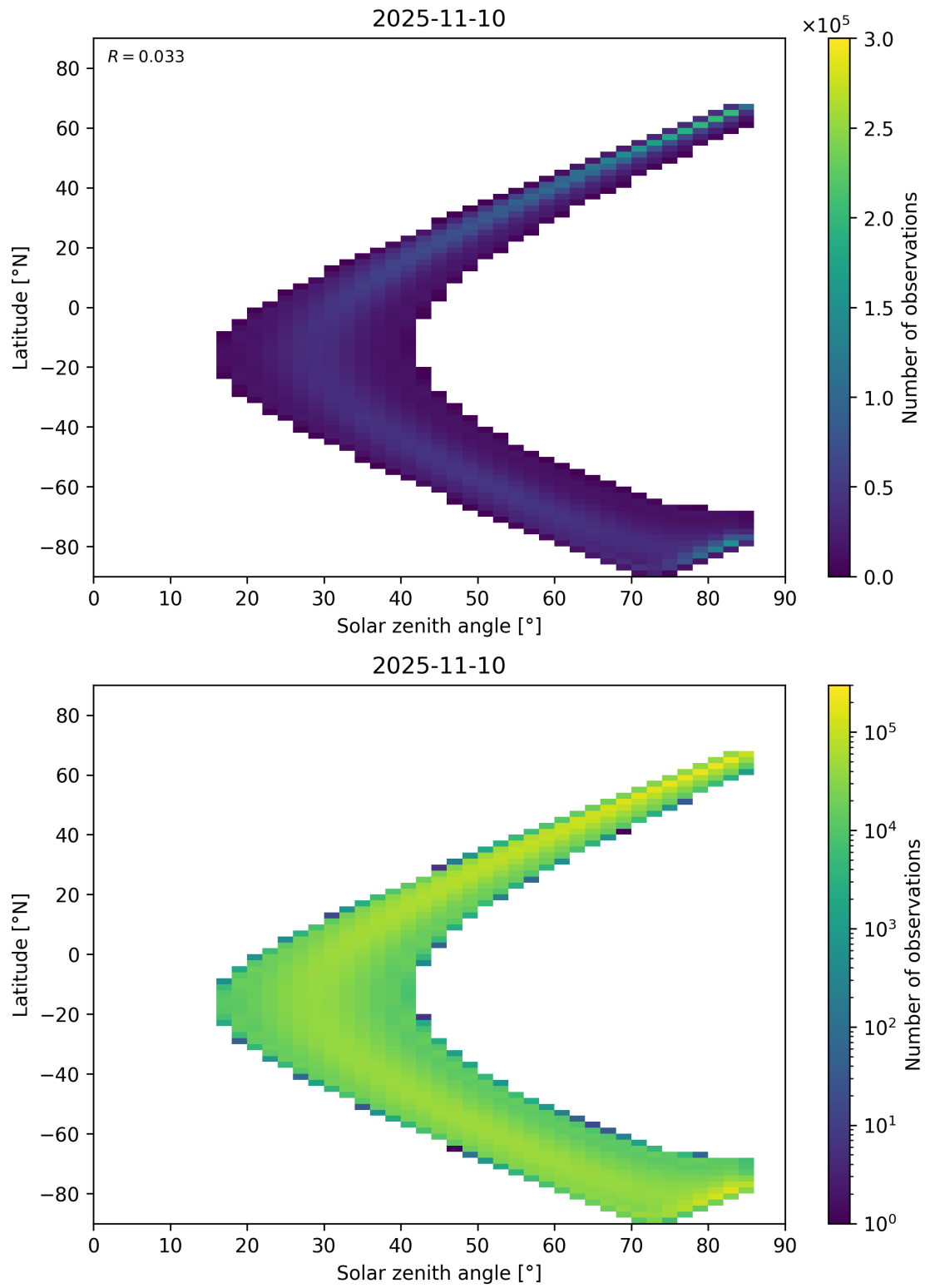
Figure 181: Scatter density plot of “Solar zenith angle” against “Latitude” for 2025-11-09 to 2025-11-11.
