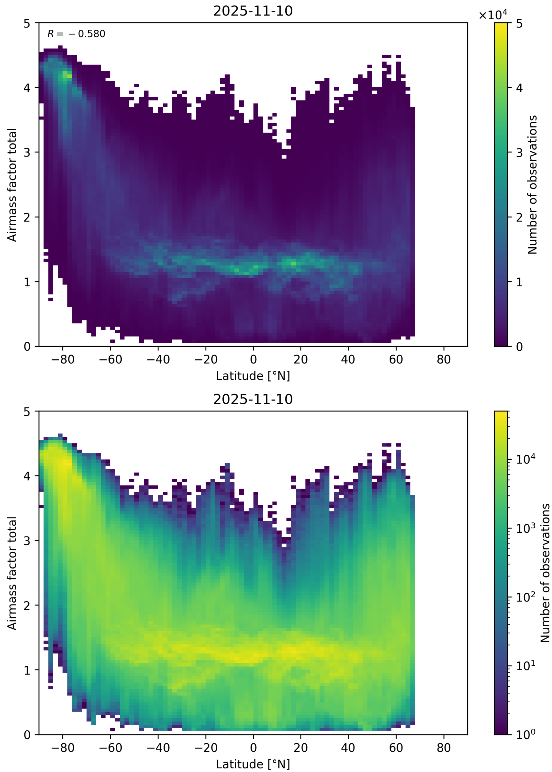
Figure 161: Scatter density plot of “Latitude” against “Airmass factor total” for 2025-11-09 to 2025-11-11.
