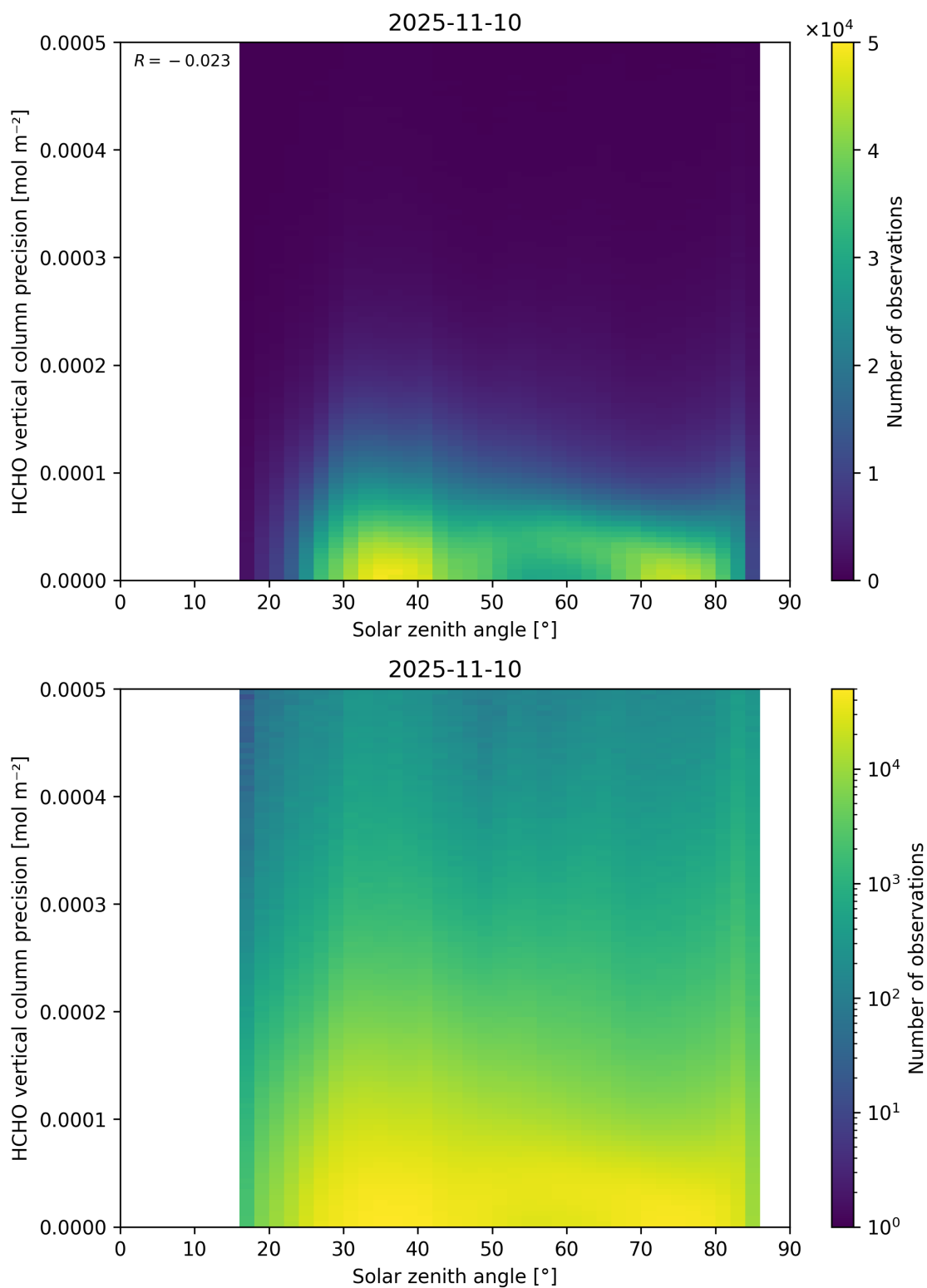
Figure 179: Scatter density plot of “Solar zenith angle” against “HCHO vertical column precision” for 2025-11-09 to 2025-11-11.
