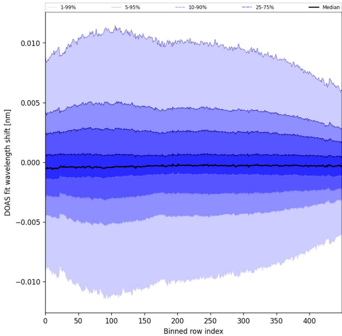
Figure 58: Along track statistics of “DOAS fit wavelength shift” for 2025-11-09 to 2025-11-11
