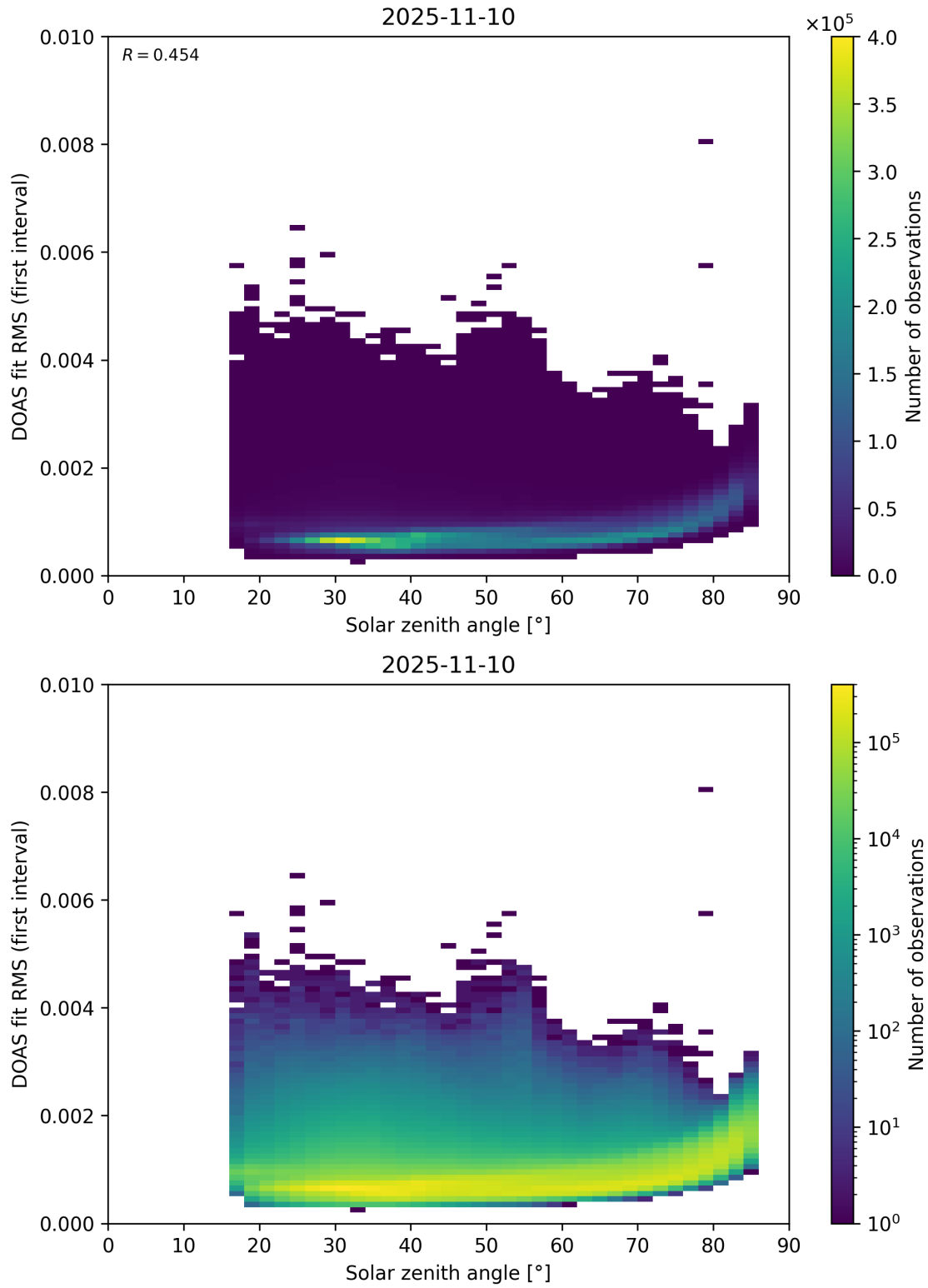
Figure 167: Scatter density plot of “Solar zenith angle” against “DOAS fit RMS (first interval)” for 2025-11-09 to 2025-11-11.
