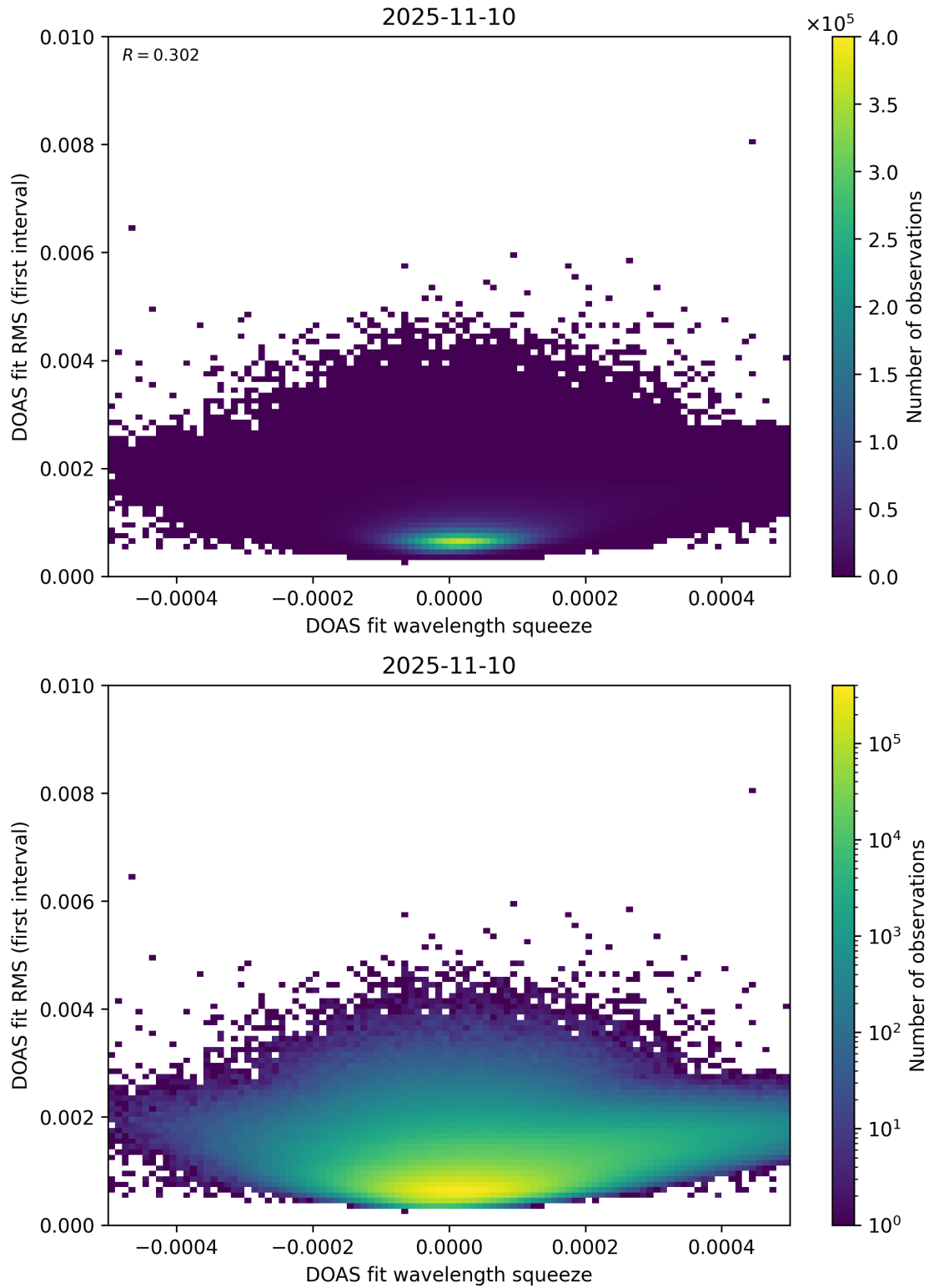
Figure 68: Scatter density plot of “DOAS fit wavelength squeeze” against “DOAS fit RMS (first interval)” for 2025-11-09 to 2025-11-11.
