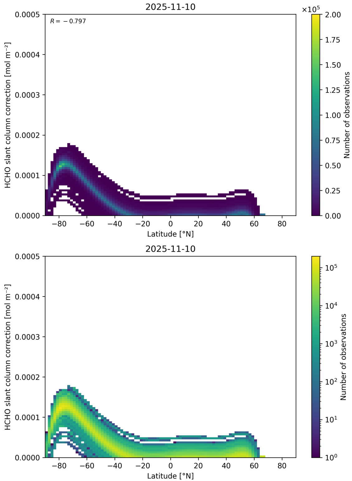
Figure 158: Scatter density plot of “Latitude” against “HCHO slant column correction” for 2025-11-09 to 2025-11-11.
