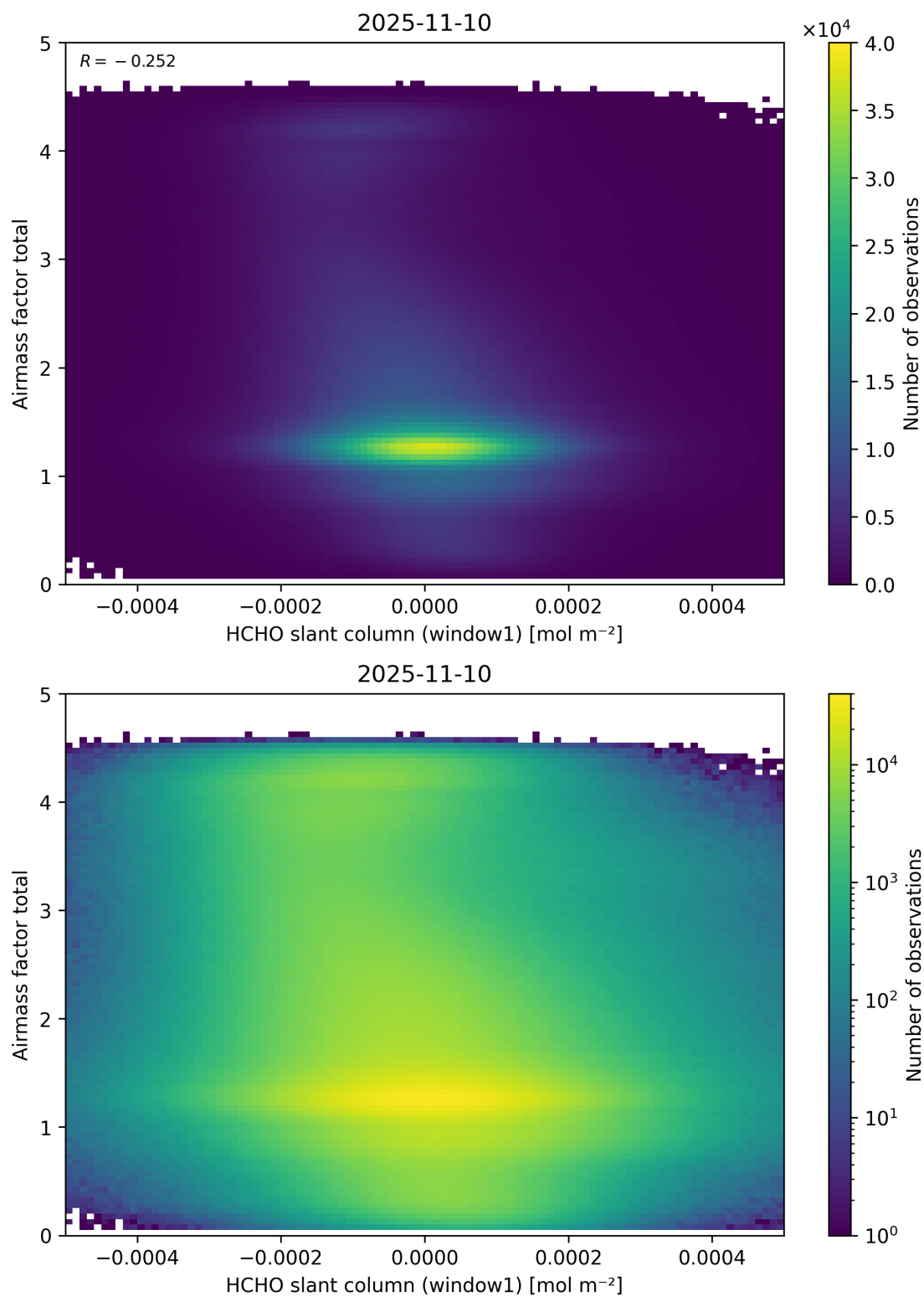
Figure 85: Scatter density plot of “HCHO slant column (window1)” against “Airmass factor total” for 2025-11-09 to 2025-11-11.
