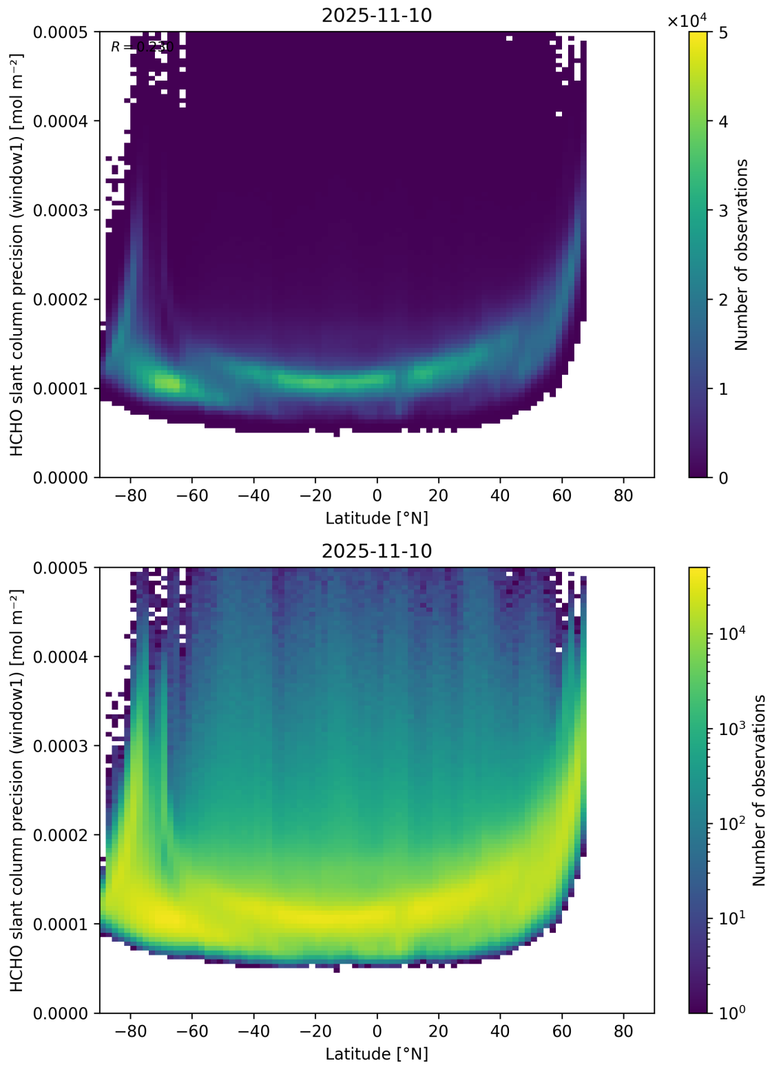
Figure 160: Scatter density plot of “Latitude” against “HCHO slant column precision (window1)” for 2025-11-09 to 2025-11-11.
