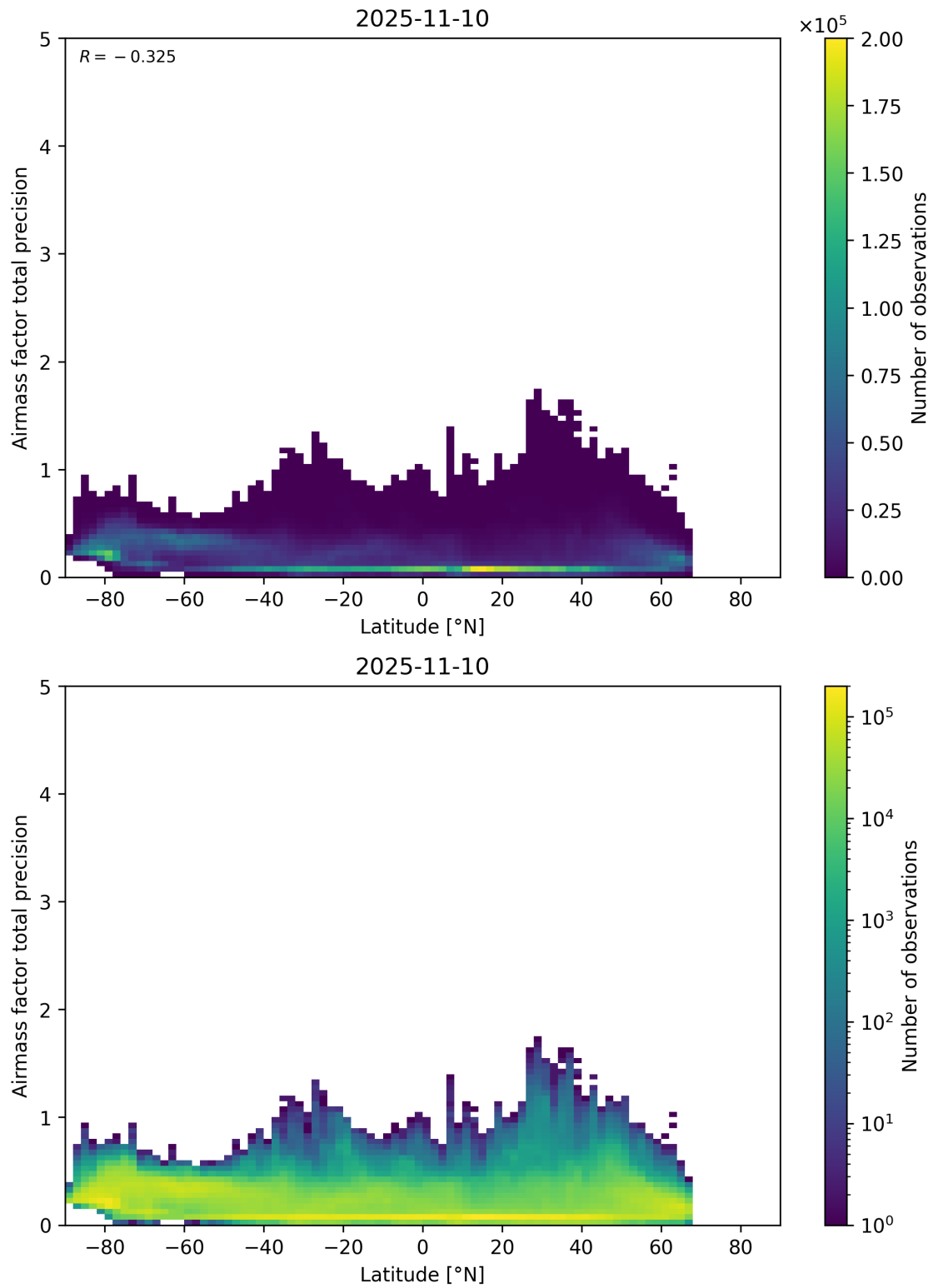
Figure 162: Scatter density plot of “Latitude” against “Airmass factor total precision” for 2025-11-09 to 2025-11-11.
