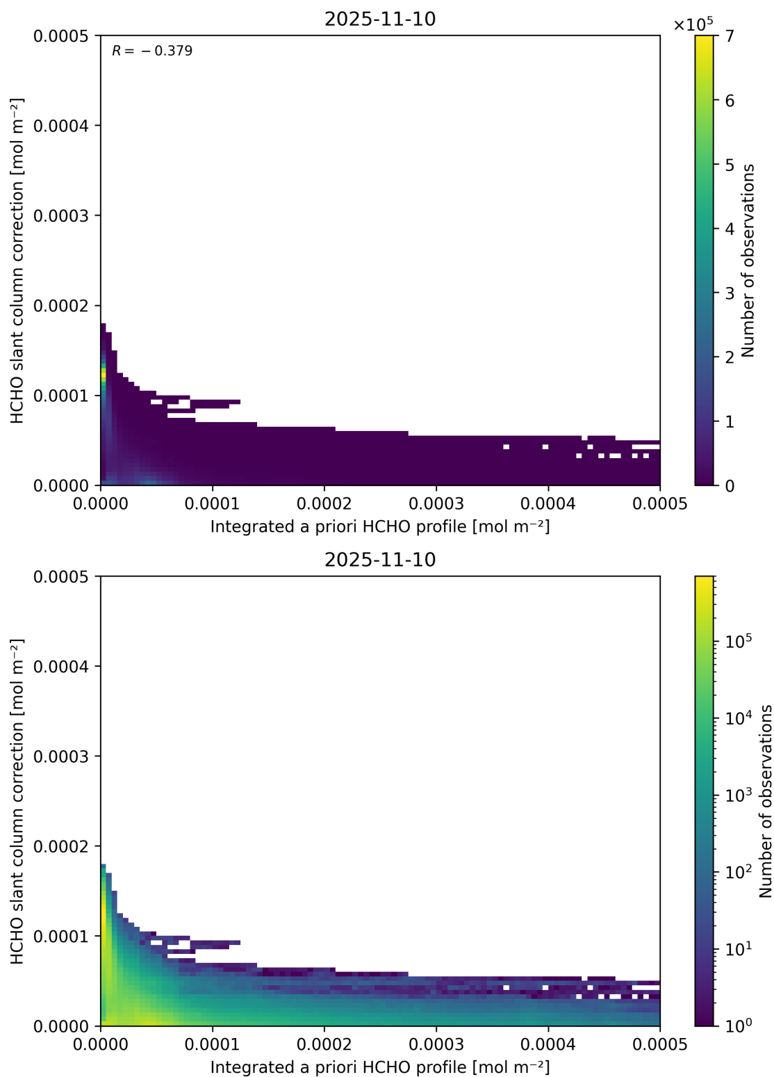
Figure 152: Scatter density plot of “Integrated a priori HCHO profile” against “HCHO slant column correction” for 2025-11-09 to 2025-11-11.
