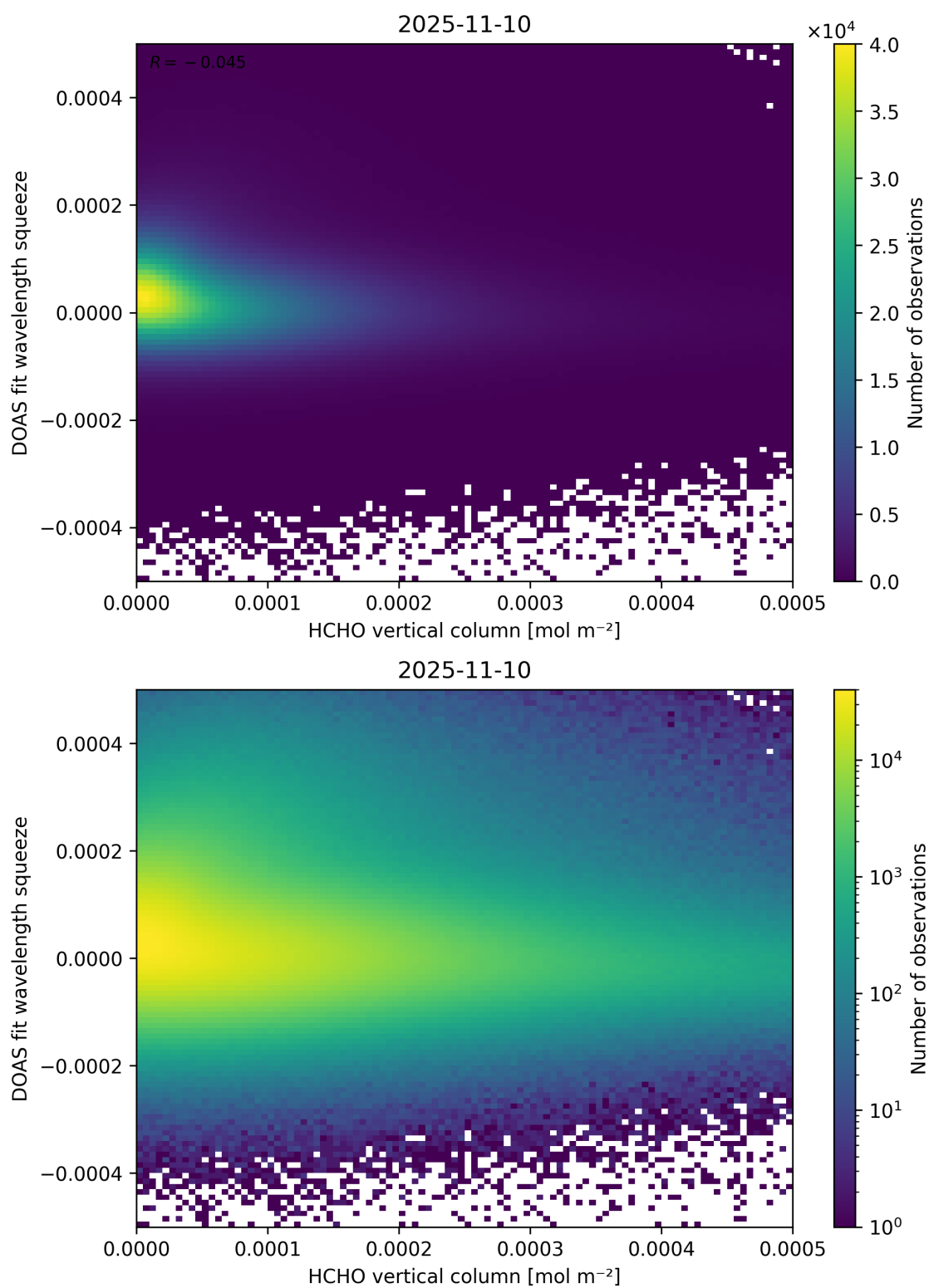
Figure 125: Scatter density plot of “HCHO vertical column” against “DOAS fit wavelength squeeze” for 2025-11-09 to 2025-11-11.
