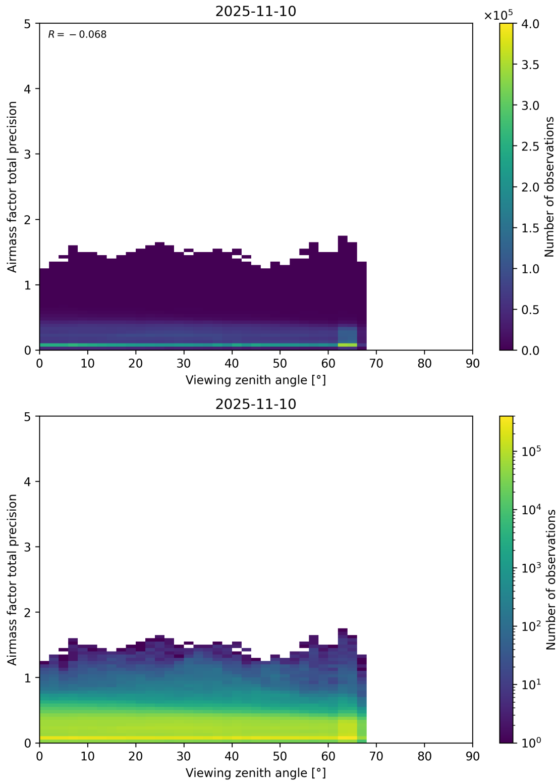
Figure 191: Scatter density plot of “Viewing zenith angle” against “Airmass factor total precision” for 2025-11-09 to 2025-11-11.
