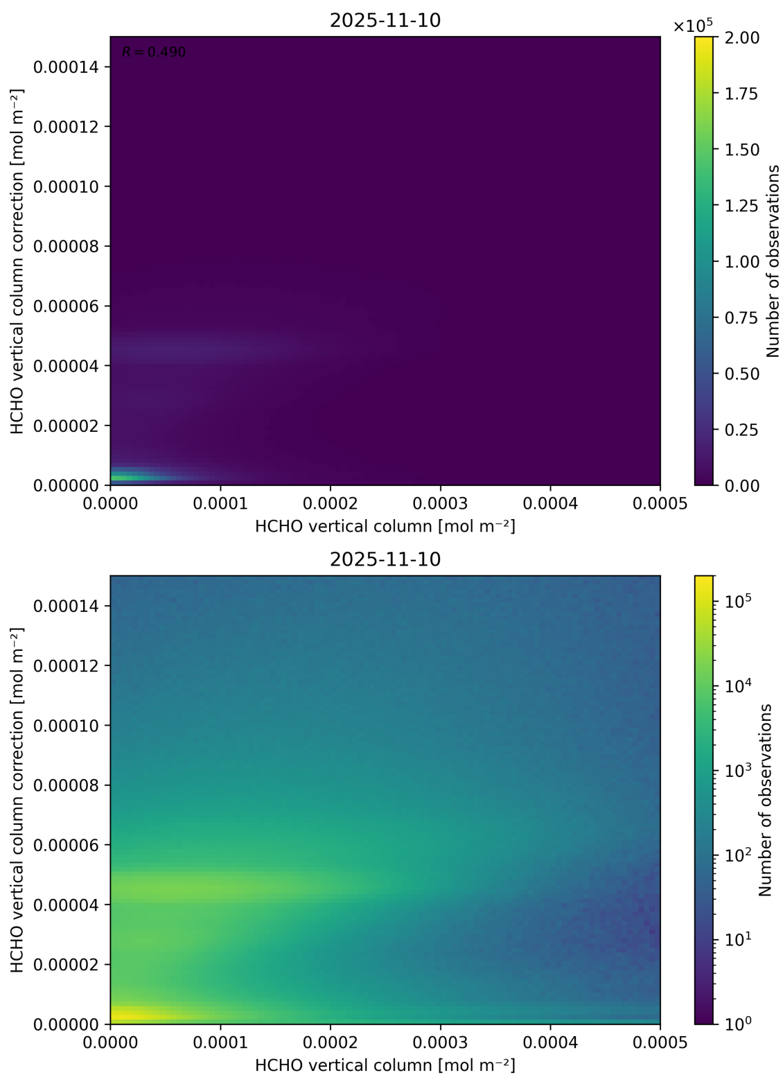
Figure 133: Scatter density plot of “HCHO vertical column” against “HCHO vertical column correction” for 2025-11-09 to 2025-11-11.
