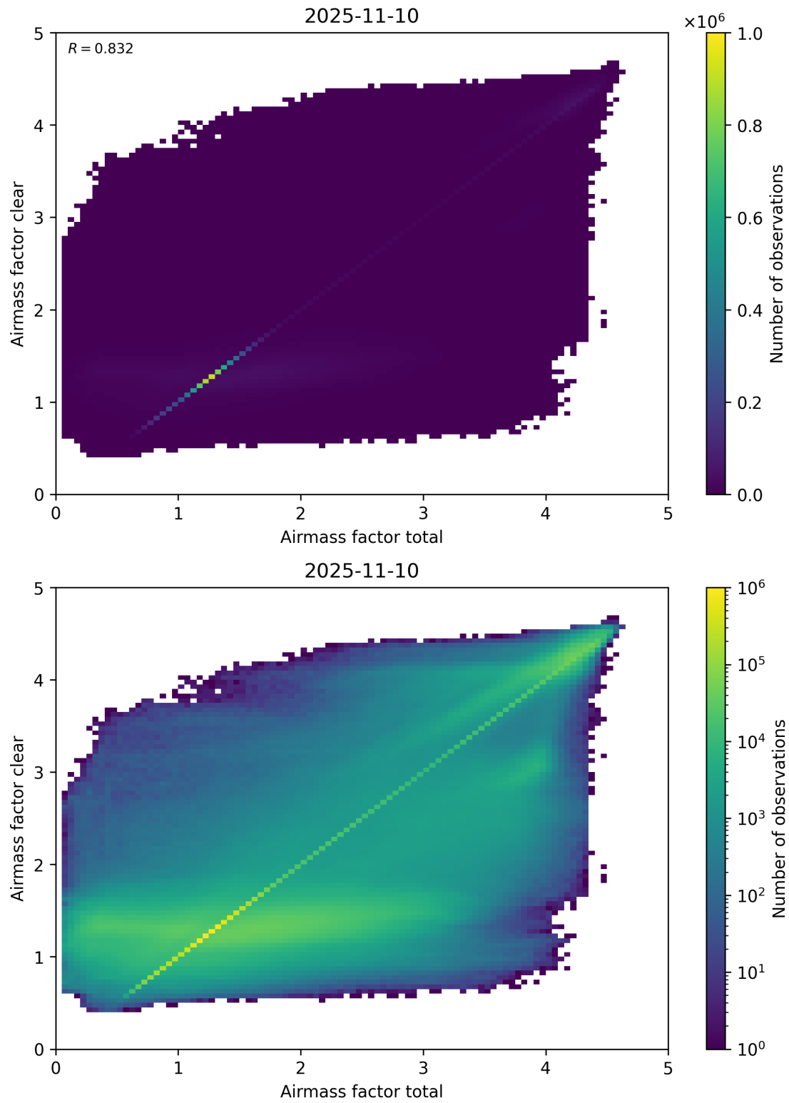
Figure 100: Scatter density plot of “Airmass factor total” against “Airmass factor clear” for 2025-11-09 to 2025-11-11.
