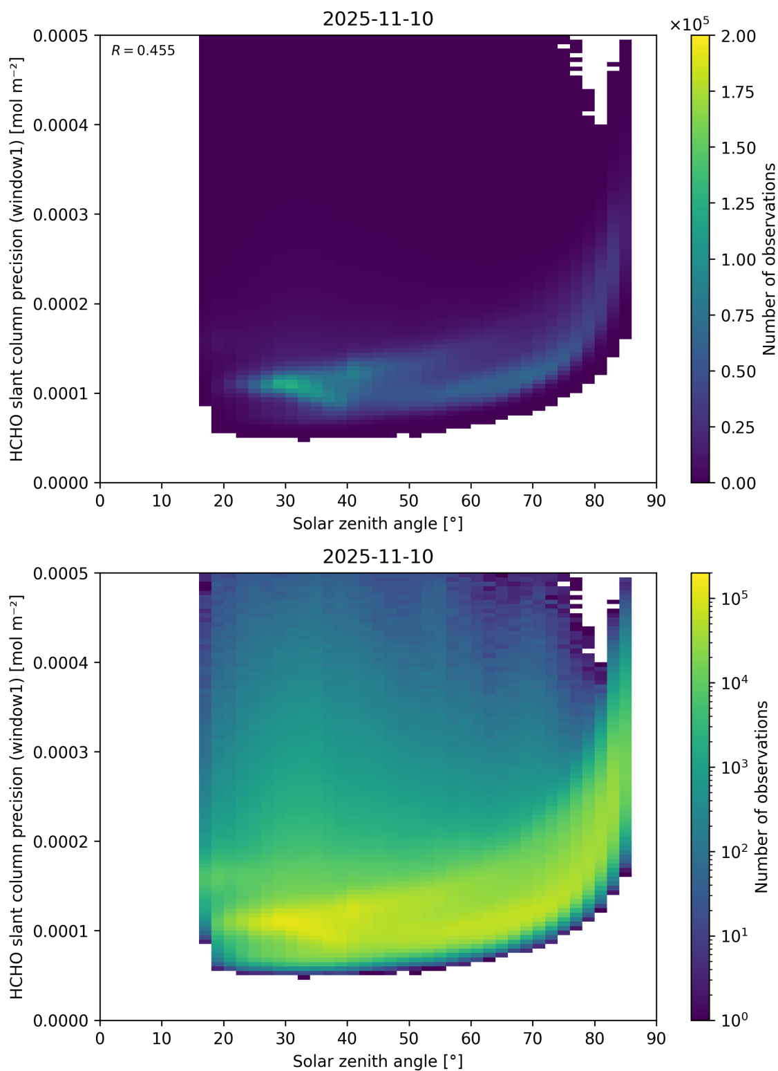
Figure 174: Scatter density plot of “Solar zenith angle” against “HCHO slant column precision (window1)” for 2025-11-09 to 2025-11-11.
