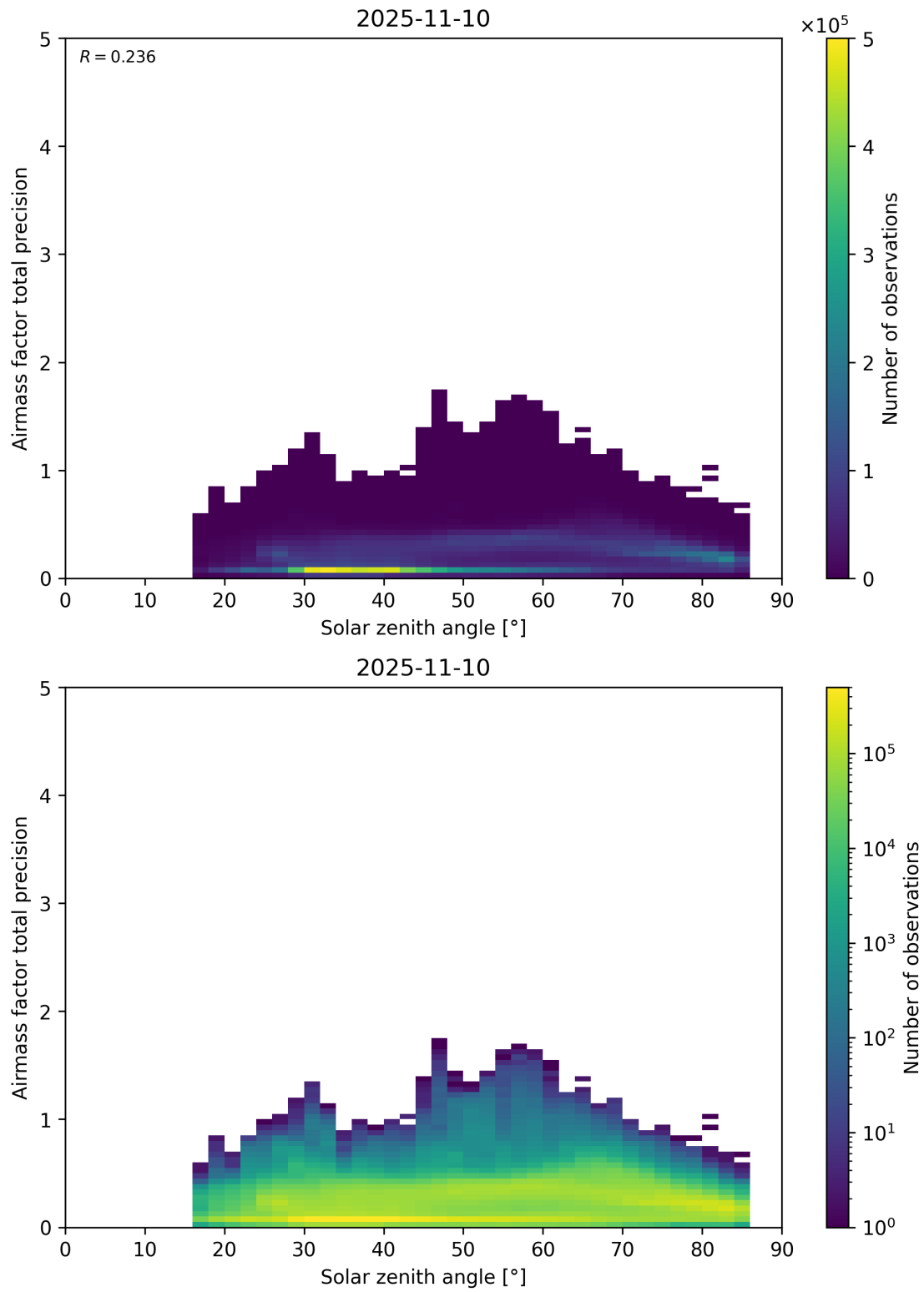
Figure 176: Scatter density plot of “Solar zenith angle” against “Airmass factor total precision” for 2025-11-09 to 2025-11-11.
