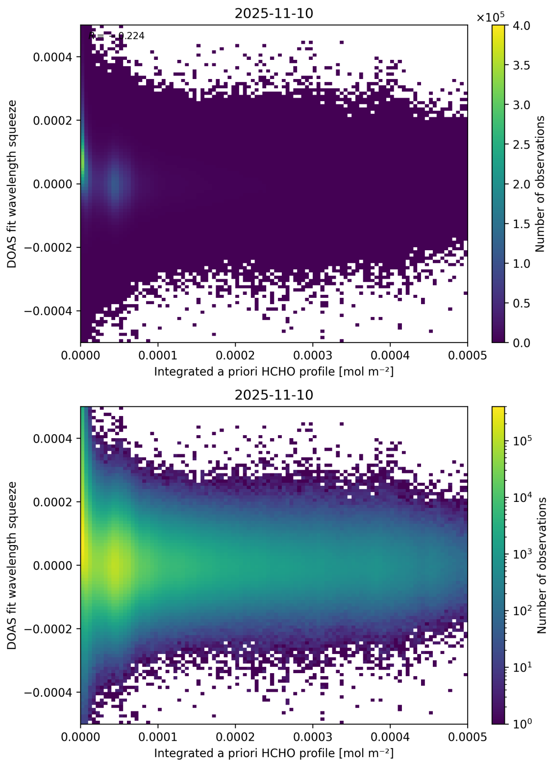
Figure 150: Scatter density plot of “Integrated a priori HCHO profile” against “DOAS fit wavelength squeeze” for 2025-11-09 to 2025-11-11.
