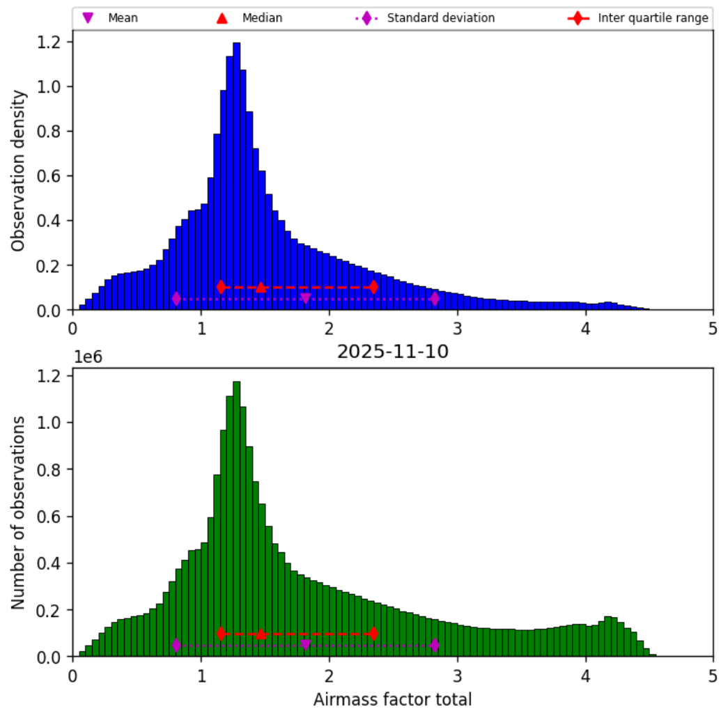
Figure 40: Histogram of “Airmass factor total” for 2025-11-09 to 2025-11-11
