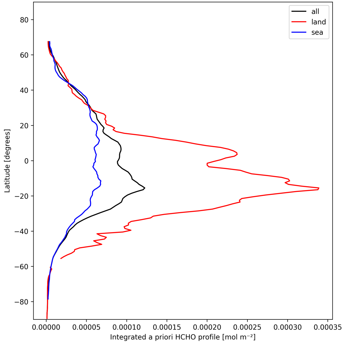
Figure 29: Zonal average of “Integrated a priori HCHO profile” for 2025-11-09 to 2025-11-11.
