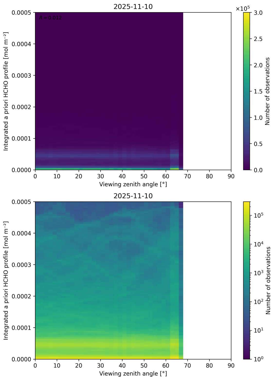
Figure 195: Scatter density plot of “Viewing zenith angle” against “Integrated a priori HCHO profile” for 2025-11-09 to 2025-11-11.
