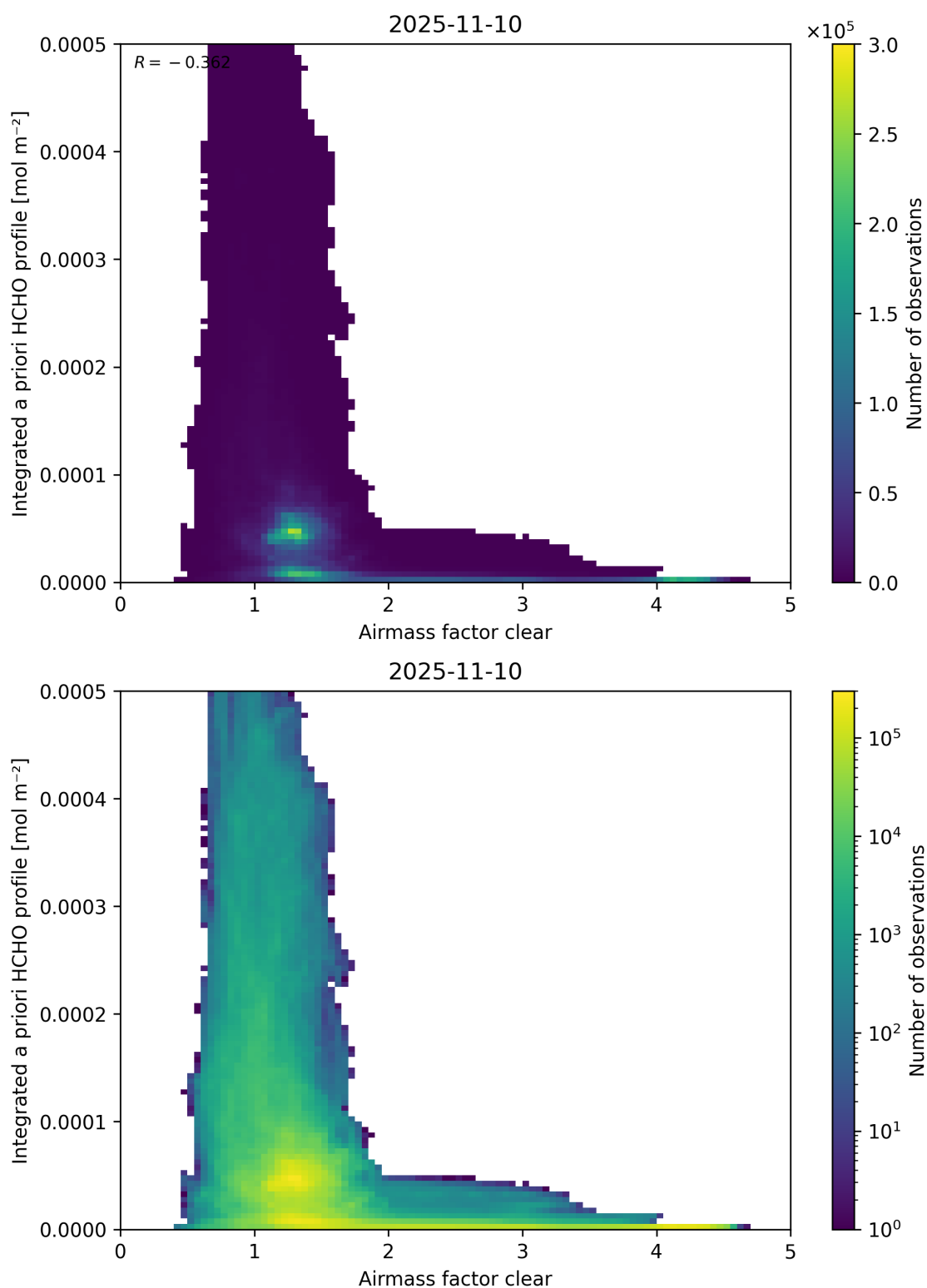
Figure 76: Scatter density plot of “Airmass factor clear” against “Integrated a priori HCHO profile” for 2025-11-09 to 2025-11-11.
