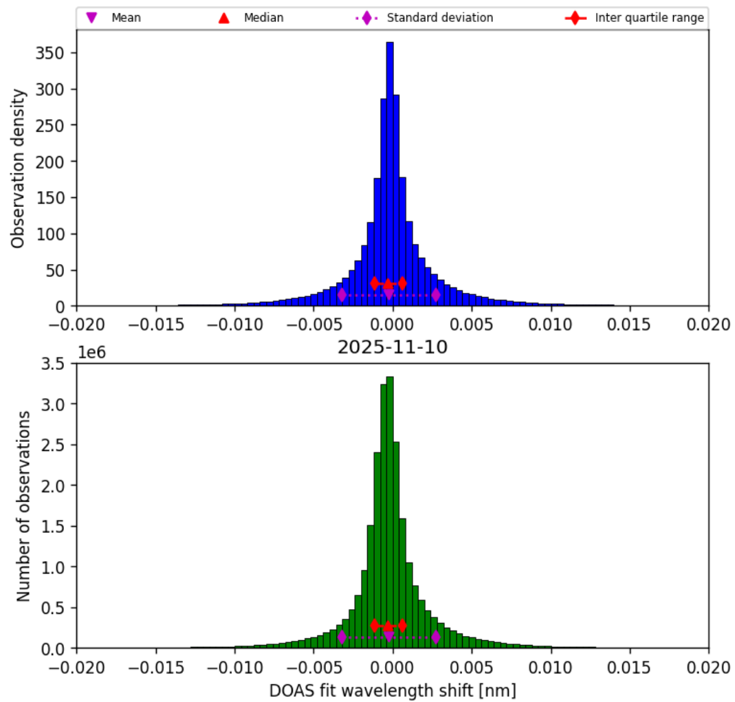
Figure 44: Histogram of “DOAS fit wavelength shift” for 2025-11-09 to 2025-11-11
