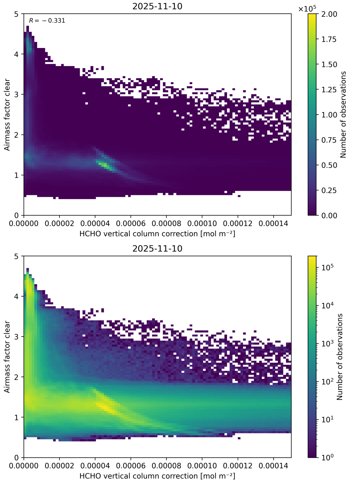
Figure 115: Scatter density plot of “HCHO vertical column correction” against “Airmass factor clear” for 2025-11-09 to 2025-11-11.
