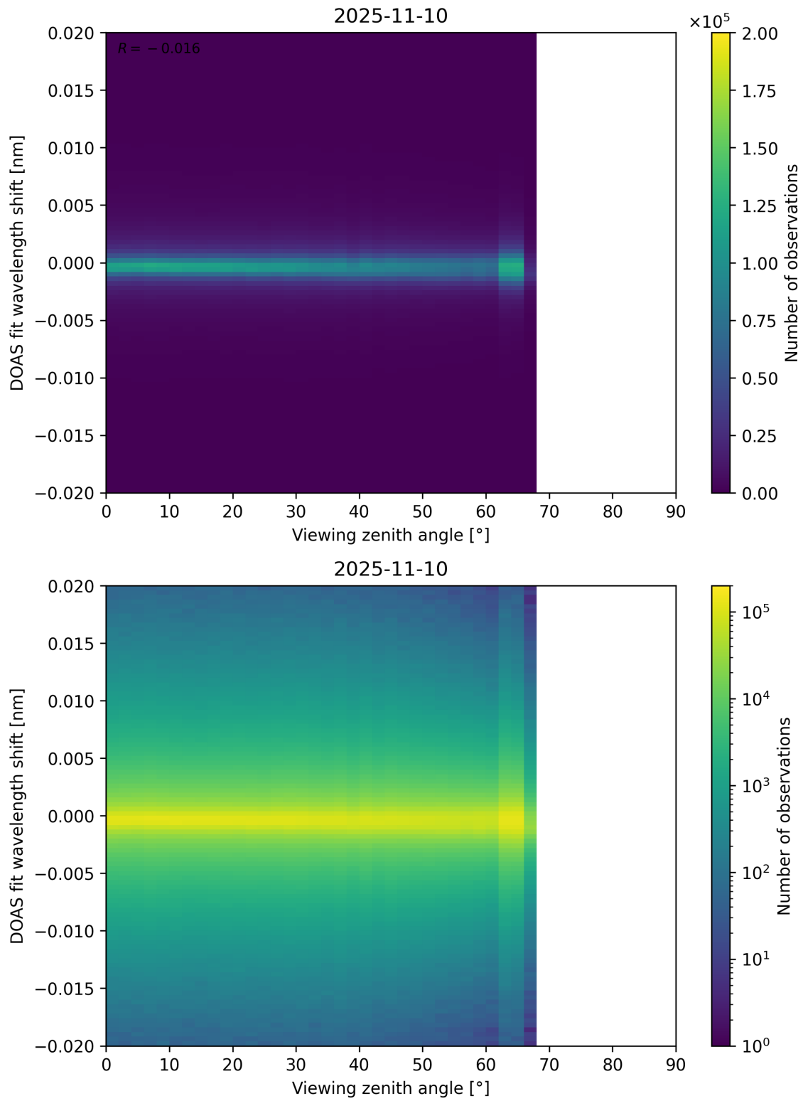
Figure 183: Scatter density plot of “Viewing zenith angle” against “DOAS fit wavelength shift” for 2025-11-09 to 2025-11-11.
