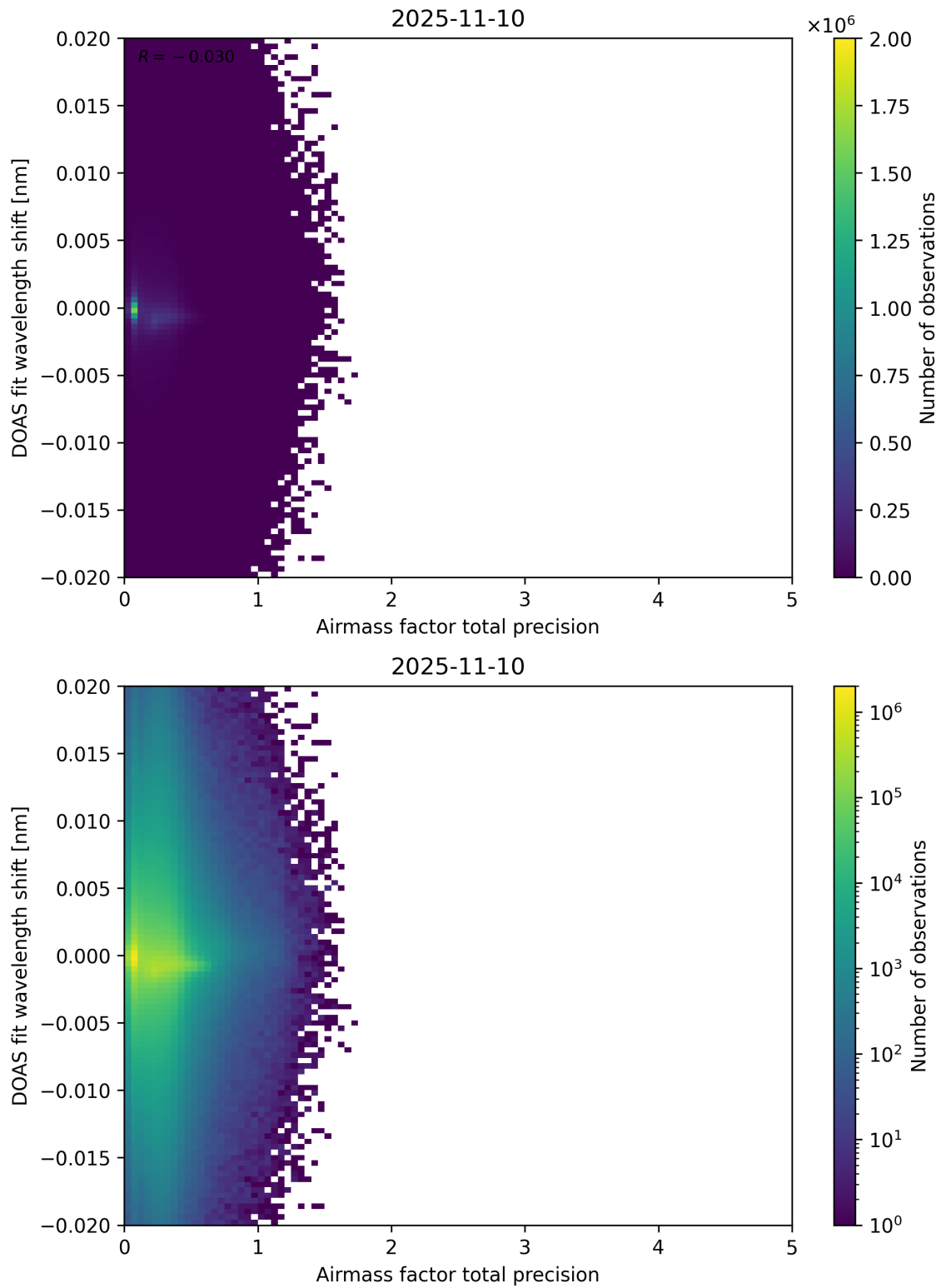
Figure 106: Scatter density plot of “Airmass factor total precision” against “DOAS fit wavelength shift” for 2025-11-09 to 2025-11-11.
