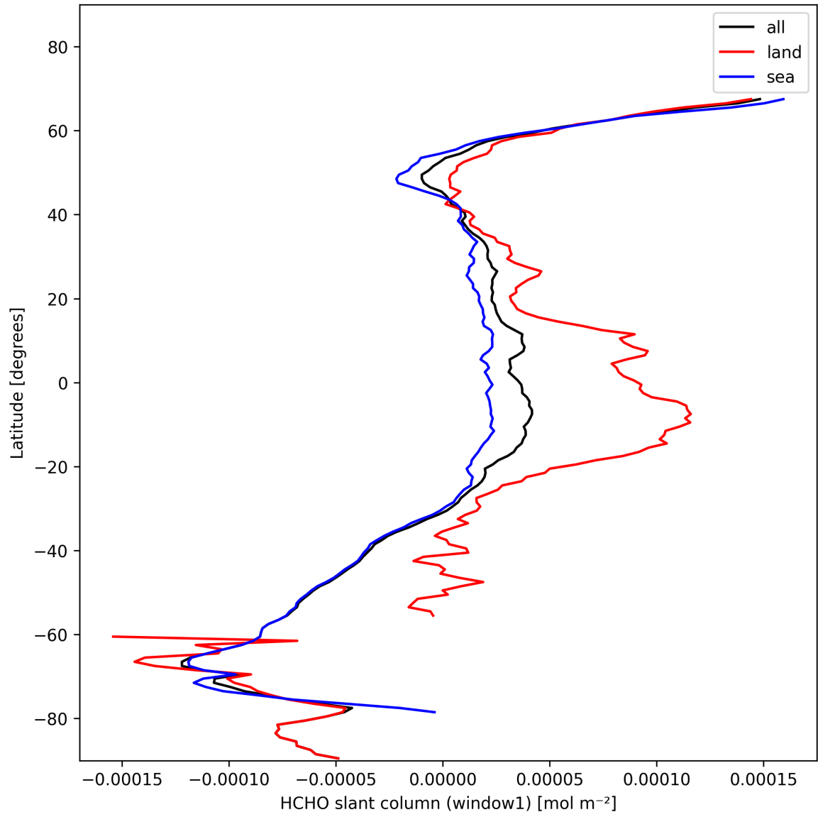
Figure 24: Zonal average of “HCHO slant column (window1)” for 2025-11-09 to 2025-11-11.
