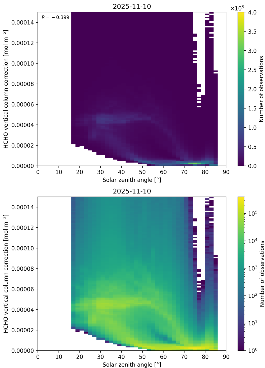
Figure 178: Scatter density plot of “Solar zenith angle” against “HCHO vertical column correction” for 2025-11-09 to 2025-11-11.
