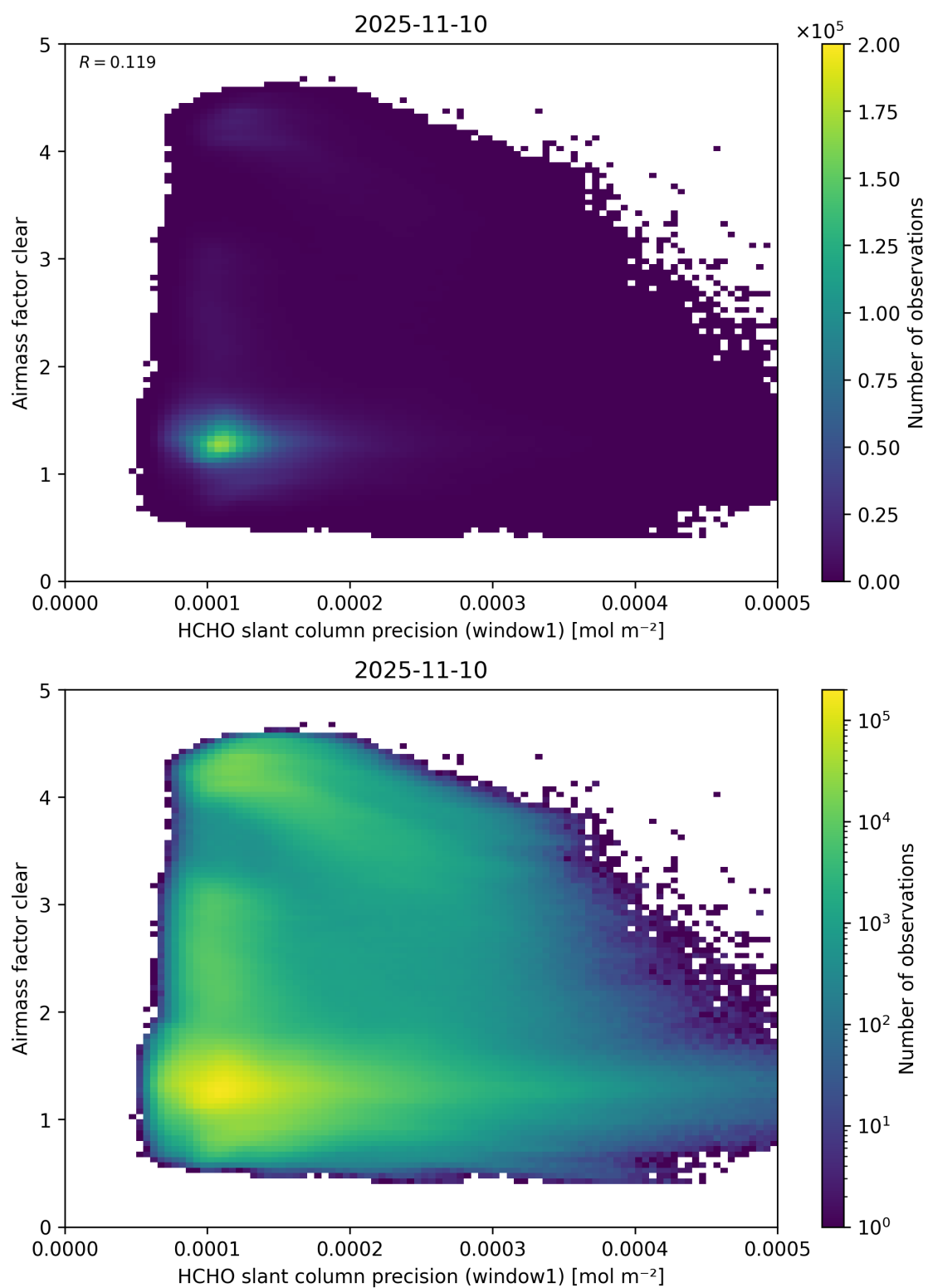
Figure 91: Scatter density plot of “HCHO slant column precision (window1)” against “Airmass factor clear” for 2025-11-09 to 2025-11-11.
