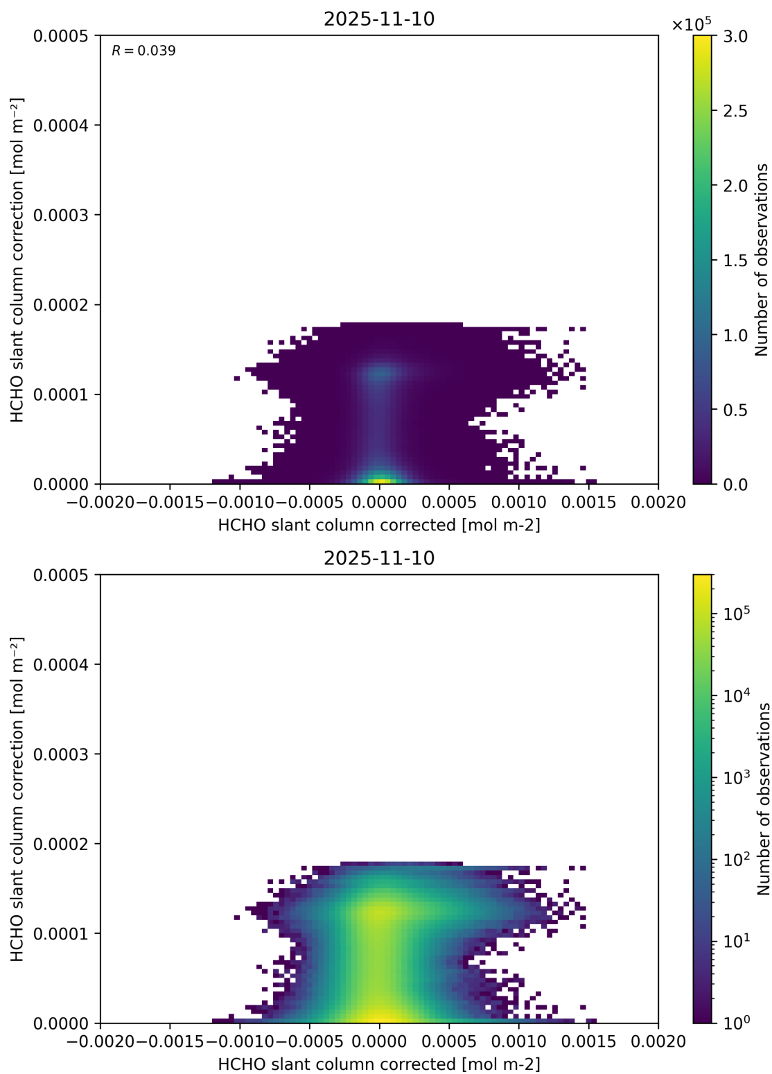
Figure 77: Scatter density plot of “HCHO slant column corrected” against “HCHO slant column correction” for 2025-11-09 to 2025-11-11.
