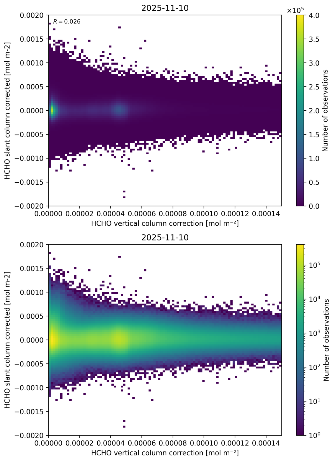
Figure 116: Scatter density plot of “HCHO vertical column correction” against “HCHO slant column corrected” for 2025-11-09 to 2025-11-11.
