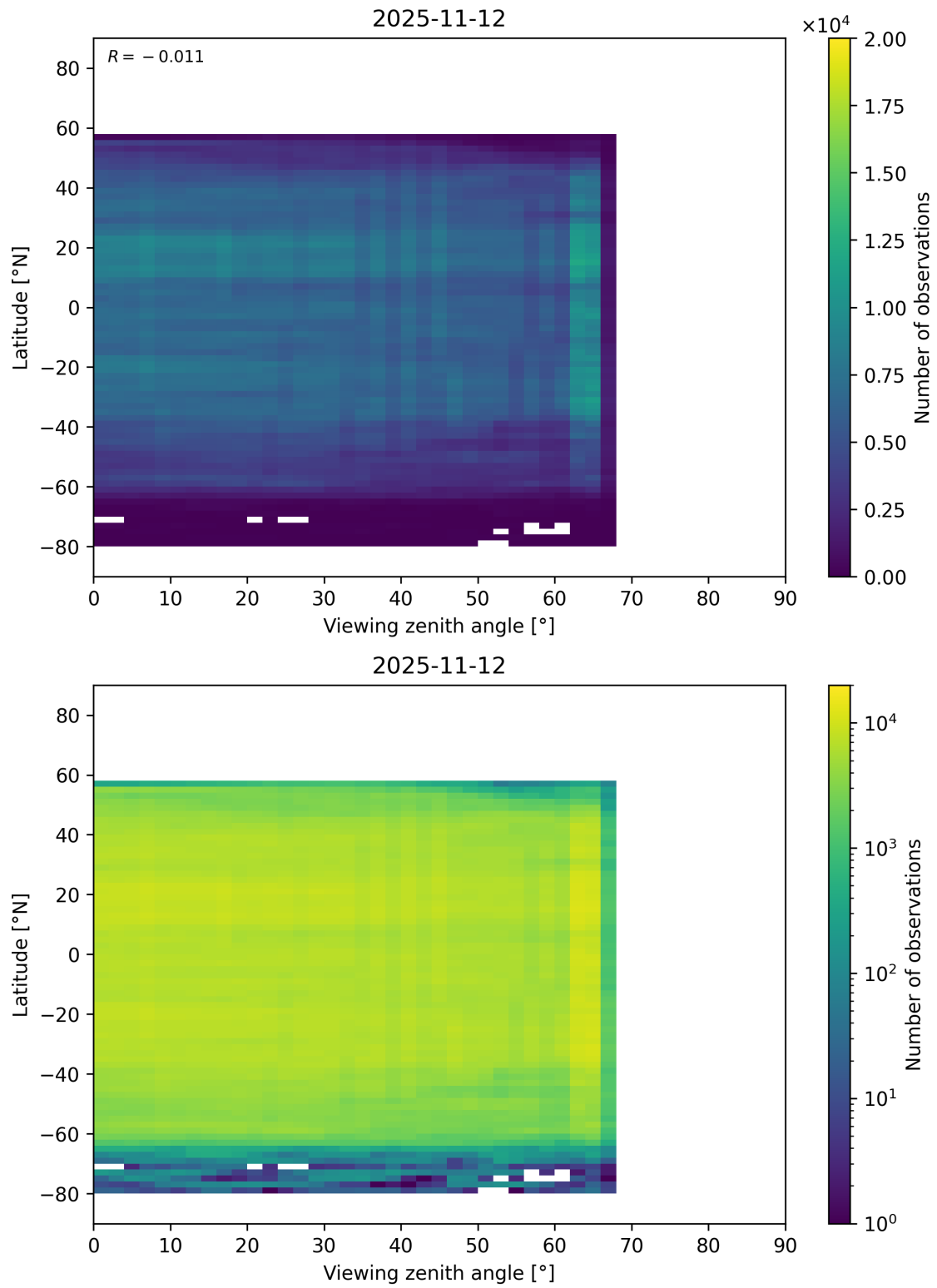
Figure 217: Scatter density plot of “Viewing zenith angle” against “Latitude” for 2025-11-12 to 2025-11-13.
