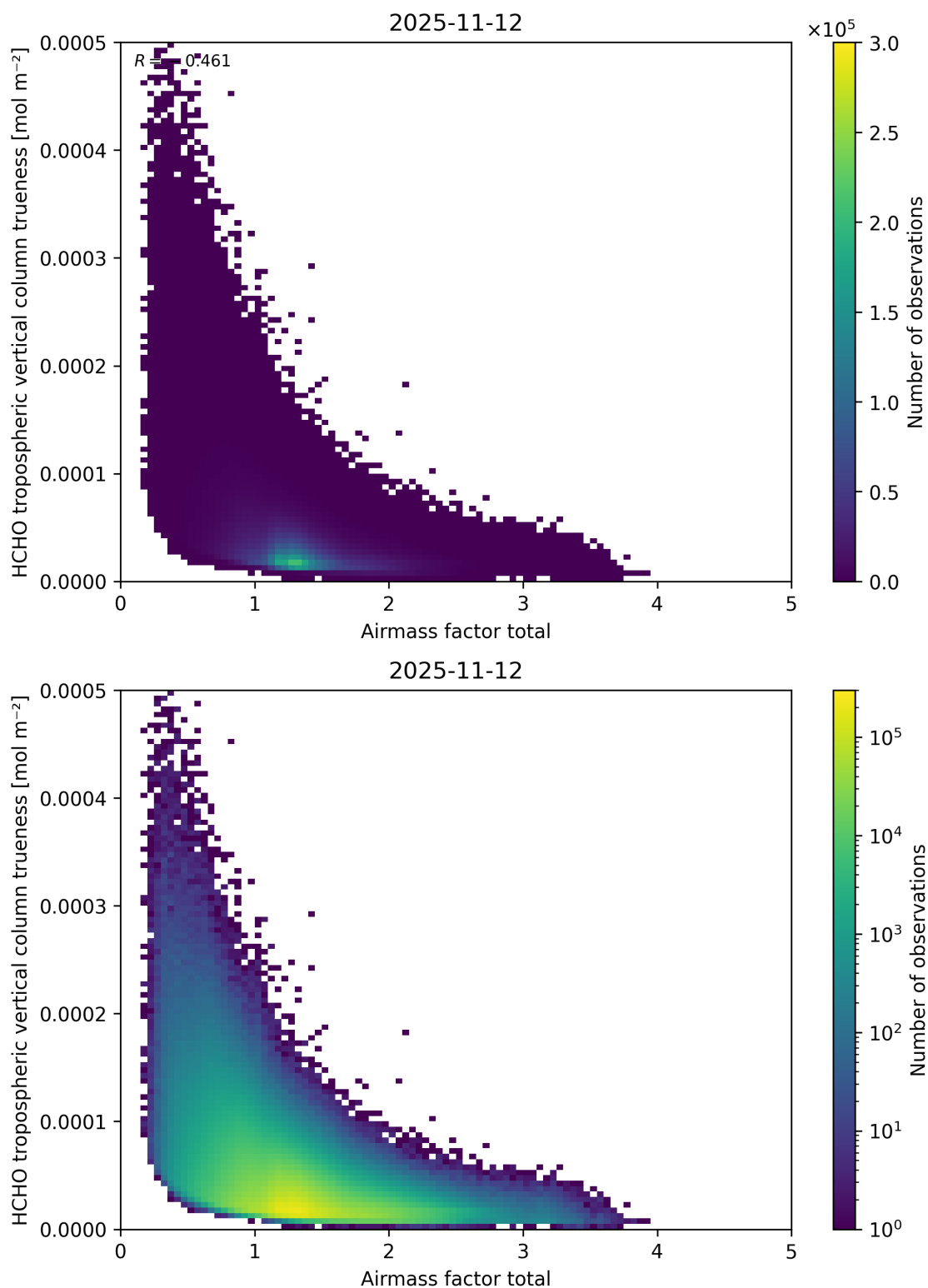
Figure 116: Scatter density plot of “Airmass factor total” against “HCHO tropospheric vertical column truiness” for 2025-11-12 to 2025-11-13.
