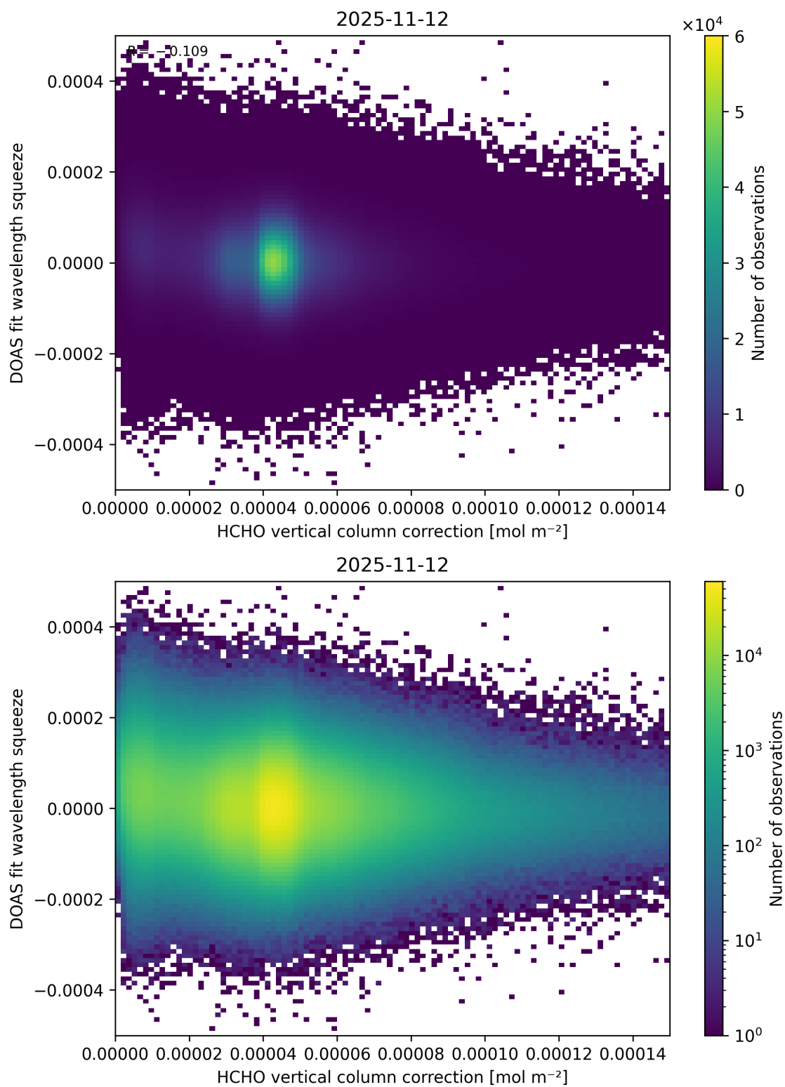
Figure 128: Scatter density plot of “HCHO vertical column correction” against “DOAS fit wavelength squeeze” for 2025-11-12 to 2025-11-13.
