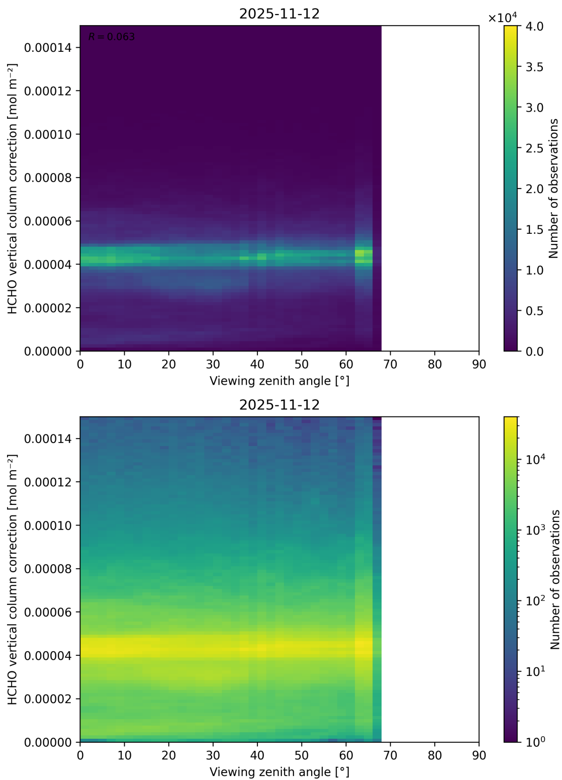
Figure 213: Scatter density plot of “Viewing zenith angle” against “HCHO vertical column correction” for 2025-11-12 to 2025-11-13.
