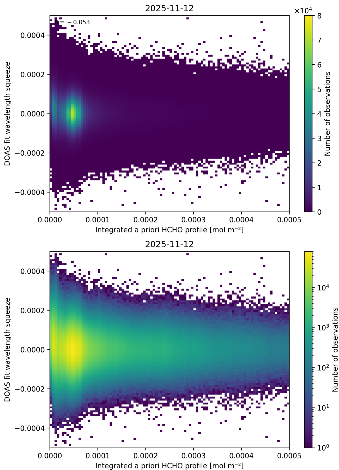
Figure 167: Scatter density plot of “Integrated a priori HCHO profile” against “DOAS fit wavelength squeeze” for 2025-11-12 to 2025-11-13.
