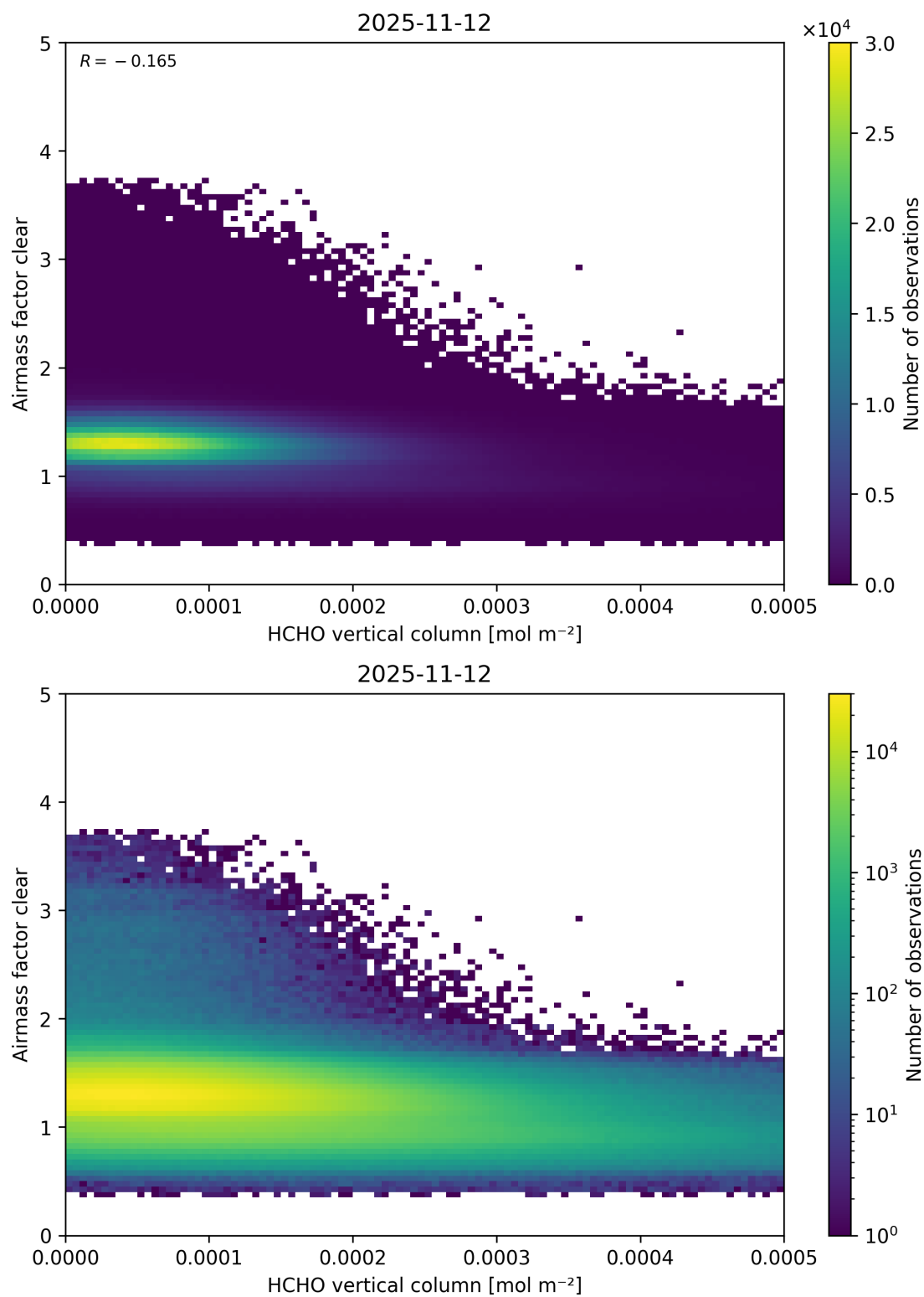
Figure 141: Scatter density plot of “HCHO vertical column” against “Airmass factor clear” for 2025-11-12 to 2025-11-13.
