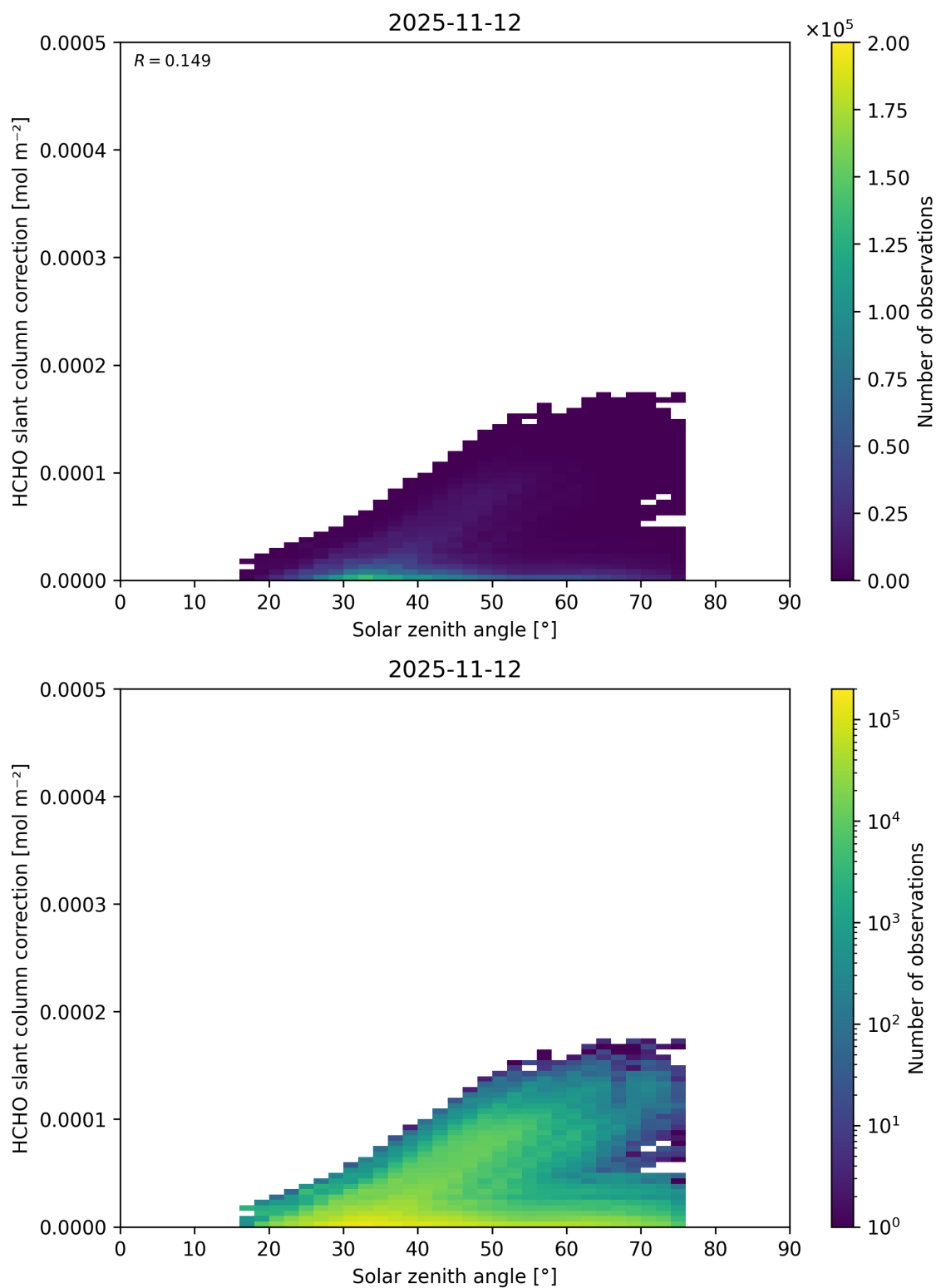
Figure 191: Scatter density plot of “Solar zenith angle” against “HCHO slant column correction” for 2025-11-12 to 2025-11-13.
