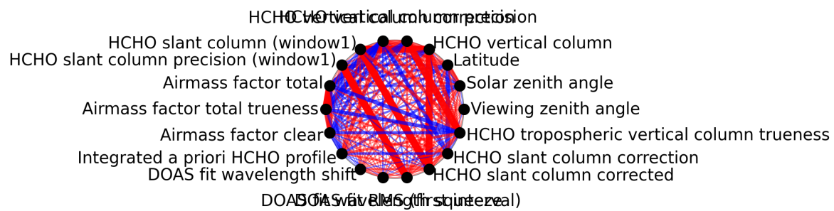
Figure 1: Map of correlation graph for 2025-11-12 to 2025-11-13.
