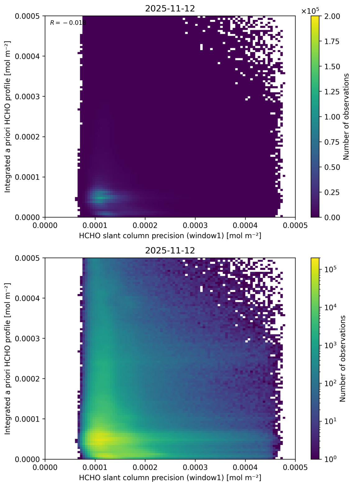
Figure 108: Scatter density plot of “HCHO slant column precision (window1)” against “Integrated a priori HCHO profile” for 2025-11-12 to 2025-11-13.
