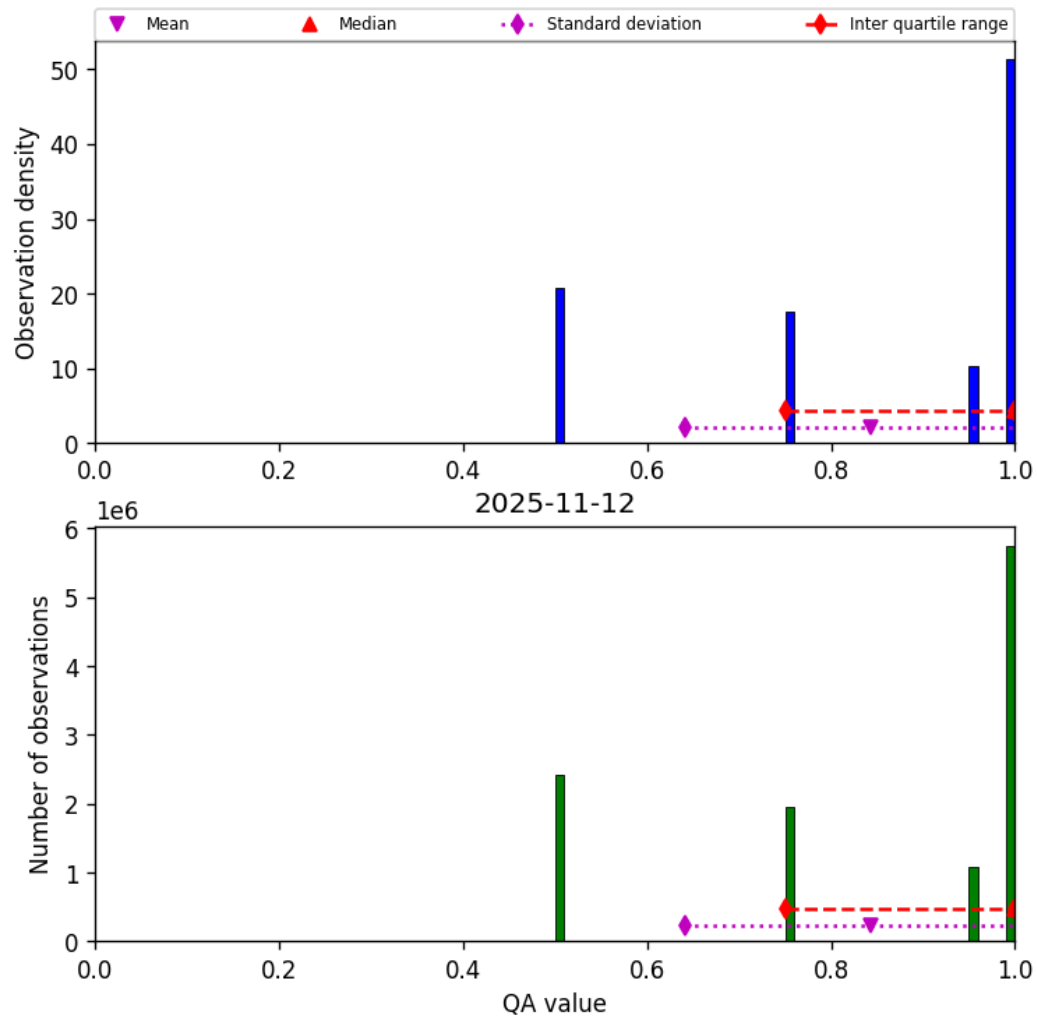
Figure 36: Histogram of “QA value” for 2025-11-12 to 2025-11-13
