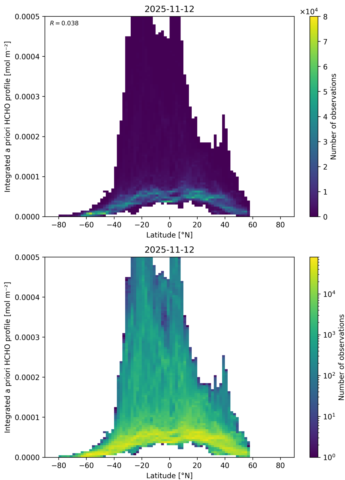
Figure 185: Scatter density plot of “Latitude” against “Integrated a priori HCHO profile” for 2025-11-12 to 2025-11-13.
