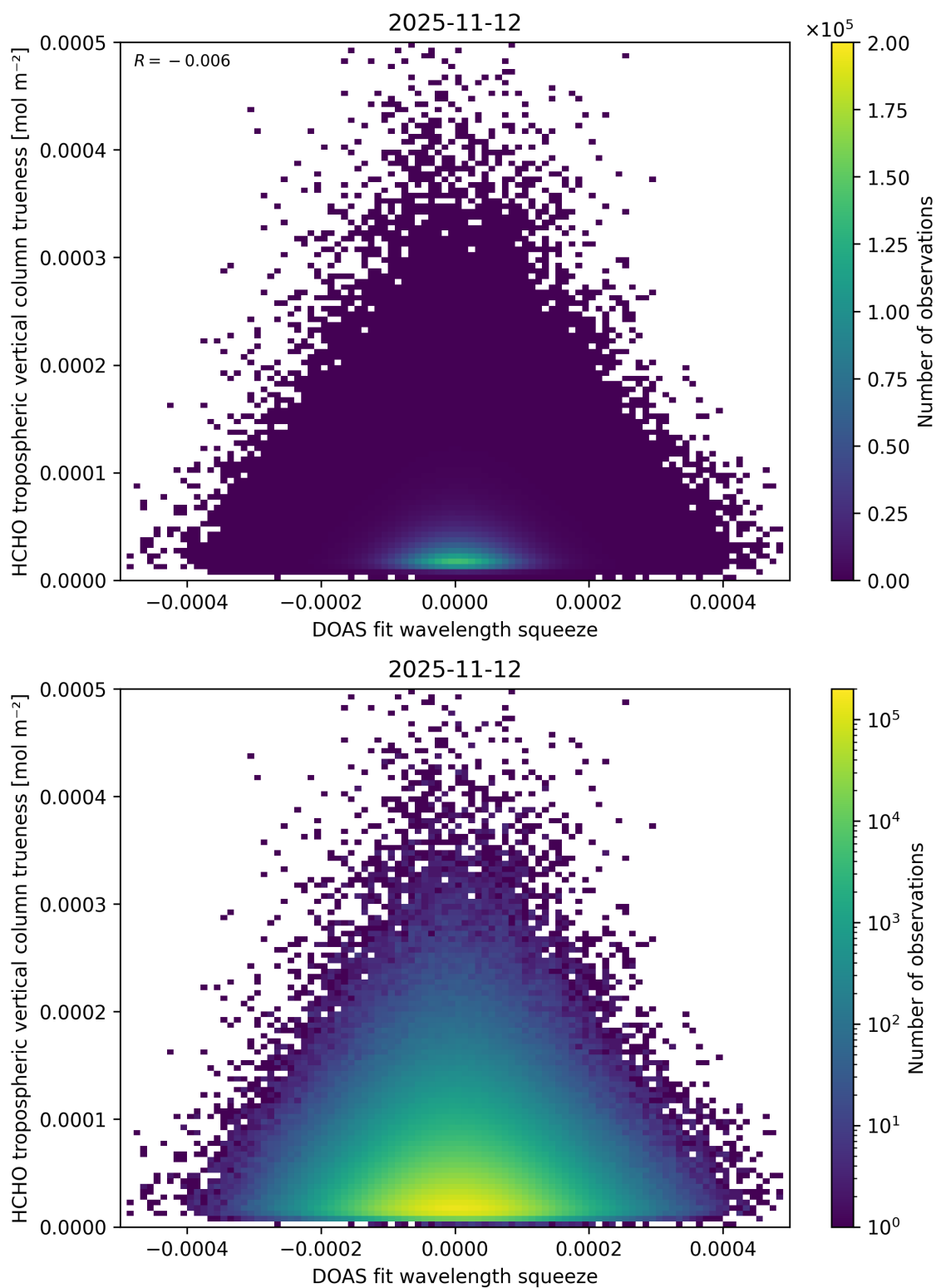
Figure 77: Scatter density plot of “DOAS fit wavelength squeeze” against “HCHO tropospheric vertical column trueness” for 2025-11-12 to 2025-11-13.
