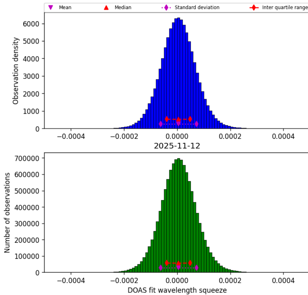
Figure 47: Histogram of “DOAS fit wavelength squeeze” for 2025-11-12 to 2025-11-13
