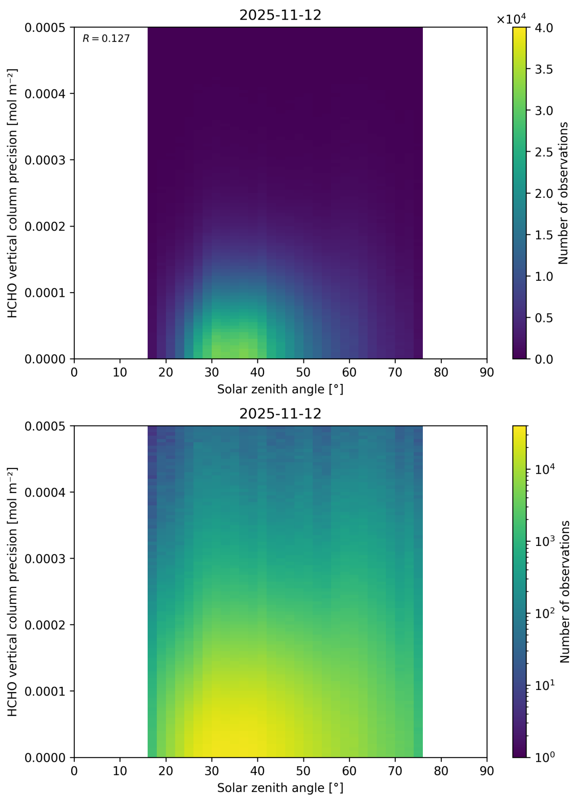
Figure 198: Scatter density plot of “Solar zenith angle” against “HCHO vertical column precision” for 2025-11-12 to 2025-11-13.
