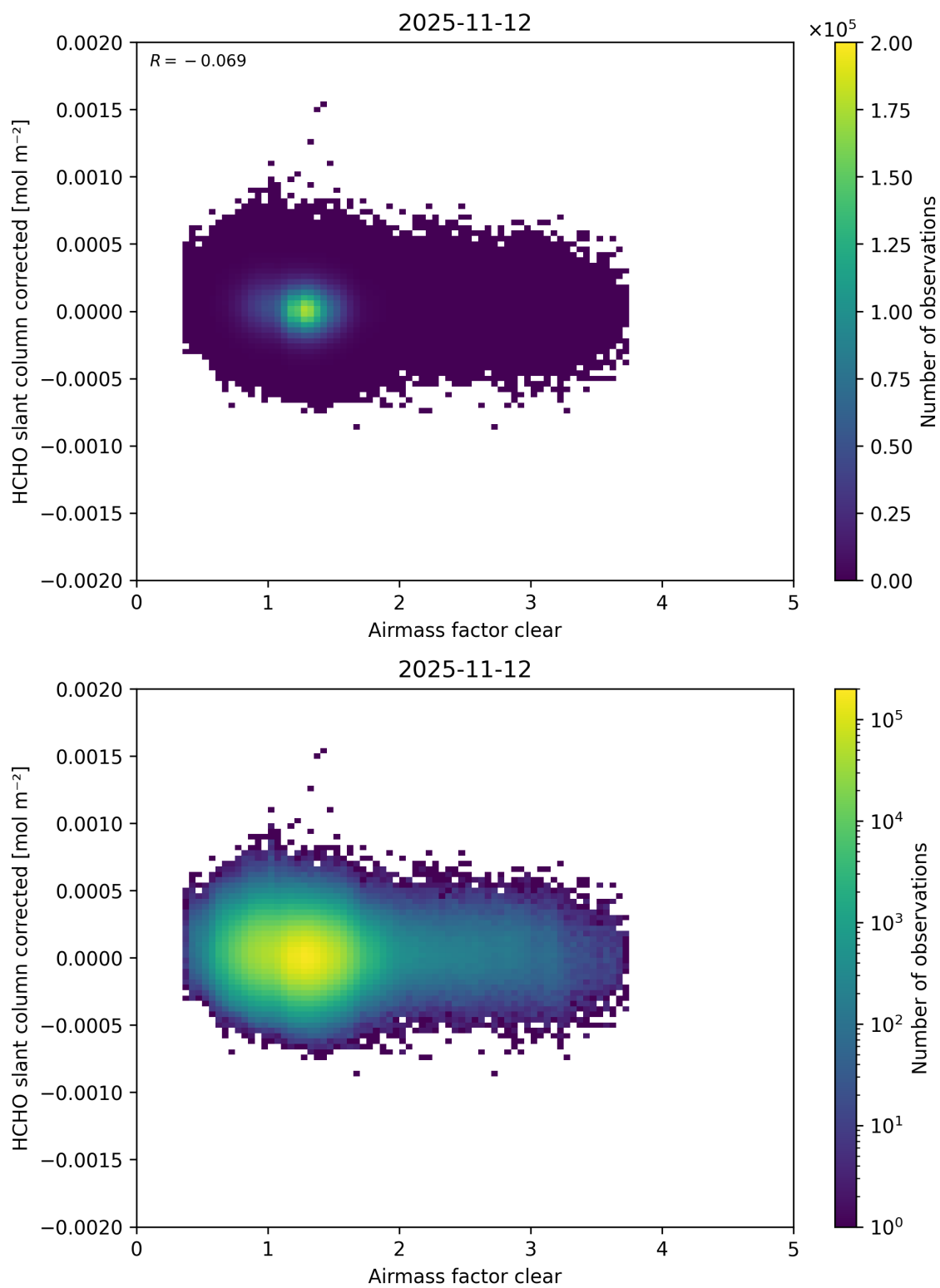
Figure 81: Scatter density plot of “Airmass factor clear” against “HCHO slant column corrected” for 2025-11-12 to 2025-11-13.
