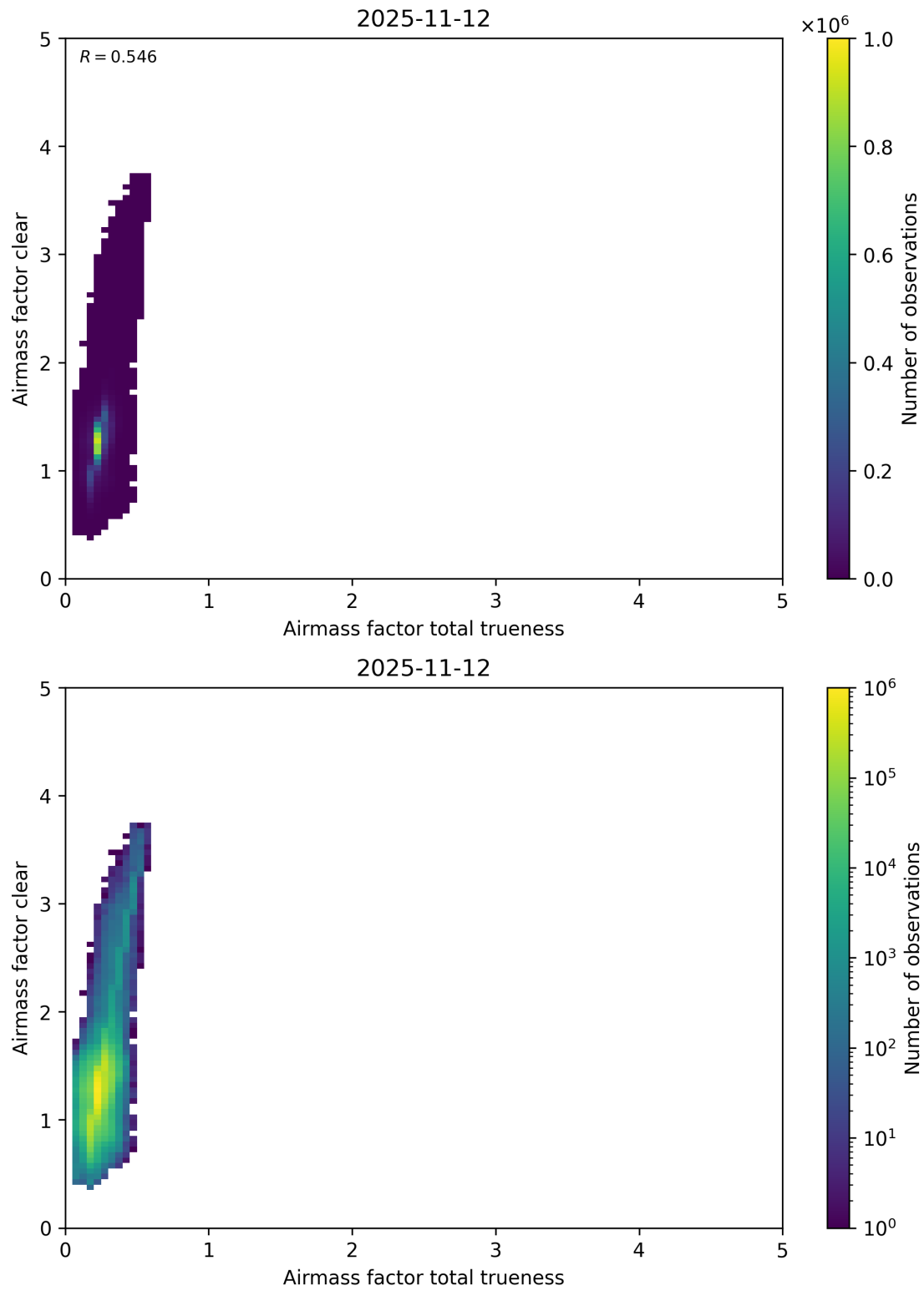
Figure 121: Scatter density plot of “Airmass factor total trueness” against “Airmass factor clear” for 2025-11-12 to 2025-11-13.
