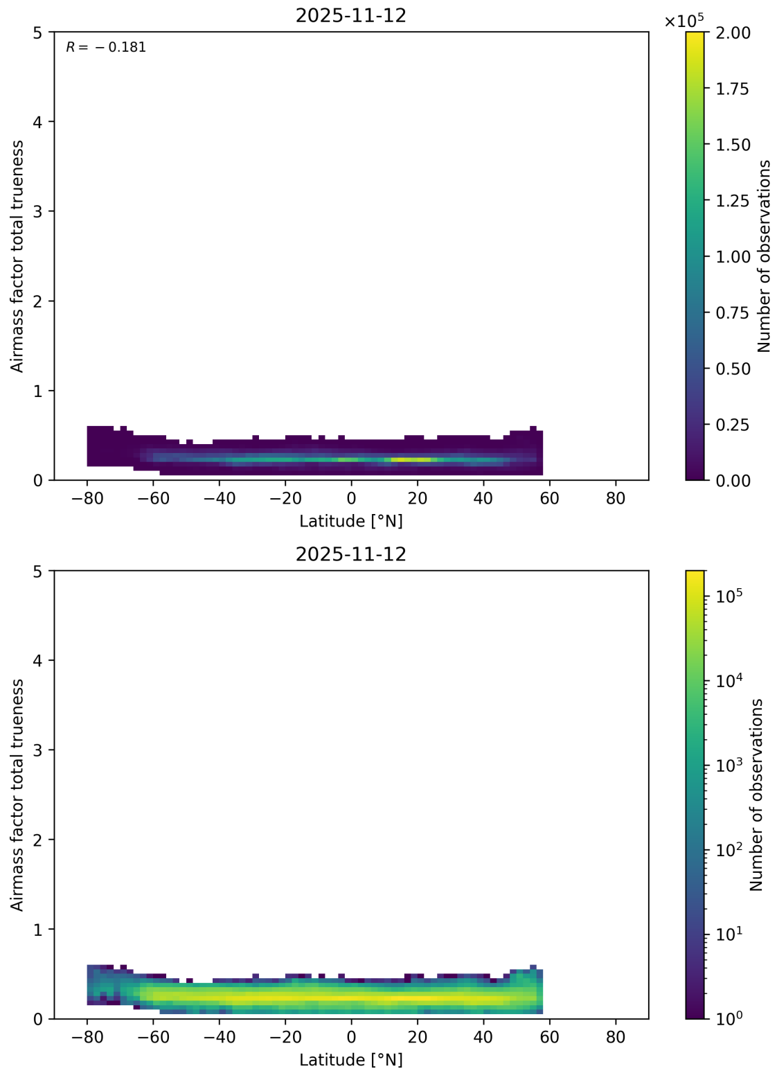
Figure 180: Scatter density plot of “Latitude” against “Airmass factor total trueness” for 2025-11-12 to 2025-11-13.
