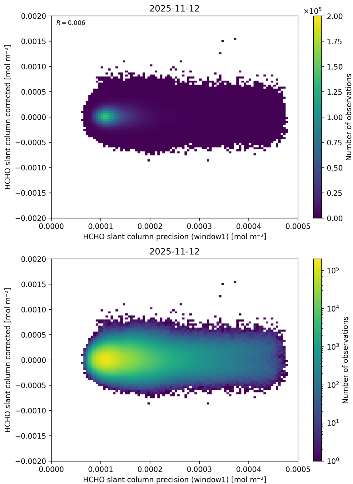
Figure 103: Scatter density plot of “HCHO slant column precision (window1)” against “HCHO slant column corrected” for 2025-11-12 to 2025-11-13.
