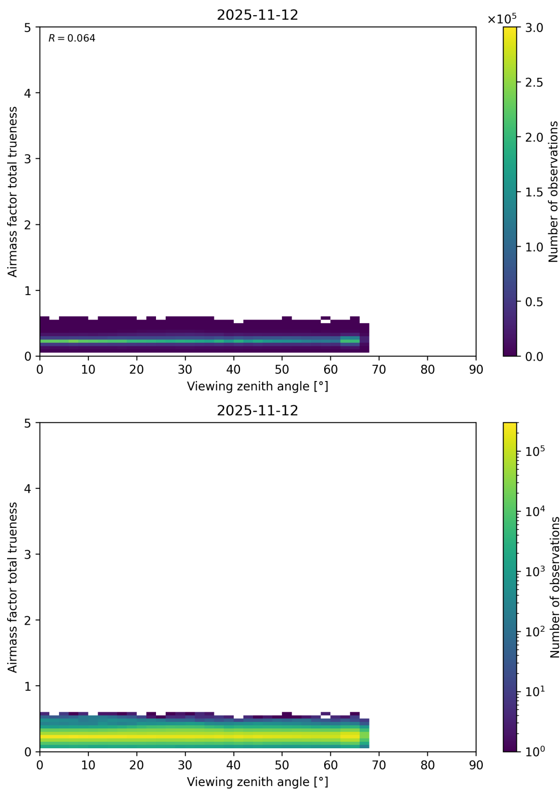
Figure 211: Scatter density plot of “Viewing zenith angle” against “Airmass factor total truiness” for 2025-11-12 to 2025-11-13.
