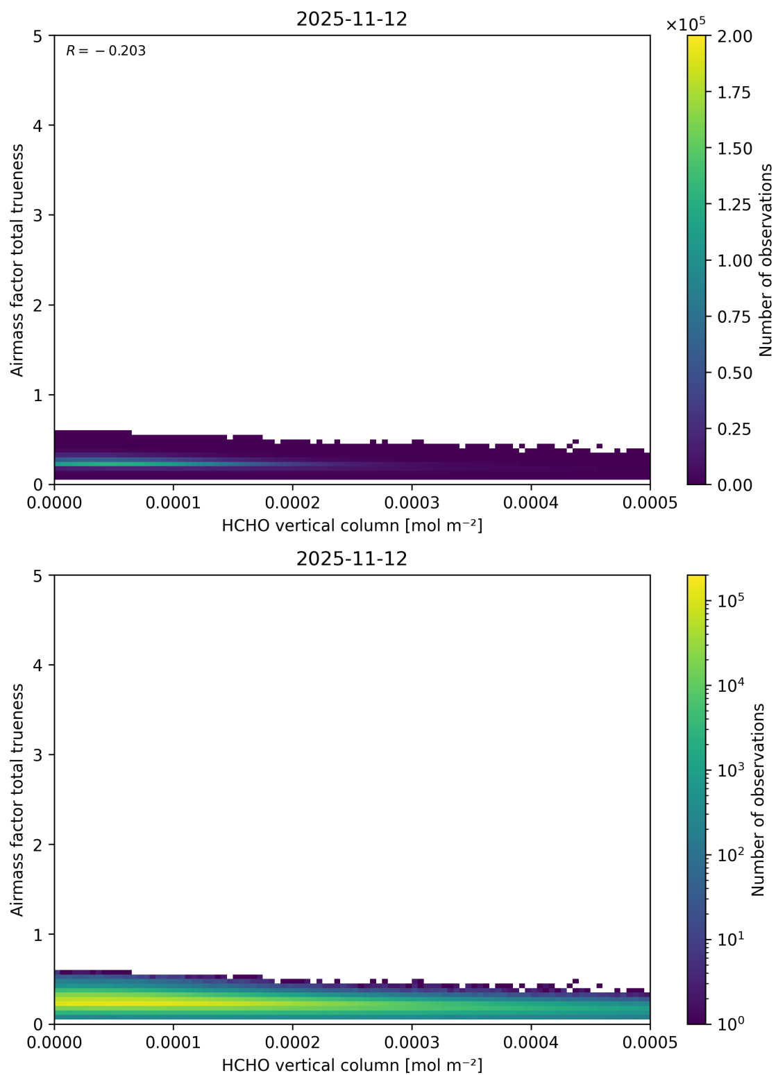
Figure 147: Scatter density plot of “HCHO vertical column” against “Airmass factor total trueneess” for 2025-11-12 to 2025-11-13.
