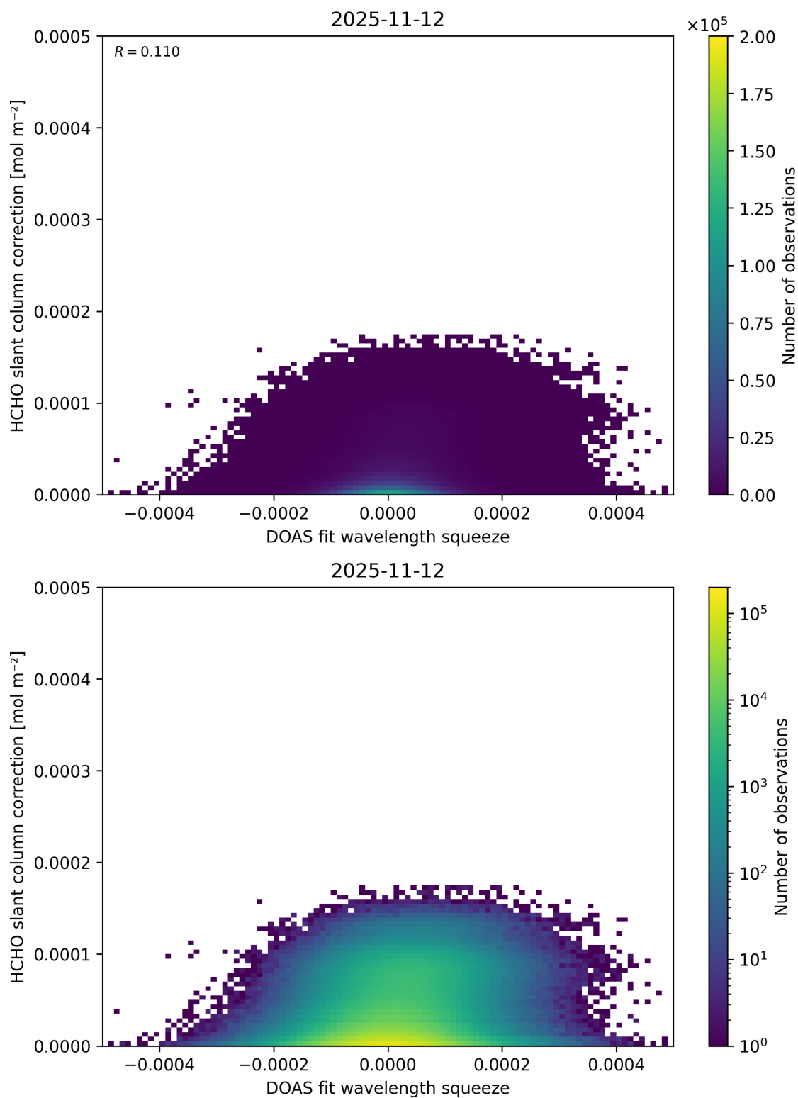
Figure 76: Scatter density plot of “DOAS fit wavelength squeeze” against “HCHO slant column correction” for 2025-11-12 to 2025-11-13.
