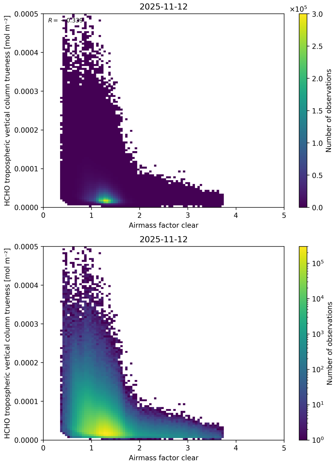
Figure 83: Scatter density plot of “Airmass factor clear” against “HCHO tropospheric vertical column trueness” for 2025-11-12 to 2025-11-13.
