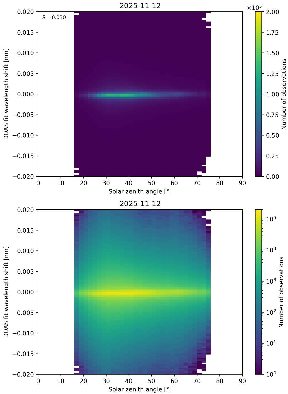
Figure 187: Scatter density plot of “Solar zenith angle” against “DOAS fit wavelength shift” for 2025-11-12 to 2025-11-13.
