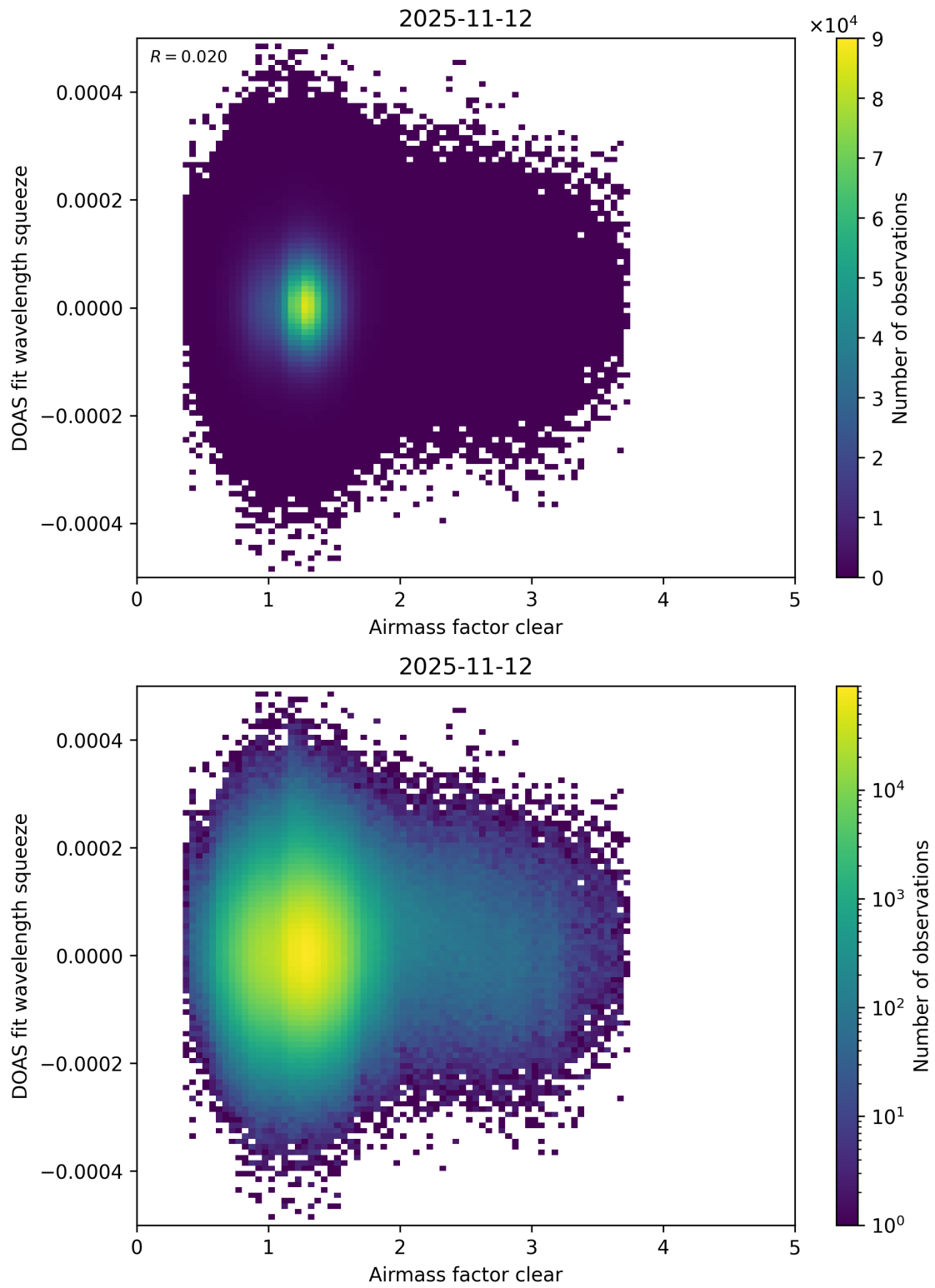
Figure 80: Scatter density plot of “Airmass factor clear” against “DOAS fit wavelength squeeze” for 2025-11-12 to 2025-11-13.
