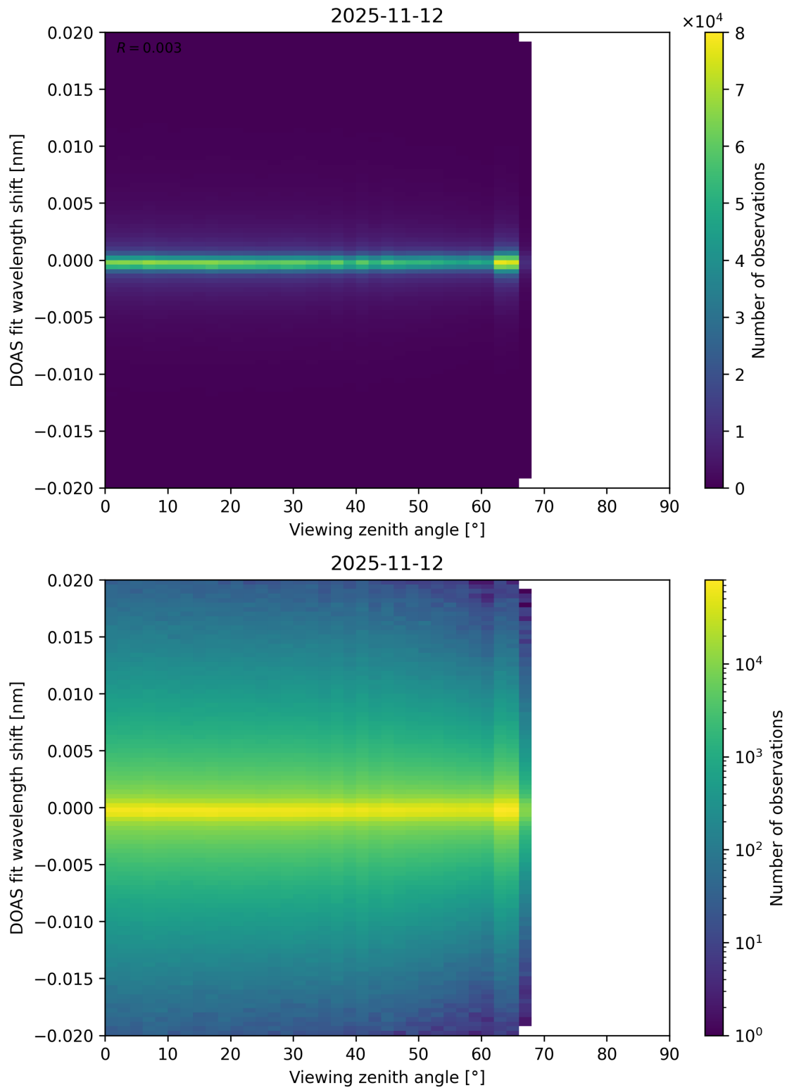
Figure 203: Scatter density plot of “Viewing zenith angle” against “DOAS fit wavelength shift” for 2025-11-12 to 2025-11-13.
