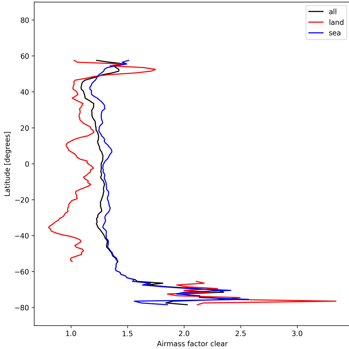
Figure 29: Zonal average of “Airmass factor clear” for 2025-11-12 to 2025-11-13.
