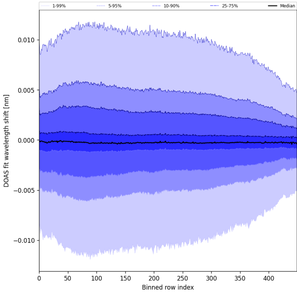
Figure 61: Along track statistics of “DOAS fit wavelength shift” for 2025-11-12 to 2025-11-13
