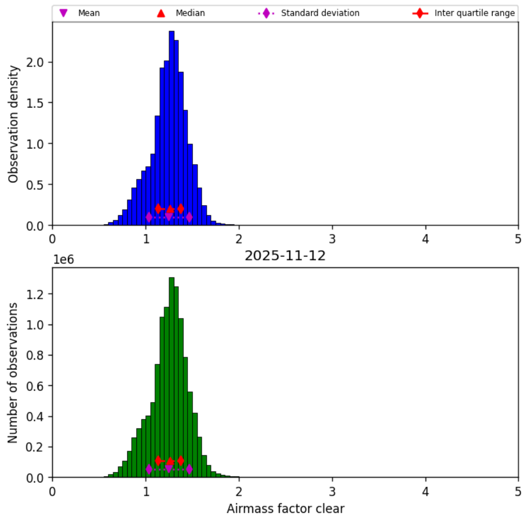
Figure 44: Histogram of “Airmass factor clear” for 2025-11-12 to 2025-11-13
