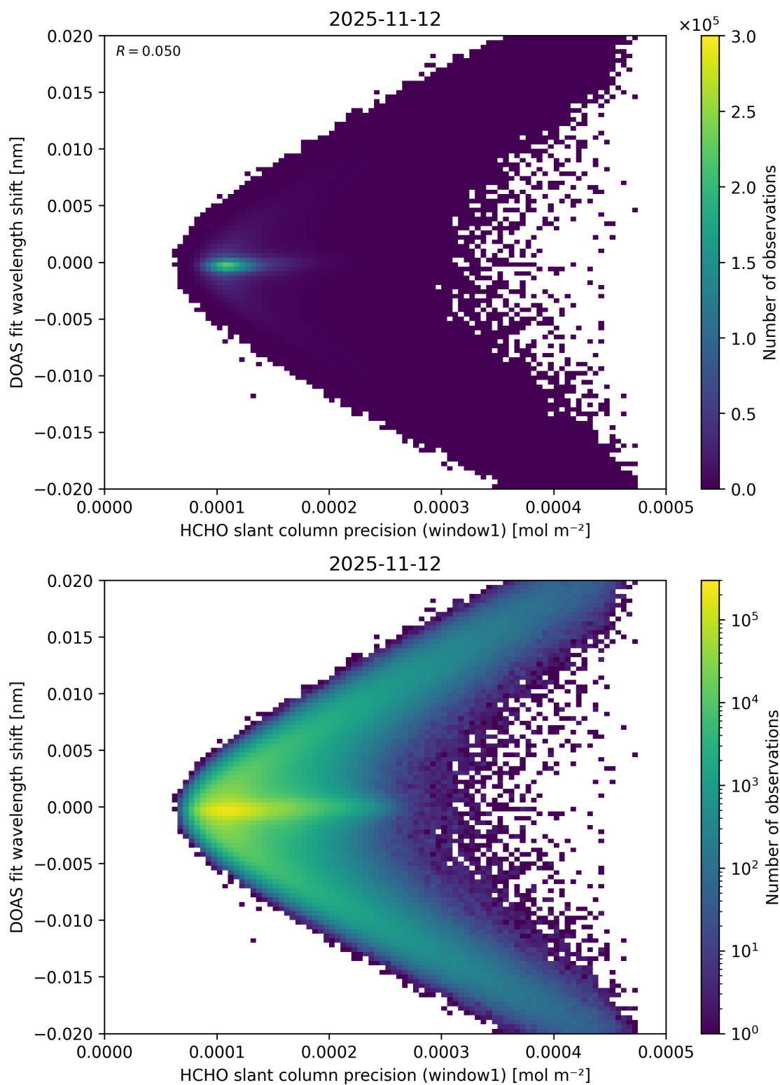
Figure 100: Scatter density plot of “HCHO slant column precision (window1)” against “DOAS fit wavelength shift” for 2025-11-12 to 2025-11-13.
