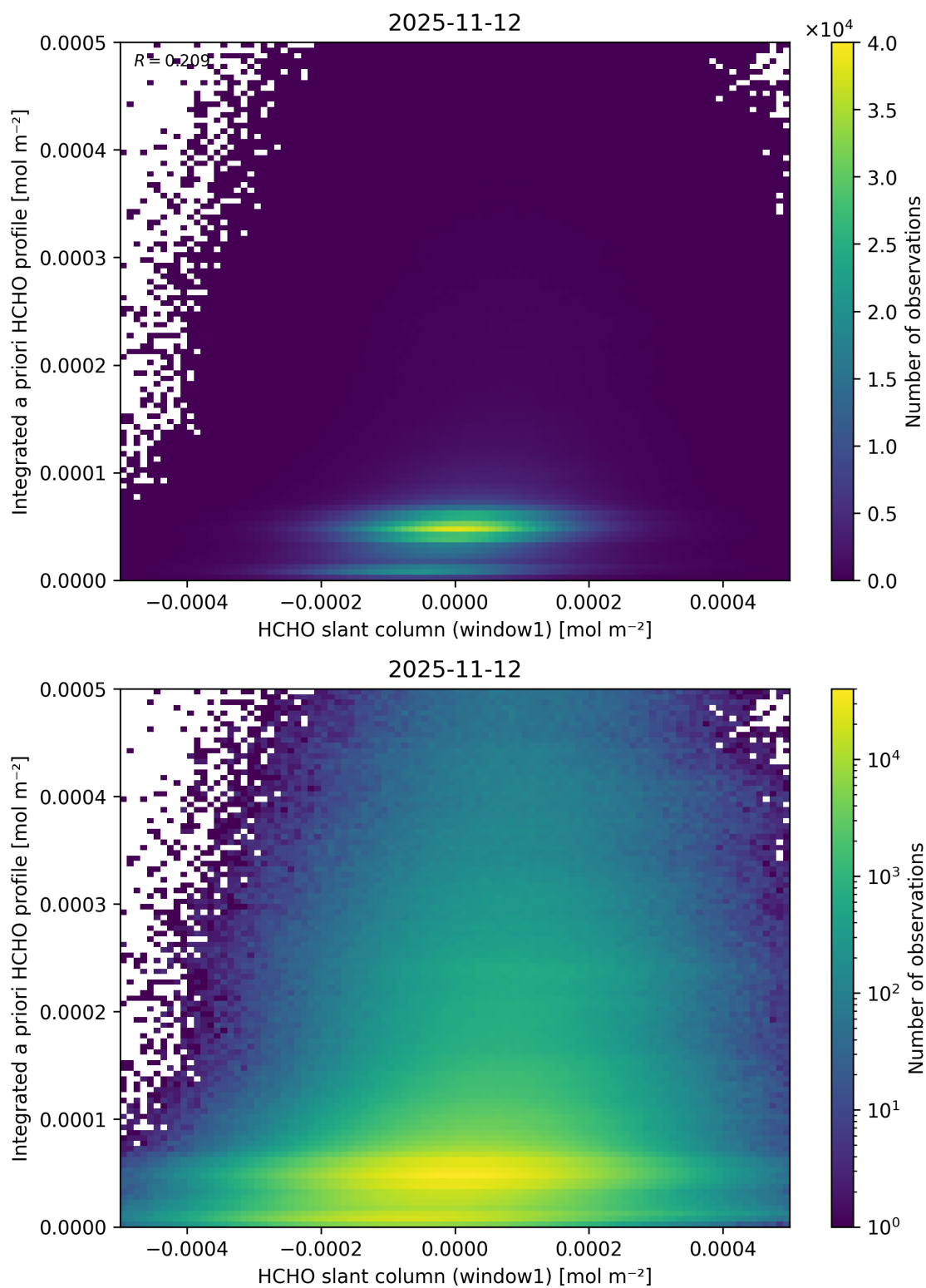
Figure 98: Scatter density plot of “HCHO slant column (window1)” against “Integrated a priori HCHO profile” for 2025-11-12 to 2025-11-13.
