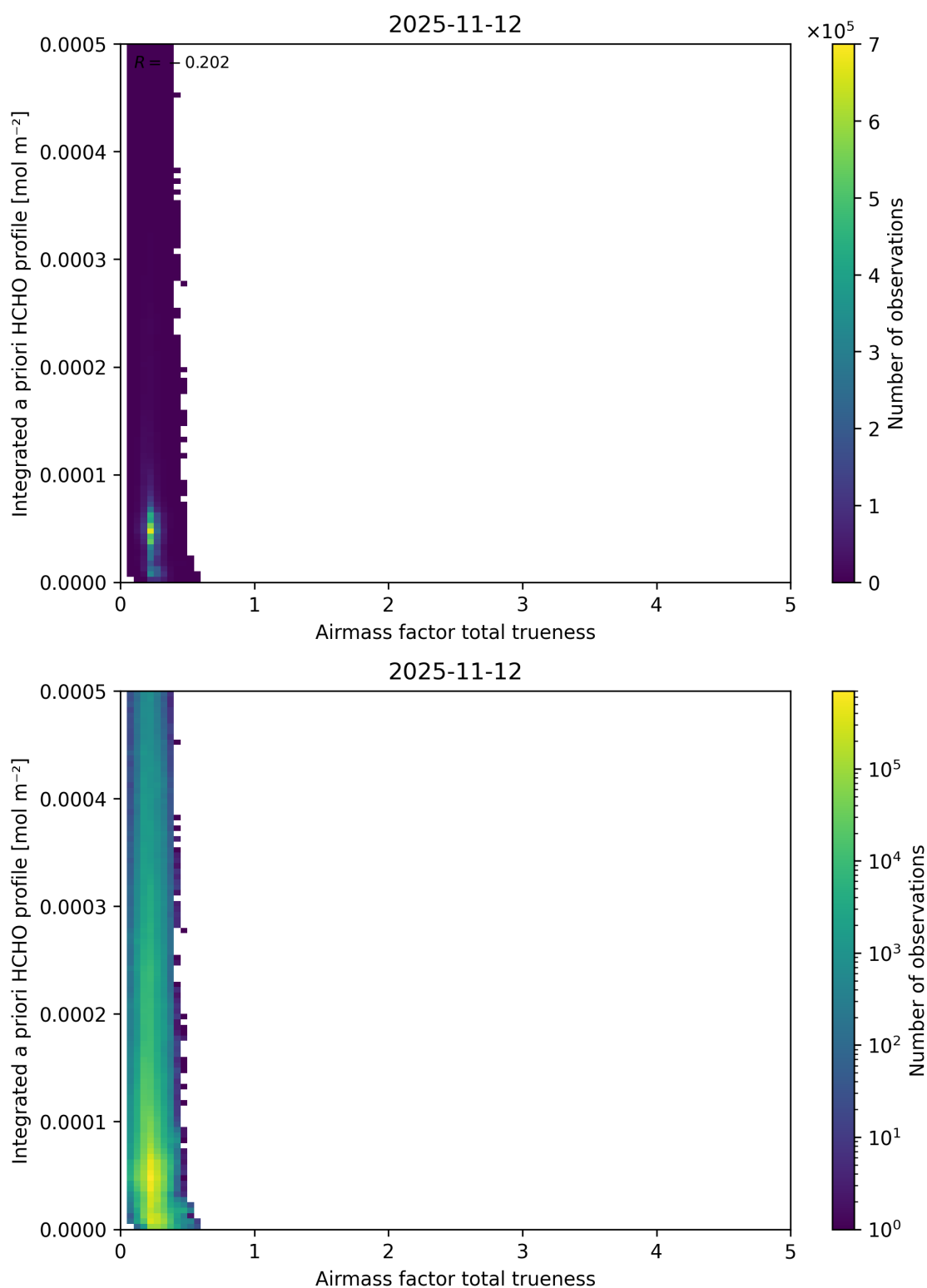
Figure 125: Scatter density plot of “Airmass factor total trueness” against “Integrated a priori HCHO profile” for 2025-11-12 to 2025-11-13.
