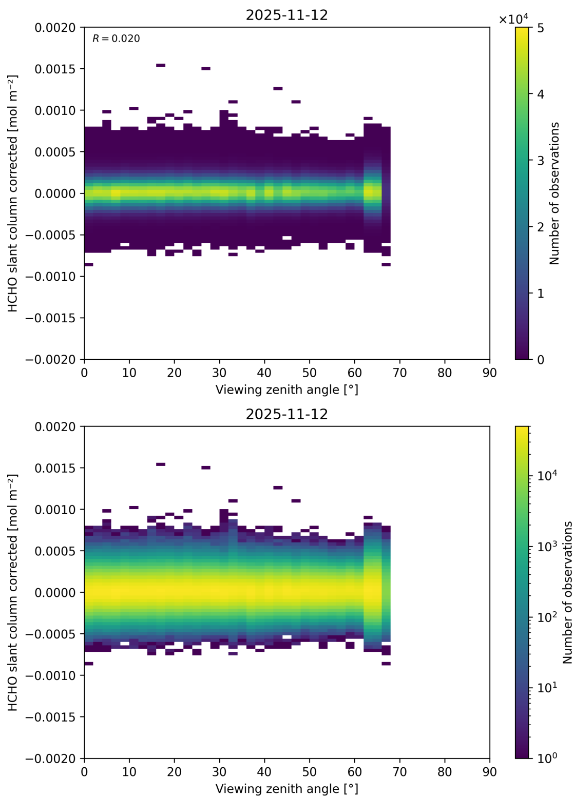
Figure 206: Scatter density plot of “Viewing zenith angle” against “HCHO slant column corrected” for 2025-11-12 to 2025-11-13.
