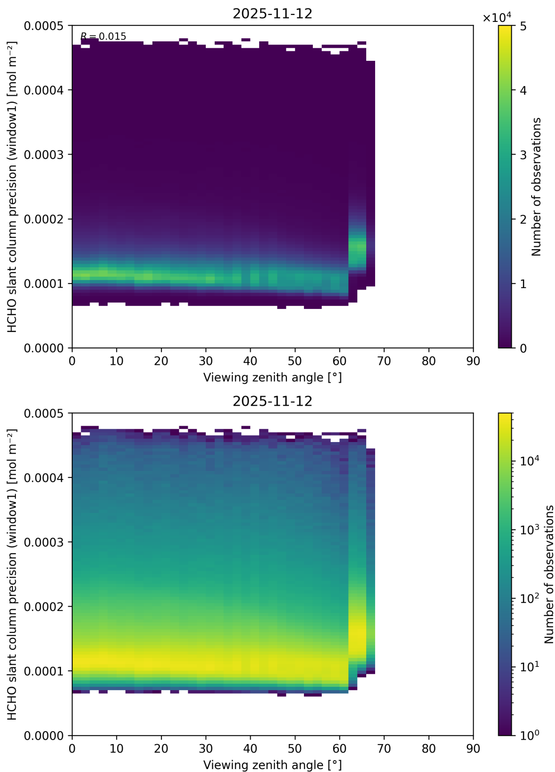
Figure 209: Scatter density plot of “Viewing zenith angle” against “HCHO slant column precision (window1)” for 2025-11-12 to 2025-11-13.
