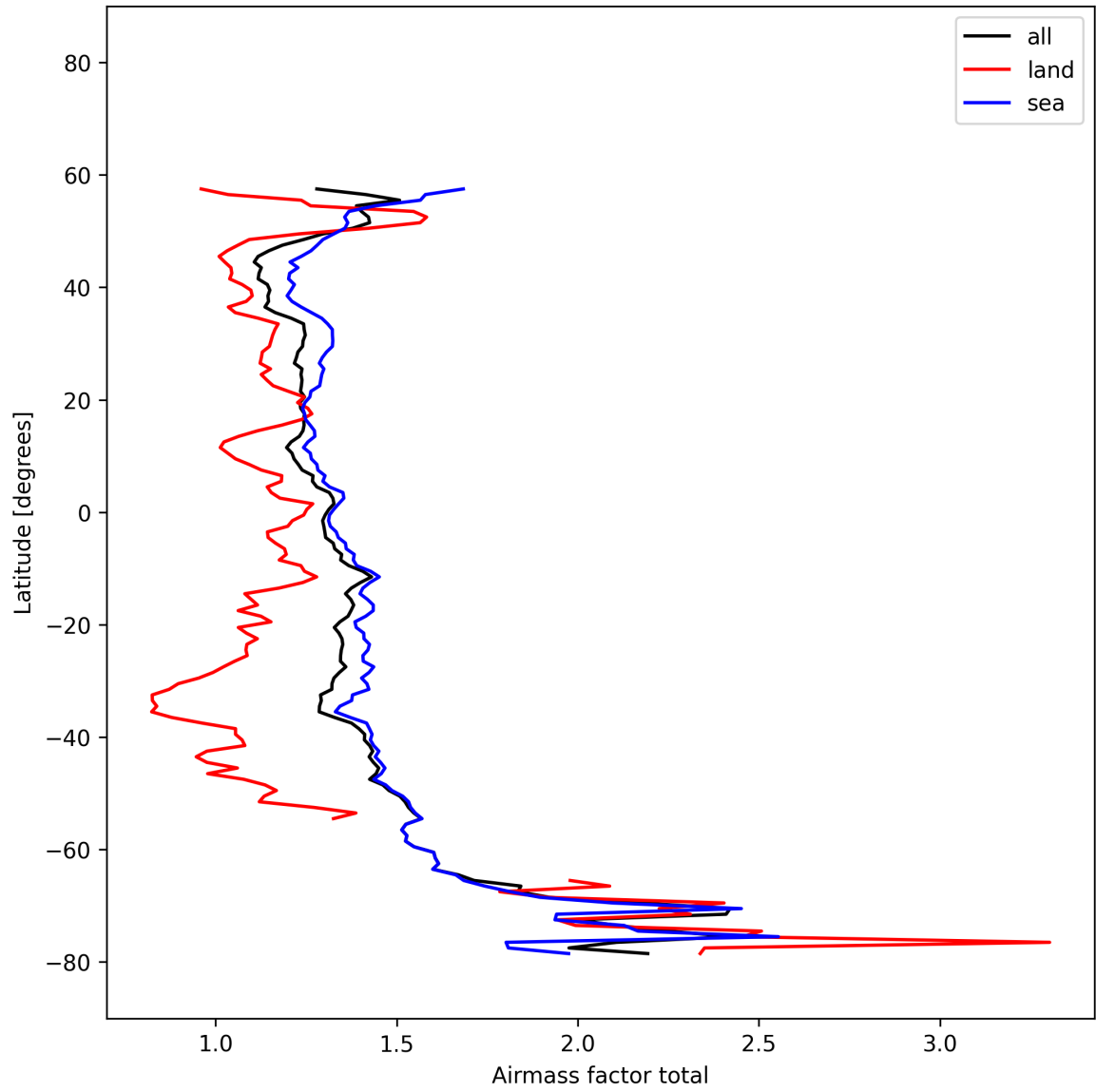
Figure 27: Zonal average of “Airmass factor total” for 2025-11-12 to 2025-11-13.
