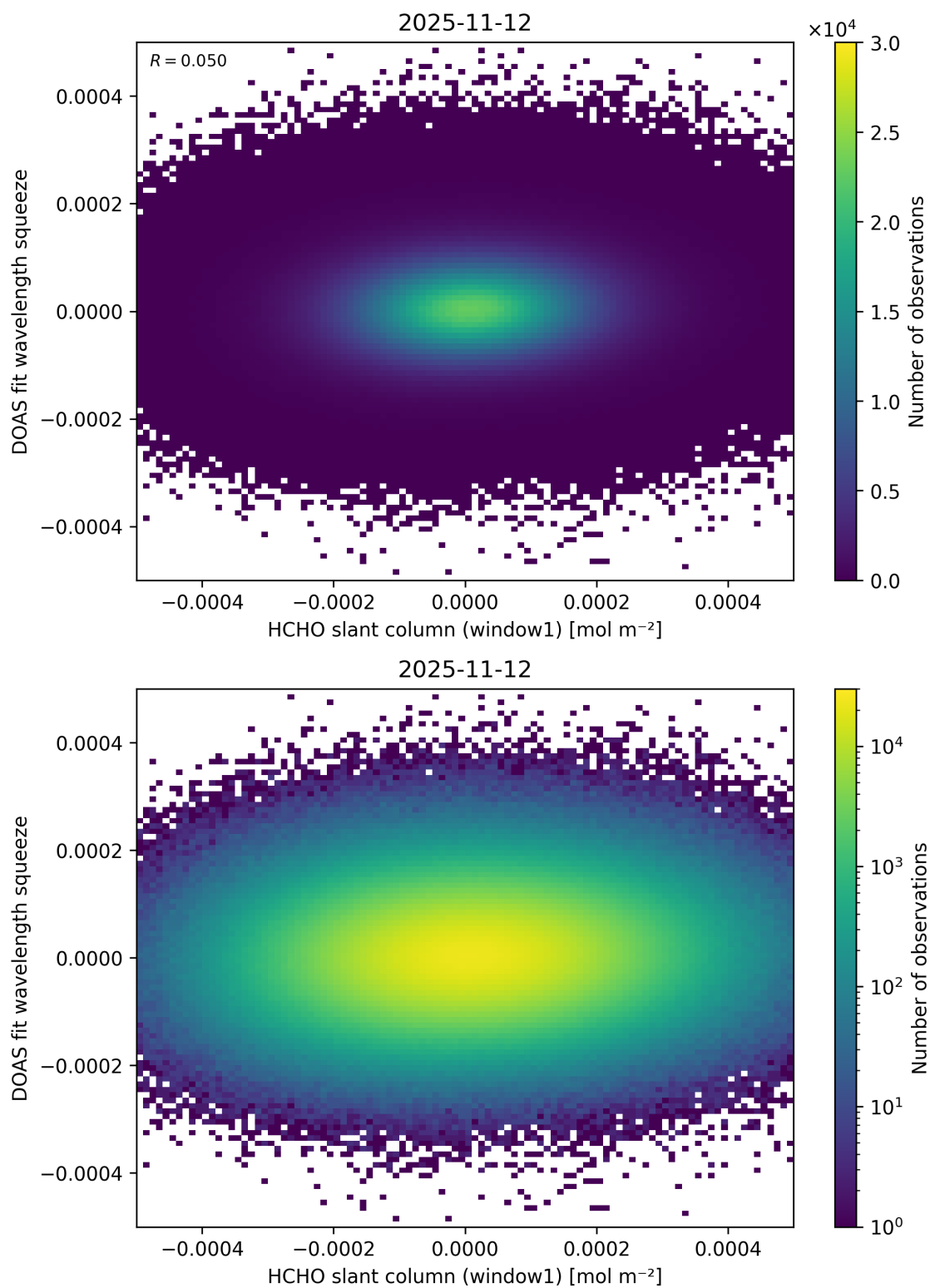
Figure 90: Scatter density plot of “HCHO slant column (window1)” against “DOAS fit wavelength squeeze” for 2025-11-12 to 2025-11-13.
