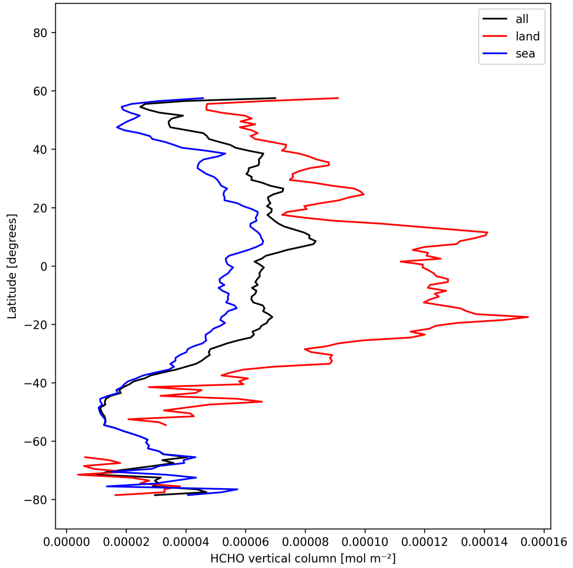
Figure 22: Zonal average of “HCHO vertical column” for 2025-11-12 to 2025-11-13.
