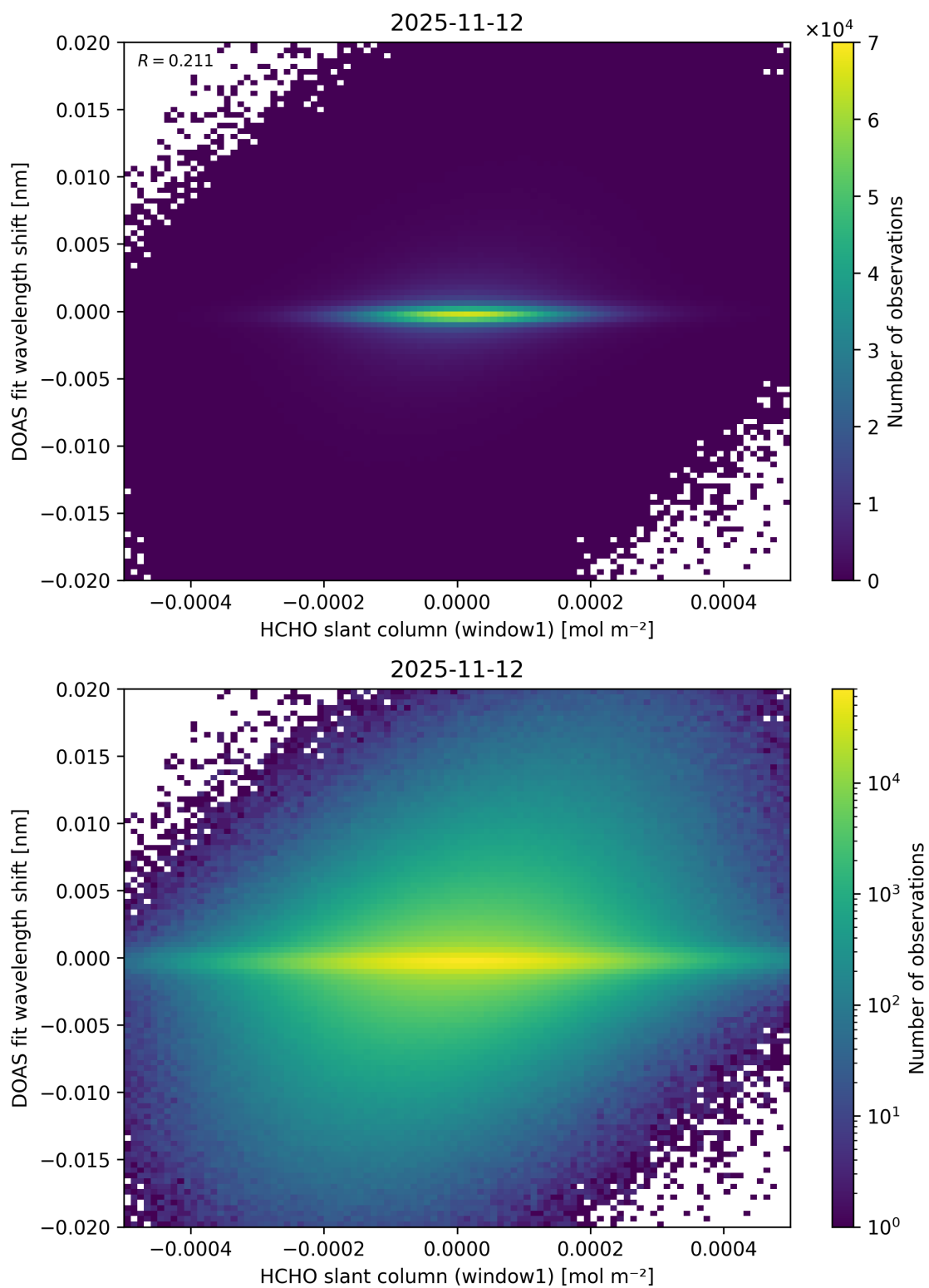
Figure 89: Scatter density plot of “HCHO slant column (window1)” against “DOAS fit wavelength shift” for 2025-11-12 to 2025-11-13.
