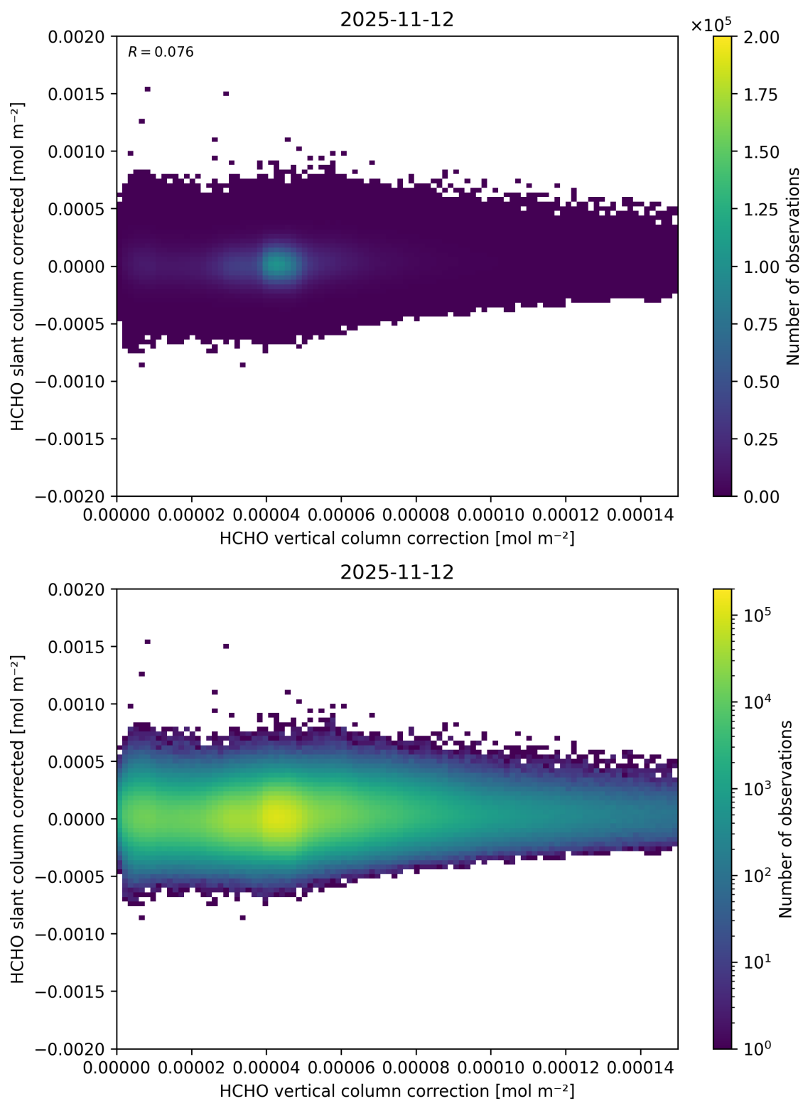
Figure 130: Scatter density plot of “HCHO vertical column correction” against “HCHO slant column corrected” for 2025-11-12 to 2025-11-13.
