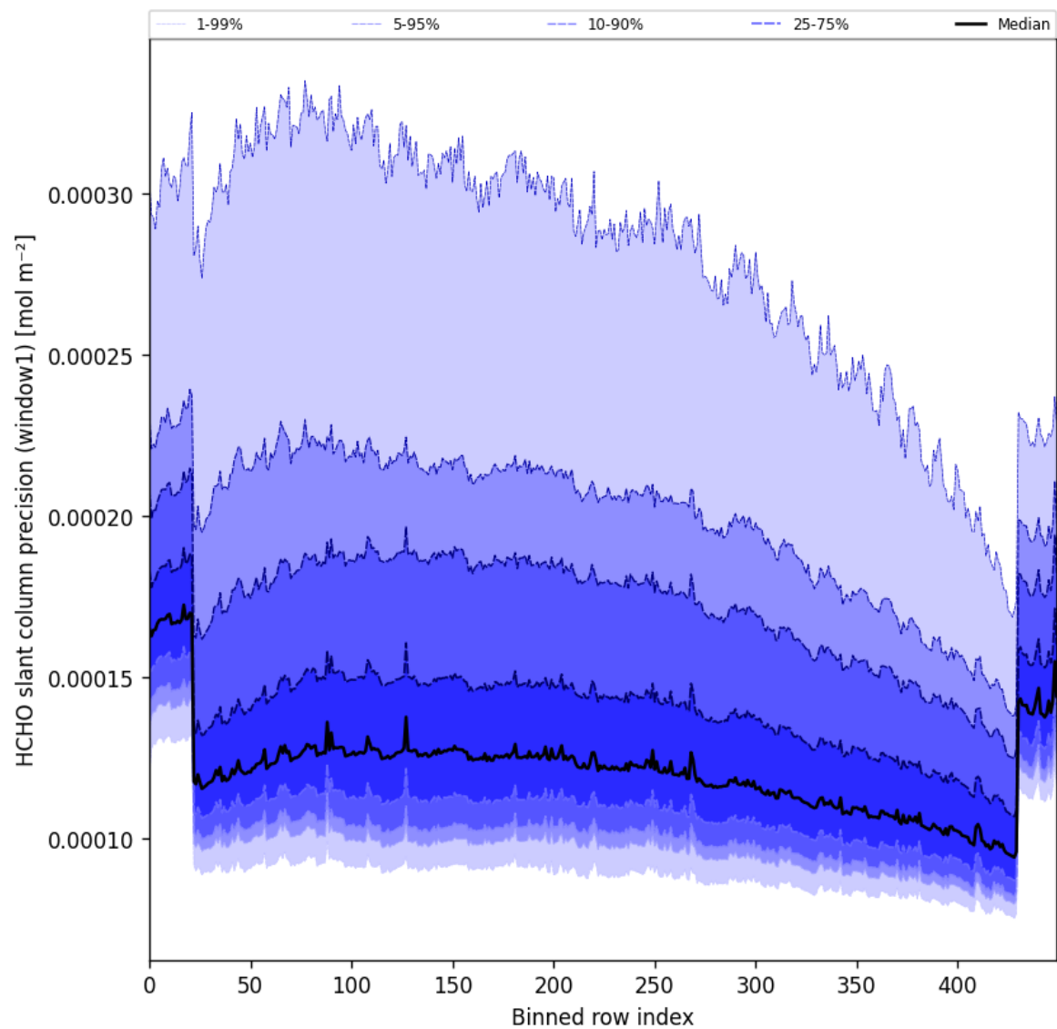
Figure 56: Along track statistics of “HCHO slant column precision (window1)” for 2025-11-12 to 2025-11-13
