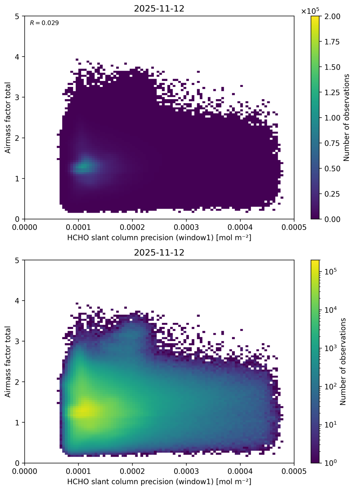
Figure 105: Scatter density plot of “HCHO slant column precision (window1)” against “Airmass factor total” for 2025-11-12 to 2025-11-13.
