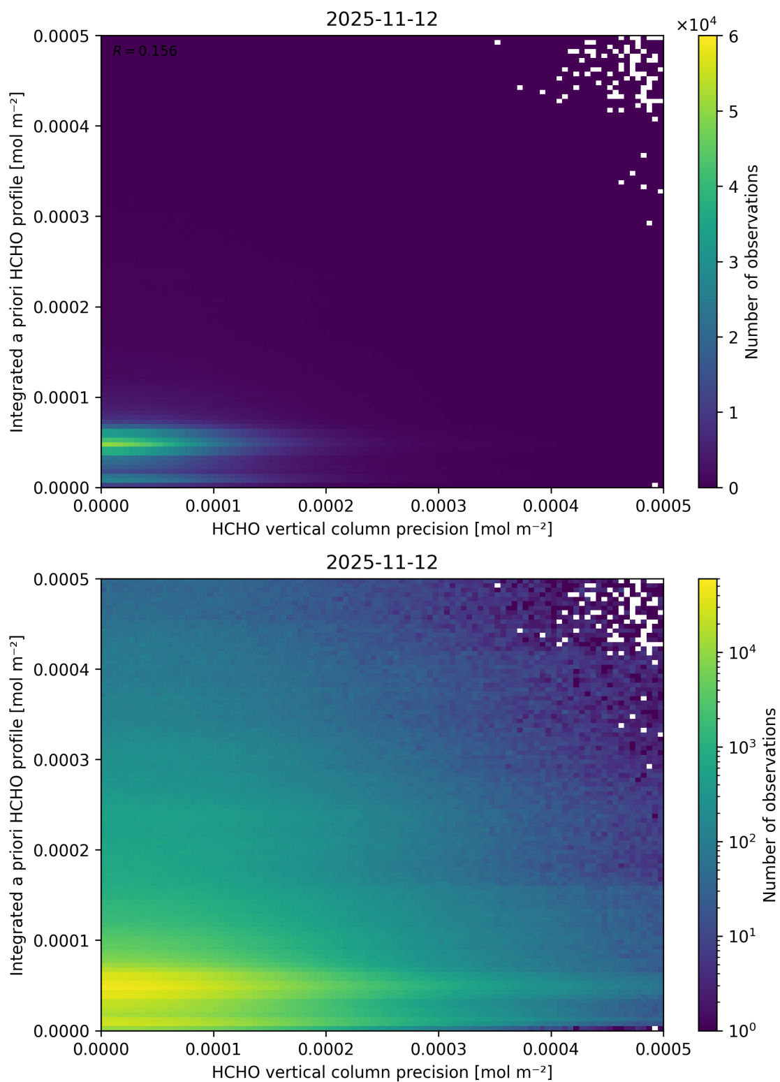
Figure 164: Scatter density plot of “HCHO vertical column precision” against “Integrated a priori HCHO profile” for 2025-11-12 to 2025-11-13.
