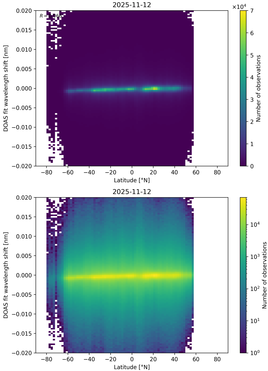
Figure 172: Scatter density plot of “Latitude” against “DOAS fit wavelength shift” for 2025-11-12 to 2025-11-13.
