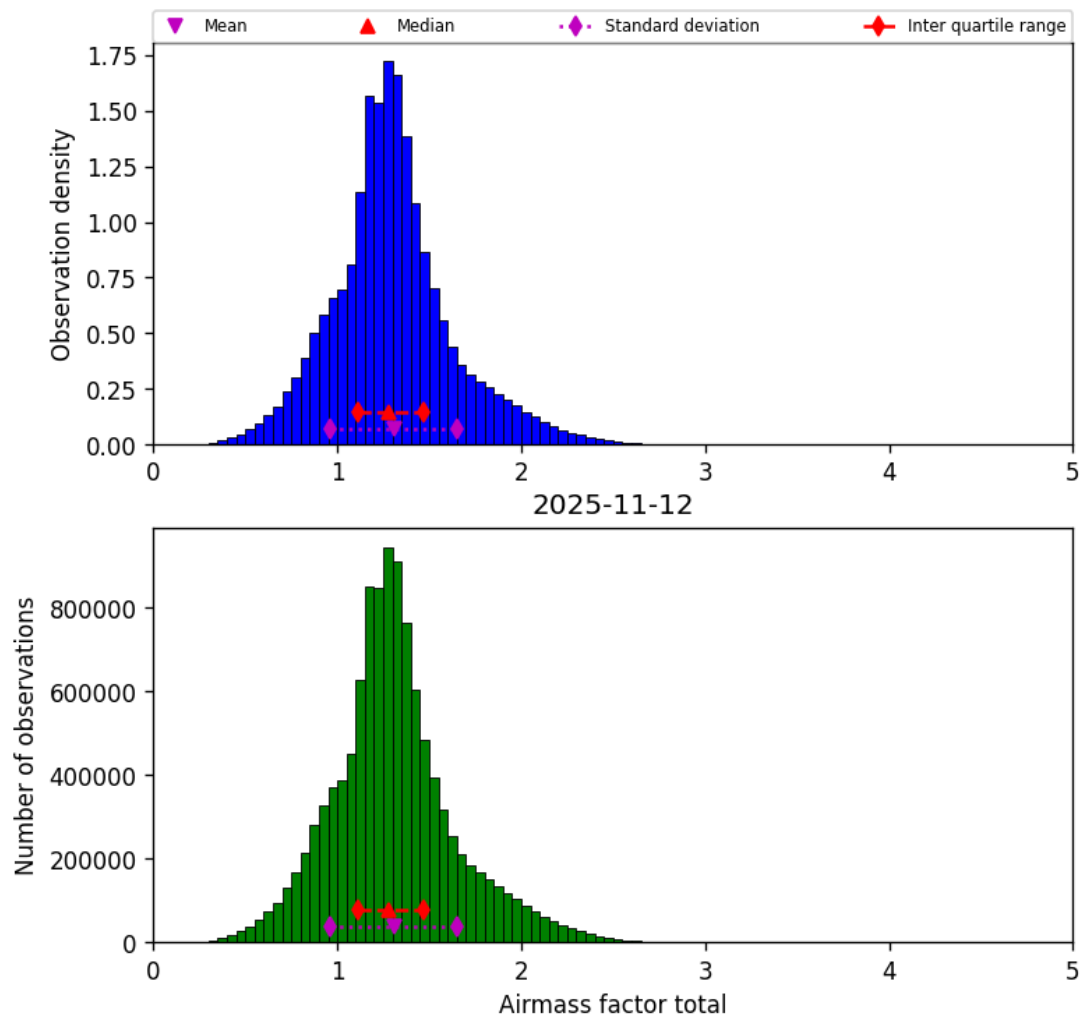
Figure 42: Histogram of “Airmass factor total” for 2025-11-12 to 2025-11-13
