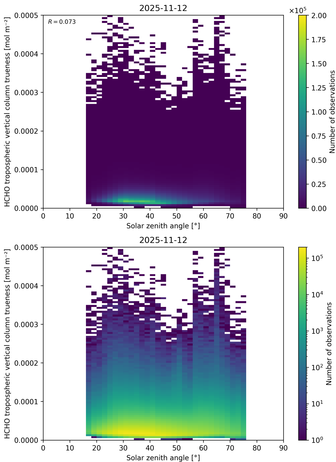
Figure 199: Scatter density plot of “Solar zenith angle” against “HCHO tropospheric vertical column trueness” for 2025-11-12 to 2025-11-13.
