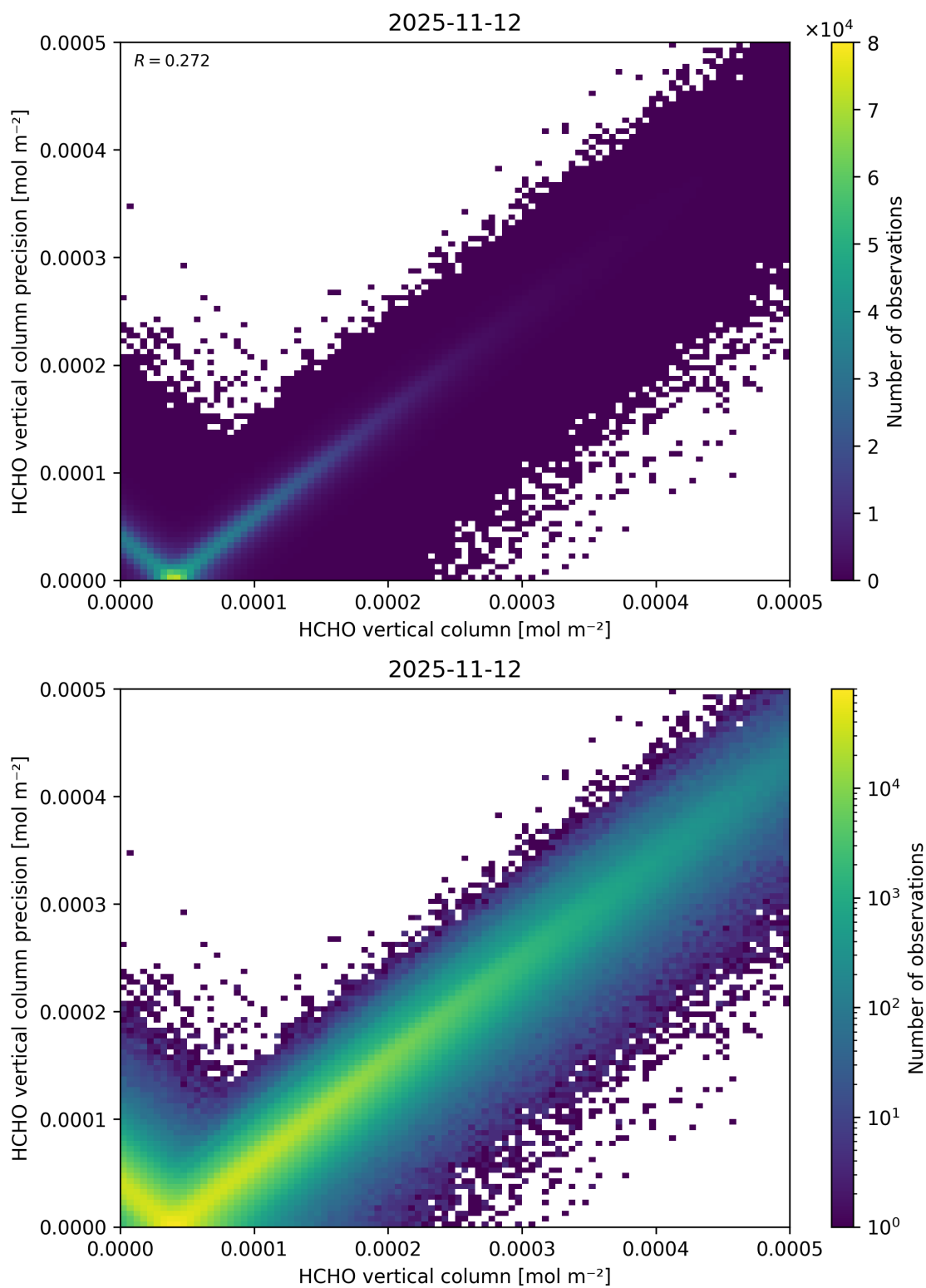
Figure 149: Scatter density plot of “HCHO vertical column” against “HCHO vertical column precision” for 2025-11-12 to 2025-11-13.
