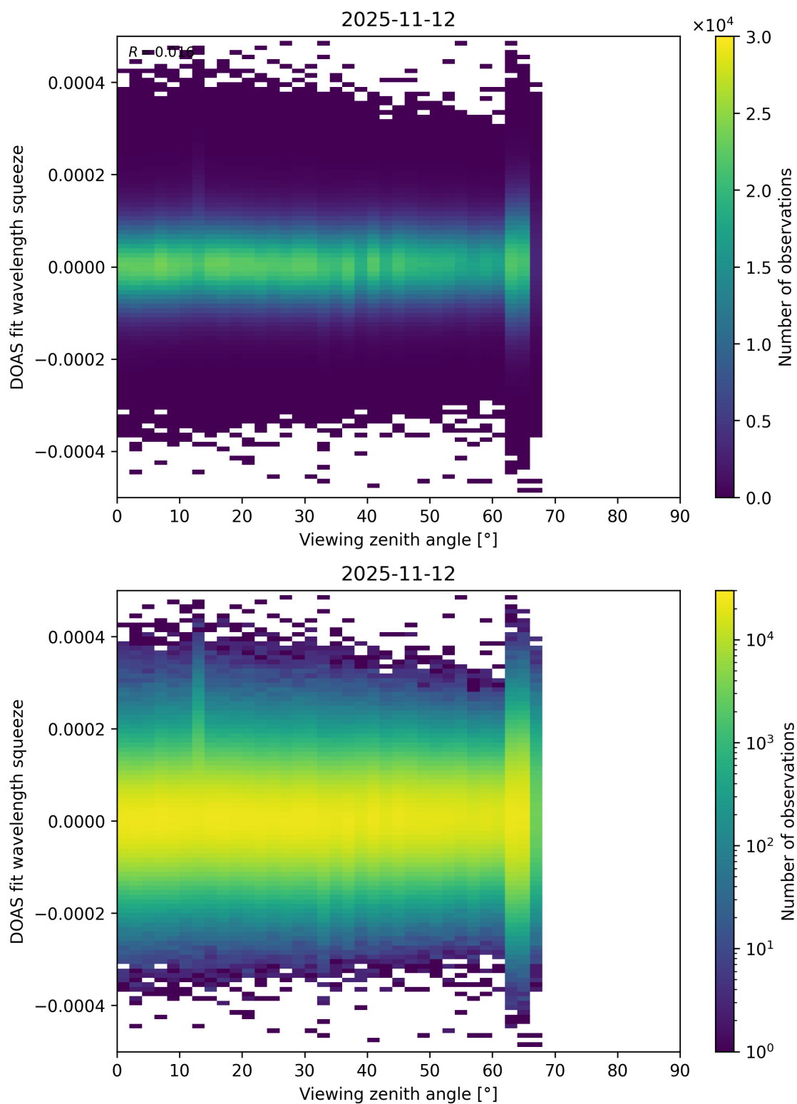
Figure 204: Scatter density plot of “Viewing zenith angle” against “DOAS fit wavelength squeeze” for 2025-11-12 to 2025-11-13.
