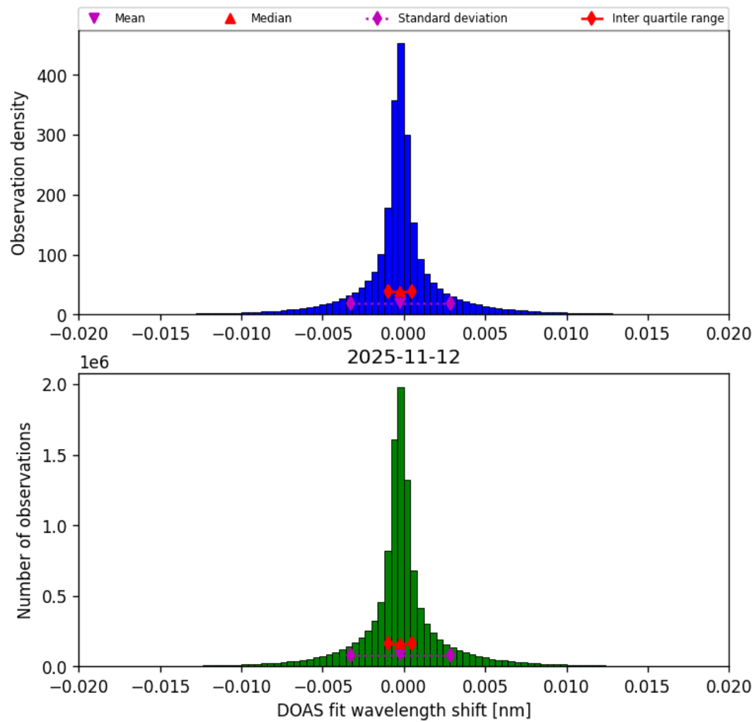
Figure 46: Histogram of “DOAS fit wavelength shift” for 2025-11-12 to 2025-11-13
