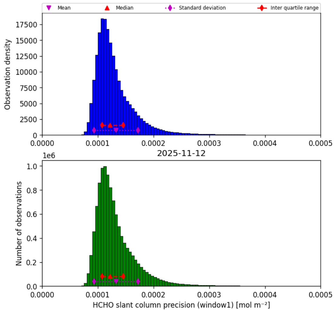
Figure 41: Histogram of “HCHO slant column precision (window1)” for 2025-11-12 to 2025-11-13
