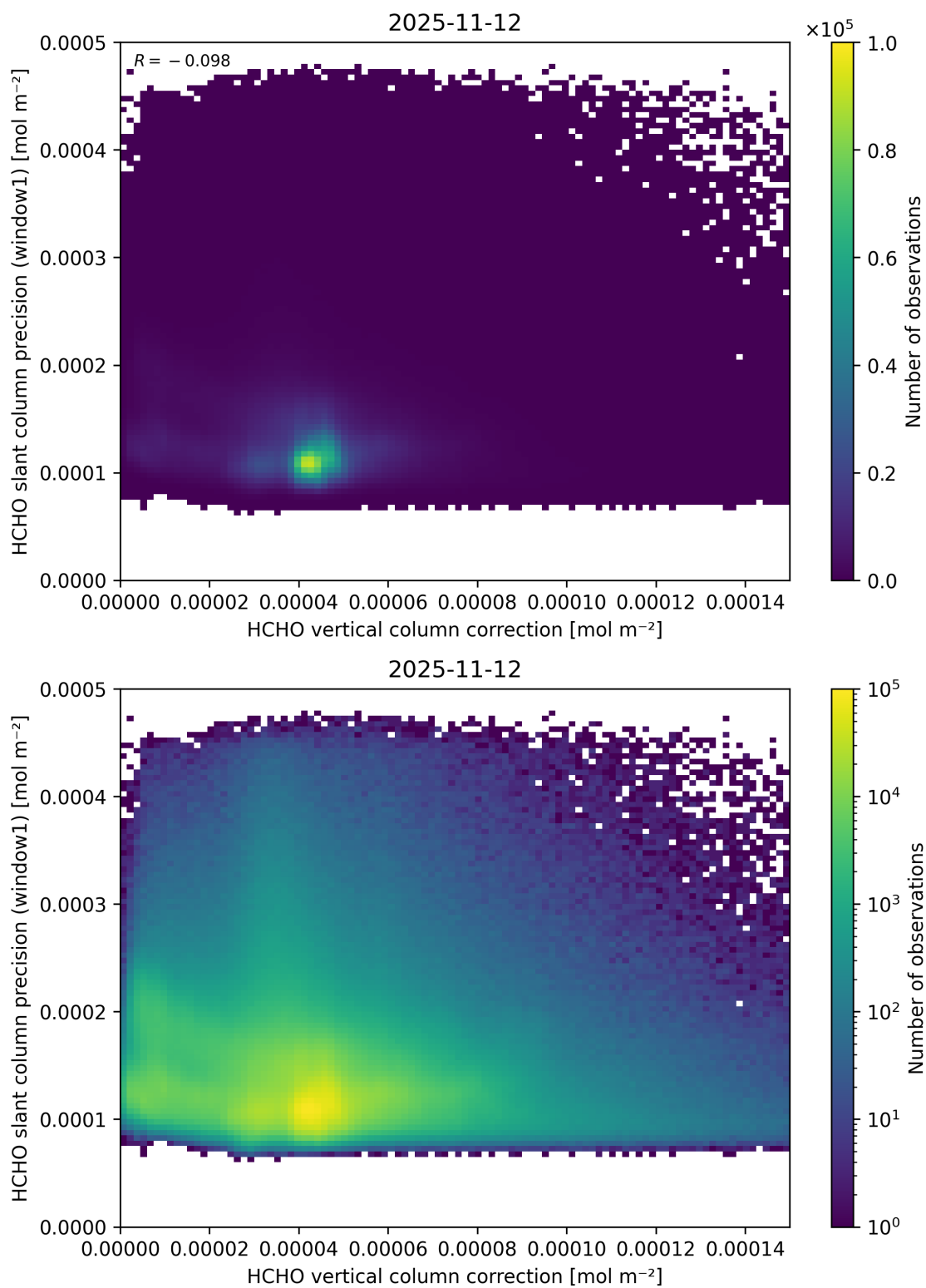
Figure 133: Scatter density plot of “HCHO vertical column correction” against “HCHO slant column precision (window1)” for 2025-11-12 to 2025-11-13.
