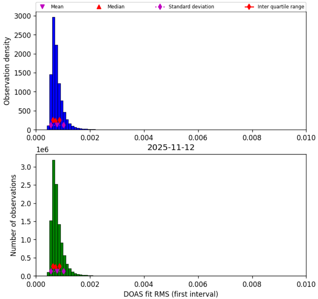
Figure 48: Histogram of “DOAS fit RMS (first interval)” for 2025-11-12 to 2025-11-13
