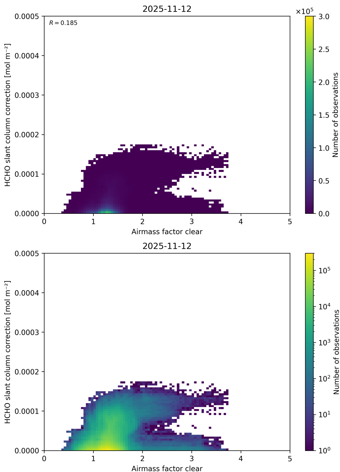
Figure 82: Scatter density plot of “Airmass factor clear” against “HCHO slant column correction” for 2025-11-12 to 2025-11-13.
