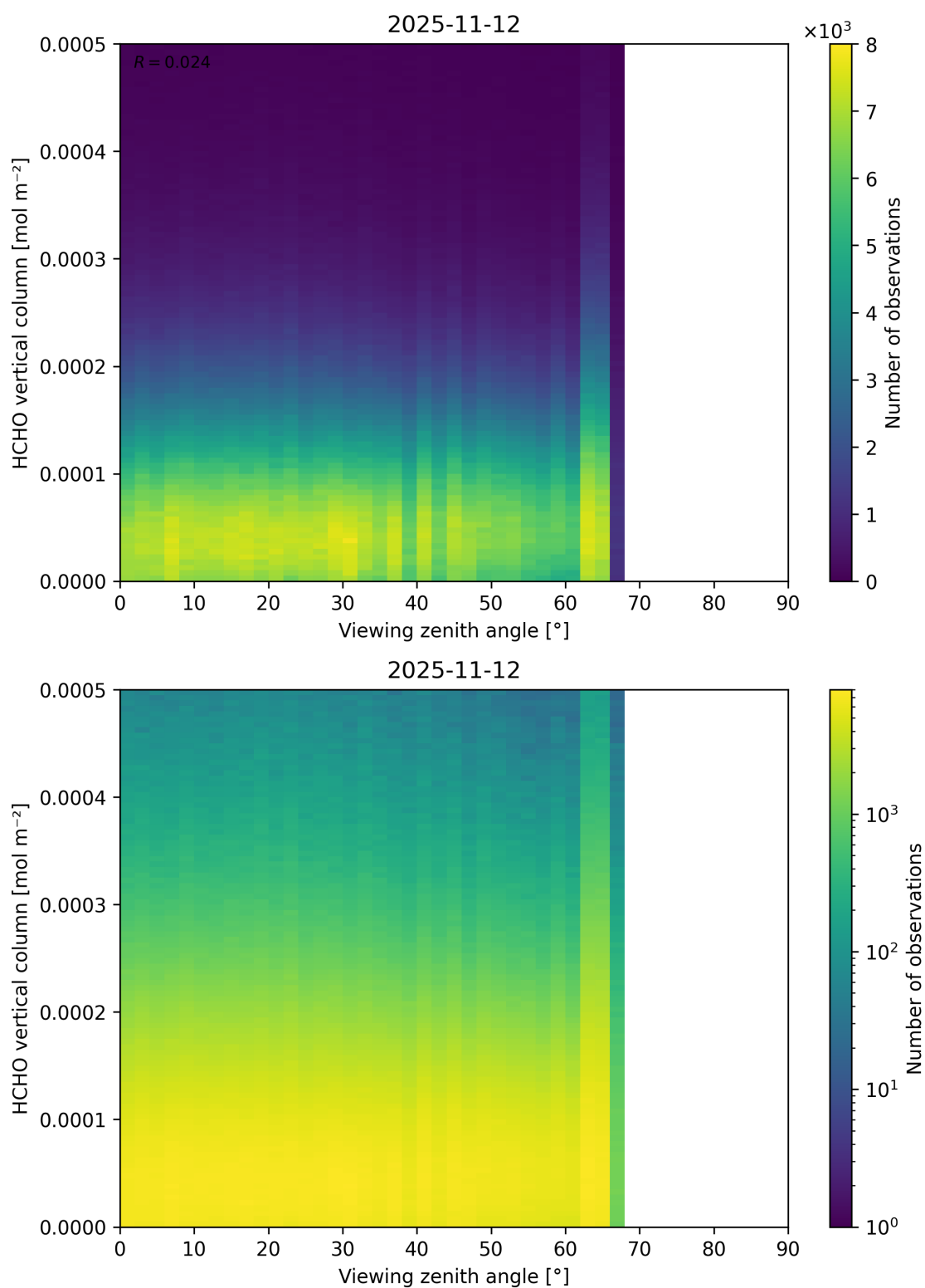
Figure 212: Scatter density plot of “Viewing zenith angle” against “HCHO vertical column” for 2025-11-12 to 2025-11-13.
