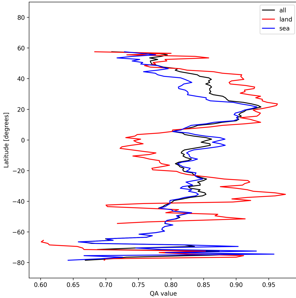
Figure 21: Zonal average of “QA value” for 2025-11-12 to 2025-11-13.
