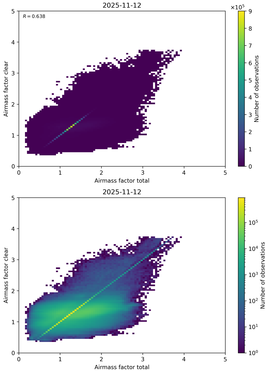
Figure 112: Scatter density plot of “Airmass factor total” against “Airmass factor clear” for 2025-11-12 to 2025-11-13.
