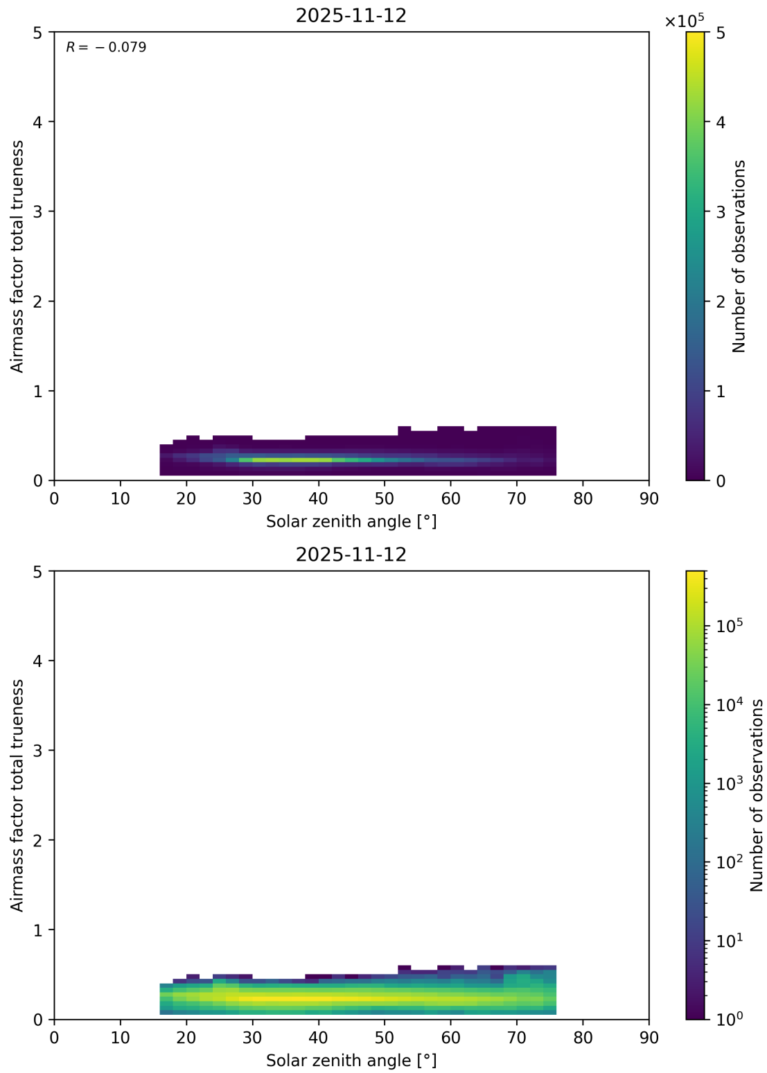
Figure 195: Scatter density plot of “Solar zenith angle” against “Airmass factor total trueness” for 2025-11-12 to 2025-11-13.
