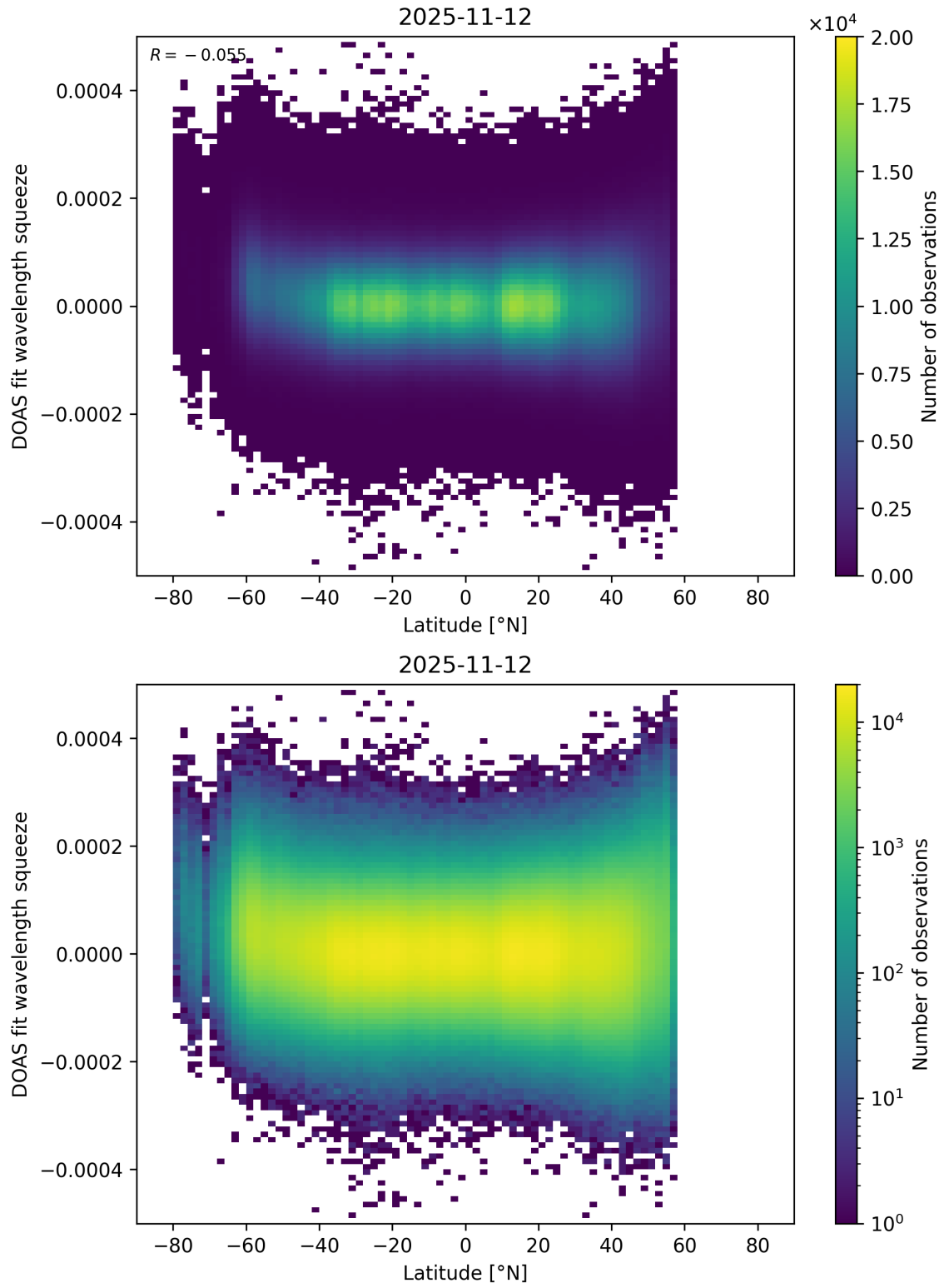
Figure 173: Scatter density plot of “Latitude” against “DOAS fit wavelength squeeze” for 2025-11-12 to 2025-11-13.
