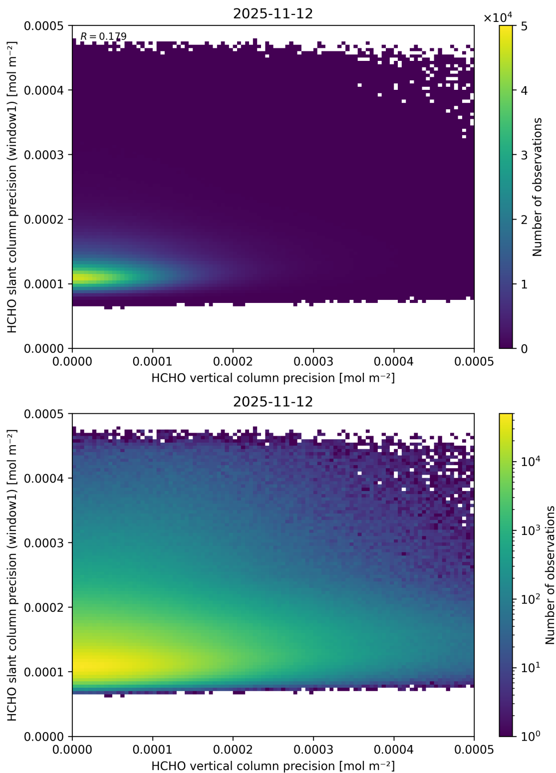
Figure 159: Scatter density plot of “HCHO vertical column precision” against “HCHO slant column precision (window1)” for 2025-11-12 to 2025-11-13.
