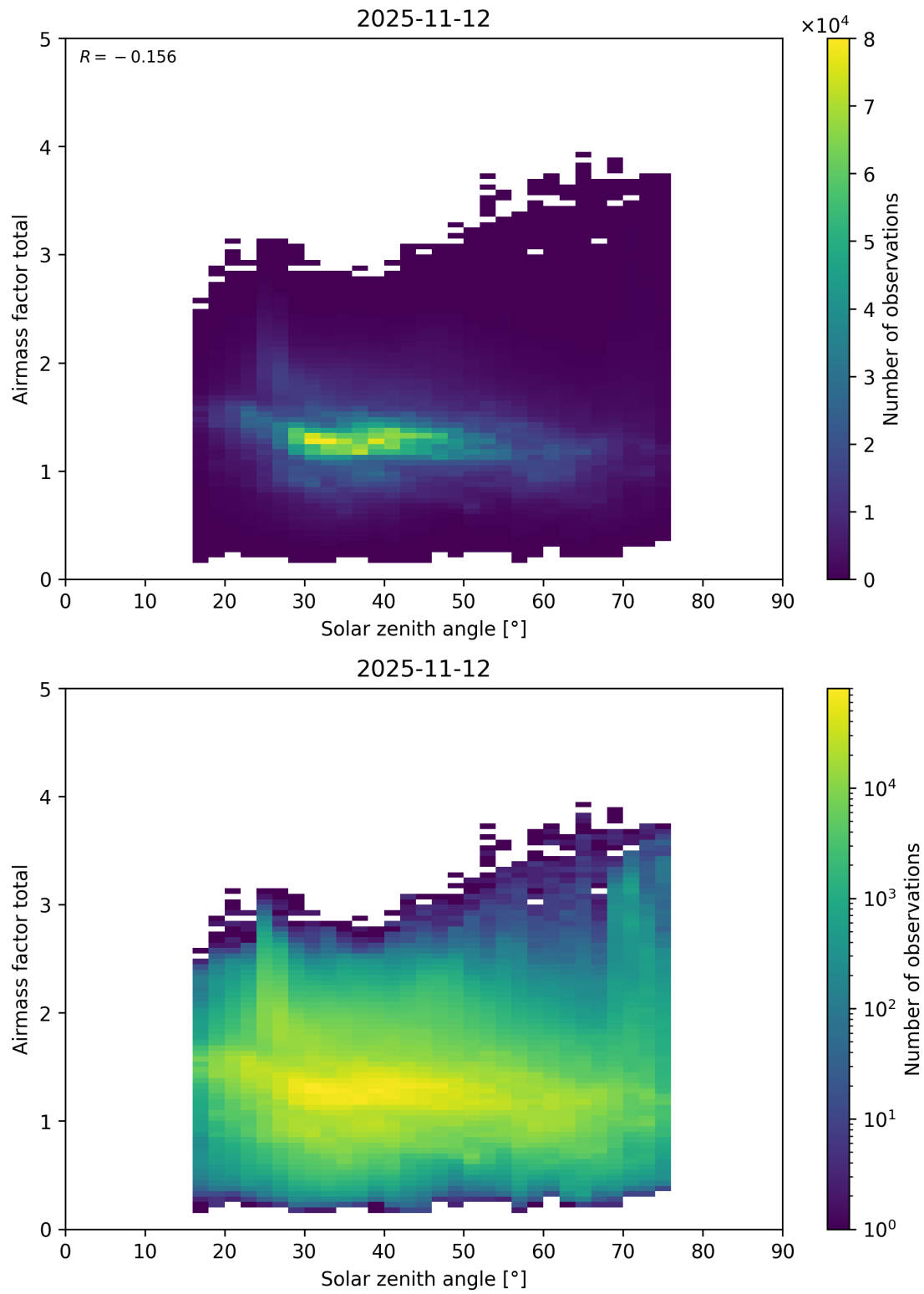
Figure 194: Scatter density plot of “Solar zenith angle” against “Airmass factor total” for 2025-11-12 to 2025-11-13.
