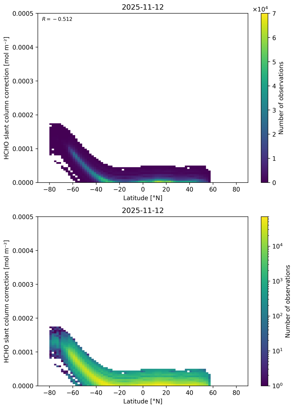
Figure 176: Scatter density plot of “Latitude” against “HCHO slant column correction” for 2025-11-12 to 2025-11-13.
