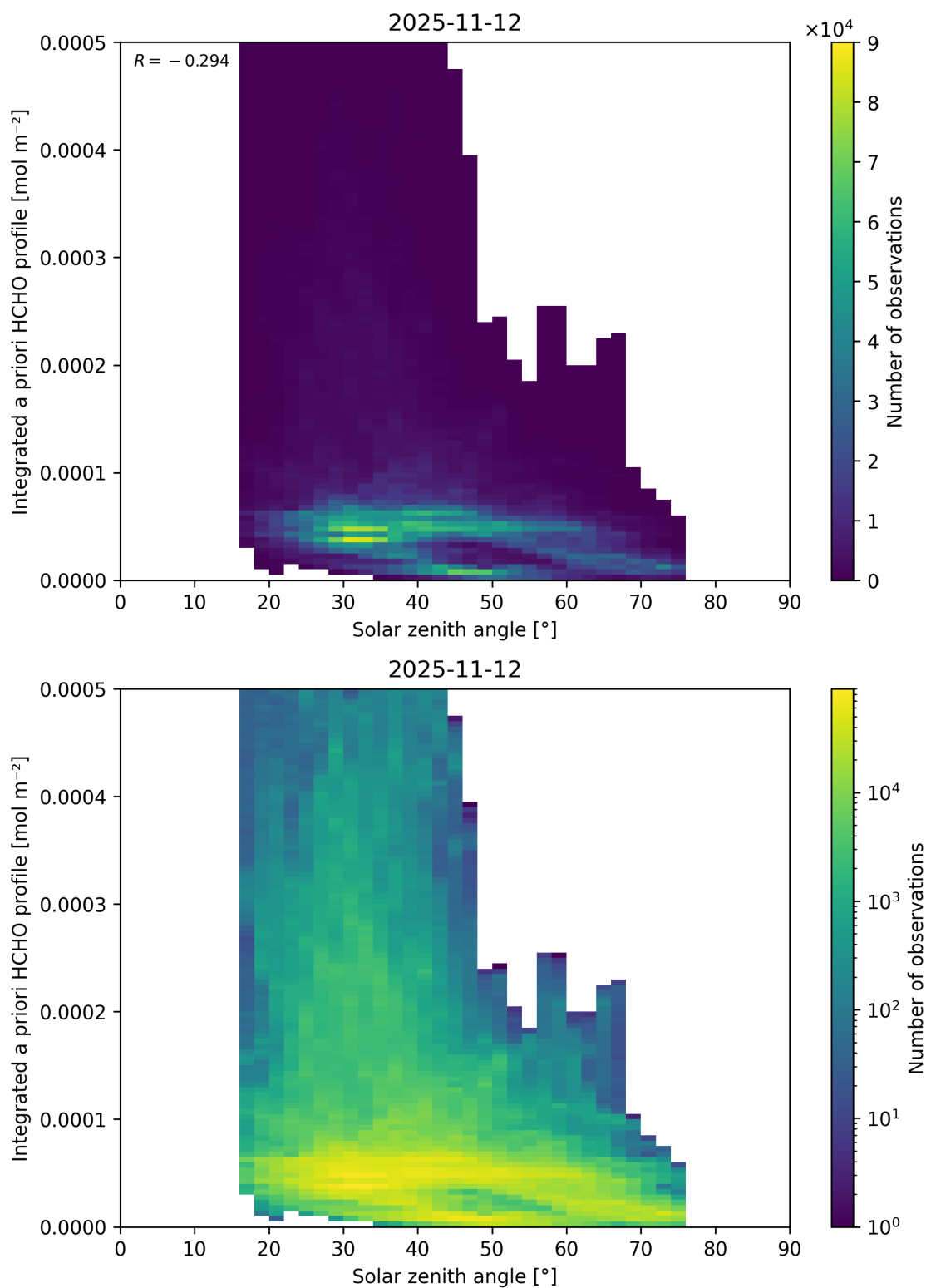
Figure 200: Scatter density plot of “Solar zenith angle” against “Integrated a priori HCHO profile” for 2025-11-12 to 2025-11-13.
