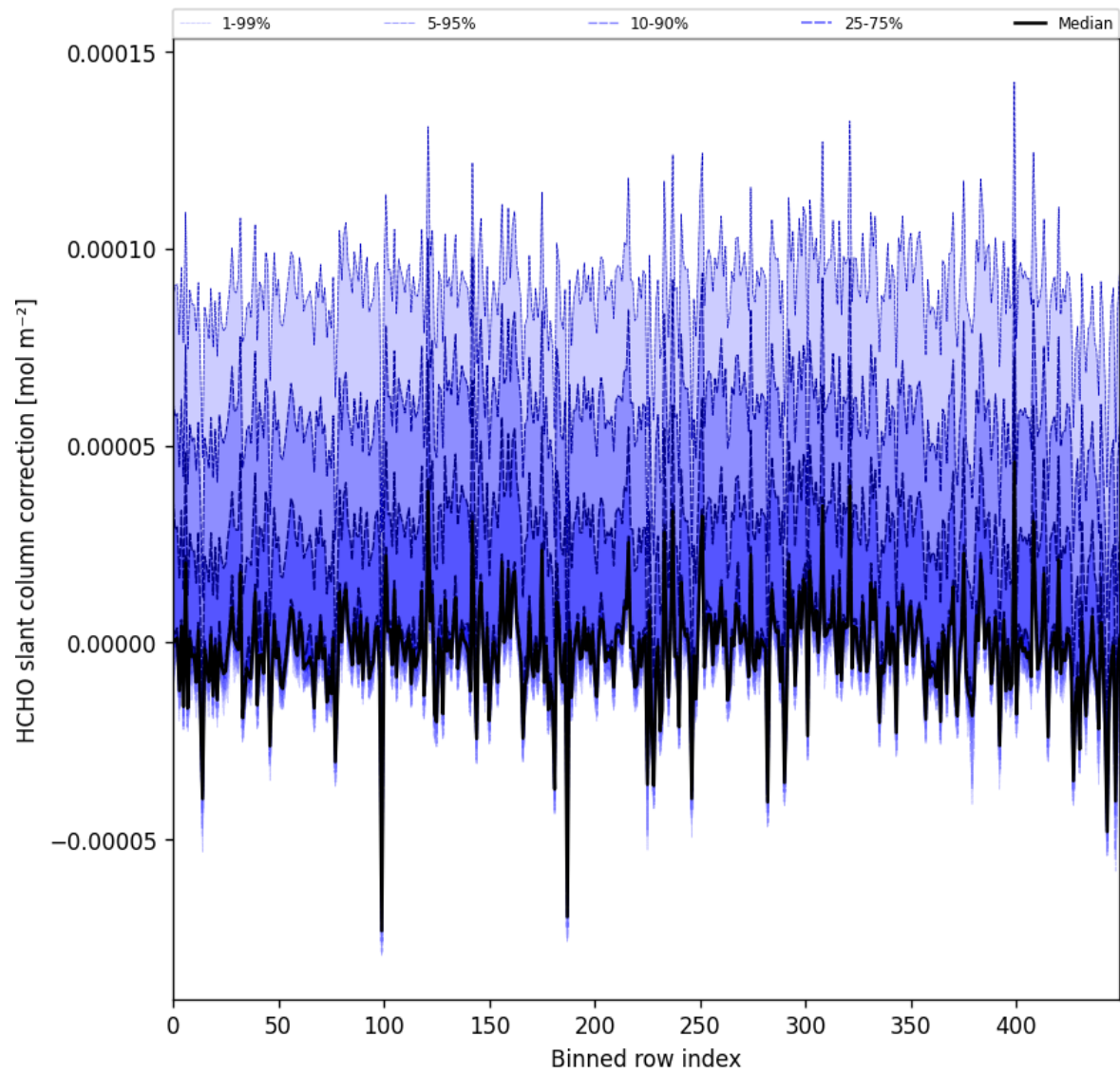
Figure 64: Along track statistics of “HCHO slant column correction” for 2025-11-12 to 2025-11-13
