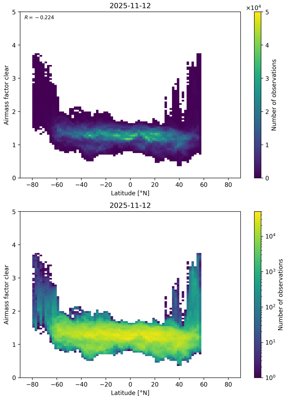
Figure 174: Scatter density plot of “Latitude” against “Airmass factor clear” for 2025-11-12 to 2025-11-13.
