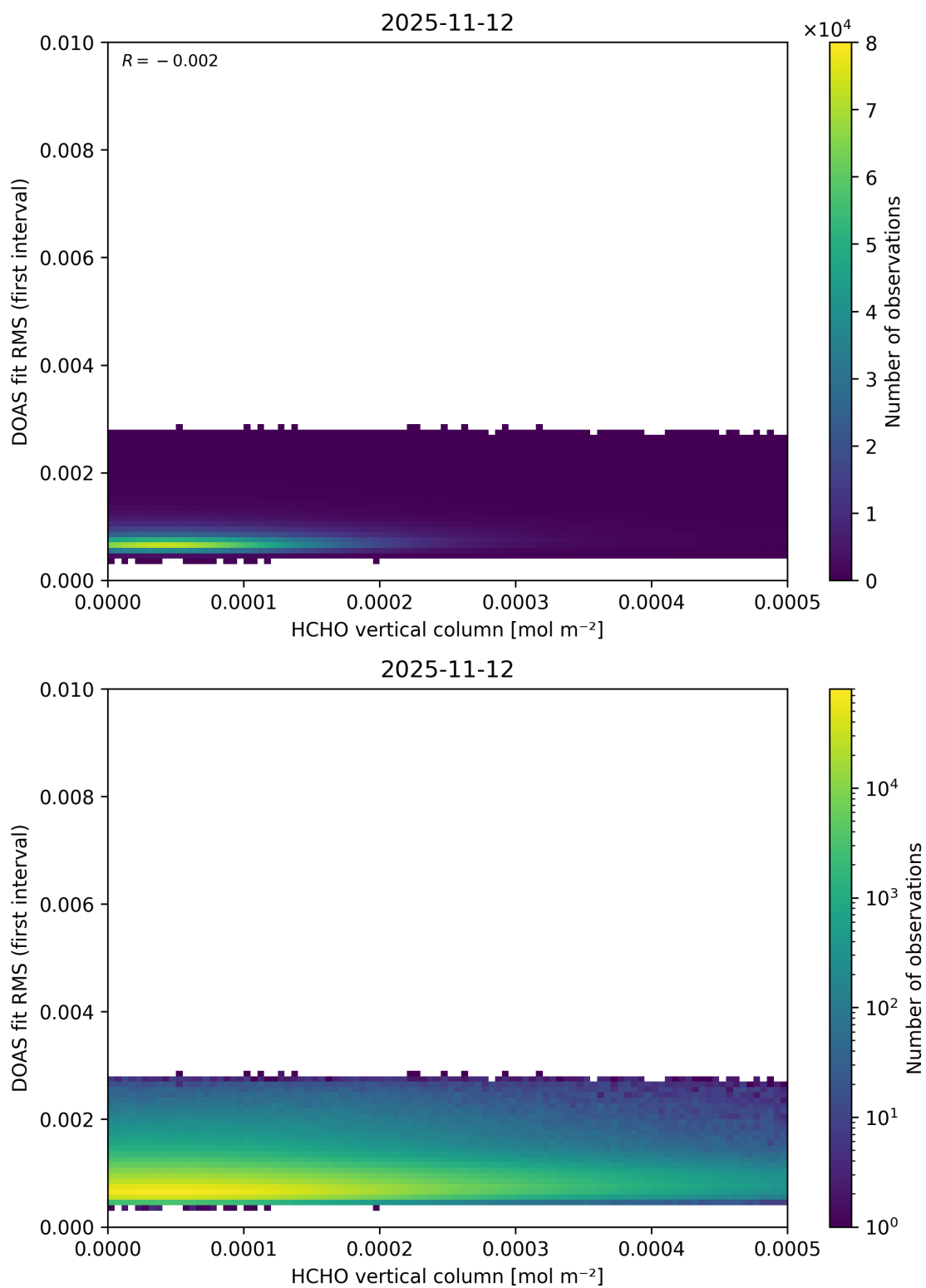
Figure 138: Scatter density plot of “HCHO vertical column” against “DOAS fit RMS (first interval)” for 2025-11-12 to 2025-11-13.
