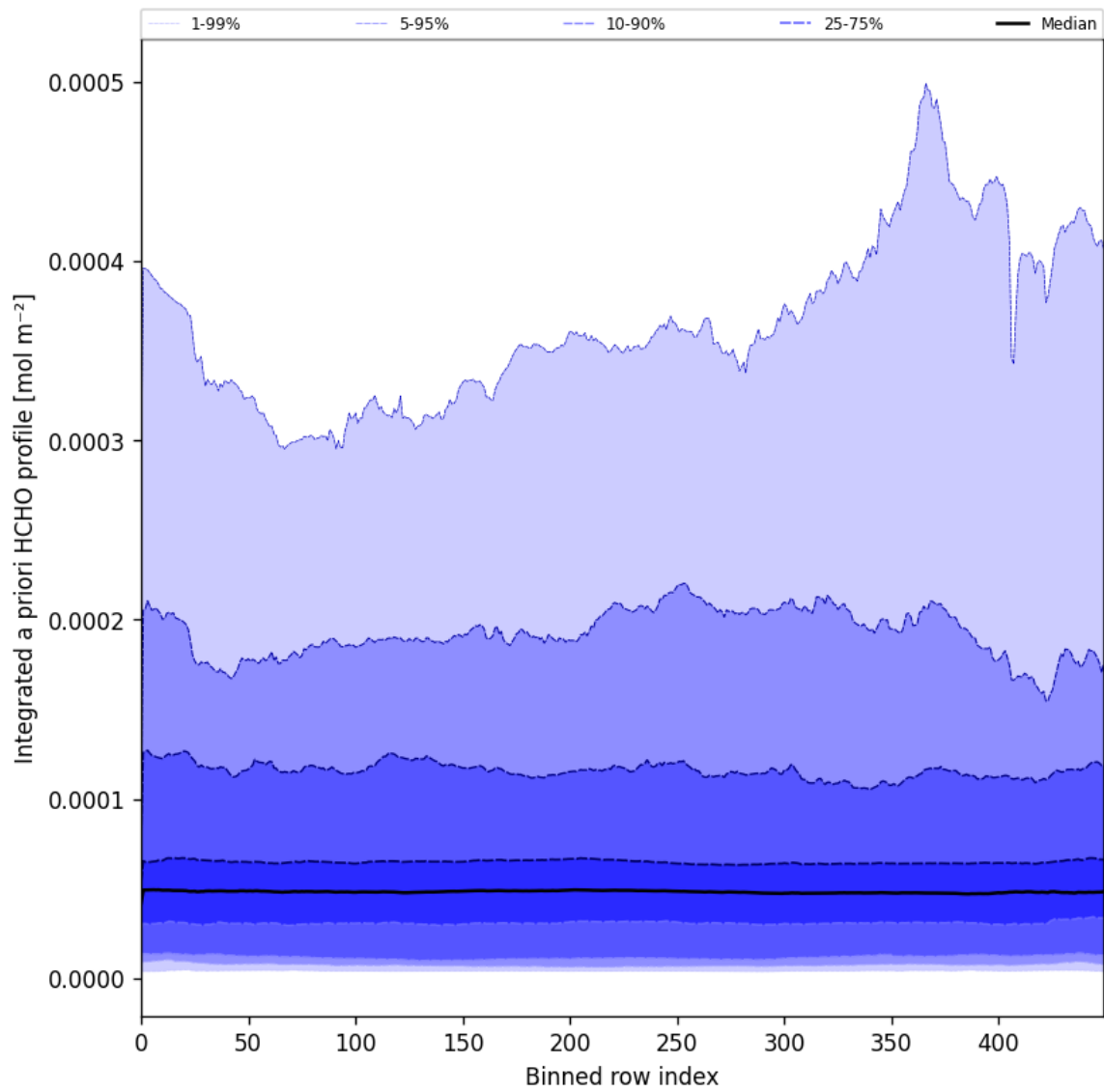
Figure 60: Along track statistics of “Integrated a priori HCHO profile” for 2025-11-12 to 2025-11-13
