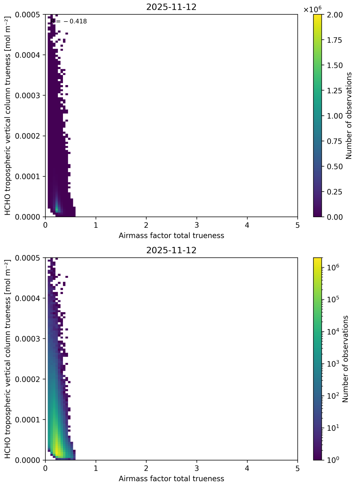
Figure 124: Scatter density plot of “Airmass factor total trueness” against “HCHO tropospheric vertical column trueness” for 2025-11-12 to 2025-11-13.
