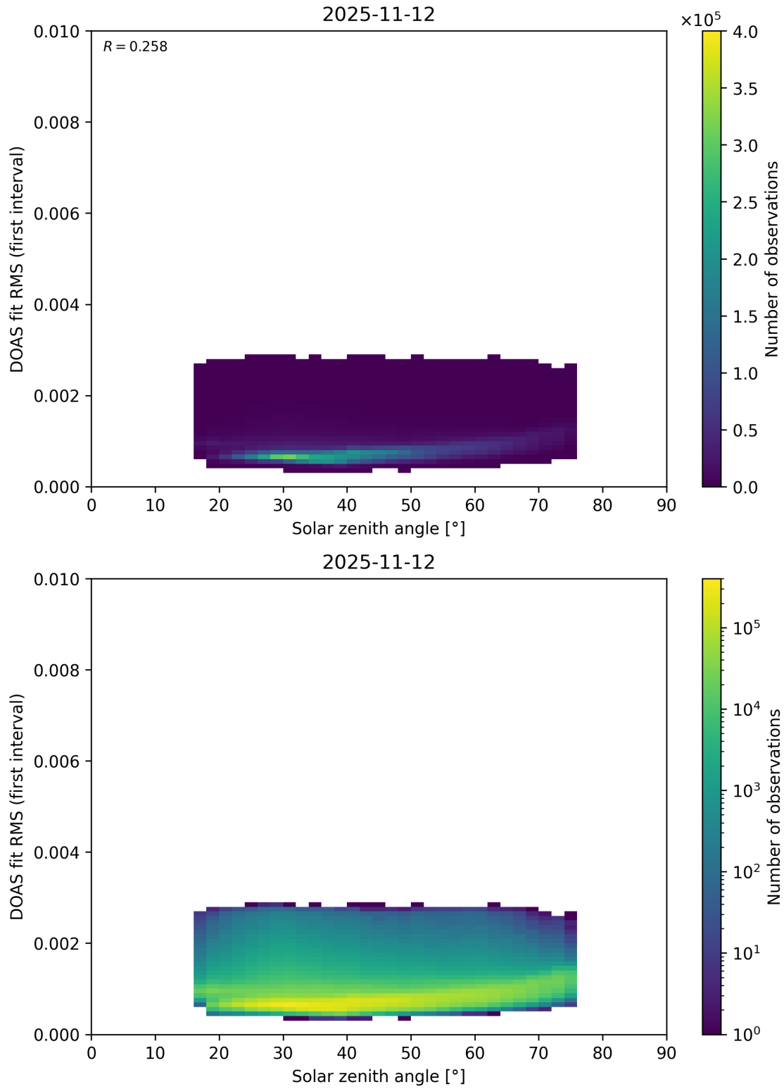
Figure 186: Scatter density plot of “Solar zenith angle” against “DOAS fit RMS (first interval)” for 2025-11-12 to 2025-11-13.
