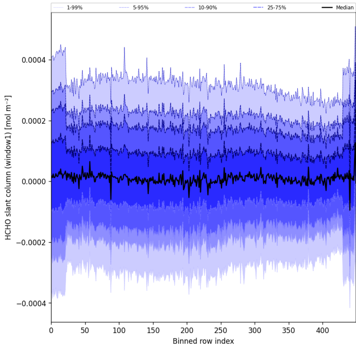
Figure 55: Along track statistics of “HCHO slant column (window1)” for 2025-11-12 to 2025-11-13
