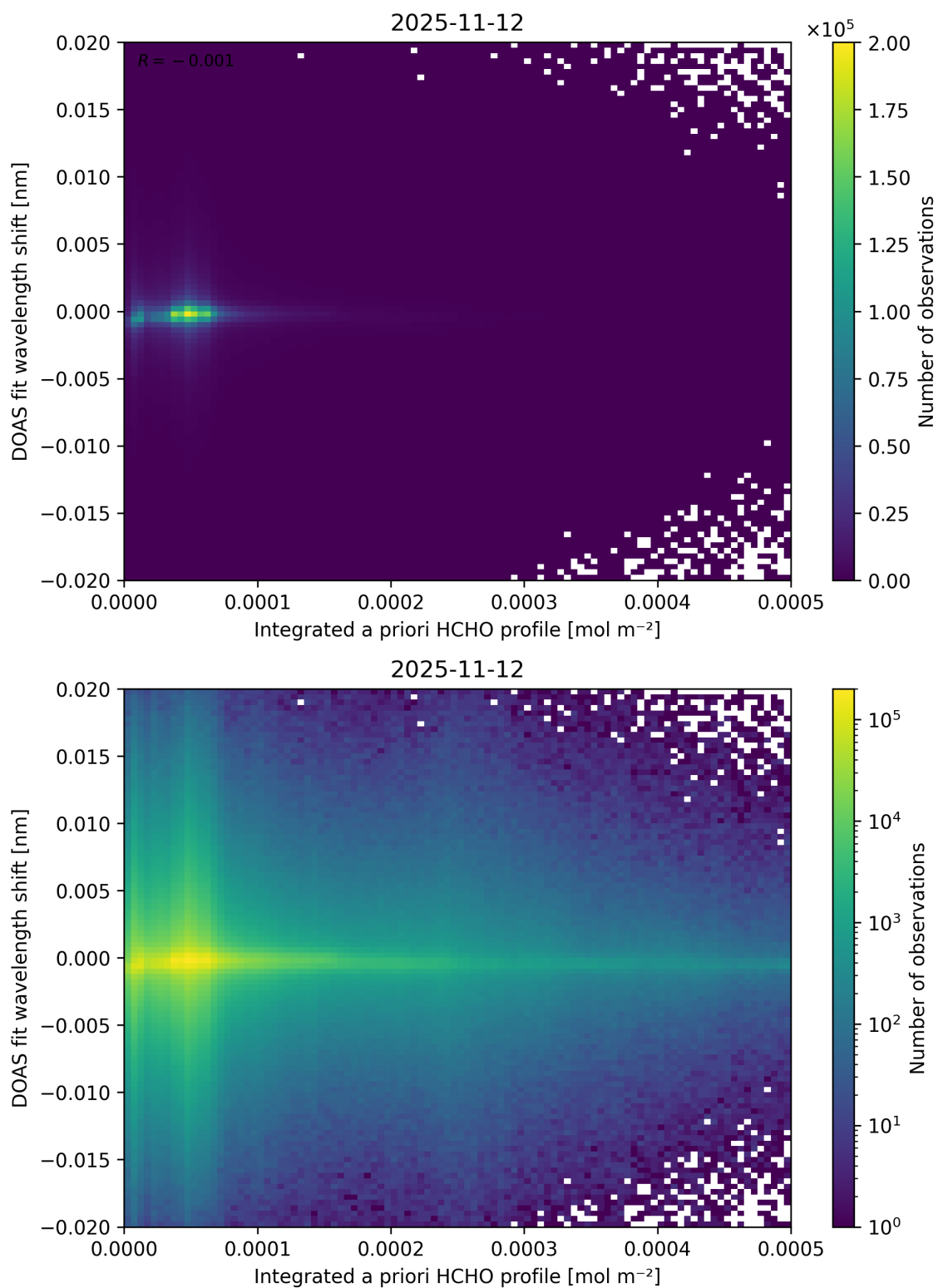
Figure 166: Scatter density plot of “Integrated a priori HCHO profile” against “DOAS fit wavelength shift” for 2025-11-12 to 2025-11-13.
