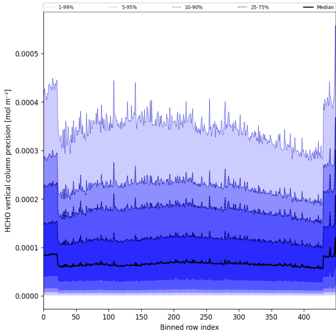
Figure 53: Along track statistics of “HCHO vertical column precision” for 2025-11-12 to 2025-11-13
