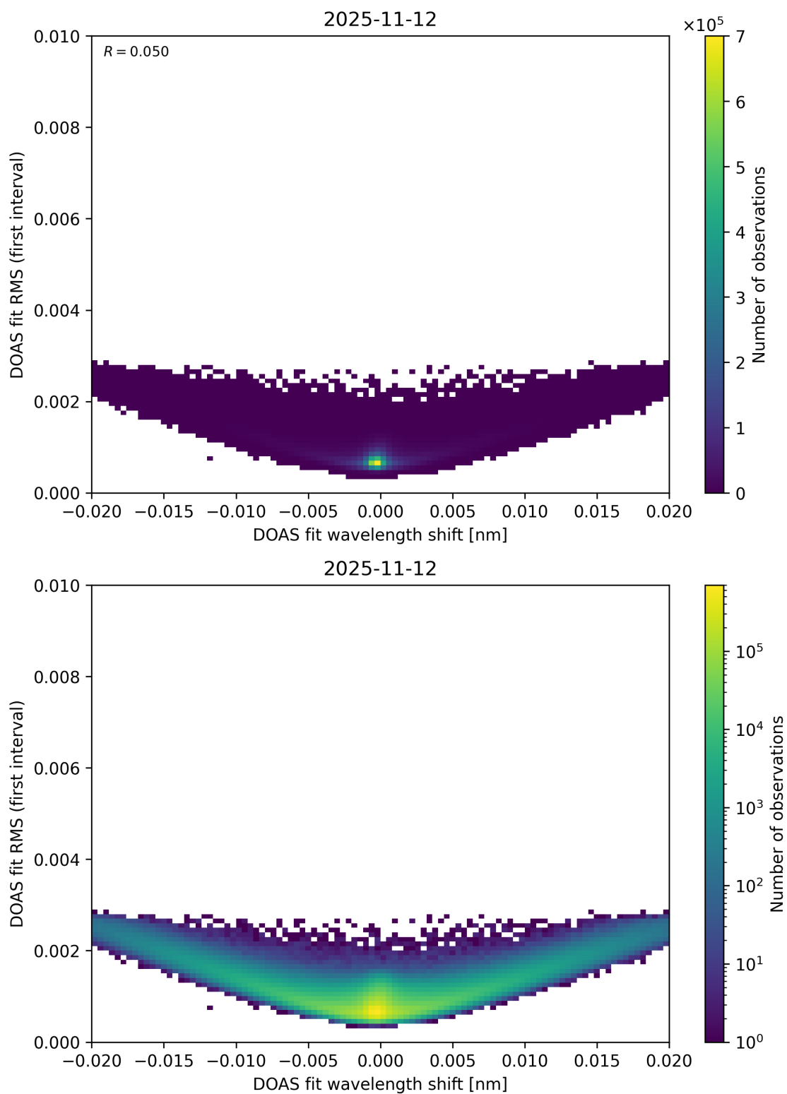
Figure 69: Scatter density plot of “DOAS fit wavelength shift” against “DOAS fit RMS (first interval)” for 2025-11-12 to 2025-11-13.
