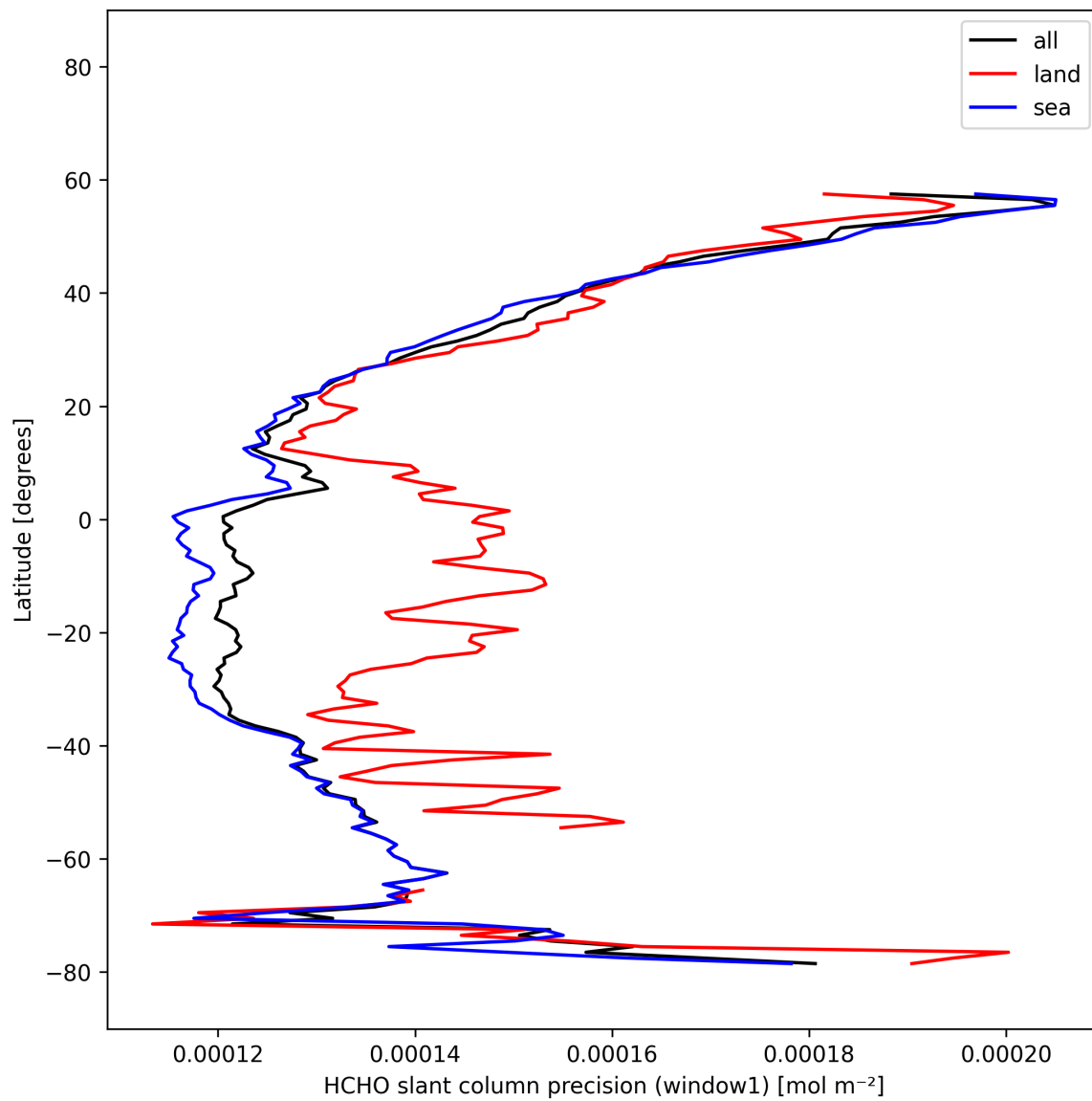
Figure 26: Zonal average of “HCHO slant column precision (window1)” for 2025-11-12 to 2025-11-13.
