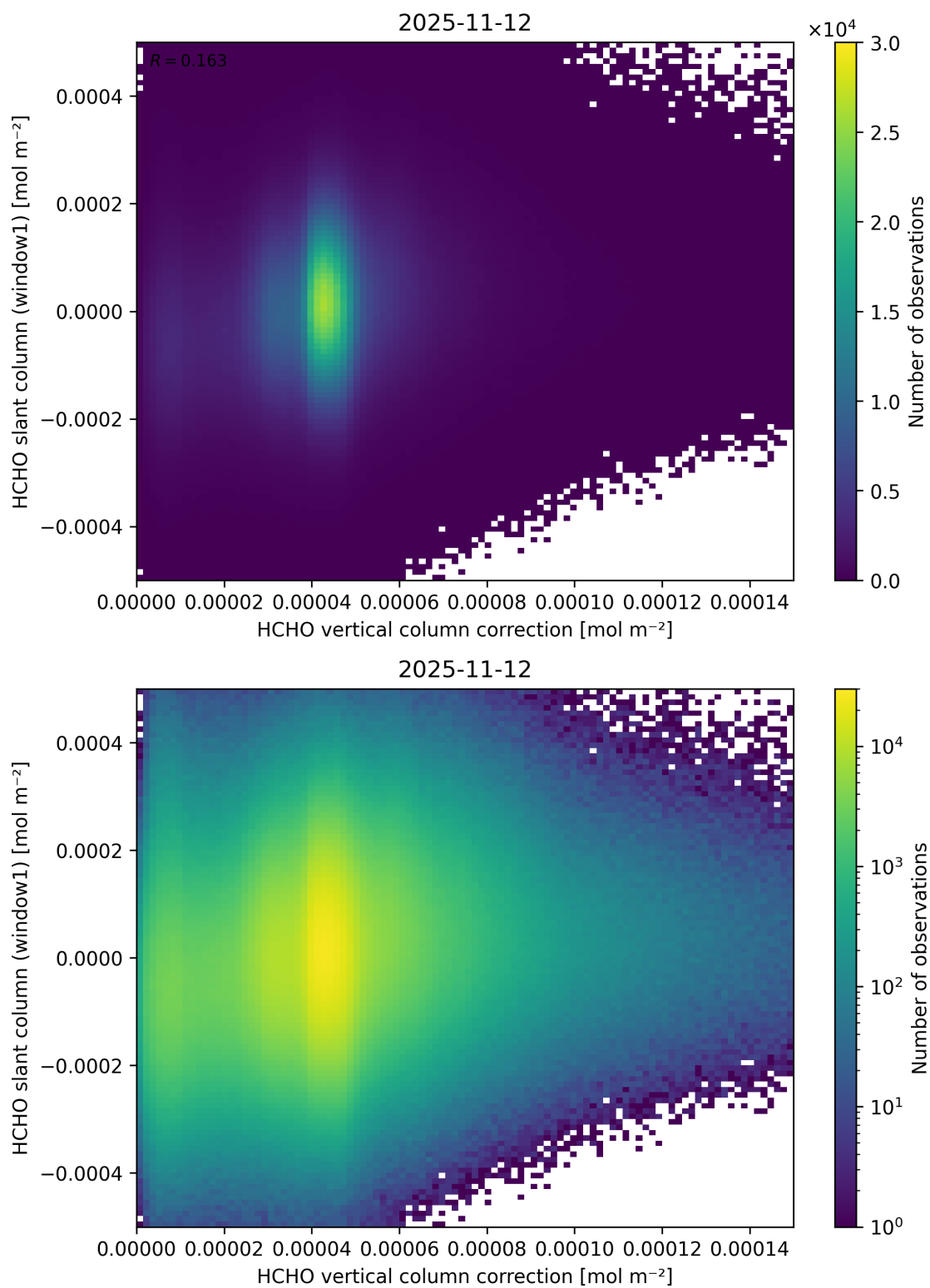
Figure 132: Scatter density plot of “HCHO vertical column correction” against “HCHO slant column (window1)” for 2025-11-12 to 2025-11-13.
