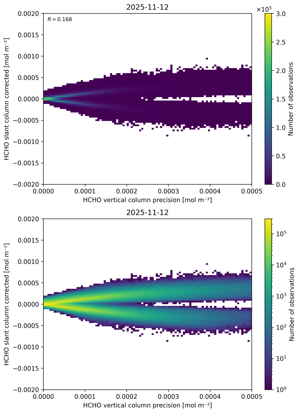
Figure 156: Scatter density plot of “HCHO vertical column precision” against “HCHO slant column corrected” for 2025-11-12 to 2025-11-13.
