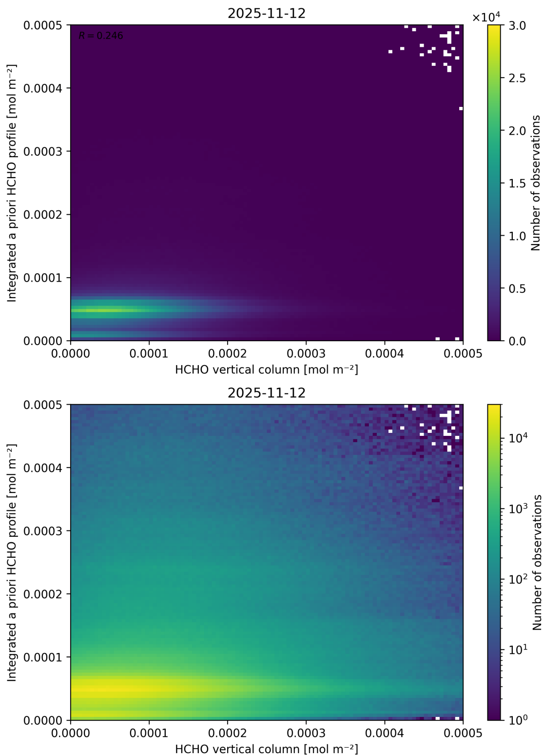
Figure 151: Scatter density plot of “HCHO vertical column” against “Integrated a priori HCHO profile” for 2025-11-12 to 2025-11-13.
