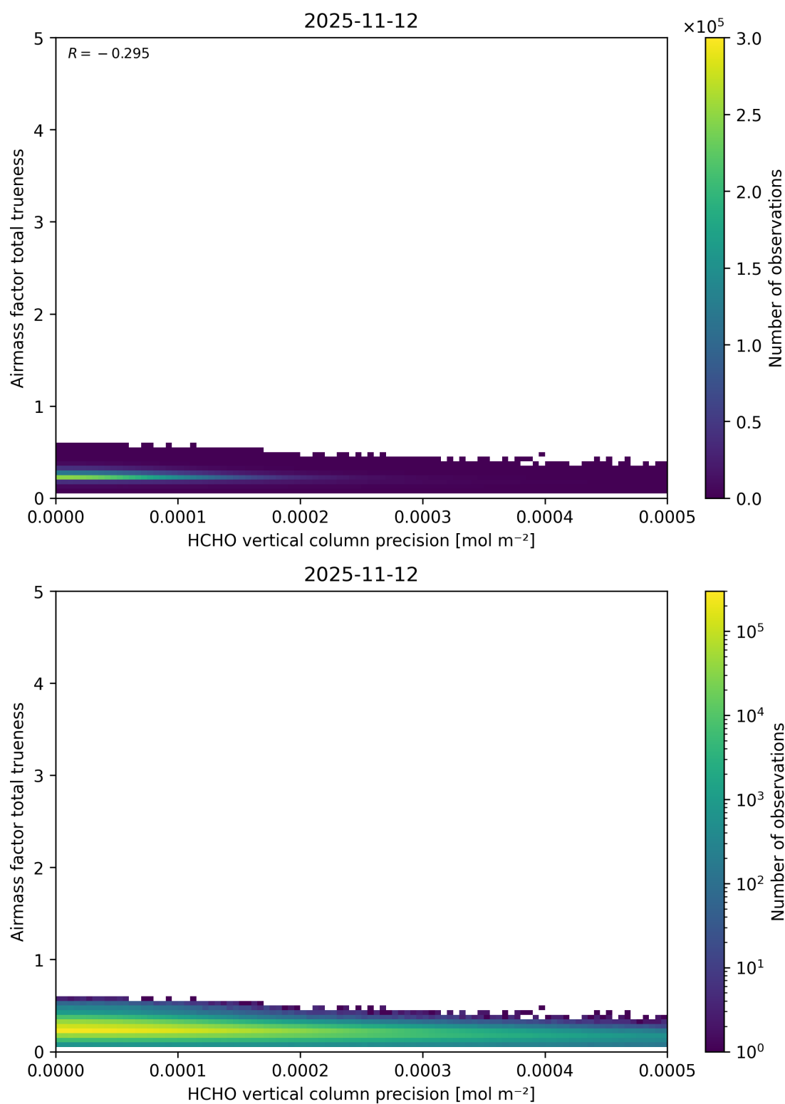
Figure 161: Scatter density plot of “HCHO vertical column precision” against “Airmass factor total trueness” for 2025-11-12 to 2025-11-13.
