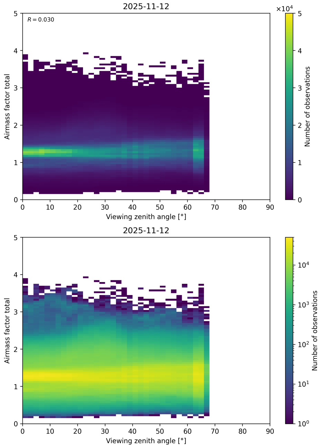
Figure 210: Scatter density plot of “Viewing zenith angle” against “Airmass factor total” for 2025-11-12 to 2025-11-13.
