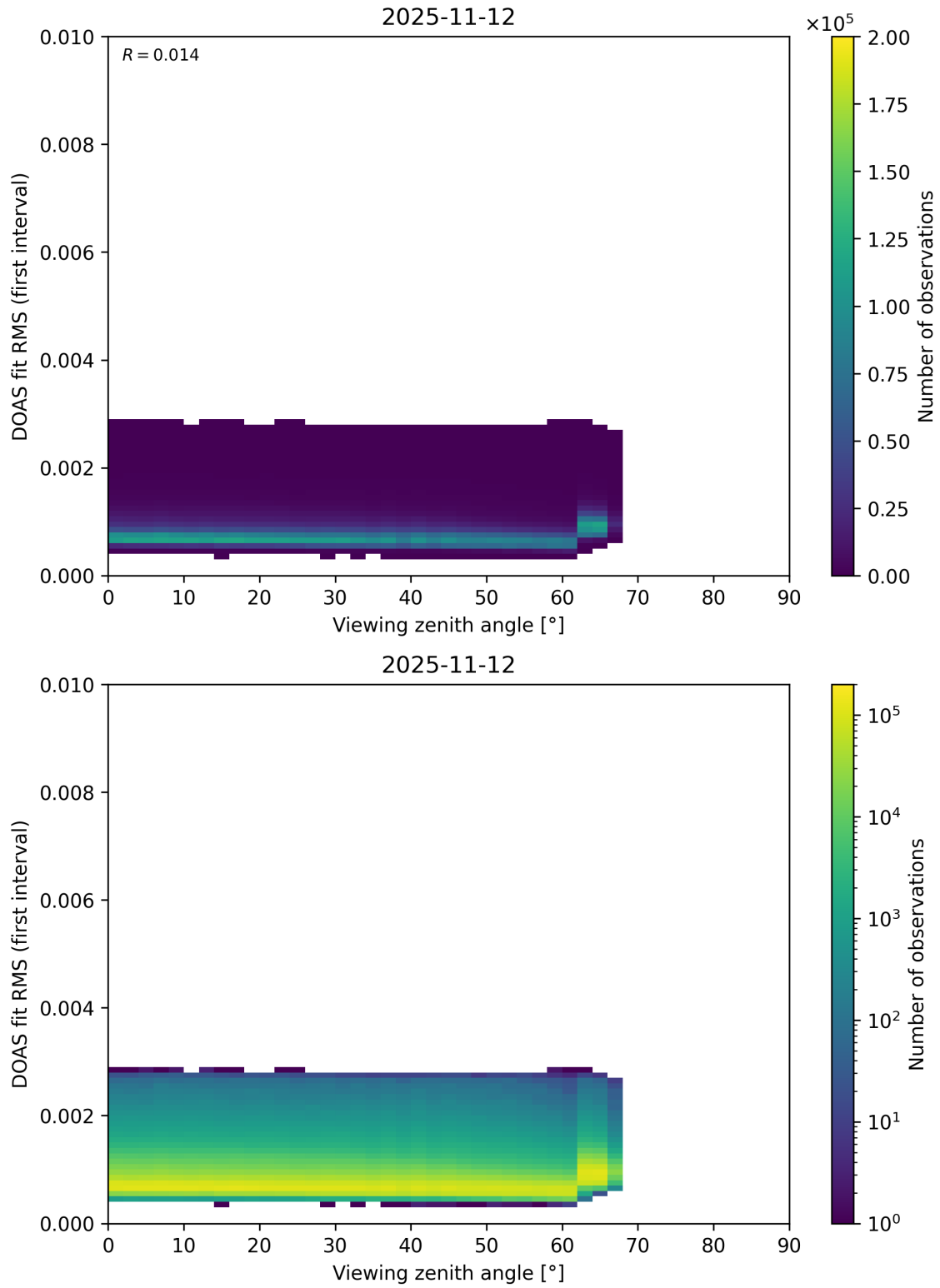
Figure 202: Scatter density plot of “Viewing zenith angle” against “DOAS fit RMS (first interval)” for 2025-11-12 to 2025-11-13.
