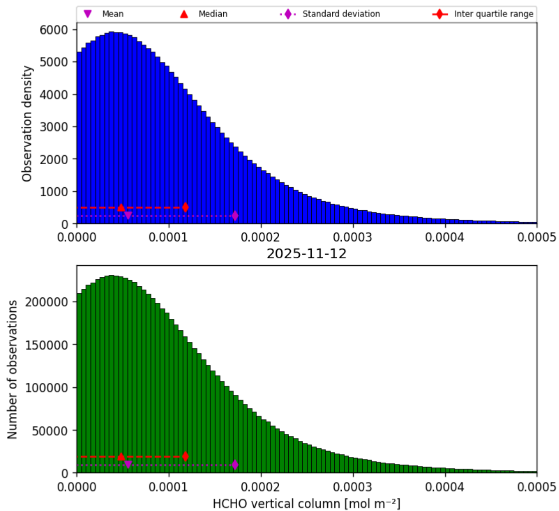
Figure 37: Histogram of “HCHO vertical column” for 2025-11-12 to 2025-11-13
