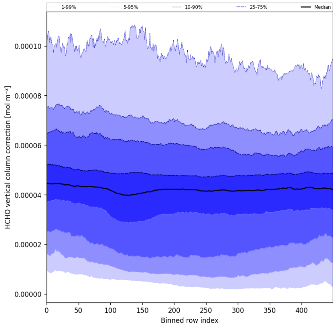
Figure 54: Along track statistics of “HCHO vertical column correction” for 2025-11-12 to 2025-11-13
