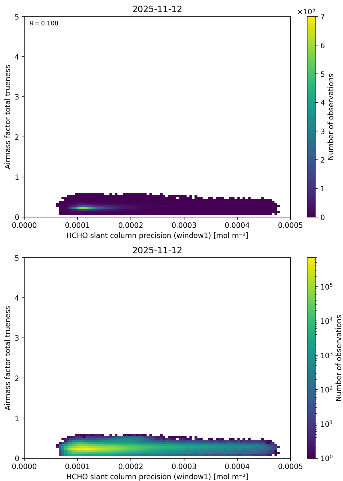
Figure 106: Scatter density plot of “HCHO slant column precision (window1)” against “Airmass factor total trueness” for 2025-11-12 to 2025-11-13.
