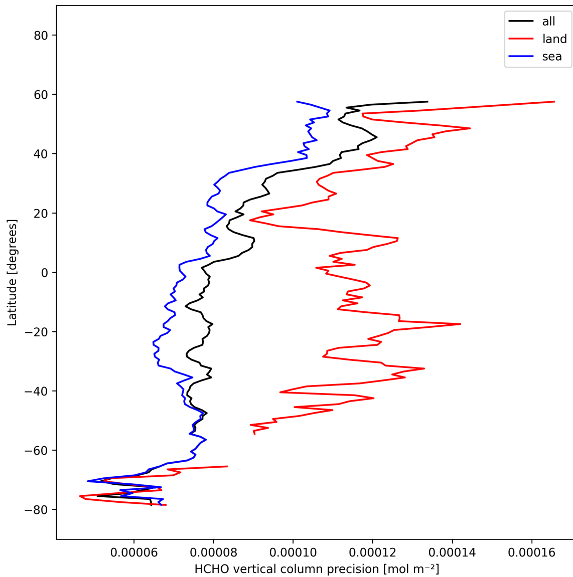
Figure 23: Zonal average of “HCHO vertical column precision” for 2025-11-12 to 2025-11-13.
