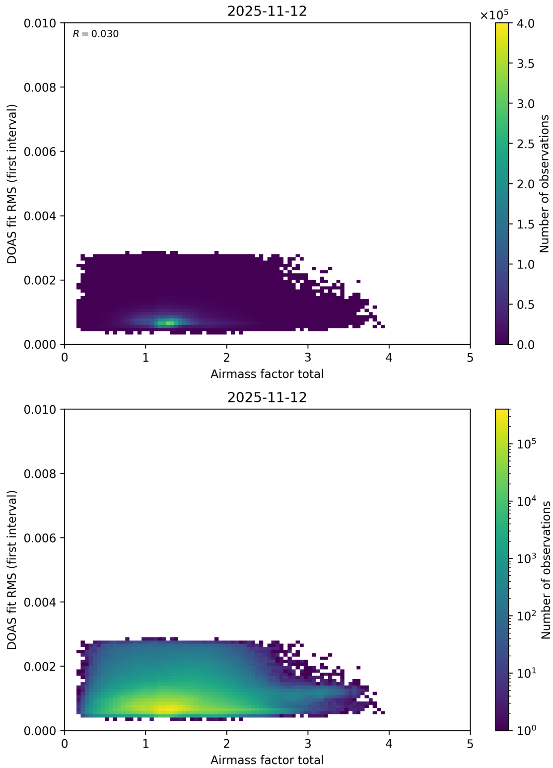
Figure 109: Scatter density plot of “Airmass factor total” against “DOAS fit RMS (first interval)” for 2025-11-12 to 2025-11-13.
