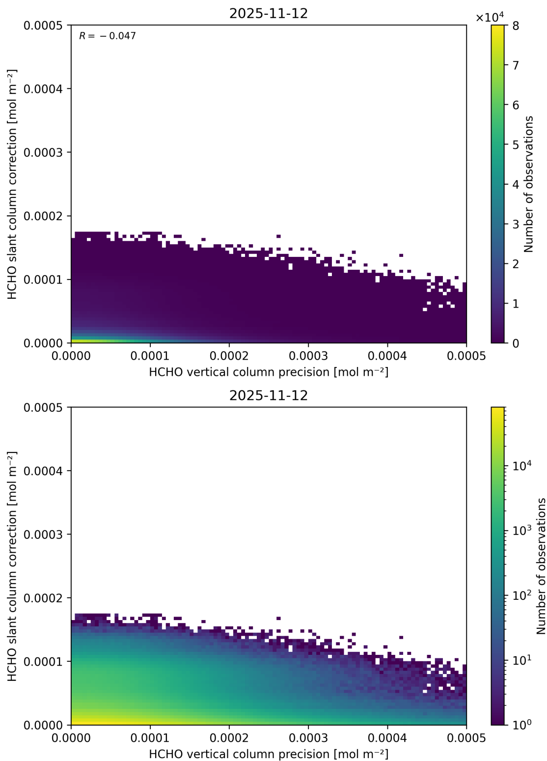
Figure 157: Scatter density plot of “HCHO vertical column precision” against “HCHO slant column correction” for 2025-11-12 to 2025-11-13.
