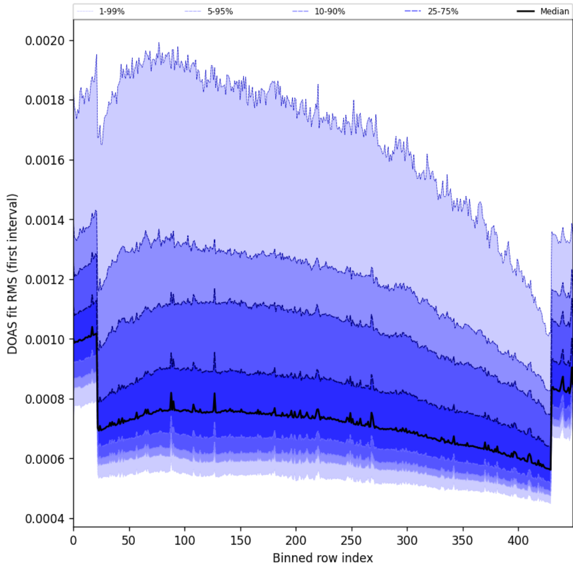
Figure 63: Along track statistics of “DOAS fit RMS (first interval)” for 2025-11-12 to 2025-11-13
