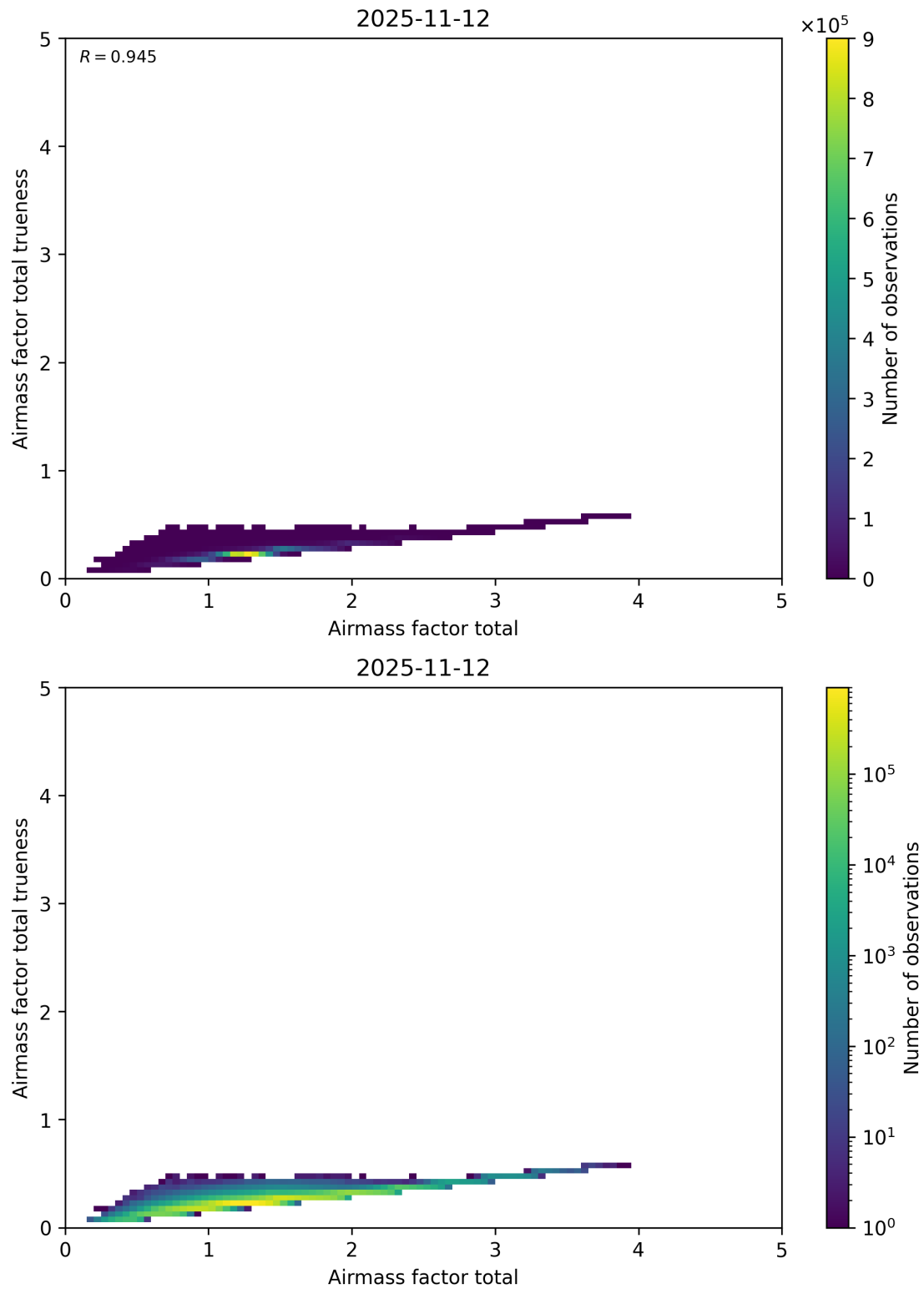
Figure 115: Scatter density plot of “Airmass factor total” against “Airmass factor total trueness” for 2025-11-12 to 2025-11-13.
