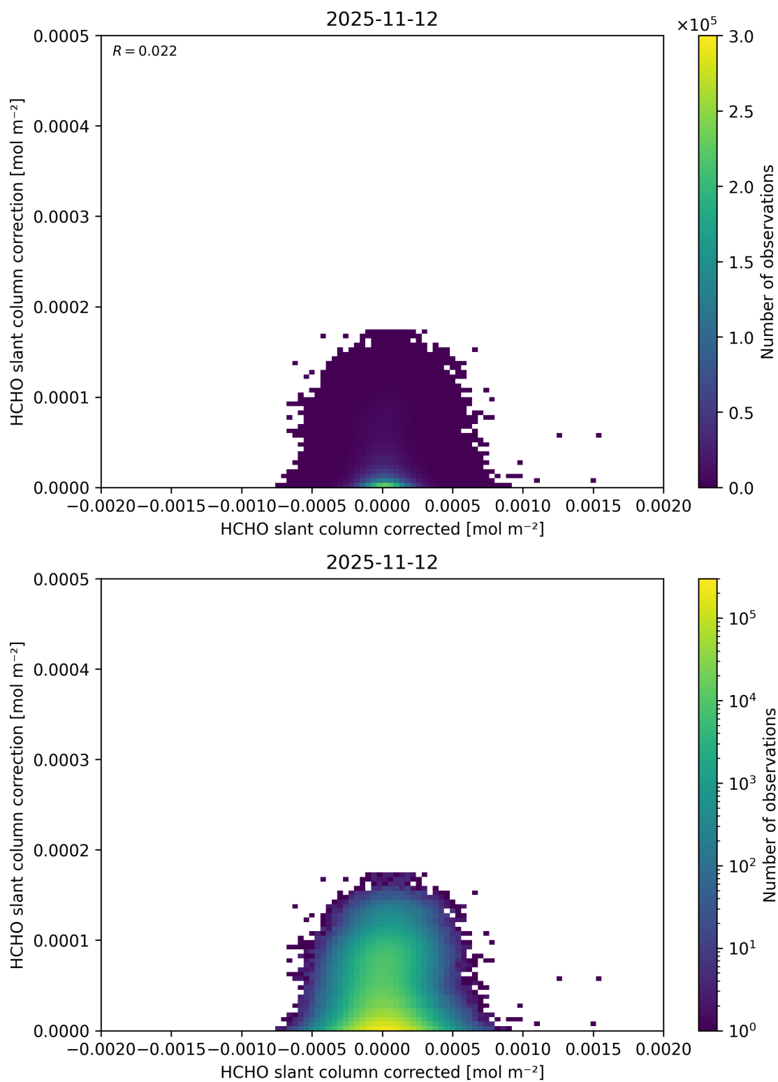
Figure 85: Scatter density plot of “HCHO slant column corrected” against “HCHO slant column correction” for 2025-11-12 to 2025-11-13.
