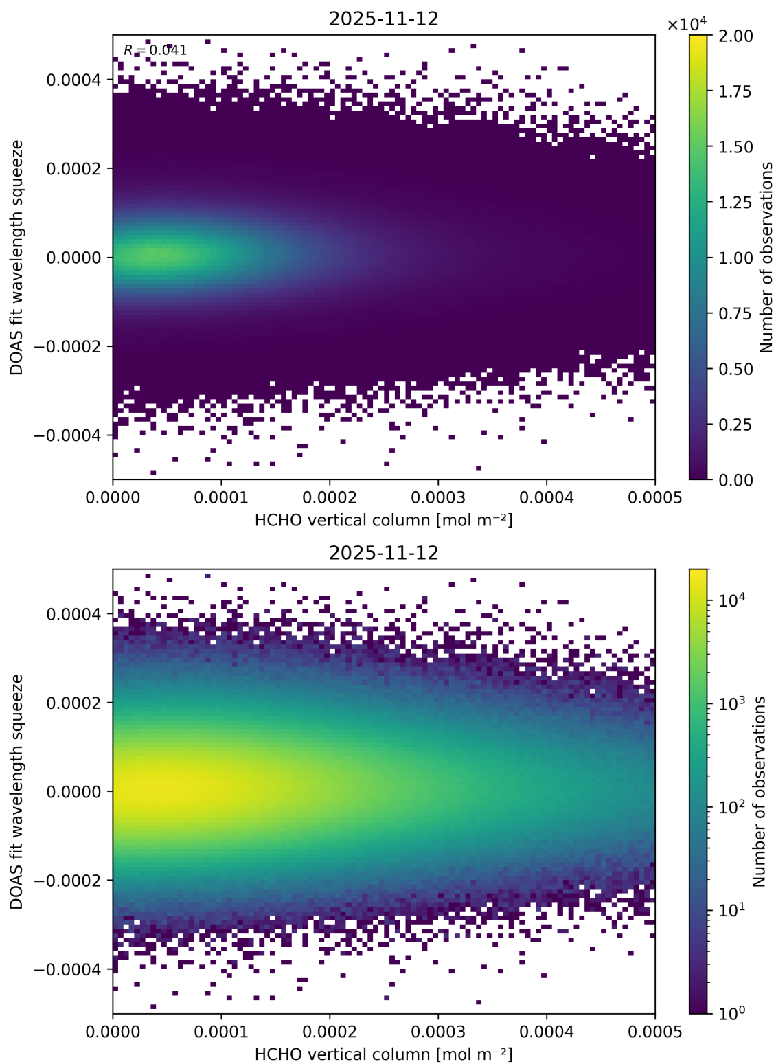
Figure 140: Scatter density plot of “HCHO vertical column” against “DOAS fit wavelength squeeze” for 2025-11-12 to 2025-11-13.
