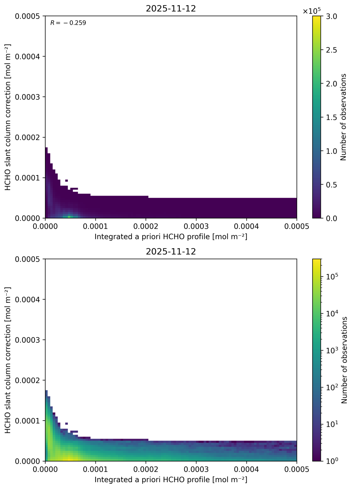
Figure 169: Scatter density plot of “Integrated a priori HCHO profile” against “HCHO slant column correction” for 2025-11-12 to 2025-11-13.
