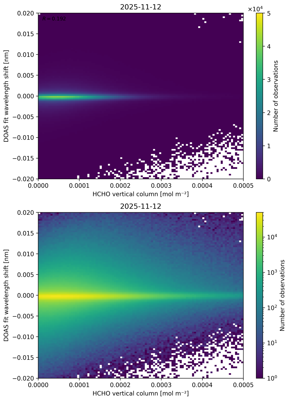
Figure 139: Scatter density plot of “HCHO vertical column” against “DOAS fit wavelength shift” for 2025-11-12 to 2025-11-13.
