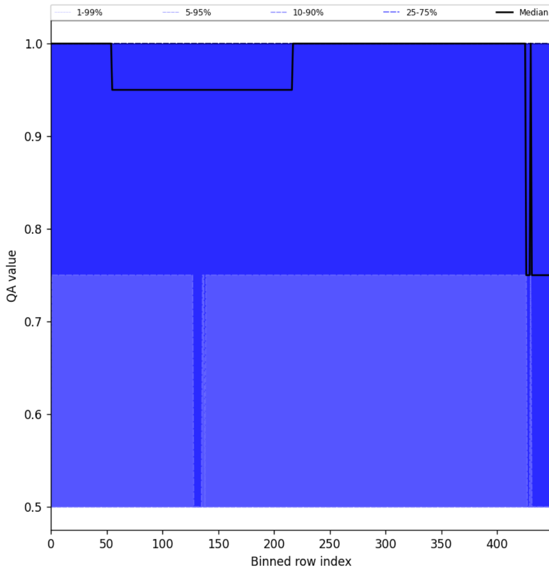
Figure 51: Along track statistics of “QA value” for 2025-11-12 to 2025-11-13
