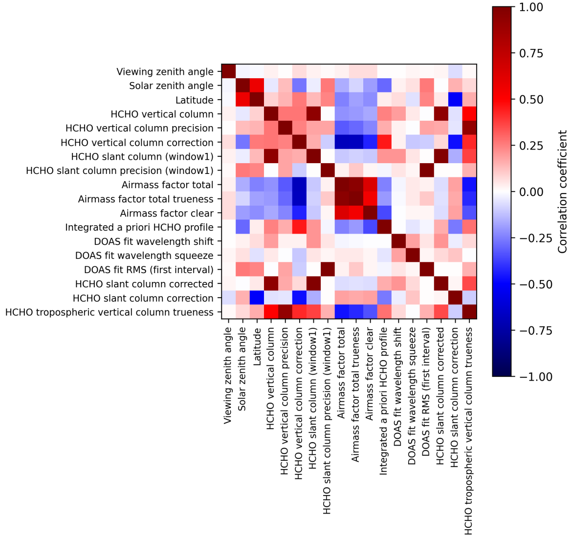
Figure 2: Map of correlation matrix for 2025-11-12 to 2025-11-13.
