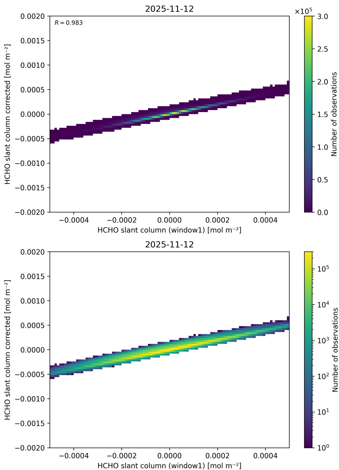
Figure 92: Scatter density plot of “HCHO slant column (window1)” against “HCHO slant column corrected” for 2025-11-12 to 2025-11-13.
