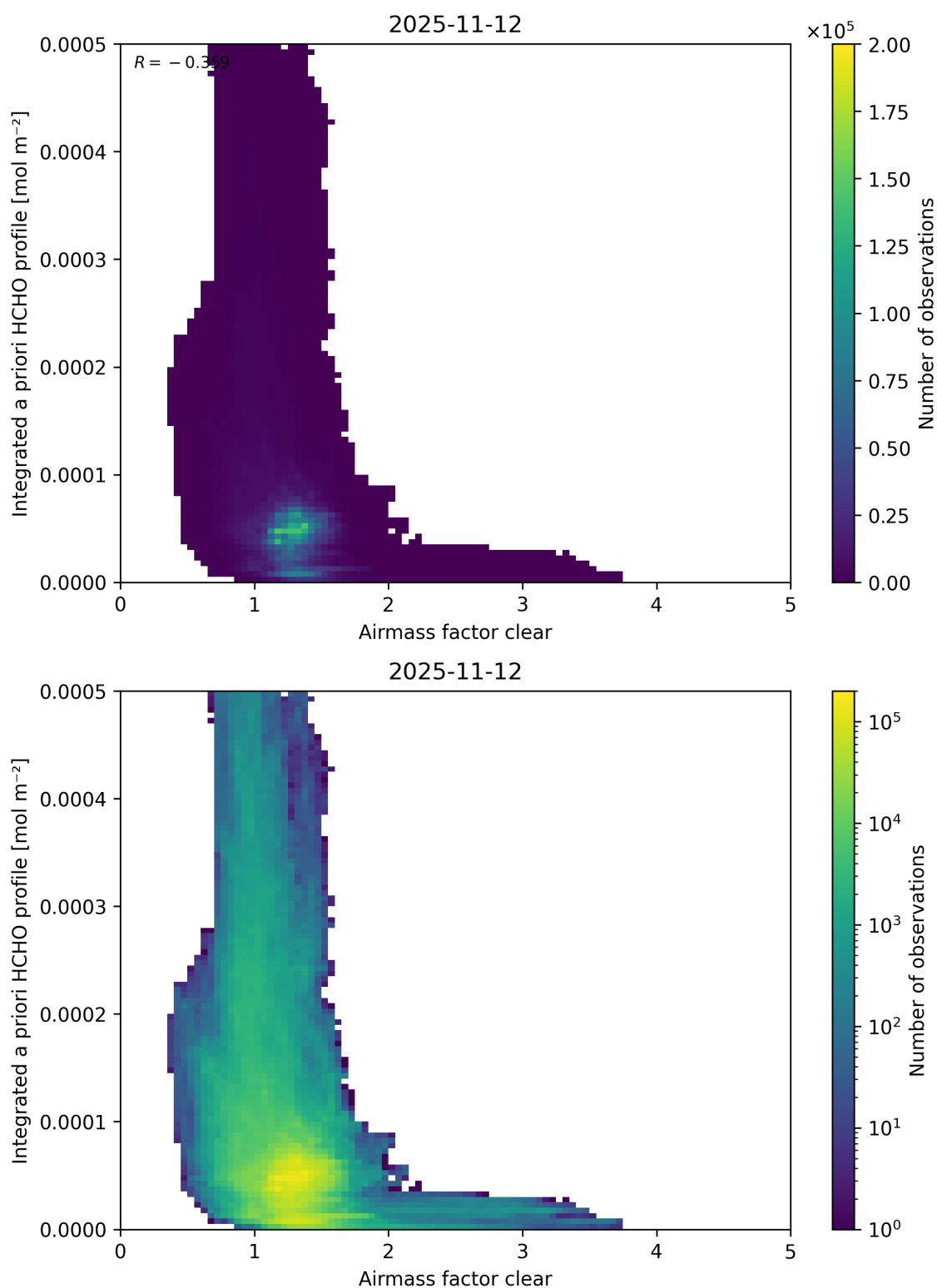
Figure 84: Scatter density plot of “Airmass factor clear” against “Integrated a priori HCHO profile” for 2025-11-12 to 2025-11-13.
