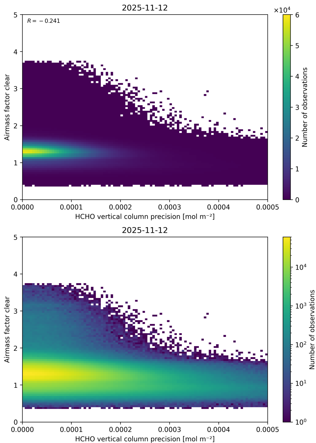
Figure 155: Scatter density plot of “HCHO vertical column precision” against “Airmass factor clear” for 2025-11-12 to 2025-11-13.
