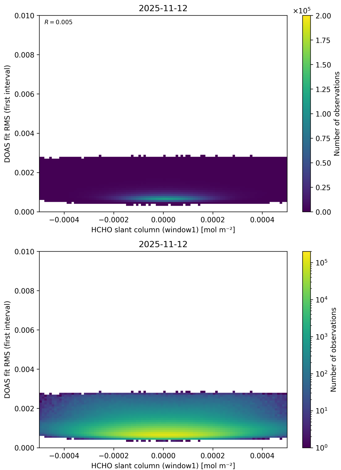
Figure 88: Scatter density plot of “HCHO slant column (window1)” against “DOAS fit RMS (first interval)” for 2025-11-12 to 2025-11-13.
