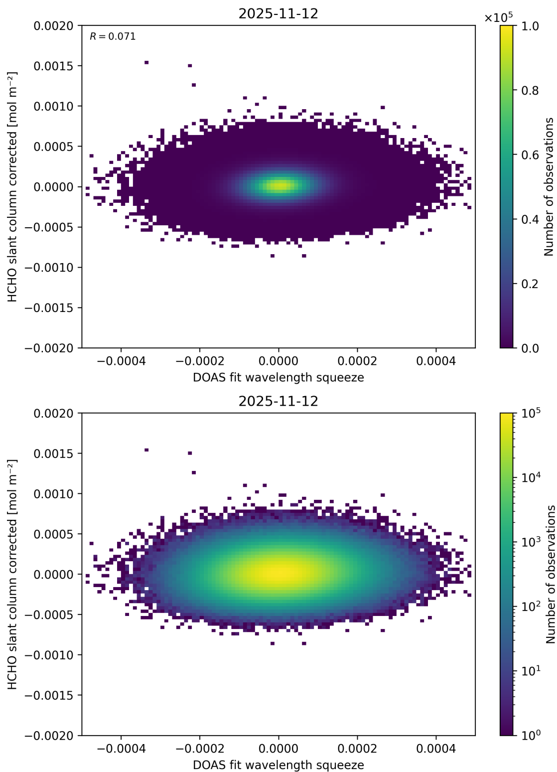
Figure 75: Scatter density plot of “DOAS fit wavelength squeeze” against “HCHO slant column corrected” for 2025-11-12 to 2025-11-13.
