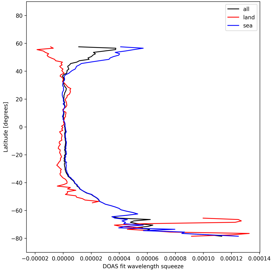
Figure 32: Zonal average of “DOAS fit wavelength squeeze” for 2025-11-12 to 2025-11-13.
