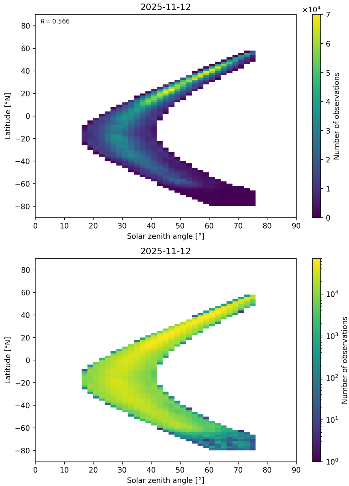
Figure 201: Scatter density plot of “Solar zenith angle” against “Latitude” for 2025-11-12 to 2025-11-13.
