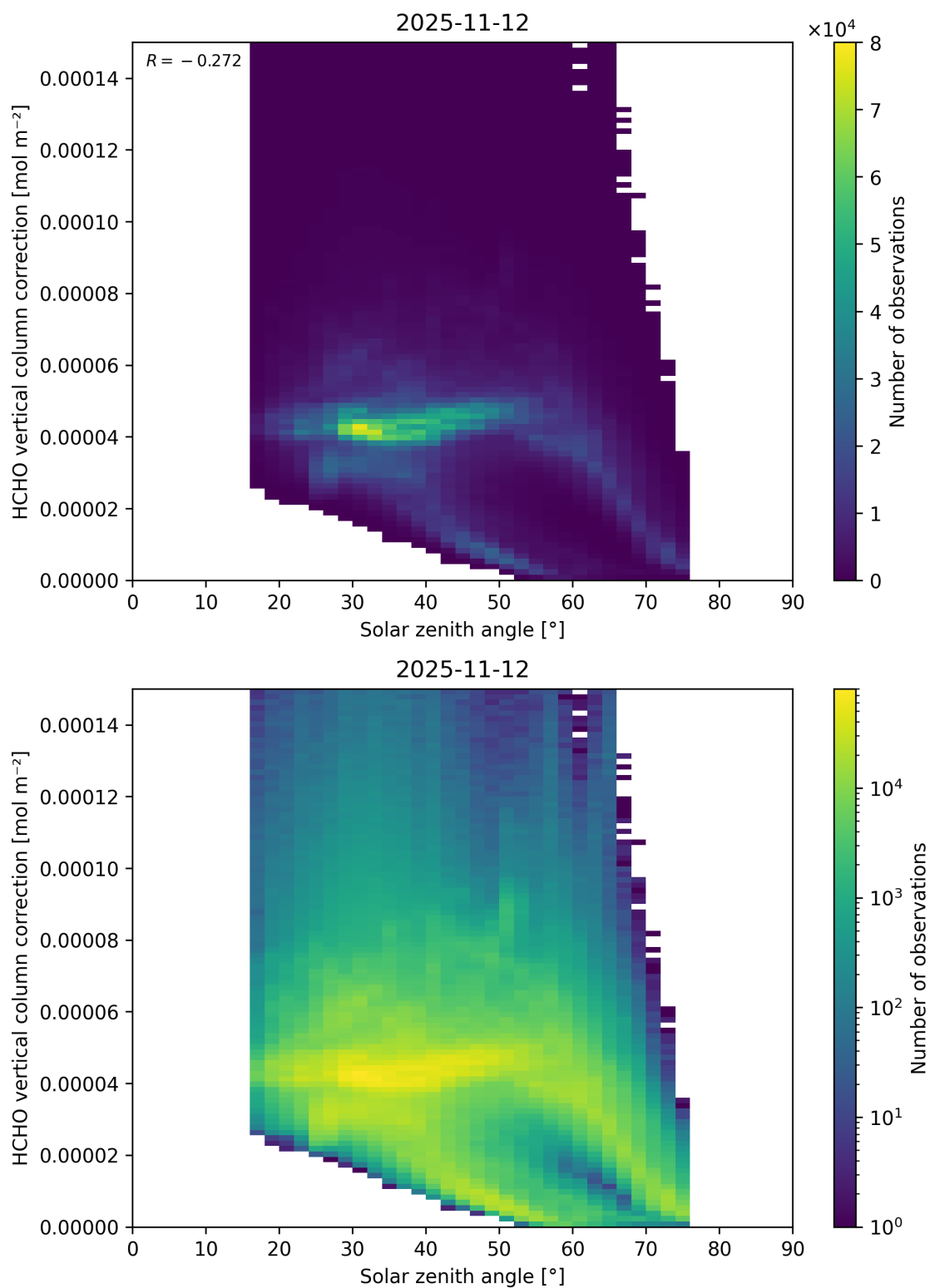
Figure 197: Scatter density plot of “Solar zenith angle” against “HCHO vertical column correction” for 2025-11-12 to 2025-11-13.
