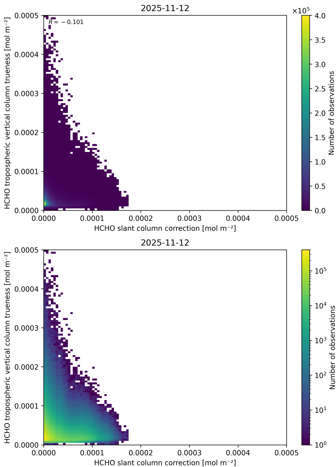
Figure 87: Scatter density plot of “HCHO slant column correction” against “HCHO tropospheric vertical column trueness” for 2025-11-12 to 2025-11-13.
