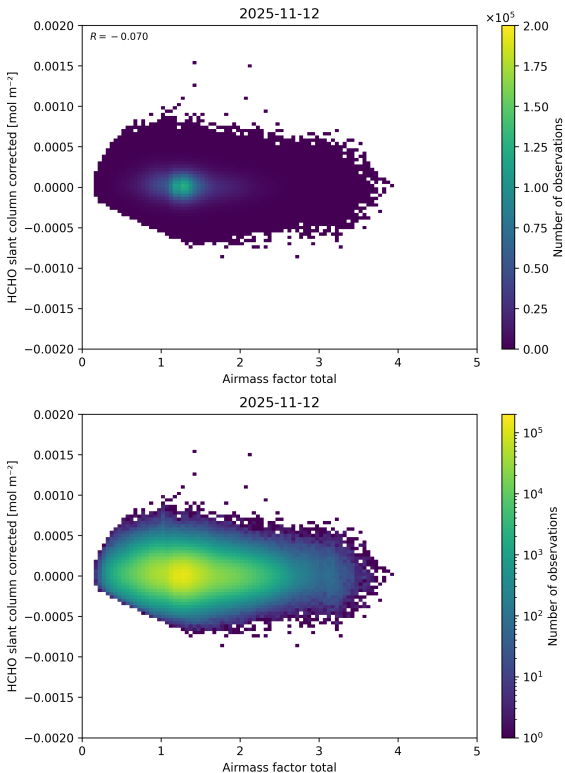
Figure 113: Scatter density plot of “Airmass factor total” against “HCHO slant column corrected” for 2025-11-12 to 2025-11-13.
