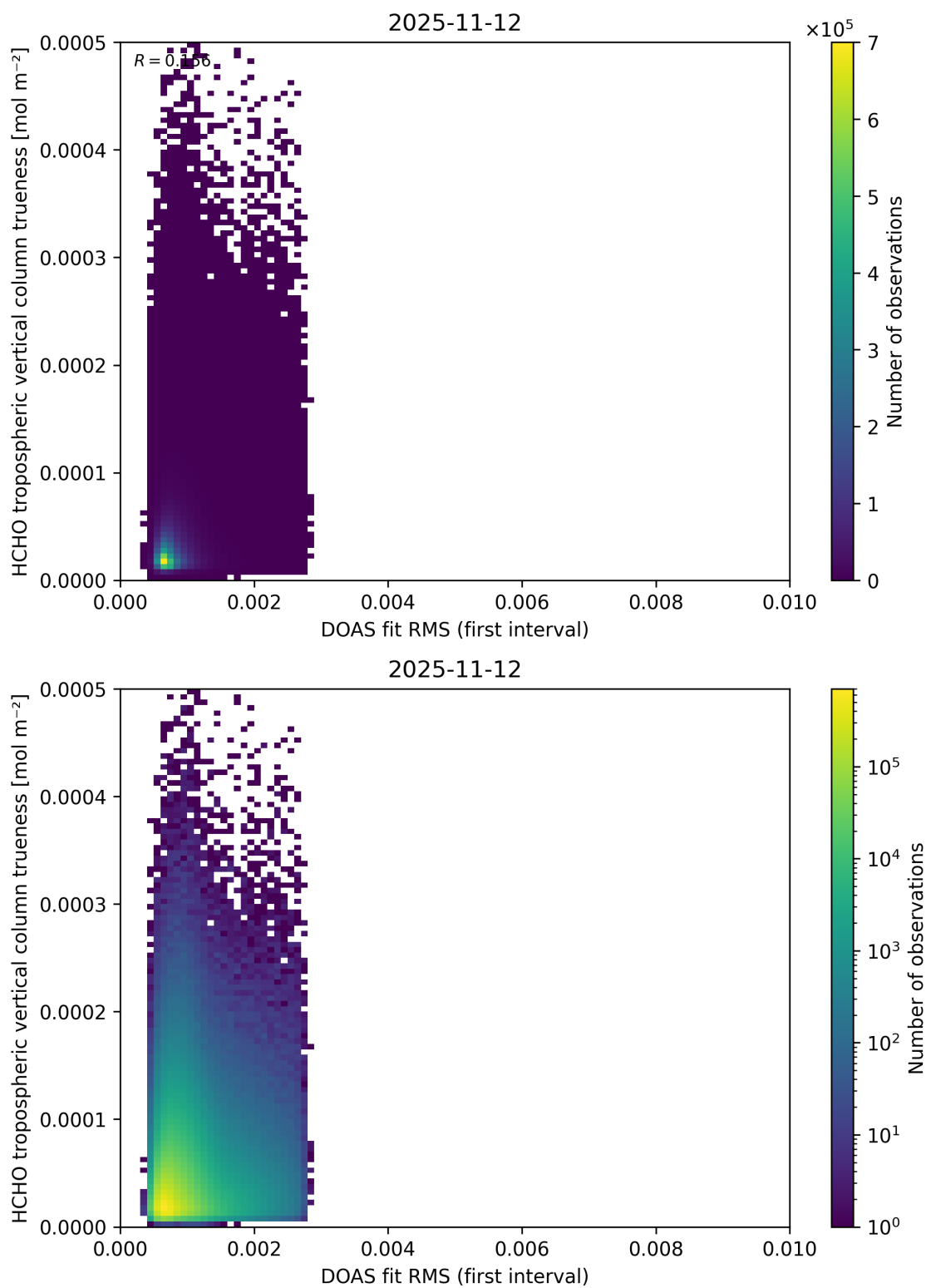
Figure 68: Scatter density plot of “DOAS fit RMS (first interval)” against “HCHO tropospheric vertical column trueness” for 2025-11-12 to 2025-11-13.
