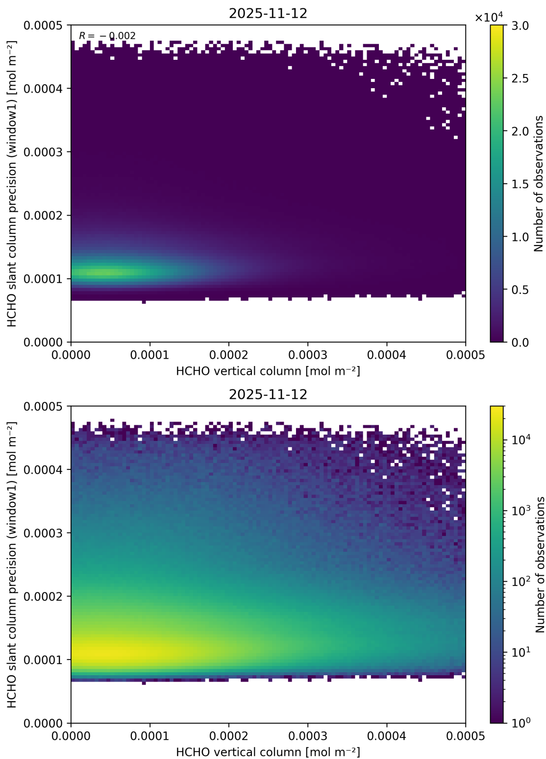
Figure 145: Scatter density plot of “HCHO vertical column” against “HCHO slant column precision (window1)” for 2025-11-12 to 2025-11-13.
