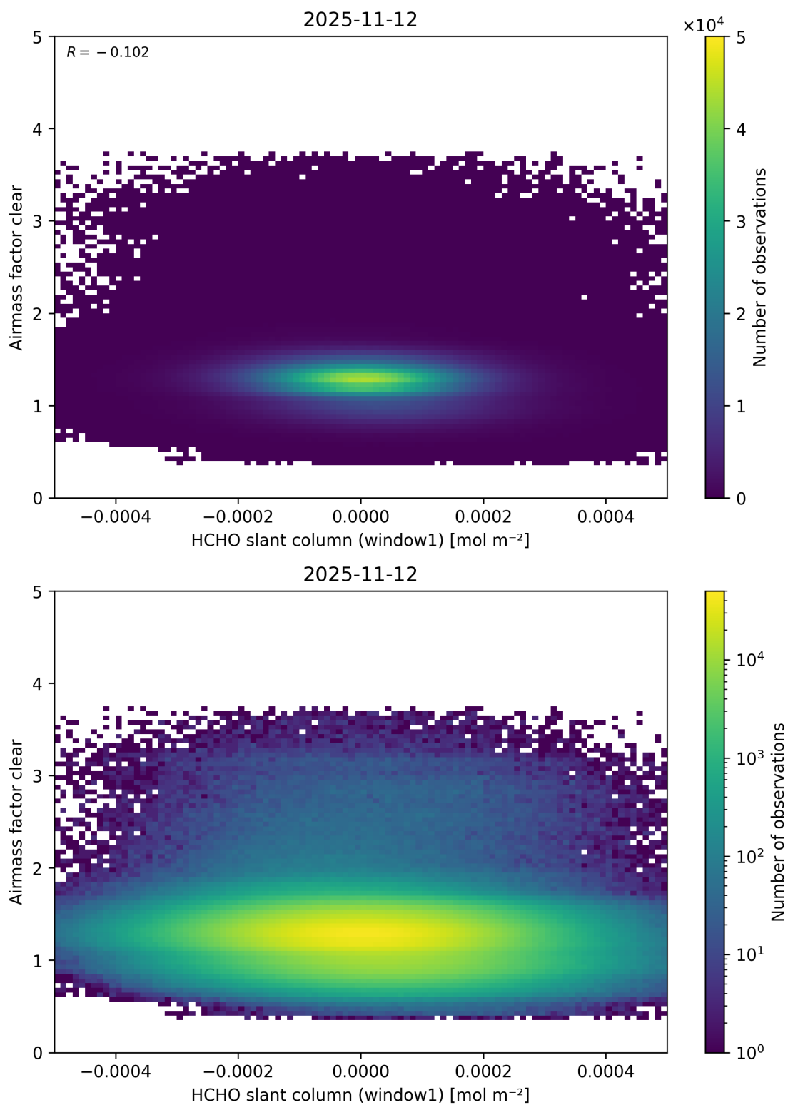
Figure 91: Scatter density plot of “HCHO slant column (window1)” against “Airmass factor clear” for 2025-11-12 to 2025-11-13.
