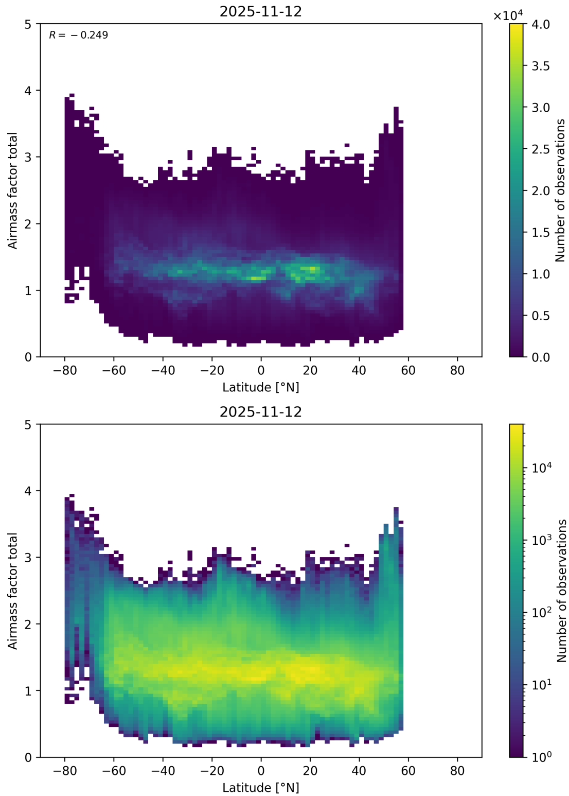
Figure 179: Scatter density plot of “Latitude” against “Airmass factor total” for 2025-11-12 to 2025-11-13.
