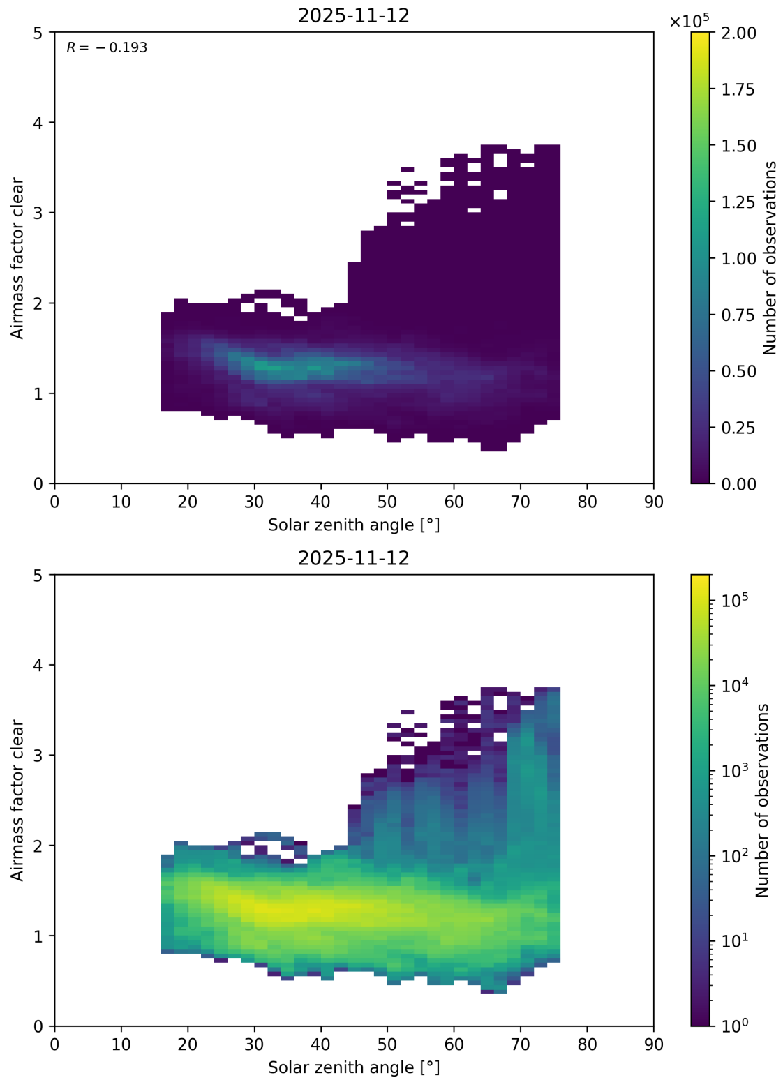
Figure 189: Scatter density plot of “Solar zenith angle” against “Airmass factor clear” for 2025-11-12 to 2025-11-13.
