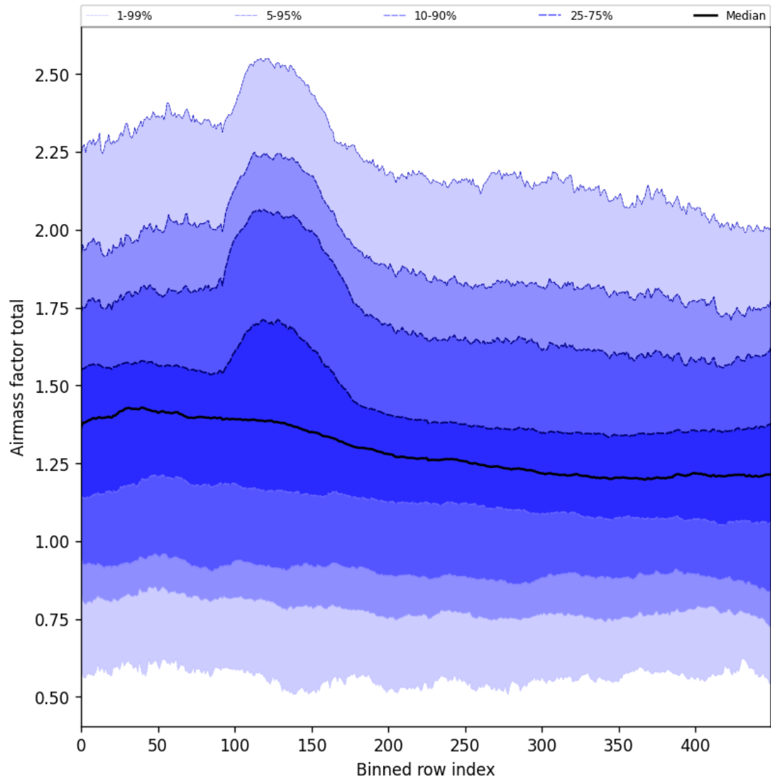
Figure 57: Along track statistics of “Airmass factor total” for 2025-11-12 to 2025-11-13
