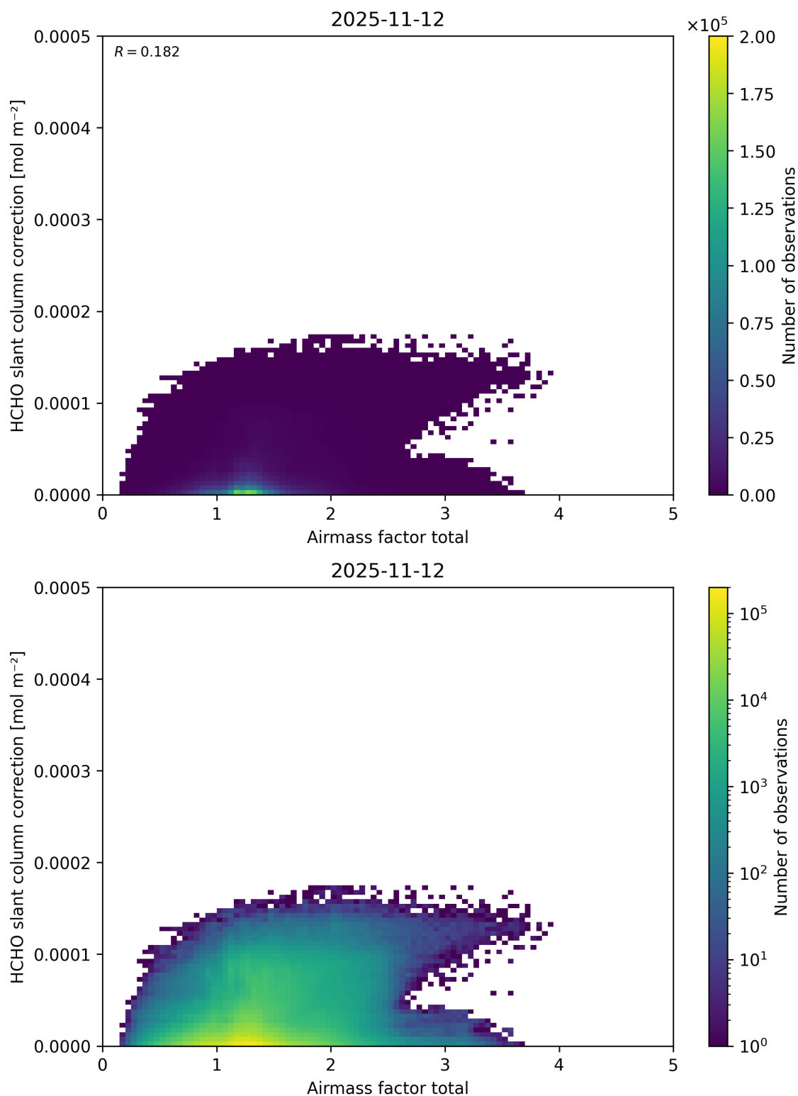
Figure 114: Scatter density plot of “Airmass factor total” against “HCHO slant column correction” for 2025-11-12 to 2025-11-13.
