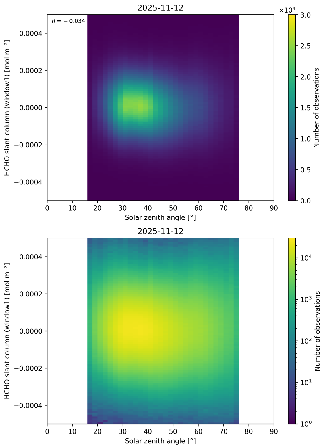
Figure 192: Scatter density plot of “Solar zenith angle” against “HCHO slant column (window1)” for 2025-11-12 to 2025-11-13.
