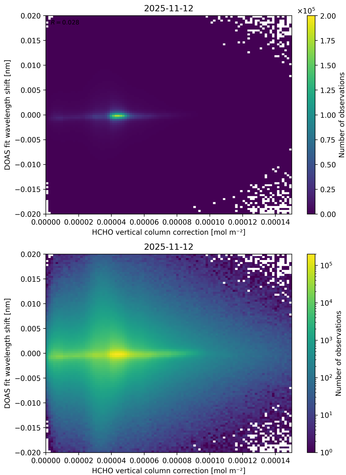
Figure 127: Scatter density plot of “HCHO vertical column correction” against “DOAS fit wavelength shift” for 2025-11-12 to 2025-11-13.
