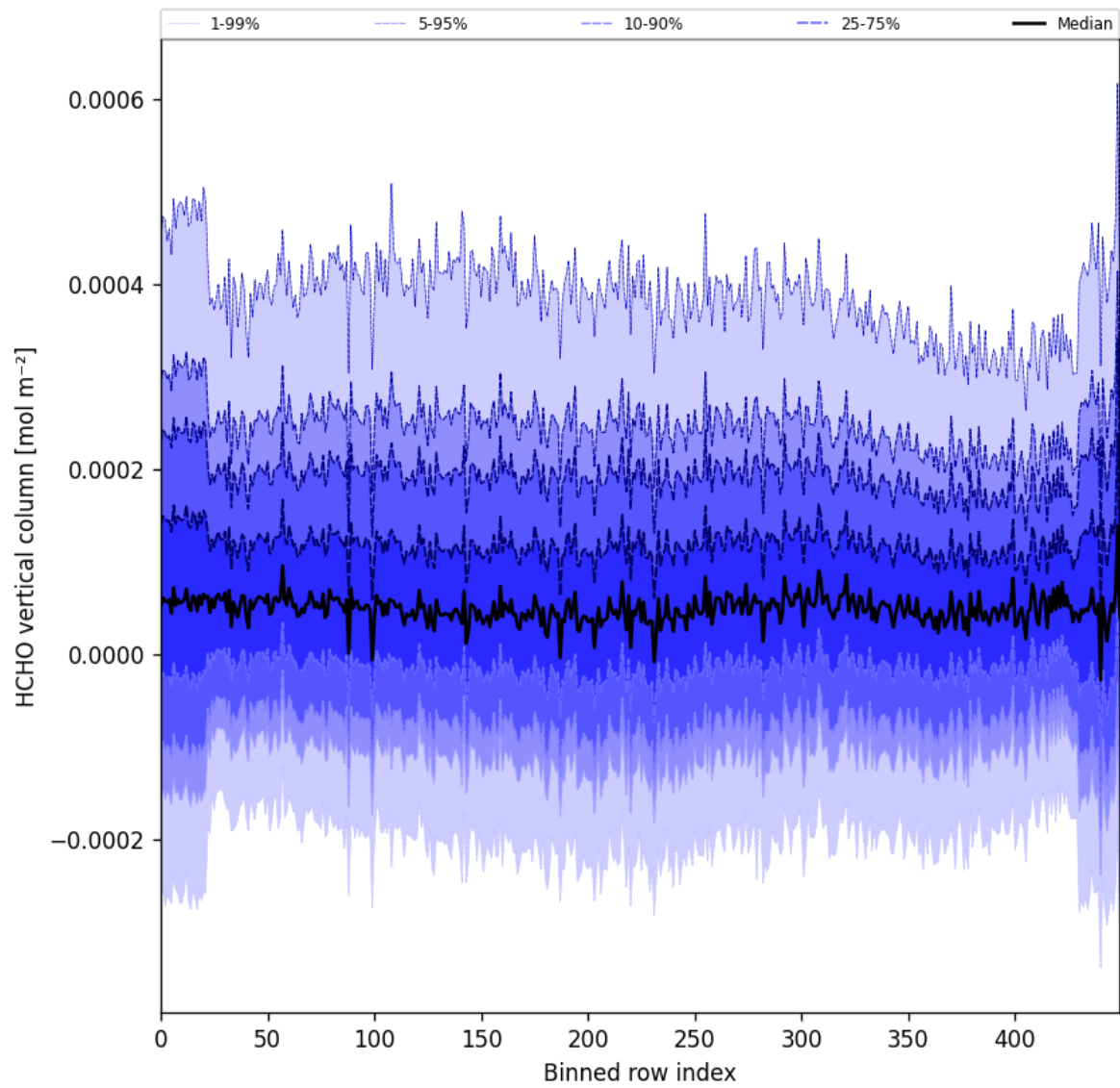
Figure 52: Along track statistics of “HCHO vertical column” for 2025-11-12 to 2025-11-13
