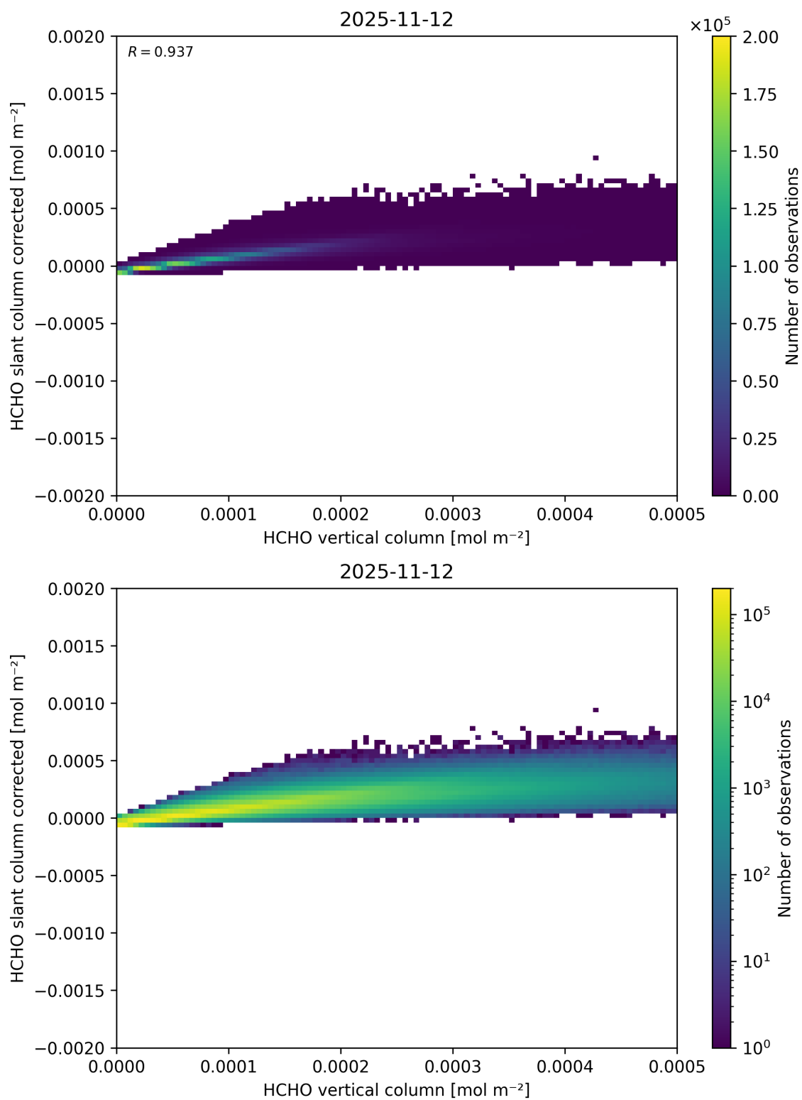
Figure 142: Scatter density plot of “HCHO vertical column” against “HCHO slant column corrected” for 2025-11-12 to 2025-11-13.
