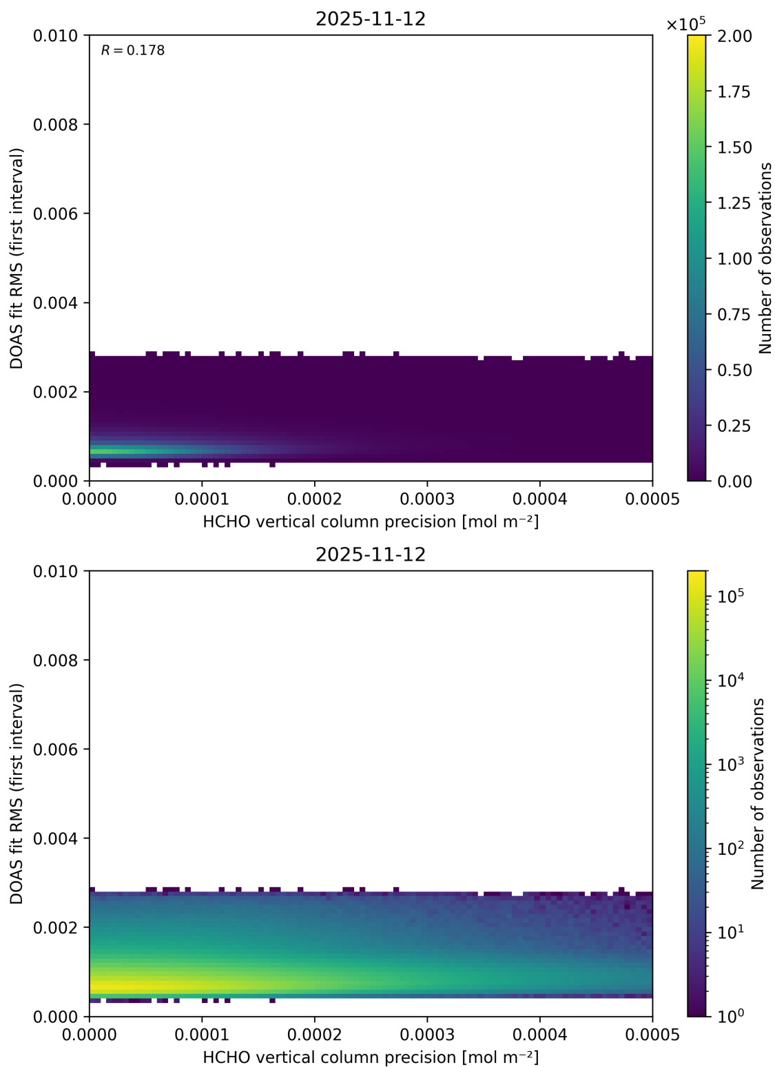
Figure 152: Scatter density plot of “HCHO vertical column precision” against “DOAS fit RMS (first interval)” for 2025-11-12 to 2025-11-13.
