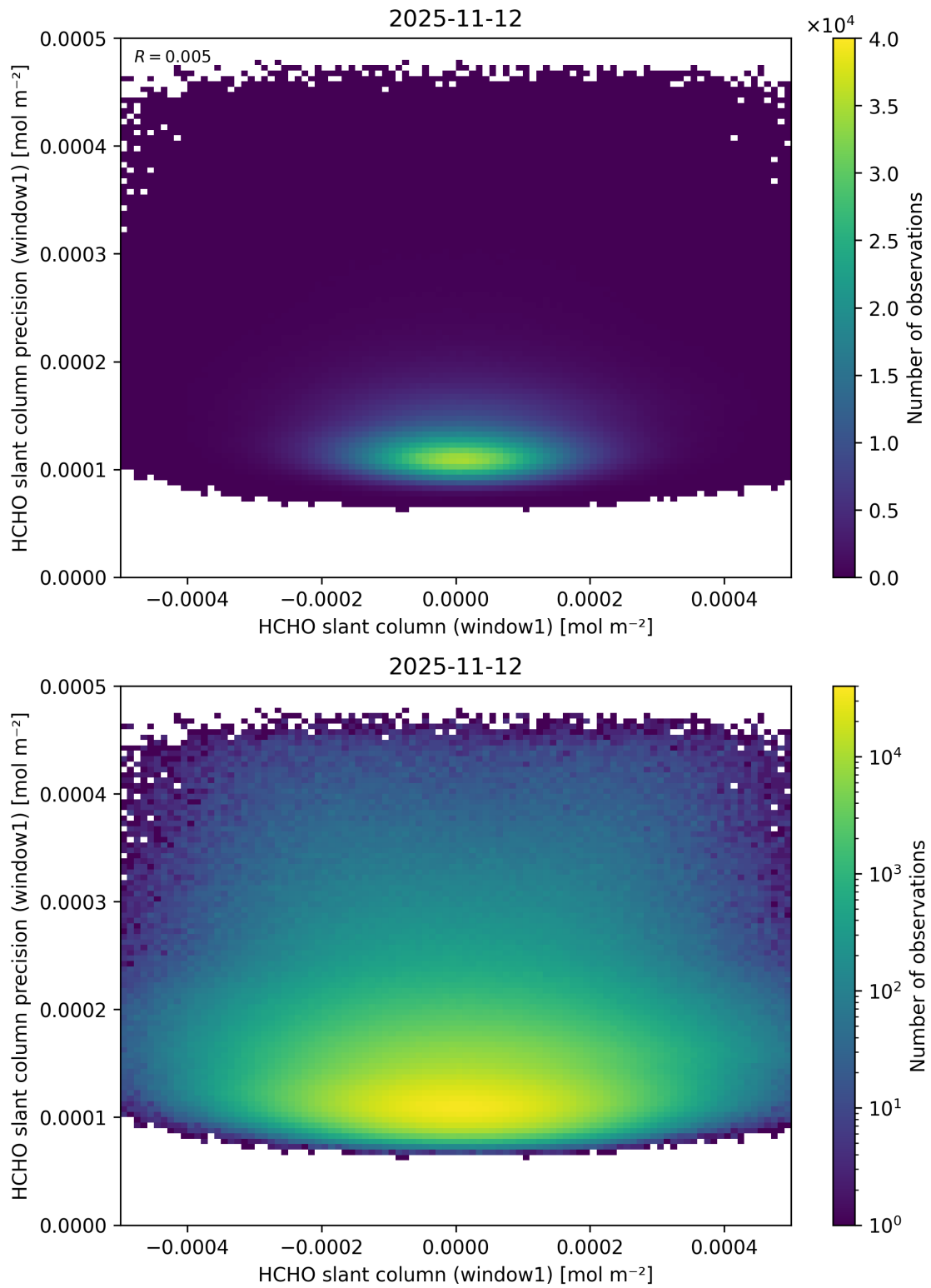
Figure 94: Scatter density plot of “HCHO slant column (window1)” against “HCHO slant column precision (window1)” for 2025-11-12 to 2025-11-13.
