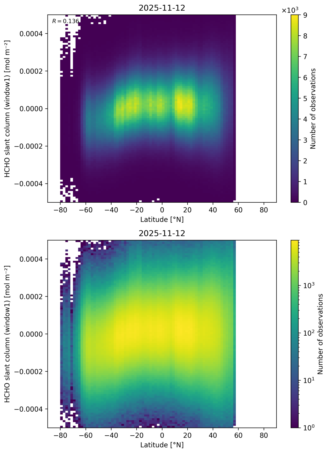
Figure 177: Scatter density plot of “Latitude” against “HCHO slant column (window1)” for 2025-11-12 to 2025-11-13.
