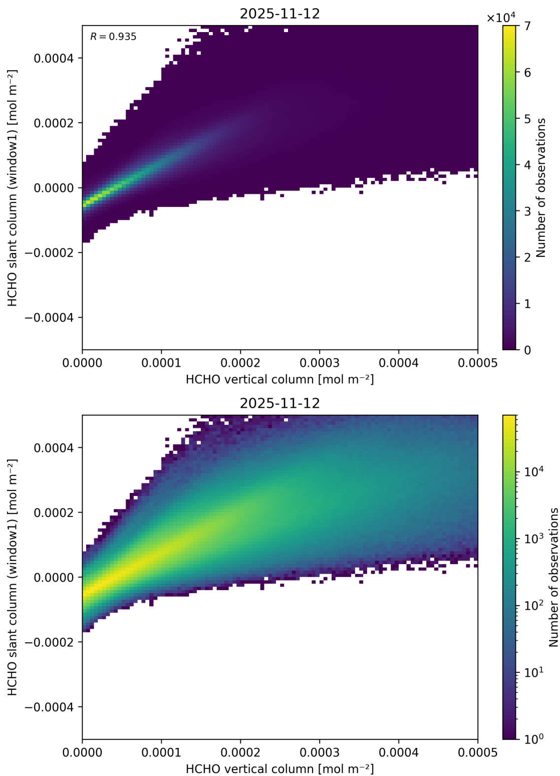
Figure 144: Scatter density plot of “HCHO vertical column” against “HCHO slant column (window1)” for 2025-11-12 to 2025-11-13.
