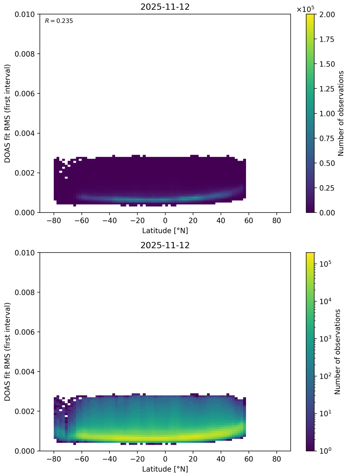
Figure 171: Scatter density plot of “Latitude” against “DOAS fit RMS (first interval)” for 2025-11-12 to 2025-11-13.
