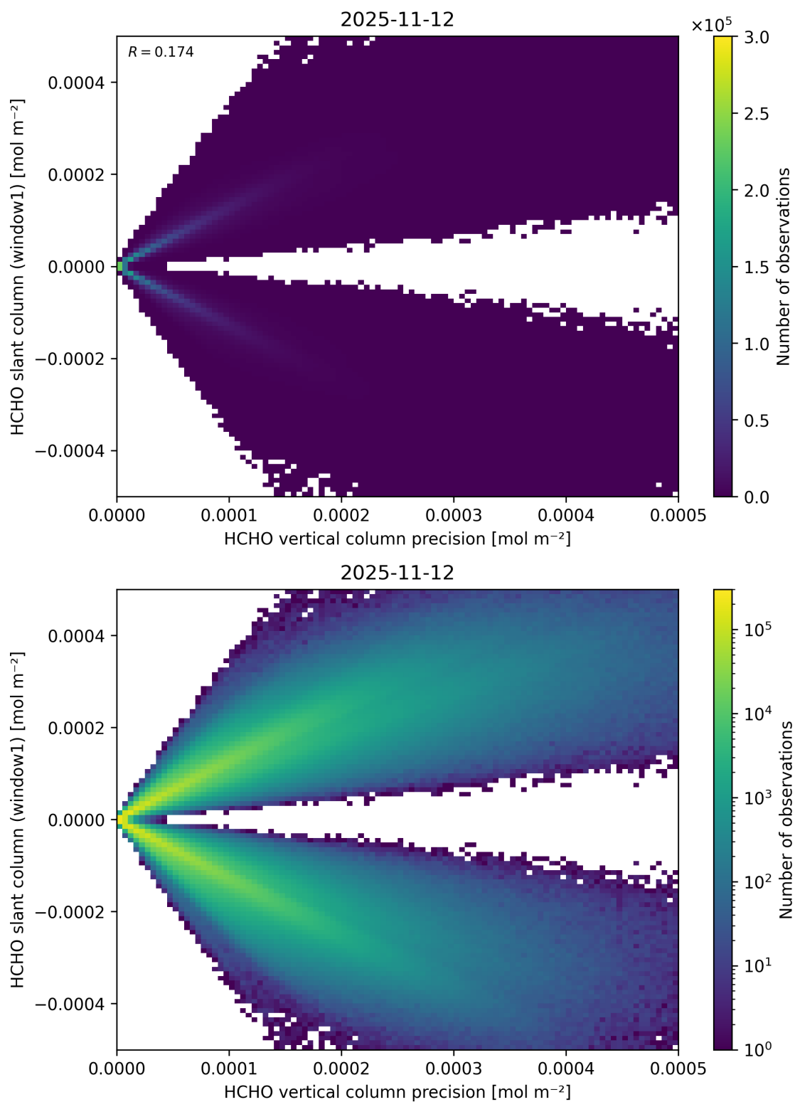
Figure 158: Scatter density plot of “HCHO vertical column precision” against “HCHO slant column (window1)” for 2025-11-12 to 2025-11-13.
