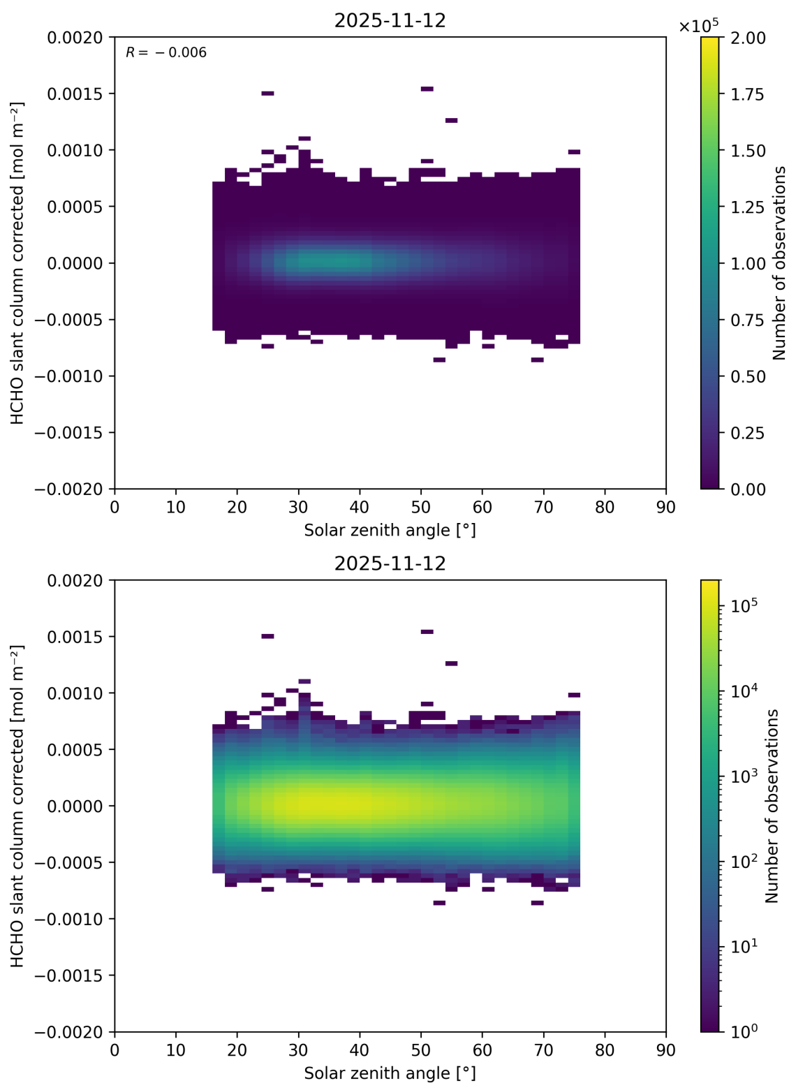
Figure 190: Scatter density plot of “Solar zenith angle” against “HCHO slant column corrected” for 2025-11-12 to 2025-11-13.
