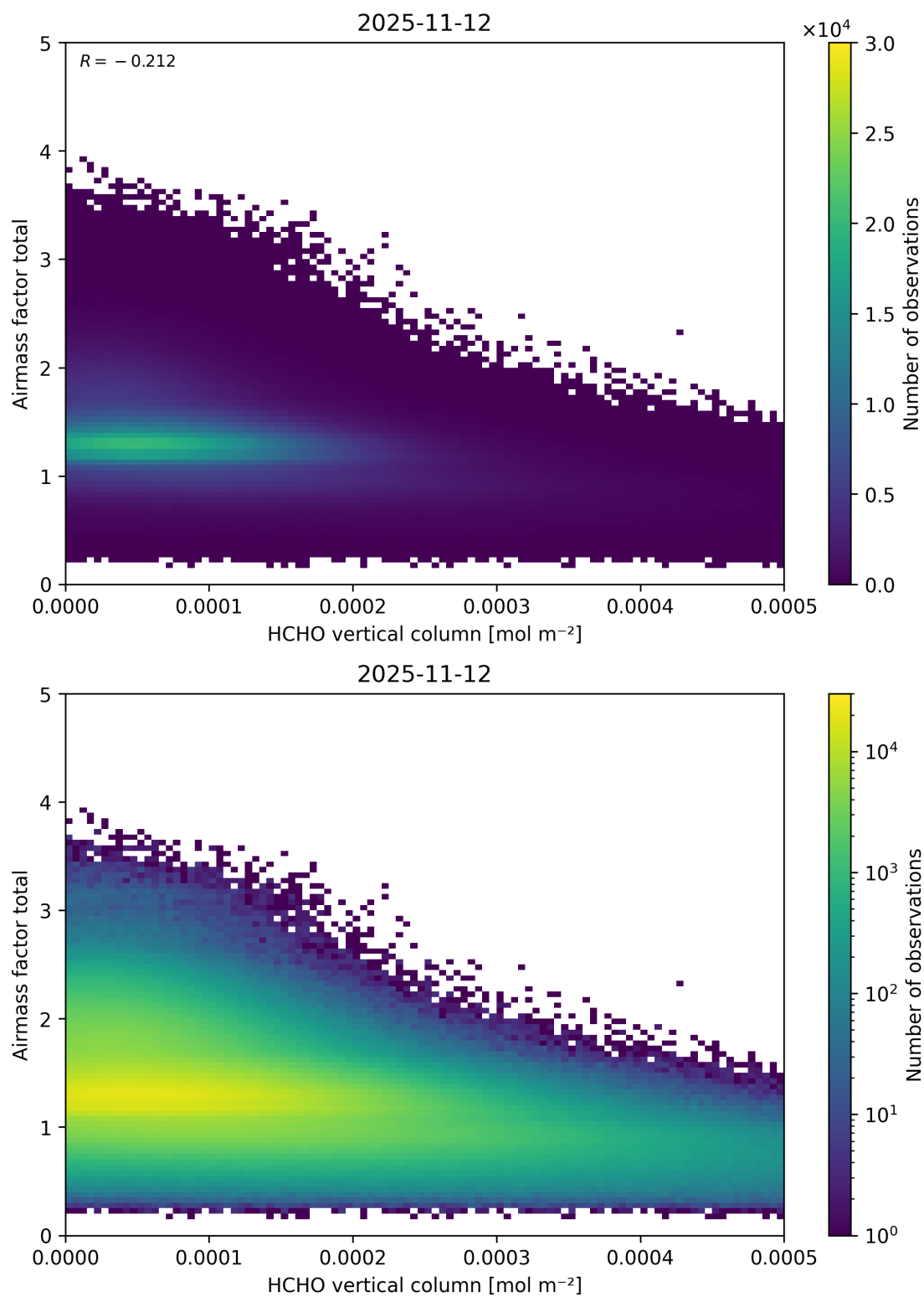
Figure 146: Scatter density plot of “HCHO vertical column” against “Airmass factor total” for 2025-11-12 to 2025-11-13.
