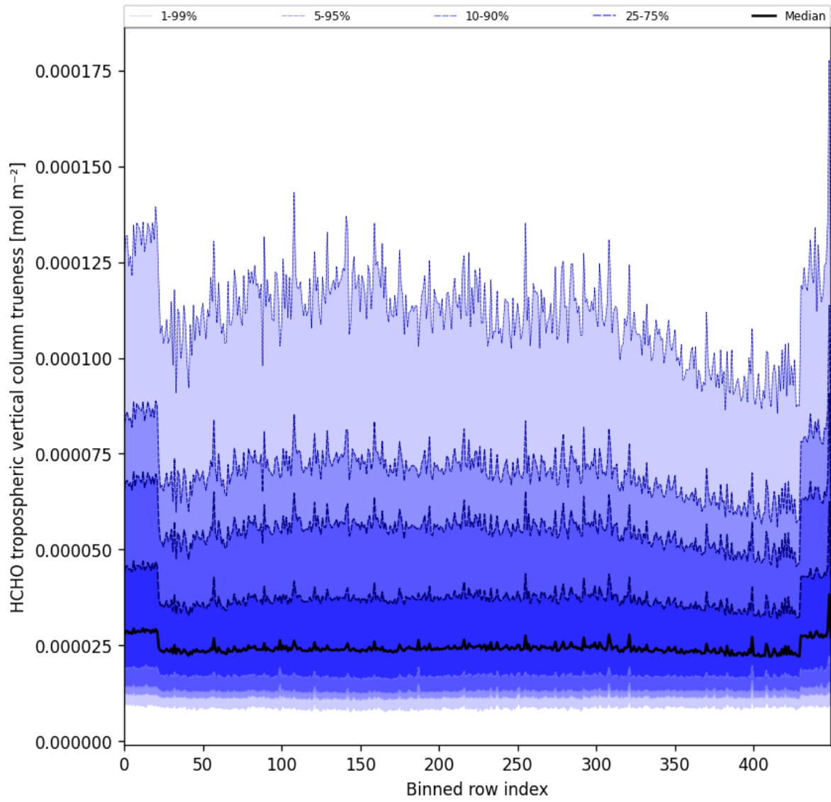
Figure 65: Along track statistics of “HCHO tropospheric vertical column trueness” for 2025-11-12 to 2025-11-13
