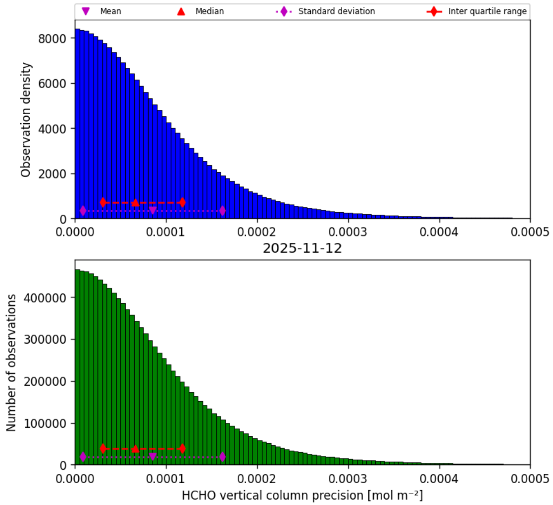
Figure 38: Histogram of “HCHO vertical column precision” for 2025-11-12 to 2025-11-13
