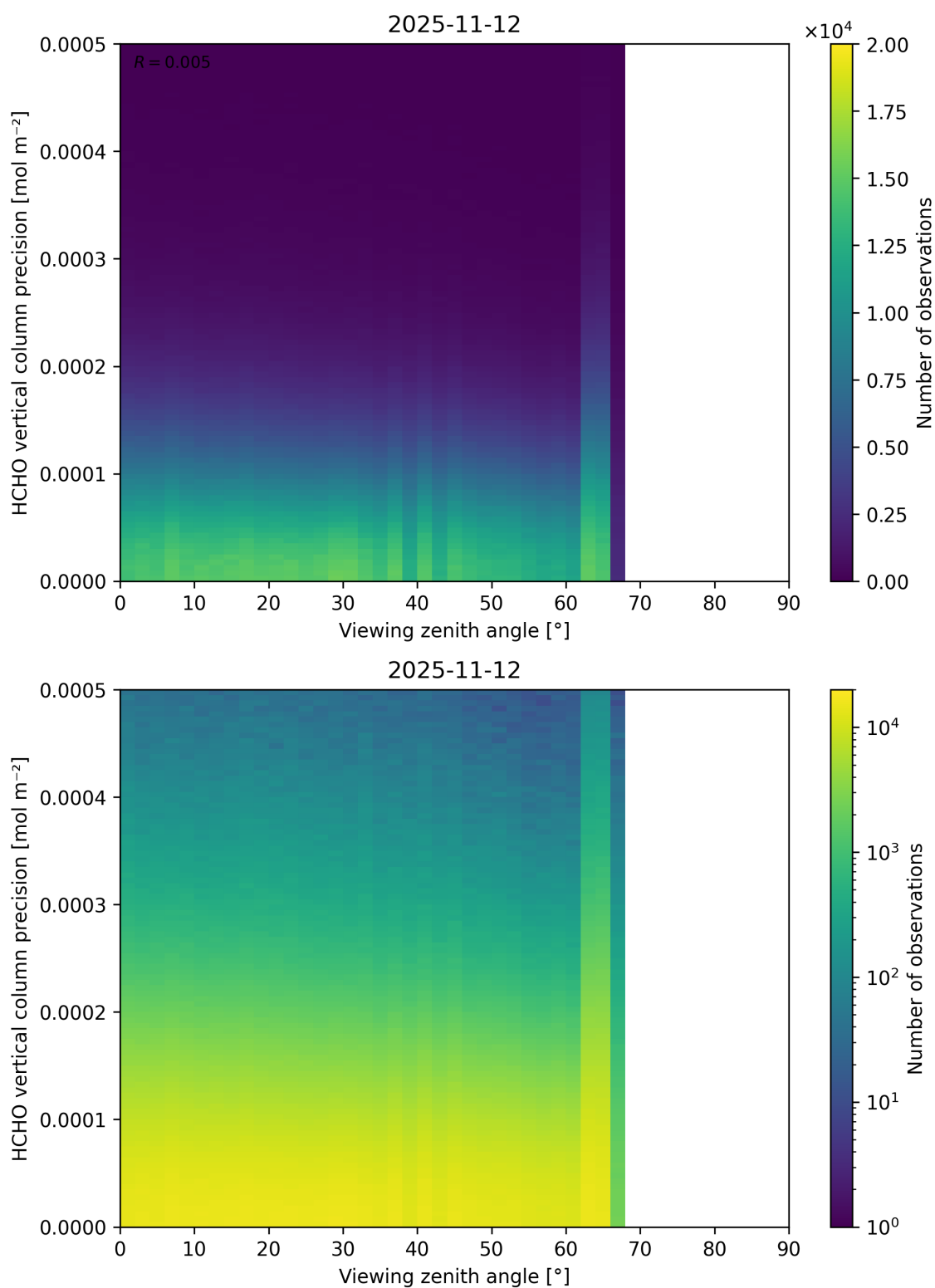
Figure 214: Scatter density plot of “Viewing zenith angle” against “HCHO vertical column precision” for 2025-11-12 to 2025-11-13.
