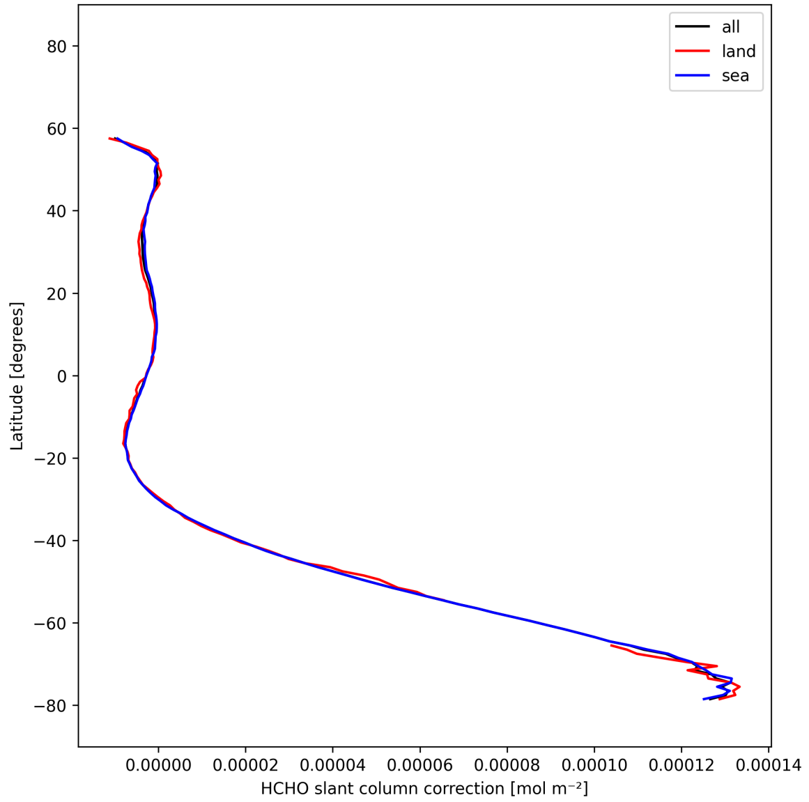
Figure 34: Zonal average of “HCHO slant column correction” for 2025-11-12 to 2025-11-13.
