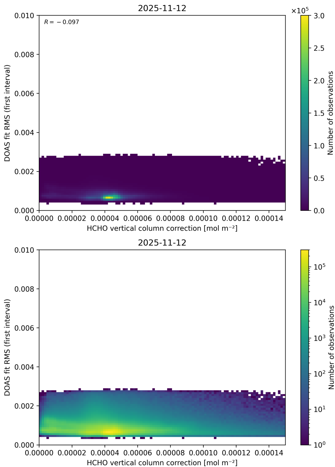
Figure 126: Scatter density plot of “HCHO vertical column correction” against “DOAS fit RMS (first interval)” for 2025-11-12 to 2025-11-13.
