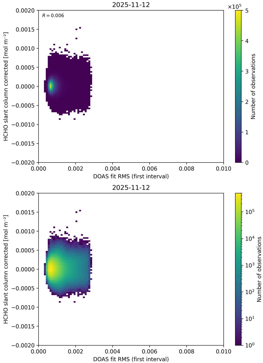
Figure 66: Scatter density plot of “DOAS fit RMS (first interval)” against “HCHO slant column corrected” for 2025-11-12 to 2025-11-13.
