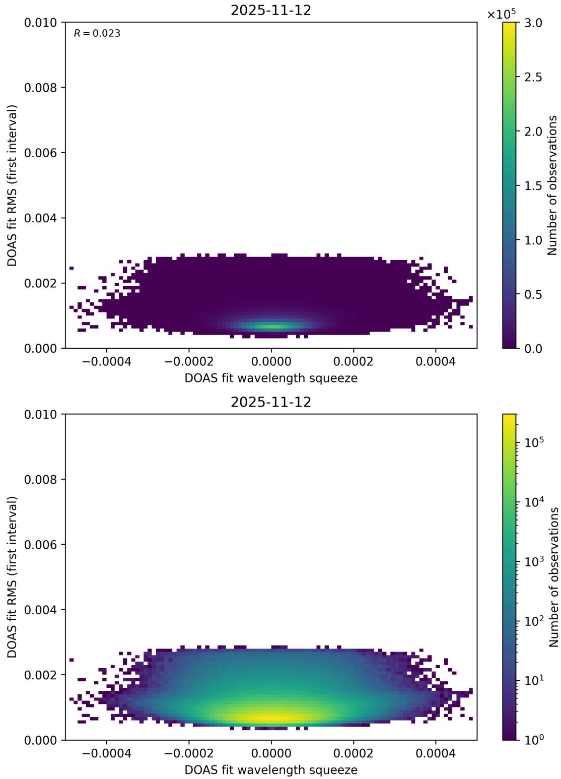
Figure 74: Scatter density plot of “DOAS fit wavelength squeeze” against “DOAS fit RMS (first interval)” for 2025-11-12 to 2025-11-13.
