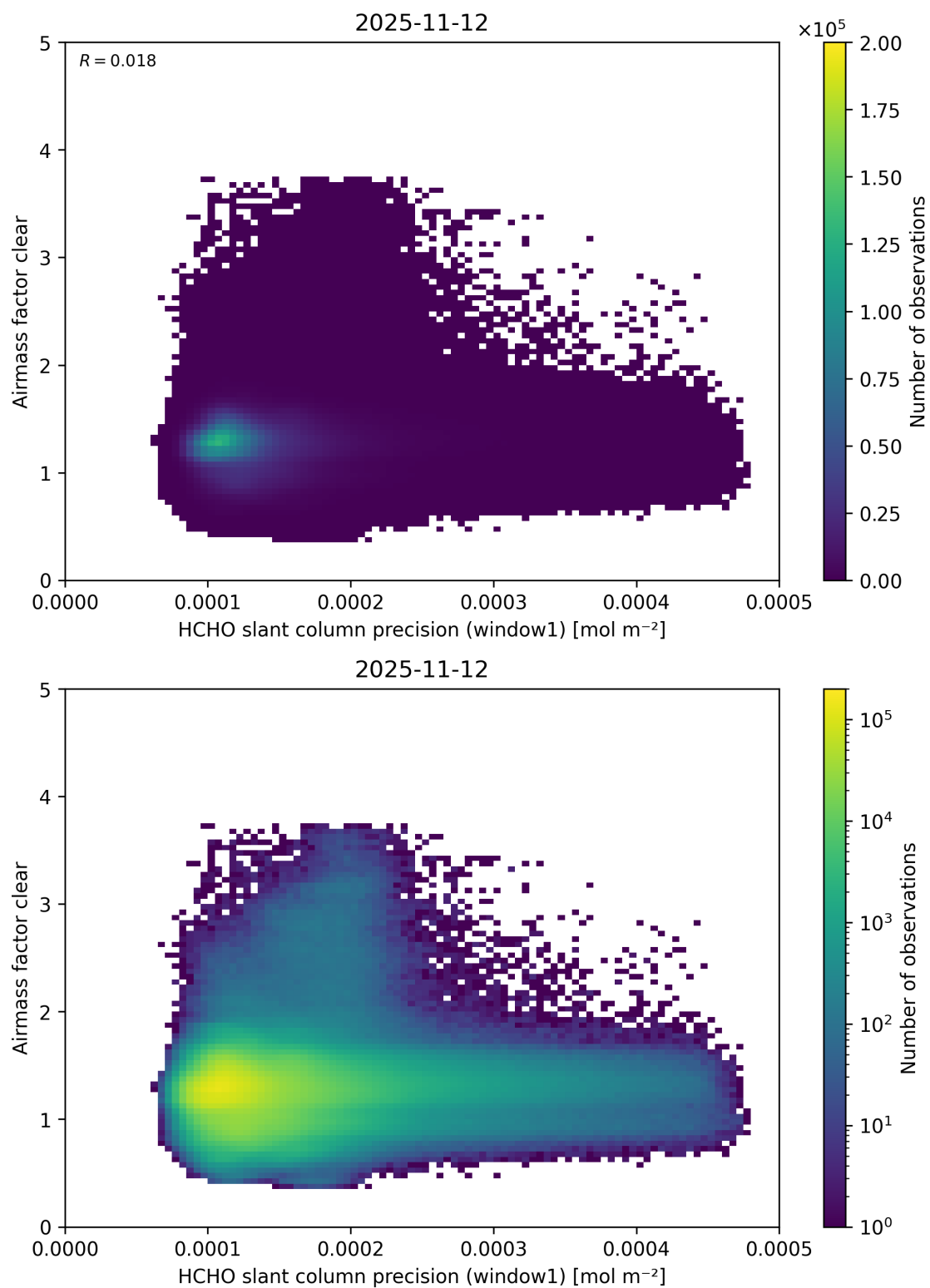
Figure 102: Scatter density plot of “HCHO slant column precision (window1)” against “Airmass factor clear” for 2025-11-12 to 2025-11-13.
