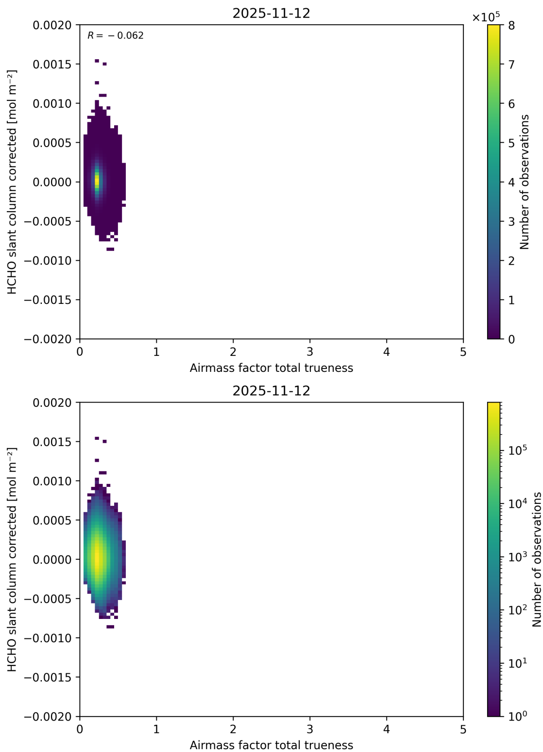
Figure 122: Scatter density plot of “Airmass factor total trueness” against “HCHO slant column corrected” for 2025-11-12 to 2025-11-13.
