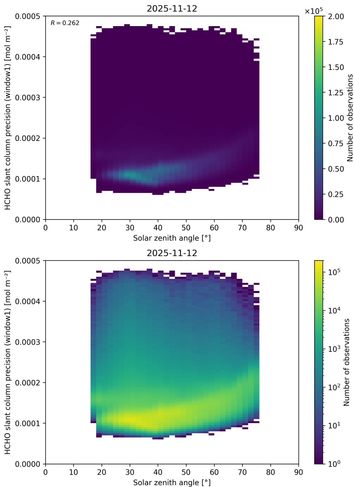
Figure 193: Scatter density plot of “Solar zenith angle” against “HCHO slant column precision (window1)” for 2025-11-12 to 2025-11-13.
