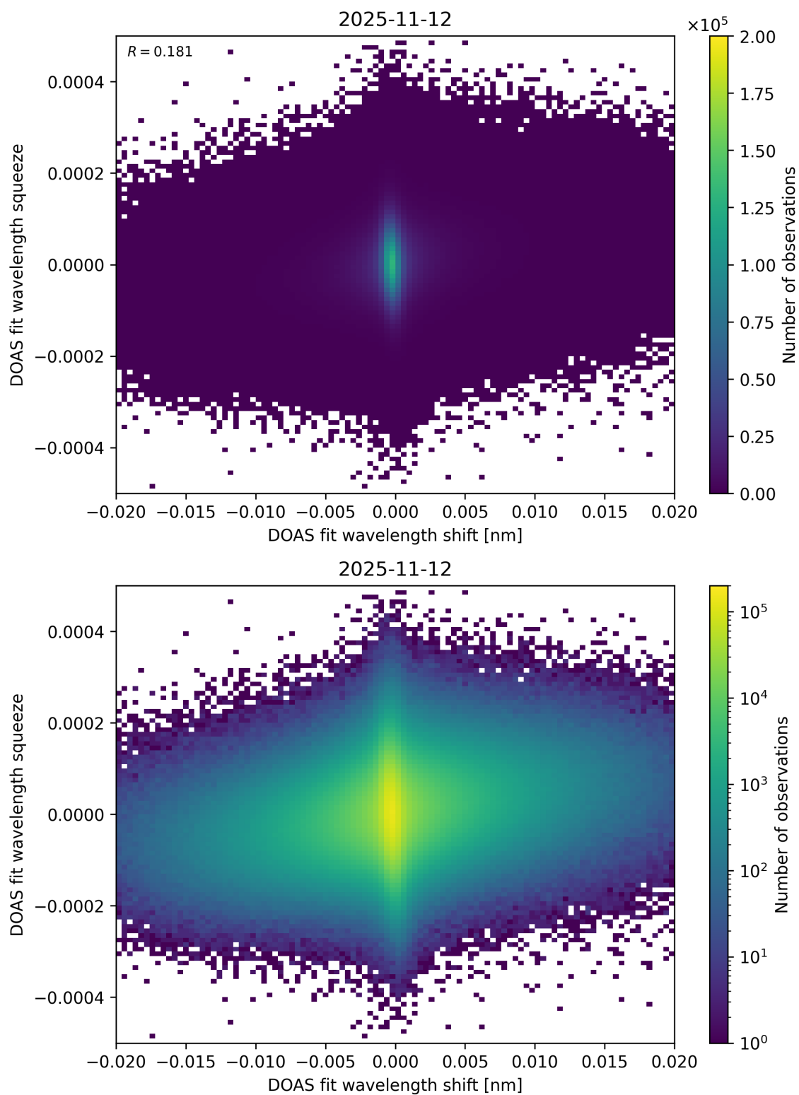
Figure 70: Scatter density plot of “DOAS fit wavelength shift” against “DOAS fit wavelength squeeze” for 2025-11-12 to 2025-11-13.
