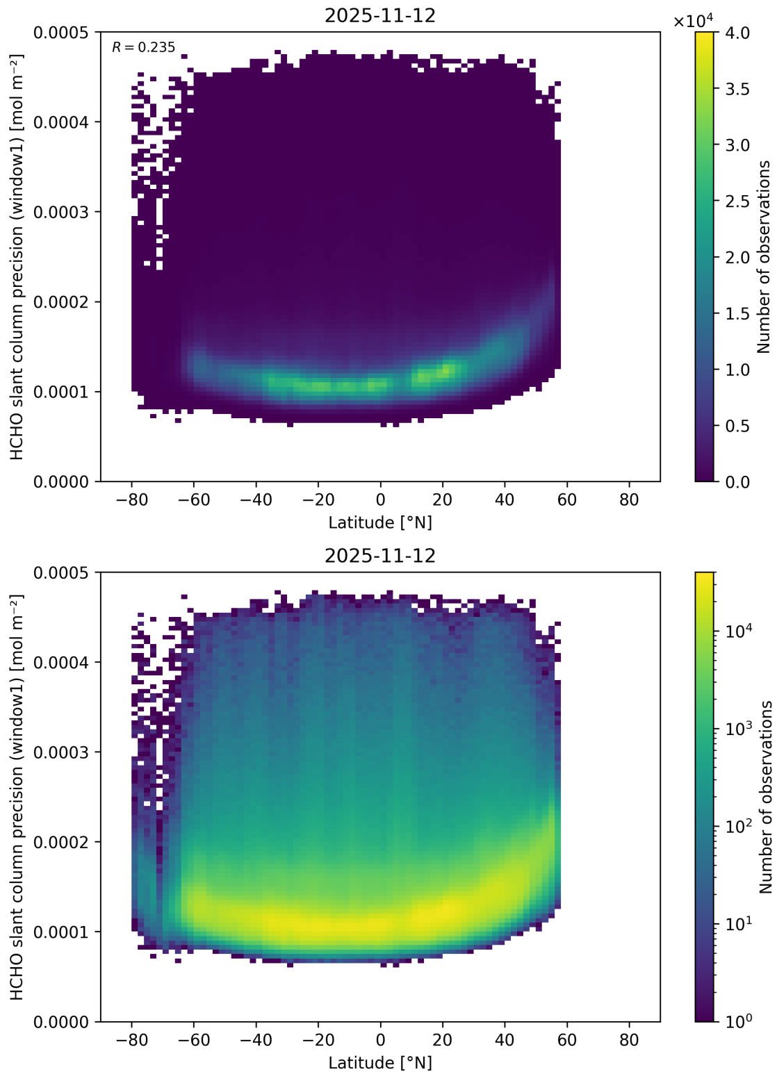
Figure 178: Scatter density plot of “Latitude” against “HCHO slant column precision (window1)” for 2025-11-12 to 2025-11-13.
