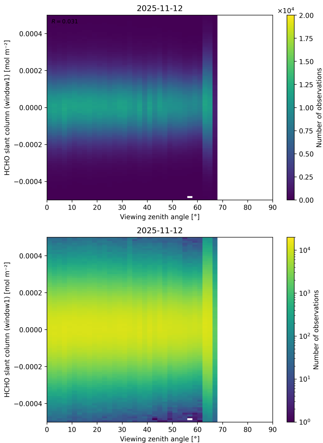
Figure 208: Scatter density plot of “Viewing zenith angle” against “HCHO slant column (window1)” for 2025-11-12 to 2025-11-13.
