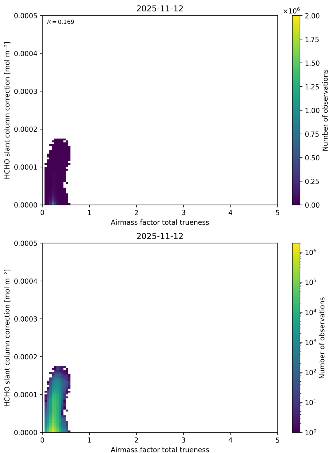
Figure 123: Scatter density plot of “Airmass factor total trueness” against “HCHO slant column correction” for 2025-11-12 to 2025-11-13.
