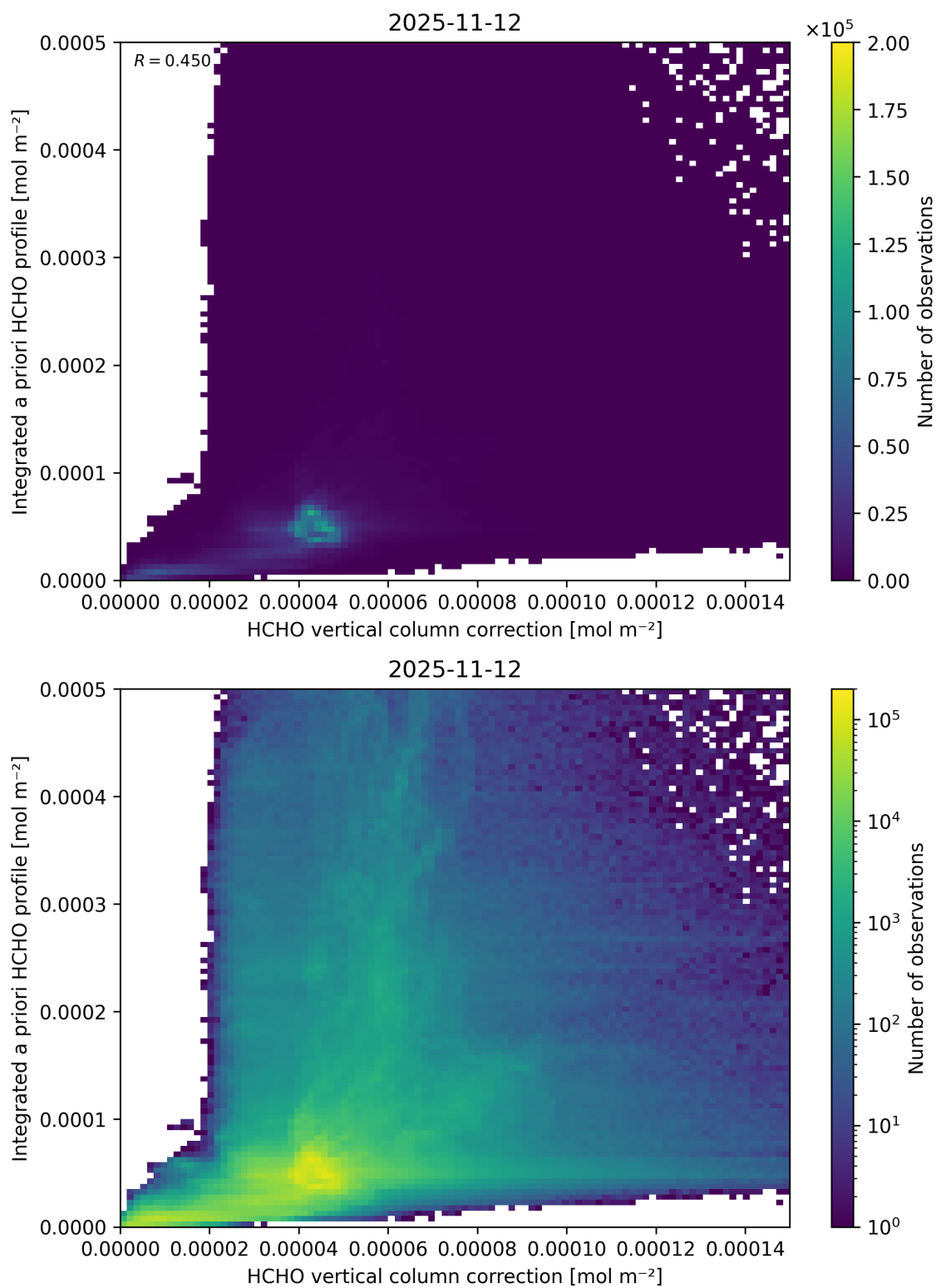
Figure 137: Scatter density plot of “HCHO vertical column correction” against “Integrated a priori HCHO profile” for 2025-11-12 to 2025-11-13.
