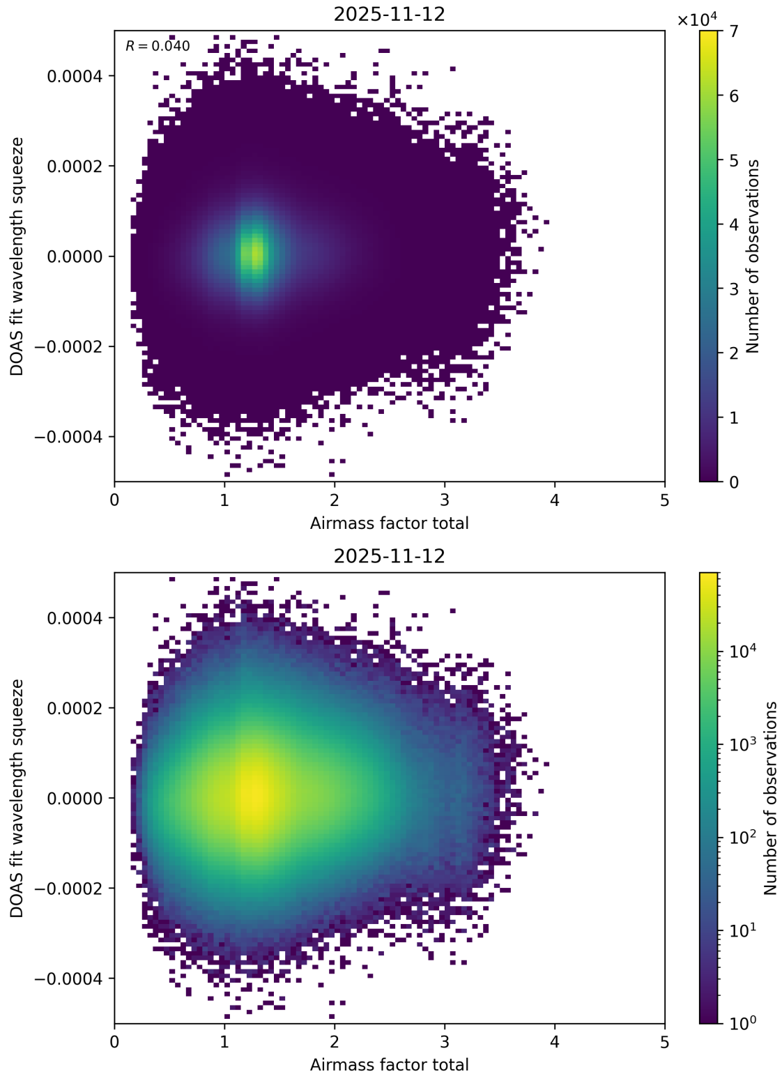
Figure 111: Scatter density plot of “Airmass factor total” against “DOAS fit wavelength squeeze” for 2025-11-12 to 2025-11-13.
