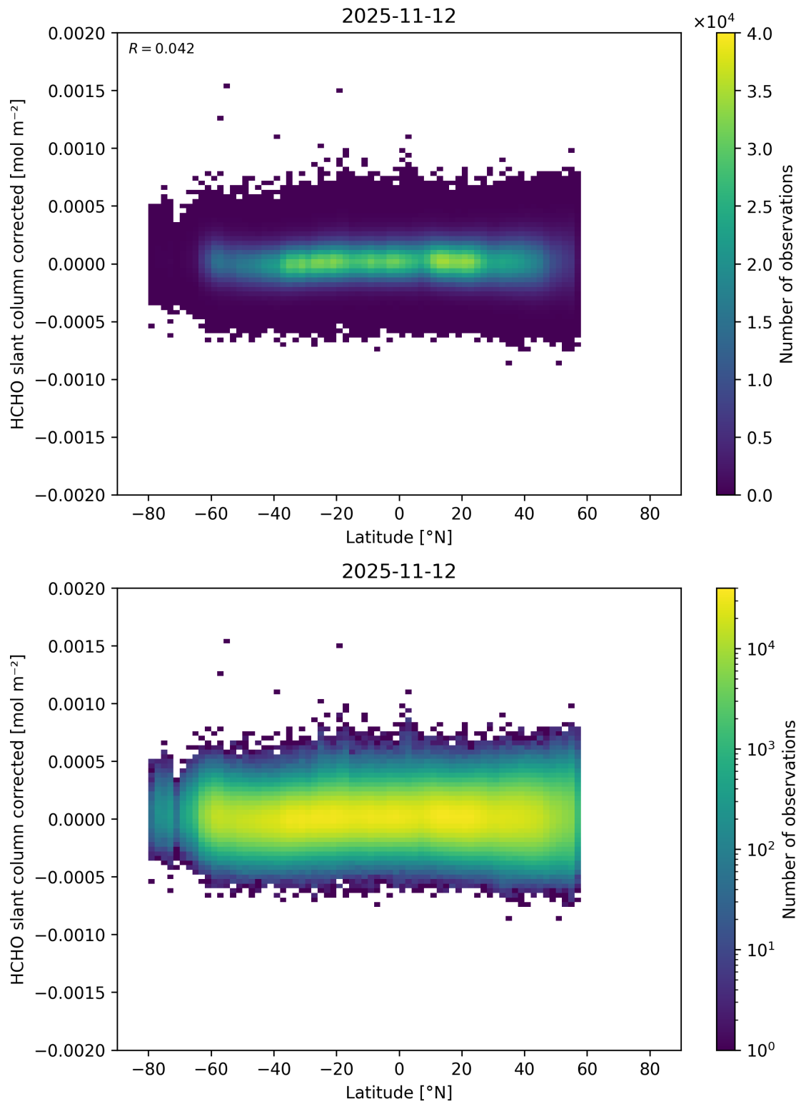
Figure 175: Scatter density plot of “Latitude” against “HCHO slant column corrected” for 2025-11-12 to 2025-11-13.
