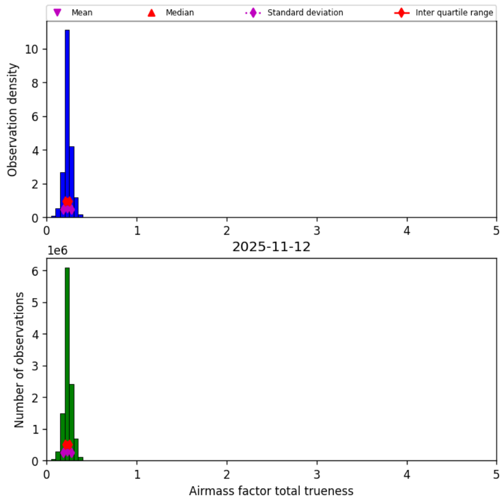
Figure 43: Histogram of “Airmass factor total trueness” for 2025-11-12 to 2025-11-13
