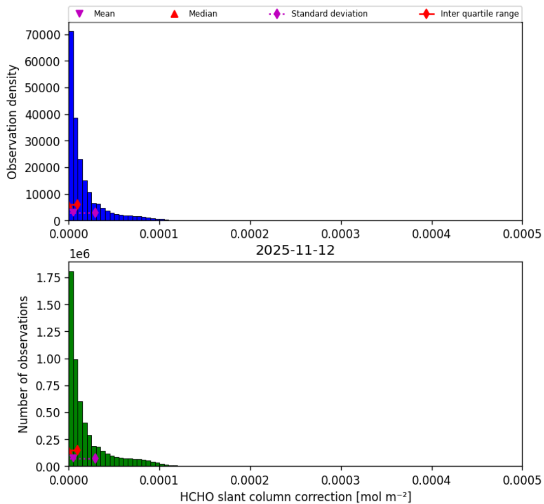
Figure 49: Histogram of “HCHO slant column correction” for 2025-11-12 to 2025-11-13
