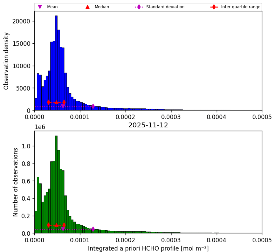
Figure 45: Histogram of “Integrated a priori HCHO profile” for 2025-11-12 to 2025-11-13
