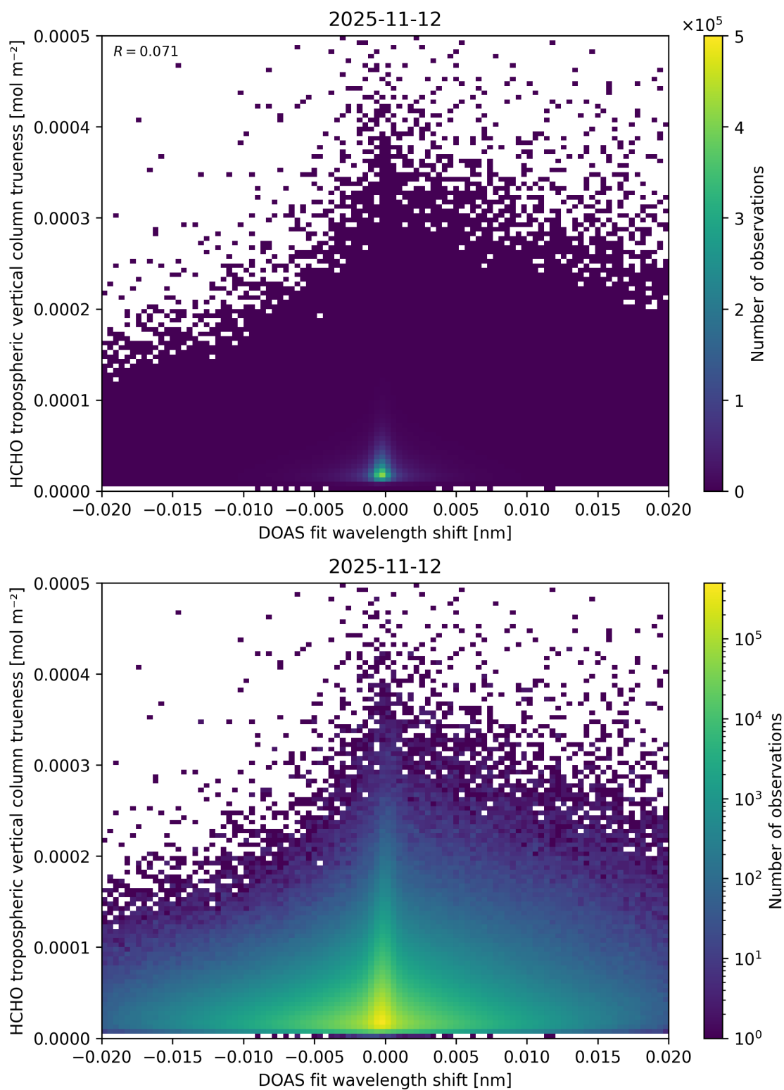
Figure 73: Scatter density plot of “DOAS fit wavelength shift” against “HCHO tropospheric vertical column trueness” for 2025-11-12 to 2025-11-13.
