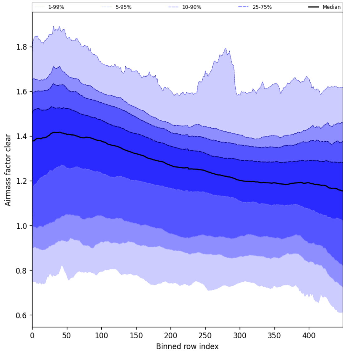
Figure 59: Along track statistics of “Airmass factor clear” for 2025-11-12 to 2025-11-13
