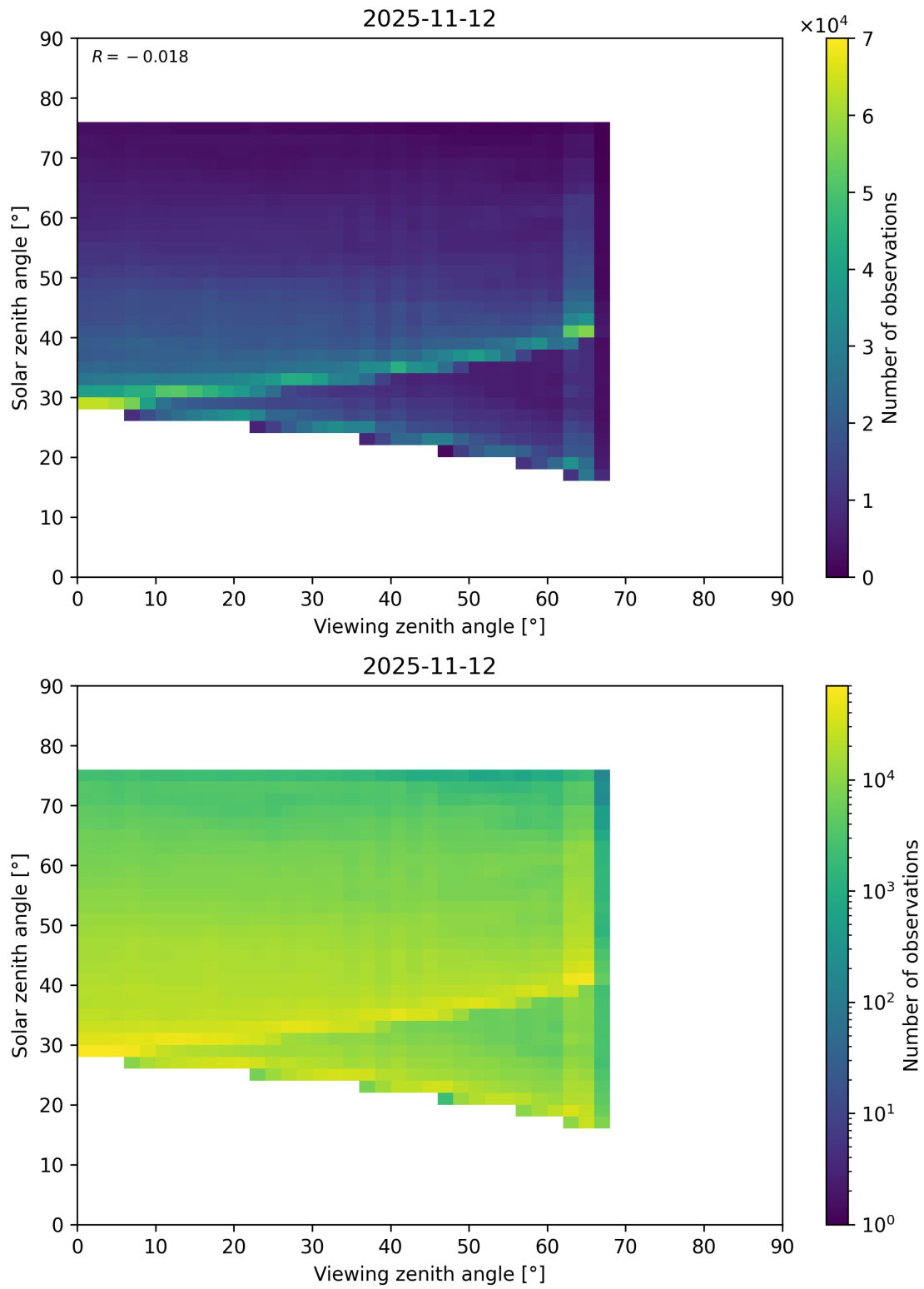
Figure 218: Scatter density plot of “Viewing zenith angle” against “Solar zenith angle” for 2025-11-12 to 2025-11-13.
