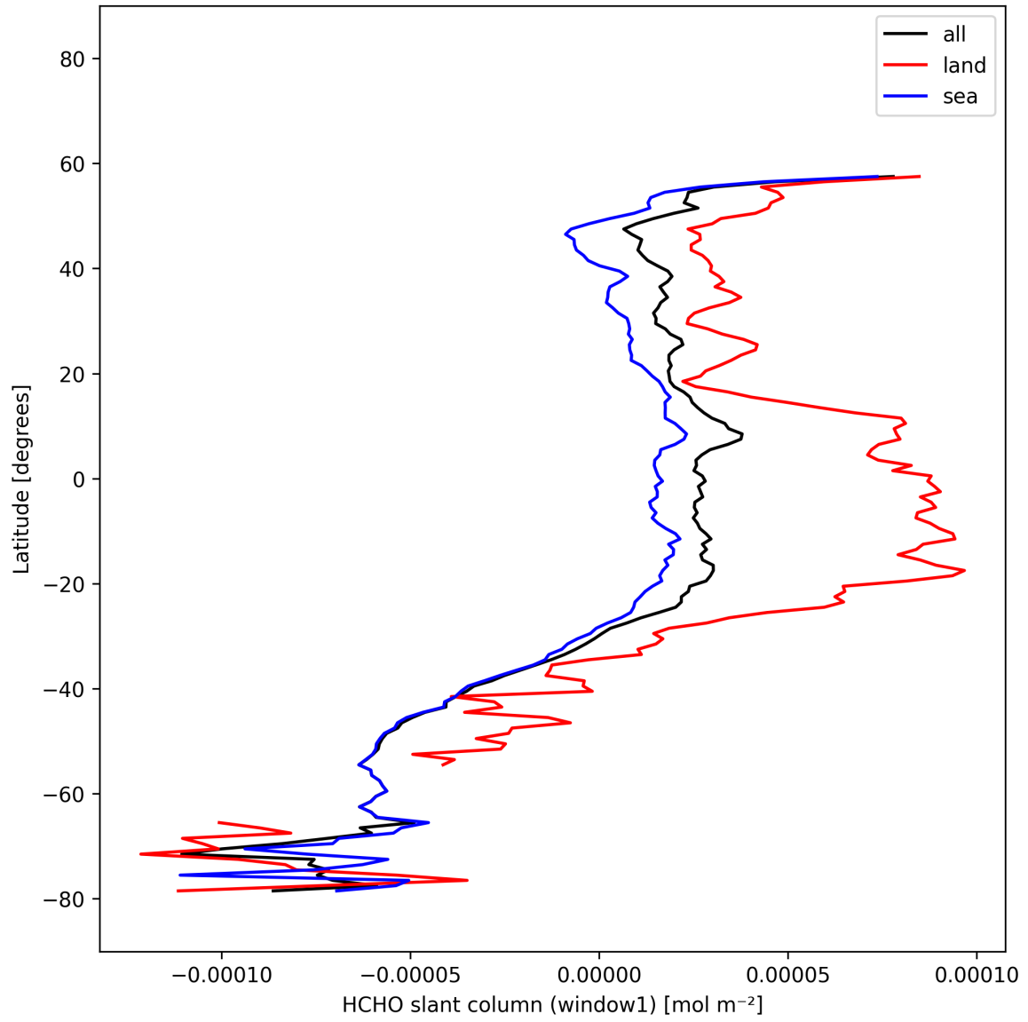
Figure 25: Zonal average of “HCHO slant column (window1)” for 2025-11-12 to 2025-11-13.
