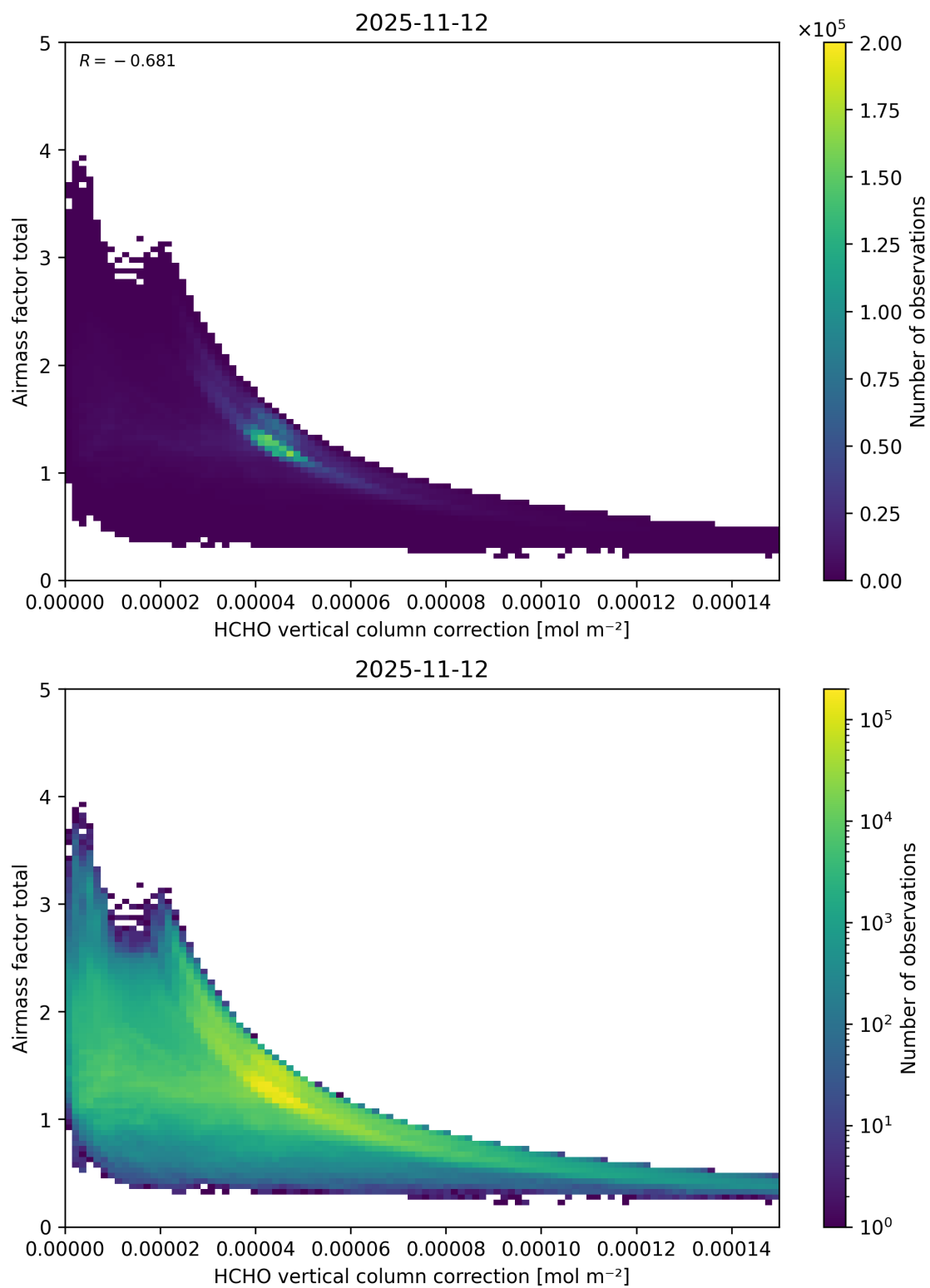
Figure 134: Scatter density plot of “HCHO vertical column correction” against “Airmass factor total” for 2025-11-12 to 2025-11-13.
