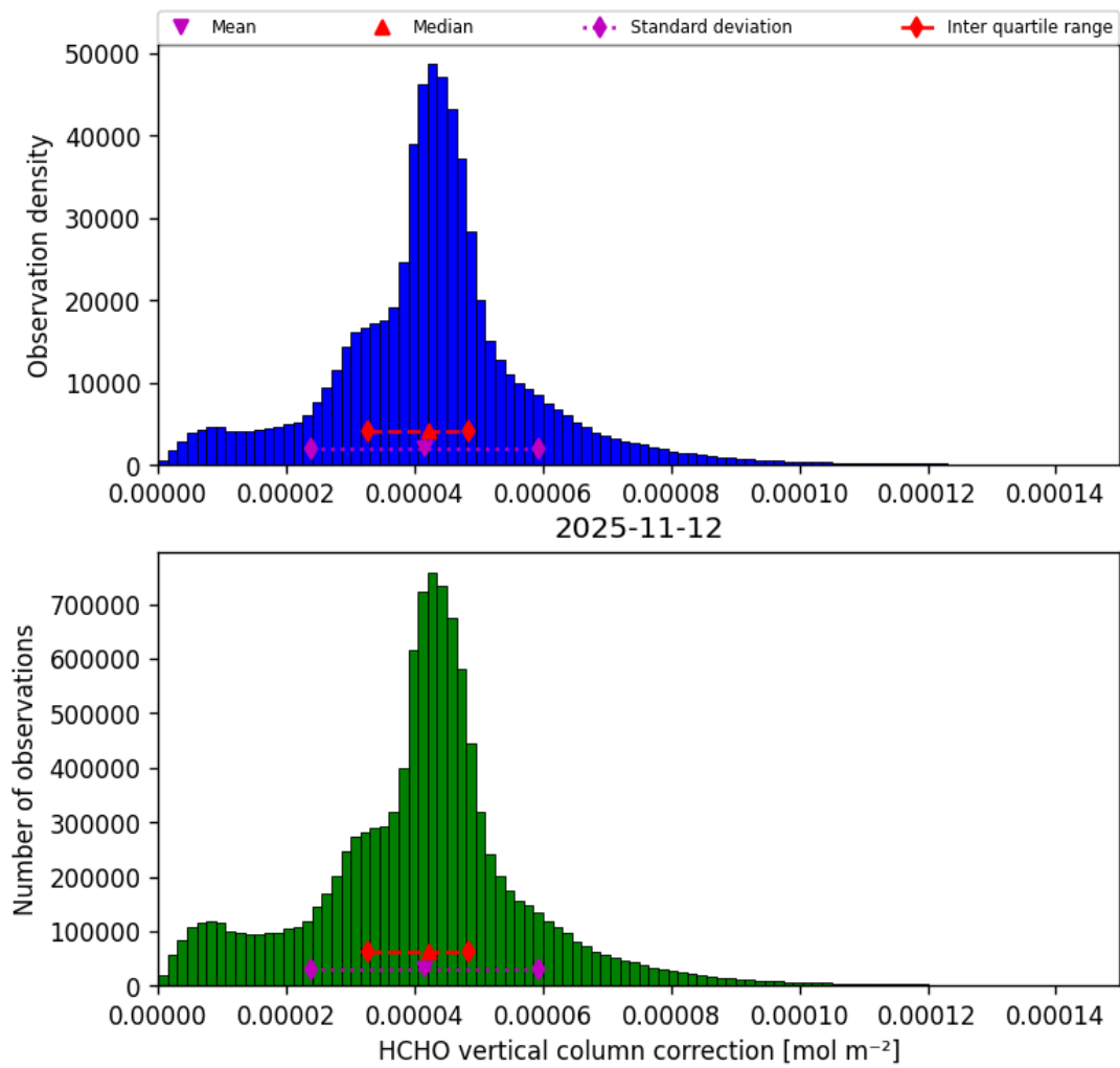
Figure 39: Histogram of “HCHO vertical column correction” for 2025-11-12 to 2025-11-13
