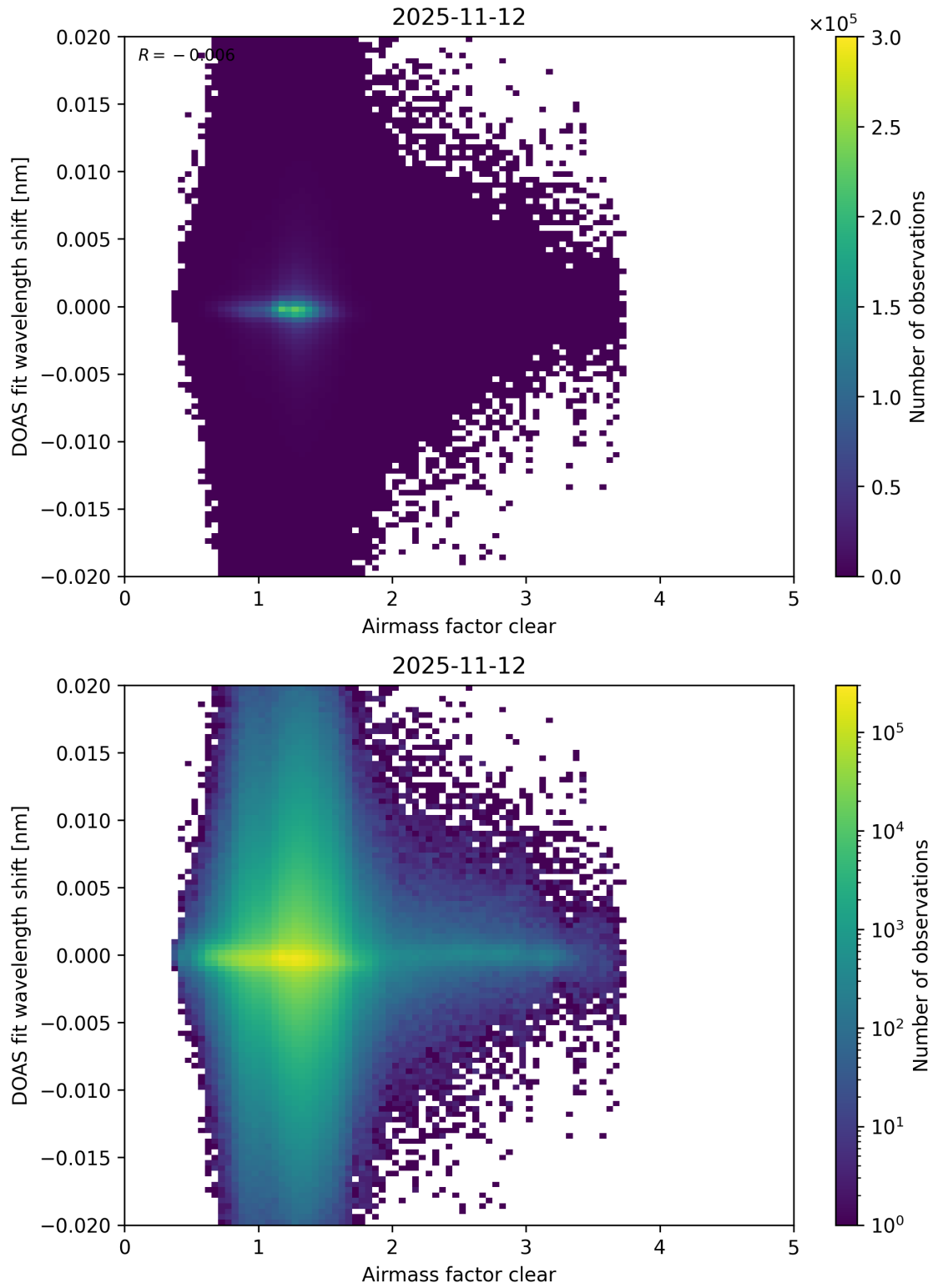
Figure 79: Scatter density plot of “Airmass factor clear” against “DOAS fit wavelength shift” for 2025-11-12 to 2025-11-13.
