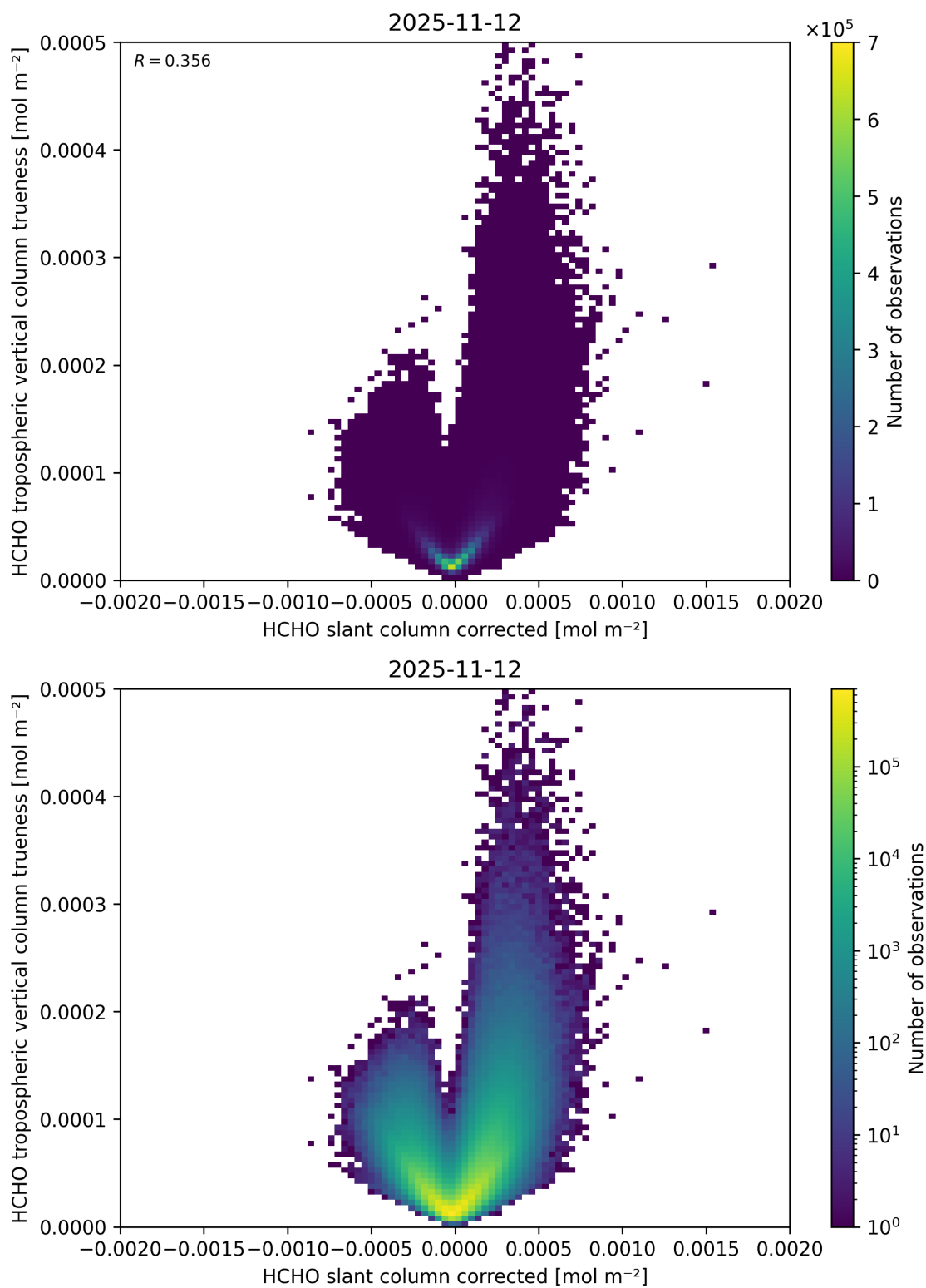
Figure 86: Scatter density plot of “HCHO slant column corrected” against “HCHO tropospheric vertical column trueness” for 2025-11-12 to 2025-11-13.
