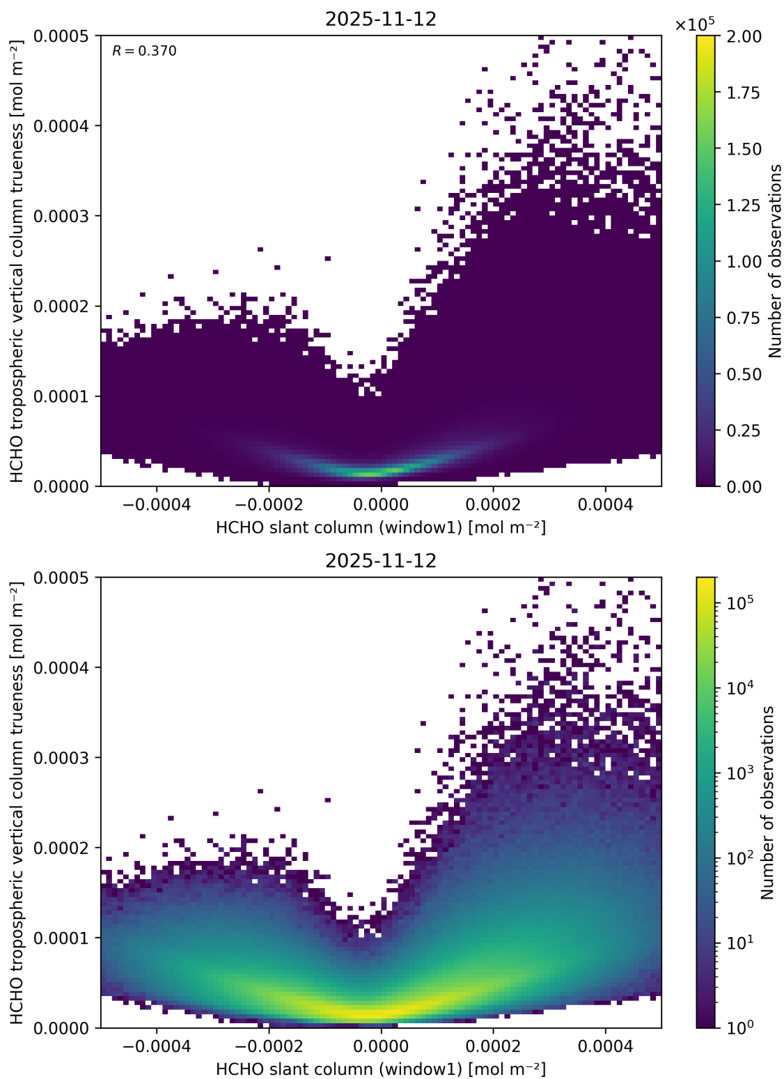
Figure 97: Scatter density plot of “HCHO slant column (window1)” against “HCHO tropospheric vertical column trueness” for 2025-11-12 to 2025-11-13.
