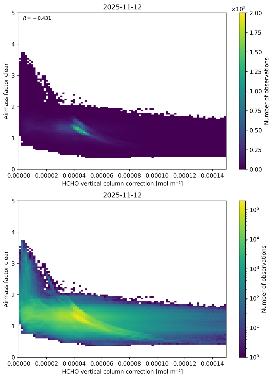
Figure 129: Scatter density plot of “HCHO vertical column correction” against “Airmass factor clear” for 2025-11-12 to 2025-11-13.
