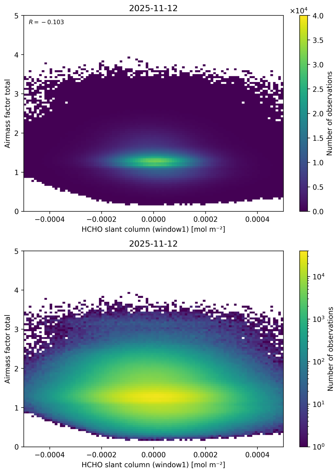
Figure 95: Scatter density plot of “HCHO slant column (window1)” against “Airmass factor total” for 2025-11-12 to 2025-11-13.
