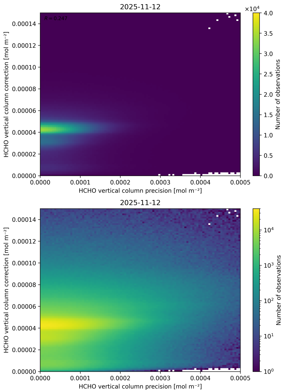
Figure 162: Scatter density plot of “HCHO vertical column precision” against “HCHO vertical column correction” for 2025-11-12 to 2025-11-13.
