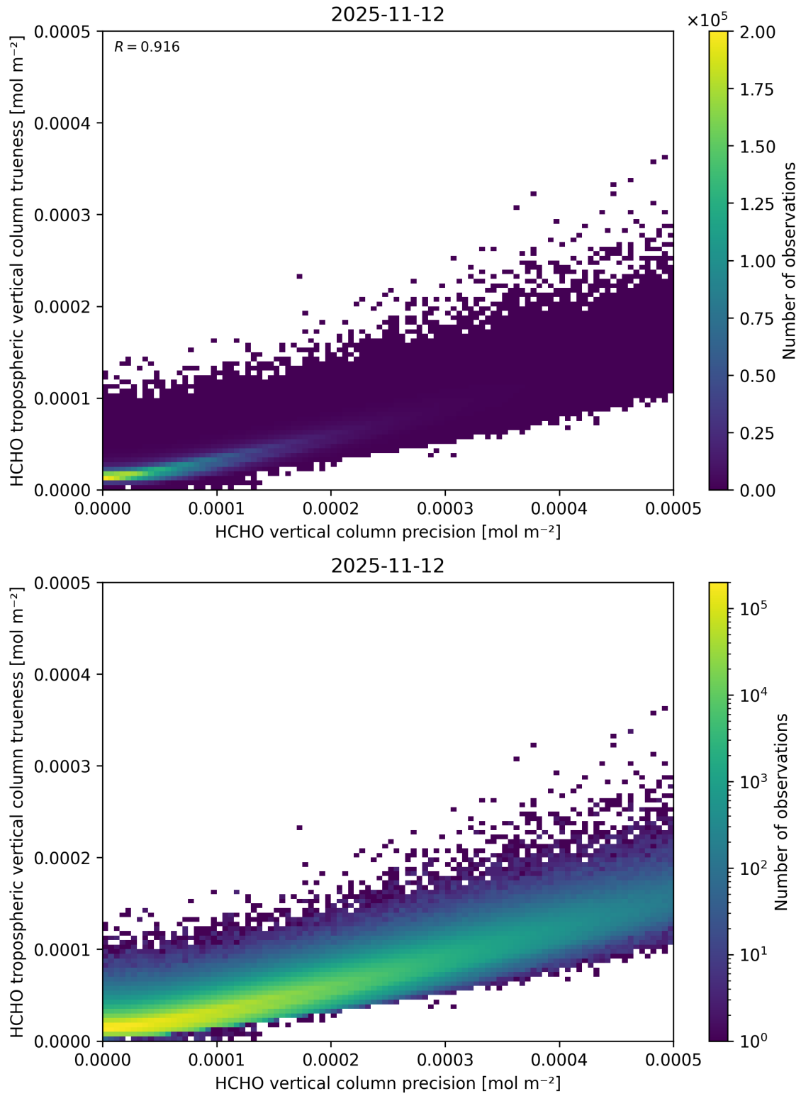
Figure 163: Scatter density plot of “HCHO vertical column precision” against “HCHO tropospheric vertical column true-ness” for 2025-11-12 to 2025-11-13.
