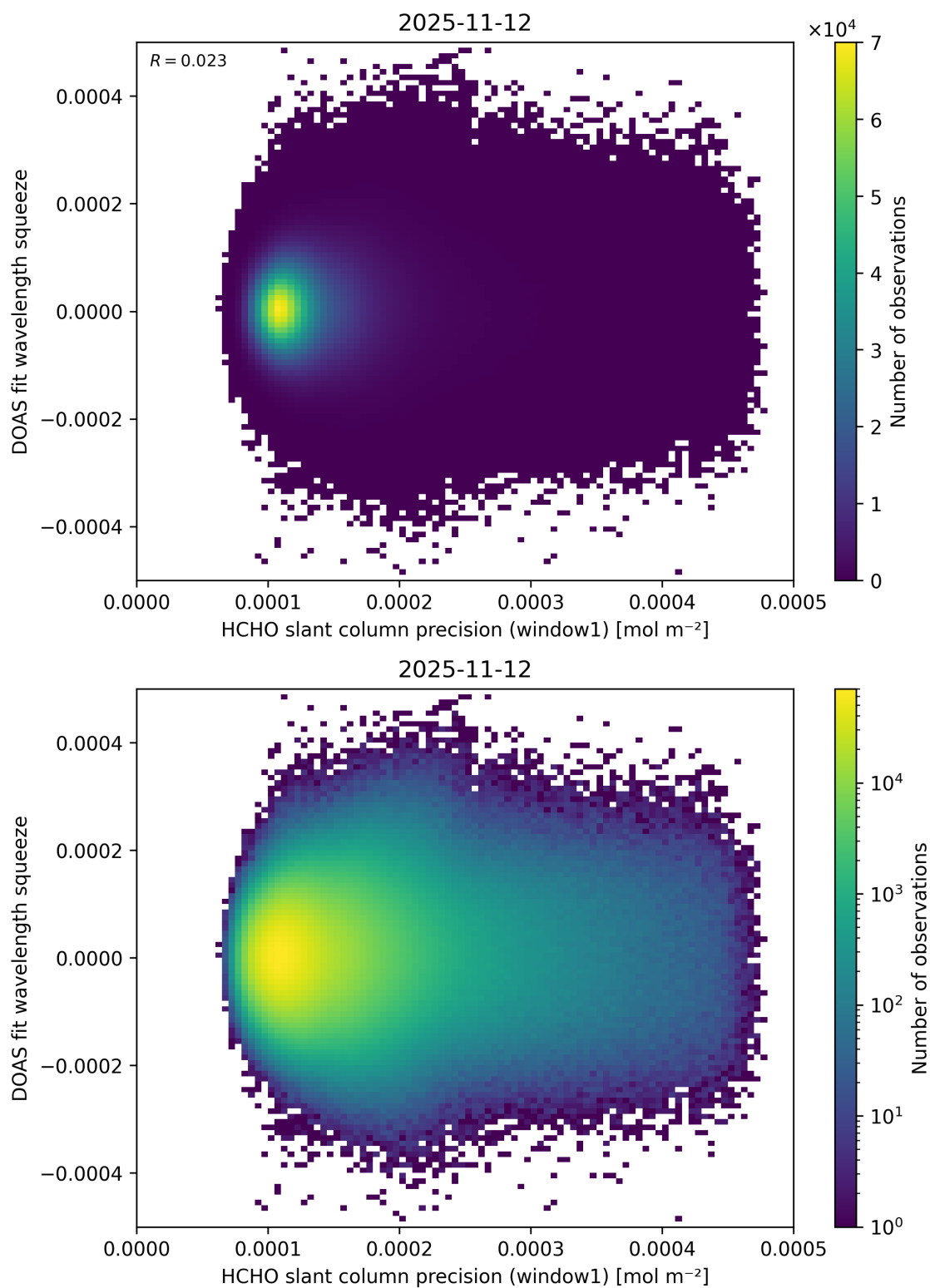
Figure 101: Scatter density plot of “HCHO slant column precision (window1)” against “DOAS fit wavelength squeeze” for 2025-11-12 to 2025-11-13.
