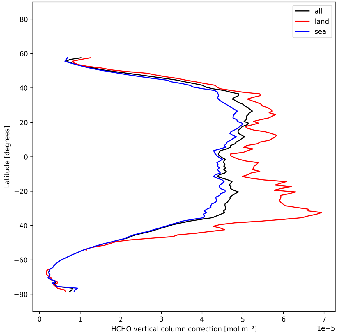
Figure 24: Zonal average of "HCHO vertical column correction" for 2025-11-12 to 2025-11-13.
