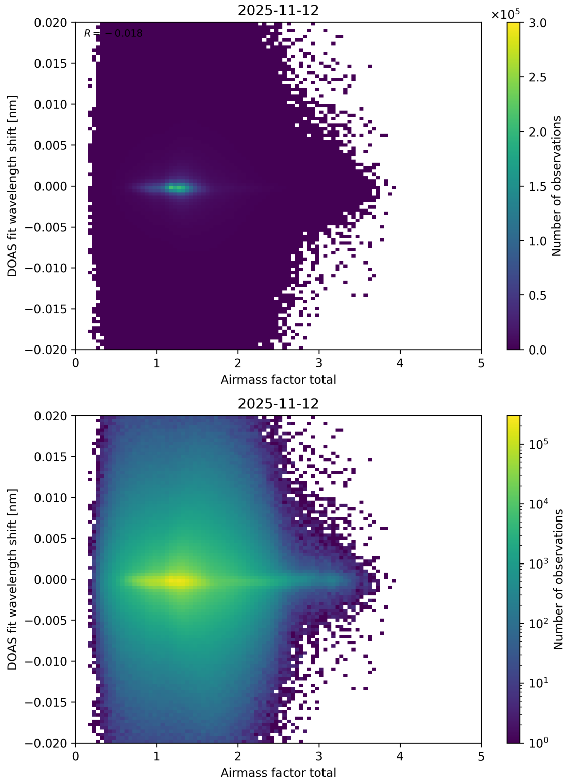
Figure 110: Scatter density plot of “Airmass factor total” against “DOAS fit wavelength shift” for 2025-11-12 to 2025-11-13.
