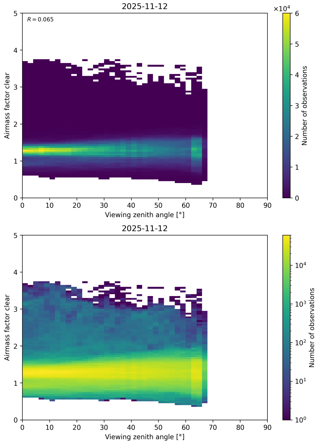
Figure 205: Scatter density plot of “Viewing zenith angle” against “Airmass factor clear” for 2025-11-12 to 2025-11-13.
