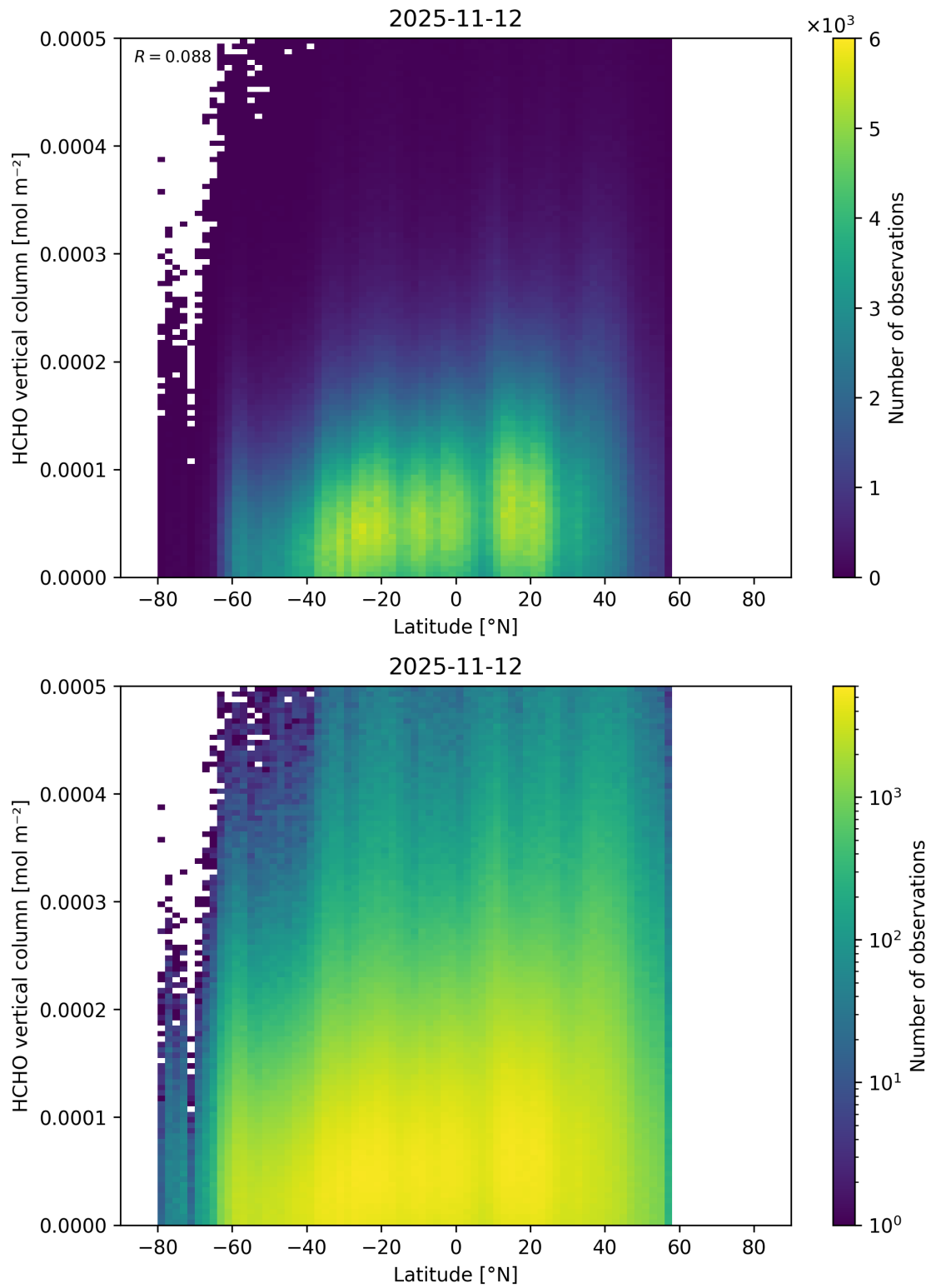
Figure 181: Scatter density plot of “Latitude” against “HCHO vertical column” for 2025-11-12 to 2025-11-13.
