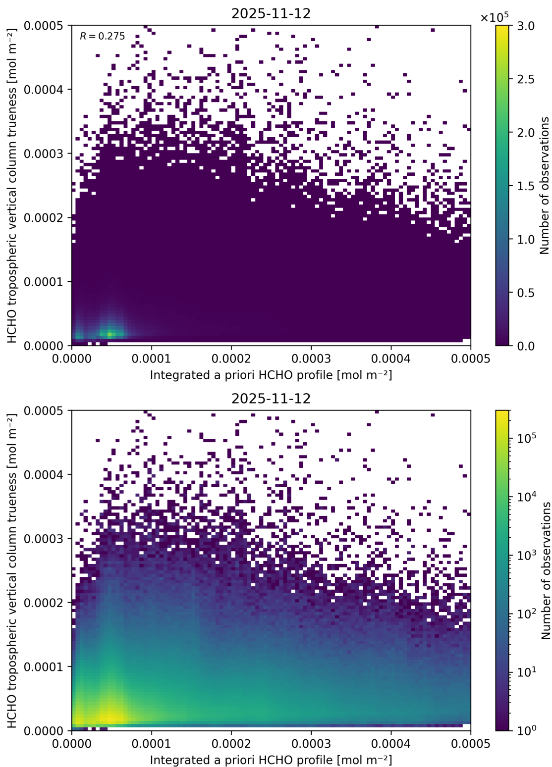
Figure 170: Scatter density plot of “Integrated a priori HCHO profile” against “HCHO tropospheric vertical column trueness” for 2025-11-12 to 2025-11-13.
