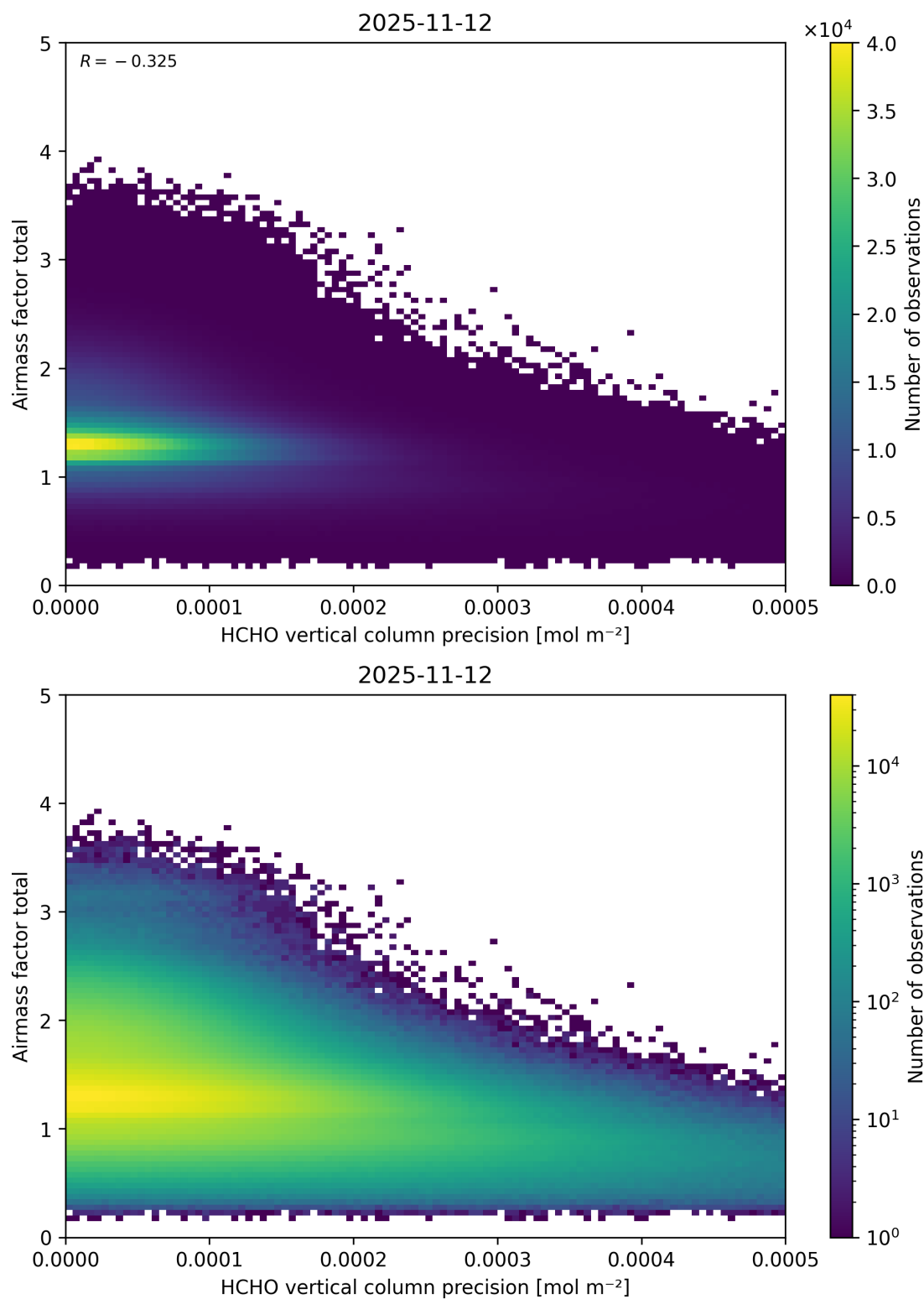
Figure 160: Scatter density plot of “HCHO vertical column precision” against “Airmass factor total” for 2025-11-12 to 2025-11-13.
