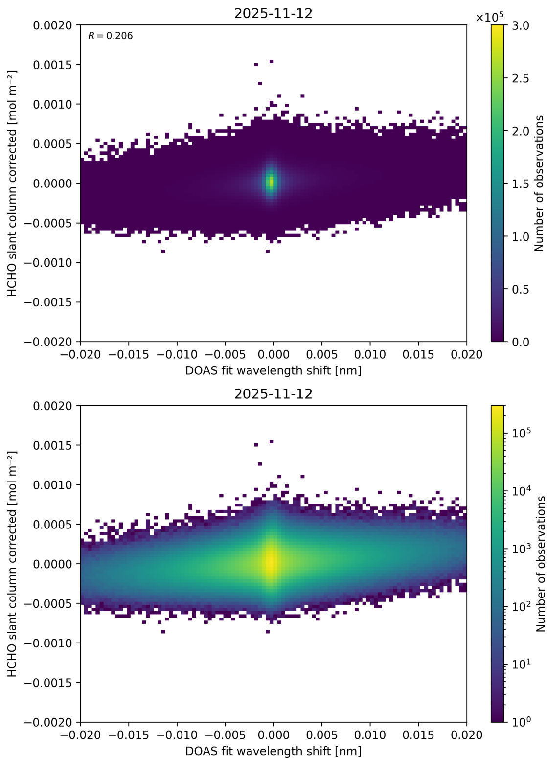
Figure 71: Scatter density plot of “DOAS fit wavelength shift” against “HCHO slant column corrected” for 2025-11-12 to 2025-11-13.
