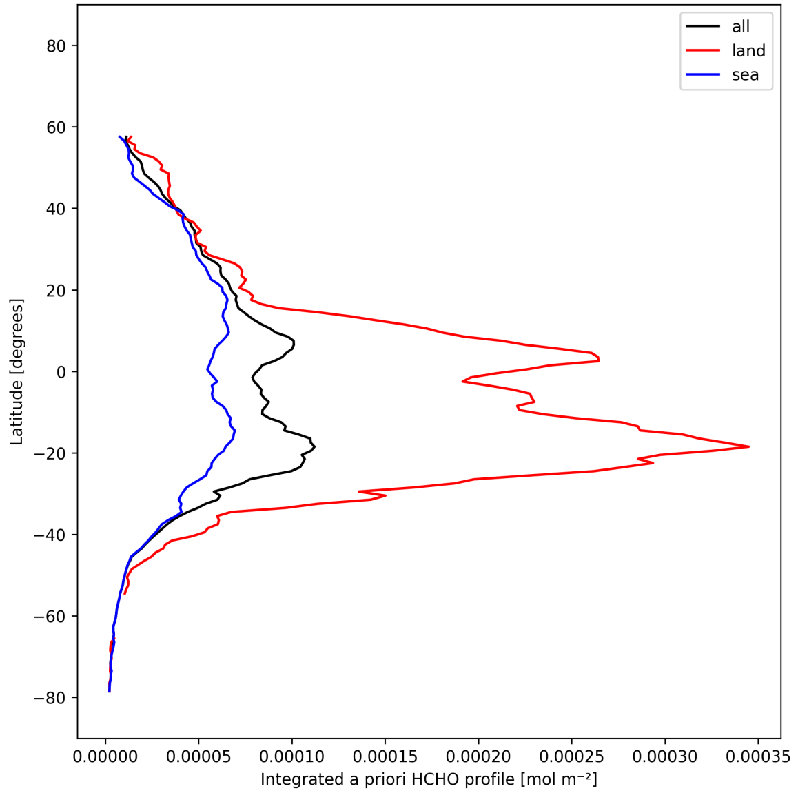
Figure 30: Zonal average of “Integrated a priori HCHO profile” for 2025-11-12 to 2025-11-13.
