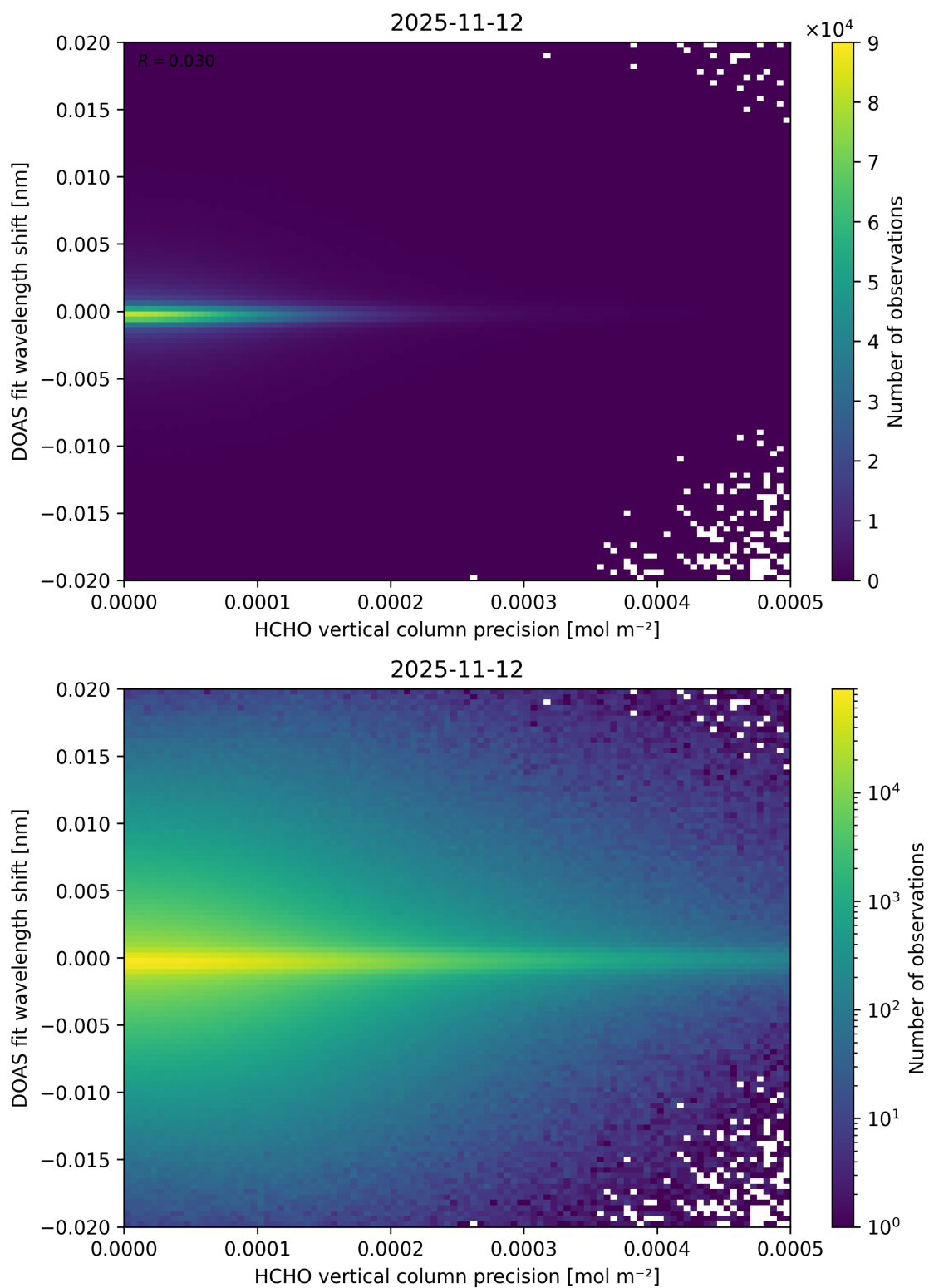
Figure 153: Scatter density plot of “HCHO vertical column precision” against “DOAS fit wavelength shift” for 2025-11-12 to 2025-11-13.
