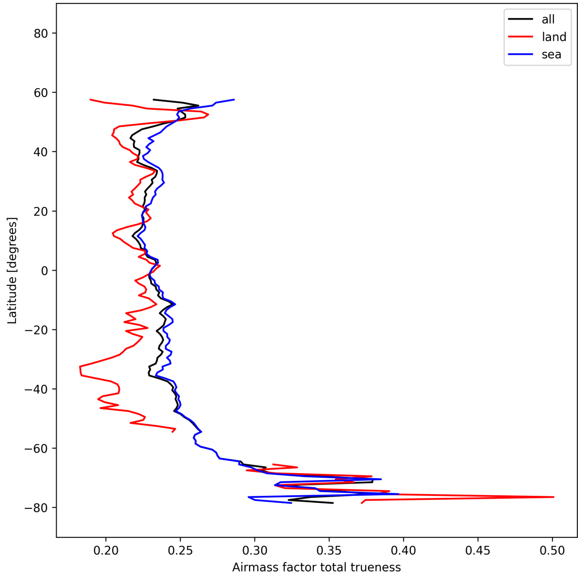
Figure 28: Zonal average of “Airmass factor total truiness” for 2025-11-12 to 2025-11-13.
