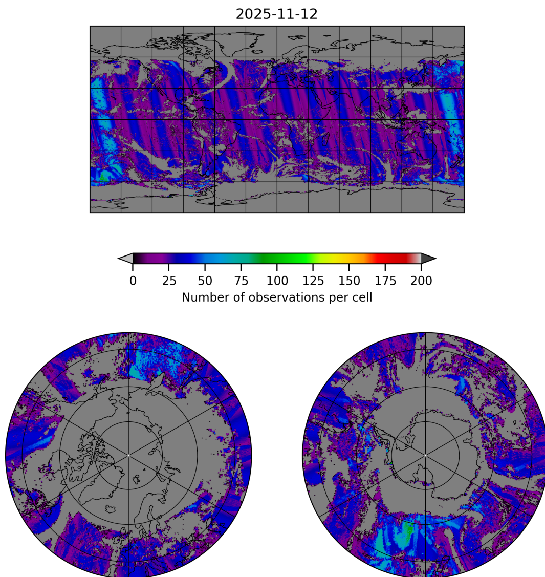
Figure 20: Map of the number of observations for 2025-11-12 to 2025-11-13
