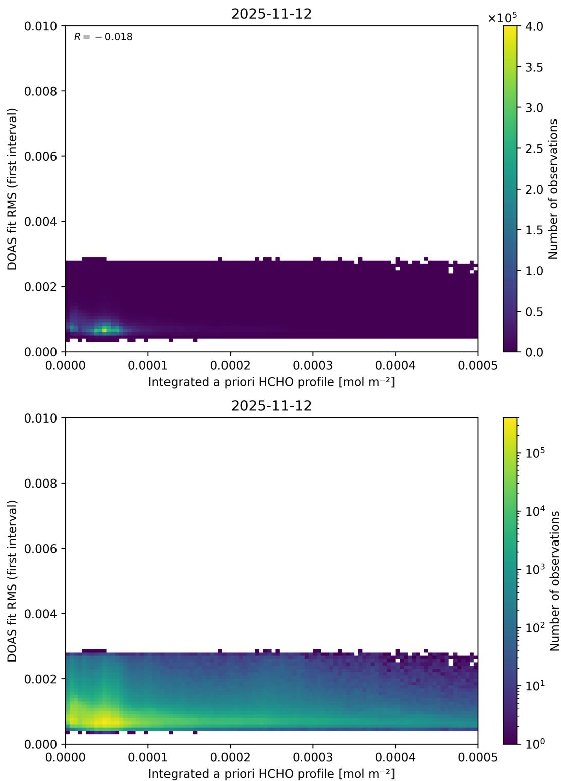
Figure 165: Scatter density plot of “Integrated a priori HCHO profile” against “DOAS fit RMS (first interval)” for 2025-11-12 to 2025-11-13.
