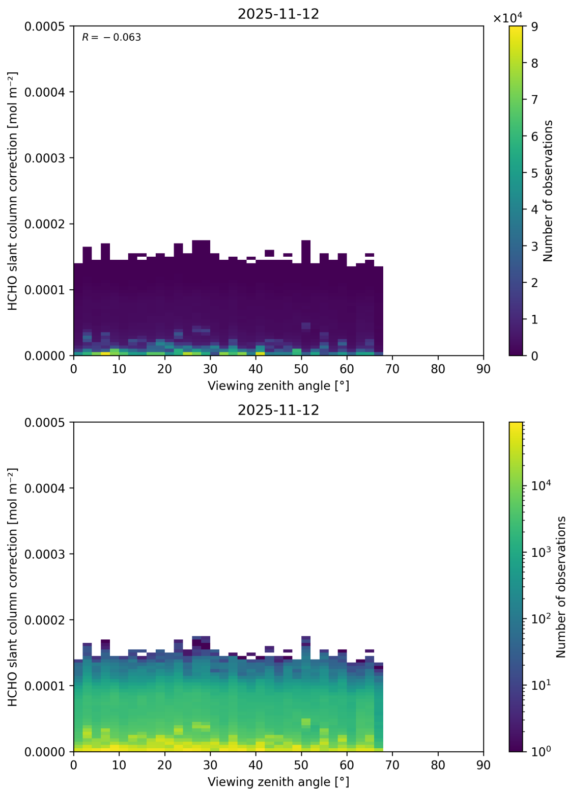
Figure 207: Scatter density plot of “Viewing zenith angle” against “HCHO slant column correction” for 2025-11-12 to 2025-11-13.
