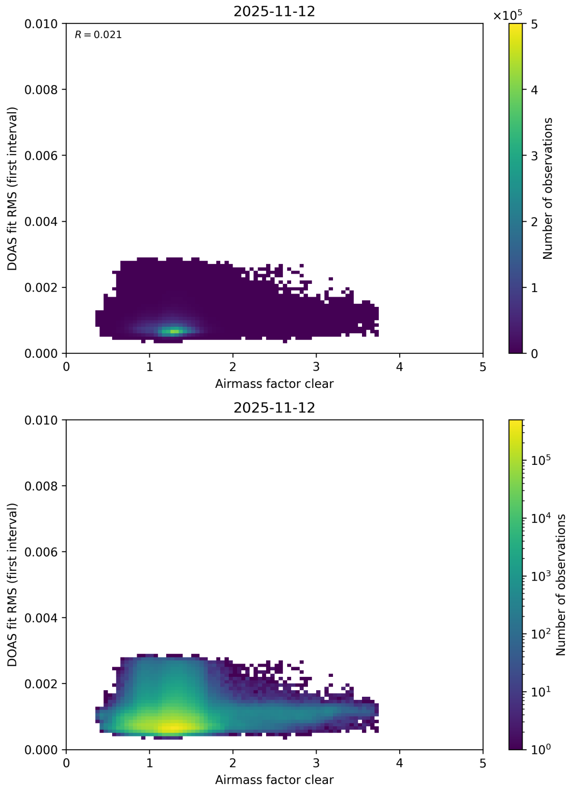
Figure 78: Scatter density plot of “Airmass factor clear” against “DOAS fit RMS (first interval)” for 2025-11-12 to 2025-11-13.
