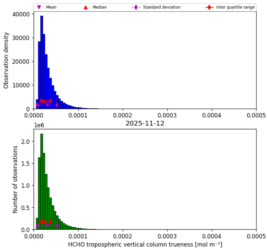
Figure 50: Histogram of “HCHO tropospheric vertical column trueness” for 2025-11-12 to 2025-11-13
