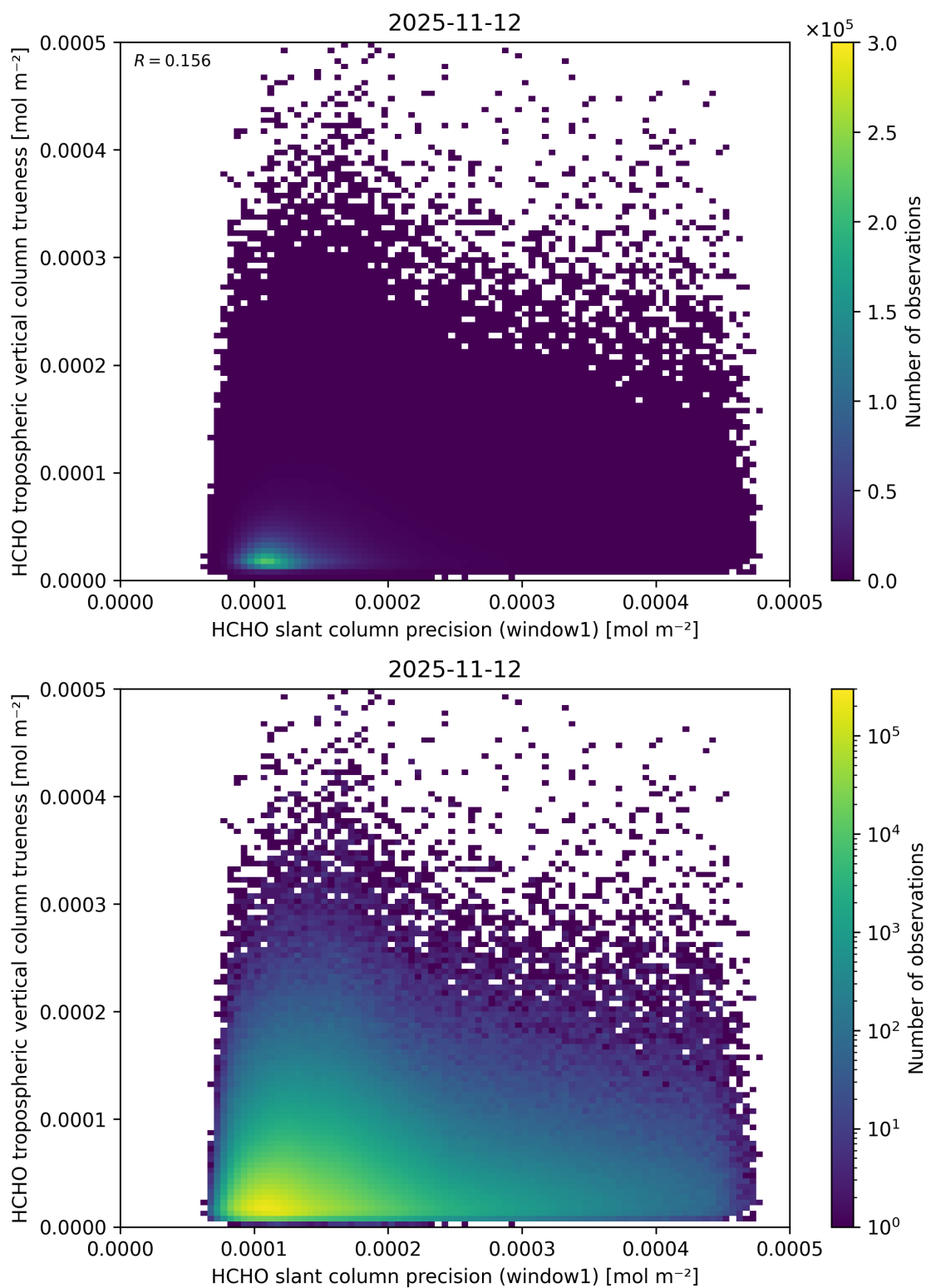
Figure 107: Scatter density plot of “HCHO slant column precision (window1)” against “HCHO tropospheric vertical column trueness” for 2025-11-12 to 2025-11-13.
