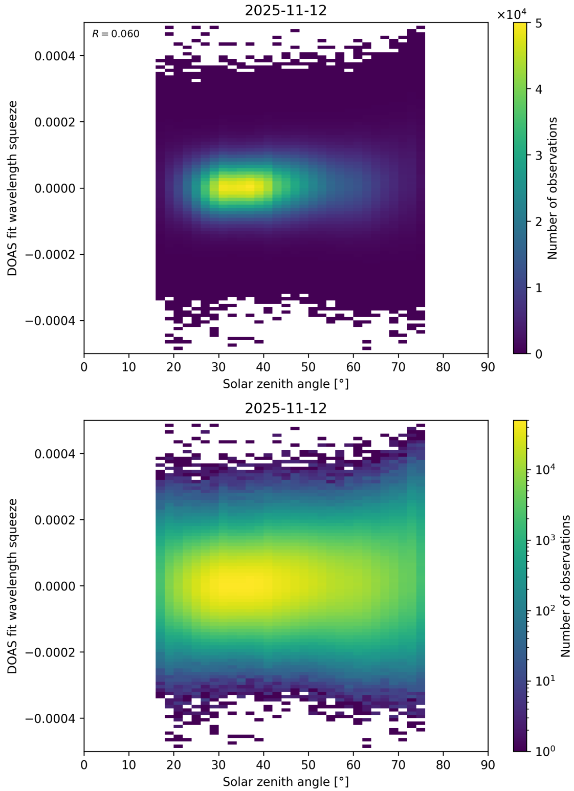
Figure 188: Scatter density plot of “Solar zenith angle” against “DOAS fit wavelength squeeze” for 2025-11-12 to 2025-11-13.
