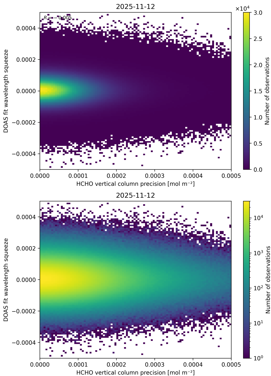
Figure 154: Scatter density plot of “HCHO vertical column precision” against “DOAS fit wavelength squeeze” for 2025-11-12 to 2025-11-13.
