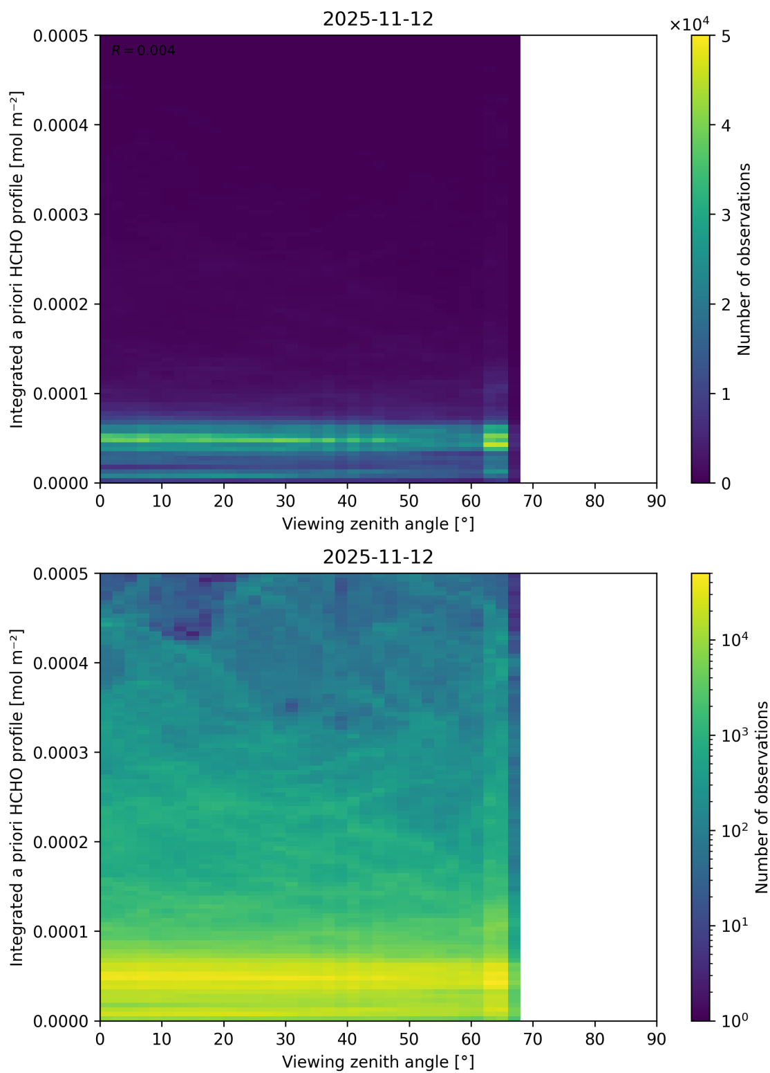
Figure 216: Scatter density plot of “Viewing zenith angle” against “Integrated a priori HCHO profile” for 2025-11-12 to 2025-11-13.
