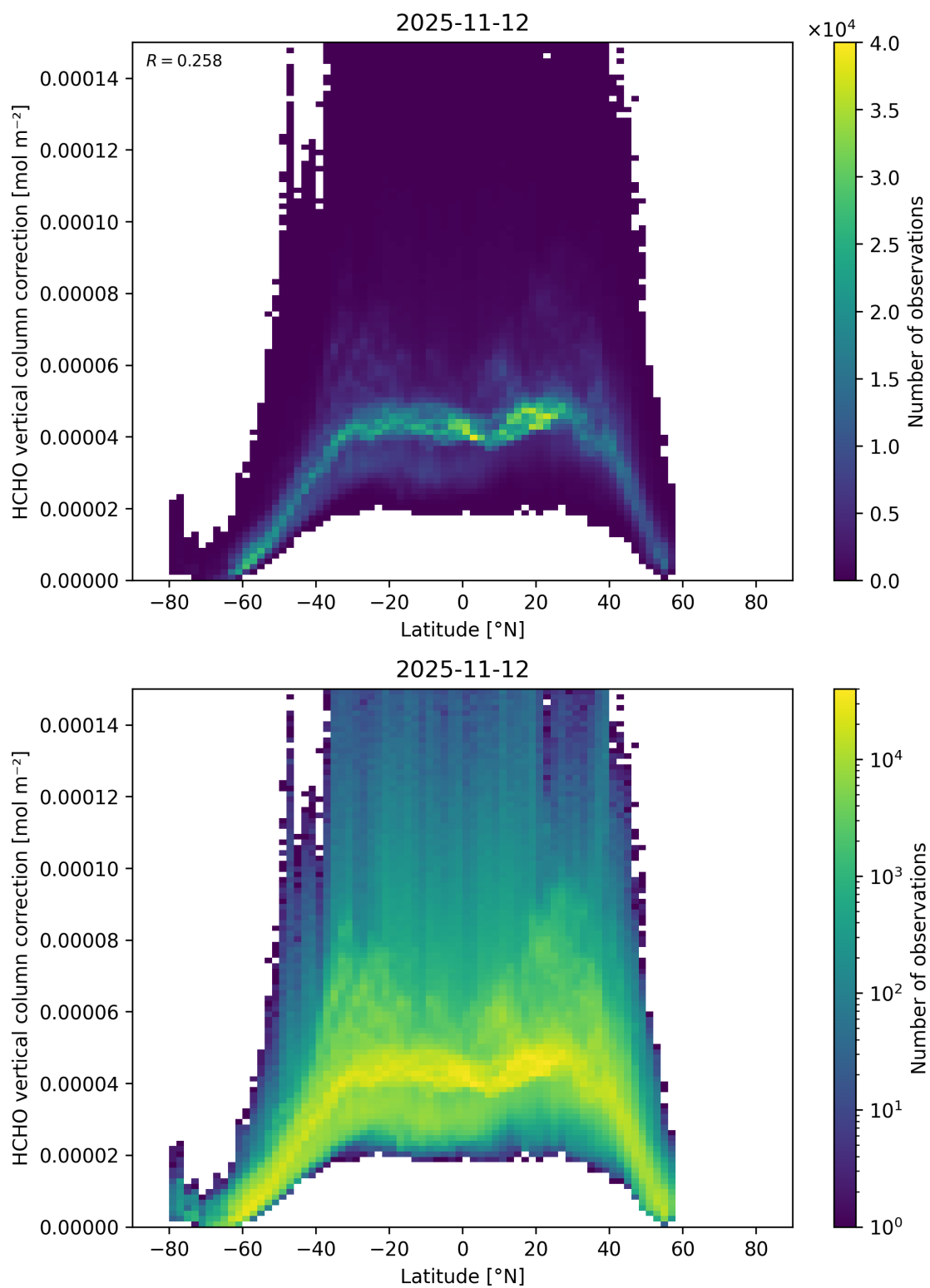
Figure 182: Scatter density plot of “Latitude” against “HCHO vertical column correction” for 2025-11-12 to 2025-11-13.
