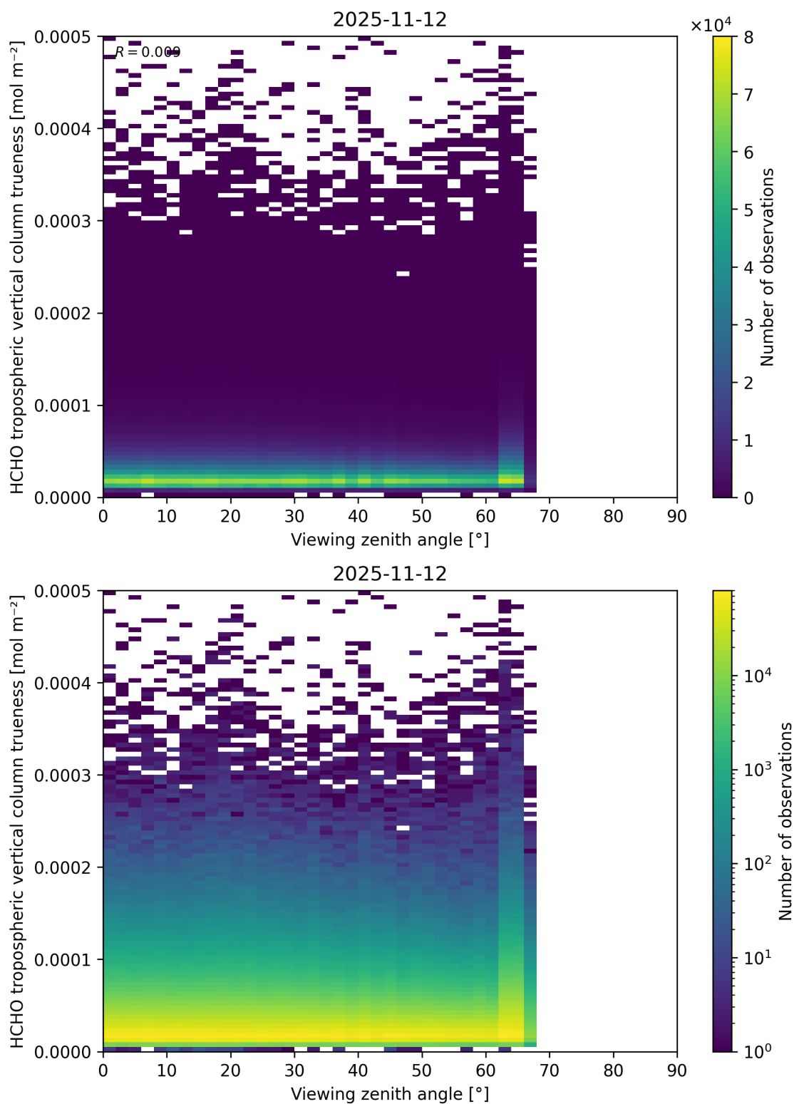
Figure 215: Scatter density plot of “Viewing zenith angle” against “HCHO tropospheric vertical column trueeness” for 2025-11-12 to 2025-11-13.
