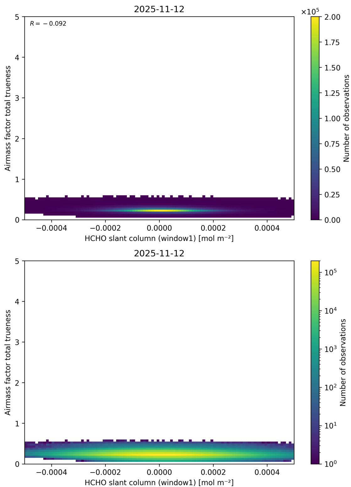
Figure 96: Scatter density plot of “HCHO slant column (window1)” against “Airmass factor total trueneess” for 2025-11-12 to 2025-11-13.
