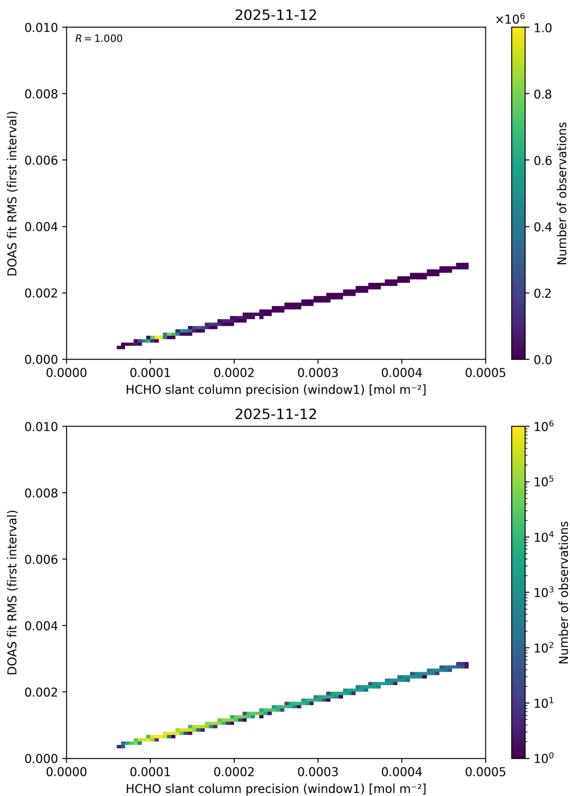
Figure 99: Scatter density plot of “HCHO slant column precision (window1)” against “DOAS fit RMS (first interval)” for 2025-11-12 to 2025-11-13.
