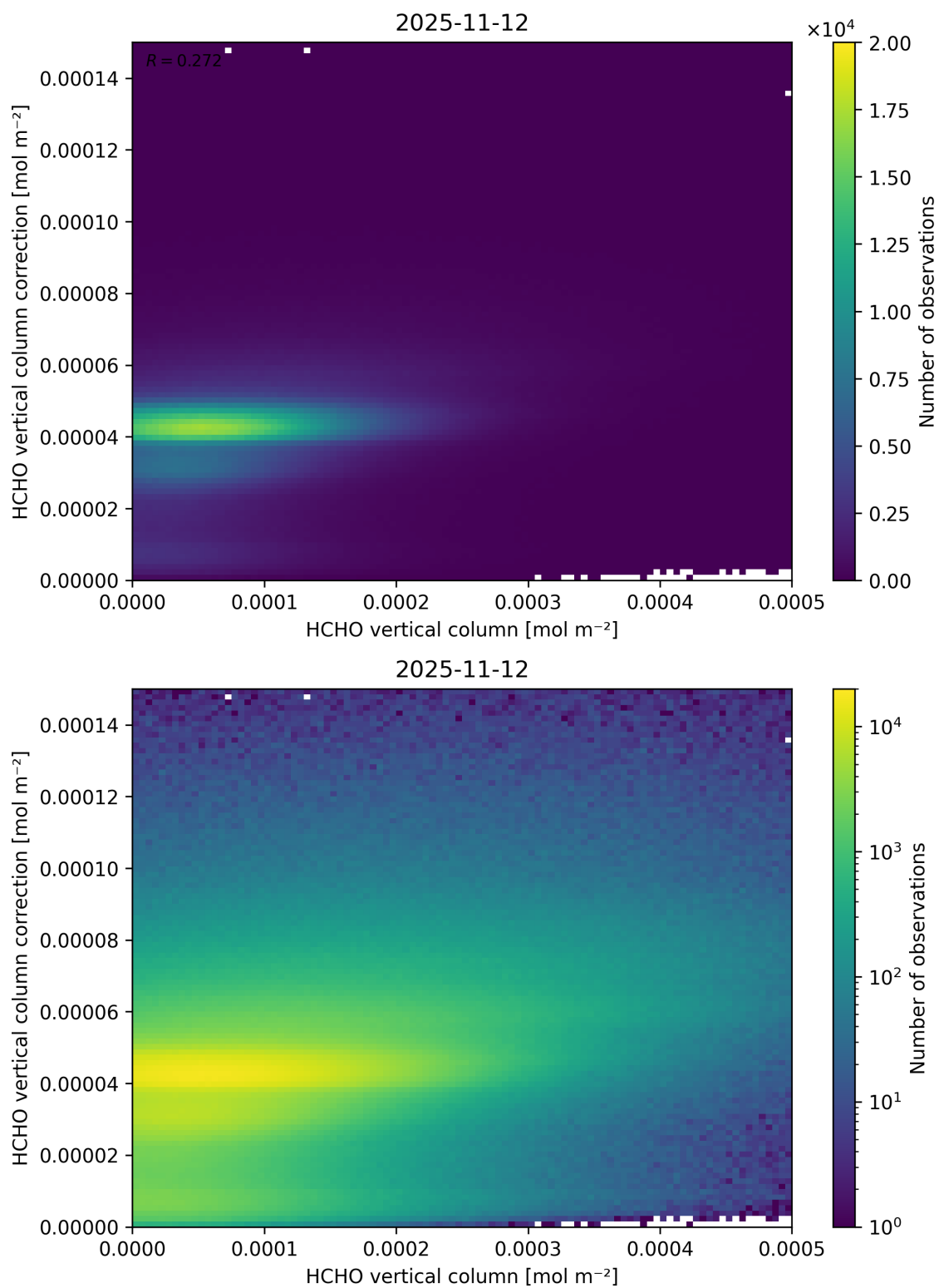
Figure 148: Scatter density plot of “HCHO vertical column” against “HCHO vertical column correction” for 2025-11-12 to 2025-11-13.
