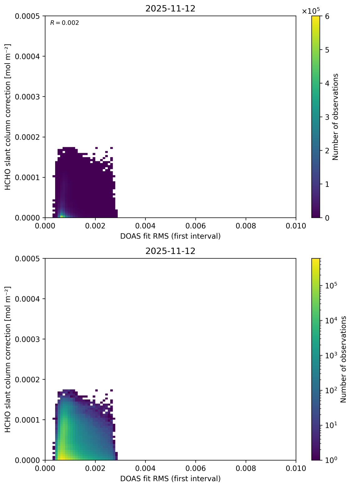
Figure 67: Scatter density plot of “DOAS fit RMS (first interval)” against “HCHO slant column correction” for 2025-11-12 to 2025-11-13.
