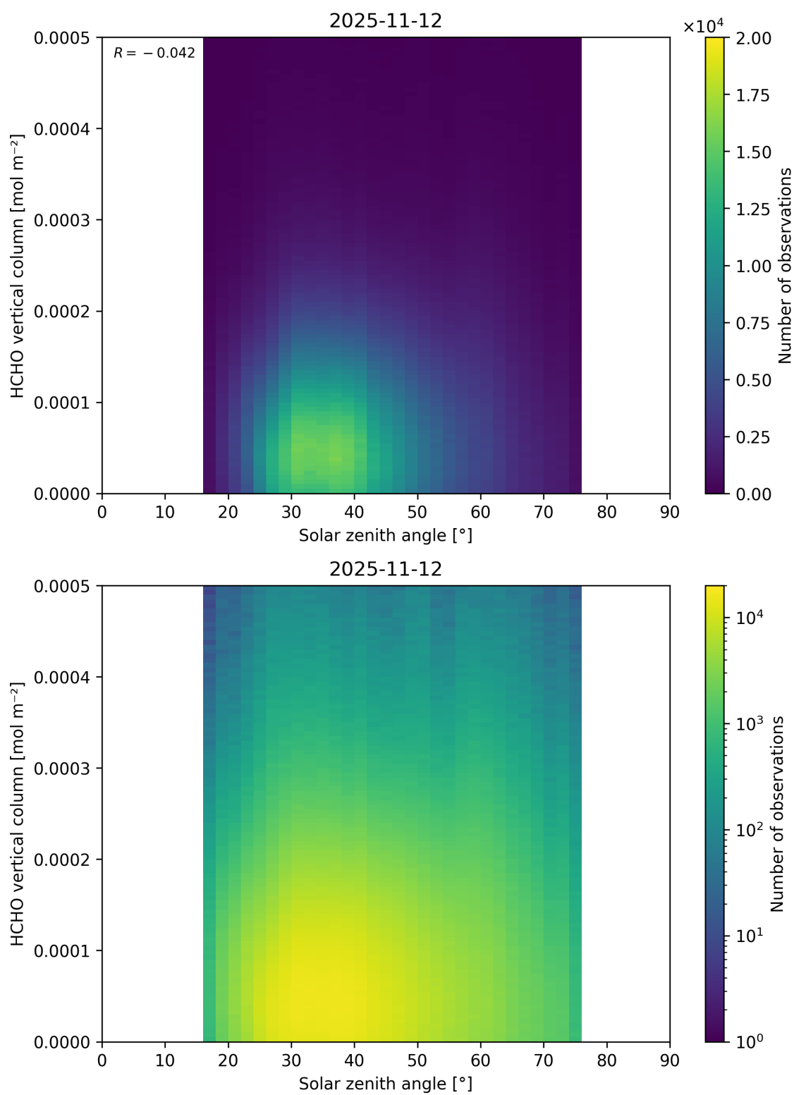
Figure 196: Scatter density plot of “Solar zenith angle” against “HCHO vertical column” for 2025-11-12 to 2025-11-13.
