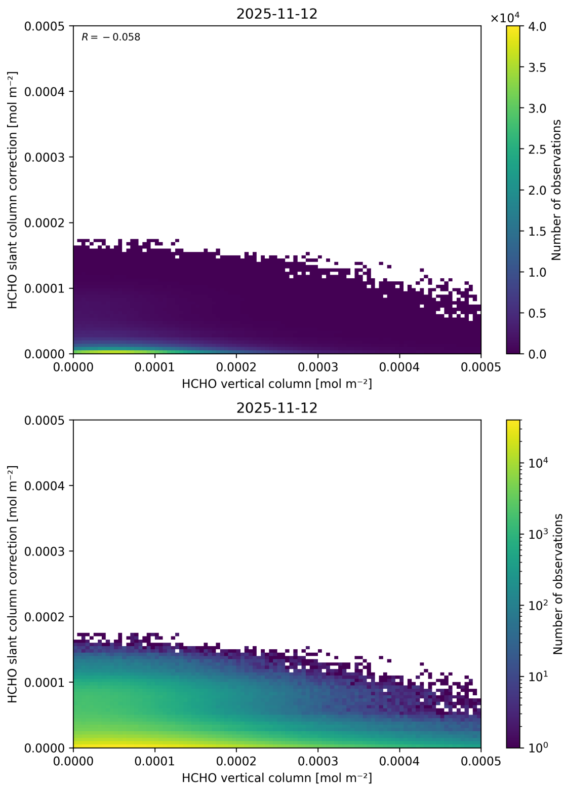
Figure 143: Scatter density plot of “HCHO vertical column” against “HCHO slant column correction” for 2025-11-12 to 2025-11-13.
