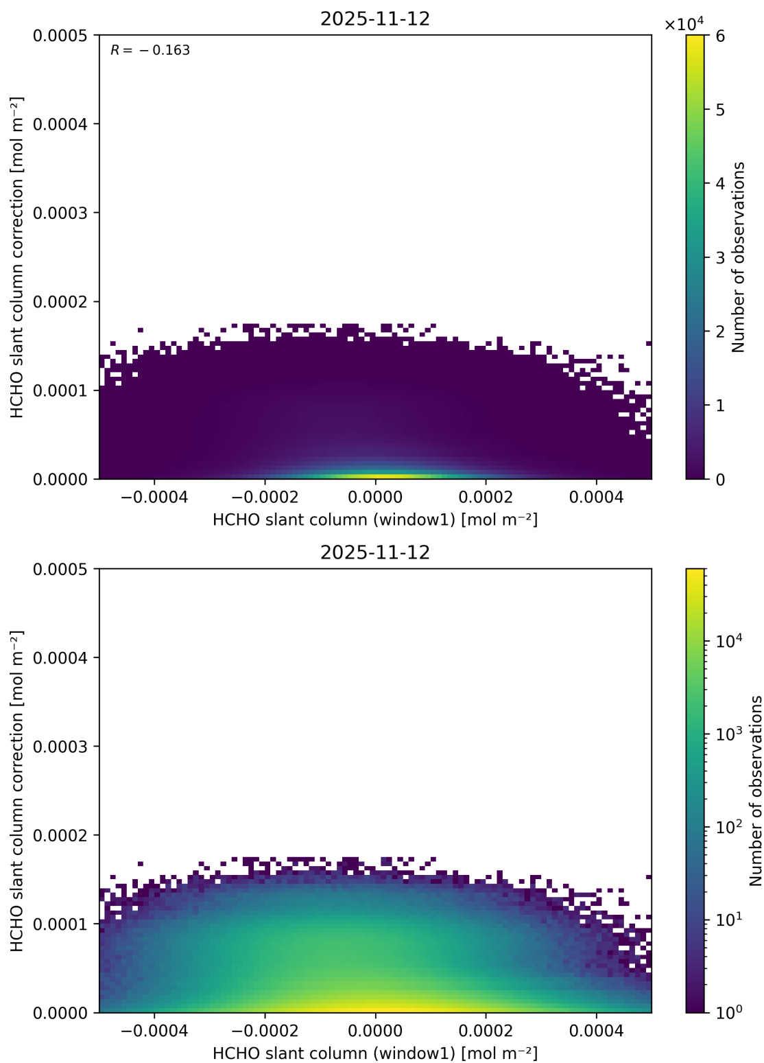
Figure 93: Scatter density plot of “HCHO slant column (window1)” against “HCHO slant column correction” for 2025-11-12 to 2025-11-13.
