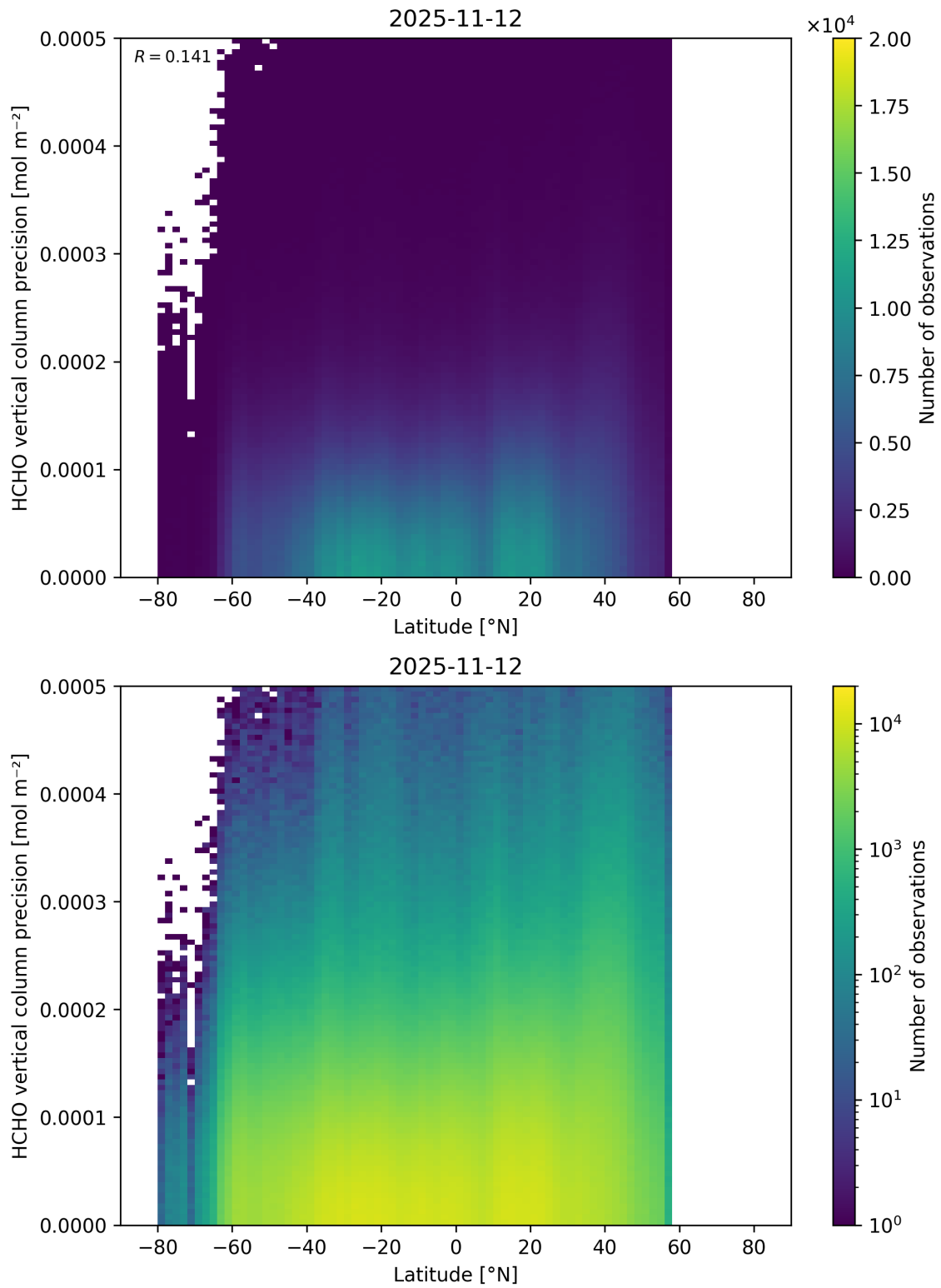
Figure 183: Scatter density plot of “Latitude” against “HCHO vertical column precision” for 2025-11-12 to 2025-11-13.
