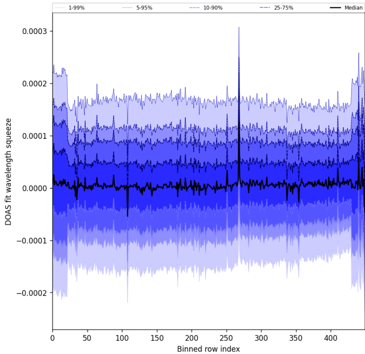
Figure 62: Along track statistics of “DOAS fit wavelength squeeze” for 2025-11-12 to 2025-11-13
