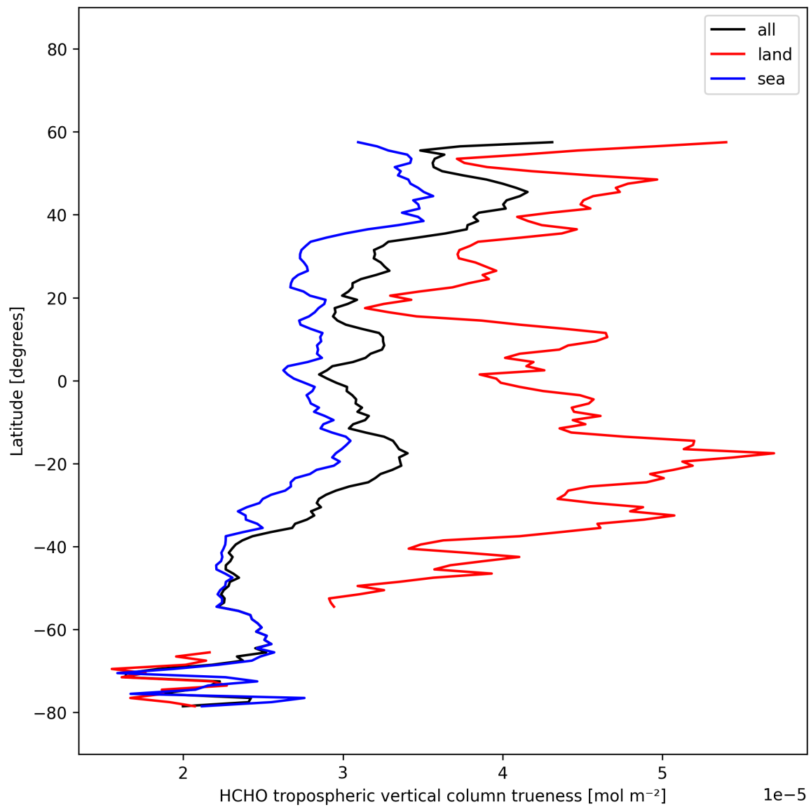
Figure 35: Zonal average of “HCHO tropospheric vertical column trueness” for 2025-11-12 to 2025-11-13.
