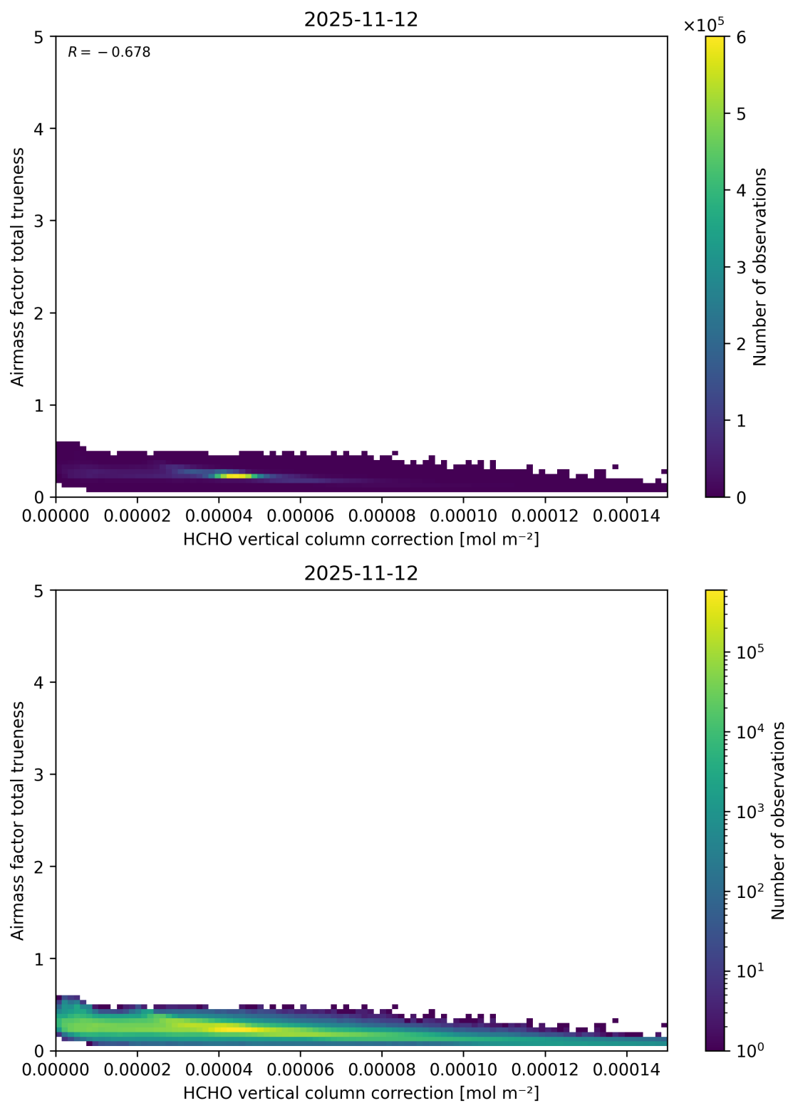
Figure 135: Scatter density plot of “HCHO vertical column correction” against “Airmass factor total trueneess” for 2025-11-12 to 2025-11-13.
