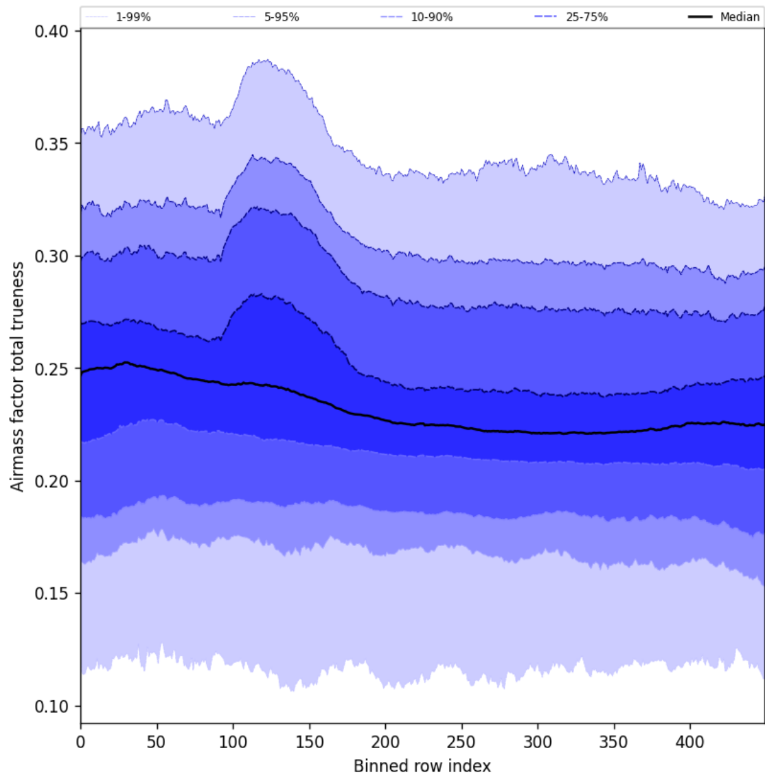
Figure 58: Along track statistics of “Airmass factor total trueness” for 2025-11-12 to 2025-11-13
