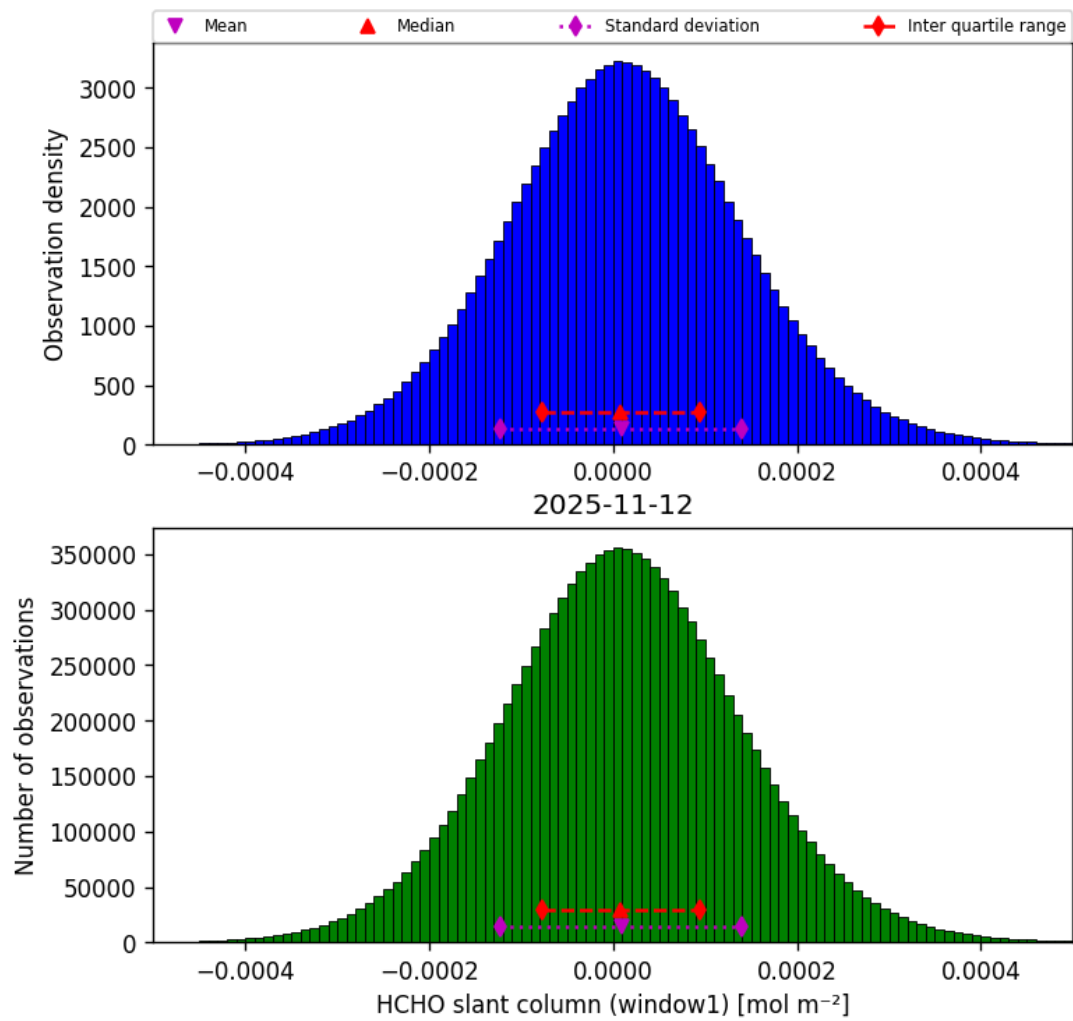
Figure 40: Histogram of “HCHO slant column (window1)” for 2025-11-12 to 2025-11-13
