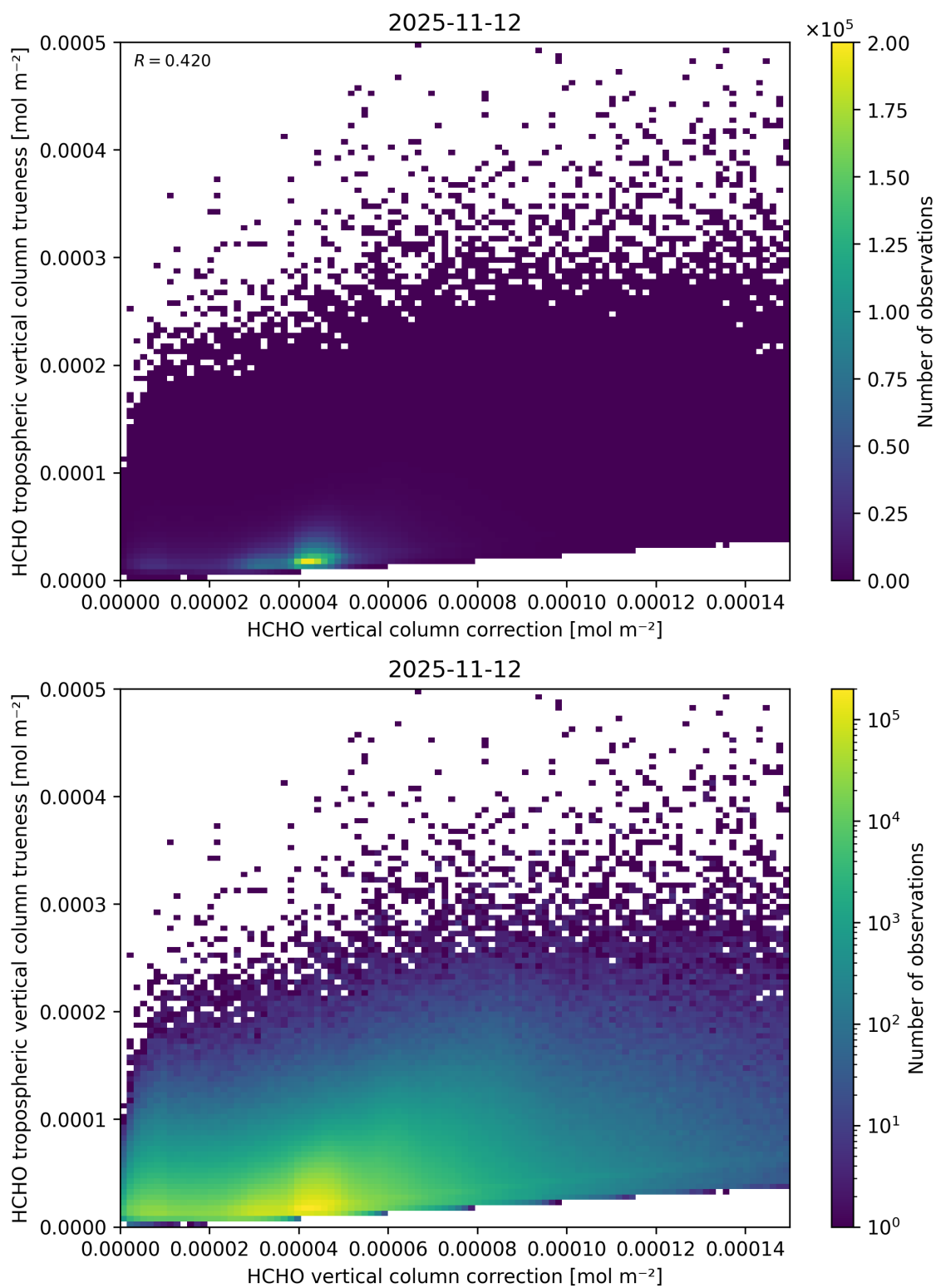
Figure 136: Scatter density plot of “HCHO vertical column correction” against “HCHO tropospheric vertical column true-ness” for 2025-11-12 to 2025-11-13.
