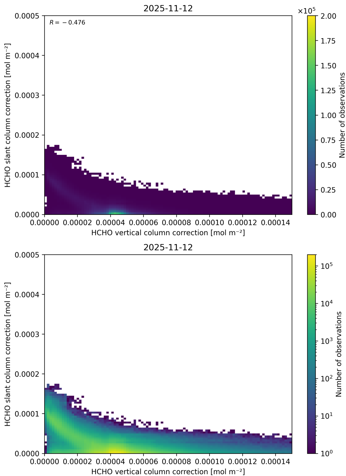
Figure 131: Scatter density plot of “HCHO vertical column correction” against “HCHO slant column correction” for 2025-11-12 to 2025-11-13.
