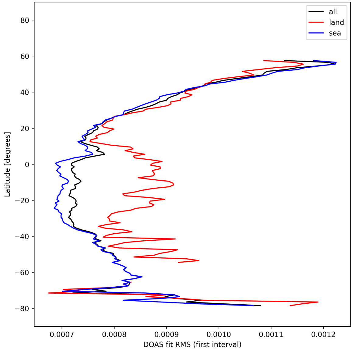
Figure 33: Zonal average of “DOAS fit RMS (first interval)” for 2025-11-12 to 2025-11-13.
