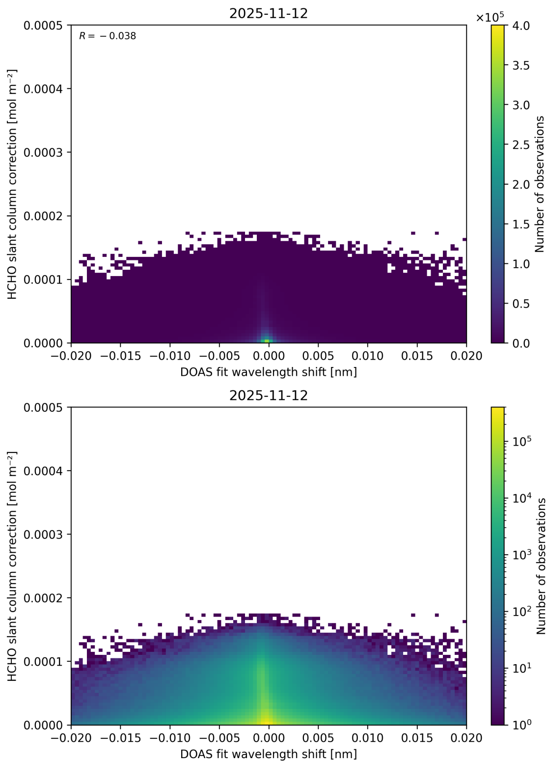
Figure 72: Scatter density plot of “DOAS fit wavelength shift” against “HCHO slant column correction” for 2025-11-12 to 2025-11-13.
