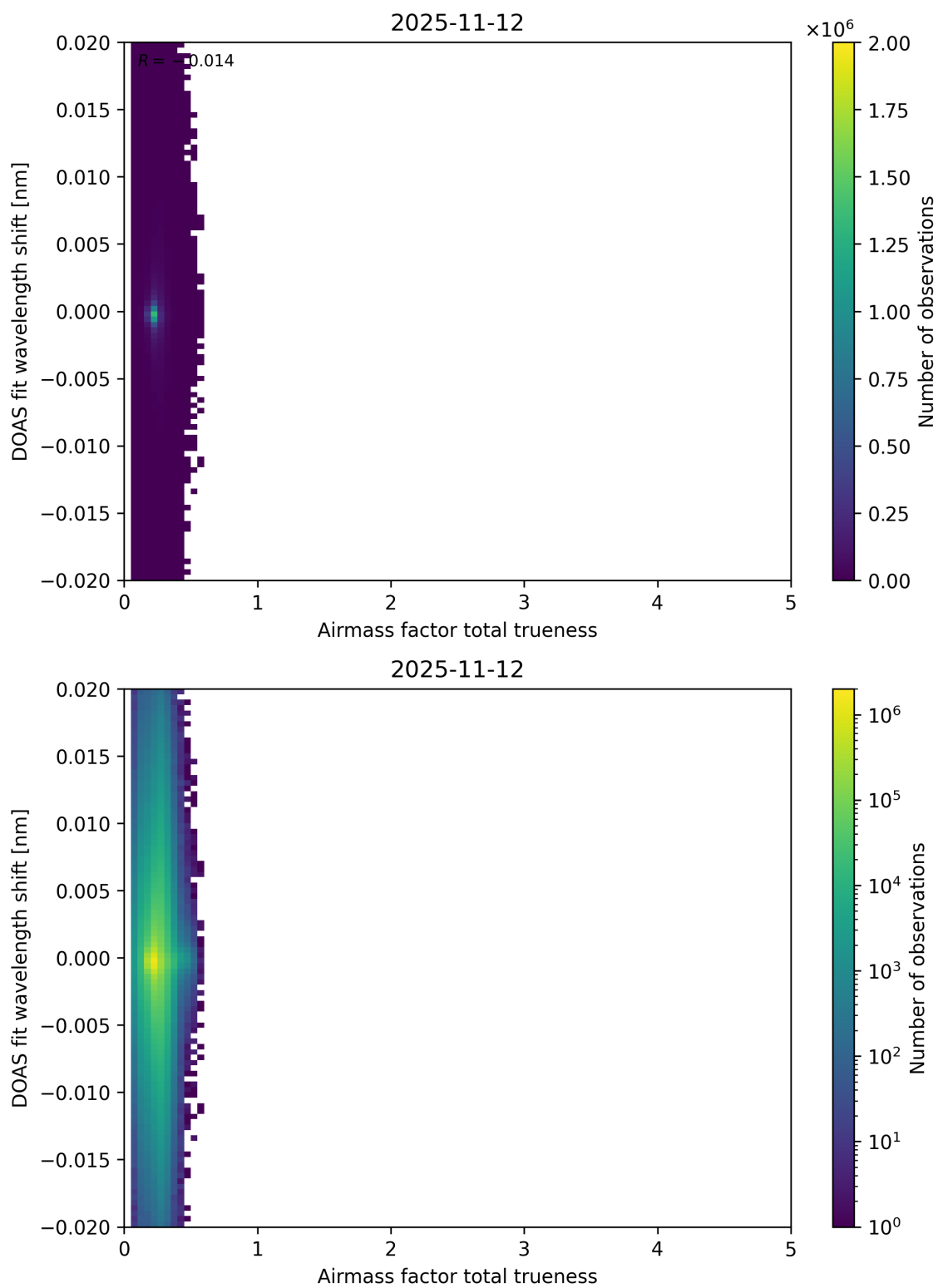
Figure 119: Scatter density plot of “Airmass factor total trueness” against “DOAS fit wavelength shift” for 2025-11-12 to 2025-11-13.
