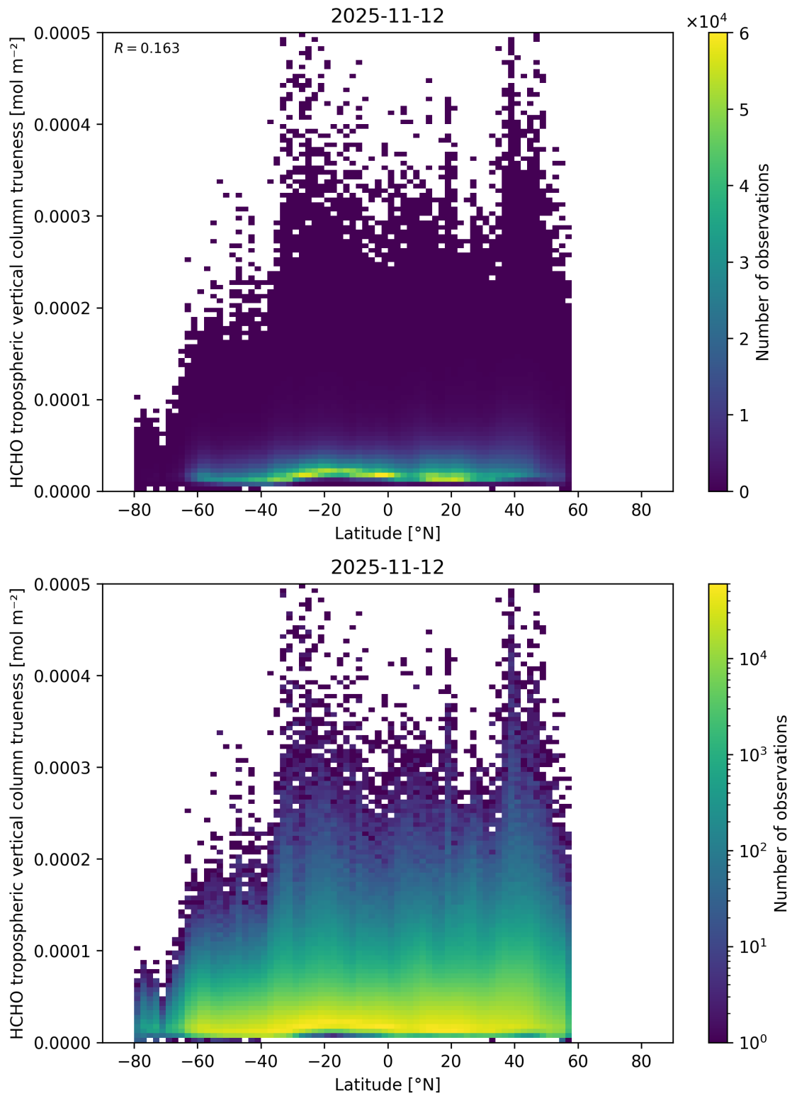
Figure 184: Scatter density plot of “Latitude” against “HCHO tropospheric vertical column trueness” for 2025-11-12 to 2025-11-13.
