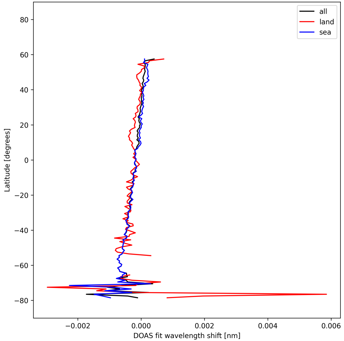
Figure 31: Zonal average of "DOAS fit wavelength shift" for 2025-11-12 to 2025-11-13.
