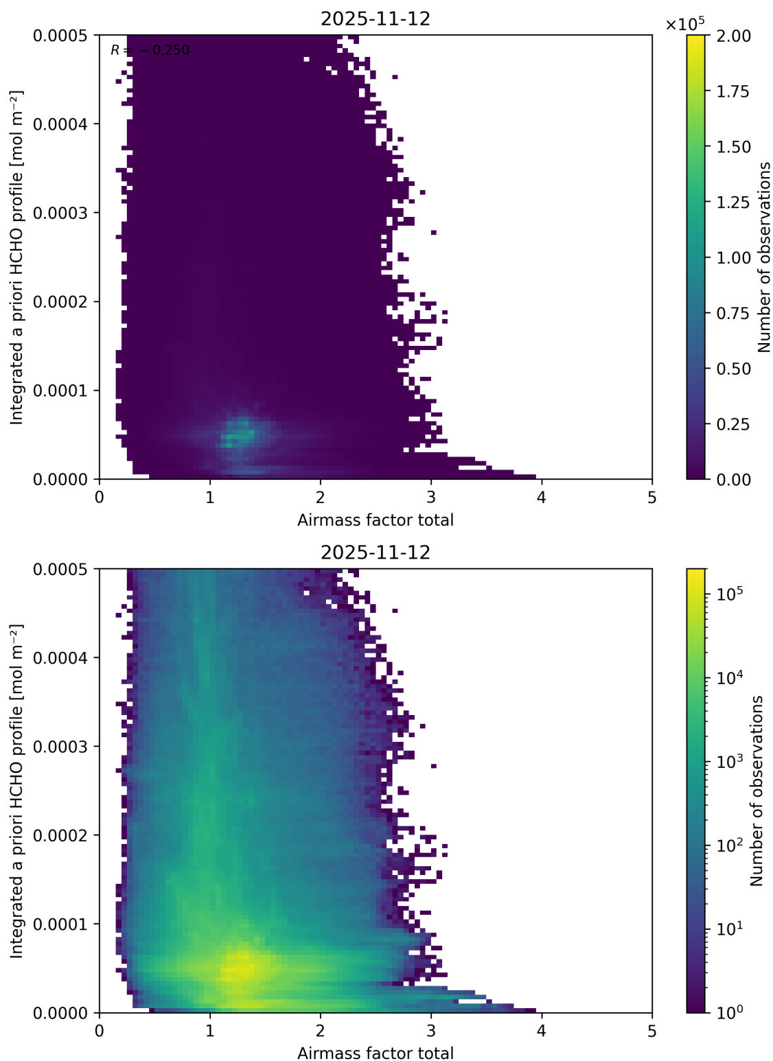
Figure 117: Scatter density plot of “Airmass factor total” against “Integrated a priori HCHO profile” for 2025-11-12 to 2025-11-13.
