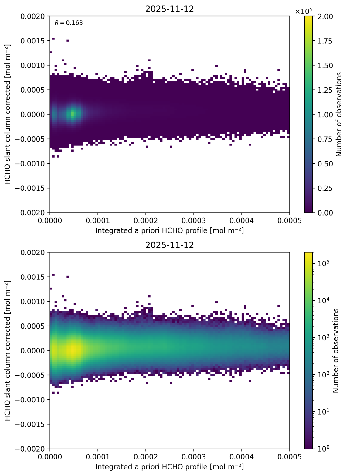
Figure 168: Scatter density plot of “Integrated a priori HCHO profile” against “HCHO slant column corrected” for 2025-11-12 to 2025-11-13.
