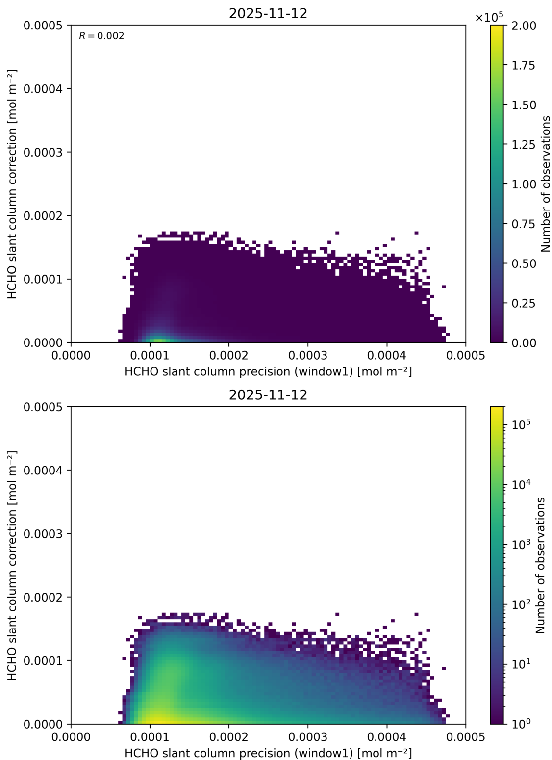
Figure 104: Scatter density plot of “HCHO slant column precision (window1)” against “HCHO slant column correction” for 2025-11-12 to 2025-11-13.
