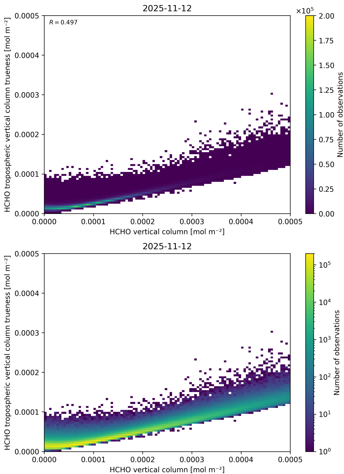
Figure 150: Scatter density plot of “HCHO vertical column” against “HCHO tropospheric vertical column trueness” for 2025-11-12 to 2025-11-13.
