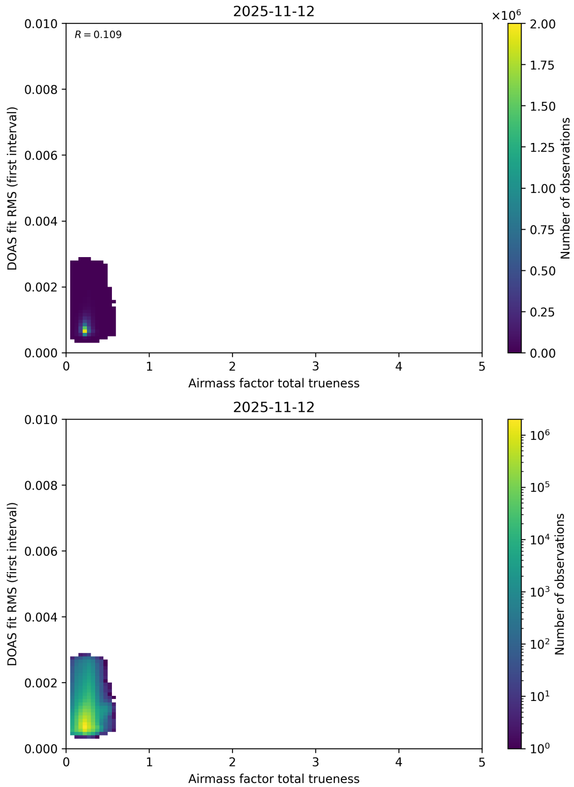
Figure 118: Scatter density plot of “Airmass factor total trueness” against “DOAS fit RMS (first interval)” for 2025-11-12 to 2025-11-13.
