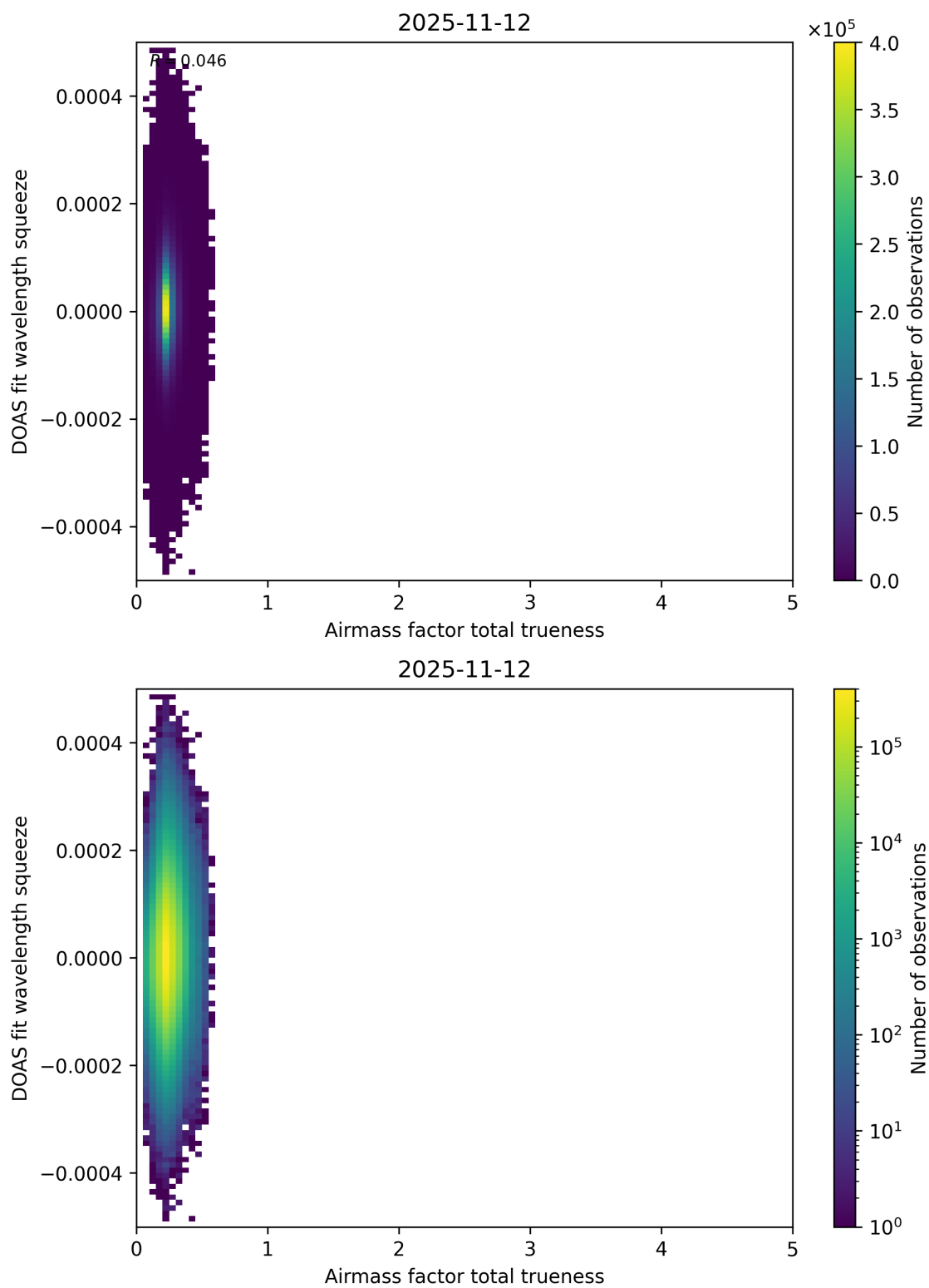
Figure 120: Scatter density plot of “Airmass factor total trueness” against “DOAS fit wavelength squeeze” for 2025-11-12 to 2025-11-13.
