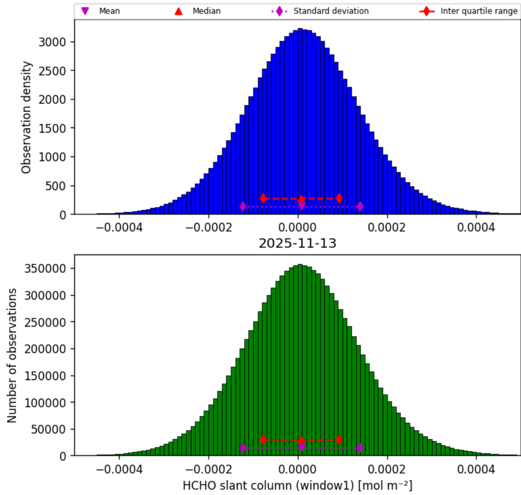
Figure 40: Histogram of “HCHO slant column (window1)” for 2025-11-12 to 2025-11-14
