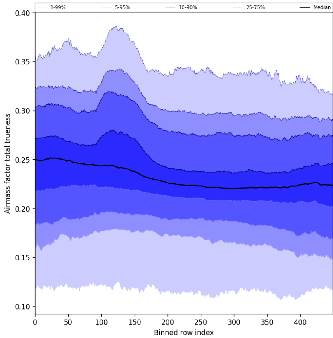
Figure 58: Along track statistics of “Airmass factor total trueness” for 2025-11-12 to 2025-11-14
