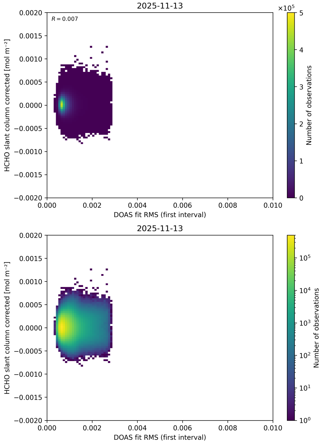
Figure 66: Scatter density plot of “DOAS fit RMS (first interval)” against “HCHO slant column corrected” for 2025-11-12 to 2025-11-14.
