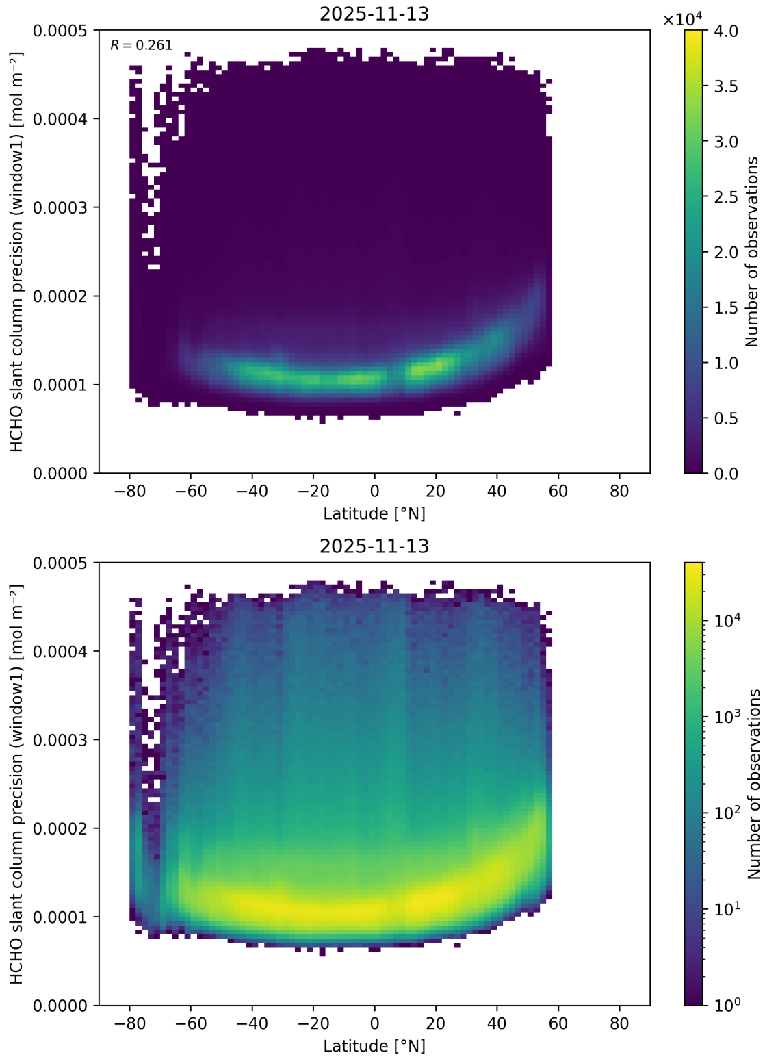
Figure 178: Scatter density plot of “Latitude” against “HCHO slant column precision (window1)” for 2025-11-12 to 2025-11-14.
