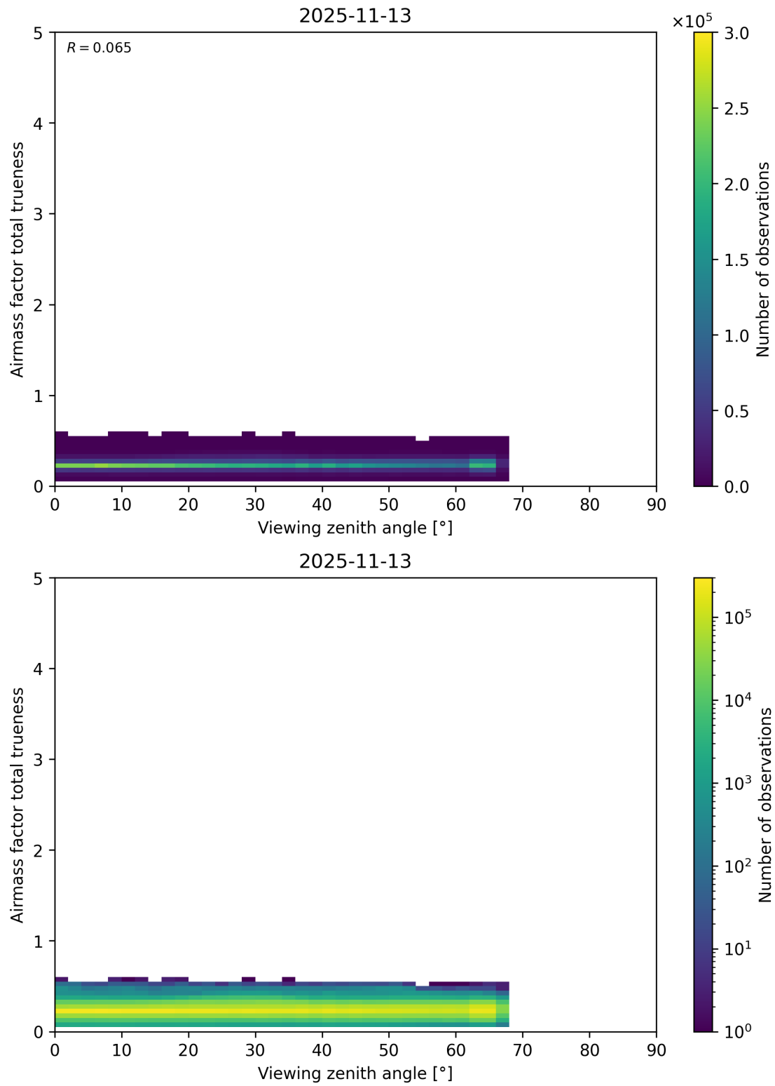
Figure 211: Scatter density plot of “Viewing zenith angle” against “Airmass factor total trueness” for 2025-11-12 to 2025-11-14.
