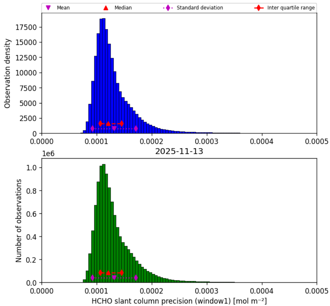
Figure 41: Histogram of “HCHO slant column precision (window1)” for 2025-11-12 to 2025-11-14
