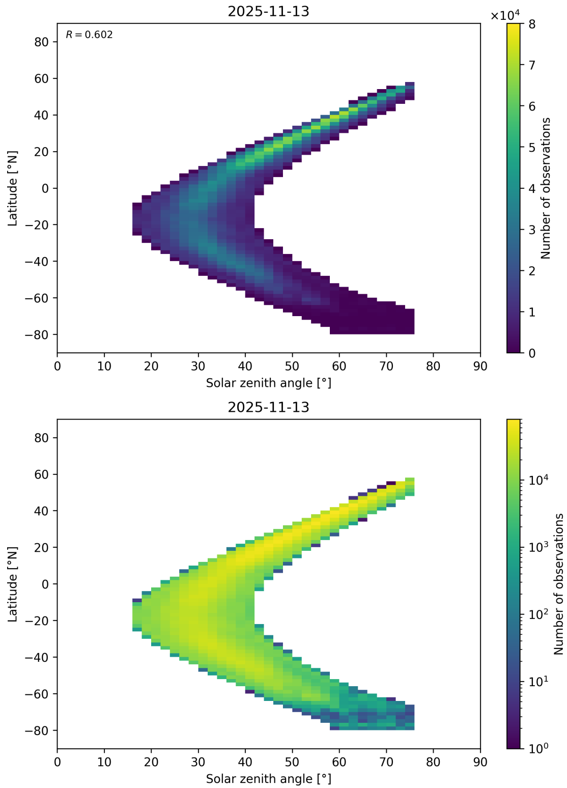
Figure 201: Scatter density plot of “Solar zenith angle” against “Latitude” for 2025-11-12 to 2025-11-14.
