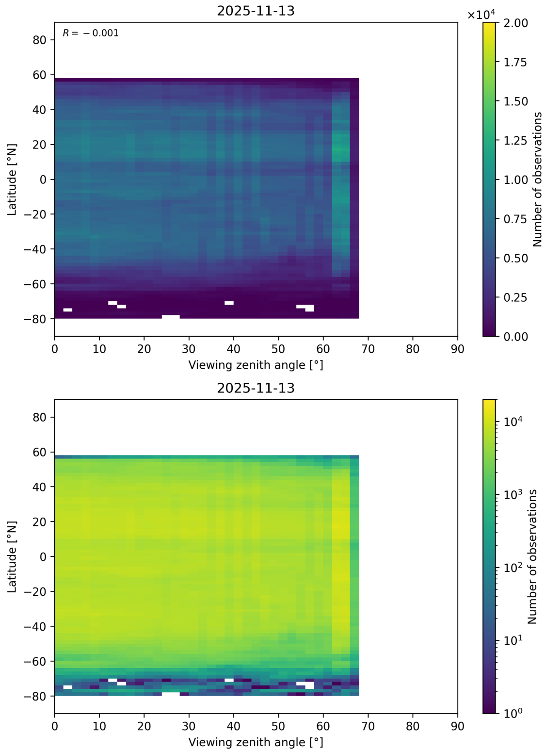
Figure 217: Scatter density plot of “Viewing zenith angle” against “Latitude” for 2025-11-12 to 2025-11-14.
