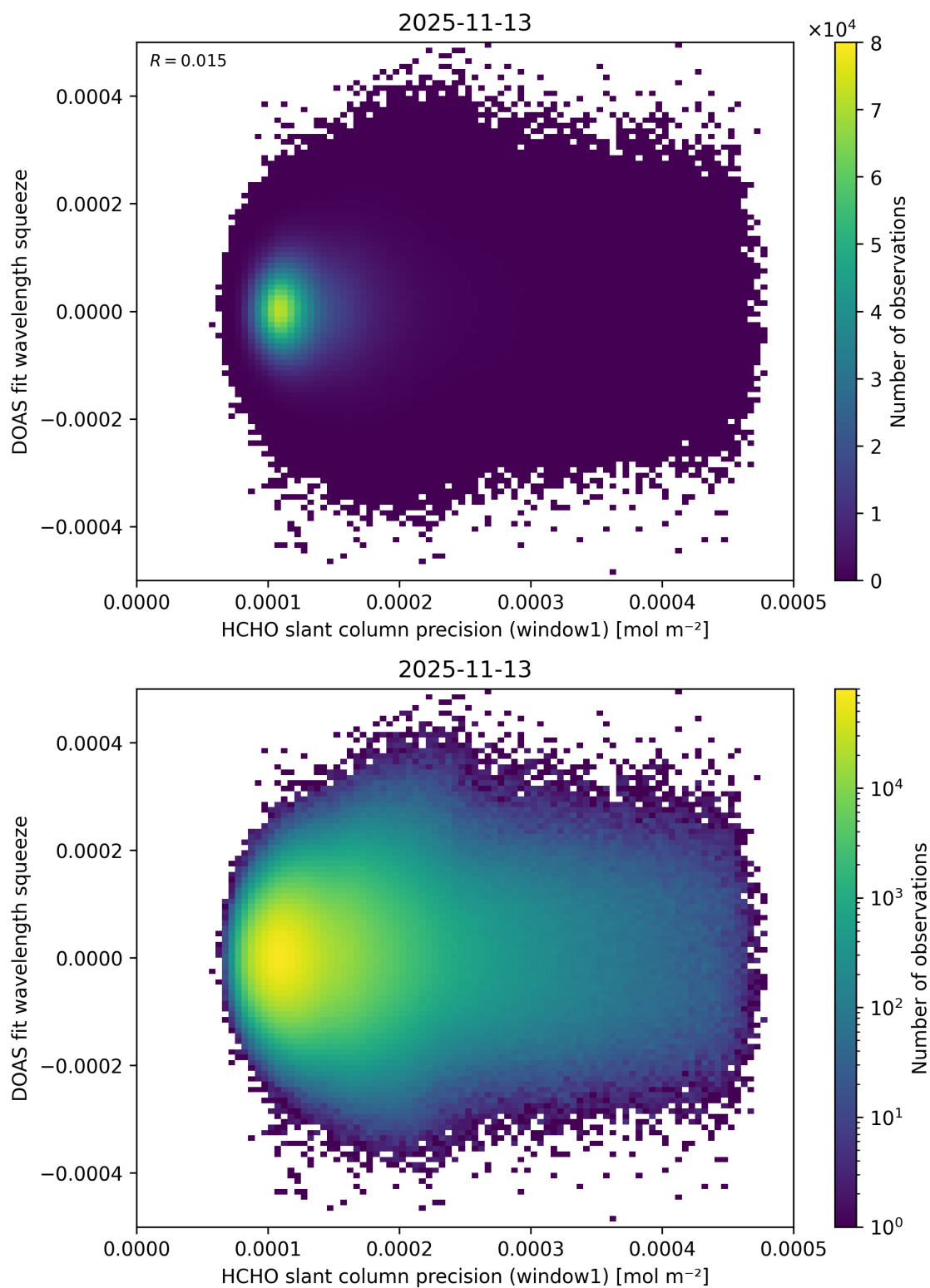
Figure 101: Scatter density plot of “HCHO slant column precision (window1)” against “DOAS fit wavelength squeeze” for 2025-11-12 to 2025-11-14.
