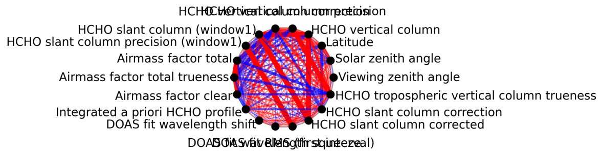
Figure 1: Map of correlation graph for 2025-11-12 to 2025-11-14.
