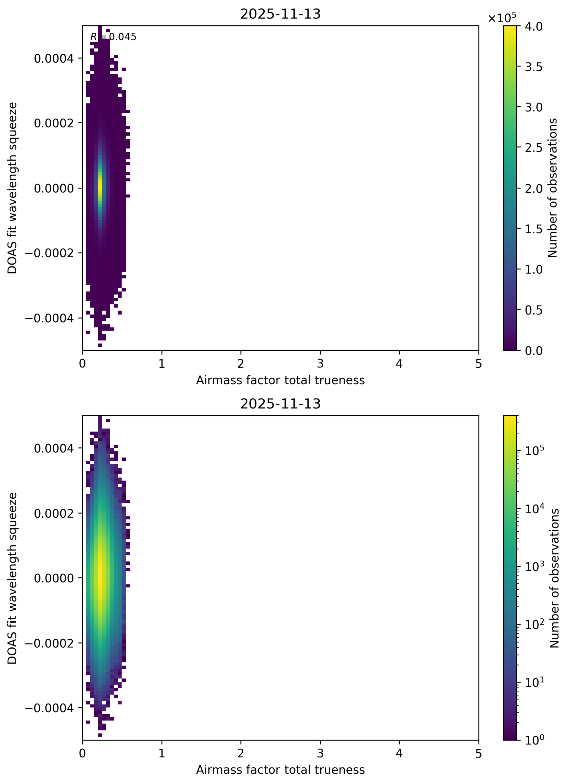
Figure 120: Scatter density plot of “Airmass factor total trueness” against “DOAS fit wavelength squeeze” for 2025-11-12 to 2025-11-14.
