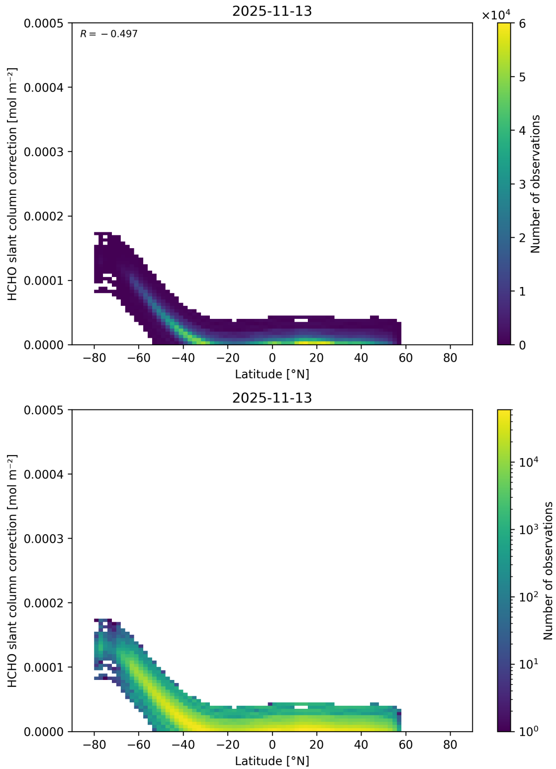
Figure 176: Scatter density plot of “Latitude” against “HCHO slant column correction” for 2025-11-12 to 2025-11-14.
