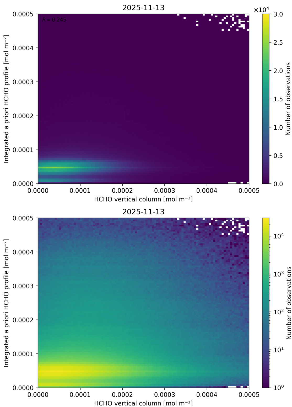
Figure 151: Scatter density plot of “HCHO vertical column” against “Integrated a priori HCHO profile” for 2025-11-12 to 2025-11-14.
