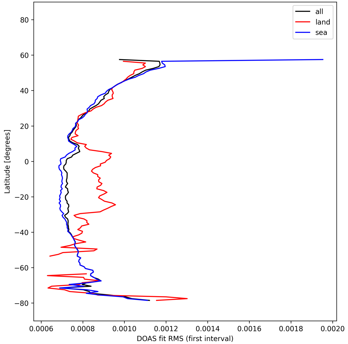
Figure 33: Zonal average of “DOAS fit RMS (first interval)” for 2025-11-12 to 2025-11-14.
