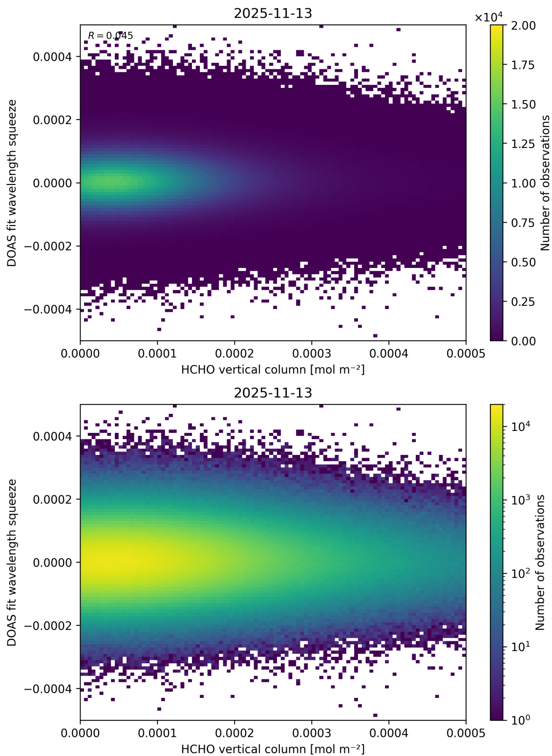
Figure 140: Scatter density plot of “HCHO vertical column” against “DOAS fit wavelength squeeze” for 2025-11-12 to 2025-11-14.
