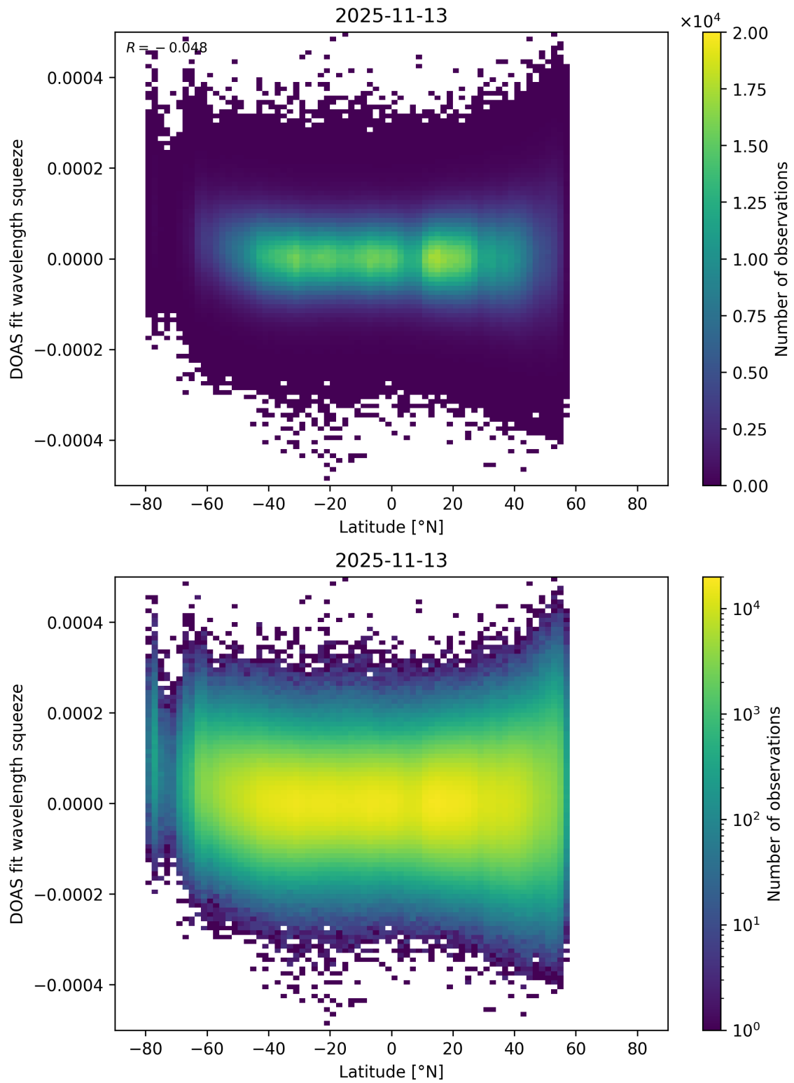
Figure 173: Scatter density plot of “Latitude” against “DOAS fit wavelength squeeze” for 2025-11-12 to 2025-11-14.
