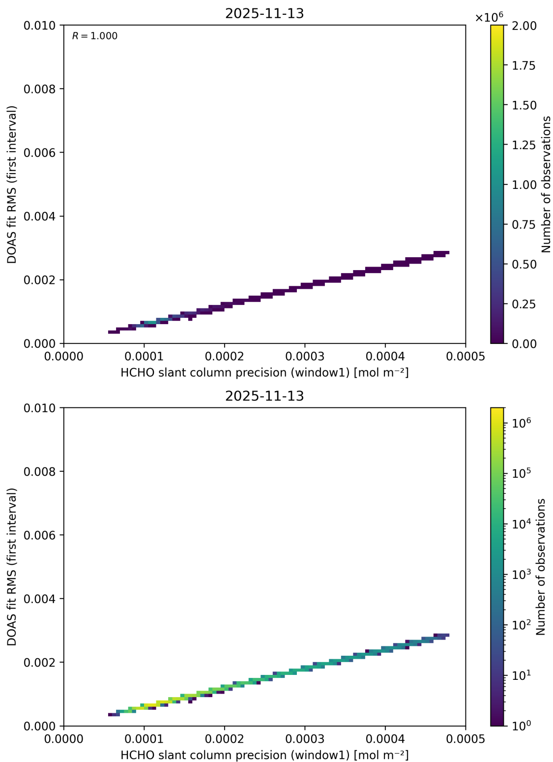
Figure 99: Scatter density plot of “HCHO slant column precision (window1)” against “DOAS fit RMS (first interval)” for 2025-11-12 to 2025-11-14.
