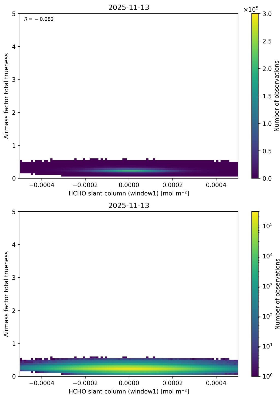
Figure 96: Scatter density plot of “HCHO slant column (window1)” against “Airmass factor total trueneess” for 2025-11-12 to 2025-11-14.
