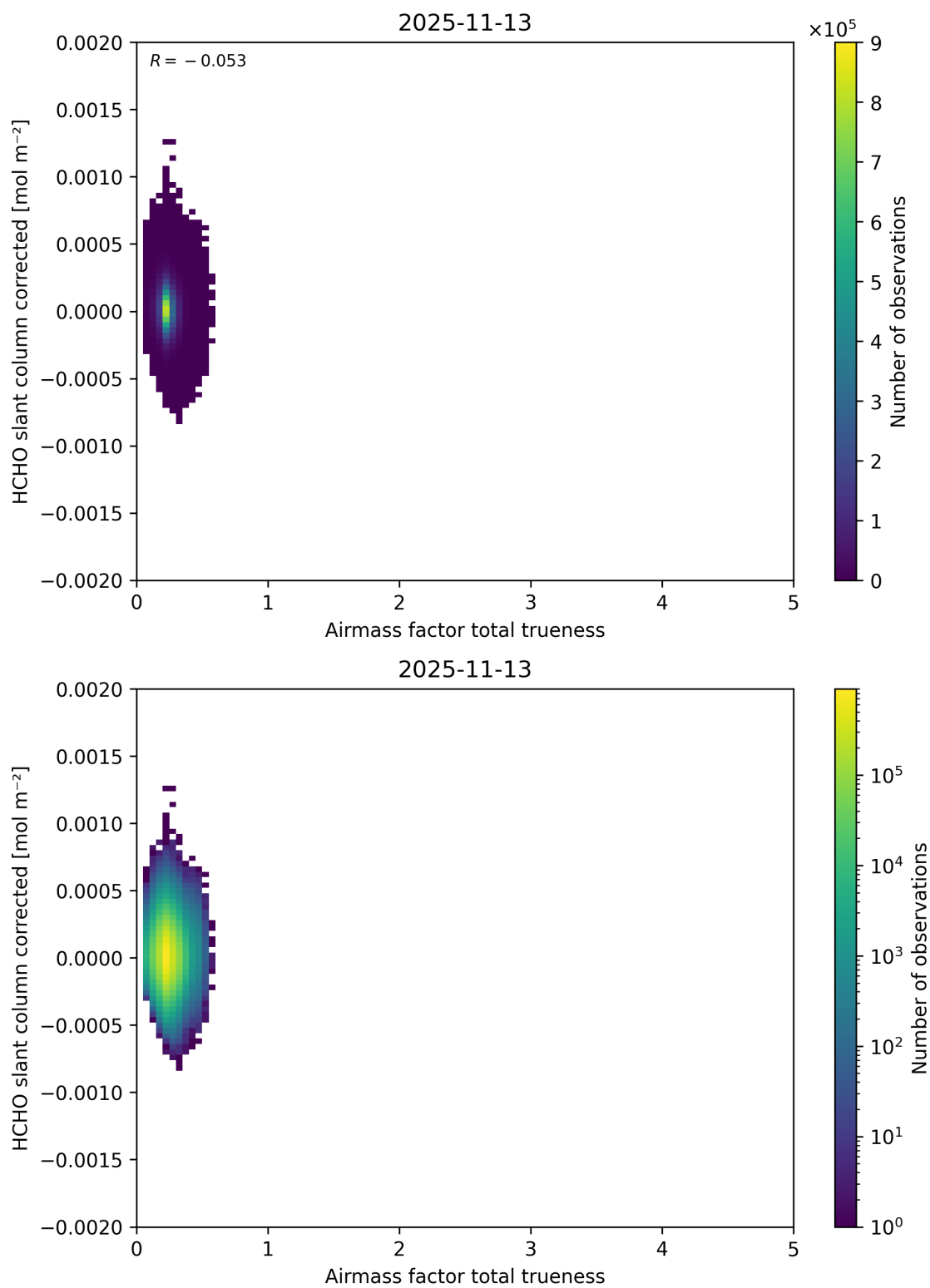
Figure 122: Scatter density plot of “Airmass factor total trueness” against “HCHO slant column corrected” for 2025-11-12 to 2025-11-14.
