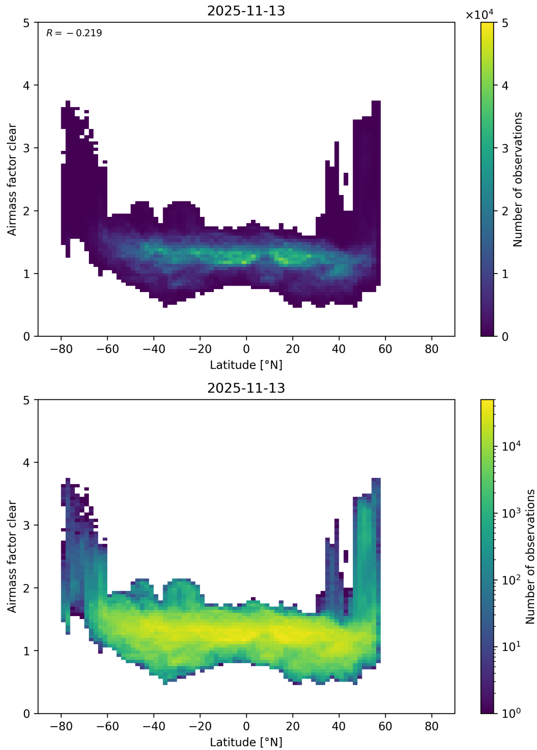
Figure 174: Scatter density plot of “Latitude” against “Airmass factor clear” for 2025-11-12 to 2025-11-14.
