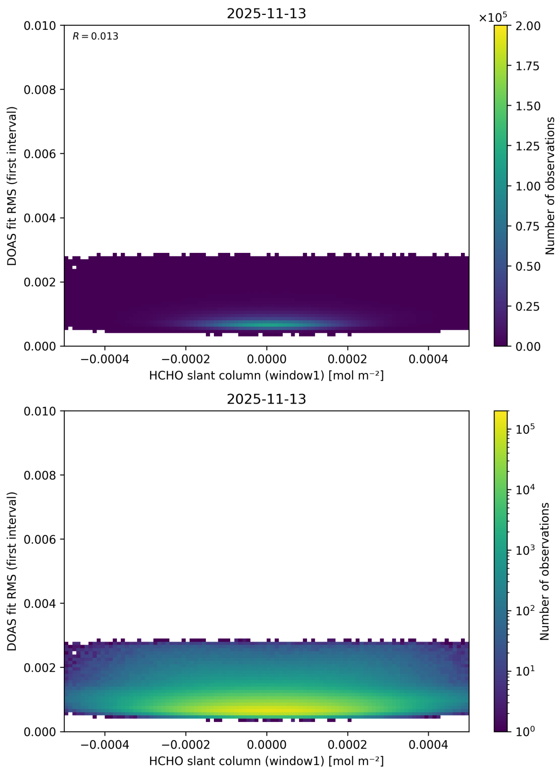
Figure 88: Scatter density plot of “HCHO slant column (window1)” against “DOAS fit RMS (first interval)” for 2025-11-12 to 2025-11-14.
