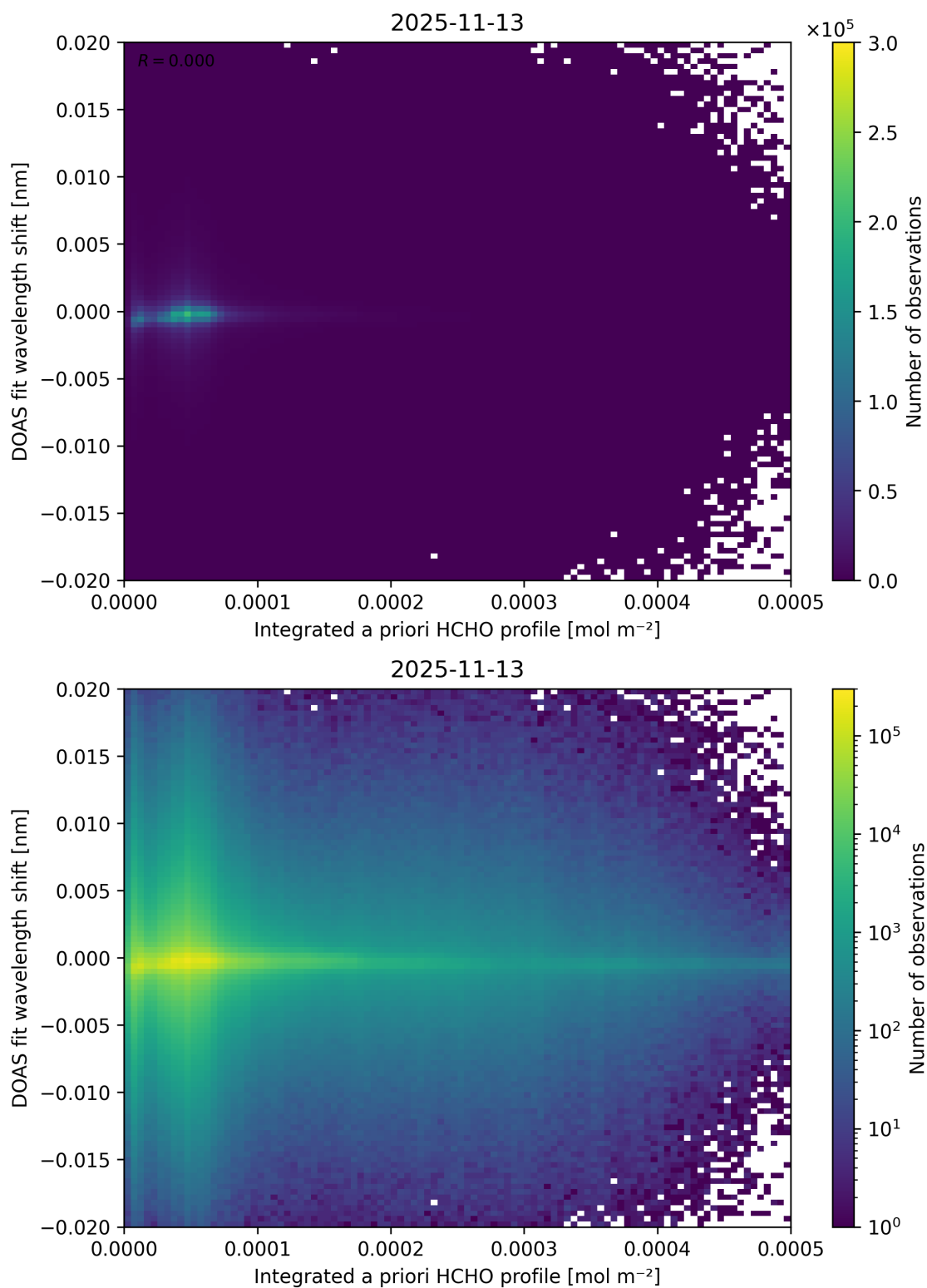
Figure 166: Scatter density plot of “Integrated a priori HCHO profile” against “DOAS fit wavelength shift” for 2025-11-12 to 2025-11-14.
