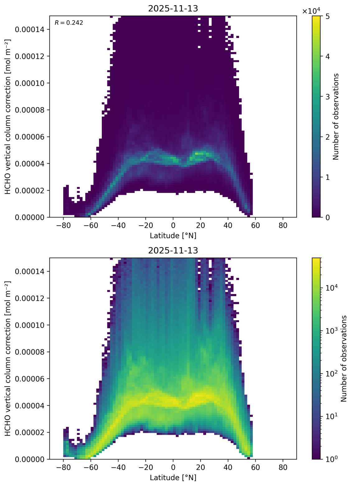
Figure 182: Scatter density plot of “Latitude” against “HCHO vertical column correction” for 2025-11-12 to 2025-11-14.
