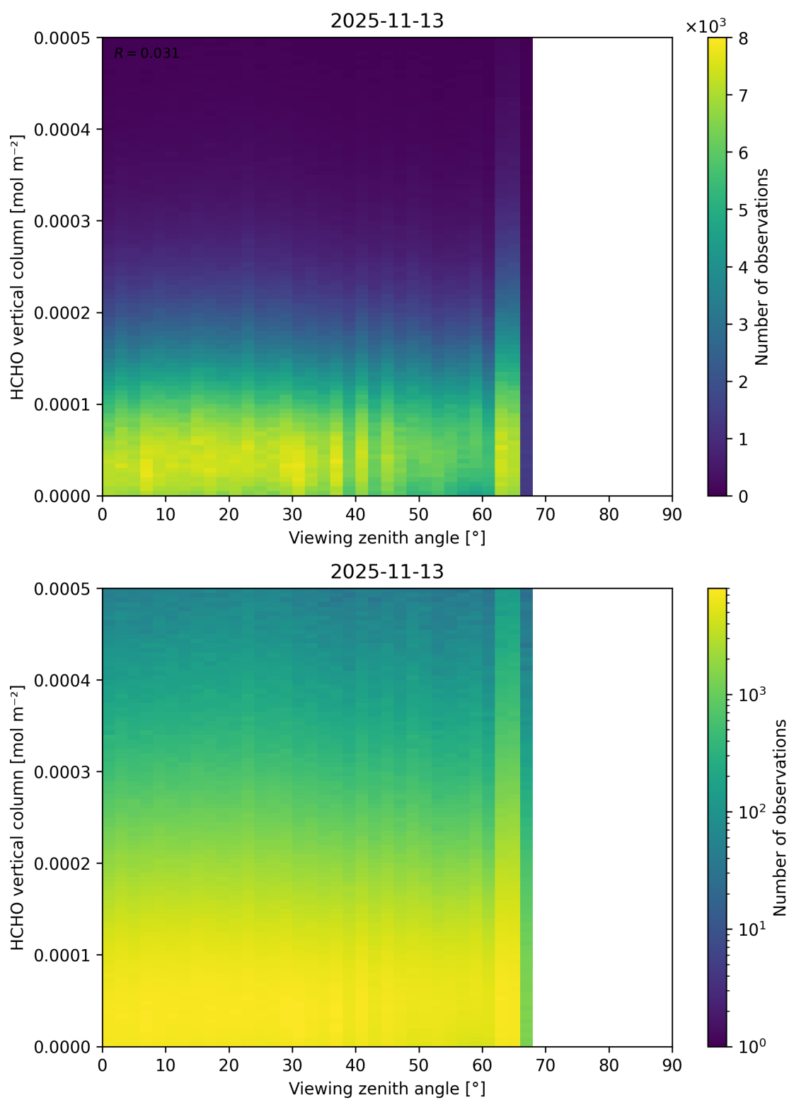
Figure 212: Scatter density plot of “Viewing zenith angle” against “HCHO vertical column” for 2025-11-12 to 2025-11-14.
