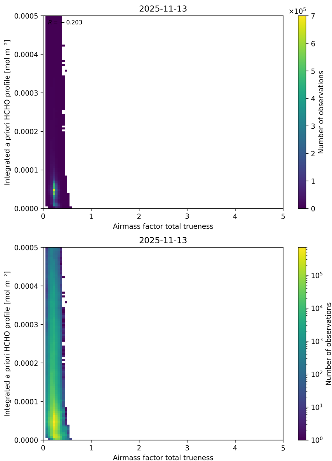
Figure 125: Scatter density plot of “Airmass factor total trueness” against “Integrated a priori HCHO profile” for 2025-11-12 to 2025-11-14.
