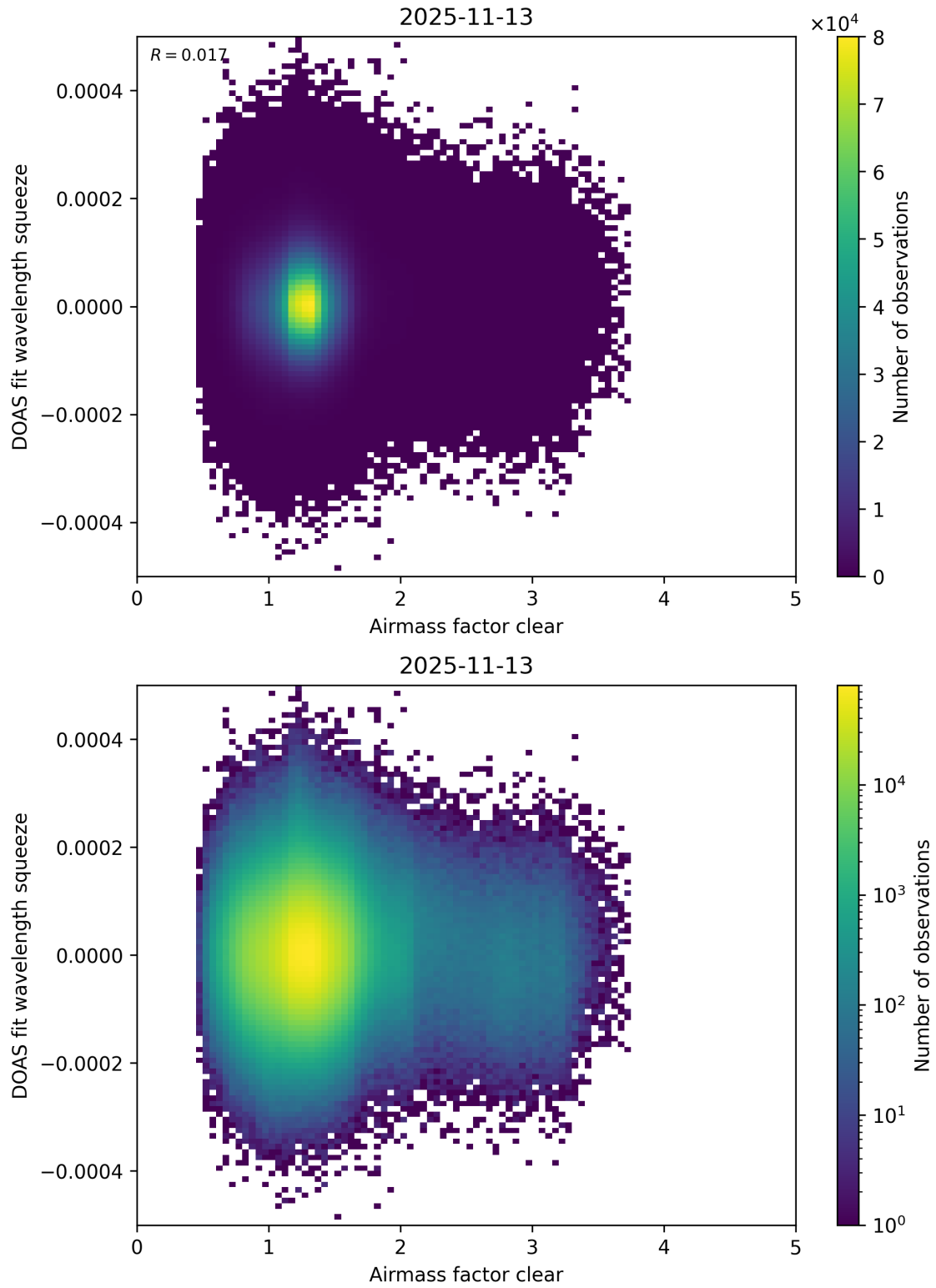
Figure 80: Scatter density plot of “Airmass factor clear” against “DOAS fit wavelength squeeze” for 2025-11-12 to 2025-11-14.
