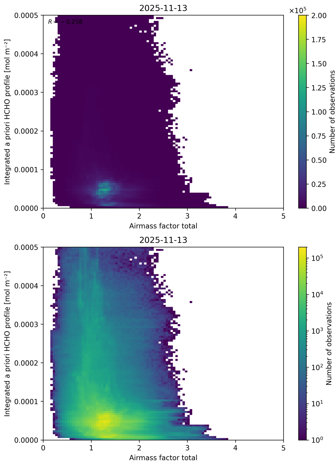
Figure 117: Scatter density plot of “Airmass factor total” against “Integrated a priori HCHO profile” for 2025-11-12 to 2025-11-14.
