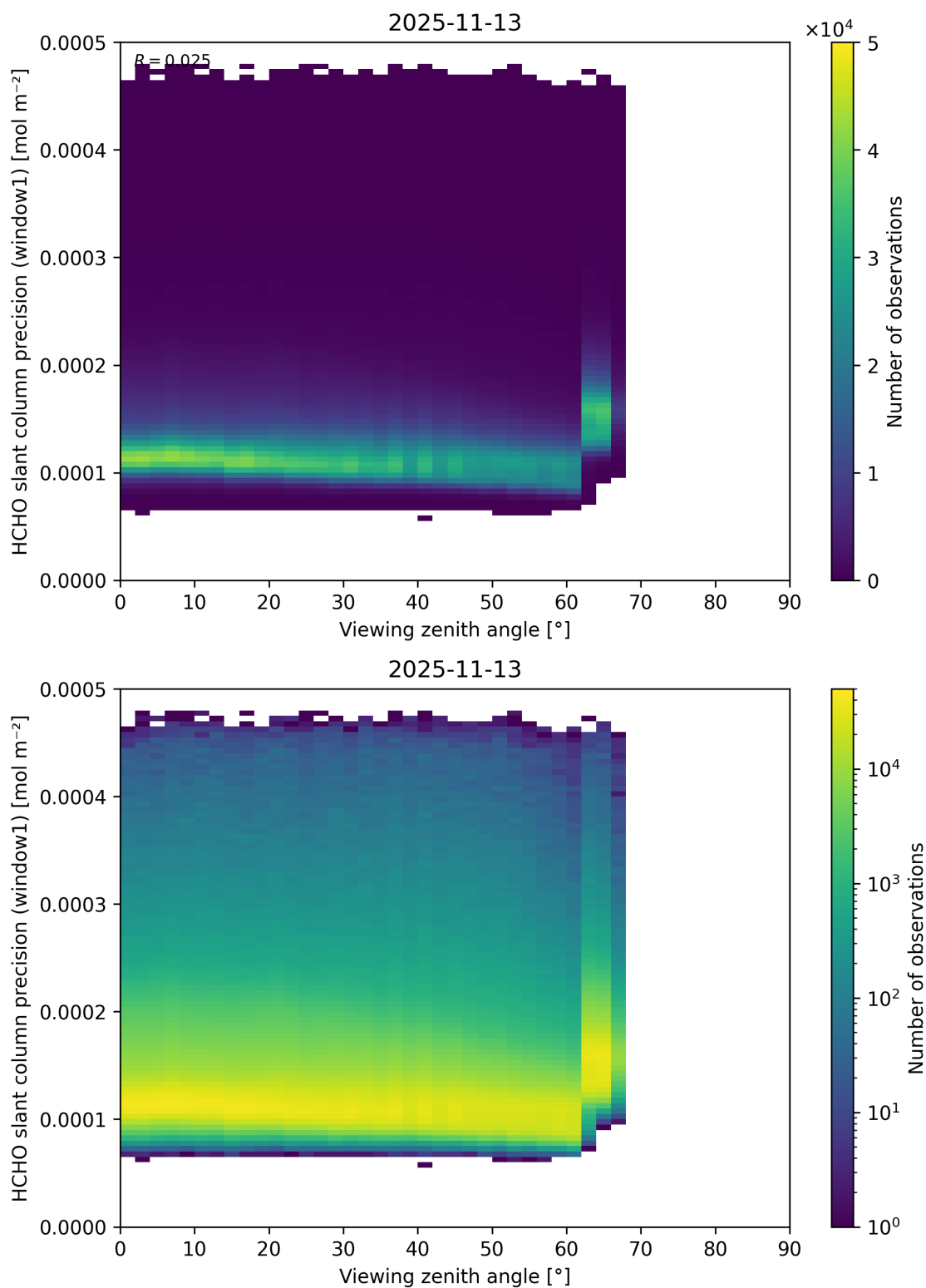
Figure 209: Scatter density plot of “Viewing zenith angle” against “HCHO slant column precision (window1)” for 2025-11-12 to 2025-11-14.
