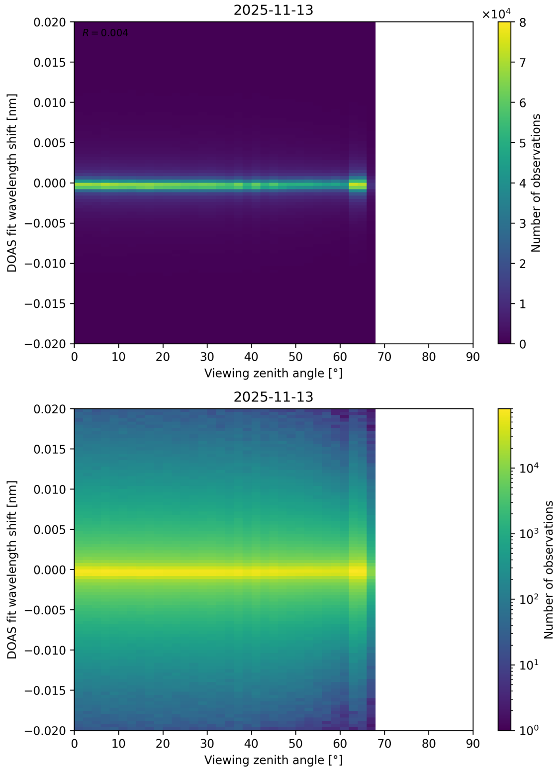
Figure 203: Scatter density plot of “Viewing zenith angle” against “DOAS fit wavelength shift” for 2025-11-12 to 2025-11-14.
