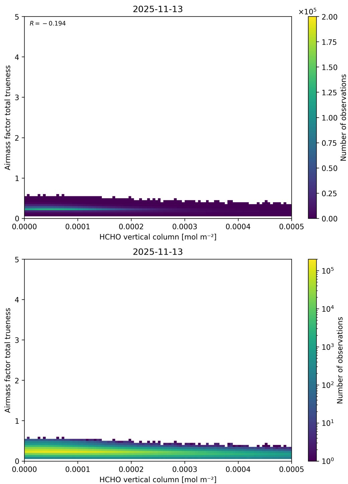
Figure 147: Scatter density plot of “HCHO vertical column” against “Airmass factor total truiness” for 2025-11-12 to 2025-11-14.
