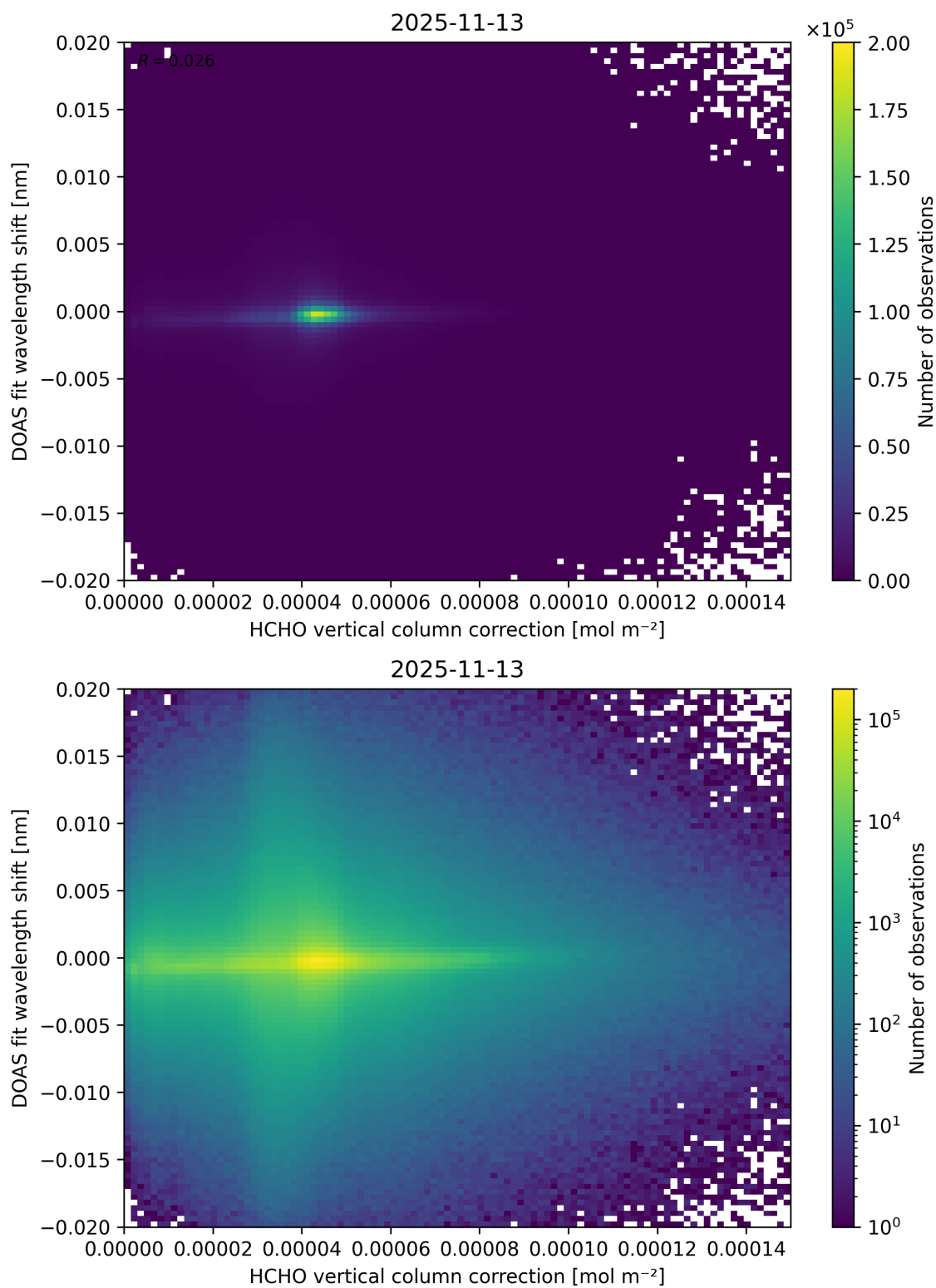
Figure 127: Scatter density plot of “HCHO vertical column correction” against “DOAS fit wavelength shift” for 2025-11-12 to 2025-11-14.
