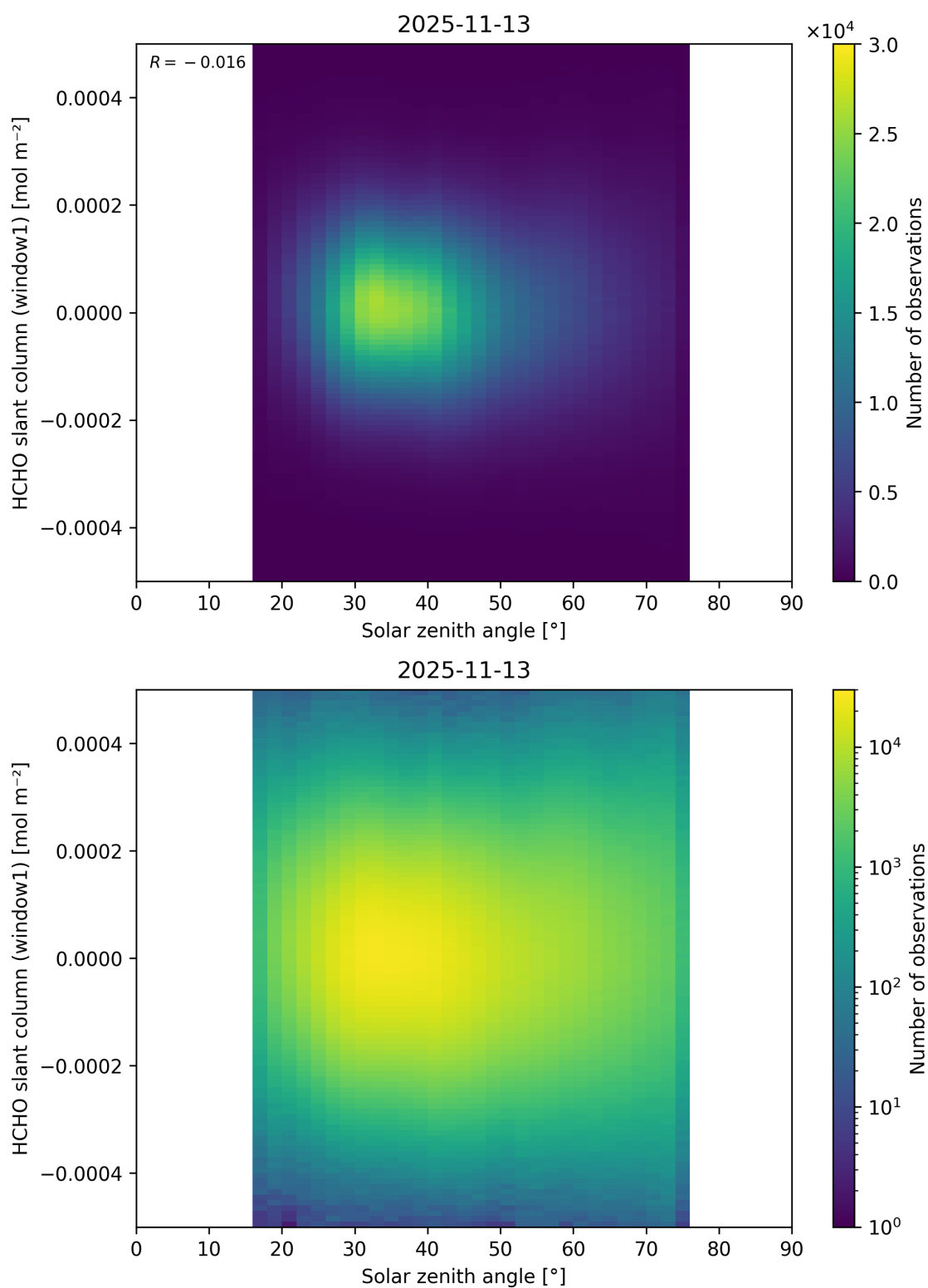
Figure 192: Scatter density plot of “Solar zenith angle” against “HCHO slant column (window1)” for 2025-11-12 to 2025-11-14.
