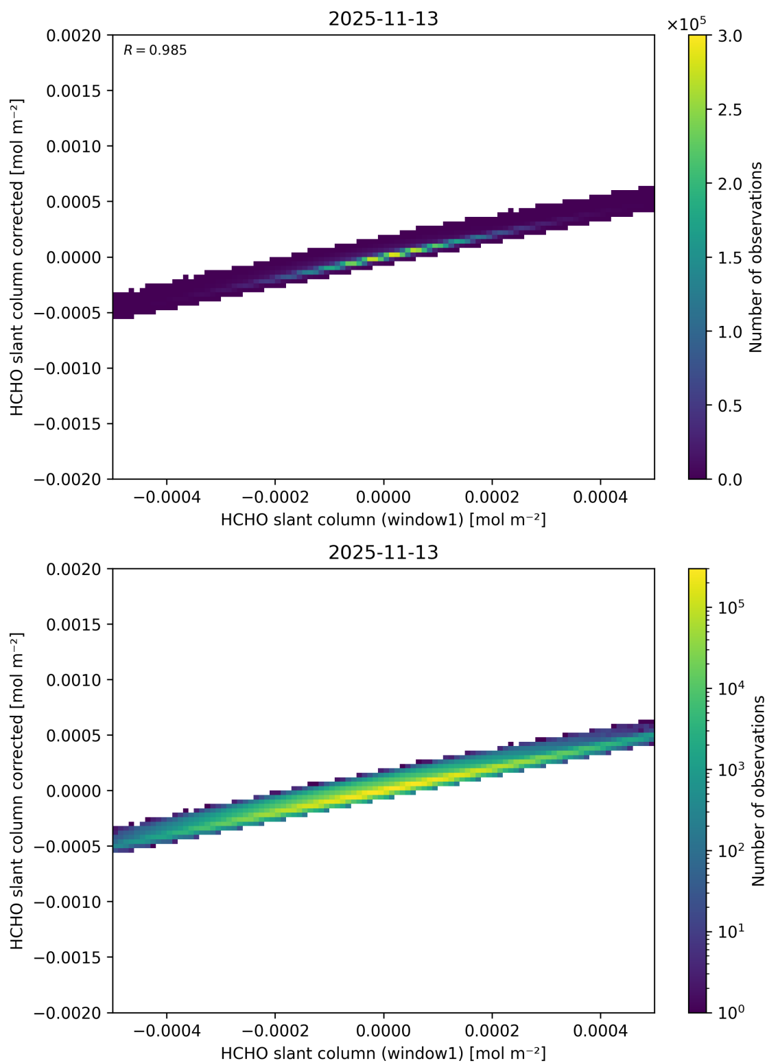
Figure 92: Scatter density plot of “HCHO slant column (window1)” against “HCHO slant column corrected” for 2025-11-12 to 2025-11-14.
