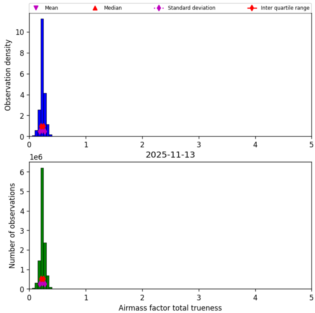
Figure 43: Histogram of “Airmass factor total trueness” for 2025-11-12 to 2025-11-14
