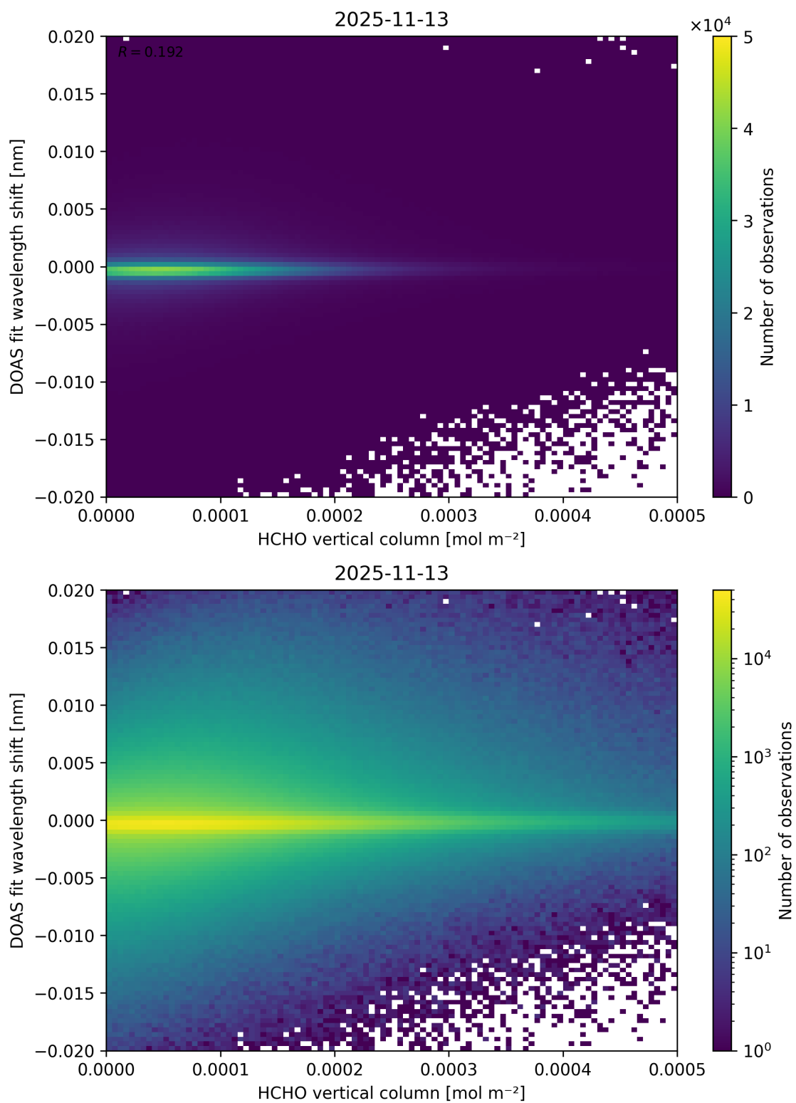
Figure 139: Scatter density plot of “HCHO vertical column” against “DOAS fit wavelength shift” for 2025-11-12 to 2025-11-14.
