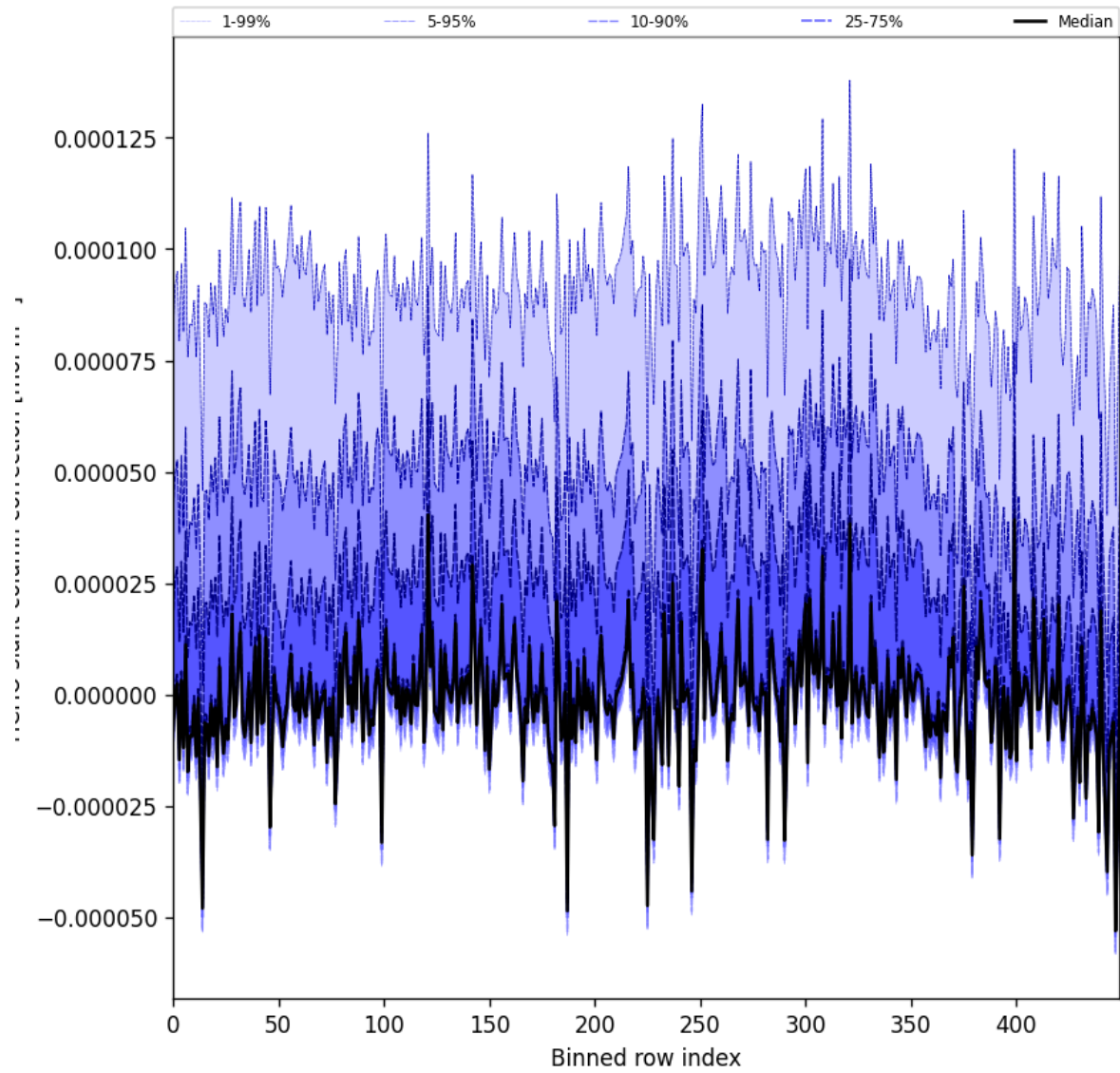
Figure 64: Along track statistics of “HCHO slant column correction” for 2025-11-12 to 2025-11-14
