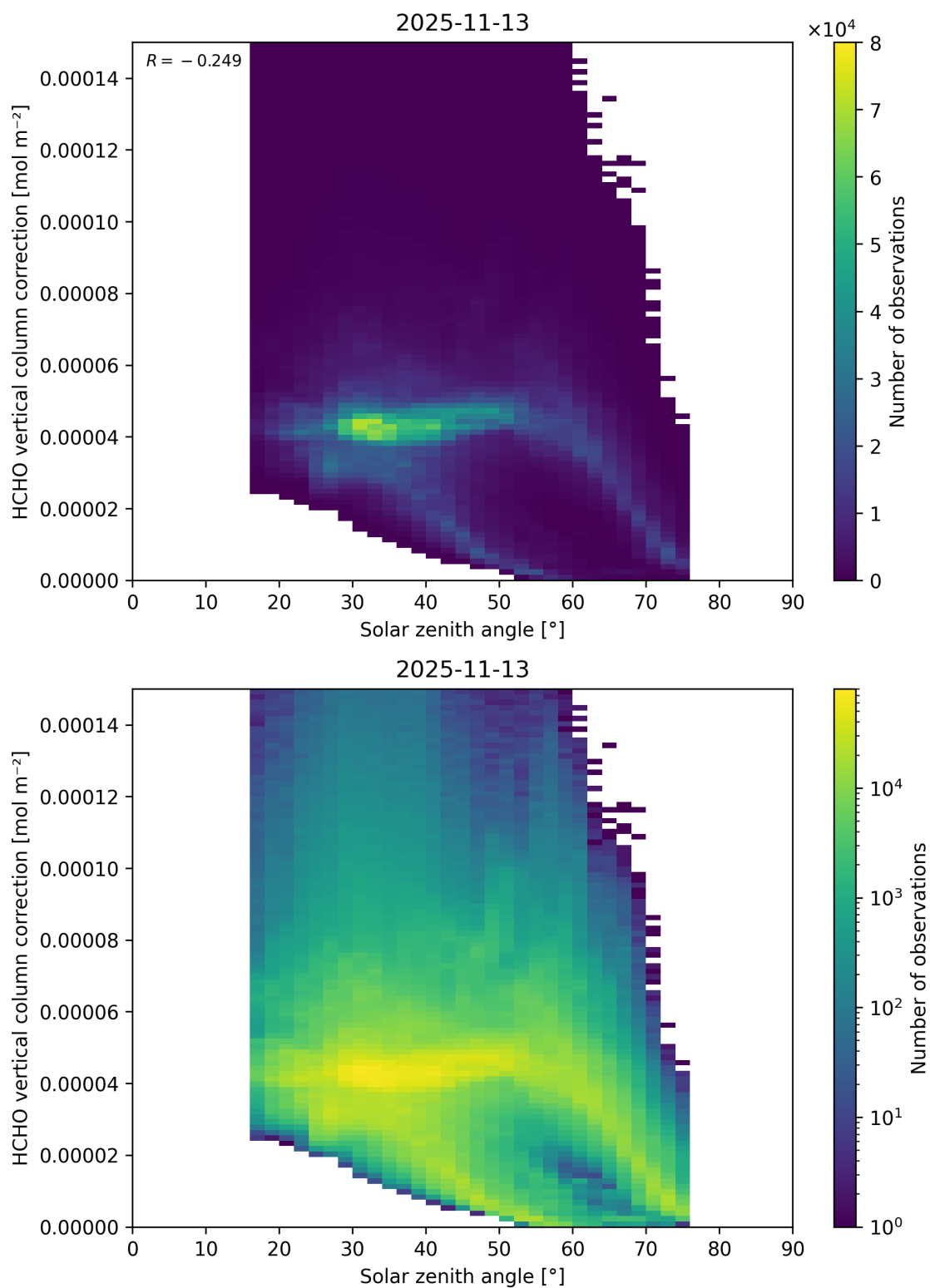
Figure 197: Scatter density plot of “Solar zenith angle” against “HCHO vertical column correction” for 2025-11-12 to 2025-11-14.
