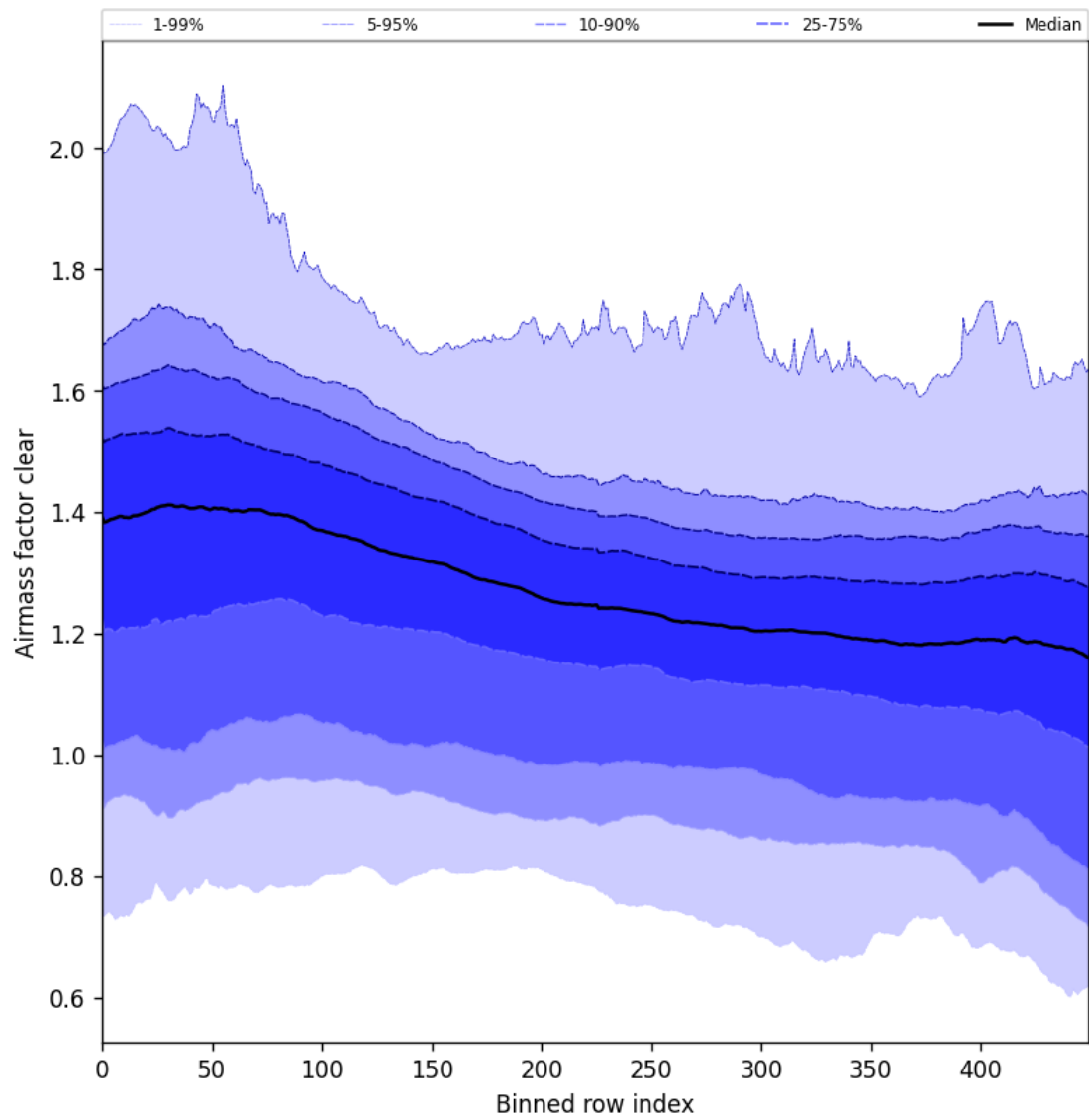
Figure 59: Along track statistics of “Airmass factor clear” for 2025-11-12 to 2025-11-14
