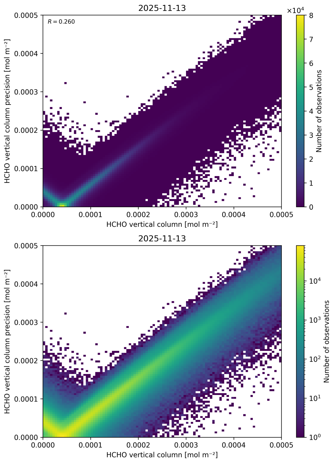
Figure 149: Scatter density plot of “HCHO vertical column” against “HCHO vertical column precision” for 2025-11-12 to 2025-11-14.
