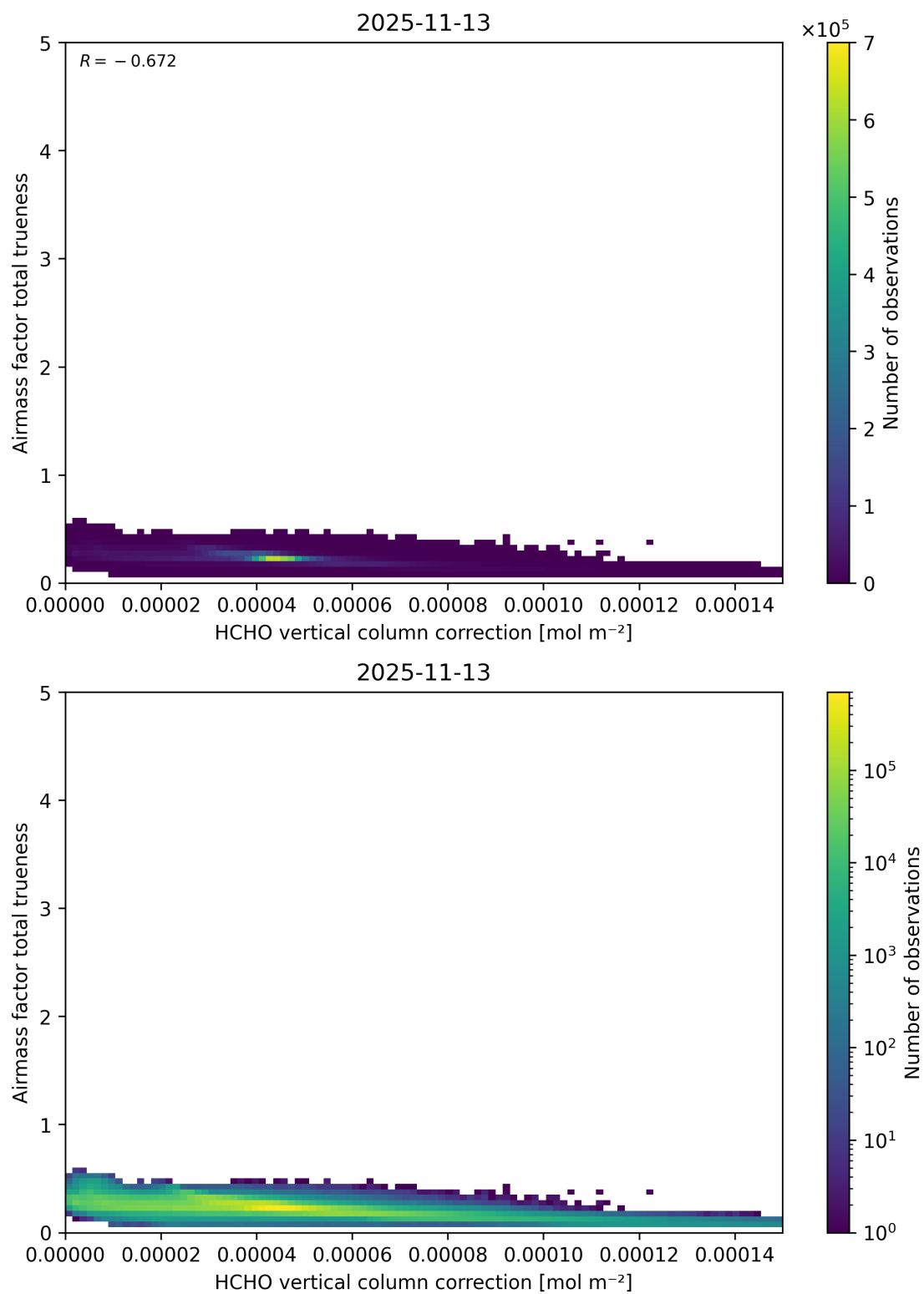
Figure 135: Scatter density plot of “HCHO vertical column correction” against “Airmass factor total trueness” for 2025-11-12 to 2025-11-14.
