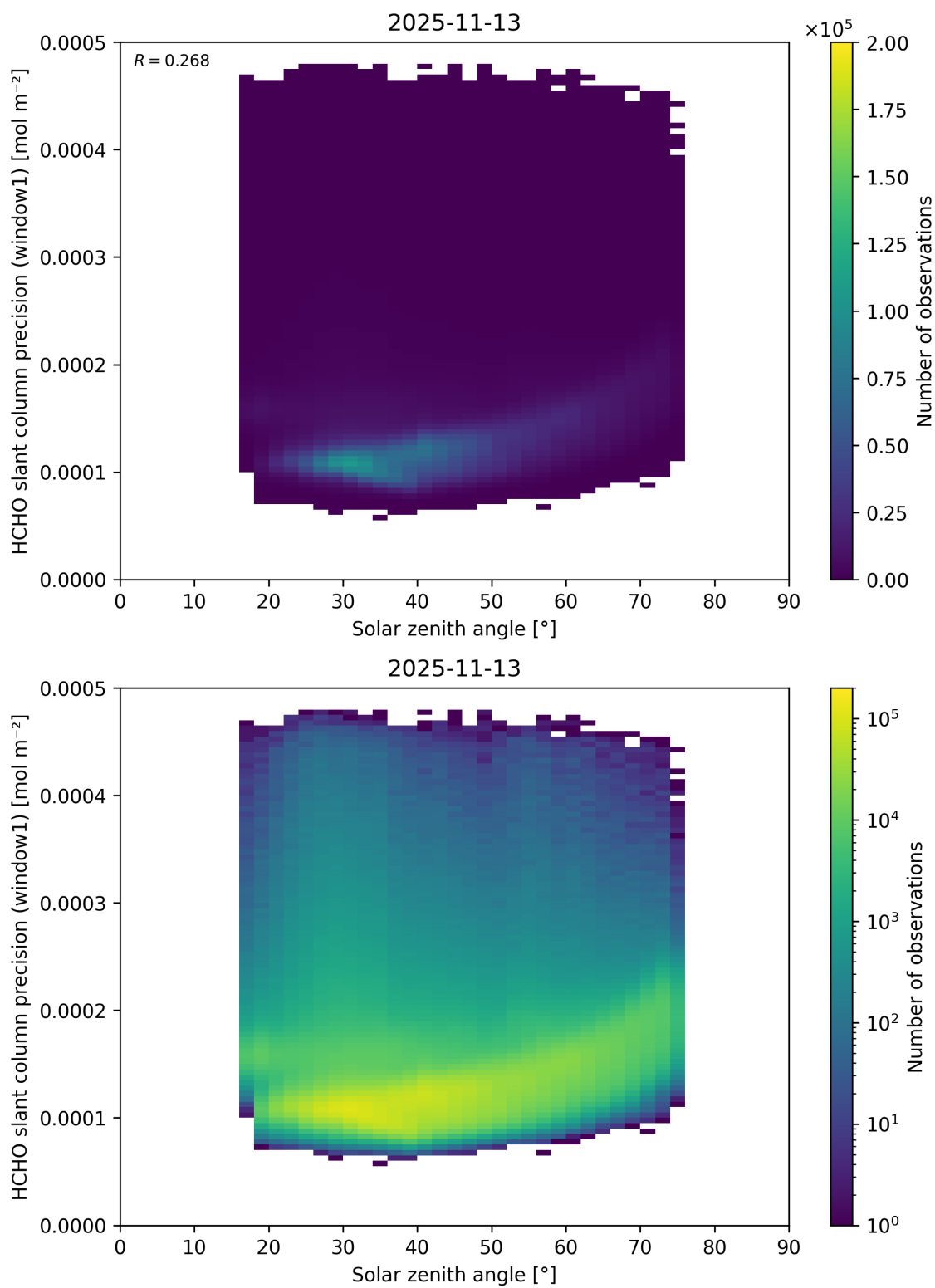
Figure 193: Scatter density plot of “Solar zenith angle” against “HCHO slant column precision (window1)” for 2025-11-12 to 2025-11-14.
