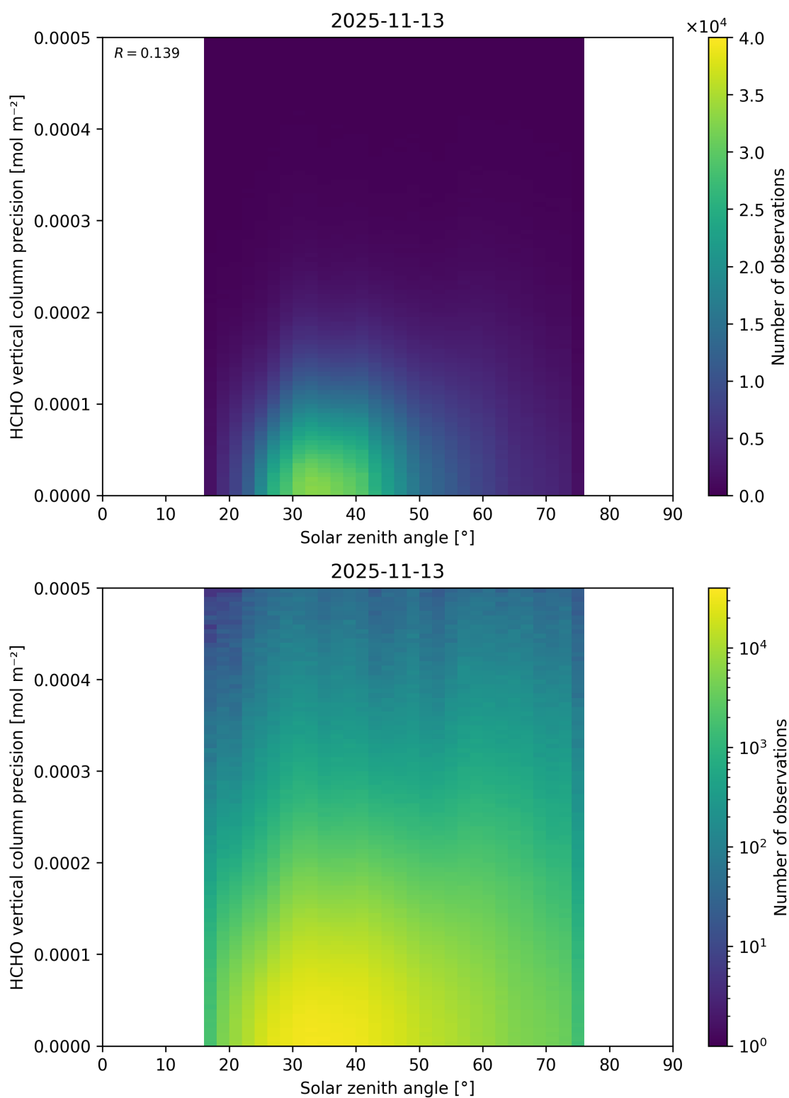
Figure 198: Scatter density plot of “Solar zenith angle” against “HCHO vertical column precision” for 2025-11-12 to 2025-11-14.
