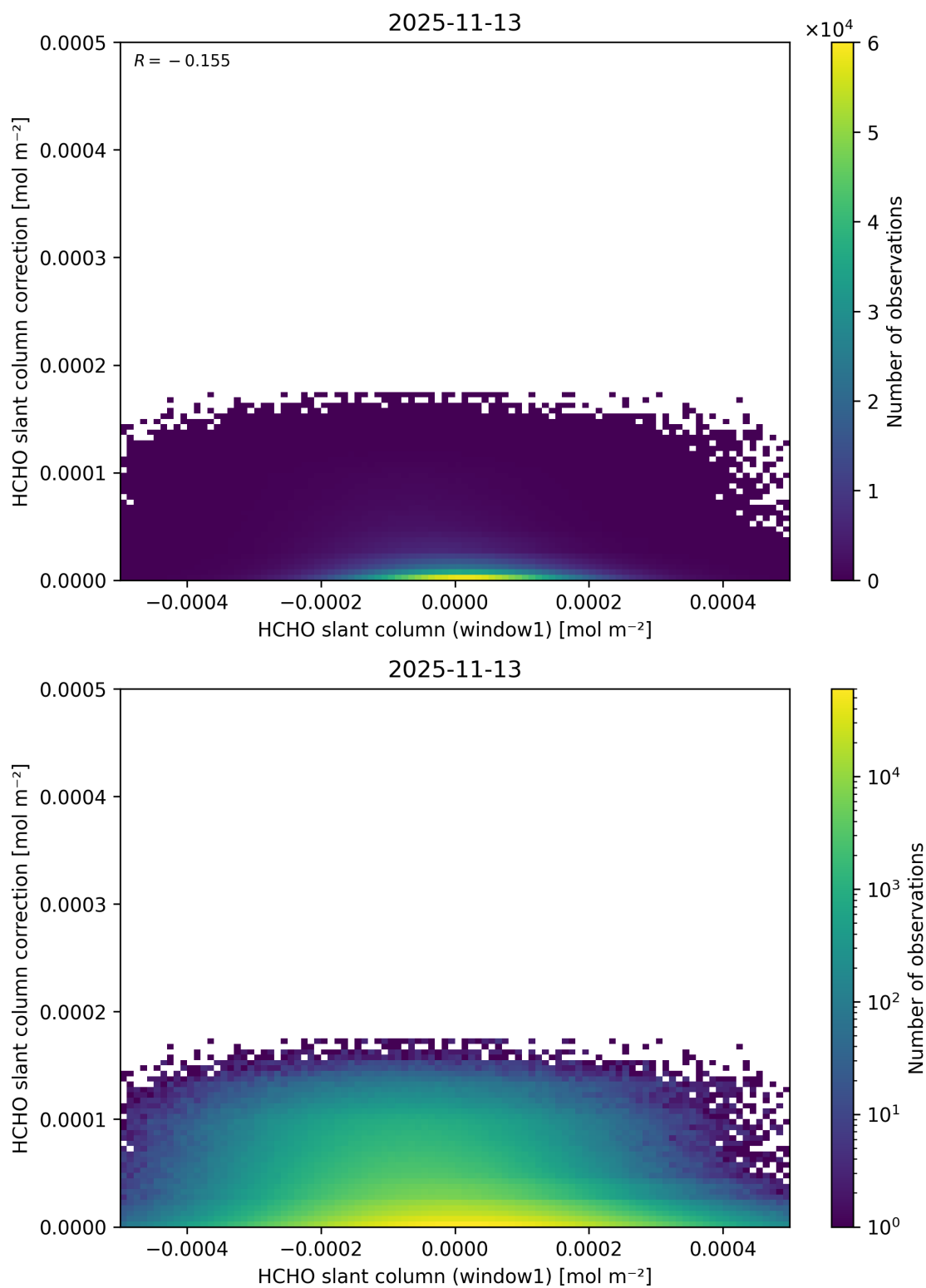
Figure 93: Scatter density plot of “HCHO slant column (window1)” against “HCHO slant column correction” for 2025-11-12 to 2025-11-14.
