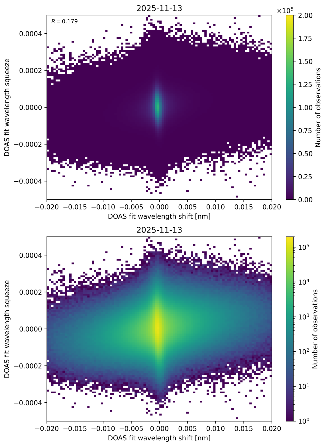
Figure 70: Scatter density plot of “DOAS fit wavelength shift” against “DOAS fit wavelength squeeze” for 2025-11-12 to 2025-11-14.
