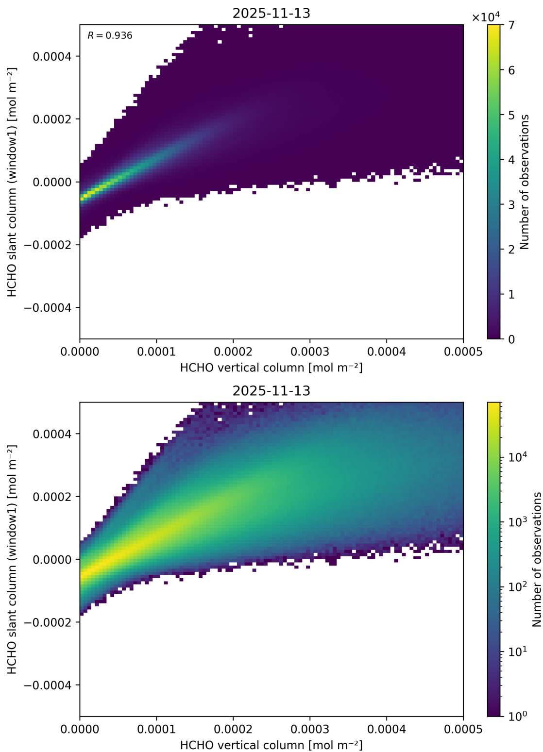
Figure 144: Scatter density plot of “HCHO vertical column” against “HCHO slant column (window1)” for 2025-11-12 to 2025-11-14.
