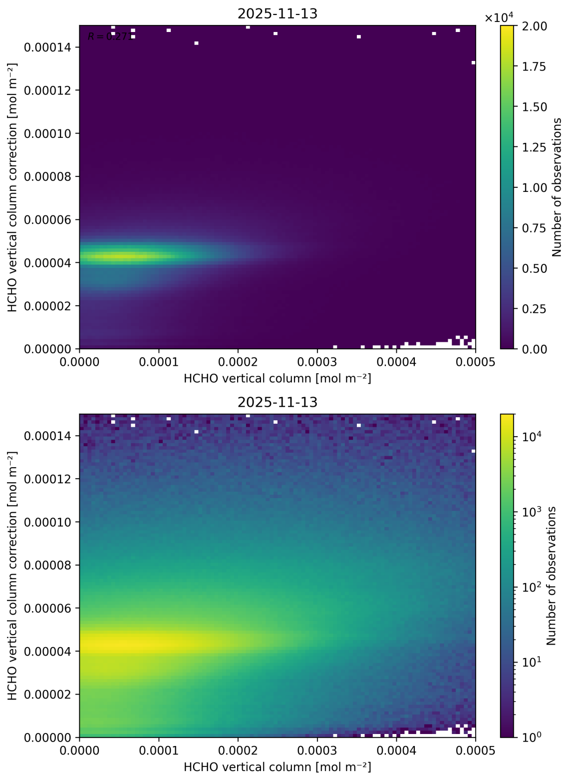
Figure 148: Scatter density plot of “HCHO vertical column” against “HCHO vertical column correction” for 2025-11-12 to 2025-11-14.
