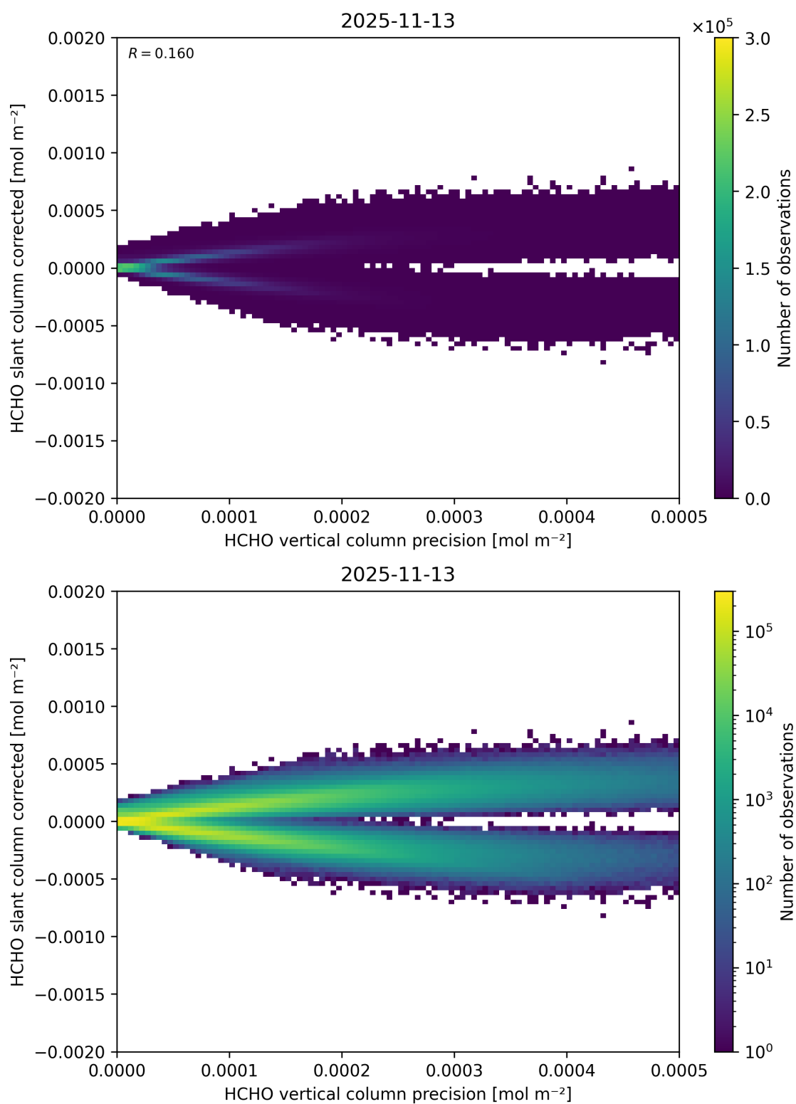
Figure 156: Scatter density plot of “HCHO vertical column precision” against “HCHO slant column corrected” for 2025-11-12 to 2025-11-14.
