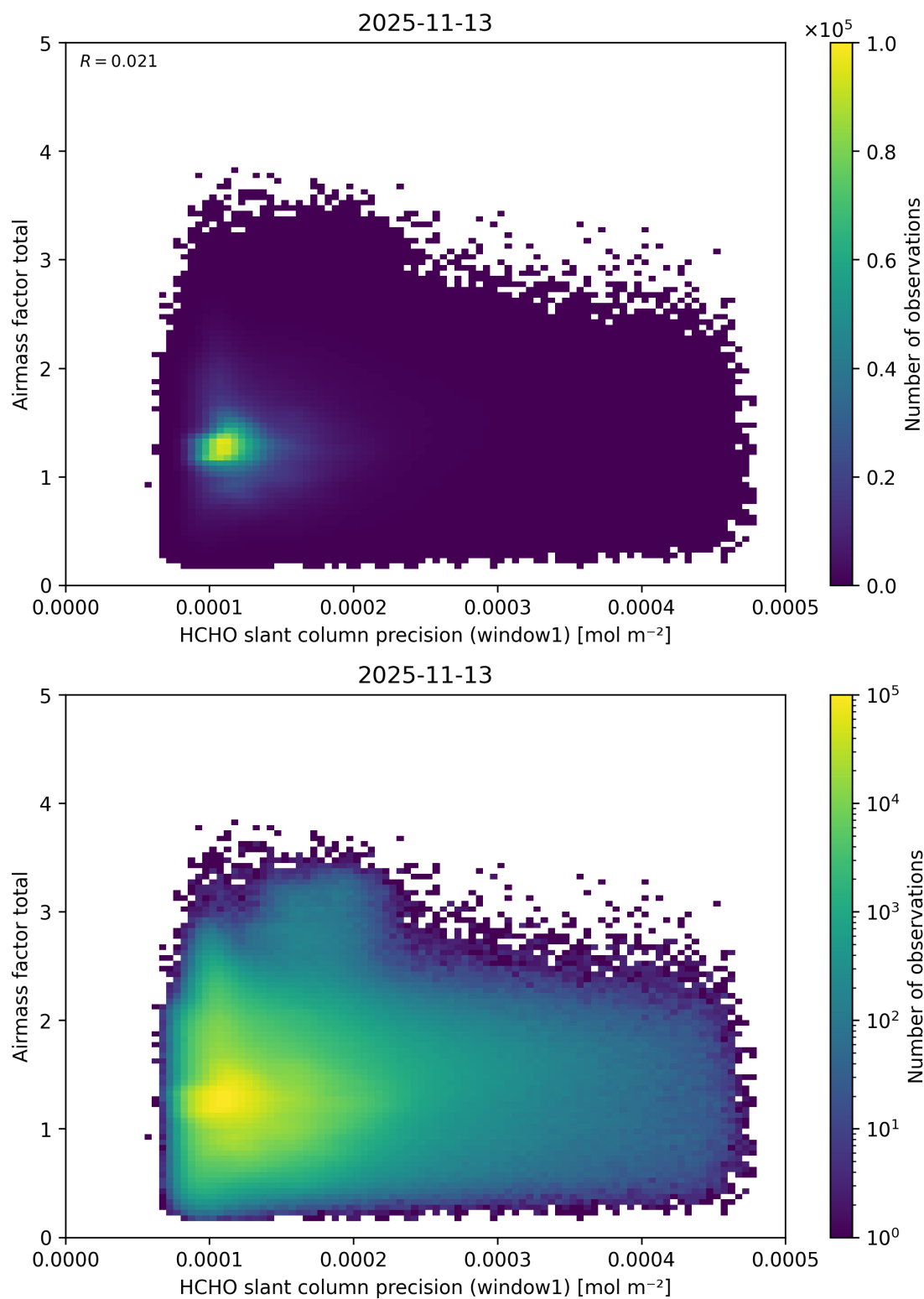
Figure 105: Scatter density plot of “HCHO slant column precision (window1)” against “Airmass factor total” for 2025-11-12 to 2025-11-14.
