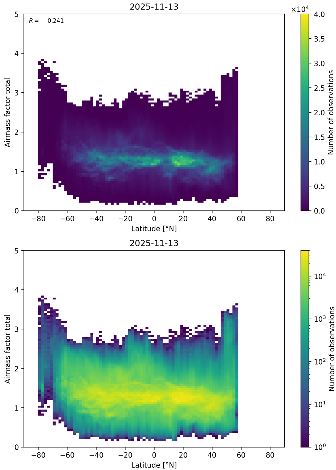
Figure 179: Scatter density plot of “Latitude” against “Airmass factor total” for 2025-11-12 to 2025-11-14.
