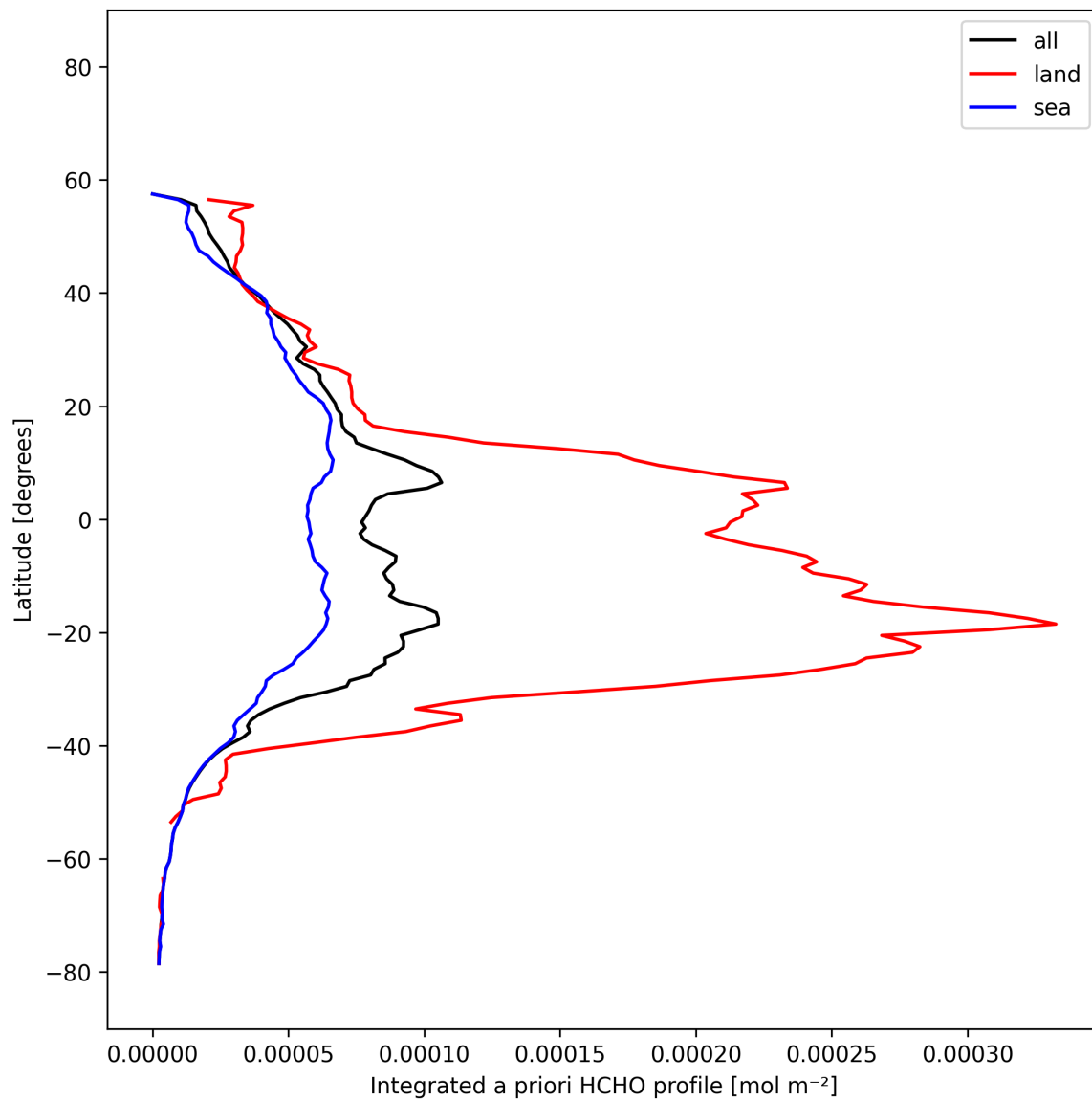
Figure 30: Zonal average of “Integrated a priori HCHO profile” for 2025-11-12 to 2025-11-14.
