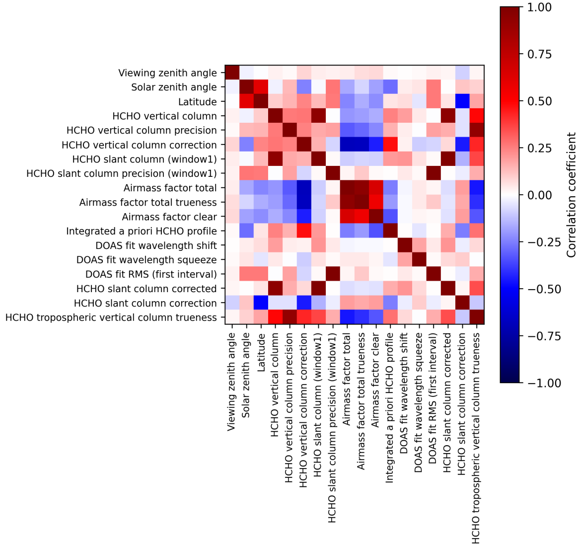
Figure 2: Map of correlation matrix for 2025-11-12 to 2025-11-14.
