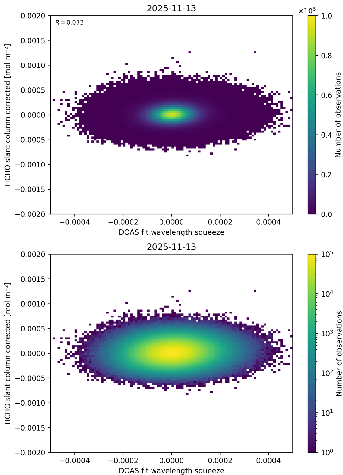
Figure 75: Scatter density plot of “DOAS fit wavelength squeeze” against “HCHO slant column corrected” for 2025-11-12 to 2025-11-14.
