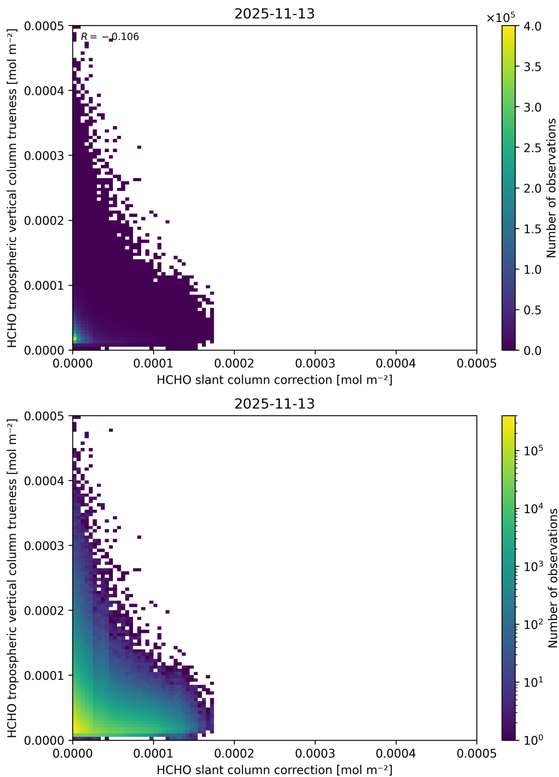
Figure 87: Scatter density plot of “HCHO slant column correction” against “HCHO tropospheric vertical column trueness” for 2025-11-12 to 2025-11-14.
