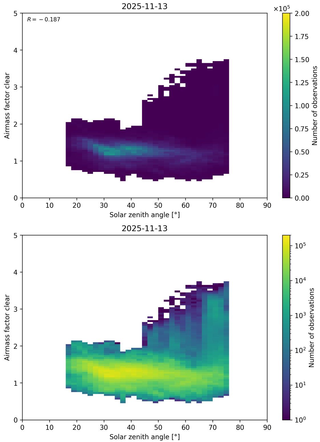
Figure 189: Scatter density plot of “Solar zenith angle” against “Airmass factor clear” for 2025-11-12 to 2025-11-14.
