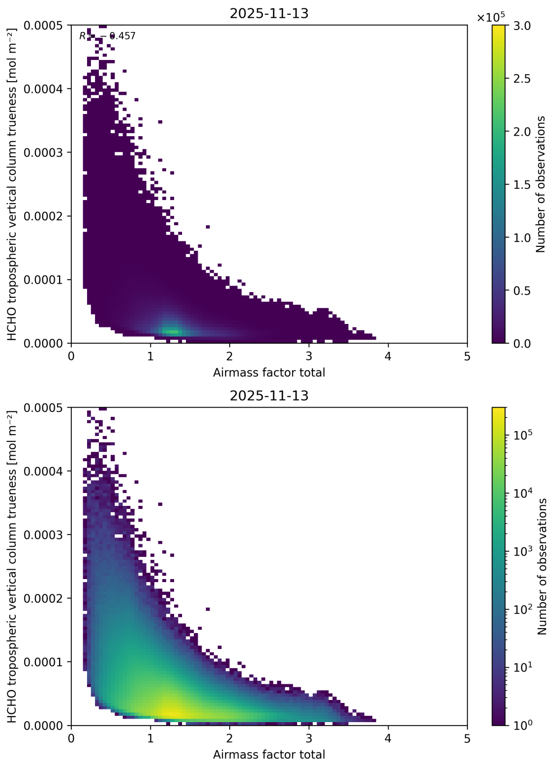
Figure 116: Scatter density plot of “Air mass factor total” against “HCHO tropospheric vertical column trueiness” for 2025-11-12 to 2025-11-14.
