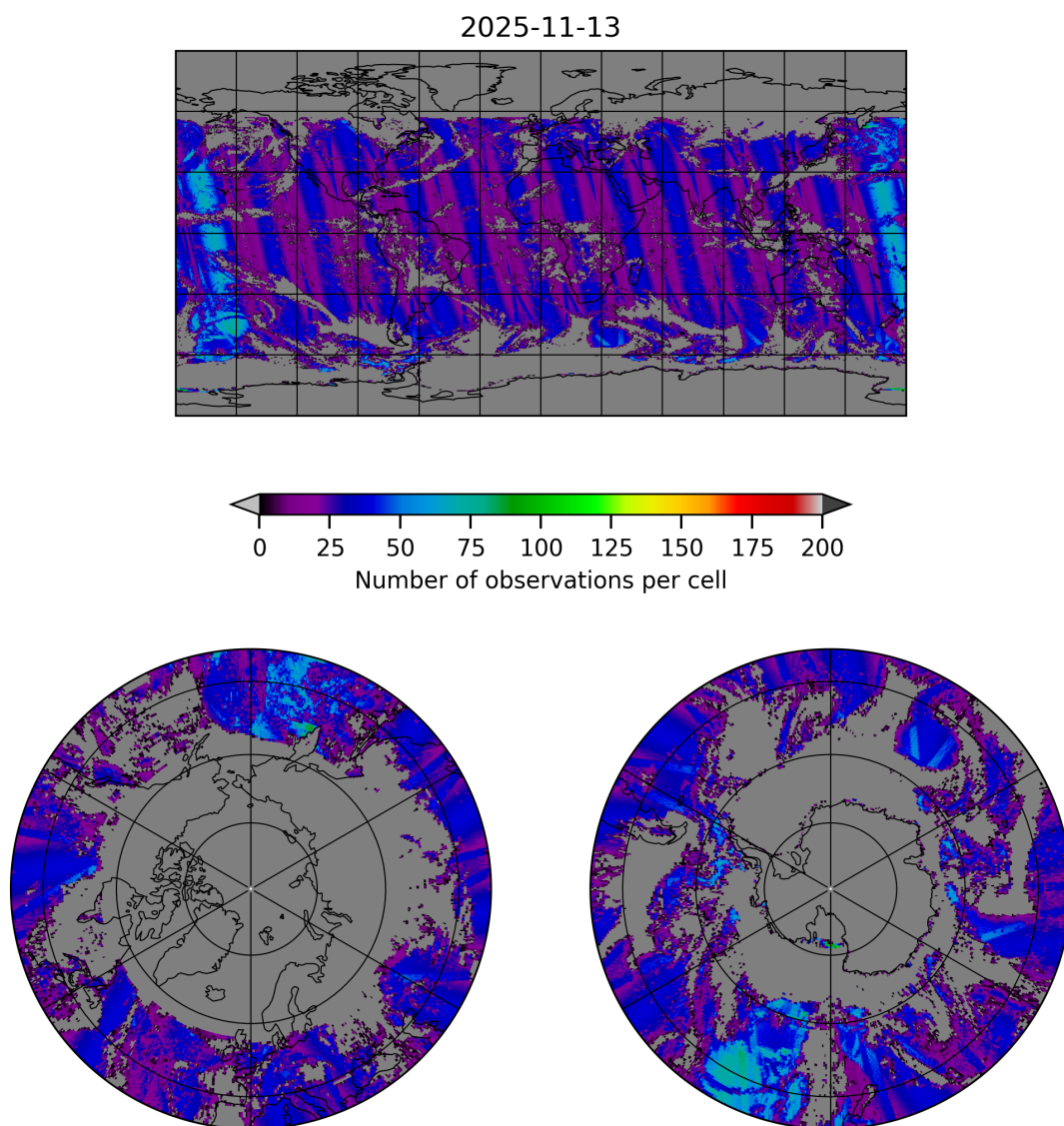
Figure 20: Map of the number of observations for 2025-11-12 to 2025-11-14
