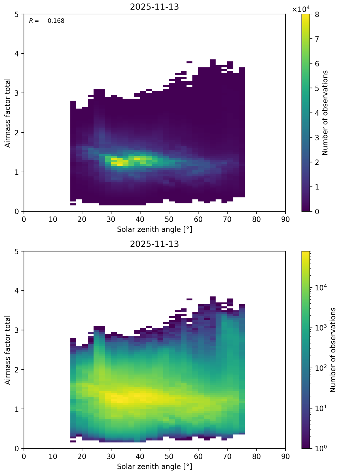
Figure 194: Scatter density plot of “Solar zenith angle” against “Airmass factor total” for 2025-11-12 to 2025-11-14.
