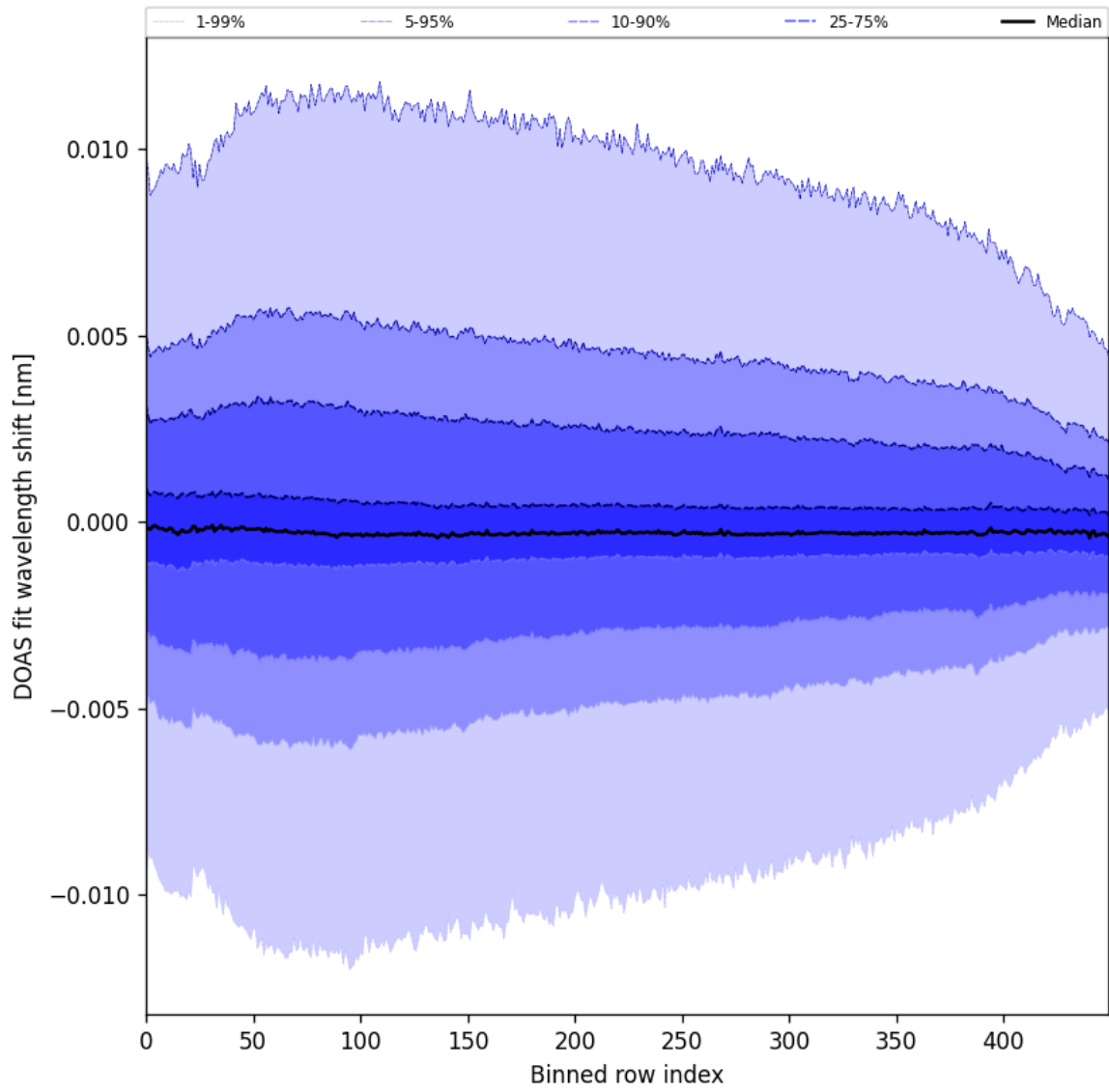
Figure 61: Along track statistics of “DOAS fit wavelength shift” for 2025-11-12 to 2025-11-14
