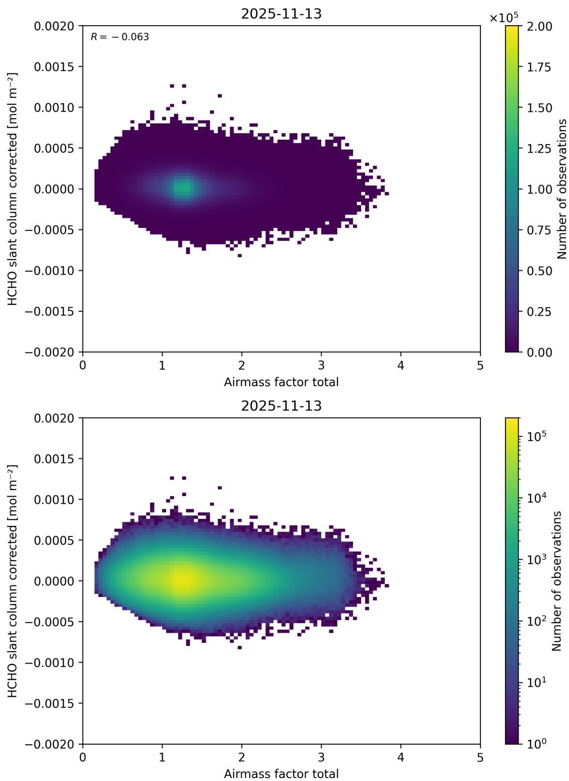
Figure 113: Scatter density plot of “Airmass factor total” against “HCHO slant column corrected” for 2025-11-12 to 2025-11-14.
