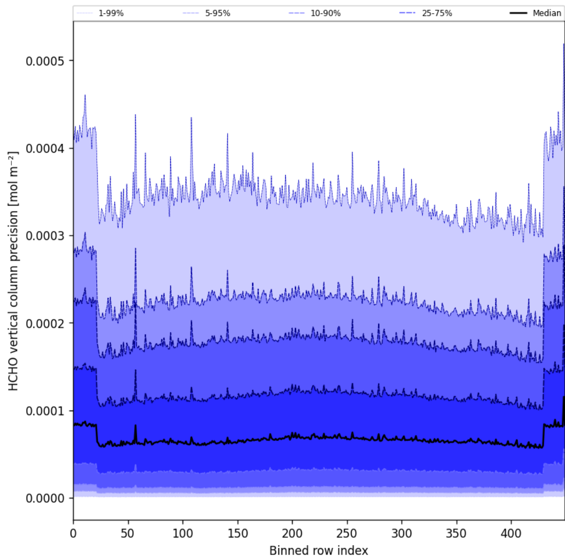
Figure 53: Along track statistics of "HCHO vertical column precision" for 2025-11-12 to 2025-11-14
