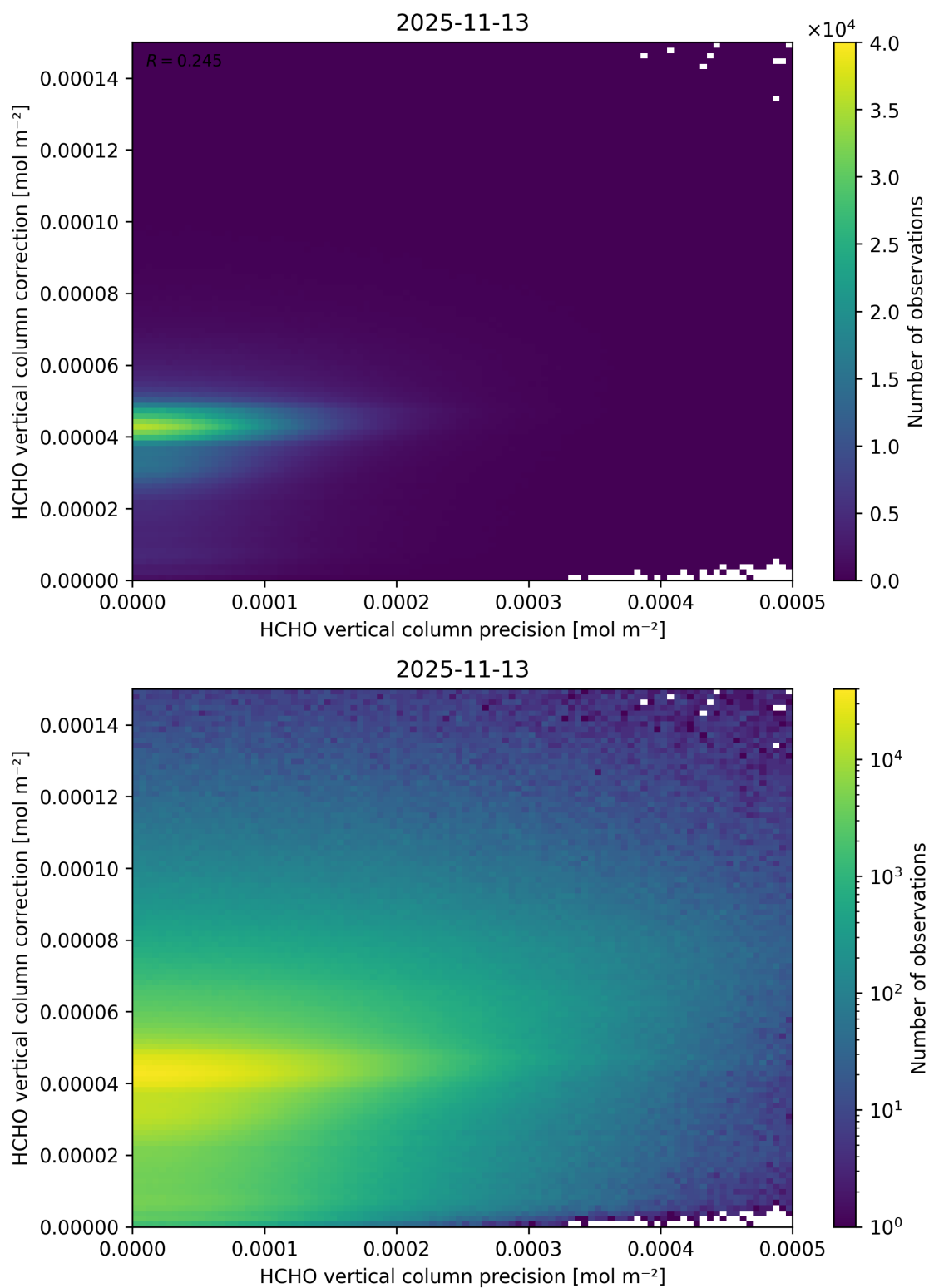
Figure 162: Scatter density plot of “HCHO vertical column precision” against “HCHO vertical column correction” for 2025-11-12 to 2025-11-14.
