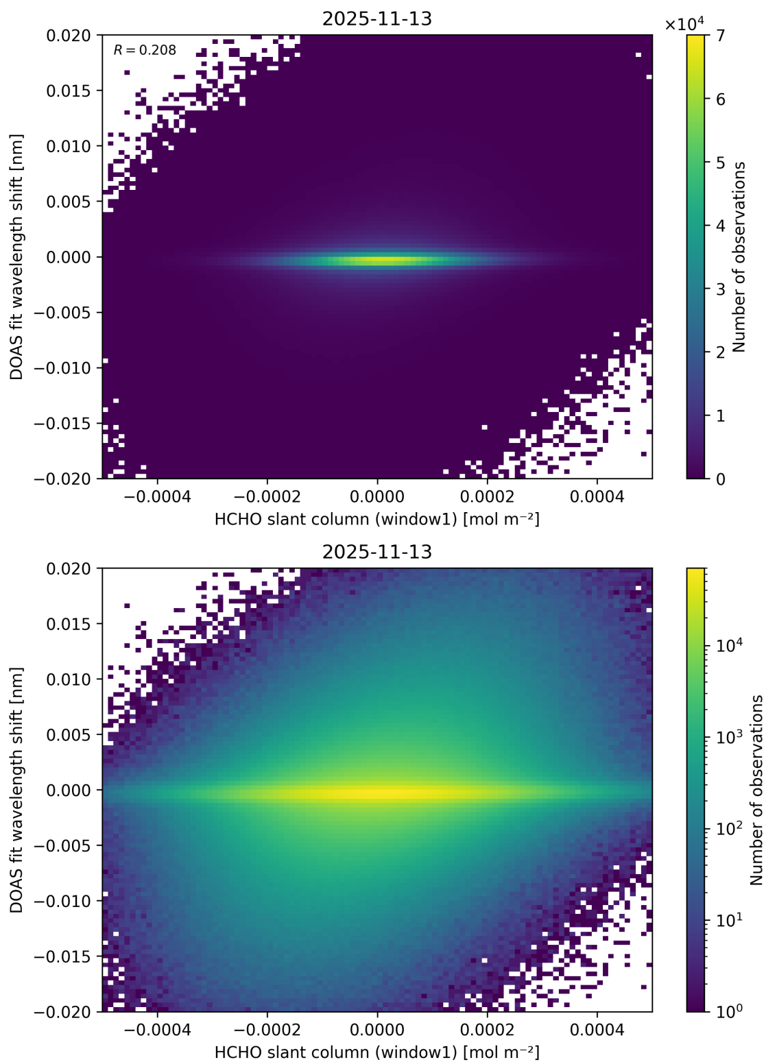
Figure 89: Scatter density plot of “HCHO slant column (window1)” against “DOAS fit wavelength shift” for 2025-11-12 to 2025-11-14.
