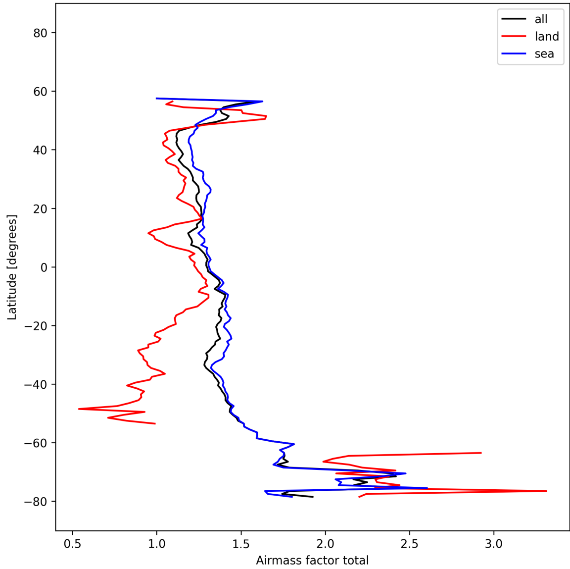
Figure 27: Zonal average of “Airmass factor total” for 2025-11-12 to 2025-11-14.
