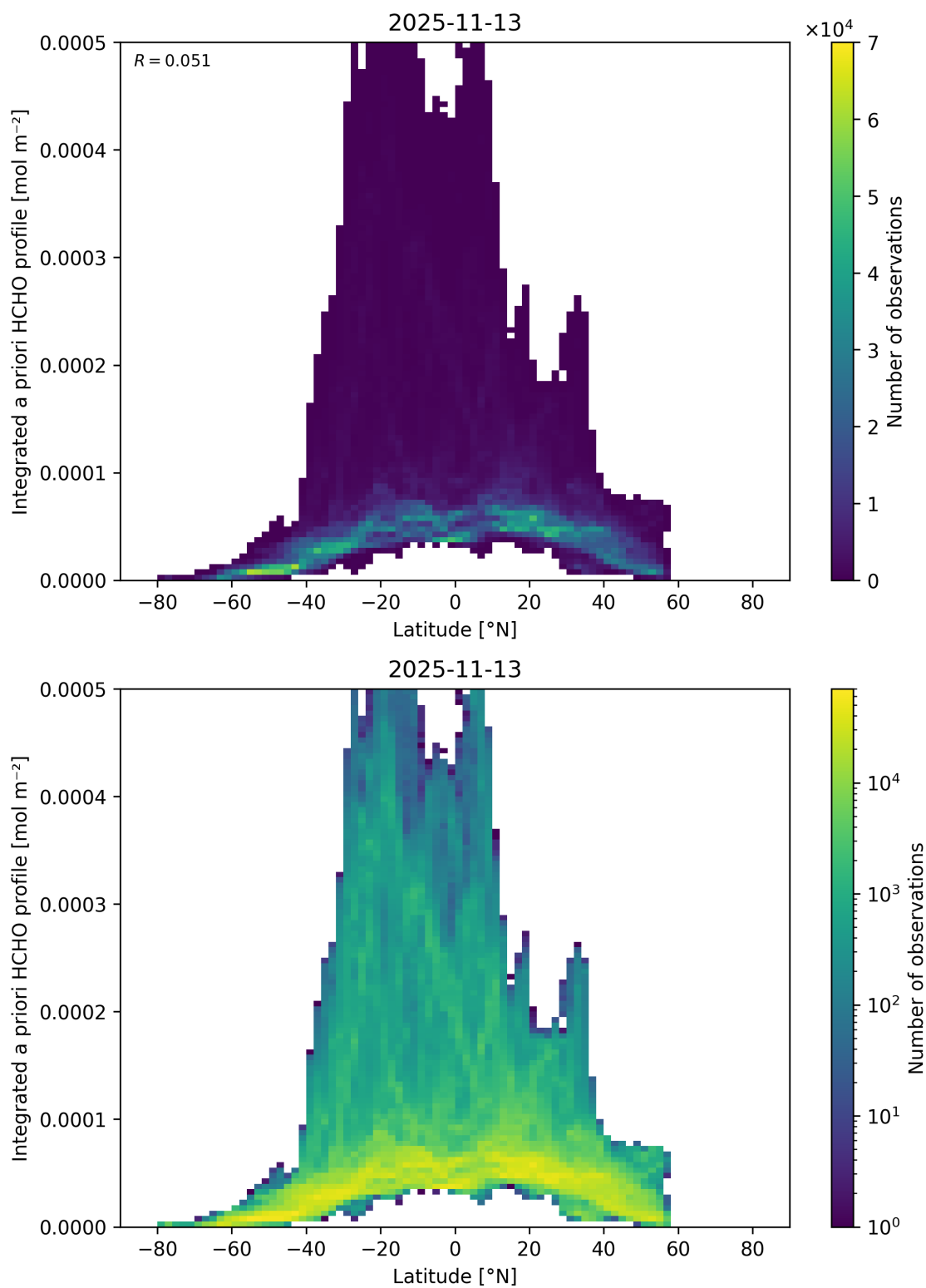
Figure 185: Scatter density plot of “Latitude” against “Integrated a priori HCHO profile” for 2025-11-12 to 2025-11-14.
