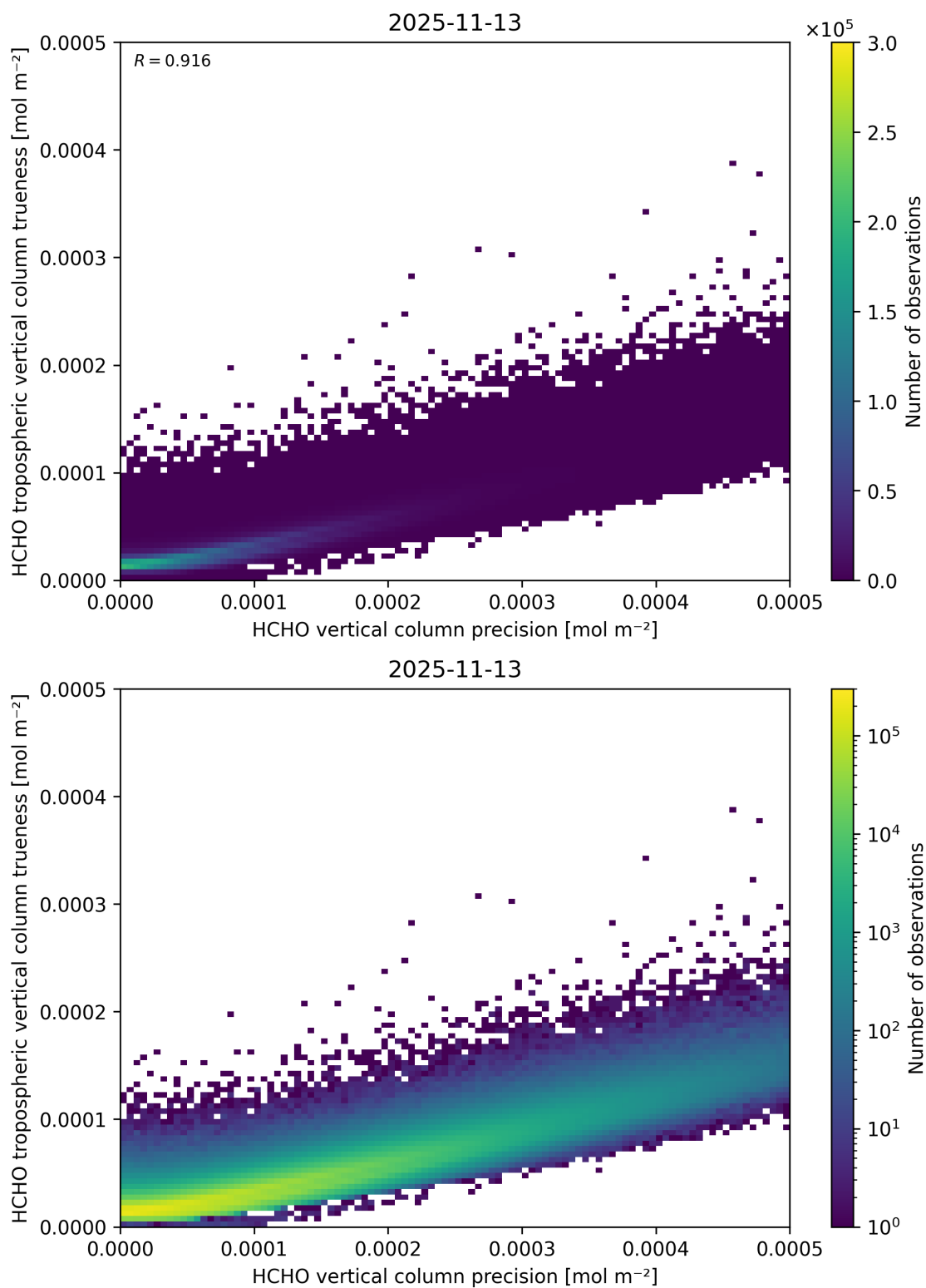
Figure 163: Scatter density plot of “HCHO vertical column precision” against “HCHO tropospheric vertical column true-ness” for 2025-11-12 to 2025-11-14.
