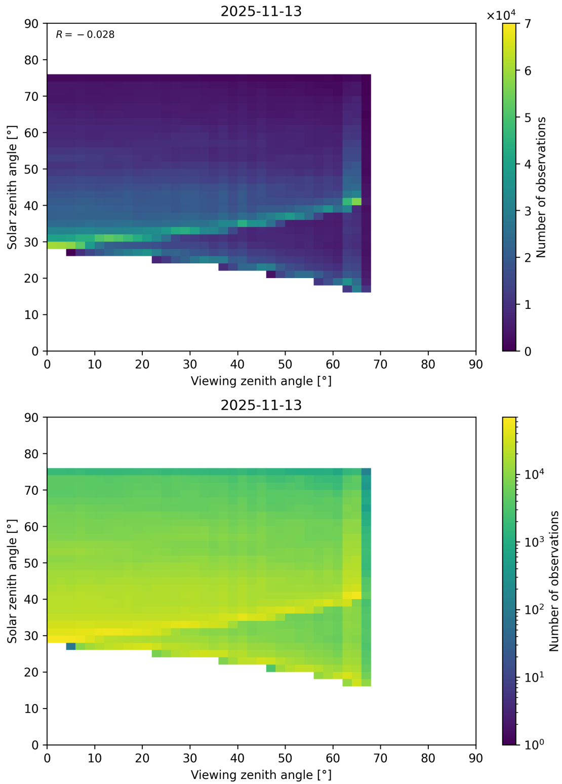
Figure 218: Scatter density plot of “Viewing zenith angle” against “Solar zenith angle” for 2025-11-12 to 2025-11-14.
