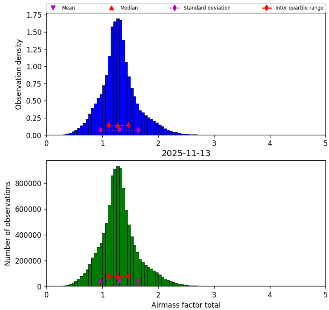
Figure 42: Histogram of “Airmass factor total” for 2025-11-12 to 2025-11-14
