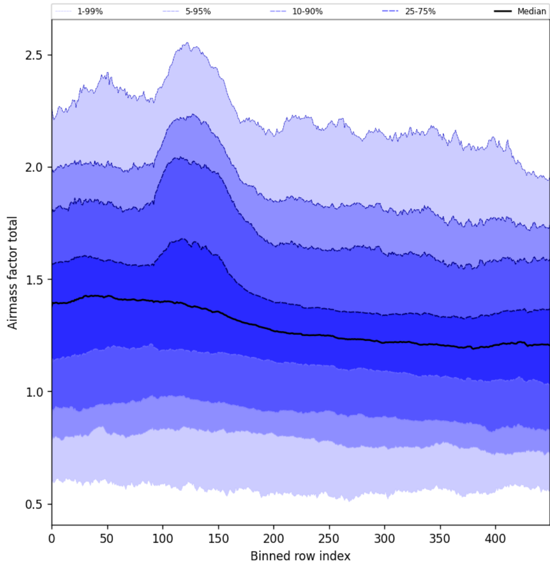
Figure 57: Along track statistics of “Airmass factor total” for 2025-11-12 to 2025-11-14
