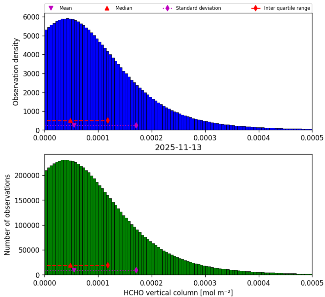
Figure 37: Histogram of “HCHO vertical column” for 2025-11-12 to 2025-11-14
