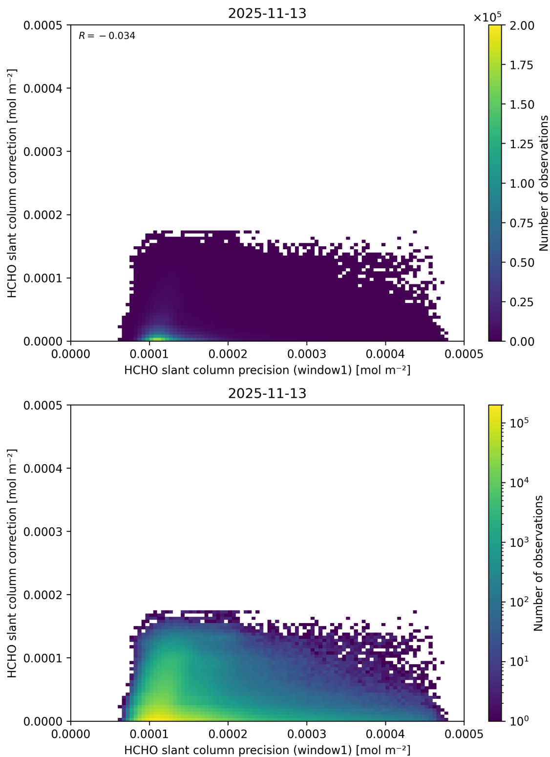
Figure 104: Scatter density plot of “HCHO slant column precision (window1)” against “HCHO slant column correction” for 2025-11-12 to 2025-11-14.
