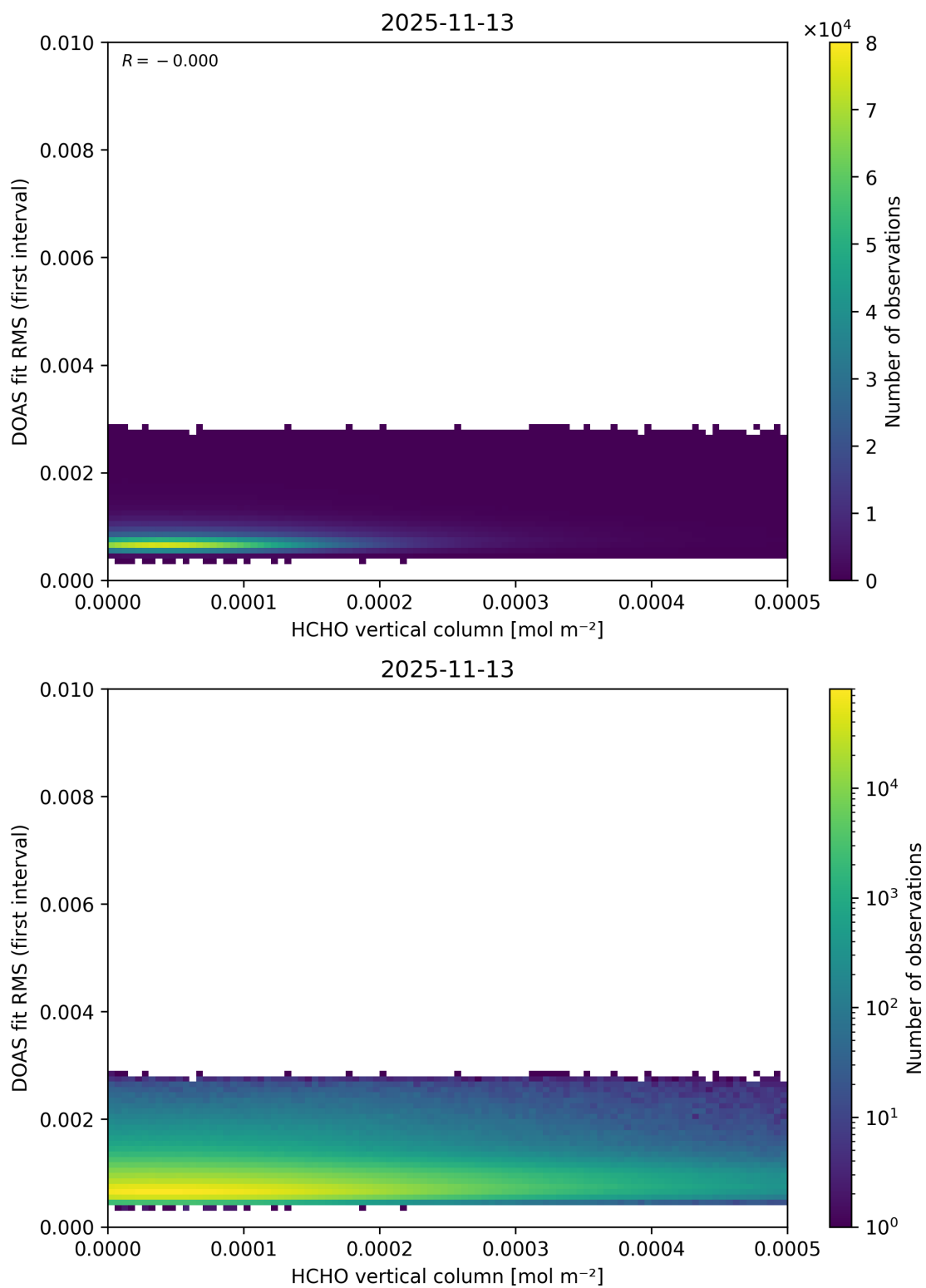
Figure 138: Scatter density plot of “HCHO vertical column” against “DOAS fit RMS (first interval)” for 2025-11-12 to 2025-11-14.
