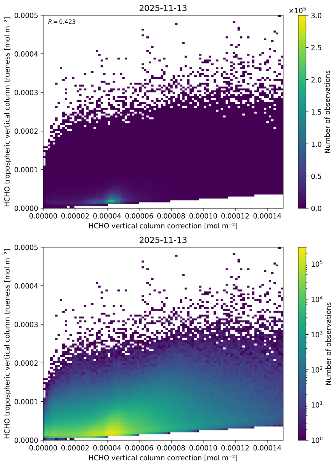
Figure 136: Scatter density plot of “HCHO vertical column correction” against “HCHO tropospheric vertical column true-ness” for 2025-11-12 to 2025-11-14.
