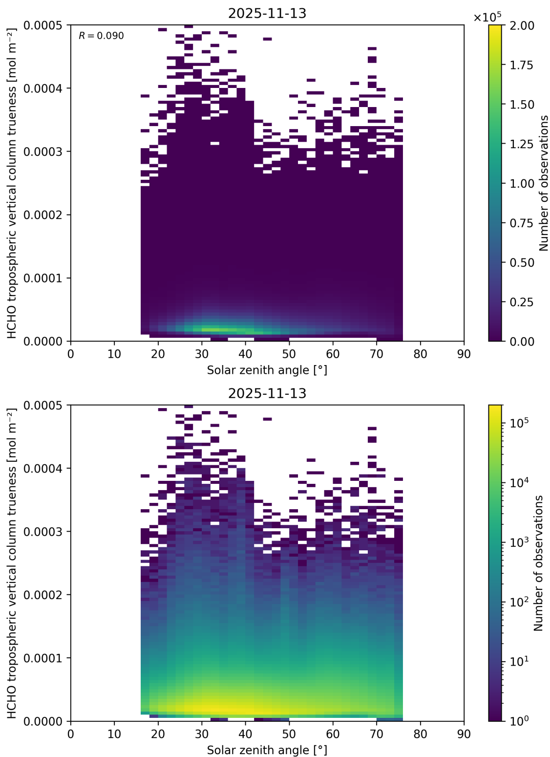
Figure 199: Scatter density plot of “Solar zenith angle” against “HCHO tropospheric vertical column trueness” for 2025-11-12 to 2025-11-14.
