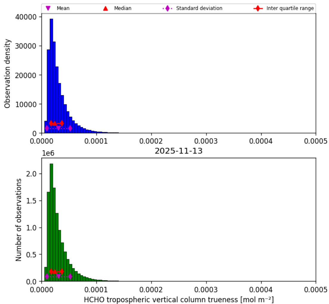
Figure 50: Histogram of “HCHO tropospheric vertical column trueness” for 2025-11-12 to 2025-11-14
