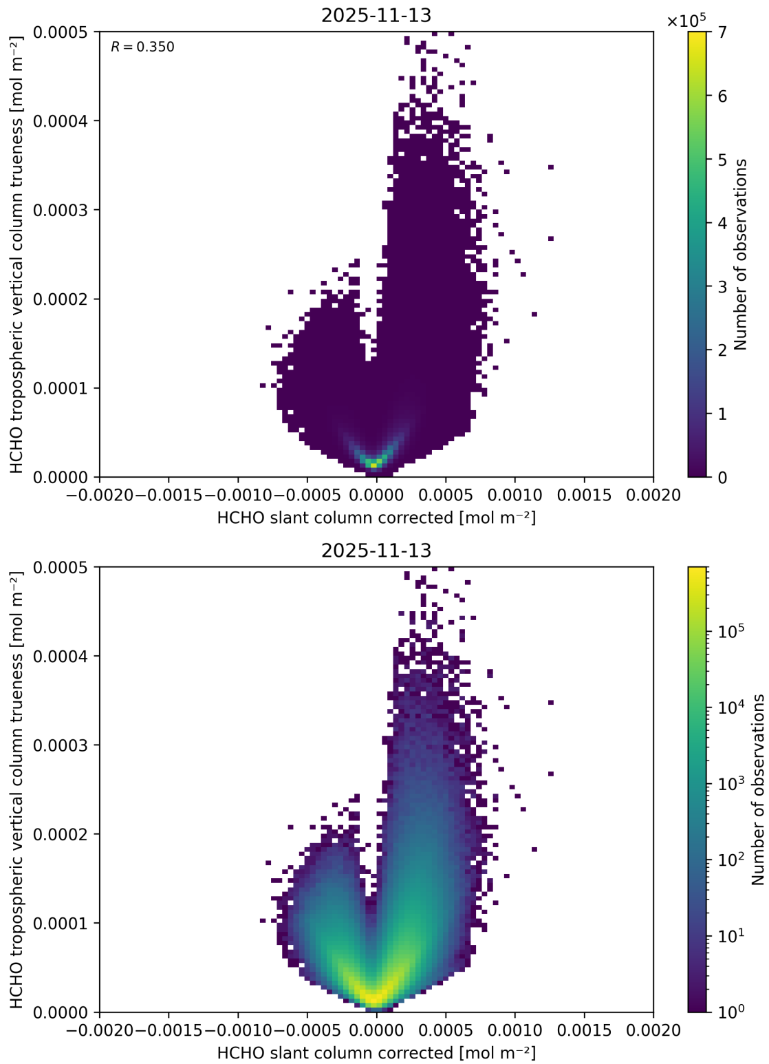
Figure 86: Scatter density plot of “HCHO slant column corrected” against “HCHO tropospheric vertical column trueness” for 2025-11-12 to 2025-11-14.
