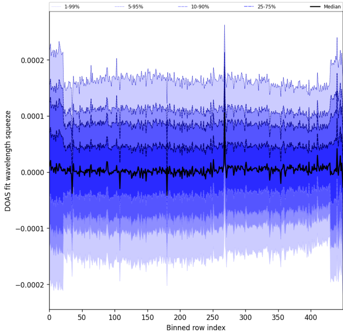
Figure 62: Along track statistics of “DOAS fit wavelength squeeze” for 2025-11-12 to 2025-11-14
