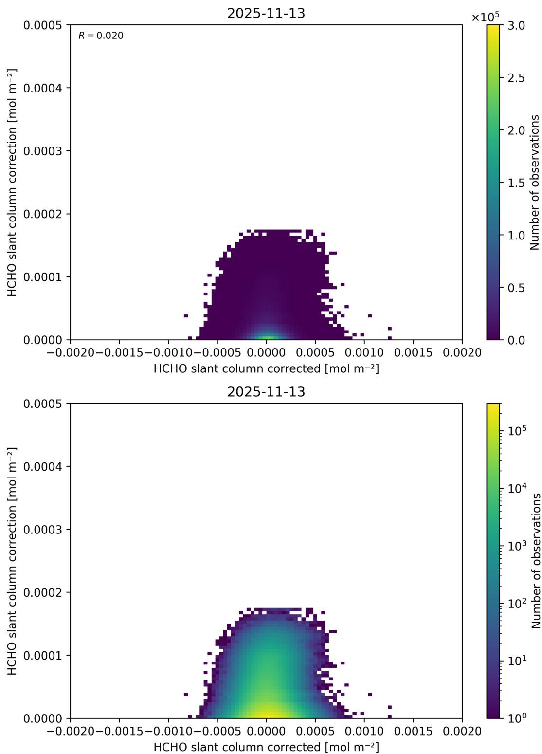
Figure 85: Scatter density plot of “HCHO slant column corrected” against “HCHO slant column correction” for 2025-11-12 to 2025-11-14.
