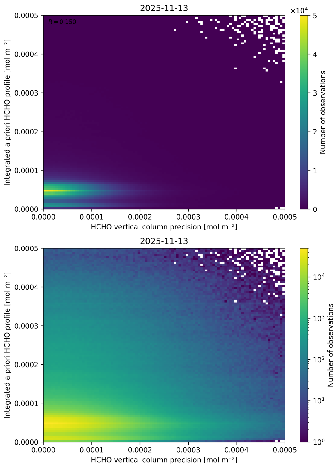
Figure 164: Scatter density plot of “HCHO vertical column precision” against “Integrated a priori HCHO profile” for 2025-11-12 to 2025-11-14.
