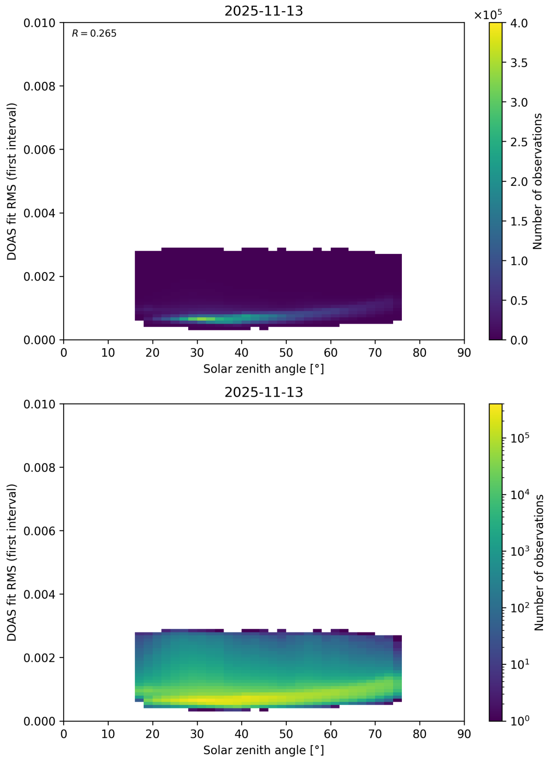
Figure 186: Scatter density plot of “Solar zenith angle” against “DOAS fit RMS (first interval)” for 2025-11-12 to 2025-11-14.
