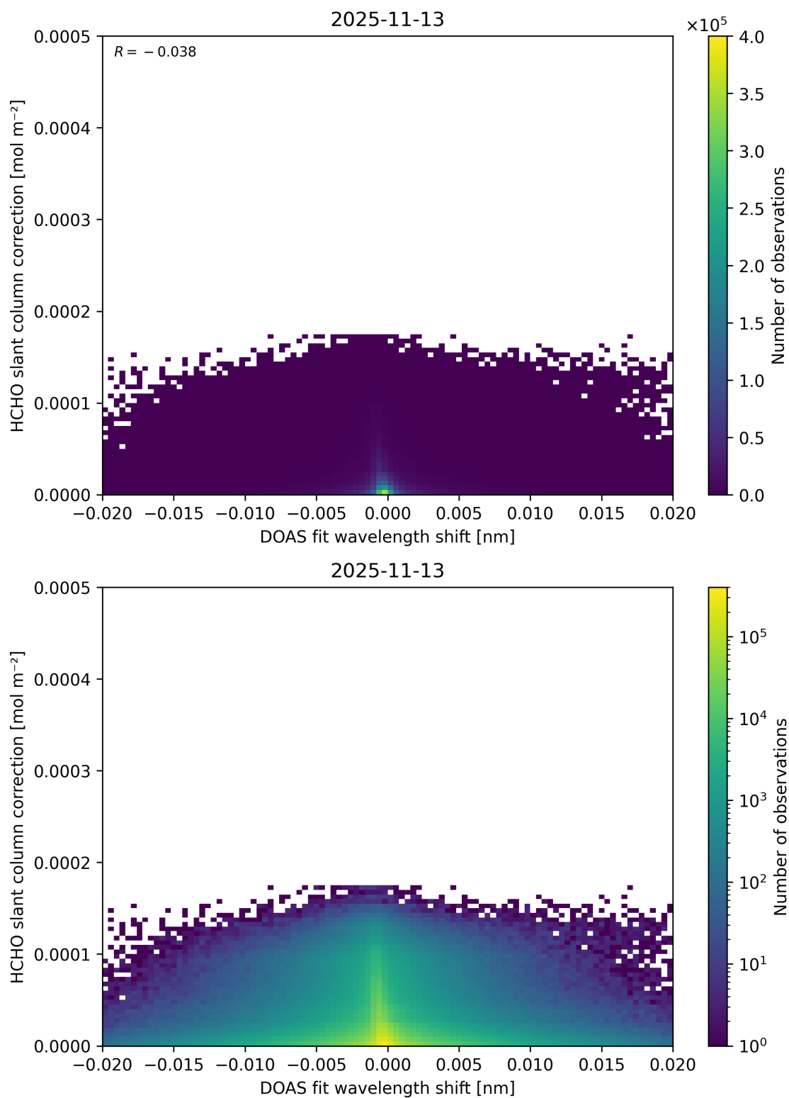
Figure 72: Scatter density plot of “DOAS fit wavelength shift” against “HCHO slant column correction” for 2025-11-12 to 2025-11-14.
