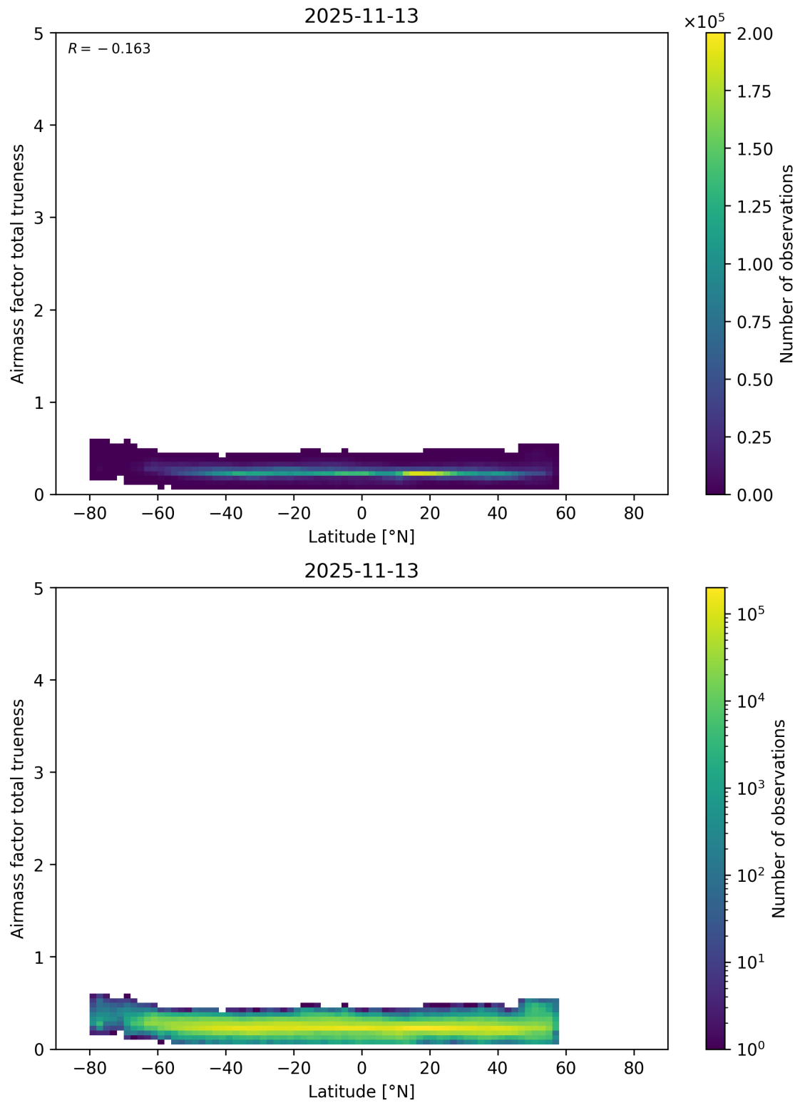
Figure 180: Scatter density plot of “Latitude” against “Airmass factor total trueness” for 2025-11-12 to 2025-11-14.
