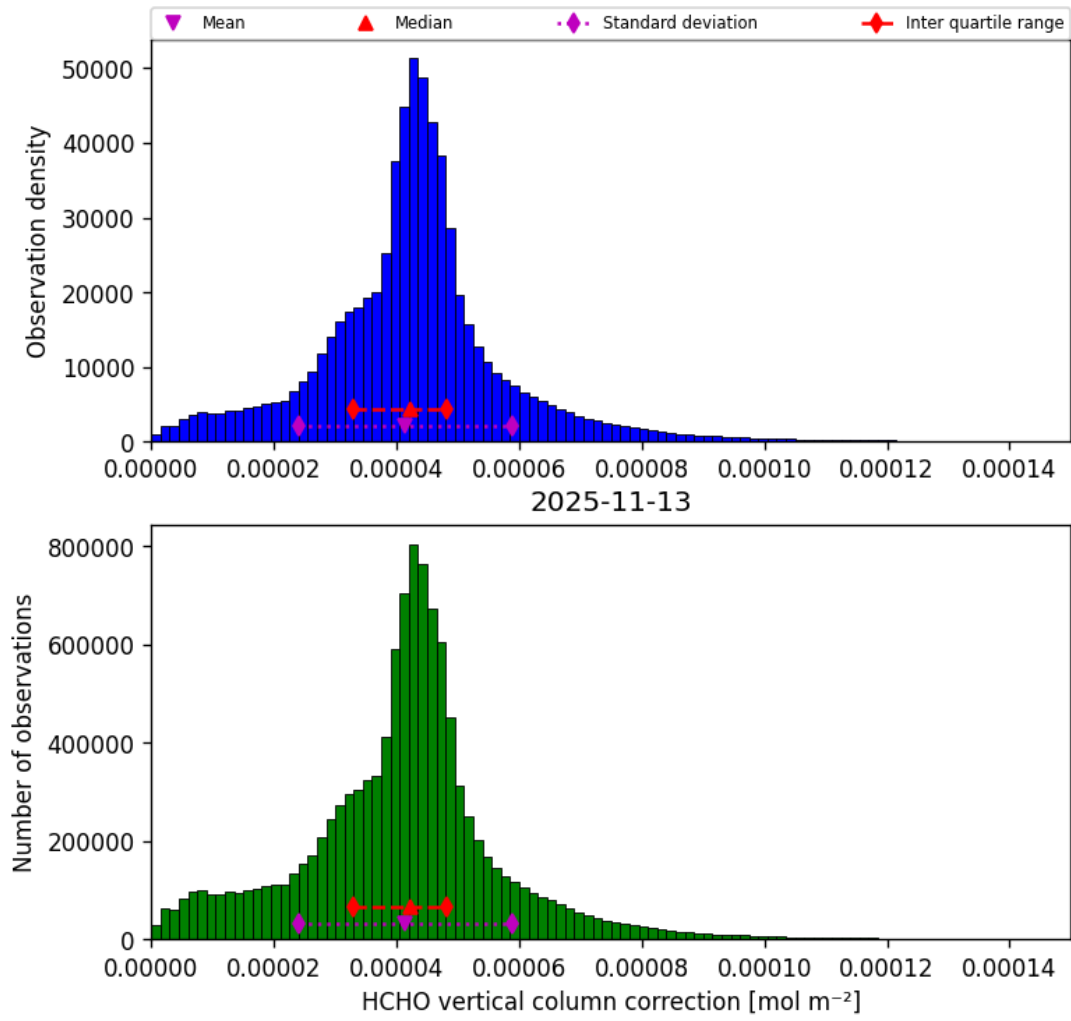
Figure 39: Histogram of “HCHO vertical column correction” for 2025-11-12 to 2025-11-14
