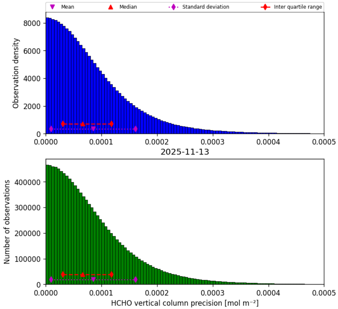
Figure 38: Histogram of “HCHO vertical column precision” for 2025-11-12 to 2025-11-14
