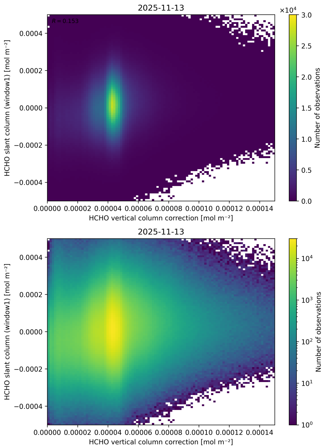
Figure 132: Scatter density plot of “HCHO vertical column correction” against “HCHO slant column (window1)” for 2025-11-12 to 2025-11-14.
