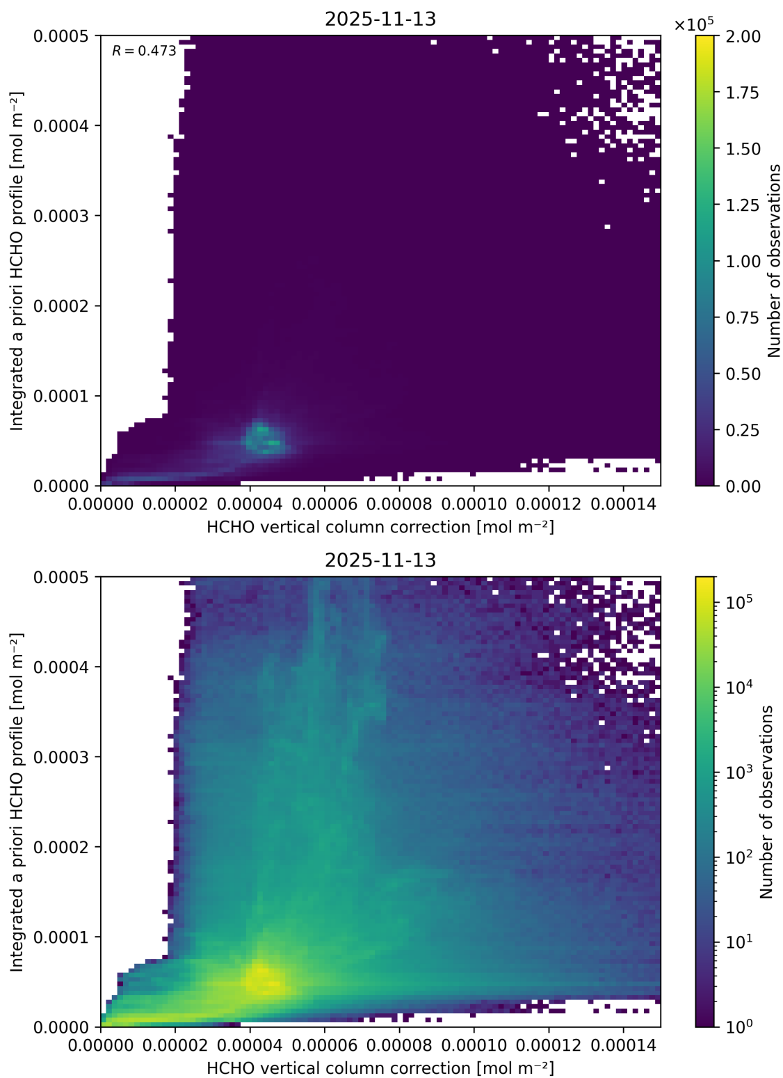
Figure 137: Scatter density plot of “HCHO vertical column correction” against “Integrated a priori HCHO profile” for 2025-11-12 to 2025-11-14.
