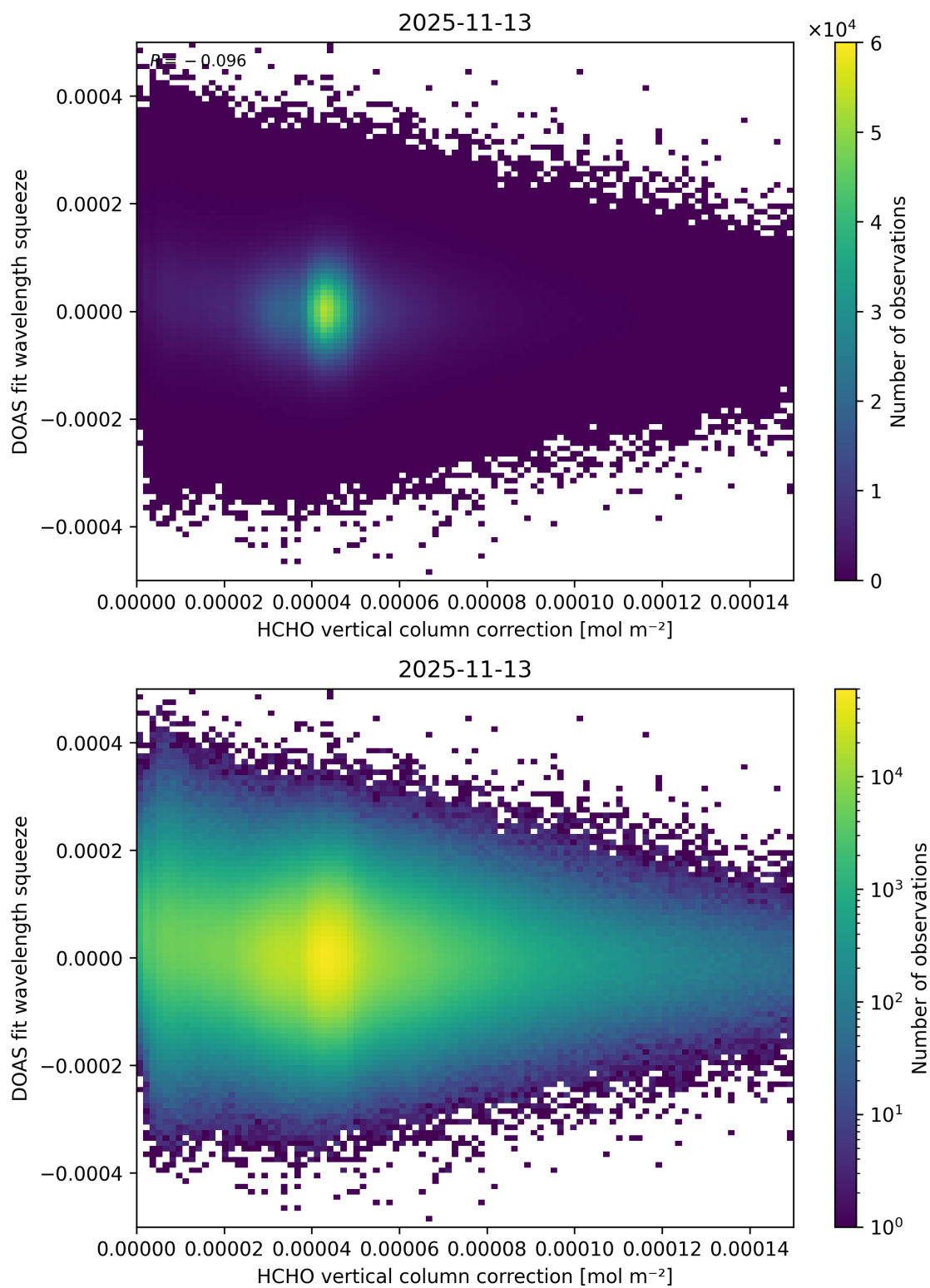
Figure 128: Scatter density plot of “HCHO vertical column correction” against “DOAS fit wavelength squeeze” for 2025-11-12 to 2025-11-14.
