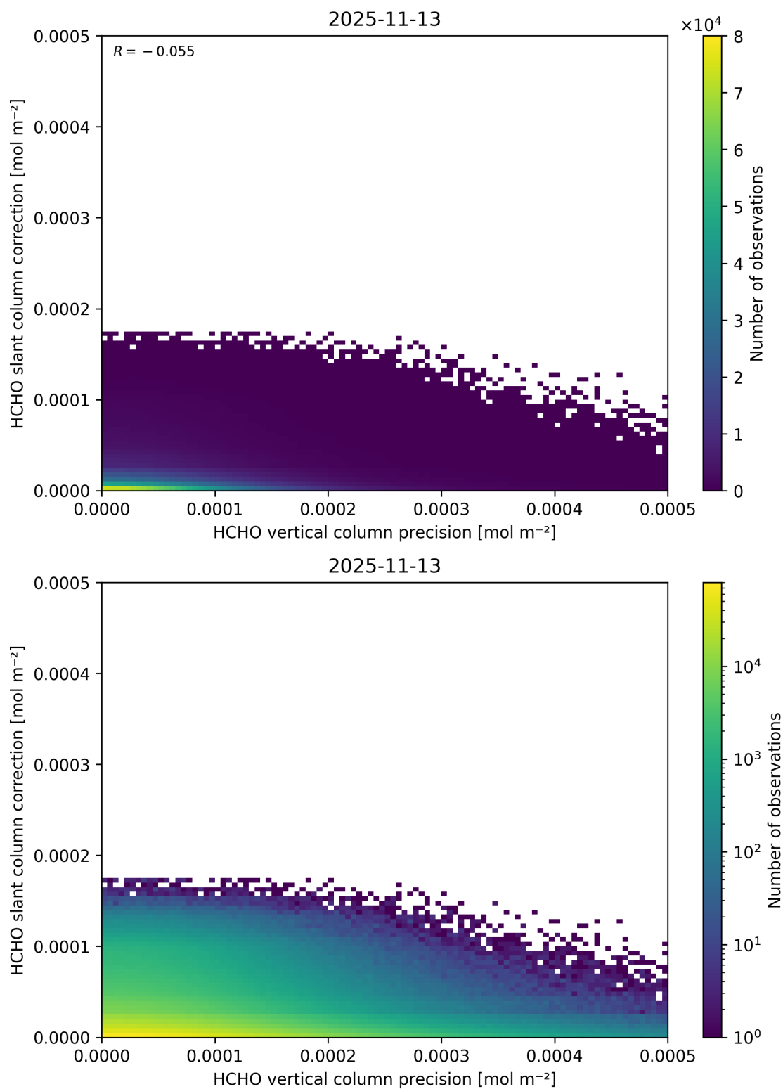
Figure 157: Scatter density plot of “HCHO vertical column precision” against “HCHO slant column correction” for 2025-11-12 to 2025-11-14.
