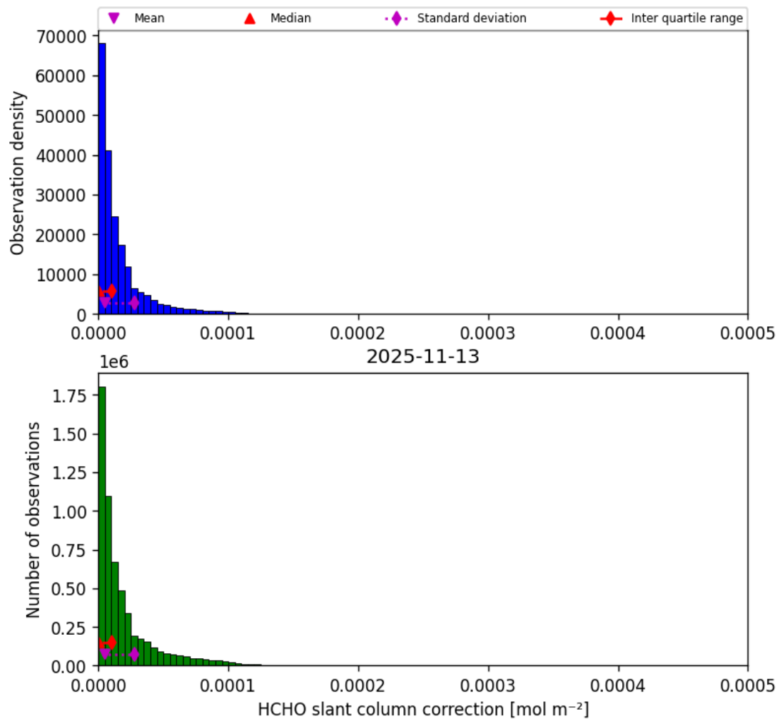
Figure 49: Histogram of “HCHO slant column correction” for 2025-11-12 to 2025-11-14
