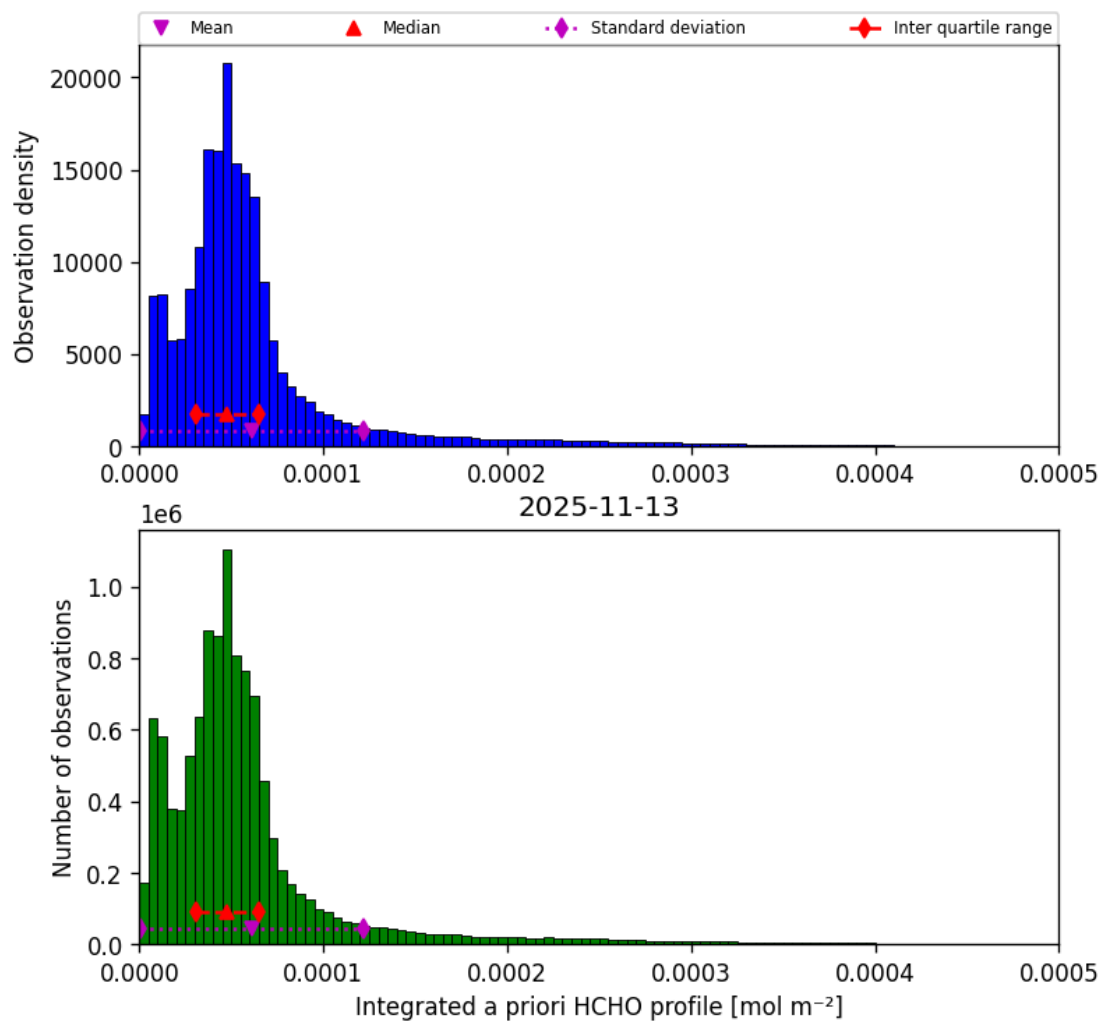
Figure 45: Histogram of “Integrated a priori HCHO profile” for 2025-11-12 to 2025-11-14
