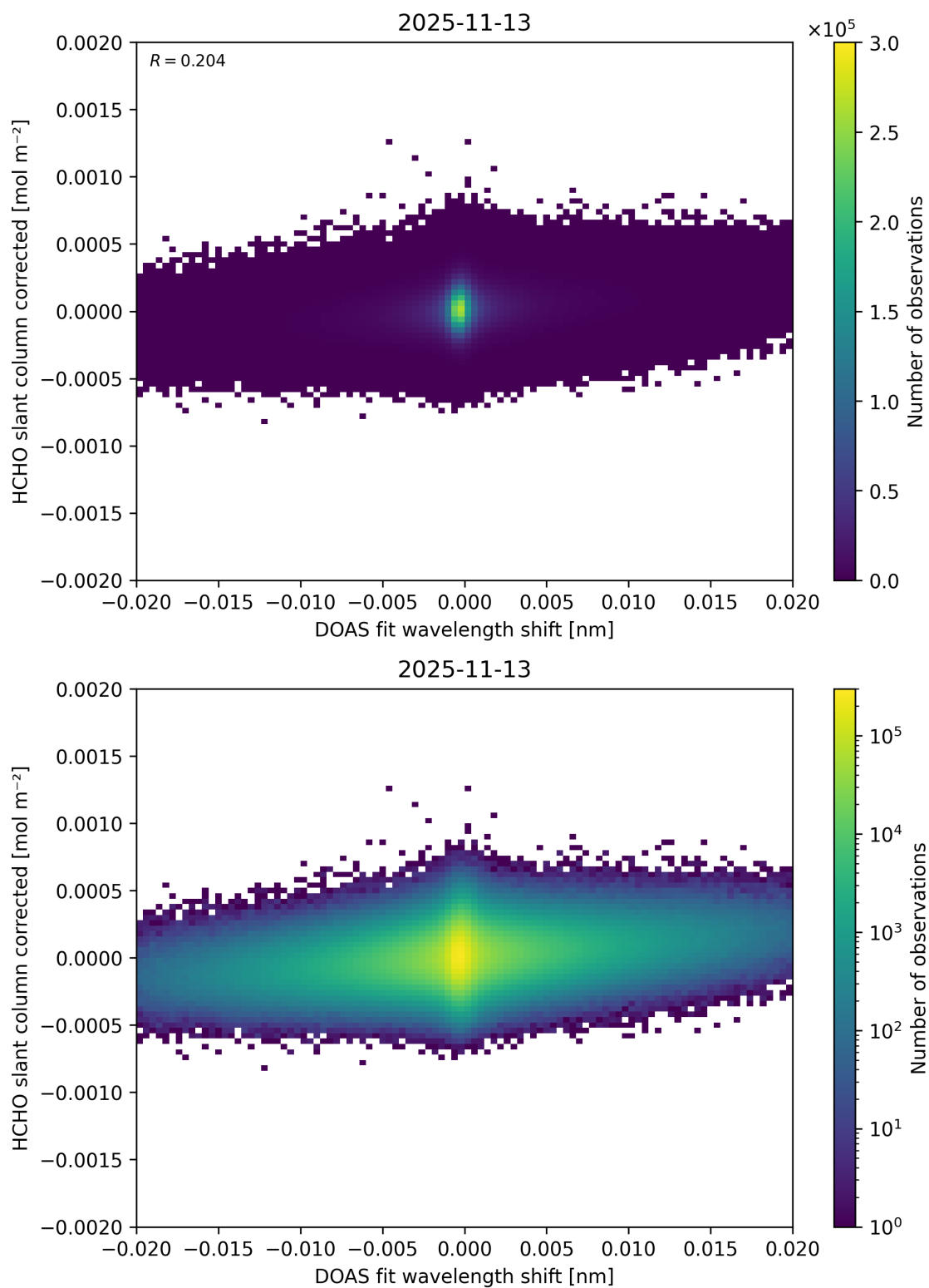
Figure 71: Scatter density plot of “DOAS fit wavelength shift” against “HCHO slant column corrected” for 2025-11-12 to 2025-11-14.
