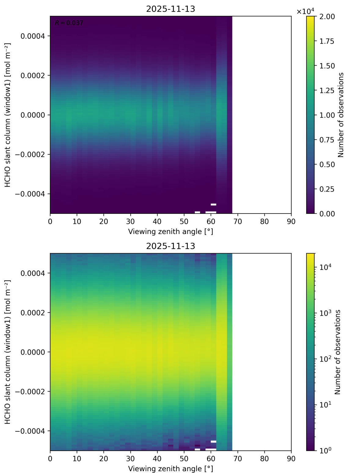
Figure 208: Scatter density plot of “Viewing zenith angle” against “HCHO slant column (window1)” for 2025-11-12 to 2025-11-14.
