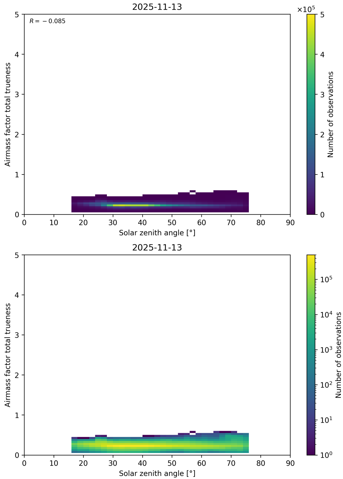
Figure 195: Scatter density plot of “Solar zenith angle” against “Airmass factor total trueneess” for 2025-11-12 to 2025-11-14.
