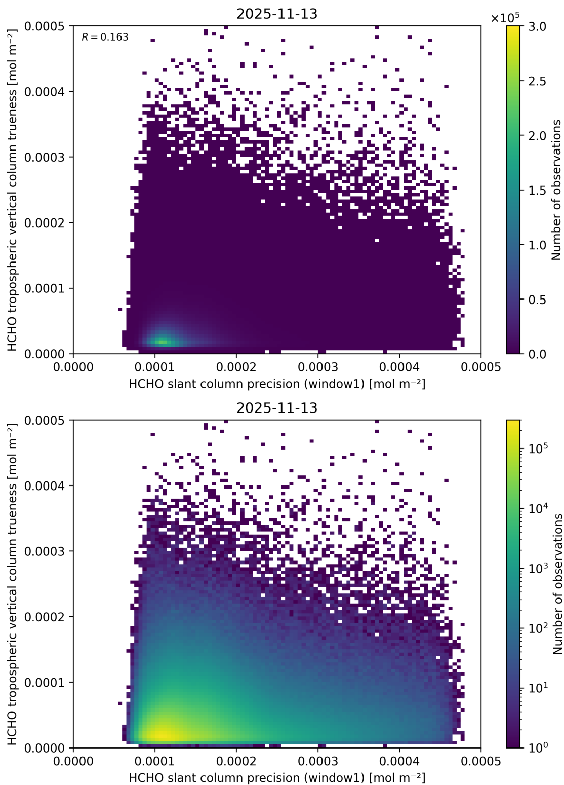
Figure 107: Scatter density plot of “HCHO slant column precision (window1)” against “HCHO tropospheric vertical column trueness” for 2025-11-12 to 2025-11-14.
