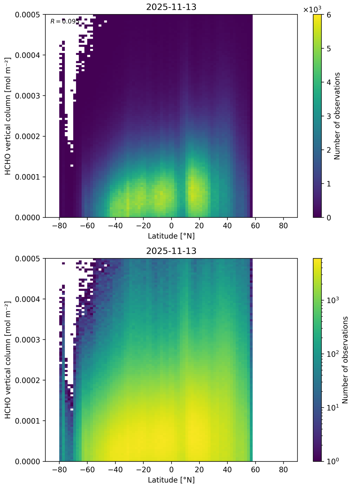
Figure 181: Scatter density plot of “Latitude” against “HCHO vertical column” for 2025-11-12 to 2025-11-14.
