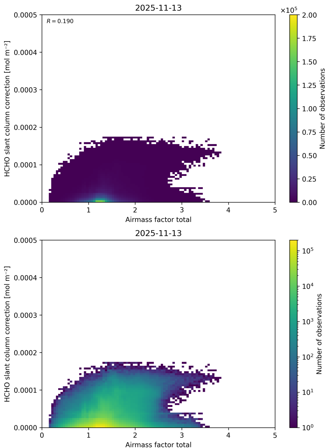
Figure 114: Scatter density plot of “Airmass factor total” against “HCHO slant column correction” for 2025-11-12 to 2025-11-14.
