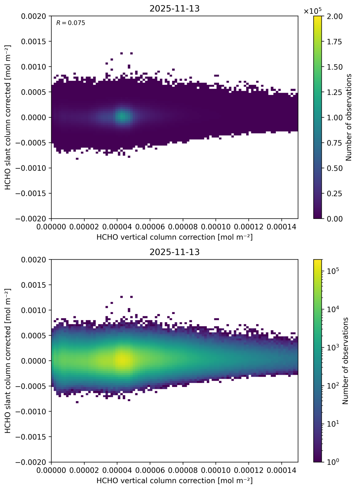
Figure 130: Scatter density plot of “HCHO vertical column correction” against “HCHO slant column corrected” for 2025-11-12 to 2025-11-14.
