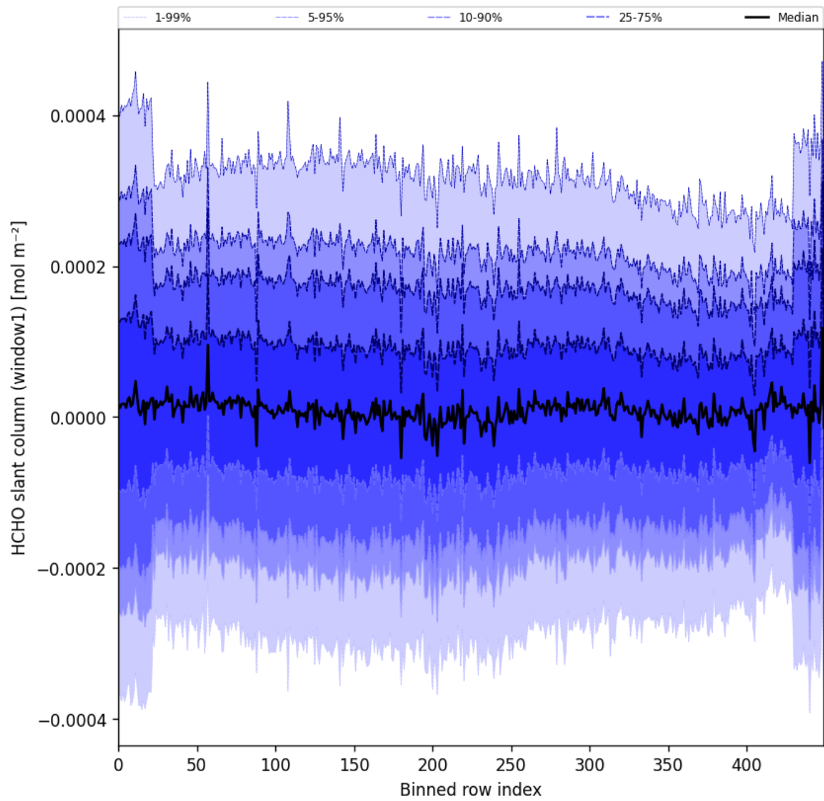
Figure 55: Along track statistics of “HCHO slant column (window1)” for 2025-11-12 to 2025-11-14
