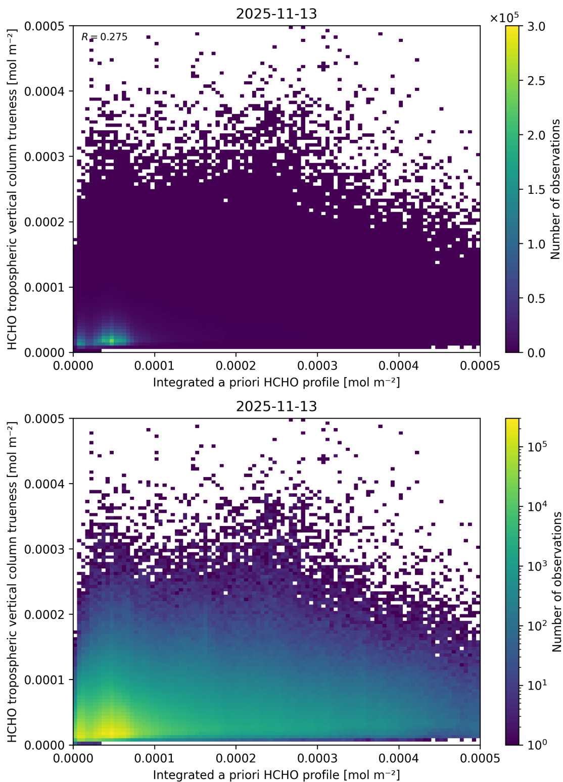
Figure 170: Scatter density plot of “Integrated a priori HCHO profile” against “HCHO tropospheric vertical column trueness” for 2025-11-12 to 2025-11-14.
