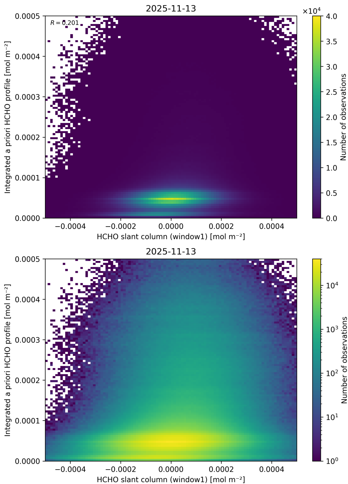
Figure 98: Scatter density plot of “HCHO slant column (window1)” against “Integrated a priori HCHO profile” for 2025-11-12 to 2025-11-14.
