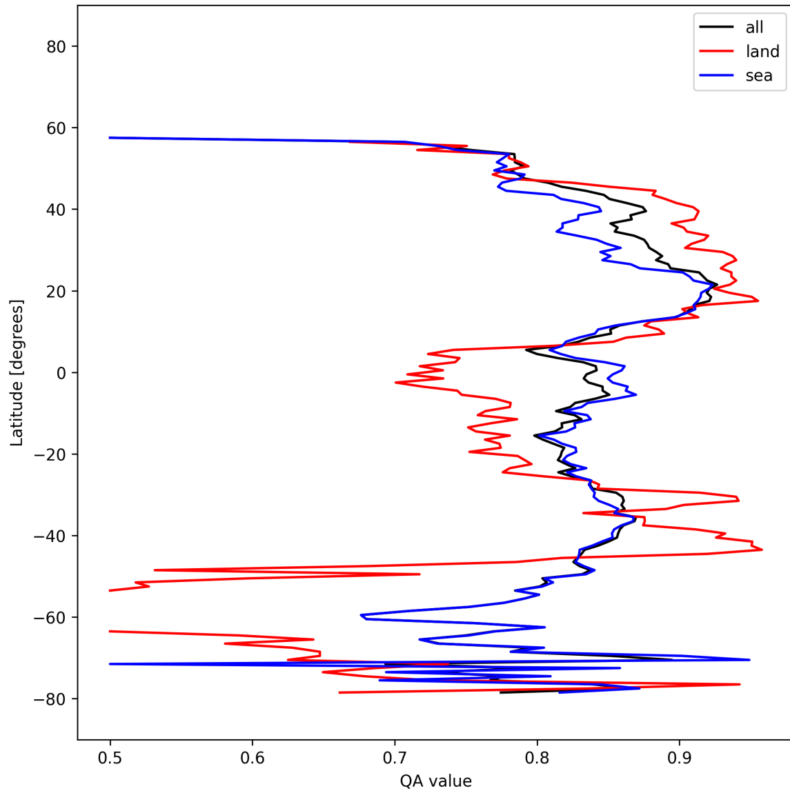
Figure 21: Zonal average of “QA value” for 2025-11-12 to 2025-11-14.
