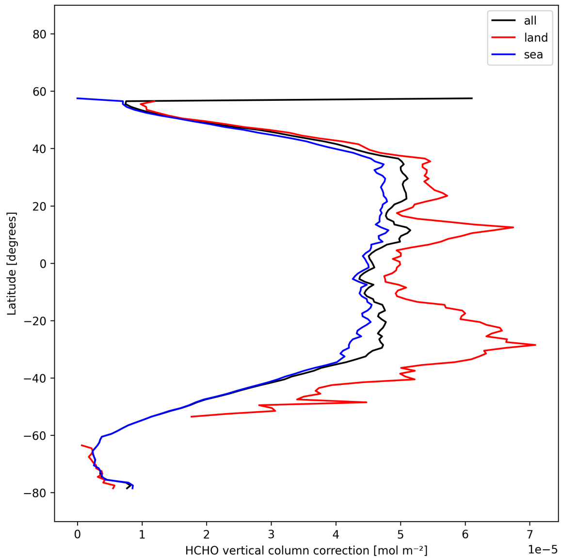
Figure 24: Zonal average of “HCHO vertical column correction” for 2025-11-12 to 2025-11-14.
