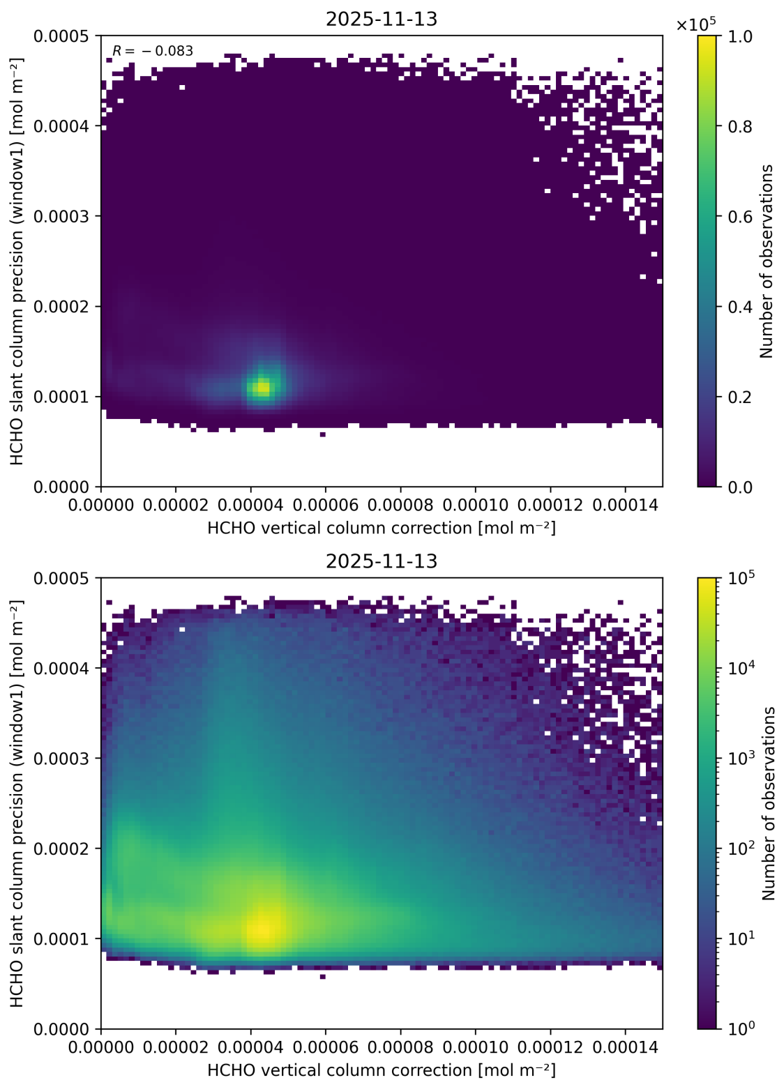
Figure 133: Scatter density plot of “HCHO vertical column correction” against “HCHO slant column precision (window1)” for 2025-11-12 to 2025-11-14.
