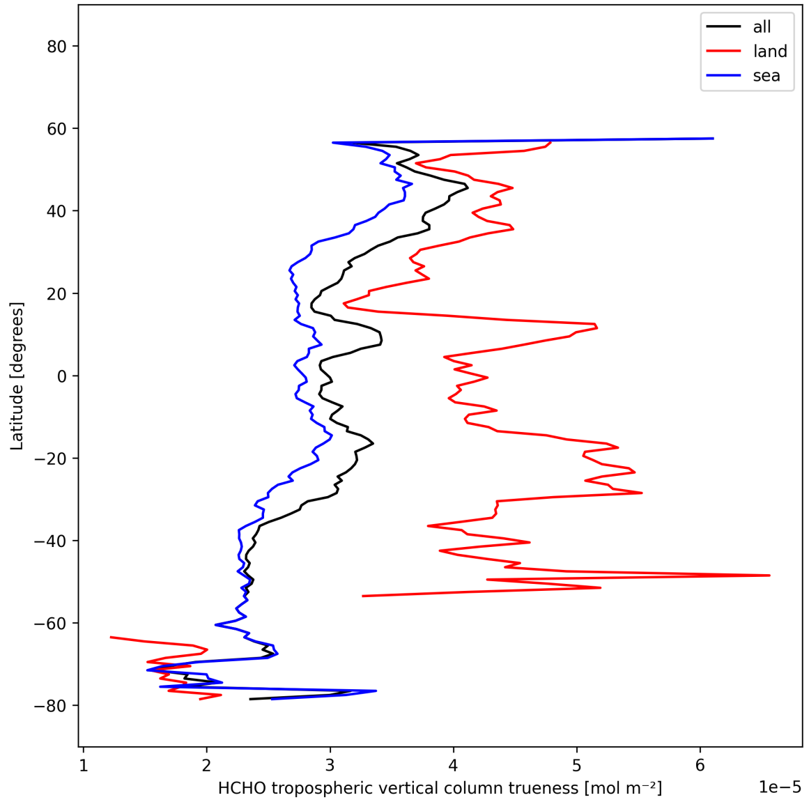
Figure 35: Zonal average of "HCHO tropospheric vertical column trueness" for 2025-11-12 to 2025-11-14.
