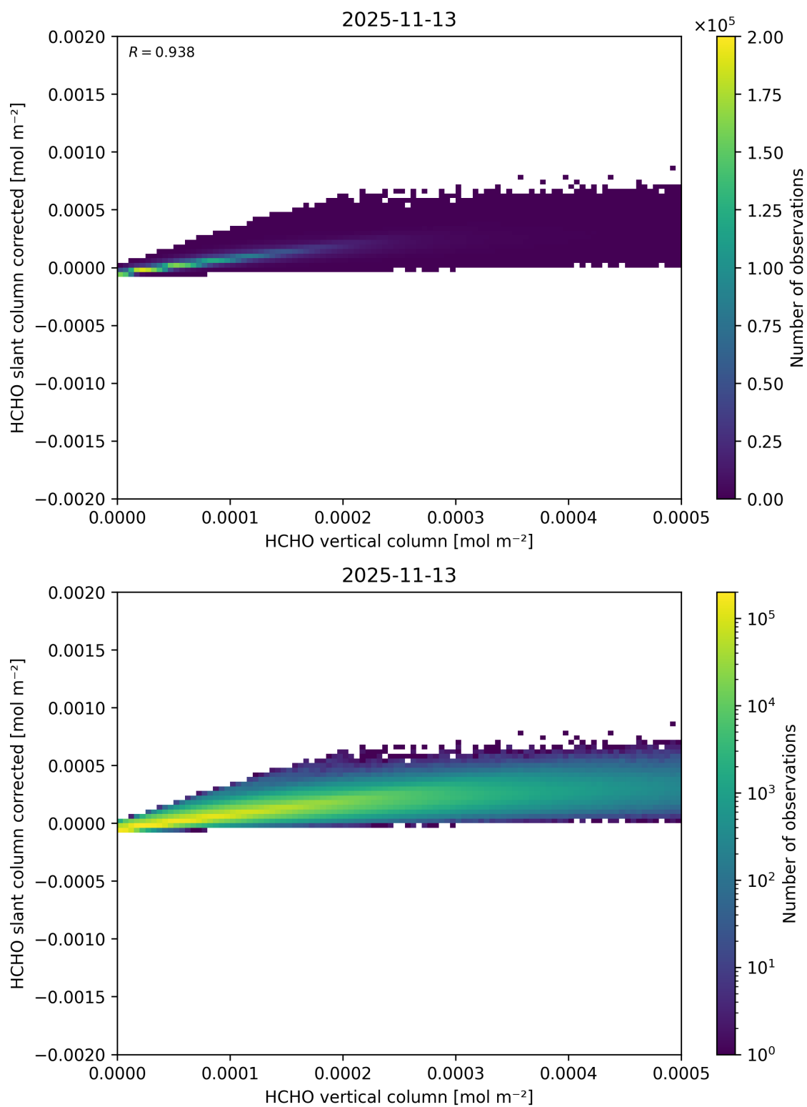
Figure 142: Scatter density plot of “HCHO vertical column” against “HCHO slant column corrected” for 2025-11-12 to 2025-11-14.
