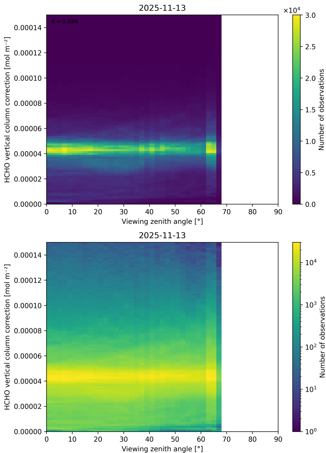
Figure 213: Scatter density plot of “Viewing zenith angle” against “HCHO vertical column correction” for 2025-11-12 to 2025-11-14.
