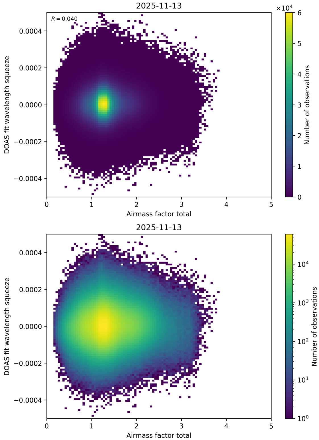
Figure 111: Scatter density plot of “Airmass factor total” against “DOAS fit wavelength squeeze” for 2025-11-12 to 2025-11-14.
