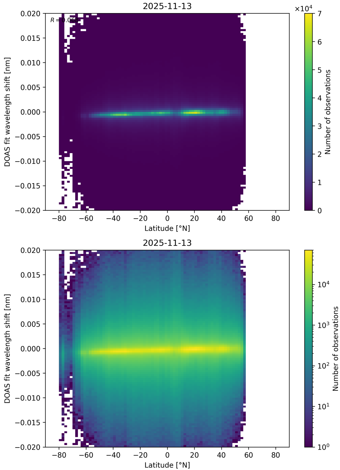
Figure 172: Scatter density plot of “Latitude” against “DOAS fit wavelength shift” for 2025-11-12 to 2025-11-14.
