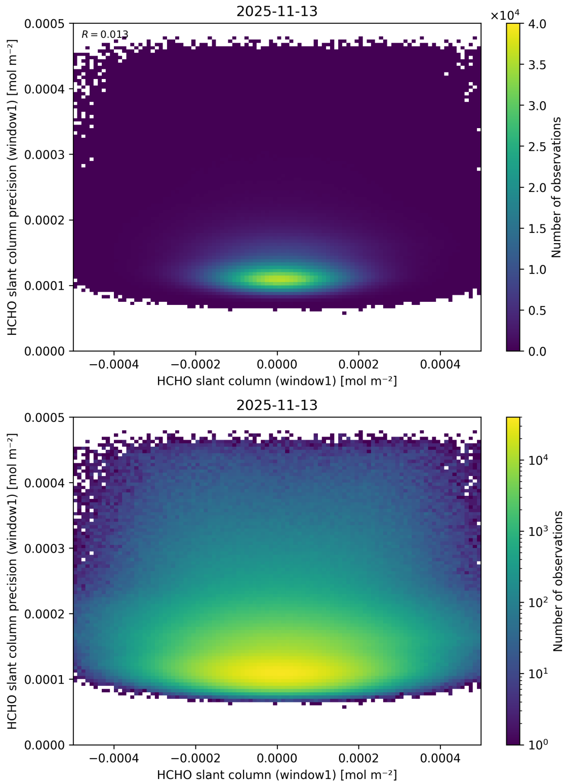
Figure 94: Scatter density plot of “HCHO slant column (window1)” against “HCHO slant column precision (window1)” for 2025-11-12 to 2025-11-14.
