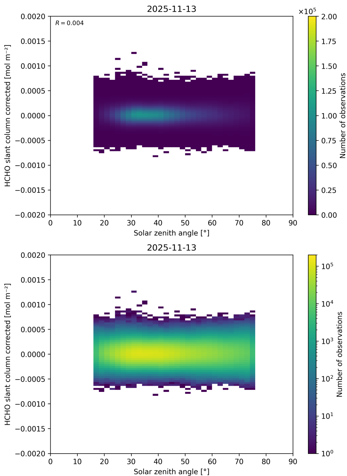
Figure 190: Scatter density plot of “Solar zenith angle” against “HCHO slant column corrected” for 2025-11-12 to 2025-11-14.
