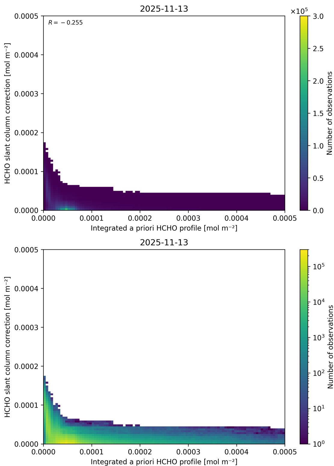
Figure 169: Scatter density plot of “Integrated a priori HCHO profile” against “HCHO slant column correction” for 2025-11-12 to 2025-11-14.
