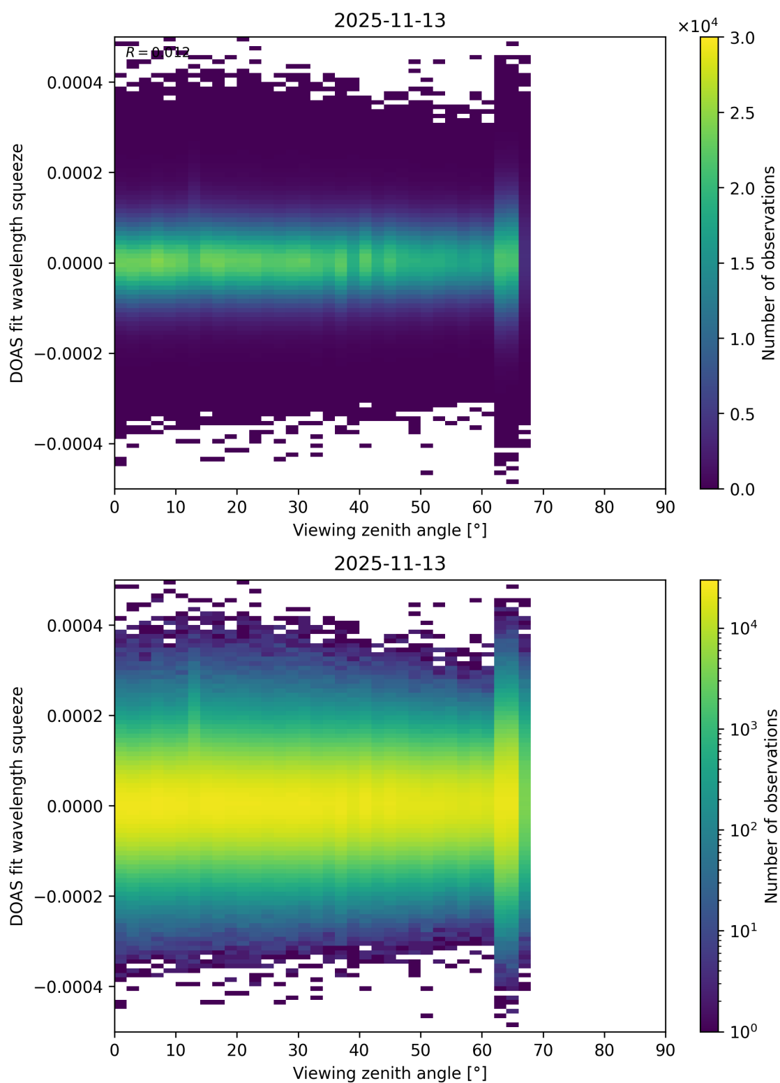
Figure 204: Scatter density plot of “Viewing zenith angle” against “DOAS fit wavelength squeeze” for 2025-11-12 to 2025-11-14.
