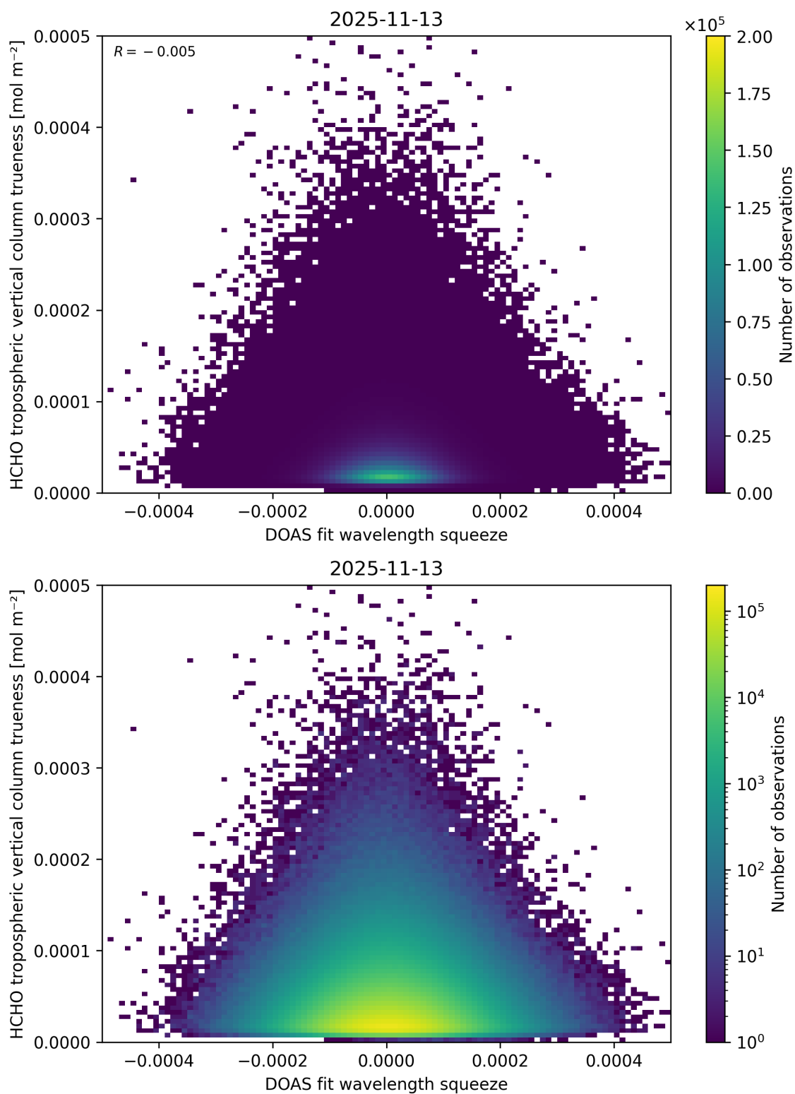
Figure 77: Scatter density plot of “DOAS fit wavelength squeeze” against “HCHO tropospheric vertical column trueness” for 2025-11-12 to 2025-11-14.
