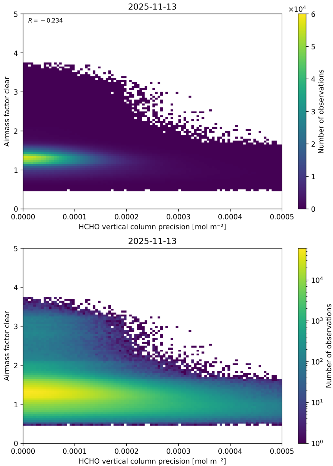
Figure 155: Scatter density plot of “HCHO vertical column precision” against “Airmass factor clear” for 2025-11-12 to 2025-11-14.
