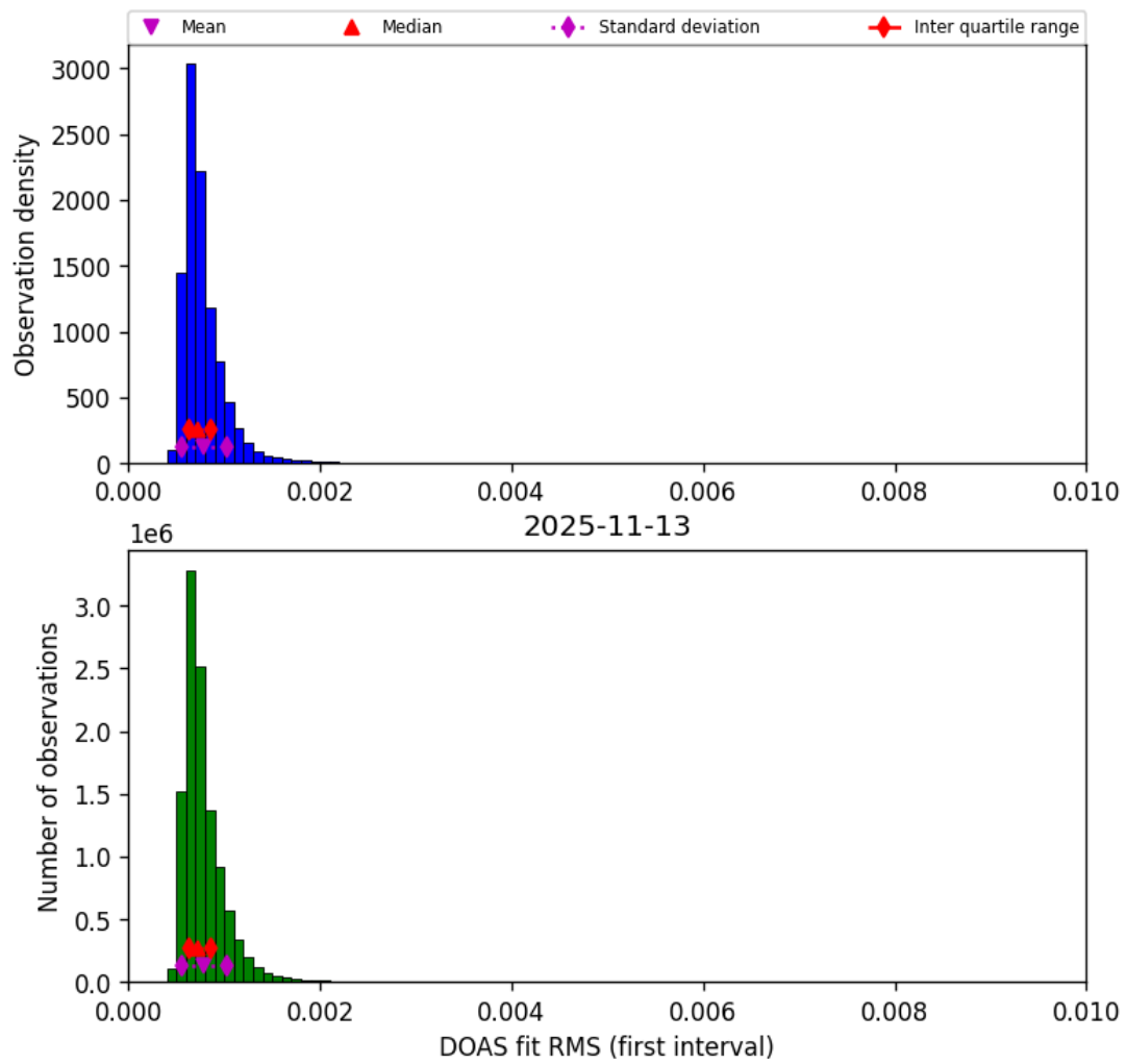
Figure 48: Histogram of “DOAS fit RMS (first interval)” for 2025-11-12 to 2025-11-14
