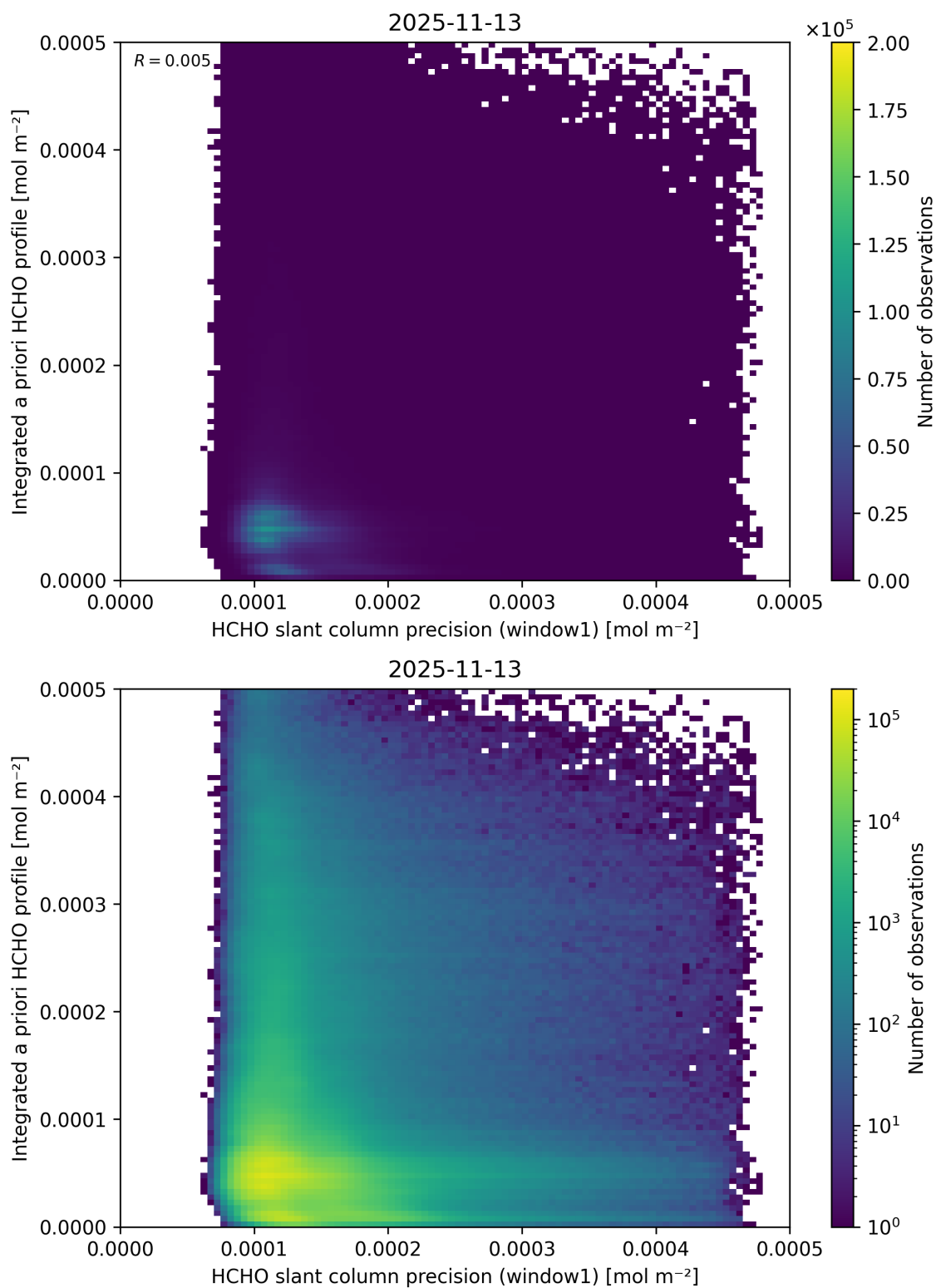
Figure 108: Scatter density plot of “HCHO slant column precision (window1)” against “Integrated a priori HCHO profile” for 2025-11-12 to 2025-11-14.
