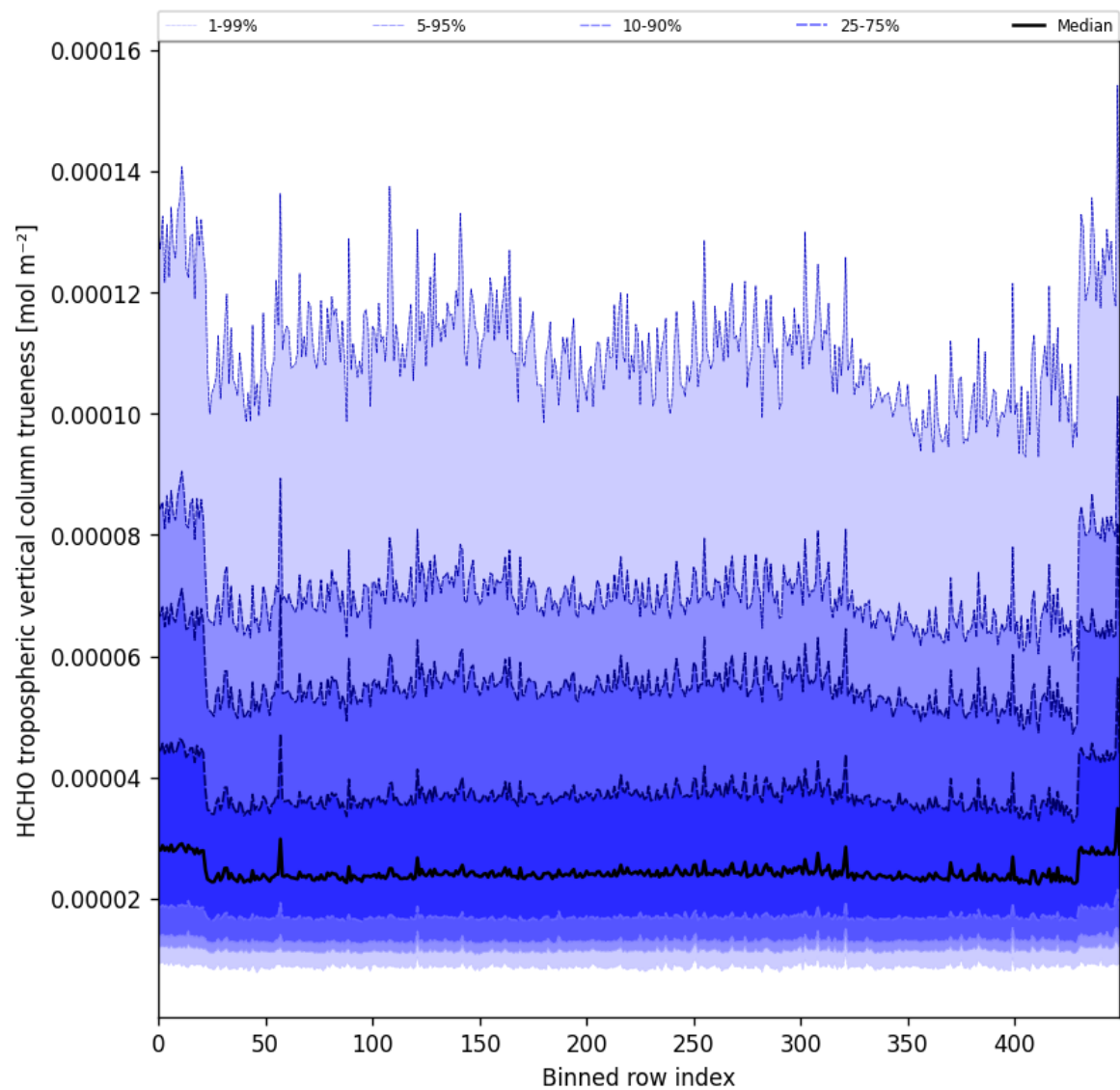
Figure 65: Along track statistics of “HCHO tropospheric vertical column trueness” for 2025-11-12 to 2025-11-14
