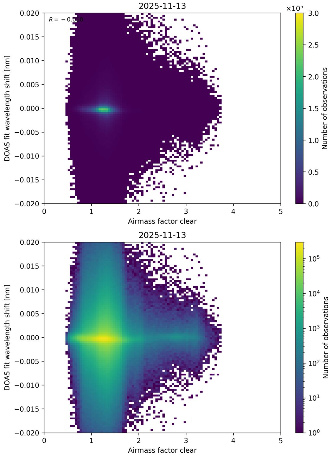
Figure 79: Scatter density plot of “Airmass factor clear” against “DOAS fit wavelength shift” for 2025-11-12 to 2025-11-14.
