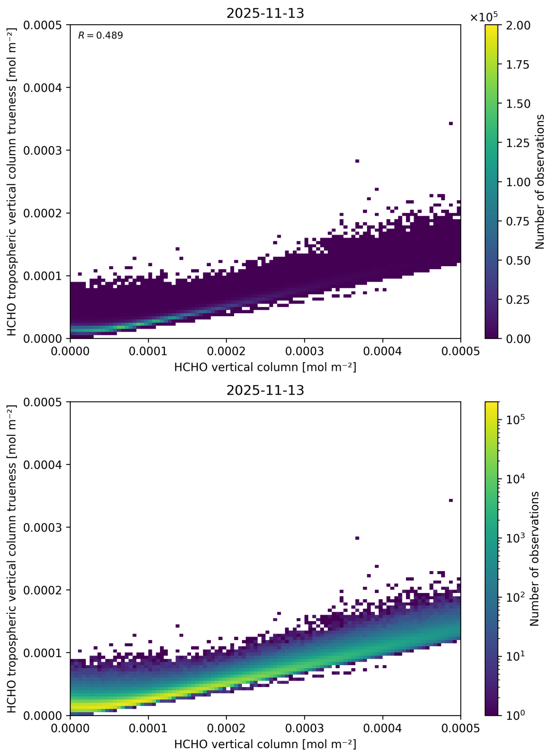
Figure 150: Scatter density plot of “HCHO vertical column” against “HCHO tropospheric vertical column trueness” for 2025-11-12 to 2025-11-14.
