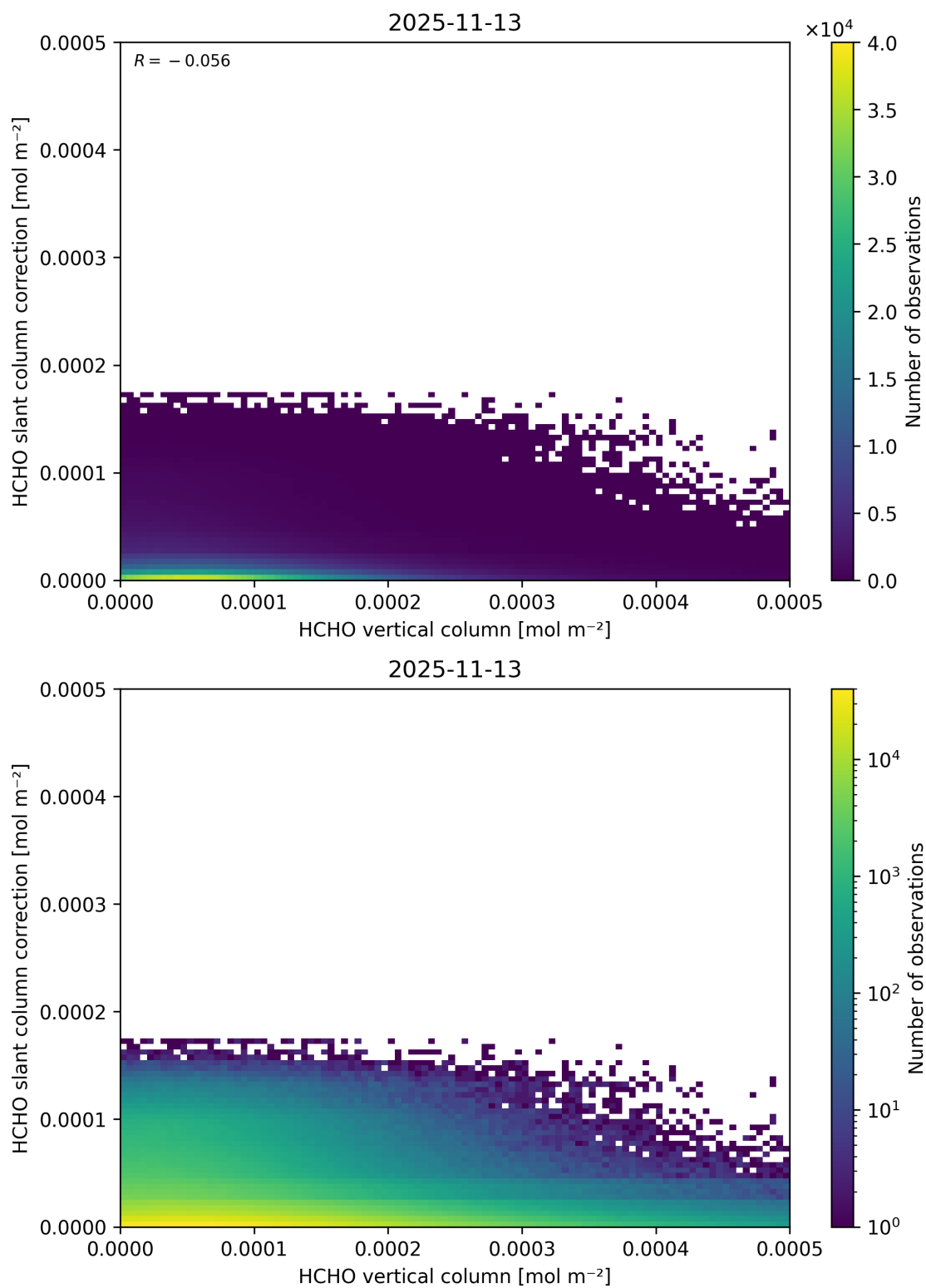
Figure 143: Scatter density plot of “HCHO vertical column” against “HCHO slant column correction” for 2025-11-12 to 2025-11-14.
