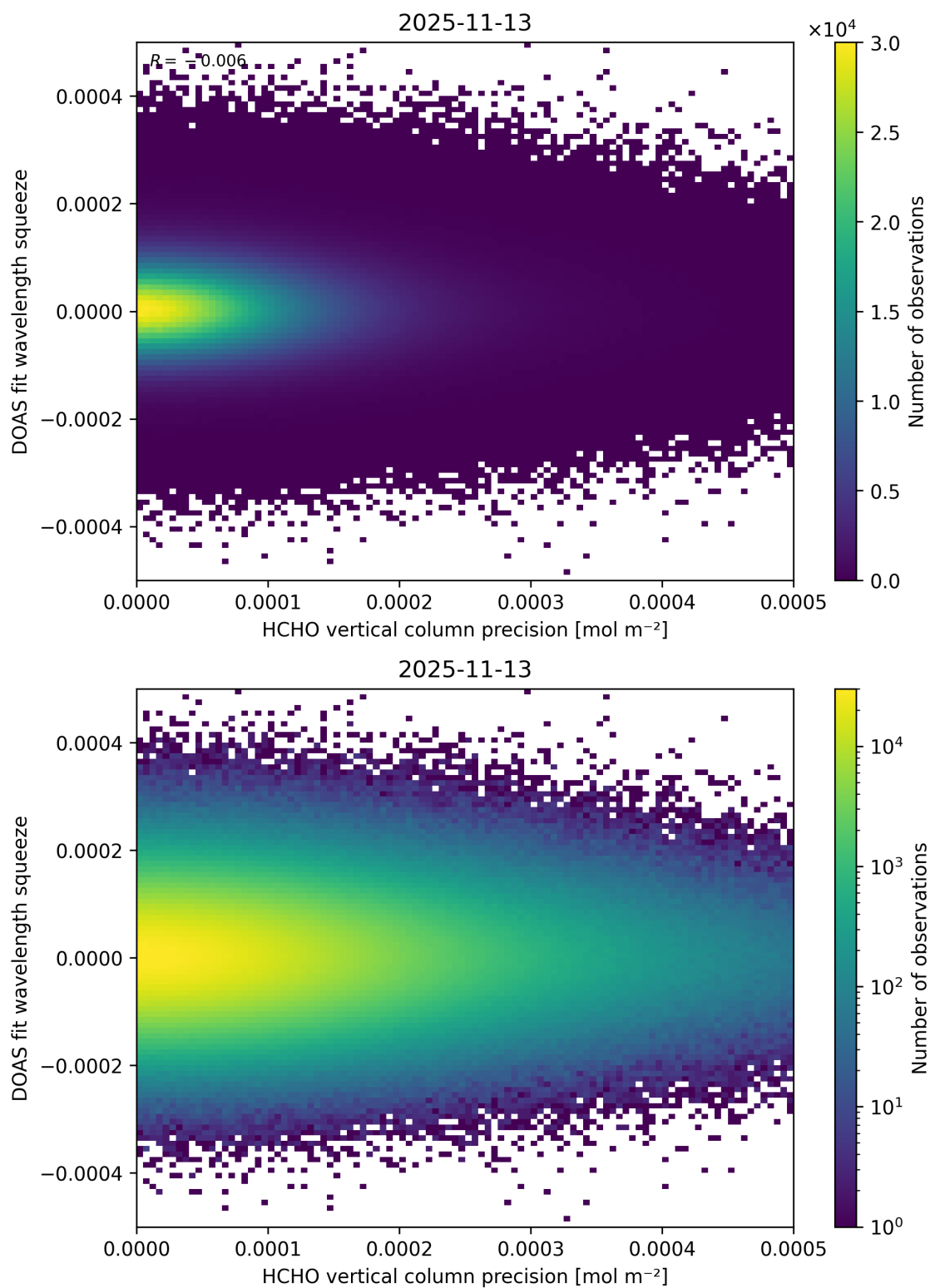
Figure 154: Scatter density plot of “HCHO vertical column precision” against “DOAS fit wavelength squeeze” for 2025-11-12 to 2025-11-14.
