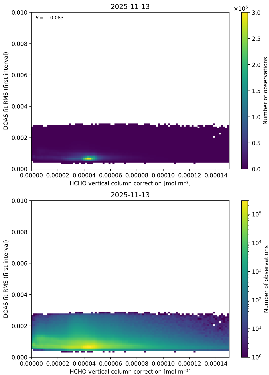
Figure 126: Scatter density plot of “HCHO vertical column correction” against “DOAS fit RMS (first interval)” for 2025-11-12 to 2025-11-14.
