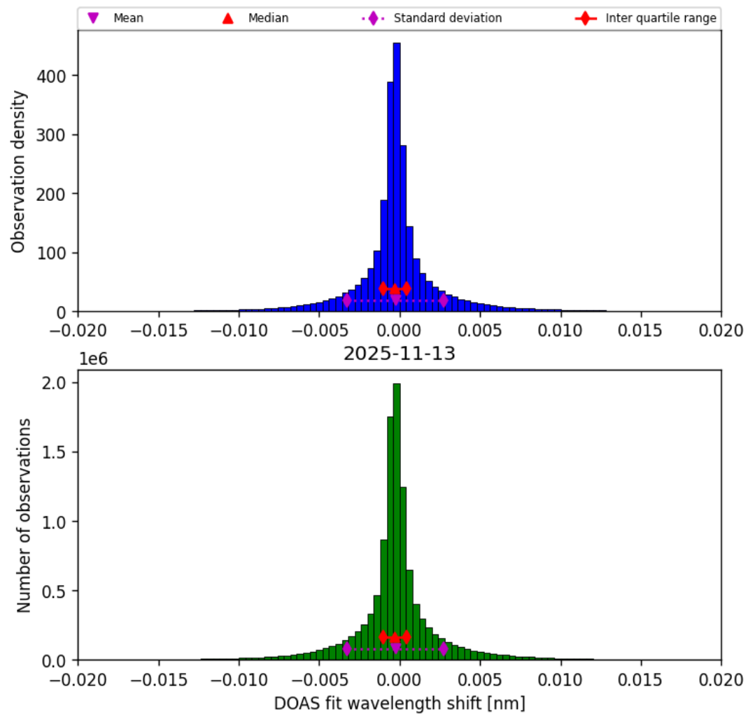
Figure 46: Histogram of “DOAS fit wavelength shift” for 2025-11-12 to 2025-11-14
