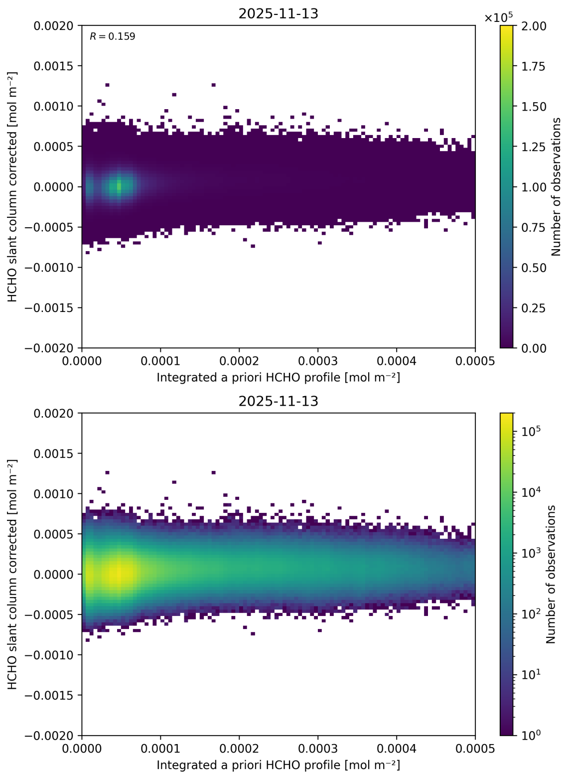
Figure 168: Scatter density plot of “Integrated a priori HCHO profile” against “HCHO slant column corrected” for 2025-11-12 to 2025-11-14.
