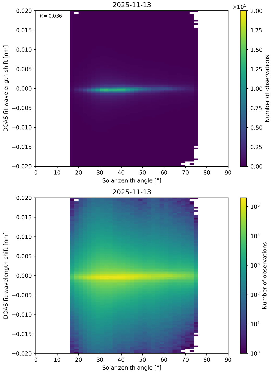
Figure 187: Scatter density plot of “Solar zenith angle” against “DOAS fit wavelength shift” for 2025-11-12 to 2025-11-14.
