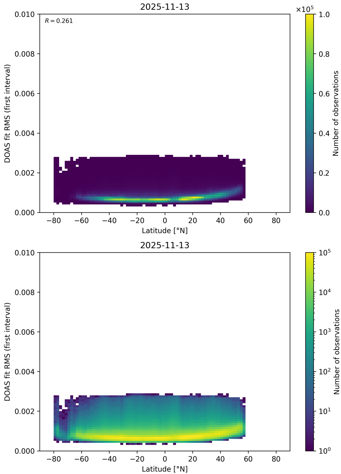
Figure 171: Scatter density plot of “Latitude” against “DOAS fit RMS (first interval)” for 2025-11-12 to 2025-11-14.
