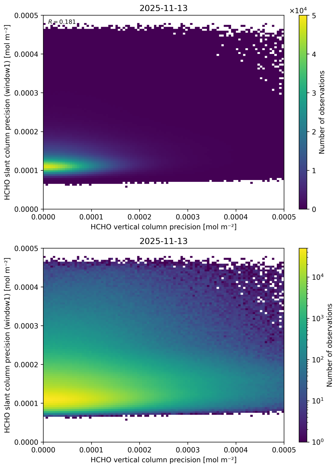
Figure 159: Scatter density plot of “HCHO vertical column precision” against “HCHO slant column precision (window1)” for 2025-11-12 to 2025-11-14.
