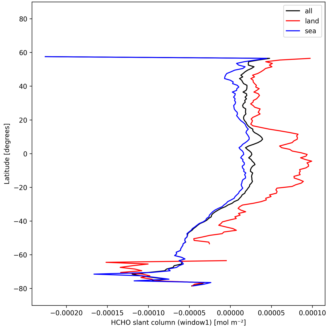
Figure 25: Zonal average of “HCHO slant column (window1)” for 2025-11-12 to 2025-11-14.
