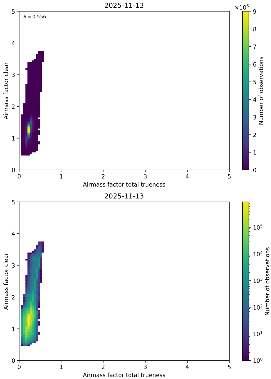
Figure 121: Scatter density plot of “Airmass factor total trueness” against “Airmass factor clear” for 2025-11-12 to 2025-11-14.
