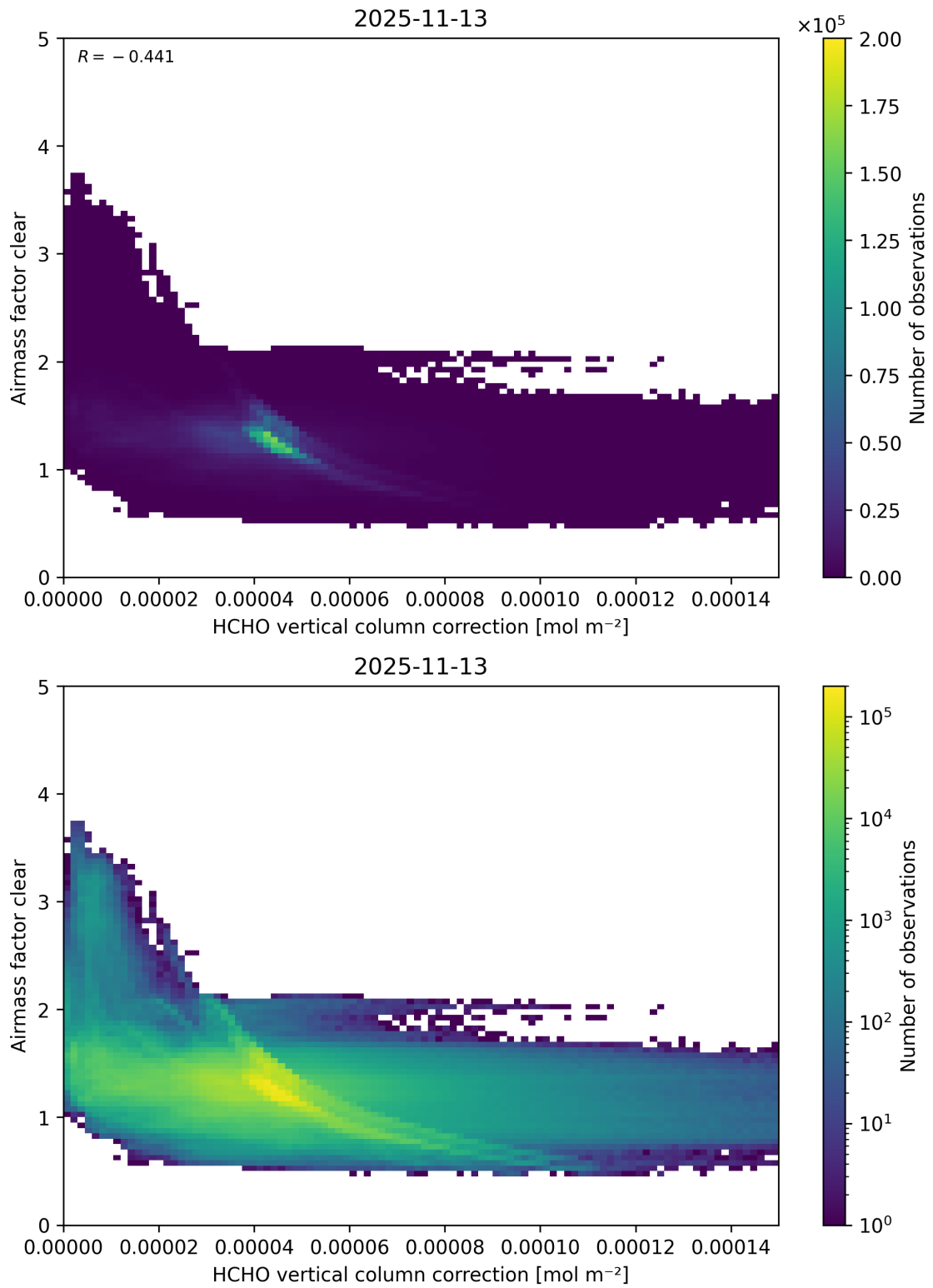
Figure 129: Scatter density plot of “HCHO vertical column correction” against “Airmass factor clear” for 2025-11-12 to 2025-11-14.
