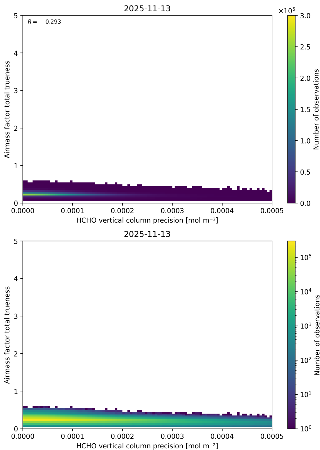
Figure 161: Scatter density plot of “HCHO vertical column precision” against “Airmass factor total trueness” for 2025-11-12 to 2025-11-14.
