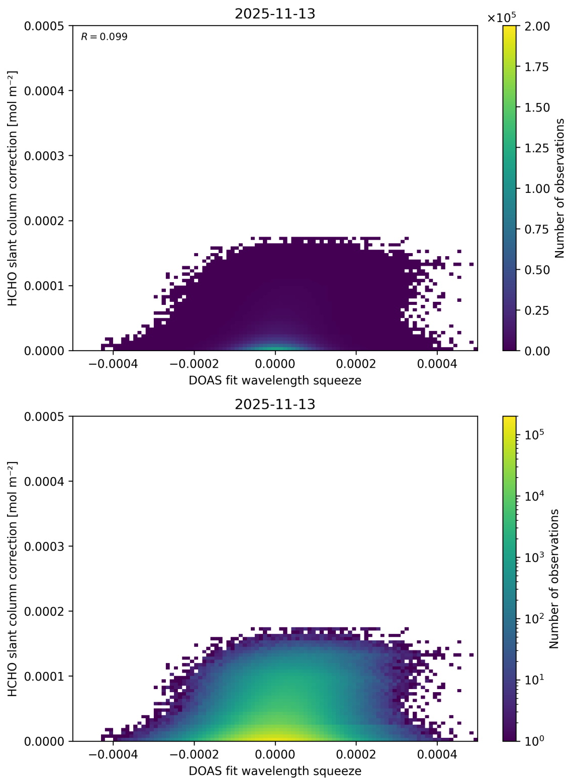
Figure 76: Scatter density plot of “DOAS fit wavelength squeeze” against “HCHO slant column correction” for 2025-11-12 to 2025-11-14.
