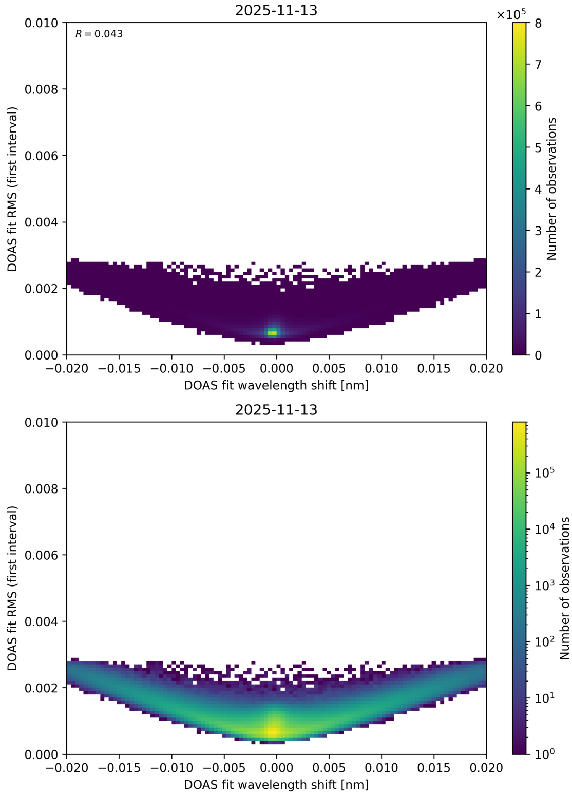
Figure 69: Scatter density plot of “DOAS fit wavelength shift” against “DOAS fit RMS (first interval)” for 2025-11-12 to 2025-11-14.
