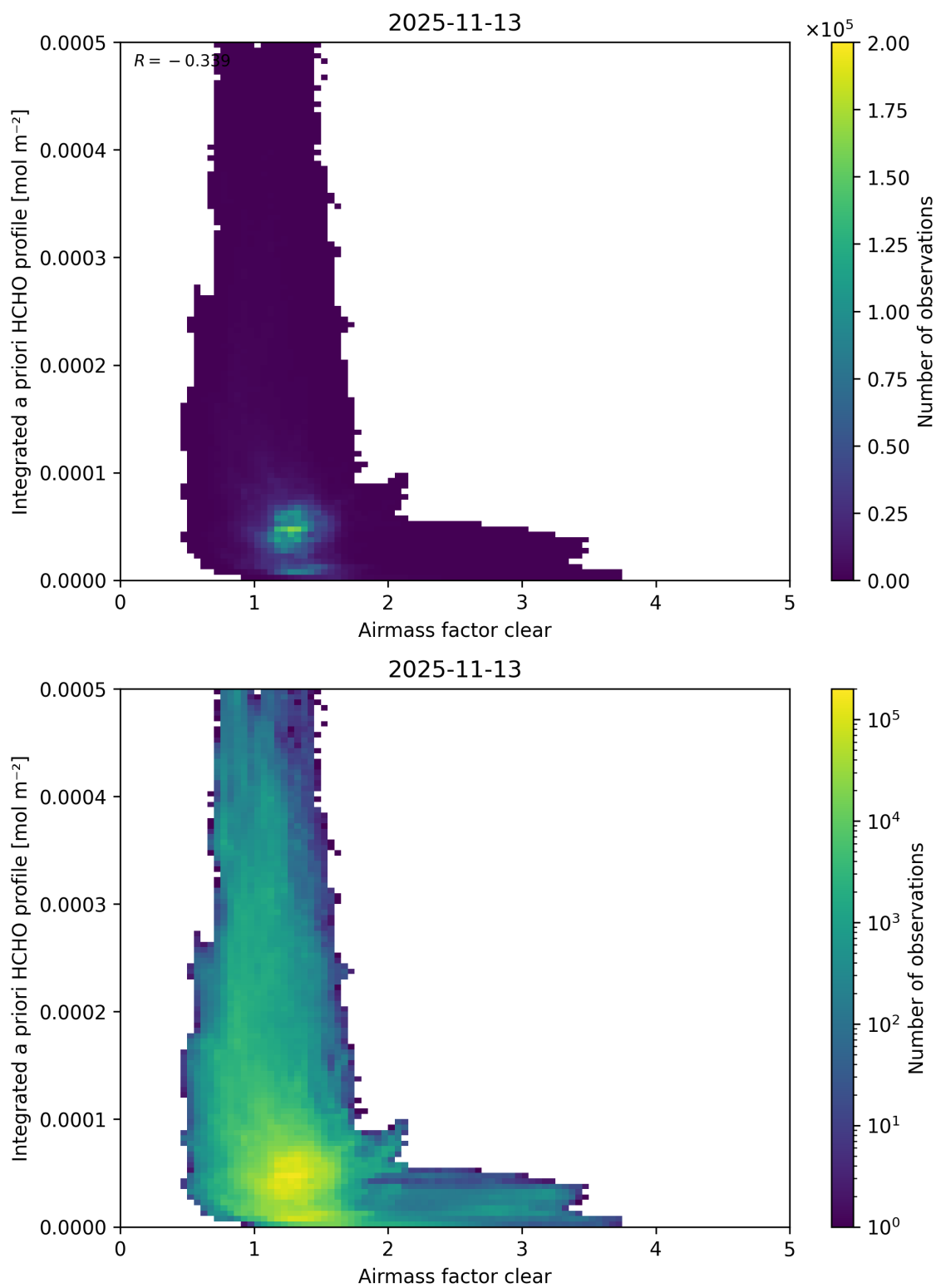
Figure 84: Scatter density plot of “Airmass factor clear” against “Integrated a priori HCHO profile” for 2025-11-12 to 2025-11-14.
