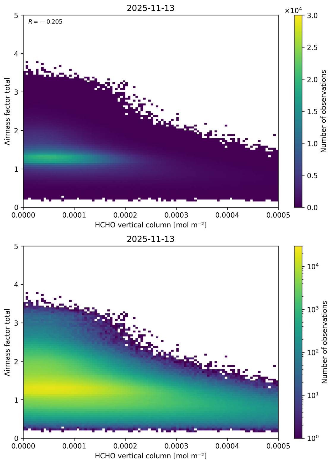
Figure 146: Scatter density plot of “HCHO vertical column” against “Airmass factor total” for 2025-11-12 to 2025-11-14.
