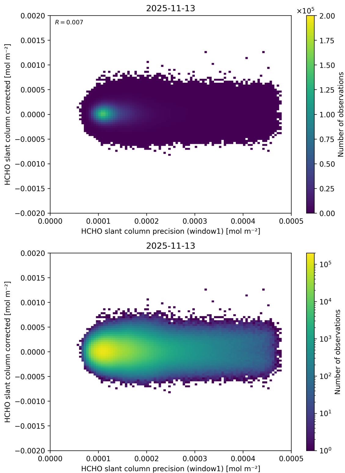
Figure 103: Scatter density plot of “HCHO slant column precision (window1)” against “HCHO slant column corrected” for 2025-11-12 to 2025-11-14.
