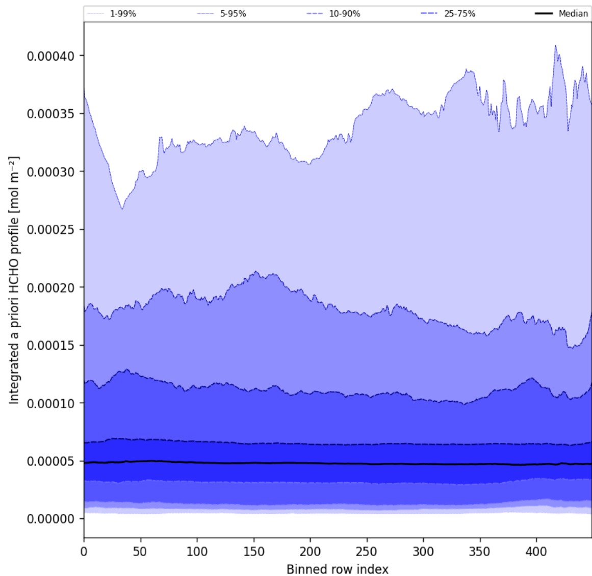
Figure 60: Along track statistics of “Integrated a priori HCHO profile” for 2025-11-12 to 2025-11-14
