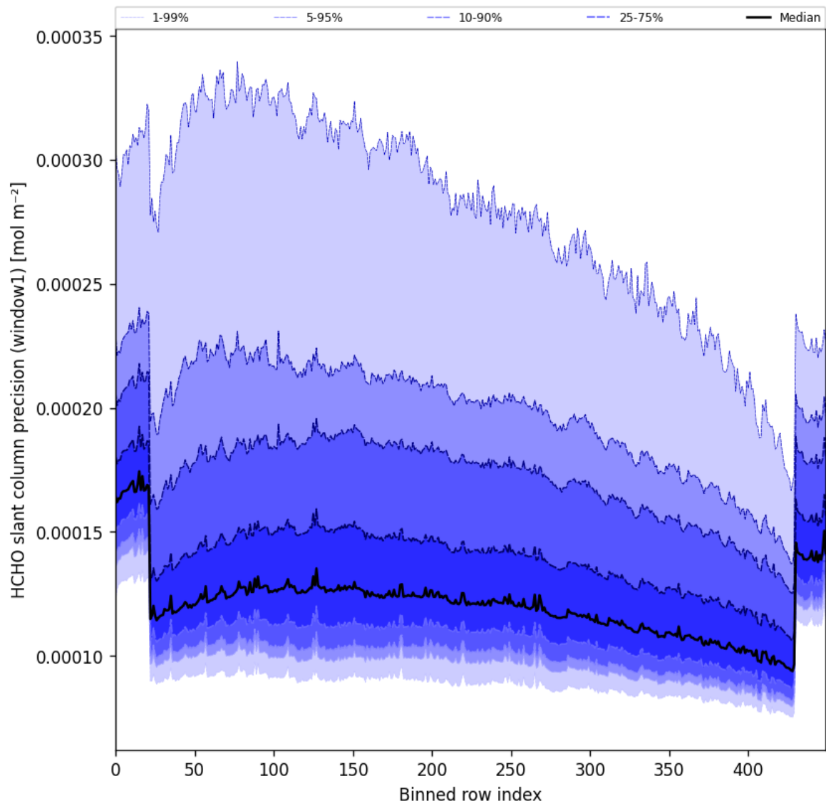
Figure 56: Along track statistics of “HCHO slant column precision (window1)” for 2025-11-12 to 2025-11-14
