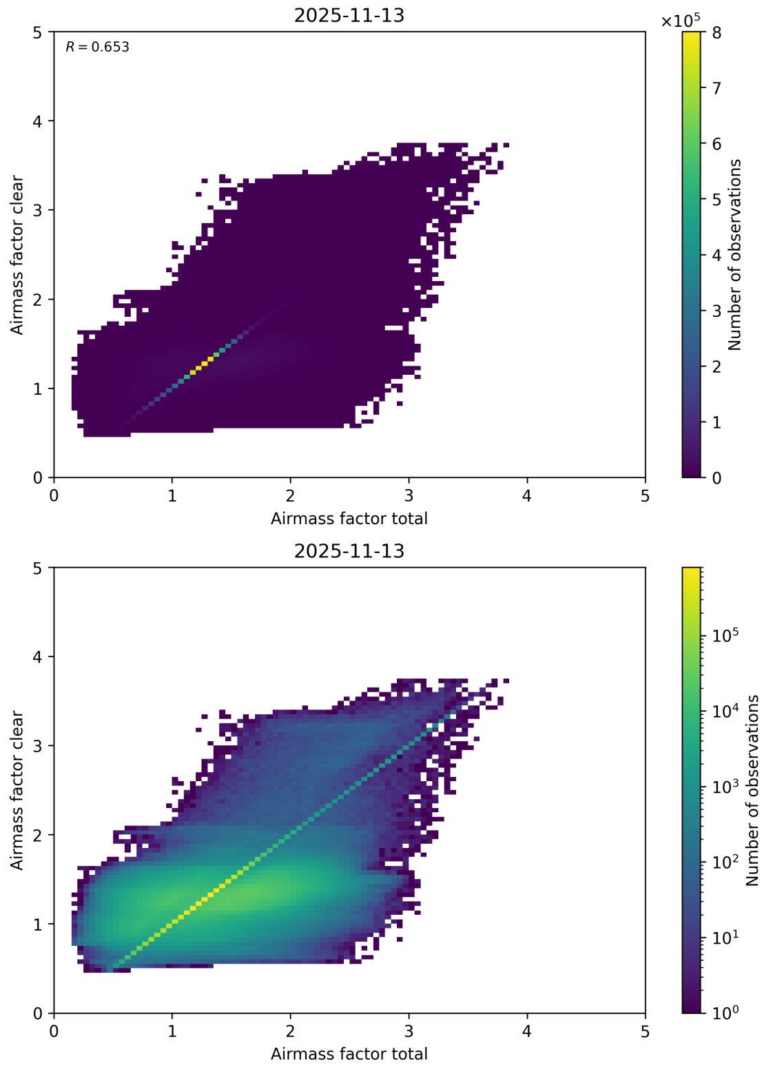
Figure 112: Scatter density plot of “Airmass factor total” against “Airmass factor clear” for 2025-11-12 to 2025-11-14.
