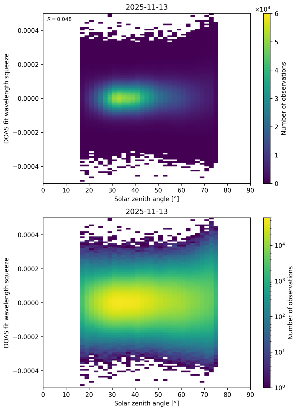
Figure 188: Scatter density plot of “Solar zenith angle” against “DOAS fit wavelength squeeze” for 2025-11-12 to 2025-11-14.
