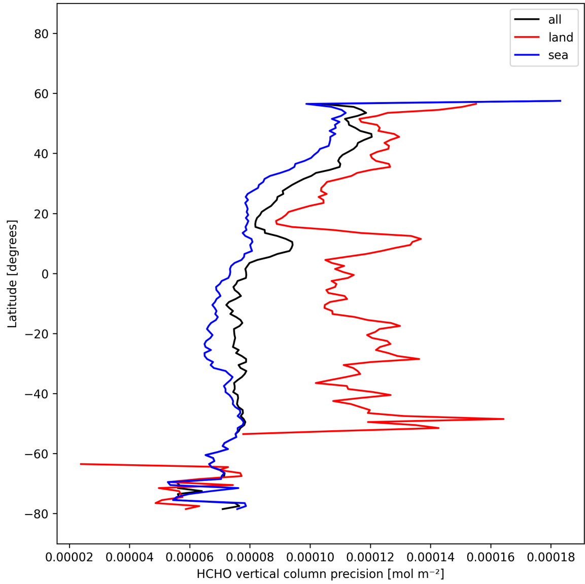
Figure 23: Zonal average of “HCHO vertical column precision” for 2025-11-12 to 2025-11-14.
