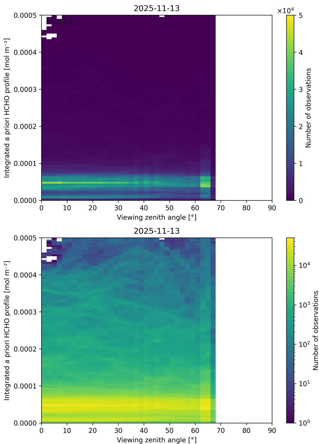
Figure 216: Scatter density plot of “Viewing zenith angle” against “Integrated a priori HCHO profile” for 2025-11-12 to 2025-11-14.
