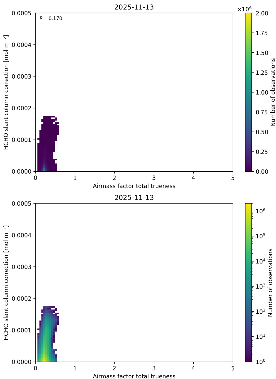
Figure 123: Scatter density plot of “Airmass factor total trueness” against “HCHO slant column correction” for 2025-11-12 to 2025-11-14.
