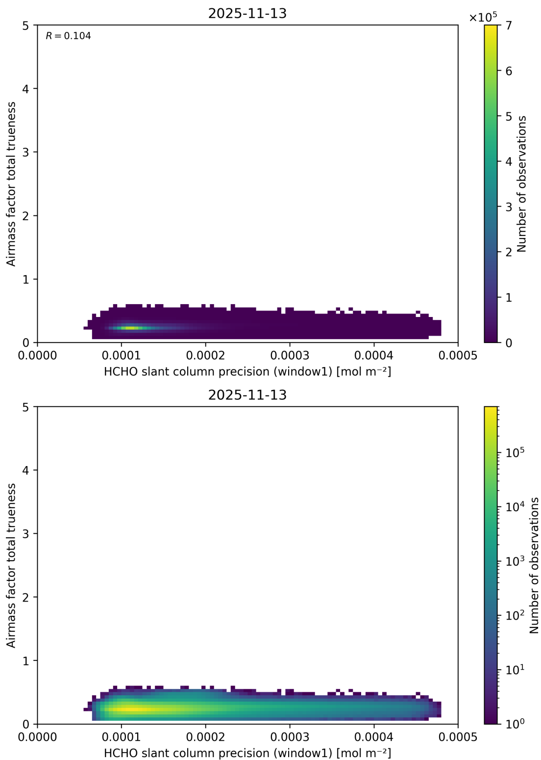
Figure 106: Scatter density plot of “HCHO slant column precision (window1)” against “Airmass factor total trueness” for 2025-11-12 to 2025-11-14.
