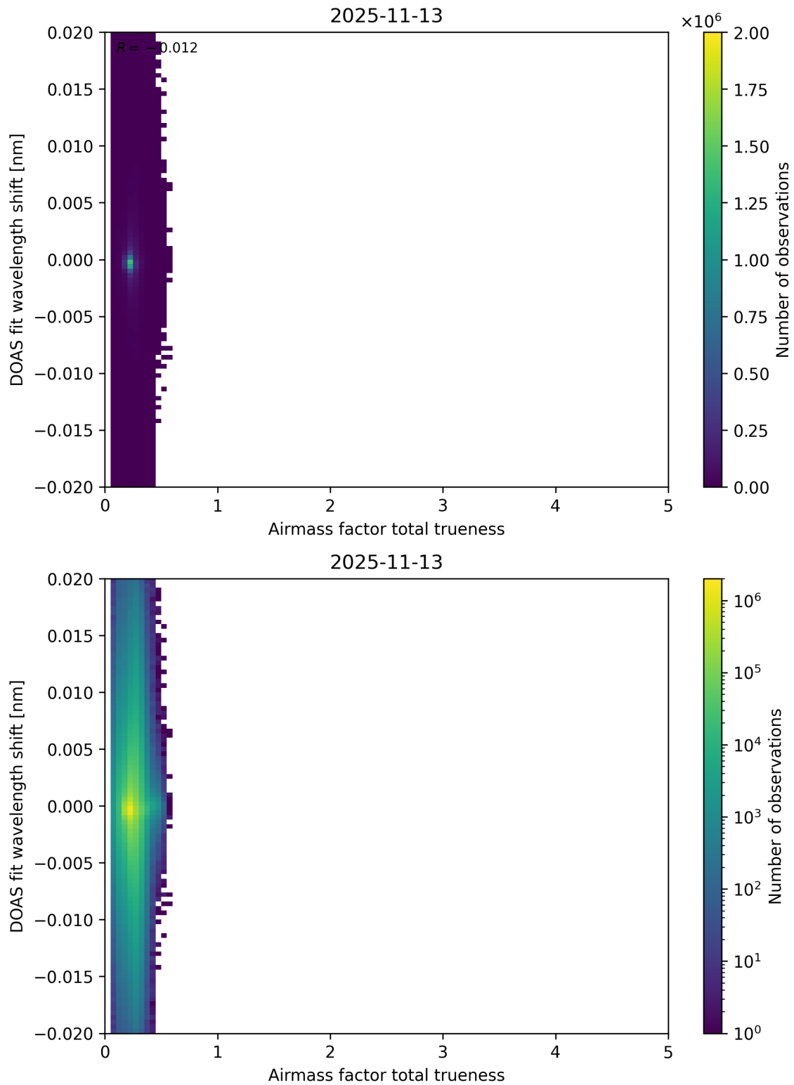
Figure 119: Scatter density plot of “Airmass factor total trueness” against “DOAS fit wavelength shift” for 2025-11-12 to 2025-11-14.
