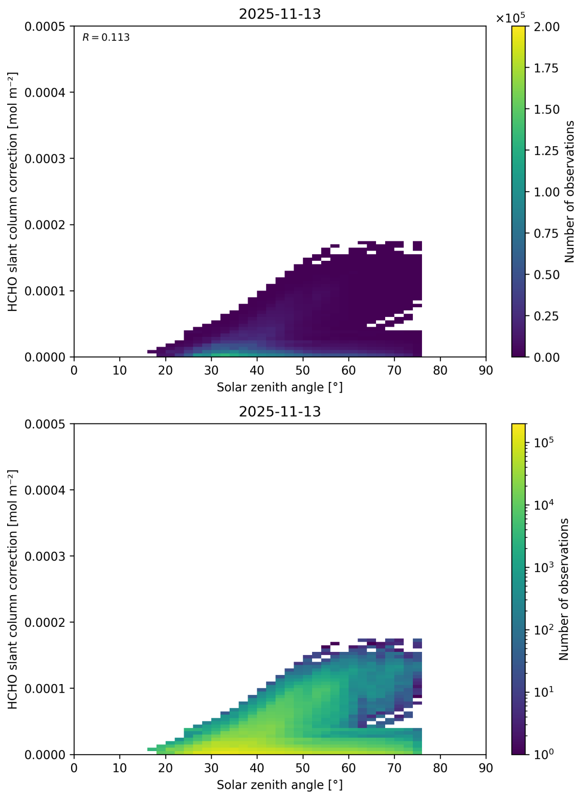
Figure 191: Scatter density plot of “Solar zenith angle” against “HCHO slant column correction” for 2025-11-12 to 2025-11-14.
