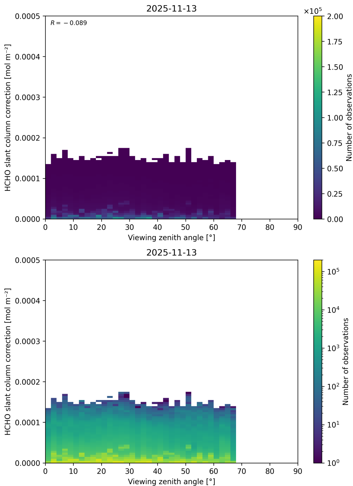
Figure 207: Scatter density plot of “Viewing zenith angle” against “HCHO slant column correction” for 2025-11-12 to 2025-11-14.
