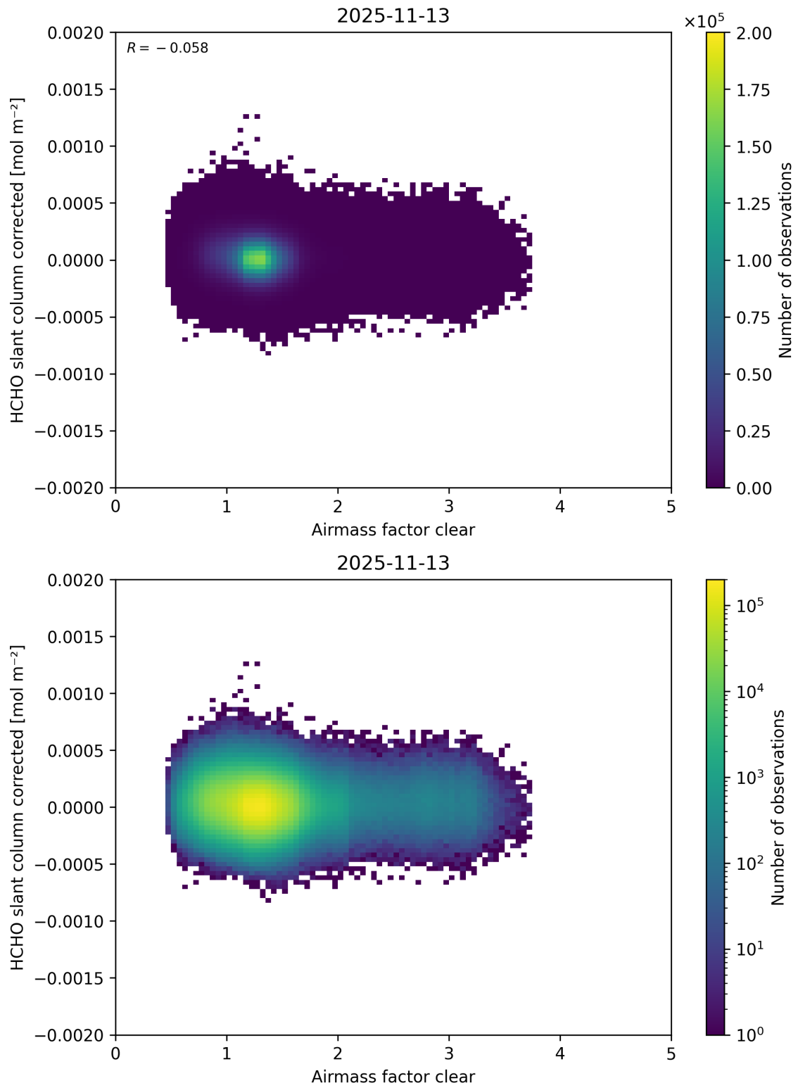
Figure 81: Scatter density plot of “Airmass factor clear” against “HCHO slant column corrected” for 2025-11-12 to 2025-11-14.
