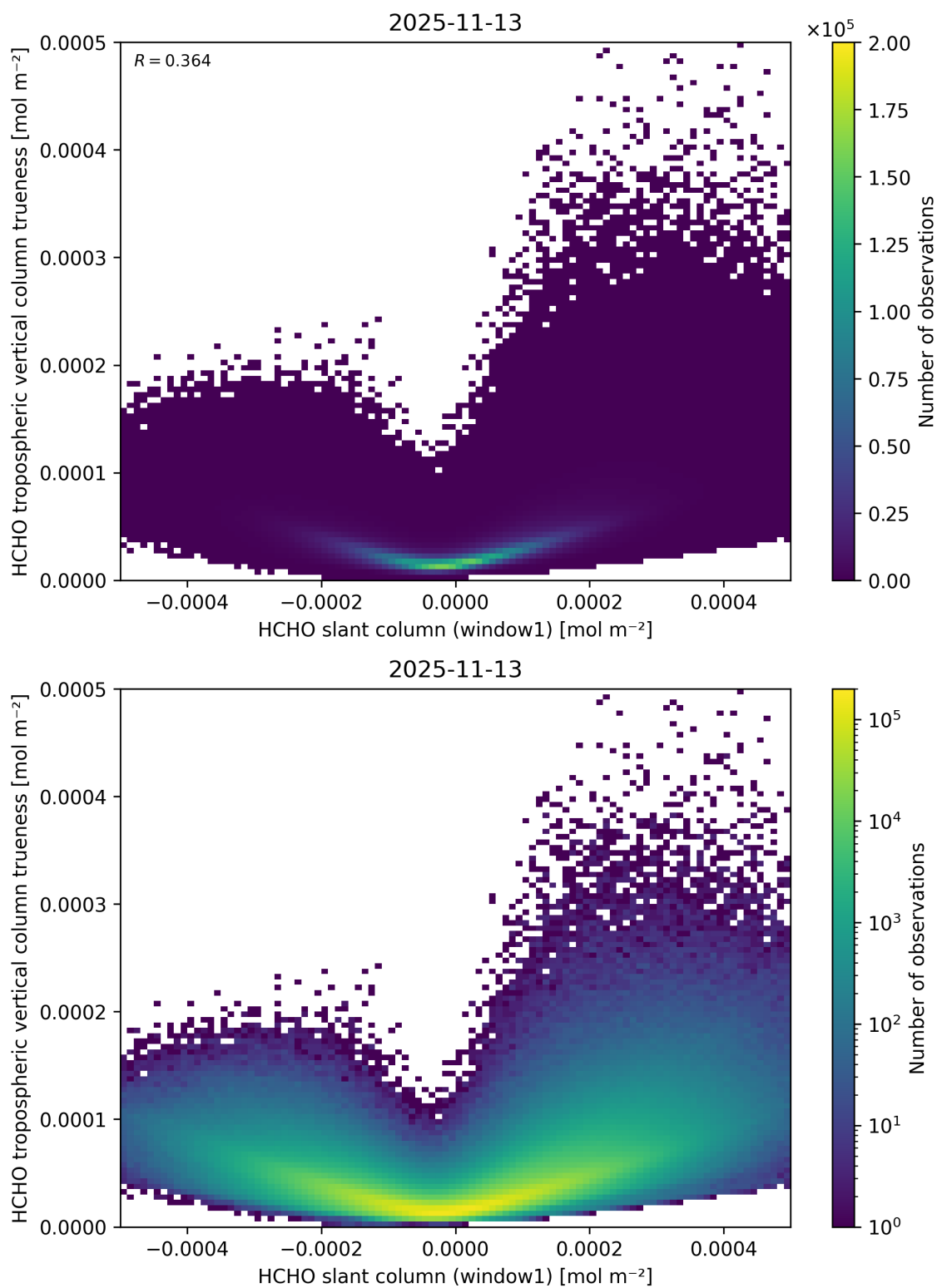
Figure 97: Scatter density plot of “HCHO slant column (window1)” against “HCHO tropospheric vertical column trueness” for 2025-11-12 to 2025-11-14.
