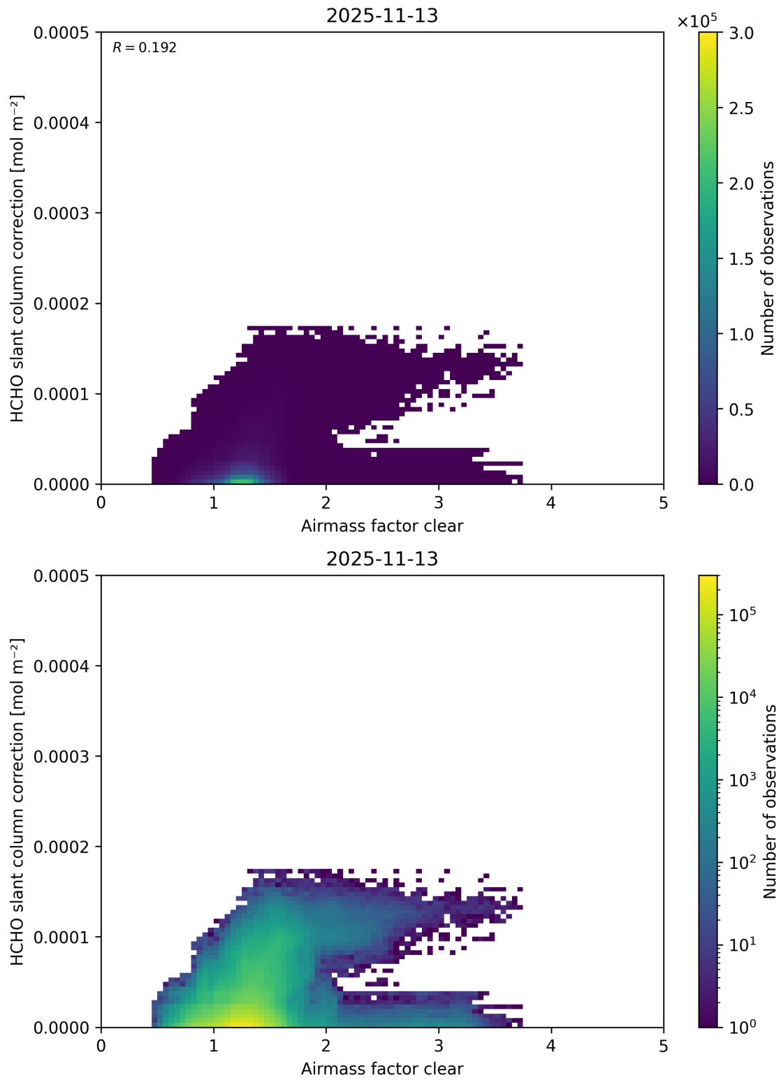
Figure 82: Scatter density plot of “Airmass factor clear” against “HCHO slant column correction” for 2025-11-12 to 2025-11-14.
