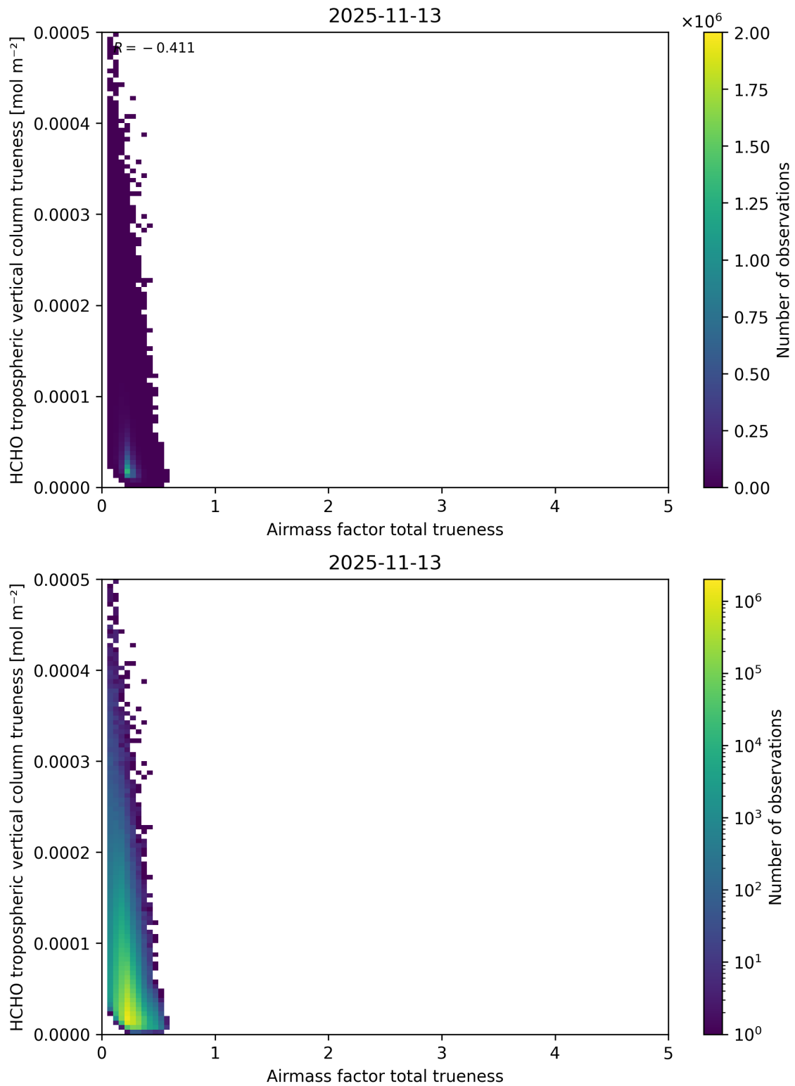
Figure 124: Scatter density plot of “Airmass factor total trueness” against “HCHO tropospheric vertical column trueness” for 2025-11-12 to 2025-11-14.
