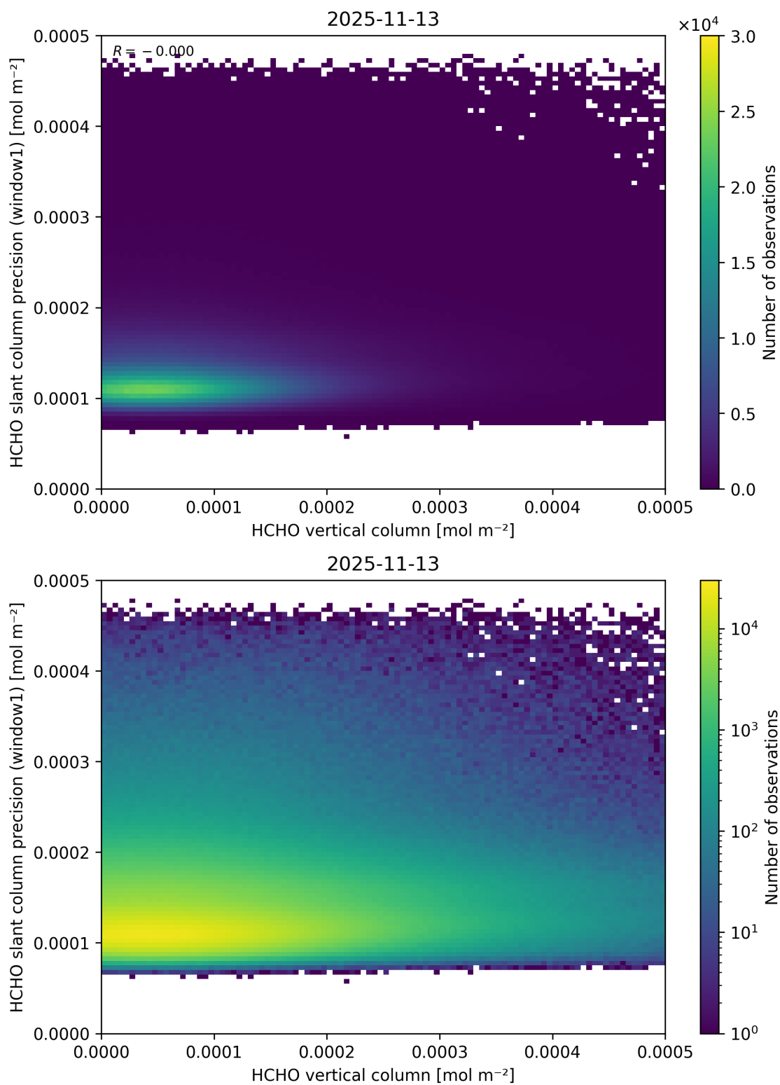
Figure 145: Scatter density plot of “HCHO vertical column” against “HCHO slant column precision (window1)” for 2025-11-12 to 2025-11-14.
