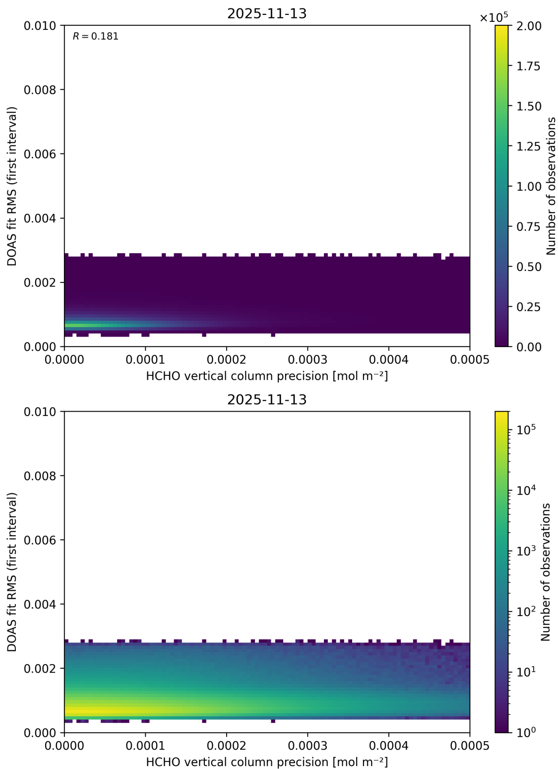
Figure 152: Scatter density plot of “HCHO vertical column precision” against “DOAS fit RMS (first interval)” for 2025-11-12 to 2025-11-14.
