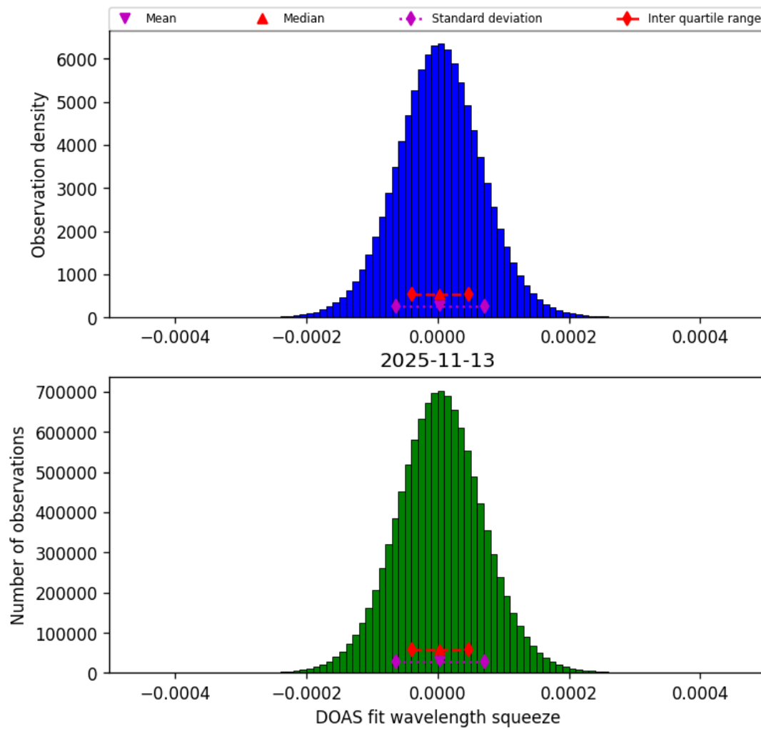
Figure 47: Histogram of “DOAS fit wavelength squeeze” for 2025-11-12 to 2025-11-14
