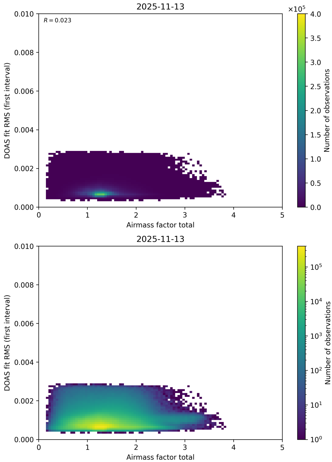
Figure 109: Scatter density plot of “Airmass factor total” against “DOAS fit RMS (first interval)” for 2025-11-12 to 2025-11-14.
