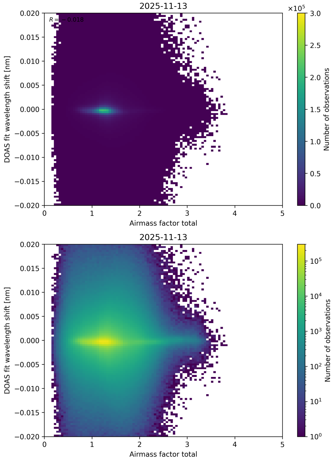
Figure 110: Scatter density plot of “Airmass factor total” against “DOAS fit wavelength shift” for 2025-11-12 to 2025-11-14.
