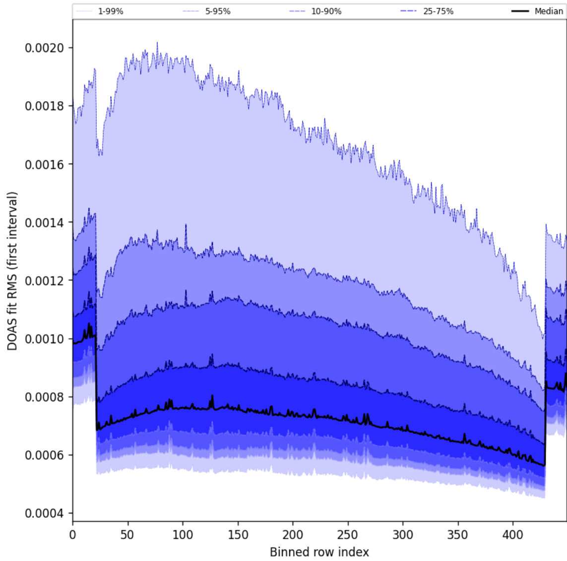
Figure 63: Along track statistics of “DOAS fit RMS (first interval)” for 2025-11-12 to 2025-11-14
