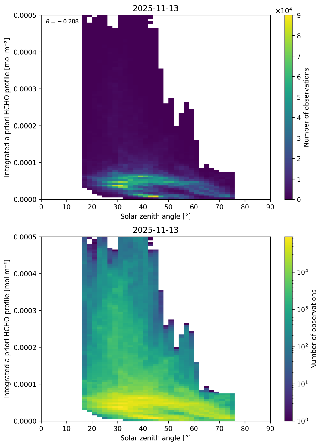
Figure 200: Scatter density plot of “Solar zenith angle” against “Integrated a priori HCHO profile” for 2025-11-12 to 2025-11-14.
