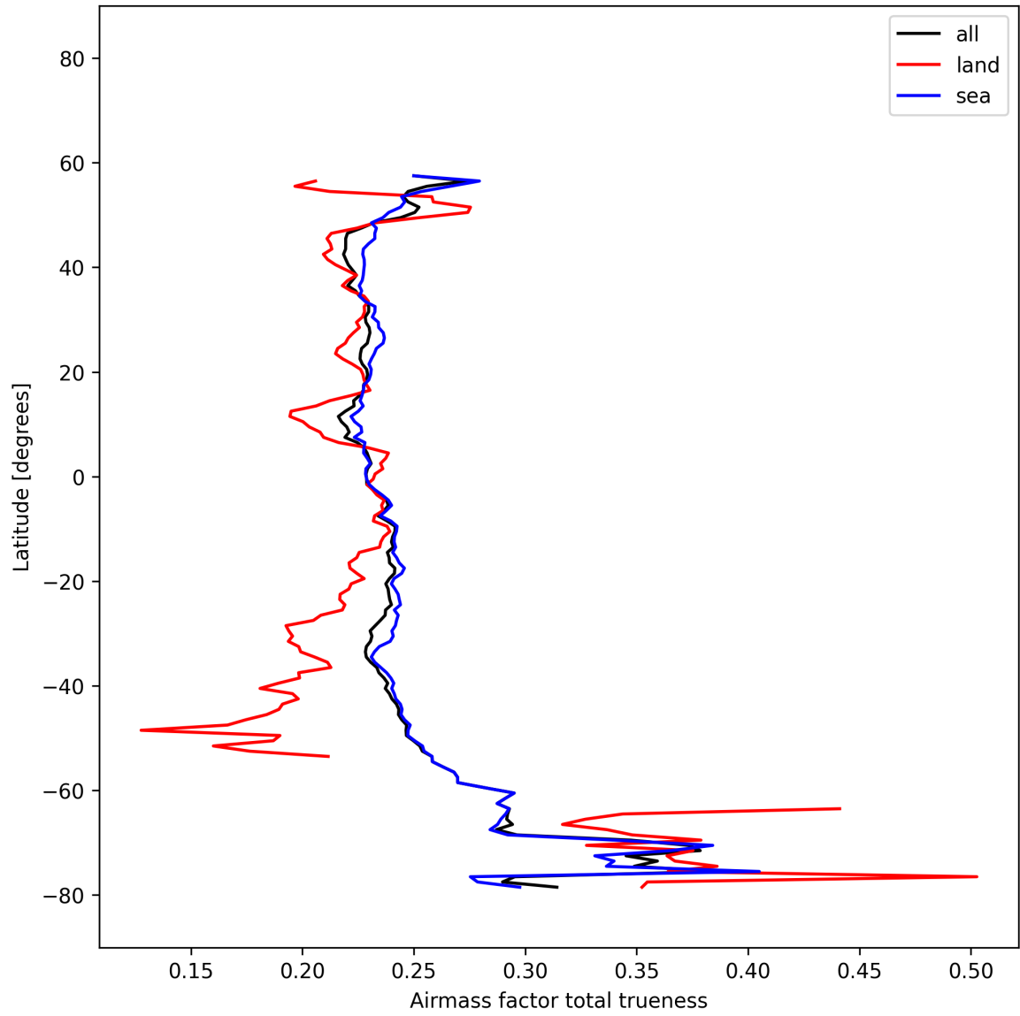
Figure 28: Zonal average of “Airmass factor total trueness” for 2025-11-12 to 2025-11-14.
