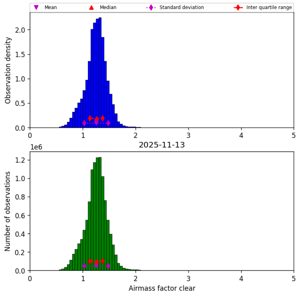
Figure 44: Histogram of “Airmass factor clear” for 2025-11-12 to 2025-11-14
