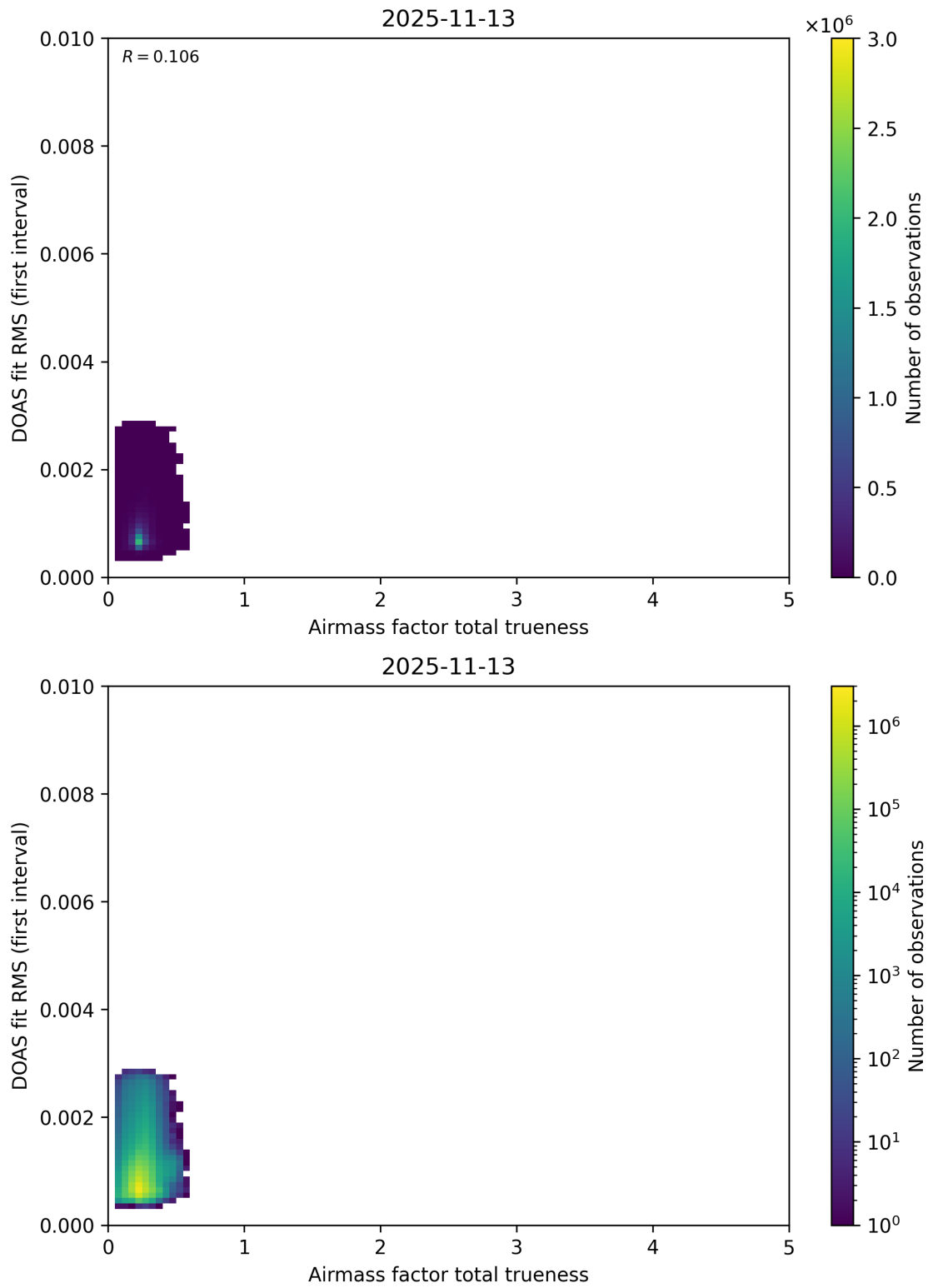
Figure 118: Scatter density plot of “Airmass factor total trueness” against “DOAS fit RMS (first interval)” for 2025-11-12 to 2025-11-14.
