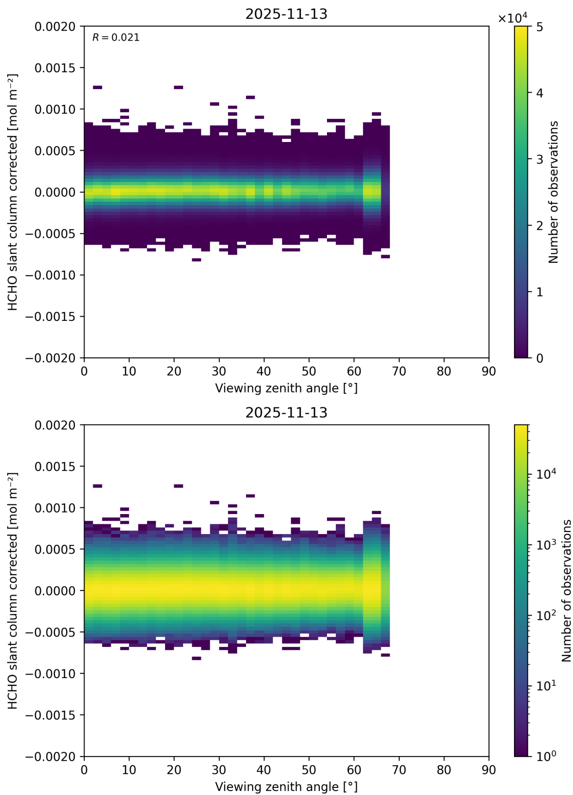
Figure 206: Scatter density plot of “Viewing zenith angle” against “HCHO slant column corrected” for 2025-11-12 to 2025-11-14.
