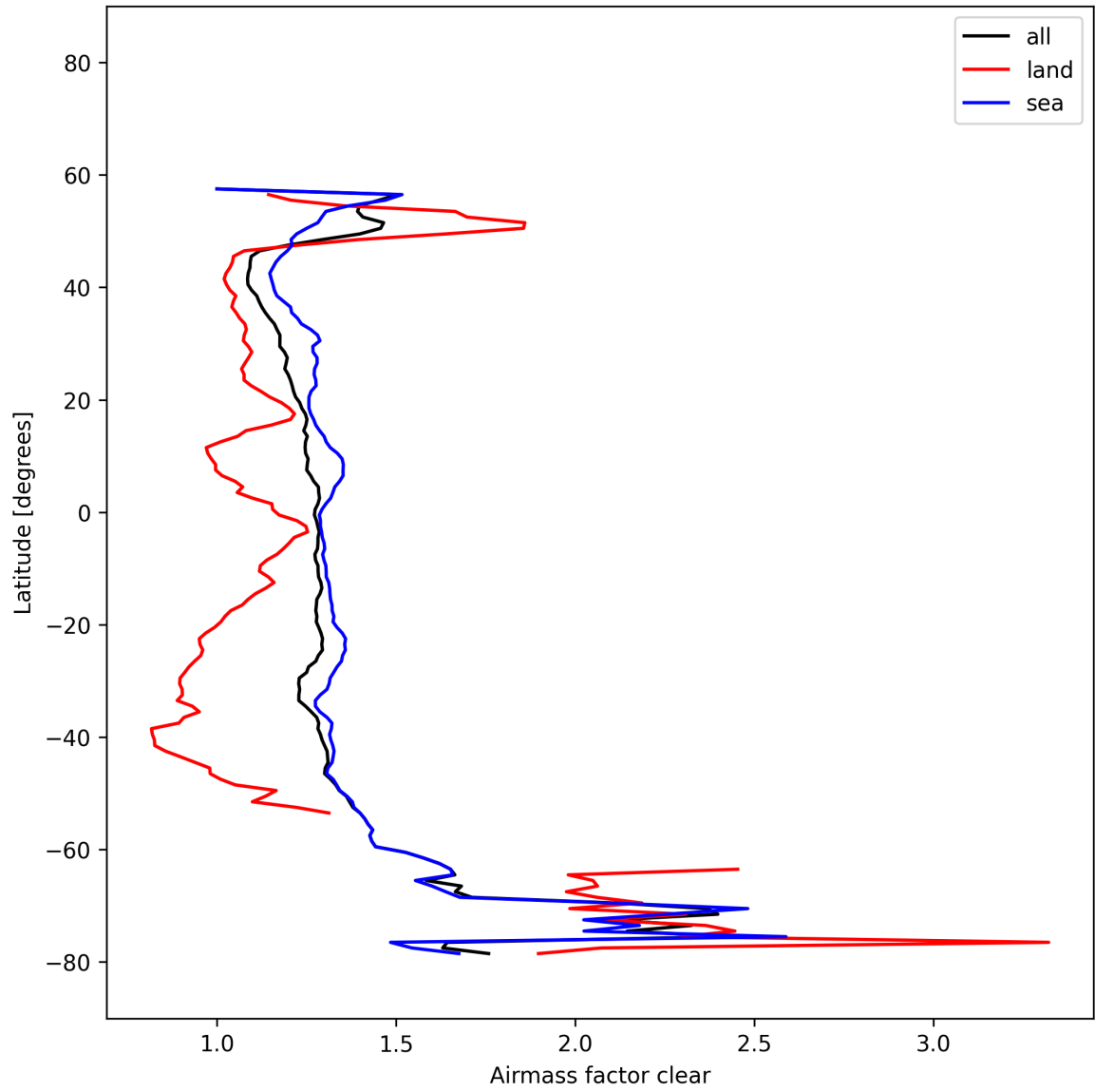
Figure 29: Zonal average of “Airmass factor clear” for 2025-11-12 to 2025-11-14.
