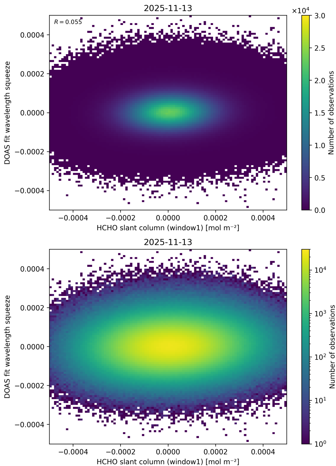
Figure 90: Scatter density plot of “HCHO slant column (window1)” against “DOAS fit wavelength squeeze” for 2025-11-12 to 2025-11-14.
