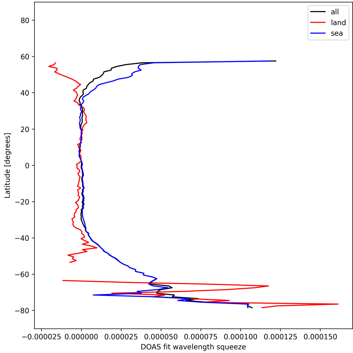
Figure 32: Zonal average of “DOAS fit wavelength squeeze” for 2025-11-12 to 2025-11-14.
