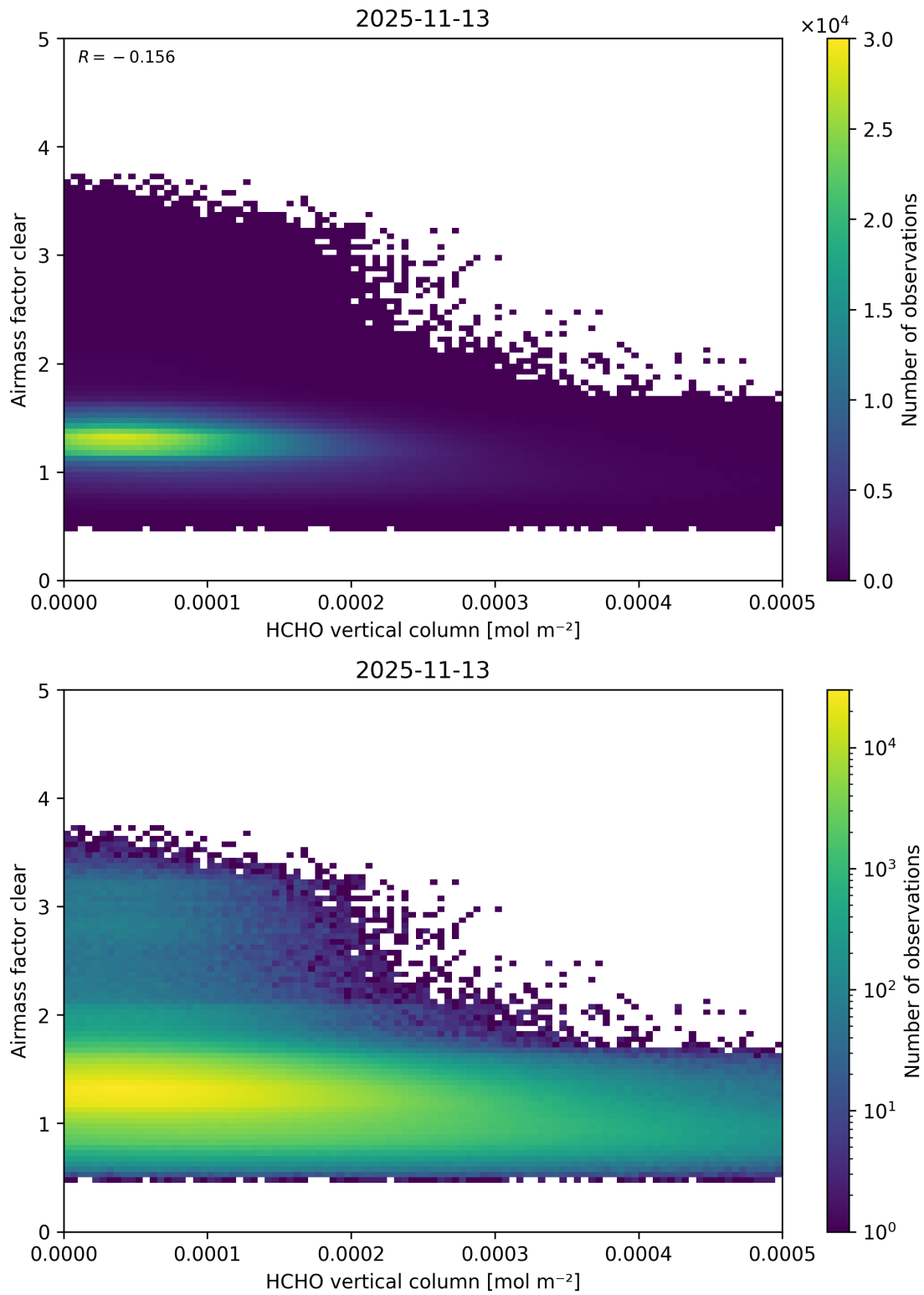
Figure 141: Scatter density plot of “HCHO vertical column” against “Airmass factor clear” for 2025-11-12 to 2025-11-14.
