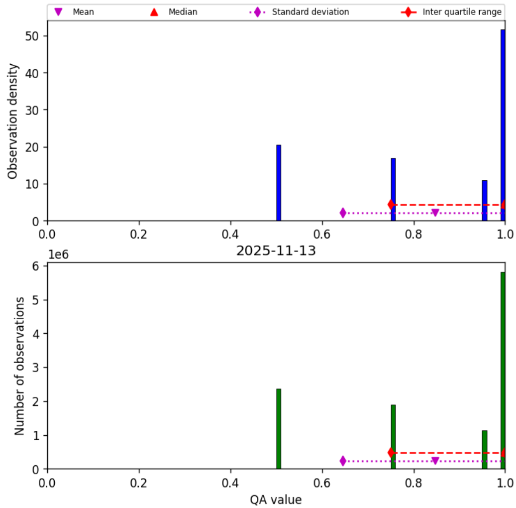
Figure 36: Histogram of “QA value” for 2025-11-12 to 2025-11-14
