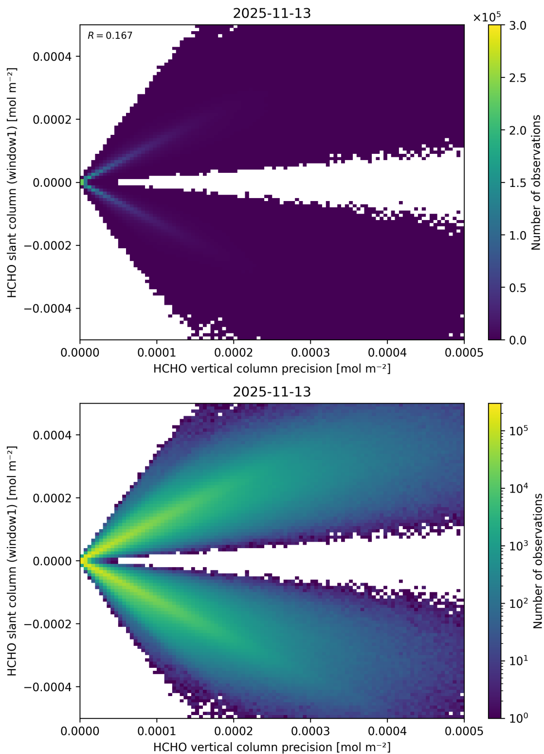
Figure 158: Scatter density plot of “HCHO vertical column precision” against “HCHO slant column (window1)” for 2025-11-12 to 2025-11-14.
