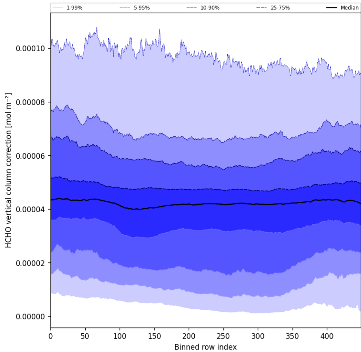
Figure 54: Along track statistics of “HCHO vertical column correction” for 2025-11-12 to 2025-11-14
