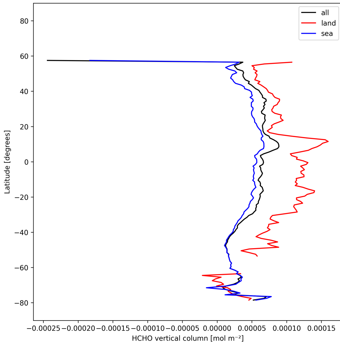
Figure 22: Zonal average of “HCHO vertical column” for 2025-11-12 to 2025-11-14.
