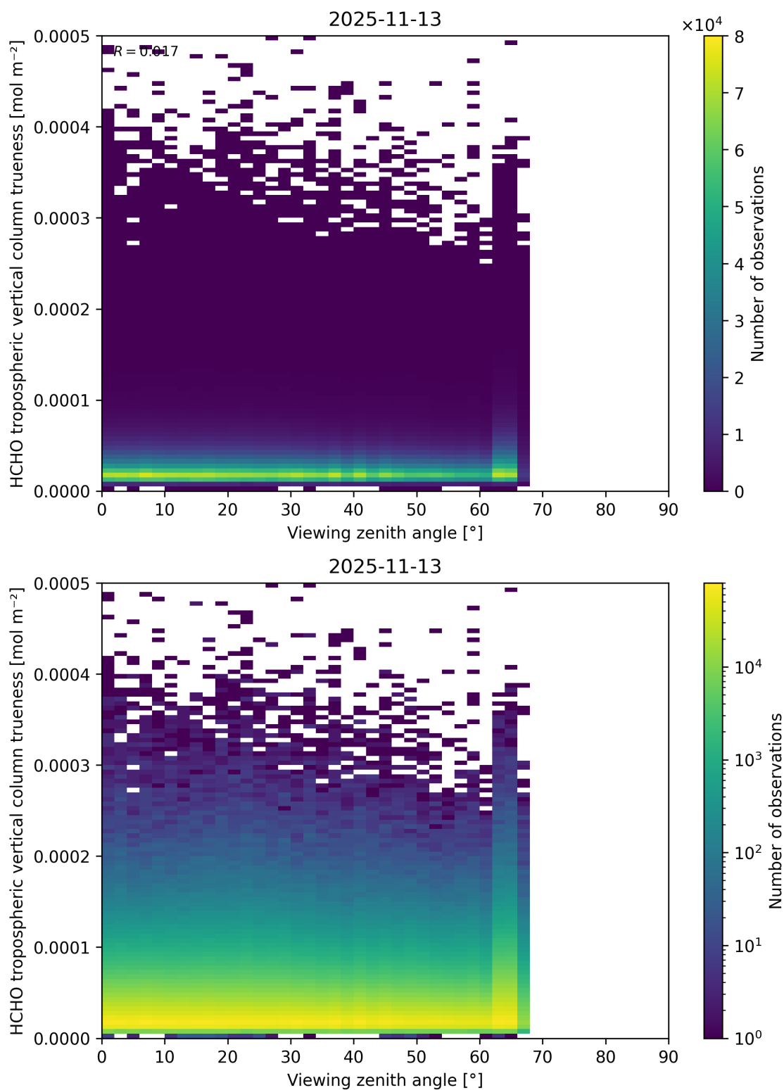
Figure 215: Scatter density plot of “Viewing zenith angle” against “HCHO tropospheric vertical column trueness” for 2025-11-12 to 2025-11-14.
