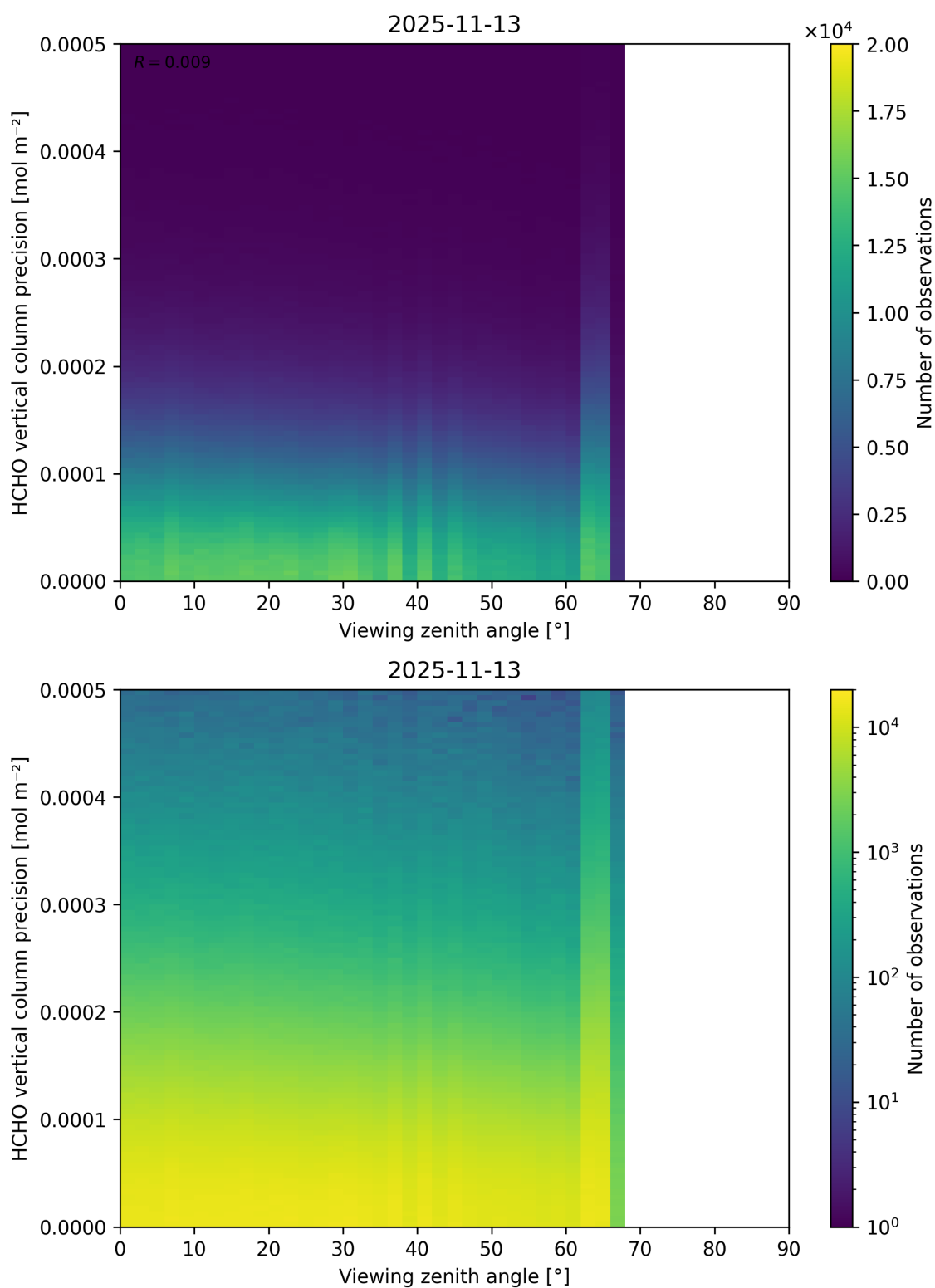
Figure 214: Scatter density plot of “Viewing zenith angle” against “HCHO vertical column precision” for 2025-11-12 to 2025-11-14.
