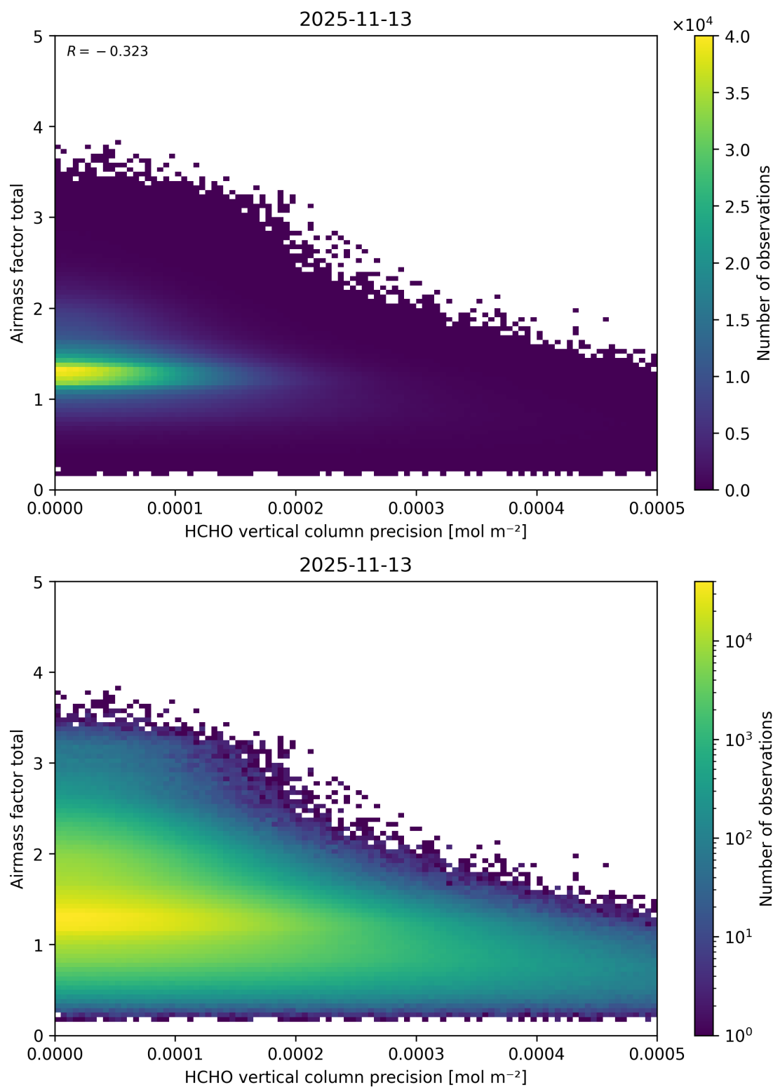
Figure 160: Scatter density plot of “HCHO vertical column precision” against “Airmass factor total” for 2025-11-12 to 2025-11-14.
