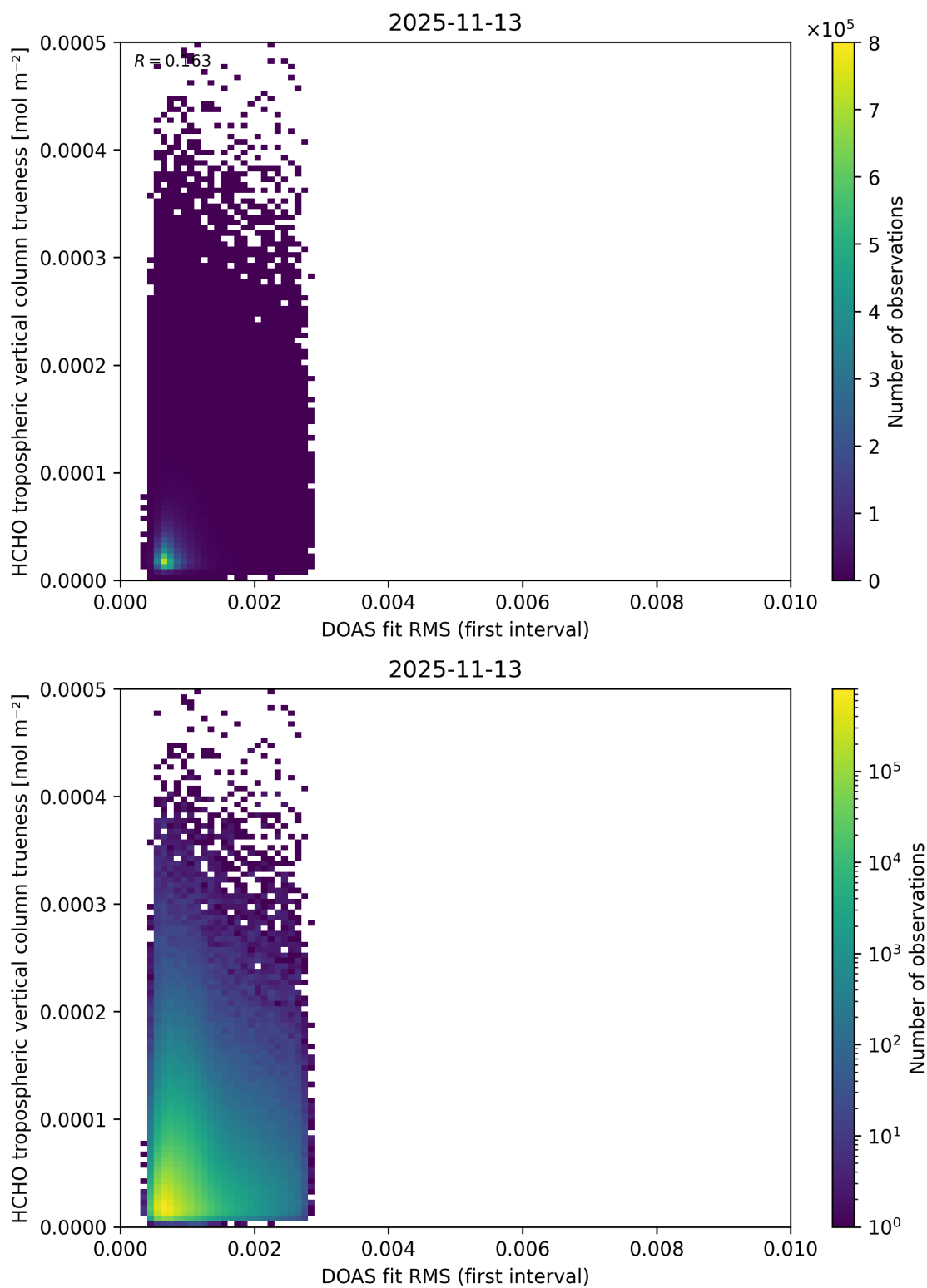
Figure 68: Scatter density plot of “DOAS fit RMS (first interval)” against “HCHO tropospheric vertical column trueness” for 2025-11-12 to 2025-11-14.
