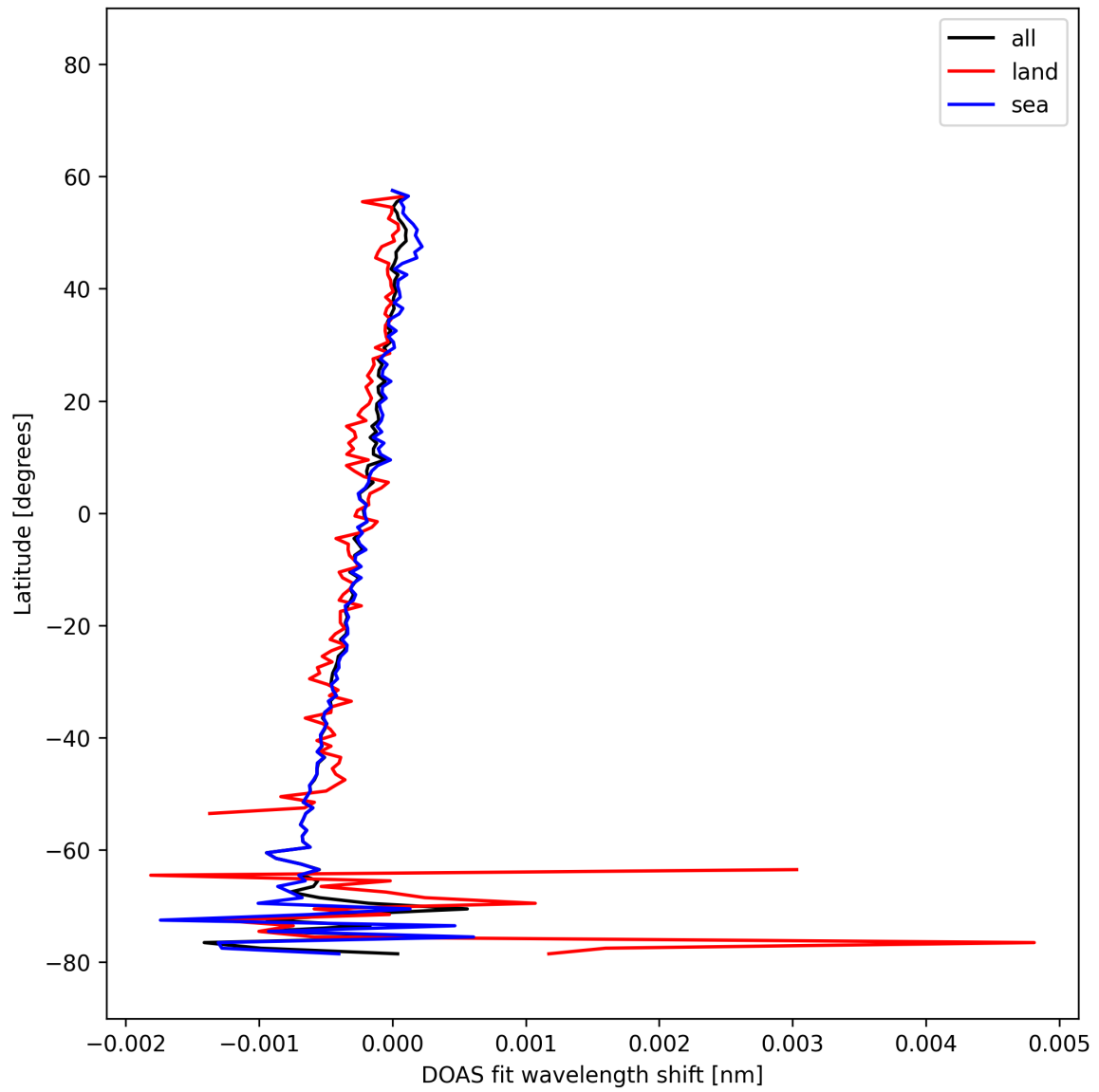
Figure 31: Zonal average of “DOAS fit wavelength shift” for 2025-11-12 to 2025-11-14.
