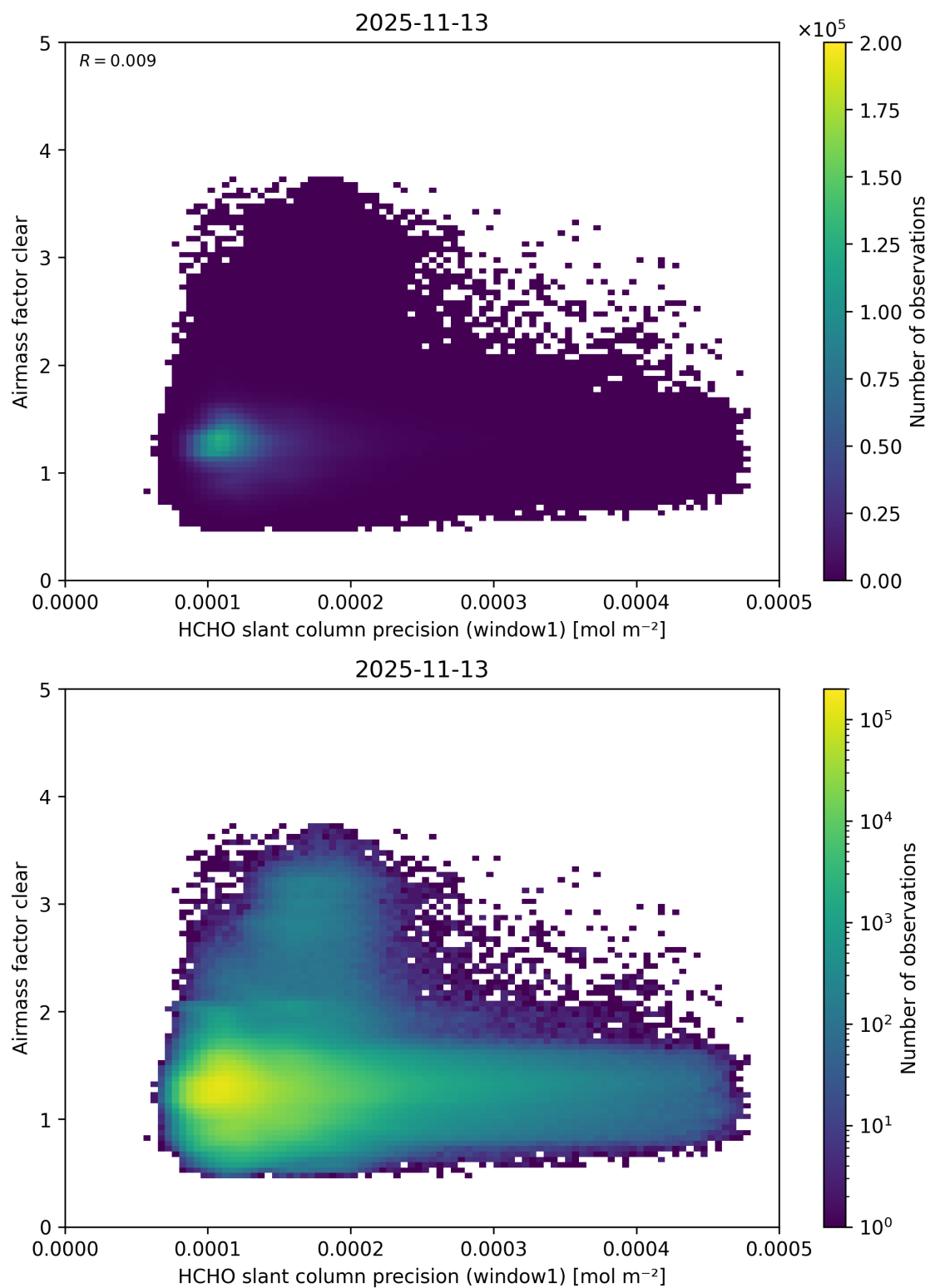
Figure 102: Scatter density plot of “HCHO slant column precision (window1)” against “Airmass factor clear” for 2025-11-12 to 2025-11-14.
