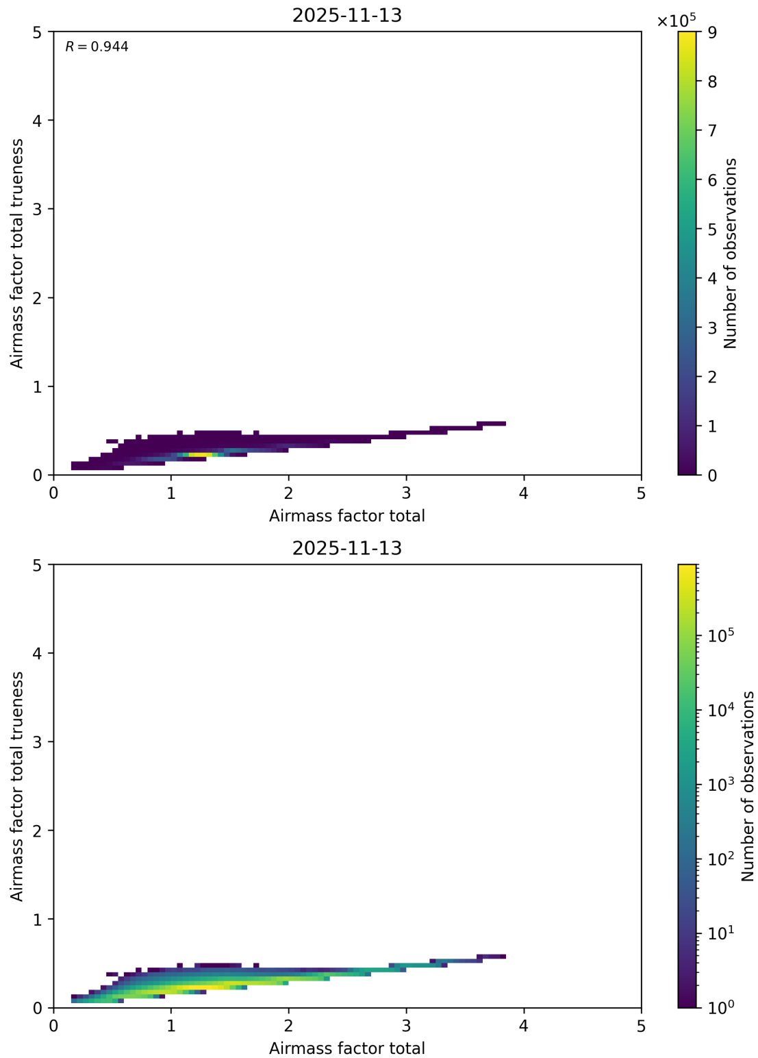
Figure 115: Scatter density plot of “Airmass factor total” against “Airmass factor total trueness” for 2025-11-12 to 2025-11-14.
