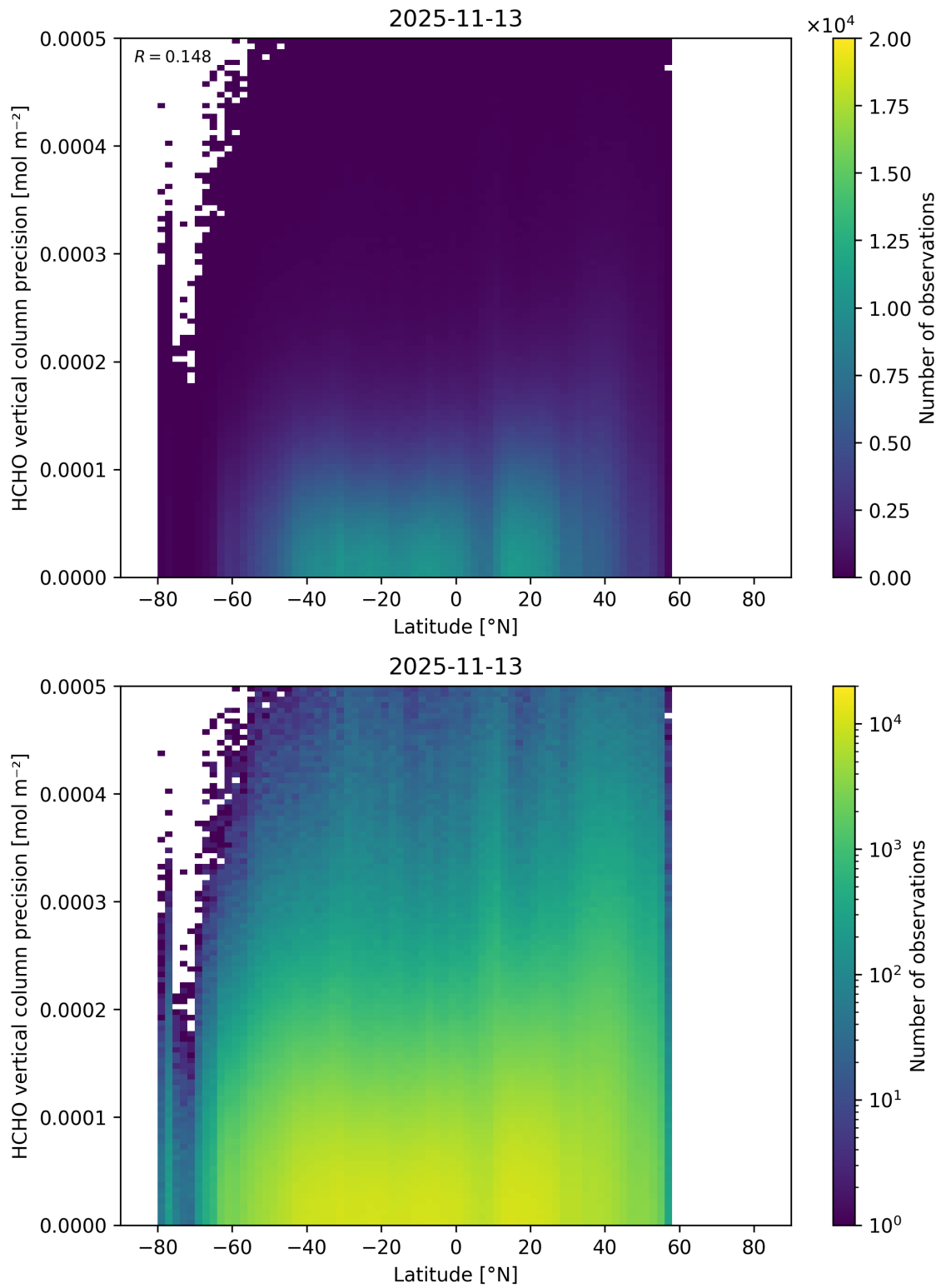
Figure 183: Scatter density plot of “Latitude” against “HCHO vertical column precision” for 2025-11-12 to 2025-11-14.
