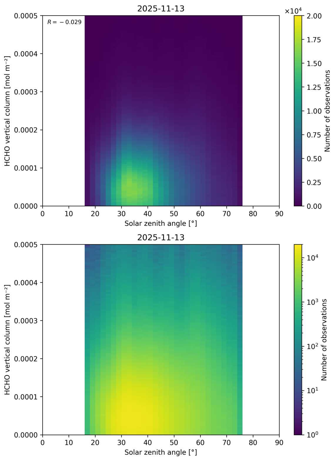
Figure 196: Scatter density plot of “Solar zenith angle” against “HCHO vertical column” for 2025-11-12 to 2025-11-14.
