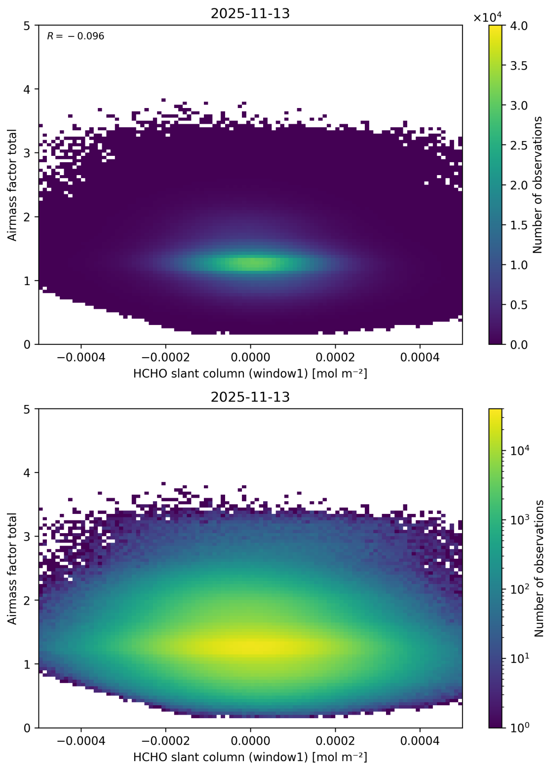
Figure 95: Scatter density plot of “HCHO slant column (window1)” against “Airmass factor total” for 2025-11-12 to 2025-11-14.
