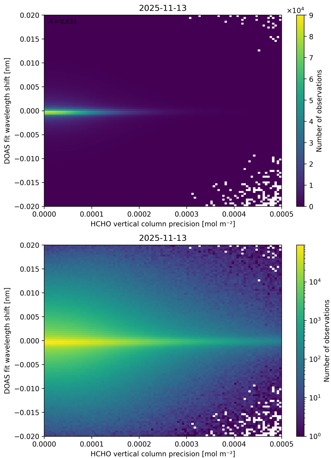
Figure 153: Scatter density plot of “HCHO vertical column precision” against “DOAS fit wavelength shift” for 2025-11-12 to 2025-11-14.
