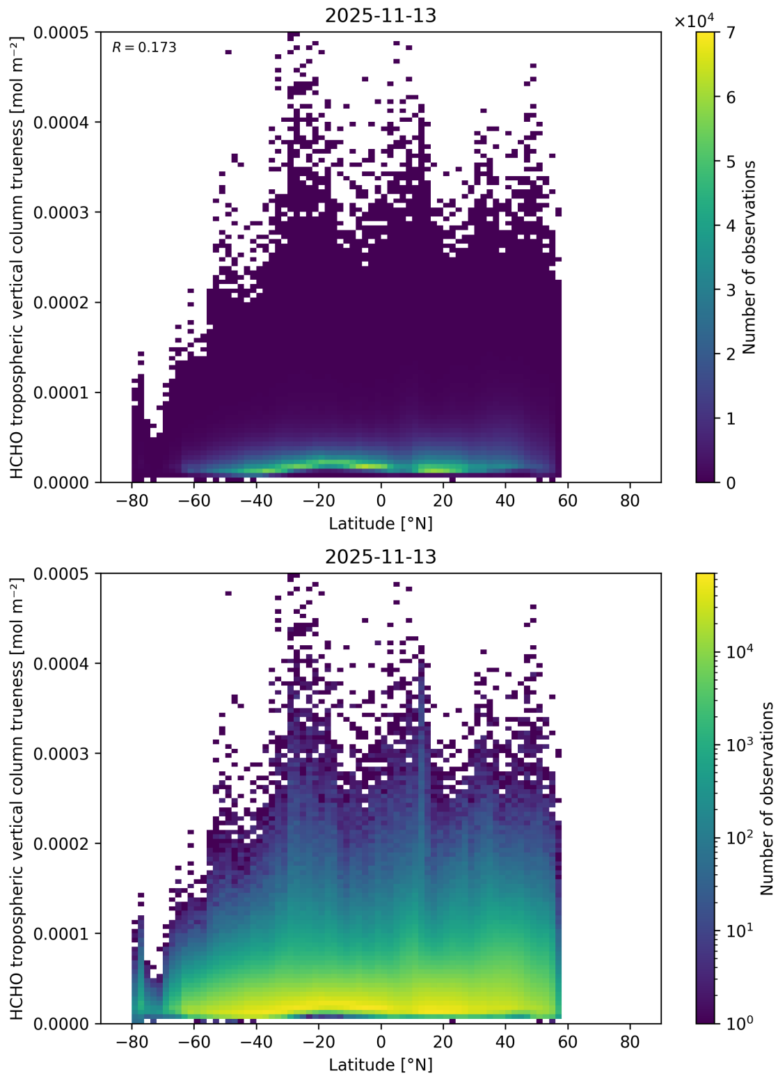
Figure 184: Scatter density plot of “Latitude” against “HCHO tropospheric vertical column trueness” for 2025-11-12 to 2025-11-14.
