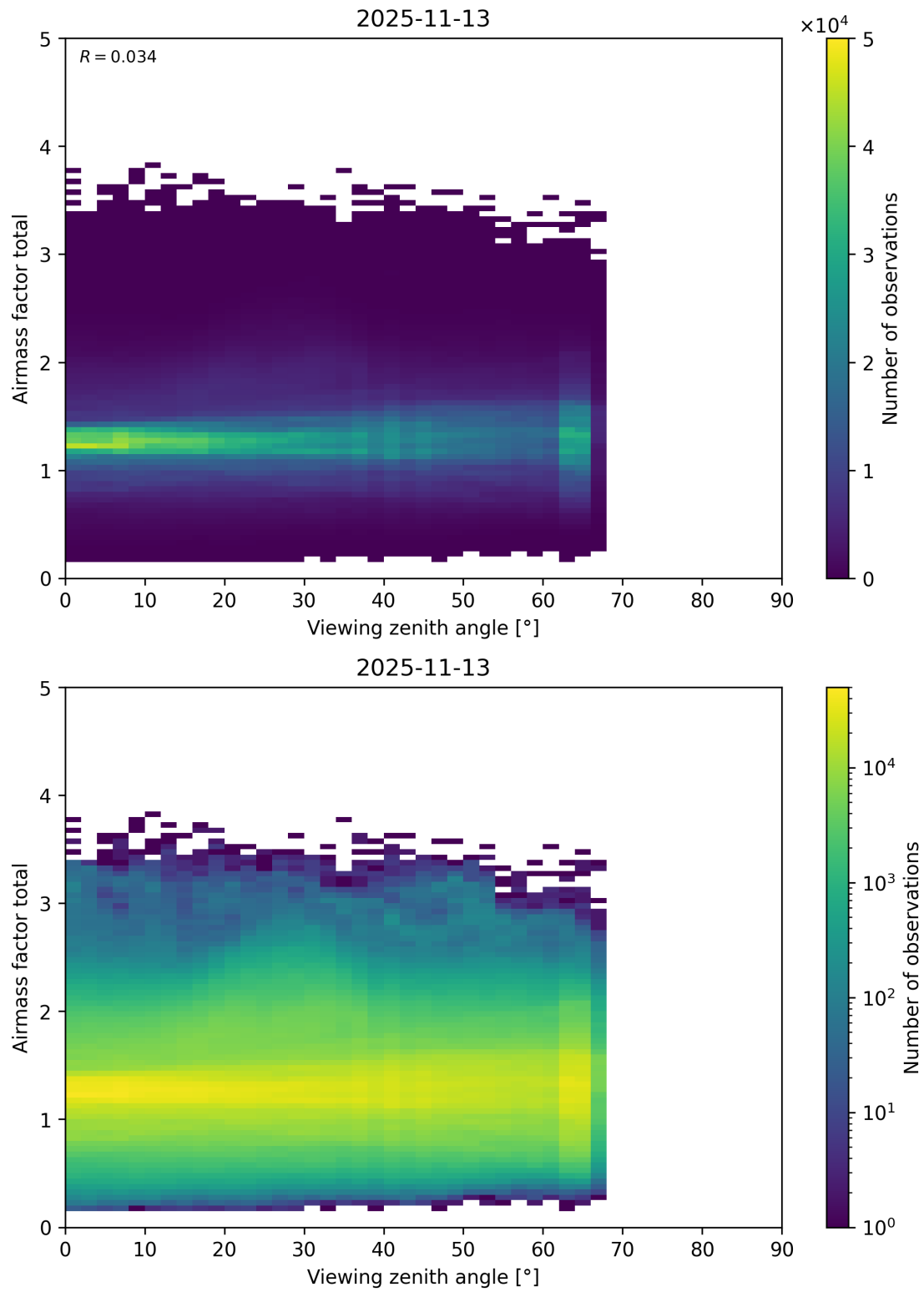
Figure 210: Scatter density plot of “Viewing zenith angle” against “Airmass factor total” for 2025-11-12 to 2025-11-14.
