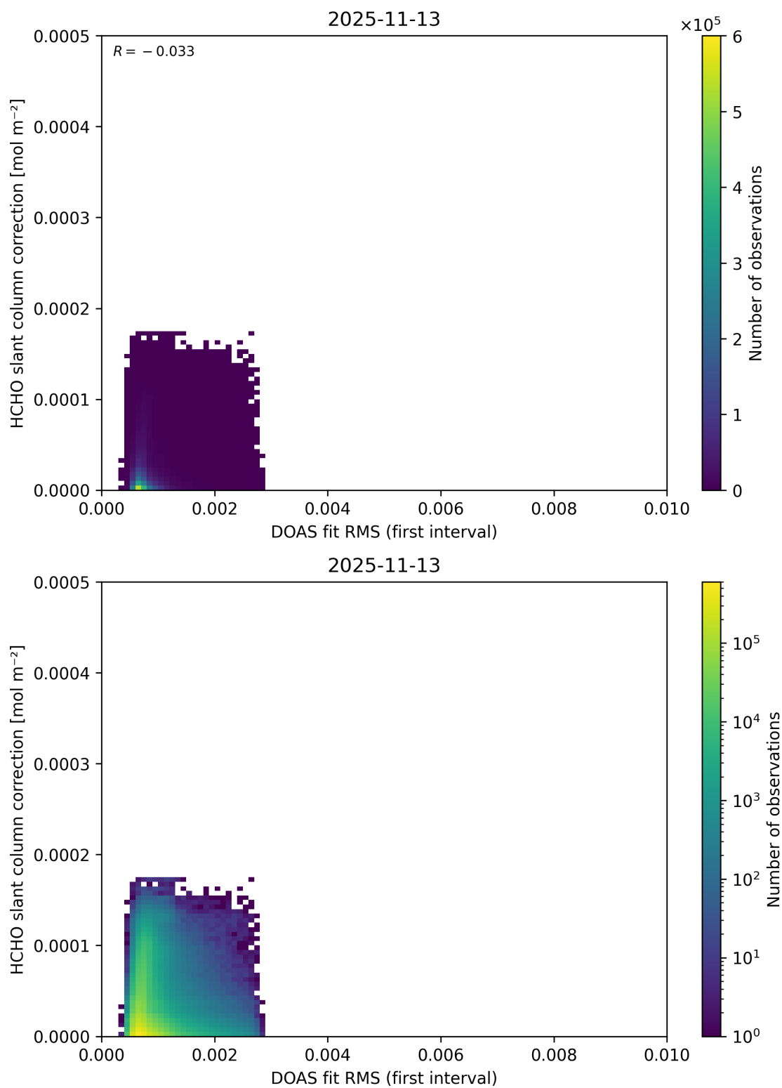
Figure 67: Scatter density plot of “DOAS fit RMS (first interval)” against “HCHO slant column correction” for 2025-11-12 to 2025-11-14.
