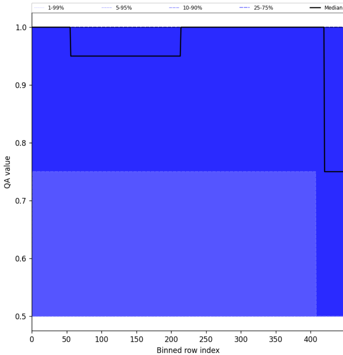
Figure 51: Along track statistics of “QA value” for 2025-11-12 to 2025-11-14
