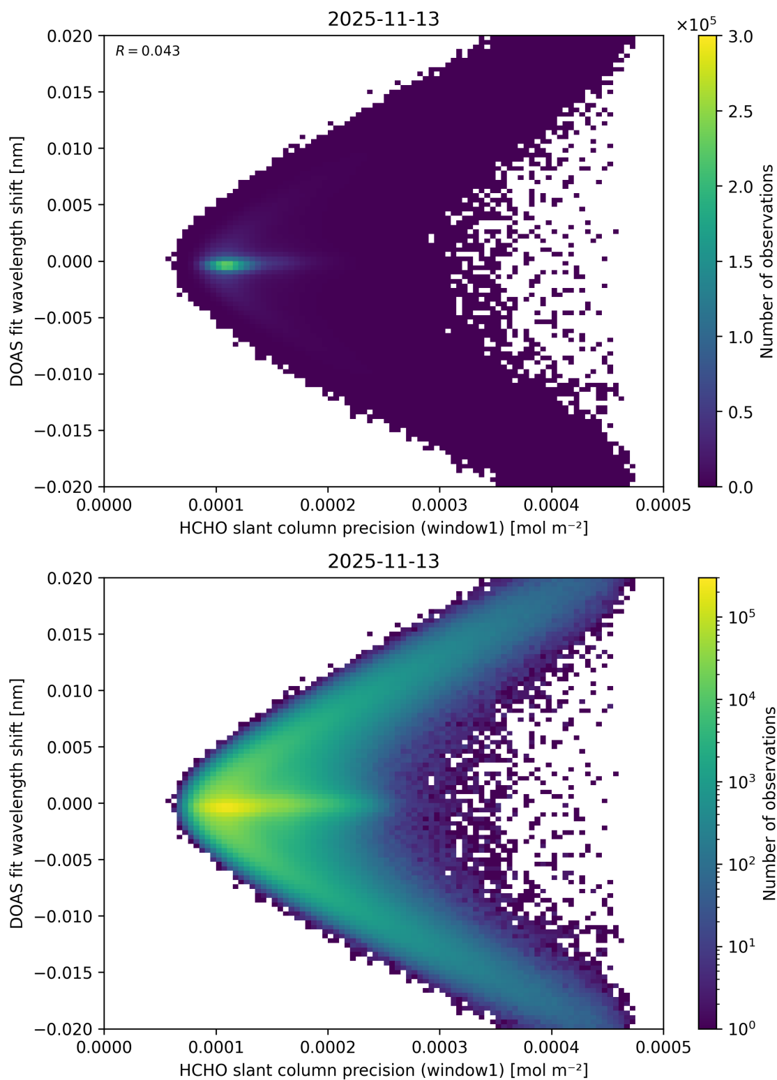
Figure 100: Scatter density plot of “HCHO slant column precision (window1)” against “DOAS fit wavelength shift” for 2025-11-12 to 2025-11-14.
