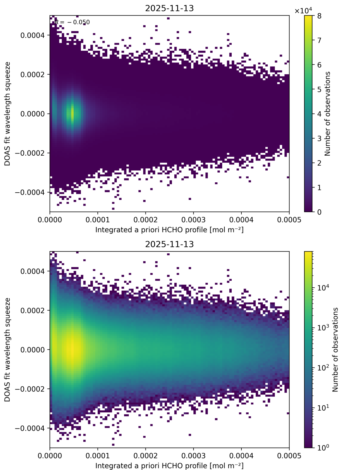
Figure 167: Scatter density plot of “Integrated a priori HCHO profile” against “DOAS fit wavelength squeeze” for 2025-11-12 to 2025-11-14.
