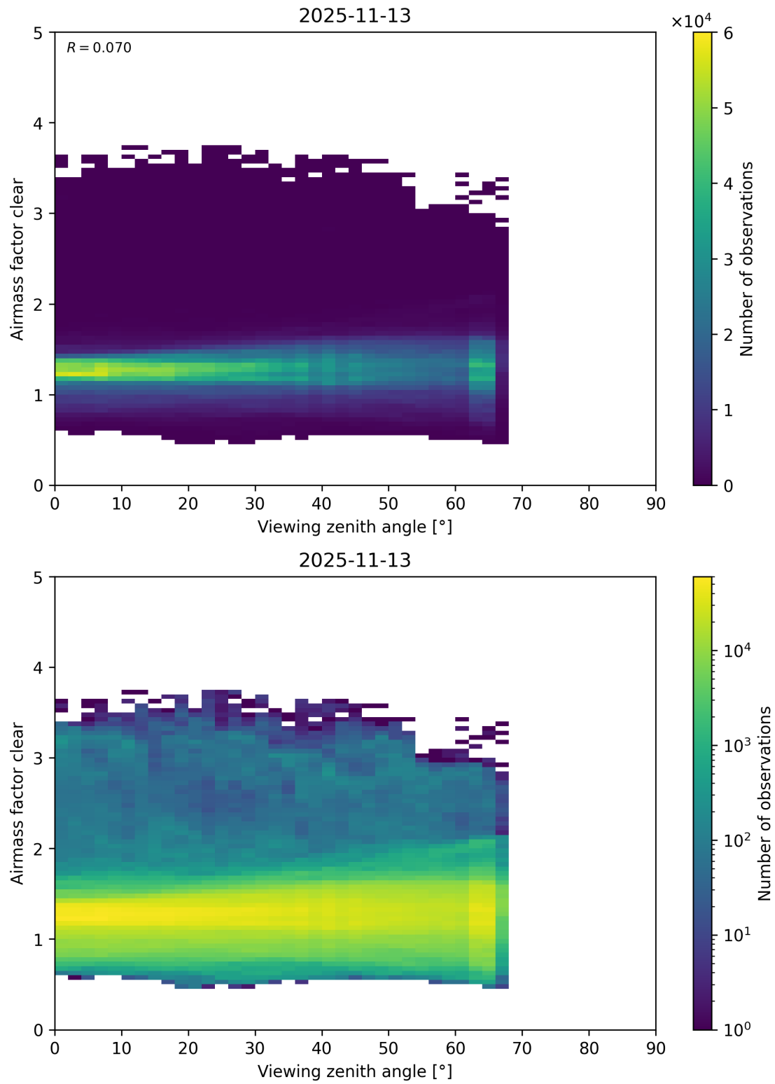
Figure 205: Scatter density plot of “Viewing zenith angle” against “Airmass factor clear” for 2025-11-12 to 2025-11-14.
