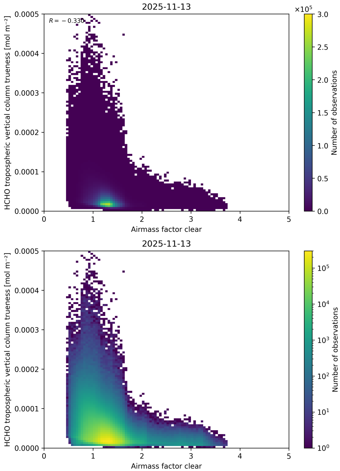
Figure 83: Scatter density plot of “Airmass factor clear” against “HCHO tropospheric vertical column trueness” for 2025-11-12 to 2025-11-14.
