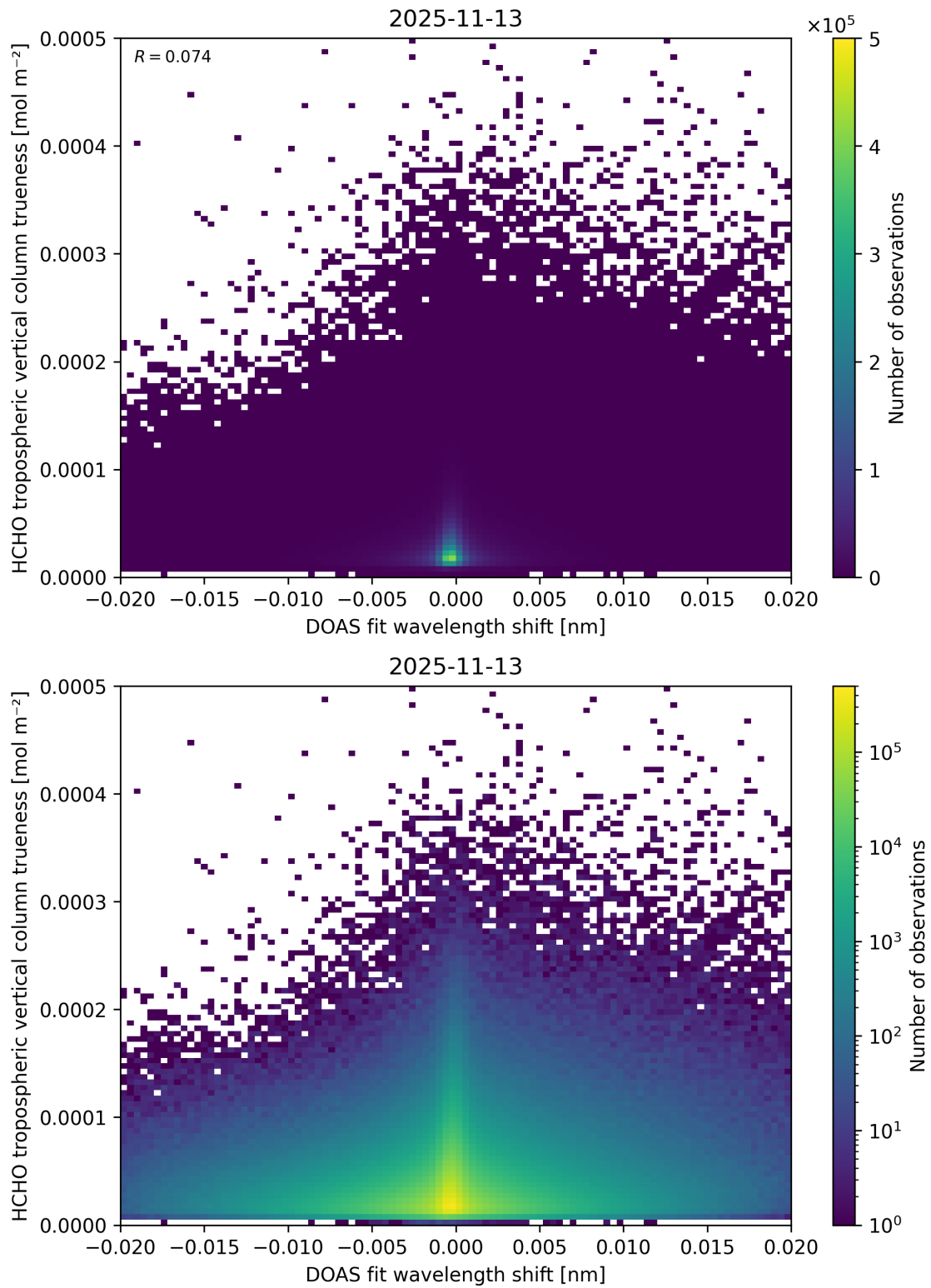
Figure 73: Scatter density plot of “DOAS fit wavelength shift” against “HCHO tropospheric vertical column trueness” for 2025-11-12 to 2025-11-14.
