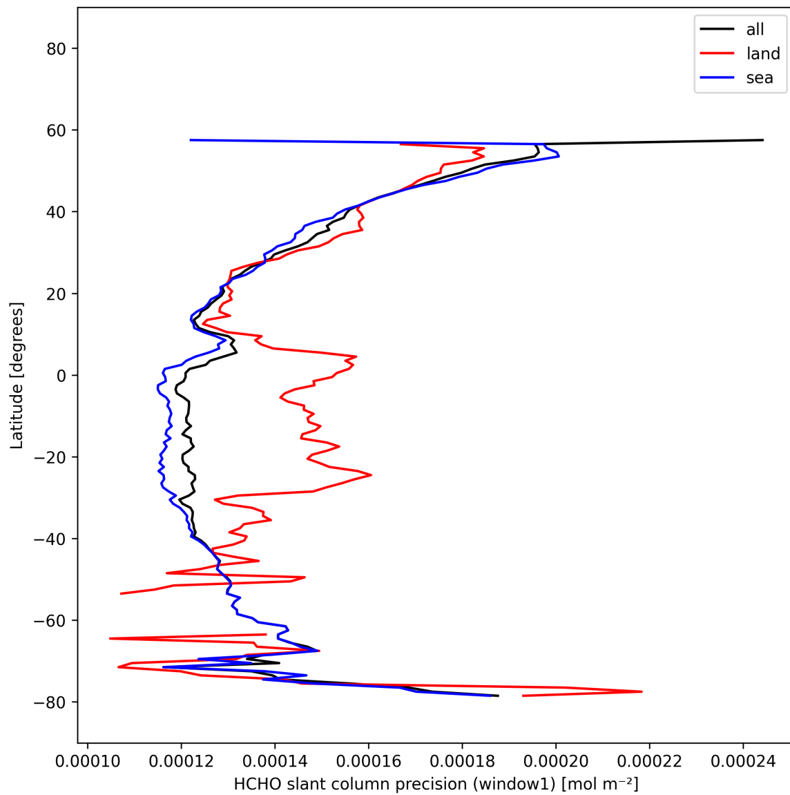
Figure 26: Zonal average of “HCHO slant column precision (window1)” for 2025-11-12 to 2025-11-14.
