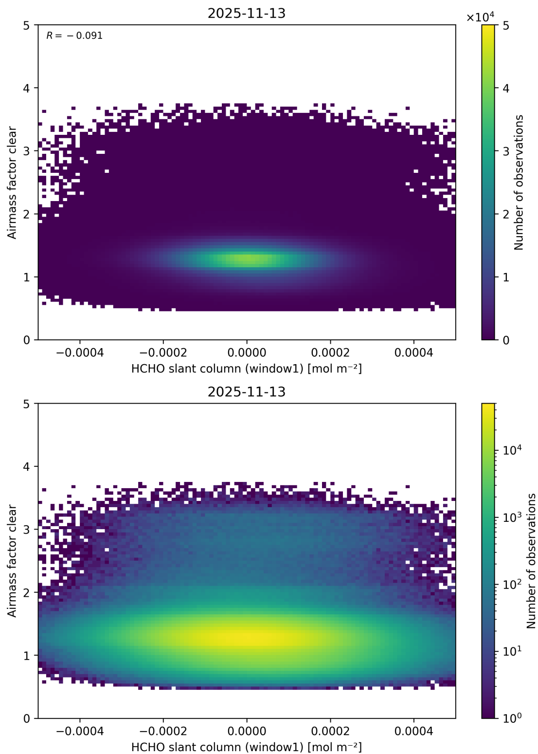
Figure 91: Scatter density plot of “HCHO slant column (window1)” against “Airmass factor clear” for 2025-11-12 to 2025-11-14.
