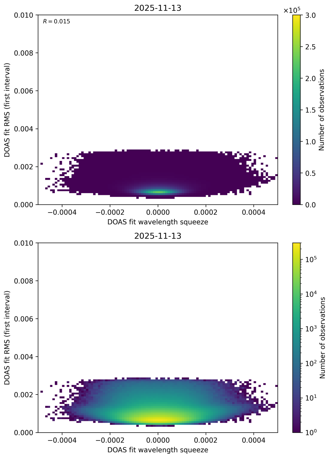
Figure 74: Scatter density plot of “DOAS fit wavelength squeeze” against “DOAS fit RMS (first interval)” for 2025-11-12 to 2025-11-14.
