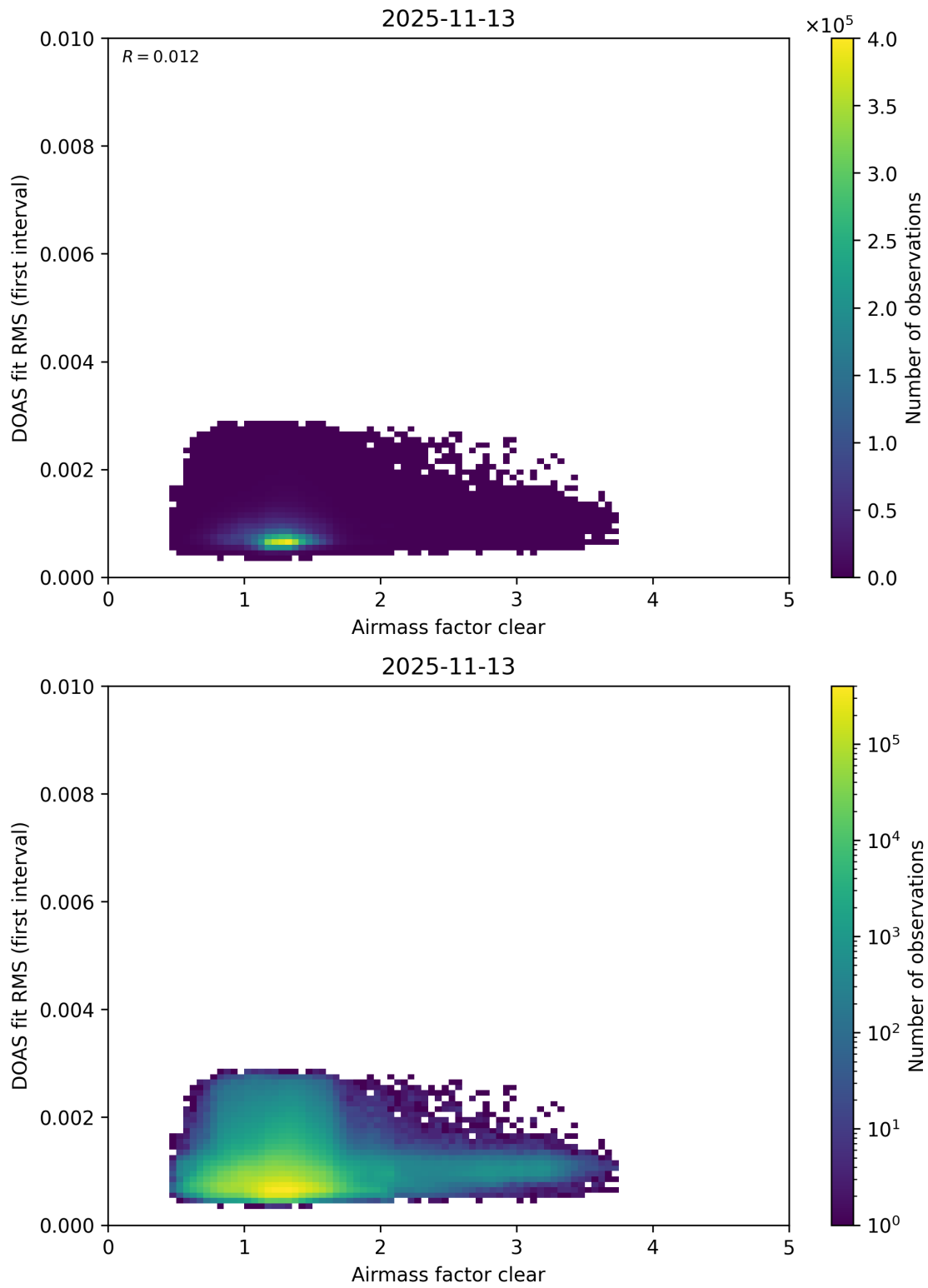
Figure 78: Scatter density plot of “Airmass factor clear” against “DOAS fit RMS (first interval)” for 2025-11-12 to 2025-11-14.
