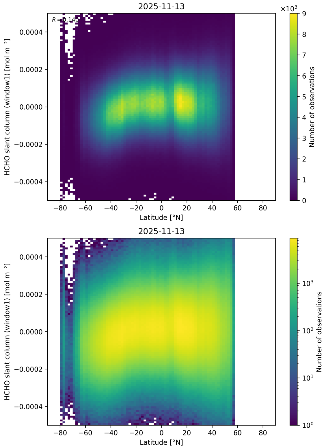
Figure 177: Scatter density plot of “Latitude” against “HCHO slant column (window1)” for 2025-11-12 to 2025-11-14.
