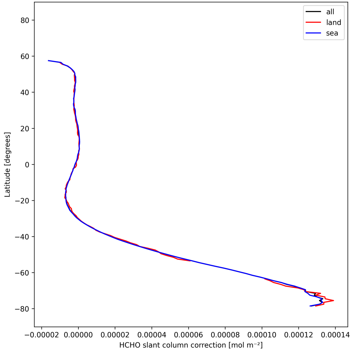
Figure 34: Zonal average of “HCHO slant column correction” for 2025-11-12 to 2025-11-14.
