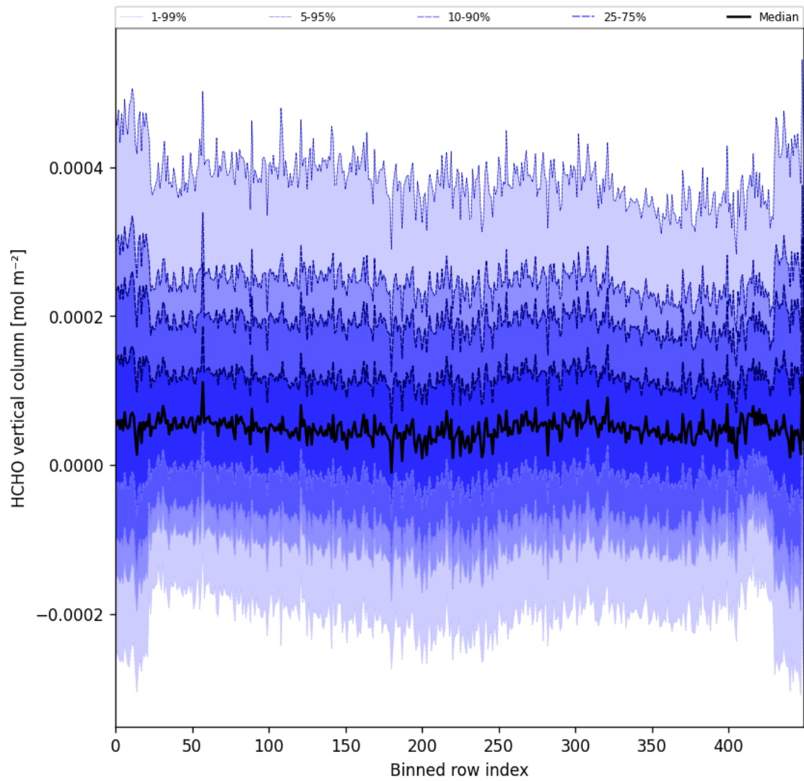
Figure 52: Along track statistics of “HCHO vertical column” for 2025-11-12 to 2025-11-14
