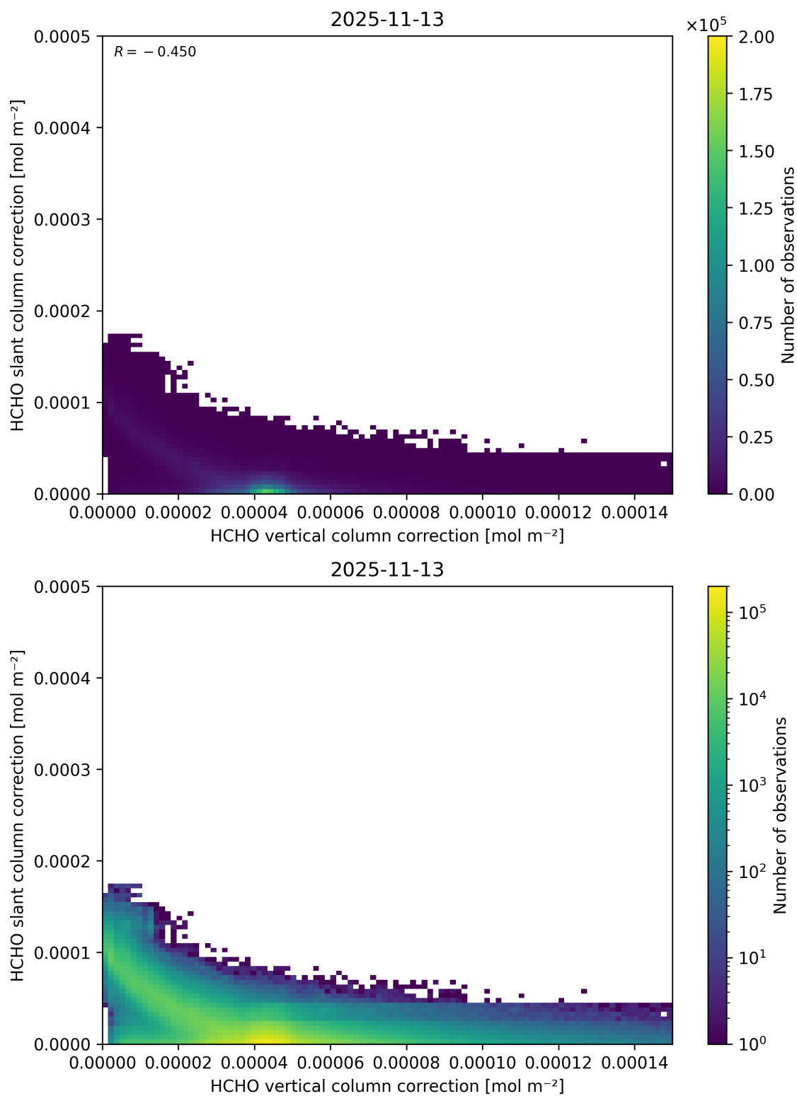
Figure 131: Scatter density plot of “HCHO vertical column correction” against “HCHO slant column correction” for 2025-11-12 to 2025-11-14.
