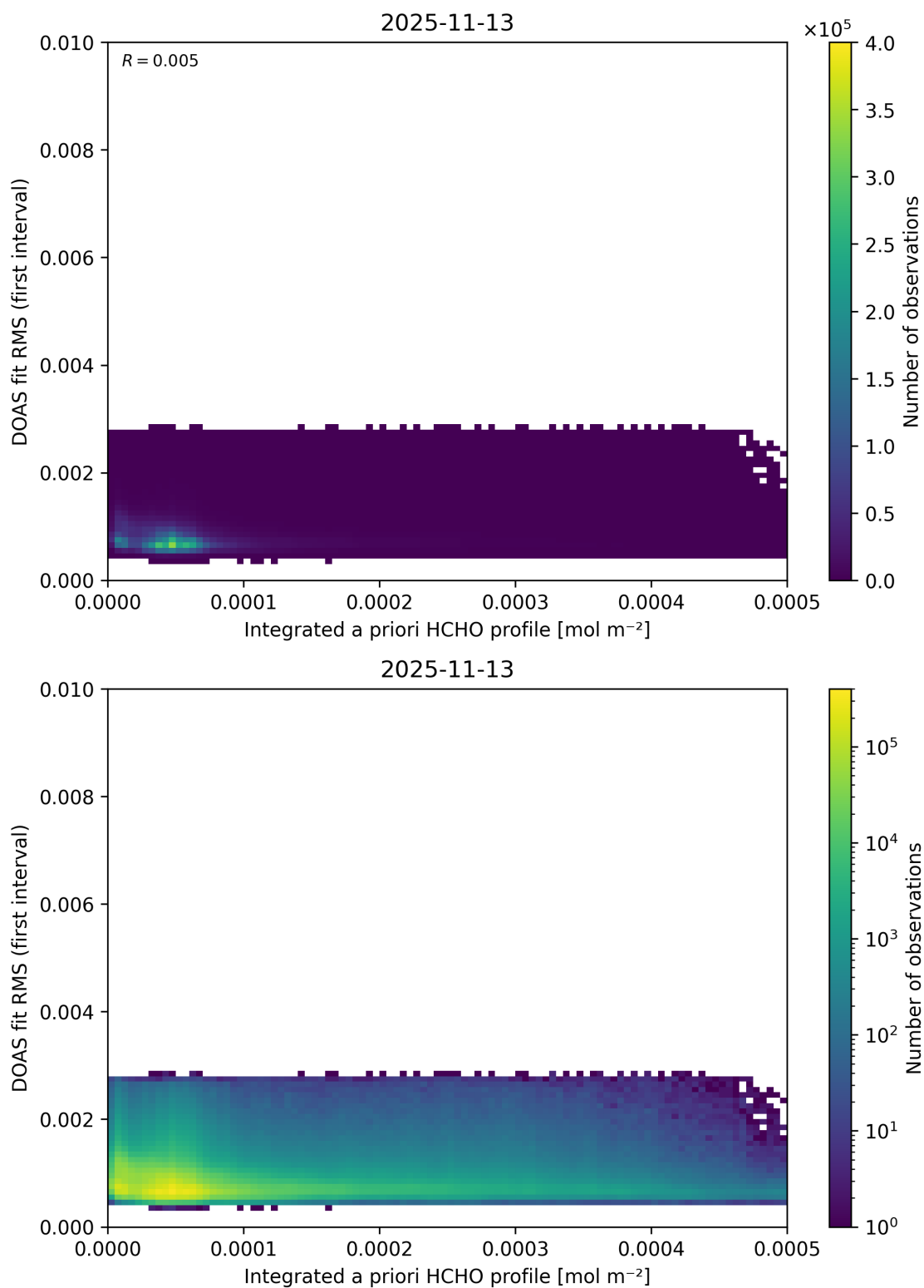
Figure 165: Scatter density plot of “Integrated a priori HCHO profile” against “DOAS fit RMS (first interval)” for 2025-11-12 to 2025-11-14.
