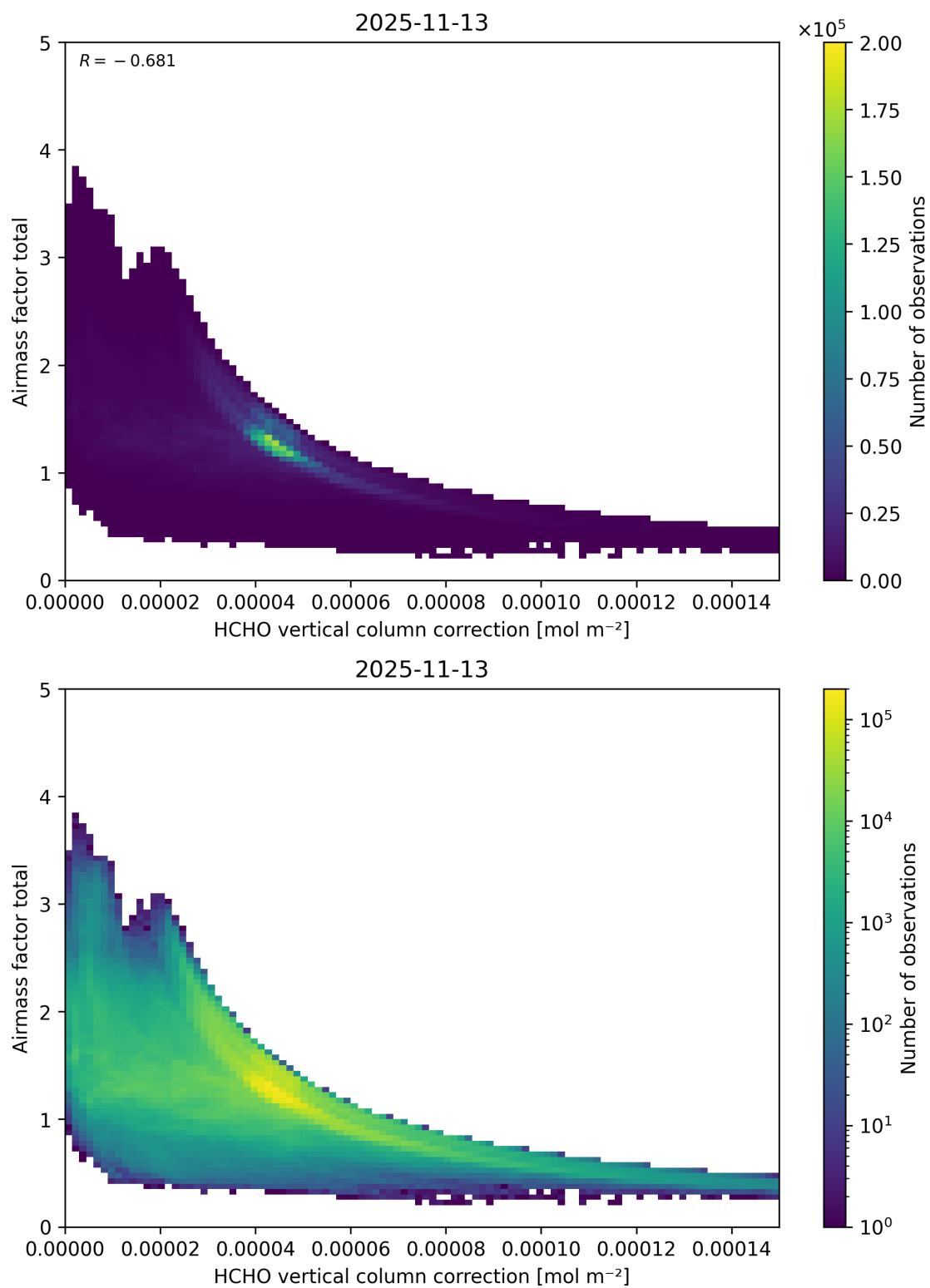
Figure 134: Scatter density plot of “HCHO vertical column correction” against “Airmass factor total” for 2025-11-12 to 2025-11-14.
