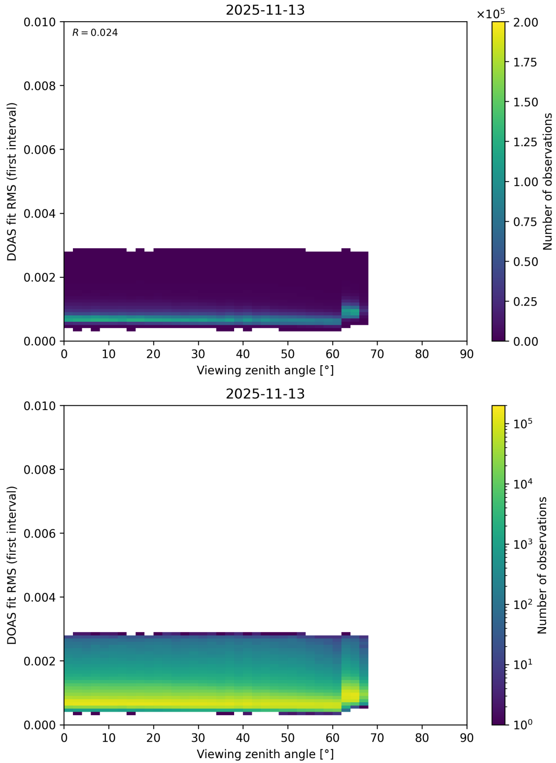
Figure 202: Scatter density plot of “Viewing zenith angle” against “DOAS fit RMS (first interval)” for 2025-11-12 to 2025-11-14.
