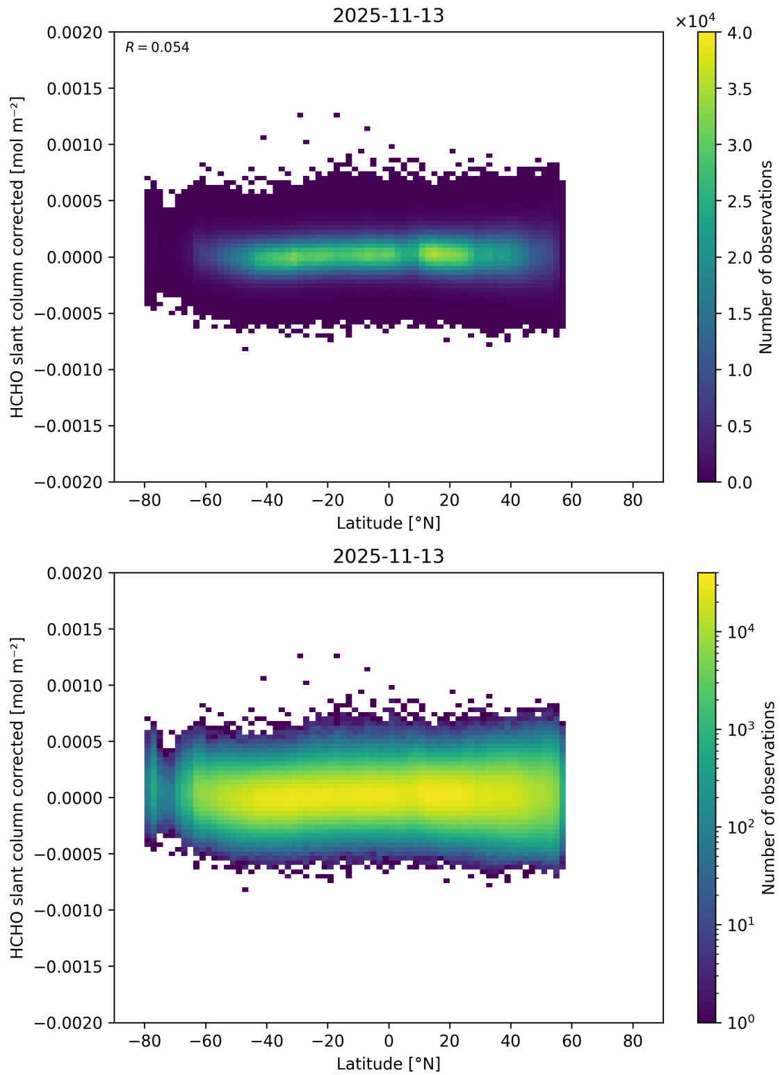
Figure 175: Scatter density plot of “Latitude” against “HCHO slant column corrected” for 2025-11-12 to 2025-11-14.
