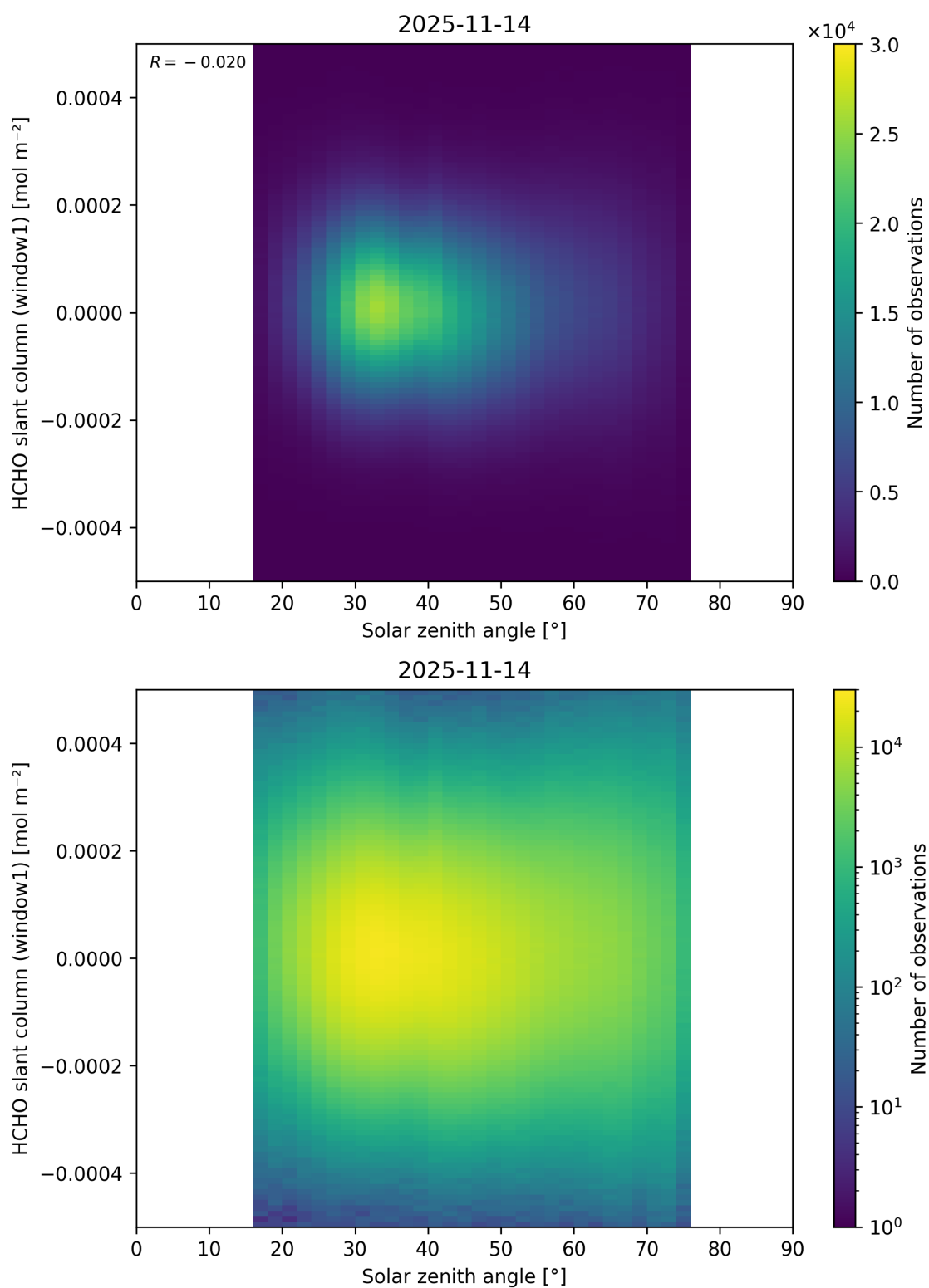
Figure 192: Scatter density plot of “Solar zenith angle” against “HCHO slant column (window1)” for 2025-11-13 to 2025-11-15.
