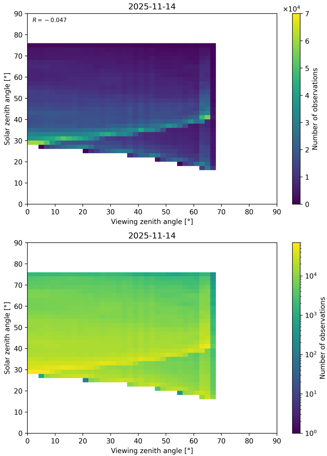
Figure 218: Scatter density plot of “Viewing zenith angle” against “Solar zenith angle” for 2025-11-13 to 2025-11-15.
