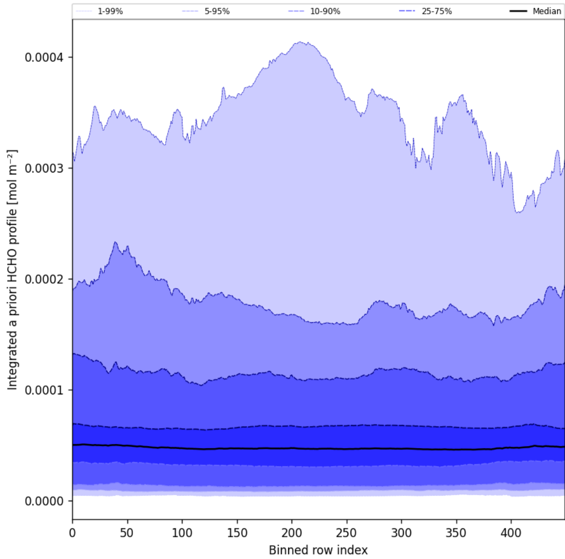
Figure 60: Along track statistics of “Integrated a priori HCHO profile” for 2025-11-13 to 2025-11-15
