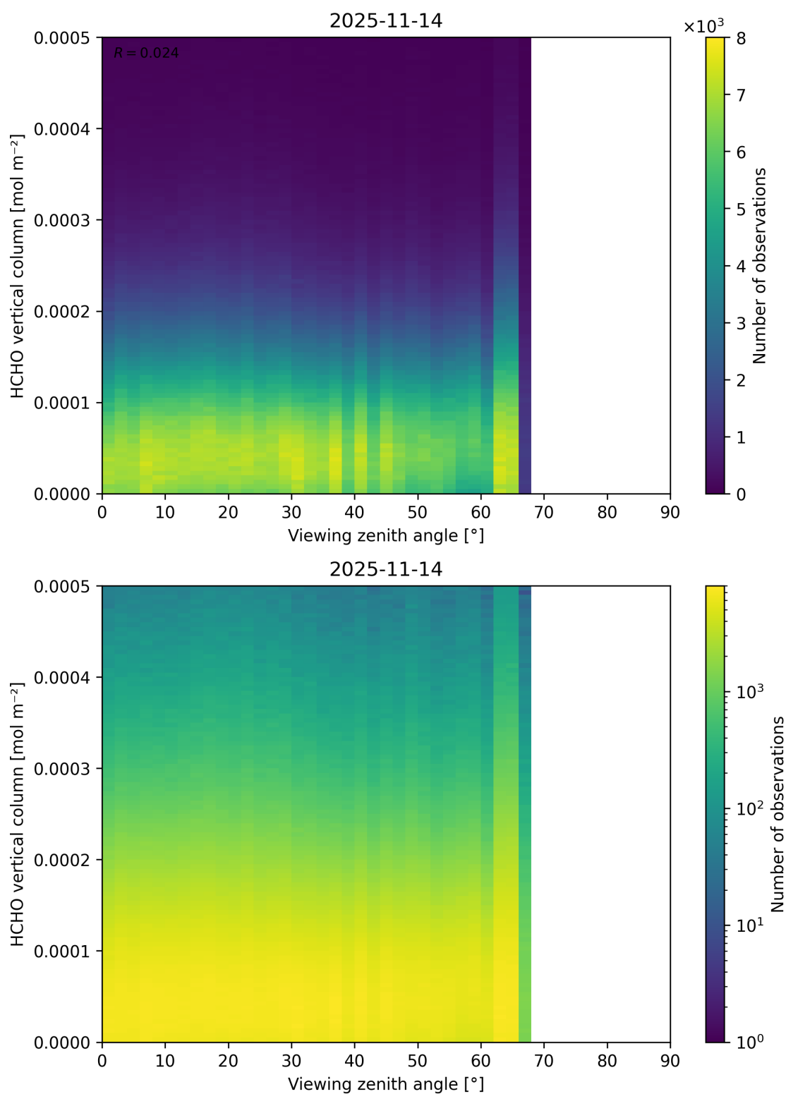
Figure 212: Scatter density plot of “Viewing zenith angle” against “HCHO vertical column” for 2025-11-13 to 2025-11-15.
