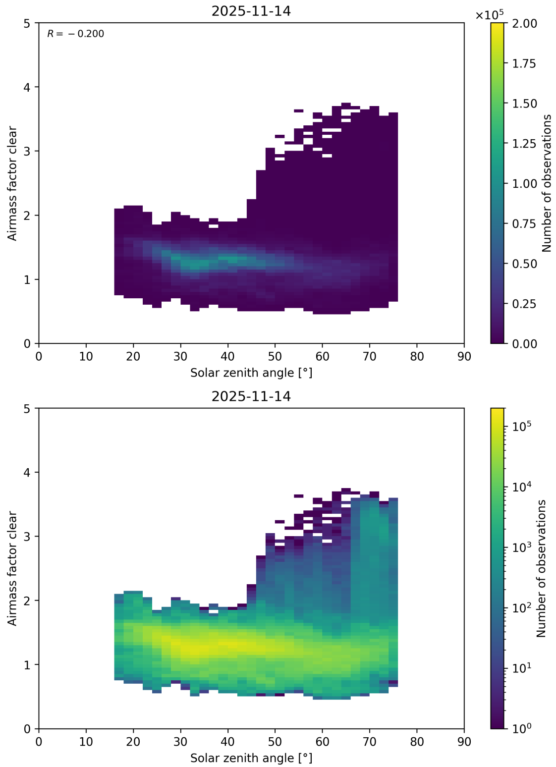
Figure 189: Scatter density plot of “Solar zenith angle” against “Airmass factor clear” for 2025-11-13 to 2025-11-15.
