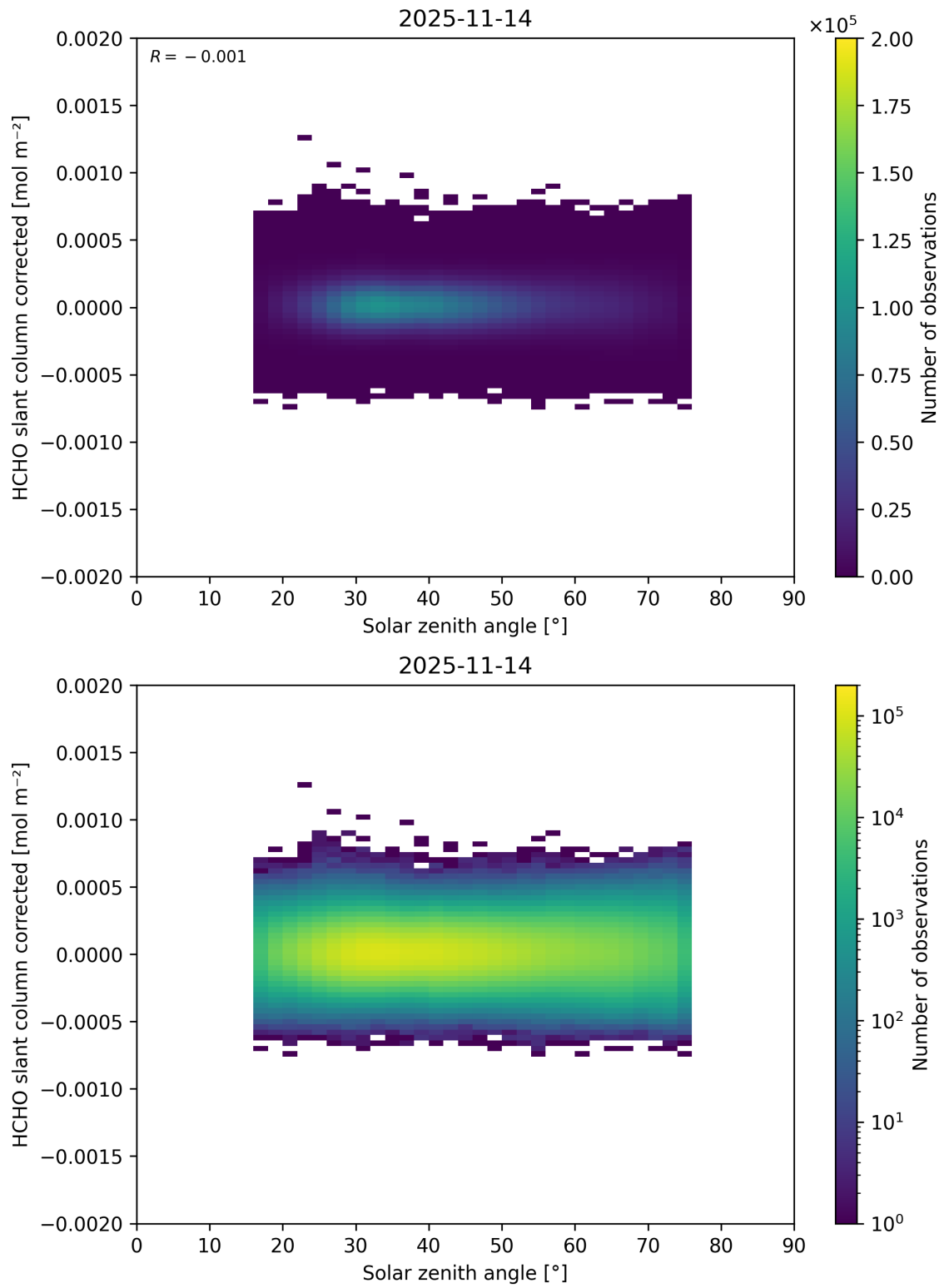
Figure 190: Scatter density plot of “Solar zenith angle” against “HCHO slant column corrected” for 2025-11-13 to 2025-11-15.
