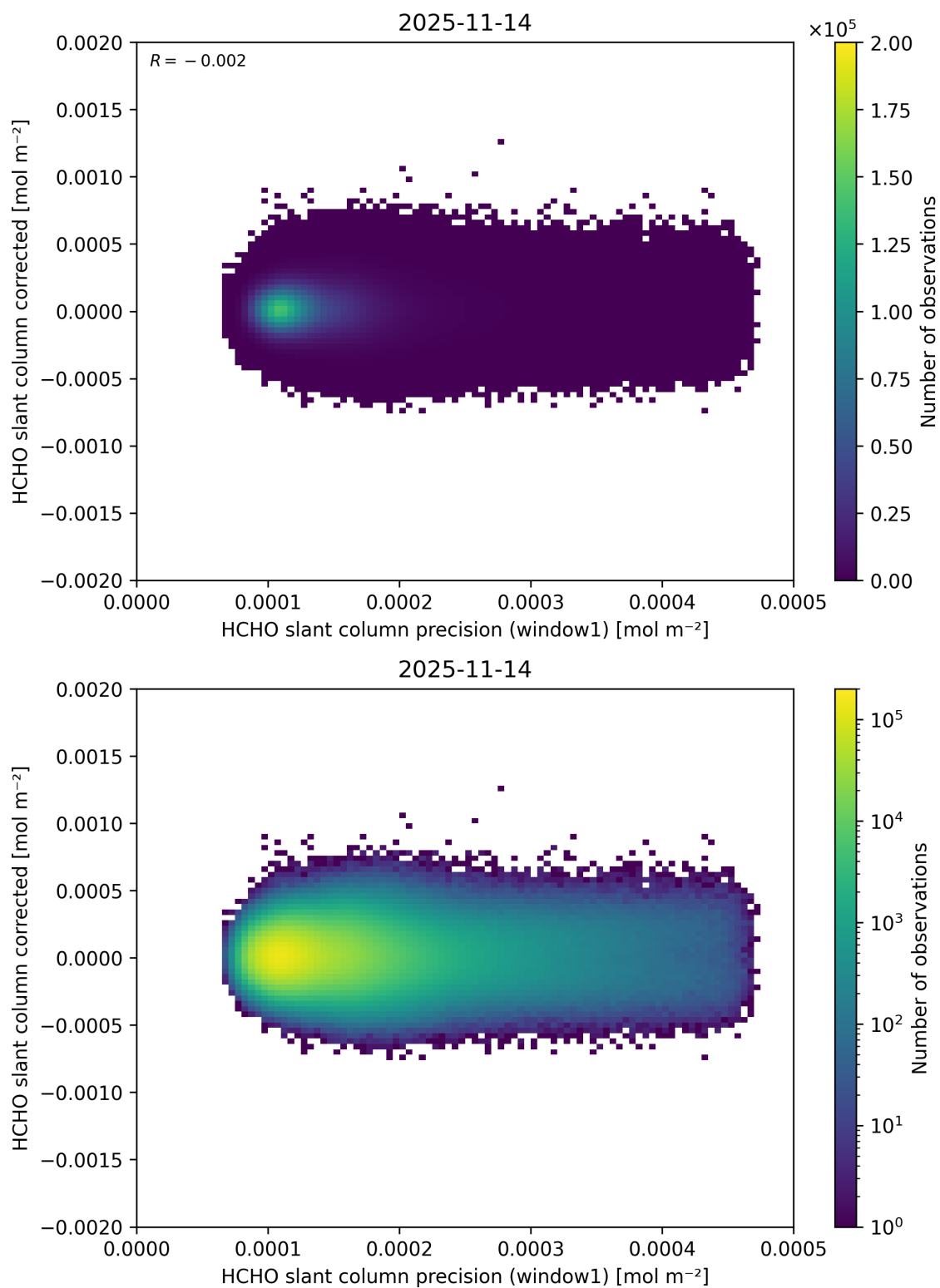
Figure 103: Scatter density plot of “HCHO slant column precision (window1)” against “HCHO slant column corrected” for 2025-11-13 to 2025-11-15.
