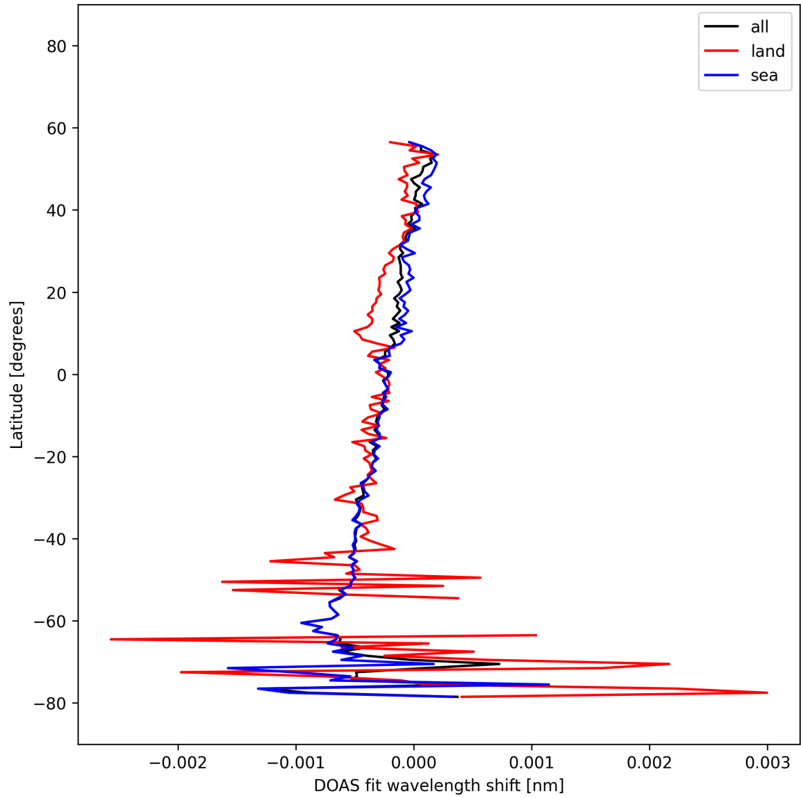
Figure 31: Zonal average of "DOAS fit wavelength shift" for 2025-11-13 to 2025-11-15.
