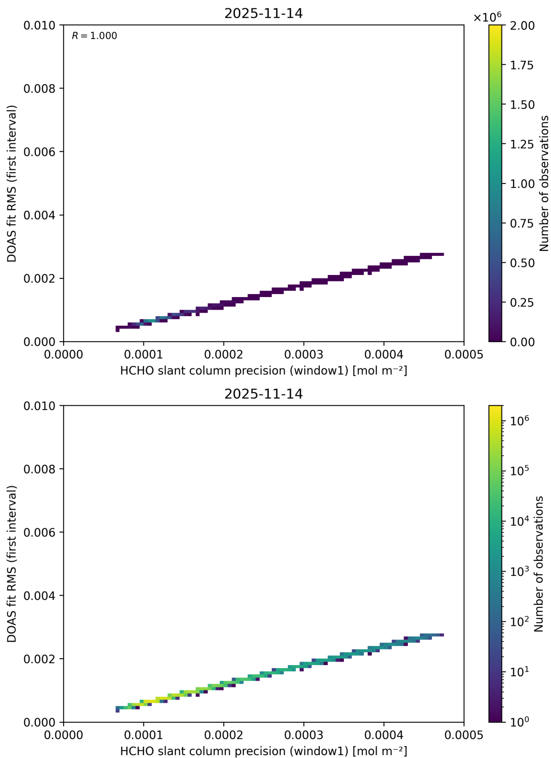
Figure 99: Scatter density plot of “HCHO slant column precision (window1)” against “DOAS fit RMS (first interval)” for 2025-11-13 to 2025-11-15.
