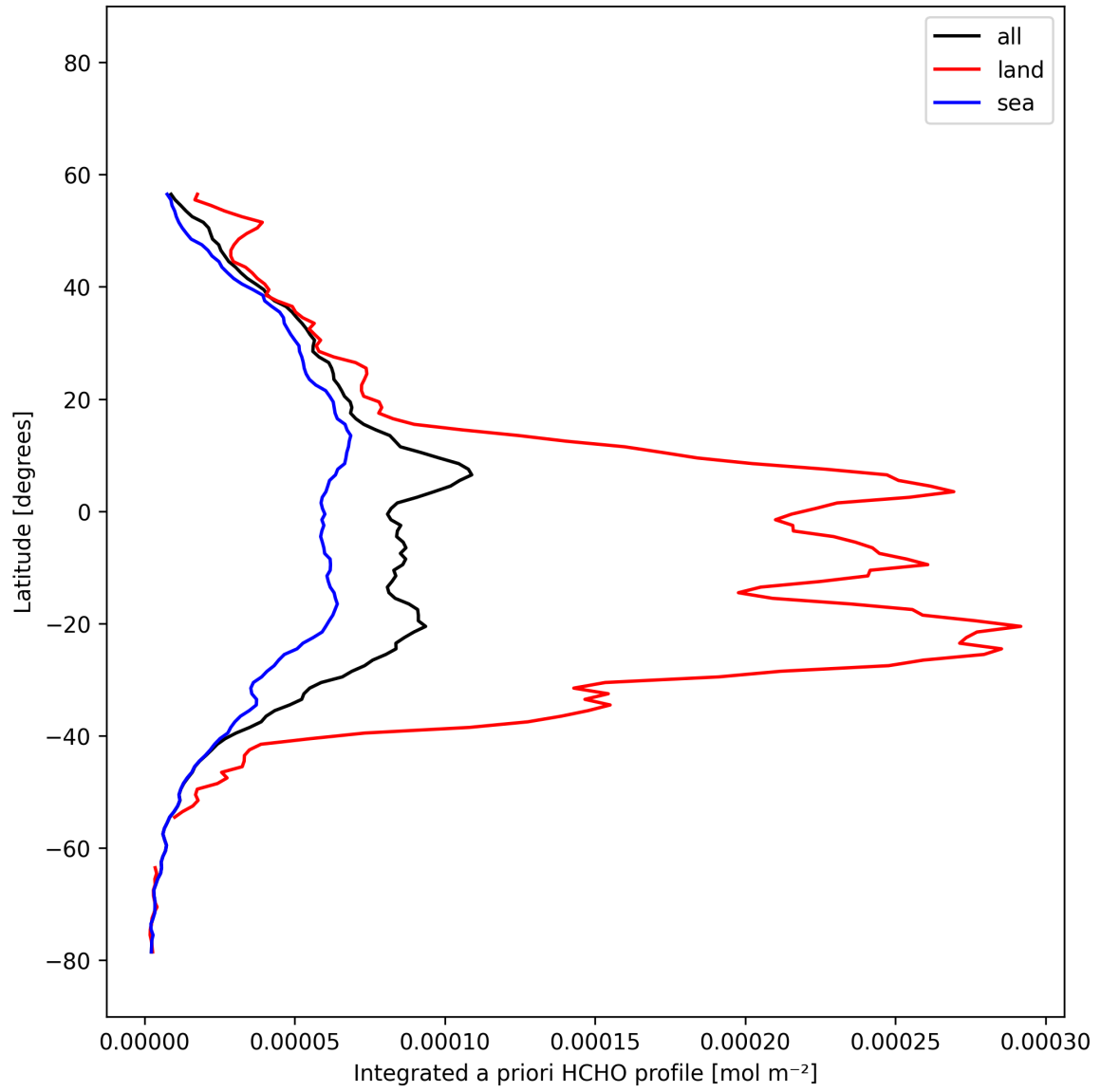
Figure 30: Zonal average of “Integrated a priori HCHO profile” for 2025-11-13 to 2025-11-15.
