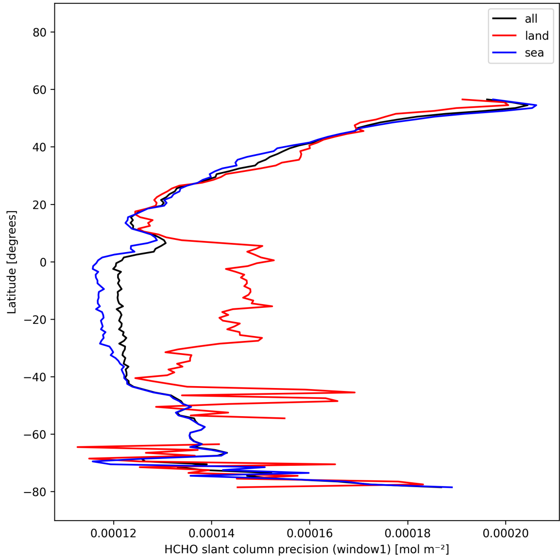
Figure 26: Zonal average of "HCHO slant column precision (window1)" for 2025-11-13 to 2025-11-15.
