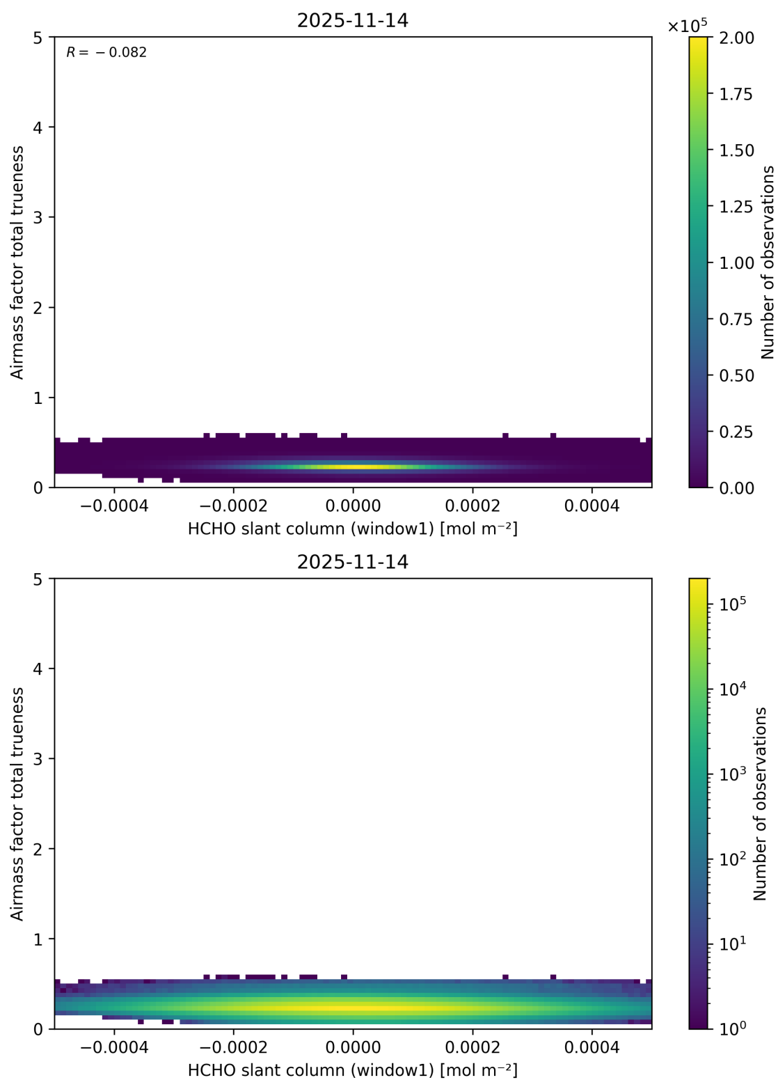
Figure 96: Scatter density plot of “HCHO slant column (window1)” against “Airmass factor total trueneess” for 2025-11-13 to 2025-11-15.
