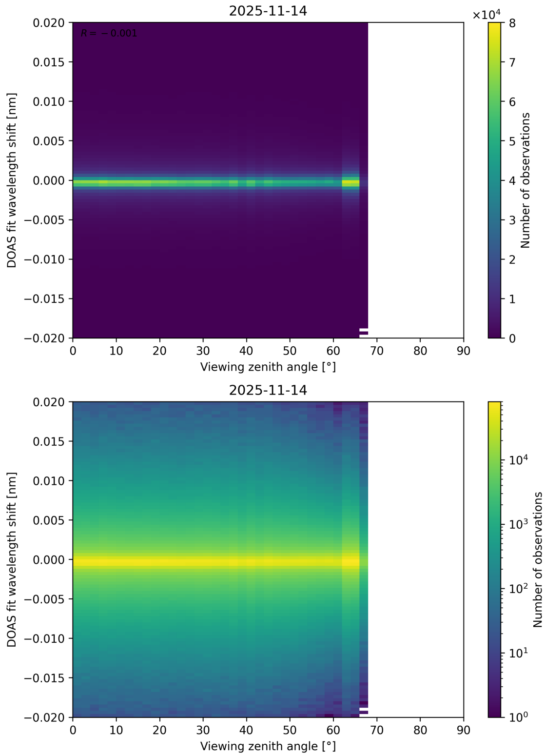
Figure 203: Scatter density plot of “Viewing zenith angle” against “DOAS fit wavelength shift” for 2025-11-13 to 2025-11-15.
