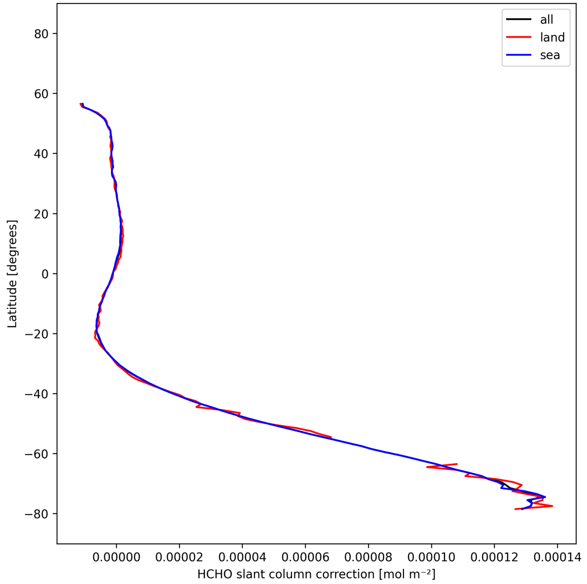
Figure 34: Zonal average of “HCHO slant column correction” for 2025-11-13 to 2025-11-15.
