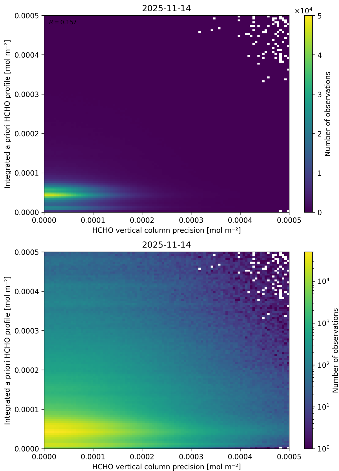
Figure 164: Scatter density plot of “HCHO vertical column precision” against “Integrated a priori HCHO profile” for 2025-11-13 to 2025-11-15.
