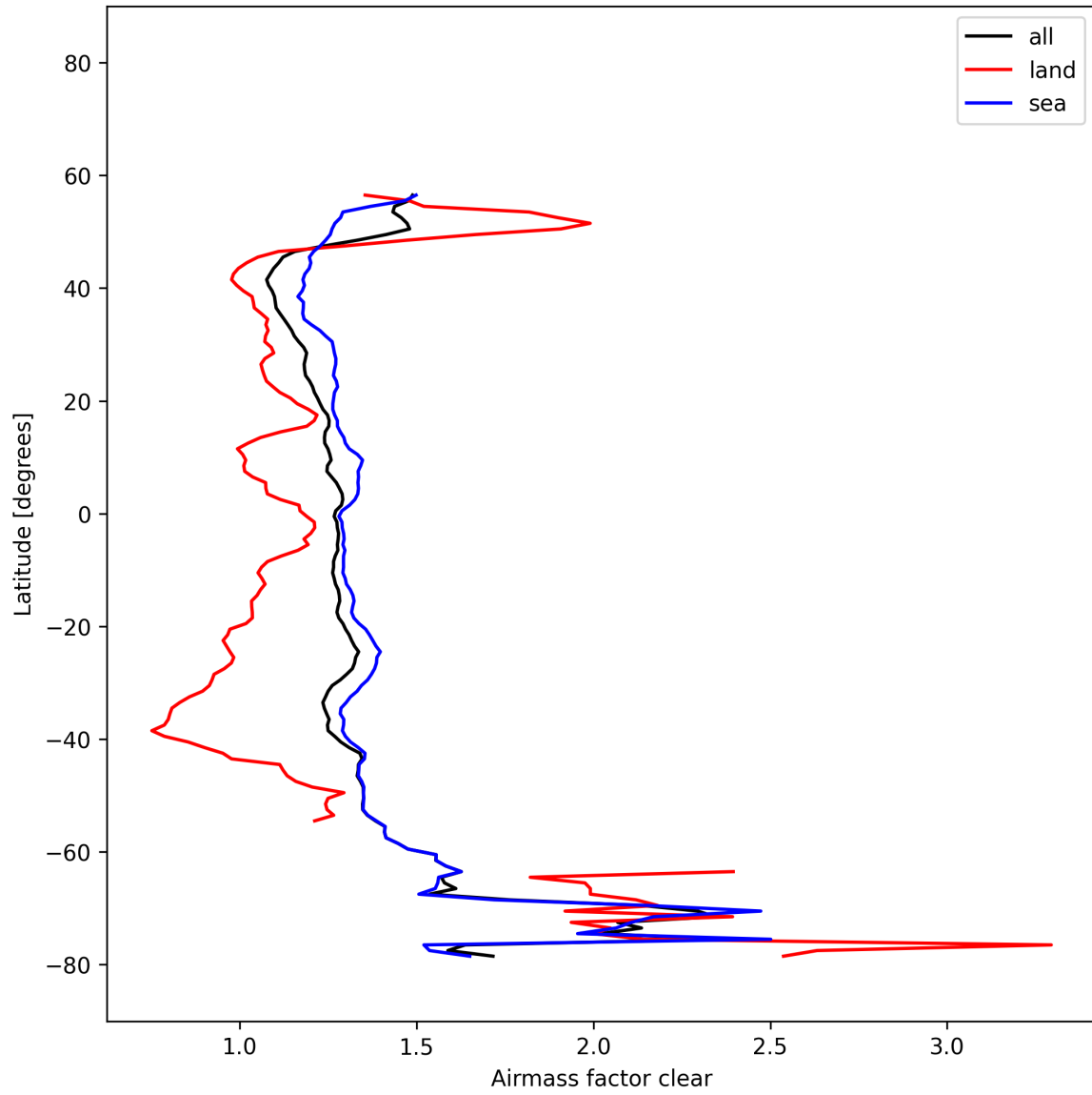
Figure 29: Zonal average of “Airmass factor clear” for 2025-11-13 to 2025-11-15.
