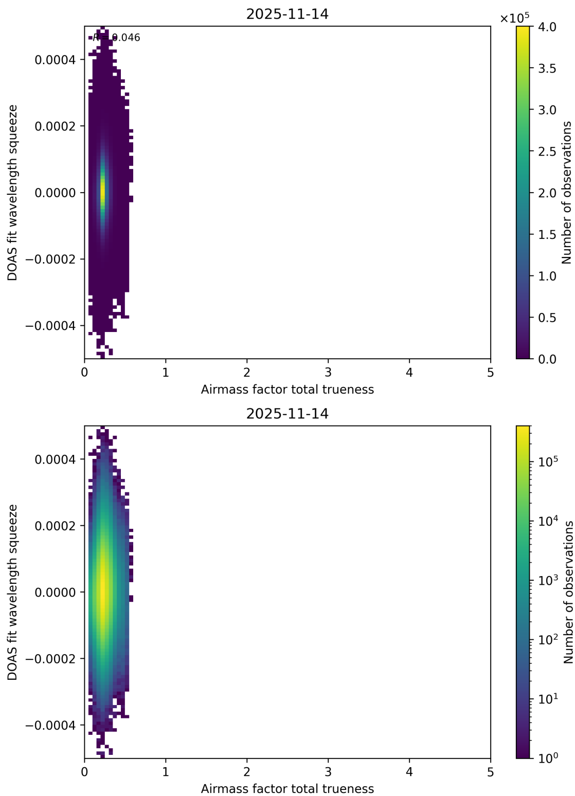
Figure 120: Scatter density plot of “Airmass factor total trueness” against “DOAS fit wavelength squeeze” for 2025-11-13 to 2025-11-15.
