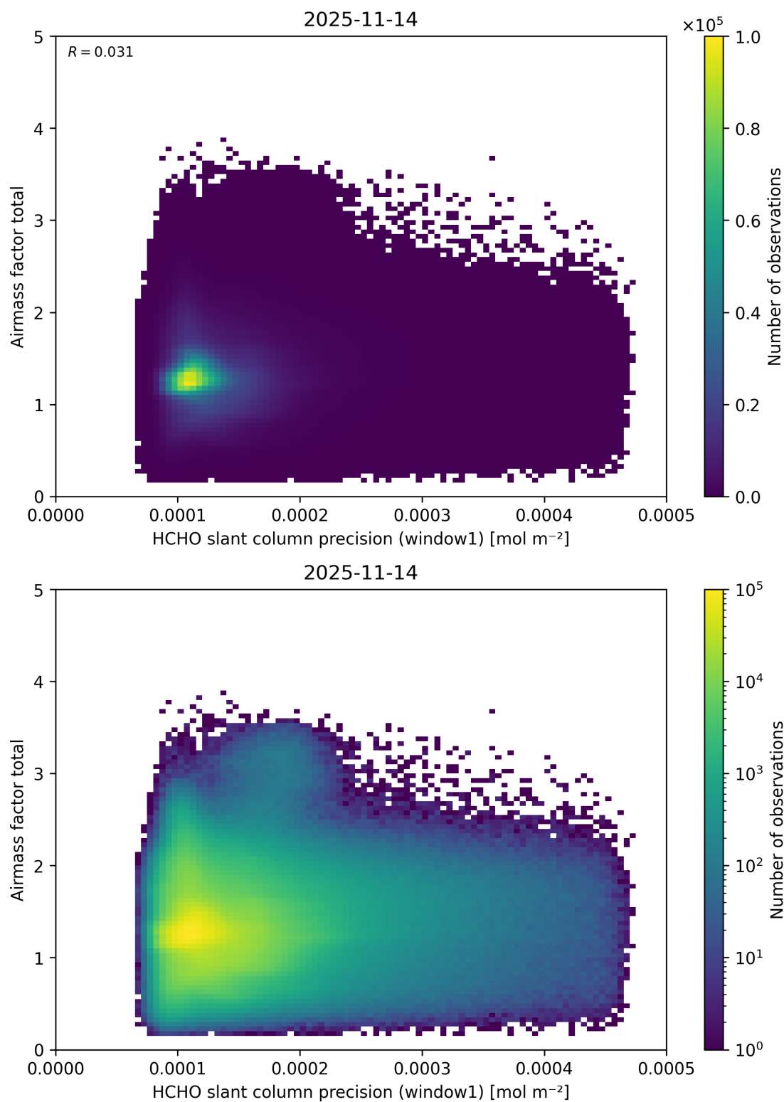
Figure 105: Scatter density plot of “HCHO slant column precision (window1)” against “Airmass factor total” for 2025-11-13 to 2025-11-15.
