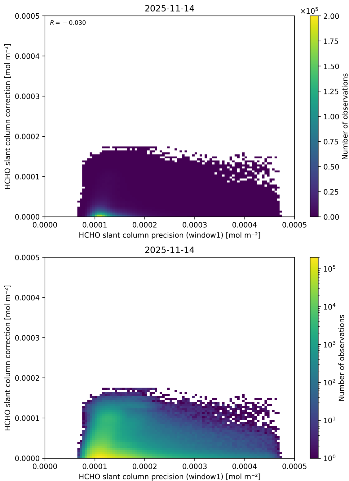
Figure 104: Scatter density plot of “HCHO slant column precision (window1)” against “HCHO slant column correction” for 2025-11-13 to 2025-11-15.
