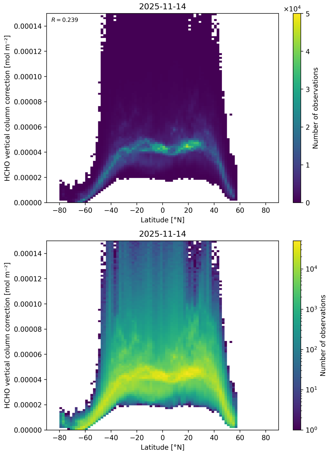
Figure 182: Scatter density plot of “Latitude” against “HCHO vertical column correction” for 2025-11-13 to 2025-11-15.
