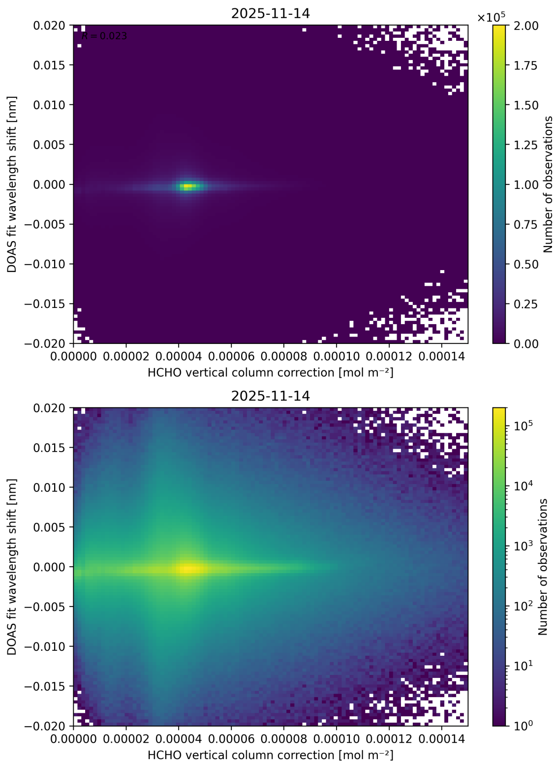
Figure 127: Scatter density plot of “HCHO vertical column correction” against “DOAS fit wavelength shift” for 2025-11-13 to 2025-11-15.
