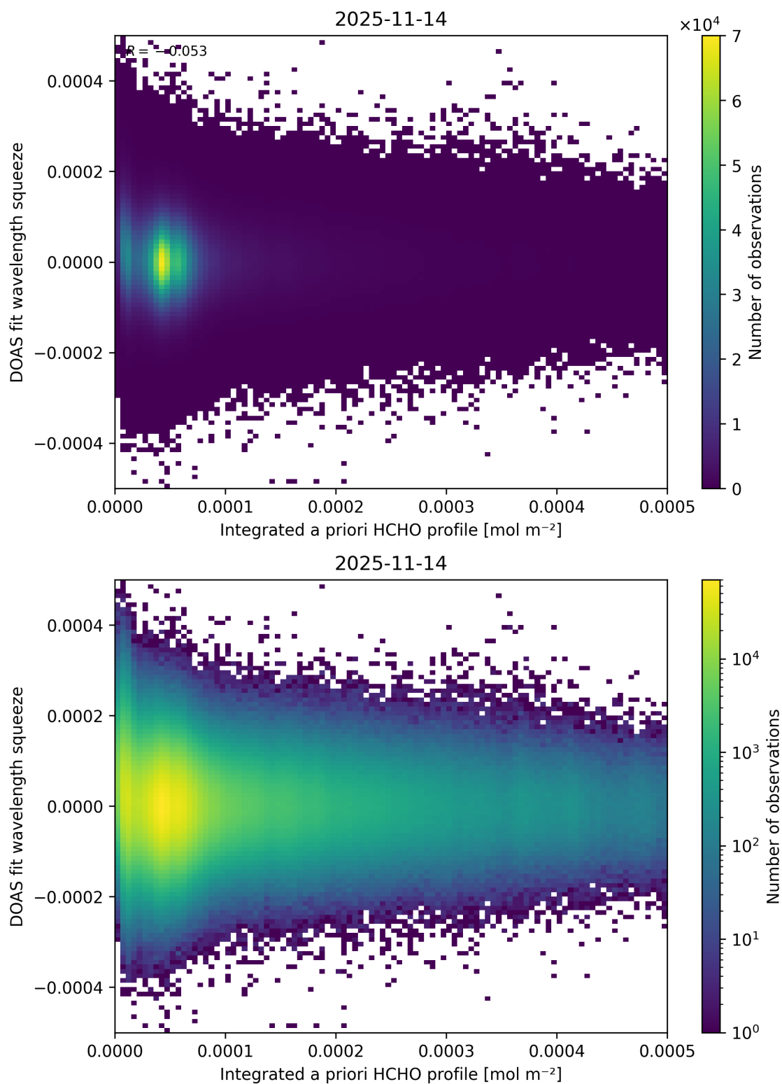
Figure 167: Scatter density plot of “Integrated a priori HCHO profile” against “DOAS fit wavelength squeeze” for 2025-11-13 to 2025-11-15.
