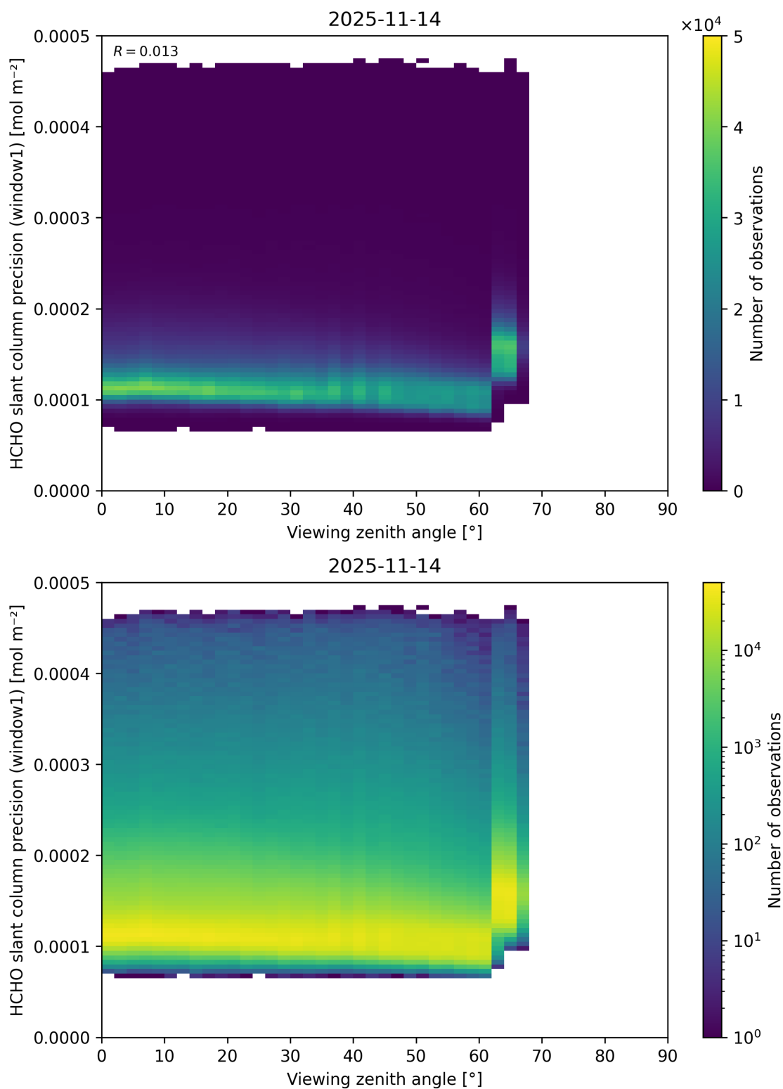
Figure 209: Scatter density plot of “Viewing zenith angle” against “HCHO slant column precision (window1)” for 2025-11-13 to 2025-11-15.
