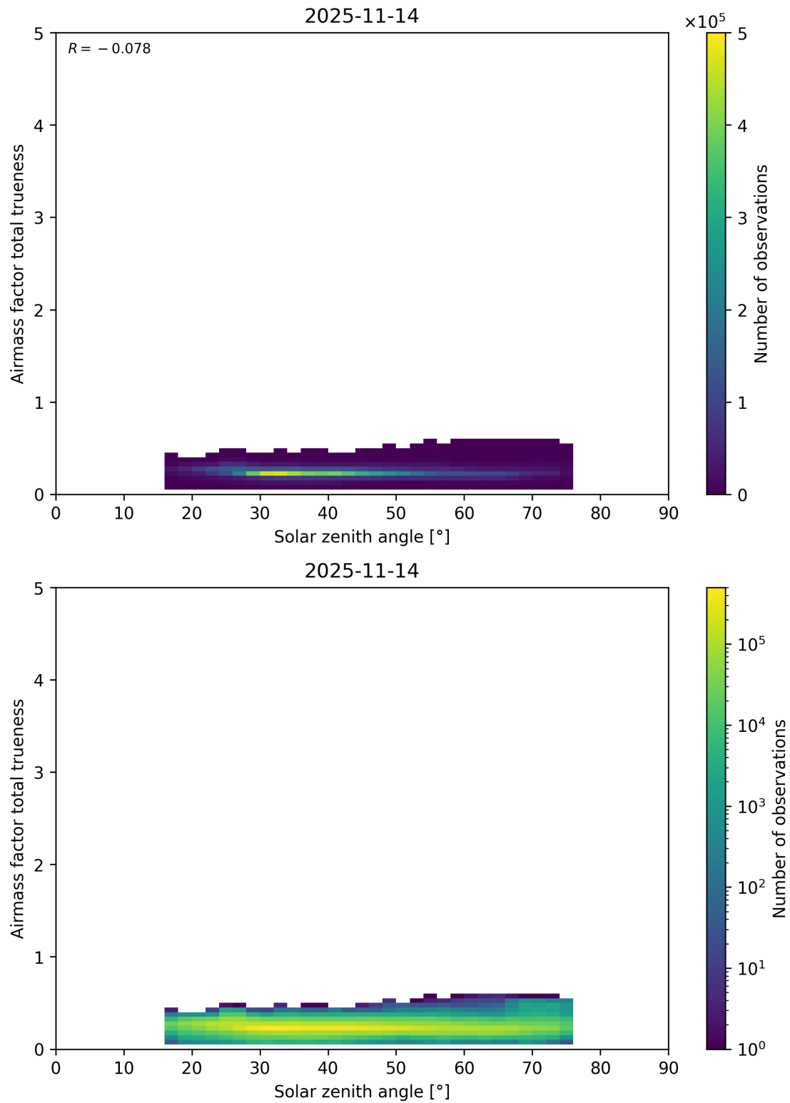
Figure 195: Scatter density plot of “Solar zenith angle” against “Airmass factor total trueneess” for 2025-11-13 to 2025-11-15.
