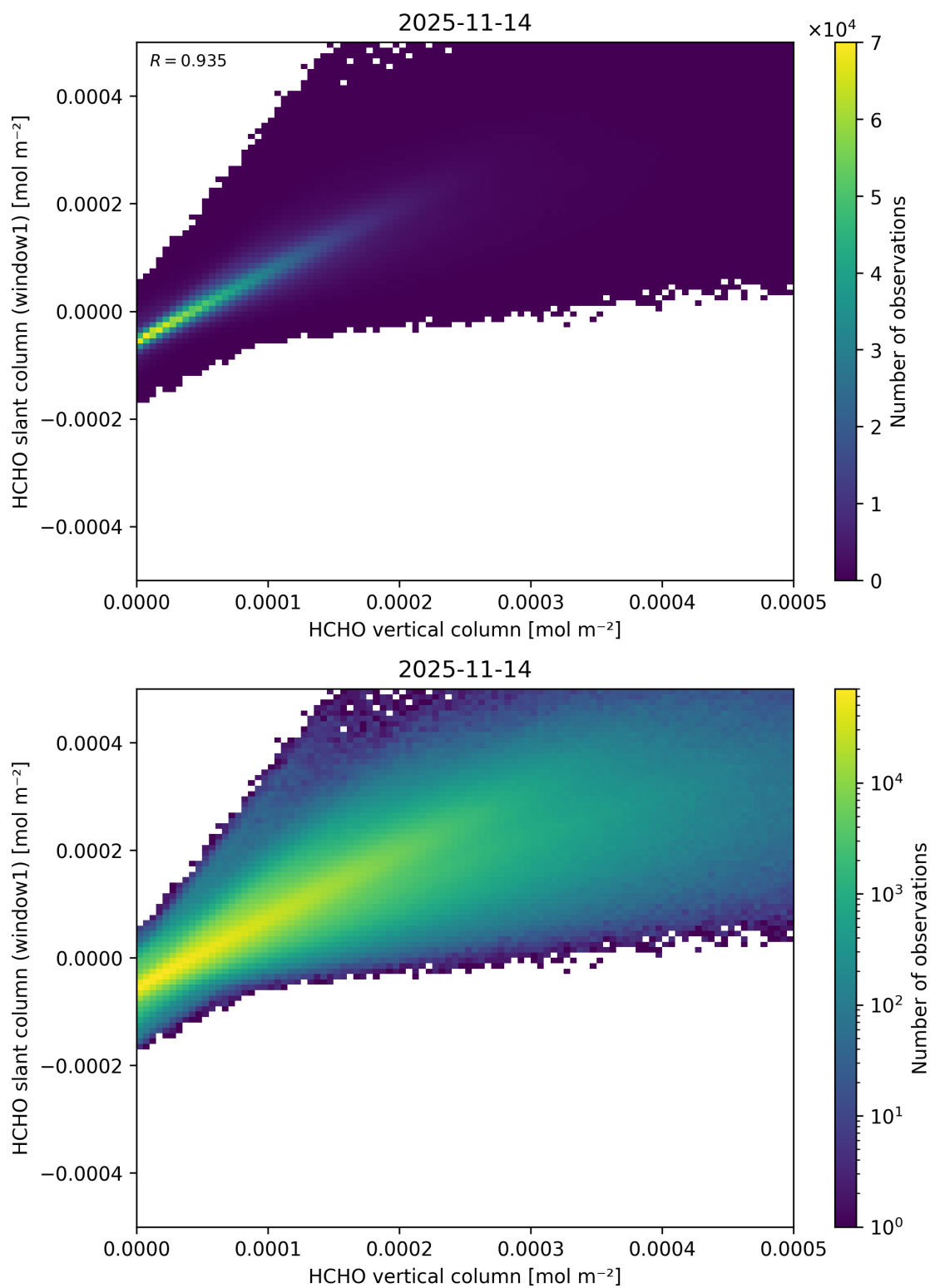
Figure 144: Scatter density plot of “HCHO vertical column” against “HCHO slant column (window1)” for 2025-11-13 to 2025-11-15.
