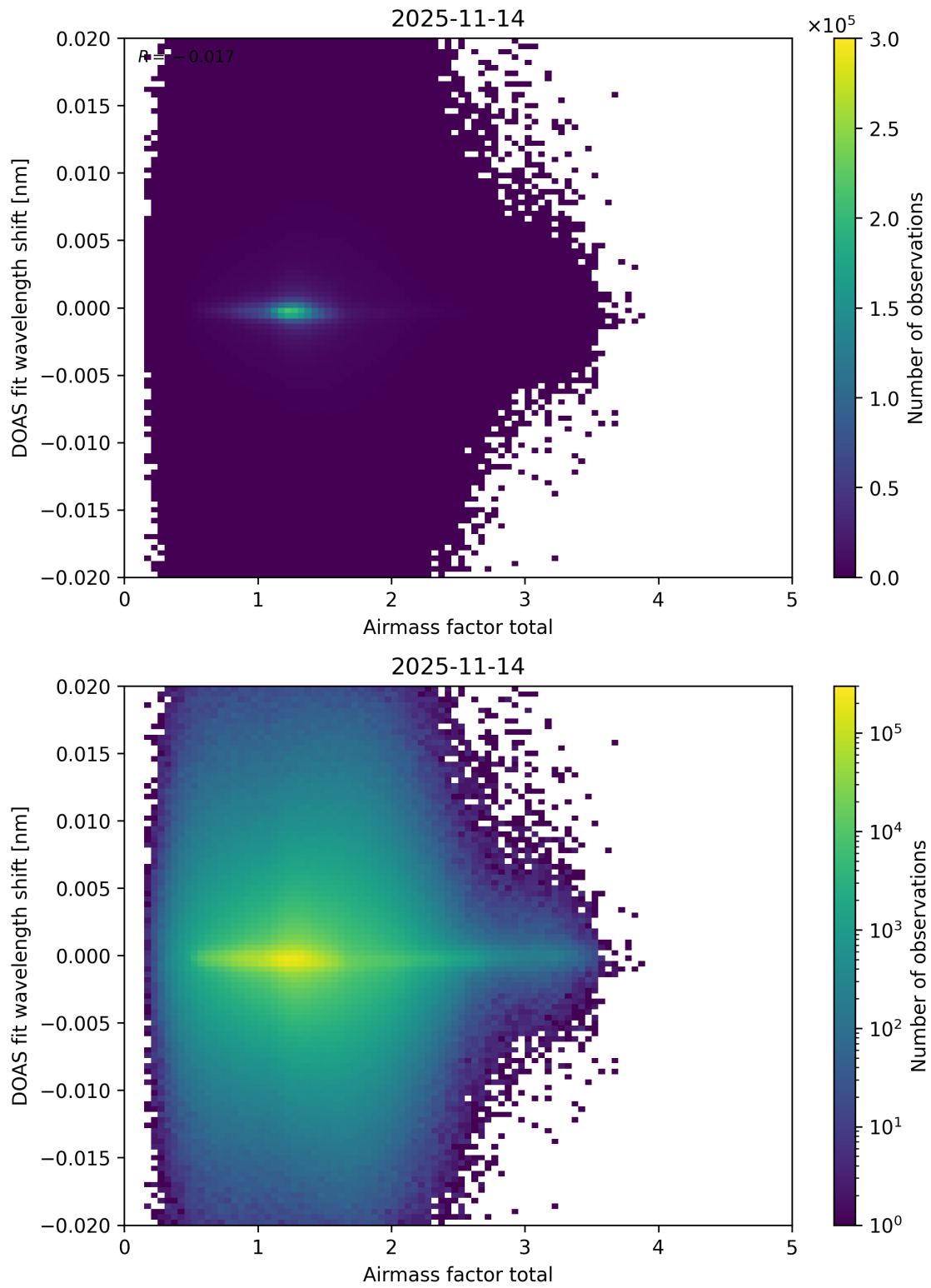
Figure 110: Scatter density plot of “Airmass factor total” against “DOAS fit wavelength shift” for 2025-11-13 to 2025-11-15.
