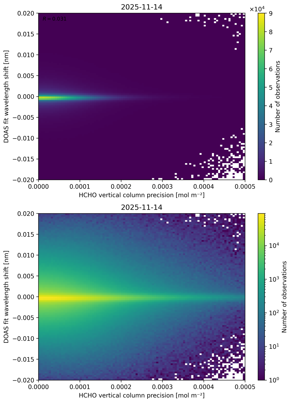
Figure 153: Scatter density plot of “HCHO vertical column precision” against “DOAS fit wavelength shift” for 2025-11-13 to 2025-11-15.
