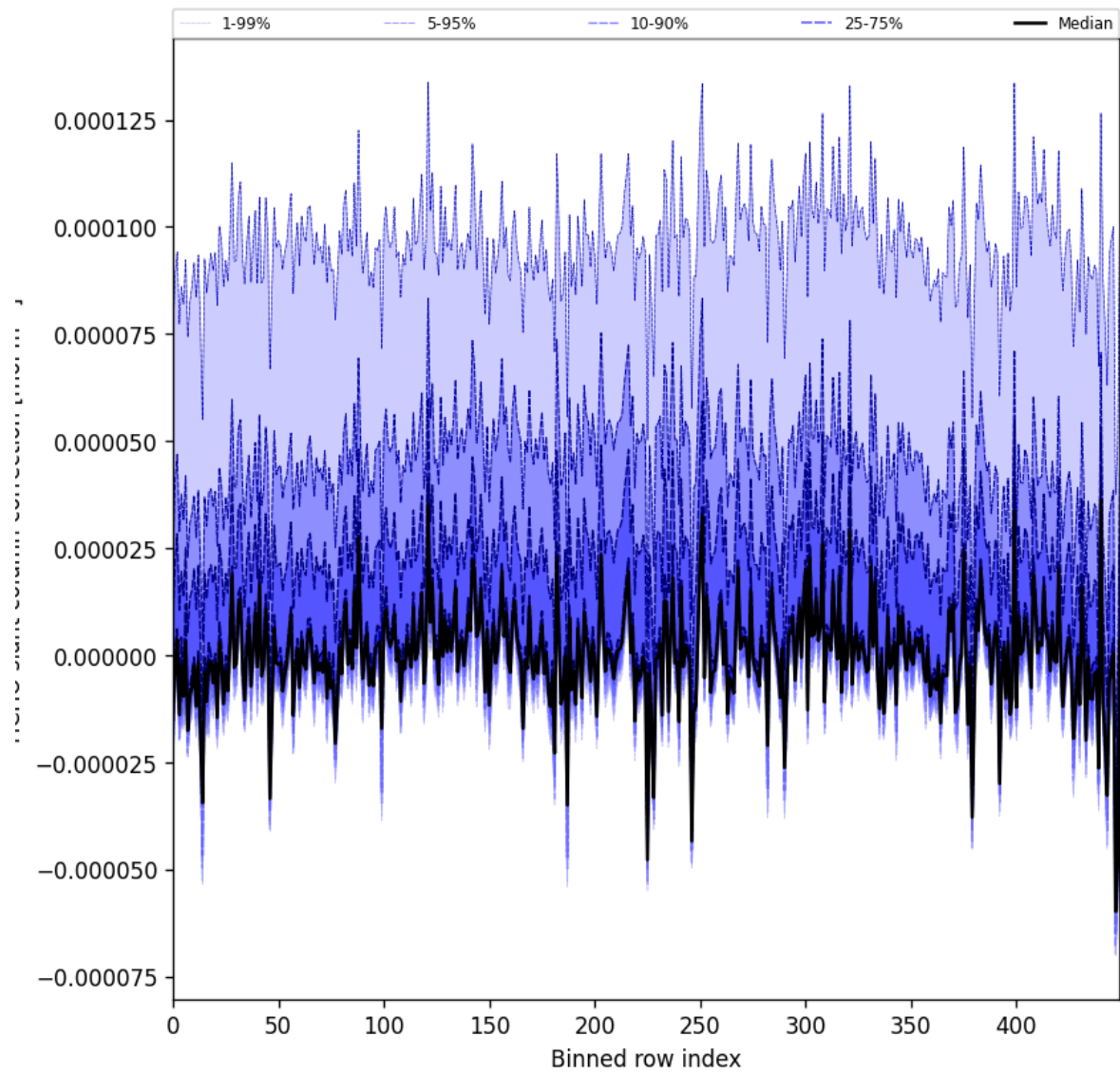
Figure 64: Along track statistics of “HCHO slant column correction” for 2025-11-13 to 2025-11-15
