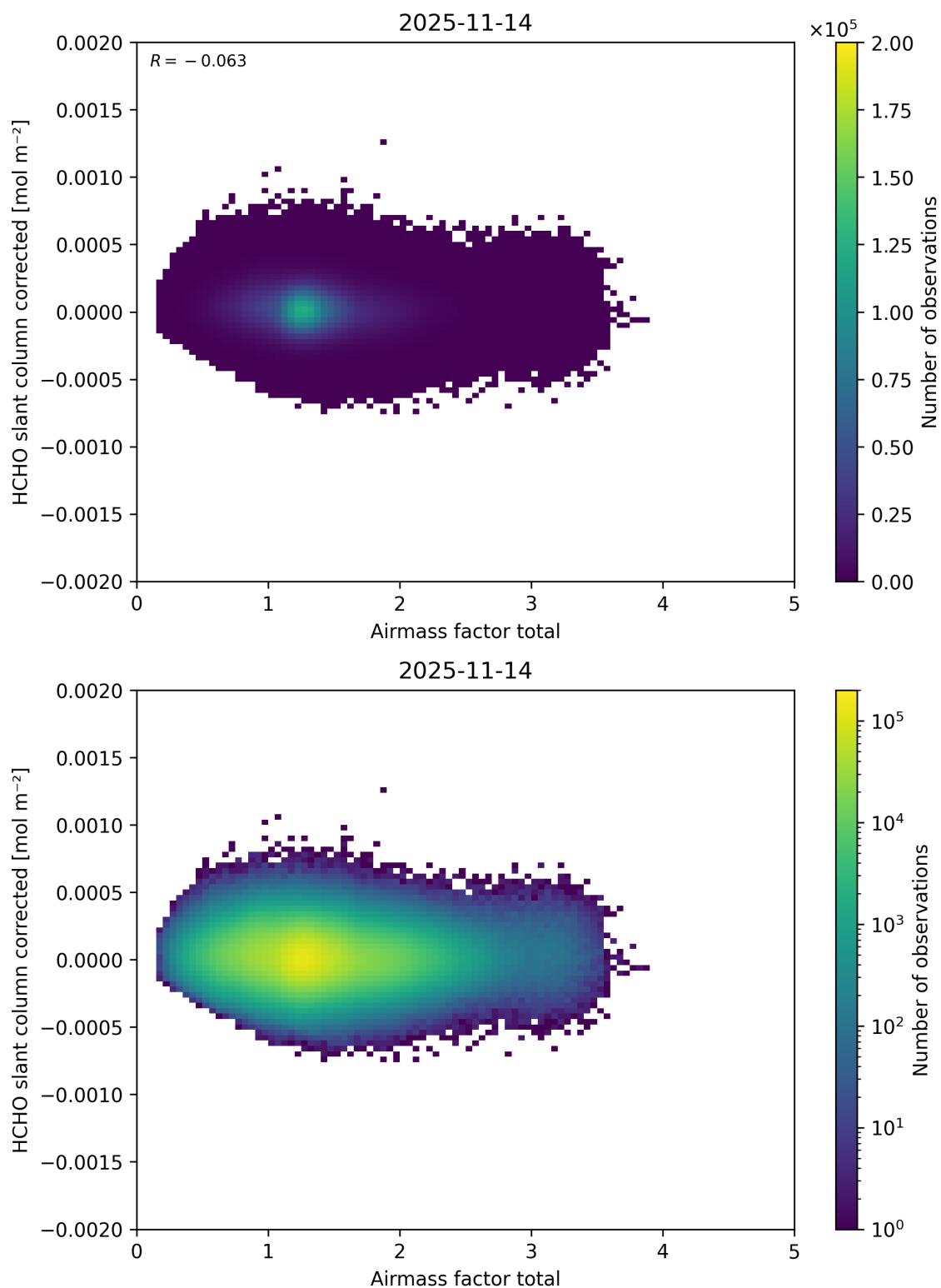
Figure 113: Scatter density plot of “Airmass factor total” against “HCHO slant column corrected” for 2025-11-13 to 2025-11-15.
