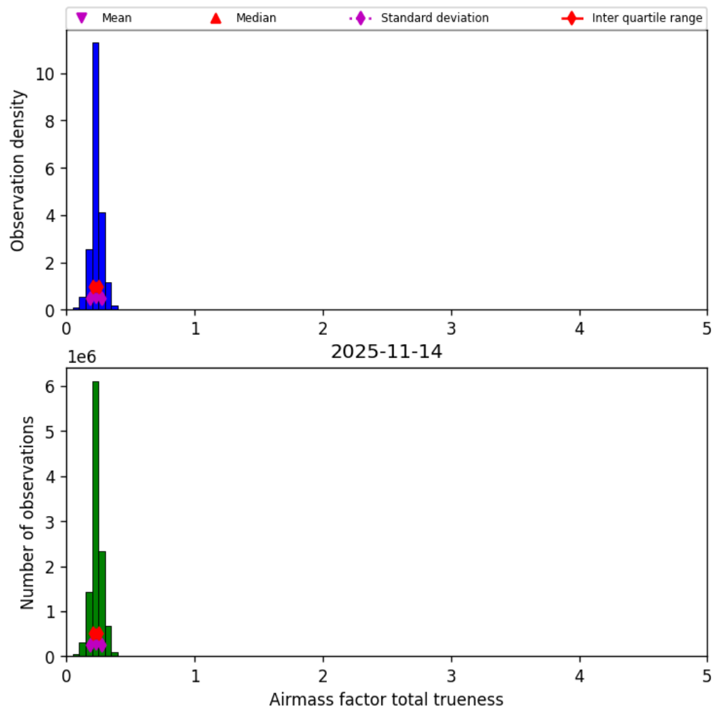
Figure 43: Histogram of “Airmass factor total trueness” for 2025-11-13 to 2025-11-15
