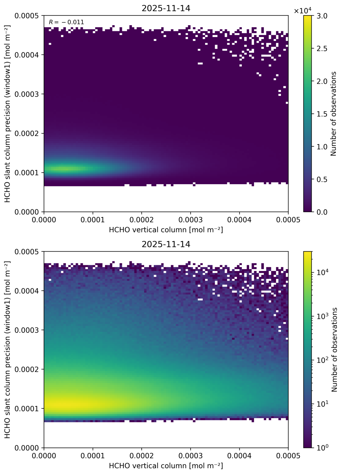
Figure 145: Scatter density plot of “HCHO vertical column” against “HCHO slant column precision (window1)” for 2025-11-13 to 2025-11-15.
