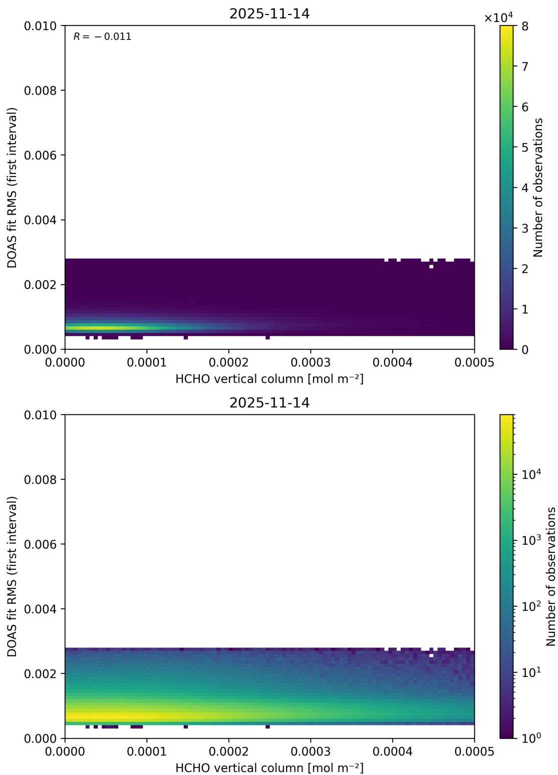
Figure 138: Scatter density plot of “HCHO vertical column” against “DOAS fit RMS (first interval)” for 2025-11-13 to 2025-11-15.
