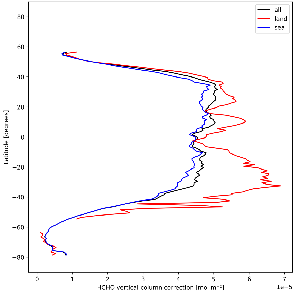
Figure 24: Zonal average of "HCHO vertical column correction" for 2025-11-13 to 2025-11-15.
