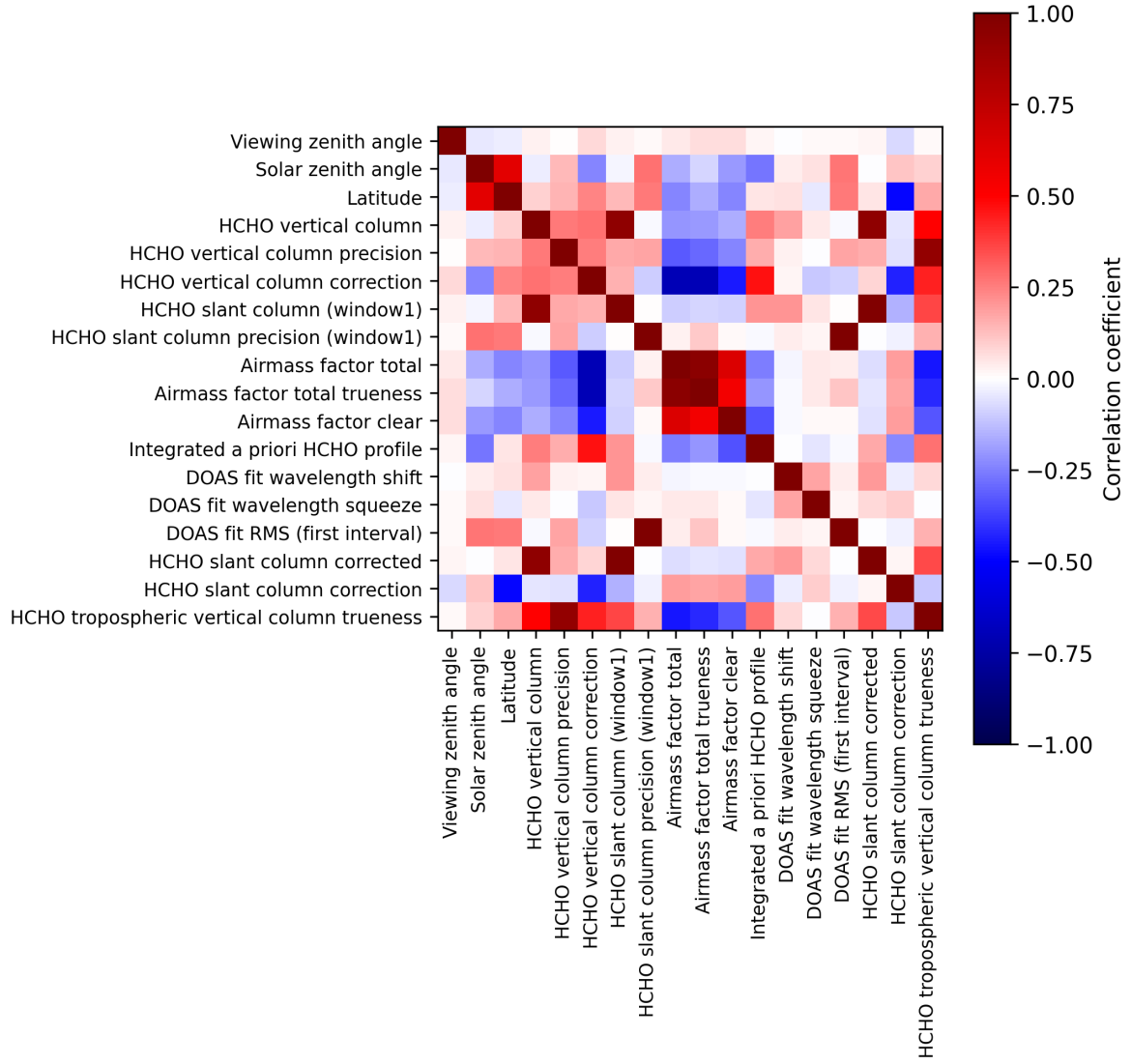
Figure 2: Map of correlation matrix for 2025-11-13 to 2025-11-15.
