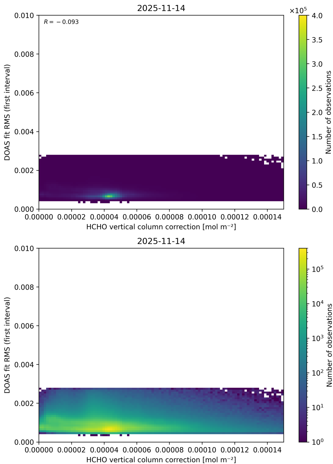
Figure 126: Scatter density plot of “HCHO vertical column correction” against “DOAS fit RMS (first interval)” for 2025-11-13 to 2025-11-15.
