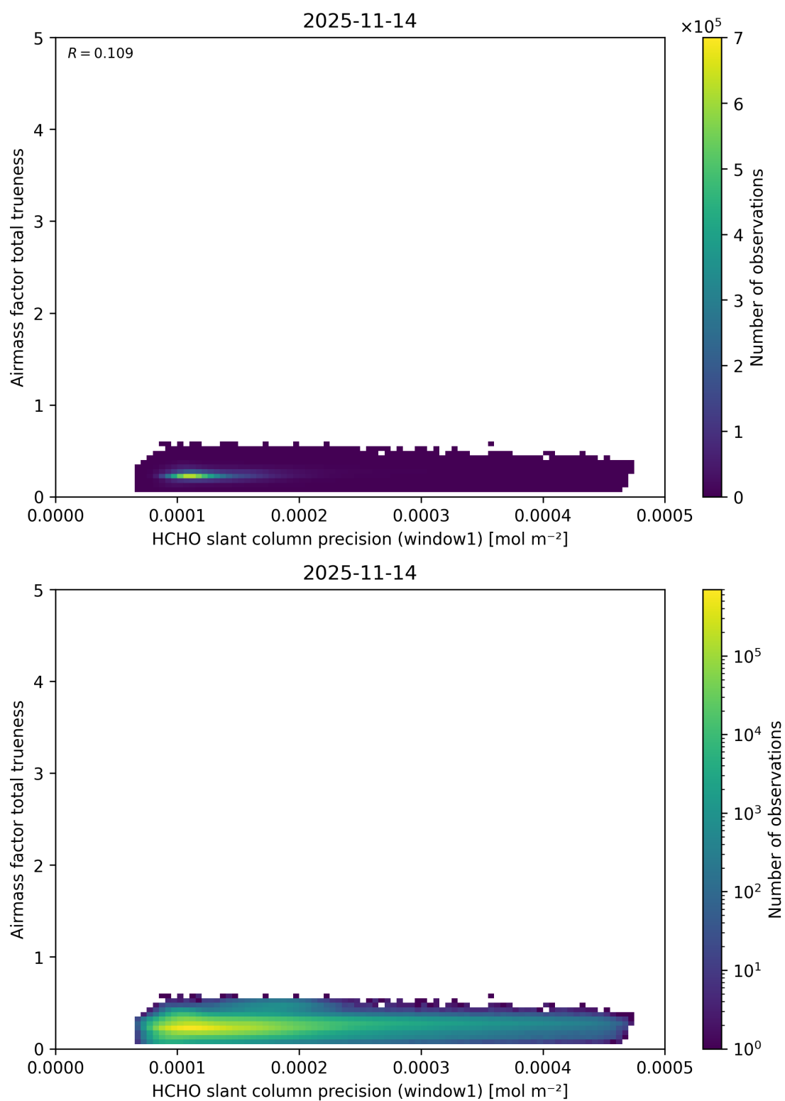
Figure 106: Scatter density plot of “HCHO slant column precision (window1)” against “Airmass factor total trueness” for 2025-11-13 to 2025-11-15.
