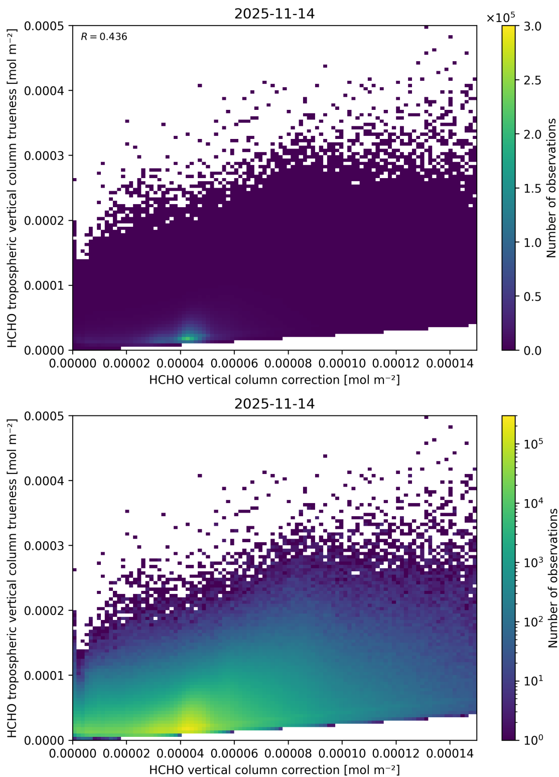
Figure 136: Scatter density plot of “HCHO vertical column correction” against “HCHO tropospheric vertical column true-ness” for 2025-11-13 to 2025-11-15.
