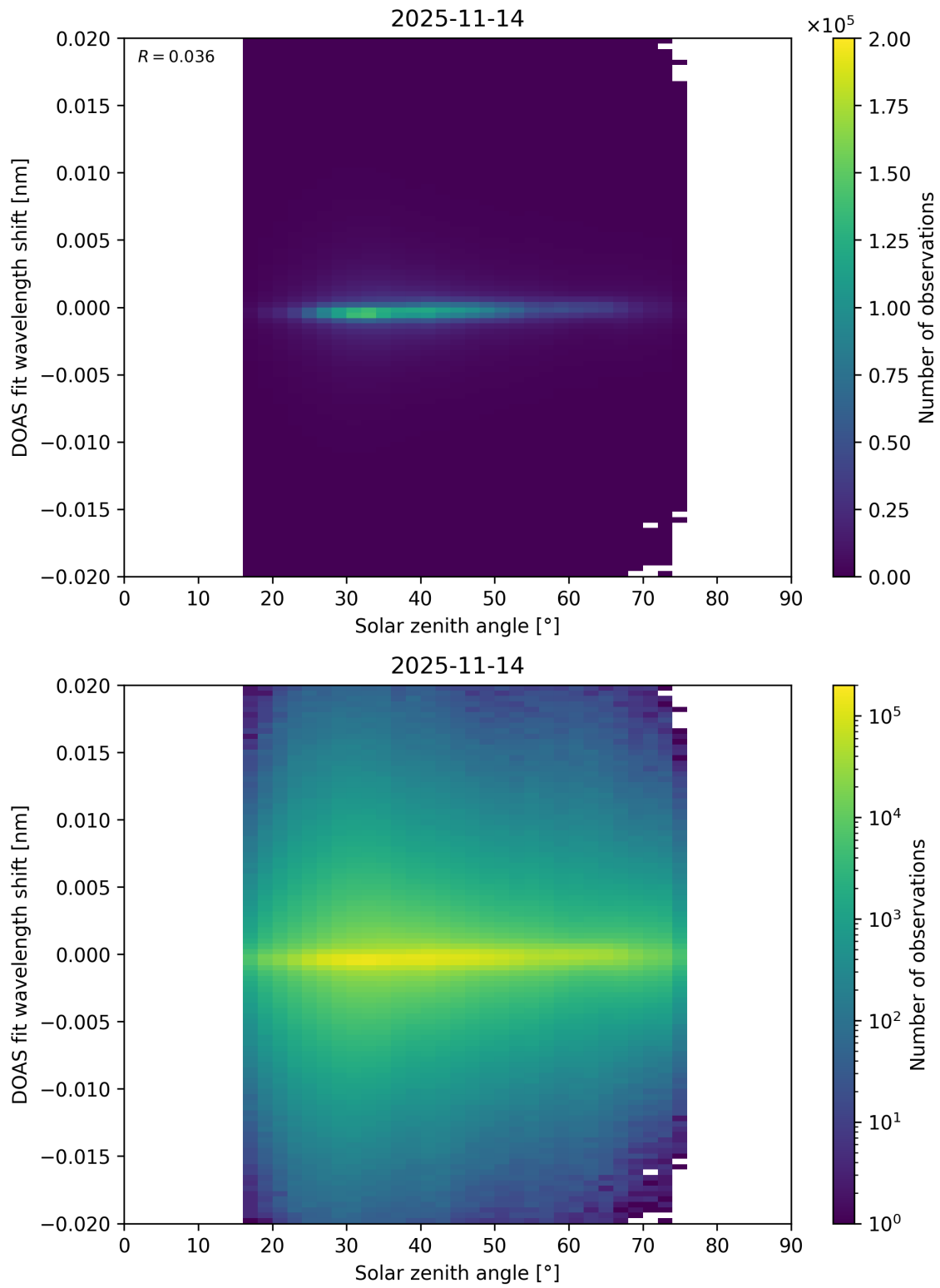
Figure 187: Scatter density plot of “Solar zenith angle” against “DOAS fit wavelength shift” for 2025-11-13 to 2025-11-15.
