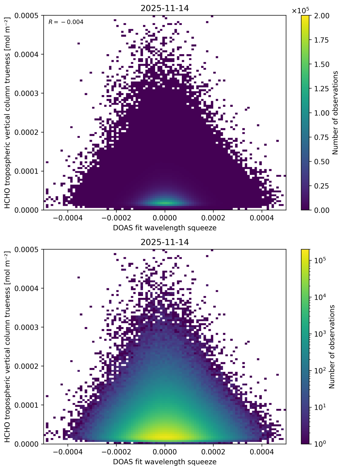
Figure 77: Scatter density plot of “DOAS fit wavelength squeeze” against “HCHO tropospheric vertical column trueness” for 2025-11-13 to 2025-11-15.
