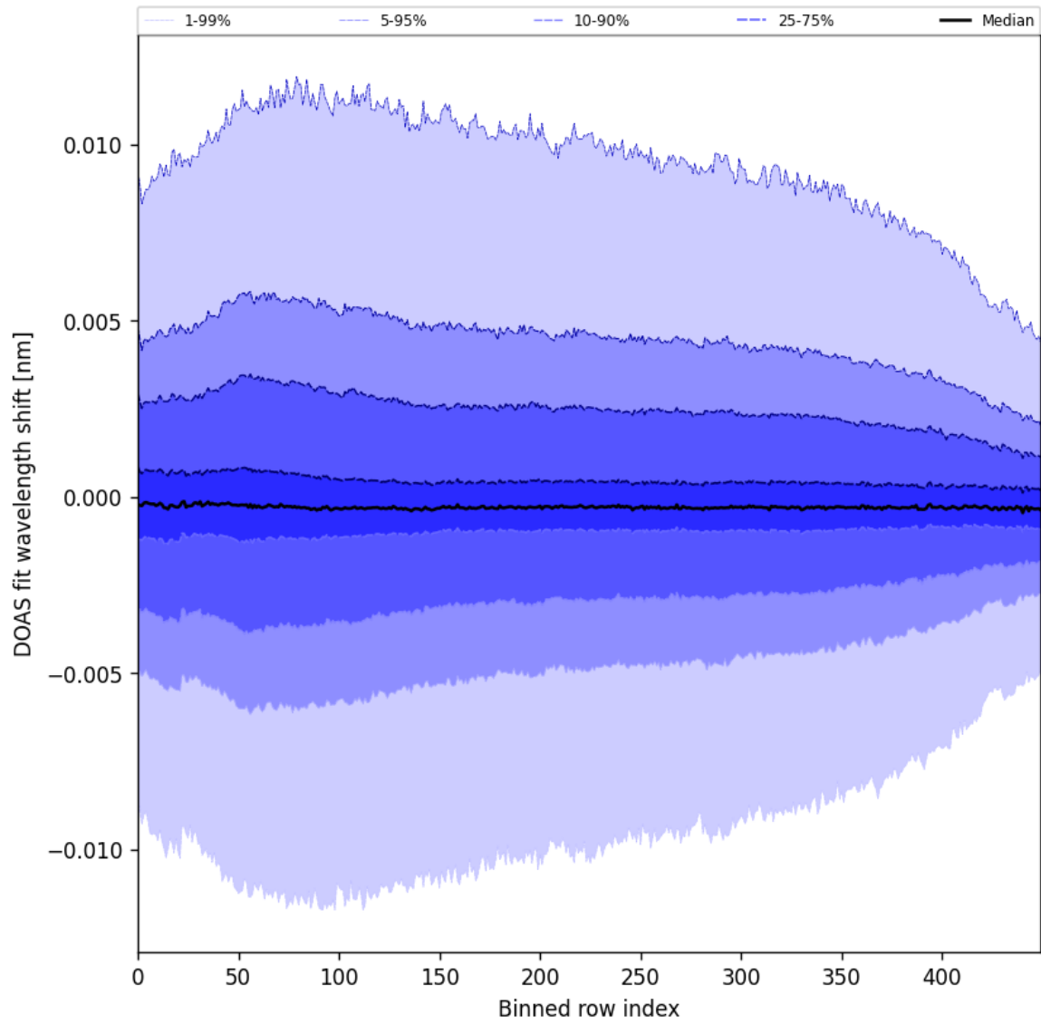
Figure 61: Along track statistics of “DOAS fit wavelength shift” for 2025-11-13 to 2025-11-15
