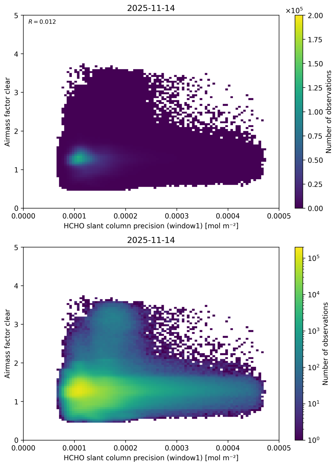
Figure 102: Scatter density plot of “HCHO slant column precision (window1)” against “Airmass factor clear” for 2025-11-13 to 2025-11-15.
