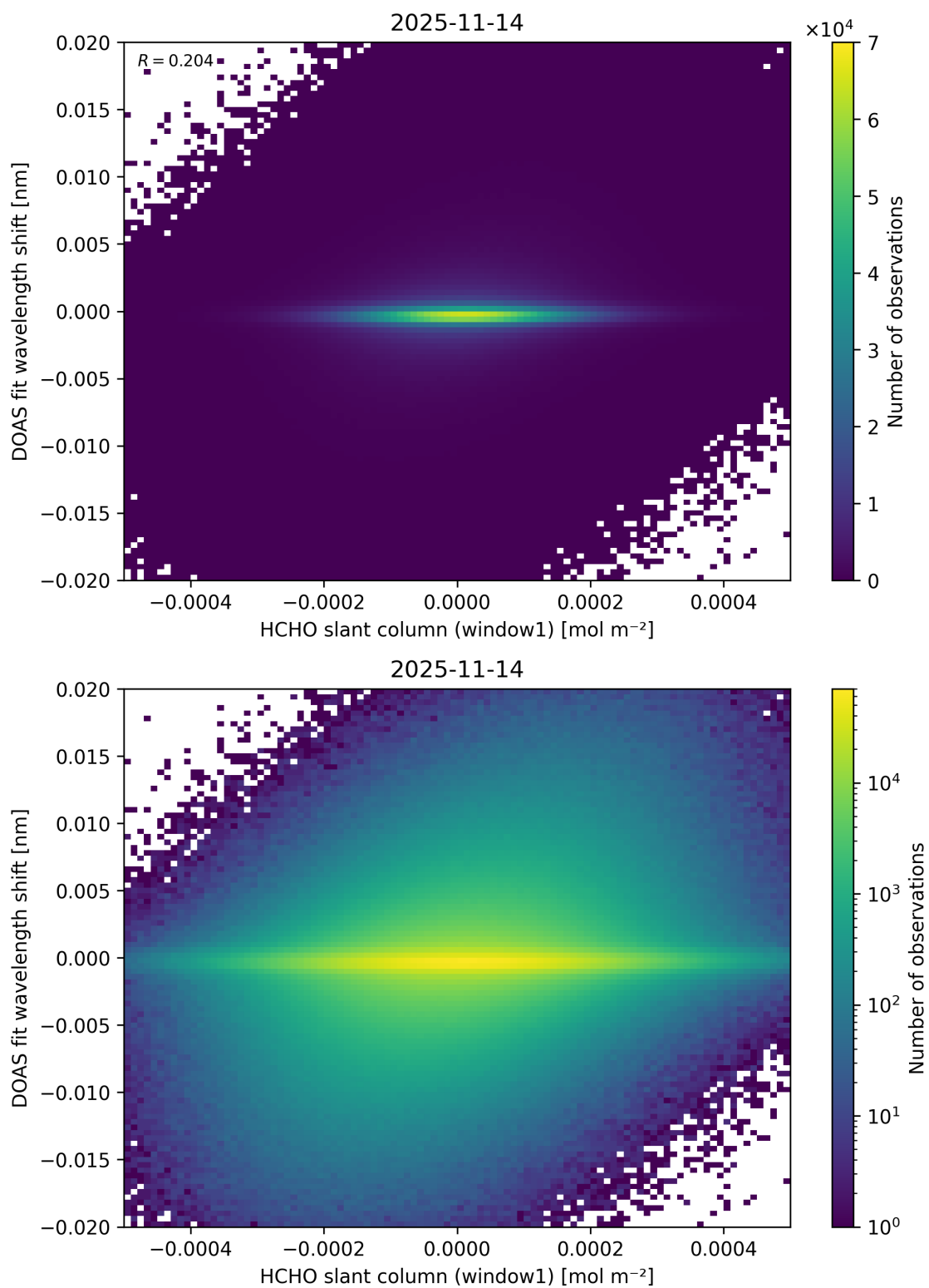
Figure 89: Scatter density plot of “HCHO slant column (window1)” against “DOAS fit wavelength shift” for 2025-11-13 to 2025-11-15.
