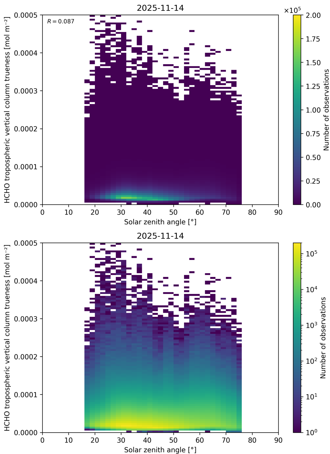
Figure 199: Scatter density plot of “Solar zenith angle” against “HCHO tropospheric vertical column trueness” for 2025-11-13 to 2025-11-15.
