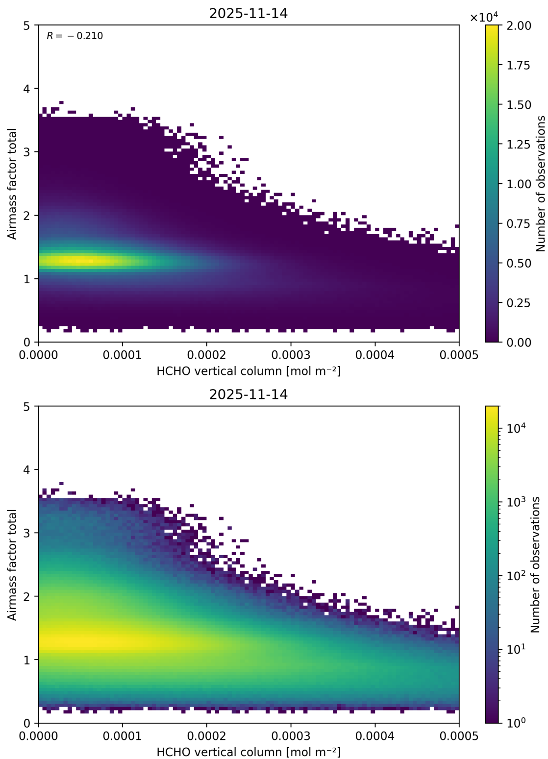
Figure 146: Scatter density plot of “HCHO vertical column” against “Airmass factor total” for 2025-11-13 to 2025-11-15.
