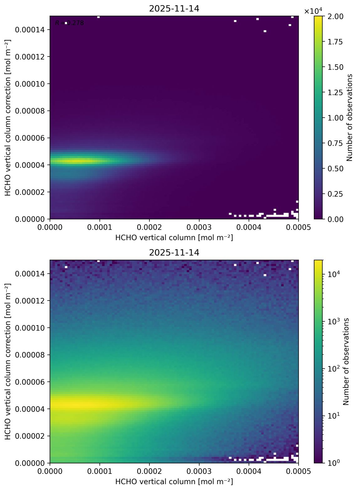
Figure 148: Scatter density plot of “HCHO vertical column” against “HCHO vertical column correction” for 2025-11-13 to 2025-11-15.
