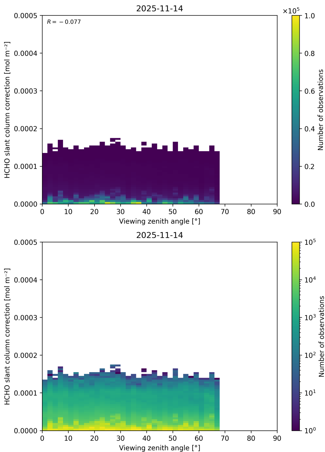
Figure 207: Scatter density plot of “Viewing zenith angle” against “HCHO slant column correction” for 2025-11-13 to 2025-11-15.
