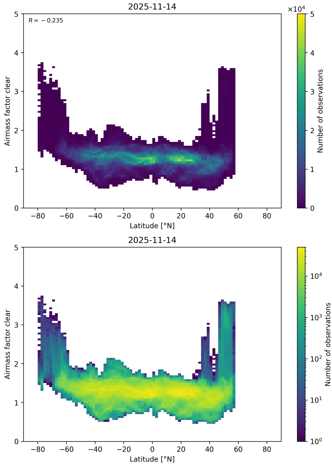
Figure 174: Scatter density plot of “Latitude” against “Airmass factor clear” for 2025-11-13 to 2025-11-15.
