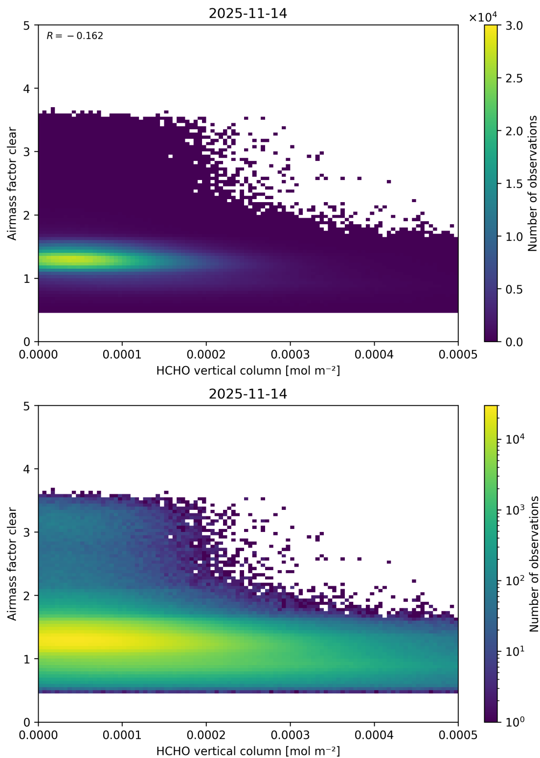
Figure 141: Scatter density plot of “HCHO vertical column” against “Airmass factor clear” for 2025-11-13 to 2025-11-15.
