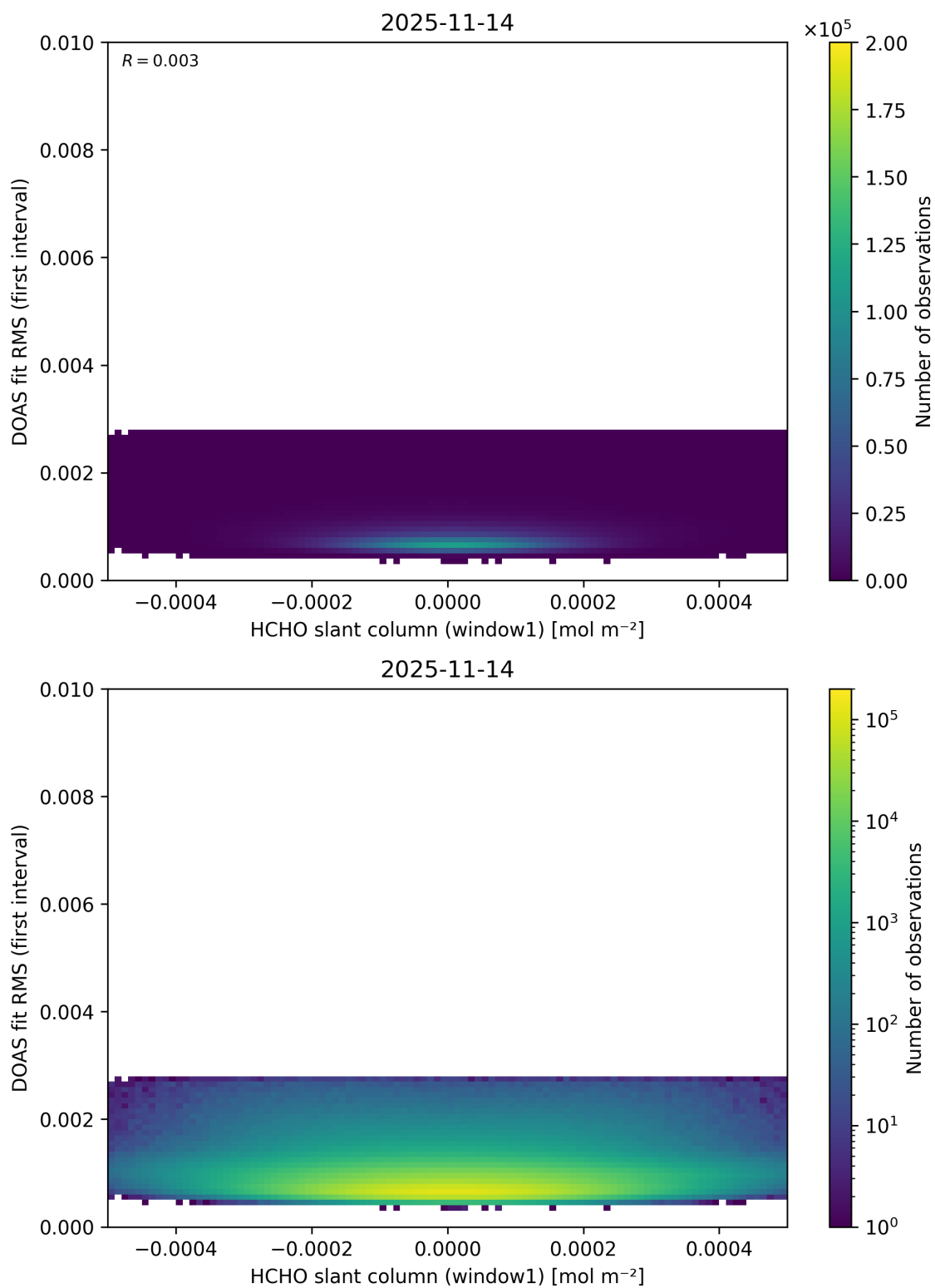
Figure 88: Scatter density plot of “HCHO slant column (window1)” against “DOAS fit RMS (first interval)” for 2025-11-13 to 2025-11-15.
