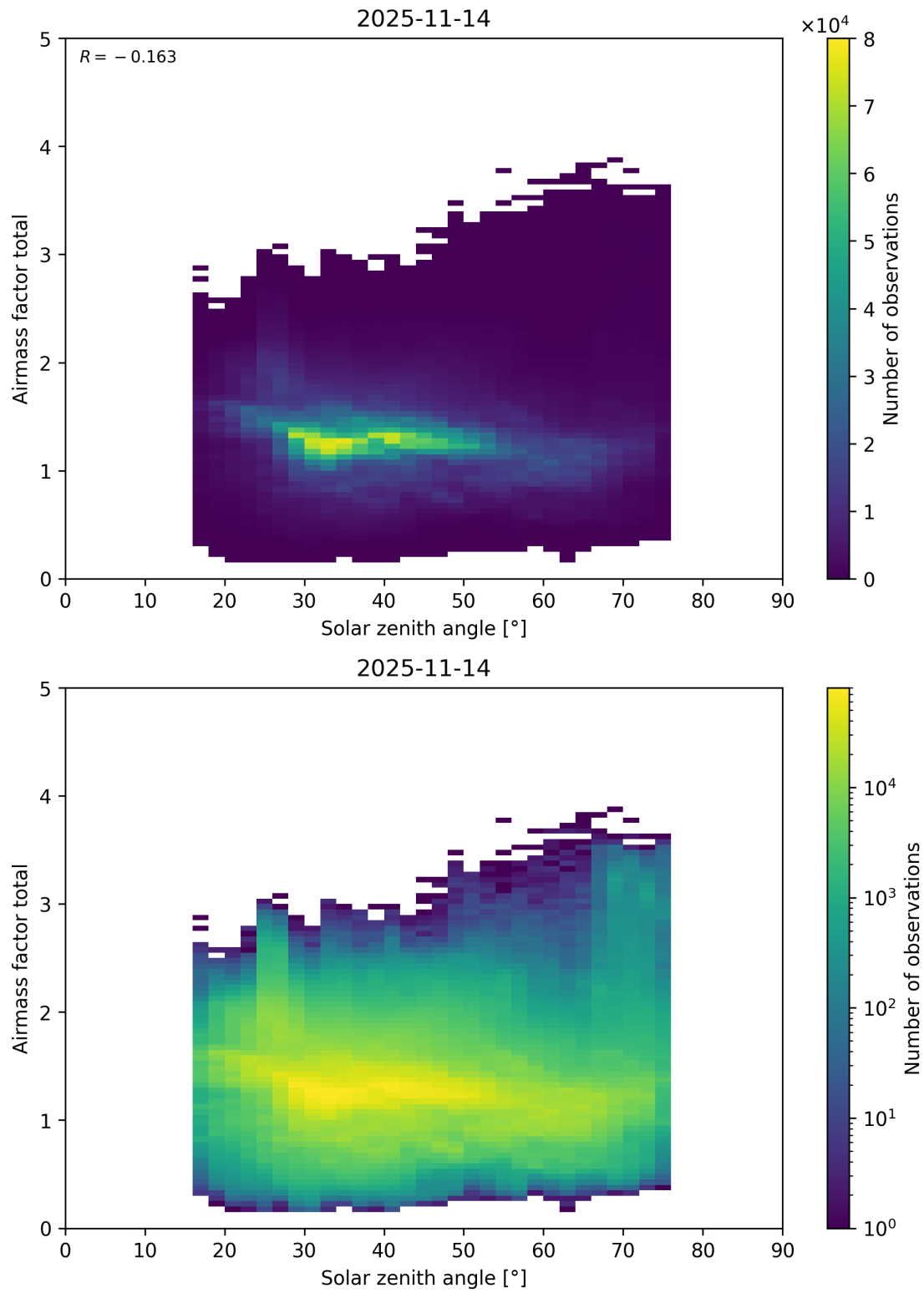
Figure 194: Scatter density plot of “Solar zenith angle” against “Airmass factor total” for 2025-11-13 to 2025-11-15.
