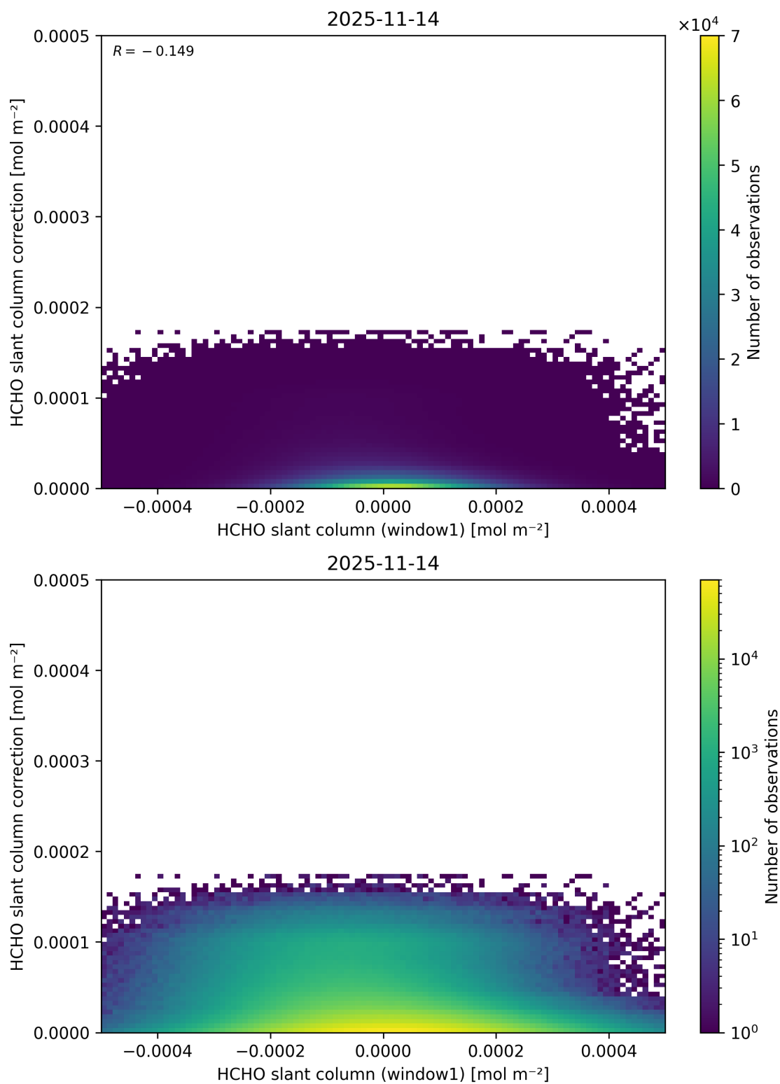
Figure 93: Scatter density plot of “HCHO slant column (window1)” against “HCHO slant column correction” for 2025-11-13 to 2025-11-15.
