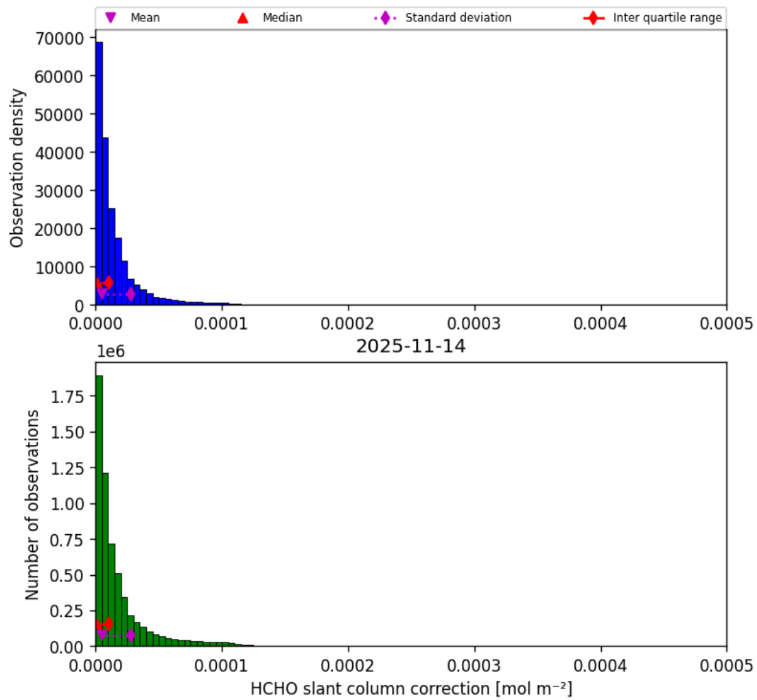
Figure 49: Histogram of “HCHO slant column correction” for 2025-11-13 to 2025-11-15
