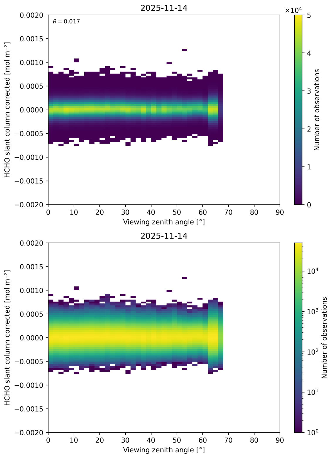
Figure 206: Scatter density plot of “Viewing zenith angle” against “HCHO slant column corrected” for 2025-11-13 to 2025-11-15.
