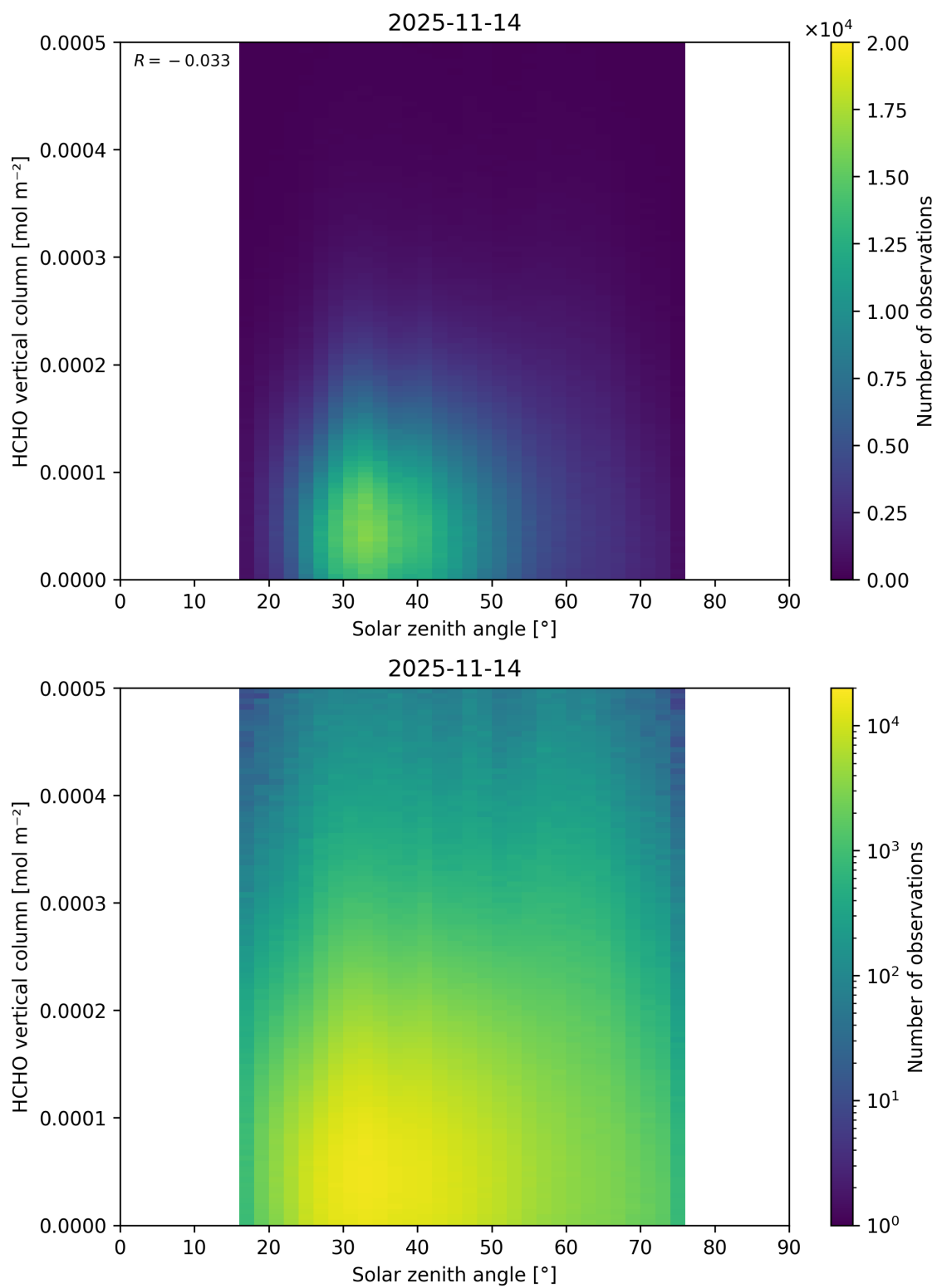
Figure 196: Scatter density plot of “Solar zenith angle” against “HCHO vertical column” for 2025-11-13 to 2025-11-15.
