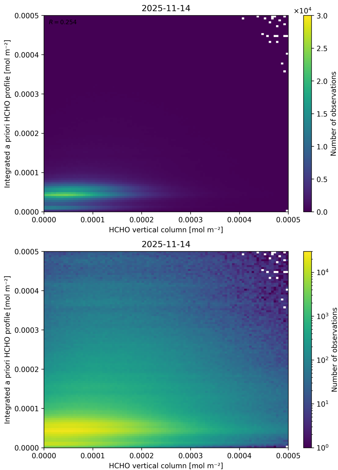
Figure 151: Scatter density plot of “HCHO vertical column” against “Integrated a priori HCHO profile” for 2025-11-13 to 2025-11-15.
