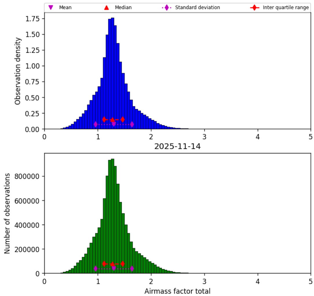
Figure 42: Histogram of “Airmass factor total” for 2025-11-13 to 2025-11-15
