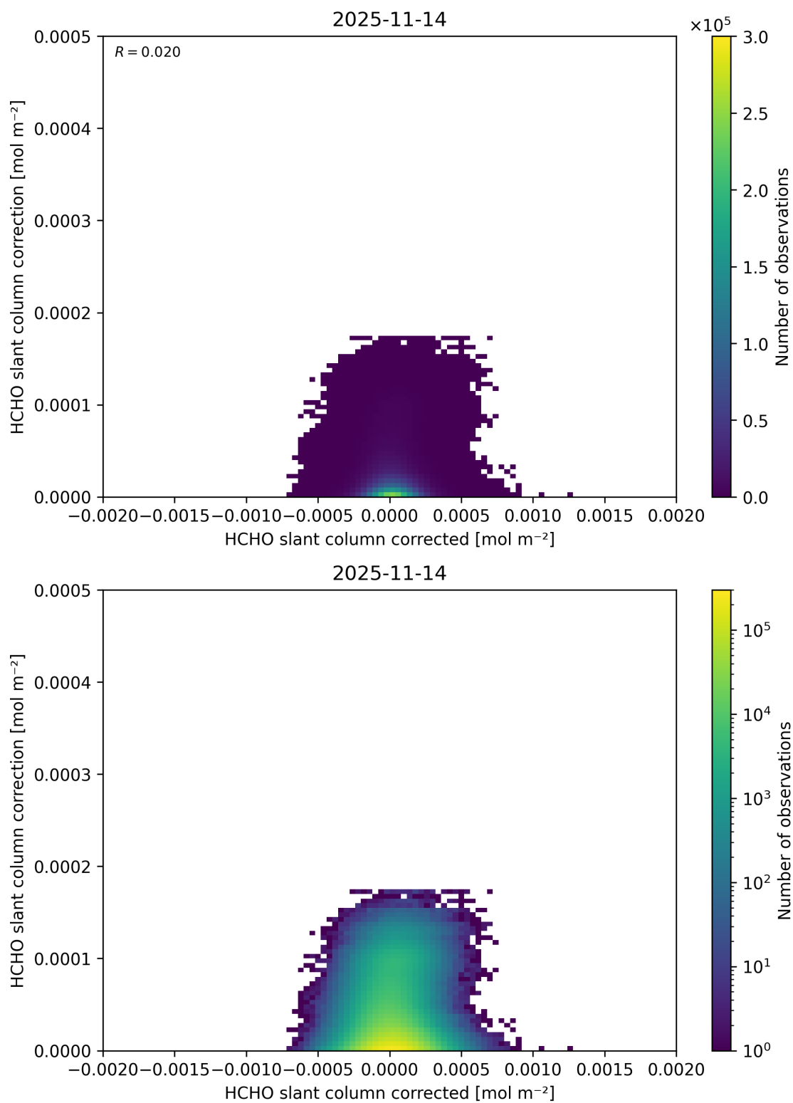
Figure 85: Scatter density plot of “HCHO slant column corrected” against “HCHO slant column correction” for 2025-11-13 to 2025-11-15.
