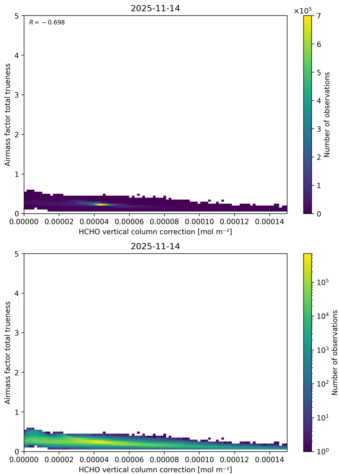
Figure 135: Scatter density plot of “HCHO vertical column correction” against “Airmass factor total trueness” for 2025-11-13 to 2025-11-15.
