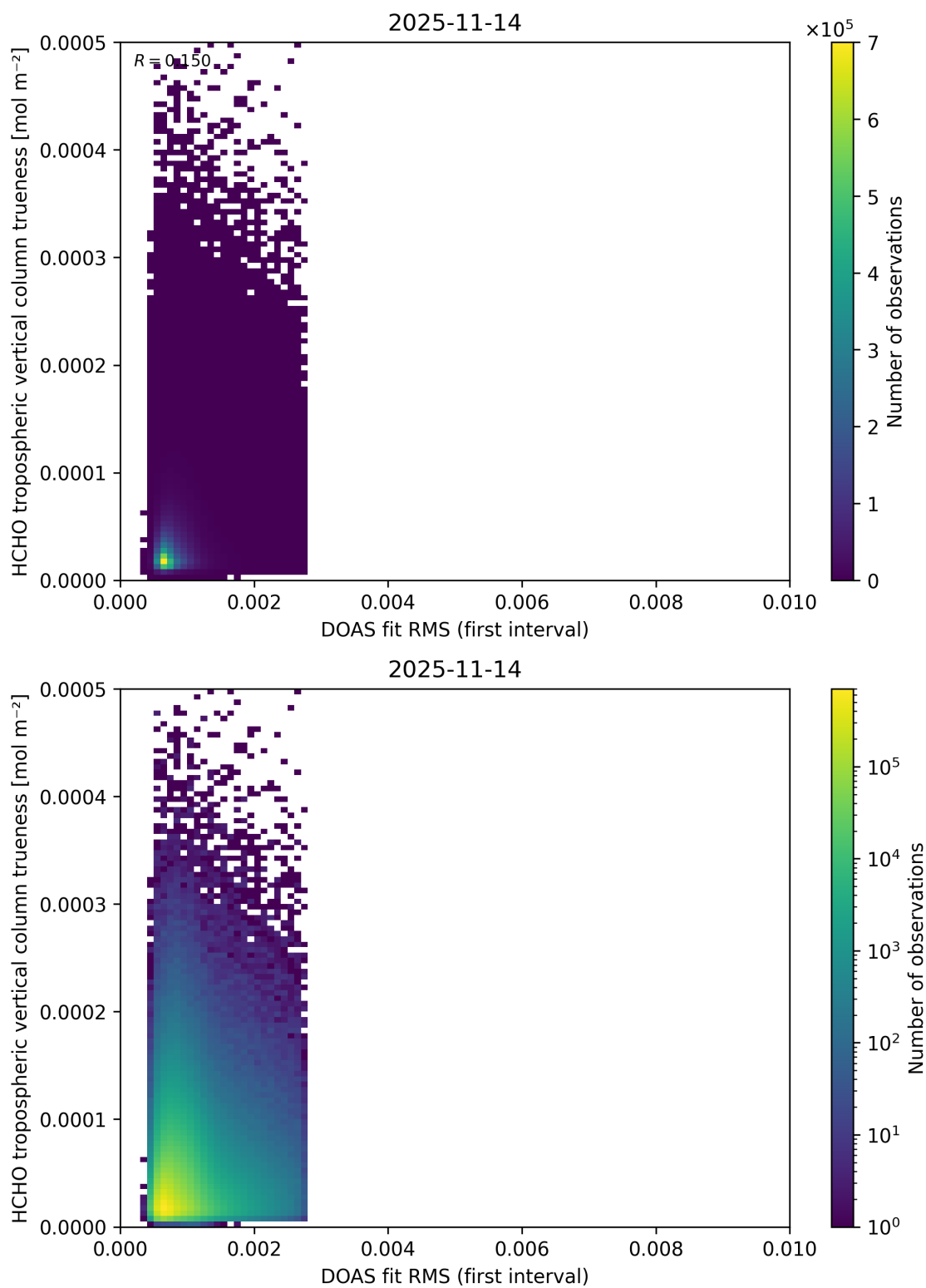
Figure 68: Scatter density plot of “DOAS fit RMS (first interval)” against “HCHO tropospheric vertical column trueness” for 2025-11-13 to 2025-11-15.
