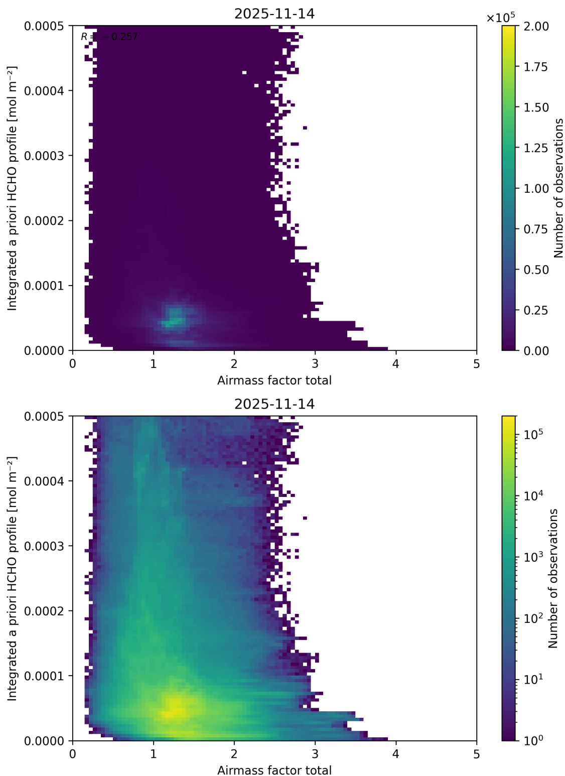
Figure 117: Scatter density plot of “Airmass factor total” against “Integrated a priori HCHO profile” for 2025-11-13 to 2025-11-15.
