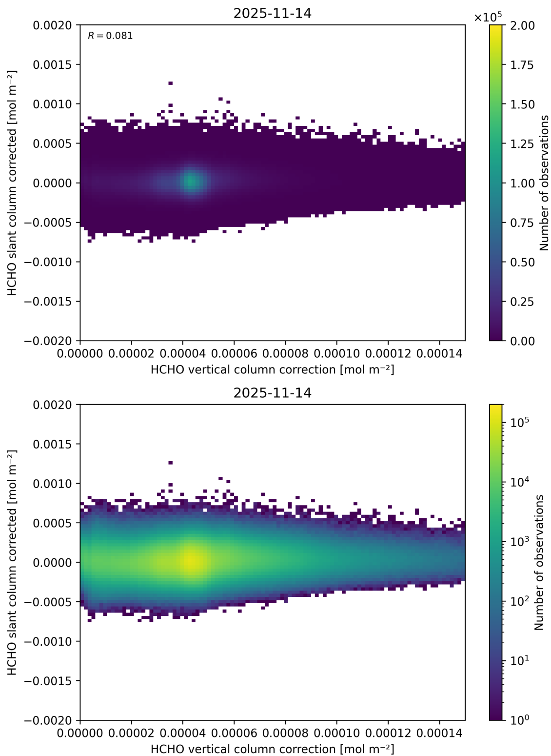
Figure 130: Scatter density plot of “HCHO vertical column correction” against “HCHO slant column corrected” for 2025-11-13 to 2025-11-15.
