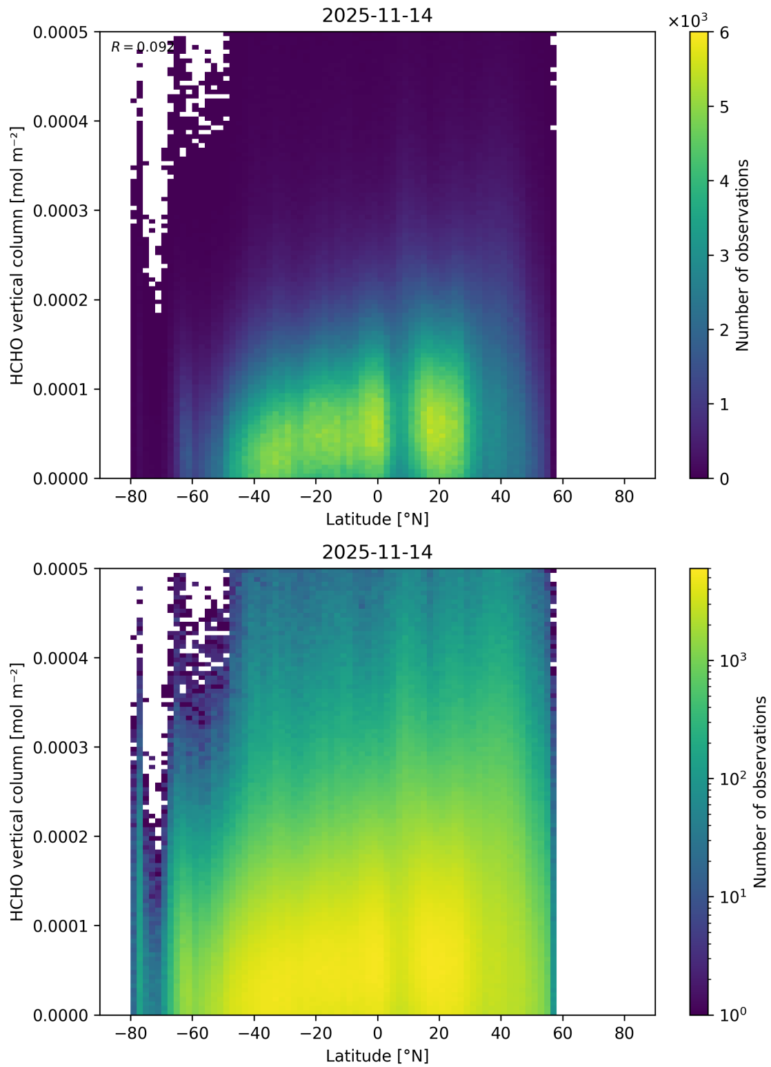
Figure 181: Scatter density plot of “Latitude” against “HCHO vertical column” for 2025-11-13 to 2025-11-15.
