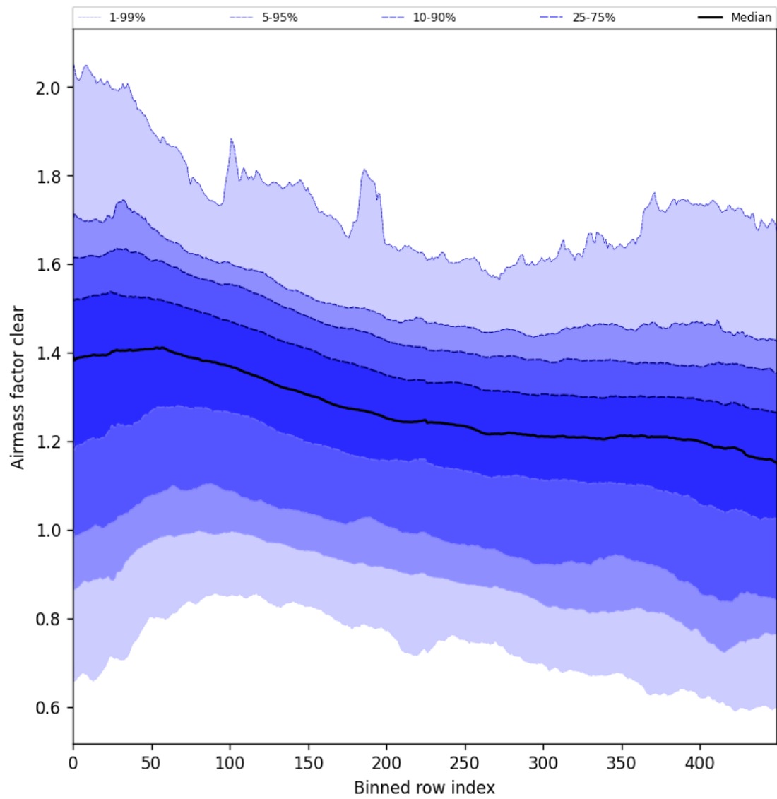
Figure 59: Along track statistics of “Airmass factor clear” for 2025-11-13 to 2025-11-15
