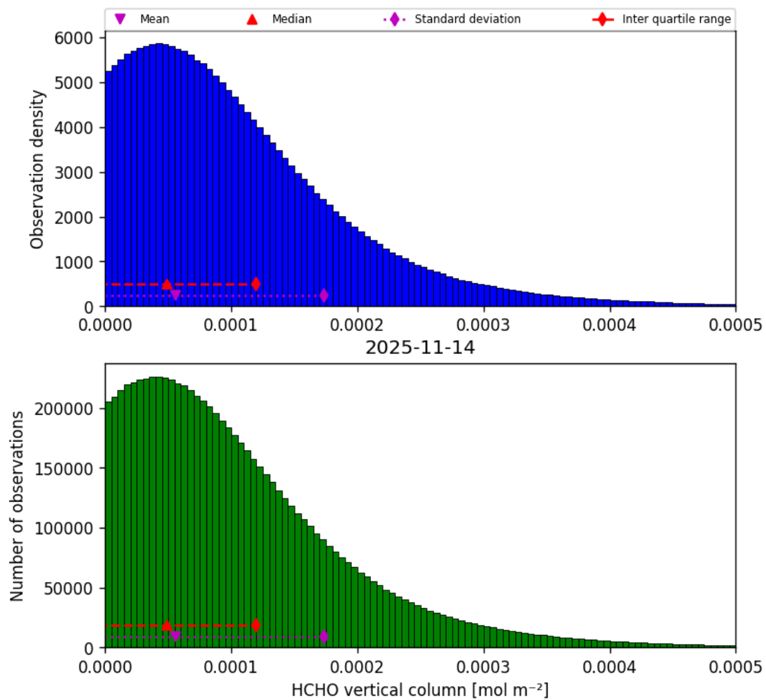
Figure 37: Histogram of “HCHO vertical column” for 2025-11-13 to 2025-11-15
