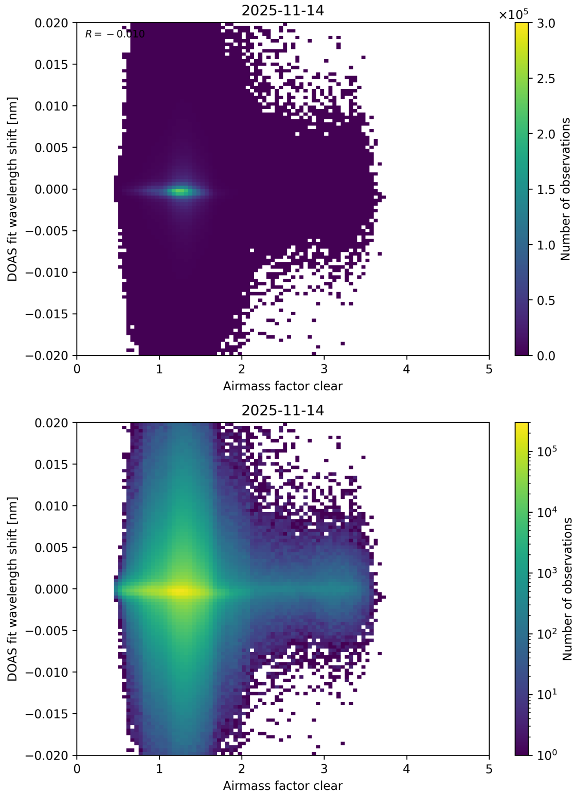
Figure 79: Scatter density plot of “Airmass factor clear” against “DOAS fit wavelength shift” for 2025-11-13 to 2025-11-15.
