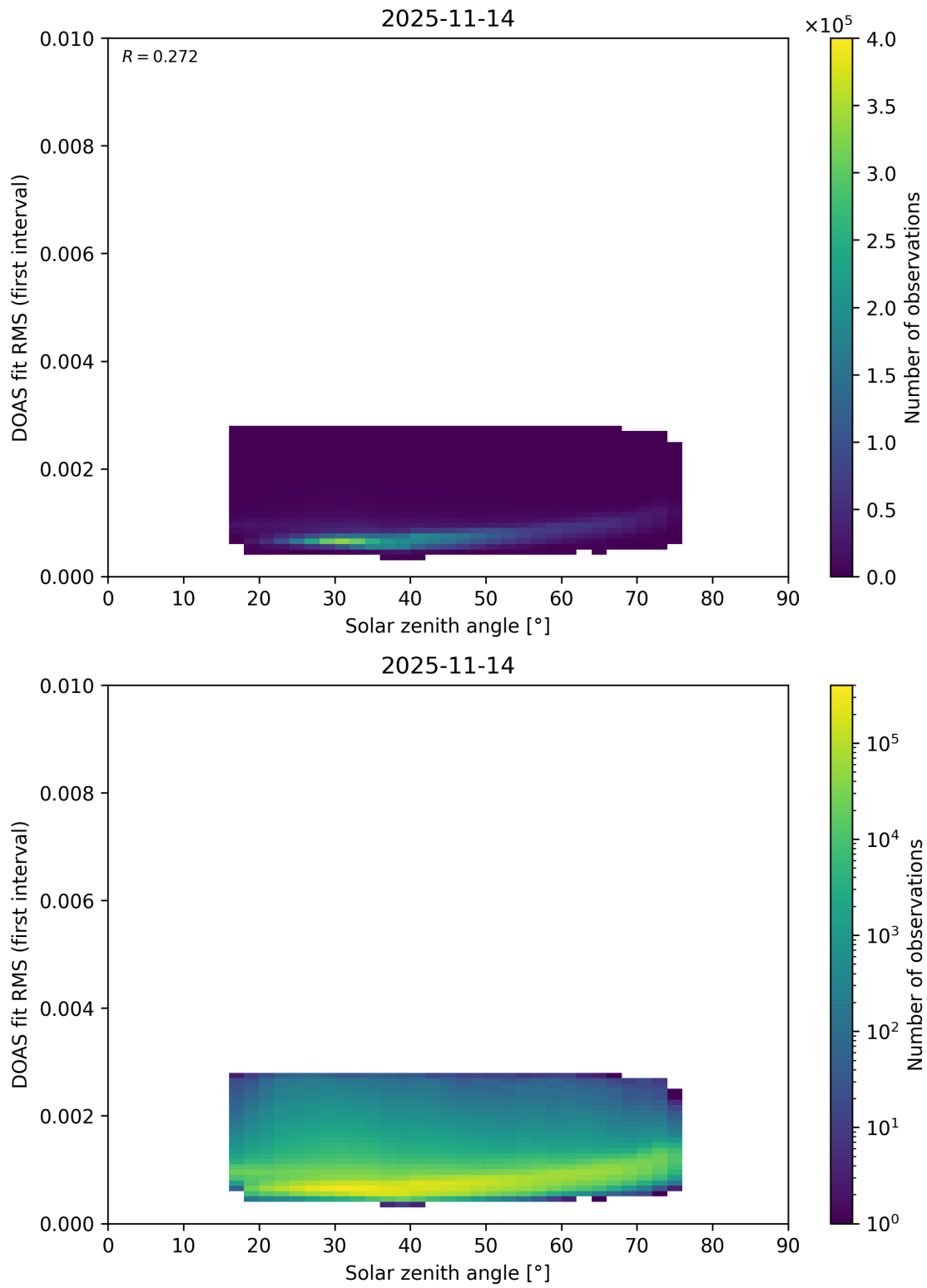
Figure 186: Scatter density plot of “Solar zenith angle” against “DOAS fit RMS (first interval)” for 2025-11-13 to 2025-11-15.
