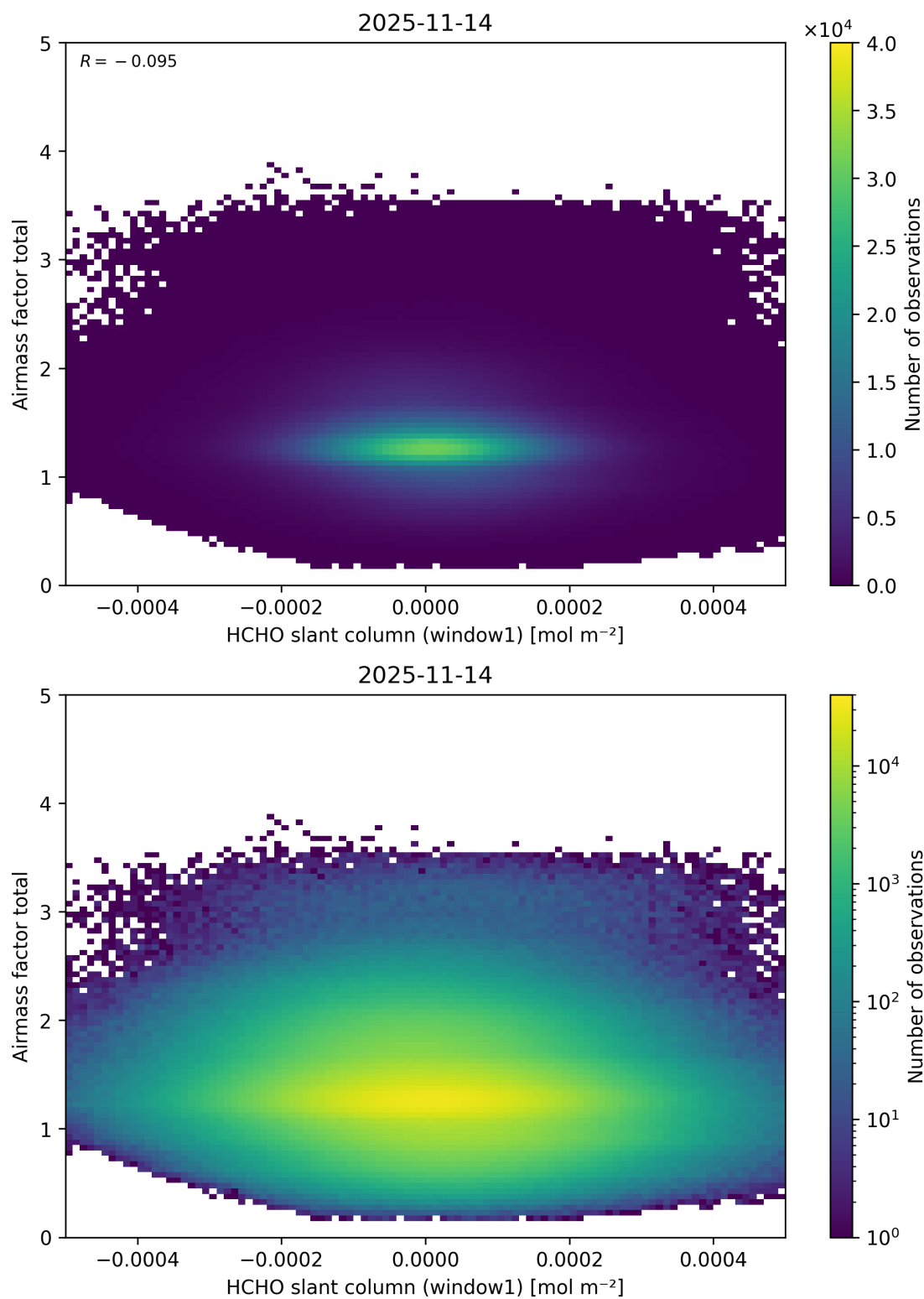
Figure 95: Scatter density plot of “HCHO slant column (window1)” against “Airmass factor total” for 2025-11-13 to 2025-11-15.
