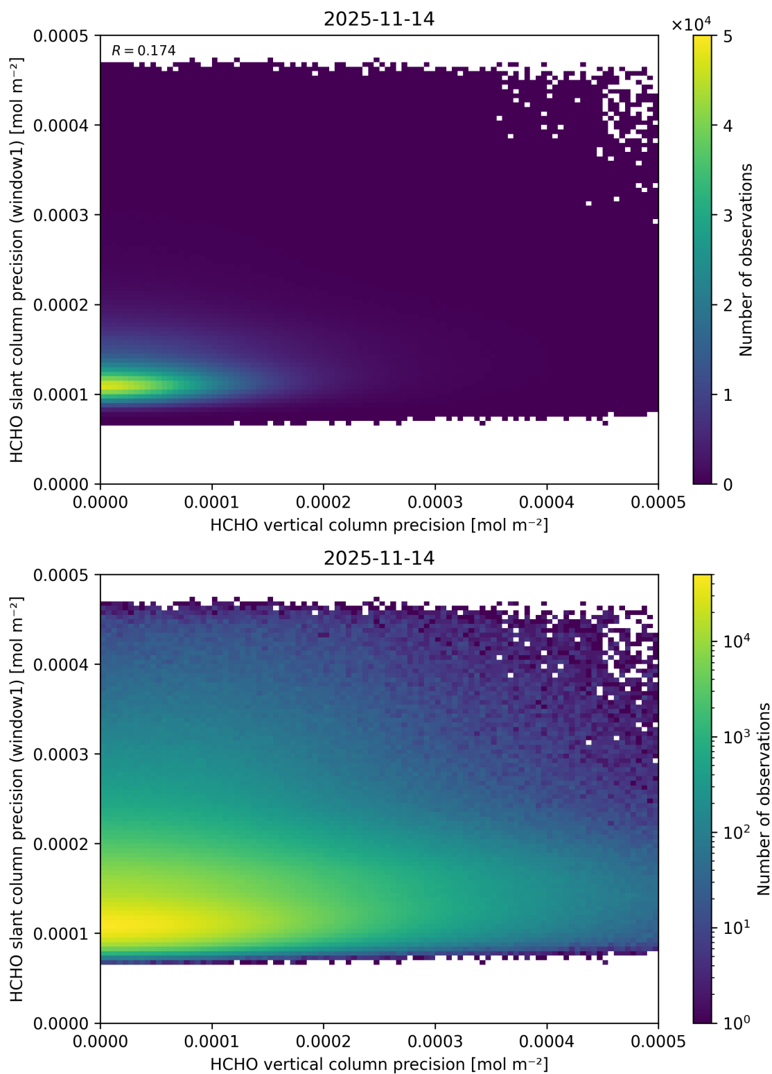
Figure 159: Scatter density plot of “HCHO vertical column precision” against “HCHO slant column precision (window1)” for 2025-11-13 to 2025-11-15.
