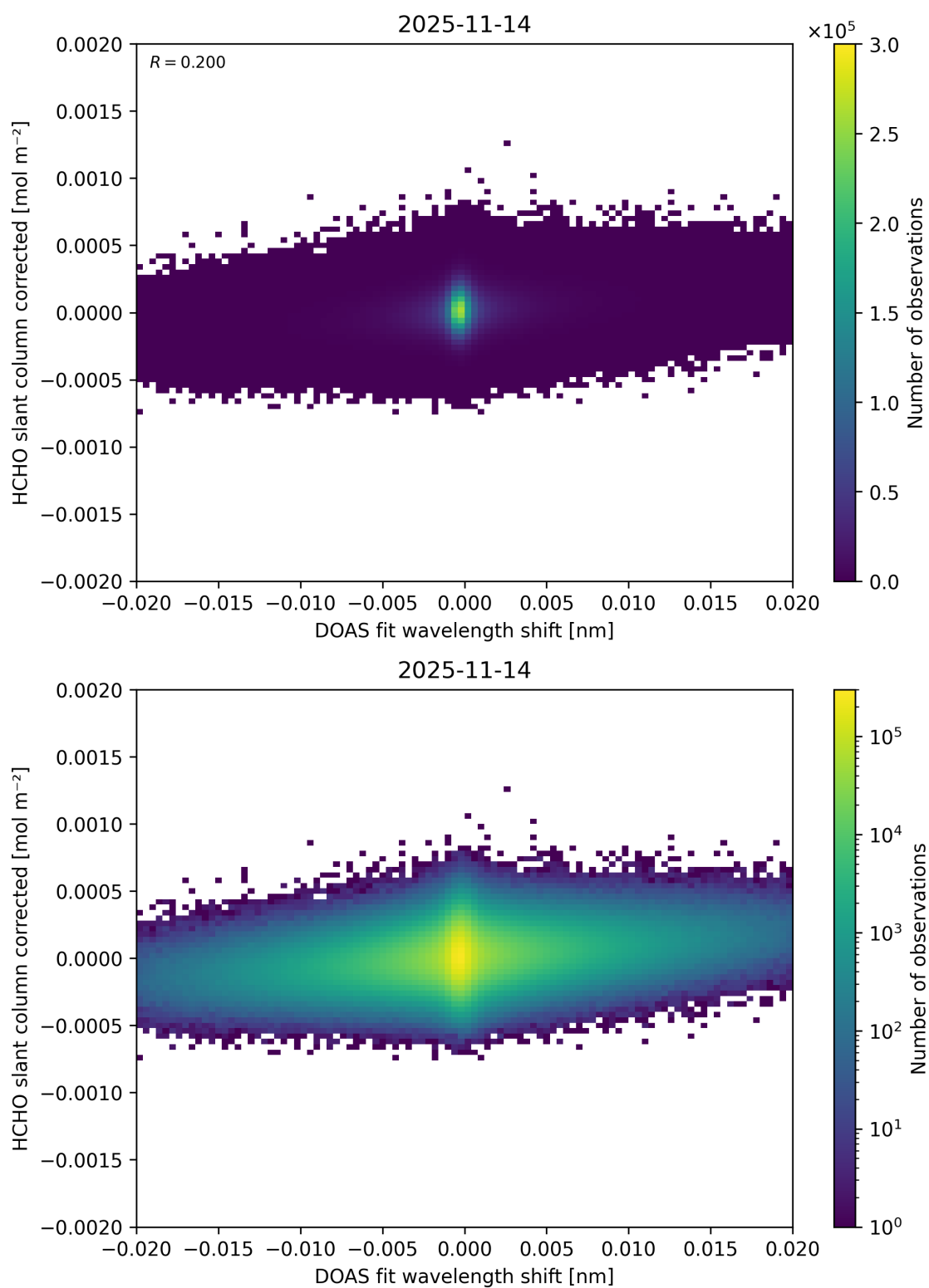
Figure 71: Scatter density plot of “DOAS fit wavelength shift” against “HCHO slant column corrected” for 2025-11-13 to 2025-11-15.
