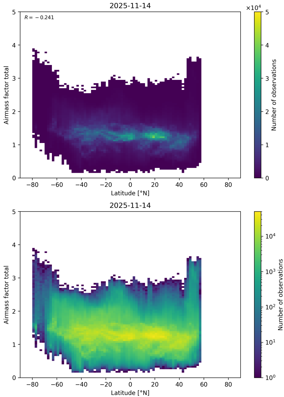
Figure 179: Scatter density plot of “Latitude” against “Airmass factor total” for 2025-11-13 to 2025-11-15.
