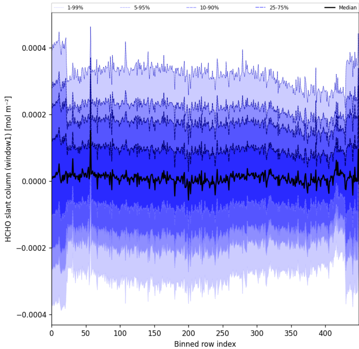
Figure 55: Along track statistics of “HCHO slant column (window1)” for 2025-11-13 to 2025-11-15
