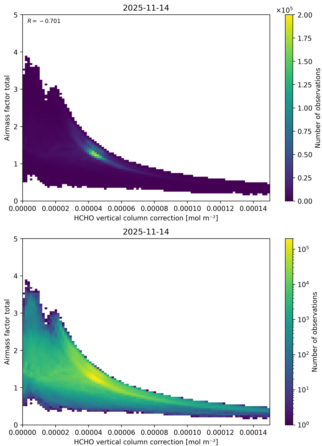
Figure 134: Scatter density plot of “HCHO vertical column correction” against “Airmass factor total” for 2025-11-13 to 2025-11-15.
