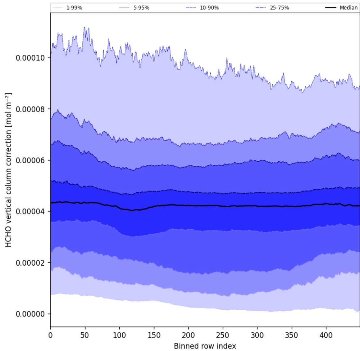
Figure 54: Along track statistics of “HCHO vertical column correction” for 2025-11-13 to 2025-11-15
