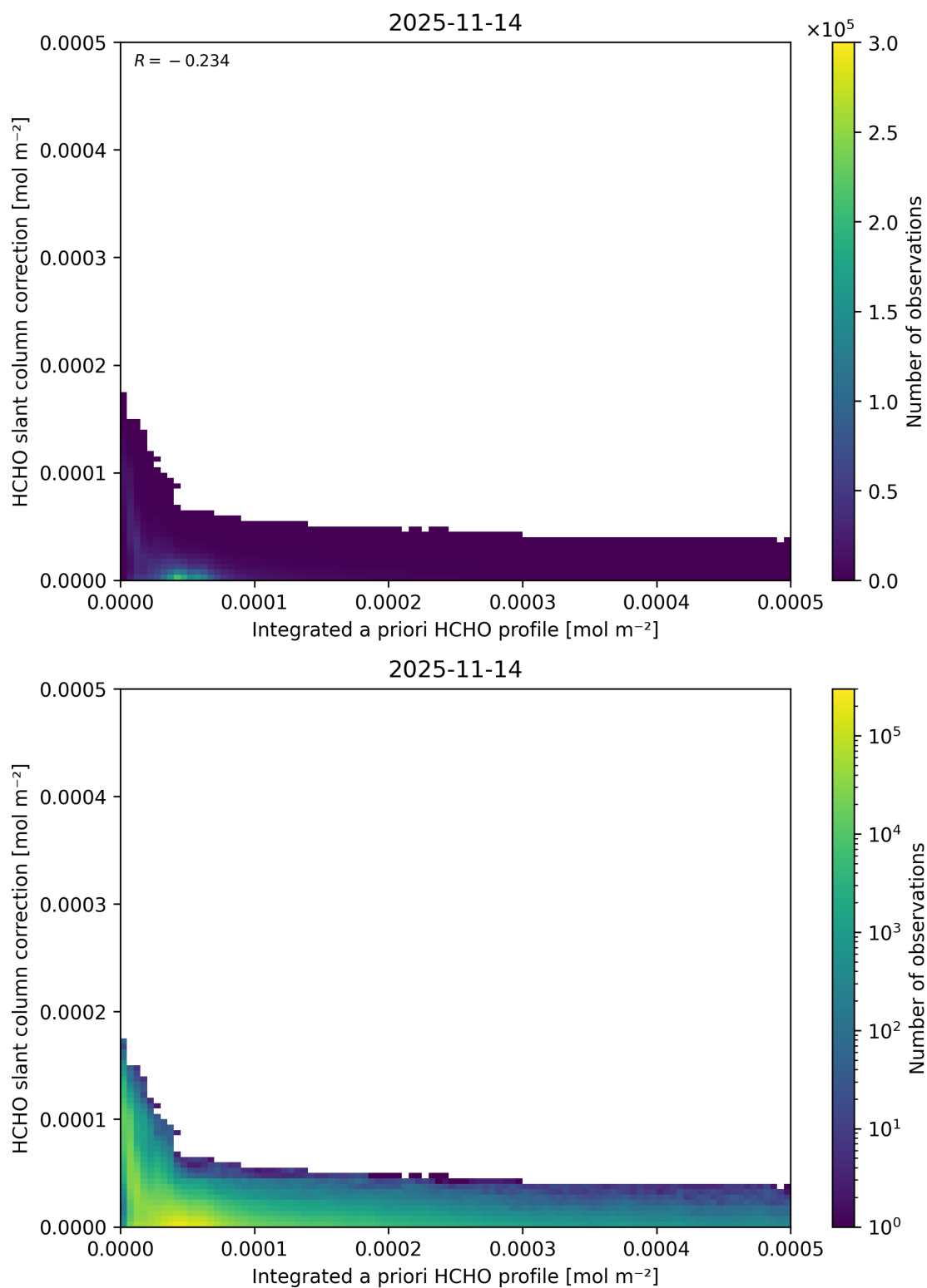
Figure 169: Scatter density plot of “Integrated a priori HCHO profile” against “HCHO slant column correction” for 2025-11-13 to 2025-11-15.
