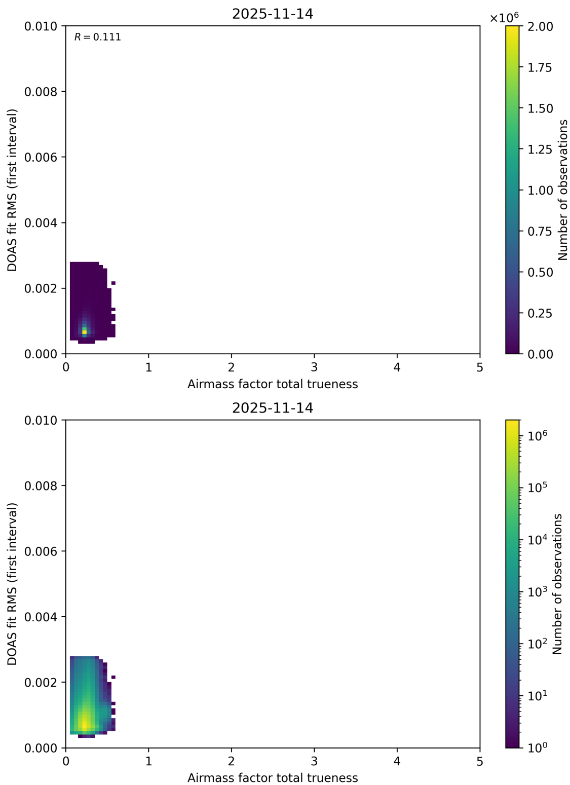
Figure 118: Scatter density plot of “Airmass factor total trueness” against “DOAS fit RMS (first interval)” for 2025-11-13 to 2025-11-15.
