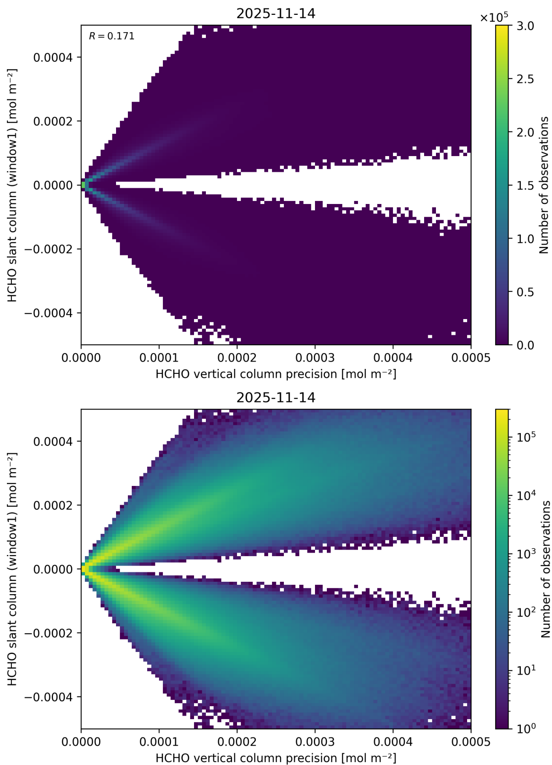
Figure 158: Scatter density plot of “HCHO vertical column precision” against “HCHO slant column (window1)” for 2025-11-13 to 2025-11-15.
