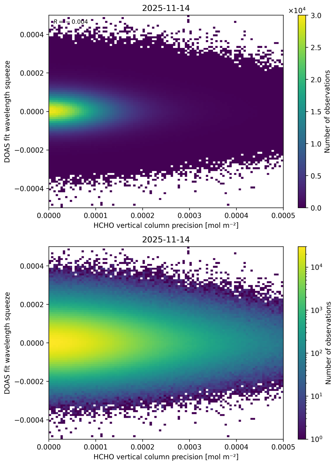
Figure 154: Scatter density plot of “HCHO vertical column precision” against “DOAS fit wavelength squeeze” for 2025-11-13 to 2025-11-15.
