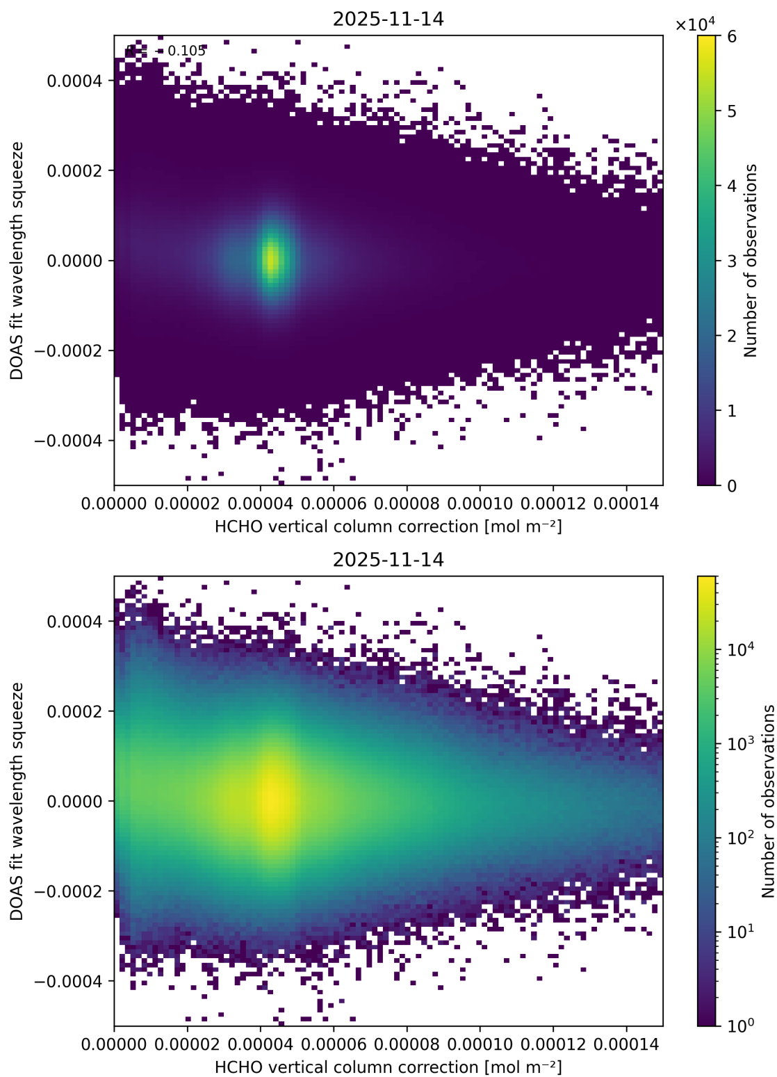
Figure 128: Scatter density plot of “HCHO vertical column correction” against “DOAS fit wavelength squeeze” for 2025-11-13 to 2025-11-15.
