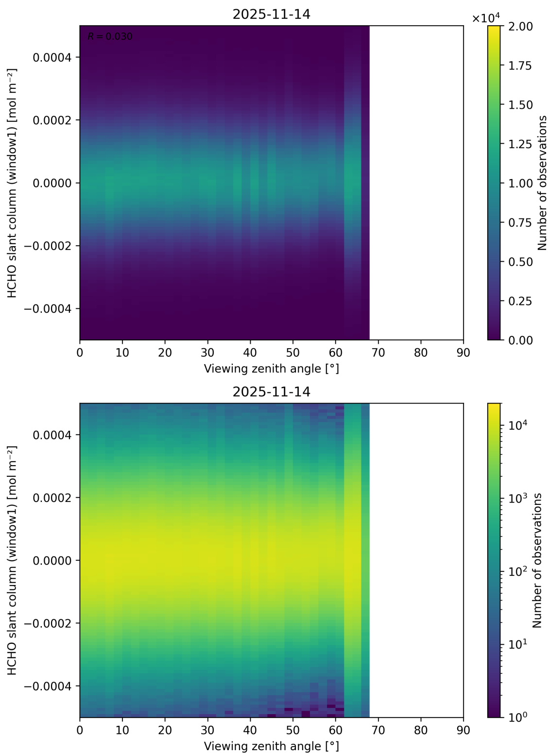
Figure 208: Scatter density plot of “Viewing zenith angle” against “HCHO slant column (window1)” for 2025-11-13 to 2025-11-15.
