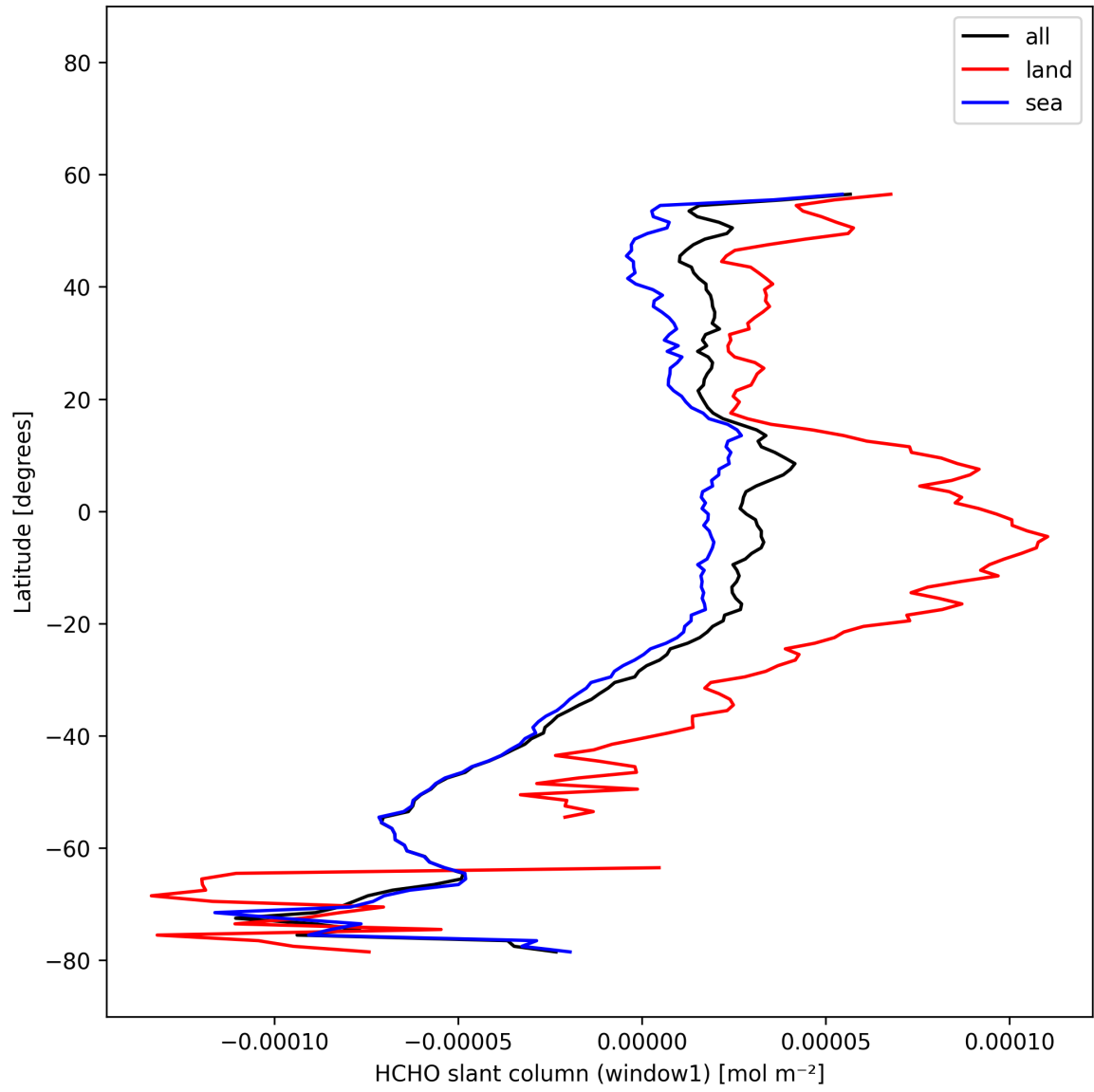
Figure 25: Zonal average of “HCHO slant column (window1)” for 2025-11-13 to 2025-11-15.
