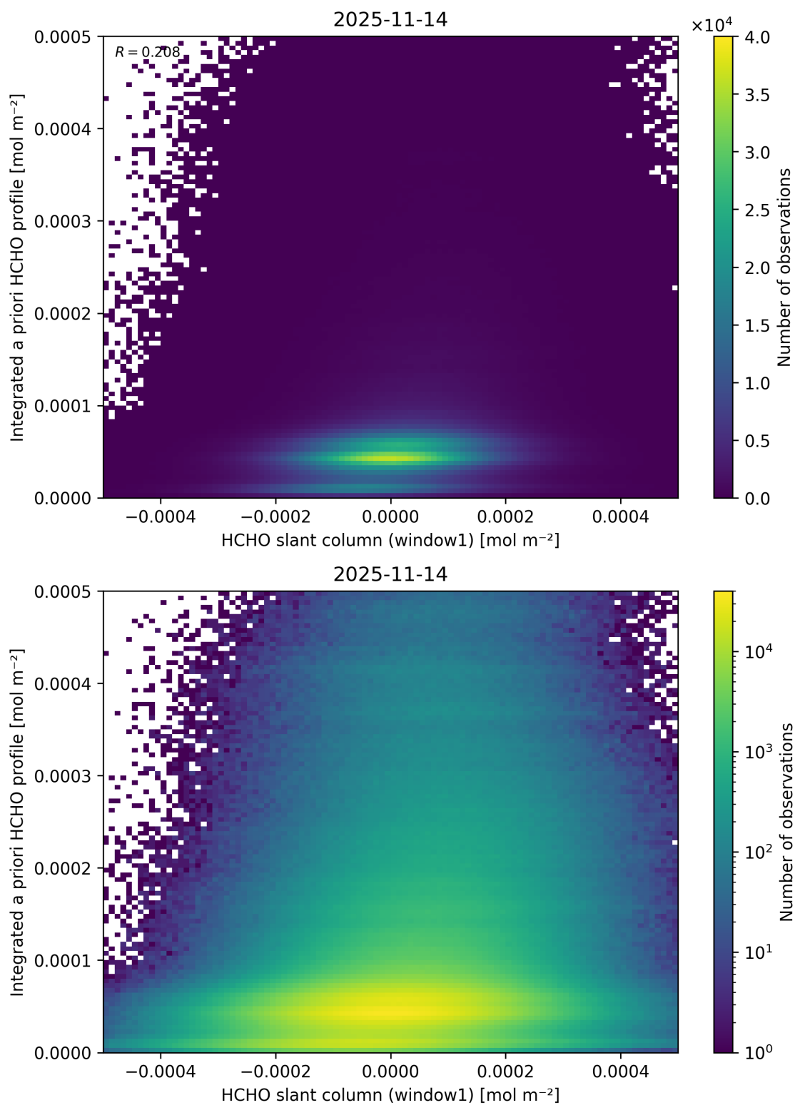
Figure 98: Scatter density plot of “HCHO slant column (window1)” against “Integrated a priori HCHO profile” for 2025-11-13 to 2025-11-15.
