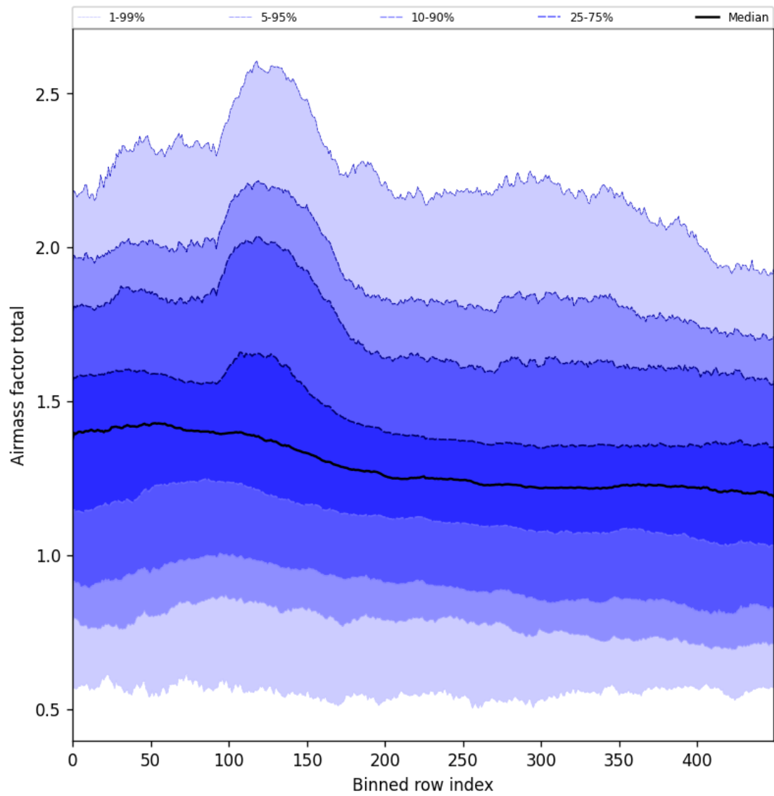
Figure 57: Along track statistics of “Airmass factor total” for 2025-11-13 to 2025-11-15
