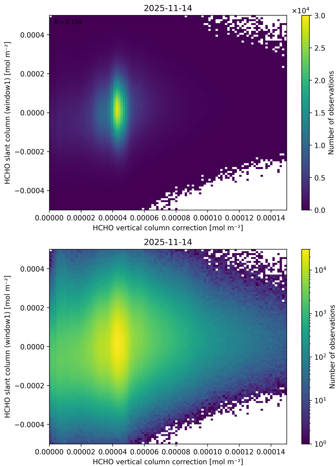
Figure 132: Scatter density plot of “HCHO vertical column correction” against “HCHO slant column (window1)” for 2025-11-13 to 2025-11-15.
