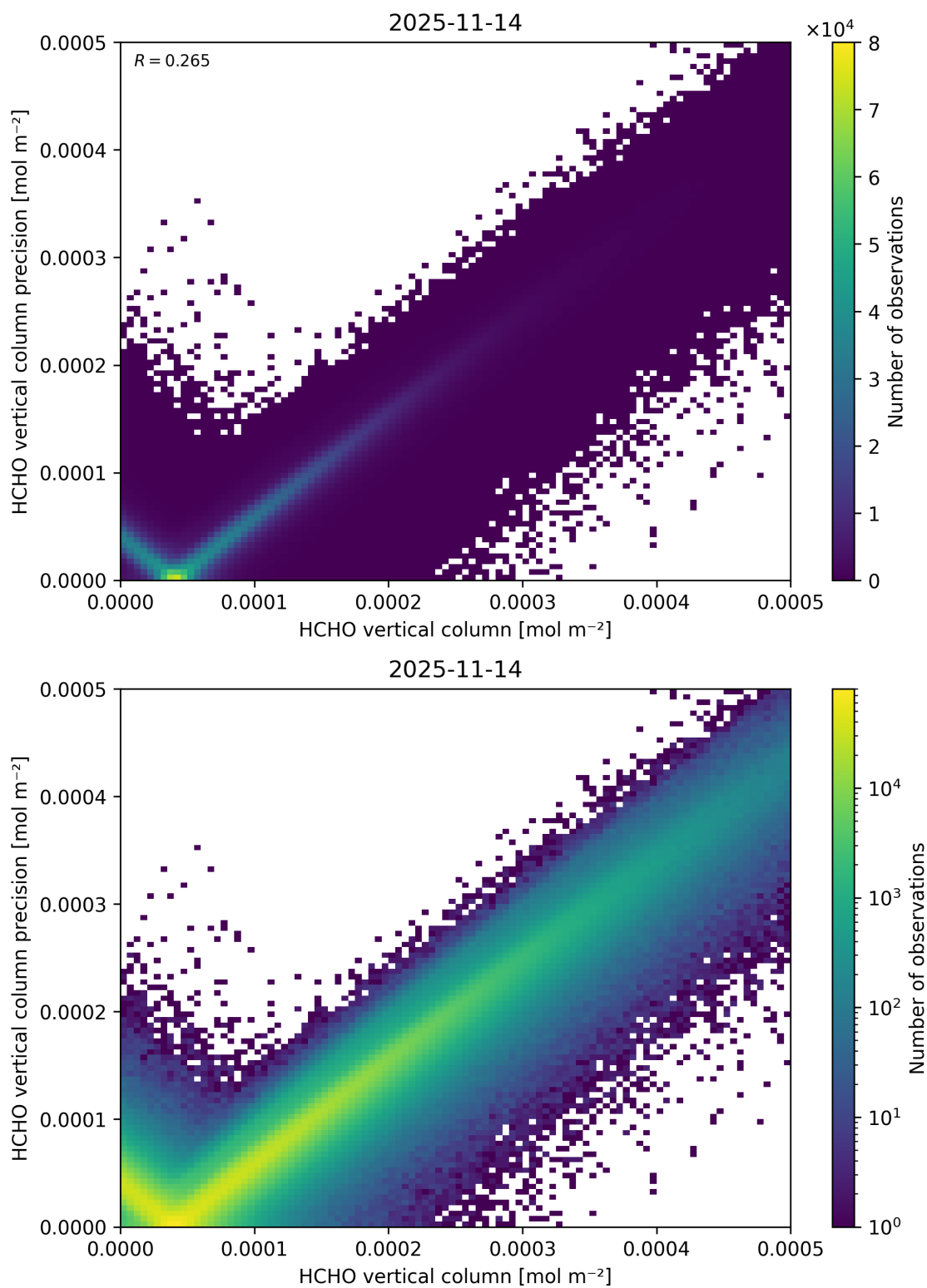
Figure 149: Scatter density plot of “HCHO vertical column” against “HCHO vertical column precision” for 2025-11-13 to 2025-11-15.
