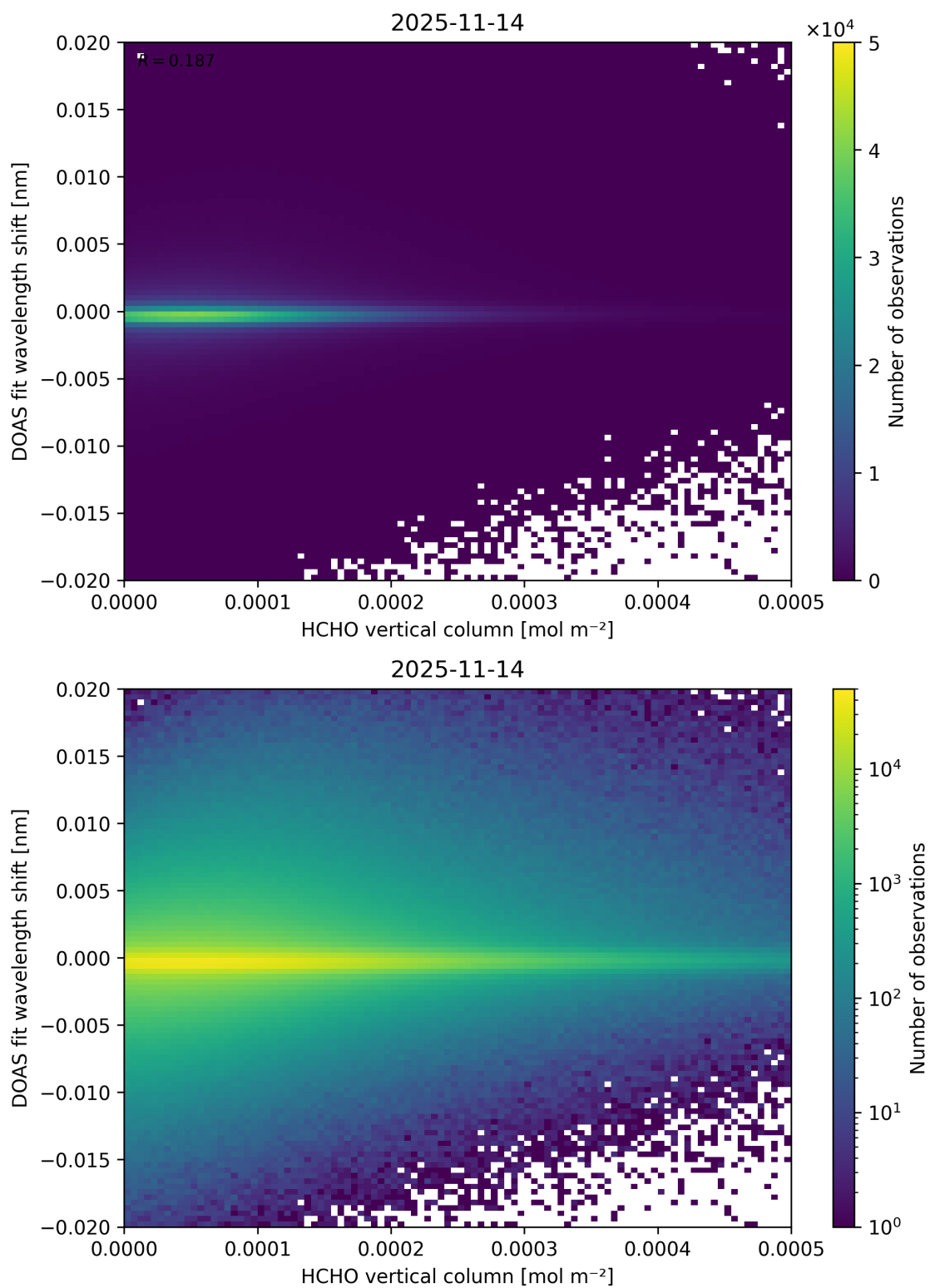
Figure 139: Scatter density plot of “HCHO vertical column” against “DOAS fit wavelength shift” for 2025-11-13 to 2025-11-15.
