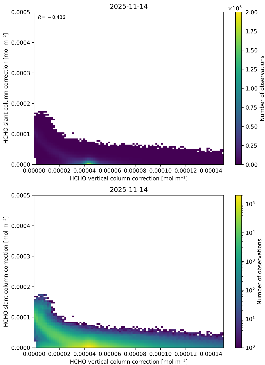
Figure 131: Scatter density plot of “HCHO vertical column correction” against “HCHO slant column correction” for 2025-11-13 to 2025-11-15.
