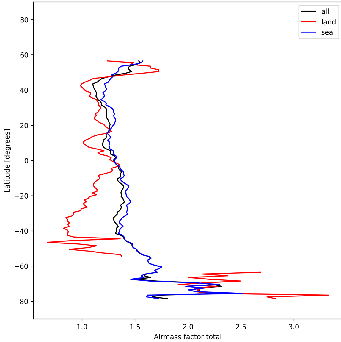
Figure 27: Zonal average of “Airmass factor total” for 2025-11-13 to 2025-11-15.
