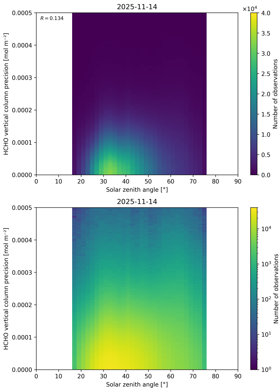
Figure 198: Scatter density plot of “Solar zenith angle” against “HCHO vertical column precision” for 2025-11-13 to 2025-11-15.
