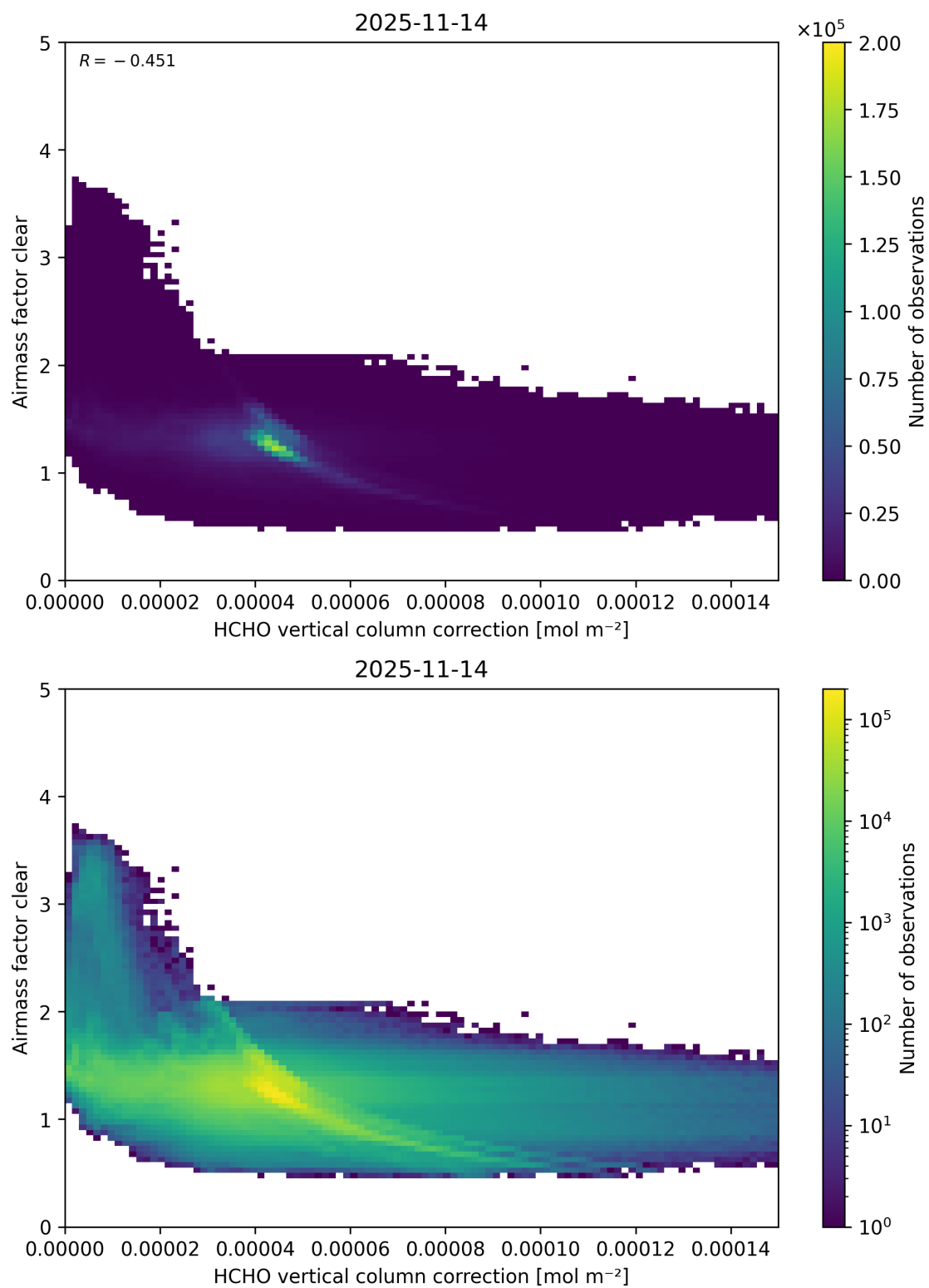
Figure 129: Scatter density plot of “HCHO vertical column correction” against “Airmass factor clear” for 2025-11-13 to 2025-11-15.
