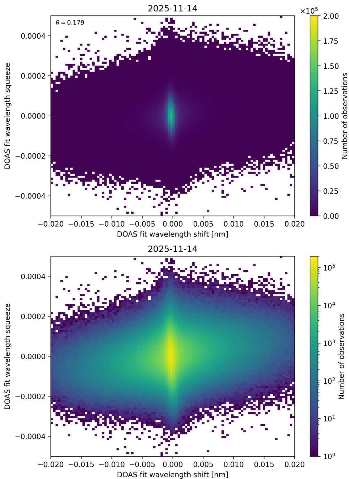
Figure 70: Scatter density plot of “DOAS fit wavelength shift” against “DOAS fit wavelength squeeze” for 2025-11-13 to 2025-11-15.
