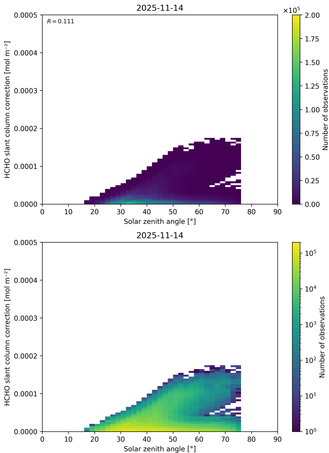
Figure 191: Scatter density plot of “Solar zenith angle” against “HCHO slant column correction” for 2025-11-13 to 2025-11-15.
