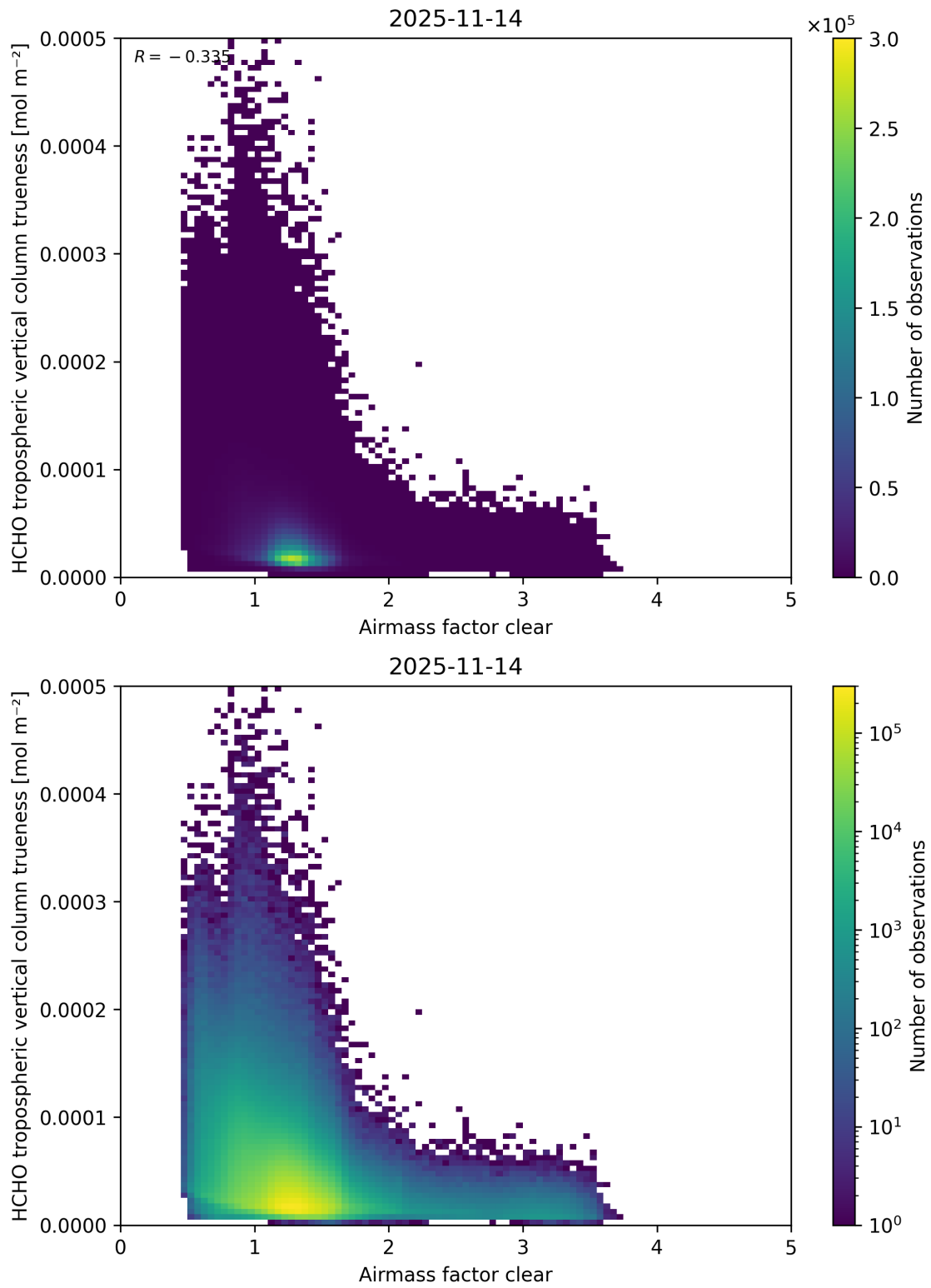
Figure 83: Scatter density plot of “Airmass factor clear” against “HCHO tropospheric vertical column trueness” for 2025-11-13 to 2025-11-15.
