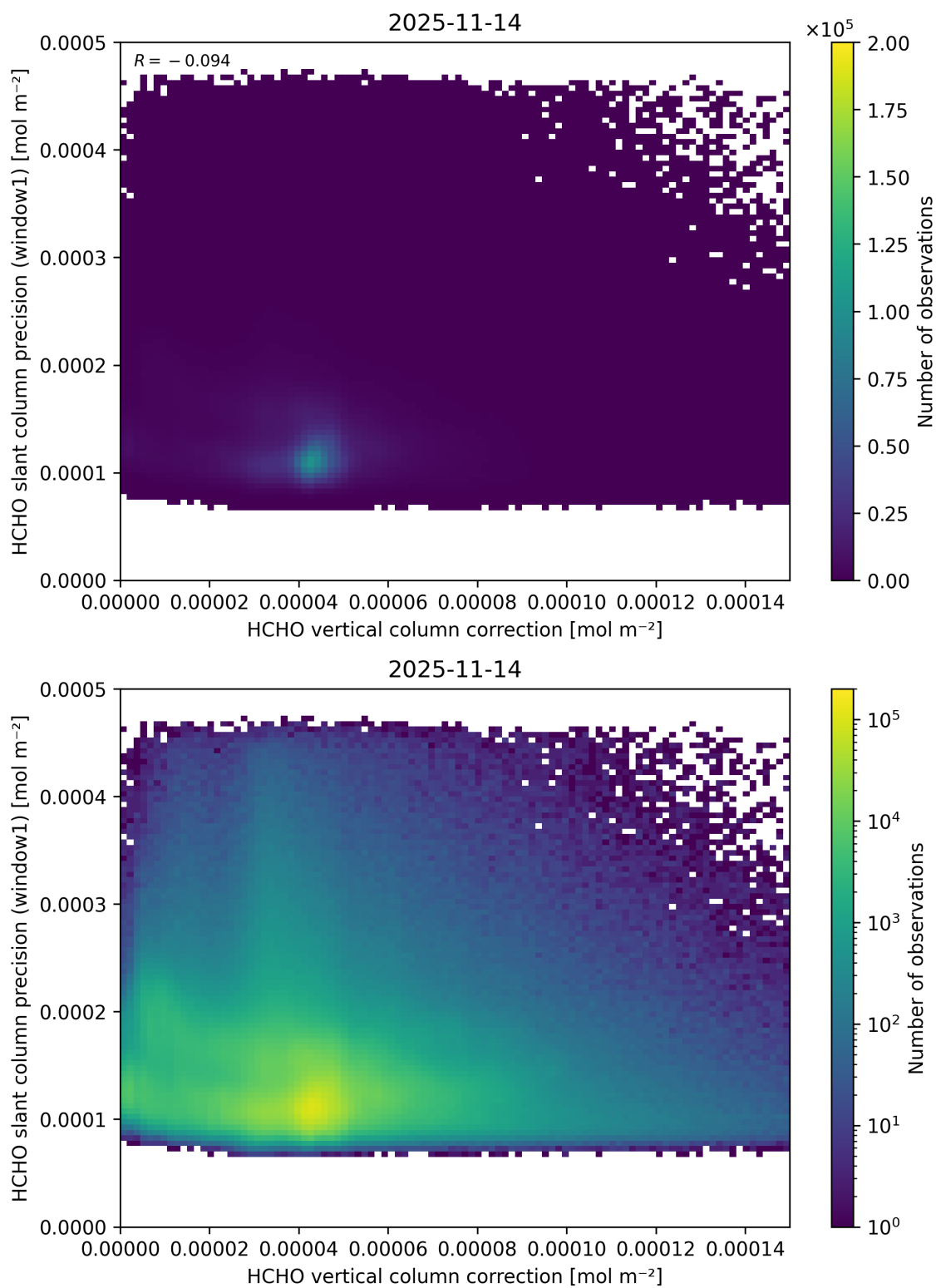
Figure 133: Scatter density plot of “HCHO vertical column correction” against “HCHO slant column precision (window1)” for 2025-11-13 to 2025-11-15.
