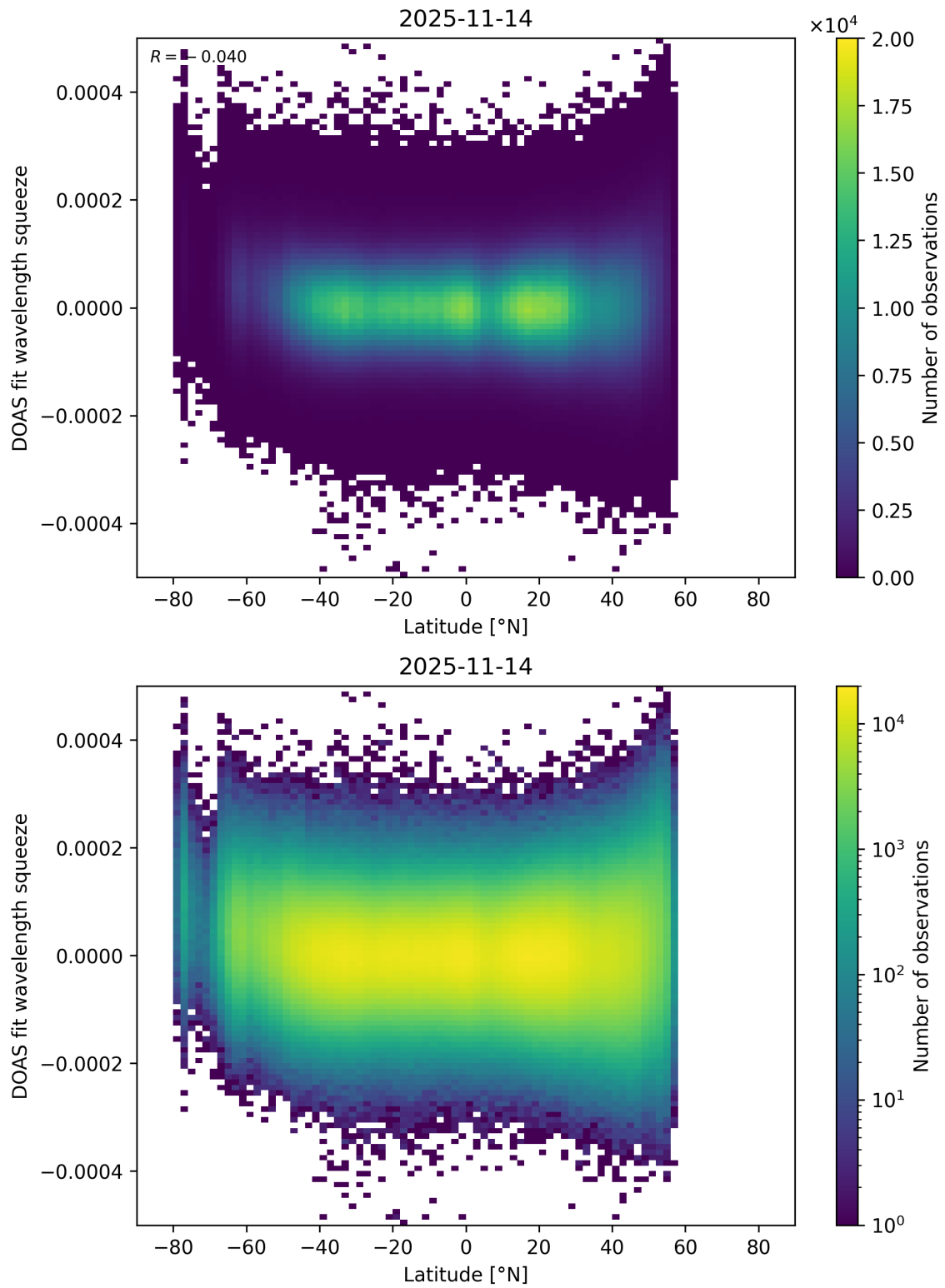
Figure 173: Scatter density plot of “Latitude” against “DOAS fit wavelength squeeze” for 2025-11-13 to 2025-11-15.
