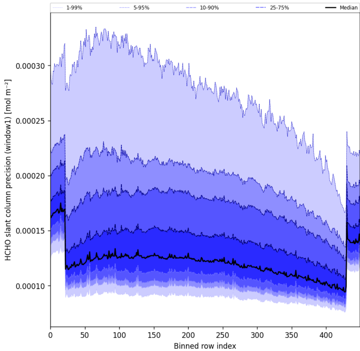
Figure 56: Along track statistics of “HCHO slant column precision (window1)” for 2025-11-13 to 2025-11-15
