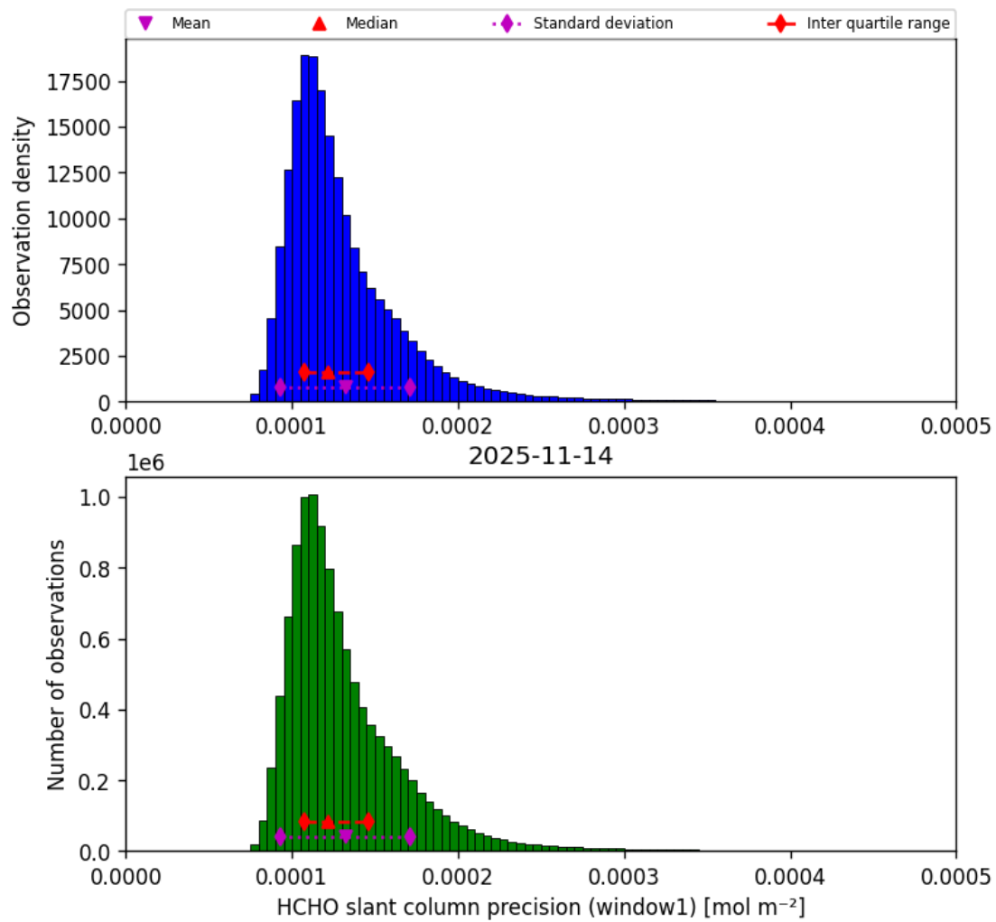
Figure 41: Histogram of “HCHO slant column precision (window1)” for 2025-11-13 to 2025-11-15
