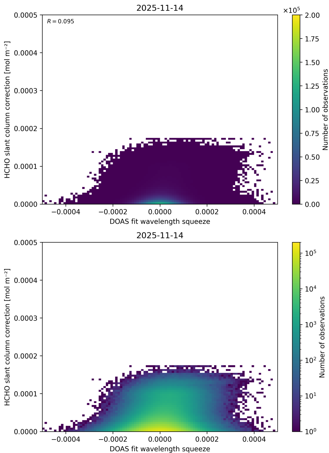
Figure 76: Scatter density plot of “DOAS fit wavelength squeeze” against “HCHO slant column correction” for 2025-11-13 to 2025-11-15.
