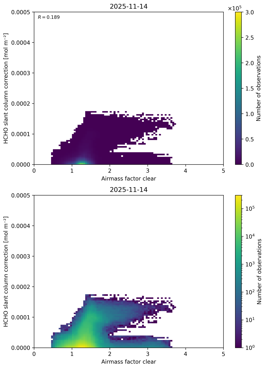
Figure 82: Scatter density plot of “Airmass factor clear” against “HCHO slant column correction” for 2025-11-13 to 2025-11-15.
