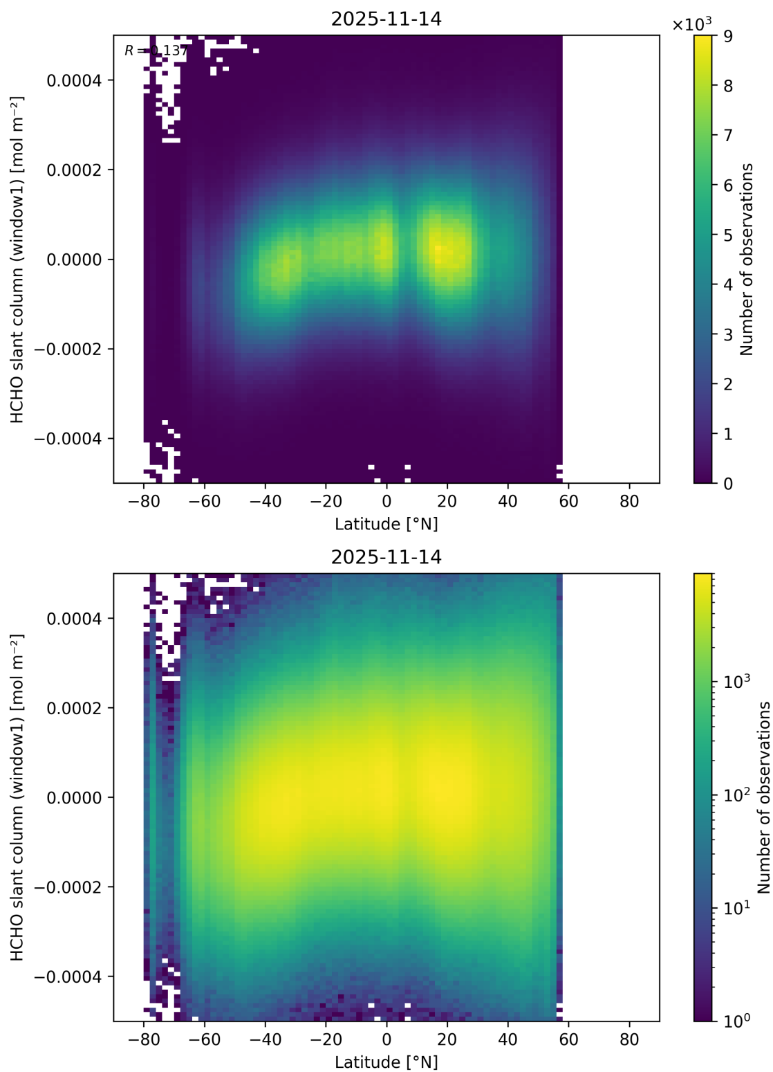
Figure 177: Scatter density plot of “Latitude” against “HCHO slant column (window1)” for 2025-11-13 to 2025-11-15.
