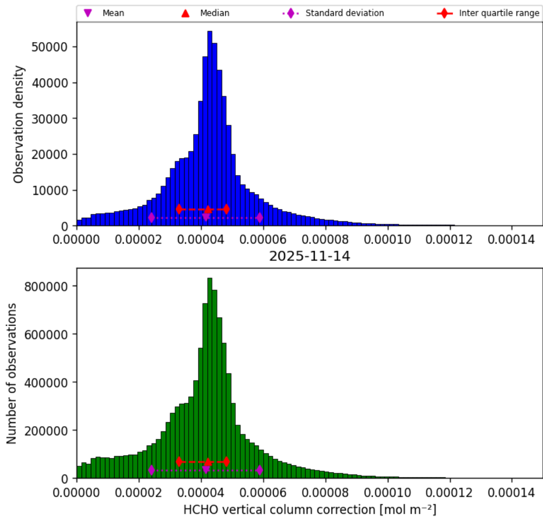
Figure 39: Histogram of “HCHO vertical column correction” for 2025-11-13 to 2025-11-15
