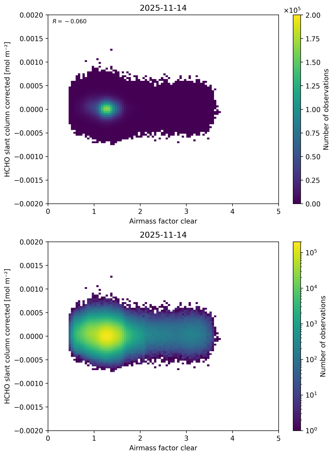
Figure 81: Scatter density plot of “Airmass factor clear” against “HCHO slant column corrected” for 2025-11-13 to 2025-11-15.
