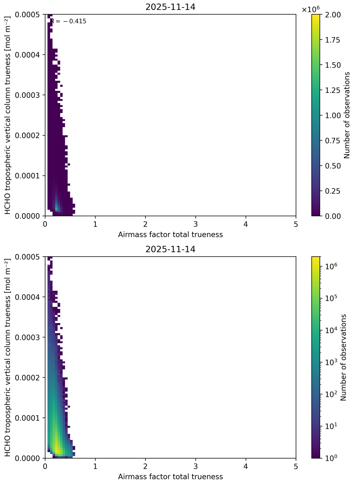
Figure 124: Scatter density plot of “Airmass factor total trueness” against “HCHO tropospheric vertical column trueness” for 2025-11-13 to 2025-11-15.
