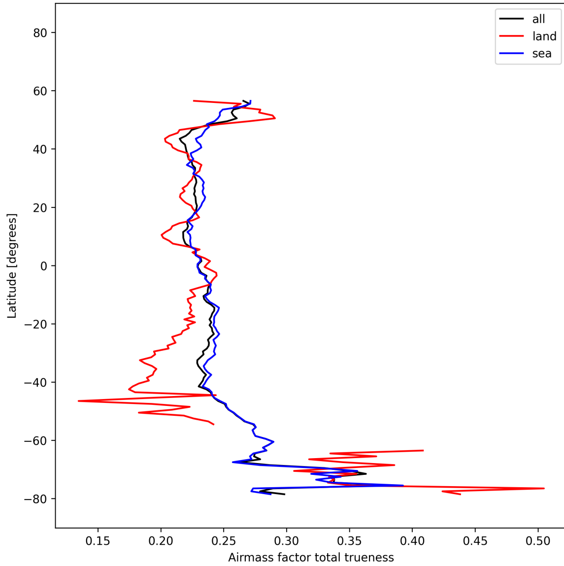
Figure 28: Zonal average of “Airmass factor total trueness” for 2025-11-13 to 2025-11-15.
