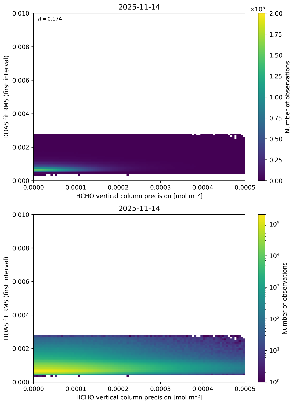
Figure 152: Scatter density plot of “HCHO vertical column precision” against “DOAS fit RMS (first interval)” for 2025-11-13 to 2025-11-15.
