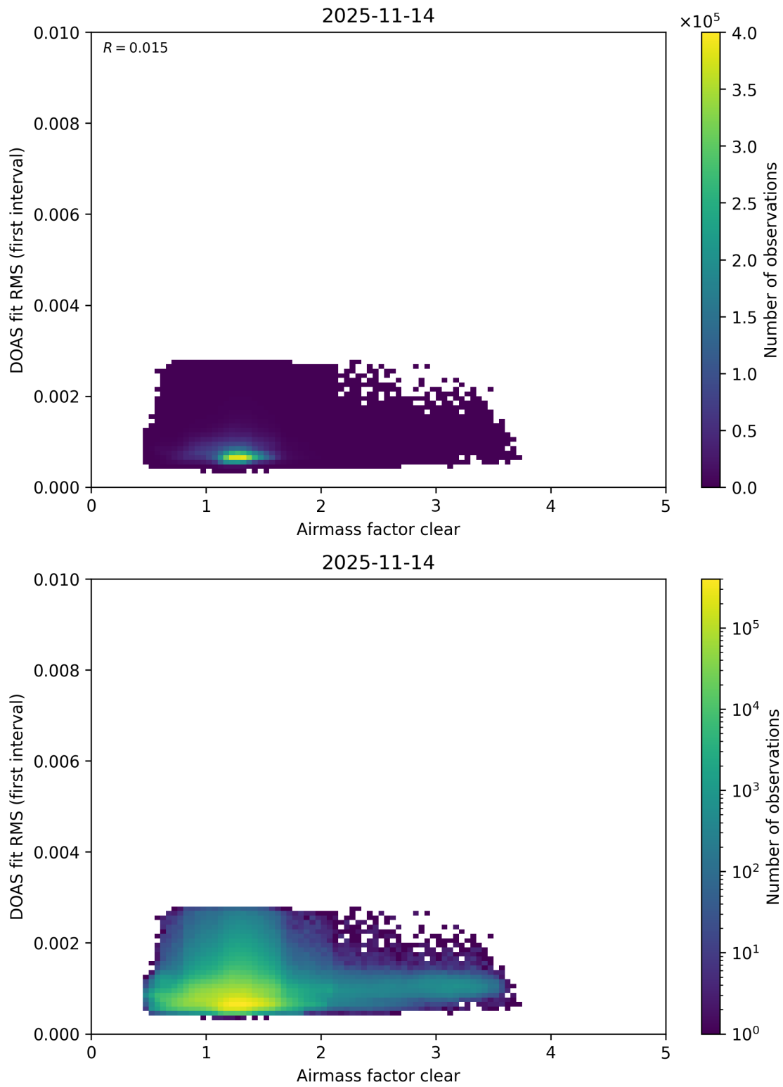
Figure 78: Scatter density plot of “Airmass factor clear” against “DOAS fit RMS (first interval)” for 2025-11-13 to 2025-11-15.
