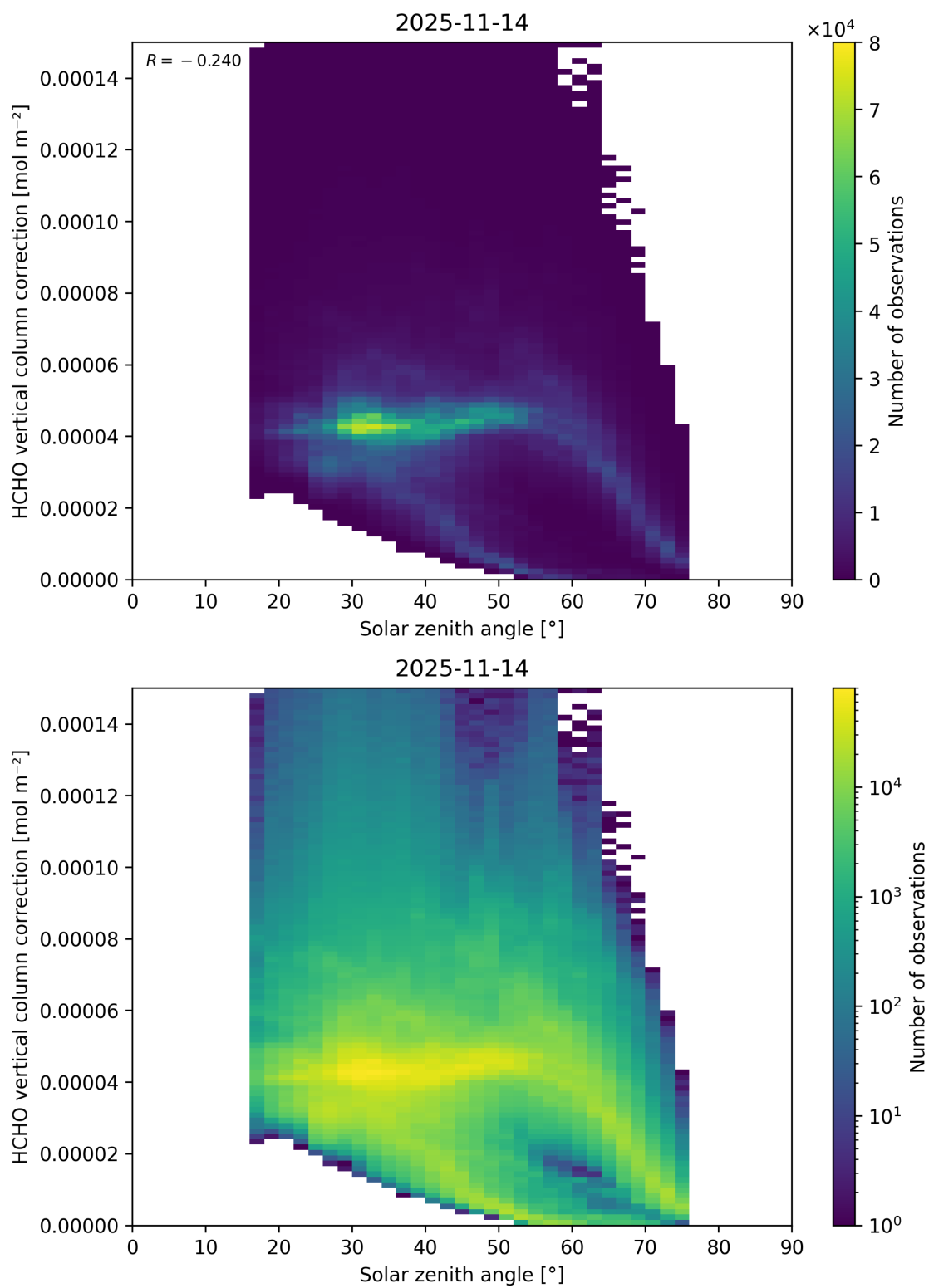
Figure 197: Scatter density plot of “Solar zenith angle” against “HCHO vertical column correction” for 2025-11-13 to 2025-11-15.
