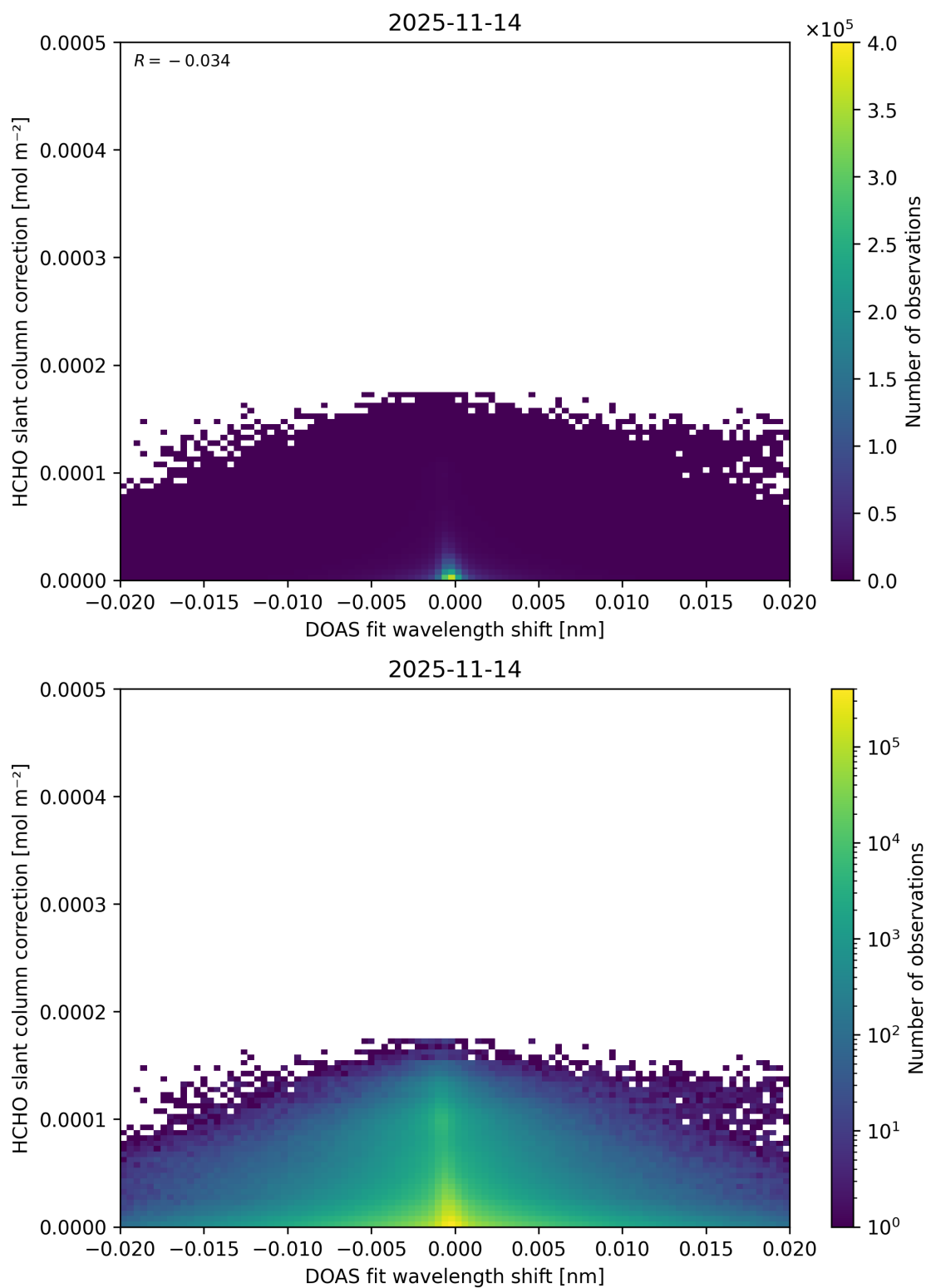
Figure 72: Scatter density plot of “DOAS fit wavelength shift” against “HCHO slant column correction” for 2025-11-13 to 2025-11-15.
