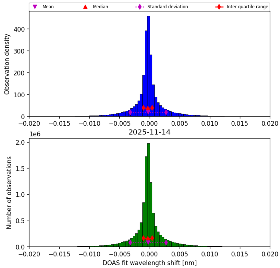
Figure 46: Histogram of “DOAS fit wavelength shift” for 2025-11-13 to 2025-11-15
