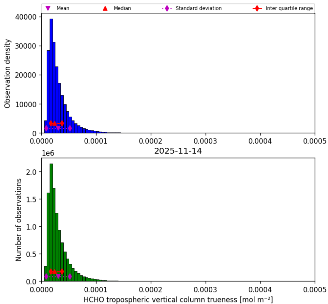
Figure 50: Histogram of “HCHO tropospheric vertical column trueness” for 2025-11-13 to 2025-11-15
