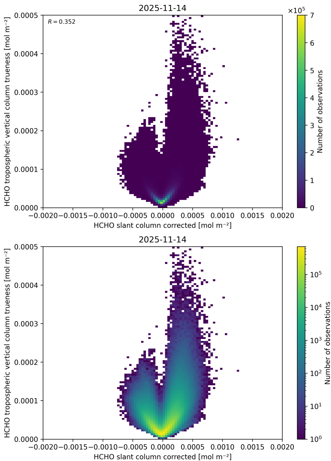
Figure 86: Scatter density plot of “HCHO slant column corrected” against “HCHO tropospheric vertical column trueness” for 2025-11-13 to 2025-11-15.
