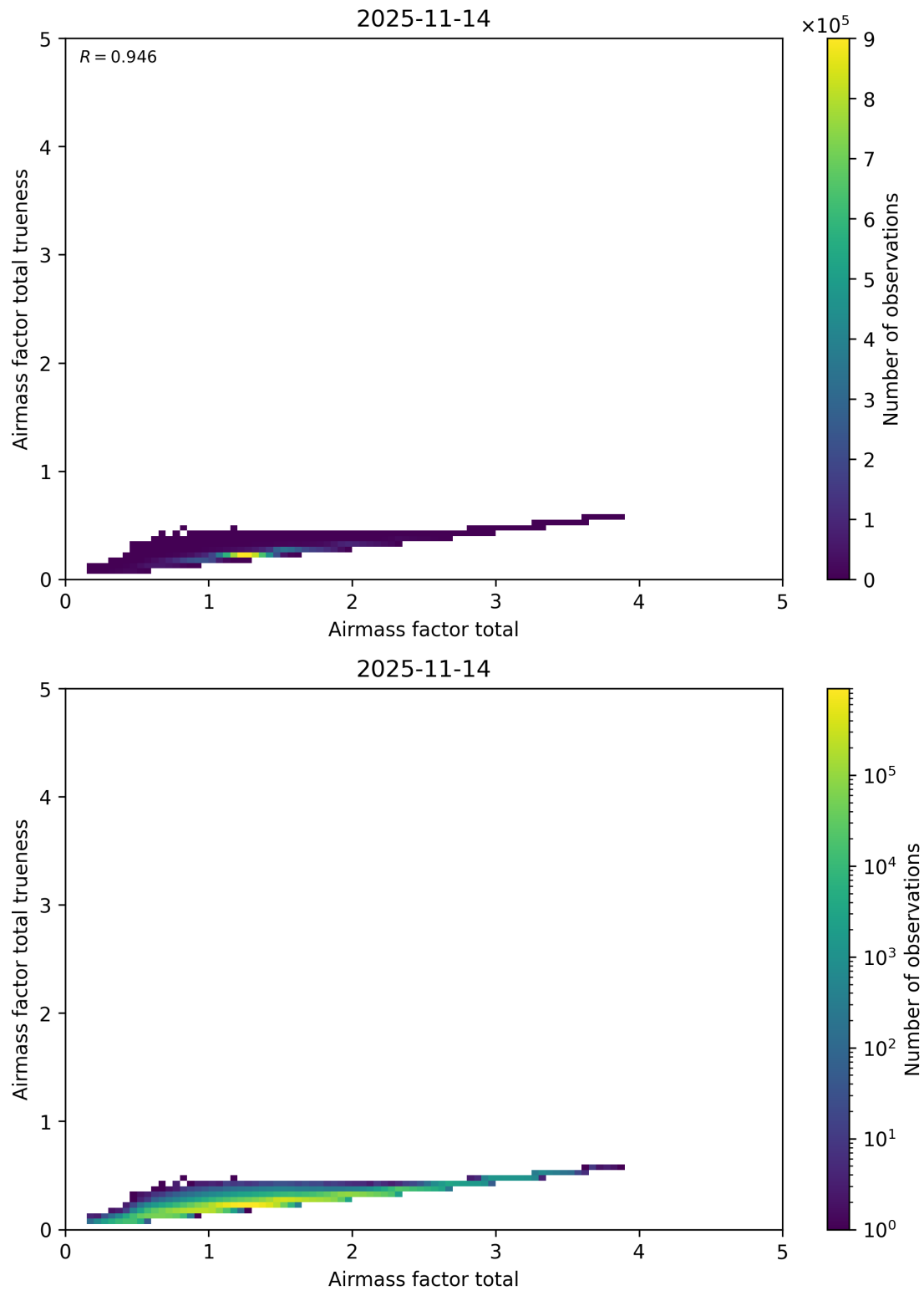
Figure 115: Scatter density plot of “Airmass factor total” against “Airmass factor total trueness” for 2025-11-13 to 2025-11-15.
