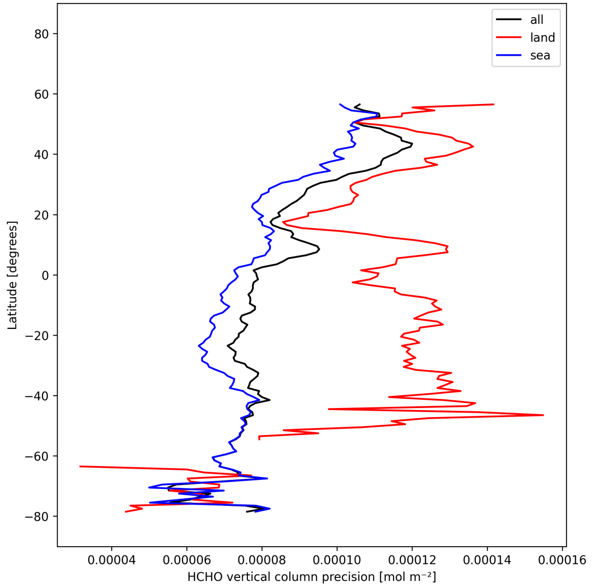
Figure 23: Zonal average of “HCHO vertical column precision” for 2025-11-13 to 2025-11-15.
