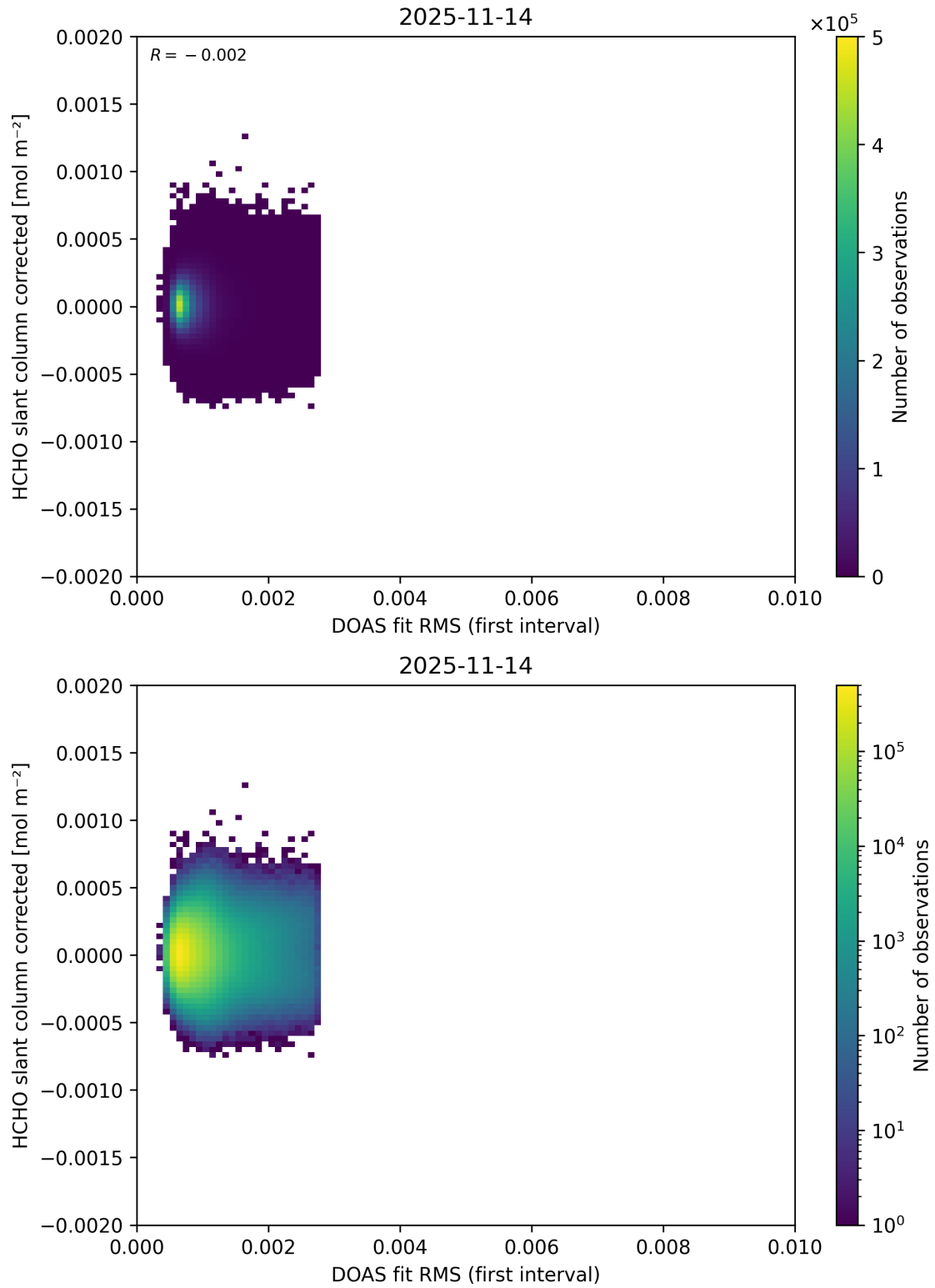
Figure 66: Scatter density plot of “DOAS fit RMS (first interval)” against “HCHO slant column corrected” for 2025-11-13 to 2025-11-15.
