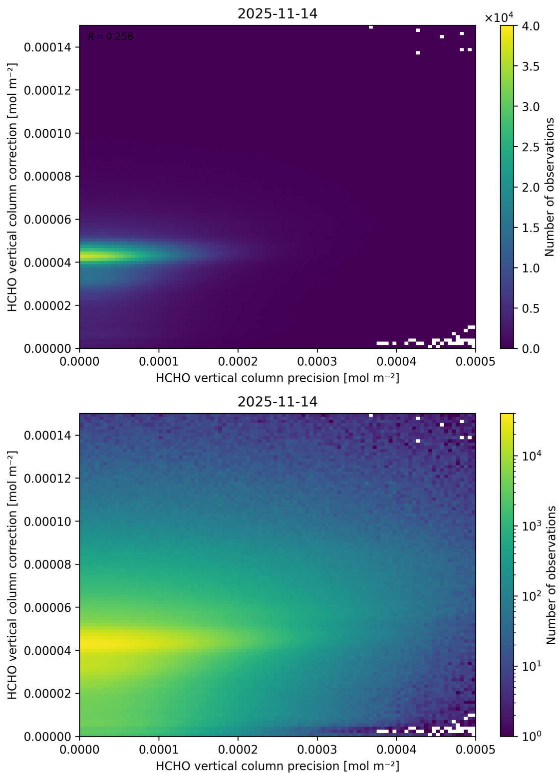
Figure 162: Scatter density plot of “HCHO vertical column precision” against “HCHO vertical column correction” for 2025-11-13 to 2025-11-15.
