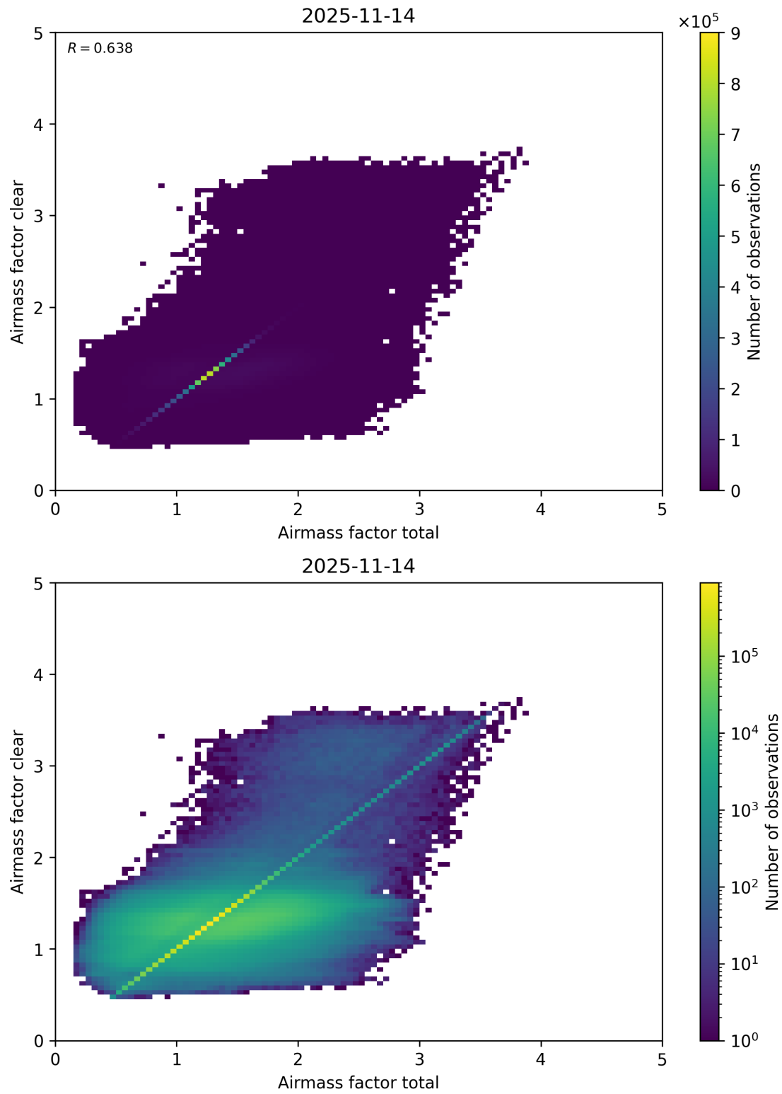
Figure 112: Scatter density plot of “Airmass factor total” against “Airmass factor clear” for 2025-11-13 to 2025-11-15.
