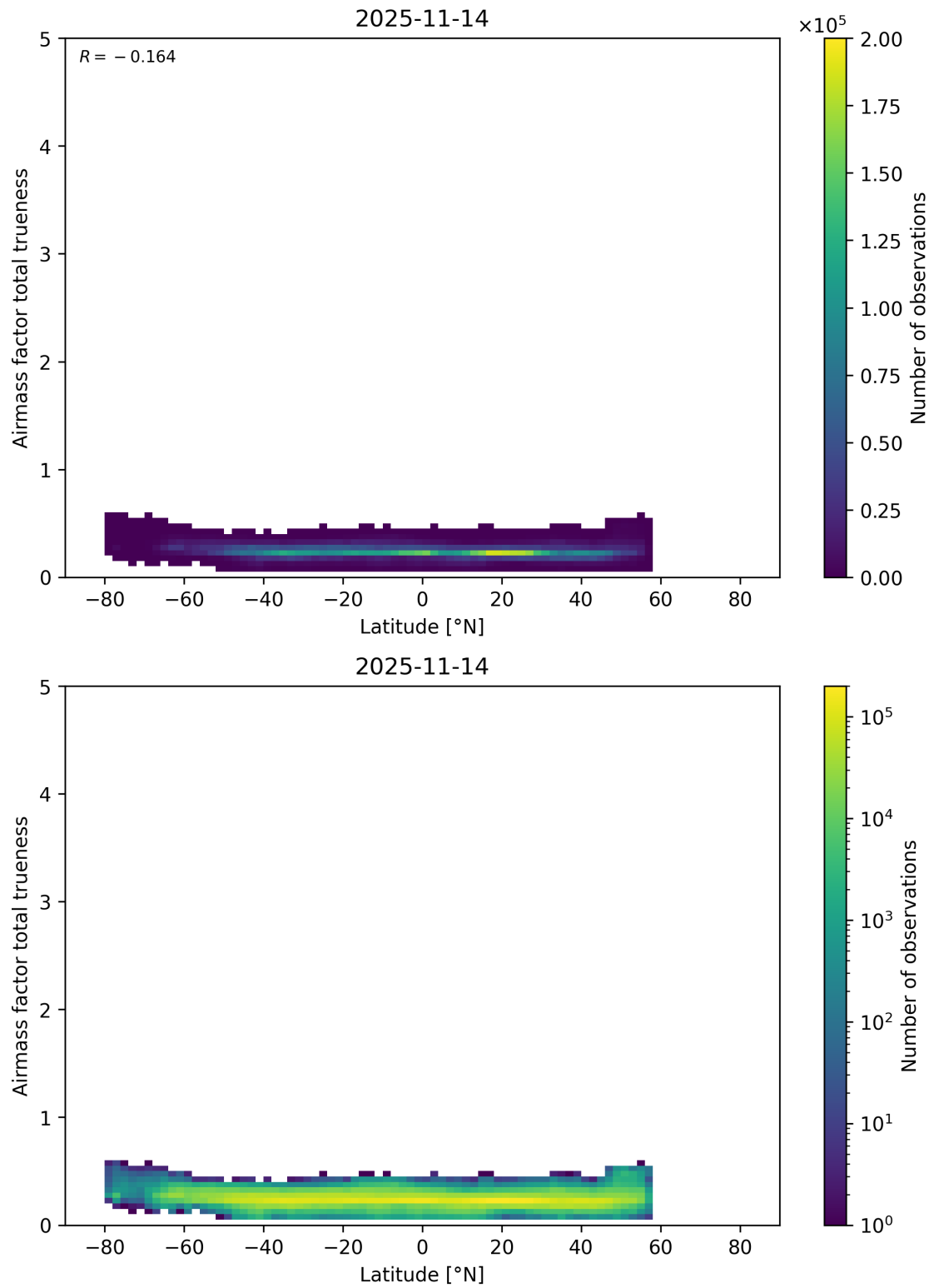
Figure 180: Scatter density plot of “Latitude” against “Airmass factor total trueness” for 2025-11-13 to 2025-11-15.
