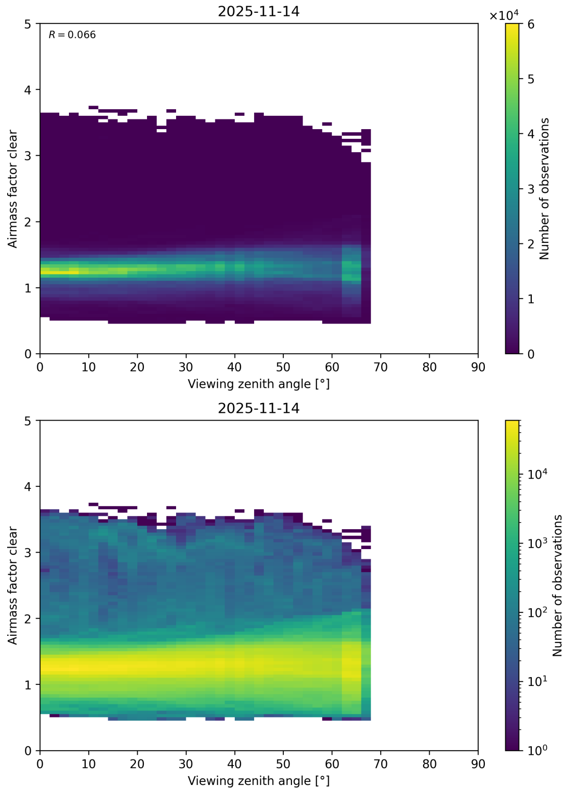
Figure 205: Scatter density plot of “Viewing zenith angle” against “Airmass factor clear” for 2025-11-13 to 2025-11-15.
