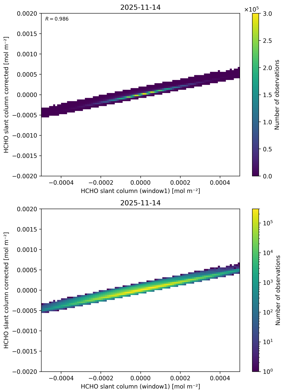
Figure 92: Scatter density plot of “HCHO slant column (window1)” against “HCHO slant column corrected” for 2025-11-13 to 2025-11-15.
