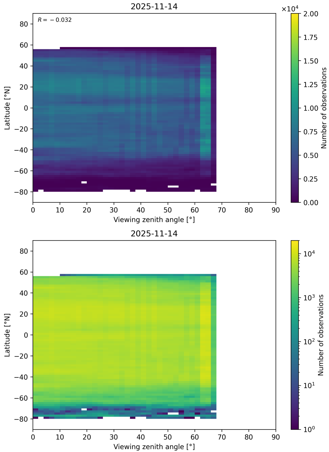
Figure 217: Scatter density plot of “Viewing zenith angle” against “Latitude” for 2025-11-13 to 2025-11-15.
