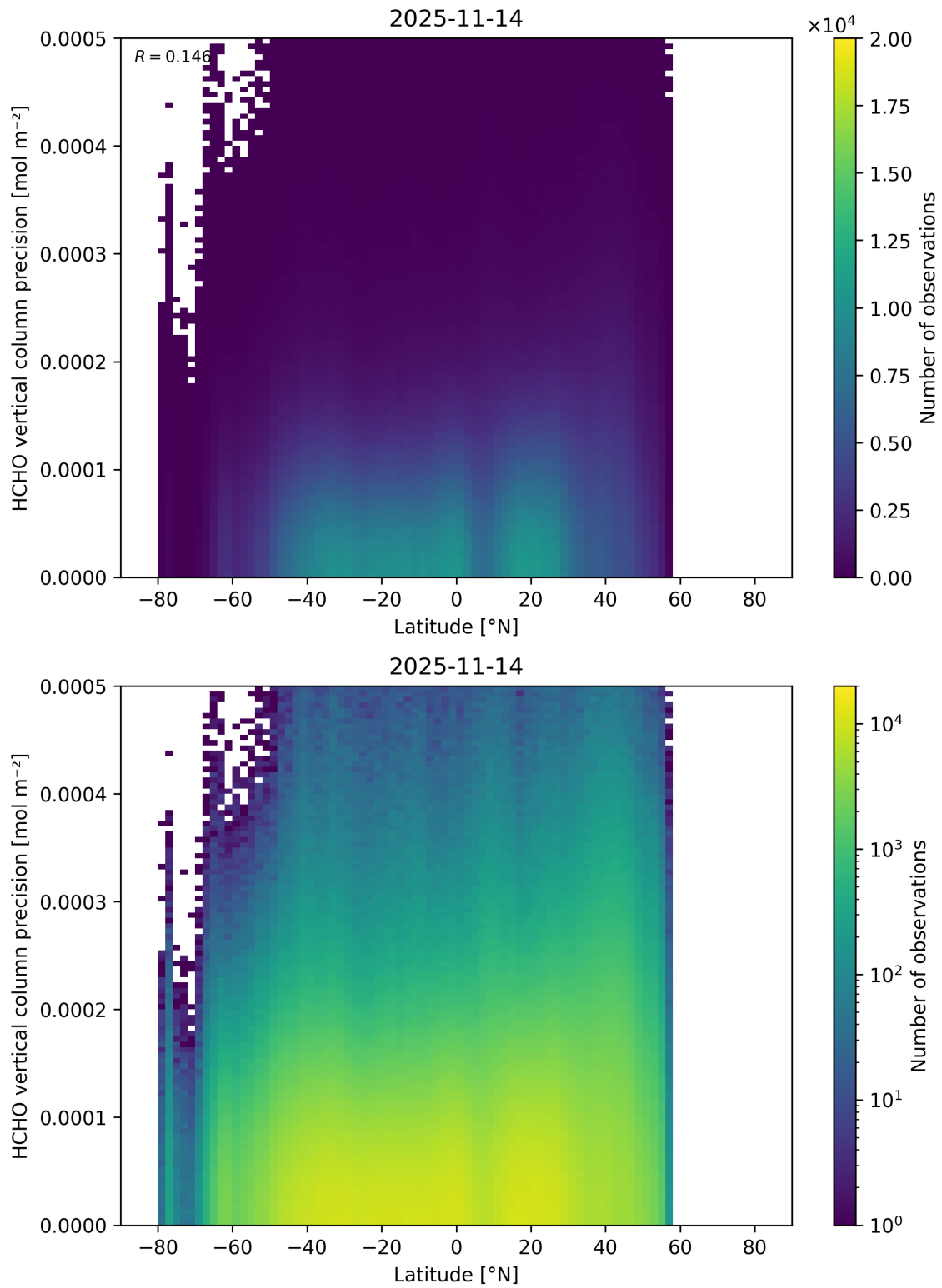
Figure 183: Scatter density plot of “Latitude” against “HCHO vertical column precision” for 2025-11-13 to 2025-11-15.
