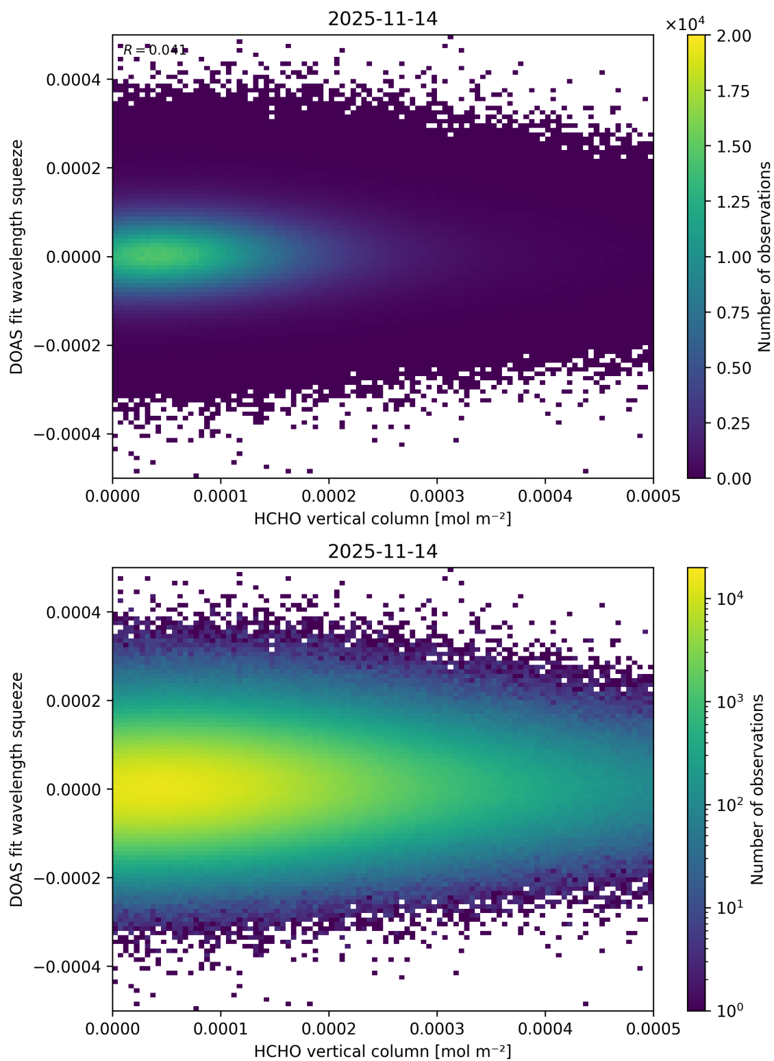
Figure 140: Scatter density plot of “HCHO vertical column” against “DOAS fit wavelength squeeze” for 2025-11-13 to 2025-11-15.
