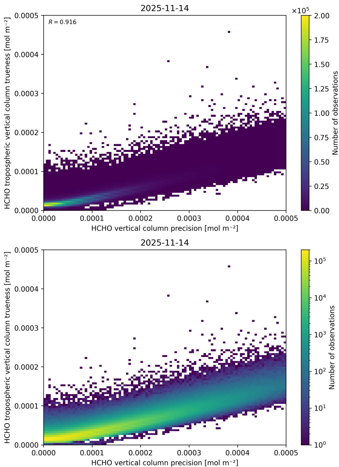
Figure 163: Scatter density plot of “HCHO vertical column precision” against “HCHO tropospheric vertical column true-ness” for 2025-11-13 to 2025-11-15.
