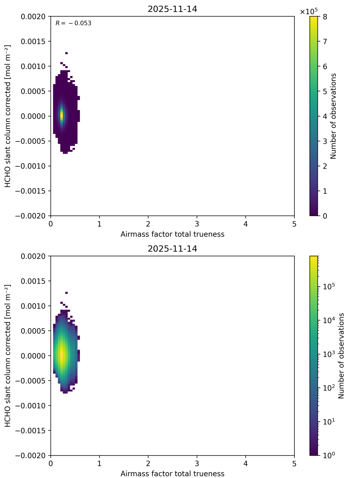
Figure 122: Scatter density plot of “Airmass factor total trueness” against “HCHO slant column corrected” for 2025-11-13 to 2025-11-15.
