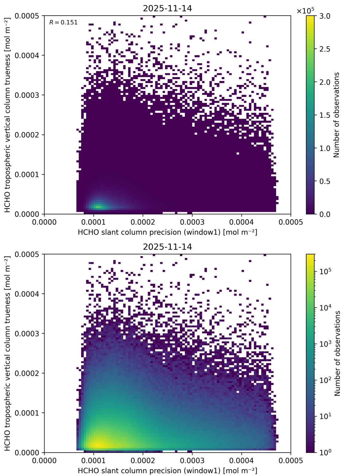
Figure 107: Scatter density plot of “HCHO slant column precision (window1)” against “HCHO tropospheric vertical column trueness” for 2025-11-13 to 2025-11-15.
