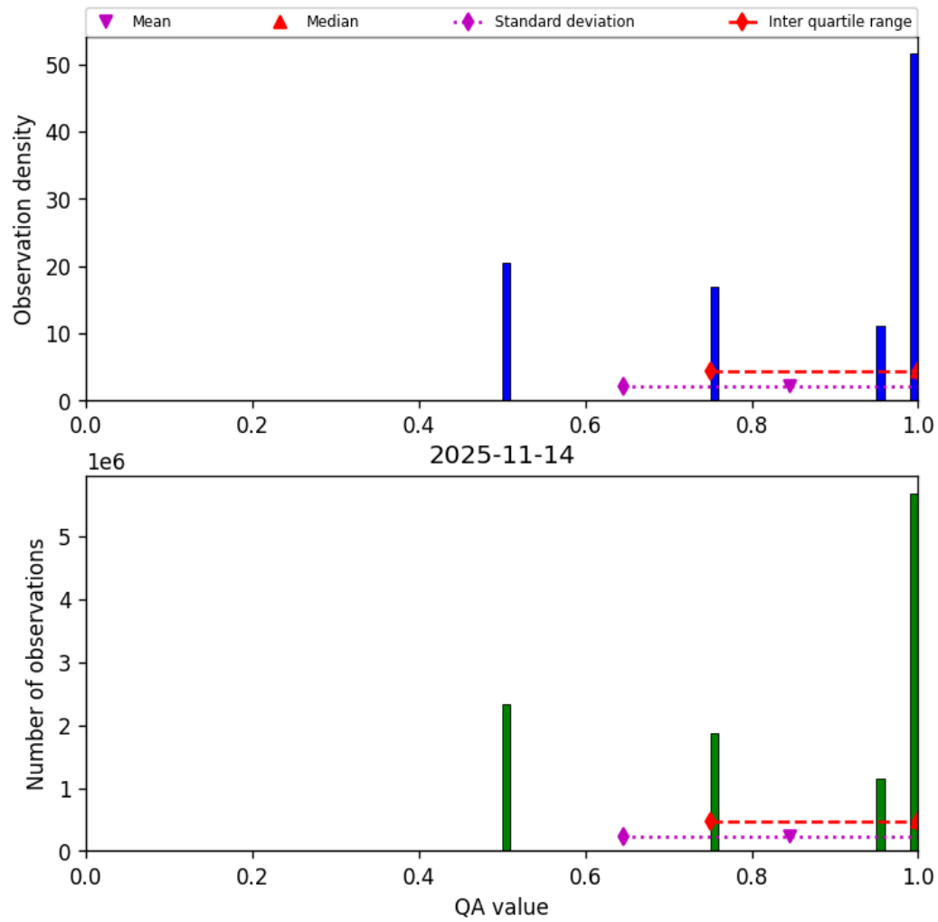
Figure 36: Histogram of “QA value” for 2025-11-13 to 2025-11-15
