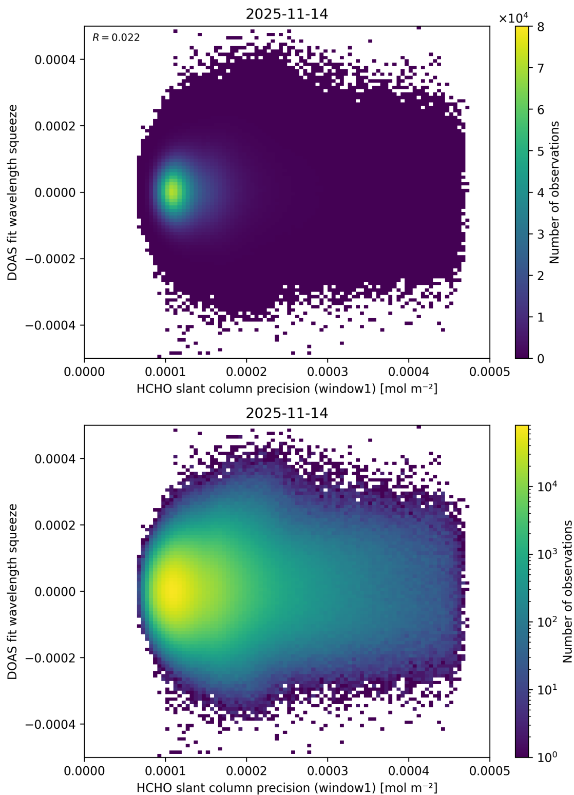
Figure 101: Scatter density plot of “HCHO slant column precision (window1)” against “DOAS fit wavelength squeeze” for 2025-11-13 to 2025-11-15.
