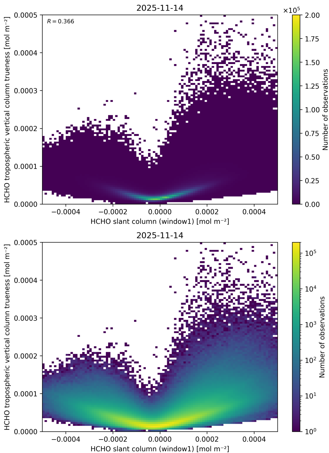
Figure 97: Scatter density plot of “HCHO slant column (window1)” against “HCHO tropospheric vertical column trueness” for 2025-11-13 to 2025-11-15.
