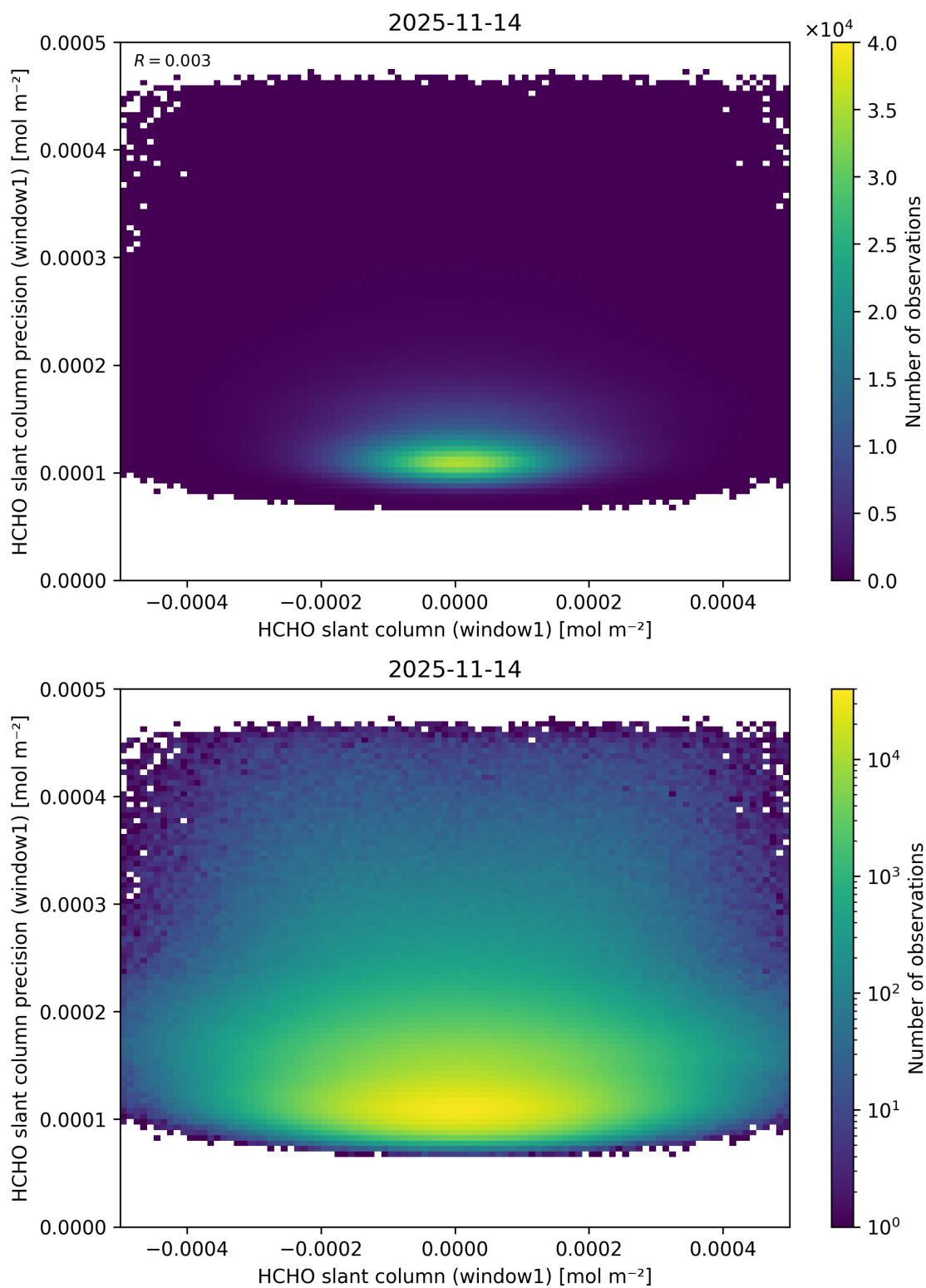
Figure 94: Scatter density plot of “HCHO slant column (window1)” against “HCHO slant column precision (window1)” for 2025-11-13 to 2025-11-15.
