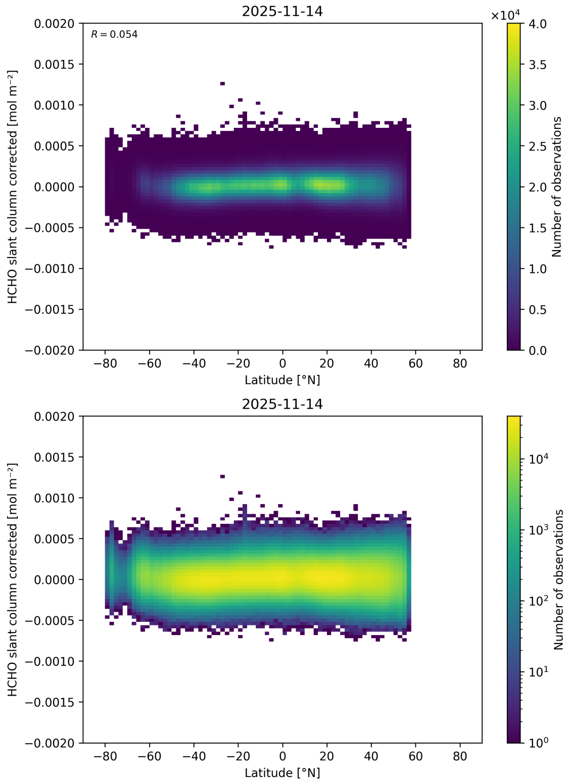
Figure 175: Scatter density plot of “Latitude” against “HCHO slant column corrected” for 2025-11-13 to 2025-11-15.
