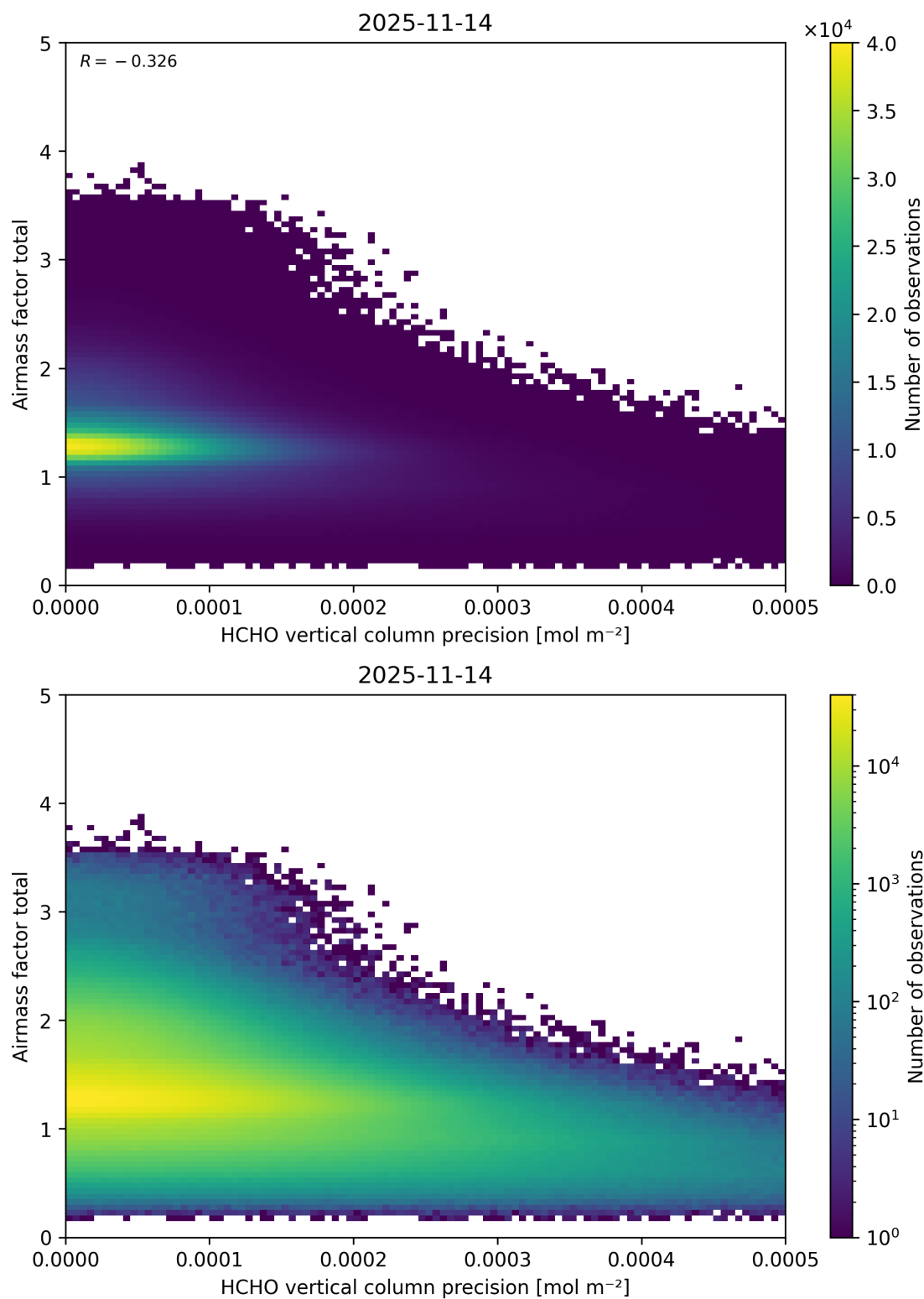
Figure 160: Scatter density plot of “HCHO vertical column precision” against “Airmass factor total” for 2025-11-13 to 2025-11-15.
