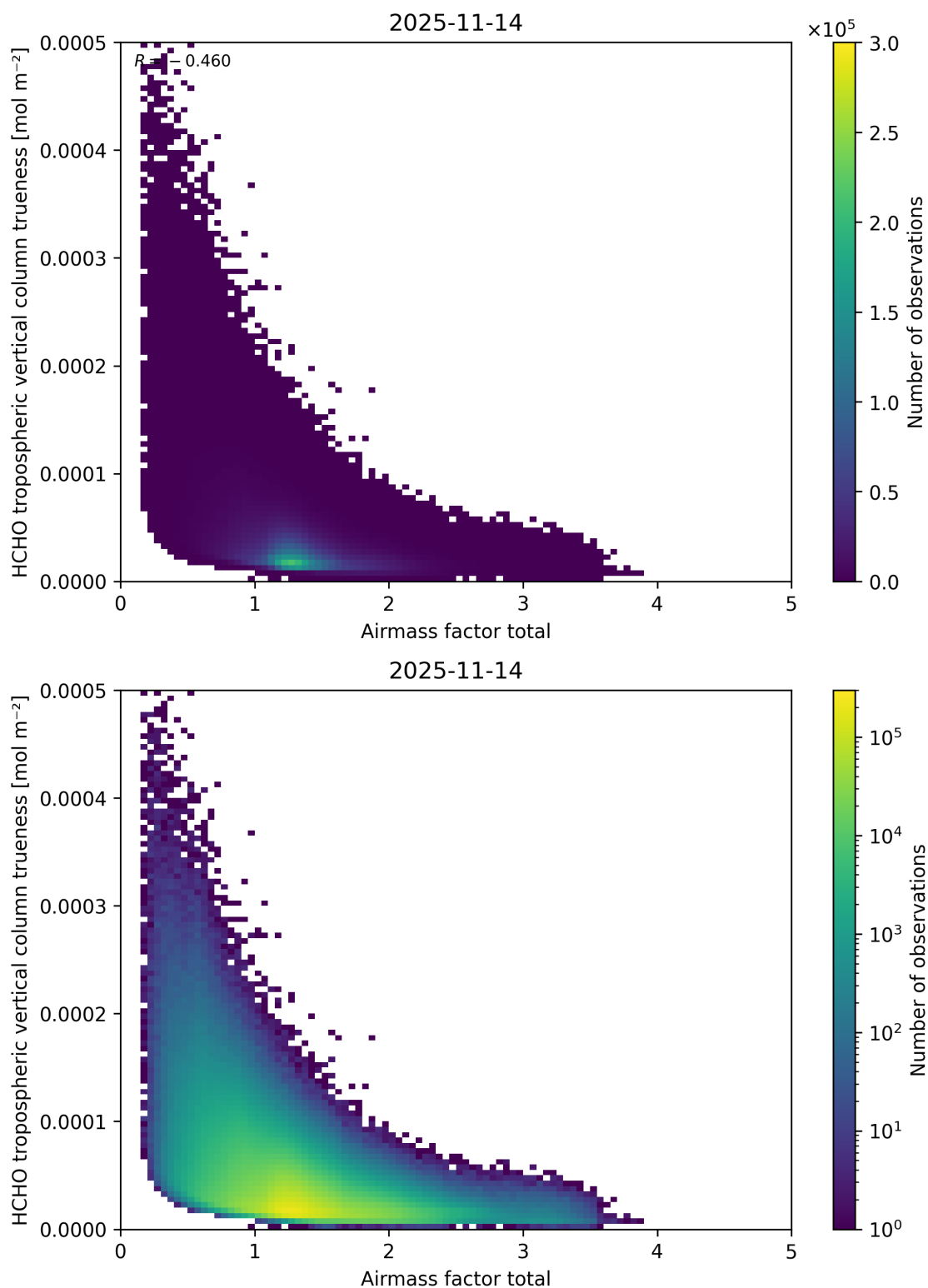
Figure 116: Scatter density plot of “Airmass factor total” against “HCHO tropospheric vertical column trueness” for 2025-11-13 to 2025-11-15.
