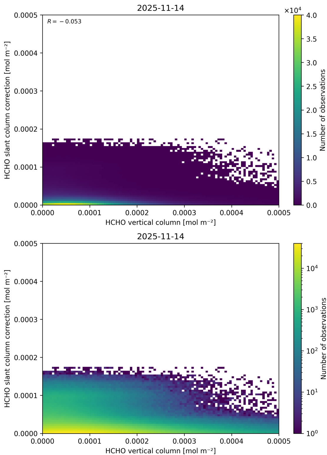
Figure 143: Scatter density plot of “HCHO vertical column” against “HCHO slant column correction” for 2025-11-13 to 2025-11-15.
