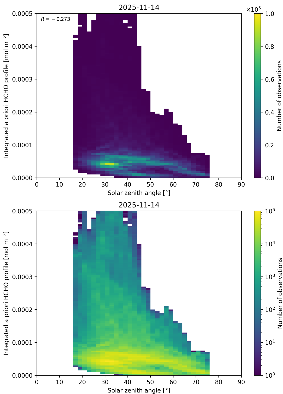
Figure 200: Scatter density plot of “Solar zenith angle” against “Integrated a priori HCHO profile” for 2025-11-13 to 2025-11-15.
