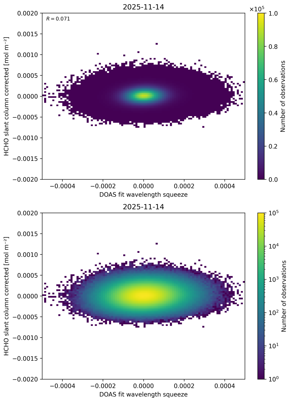
Figure 75: Scatter density plot of “DOAS fit wavelength squeeze” against “HCHO slant column corrected” for 2025-11-13 to 2025-11-15.
