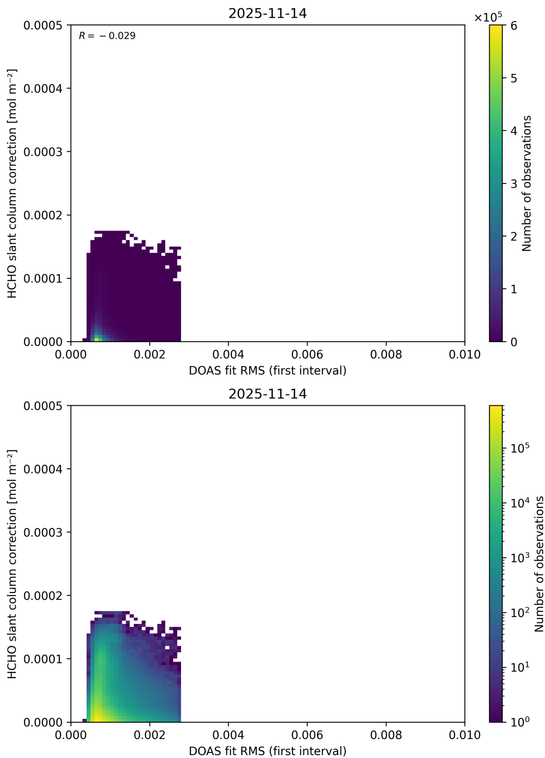
Figure 67: Scatter density plot of “DOAS fit RMS (first interval)” against “HCHO slant column correction” for 2025-11-13 to 2025-11-15.
