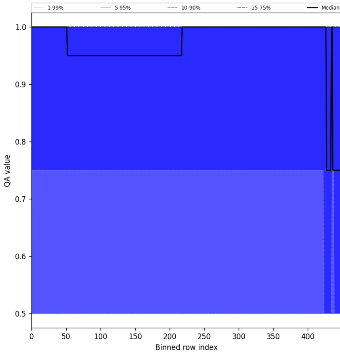
Figure 51: Along track statistics of “QA value” for 2025-11-13 to 2025-11-15
