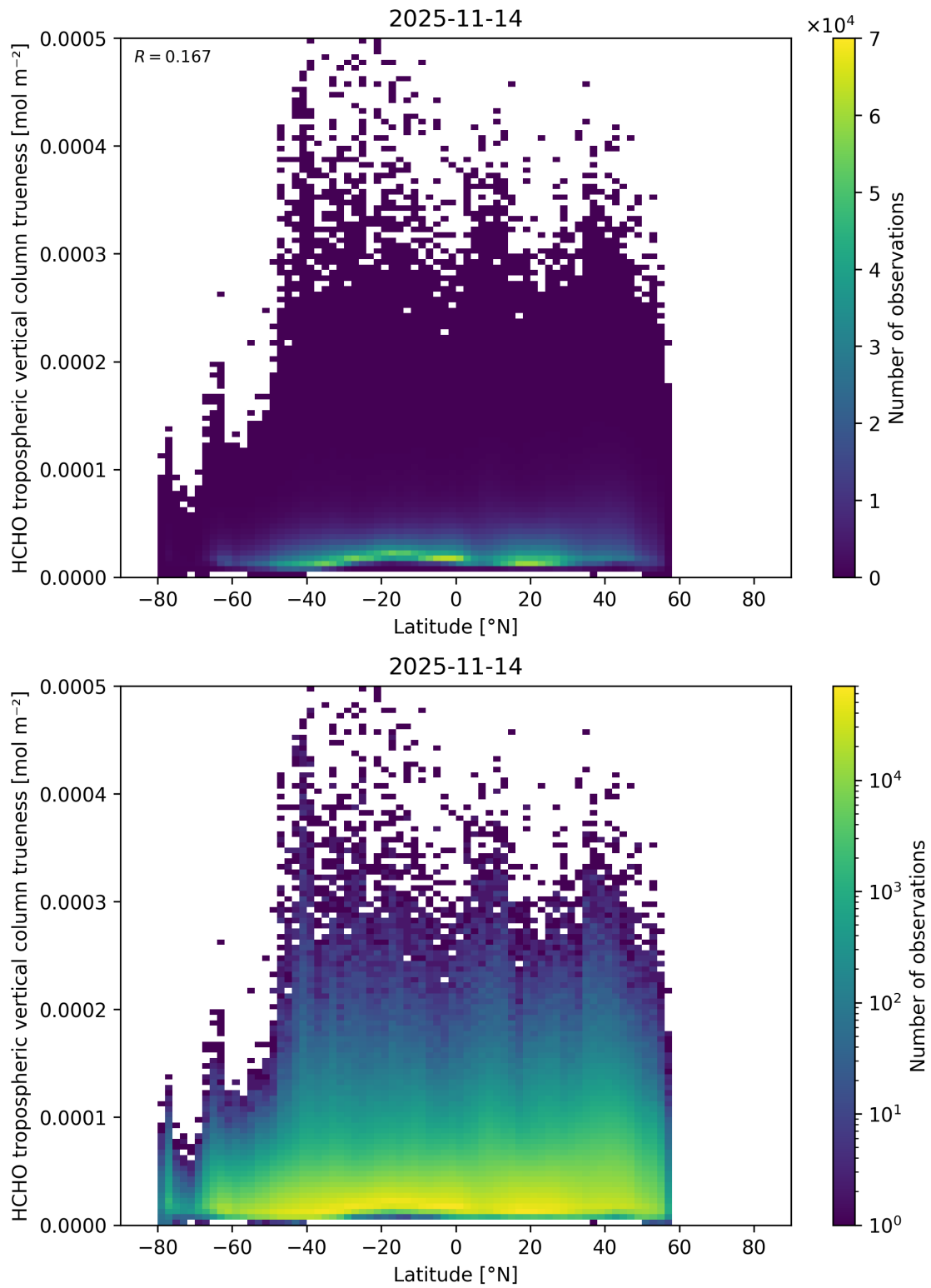
Figure 184: Scatter density plot of “Latitude” against “HCHO tropospheric vertical column trueness” for 2025-11-13 to 2025-11-15.
