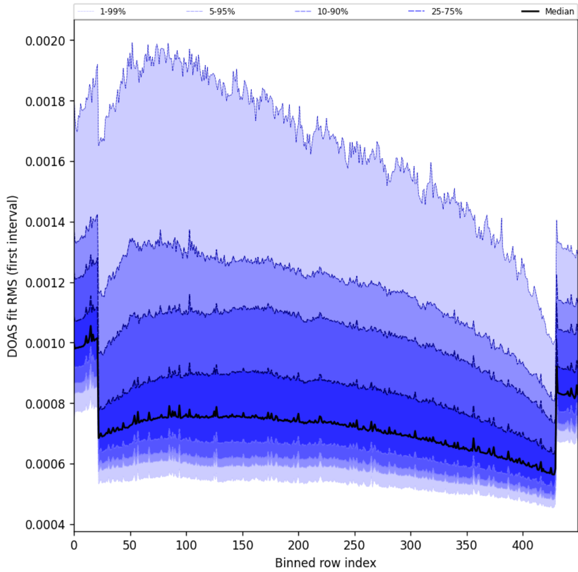
Figure 63: Along track statistics of “DOAS fit RMS (first interval)” for 2025-11-13 to 2025-11-15
