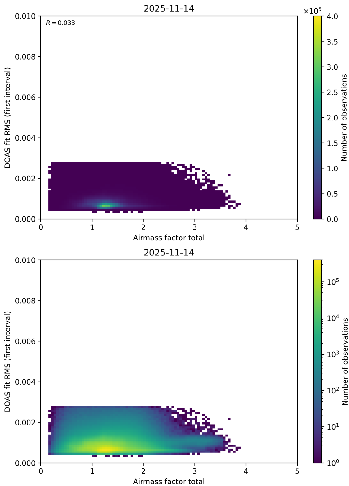
Figure 109: Scatter density plot of “Airmass factor total” against “DOAS fit RMS (first interval)” for 2025-11-13 to 2025-11-15.
