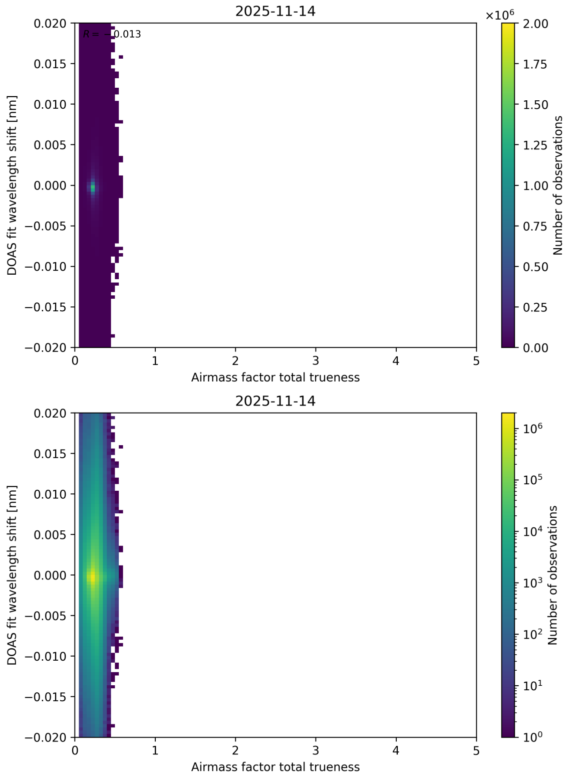
Figure 119: Scatter density plot of “Airmass factor total trueness” against “DOAS fit wavelength shift” for 2025-11-13 to 2025-11-15.
