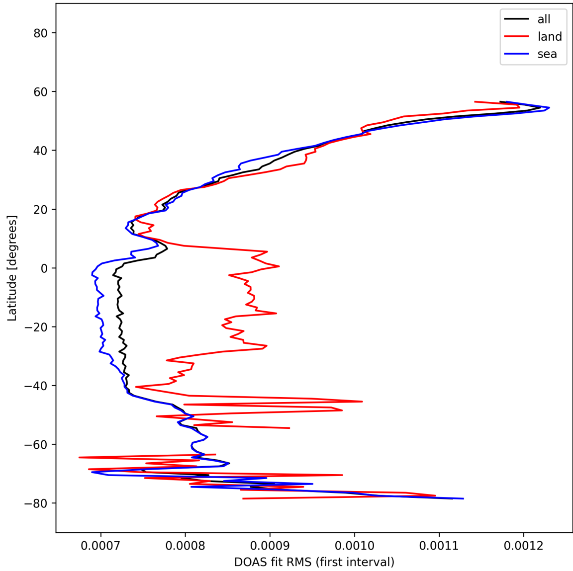
Figure 33: Zonal average of “DOAS fit RMS (first interval)” for 2025-11-13 to 2025-11-15.
