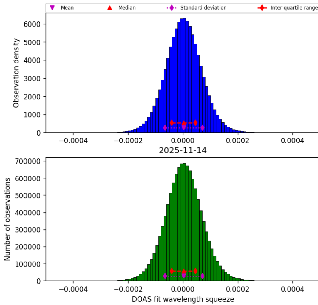
Figure 47: Histogram of “DOAS fit wavelength squeeze” for 2025-11-13 to 2025-11-15
