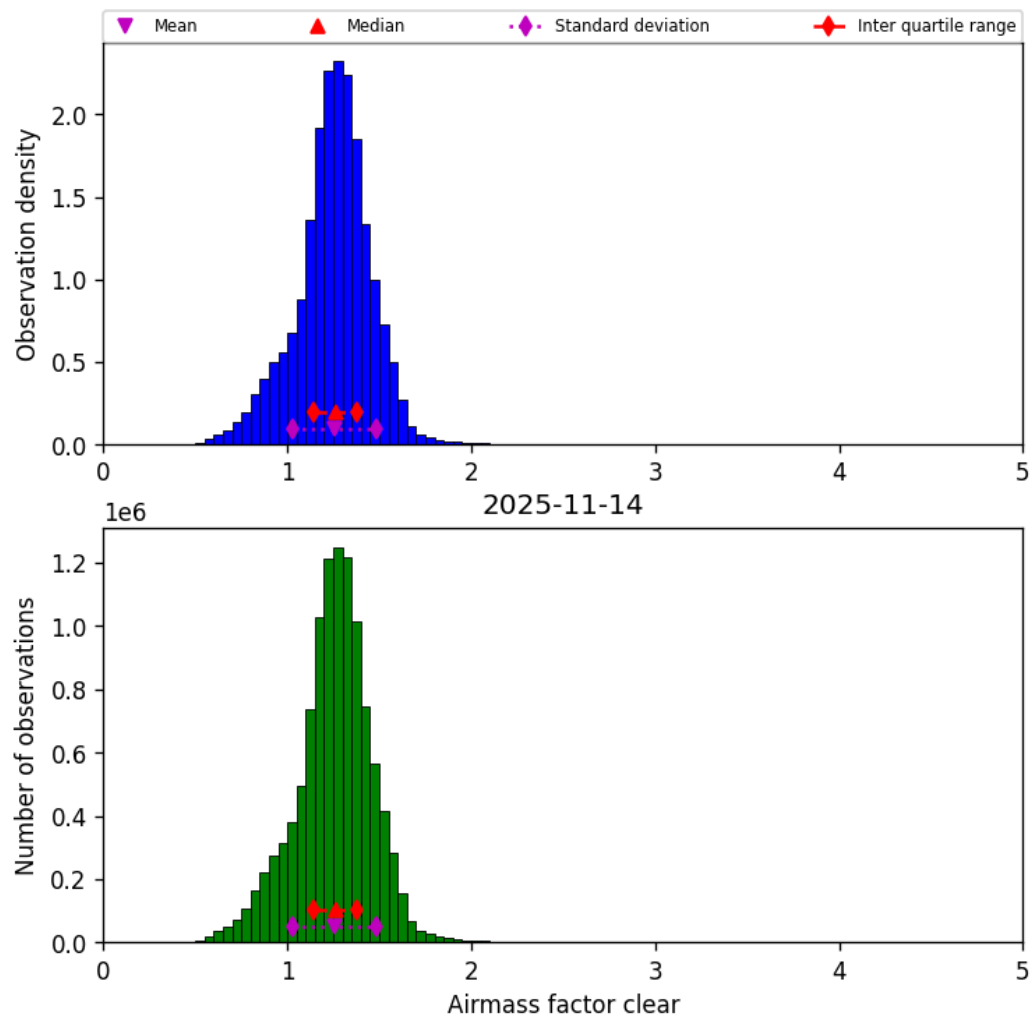
Figure 44: Histogram of “Airmass factor clear” for 2025-11-13 to 2025-11-15
