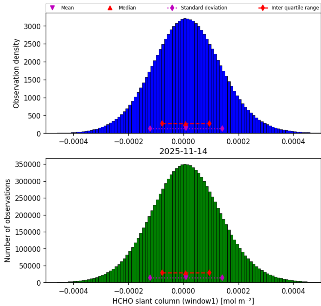
Figure 40: Histogram of “HCHO slant column (window1)” for 2025-11-13 to 2025-11-15
