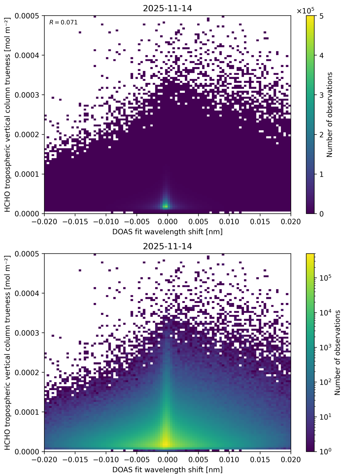
Figure 73: Scatter density plot of “DOAS fit wavelength shift” against “HCHO tropospheric vertical column trueness” for 2025-11-13 to 2025-11-15.
