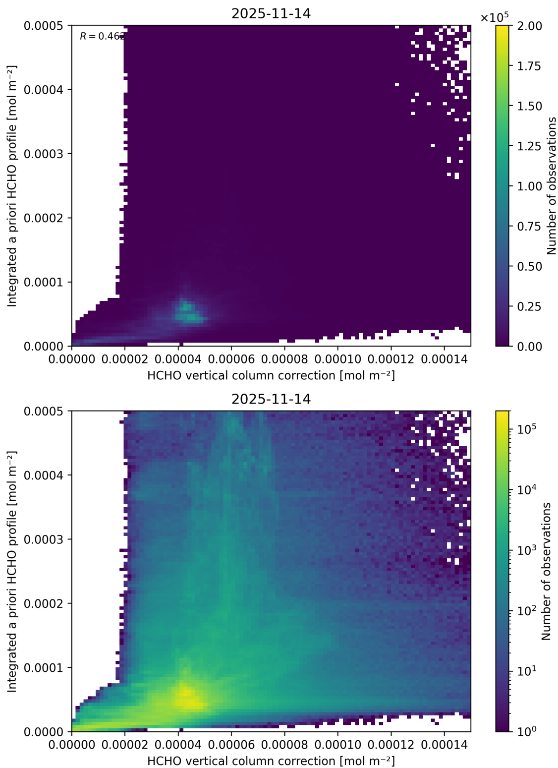
Figure 137: Scatter density plot of “HCHO vertical column correction” against “Integrated a priori HCHO profile” for 2025-11-13 to 2025-11-15.
