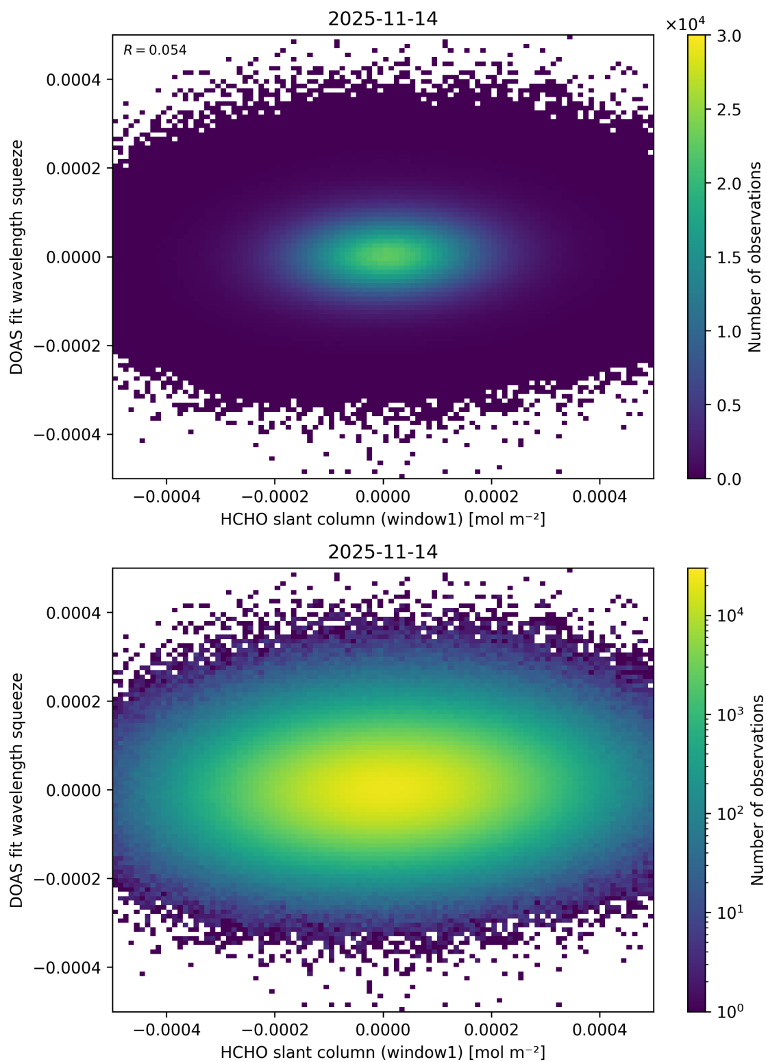
Figure 90: Scatter density plot of “HCHO slant column (window1)” against “DOAS fit wavelength squeeze” for 2025-11-13 to 2025-11-15.
