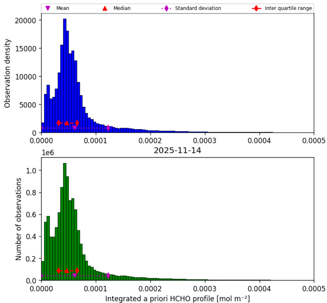
Figure 45: Histogram of “Integrated a priori HCHO profile” for 2025-11-13 to 2025-11-15
