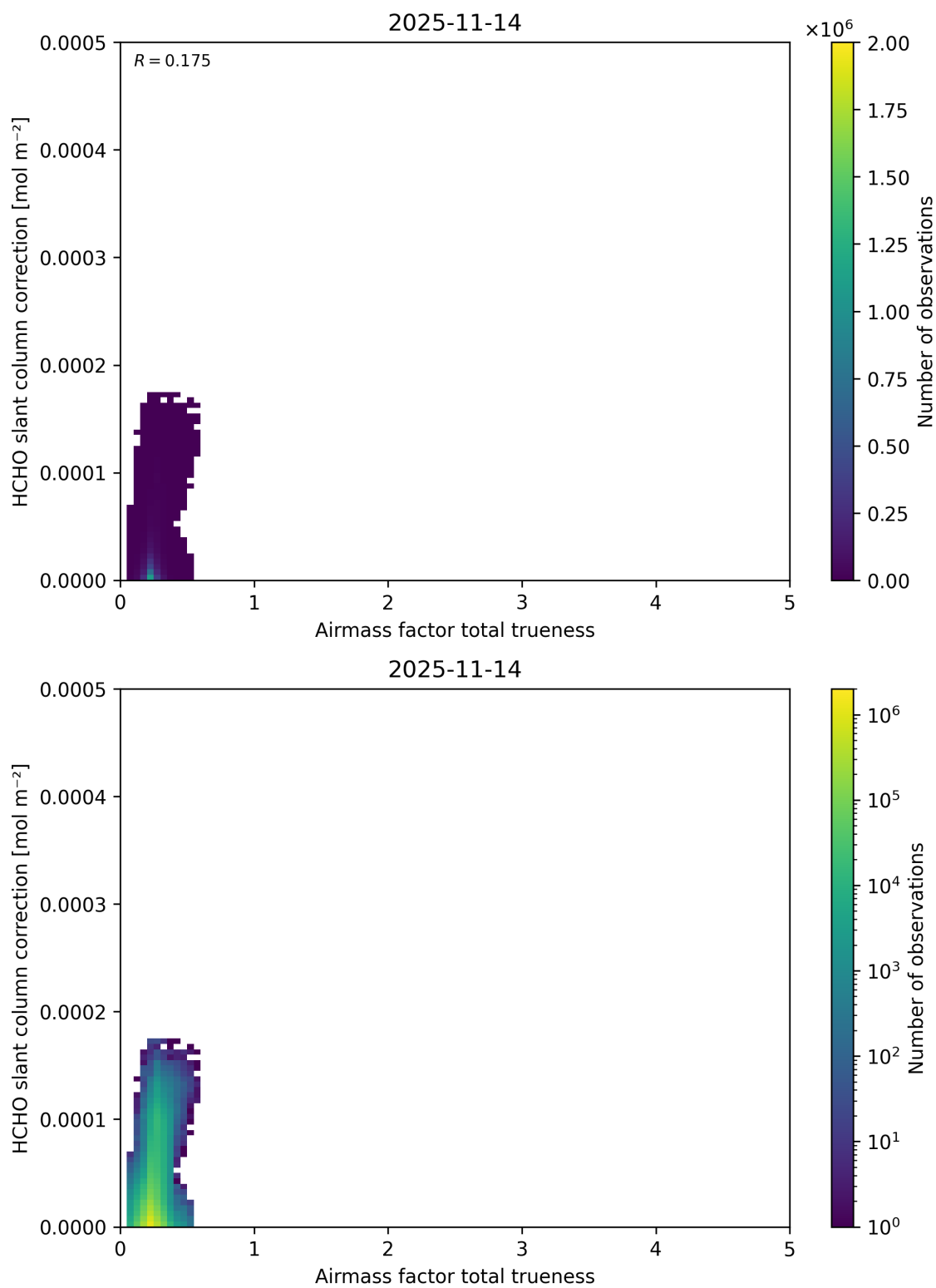
Figure 123: Scatter density plot of “Airmass factor total trueness” against “HCHO slant column correction” for 2025-11-13 to 2025-11-15.
