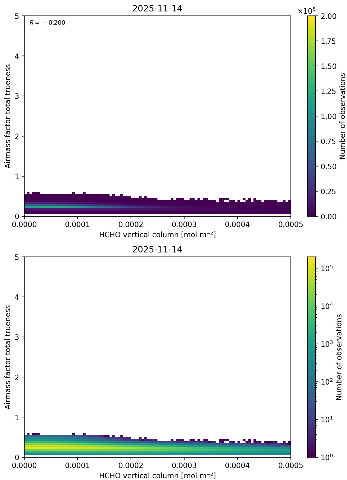
Figure 147: Scatter density plot of “HCHO vertical column” against “Airmass factor total trueneess” for 2025-11-13 to 2025-11-15.
