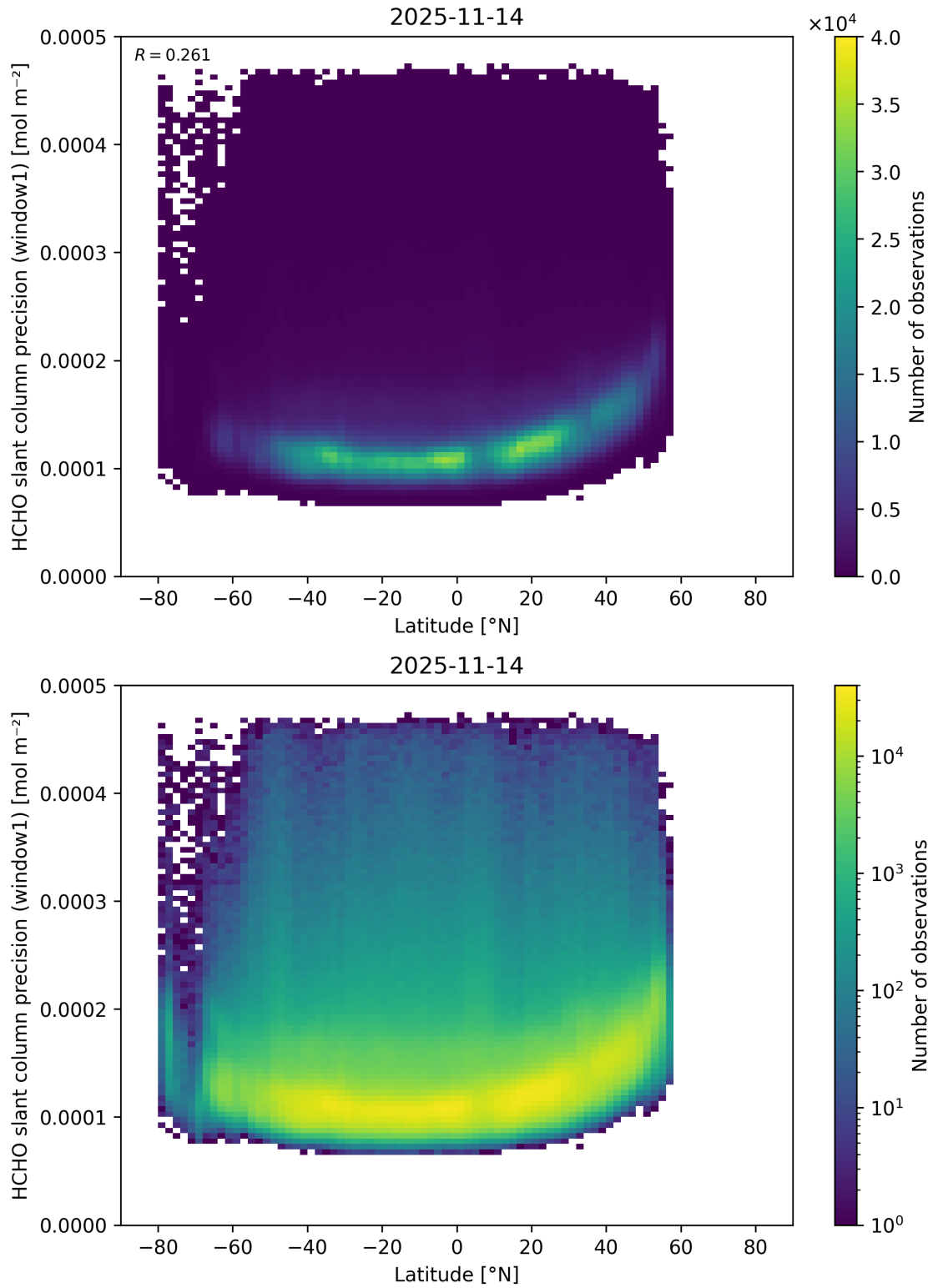
Figure 178: Scatter density plot of “Latitude” against “HCHO slant column precision (window1)” for 2025-11-13 to 2025-11-15.
