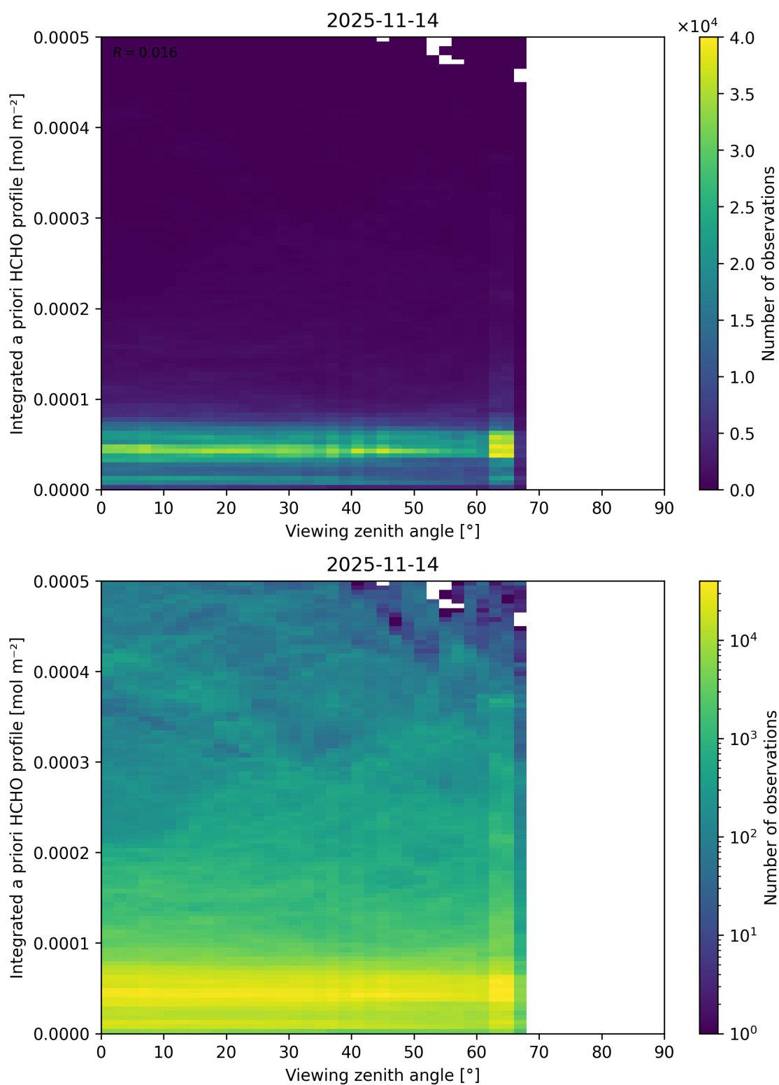
Figure 216: Scatter density plot of “Viewing zenith angle” against “Integrated a priori HCHO profile” for 2025-11-13 to 2025-11-15.
