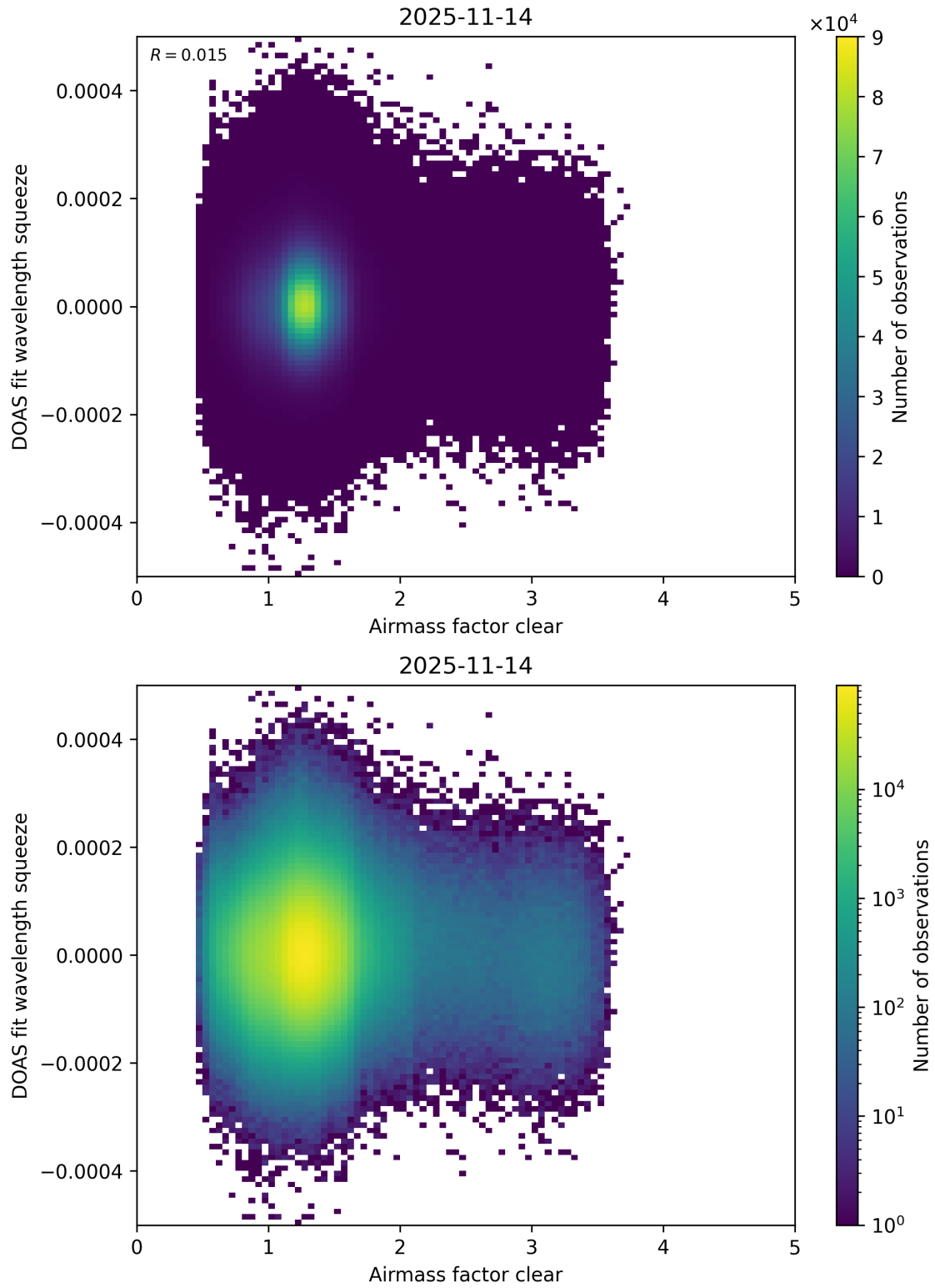
Figure 80: Scatter density plot of “Airmass factor clear” against “DOAS fit wavelength squeeze” for 2025-11-13 to 2025-11-15.
