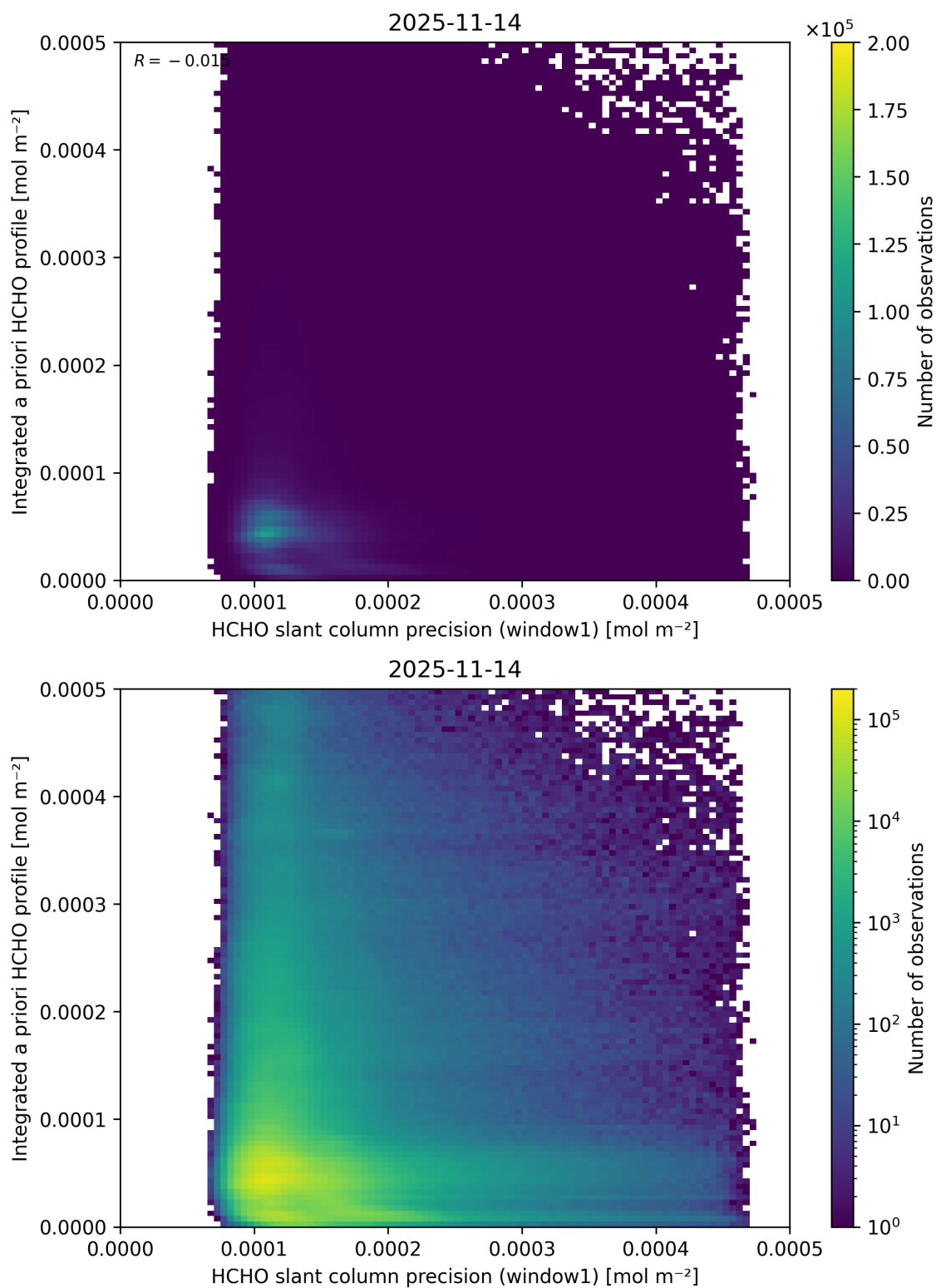
Figure 108: Scatter density plot of “HCHO slant column precision (window1)” against “Integrated a priori HCHO profile” for 2025-11-13 to 2025-11-15.
