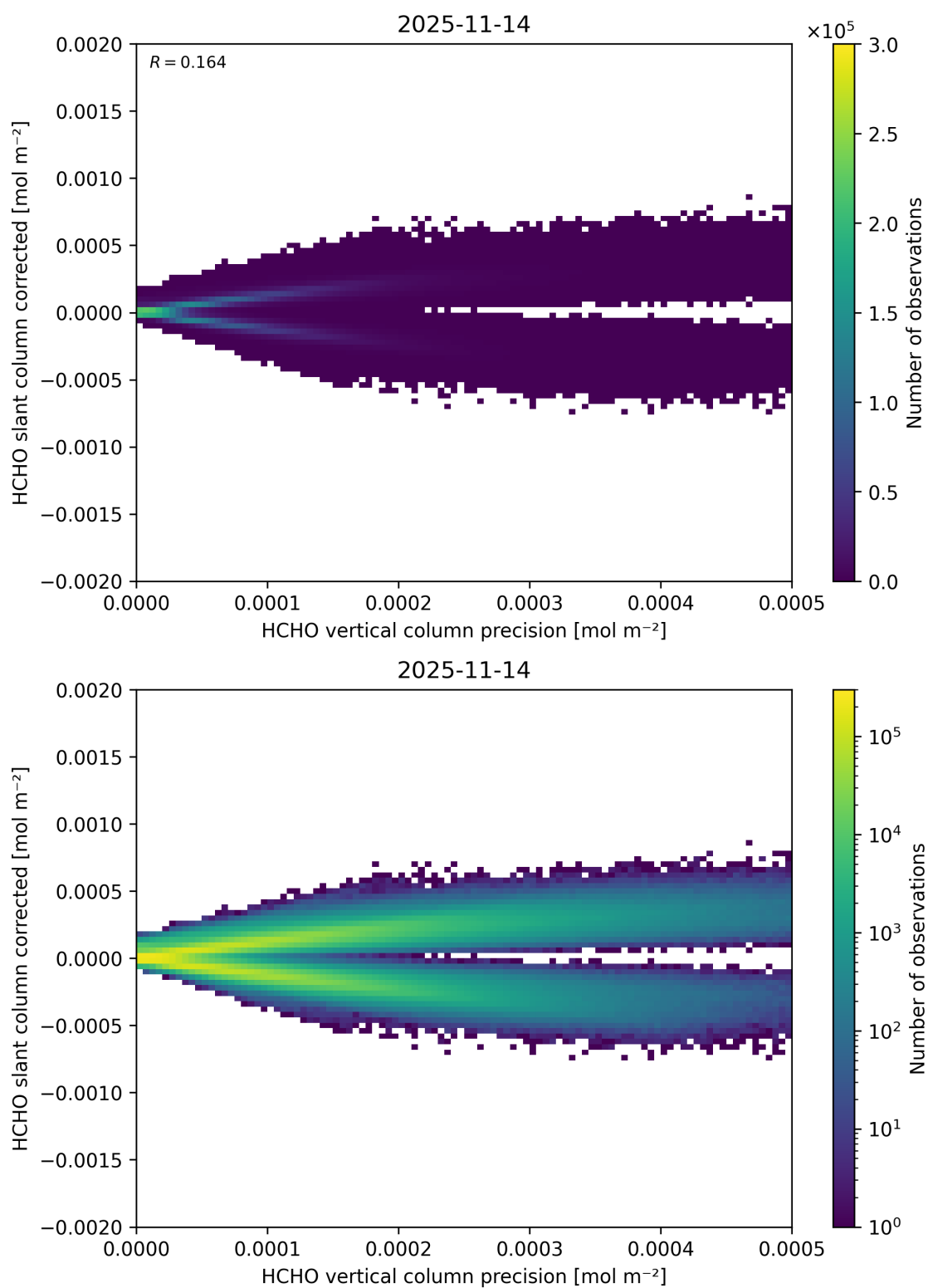
Figure 156: Scatter density plot of “HCHO vertical column precision” against “HCHO slant column corrected” for 2025-11-13 to 2025-11-15.
