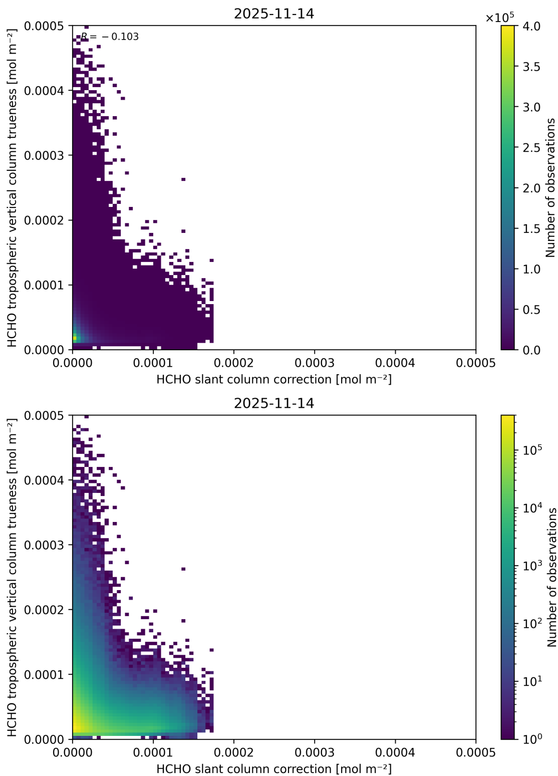
Figure 87: Scatter density plot of “HCHO slant column correction” against “HCHO tropospheric vertical column trueness” for 2025-11-13 to 2025-11-15.
