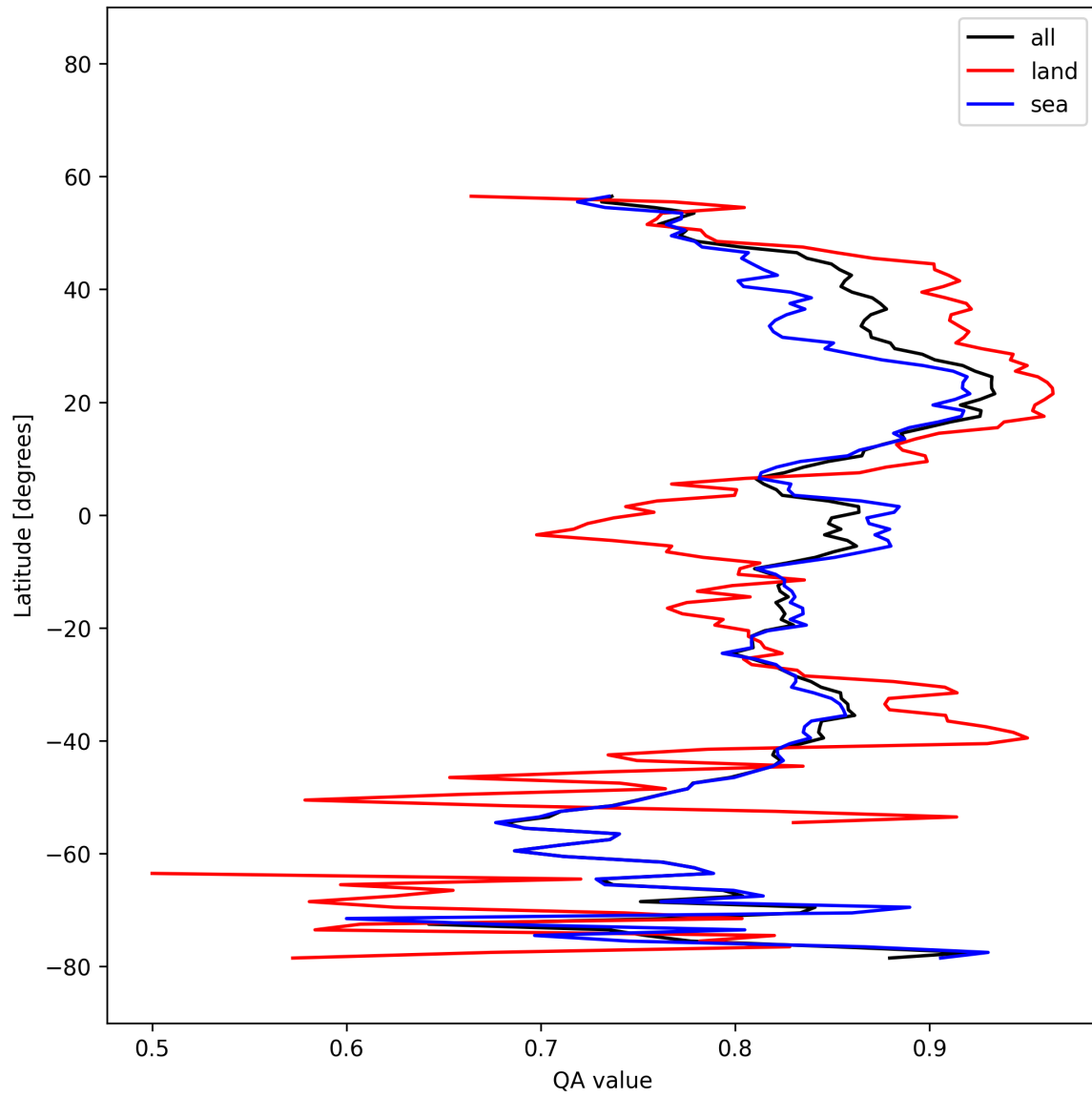
Figure 21: Zonal average of “QA value” for 2025-11-13 to 2025-11-15.
