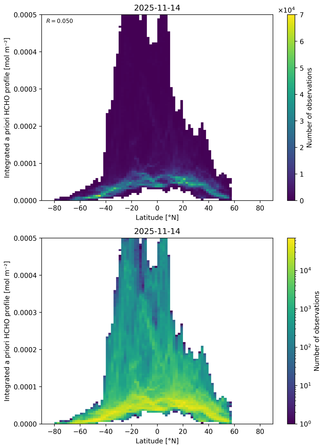
Figure 185: Scatter density plot of “Latitude” against “Integrated a priori HCHO profile” for 2025-11-13 to 2025-11-15.
