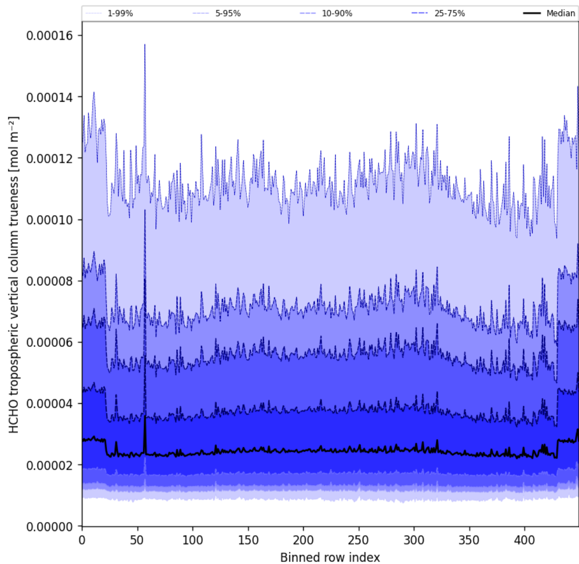
Figure 65: Along track statistics of “HCHO tropospheric vertical column trueness” for 2025-11-13 to 2025-11-15
