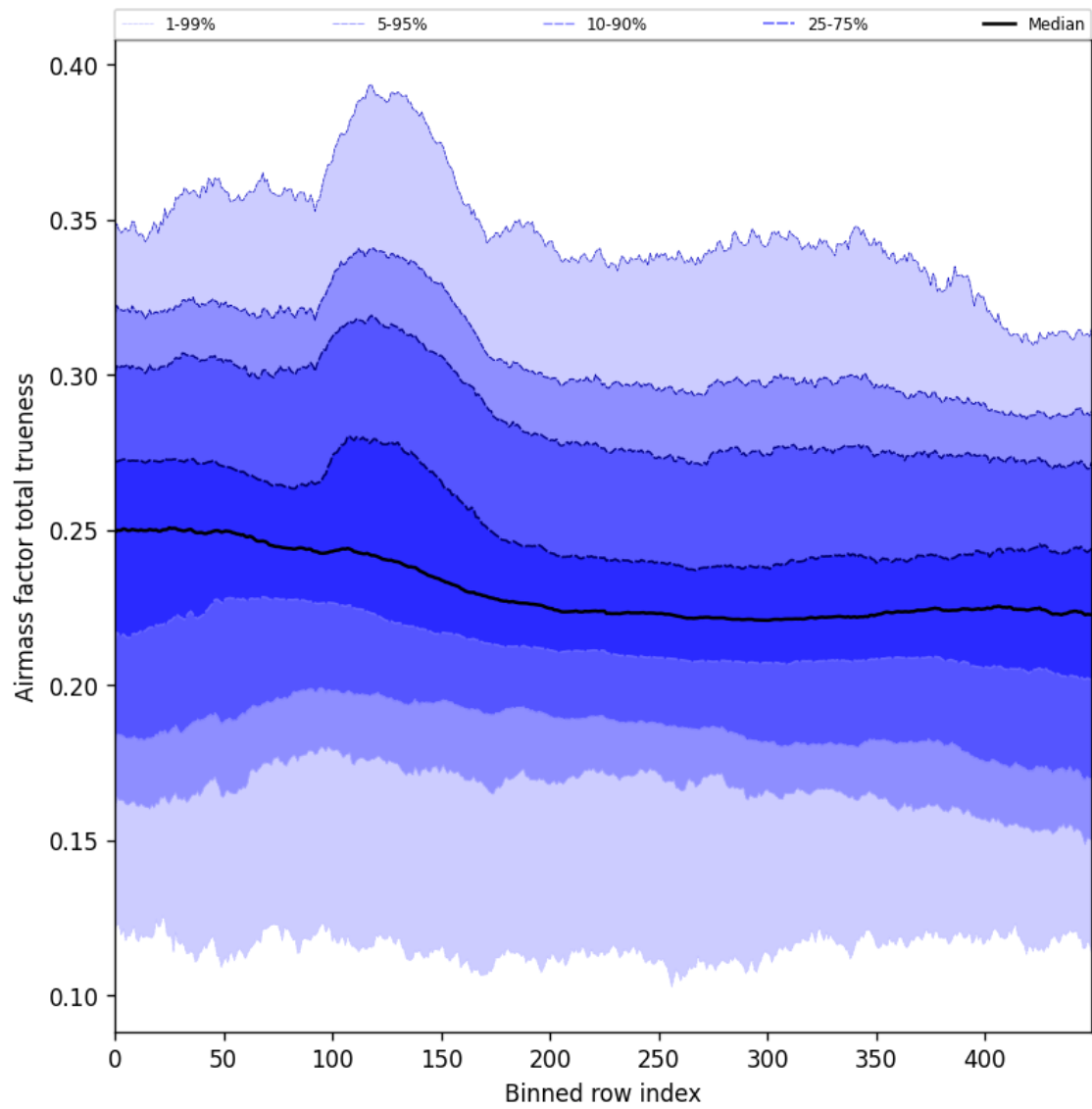
Figure 58: Along track statistics of “Airmass factor total trueness” for 2025-11-13 to 2025-11-15
