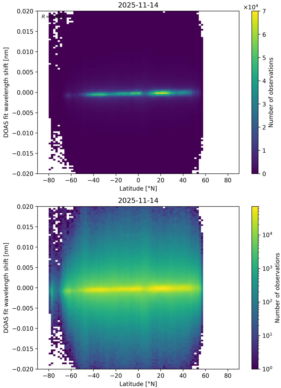
Figure 172: Scatter density plot of “Latitude” against “DOAS fit wavelength shift” for 2025-11-13 to 2025-11-15.
