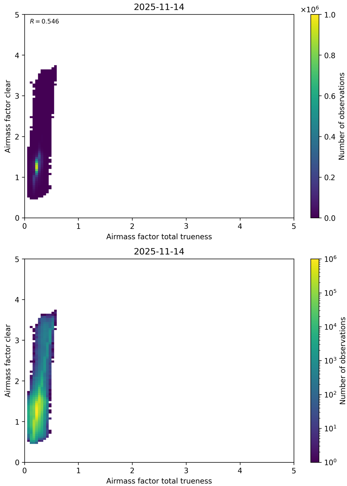
Figure 121: Scatter density plot of “Airmass factor total trueness” against “Airmass factor clear” for 2025-11-13 to 2025-11-15.
