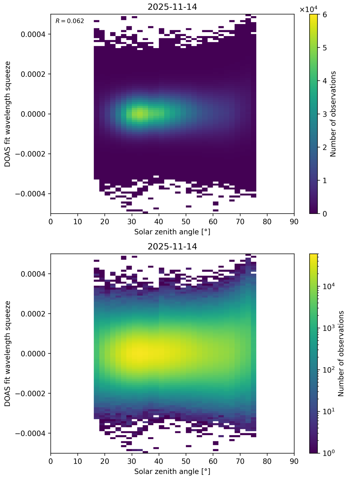
Figure 188: Scatter density plot of “Solar zenith angle” against “DOAS fit wavelength squeeze” for 2025-11-13 to 2025-11-15.
