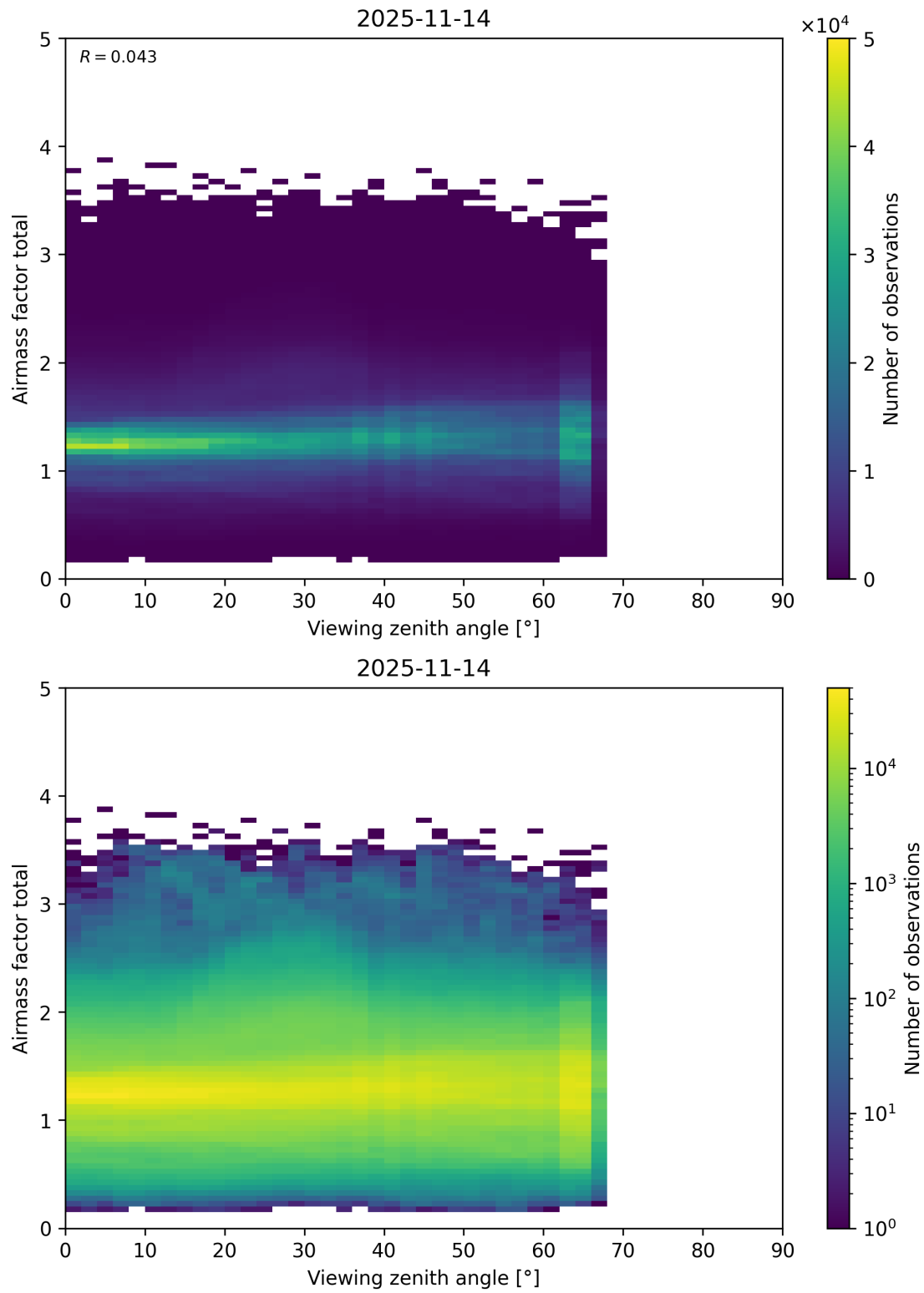
Figure 210: Scatter density plot of “Viewing zenith angle” against “Airmass factor total” for 2025-11-13 to 2025-11-15.
