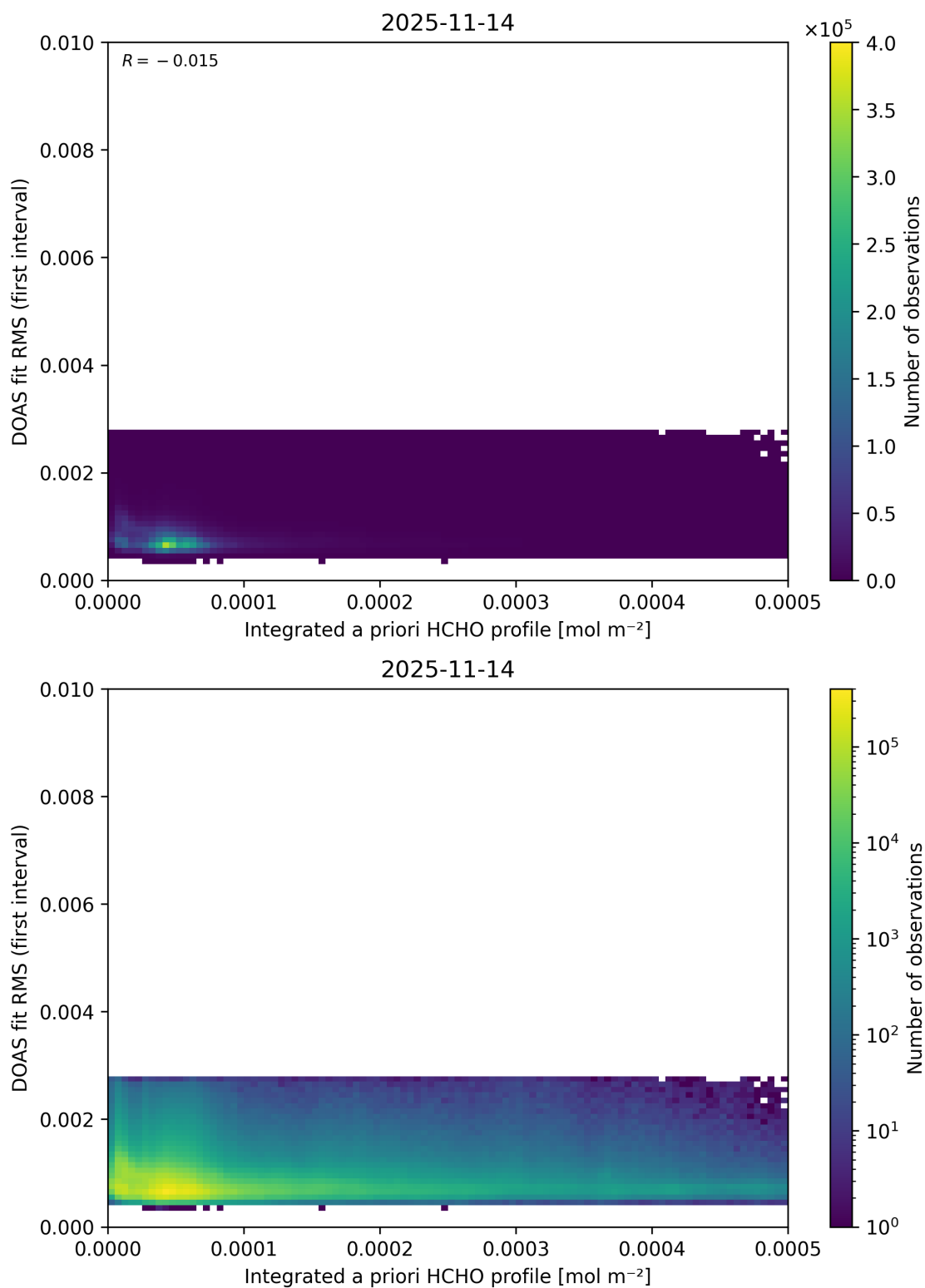
Figure 165: Scatter density plot of “Integrated a priori HCHO profile” against “DOAS fit RMS (first interval)” for 2025-11-13 to 2025-11-15.
