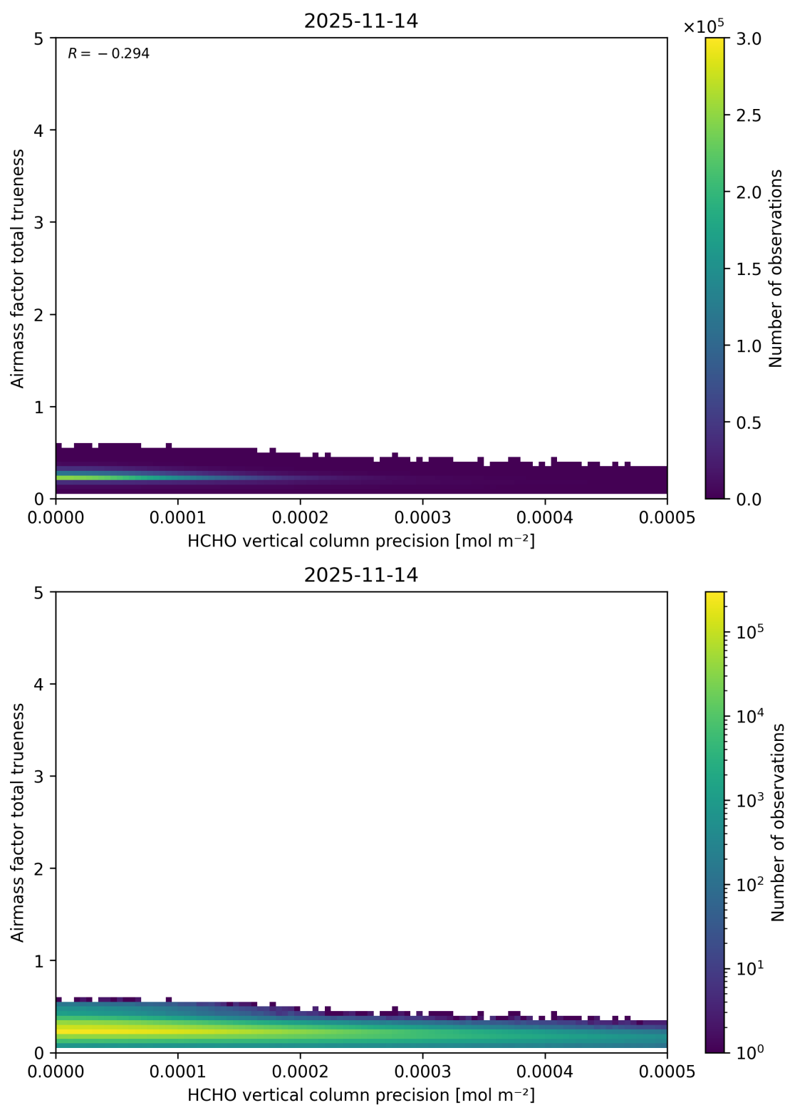
Figure 161: Scatter density plot of “HCHO vertical column precision” against “Airmass factor total trueness” for 2025-11-13 to 2025-11-15.
