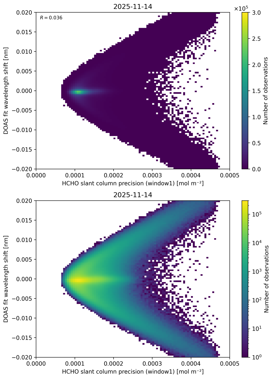
Figure 100: Scatter density plot of “HCHO slant column precision (window1)” against “DOAS fit wavelength shift” for 2025-11-13 to 2025-11-15.
