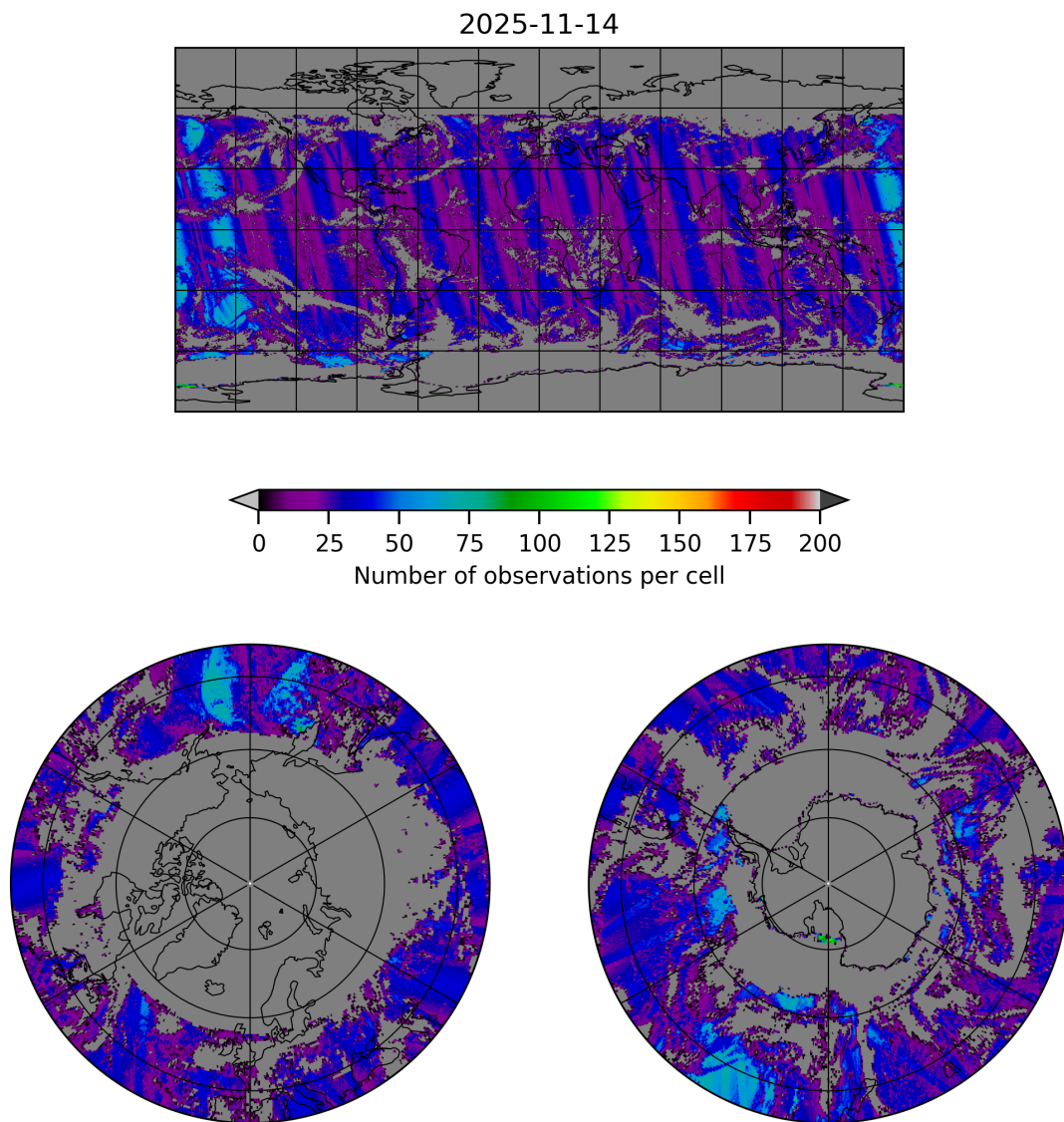
Figure 20: Map of the number of observations for 2025-11-13 to 2025-11-15
