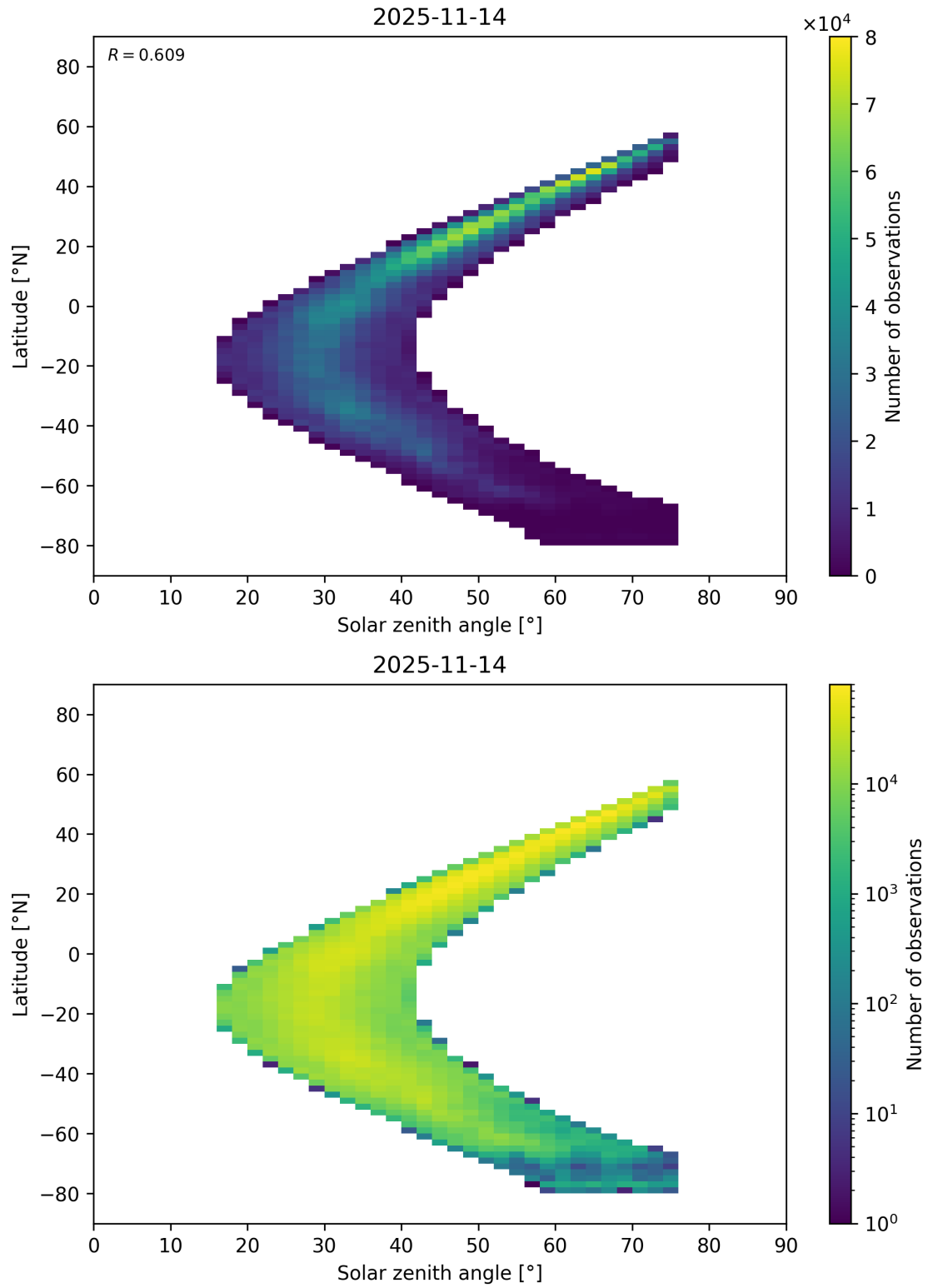
Figure 201: Scatter density plot of “Solar zenith angle” against “Latitude” for 2025-11-13 to 2025-11-15.
