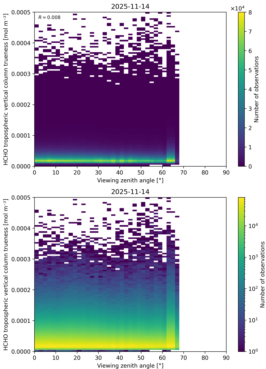
Figure 215: Scatter density plot of “Viewing zenith angle” against “HCHO tropospheric vertical column trueness” for 2025-11-13 to 2025-11-15.
