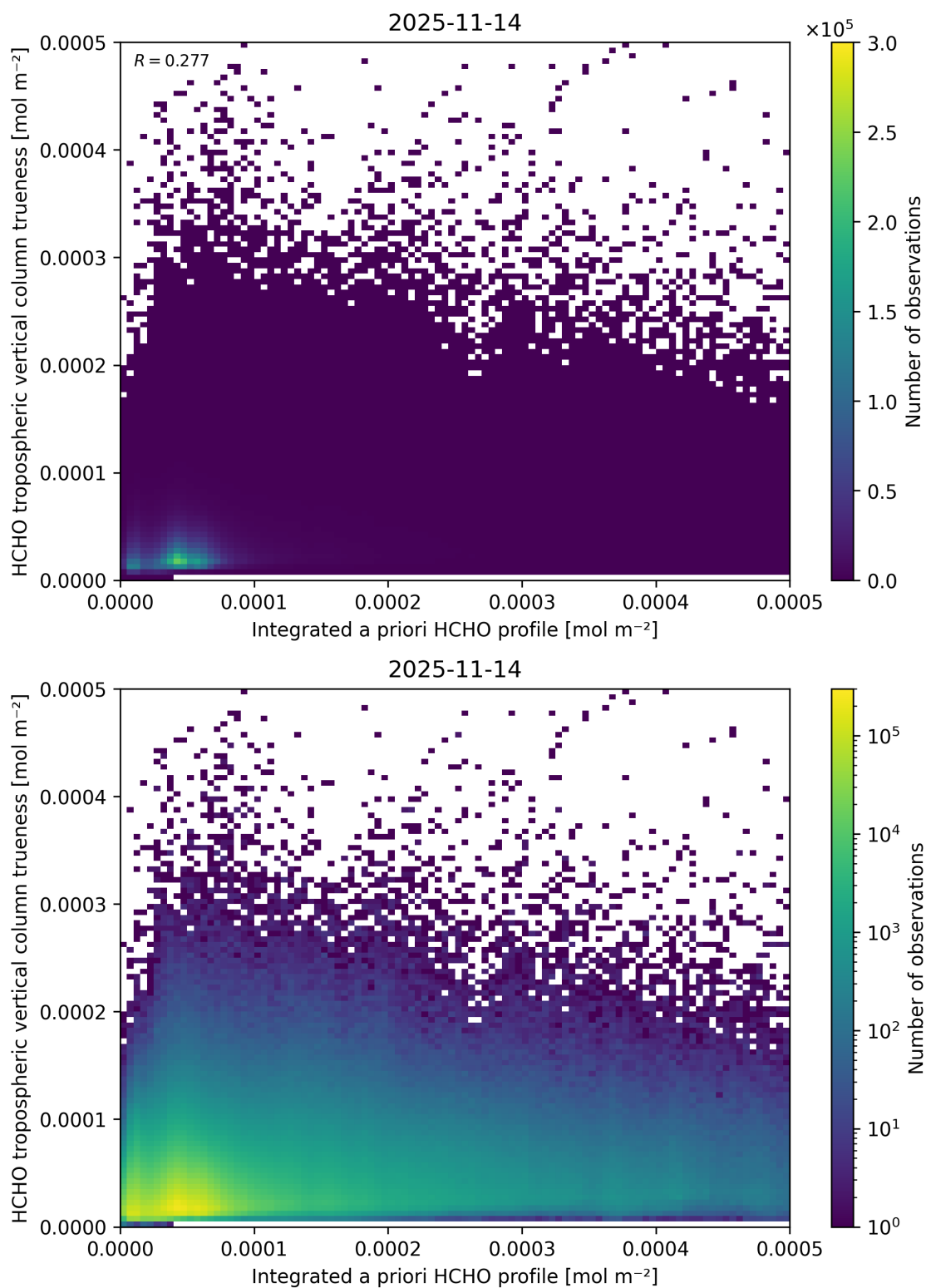
Figure 170: Scatter density plot of “Integrated a priori HCHO profile” against “HCHO tropospheric vertical column truthness” for 2025-11-13 to 2025-11-15.
