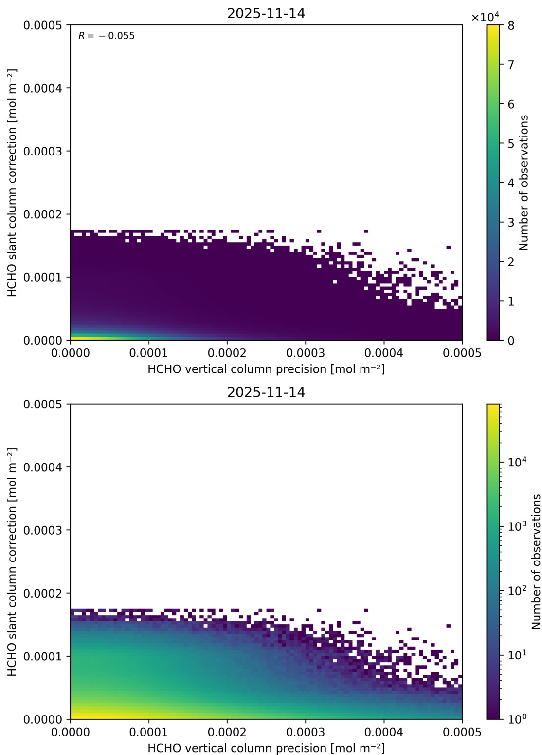
Figure 157: Scatter density plot of “HCHO vertical column precision” against “HCHO slant column correction” for 2025-11-13 to 2025-11-15.
