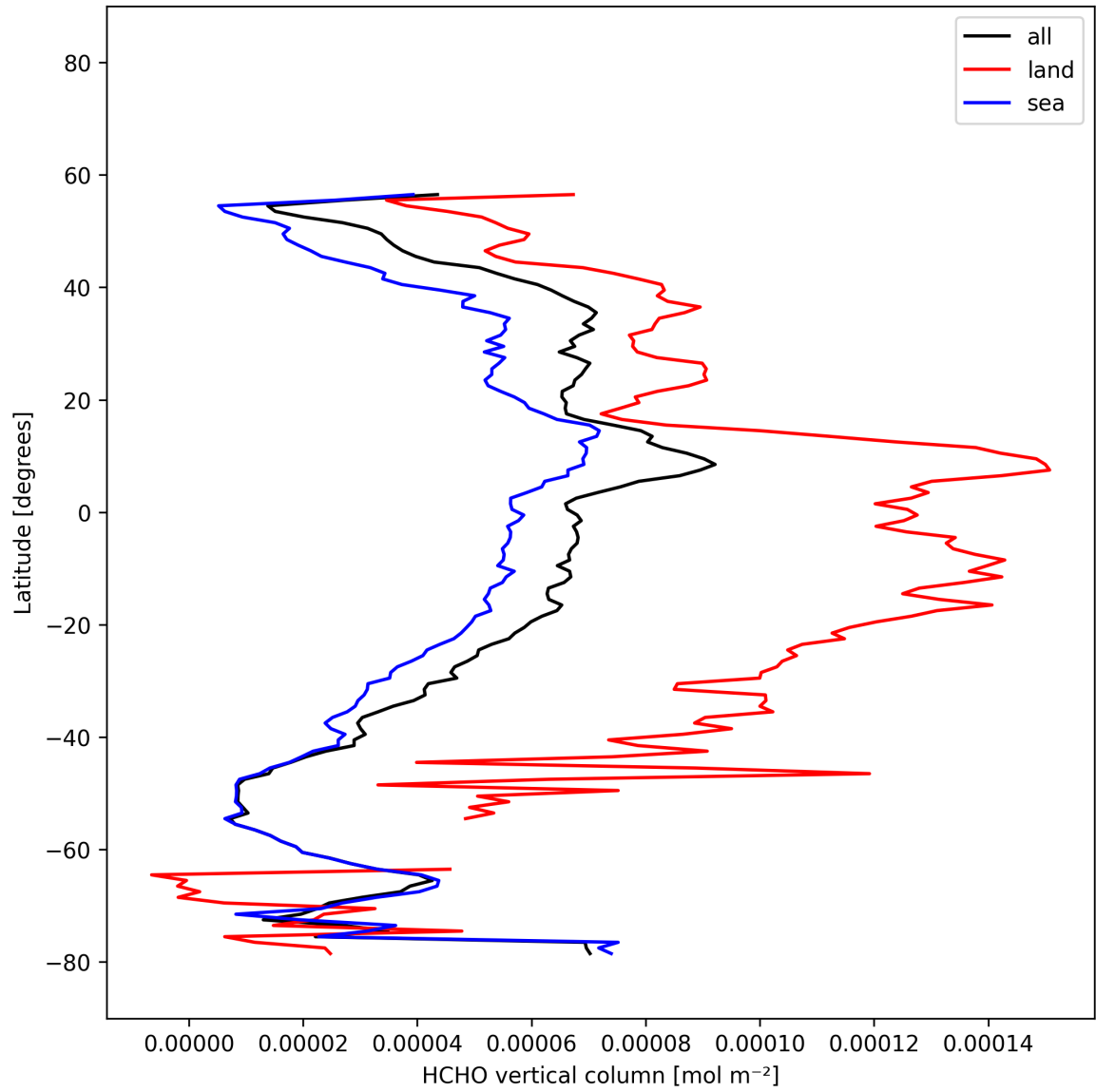
Figure 22: Zonal average of “HCHO vertical column” for 2025-11-13 to 2025-11-15.
