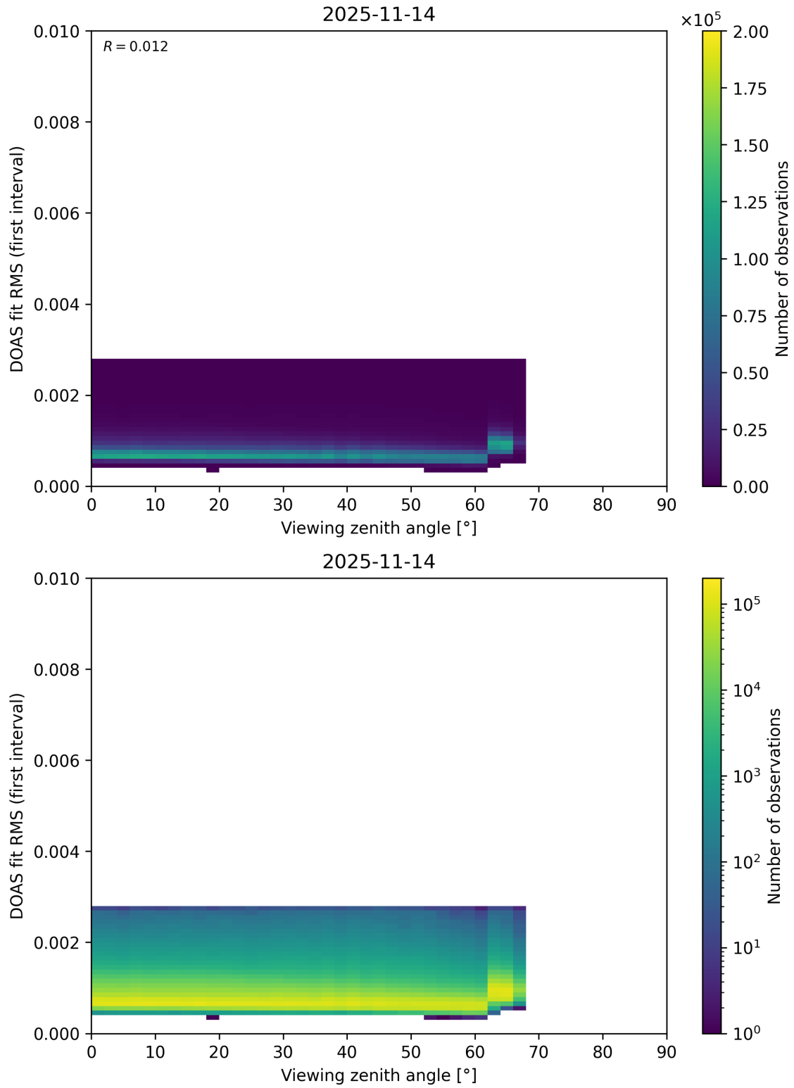
Figure 202: Scatter density plot of “Viewing zenith angle” against “DOAS fit RMS (first interval)” for 2025-11-13 to 2025-11-15.
