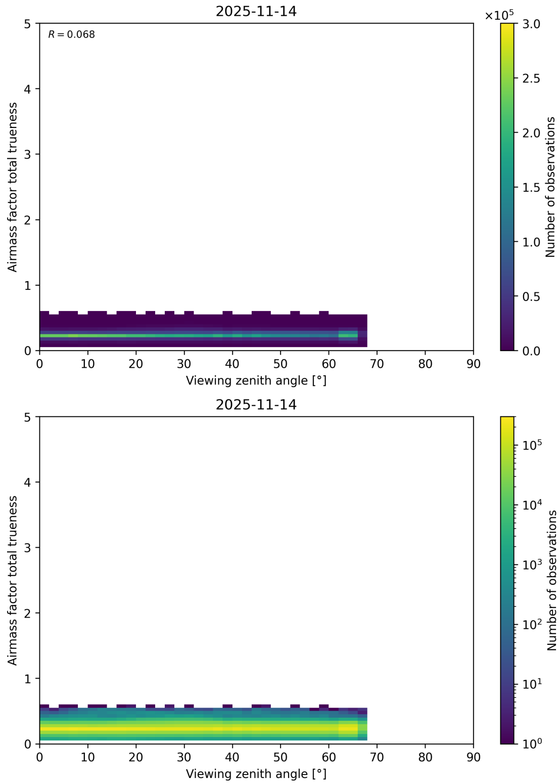
Figure 211: Scatter density plot of “Viewing zenith angle” against “Airmass factor total trueness” for 2025-11-13 to 2025-11-15.
