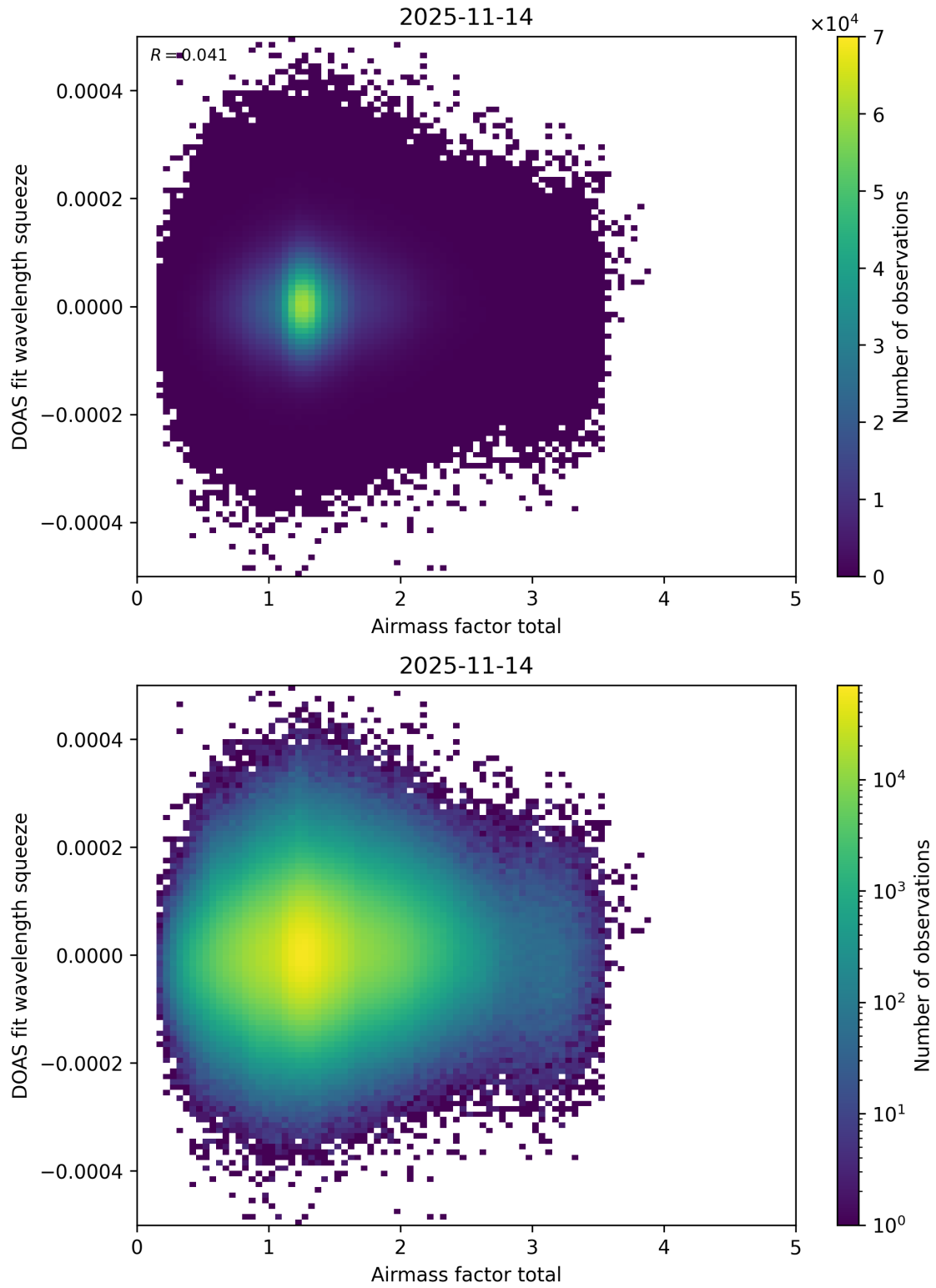
Figure 111: Scatter density plot of “Airmass factor total” against “DOAS fit wavelength squeeze” for 2025-11-13 to 2025-11-15.
