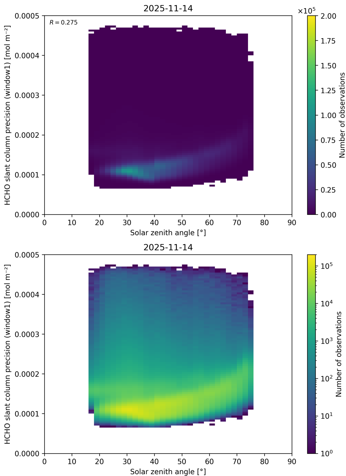
Figure 193: Scatter density plot of “Solar zenith angle” against “HCHO slant column precision (window1)” for 2025-11-13 to 2025-11-15.
