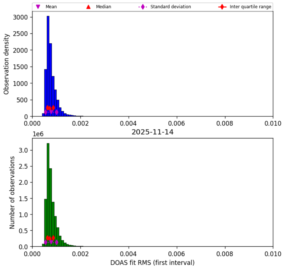
Figure 48: Histogram of “DOAS fit RMS (first interval)” for 2025-11-13 to 2025-11-15
