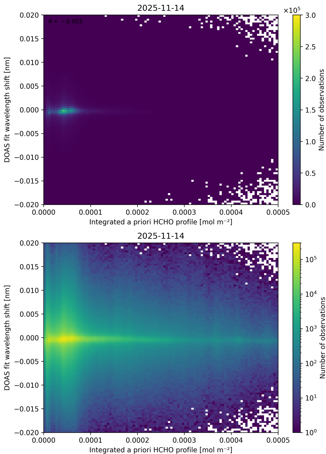
Figure 166: Scatter density plot of “Integrated a priori HCHO profile” against “DOAS fit wavelength shift” for 2025-11-13 to 2025-11-15.
