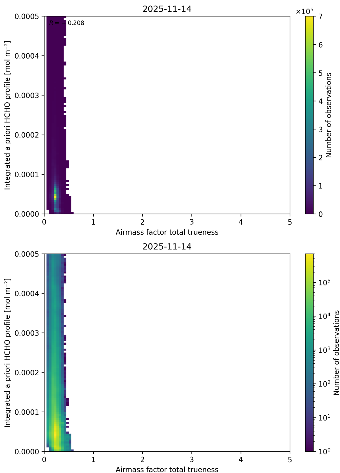
Figure 125: Scatter density plot of “Airmass factor total trueness” against “Integrated a priori HCHO profile” for 2025-11-13 to 2025-11-15.
