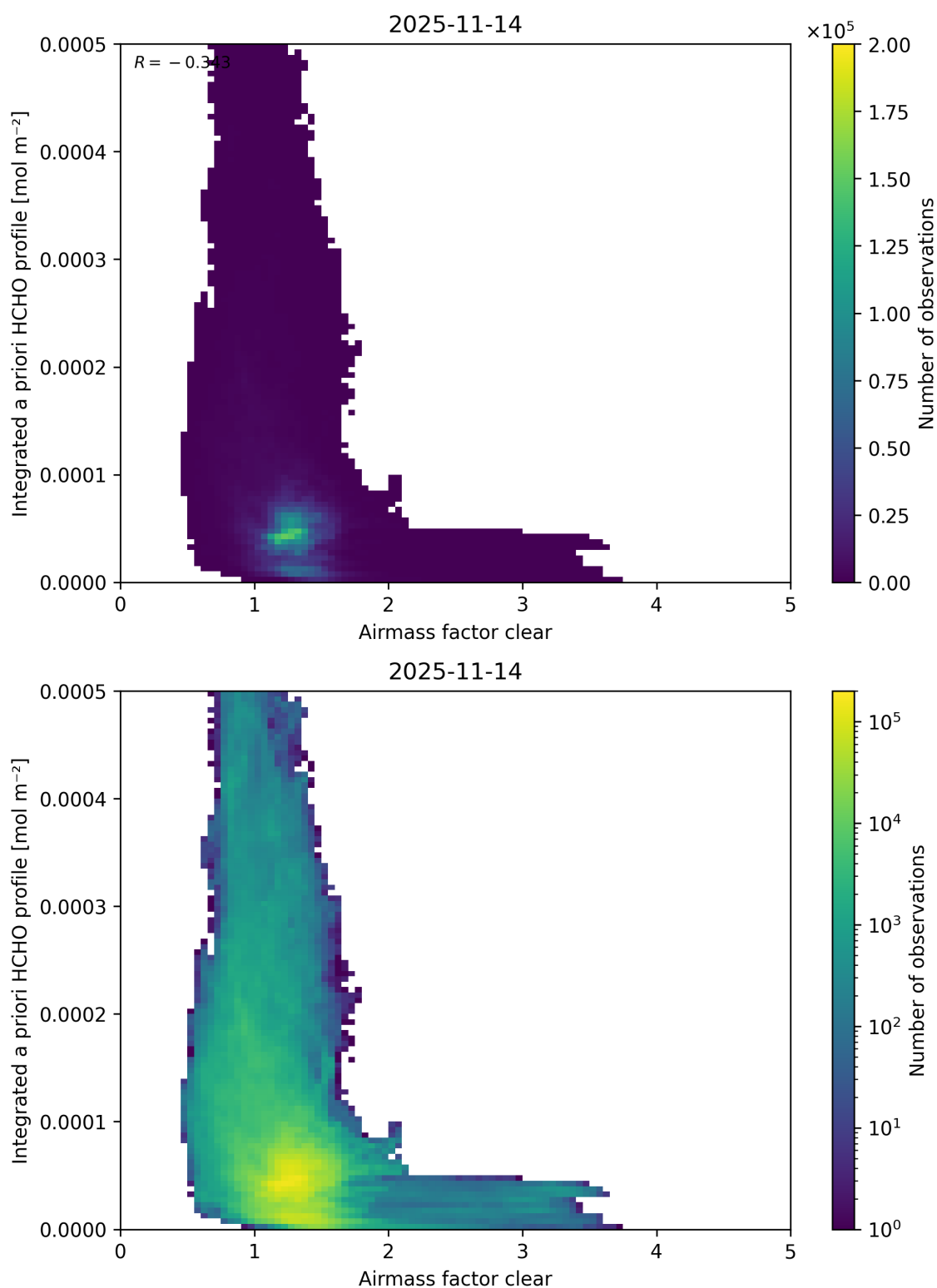
Figure 84: Scatter density plot of “Airmass factor clear” against “Integrated a priori HCHO profile” for 2025-11-13 to 2025-11-15.
