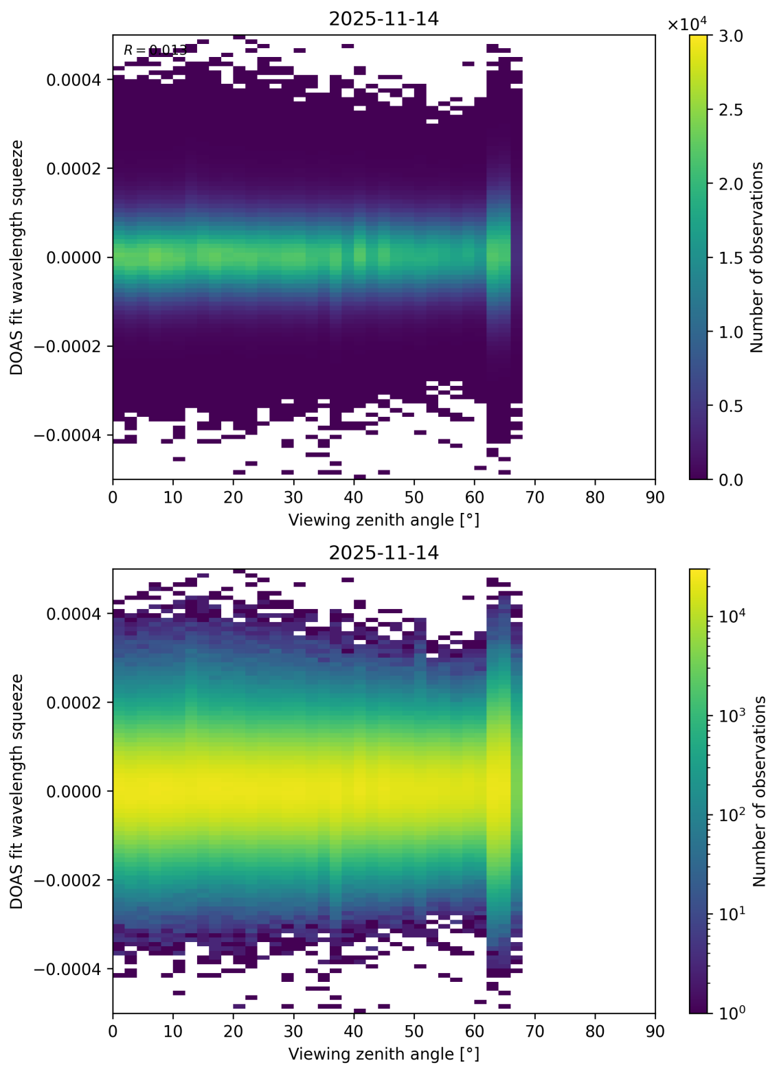
Figure 204: Scatter density plot of “Viewing zenith angle” against “DOAS fit wavelength squeeze” for 2025-11-13 to 2025-11-15.
