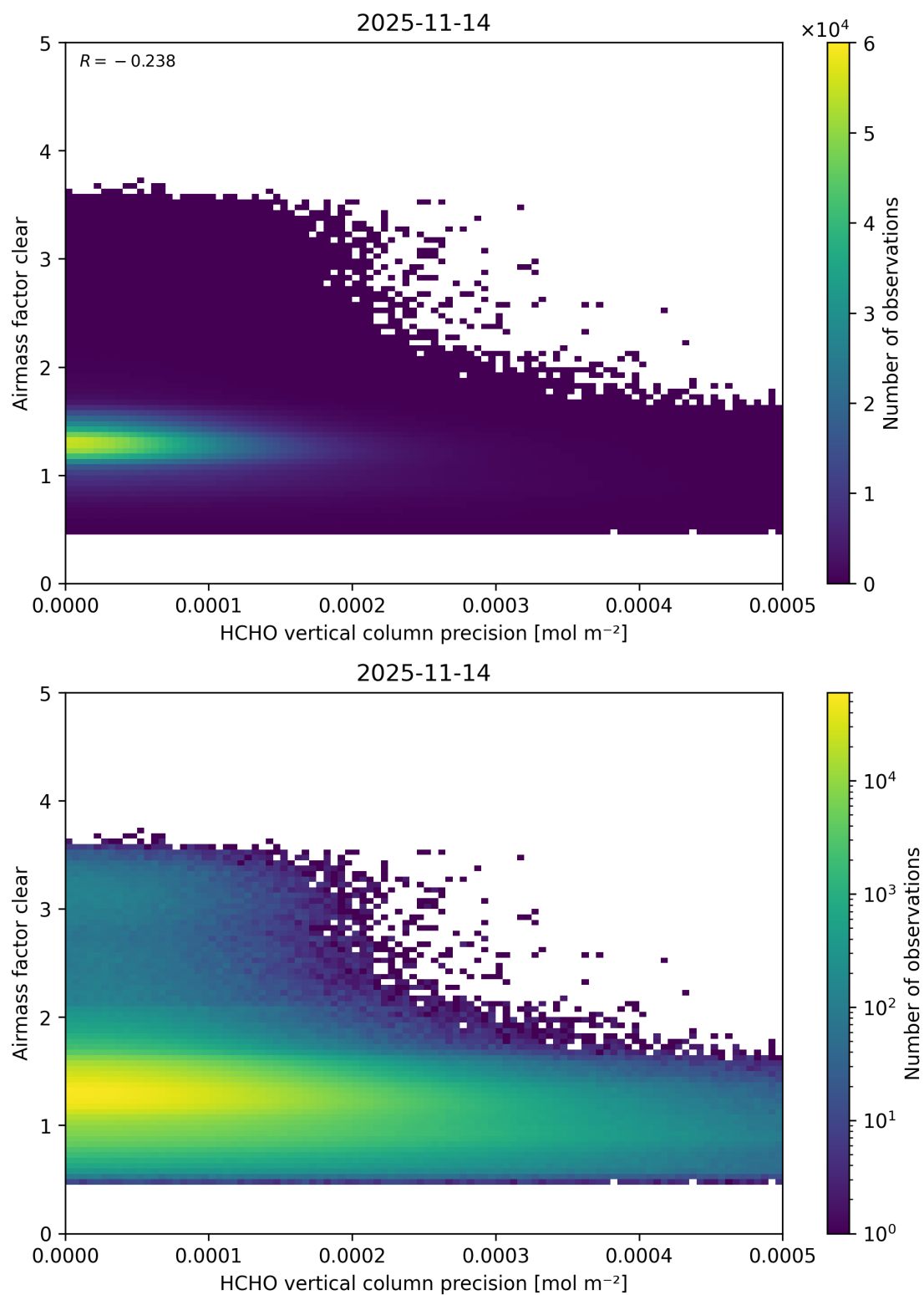
Figure 155: Scatter density plot of “HCHO vertical column precision” against “Airmass factor clear” for 2025-11-13 to 2025-11-15.
