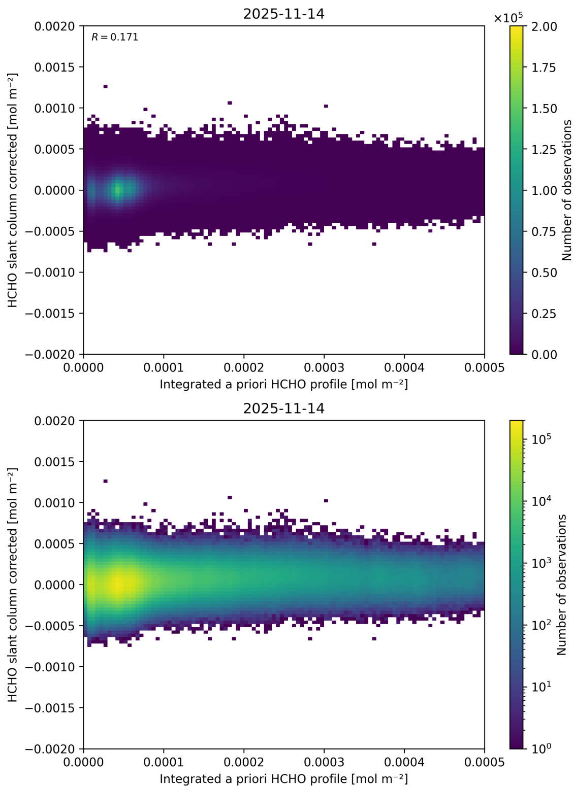
Figure 168: Scatter density plot of “Integrated a priori HCHO profile” against “HCHO slant column corrected” for 2025-11-13 to 2025-11-15.
