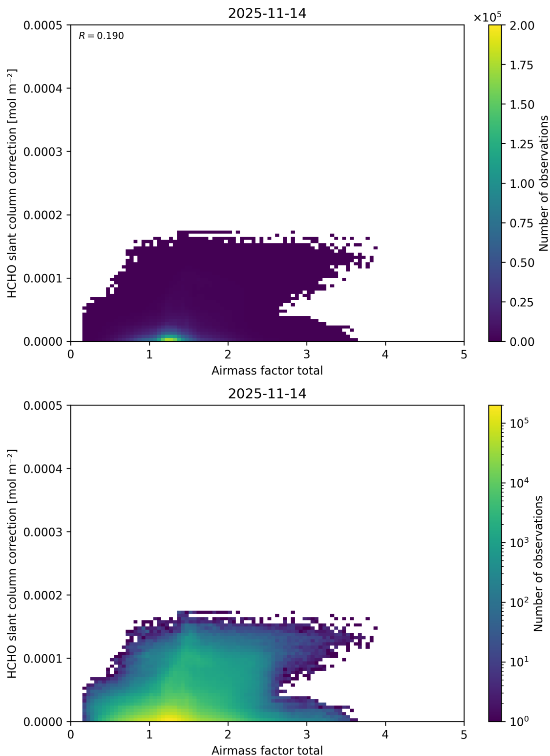
Figure 114: Scatter density plot of “Airmass factor total” against “HCHO slant column correction” for 2025-11-13 to 2025-11-15.
