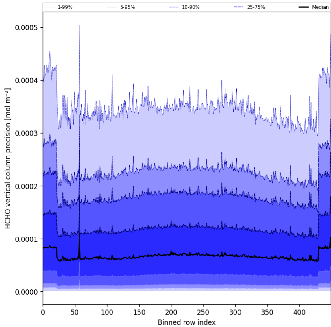
Figure 53: Along track statistics of “HCHO vertical column precision” for 2025-11-13 to 2025-11-15
