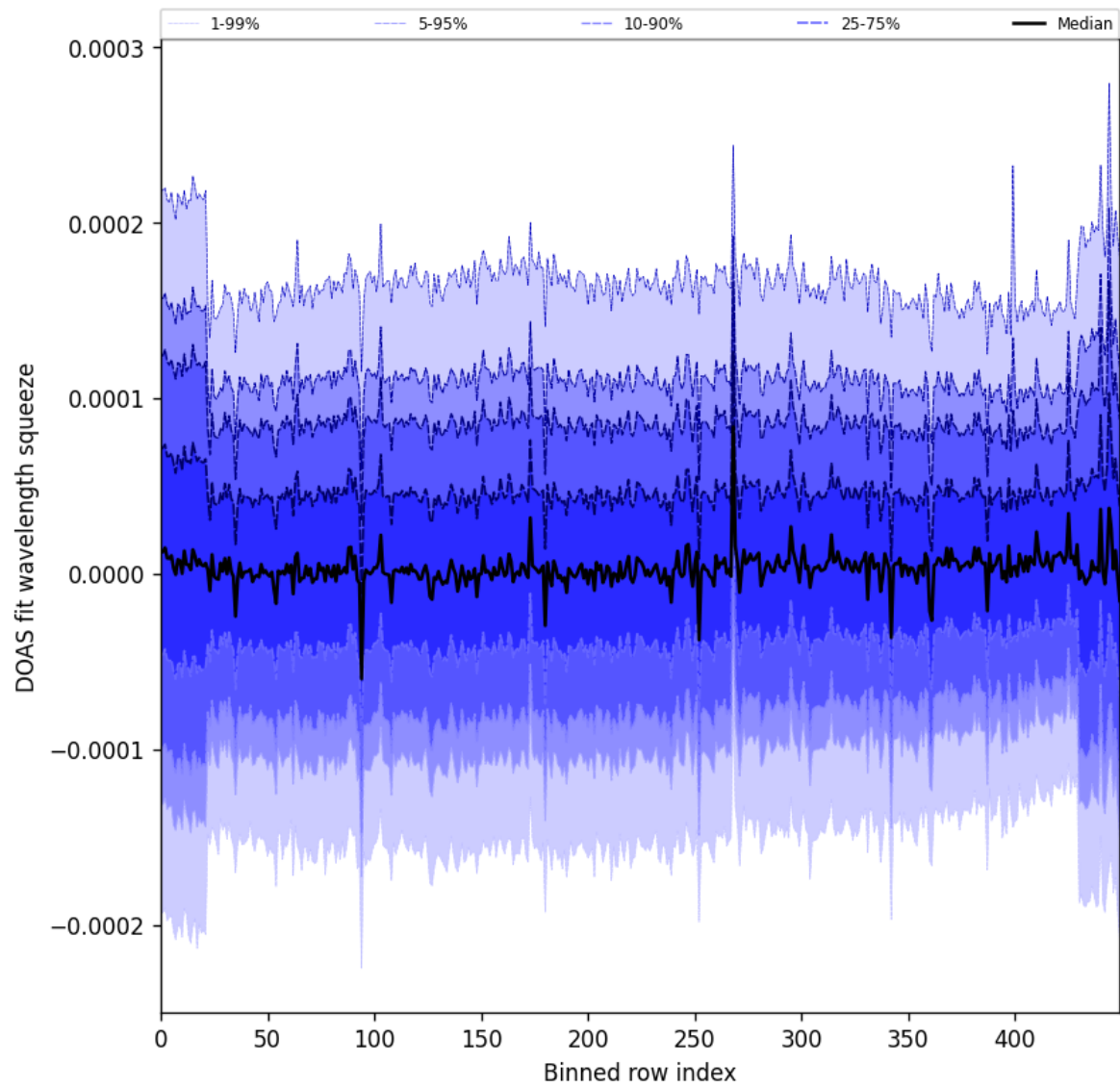
Figure 62: Along track statistics of “DOAS fit wavelength squeeze” for 2025-11-13 to 2025-11-15
