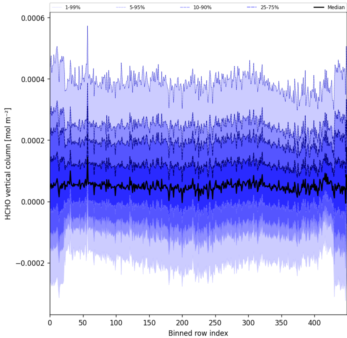
Figure 52: Along track statistics of “HCHO vertical column” for 2025-11-13 to 2025-11-15
