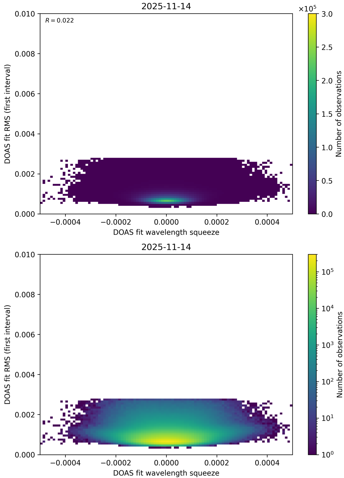
Figure 74: Scatter density plot of “DOAS fit wavelength squeeze” against “DOAS fit RMS (first interval)” for 2025-11-13 to 2025-11-15.
