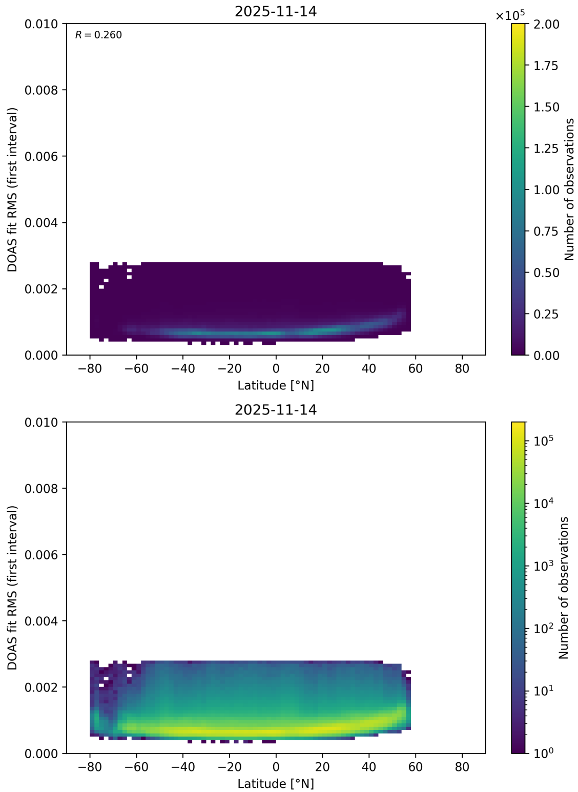
Figure 171: Scatter density plot of “Latitude” against “DOAS fit RMS (first interval)” for 2025-11-13 to 2025-11-15.
