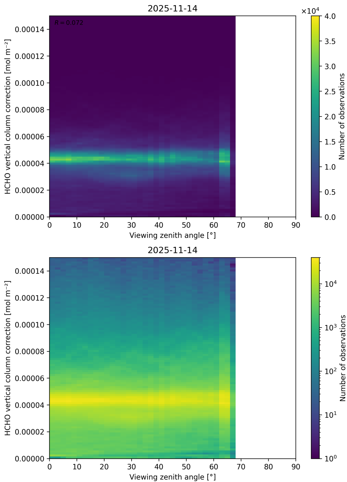
Figure 213: Scatter density plot of “Viewing zenith angle” against “HCHO vertical column correction” for 2025-11-13 to 2025-11-15.
