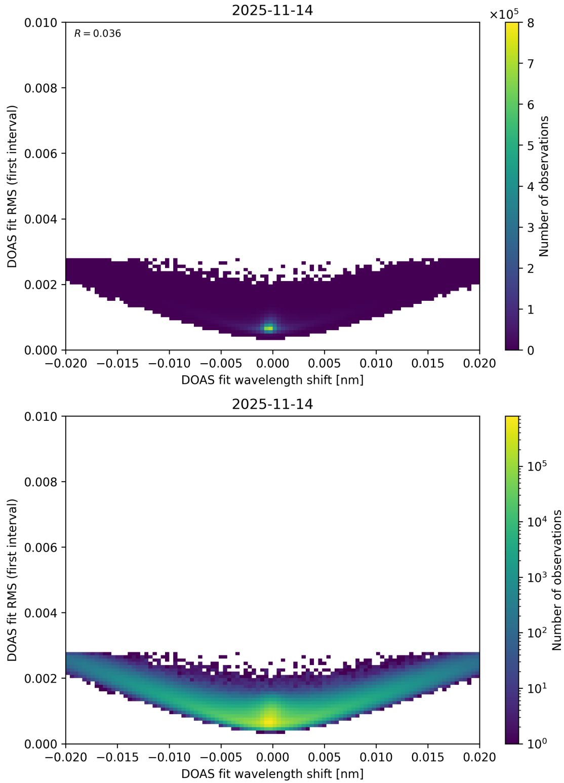
Figure 69: Scatter density plot of “DOAS fit wavelength shift” against “DOAS fit RMS (first interval)” for 2025-11-13 to 2025-11-15.
