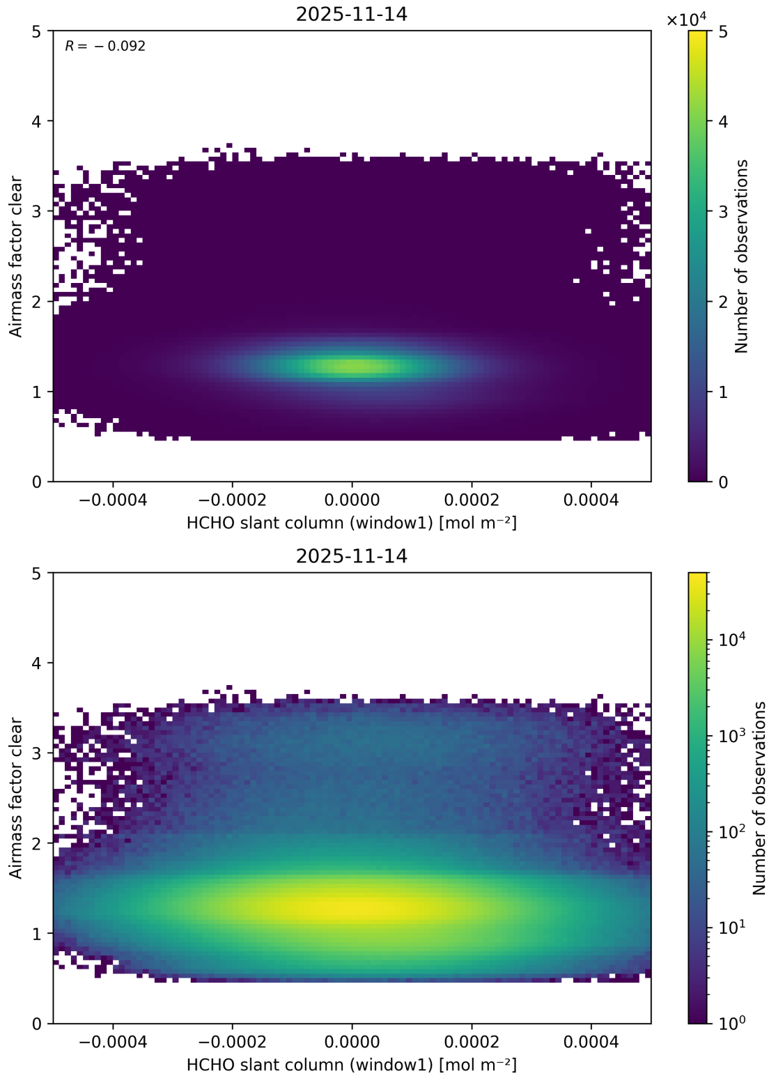
Figure 91: Scatter density plot of “HCHO slant column (window1)” against “Airmass factor clear” for 2025-11-13 to 2025-11-15.
