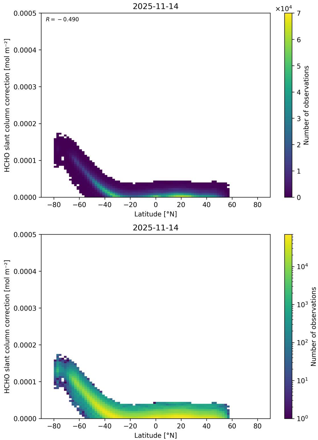
Figure 176: Scatter density plot of “Latitude” against “HCHO slant column correction” for 2025-11-13 to 2025-11-15.
