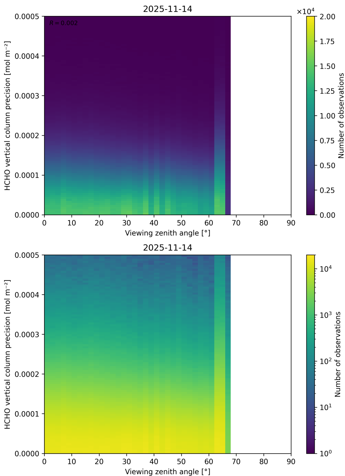
Figure 214: Scatter density plot of “Viewing zenith angle” against “HCHO vertical column precision” for 2025-11-13 to 2025-11-15.
