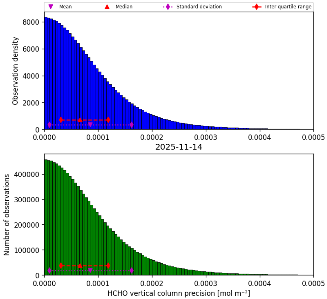
Figure 38: Histogram of “HCHO vertical column precision” for 2025-11-13 to 2025-11-15
