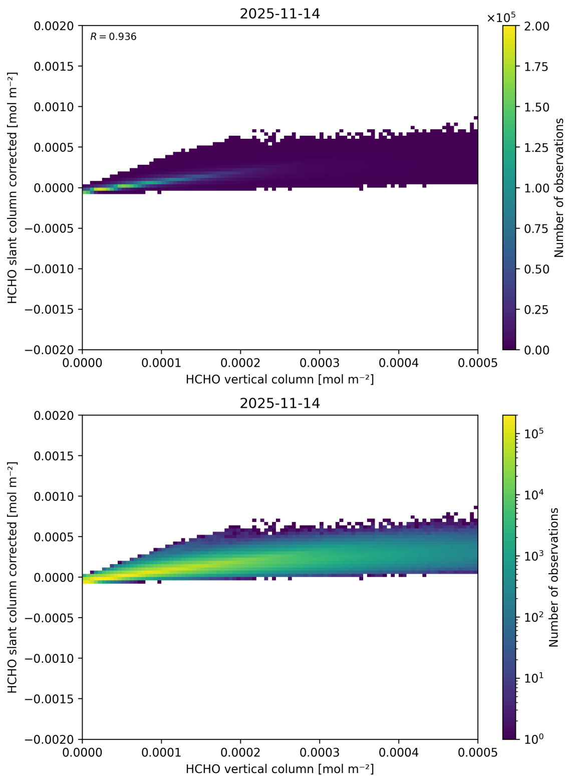
Figure 142: Scatter density plot of “HCHO vertical column” against “HCHO slant column corrected” for 2025-11-13 to 2025-11-15.
