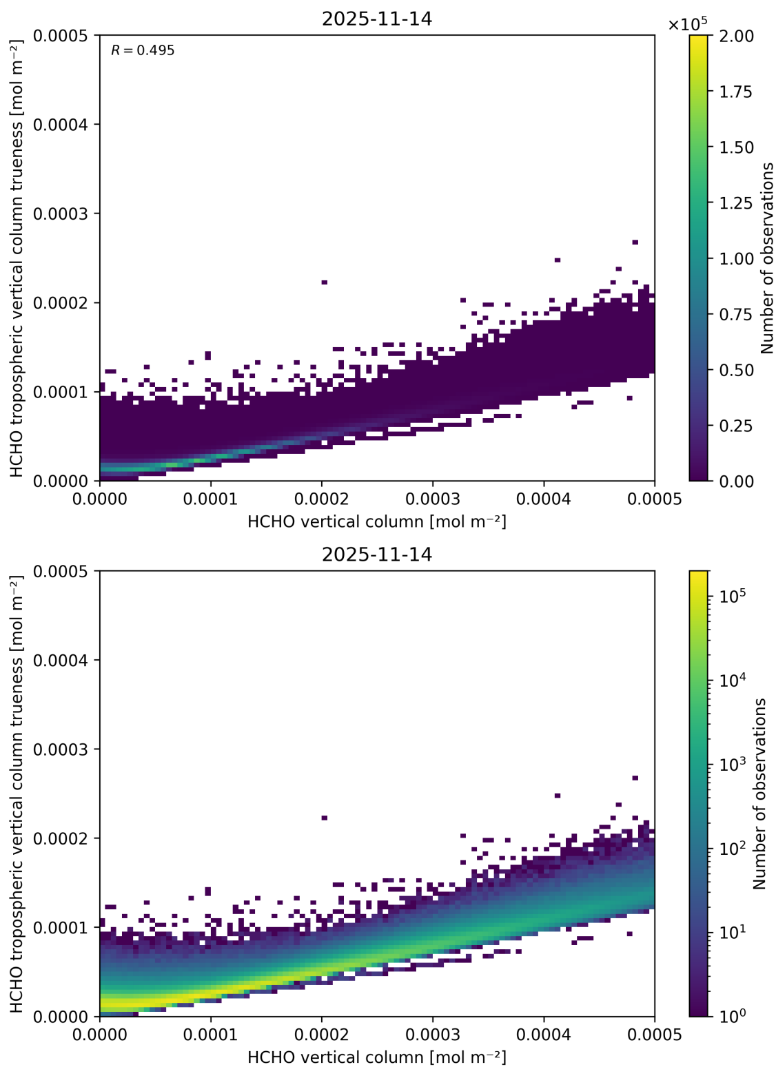
Figure 150: Scatter density plot of “HCHO vertical column” against “HCHO tropospheric vertical column trueness” for 2025-11-13 to 2025-11-15.
