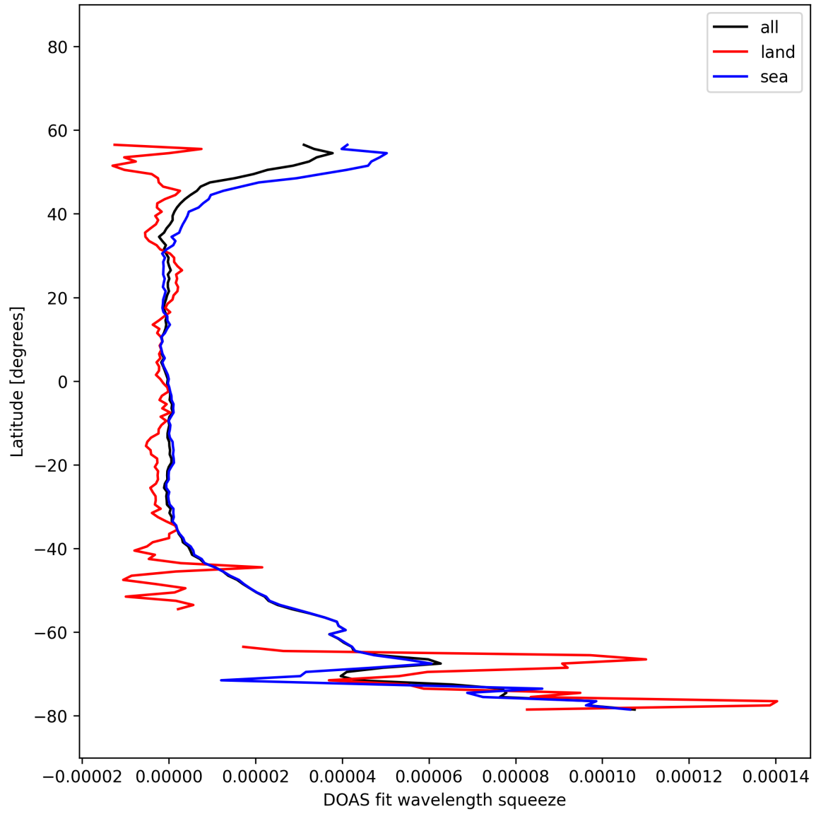
Figure 32: Zonal average of “DOAS fit wavelength squeeze” for 2025-11-13 to 2025-11-15.
