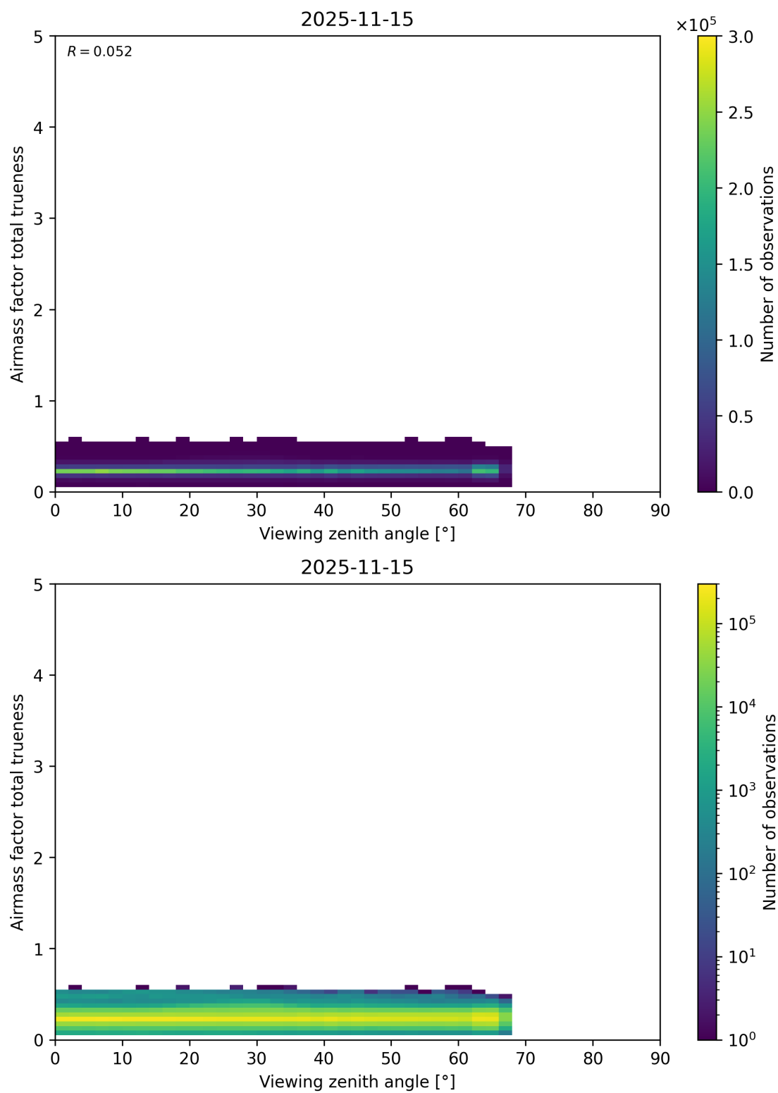
Figure 211: Scatter density plot of “Viewing zenith angle” against “Airmass factor total trueness” for 2025-11-14 to 2025-11-16.
