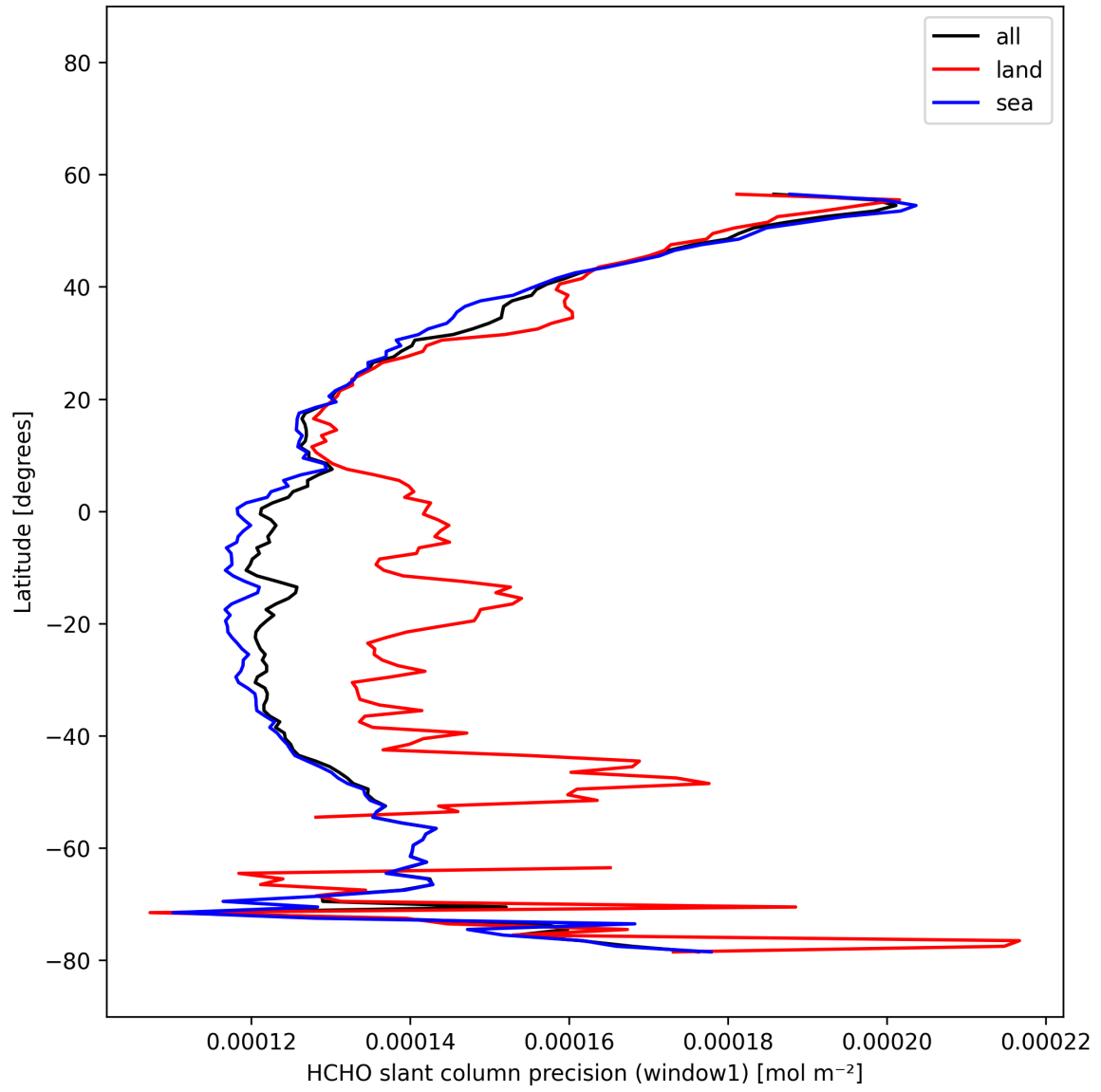
Figure 26: Zonal average of "HCHO slant column precision (window1)" for 2025-11-14 to 2025-11-16.
