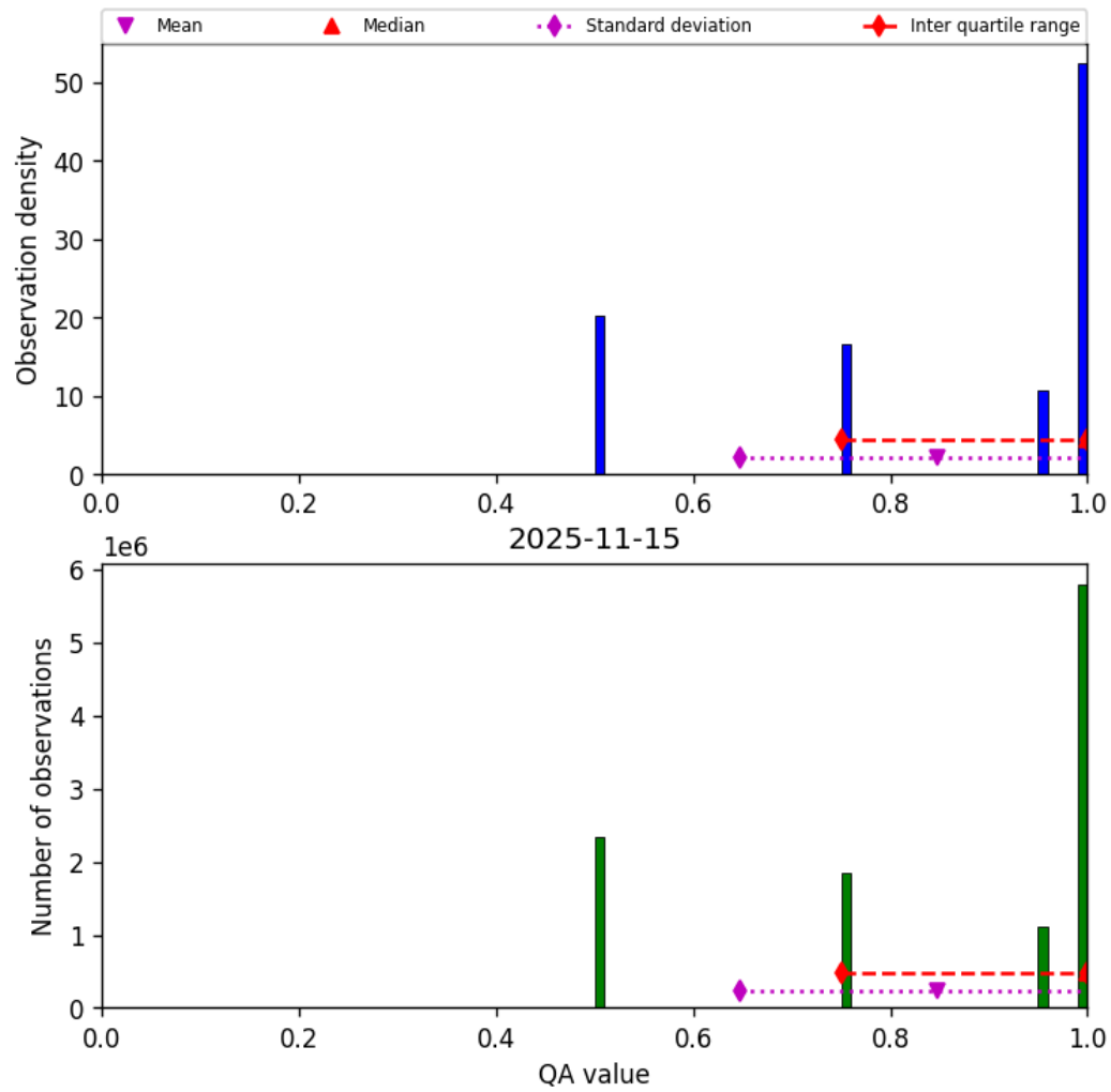
Figure 36: Histogram of “QA value” for 2025-11-14 to 2025-11-16
