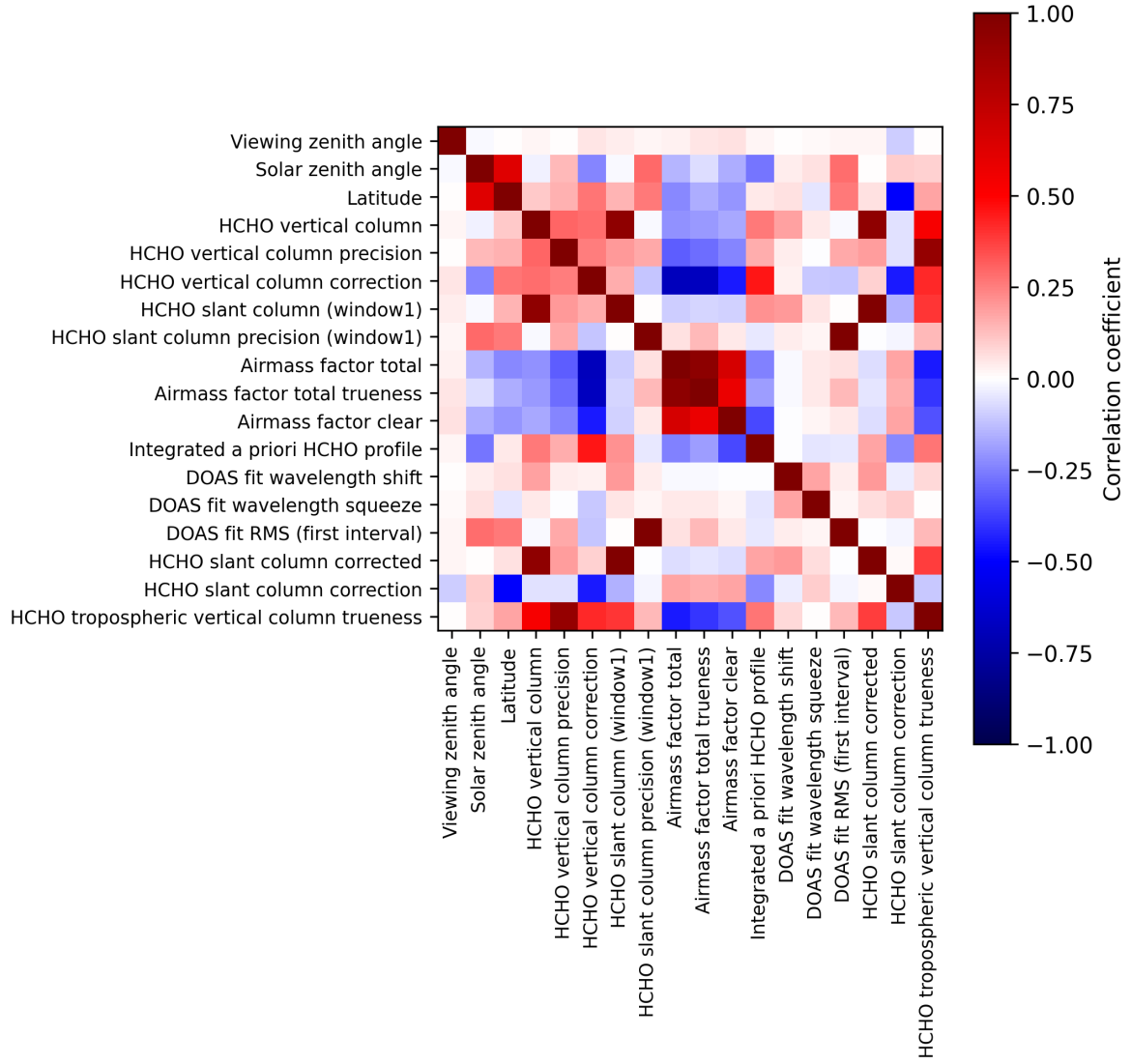
Figure 2: Map of correlation matrix for 2025-11-14 to 2025-11-16.
