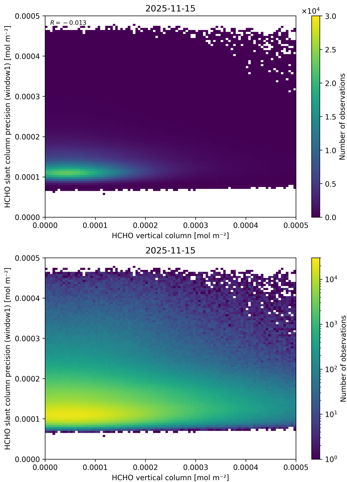
Figure 145: Scatter density plot of “HCHO vertical column” against “HCHO slant column precision (window1)” for 2025-11-14 to 2025-11-16.
