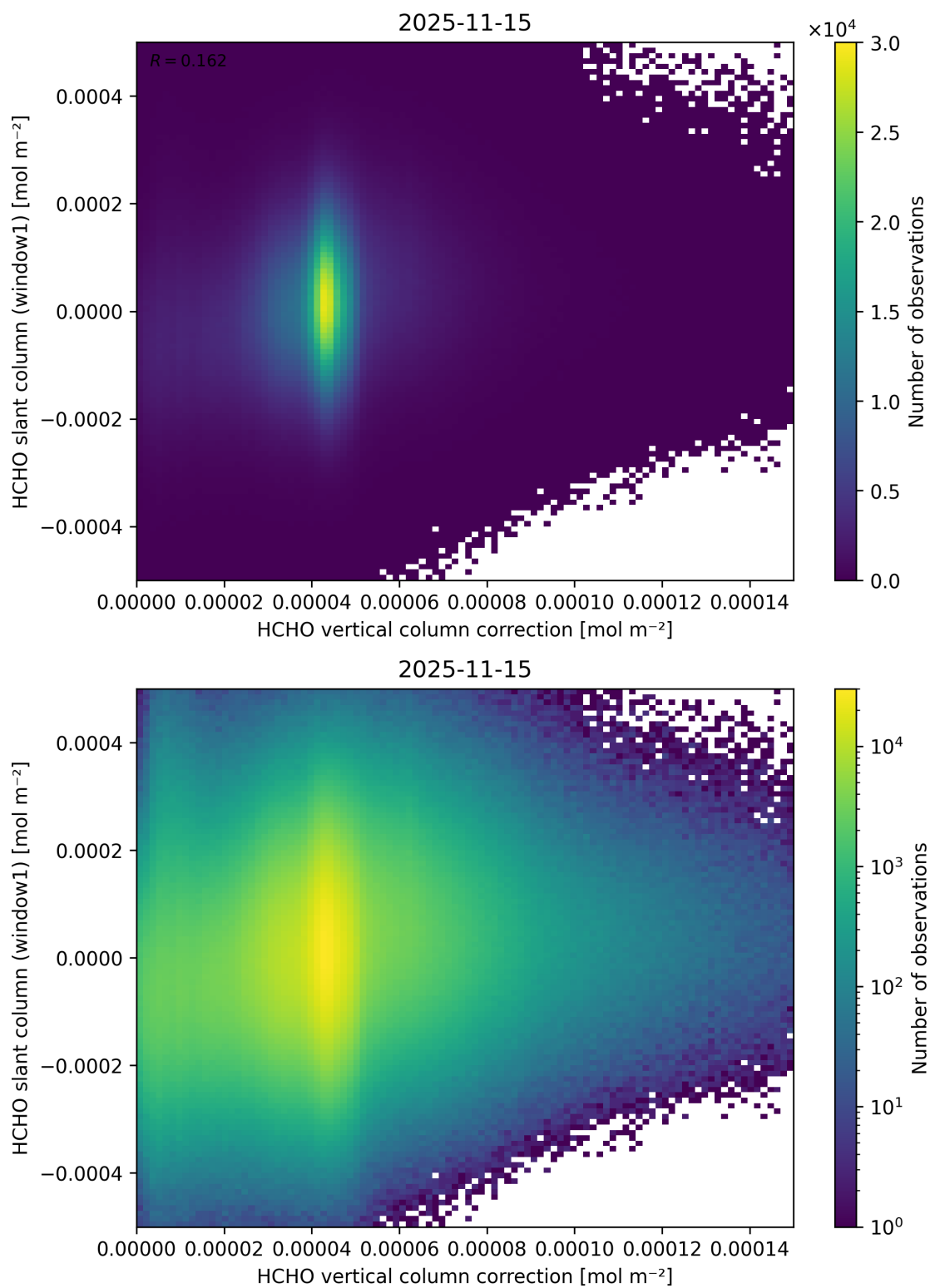
Figure 132: Scatter density plot of “HCHO vertical column correction” against “HCHO slant column (window1)” for 2025-11-14 to 2025-11-16.
