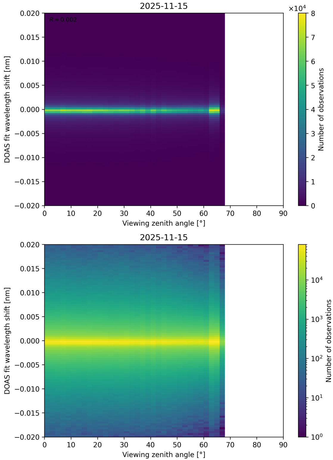
Figure 203: Scatter density plot of “Viewing zenith angle” against “DOAS fit wavelength shift” for 2025-11-14 to 2025-11-16.
