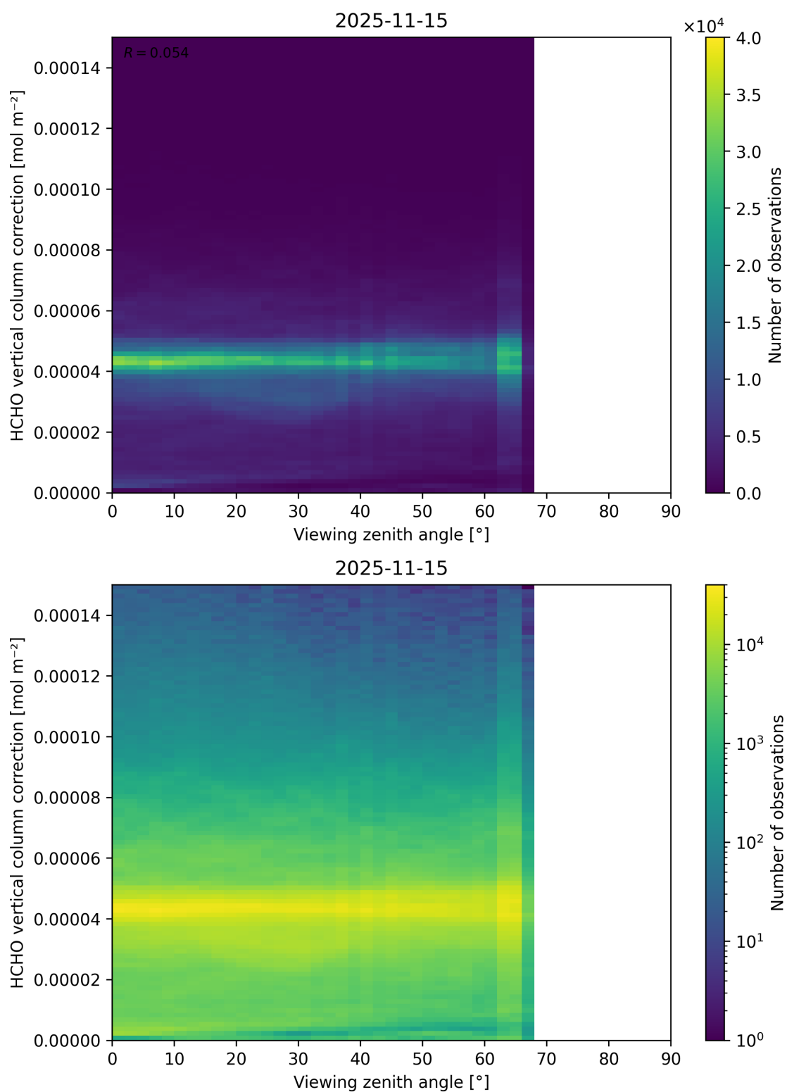
Figure 213: Scatter density plot of “Viewing zenith angle” against “HCHO vertical column correction” for 2025-11-14 to 2025-11-16.
