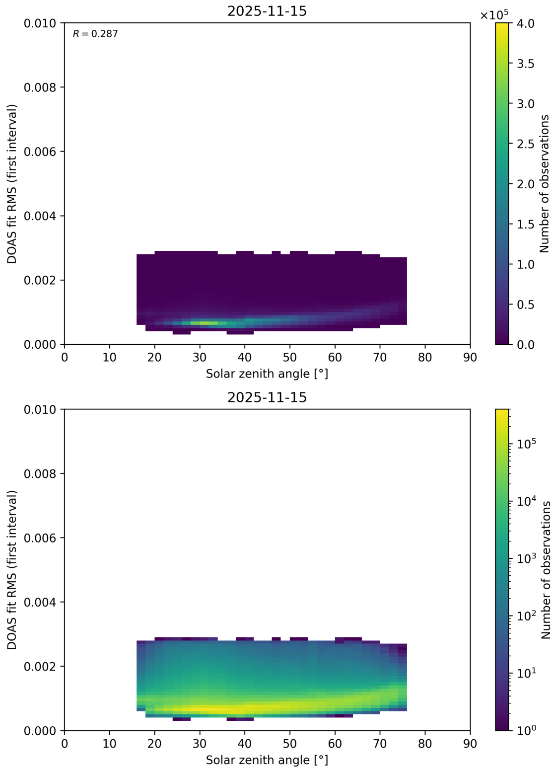
Figure 186: Scatter density plot of “Solar zenith angle” against “DOAS fit RMS (first interval)” for 2025-11-14 to 2025-11-16.
