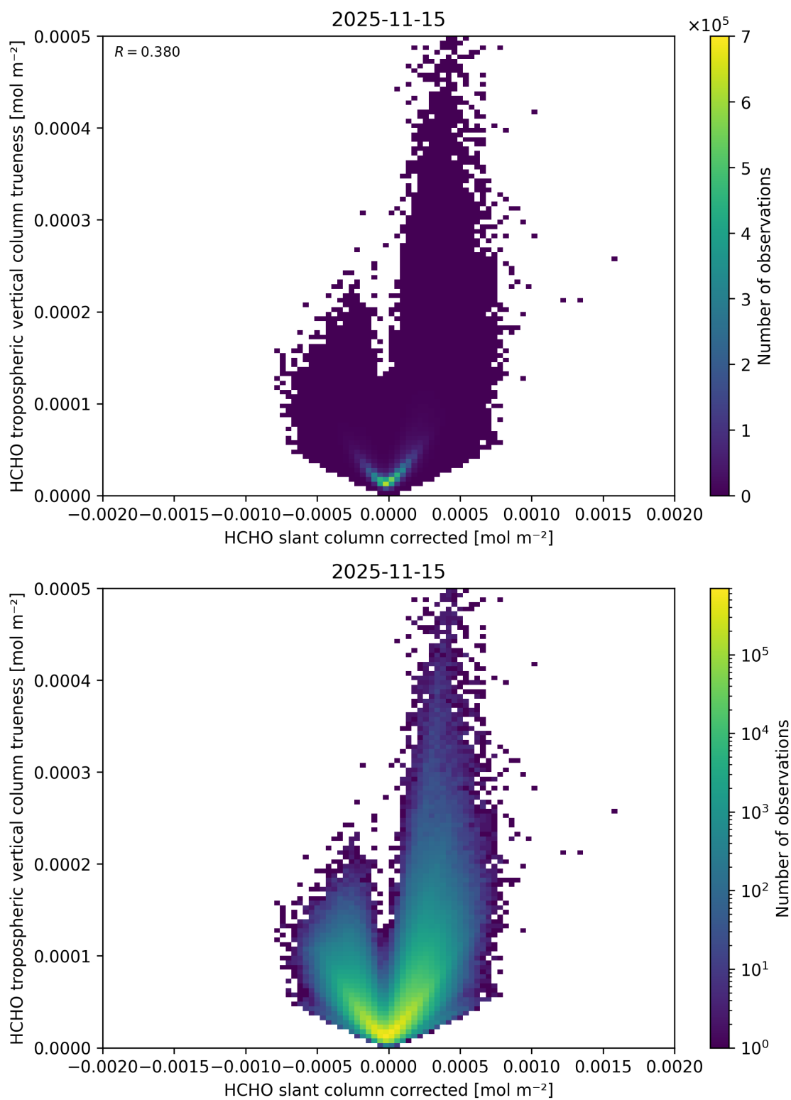
Figure 86: Scatter density plot of “HCHO slant column corrected” against “HCHO tropospheric vertical column trueness” for 2025-11-14 to 2025-11-16.
