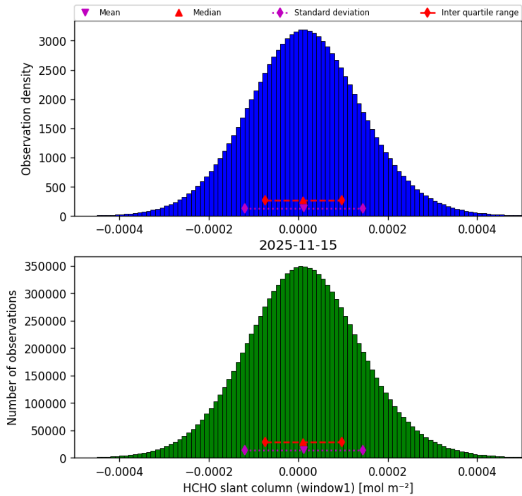
Figure 40: Histogram of “HCHO slant column (window1)” for 2025-11-14 to 2025-11-16
