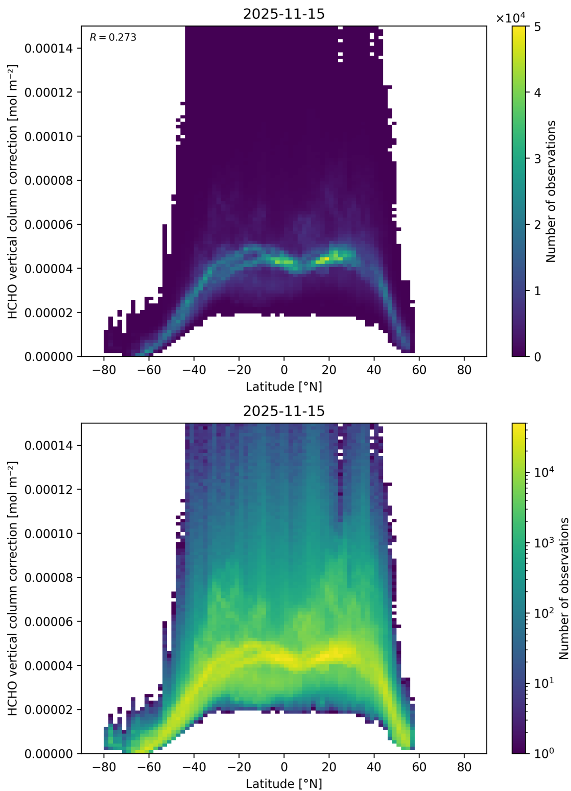
Figure 182: Scatter density plot of “Latitude” against “HCHO vertical column correction” for 2025-11-14 to 2025-11-16.
