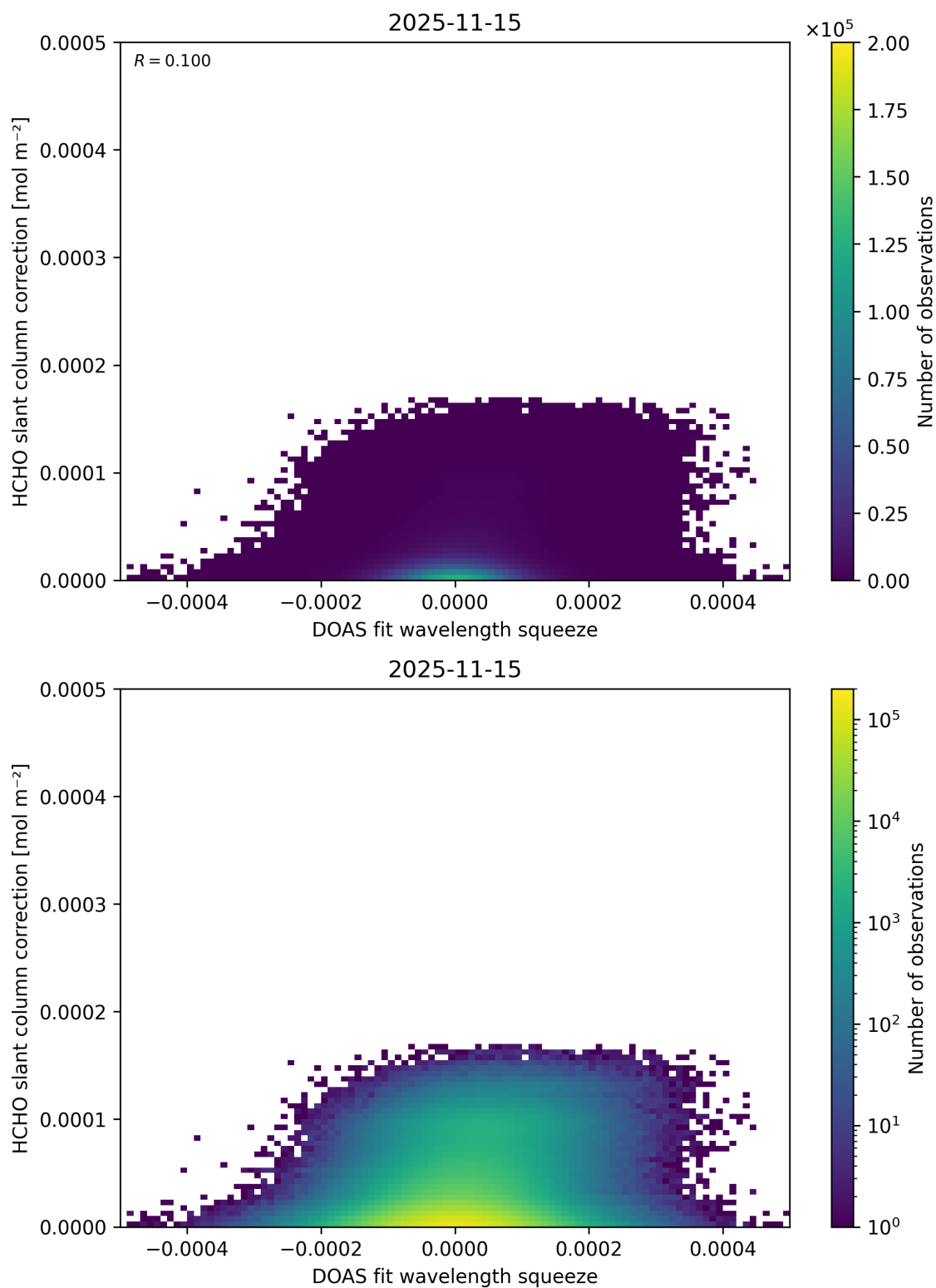
Figure 76: Scatter density plot of “DOAS fit wavelength squeeze” against “HCHO slant column correction” for 2025-11-14 to 2025-11-16.
