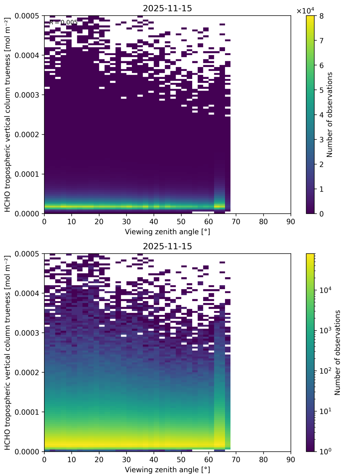
Figure 215: Scatter density plot of “Viewing zenith angle” against “HCHO tropospheric vertical column trueness” for 2025-11-14 to 2025-11-16.
