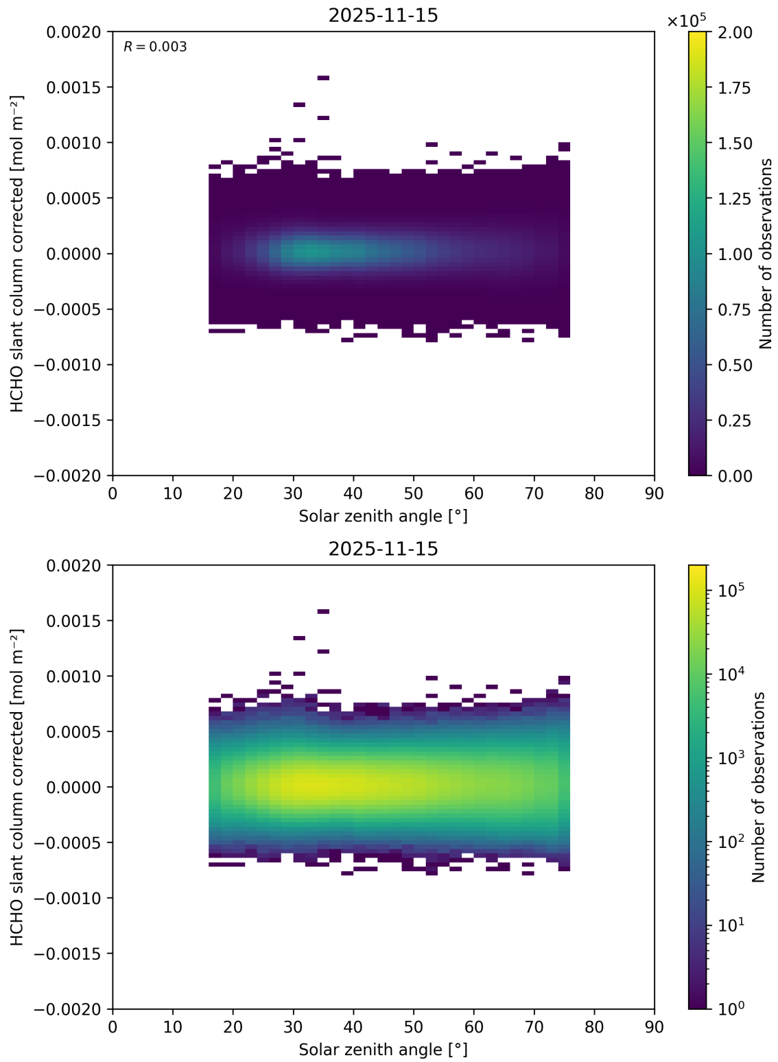
Figure 190: Scatter density plot of “Solar zenith angle” against “HCHO slant column corrected” for 2025-11-14 to 2025-11-16.
