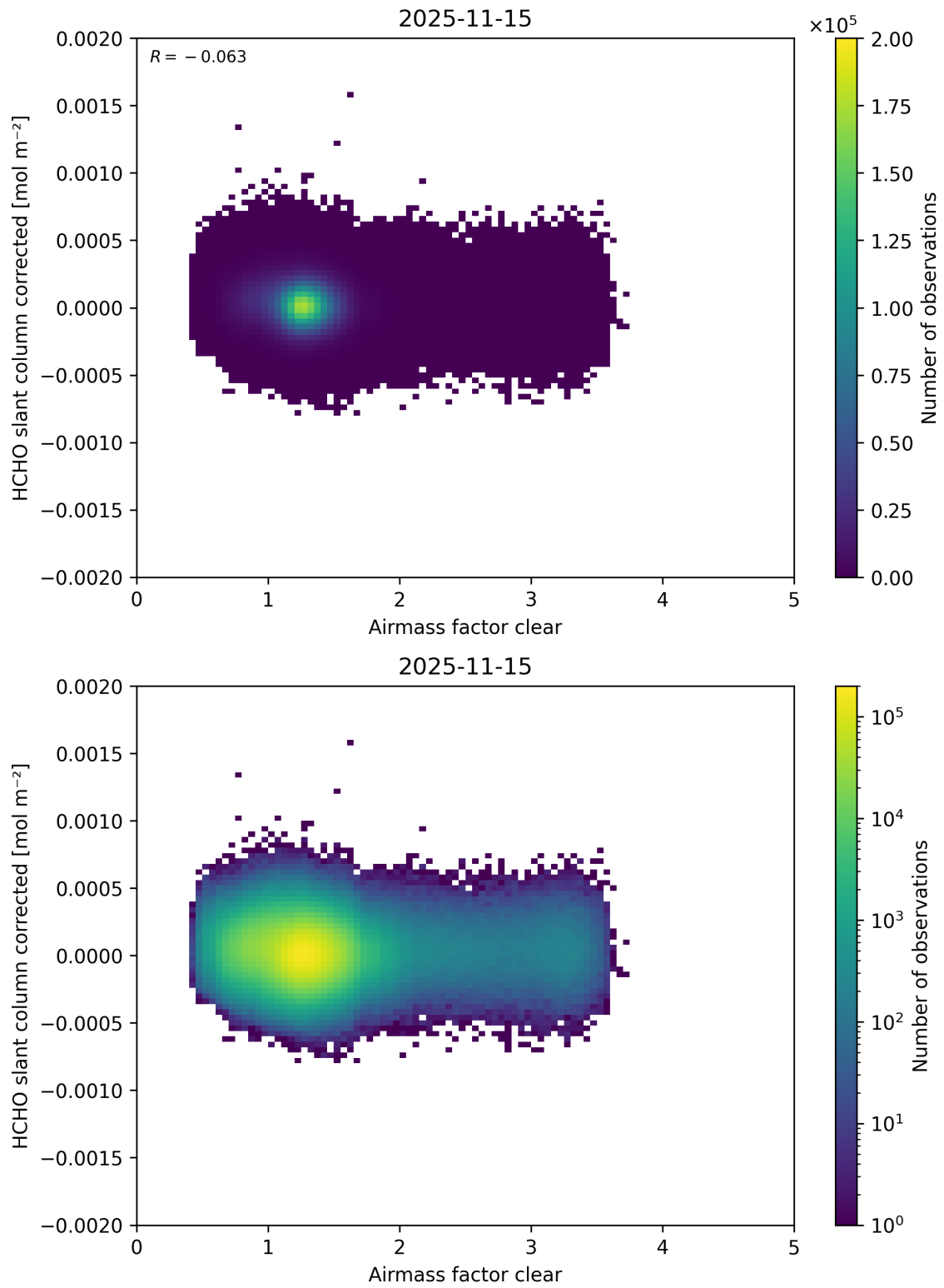
Figure 81: Scatter density plot of “Airmass factor clear” against “HCHO slant column corrected” for 2025-11-14 to 2025-11-16.
