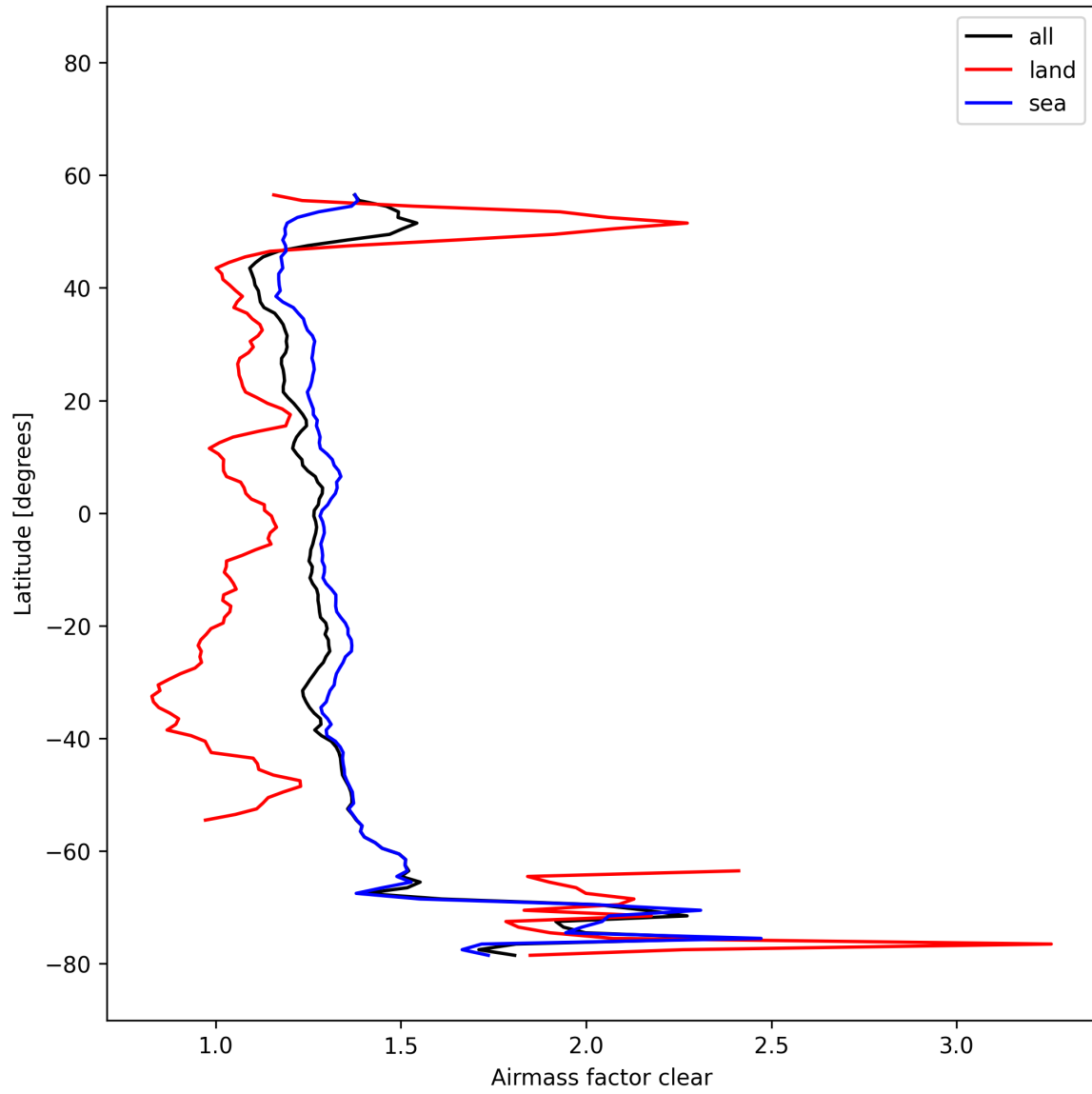
Figure 29: Zonal average of “Airmass factor clear” for 2025-11-14 to 2025-11-16.
