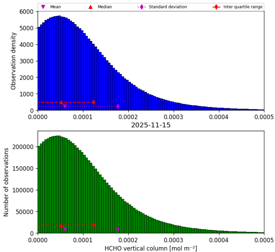
Figure 37: Histogram of “HCHO vertical column” for 2025-11-14 to 2025-11-16
