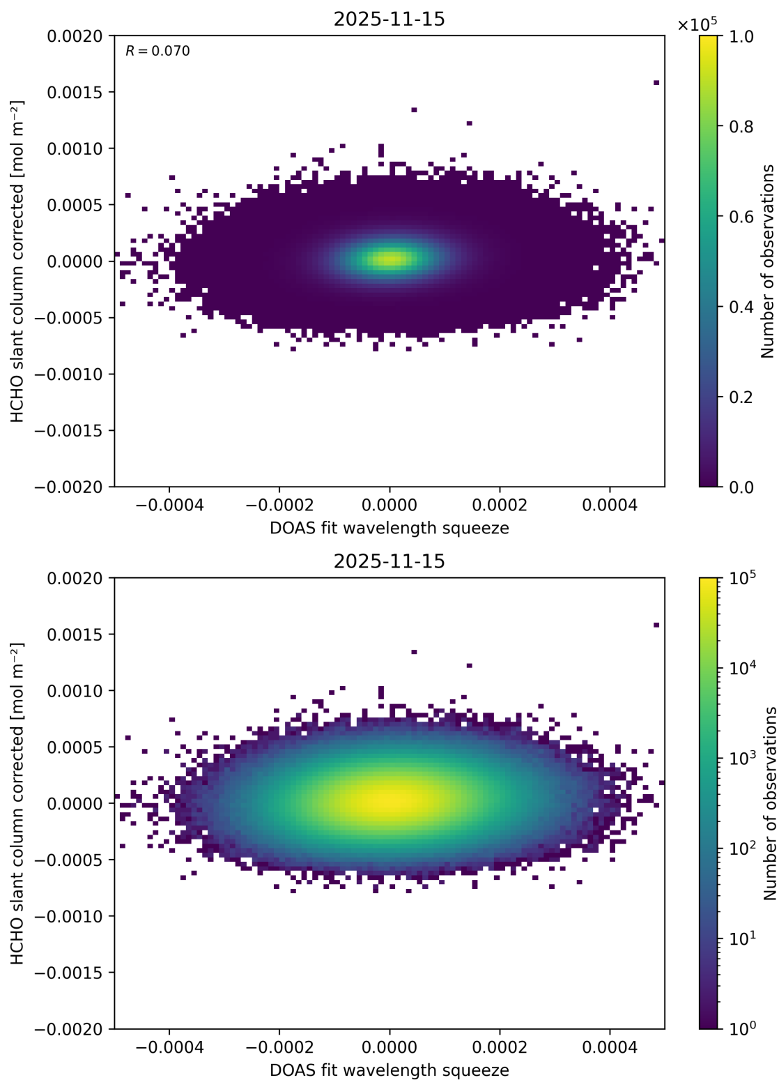
Figure 75: Scatter density plot of “DOAS fit wavelength squeeze” against “HCHO slant column corrected” for 2025-11-14 to 2025-11-16.
