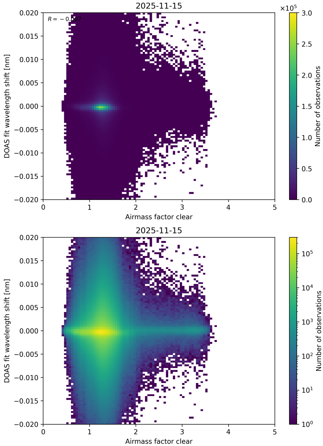
Figure 79: Scatter density plot of “Airmass factor clear” against “DOAS fit wavelength shift” for 2025-11-14 to 2025-11-16.
