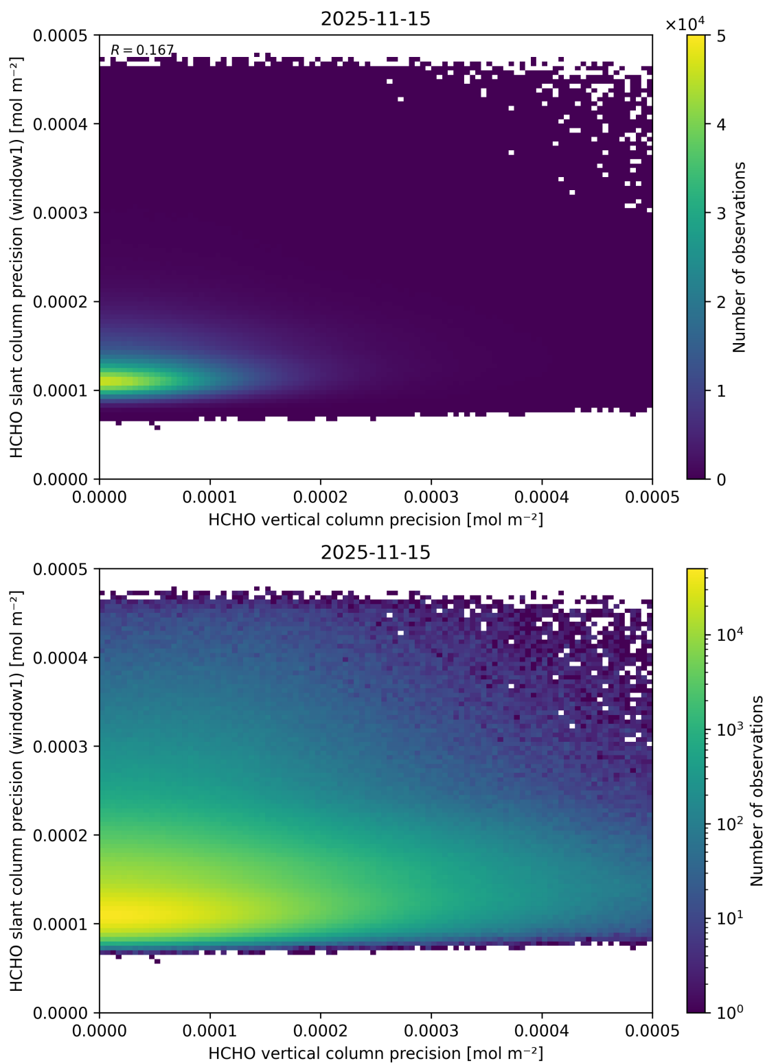
Figure 159: Scatter density plot of “HCHO vertical column precision” against “HCHO slant column precision (window1)” for 2025-11-14 to 2025-11-16.
