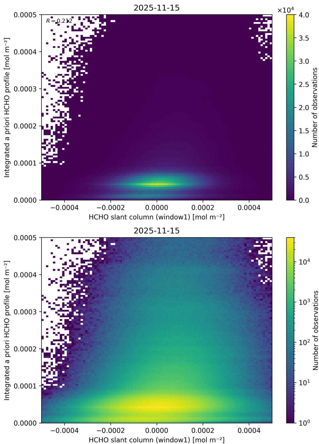
Figure 98: Scatter density plot of “HCHO slant column (window1)” against “Integrated a priori HCHO profile” for 2025-11-14 to 2025-11-16.
