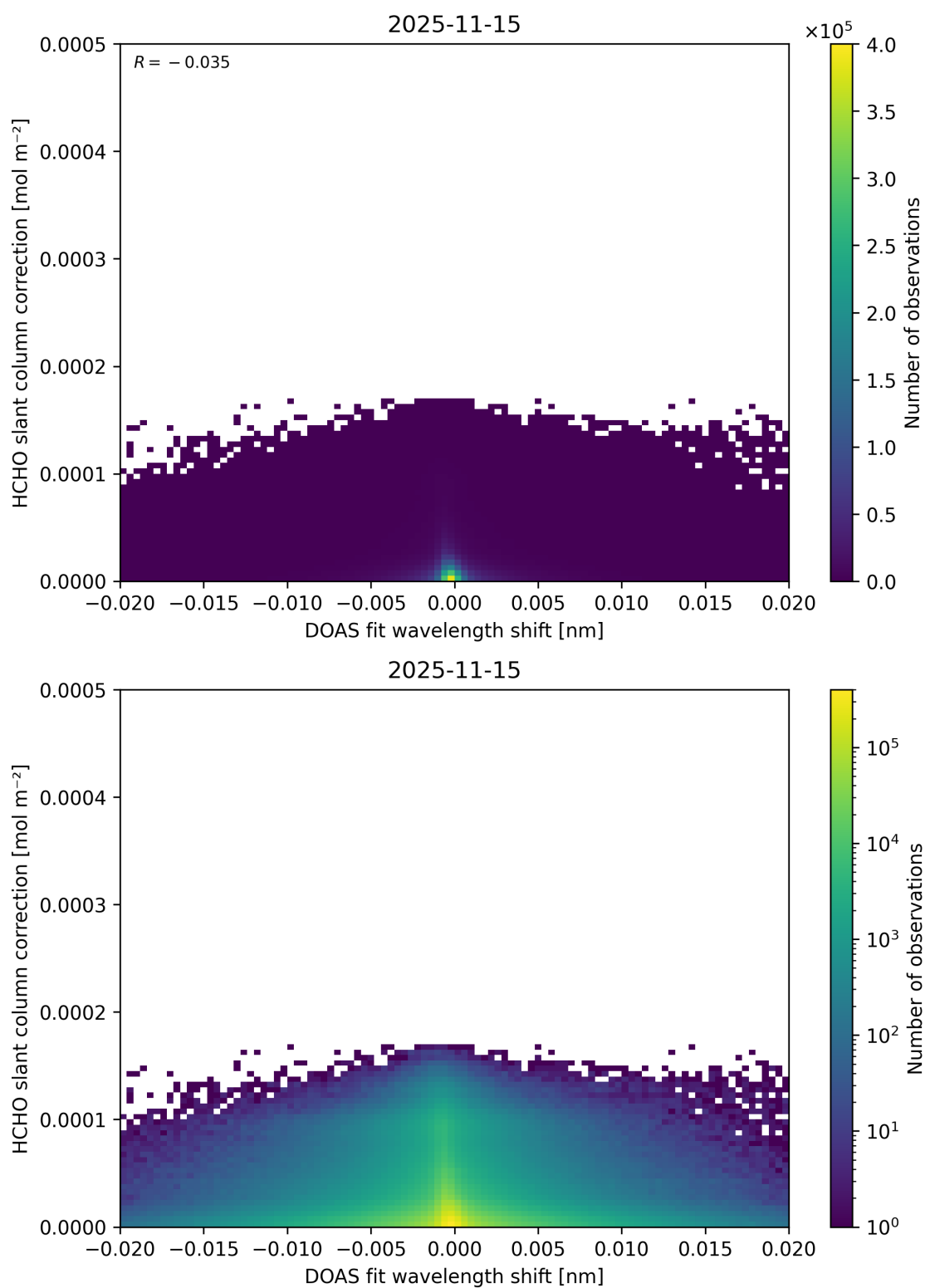
Figure 72: Scatter density plot of “DOAS fit wavelength shift” against “HCHO slant column correction” for 2025-11-14 to 2025-11-16.
