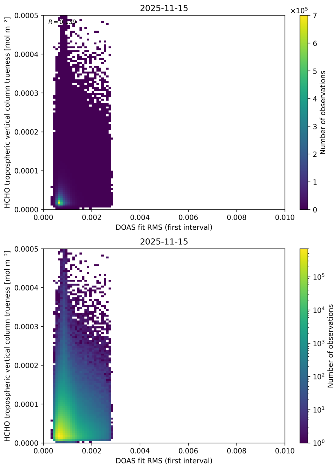
Figure 68: Scatter density plot of “DOAS fit RMS (first interval)” against “HCHO tropospheric vertical column trueness” for 2025-11-14 to 2025-11-16.
