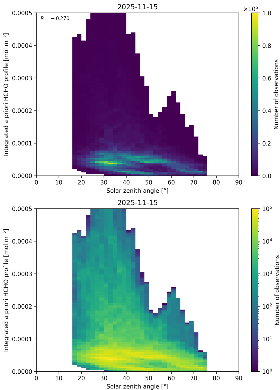
Figure 200: Scatter density plot of “Solar zenith angle” against “Integrated a priori HCHO profile” for 2025-11-14 to 2025-11-16.
