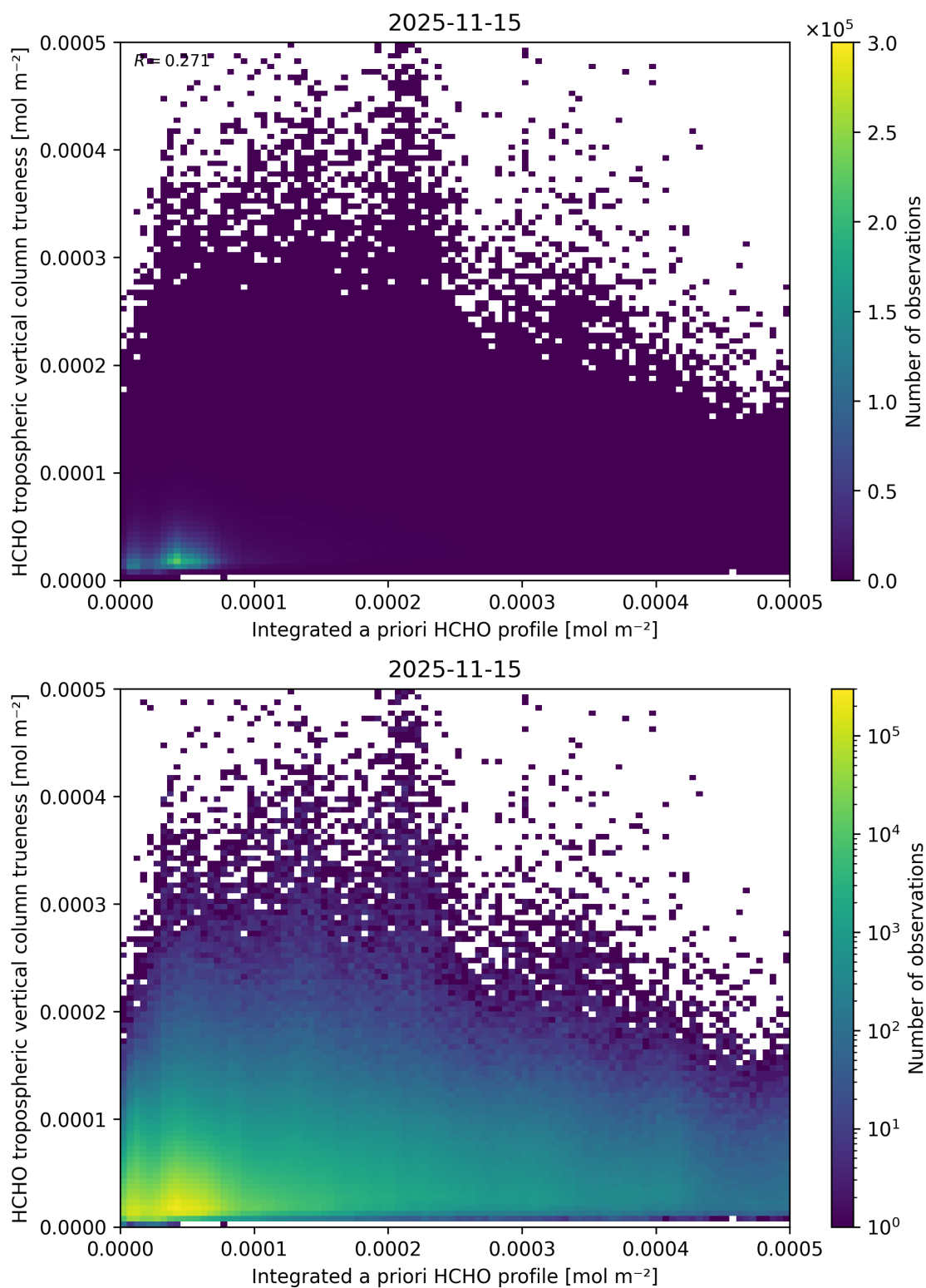
Figure 170: Scatter density plot of “Integrated a priori HCHO profile” against “HCHO tropospheric vertical column trueness” for 2025-11-14 to 2025-11-16.
