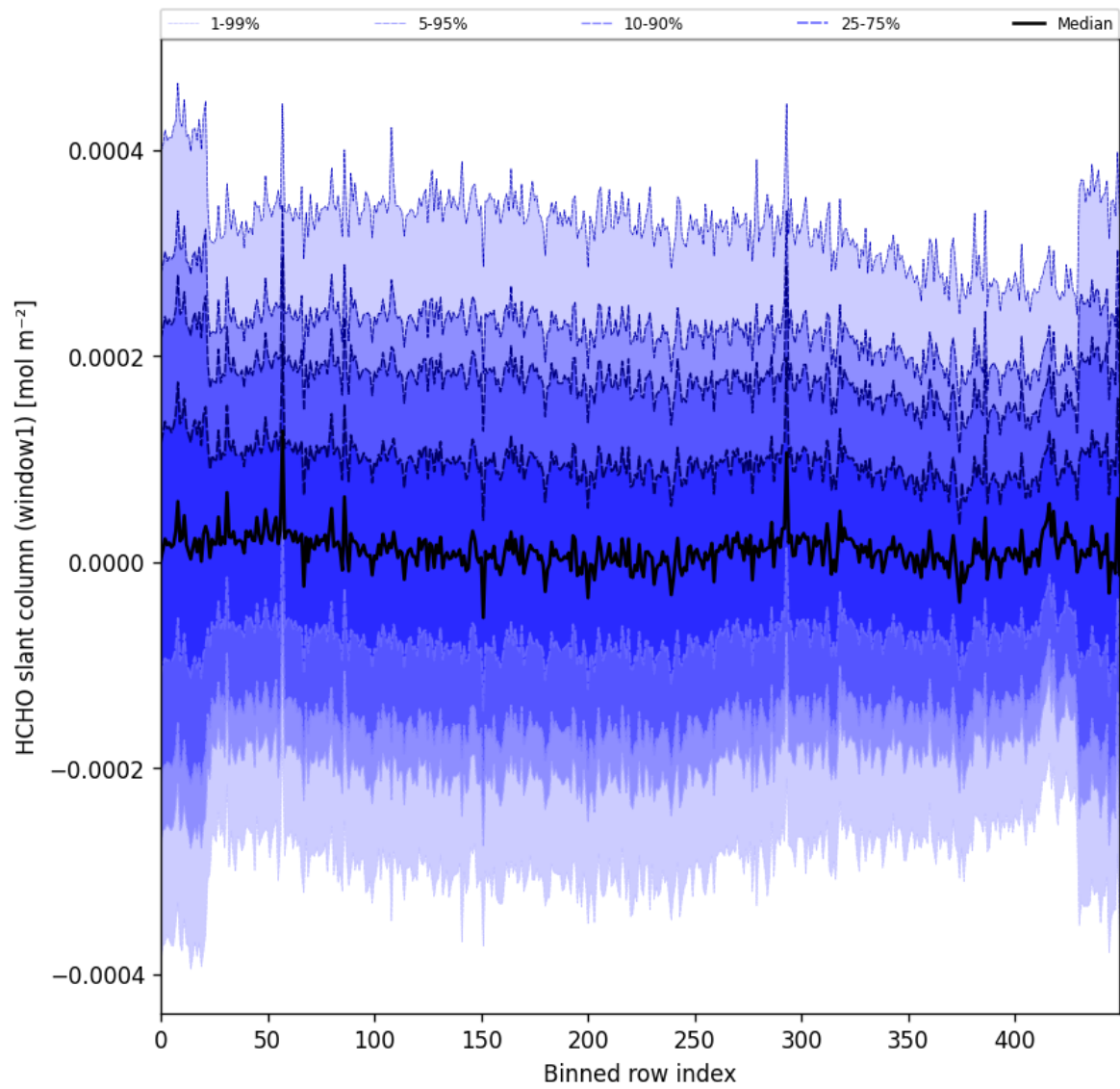
Figure 55: Along track statistics of “HCHO slant column (window1)” for 2025-11-14 to 2025-11-16
