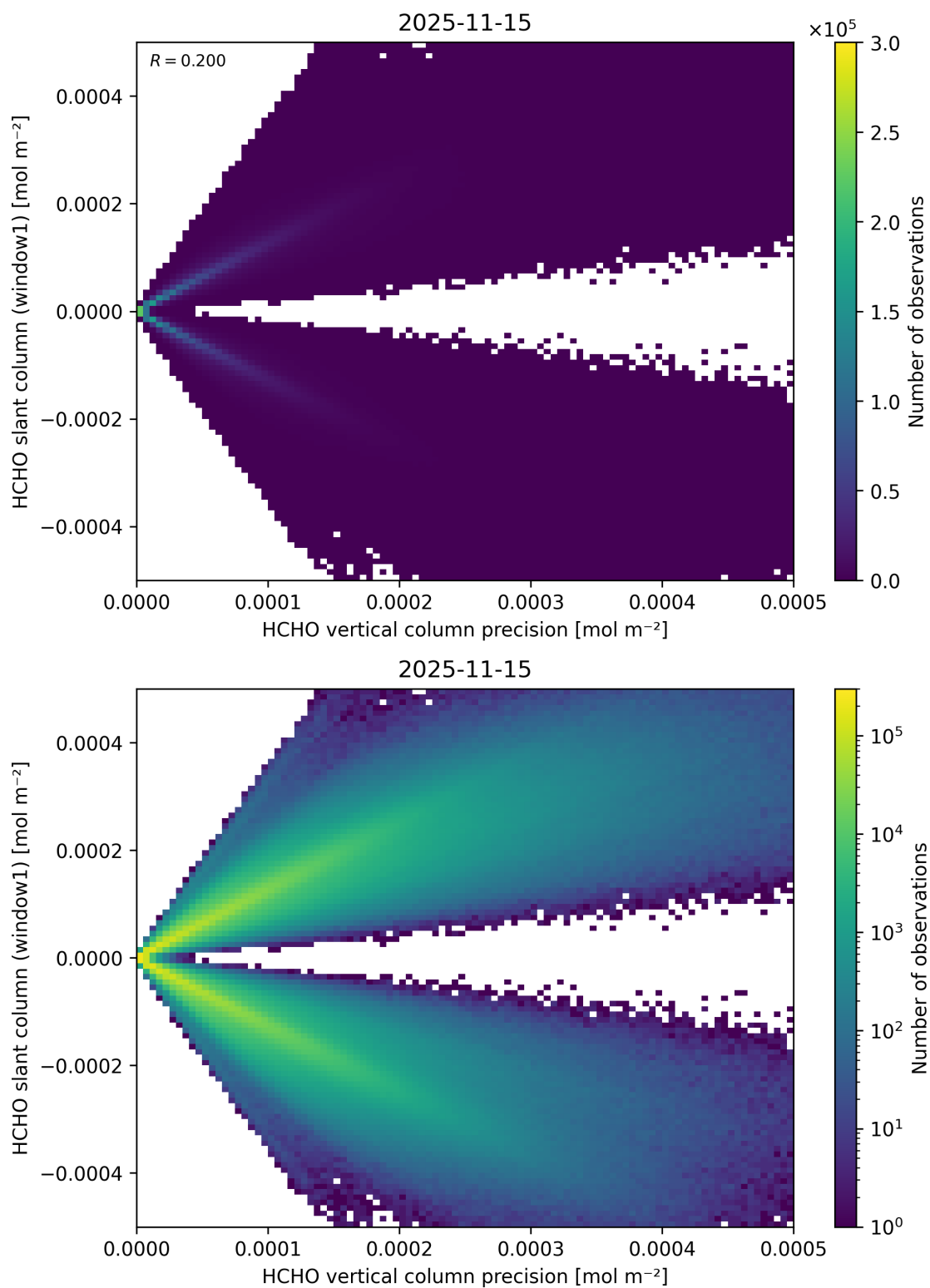
Figure 158: Scatter density plot of “HCHO vertical column precision” against “HCHO slant column (window1)” for 2025-11-14 to 2025-11-16.
