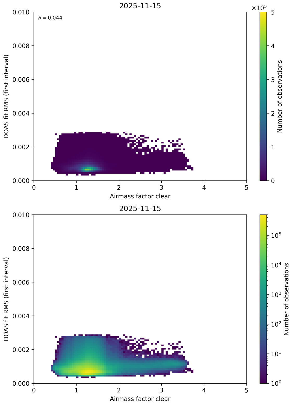
Figure 78: Scatter density plot of “Airmass factor clear” against “DOAS fit RMS (first interval)” for 2025-11-14 to 2025-11-16.
