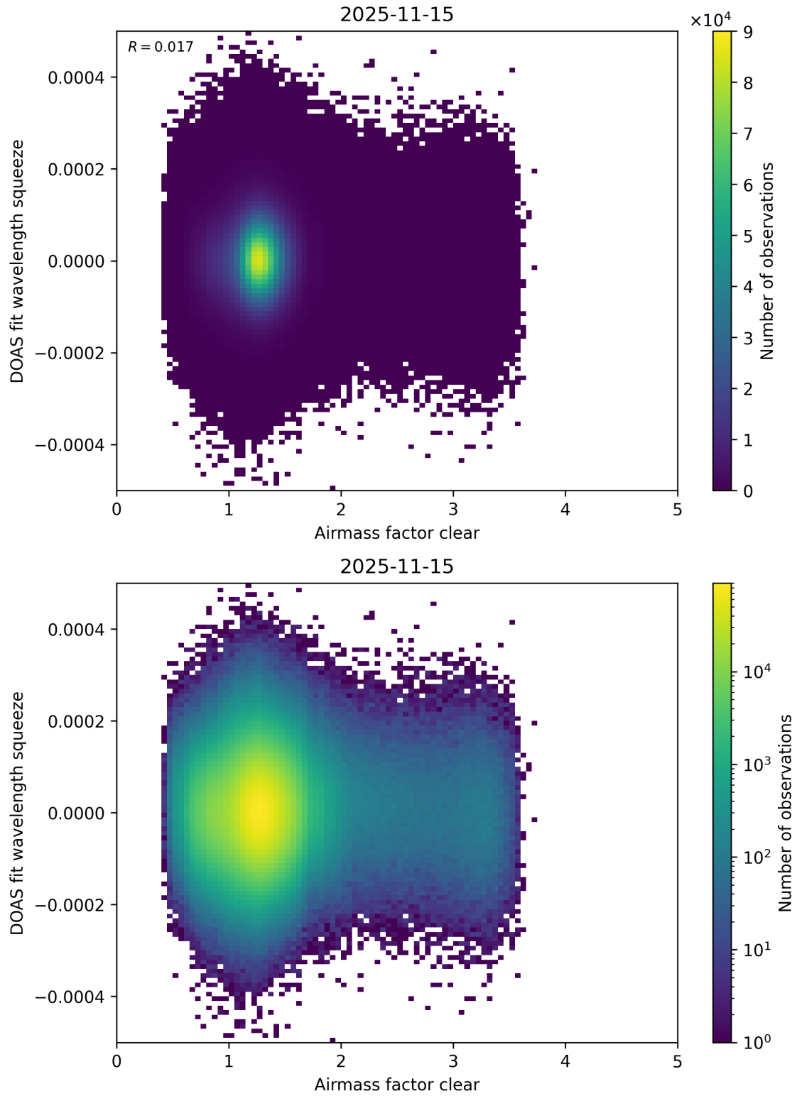
Figure 80: Scatter density plot of “Airmass factor clear” against “DOAS fit wavelength squeeze” for 2025-11-14 to 2025-11-16.
