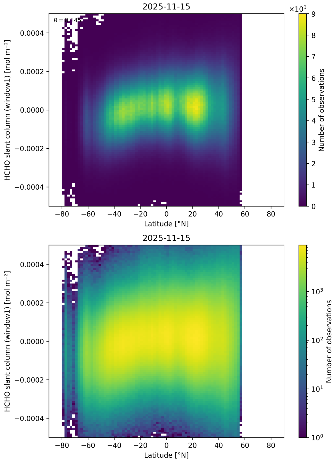
Figure 177: Scatter density plot of “Latitude” against “HCHO slant column (window1)” for 2025-11-14 to 2025-11-16.
