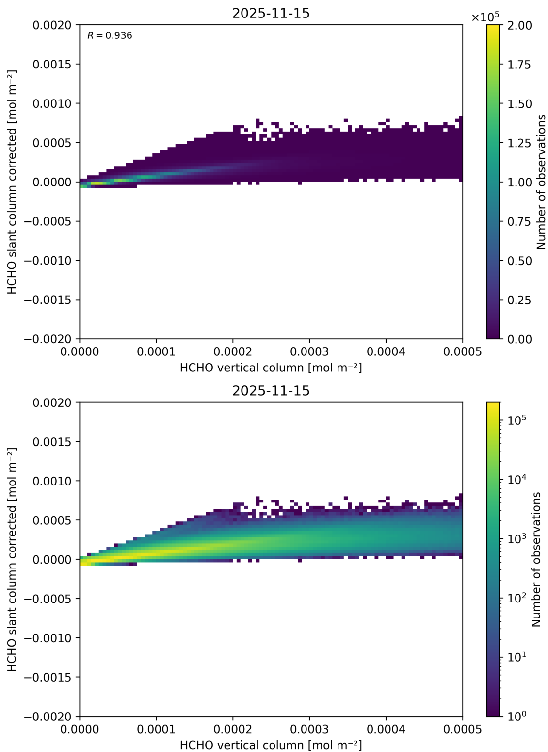
Figure 142: Scatter density plot of “HCHO vertical column” against “HCHO slant column corrected” for 2025-11-14 to 2025-11-16.
