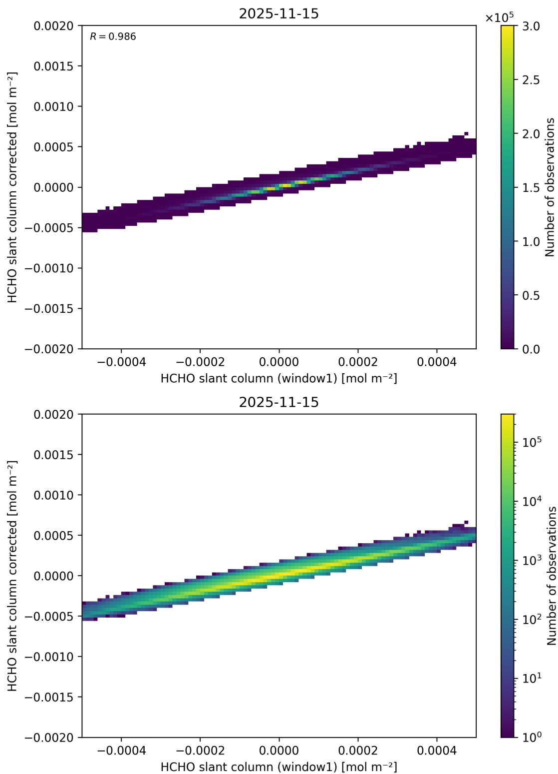
Figure 92: Scatter density plot of “HCHO slant column (window1)” against “HCHO slant column corrected” for 2025-11-14 to 2025-11-16.
