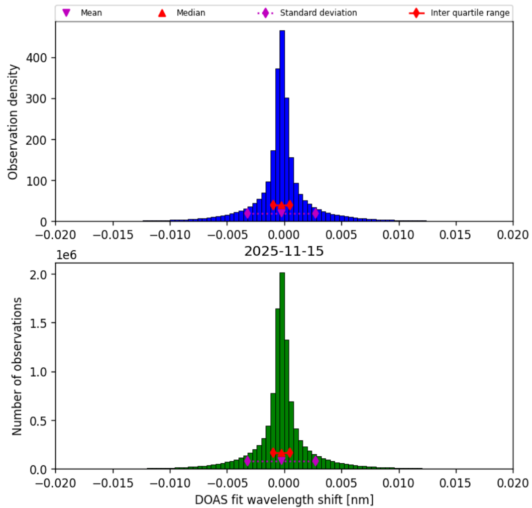
Figure 46: Histogram of “DOAS fit wavelength shift” for 2025-11-14 to 2025-11-16
