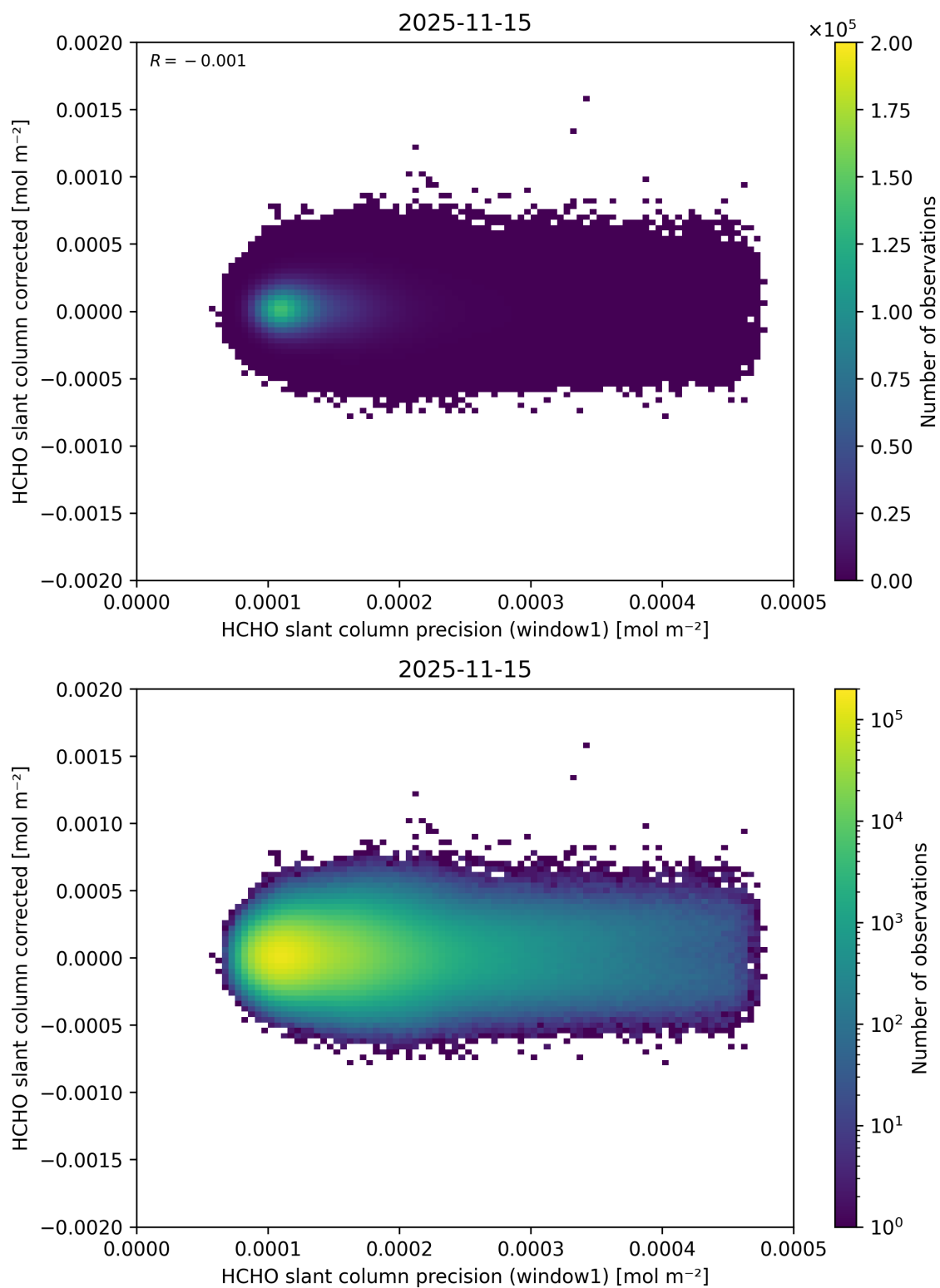
Figure 103: Scatter density plot of “HCHO slant column precision (window1)” against “HCHO slant column corrected” for 2025-11-14 to 2025-11-16.
