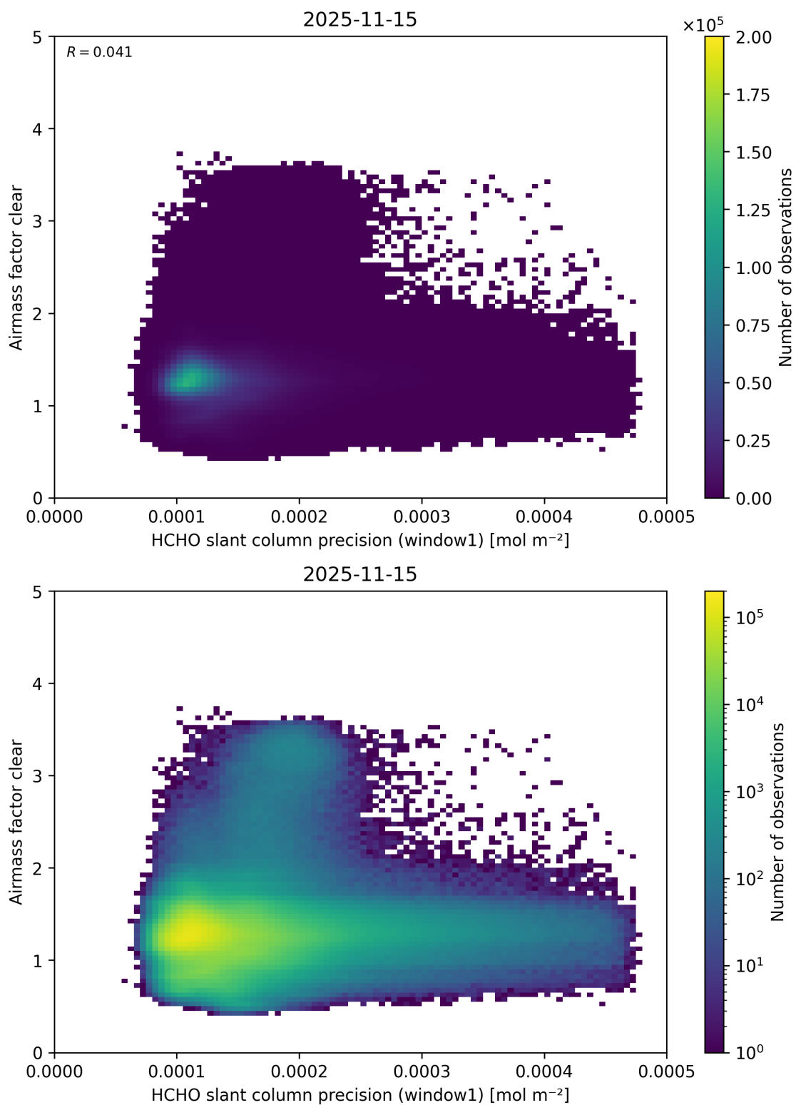
Figure 102: Scatter density plot of “HCHO slant column precision (window1)” against “Airmass factor clear” for 2025-11-14 to 2025-11-16.
