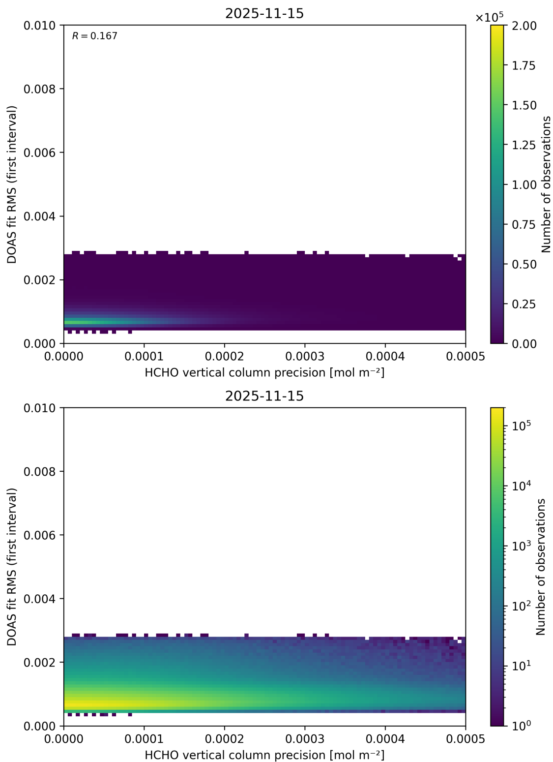
Figure 152: Scatter density plot of “HCHO vertical column precision” against “DOAS fit RMS (first interval)” for 2025-11-14 to 2025-11-16.
