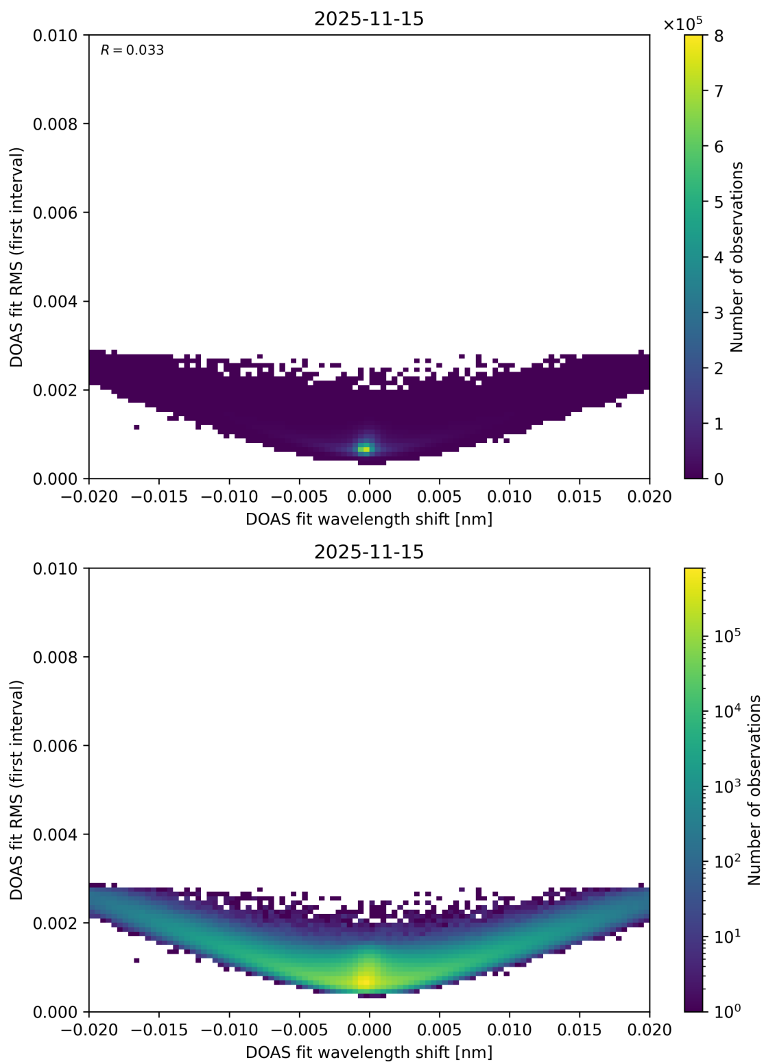
Figure 69: Scatter density plot of “DOAS fit wavelength shift” against “DOAS fit RMS (first interval)” for 2025-11-14 to 2025-11-16.
