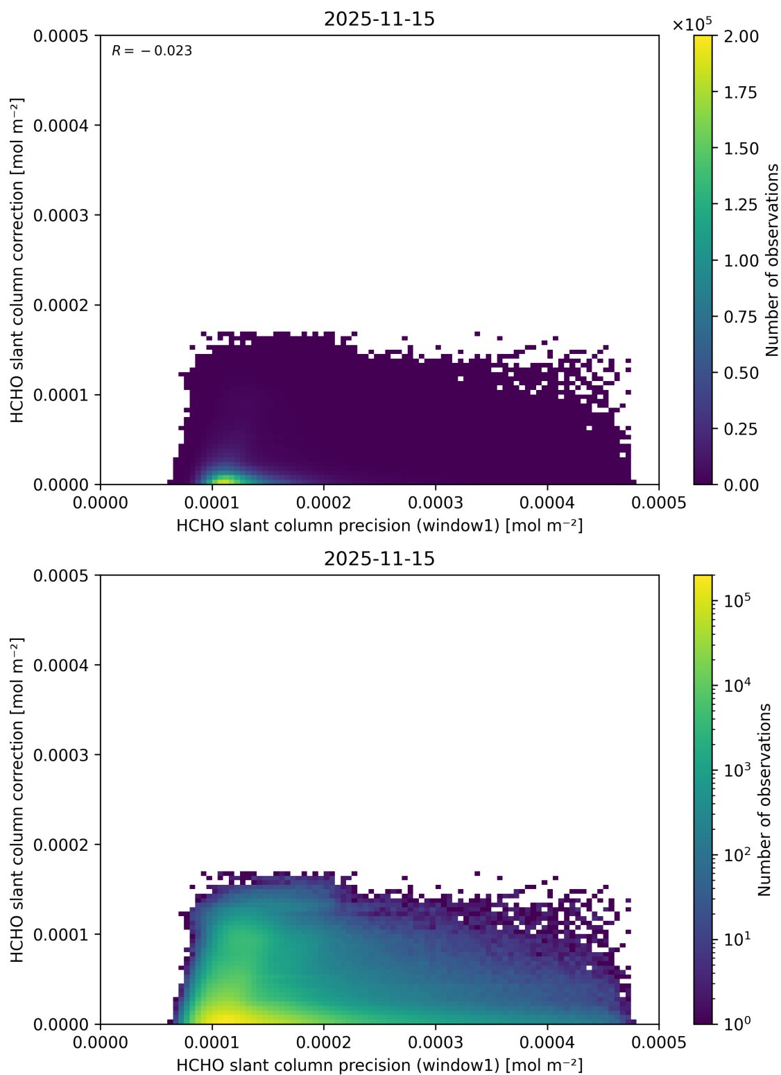
Figure 104: Scatter density plot of “HCHO slant column precision (window1)” against “HCHO slant column correction” for 2025-11-14 to 2025-11-16.
