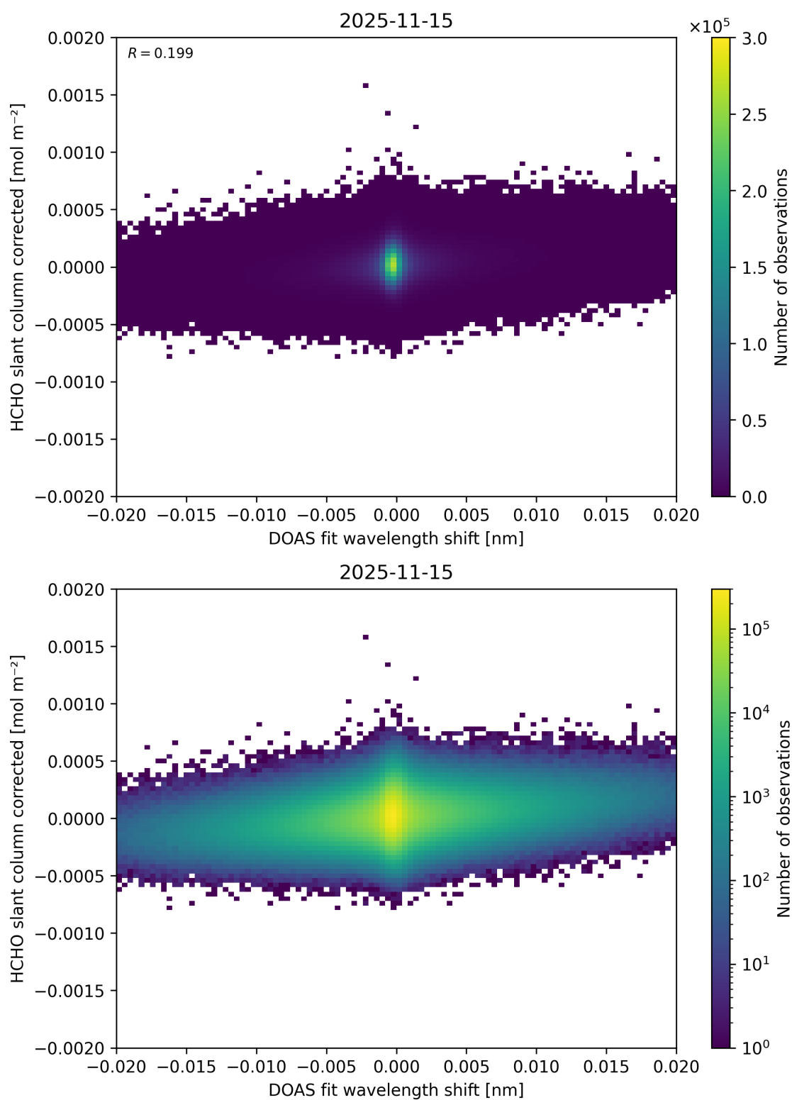
Figure 71: Scatter density plot of “DOAS fit wavelength shift” against “HCHO slant column corrected” for 2025-11-14 to 2025-11-16.
