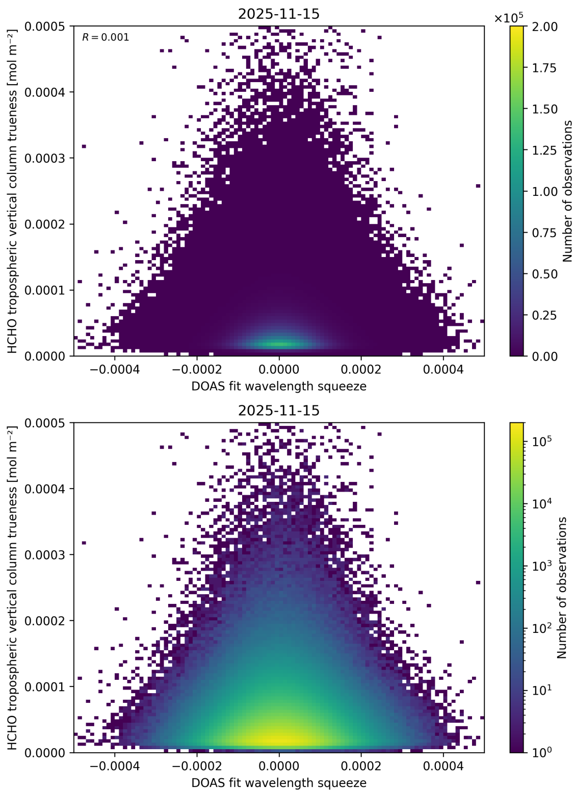
Figure 77: Scatter density plot of “DOAS fit wavelength squeeze” against “HCHO tropospheric vertical column trueness” for 2025-11-14 to 2025-11-16.
