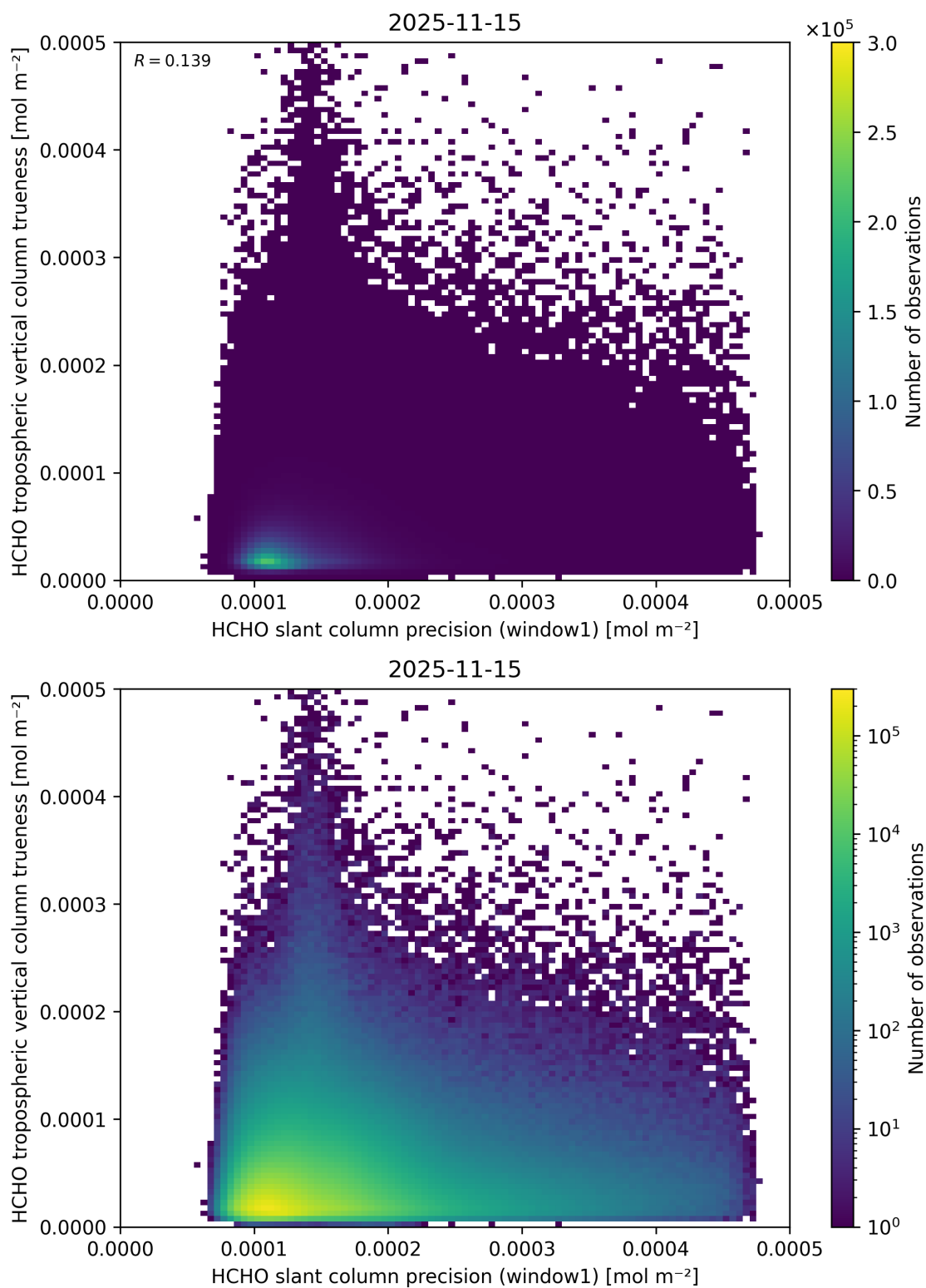
Figure 107: Scatter density plot of “HCHO slant column precision (window1)” against “HCHO tropospheric vertical column trueness” for 2025-11-14 to 2025-11-16.
