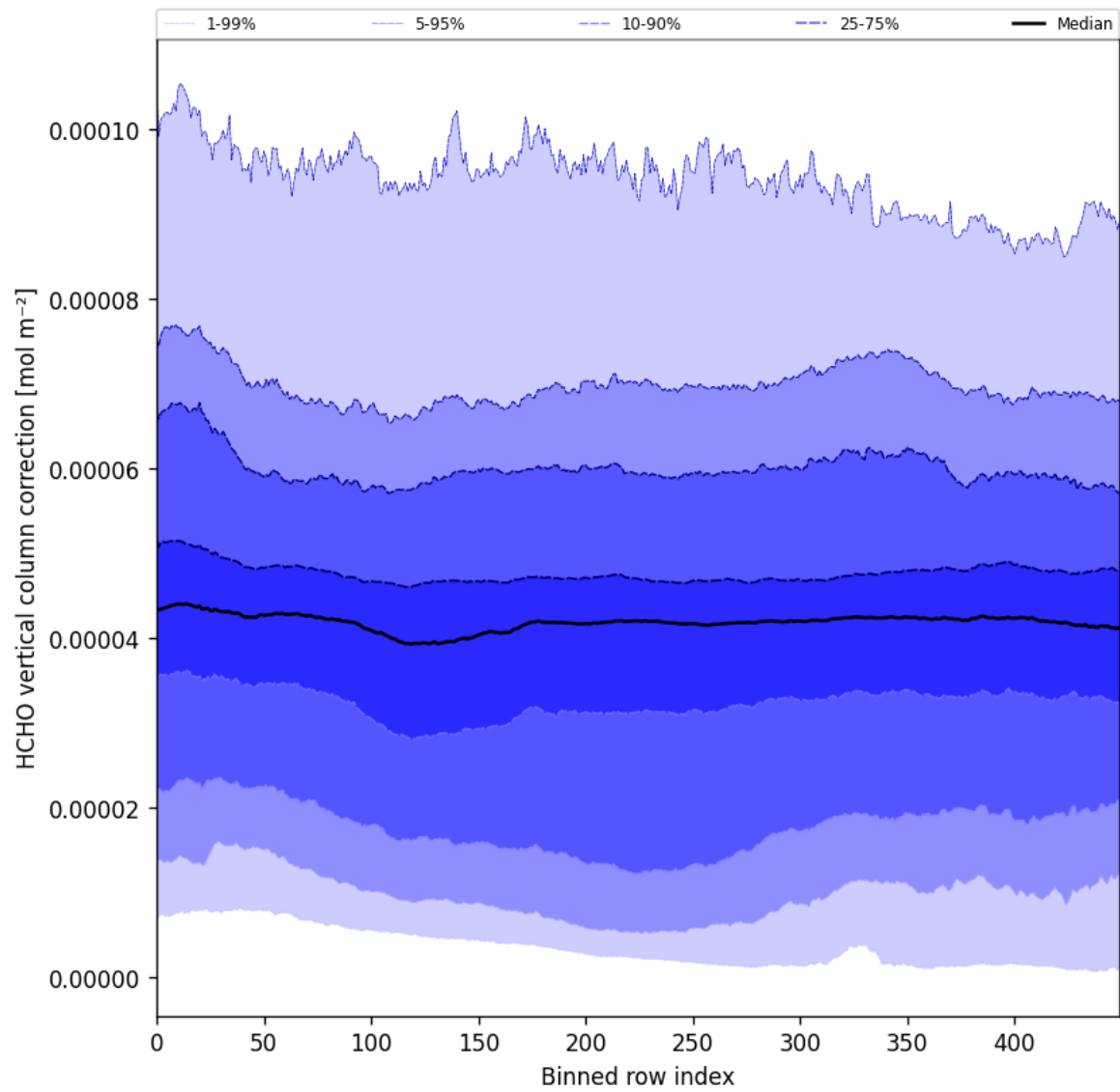
Figure 54: Along track statistics of “HCHO vertical column correction” for 2025-11-14 to 2025-11-16
