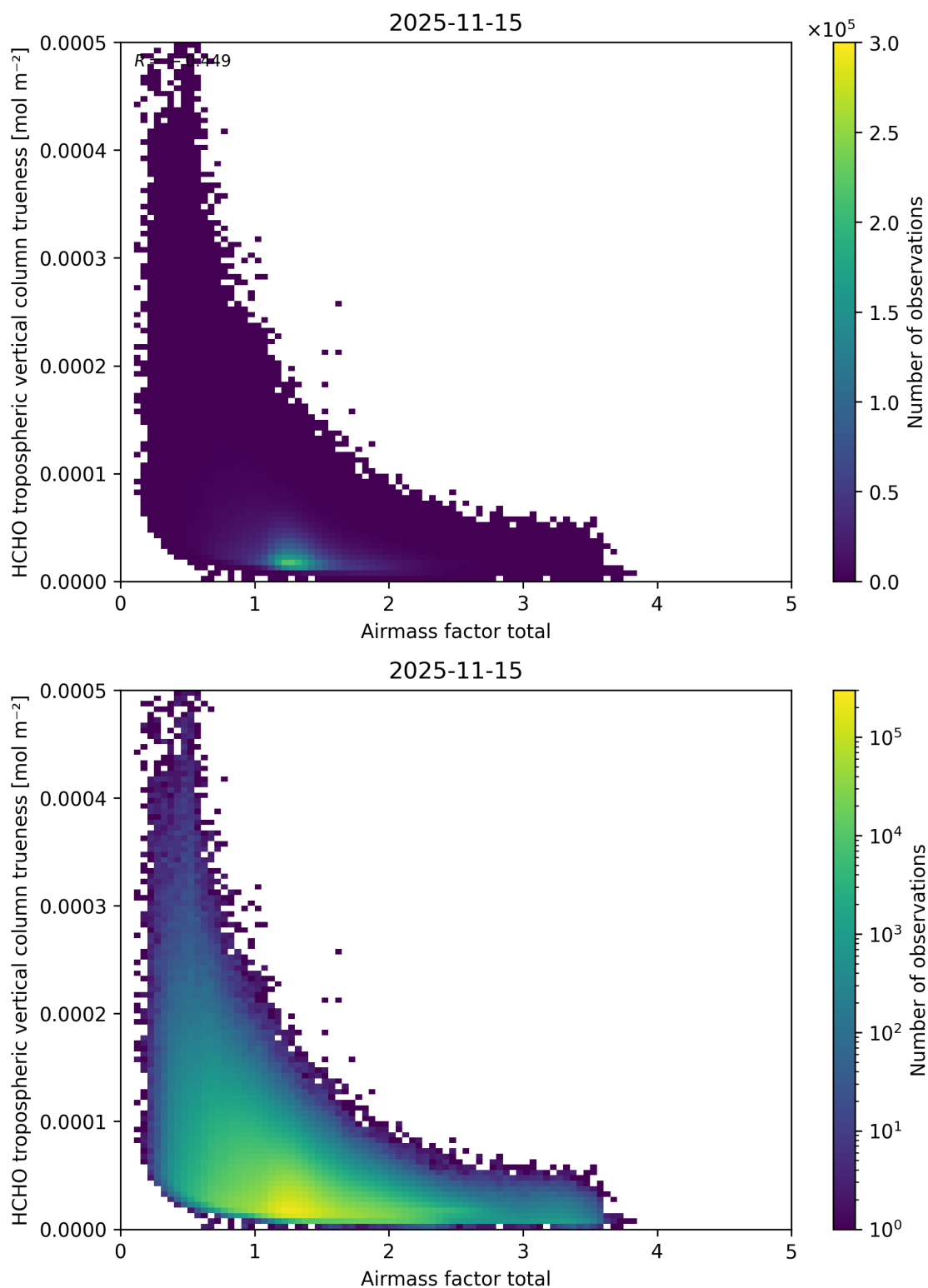
Figure 116: Scatter density plot of “Airmass factor total” against “HCHO tropospheric vertical column trueness” for 2025-11-14 to 2025-11-16.
