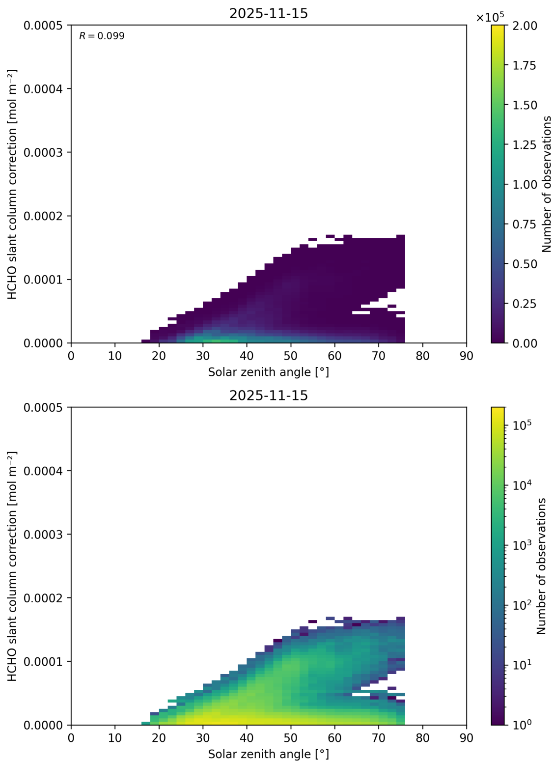
Figure 191: Scatter density plot of “Solar zenith angle” against “HCHO slant column correction” for 2025-11-14 to 2025-11-16.
