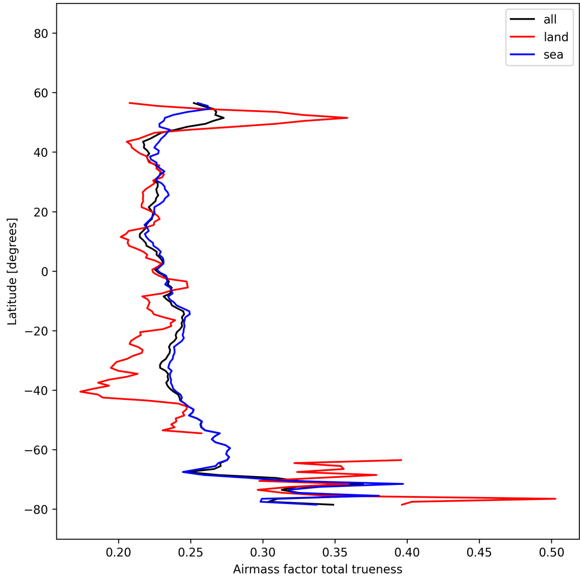
Figure 28: Zonal average of “Airmass factor total truiness” for 2025-11-14 to 2025-11-16.
