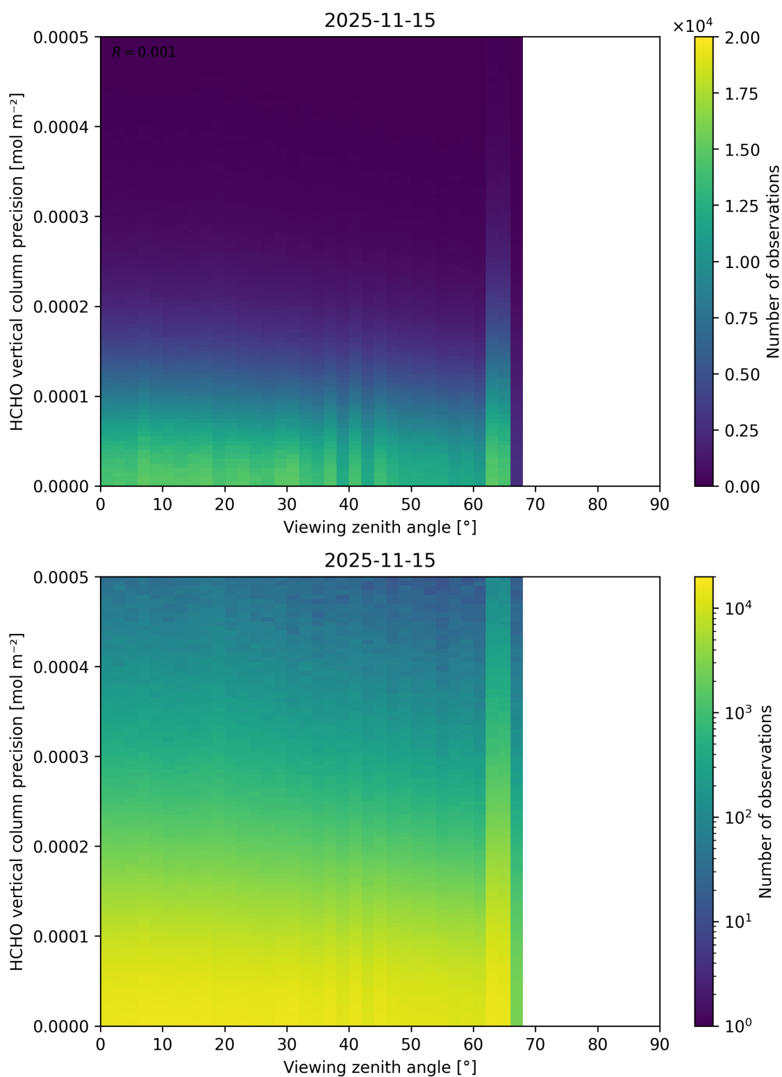
Figure 214: Scatter density plot of “Viewing zenith angle” against “HCHO vertical column precision” for 2025-11-14 to 2025-11-16.
