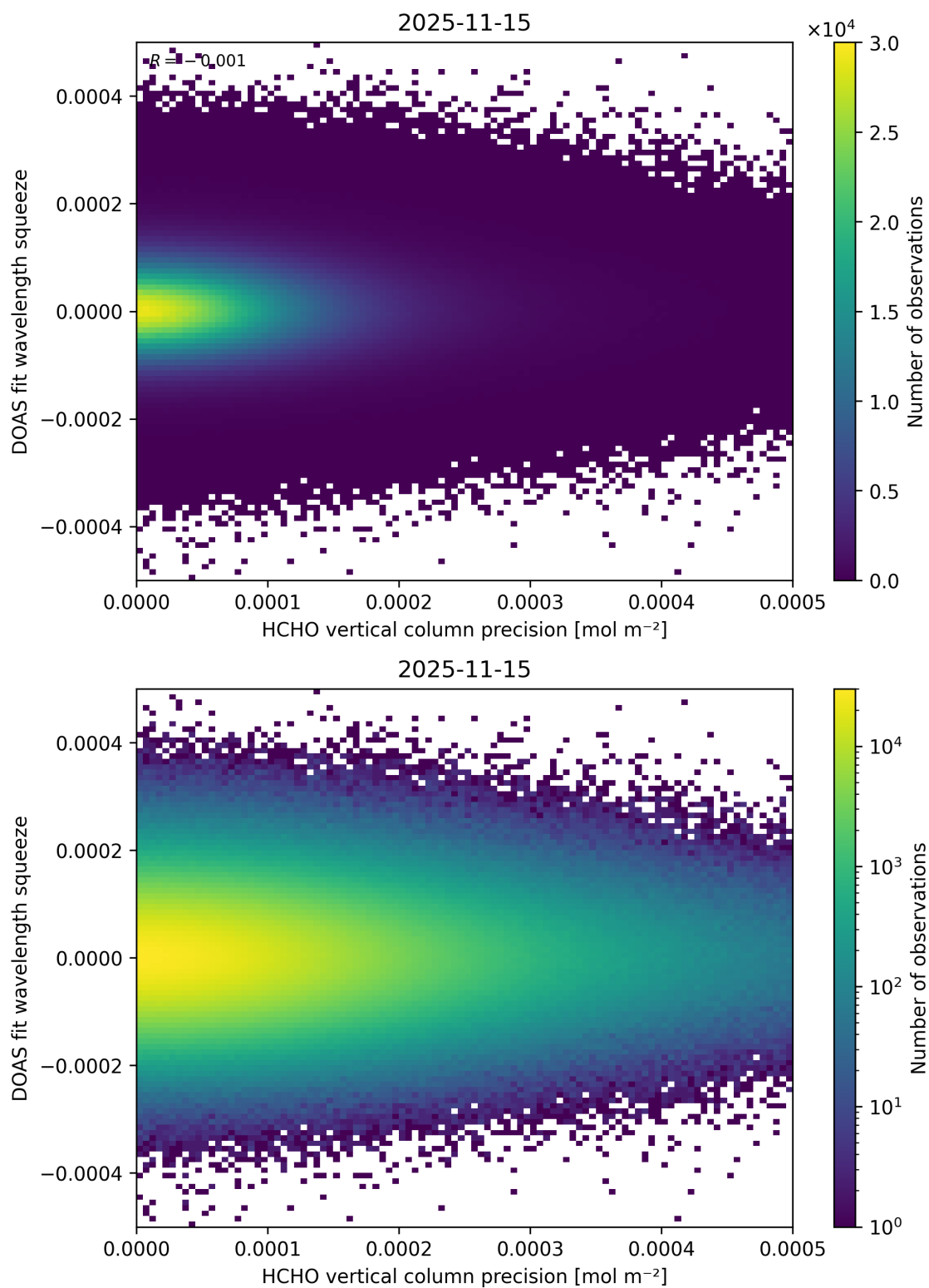
Figure 154: Scatter density plot of “HCHO vertical column precision” against “DOAS fit wavelength squeeze” for 2025-11-14 to 2025-11-16.
