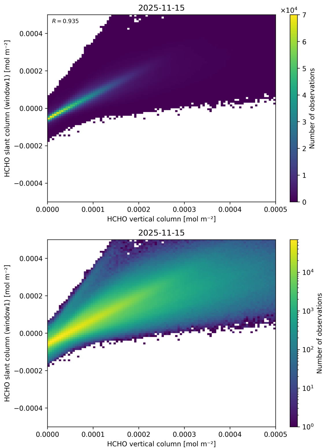
Figure 144: Scatter density plot of “HCHO vertical column” against “HCHO slant column (window1)” for 2025-11-14 to 2025-11-16.
