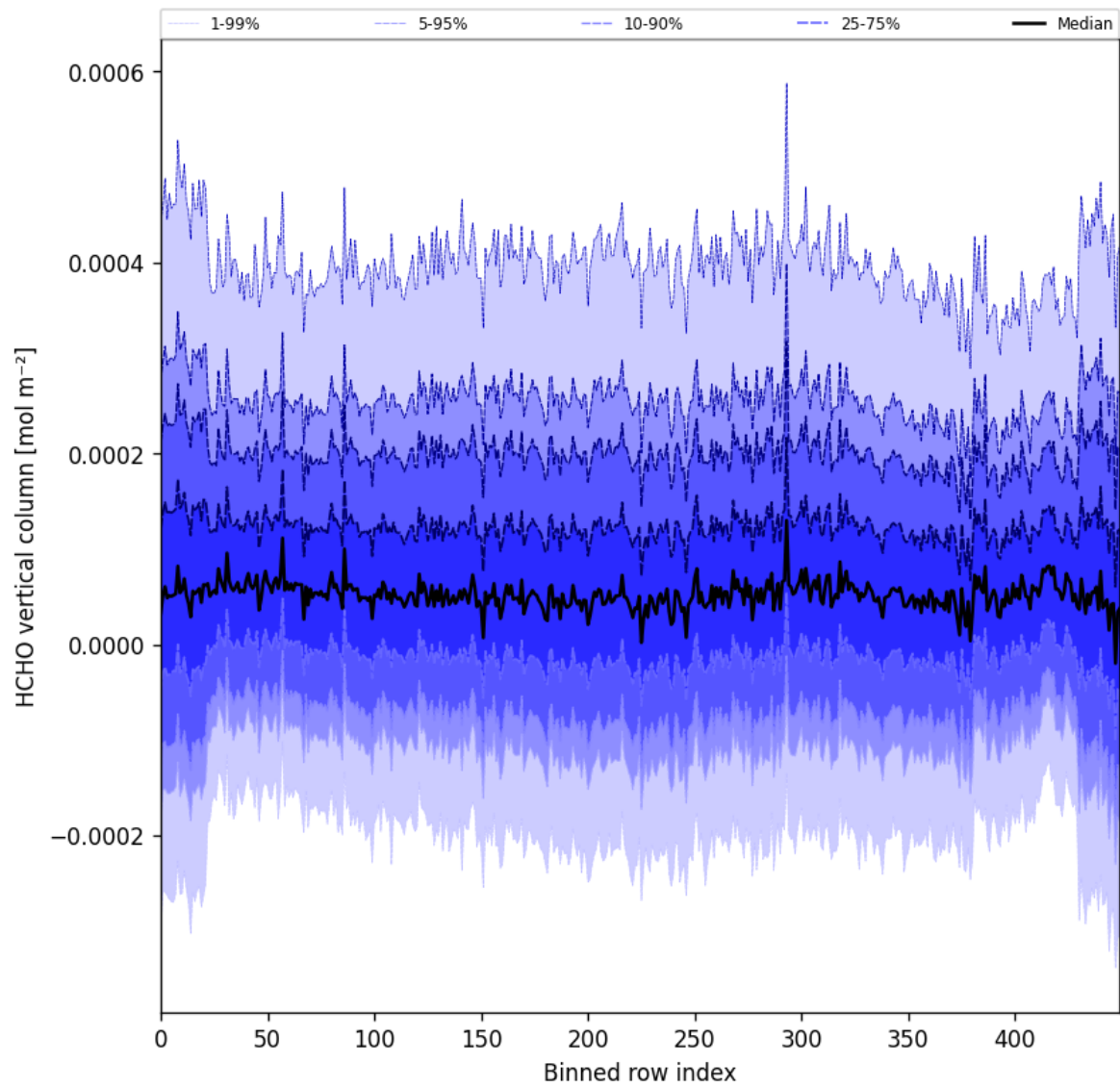
Figure 52: Along track statistics of “HCHO vertical column” for 2025-11-14 to 2025-11-16
