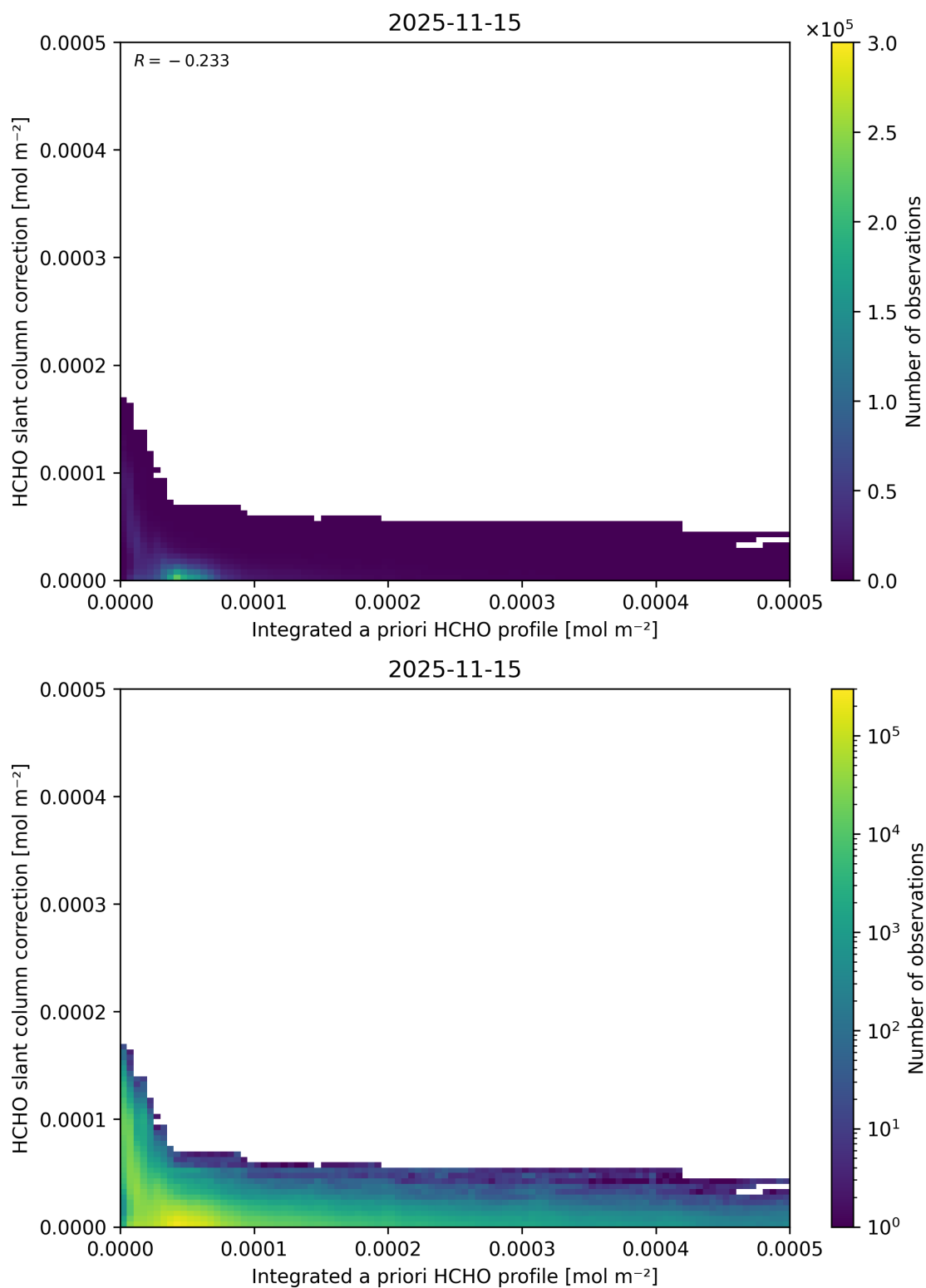
Figure 169: Scatter density plot of “Integrated a priori HCHO profile” against “HCHO slant column correction” for 2025-11-14 to 2025-11-16.
