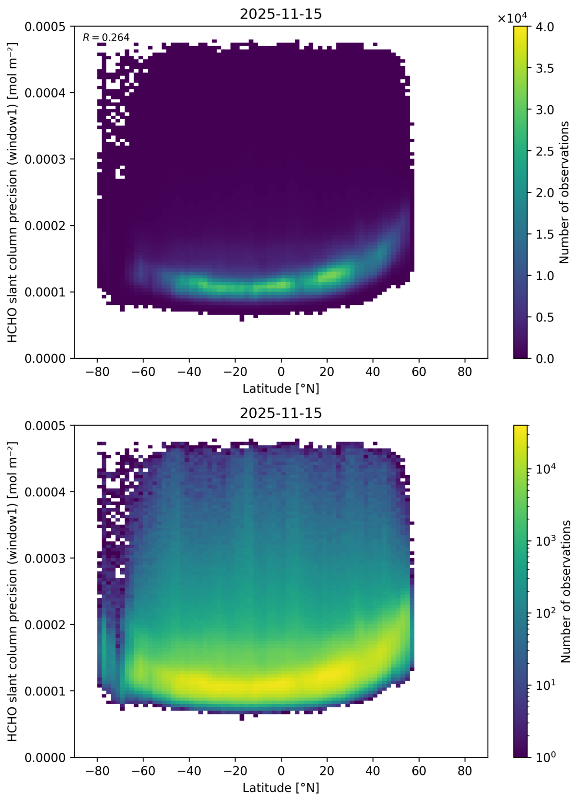
Figure 178: Scatter density plot of “Latitude” against “HCHO slant column precision (window1)” for 2025-11-14 to 2025-11-16.
