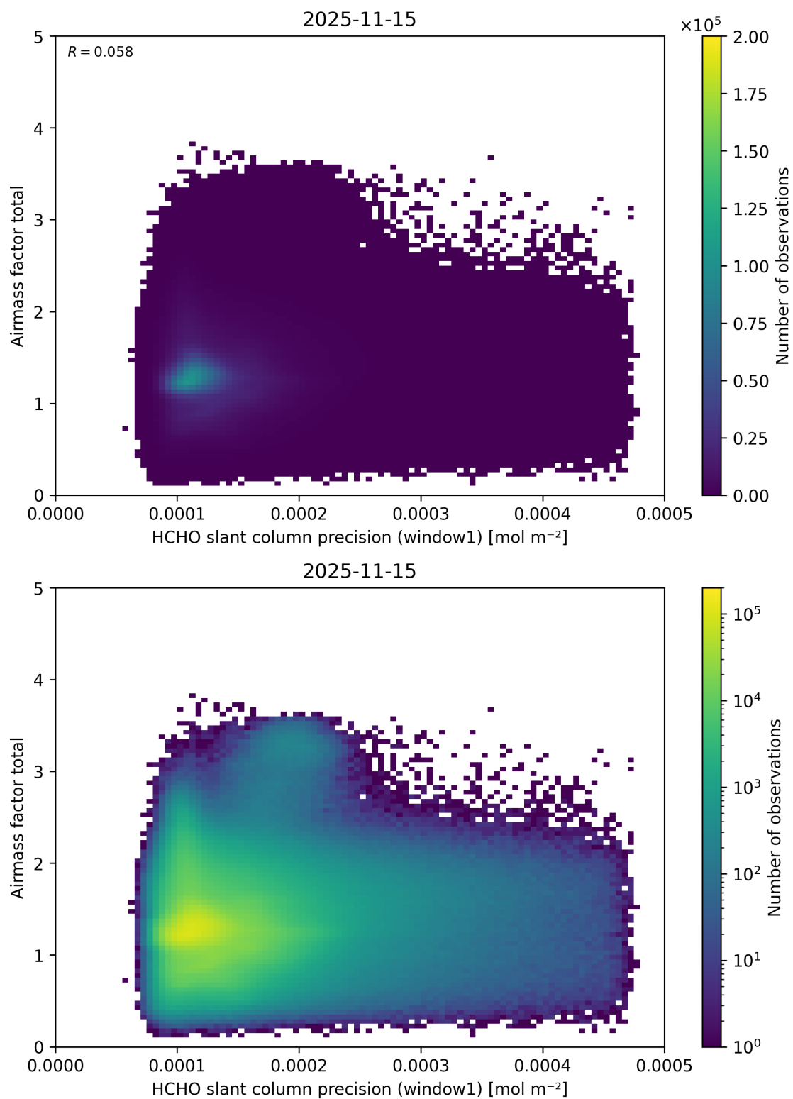
Figure 105: Scatter density plot of “HCHO slant column precision (window1)” against “Airmass factor total” for 2025-11-14 to 2025-11-16.
