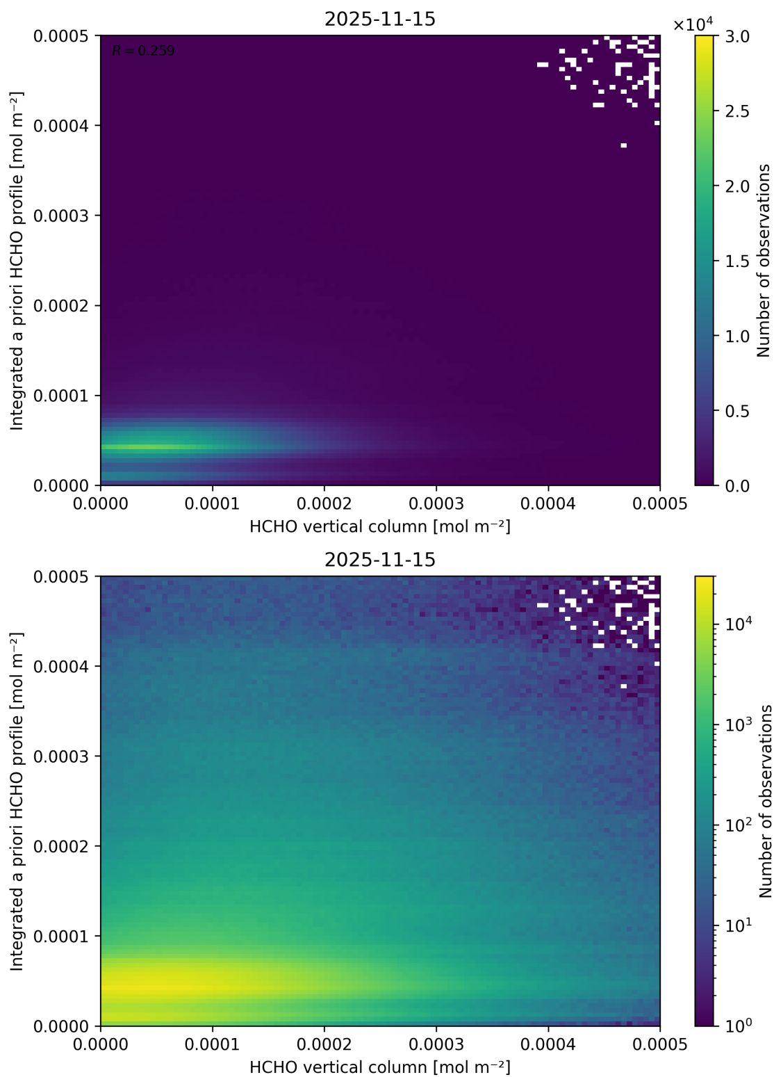
Figure 151: Scatter density plot of “HCHO vertical column” against “Integrated a priori HCHO profile” for 2025-11-14 to 2025-11-16.
