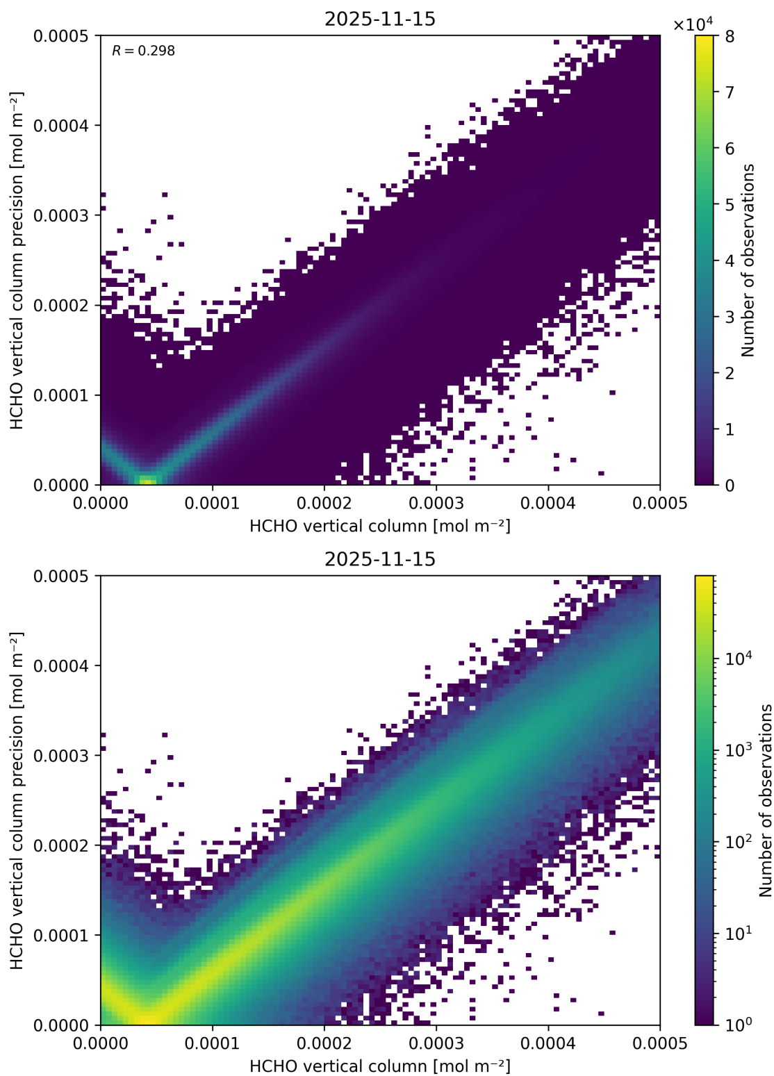
Figure 149: Scatter density plot of “HCHO vertical column” against “HCHO vertical column precision” for 2025-11-14 to 2025-11-16.
