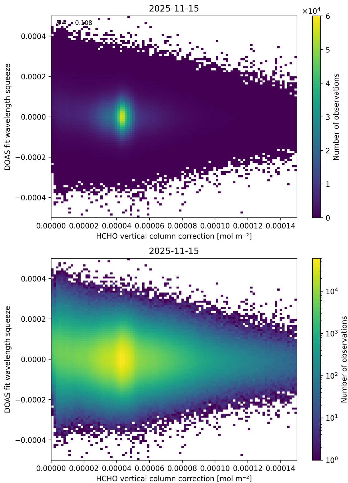
Figure 128: Scatter density plot of “HCHO vertical column correction” against “DOAS fit wavelength squeeze” for 2025-11-14 to 2025-11-16.
