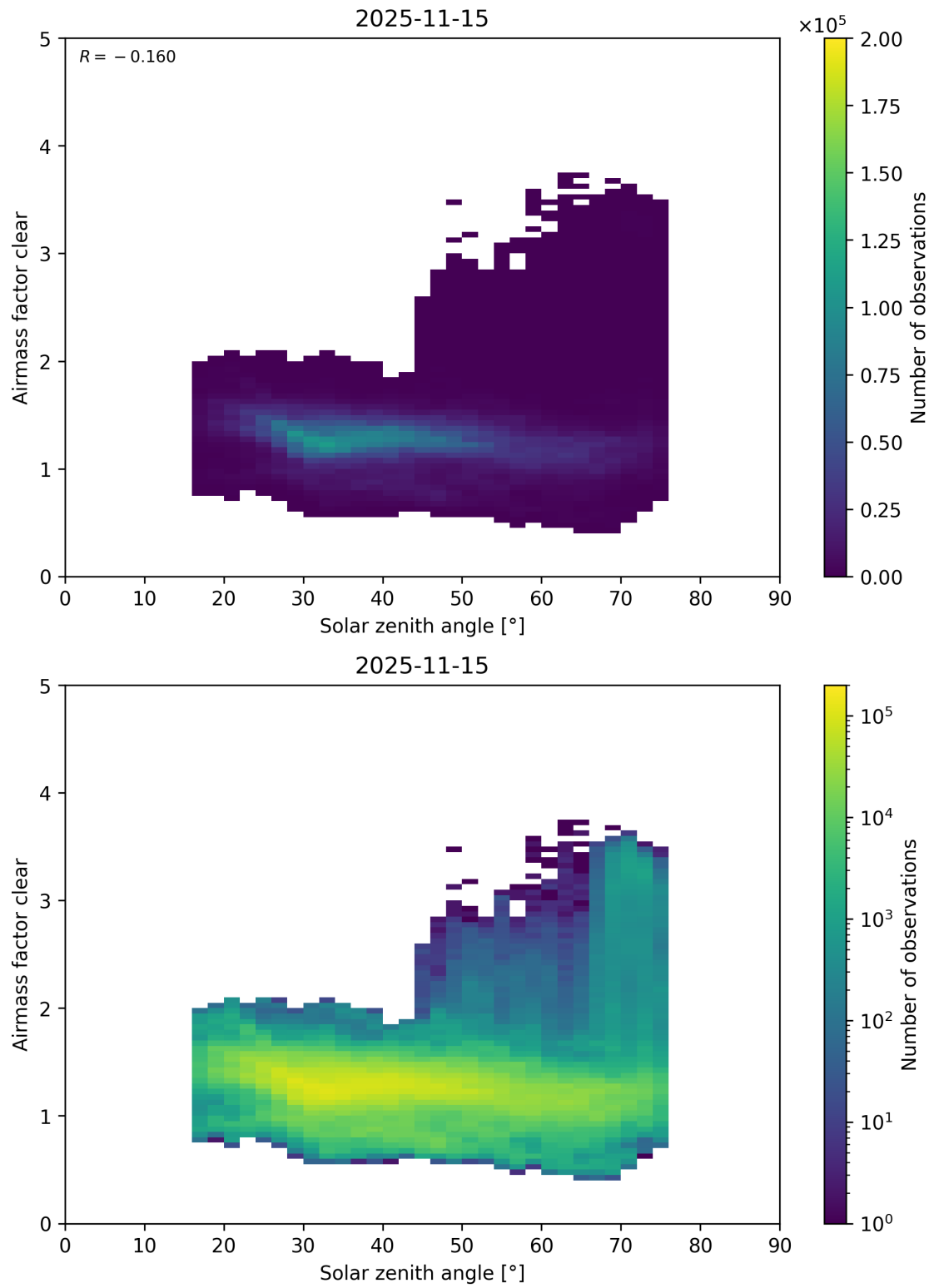
Figure 189: Scatter density plot of “Solar zenith angle” against “Airmass factor clear” for 2025-11-14 to 2025-11-16.
