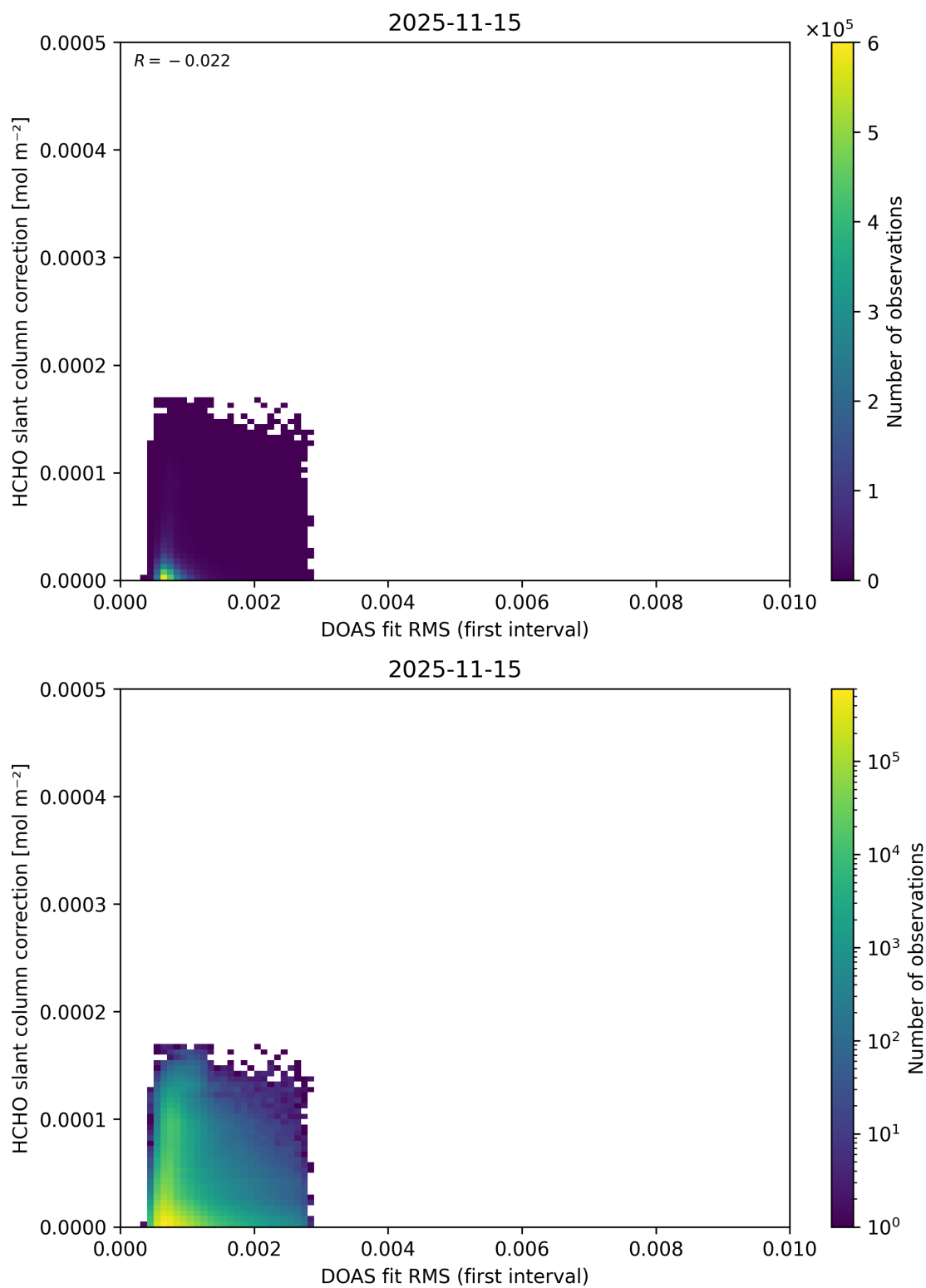
Figure 67: Scatter density plot of “DOAS fit RMS (first interval)” against “HCHO slant column correction” for 2025-11-14 to 2025-11-16.
