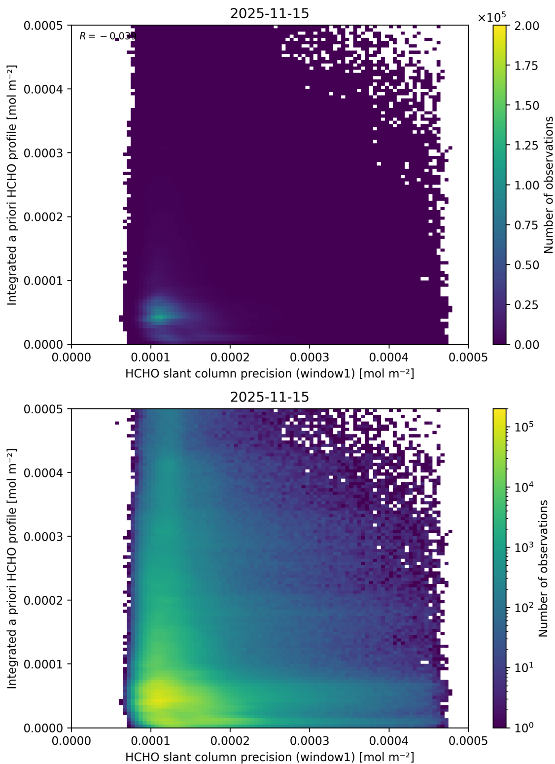
Figure 108: Scatter density plot of “HCHO slant column precision (window1)” against “Integrated a priori HCHO profile” for 2025-11-14 to 2025-11-16.
