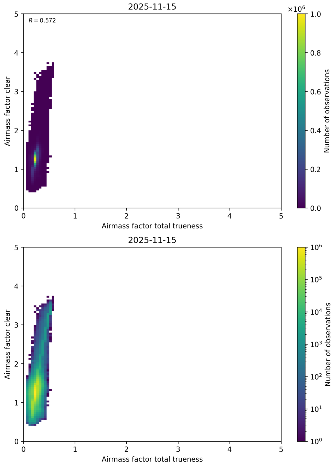
Figure 121: Scatter density plot of “Airmass factor total trueness” against “Airmass factor clear” for 2025-11-14 to 2025-11-16.
