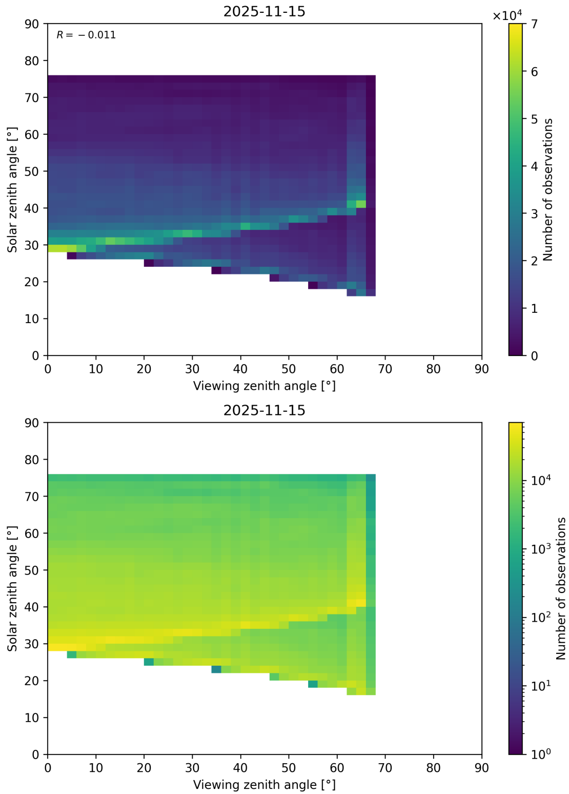
Figure 218: Scatter density plot of “Viewing zenith angle” against “Solar zenith angle” for 2025-11-14 to 2025-11-16.
