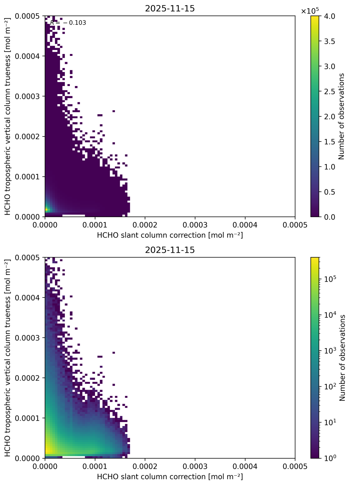
Figure 87: Scatter density plot of “HCHO slant column correction” against “HCHO tropospheric vertical column trueness” for 2025-11-14 to 2025-11-16.
