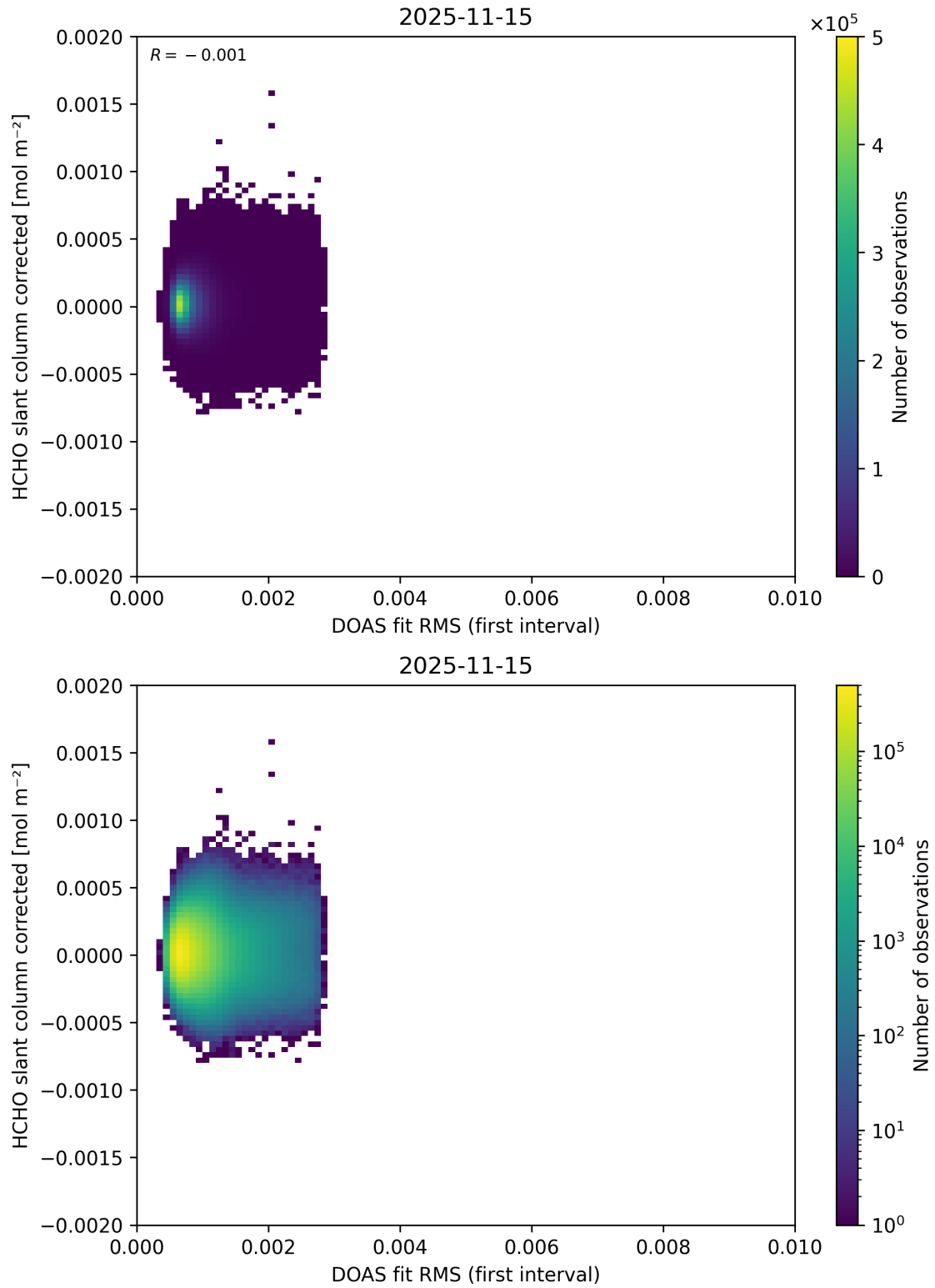
Figure 66: Scatter density plot of “DOAS fit RMS (first interval)” against “HCHO slant column corrected” for 2025-11-14 to 2025-11-16.
