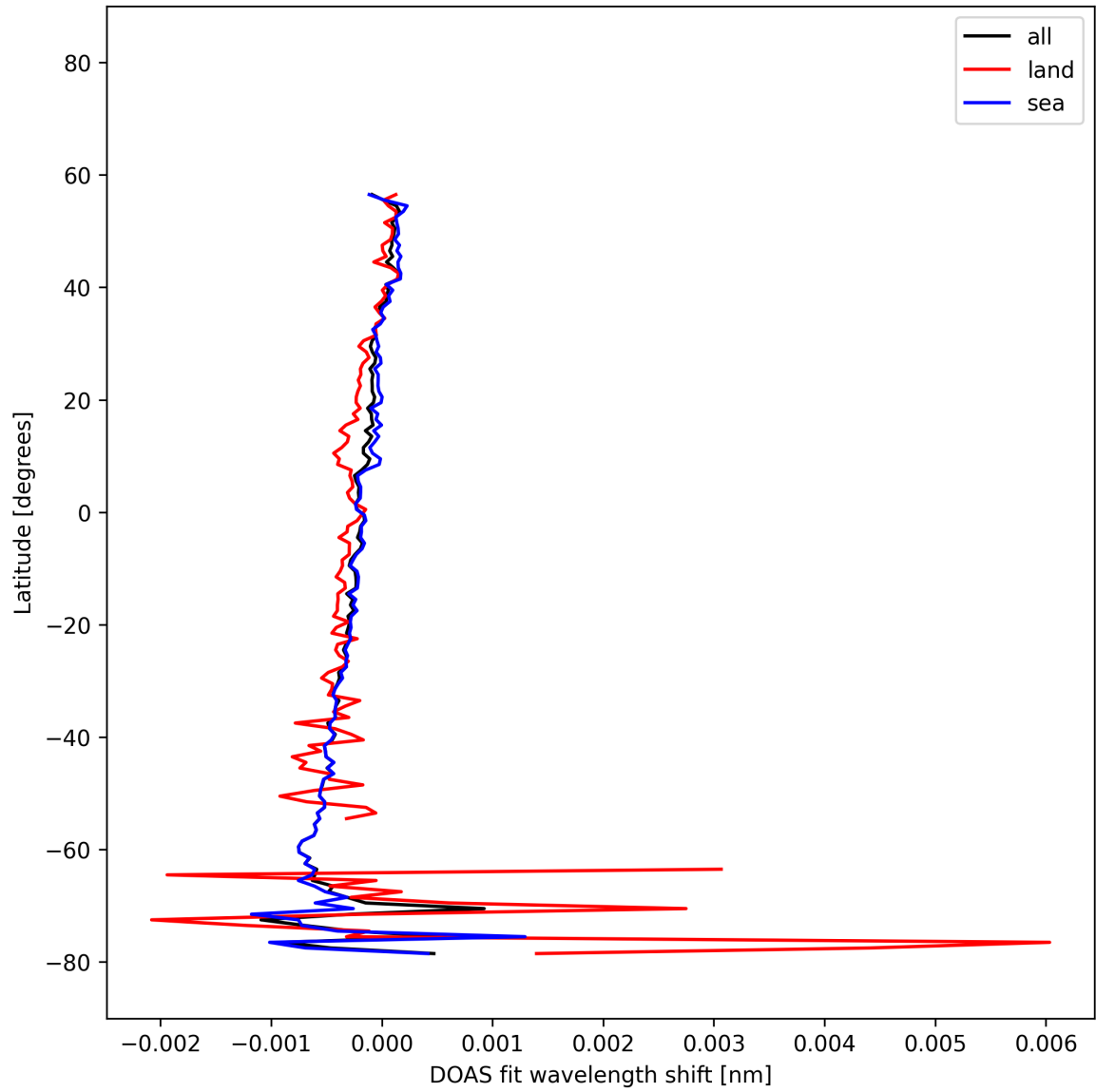
Figure 31: Zonal average of “DOAS fit wavelength shift” for 2025-11-14 to 2025-11-16.
