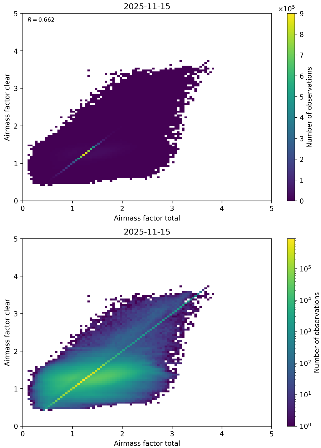
Figure 112: Scatter density plot of “Airmass factor total” against “Airmass factor clear” for 2025-11-14 to 2025-11-16.
