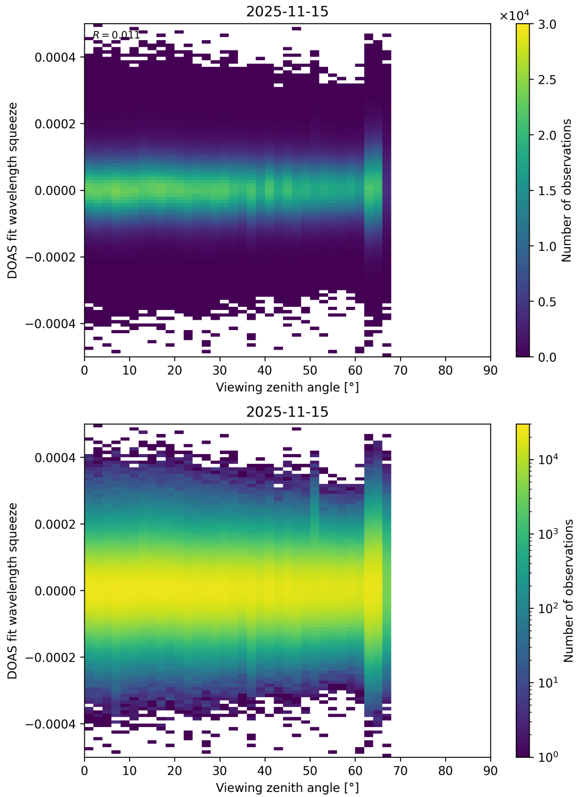
Figure 204: Scatter density plot of “Viewing zenith angle” against “DOAS fit wavelength squeeze” for 2025-11-14 to 2025-11-16.
