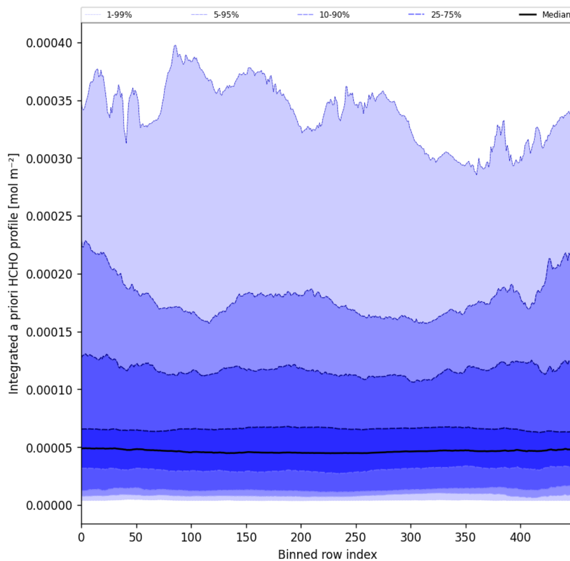
Figure 60: Along track statistics of “Integrated a priori HCHO profile” for 2025-11-14 to 2025-11-16
