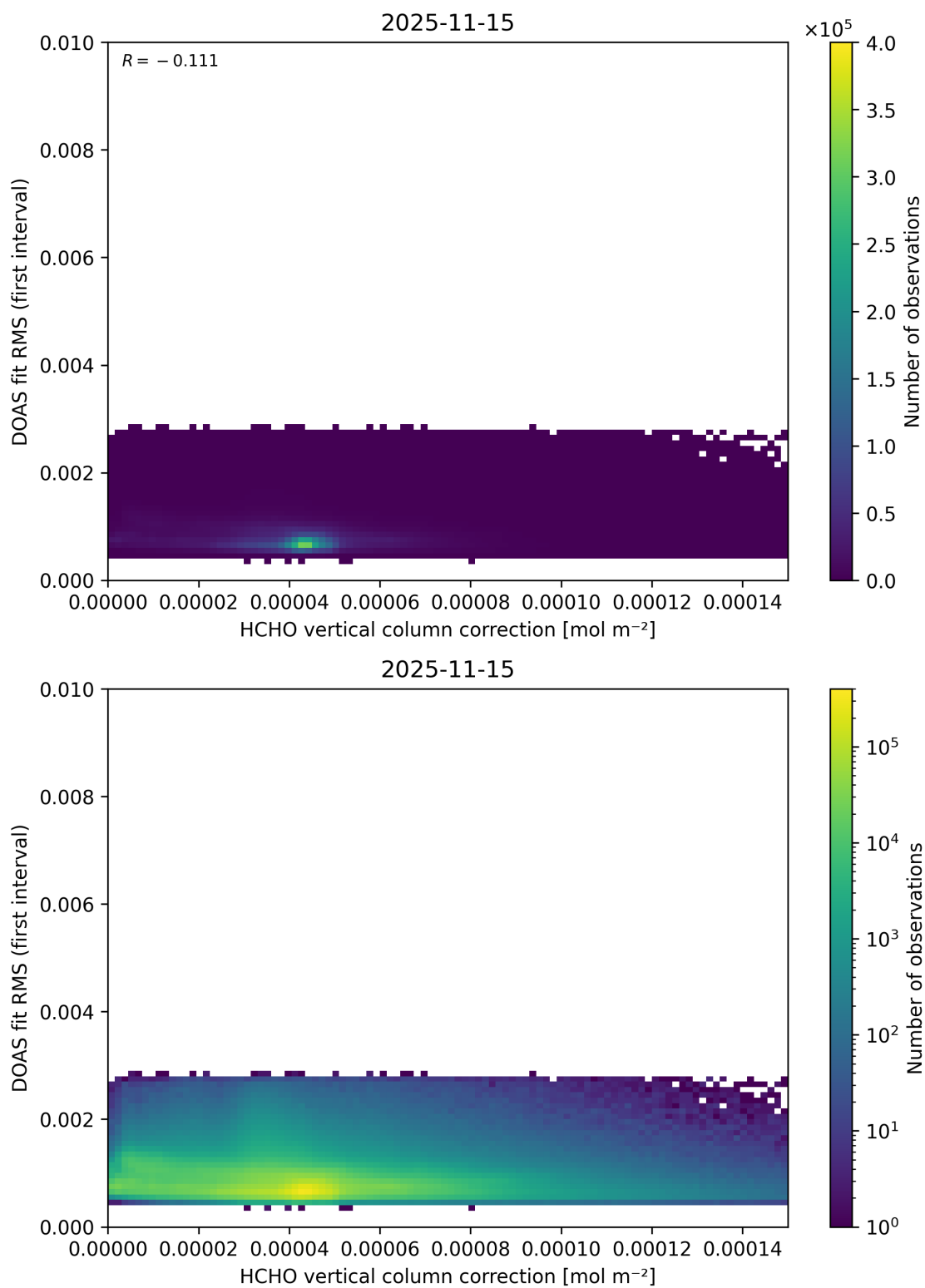
Figure 126: Scatter density plot of “HCHO vertical column correction” against “DOAS fit RMS (first interval)” for 2025-11-14 to 2025-11-16.
