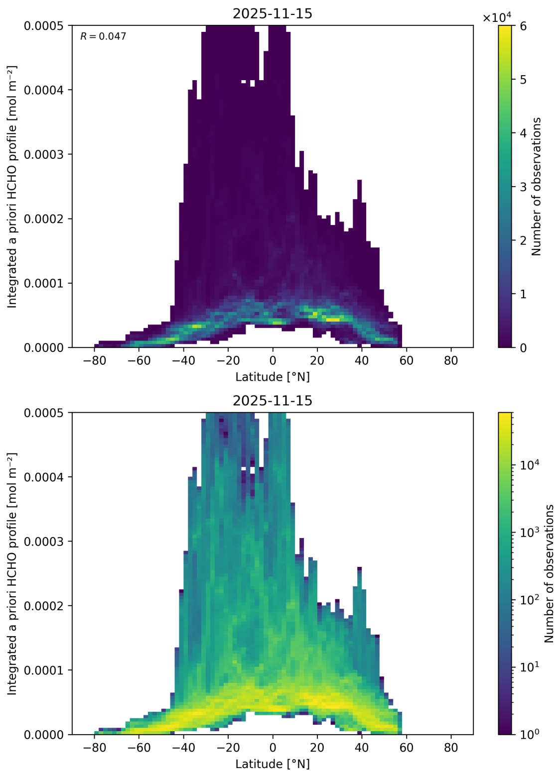
Figure 185: Scatter density plot of “Latitude” against “Integrated a priori HCHO profile” for 2025-11-14 to 2025-11-16.
