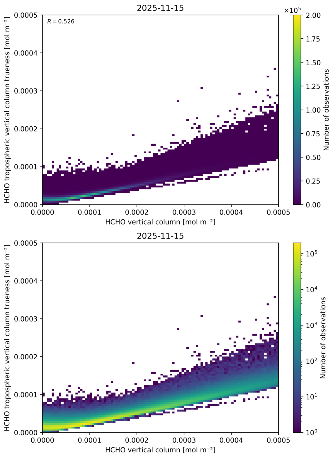
Figure 150: Scatter density plot of “HCHO vertical column” against “HCHO tropospheric vertical column trueness” for 2025-11-14 to 2025-11-16.
