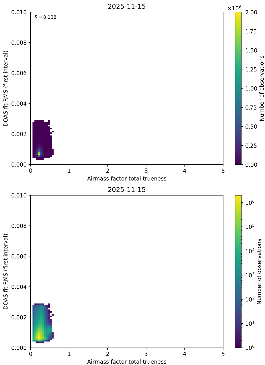
Figure 118: Scatter density plot of “Airmass factor total trueness” against “DOAS fit RMS (first interval)” for 2025-11-14 to 2025-11-16.
