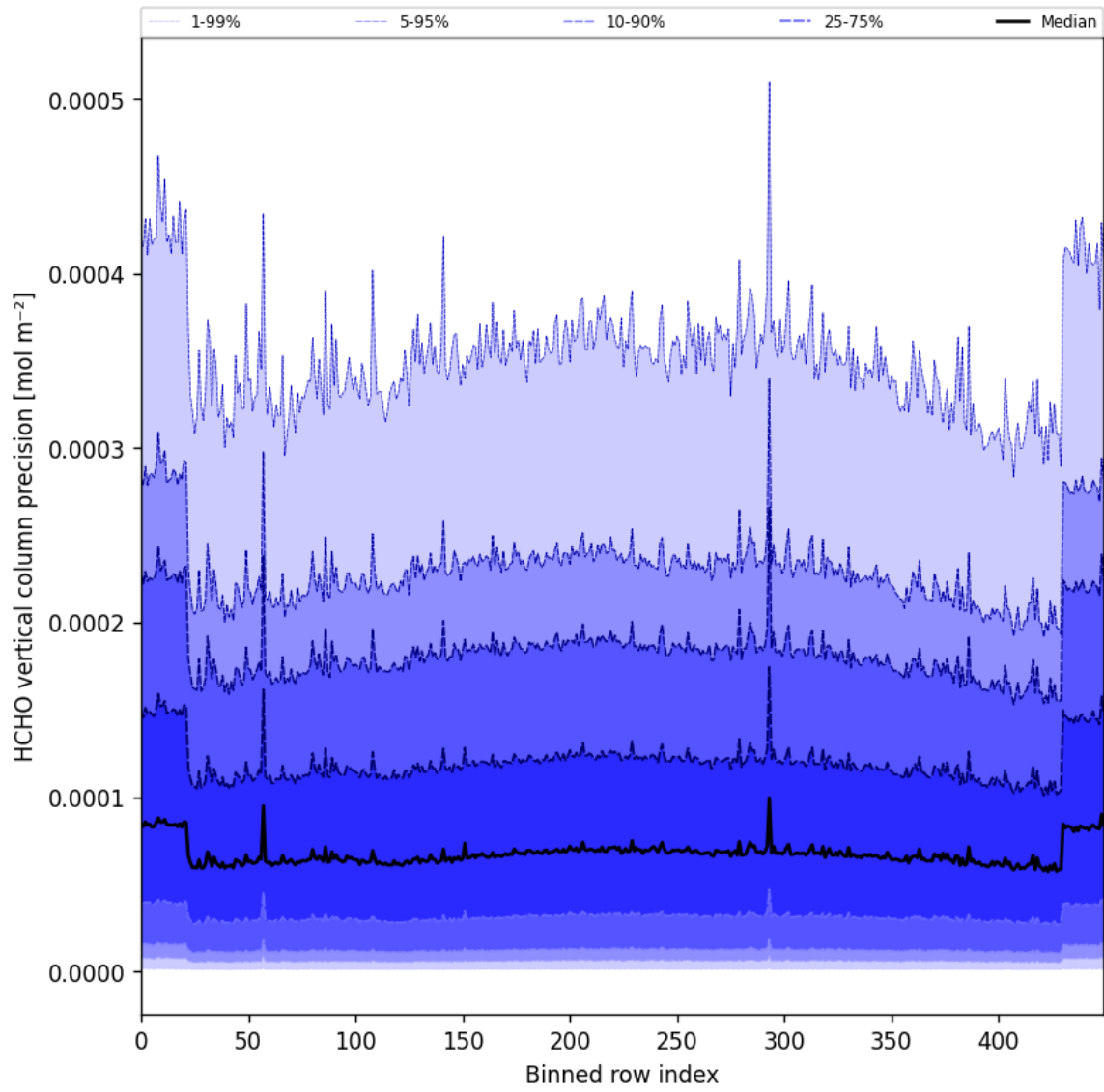
Figure 53: Along track statistics of "HCHO vertical column precision" for 2025-11-14 to 2025-11-16
