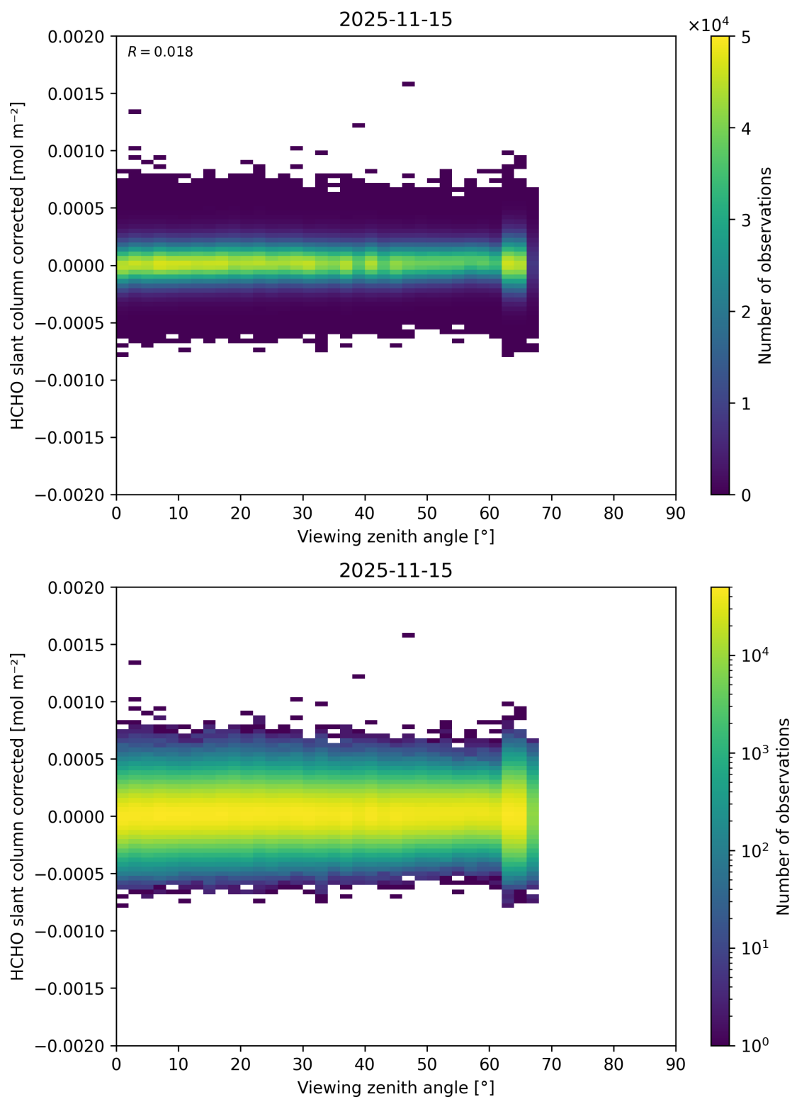
Figure 206: Scatter density plot of “Viewing zenith angle” against “HCHO slant column corrected” for 2025-11-14 to 2025-11-16.
