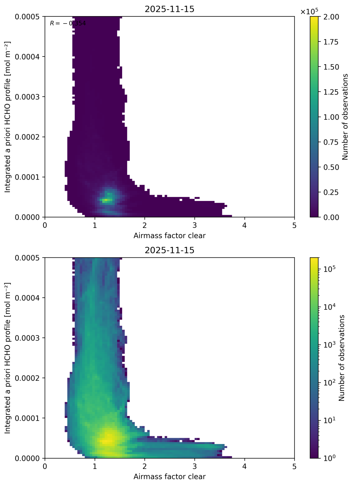
Figure 84: Scatter density plot of “Airmass factor clear” against “Integrated a priori HCHO profile” for 2025-11-14 to 2025-11-16.
