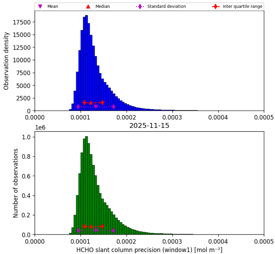
Figure 41: Histogram of “HCHO slant column precision (window1)” for 2025-11-14 to 2025-11-16
