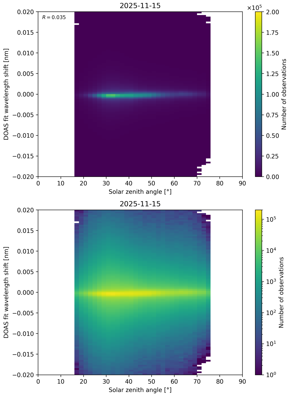
Figure 187: Scatter density plot of “Solar zenith angle” against “DOAS fit wavelength shift” for 2025-11-14 to 2025-11-16.
