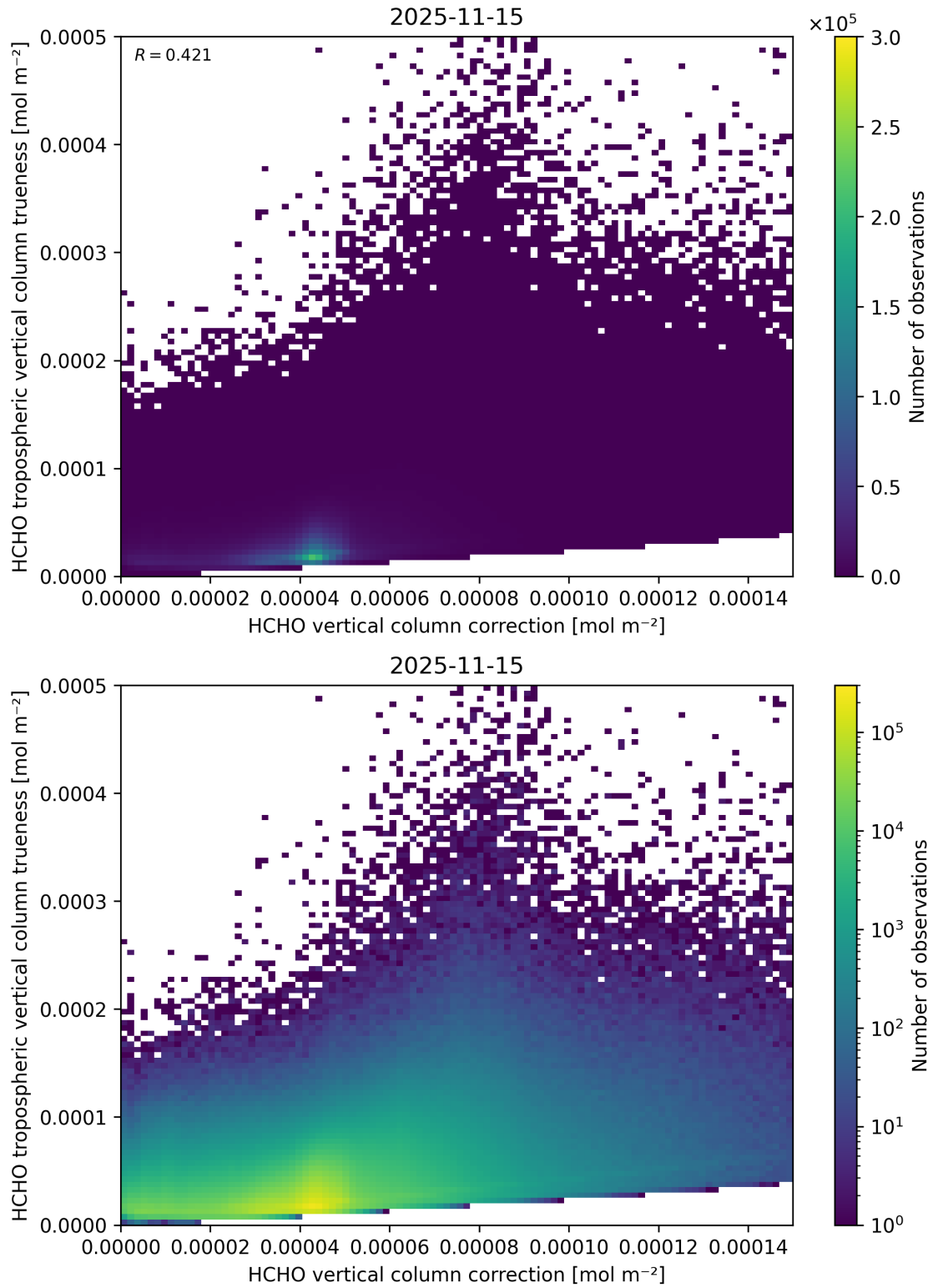
Figure 136: Scatter density plot of “HCHO vertical column correction” against “HCHO tropospheric vertical column truthness” for 2025-11-14 to 2025-11-16.
