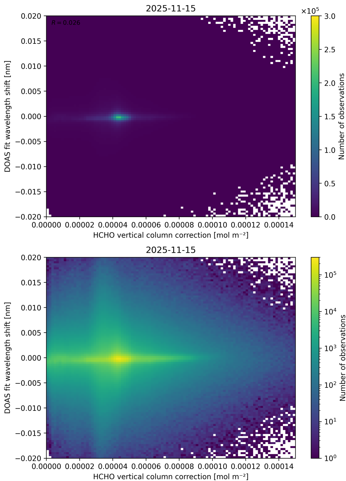
Figure 127: Scatter density plot of “HCHO vertical column correction” against “DOAS fit wavelength shift” for 2025-11-14 to 2025-11-16.
