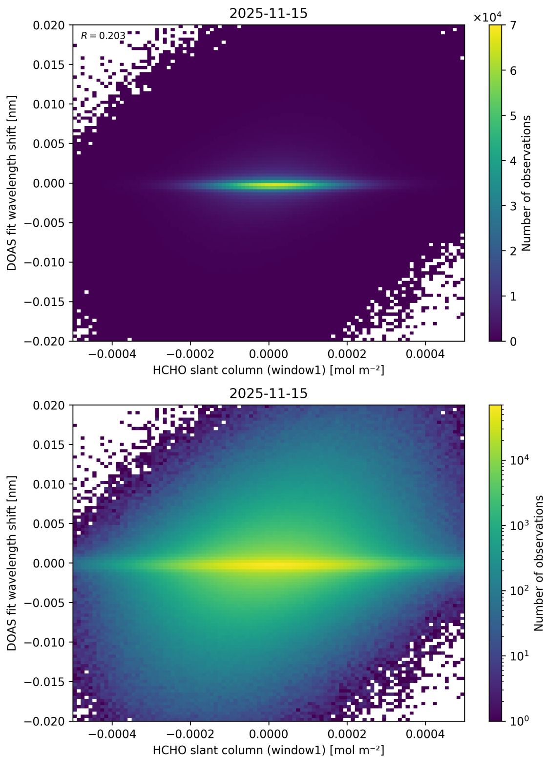
Figure 89: Scatter density plot of “HCHO slant column (window1)” against “DOAS fit wavelength shift” for 2025-11-14 to 2025-11-16.
