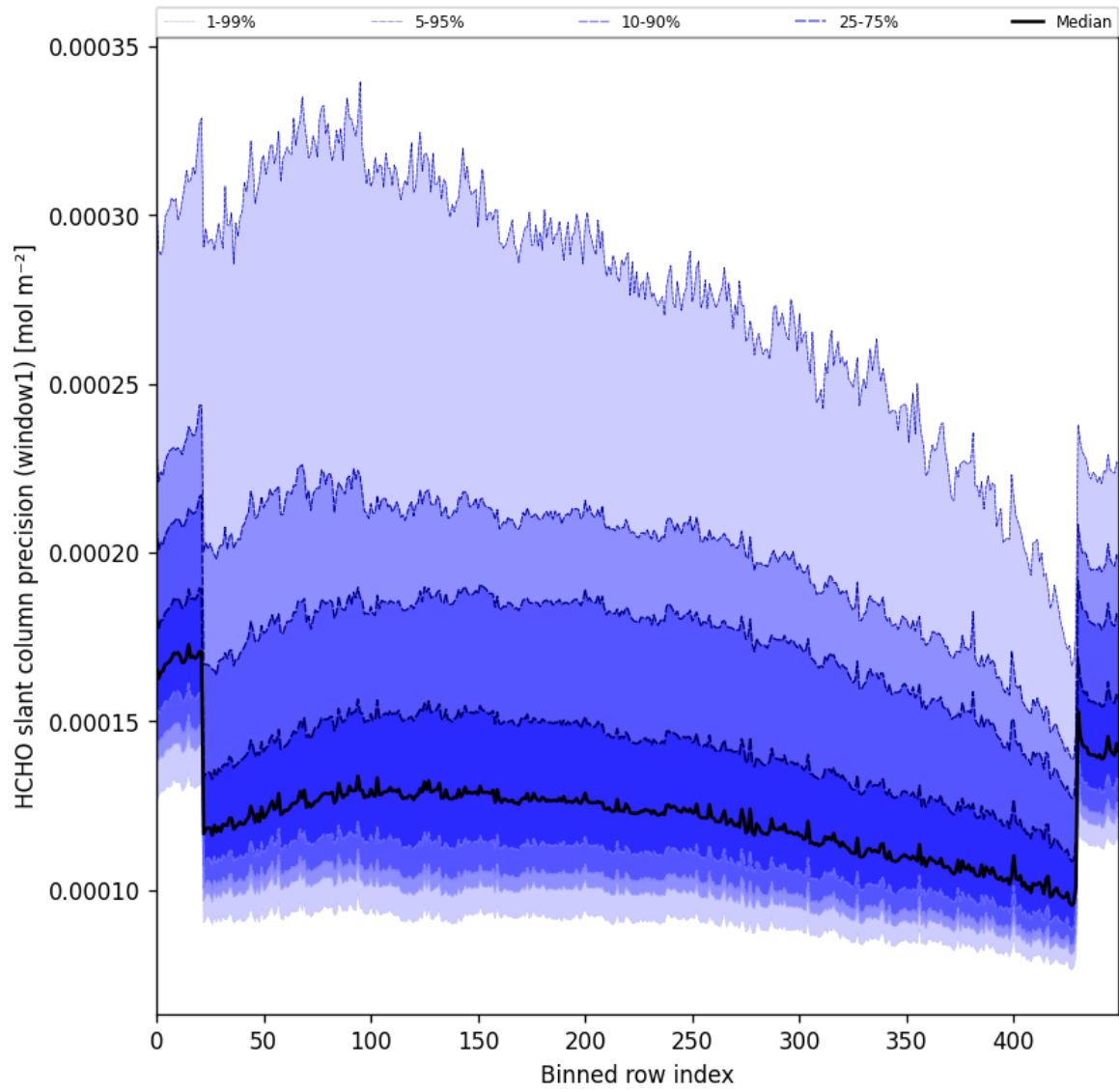
Figure 56: Along track statistics of “HCHO slant column precision (window1)” for 2025-11-14 to 2025-11-16
