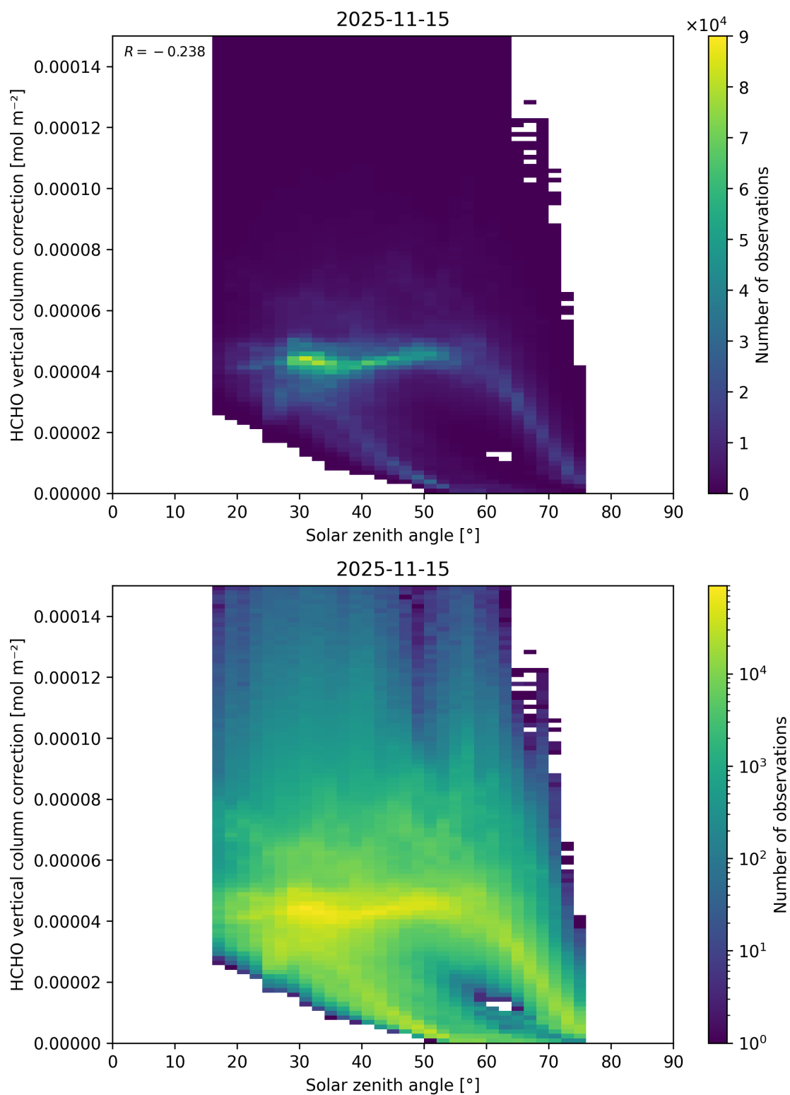
Figure 197: Scatter density plot of “Solar zenith angle” against “HCHO vertical column correction” for 2025-11-14 to 2025-11-16.
