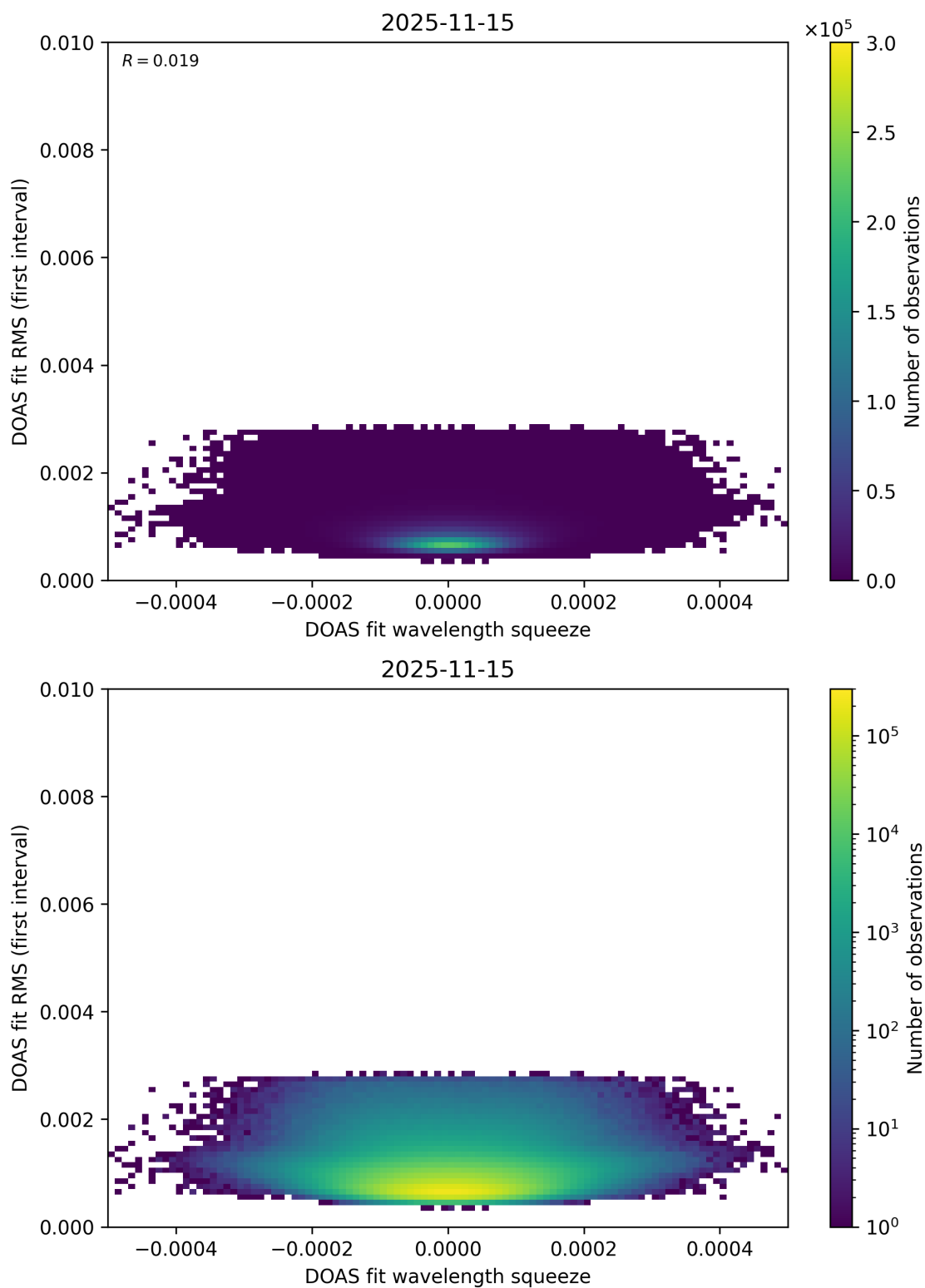
Figure 74: Scatter density plot of “DOAS fit wavelength squeeze” against “DOAS fit RMS (first interval)” for 2025-11-14 to 2025-11-16.
