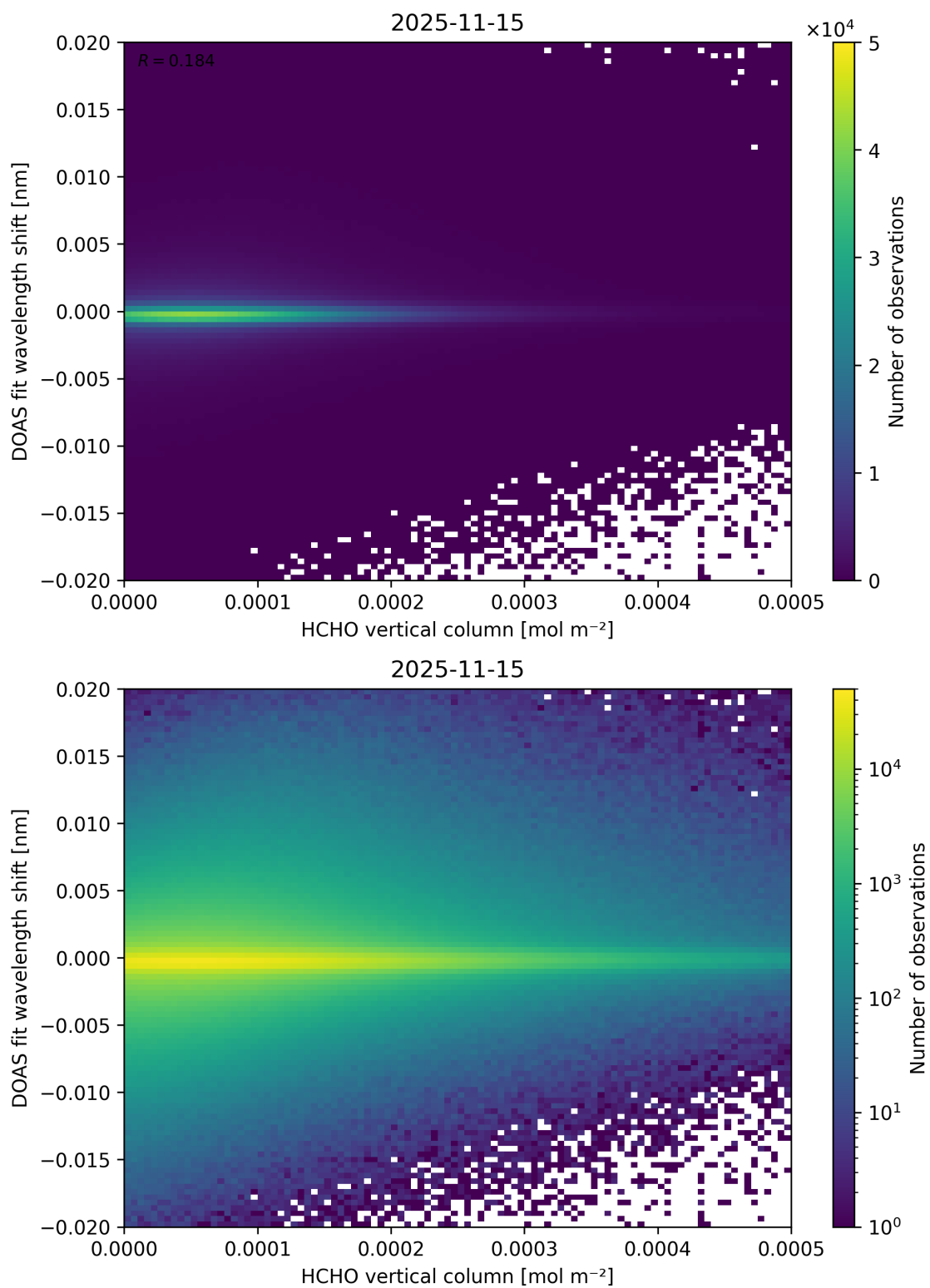
Figure 139: Scatter density plot of “HCHO vertical column” against “DOAS fit wavelength shift” for 2025-11-14 to 2025-11-16.
