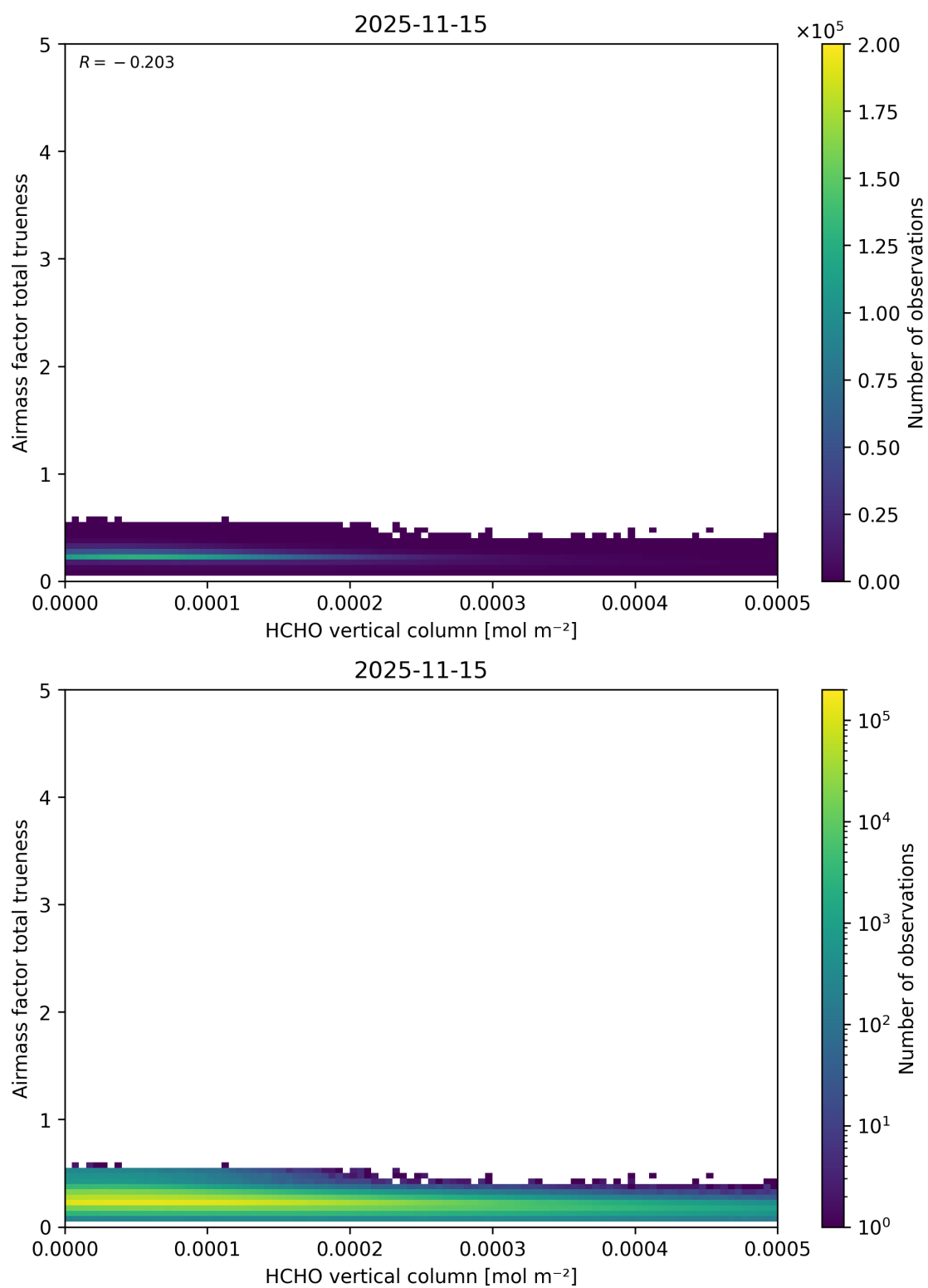
Figure 147: Scatter density plot of “HCHO vertical column” against “Airmass factor total truiness” for 2025-11-14 to 2025-11-16.
