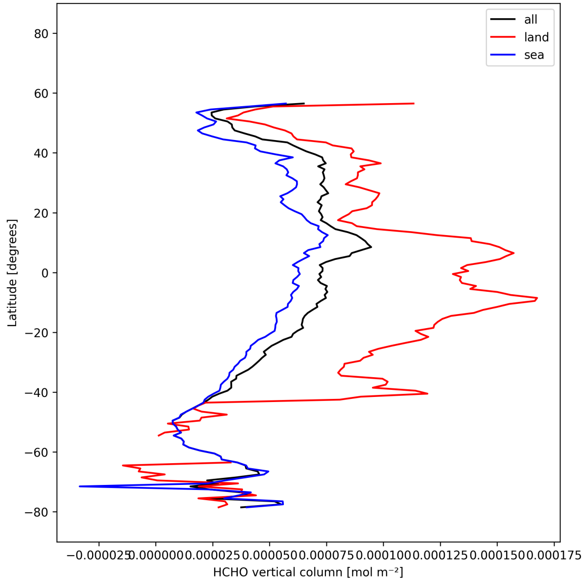
Figure 22: Zonal average of “HCHO vertical column” for 2025-11-14 to 2025-11-16.
