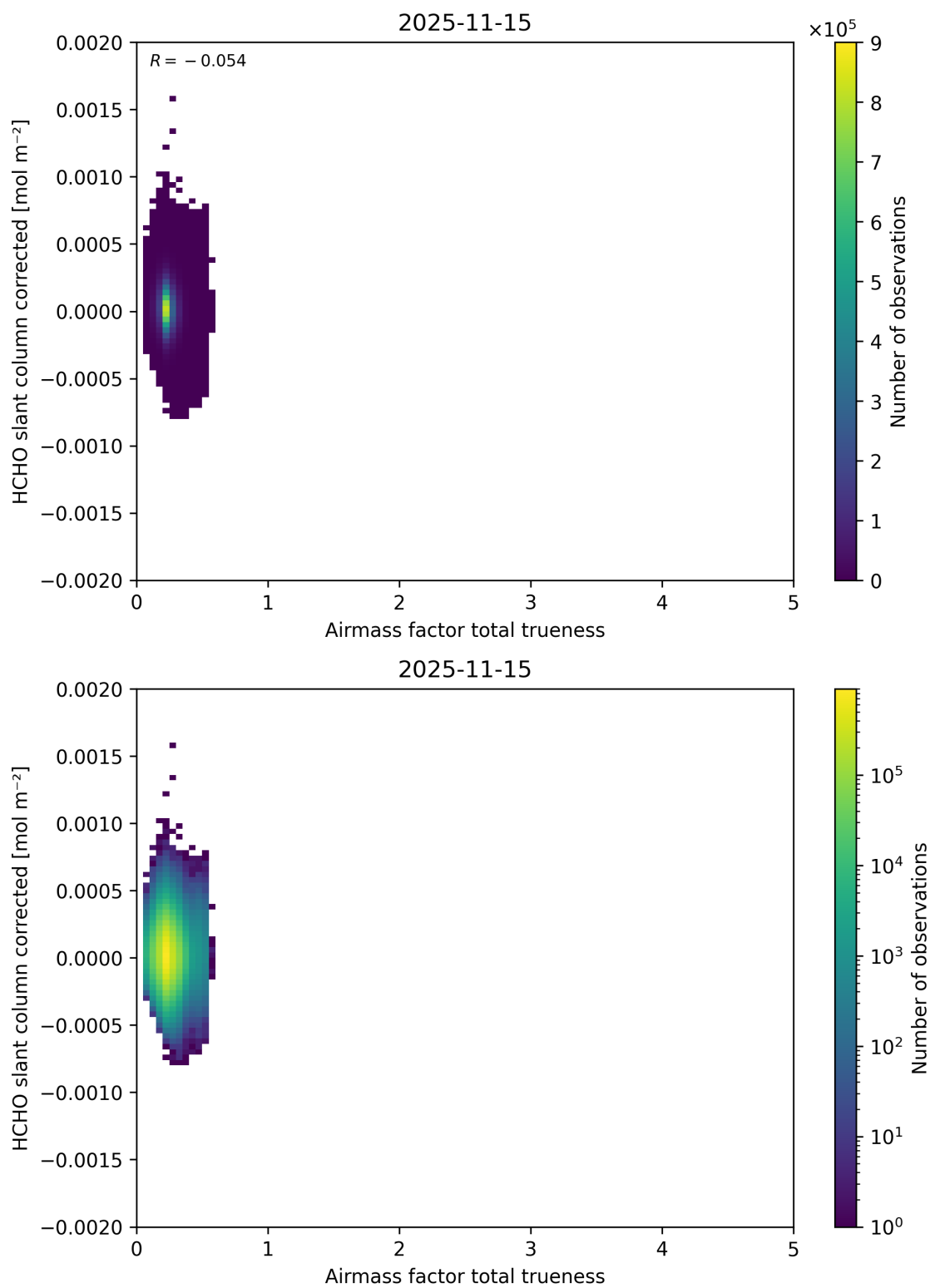
Figure 122: Scatter density plot of “Airmass factor total trueness” against “HCHO slant column corrected” for 2025-11-14 to 2025-11-16.
