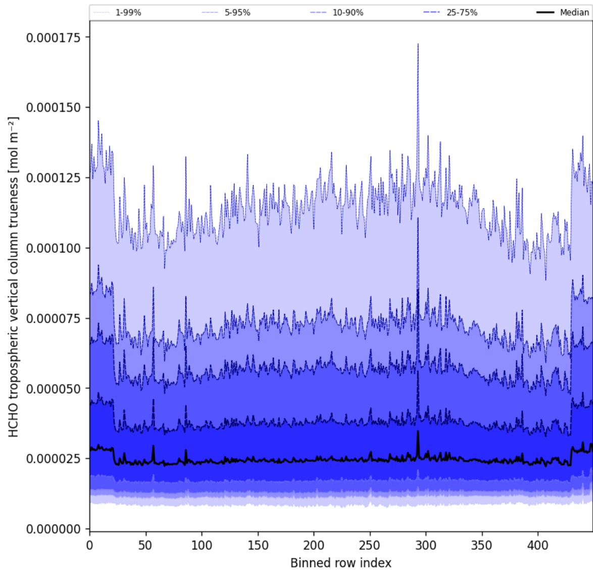
Figure 65: Along track statistics of "HCHO tropospheric vertical column trueness" for 2025-11-14 to 2025-11-16
