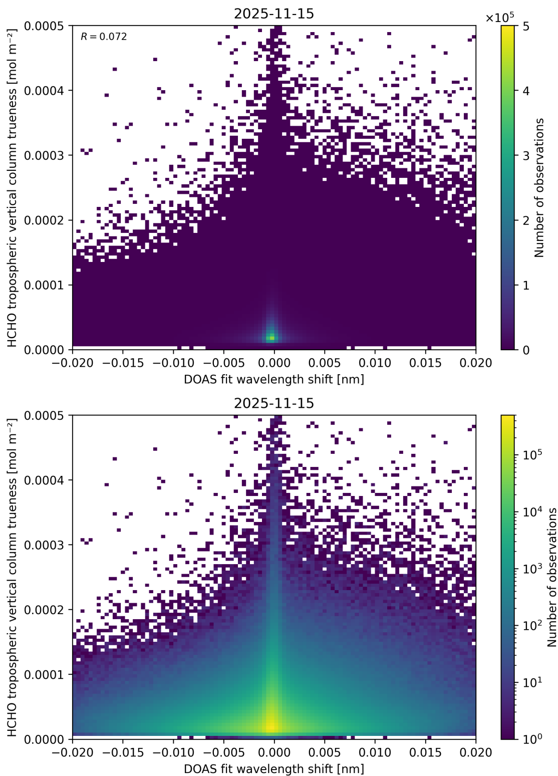
Figure 73: Scatter density plot of “DOAS fit wavelength shift” against “HCHO tropospheric vertical column trueness” for 2025-11-14 to 2025-11-16.
