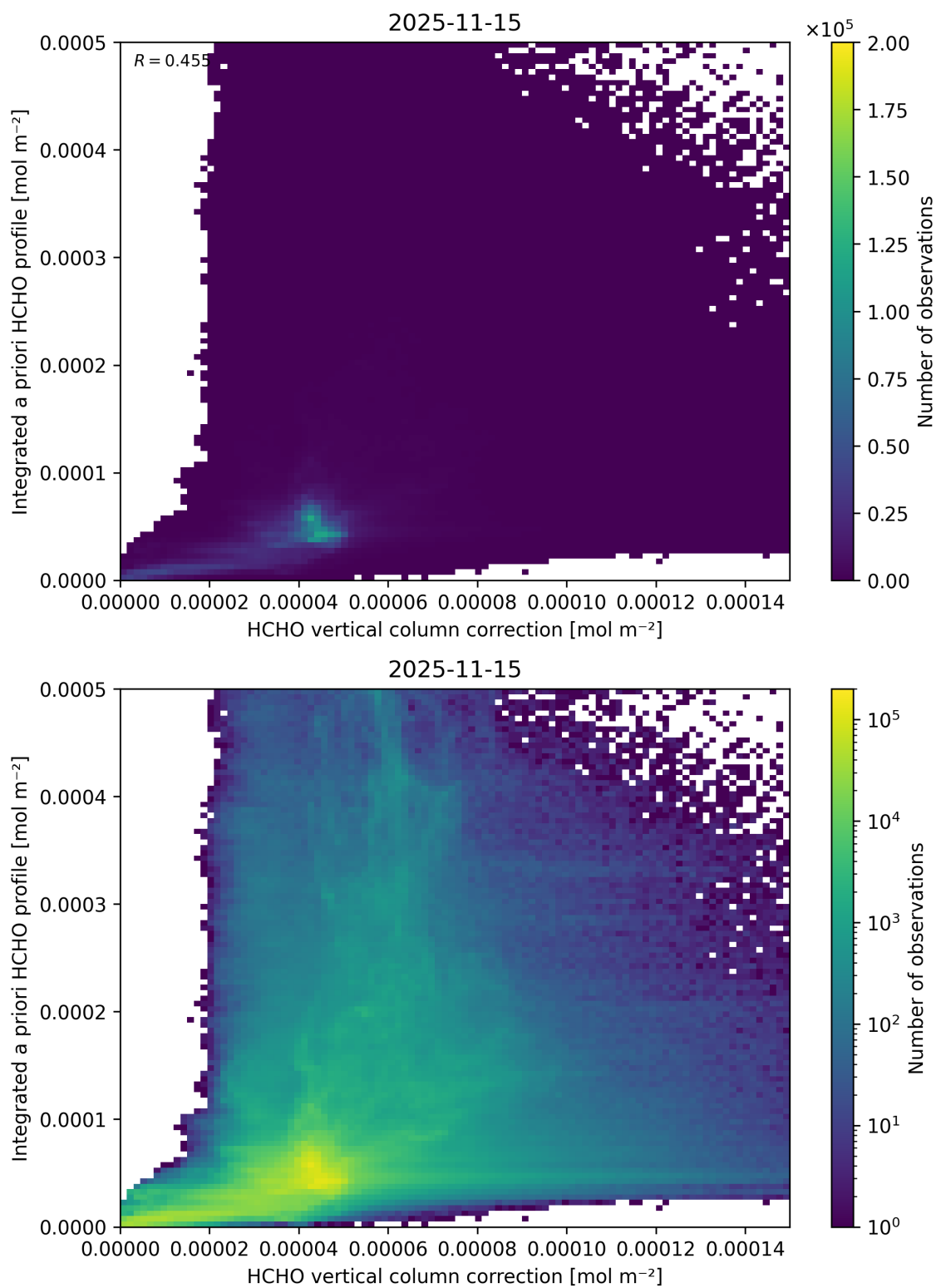
Figure 137: Scatter density plot of “HCHO vertical column correction” against “Integrated a priori HCHO profile” for 2025-11-14 to 2025-11-16.
