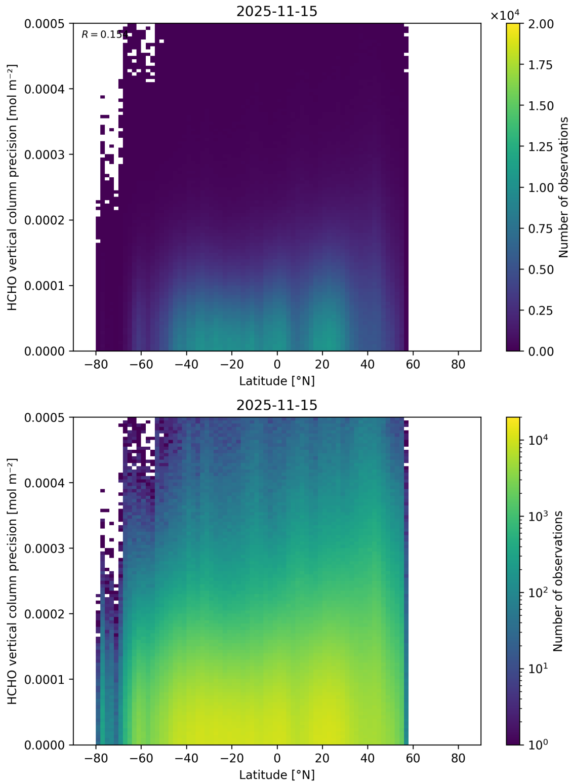
Figure 183: Scatter density plot of “Latitude” against “HCHO vertical column precision” for 2025-11-14 to 2025-11-16.
