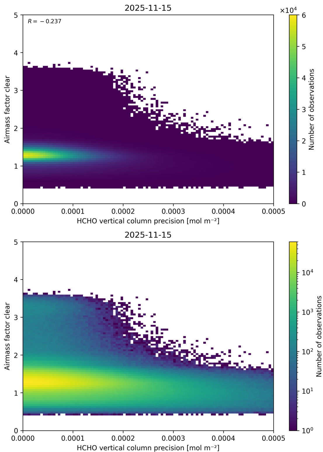
Figure 155: Scatter density plot of “HCHO vertical column precision” against “Airmass factor clear” for 2025-11-14 to 2025-11-16.
