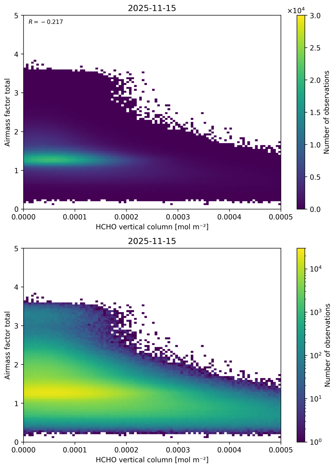
Figure 146: Scatter density plot of “HCHO vertical column” against “Airmass factor total” for 2025-11-14 to 2025-11-16.
