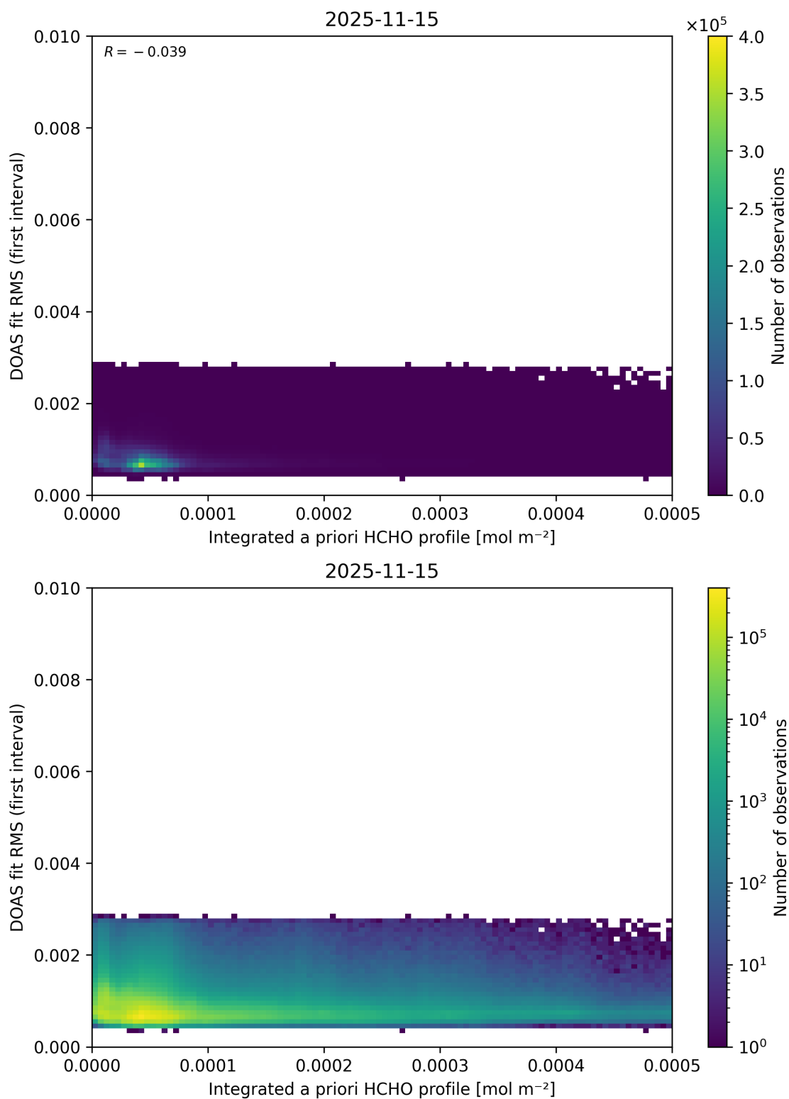
Figure 165: Scatter density plot of “Integrated a priori HCHO profile” against “DOAS fit RMS (first interval)” for 2025-11-14 to 2025-11-16.
