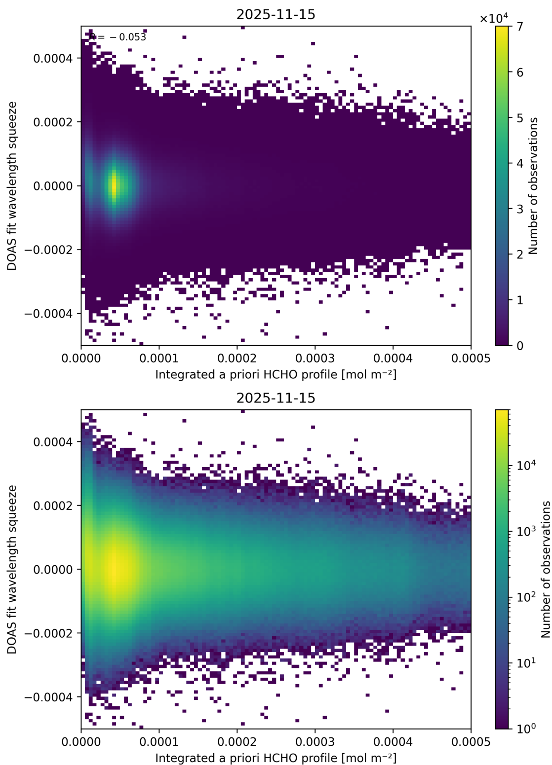
Figure 167: Scatter density plot of “Integrated a priori HCHO profile” against “DOAS fit wavelength squeeze” for 2025-11-14 to 2025-11-16.
