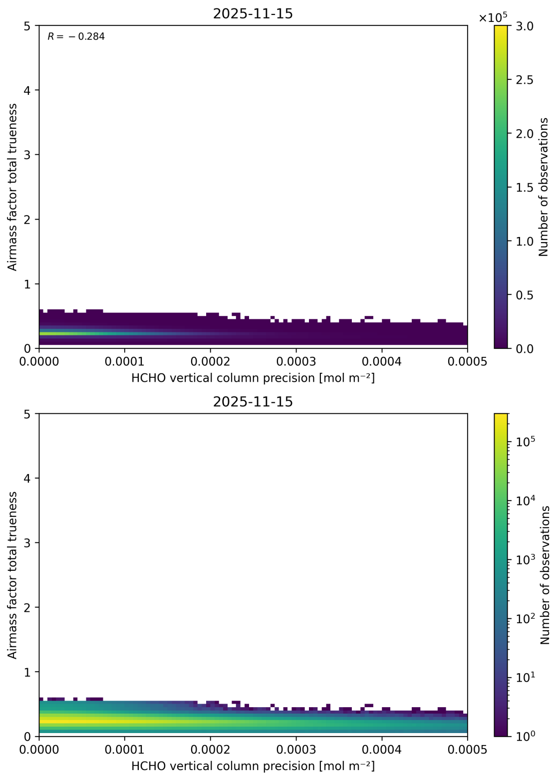
Figure 161: Scatter density plot of “HCHO vertical column precision” against “Airmass factor total trueness” for 2025-11-14 to 2025-11-16.
