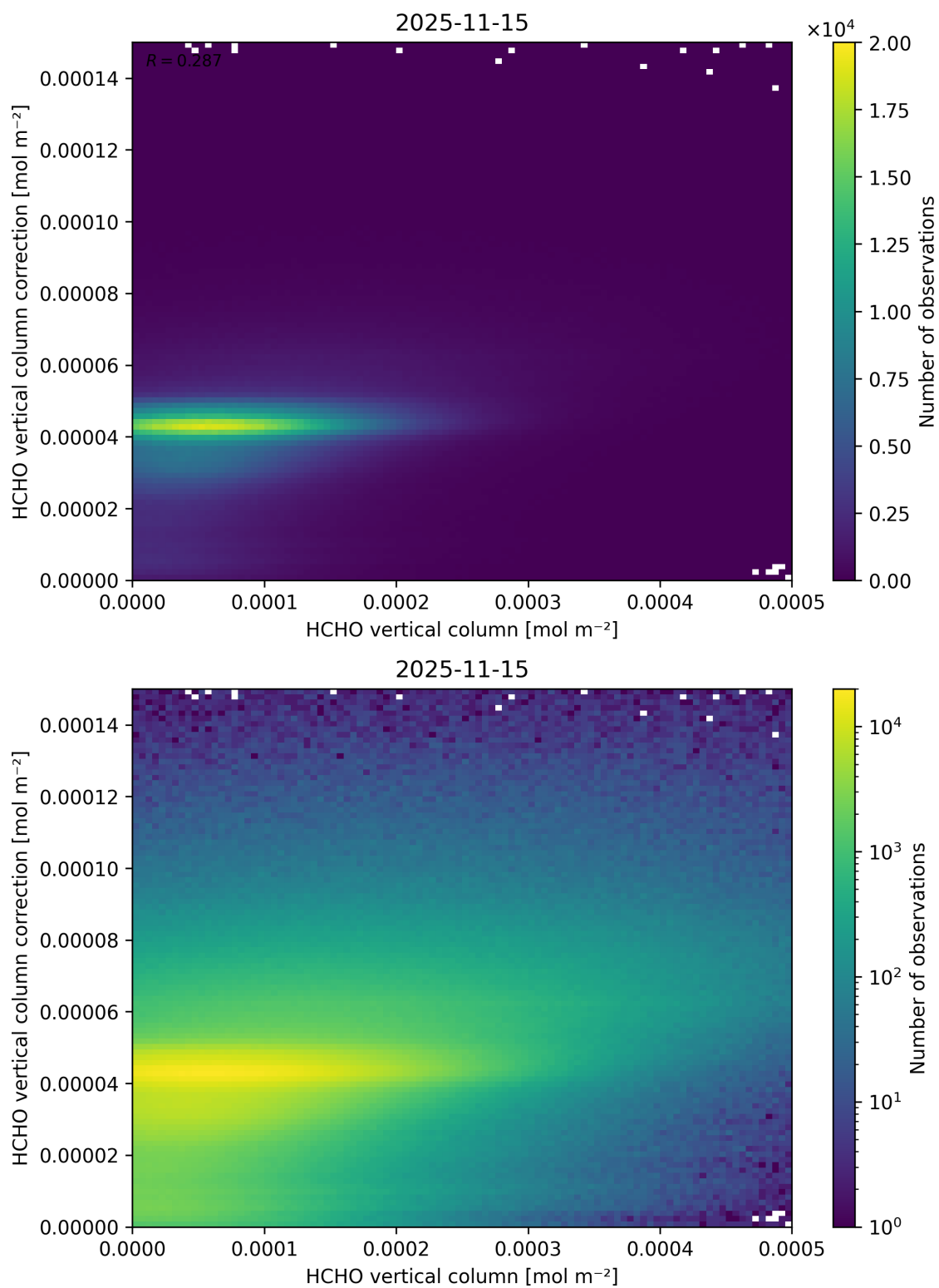
Figure 148: Scatter density plot of “HCHO vertical column” against “HCHO vertical column correction” for 2025-11-14 to 2025-11-16.
