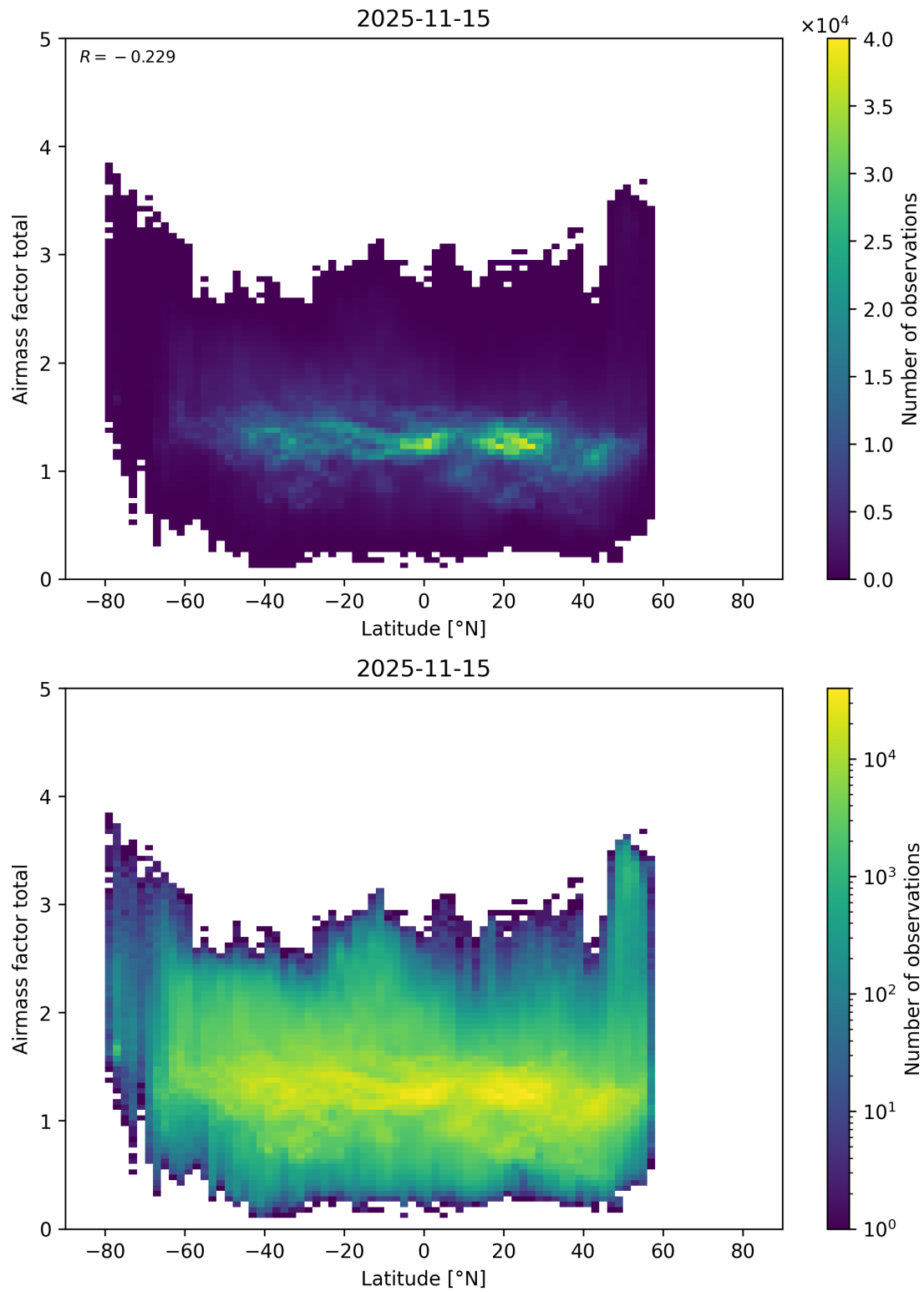
Figure 179: Scatter density plot of “Latitude” against “Airmass factor total” for 2025-11-14 to 2025-11-16.
