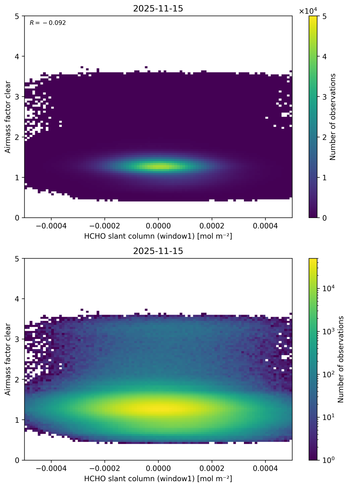
Figure 91: Scatter density plot of “HCHO slant column (window1)” against “Airmass factor clear” for 2025-11-14 to 2025-11-16.
