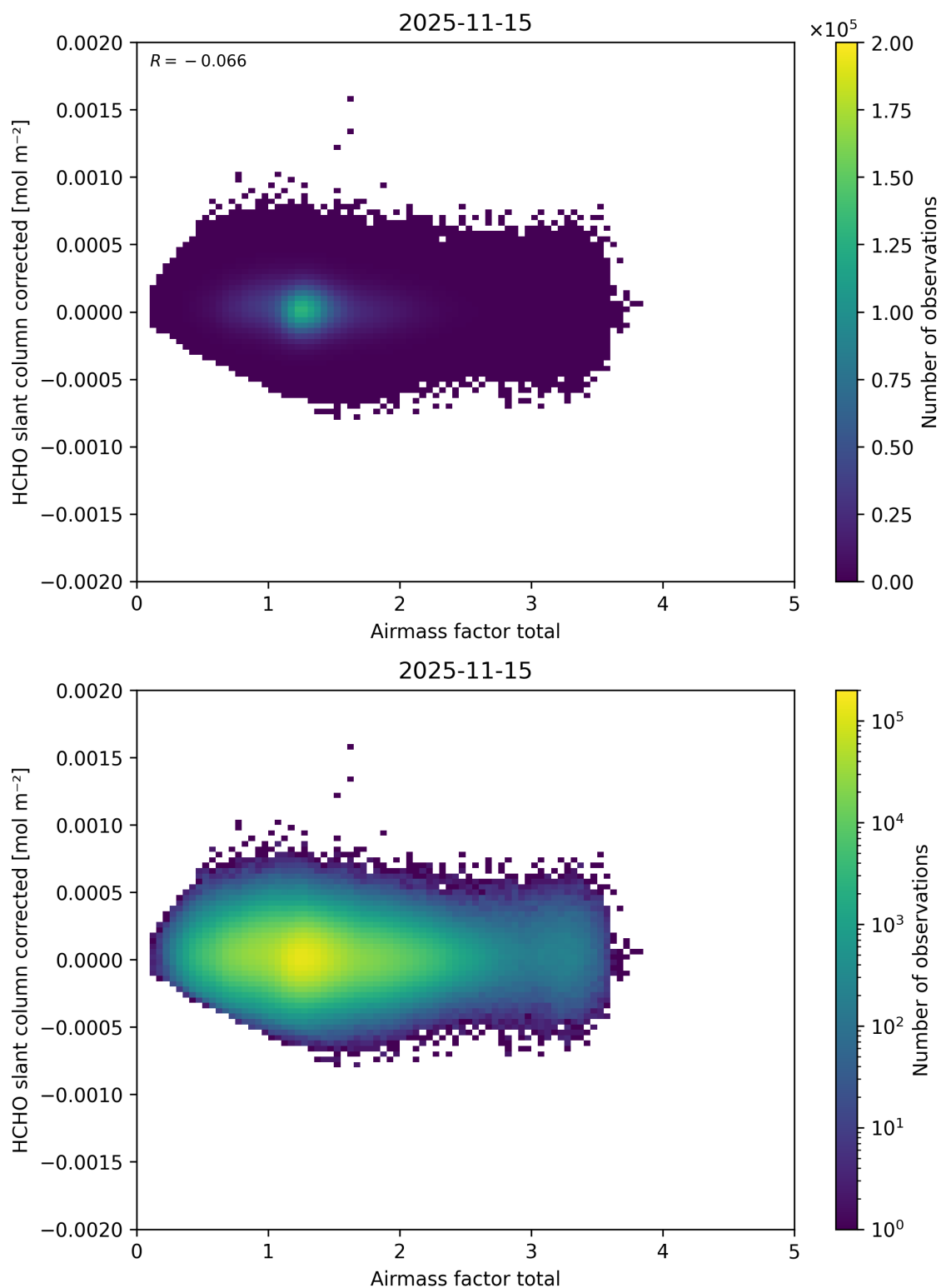
Figure 113: Scatter density plot of “Airmass factor total” against “HCHO slant column corrected” for 2025-11-14 to 2025-11-16.
