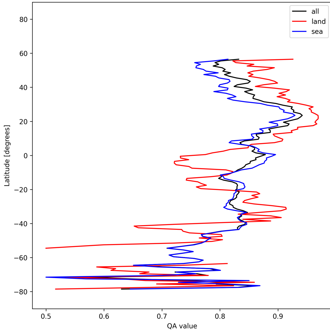
Figure 21: Zonal average of “QA value” for 2025-11-14 to 2025-11-16.
