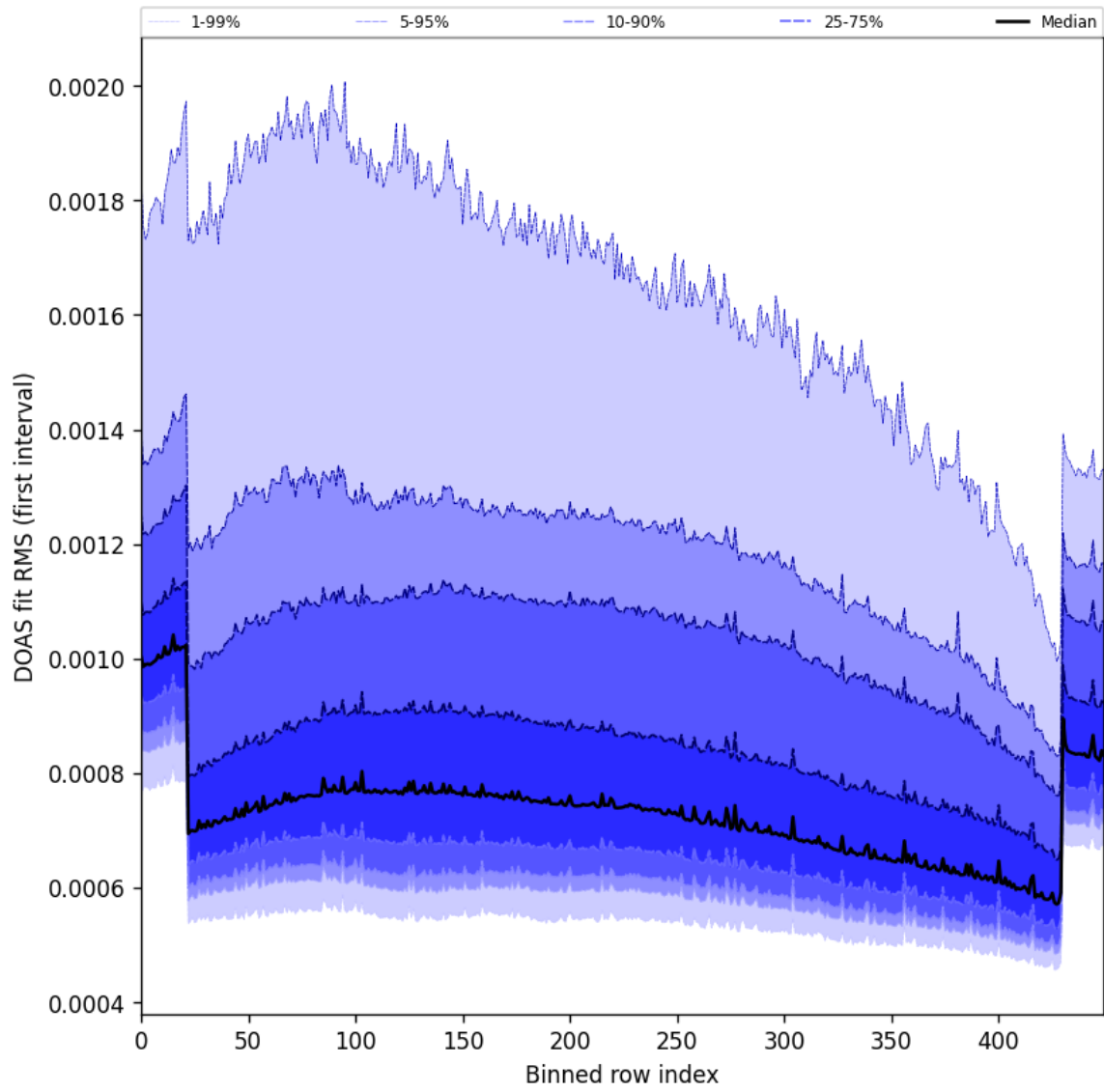
Figure 63: Along track statistics of “DOAS fit RMS (first interval)” for 2025-11-14 to 2025-11-16
