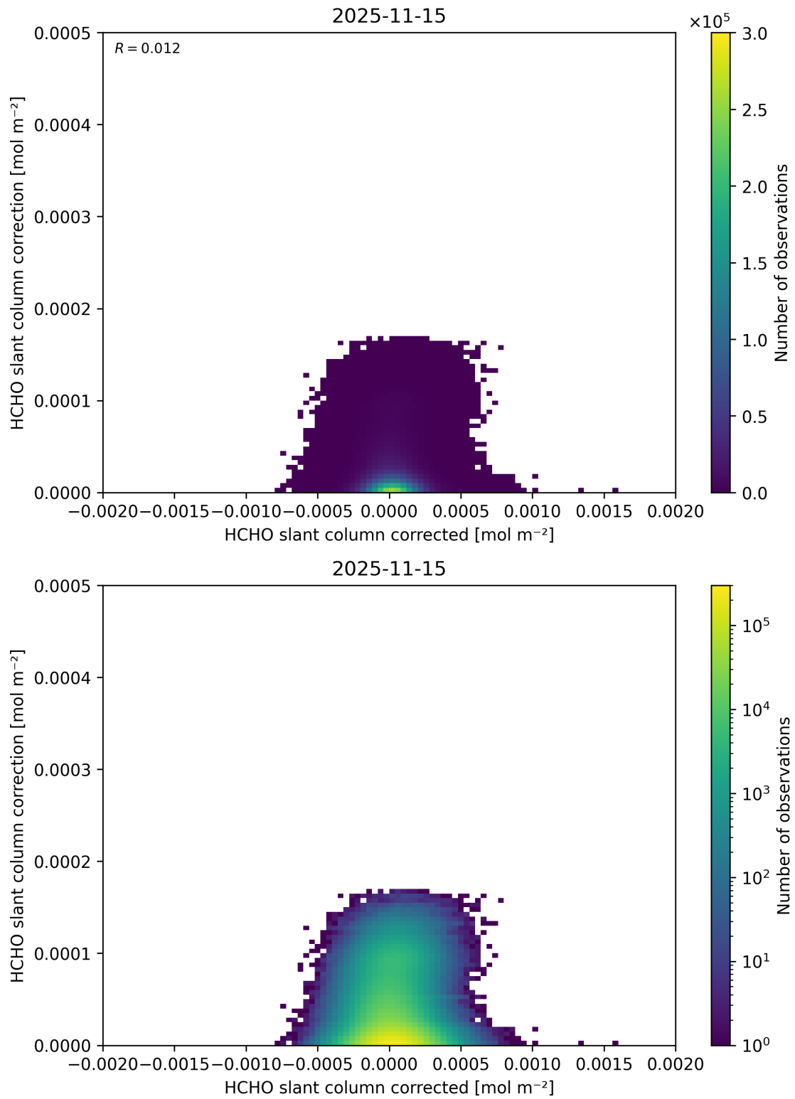
Figure 85: Scatter density plot of “HCHO slant column corrected” against “HCHO slant column correction” for 2025-11-14 to 2025-11-16.
