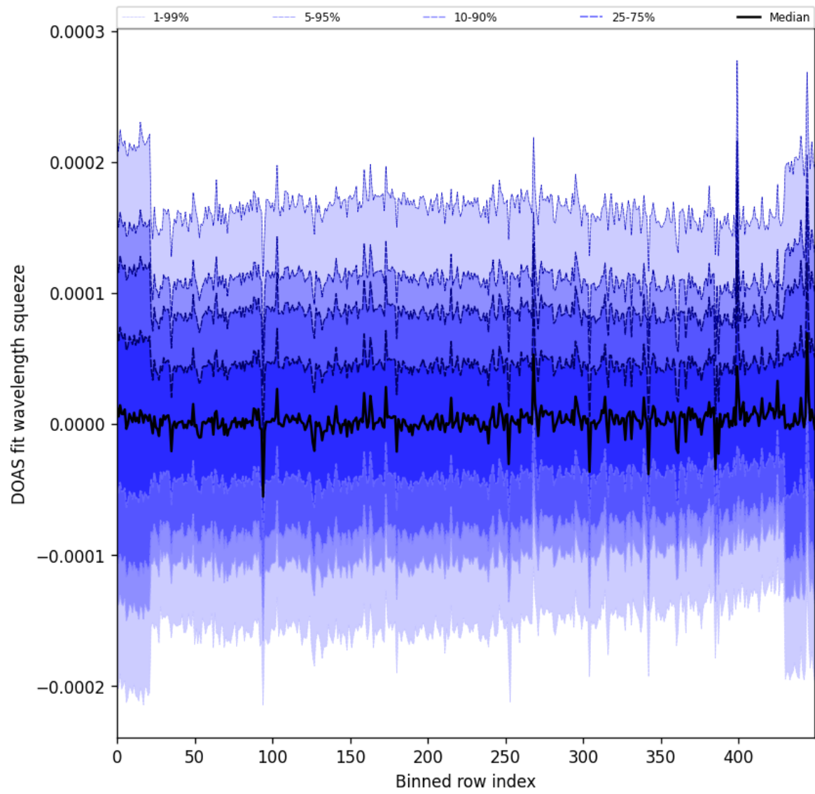
Figure 62: Along track statistics of “DOAS fit wavelength squeeze” for 2025-11-14 to 2025-11-16
