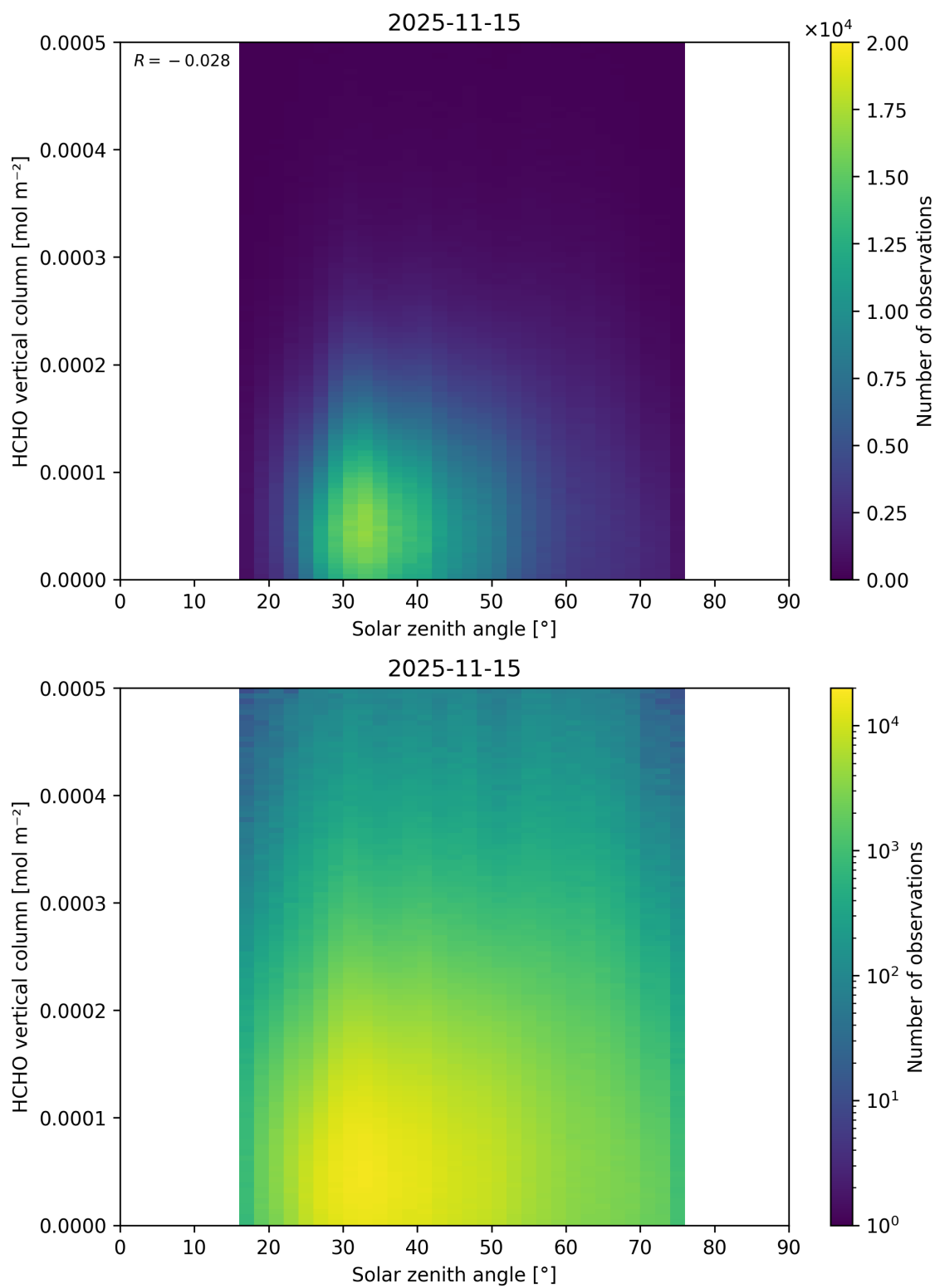
Figure 196: Scatter density plot of “Solar zenith angle” against “HCHO vertical column” for 2025-11-14 to 2025-11-16.
