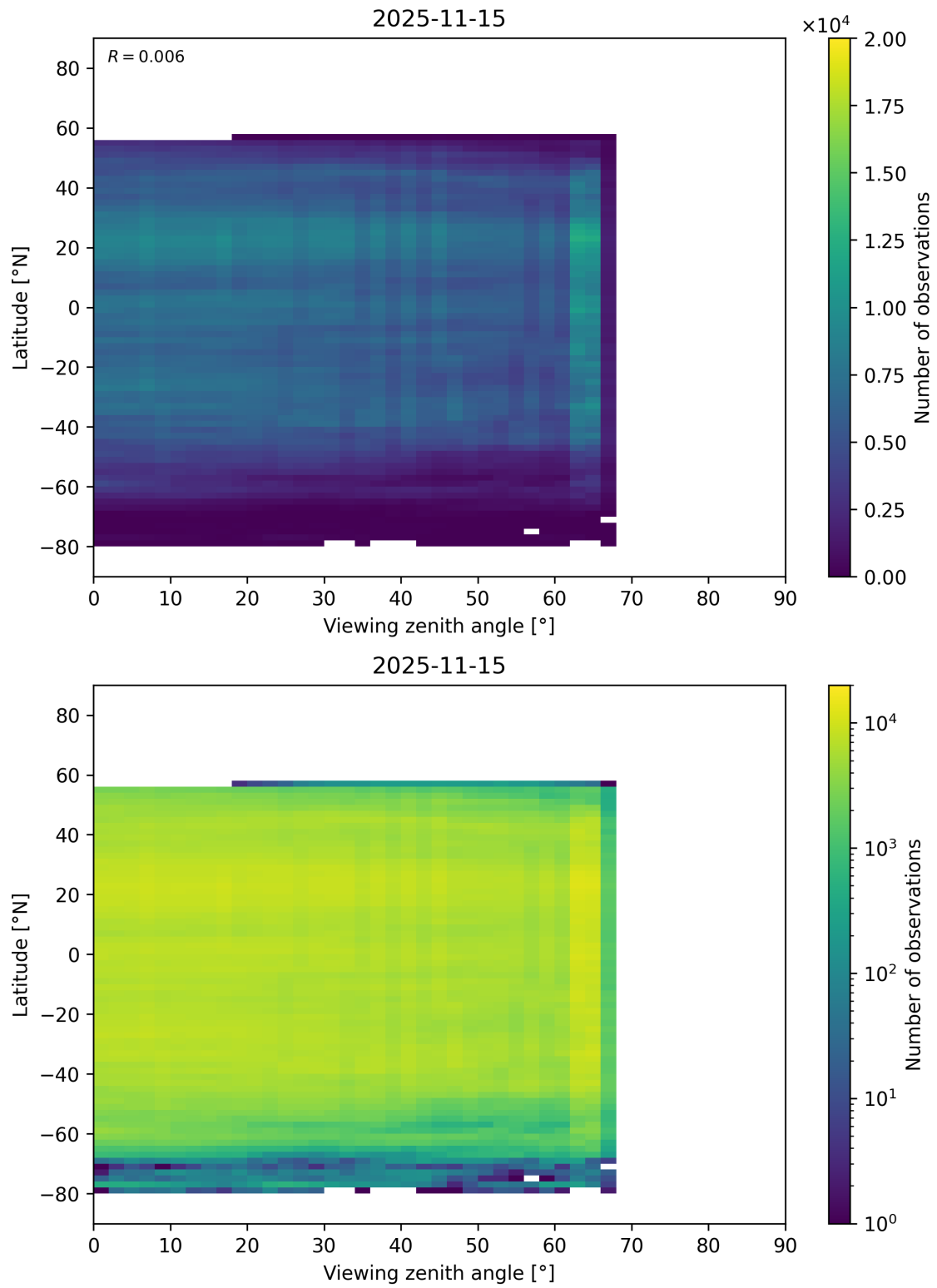
Figure 217: Scatter density plot of “Viewing zenith angle” against “Latitude” for 2025-11-14 to 2025-11-16.
