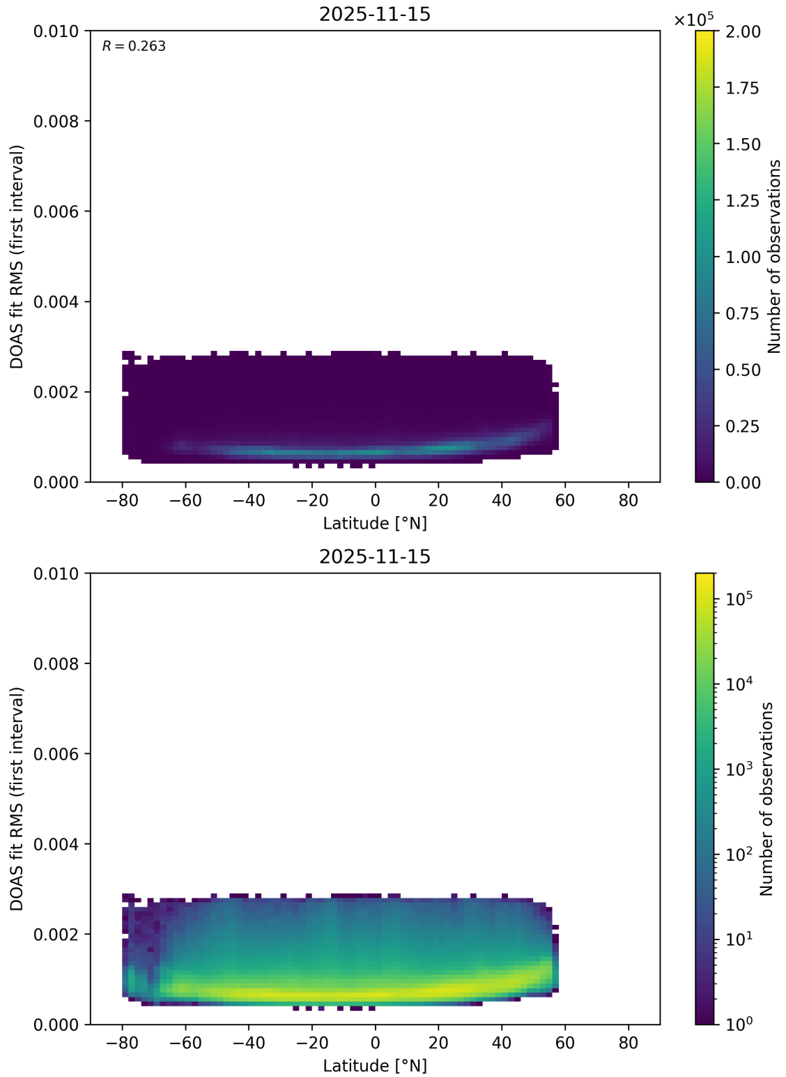
Figure 171: Scatter density plot of “Latitude” against “DOAS fit RMS (first interval)” for 2025-11-14 to 2025-11-16.
