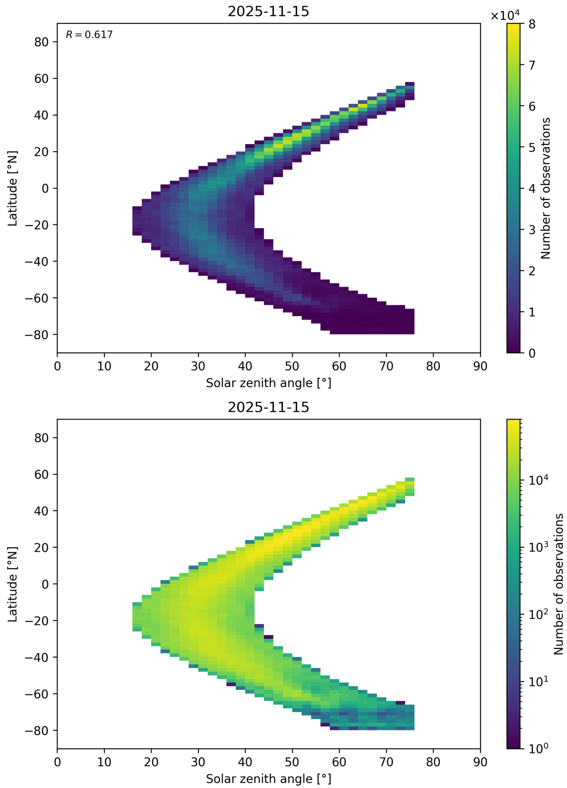
Figure 201: Scatter density plot of “Solar zenith angle” against “Latitude” for 2025-11-14 to 2025-11-16.
