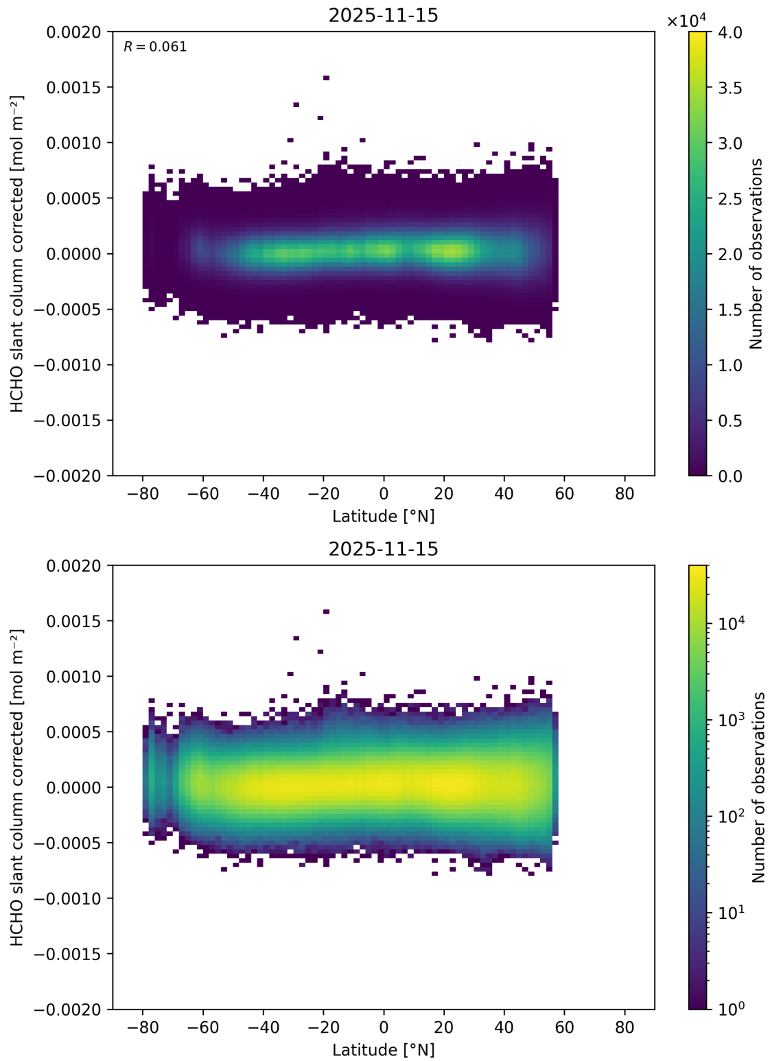
Figure 175: Scatter density plot of “Latitude” against “HCHO slant column corrected” for 2025-11-14 to 2025-11-16.
