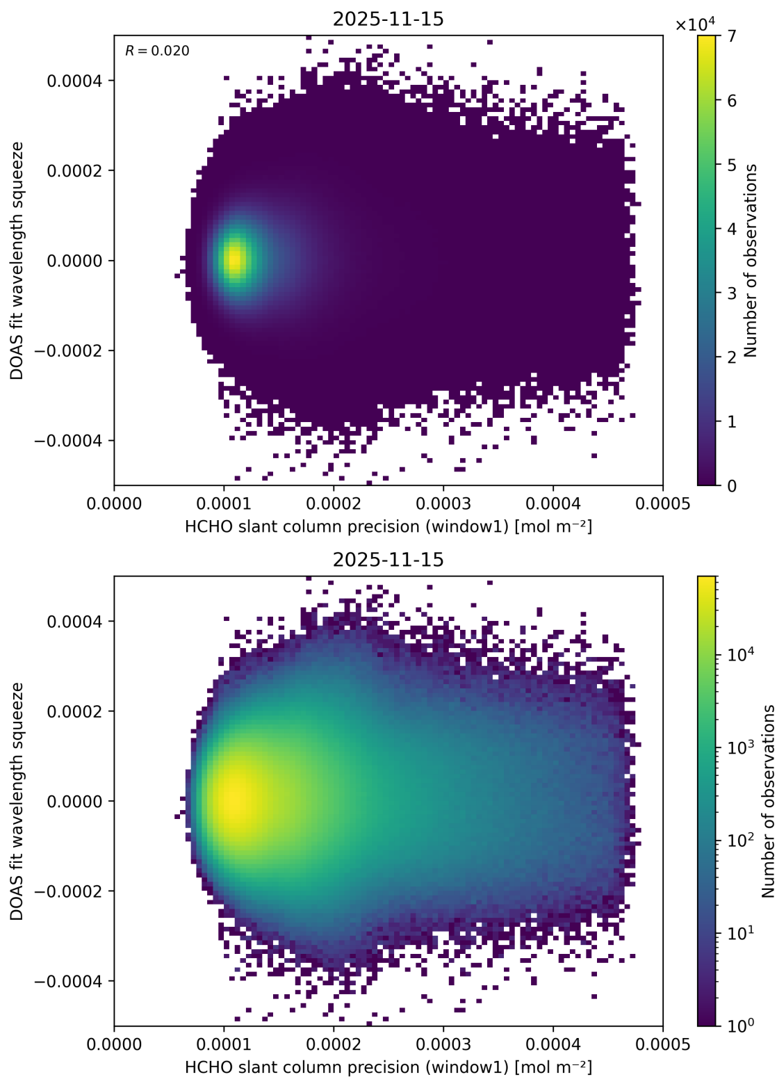
Figure 101: Scatter density plot of “HCHO slant column precision (window1)” against “DOAS fit wavelength squeeze” for 2025-11-14 to 2025-11-16.
