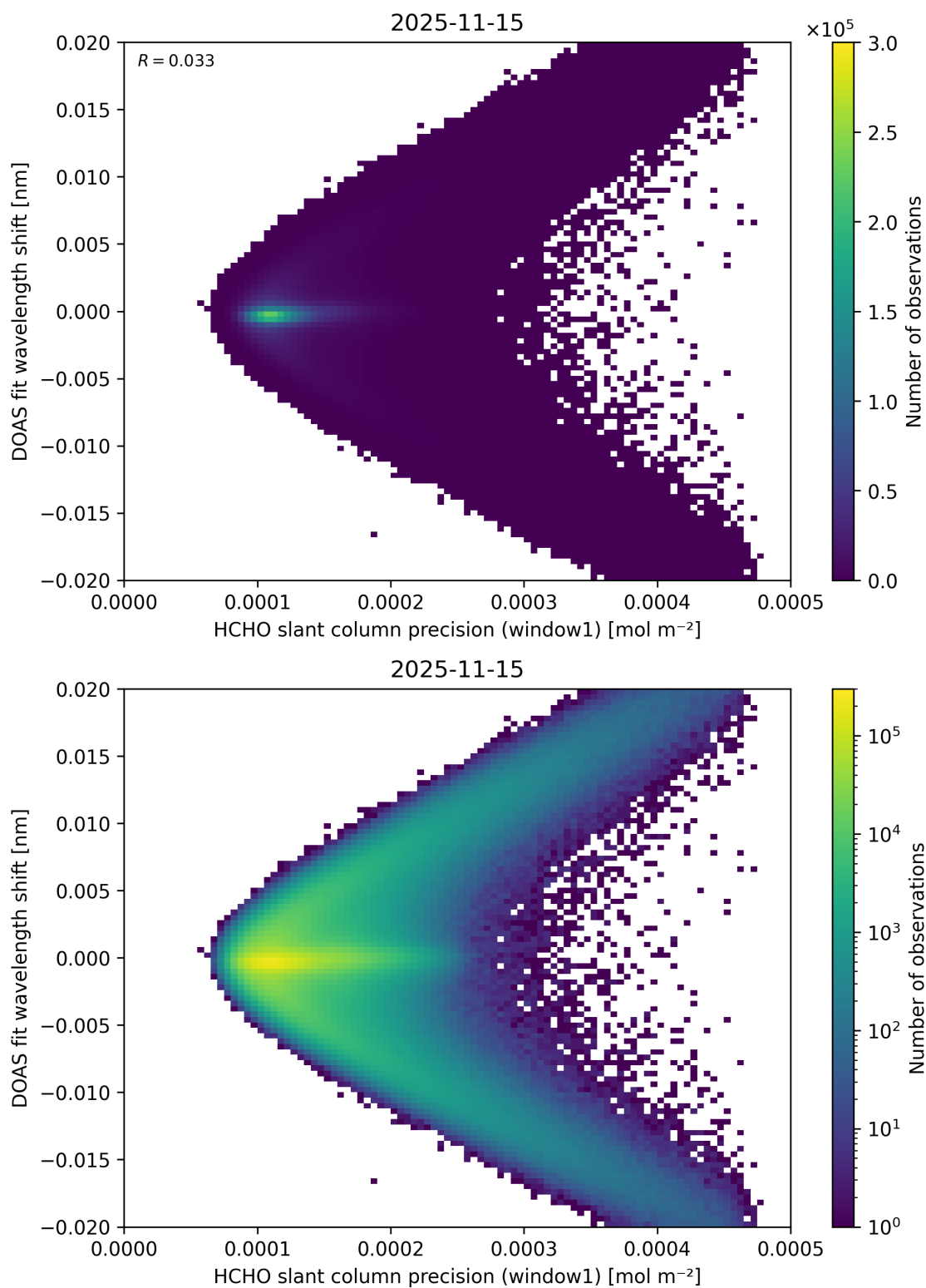
Figure 100: Scatter density plot of “HCHO slant column precision (window1)” against “DOAS fit wavelength shift” for 2025-11-14 to 2025-11-16.
