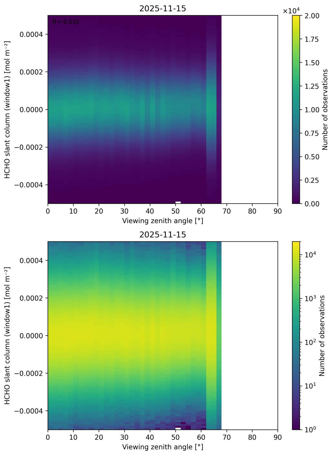
Figure 208: Scatter density plot of “Viewing zenith angle” against “HCHO slant column (window1)” for 2025-11-14 to 2025-11-16.
