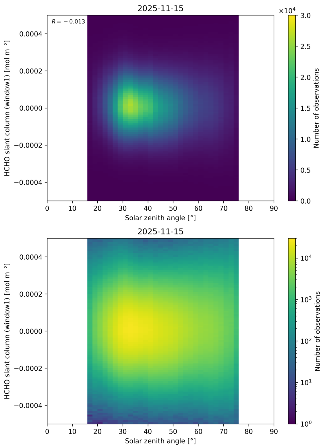
Figure 192: Scatter density plot of “Solar zenith angle” against “HCHO slant column (window1)” for 2025-11-14 to 2025-11-16.
