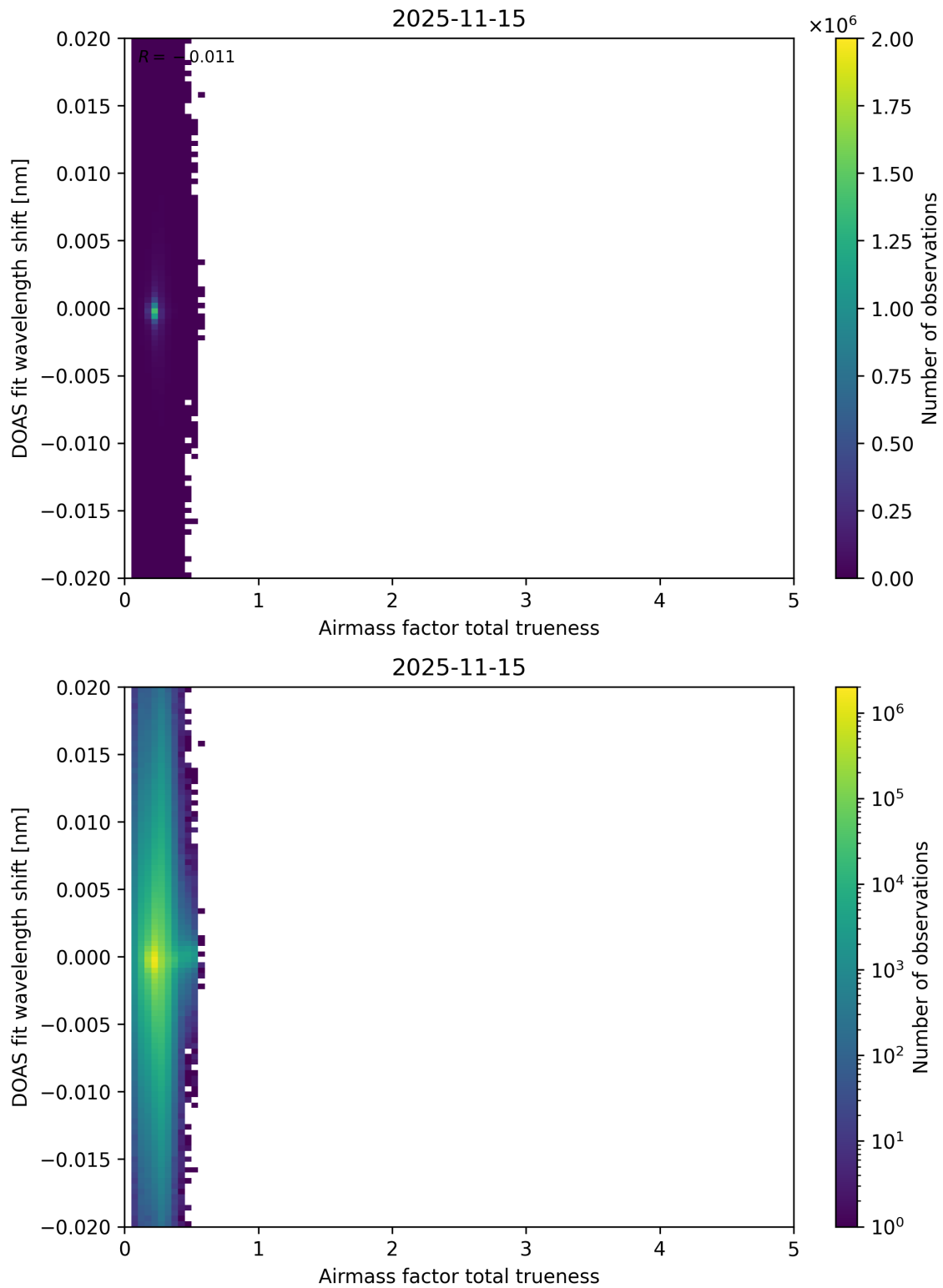
Figure 119: Scatter density plot of “Airmass factor total trueness” against “DOAS fit wavelength shift” for 2025-11-14 to 2025-11-16.
