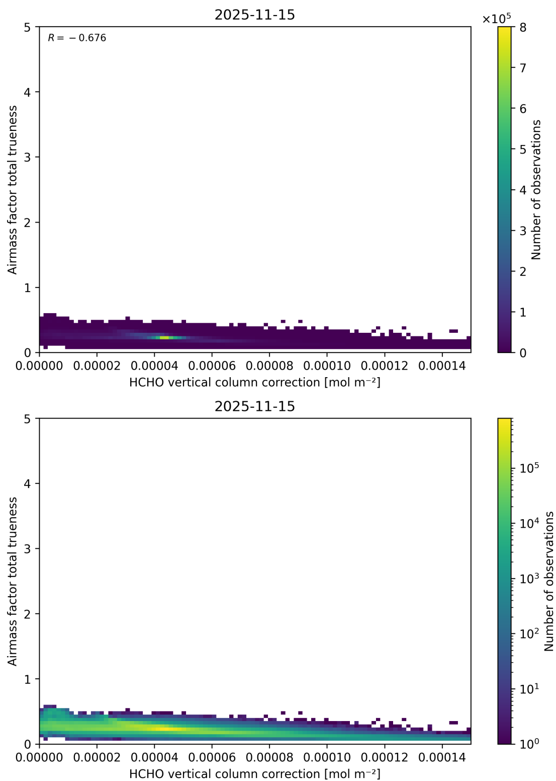
Figure 135: Scatter density plot of “HCHO vertical column correction” against “Airmass factor total trueness” for 2025-11-14 to 2025-11-16.
