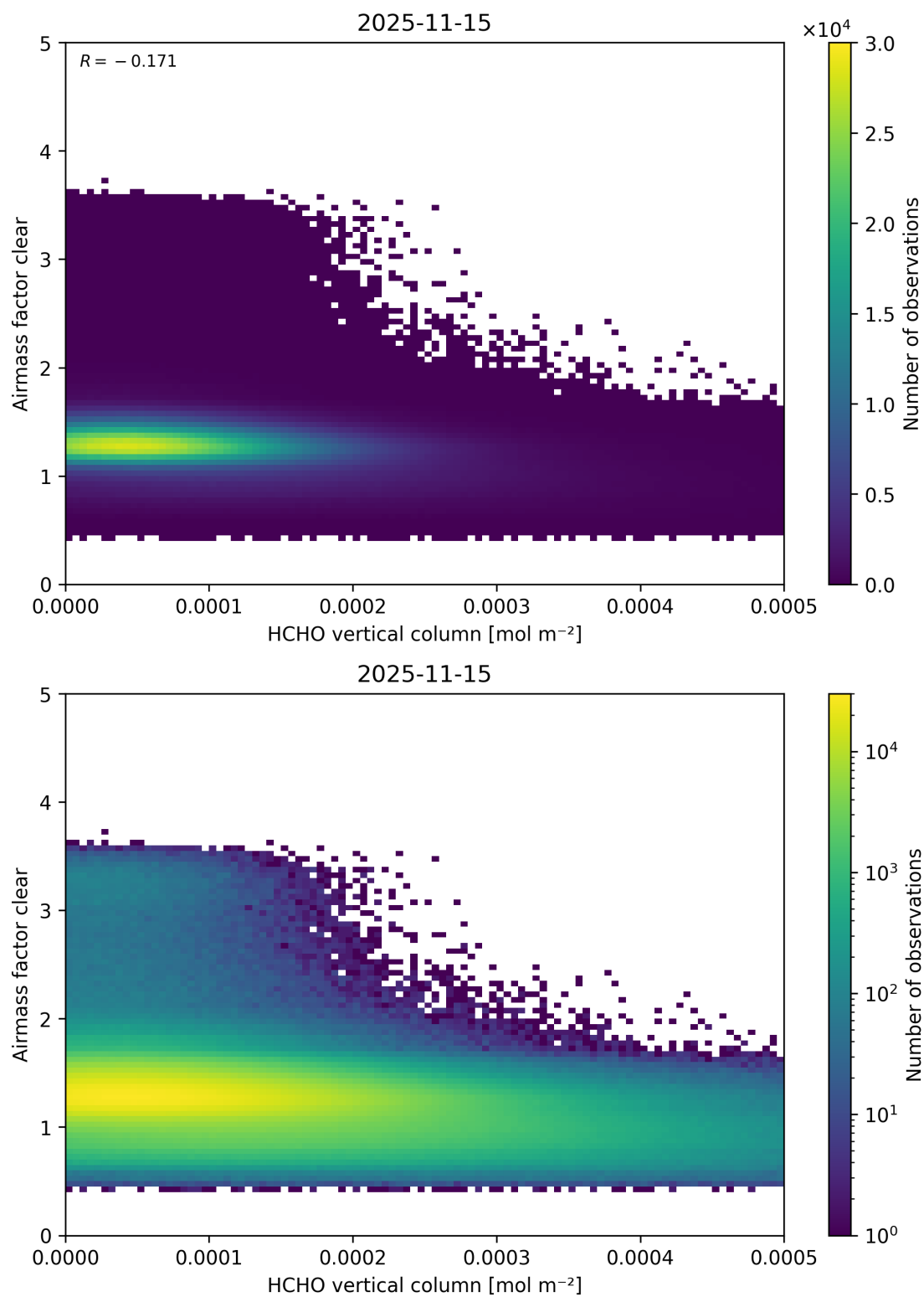
Figure 141: Scatter density plot of “HCHO vertical column” against “Airmass factor clear” for 2025-11-14 to 2025-11-16.
