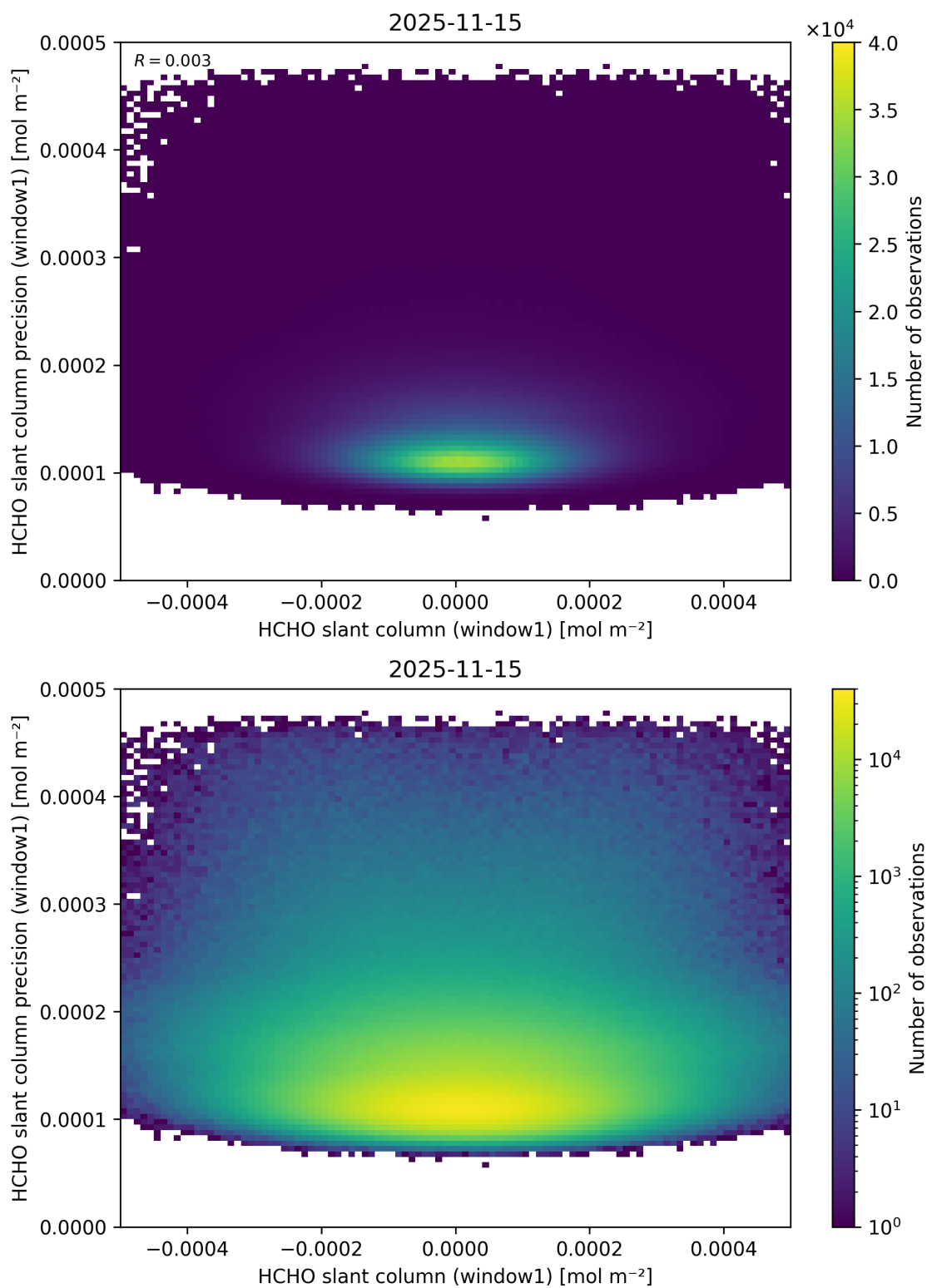
Figure 94: Scatter density plot of “HCHO slant column (window1)” against “HCHO slant column precision (window1)” for 2025-11-14 to 2025-11-16.
