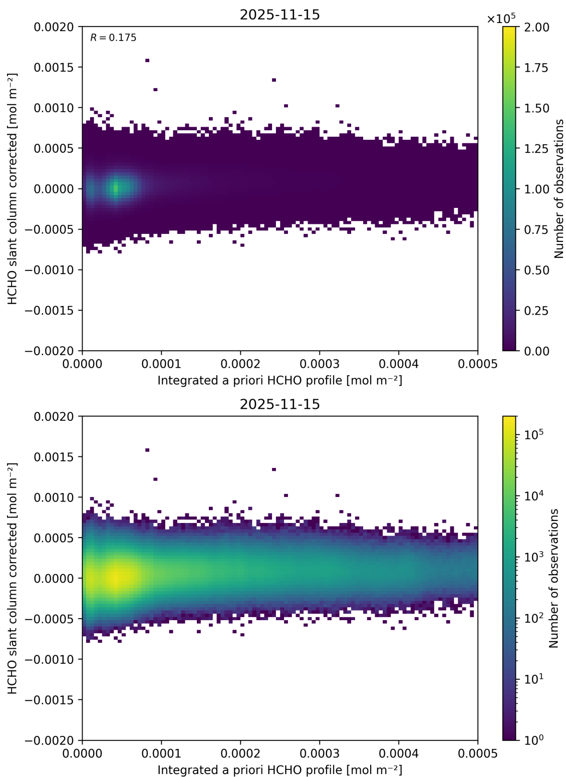
Figure 168: Scatter density plot of “Integrated a priori HCHO profile” against “HCHO slant column corrected” for 2025-11-14 to 2025-11-16.
