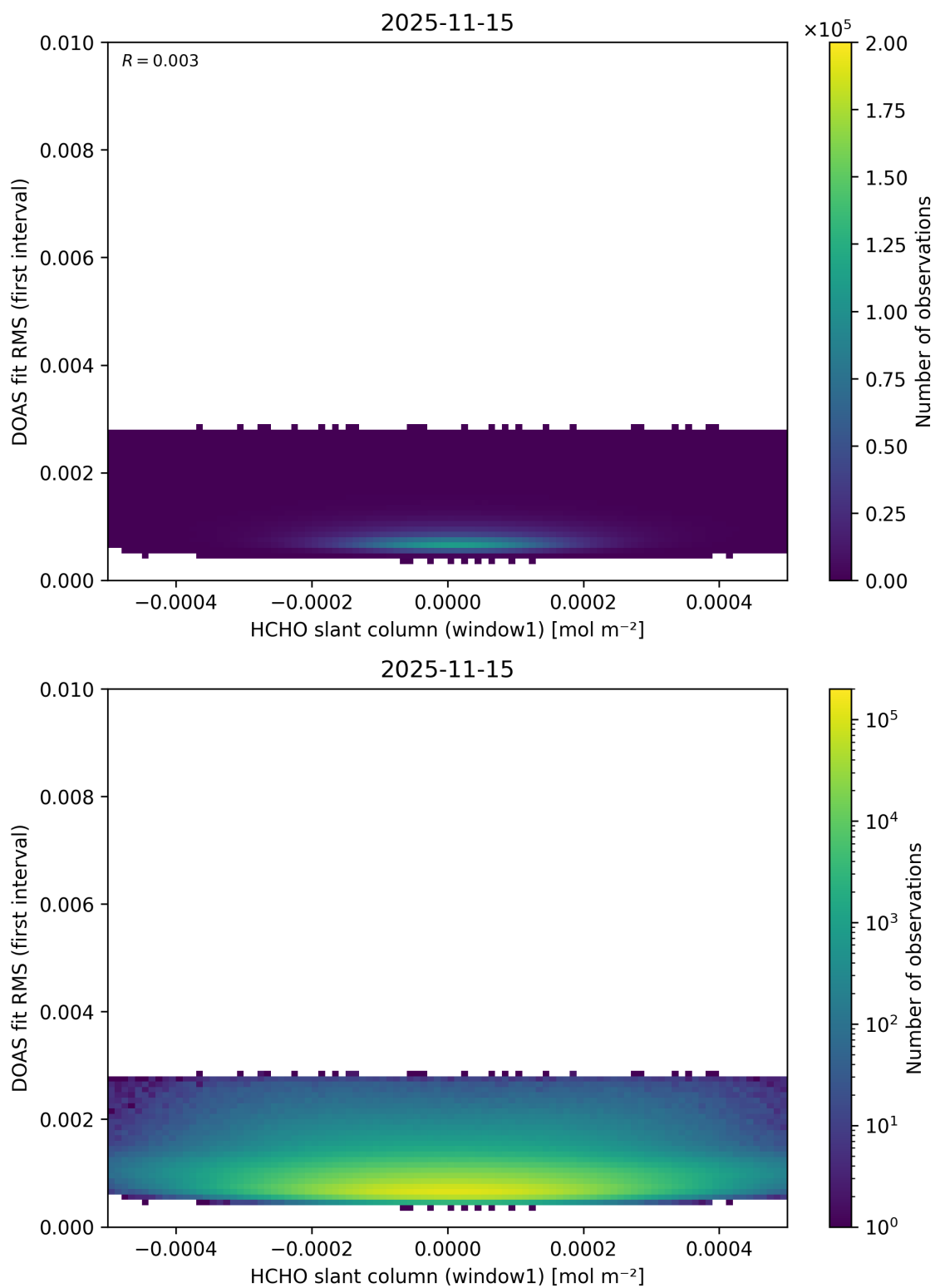
Figure 88: Scatter density plot of “HCHO slant column (window1)” against “DOAS fit RMS (first interval)” for 2025-11-14 to 2025-11-16.
