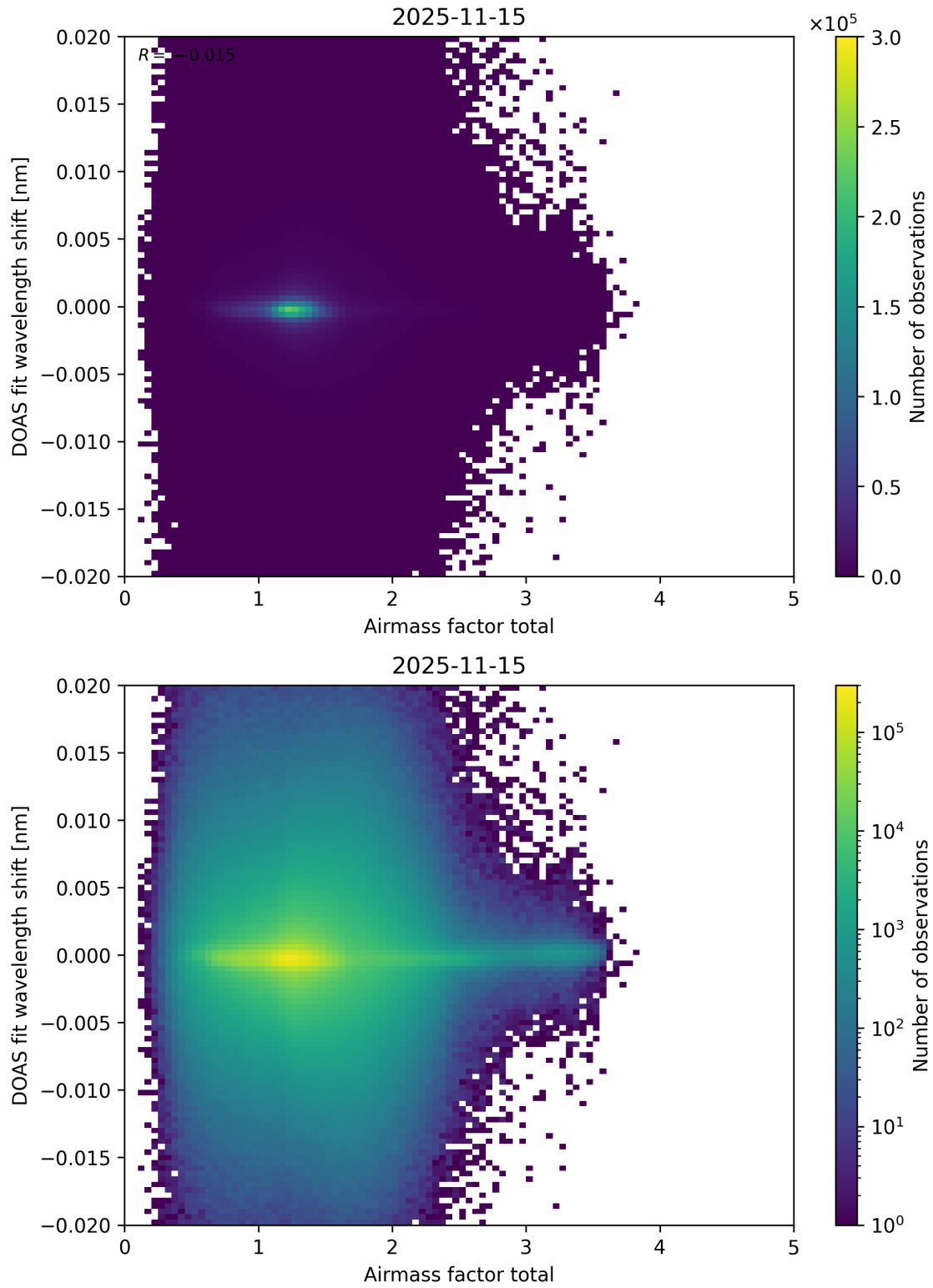
Figure 110: Scatter density plot of “Airmass factor total” against “DOAS fit wavelength shift” for 2025-11-14 to 2025-11-16.
