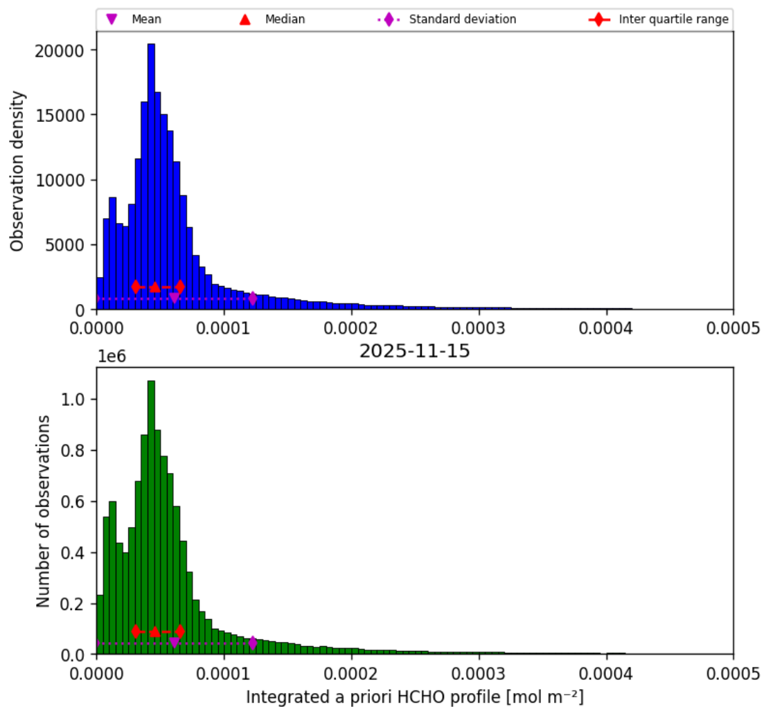
Figure 45: Histogram of “Integrated a priori HCHO profile” for 2025-11-14 to 2025-11-16
