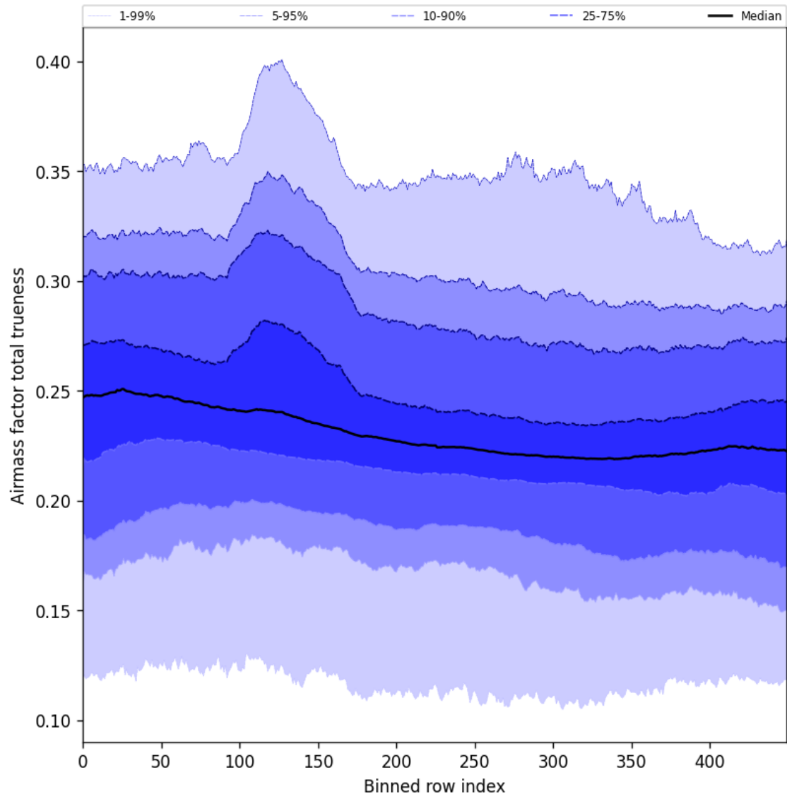
Figure 58: Along track statistics of “Airmass factor total trueness” for 2025-11-14 to 2025-11-16
