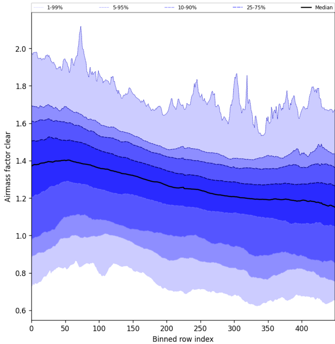
Figure 59: Along track statistics of “Airmass factor clear” for 2025-11-14 to 2025-11-16
