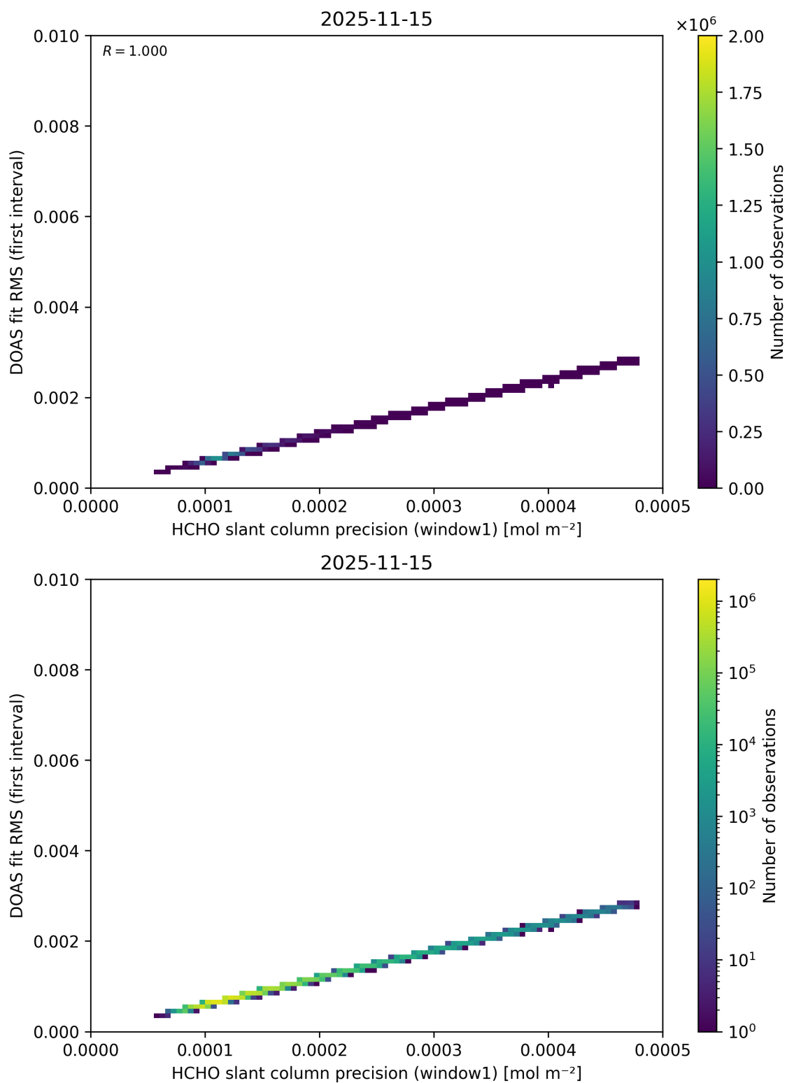
Figure 99: Scatter density plot of “HCHO slant column precision (window1)” against “DOAS fit RMS (first interval)” for 2025-11-14 to 2025-11-16.
