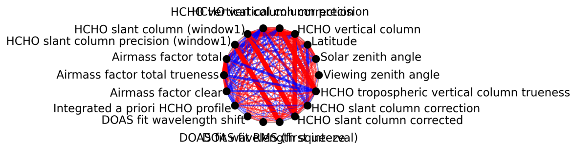
Figure 1: Map of correlation graph for 2025-11-14 to 2025-11-16.
