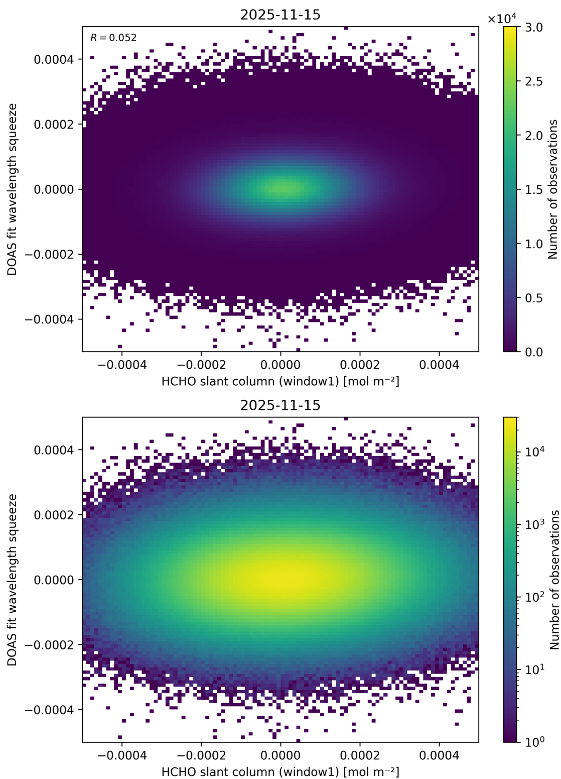
Figure 90: Scatter density plot of “HCHO slant column (window1)” against “DOAS fit wavelength squeeze” for 2025-11-14 to 2025-11-16.
