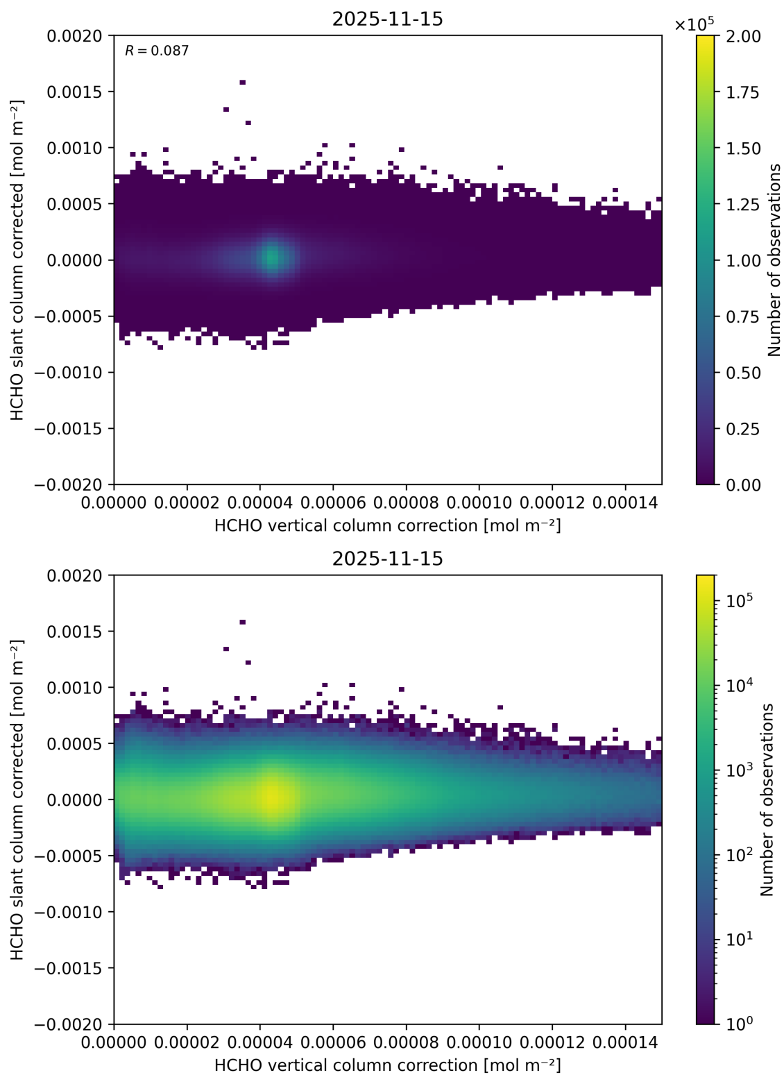
Figure 130: Scatter density plot of “HCHO vertical column correction” against “HCHO slant column corrected” for 2025-11-14 to 2025-11-16.
