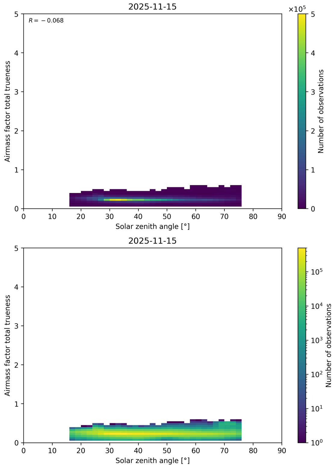
Figure 195: Scatter density plot of “Solar zenith angle” against “Airmass factor total trueneess” for 2025-11-14 to 2025-11-16.
