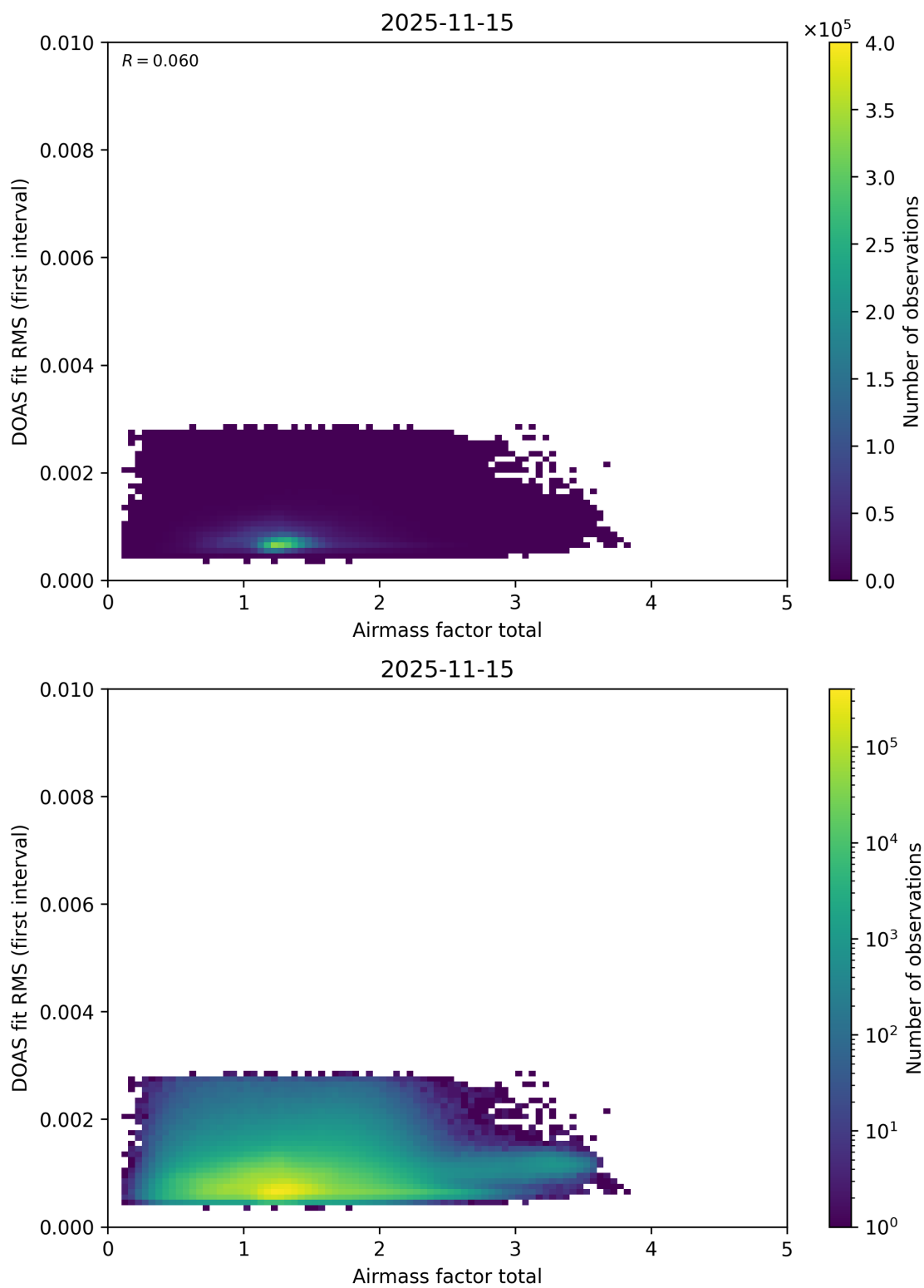
Figure 109: Scatter density plot of “Airmass factor total” against “DOAS fit RMS (first interval)” for 2025-11-14 to 2025-11-16.
