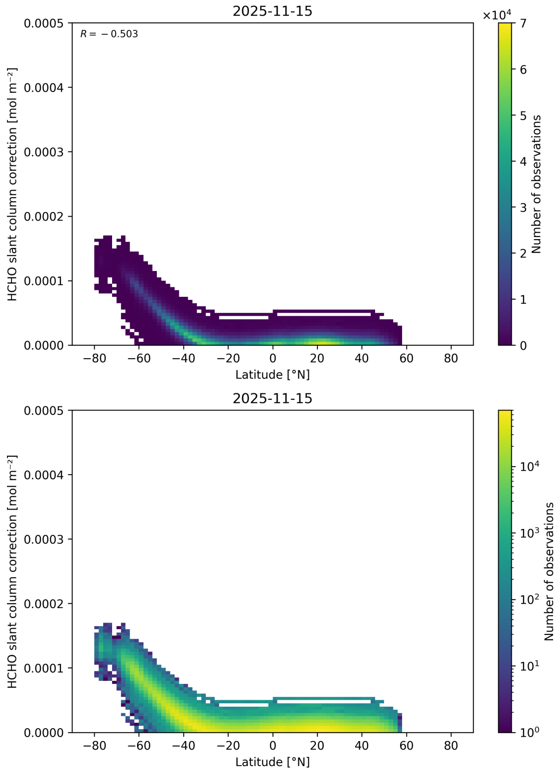
Figure 176: Scatter density plot of “Latitude” against “HCHO slant column correction” for 2025-11-14 to 2025-11-16.
