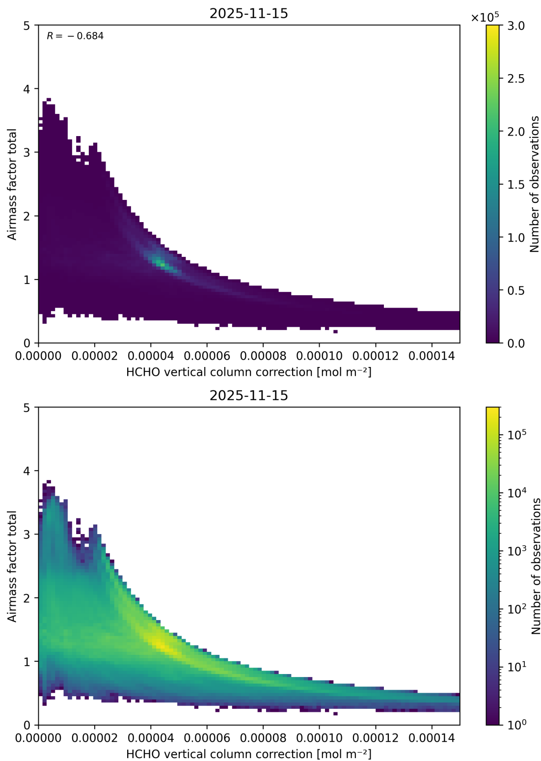
Figure 134: Scatter density plot of “HCHO vertical column correction” against “Airmass factor total” for 2025-11-14 to 2025-11-16.
