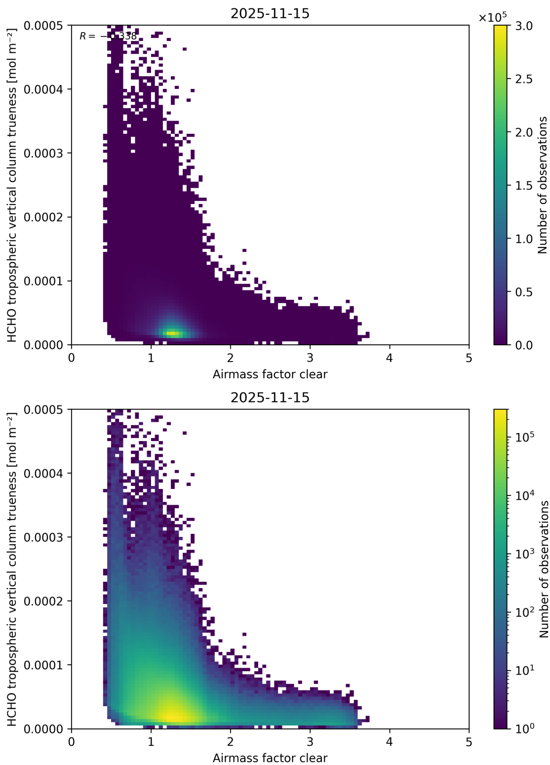
Figure 83: Scatter density plot of “Airmass factor clear” against “HCHO tropospheric vertical column trueeness” for 2025-11-14 to 2025-11-16.
