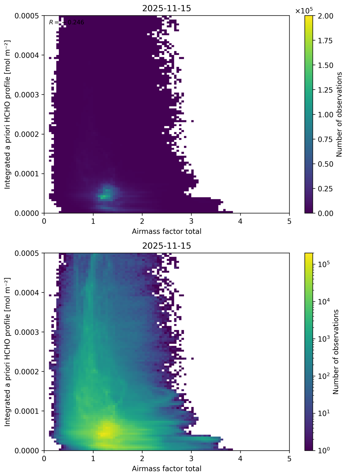
Figure 117: Scatter density plot of “Airmass factor total” against “Integrated a priori HCHO profile” for 2025-11-14 to 2025-11-16.
