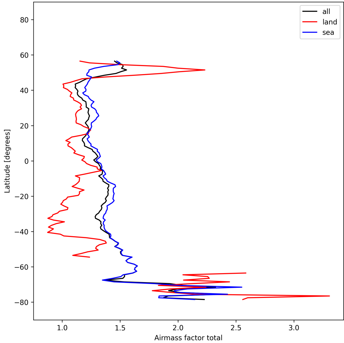
Figure 27: Zonal average of “Airmass factor total” for 2025-11-14 to 2025-11-16.
