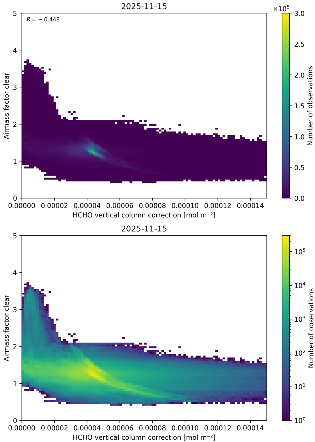
Figure 129: Scatter density plot of “HCHO vertical column correction” against “Airmass factor clear” for 2025-11-14 to 2025-11-16.
