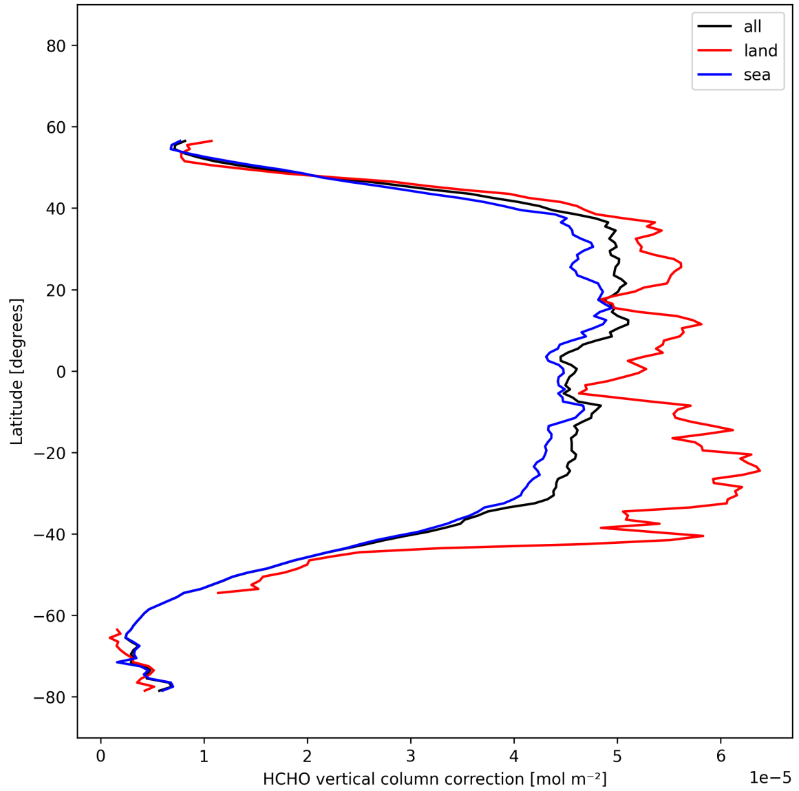
Figure 24: Zonal average of “HCHO vertical column correction” for 2025-11-14 to 2025-11-16.
