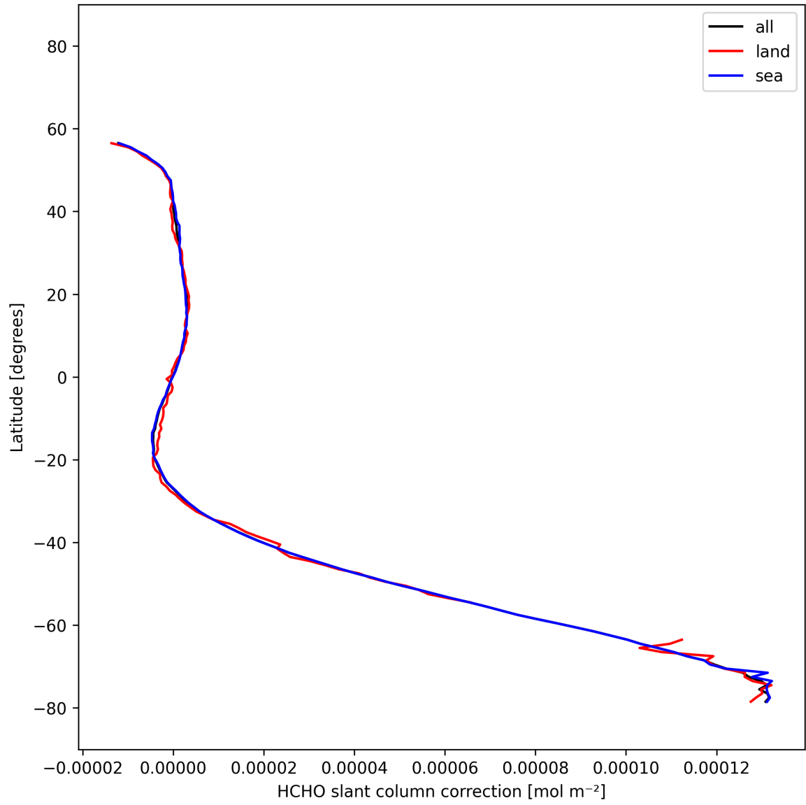
Figure 34: Zonal average of “HCHO slant column correction” for 2025-11-14 to 2025-11-16.
