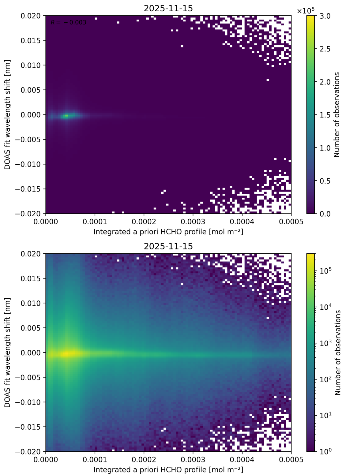
Figure 166: Scatter density plot of “Integrated a priori HCHO profile” against “DOAS fit wavelength shift” for 2025-11-14 to 2025-11-16.
