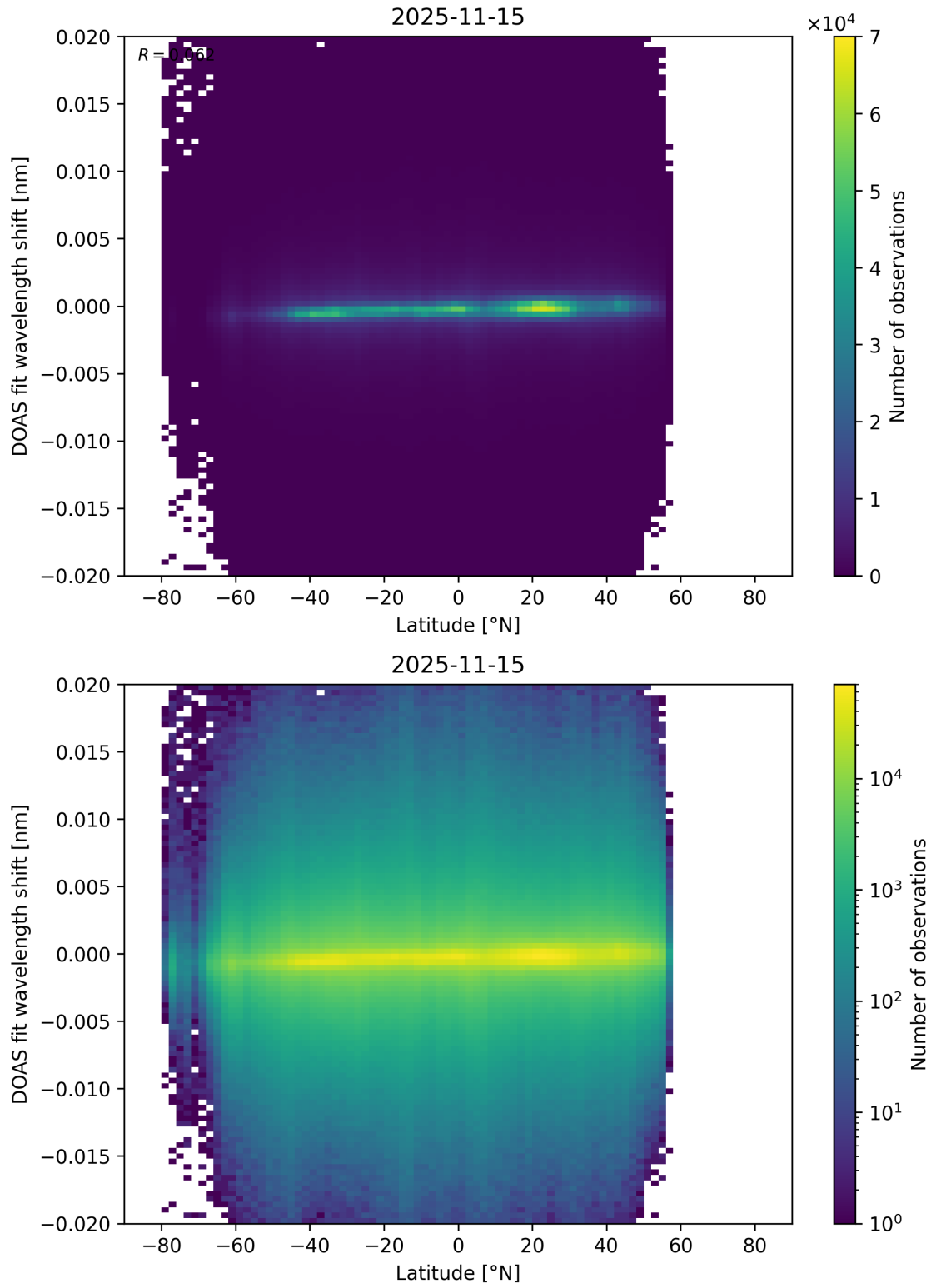
Figure 172: Scatter density plot of “Latitude” against “DOAS fit wavelength shift” for 2025-11-14 to 2025-11-16.
