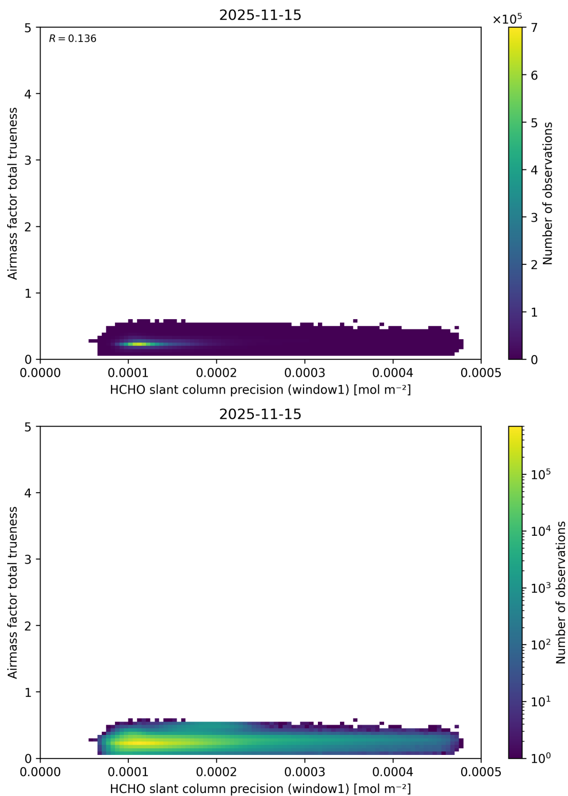
Figure 106: Scatter density plot of “HCHO slant column precision (window1)” against “Airmass factor total trueness” for 2025-11-14 to 2025-11-16.
