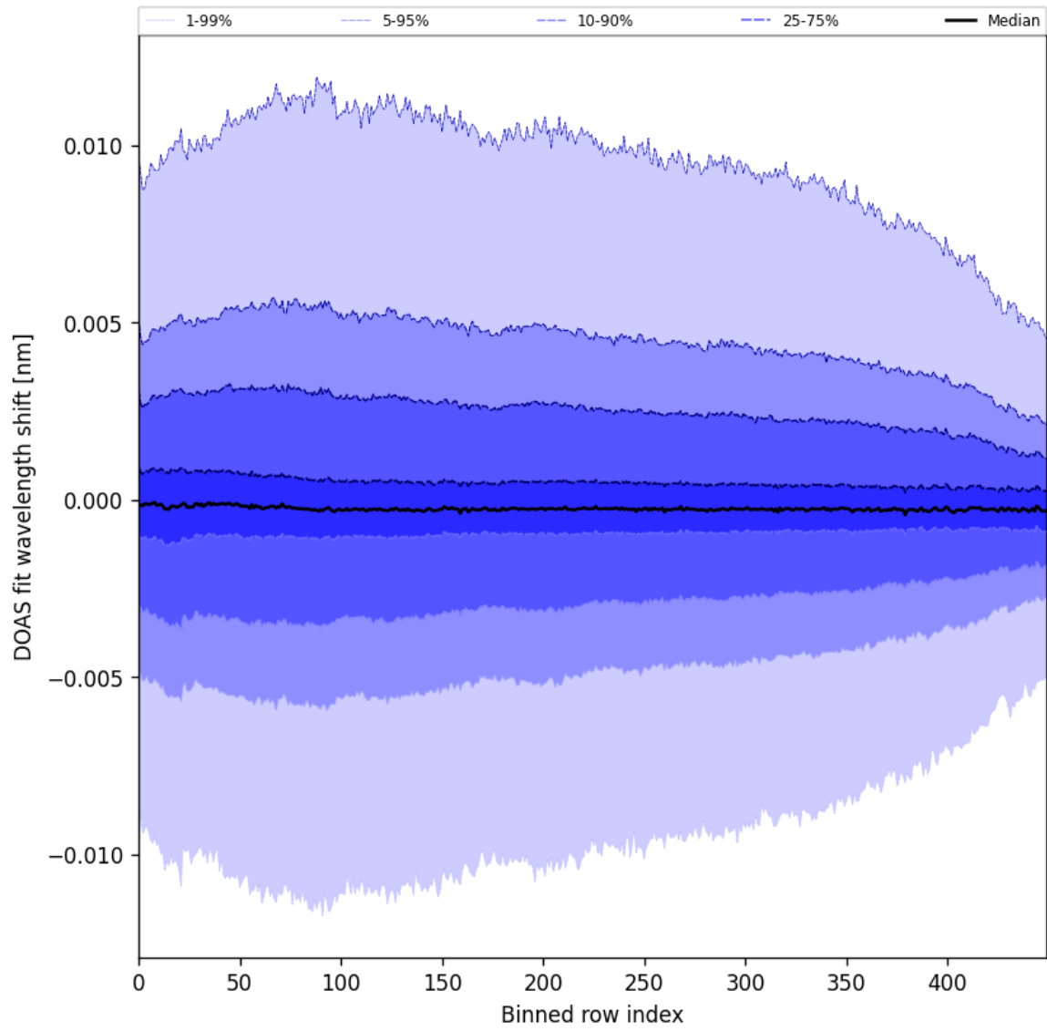
Figure 61: Along track statistics of “DOAS fit wavelength shift” for 2025-11-14 to 2025-11-16
