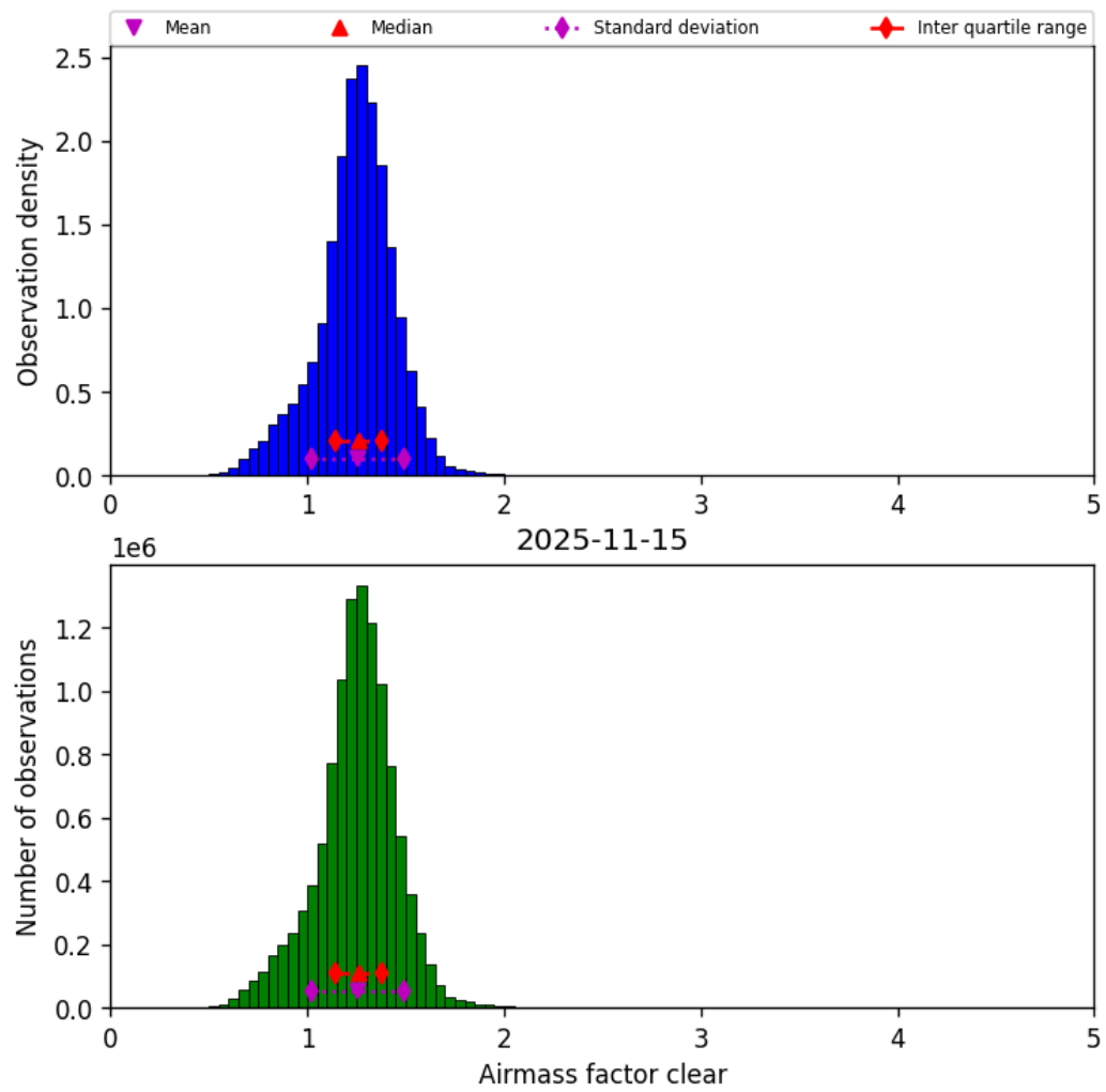
Figure 44: Histogram of “Airmass factor clear” for 2025-11-14 to 2025-11-16
