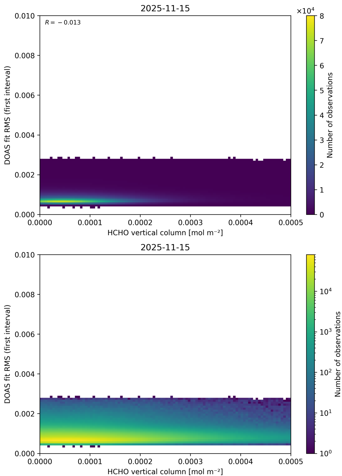
Figure 138: Scatter density plot of “HCHO vertical column” against “DOAS fit RMS (first interval)” for 2025-11-14 to 2025-11-16.
