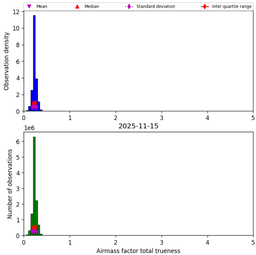
Figure 43: Histogram of “Airmass factor total trueness” for 2025-11-14 to 2025-11-16
