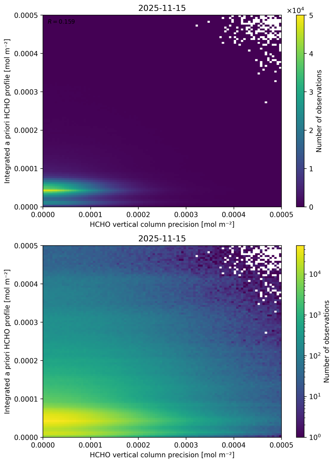
Figure 164: Scatter density plot of “HCHO vertical column precision” against “Integrated a priori HCHO profile” for 2025-11-14 to 2025-11-16.
