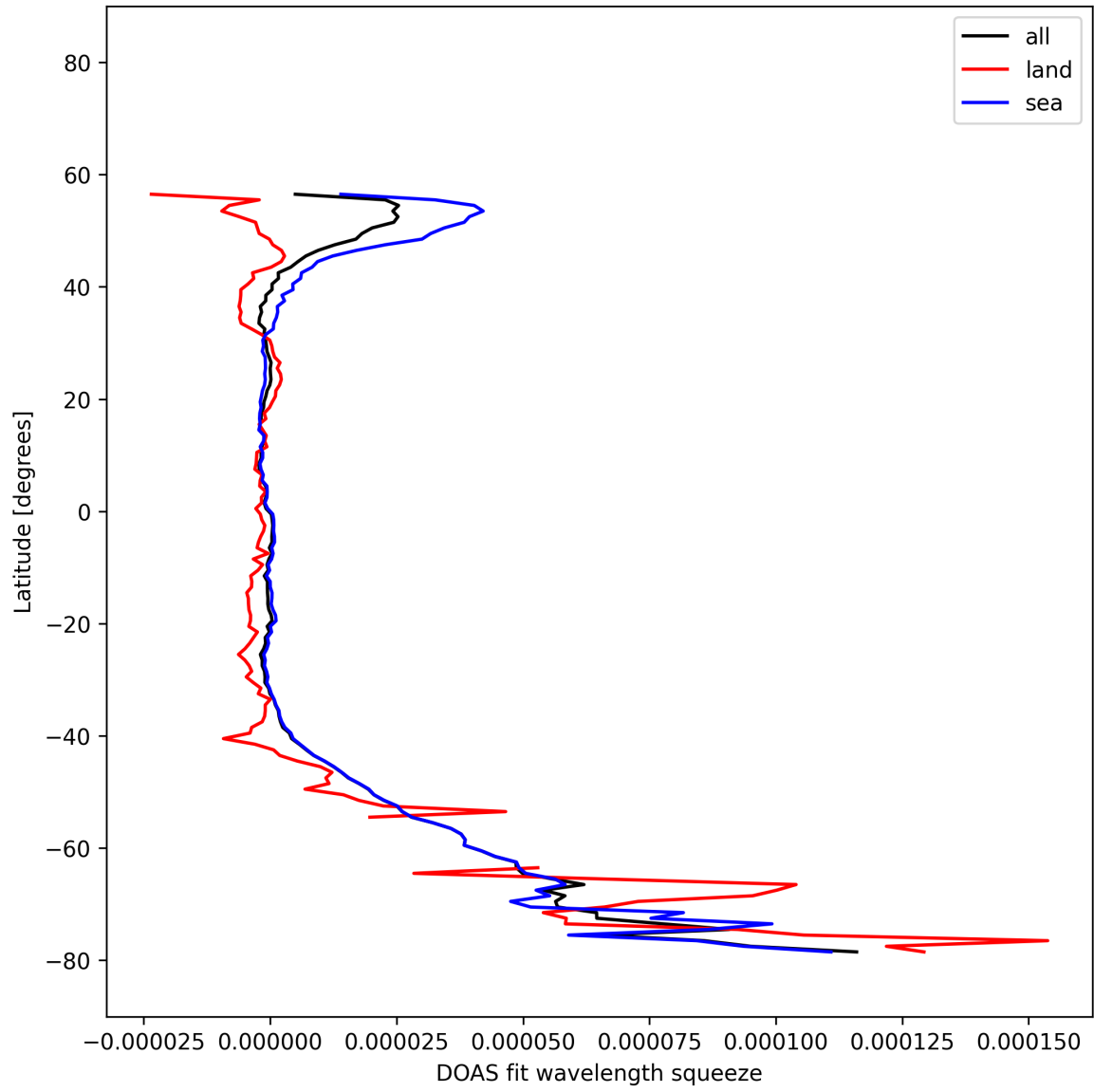
Figure 32: Zonal average of “DOAS fit wavelength squeeze” for 2025-11-14 to 2025-11-16.
