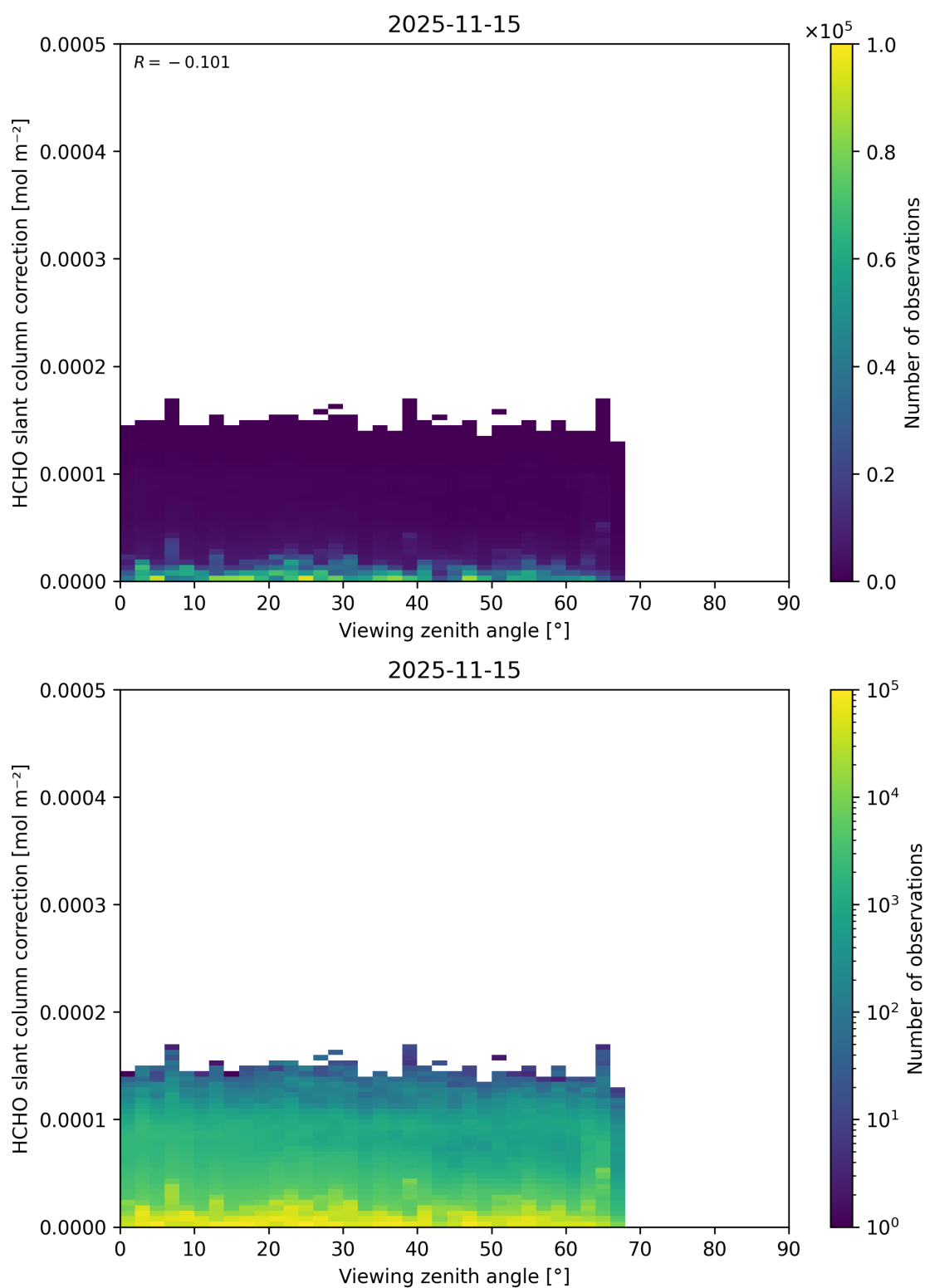
Figure 207: Scatter density plot of “Viewing zenith angle” against “HCHO slant column correction” for 2025-11-14 to 2025-11-16.
