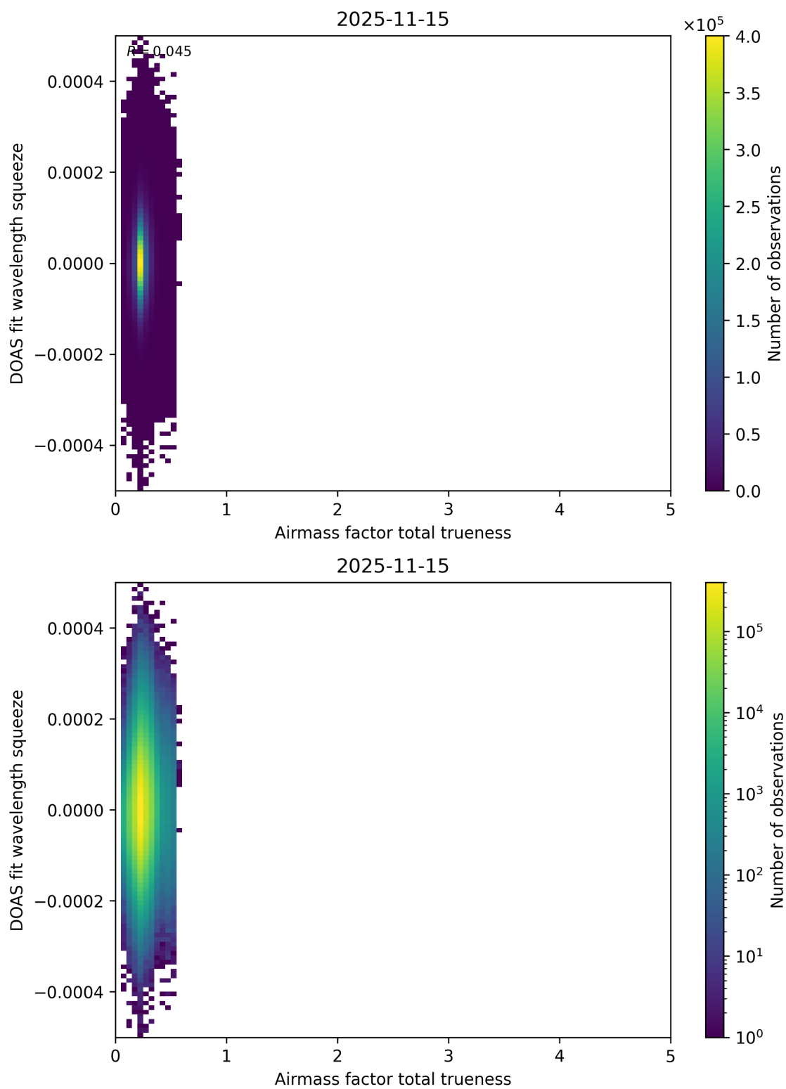
Figure 120: Scatter density plot of “Airmass factor total trueness” against “DOAS fit wavelength squeeze” for 2025-11-14 to 2025-11-16.
