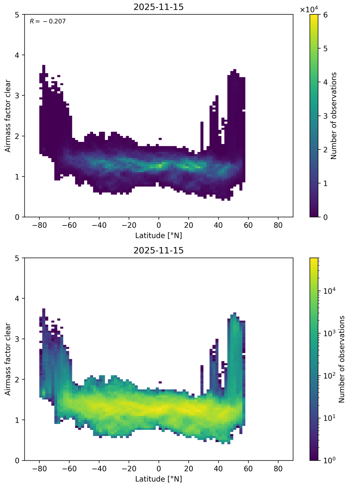
Figure 174: Scatter density plot of “Latitude” against “Airmass factor clear” for 2025-11-14 to 2025-11-16.
