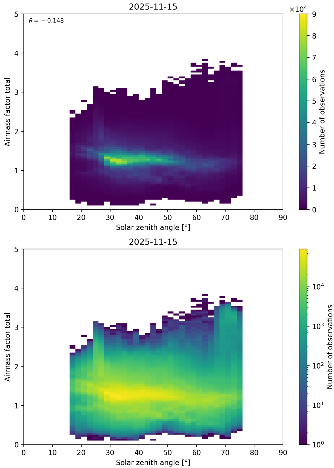
Figure 194: Scatter density plot of “Solar zenith angle” against “Airmass factor total” for 2025-11-14 to 2025-11-16.
