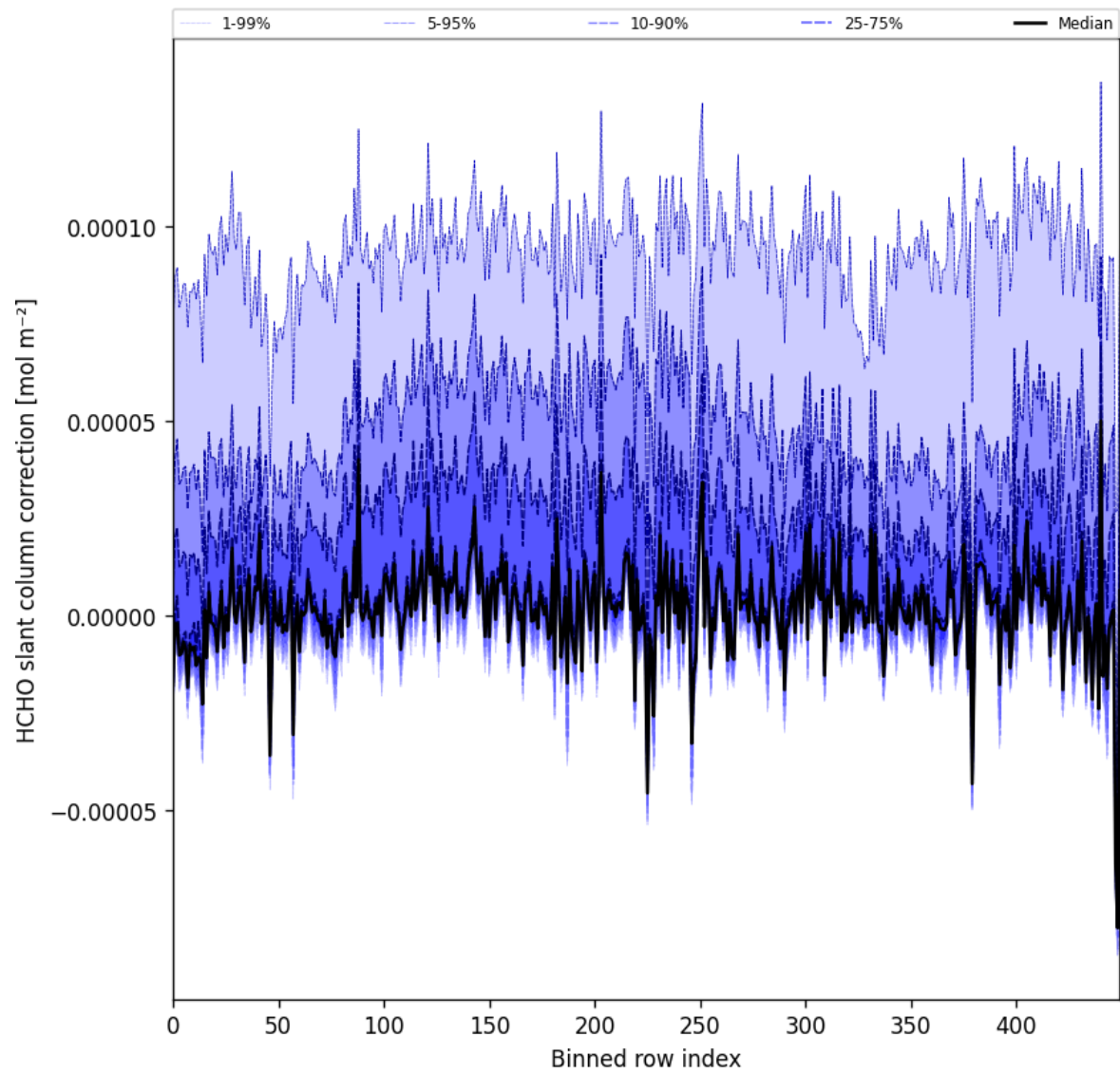
Figure 64: Along track statistics of “HCHO slant column correction” for 2025-11-14 to 2025-11-16
