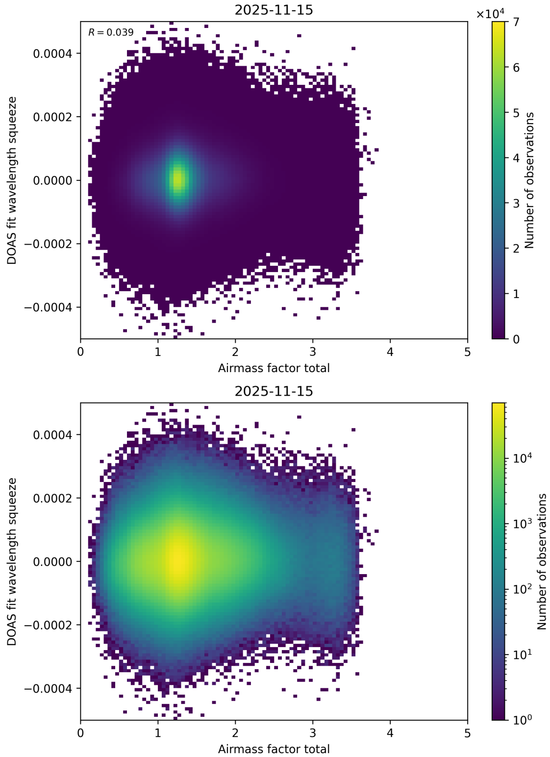
Figure 111: Scatter density plot of “Airmass factor total” against “DOAS fit wavelength squeeze” for 2025-11-14 to 2025-11-16.
