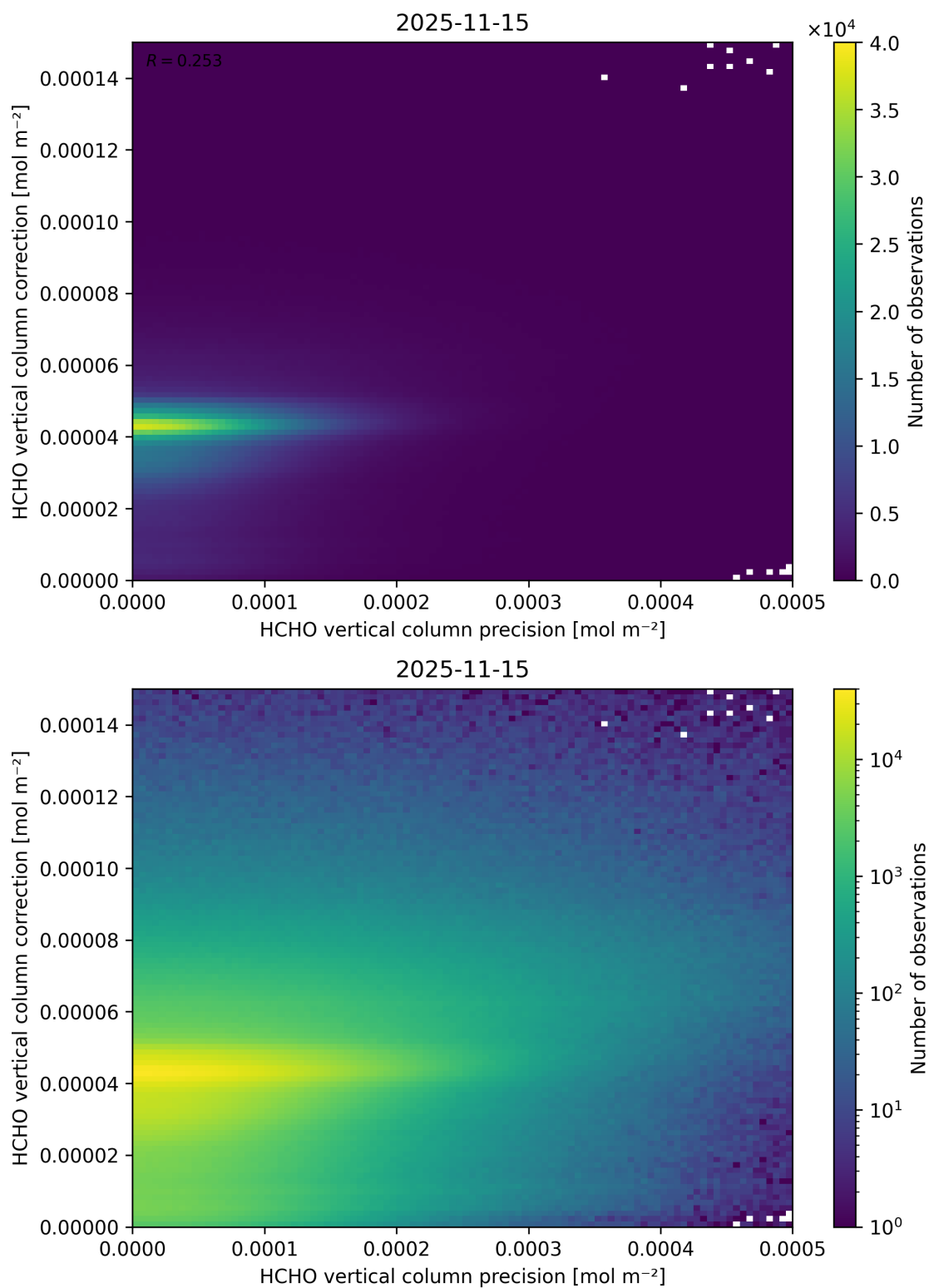
Figure 162: Scatter density plot of “HCHO vertical column precision” against “HCHO vertical column correction” for 2025-11-14 to 2025-11-16.
