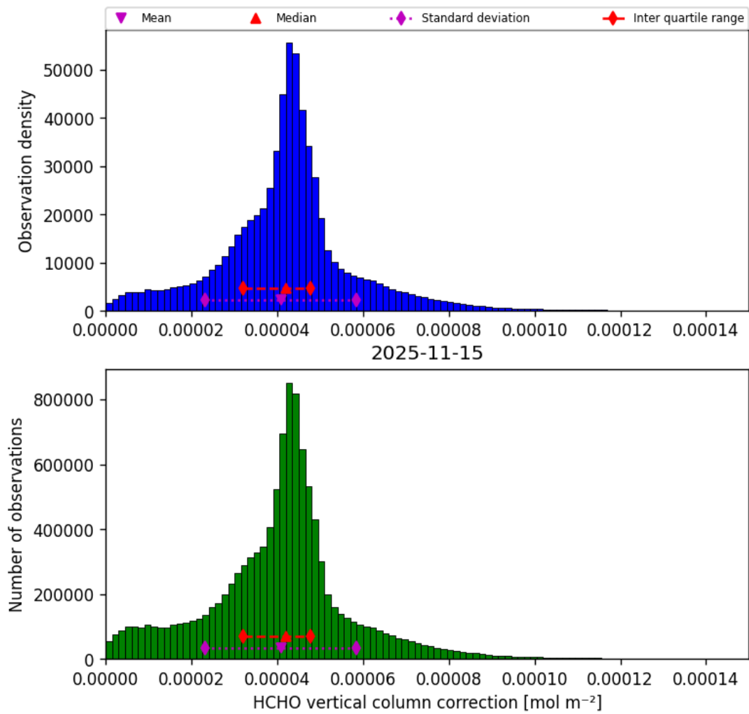
Figure 39: Histogram of “HCHO vertical column correction” for 2025-11-14 to 2025-11-16
