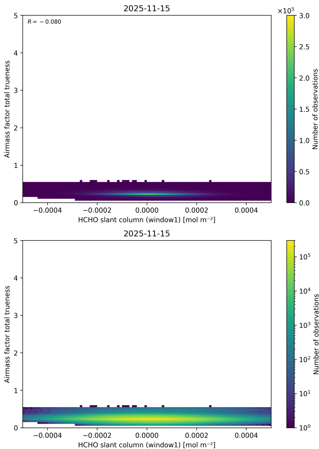
Figure 96: Scatter density plot of “HCHO slant column (window1)” against “Airmass factor total trueneess” for 2025-11-14 to 2025-11-16.
