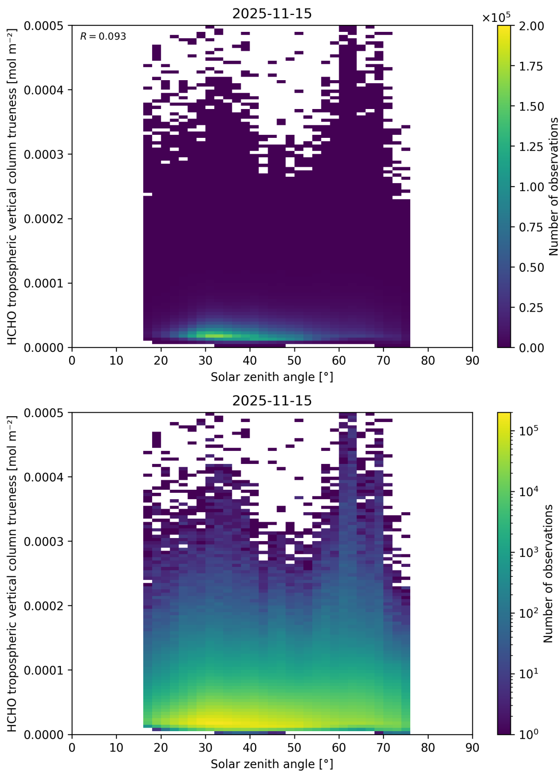
Figure 199: Scatter density plot of “Solar zenith angle” against “HCHO tropospheric vertical column trueness” for 2025-11-14 to 2025-11-16.
