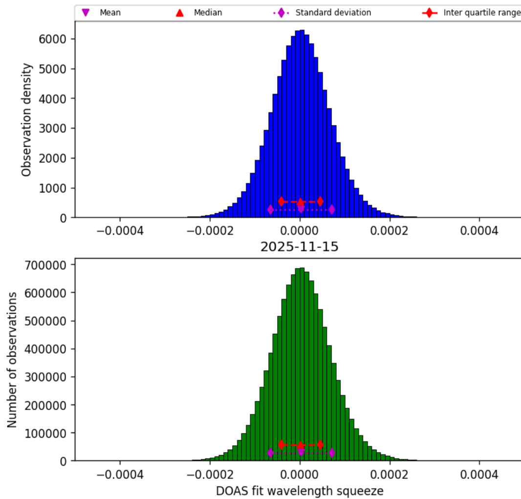
Figure 47: Histogram of “DOAS fit wavelength squeeze” for 2025-11-14 to 2025-11-16
