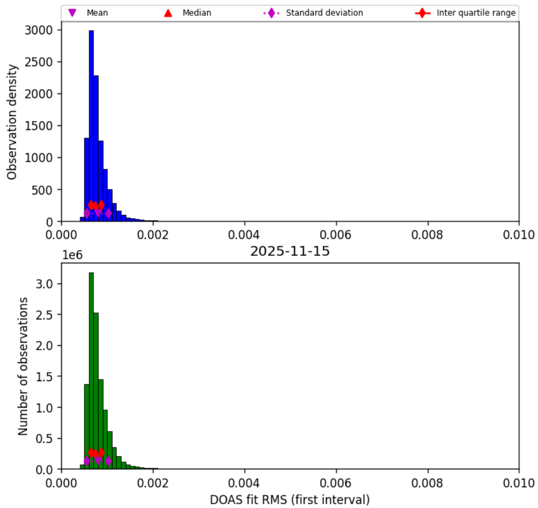
Figure 48: Histogram of “DOAS fit RMS (first interval)” for 2025-11-14 to 2025-11-16
