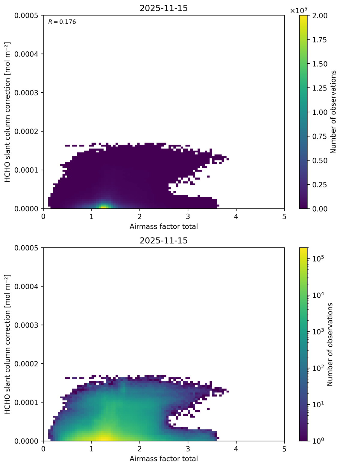
Figure 114: Scatter density plot of “Airmass factor total” against “HCHO slant column correction” for 2025-11-14 to 2025-11-16.
