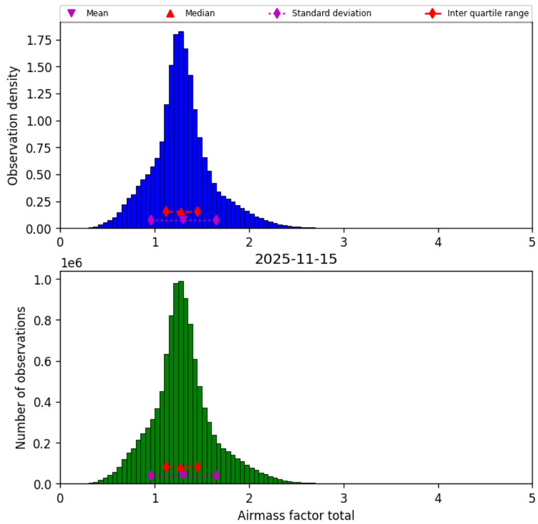
Figure 42: Histogram of “Airmass factor total” for 2025-11-14 to 2025-11-16
