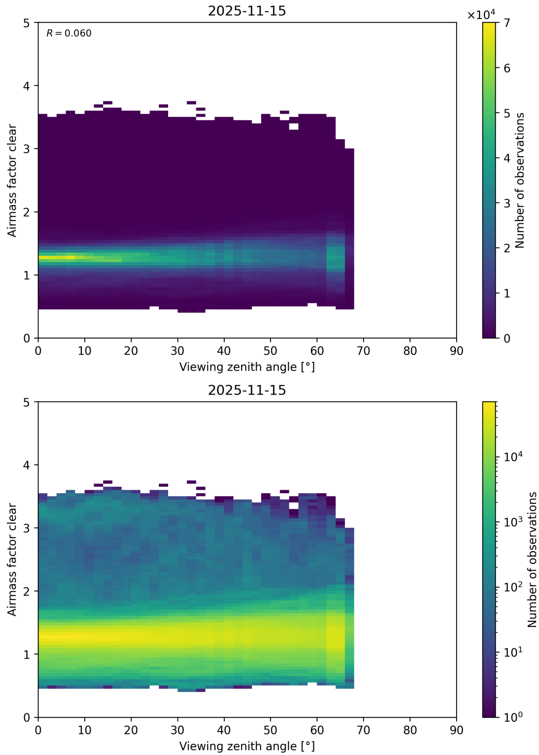
Figure 205: Scatter density plot of “Viewing zenith angle” against “Airmass factor clear” for 2025-11-14 to 2025-11-16.
