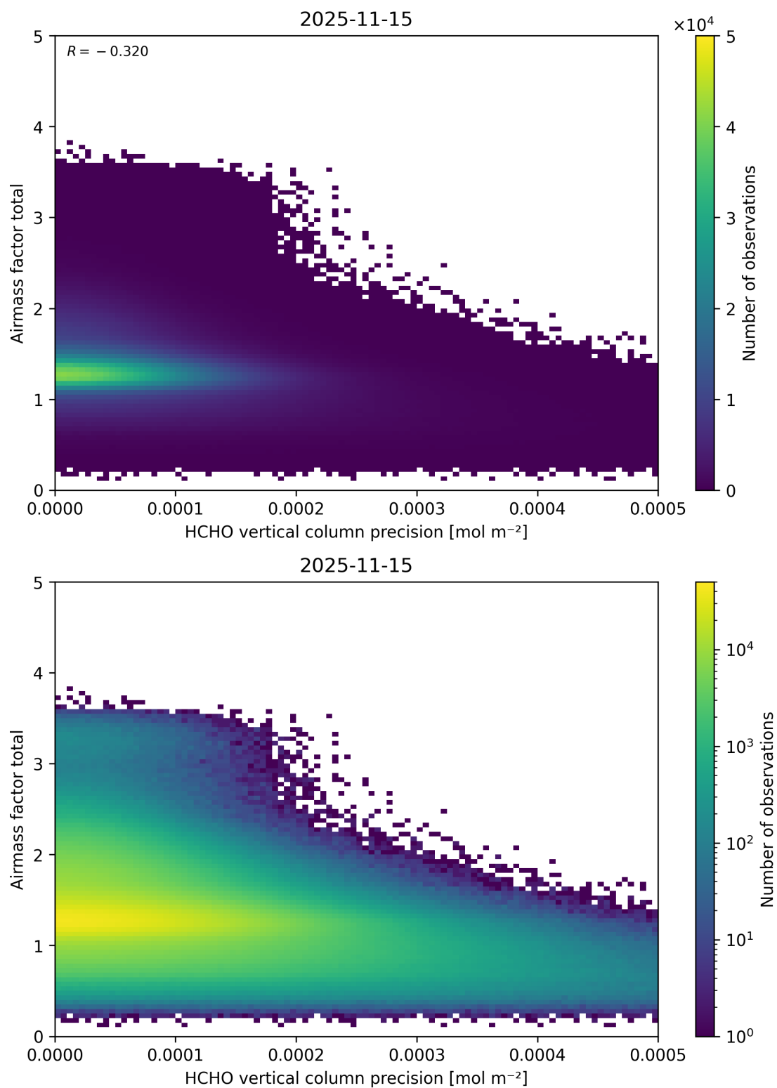
Figure 160: Scatter density plot of “HCHO vertical column precision” against “Airmass factor total” for 2025-11-14 to 2025-11-16.
