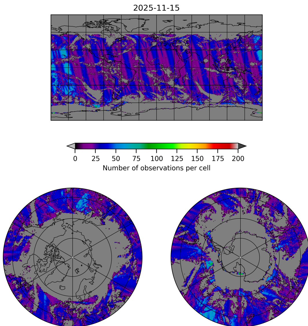
Figure 20: Map of the number of observations for 2025-11-14 to 2025-11-16
