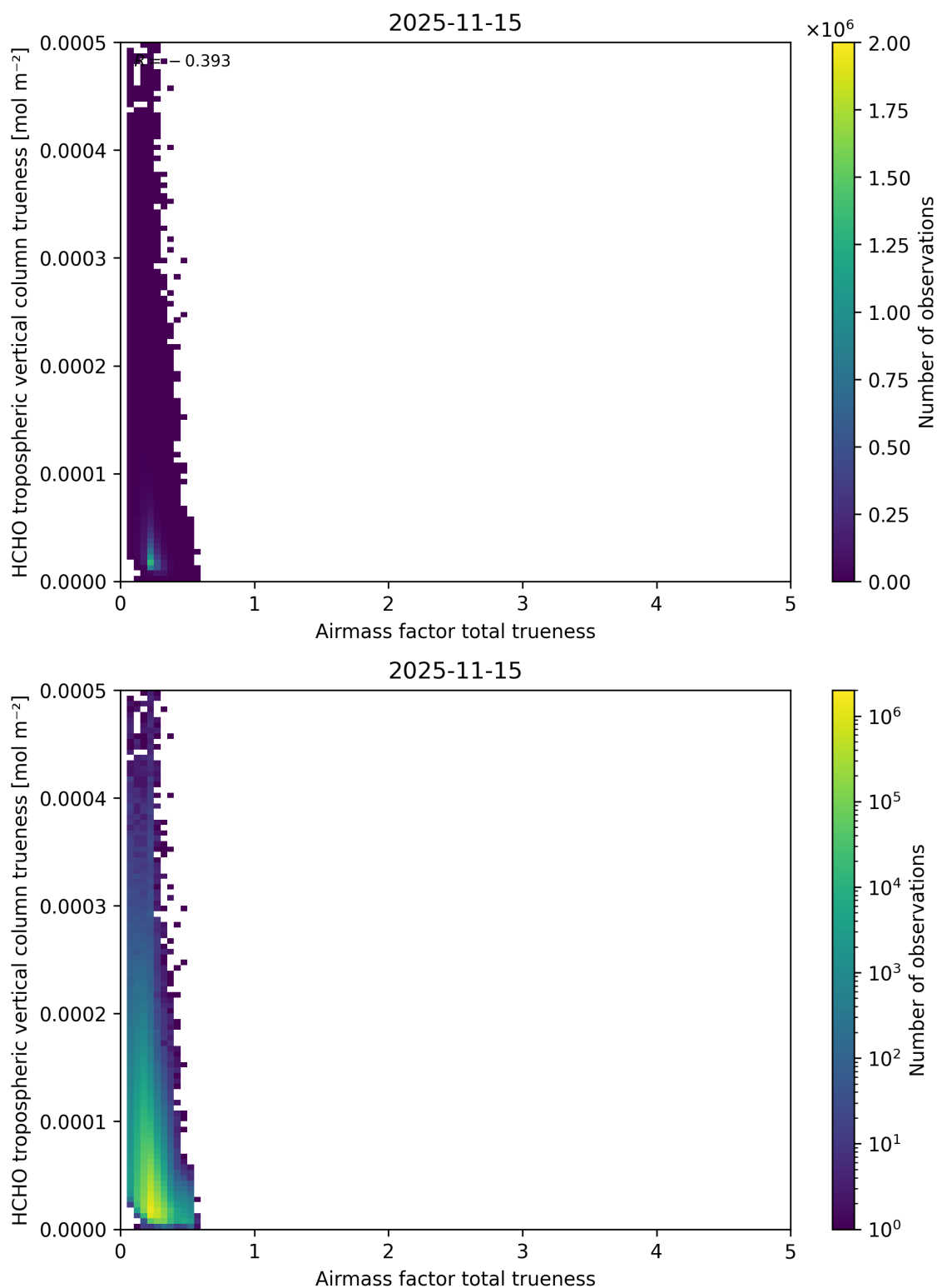
Figure 124: Scatter density plot of “Airmass factor total truiness” against “HCHO tropospheric vertical column truiness” for 2025-11-14 to 2025-11-16.
