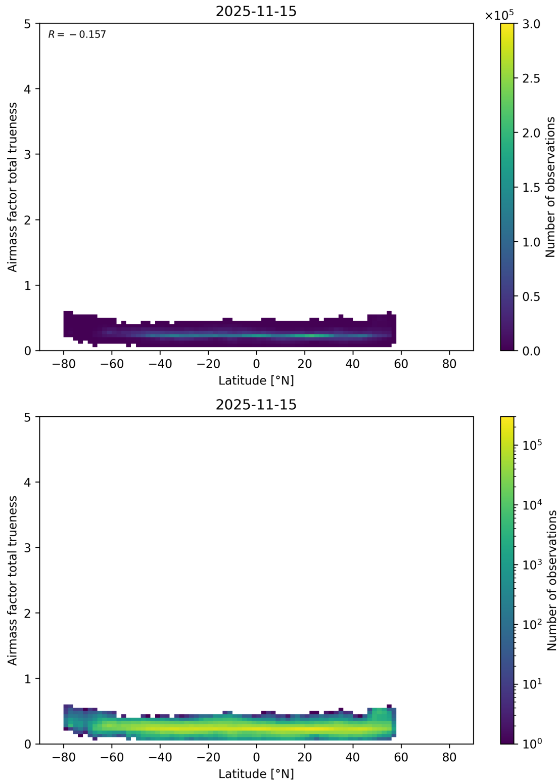
Figure 180: Scatter density plot of “Latitude” against “Airmass factor total trueness” for 2025-11-14 to 2025-11-16.
