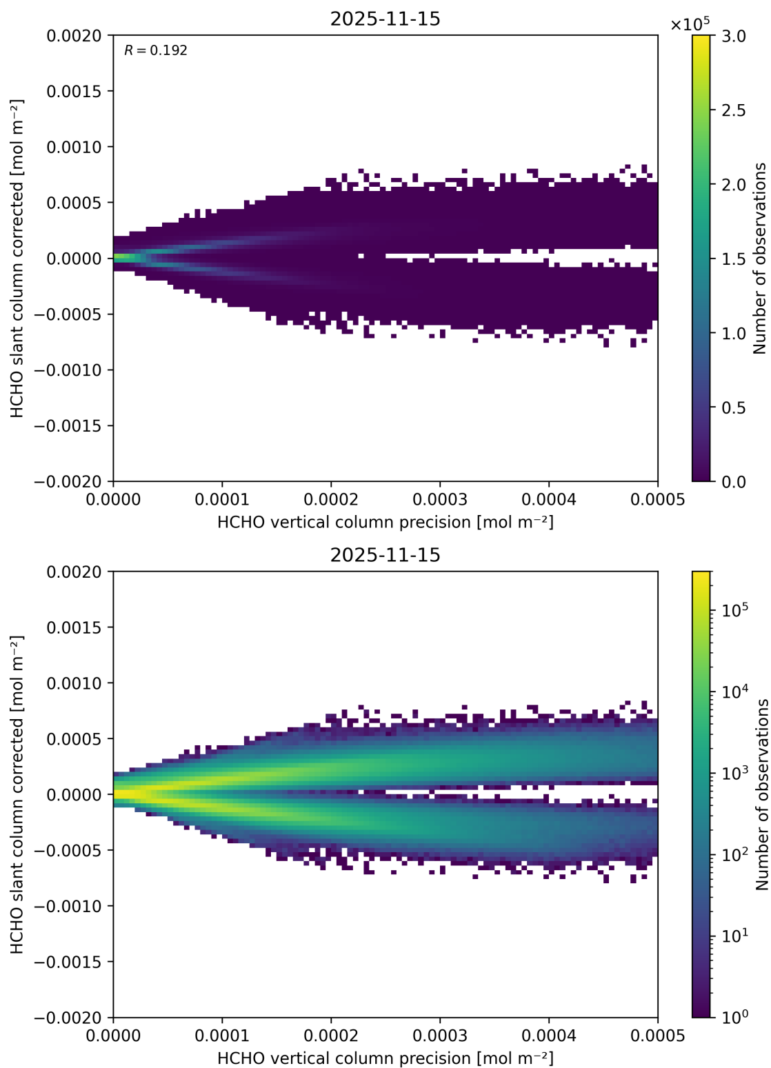
Figure 156: Scatter density plot of “HCHO vertical column precision” against “HCHO slant column corrected” for 2025-11-14 to 2025-11-16.
