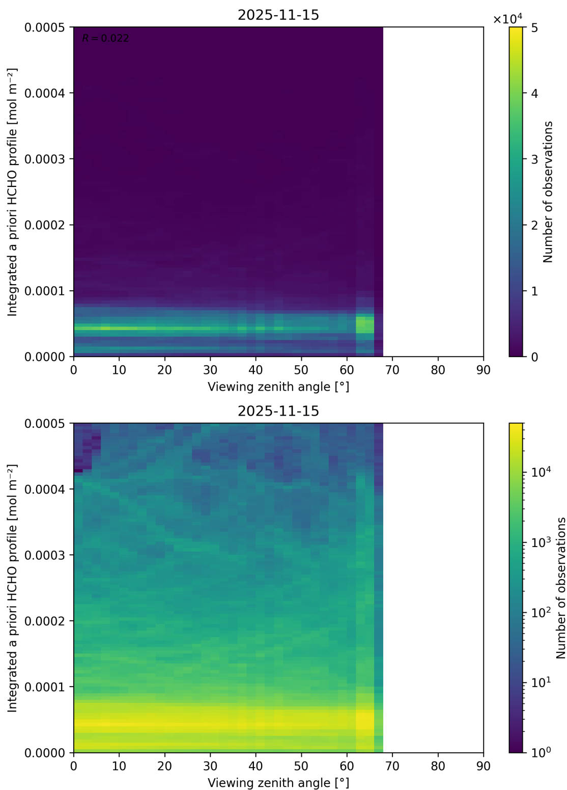
Figure 216: Scatter density plot of “Viewing zenith angle” against “Integrated a priori HCHO profile” for 2025-11-14 to 2025-11-16.
