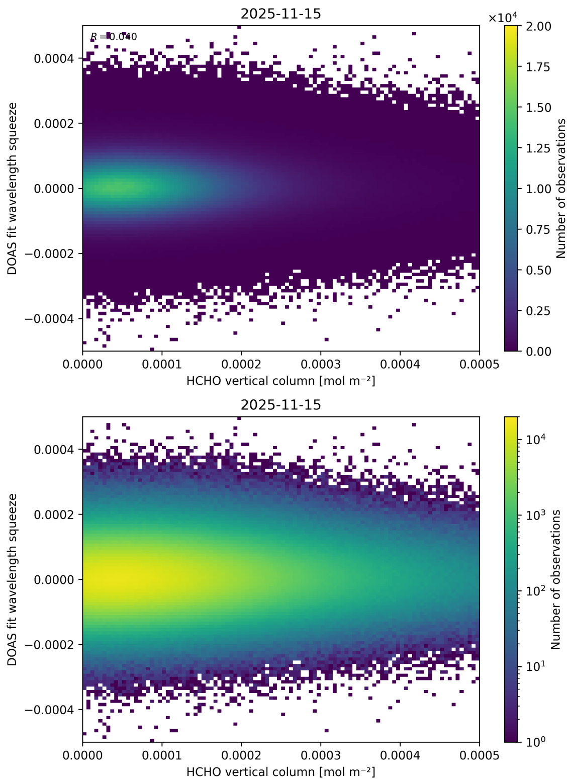
Figure 140: Scatter density plot of “HCHO vertical column” against “DOAS fit wavelength squeeze” for 2025-11-14 to 2025-11-16.
