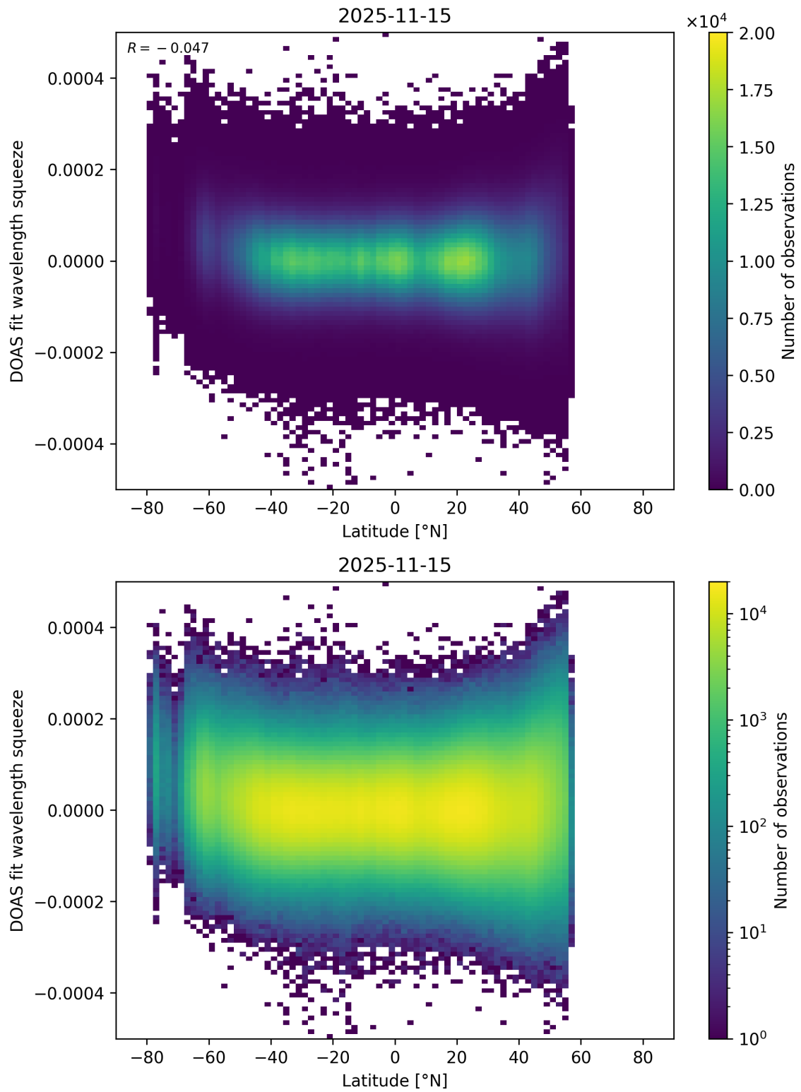
Figure 173: Scatter density plot of “Latitude” against “DOAS fit wavelength squeeze” for 2025-11-14 to 2025-11-16.
