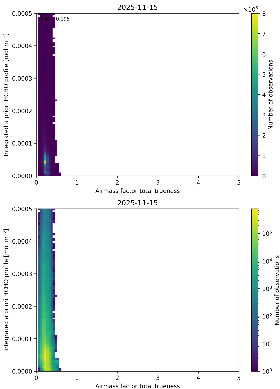
Figure 125: Scatter density plot of “Airmass factor total trueness” against “Integrated a priori HCHO profile” for 2025-11-14 to 2025-11-16.
