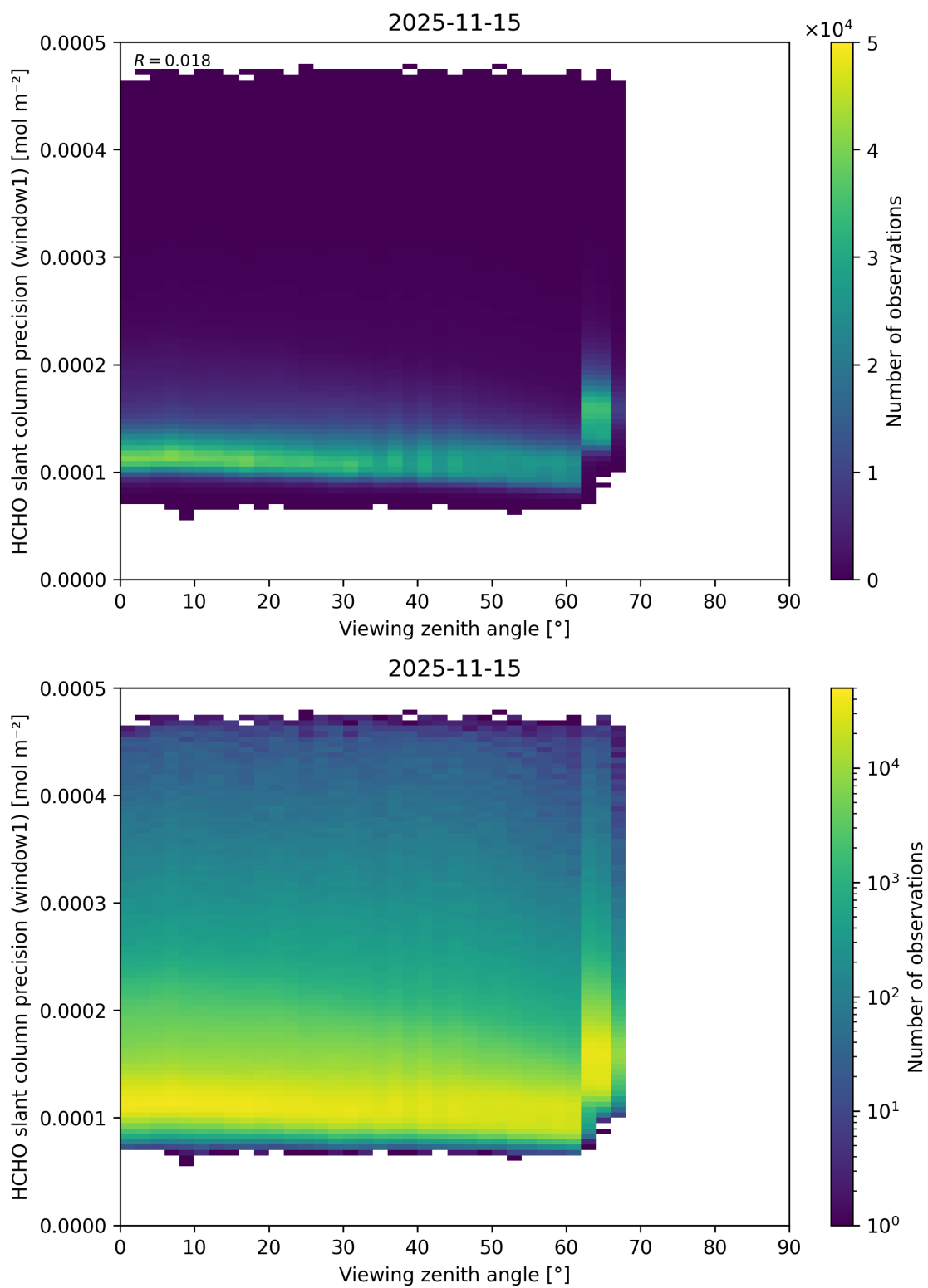
Figure 209: Scatter density plot of “Viewing zenith angle” against “HCHO slant column precision (window1)” for 2025-11-14 to 2025-11-16.
