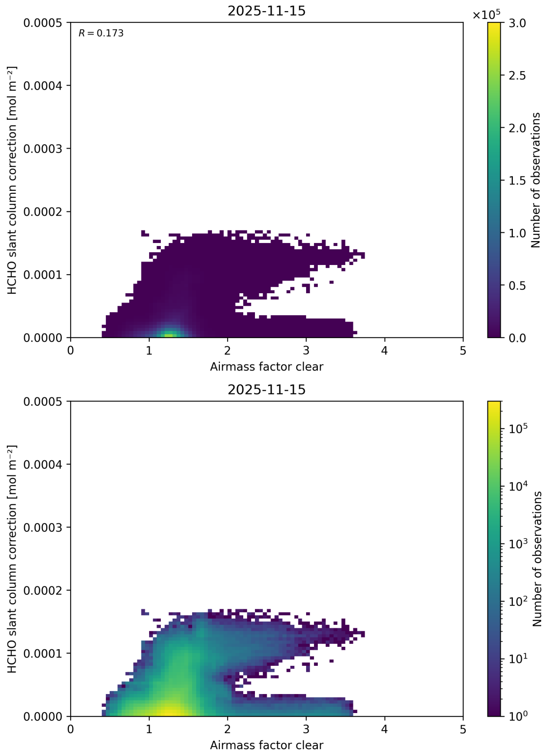
Figure 82: Scatter density plot of “Airmass factor clear” against “HCHO slant column correction” for 2025-11-14 to 2025-11-16.
