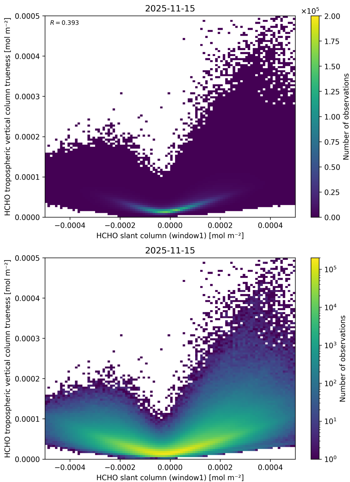
Figure 97: Scatter density plot of “HCHO slant column (window1)” against “HCHO tropospheric vertical column trueness” for 2025-11-14 to 2025-11-16.
