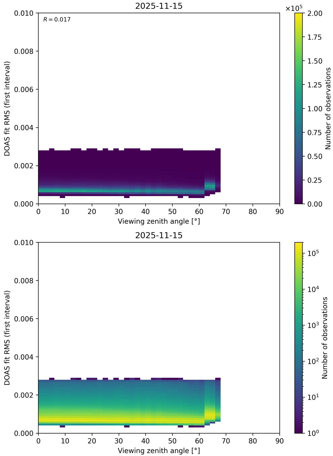
Figure 202: Scatter density plot of “Viewing zenith angle” against “DOAS fit RMS (first interval)” for 2025-11-14 to 2025-11-16.
