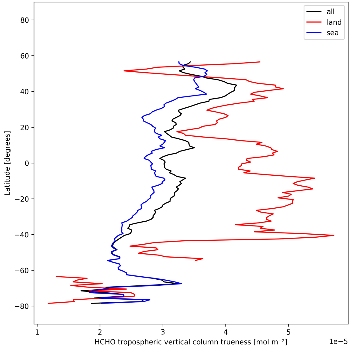
Figure 35: Zonal average of “HCHO tropospheric vertical column density” for 2025-11-14 to 2025-11-16.
