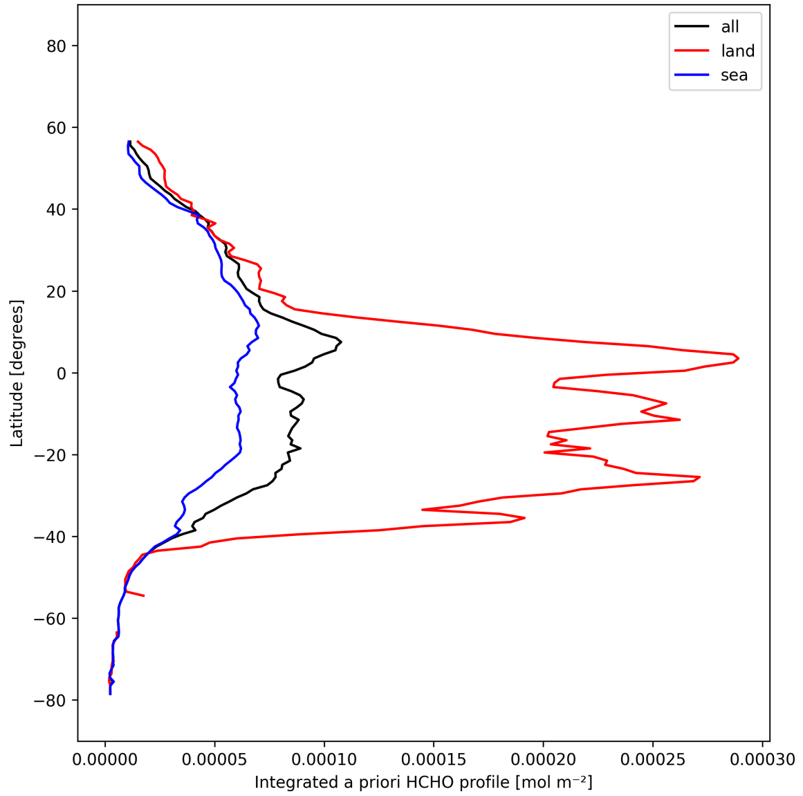
Figure 30: Zonal average of “Integrated a priori HCHO profile” for 2025-11-14 to 2025-11-16.
