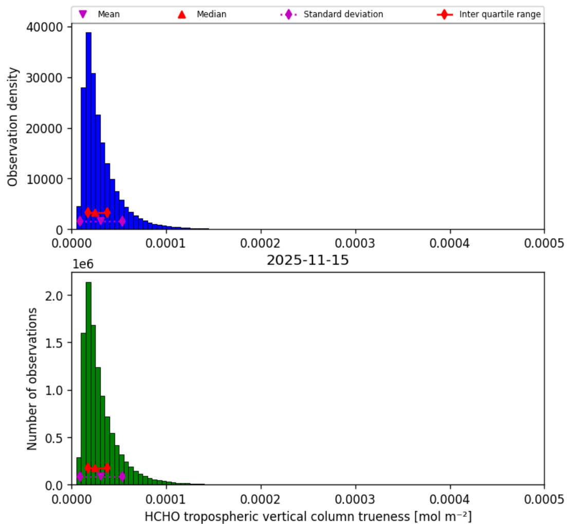
Figure 50: Histogram of “HCHO tropospheric vertical column trueness” for 2025-11-14 to 2025-11-16
