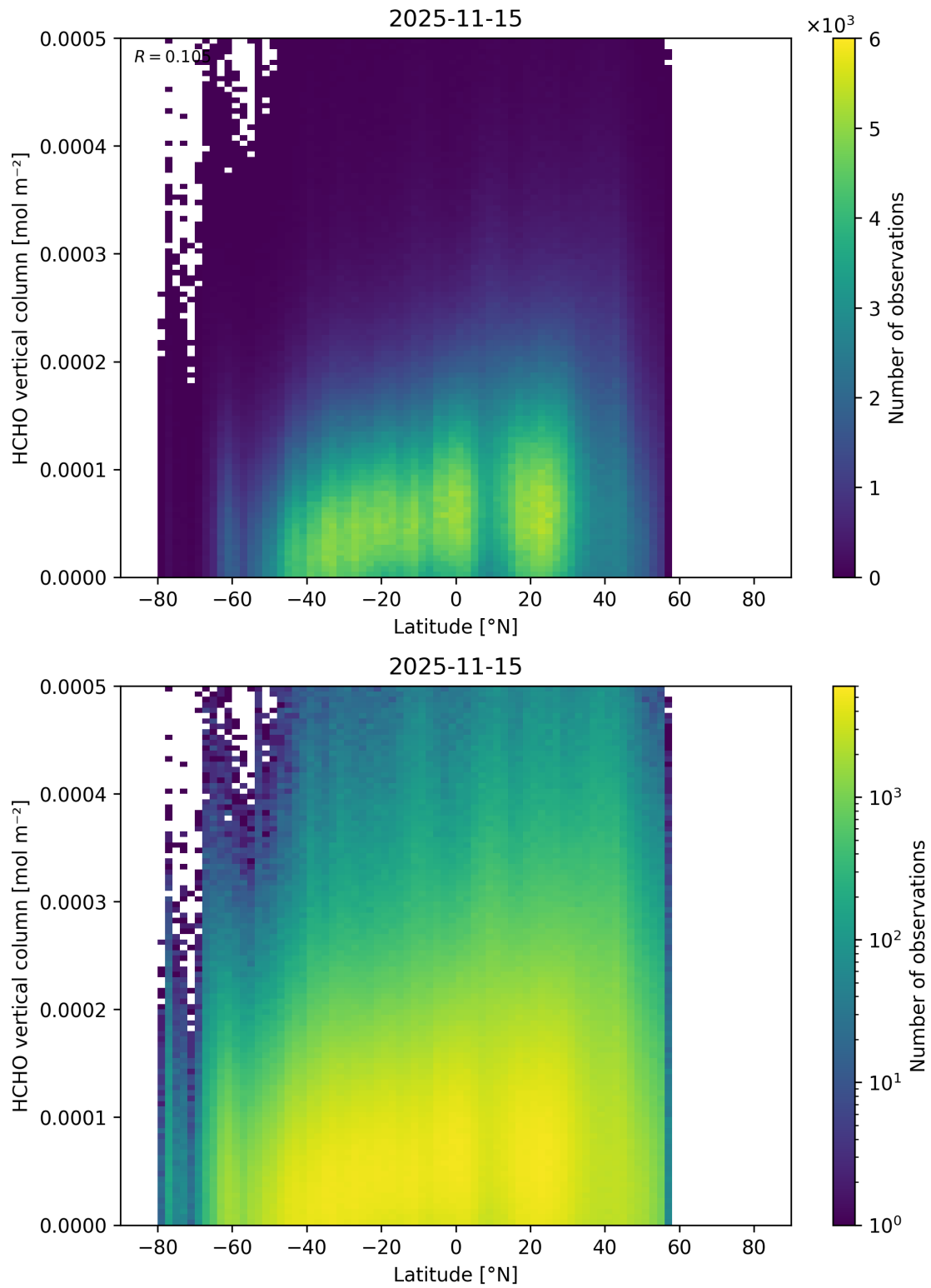
Figure 181: Scatter density plot of “Latitude” against “HCHO vertical column” for 2025-11-14 to 2025-11-16.
