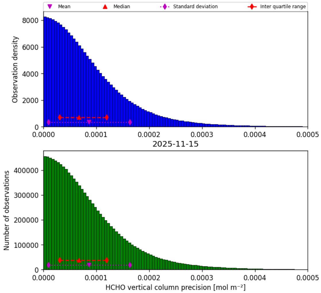
Figure 38: Histogram of “HCHO vertical column precision” for 2025-11-14 to 2025-11-16
