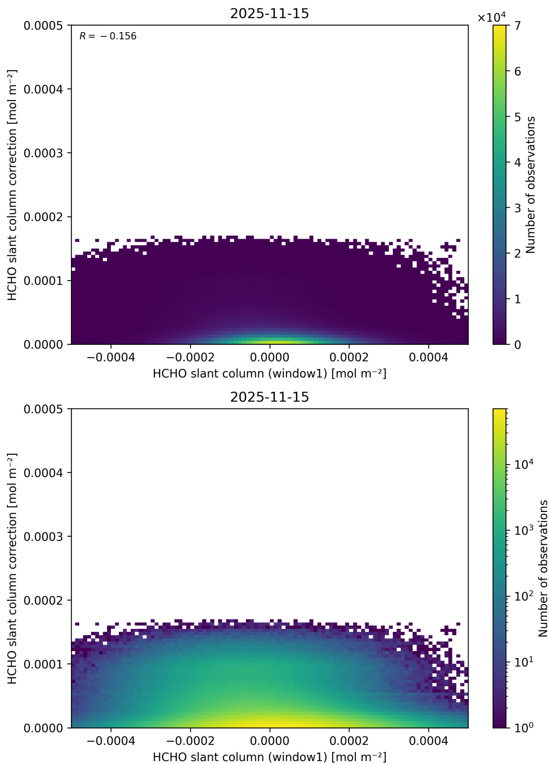
Figure 93: Scatter density plot of “HCHO slant column (window1)” against “HCHO slant column correction” for 2025-11-14 to 2025-11-16.
