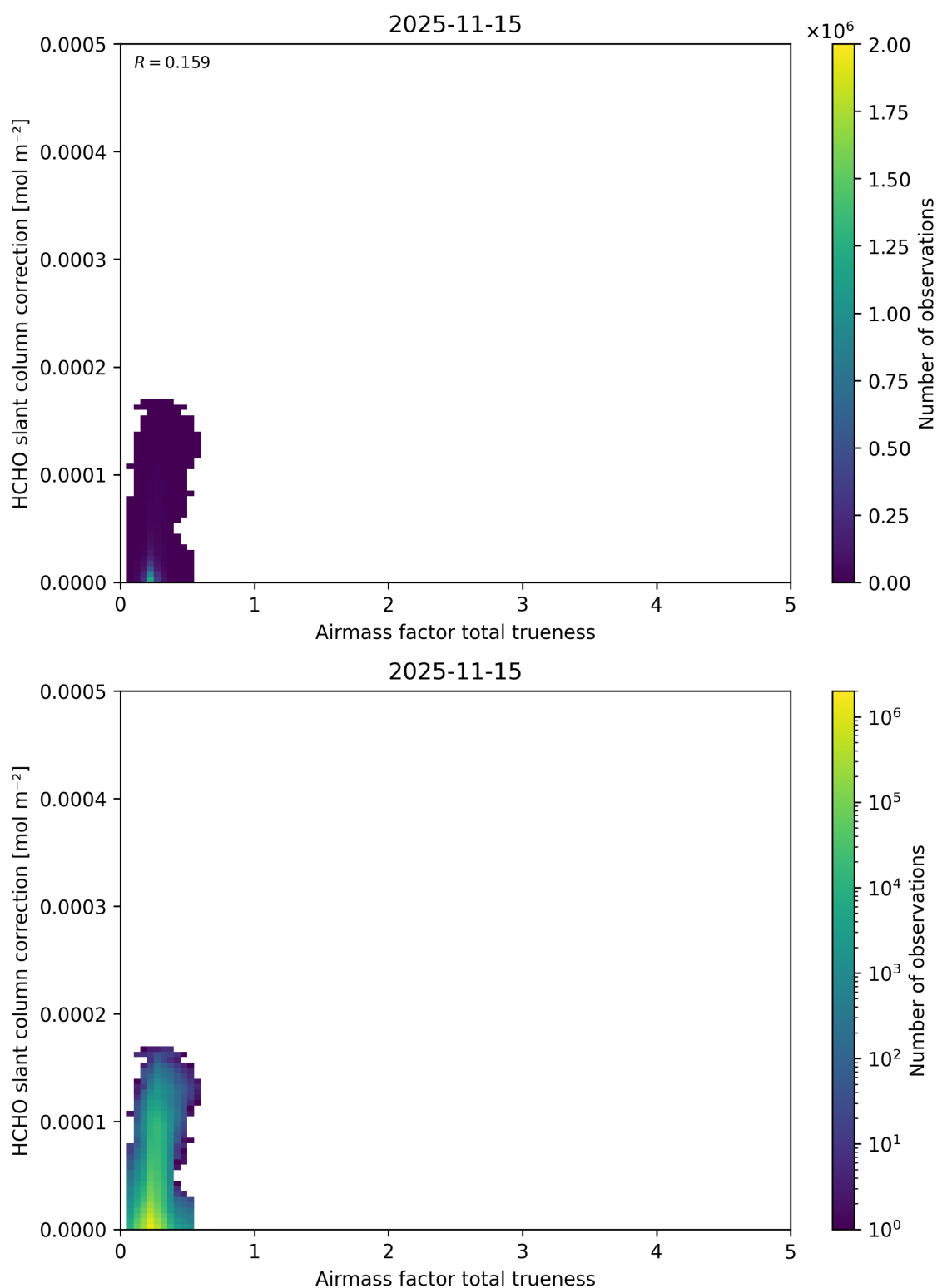
Figure 123: Scatter density plot of “Airmass factor total trueness” against “HCHO slant column correction” for 2025-11-14 to 2025-11-16.
