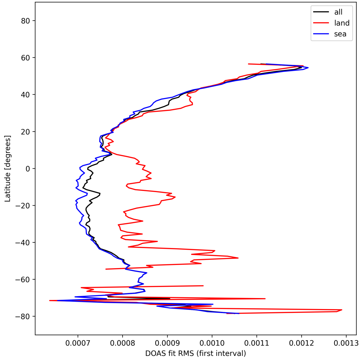
Figure 33: Zonal average of “DOAS fit RMS (first interval)” for 2025-11-14 to 2025-11-16.
