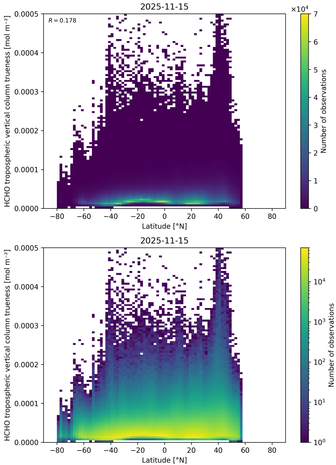
Figure 184: Scatter density plot of “Latitude” against “HCHO tropospheric vertical column trueness” for 2025-11-14 to 2025-11-16.
