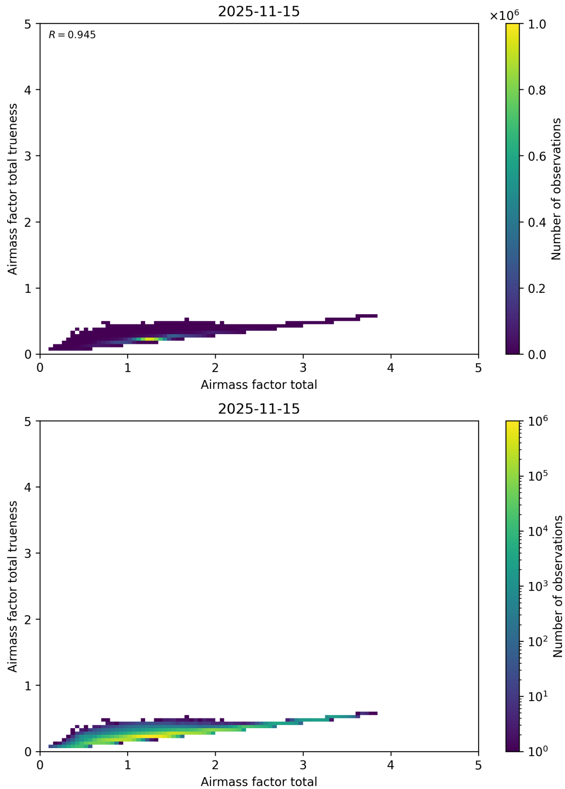
Figure 115: Scatter density plot of “Airmass factor total” against “Airmass factor total trueness” for 2025-11-14 to 2025-11-16.
