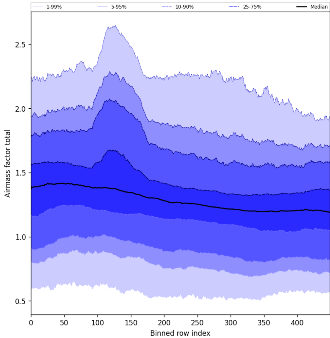
Figure 57: Along track statistics of “Airmass factor total” for 2025-11-14 to 2025-11-16
