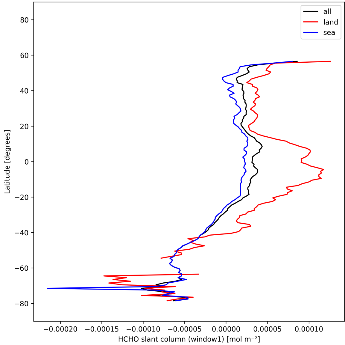
Figure 25: Zonal average of “HCHO slant column (window1)” for 2025-11-14 to 2025-11-16.
