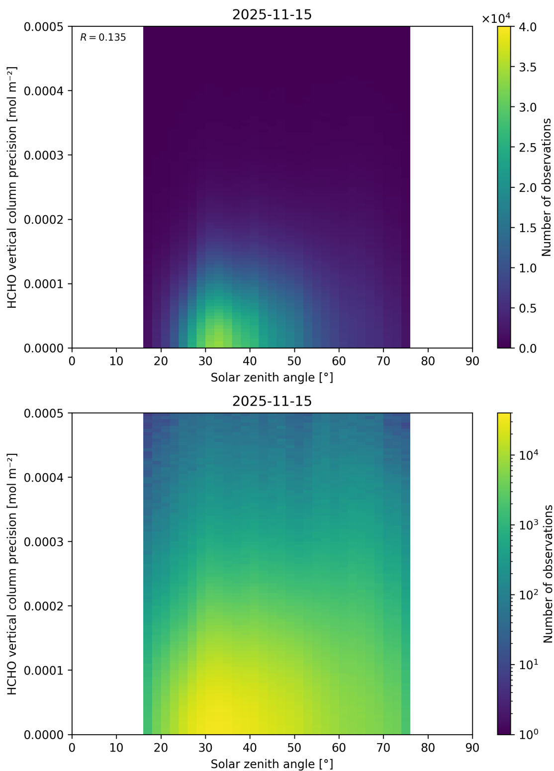
Figure 198: Scatter density plot of “Solar zenith angle” against “HCHO vertical column precision” for 2025-11-14 to 2025-11-16.
