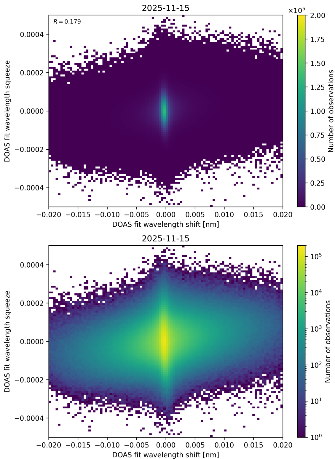
Figure 70: Scatter density plot of “DOAS fit wavelength shift” against “DOAS fit wavelength squeeze” for 2025-11-14 to 2025-11-16.
