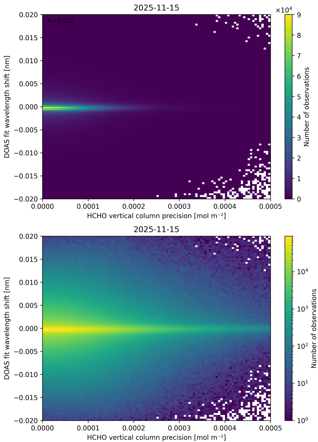
Figure 153: Scatter density plot of “HCHO vertical column precision” against “DOAS fit wavelength shift” for 2025-11-14 to 2025-11-16.
