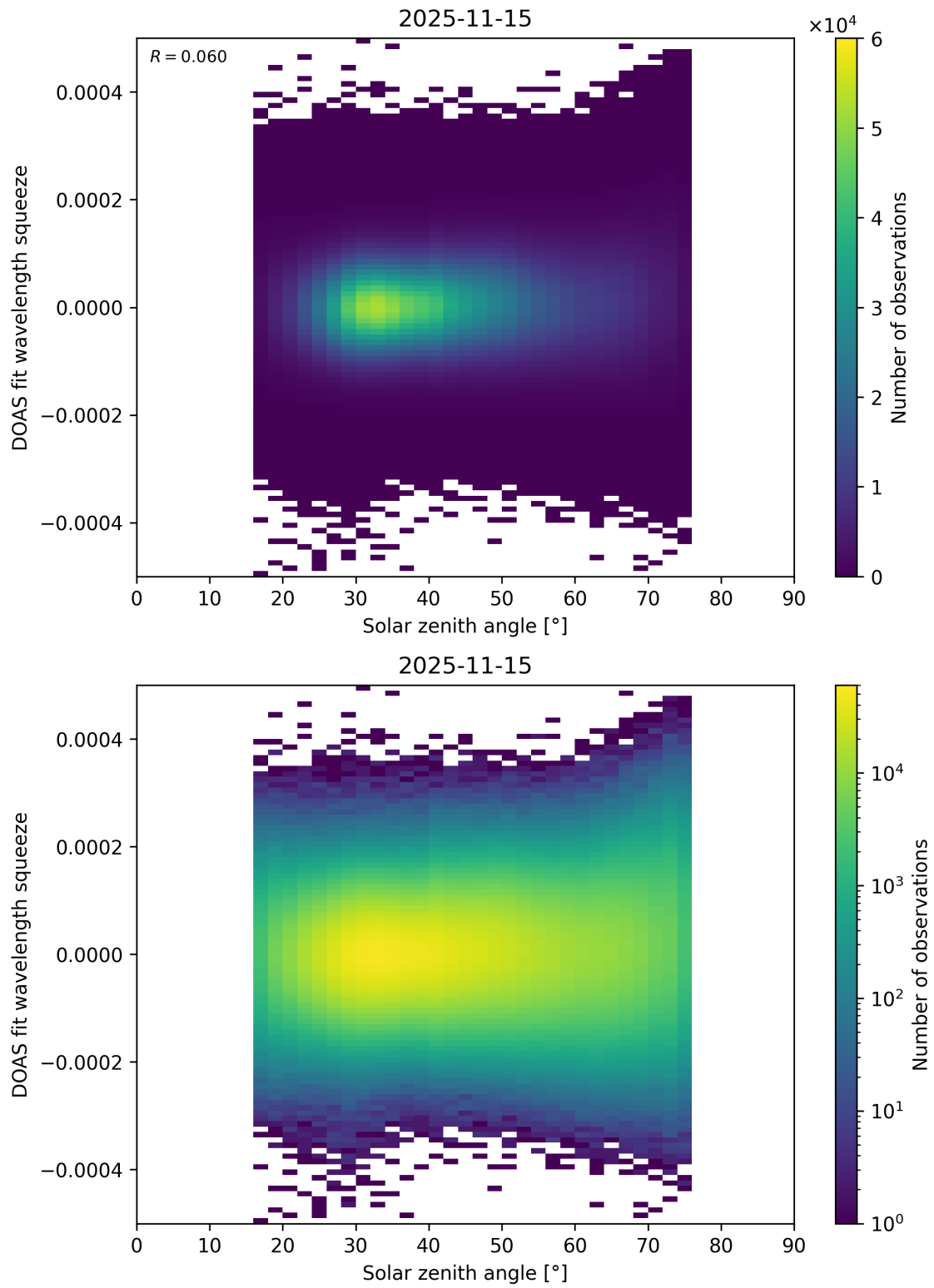
Figure 188: Scatter density plot of “Solar zenith angle” against “DOAS fit wavelength squeeze” for 2025-11-14 to 2025-11-16.
