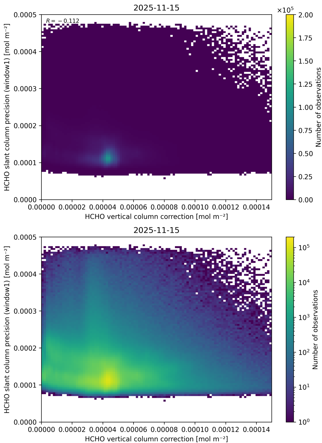
Figure 133: Scatter density plot of “HCHO vertical column correction” against “HCHO slant column precision (window1)” for 2025-11-14 to 2025-11-16.
