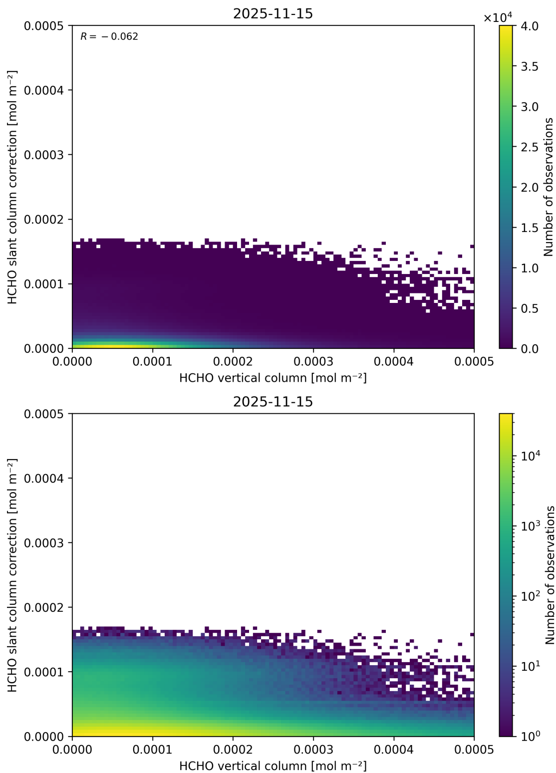
Figure 143: Scatter density plot of “HCHO vertical column” against “HCHO slant column correction” for 2025-11-14 to 2025-11-16.
