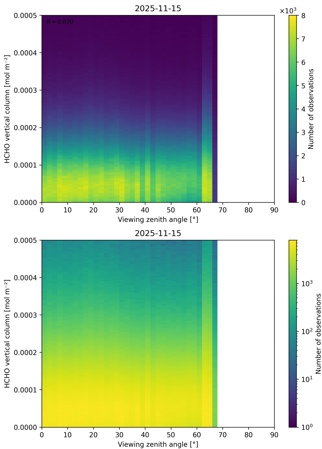
Figure 212: Scatter density plot of “Viewing zenith angle” against “HCHO vertical column” for 2025-11-14 to 2025-11-16.
