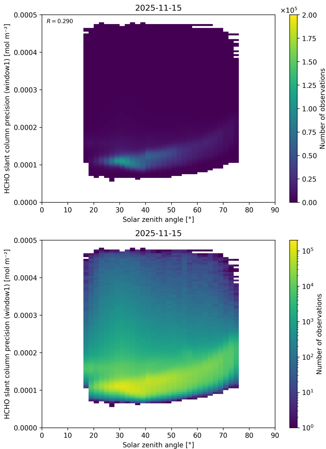
Figure 193: Scatter density plot of “Solar zenith angle” against “HCHO slant column precision (window1)” for 2025-11-14 to 2025-11-16.
