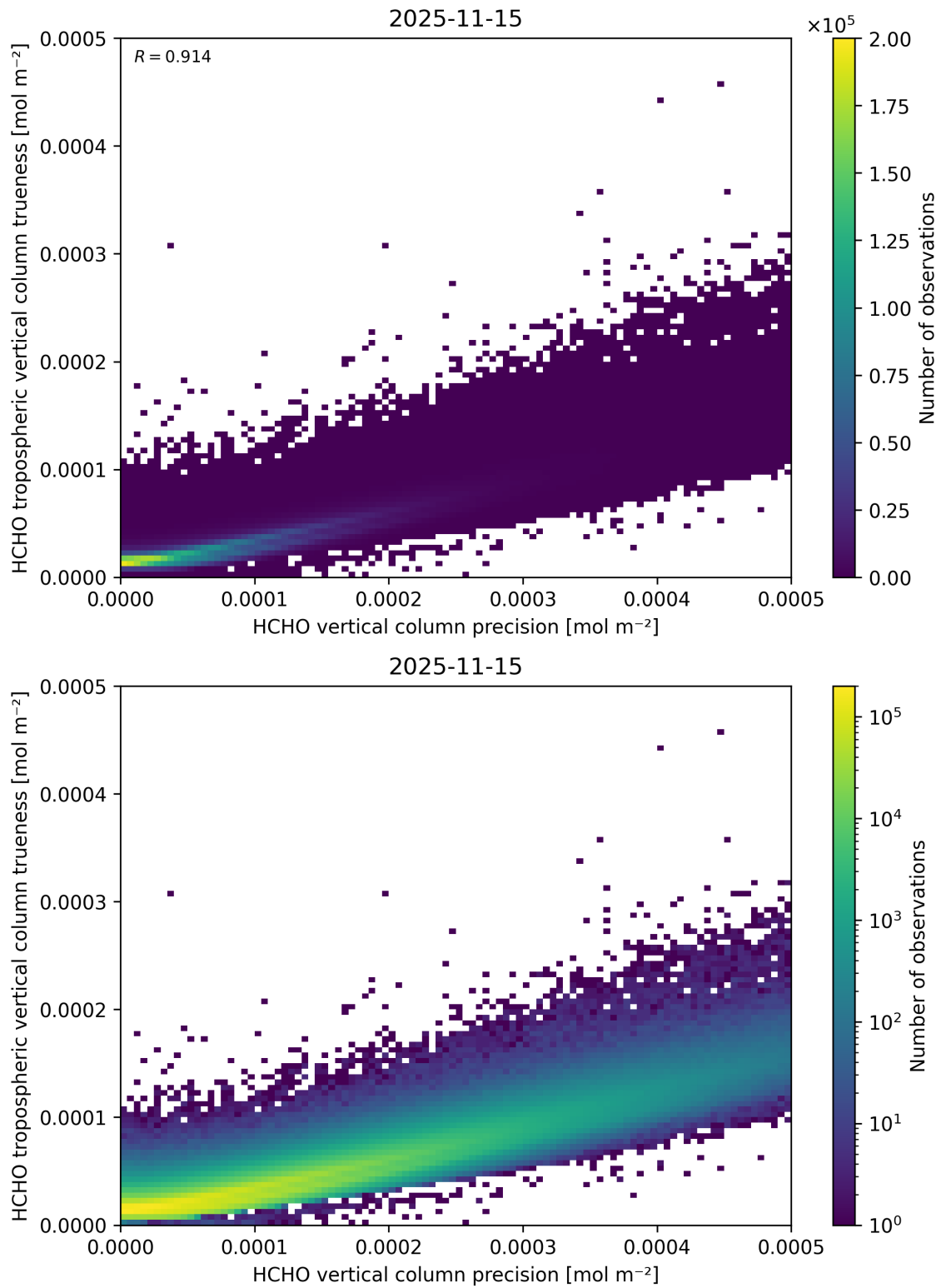
Figure 163: Scatter density plot of “HCHO vertical column precision” against “HCHO tropospheric vertical column trueness” for 2025-11-14 to 2025-11-16.
