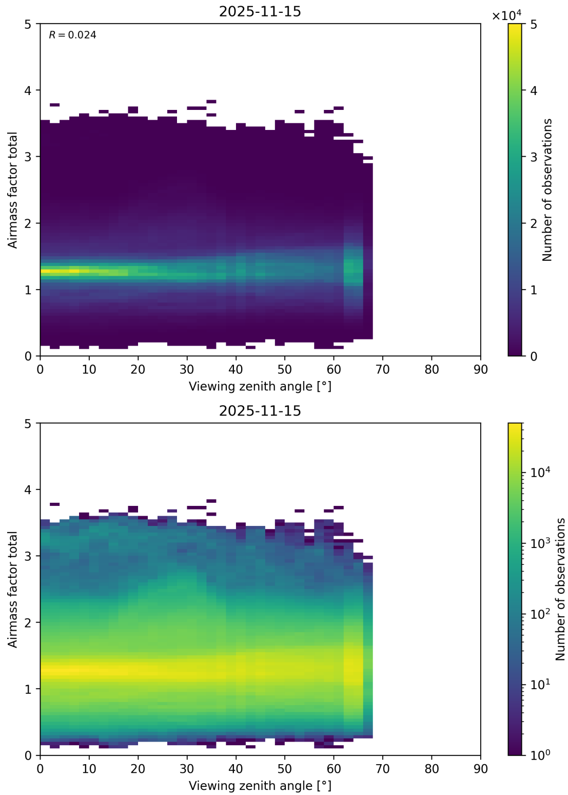
Figure 210: Scatter density plot of “Viewing zenith angle” against “Airmass factor total” for 2025-11-14 to 2025-11-16.
