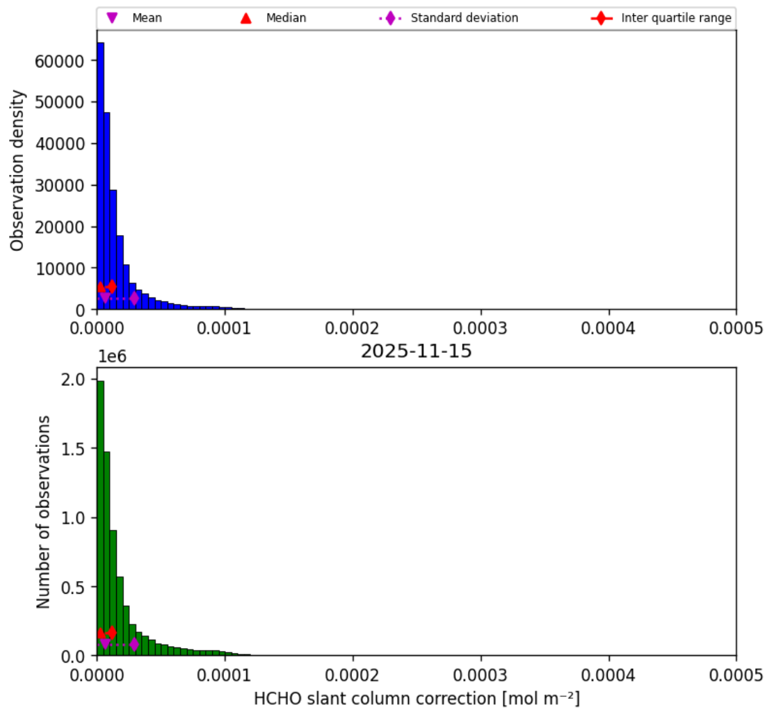
Figure 49: Histogram of “HCHO slant column correction” for 2025-11-14 to 2025-11-16
