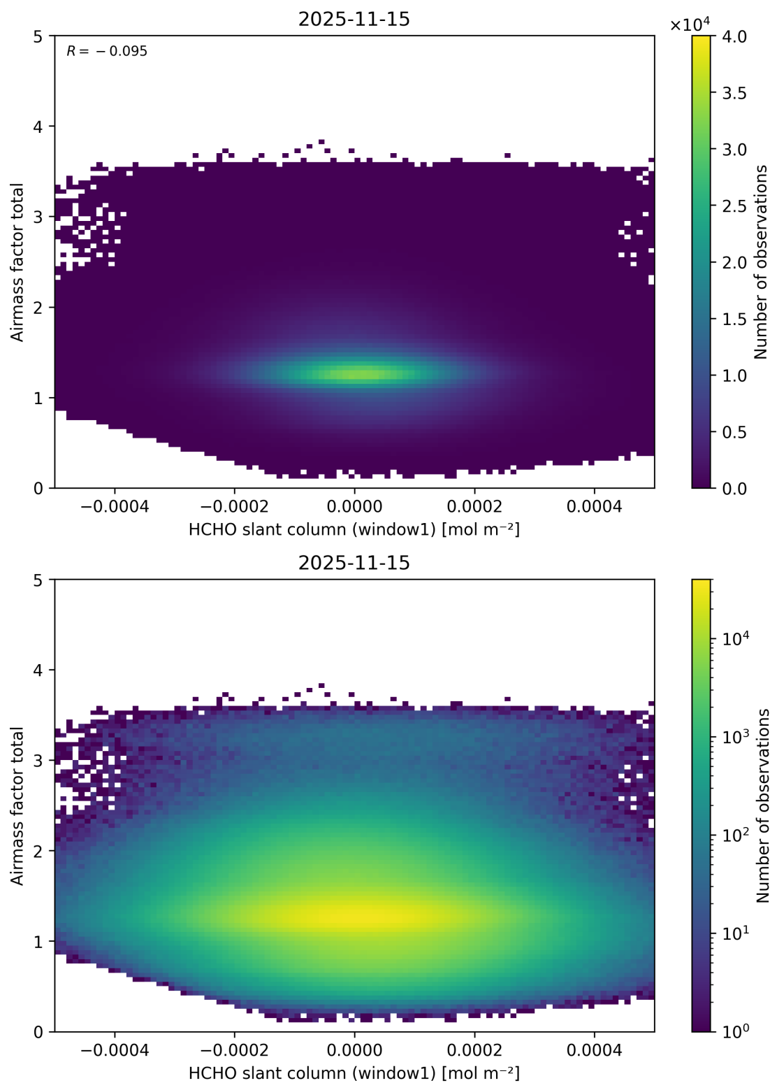
Figure 95: Scatter density plot of “HCHO slant column (window1)” against “Airmass factor total” for 2025-11-14 to 2025-11-16.
