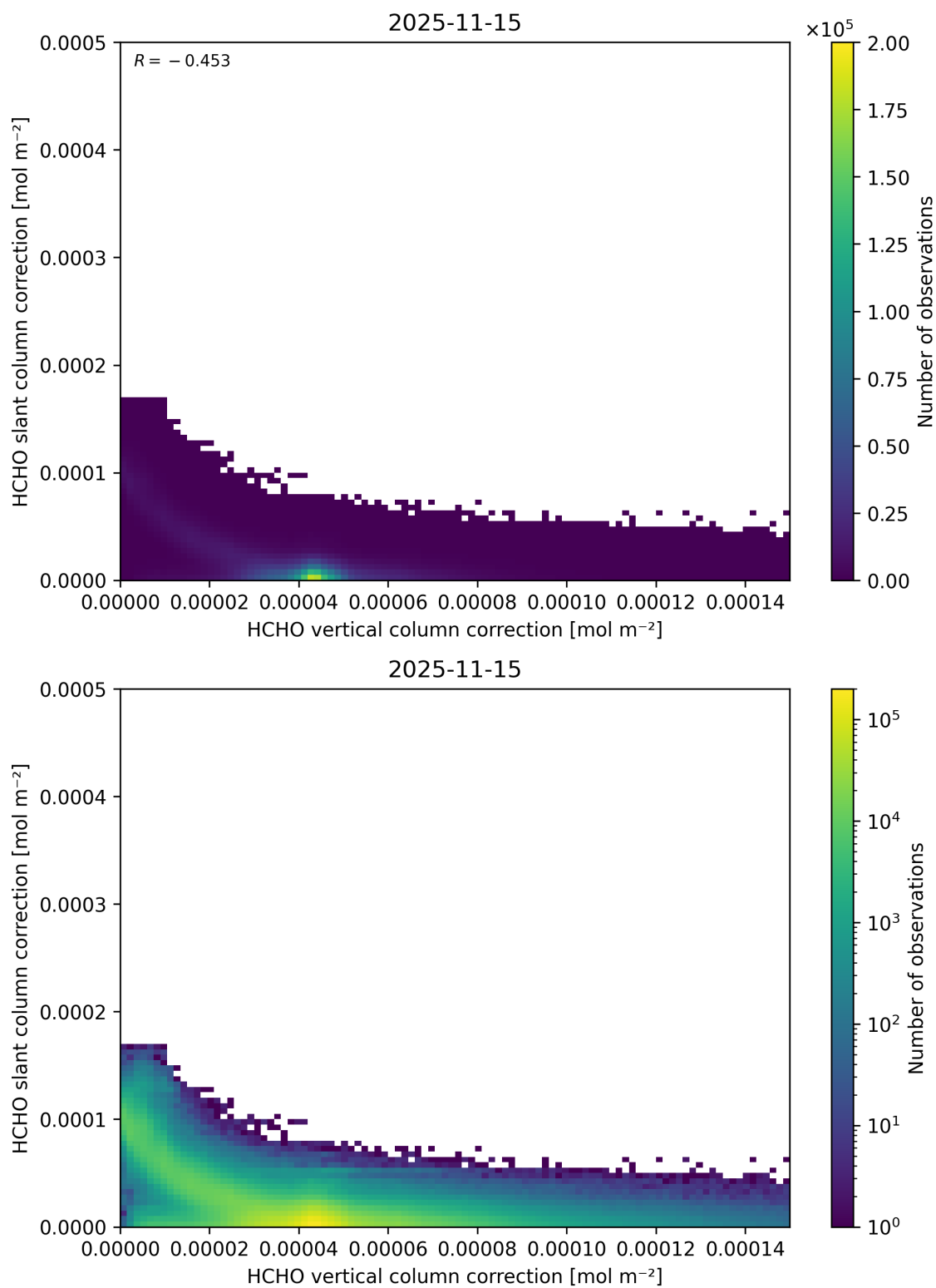
Figure 131: Scatter density plot of “HCHO vertical column correction” against “HCHO slant column correction” for 2025-11-14 to 2025-11-16.
