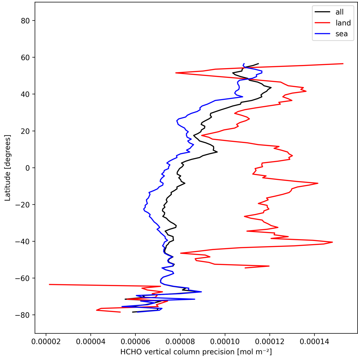
Figure 23: Zonal average of “HCHO vertical column precision” for 2025-11-14 to 2025-11-16.
