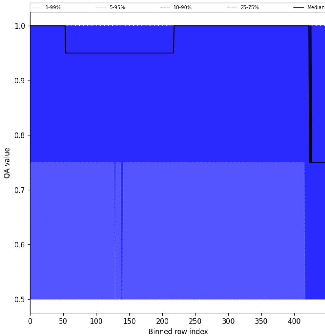
Figure 51: Along track statistics of “QA value” for 2025-11-14 to 2025-11-16
