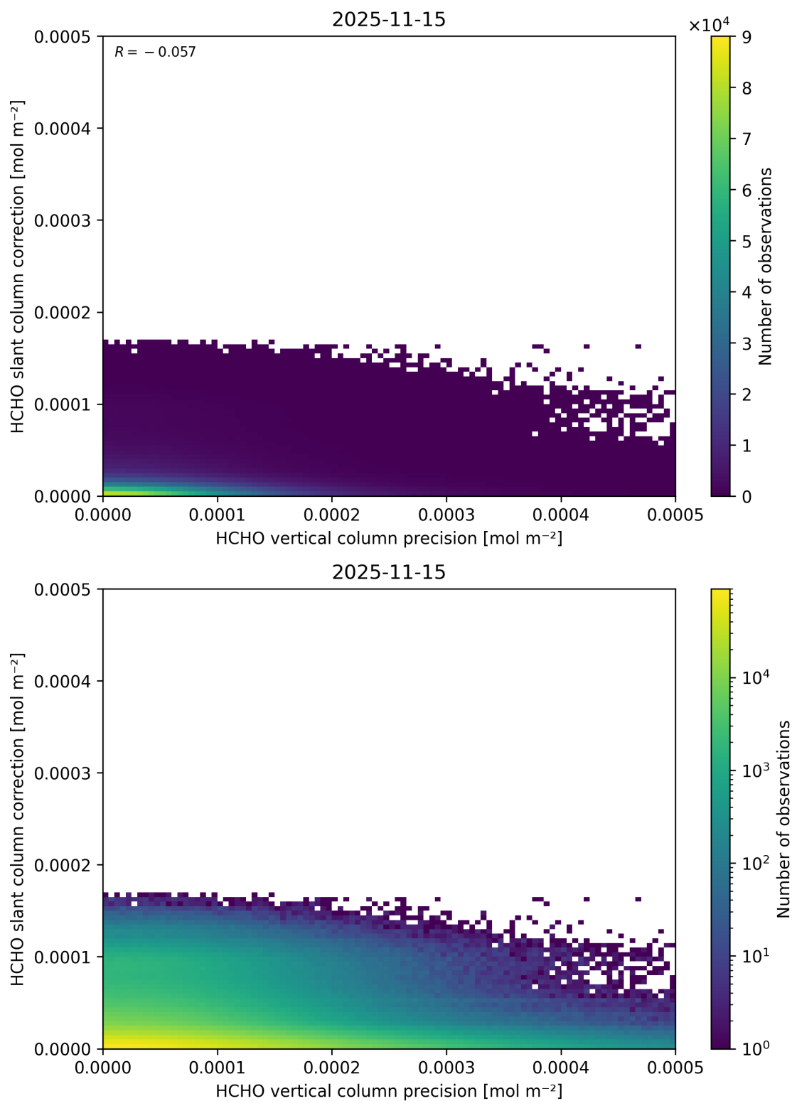
Figure 157: Scatter density plot of “HCHO vertical column precision” against “HCHO slant column correction” for 2025-11-14 to 2025-11-16.
