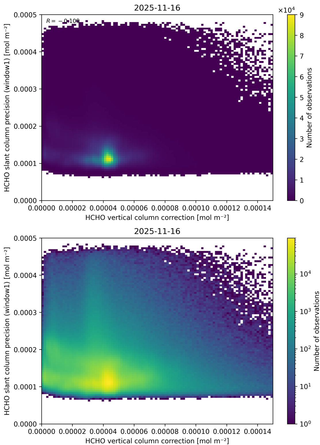
Figure 133: Scatter density plot of “HCHO vertical column correction” against “HCHO slant column precision (window1)” for 2025-11-15 to 2025-11-17.
