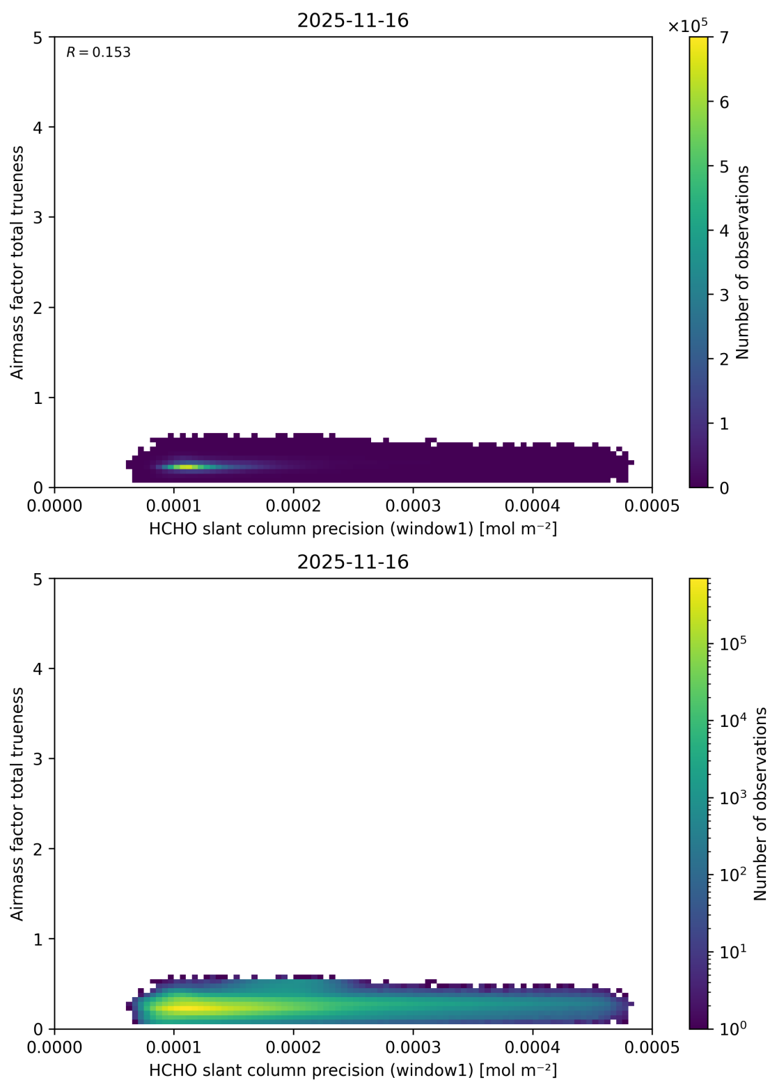
Figure 106: Scatter density plot of “HCHO slant column precision (window1)” against “Airmass factor total trueness” for 2025-11-15 to 2025-11-17.
