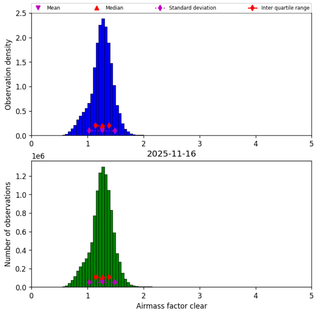
Figure 44: Histogram of “Airmass factor clear” for 2025-11-15 to 2025-11-17
