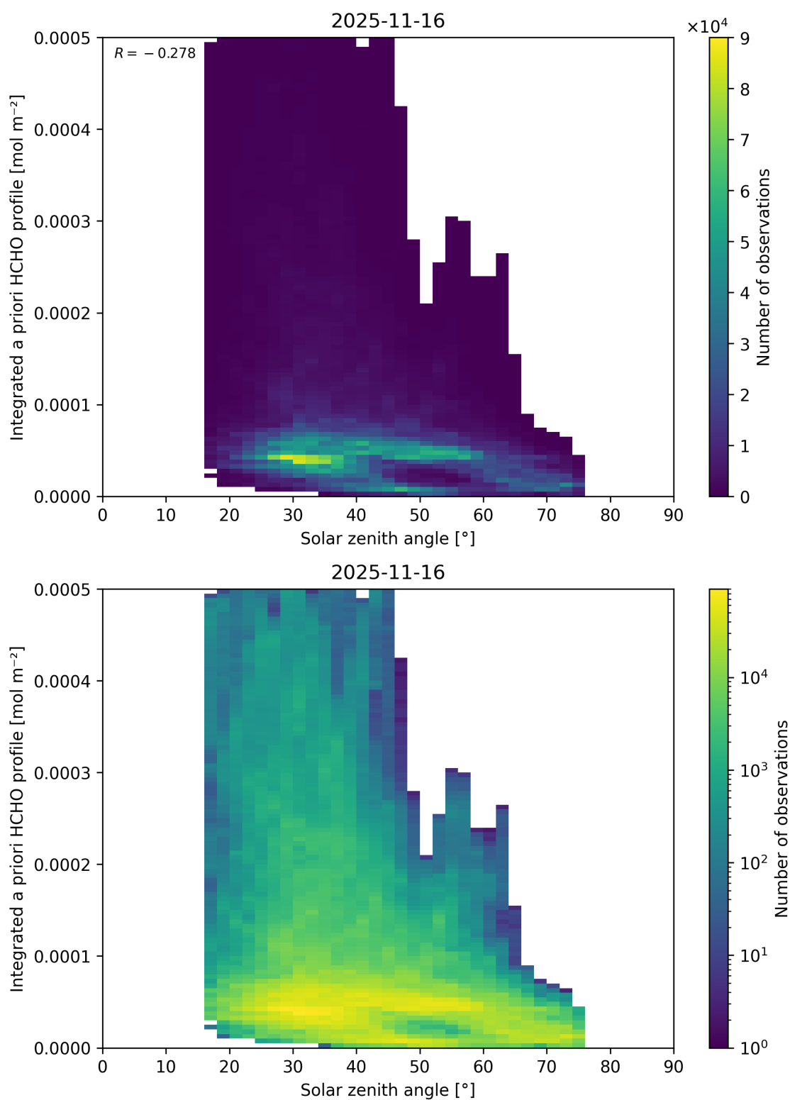
Figure 200: Scatter density plot of “Solar zenith angle” against “Integrated a priori HCHO profile” for 2025-11-15 to 2025-11-17.
