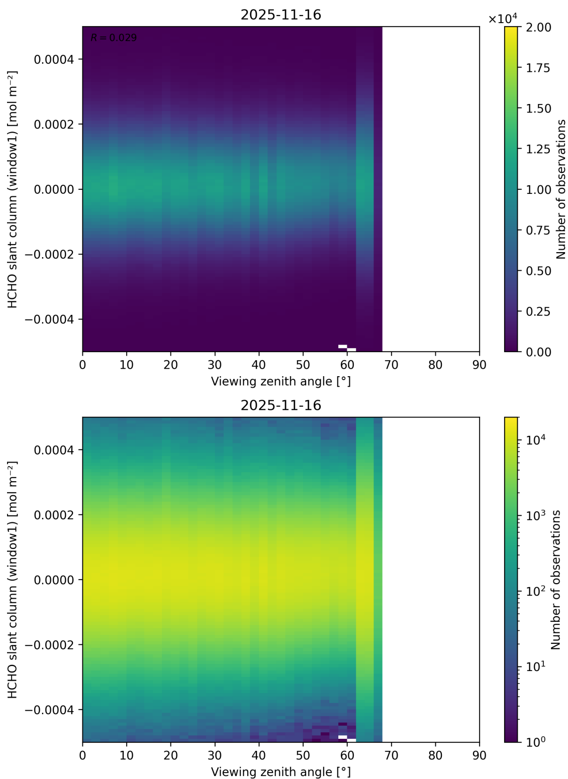
Figure 208: Scatter density plot of “Viewing zenith angle” against “HCHO slant column (window1)” for 2025-11-15 to 2025-11-17.
