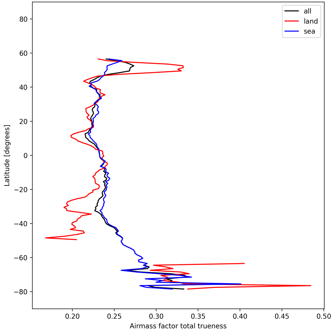
Figure 28: Zonal average of “Airmass factor total trueness” for 2025-11-15 to 2025-11-17.
