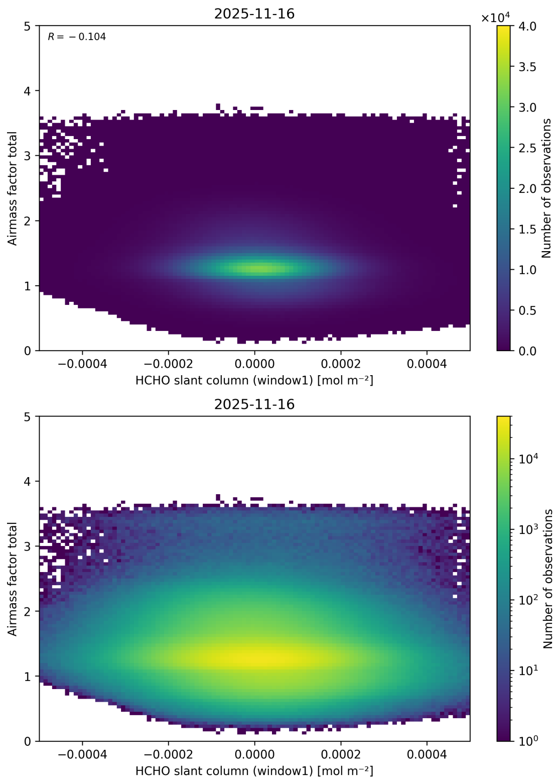
Figure 95: Scatter density plot of “HCHO slant column (window1)” against “Airmass factor total” for 2025-11-15 to 2025-11-17.
