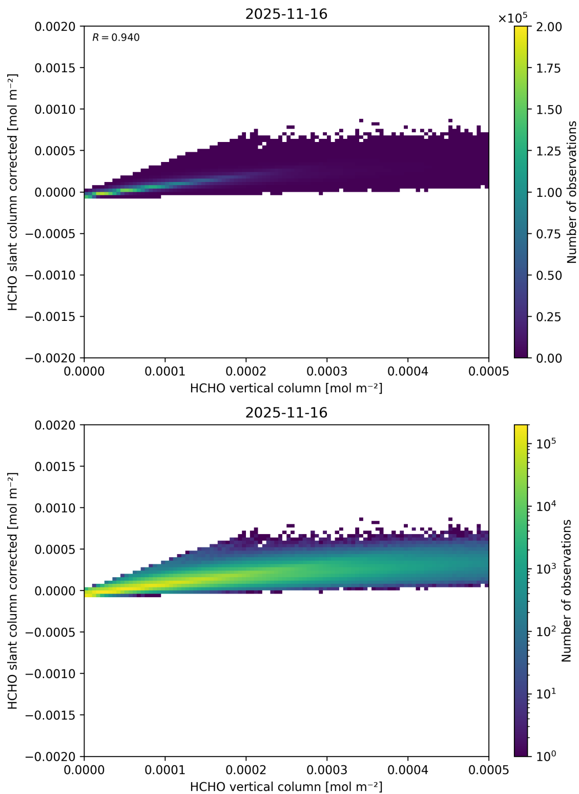
Figure 142: Scatter density plot of “HCHO vertical column” against “HCHO slant column corrected” for 2025-11-15 to 2025-11-17.
