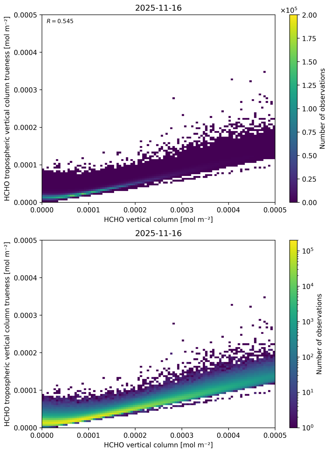
Figure 150: Scatter density plot of “HCHO vertical column” against “HCHO tropospheric vertical column trueness” for 2025-11-15 to 2025-11-17.
