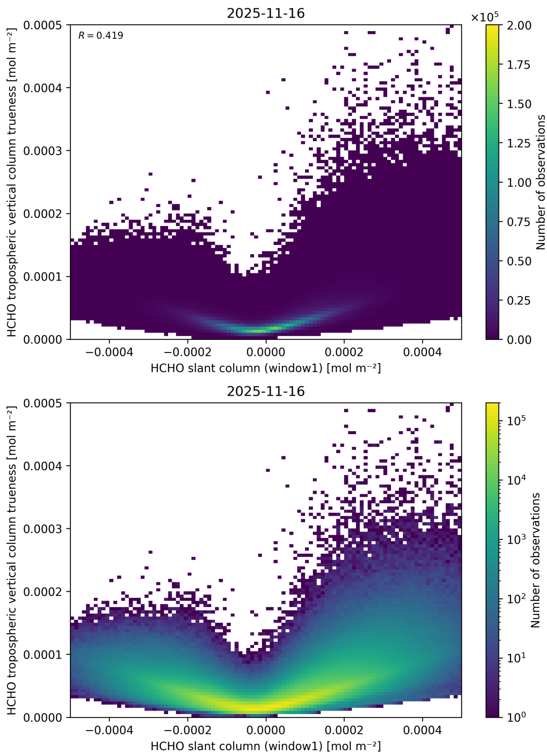
Figure 97: Scatter density plot of “HCHO slant column (window1)” against “HCHO tropospheric vertical column trueness” for 2025-11-15 to 2025-11-17.
