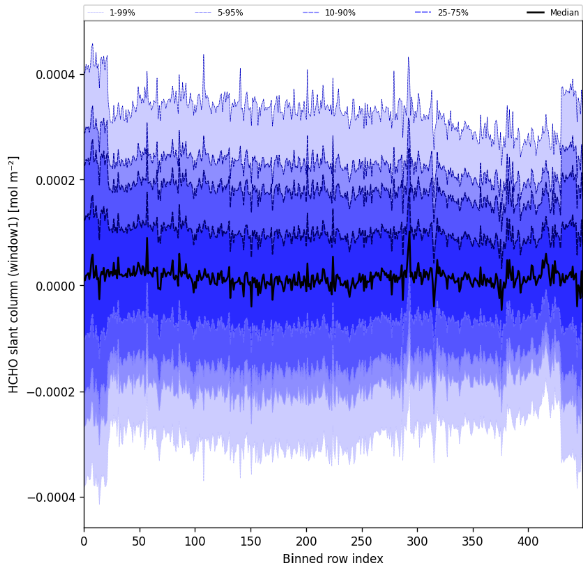
Figure 55: Along track statistics of “HCHO slant column (window1)” for 2025-11-15 to 2025-11-17
