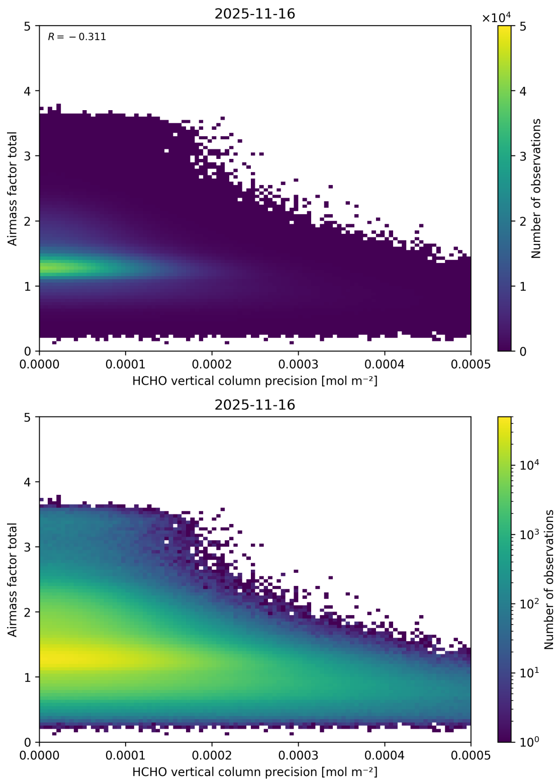
Figure 160: Scatter density plot of “HCHO vertical column precision” against “Airmass factor total” for 2025-11-15 to 2025-11-17.
