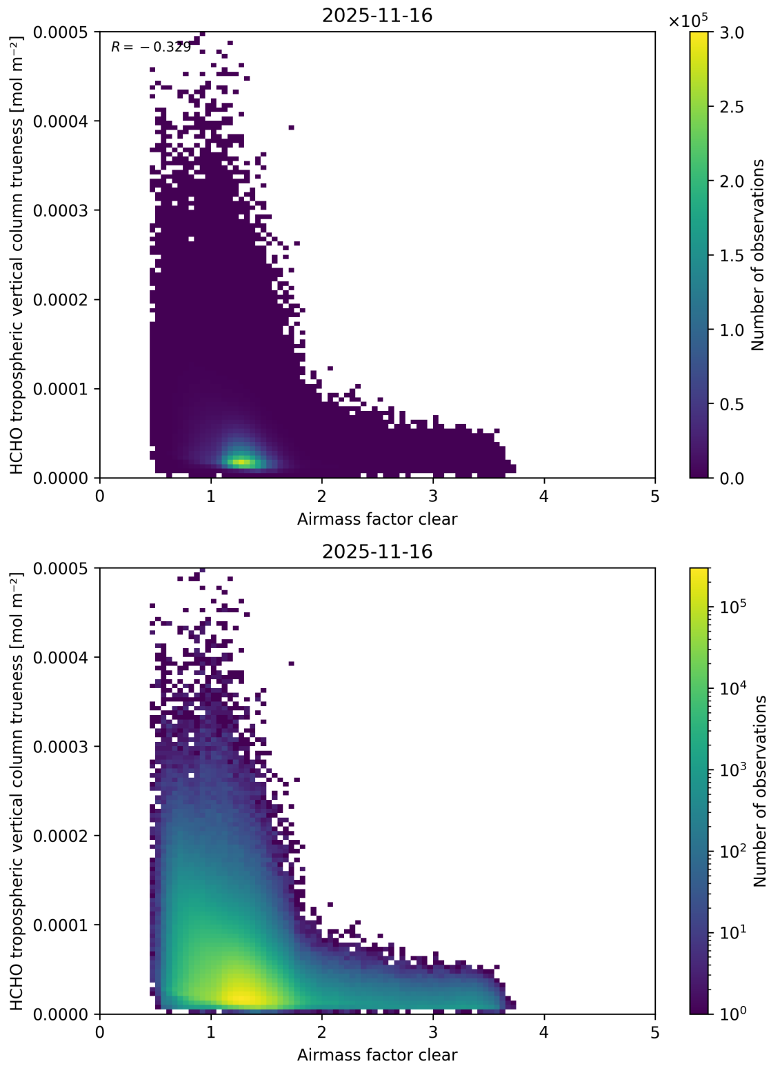
Figure 83: Scatter density plot of “Airmass factor clear” against “HCHO tropospheric vertical column trueness” for 2025-11-15 to 2025-11-17.
