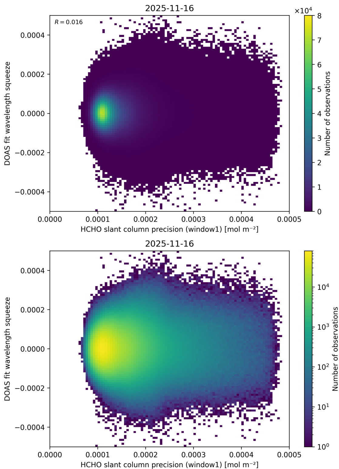
Figure 101: Scatter density plot of “HCHO slant column precision (window1)” against “DOAS fit wavelength squeeze” for 2025-11-15 to 2025-11-17.
