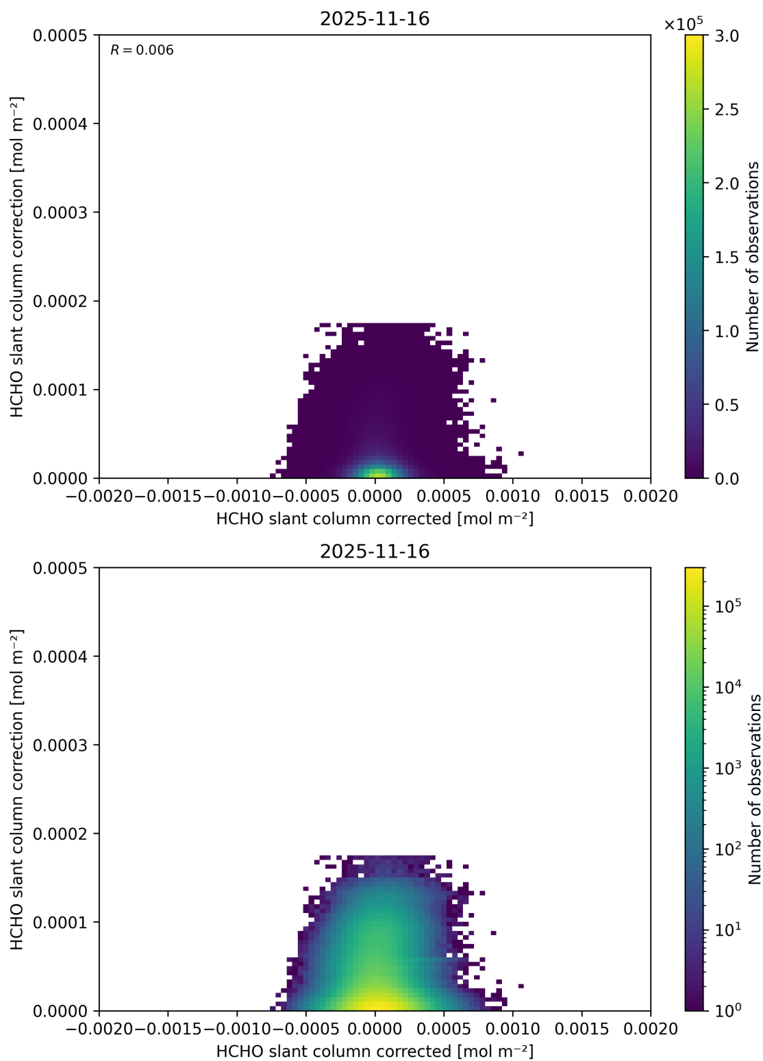
Figure 85: Scatter density plot of “HCHO slant column corrected” against “HCHO slant column correction” for 2025-11-15 to 2025-11-17.
