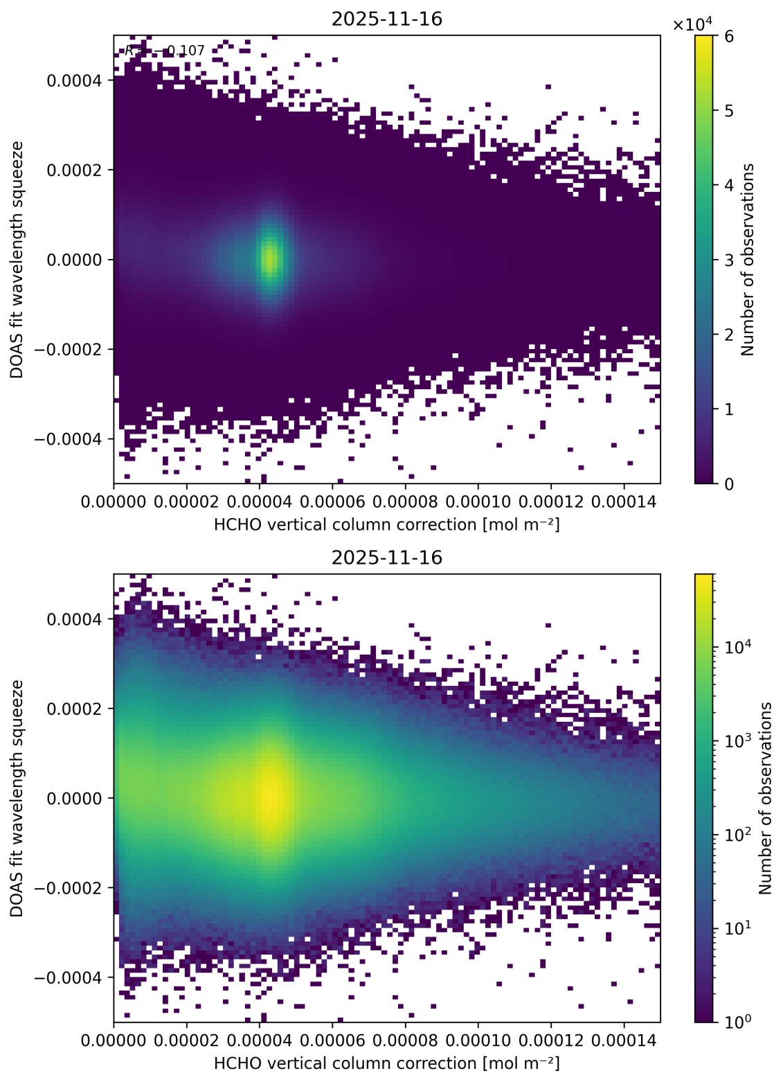
Figure 128: Scatter density plot of “HCHO vertical column correction” against “DOAS fit wavelength squeeze” for 2025-11-15 to 2025-11-17.
