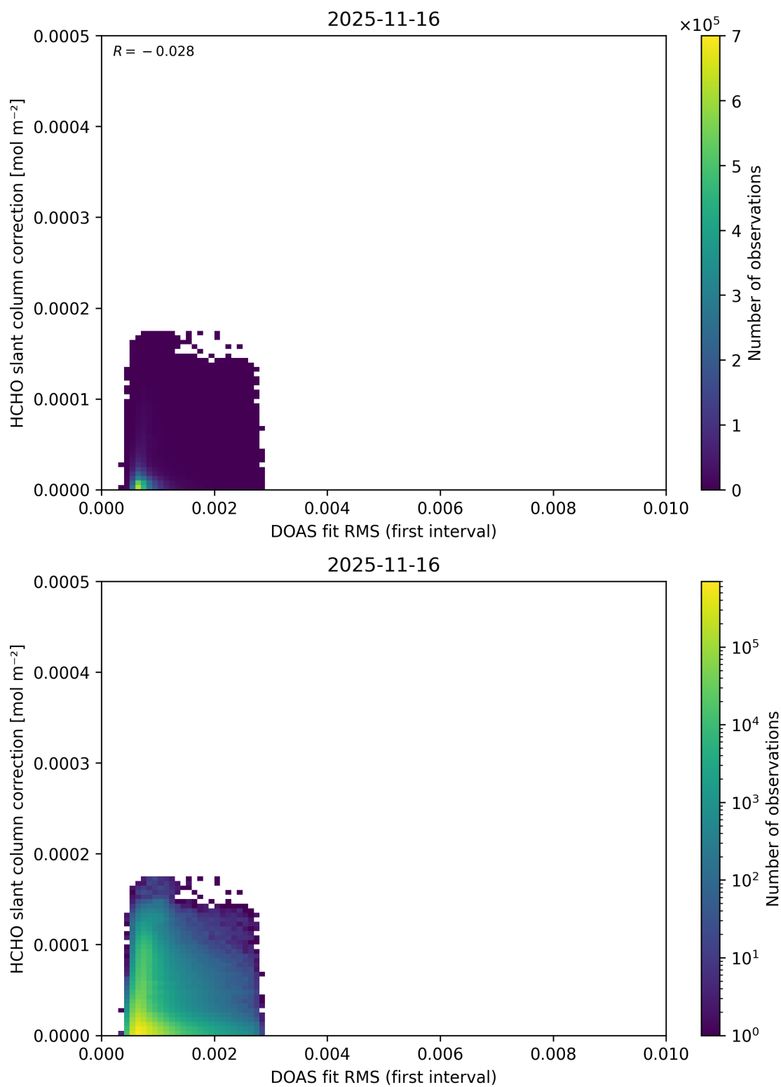
Figure 67: Scatter density plot of “DOAS fit RMS (first interval)” against “HCHO slant column correction” for 2025-11-15 to 2025-11-17.
