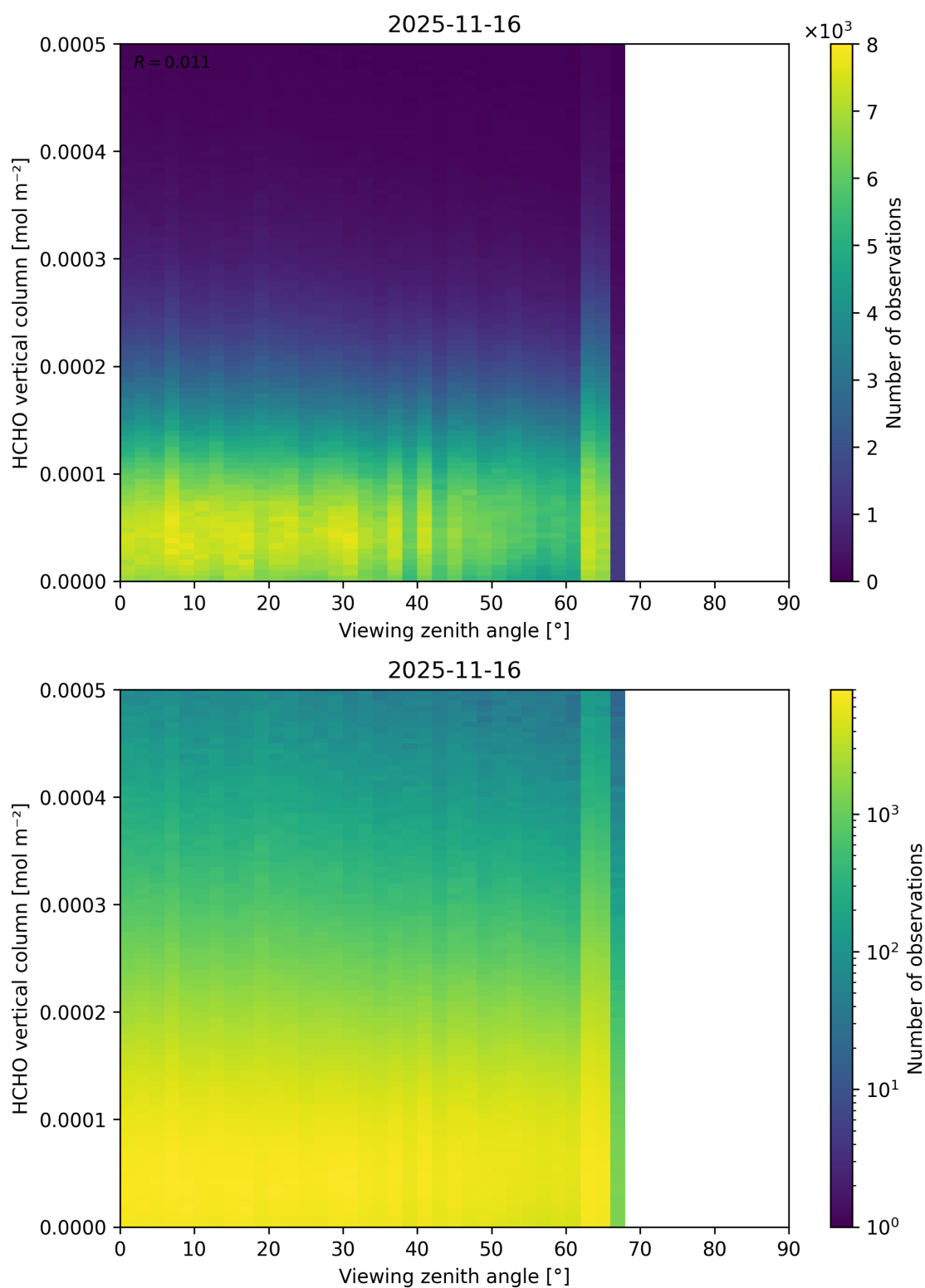
Figure 212: Scatter density plot of “Viewing zenith angle” against “HCHO vertical column” for 2025-11-15 to 2025-11-17.
