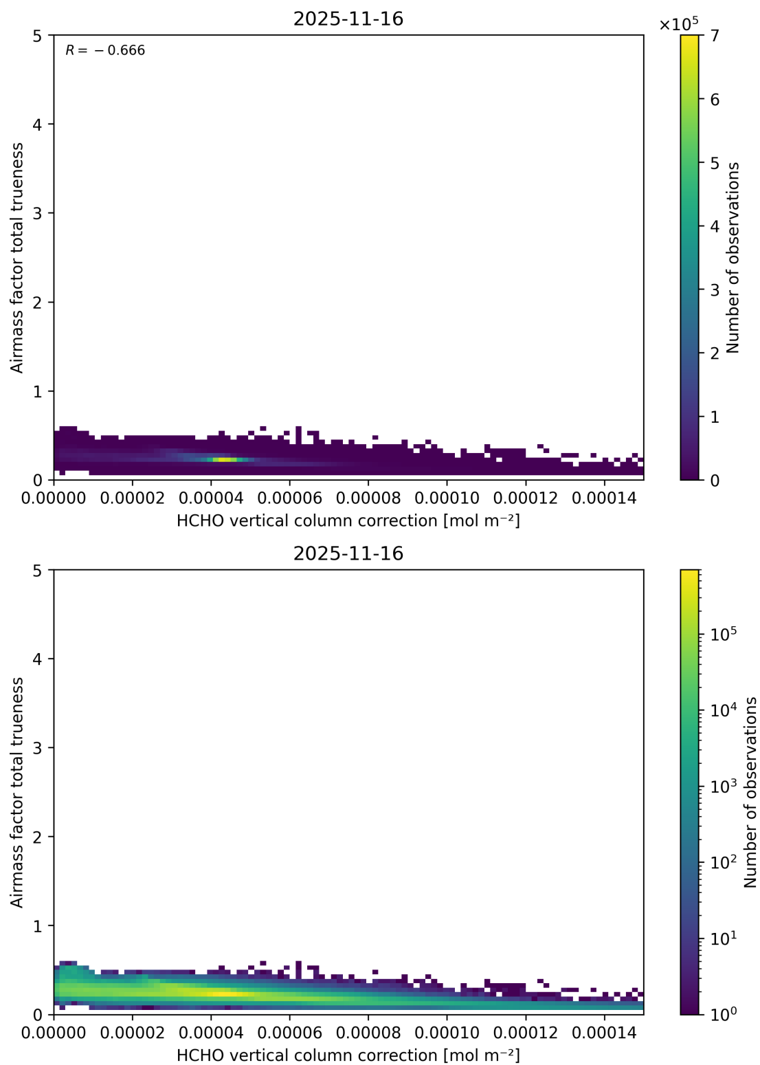
Figure 135: Scatter density plot of “HCHO vertical column correction” against “Airmass factor total truiness” for 2025-11-15 to 2025-11-17.
