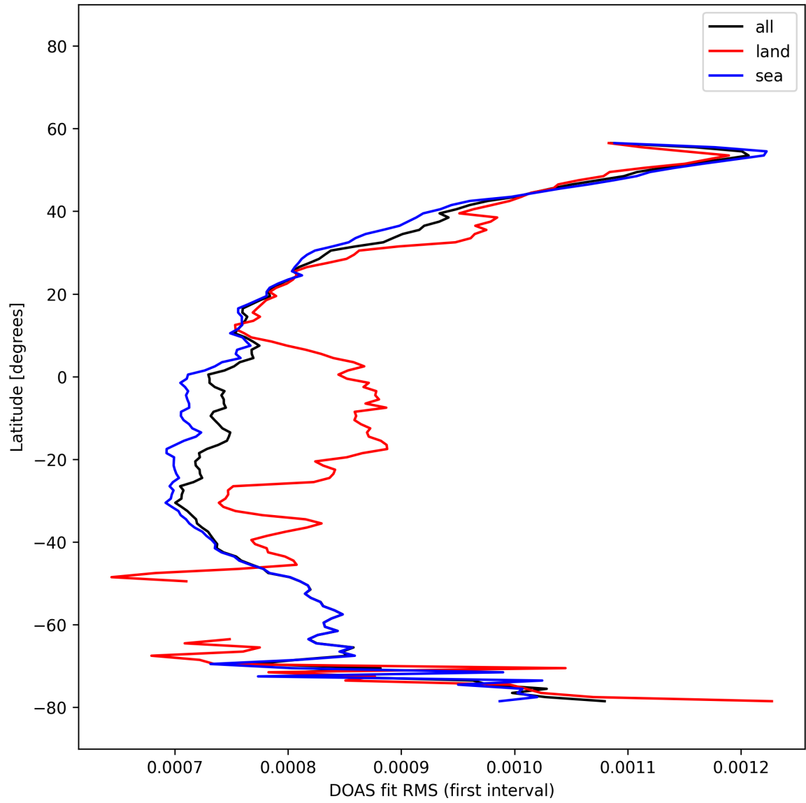
Figure 33: Zonal average of “DOAS fit RMS (first interval)” for 2025-11-15 to 2025-11-17.
