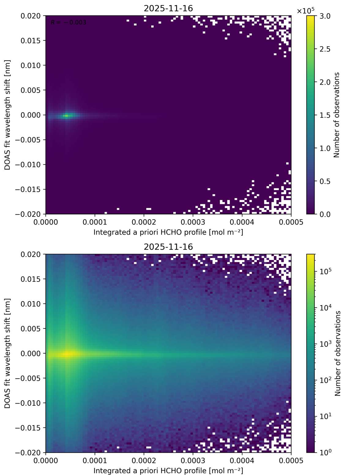
Figure 166: Scatter density plot of “Integrated a priori HCHO profile” against “DOAS fit wavelength shift” for 2025-11-15 to 2025-11-17.
