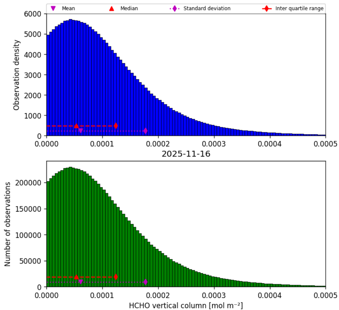
Figure 37: Histogram of “HCHO vertical column” for 2025-11-15 to 2025-11-17
