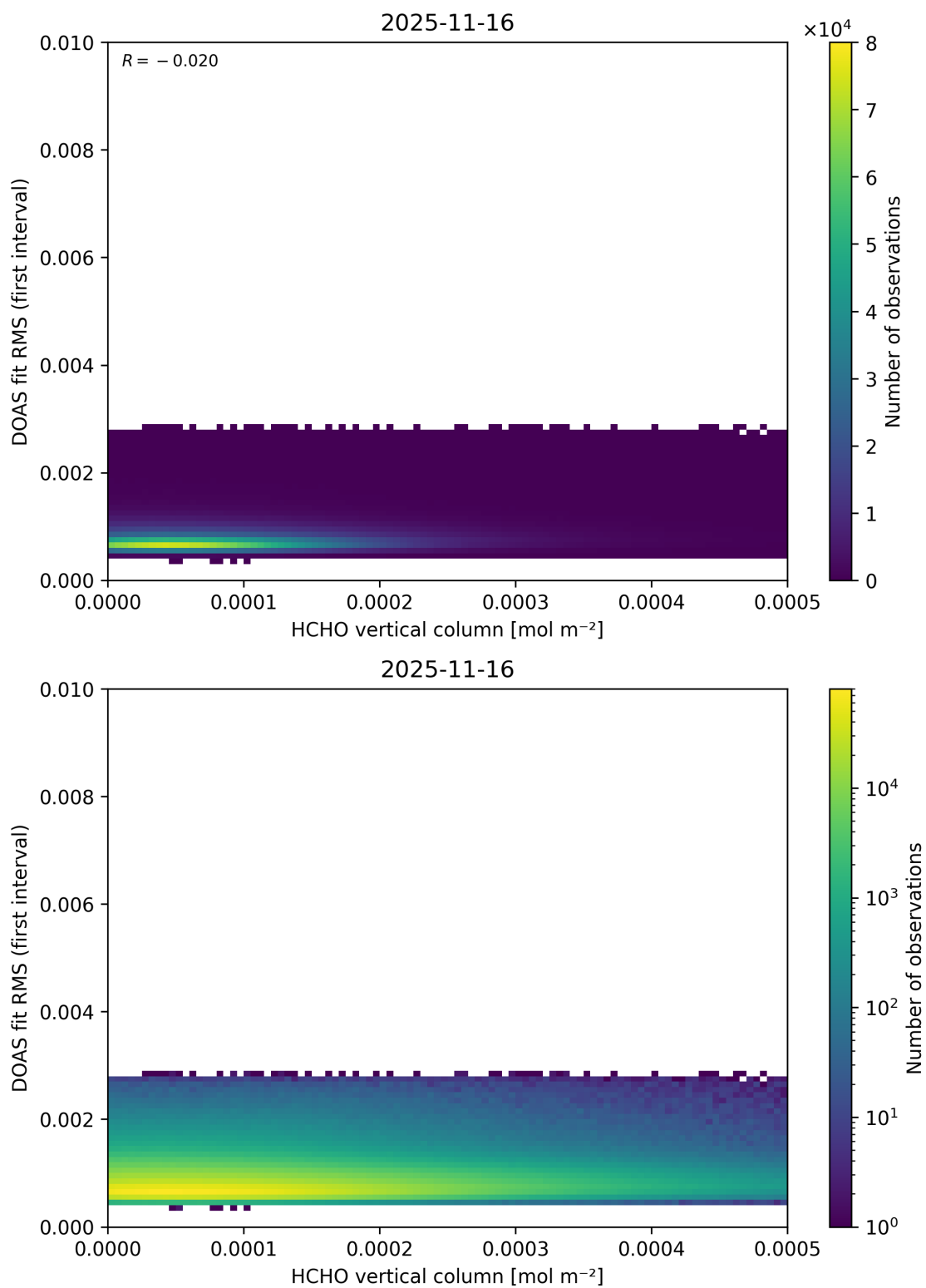
Figure 138: Scatter density plot of “HCHO vertical column” against “DOAS fit RMS (first interval)” for 2025-11-15 to 2025-11-17.
