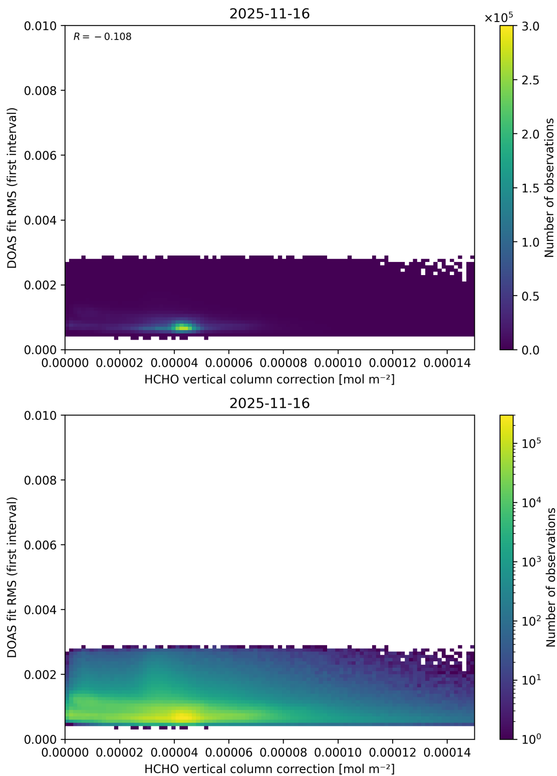
Figure 126: Scatter density plot of “HCHO vertical column correction” against “DOAS fit RMS (first interval)” for 2025-11-15 to 2025-11-17.
