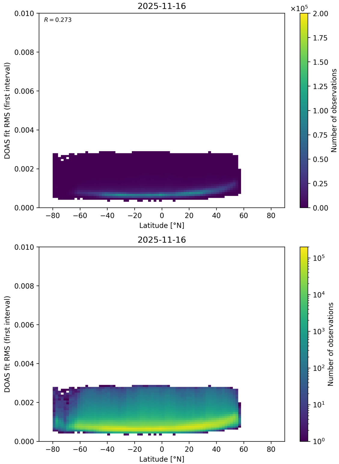
Figure 171: Scatter density plot of “Latitude” against “DOAS fit RMS (first interval)” for 2025-11-15 to 2025-11-17.
