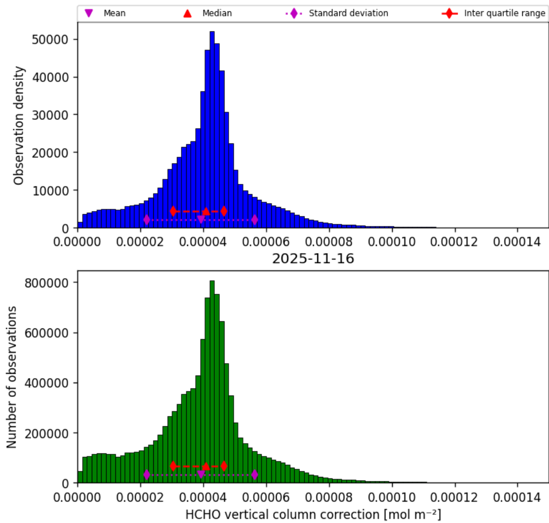
Figure 39: Histogram of “HCHO vertical column correction” for 2025-11-15 to 2025-11-17
