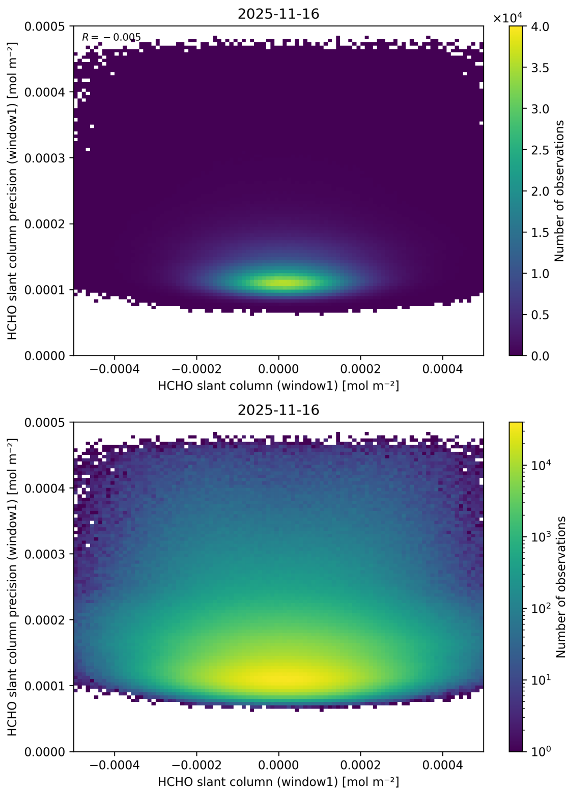
Figure 94: Scatter density plot of “HCHO slant column (window1)” against “HCHO slant column precision (window1)” for 2025-11-15 to 2025-11-17.
