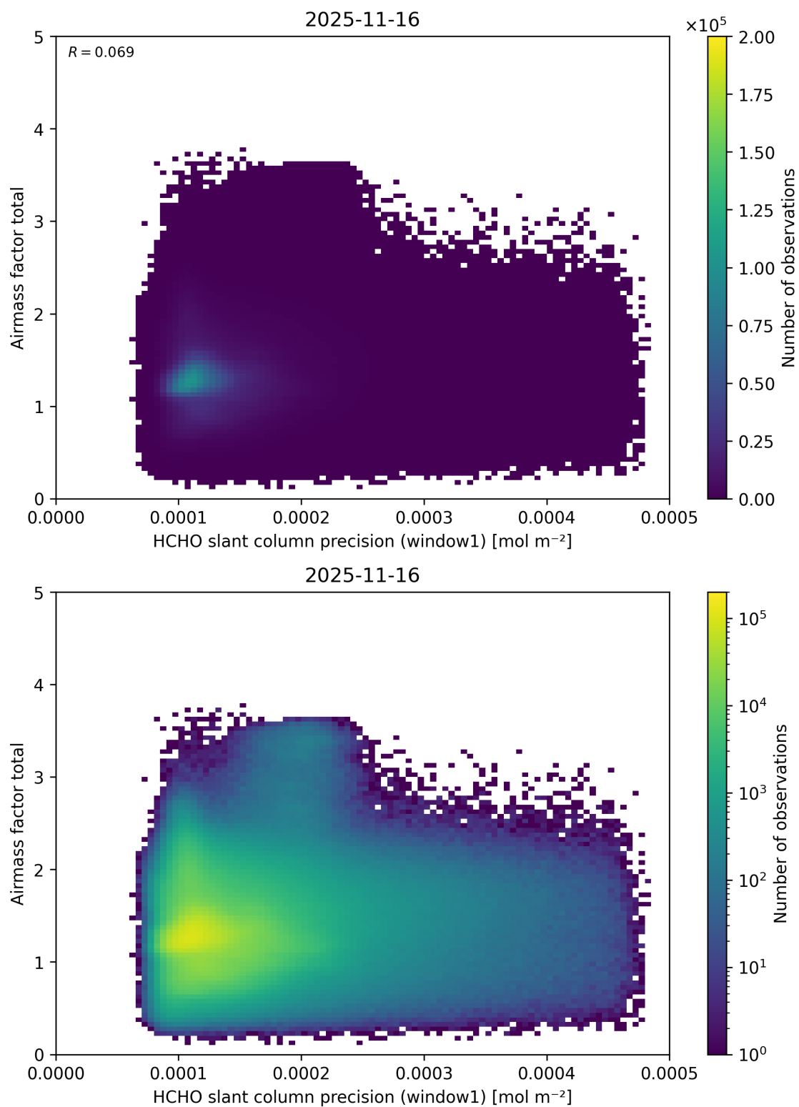
Figure 105: Scatter density plot of “HCHO slant column precision (window1)” against “Airmass factor total” for 2025-11-15 to 2025-11-17.
