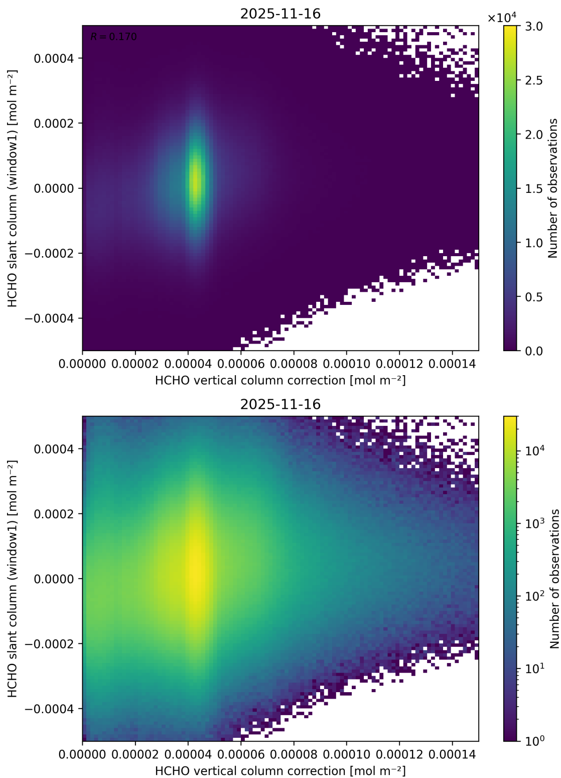
Figure 132: Scatter density plot of “HCHO vertical column correction” against “HCHO slant column (window1)” for 2025-11-15 to 2025-11-17.
