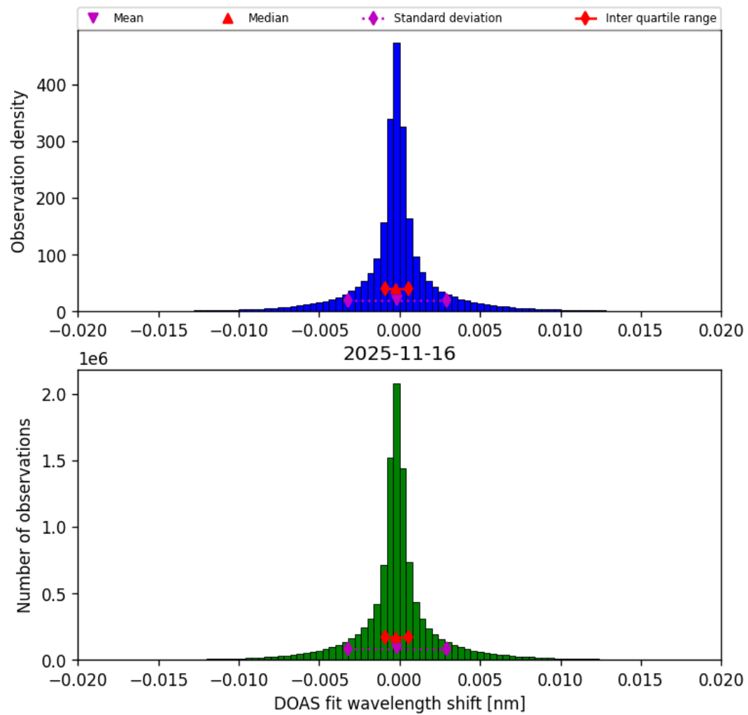
Figure 46: Histogram of “DOAS fit wavelength shift” for 2025-11-15 to 2025-11-17
