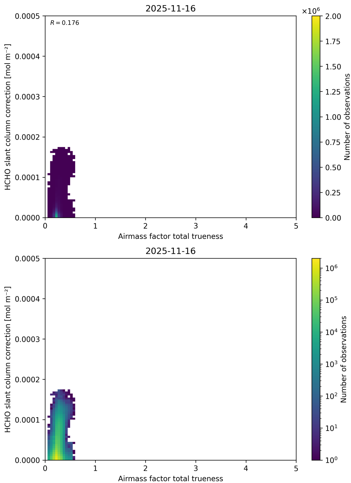
Figure 123: Scatter density plot of “Airmass factor total truiness” against “HCHO slant column correction” for 2025-11-15 to 2025-11-17.
