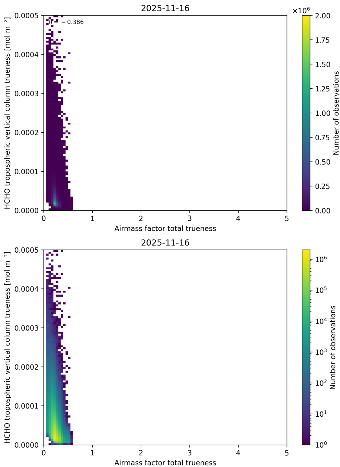
Figure 124: Scatter density plot of “Airmass factor total truiness” against “HCHO tropospheric vertical column truiness” for 2025-11-15 to 2025-11-17.
