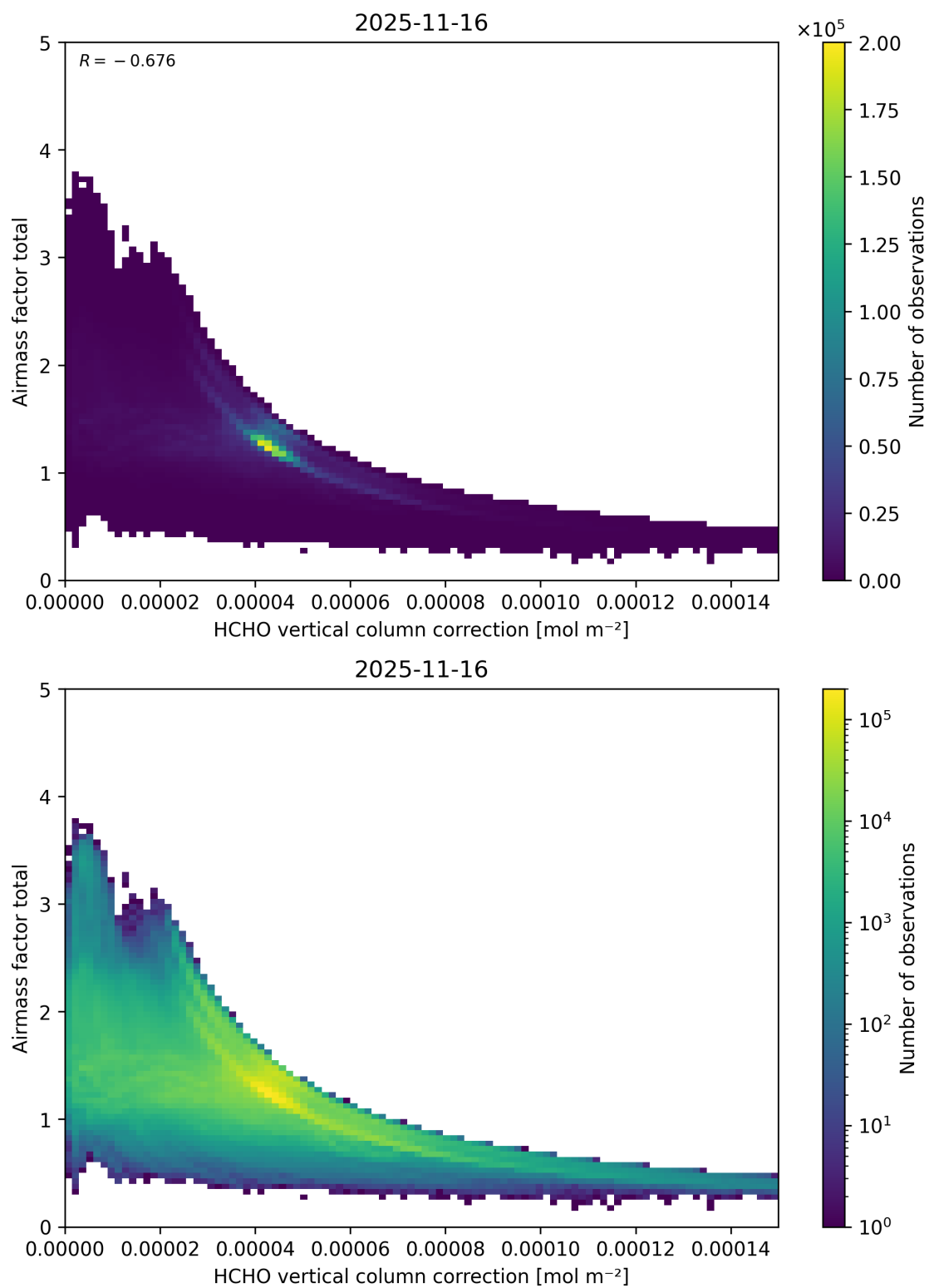
Figure 134: Scatter density plot of “HCHO vertical column correction” against “Airmass factor total” for 2025-11-15 to 2025-11-17.
