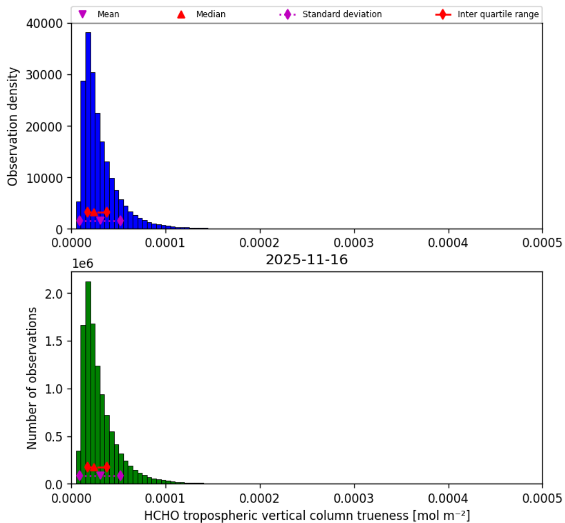
Figure 50: Histogram of “HCHO tropospheric vertical column trueness” for 2025-11-15 to 2025-11-17
