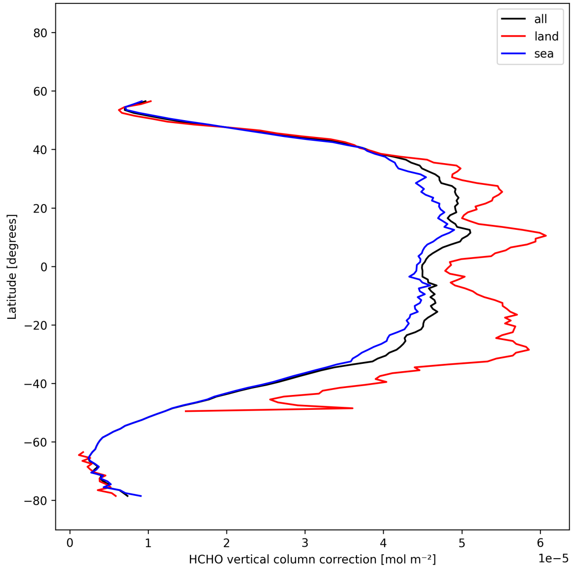
Figure 24: Zonal average of “HCHO vertical column correction” for 2025-11-15 to 2025-11-17.
