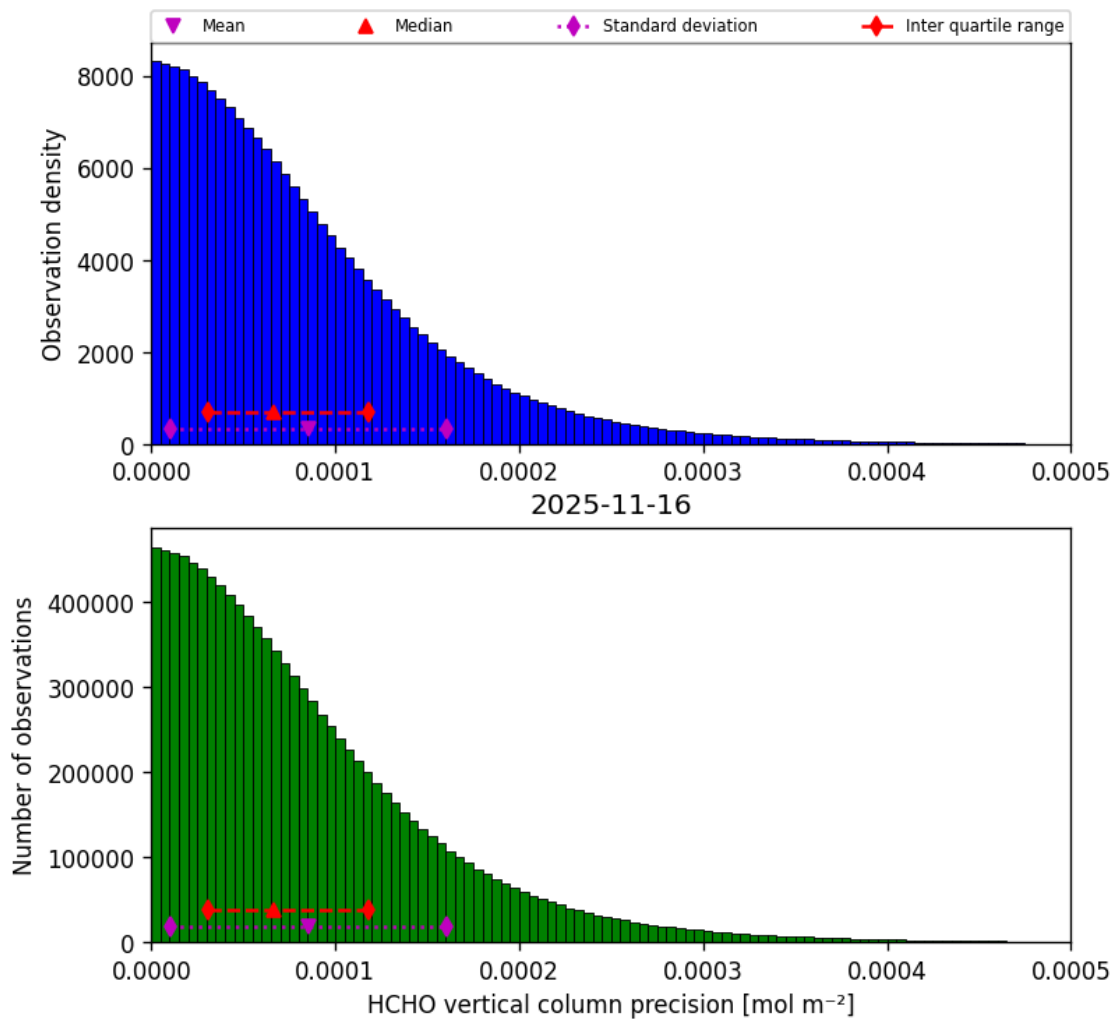
Figure 38: Histogram of “HCHO vertical column precision” for 2025-11-15 to 2025-11-17
