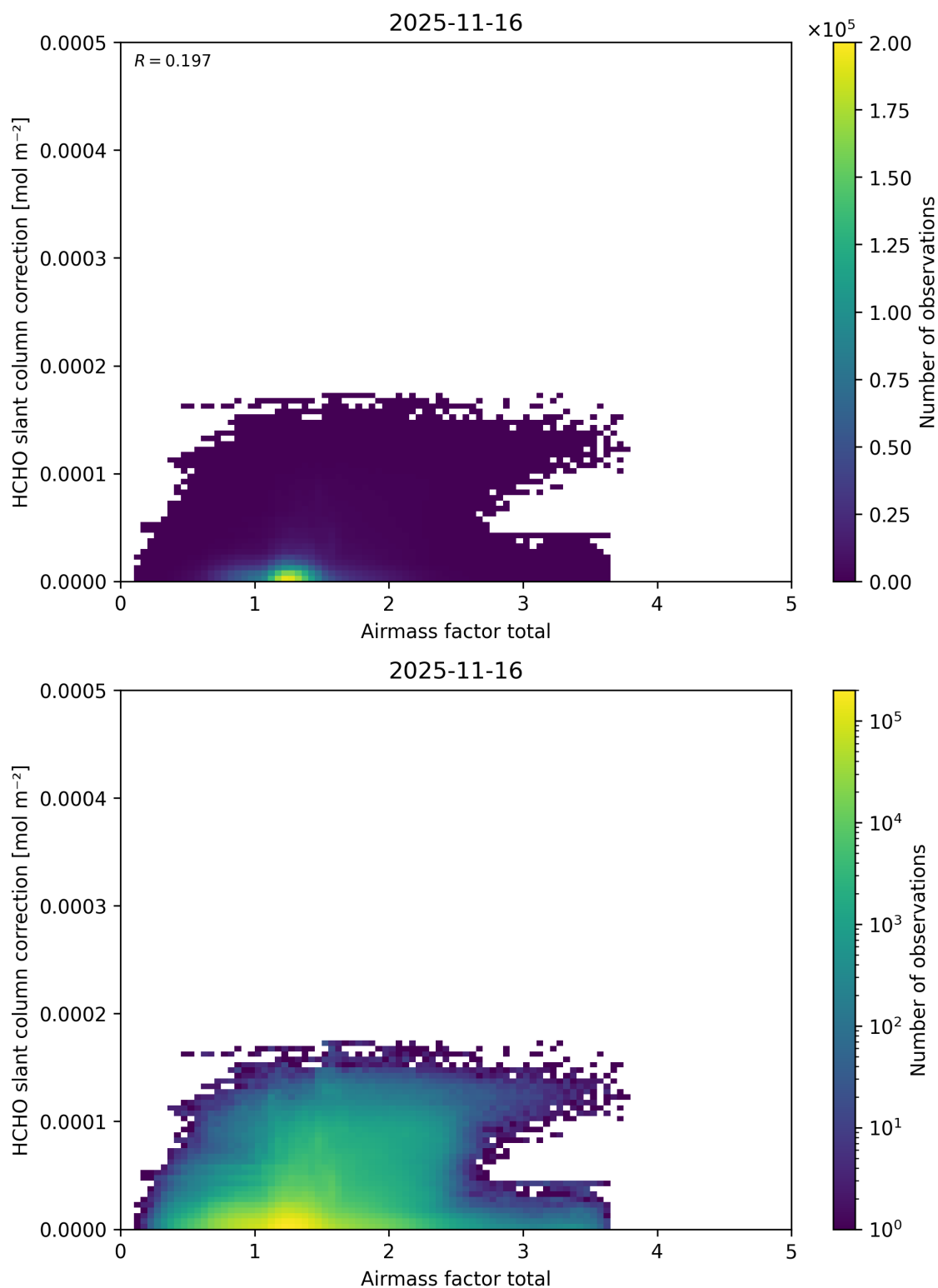
Figure 114: Scatter density plot of “Airmass factor total” against “HCHO slant column correction” for 2025-11-15 to 2025-11-17.
