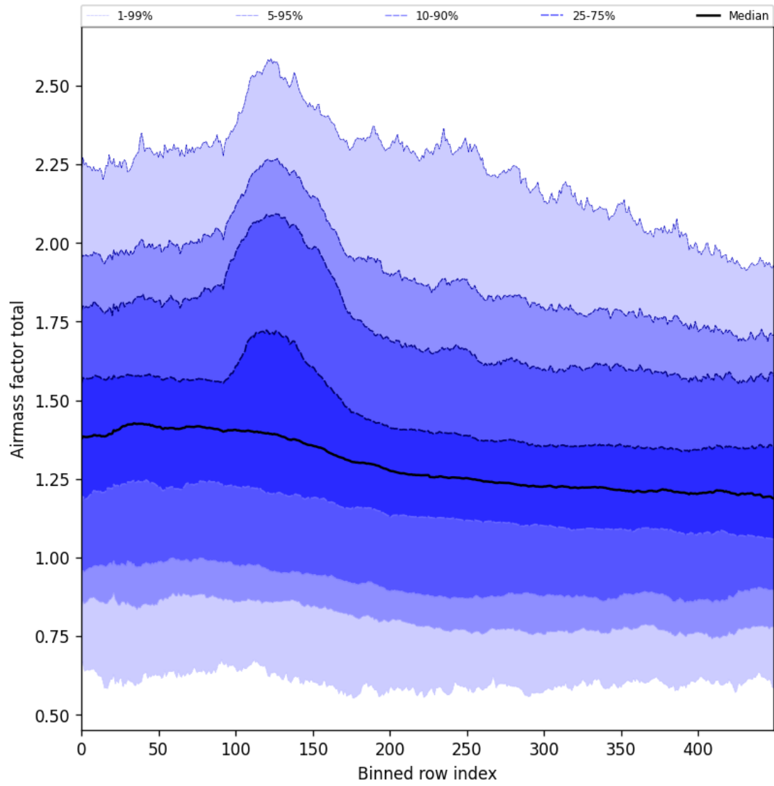
Figure 57: Along track statistics of “Airmass factor total” for 2025-11-15 to 2025-11-17
