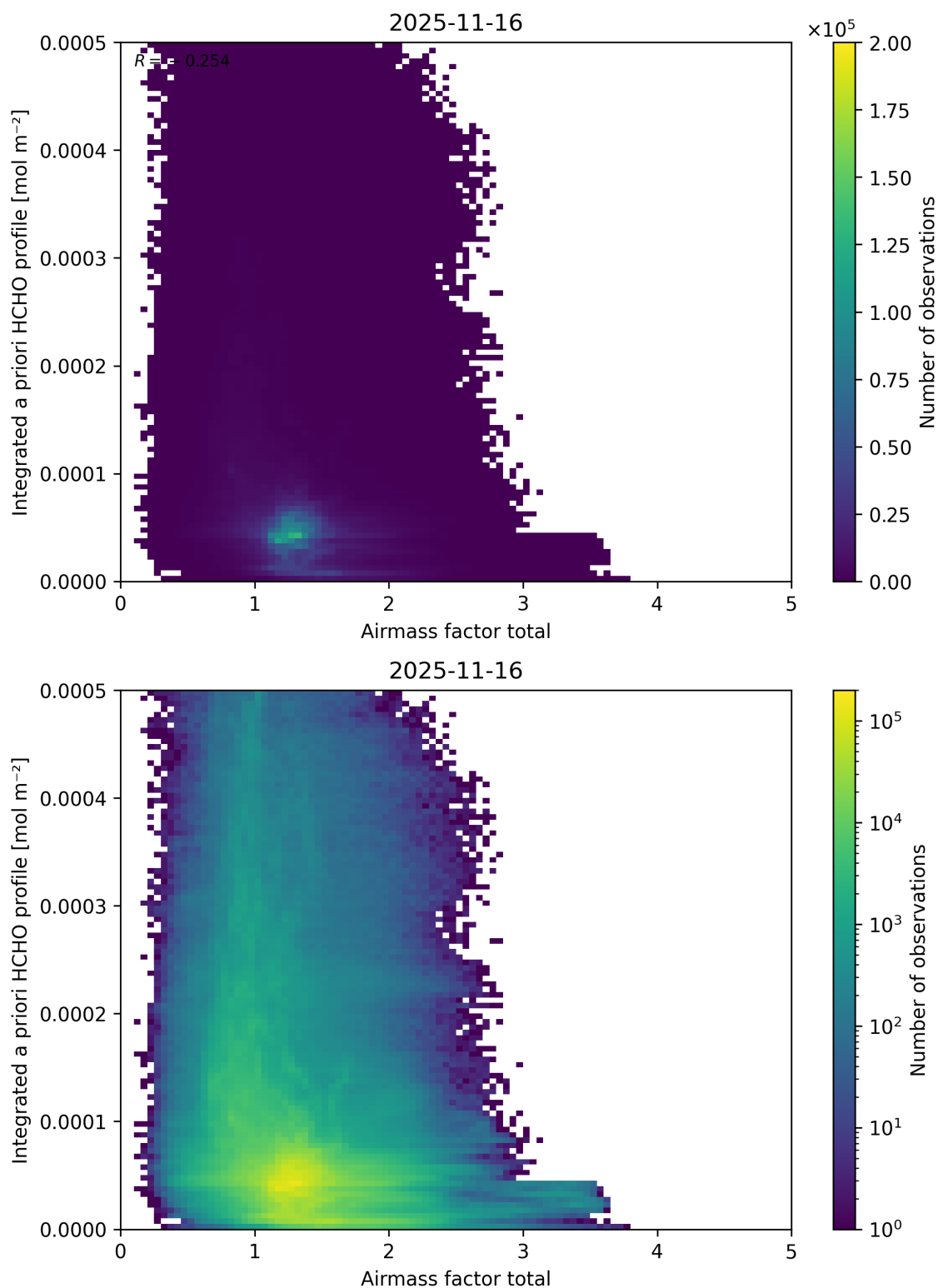
Figure 117: Scatter density plot of “Airmass factor total” against “Integrated a priori HCHO profile” for 2025-11-15 to 2025-11-17.
