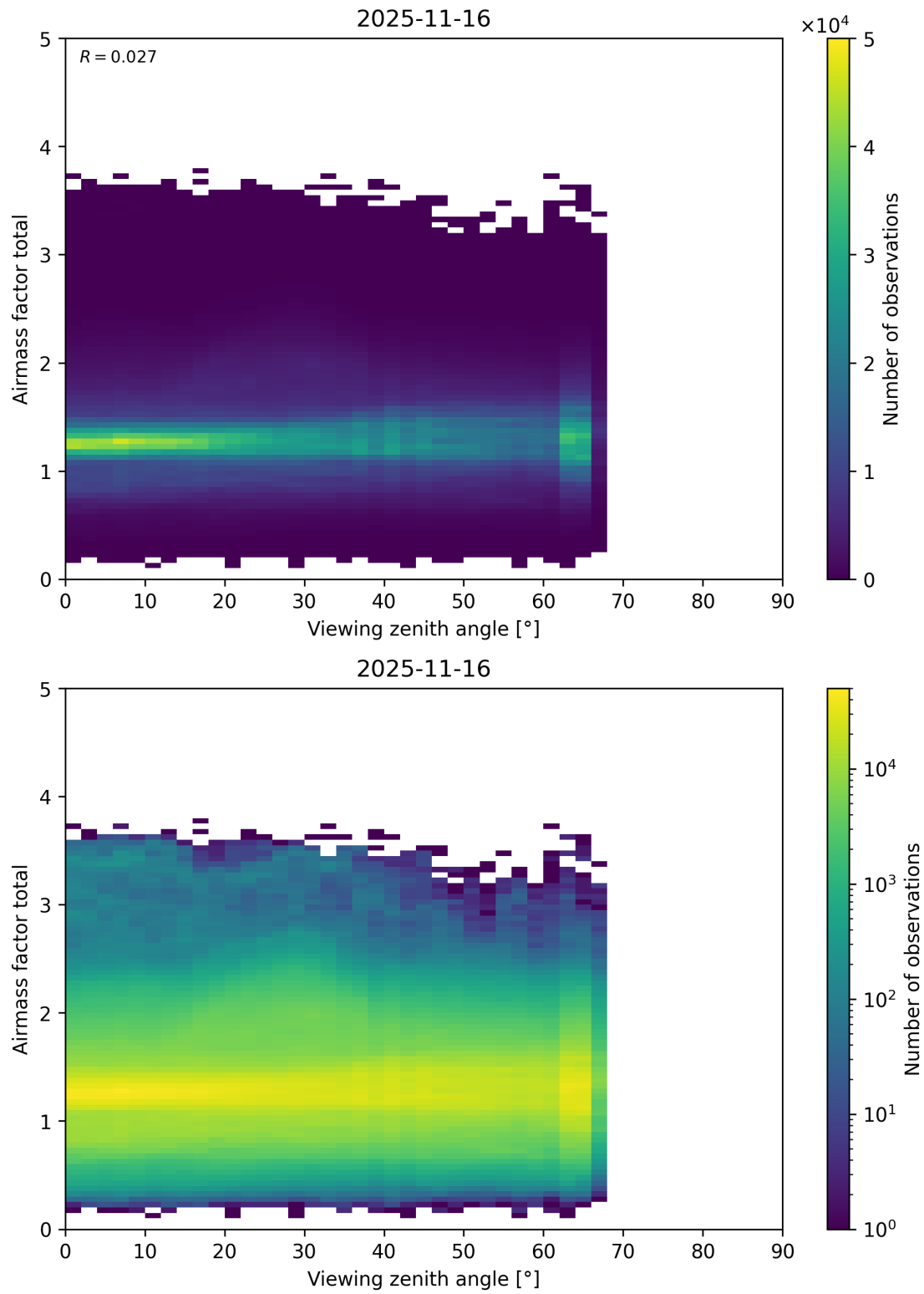
Figure 210: Scatter density plot of “Viewing zenith angle” against “Airmass factor total” for 2025-11-15 to 2025-11-17.
