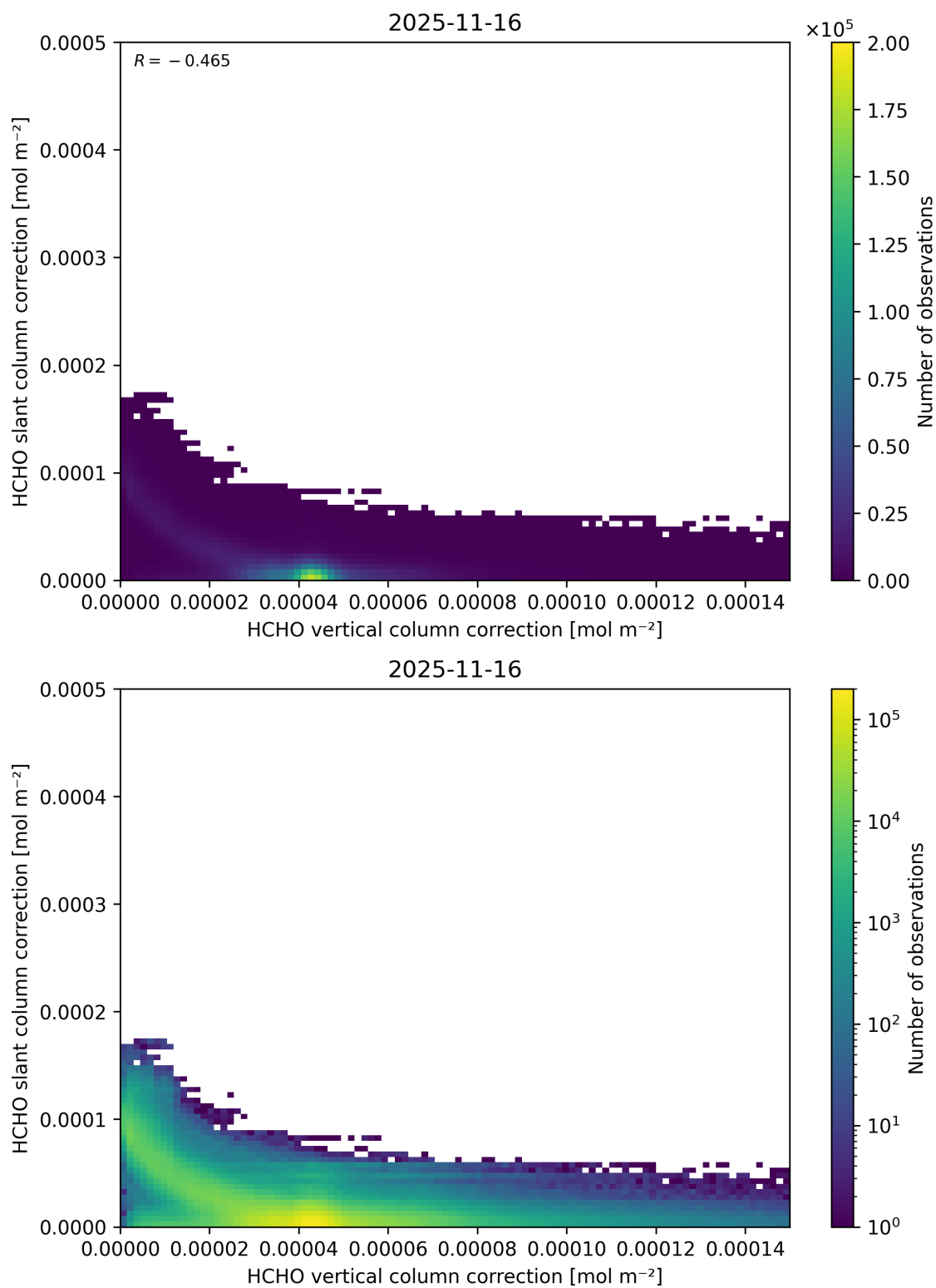
Figure 131: Scatter density plot of “HCHO vertical column correction” against “HCHO slant column correction” for 2025-11-15 to 2025-11-17.
