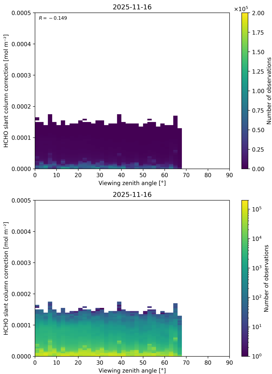
Figure 207: Scatter density plot of “Viewing zenith angle” against “HCHO slant column correction” for 2025-11-15 to 2025-11-17.
