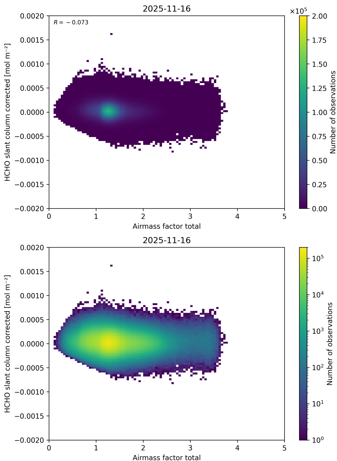
Figure 113: Scatter density plot of “Airmass factor total” against “HCHO slant column corrected” for 2025-11-15 to 2025-11-17.
