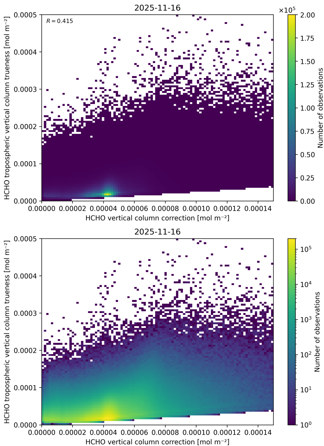
Figure 136: Scatter density plot of “HCHO vertical column correction” against “HCHO tropospheric vertical column true-ness” for 2025-11-15 to 2025-11-17.
