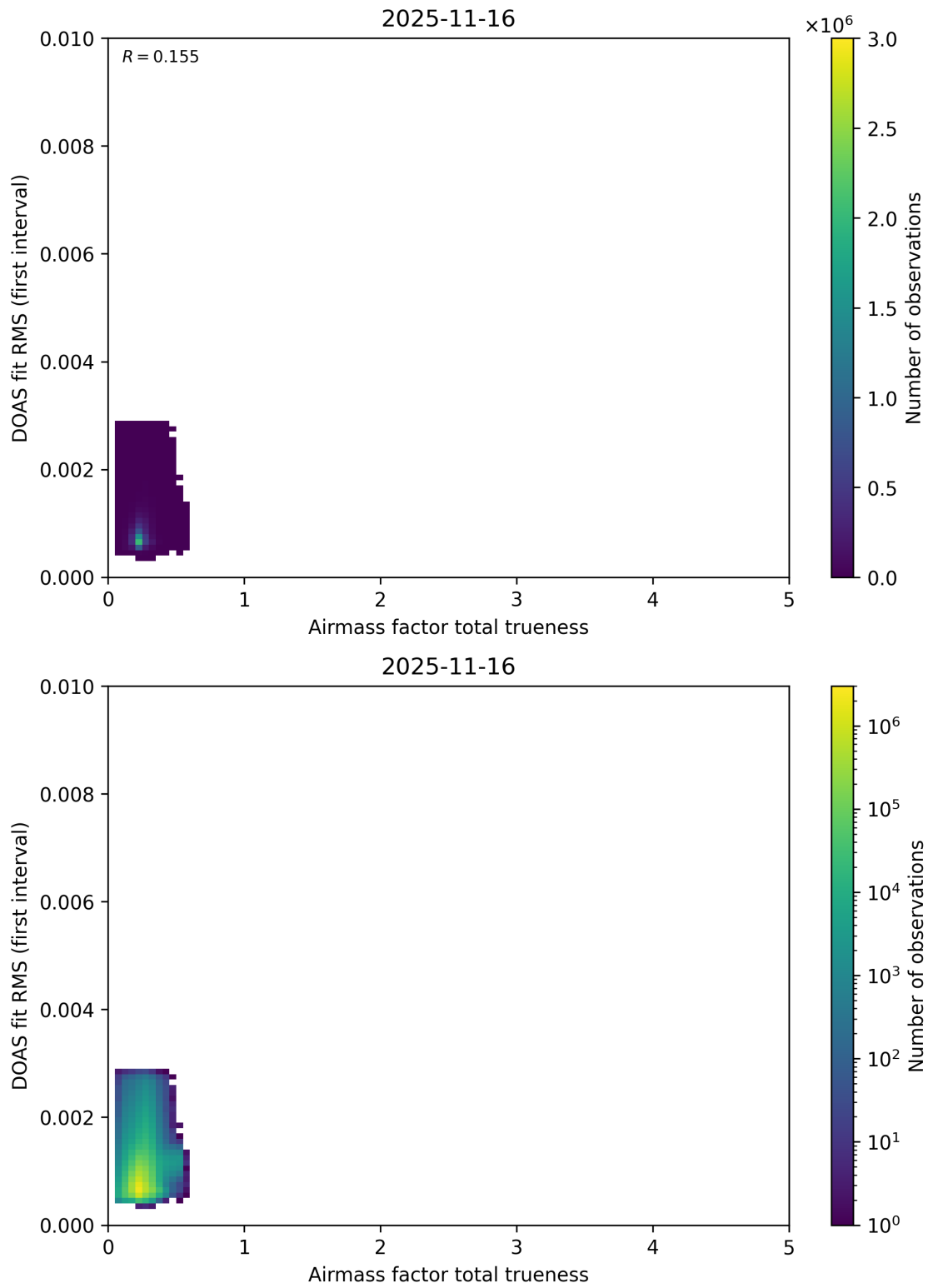
Figure 118: Scatter density plot of “Airmass factor total trueness” against “DOAS fit RMS (first interval)” for 2025-11-15 to 2025-11-17.
