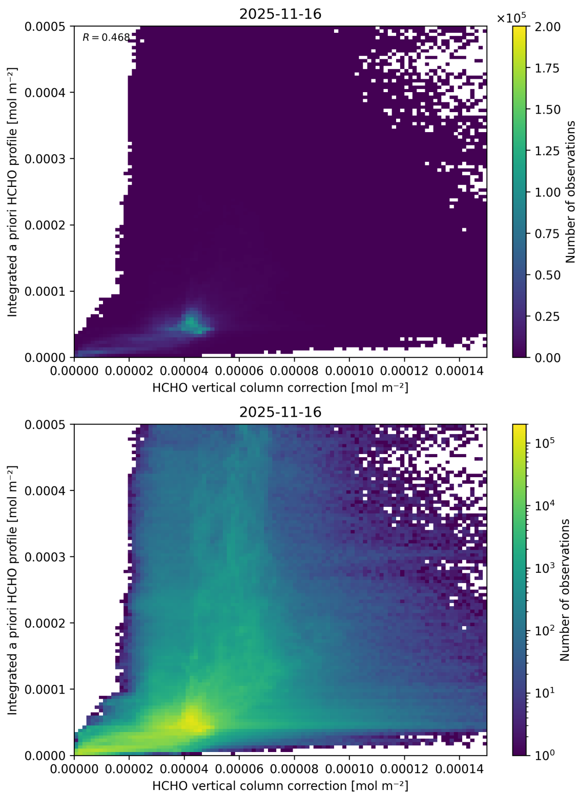
Figure 137: Scatter density plot of “HCHO vertical column correction” against “Integrated a priori HCHO profile” for 2025-11-15 to 2025-11-17.
