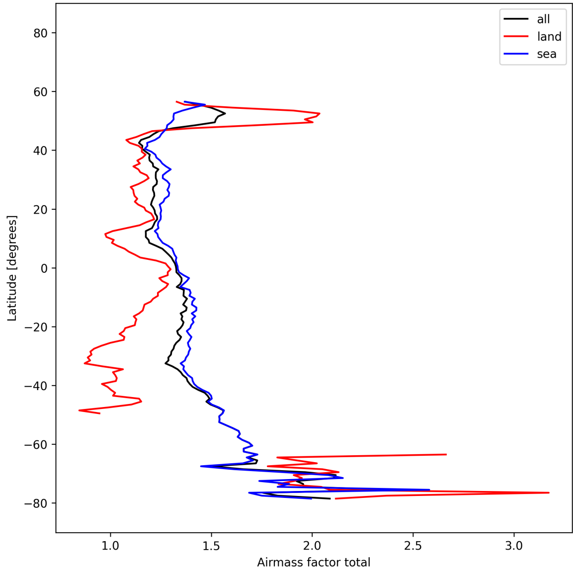
Figure 27: Zonal average of “Airmass factor total” for 2025-11-15 to 2025-11-17.
