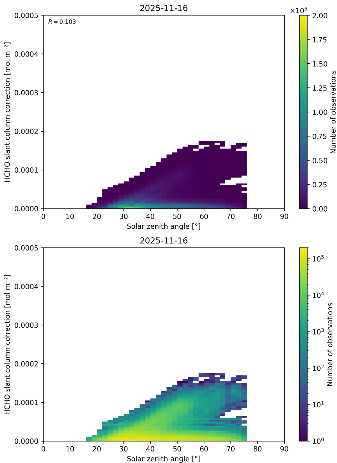
Figure 191: Scatter density plot of “Solar zenith angle” against “HCHO slant column correction” for 2025-11-15 to 2025-11-17.
