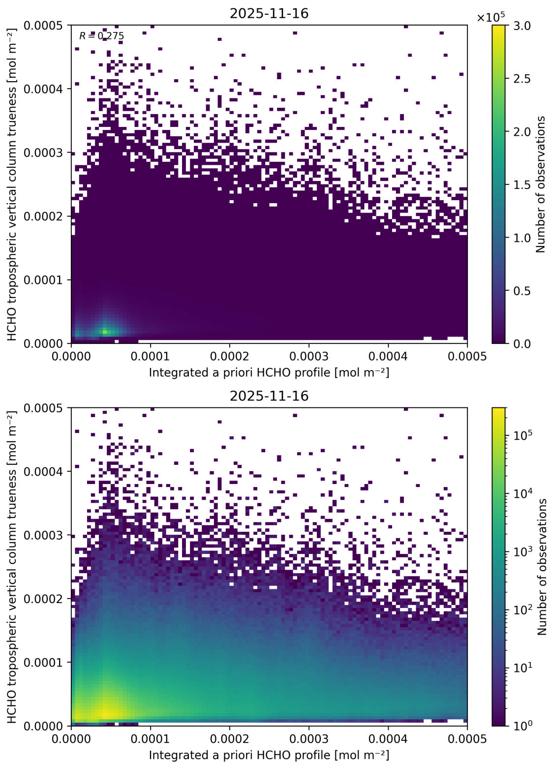
Figure 170: Scatter density plot of “Integrated a priori HCHO profile” against “HCHO tropospheric vertical column trueness” for 2025-11-15 to 2025-11-17.
