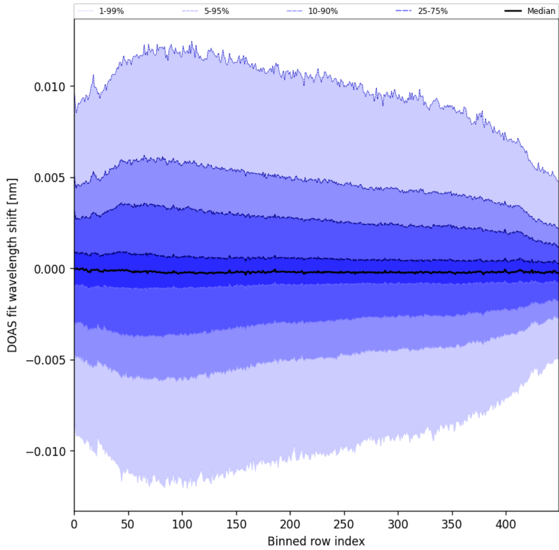
Figure 61: Along track statistics of “DOAS fit wavelength shift” for 2025-11-15 to 2025-11-17
