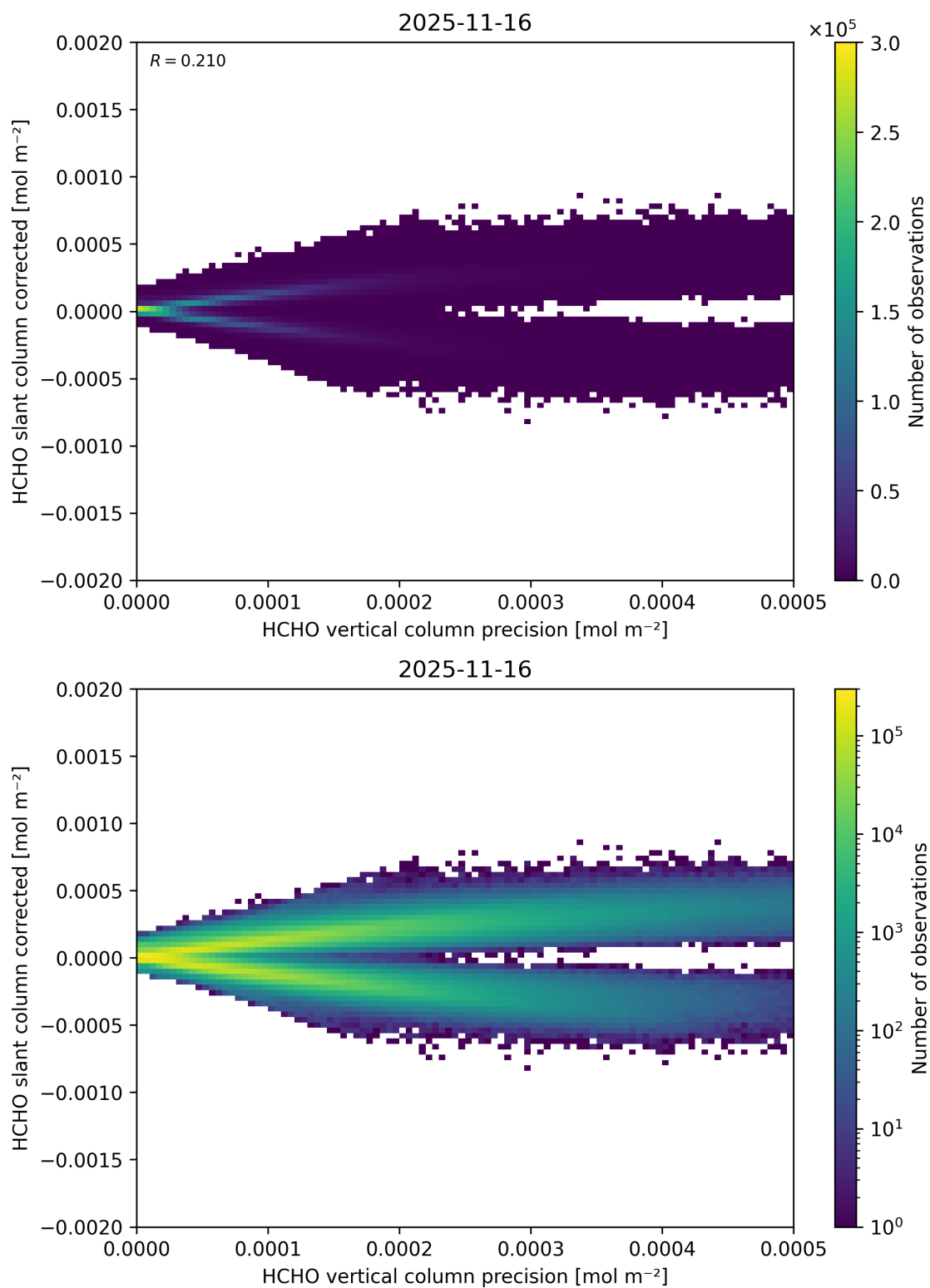
Figure 156: Scatter density plot of “HCHO vertical column precision” against “HCHO slant column corrected” for 2025-11-15 to 2025-11-17.
