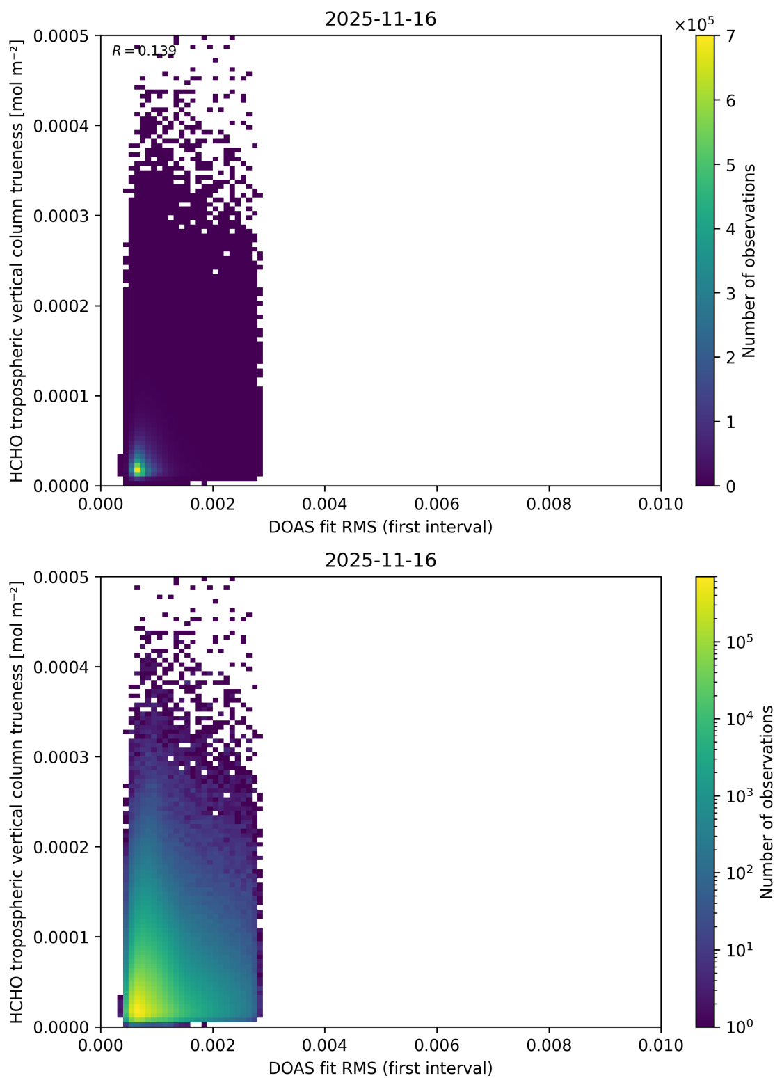
Figure 68: Scatter density plot of “DOAS fit RMS (first interval)” against “HCHO tropospheric vertical column trueness” for 2025-11-15 to 2025-11-17.
