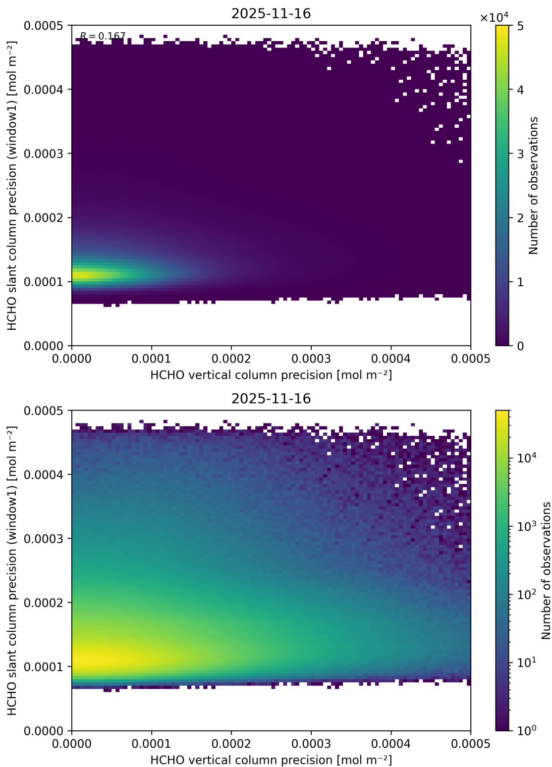
Figure 159: Scatter density plot of “HCHO vertical column precision” against “HCHO slant column precision (window1)” for 2025-11-15 to 2025-11-17.
