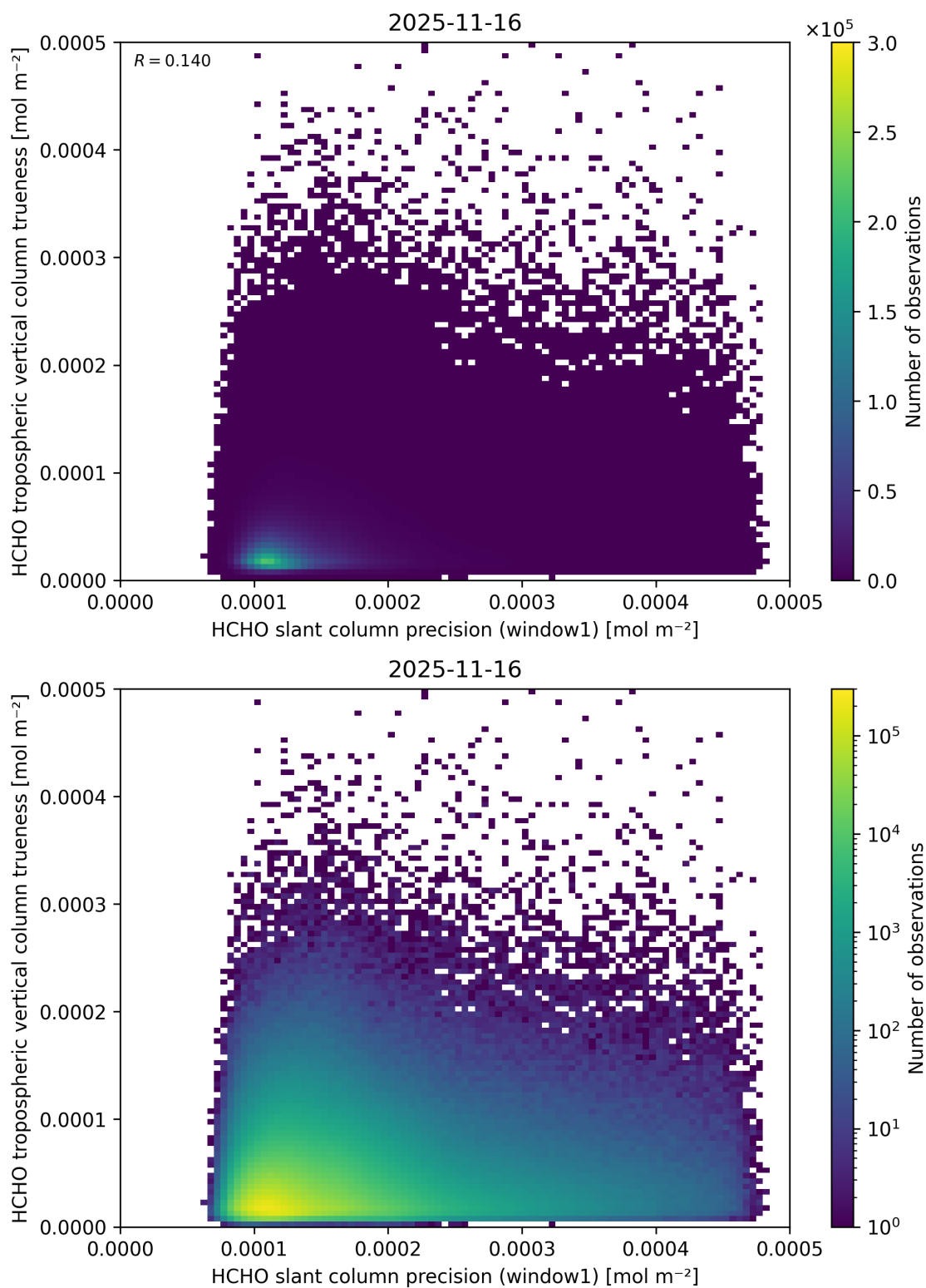
Figure 107: Scatter density plot of “HCHO slant column precision (window1)” against “HCHO tropospheric vertical column trueness” for 2025-11-15 to 2025-11-17.
