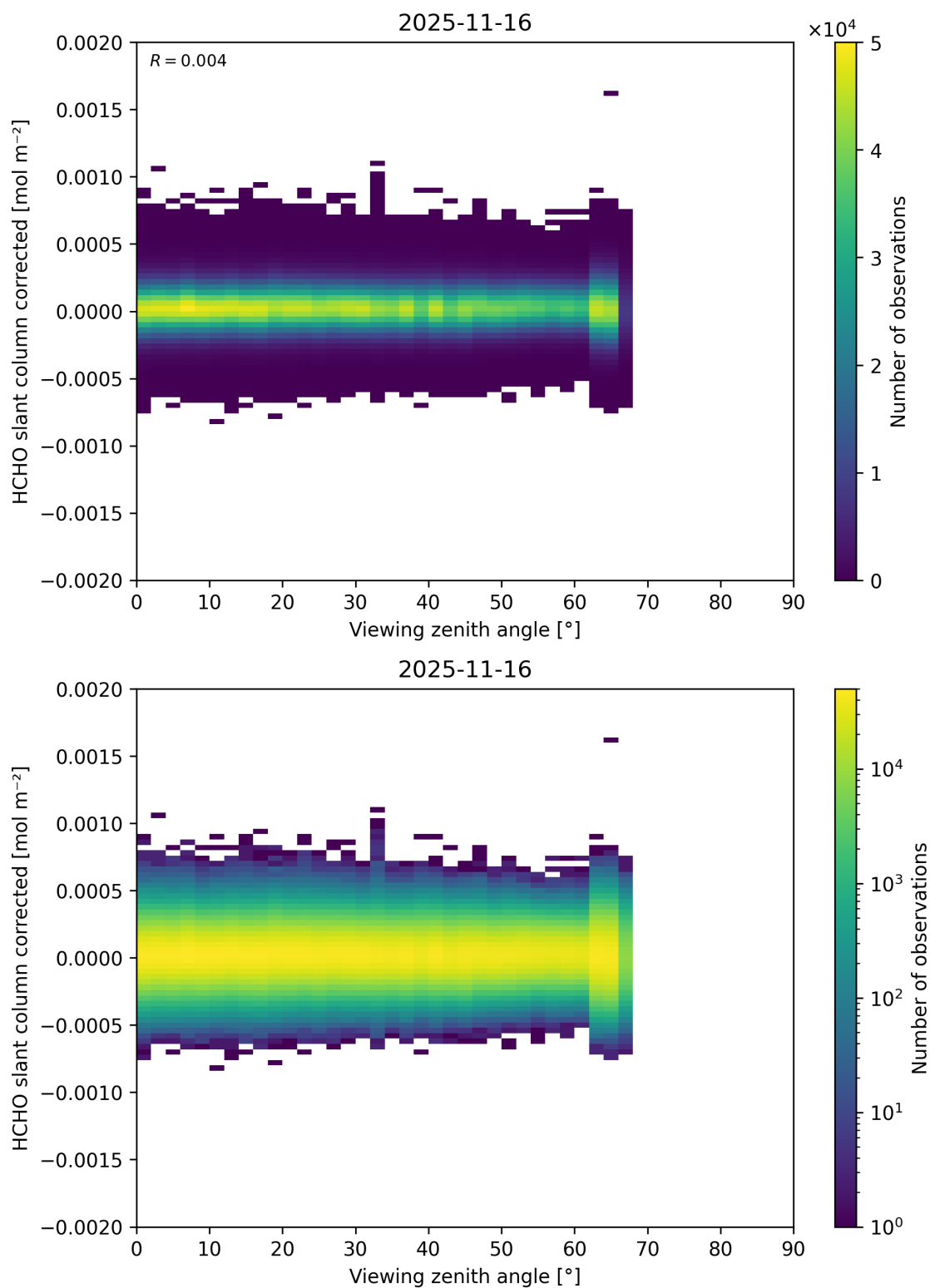
Figure 206: Scatter density plot of “Viewing zenith angle” against “HCHO slant column corrected” for 2025-11-15 to 2025-11-17.
