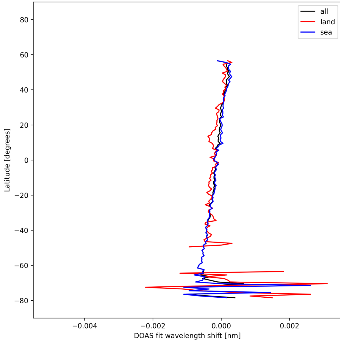
Figure 31: Zonal average of "DOAS fit wavelength shift" for 2025-11-15 to 2025-11-17.
