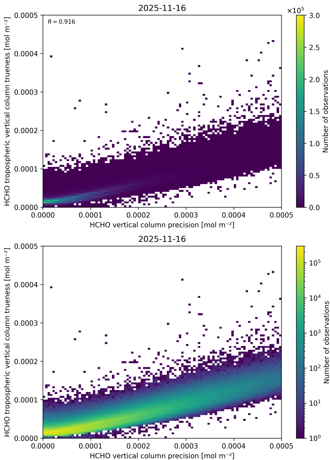
Figure 163: Scatter density plot of “HCHO vertical column precision” against “HCHO tropospheric vertical column true-ness” for 2025-11-15 to 2025-11-17.
