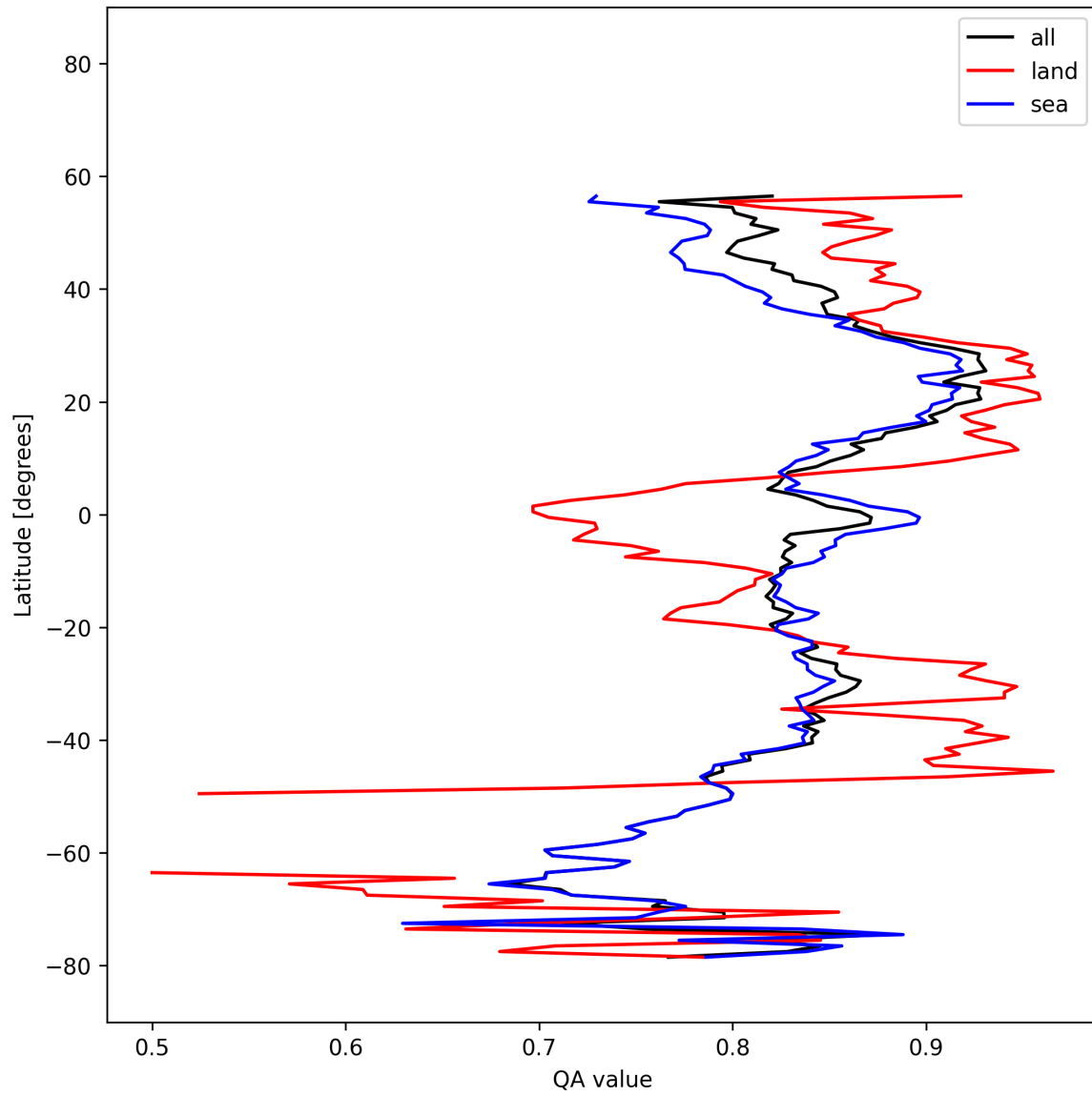
Figure 21: Zonal average of “QA value” for 2025-11-15 to 2025-11-17.
