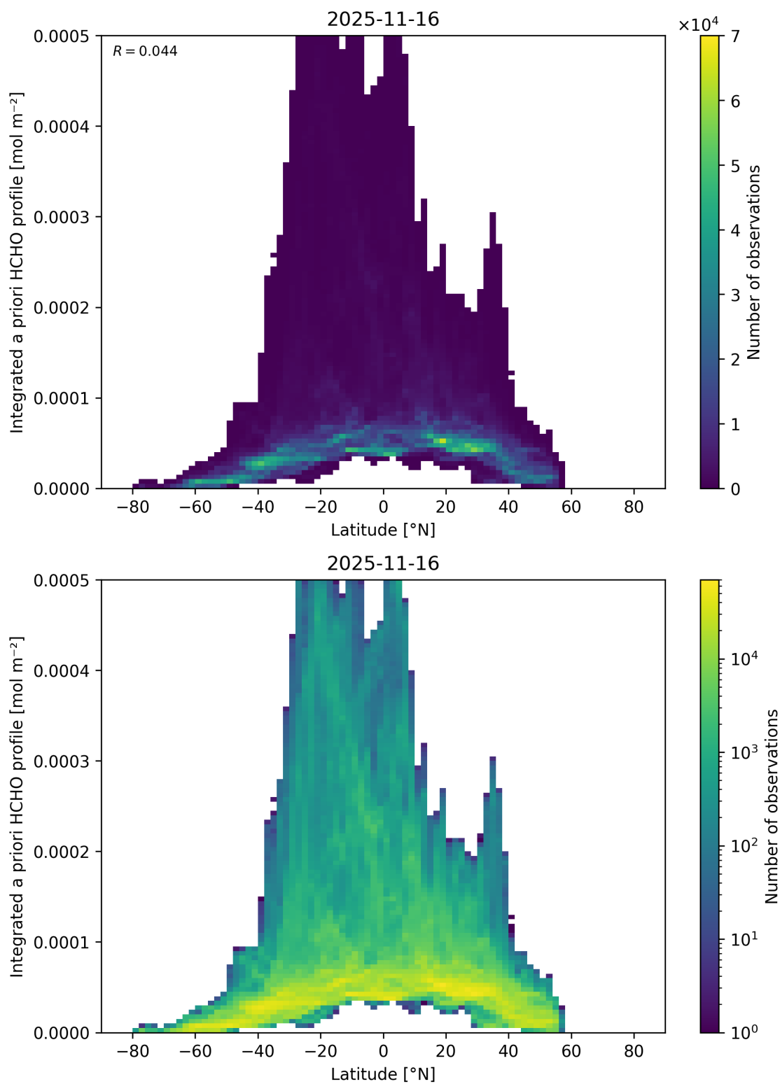
Figure 185: Scatter density plot of “Latitude” against “Integrated a priori HCHO profile” for 2025-11-15 to 2025-11-17.
