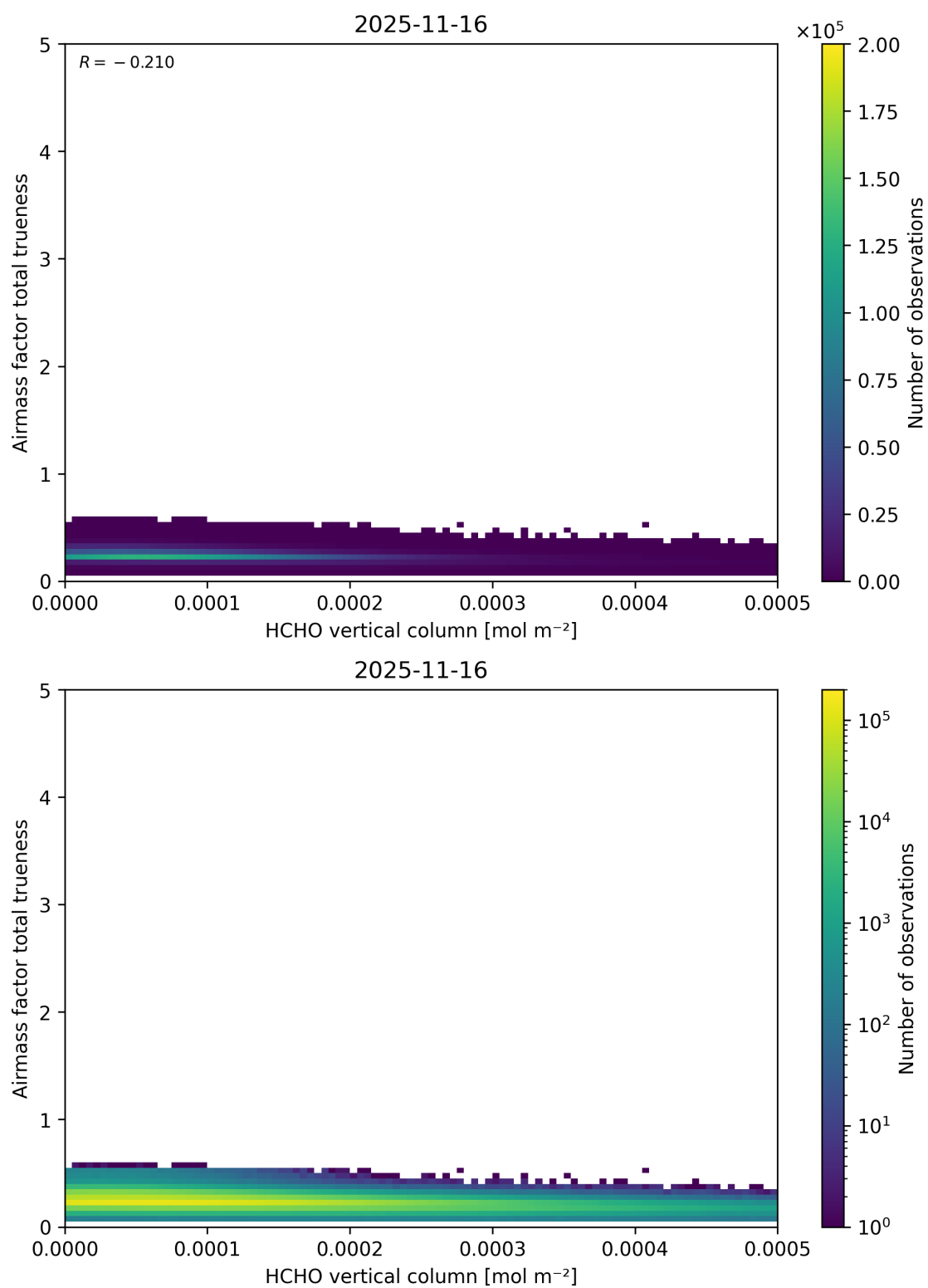
Figure 147: Scatter density plot of “HCHO vertical column” against “Airmass factor total truiness” for 2025-11-15 to 2025-11-17.
