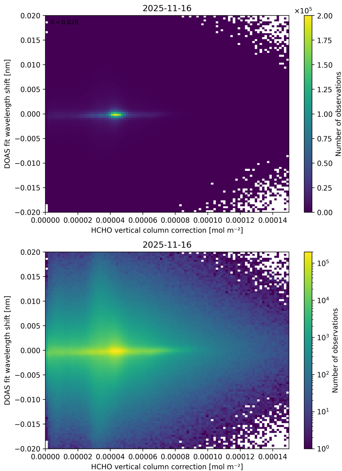
Figure 127: Scatter density plot of “HCHO vertical column correction” against “DOAS fit wavelength shift” for 2025-11-15 to 2025-11-17.
