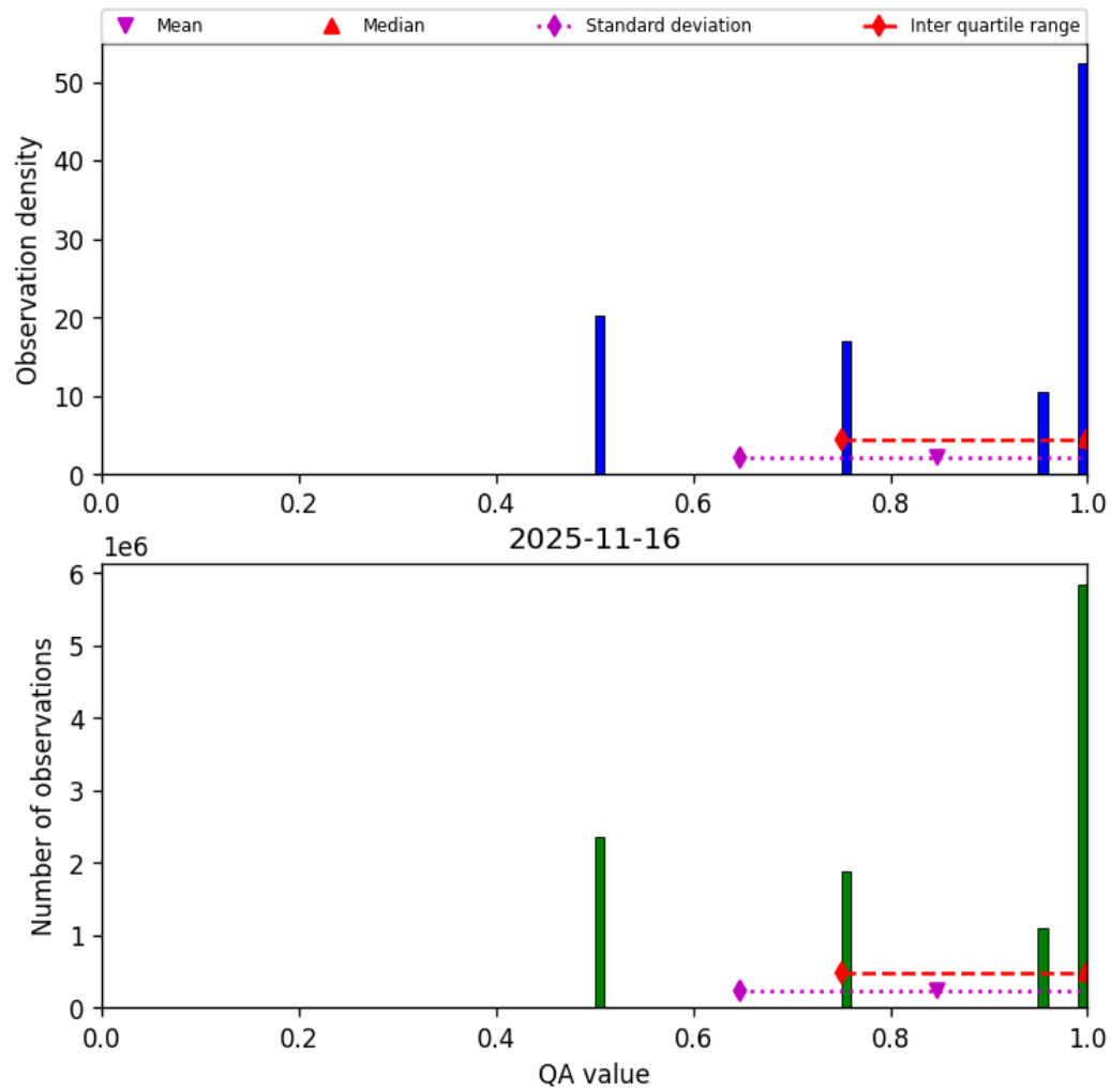
Figure 36: Histogram of “QA value” for 2025-11-15 to 2025-11-17
