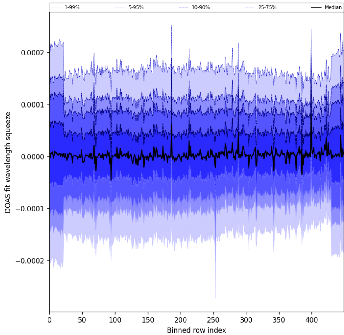
Figure 62: Along track statistics of “DOAS fit wavelength squeeze” for 2025-11-15 to 2025-11-17
