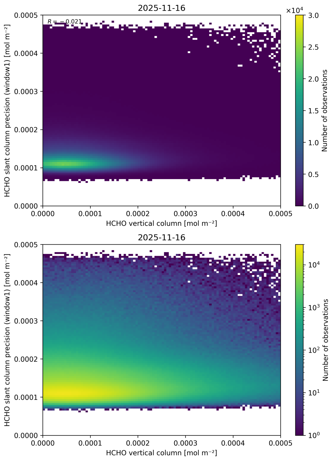
Figure 145: Scatter density plot of “HCHO vertical column” against “HCHO slant column precision (window1)” for 2025-11-15 to 2025-11-17.
