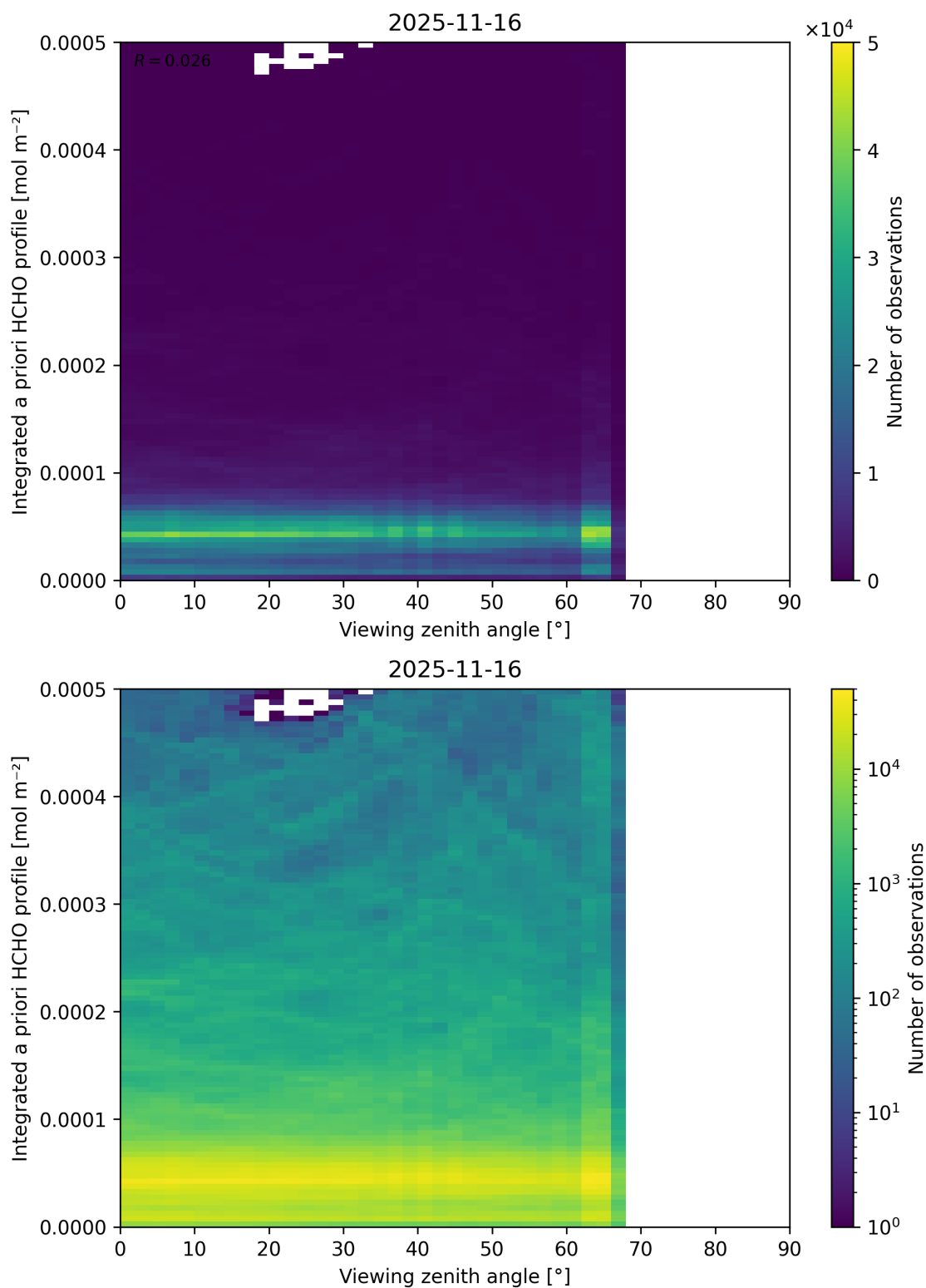
Figure 216: Scatter density plot of “Viewing zenith angle” against “Integrated a priori HCHO profile” for 2025-11-15 to 2025-11-17.
