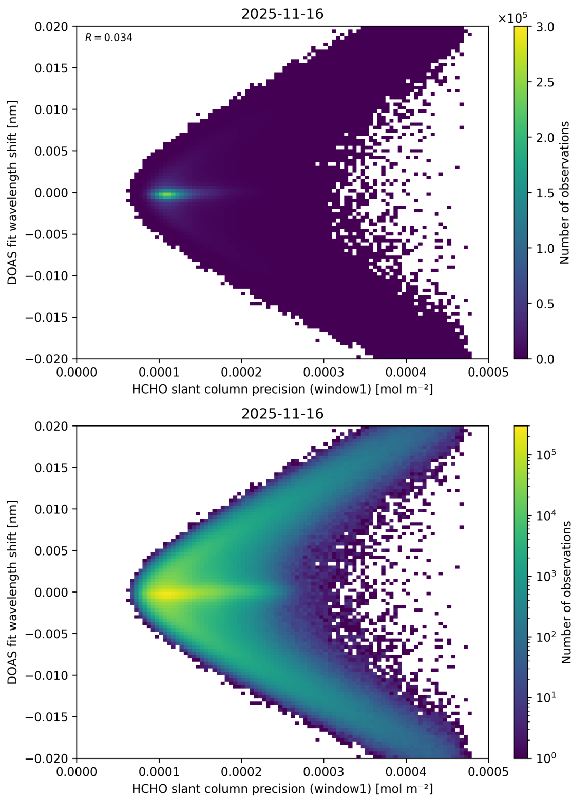
Figure 100: Scatter density plot of “HCHO slant column precision (window1)” against “DOAS fit wavelength shift” for 2025-11-15 to 2025-11-17.
