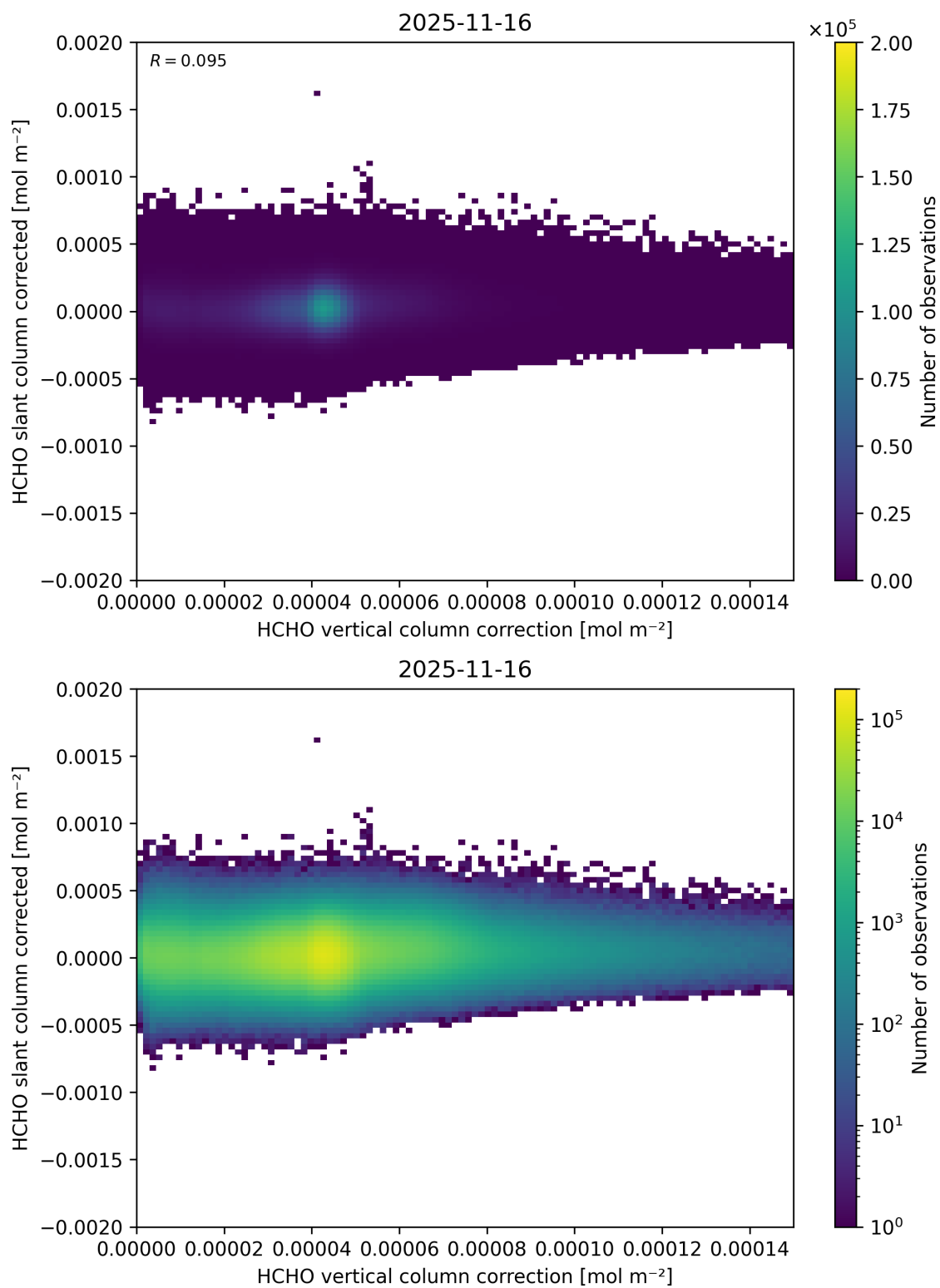
Figure 130: Scatter density plot of “HCHO vertical column correction” against “HCHO slant column corrected” for 2025-11-15 to 2025-11-17.
