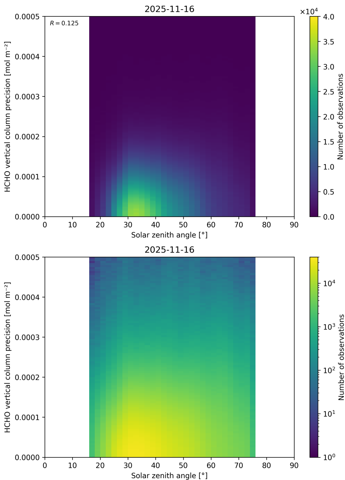
Figure 198: Scatter density plot of “Solar zenith angle” against “HCHO vertical column precision” for 2025-11-15 to 2025-11-17.
