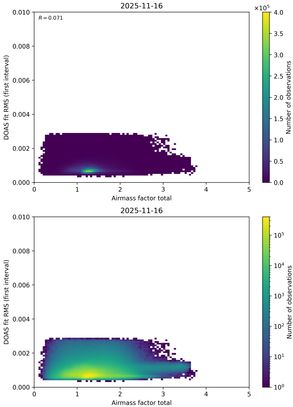
Figure 109: Scatter density plot of “Airmass factor total” against “DOAS fit RMS (first interval)” for 2025-11-15 to 2025-11-17.
