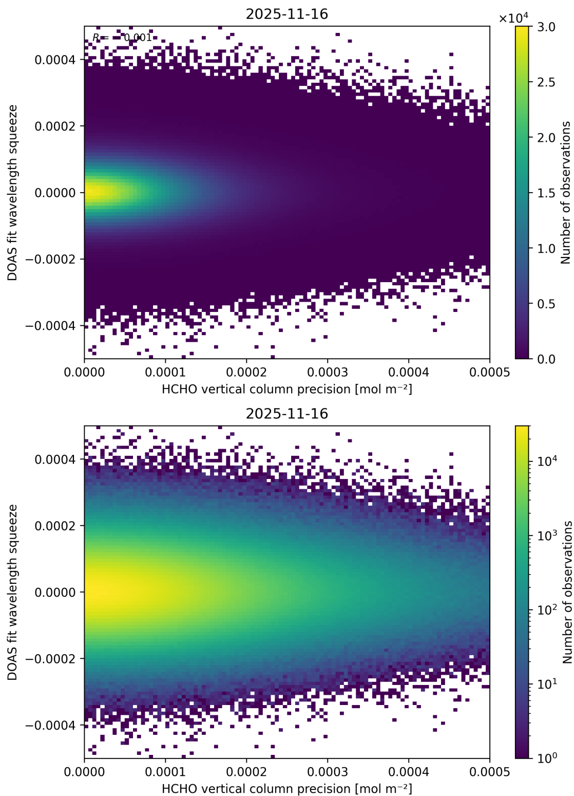
Figure 154: Scatter density plot of “HCHO vertical column precision” against “DOAS fit wavelength squeeze” for 2025-11-15 to 2025-11-17.
