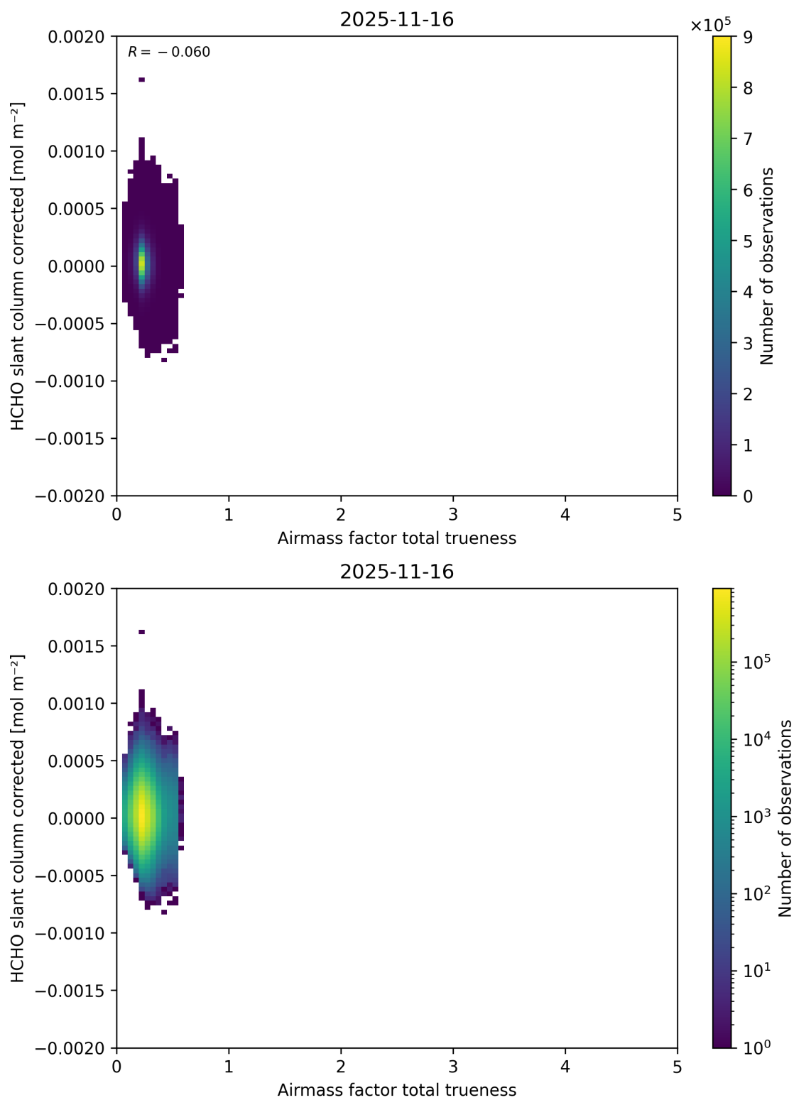
Figure 122: Scatter density plot of “Airmass factor total trueness” against “HCHO slant column corrected” for 2025-11-15 to 2025-11-17.
