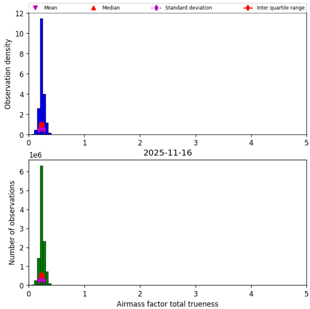
Figure 43: Histogram of “Airmass factor total trueness” for 2025-11-15 to 2025-11-17
