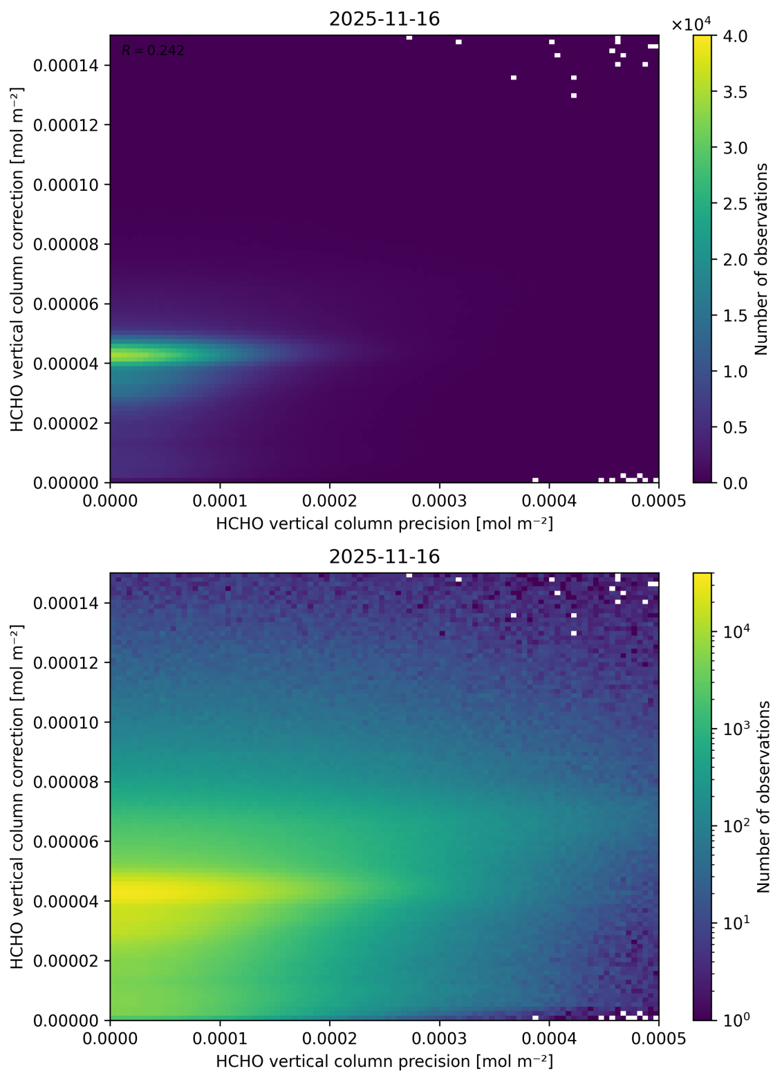
Figure 162: Scatter density plot of “HCHO vertical column precision” against “HCHO vertical column correction” for 2025-11-15 to 2025-11-17.
