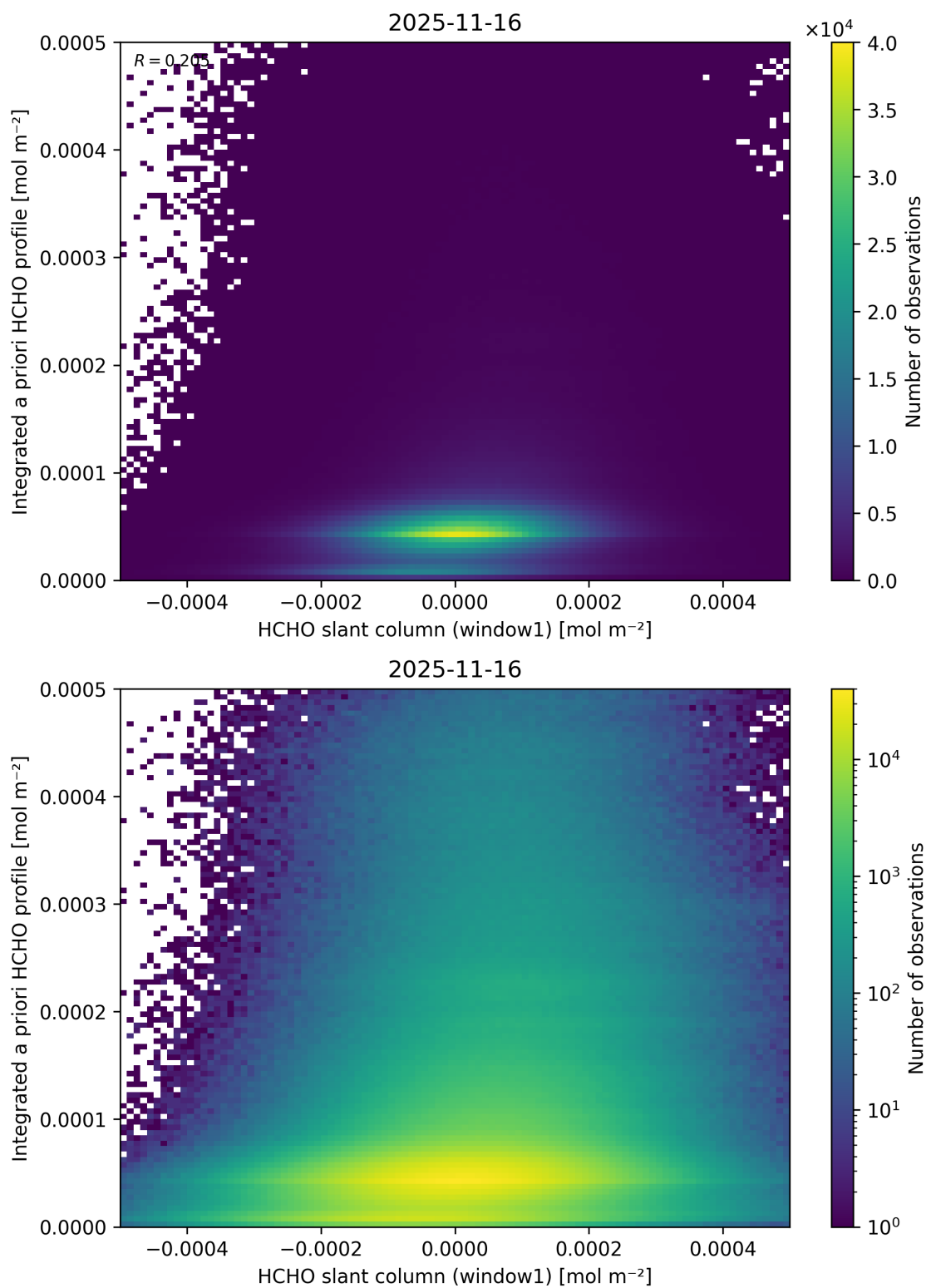
Figure 98: Scatter density plot of “HCHO slant column (window1)” against “Integrated a priori HCHO profile” for 2025-11-15 to 2025-11-17.
