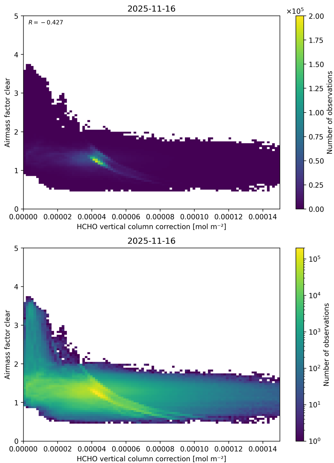
Figure 129: Scatter density plot of “HCHO vertical column correction” against “Airmass factor clear” for 2025-11-15 to 2025-11-17.
