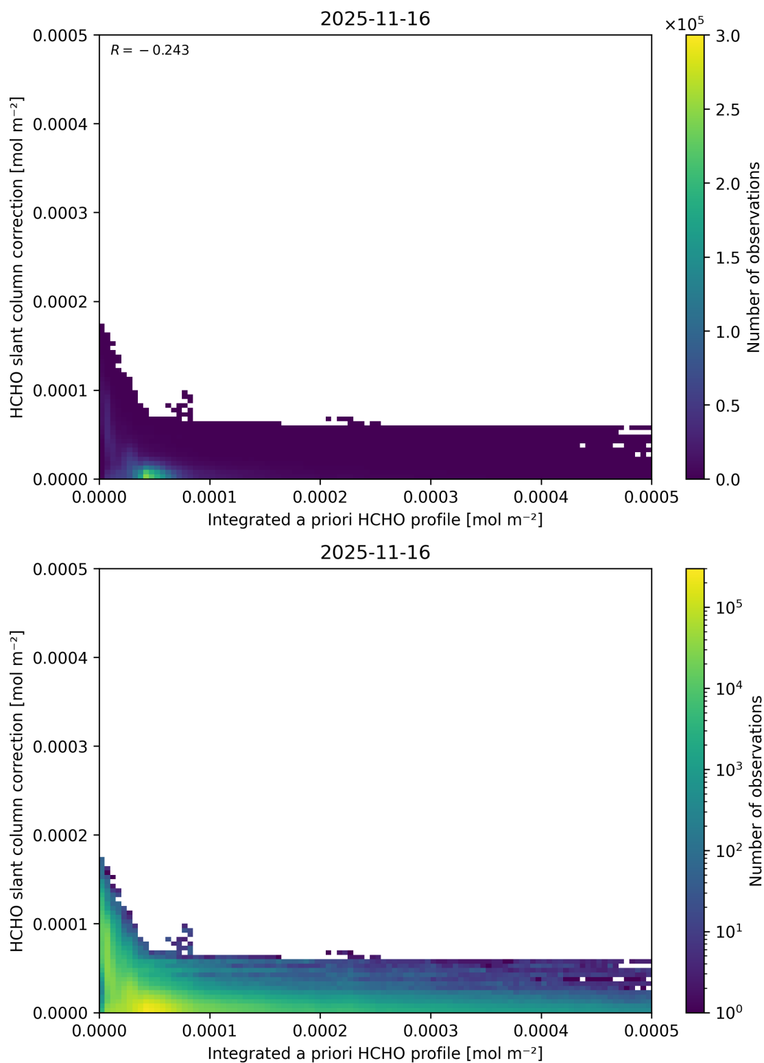
Figure 169: Scatter density plot of “Integrated a priori HCHO profile” against “HCHO slant column correction” for 2025-11-15 to 2025-11-17.
