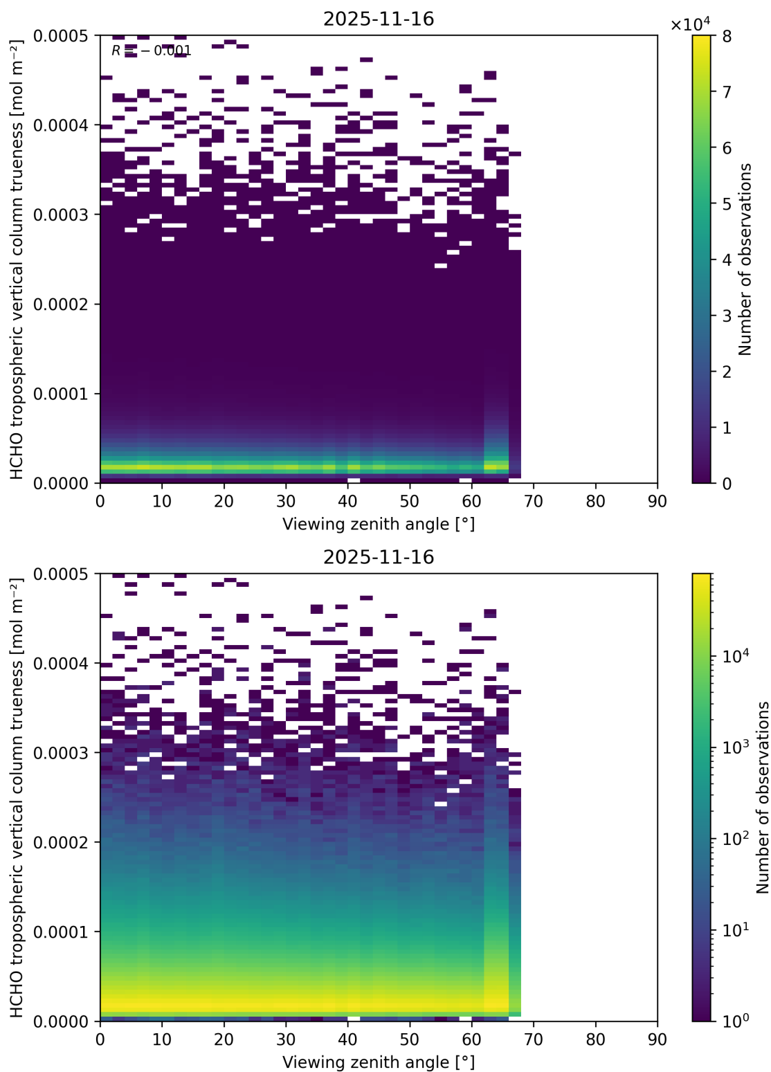
Figure 215: Scatter density plot of “Viewing zenith angle” against “HCHO tropospheric vertical column trueness” for 2025-11-15 to 2025-11-17.
