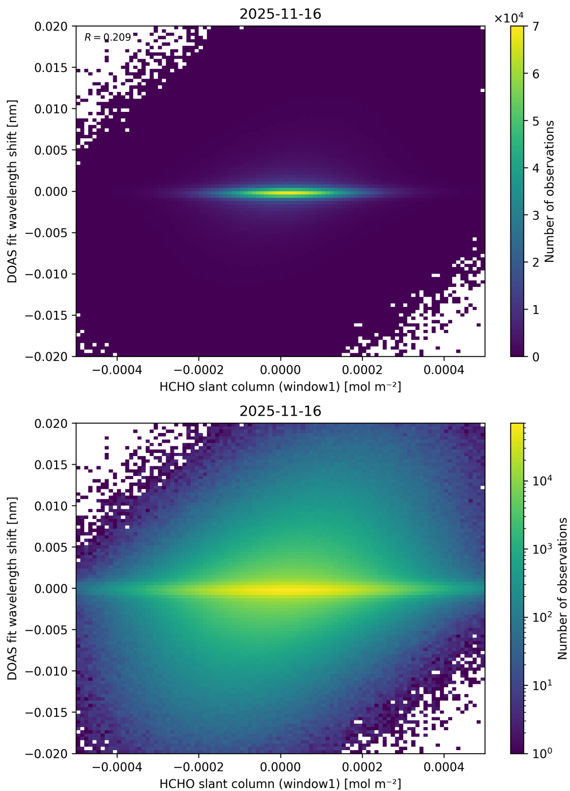
Figure 89: Scatter density plot of “HCHO slant column (window1)” against “DOAS fit wavelength shift” for 2025-11-15 to 2025-11-17.
