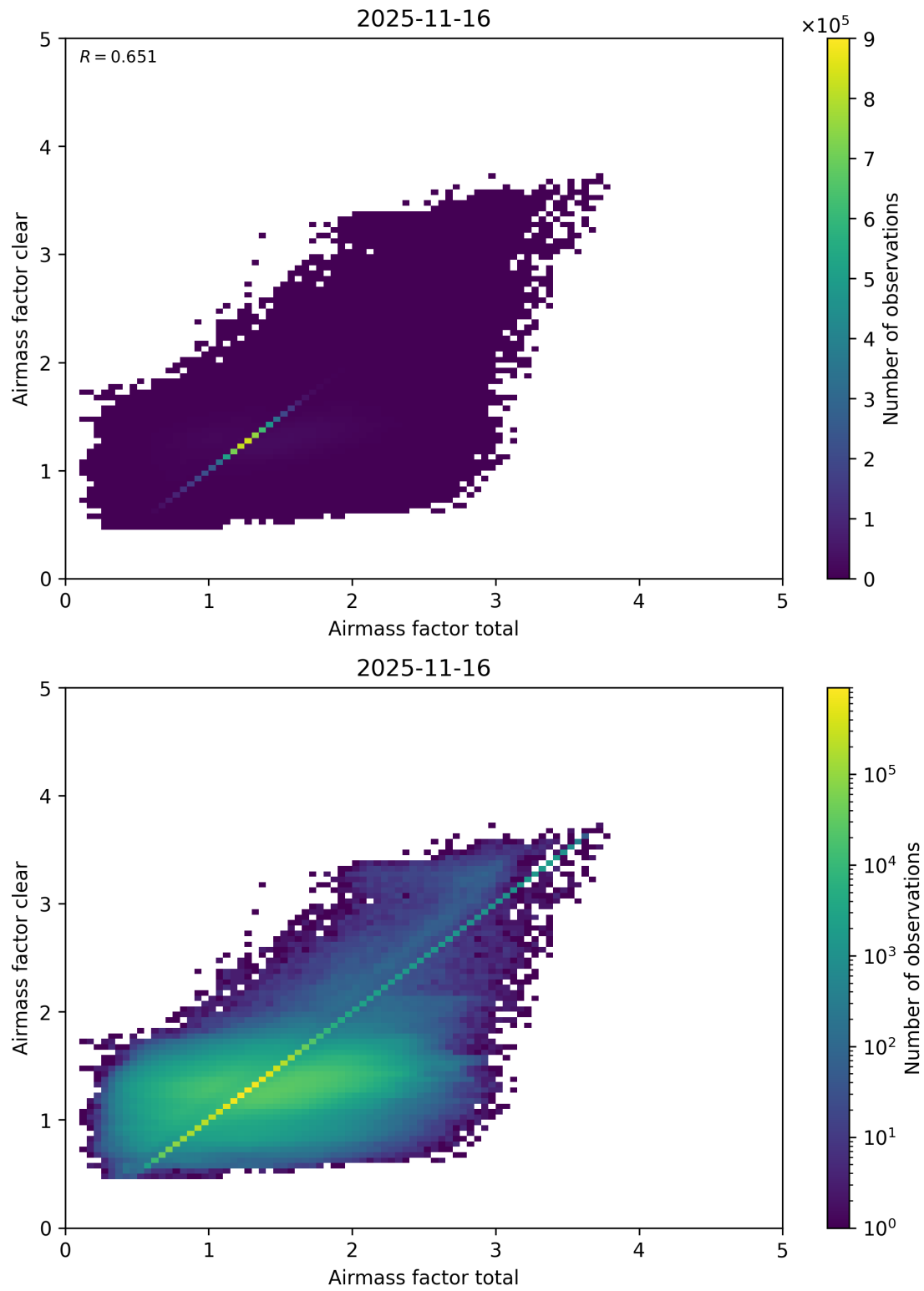
Figure 112: Scatter density plot of “Airmass factor total” against “Airmass factor clear” for 2025-11-15 to 2025-11-17.
