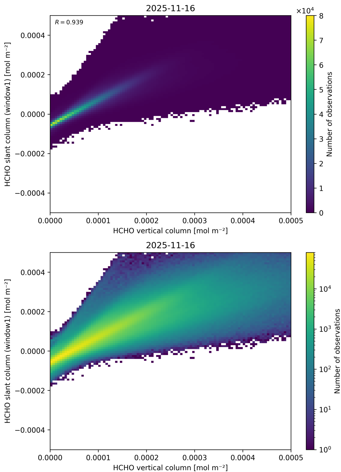
Figure 144: Scatter density plot of “HCHO vertical column” against “HCHO slant column (window1)” for 2025-11-15 to 2025-11-17.
