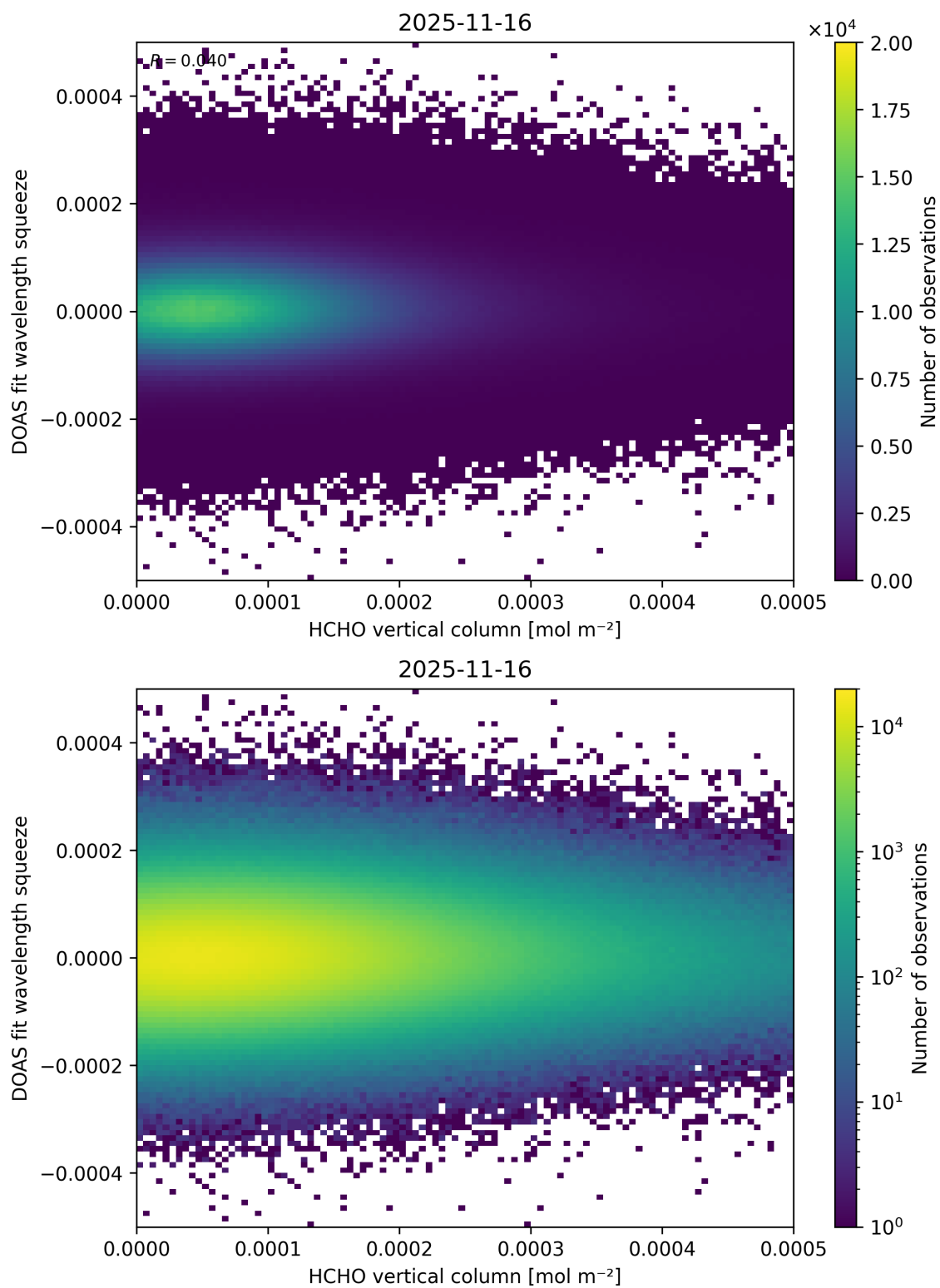
Figure 140: Scatter density plot of “HCHO vertical column” against “DOAS fit wavelength squeeze” for 2025-11-15 to 2025-11-17.
