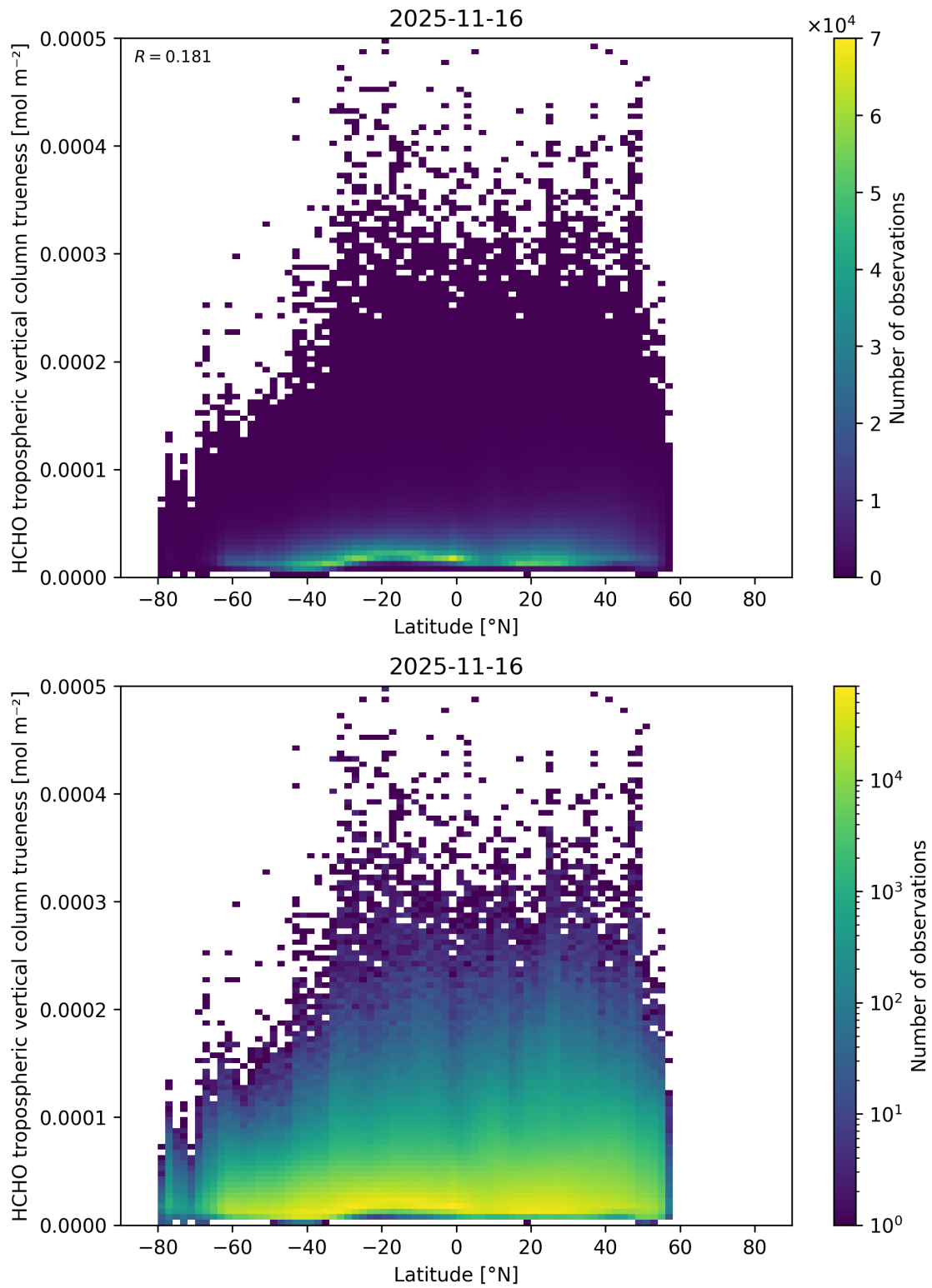
Figure 184: Scatter density plot of “Latitude” against “HCHO tropospheric vertical column trueeness” for 2025-11-15 to 2025-11-17.
