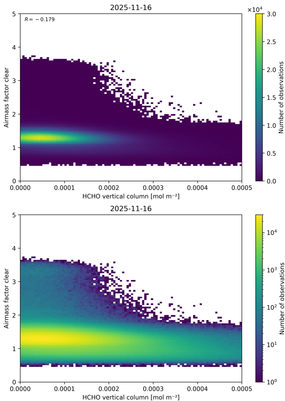
Figure 141: Scatter density plot of “HCHO vertical column” against “Airmass factor clear” for 2025-11-15 to 2025-11-17.
