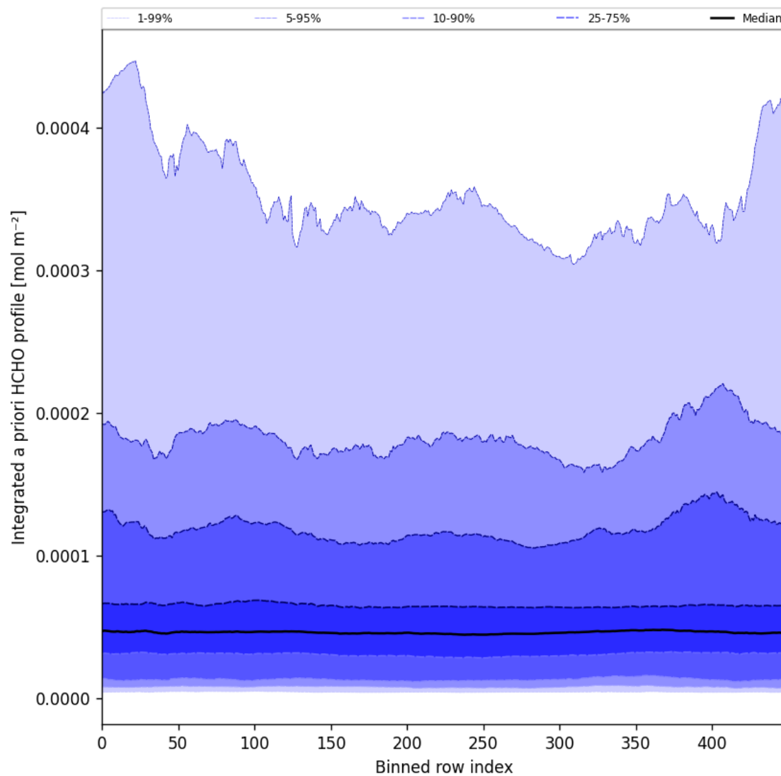
Figure 60: Along track statistics of “Integrated a priori HCHO profile” for 2025-11-15 to 2025-11-17
