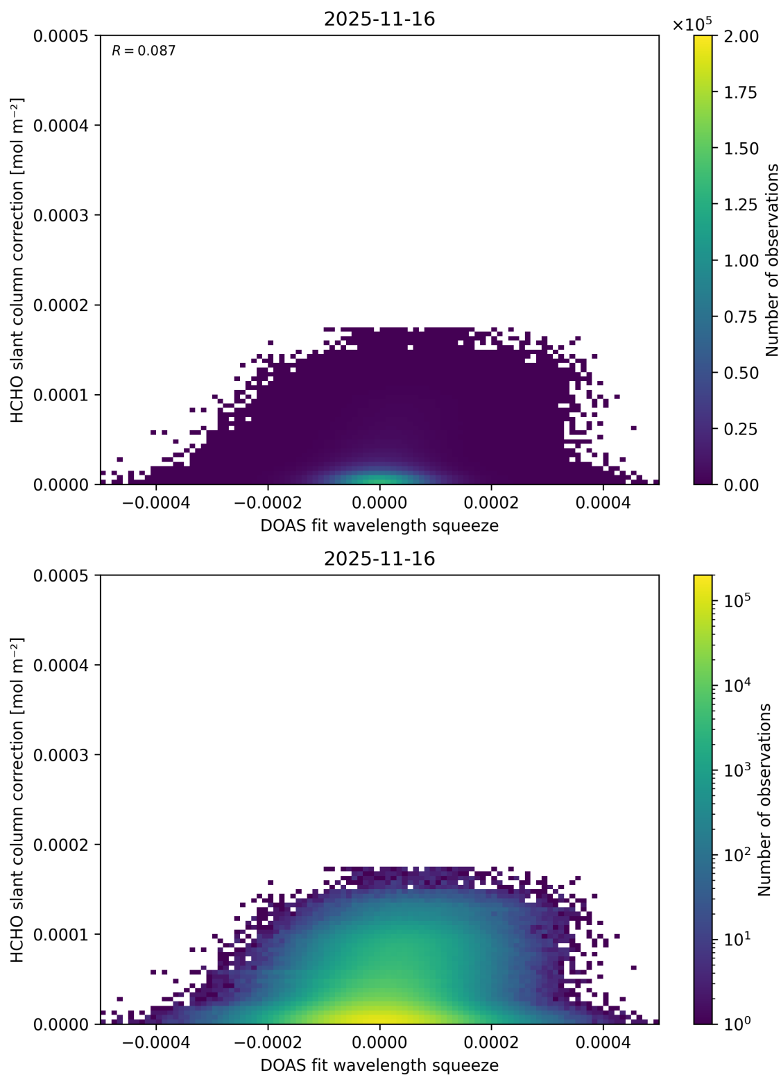
Figure 76: Scatter density plot of “DOAS fit wavelength squeeze” against “HCHO slant column correction” for 2025-11-15 to 2025-11-17.
