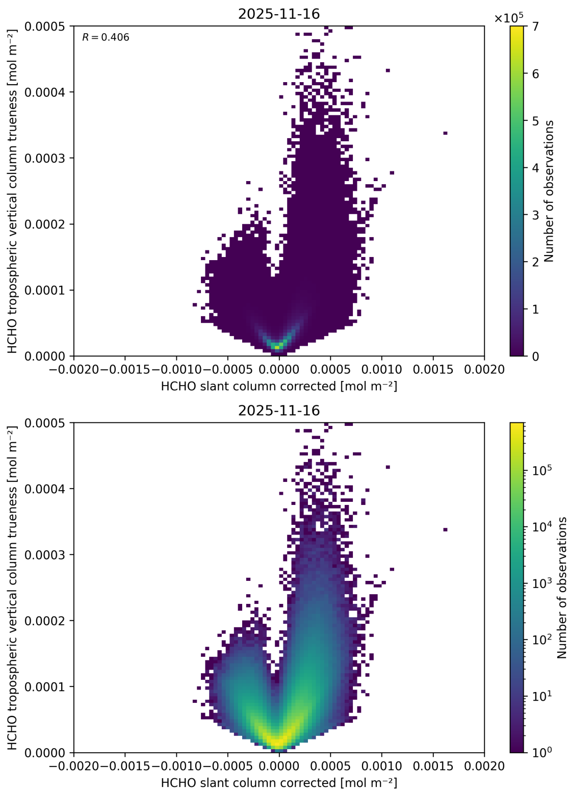
Figure 86: Scatter density plot of “HCHO slant column corrected” against “HCHO tropospheric vertical column trueness” for 2025-11-15 to 2025-11-17.
