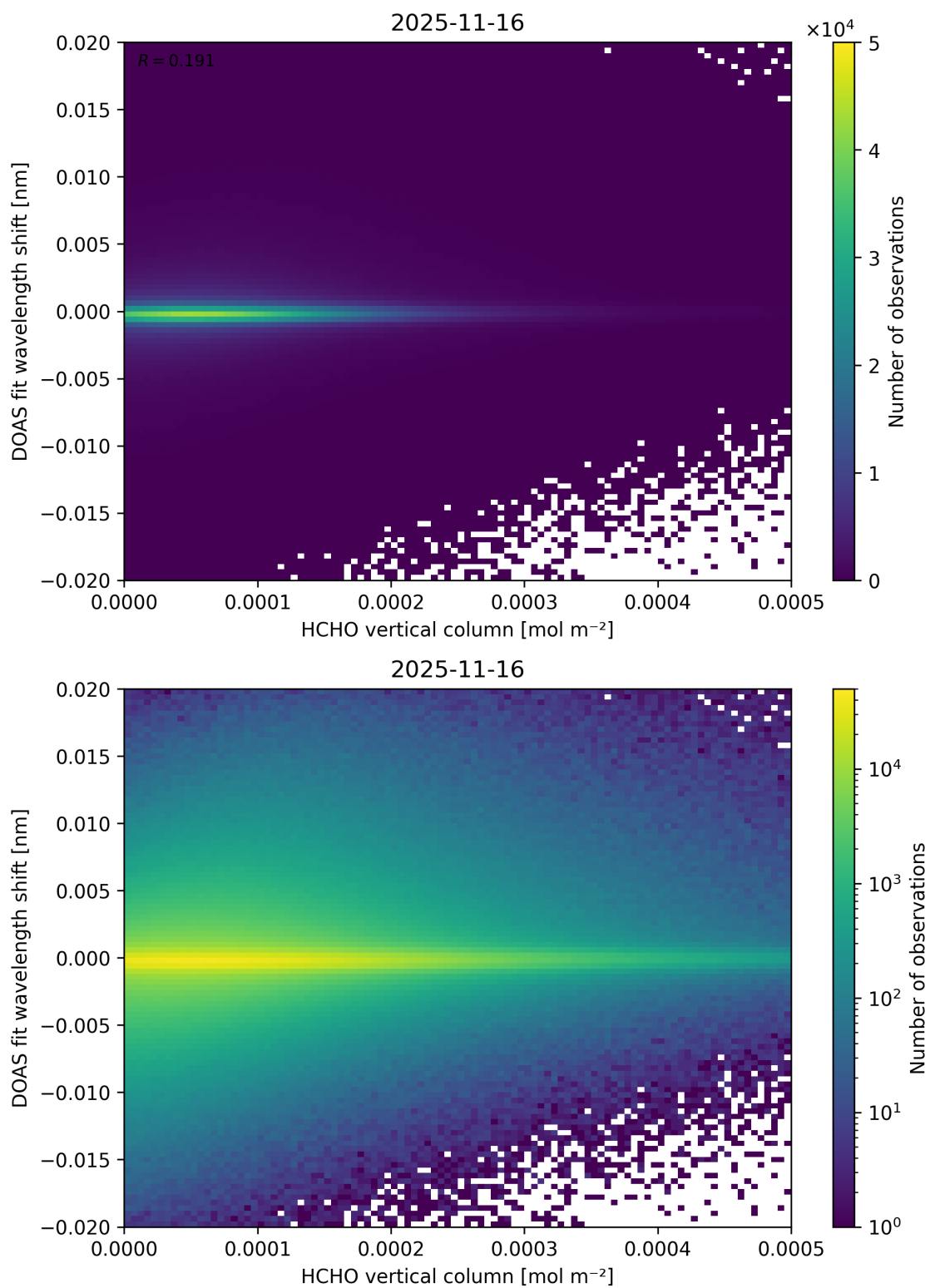
Figure 139: Scatter density plot of “HCHO vertical column” against “DOAS fit wavelength shift” for 2025-11-15 to 2025-11-17.
