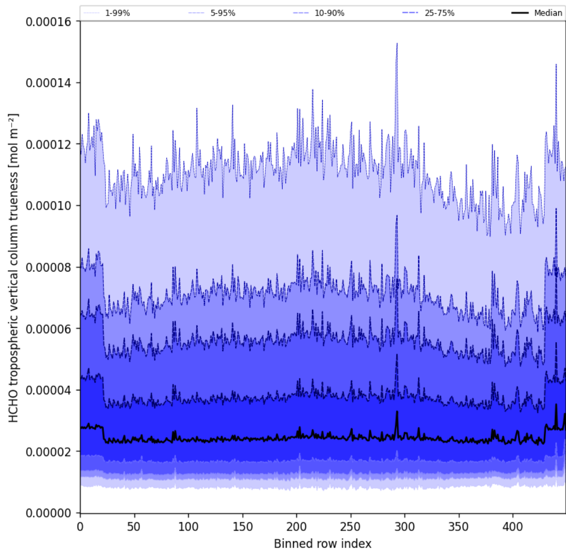
Figure 65: Along track statistics of “HCHO tropospheric vertical column trueness” for 2025-11-15 to 2025-11-17
