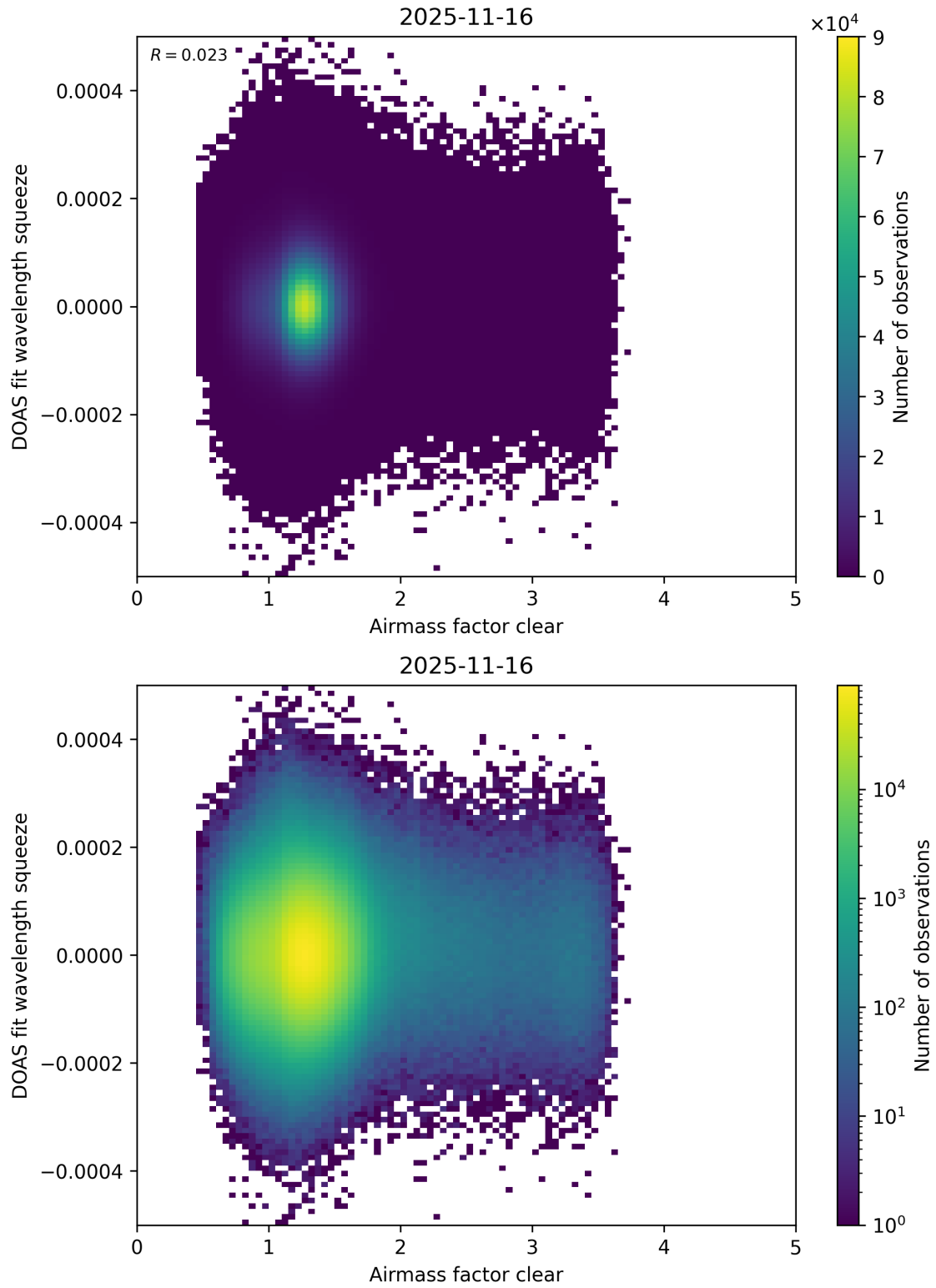
Figure 80: Scatter density plot of “Airmass factor clear” against “DOAS fit wavelength squeeze” for 2025-11-15 to 2025-11-17.
