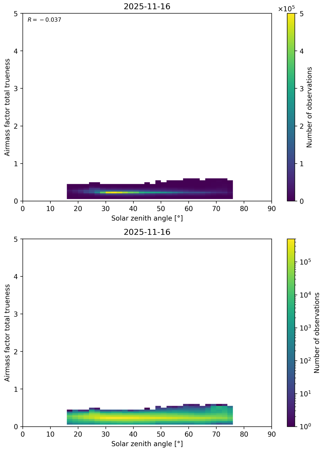
Figure 195: Scatter density plot of “Solar zenith angle” against “Airmass factor total truiness” for 2025-11-15 to 2025-11-17.
