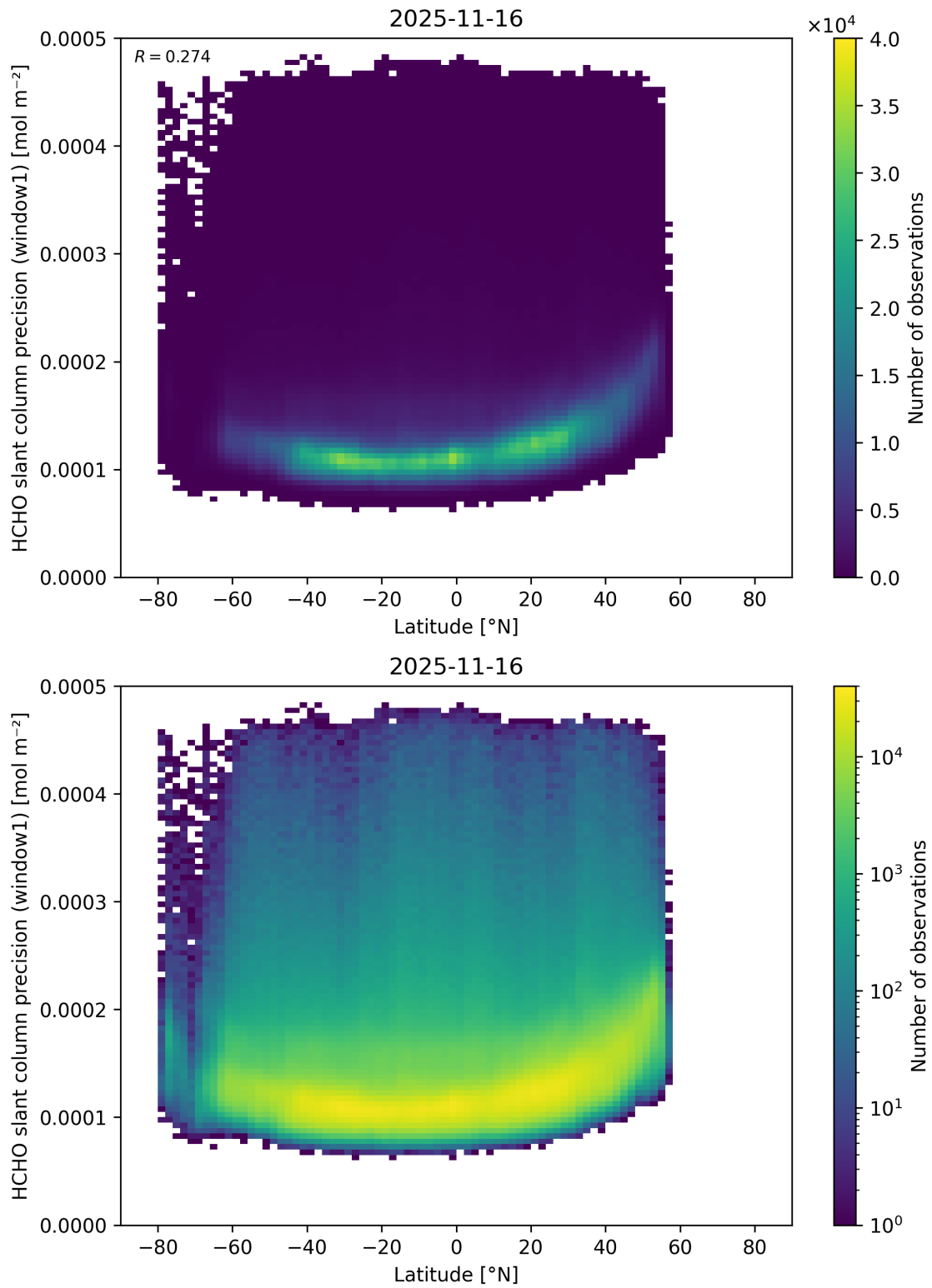
Figure 178: Scatter density plot of “Latitude” against “HCHO slant column precision (window1)” for 2025-11-15 to 2025-11-17.
