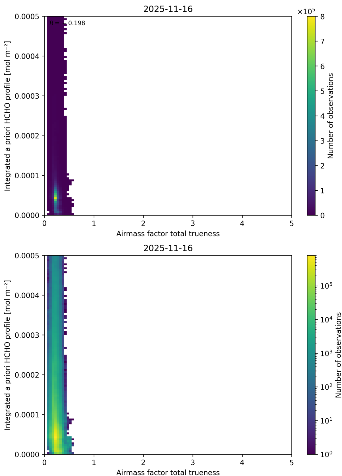
Figure 125: Scatter density plot of “Airmass factor total trueness” against “Integrated a priori HCHO profile” for 2025-11-15 to 2025-11-17.
