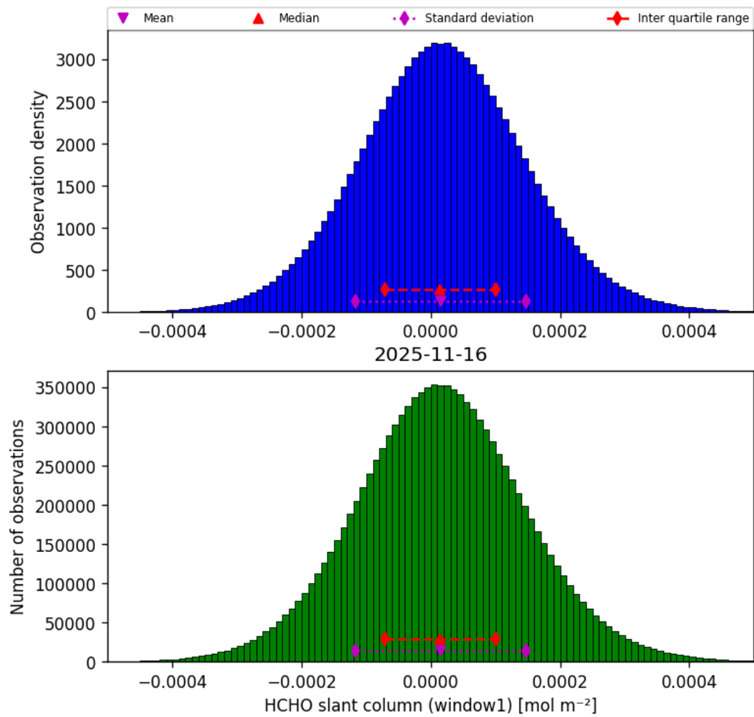
Figure 40: Histogram of “HCHO slant column (window1)” for 2025-11-15 to 2025-11-17
