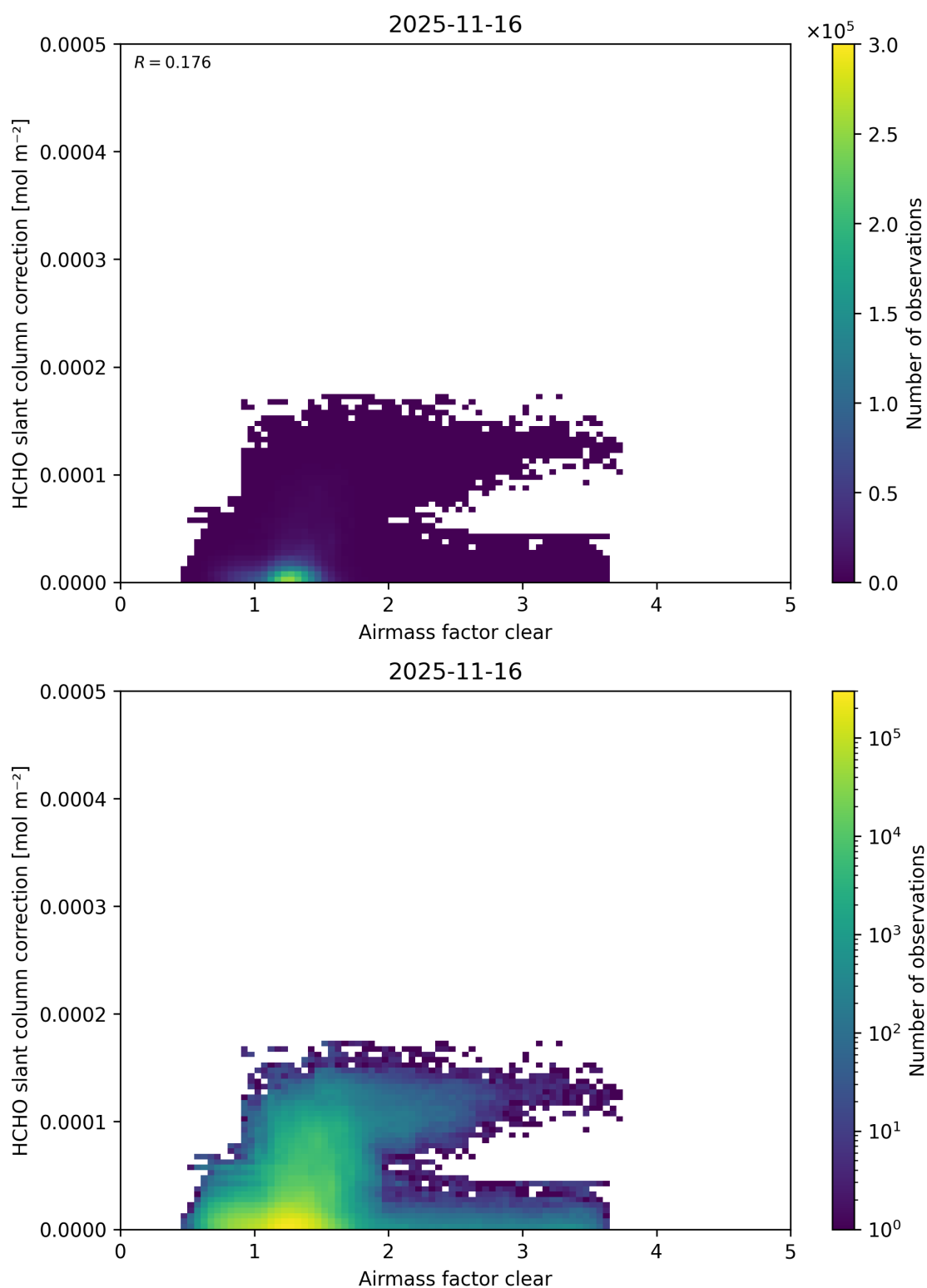
Figure 82: Scatter density plot of “Airmass factor clear” against “HCHO slant column correction” for 2025-11-15 to 2025-11-17.
