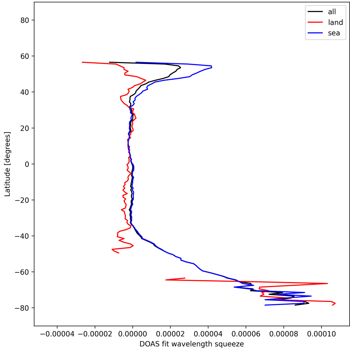
Figure 32: Zonal average of “DOAS fit wavelength squeeze” for 2025-11-15 to 2025-11-17.
