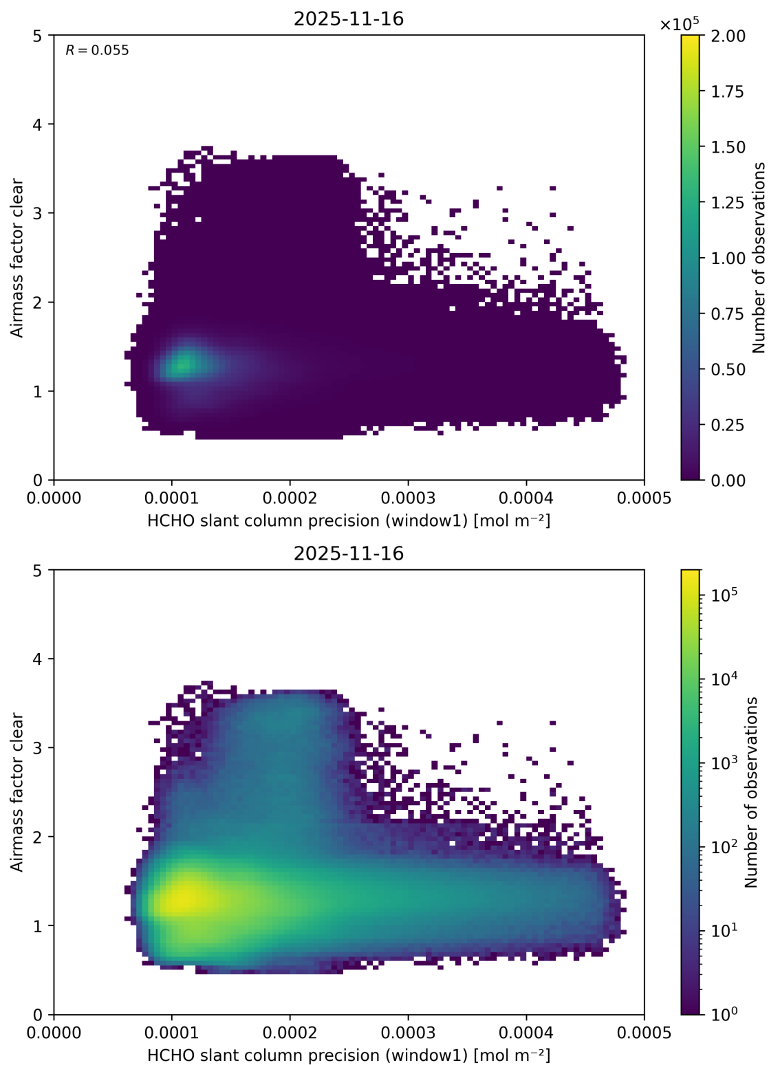
Figure 102: Scatter density plot of “HCHO slant column precision (window1)” against “Airmass factor clear” for 2025-11-15 to 2025-11-17.
