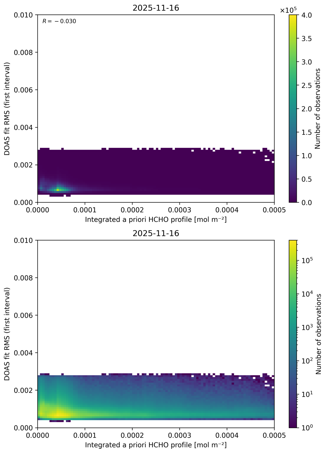
Figure 165: Scatter density plot of “Integrated a priori HCHO profile” against “DOAS fit RMS (first interval)” for 2025-11-15 to 2025-11-17.
