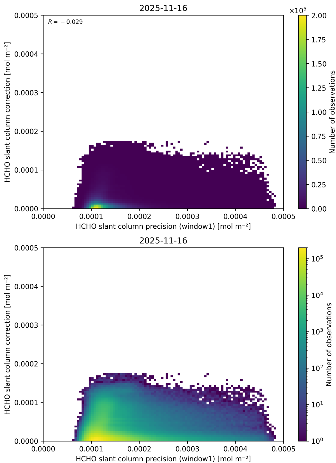
Figure 104: Scatter density plot of “HCHO slant column precision (window1)” against “HCHO slant column correction” for 2025-11-15 to 2025-11-17.
