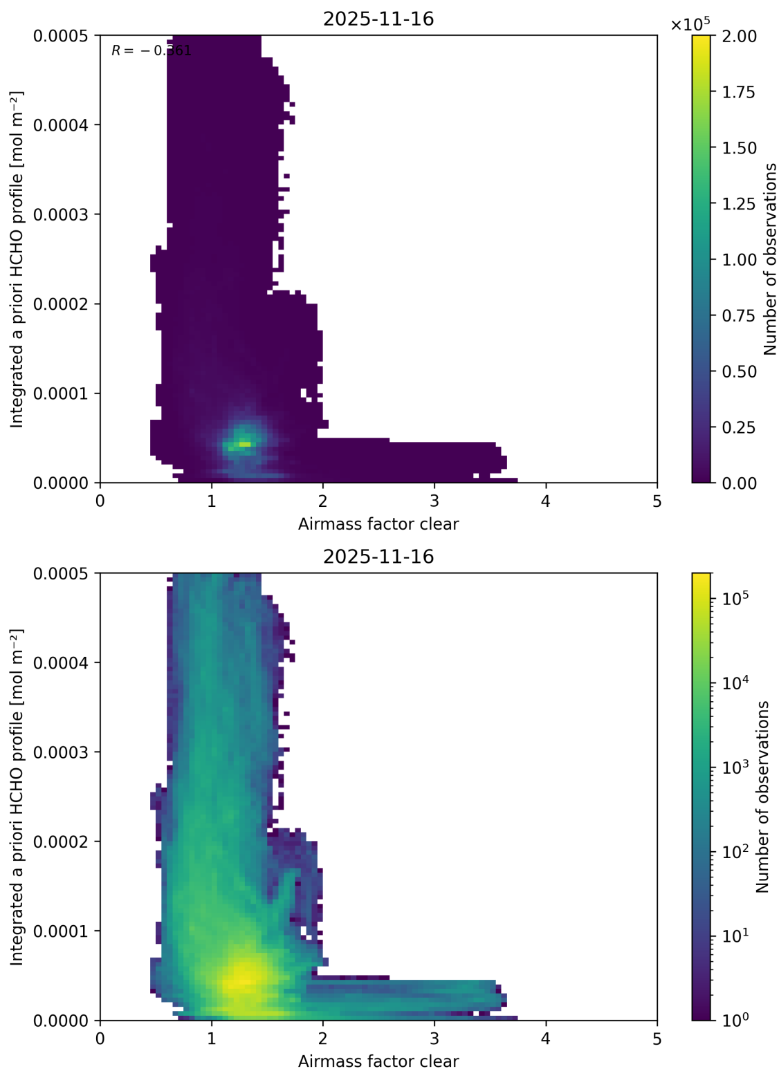
Figure 84: Scatter density plot of “Airmass factor clear” against “Integrated a priori HCHO profile” for 2025-11-15 to 2025-11-17.
