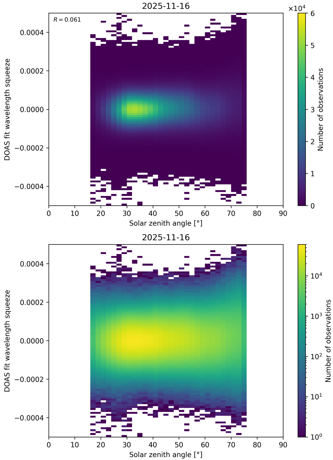
Figure 188: Scatter density plot of “Solar zenith angle” against “DOAS fit wavelength squeeze” for 2025-11-15 to 2025-11-17.
