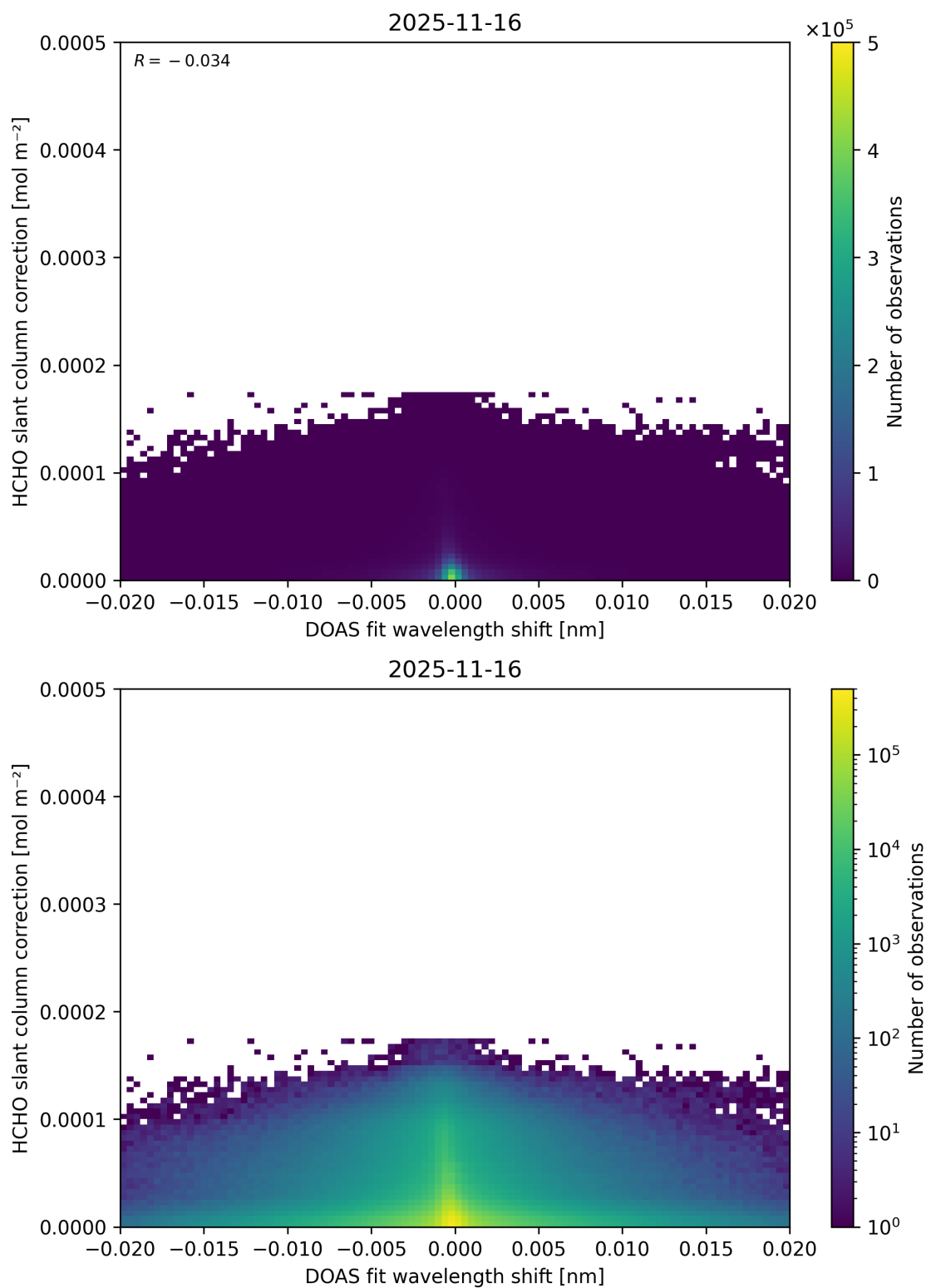
Figure 72: Scatter density plot of “DOAS fit wavelength shift” against “HCHO slant column correction” for 2025-11-15 to 2025-11-17.
