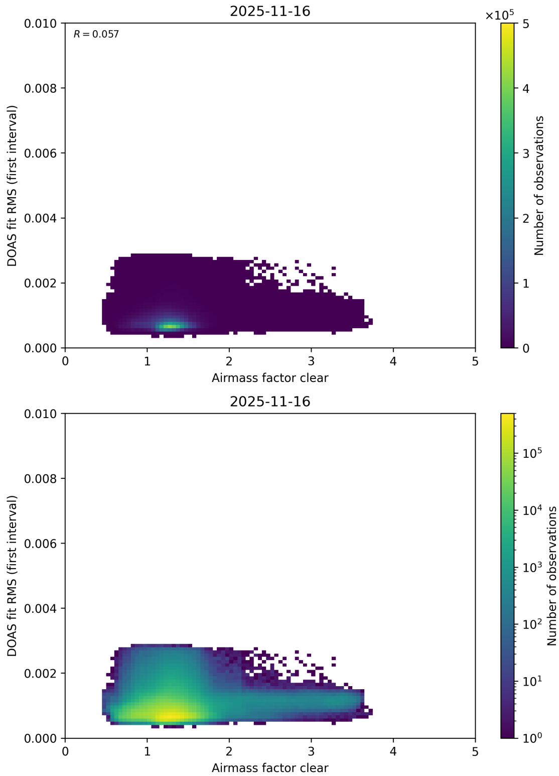
Figure 78: Scatter density plot of “Airmass factor clear” against “DOAS fit RMS (first interval)” for 2025-11-15 to 2025-11-17.
