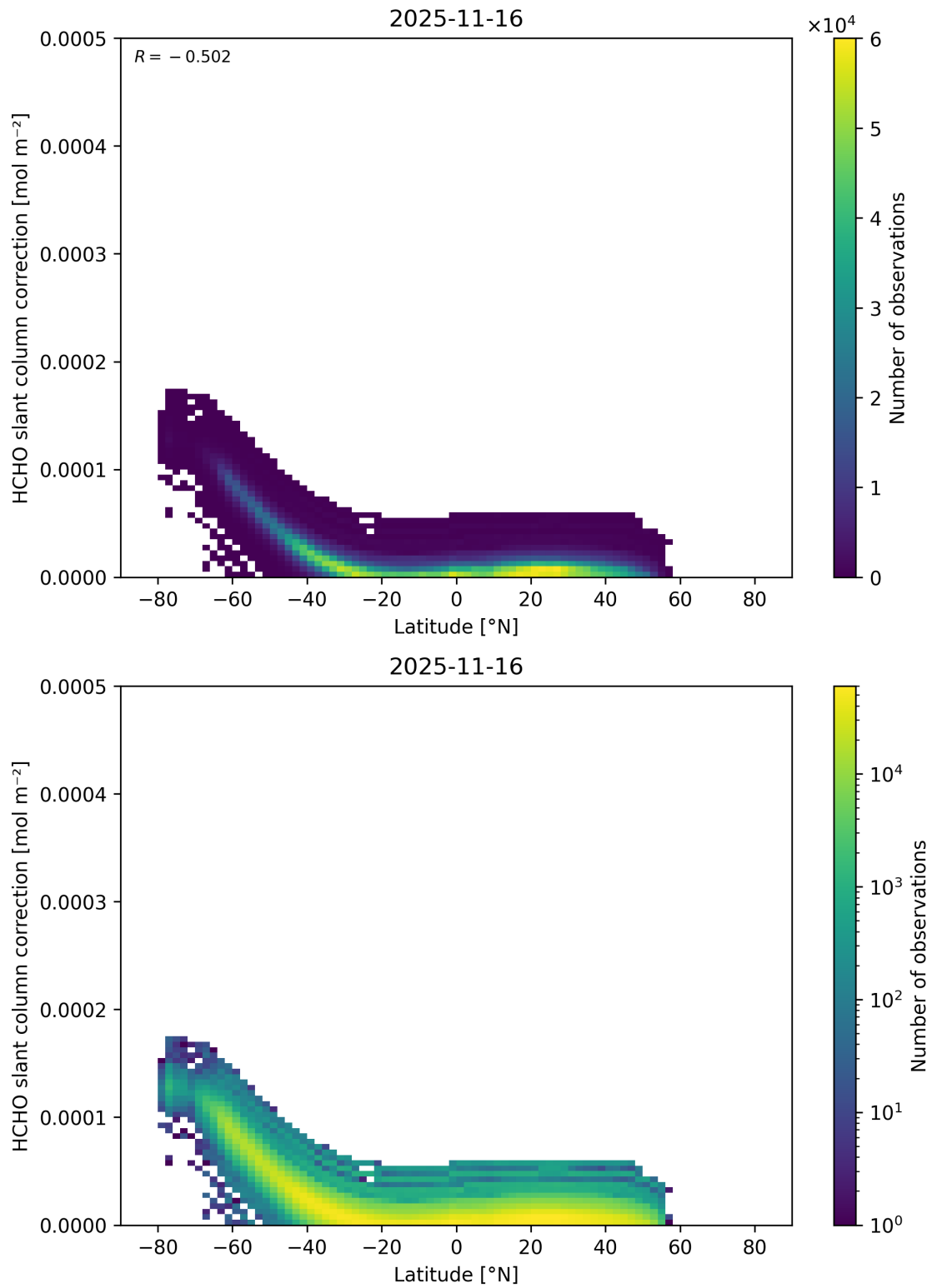
Figure 176: Scatter density plot of “Latitude” against “HCHO slant column correction” for 2025-11-15 to 2025-11-17.
