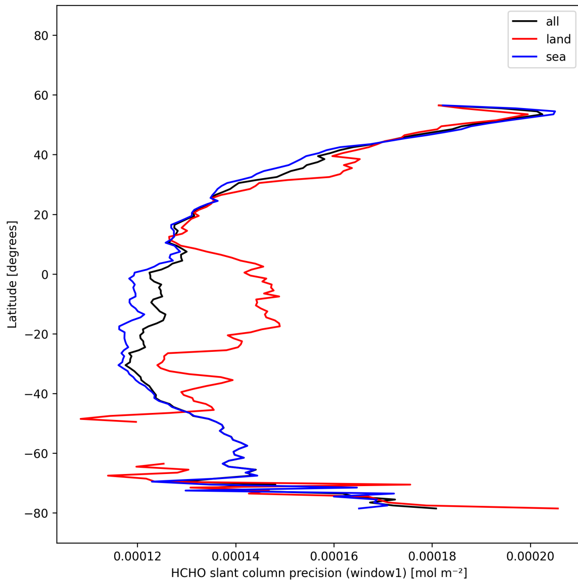
Figure 26: Zonal average of "HCHO slant column precision (window1)" for 2025-11-15 to 2025-11-17.
