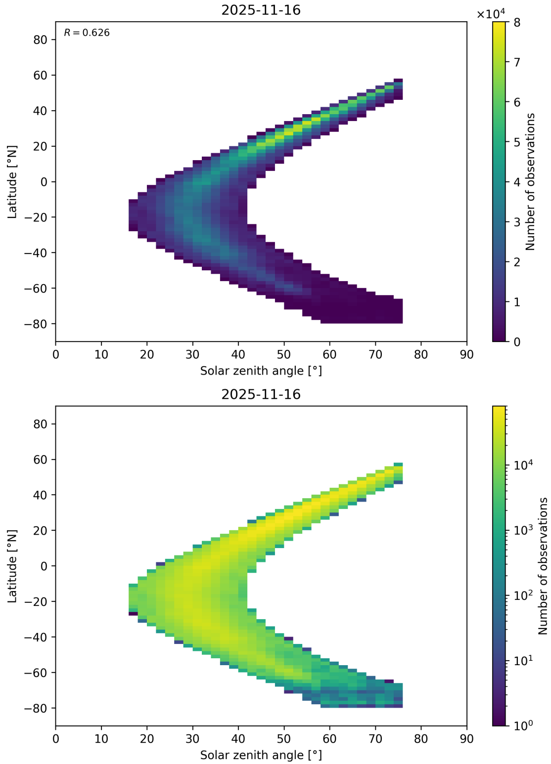
Figure 201: Scatter density plot of “Solar zenith angle” against “Latitude” for 2025-11-15 to 2025-11-17.
