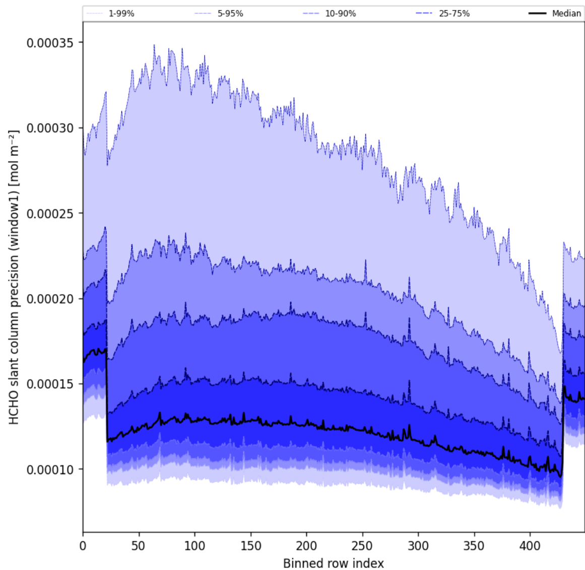
Figure 56: Along track statistics of “HCHO slant column precision (window1)” for 2025-11-15 to 2025-11-17
