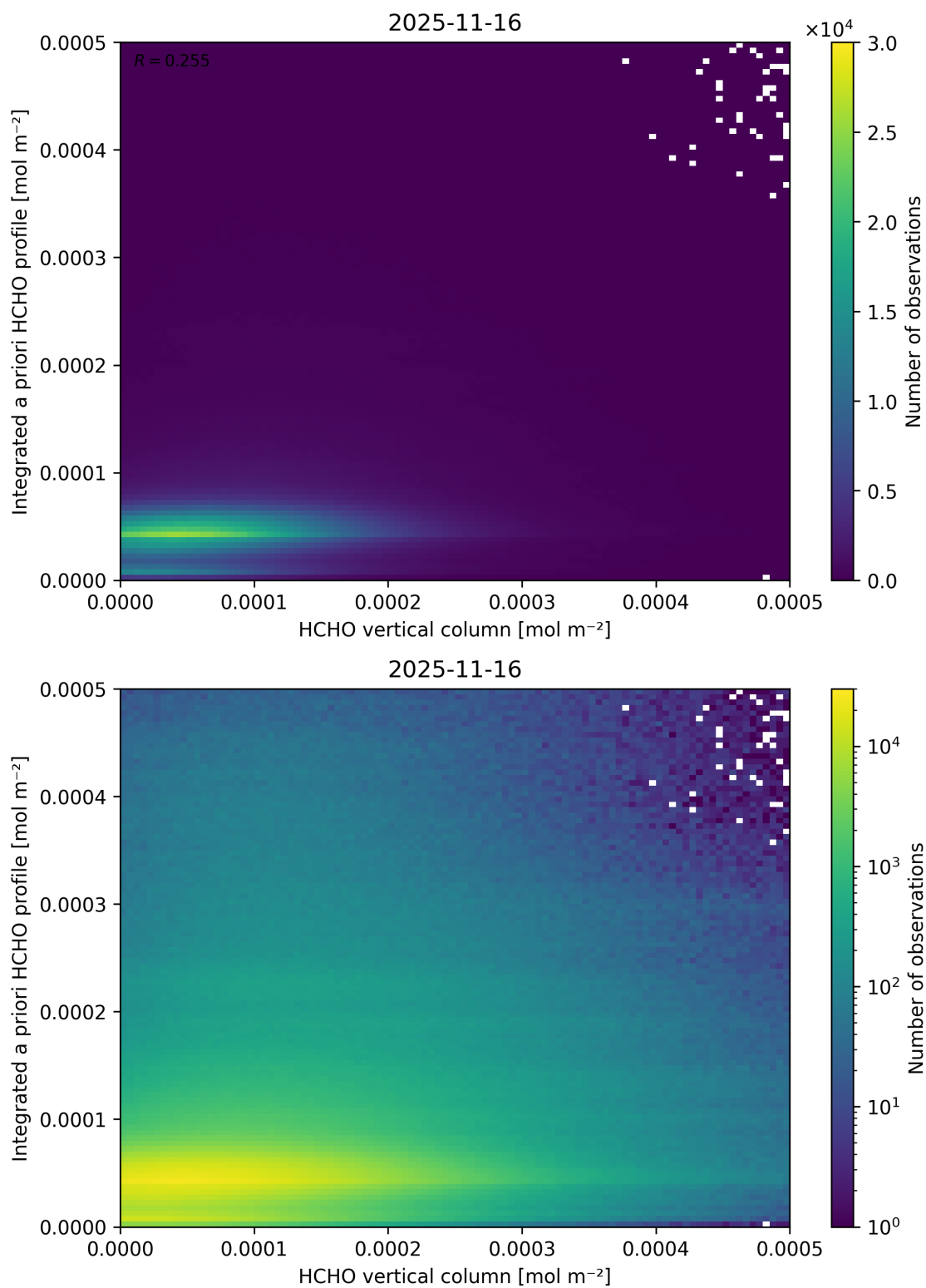
Figure 151: Scatter density plot of “HCHO vertical column” against “Integrated a priori HCHO profile” for 2025-11-15 to 2025-11-17.
