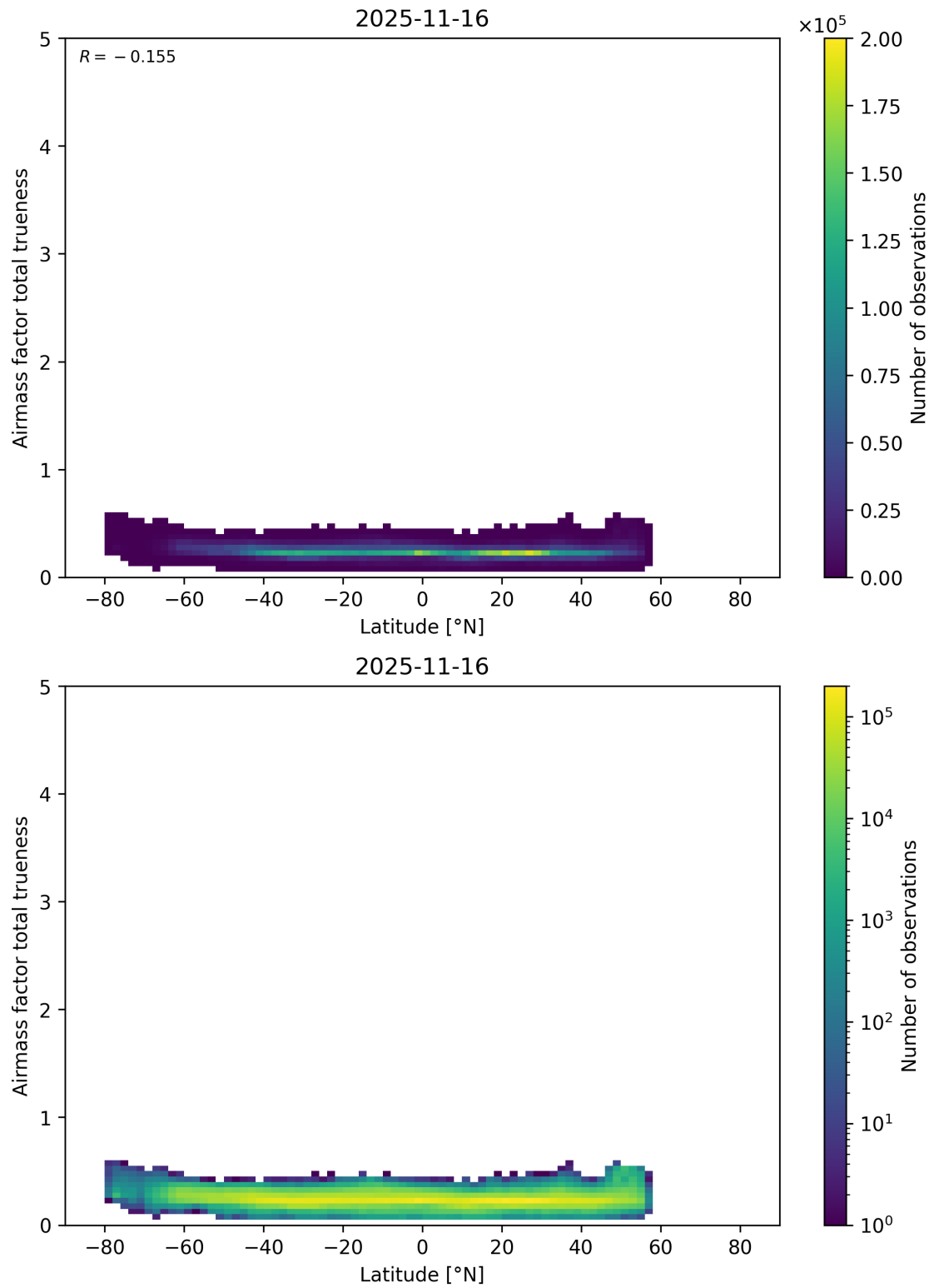
Figure 180: Scatter density plot of “Latitude” against “Airmass factor total trueneess” for 2025-11-15 to 2025-11-17.
