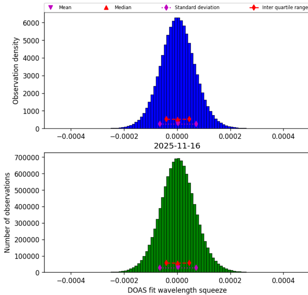
Figure 47: Histogram of “DOAS fit wavelength squeeze” for 2025-11-15 to 2025-11-17
