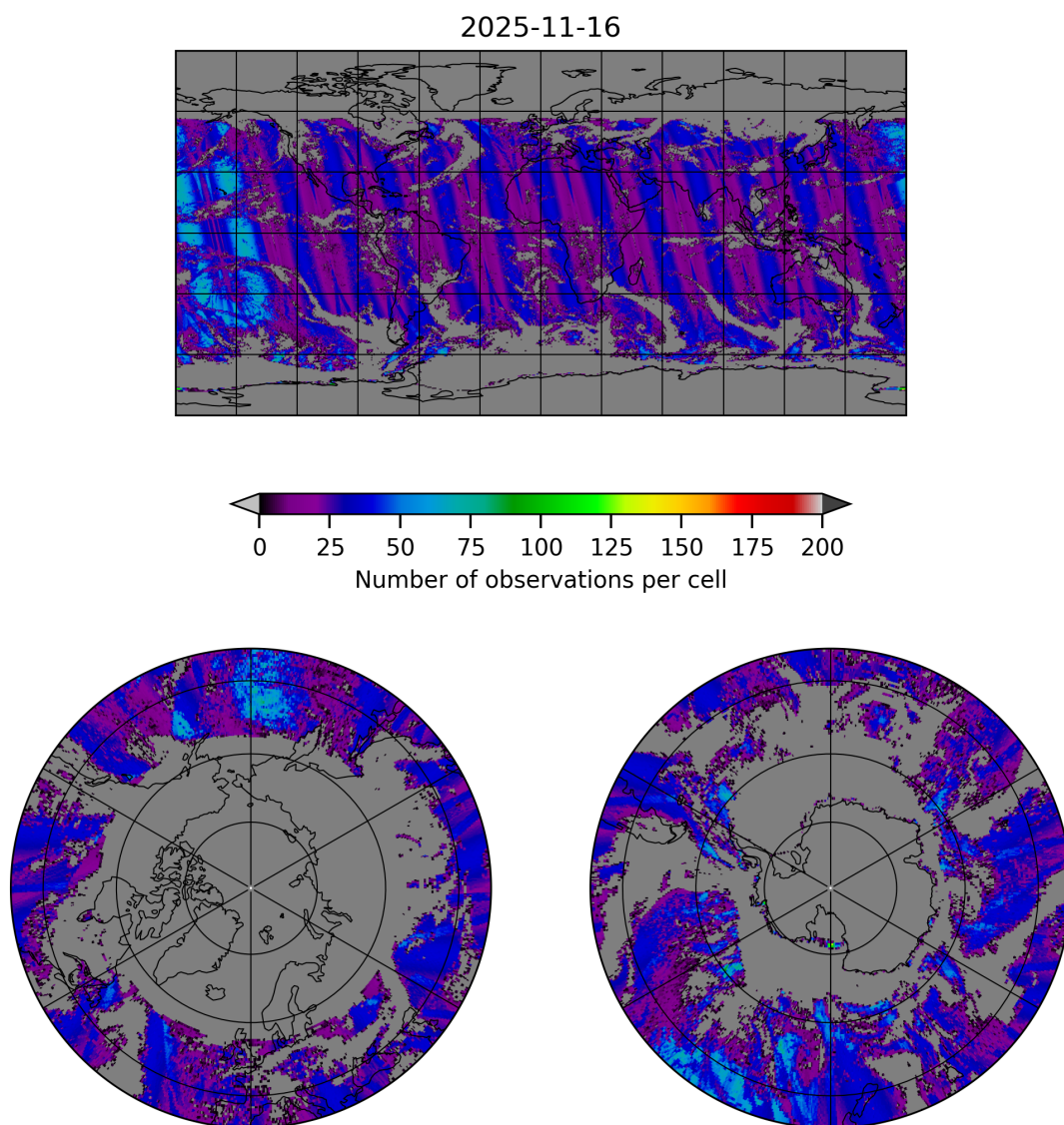
Figure 20: Map of the number of observations for 2025-11-15 to 2025-11-17
