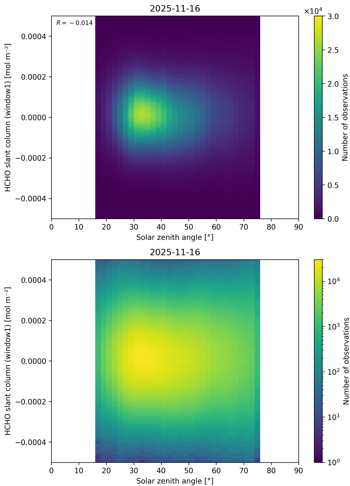
Figure 192: Scatter density plot of “Solar zenith angle” against “HCHO slant column (window1)” for 2025-11-15 to 2025-11-17.
