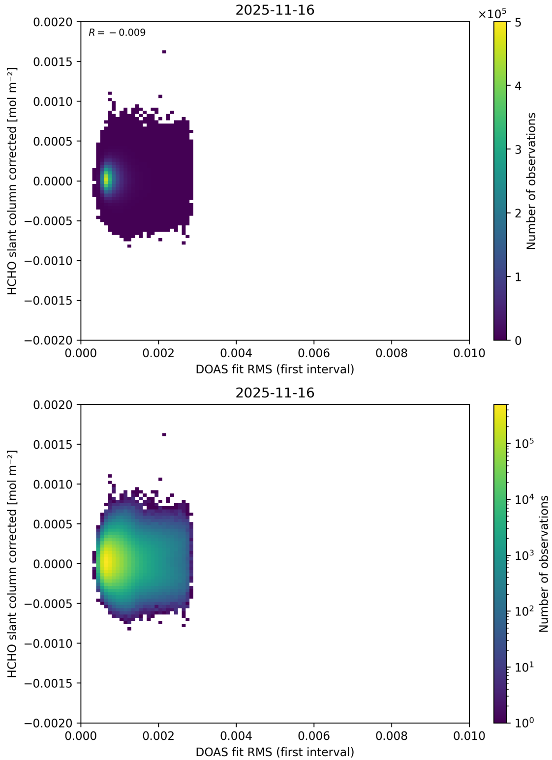
Figure 66: Scatter density plot of “DOAS fit RMS (first interval)” against “HCHO slant column corrected” for 2025-11-15 to 2025-11-17.
