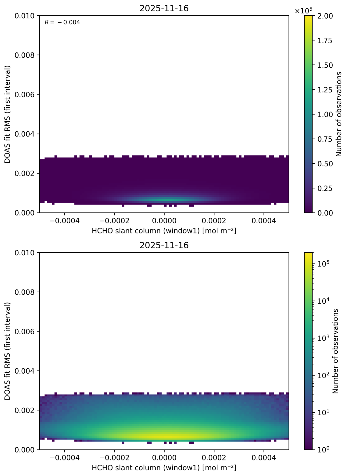
Figure 88: Scatter density plot of “HCHO slant column (window1)” against “DOAS fit RMS (first interval)” for 2025-11-15 to 2025-11-17.
