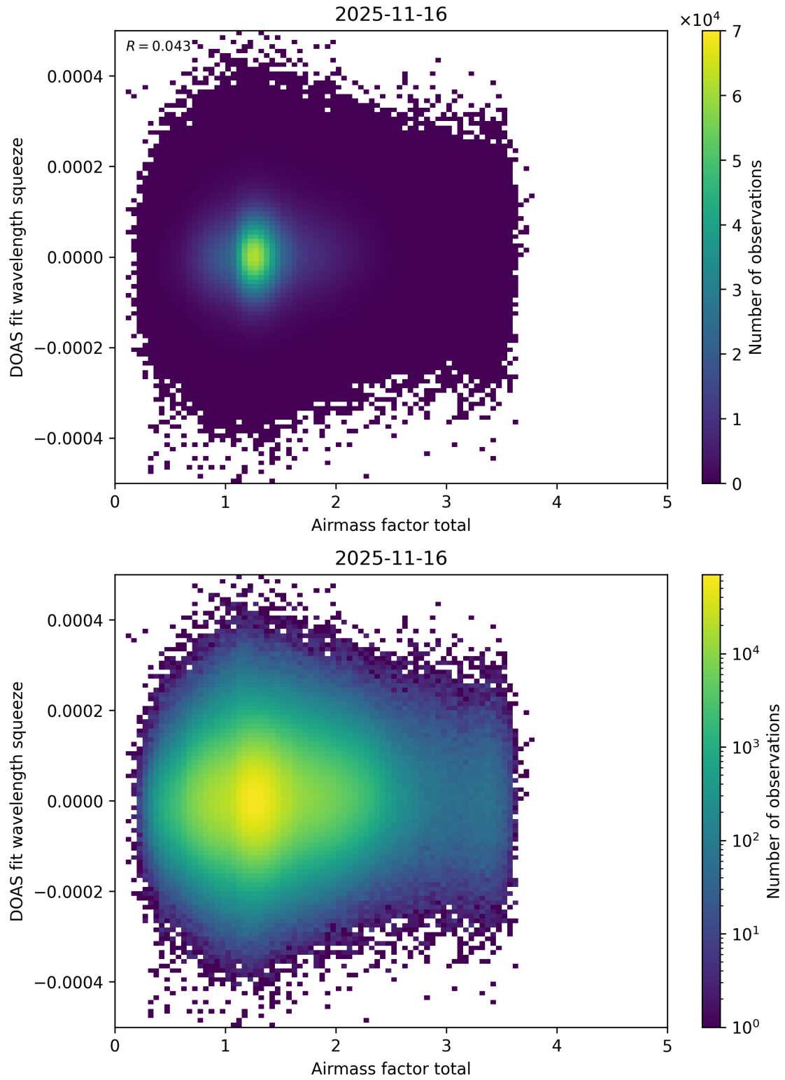
Figure 111: Scatter density plot of “Airmass factor total” against “DOAS fit wavelength squeeze” for 2025-11-15 to 2025-11-17.
