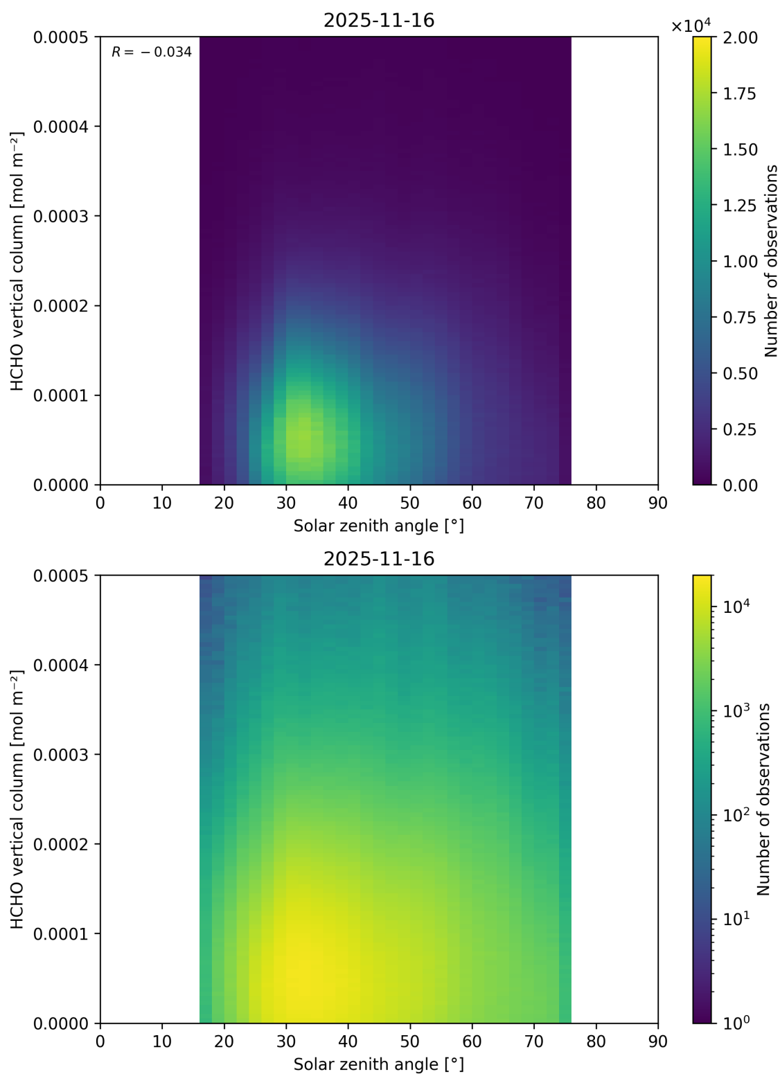
Figure 196: Scatter density plot of “Solar zenith angle” against “HCHO vertical column” for 2025-11-15 to 2025-11-17.
