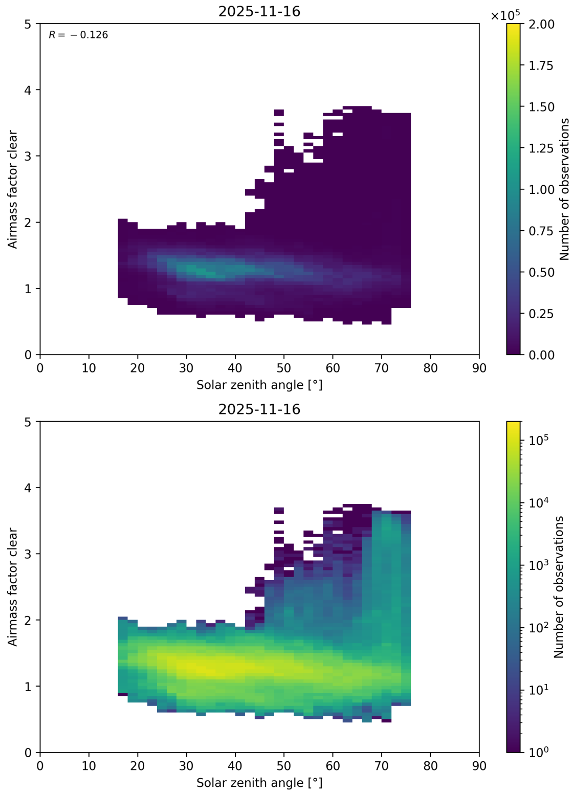
Figure 189: Scatter density plot of “Solar zenith angle” against “Airmass factor clear” for 2025-11-15 to 2025-11-17.
