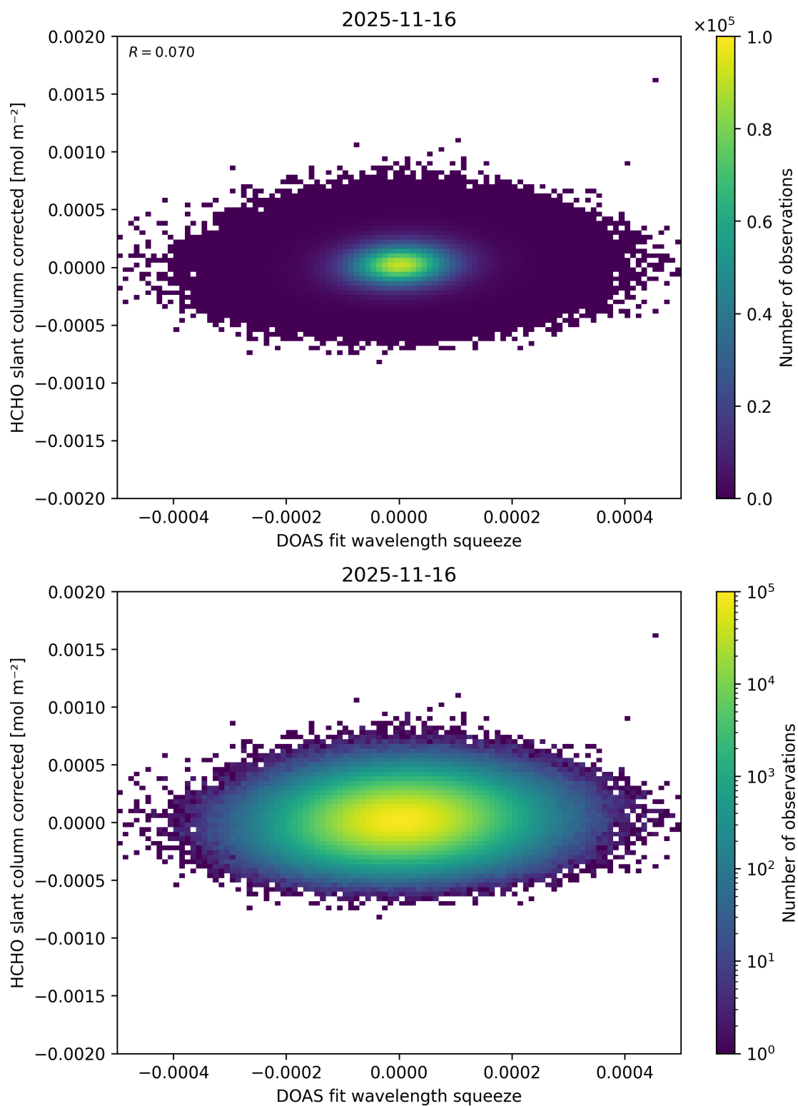
Figure 75: Scatter density plot of “DOAS fit wavelength squeeze” against “HCHO slant column corrected” for 2025-11-15 to 2025-11-17.
