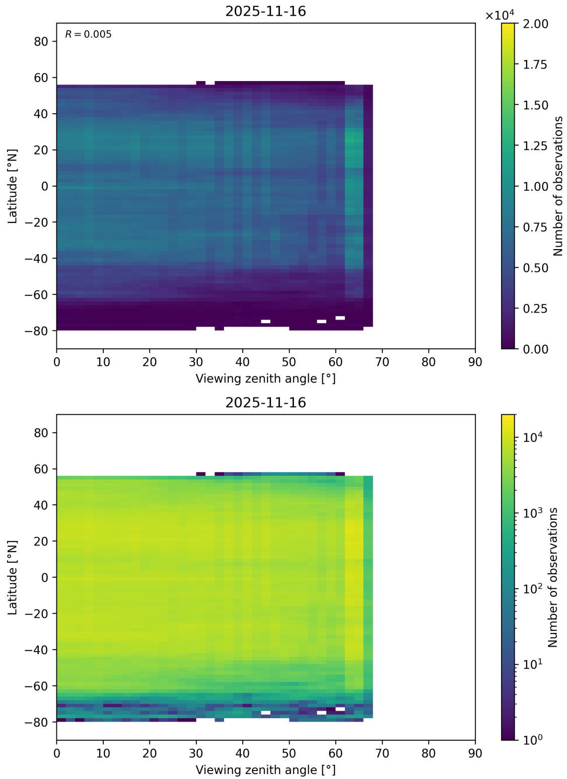
Figure 217: Scatter density plot of “Viewing zenith angle” against “Latitude” for 2025-11-15 to 2025-11-17.
