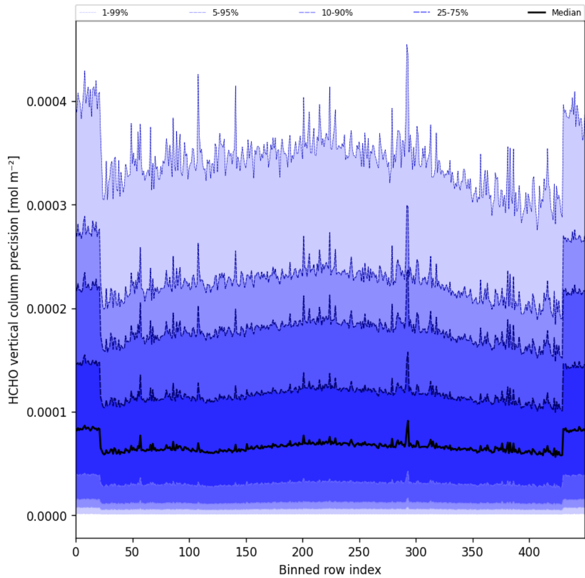
Figure 53: Along track statistics of “HCHO vertical column precision” for 2025-11-15 to 2025-11-17
