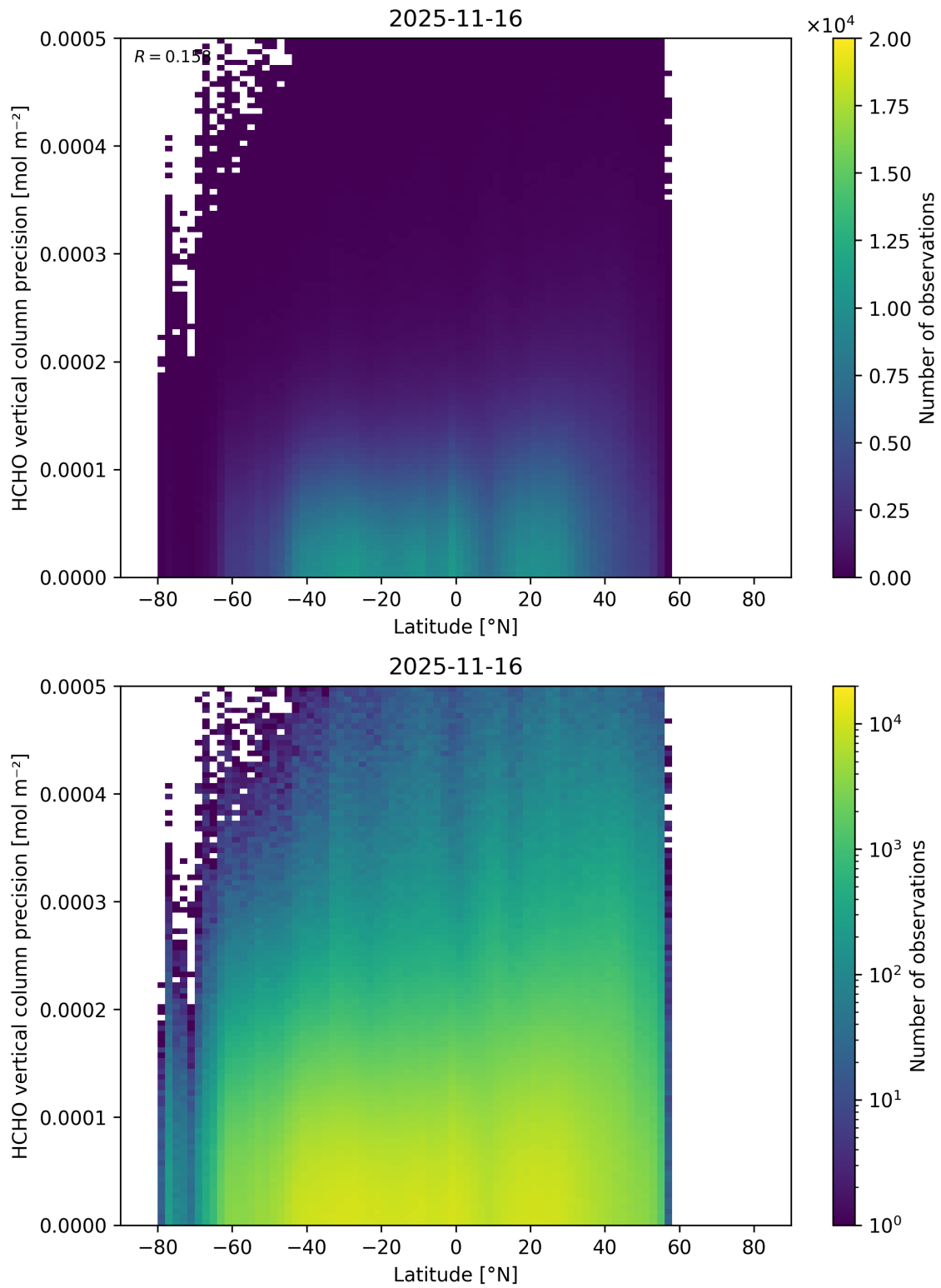
Figure 183: Scatter density plot of “Latitude” against “HCHO vertical column precision” for 2025-11-15 to 2025-11-17.
