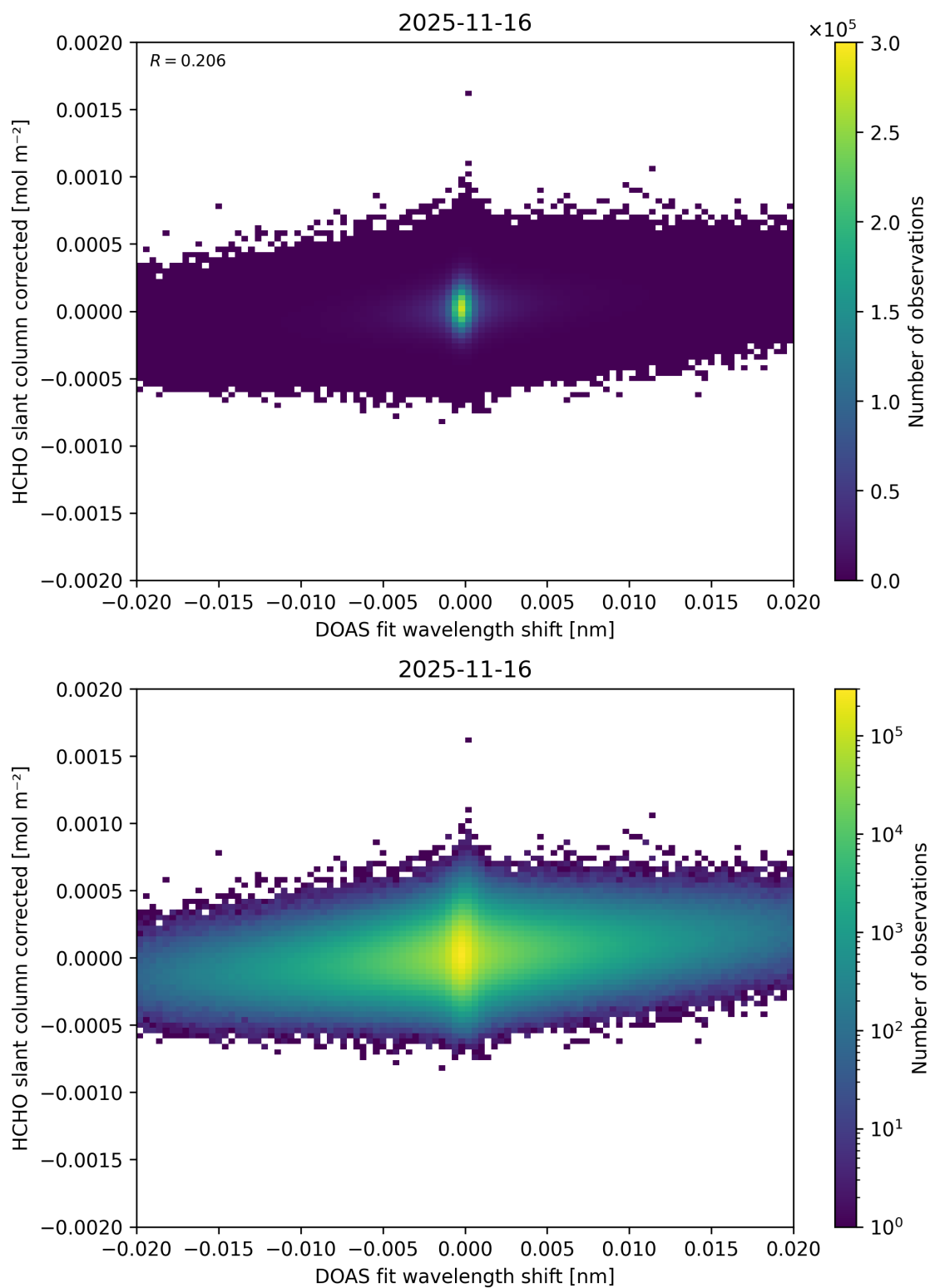
Figure 71: Scatter density plot of “DOAS fit wavelength shift” against “HCHO slant column corrected” for 2025-11-15 to 2025-11-17.
