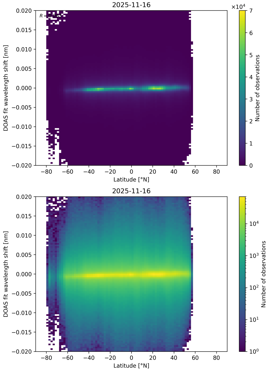
Figure 172: Scatter density plot of “Latitude” against “DOAS fit wavelength shift” for 2025-11-15 to 2025-11-17.
