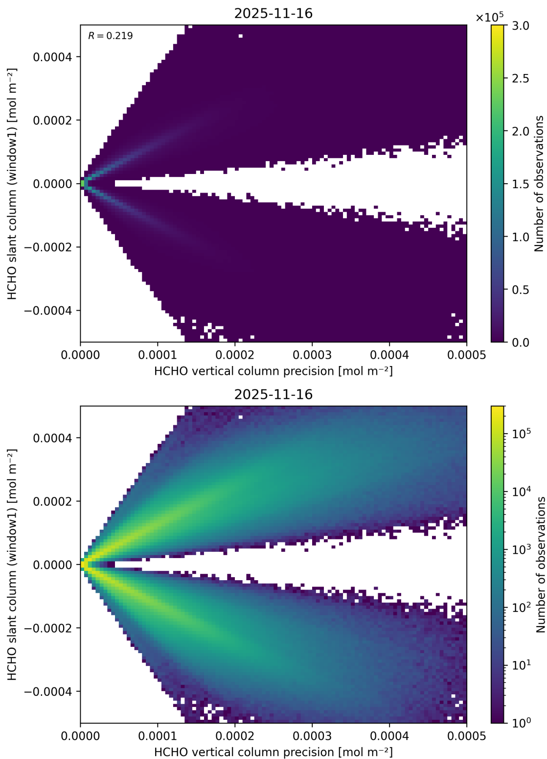
Figure 158: Scatter density plot of “HCHO vertical column precision” against “HCHO slant column (window1)” for 2025-11-15 to 2025-11-17.
