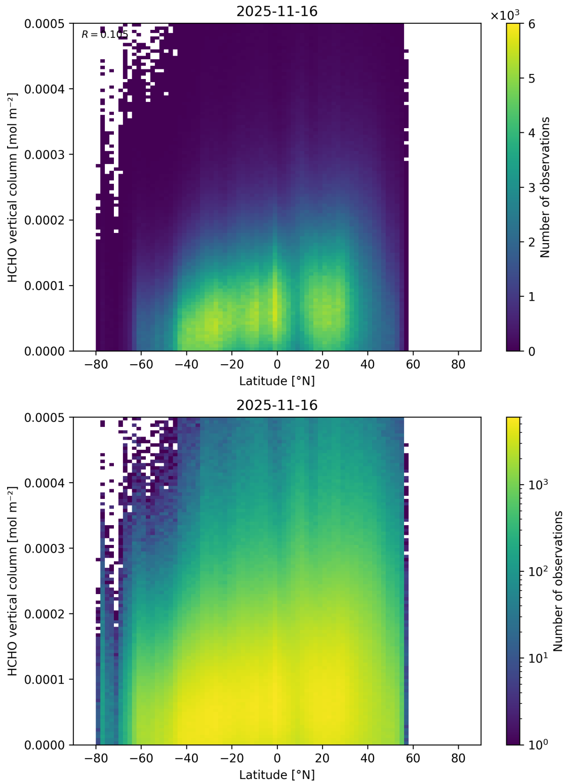
Figure 181: Scatter density plot of “Latitude” against “HCHO vertical column” for 2025-11-15 to 2025-11-17.
