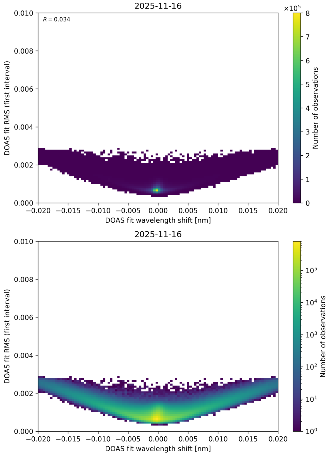
Figure 69: Scatter density plot of “DOAS fit wavelength shift” against “DOAS fit RMS (first interval)” for 2025-11-15 to 2025-11-17.
