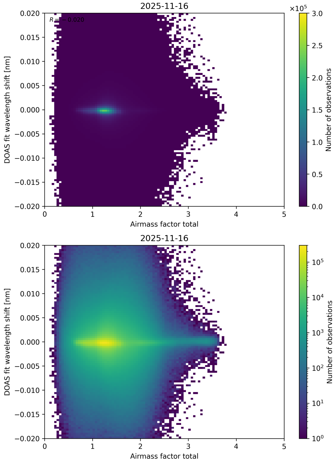
Figure 110: Scatter density plot of “Airmass factor total” against “DOAS fit wavelength shift” for 2025-11-15 to 2025-11-17.
