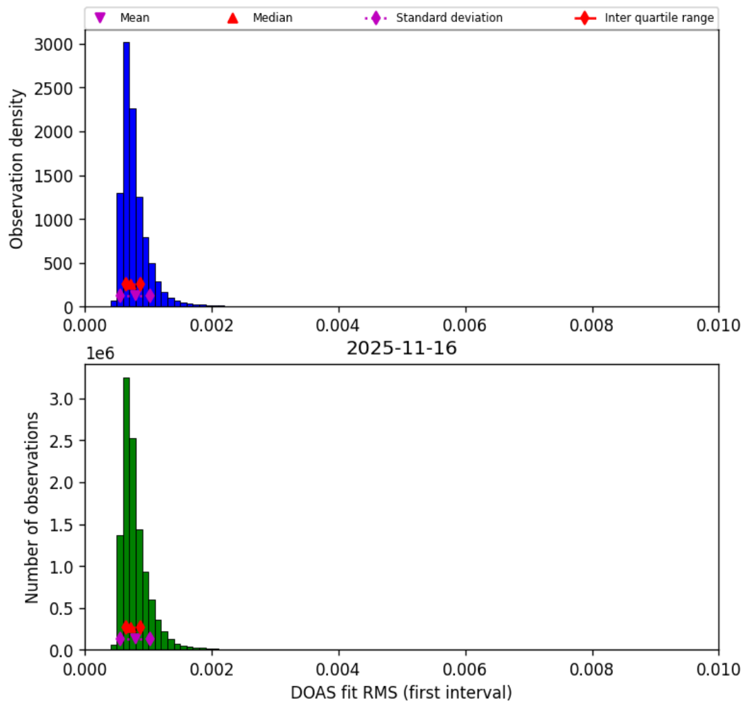
Figure 48: Histogram of “DOAS fit RMS (first interval)” for 2025-11-15 to 2025-11-17
