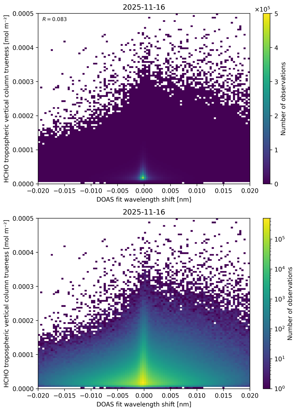
Figure 73: Scatter density plot of “DOAS fit wavelength shift” against “HCHO tropospheric vertical column trueness” for 2025-11-15 to 2025-11-17.
