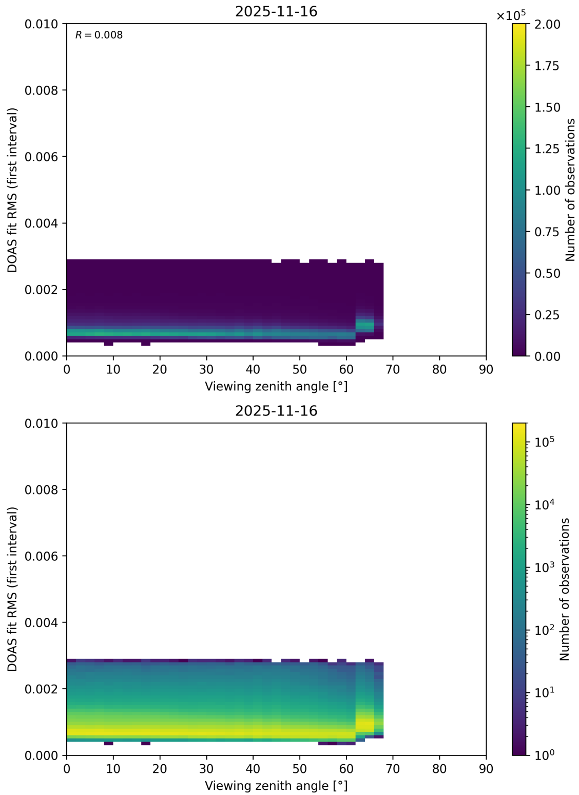
Figure 202: Scatter density plot of “Viewing zenith angle” against “DOAS fit RMS (first interval)” for 2025-11-15 to 2025-11-17.
