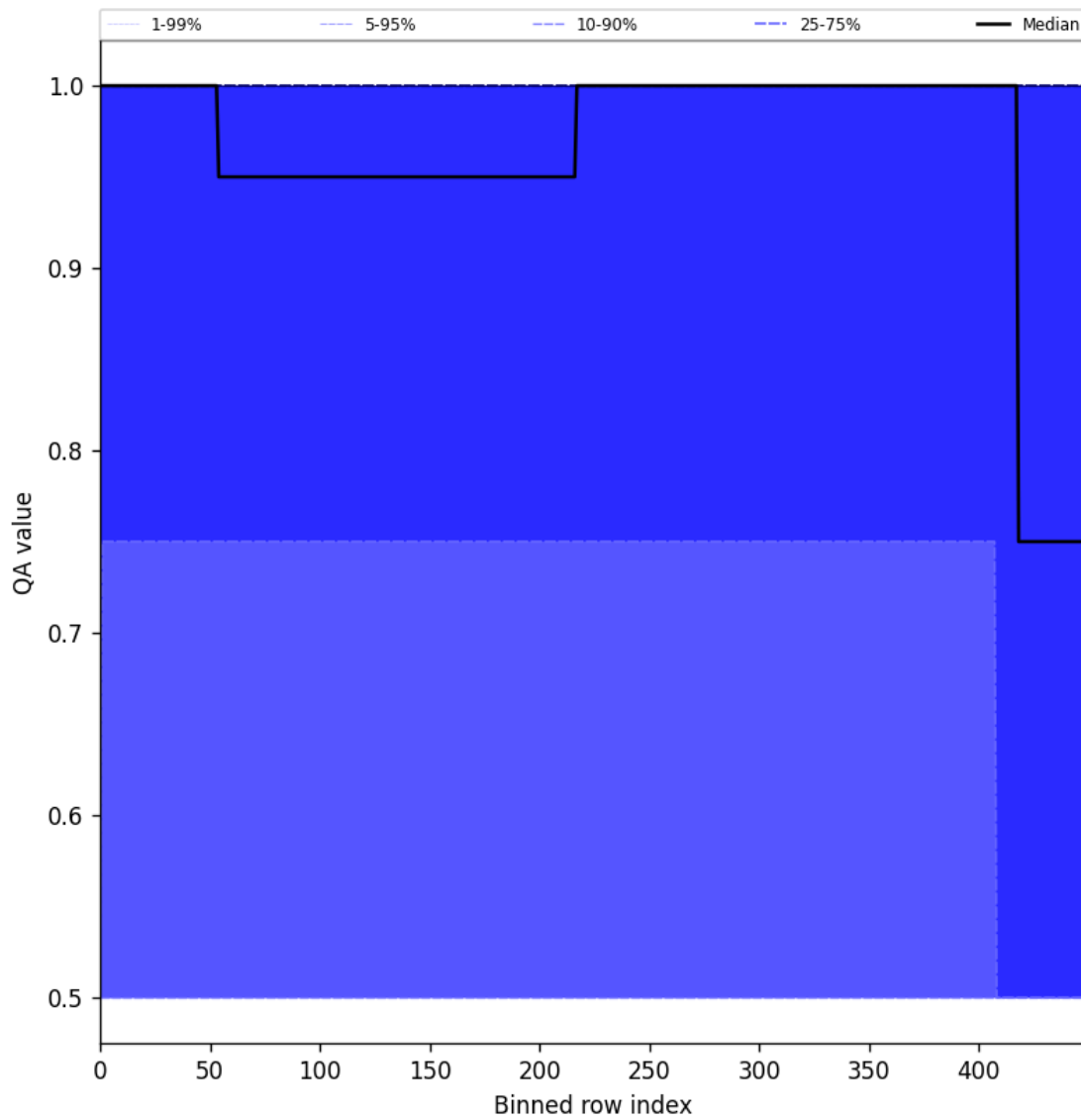
Figure 51: Along track statistics of “QA value” for 2025-11-15 to 2025-11-17
