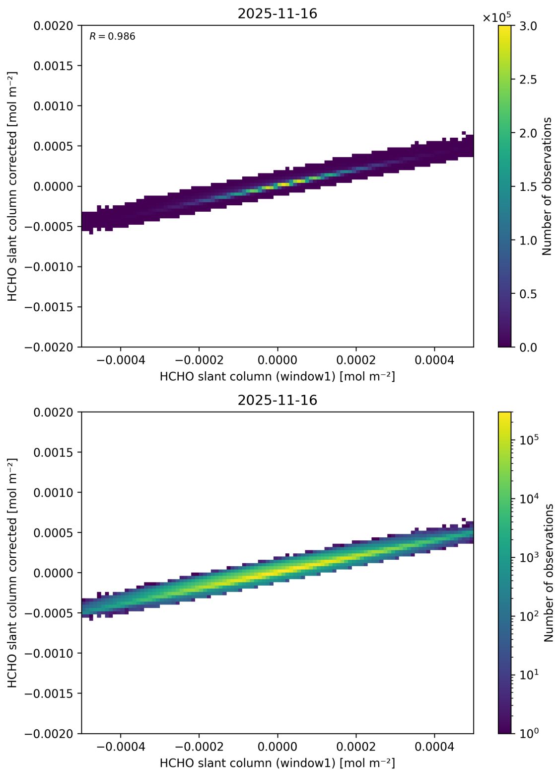
Figure 92: Scatter density plot of “HCHO slant column (window1)” against “HCHO slant column corrected” for 2025-11-15 to 2025-11-17.
