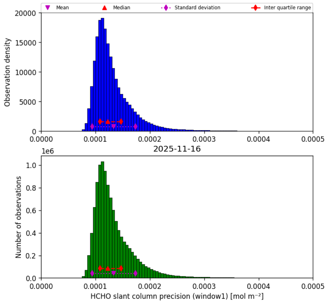
Figure 41: Histogram of “HCHO slant column precision (window1)” for 2025-11-15 to 2025-11-17
