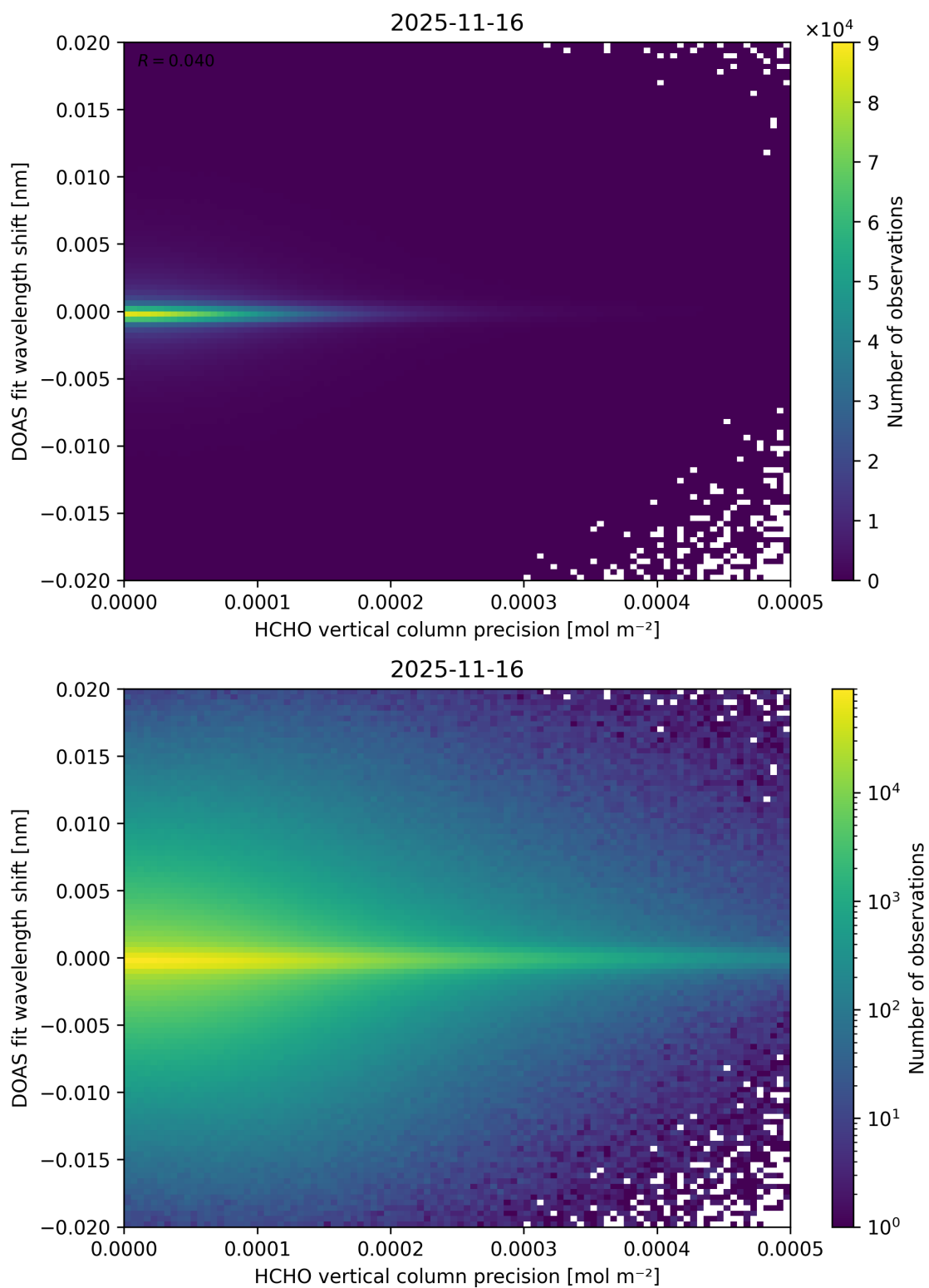
Figure 153: Scatter density plot of “HCHO vertical column precision” against “DOAS fit wavelength shift” for 2025-11-15 to 2025-11-17.
