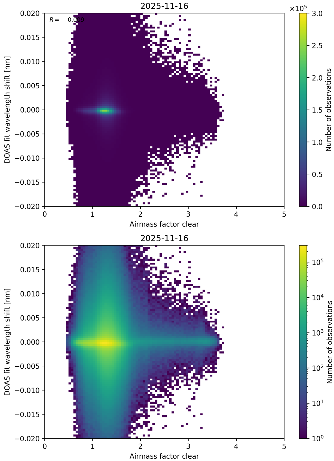
Figure 79: Scatter density plot of “Airmass factor clear” against “DOAS fit wavelength shift” for 2025-11-15 to 2025-11-17.
