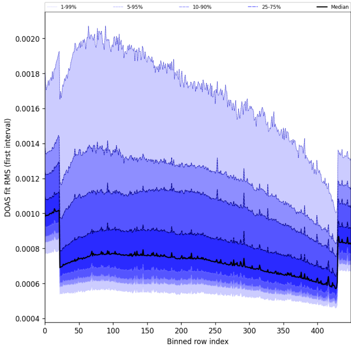
Figure 63: Along track statistics of “DOAS fit RMS (first interval)” for 2025-11-15 to 2025-11-17
