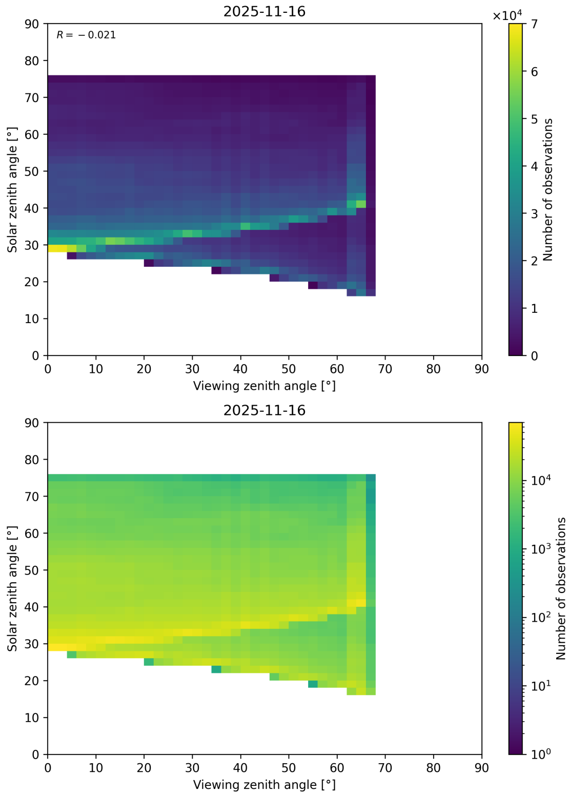
Figure 218: Scatter density plot of “Viewing zenith angle” against “Solar zenith angle” for 2025-11-15 to 2025-11-17.
