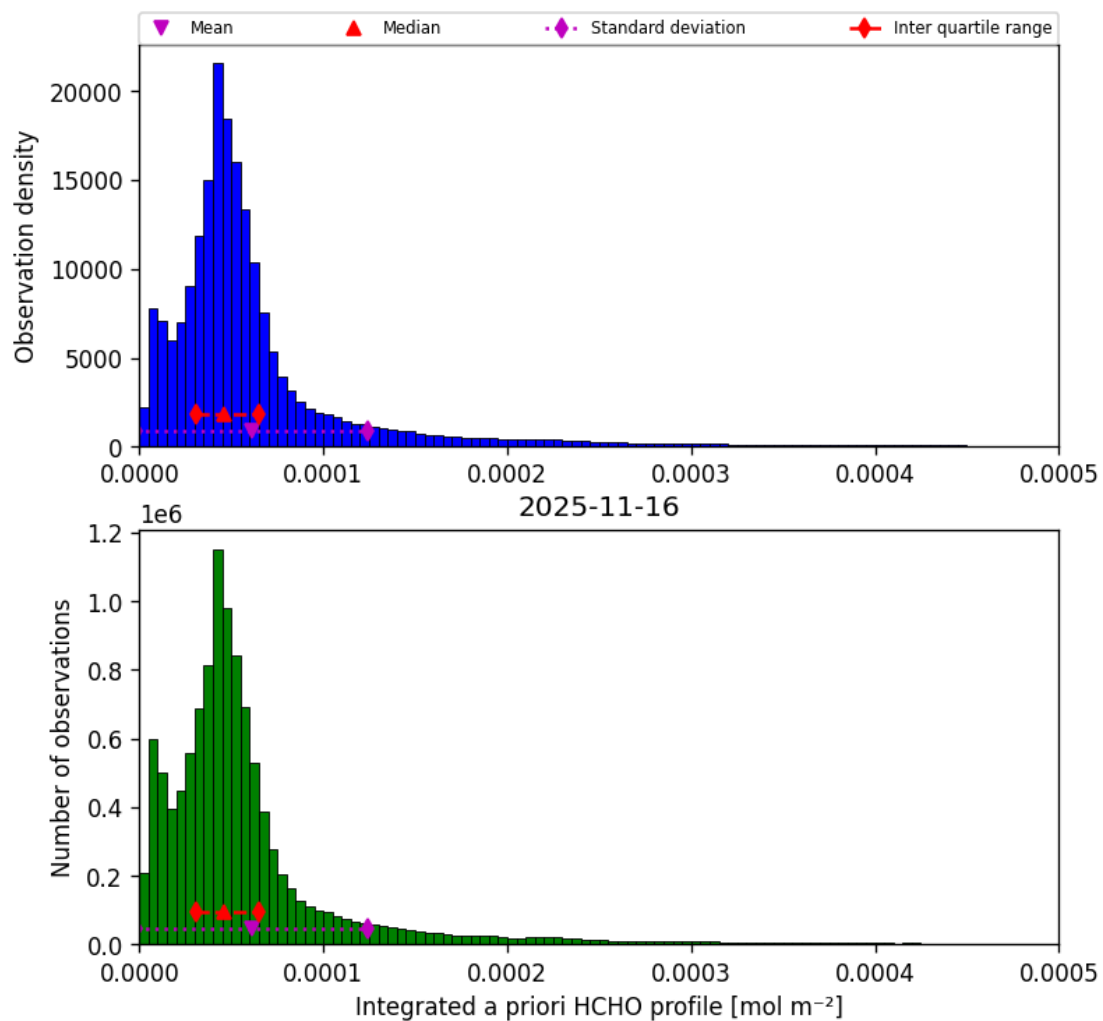
Figure 45: Histogram of “Integrated a priori HCHO profile” for 2025-11-15 to 2025-11-17
