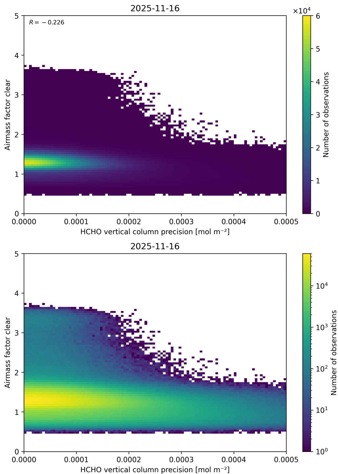
Figure 155: Scatter density plot of “HCHO vertical column precision” against “Airmass factor clear” for 2025-11-15 to 2025-11-17.
