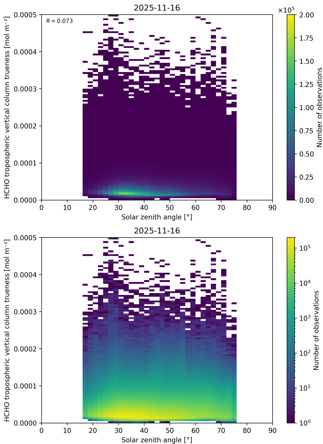
Figure 199: Scatter density plot of “Solar zenith angle” against “HCHO tropospheric vertical column trueness” for 2025-11-15 to 2025-11-17.
