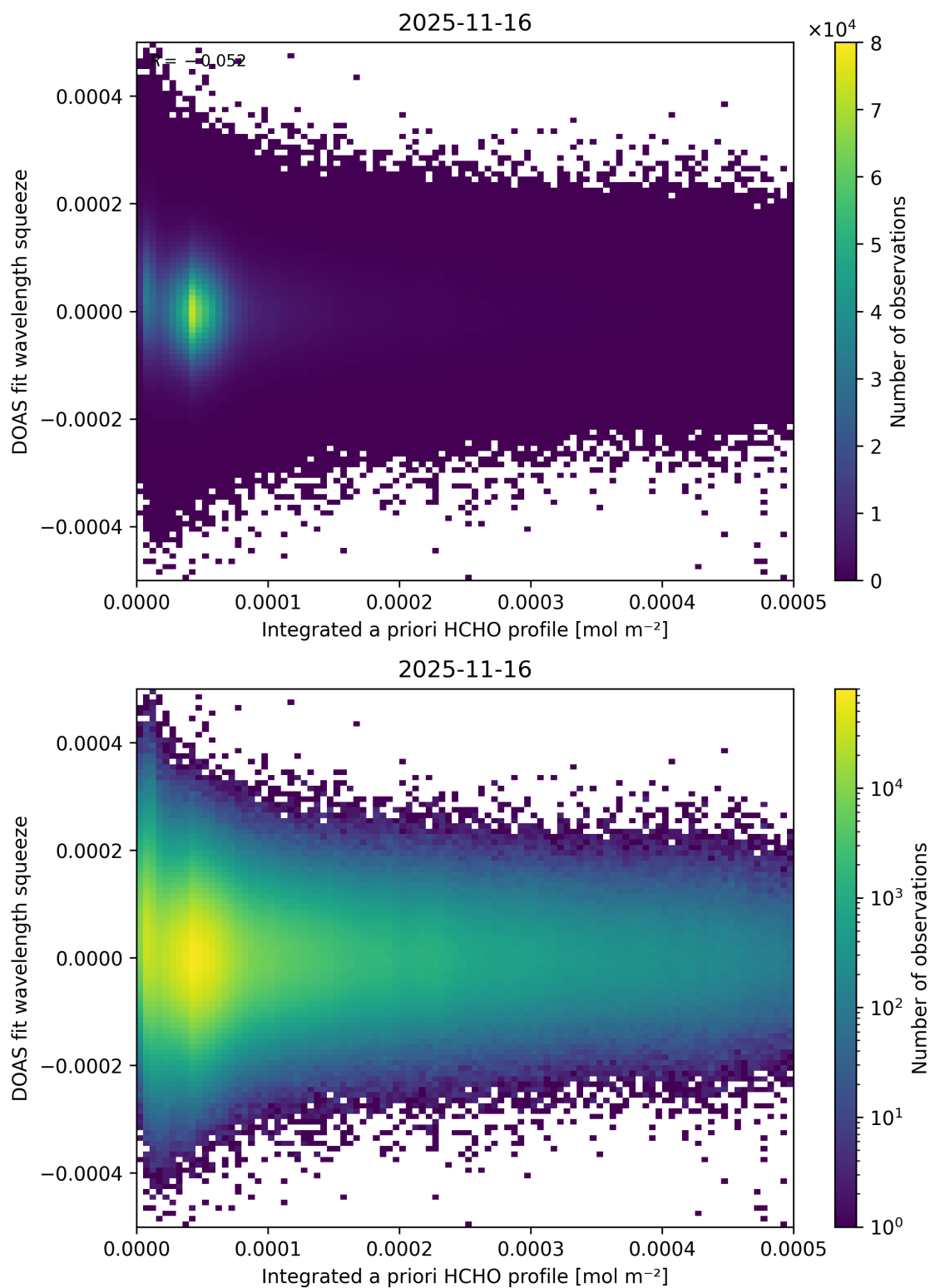
Figure 167: Scatter density plot of “Integrated a priori HCHO profile” against “DOAS fit wavelength squeeze” for 2025-11-15 to 2025-11-17.
