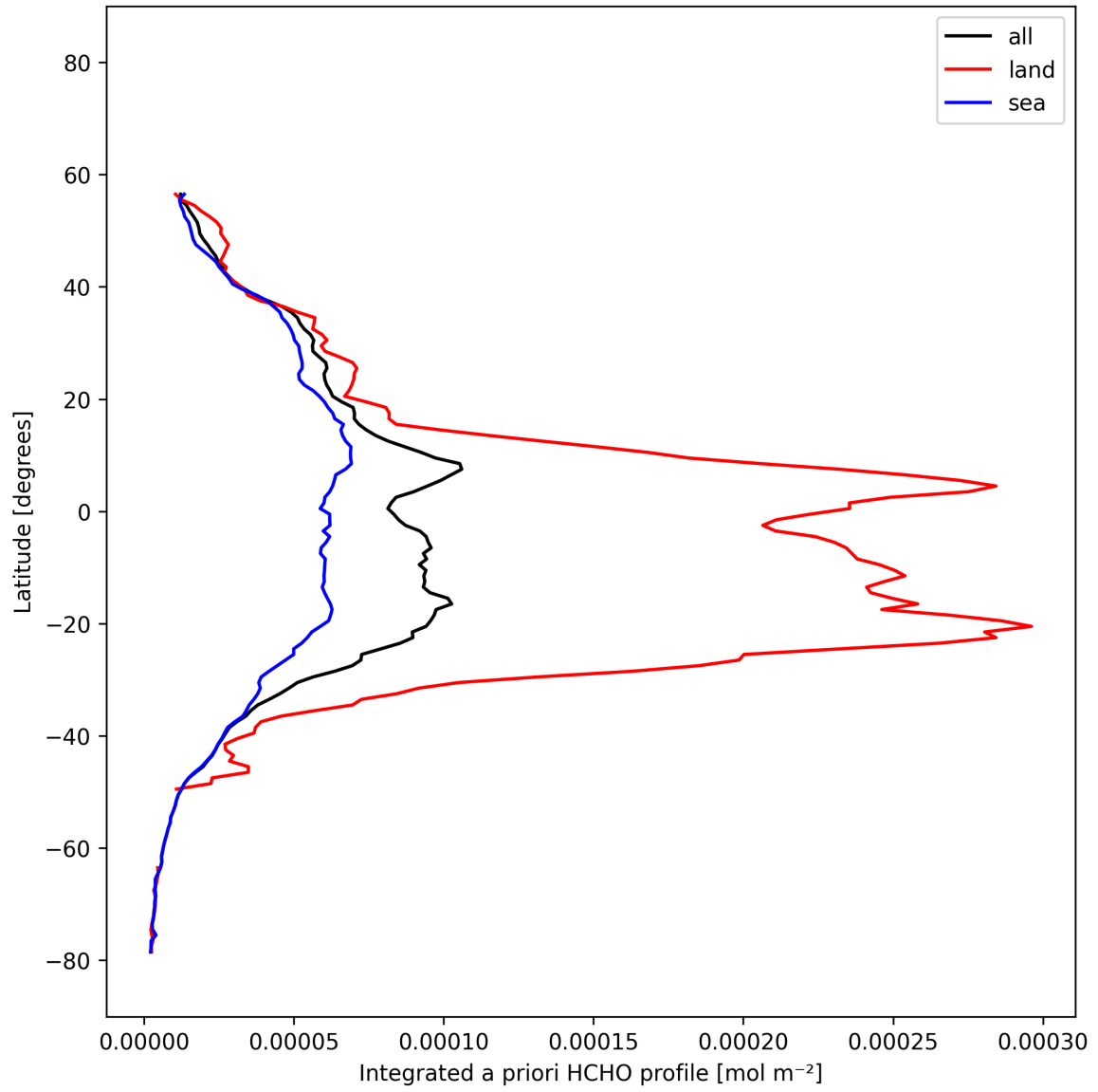
Figure 30: Zonal average of “Integrated a priori HCHO profile” for 2025-11-15 to 2025-11-17.
