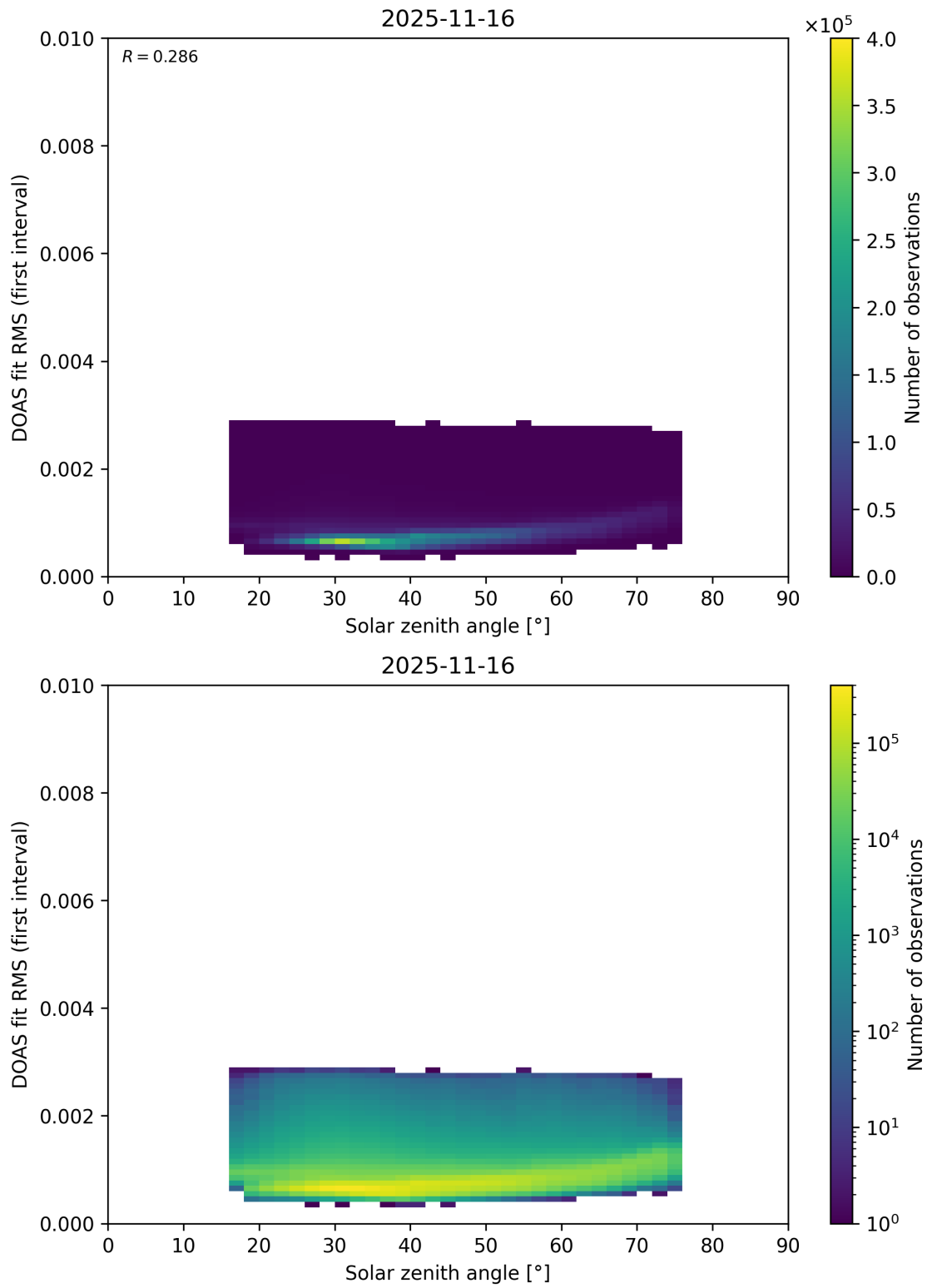
Figure 186: Scatter density plot of “Solar zenith angle” against “DOAS fit RMS (first interval)” for 2025-11-15 to 2025-11-17.
