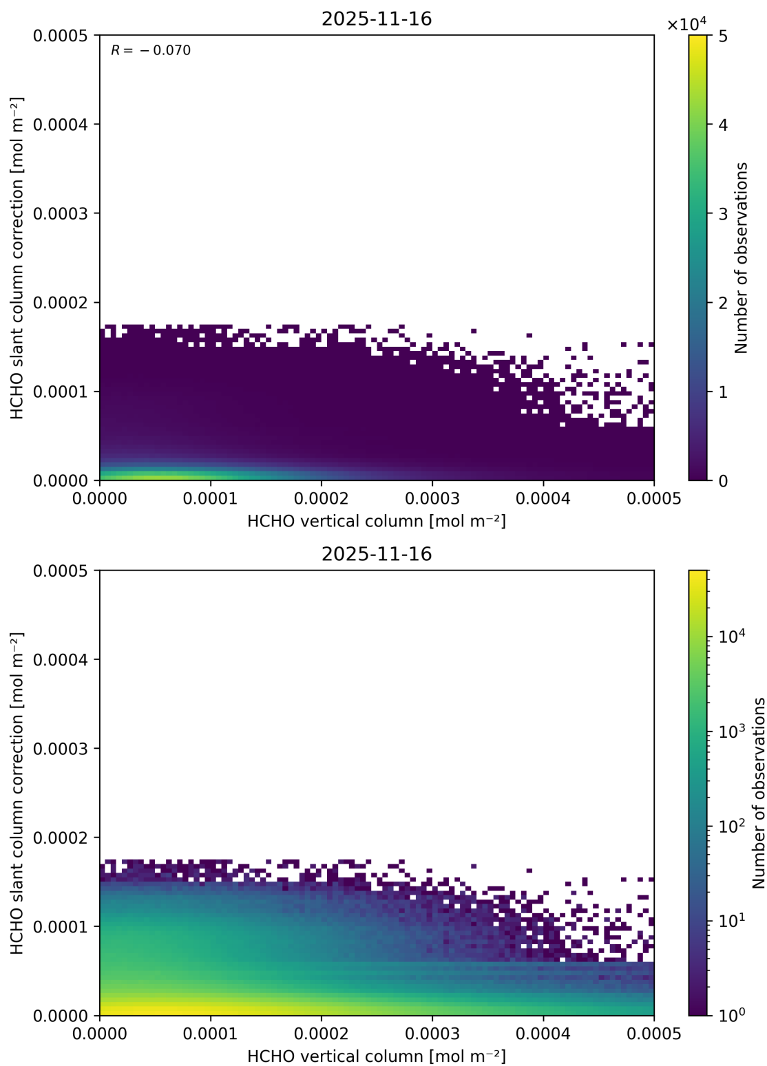
Figure 143: Scatter density plot of “HCHO vertical column” against “HCHO slant column correction” for 2025-11-15 to 2025-11-17.
