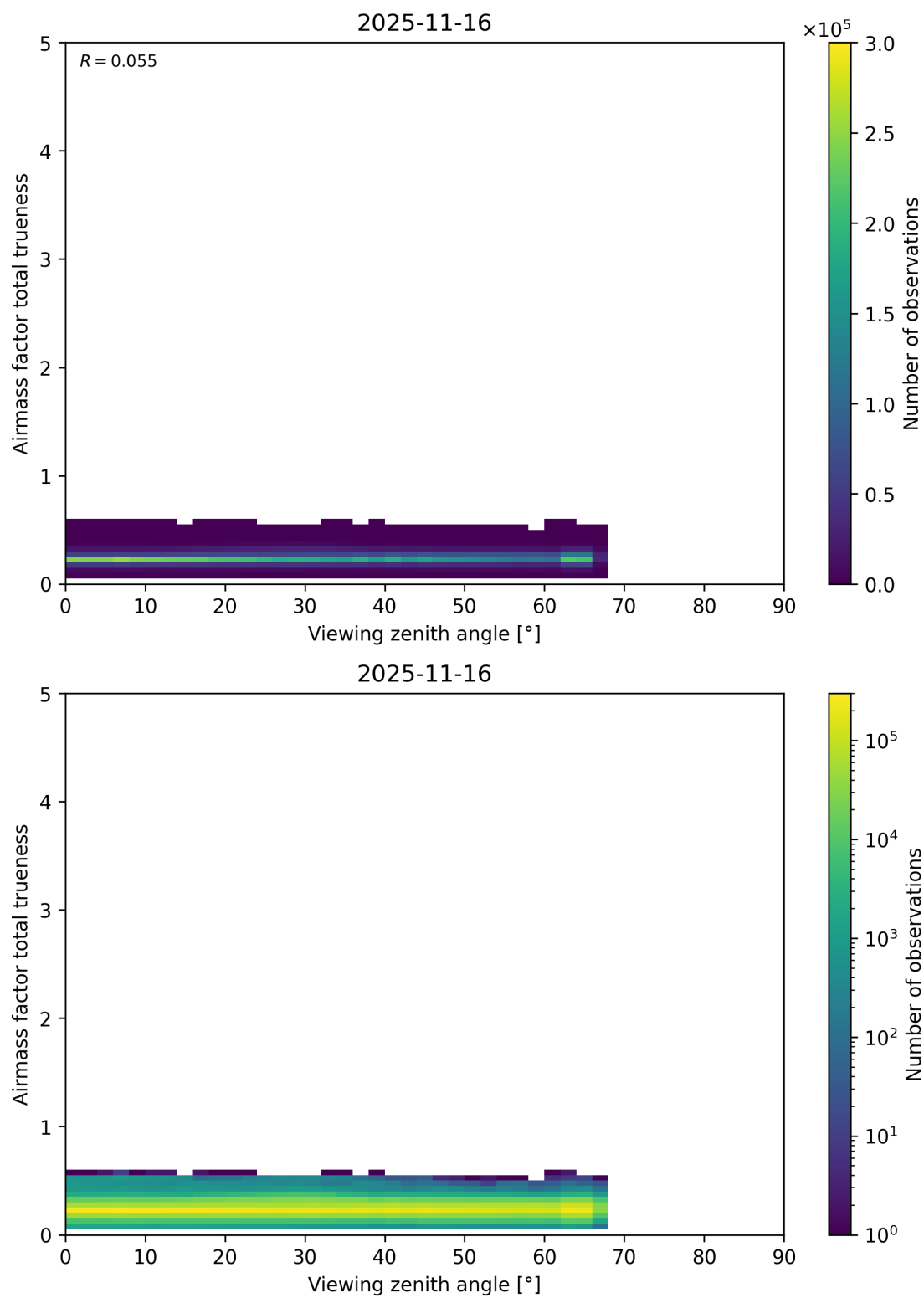
Figure 211: Scatter density plot of “Viewing zenith angle” against “Airmass factor total trueness” for 2025-11-15 to 2025-11-17.
