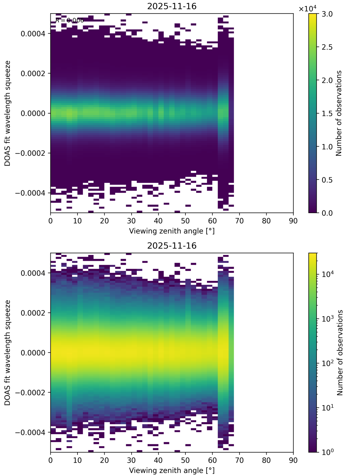
Figure 204: Scatter density plot of “Viewing zenith angle” against “DOAS fit wavelength squeeze” for 2025-11-15 to 2025-11-17.
