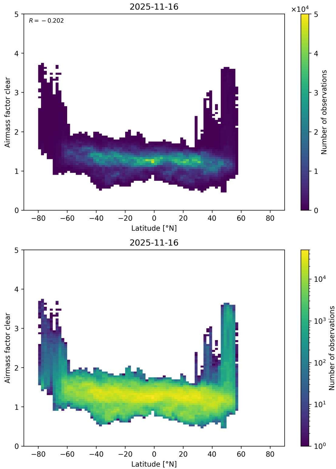
Figure 174: Scatter density plot of “Latitude” against “Airmass factor clear” for 2025-11-15 to 2025-11-17.
