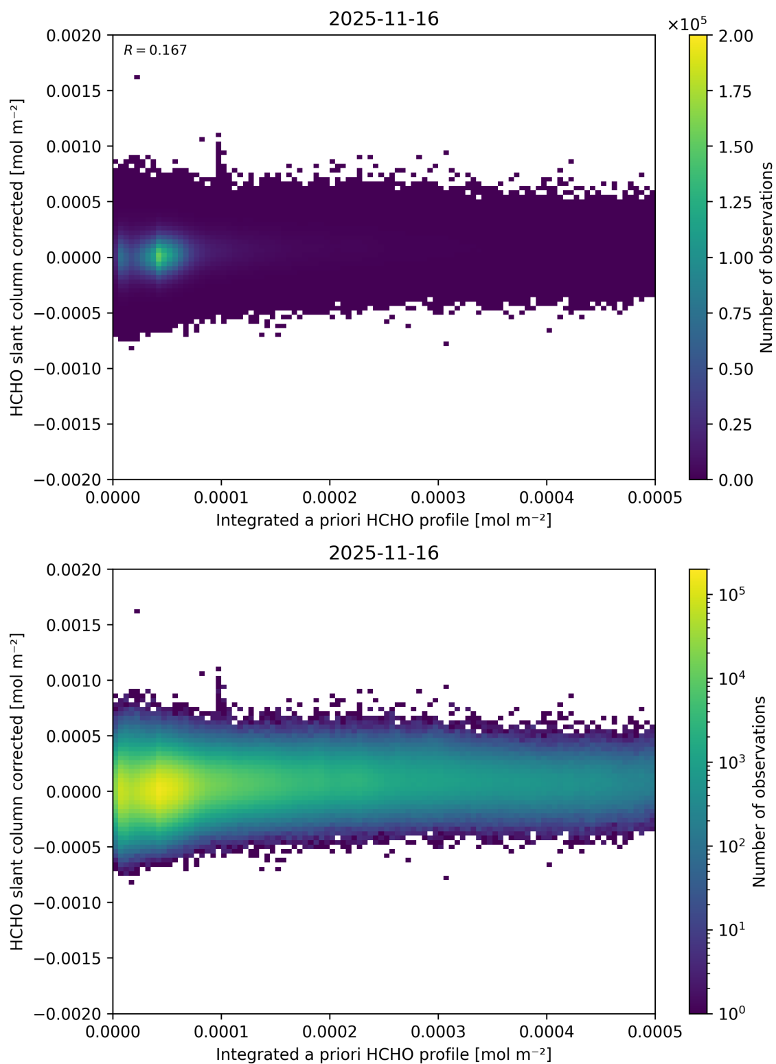
Figure 168: Scatter density plot of “Integrated a priori HCHO profile” against “HCHO slant column corrected” for 2025-11-15 to 2025-11-17.
