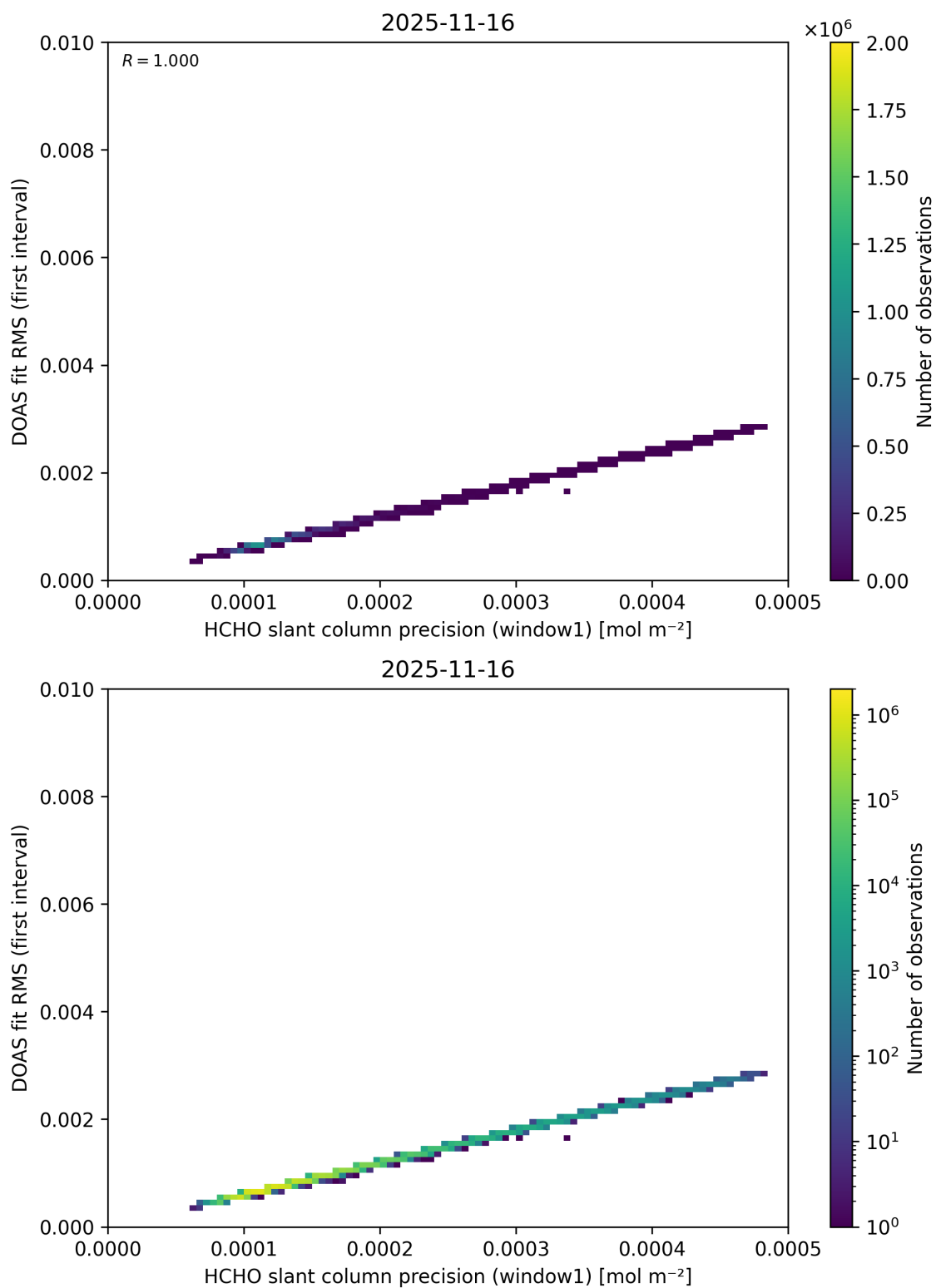
Figure 99: Scatter density plot of “HCHO slant column precision (window1)” against “DOAS fit RMS (first interval)” for 2025-11-15 to 2025-11-17.
