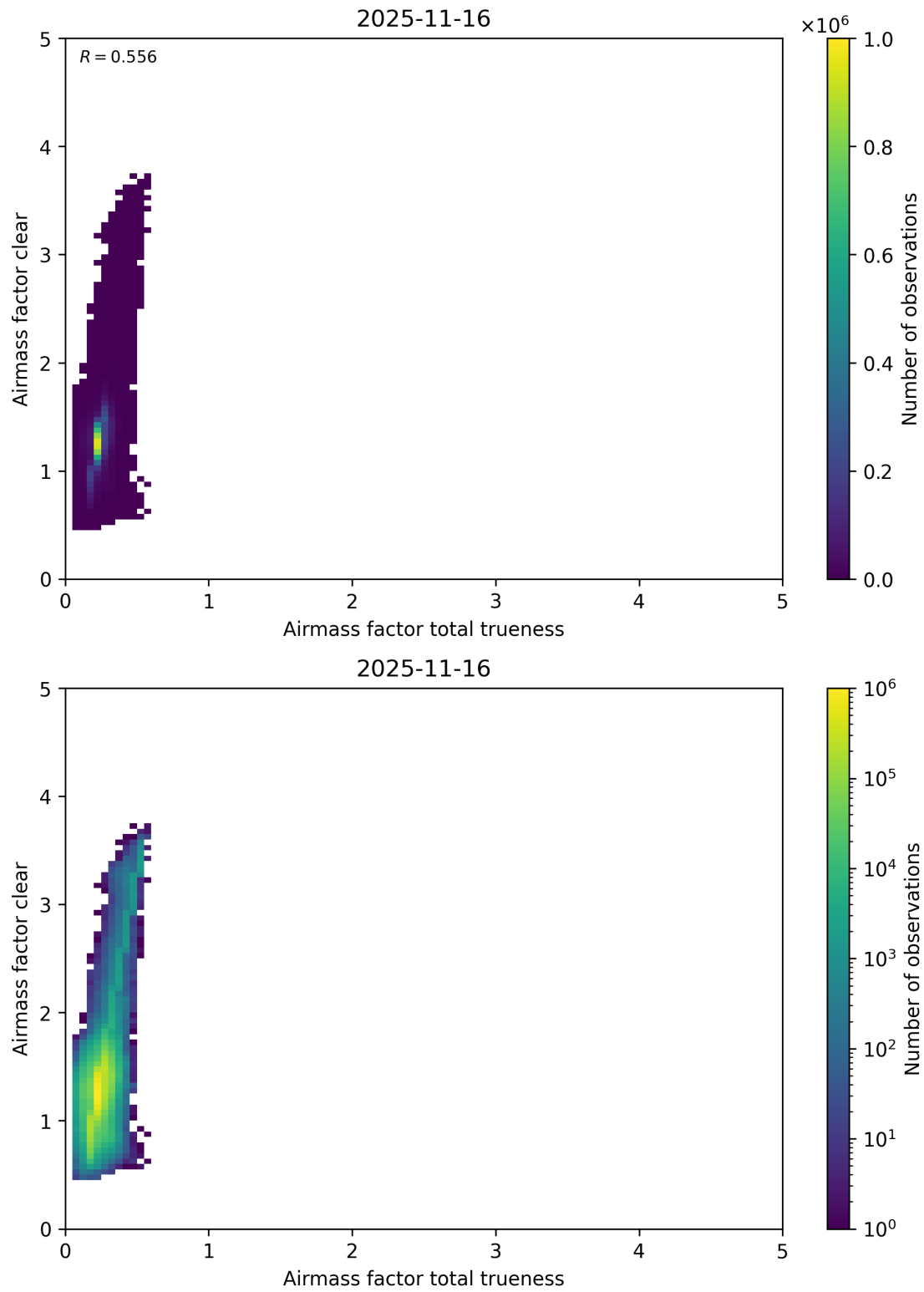
Figure 121: Scatter density plot of “Airmass factor total trueness” against “Airmass factor clear” for 2025-11-15 to 2025-11-17.
