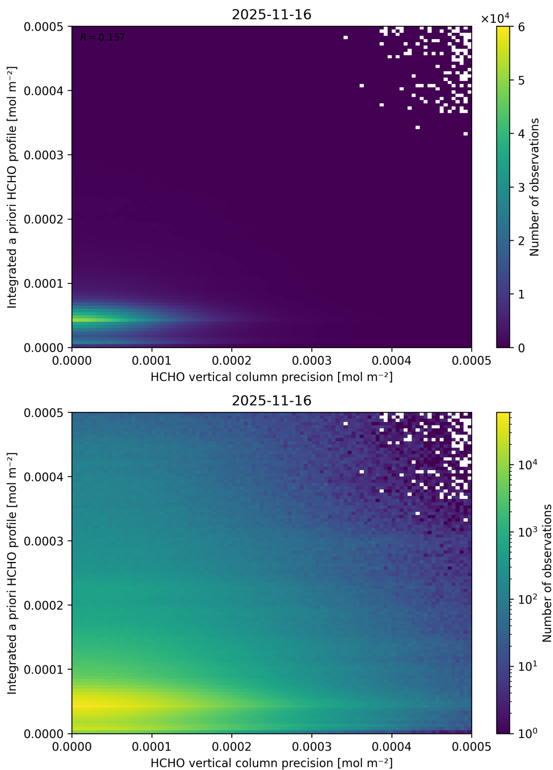
Figure 164: Scatter density plot of “HCHO vertical column precision” against “Integrated a priori HCHO profile” for 2025-11-15 to 2025-11-17.
