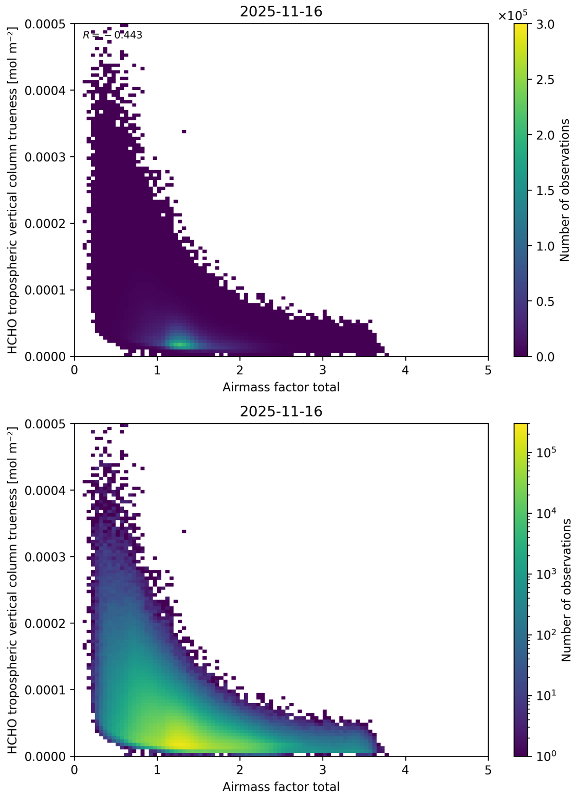
Figure 116: Scatter density plot of “Airmass factor total” against “HCHO tropospheric vertical column trueness” for 2025-11-15 to 2025-11-17.
