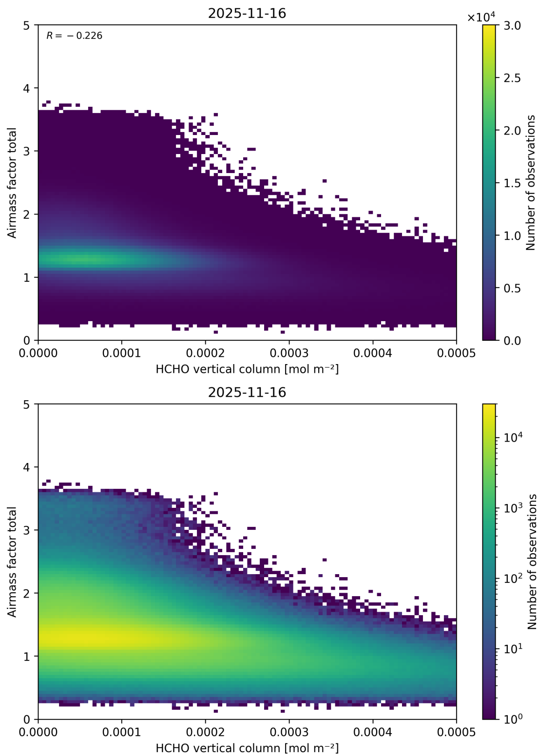
Figure 146: Scatter density plot of “HCHO vertical column” against “Airmass factor total” for 2025-11-15 to 2025-11-17.
