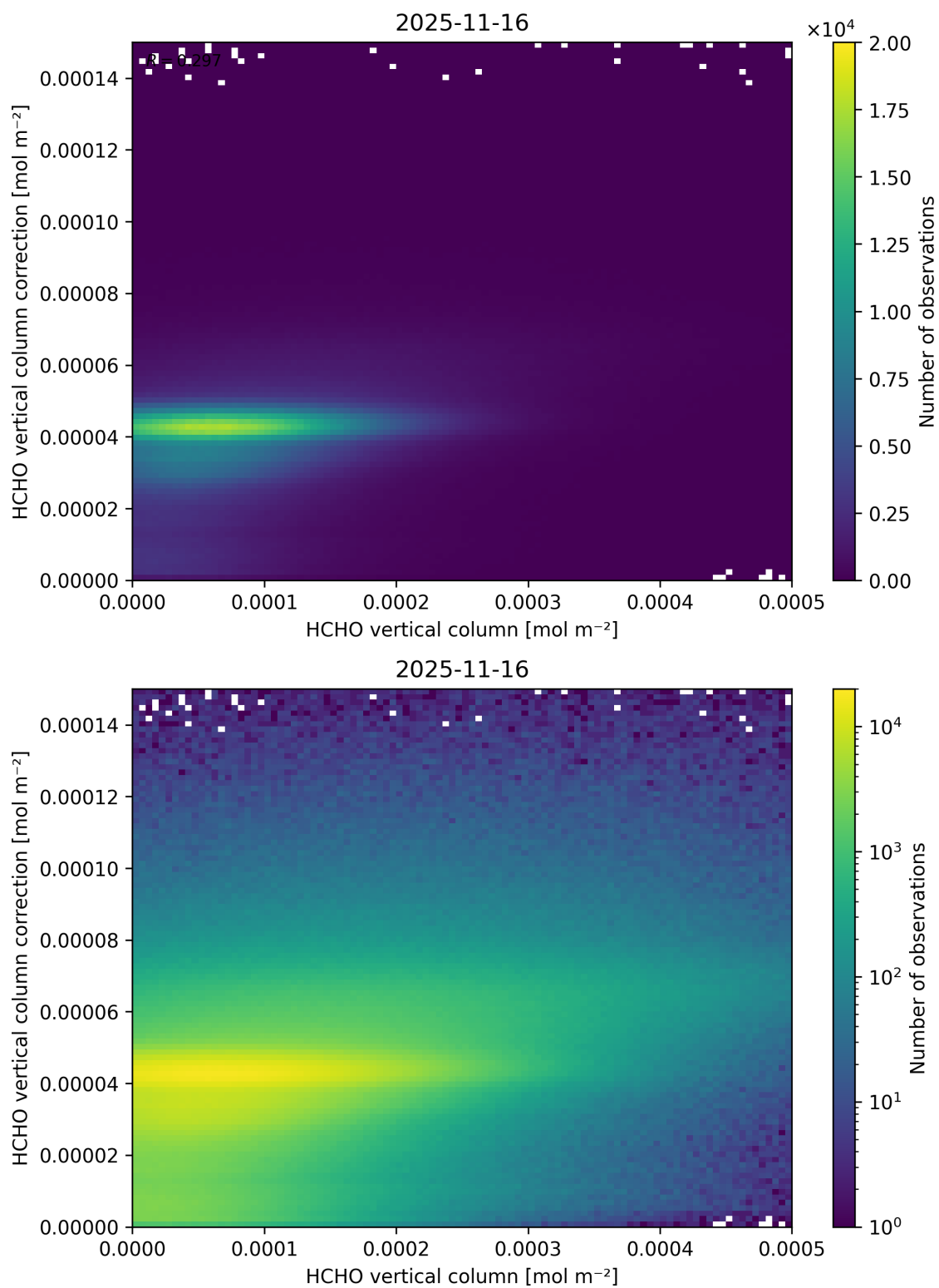
Figure 148: Scatter density plot of “HCHO vertical column” against “HCHO vertical column correction” for 2025-11-15 to 2025-11-17.
