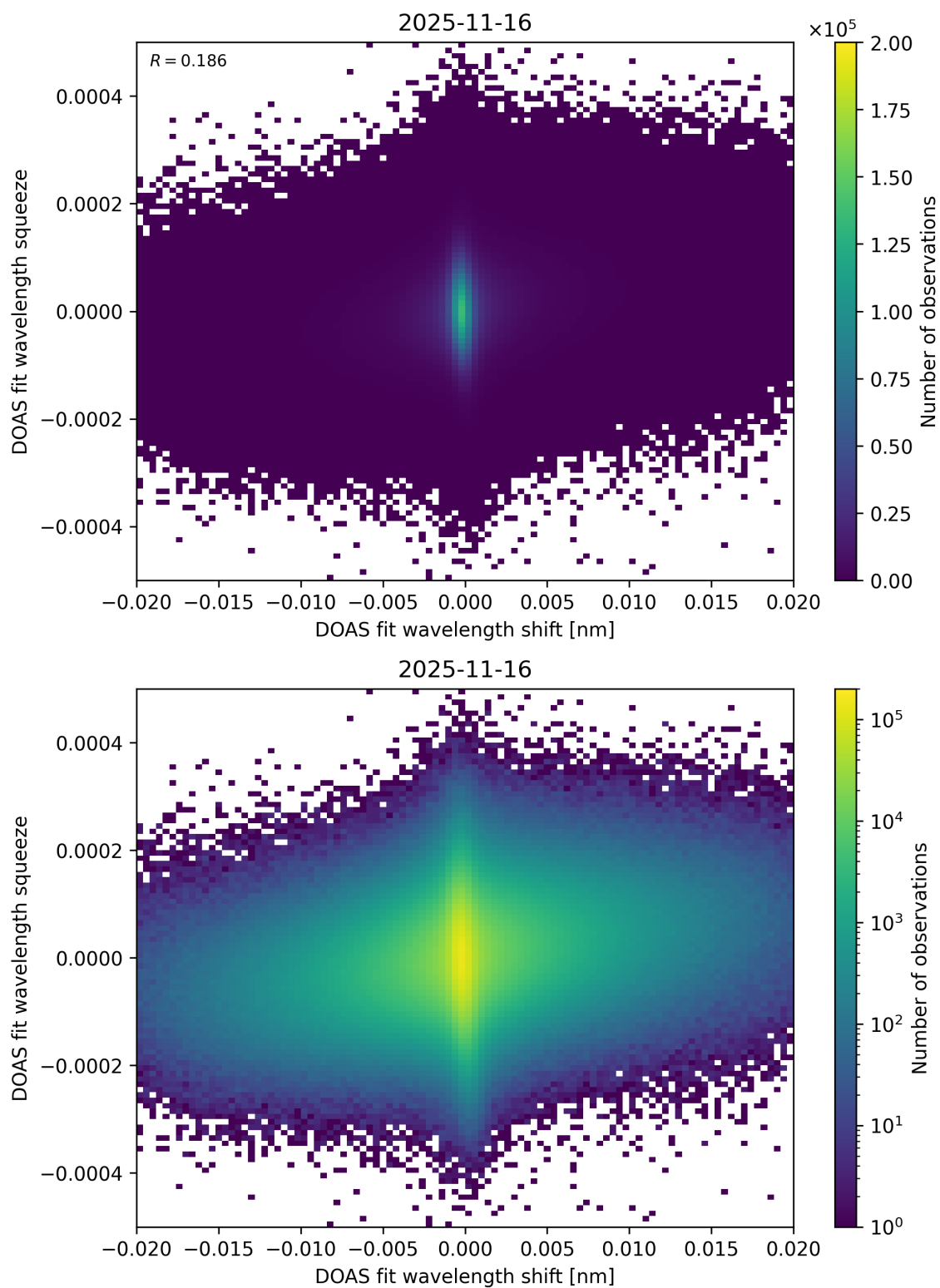
Figure 70: Scatter density plot of “DOAS fit wavelength shift” against “DOAS fit wavelength squeeze” for 2025-11-15 to 2025-11-17.
