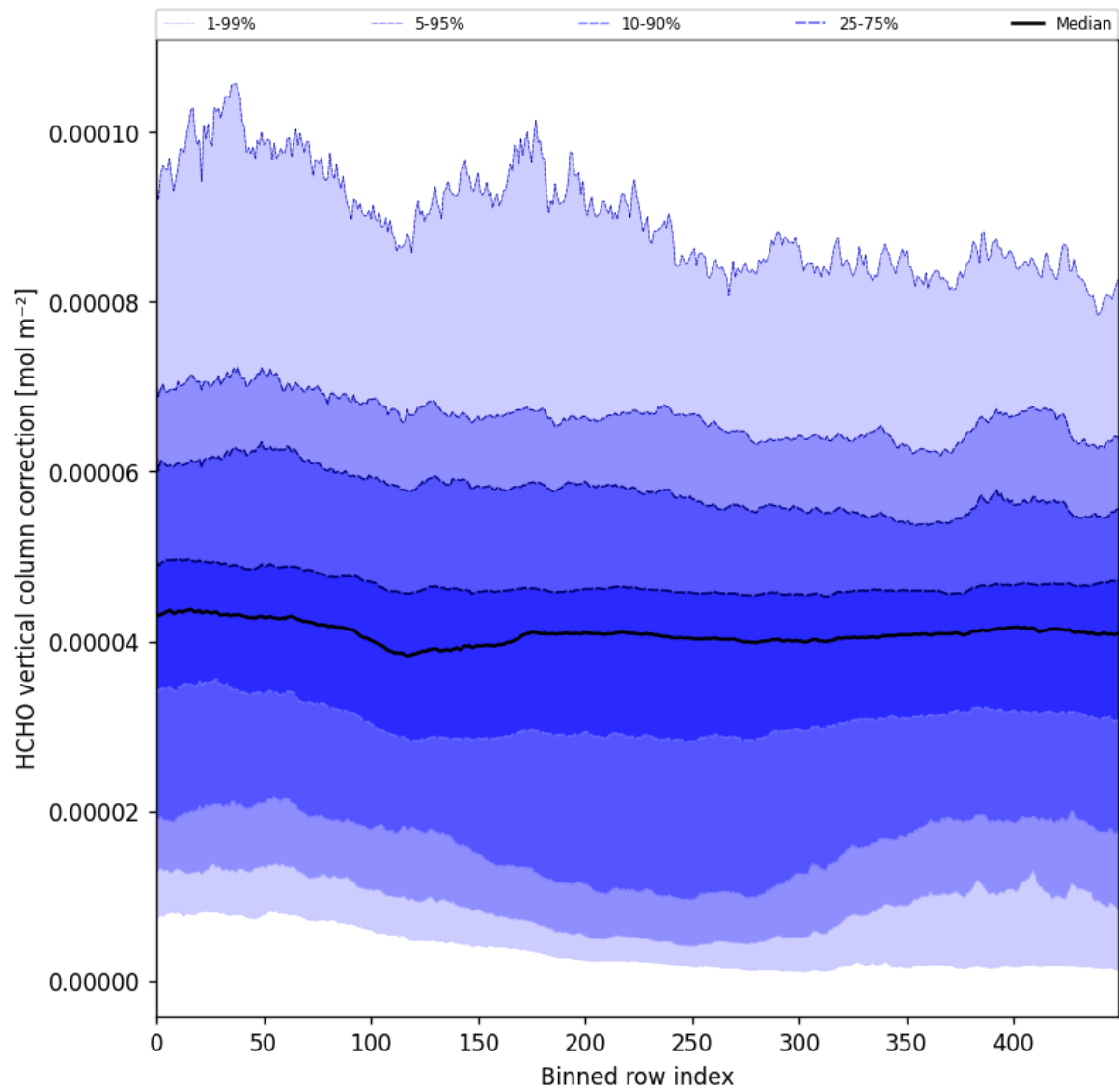
Figure 54: Along track statistics of “HCHO vertical column correction” for 2025-11-15 to 2025-11-17
