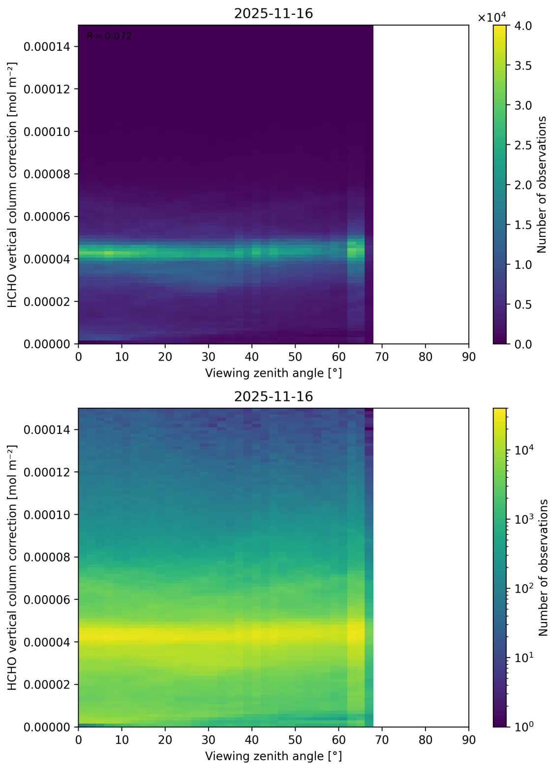
Figure 213: Scatter density plot of “Viewing zenith angle” against “HCHO vertical column correction” for 2025-11-15 to 2025-11-17.
