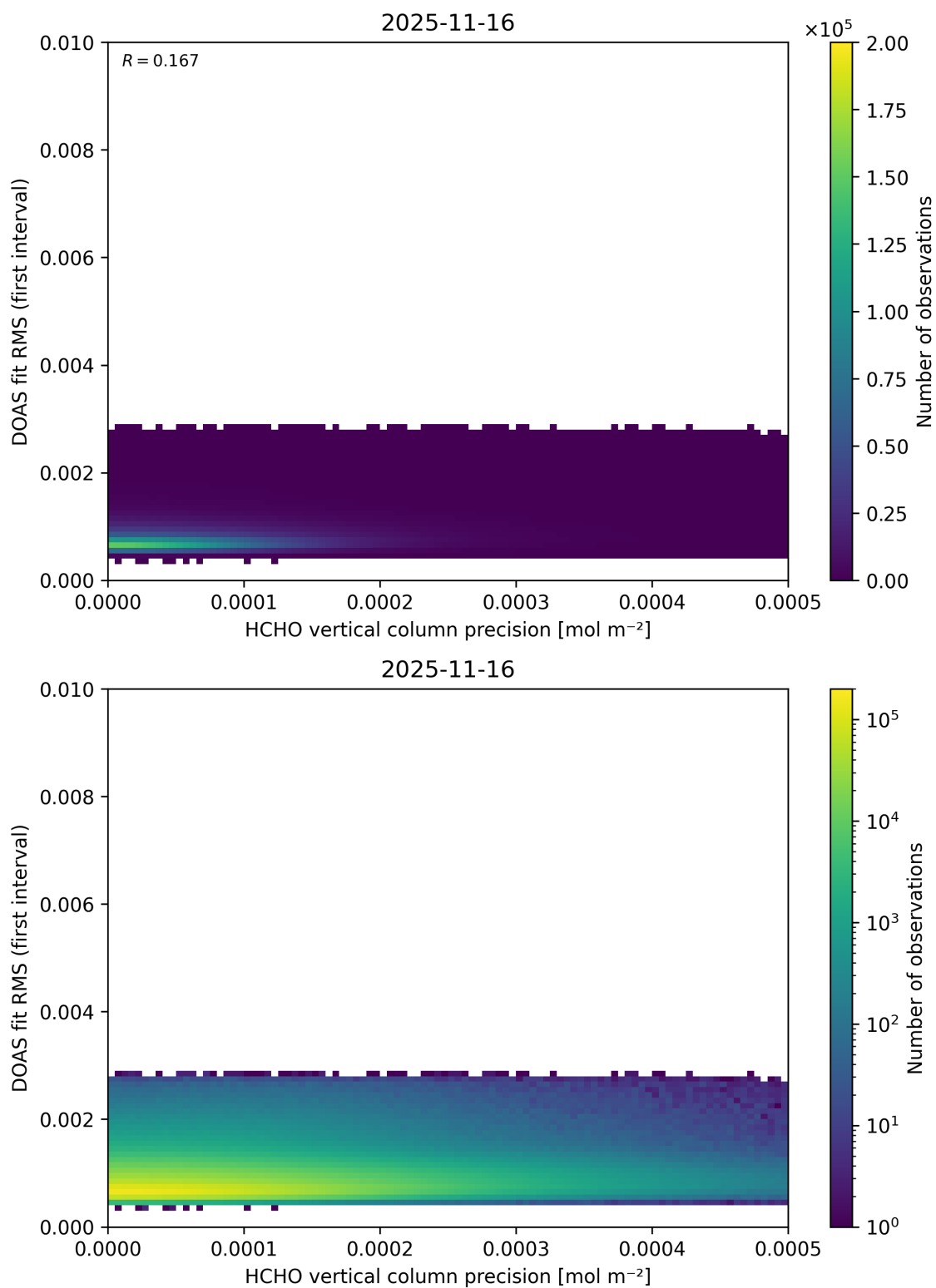
Figure 152: Scatter density plot of “HCHO vertical column precision” against “DOAS fit RMS (first interval)” for 2025-11-15 to 2025-11-17.
