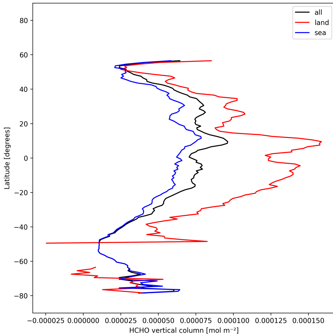
Figure 22: Zonal average of “HCHO vertical column” for 2025-11-15 to 2025-11-17.
