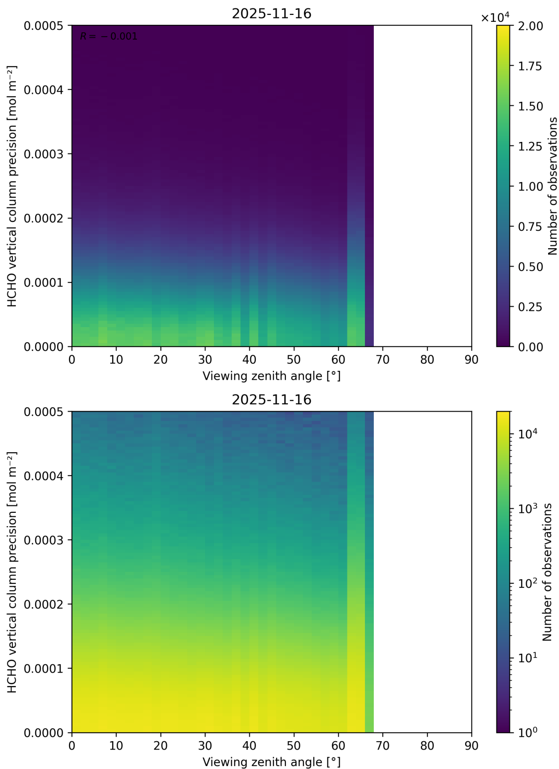
Figure 214: Scatter density plot of “Viewing zenith angle” against “HCHO vertical column precision” for 2025-11-15 to 2025-11-17.
