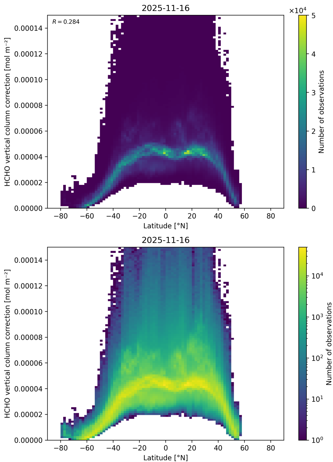
Figure 182: Scatter density plot of “Latitude” against “HCHO vertical column correction” for 2025-11-15 to 2025-11-17.
