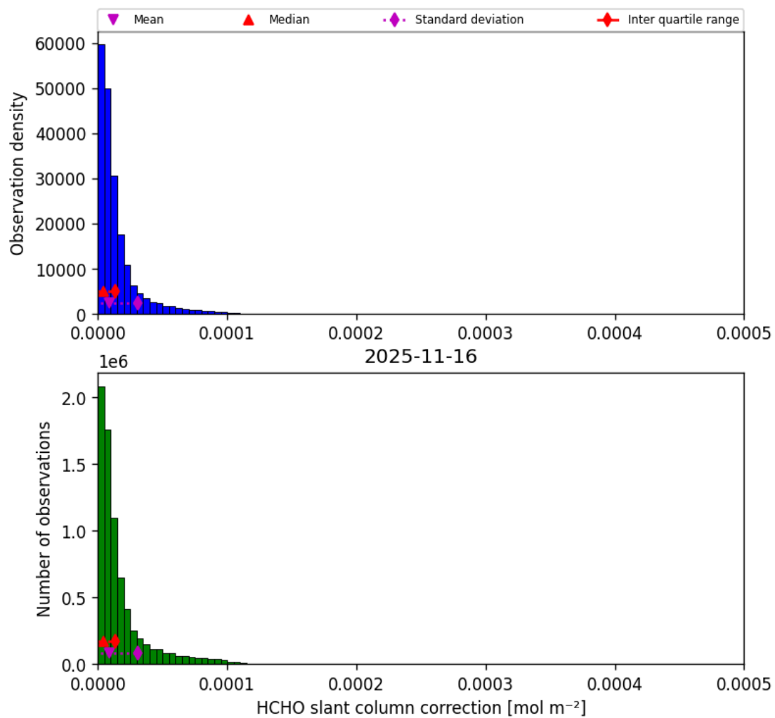
Figure 49: Histogram of “HCHO slant column correction” for 2025-11-15 to 2025-11-17
