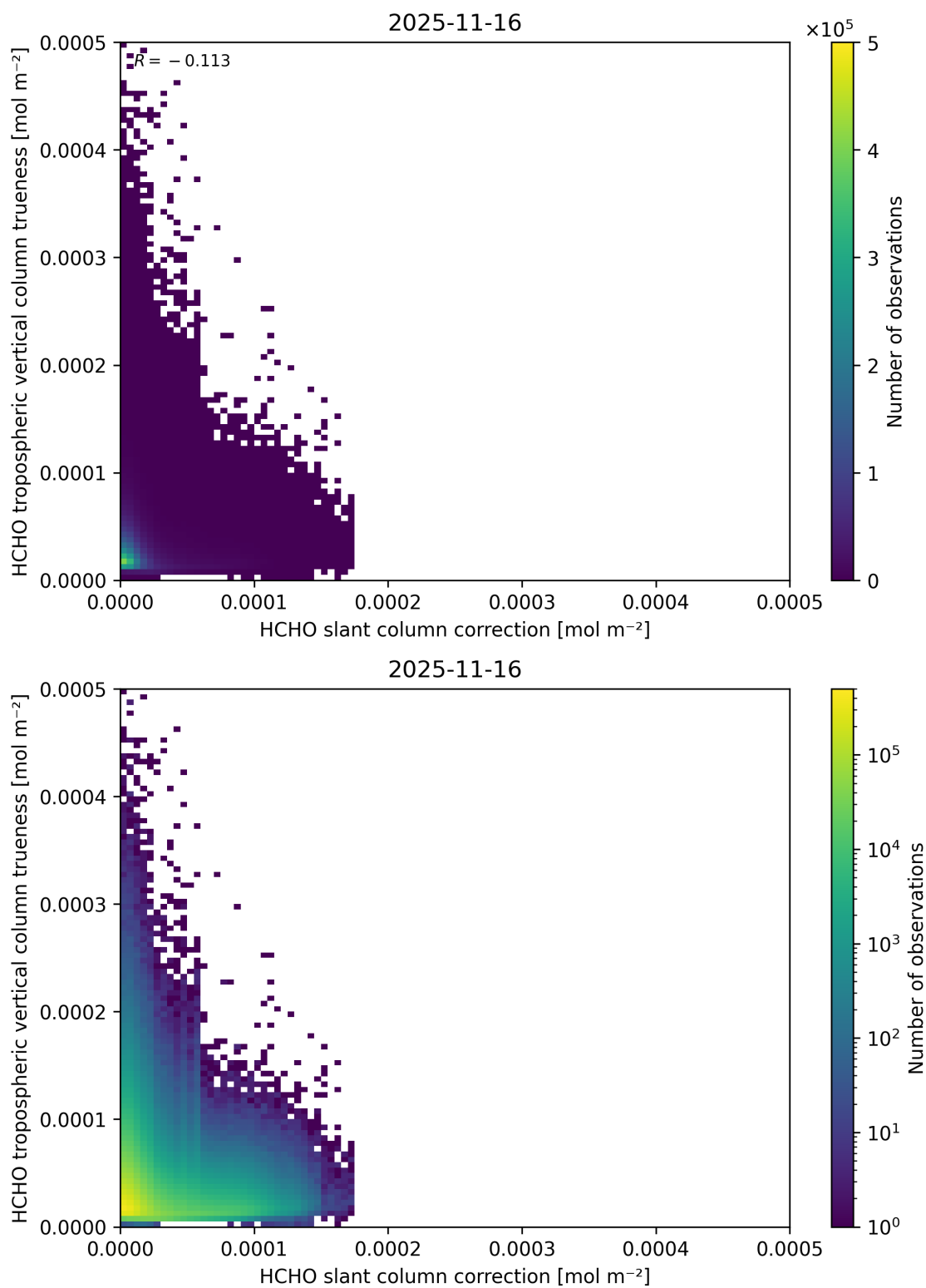
Figure 87: Scatter density plot of “HCHO slant column correction” against “HCHO tropospheric vertical column trueness” for 2025-11-15 to 2025-11-17.
