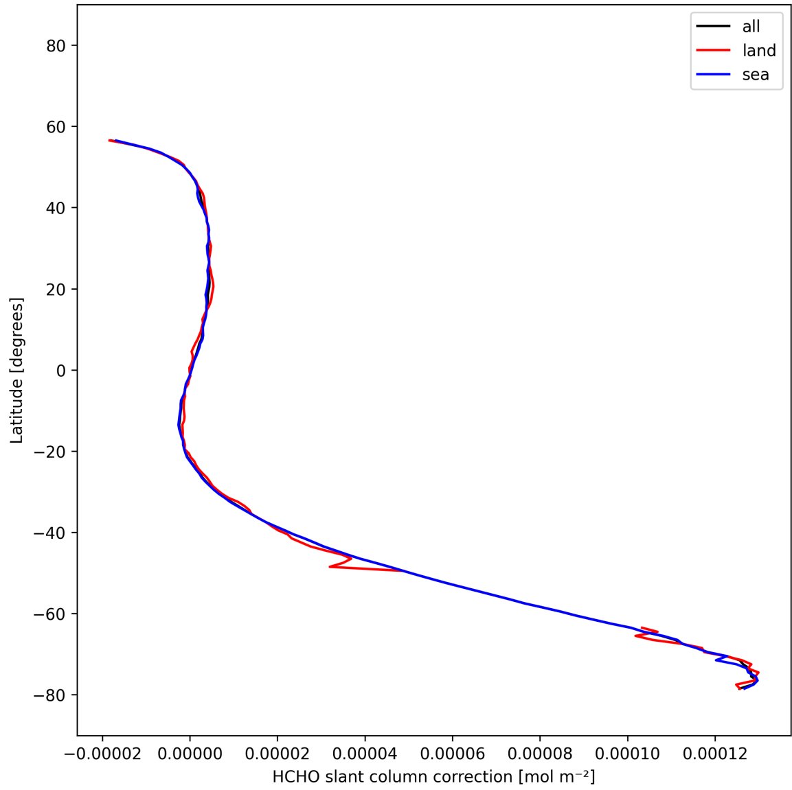
Figure 34: Zonal average of “HCHO slant column correction” for 2025-11-15 to 2025-11-17.
