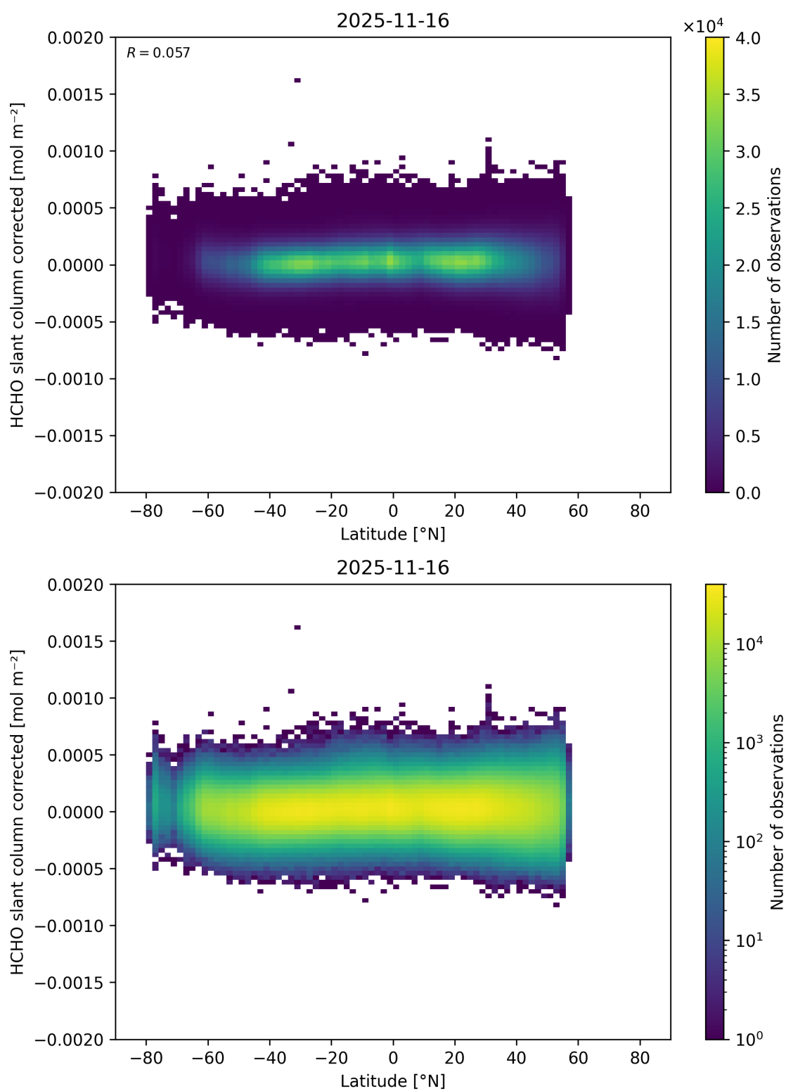
Figure 175: Scatter density plot of “Latitude” against “HCHO slant column corrected” for 2025-11-15 to 2025-11-17.
