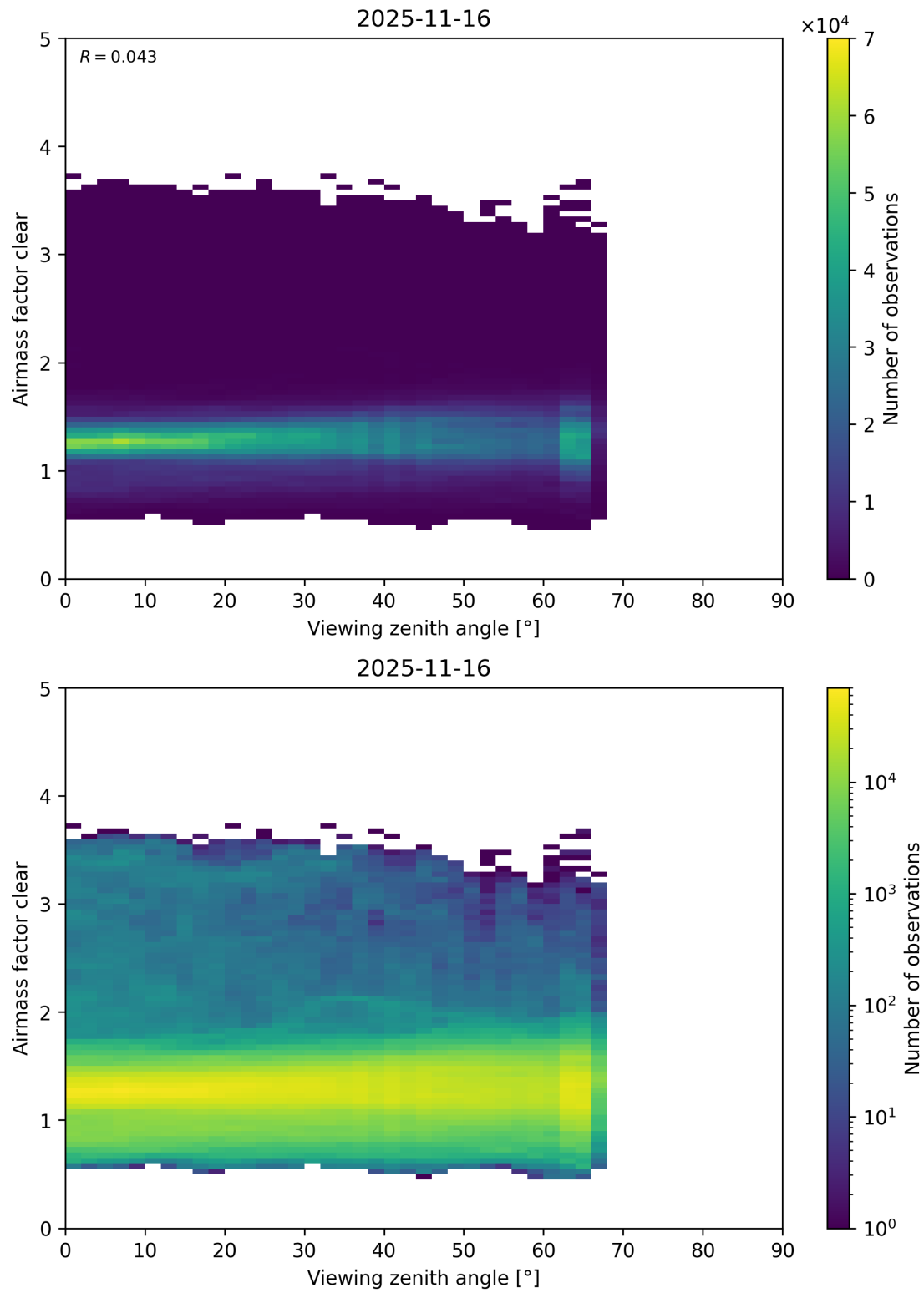
Figure 205: Scatter density plot of “Viewing zenith angle” against “Airmass factor clear” for 2025-11-15 to 2025-11-17.
