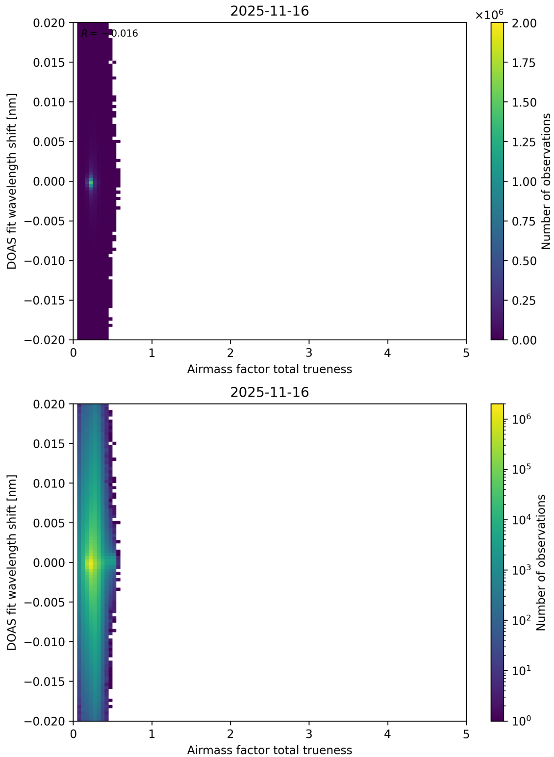
Figure 119: Scatter density plot of “Airmass factor total trueness” against “DOAS fit wavelength shift” for 2025-11-15 to 2025-11-17.
