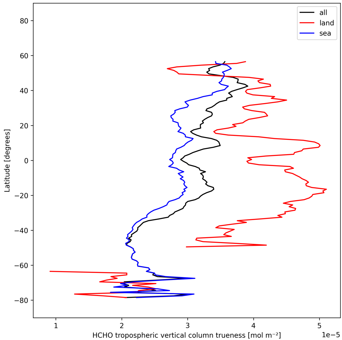
Figure 35: Zonal average of “HCHO tropospheric vertical column density” for 2025-11-15 to 2025-11-17.
