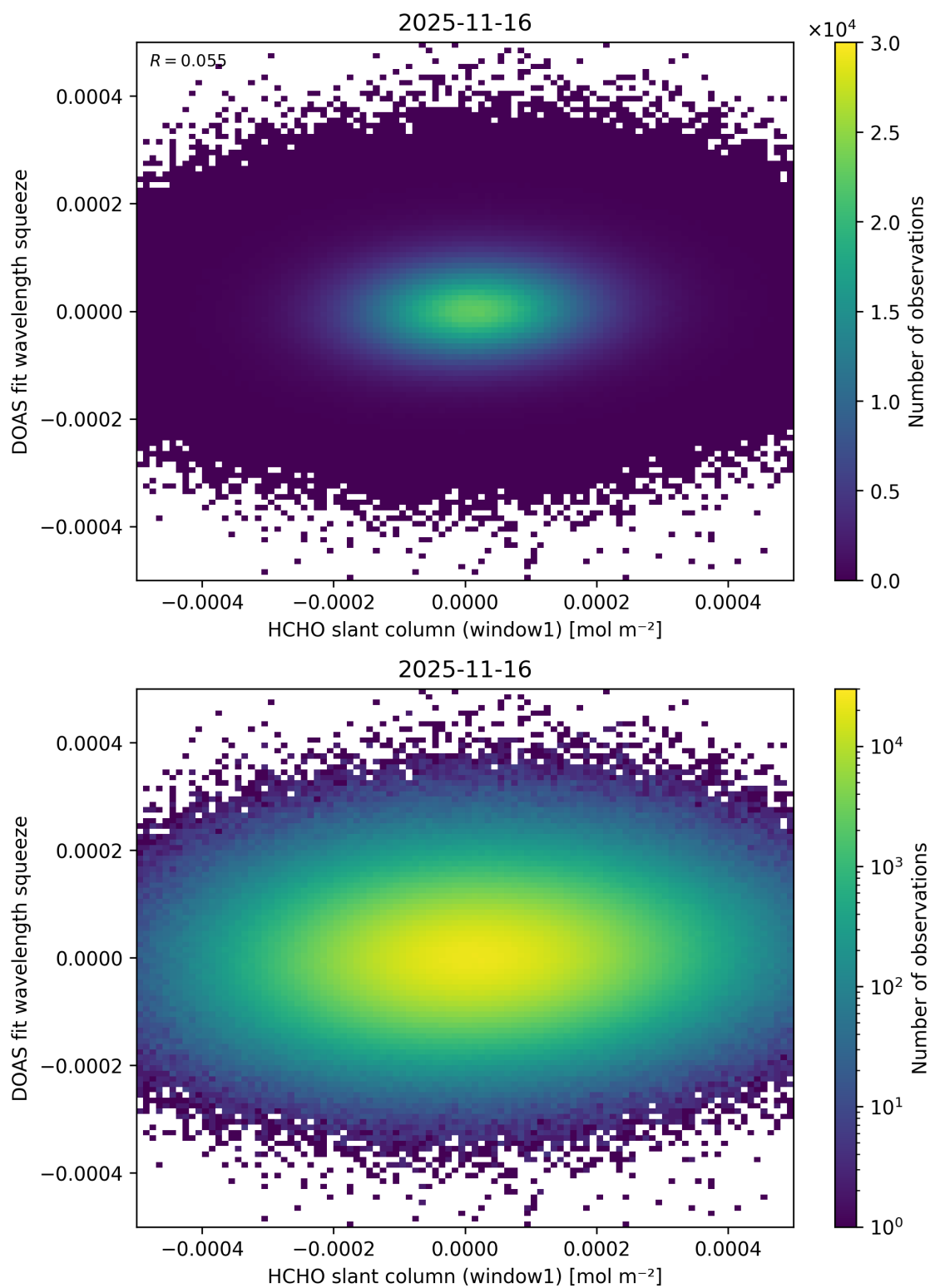
Figure 90: Scatter density plot of “HCHO slant column (window1)” against “DOAS fit wavelength squeeze” for 2025-11-15 to 2025-11-17.
