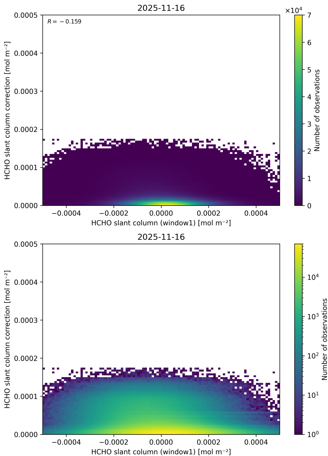
Figure 93: Scatter density plot of “HCHO slant column (window1)” against “HCHO slant column correction” for 2025-11-15 to 2025-11-17.
