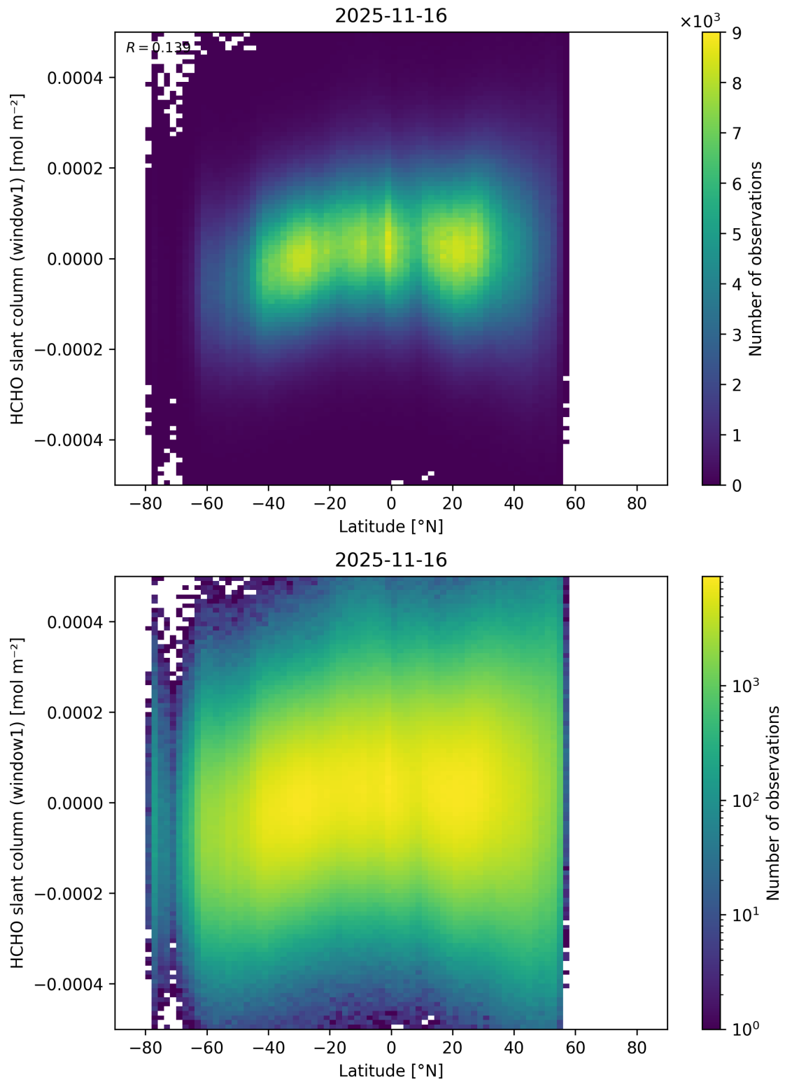
Figure 177: Scatter density plot of “Latitude” against “HCHO slant column (window1)” for 2025-11-15 to 2025-11-17.
