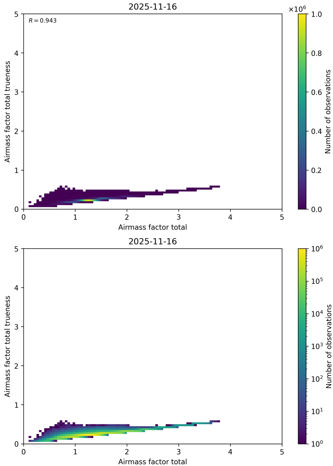
Figure 115: Scatter density plot of “Airmass factor total” against “Airmass factor total trueness” for 2025-11-15 to 2025-11-17.
