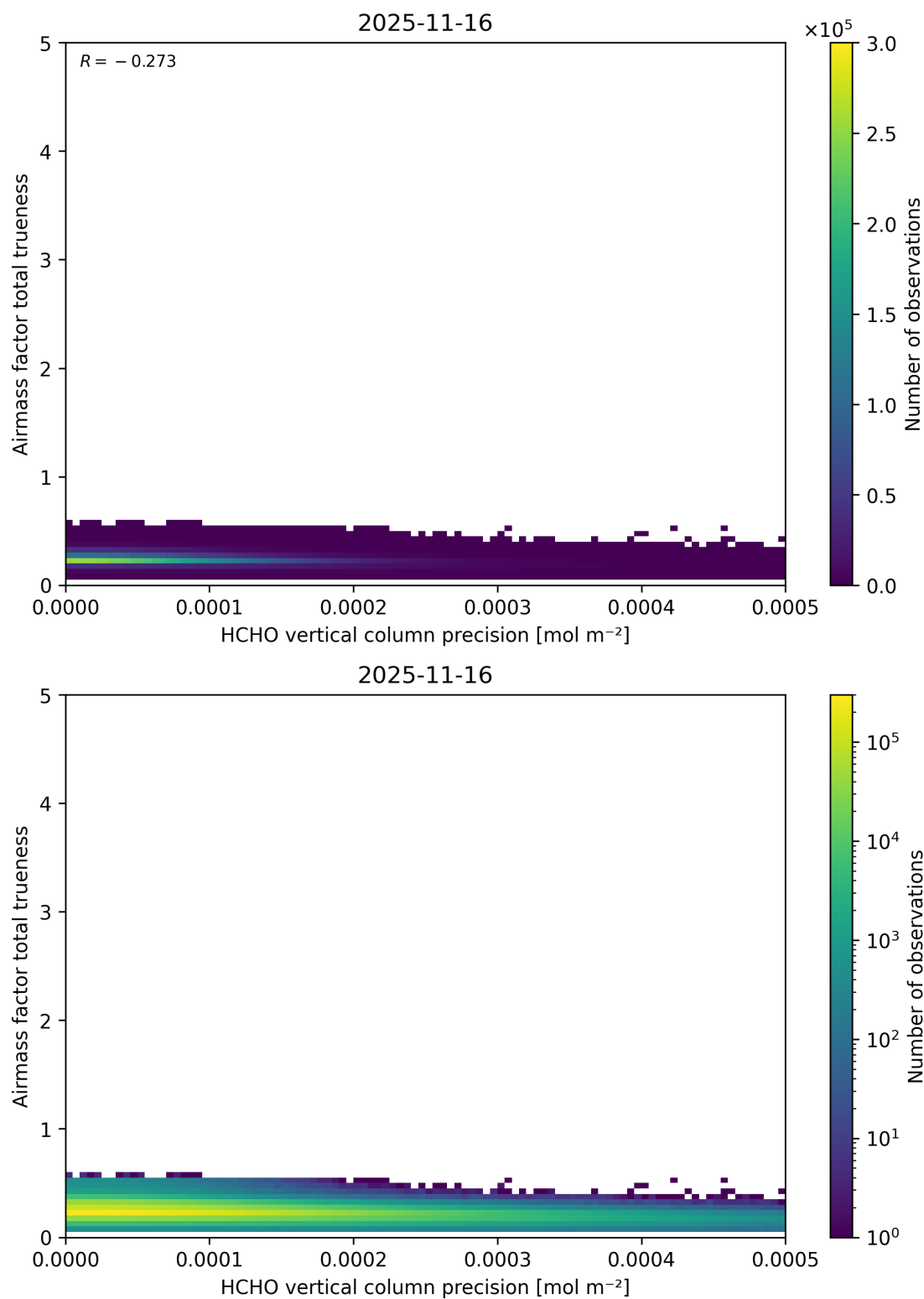
Figure 161: Scatter density plot of “HCHO vertical column precision” against “Airmass factor total trueness” for 2025-11-15 to 2025-11-17.
