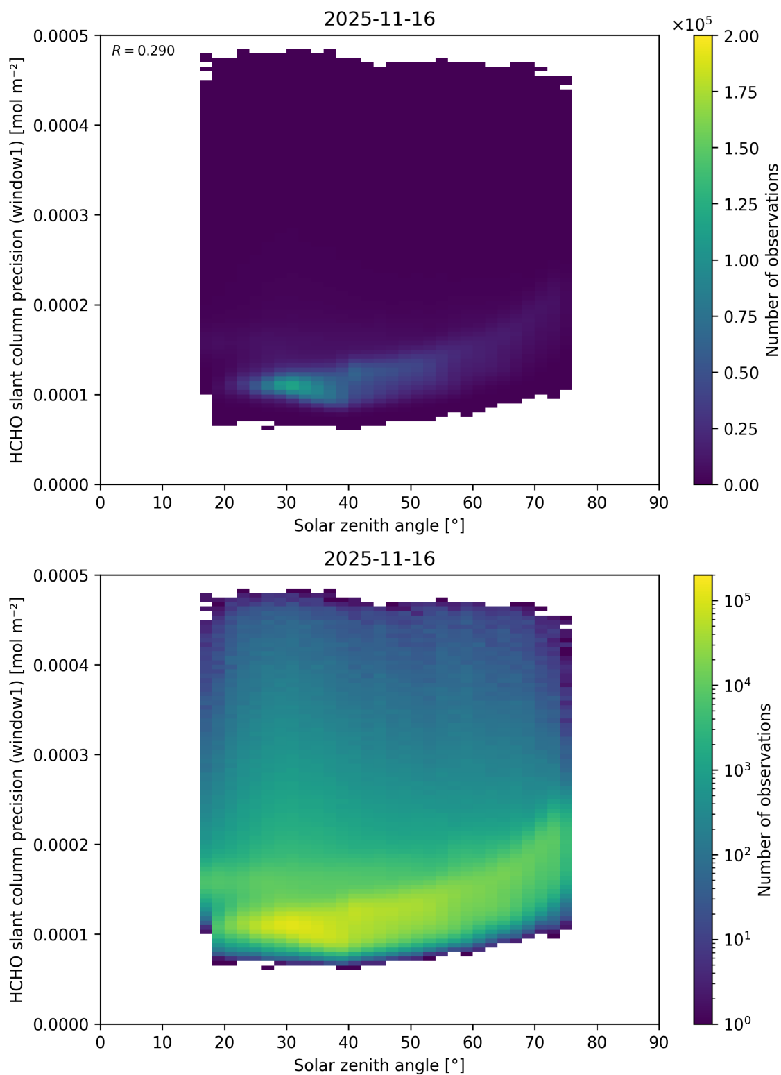
Figure 193: Scatter density plot of “Solar zenith angle” against “HCHO slant column precision (window1)” for 2025-11-15 to 2025-11-17.
