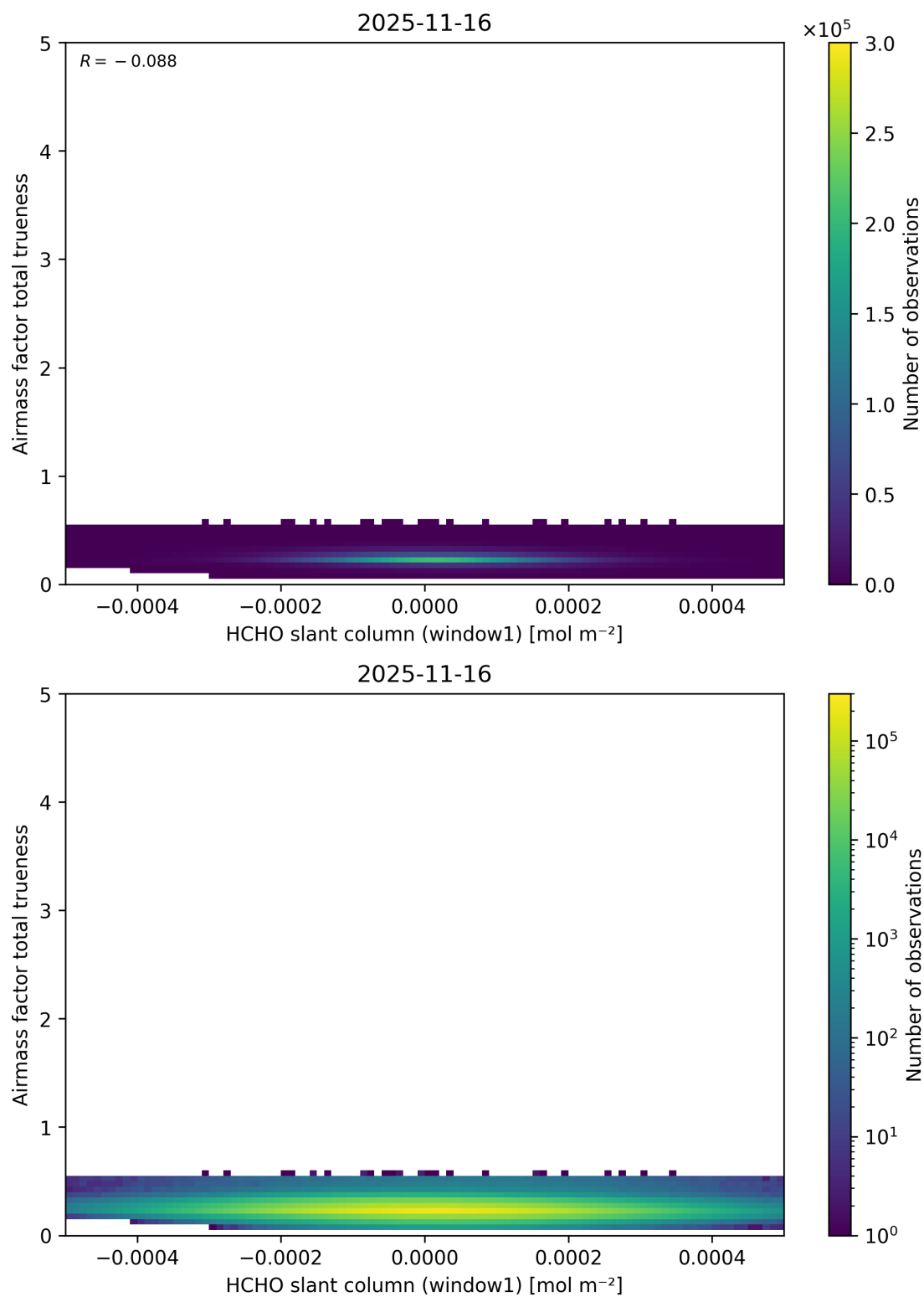
Figure 96: Scatter density plot of “HCHO slant column (window1)” against “Airmass factor total trueneess” for 2025-11-15 to 2025-11-17.
