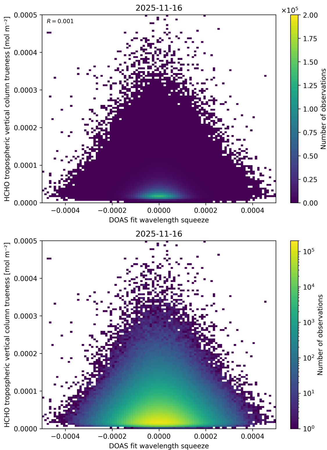
Figure 77: Scatter density plot of “DOAS fit wavelength squeeze” against “HCHO tropospheric vertical column trueness” for 2025-11-15 to 2025-11-17.
