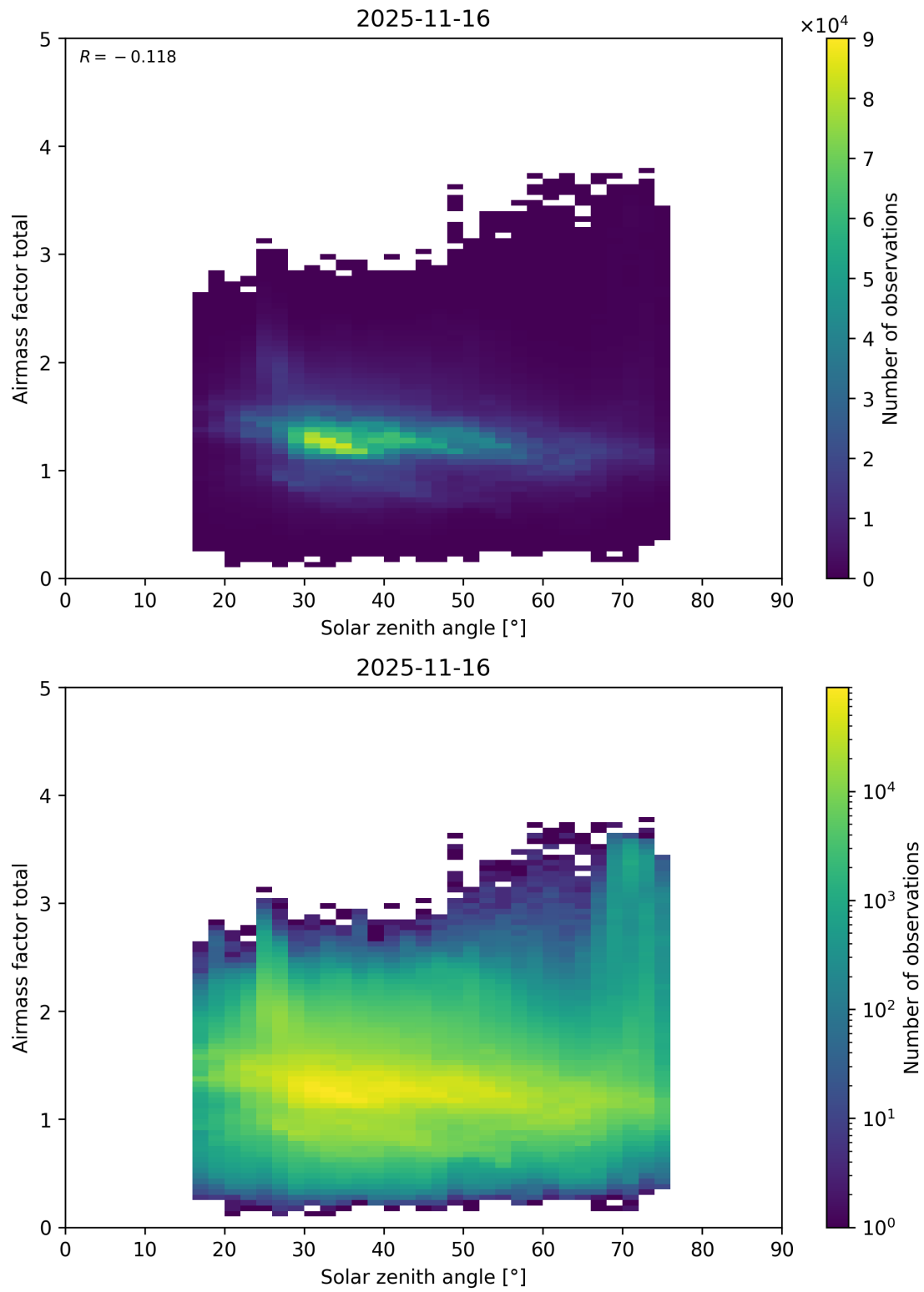
Figure 194: Scatter density plot of “Solar zenith angle” against “Airmass factor total” for 2025-11-15 to 2025-11-17.
