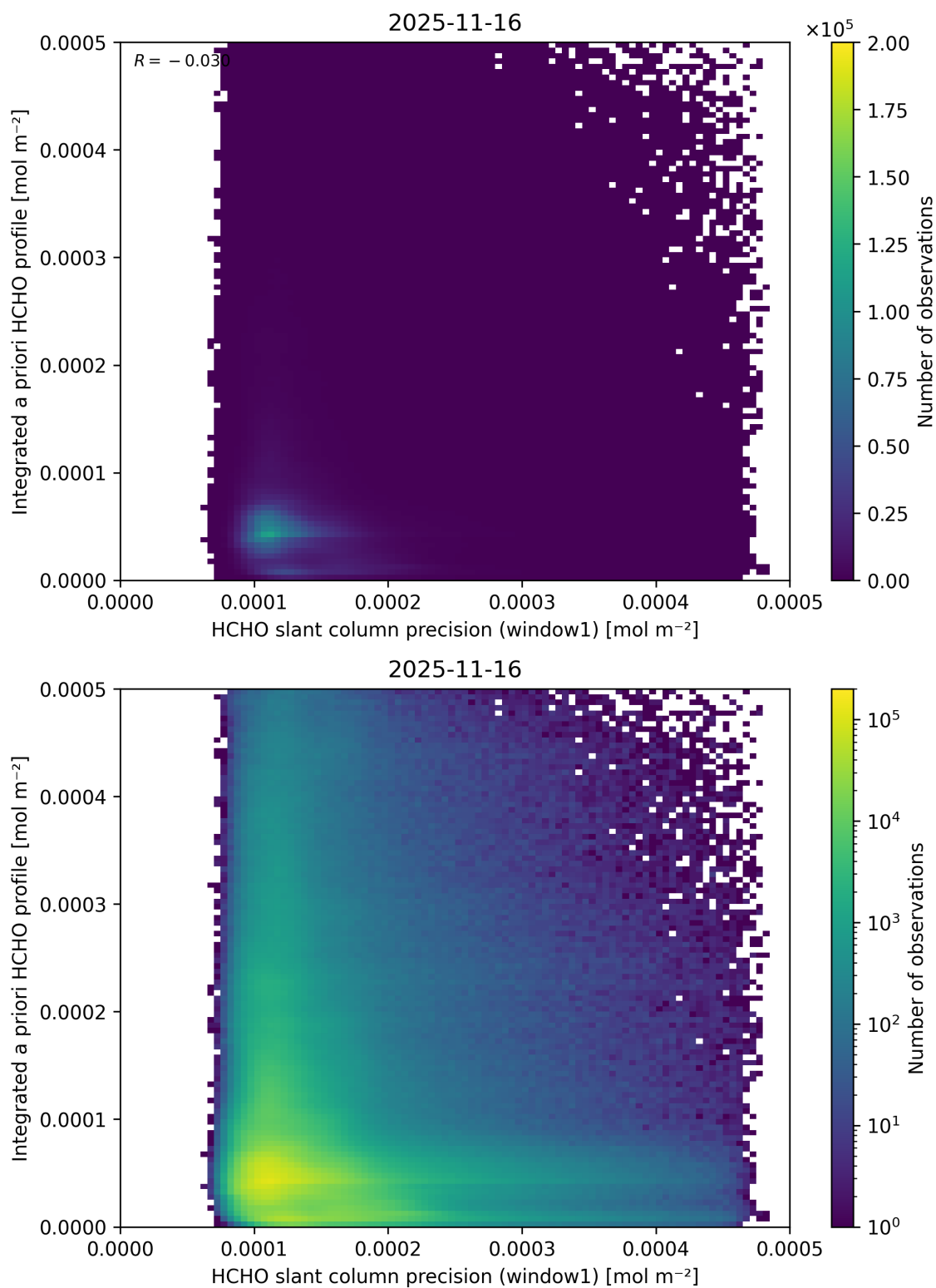
Figure 108: Scatter density plot of “HCHO slant column precision (window1)” against “Integrated a priori HCHO profile” for 2025-11-15 to 2025-11-17.
