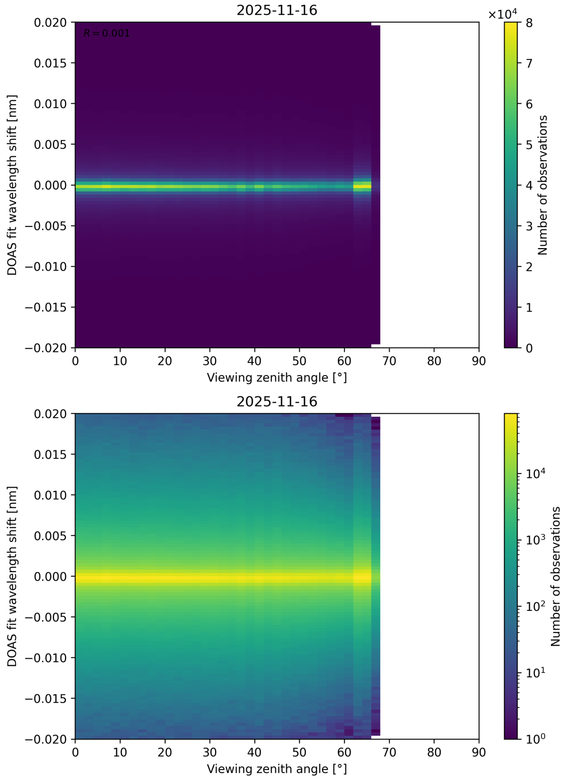
Figure 203: Scatter density plot of “Viewing zenith angle” against “DOAS fit wavelength shift” for 2025-11-15 to 2025-11-17.
