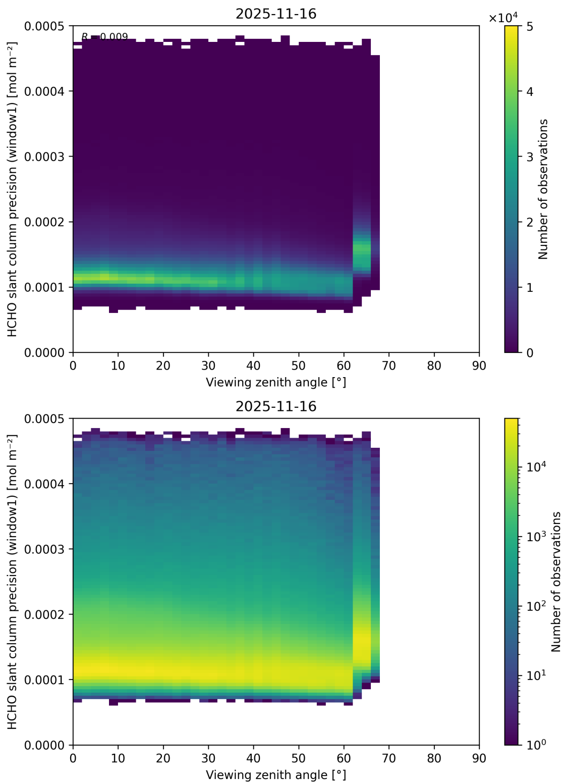
Figure 209: Scatter density plot of “Viewing zenith angle” against “HCHO slant column precision (window1)” for 2025-11-15 to 2025-11-17.
