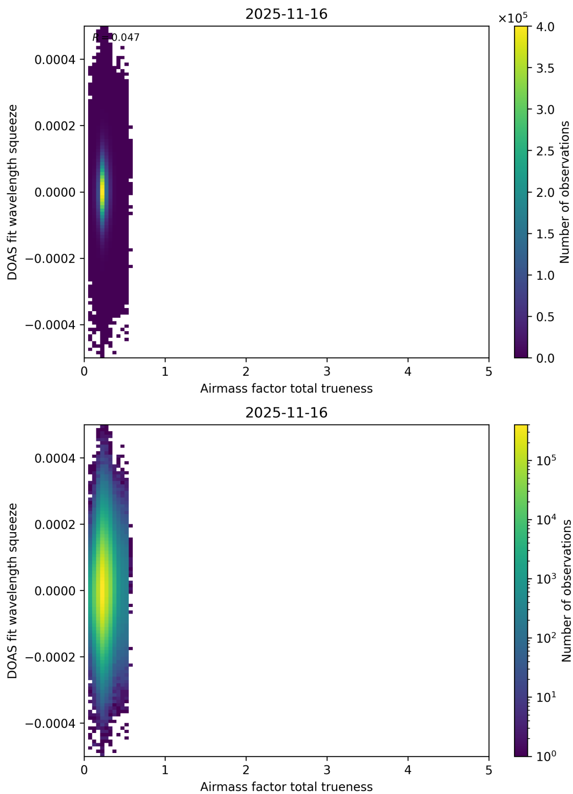
Figure 120: Scatter density plot of “Airmass factor total trueness” against “DOAS fit wavelength squeeze” for 2025-11-15 to 2025-11-17.
