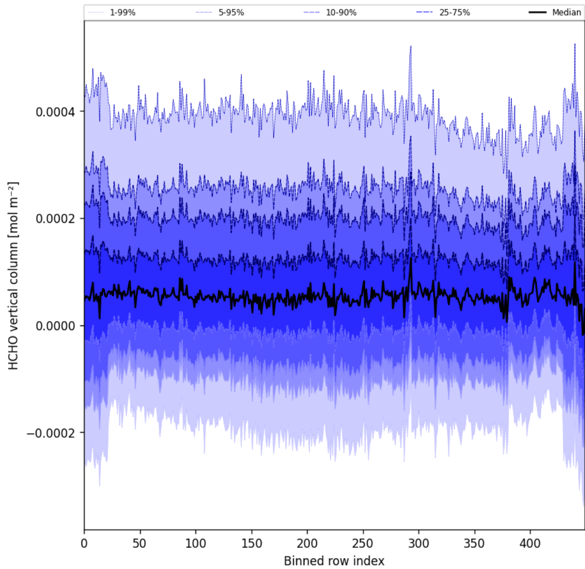
Figure 52: Along track statistics of “HCHO vertical column” for 2025-11-15 to 2025-11-17
