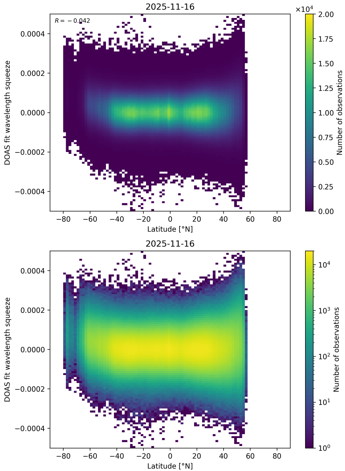
Figure 173: Scatter density plot of “Latitude” against “DOAS fit wavelength squeeze” for 2025-11-15 to 2025-11-17.
