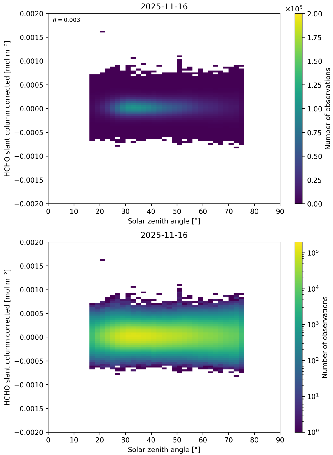
Figure 190: Scatter density plot of “Solar zenith angle” against “HCHO slant column corrected” for 2025-11-15 to 2025-11-17.
