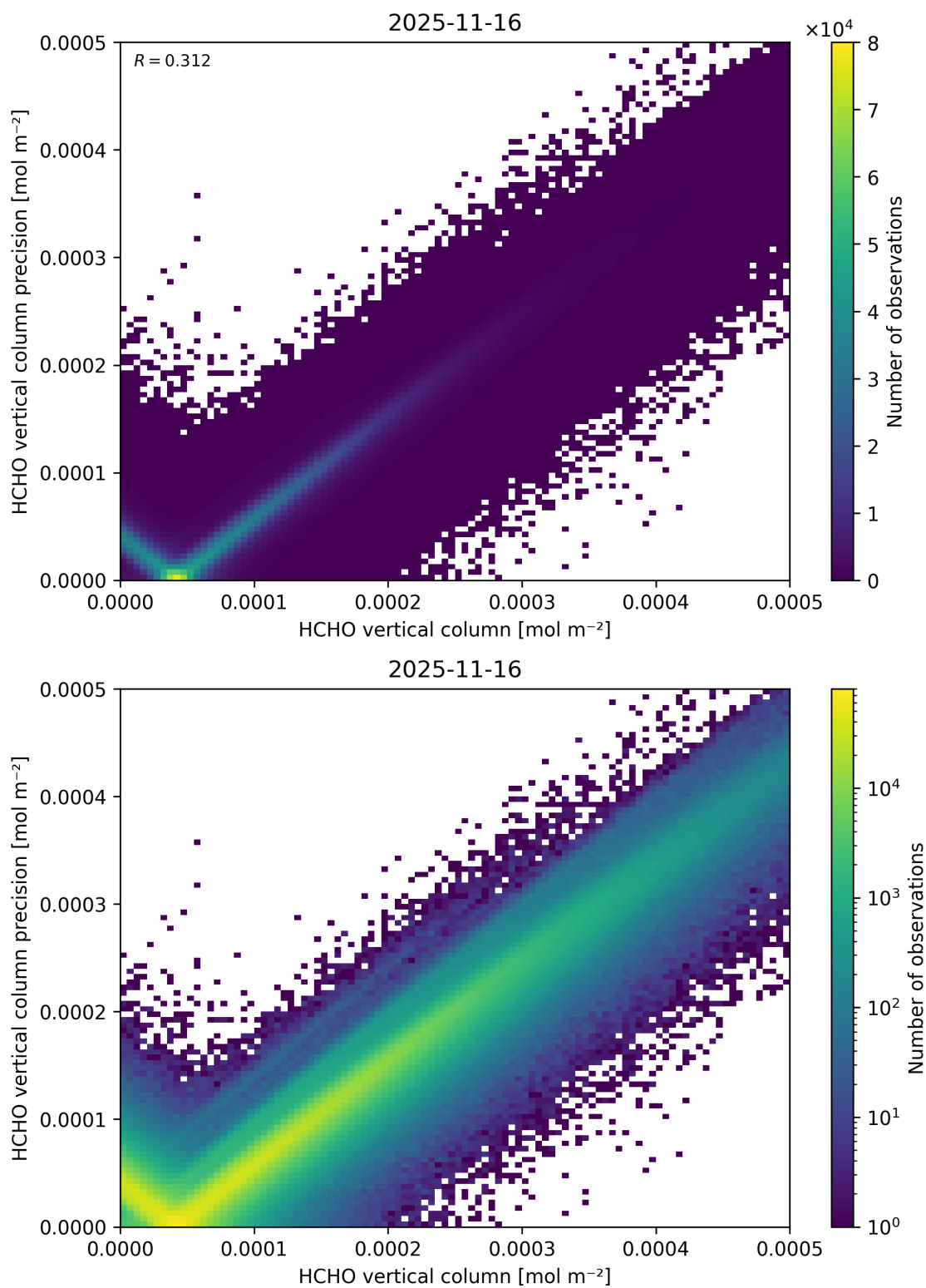
Figure 149: Scatter density plot of “HCHO vertical column” against “HCHO vertical column precision” for 2025-11-15 to 2025-11-17.
