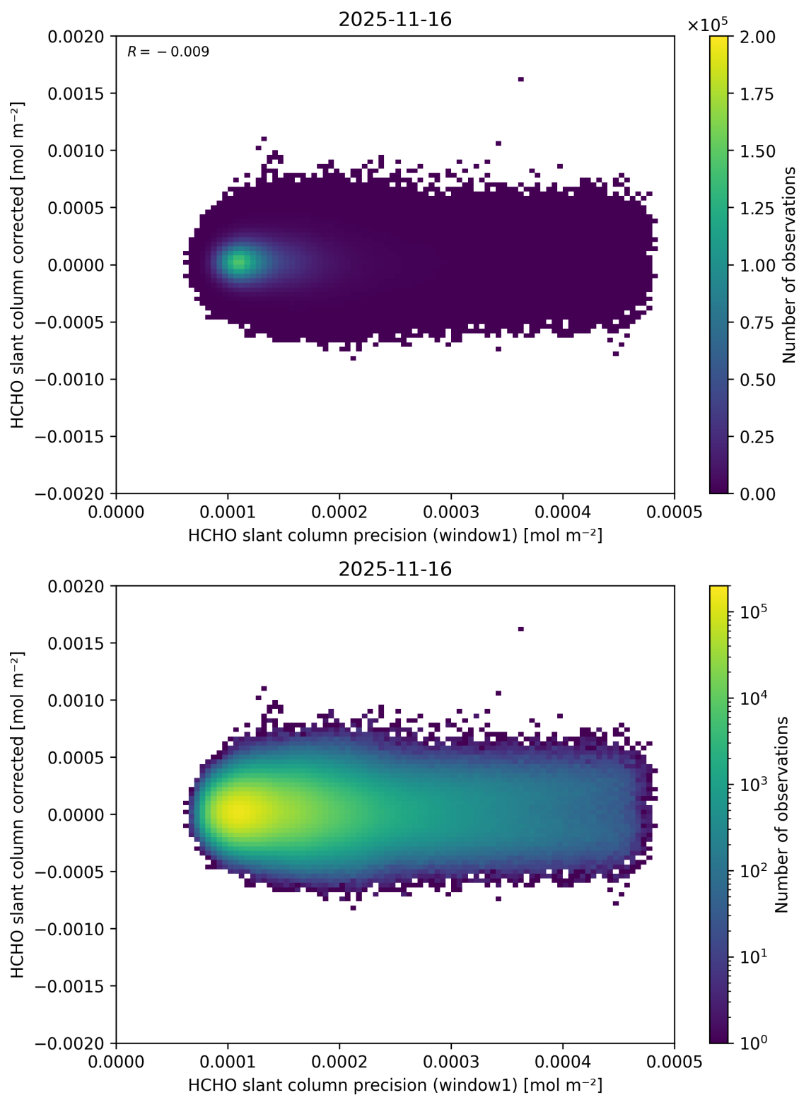
Figure 103: Scatter density plot of “HCHO slant column precision (window1)” against “HCHO slant column corrected” for 2025-11-15 to 2025-11-17.
