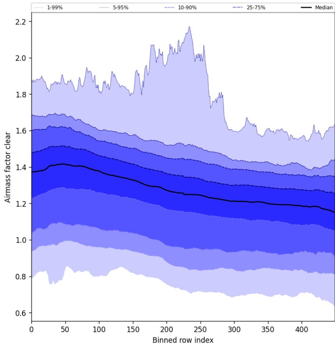
Figure 59: Along track statistics of “Airmass factor clear” for 2025-11-15 to 2025-11-17
