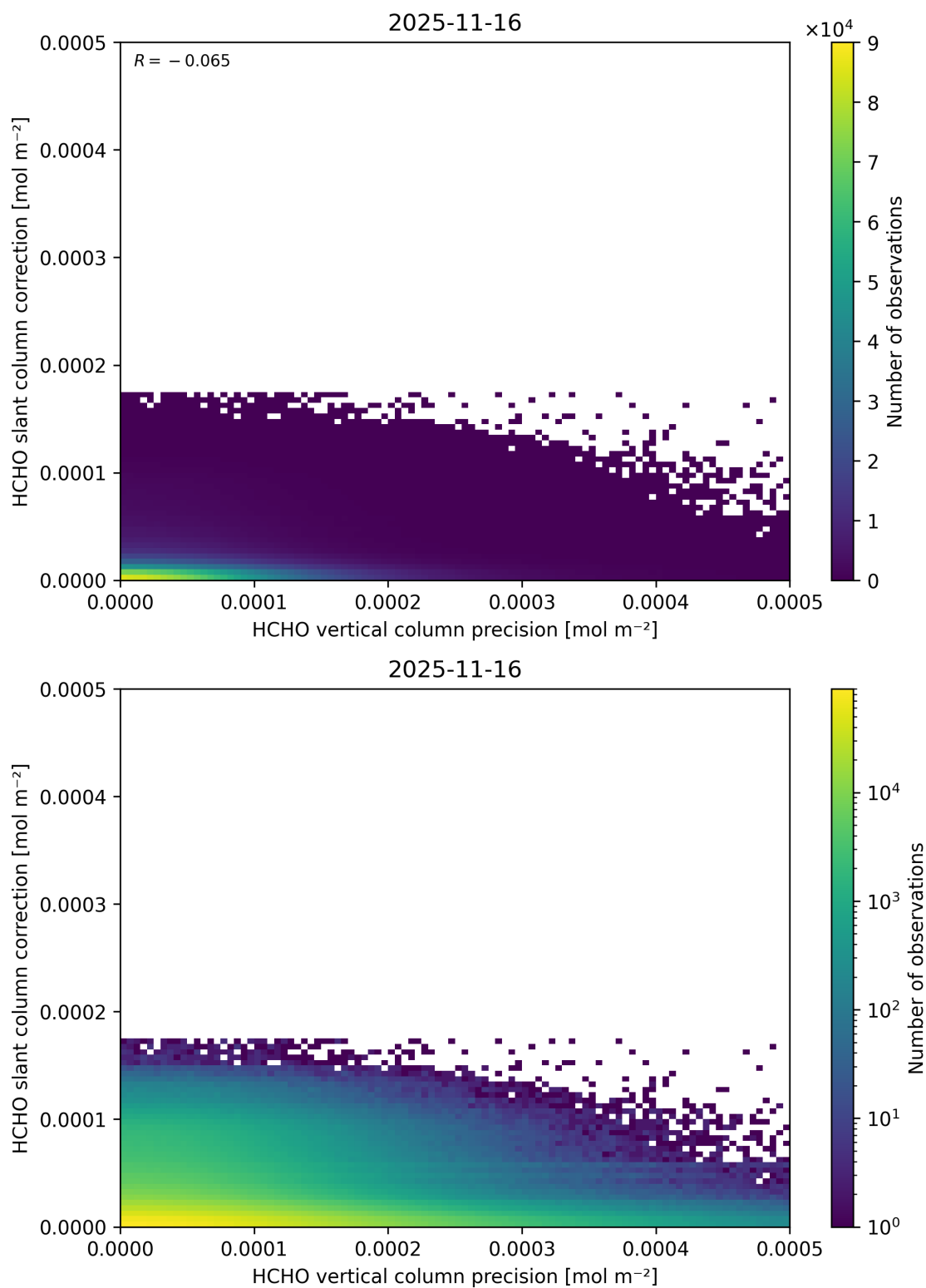
Figure 157: Scatter density plot of “HCHO vertical column precision” against “HCHO slant column correction” for 2025-11-15 to 2025-11-17.
