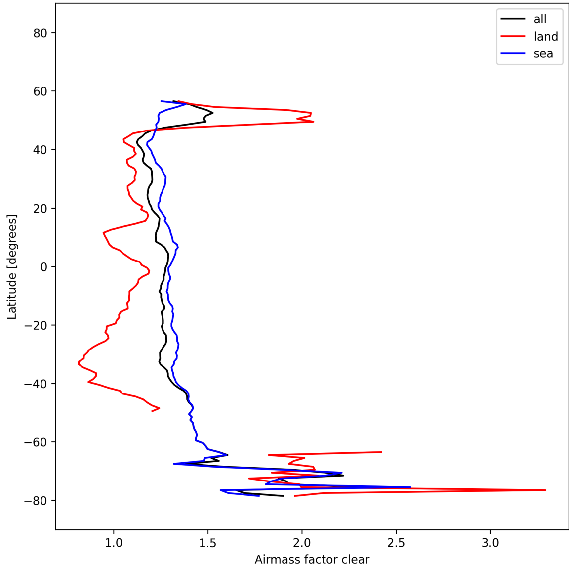
Figure 29: Zonal average of “Airmass factor clear” for 2025-11-15 to 2025-11-17.
