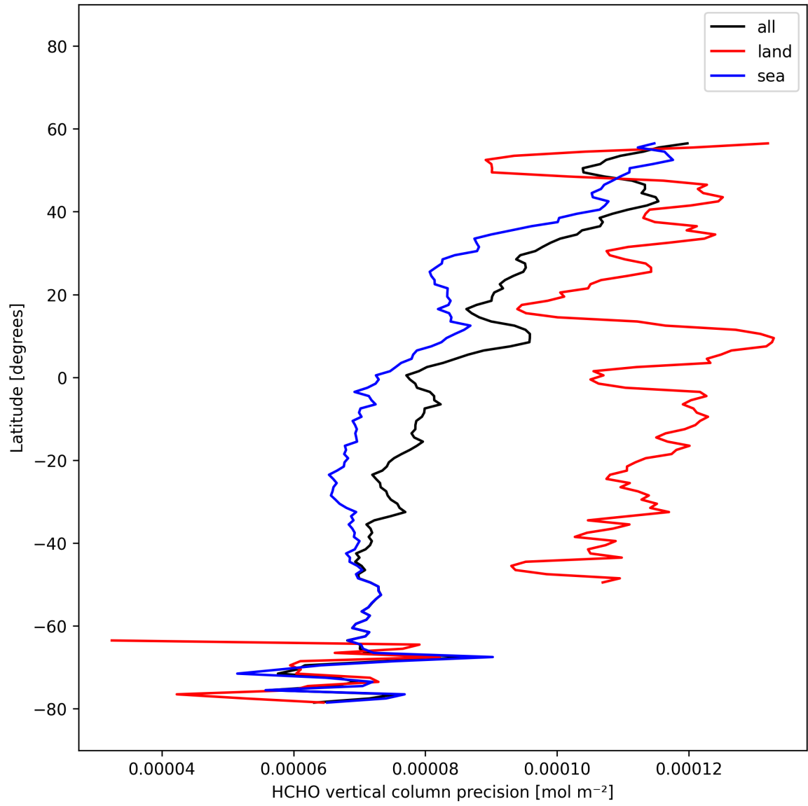
Figure 23: Zonal average of “HCHO vertical column precision” for 2025-11-15 to 2025-11-17.
