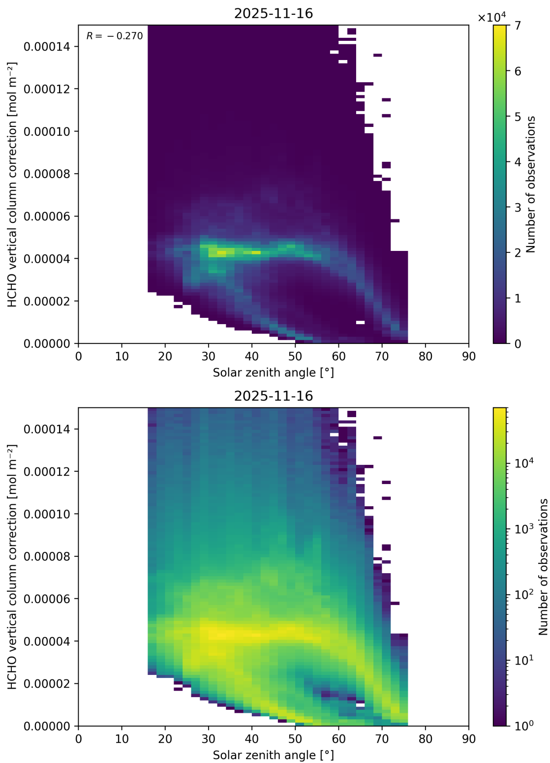
Figure 197: Scatter density plot of “Solar zenith angle” against “HCHO vertical column correction” for 2025-11-15 to 2025-11-17.
