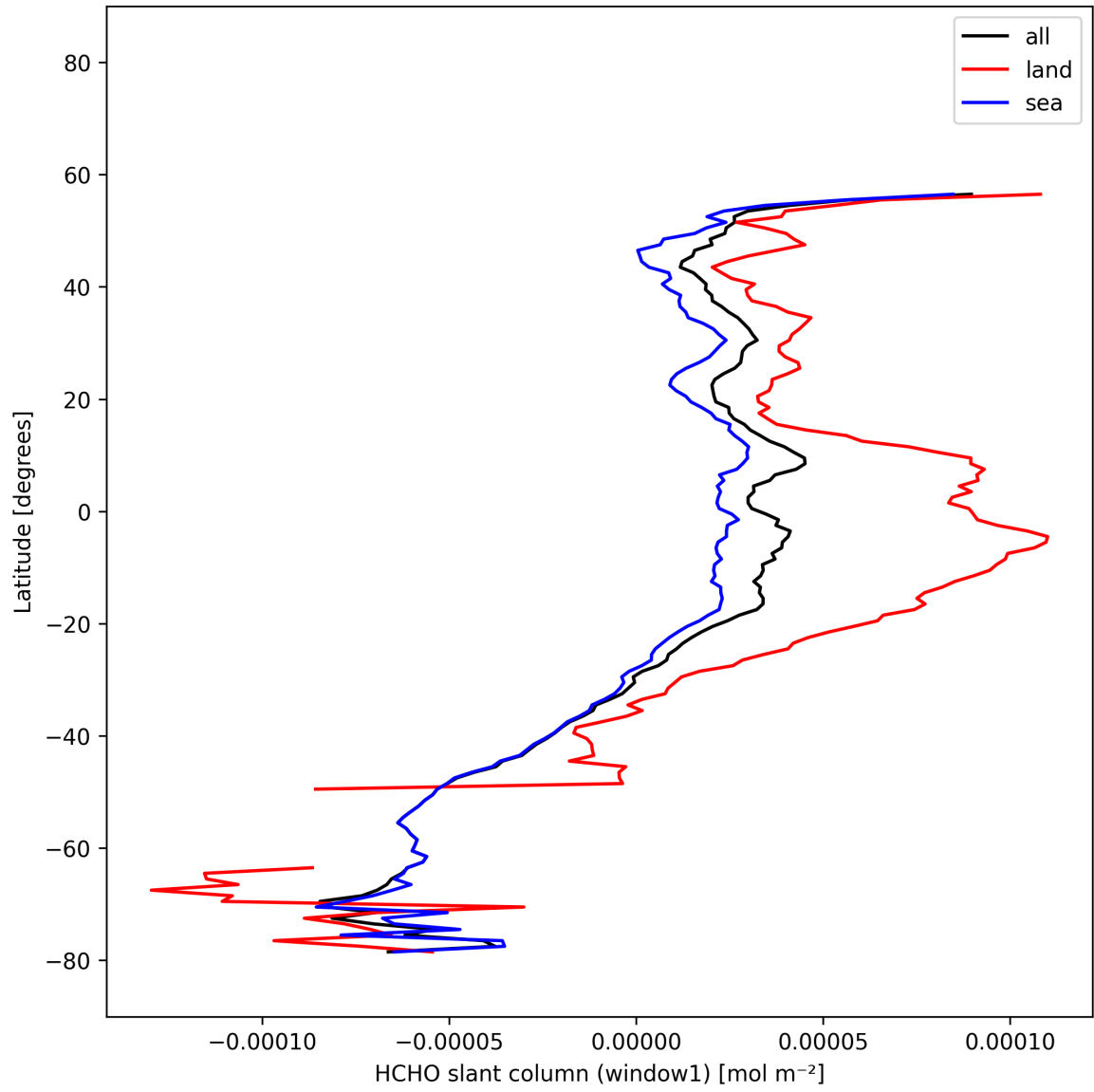
Figure 25: Zonal average of “HCHO slant column (window1)” for 2025-11-15 to 2025-11-17.
