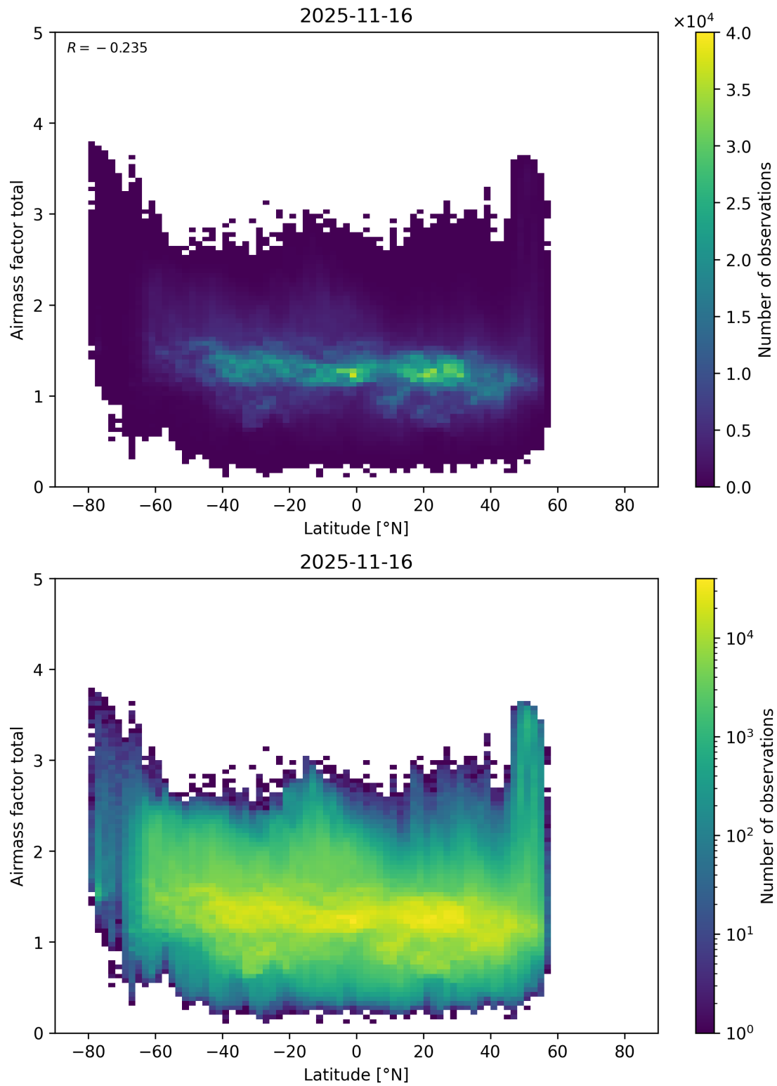
Figure 179: Scatter density plot of “Latitude” against “Airmass factor total” for 2025-11-15 to 2025-11-17.
