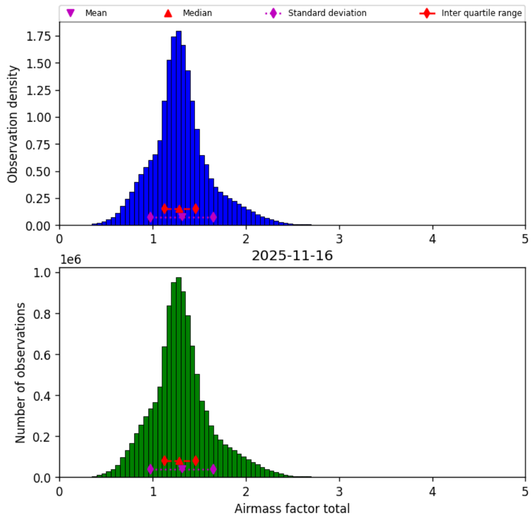
Figure 42: Histogram of “Airmass factor total” for 2025-11-15 to 2025-11-17
