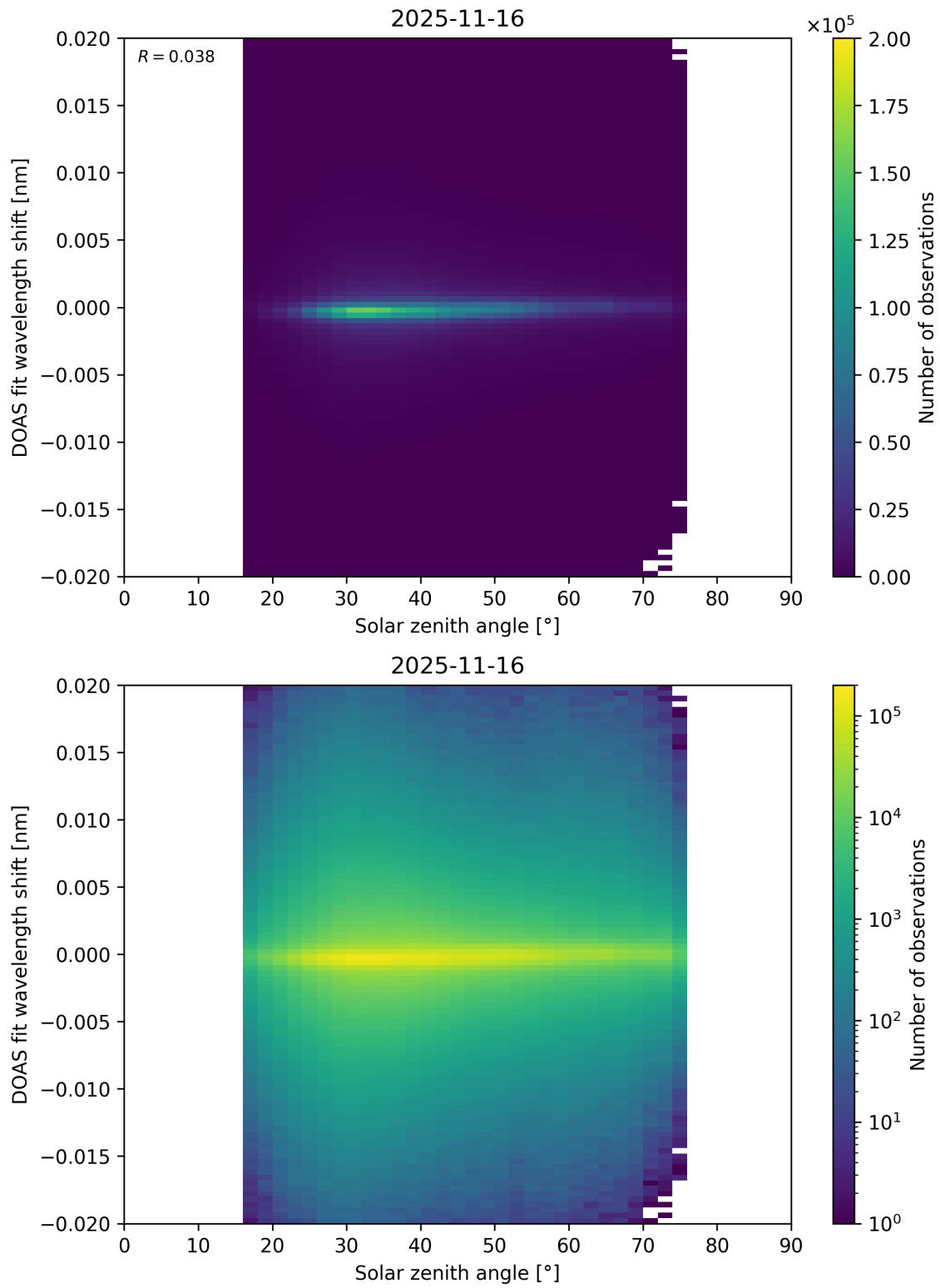
Figure 187: Scatter density plot of “Solar zenith angle” against “DOAS fit wavelength shift” for 2025-11-15 to 2025-11-17.
