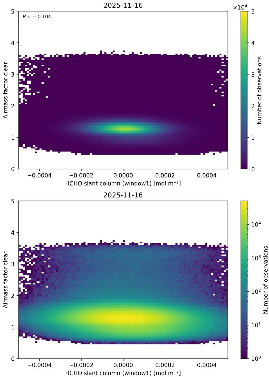
Figure 91: Scatter density plot of “HCHO slant column (window1)” against “Airmass factor clear” for 2025-11-15 to 2025-11-17.
