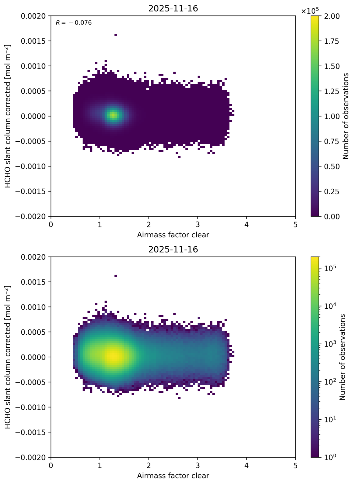
Figure 81: Scatter density plot of “Airmass factor clear” against “HCHO slant column corrected” for 2025-11-15 to 2025-11-17.
