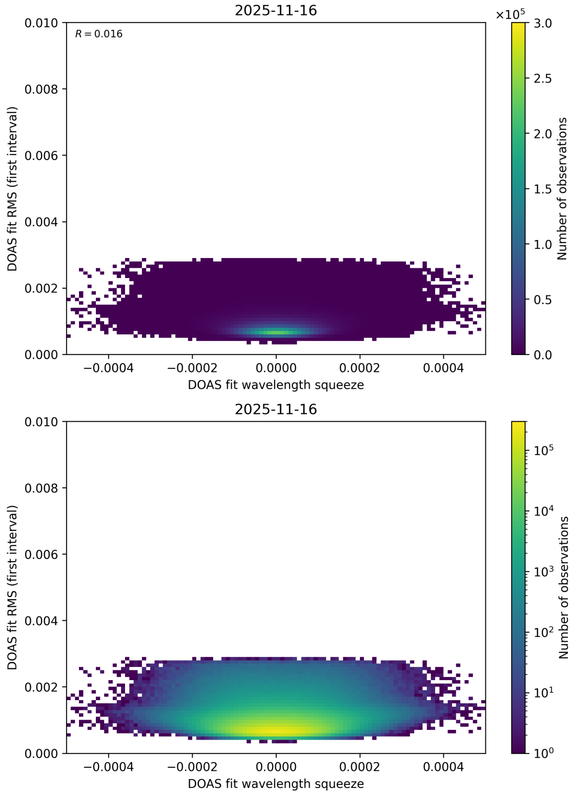
Figure 74: Scatter density plot of “DOAS fit wavelength squeeze” against “DOAS fit RMS (first interval)” for 2025-11-15 to 2025-11-17.
