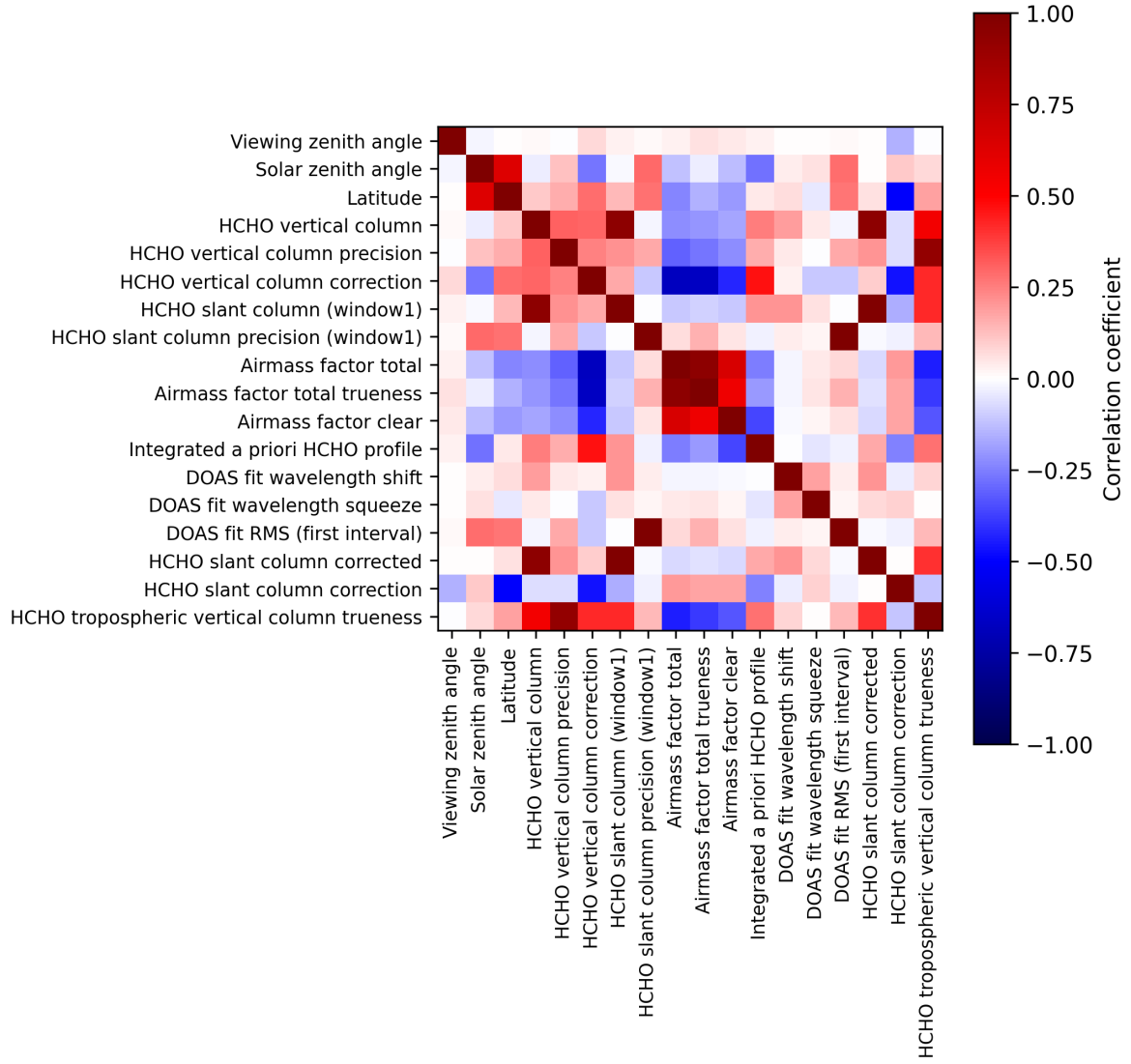
Figure 2: Map of correlation matrix for 2025-11-15 to 2025-11-17.
