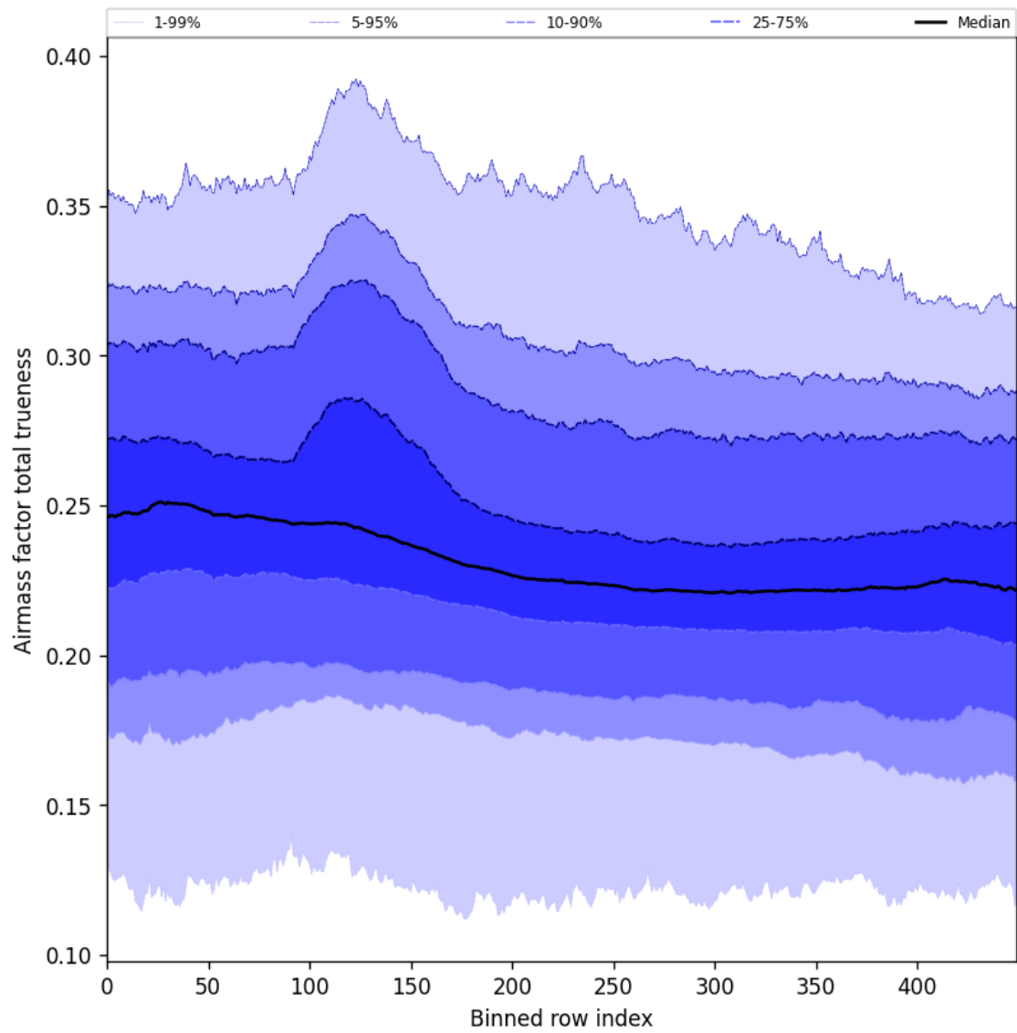
Figure 58: Along track statistics of “Airmass factor total trueness” for 2025-11-15 to 2025-11-17
