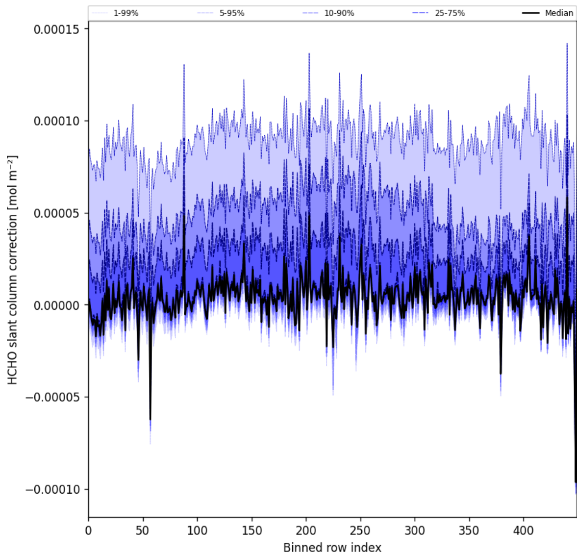
Figure 64: Along track statistics of “HCHO slant column correction” for 2025-11-15 to 2025-11-17
