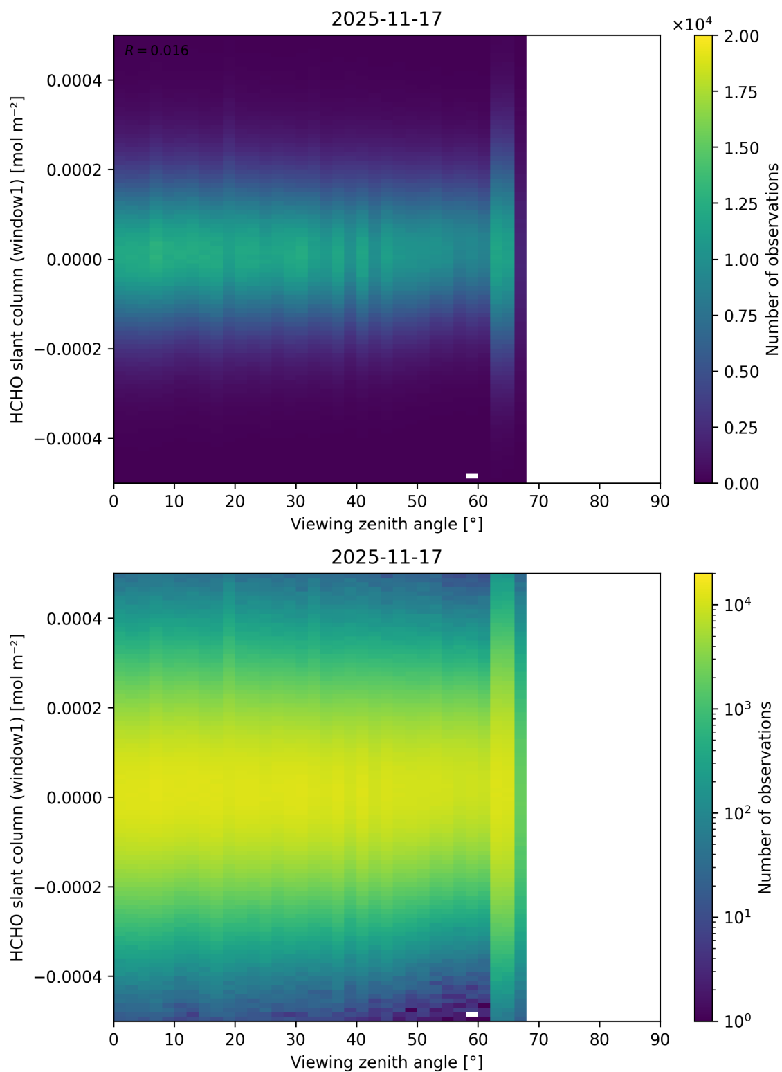
Figure 208: Scatter density plot of “Viewing zenith angle” against “HCHO slant column (window1)” for 2025-11-16 to 2025-11-18.
