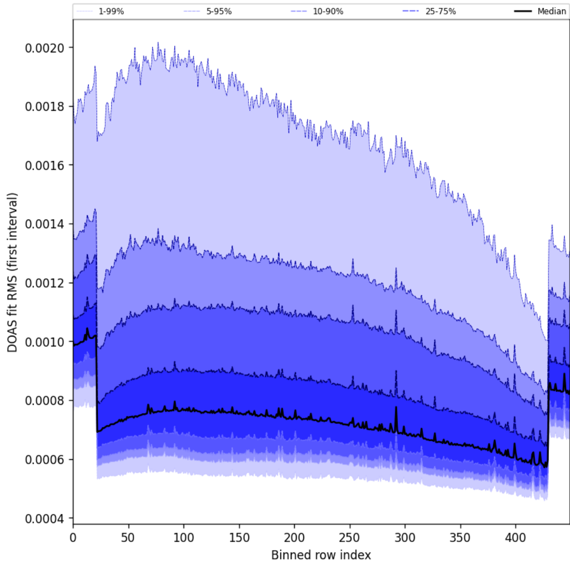
Figure 63: Along track statistics of “DOAS fit RMS (first interval)” for 2025-11-16 to 2025-11-18
