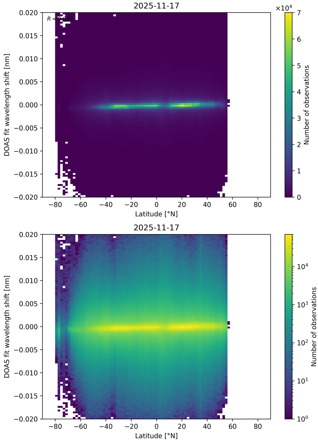
Figure 172: Scatter density plot of “Latitude” against “DOAS fit wavelength shift” for 2025-11-16 to 2025-11-18.
