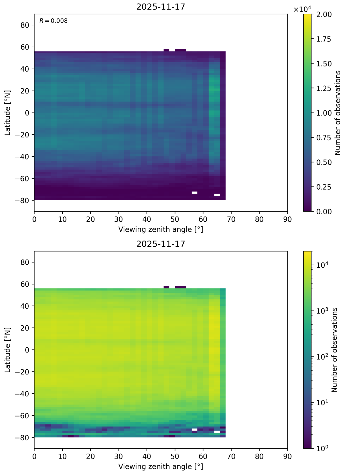
Figure 217: Scatter density plot of “Viewing zenith angle” against “Latitude” for 2025-11-16 to 2025-11-18.
