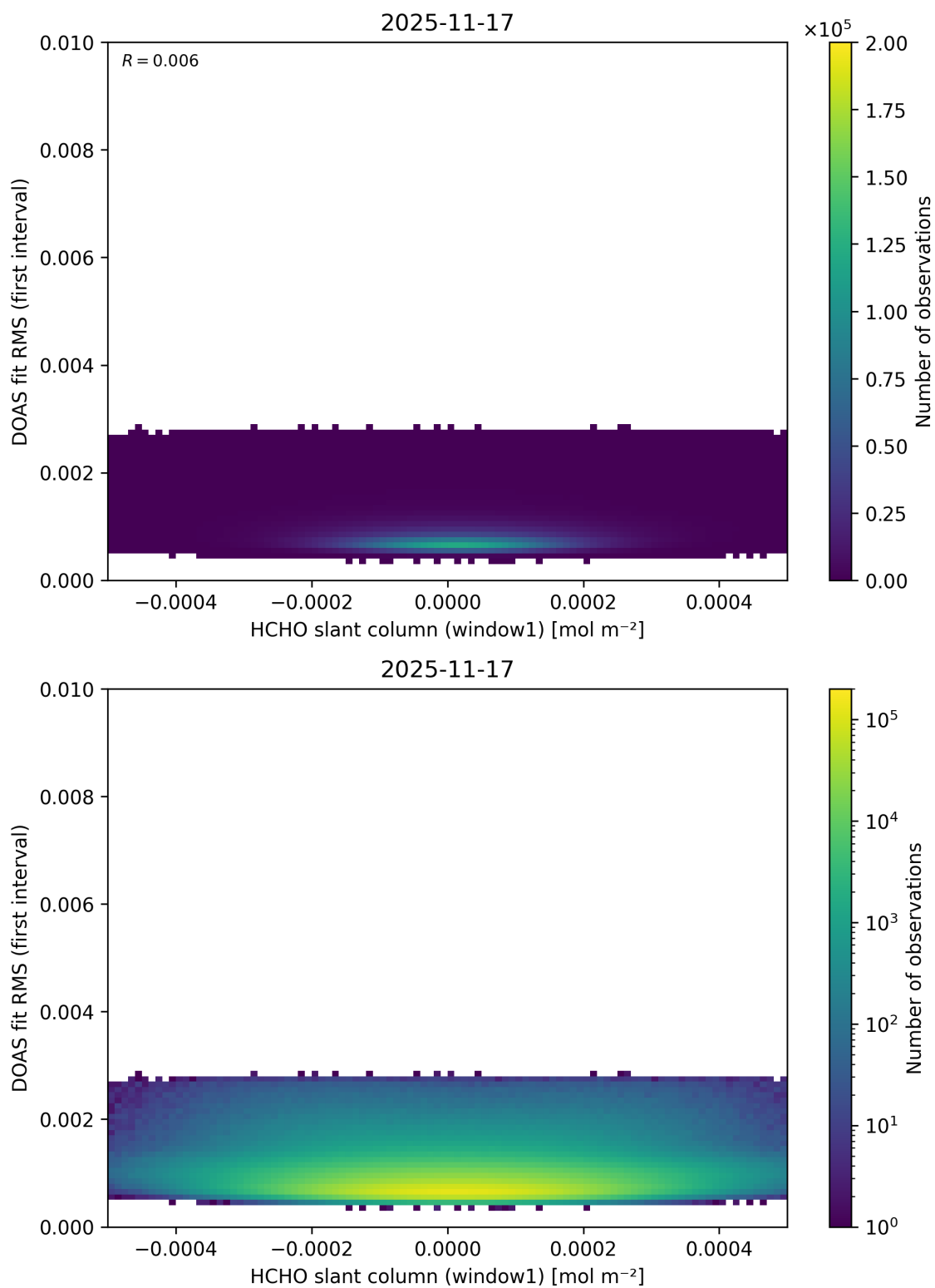
Figure 88: Scatter density plot of “HCHO slant column (window1)” against “DOAS fit RMS (first interval)” for 2025-11-16 to 2025-11-18.
