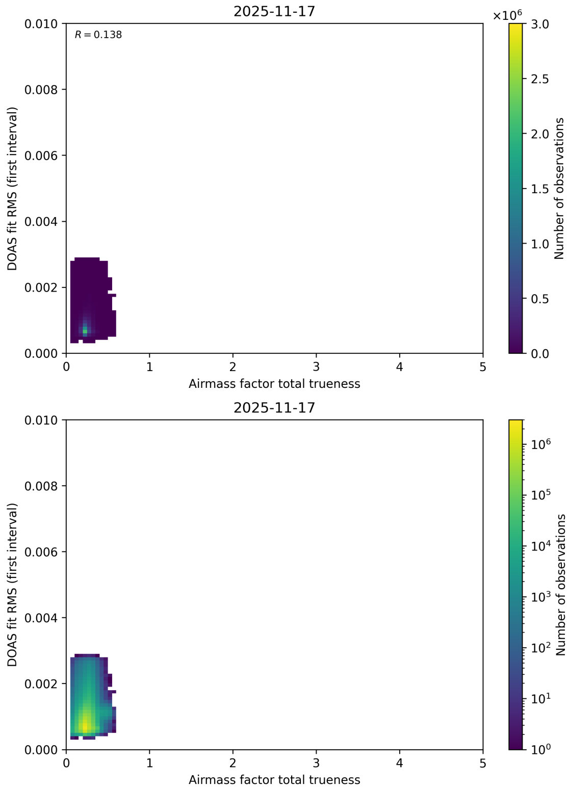
Figure 118: Scatter density plot of “Airmass factor total trueness” against “DOAS fit RMS (first interval)” for 2025-11-16 to 2025-11-18.
