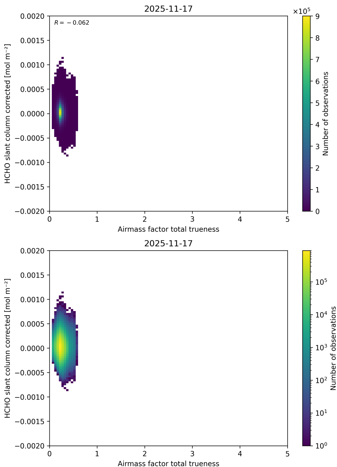
Figure 122: Scatter density plot of “Airmass factor total trueness” against “HCHO slant column corrected” for 2025-11-16 to 2025-11-18.
