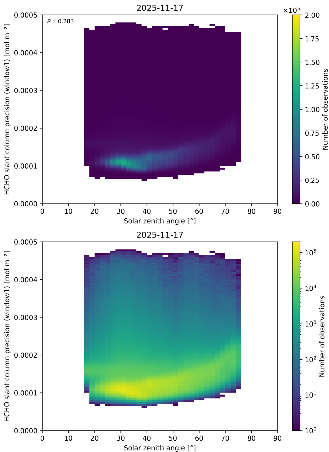
Figure 193: Scatter density plot of “Solar zenith angle” against “HCHO slant column precision (window1)” for 2025-11-16 to 2025-11-18.
