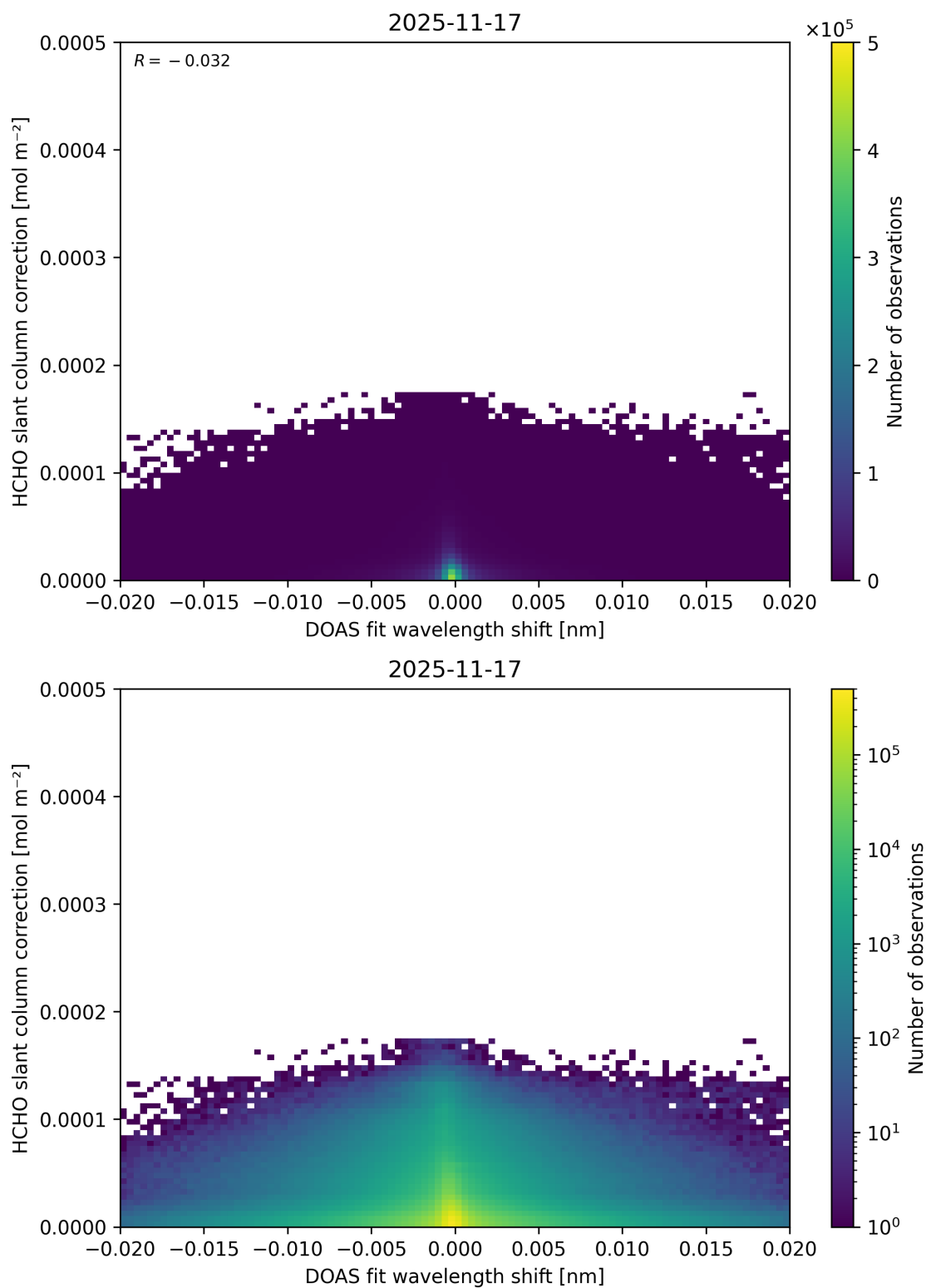
Figure 72: Scatter density plot of “DOAS fit wavelength shift” against “HCHO slant column correction” for 2025-11-16 to 2025-11-18.
