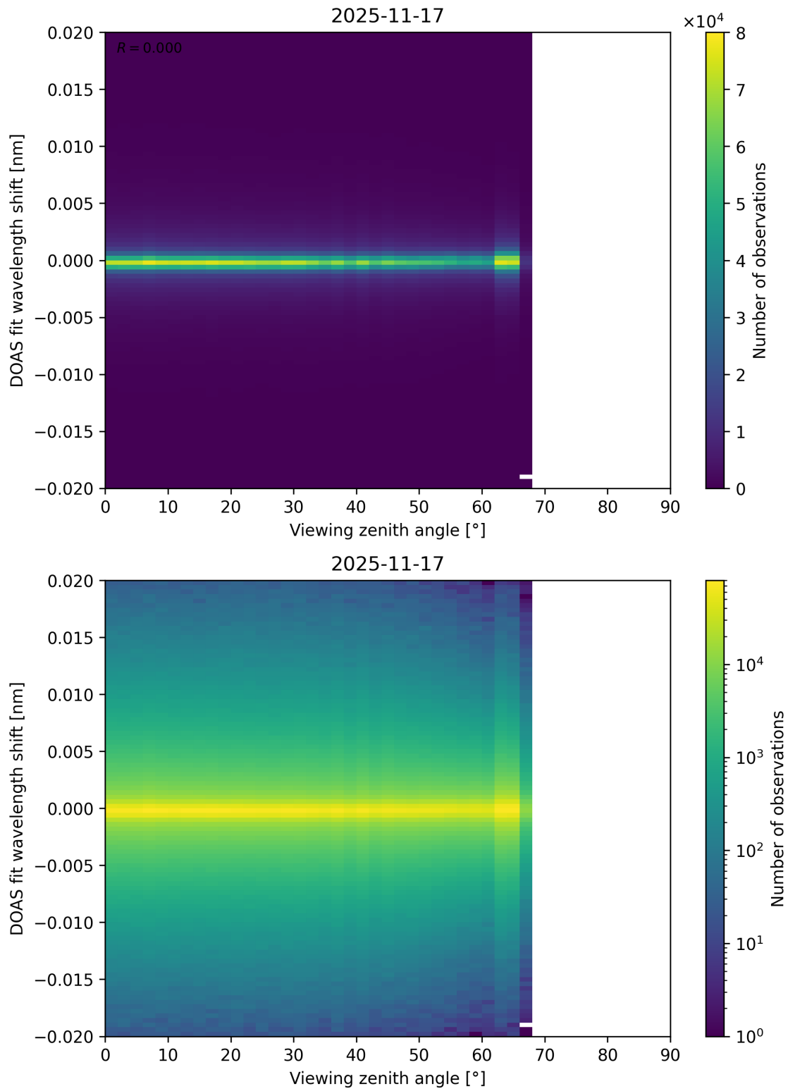
Figure 203: Scatter density plot of “Viewing zenith angle” against “DOAS fit wavelength shift” for 2025-11-16 to 2025-11-18.
