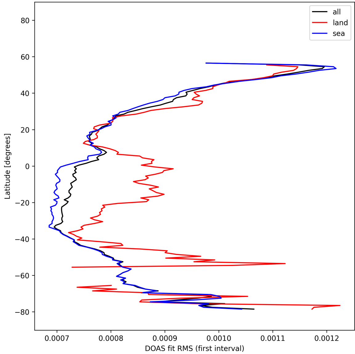
Figure 33: Zonal average of “DOAS fit RMS (first interval)” for 2025-11-16 to 2025-11-18.
