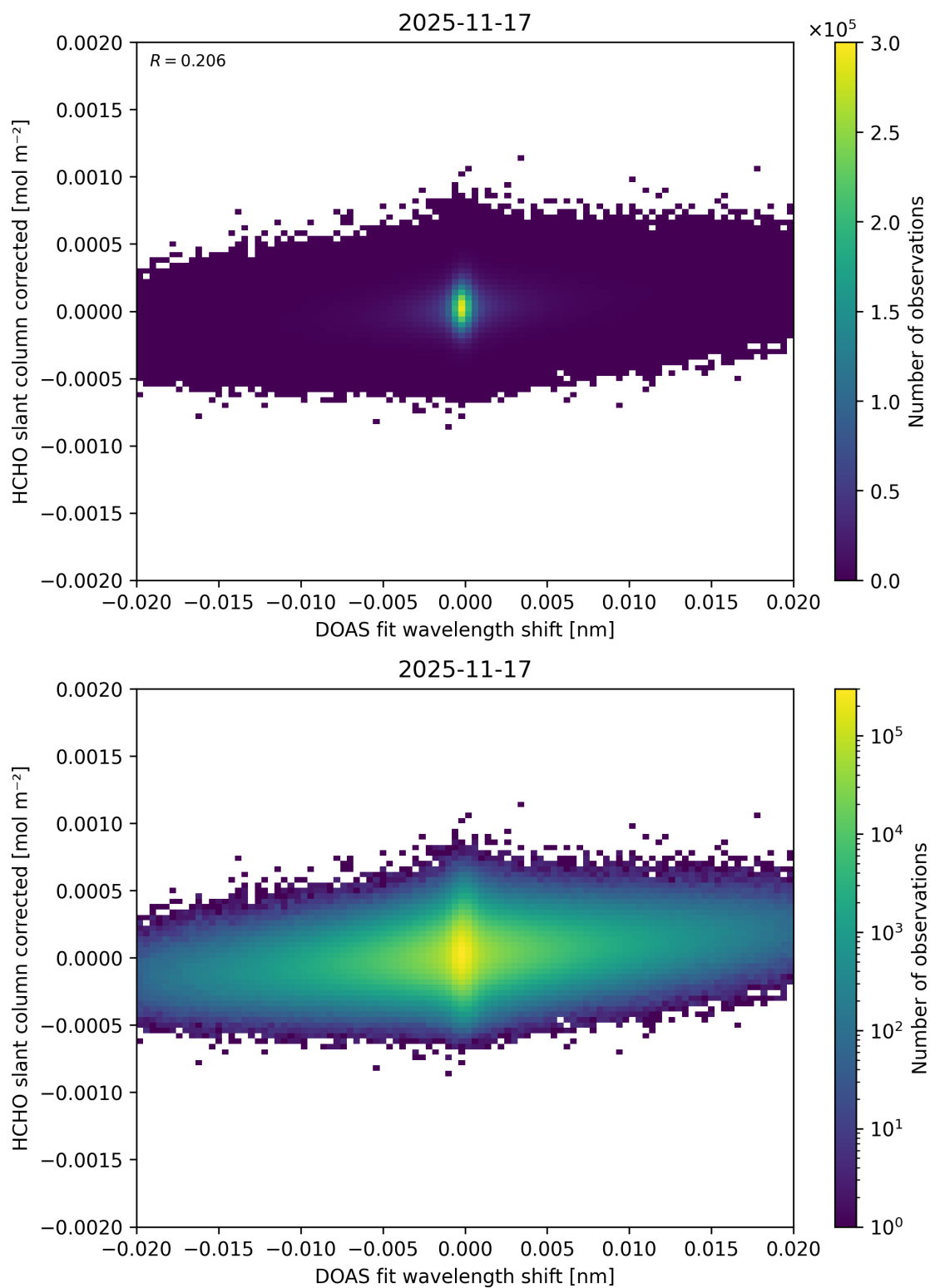
Figure 71: Scatter density plot of “DOAS fit wavelength shift” against “HCHO slant column corrected” for 2025-11-16 to 2025-11-18.
