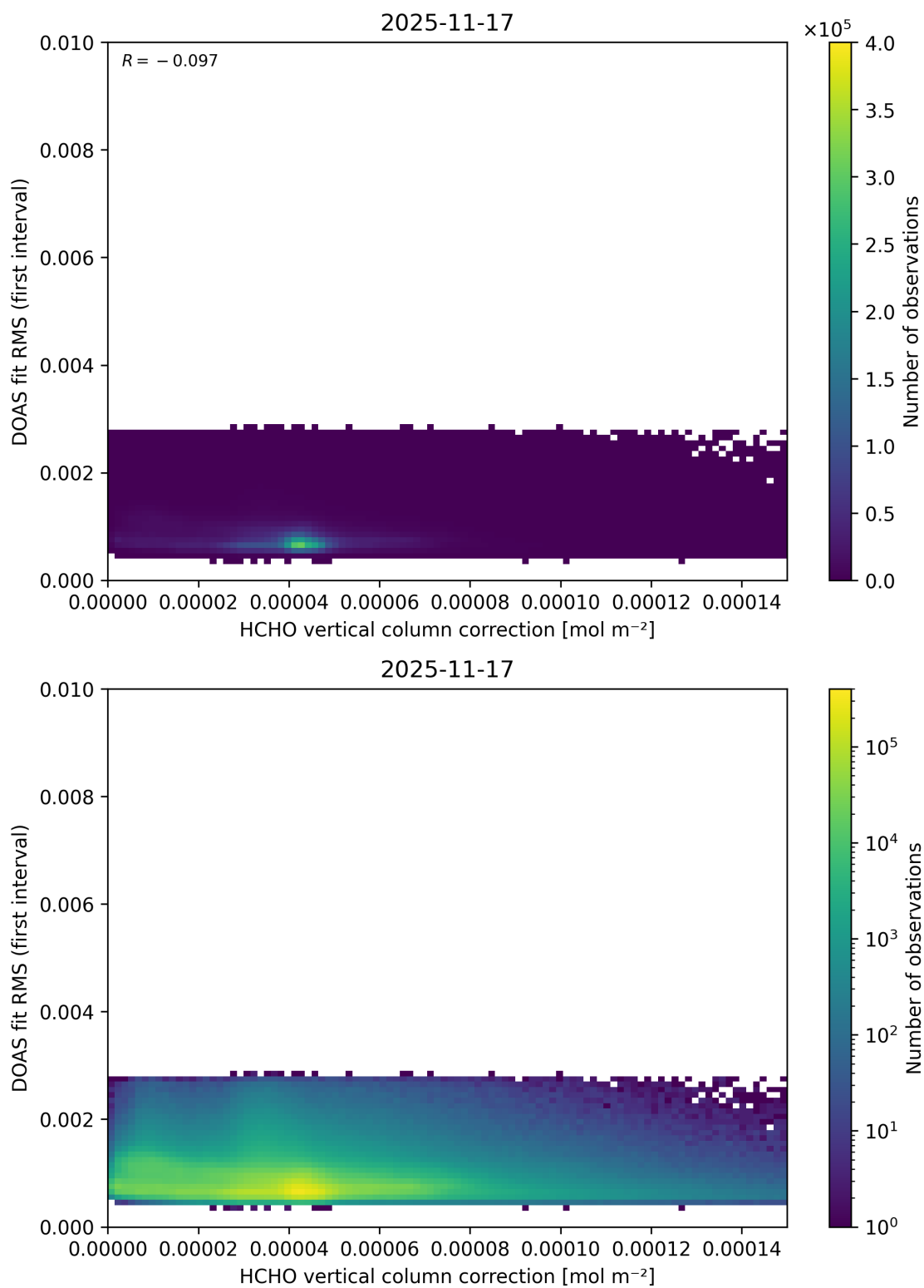
Figure 126: Scatter density plot of “HCHO vertical column correction” against “DOAS fit RMS (first interval)” for 2025-11-16 to 2025-11-18.
