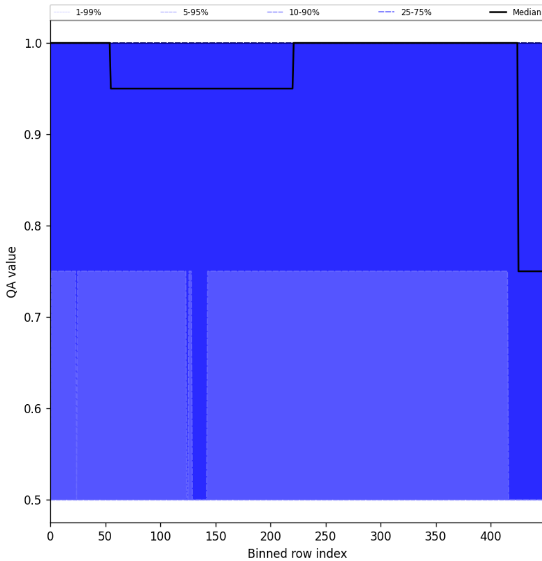
Figure 51: Along track statistics of “QA value” for 2025-11-16 to 2025-11-18
