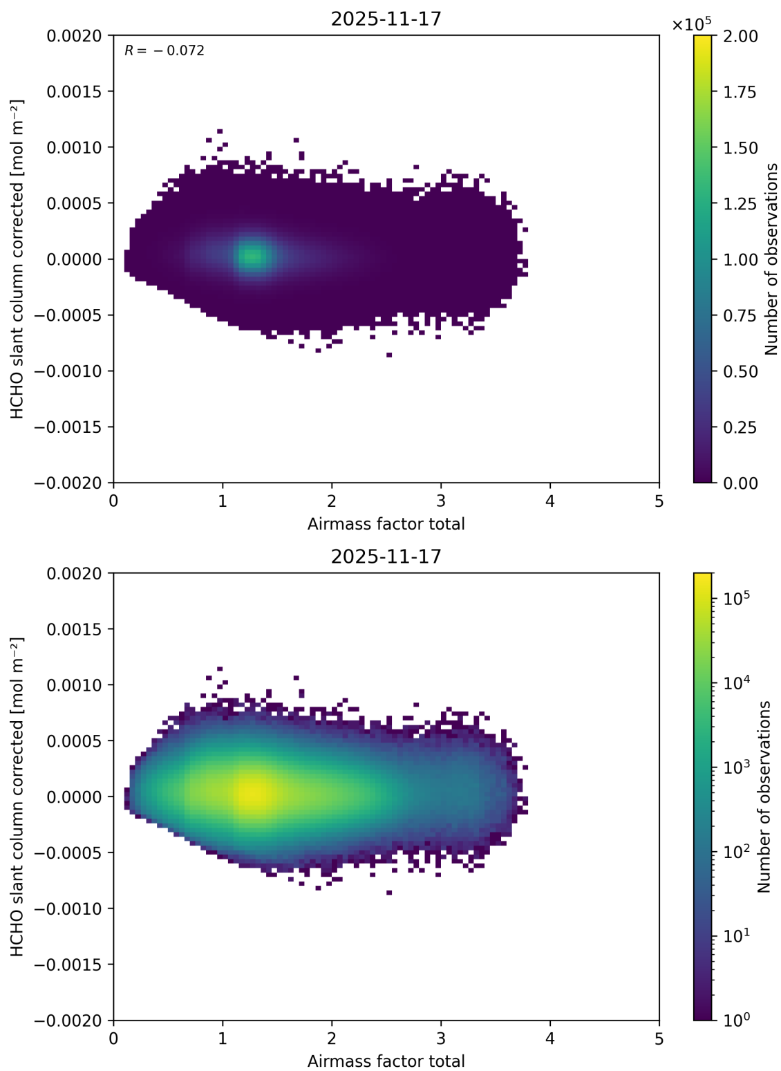
Figure 113: Scatter density plot of “Airmass factor total” against “HCHO slant column corrected” for 2025-11-16 to 2025-11-18.
