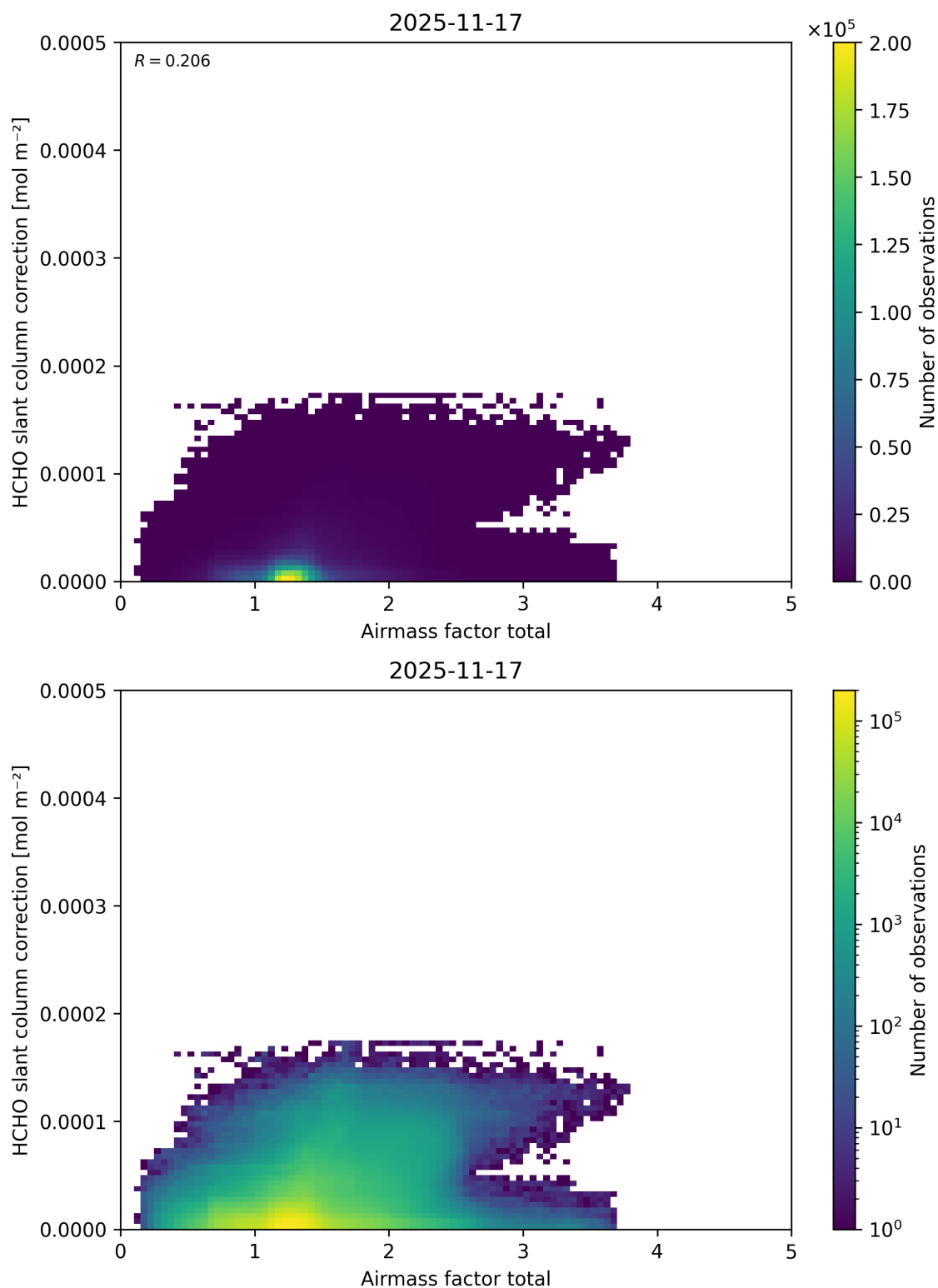
Figure 114: Scatter density plot of “Airmass factor total” against “HCHO slant column correction” for 2025-11-16 to 2025-11-18.
