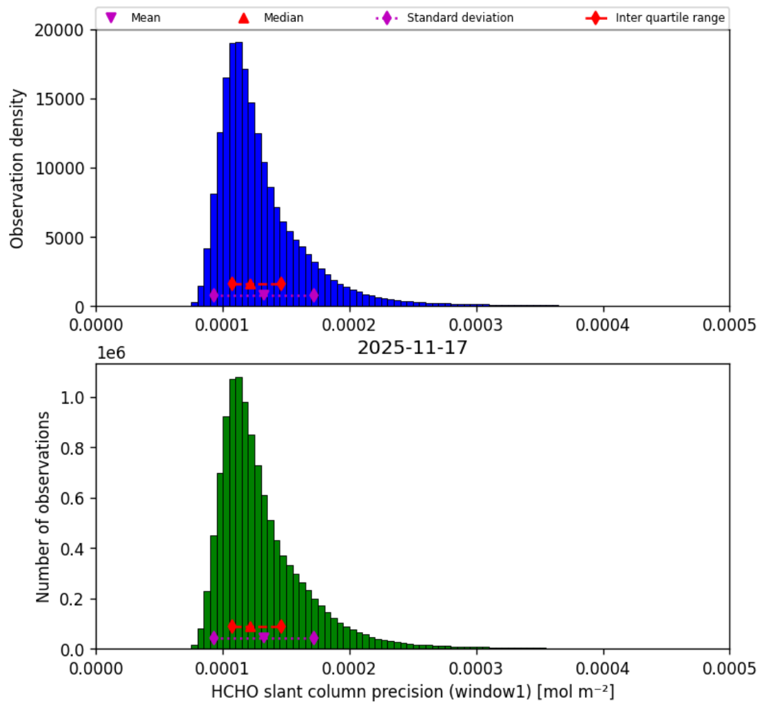
Figure 41: Histogram of “HCHO slant column precision (window1)” for 2025-11-16 to 2025-11-18
