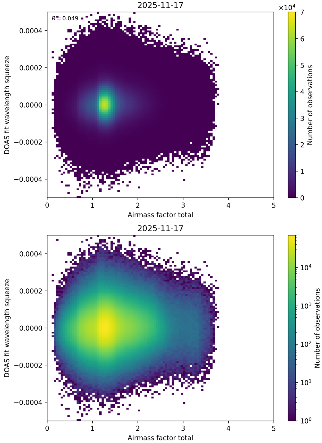
Figure 111: Scatter density plot of “Airmass factor total” against “DOAS fit wavelength squeeze” for 2025-11-16 to 2025-11-18.
