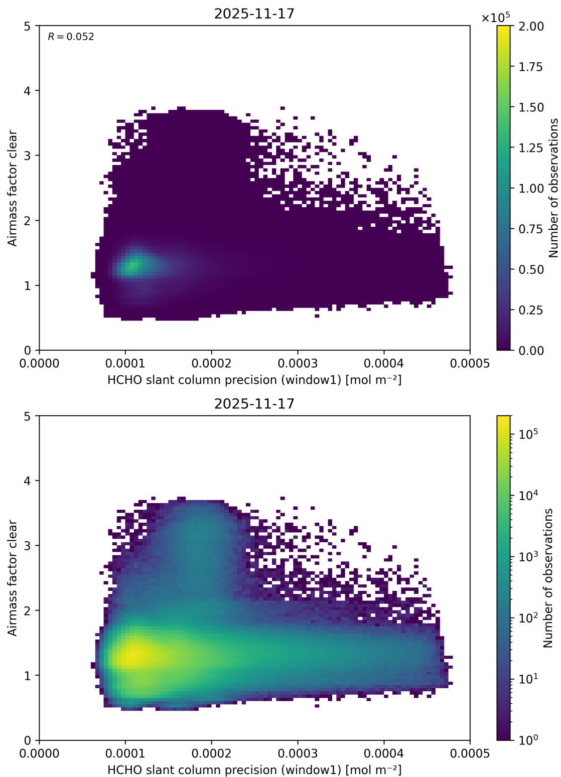
Figure 102: Scatter density plot of “HCHO slant column precision (window1)” against “Airmass factor clear” for 2025-11-16 to 2025-11-18.
