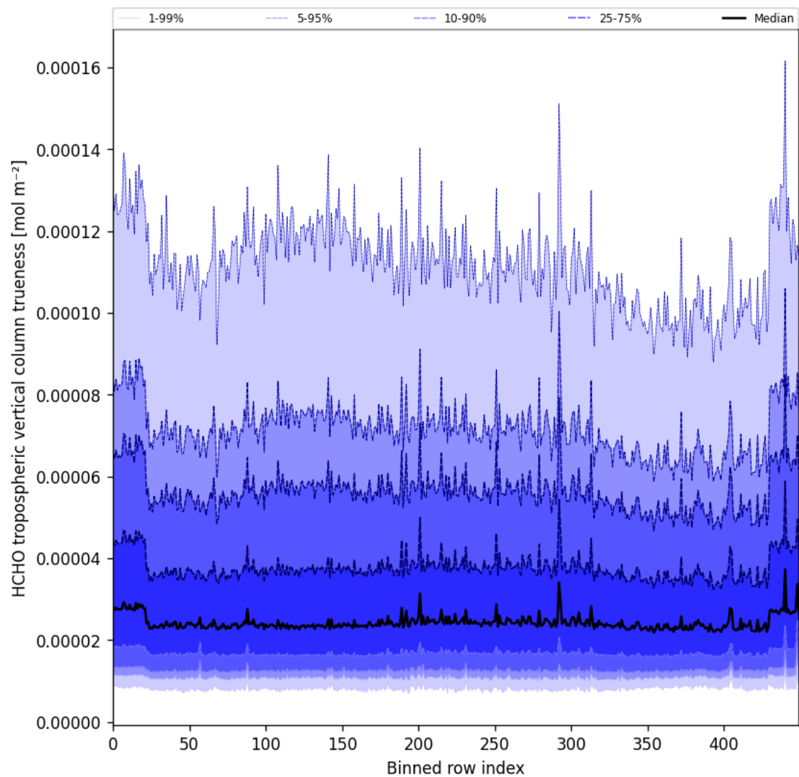
Figure 65: Along track statistics of “HCHO tropospheric vertical column trueness” for 2025-11-16 to 2025-11-18
