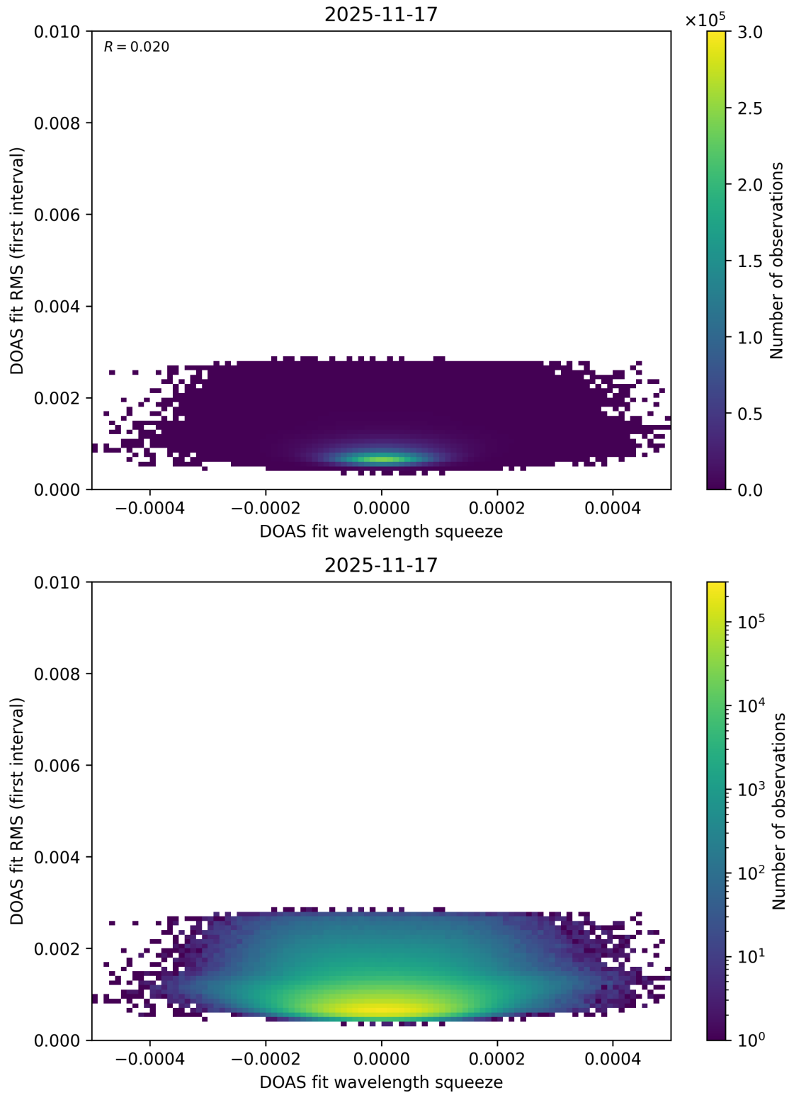
Figure 74: Scatter density plot of “DOAS fit wavelength squeeze” against “DOAS fit RMS (first interval)” for 2025-11-16 to 2025-11-18.
