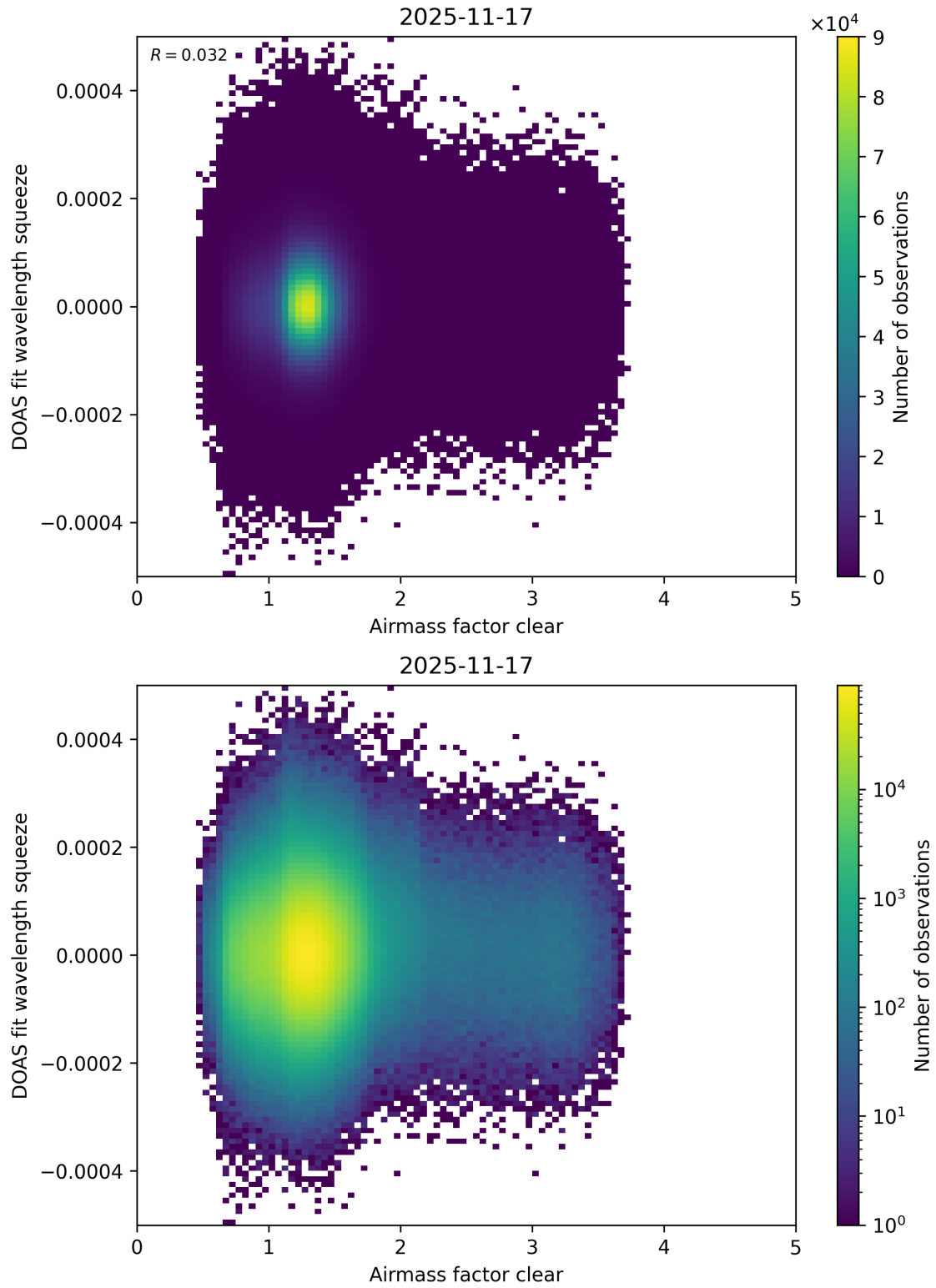
Figure 80: Scatter density plot of “Airmass factor clear” against “DOAS fit wavelength squeeze” for 2025-11-16 to 2025-11-18.
