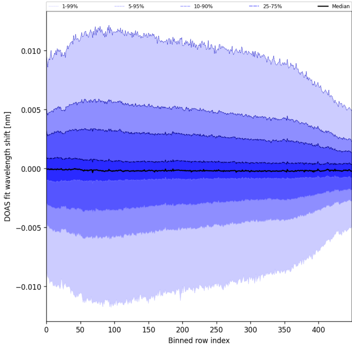
Figure 61: Along track statistics of “DOAS fit wavelength shift” for 2025-11-16 to 2025-11-18
