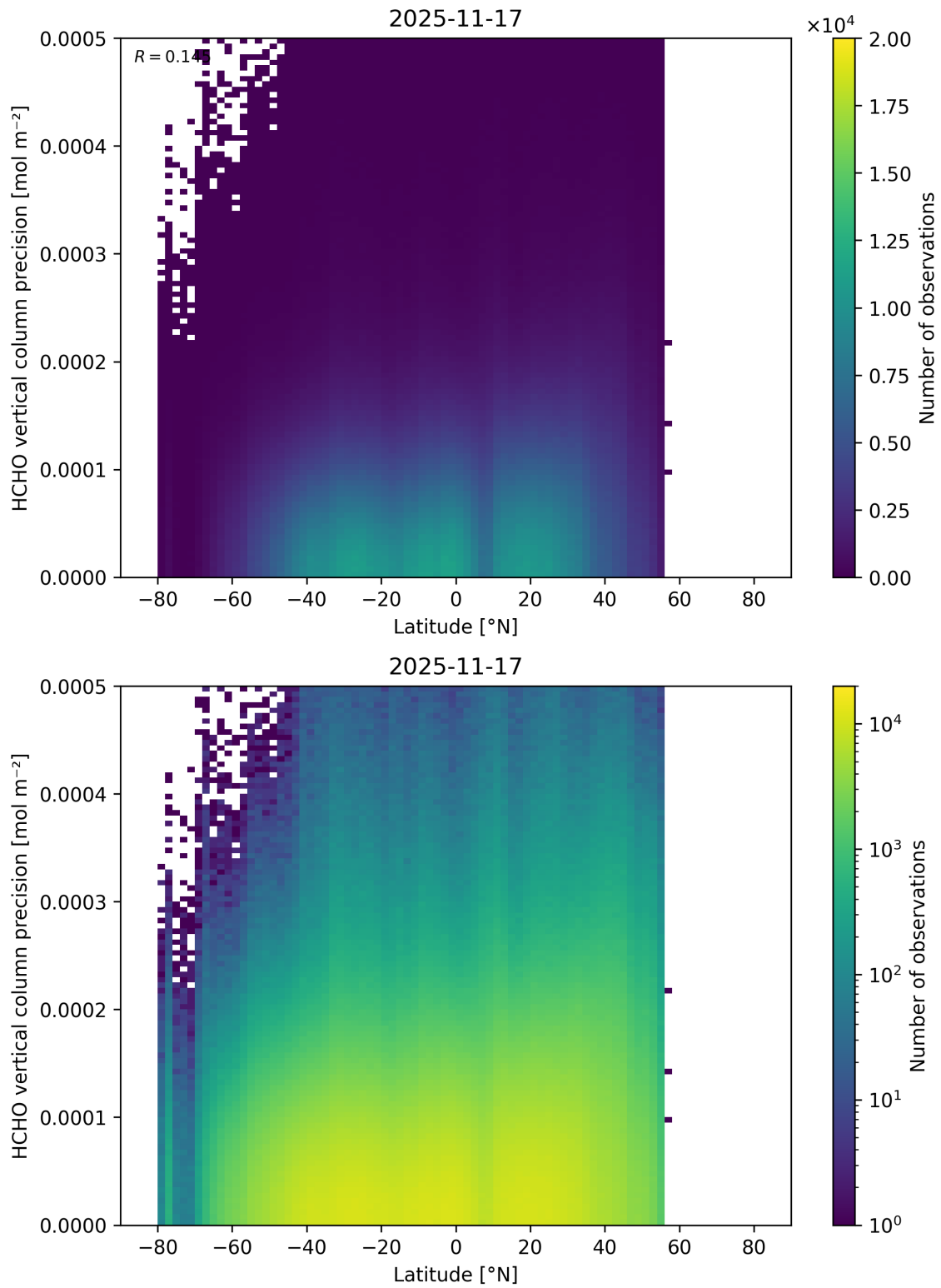
Figure 183: Scatter density plot of “Latitude” against “HCHO vertical column precision” for 2025-11-16 to 2025-11-18.
