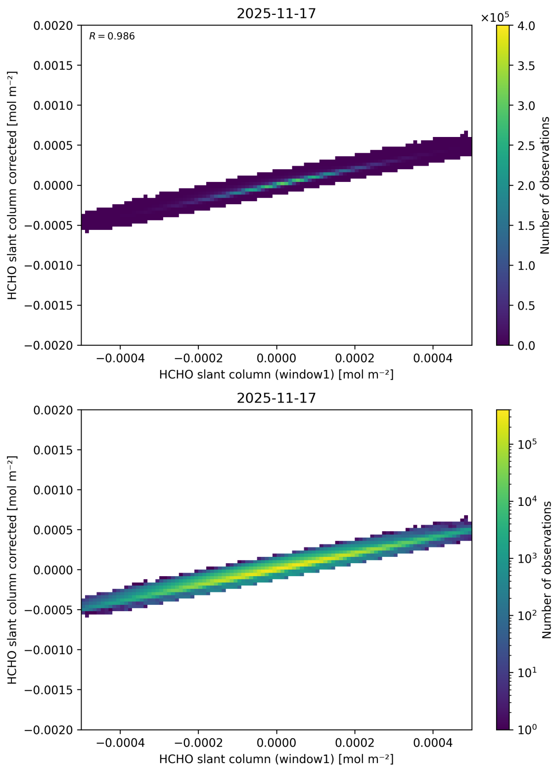
Figure 92: Scatter density plot of “HCHO slant column (window1)” against “HCHO slant column corrected” for 2025-11-16 to 2025-11-18.
