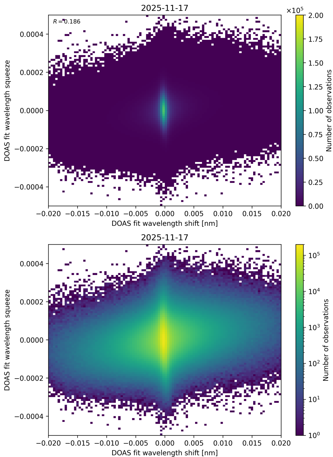
Figure 70: Scatter density plot of “DOAS fit wavelength shift” against “DOAS fit wavelength squeeze” for 2025-11-16 to 2025-11-18.
