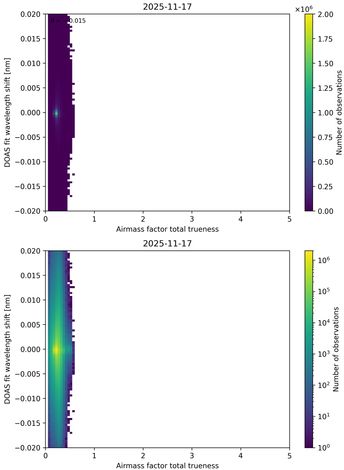
Figure 119: Scatter density plot of “Airmass factor total trueness” against “DOAS fit wavelength shift” for 2025-11-16 to 2025-11-18.
