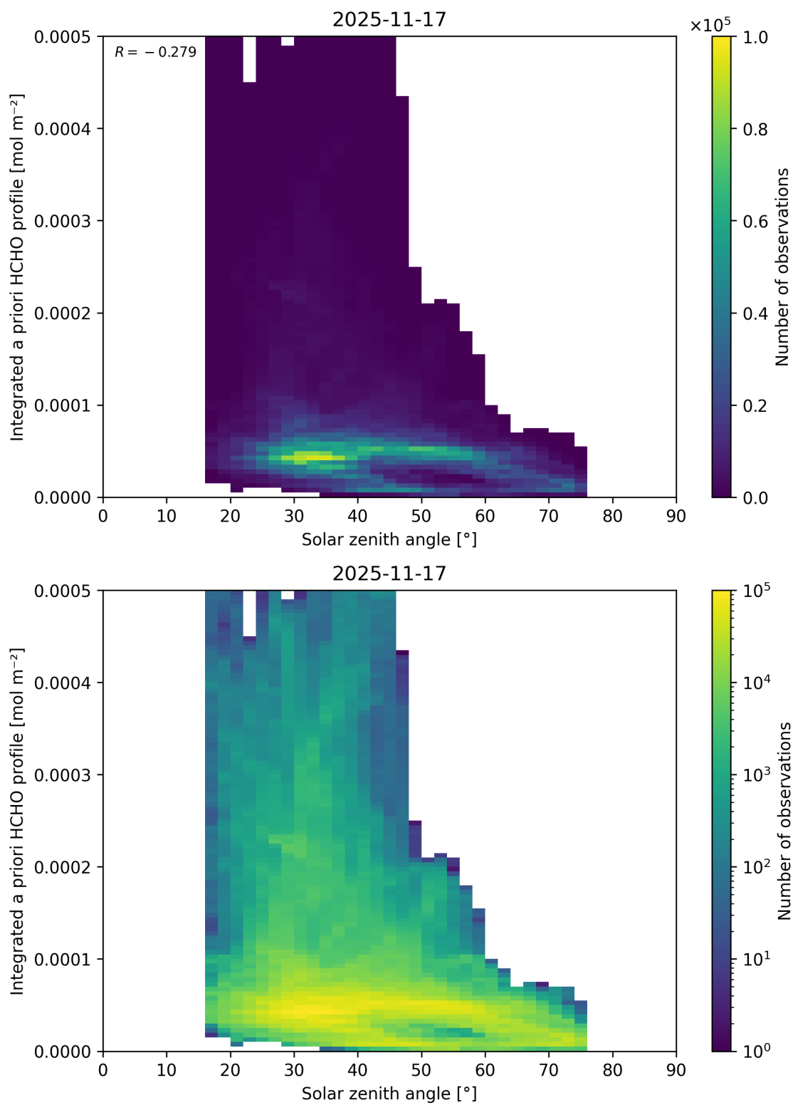
Figure 200: Scatter density plot of “Solar zenith angle” against “Integrated a priori HCHO profile” for 2025-11-16 to 2025-11-18.
