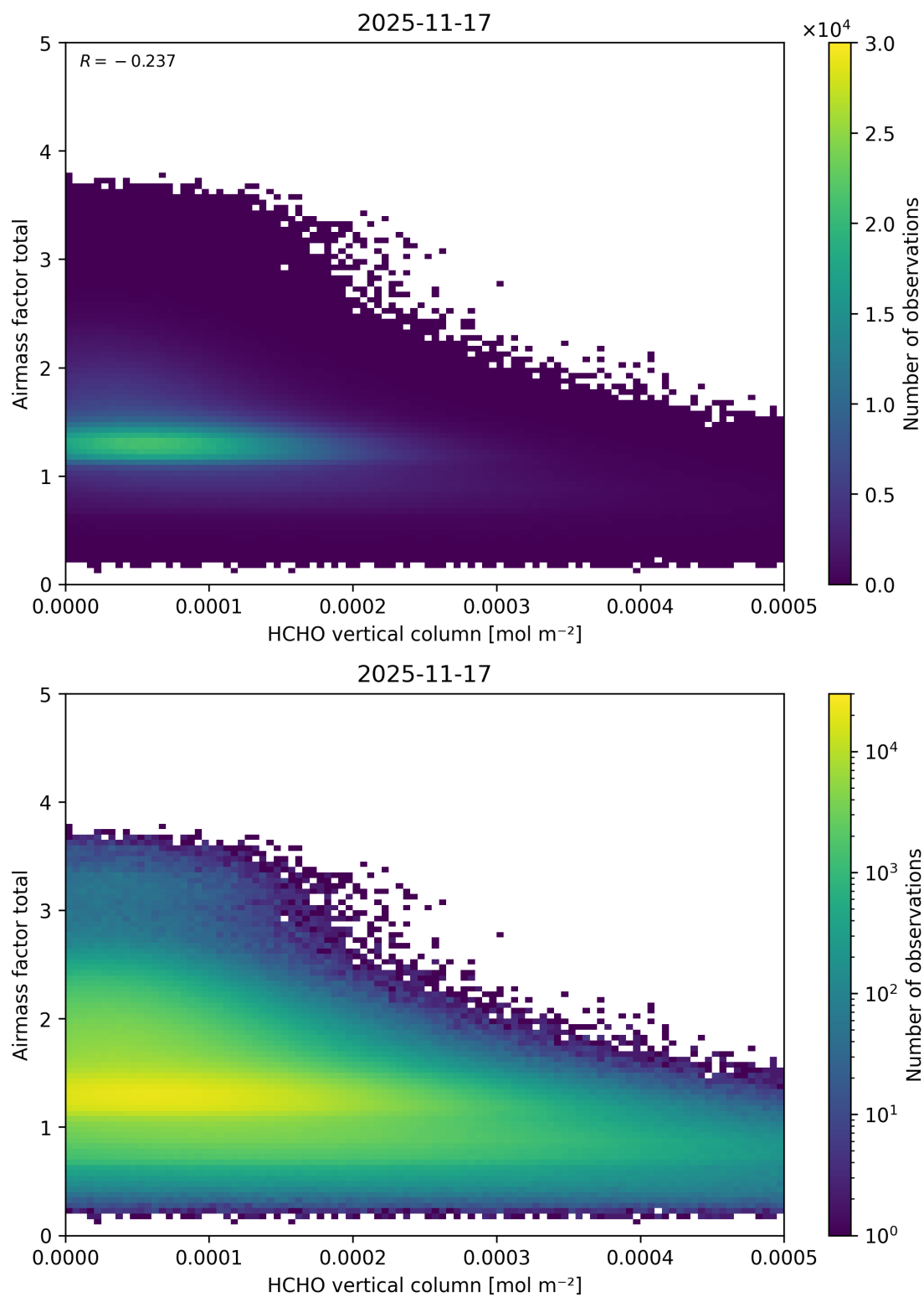
Figure 146: Scatter density plot of “HCHO vertical column” against “Airmass factor total” for 2025-11-16 to 2025-11-18.
