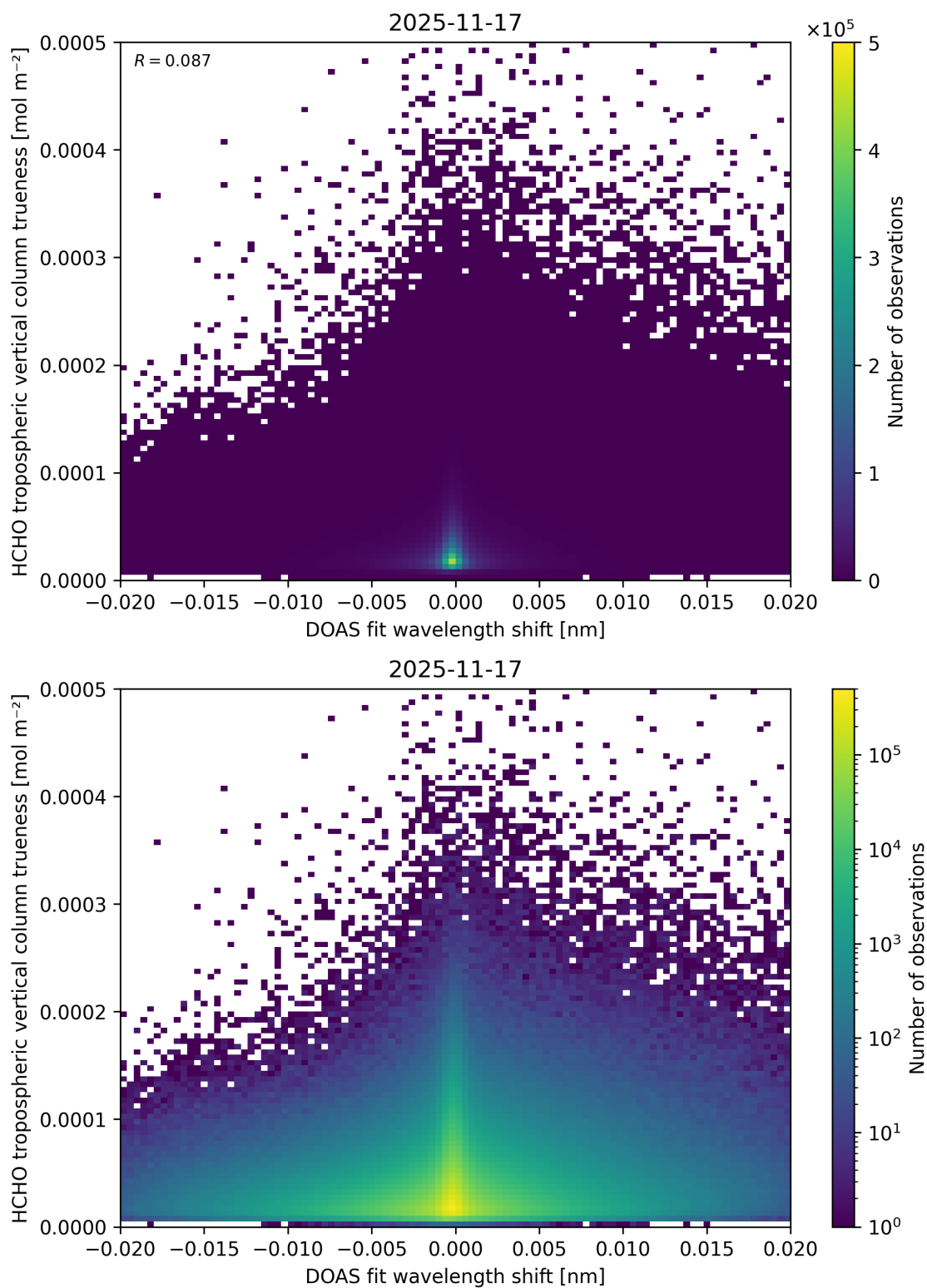
Figure 73: Scatter density plot of “DOAS fit wavelength shift” against “HCHO tropospheric vertical column trueness” for 2025-11-16 to 2025-11-18.
