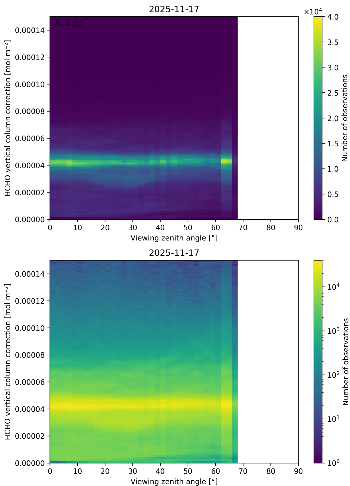
Figure 213: Scatter density plot of “Viewing zenith angle” against “HCHO vertical column correction” for 2025-11-16 to 2025-11-18.
