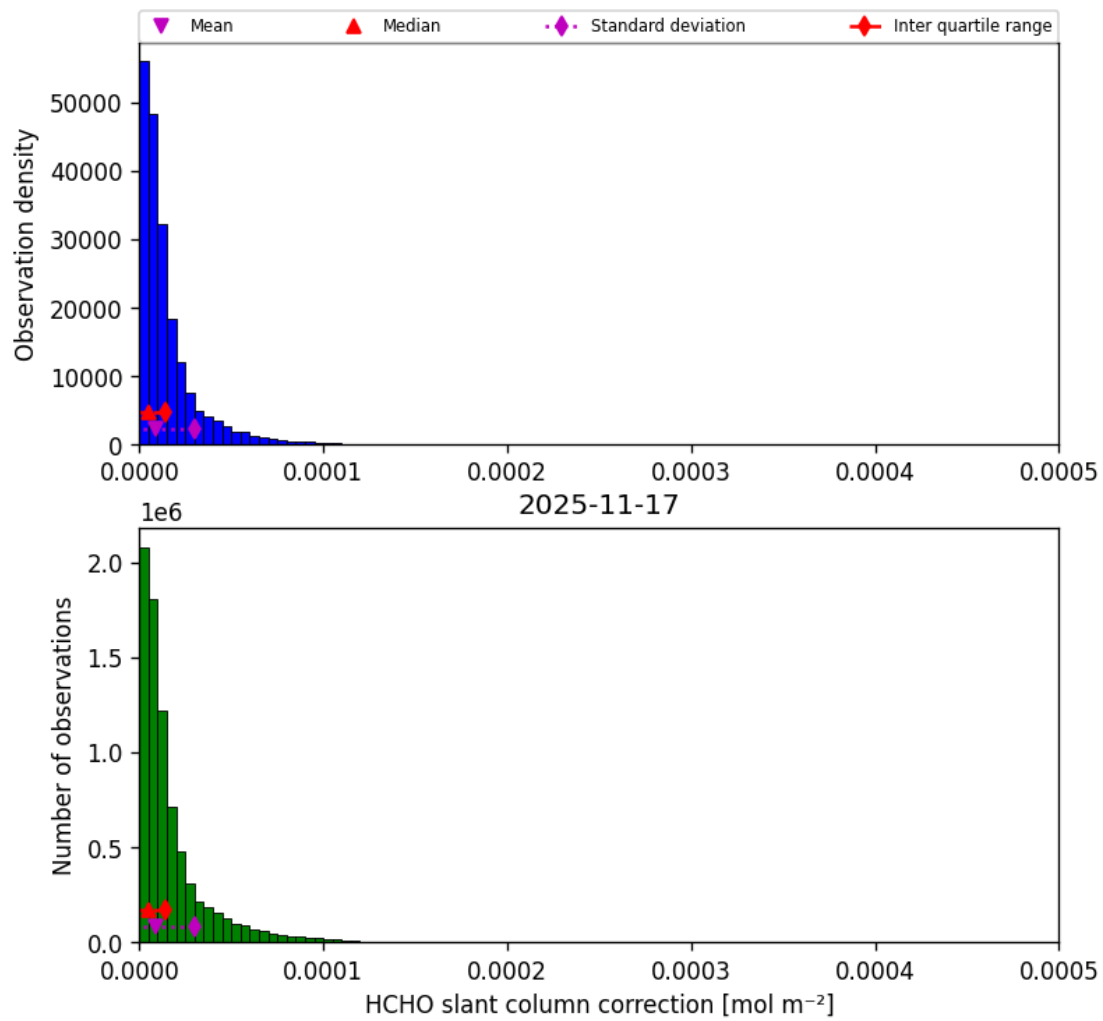
Figure 49: Histogram of “HCHO slant column correction” for 2025-11-16 to 2025-11-18
