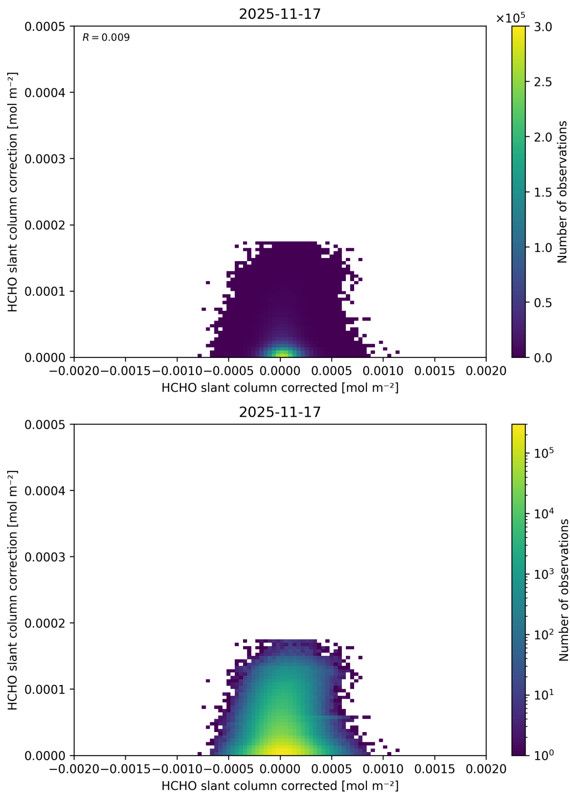
Figure 85: Scatter density plot of “HCHO slant column corrected” against “HCHO slant column correction” for 2025-11-16 to 2025-11-18.
