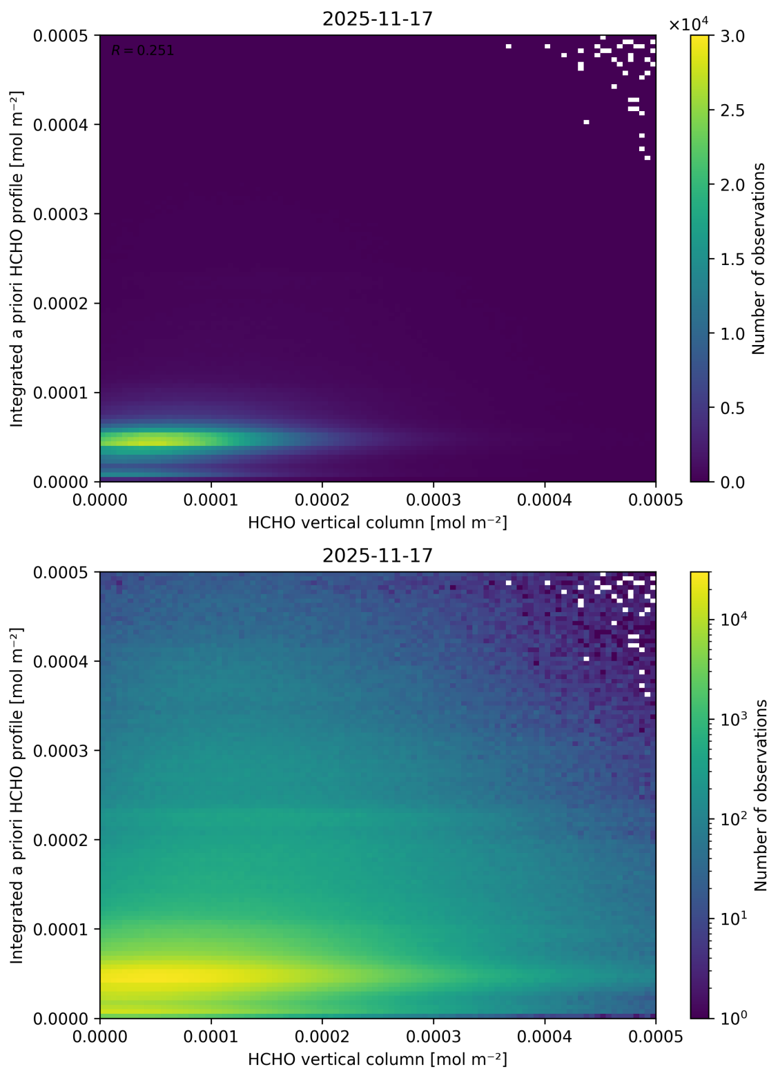
Figure 151: Scatter density plot of “HCHO vertical column” against “Integrated a priori HCHO profile” for 2025-11-16 to 2025-11-18.
