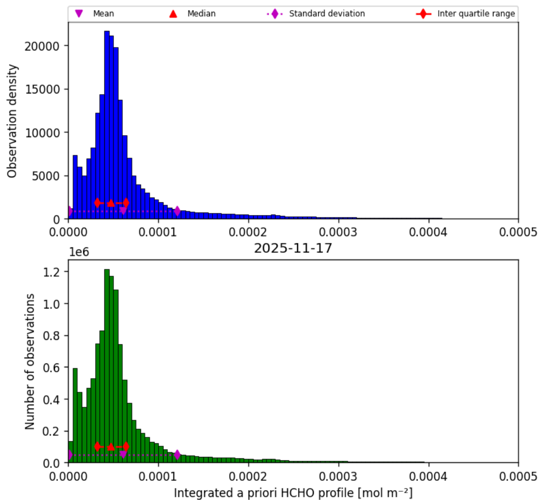
Figure 45: Histogram of “Integrated a priori HCHO profile” for 2025-11-16 to 2025-11-18
