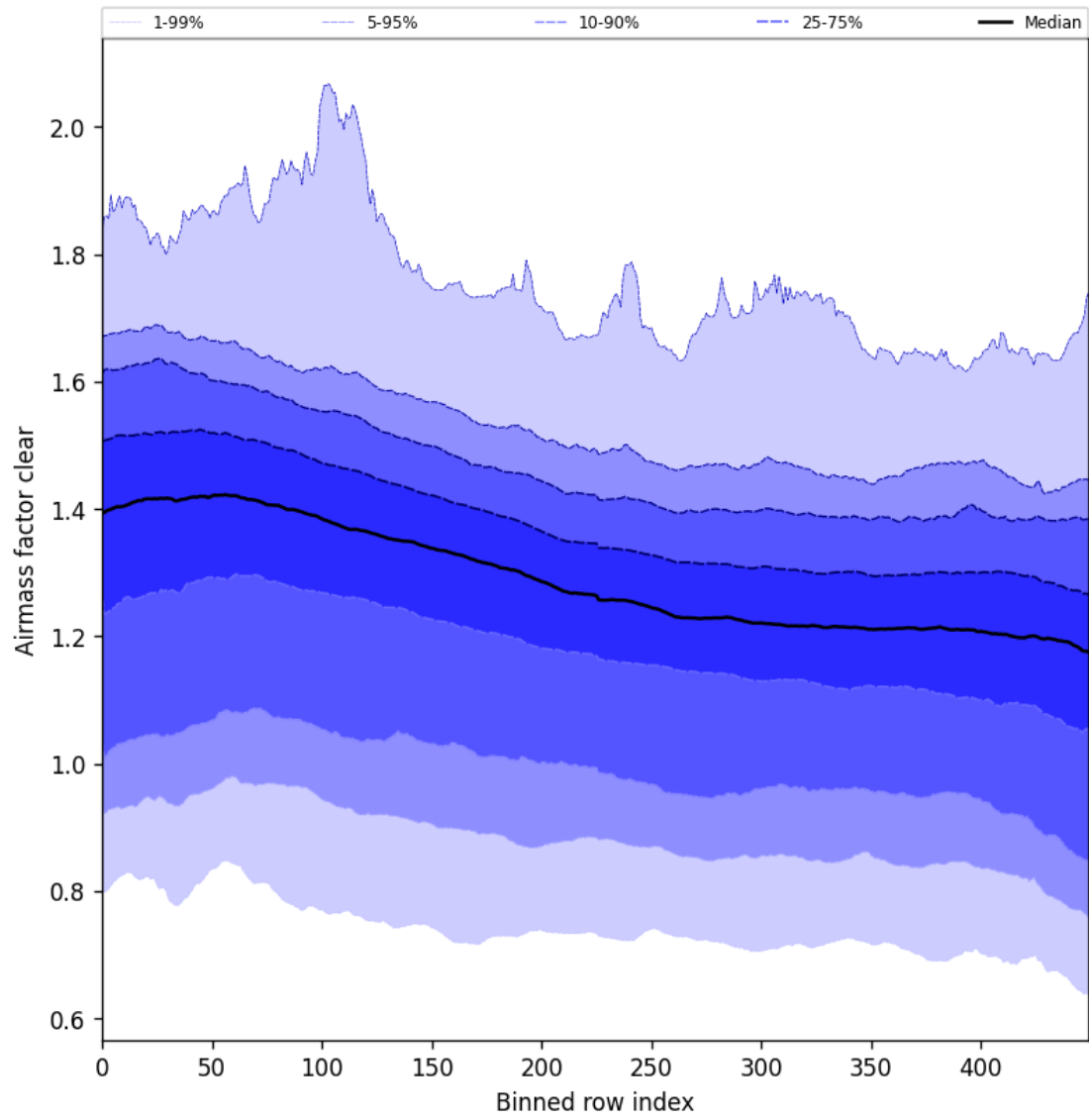
Figure 59: Along track statistics of “Airmass factor clear” for 2025-11-16 to 2025-11-18
