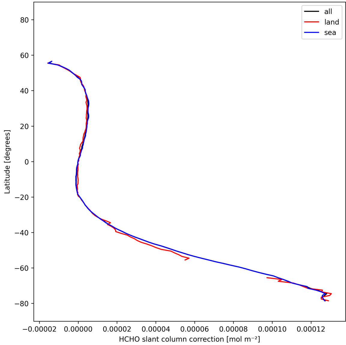
Figure 34: Zonal average of "HCHO slant column correction" for 2025-11-16 to 2025-11-18.
