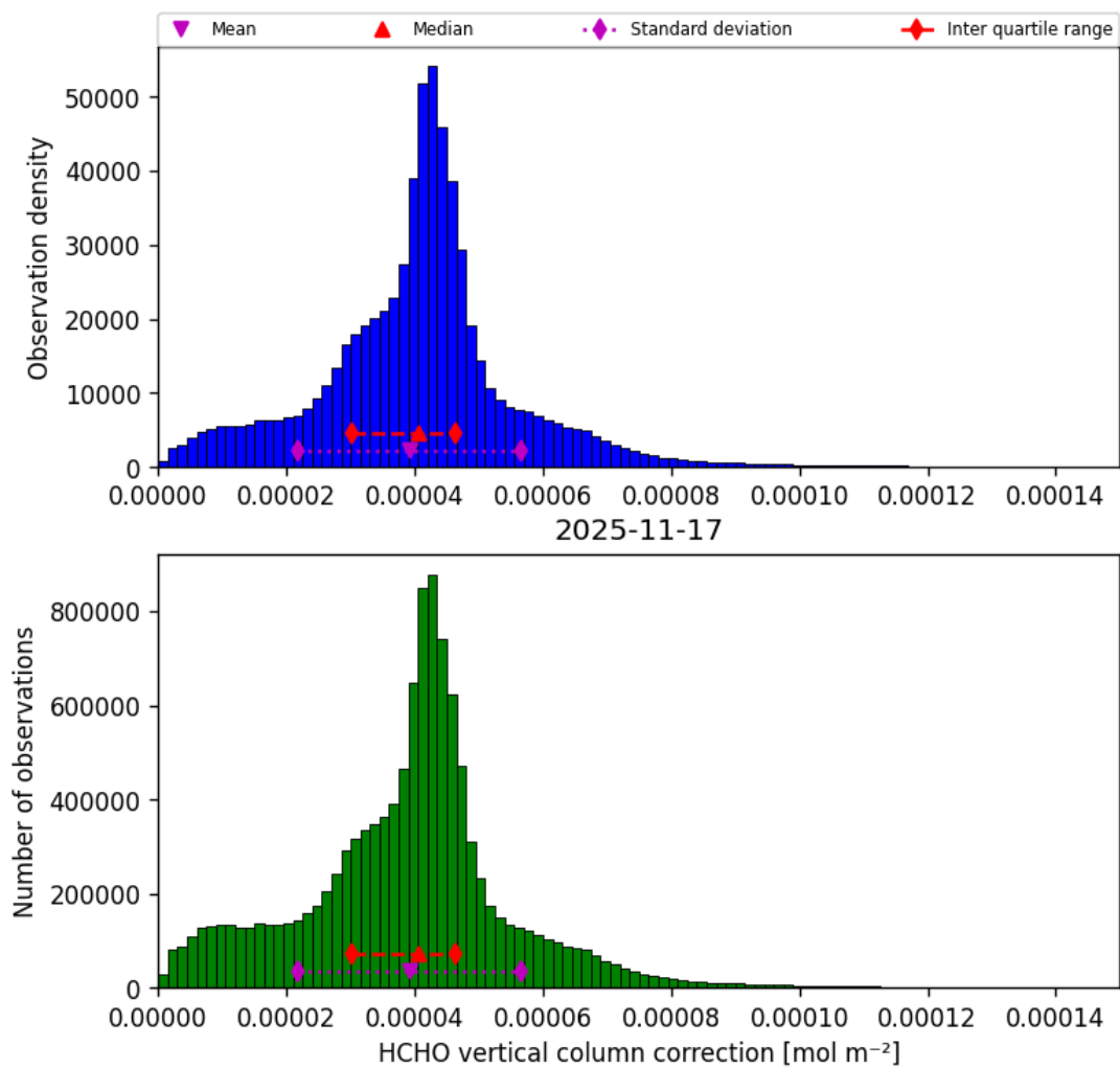
Figure 39: Histogram of “HCHO vertical column correction” for 2025-11-16 to 2025-11-18
