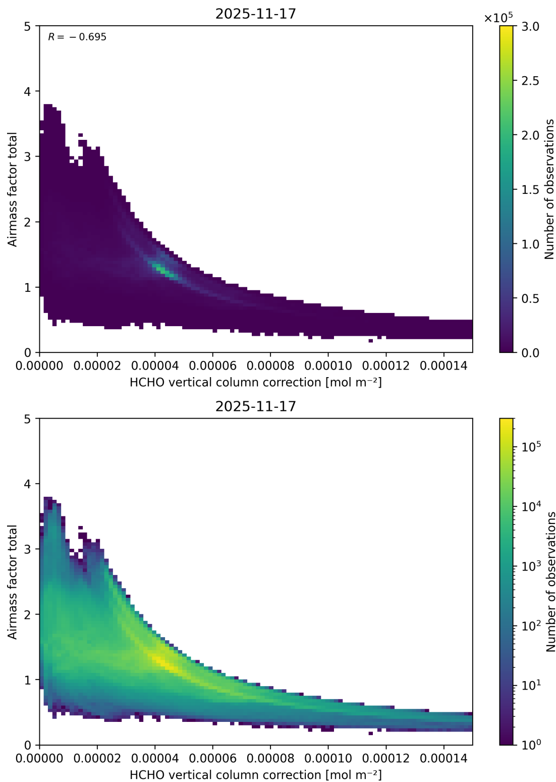
Figure 134: Scatter density plot of “HCHO vertical column correction” against “Airmass factor total” for 2025-11-16 to 2025-11-18.
