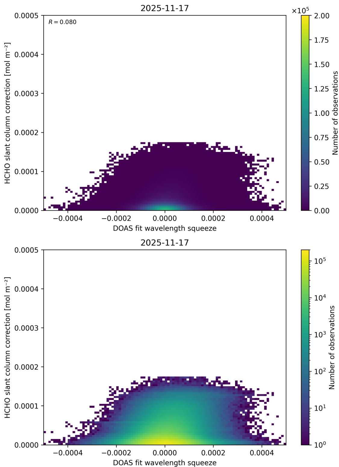
Figure 76: Scatter density plot of “DOAS fit wavelength squeeze” against “HCHO slant column correction” for 2025-11-16 to 2025-11-18.
