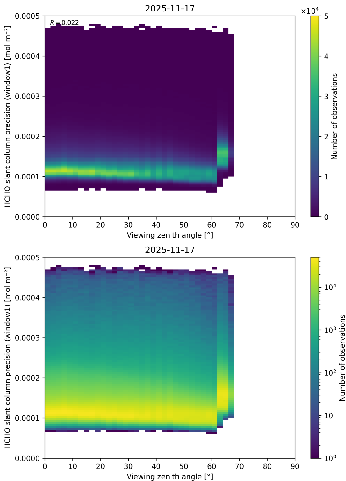
Figure 209: Scatter density plot of “Viewing zenith angle” against “HCHO slant column precision (window1)” for 2025-11-16 to 2025-11-18.
