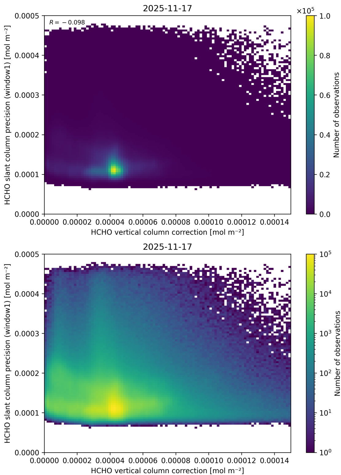
Figure 133: Scatter density plot of “HCHO vertical column correction” against “HCHO slant column precision (window1)” for 2025-11-16 to 2025-11-18.
