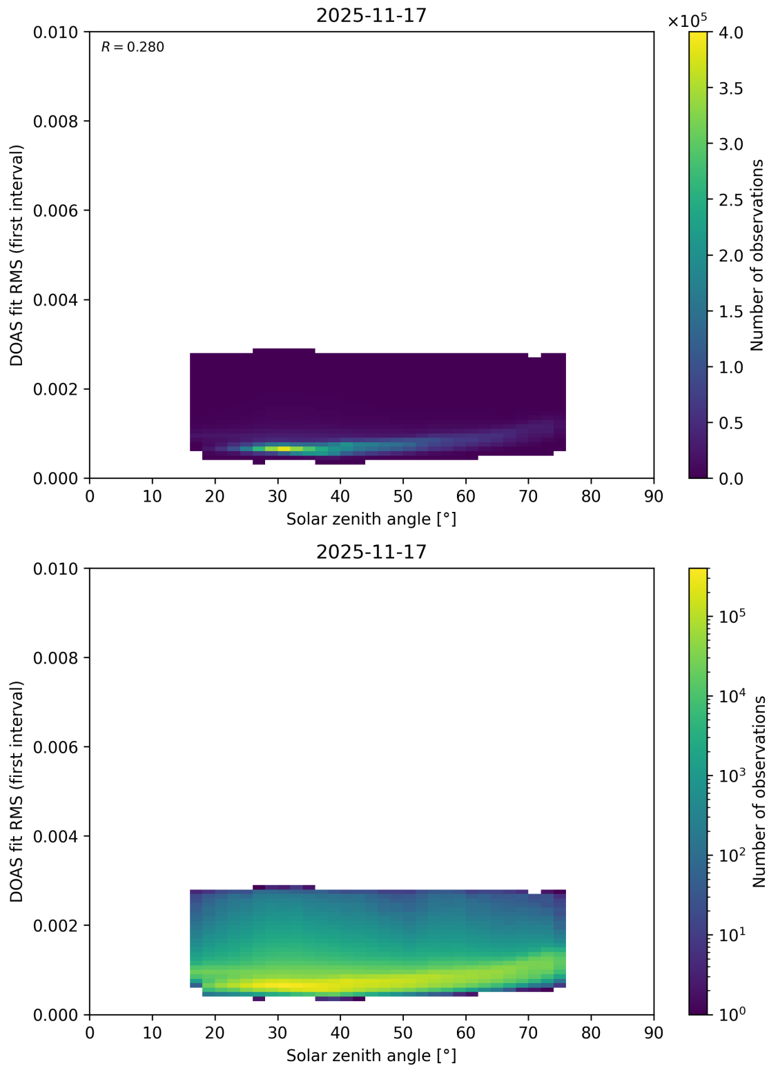
Figure 186: Scatter density plot of “Solar zenith angle” against “DOAS fit RMS (first interval)” for 2025-11-16 to 2025-11-18.
