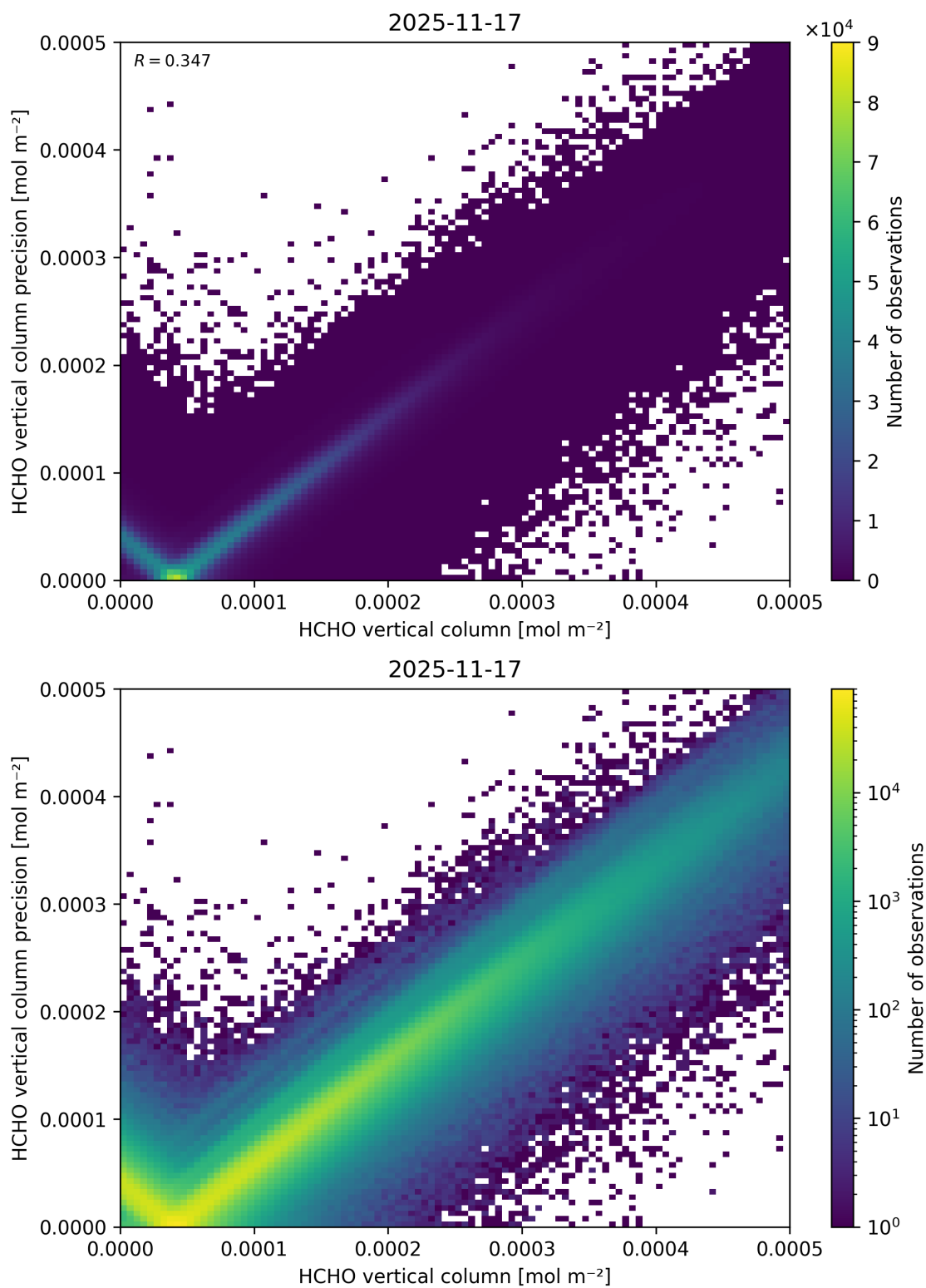
Figure 149: Scatter density plot of “HCHO vertical column” against “HCHO vertical column precision” for 2025-11-16 to 2025-11-18.
