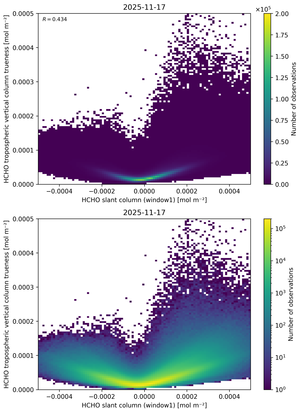
Figure 97: Scatter density plot of “HCHO slant column (window1)” against “HCHO tropospheric vertical column trueness” for 2025-11-16 to 2025-11-18.
