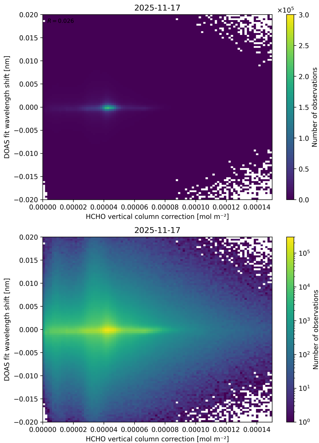
Figure 127: Scatter density plot of “HCHO vertical column correction” against “DOAS fit wavelength shift” for 2025-11-16 to 2025-11-18.
