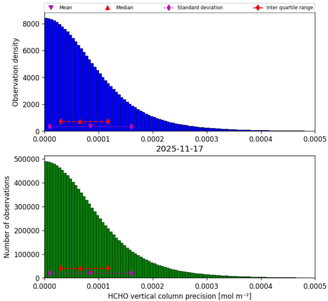
Figure 38: Histogram of “HCHO vertical column precision” for 2025-11-16 to 2025-11-18
