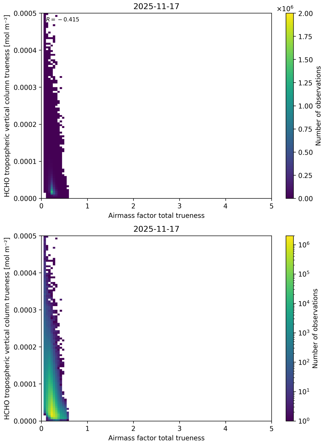
Figure 124: Scatter density plot of “Airmass factor total truiness” against “HCHO tropospheric vertical column truiness” for 2025-11-16 to 2025-11-18.
