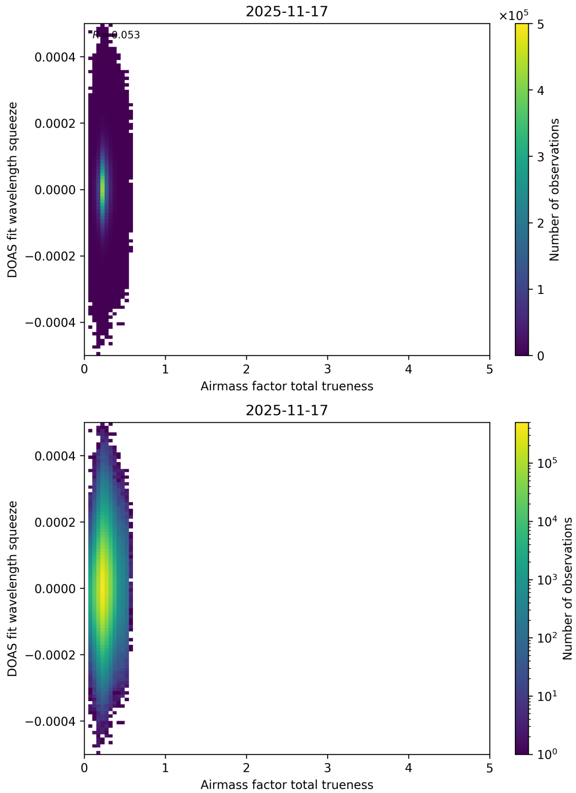
Figure 120: Scatter density plot of “Airmass factor total trueness” against “DOAS fit wavelength squeeze” for 2025-11-16 to 2025-11-18.
