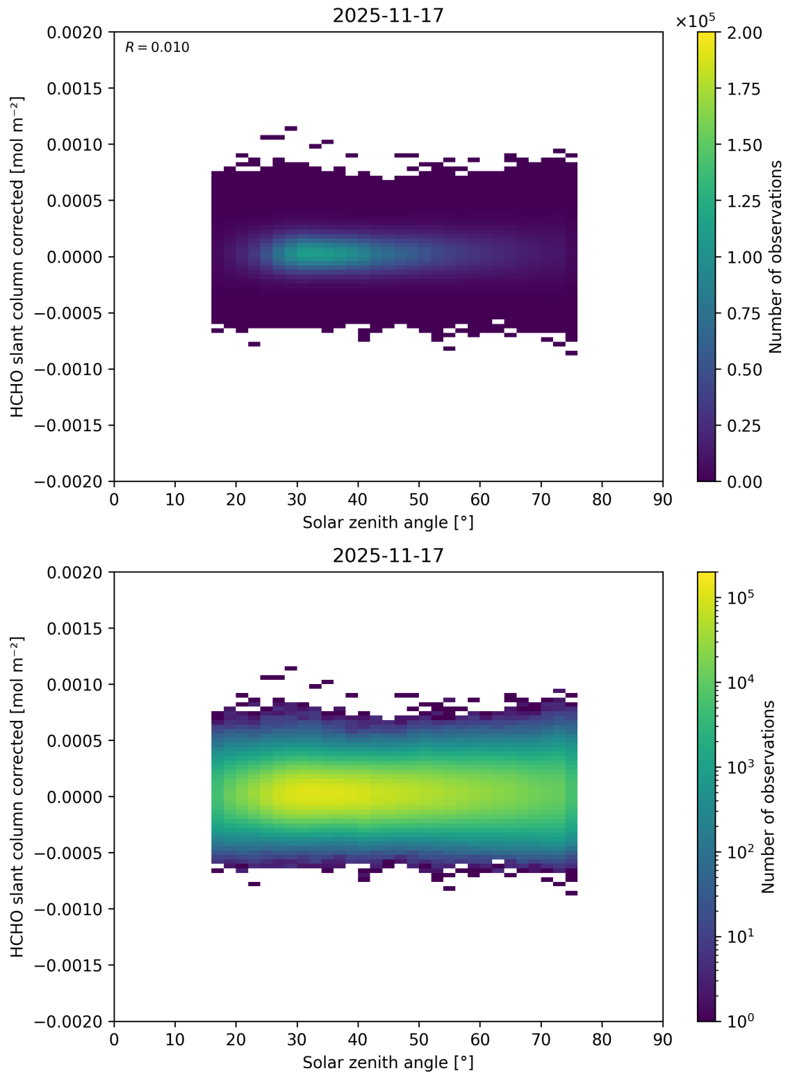
Figure 190: Scatter density plot of “Solar zenith angle” against “HCHO slant column corrected” for 2025-11-16 to 2025-11-18.
