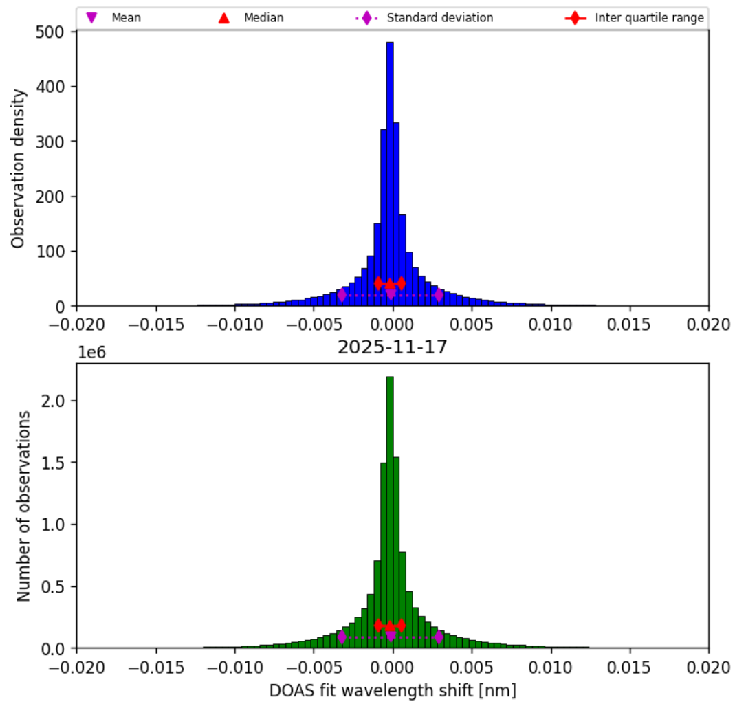
Figure 46: Histogram of “DOAS fit wavelength shift” for 2025-11-16 to 2025-11-18
