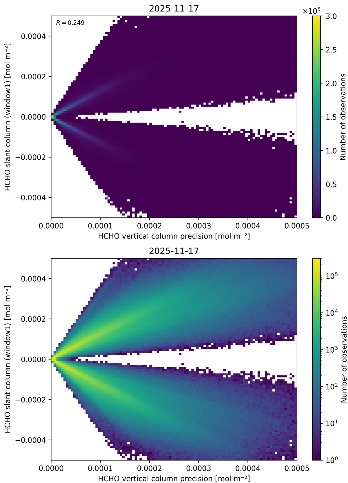
Figure 158: Scatter density plot of “HCHO vertical column precision” against “HCHO slant column (window1)” for 2025-11-16 to 2025-11-18.
