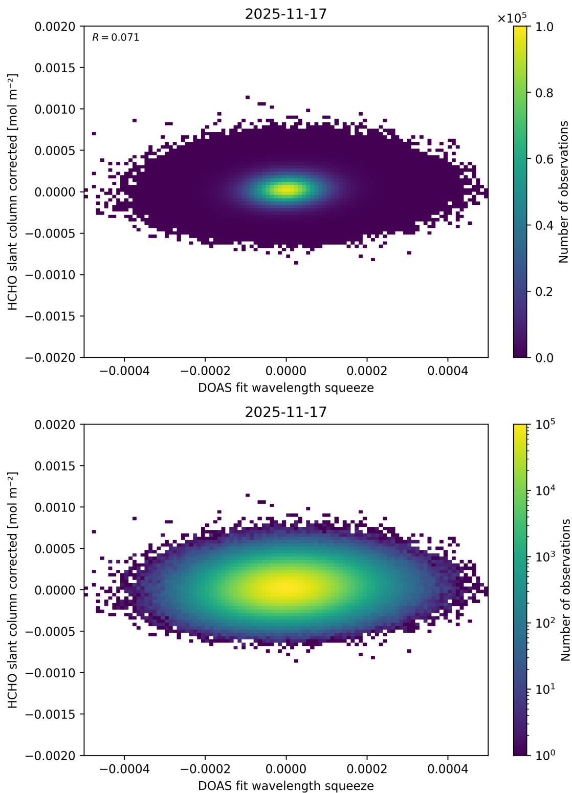
Figure 75: Scatter density plot of “DOAS fit wavelength squeeze” against “HCHO slant column corrected” for 2025-11-16 to 2025-11-18.
