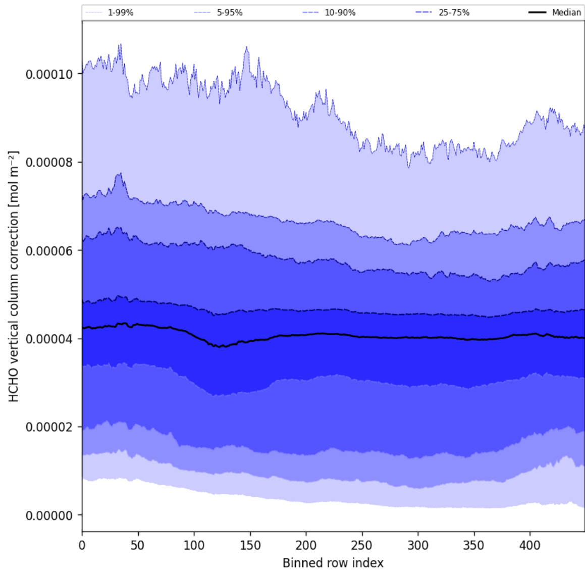
Figure 54: Along track statistics of “HCHO vertical column correction” for 2025-11-16 to 2025-11-18
