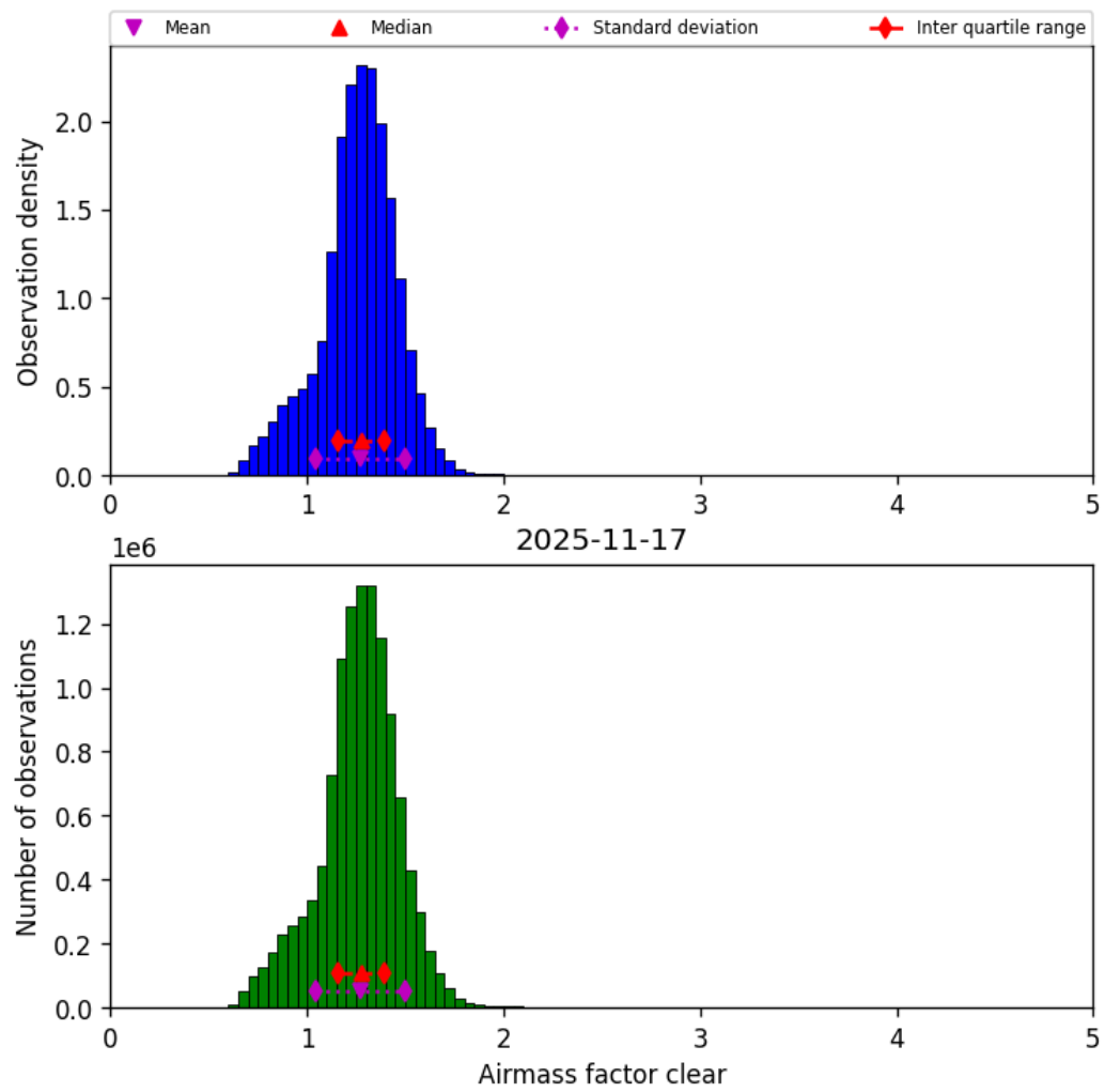
Figure 44: Histogram of “Airmass factor clear” for 2025-11-16 to 2025-11-18
