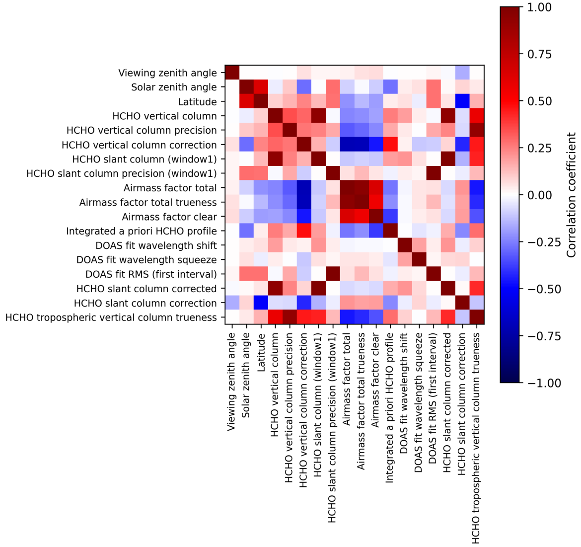
Figure 2: Map of correlation matrix for 2025-11-16 to 2025-11-18.
