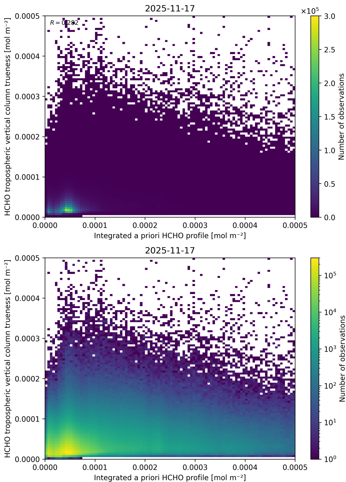
Figure 170: Scatter density plot of “Integrated a priori HCHO profile” against “HCHO tropospheric vertical column trueness” for 2025-11-16 to 2025-11-18.
