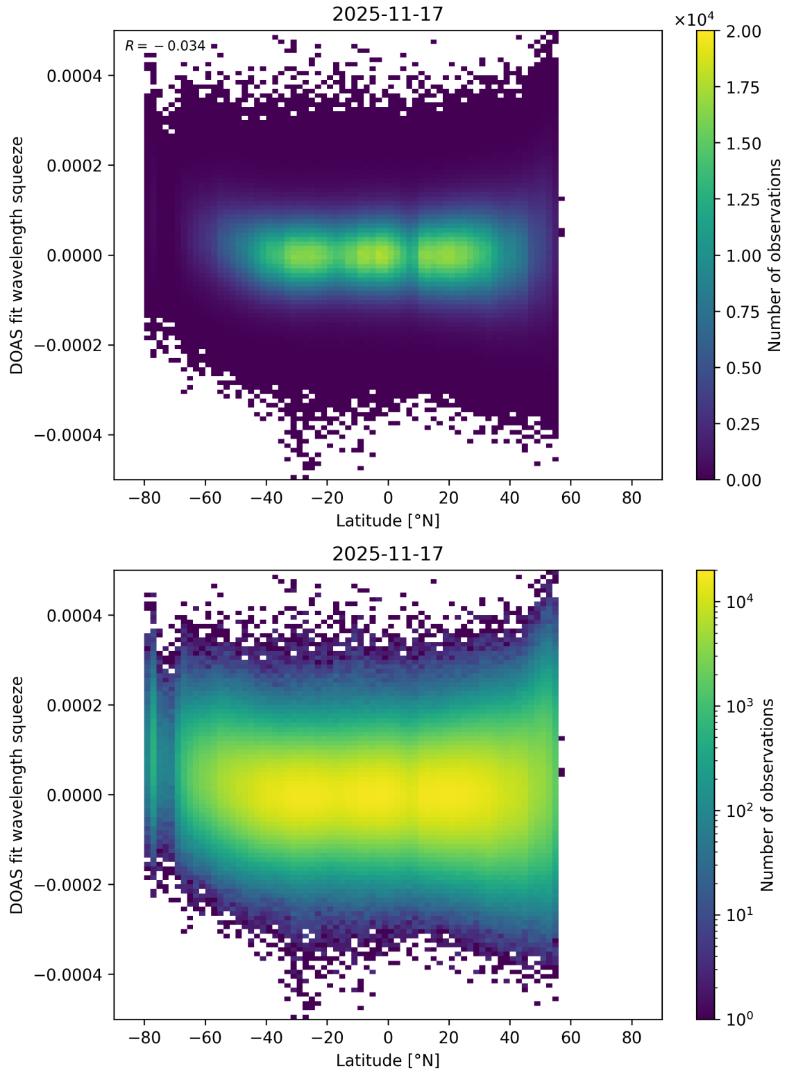
Figure 173: Scatter density plot of “Latitude” against “DOAS fit wavelength squeeze” for 2025-11-16 to 2025-11-18.
