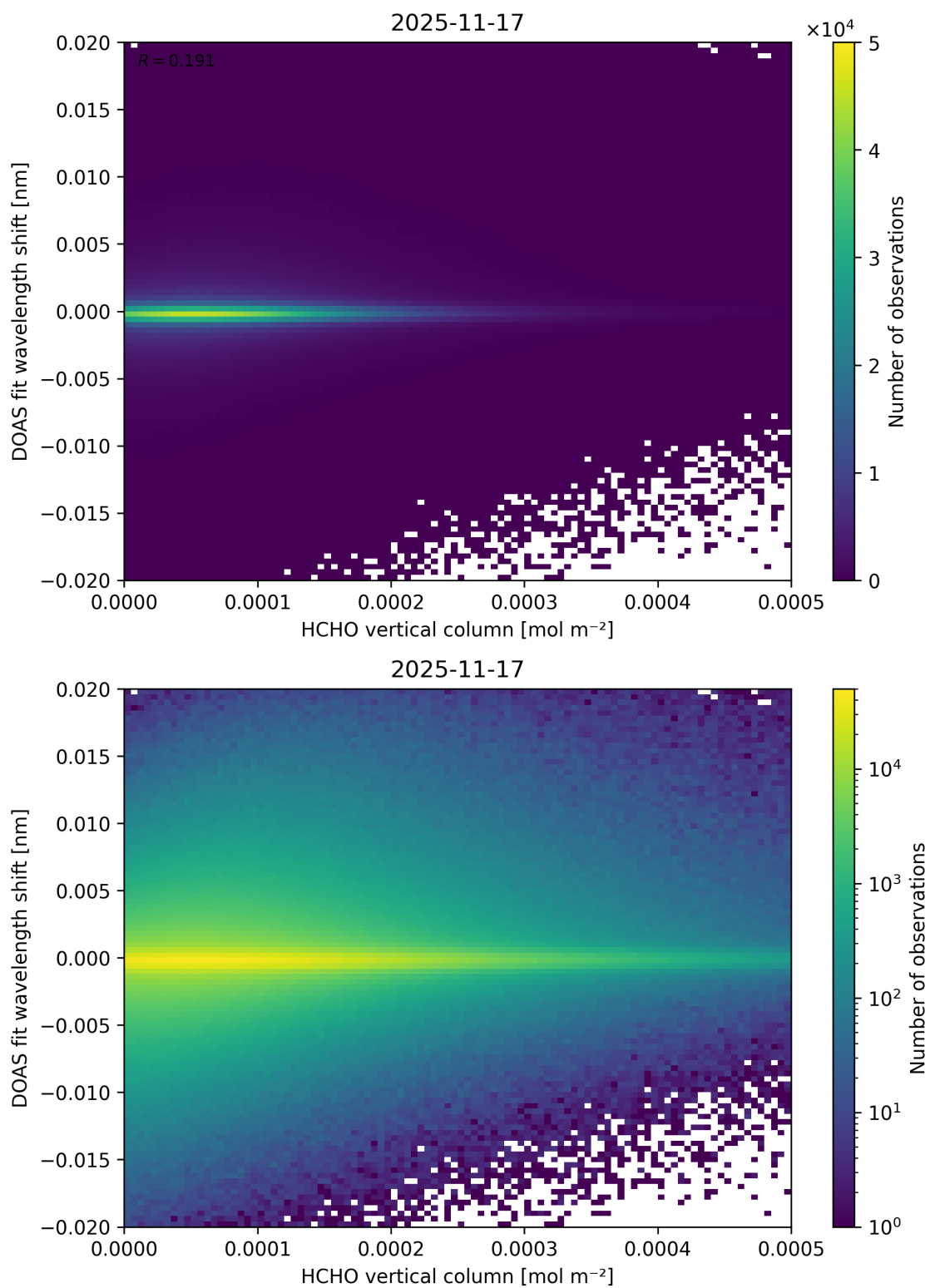
Figure 139: Scatter density plot of “HCHO vertical column” against “DOAS fit wavelength shift” for 2025-11-16 to 2025-11-18.
