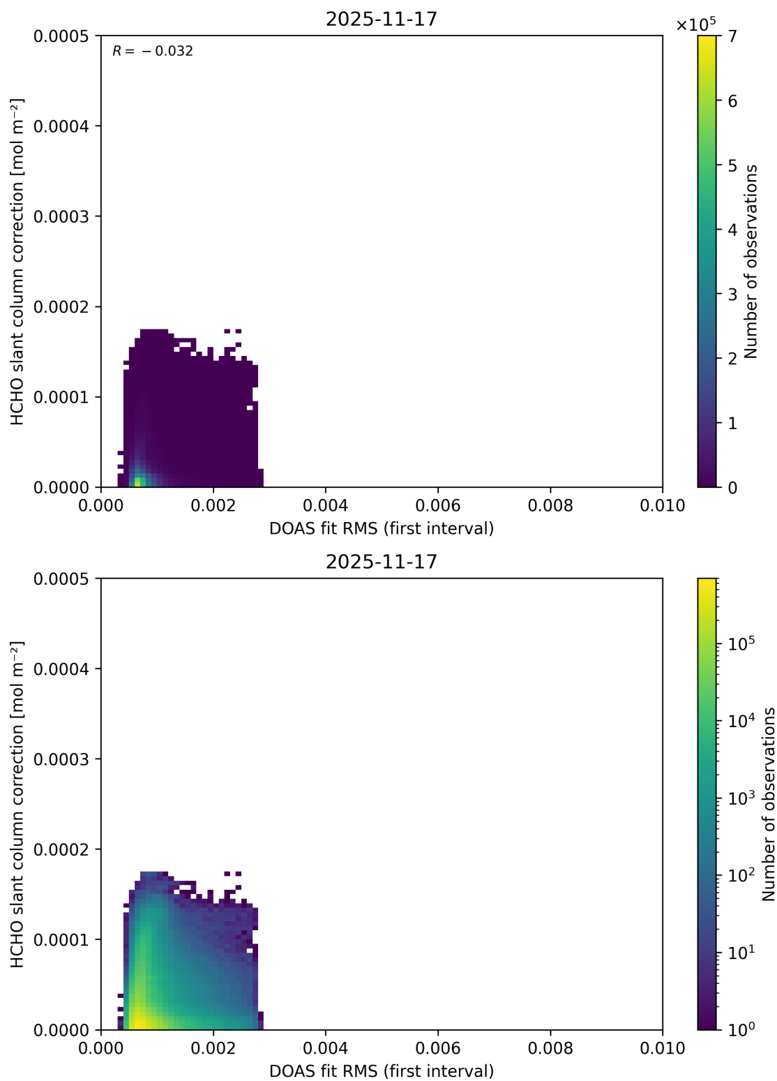
Figure 67: Scatter density plot of “DOAS fit RMS (first interval)” against “HCHO slant column correction” for 2025-11-16 to 2025-11-18.
