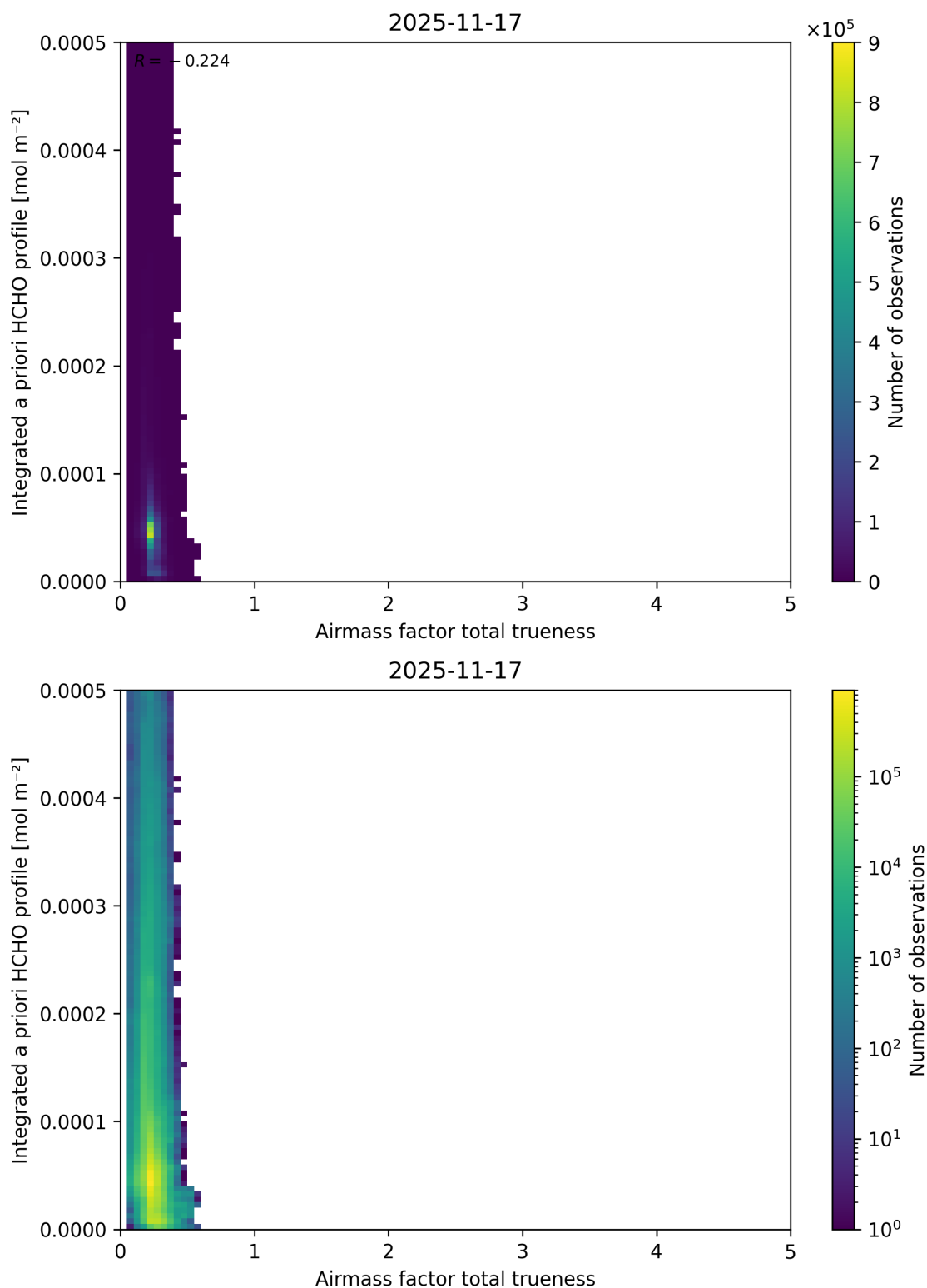
Figure 125: Scatter density plot of “Airmass factor total trueness” against “Integrated a priori HCHO profile” for 2025-11-16 to 2025-11-18.
