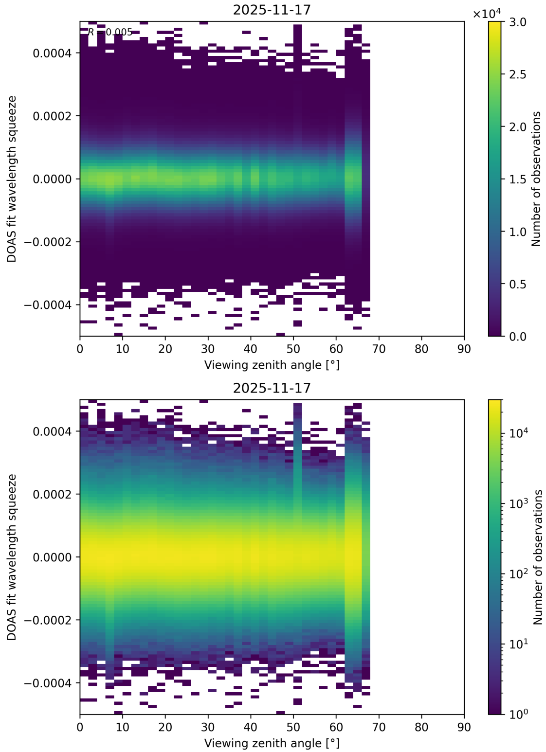
Figure 204: Scatter density plot of “Viewing zenith angle” against “DOAS fit wavelength squeeze” for 2025-11-16 to 2025-11-18.
