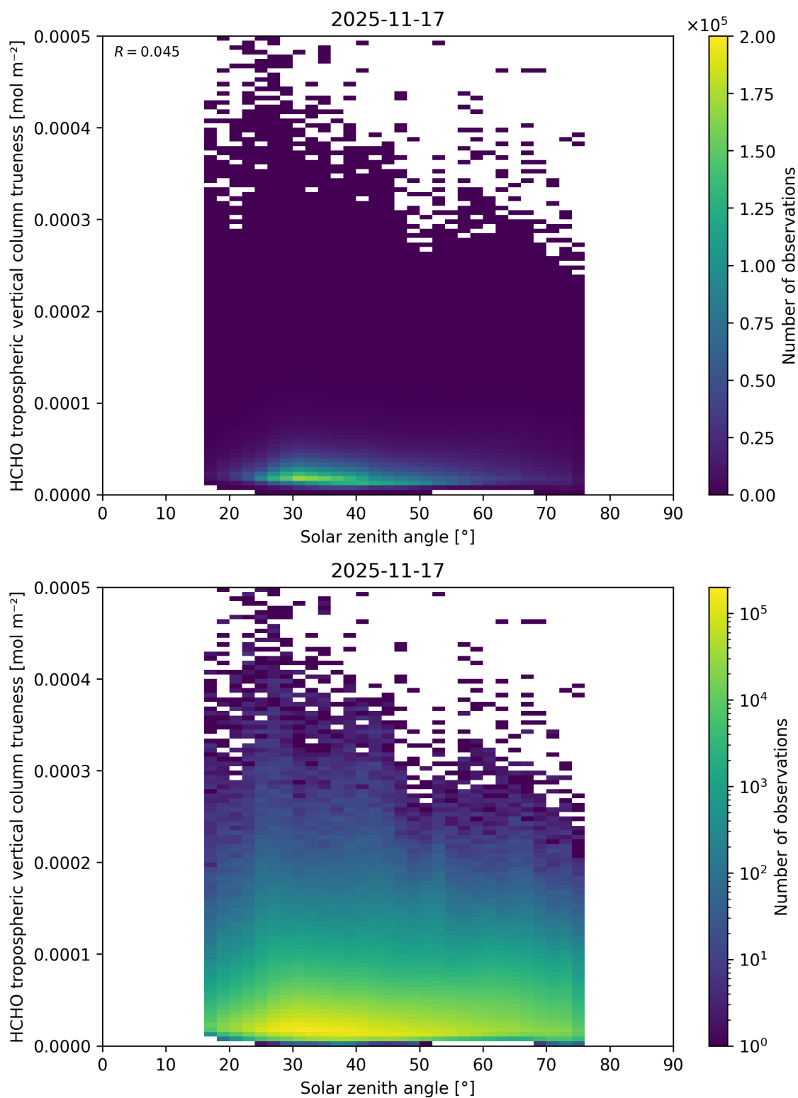
Figure 199: Scatter density plot of “Solar zenith angle” against “HCHO tropospheric vertical column trueness” for 2025-11-16 to 2025-11-18.
