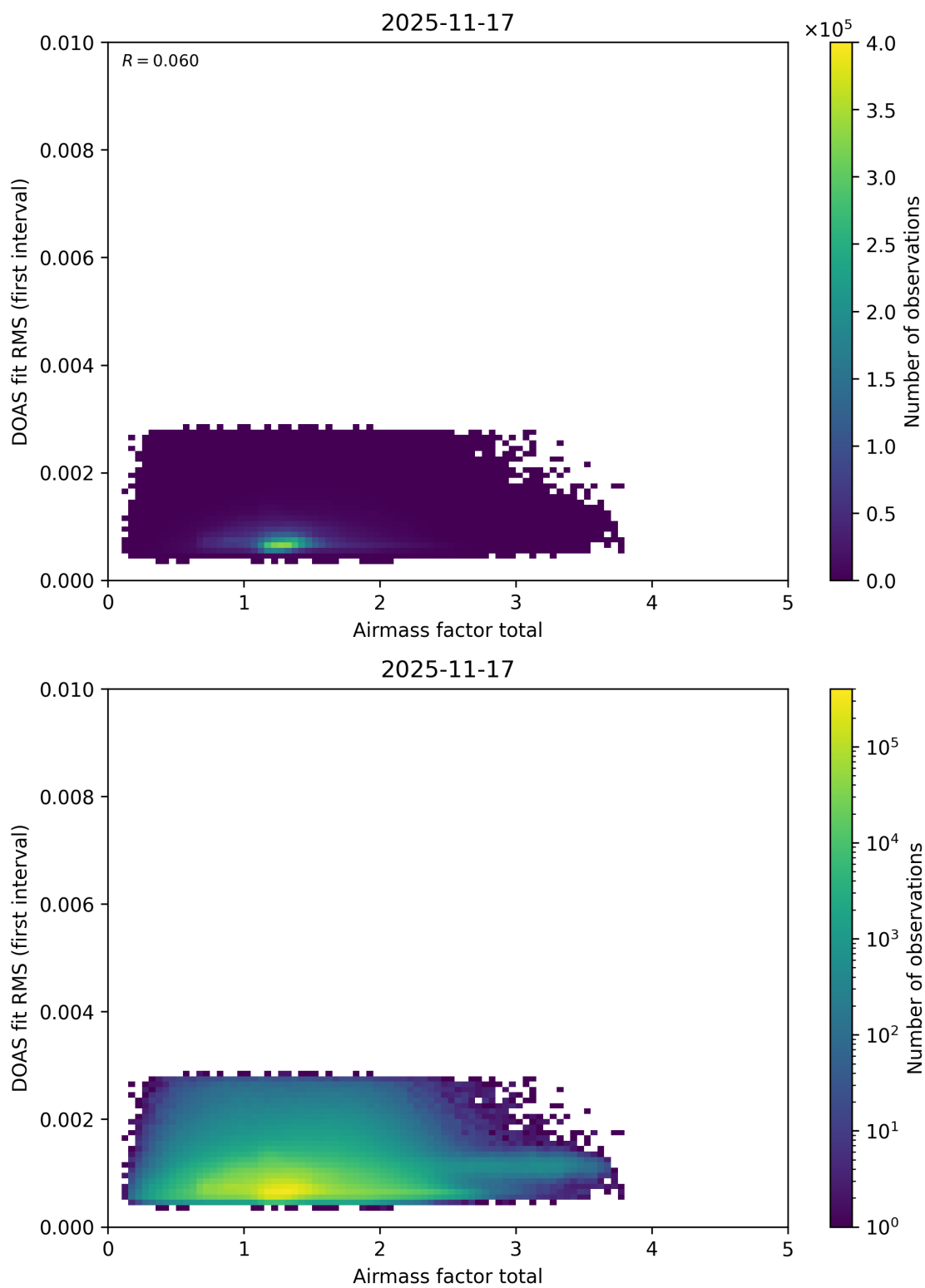
Figure 109: Scatter density plot of “Airmass factor total” against “DOAS fit RMS (first interval)” for 2025-11-16 to 2025-11-18.
