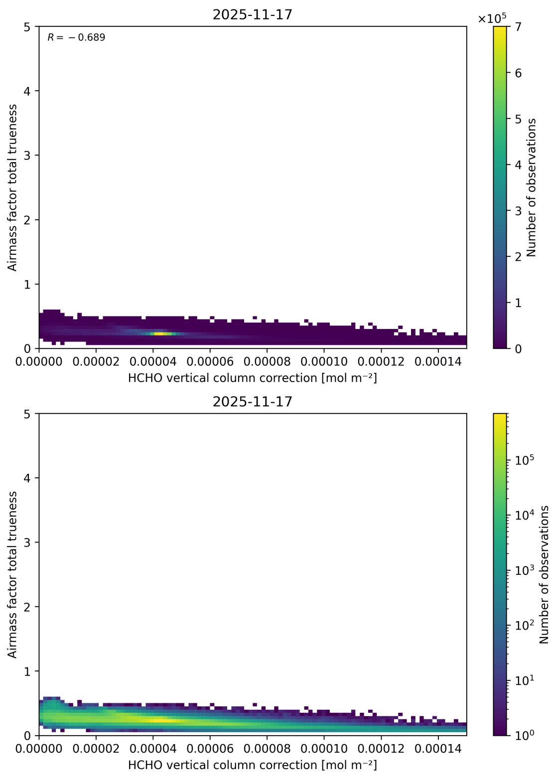
Figure 135: Scatter density plot of “HCHO vertical column correction” against “Airmass factor total trueneess” for 2025-11-16 to 2025-11-18.
