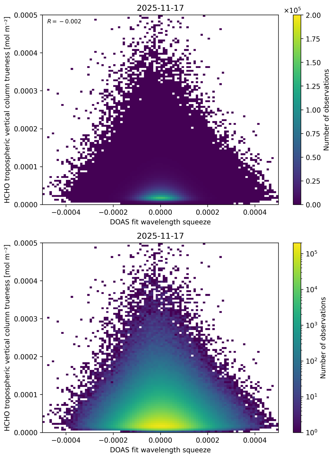
Figure 77: Scatter density plot of “DOAS fit wavelength squeeze” against “HCHO tropospheric vertical column trueness” for 2025-11-16 to 2025-11-18.
