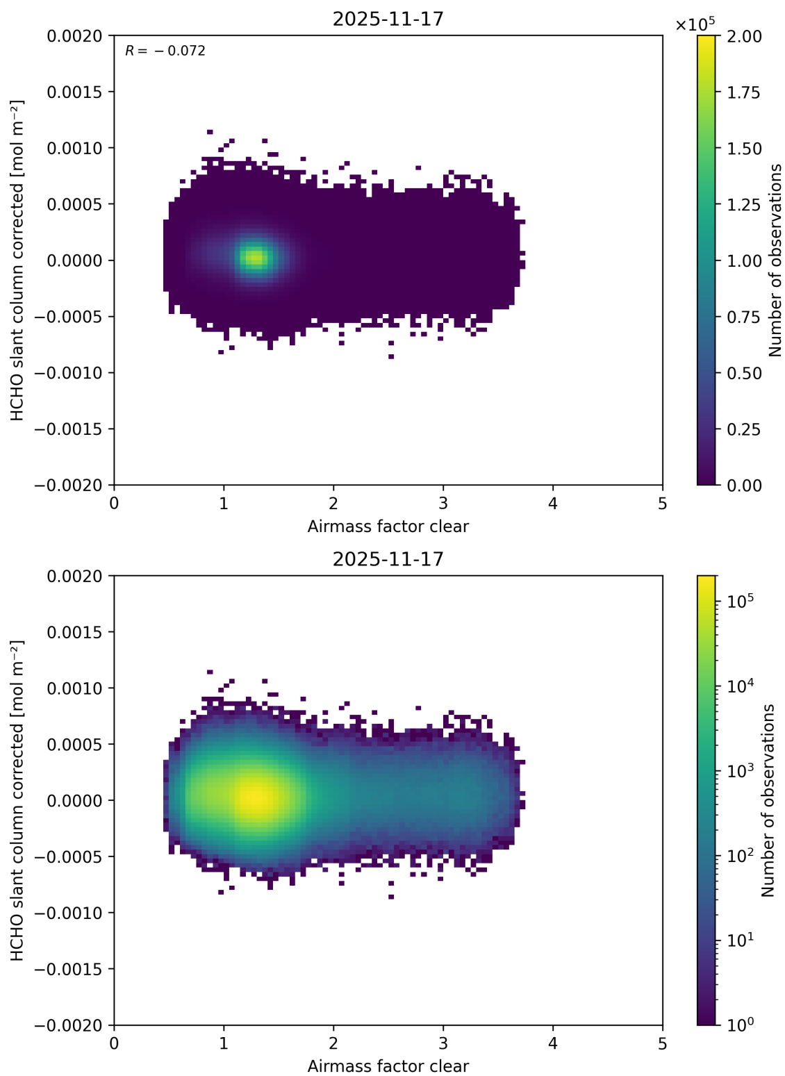
Figure 81: Scatter density plot of “Airmass factor clear” against “HCHO slant column corrected” for 2025-11-16 to 2025-11-18.
