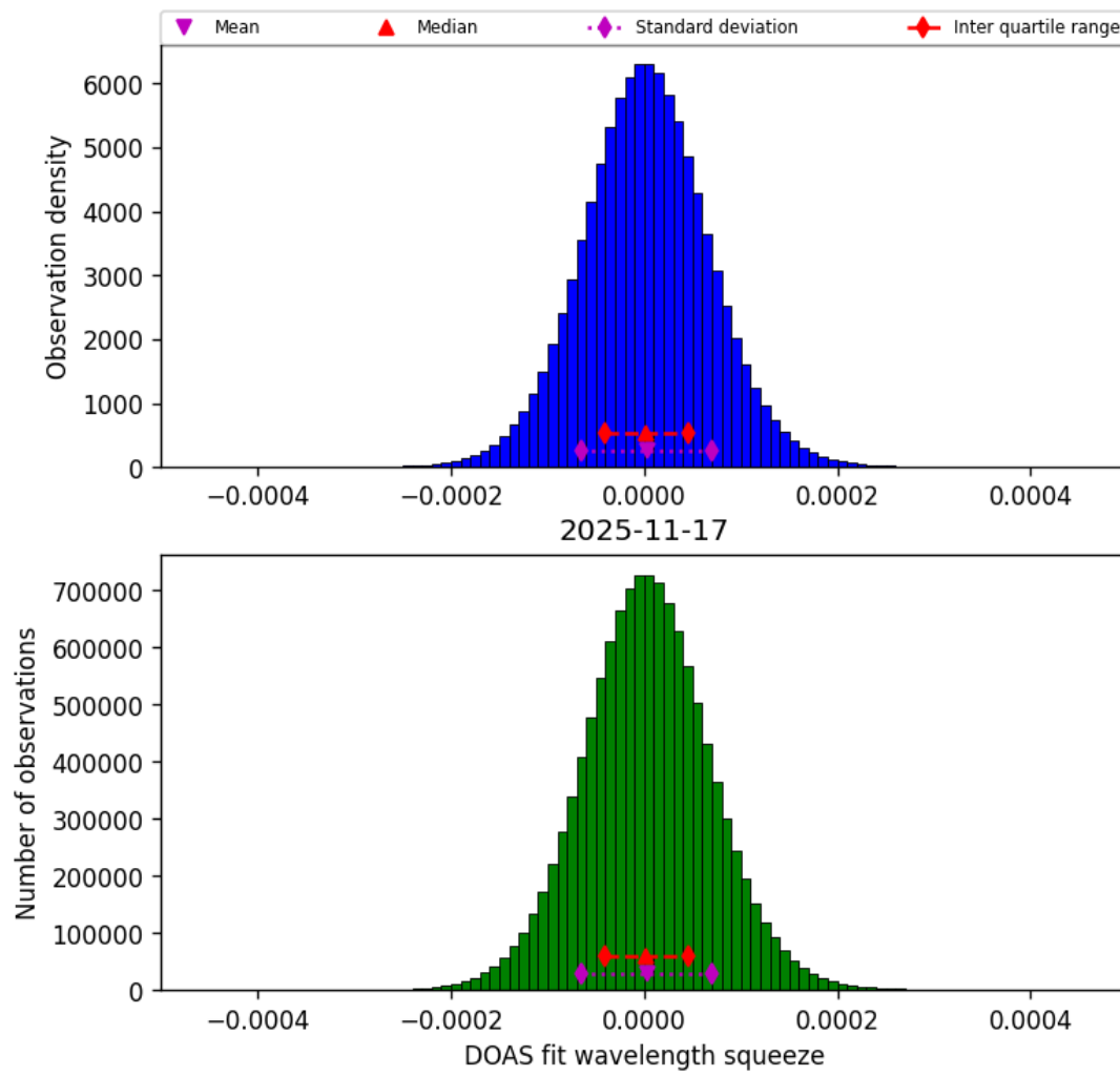
Figure 47: Histogram of “DOAS fit wavelength squeeze” for 2025-11-16 to 2025-11-18
