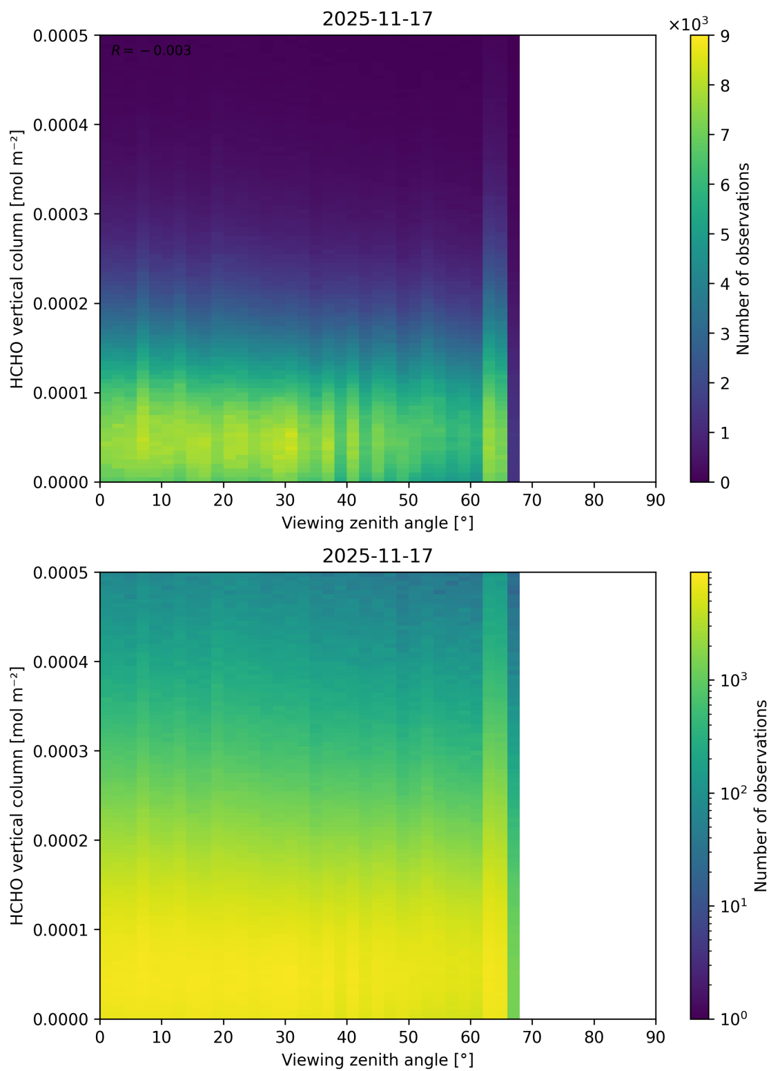
Figure 212: Scatter density plot of “Viewing zenith angle” against “HCHO vertical column” for 2025-11-16 to 2025-11-18.
