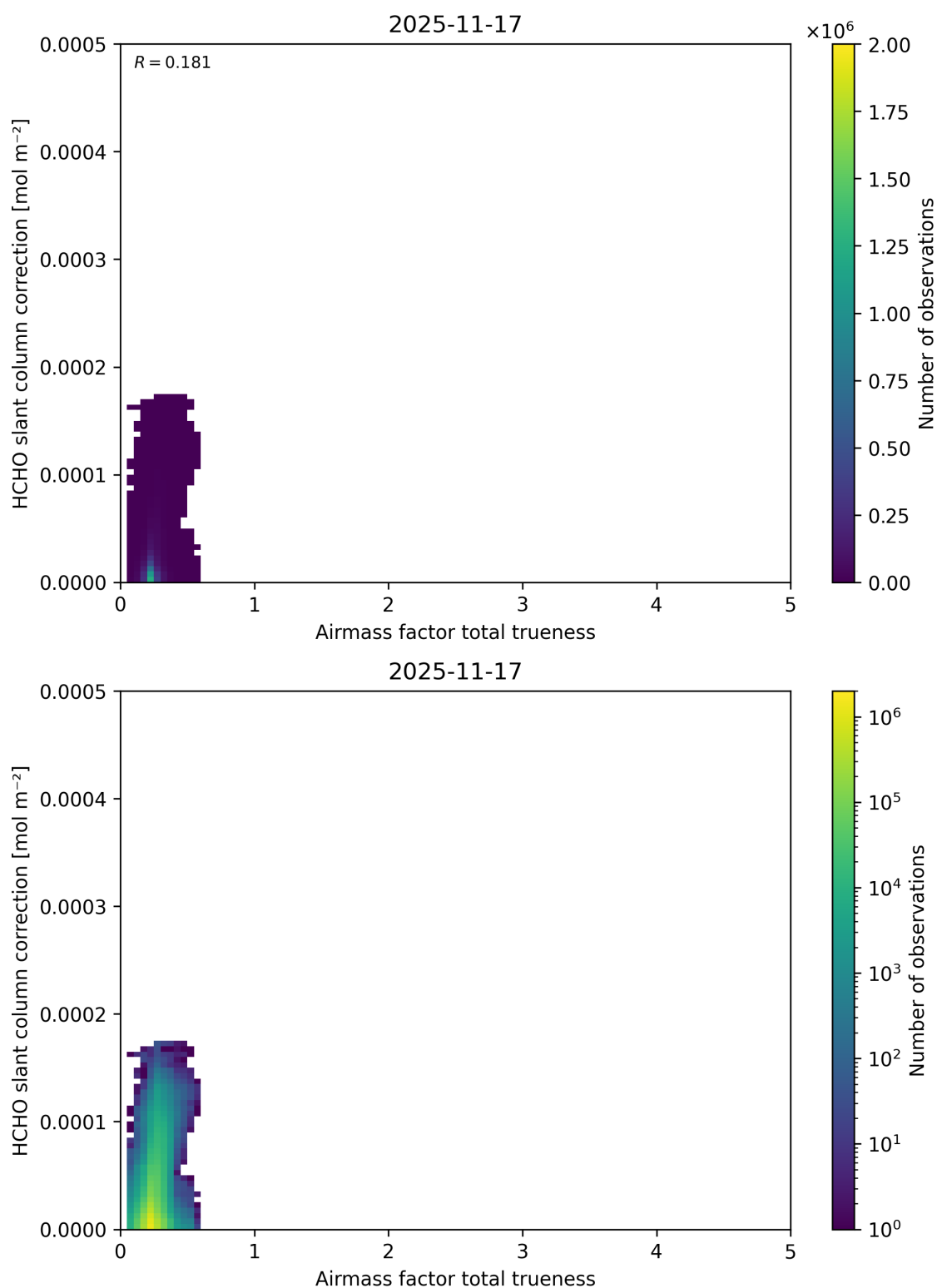
Figure 123: Scatter density plot of “Airmass factor total trueness” against “HCHO slant column correction” for 2025-11-16 to 2025-11-18.
