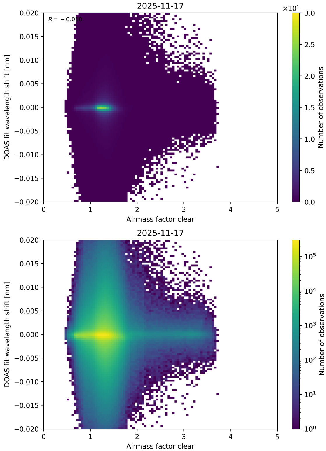
Figure 79: Scatter density plot of “Airmass factor clear” against “DOAS fit wavelength shift” for 2025-11-16 to 2025-11-18.
