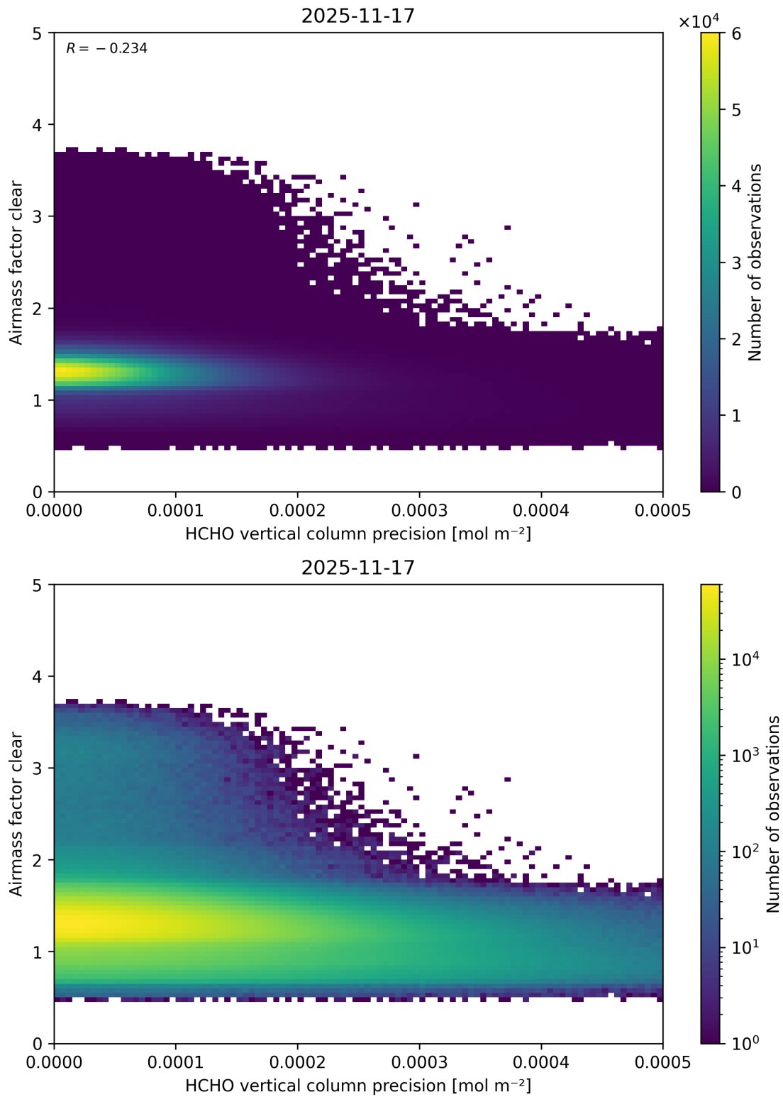
Figure 155: Scatter density plot of “HCHO vertical column precision” against “Airmass factor clear” for 2025-11-16 to 2025-11-18.
