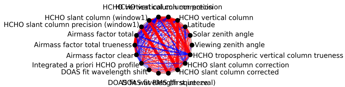
Figure 1: Map of correlation graph for 2025-11-16 to 2025-11-18.
