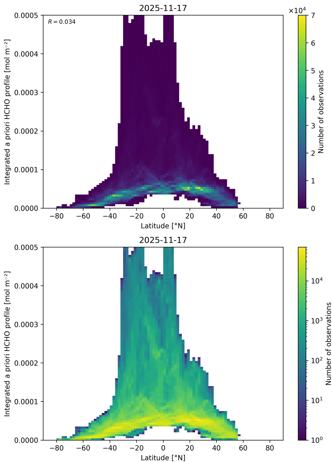
Figure 185: Scatter density plot of “Latitude” against “Integrated a priori HCHO profile” for 2025-11-16 to 2025-11-18.
