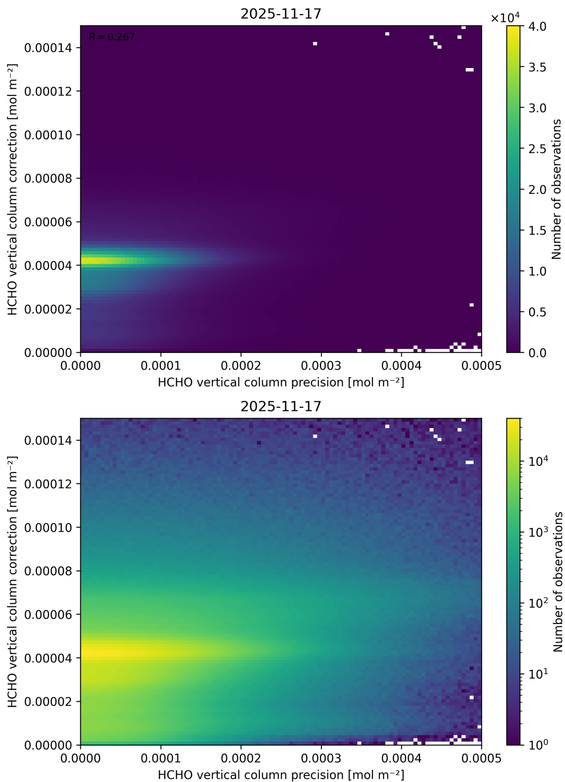
Figure 162: Scatter density plot of “HCHO vertical column precision” against “HCHO vertical column correction” for 2025-11-16 to 2025-11-18.
