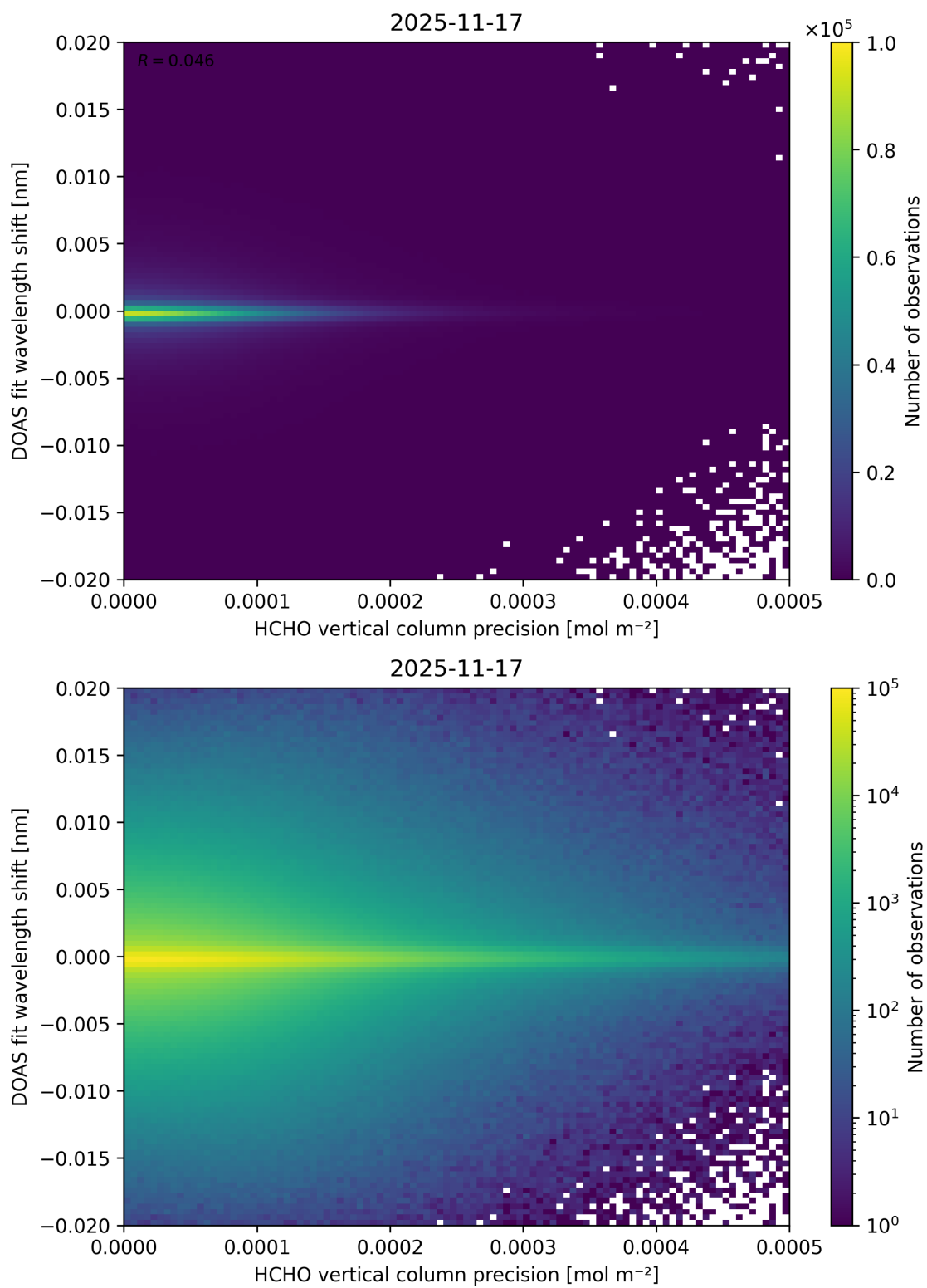
Figure 153: Scatter density plot of “HCHO vertical column precision” against “DOAS fit wavelength shift” for 2025-11-16 to 2025-11-18.
