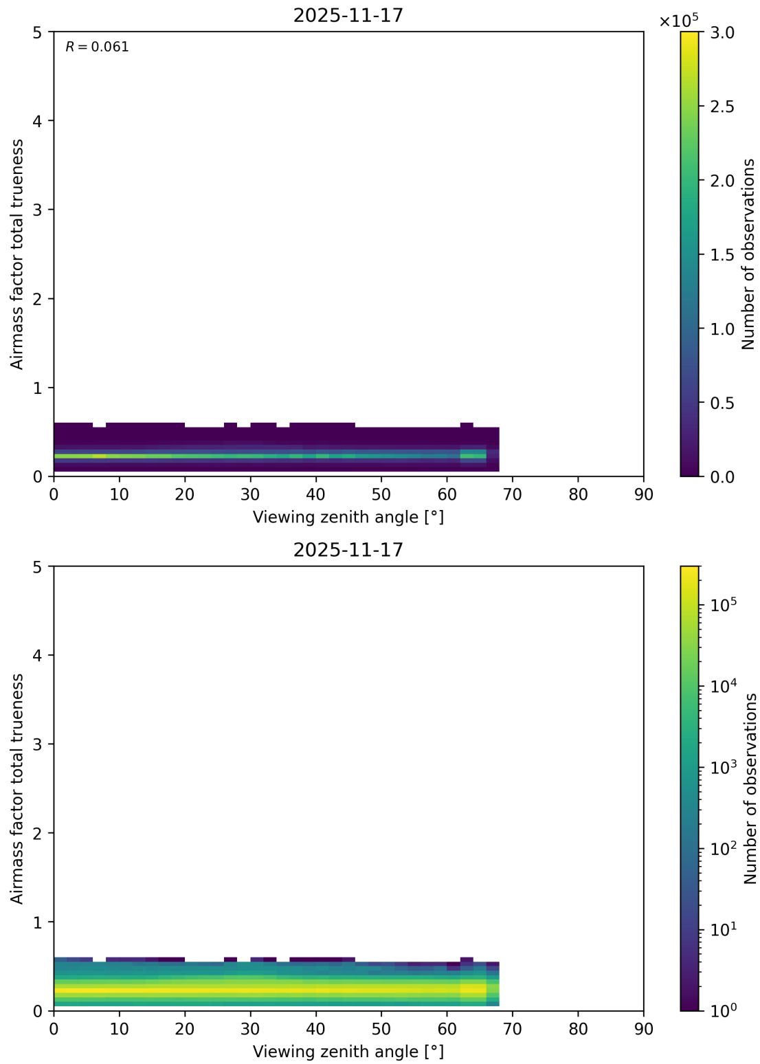
Figure 211: Scatter density plot of “Viewing zenith angle” against “Airmass factor total trueness” for 2025-11-16 to 2025-11-18.
