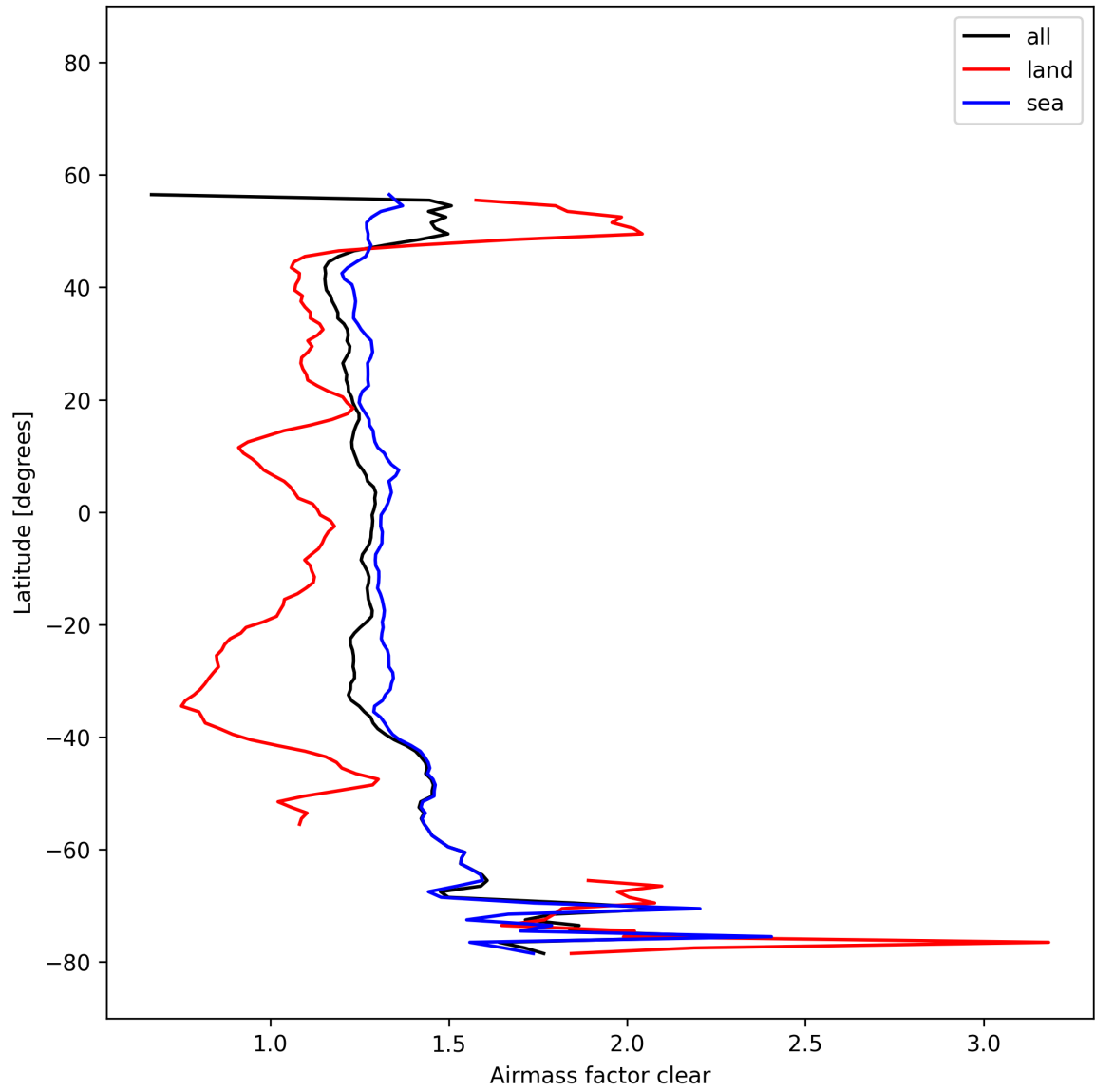
Figure 29: Zonal average of “Airmass factor clear” for 2025-11-16 to 2025-11-18.
