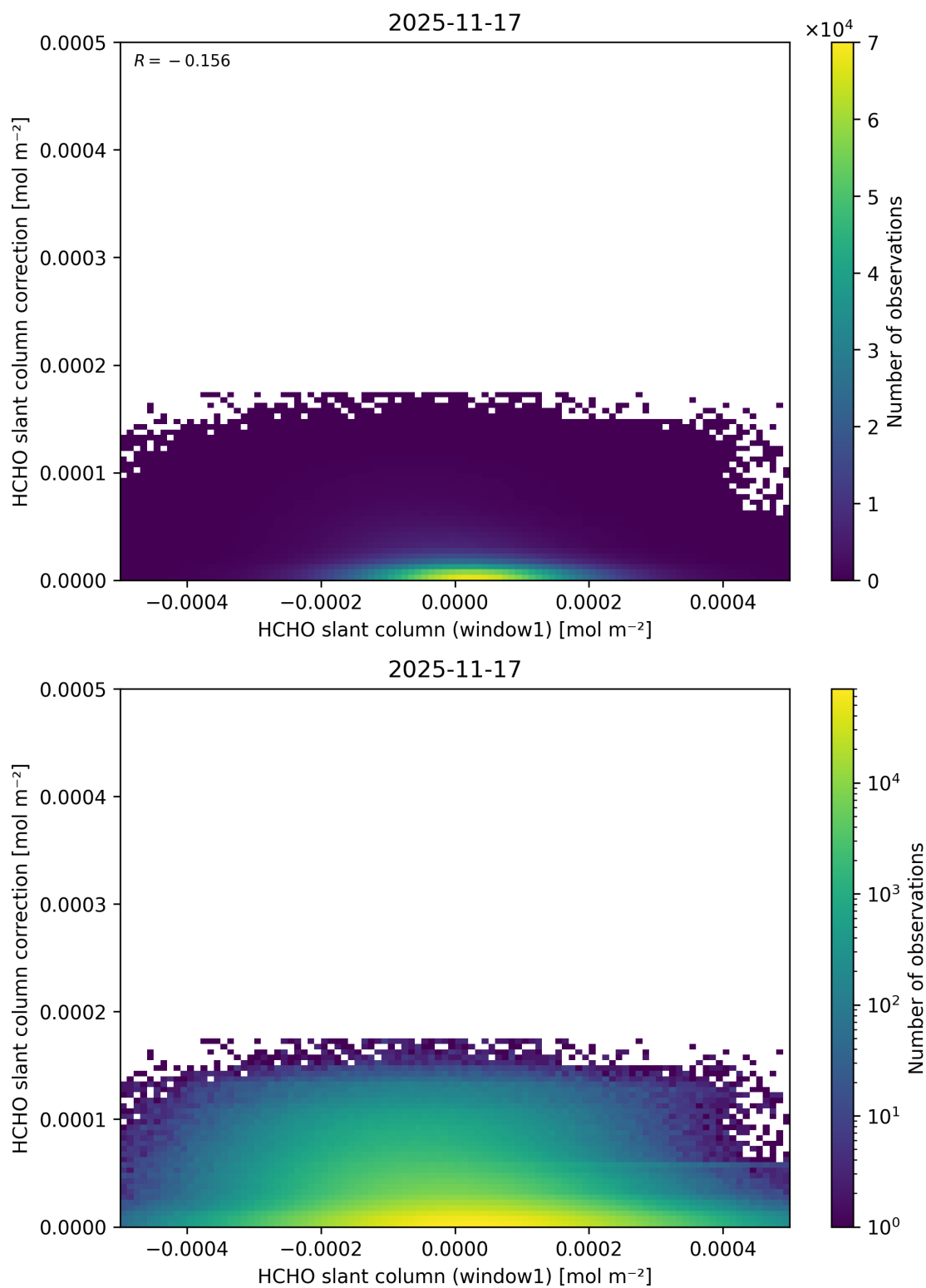
Figure 93: Scatter density plot of “HCHO slant column (window1)” against “HCHO slant column correction” for 2025-11-16 to 2025-11-18.
