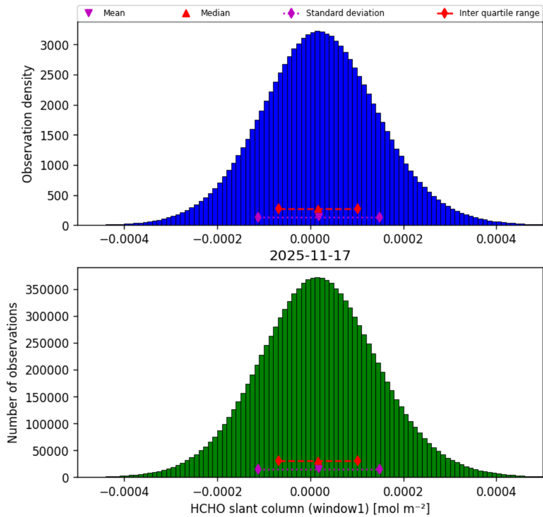
Figure 40: Histogram of “HCHO slant column (window1)” for 2025-11-16 to 2025-11-18
