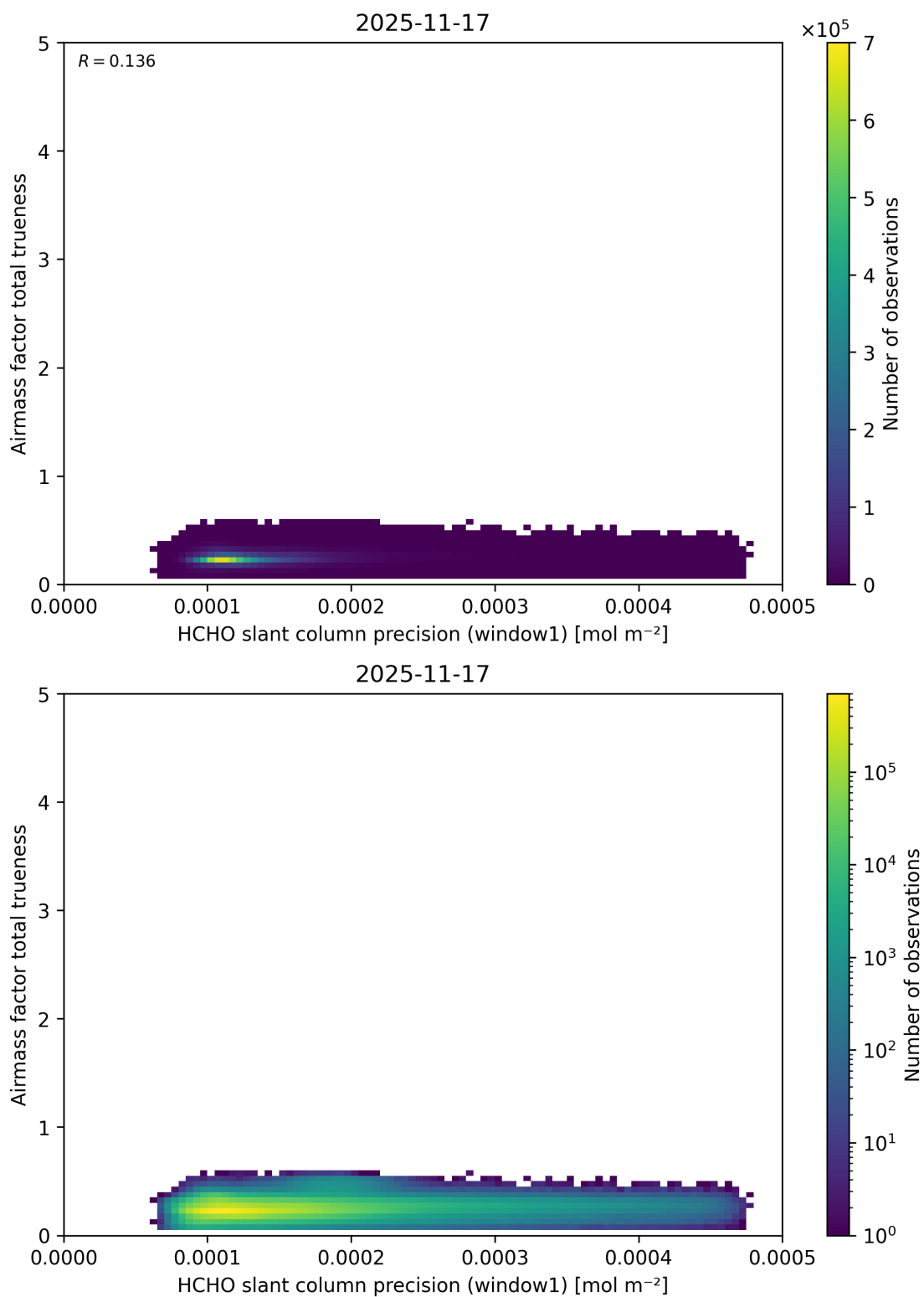
Figure 106: Scatter density plot of “HCHO slant column precision (window1)” against “Airmass factor total trueness” for 2025-11-16 to 2025-11-18.
