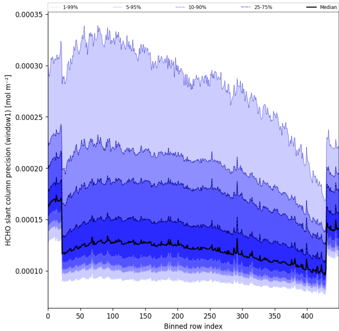
Figure 56: Along track statistics of “HCHO slant column precision (window1)” for 2025-11-16 to 2025-11-18
