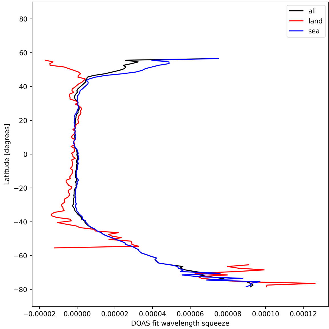
Figure 32: Zonal average of “DOAS fit wavelength squeeze” for 2025-11-16 to 2025-11-18.
