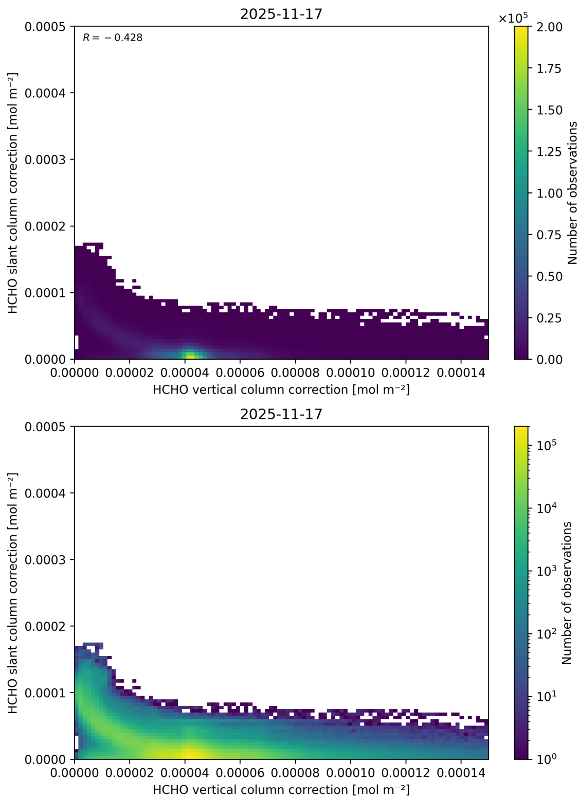
Figure 131: Scatter density plot of “HCHO vertical column correction” against “HCHO slant column correction” for 2025-11-16 to 2025-11-18.
