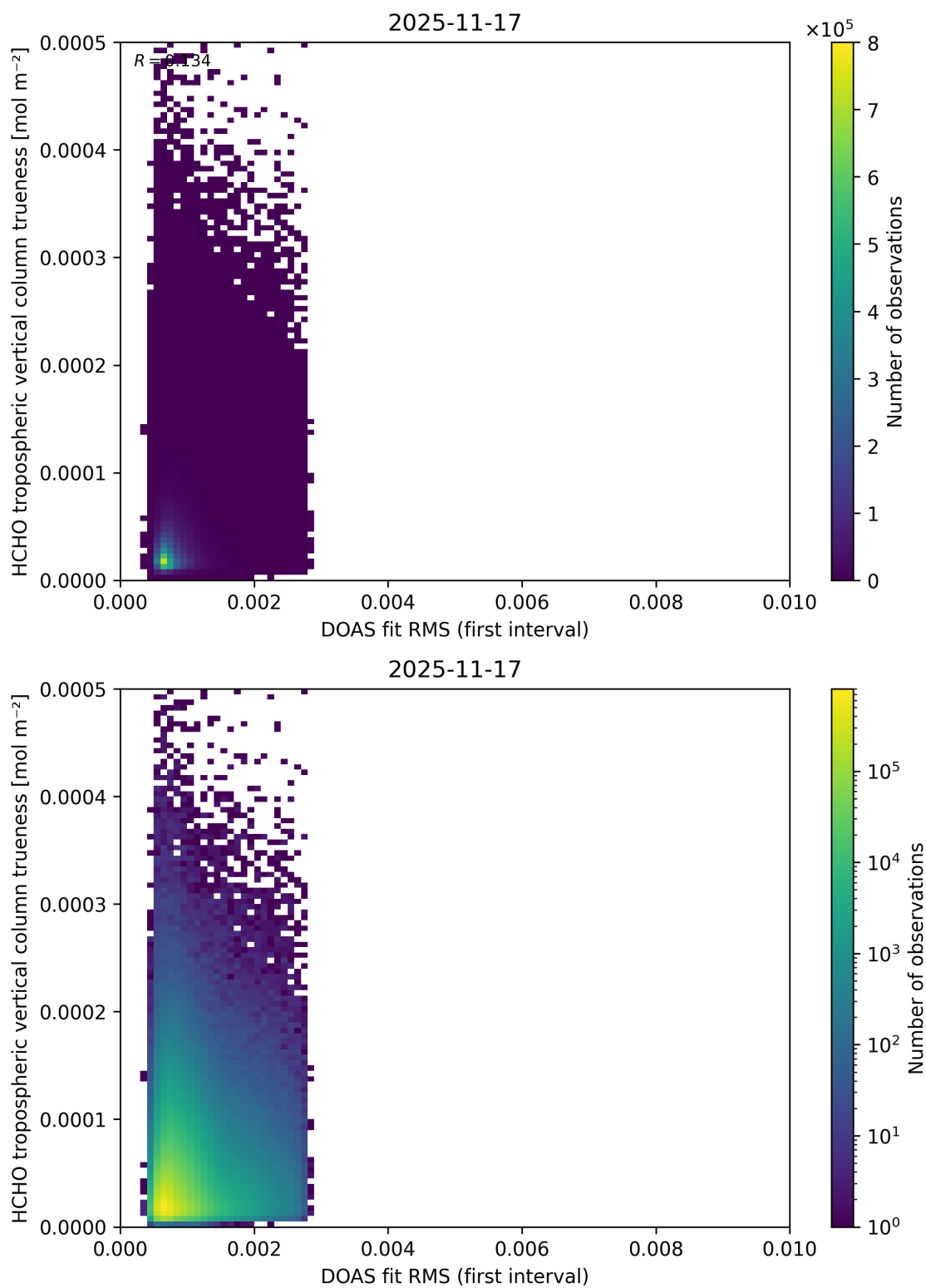
Figure 68: Scatter density plot of “DOAS fit RMS (first interval)” against “HCHO tropospheric vertical column trueness” for 2025-11-16 to 2025-11-18.
