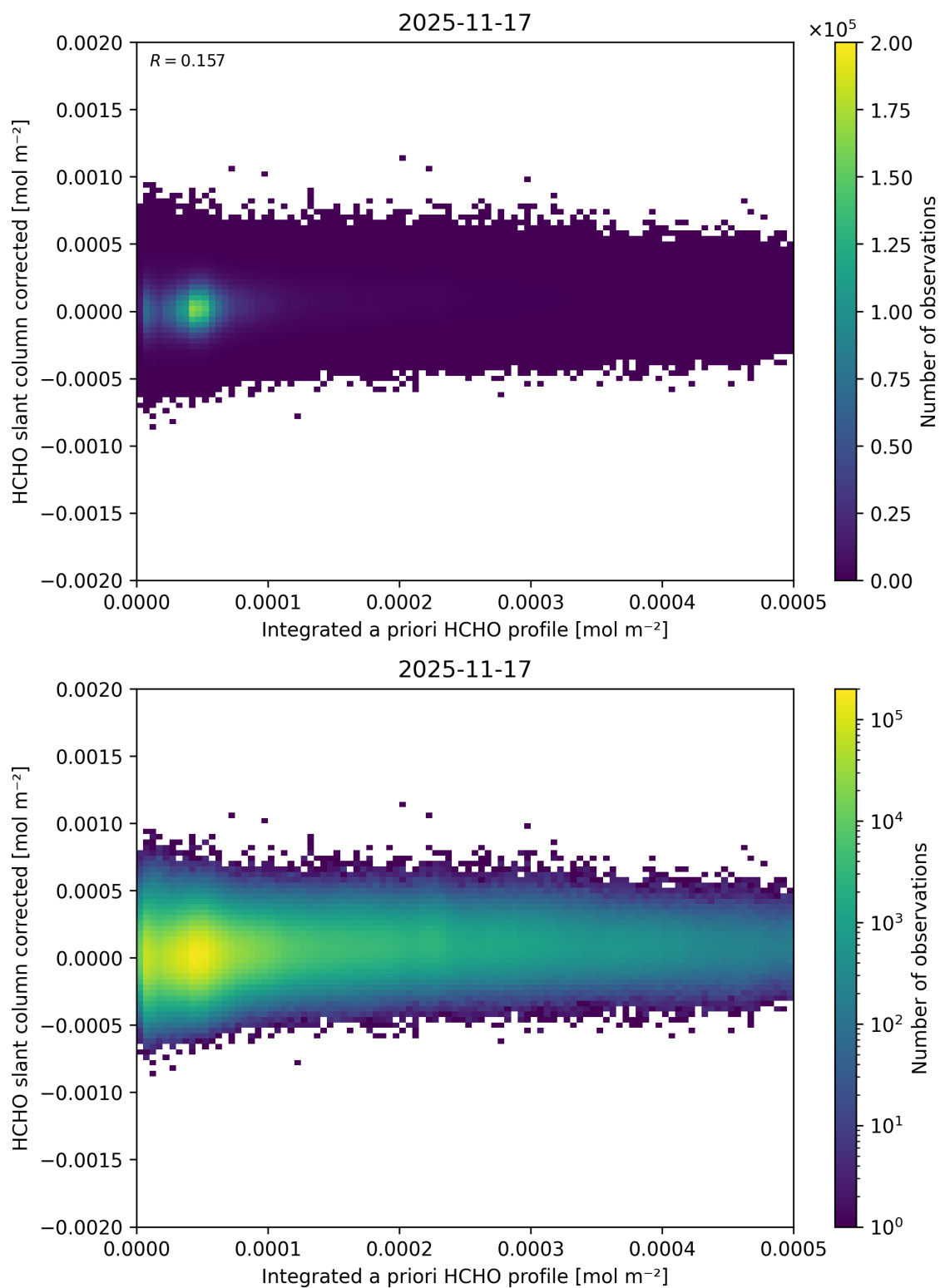
Figure 168: Scatter density plot of “Integrated a priori HCHO profile” against “HCHO slant column corrected” for 2025-11-16 to 2025-11-18.
