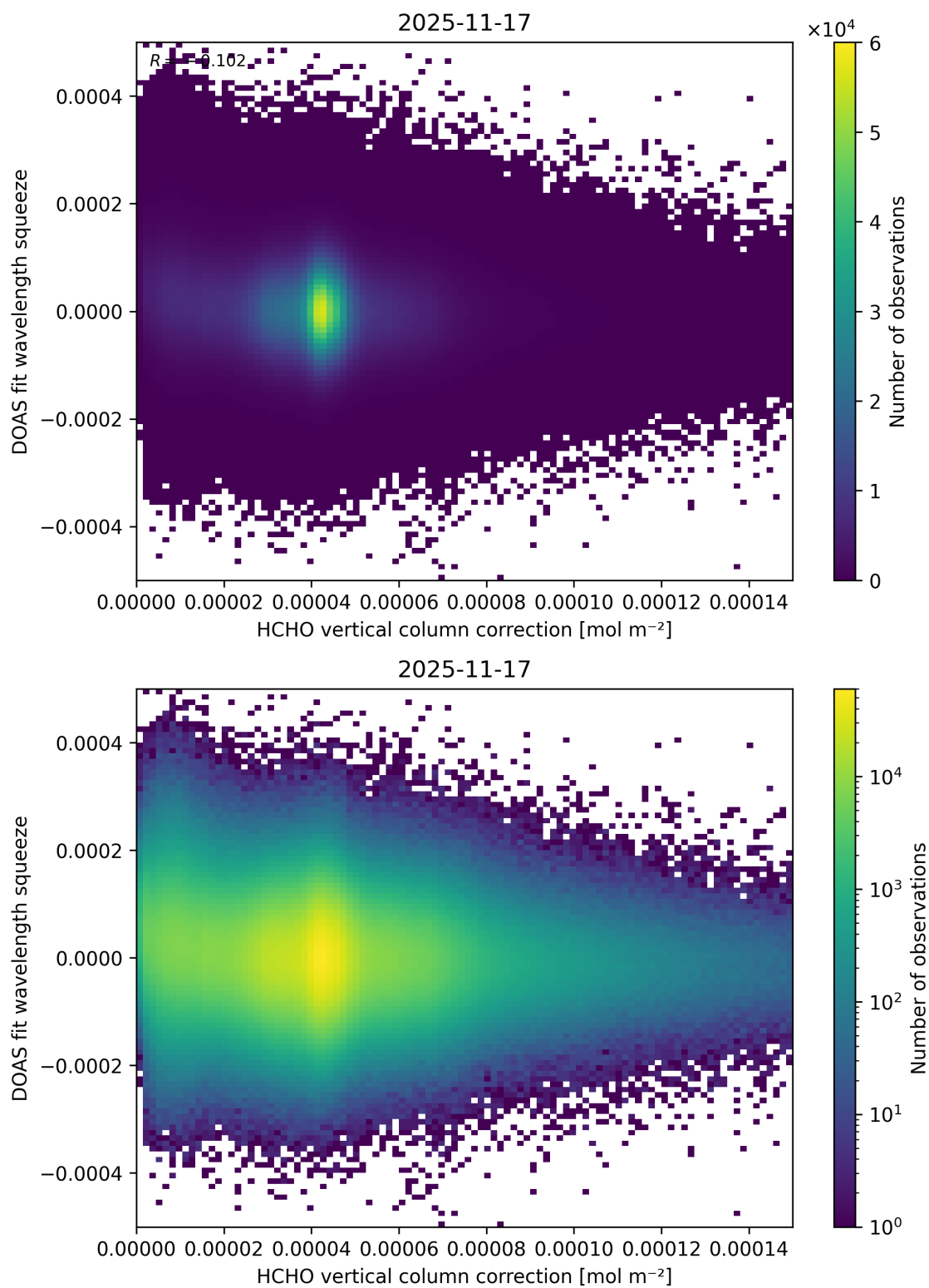
Figure 128: Scatter density plot of “HCHO vertical column correction” against “DOAS fit wavelength squeeze” for 2025-11-16 to 2025-11-18.
