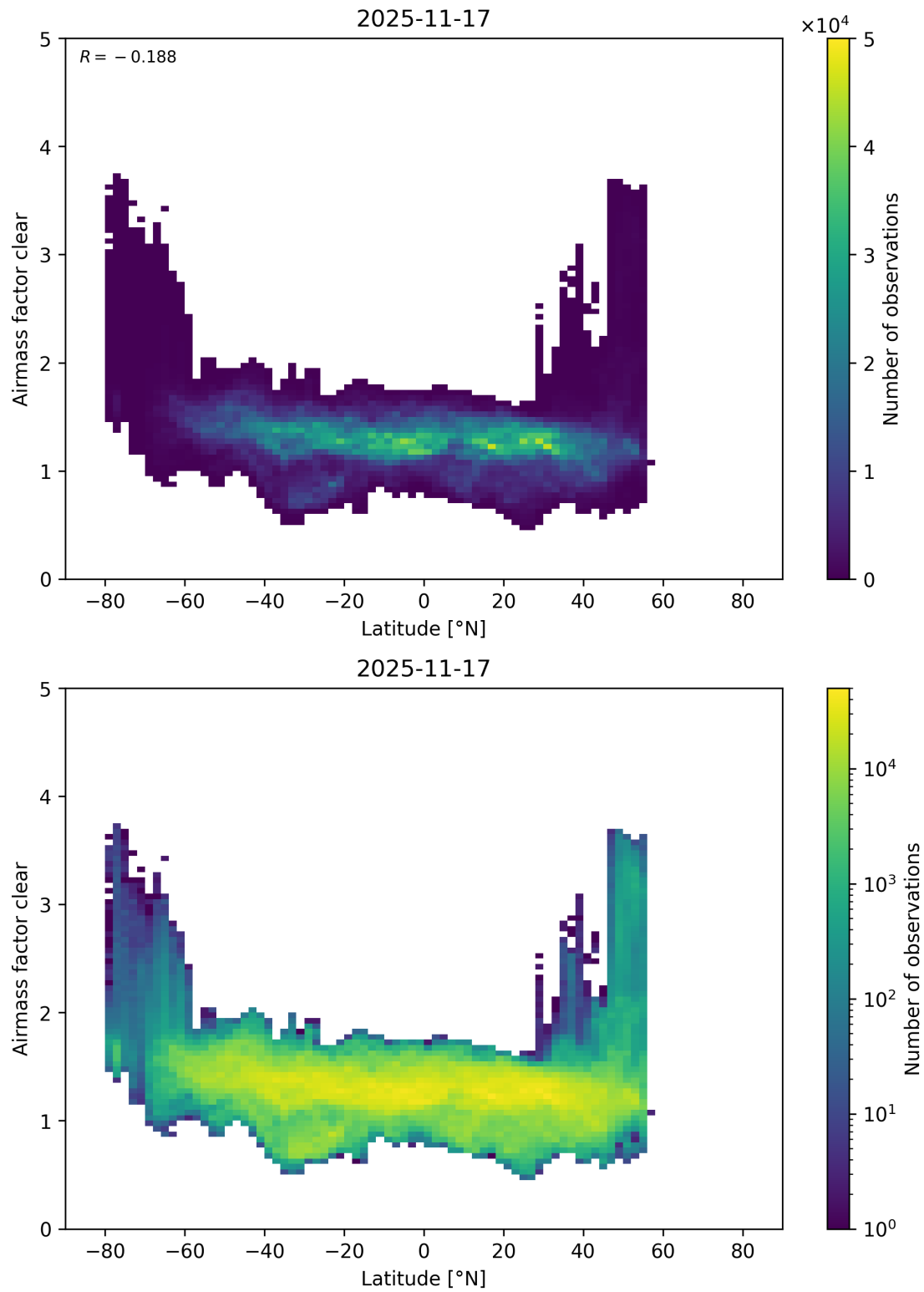
Figure 174: Scatter density plot of “Latitude” against “Airmass factor clear” for 2025-11-16 to 2025-11-18.
