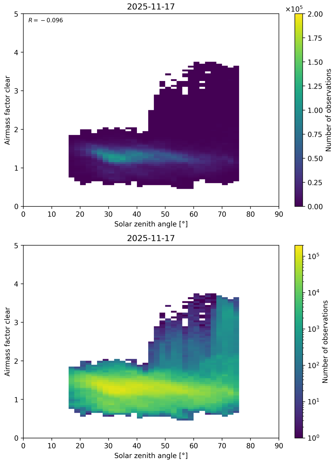
Figure 189: Scatter density plot of “Solar zenith angle” against “Airmass factor clear” for 2025-11-16 to 2025-11-18.
