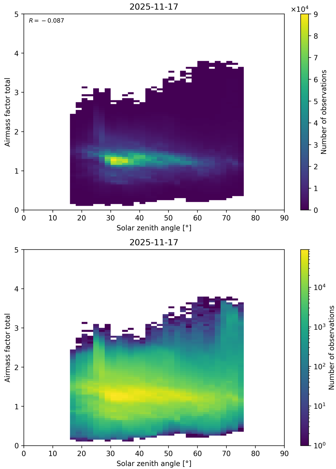
Figure 194: Scatter density plot of “Solar zenith angle” against “Airmass factor total” for 2025-11-16 to 2025-11-18.
