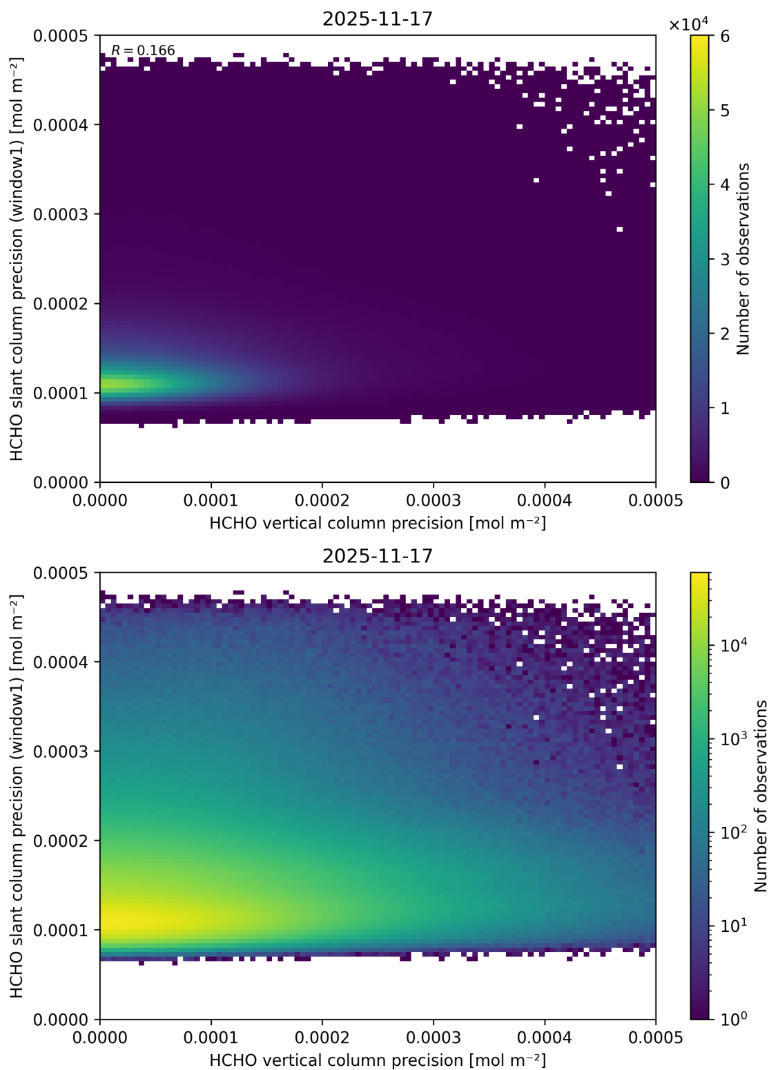
Figure 159: Scatter density plot of “HCHO vertical column precision” against “HCHO slant column precision (window1)” for 2025-11-16 to 2025-11-18.
