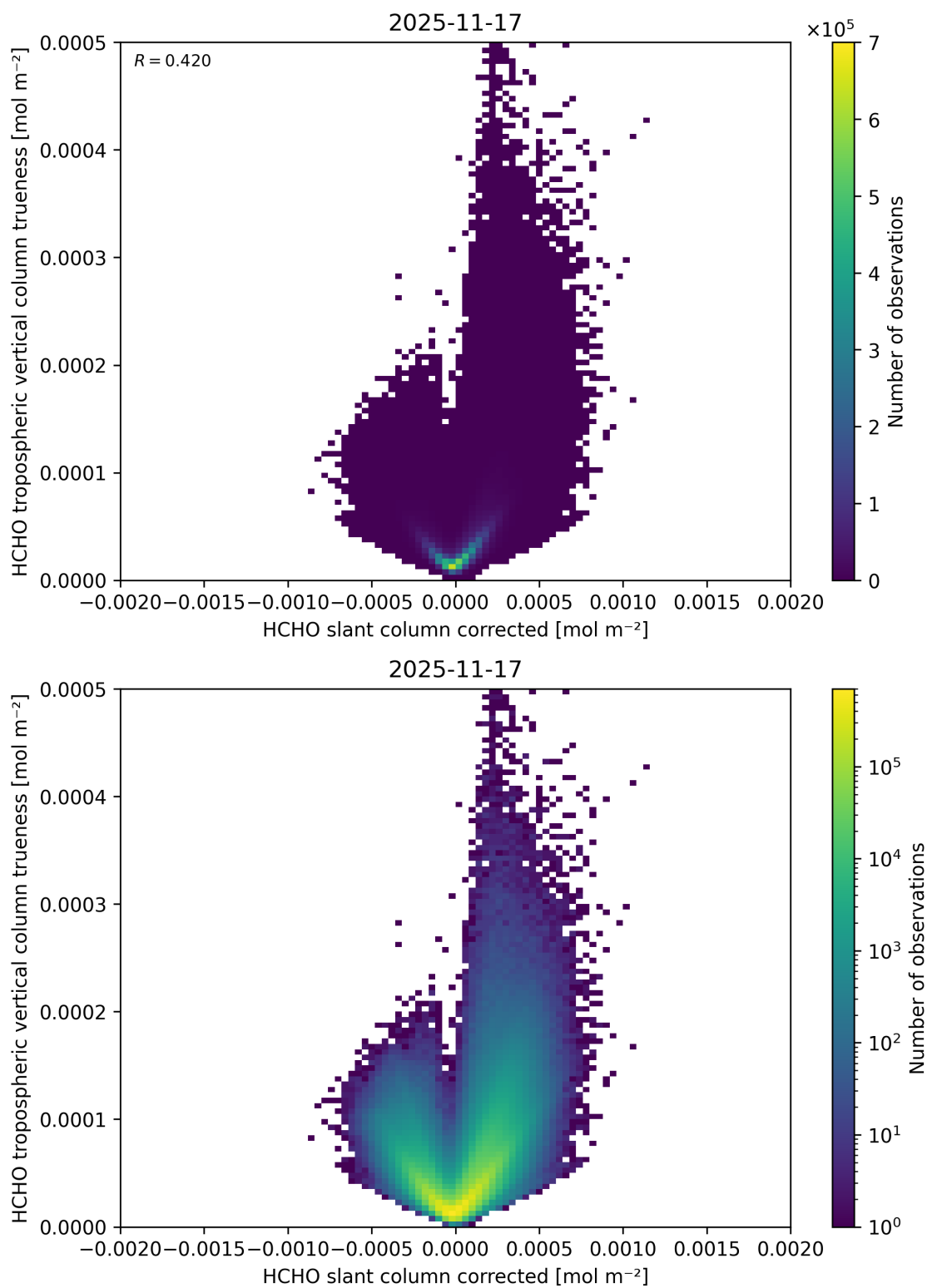
Figure 86: Scatter density plot of “HCHO slant column corrected” against “HCHO tropospheric vertical column trueness” for 2025-11-16 to 2025-11-18.
