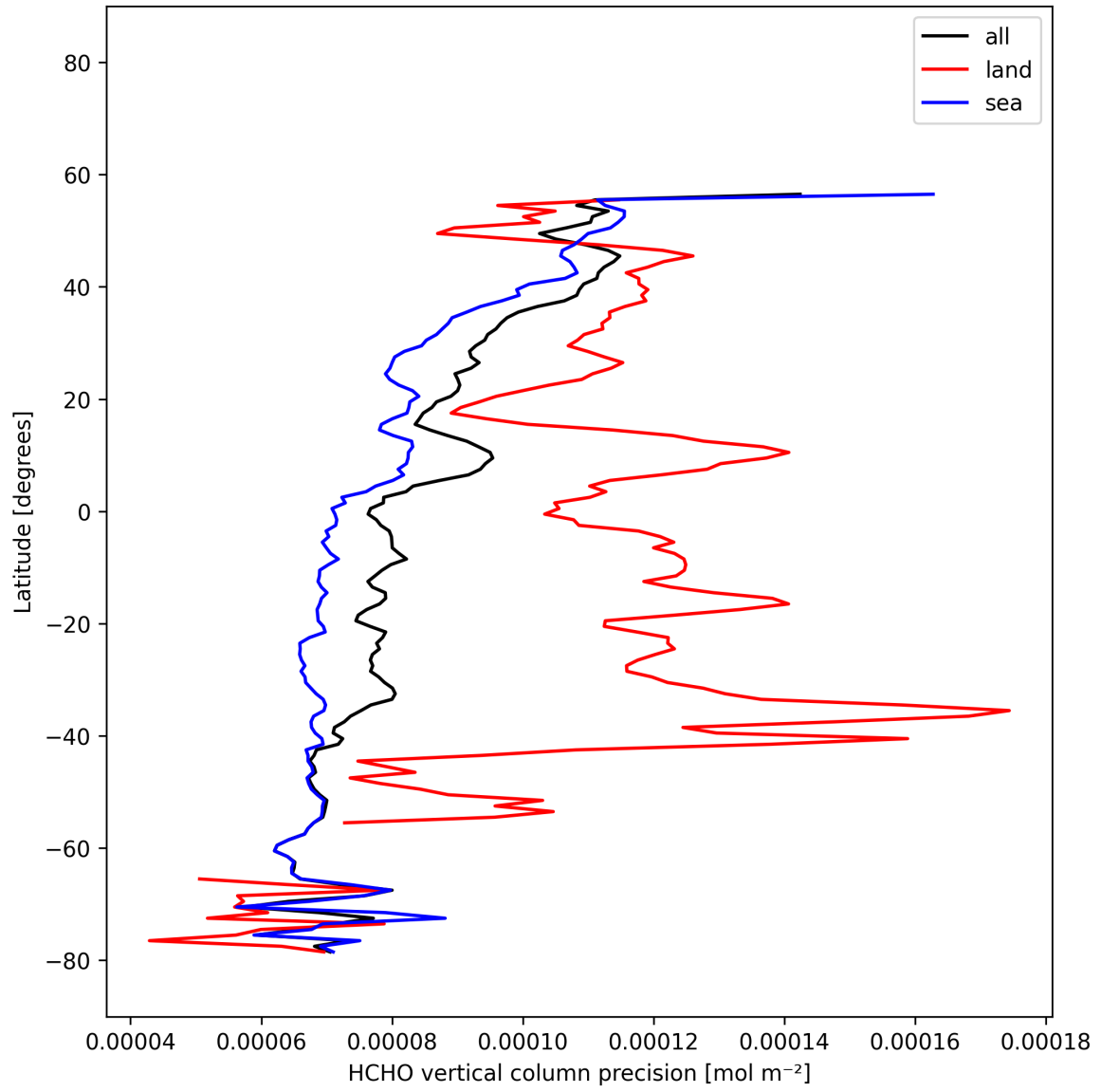
Figure 23: Zonal average of “HCHO vertical column precision” for 2025-11-16 to 2025-11-18.
