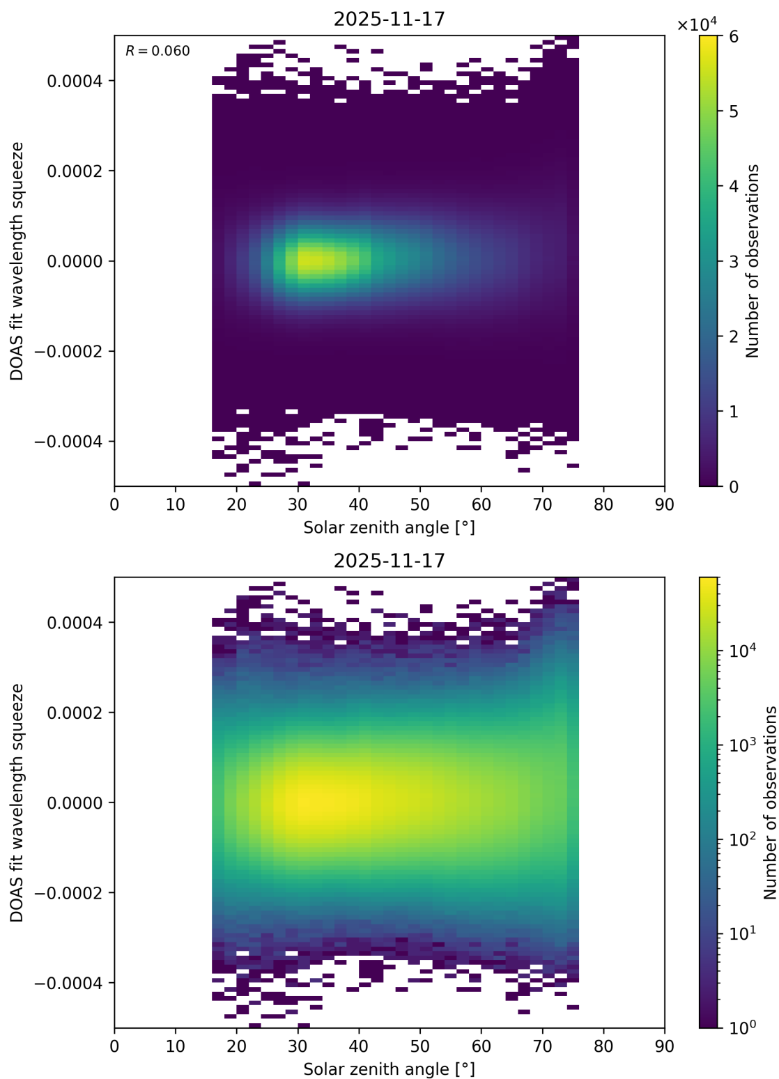
Figure 188: Scatter density plot of “Solar zenith angle” against “DOAS fit wavelength squeeze” for 2025-11-16 to 2025-11-18.
