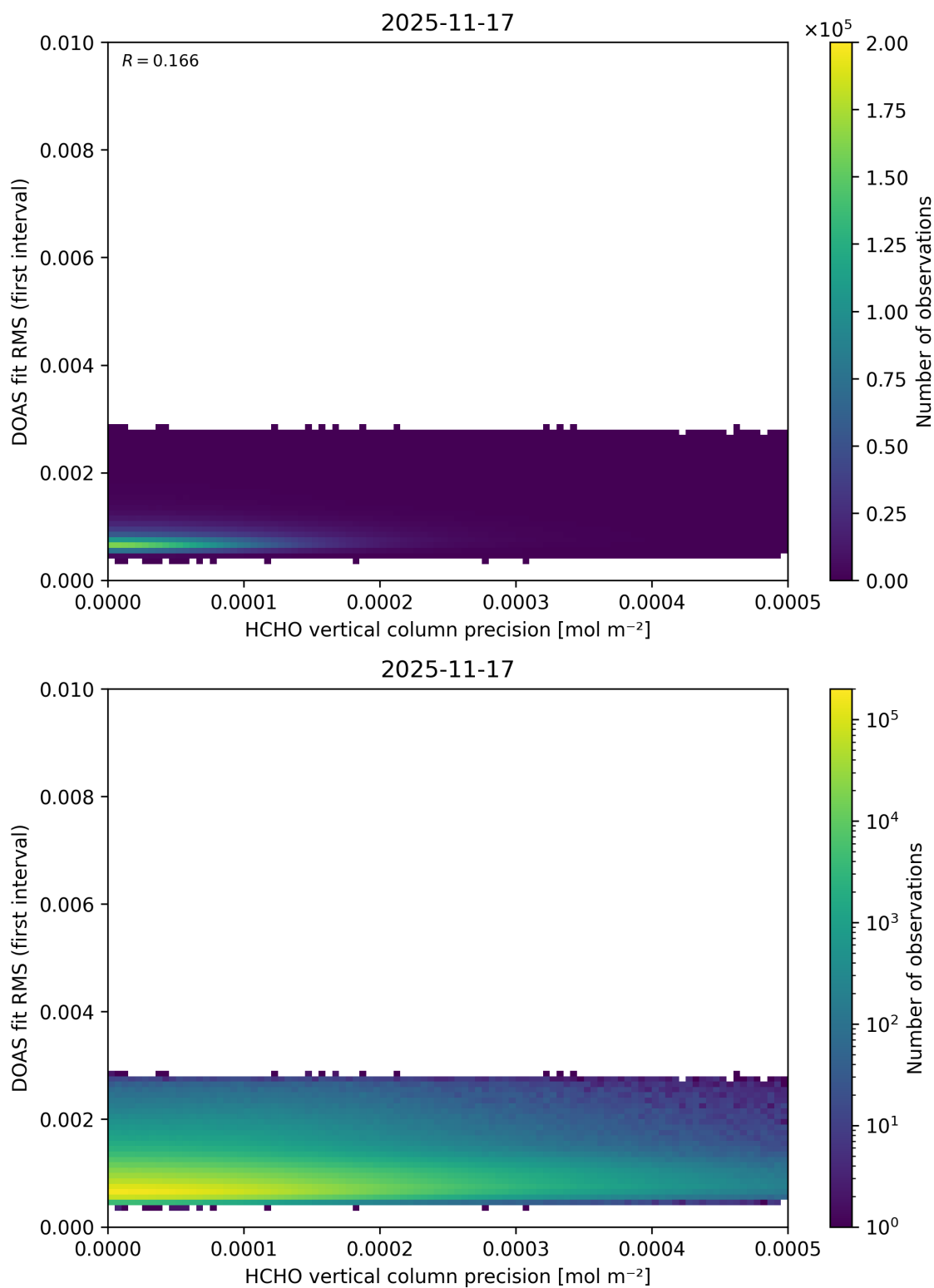
Figure 152: Scatter density plot of “HCHO vertical column precision” against “DOAS fit RMS (first interval)” for 2025-11-16 to 2025-11-18.
