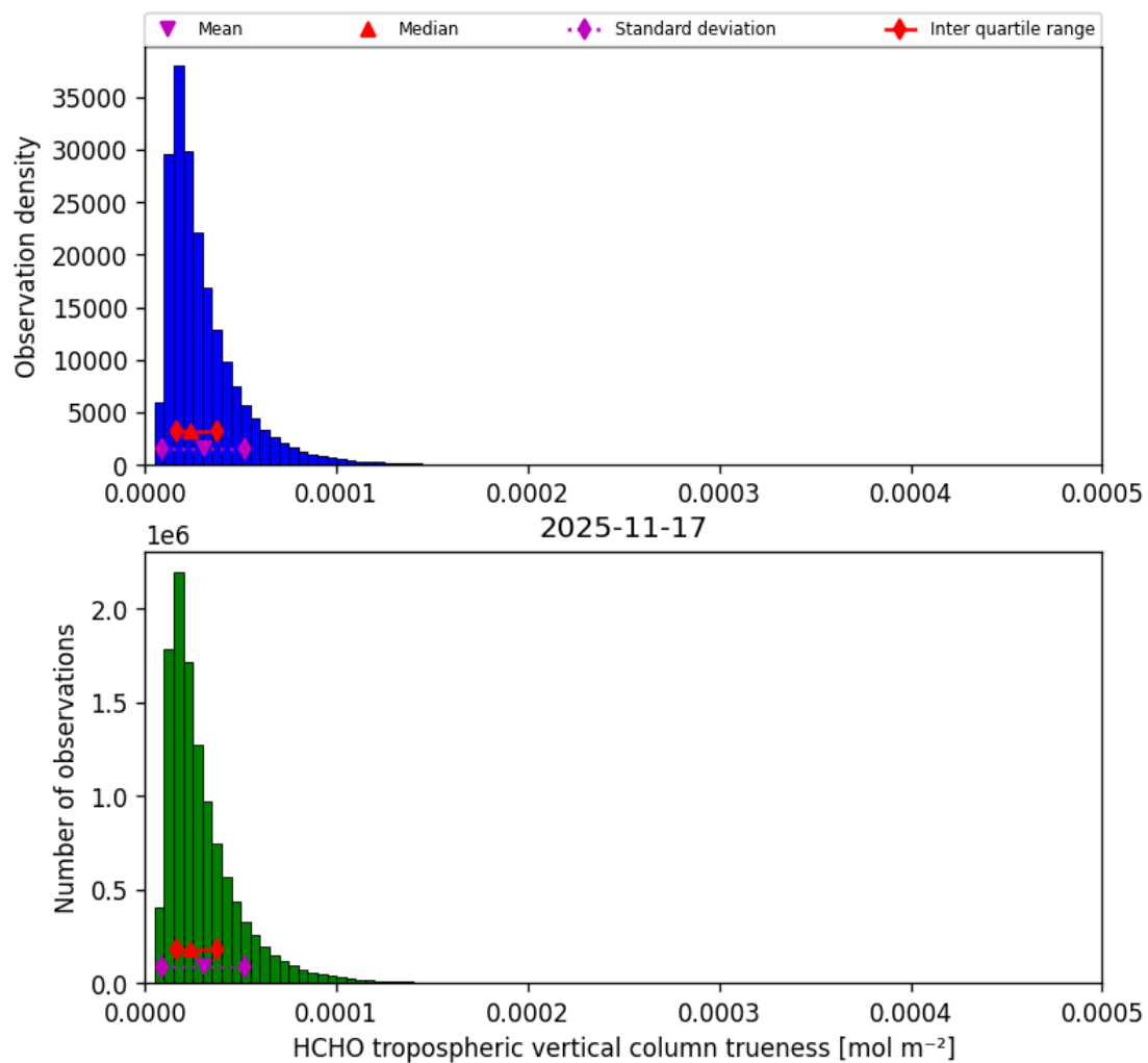
Figure 50: Histogram of “HCHO tropospheric vertical column trueness” for 2025-11-16 to 2025-11-18
