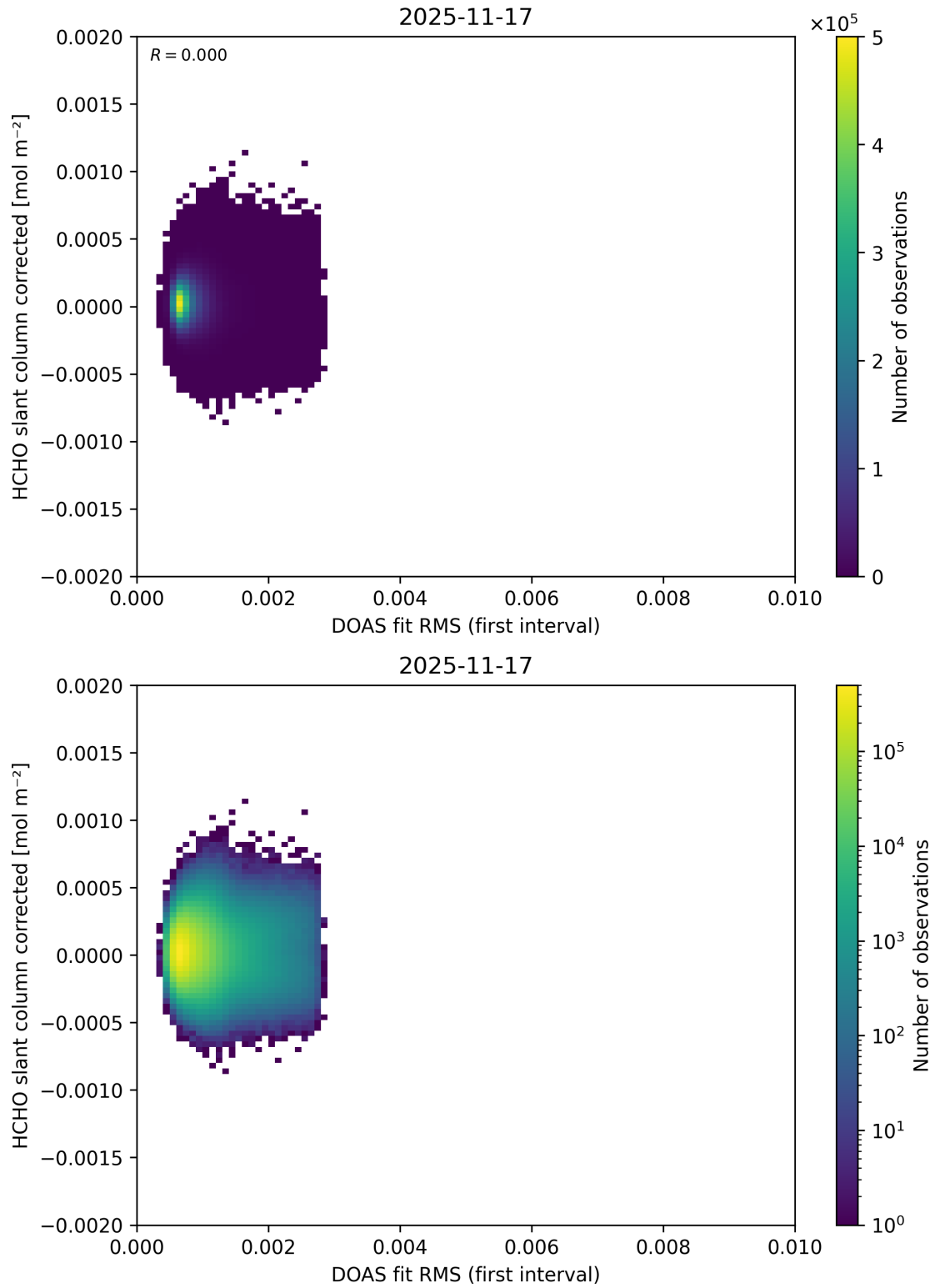
Figure 66: Scatter density plot of “DOAS fit RMS (first interval)” against “HCHO slant column corrected” for 2025-11-16 to 2025-11-18.
