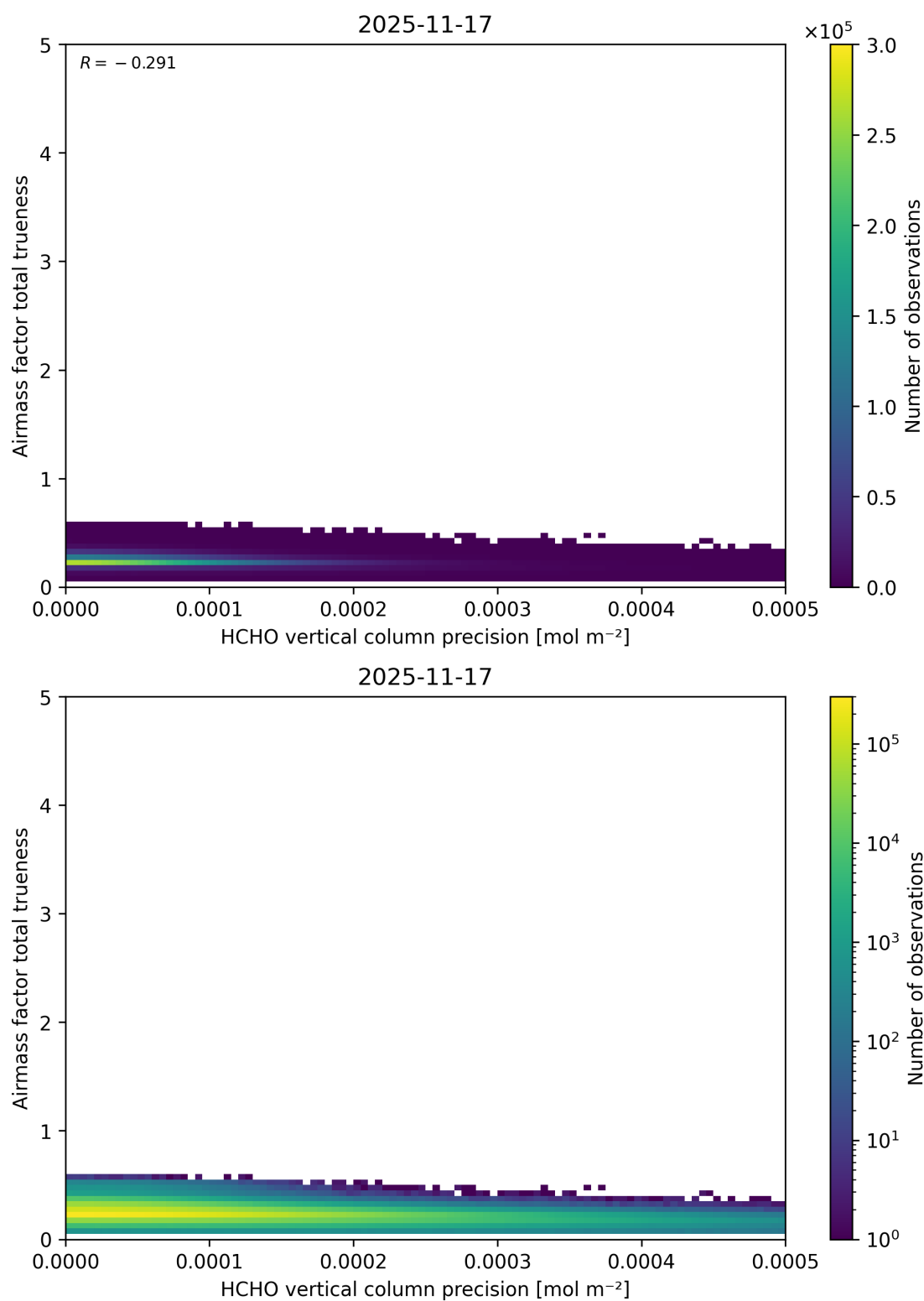
Figure 161: Scatter density plot of “HCHO vertical column precision” against “Airmass factor total trueness” for 2025-11-16 to 2025-11-18.
