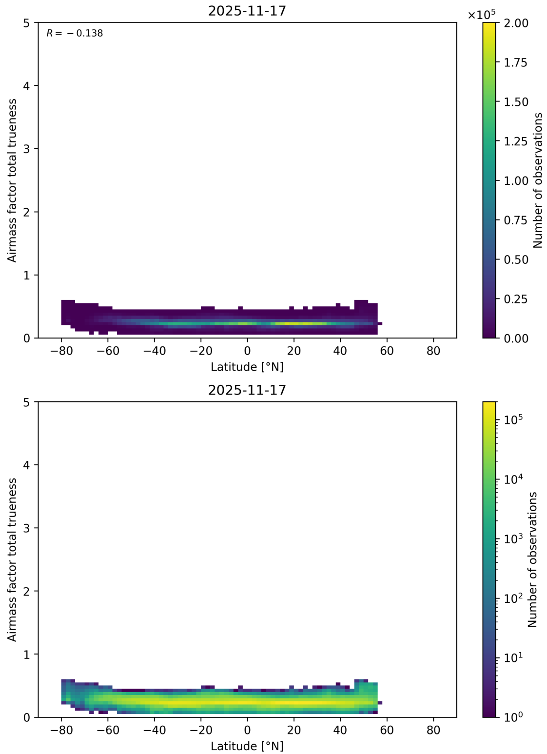
Figure 180: Scatter density plot of “Latitude” against “Airmass factor total trueness” for 2025-11-16 to 2025-11-18.
