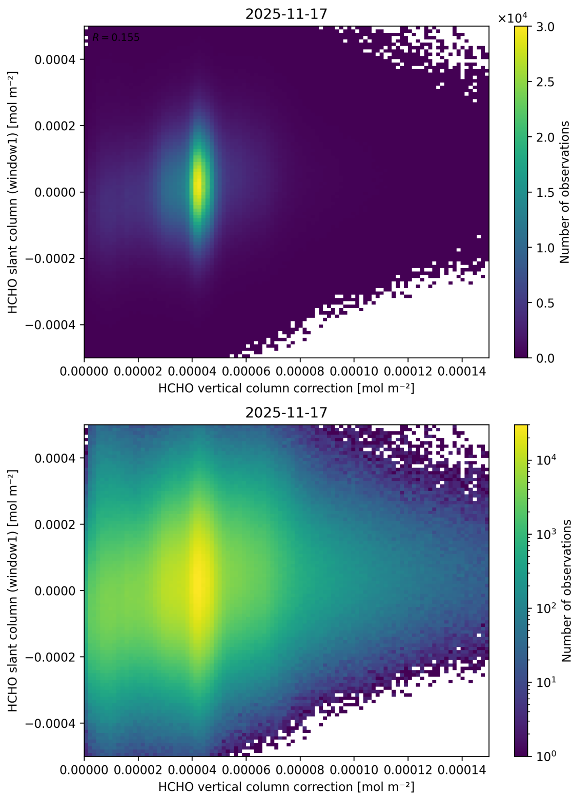
Figure 132: Scatter density plot of “HCHO vertical column correction” against “HCHO slant column (window1)” for 2025-11-16 to 2025-11-18.
