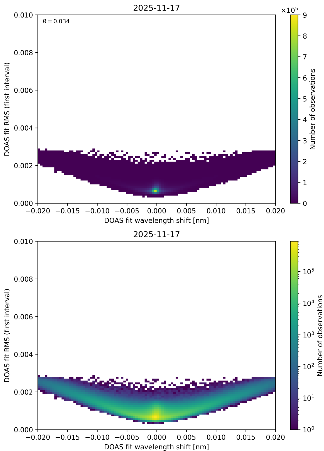
Figure 69: Scatter density plot of “DOAS fit wavelength shift” against “DOAS fit RMS (first interval)” for 2025-11-16 to 2025-11-18.
