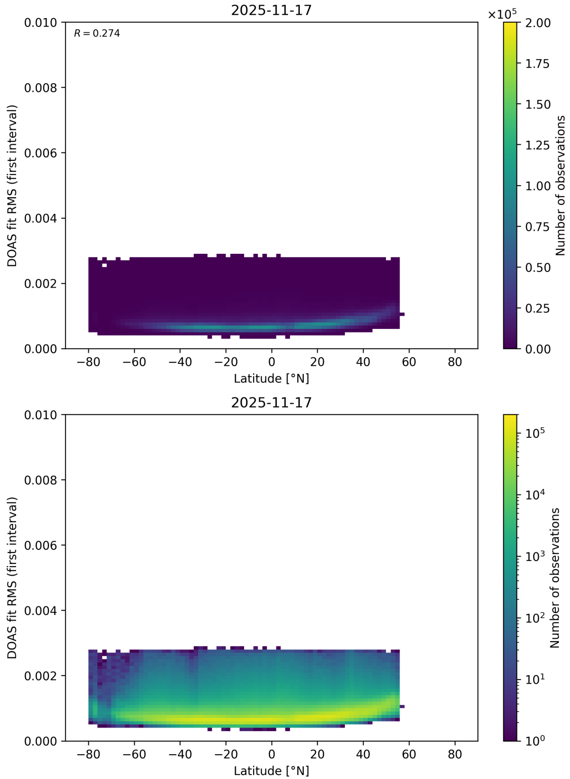
Figure 171: Scatter density plot of “Latitude” against “DOAS fit RMS (first interval)” for 2025-11-16 to 2025-11-18.
