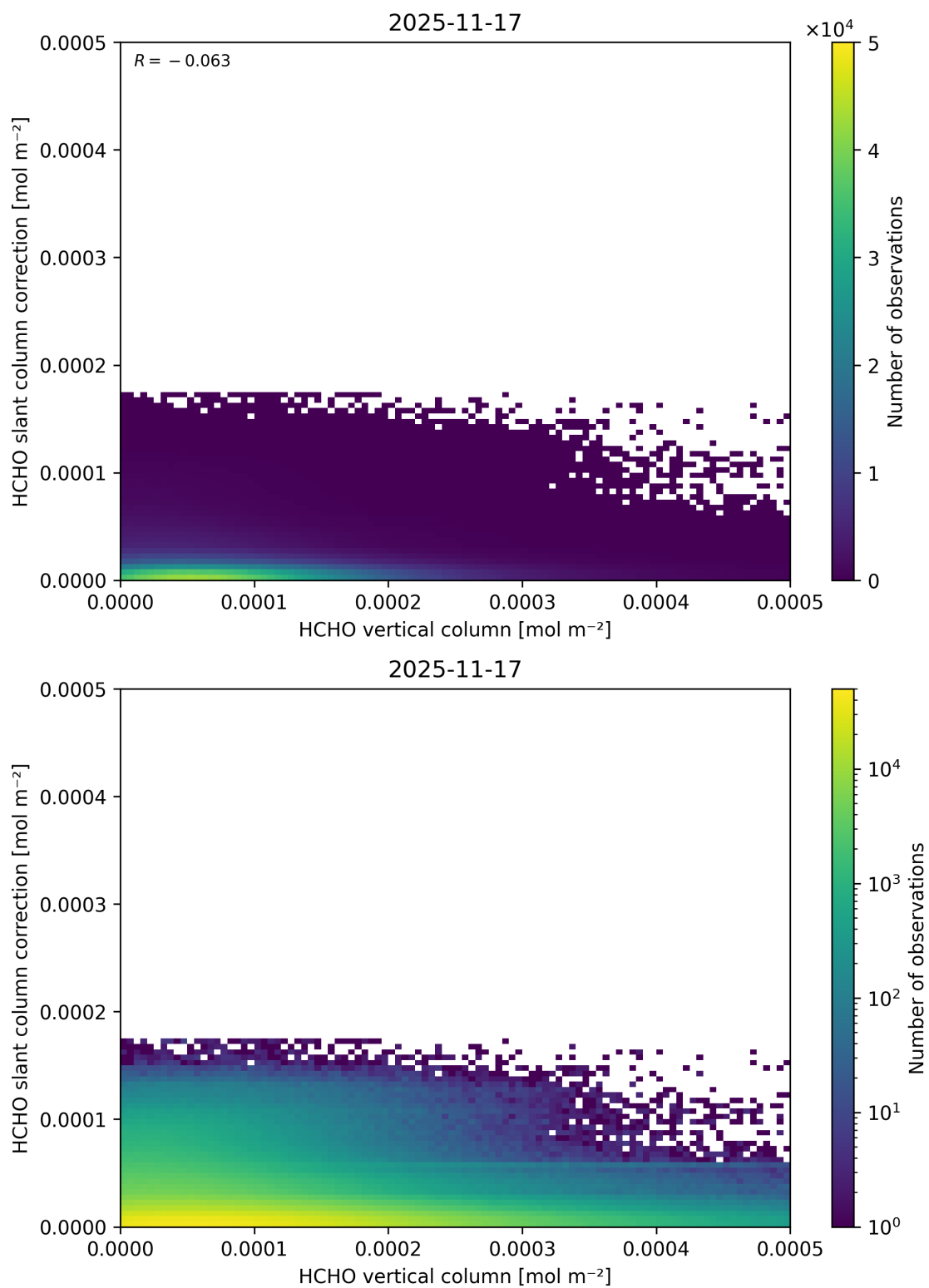
Figure 143: Scatter density plot of “HCHO vertical column” against “HCHO slant column correction” for 2025-11-16 to 2025-11-18.
