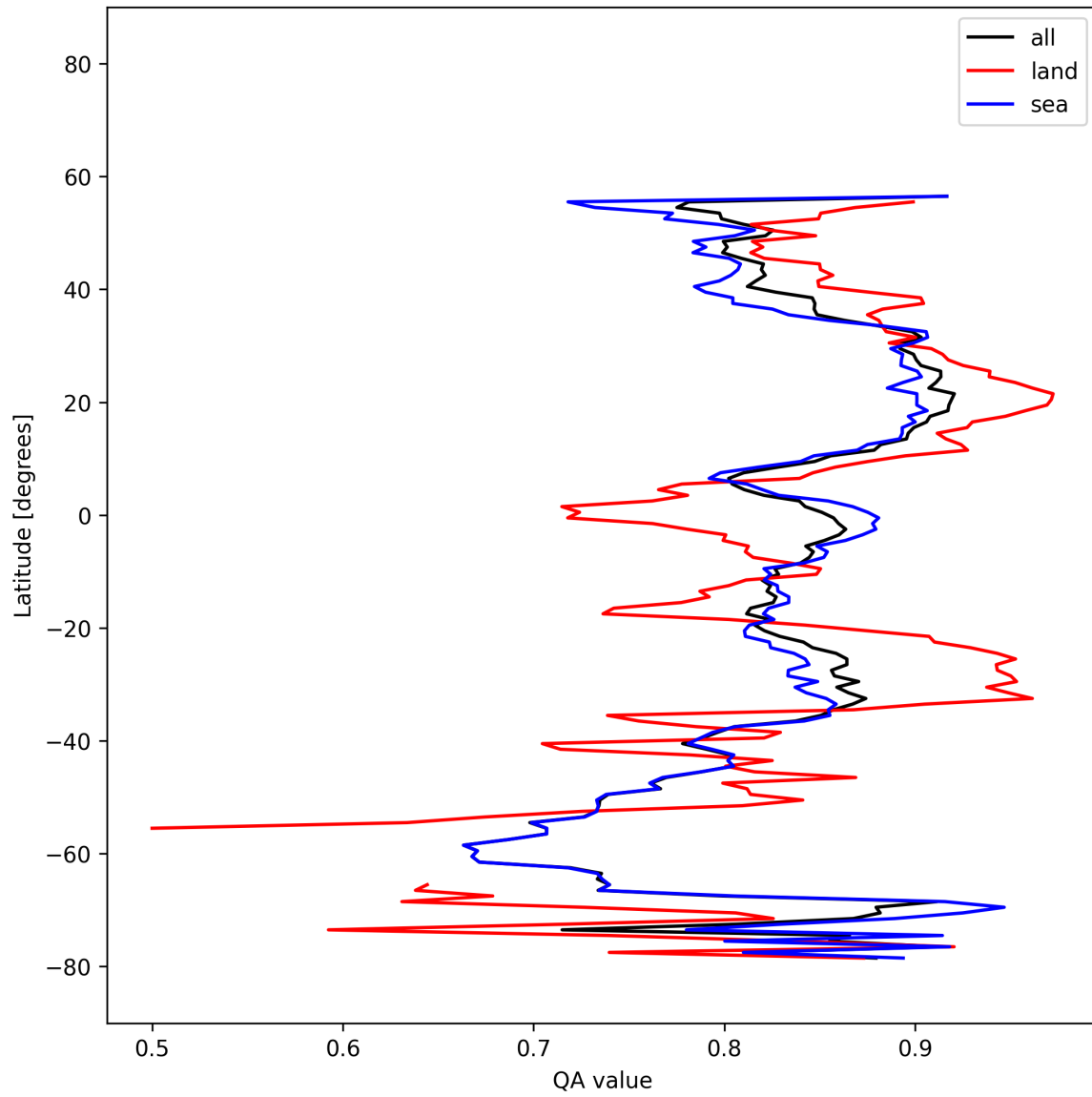
Figure 21: Zonal average of “QA value” for 2025-11-16 to 2025-11-18.
