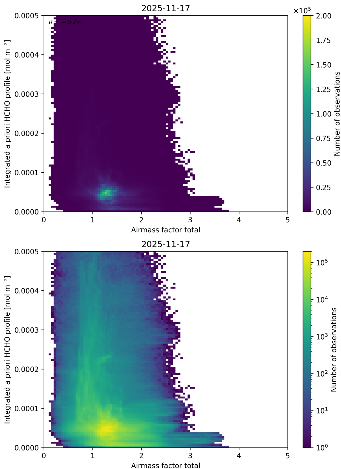
Figure 117: Scatter density plot of “Airmass factor total” against “Integrated a priori HCHO profile” for 2025-11-16 to 2025-11-18.
