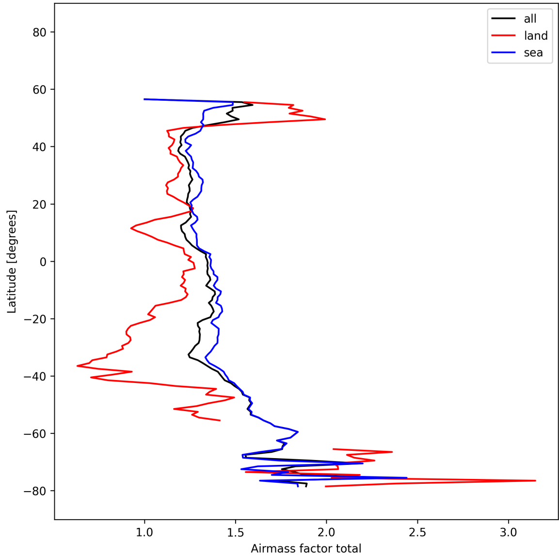
Figure 27: Zonal average of “Airmass factor total” for 2025-11-16 to 2025-11-18.
