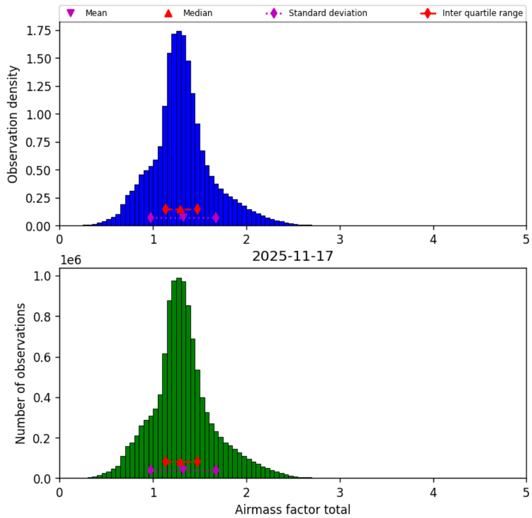
Figure 42: Histogram of “Airmass factor total” for 2025-11-16 to 2025-11-18
