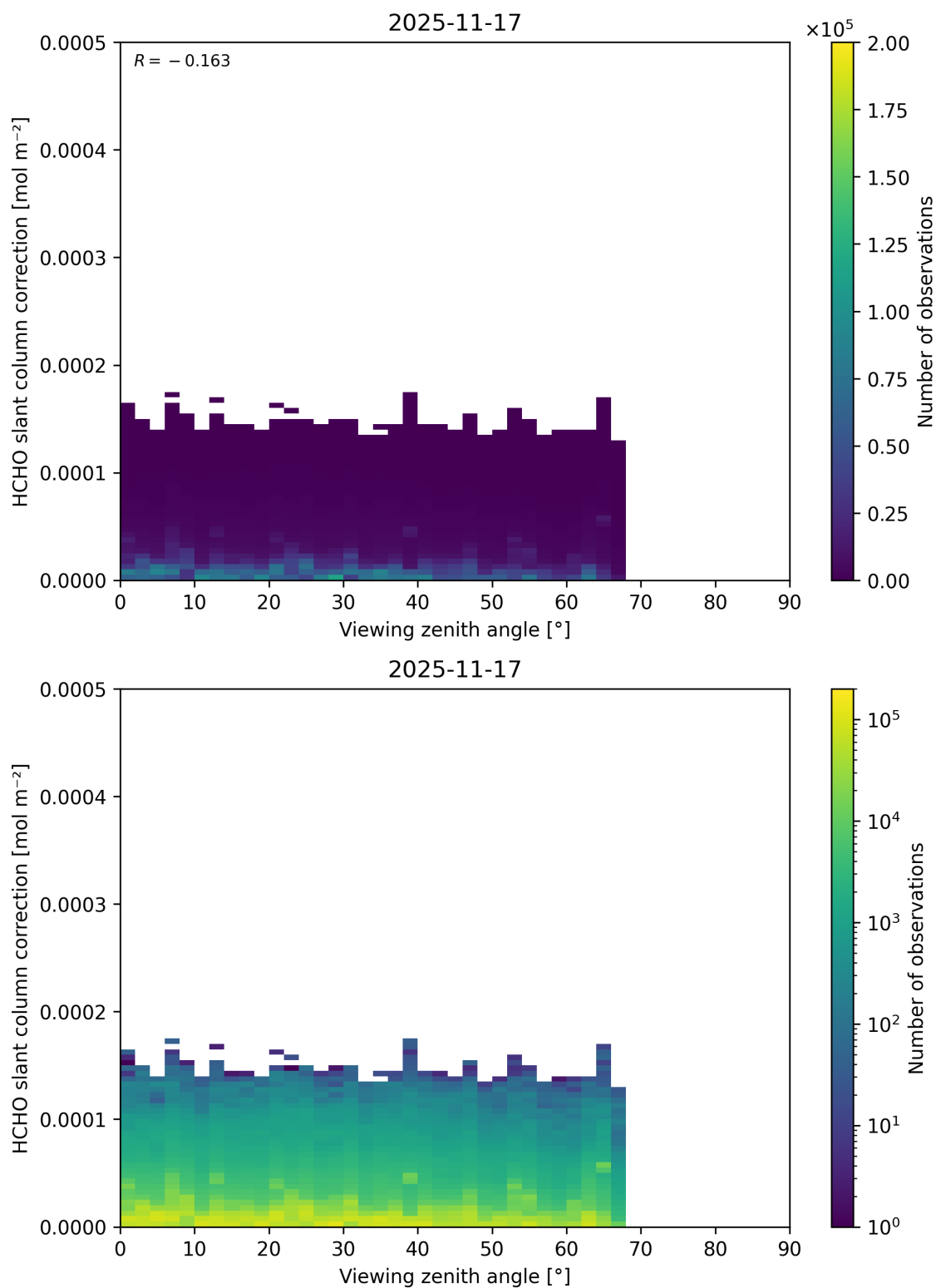
Figure 207: Scatter density plot of “Viewing zenith angle” against “HCHO slant column correction” for 2025-11-16 to 2025-11-18.
