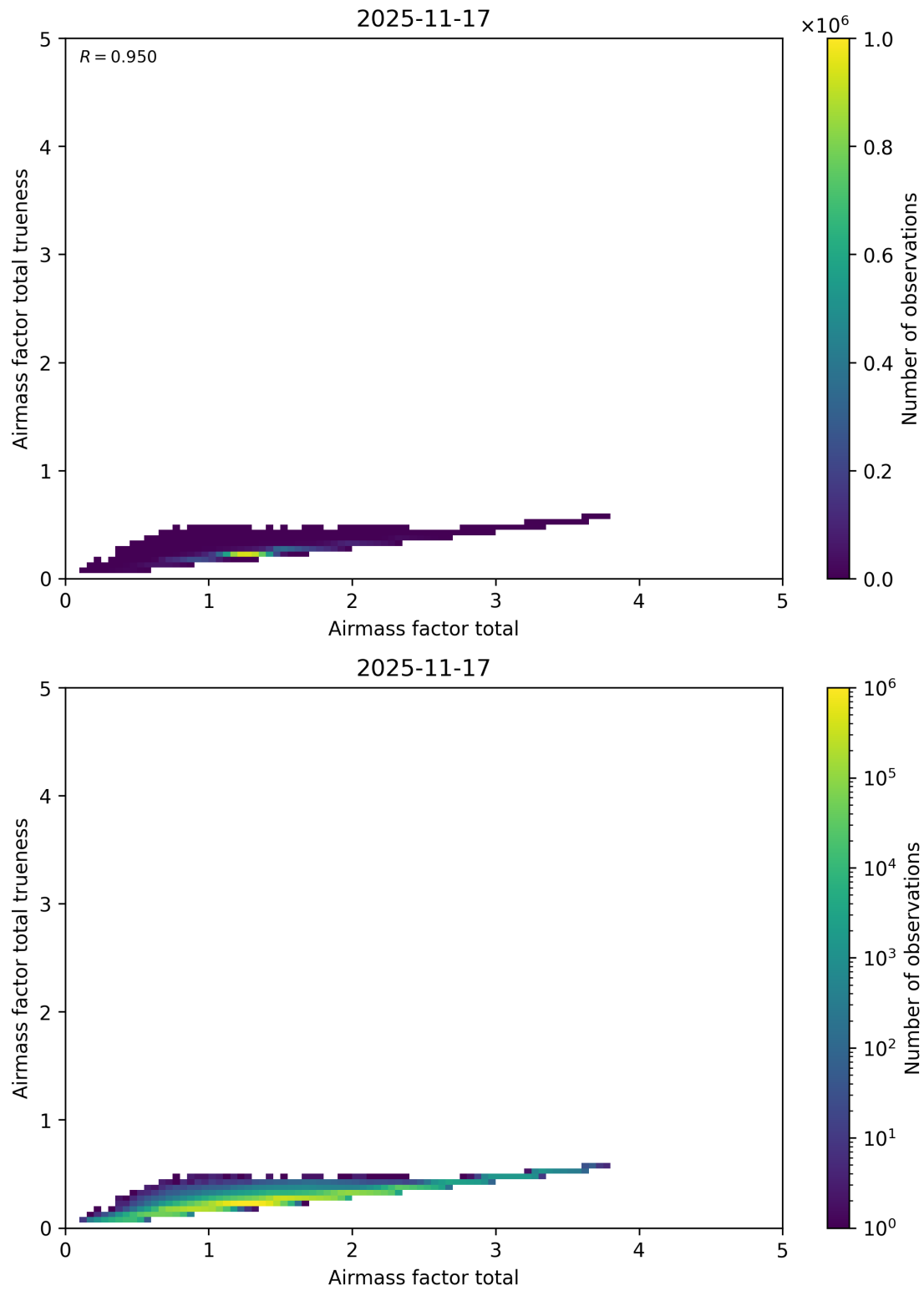
Figure 115: Scatter density plot of “Airmass factor total” against “Airmass factor total trueness” for 2025-11-16 to 2025-11-18.
