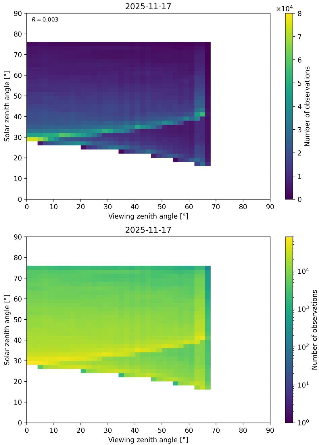
Figure 218: Scatter density plot of “Viewing zenith angle” against “Solar zenith angle” for 2025-11-16 to 2025-11-18.
