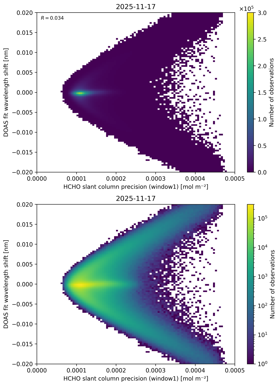
Figure 100: Scatter density plot of “HCHO slant column precision (window1)” against “DOAS fit wavelength shift” for 2025-11-16 to 2025-11-18.
