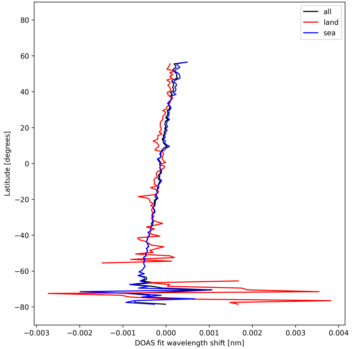
Figure 31: Zonal average of "DOAS fit wavelength shift" for 2025-11-16 to 2025-11-18.
