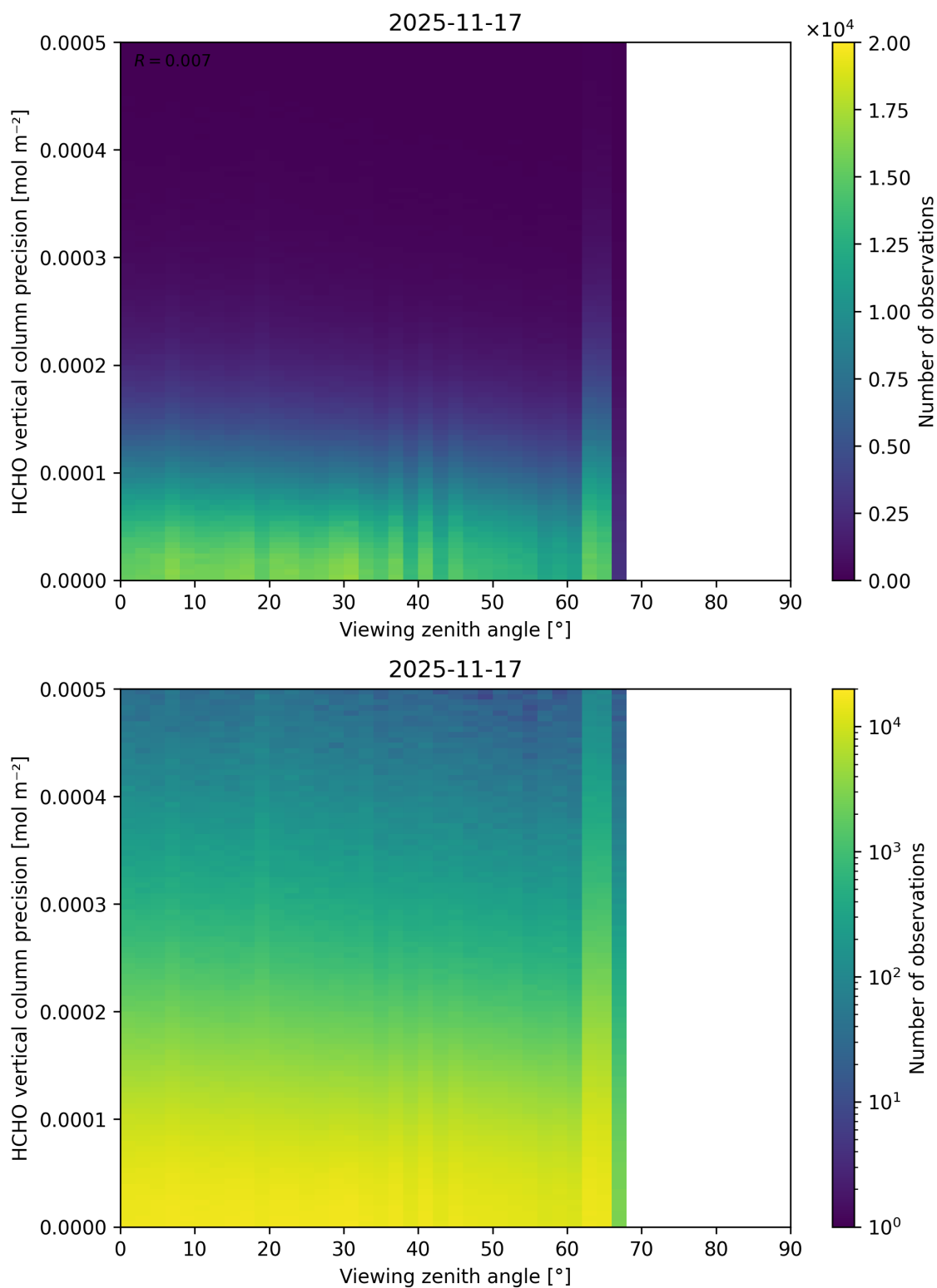
Figure 214: Scatter density plot of “Viewing zenith angle” against “HCHO vertical column precision” for 2025-11-16 to 2025-11-18.
