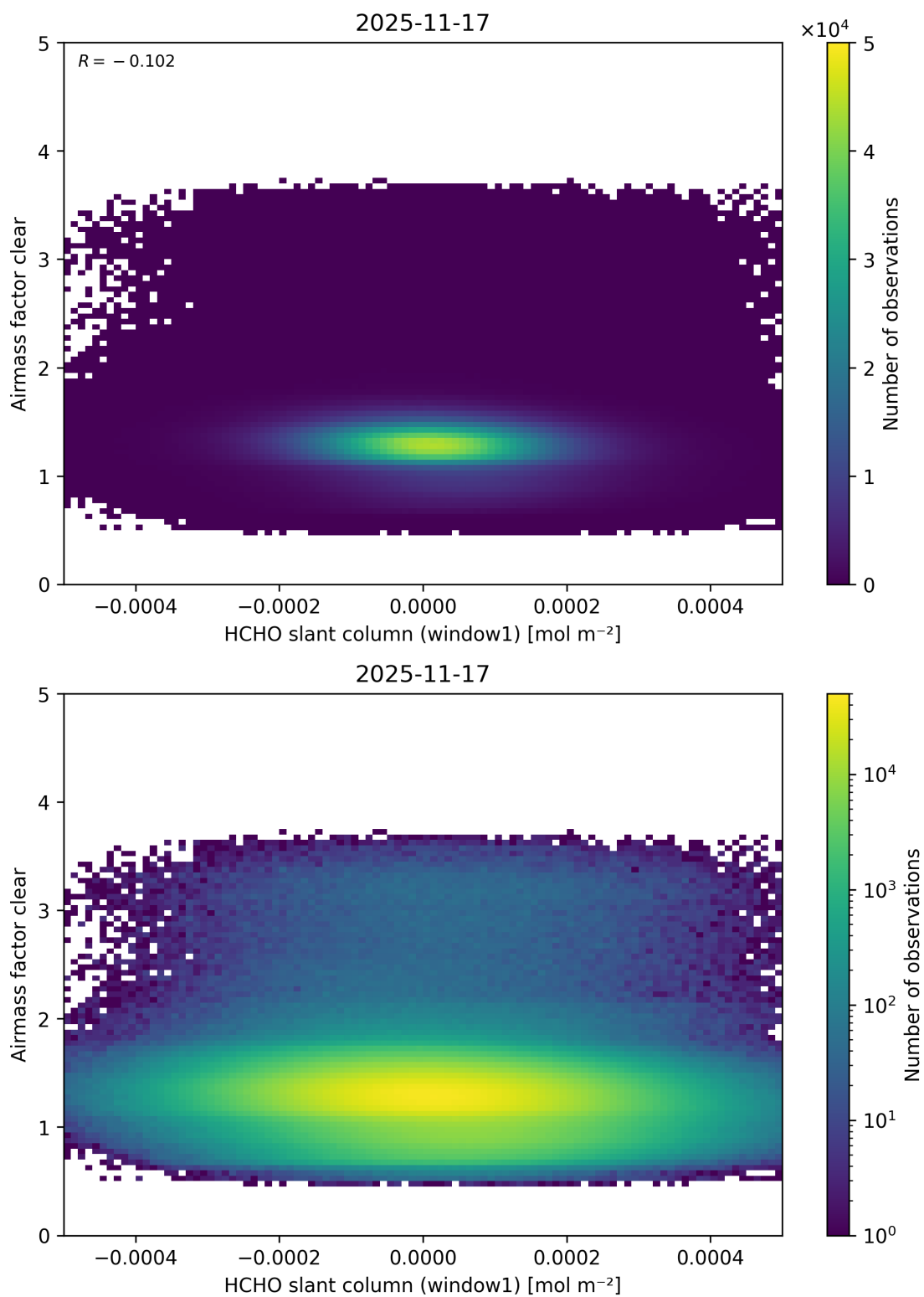
Figure 91: Scatter density plot of “HCHO slant column (window1)” against “Airmass factor clear” for 2025-11-16 to 2025-11-18.
