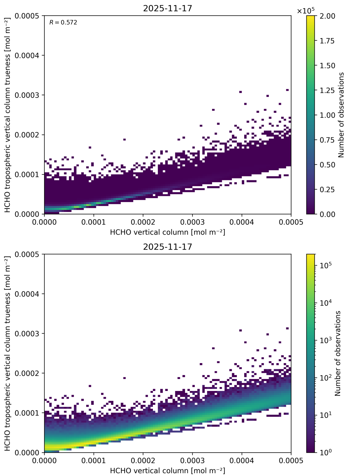
Figure 150: Scatter density plot of “HCHO vertical column” against “HCHO tropospheric vertical column trueness” for 2025-11-16 to 2025-11-18.
