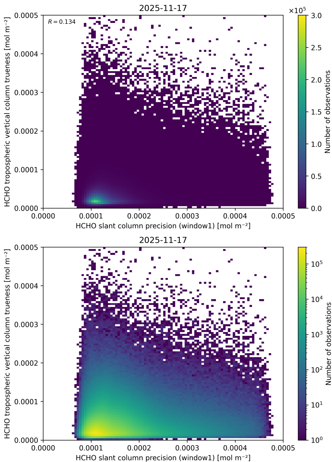
Figure 107: Scatter density plot of “HCHO slant column precision (window1)” against “HCHO tropospheric vertical column trueness” for 2025-11-16 to 2025-11-18.
