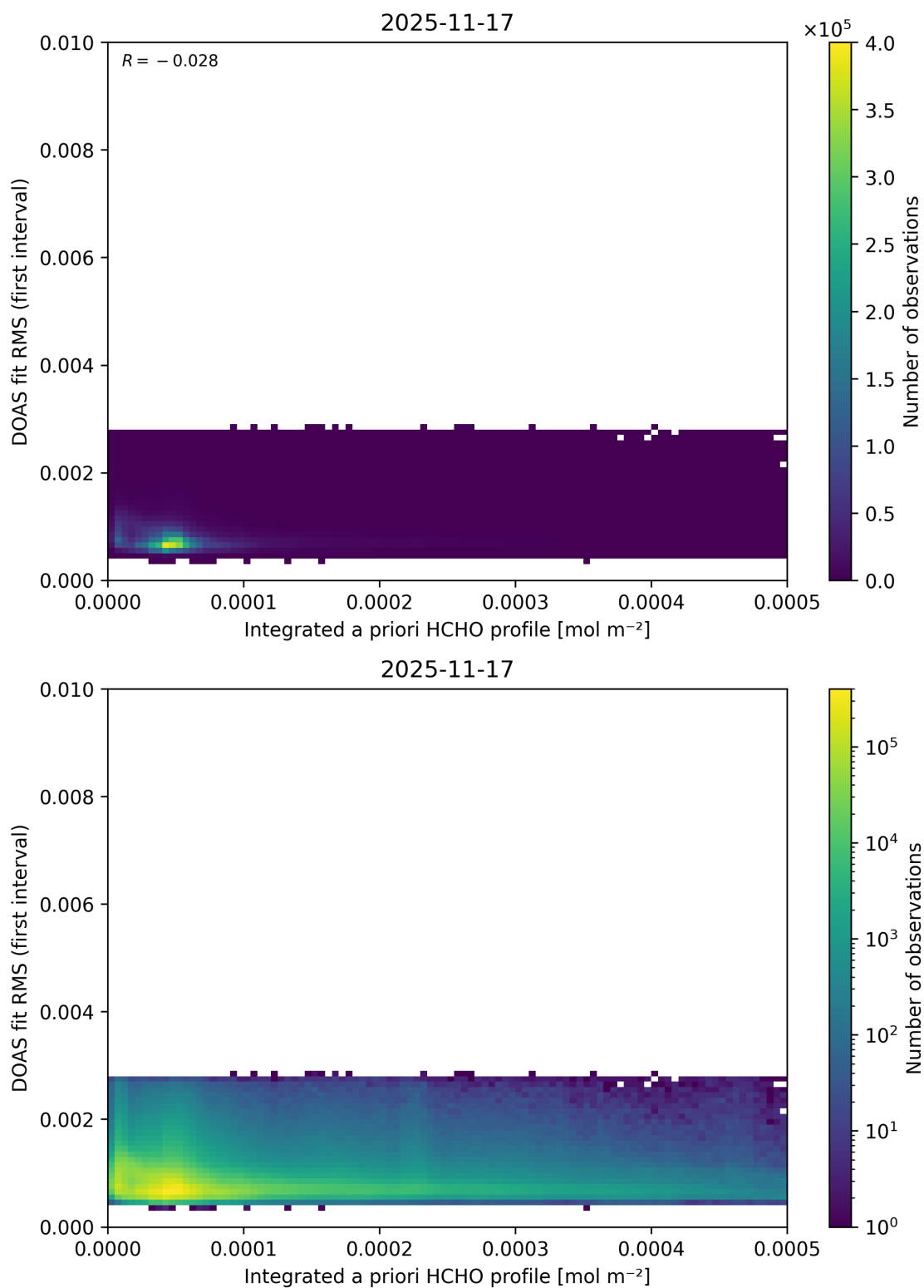
Figure 165: Scatter density plot of “Integrated a priori HCHO profile” against “DOAS fit RMS (first interval)” for 2025-11-16 to 2025-11-18.
