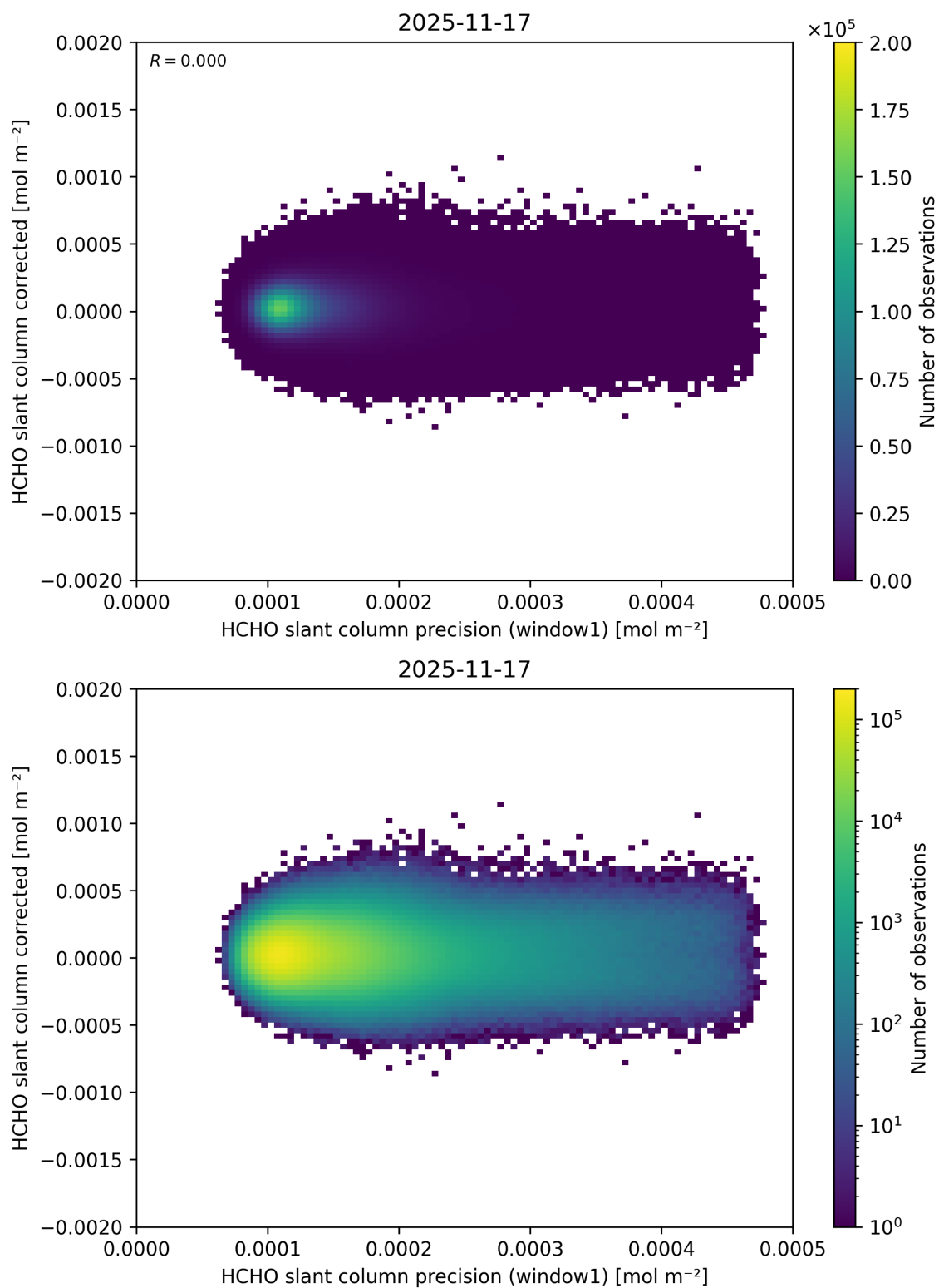
Figure 103: Scatter density plot of “HCHO slant column precision (window1)” against “HCHO slant column corrected” for 2025-11-16 to 2025-11-18.
