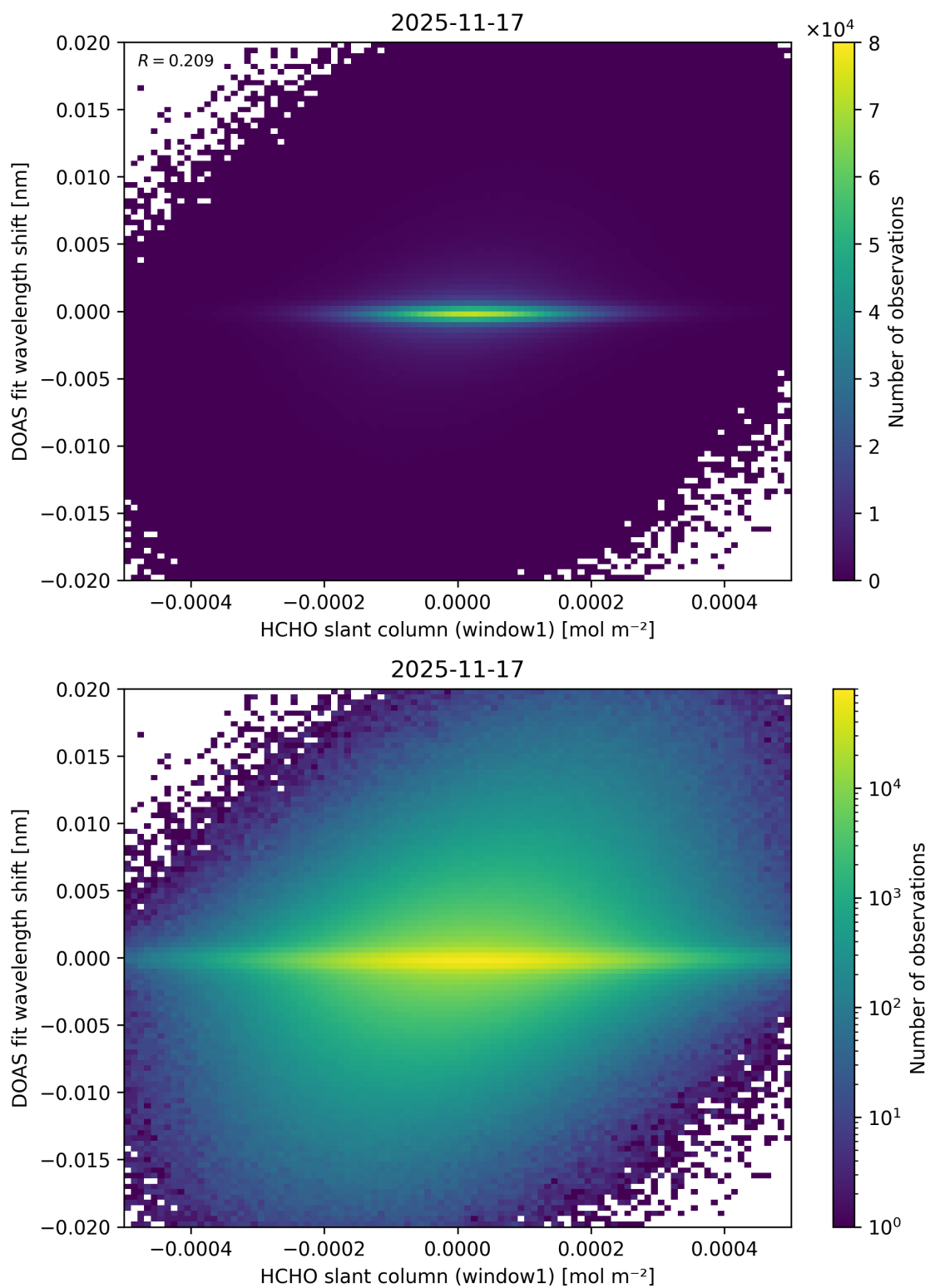
Figure 89: Scatter density plot of “HCHO slant column (window1)” against “DOAS fit wavelength shift” for 2025-11-16 to 2025-11-18.
