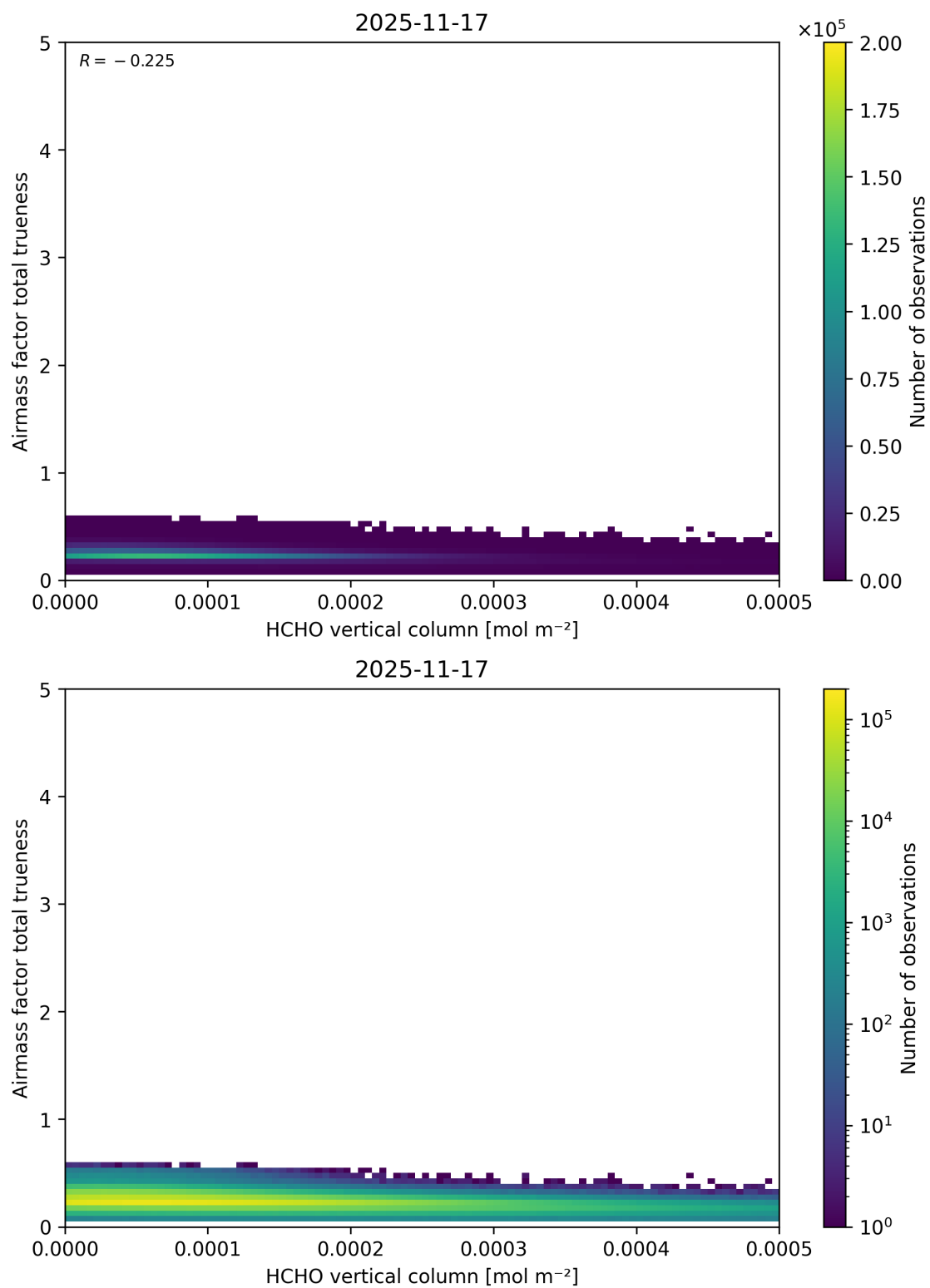
Figure 147: Scatter density plot of “HCHO vertical column” against “Airmass factor total trueneess” for 2025-11-16 to 2025-11-18.
