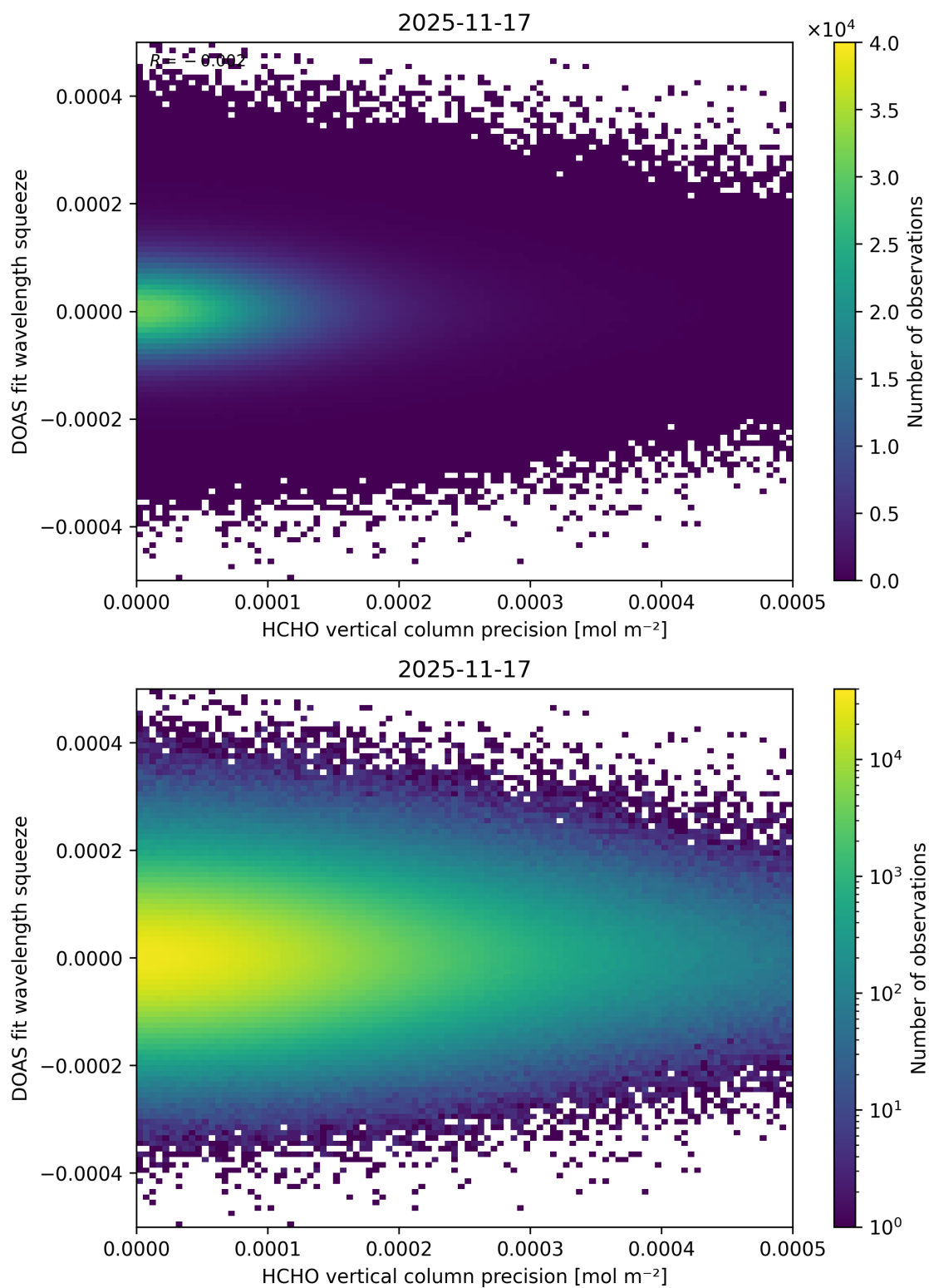
Figure 154: Scatter density plot of “HCHO vertical column precision” against “DOAS fit wavelength squeeze” for 2025-11-16 to 2025-11-18.
