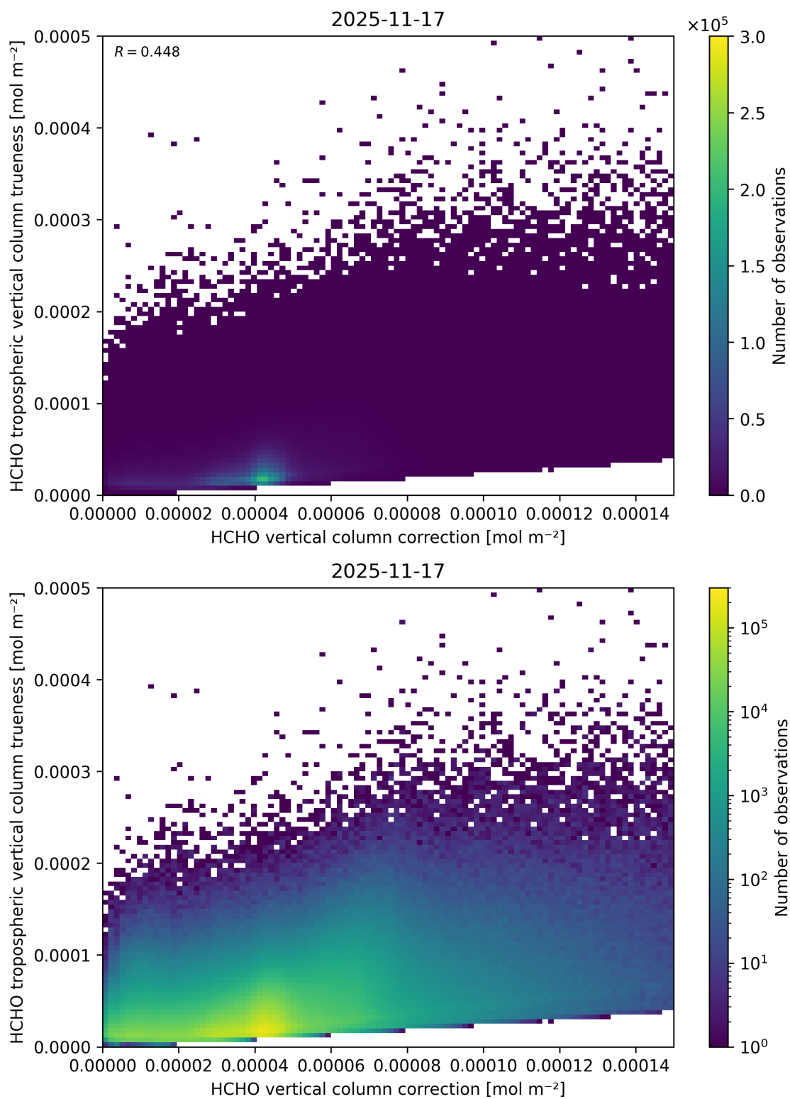
Figure 136: Scatter density plot of “HCHO vertical column correction” against “HCHO tropospheric vertical column true-ness” for 2025-11-16 to 2025-11-18.
