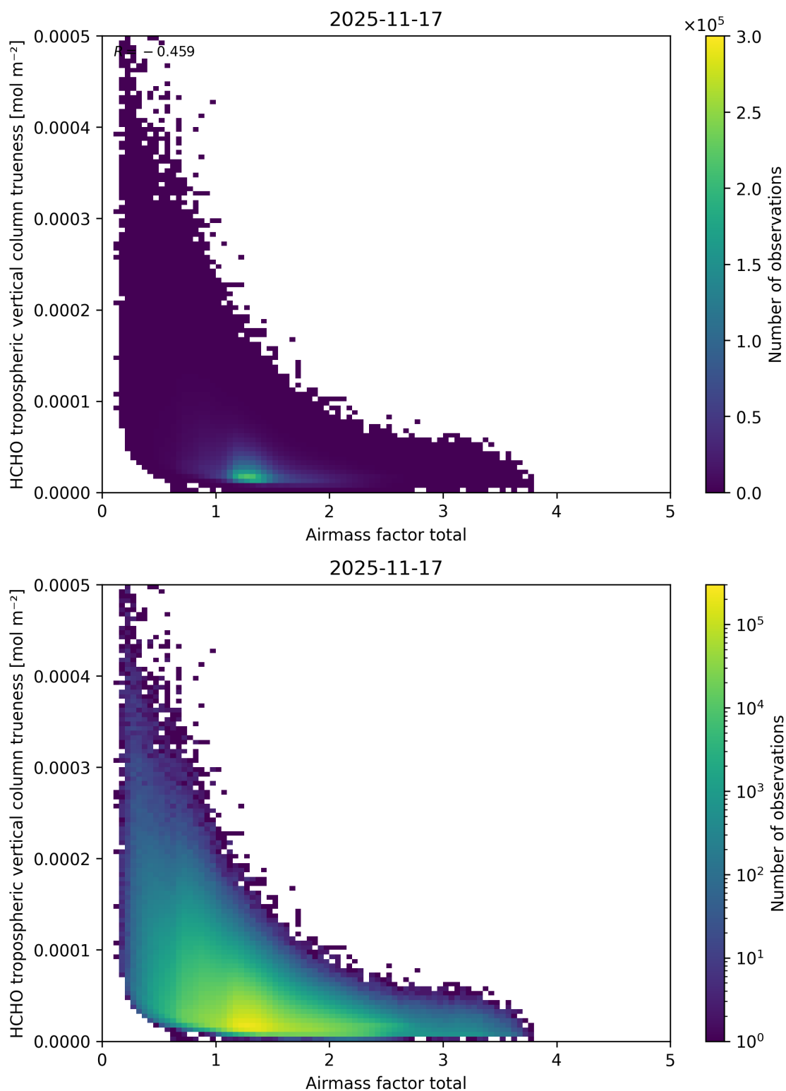
Figure 116: Scatter density plot of “Air mass factor total” against “HCHO tropospheric vertical column trueeness” for 2025-11-16 to 2025-11-18.
