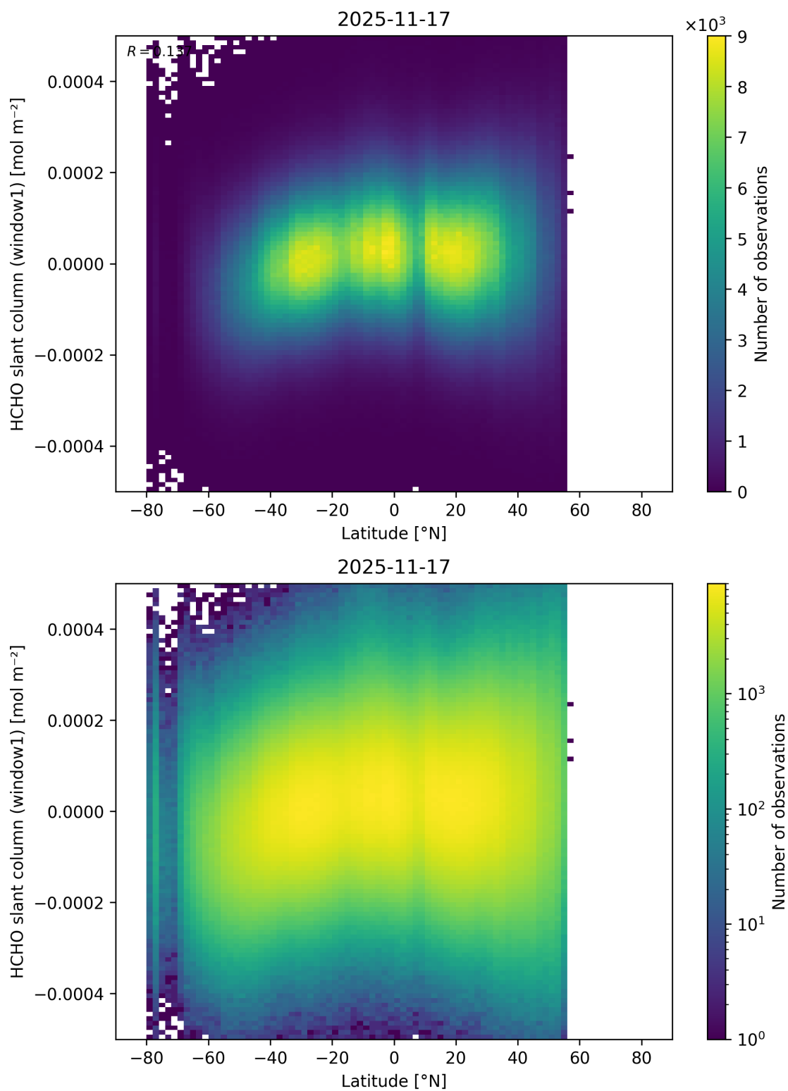
Figure 177: Scatter density plot of “Latitude” against “HCHO slant column (window1)” for 2025-11-16 to 2025-11-18.
