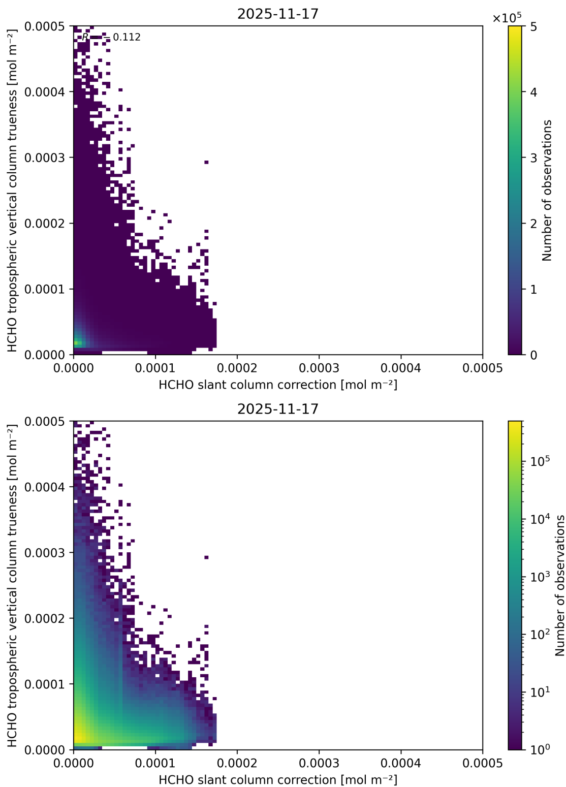
Figure 87: Scatter density plot of “HCHO slant column correction” against “HCHO tropospheric vertical column trueness” for 2025-11-16 to 2025-11-18.
