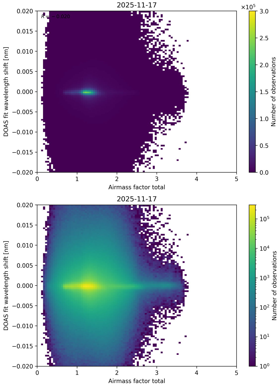
Figure 110: Scatter density plot of “Airmass factor total” against “DOAS fit wavelength shift” for 2025-11-16 to 2025-11-18.
