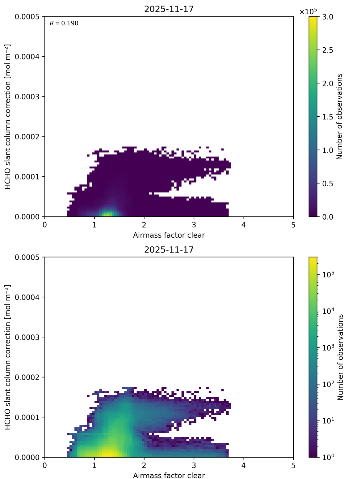
Figure 82: Scatter density plot of “Airmass factor clear” against “HCHO slant column correction” for 2025-11-16 to 2025-11-18.
