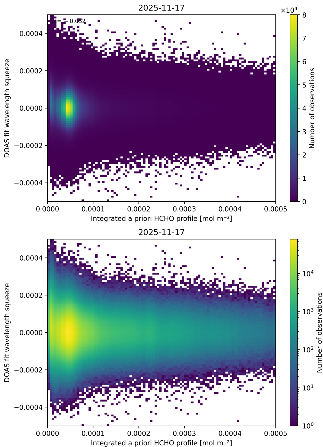
Figure 167: Scatter density plot of “Integrated a priori HCHO profile” against “DOAS fit wavelength squeeze” for 2025-11-16 to 2025-11-18.
