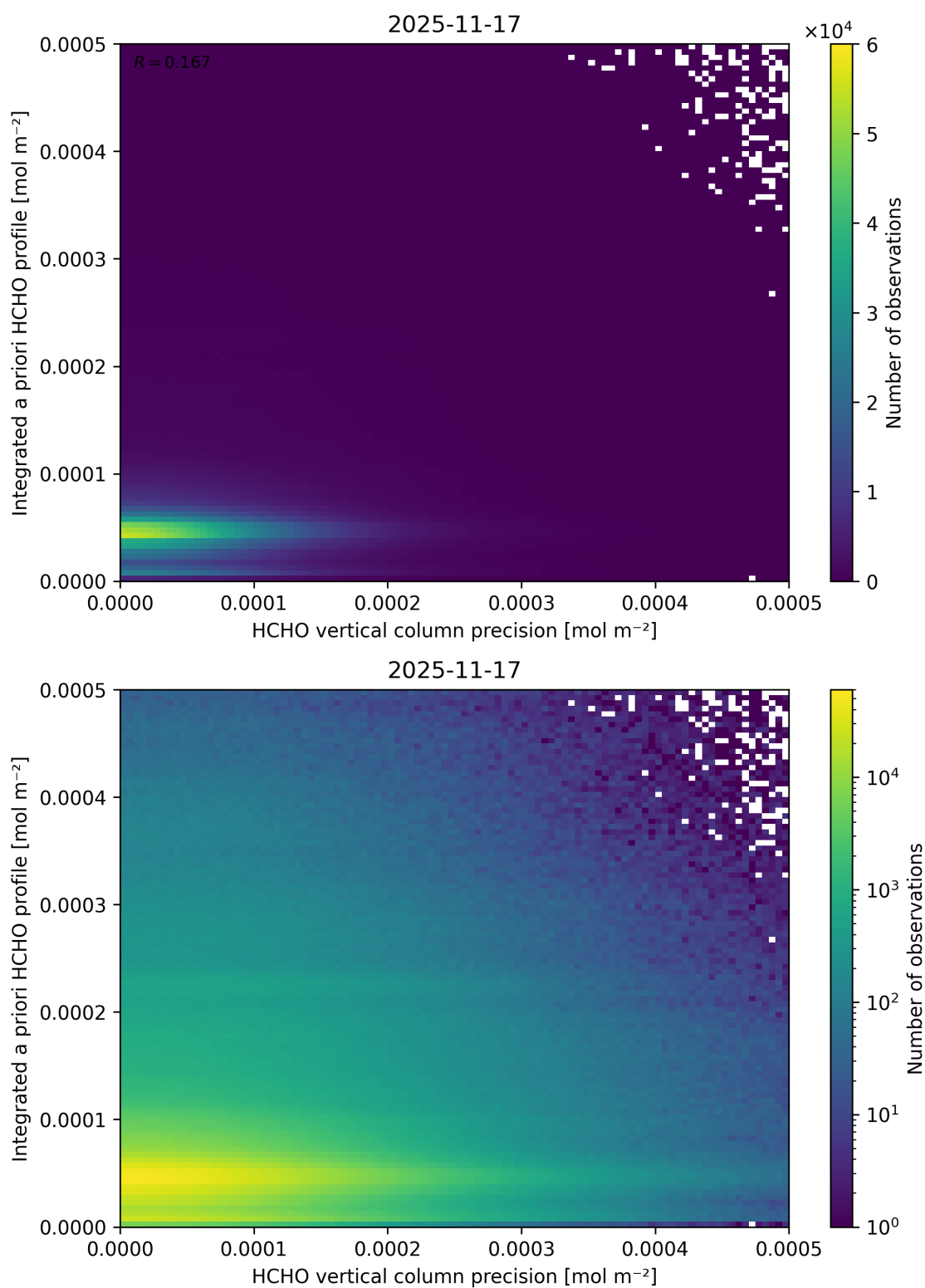
Figure 164: Scatter density plot of “HCHO vertical column precision” against “Integrated a priori HCHO profile” for 2025-11-16 to 2025-11-18.
