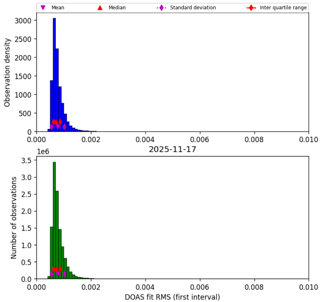
Figure 48: Histogram of “DOAS fit RMS (first interval)” for 2025-11-16 to 2025-11-18
