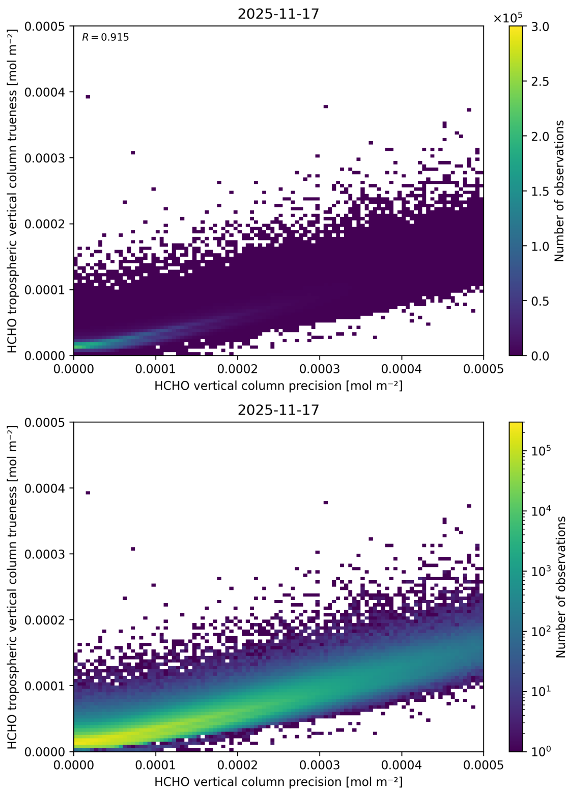
Figure 163: Scatter density plot of “HCHO vertical column precision” against “HCHO tropospheric vertical column true-ness” for 2025-11-16 to 2025-11-18.
