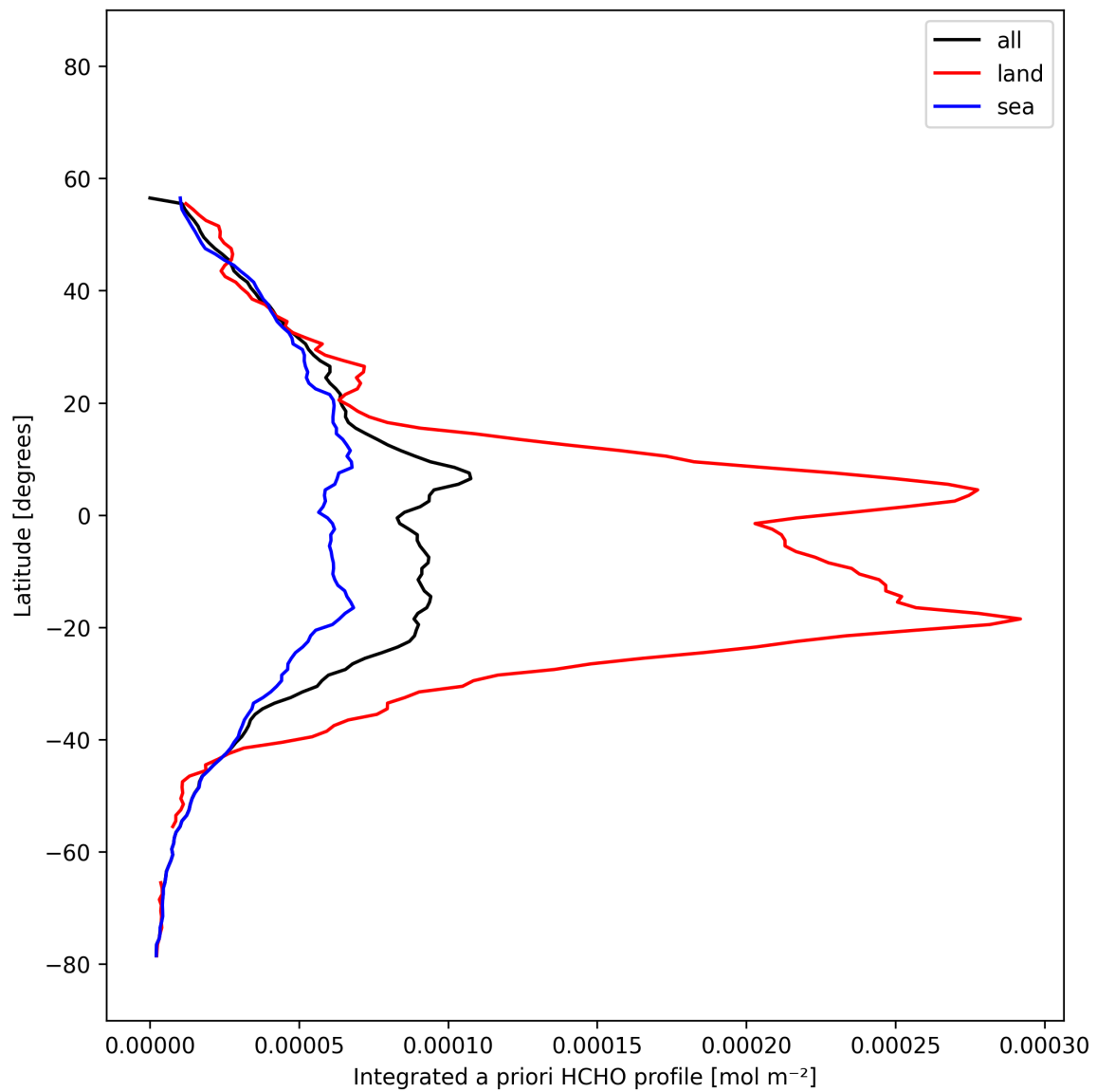
Figure 30: Zonal average of “Integrated a priori HCHO profile” for 2025-11-16 to 2025-11-18.
