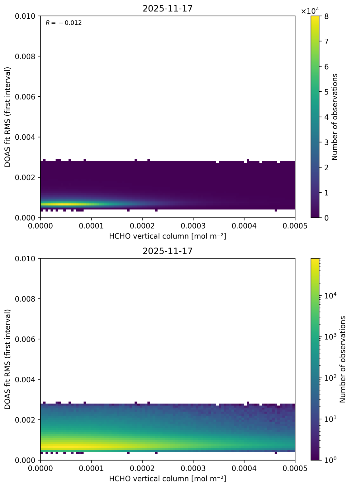
Figure 138: Scatter density plot of “HCHO vertical column” against “DOAS fit RMS (first interval)” for 2025-11-16 to 2025-11-18.
