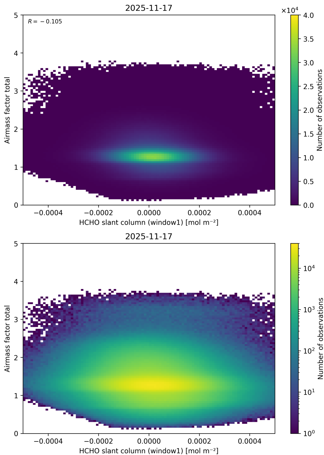
Figure 95: Scatter density plot of “HCHO slant column (window1)” against “Airmass factor total” for 2025-11-16 to 2025-11-18.
