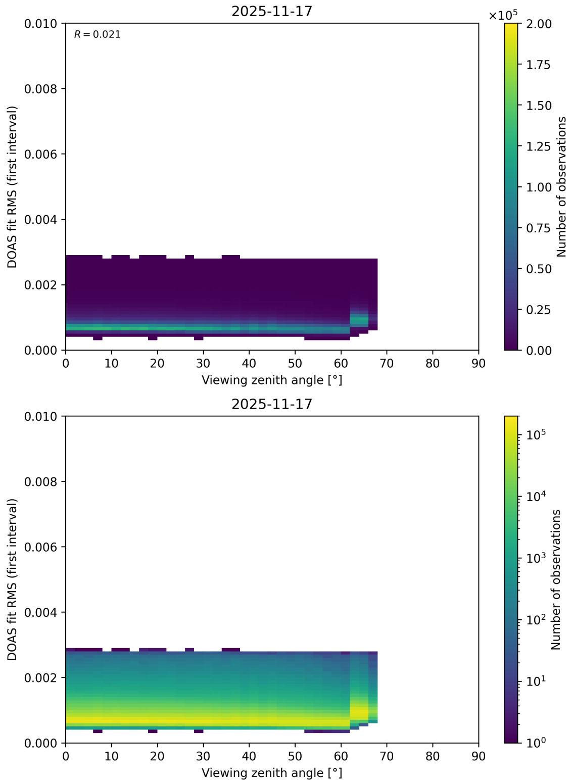
Figure 202: Scatter density plot of “Viewing zenith angle” against “DOAS fit RMS (first interval)” for 2025-11-16 to 2025-11-18.
