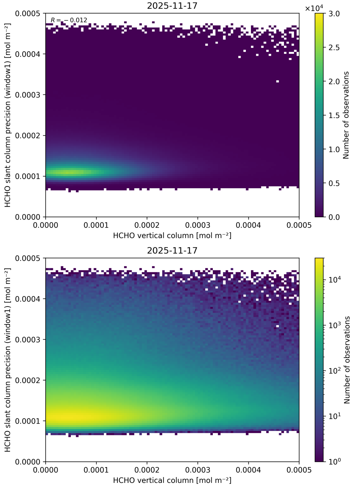
Figure 145: Scatter density plot of “HCHO vertical column” against “HCHO slant column precision (window1)” for 2025-11-16 to 2025-11-18.
