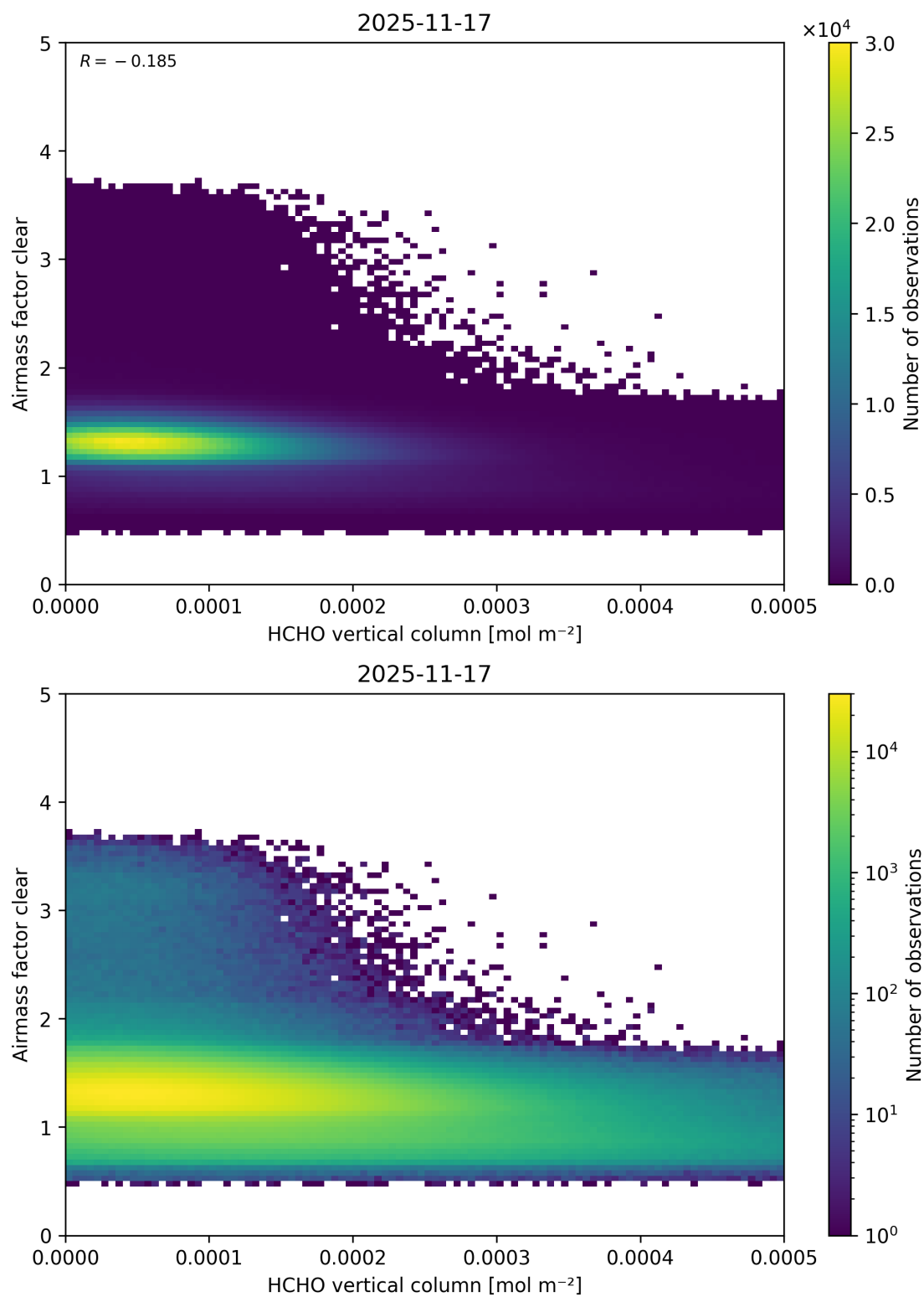
Figure 141: Scatter density plot of “HCHO vertical column” against “Airmass factor clear” for 2025-11-16 to 2025-11-18.
