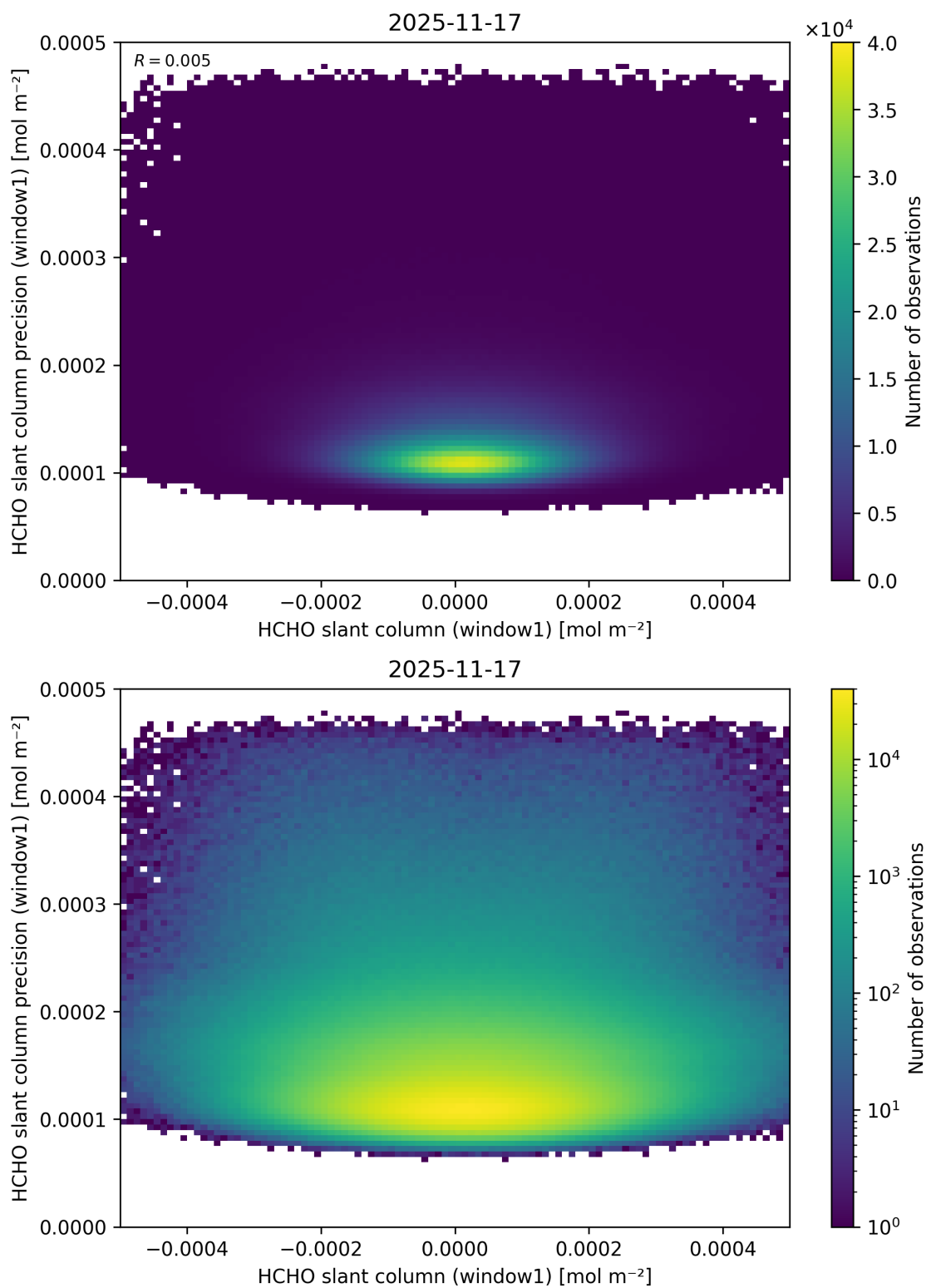
Figure 94: Scatter density plot of “HCHO slant column (window1)” against “HCHO slant column precision (window1)” for 2025-11-16 to 2025-11-18.
