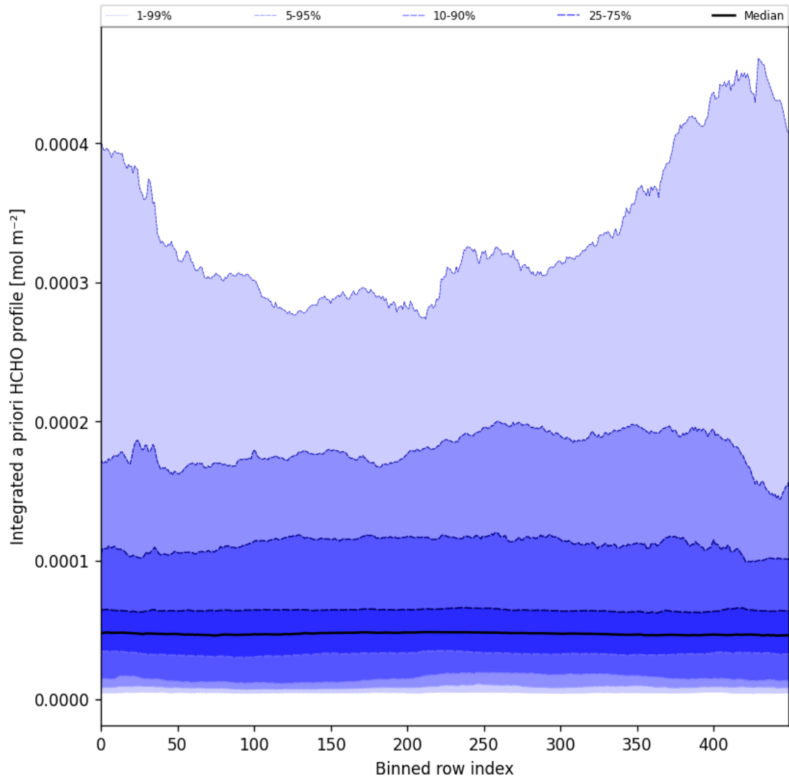
Figure 60: Along track statistics of “Integrated a priori HCHO profile” for 2025-11-16 to 2025-11-18
