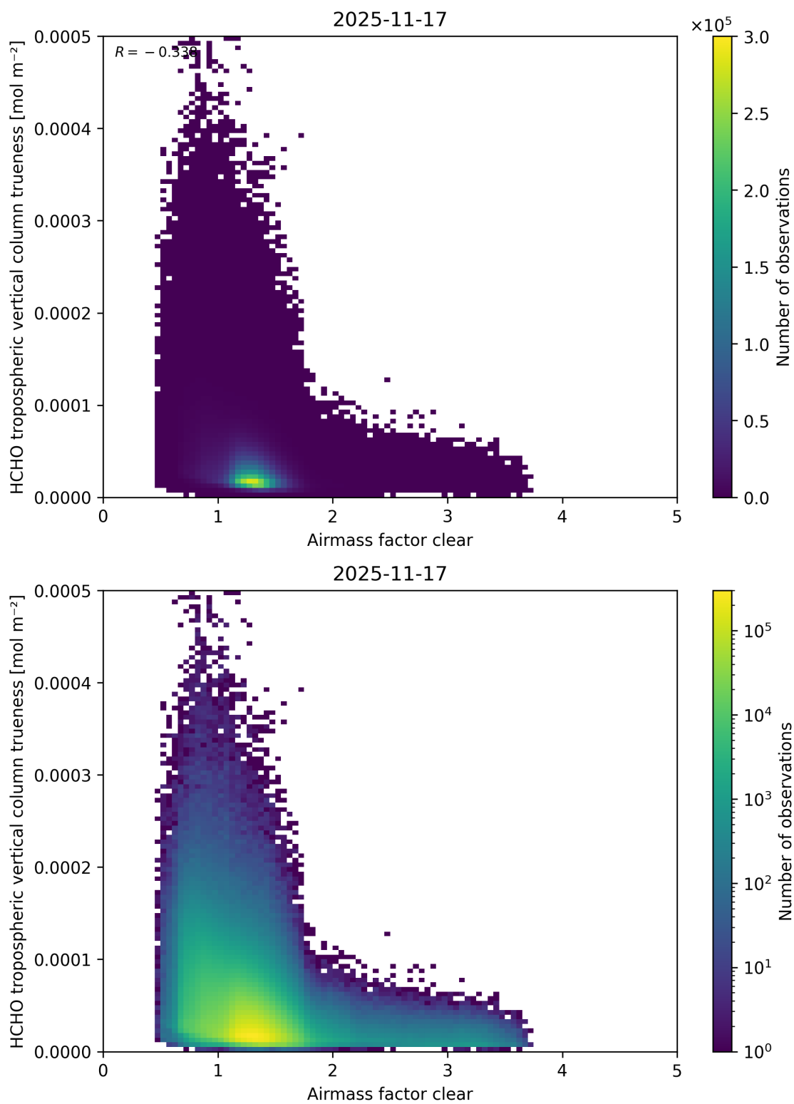
Figure 83: Scatter density plot of “Airmass factor clear” against “HCHO tropospheric vertical column trueness” for 2025-11-16 to 2025-11-18.
