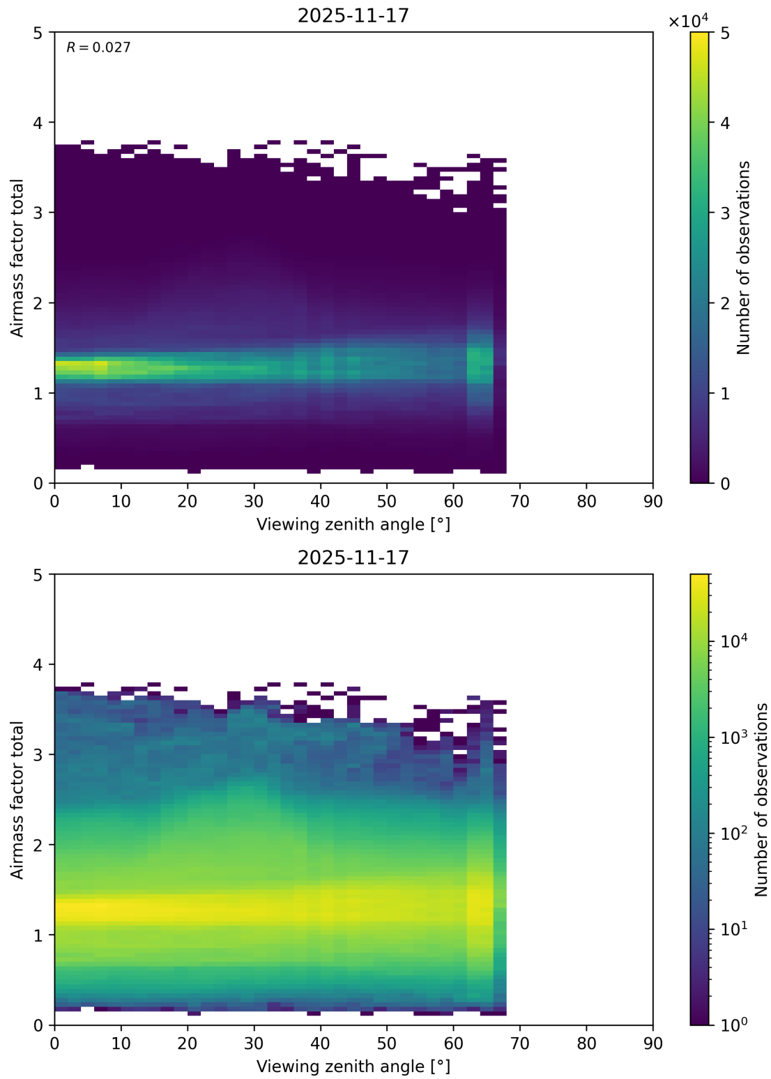
Figure 210: Scatter density plot of “Viewing zenith angle” against “Airmass factor total” for 2025-11-16 to 2025-11-18.
