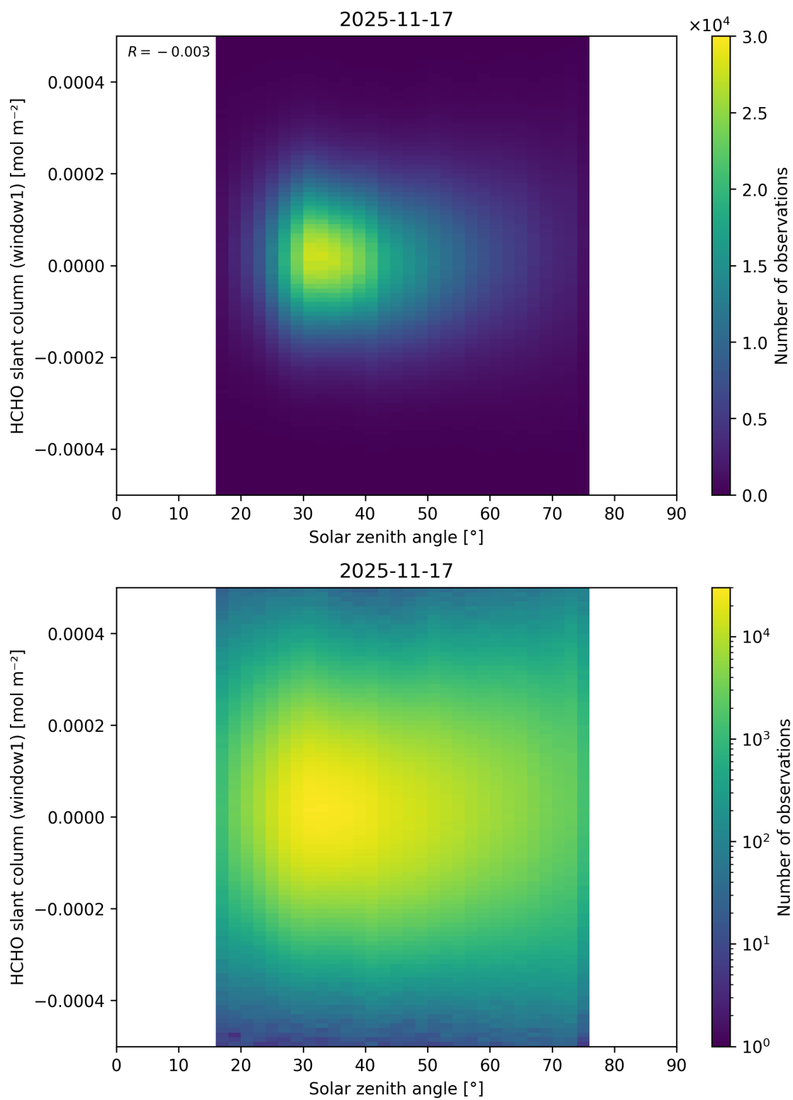
Figure 192: Scatter density plot of “Solar zenith angle” against “HCHO slant column (window1)” for 2025-11-16 to 2025-11-18.
