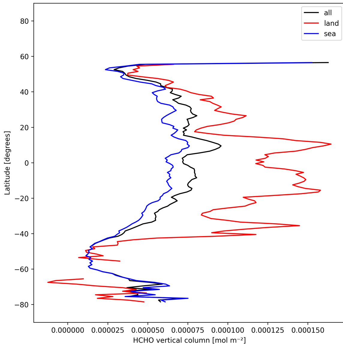
Figure 22: Zonal average of “HCHO vertical column” for 2025-11-16 to 2025-11-18.
