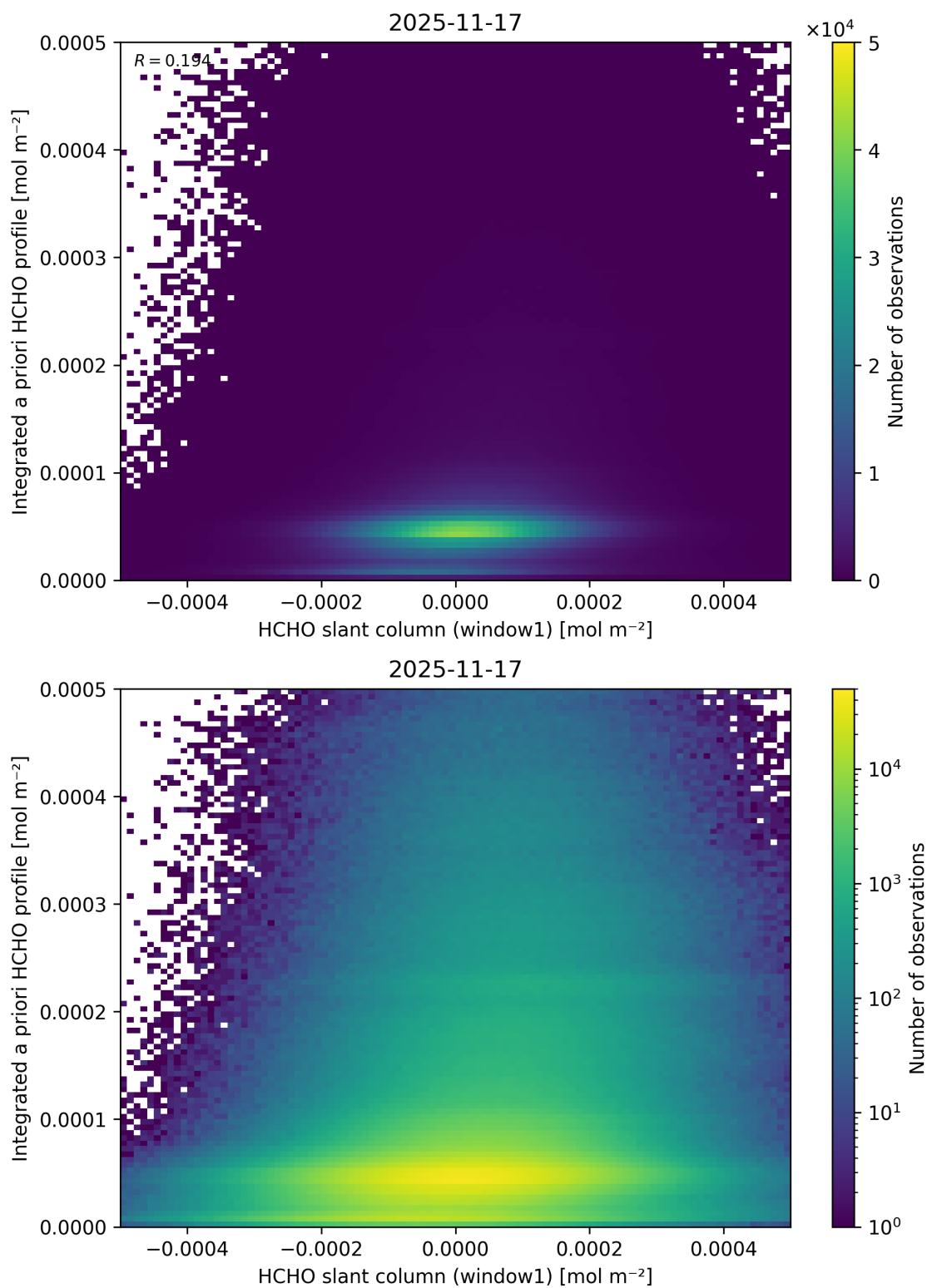
Figure 98: Scatter density plot of “HCHO slant column (window1)” against “Integrated a priori HCHO profile” for 2025-11-16 to 2025-11-18.
