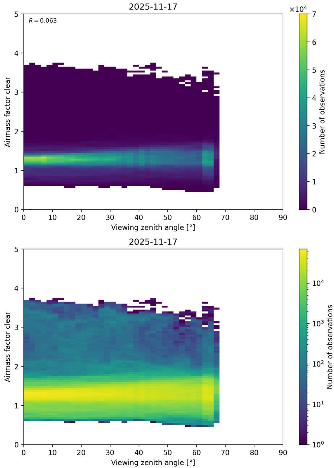
Figure 205: Scatter density plot of “Viewing zenith angle” against “Airmass factor clear” for 2025-11-16 to 2025-11-18.
