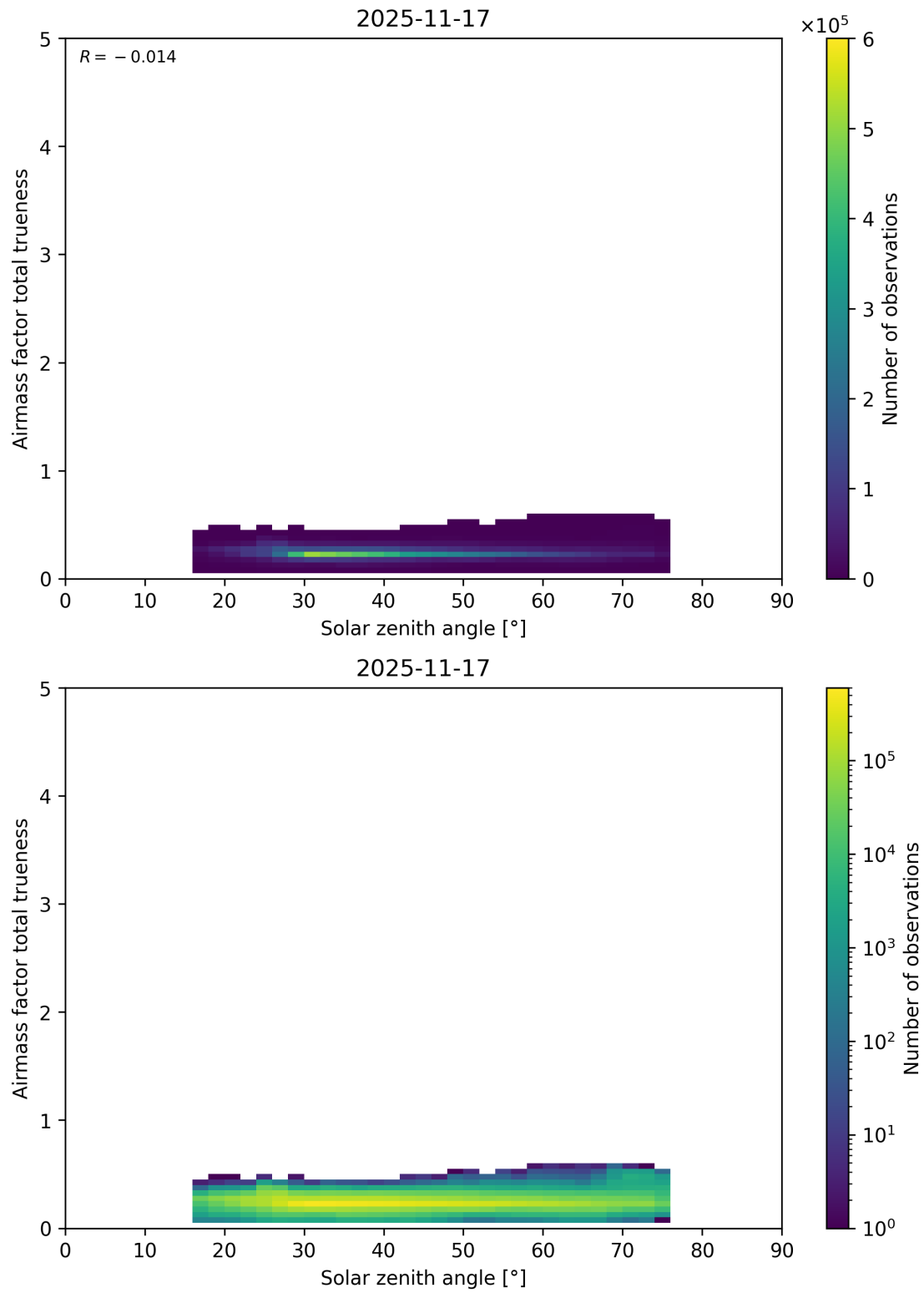
Figure 195: Scatter density plot of “Solar zenith angle” against “Airmass factor total trueneess” for 2025-11-16 to 2025-11-18.
