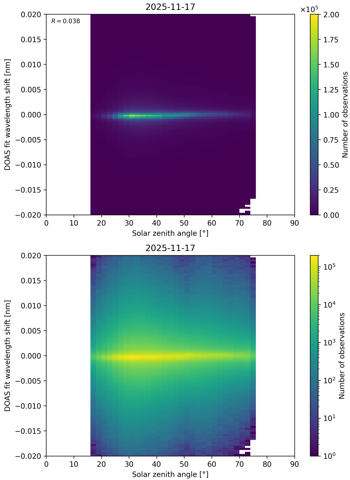
Figure 187: Scatter density plot of “Solar zenith angle” against “DOAS fit wavelength shift” for 2025-11-16 to 2025-11-18.
