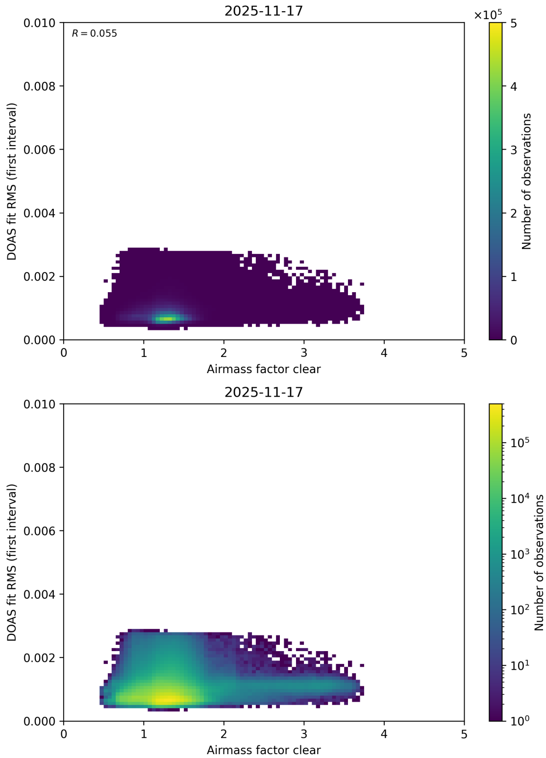
Figure 78: Scatter density plot of “Airmass factor clear” against “DOAS fit RMS (first interval)” for 2025-11-16 to 2025-11-18.
