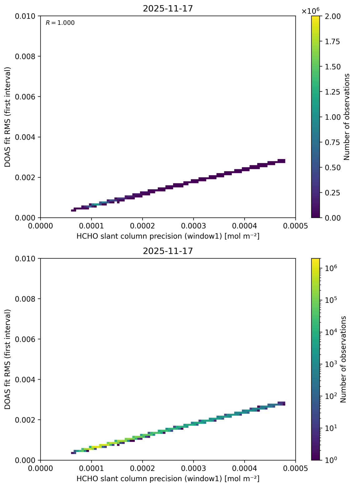
Figure 99: Scatter density plot of “HCHO slant column precision (window1)” against “DOAS fit RMS (first interval)” for 2025-11-16 to 2025-11-18.
