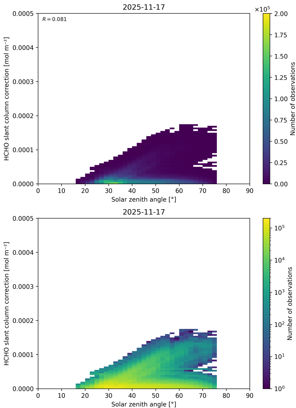
Figure 191: Scatter density plot of “Solar zenith angle” against “HCHO slant column correction” for 2025-11-16 to 2025-11-18.
