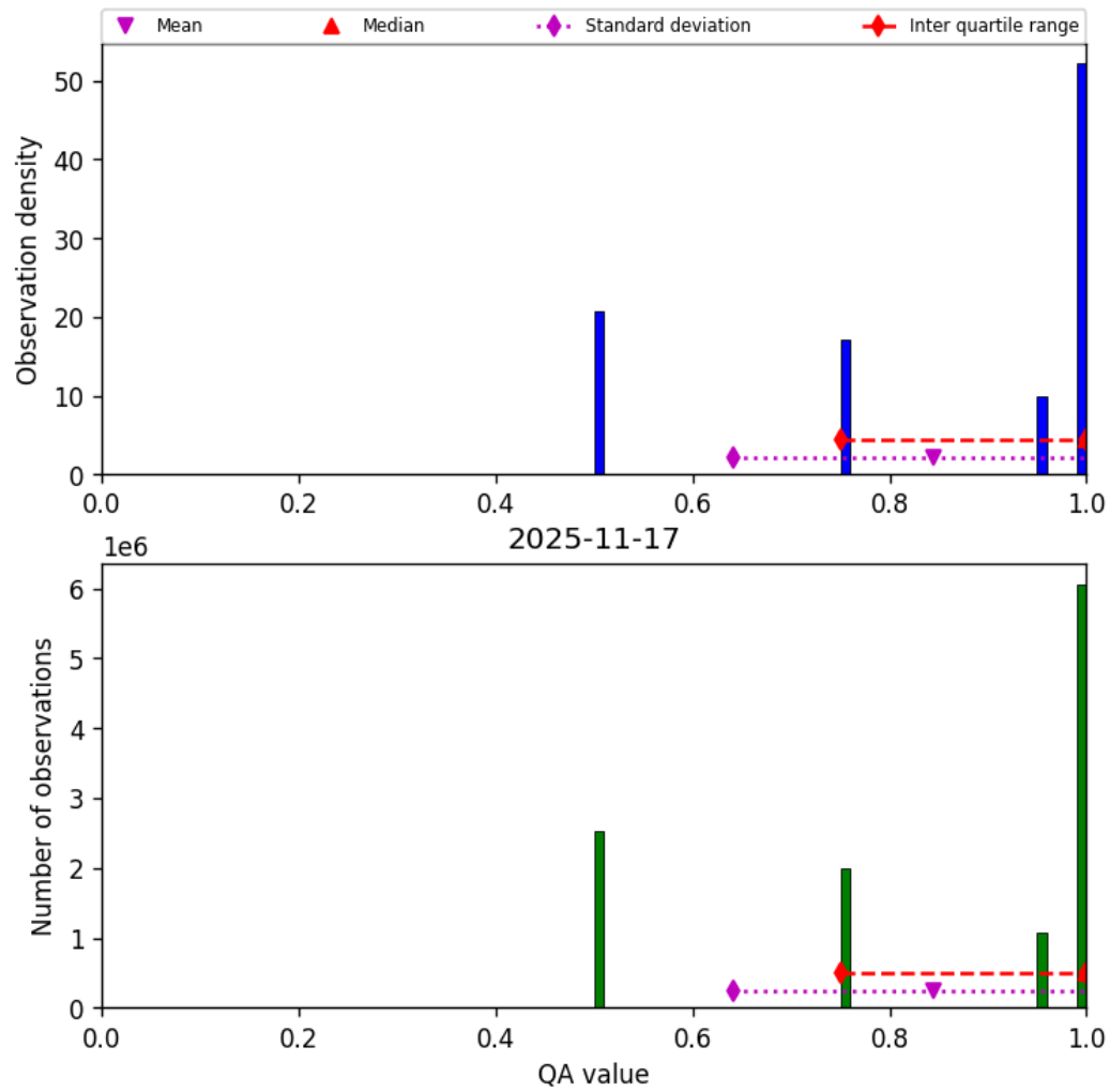
Figure 36: Histogram of “QA value” for 2025-11-16 to 2025-11-18
