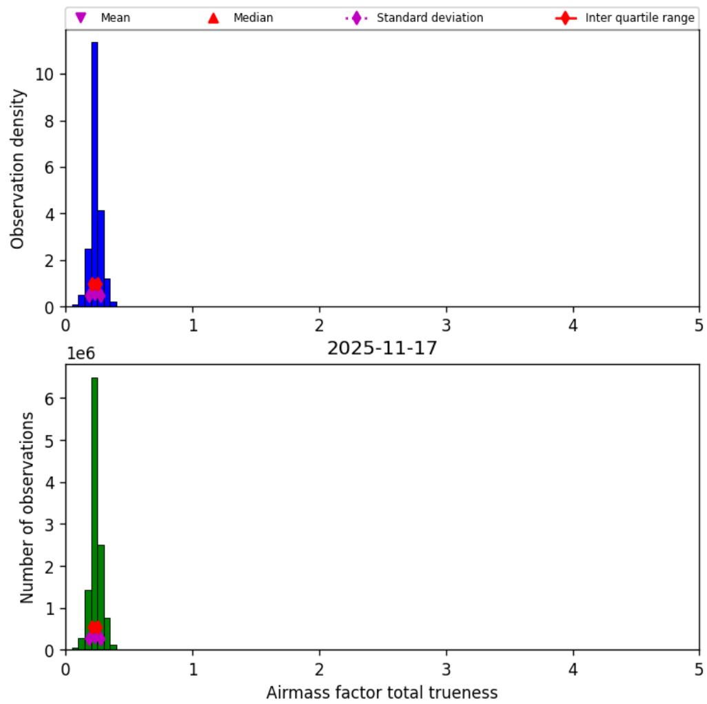
Figure 43: Histogram of “Airmass factor total trueness” for 2025-11-16 to 2025-11-18
