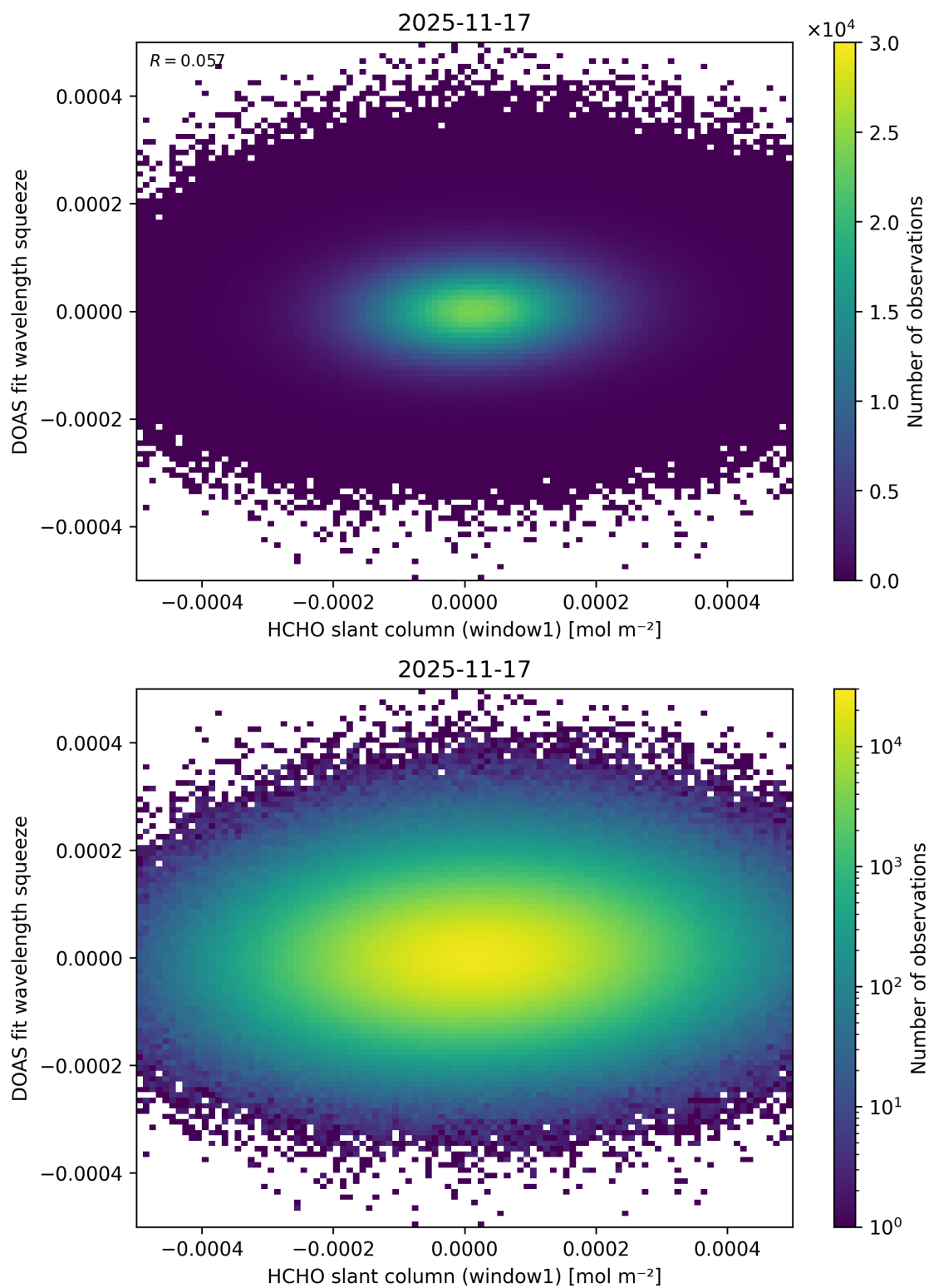
Figure 90: Scatter density plot of “HCHO slant column (window1)” against “DOAS fit wavelength squeeze” for 2025-11-16 to 2025-11-18.
