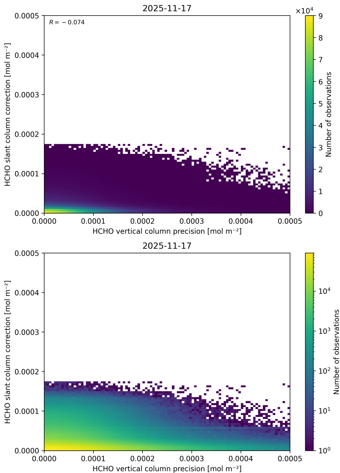
Figure 157: Scatter density plot of “HCHO vertical column precision” against “HCHO slant column correction” for 2025-11-16 to 2025-11-18.
