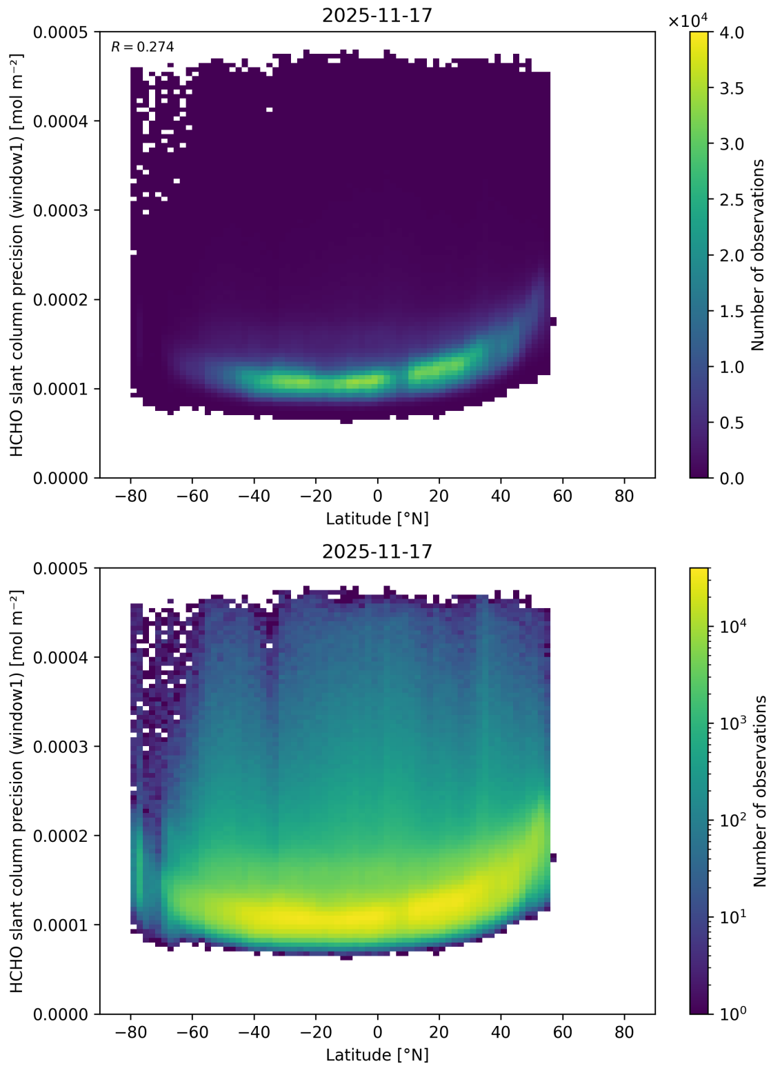
Figure 178: Scatter density plot of “Latitude” against “HCHO slant column precision (window1)” for 2025-11-16 to 2025-11-18.
