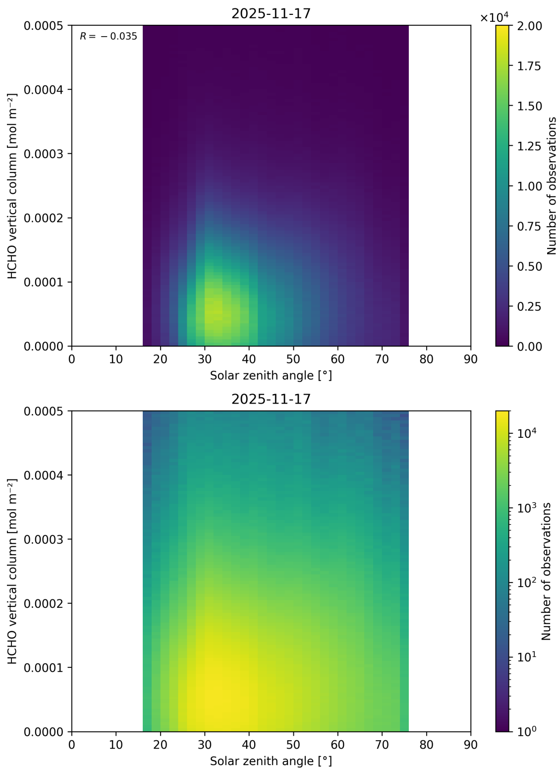
Figure 196: Scatter density plot of “Solar zenith angle” against “HCHO vertical column” for 2025-11-16 to 2025-11-18.
