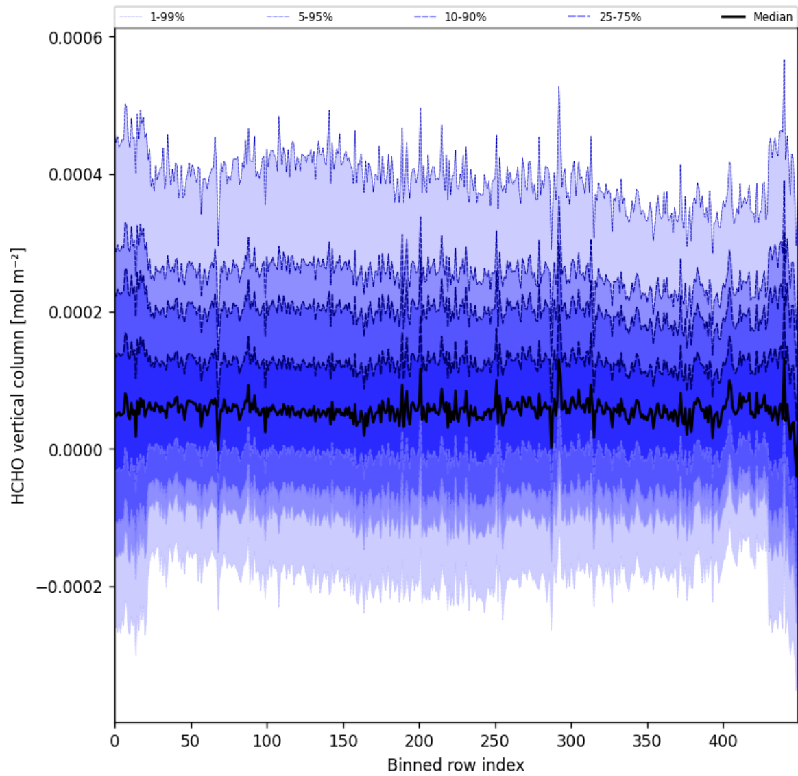
Figure 52: Along track statistics of “HCHO vertical column” for 2025-11-16 to 2025-11-18
