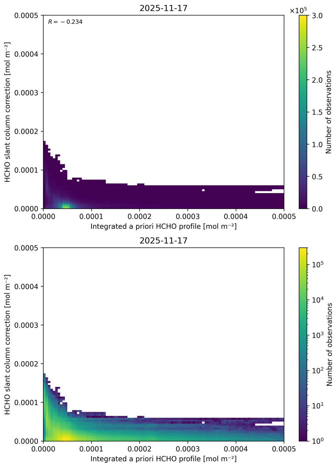
Figure 169: Scatter density plot of “Integrated a priori HCHO profile” against “HCHO slant column correction” for 2025-11-16 to 2025-11-18.
