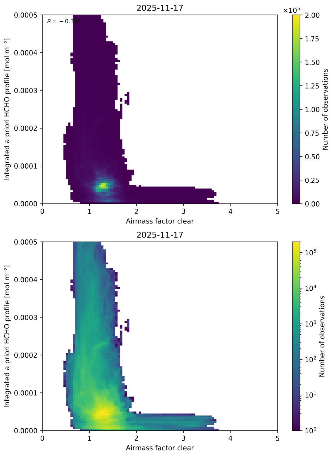
Figure 84: Scatter density plot of “Airmass factor clear” against “Integrated a priori HCHO profile” for 2025-11-16 to 2025-11-18.
