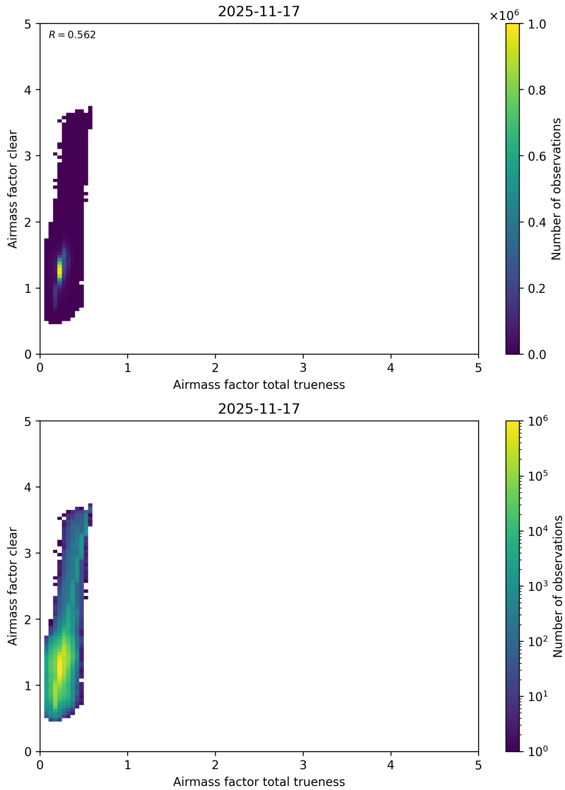
Figure 121: Scatter density plot of “Airmass factor total trueness” against “Airmass factor clear” for 2025-11-16 to 2025-11-18.
