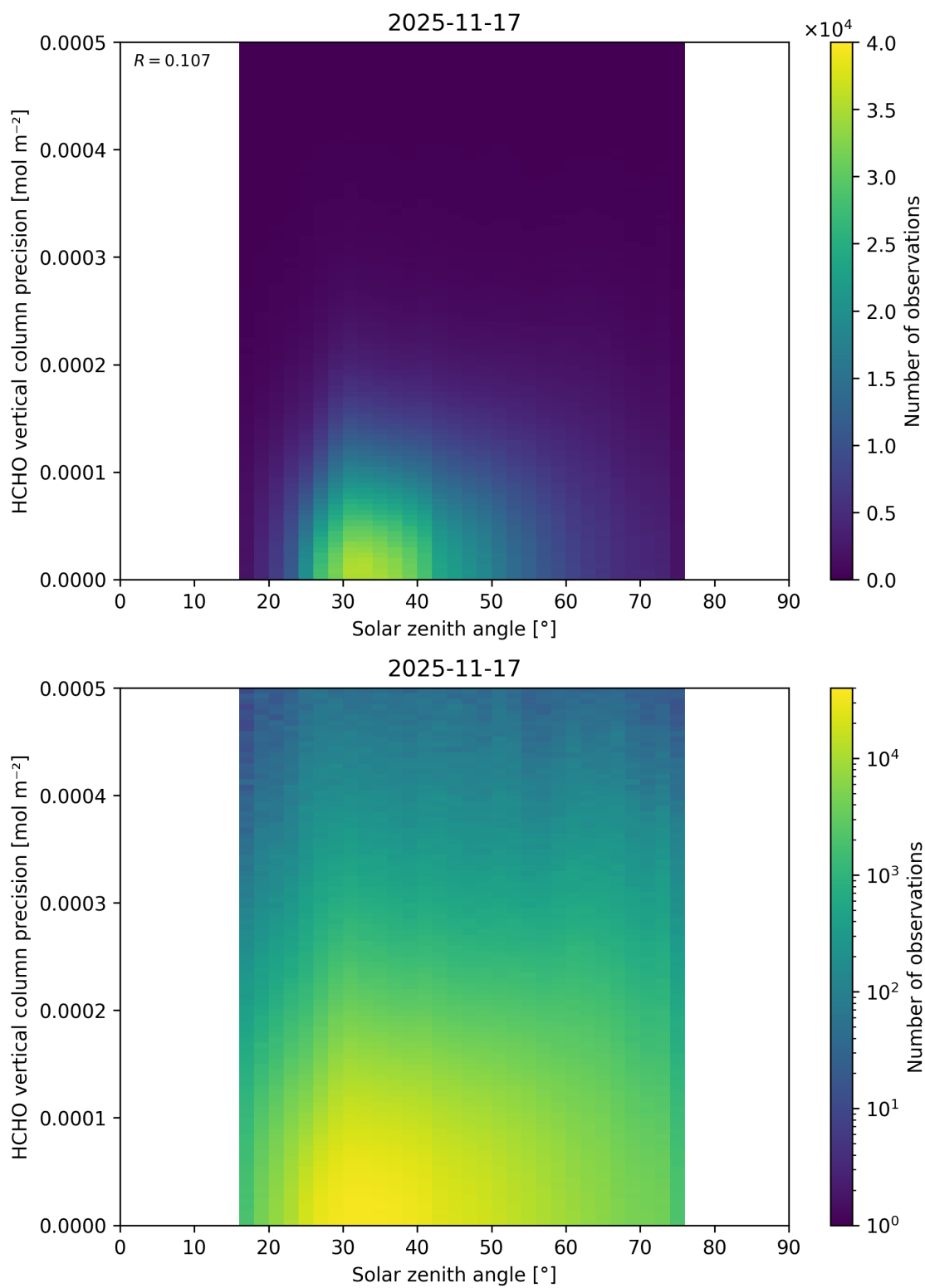
Figure 198: Scatter density plot of “Solar zenith angle” against “HCHO vertical column precision” for 2025-11-16 to 2025-11-18.
