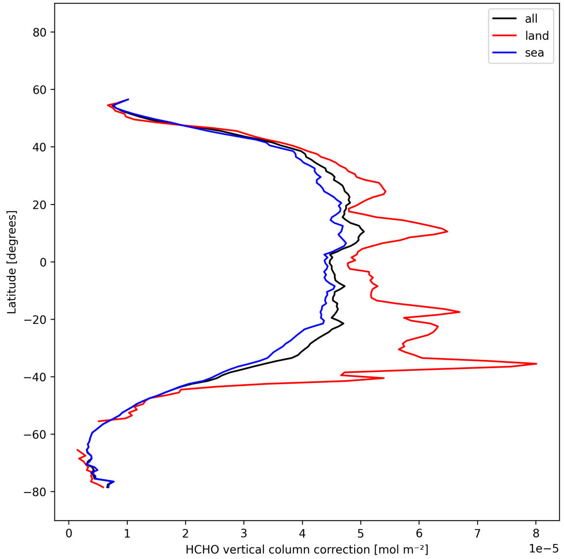
Figure 24: Zonal average of “HCHO vertical column correction” for 2025-11-16 to 2025-11-18.
