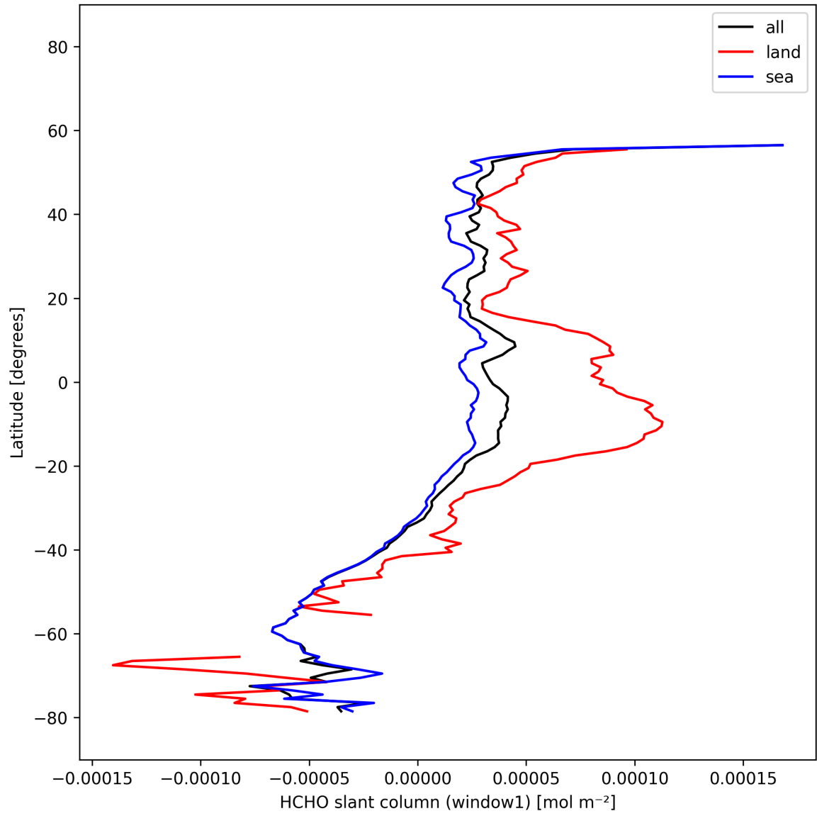
Figure 25: Zonal average of “HCHO slant column (window1)” for 2025-11-16 to 2025-11-18.
