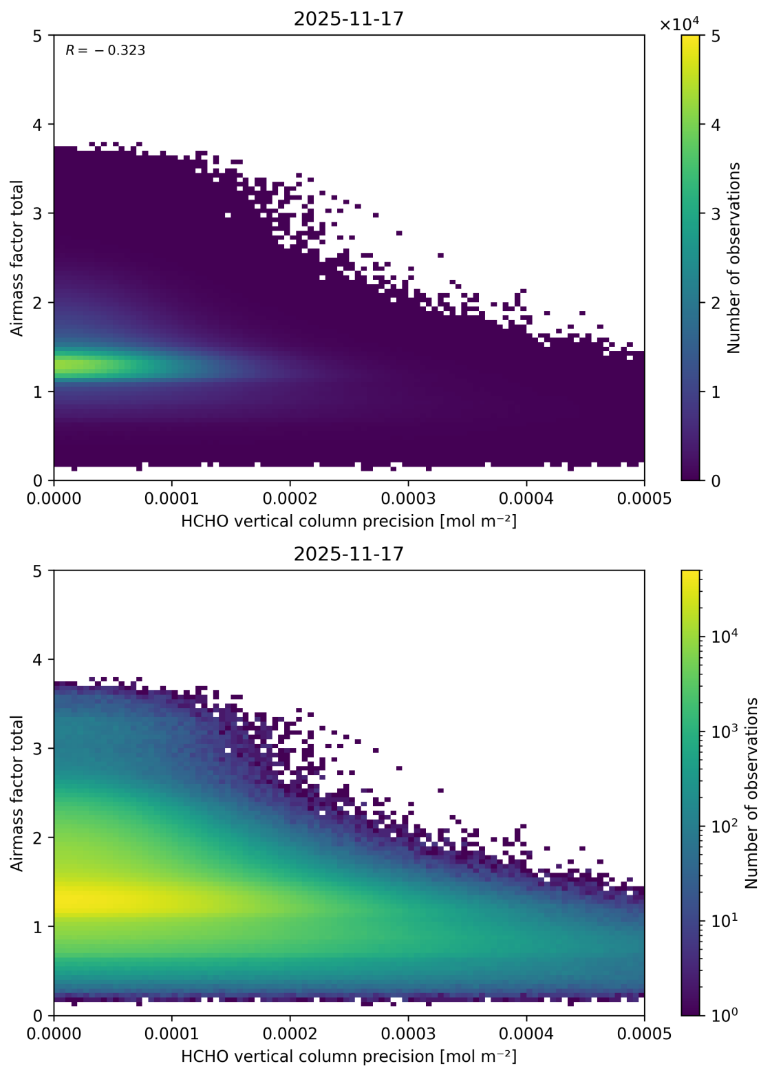
Figure 160: Scatter density plot of “HCHO vertical column precision” against “Airmass factor total” for 2025-11-16 to 2025-11-18.
