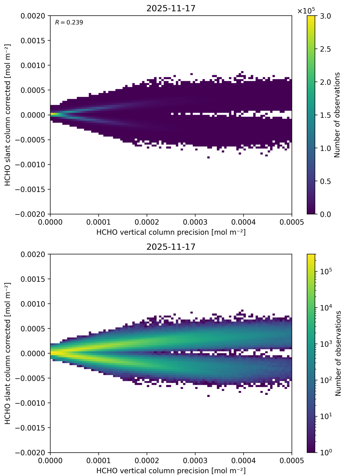
Figure 156: Scatter density plot of “HCHO vertical column precision” against “HCHO slant column corrected” for 2025-11-16 to 2025-11-18.
