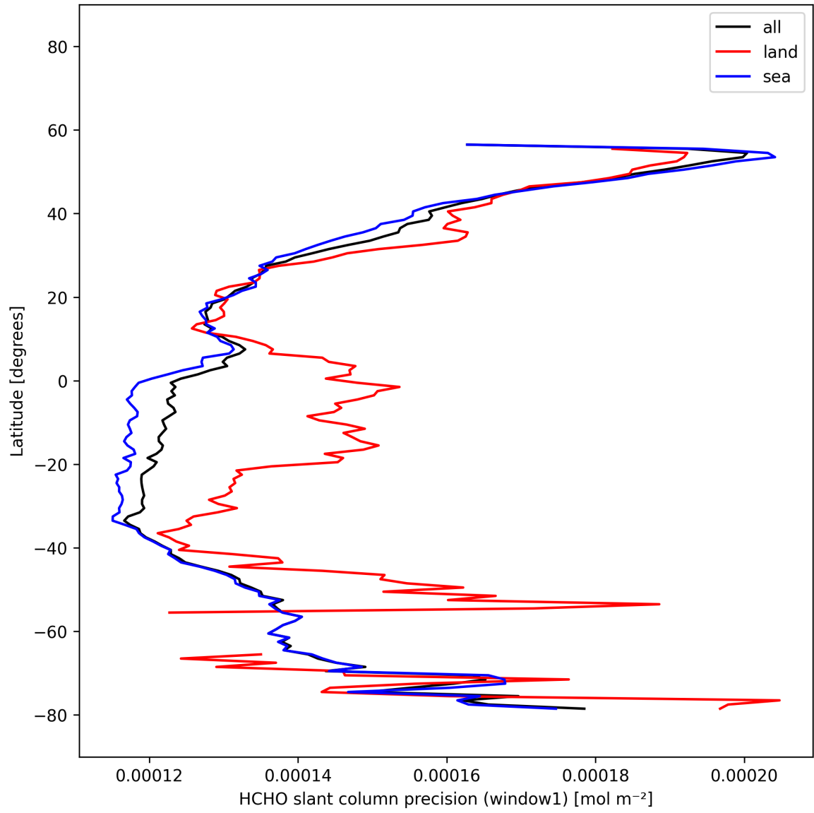
Figure 26: Zonal average of “HCHO slant column precision (window1)” for 2025-11-16 to 2025-11-18.
