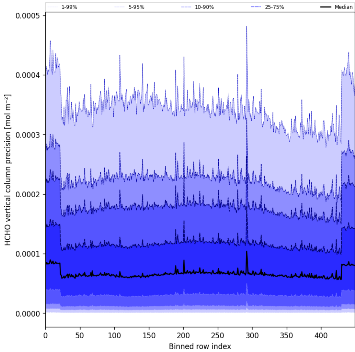
Figure 53: Along track statistics of “HCHO vertical column precision” for 2025-11-16 to 2025-11-18
