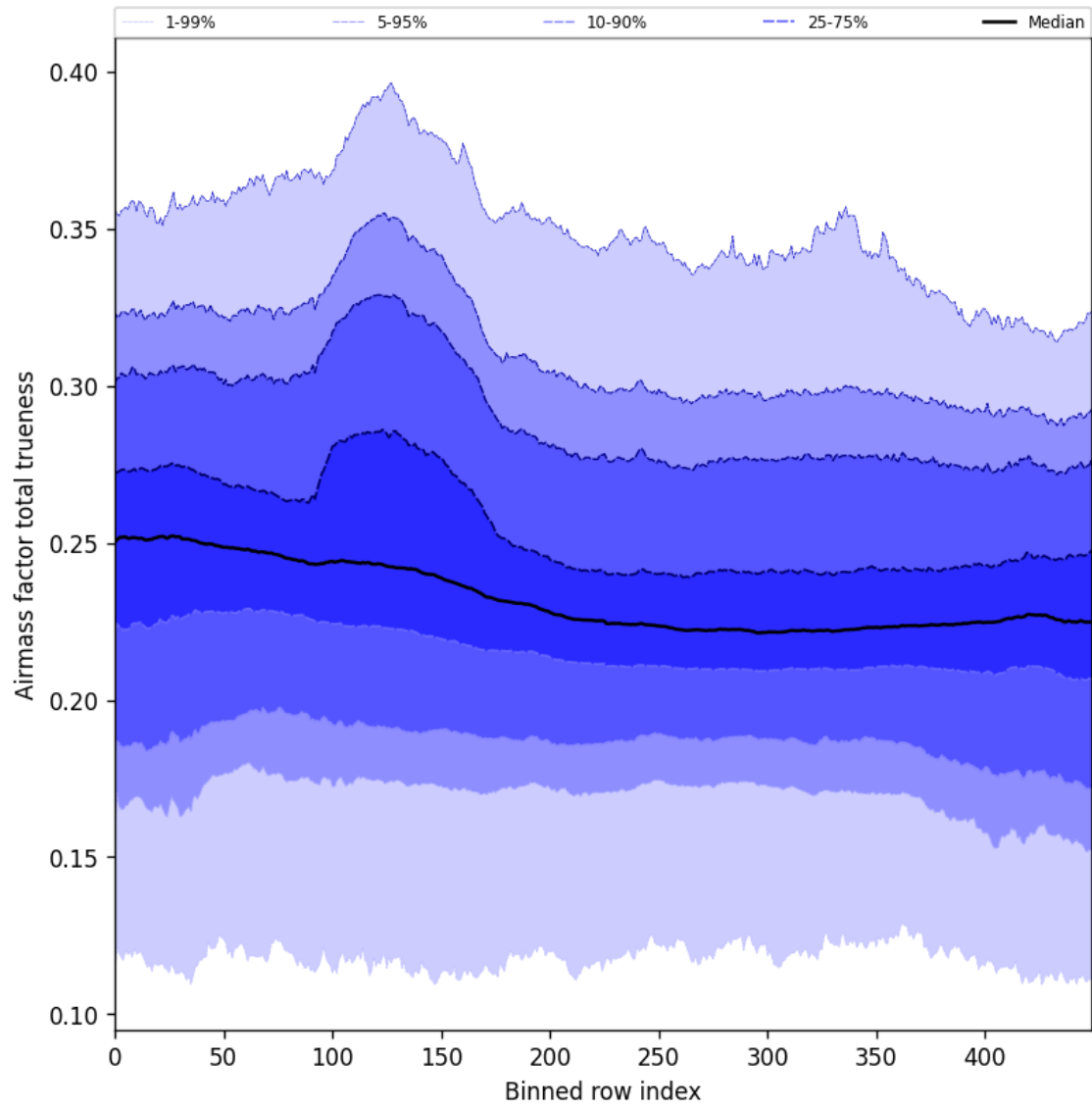
Figure 58: Along track statistics of “Airmass factor total trueness” for 2025-11-16 to 2025-11-18
