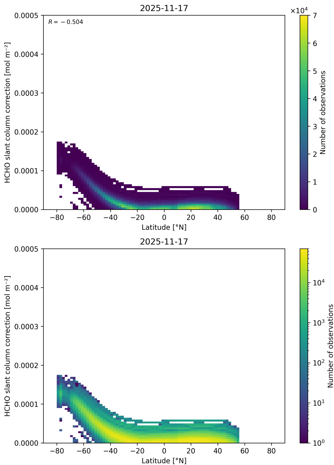
Figure 176: Scatter density plot of “Latitude” against “HCHO slant column correction” for 2025-11-16 to 2025-11-18.
