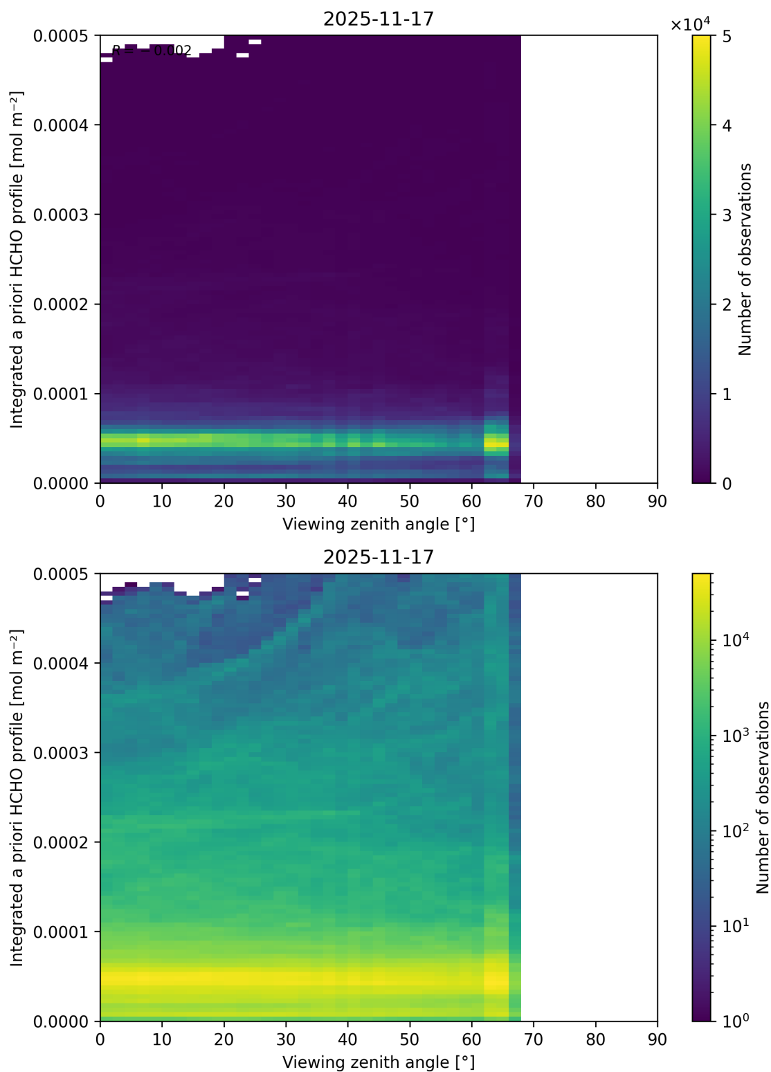
Figure 216: Scatter density plot of “Viewing zenith angle” against “Integrated a priori HCHO profile” for 2025-11-16 to 2025-11-18.
