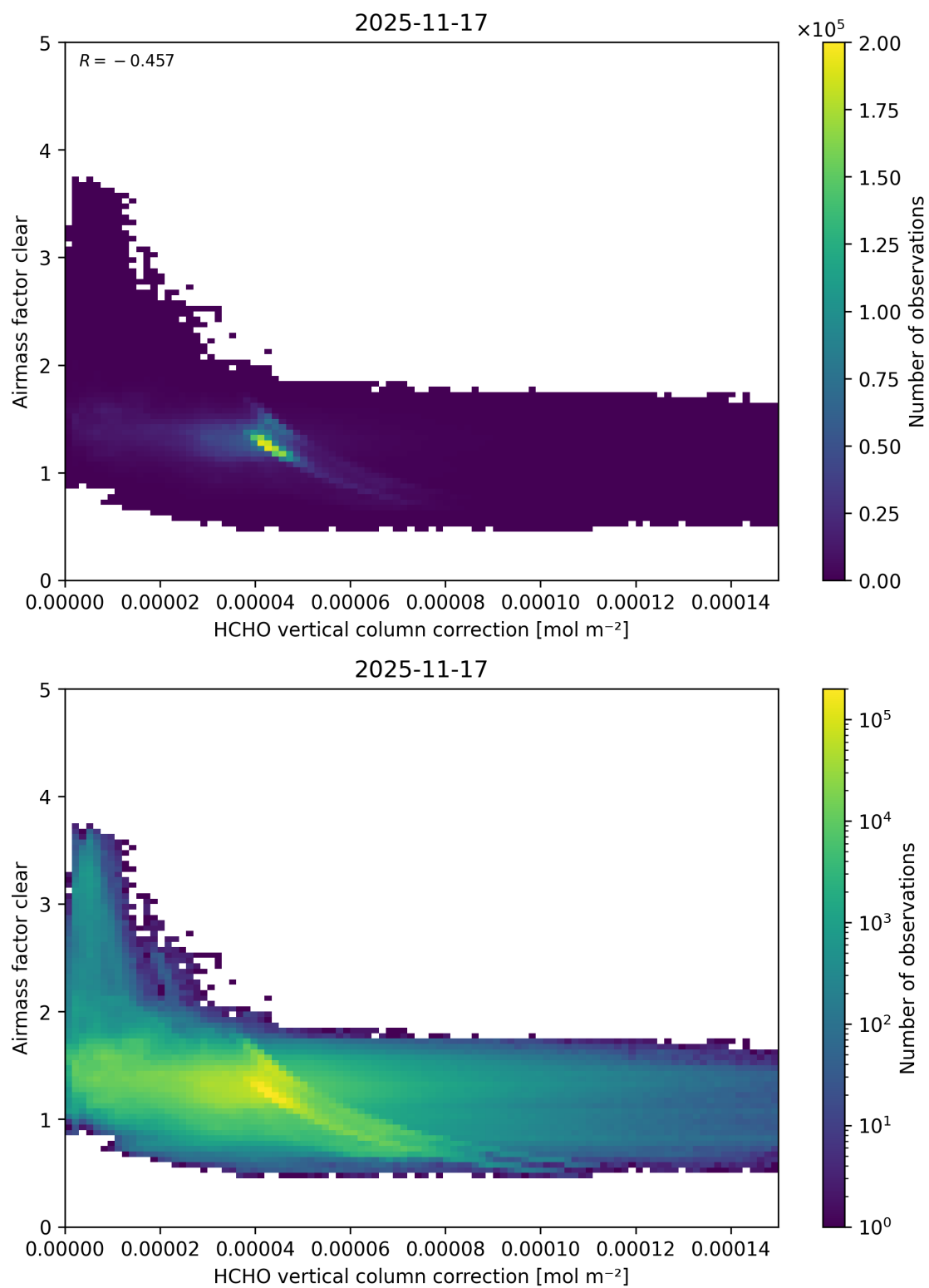
Figure 129: Scatter density plot of “HCHO vertical column correction” against “Airmass factor clear” for 2025-11-16 to 2025-11-18.
