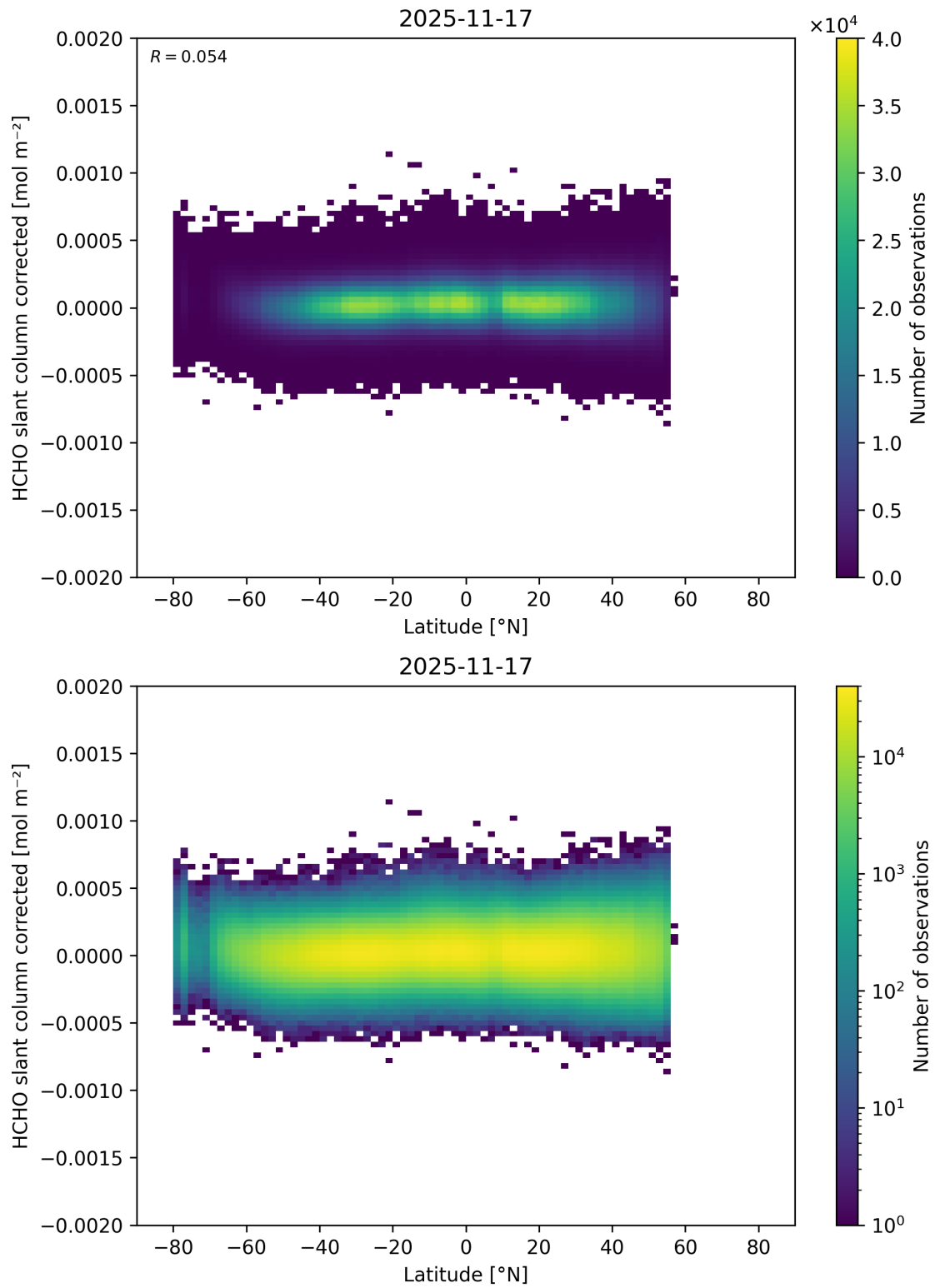
Figure 175: Scatter density plot of “Latitude” against “HCHO slant column corrected” for 2025-11-16 to 2025-11-18.
