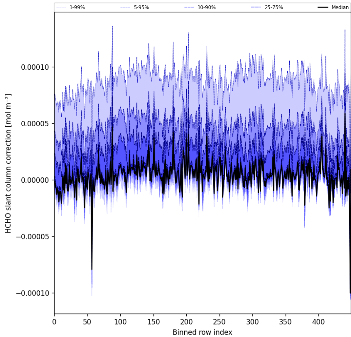
Figure 64: Along track statistics of “HCHO slant column correction” for 2025-11-16 to 2025-11-18
