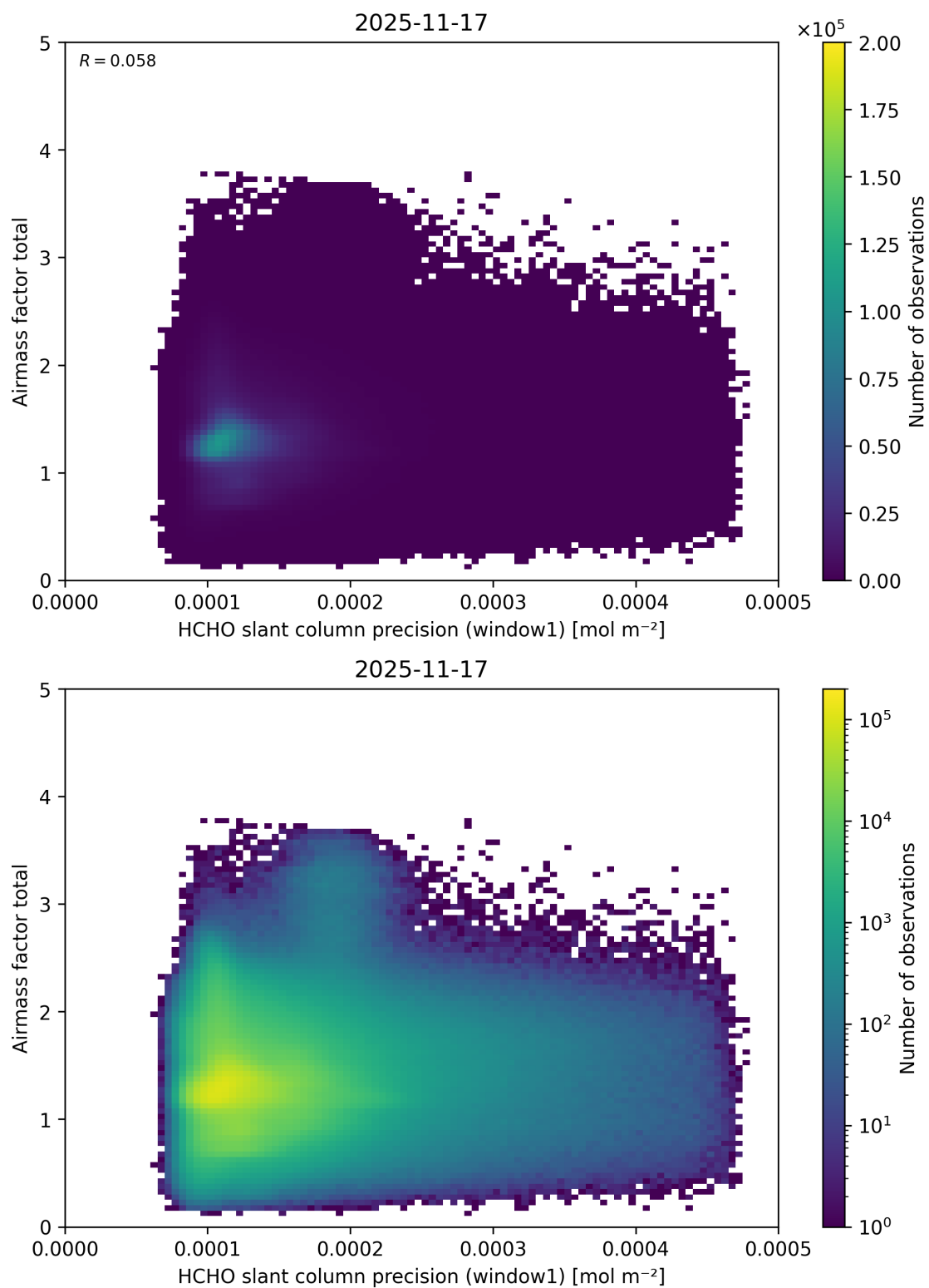
Figure 105: Scatter density plot of “HCHO slant column precision (window1)” against “Airmass factor total” for 2025-11-16 to 2025-11-18.
