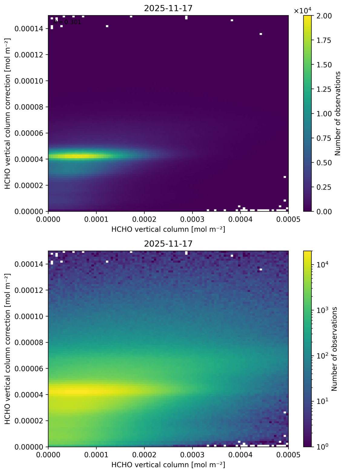
Figure 148: Scatter density plot of “HCHO vertical column” against “HCHO vertical column correction” for 2025-11-16 to 2025-11-18.
