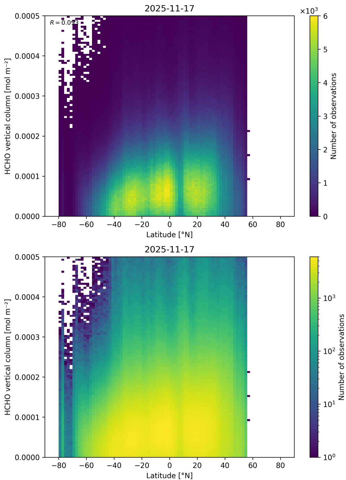
Figure 181: Scatter density plot of “Latitude” against “HCHO vertical column” for 2025-11-16 to 2025-11-18.
