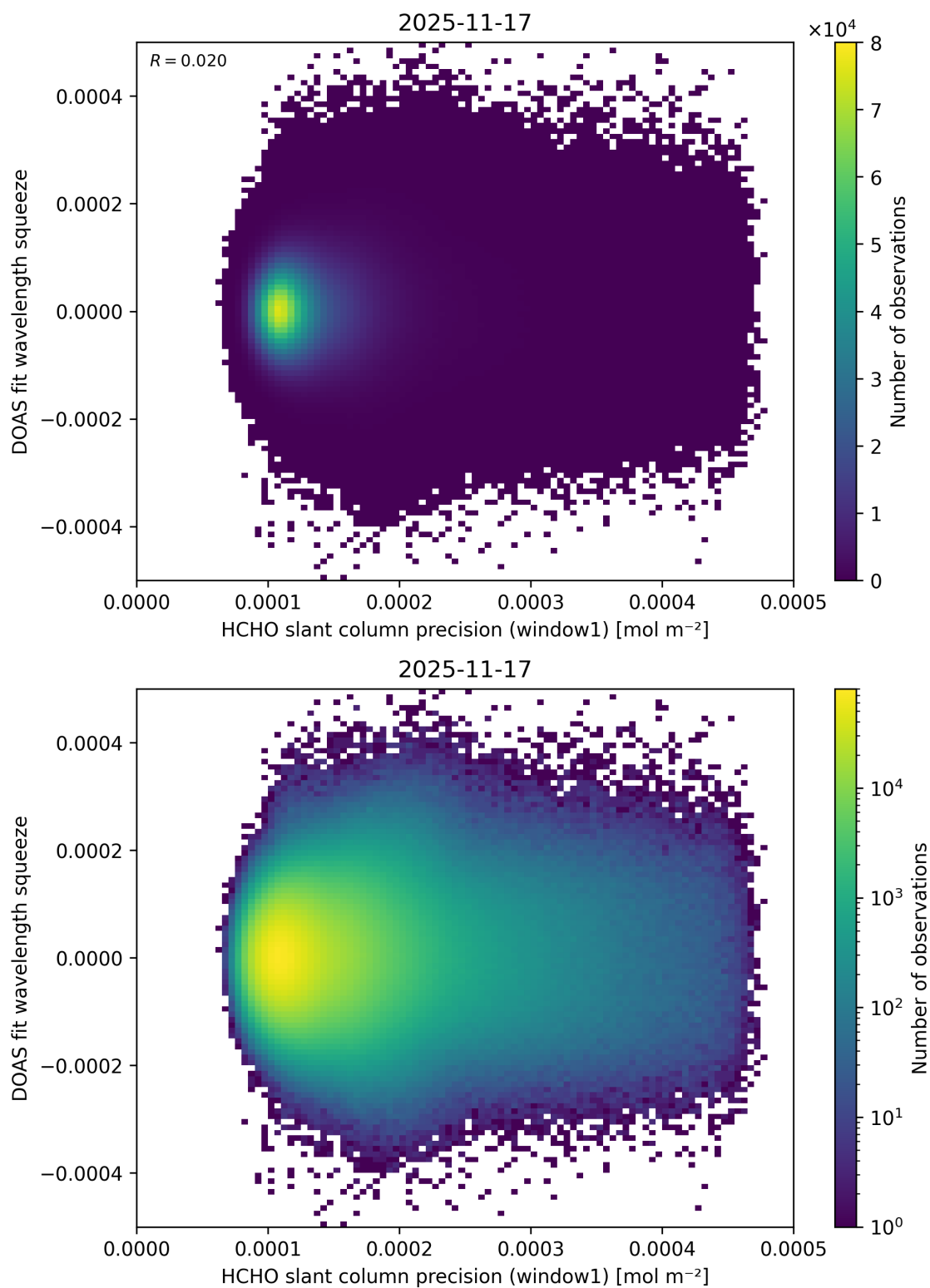
Figure 101: Scatter density plot of “HCHO slant column precision (window1)” against “DOAS fit wavelength squeeze” for 2025-11-16 to 2025-11-18.
