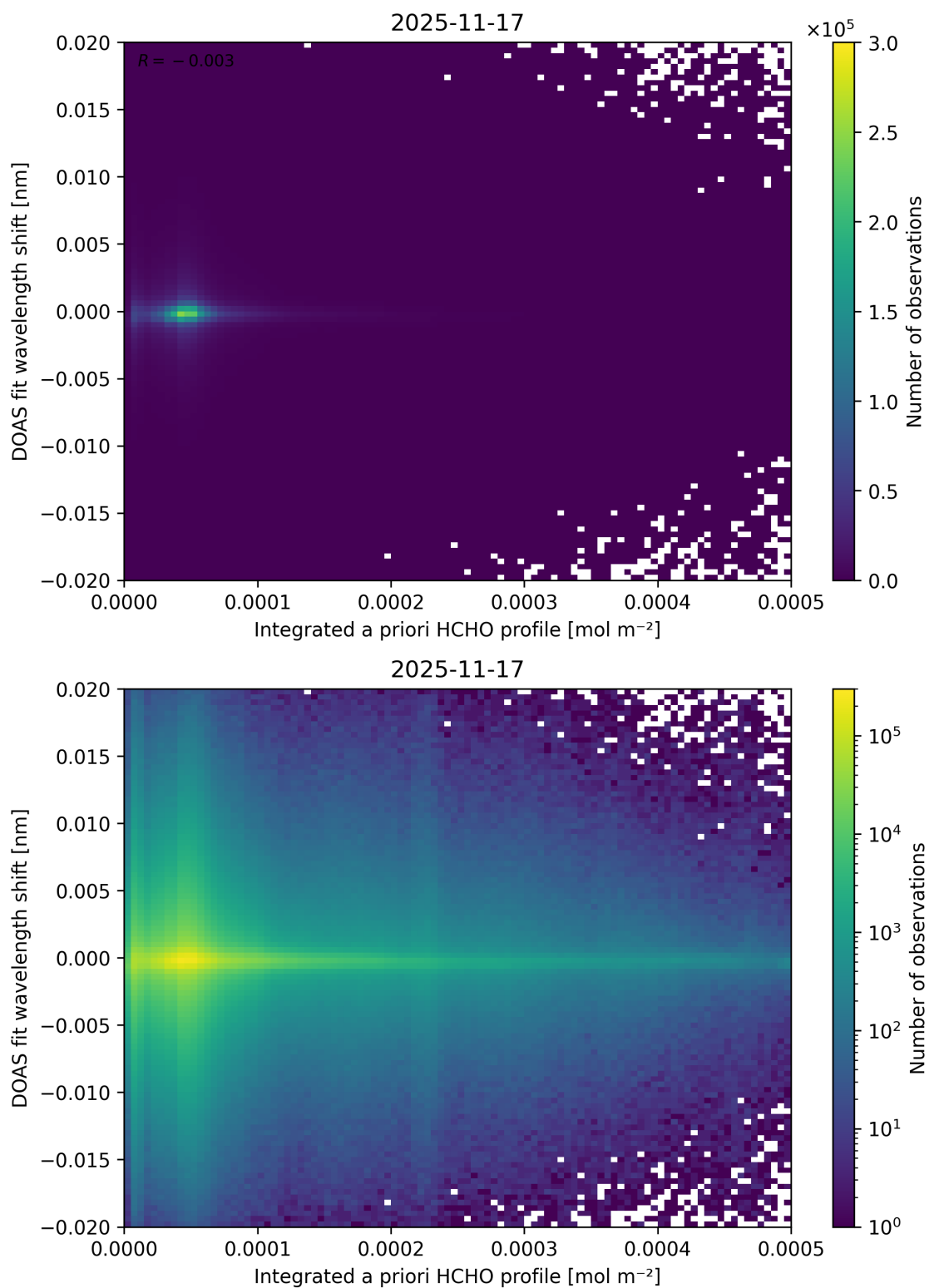
Figure 166: Scatter density plot of “Integrated a priori HCHO profile” against “DOAS fit wavelength shift” for 2025-11-16 to 2025-11-18.
