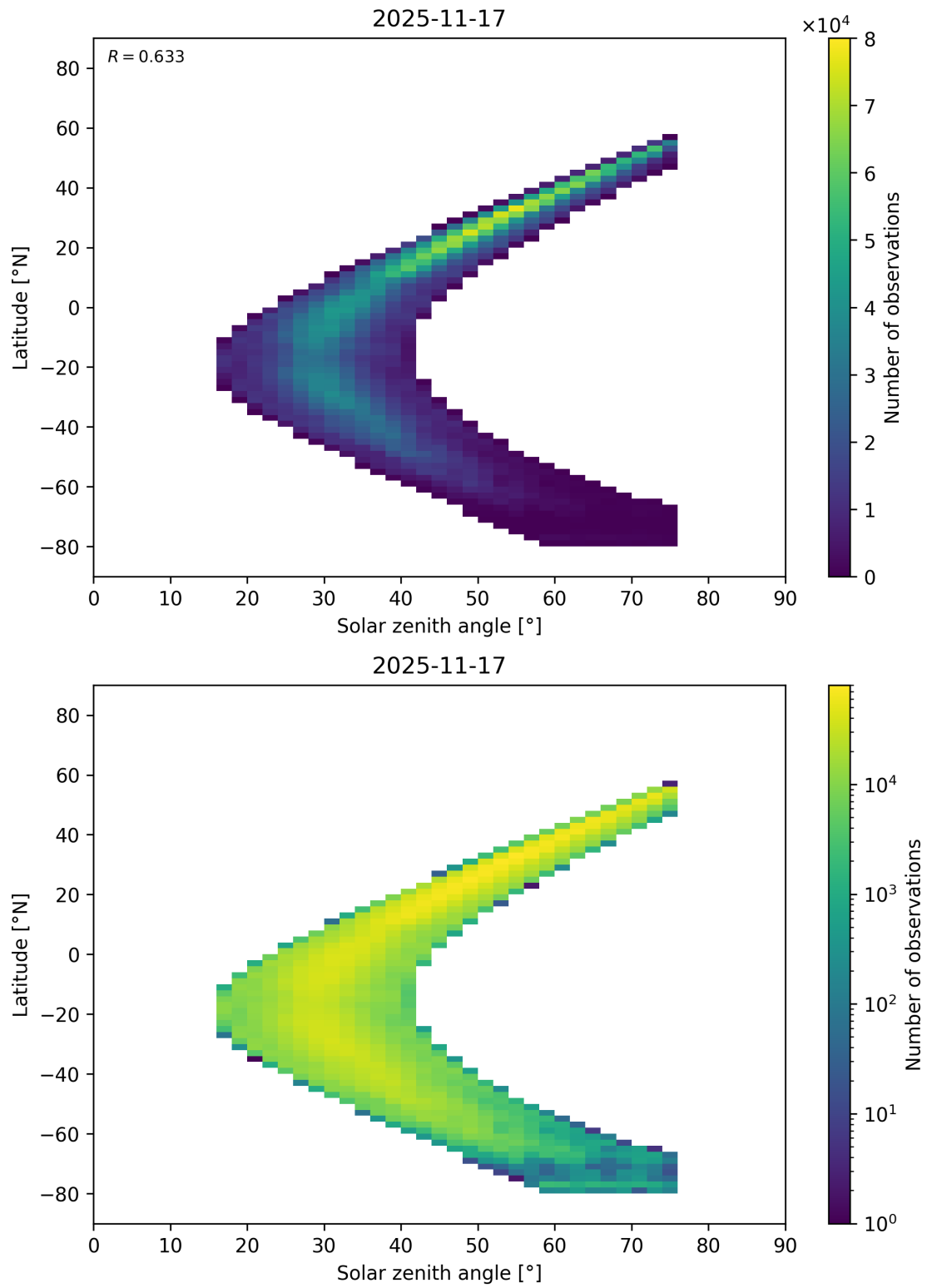
Figure 201: Scatter density plot of “Solar zenith angle” against “Latitude” for 2025-11-16 to 2025-11-18.
