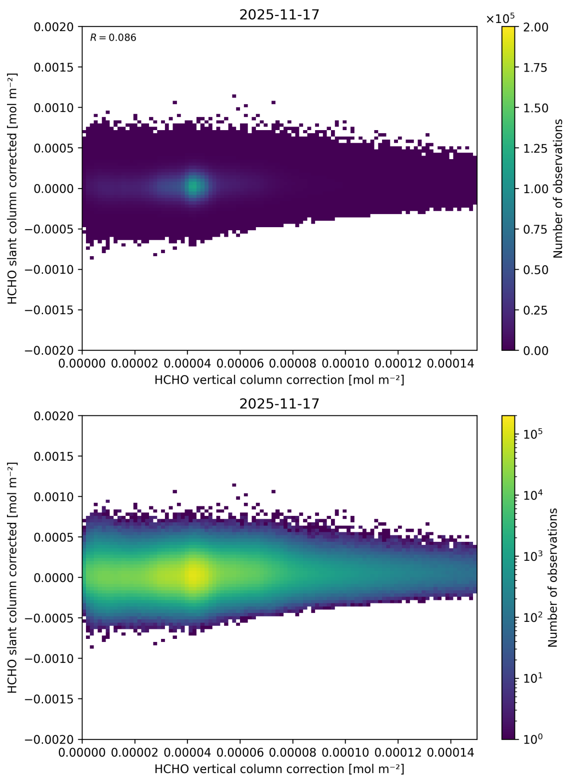
Figure 130: Scatter density plot of “HCHO vertical column correction” against “HCHO slant column corrected” for 2025-11-16 to 2025-11-18.
