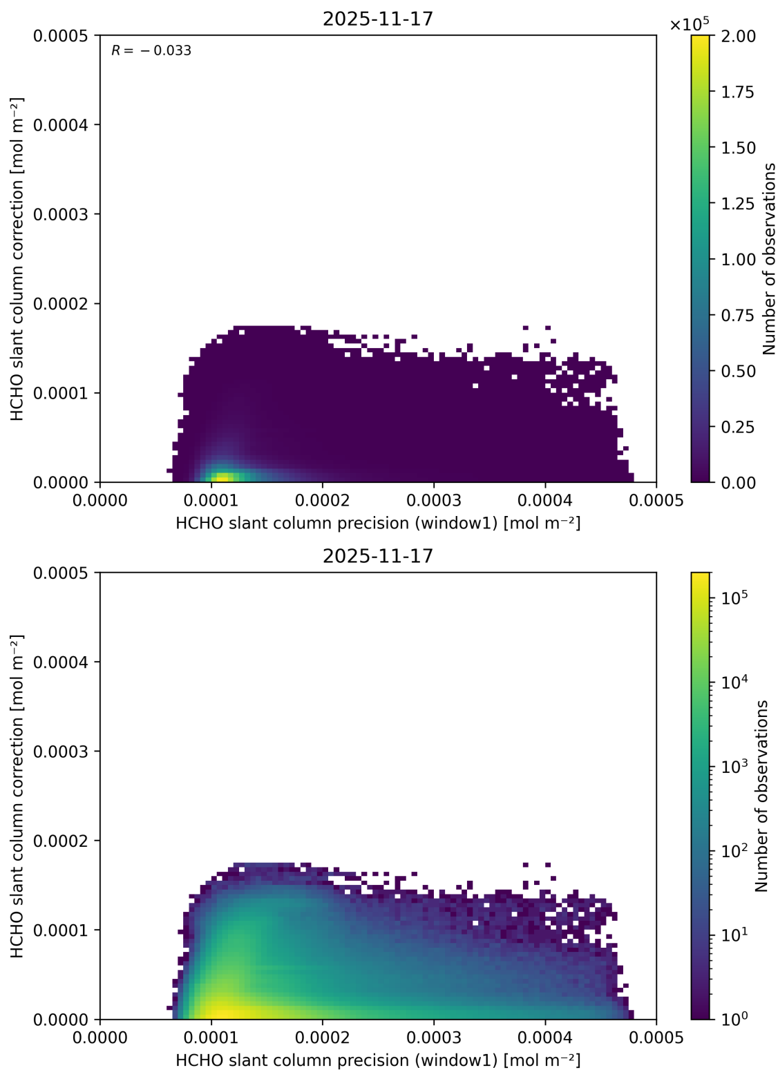
Figure 104: Scatter density plot of “HCHO slant column precision (window1)” against “HCHO slant column correction” for 2025-11-16 to 2025-11-18.
