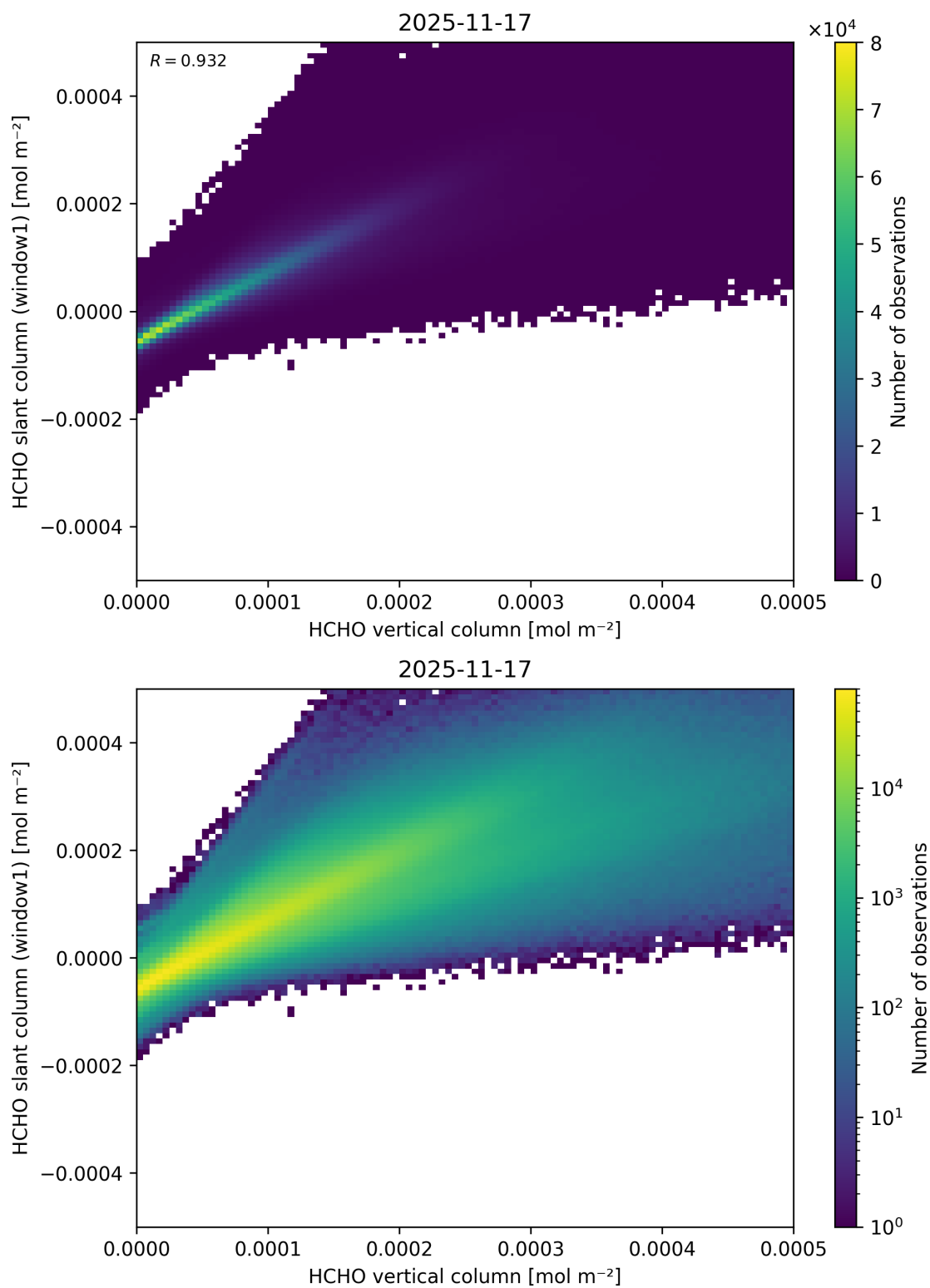
Figure 144: Scatter density plot of “HCHO vertical column” against “HCHO slant column (window1)” for 2025-11-16 to 2025-11-18.
