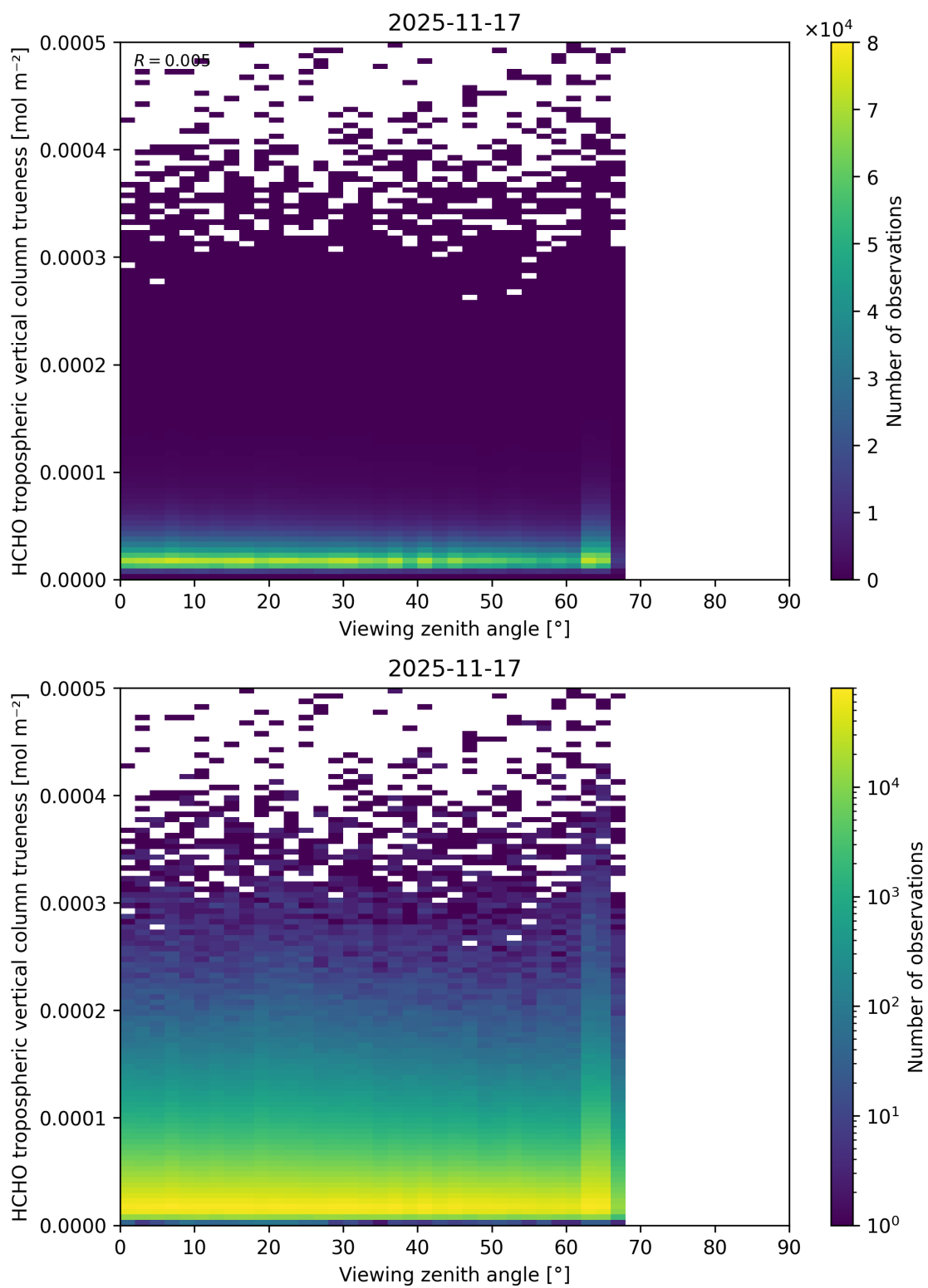
Figure 215: Scatter density plot of “Viewing zenith angle” against “HCHO tropospheric vertical column trueness” for 2025-11-16 to 2025-11-18.
