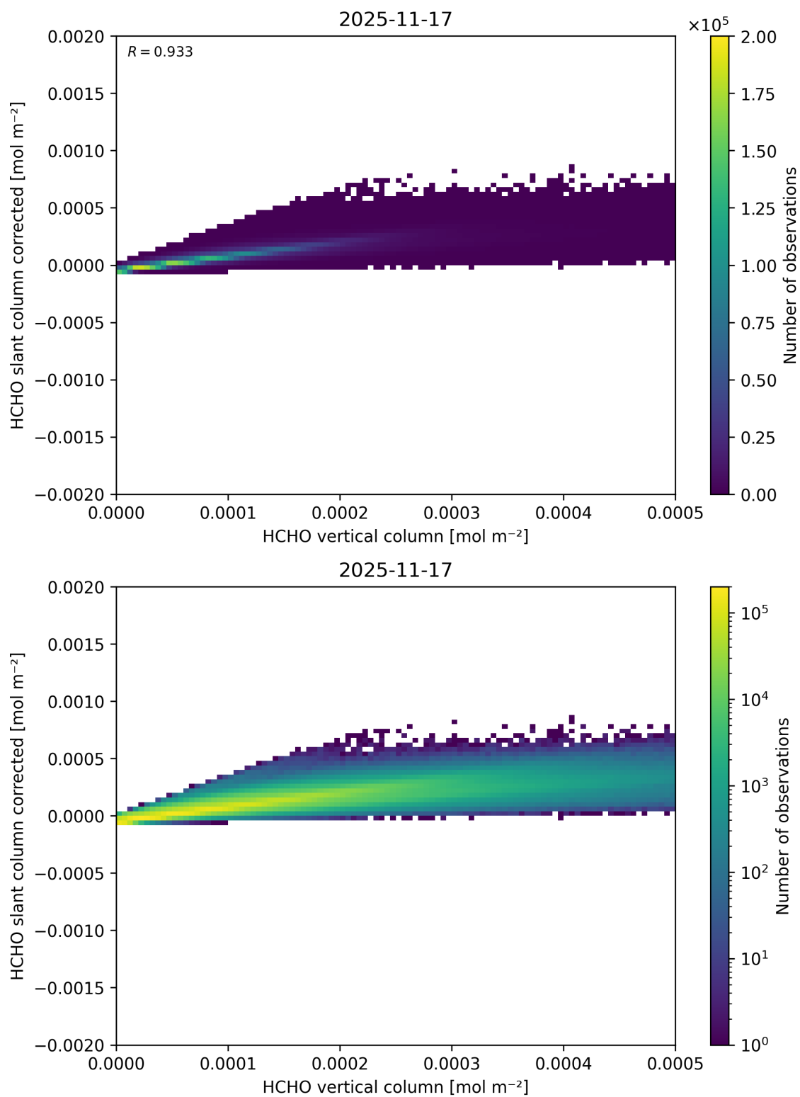
Figure 142: Scatter density plot of “HCHO vertical column” against “HCHO slant column corrected” for 2025-11-16 to 2025-11-18.
