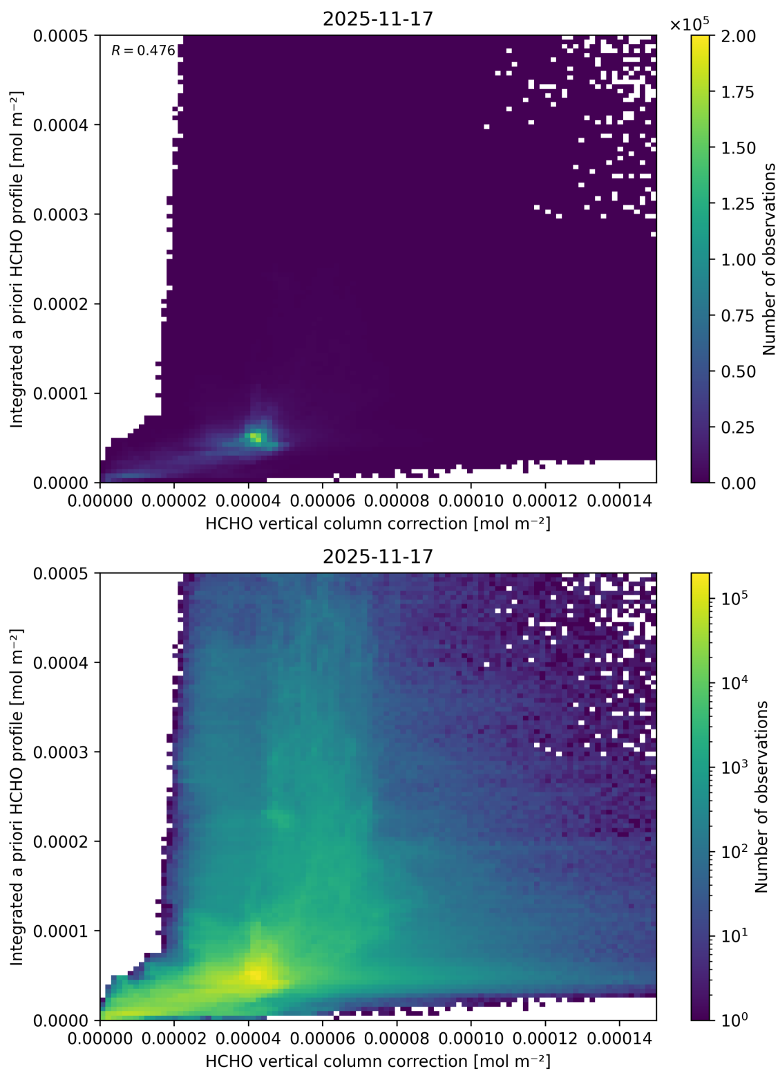
Figure 137: Scatter density plot of “HCHO vertical column correction” against “Integrated a priori HCHO profile” for 2025-11-16 to 2025-11-18.
