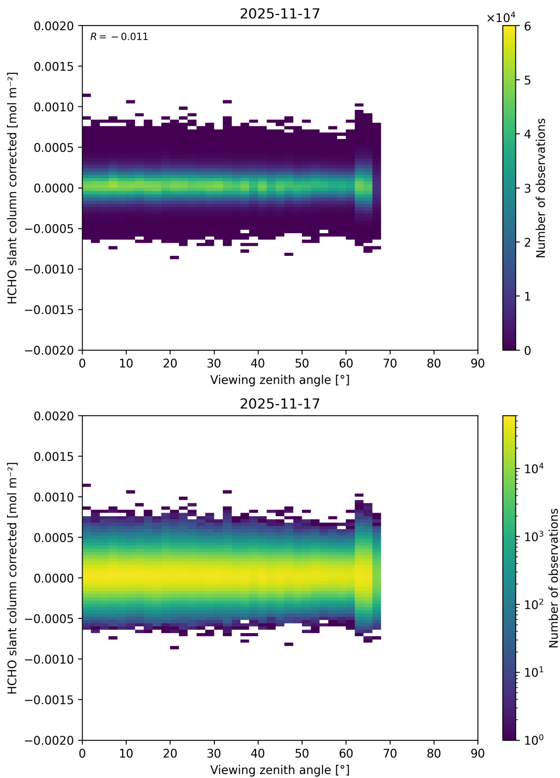
Figure 206: Scatter density plot of “Viewing zenith angle” against “HCHO slant column corrected” for 2025-11-16 to 2025-11-18.
