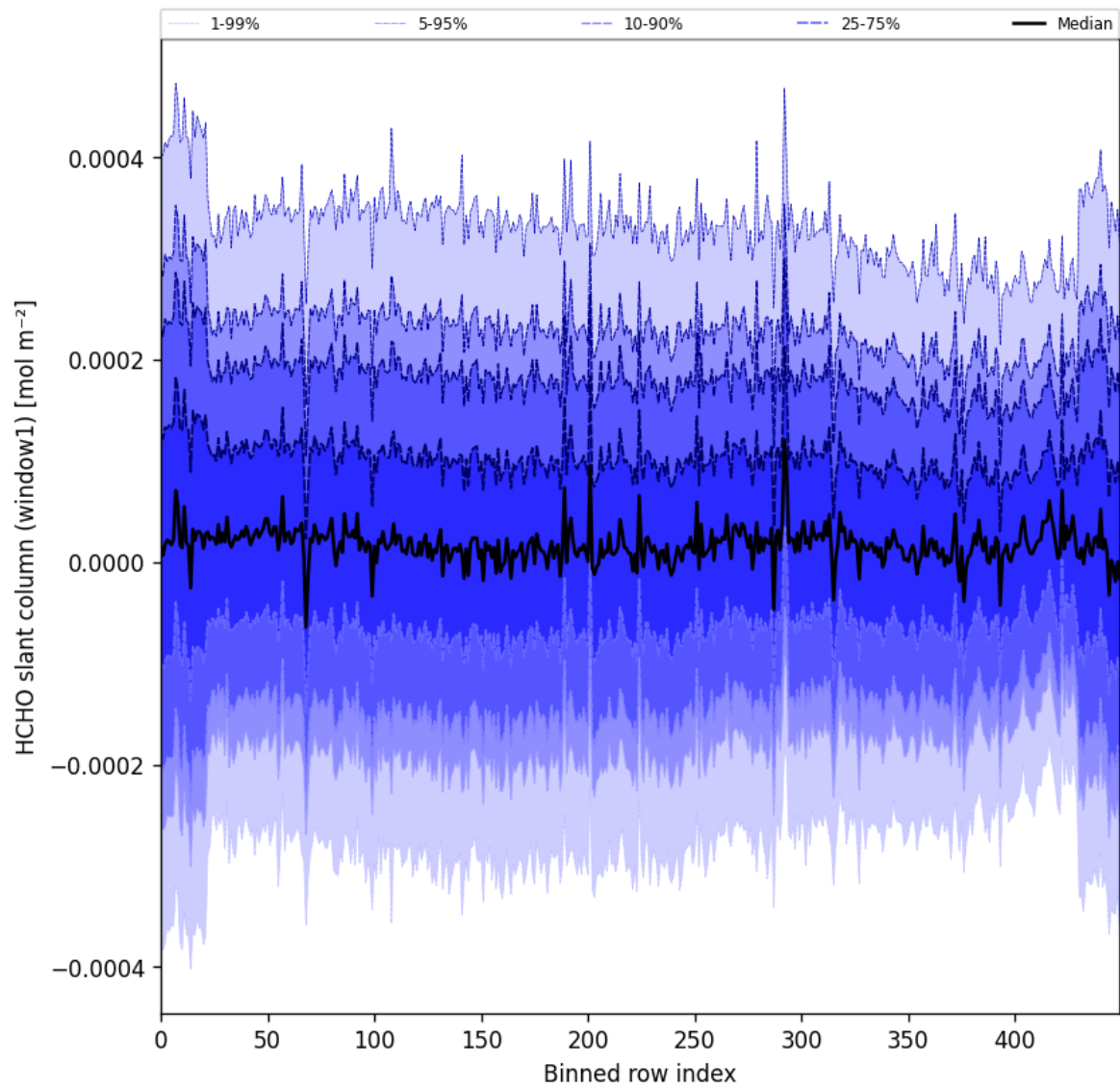
Figure 55: Along track statistics of “HCHO slant column (window1)” for 2025-11-16 to 2025-11-18
