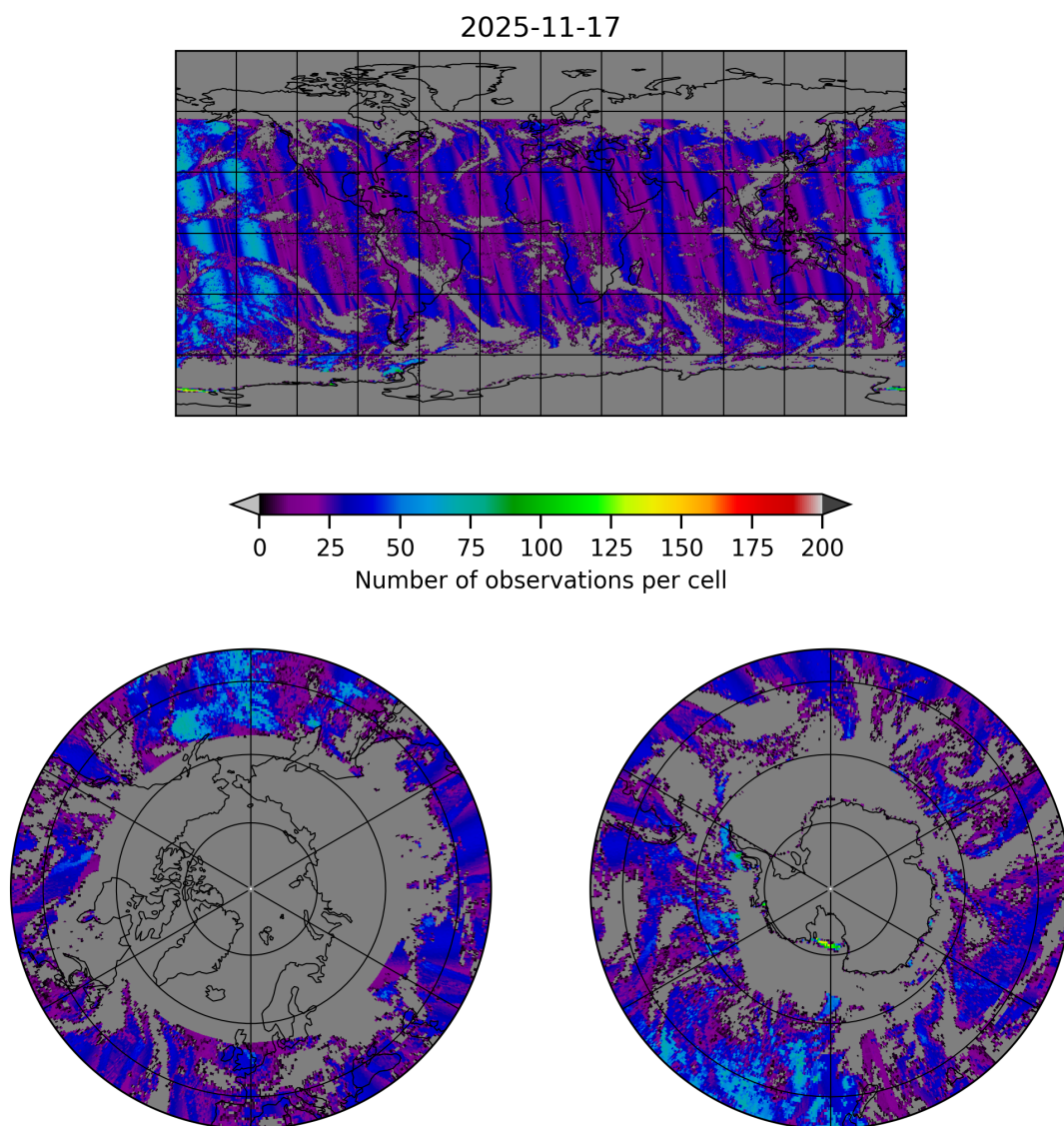
Figure 20: Map of the number of observations for 2025-11-16 to 2025-11-18
