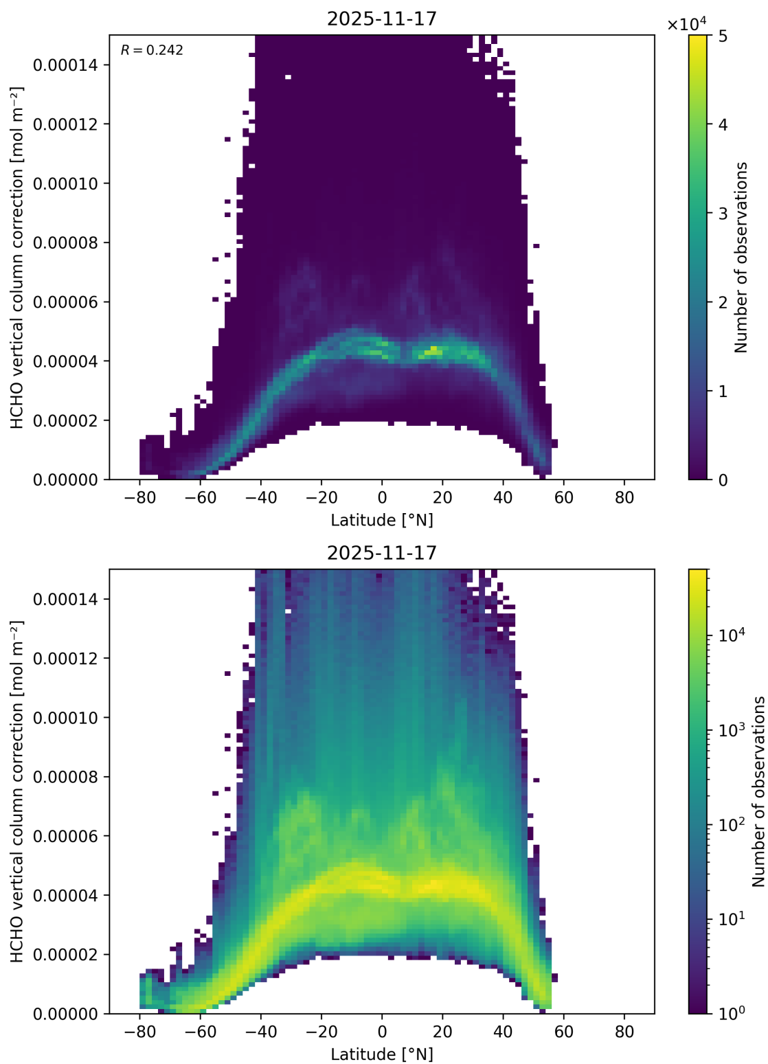
Figure 182: Scatter density plot of “Latitude” against “HCHO vertical column correction” for 2025-11-16 to 2025-11-18.
