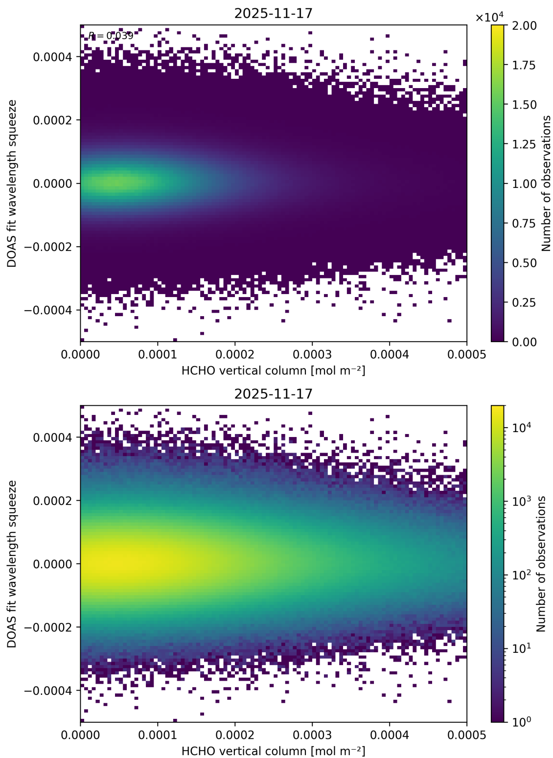
Figure 140: Scatter density plot of “HCHO vertical column” against “DOAS fit wavelength squeeze” for 2025-11-16 to 2025-11-18.
