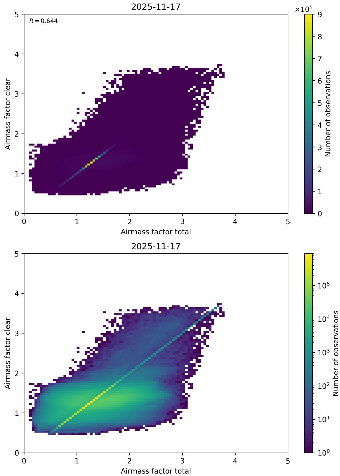
Figure 112: Scatter density plot of “Airmass factor total” against “Airmass factor clear” for 2025-11-16 to 2025-11-18.
