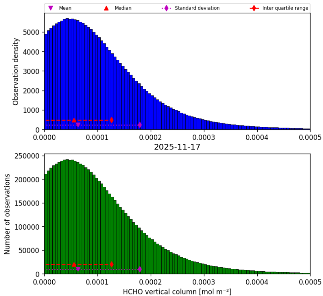
Figure 37: Histogram of “HCHO vertical column” for 2025-11-16 to 2025-11-18
