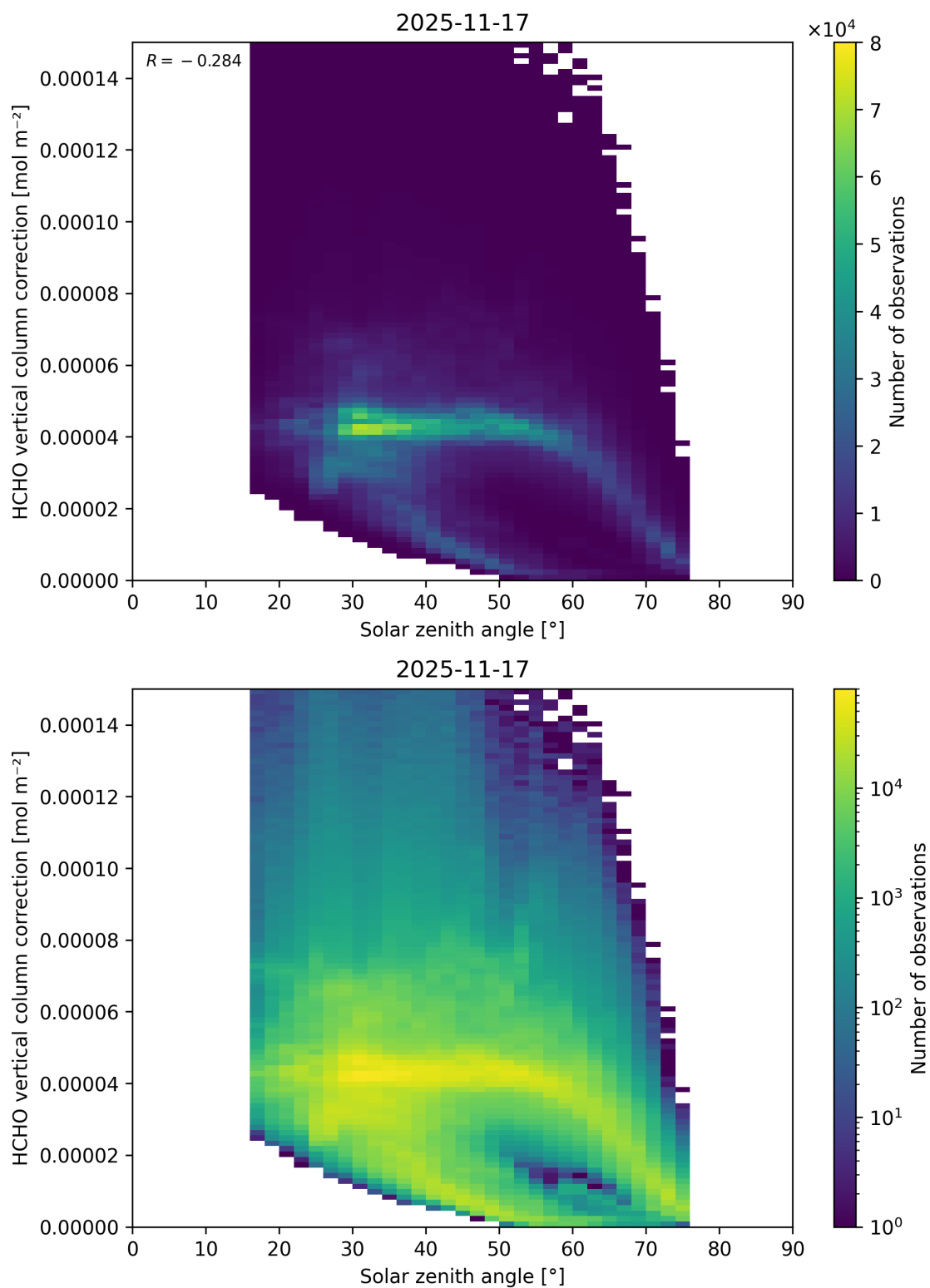
Figure 197: Scatter density plot of “Solar zenith angle” against “HCHO vertical column correction” for 2025-11-16 to 2025-11-18.
