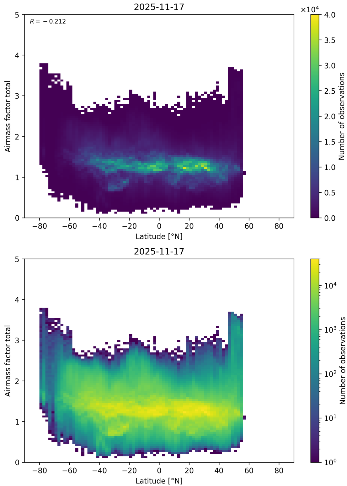
Figure 179: Scatter density plot of “Latitude” against “Airmass factor total” for 2025-11-16 to 2025-11-18.
