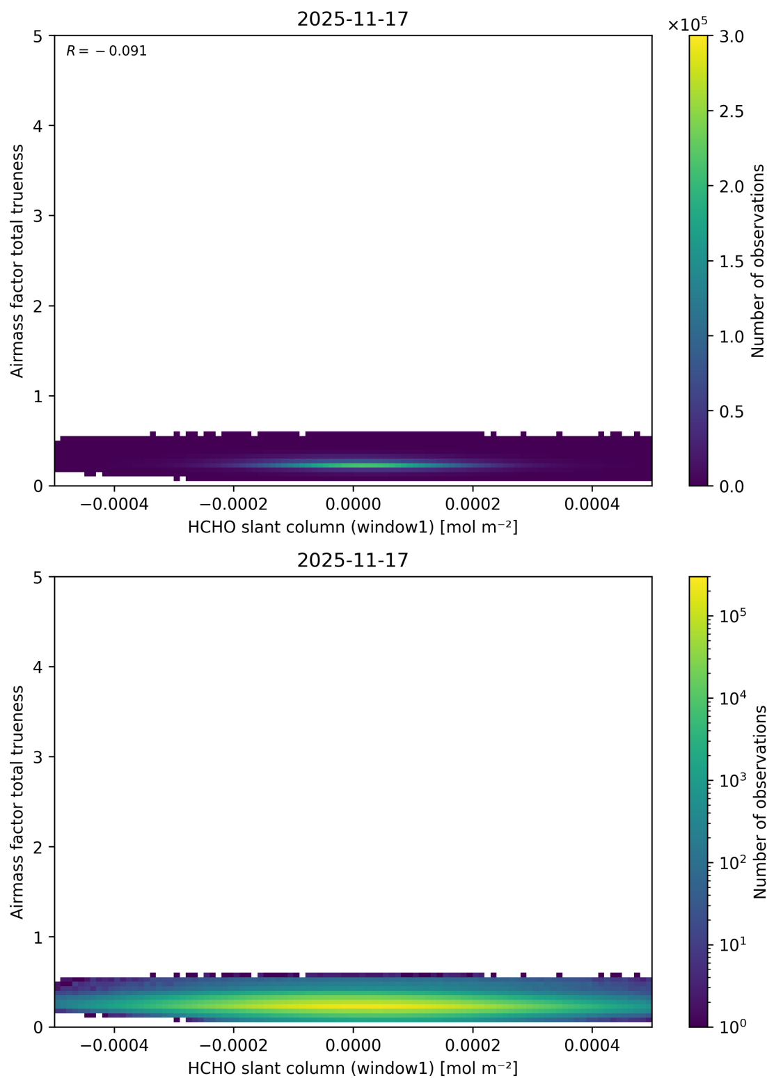
Figure 96: Scatter density plot of “HCHO slant column (window1)” against “Airmass factor total trueneess” for 2025-11-16 to 2025-11-18.
