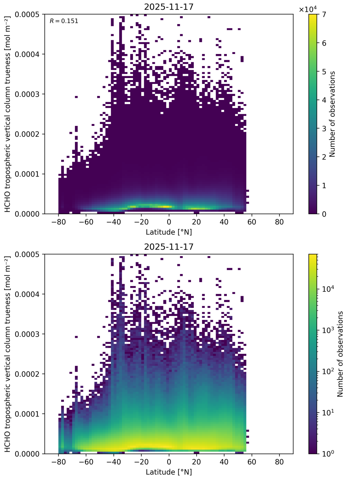
Figure 184: Scatter density plot of “Latitude” against “HCHO tropospheric vertical column trueness” for 2025-11-16 to 2025-11-18.
