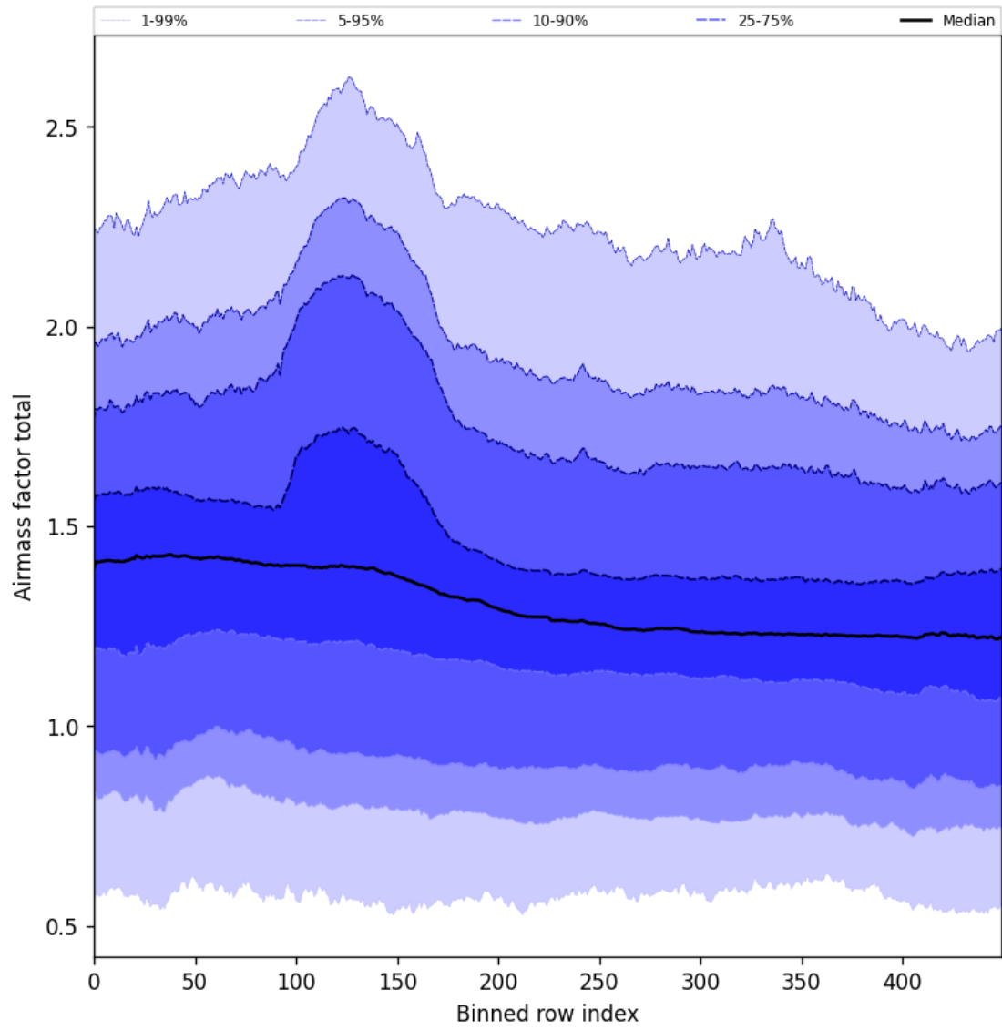
Figure 57: Along track statistics of “Airmass factor total” for 2025-11-16 to 2025-11-18
