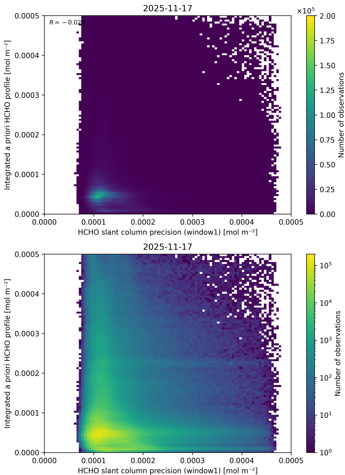
Figure 108: Scatter density plot of “HCHO slant column precision (window1)” against “Integrated a priori HCHO profile” for 2025-11-16 to 2025-11-18.
