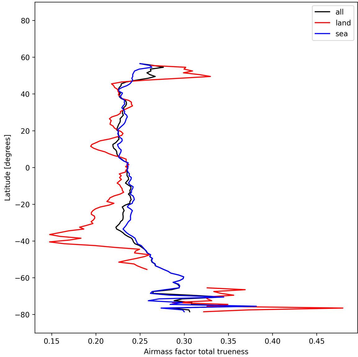
Figure 28: Zonal average of “Airmass factor total truiness” for 2025-11-16 to 2025-11-18.
