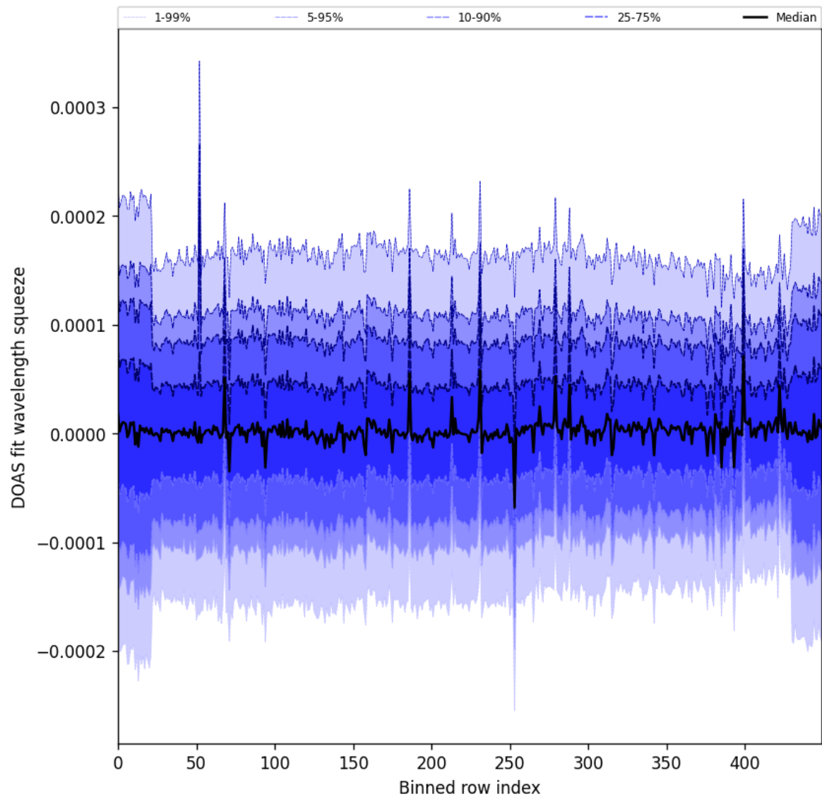
Figure 62: Along track statistics of “DOAS fit wavelength squeeze” for 2025-11-16 to 2025-11-18
