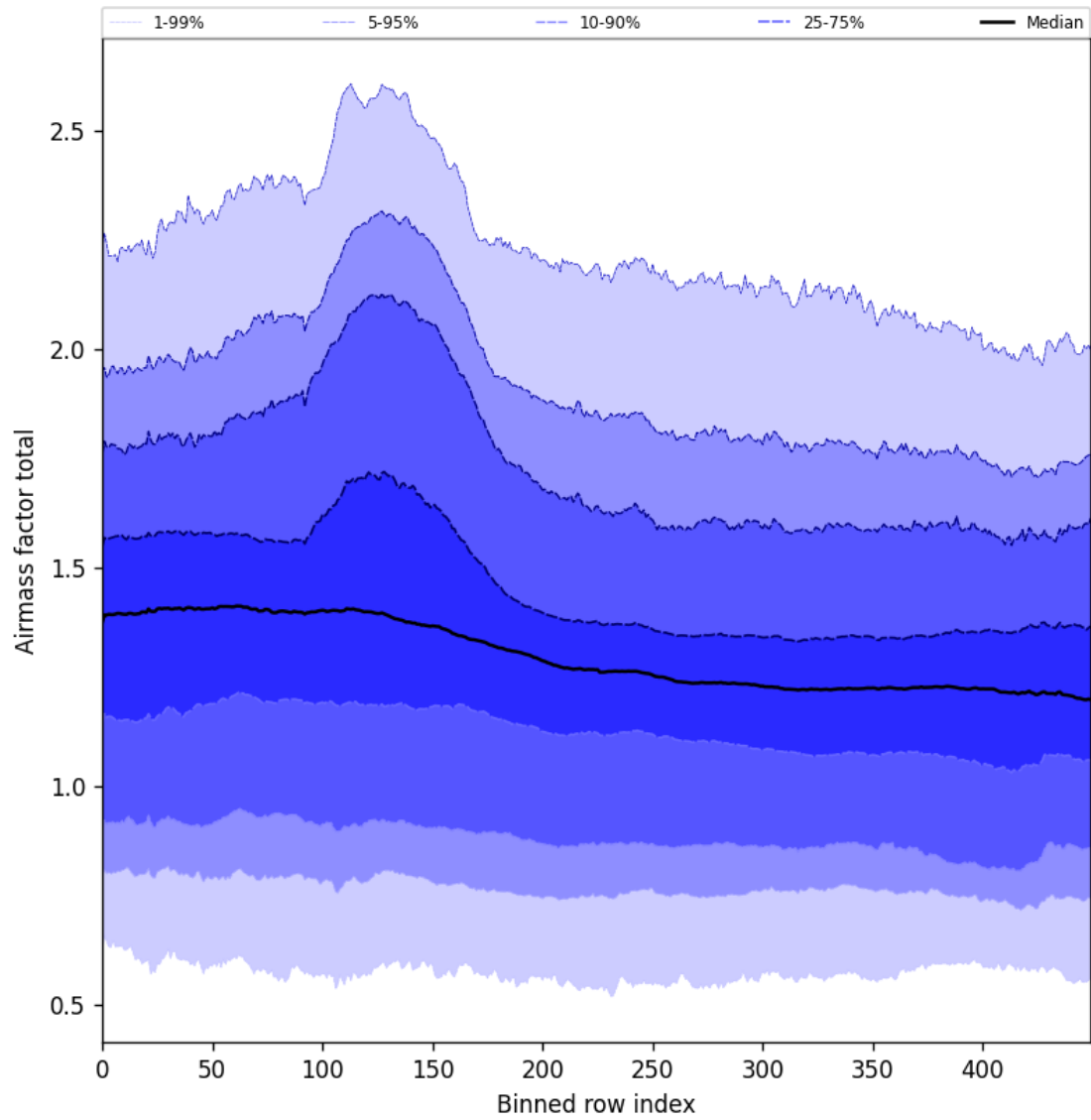
Figure 57: Along track statistics of “Airmass factor total” for 2025-11-18 to 2025-11-19
