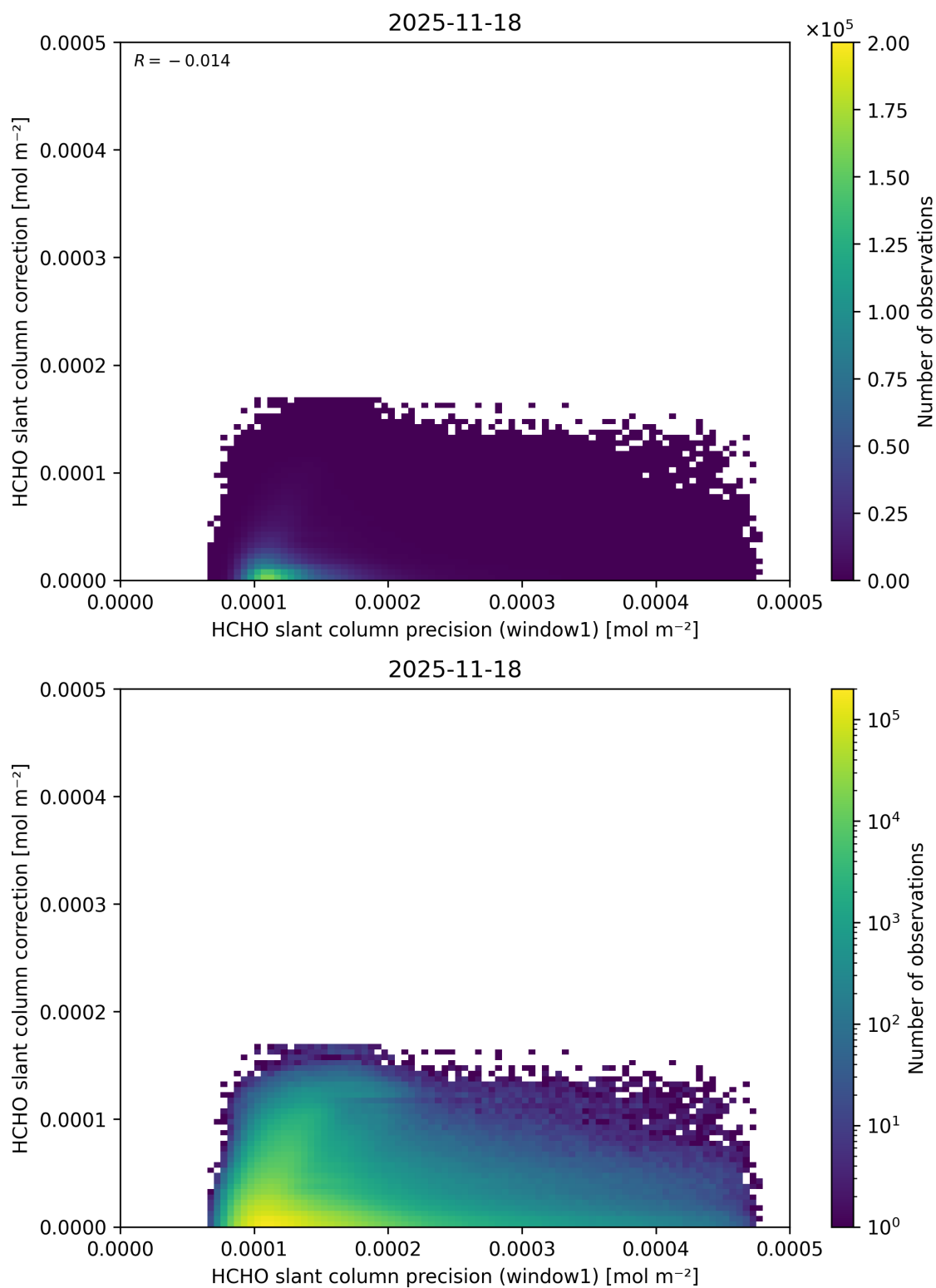
Figure 104: Scatter density plot of “HCHO slant column precision (window1)” against “HCHO slant column correction” for 2025-11-18 to 2025-11-19.
