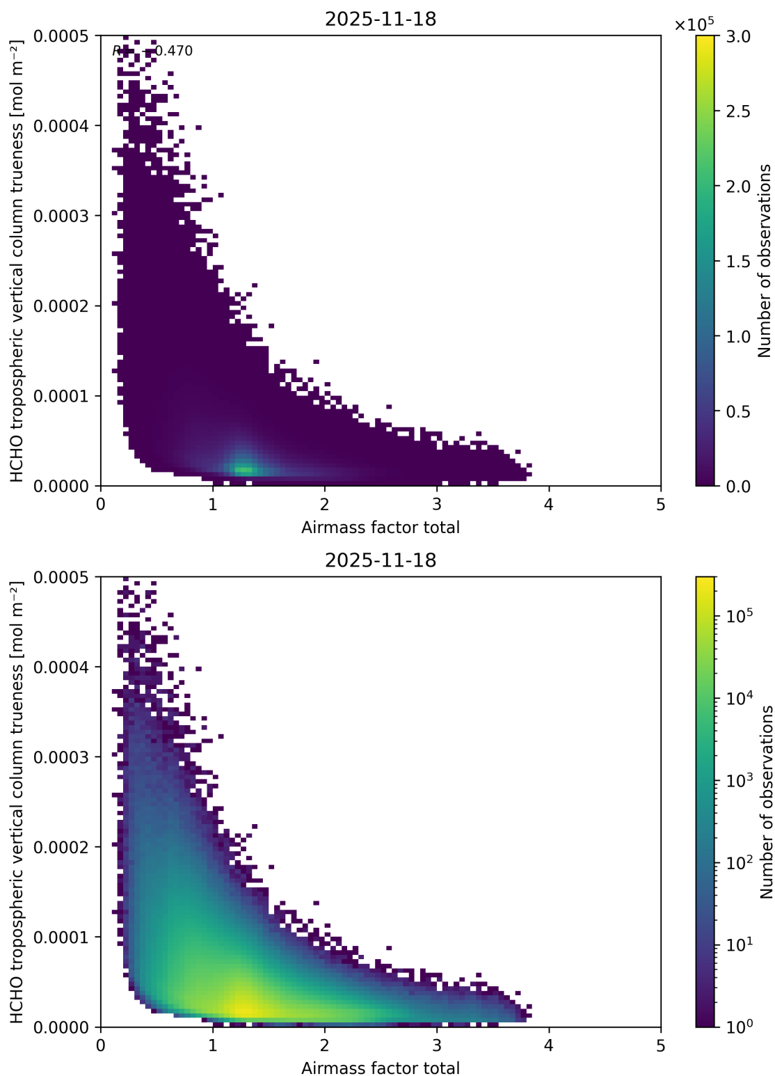
Figure 116: Scatter density plot of “Air mass factor total” against “HCHO tropospheric vertical column trueeness” for 2025-11-18 to 2025-11-19.
