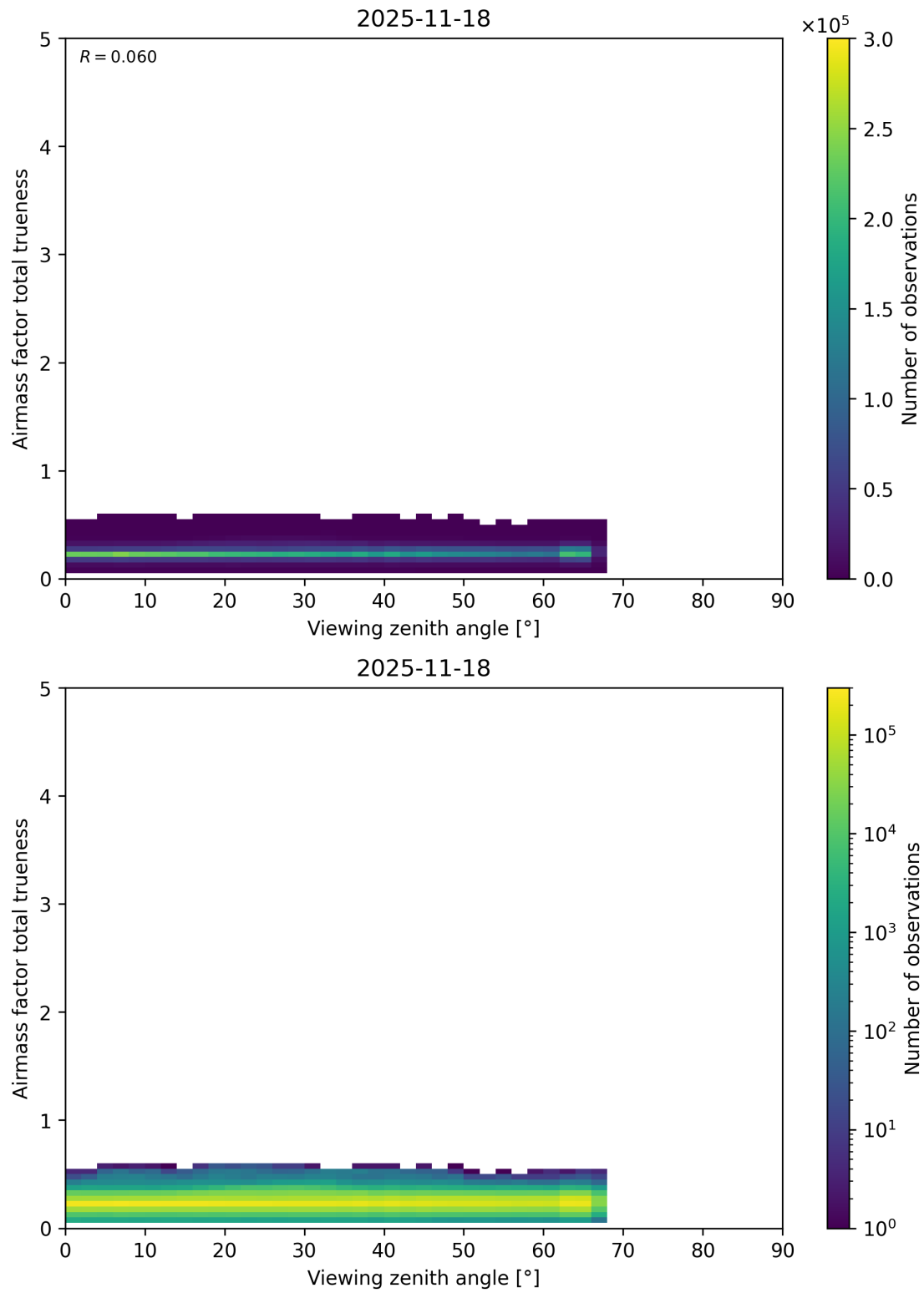
Figure 211: Scatter density plot of “Viewing zenith angle” against “Airmass factor total trueness” for 2025-11-18 to 2025-11-19.
