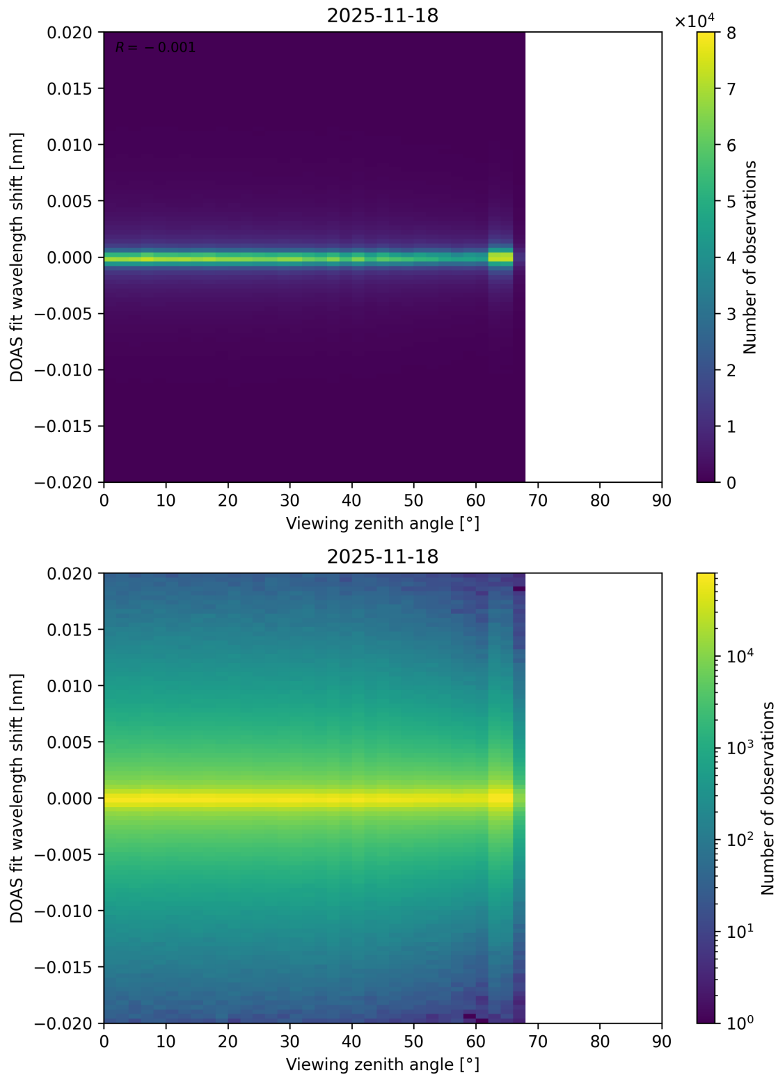
Figure 203: Scatter density plot of “Viewing zenith angle” against “DOAS fit wavelength shift” for 2025-11-18 to 2025-11-19.
