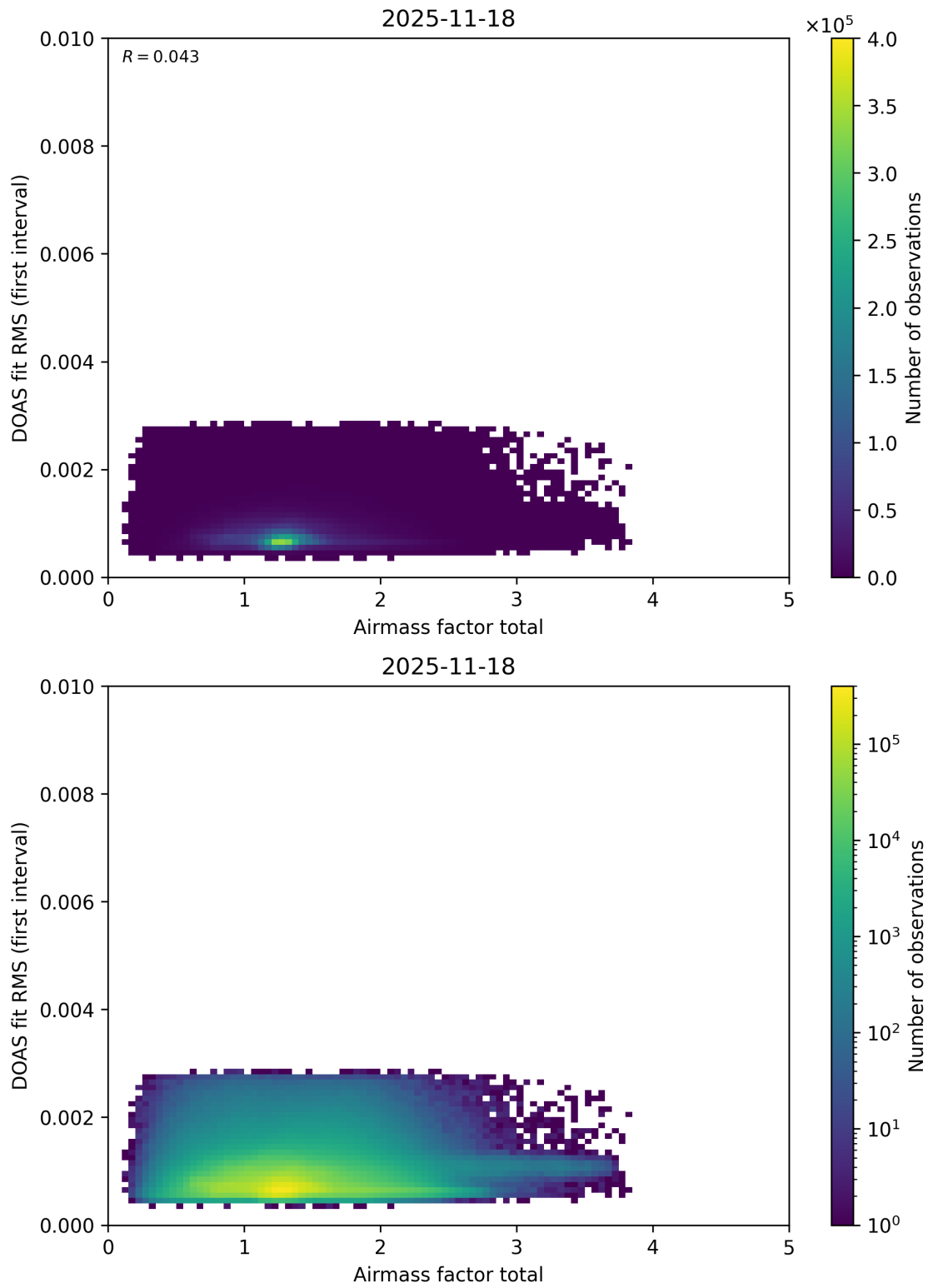
Figure 109: Scatter density plot of “Airmass factor total” against “DOAS fit RMS (first interval)” for 2025-11-18 to 2025-11-19.
