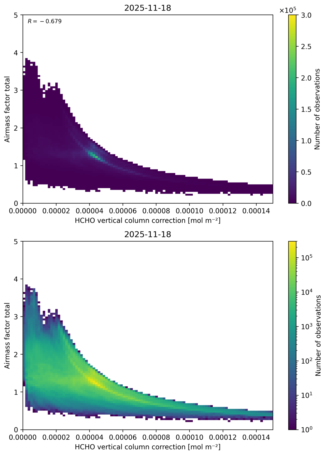
Figure 134: Scatter density plot of “HCHO vertical column correction” against “Airmass factor total” for 2025-11-18 to 2025-11-19.
