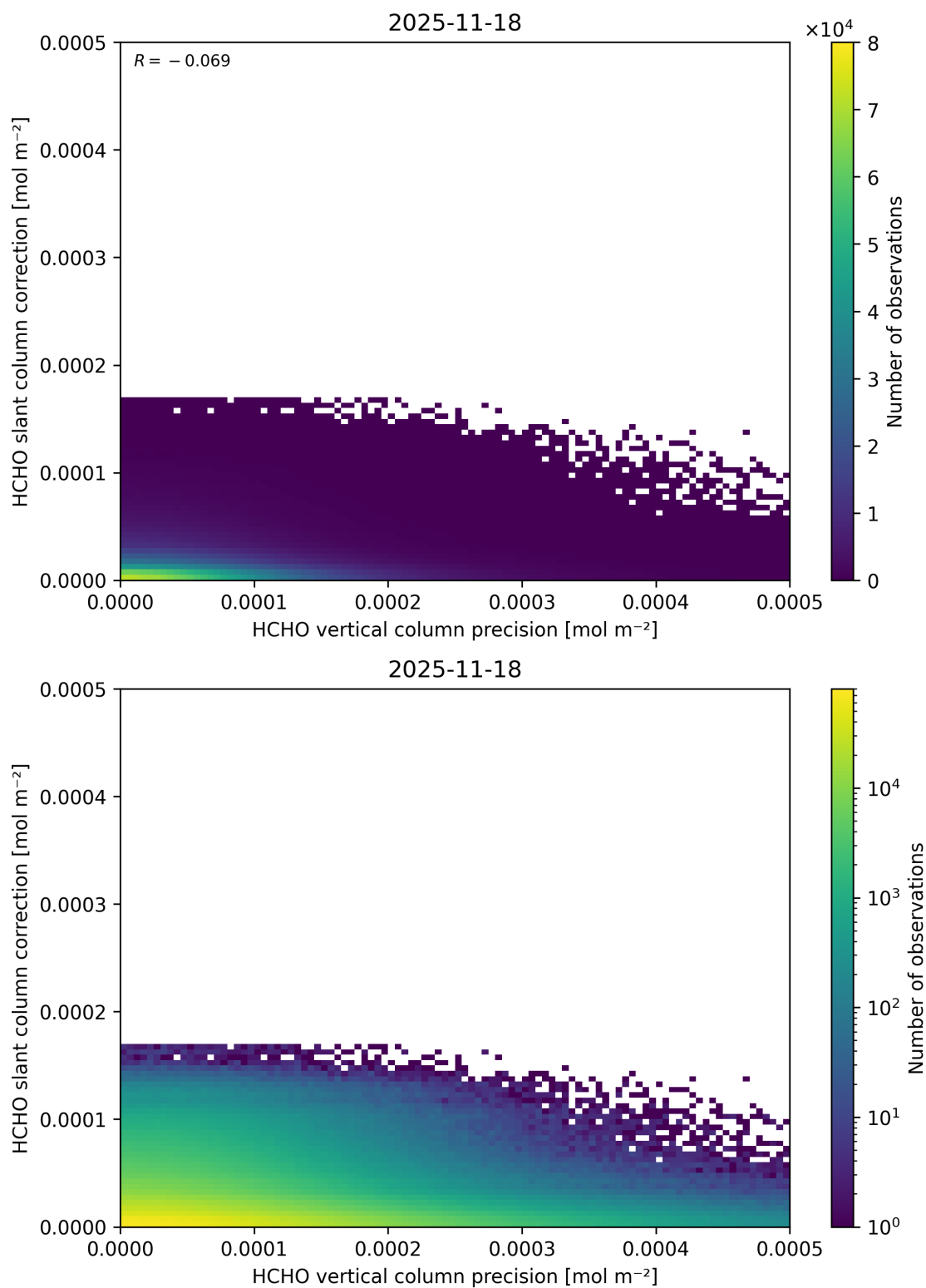
Figure 157: Scatter density plot of “HCHO vertical column precision” against “HCHO slant column correction” for 2025-11-18 to 2025-11-19.
