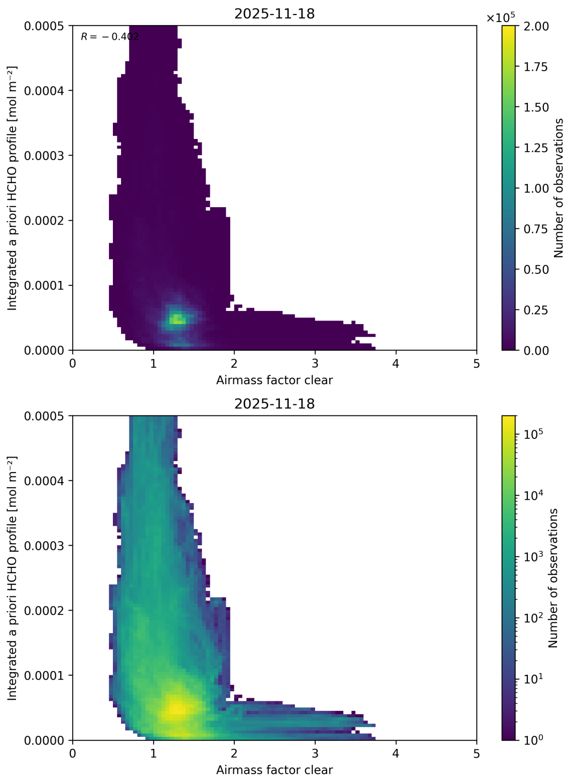
Figure 84: Scatter density plot of “Airmass factor clear” against “Integrated a priori HCHO profile” for 2025-11-18 to 2025-11-19.
