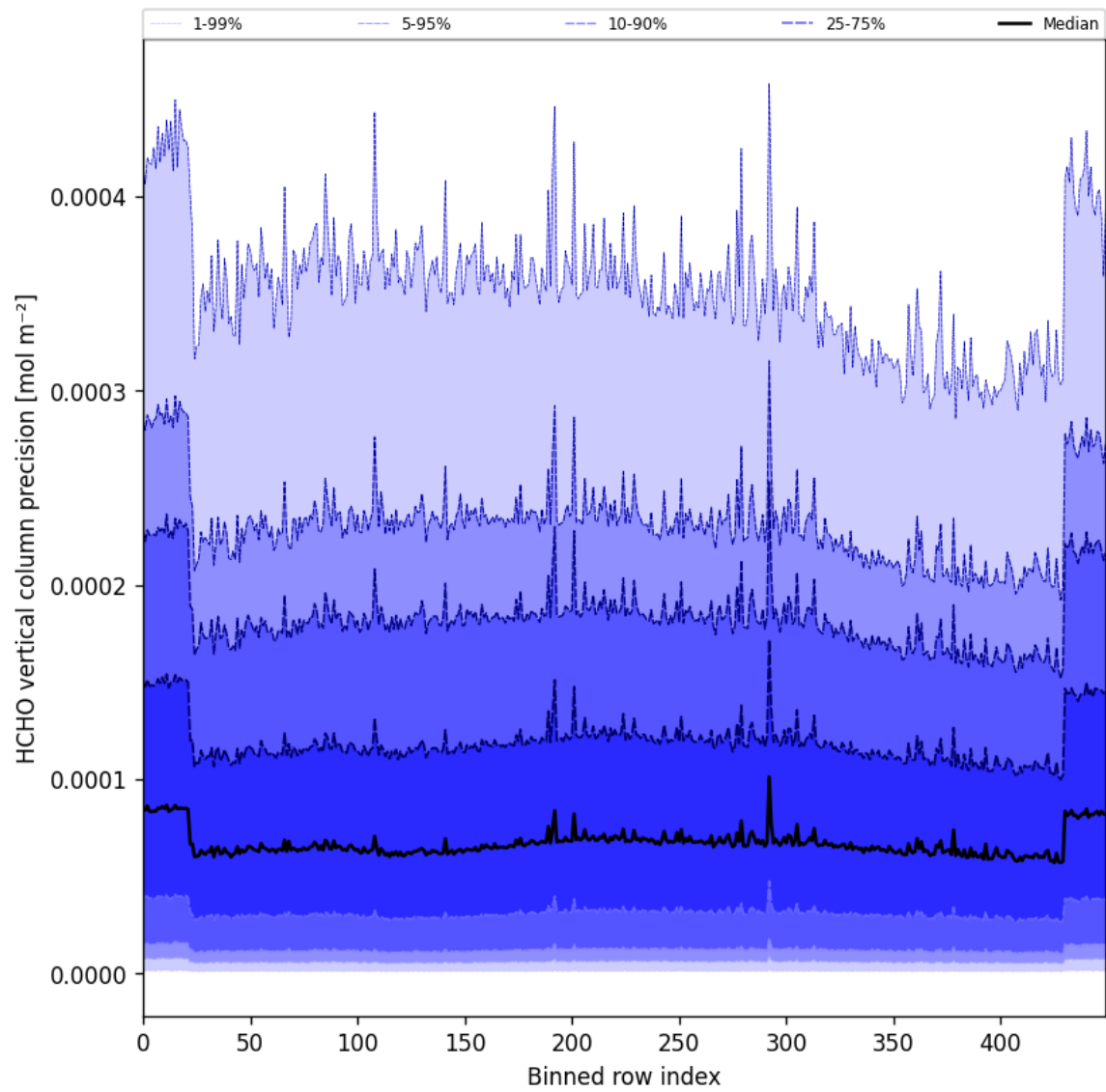
Figure 53: Along track statistics of “HCHO vertical column precision” for 2025-11-18 to 2025-11-19
