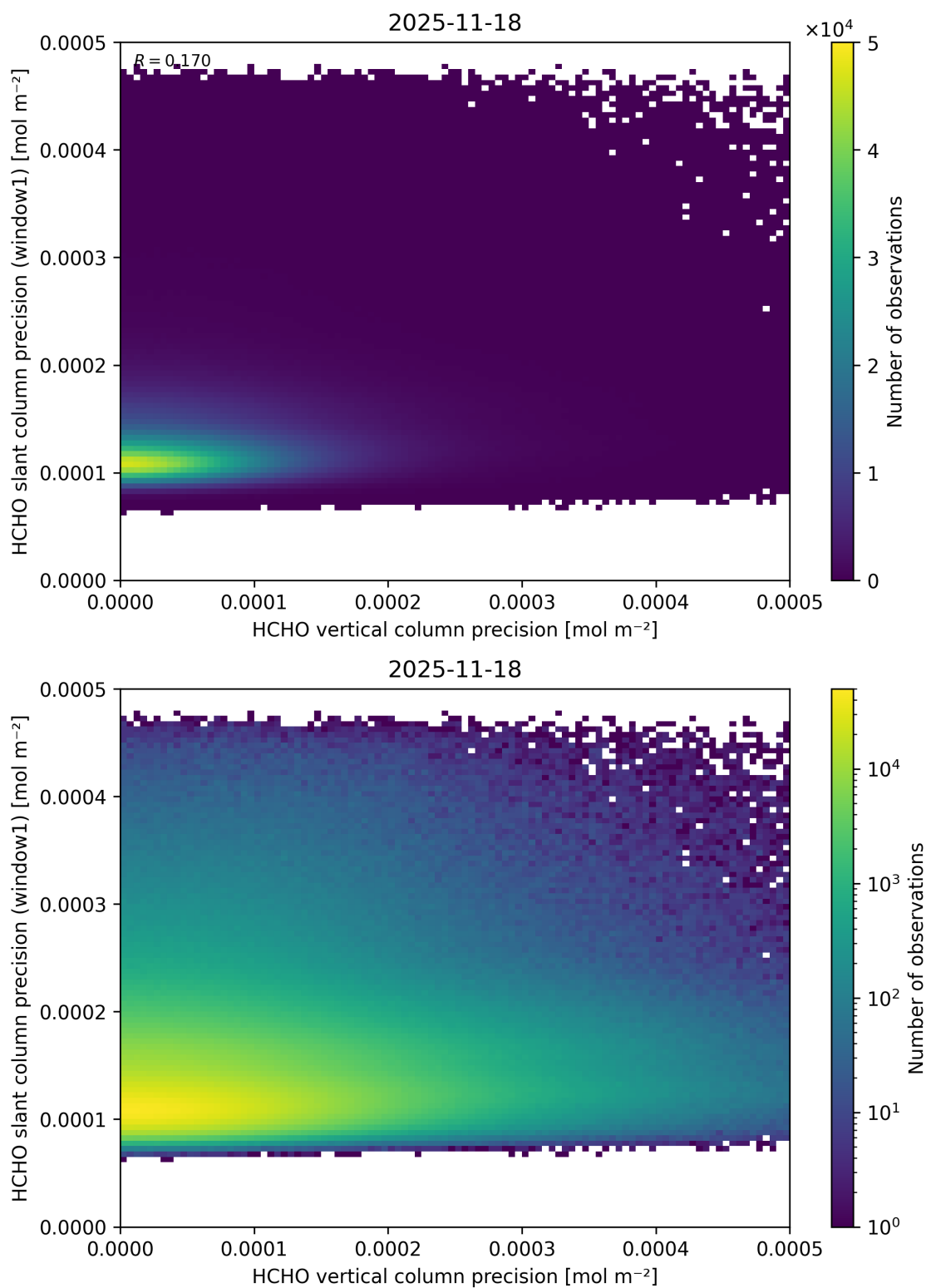
Figure 159: Scatter density plot of “HCHO vertical column precision” against “HCHO slant column precision (window1)” for 2025-11-18 to 2025-11-19.
