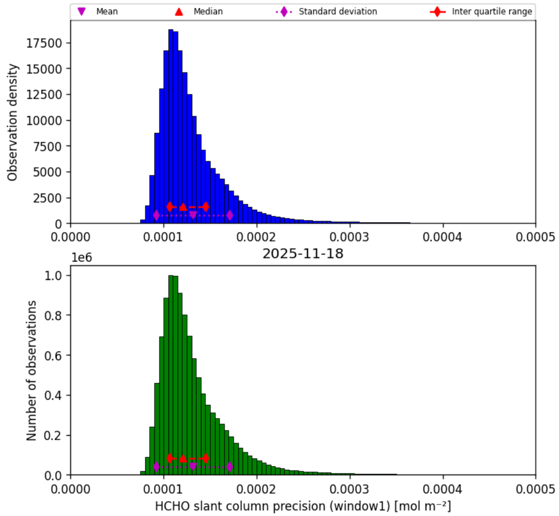
Figure 41: Histogram of “HCHO slant column precision (window1)” for 2025-11-18 to 2025-11-19
