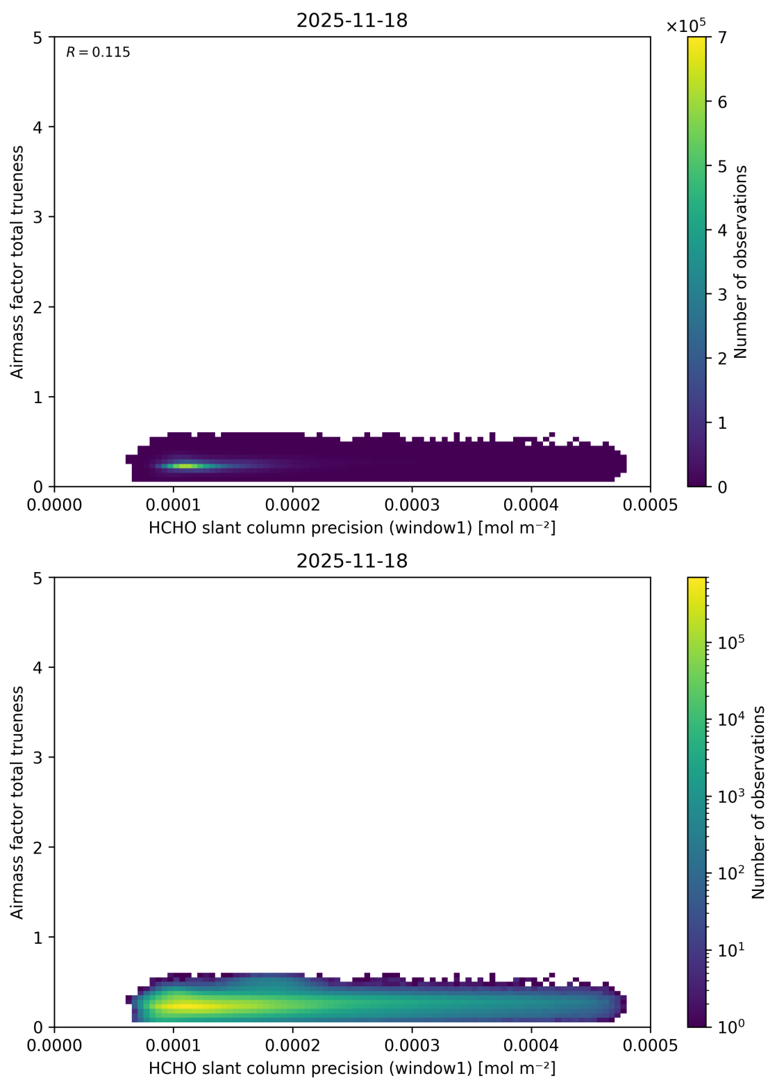
Figure 106: Scatter density plot of “HCHO slant column precision (window1)” against “Airmass factor total trueness” for 2025-11-18 to 2025-11-19.
