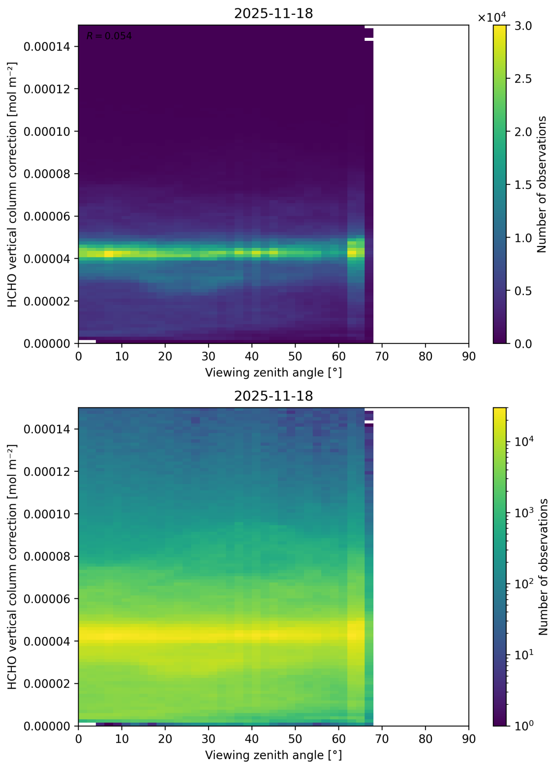
Figure 213: Scatter density plot of “Viewing zenith angle” against “HCHO vertical column correction” for 2025-11-18 to 2025-11-19.
