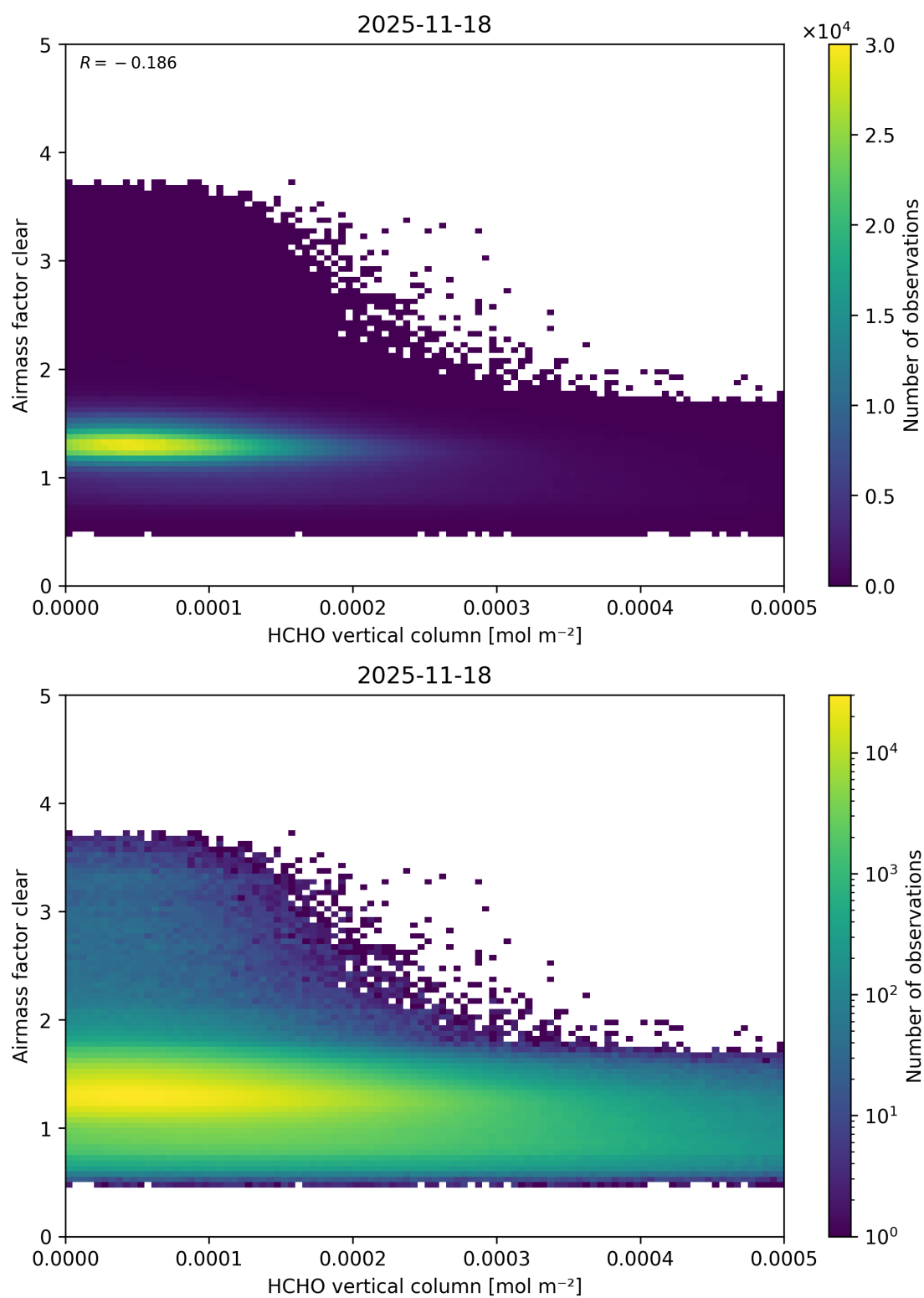
Figure 141: Scatter density plot of “HCHO vertical column” against “Airmass factor clear” for 2025-11-18 to 2025-11-19.
