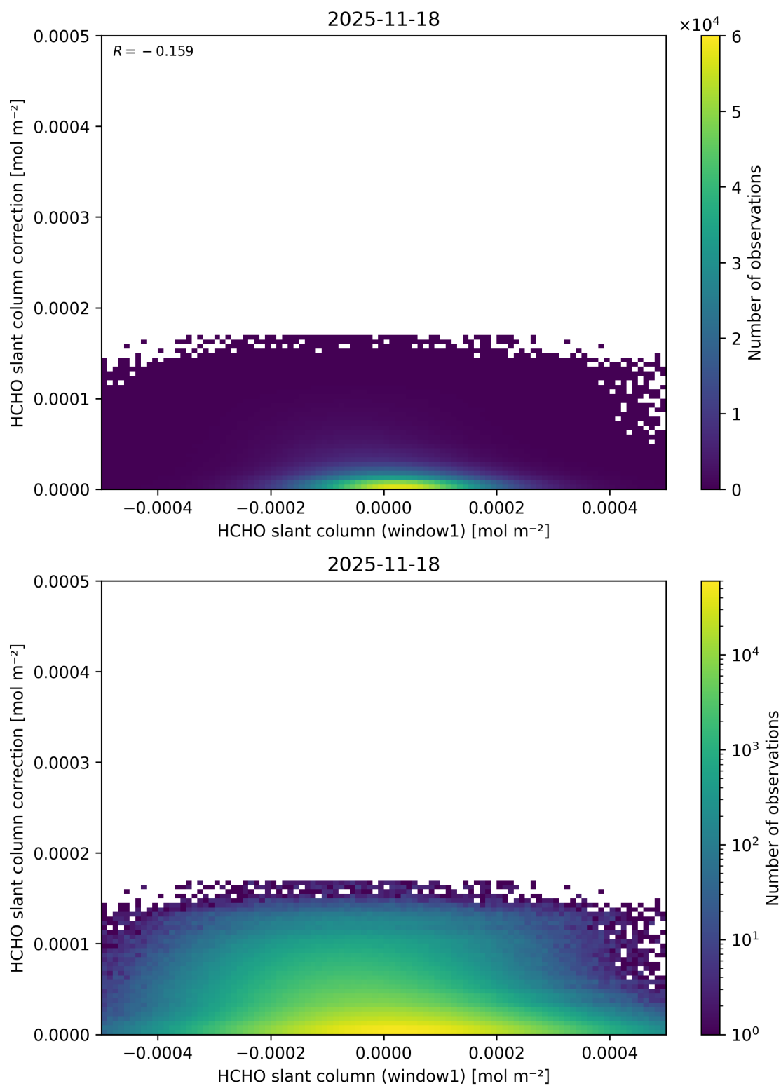
Figure 93: Scatter density plot of “HCHO slant column (window1)” against “HCHO slant column correction” for 2025-11-18 to 2025-11-19.
