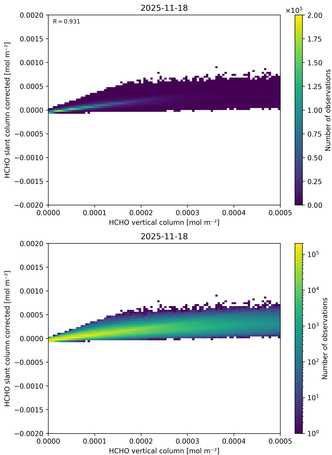
Figure 142: Scatter density plot of “HCHO vertical column” against “HCHO slant column corrected” for 2025-11-18 to 2025-11-19.
