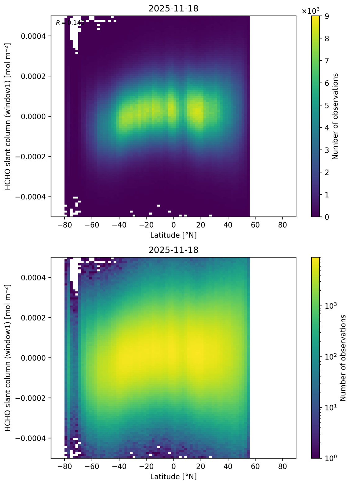
Figure 177: Scatter density plot of “Latitude” against “HCHO slant column (window1)” for 2025-11-18 to 2025-11-19.
