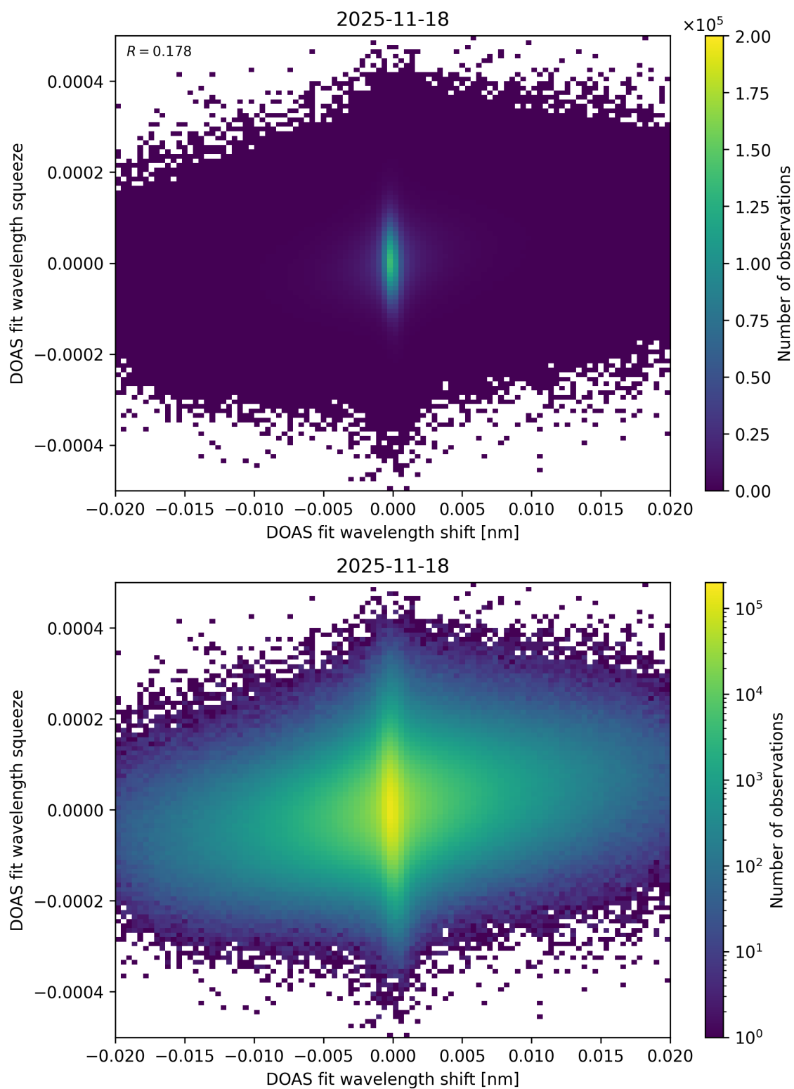
Figure 70: Scatter density plot of “DOAS fit wavelength shift” against “DOAS fit wavelength squeeze” for 2025-11-18 to 2025-11-19.
