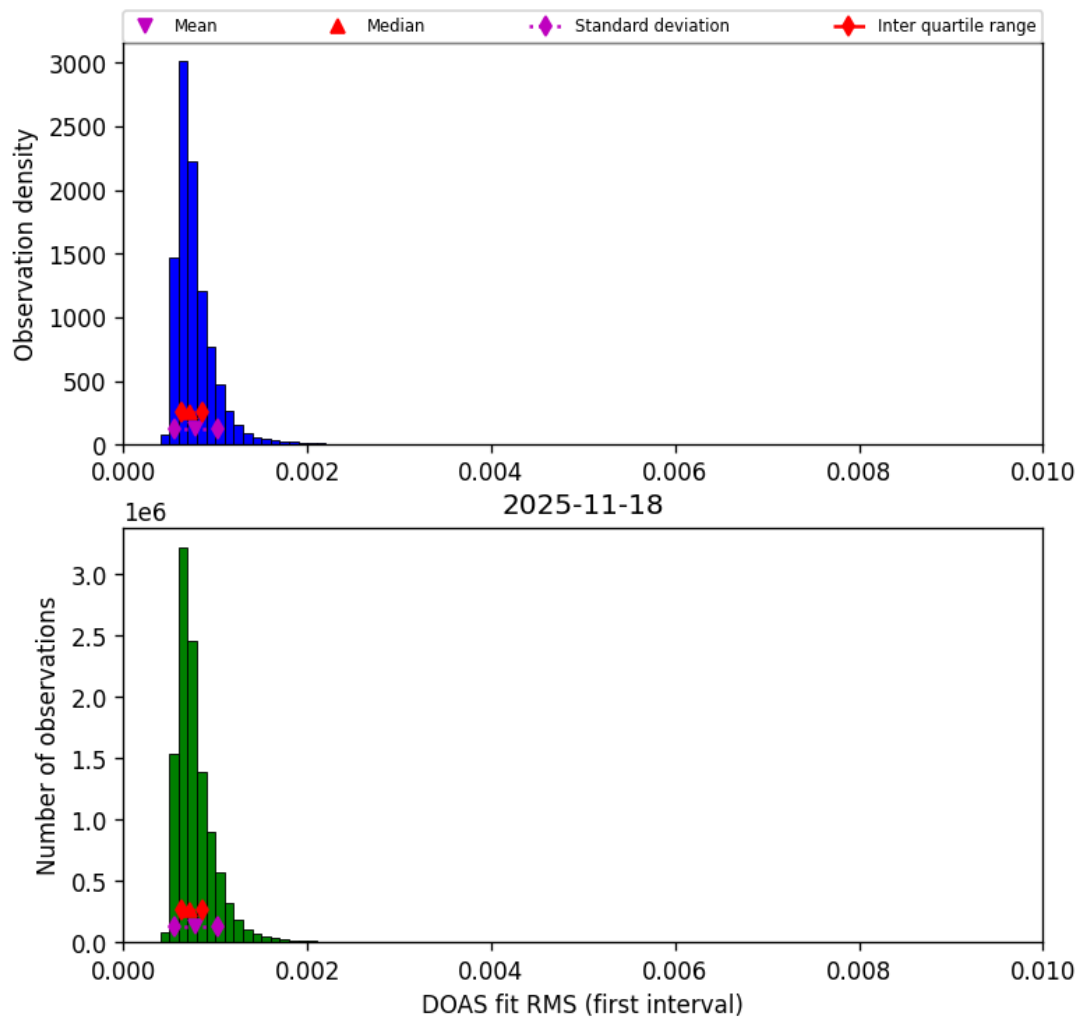
Figure 48: Histogram of “DOAS fit RMS (first interval)” for 2025-11-18 to 2025-11-19
