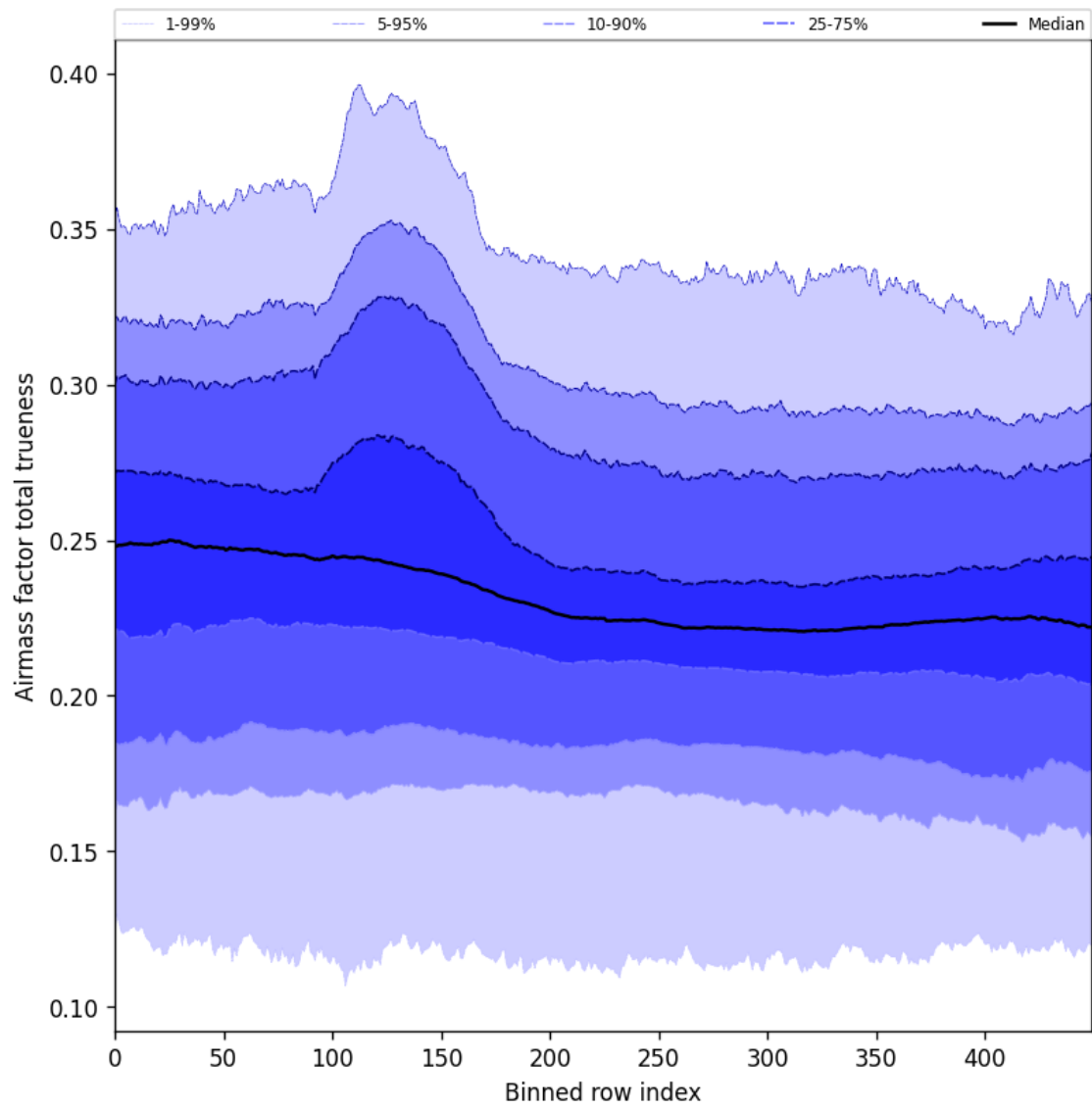
Figure 58: Along track statistics of “Airmass factor total trueness” for 2025-11-18 to 2025-11-19
