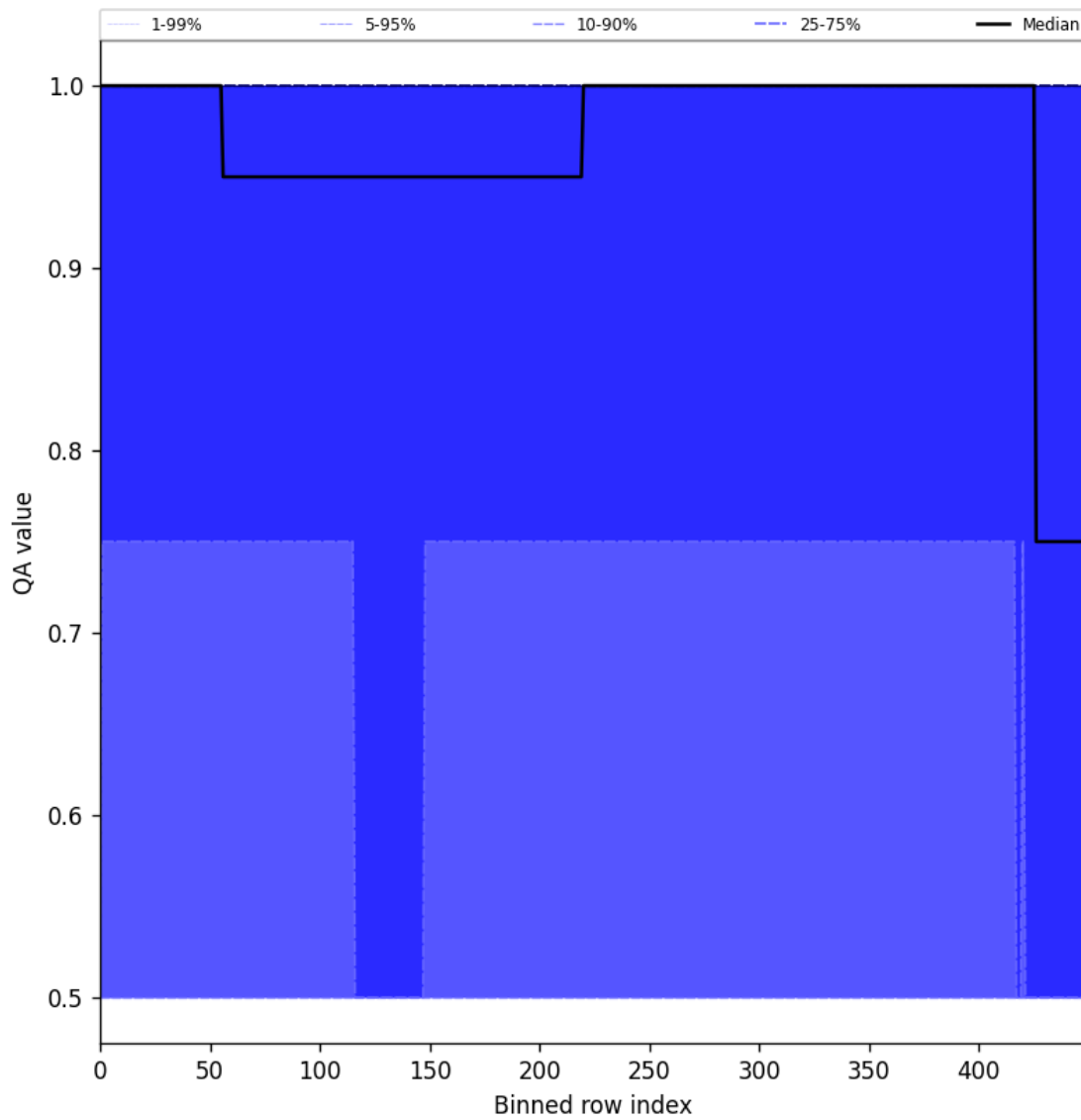
Figure 51: Along track statistics of “QA value” for 2025-11-18 to 2025-11-19
