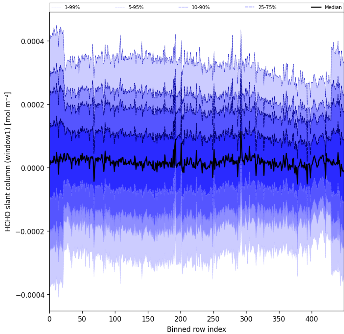
Figure 55: Along track statistics of “HCHO slant column (window1)” for 2025-11-18 to 2025-11-19
