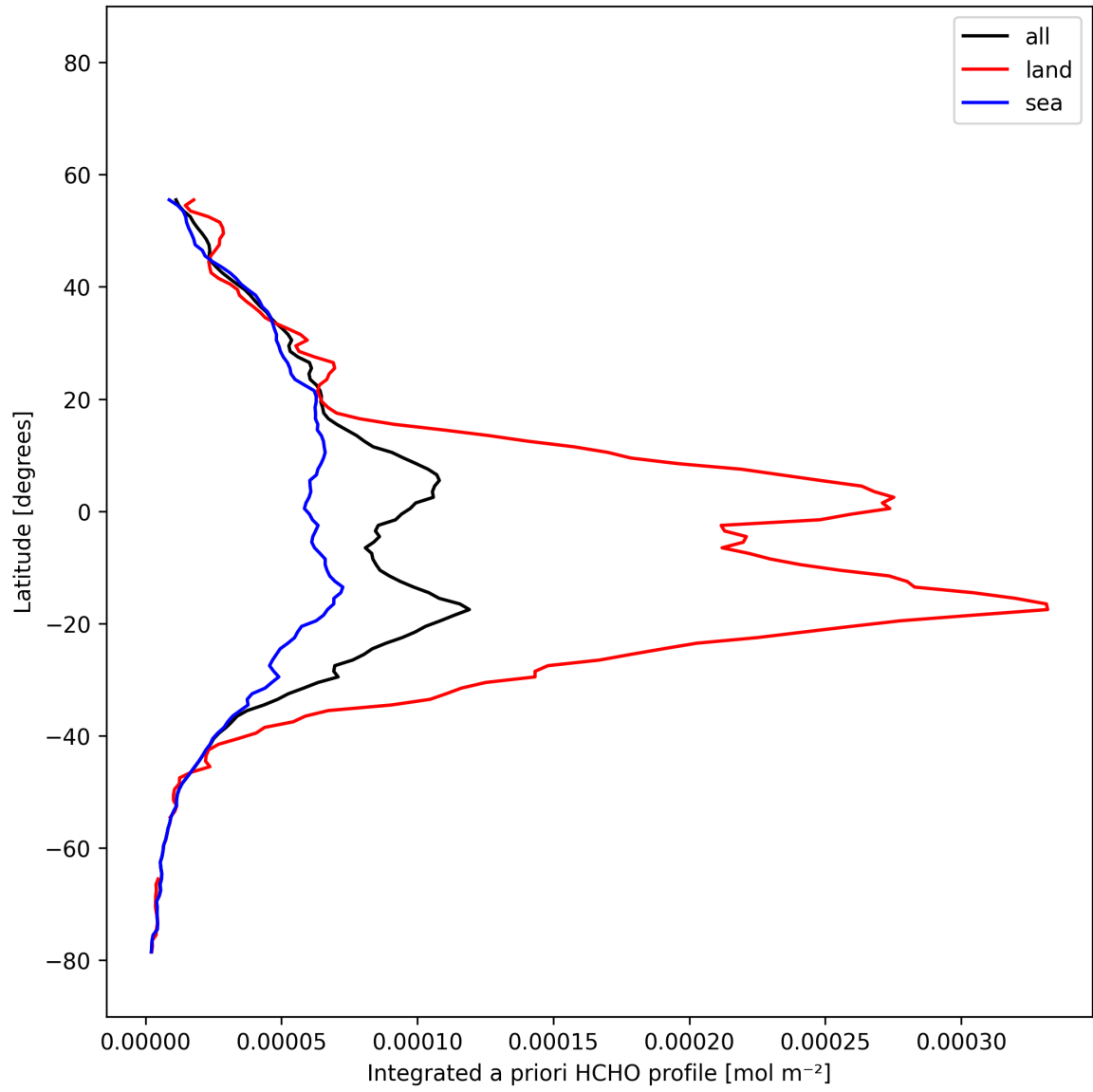
Figure 30: Zonal average of “Integrated a priori HCHO profile” for 2025-11-18 to 2025-11-19.
