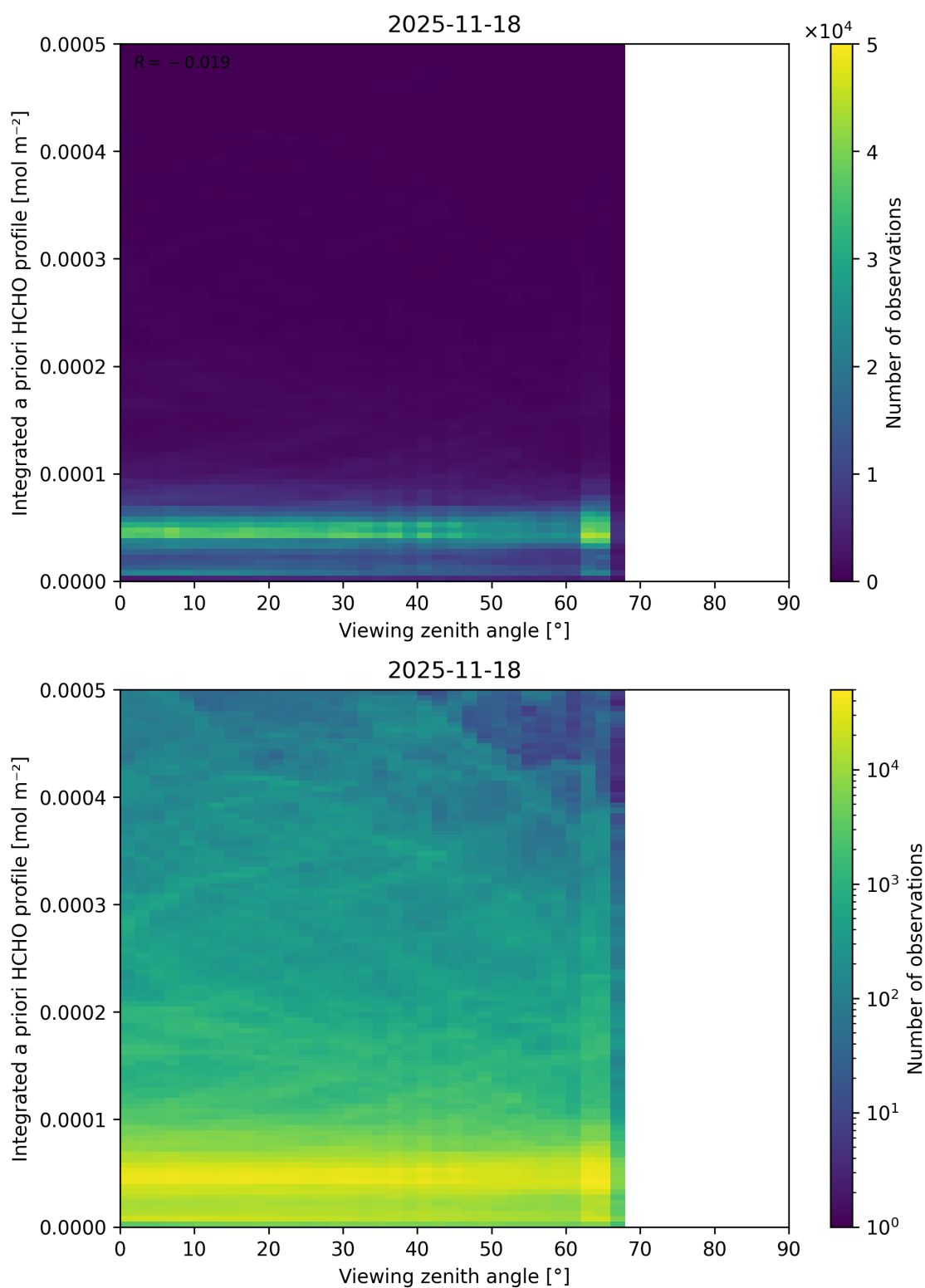
Figure 216: Scatter density plot of “Viewing zenith angle” against “Integrated a priori HCHO profile” for 2025-11-18 to 2025-11-19.
