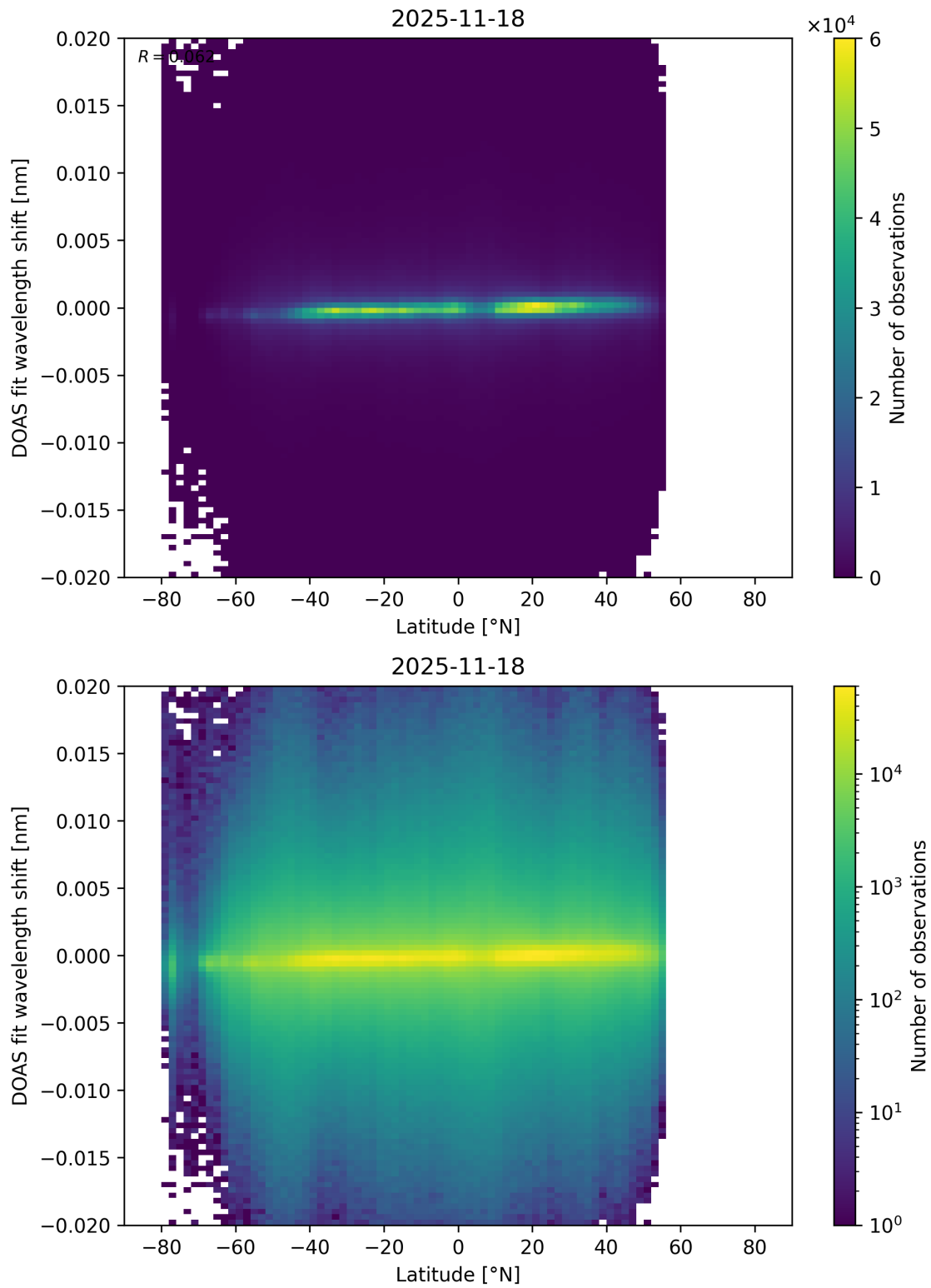
Figure 172: Scatter density plot of “Latitude” against “DOAS fit wavelength shift” for 2025-11-18 to 2025-11-19.
