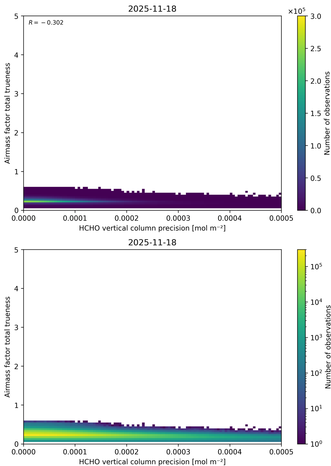
Figure 161: Scatter density plot of “HCHO vertical column precision” against “Airmass factor total trueness” for 2025-11-18 to 2025-11-19.
