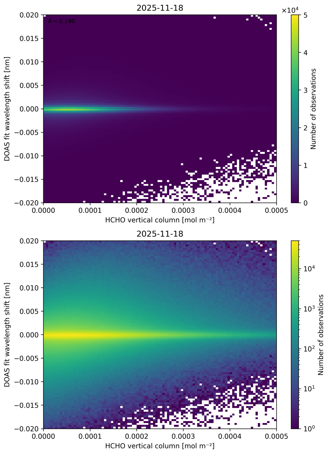
Figure 139: Scatter density plot of “HCHO vertical column” against “DOAS fit wavelength shift” for 2025-11-18 to 2025-11-19.
