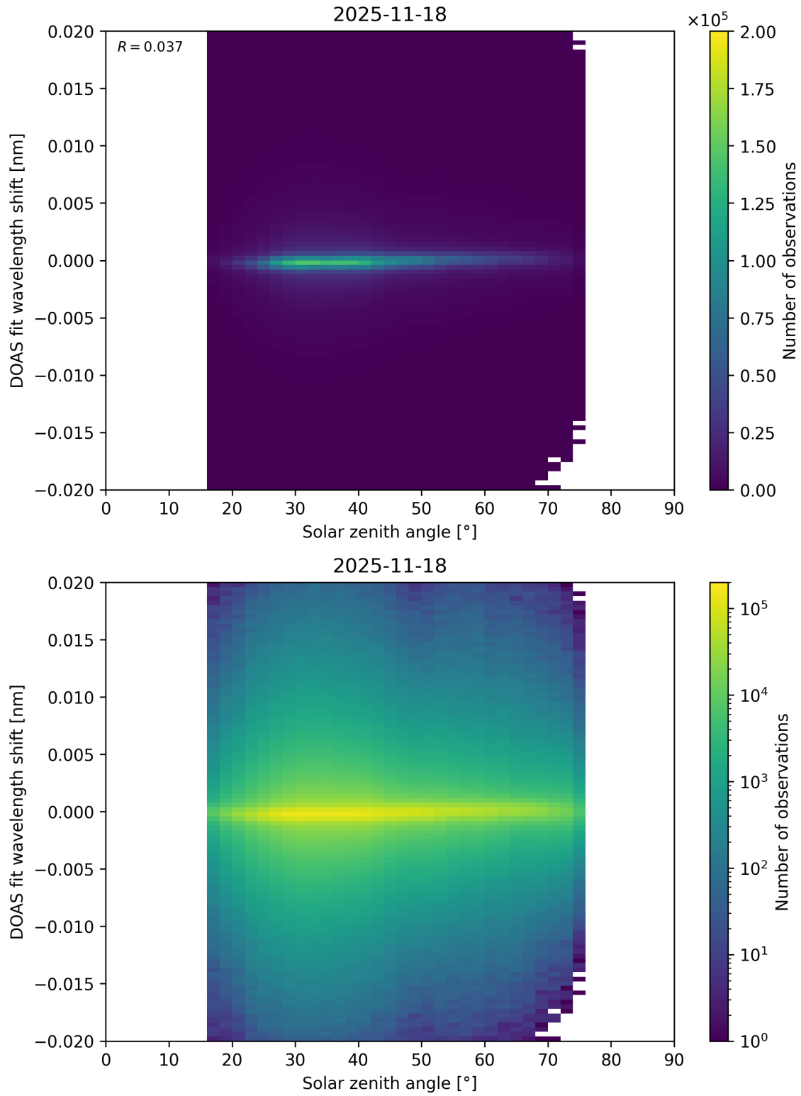
Figure 187: Scatter density plot of “Solar zenith angle” against “DOAS fit wavelength shift” for 2025-11-18 to 2025-11-19.
