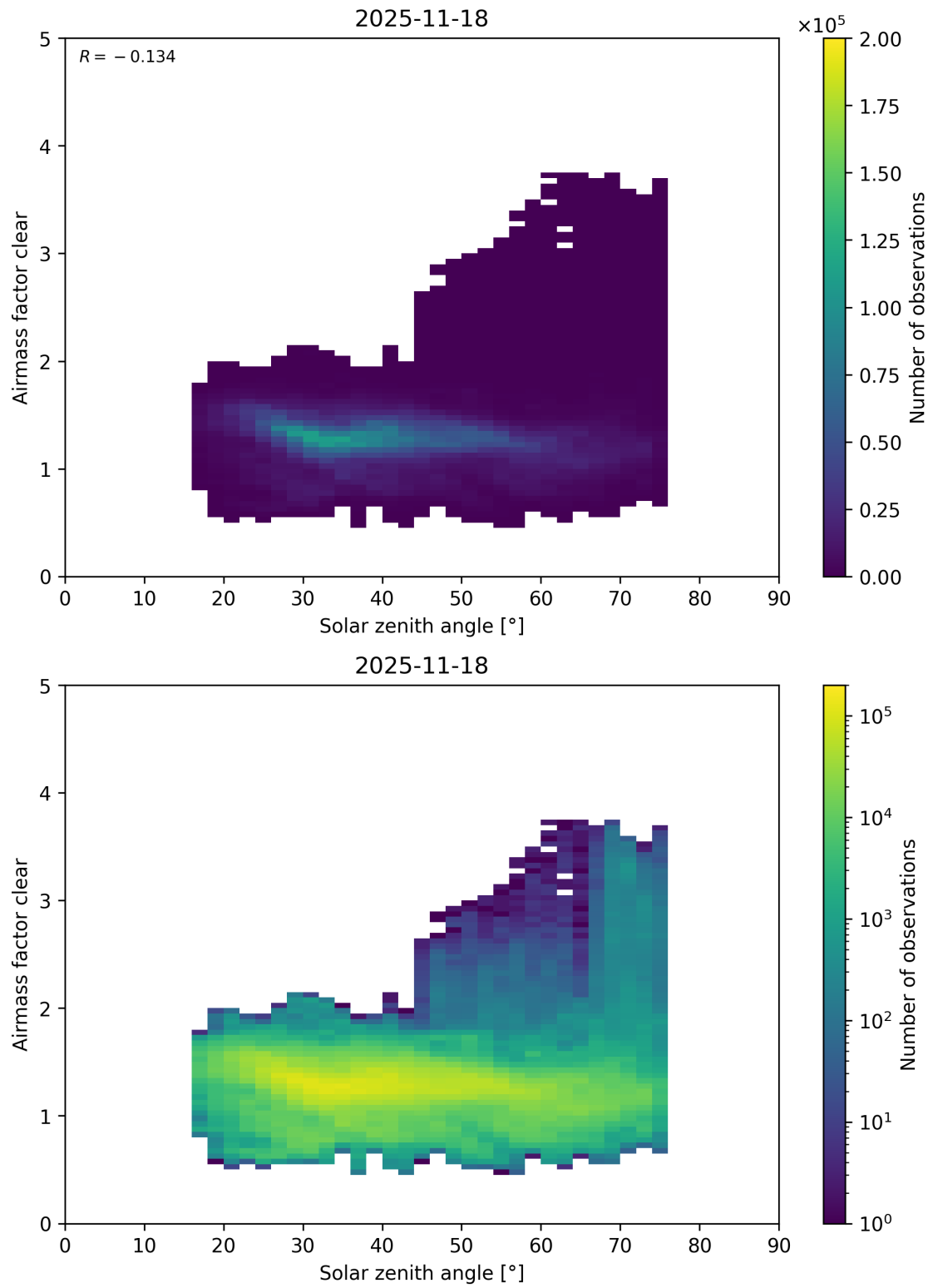
Figure 189: Scatter density plot of “Solar zenith angle” against “Airmass factor clear” for 2025-11-18 to 2025-11-19.
