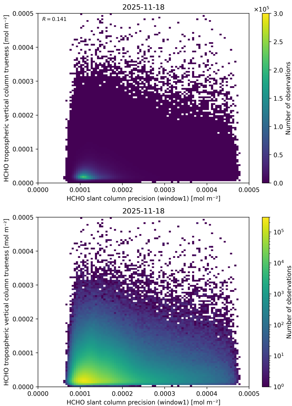
Figure 107: Scatter density plot of “HCHO slant column precision (window1)” against “HCHO tropospheric vertical column trueness” for 2025-11-18 to 2025-11-19.
