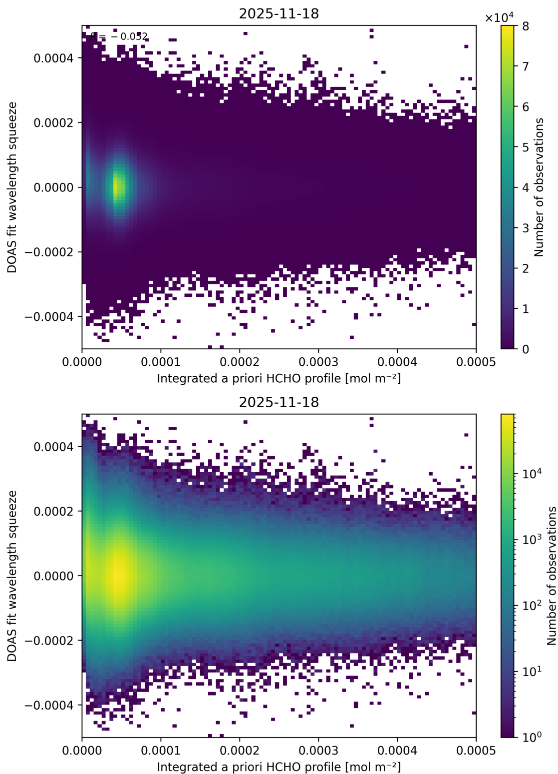
Figure 167: Scatter density plot of “Integrated a priori HCHO profile” against “DOAS fit wavelength squeeze” for 2025-11-18 to 2025-11-19.
