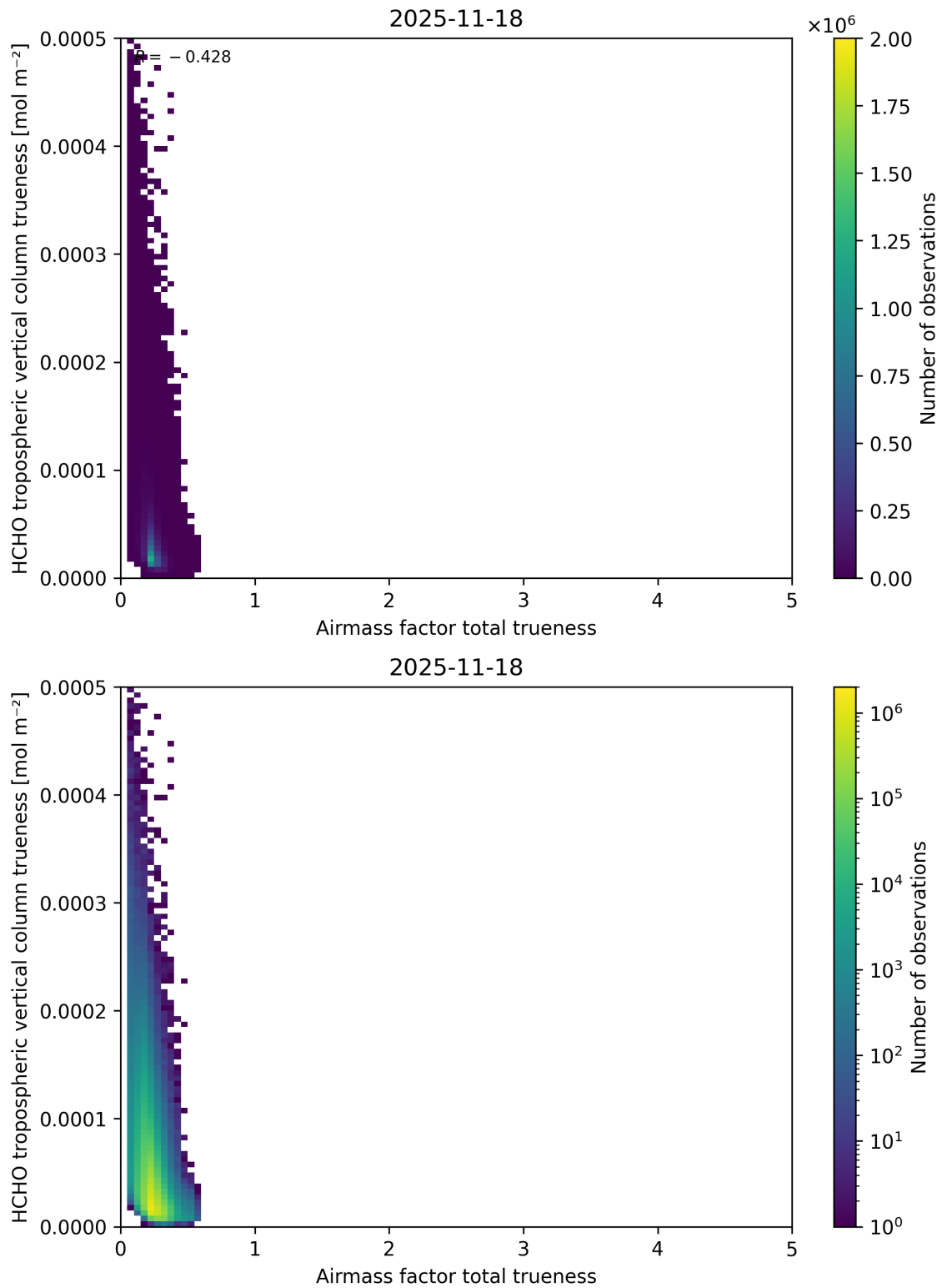
Figure 124: Scatter density plot of “Airmass factor total trueness” against “HCHO tropospheric vertical column trueness” for 2025-11-18 to 2025-11-19.
