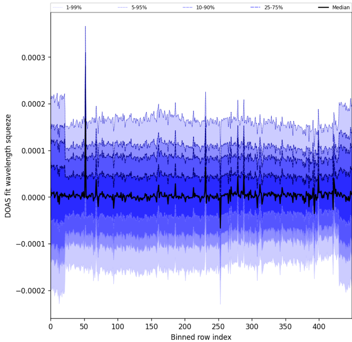
Figure 62: Along track statistics of “DOAS fit wavelength squeeze” for 2025-11-18 to 2025-11-19
