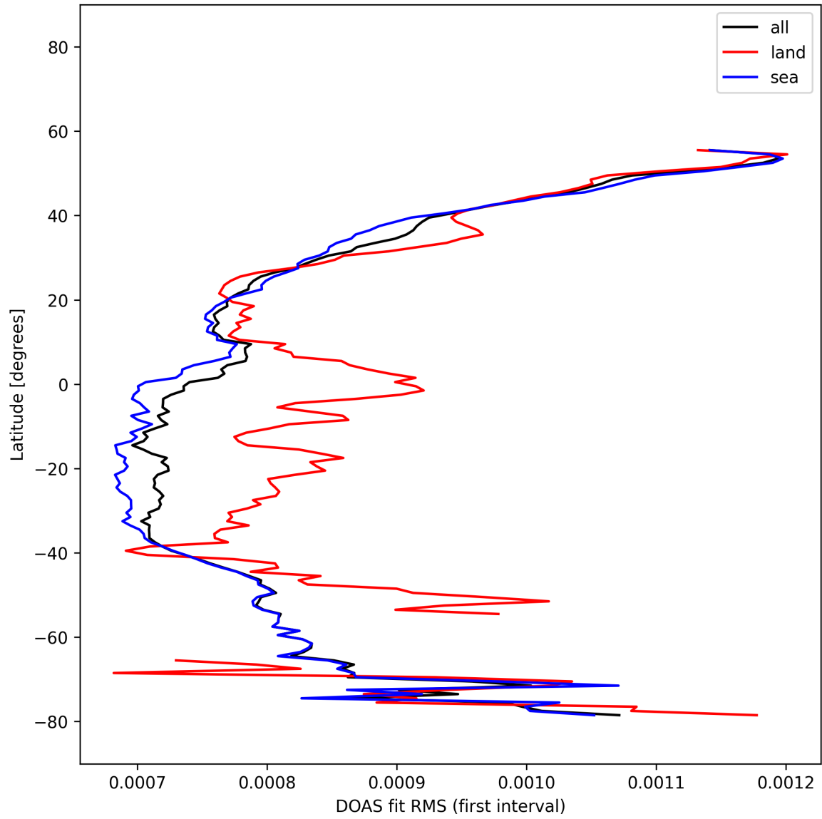
Figure 33: Zonal average of “DOAS fit RMS (first interval)” for 2025-11-18 to 2025-11-19.
