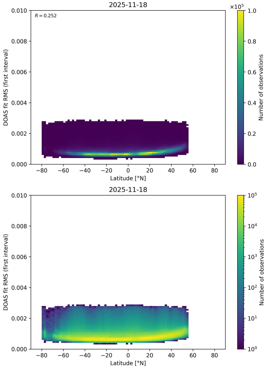
Figure 171: Scatter density plot of “Latitude” against “DOAS fit RMS (first interval)” for 2025-11-18 to 2025-11-19.
