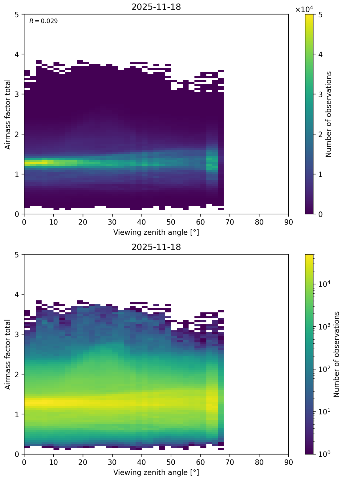
Figure 210: Scatter density plot of “Viewing zenith angle” against “Airmass factor total” for 2025-11-18 to 2025-11-19.
