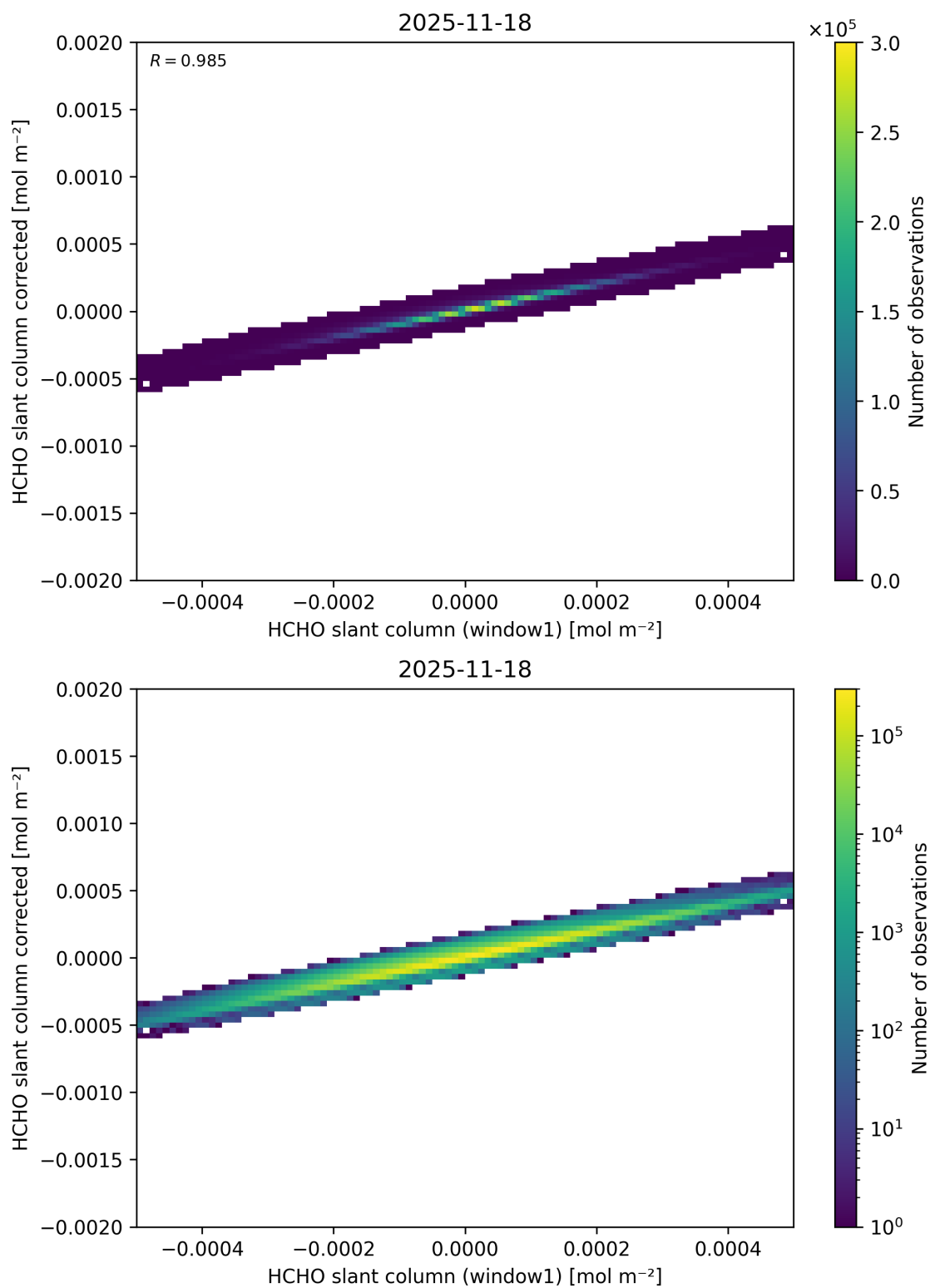
Figure 92: Scatter density plot of “HCHO slant column (window1)” against “HCHO slant column corrected” for 2025-11-18 to 2025-11-19.
