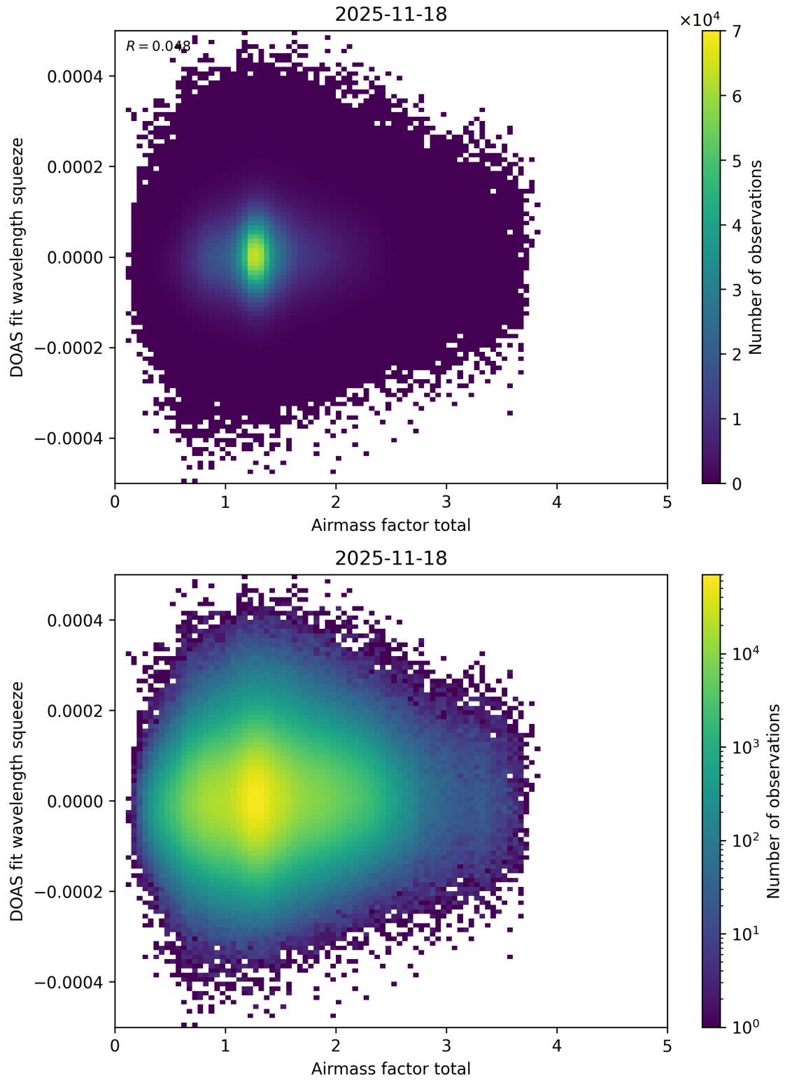
Figure 111: Scatter density plot of “Airmass factor total” against “DOAS fit wavelength squeeze” for 2025-11-18 to 2025-11-19.
