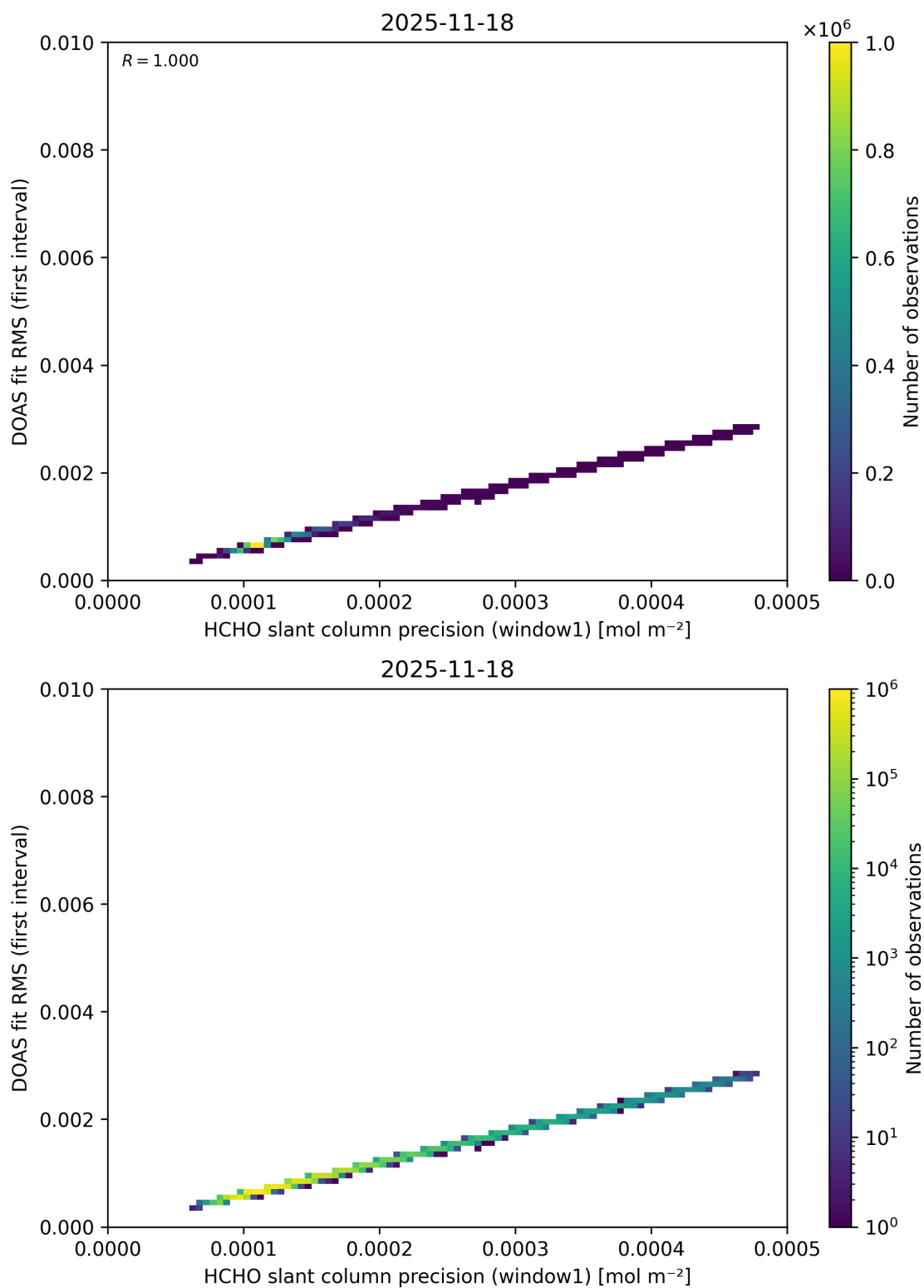
Figure 99: Scatter density plot of “HCHO slant column precision (window1)” against “DOAS fit RMS (first interval)” for 2025-11-18 to 2025-11-19.
