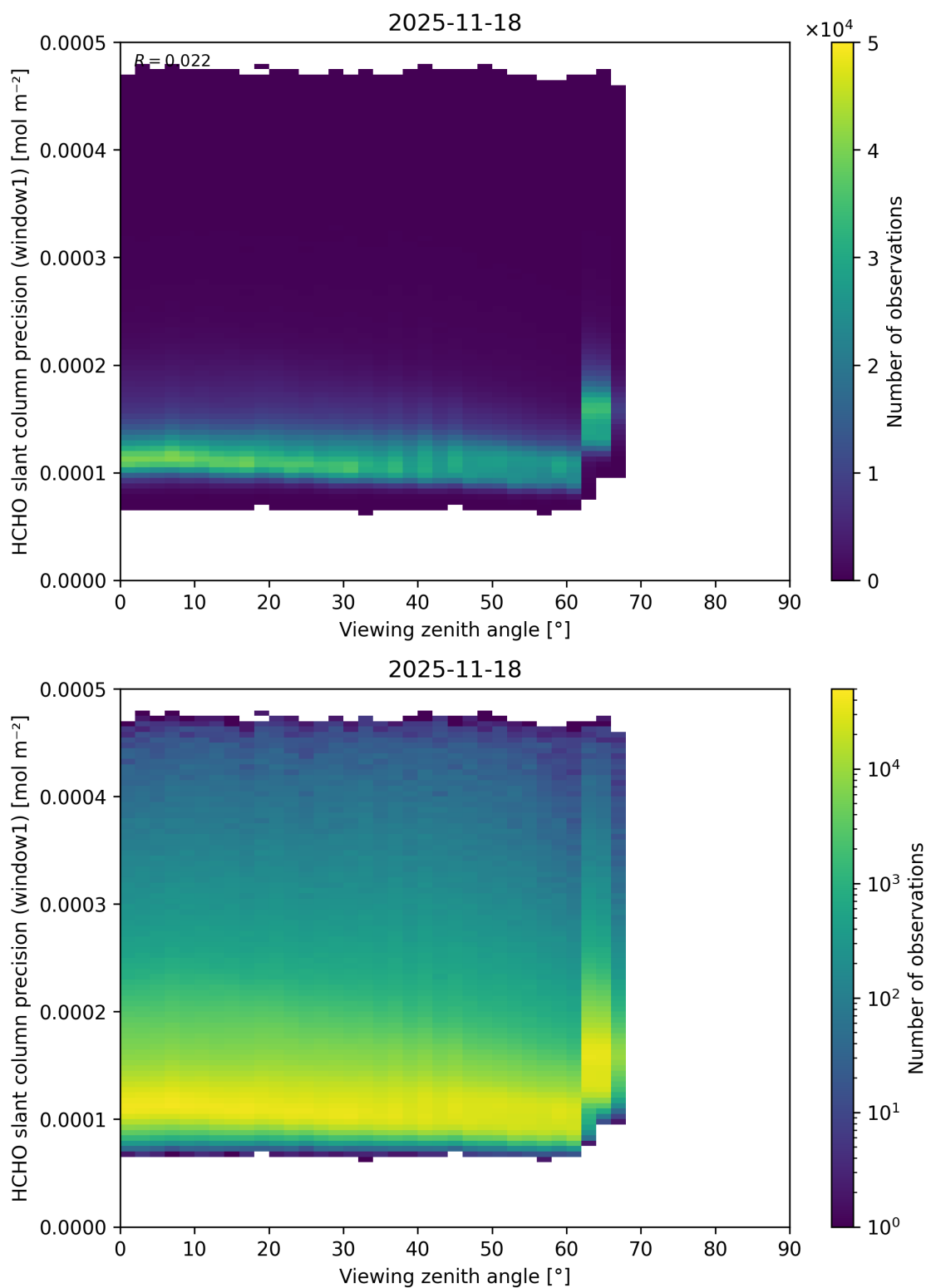
Figure 209: Scatter density plot of “Viewing zenith angle” against “HCHO slant column precision (window1)” for 2025-11-18 to 2025-11-19.
