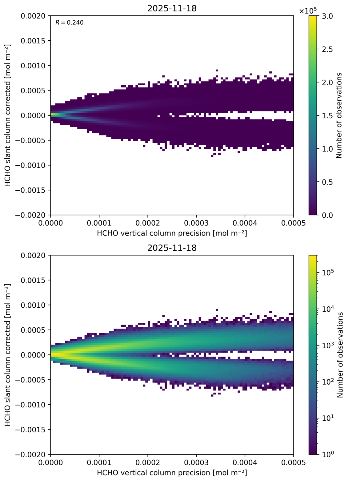
Figure 156: Scatter density plot of “HCHO vertical column precision” against “HCHO slant column corrected” for 2025-11-18 to 2025-11-19.
