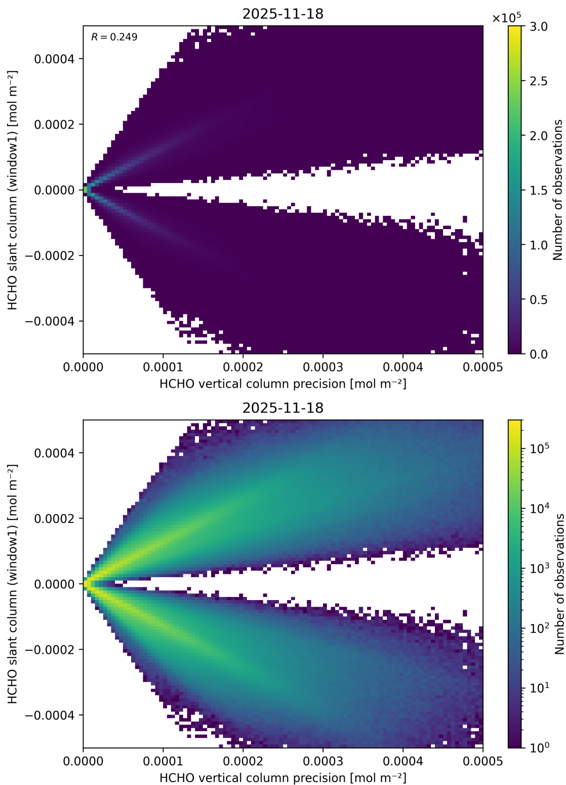
Figure 158: Scatter density plot of “HCHO vertical column precision” against “HCHO slant column (window1)” for 2025-11-18 to 2025-11-19.
