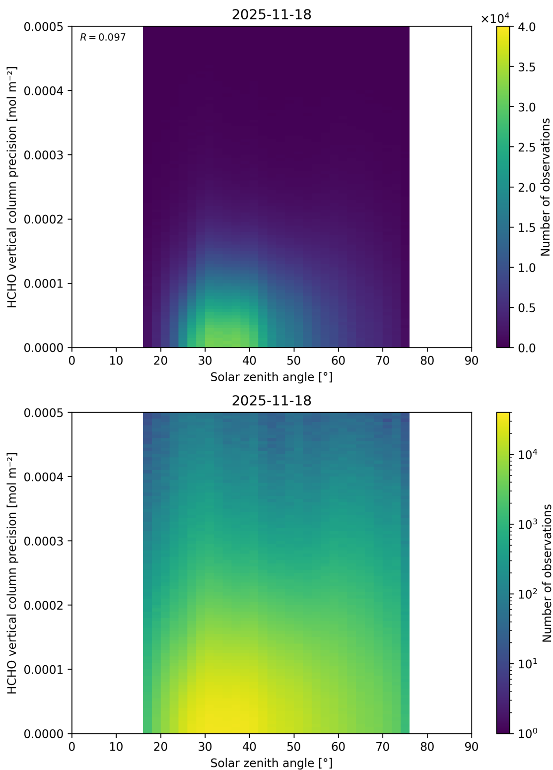
Figure 198: Scatter density plot of “Solar zenith angle” against “HCHO vertical column precision” for 2025-11-18 to 2025-11-19.
