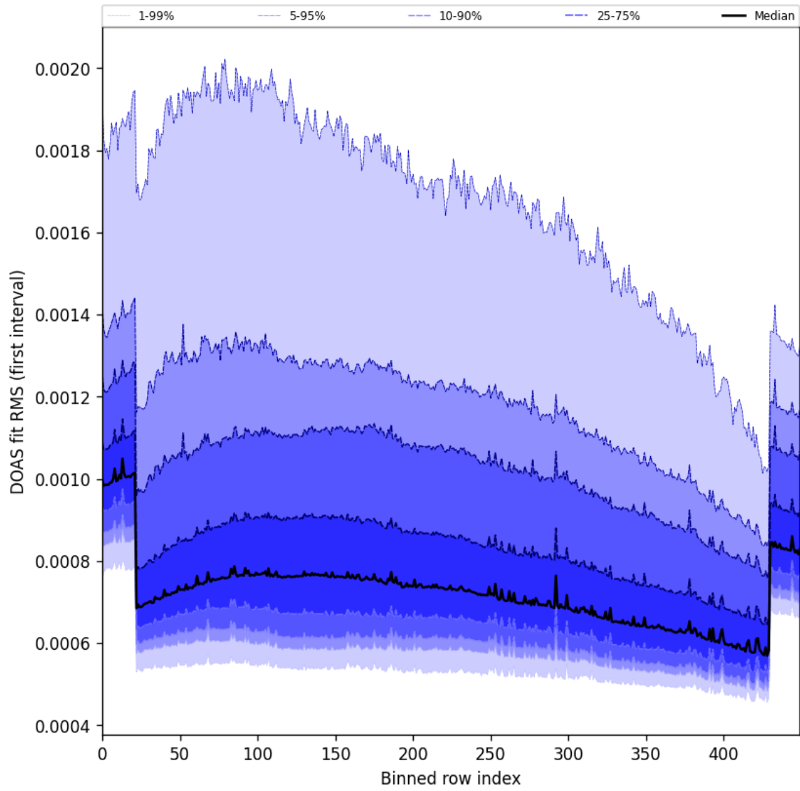
Figure 63: Along track statistics of “DOAS fit RMS (first interval)” for 2025-11-18 to 2025-11-19
