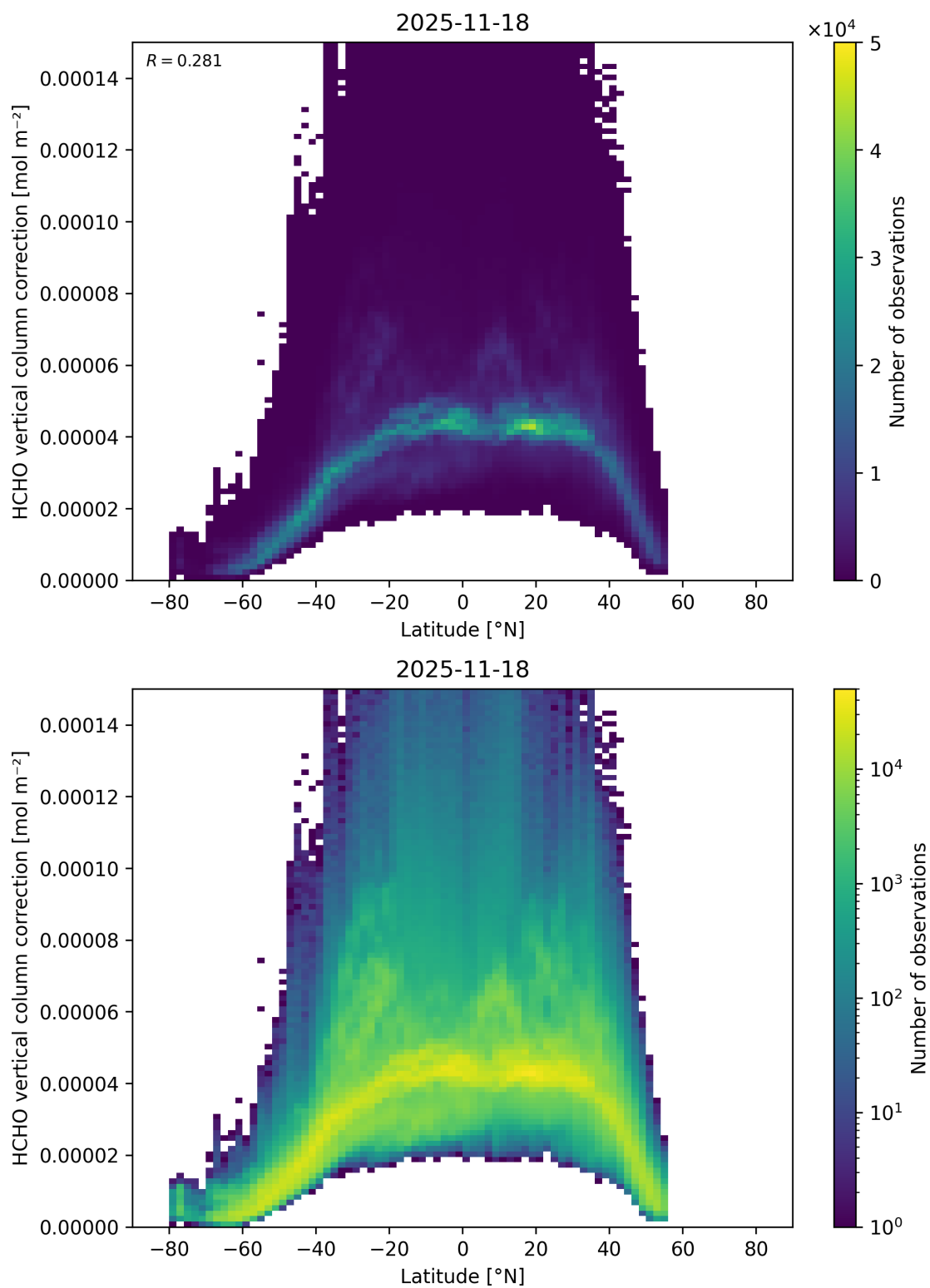
Figure 182: Scatter density plot of “Latitude” against “HCHO vertical column correction” for 2025-11-18 to 2025-11-19.
