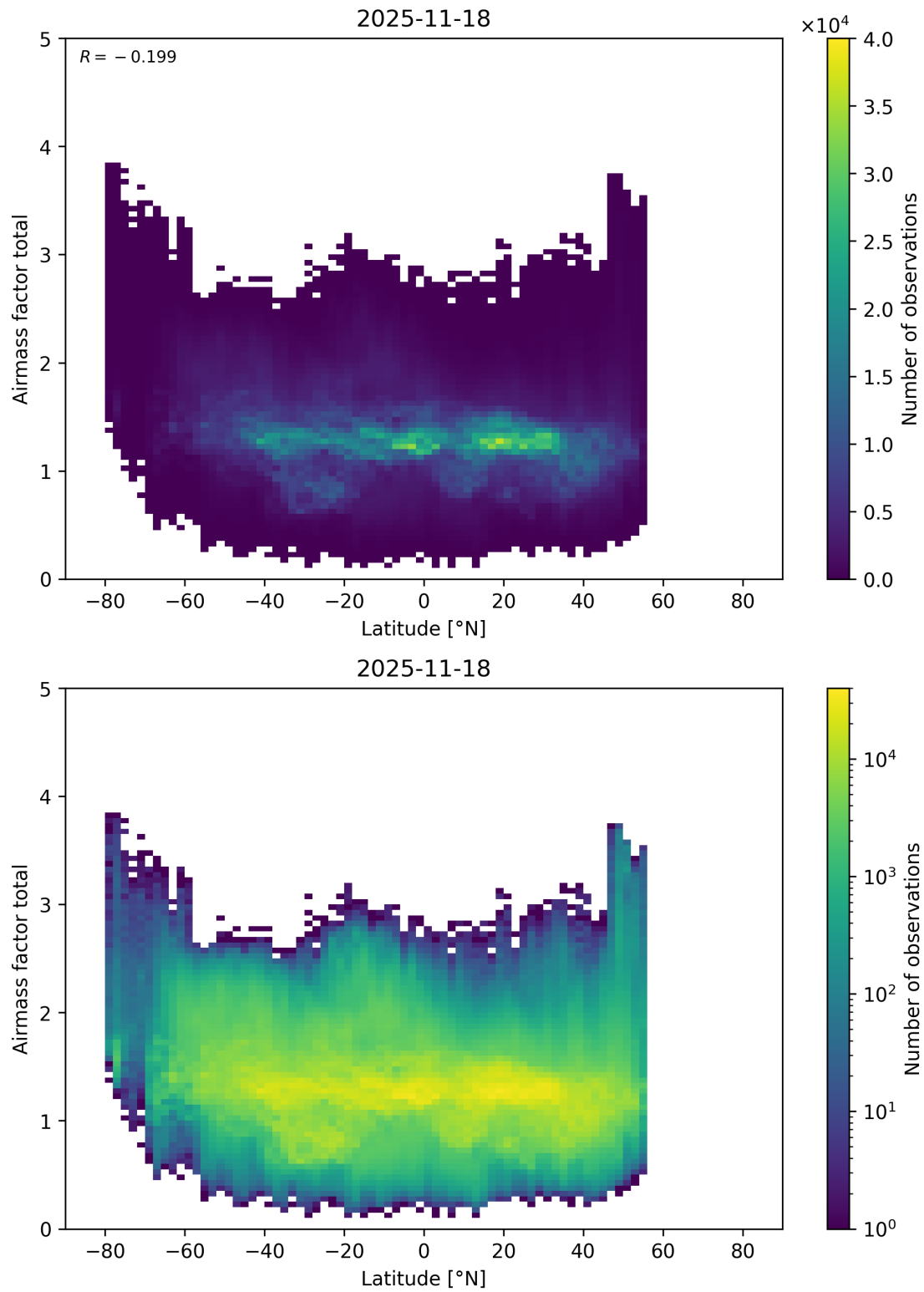
Figure 179: Scatter density plot of “Latitude” against “Airmass factor total” for 2025-11-18 to 2025-11-19.
