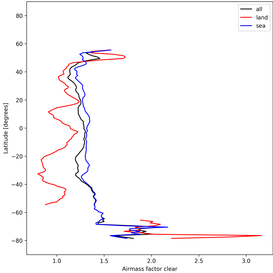
Figure 29: Zonal average of “Airmass factor clear” for 2025-11-18 to 2025-11-19.
