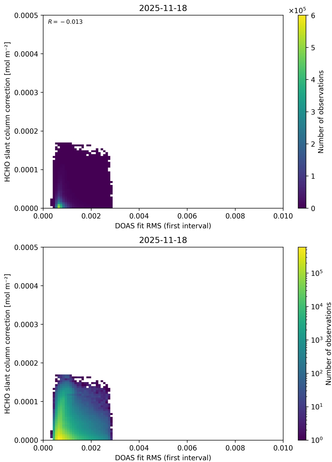
Figure 67: Scatter density plot of “DOAS fit RMS (first interval)” against “HCHO slant column correction” for 2025-11-18 to 2025-11-19.
