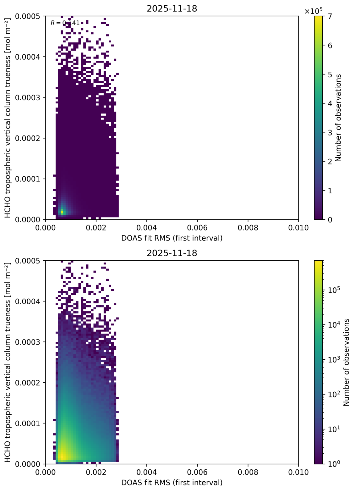
Figure 68: Scatter density plot of “DOAS fit RMS (first interval)” against “HCHO tropospheric vertical column trueness” for 2025-11-18 to 2025-11-19.
