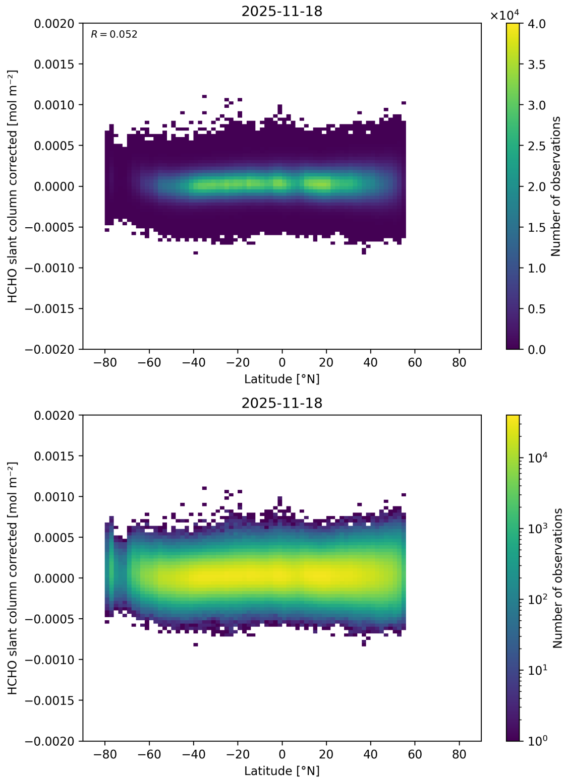
Figure 175: Scatter density plot of “Latitude” against “HCHO slant column corrected” for 2025-11-18 to 2025-11-19.
