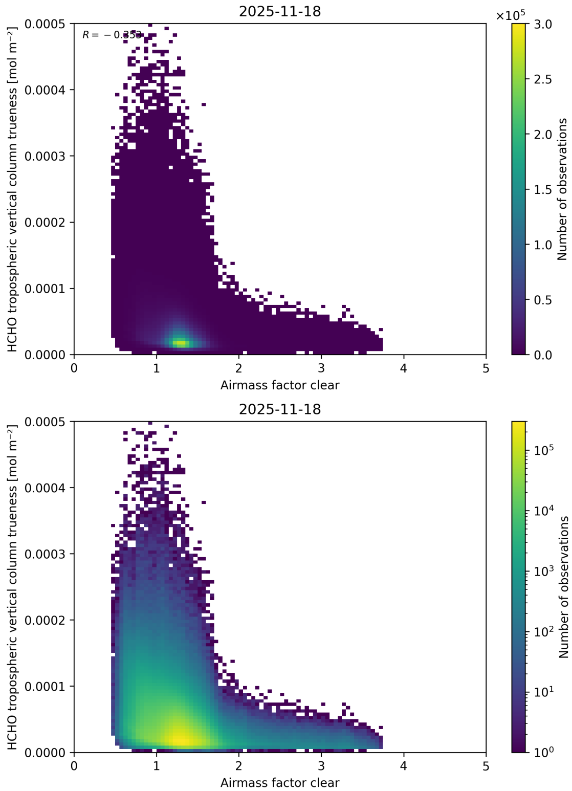
Figure 83: Scatter density plot of “Airmass factor clear” against “HCHO tropospheric vertical column truiness” for 2025-11-18 to 2025-11-19.
