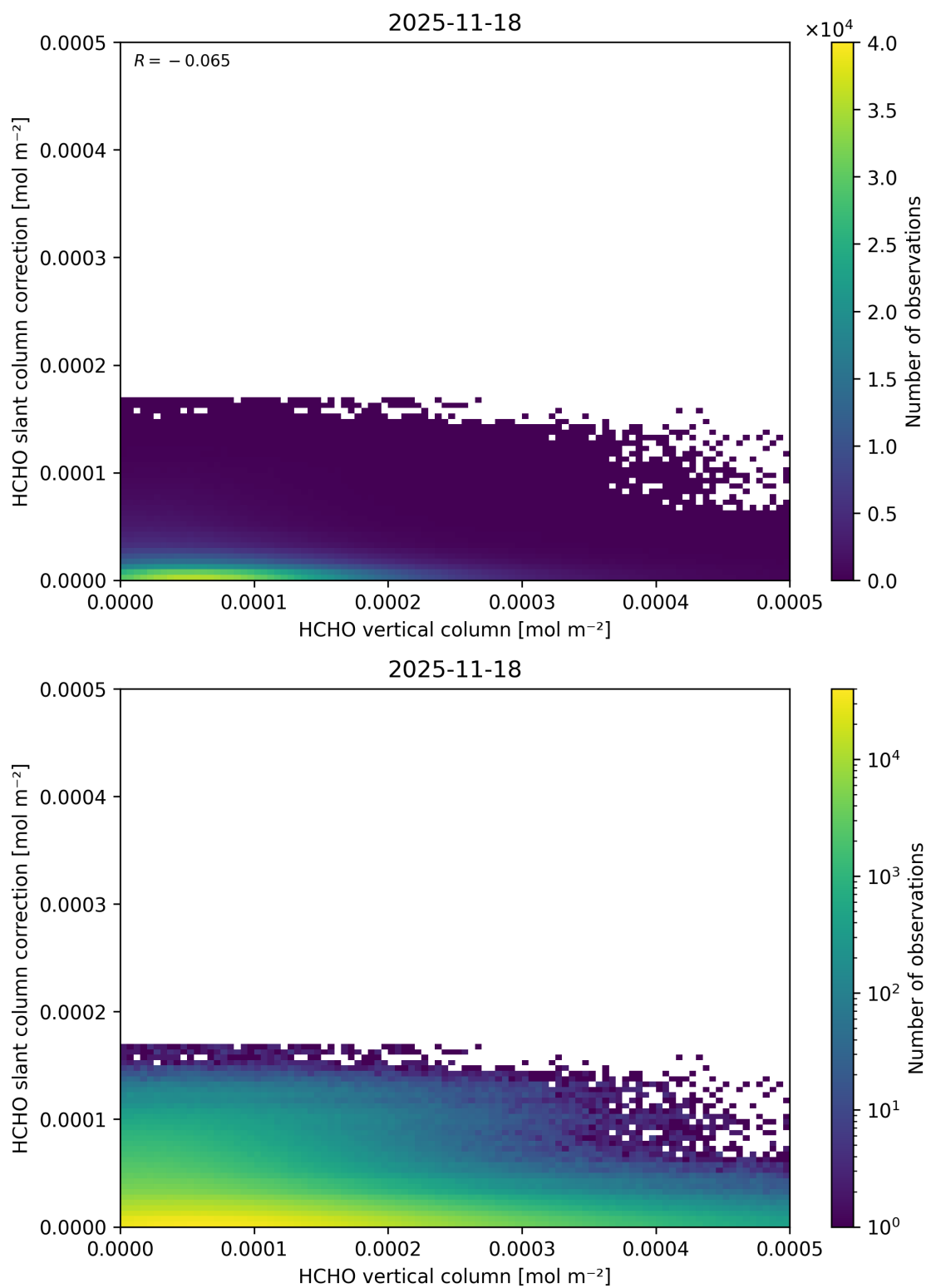
Figure 143: Scatter density plot of “HCHO vertical column” against “HCHO slant column correction” for 2025-11-18 to 2025-11-19.
