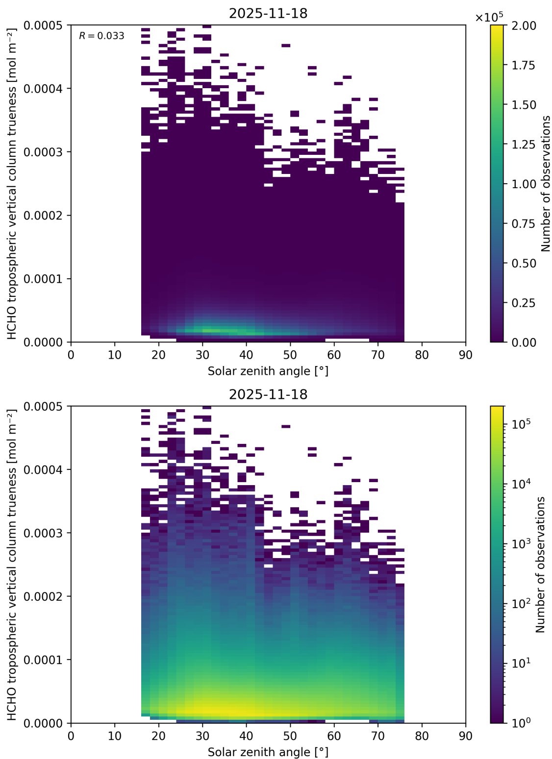
Figure 199: Scatter density plot of “Solar zenith angle” against “HCHO tropospheric vertical column trueness” for 2025-11-18 to 2025-11-19.
