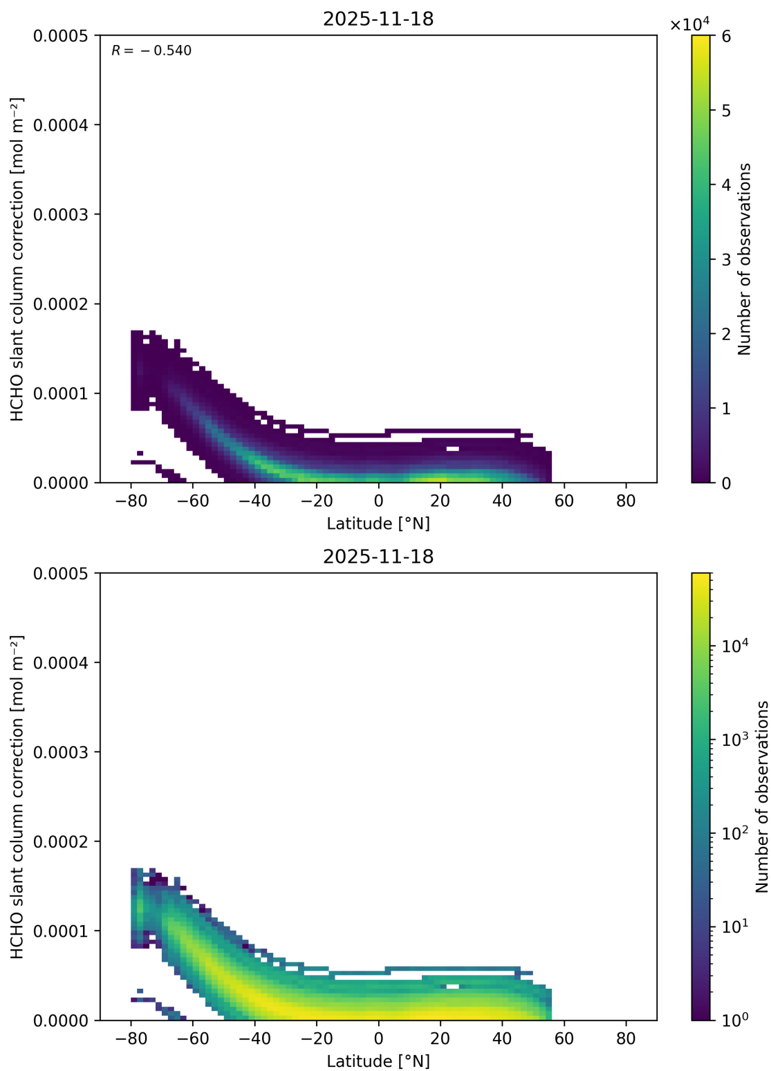
Figure 176: Scatter density plot of “Latitude” against “HCHO slant column correction” for 2025-11-18 to 2025-11-19.
