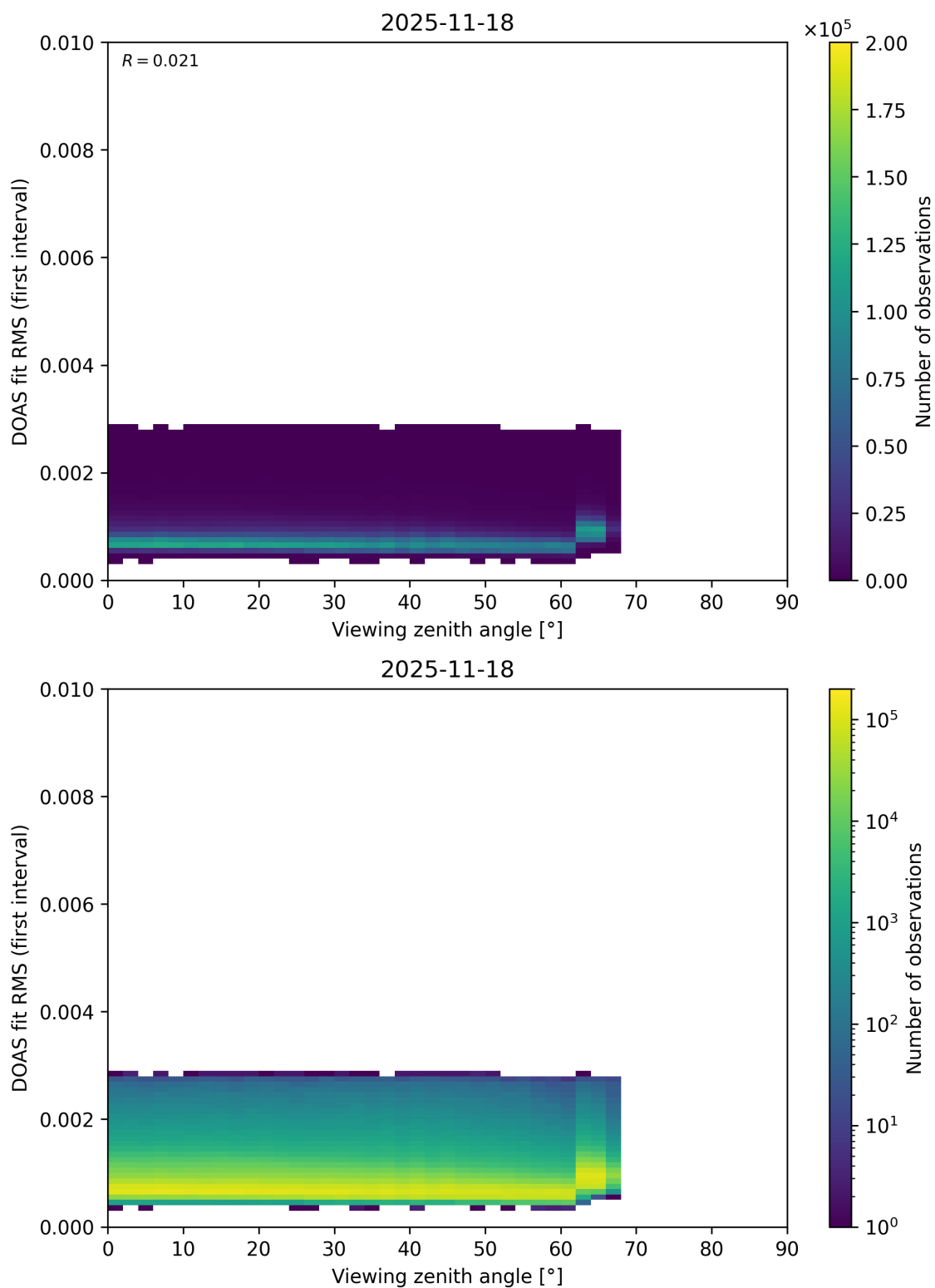
Figure 202: Scatter density plot of “Viewing zenith angle” against “DOAS fit RMS (first interval)” for 2025-11-18 to 2025-11-19.
