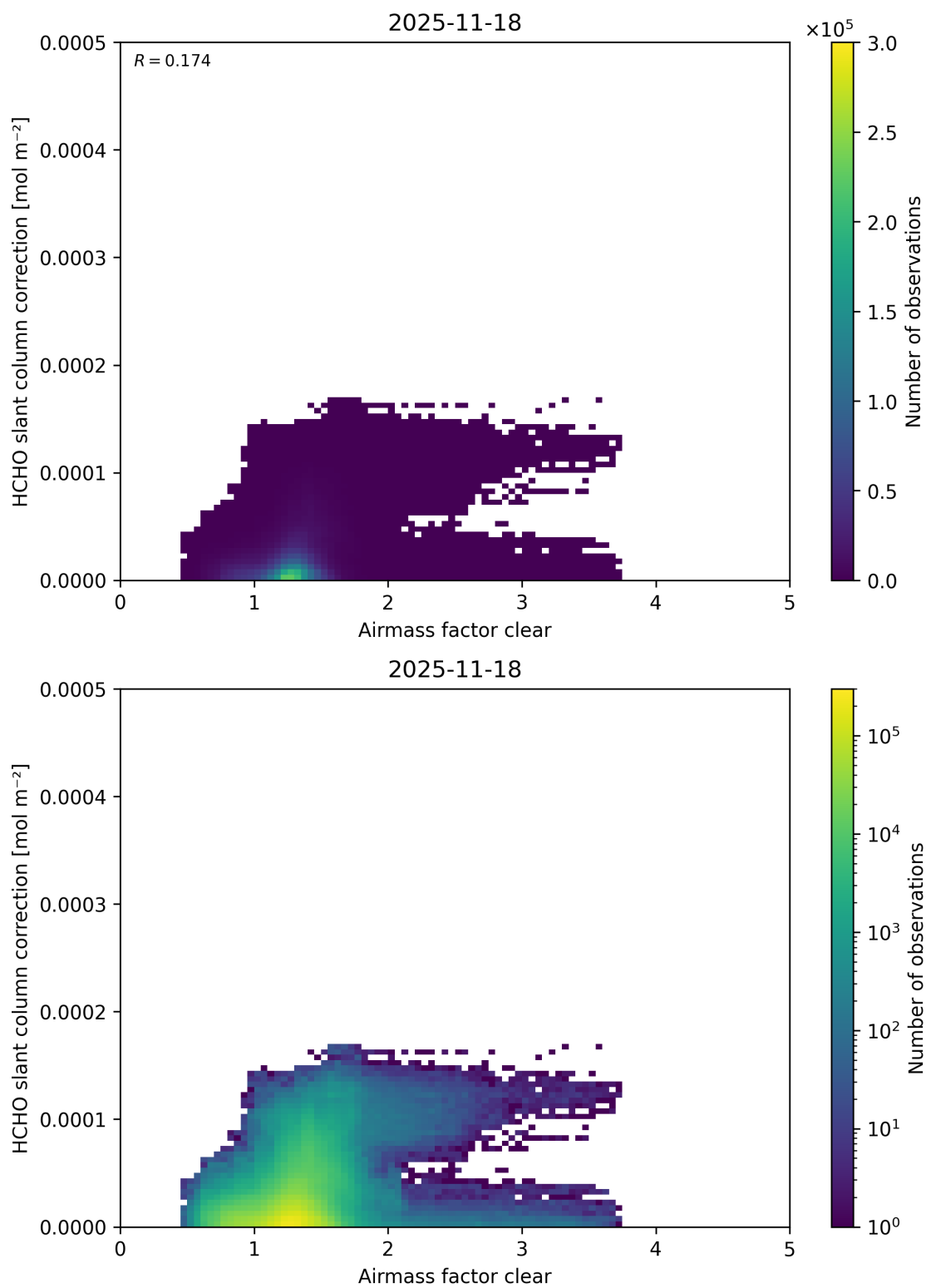
Figure 82: Scatter density plot of “Airmass factor clear” against “HCHO slant column correction” for 2025-11-18 to 2025-11-19.
