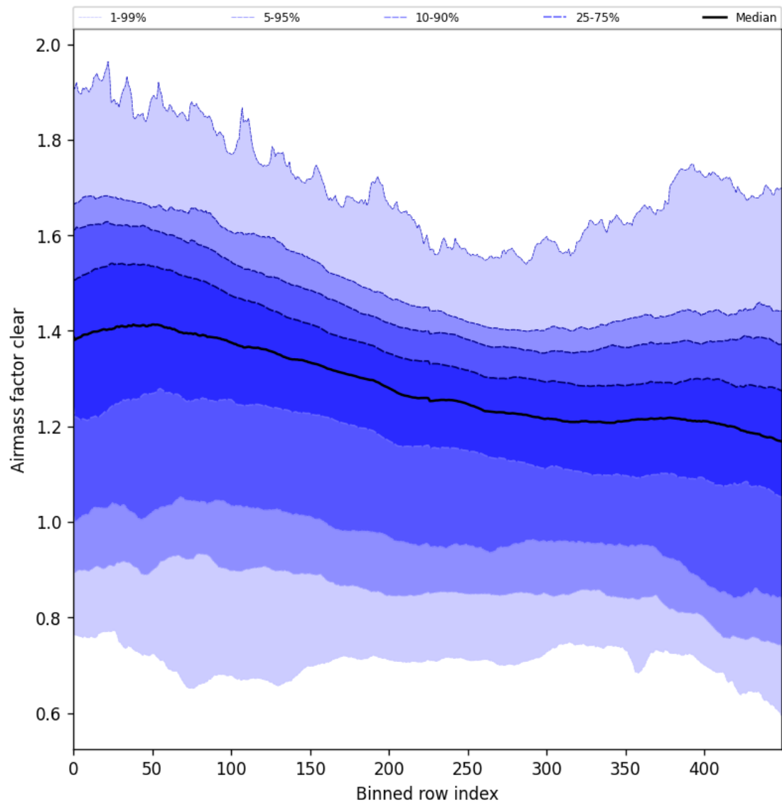
Figure 59: Along track statistics of “Airmass factor clear” for 2025-11-18 to 2025-11-19
