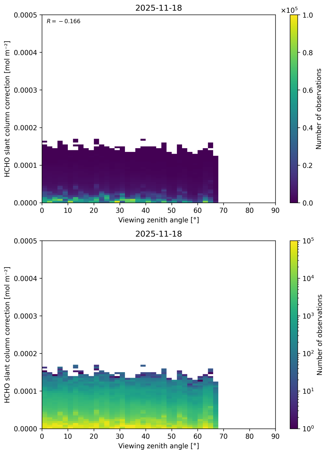
Figure 207: Scatter density plot of “Viewing zenith angle” against “HCHO slant column correction” for 2025-11-18 to 2025-11-19.
