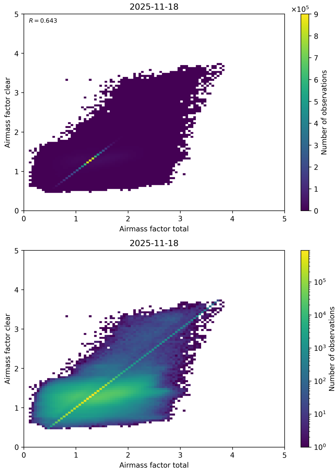
Figure 112: Scatter density plot of “Airmass factor total” against “Airmass factor clear” for 2025-11-18 to 2025-11-19.
