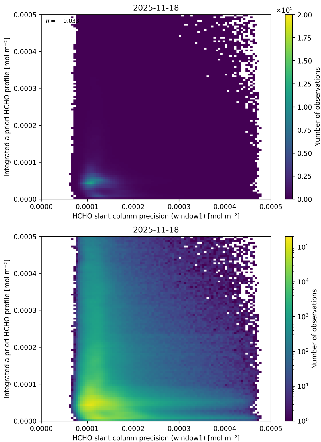
Figure 108: Scatter density plot of “HCHO slant column precision (window1)” against “Integrated a priori HCHO profile” for 2025-11-18 to 2025-11-19.
