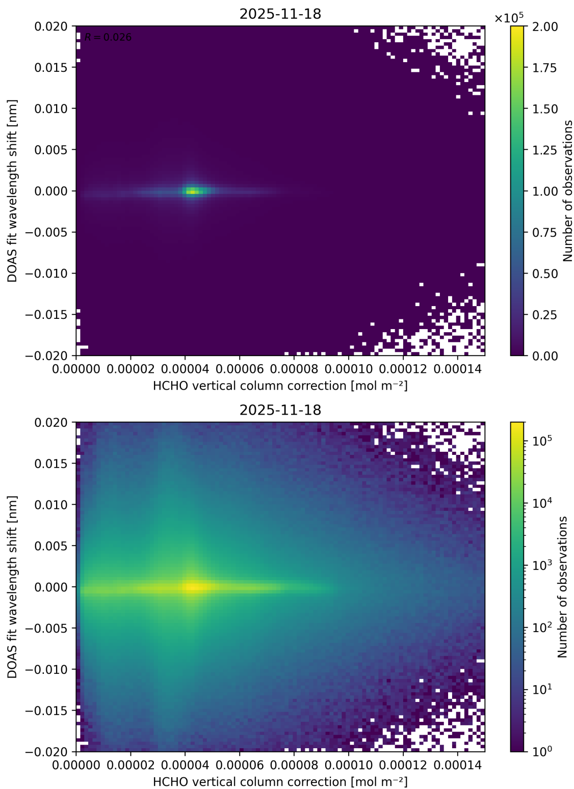
Figure 127: Scatter density plot of “HCHO vertical column correction” against “DOAS fit wavelength shift” for 2025-11-18 to 2025-11-19.
