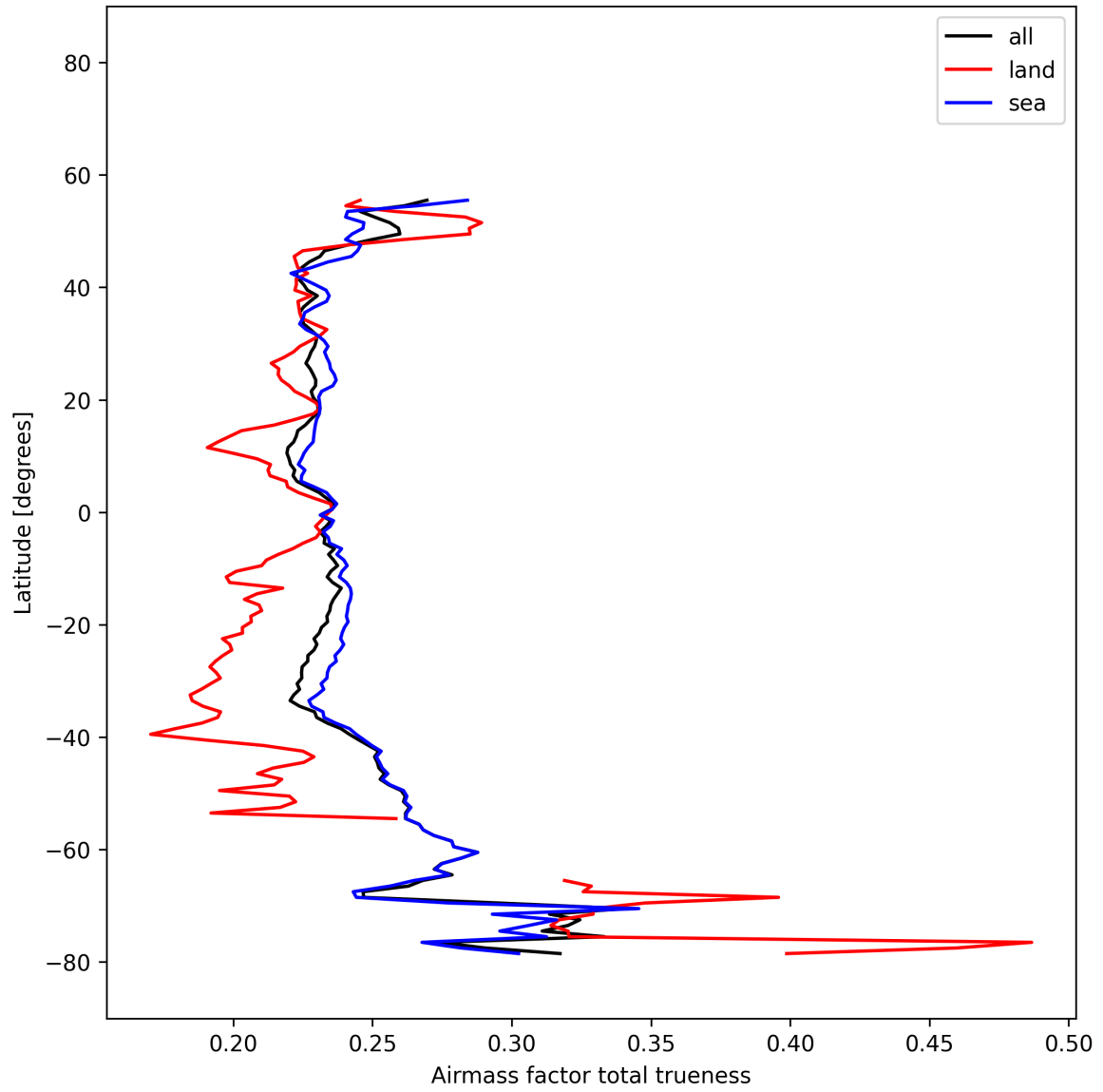
Figure 28: Zonal average of “Airmass factor total trueness” for 2025-11-18 to 2025-11-19.
