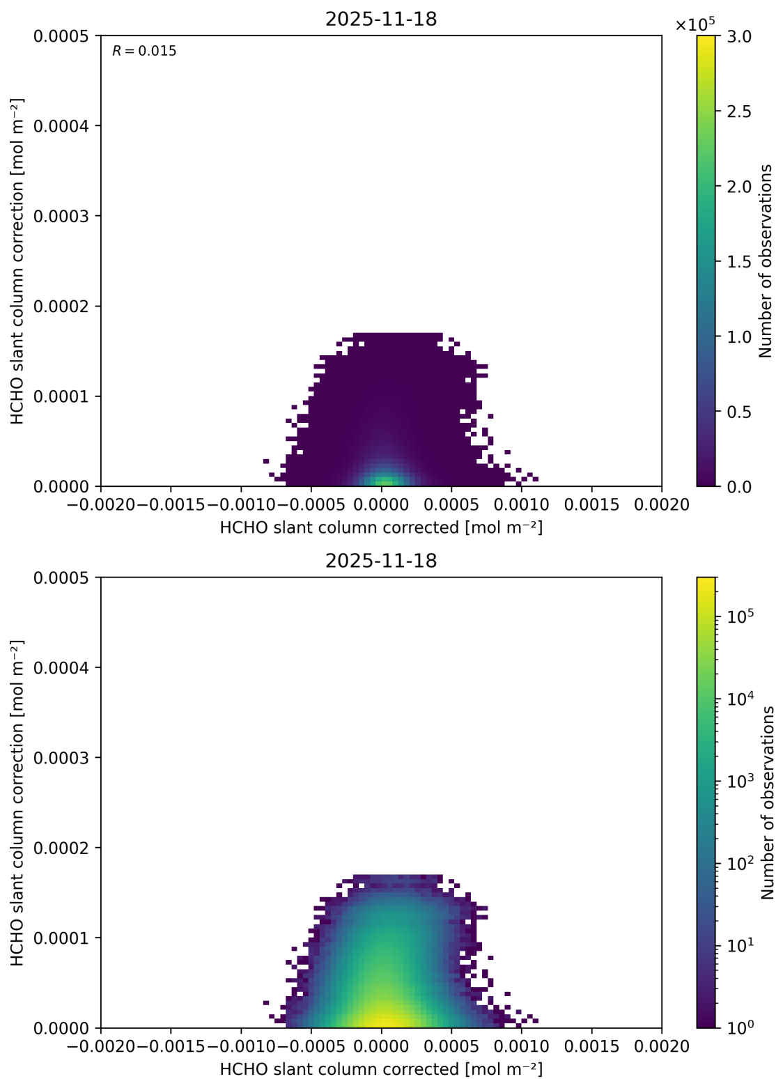
Figure 85: Scatter density plot of “HCHO slant column corrected” against “HCHO slant column correction” for 2025-11-18 to 2025-11-19.
