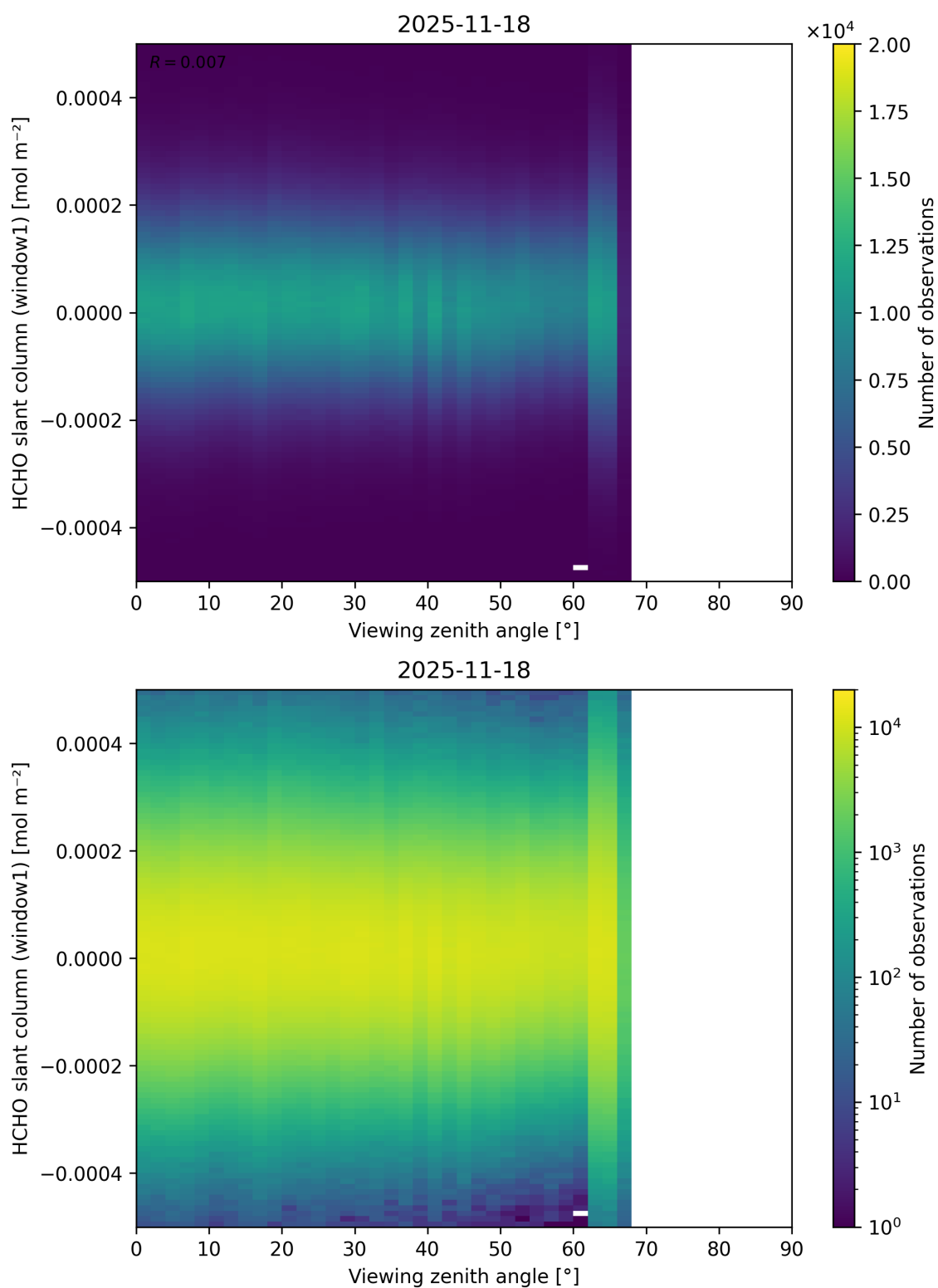
Figure 208: Scatter density plot of “Viewing zenith angle” against “HCHO slant column (window1)” for 2025-11-18 to 2025-11-19.
