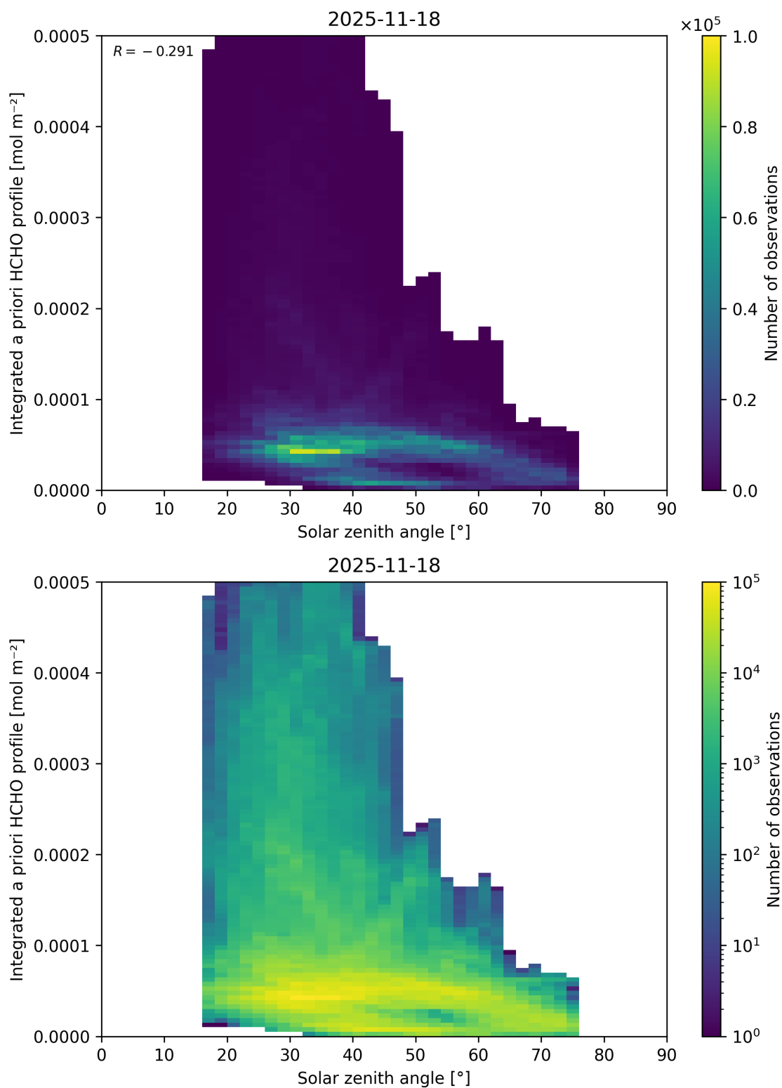
Figure 200: Scatter density plot of “Solar zenith angle” against “Integrated a priori HCHO profile” for 2025-11-18 to 2025-11-19.
