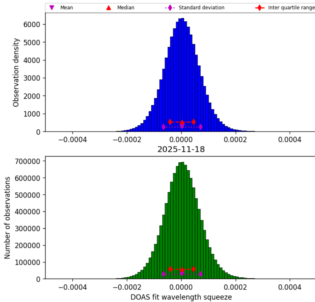
Figure 47: Histogram of “DOAS fit wavelength squeeze” for 2025-11-18 to 2025-11-19
