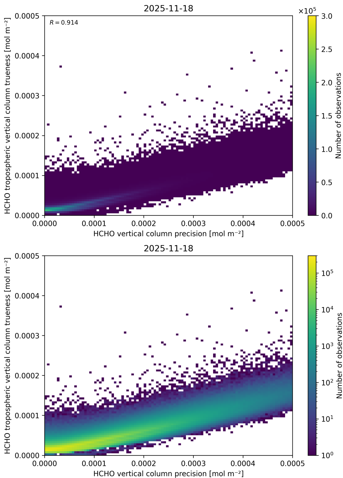
Figure 163: Scatter density plot of “HCHO vertical column precision” against “HCHO tropospheric vertical column trueness” for 2025-11-18 to 2025-11-19.
