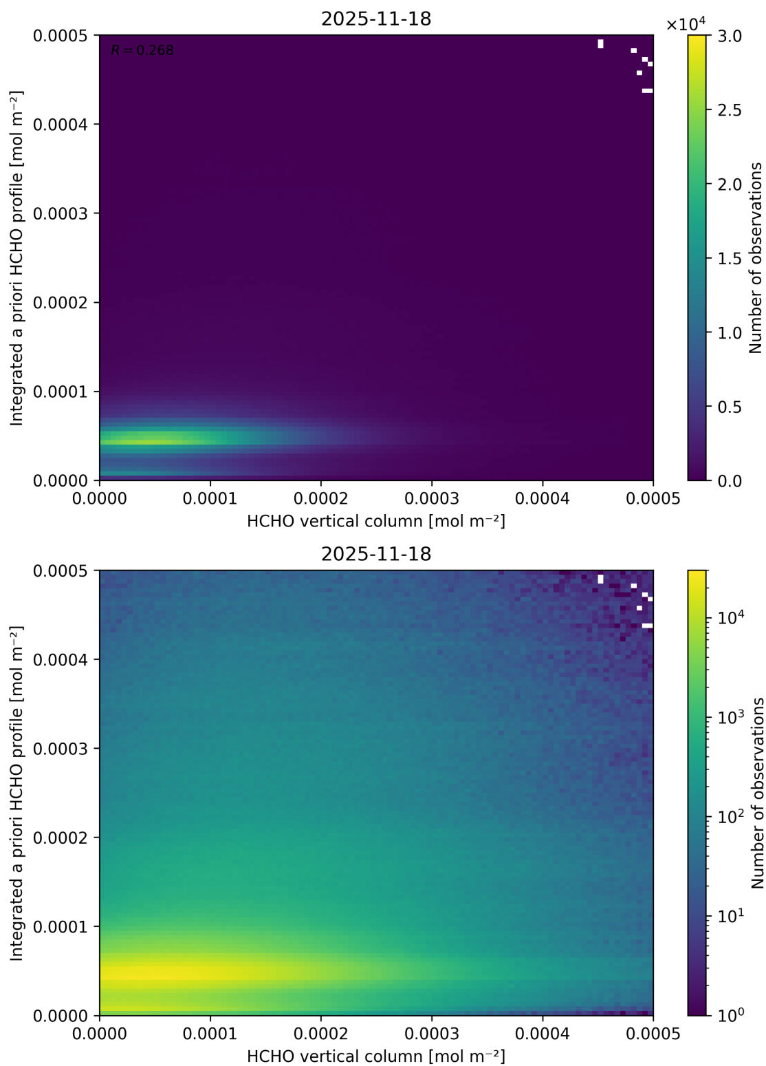
Figure 151: Scatter density plot of “HCHO vertical column” against “Integrated a priori HCHO profile” for 2025-11-18 to 2025-11-19.
