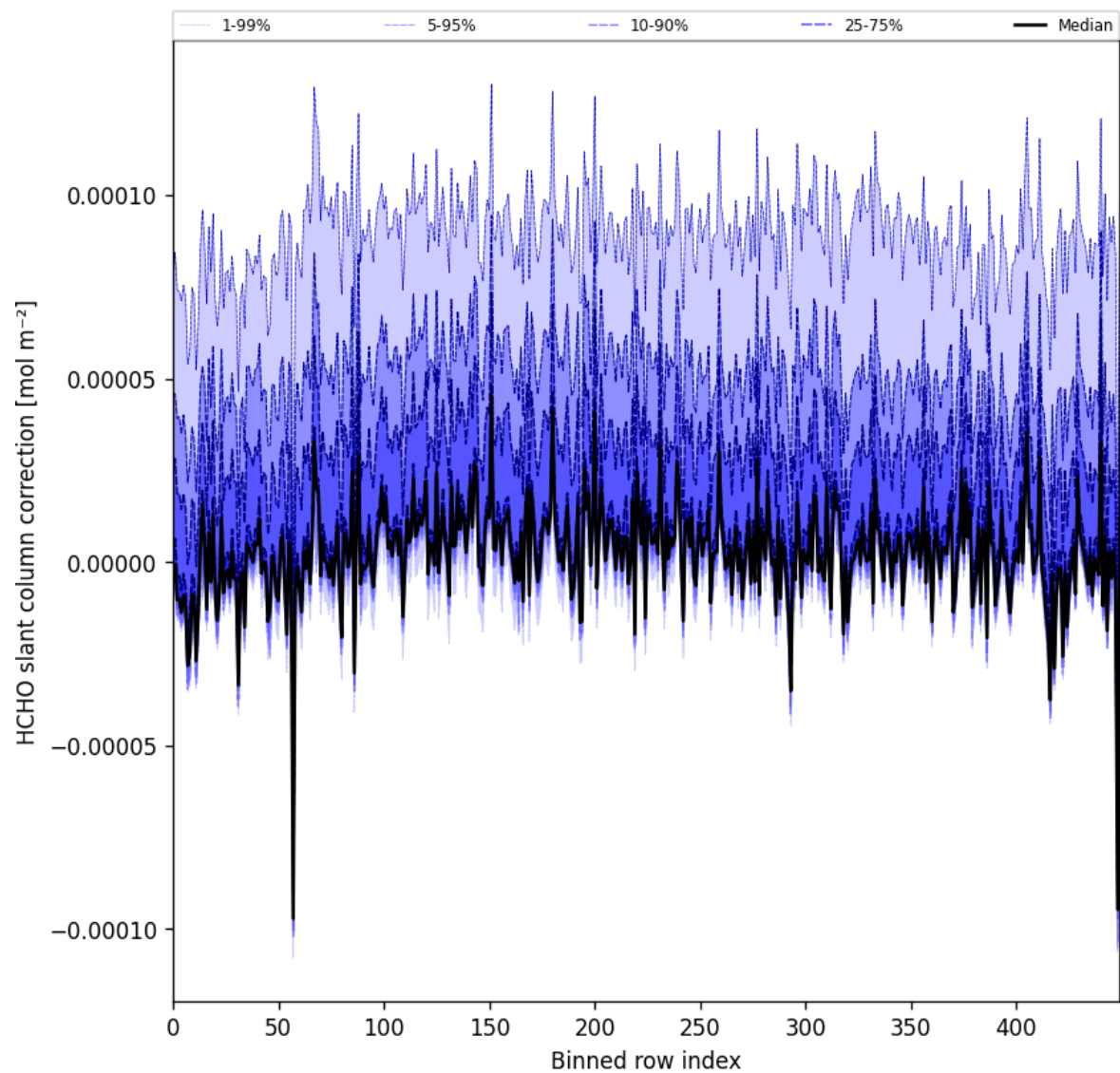
Figure 64: Along track statistics of “HCHO slant column correction” for 2025-11-18 to 2025-11-19
