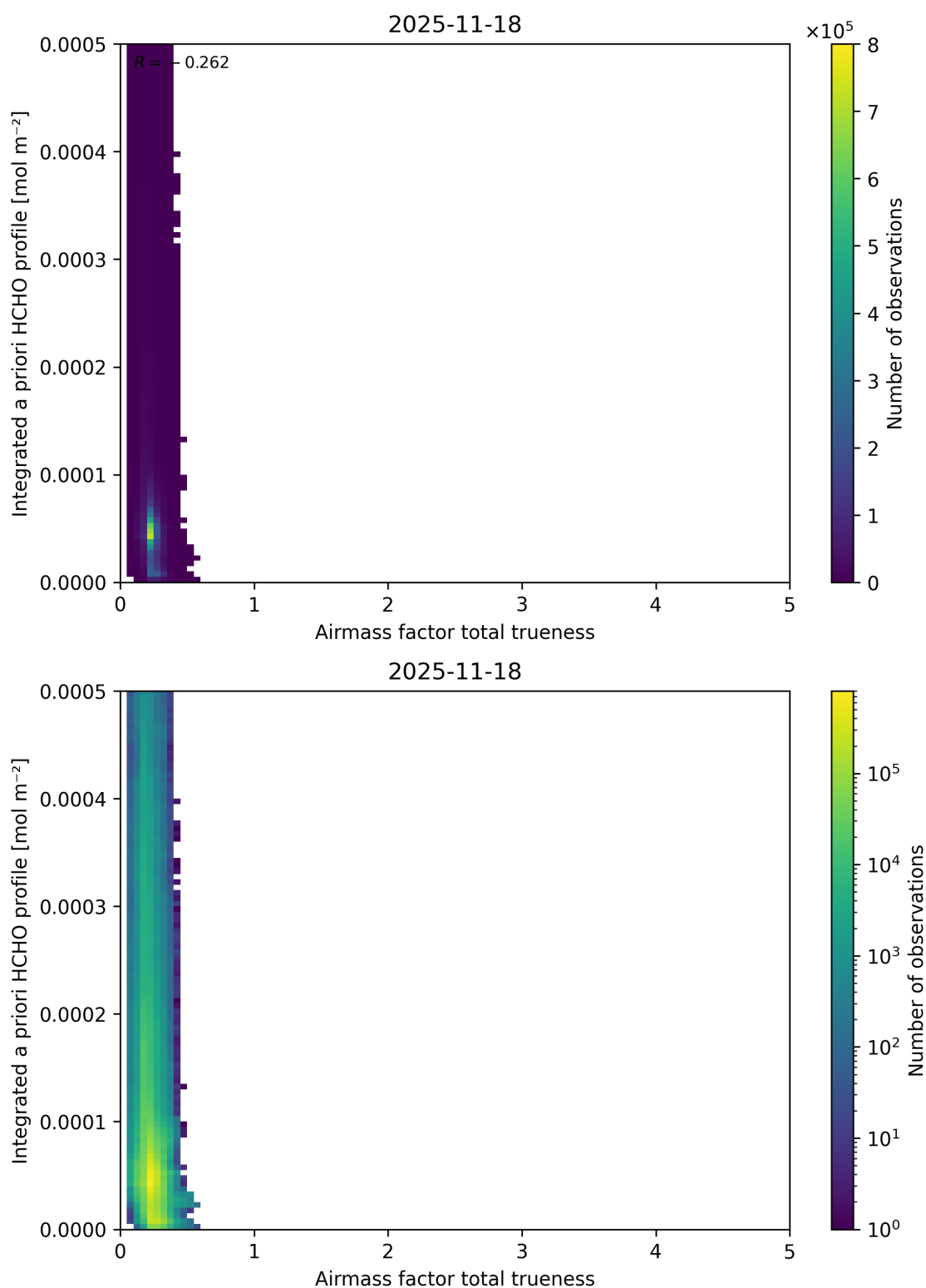
Figure 125: Scatter density plot of “Airmass factor total trueness” against “Integrated a priori HCHO profile” for 2025-11-18 to 2025-11-19.
