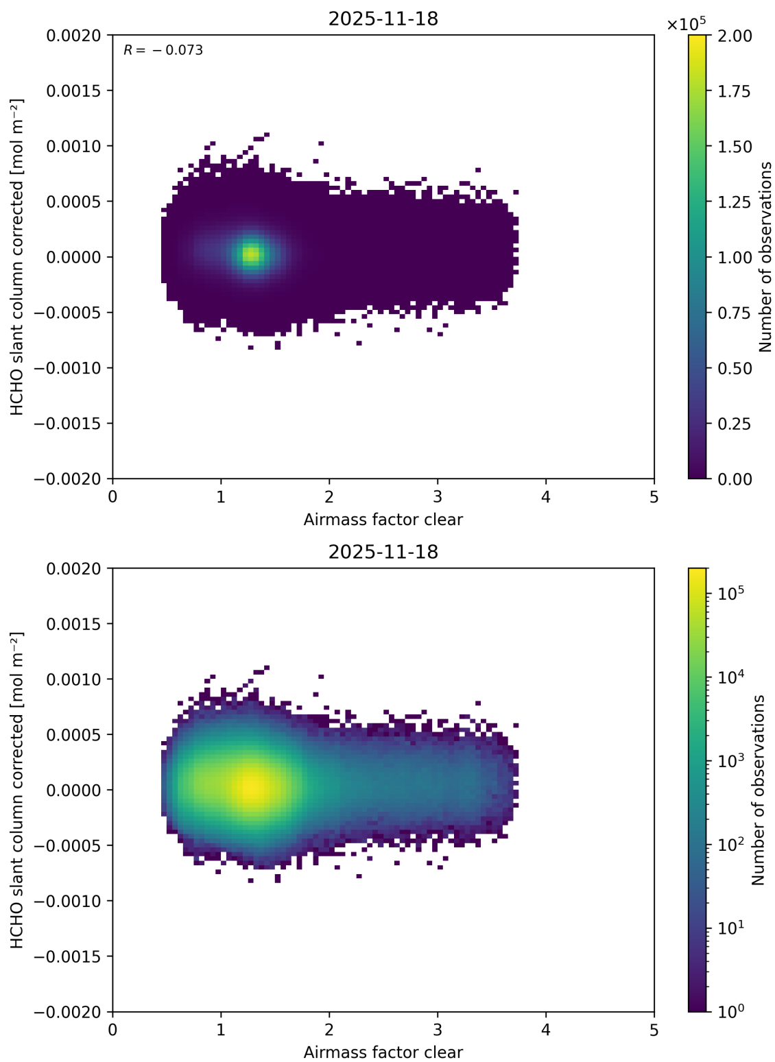
Figure 81: Scatter density plot of “Airmass factor clear” against “HCHO slant column corrected” for 2025-11-18 to 2025-11-19.
