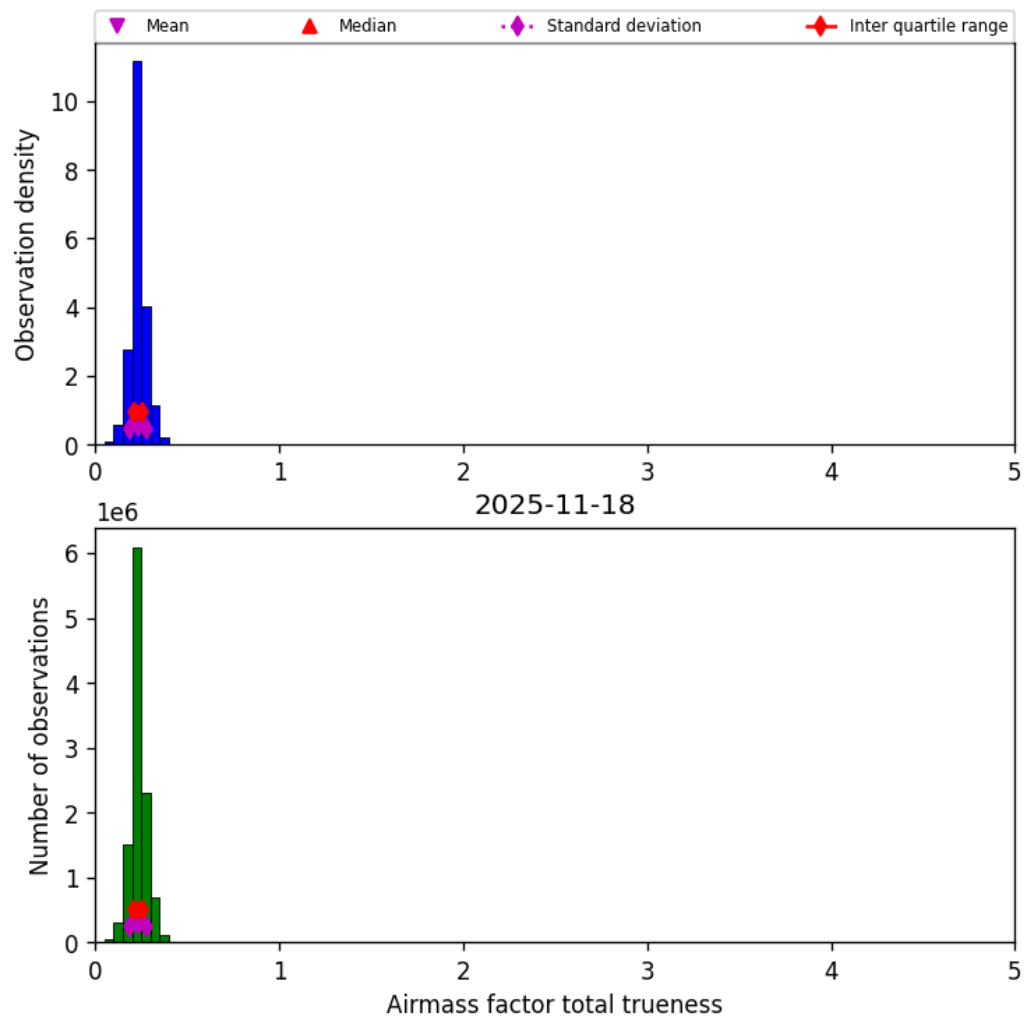
Figure 43: Histogram of “Airmass factor total trueness” for 2025-11-18 to 2025-11-19
