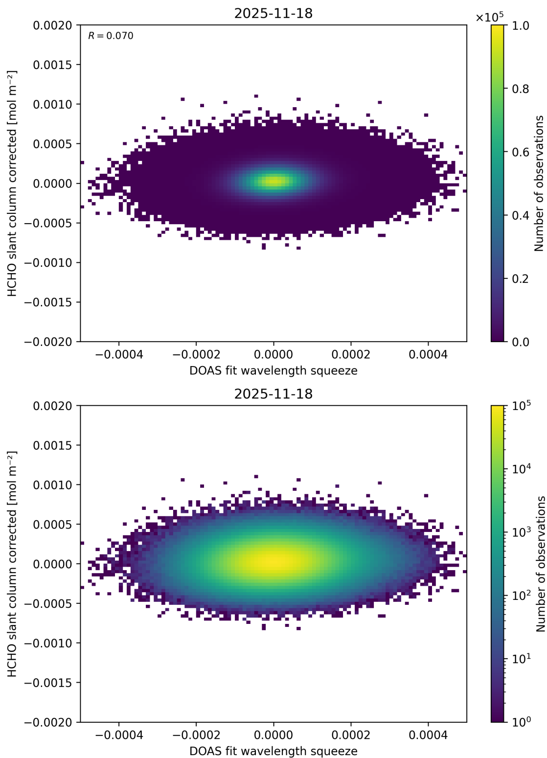
Figure 75: Scatter density plot of “DOAS fit wavelength squeeze” against “HCHO slant column corrected” for 2025-11-18 to 2025-11-19.
