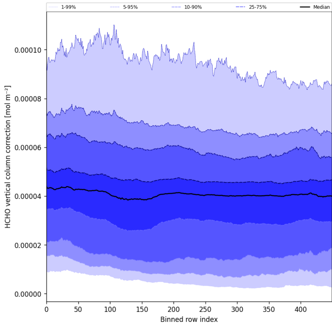
Figure 54: Along track statistics of “HCHO vertical column correction” for 2025-11-18 to 2025-11-19
