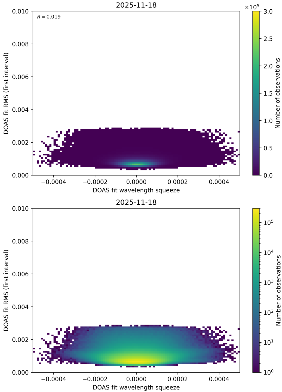
Figure 74: Scatter density plot of “DOAS fit wavelength squeeze” against “DOAS fit RMS (first interval)” for 2025-11-18 to 2025-11-19.
