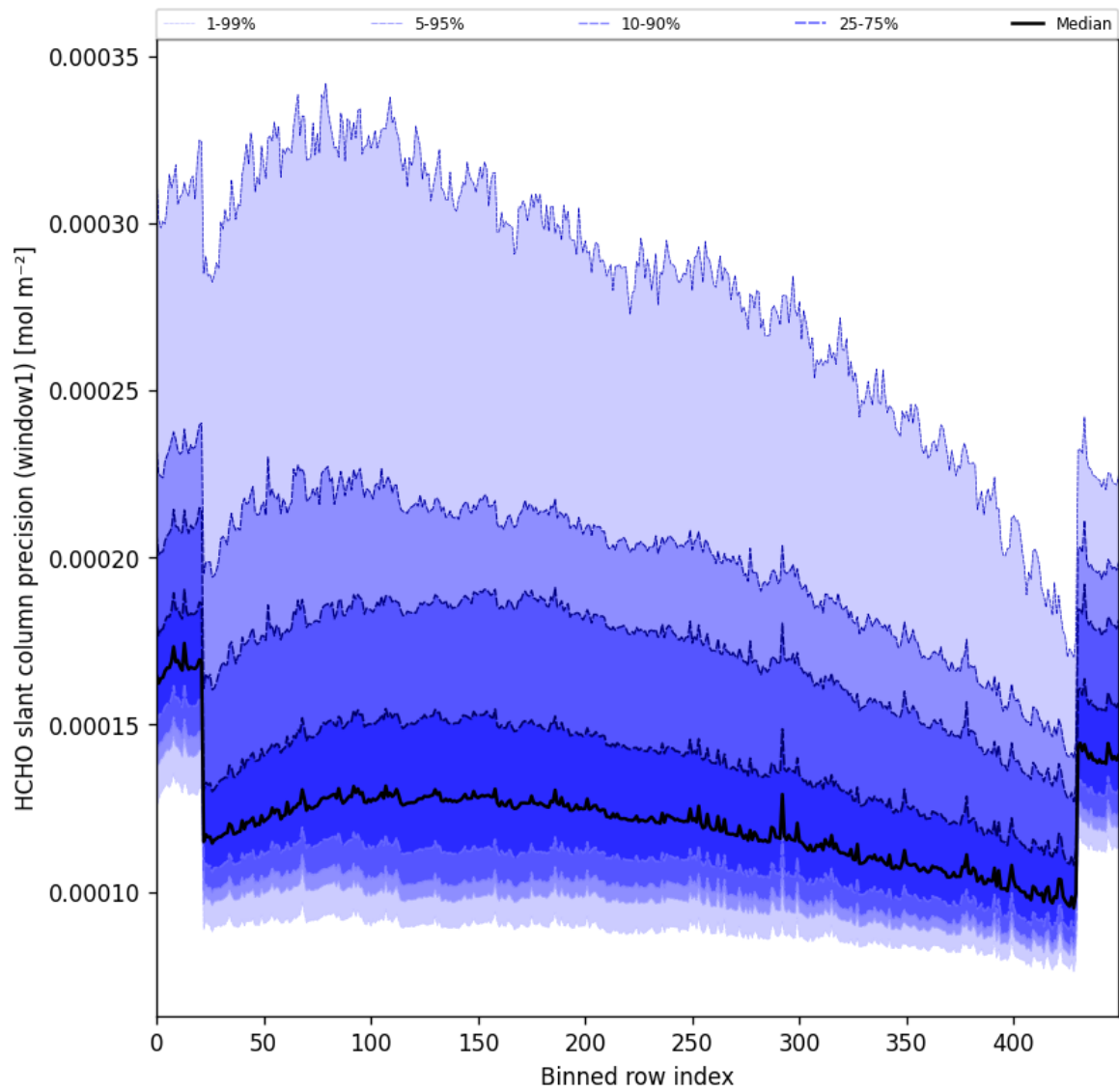
Figure 56: Along track statistics of “HCHO slant column precision (window1)” for 2025-11-18 to 2025-11-19
