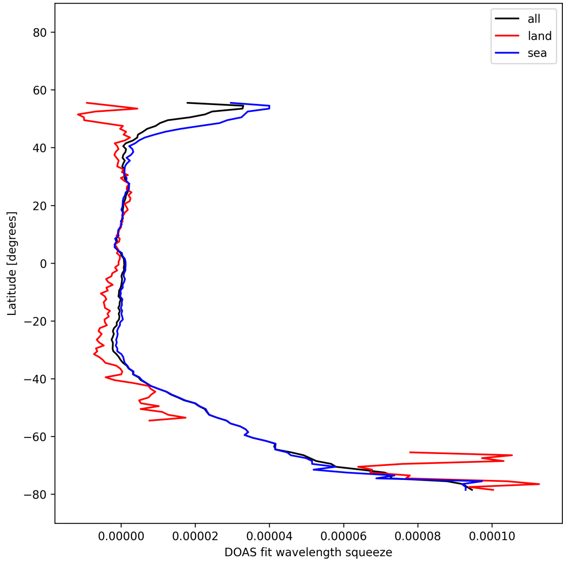
Figure 32: Zonal average of “DOAS fit wavelength squeeze” for 2025-11-18 to 2025-11-19.
