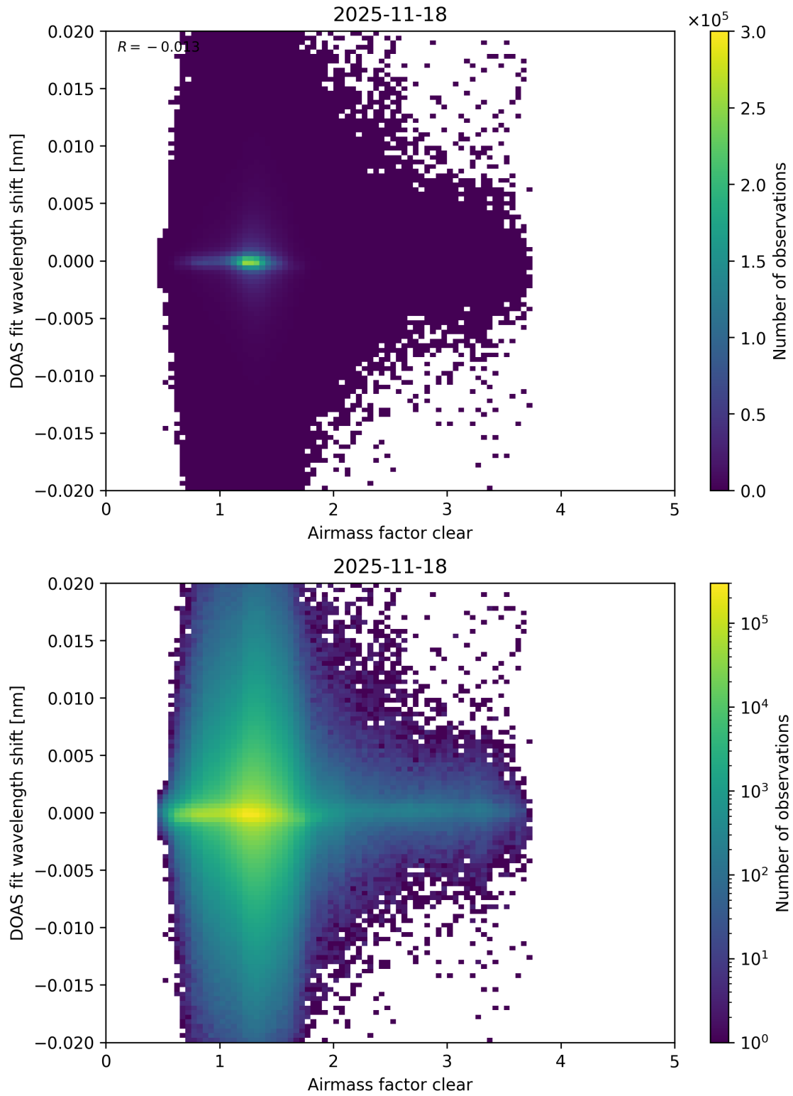
Figure 79: Scatter density plot of “Airmass factor clear” against “DOAS fit wavelength shift” for 2025-11-18 to 2025-11-19.
