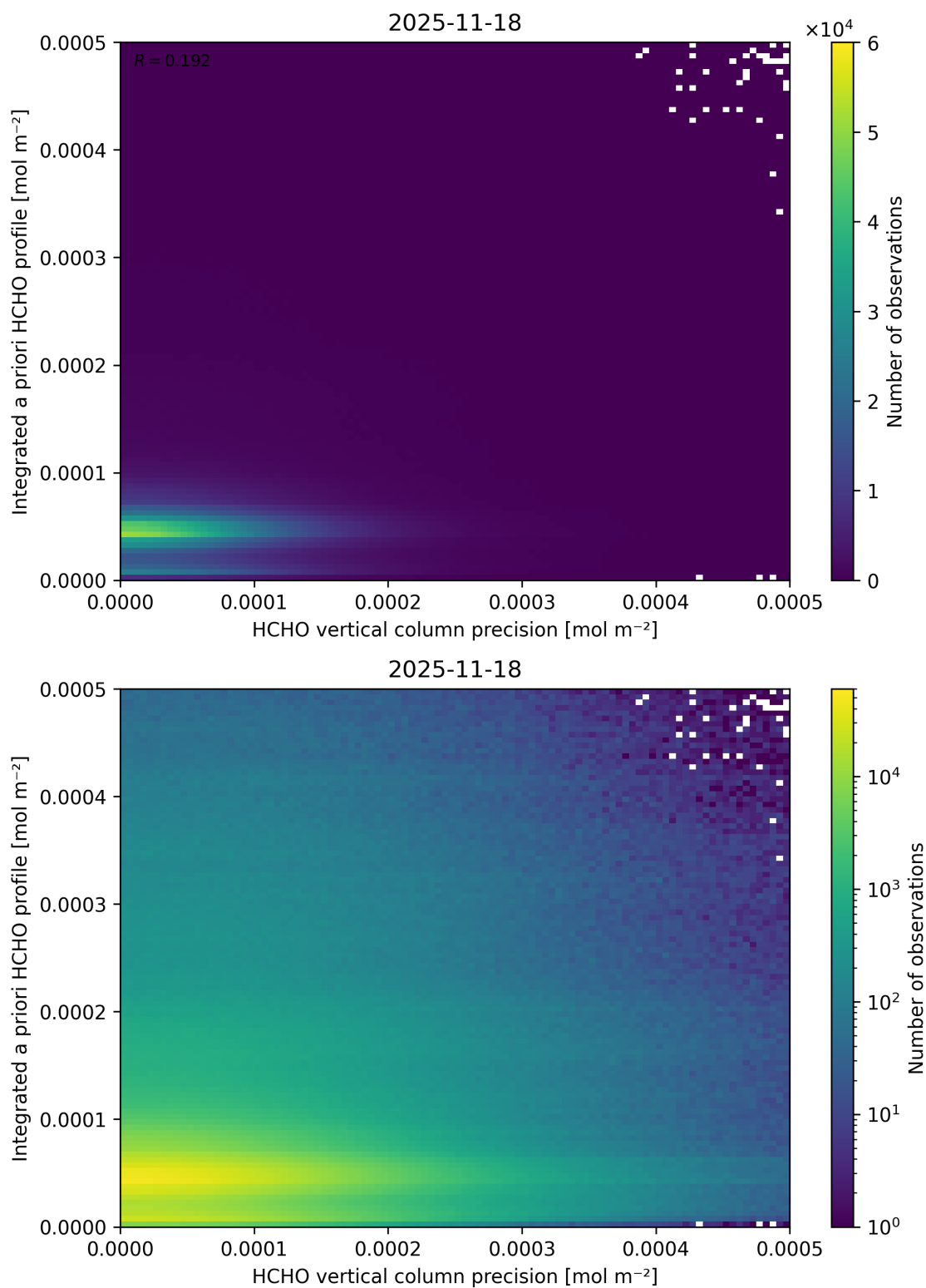
Figure 164: Scatter density plot of “HCHO vertical column precision” against “Integrated a priori HCHO profile” for 2025-11-18 to 2025-11-19.
