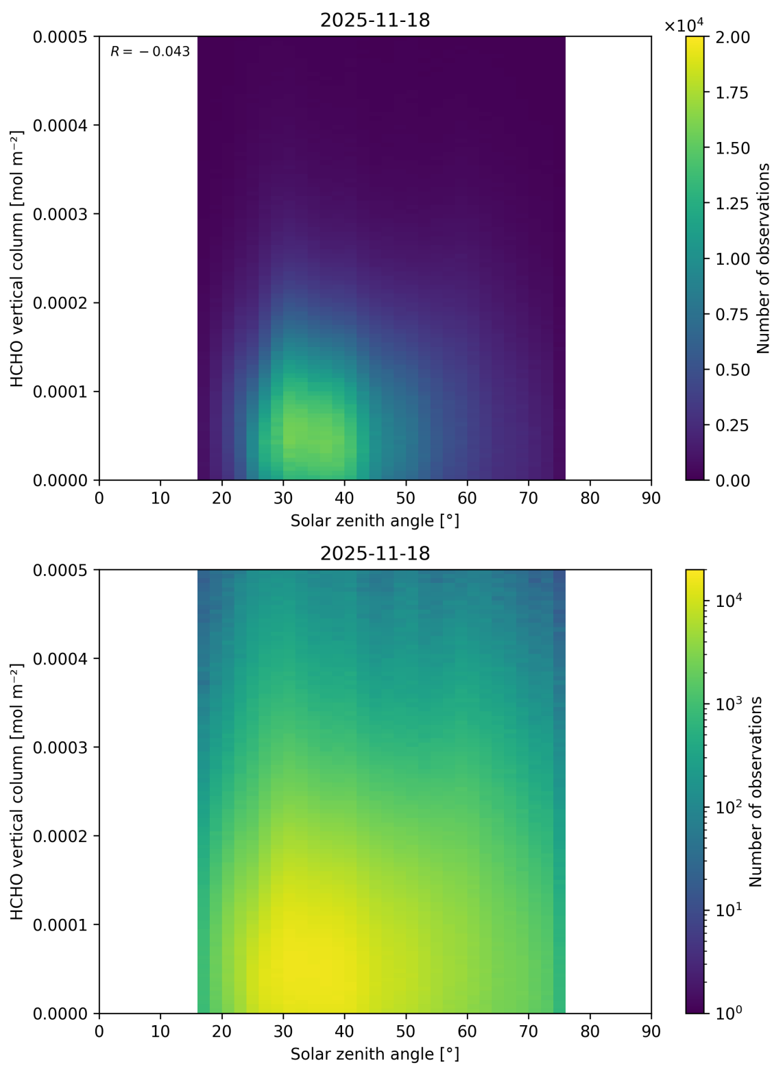
Figure 196: Scatter density plot of “Solar zenith angle” against “HCHO vertical column” for 2025-11-18 to 2025-11-19.
