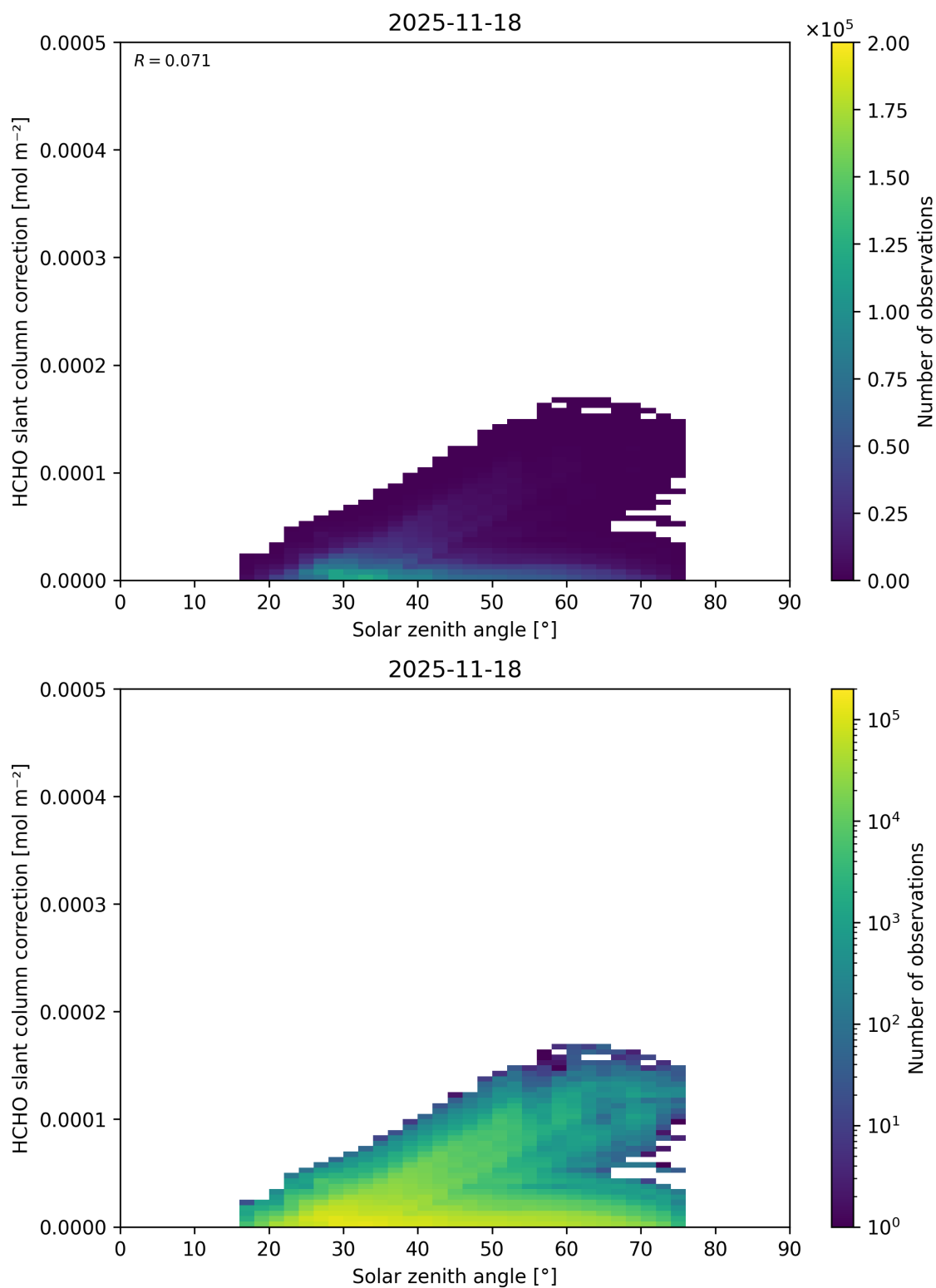
Figure 191: Scatter density plot of “Solar zenith angle” against “HCHO slant column correction” for 2025-11-18 to 2025-11-19.
