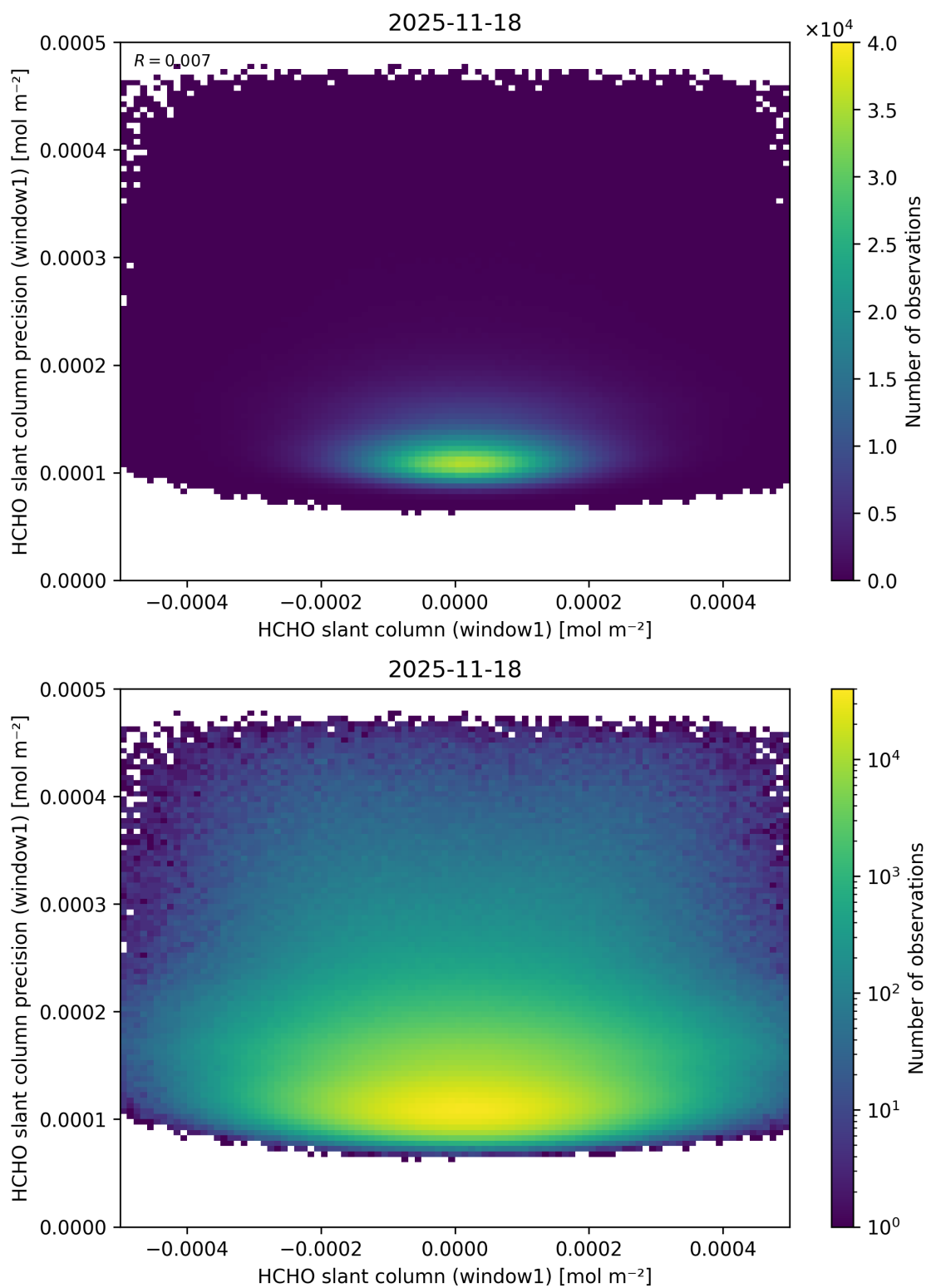
Figure 94: Scatter density plot of “HCHO slant column (window1)” against “HCHO slant column precision (window1)” for 2025-11-18 to 2025-11-19.
