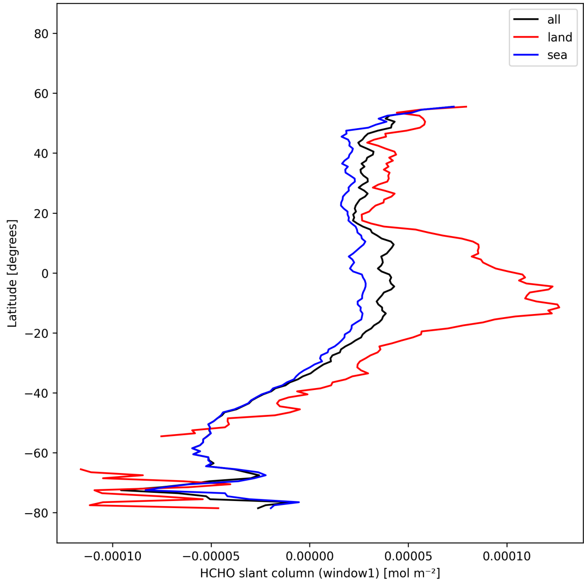
Figure 25: Zonal average of “HCHO slant column (window1)” for 2025-11-18 to 2025-11-19.
