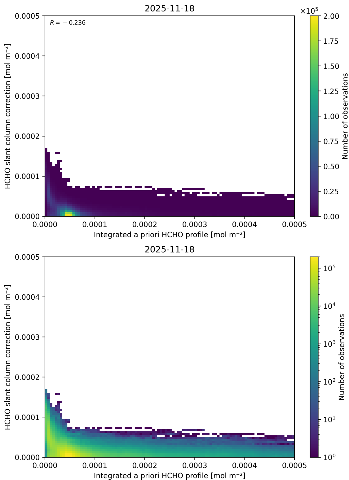
Figure 169: Scatter density plot of “Integrated a priori HCHO profile” against “HCHO slant column correction” for 2025-11-18 to 2025-11-19.
