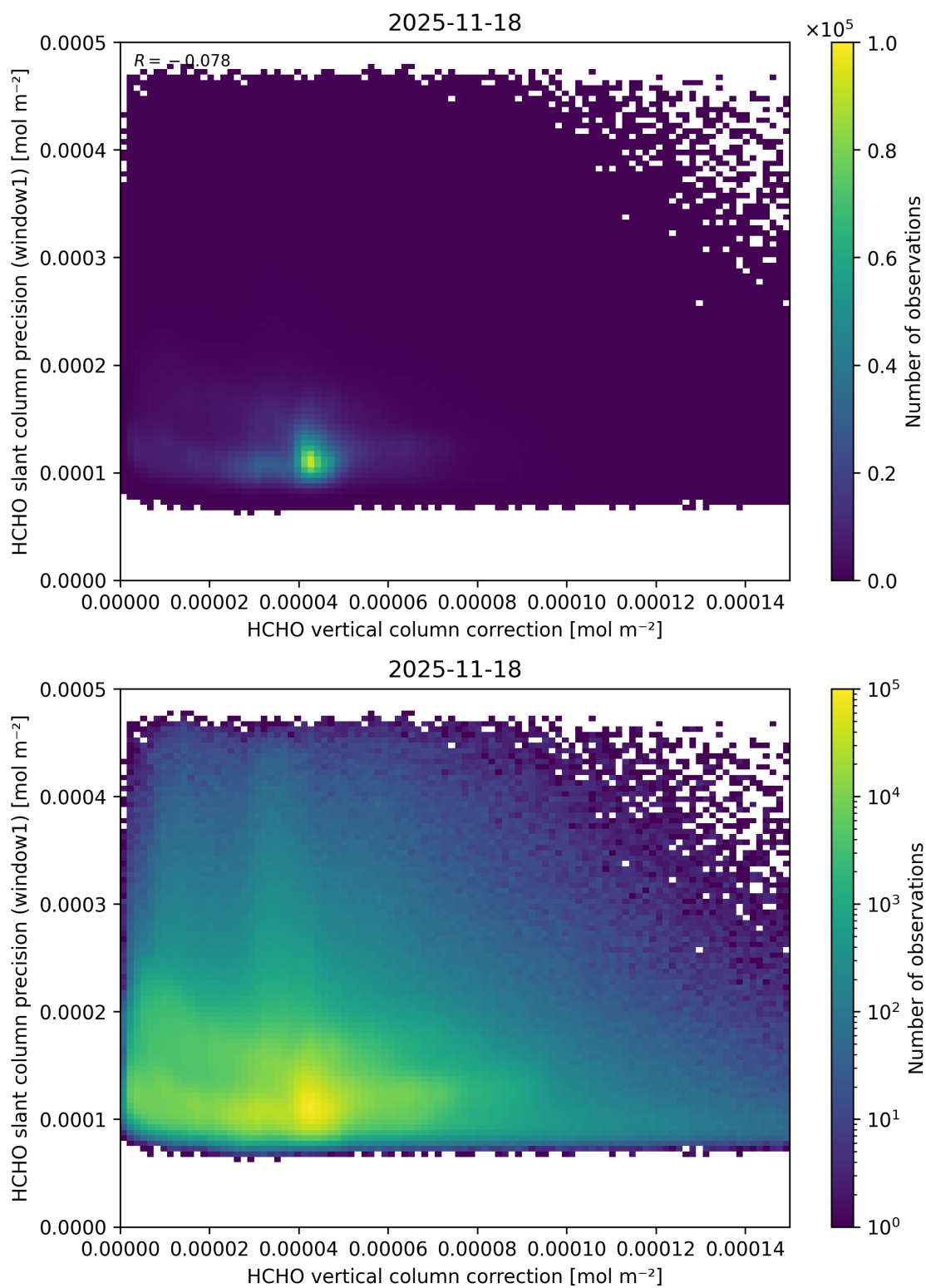
Figure 133: Scatter density plot of “HCHO vertical column correction” against “HCHO slant column precision (window1)” for 2025-11-18 to 2025-11-19.
