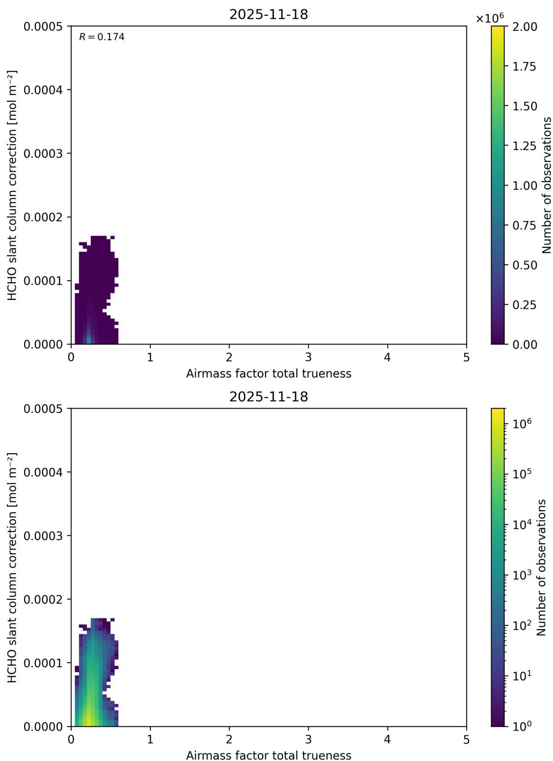
Figure 123: Scatter density plot of “Airmass factor total trueness” against “HCHO slant column correction” for 2025-11-18 to 2025-11-19.
