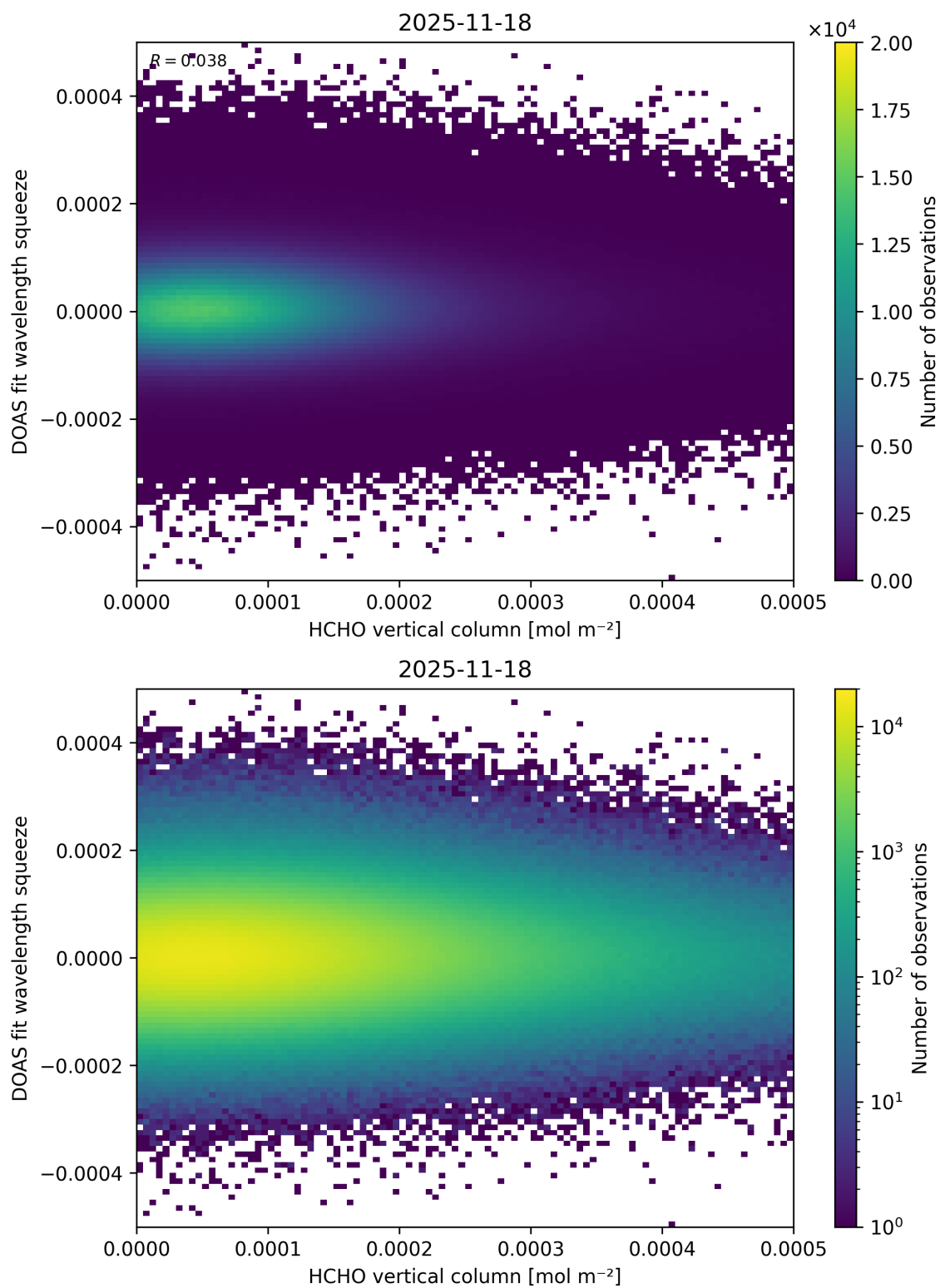
Figure 140: Scatter density plot of “HCHO vertical column” against “DOAS fit wavelength squeeze” for 2025-11-18 to 2025-11-19.
