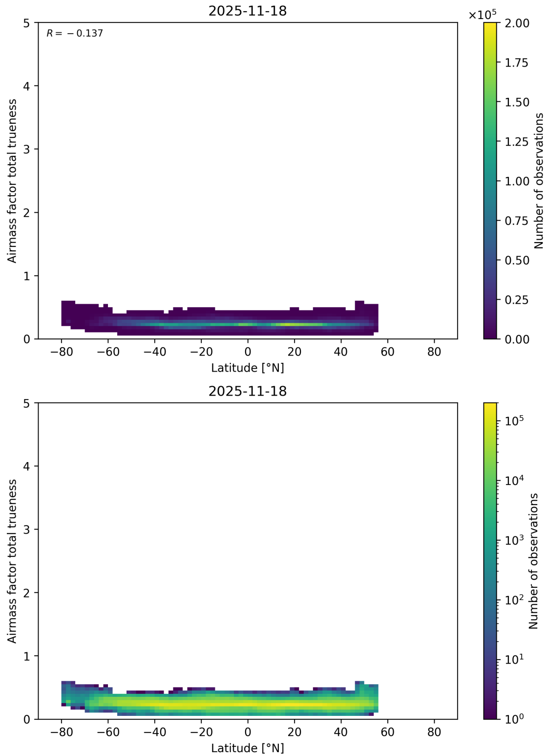
Figure 180: Scatter density plot of “Latitude” against “Airmass factor total trueneess” for 2025-11-18 to 2025-11-19.
