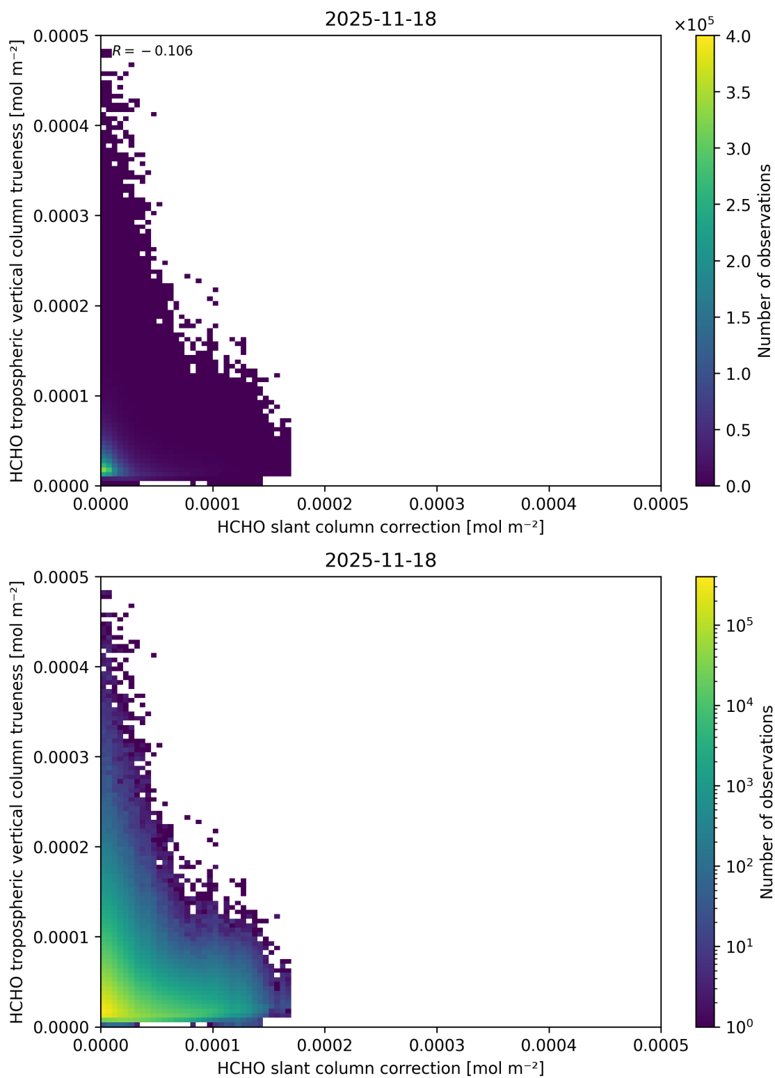
Figure 87: Scatter density plot of “HCHO slant column correction” against “HCHO tropospheric vertical column trueness” for 2025-11-18 to 2025-11-19.
