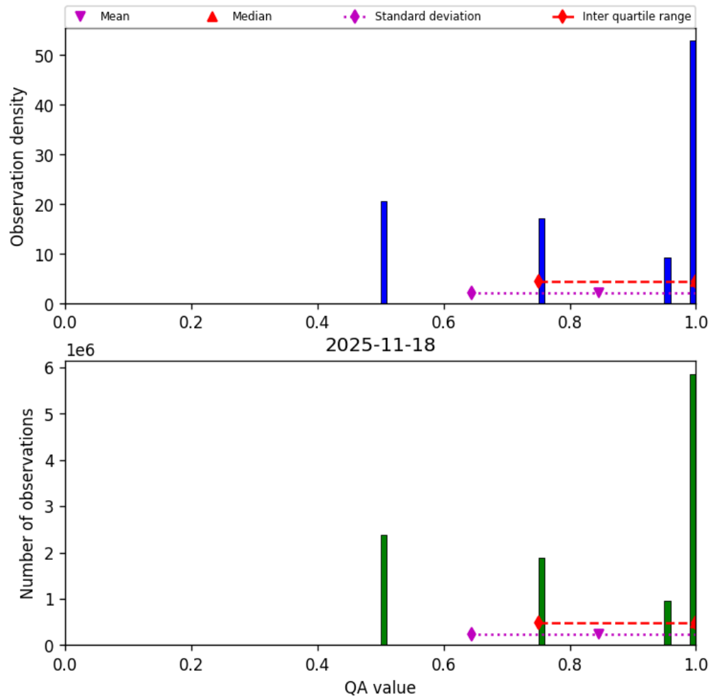
Figure 36: Histogram of “QA value” for 2025-11-18 to 2025-11-19
