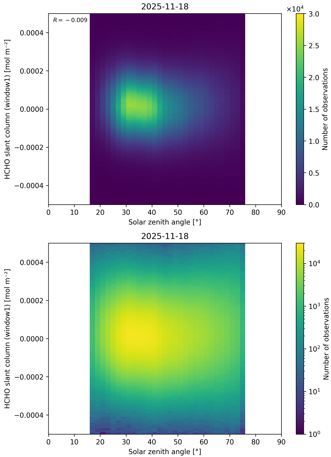
Figure 192: Scatter density plot of “Solar zenith angle” against “HCHO slant column (window1)” for 2025-11-18 to 2025-11-19.
