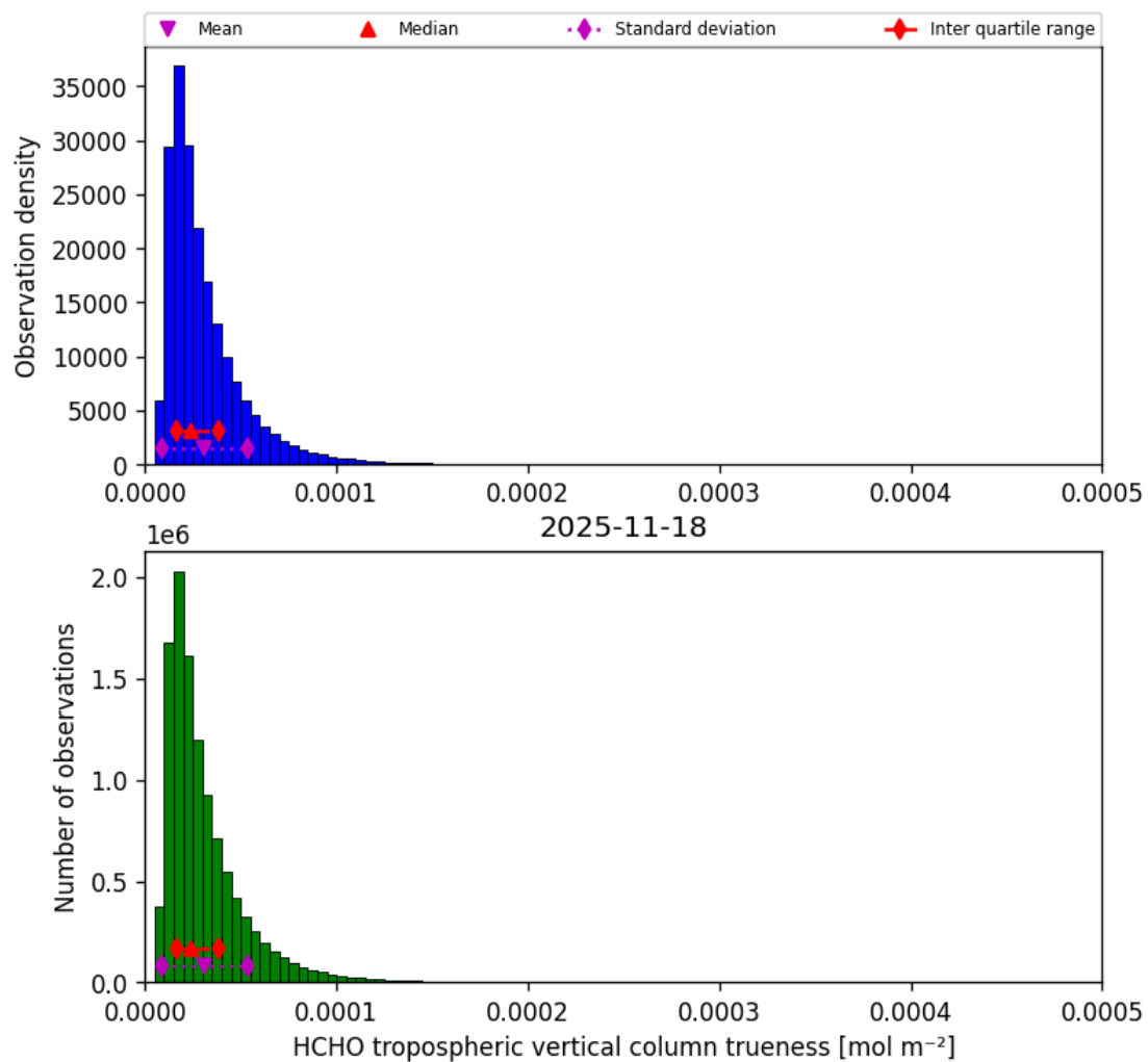
Figure 50: Histogram of “HCHO tropospheric vertical column trueness” for 2025-11-18 to 2025-11-19
