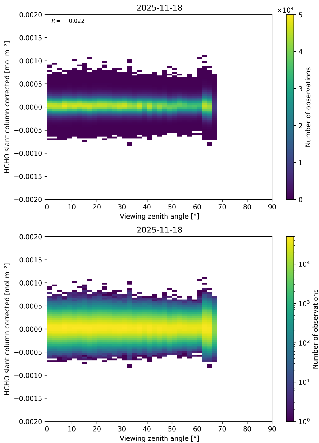
Figure 206: Scatter density plot of “Viewing zenith angle” against “HCHO slant column corrected” for 2025-11-18 to 2025-11-19.
