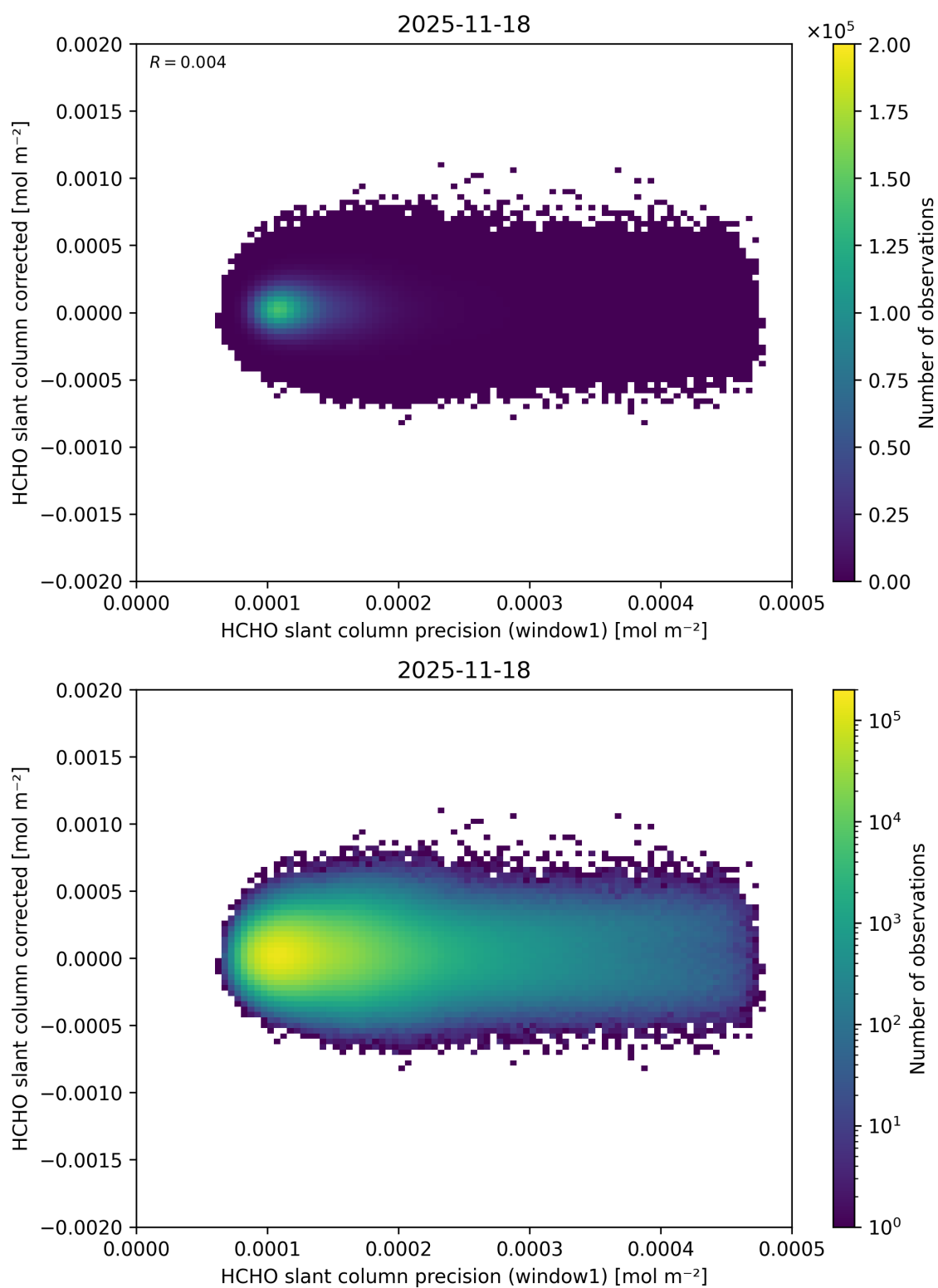
Figure 103: Scatter density plot of “HCHO slant column precision (window1)” against “HCHO slant column corrected” for 2025-11-18 to 2025-11-19.
