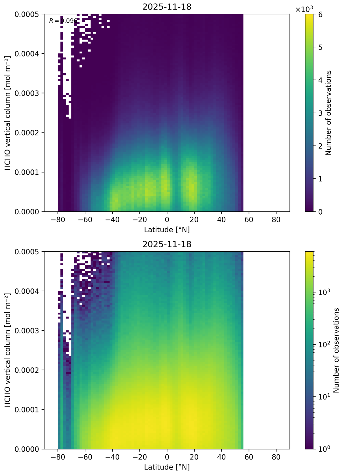
Figure 181: Scatter density plot of “Latitude” against “HCHO vertical column” for 2025-11-18 to 2025-11-19.
