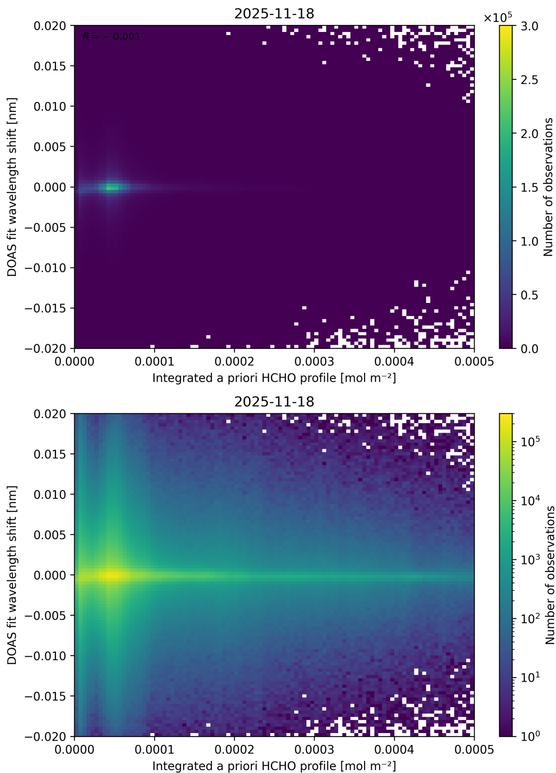
Figure 166: Scatter density plot of “Integrated a priori HCHO profile” against “DOAS fit wavelength shift” for 2025-11-18 to 2025-11-19.
