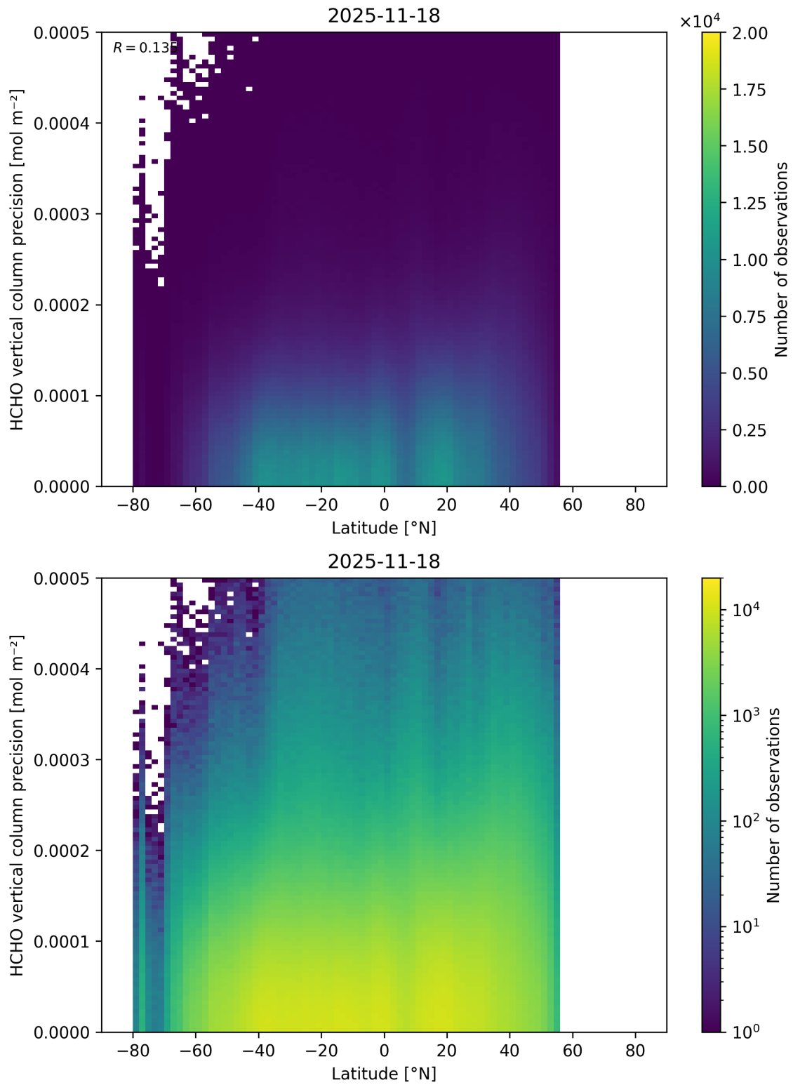
Figure 183: Scatter density plot of “Latitude” against “HCHO vertical column precision” for 2025-11-18 to 2025-11-19.
