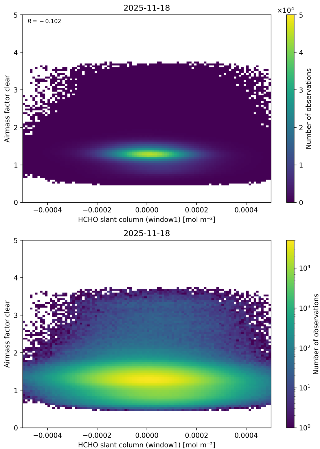
Figure 91: Scatter density plot of “HCHO slant column (window1)” against “Airmass factor clear” for 2025-11-18 to 2025-11-19.
