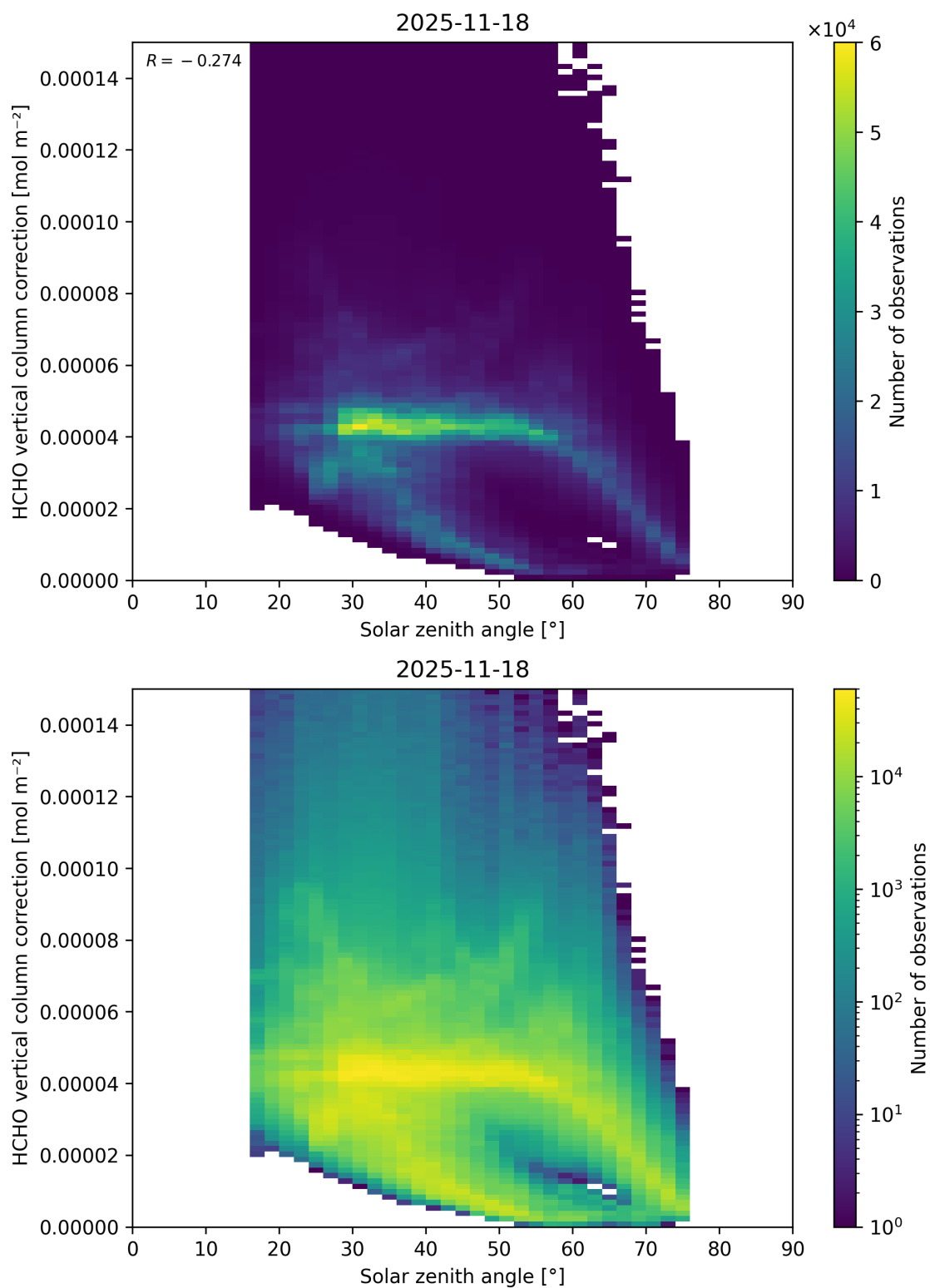
Figure 197: Scatter density plot of “Solar zenith angle” against “HCHO vertical column correction” for 2025-11-18 to 2025-11-19.
