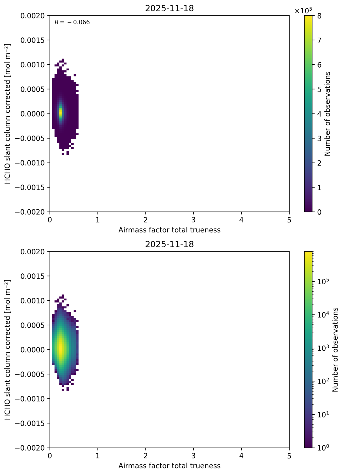
Figure 122: Scatter density plot of “Airmass factor total trueness” against “HCHO slant column corrected” for 2025-11-18 to 2025-11-19.
