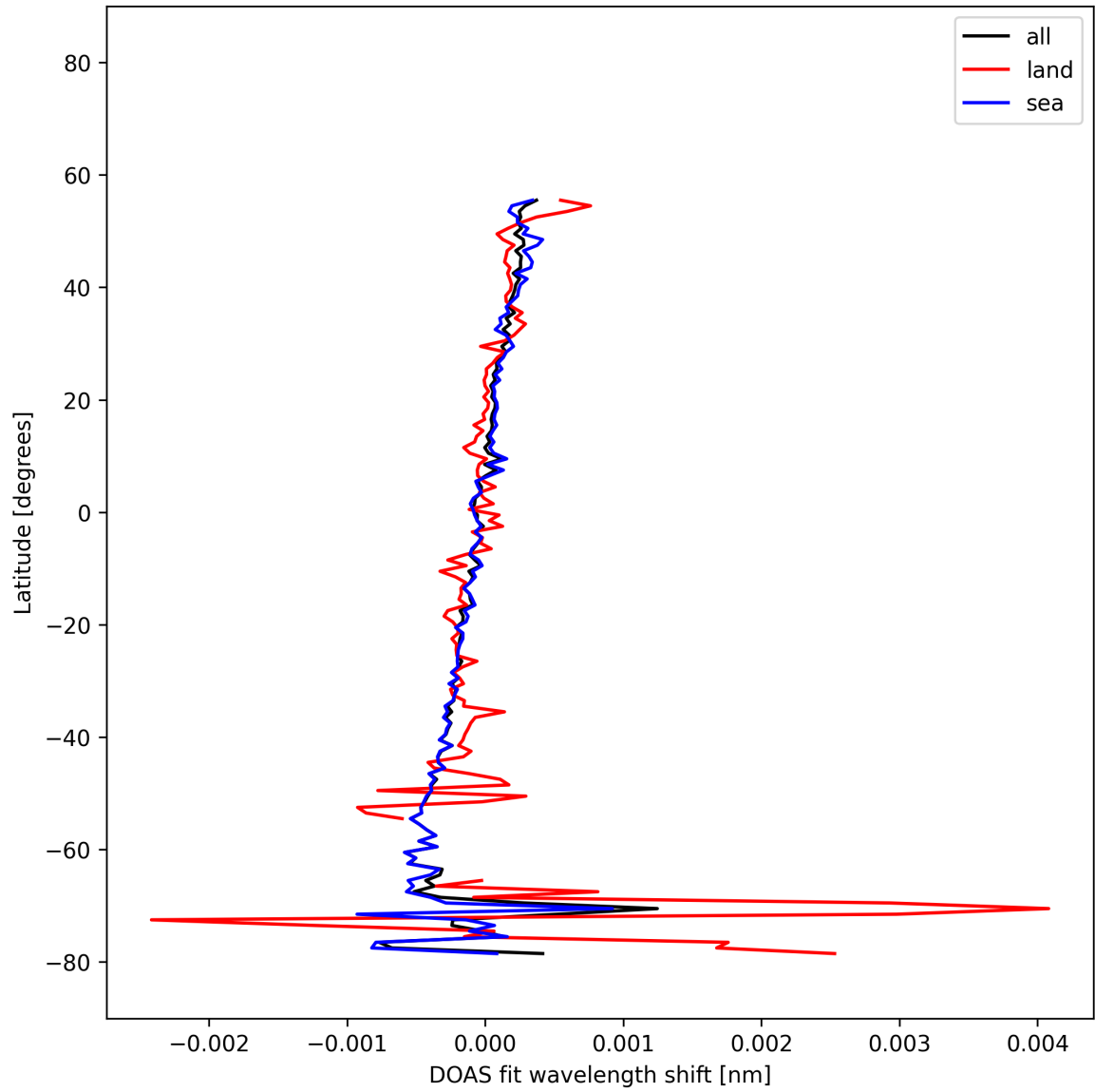
Figure 31: Zonal average of “DOAS fit wavelength shift” for 2025-11-18 to 2025-11-19.
