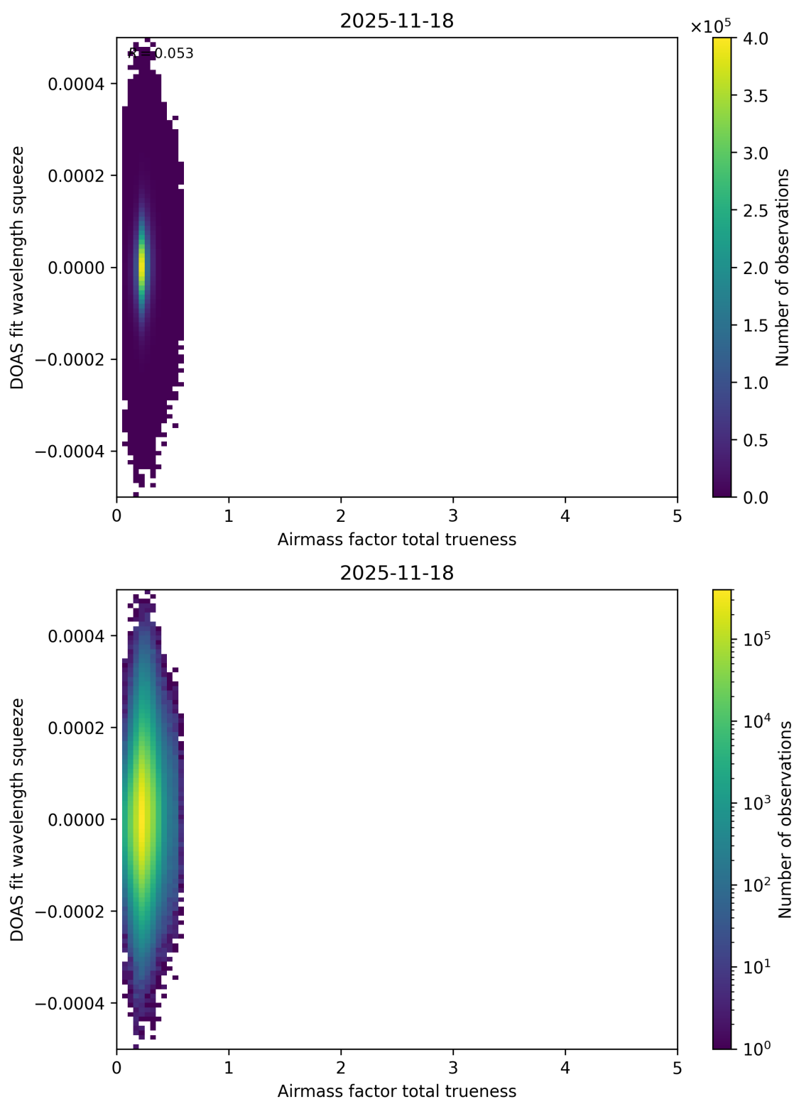
Figure 120: Scatter density plot of “Airmass factor total trueness” against “DOAS fit wavelength squeeze” for 2025-11-18 to 2025-11-19.
