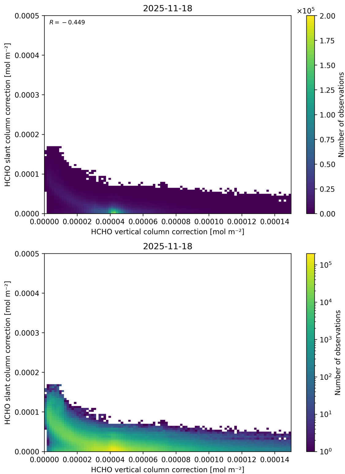
Figure 131: Scatter density plot of “HCHO vertical column correction” against “HCHO slant column correction” for 2025-11-18 to 2025-11-19.
