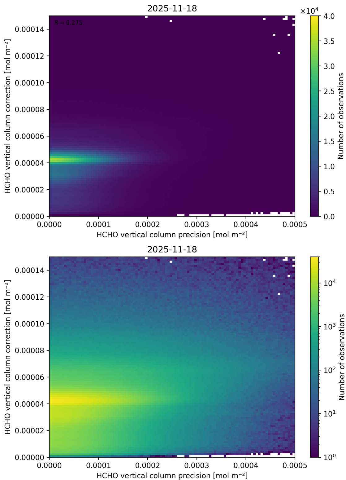
Figure 162: Scatter density plot of “HCHO vertical column precision” against “HCHO vertical column correction” for 2025-11-18 to 2025-11-19.
