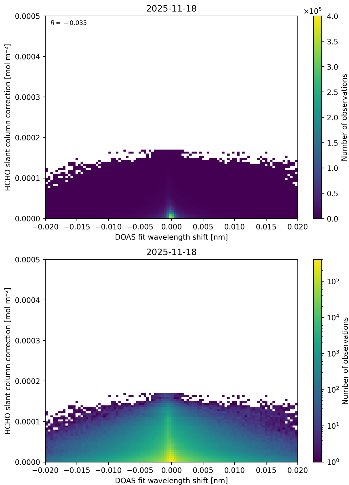
Figure 72: Scatter density plot of “DOAS fit wavelength shift” against “HCHO slant column correction” for 2025-11-18 to 2025-11-19.
