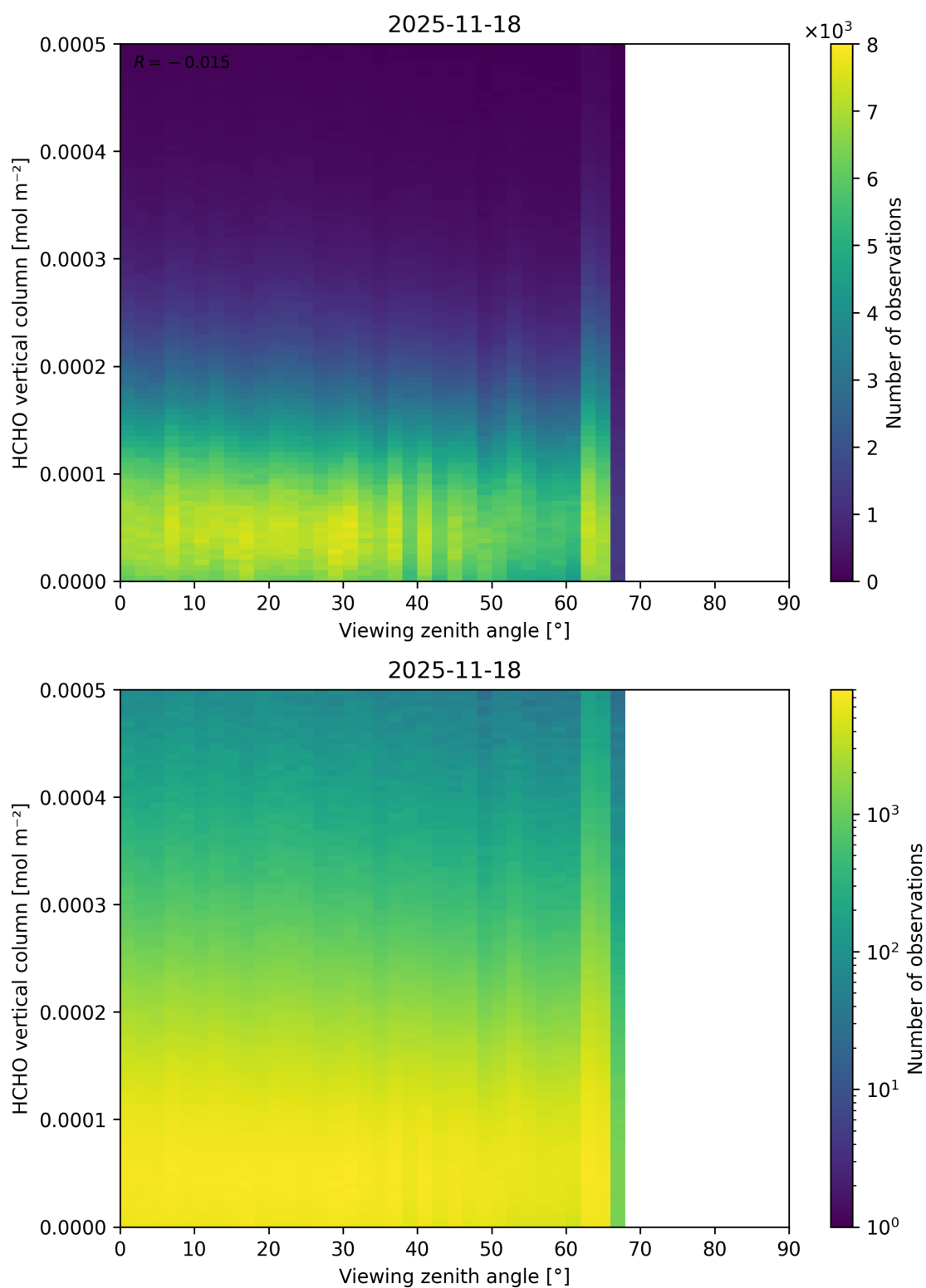
Figure 212: Scatter density plot of “Viewing zenith angle” against “HCHO vertical column” for 2025-11-18 to 2025-11-19.
