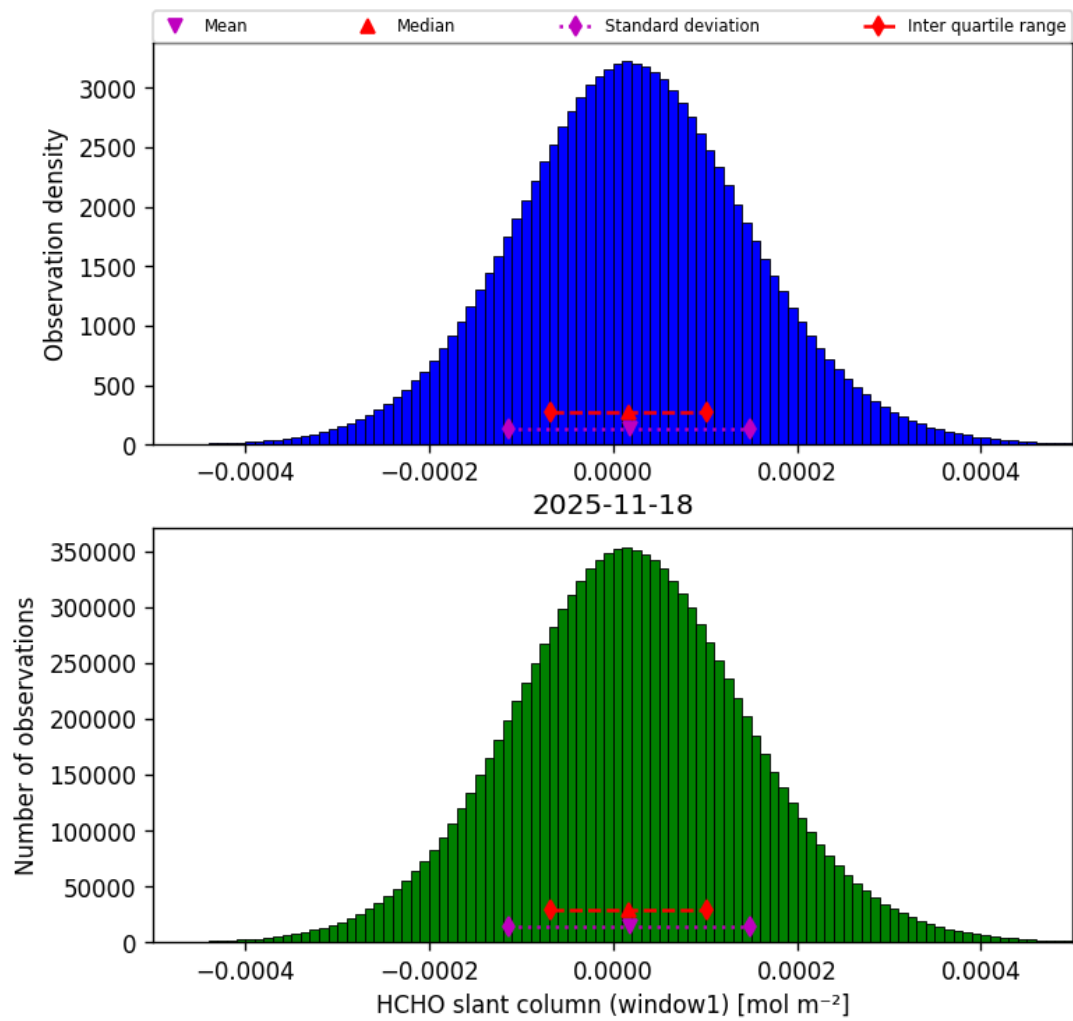
Figure 40: Histogram of “HCHO slant column (window1)” for 2025-11-18 to 2025-11-19
