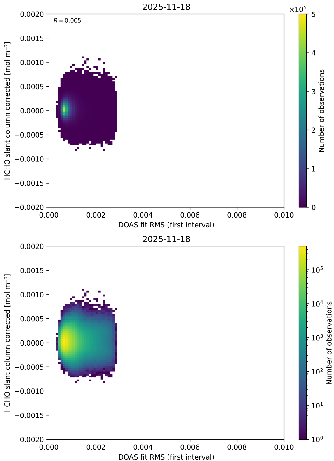
Figure 66: Scatter density plot of “DOAS fit RMS (first interval)” against “HCHO slant column corrected” for 2025-11-18 to 2025-11-19.
