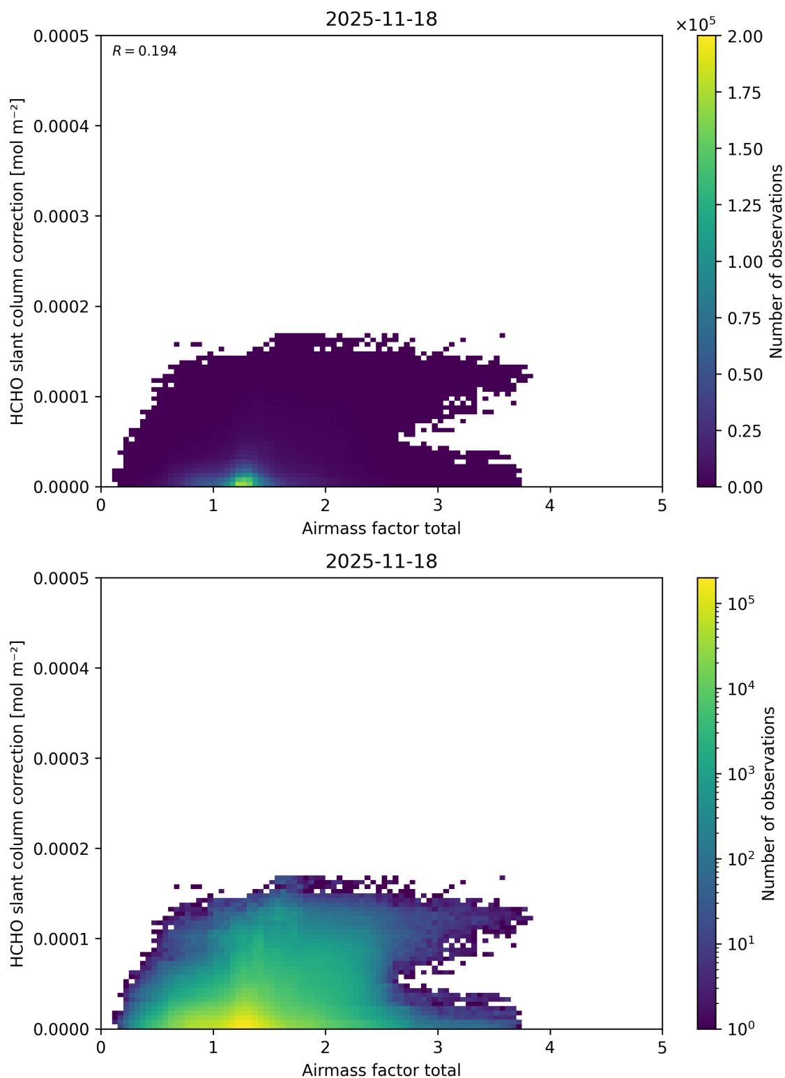
Figure 114: Scatter density plot of “Airmass factor total” against “HCHO slant column correction” for 2025-11-18 to 2025-11-19.
