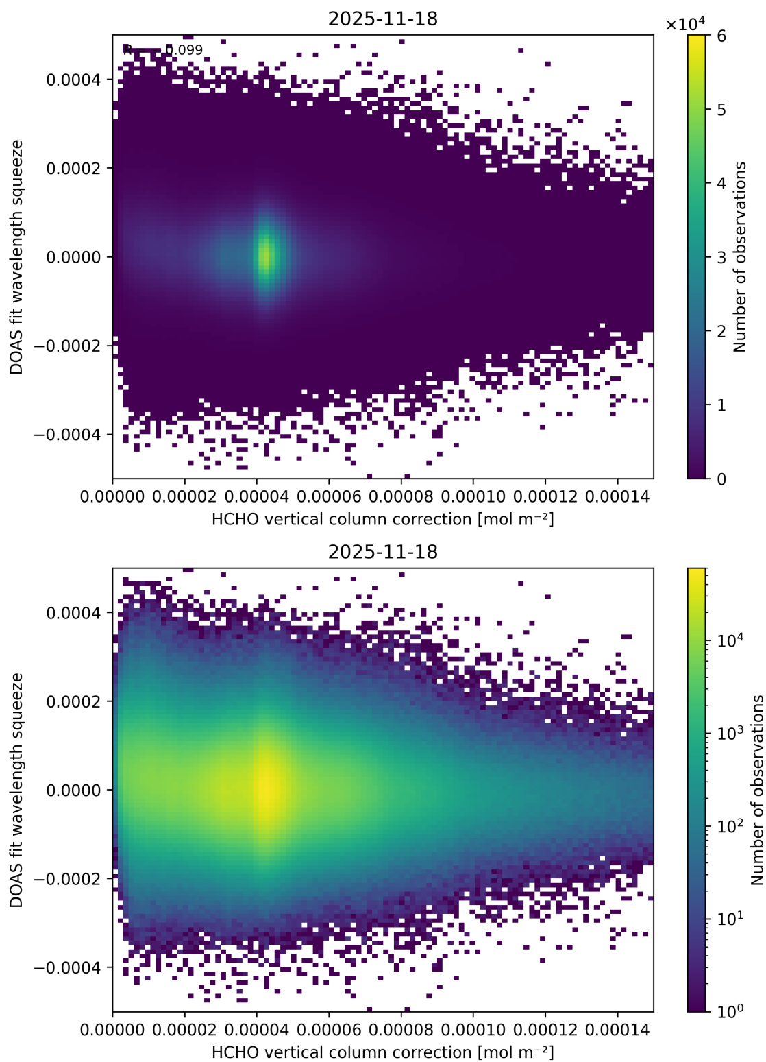
Figure 128: Scatter density plot of “HCHO vertical column correction” against “DOAS fit wavelength squeeze” for 2025-11-18 to 2025-11-19.
