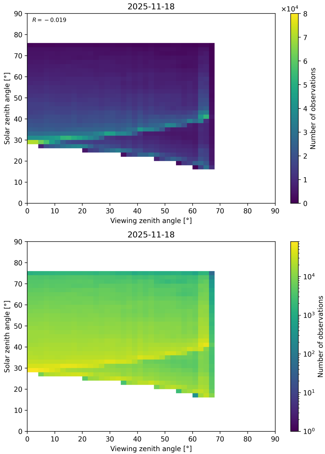
Figure 218: Scatter density plot of “Viewing zenith angle” against “Solar zenith angle” for 2025-11-18 to 2025-11-19.
