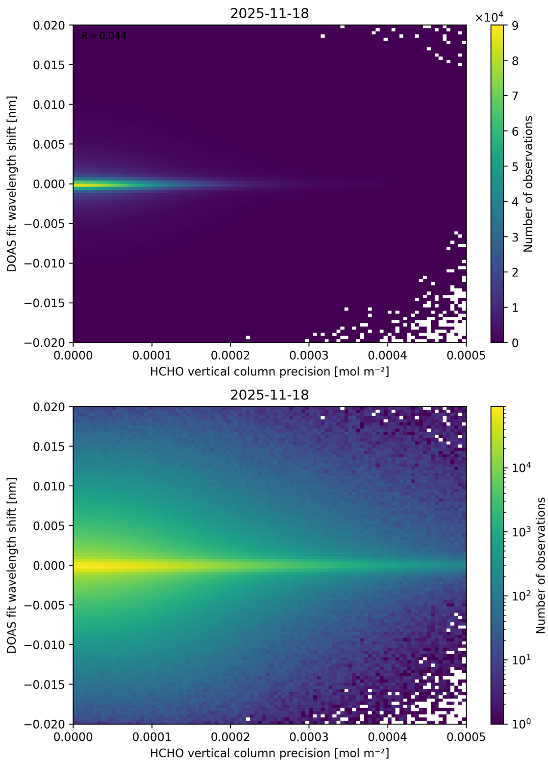
Figure 153: Scatter density plot of “HCHO vertical column precision” against “DOAS fit wavelength shift” for 2025-11-18 to 2025-11-19.
