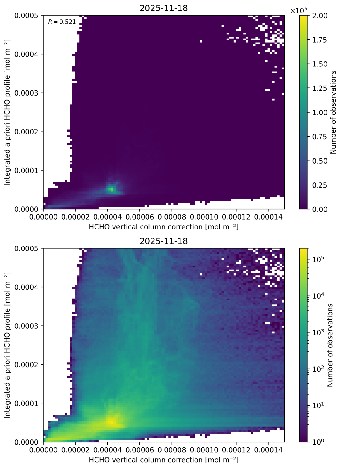
Figure 137: Scatter density plot of “HCHO vertical column correction” against “Integrated a priori HCHO profile” for 2025-11-18 to 2025-11-19.
