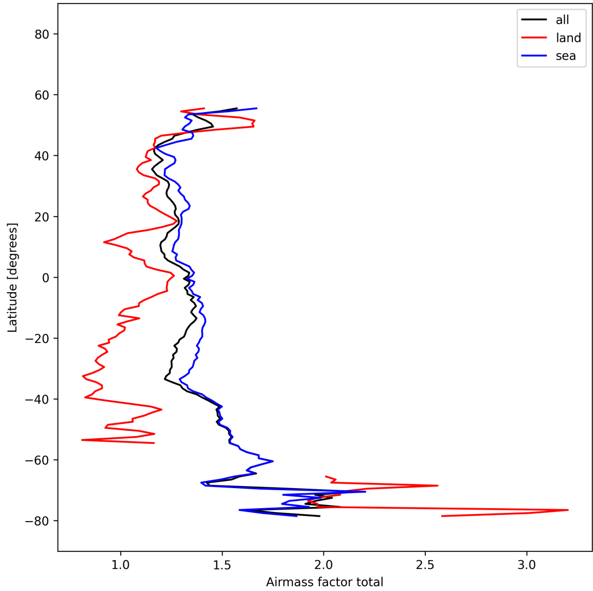
Figure 27: Zonal average of “Airmass factor total” for 2025-11-18 to 2025-11-19.
