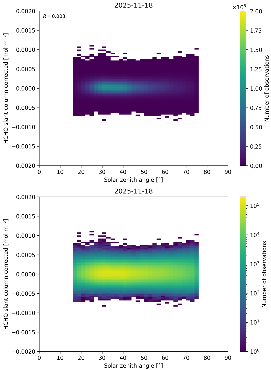
Figure 190: Scatter density plot of “Solar zenith angle” against “HCHO slant column corrected” for 2025-11-18 to 2025-11-19.
