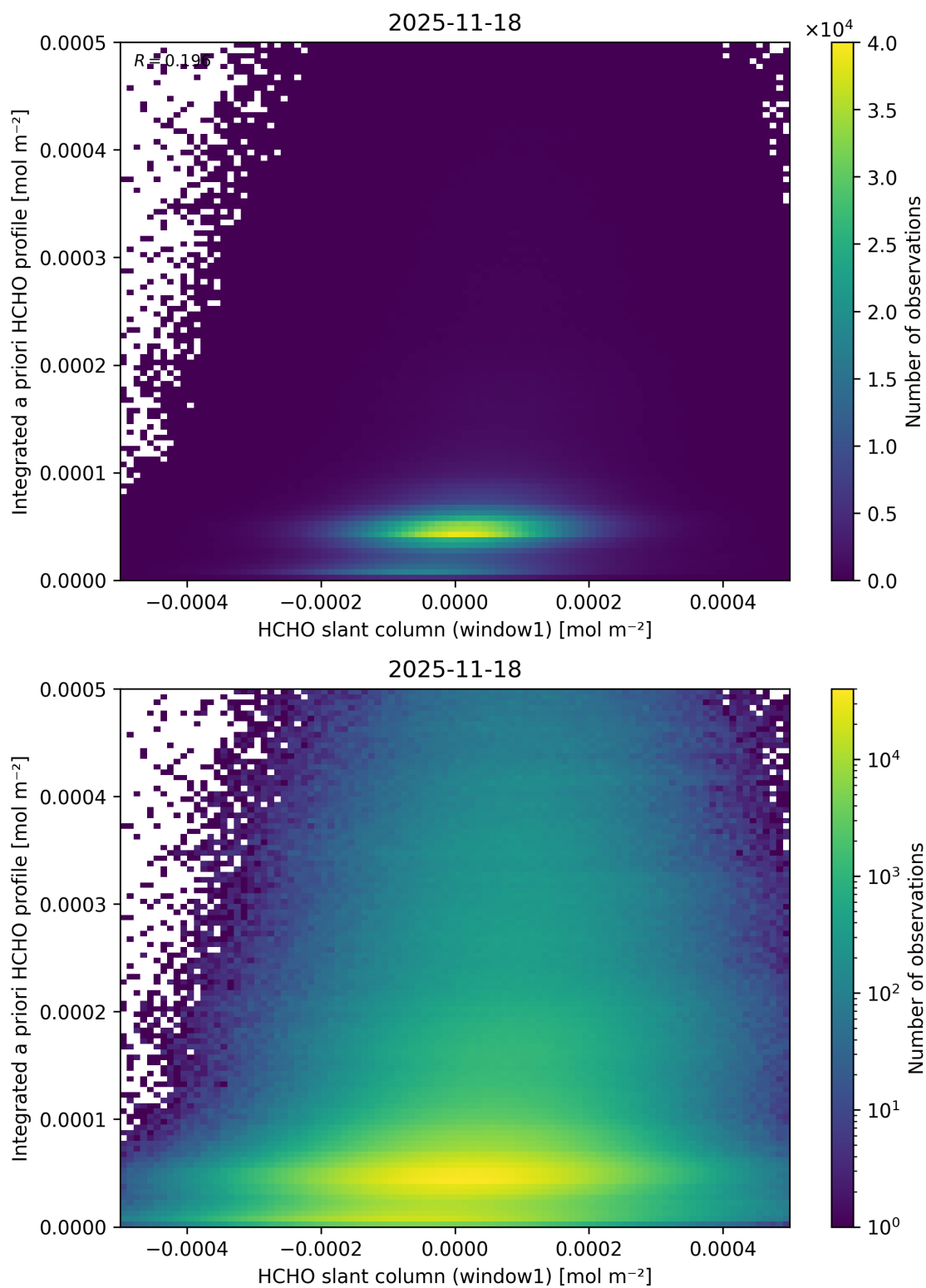
Figure 98: Scatter density plot of “HCHO slant column (window1)” against “Integrated a priori HCHO profile” for 2025-11-18 to 2025-11-19.
