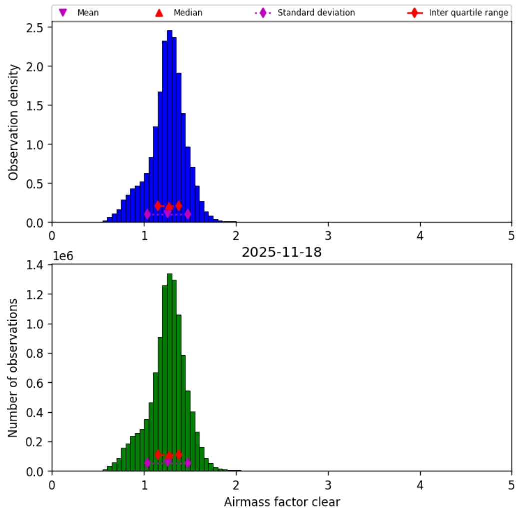
Figure 44: Histogram of “Airmass factor clear” for 2025-11-18 to 2025-11-19
