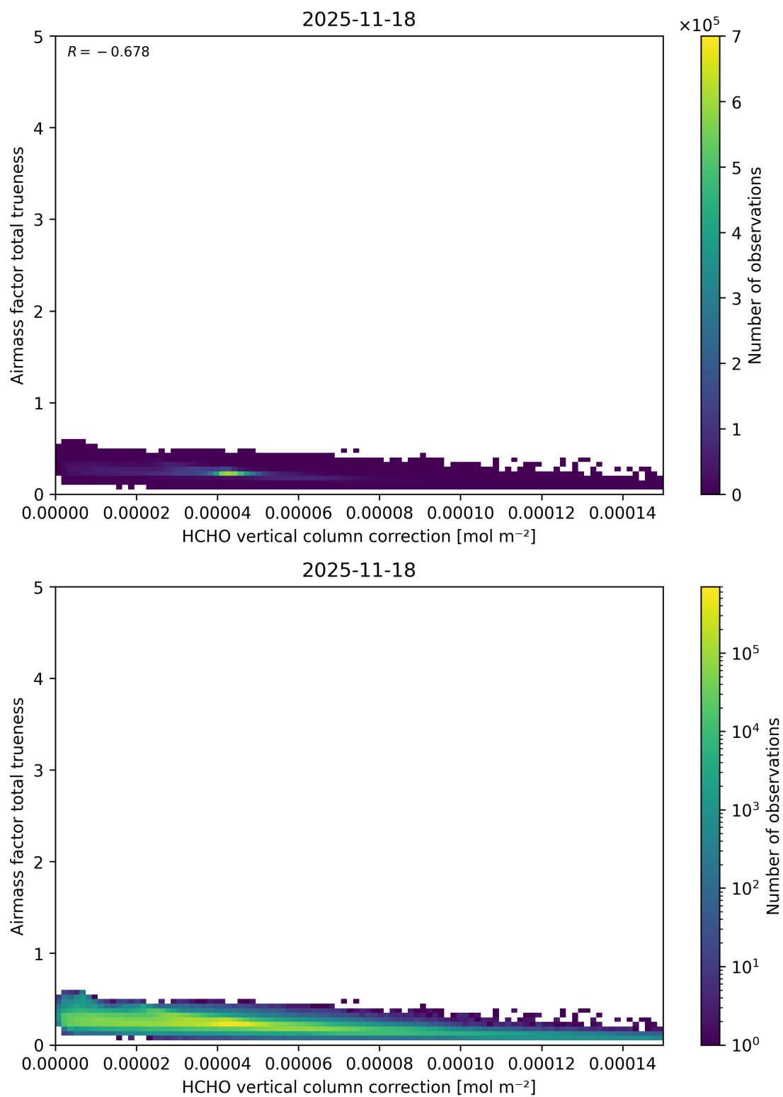
Figure 135: Scatter density plot of “HCHO vertical column correction” against “Airmass factor total trueness” for 2025-11-18 to 2025-11-19.
