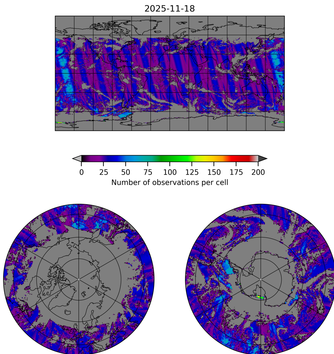
Figure 20: Map of the number of observations for 2025-11-18 to 2025-11-19
