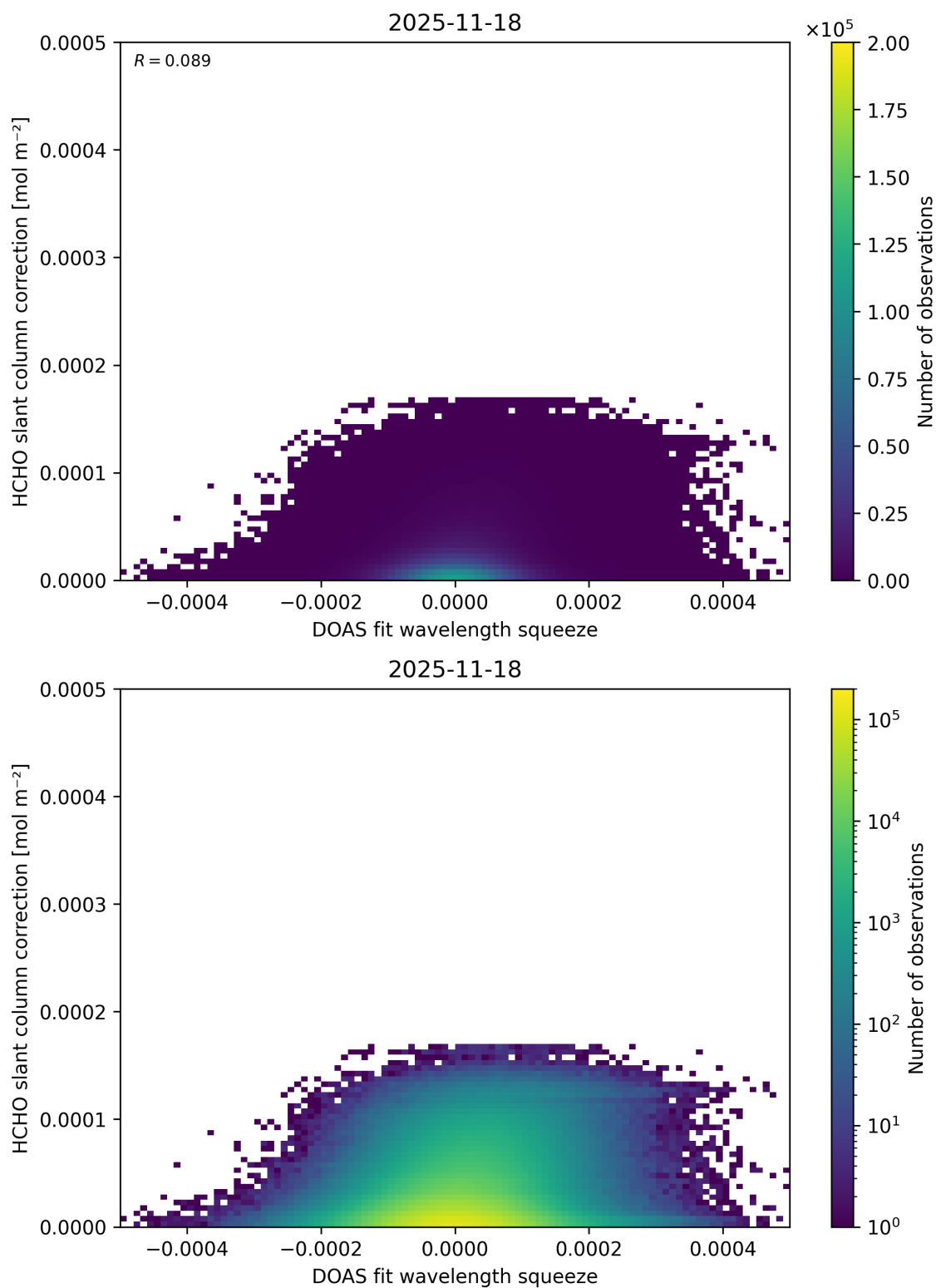
Figure 76: Scatter density plot of “DOAS fit wavelength squeeze” against “HCHO slant column correction” for 2025-11-18 to 2025-11-19.
