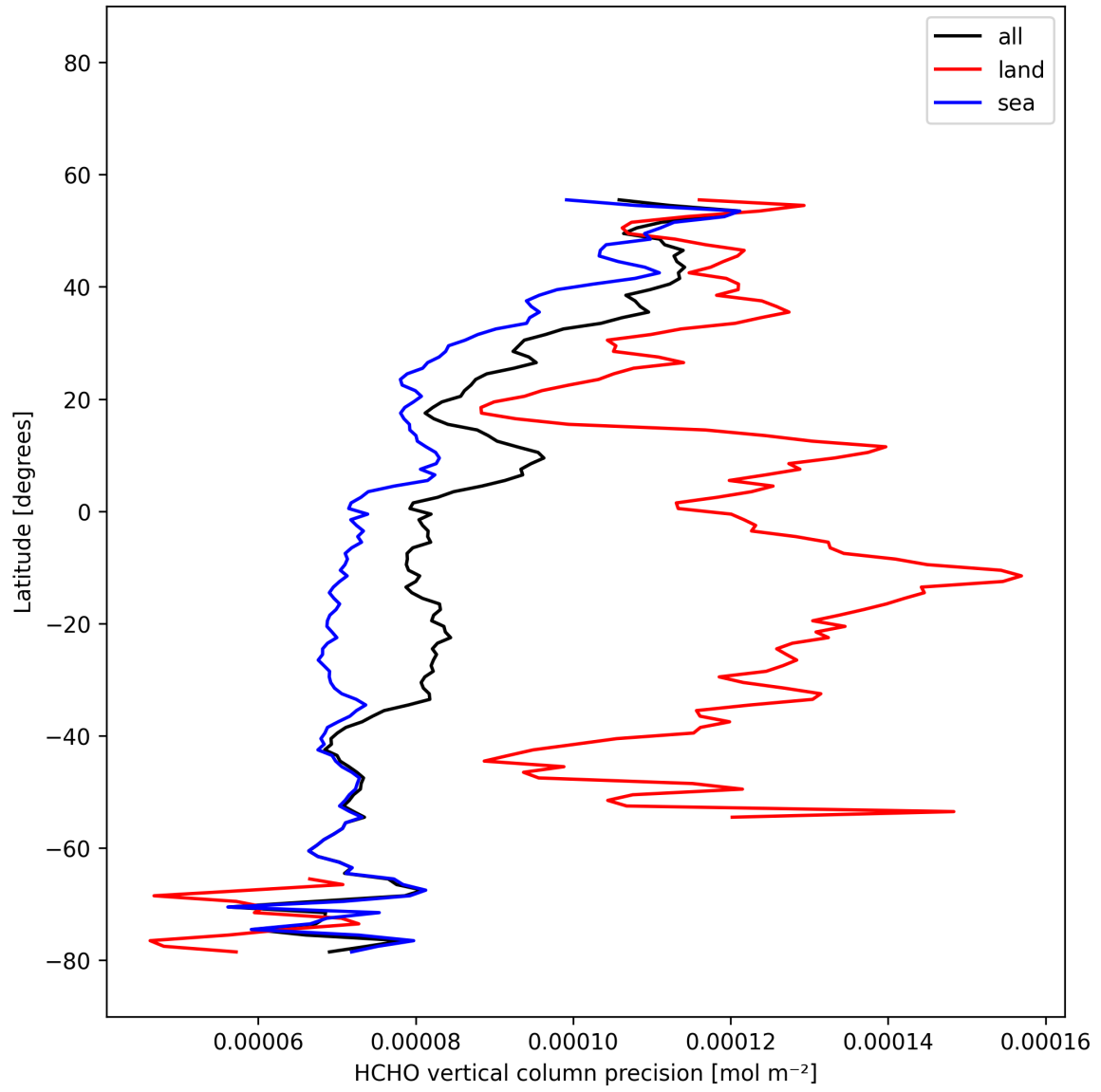
Figure 23: Zonal average of “HCHO vertical column precision” for 2025-11-18 to 2025-11-19.
