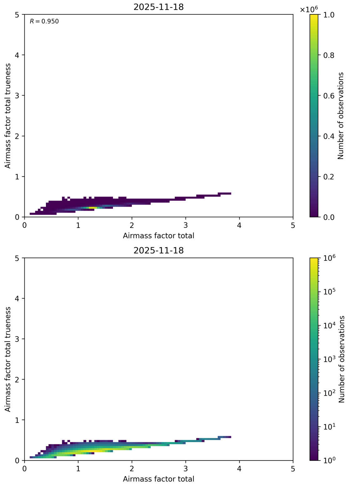
Figure 115: Scatter density plot of “Airmass factor total” against “Airmass factor total trueness” for 2025-11-18 to 2025-11-19.
