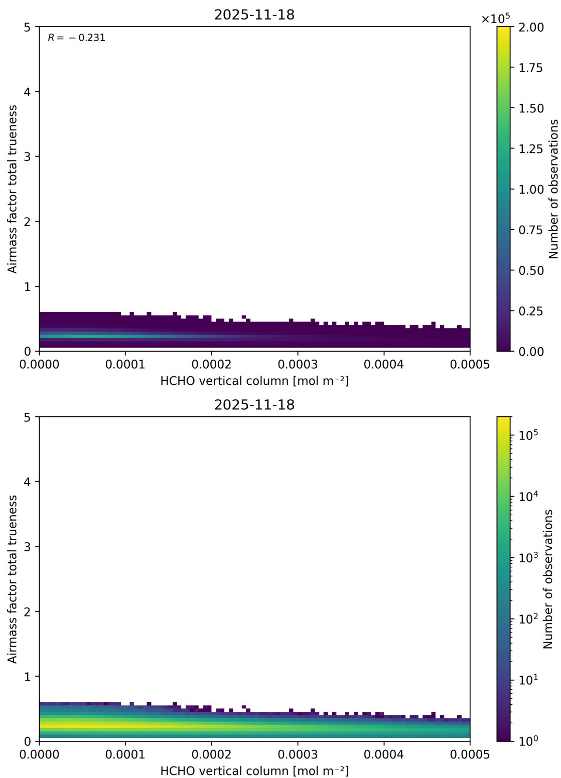
Figure 147: Scatter density plot of “HCHO vertical column” against “Airmass factor total trueneess” for 2025-11-18 to 2025-11-19.
