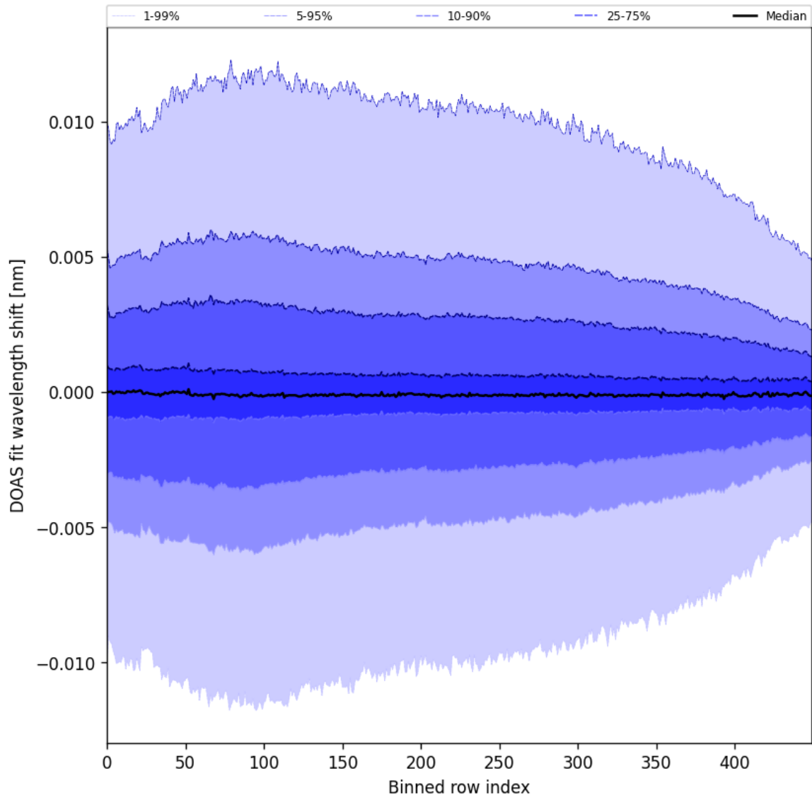
Figure 61: Along track statistics of “DOAS fit wavelength shift” for 2025-11-18 to 2025-11-19
