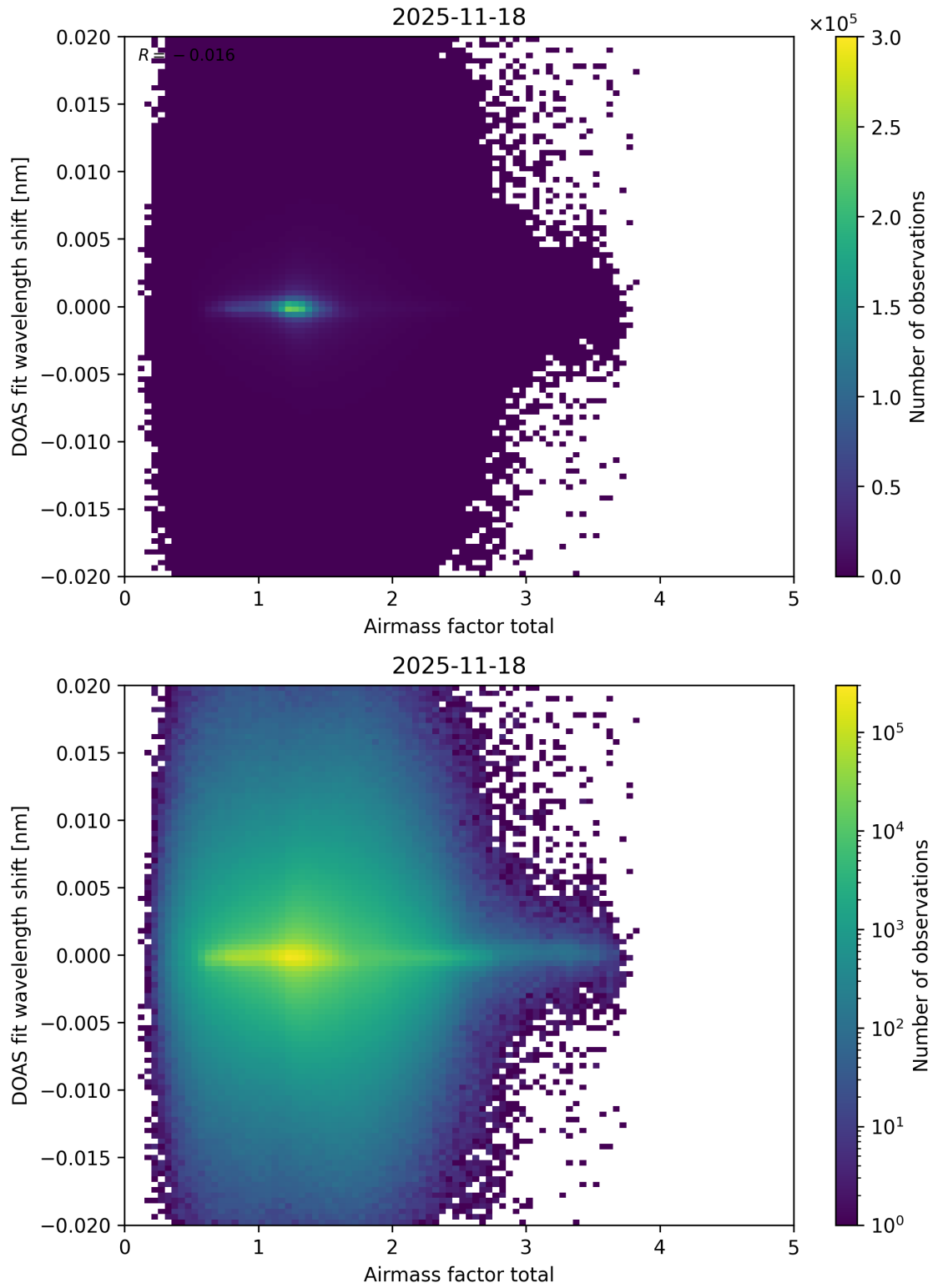
Figure 110: Scatter density plot of “Airmass factor total” against “DOAS fit wavelength shift” for 2025-11-18 to 2025-11-19.
