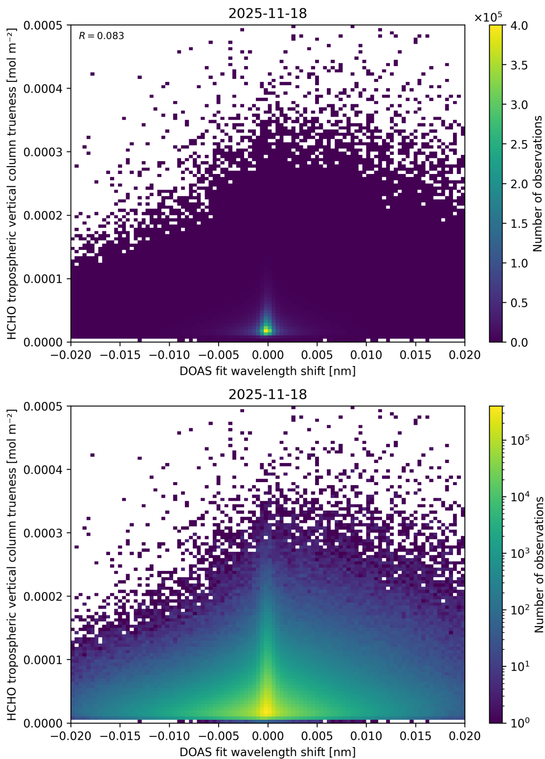
Figure 73: Scatter density plot of “DOAS fit wavelength shift” against “HCHO tropospheric vertical column trueness” for 2025-11-18 to 2025-11-19.
