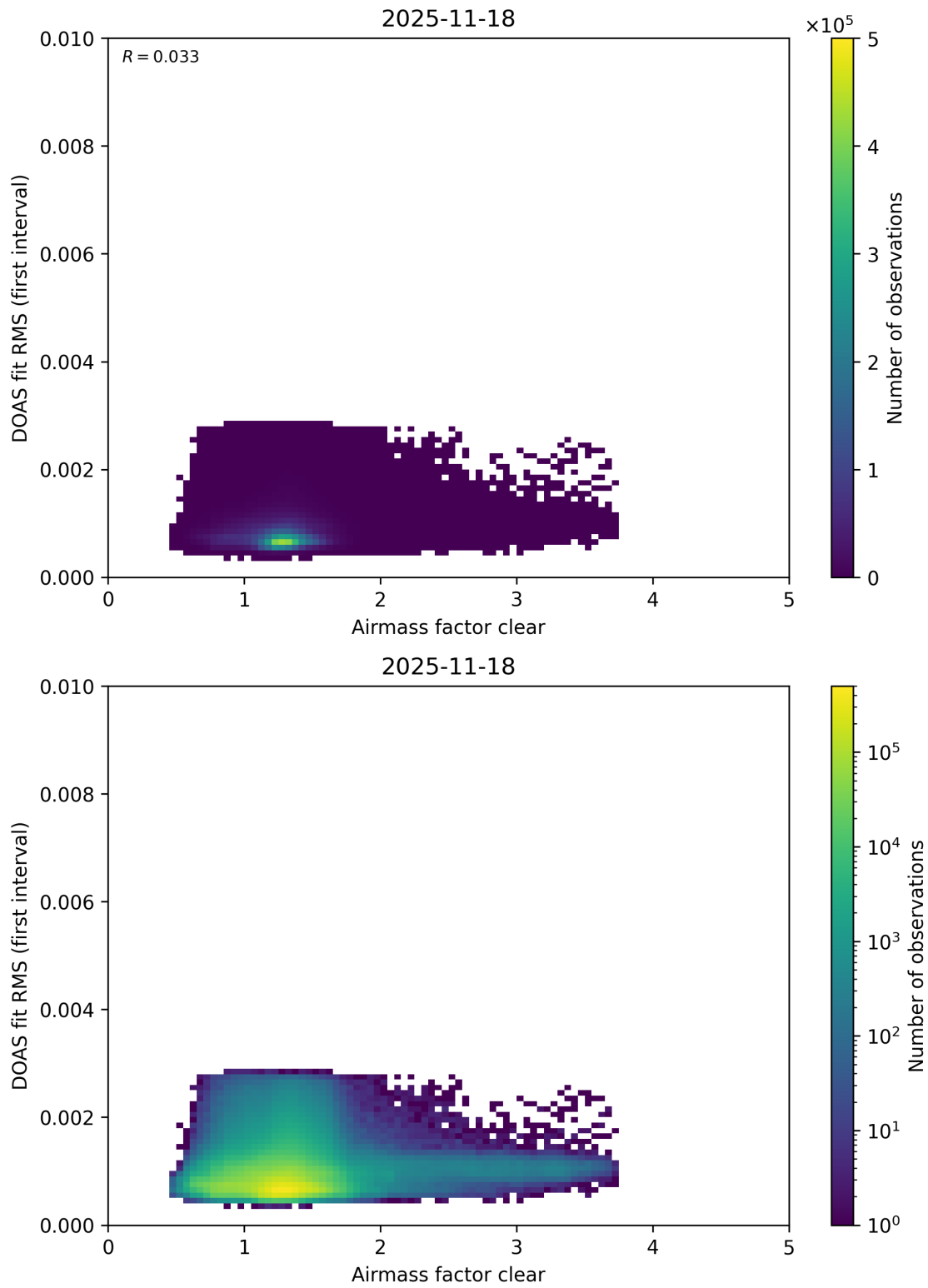
Figure 78: Scatter density plot of “Airmass factor clear” against “DOAS fit RMS (first interval)” for 2025-11-18 to 2025-11-19.
