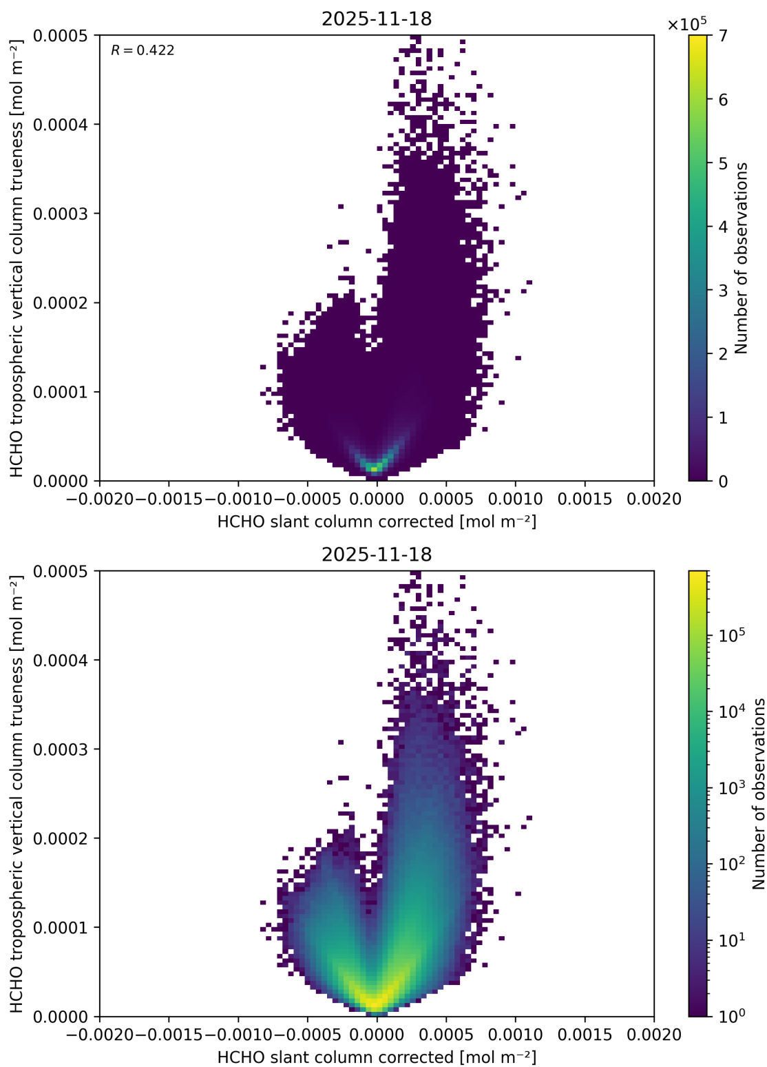
Figure 86: Scatter density plot of “HCHO slant column corrected” against “HCHO tropospheric vertical column trueness” for 2025-11-18 to 2025-11-19.
