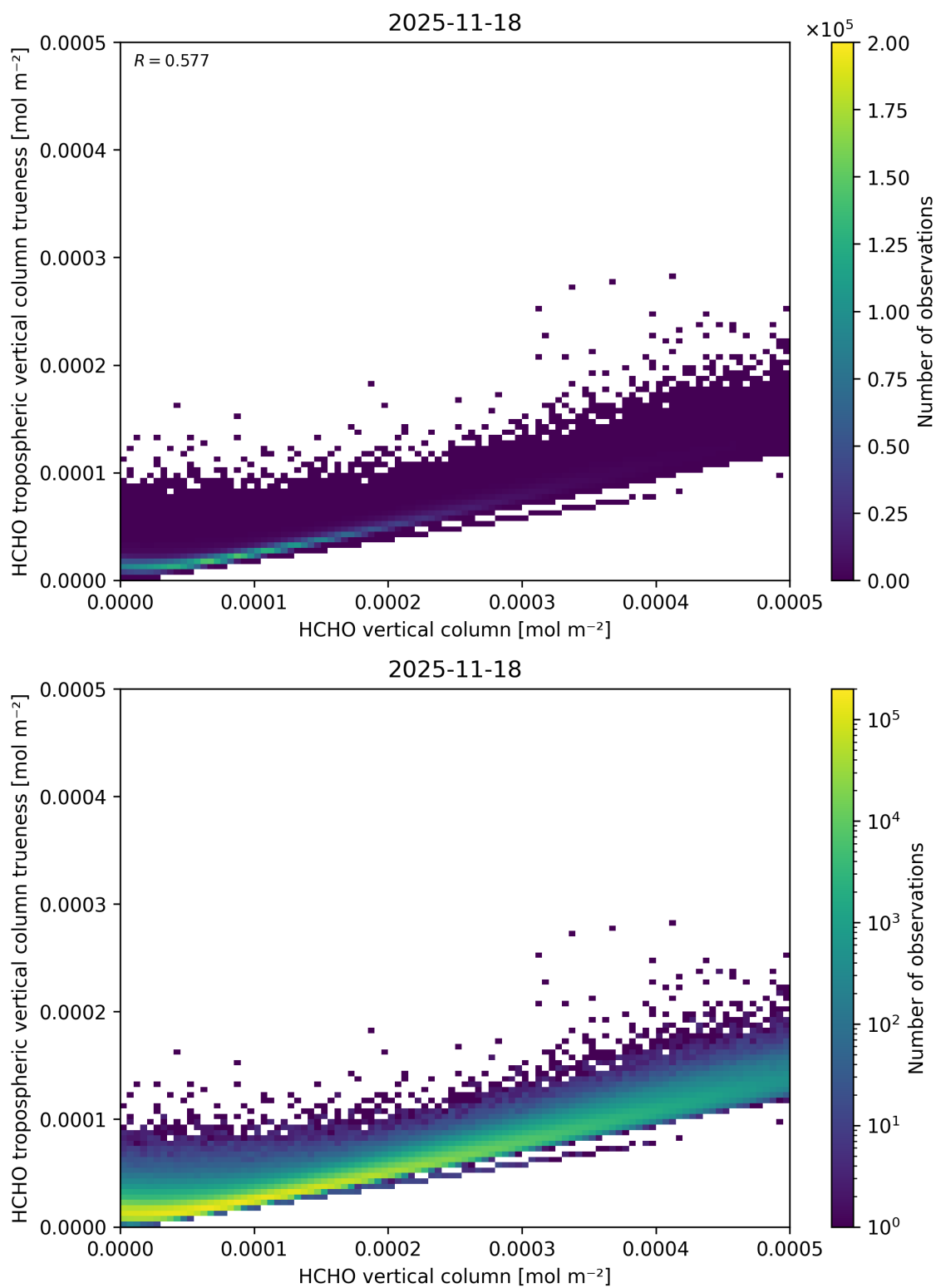
Figure 150: Scatter density plot of “HCHO vertical column” against “HCHO tropospheric vertical column trueness” for 2025-11-18 to 2025-11-19.
