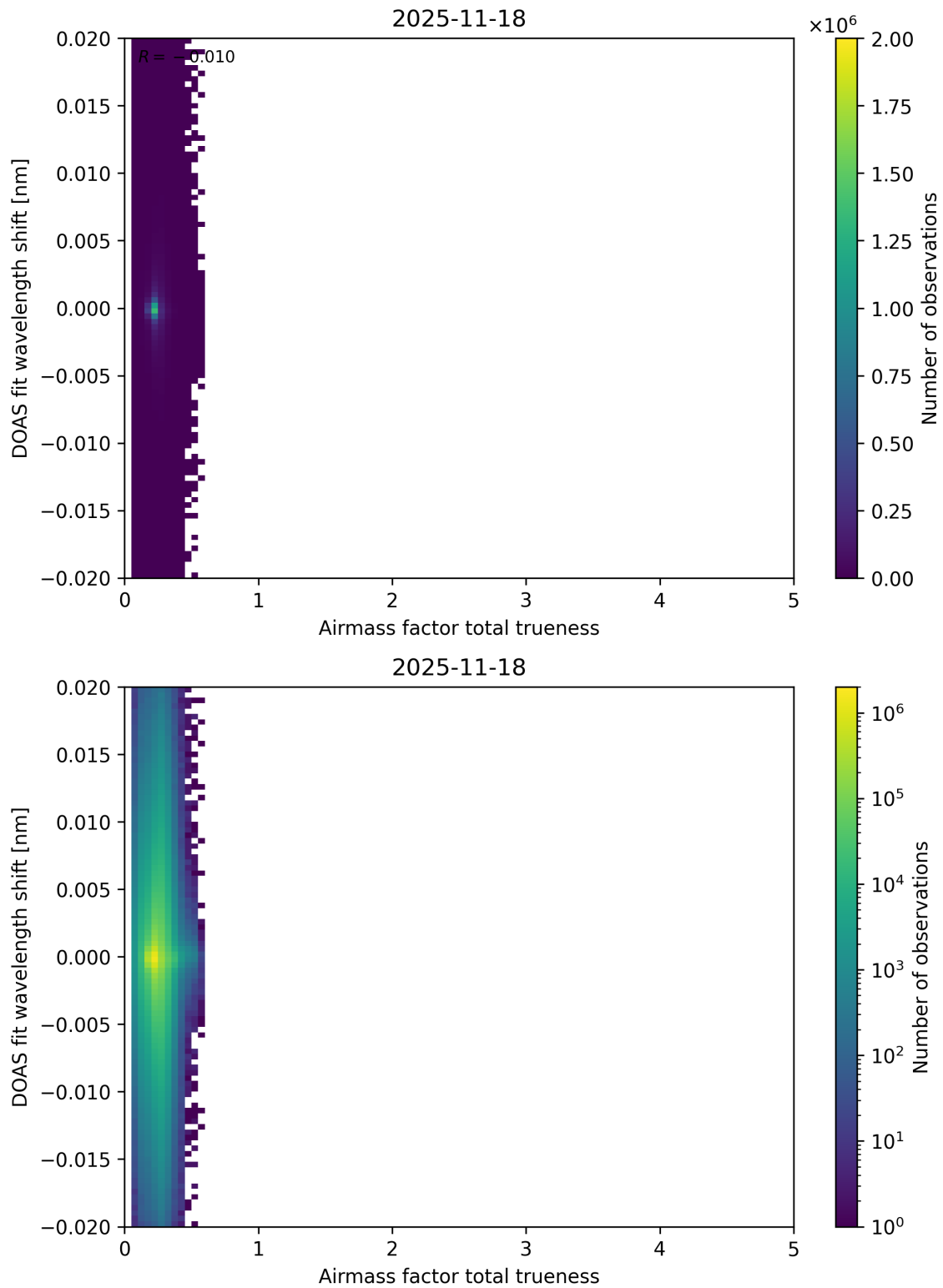
Figure 119: Scatter density plot of “Airmass factor total trueness” against “DOAS fit wavelength shift” for 2025-11-18 to 2025-11-19.
