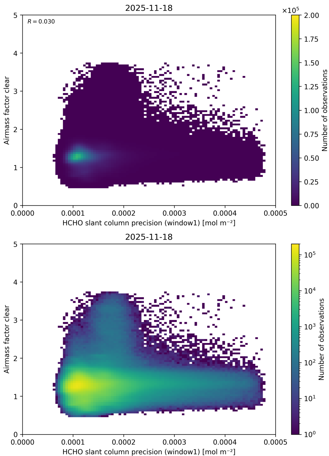
Figure 102: Scatter density plot of “HCHO slant column precision (window1)” against “Airmass factor clear” for 2025-11-18 to 2025-11-19.
