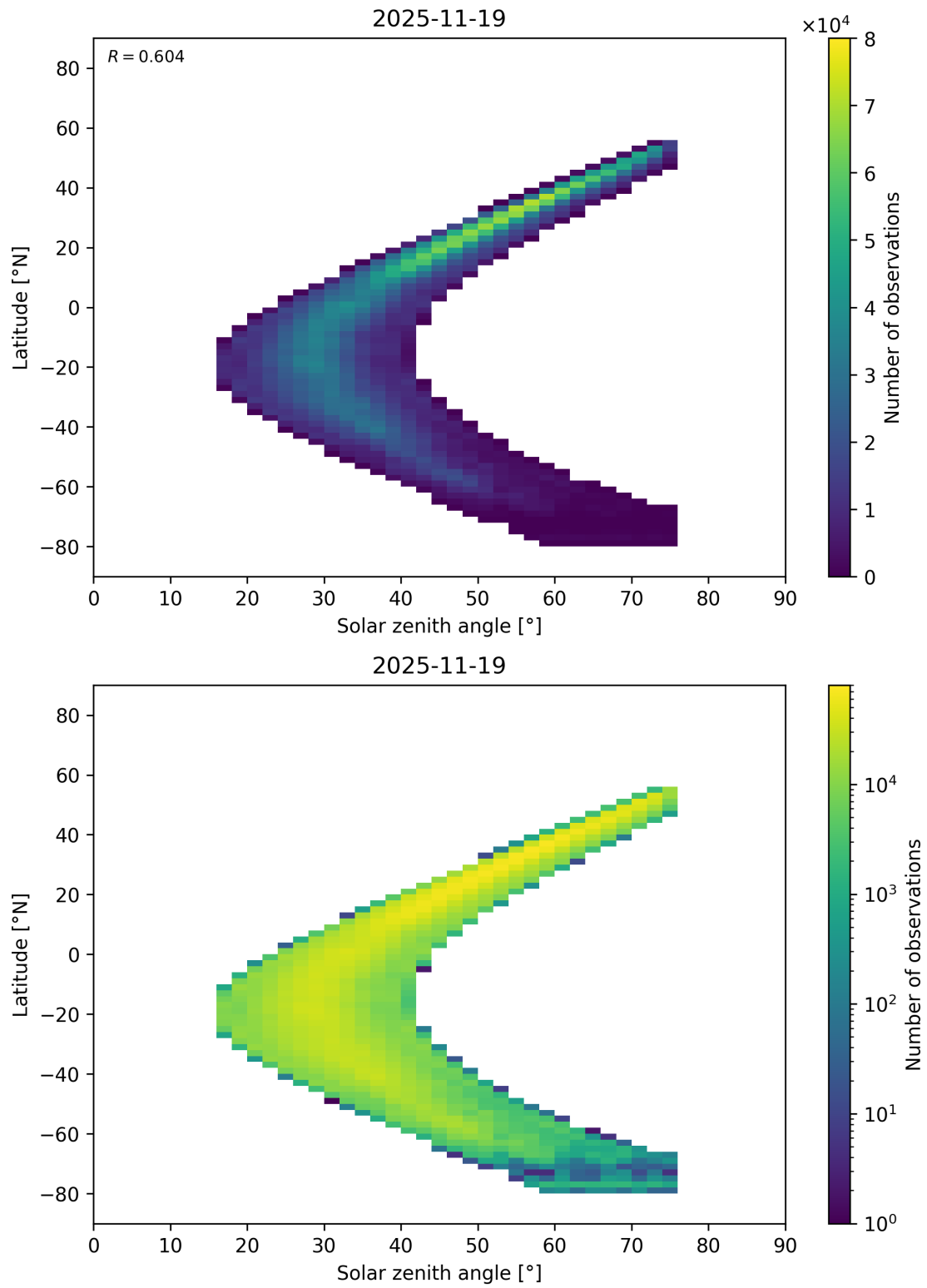
Figure 201: Scatter density plot of “Solar zenith angle” against “Latitude” for 2025-11-18 to 2025-11-20.
