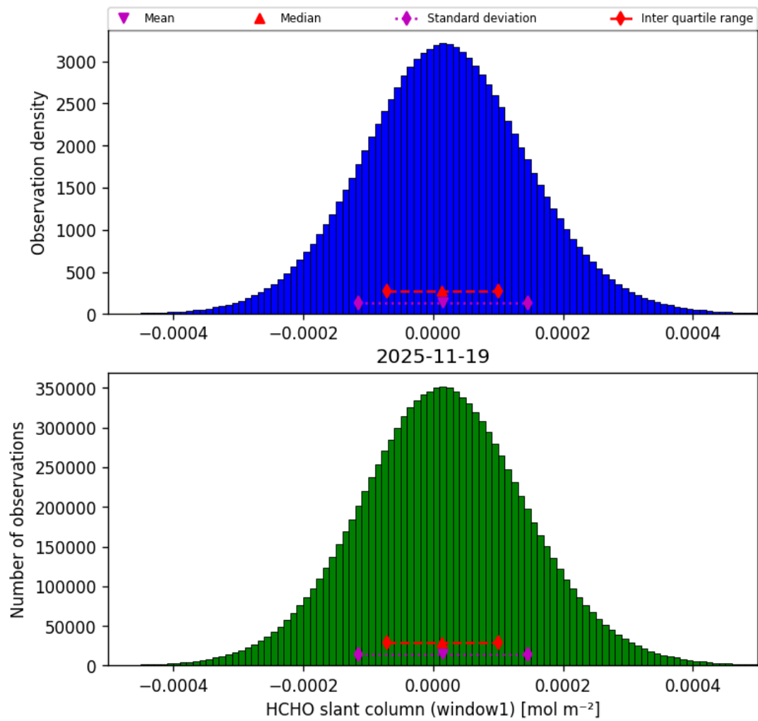
Figure 40: Histogram of “HCHO slant column (window1)” for 2025-11-18 to 2025-11-20
