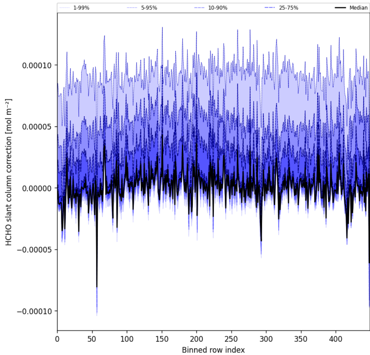
Figure 64: Along track statistics of “HCHO slant column correction” for 2025-11-18 to 2025-11-20
