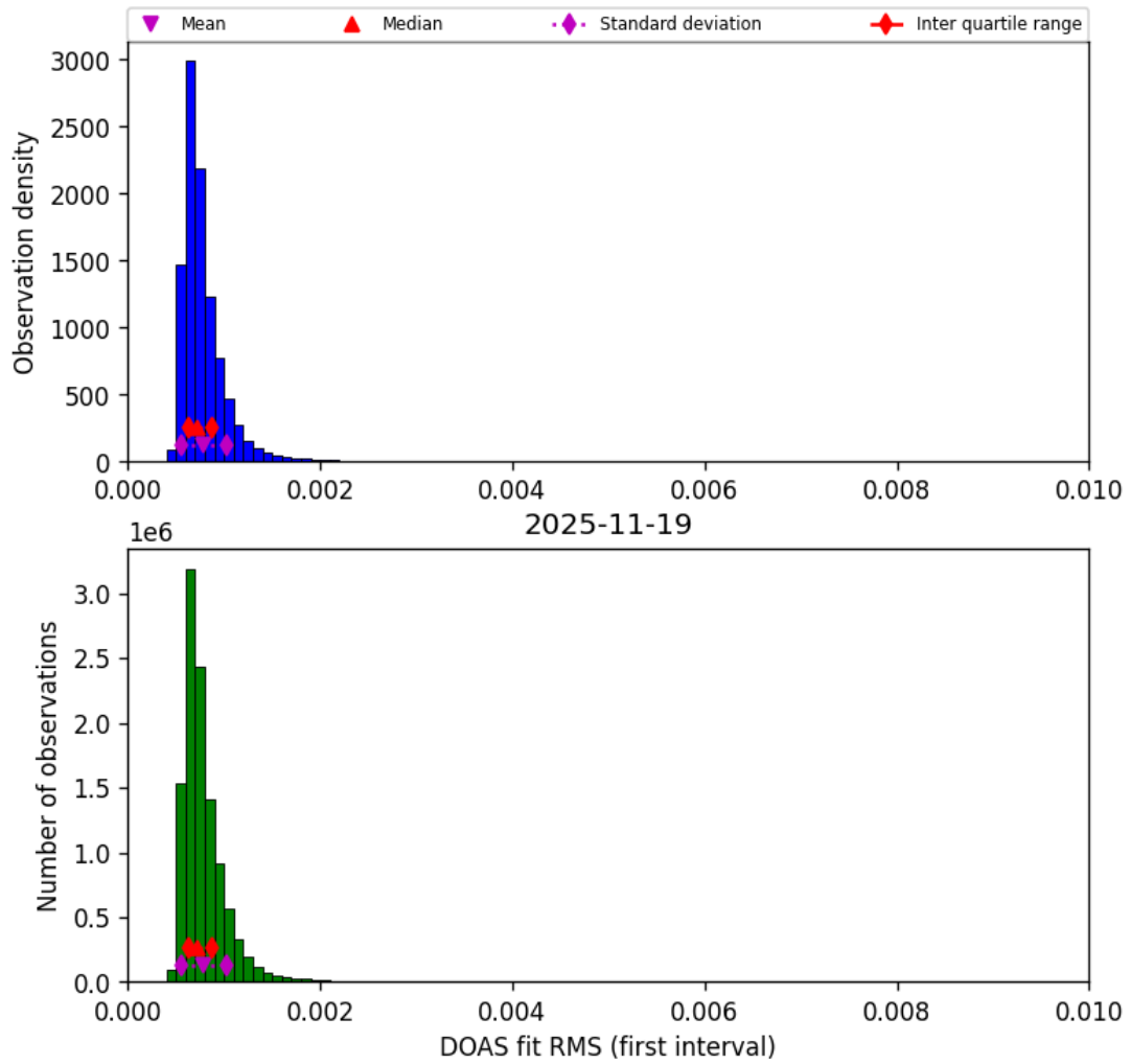
Figure 48: Histogram of “DOAS fit RMS (first interval)” for 2025-11-18 to 2025-11-20
