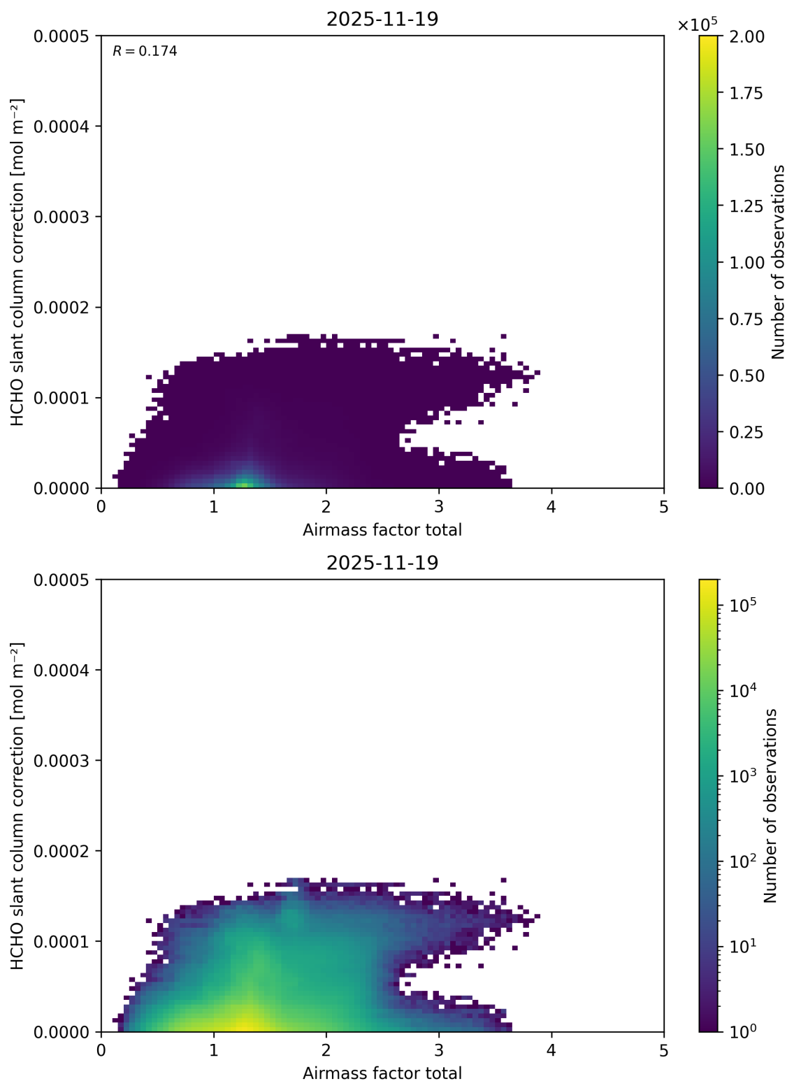
Figure 114: Scatter density plot of “Airmass factor total” against “HCHO slant column correction” for 2025-11-18 to 2025-11-20.
