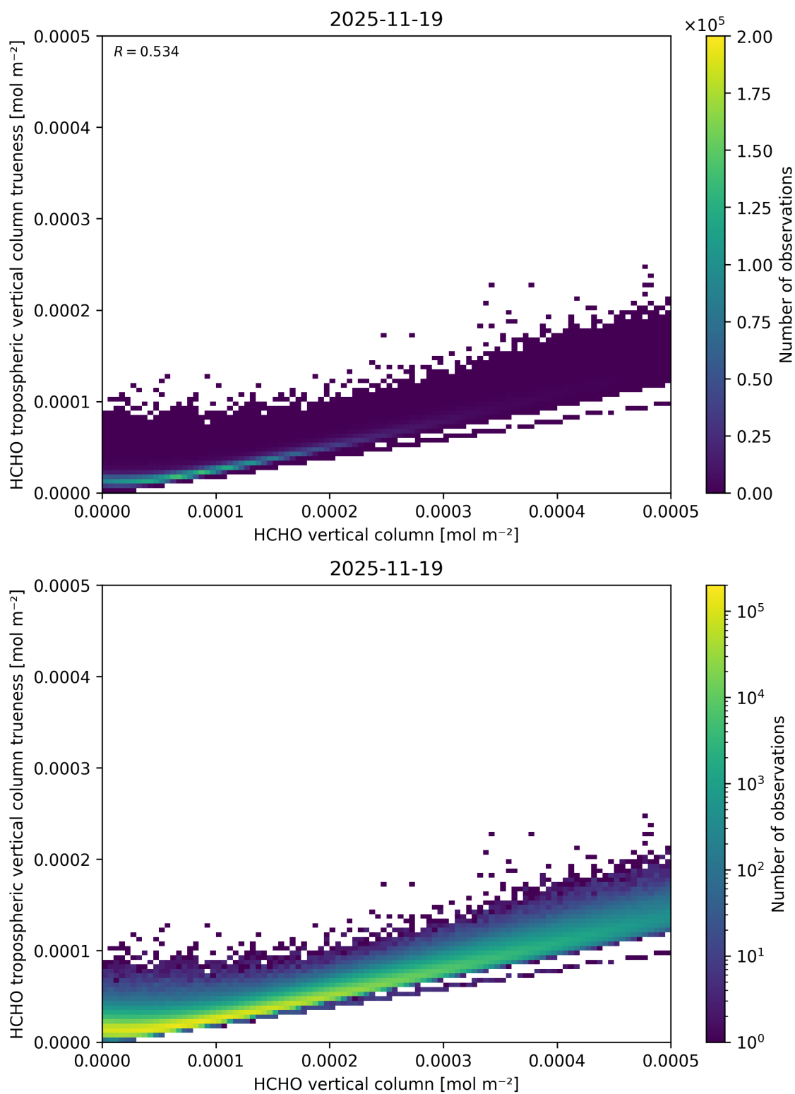
Figure 150: Scatter density plot of “HCHO vertical column” against “HCHO tropospheric vertical column trueness” for 2025-11-18 to 2025-11-20.
