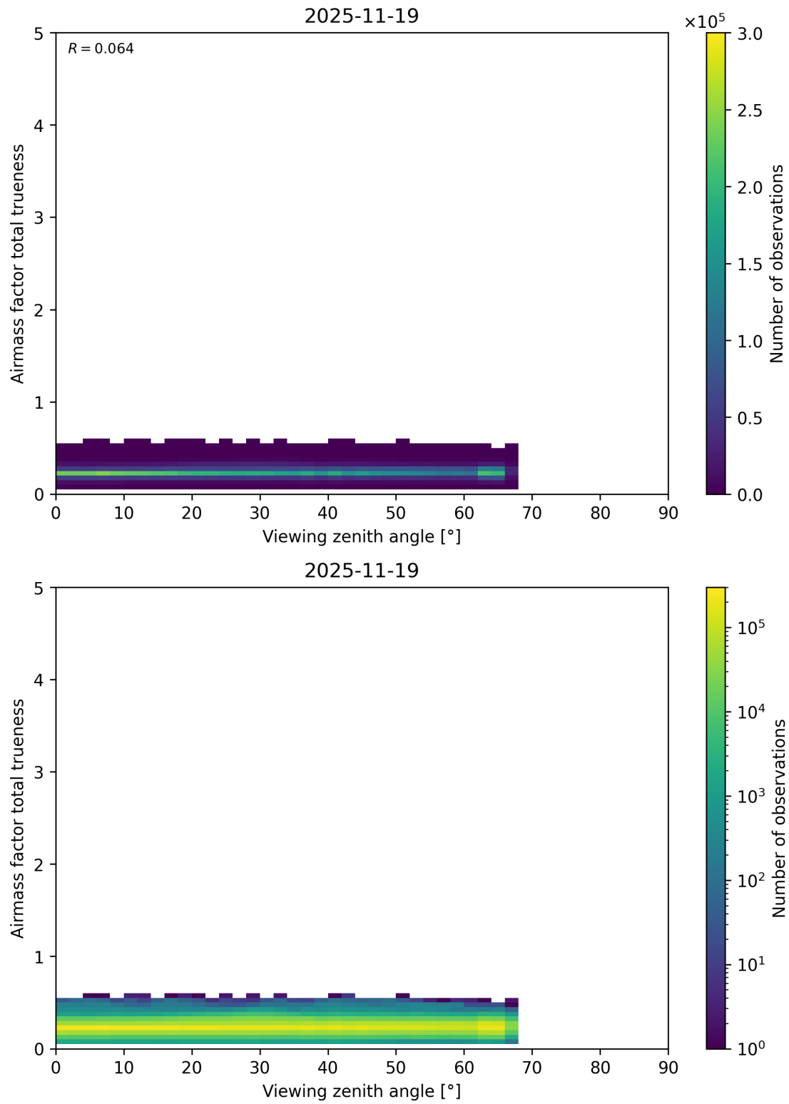
Figure 211: Scatter density plot of “Viewing zenith angle” against “Airmass factor total trueness” for 2025-11-18 to 2025-11-20.
