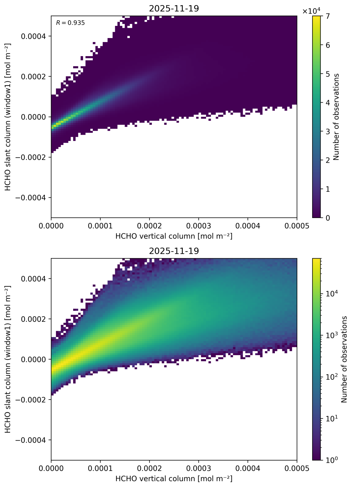
Figure 144: Scatter density plot of “HCHO vertical column” against “HCHO slant column (window1)” for 2025-11-18 to 2025-11-20.
