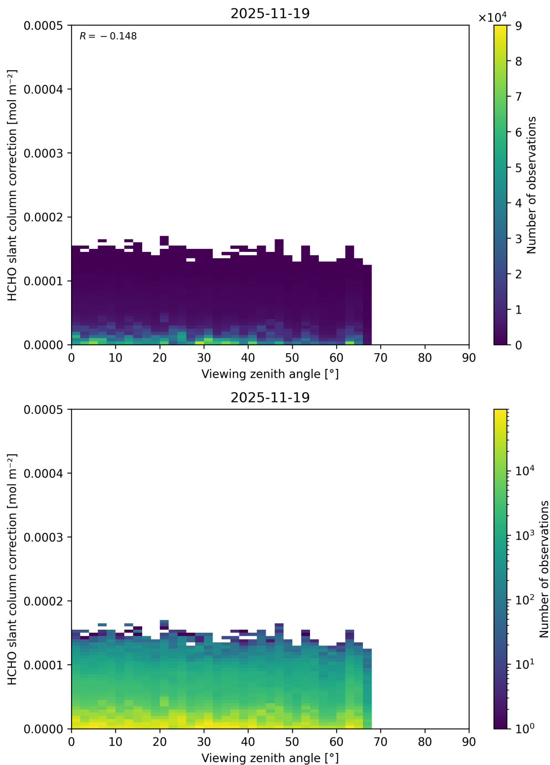
Figure 207: Scatter density plot of “Viewing zenith angle” against “HCHO slant column correction” for 2025-11-18 to 2025-11-20.
