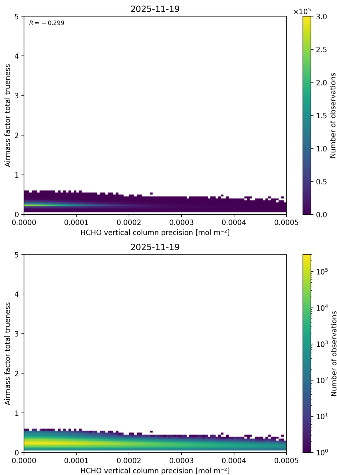
Figure 161: Scatter density plot of “HCHO vertical column precision” against “Airmass factor total trueness” for 2025-11-18 to 2025-11-20.
