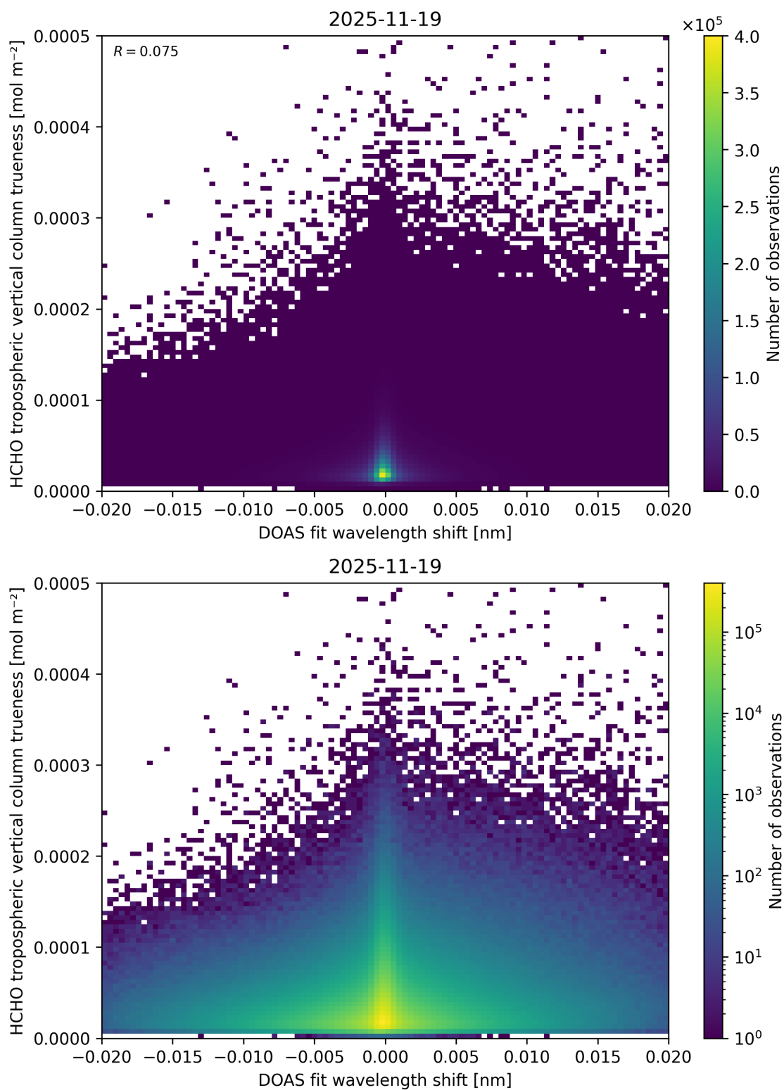
Figure 73: Scatter density plot of “DOAS fit wavelength shift” against “HCHO tropospheric vertical column trueness” for 2025-11-18 to 2025-11-20.
