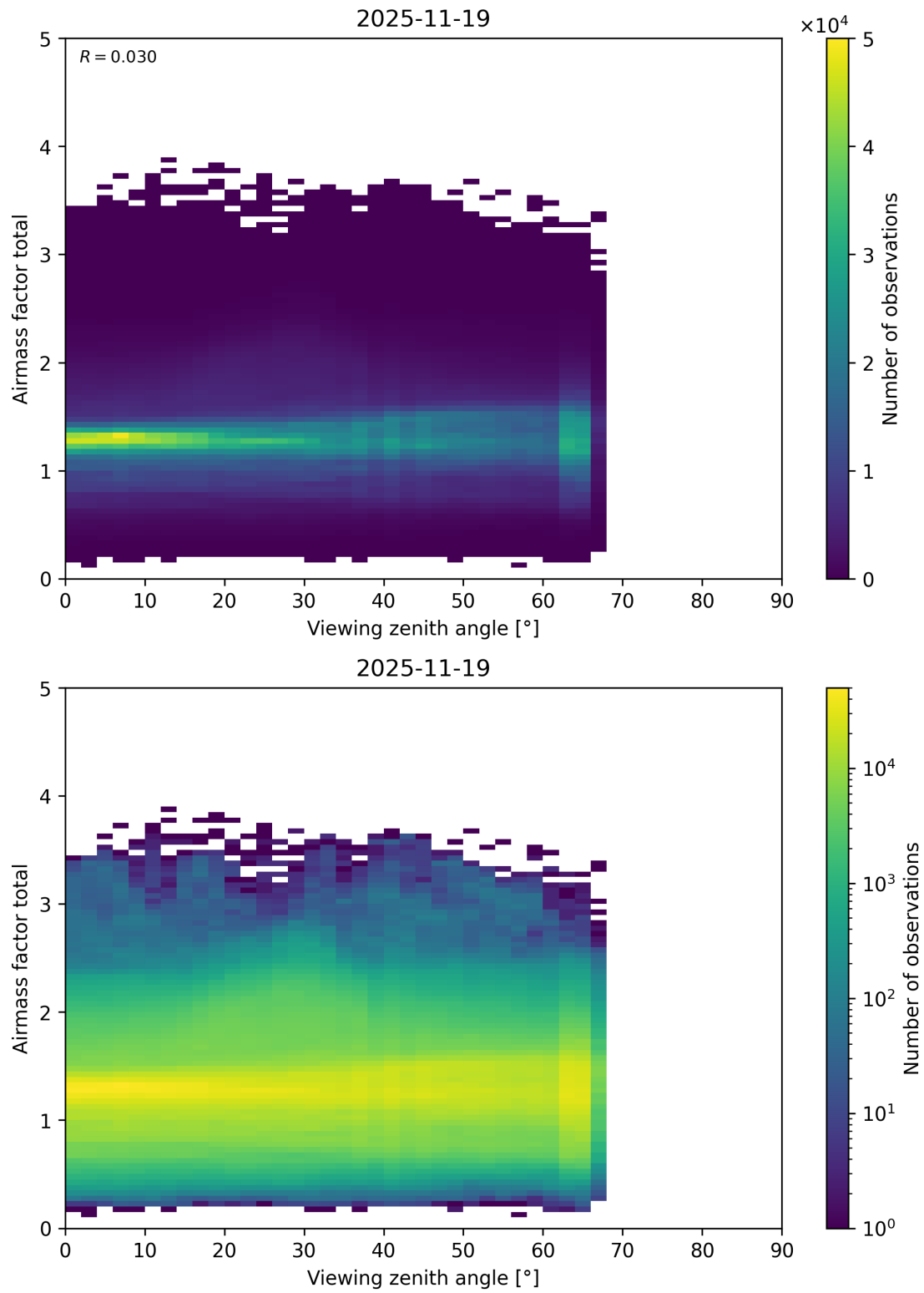
Figure 210: Scatter density plot of “Viewing zenith angle” against “Airmass factor total” for 2025-11-18 to 2025-11-20.
