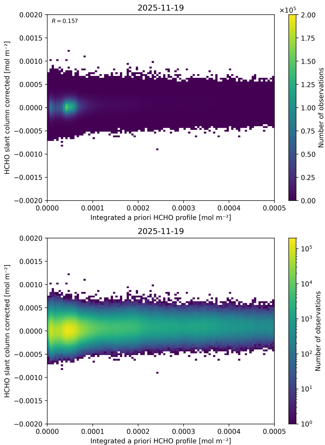
Figure 168: Scatter density plot of “Integrated a priori HCHO profile” against “HCHO slant column corrected” for 2025-11-18 to 2025-11-20.
