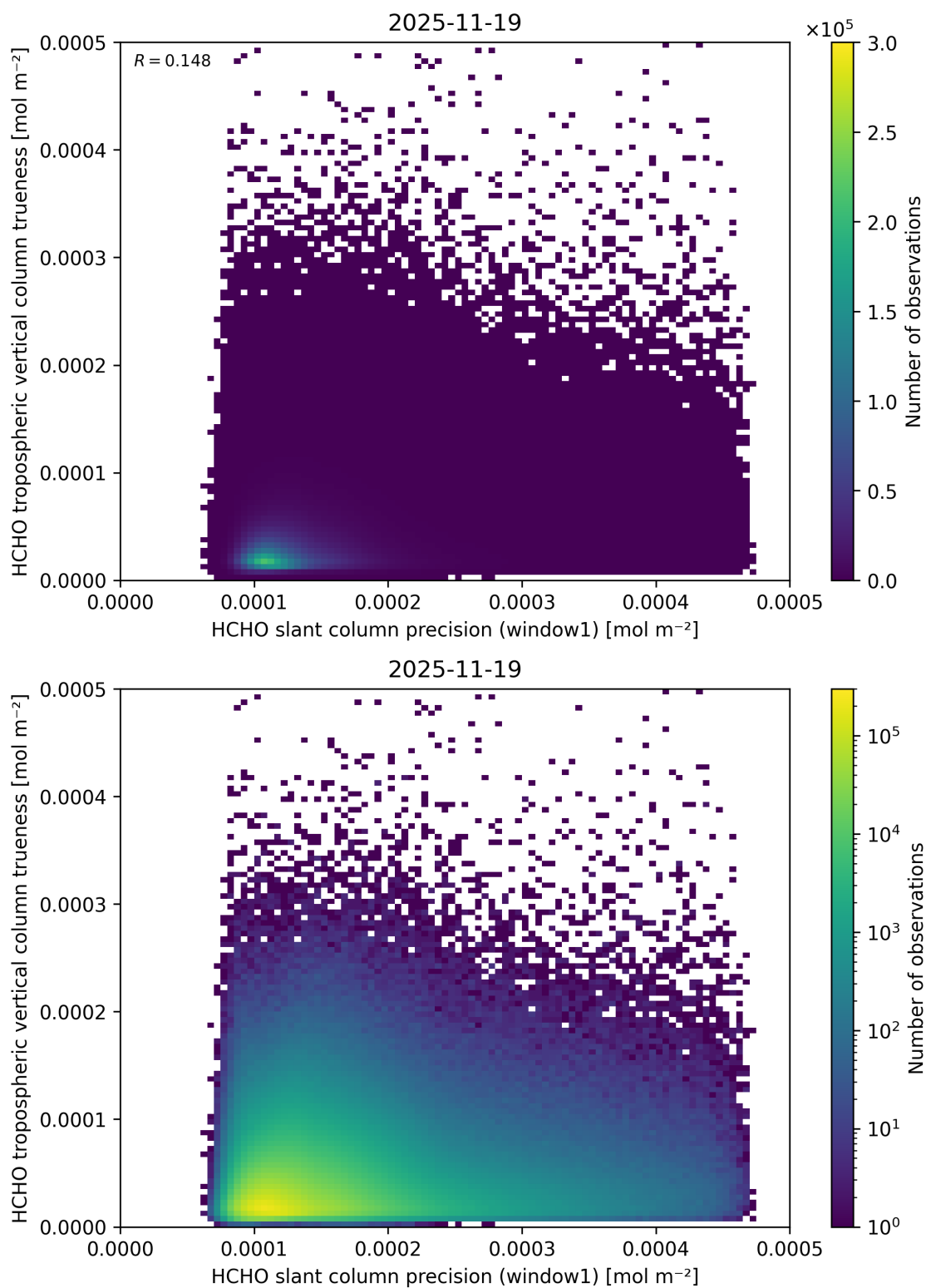
Figure 107: Scatter density plot of “HCHO slant column precision (window1)” against “HCHO tropospheric vertical column trueness” for 2025-11-18 to 2025-11-20.
