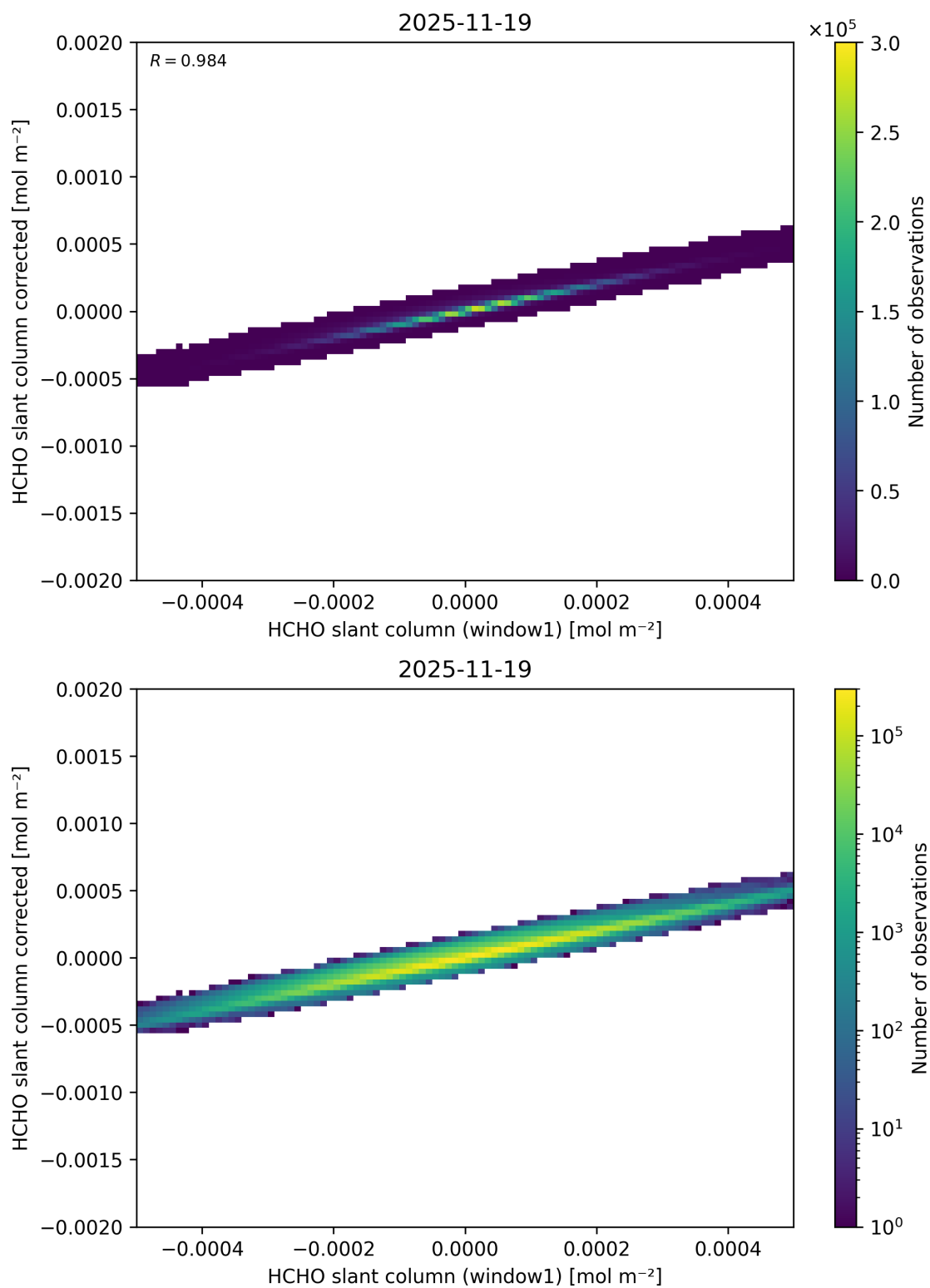
Figure 92: Scatter density plot of “HCHO slant column (window1)” against “HCHO slant column corrected” for 2025-11-18 to 2025-11-20.
