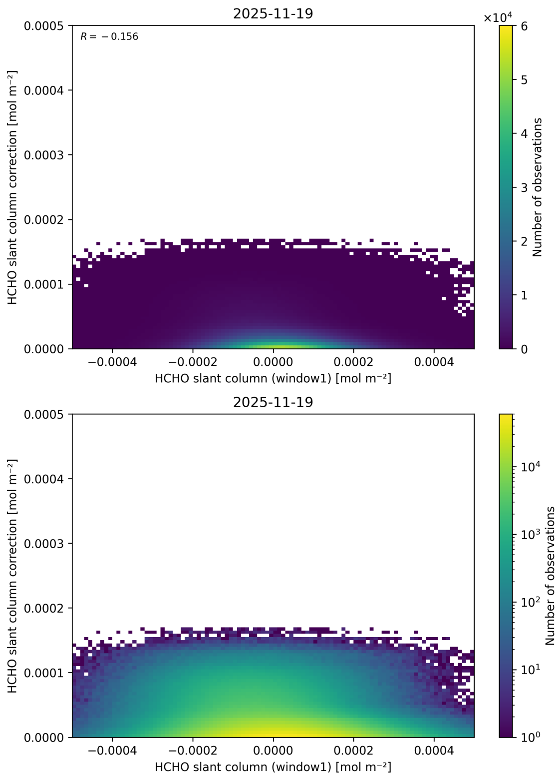
Figure 93: Scatter density plot of “HCHO slant column (window1)” against “HCHO slant column correction” for 2025-11-18 to 2025-11-20.
