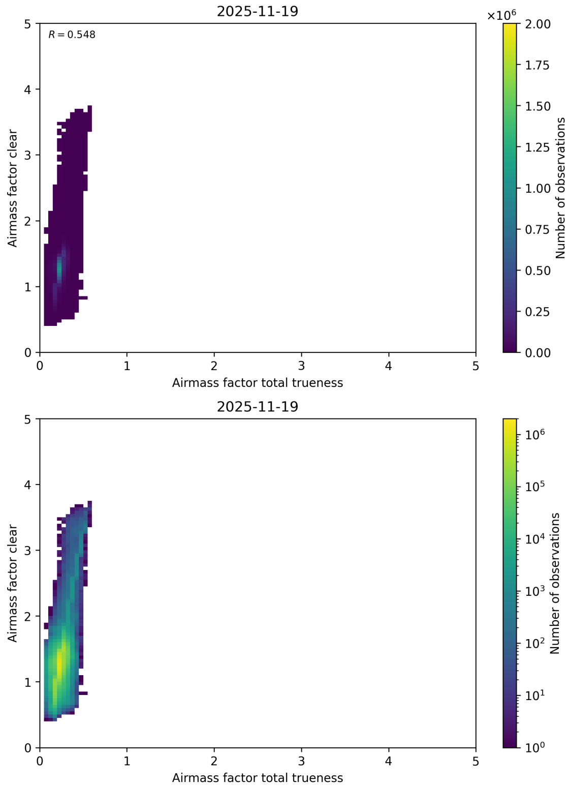
Figure 121: Scatter density plot of “Airmass factor total trueness” against “Airmass factor clear” for 2025-11-18 to 2025-11-20.
