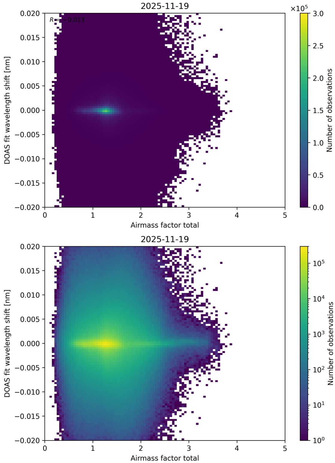
Figure 110: Scatter density plot of “Airmass factor total” against “DOAS fit wavelength shift” for 2025-11-18 to 2025-11-20.
