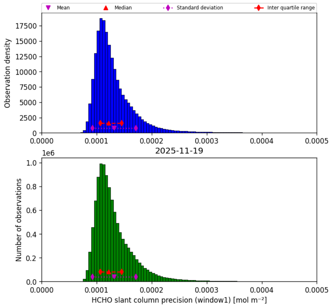
Figure 41: Histogram of “HCHO slant column precision (window1)” for 2025-11-18 to 2025-11-20
