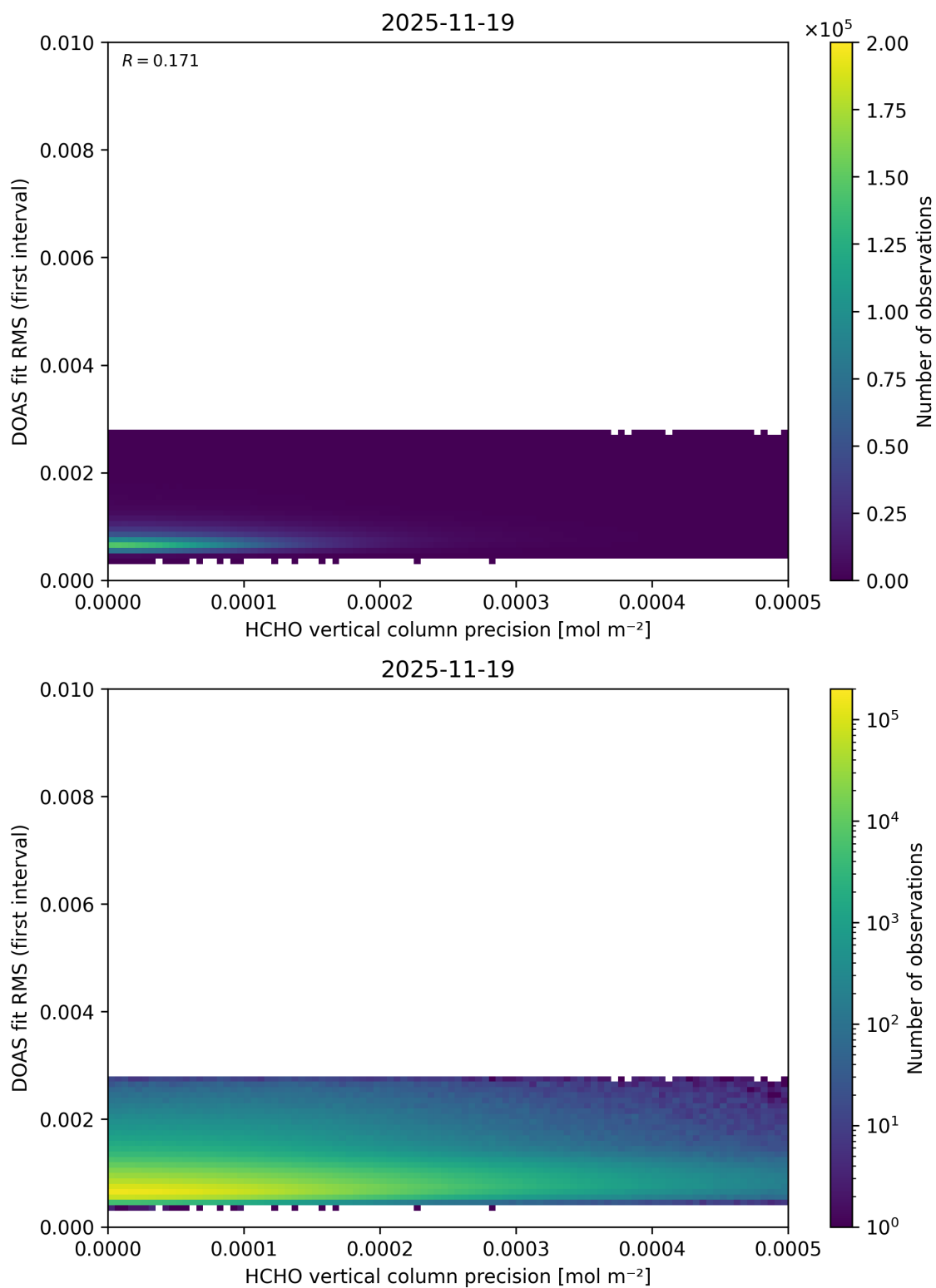
Figure 152: Scatter density plot of “HCHO vertical column precision” against “DOAS fit RMS (first interval)” for 2025-11-18 to 2025-11-20.
