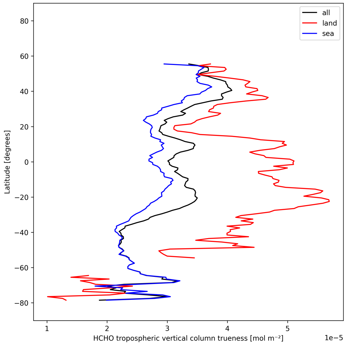
Figure 35: Zonal average of “HCHO tropospheric vertical column density” for 2025-11-18 to 2025-11-20.
