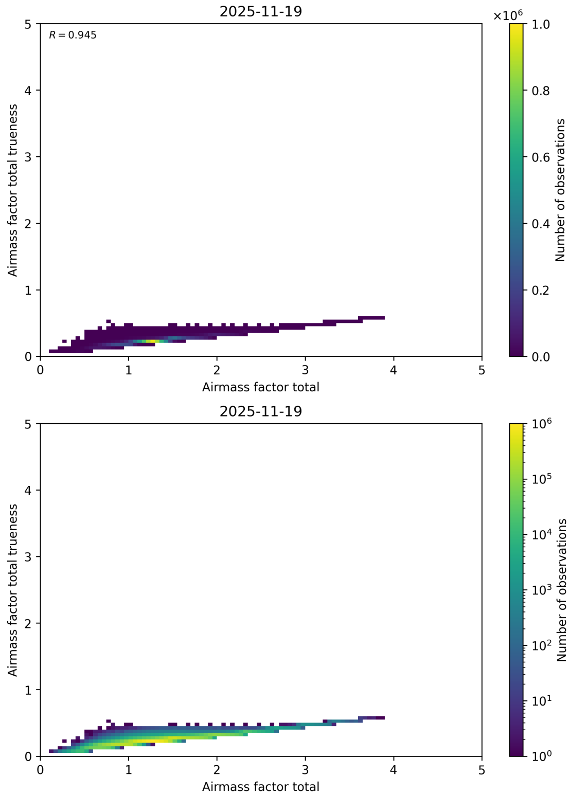
Figure 115: Scatter density plot of “Airmass factor total” against “Airmass factor total trueness” for 2025-11-18 to 2025-11-20.
