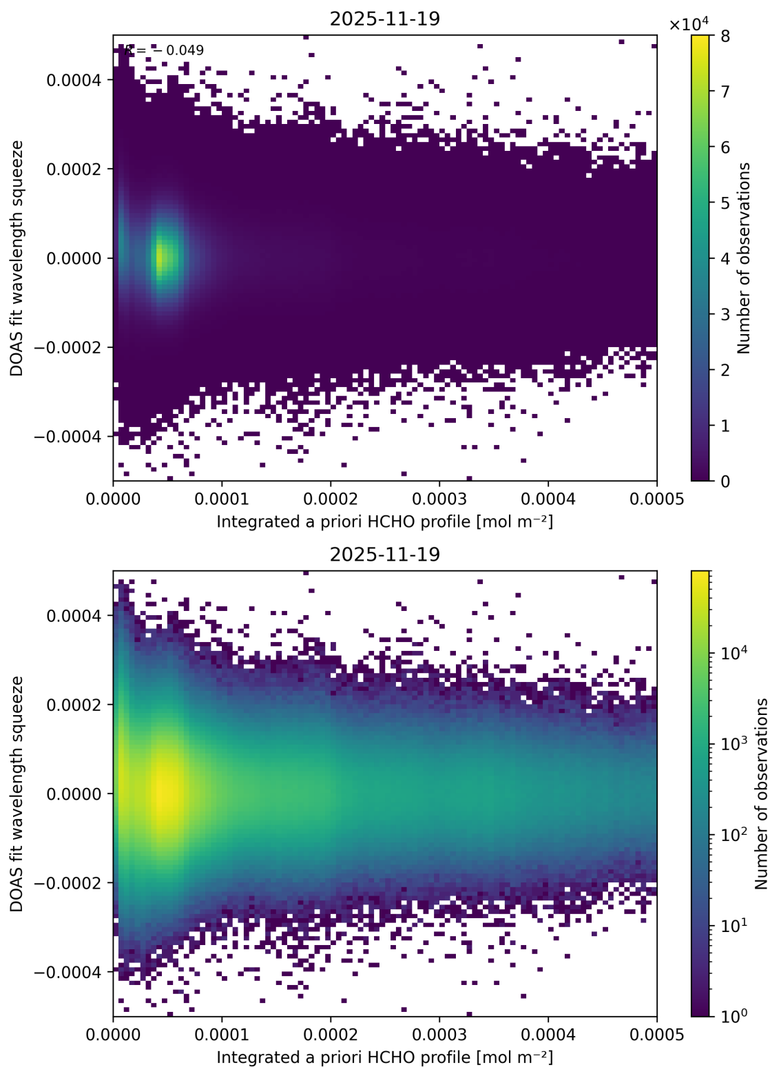
Figure 167: Scatter density plot of “Integrated a priori HCHO profile” against “DOAS fit wavelength squeeze” for 2025-11-18 to 2025-11-20.
