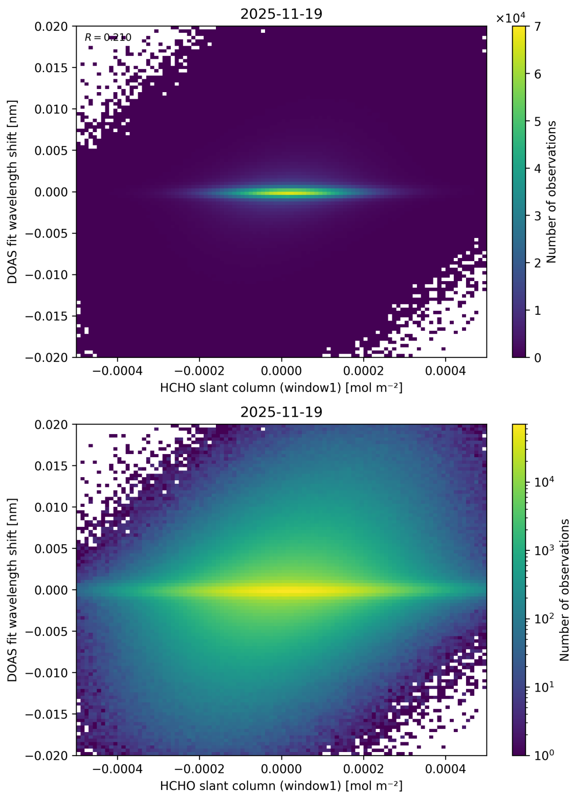
Figure 89: Scatter density plot of “HCHO slant column (window1)” against “DOAS fit wavelength shift” for 2025-11-18 to 2025-11-20.
