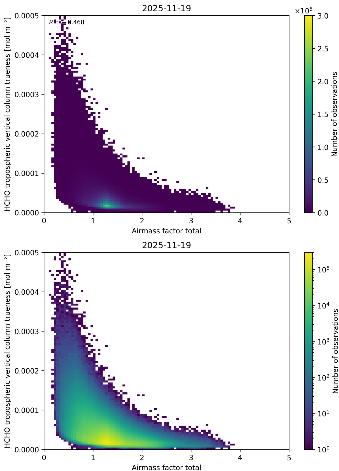
Figure 116: Scatter density plot of “Airmass factor total” against “HCHO tropospheric vertical column truiness” for 2025-11-18 to 2025-11-20.
