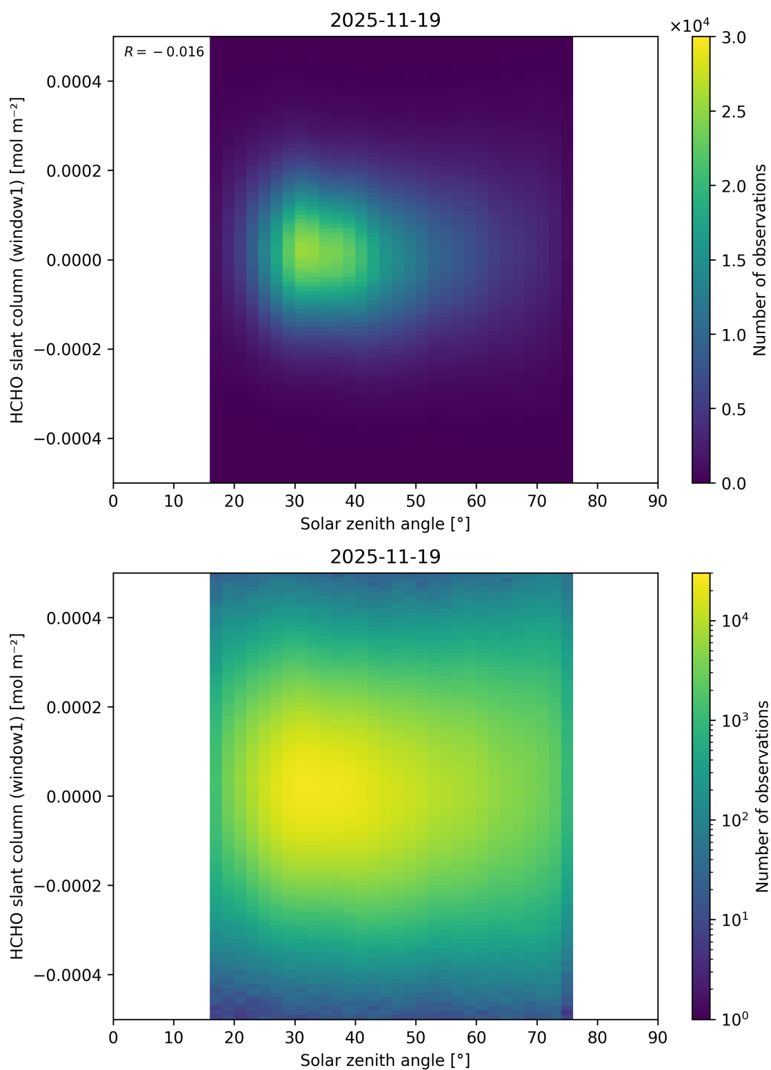
Figure 192: Scatter density plot of “Solar zenith angle” against “HCHO slant column (window1)” for 2025-11-18 to 2025-11-20.
