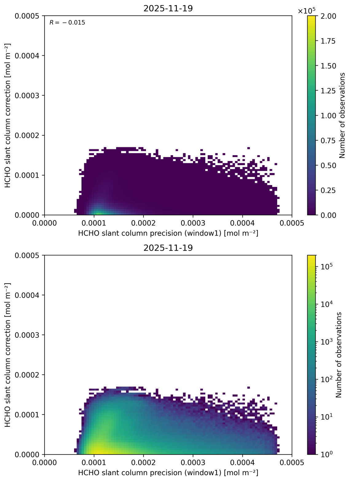
Figure 104: Scatter density plot of “HCHO slant column precision (window1)” against “HCHO slant column correction” for 2025-11-18 to 2025-11-20.
