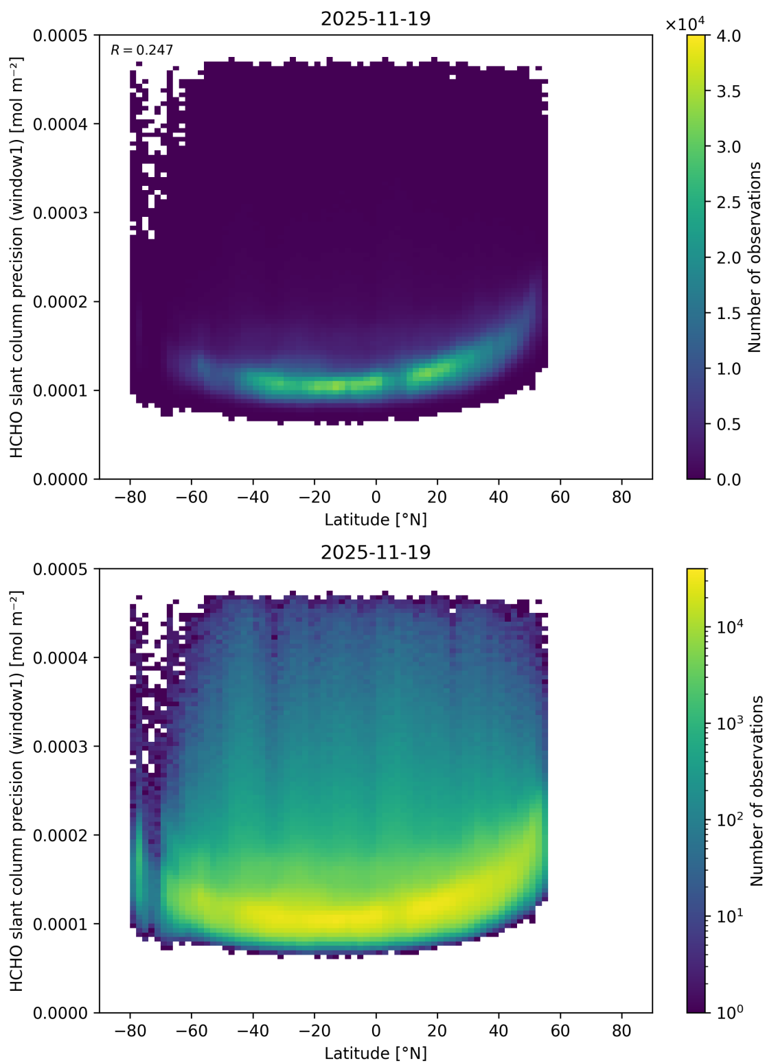
Figure 178: Scatter density plot of “Latitude” against “HCHO slant column precision (window1)” for 2025-11-18 to 2025-11-20.
