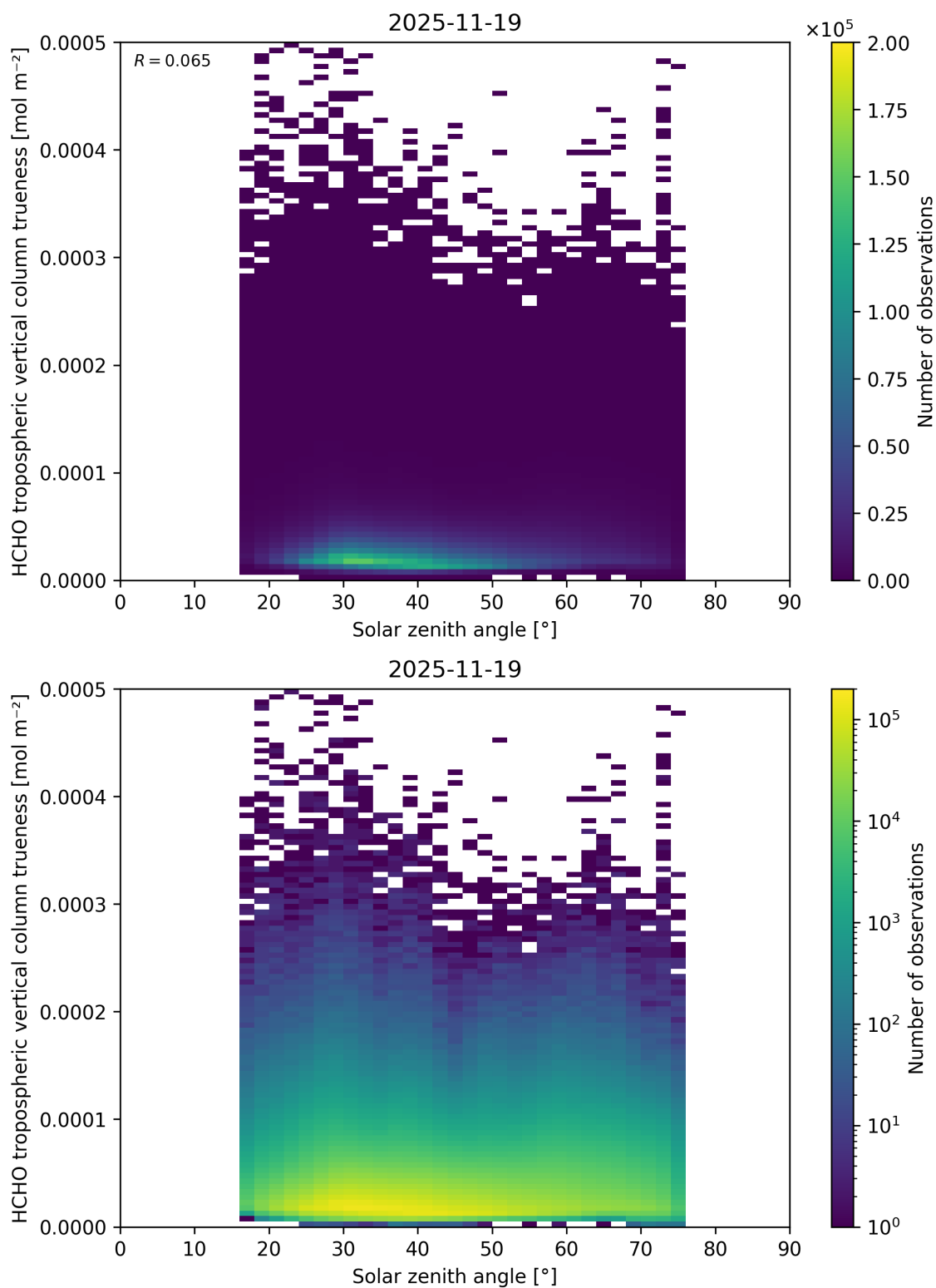
Figure 199: Scatter density plot of “Solar zenith angle” against “HCHO tropospheric vertical column trueness” for 2025-11-18 to 2025-11-20.
