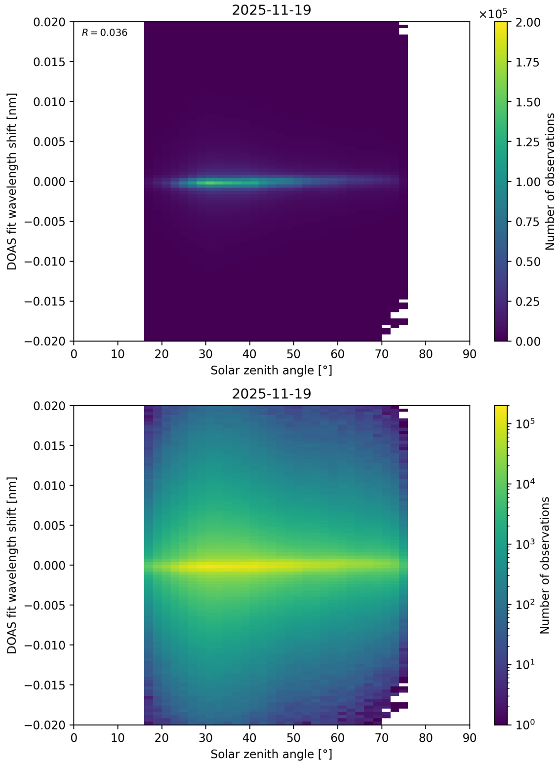
Figure 187: Scatter density plot of “Solar zenith angle” against “DOAS fit wavelength shift” for 2025-11-18 to 2025-11-20.
