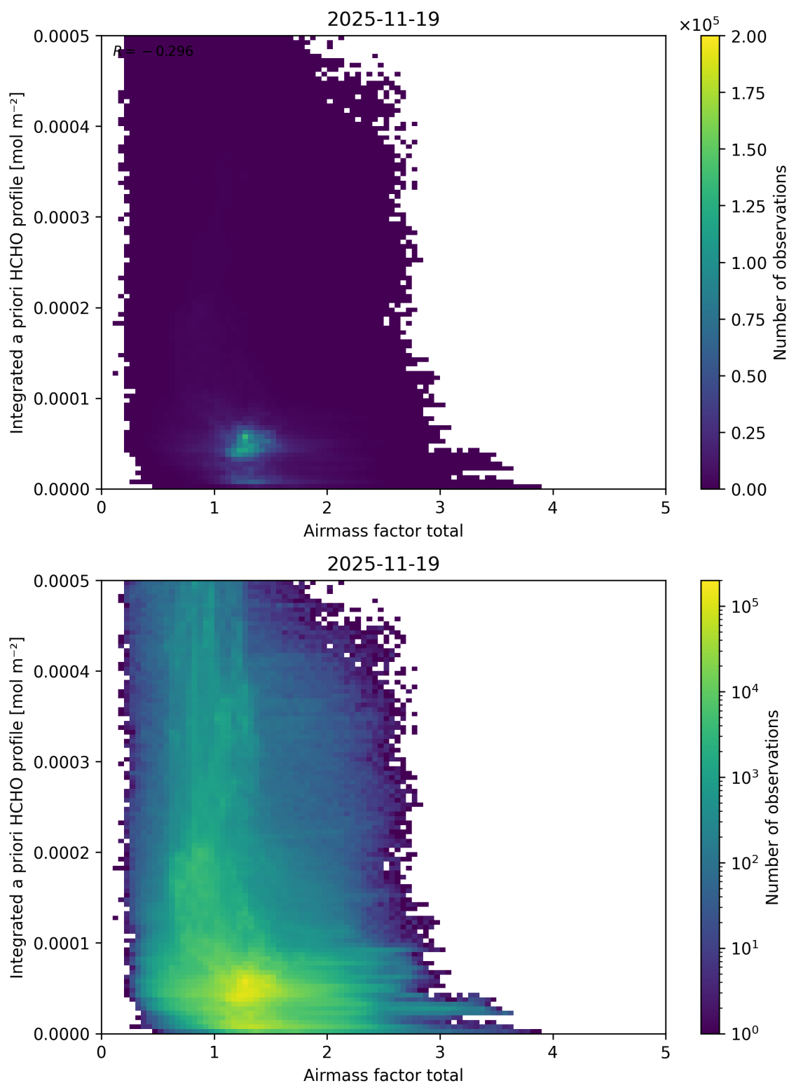
Figure 117: Scatter density plot of “Airmass factor total” against “Integrated a priori HCHO profile” for 2025-11-18 to 2025-11-20.
