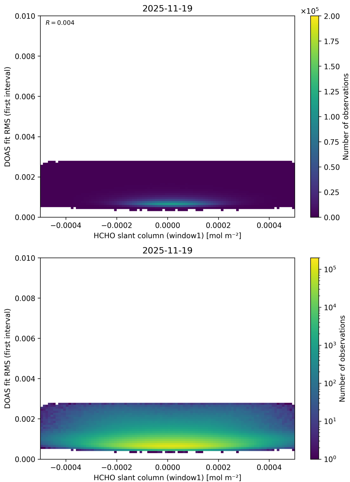
Figure 88: Scatter density plot of “HCHO slant column (window1)” against “DOAS fit RMS (first interval)” for 2025-11-18 to 2025-11-20.
