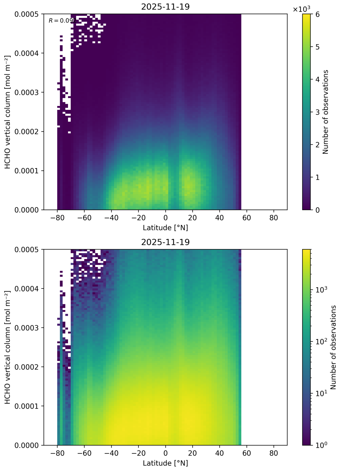
Figure 181: Scatter density plot of “Latitude” against “HCHO vertical column” for 2025-11-18 to 2025-11-20.
