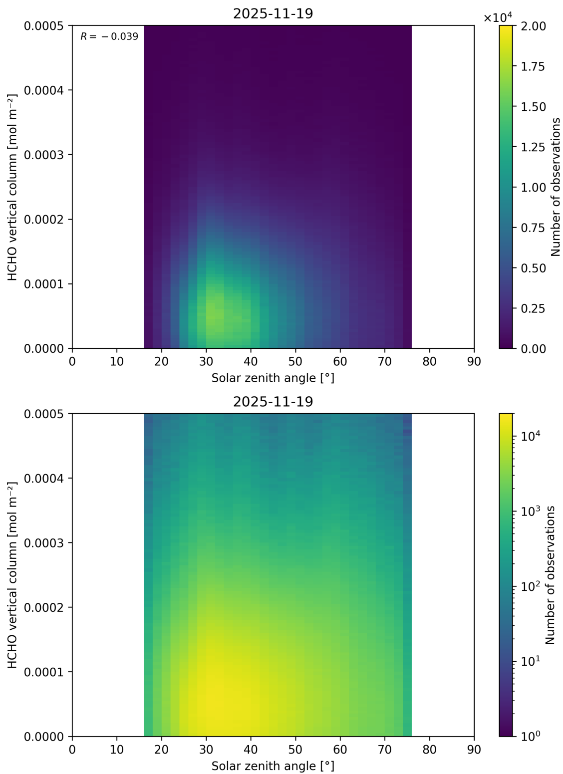
Figure 196: Scatter density plot of “Solar zenith angle” against “HCHO vertical column” for 2025-11-18 to 2025-11-20.
