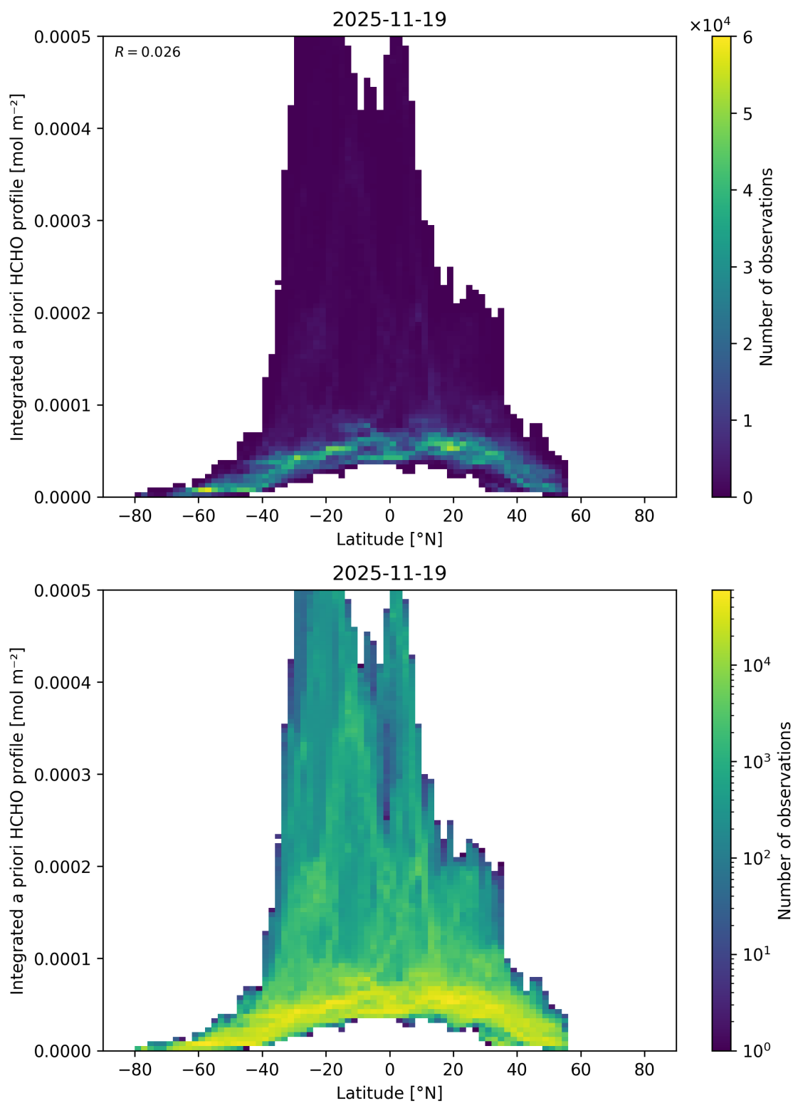
Figure 185: Scatter density plot of “Latitude” against “Integrated a priori HCHO profile” for 2025-11-18 to 2025-11-20.
