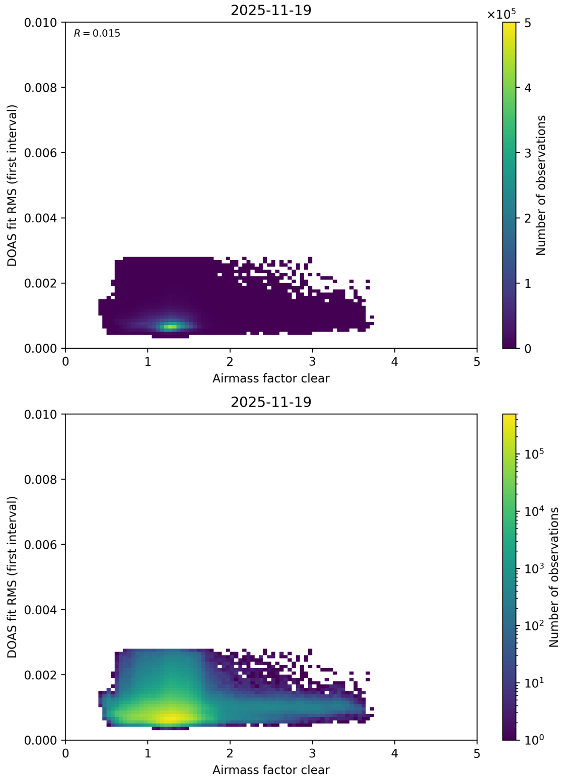
Figure 78: Scatter density plot of “Airmass factor clear” against “DOAS fit RMS (first interval)” for 2025-11-18 to 2025-11-20.
