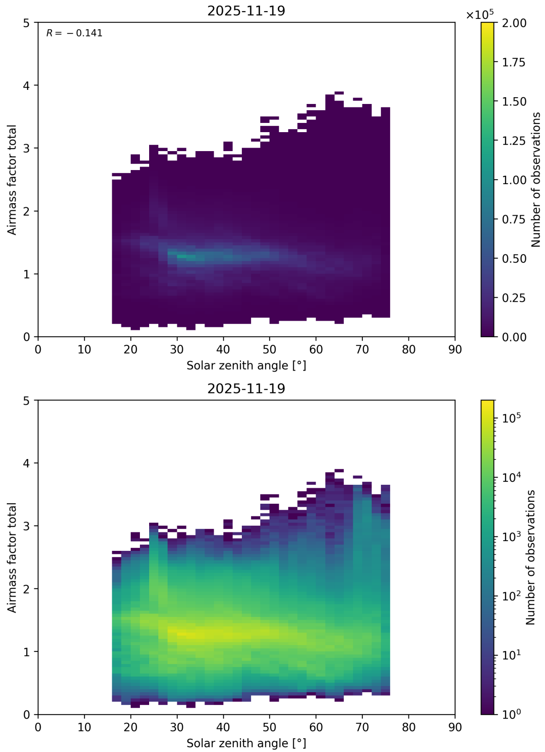
Figure 194: Scatter density plot of “Solar zenith angle” against “Airmass factor total” for 2025-11-18 to 2025-11-20.
