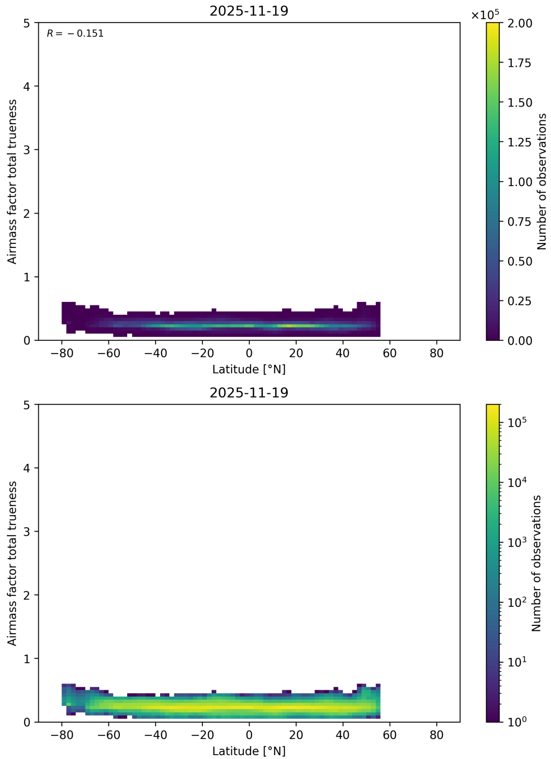
Figure 180: Scatter density plot of “Latitude” against “Airmass factor total trueness” for 2025-11-18 to 2025-11-20.
