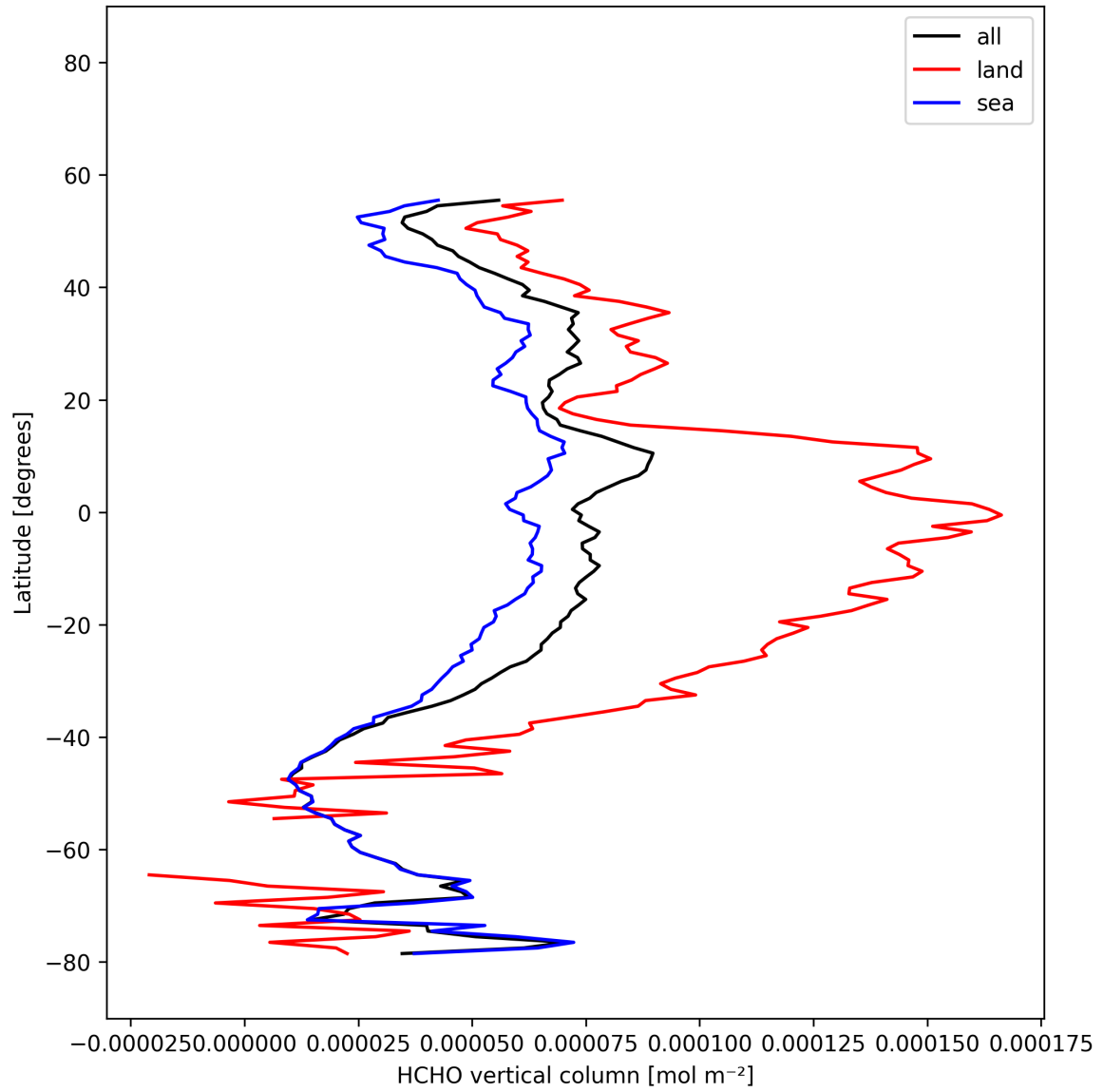
Figure 22: Zonal average of “HCHO vertical column” for 2025-11-18 to 2025-11-20.
