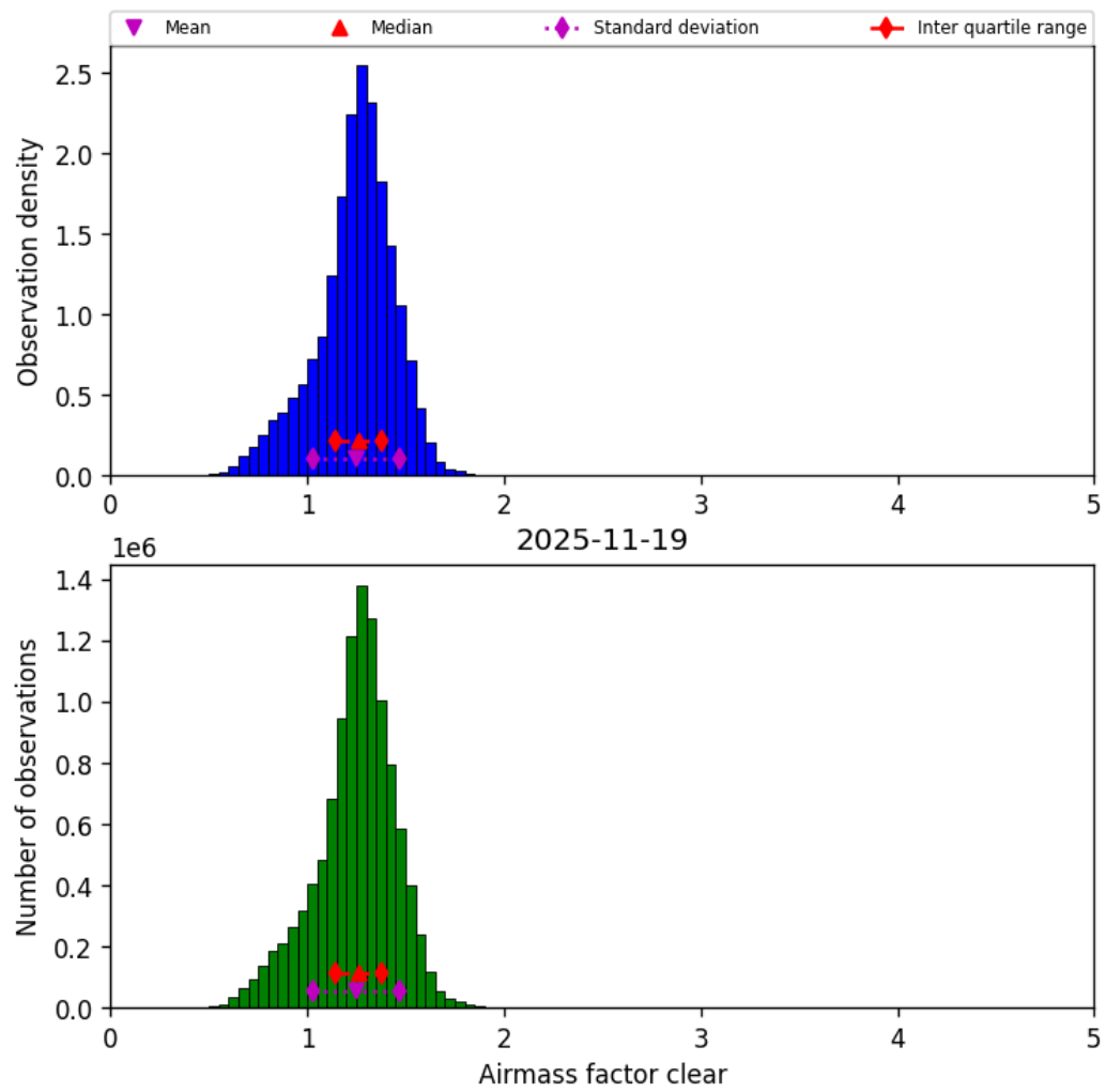
Figure 44: Histogram of “Airmass factor clear” for 2025-11-18 to 2025-11-20
