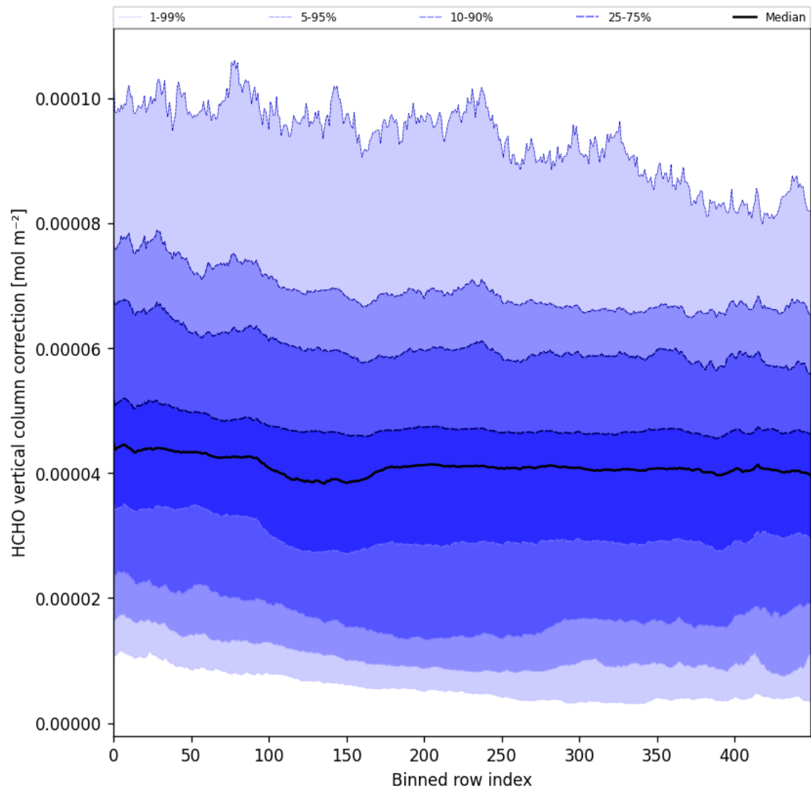
Figure 54: Along track statistics of “HCHO vertical column correction” for 2025-11-18 to 2025-11-20
