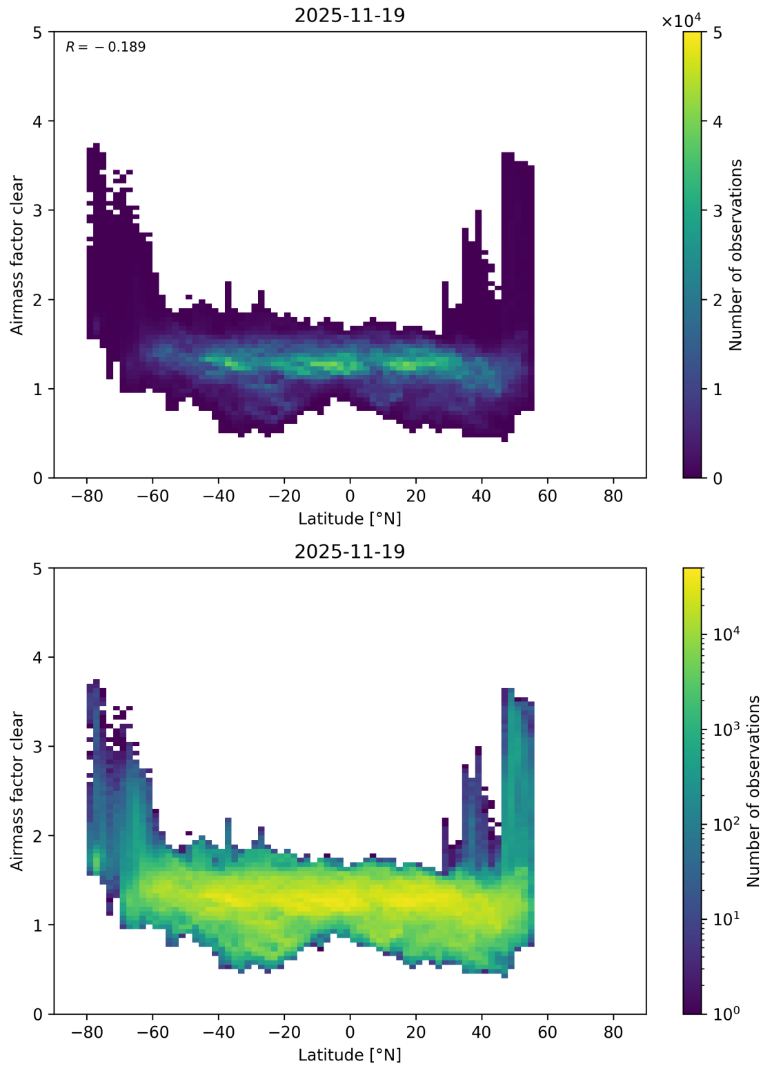
Figure 174: Scatter density plot of “Latitude” against “Airmass factor clear” for 2025-11-18 to 2025-11-20.
