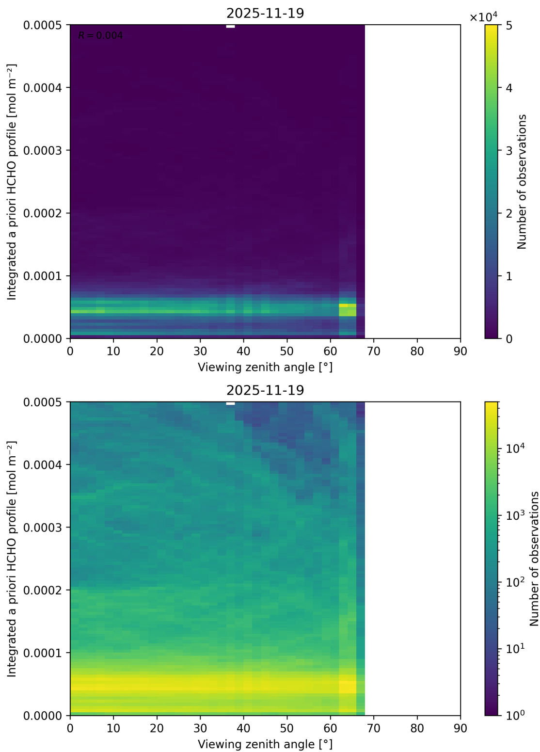
Figure 216: Scatter density plot of “Viewing zenith angle” against “Integrated a priori HCHO profile” for 2025-11-18 to 2025-11-20.
