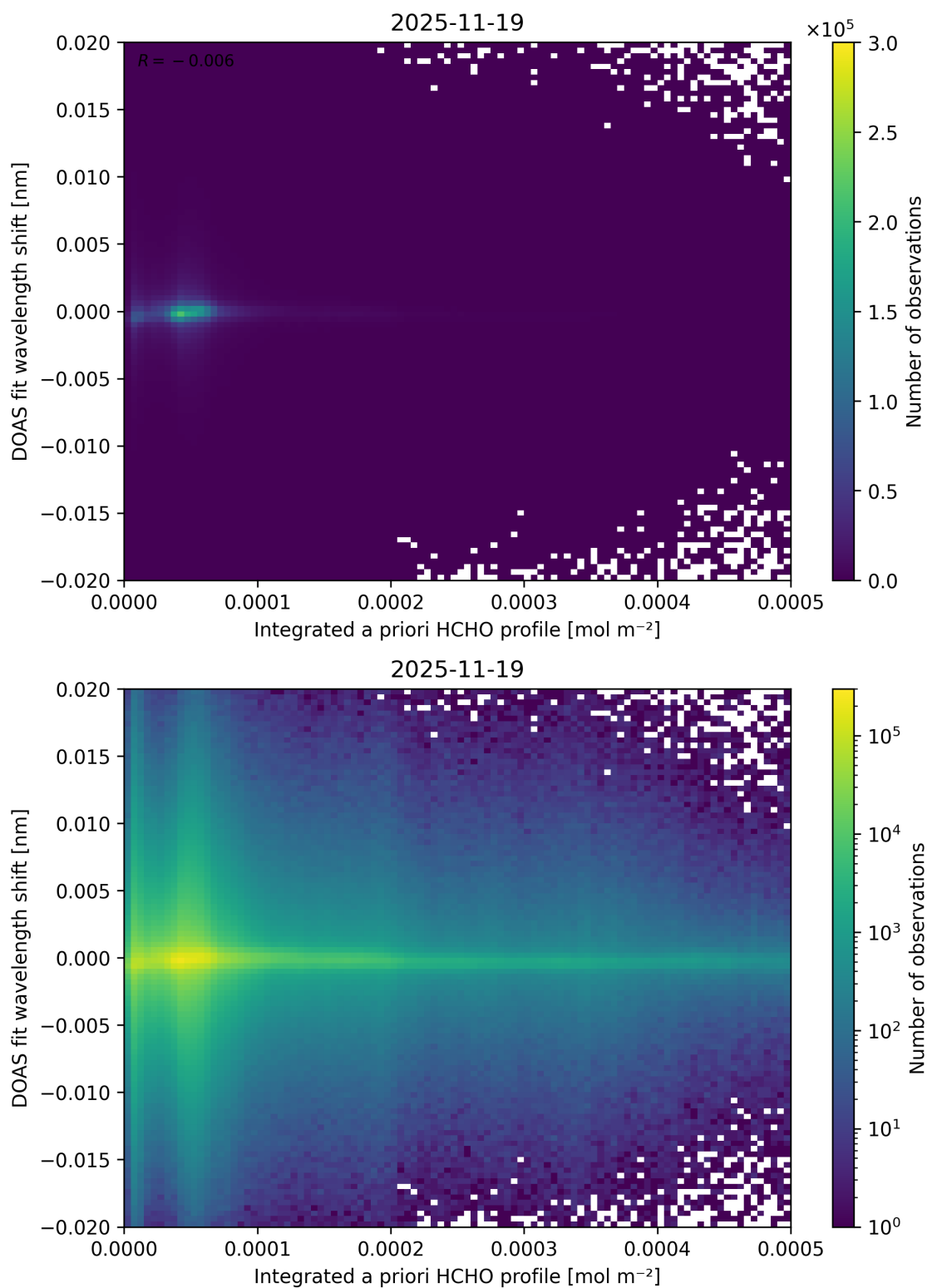
Figure 166: Scatter density plot of “Integrated a priori HCHO profile” against “DOAS fit wavelength shift” for 2025-11-18 to 2025-11-20.
