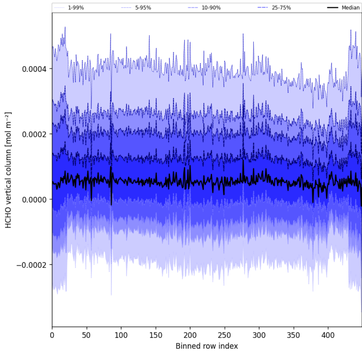
Figure 52: Along track statistics of “HCHO vertical column” for 2025-11-18 to 2025-11-20
