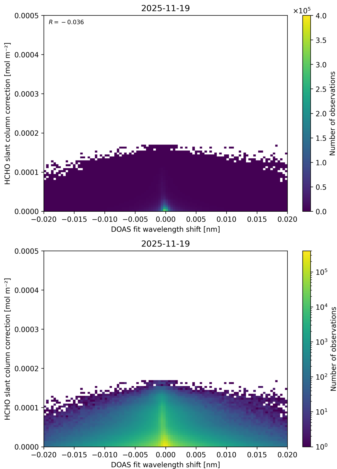
Figure 72: Scatter density plot of “DOAS fit wavelength shift” against “HCHO slant column correction” for 2025-11-18 to 2025-11-20.
