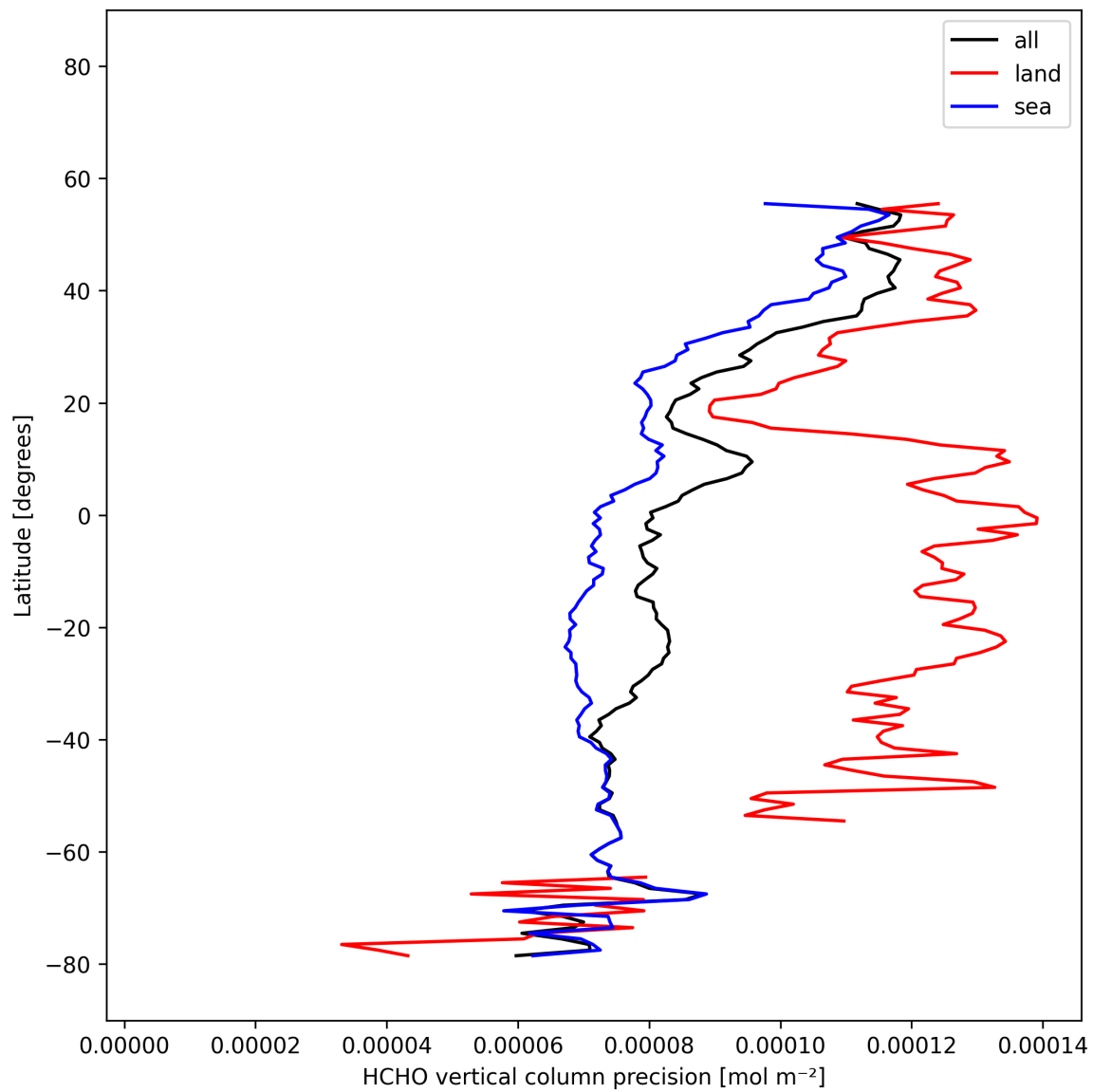
Figure 23: Zonal average of “HCHO vertical column precision” for 2025-11-18 to 2025-11-20.
