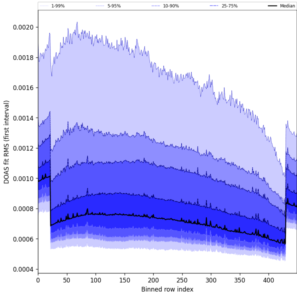
Figure 63: Along track statistics of “DOAS fit RMS (first interval)” for 2025-11-18 to 2025-11-20
