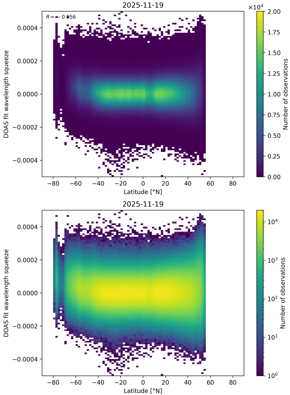
Figure 173: Scatter density plot of “Latitude” against “DOAS fit wavelength squeeze” for 2025-11-18 to 2025-11-20.
