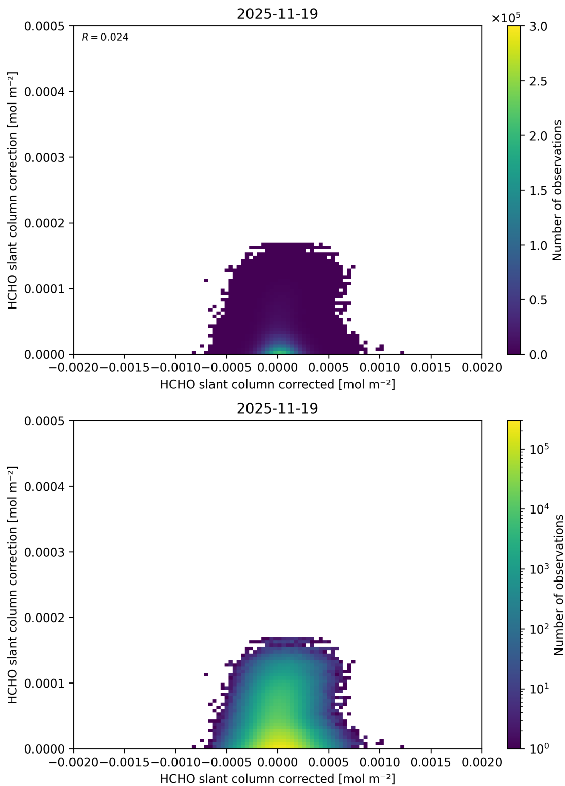
Figure 85: Scatter density plot of “HCHO slant column corrected” against “HCHO slant column correction” for 2025-11-18 to 2025-11-20.
