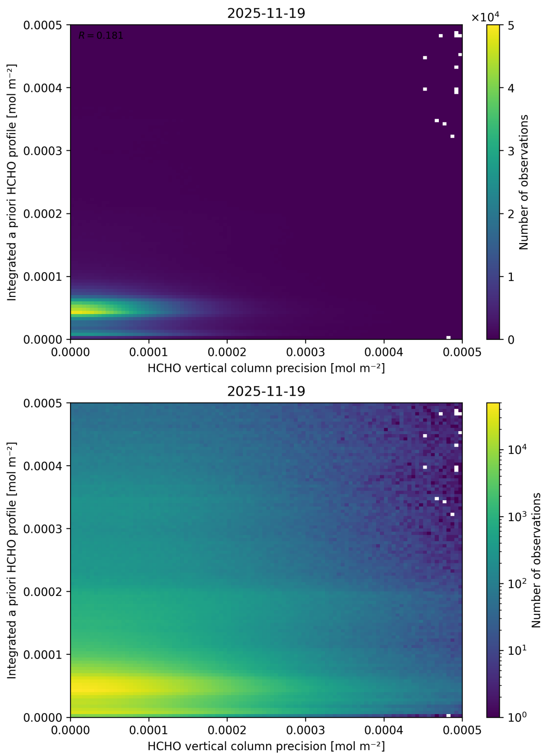
Figure 164: Scatter density plot of “HCHO vertical column precision” against “Integrated a priori HCHO profile” for 2025-11-18 to 2025-11-20.
