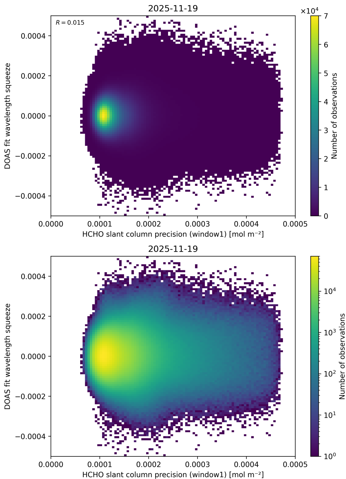
Figure 101: Scatter density plot of “HCHO slant column precision (window1)” against “DOAS fit wavelength squeeze” for 2025-11-18 to 2025-11-20.
