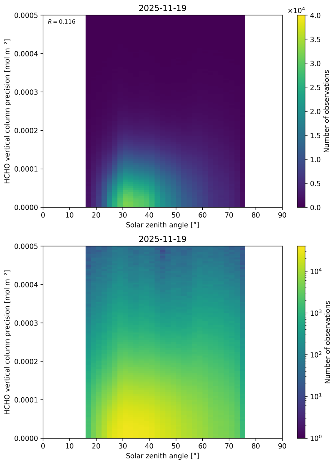
Figure 198: Scatter density plot of “Solar zenith angle” against “HCHO vertical column precision” for 2025-11-18 to 2025-11-20.
