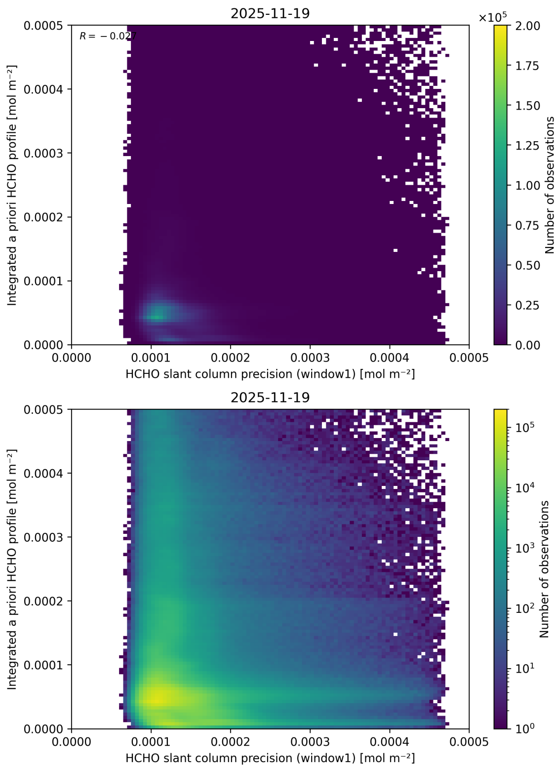
Figure 108: Scatter density plot of “HCHO slant column precision (window1)” against “Integrated a priori HCHO profile” for 2025-11-18 to 2025-11-20.
