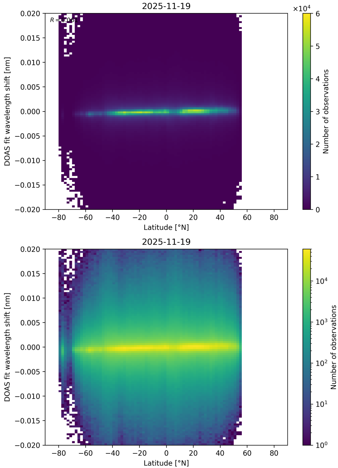
Figure 172: Scatter density plot of “Latitude” against “DOAS fit wavelength shift” for 2025-11-18 to 2025-11-20.
