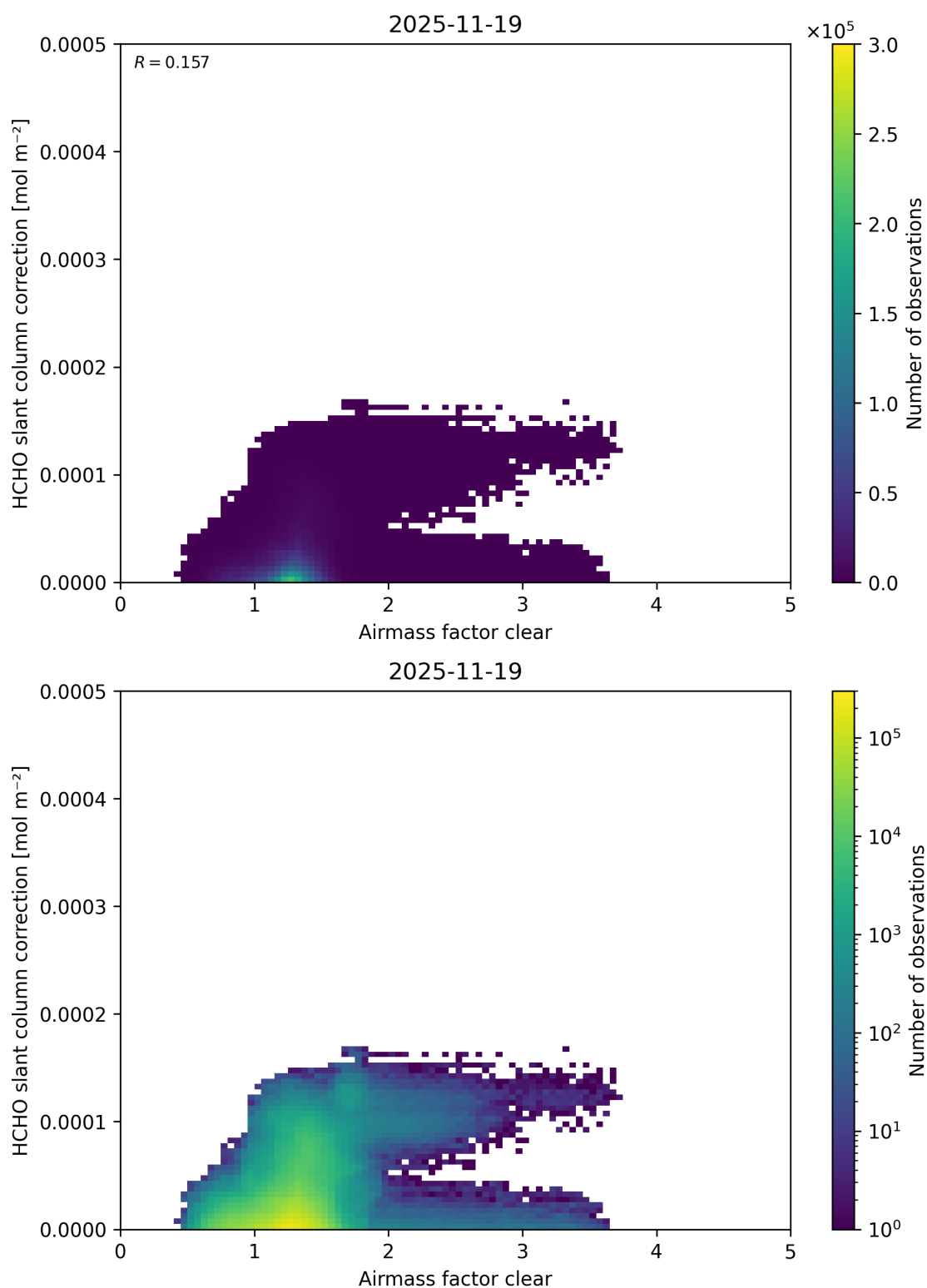
Figure 82: Scatter density plot of “Airmass factor clear” against “HCHO slant column correction” for 2025-11-18 to 2025-11-20.
