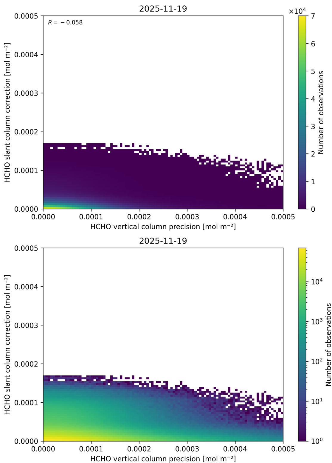
Figure 157: Scatter density plot of “HCHO vertical column precision” against “HCHO slant column correction” for 2025-11-18 to 2025-11-20.
