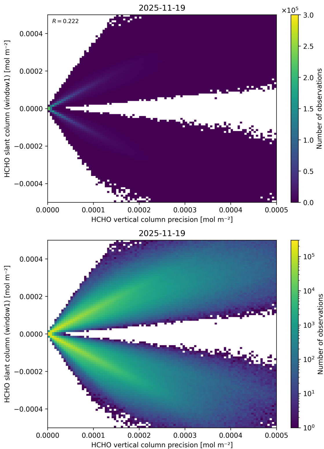
Figure 158: Scatter density plot of “HCHO vertical column precision” against “HCHO slant column (window1)” for 2025-11-18 to 2025-11-20.
