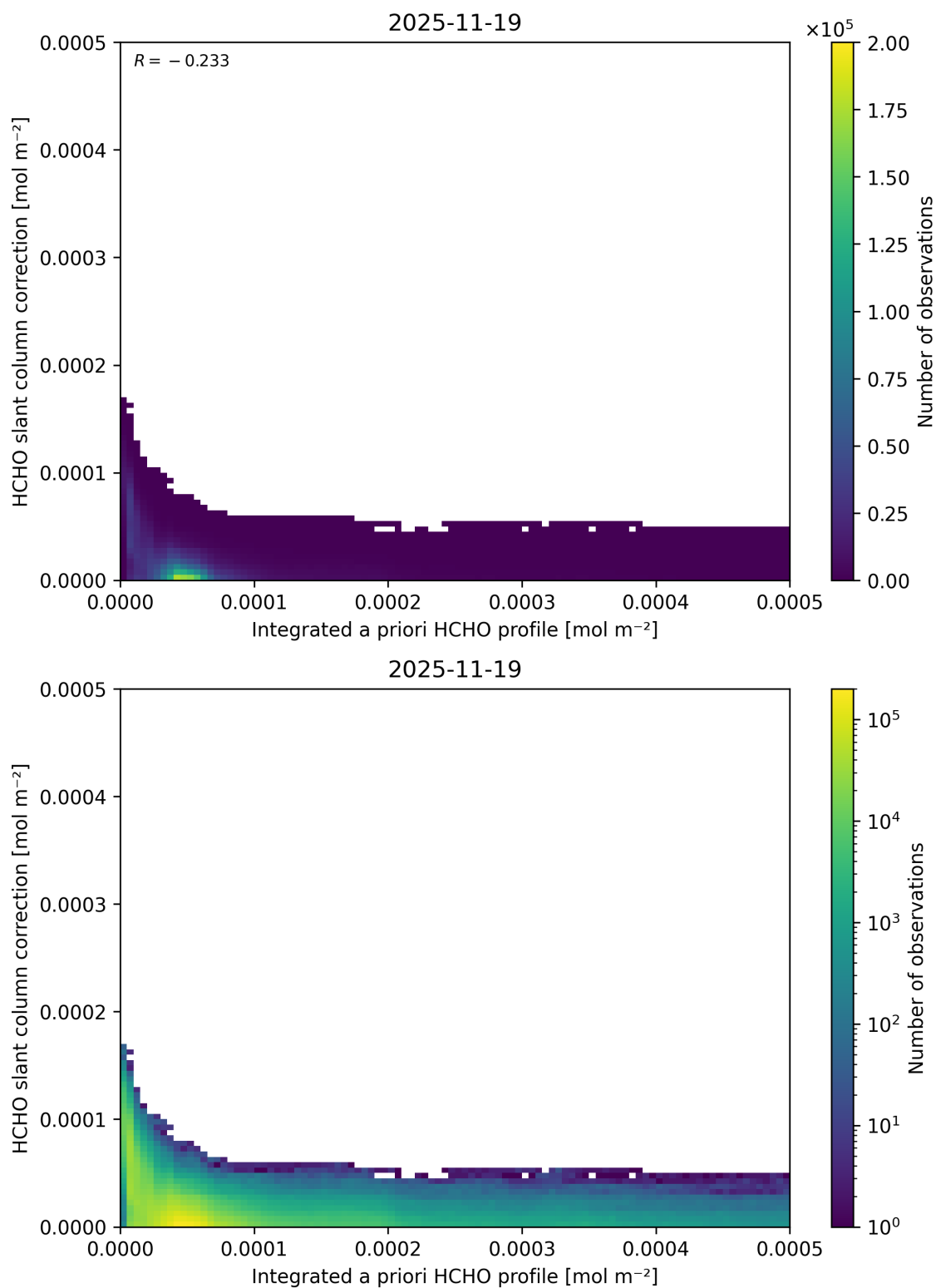
Figure 169: Scatter density plot of “Integrated a priori HCHO profile” against “HCHO slant column correction” for 2025-11-18 to 2025-11-20.
