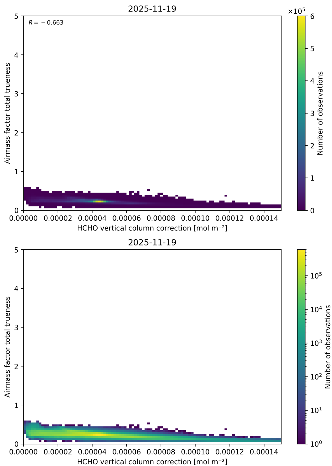
Figure 135: Scatter density plot of “HCHO vertical column correction” against “Airmass factor total truiness” for 2025-11-18 to 2025-11-20.
