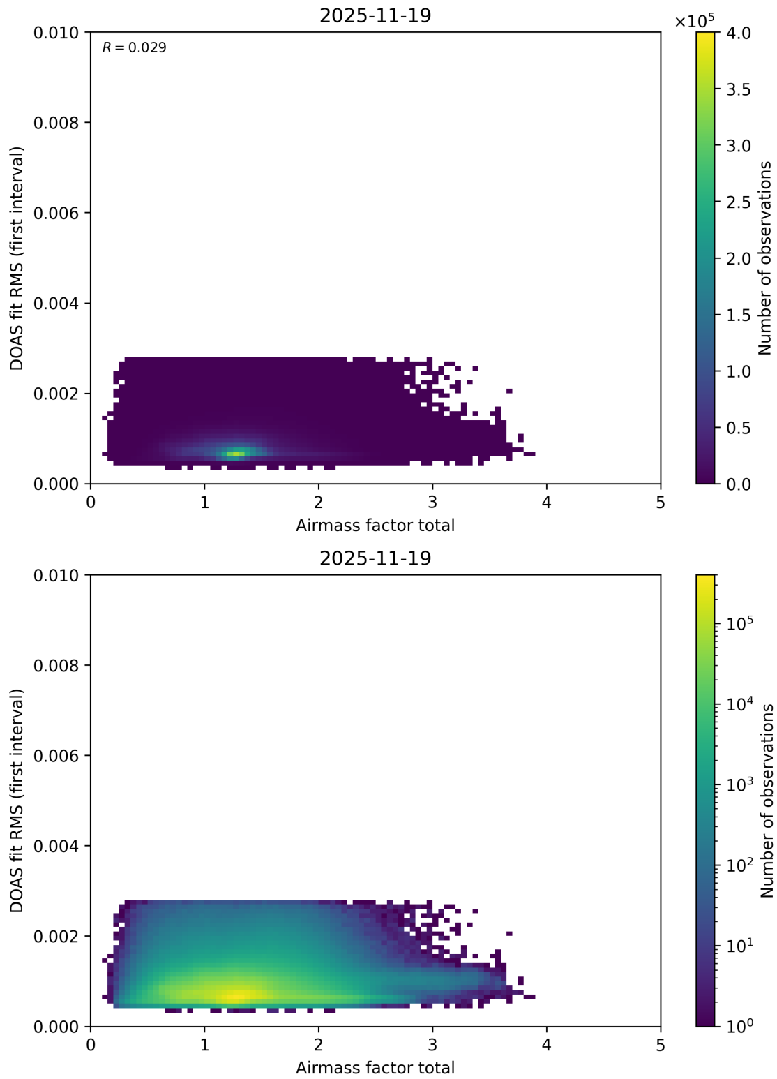
Figure 109: Scatter density plot of “Airmass factor total” against “DOAS fit RMS (first interval)” for 2025-11-18 to 2025-11-20.
