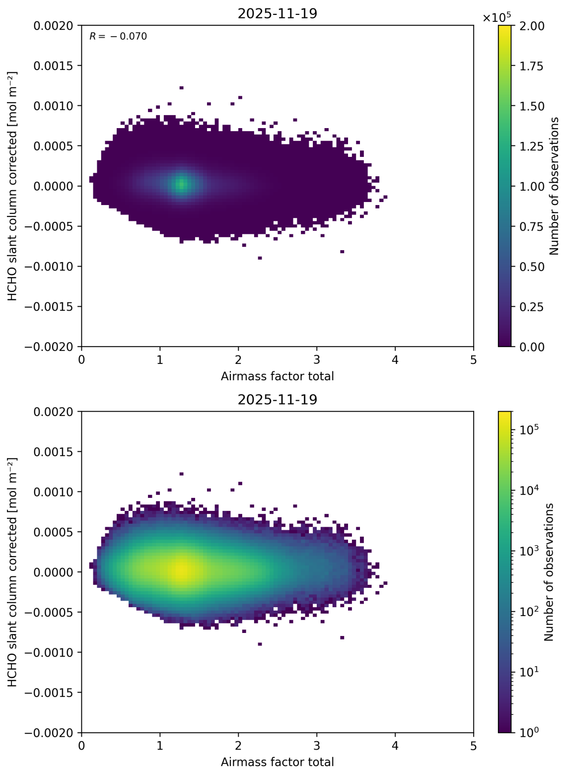
Figure 113: Scatter density plot of “Airmass factor total” against “HCHO slant column corrected” for 2025-11-18 to 2025-11-20.
