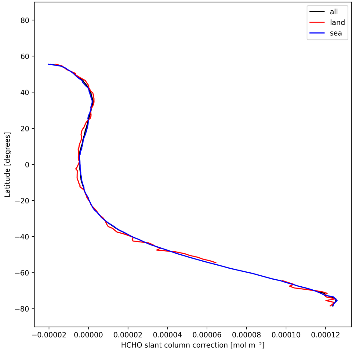
Figure 34: Zonal average of "HCHO slant column correction" for 2025-11-18 to 2025-11-20.
