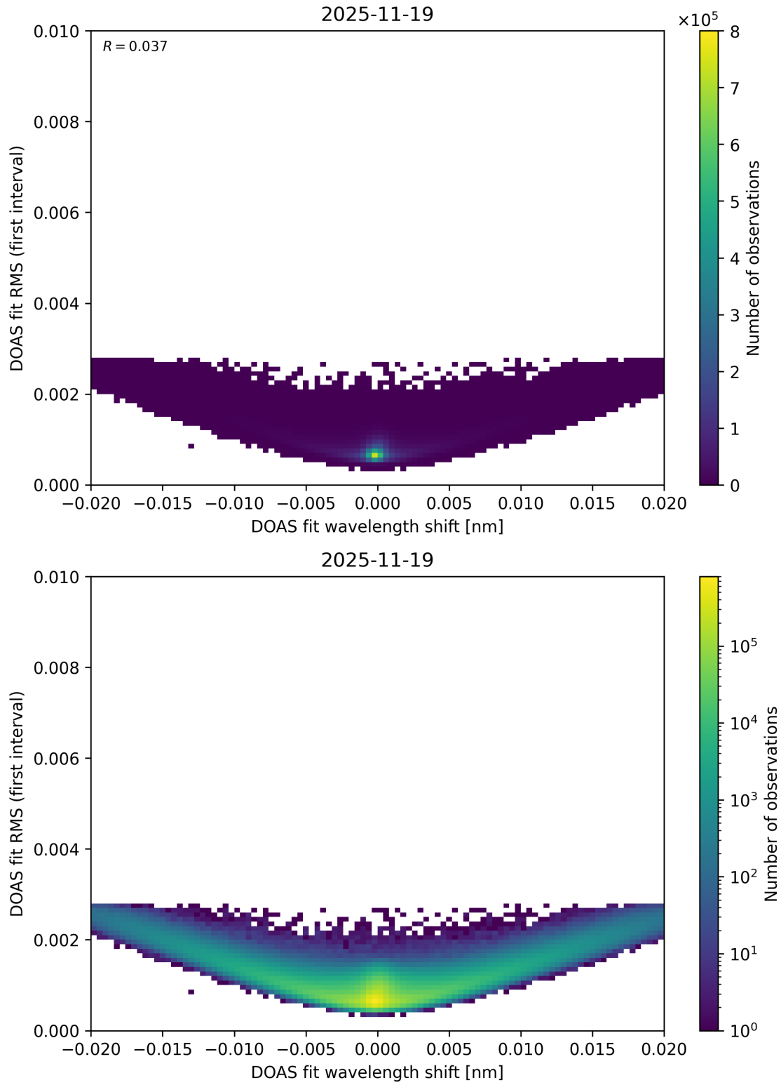
Figure 69: Scatter density plot of “DOAS fit wavelength shift” against “DOAS fit RMS (first interval)” for 2025-11-18 to 2025-11-20.
