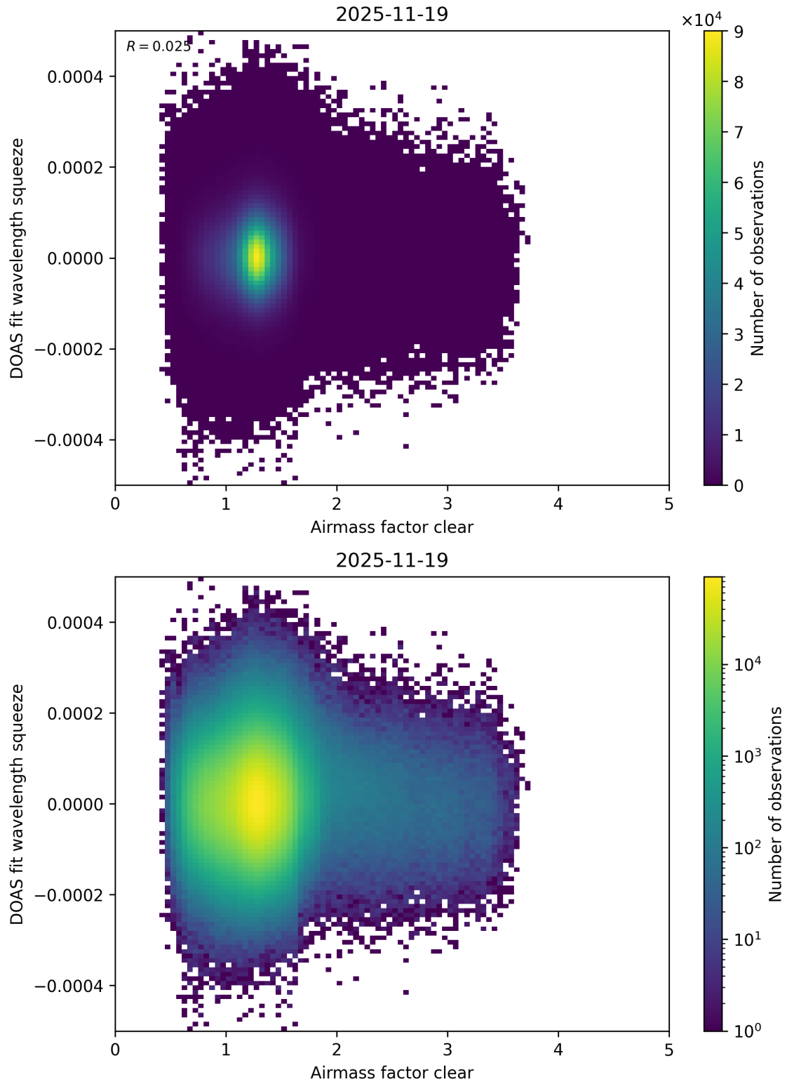
Figure 80: Scatter density plot of “Airmass factor clear” against “DOAS fit wavelength squeeze” for 2025-11-18 to 2025-11-20.
