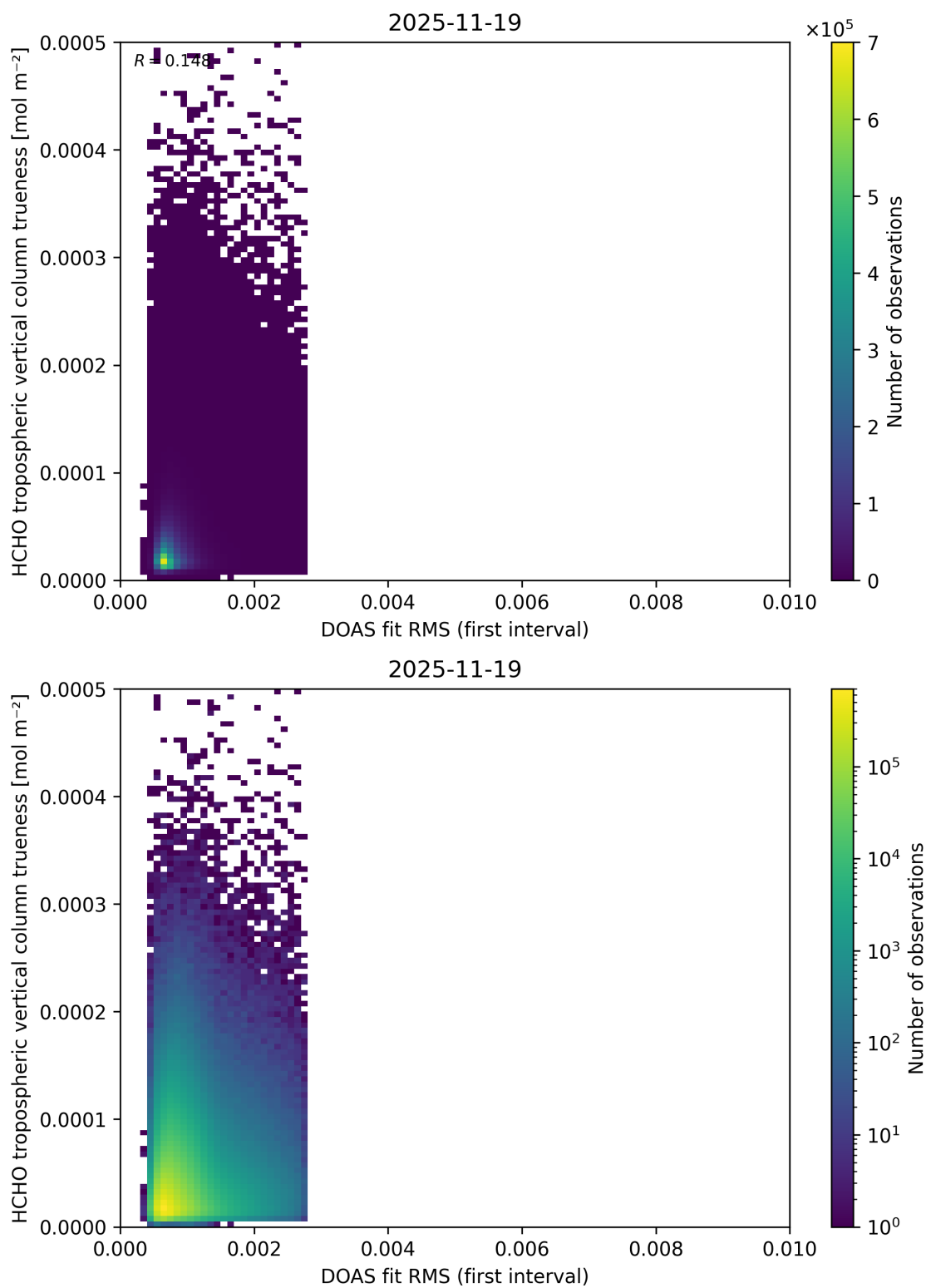
Figure 68: Scatter density plot of “DOAS fit RMS (first interval)” against “HCHO tropospheric vertical column trueness” for 2025-11-18 to 2025-11-20.
