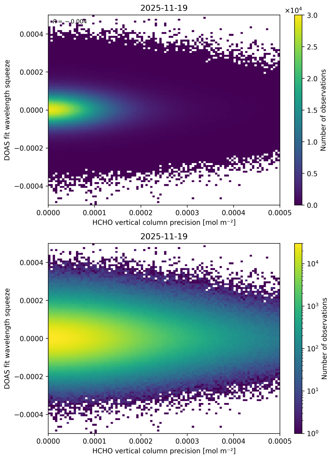
Figure 154: Scatter density plot of “HCHO vertical column precision” against “DOAS fit wavelength squeeze” for 2025-11-18 to 2025-11-20.
