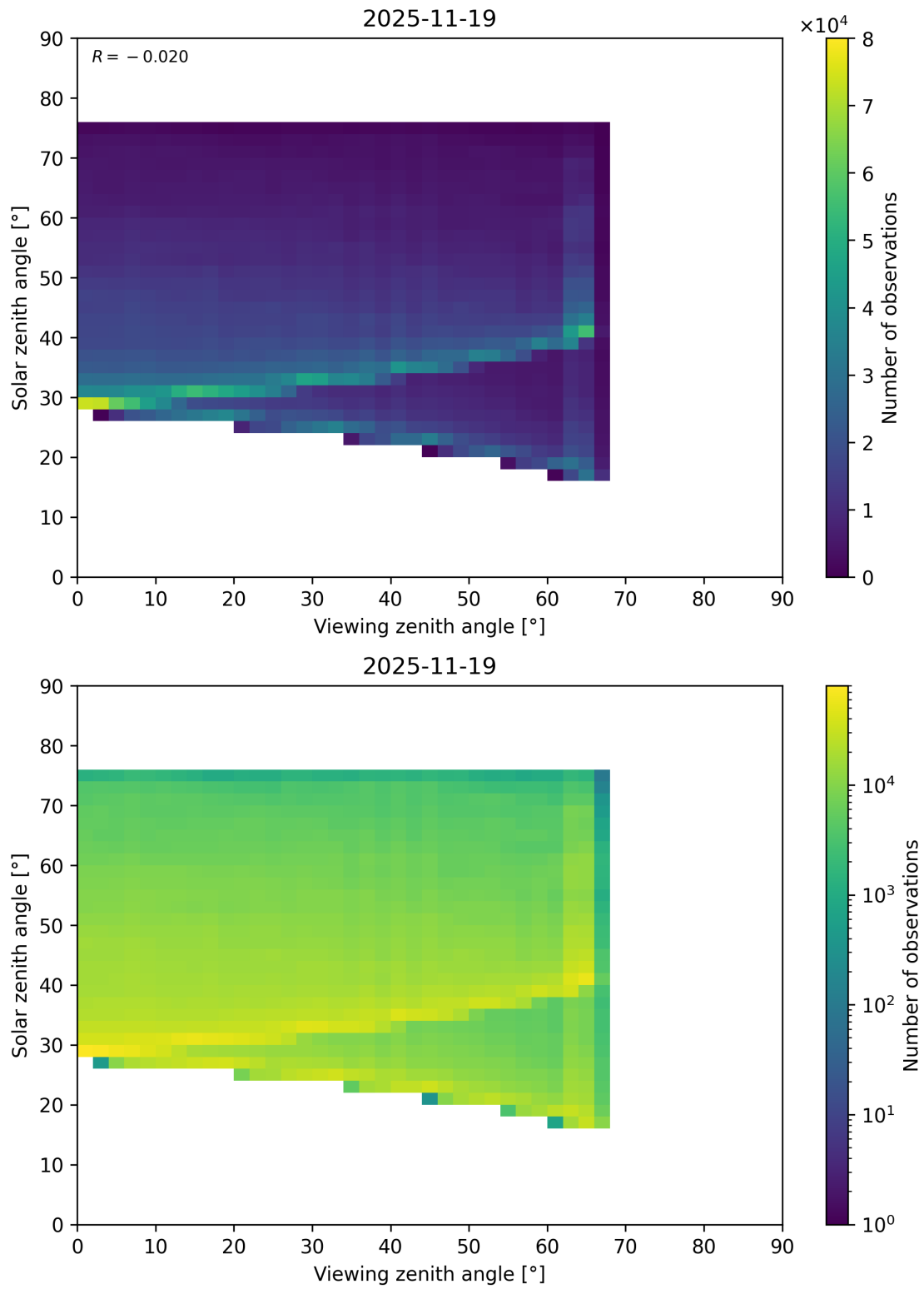
Figure 218: Scatter density plot of “Viewing zenith angle” against “Solar zenith angle” for 2025-11-18 to 2025-11-20.
