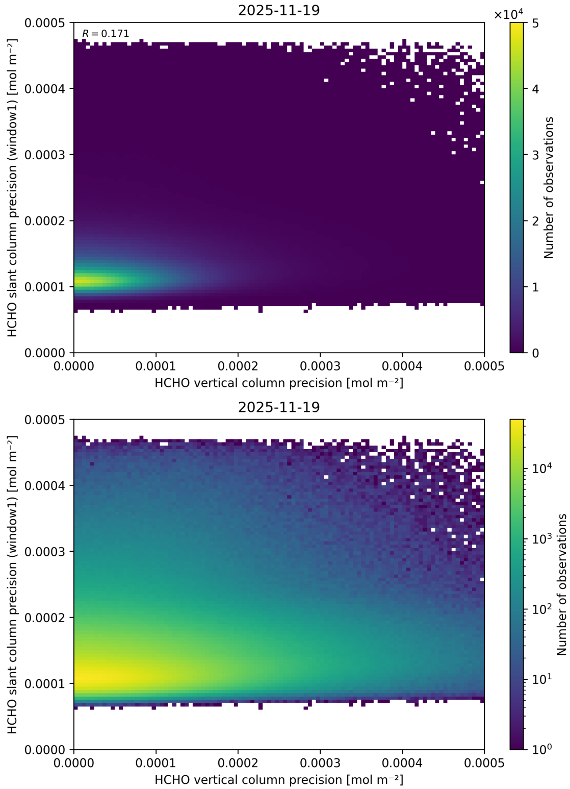
Figure 159: Scatter density plot of “HCHO vertical column precision” against “HCHO slant column precision (window1)” for 2025-11-18 to 2025-11-20.
