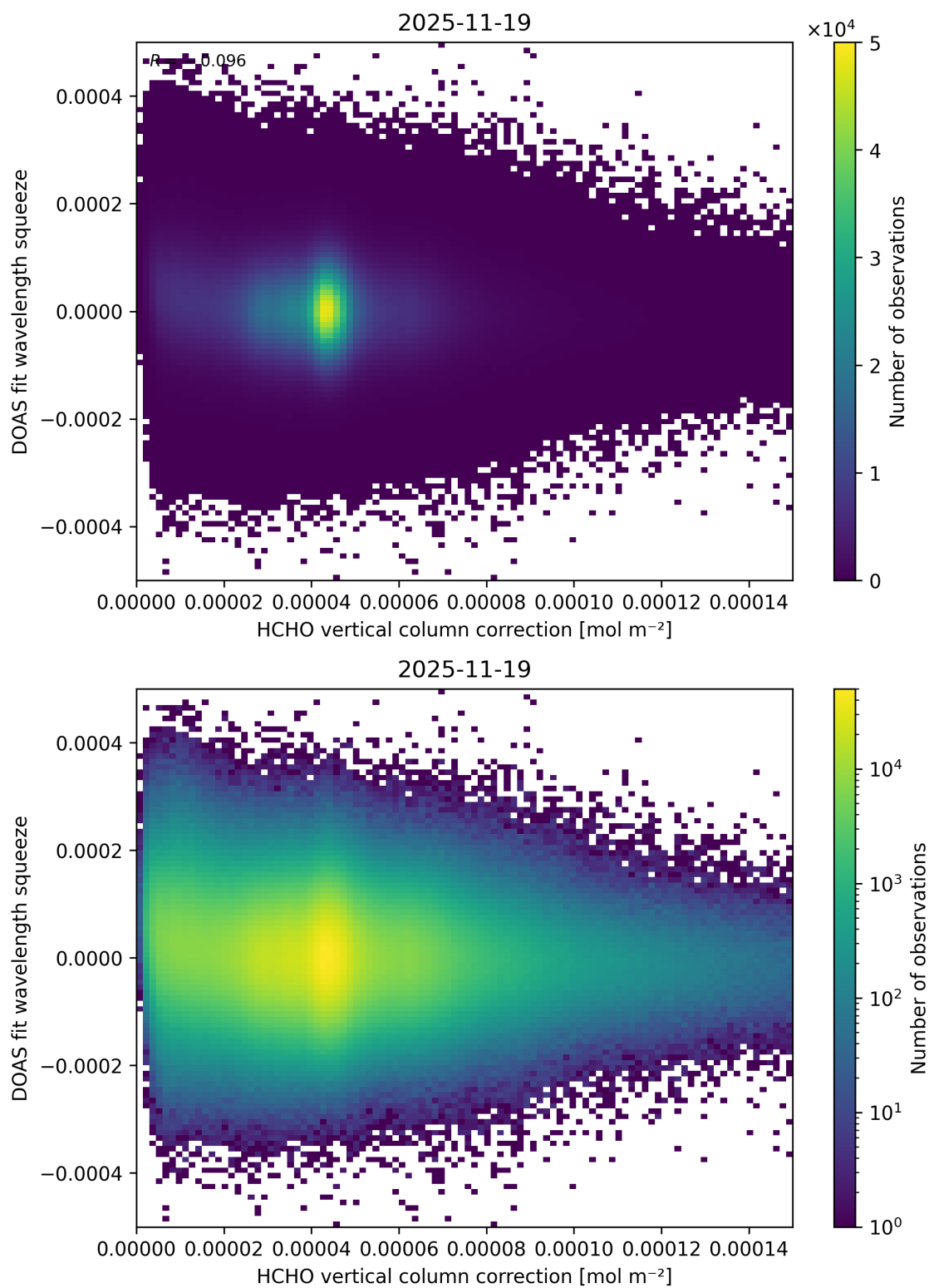
Figure 128: Scatter density plot of “HCHO vertical column correction” against “DOAS fit wavelength squeeze” for 2025-11-18 to 2025-11-20.
