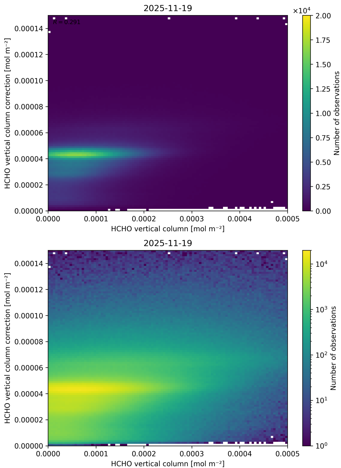
Figure 148: Scatter density plot of “HCHO vertical column” against “HCHO vertical column correction” for 2025-11-18 to 2025-11-20.
