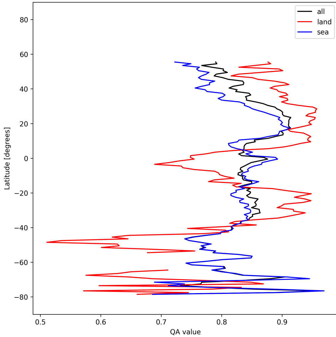
Figure 21: Zonal average of “QA value” for 2025-11-18 to 2025-11-20.
