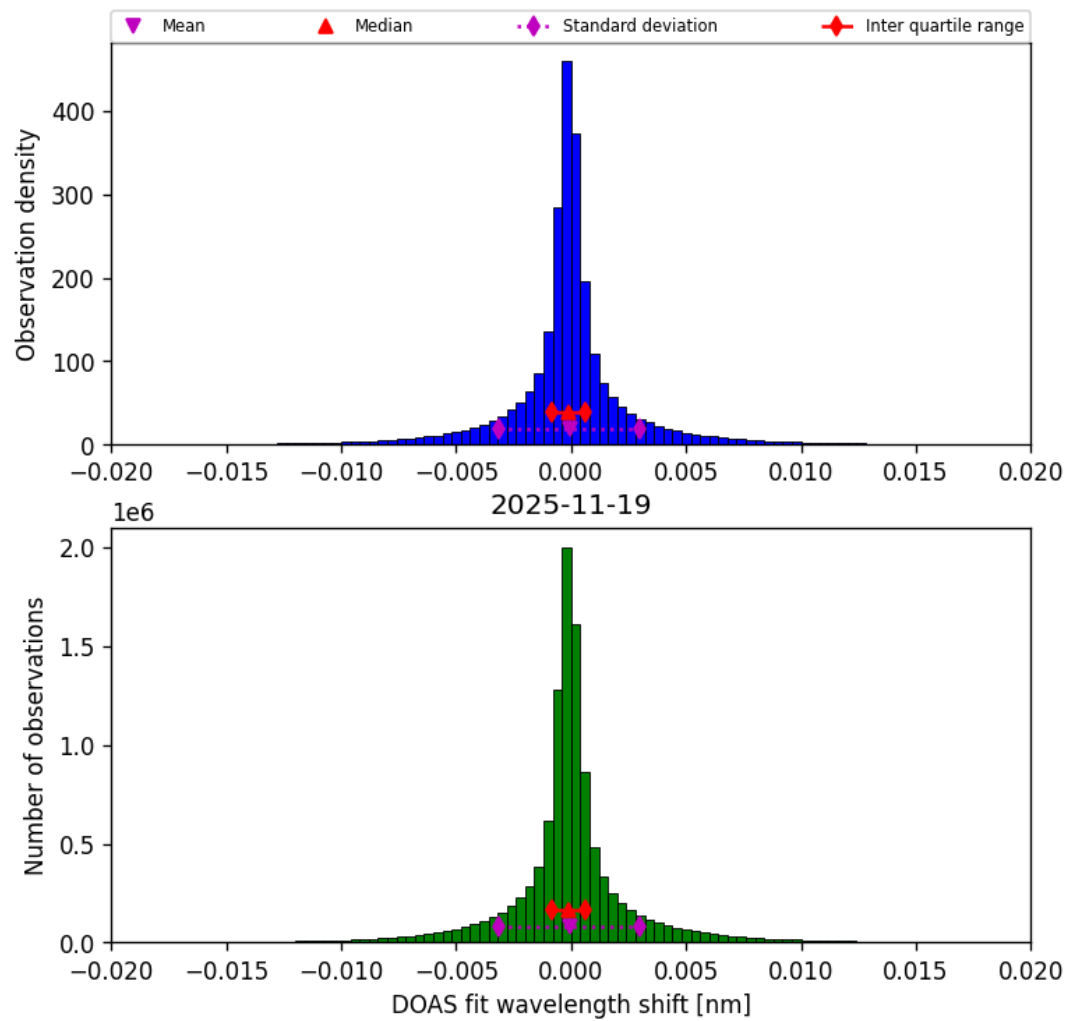
Figure 46: Histogram of “DOAS fit wavelength shift” for 2025-11-18 to 2025-11-20
