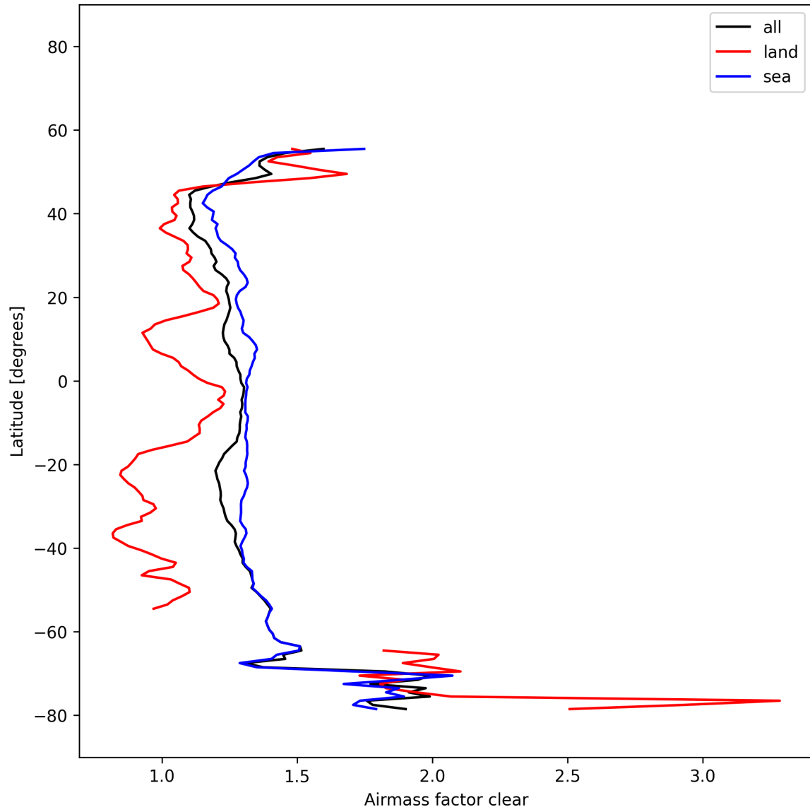
Figure 29: Zonal average of “Airmass factor clear” for 2025-11-18 to 2025-11-20.
