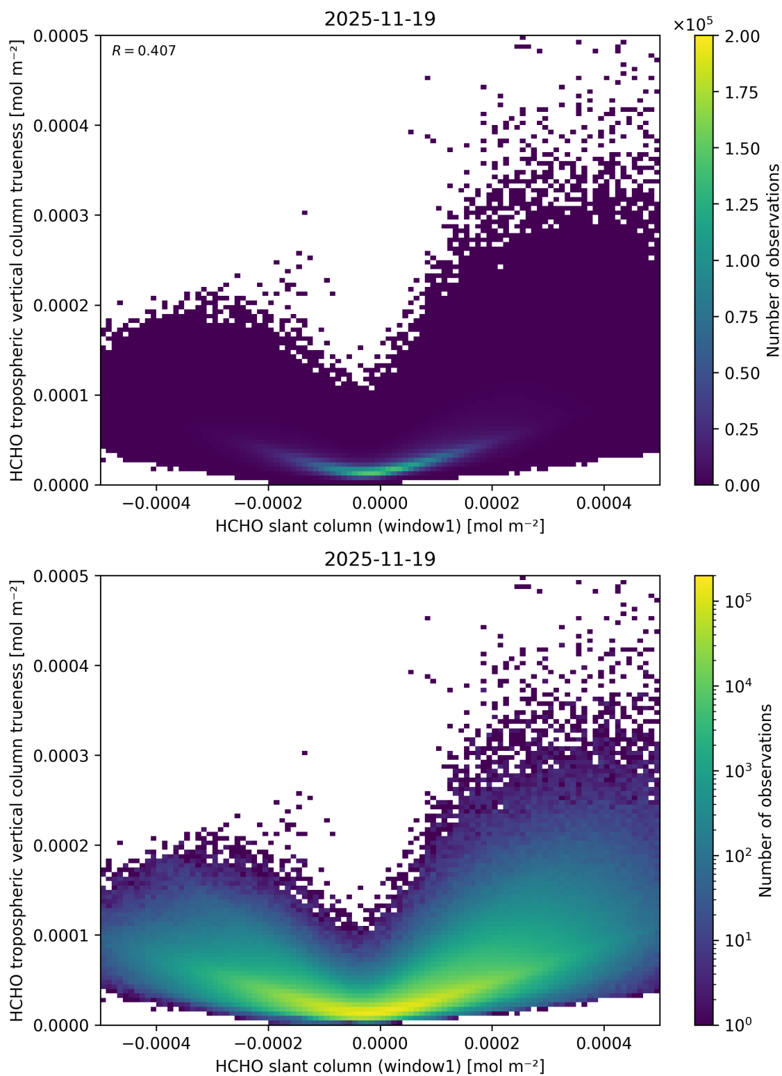
Figure 97: Scatter density plot of “HCHO slant column (window1)” against “HCHO tropospheric vertical column trueness” for 2025-11-18 to 2025-11-20.
