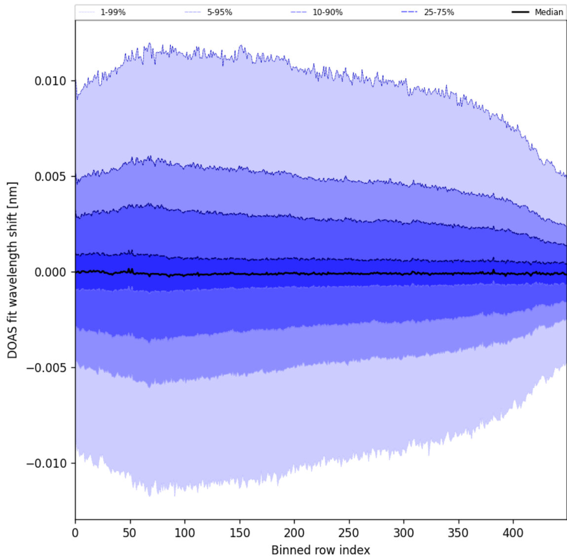
Figure 61: Along track statistics of “DOAS fit wavelength shift” for 2025-11-18 to 2025-11-20
