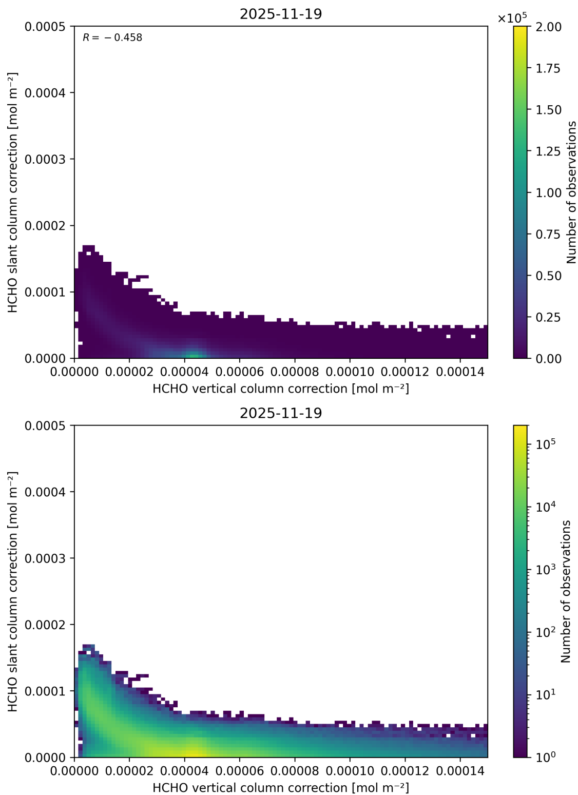
Figure 131: Scatter density plot of “HCHO vertical column correction” against “HCHO slant column correction” for 2025-11-18 to 2025-11-20.
