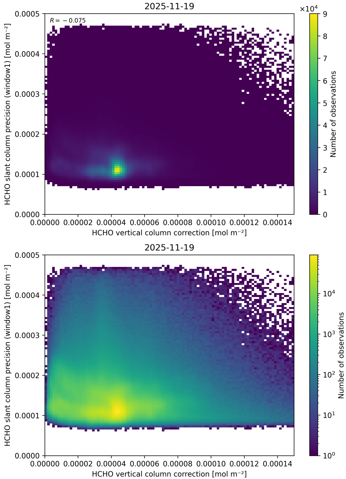
Figure 133: Scatter density plot of “HCHO vertical column correction” against “HCHO slant column precision (window1)” for 2025-11-18 to 2025-11-20.
