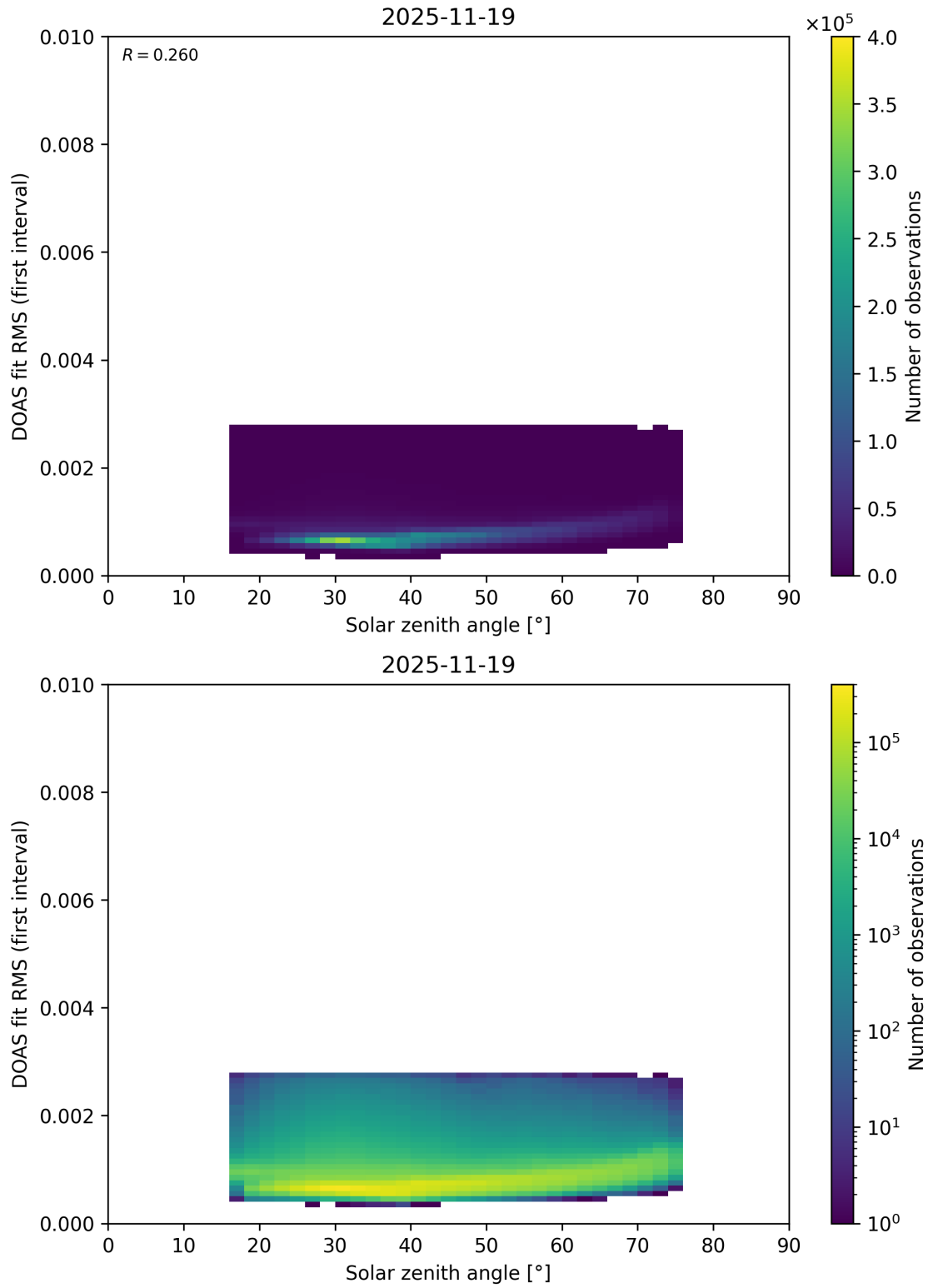
Figure 186: Scatter density plot of “Solar zenith angle” against “DOAS fit RMS (first interval)” for 2025-11-18 to 2025-11-20.
