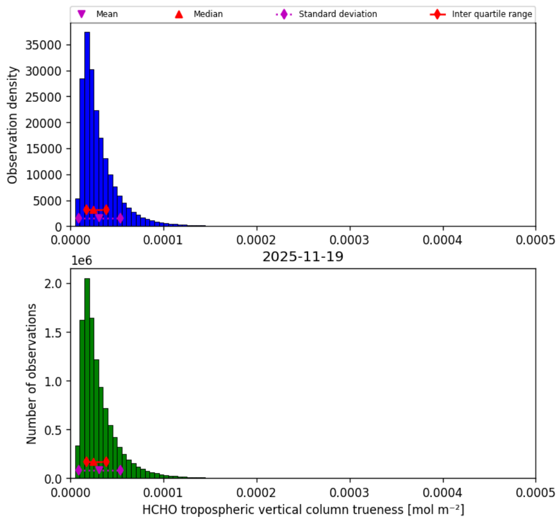
Figure 50: Histogram of “HCHO tropospheric vertical column trueness” for 2025-11-18 to 2025-11-20
