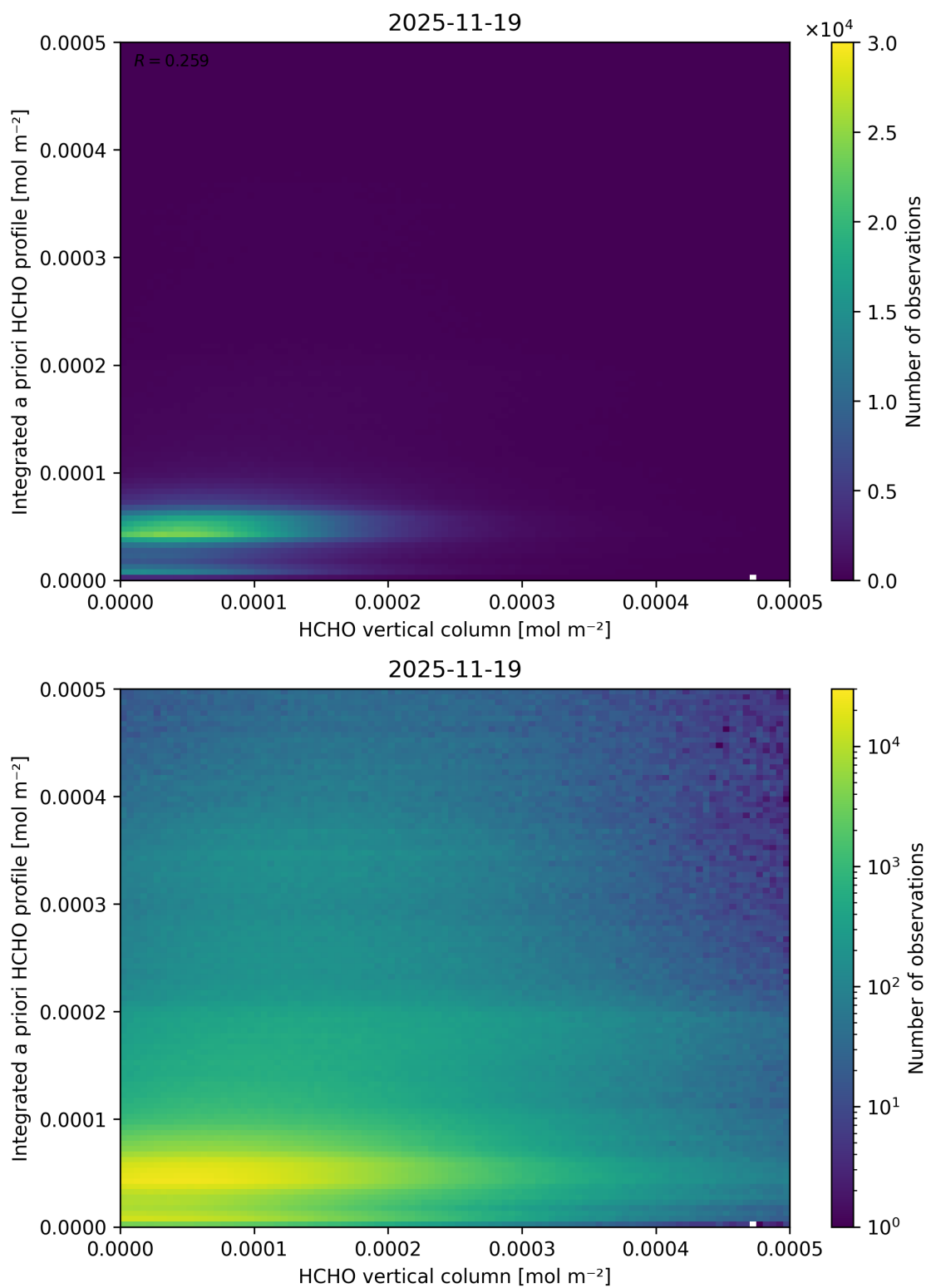
Figure 151: Scatter density plot of “HCHO vertical column” against “Integrated a priori HCHO profile” for 2025-11-18 to 2025-11-20.
