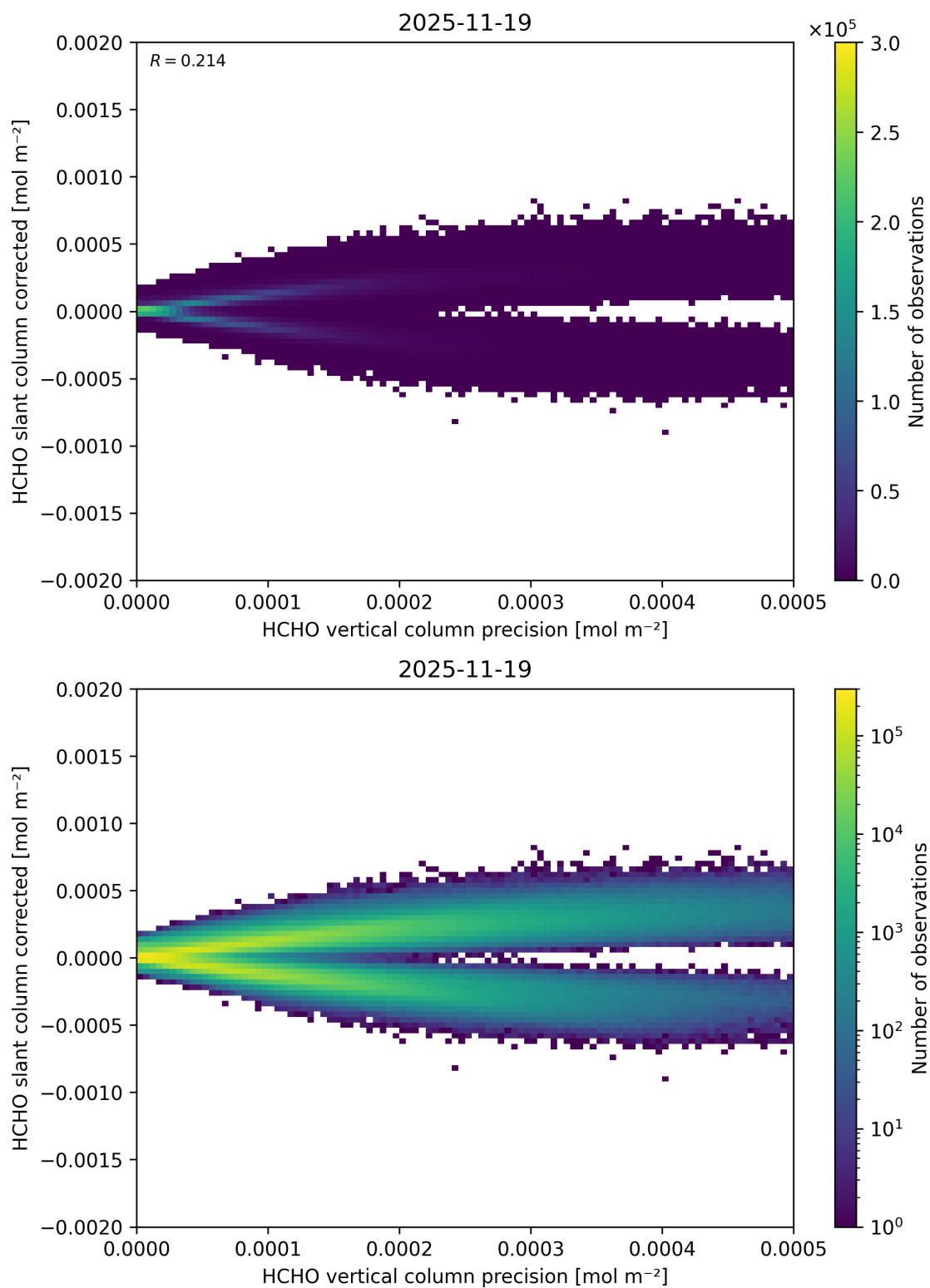
Figure 156: Scatter density plot of “HCHO vertical column precision” against “HCHO slant column corrected” for 2025-11-18 to 2025-11-20.
