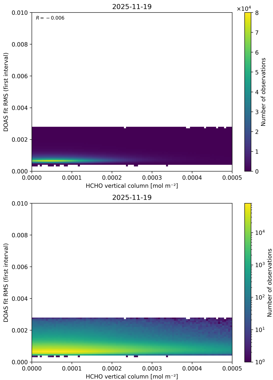
Figure 138: Scatter density plot of “HCHO vertical column” against “DOAS fit RMS (first interval)” for 2025-11-18 to 2025-11-20.
