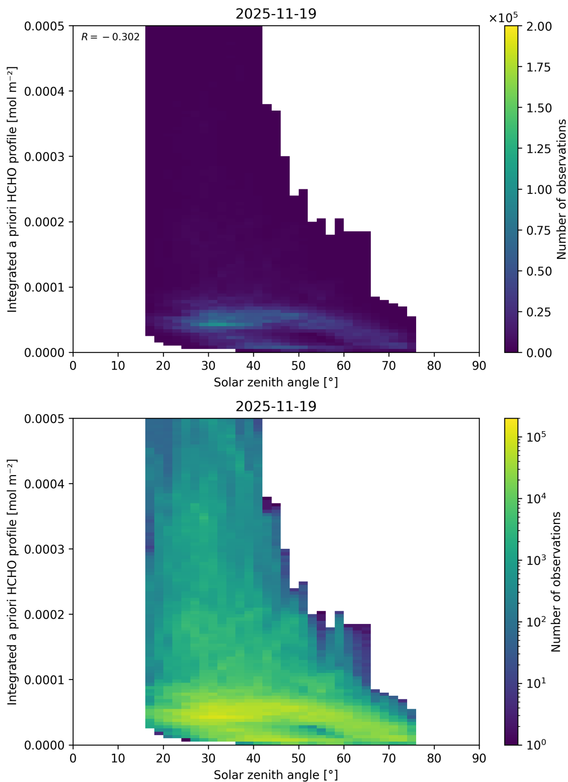
Figure 200: Scatter density plot of “Solar zenith angle” against “Integrated a priori HCHO profile” for 2025-11-18 to 2025-11-20.
