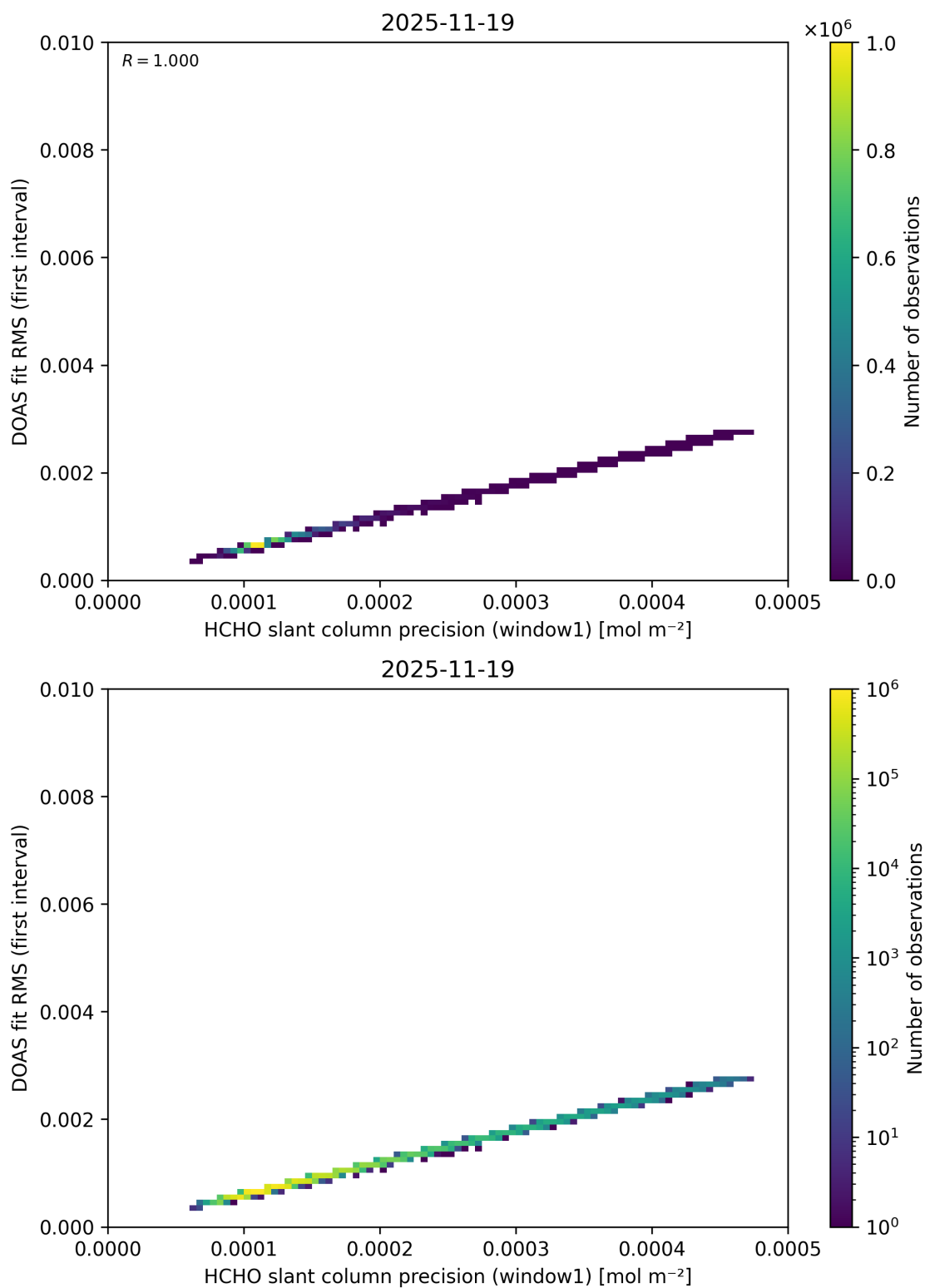
Figure 99: Scatter density plot of “HCHO slant column precision (window1)” against “DOAS fit RMS (first interval)” for 2025-11-18 to 2025-11-20.
