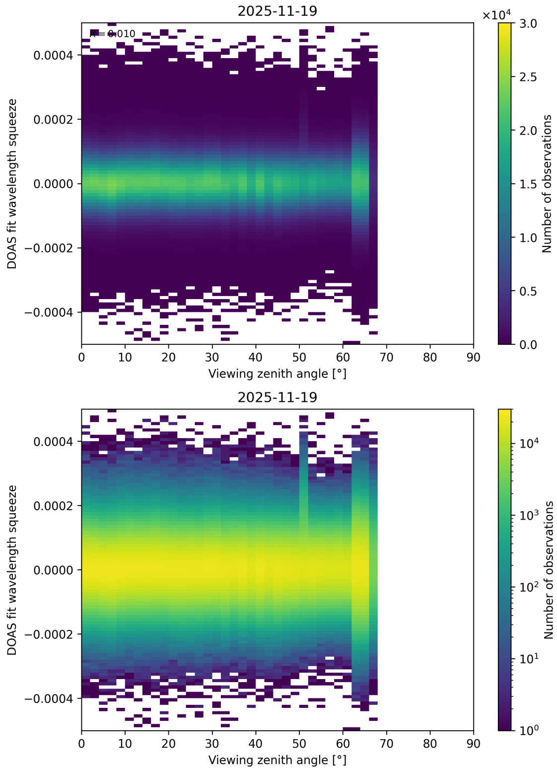
Figure 204: Scatter density plot of “Viewing zenith angle” against “DOAS fit wavelength squeeze” for 2025-11-18 to 2025-11-20.
