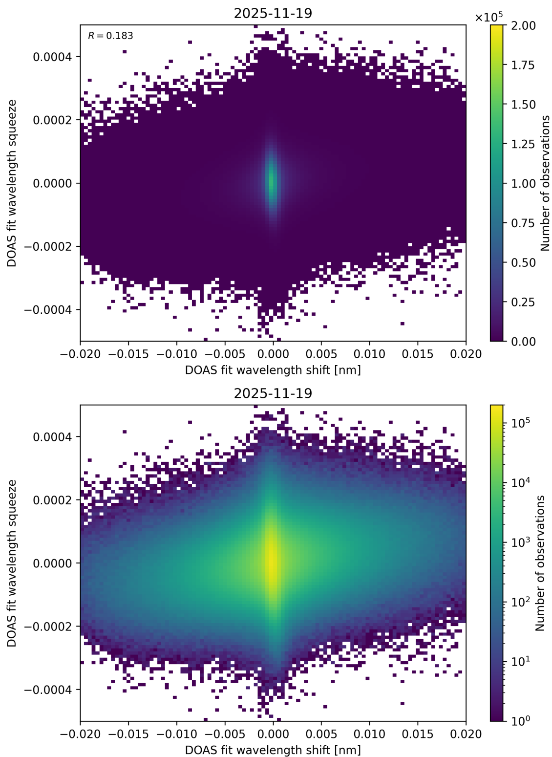
Figure 70: Scatter density plot of “DOAS fit wavelength shift” against “DOAS fit wavelength squeeze” for 2025-11-18 to 2025-11-20.
