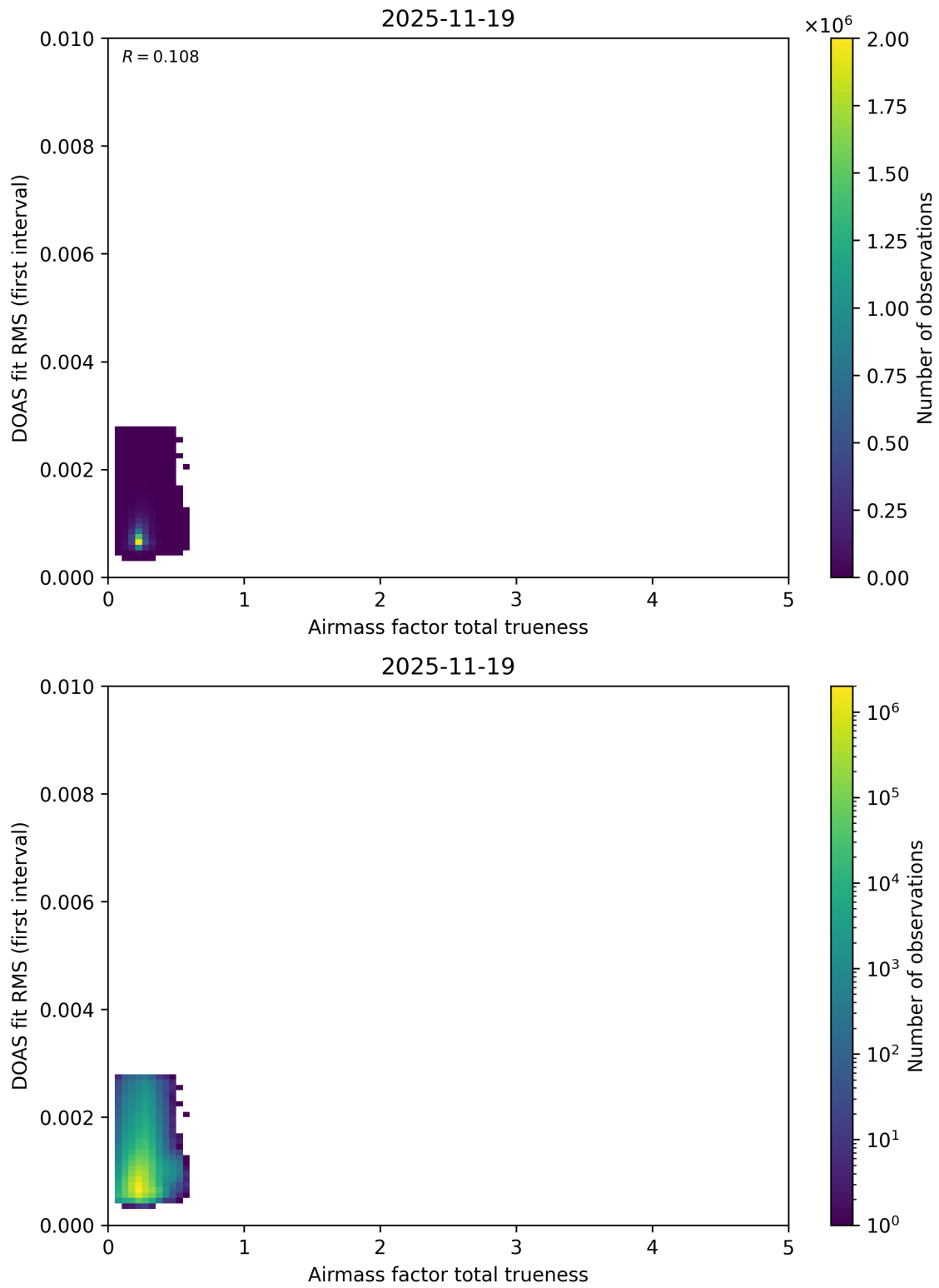
Figure 118: Scatter density plot of “Airmass factor total trueness” against “DOAS fit RMS (first interval)” for 2025-11-18 to 2025-11-20.
