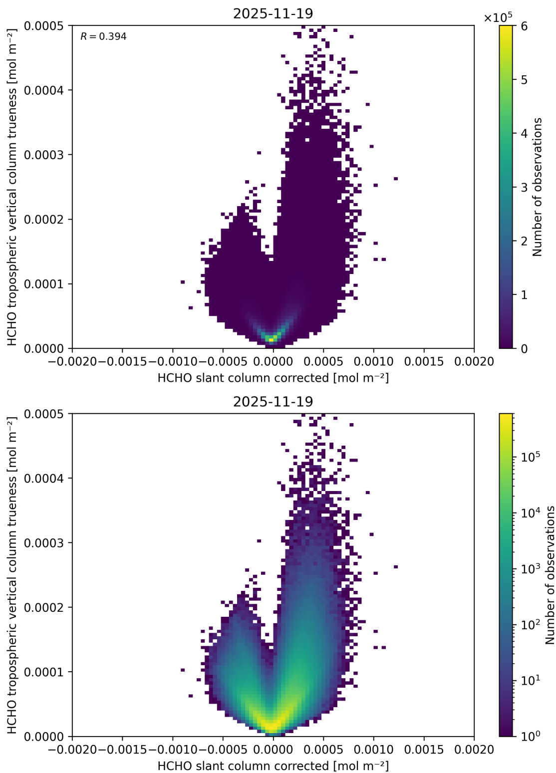
Figure 86: Scatter density plot of “HCHO slant column corrected” against “HCHO tropospheric vertical column trueness” for 2025-11-18 to 2025-11-20.
