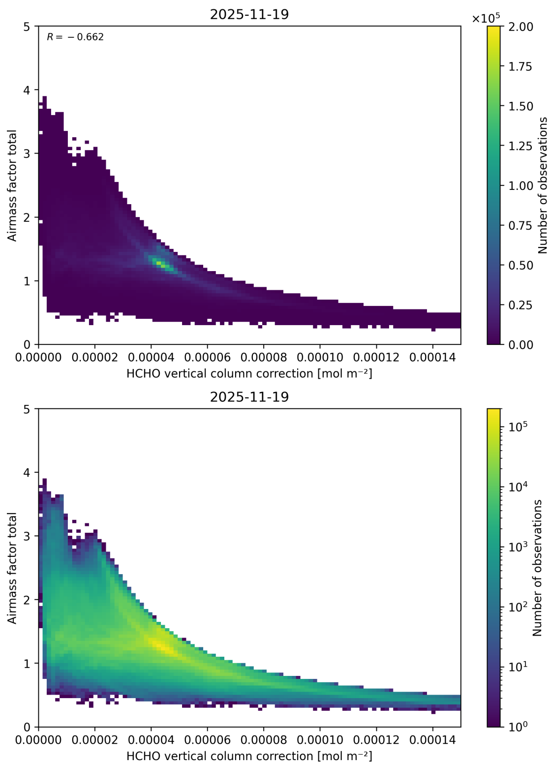
Figure 134: Scatter density plot of “HCHO vertical column correction” against “Airmass factor total” for 2025-11-18 to 2025-11-20.
