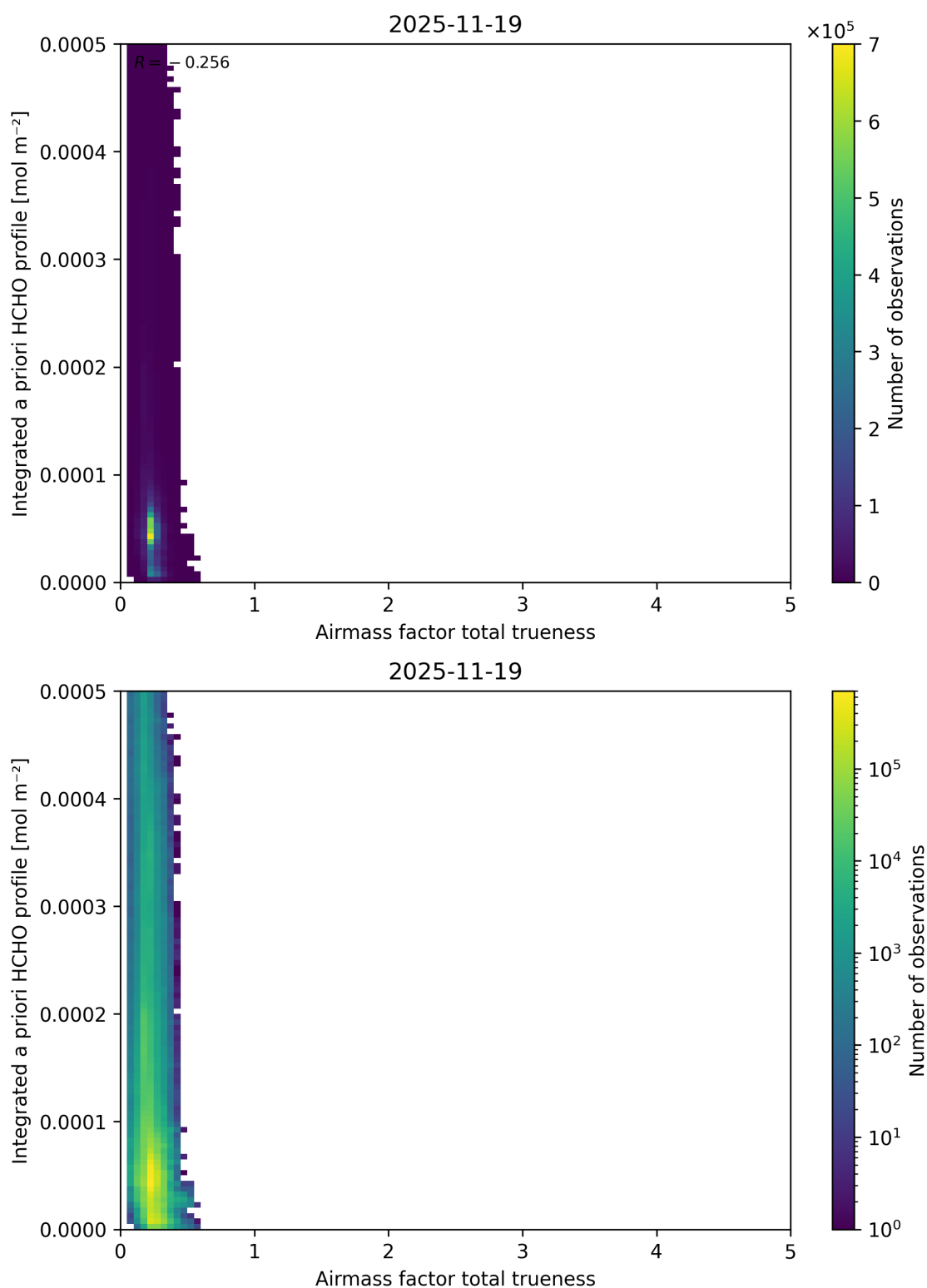
Figure 125: Scatter density plot of “Airmass factor total trueness” against “Integrated a priori HCHO profile” for 2025-11-18 to 2025-11-20.
