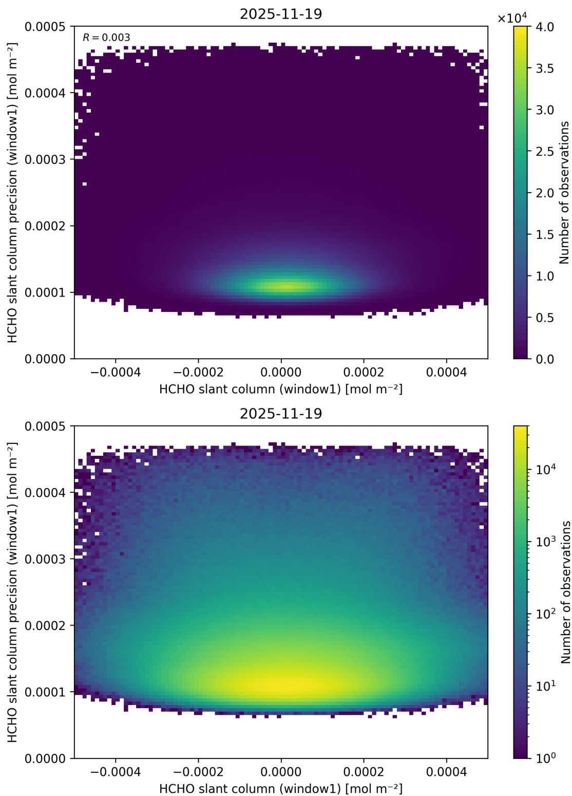
Figure 94: Scatter density plot of “HCHO slant column (window1)” against “HCHO slant column precision (window1)” for 2025-11-18 to 2025-11-20.
