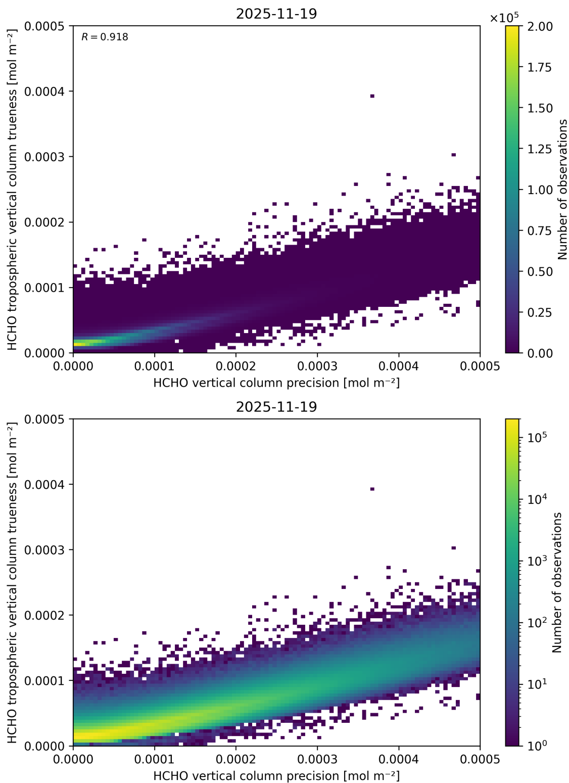
Figure 163: Scatter density plot of “HCHO vertical column precision” against “HCHO tropospheric vertical column true-ness” for 2025-11-18 to 2025-11-20.
