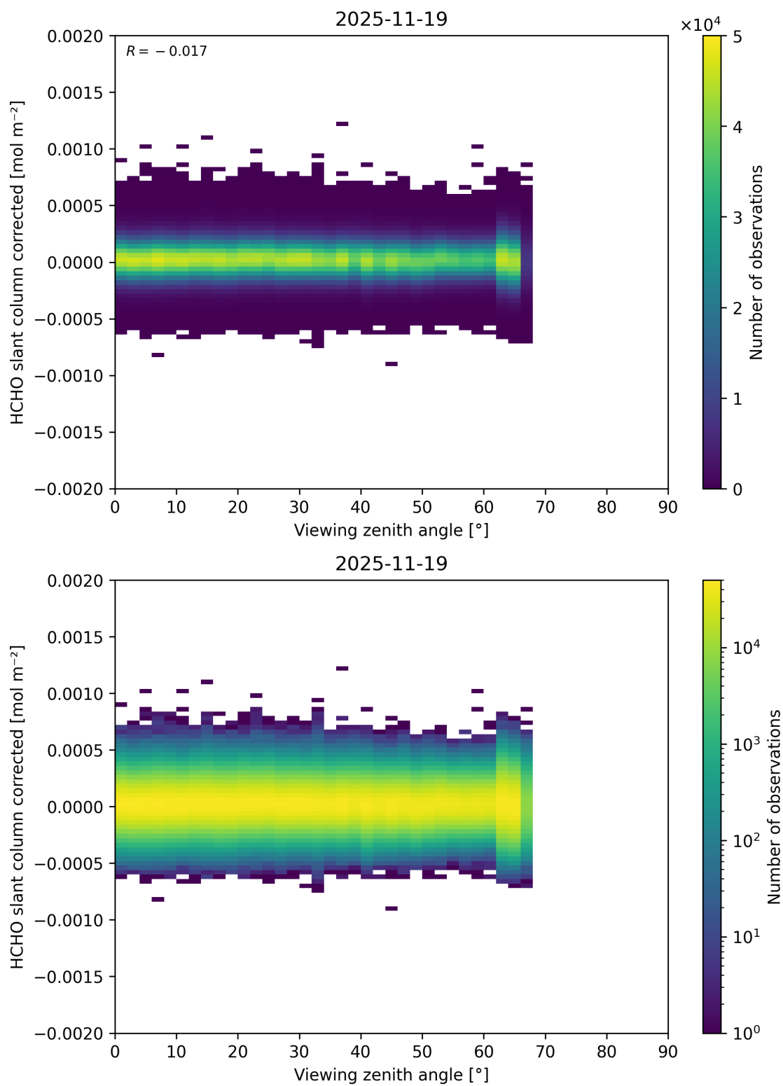
Figure 206: Scatter density plot of “Viewing zenith angle” against “HCHO slant column corrected” for 2025-11-18 to 2025-11-20.
