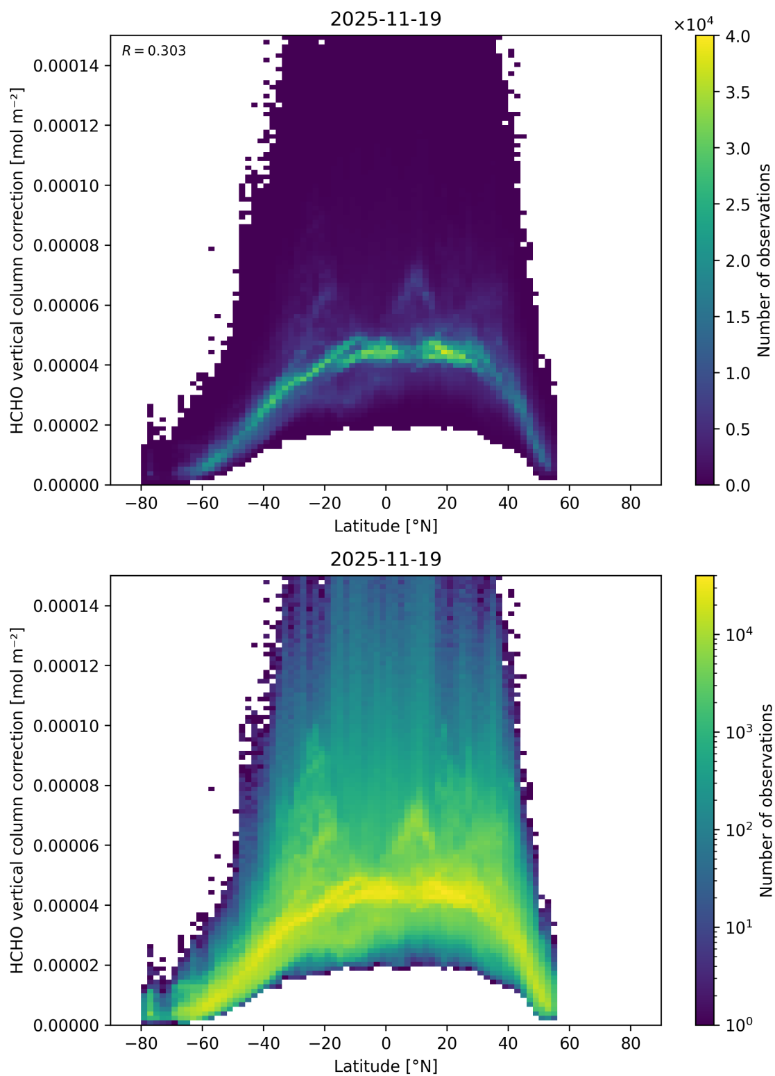
Figure 182: Scatter density plot of “Latitude” against “HCHO vertical column correction” for 2025-11-18 to 2025-11-20.
