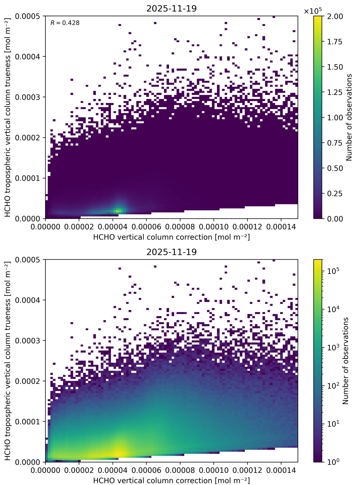
Figure 136: Scatter density plot of “HCHO vertical column correction” against “HCHO tropospheric vertical column true-ness” for 2025-11-18 to 2025-11-20.
