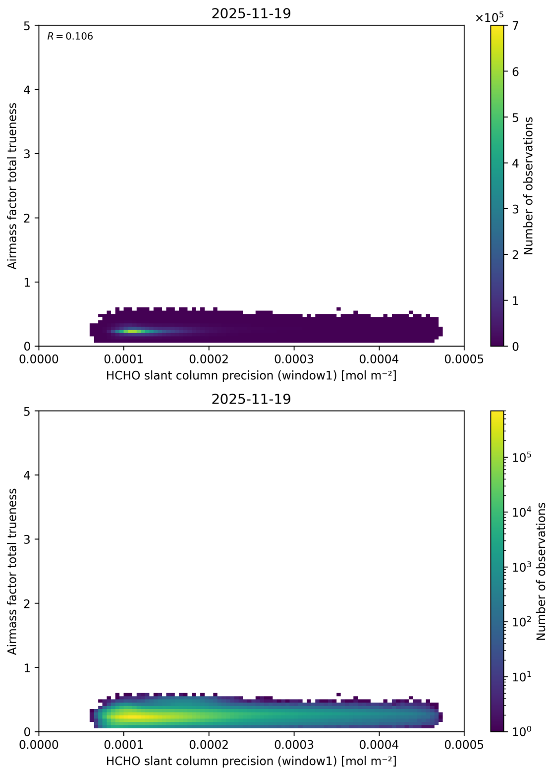
Figure 106: Scatter density plot of “HCHO slant column precision (window1)” against “Airmass factor total trueness” for 2025-11-18 to 2025-11-20.
