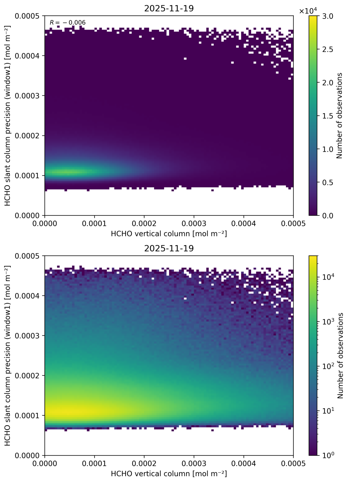
Figure 145: Scatter density plot of “HCHO vertical column” against “HCHO slant column precision (window1)” for 2025-11-18 to 2025-11-20.
