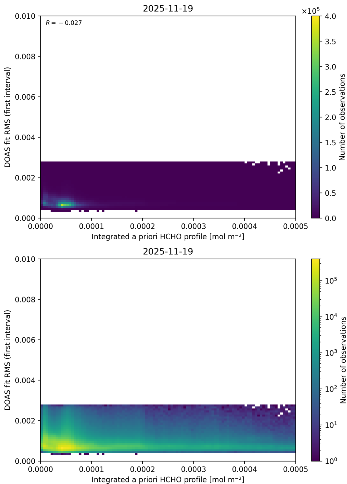
Figure 165: Scatter density plot of “Integrated a priori HCHO profile” against “DOAS fit RMS (first interval)” for 2025-11-18 to 2025-11-20.
