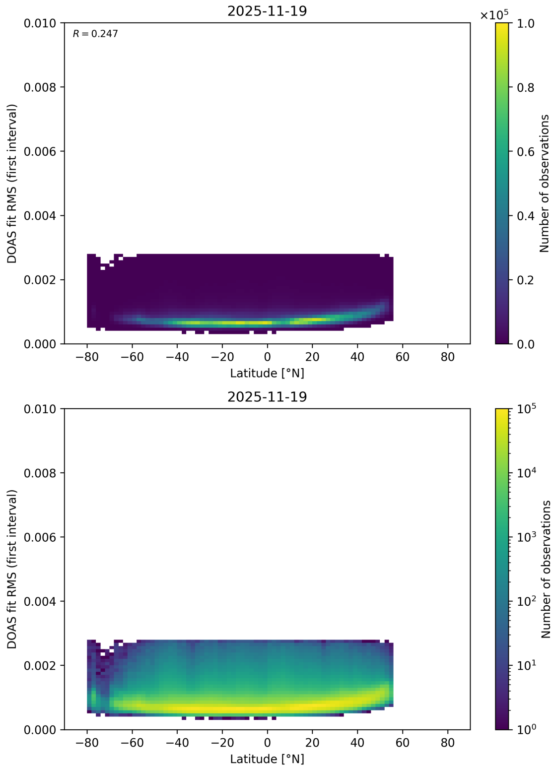
Figure 171: Scatter density plot of “Latitude” against “DOAS fit RMS (first interval)” for 2025-11-18 to 2025-11-20.
