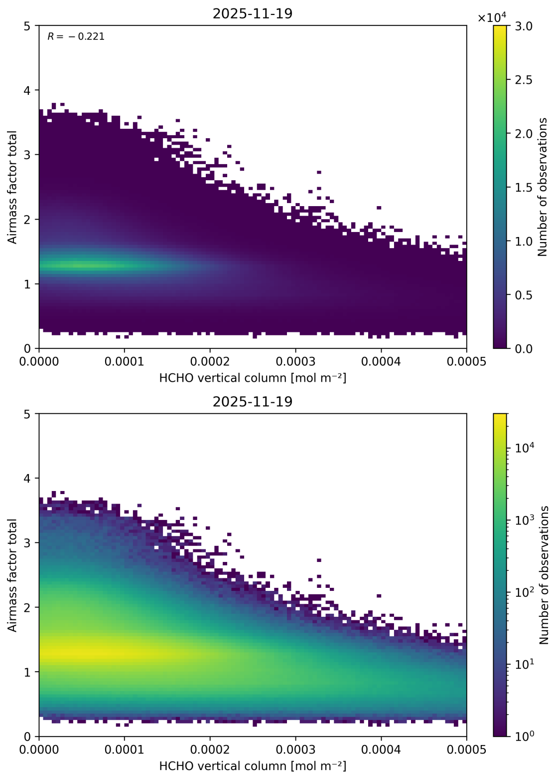
Figure 146: Scatter density plot of “HCHO vertical column” against “Airmass factor total” for 2025-11-18 to 2025-11-20.
