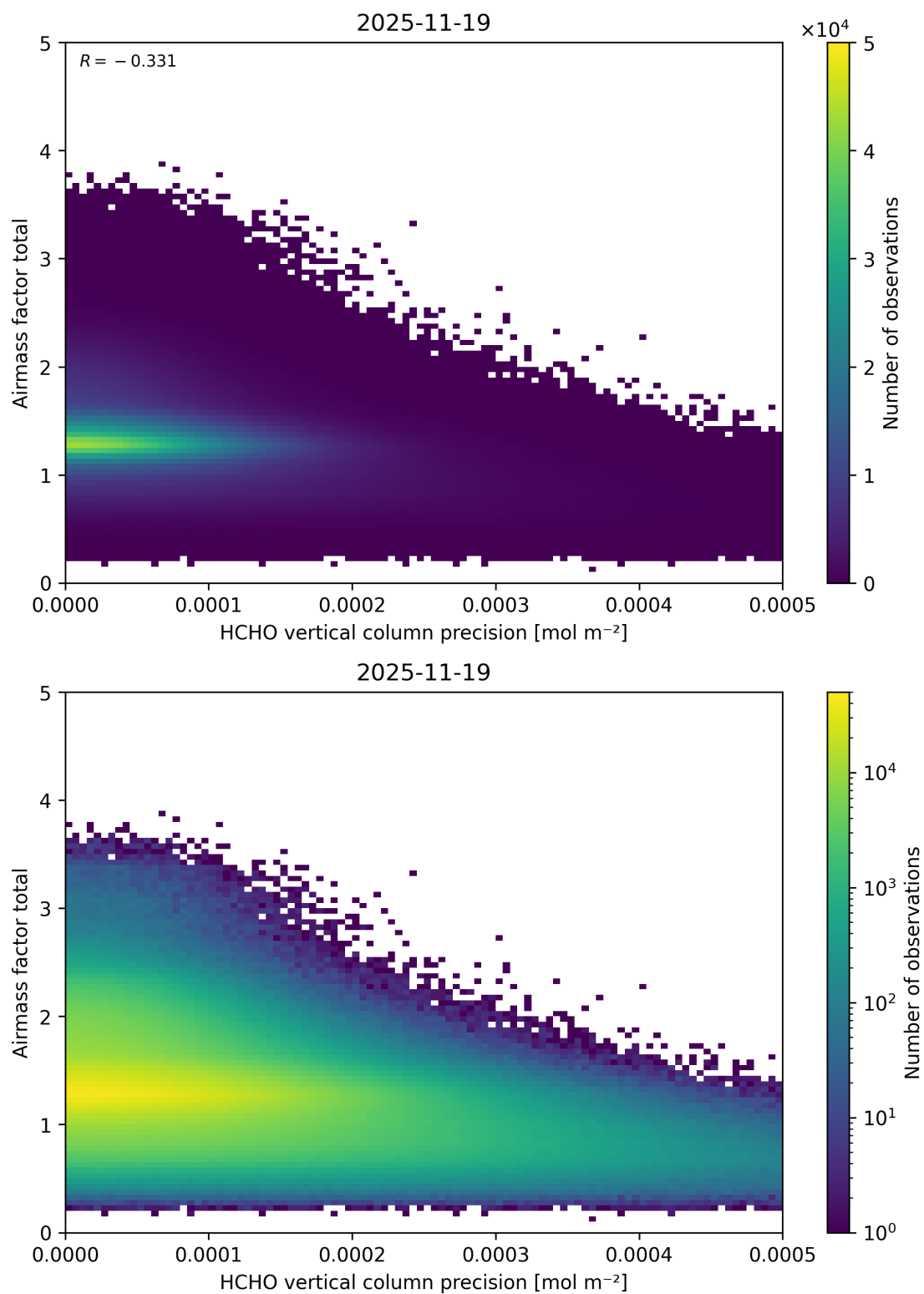
Figure 160: Scatter density plot of “HCHO vertical column precision” against “Airmass factor total” for 2025-11-18 to 2025-11-20.
