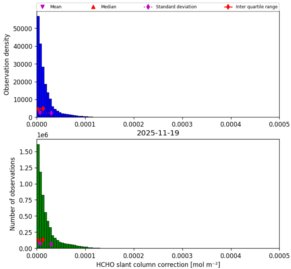
Figure 49: Histogram of “HCHO slant column correction” for 2025-11-18 to 2025-11-20
