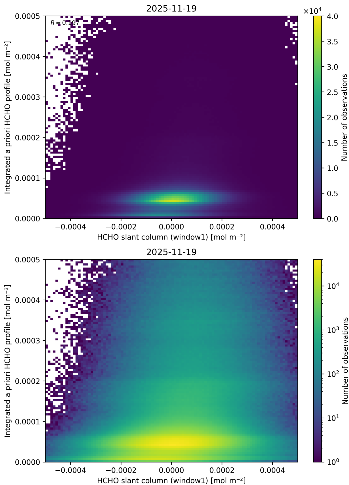
Figure 98: Scatter density plot of “HCHO slant column (window1)” against “Integrated a priori HCHO profile” for 2025-11-18 to 2025-11-20.
