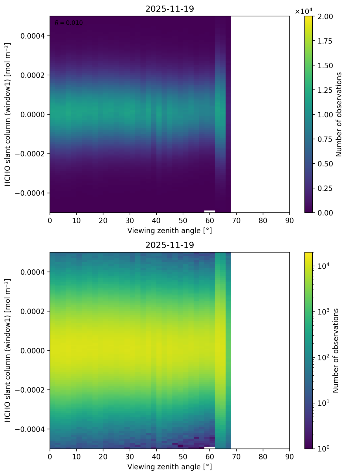
Figure 208: Scatter density plot of “Viewing zenith angle” against “HCHO slant column (window1)” for 2025-11-18 to 2025-11-20.
