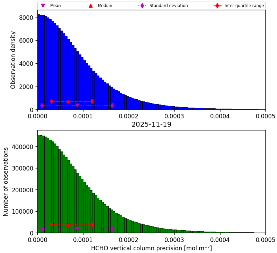
Figure 38: Histogram of “HCHO vertical column precision” for 2025-11-18 to 2025-11-20
