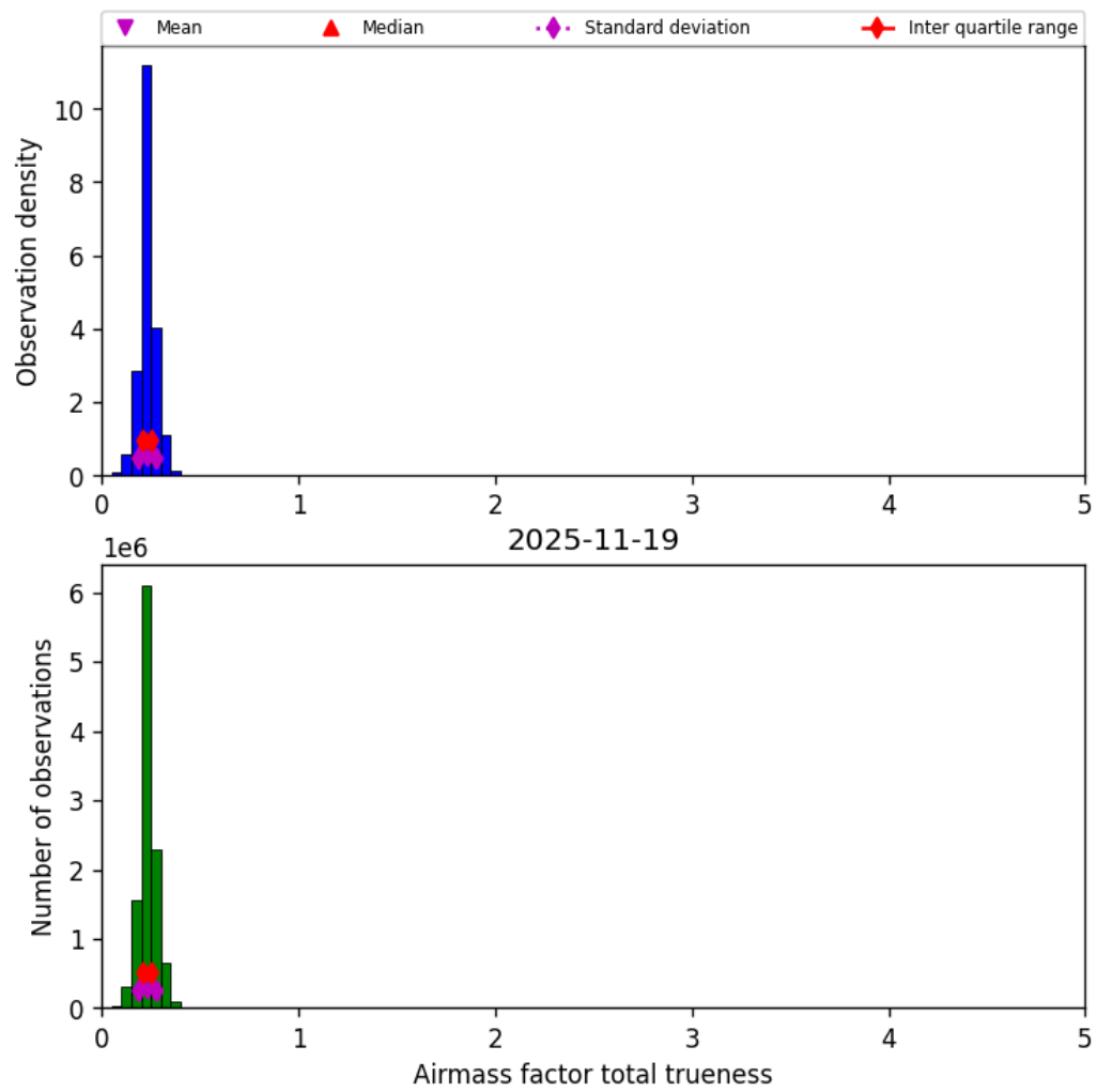
Figure 43: Histogram of “Airmass factor total trueness” for 2025-11-18 to 2025-11-20
