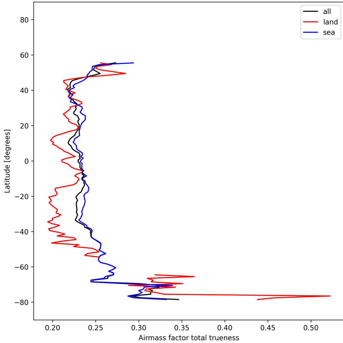
Figure 28: Zonal average of “Airmass factor total trueness” for 2025-11-18 to 2025-11-20.
