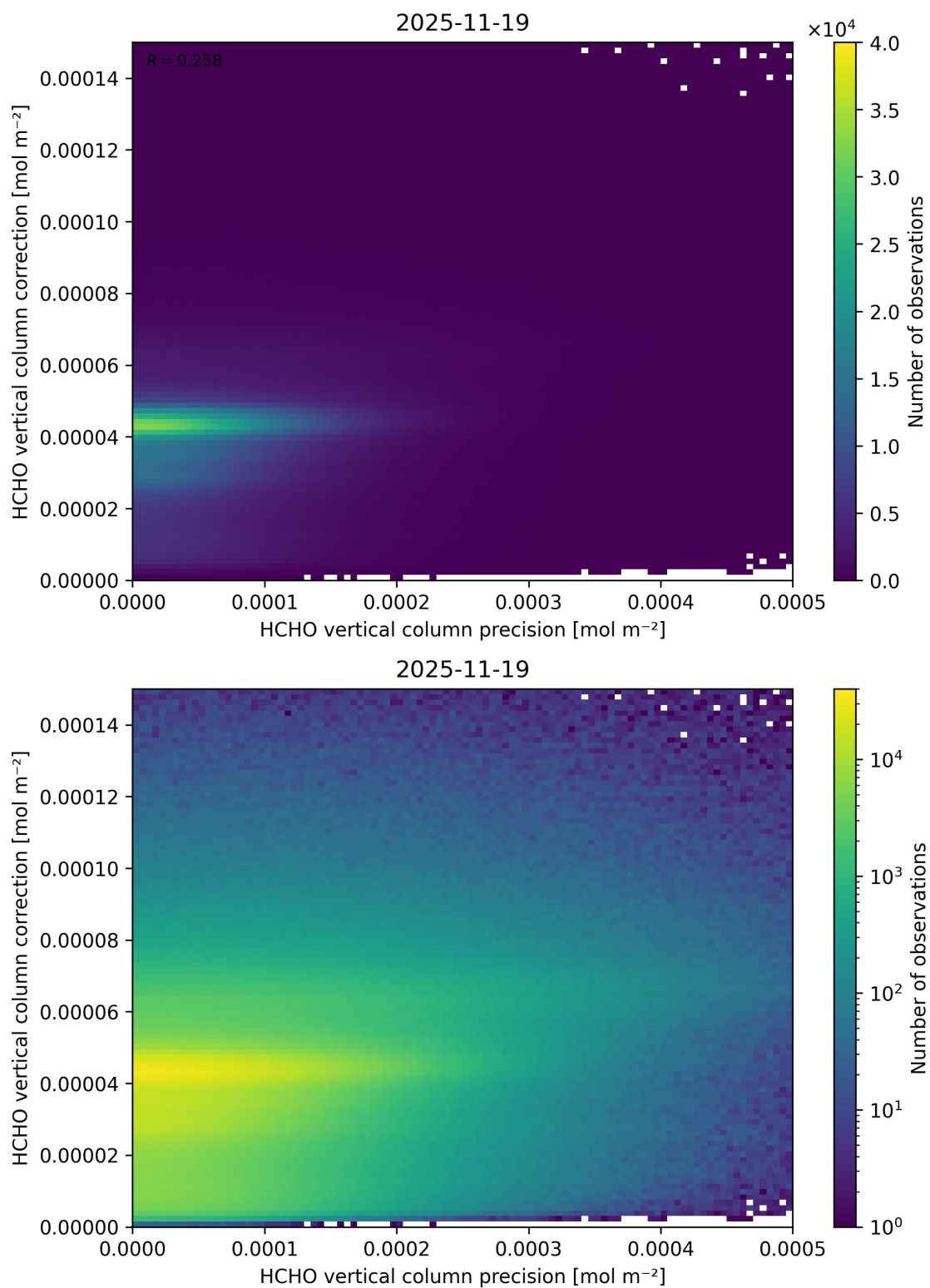
Figure 162: Scatter density plot of “HCHO vertical column precision” against “HCHO vertical column correction” for 2025-11-18 to 2025-11-20.
