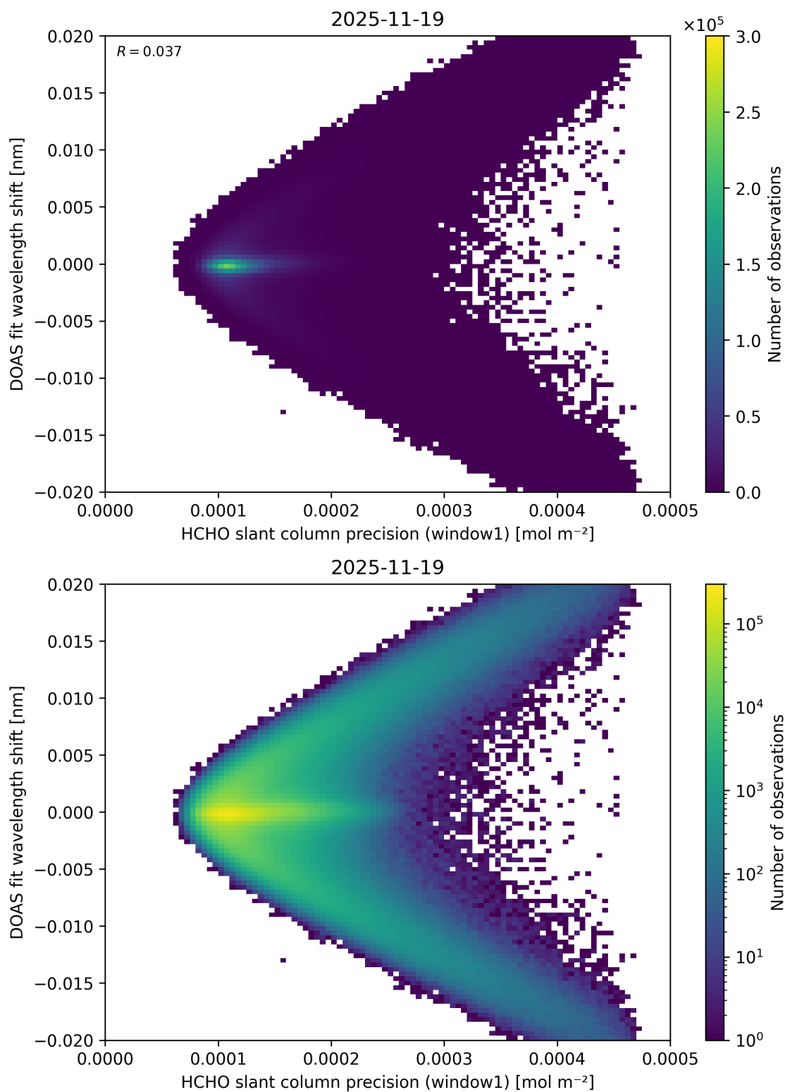
Figure 100: Scatter density plot of “HCHO slant column precision (window1)” against “DOAS fit wavelength shift” for 2025-11-18 to 2025-11-20.
