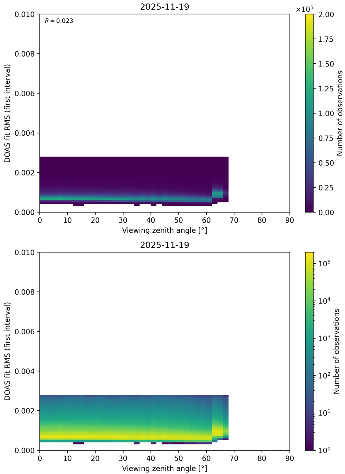
Figure 202: Scatter density plot of “Viewing zenith angle” against “DOAS fit RMS (first interval)” for 2025-11-18 to 2025-11-20.
