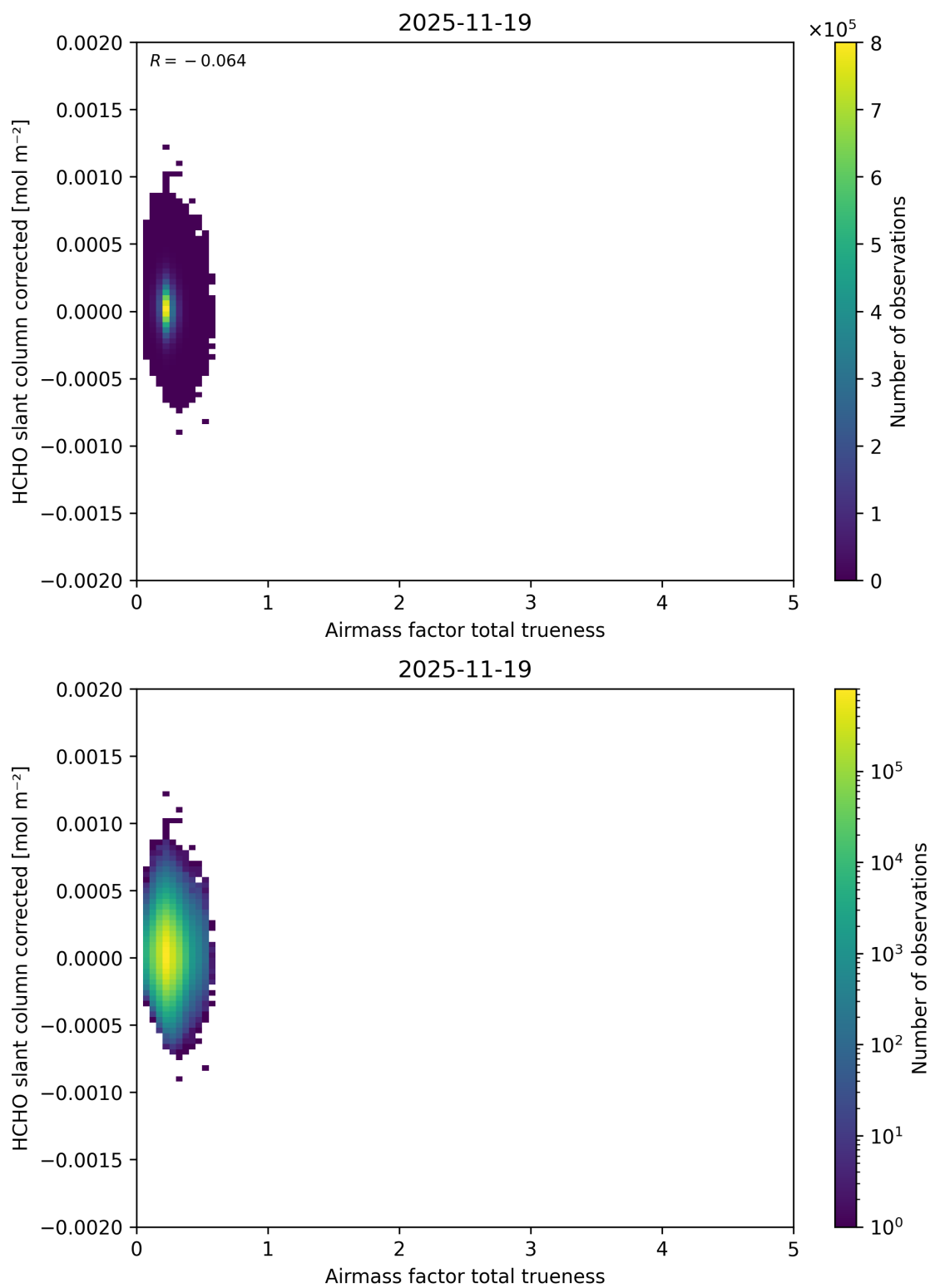
Figure 122: Scatter density plot of “Airmass factor total trueness” against “HCHO slant column corrected” for 2025-11-18 to 2025-11-20.
