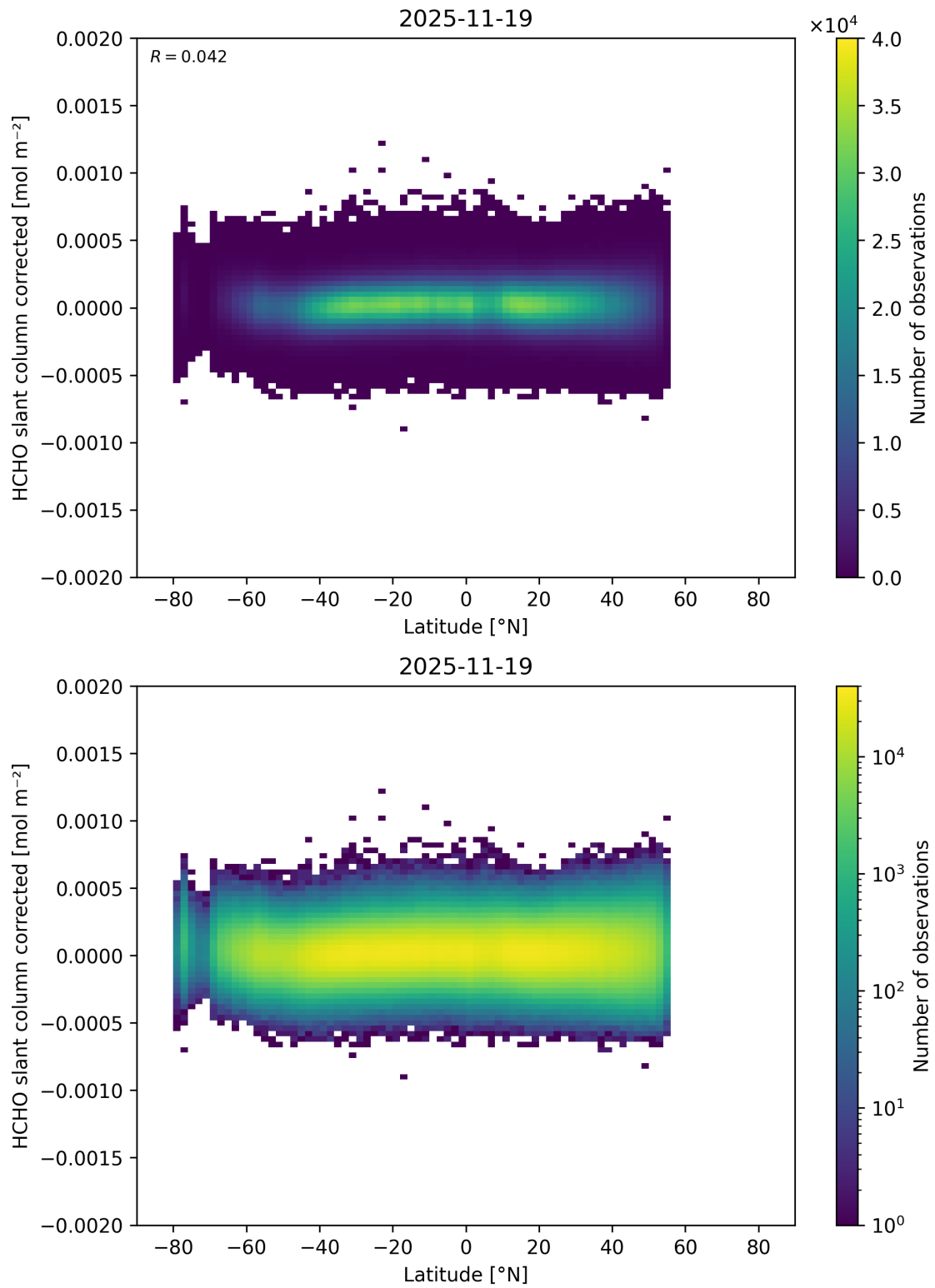
Figure 175: Scatter density plot of “Latitude” against “HCHO slant column corrected” for 2025-11-18 to 2025-11-20.
