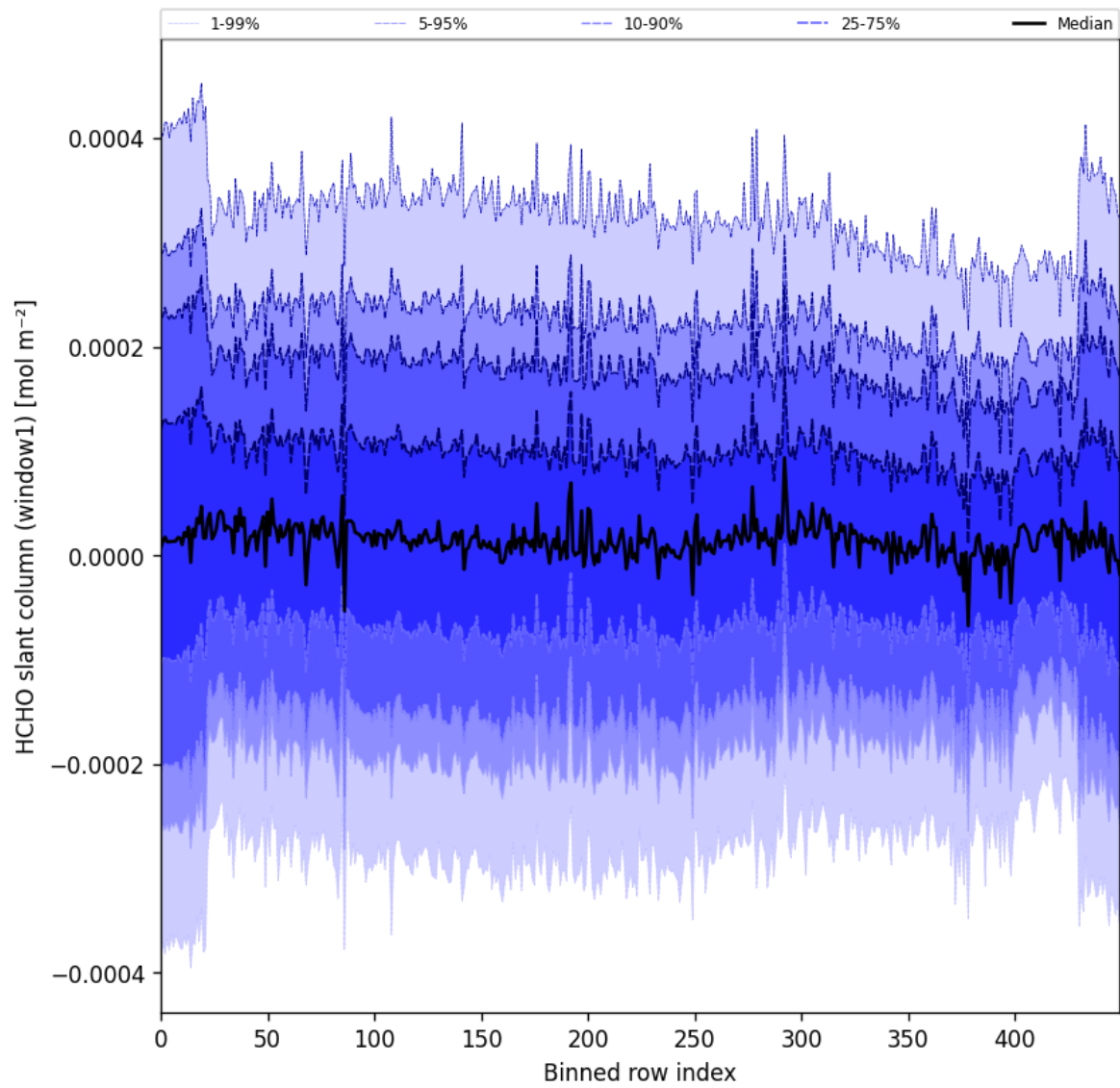
Figure 55: Along track statistics of “HCHO slant column (window1)” for 2025-11-18 to 2025-11-20
