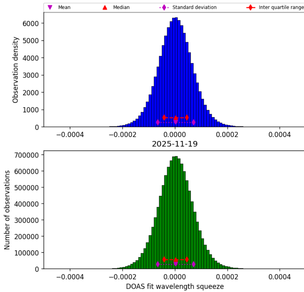
Figure 47: Histogram of “DOAS fit wavelength squeeze” for 2025-11-18 to 2025-11-20
