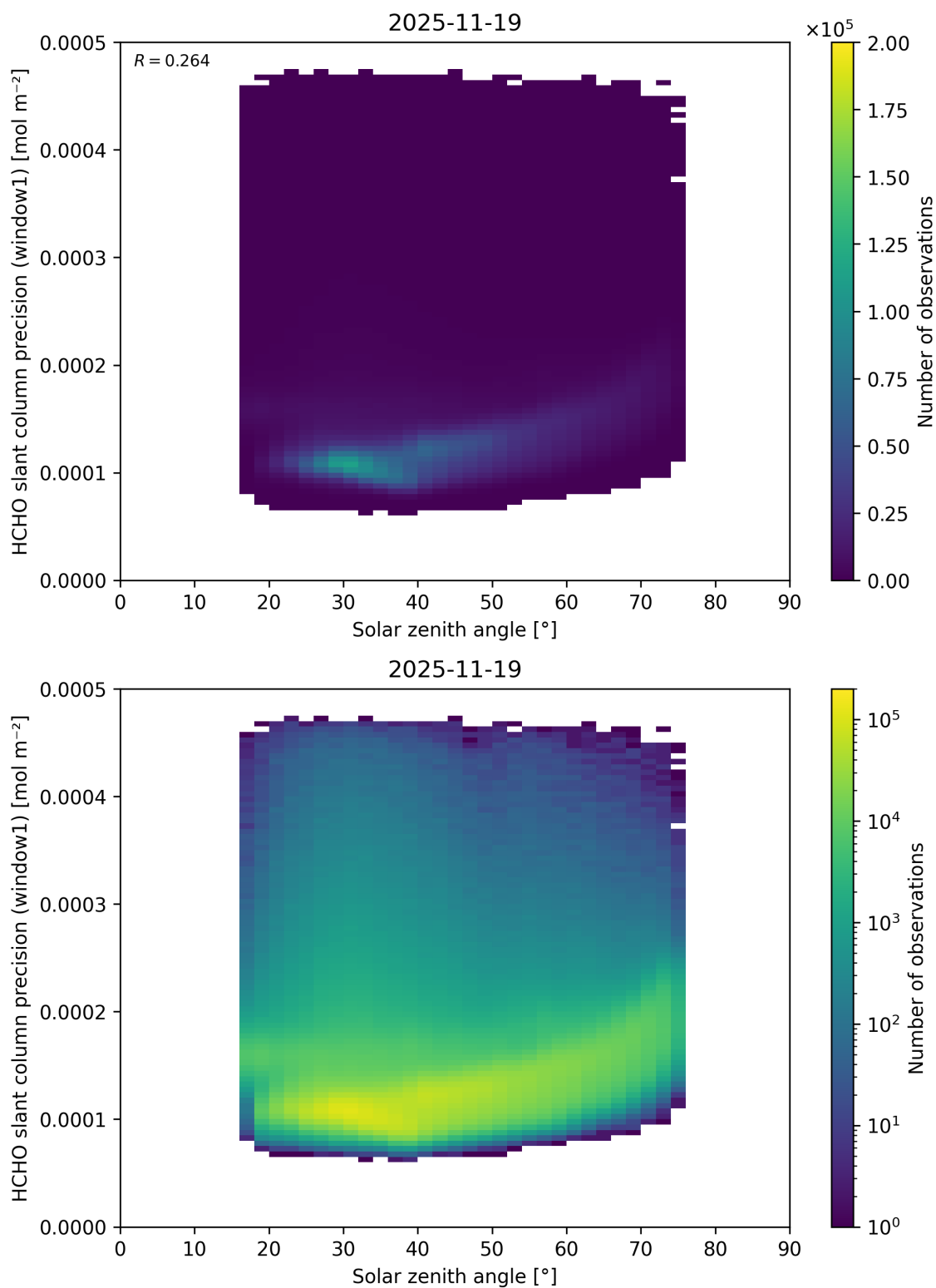
Figure 193: Scatter density plot of “Solar zenith angle” against “HCHO slant column precision (window1)” for 2025-11-18 to 2025-11-20.
