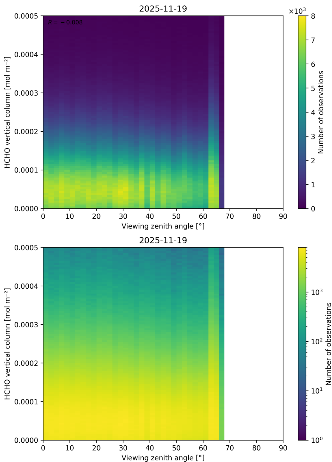
Figure 212: Scatter density plot of “Viewing zenith angle” against “HCHO vertical column” for 2025-11-18 to 2025-11-20.
