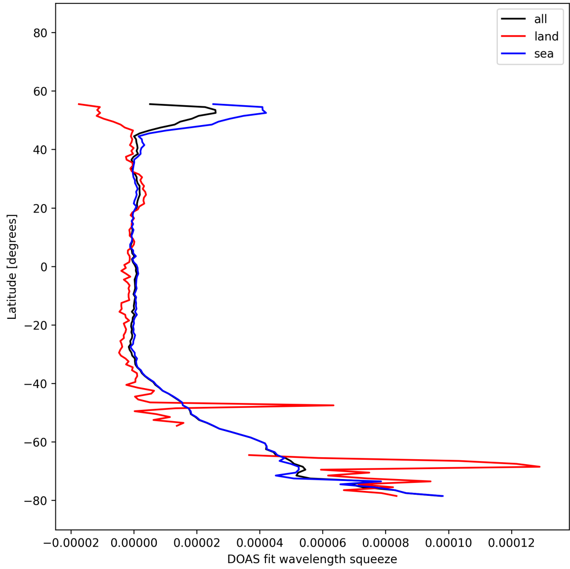
Figure 32: Zonal average of “DOAS fit wavelength squeeze” for 2025-11-18 to 2025-11-20.
