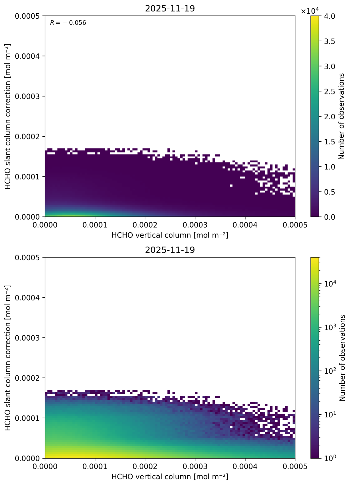
Figure 143: Scatter density plot of “HCHO vertical column” against “HCHO slant column correction” for 2025-11-18 to 2025-11-20.
