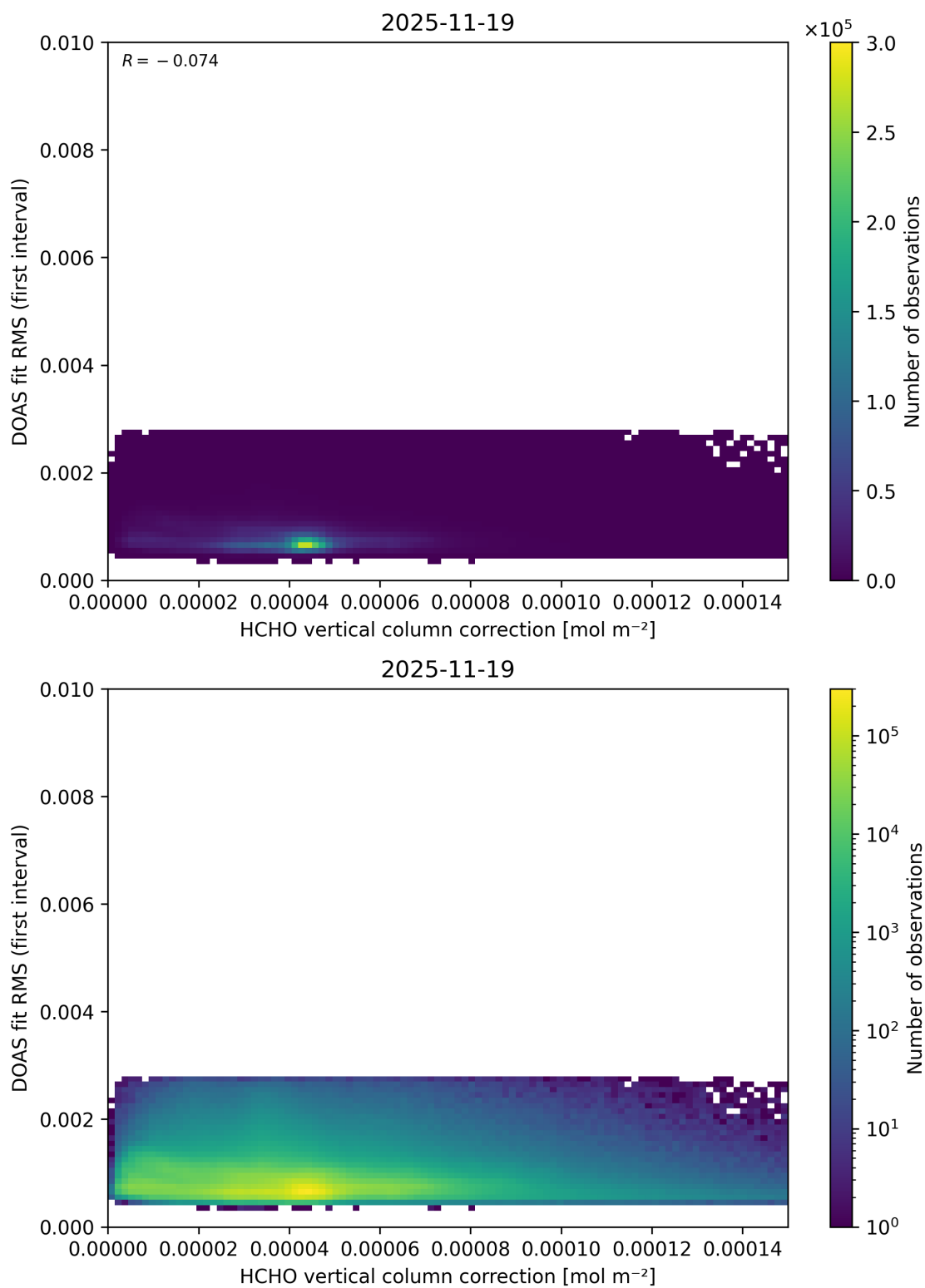
Figure 126: Scatter density plot of “HCHO vertical column correction” against “DOAS fit RMS (first interval)” for 2025-11-18 to 2025-11-20.
