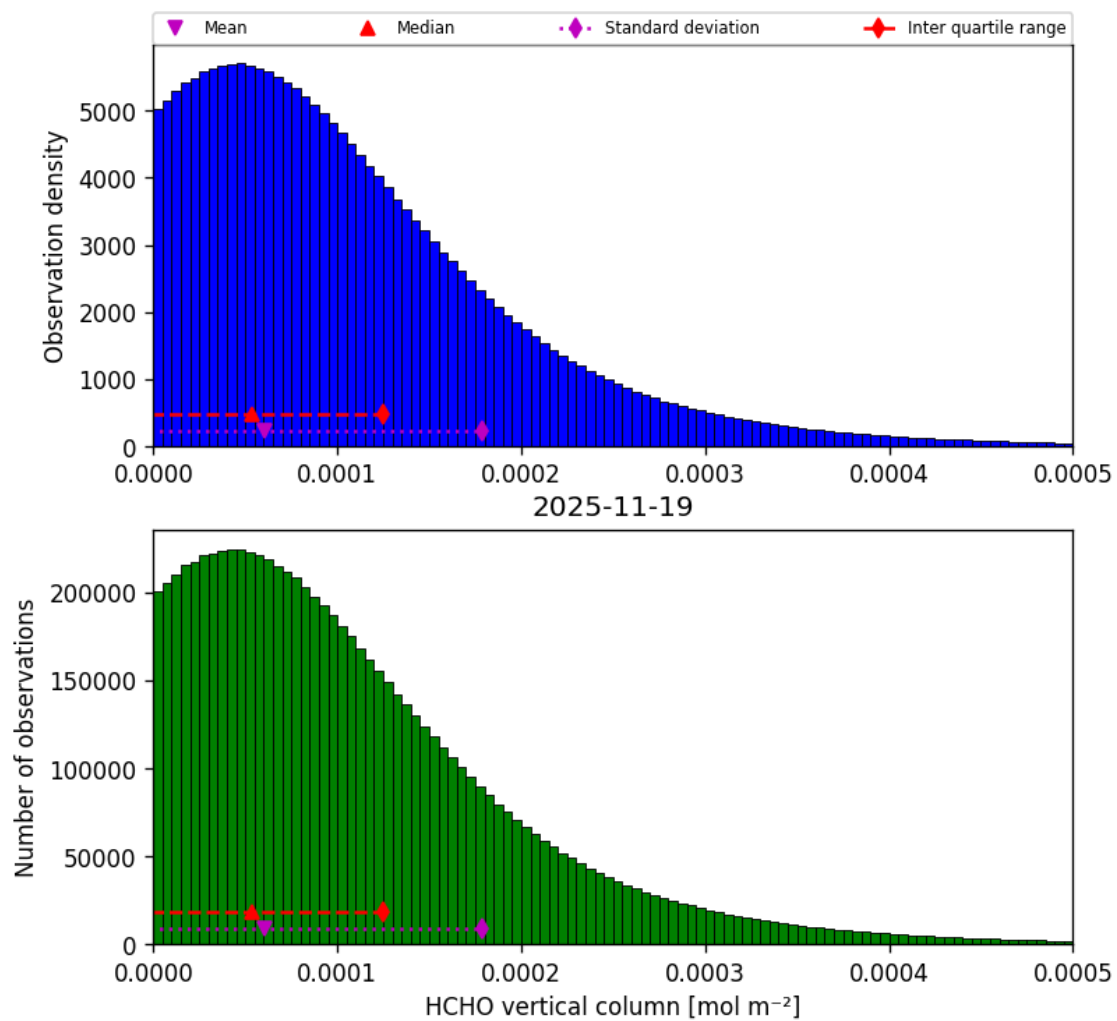
Figure 37: Histogram of “HCHO vertical column” for 2025-11-18 to 2025-11-20
