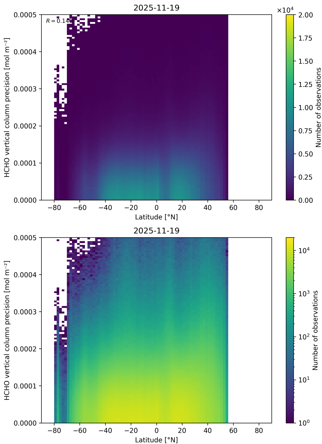
Figure 183: Scatter density plot of “Latitude” against “HCHO vertical column precision” for 2025-11-18 to 2025-11-20.
