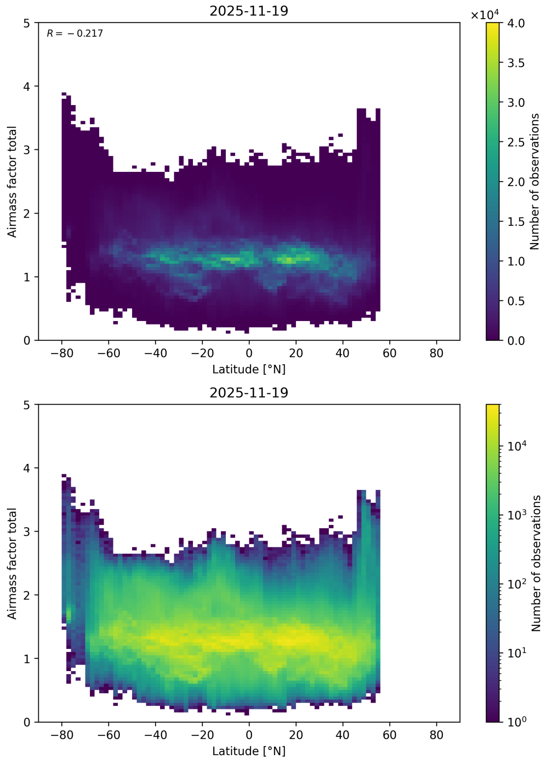
Figure 179: Scatter density plot of “Latitude” against “Airmass factor total” for 2025-11-18 to 2025-11-20.
