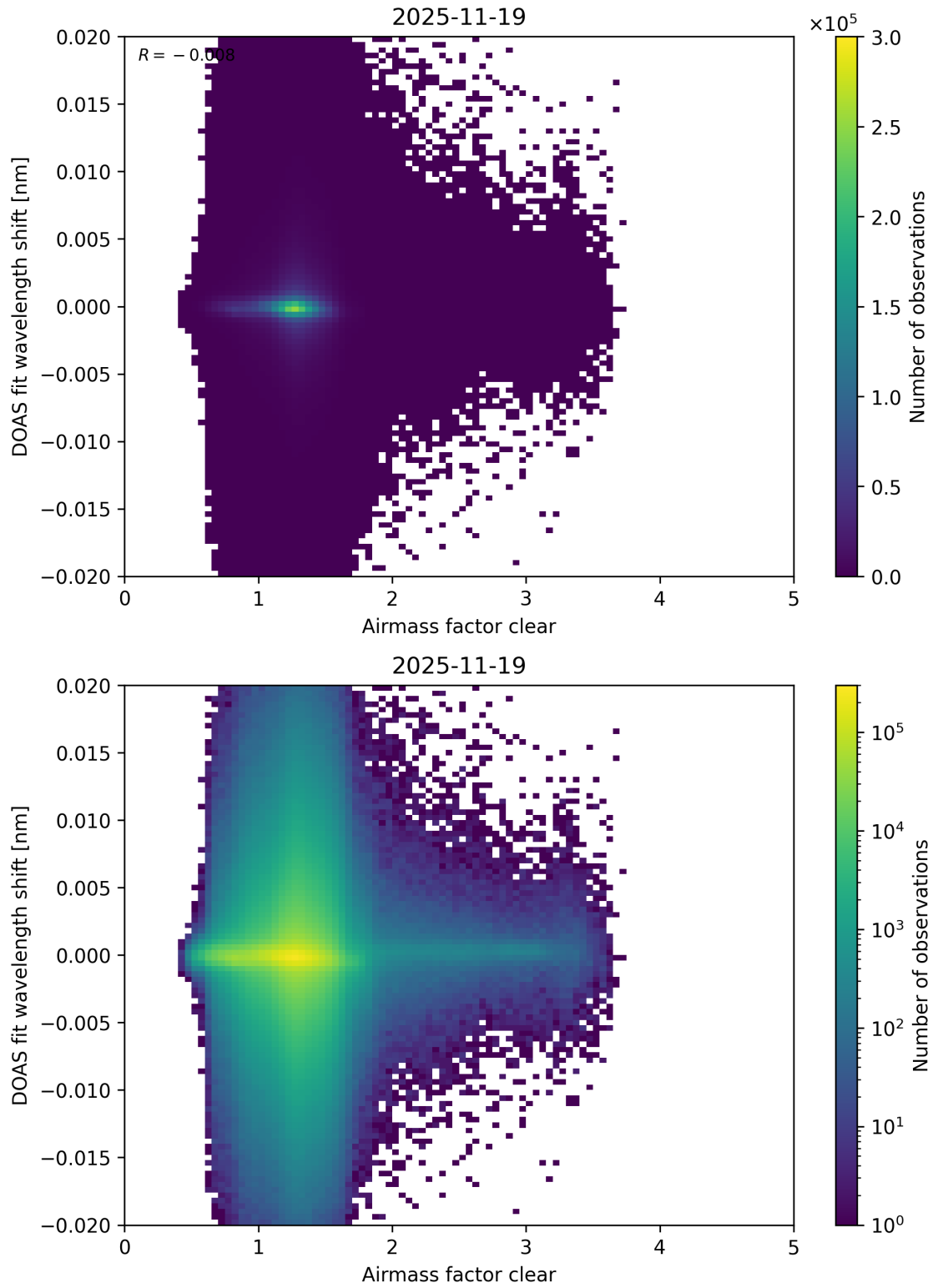
Figure 79: Scatter density plot of “Airmass factor clear” against “DOAS fit wavelength shift” for 2025-11-18 to 2025-11-20.
