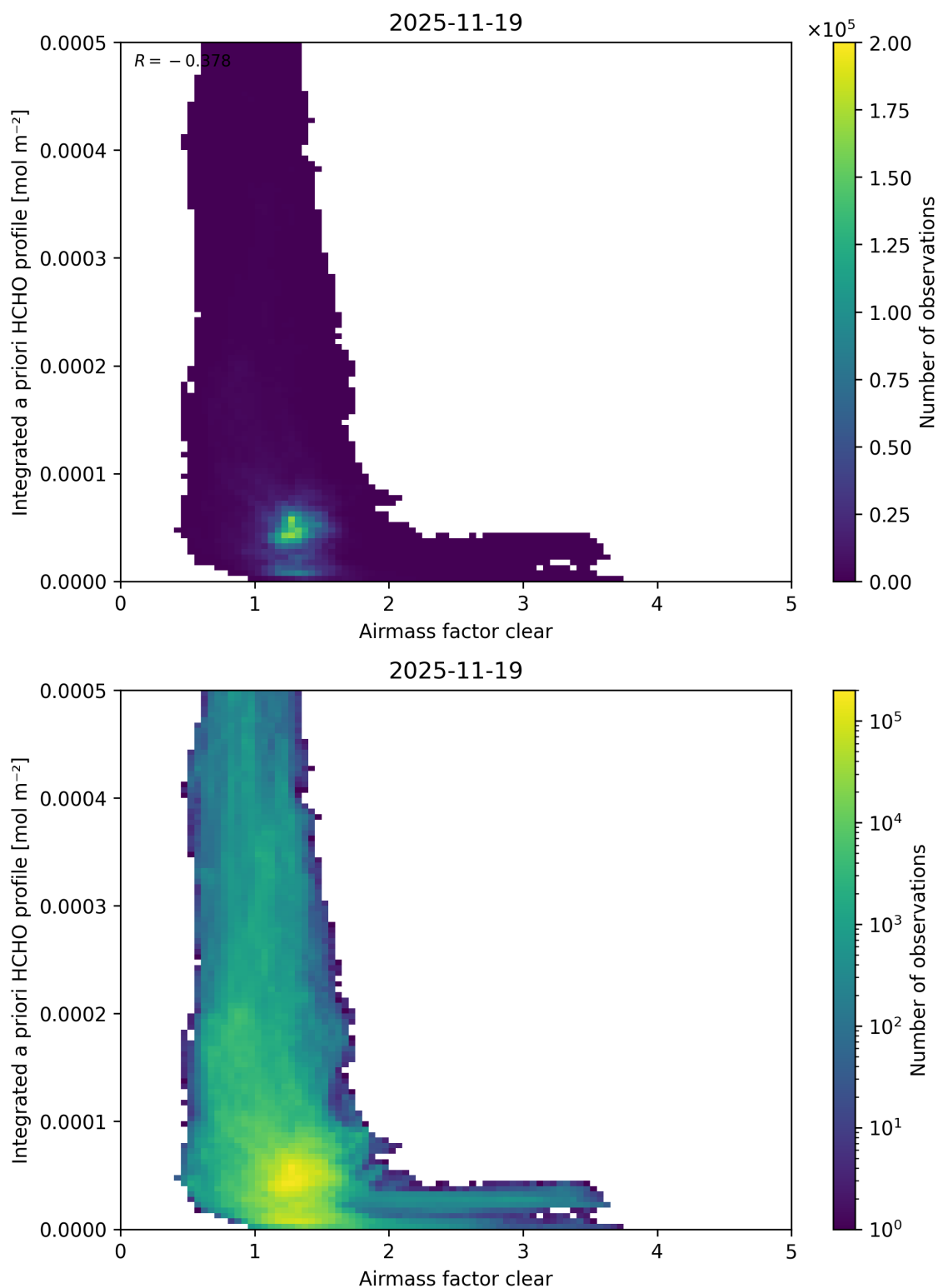
Figure 84: Scatter density plot of “Airmass factor clear” against “Integrated a priori HCHO profile” for 2025-11-18 to 2025-11-20.
