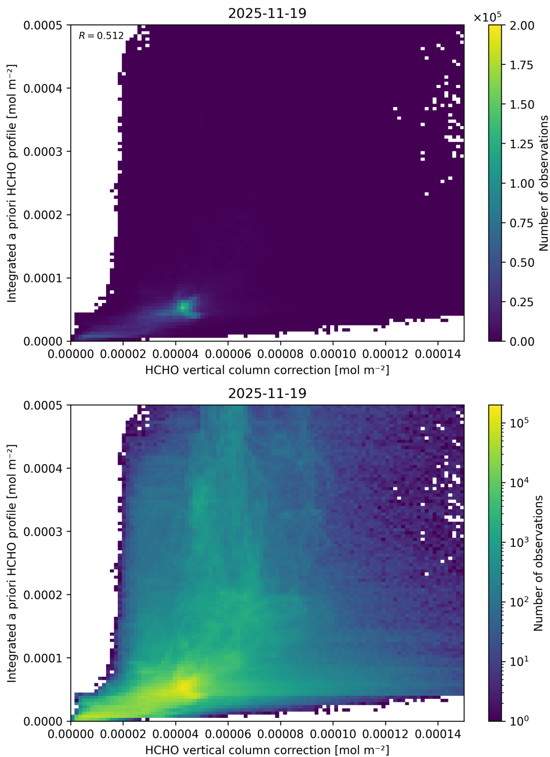
Figure 137: Scatter density plot of “HCHO vertical column correction” against “Integrated a priori HCHO profile” for 2025-11-18 to 2025-11-20.
