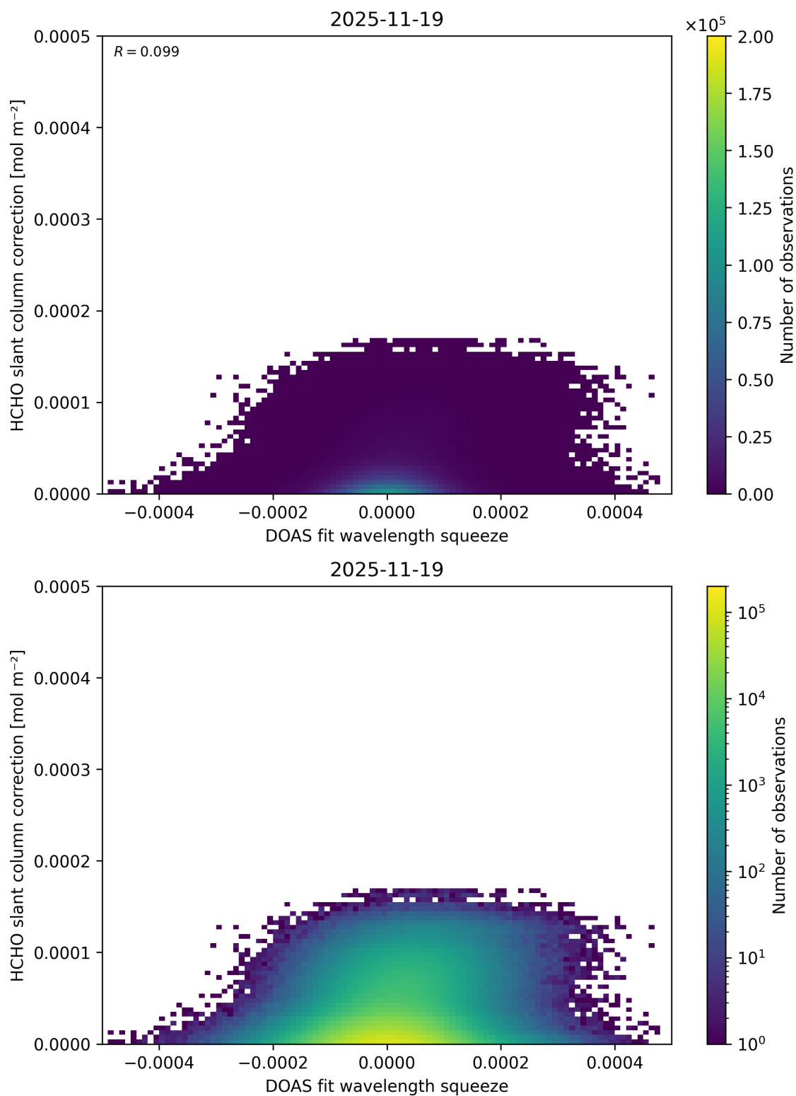
Figure 76: Scatter density plot of “DOAS fit wavelength squeeze” against “HCHO slant column correction” for 2025-11-18 to 2025-11-20.
