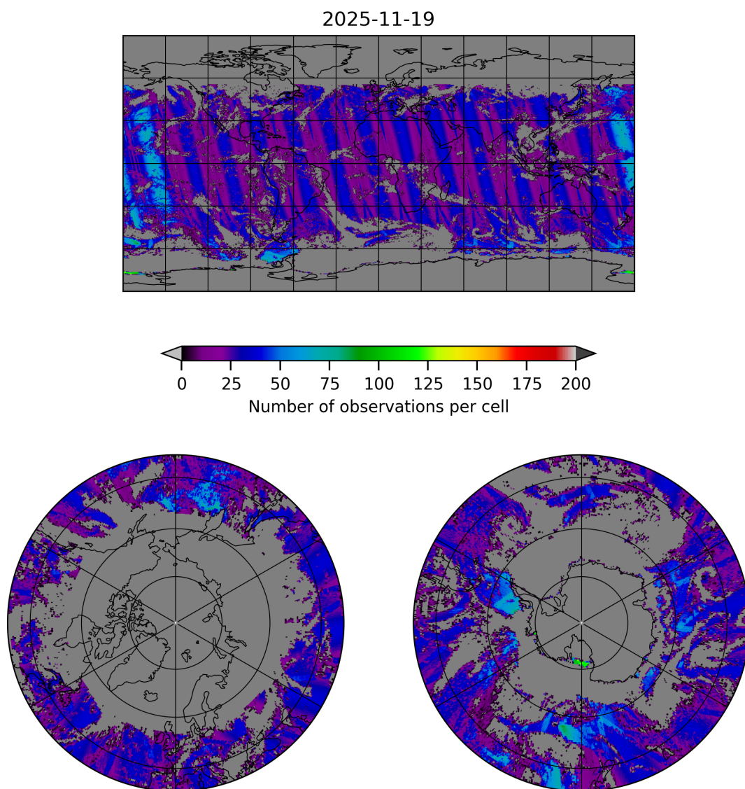
Figure 20: Map of the number of observations for 2025-11-18 to 2025-11-20
