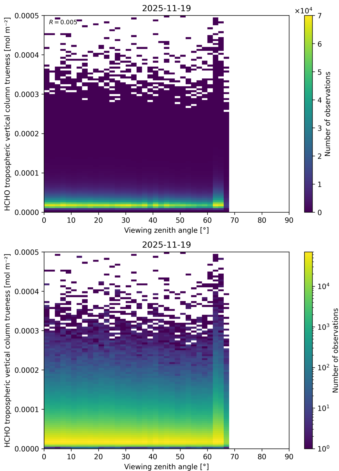
Figure 215: Scatter density plot of “Viewing zenith angle” against “HCHO tropospheric vertical column trueness” for 2025-11-18 to 2025-11-20.
