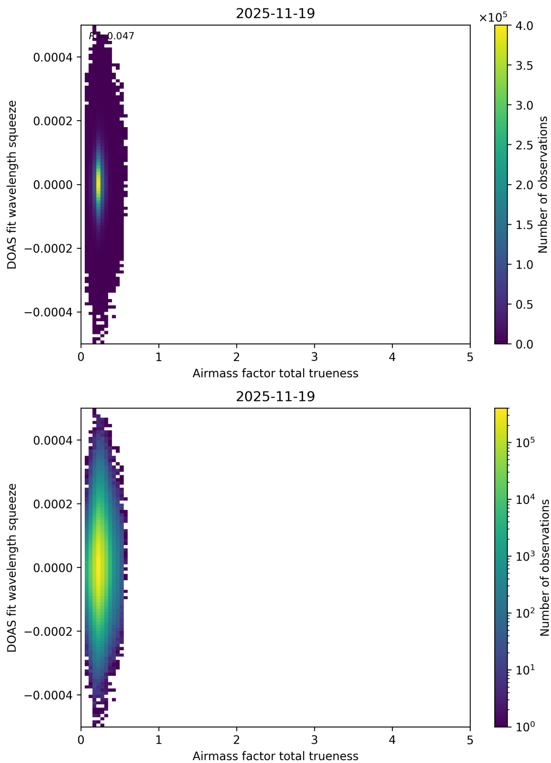
Figure 120: Scatter density plot of “Airmass factor total trueness” against “DOAS fit wavelength squeeze” for 2025-11-18 to 2025-11-20.
