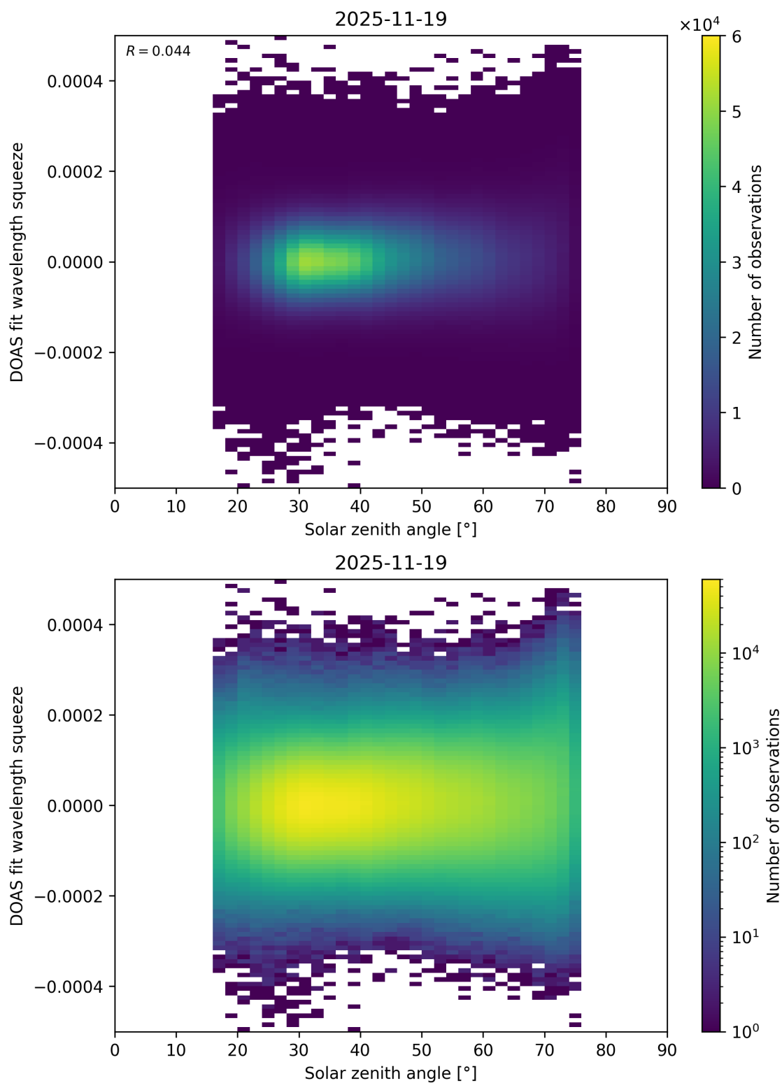
Figure 188: Scatter density plot of “Solar zenith angle” against “DOAS fit wavelength squeeze” for 2025-11-18 to 2025-11-20.
