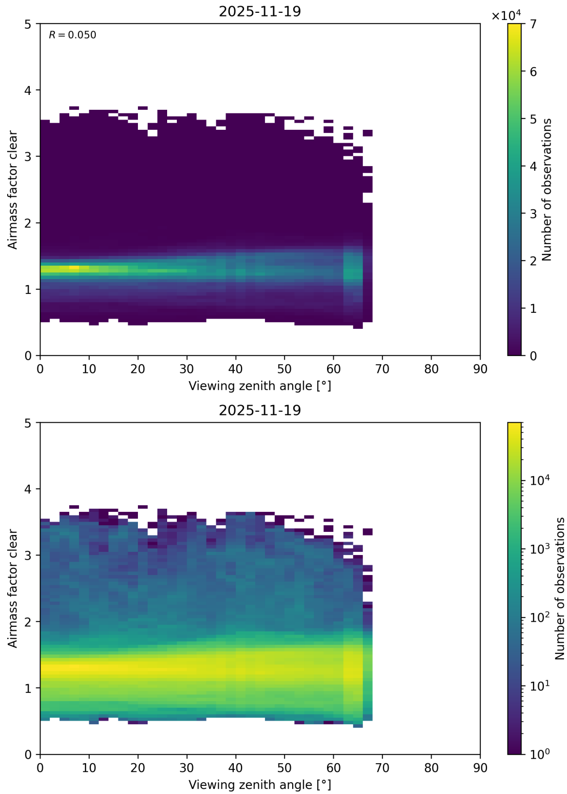
Figure 205: Scatter density plot of “Viewing zenith angle” against “Airmass factor clear” for 2025-11-18 to 2025-11-20.
