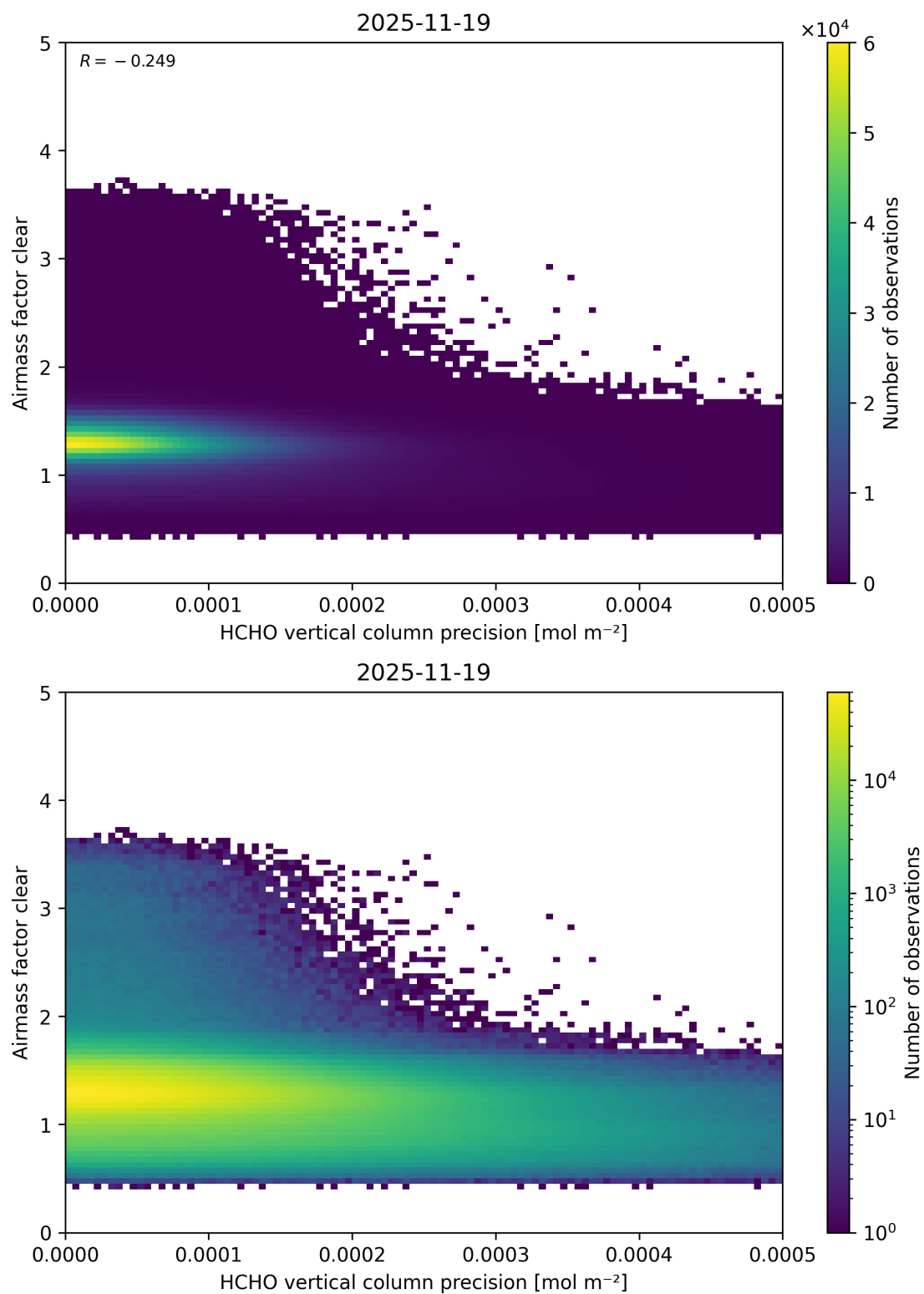
Figure 155: Scatter density plot of “HCHO vertical column precision” against “Airmass factor clear” for 2025-11-18 to 2025-11-20.
