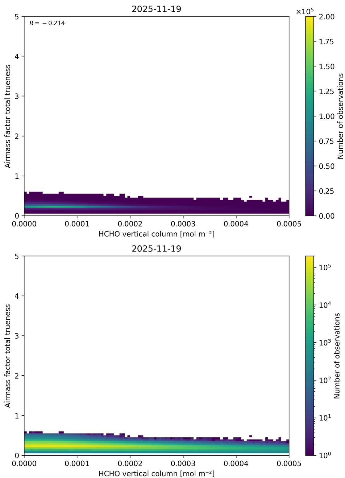
Figure 147: Scatter density plot of “HCHO vertical column” against “Airmass factor total truiness” for 2025-11-18 to 2025-11-20.
