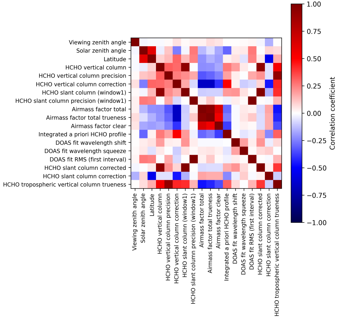
Figure 2: Map of correlation matrix for 2025-11-18 to 2025-11-20.
