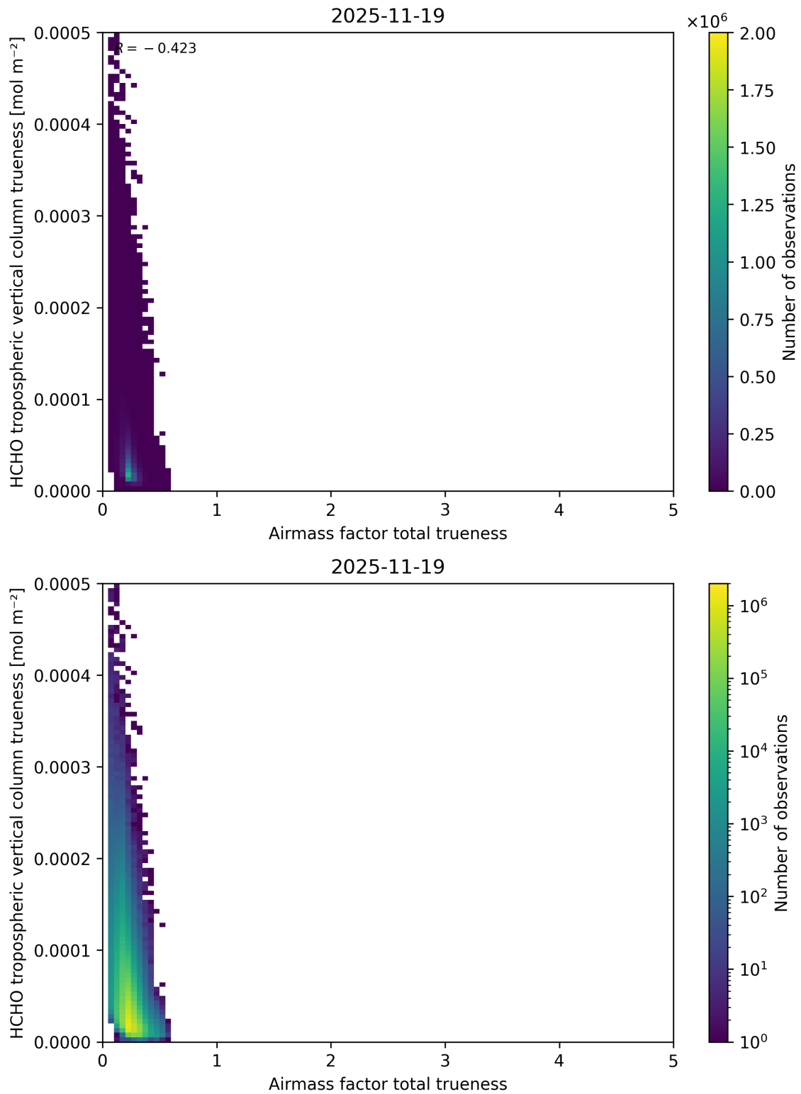
Figure 124: Scatter density plot of “Airmass factor total trueness” against “HCHO tropospheric vertical column trueness” for 2025-11-18 to 2025-11-20.
