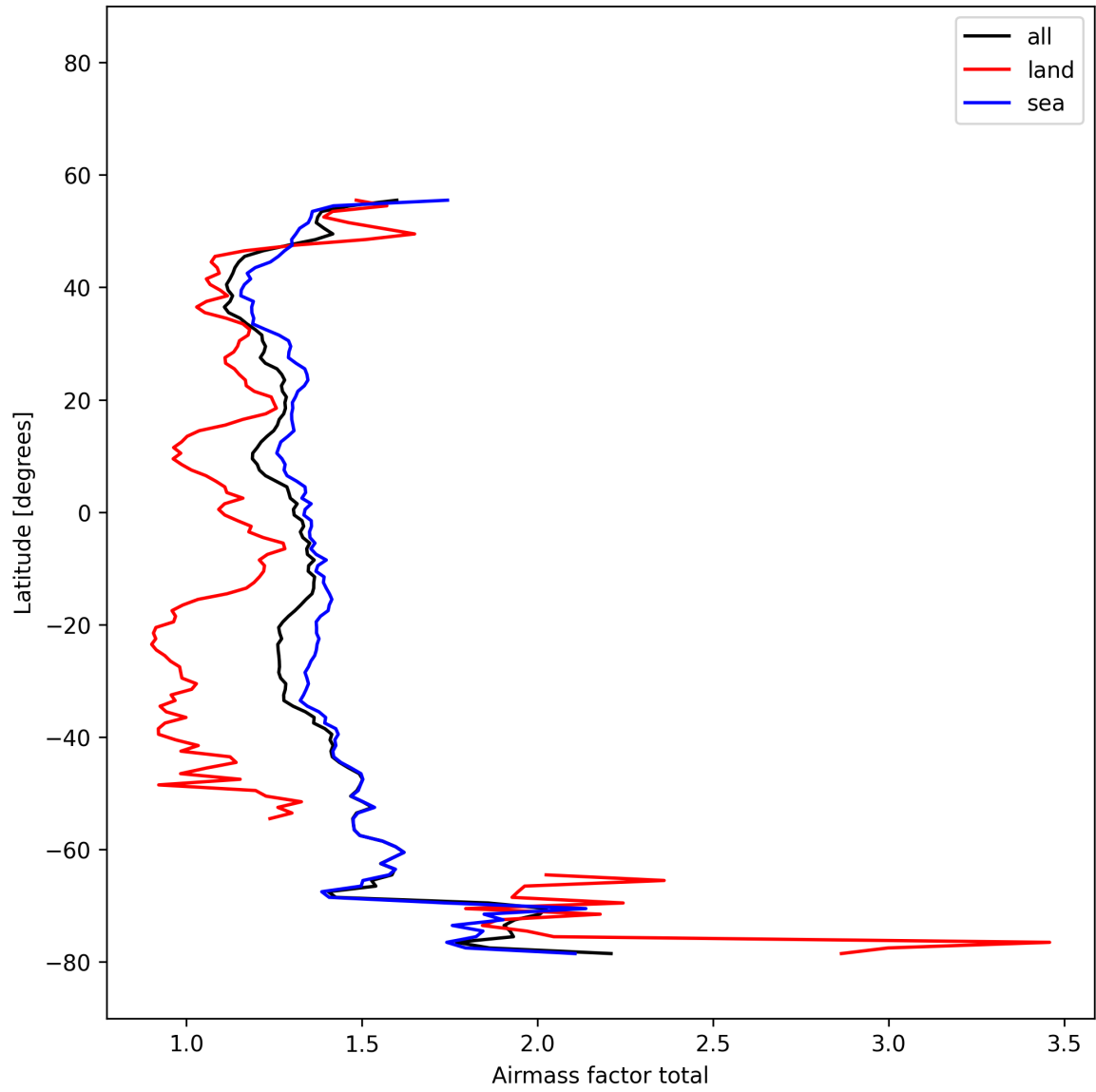
Figure 27: Zonal average of “Airmass factor total” for 2025-11-18 to 2025-11-20.
