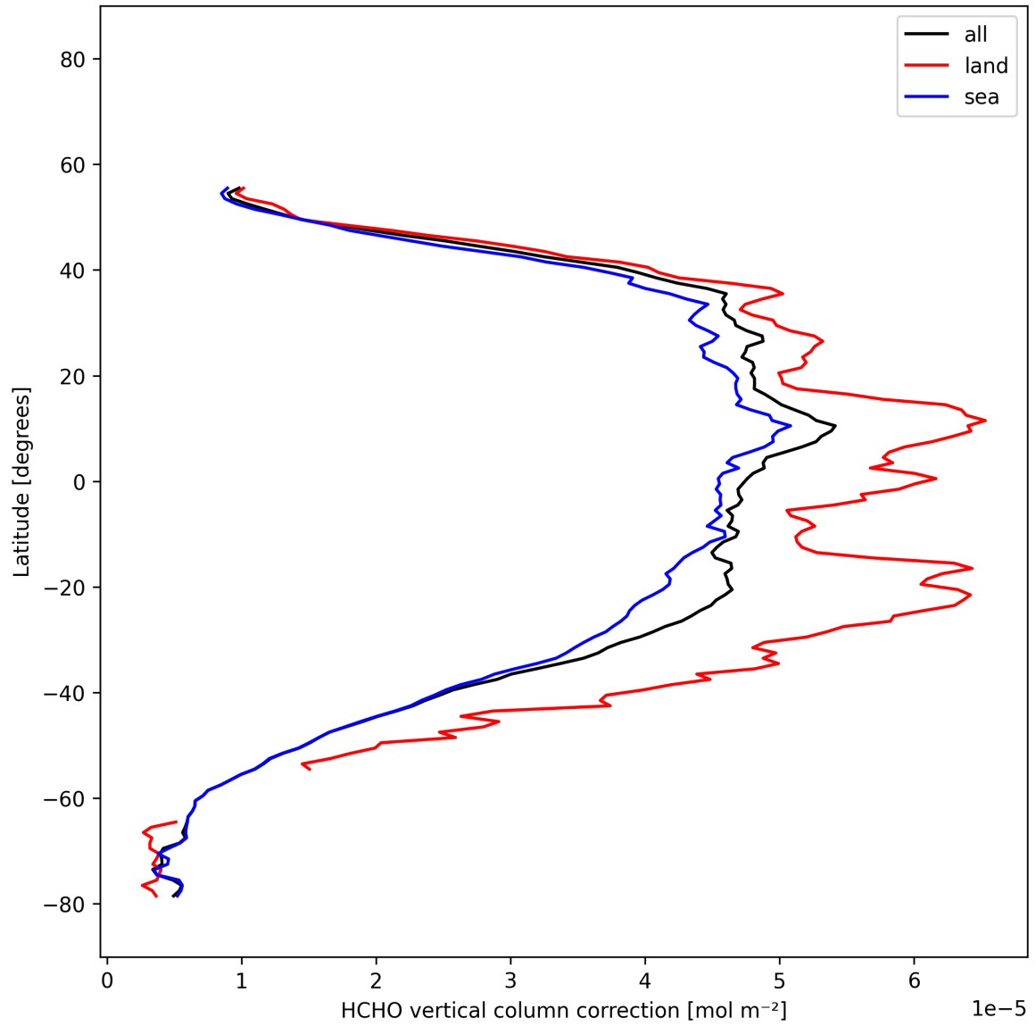
Figure 24: Zonal average of “HCHO vertical column correction” for 2025-11-18 to 2025-11-20.
