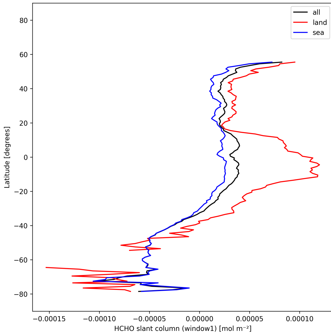
Figure 25: Zonal average of “HCHO slant column (window1)” for 2025-11-18 to 2025-11-20.
