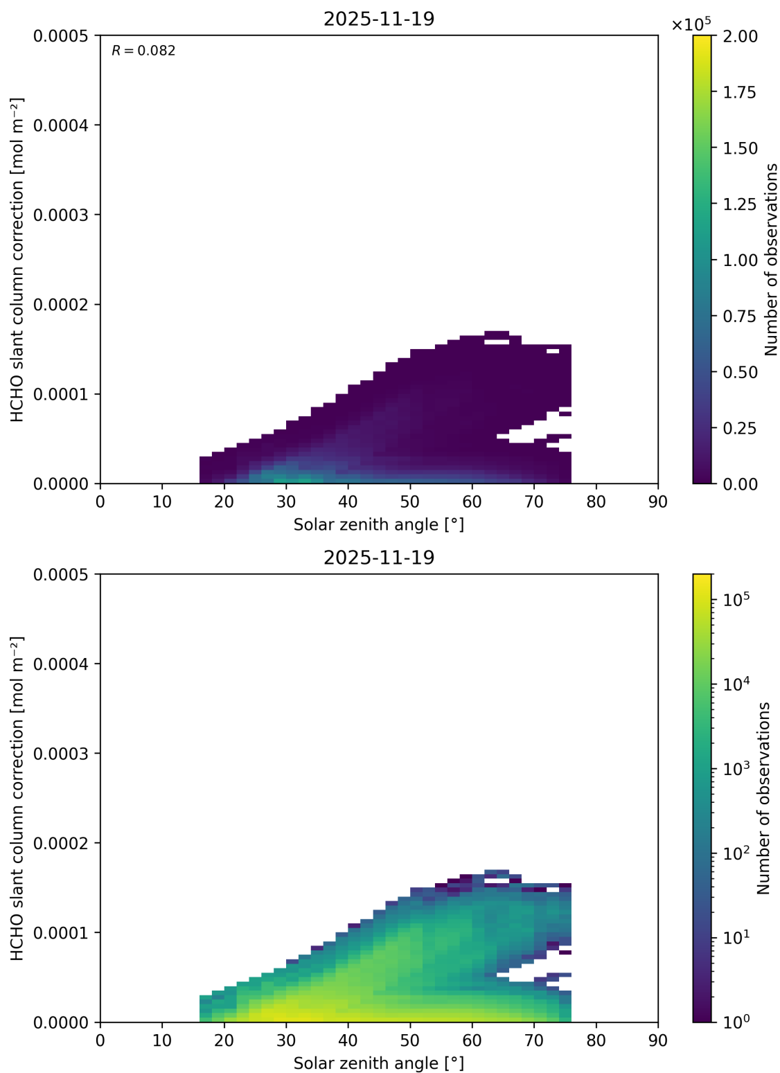
Figure 191: Scatter density plot of “Solar zenith angle” against “HCHO slant column correction” for 2025-11-18 to 2025-11-20.
