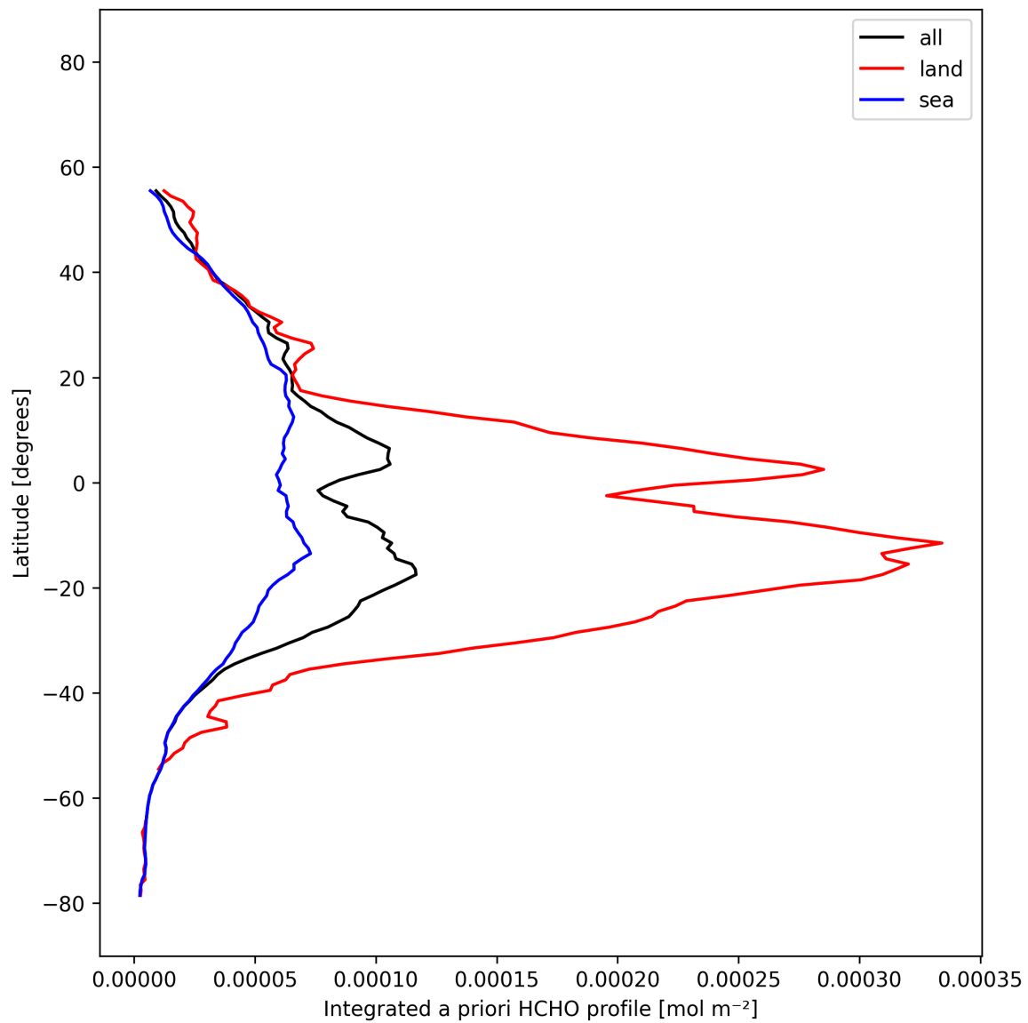
Figure 30: Zonal average of “Integrated a priori HCHO profile” for 2025-11-18 to 2025-11-20.
