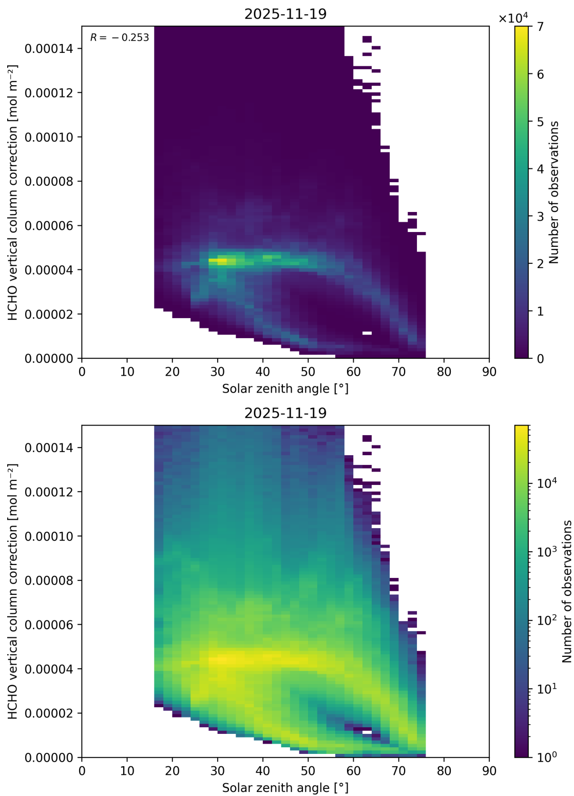
Figure 197: Scatter density plot of “Solar zenith angle” against “HCHO vertical column correction” for 2025-11-18 to 2025-11-20.
