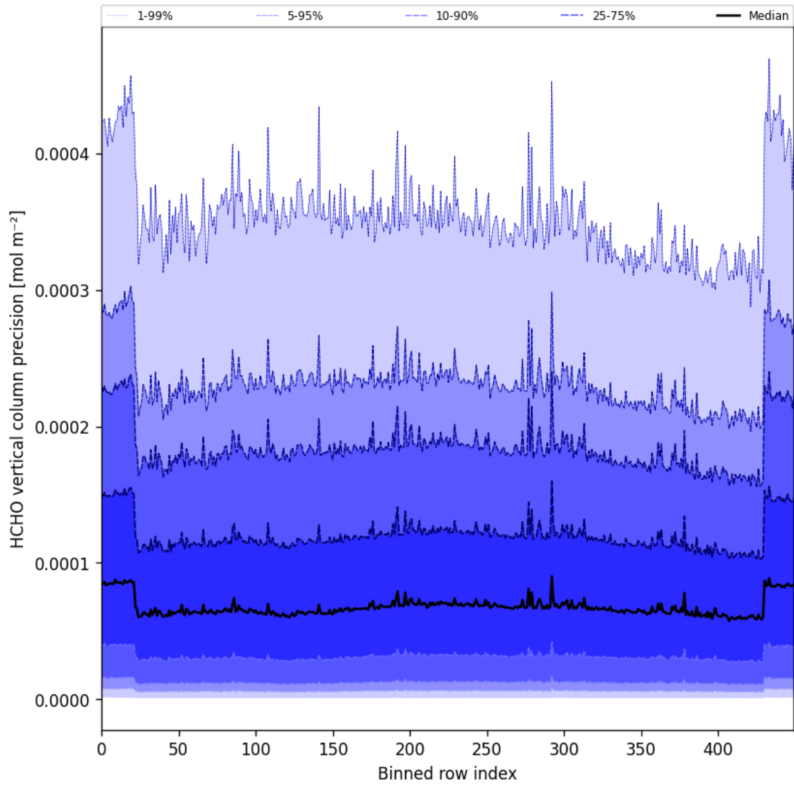
Figure 53: Along track statistics of “HCHO vertical column precision” for 2025-11-18 to 2025-11-20
