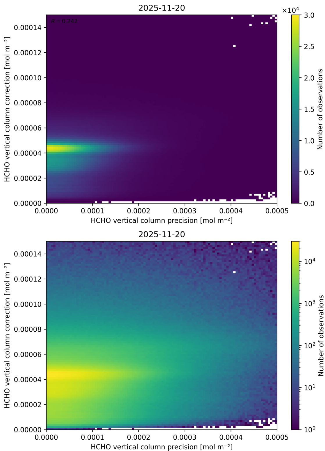
Figure 162: Scatter density plot of “HCHO vertical column precision” against “HCHO vertical column correction” for 2025-11-19 to 2025-11-21.
