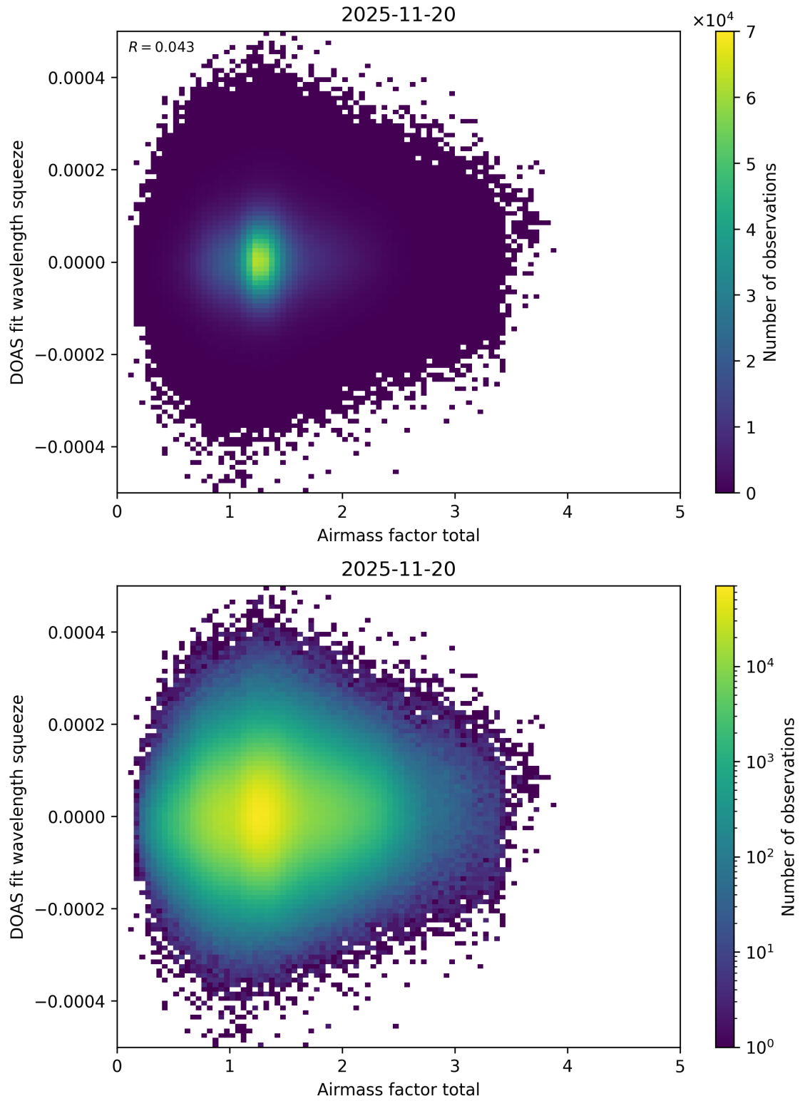
Figure 111: Scatter density plot of “Airmass factor total” against “DOAS fit wavelength squeeze” for 2025-11-19 to 2025-11-21.
