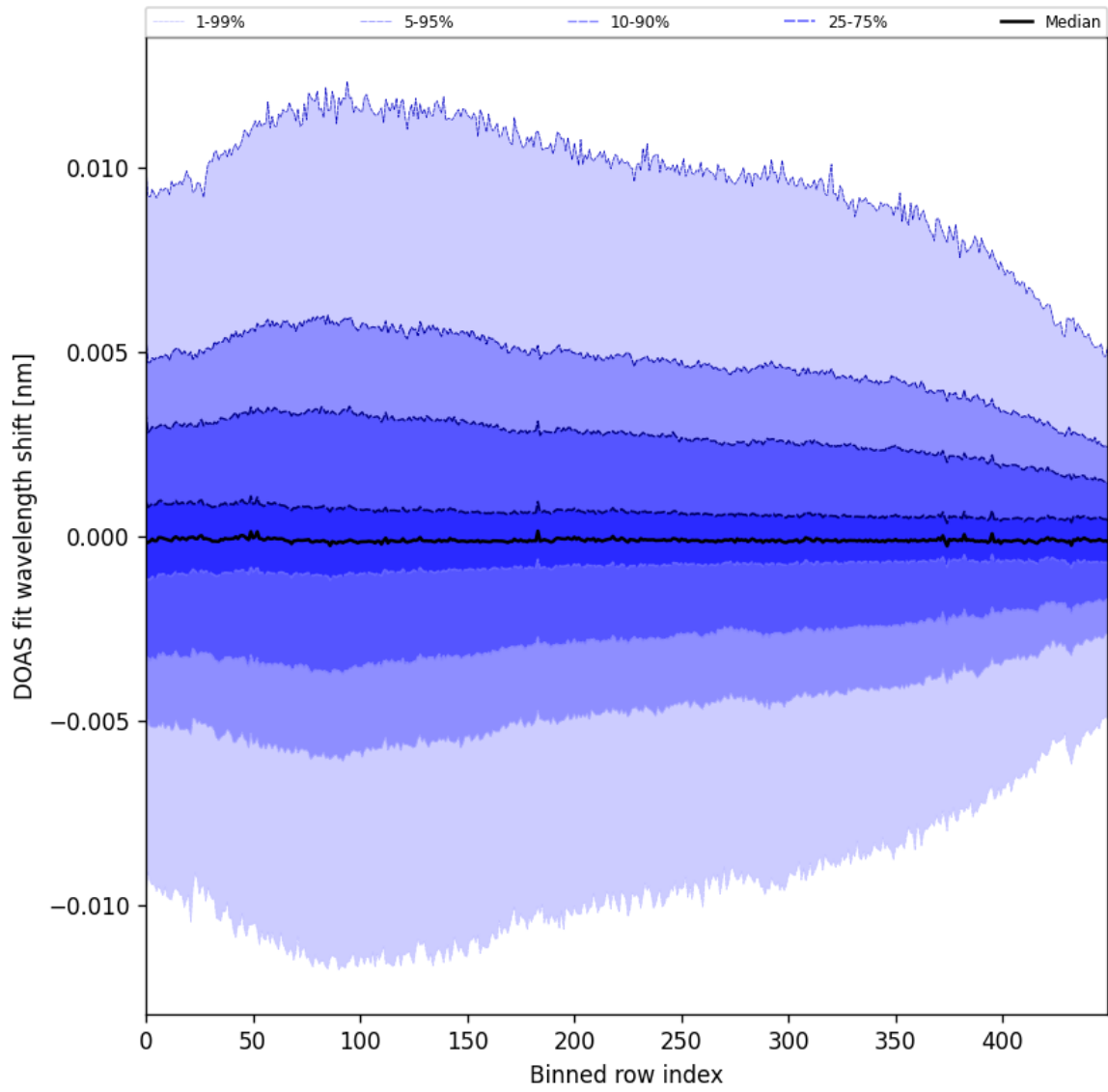
Figure 61: Along track statistics of “DOAS fit wavelength shift” for 2025-11-19 to 2025-11-21
