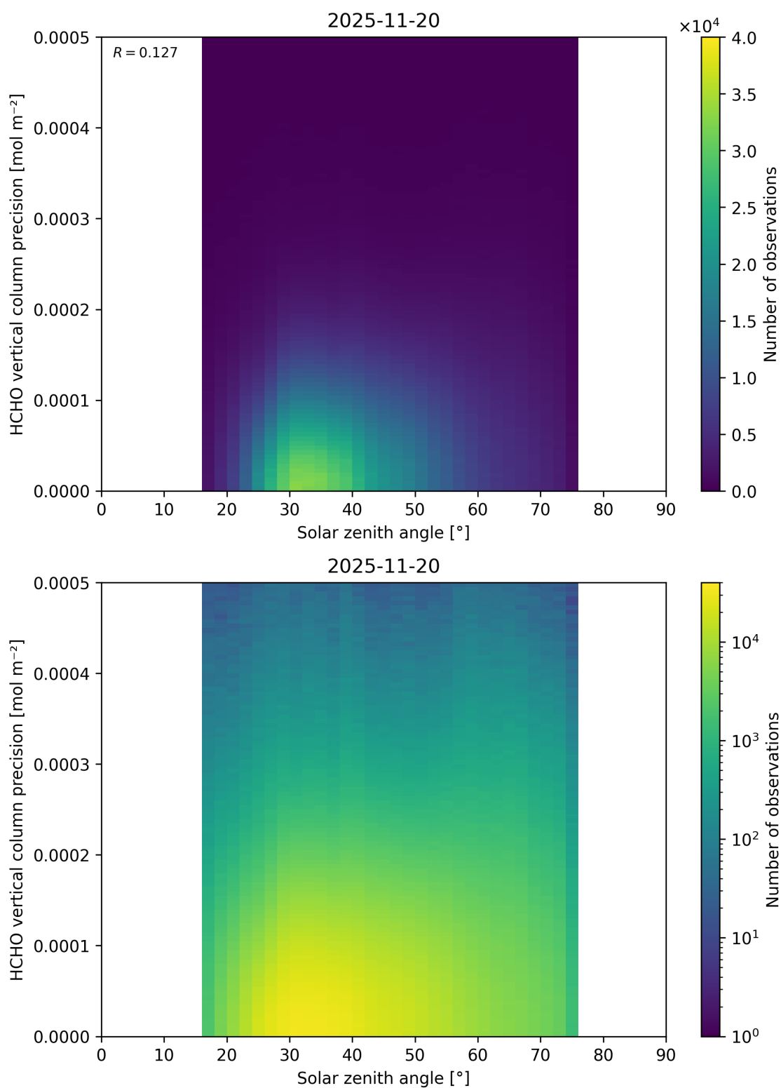
Figure 198: Scatter density plot of “Solar zenith angle” against “HCHO vertical column precision” for 2025-11-19 to 2025-11-21.
