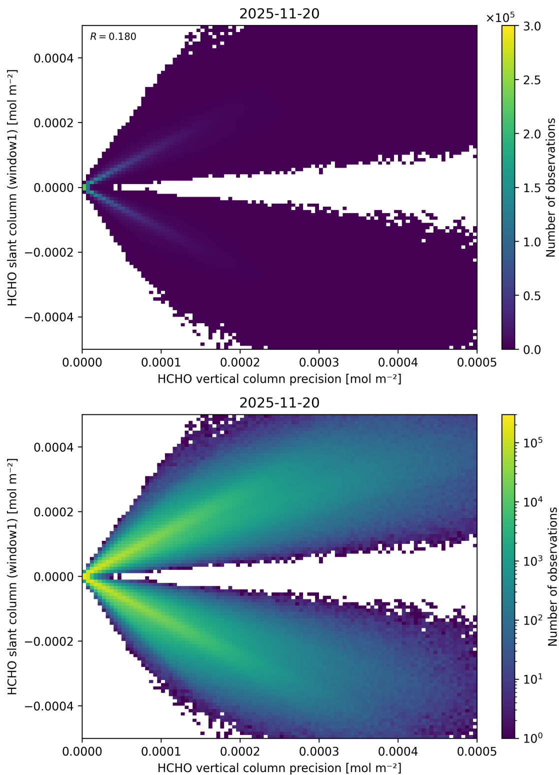
Figure 158: Scatter density plot of “HCHO vertical column precision” against “HCHO slant column (window1)” for 2025-11-19 to 2025-11-21.
