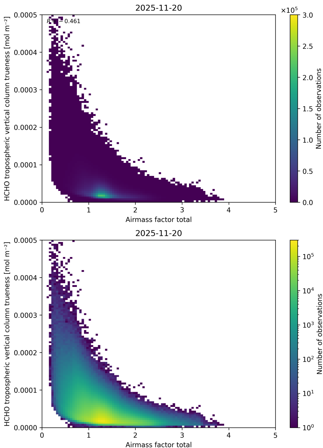
Figure 116: Scatter density plot of “Airmass factor total” against “HCHO tropospheric vertical column trueness” for 2025-11-19 to 2025-11-21.
