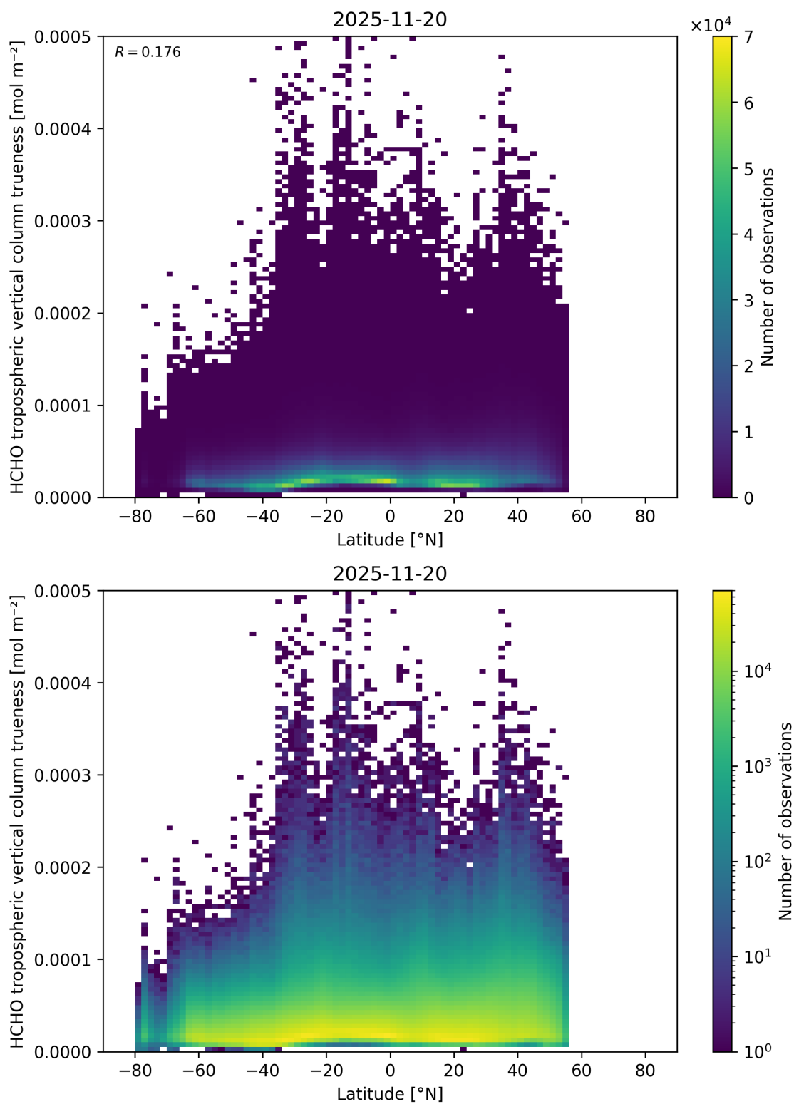
Figure 184: Scatter density plot of “Latitude” against “HCHO tropospheric vertical column trueness” for 2025-11-19 to 2025-11-21.
