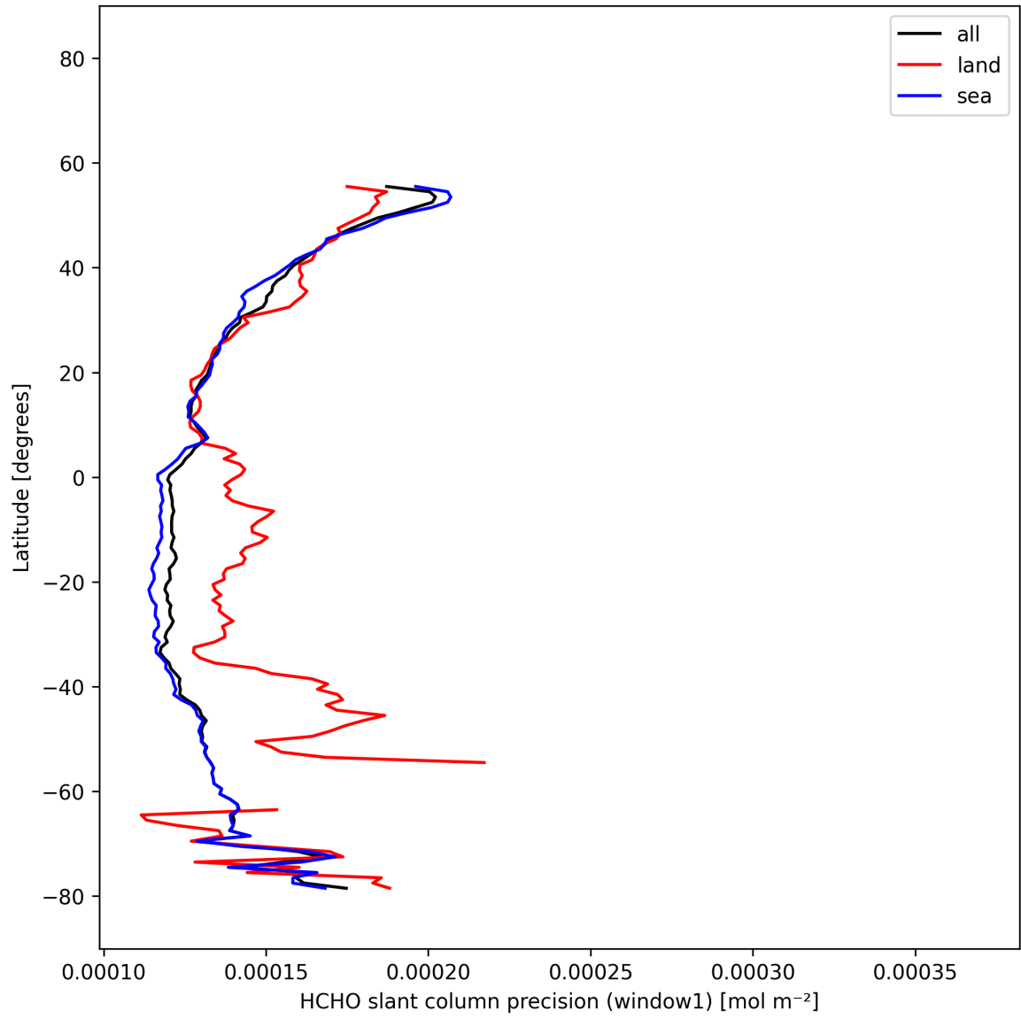
Figure 26: Zonal average of “HCHO slant column precision (window1)” for 2025-11-19 to 2025-11-21.
