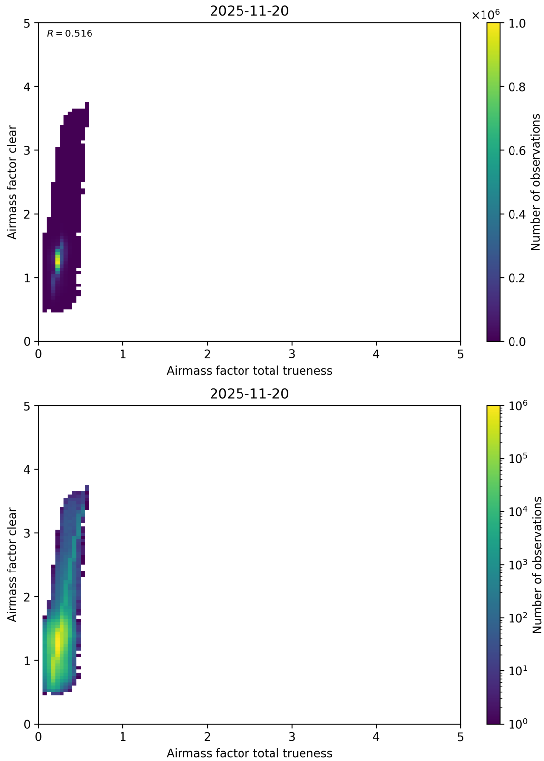
Figure 121: Scatter density plot of “Airmass factor total trueness” against “Airmass factor clear” for 2025-11-19 to 2025-11-21.
