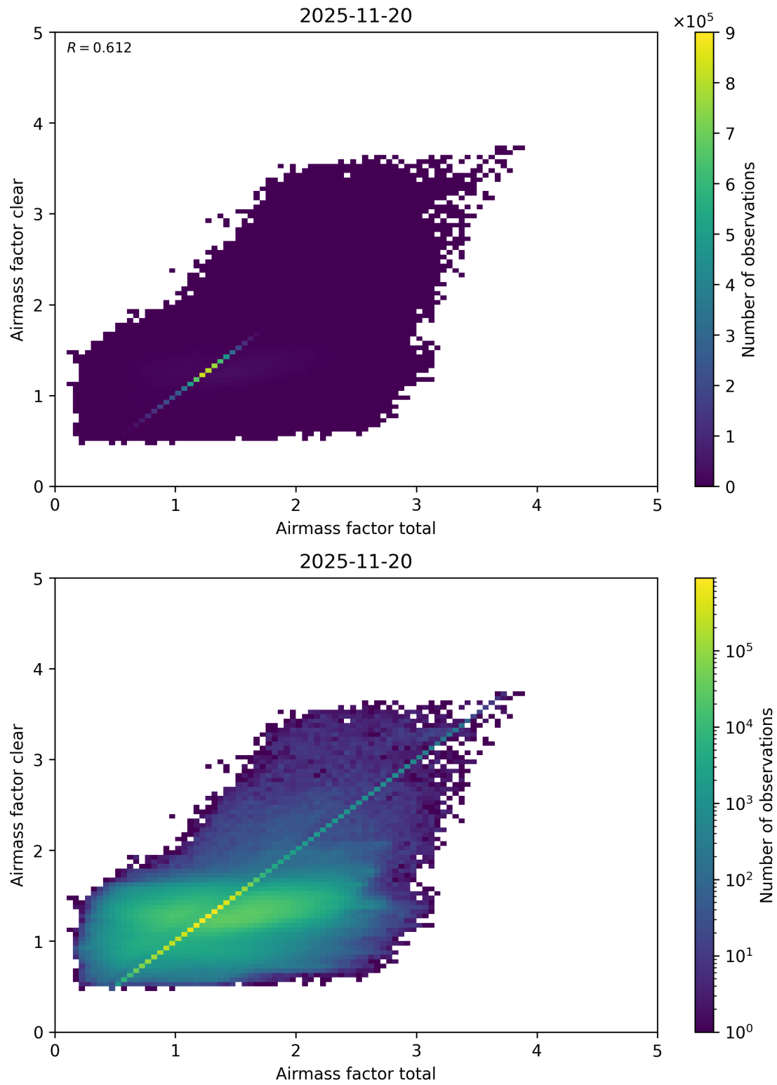
Figure 112: Scatter density plot of “Airmass factor total” against “Airmass factor clear” for 2025-11-19 to 2025-11-21.
