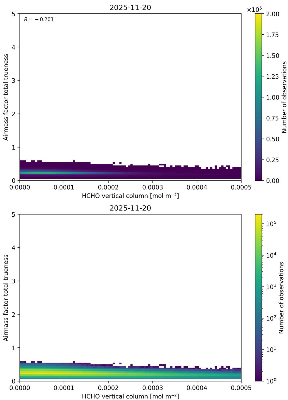
Figure 147: Scatter density plot of “HCHO vertical column” against “Airmass factor total trueneess” for 2025-11-19 to 2025-11-21.
