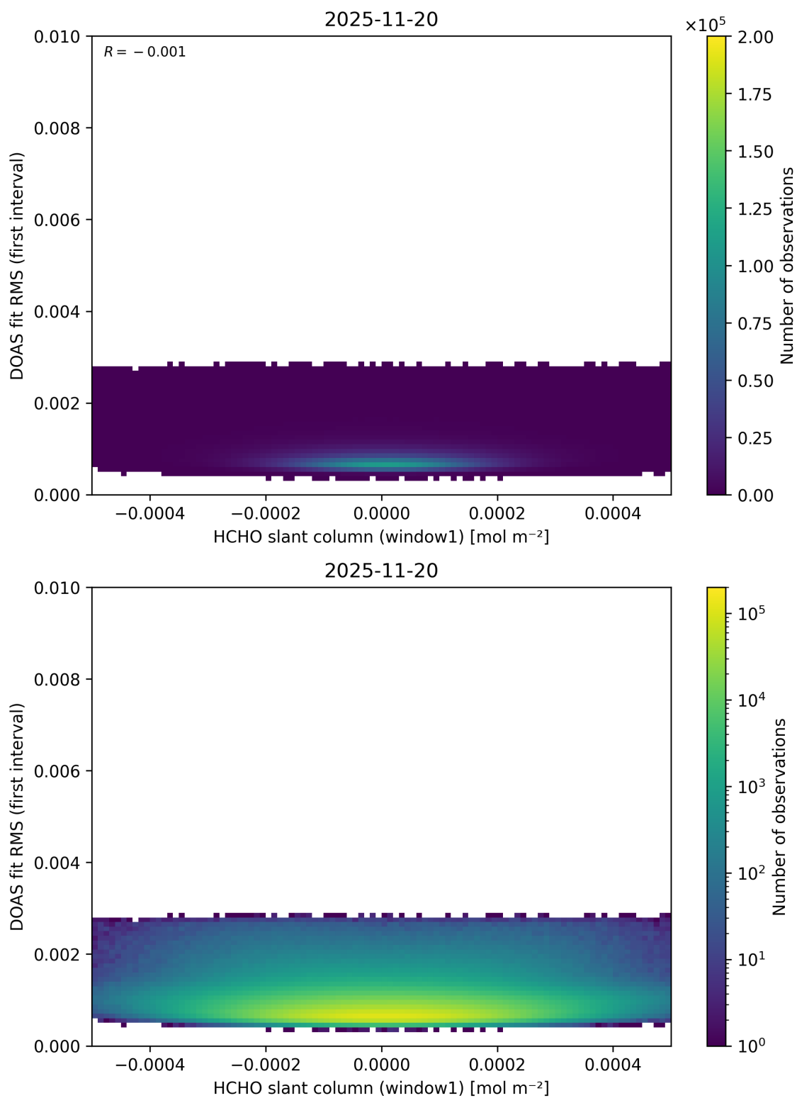
Figure 88: Scatter density plot of “HCHO slant column (window1)” against “DOAS fit RMS (first interval)” for 2025-11-19 to 2025-11-21.
