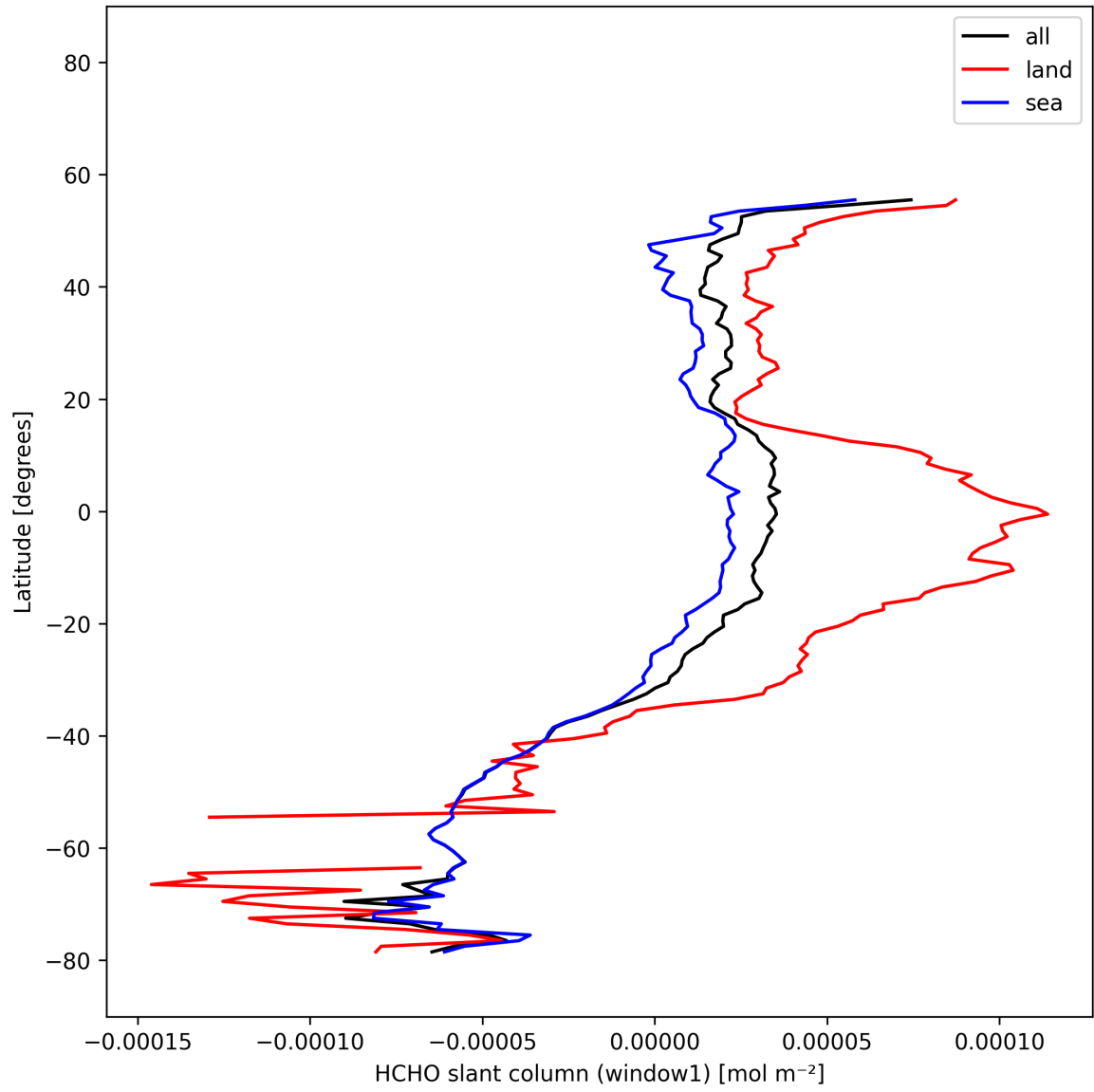
Figure 25: Zonal average of “HCHO slant column (window1)” for 2025-11-19 to 2025-11-21.
