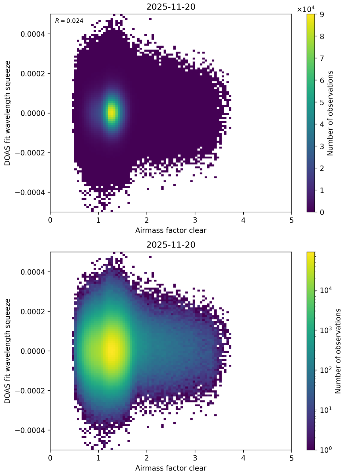
Figure 80: Scatter density plot of “Airmass factor clear” against “DOAS fit wavelength squeeze” for 2025-11-19 to 2025-11-21.
