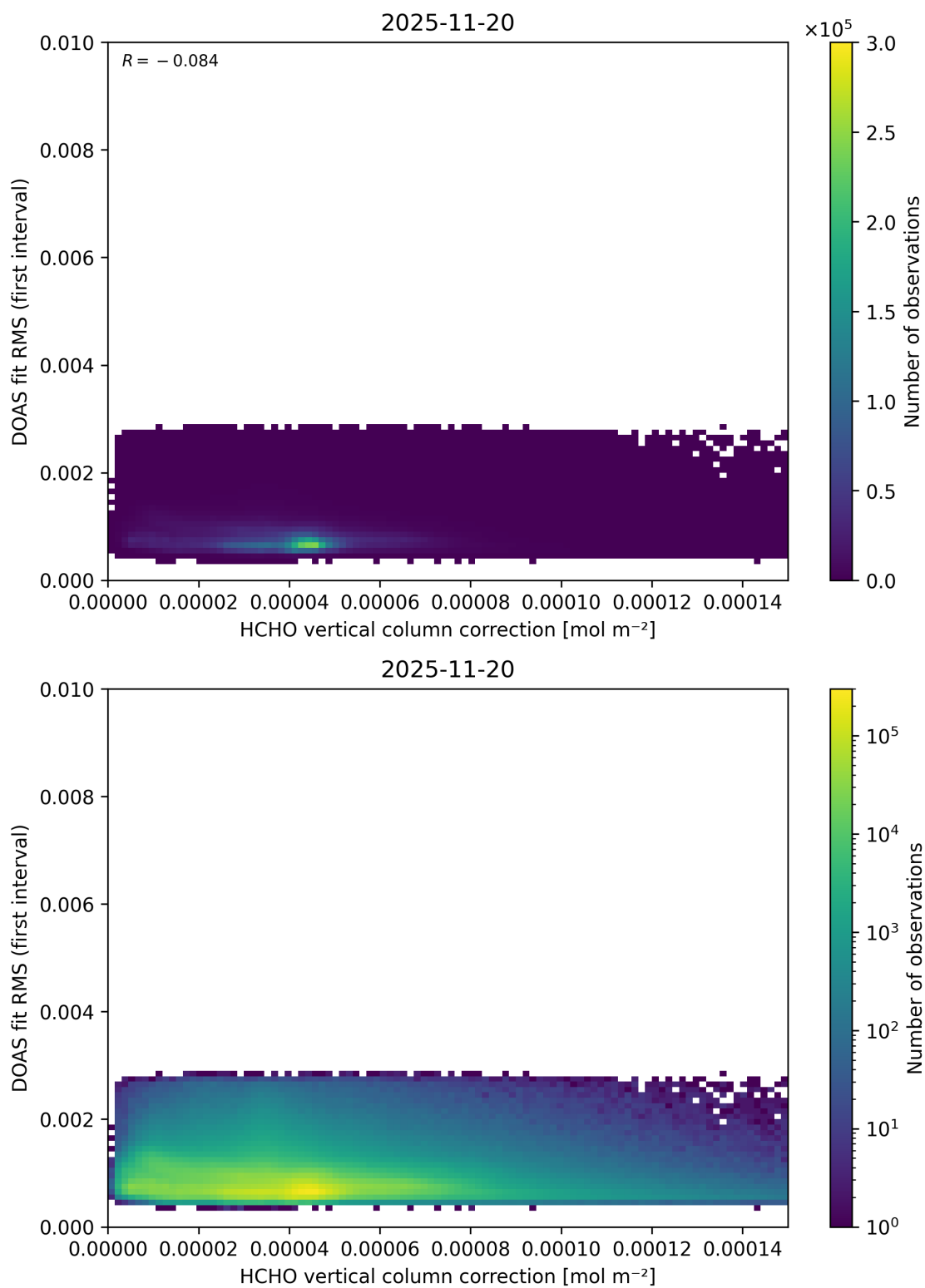
Figure 126: Scatter density plot of “HCHO vertical column correction” against “DOAS fit RMS (first interval)” for 2025-11-19 to 2025-11-21.
