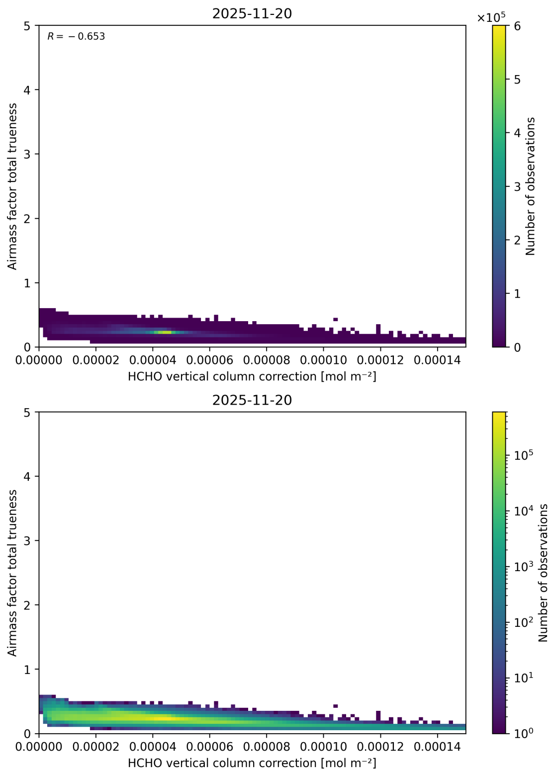
Figure 135: Scatter density plot of “HCHO vertical column correction” against “Airmass factor total trueneess” for 2025-11-19 to 2025-11-21.
