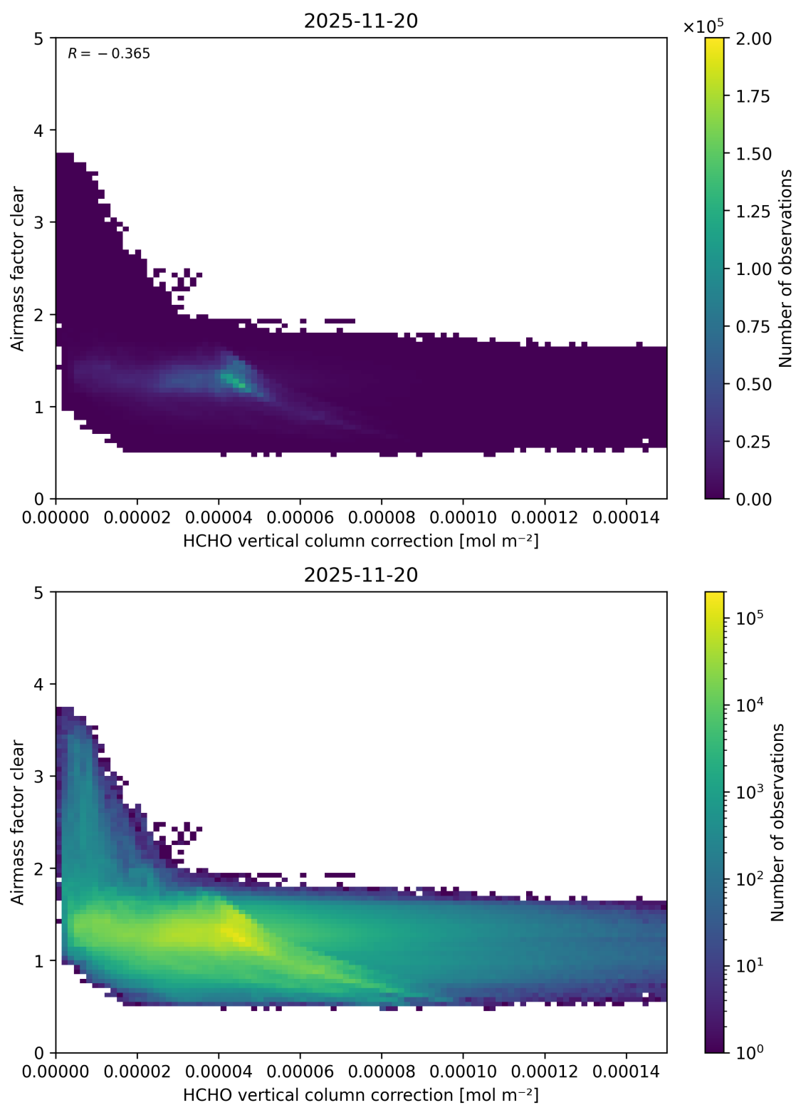
Figure 129: Scatter density plot of “HCHO vertical column correction” against “Airmass factor clear” for 2025-11-19 to 2025-11-21.
