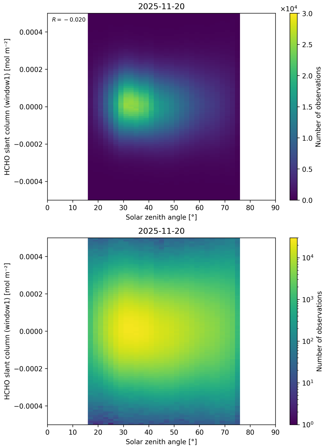
Figure 192: Scatter density plot of “Solar zenith angle” against “HCHO slant column (window1)” for 2025-11-19 to 2025-11-21.
