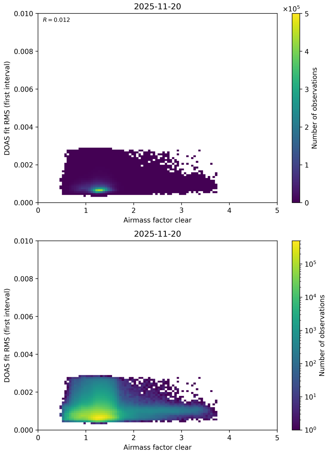
Figure 78: Scatter density plot of “Airmass factor clear” against “DOAS fit RMS (first interval)” for 2025-11-19 to 2025-11-21.
