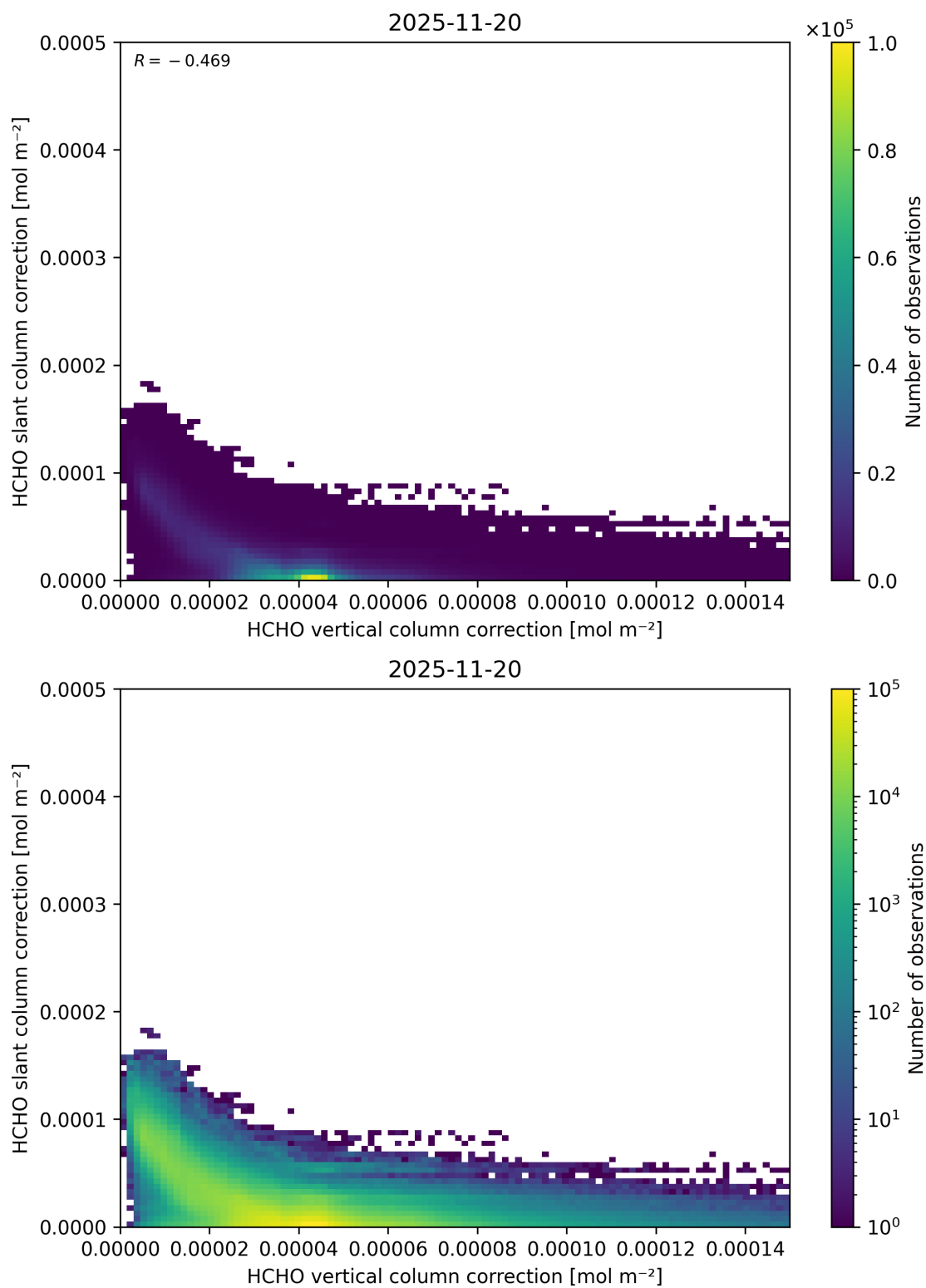
Figure 131: Scatter density plot of “HCHO vertical column correction” against “HCHO slant column correction” for 2025-11-19 to 2025-11-21.
