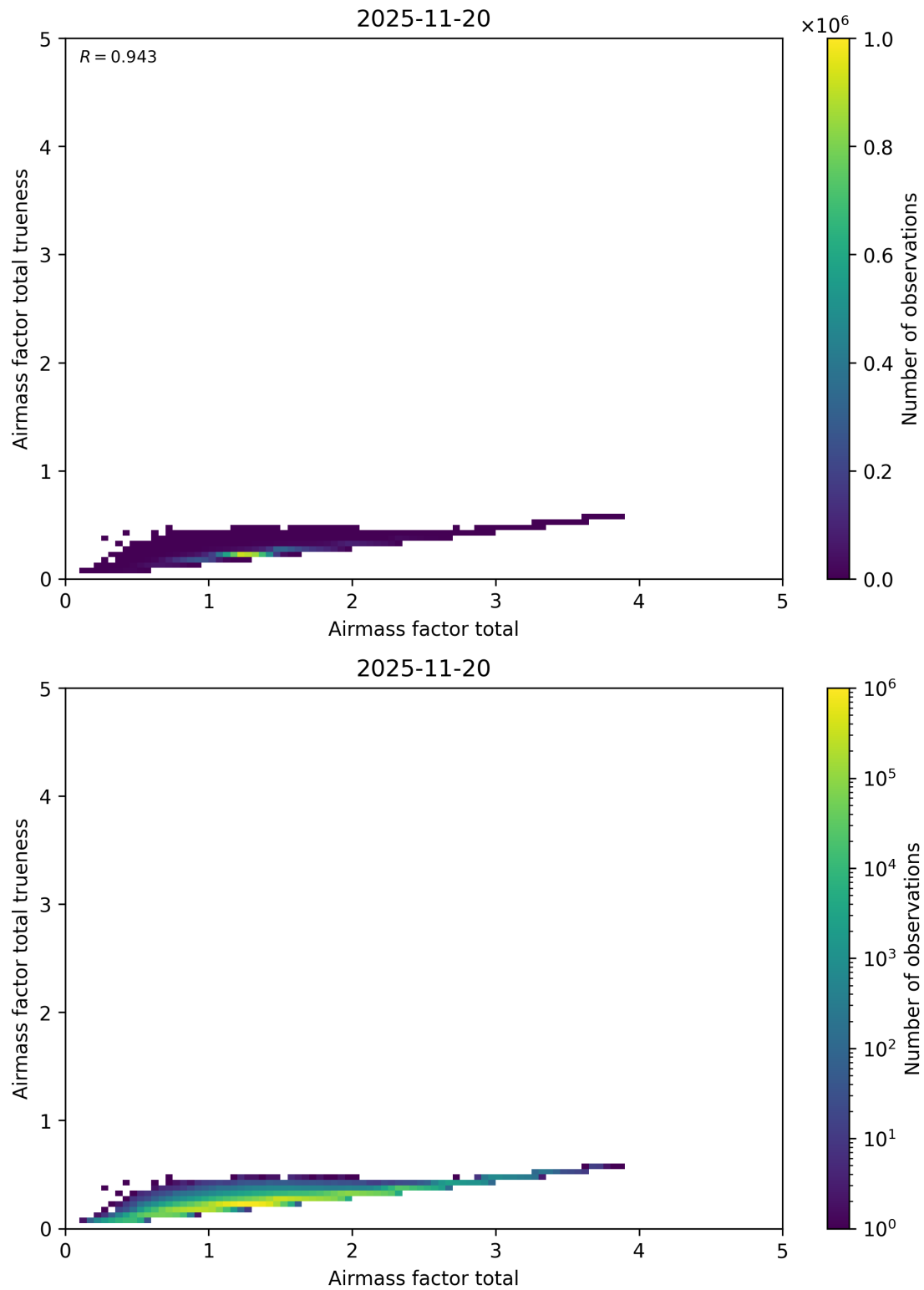
Figure 115: Scatter density plot of “Airmass factor total” against “Airmass factor total trueness” for 2025-11-19 to 2025-11-21.
