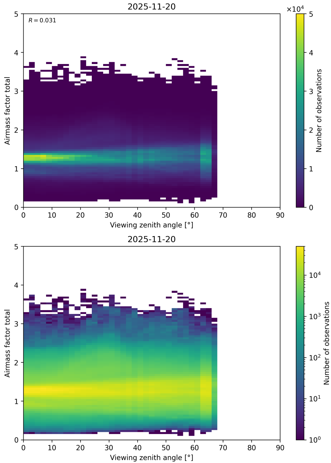
Figure 210: Scatter density plot of “Viewing zenith angle” against “Airmass factor total” for 2025-11-19 to 2025-11-21.
