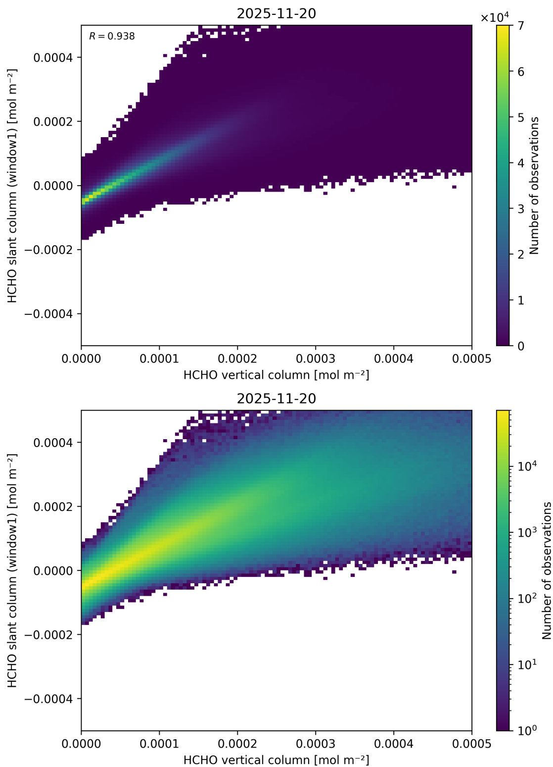
Figure 144: Scatter density plot of “HCHO vertical column” against “HCHO slant column (window1)” for 2025-11-19 to 2025-11-21.
