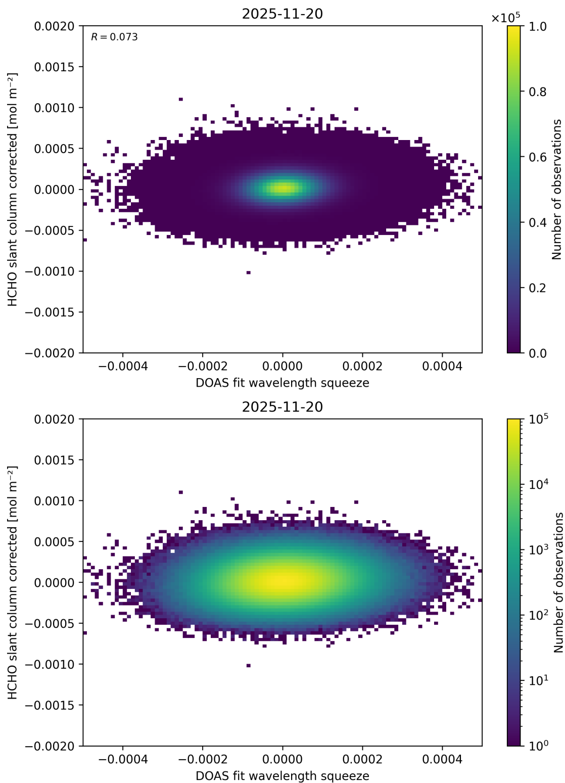
Figure 75: Scatter density plot of “DOAS fit wavelength squeeze” against “HCHO slant column corrected” for 2025-11-19 to 2025-11-21.
