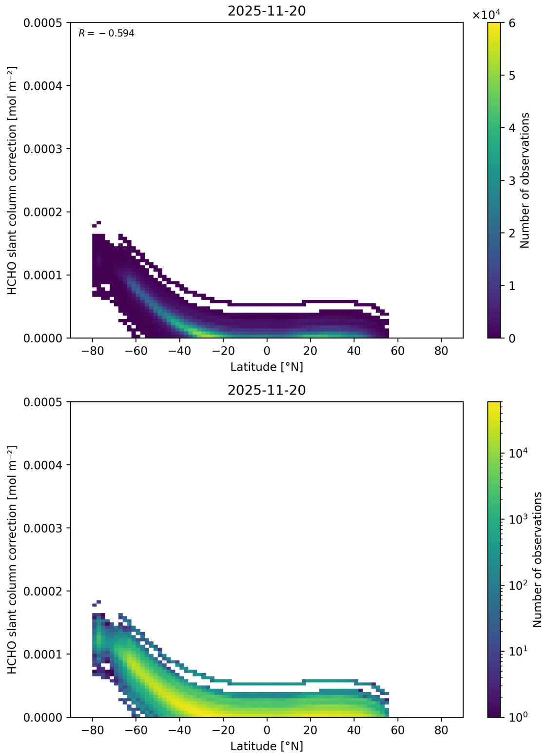
Figure 176: Scatter density plot of “Latitude” against “HCHO slant column correction” for 2025-11-19 to 2025-11-21.
