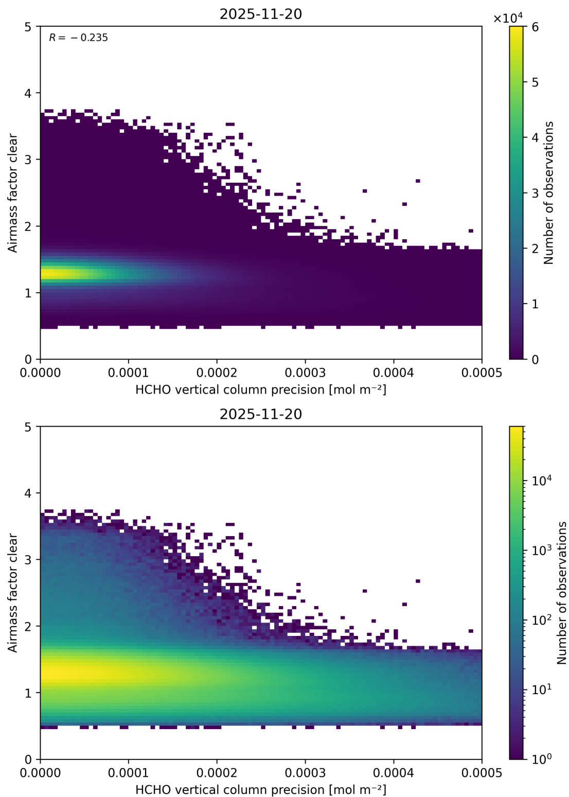
Figure 155: Scatter density plot of “HCHO vertical column precision” against “Airmass factor clear” for 2025-11-19 to 2025-11-21.
