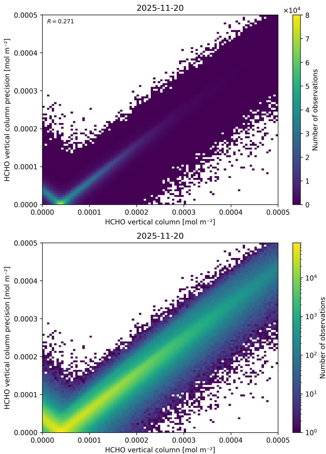
Figure 149: Scatter density plot of “HCHO vertical column” against “HCHO vertical column precision” for 2025-11-19 to 2025-11-21.
