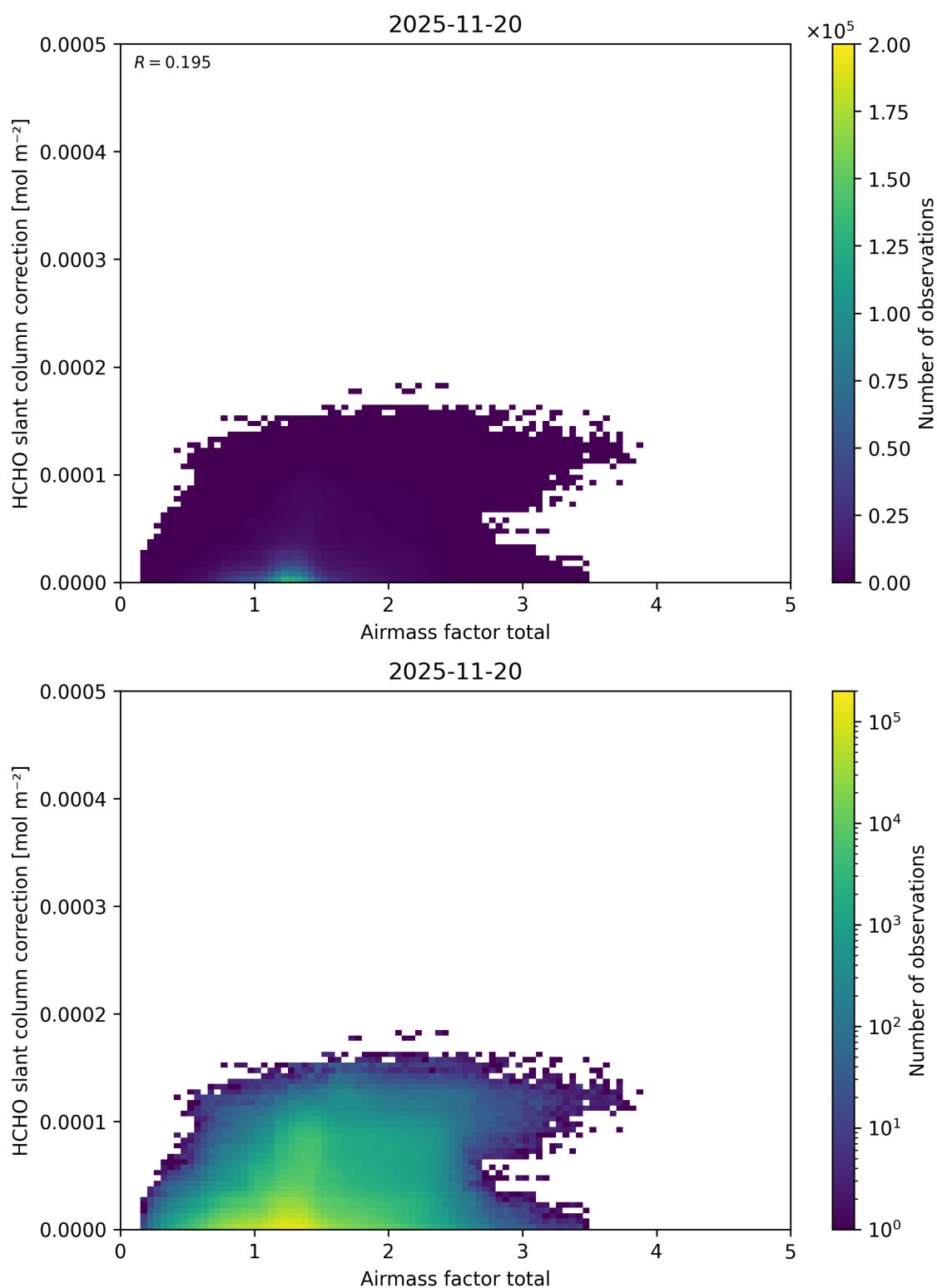
Figure 114: Scatter density plot of “Airmass factor total” against “HCHO slant column correction” for 2025-11-19 to 2025-11-21.
