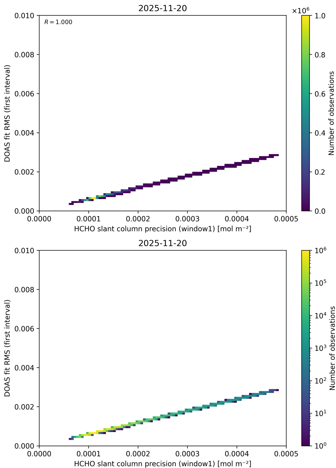
Figure 99: Scatter density plot of “HCHO slant column precision (window1)” against “DOAS fit RMS (first interval)” for 2025-11-19 to 2025-11-21.
