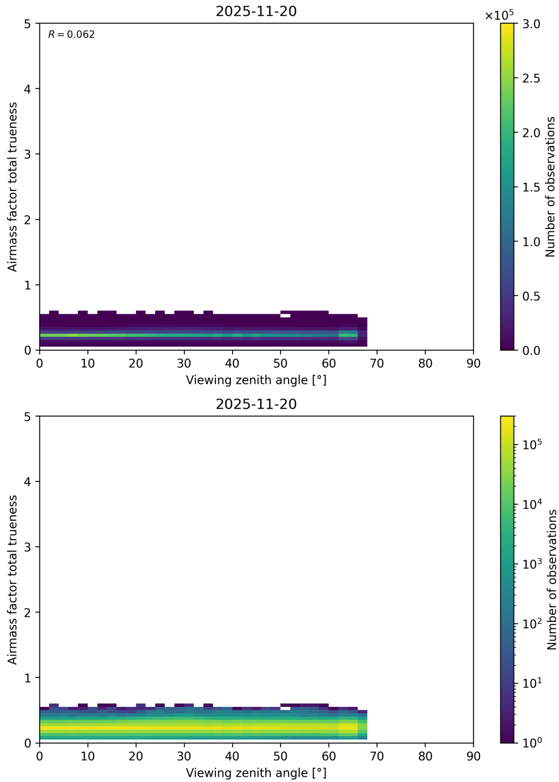
Figure 211: Scatter density plot of “Viewing zenith angle” against “Airmass factor total trueness” for 2025-11-19 to 2025-11-21.
