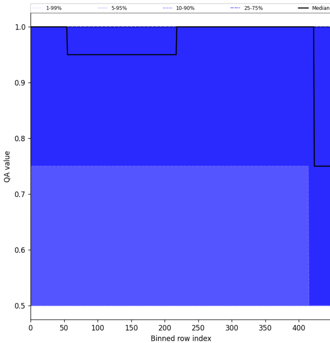
Figure 51: Along track statistics of “QA value” for 2025-11-19 to 2025-11-21
