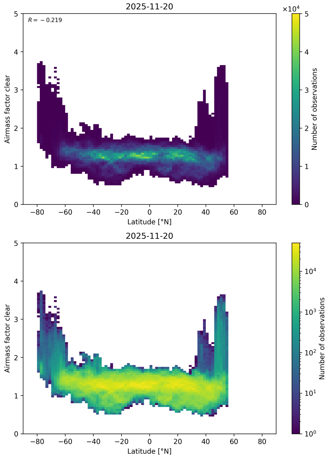
Figure 174: Scatter density plot of “Latitude” against “Airmass factor clear” for 2025-11-19 to 2025-11-21.
