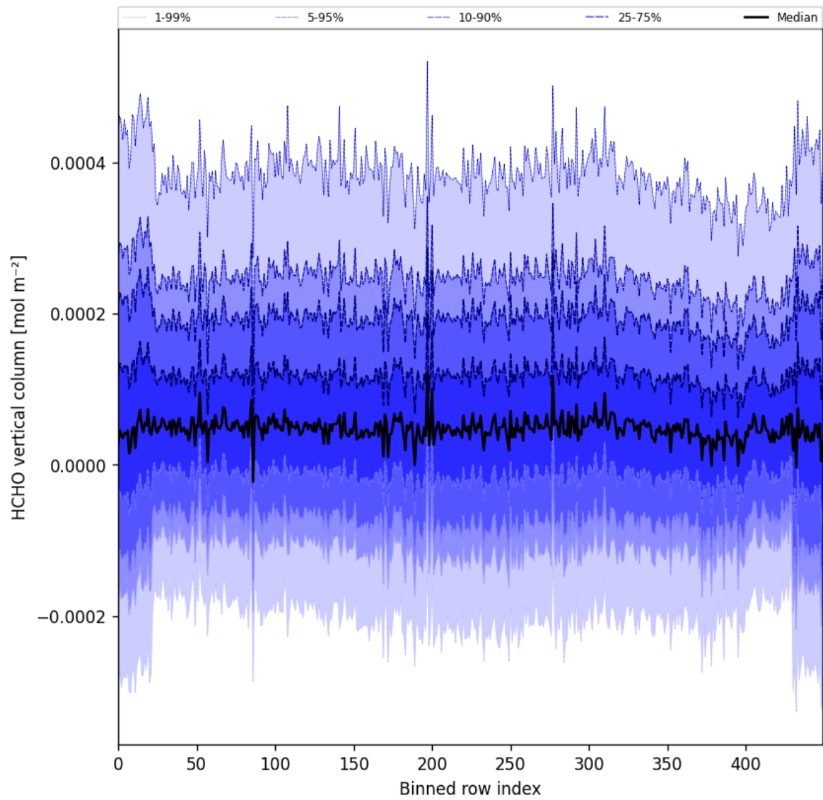
Figure 52: Along track statistics of “HCHO vertical column” for 2025-11-19 to 2025-11-21
