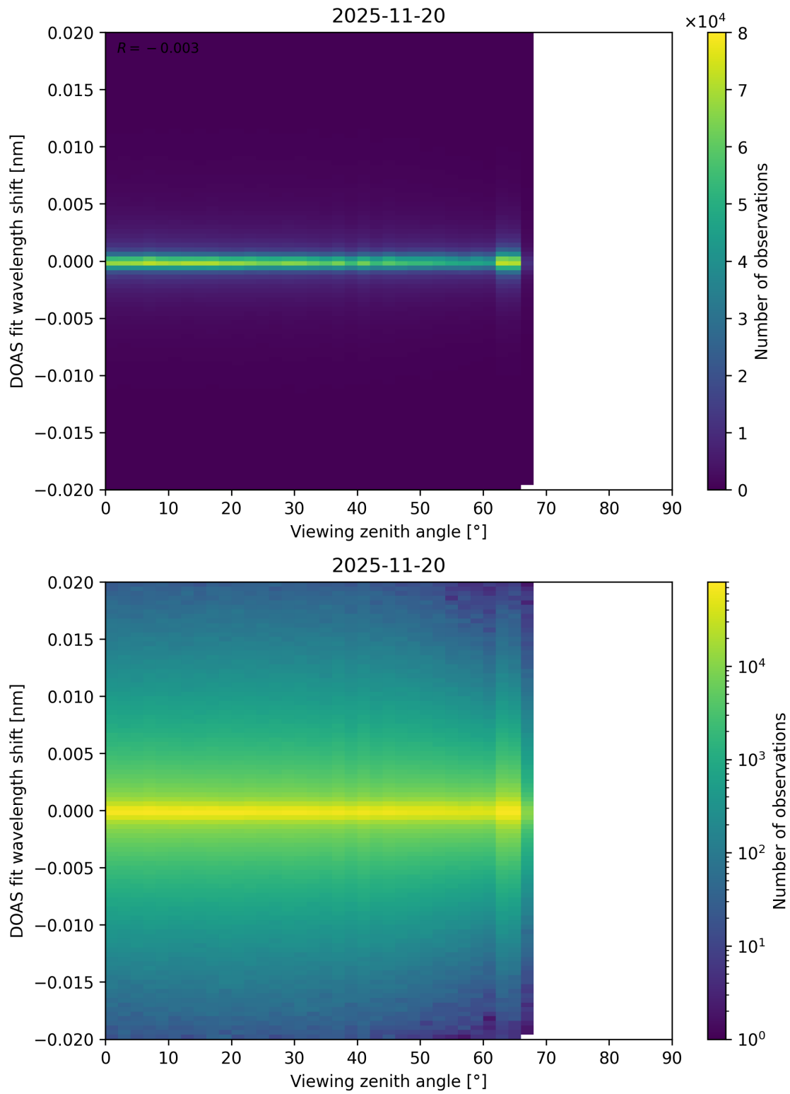
Figure 203: Scatter density plot of “Viewing zenith angle” against “DOAS fit wavelength shift” for 2025-11-19 to 2025-11-21.
