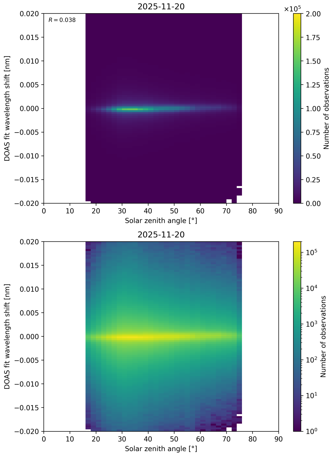
Figure 187: Scatter density plot of “Solar zenith angle” against “DOAS fit wavelength shift” for 2025-11-19 to 2025-11-21.
