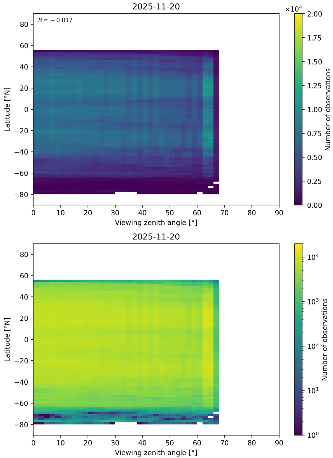
Figure 217: Scatter density plot of “Viewing zenith angle” against “Latitude” for 2025-11-19 to 2025-11-21.
