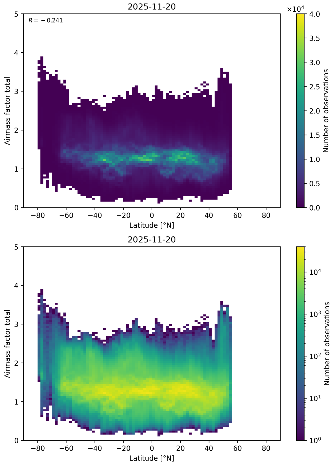
Figure 179: Scatter density plot of “Latitude” against “Airmass factor total” for 2025-11-19 to 2025-11-21.
