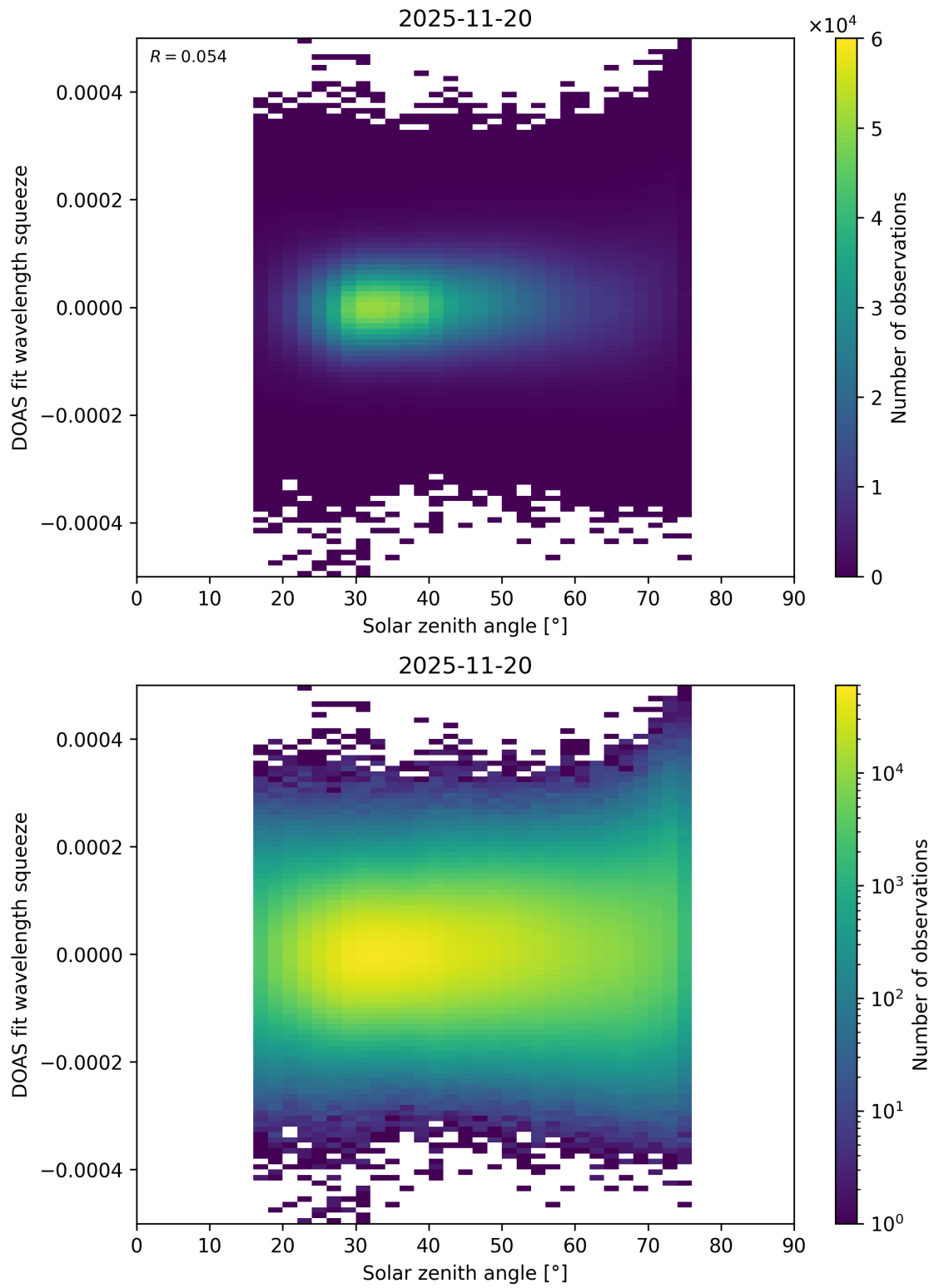
Figure 188: Scatter density plot of “Solar zenith angle” against “DOAS fit wavelength squeeze” for 2025-11-19 to 2025-11-21.
