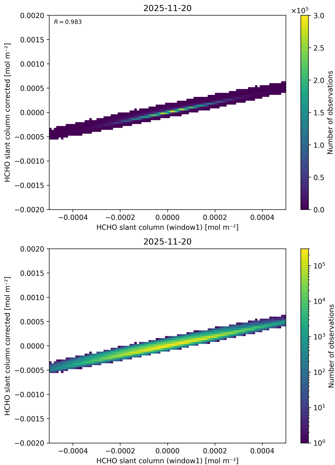
Figure 92: Scatter density plot of “HCHO slant column (window1)” against “HCHO slant column corrected” for 2025-11-19 to 2025-11-21.
