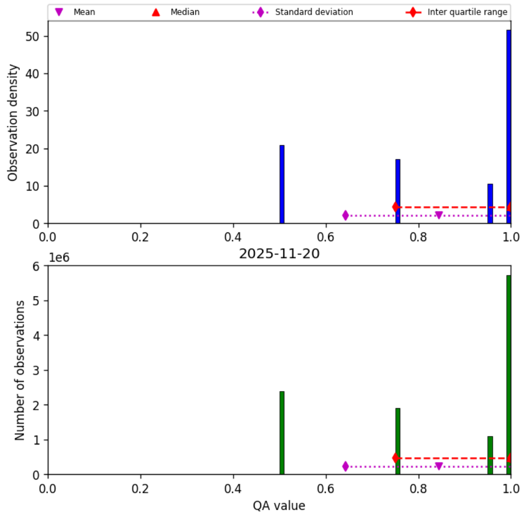
Figure 36: Histogram of “QA value” for 2025-11-19 to 2025-11-21
