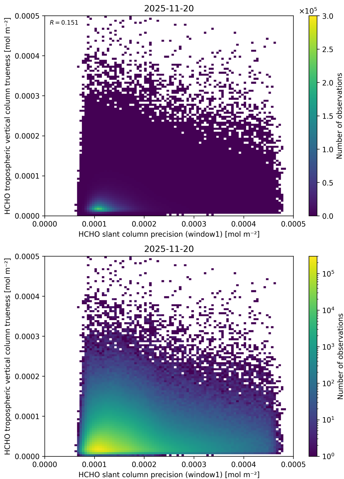
Figure 107: Scatter density plot of “HCHO slant column precision (window1)” against “HCHO tropospheric vertical column trueness” for 2025-11-19 to 2025-11-21.
