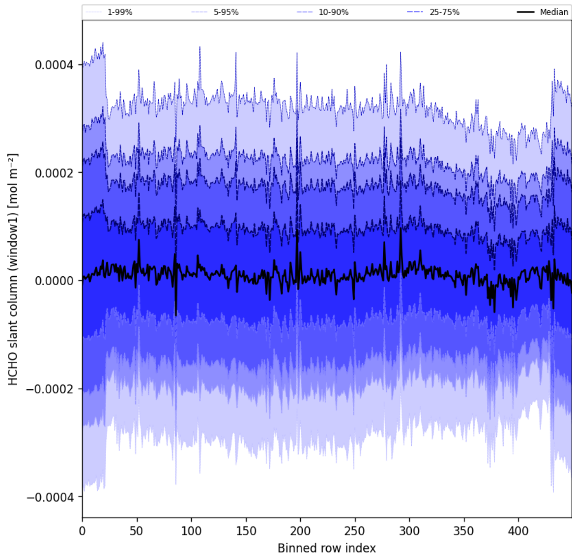
Figure 55: Along track statistics of “HCHO slant column (window1)” for 2025-11-19 to 2025-11-21
