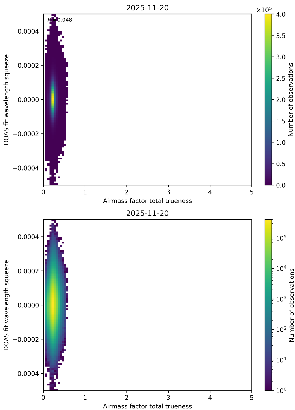
Figure 120: Scatter density plot of “Airmass factor total trueness” against “DOAS fit wavelength squeeze” for 2025-11-19 to 2025-11-21.
