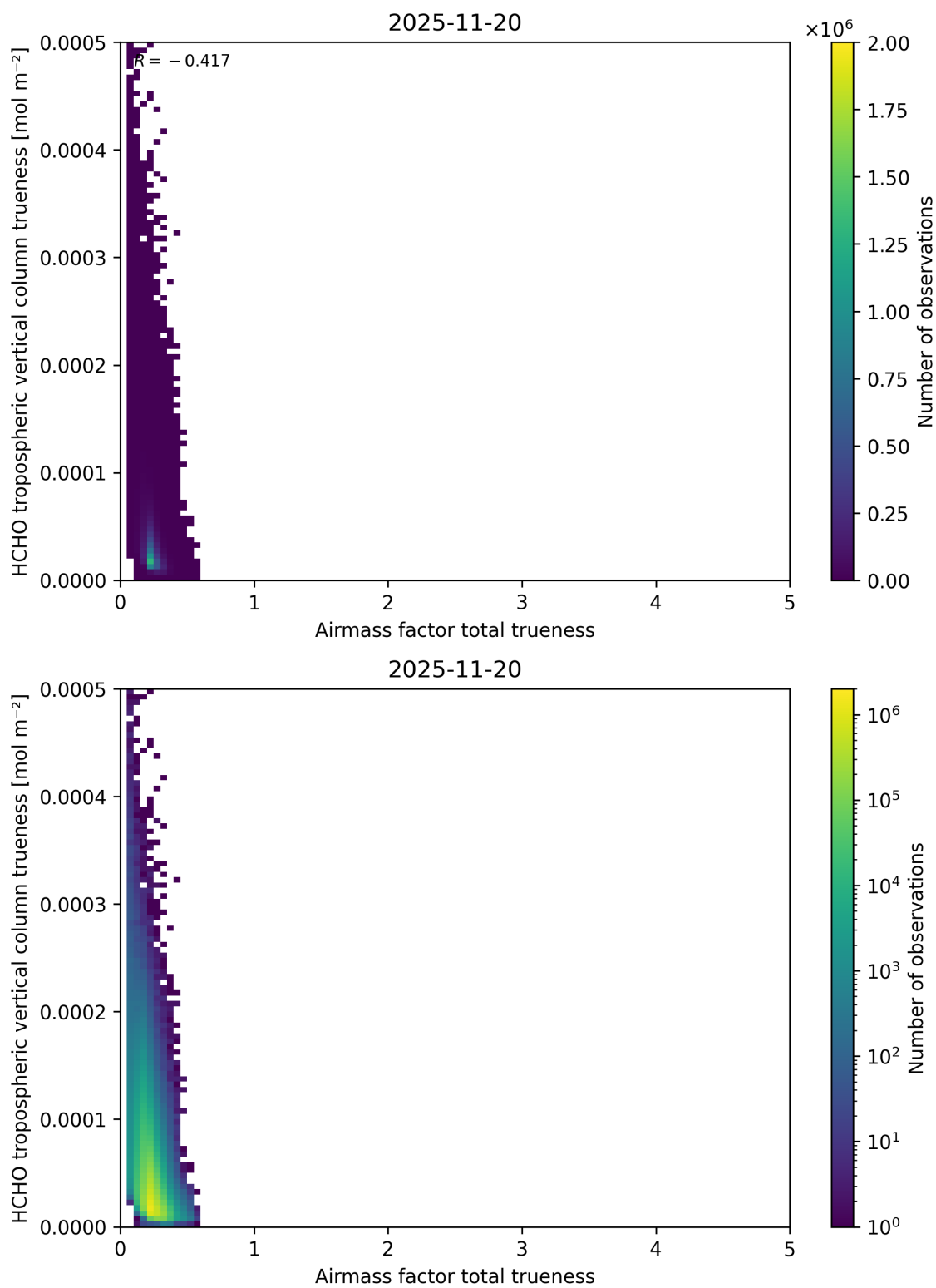
Figure 124: Scatter density plot of “Airmass factor total truiness” against “HCHO tropospheric vertical column truiness” for 2025-11-19 to 2025-11-21.
