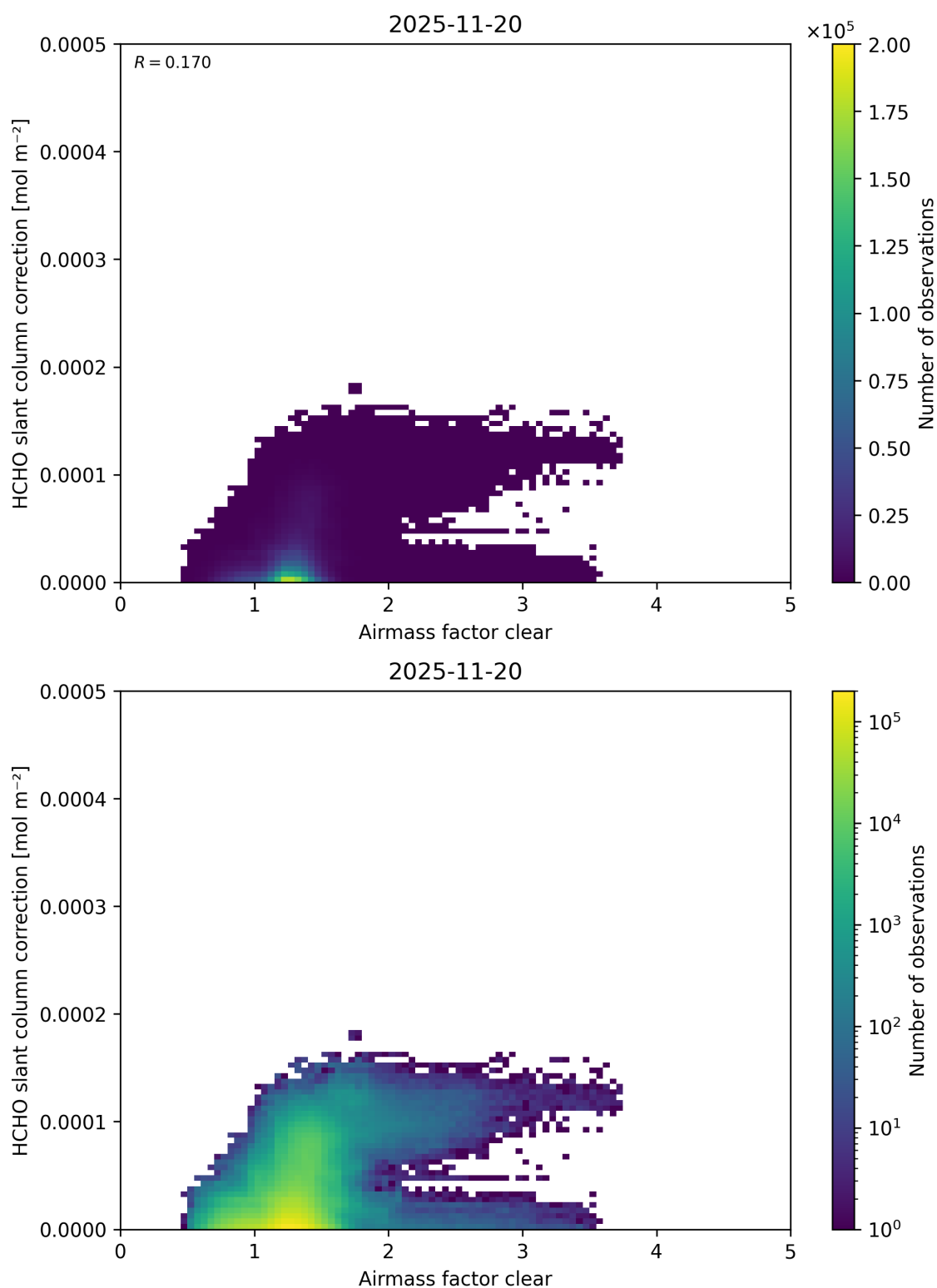
Figure 82: Scatter density plot of “Airmass factor clear” against “HCHO slant column correction” for 2025-11-19 to 2025-11-21.
