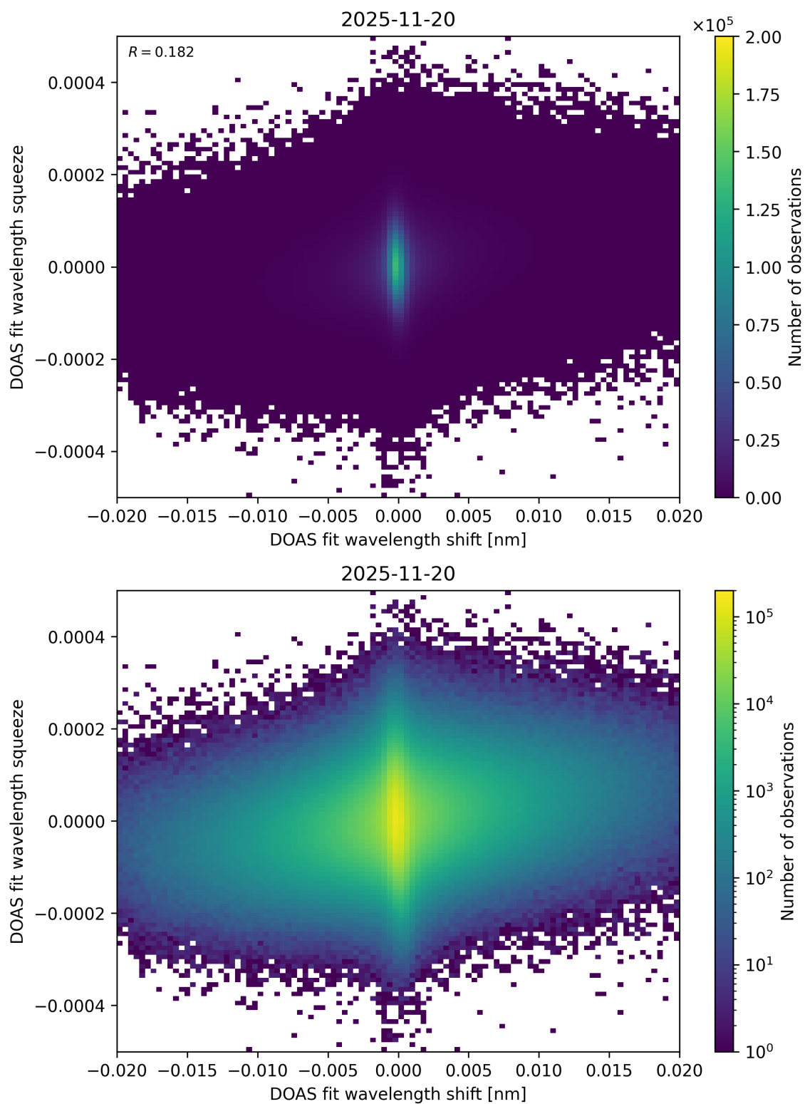
Figure 70: Scatter density plot of “DOAS fit wavelength shift” against “DOAS fit wavelength squeeze” for 2025-11-19 to 2025-11-21.
