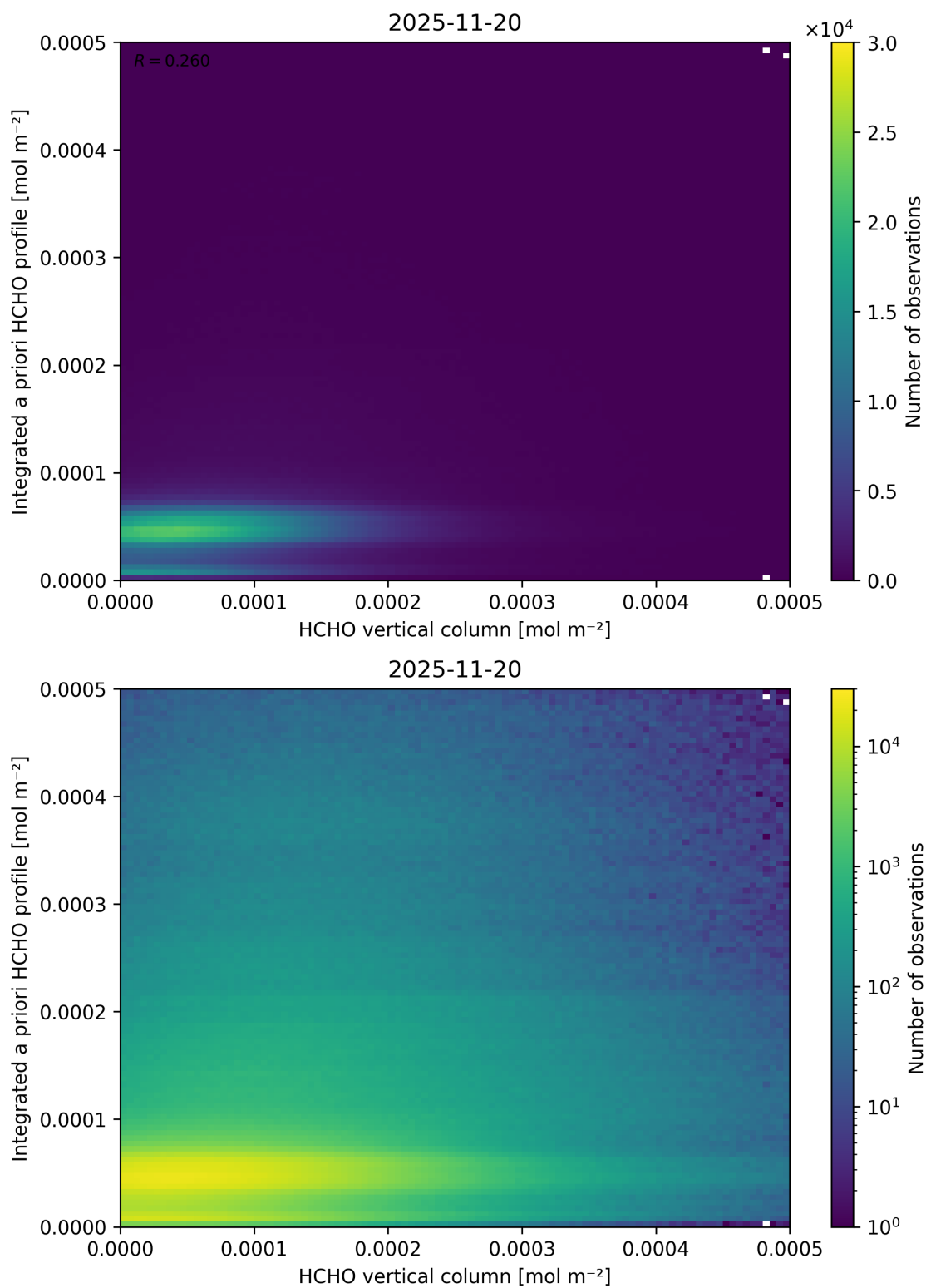
Figure 151: Scatter density plot of “HCHO vertical column” against “Integrated a priori HCHO profile” for 2025-11-19 to 2025-11-21.
