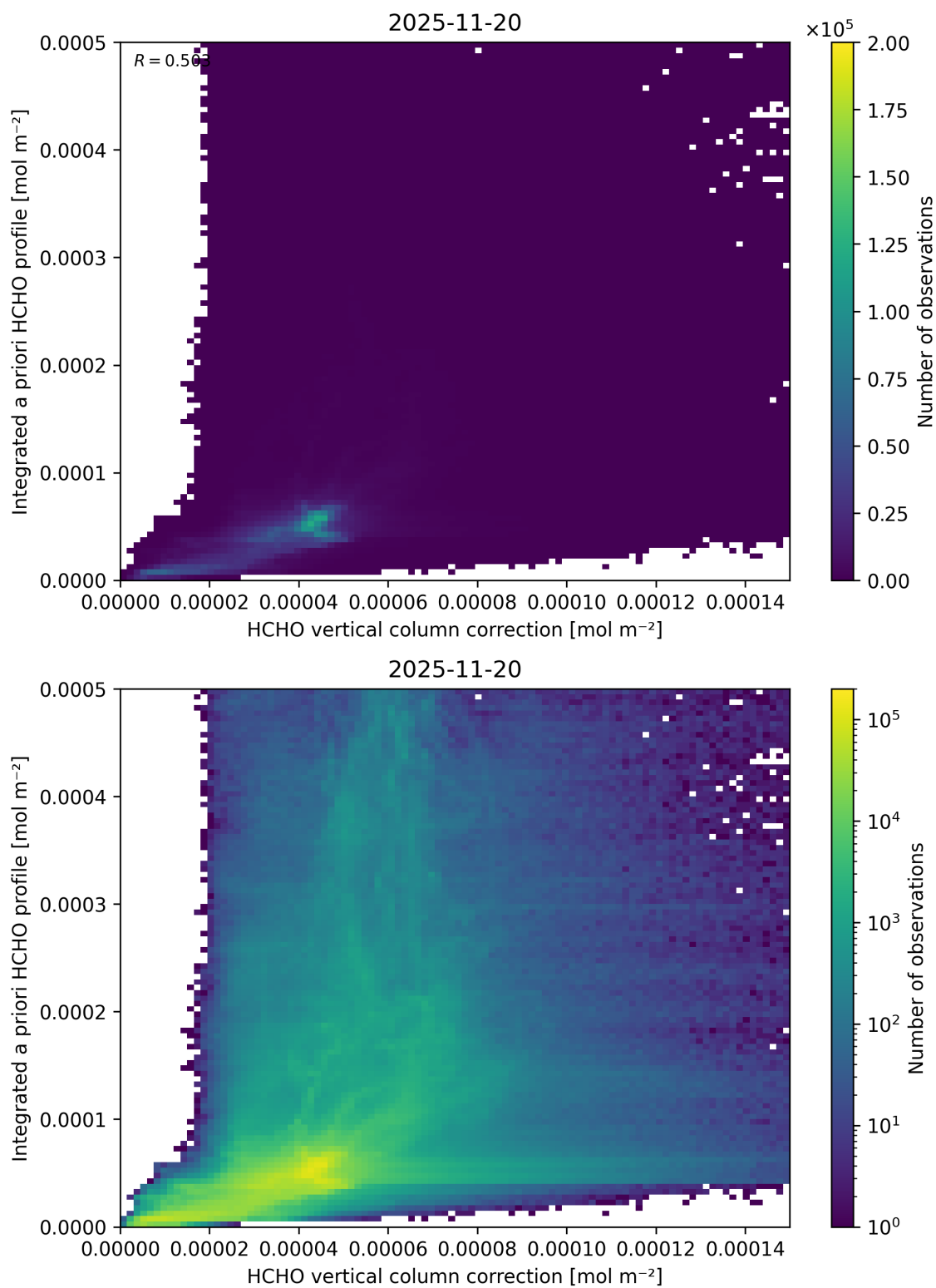
Figure 137: Scatter density plot of “HCHO vertical column correction” against “Integrated a priori HCHO profile” for 2025-11-19 to 2025-11-21.
