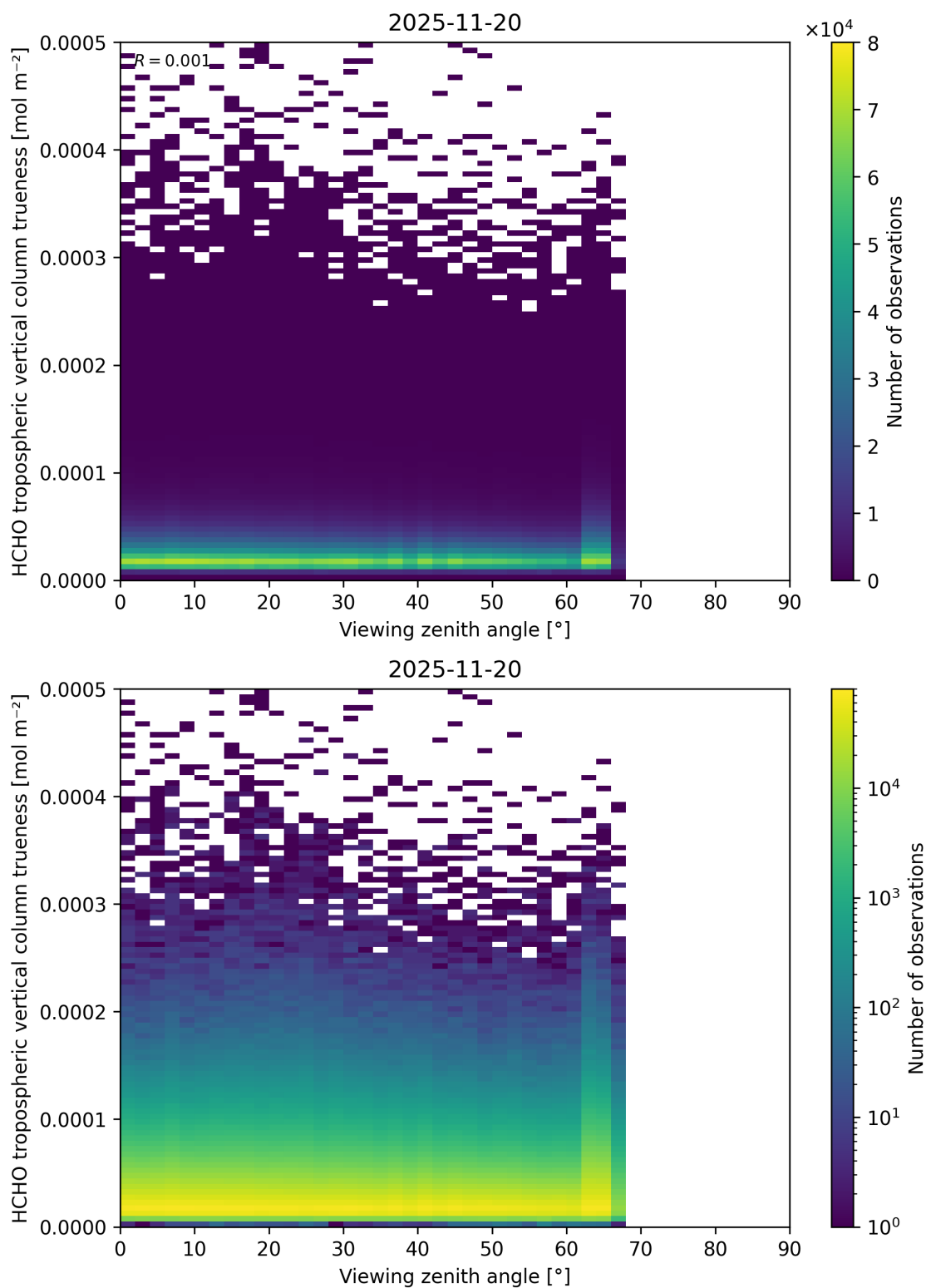
Figure 215: Scatter density plot of “Viewing zenith angle” against “HCHO tropospheric vertical column truthness” for 2025-11-19 to 2025-11-21.
