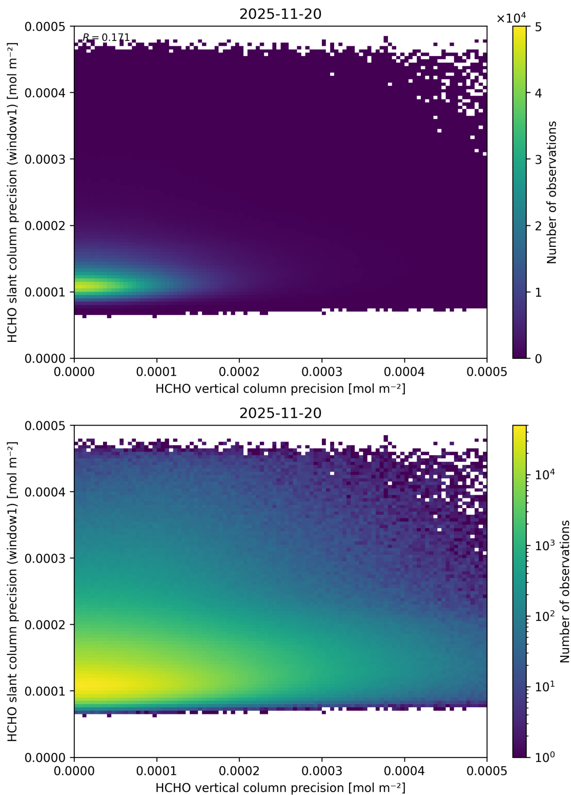
Figure 159: Scatter density plot of “HCHO vertical column precision” against “HCHO slant column precision (window1)” for 2025-11-19 to 2025-11-21.
