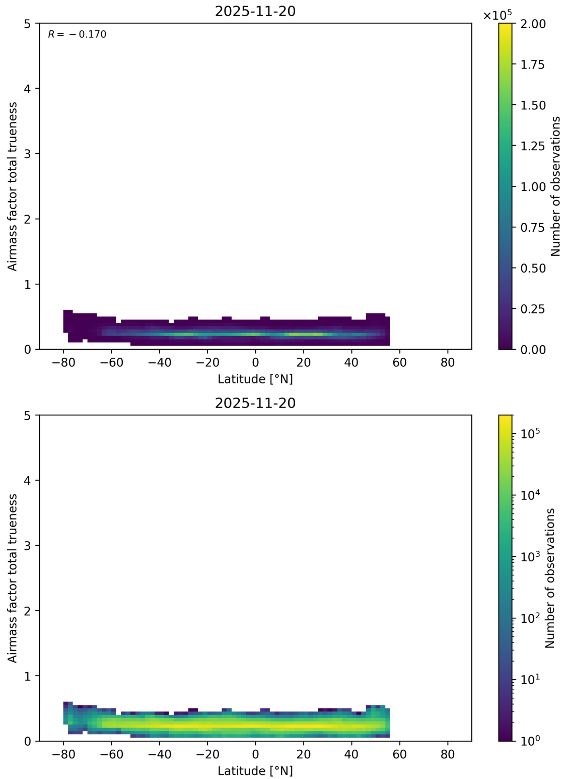
Figure 180: Scatter density plot of “Latitude” against “Airmass factor total trueneess” for 2025-11-19 to 2025-11-21.
