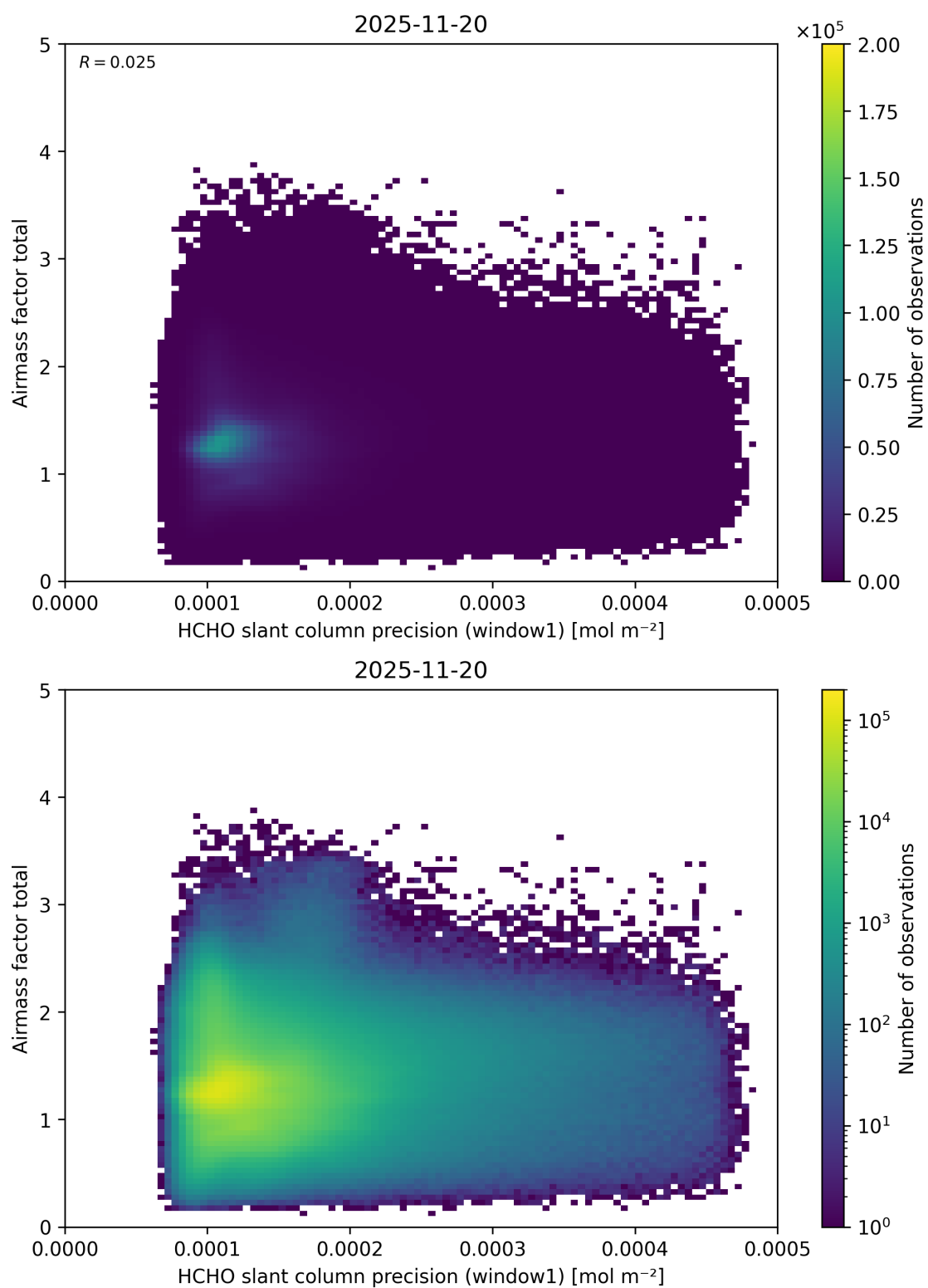
Figure 105: Scatter density plot of “HCHO slant column precision (window1)” against “Airmass factor total” for 2025-11-19 to 2025-11-21.
