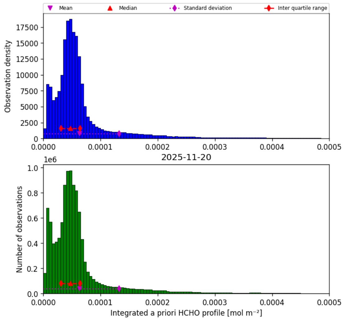
Figure 45: Histogram of “Integrated a priori HCHO profile” for 2025-11-19 to 2025-11-21
