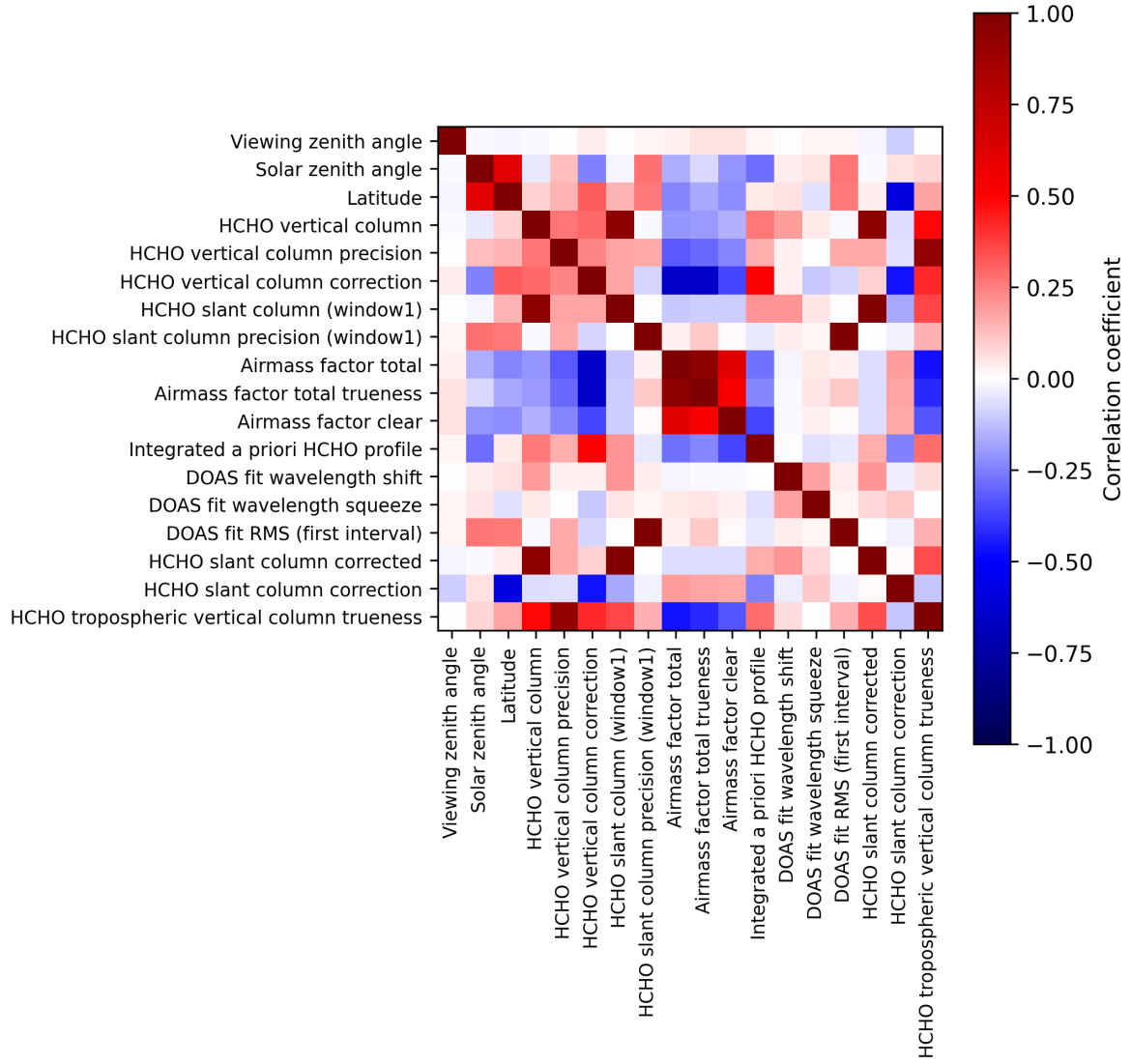
Figure 2: Map of correlation matrix for 2025-11-19 to 2025-11-21.
