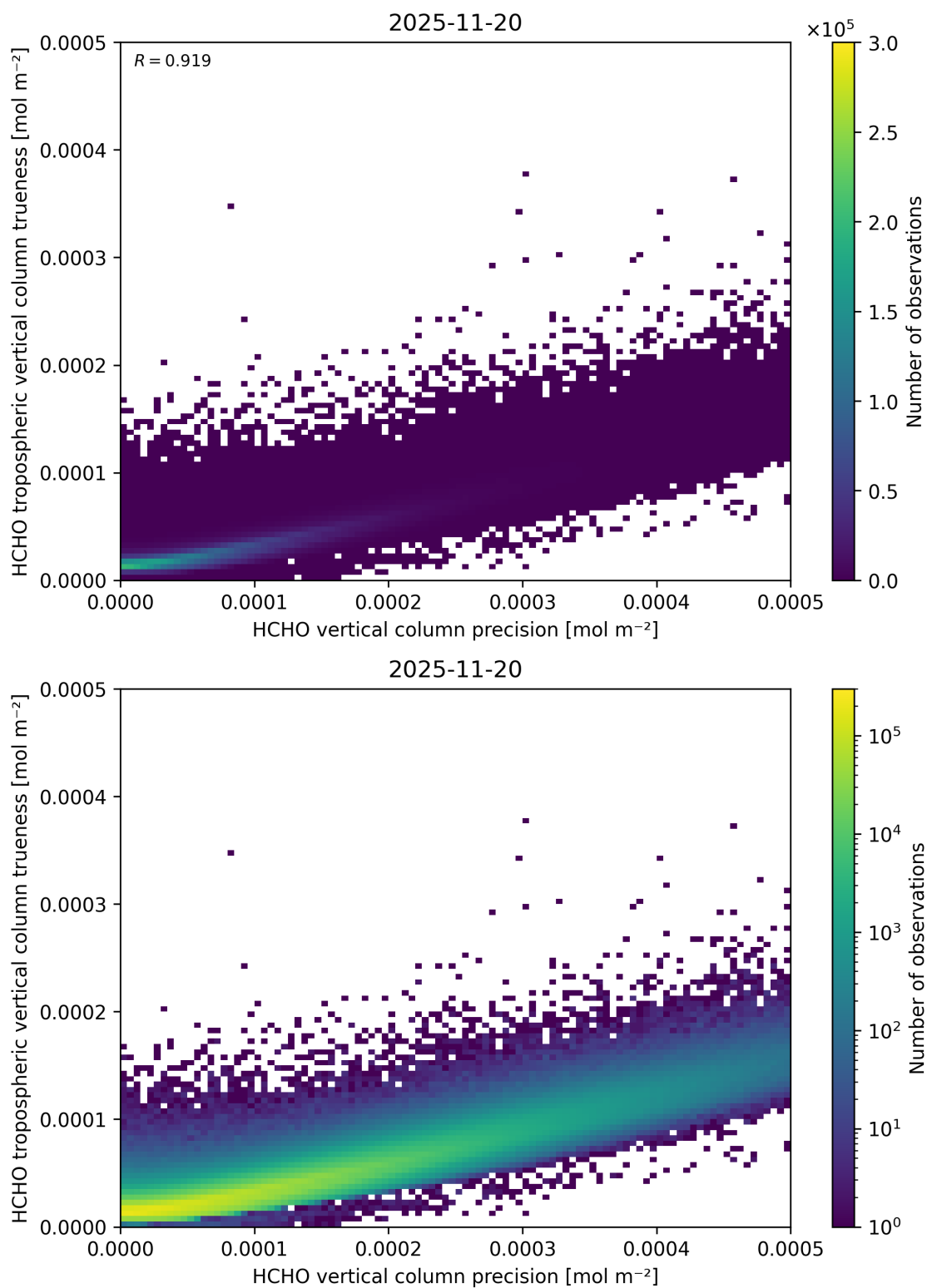
Figure 163: Scatter density plot of “HCHO vertical column precision” against “HCHO tropospheric vertical column trueness” for 2025-11-19 to 2025-11-21.
