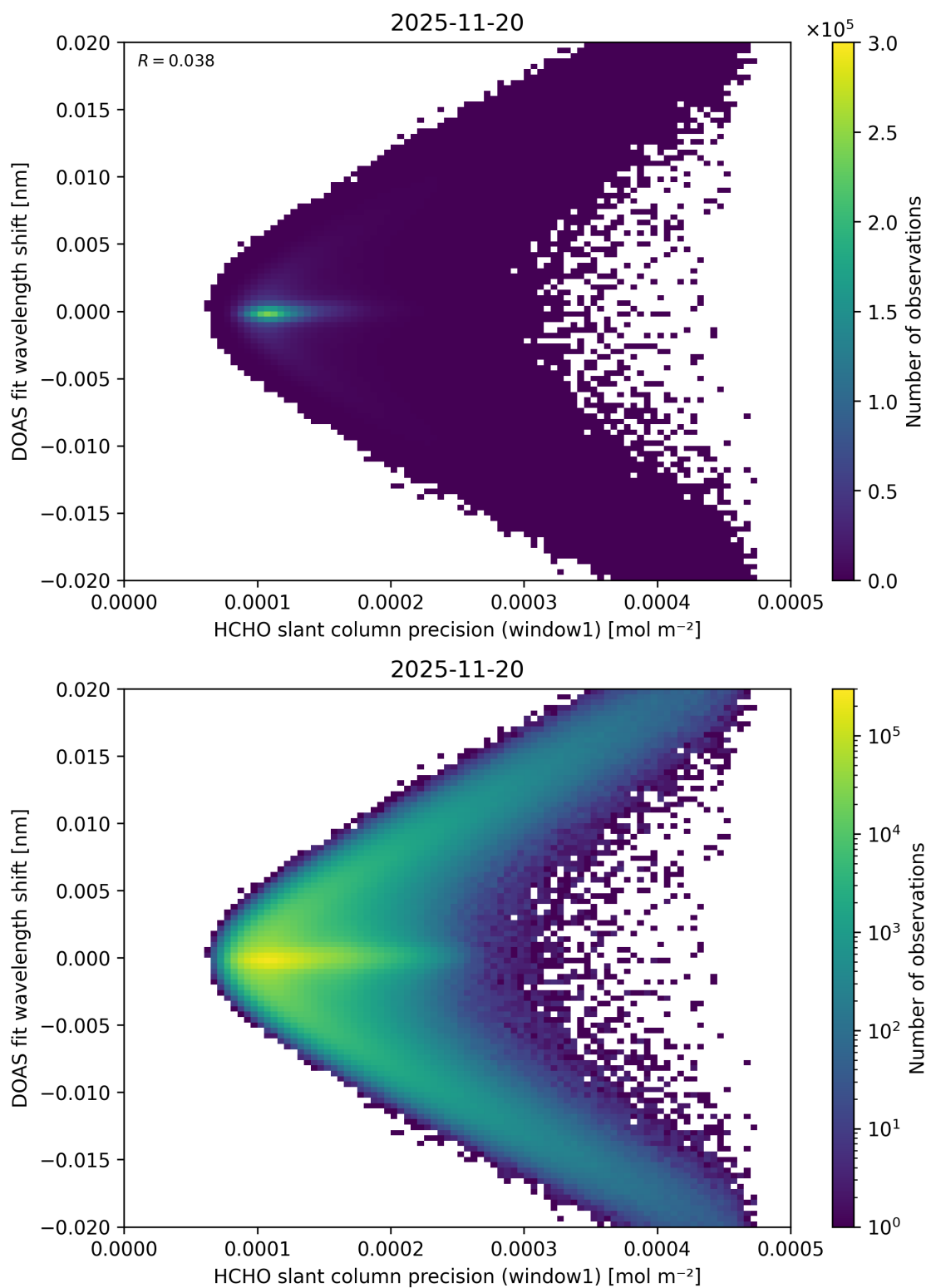
Figure 100: Scatter density plot of “HCHO slant column precision (window1)” against “DOAS fit wavelength shift” for 2025-11-19 to 2025-11-21.
