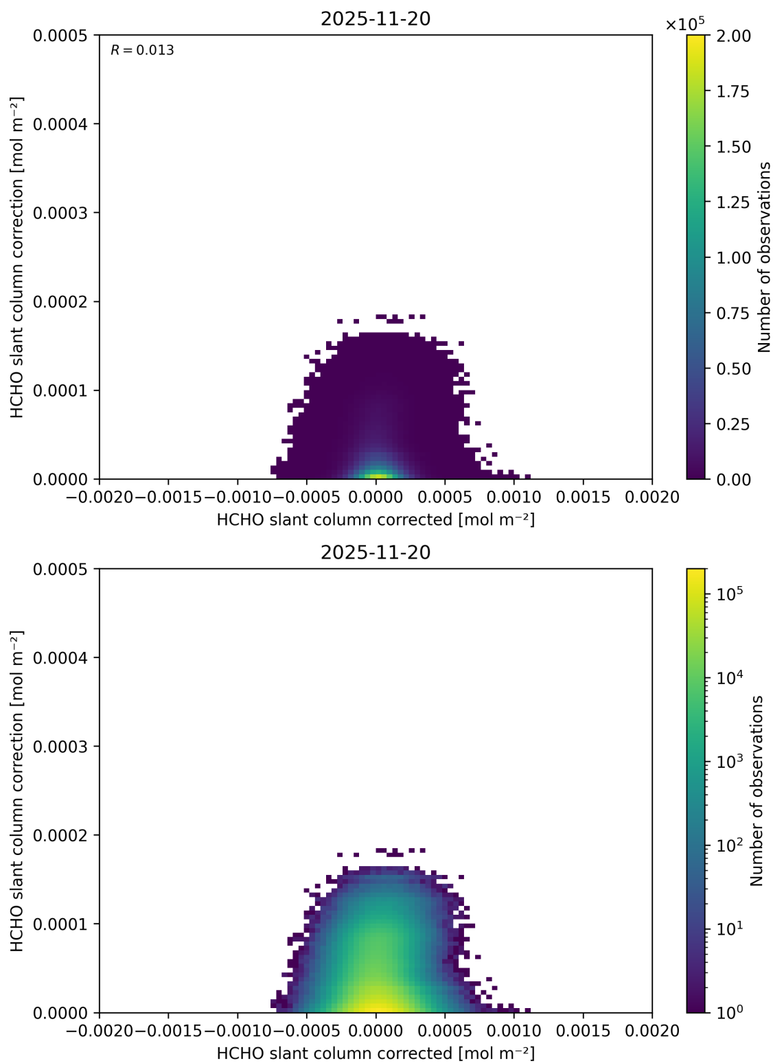
Figure 85: Scatter density plot of “HCHO slant column corrected” against “HCHO slant column correction” for 2025-11-19 to 2025-11-21.
