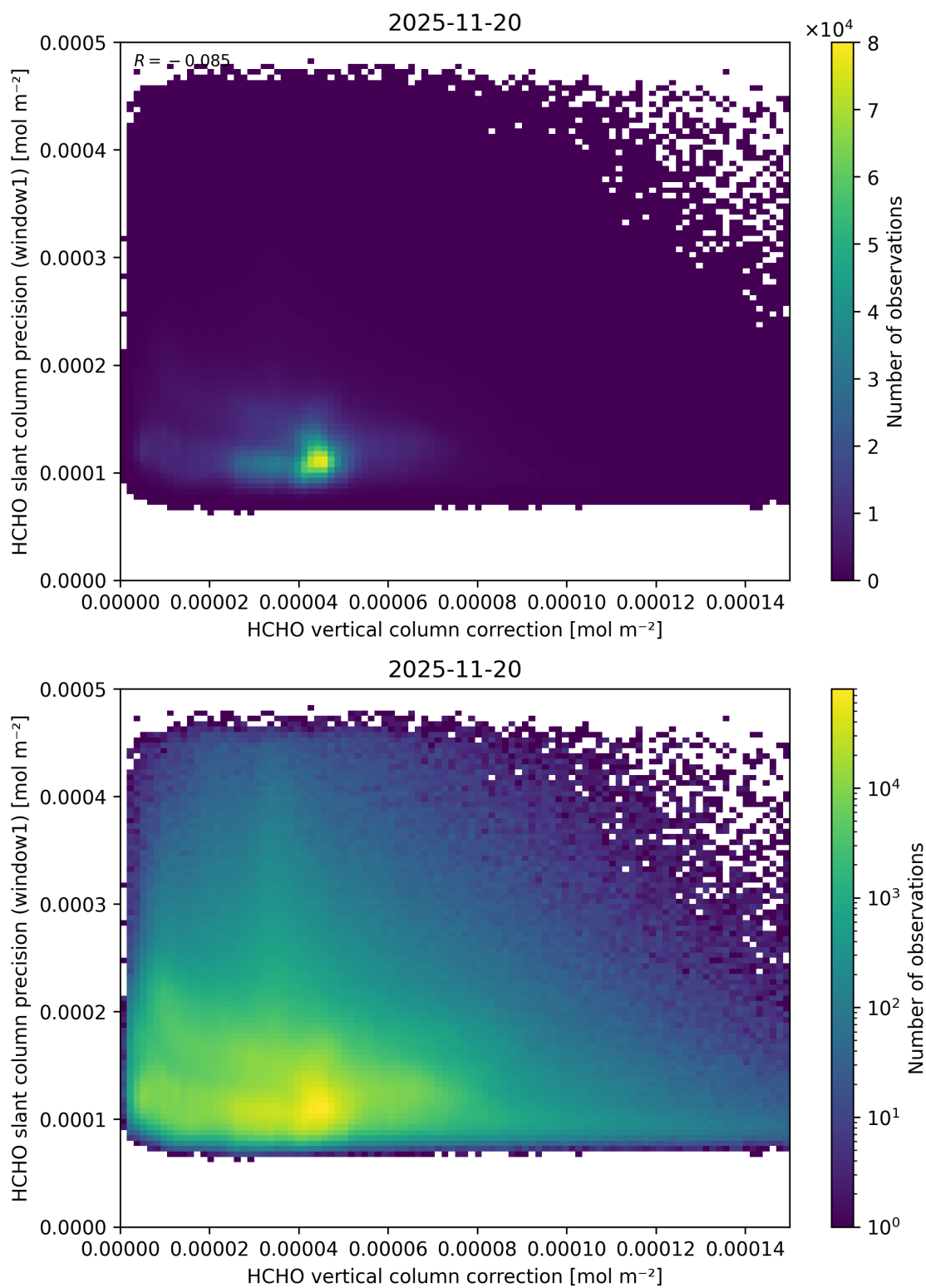
Figure 133: Scatter density plot of “HCHO vertical column correction” against “HCHO slant column precision (window1)” for 2025-11-19 to 2025-11-21.
