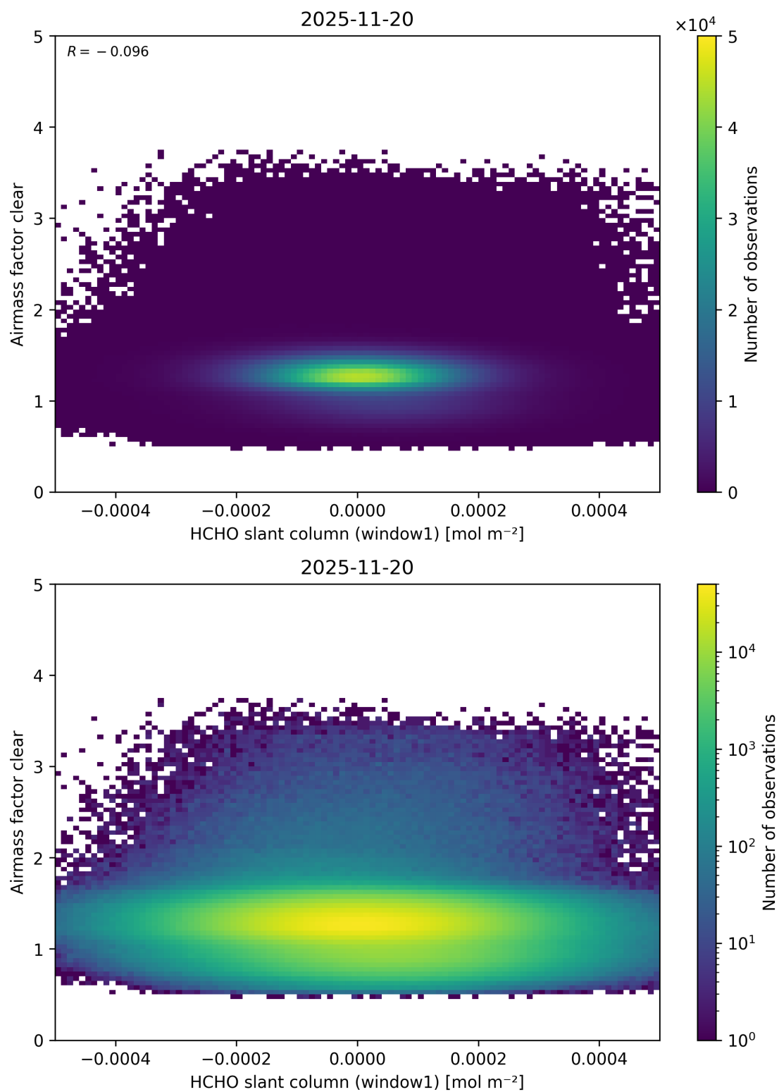
Figure 91: Scatter density plot of “HCHO slant column (window1)” against “Airmass factor clear” for 2025-11-19 to 2025-11-21.
