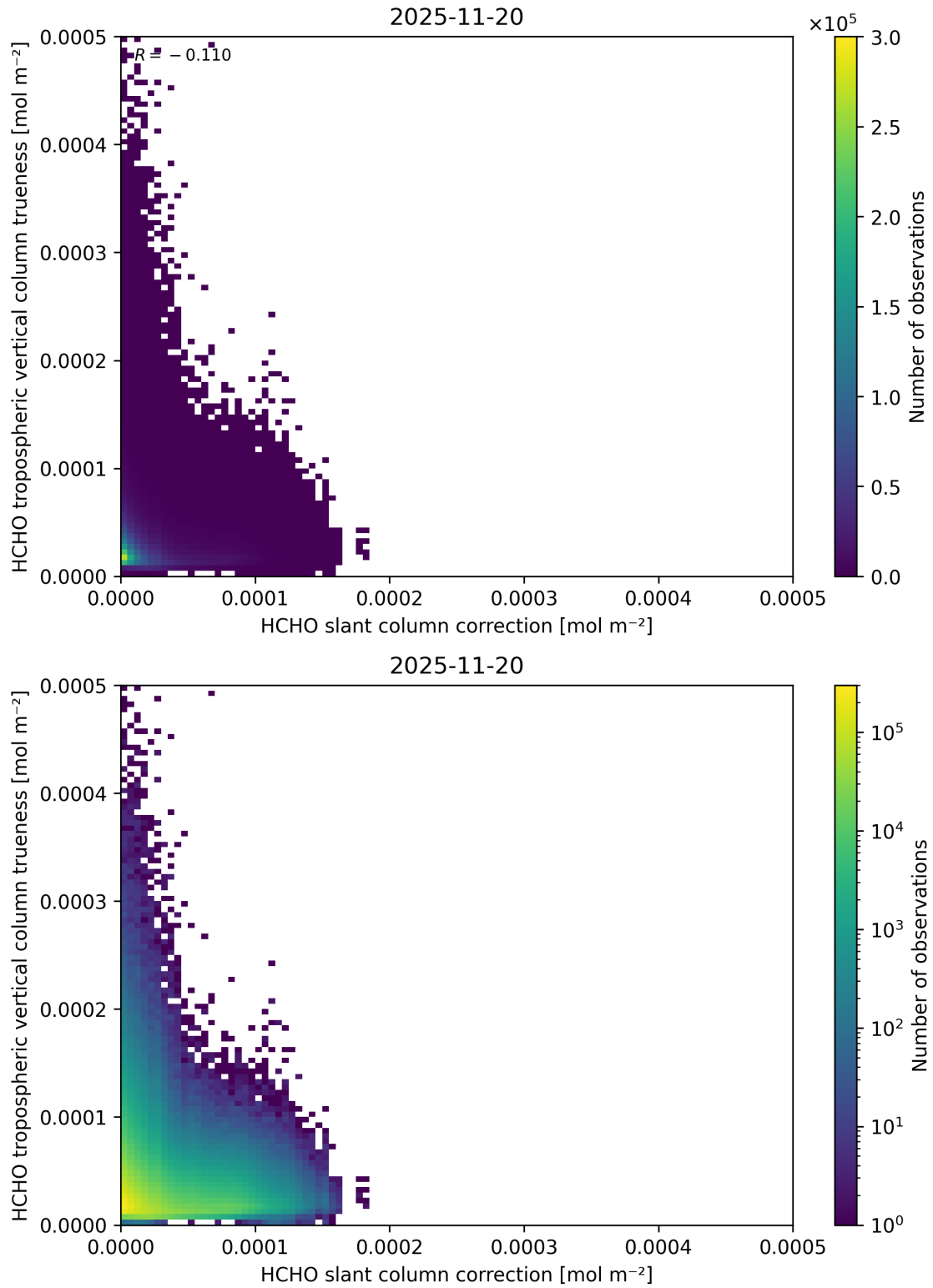
Figure 87: Scatter density plot of “HCHO slant column correction” against “HCHO tropospheric vertical column trueness” for 2025-11-19 to 2025-11-21.
