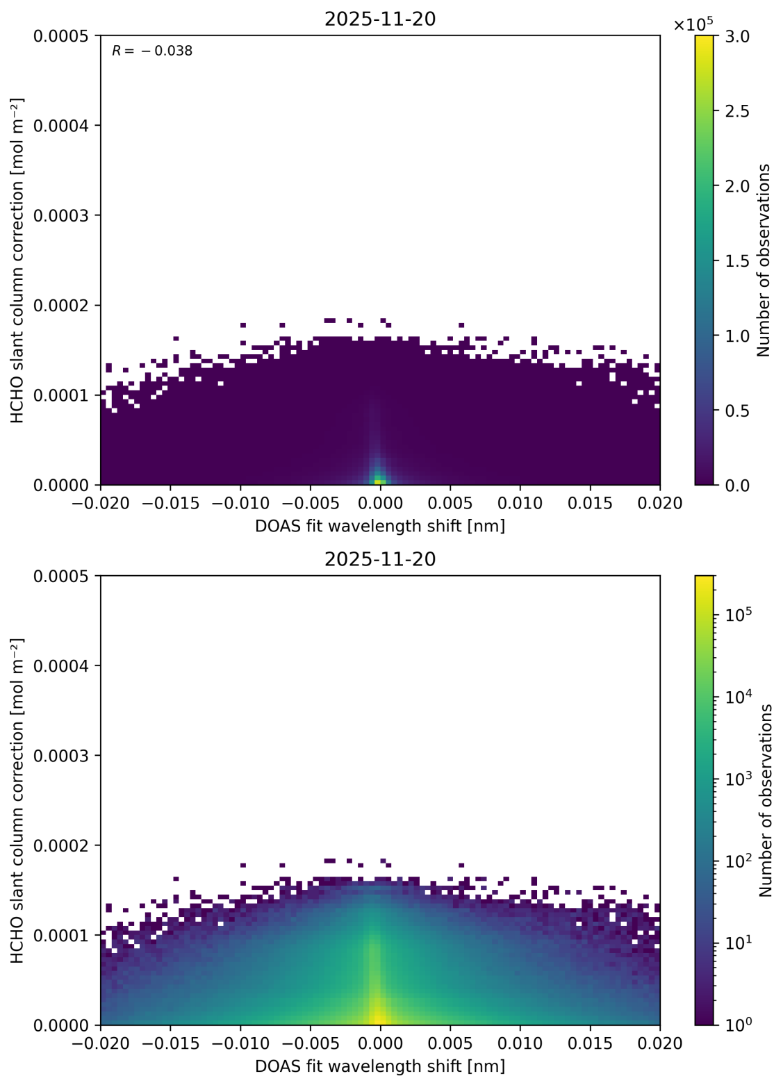
Figure 72: Scatter density plot of “DOAS fit wavelength shift” against “HCHO slant column correction” for 2025-11-19 to 2025-11-21.
