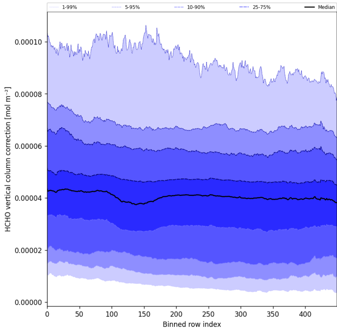
Figure 54: Along track statistics of “HCHO vertical column correction” for 2025-11-19 to 2025-11-21
