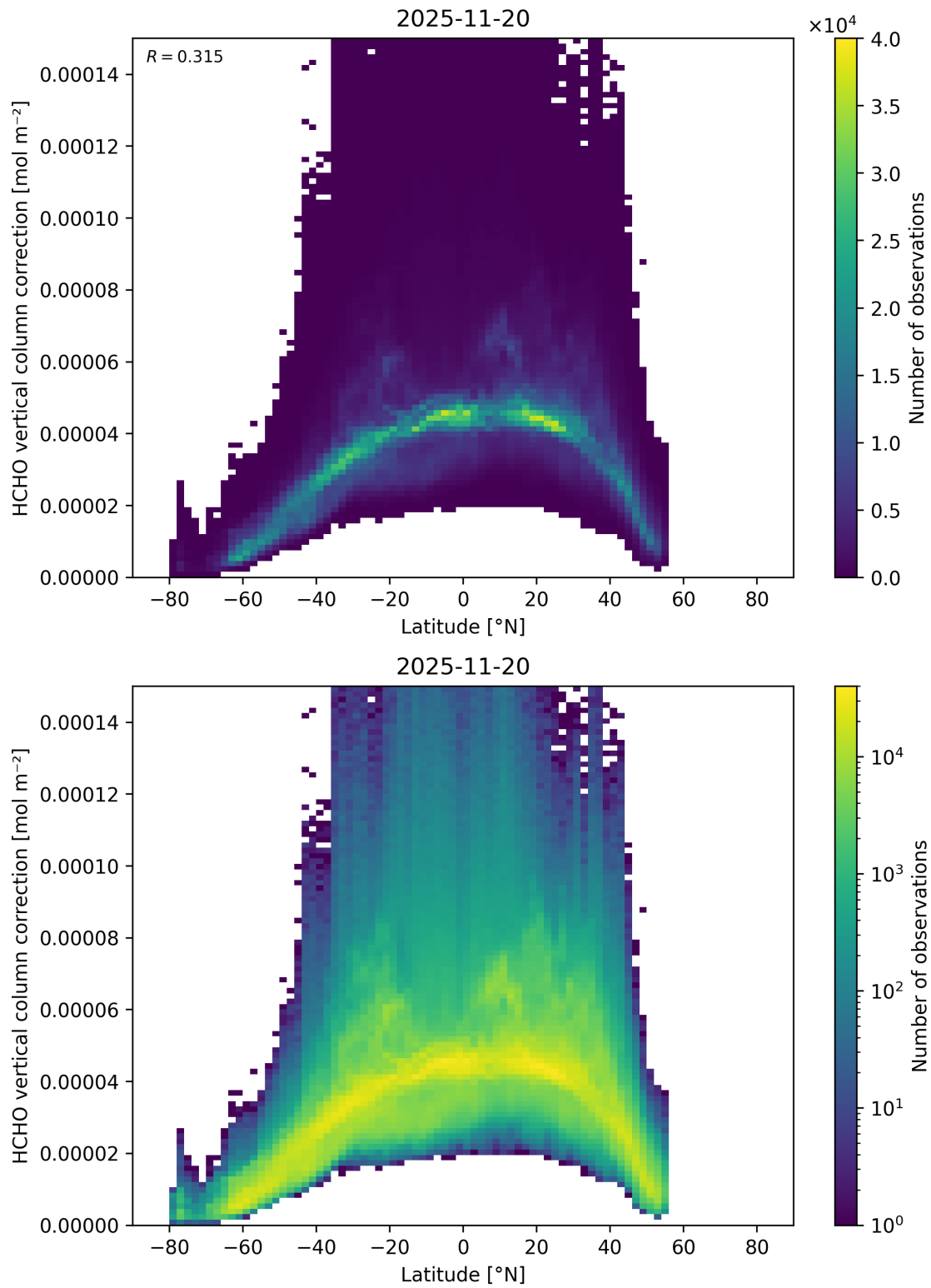
Figure 182: Scatter density plot of “Latitude” against “HCHO vertical column correction” for 2025-11-19 to 2025-11-21.
