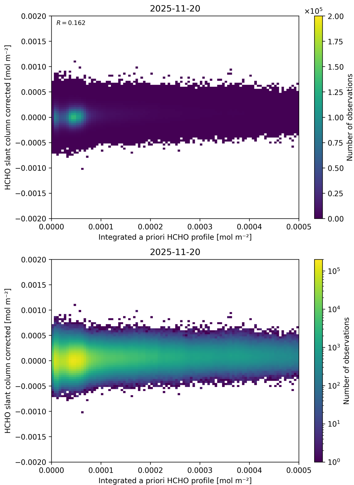
Figure 168: Scatter density plot of “Integrated a priori HCHO profile” against “HCHO slant column corrected” for 2025-11-19 to 2025-11-21.
