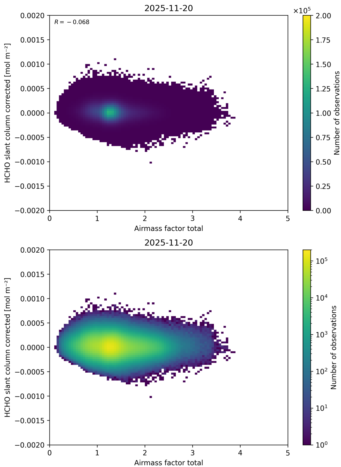
Figure 113: Scatter density plot of “Airmass factor total” against “HCHO slant column corrected” for 2025-11-19 to 2025-11-21.
