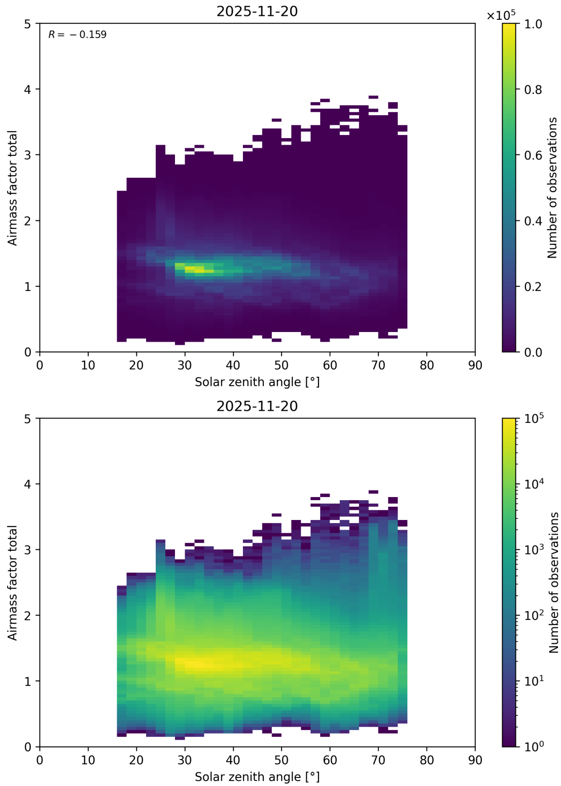
Figure 194: Scatter density plot of “Solar zenith angle” against “Airmass factor total” for 2025-11-19 to 2025-11-21.
