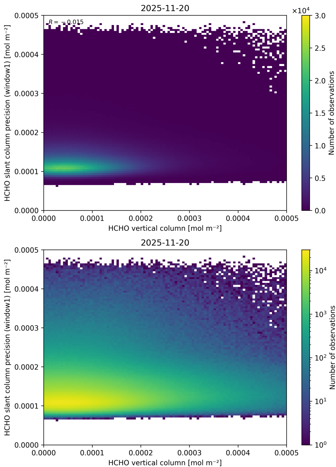
Figure 145: Scatter density plot of “HCHO vertical column” against “HCHO slant column precision (window1)” for 2025-11-19 to 2025-11-21.
