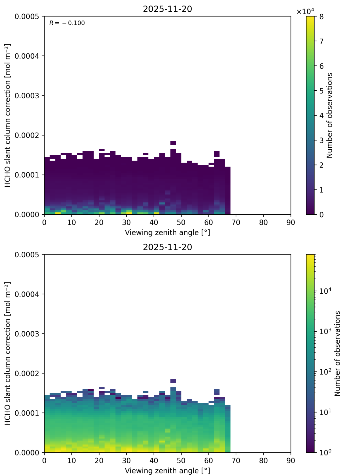
Figure 207: Scatter density plot of “Viewing zenith angle” against “HCHO slant column correction” for 2025-11-19 to 2025-11-21.
