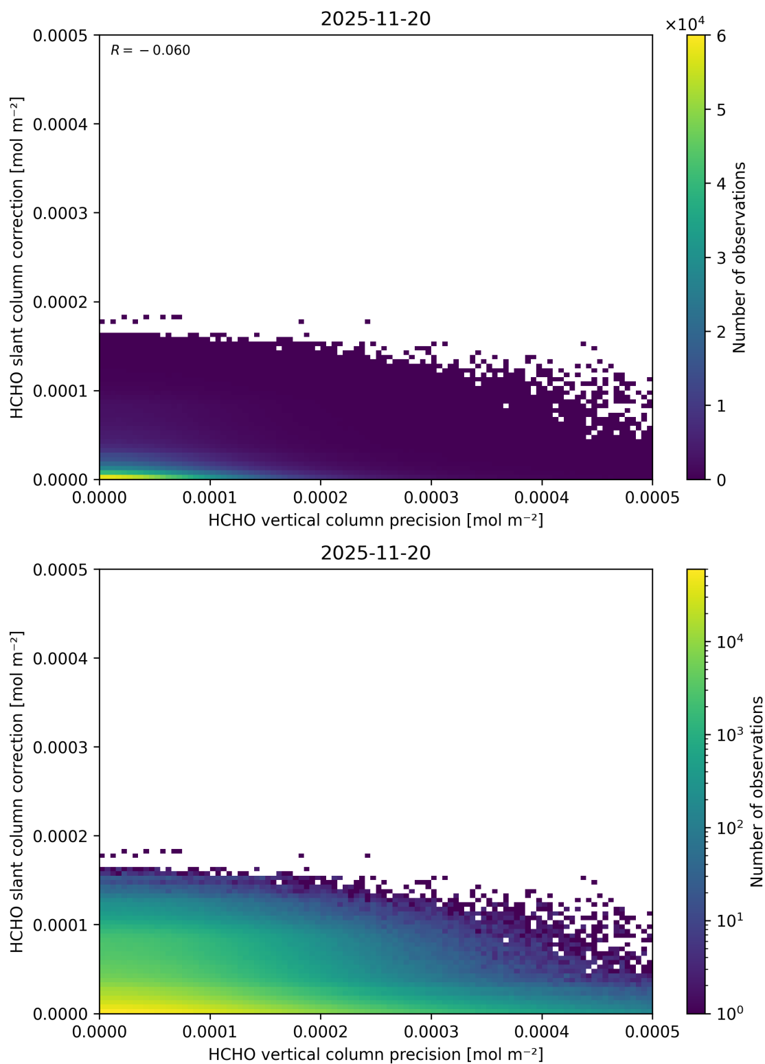
Figure 157: Scatter density plot of “HCHO vertical column precision” against “HCHO slant column correction” for 2025-11-19 to 2025-11-21.
