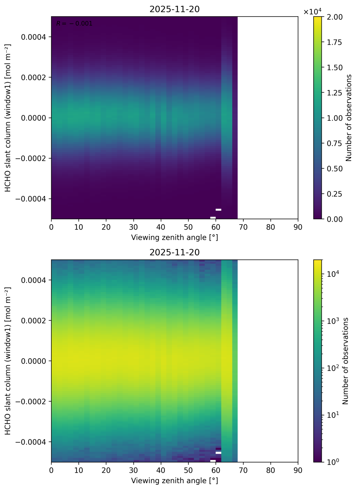
Figure 208: Scatter density plot of “Viewing zenith angle” against “HCHO slant column (window1)” for 2025-11-19 to 2025-11-21.
