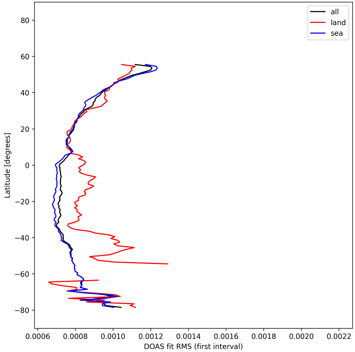
Figure 33: Zonal average of “DOAS fit RMS (first interval)” for 2025-11-19 to 2025-11-21.
