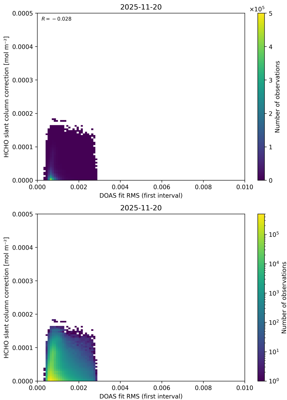
Figure 67: Scatter density plot of “DOAS fit RMS (first interval)” against “HCHO slant column correction” for 2025-11-19 to 2025-11-21.
