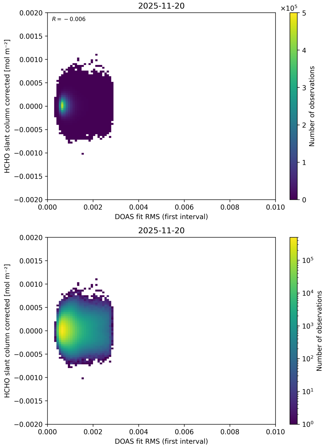
Figure 66: Scatter density plot of “DOAS fit RMS (first interval)” against “HCHO slant column corrected” for 2025-11-19 to 2025-11-21.
