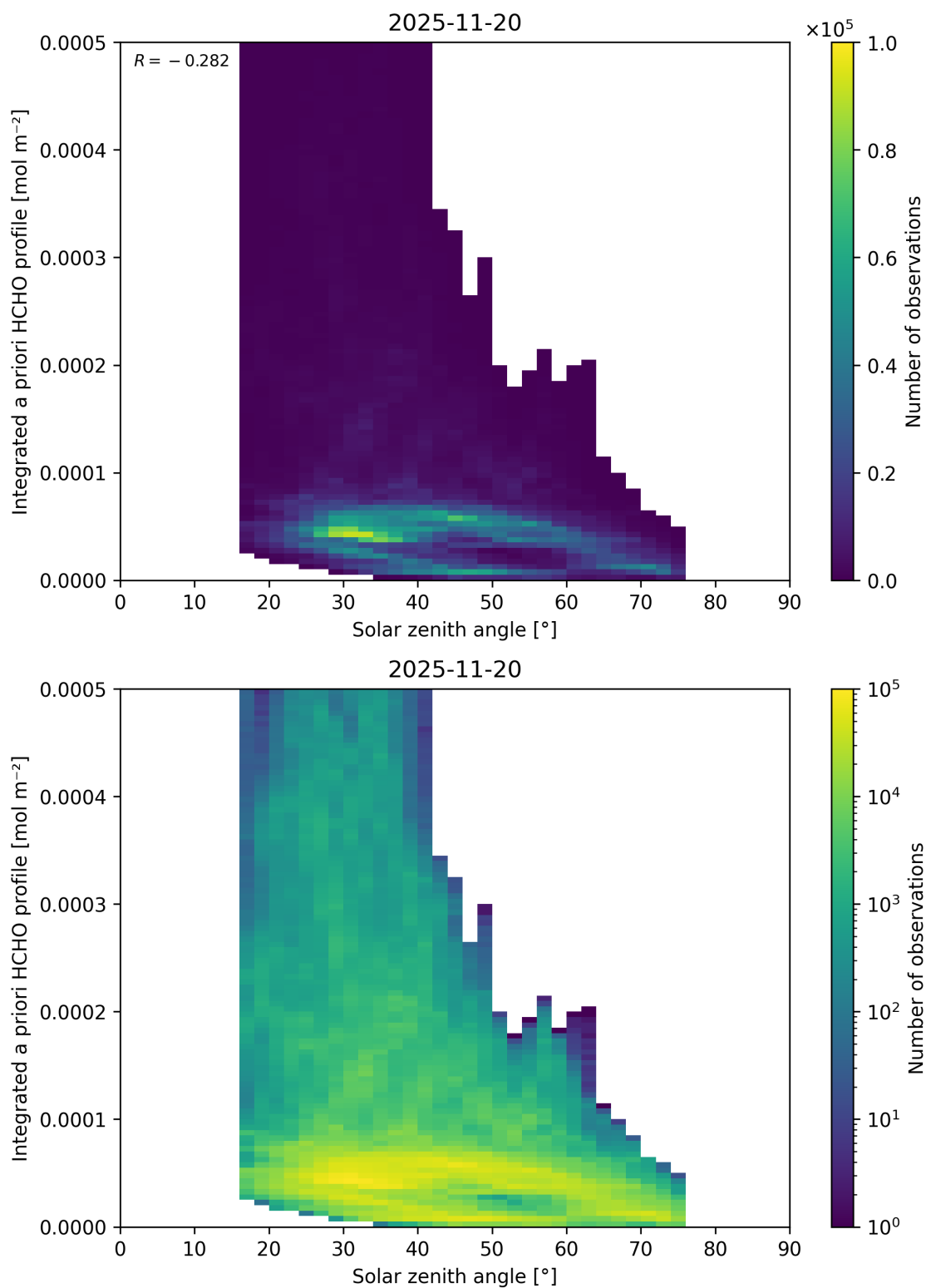
Figure 200: Scatter density plot of “Solar zenith angle” against “Integrated a priori HCHO profile” for 2025-11-19 to 2025-11-21.
