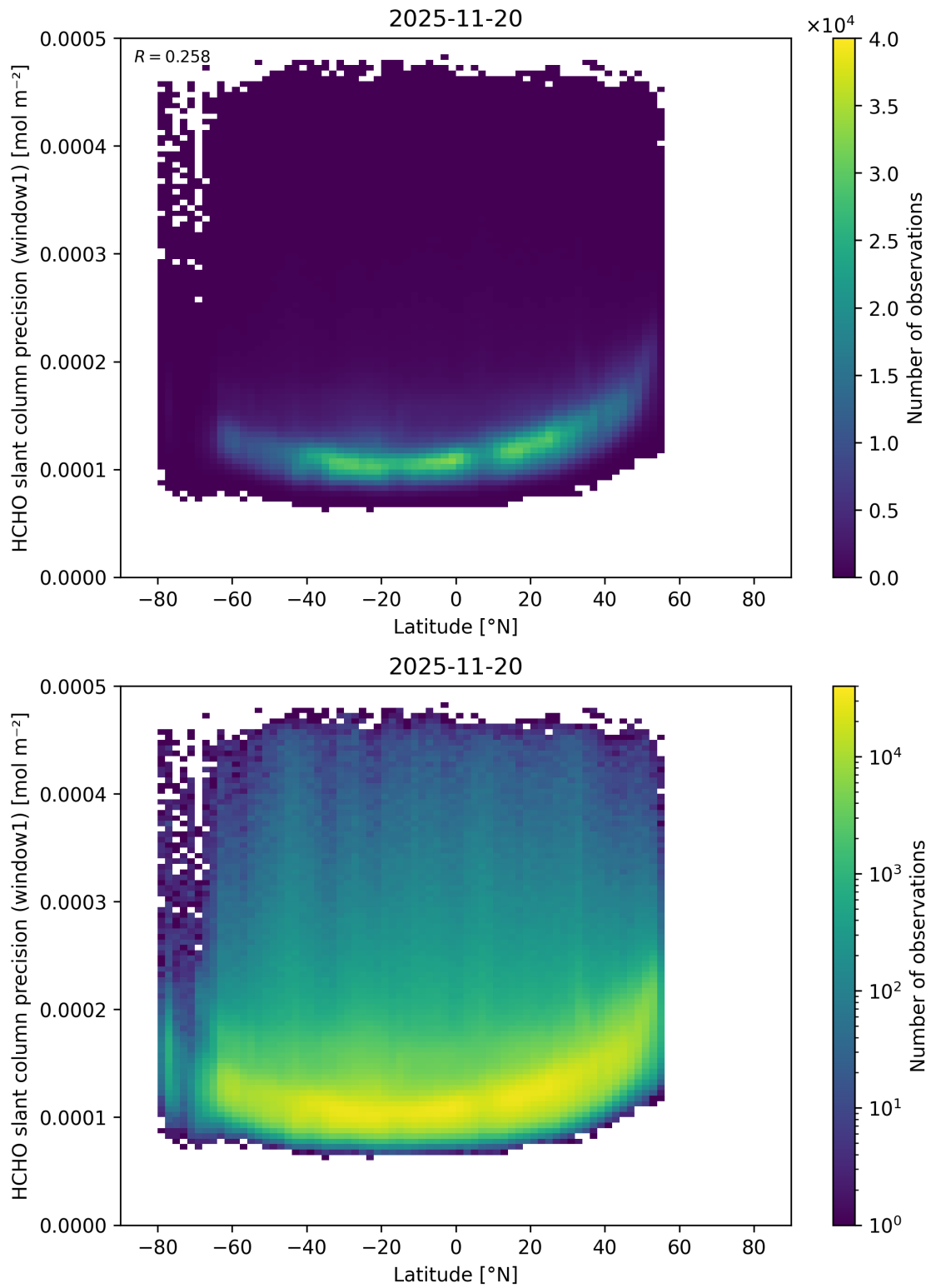
Figure 178: Scatter density plot of “Latitude” against “HCHO slant column precision (window1)” for 2025-11-19 to 2025-11-21.
