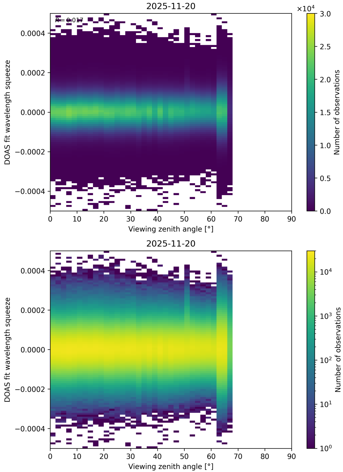
Figure 204: Scatter density plot of “Viewing zenith angle” against “DOAS fit wavelength squeeze” for 2025-11-19 to 2025-11-21.
