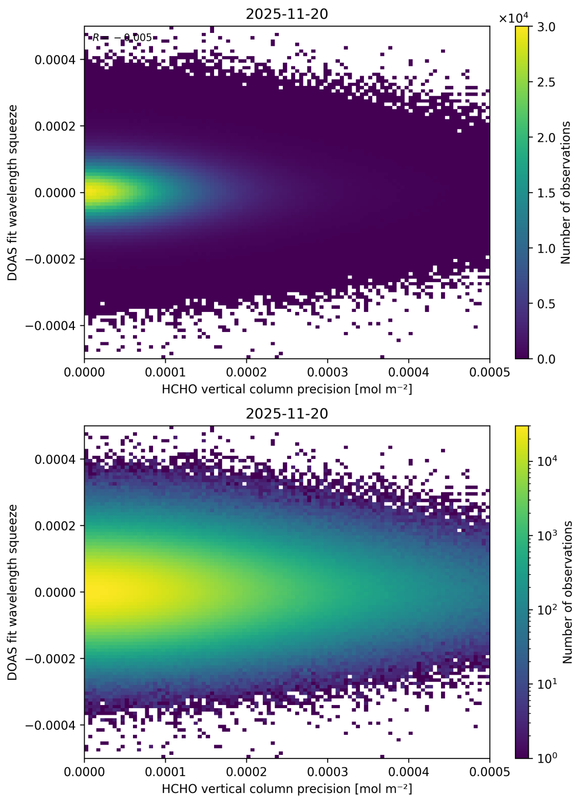
Figure 154: Scatter density plot of “HCHO vertical column precision” against “DOAS fit wavelength squeeze” for 2025-11-19 to 2025-11-21.
