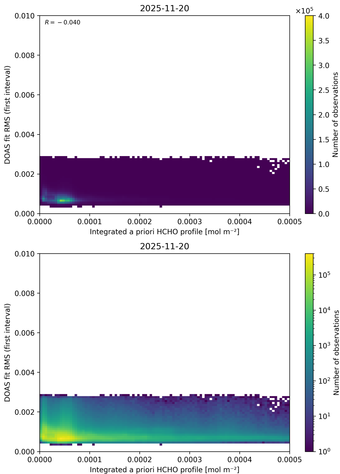
Figure 165: Scatter density plot of “Integrated a priori HCHO profile” against “DOAS fit RMS (first interval)” for 2025-11-19 to 2025-11-21.
