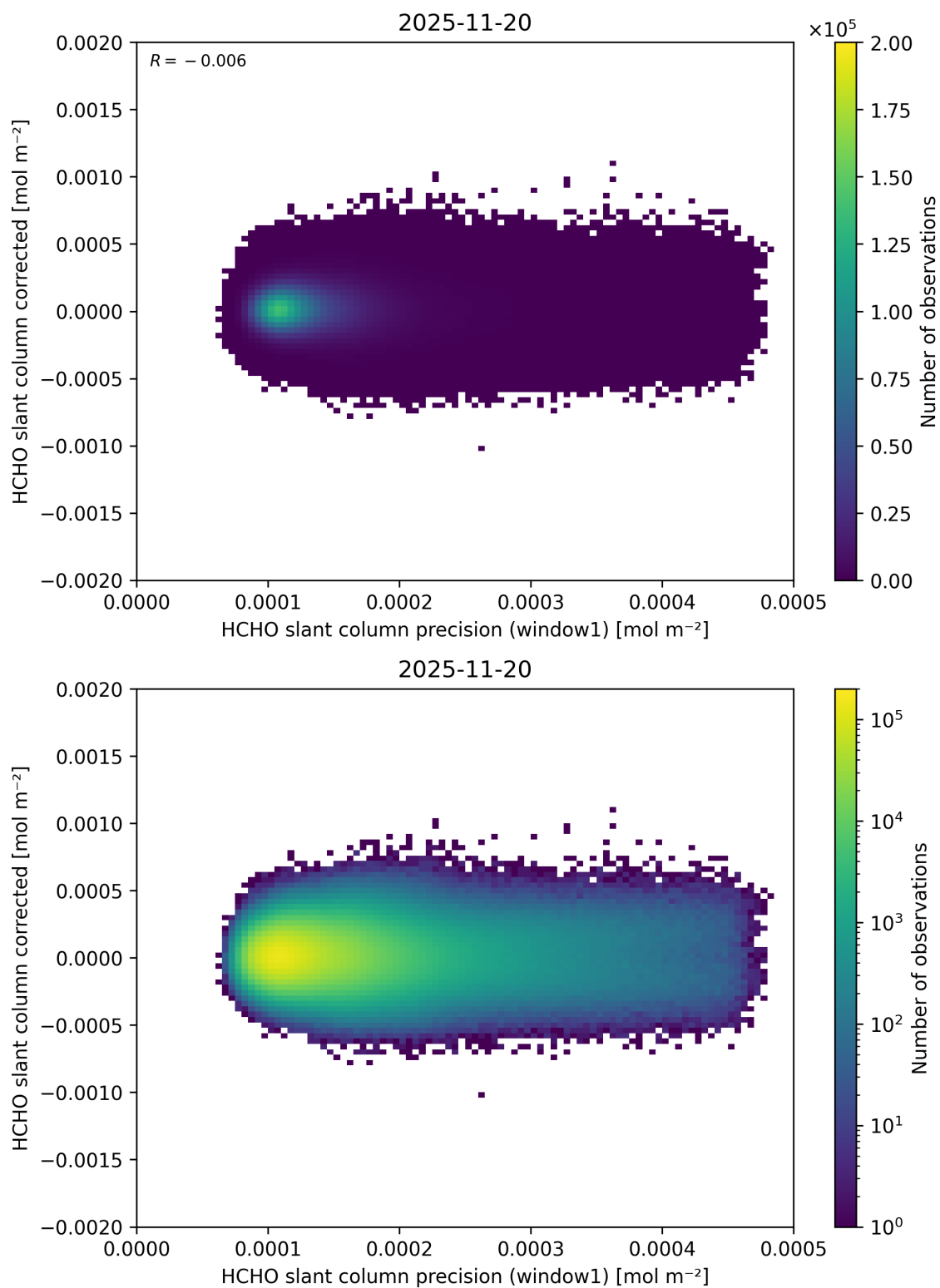
Figure 103: Scatter density plot of “HCHO slant column precision (window1)” against “HCHO slant column corrected” for 2025-11-19 to 2025-11-21.
