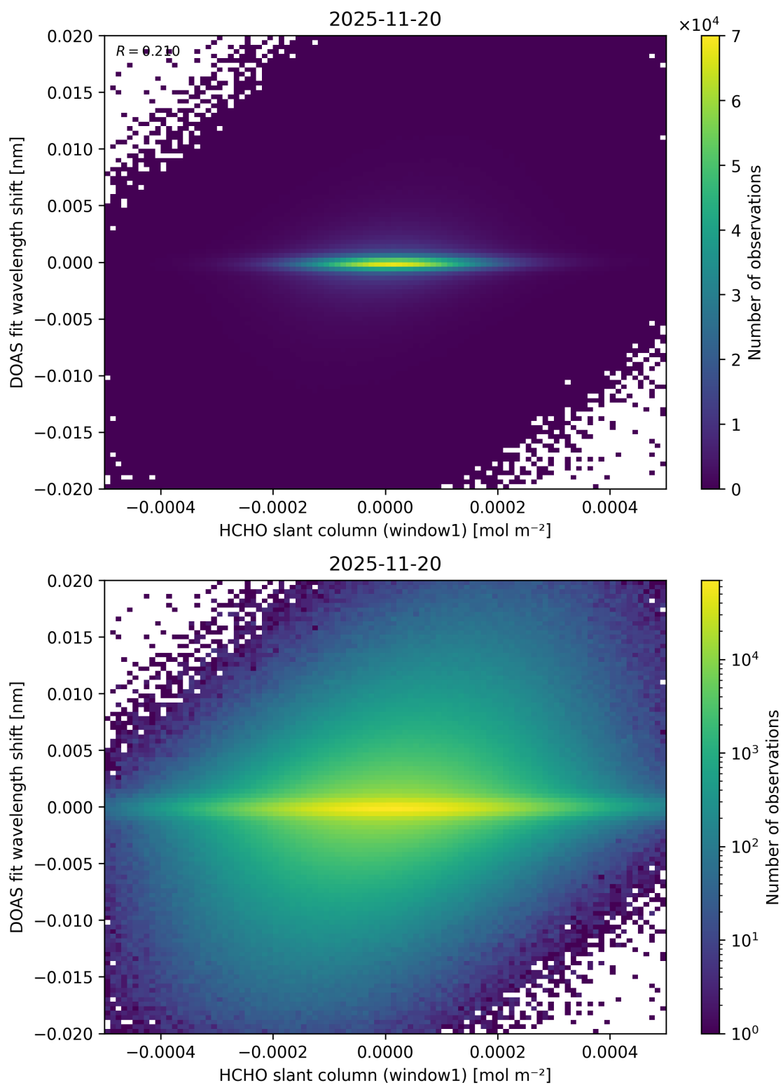
Figure 89: Scatter density plot of “HCHO slant column (window1)” against “DOAS fit wavelength shift” for 2025-11-19 to 2025-11-21.
