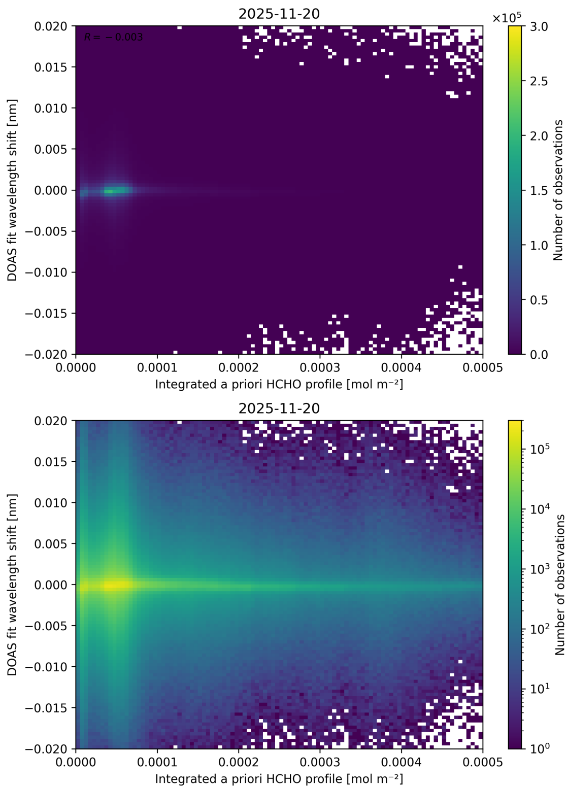
Figure 166: Scatter density plot of “Integrated a priori HCHO profile” against “DOAS fit wavelength shift” for 2025-11-19 to 2025-11-21.
