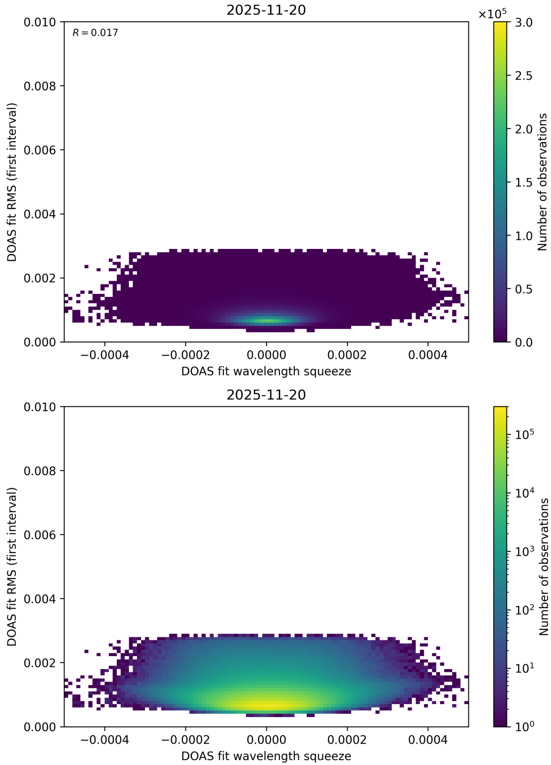
Figure 74: Scatter density plot of “DOAS fit wavelength squeeze” against “DOAS fit RMS (first interval)” for 2025-11-19 to 2025-11-21.
