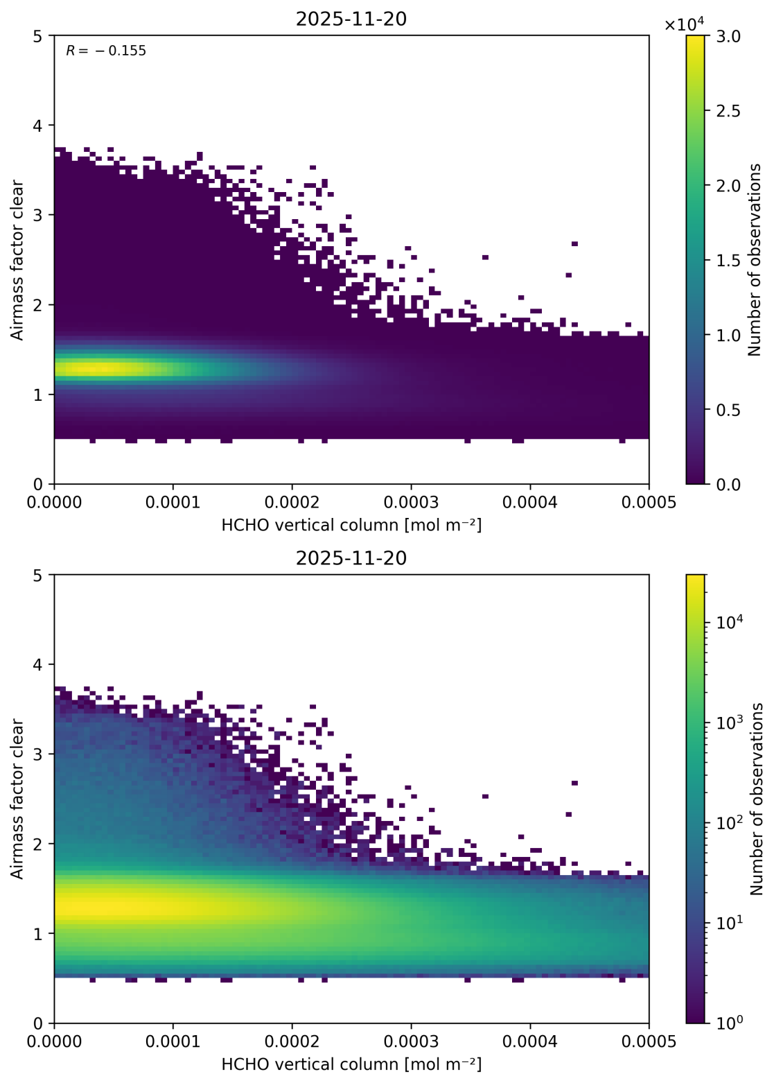
Figure 141: Scatter density plot of “HCHO vertical column” against “Airmass factor clear” for 2025-11-19 to 2025-11-21.
