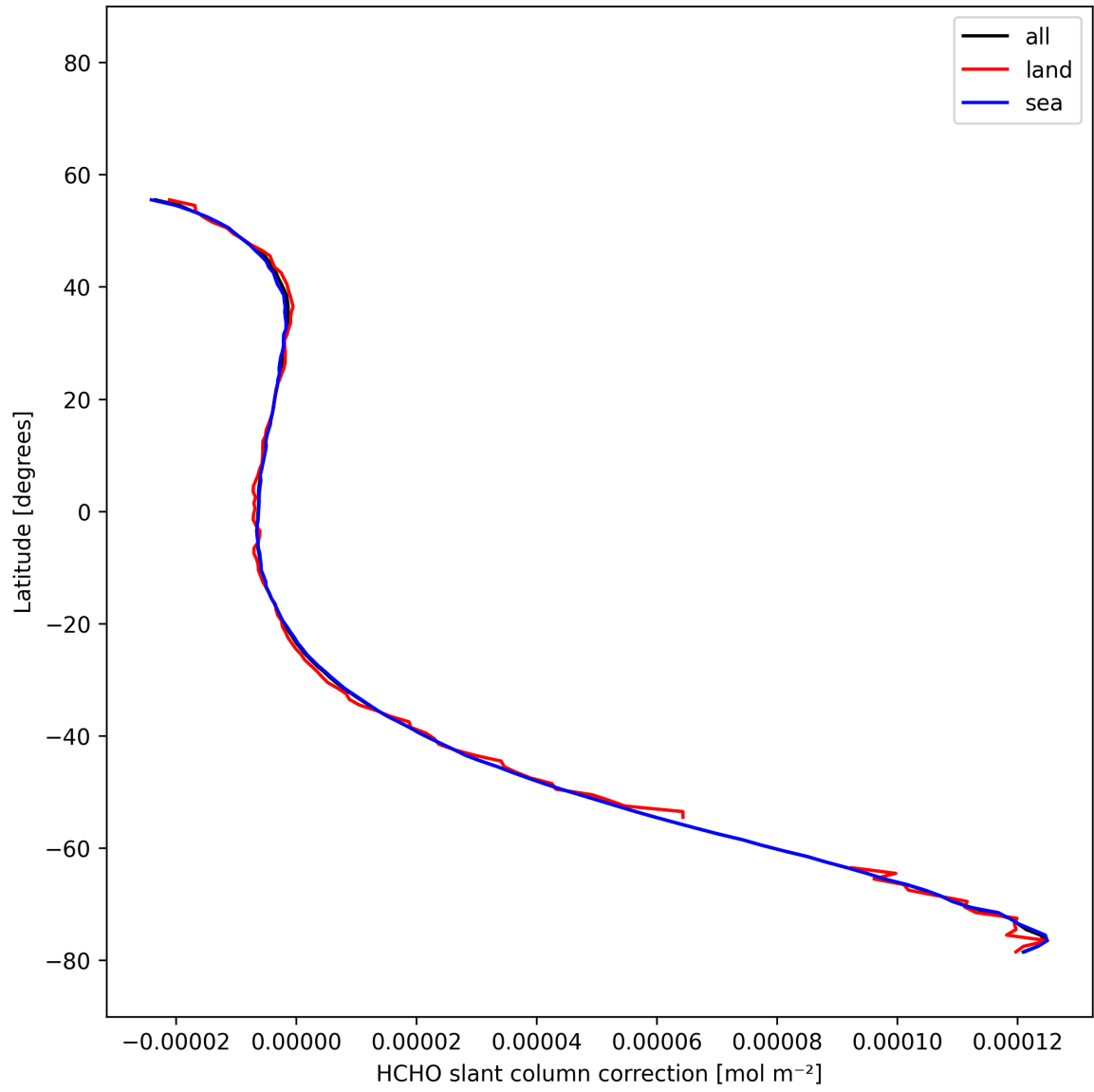
Figure 34: Zonal average of “HCHO slant column correction” for 2025-11-19 to 2025-11-21.
