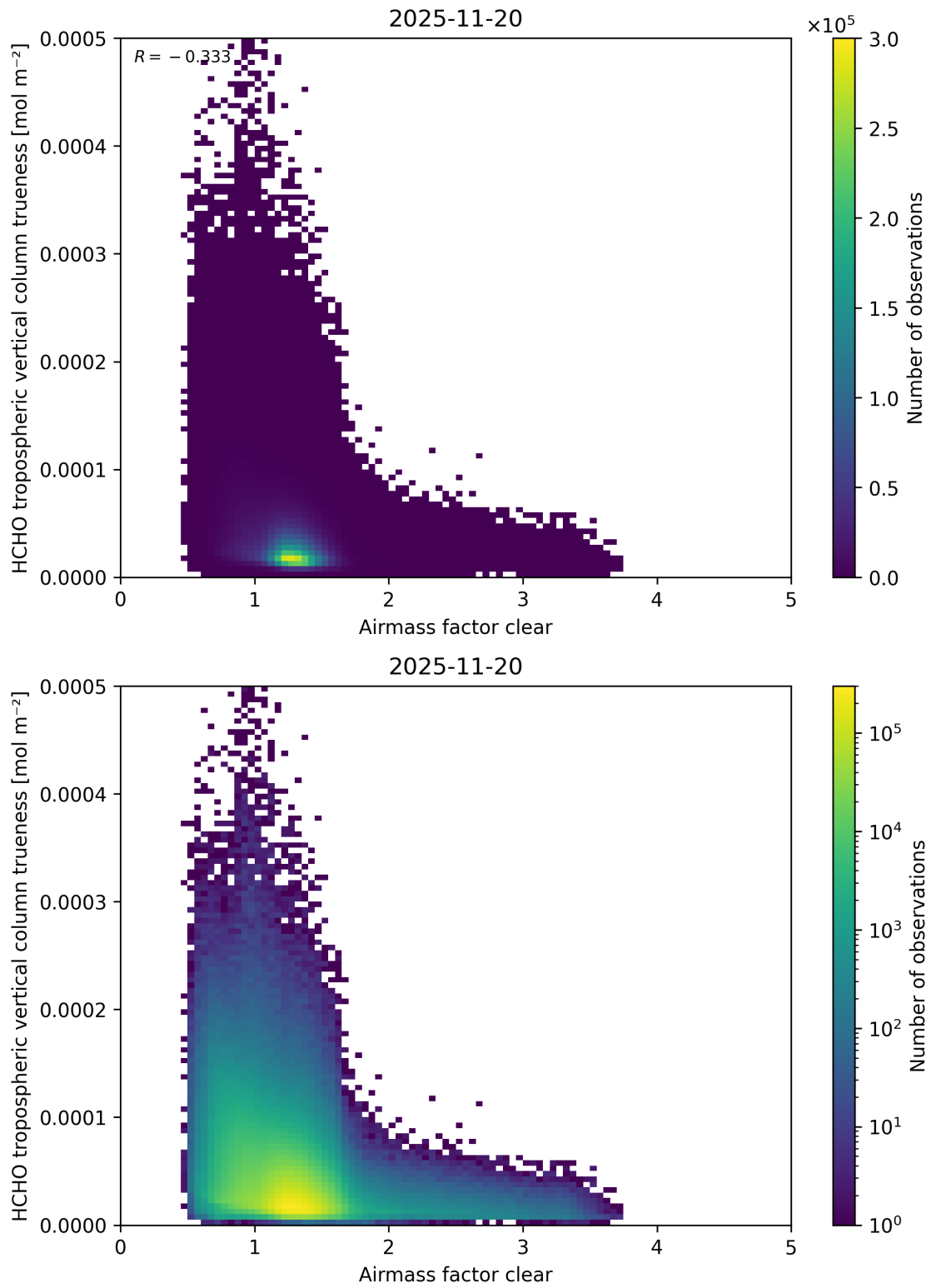
Figure 83: Scatter density plot of “Airmass factor clear” against “HCHO tropospheric vertical column trueness” for 2025-11-19 to 2025-11-21.
