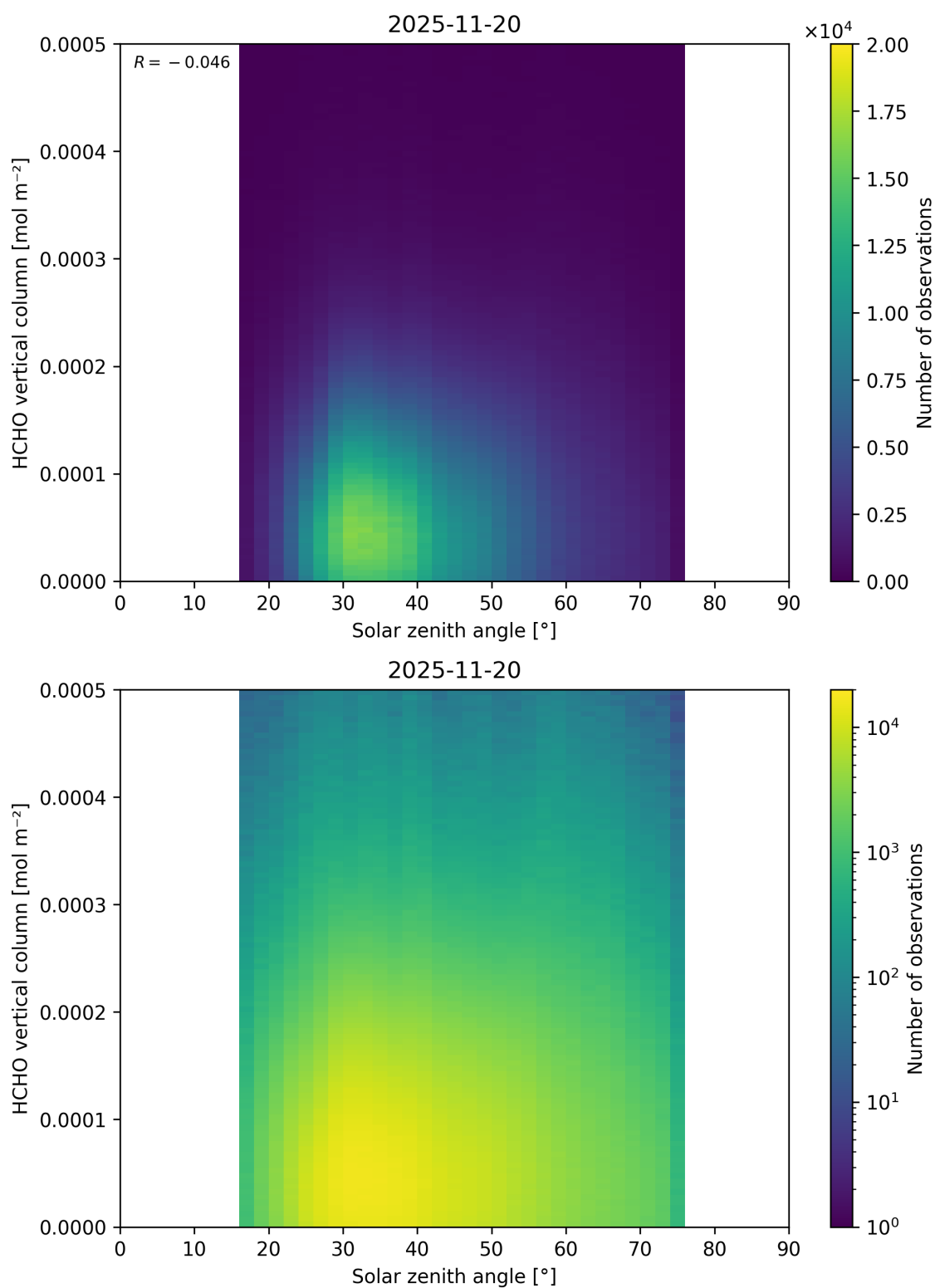
Figure 196: Scatter density plot of “Solar zenith angle” against “HCHO vertical column” for 2025-11-19 to 2025-11-21.
