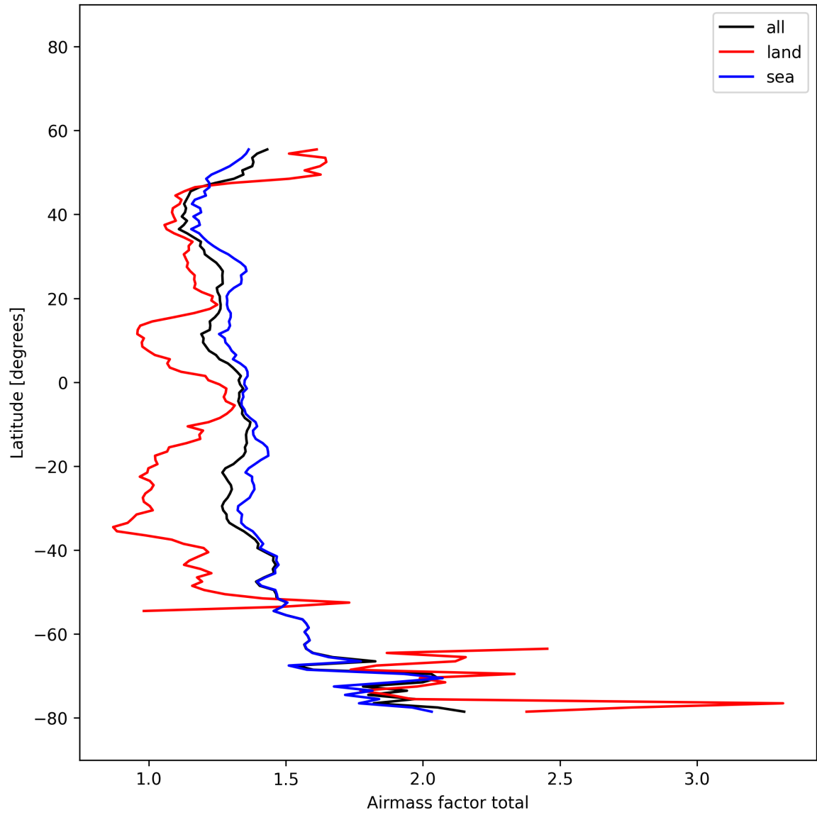
Figure 27: Zonal average of “Airmass factor total” for 2025-11-19 to 2025-11-21.
