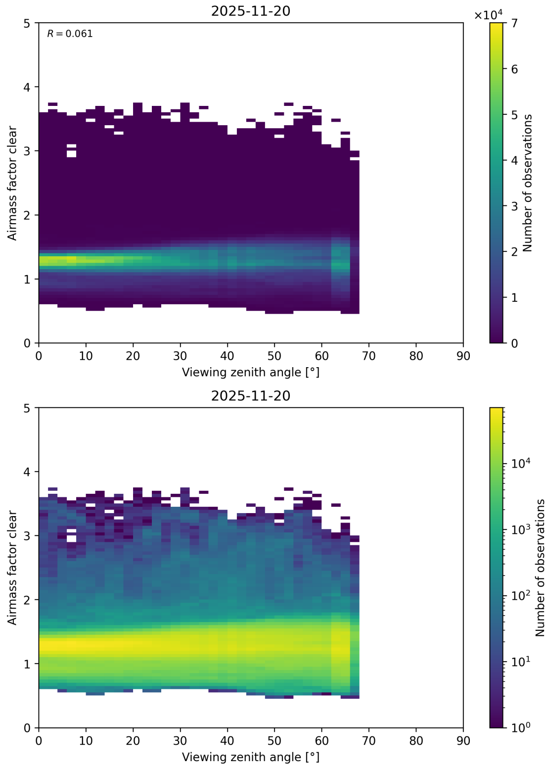
Figure 205: Scatter density plot of “Viewing zenith angle” against “Airmass factor clear” for 2025-11-19 to 2025-11-21.
