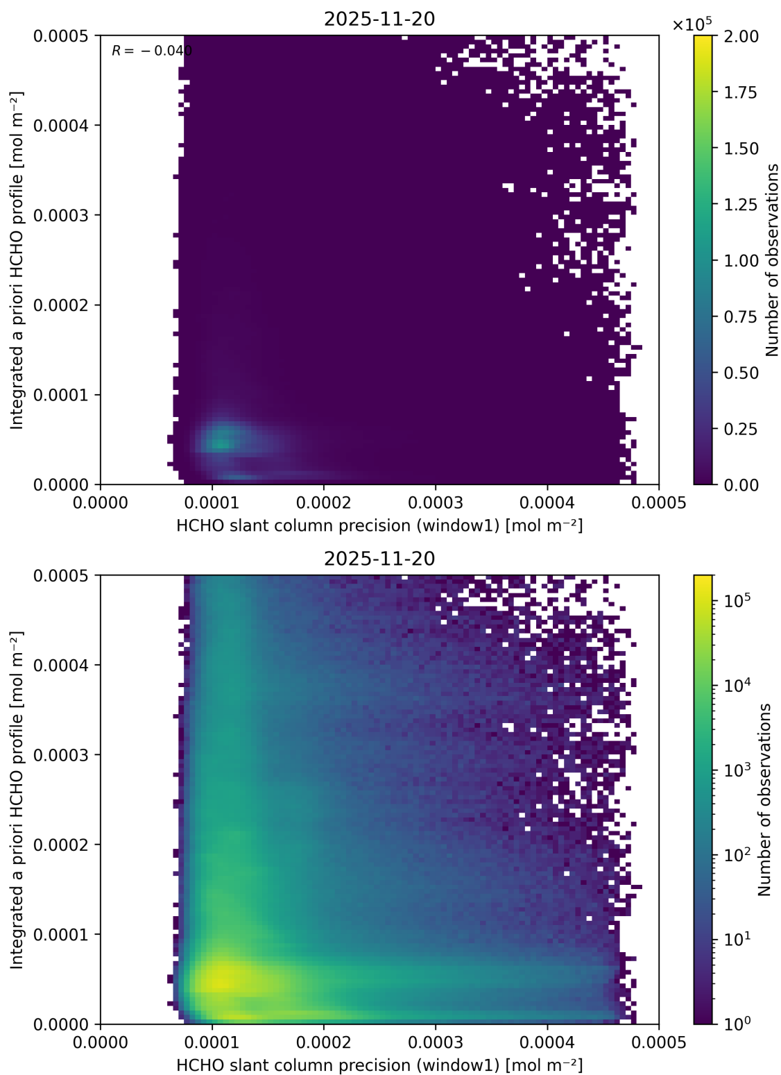
Figure 108: Scatter density plot of “HCHO slant column precision (window1)” against “Integrated a priori HCHO profile” for 2025-11-19 to 2025-11-21.
