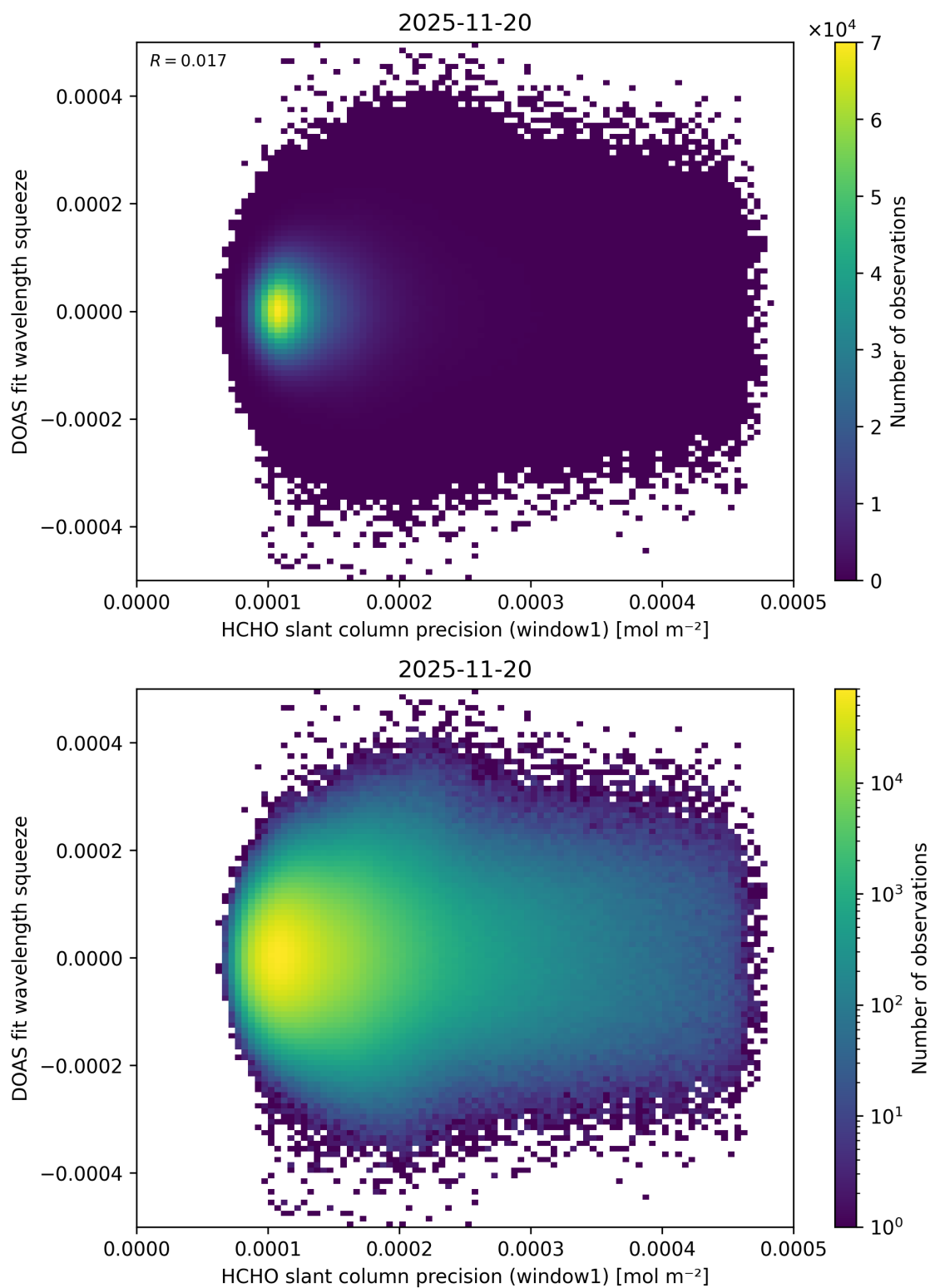
Figure 101: Scatter density plot of “HCHO slant column precision (window1)” against “DOAS fit wavelength squeeze” for 2025-11-19 to 2025-11-21.
