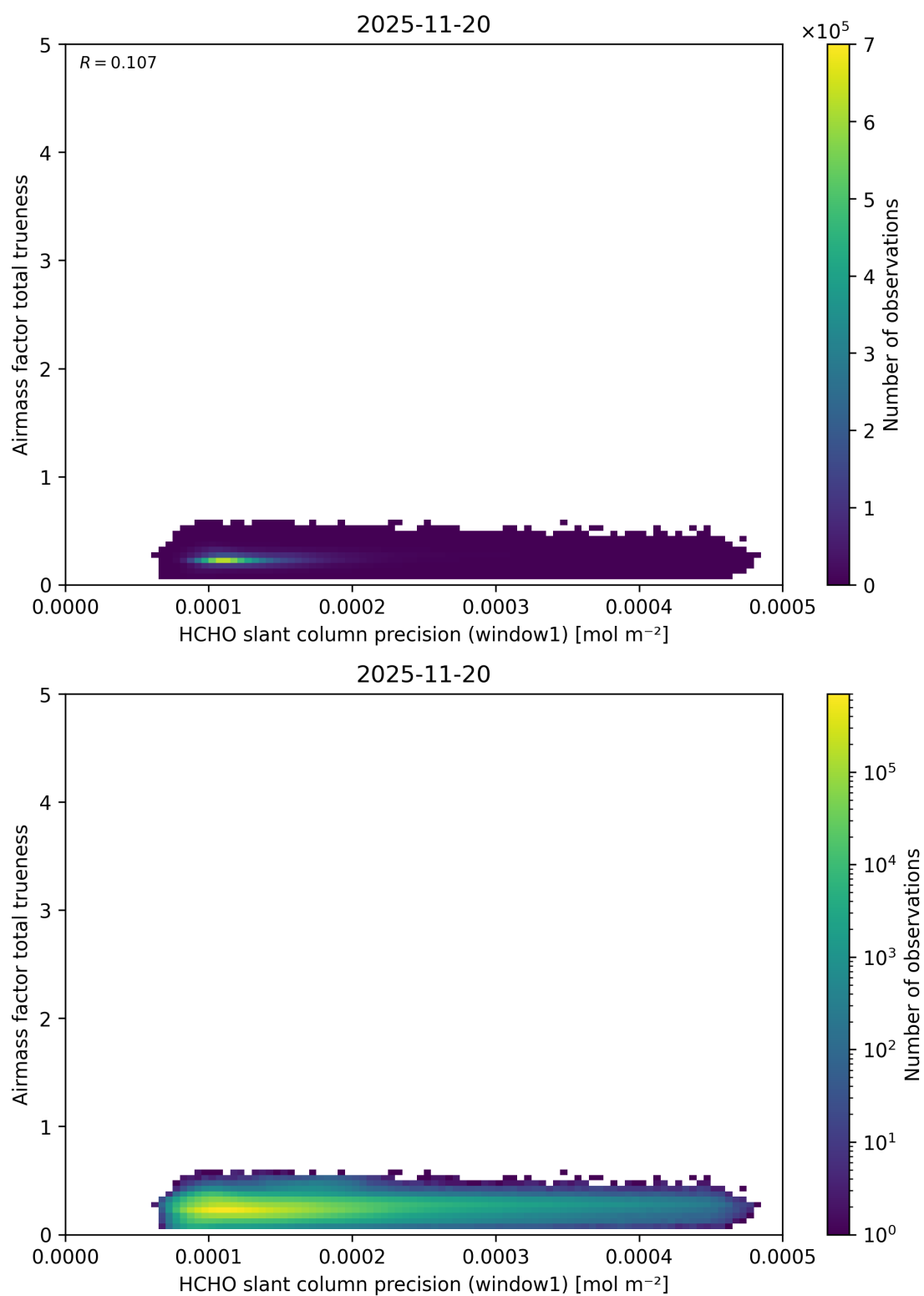
Figure 106: Scatter density plot of “HCHO slant column precision (window1)” against “Airmass factor total trueness” for 2025-11-19 to 2025-11-21.
