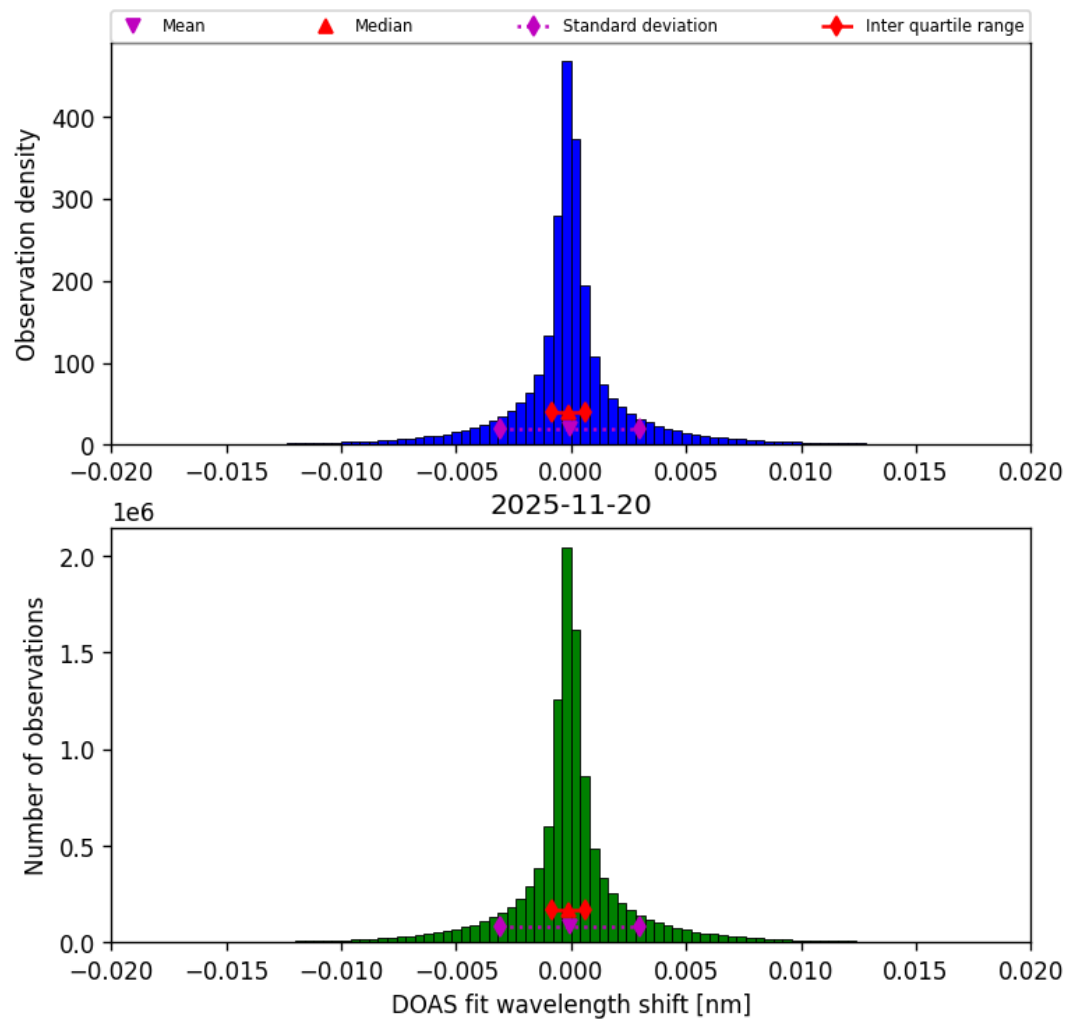
Figure 46: Histogram of “DOAS fit wavelength shift” for 2025-11-19 to 2025-11-21
