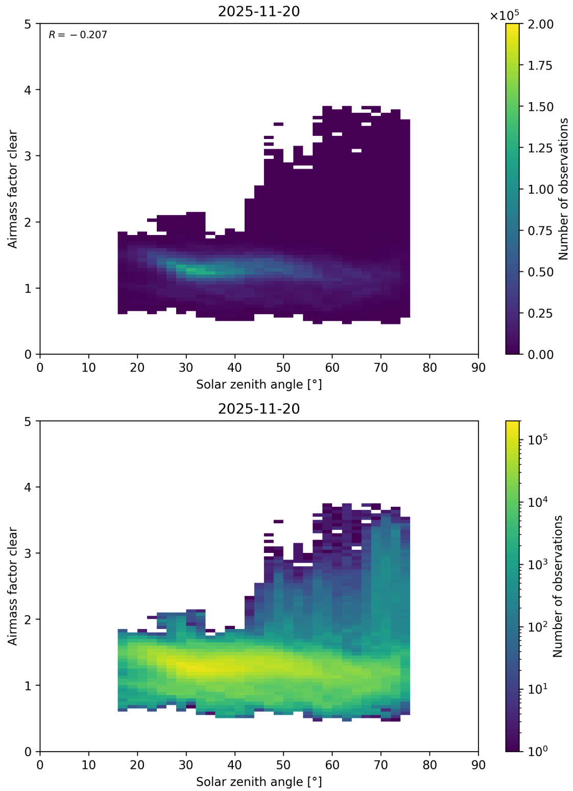
Figure 189: Scatter density plot of “Solar zenith angle” against “Airmass factor clear” for 2025-11-19 to 2025-11-21.
