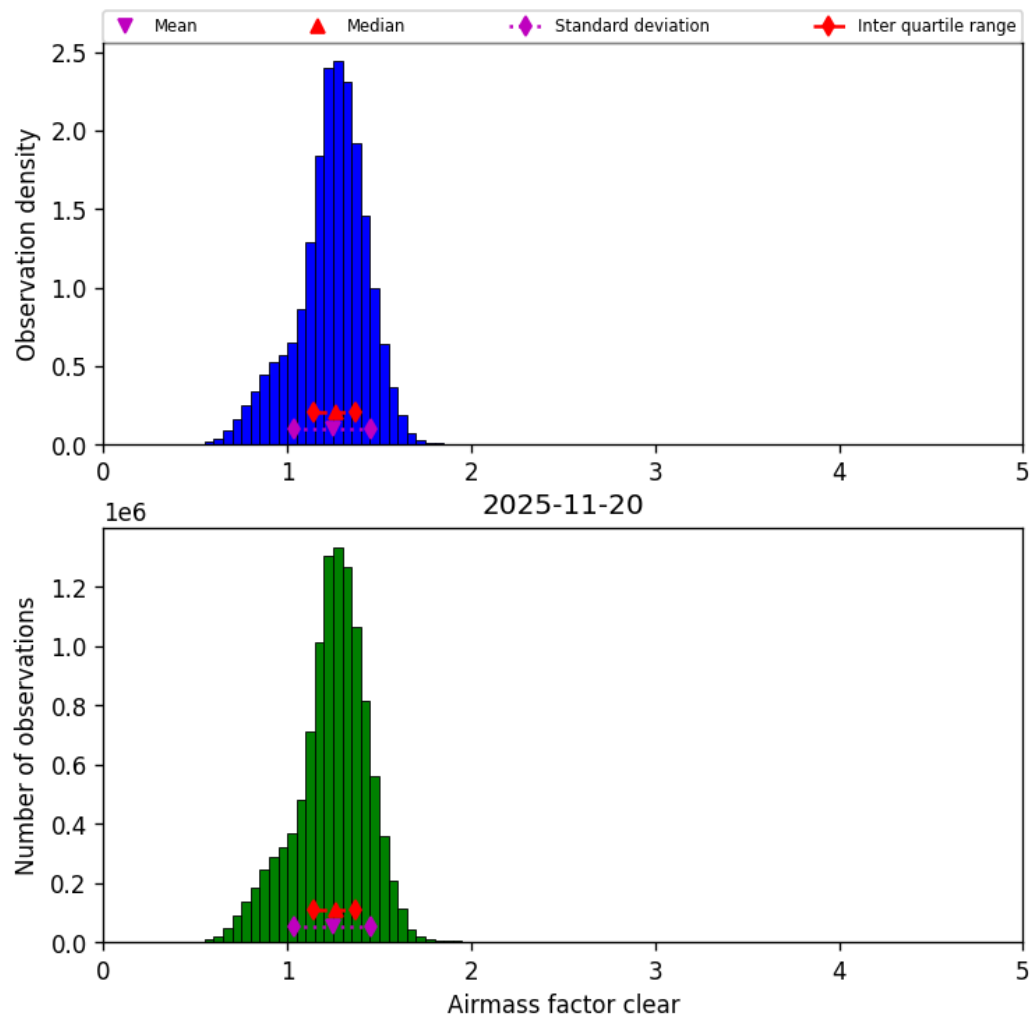
Figure 44: Histogram of “Airmass factor clear” for 2025-11-19 to 2025-11-21
