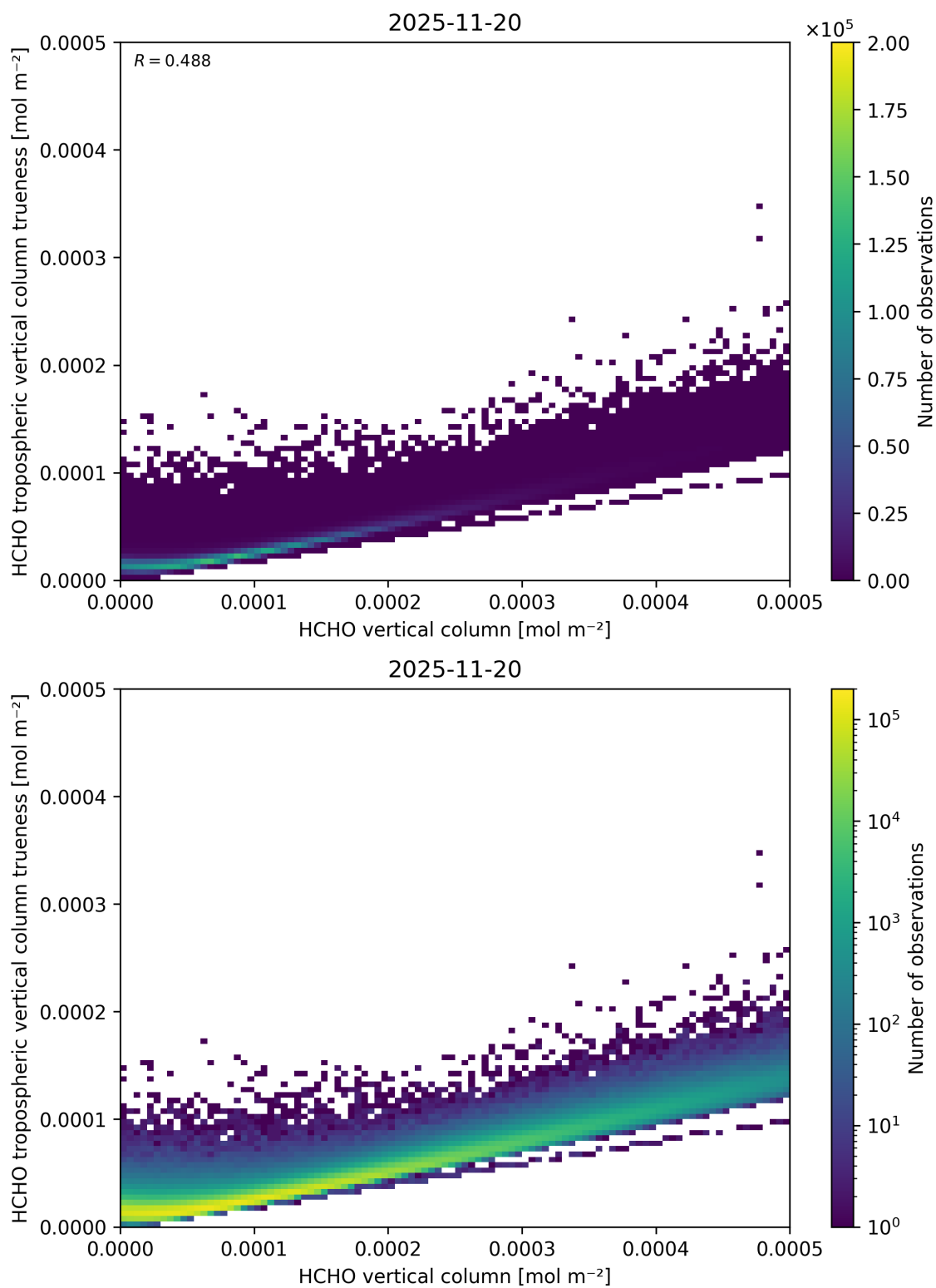
Figure 150: Scatter density plot of “HCHO vertical column” against “HCHO tropospheric vertical column trueness” for 2025-11-19 to 2025-11-21.
