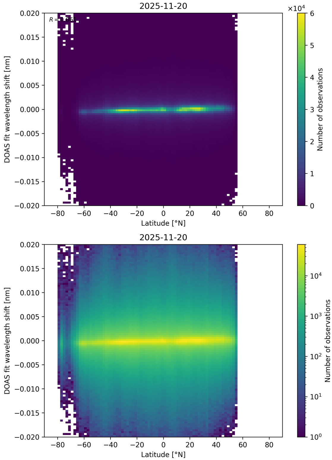
Figure 172: Scatter density plot of “Latitude” against “DOAS fit wavelength shift” for 2025-11-19 to 2025-11-21.
