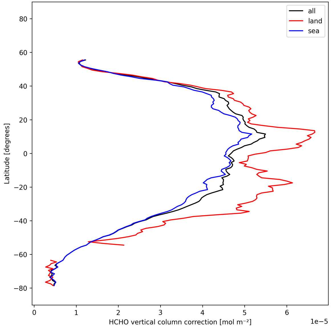
Figure 24: Zonal average of “HCHO vertical column correction” for 2025-11-19 to 2025-11-21.
