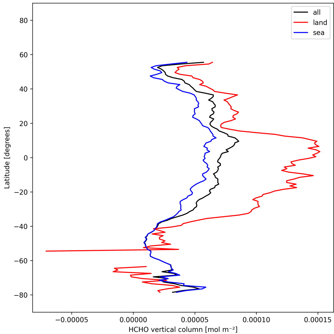
Figure 22: Zonal average of “HCHO vertical column” for 2025-11-19 to 2025-11-21.
