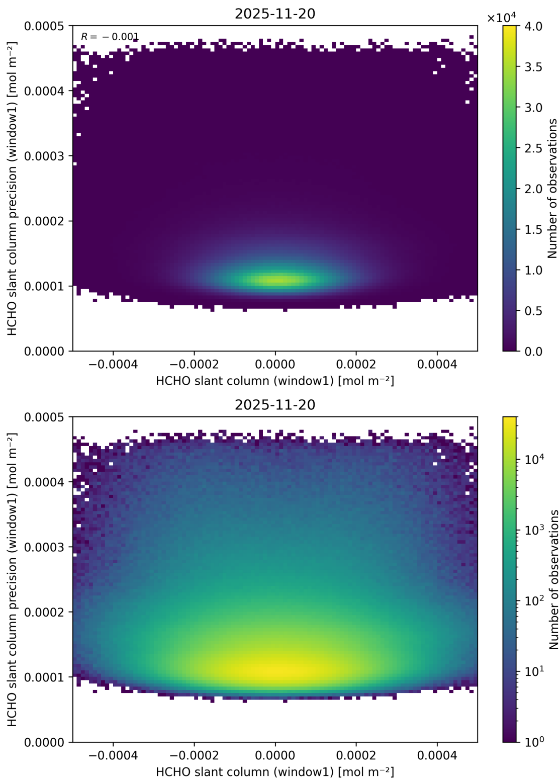
Figure 94: Scatter density plot of “HCHO slant column (window1)” against “HCHO slant column precision (window1)” for 2025-11-19 to 2025-11-21.
