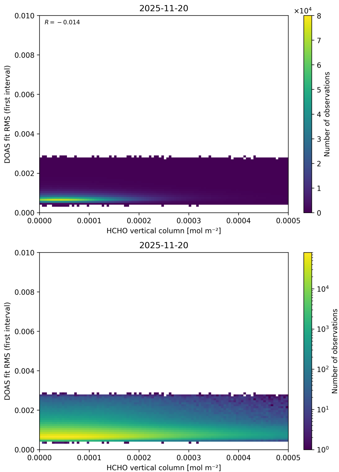
Figure 138: Scatter density plot of “HCHO vertical column” against “DOAS fit RMS (first interval)” for 2025-11-19 to 2025-11-21.
