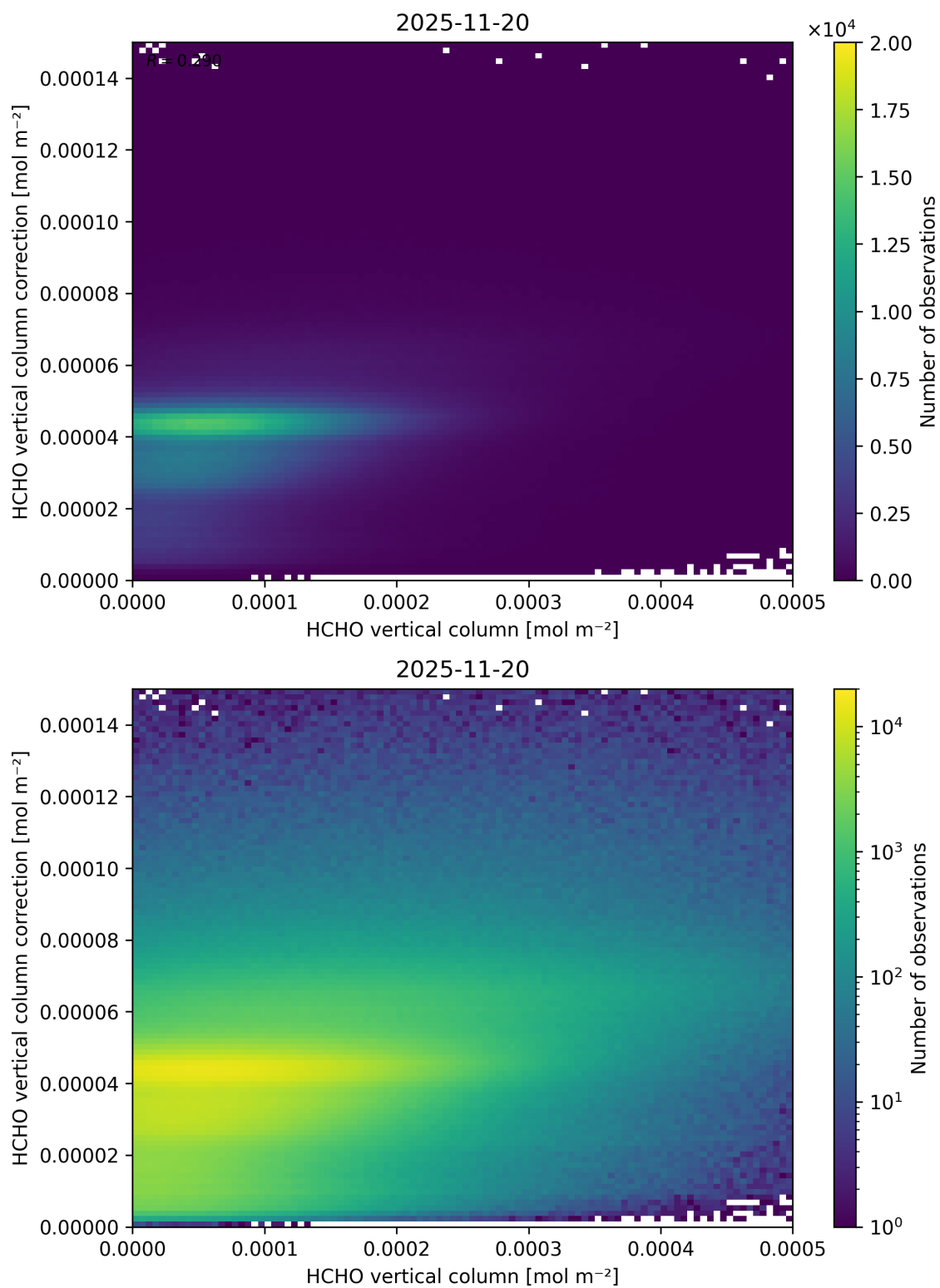
Figure 148: Scatter density plot of “HCHO vertical column” against “HCHO vertical column correction” for 2025-11-19 to 2025-11-21.
