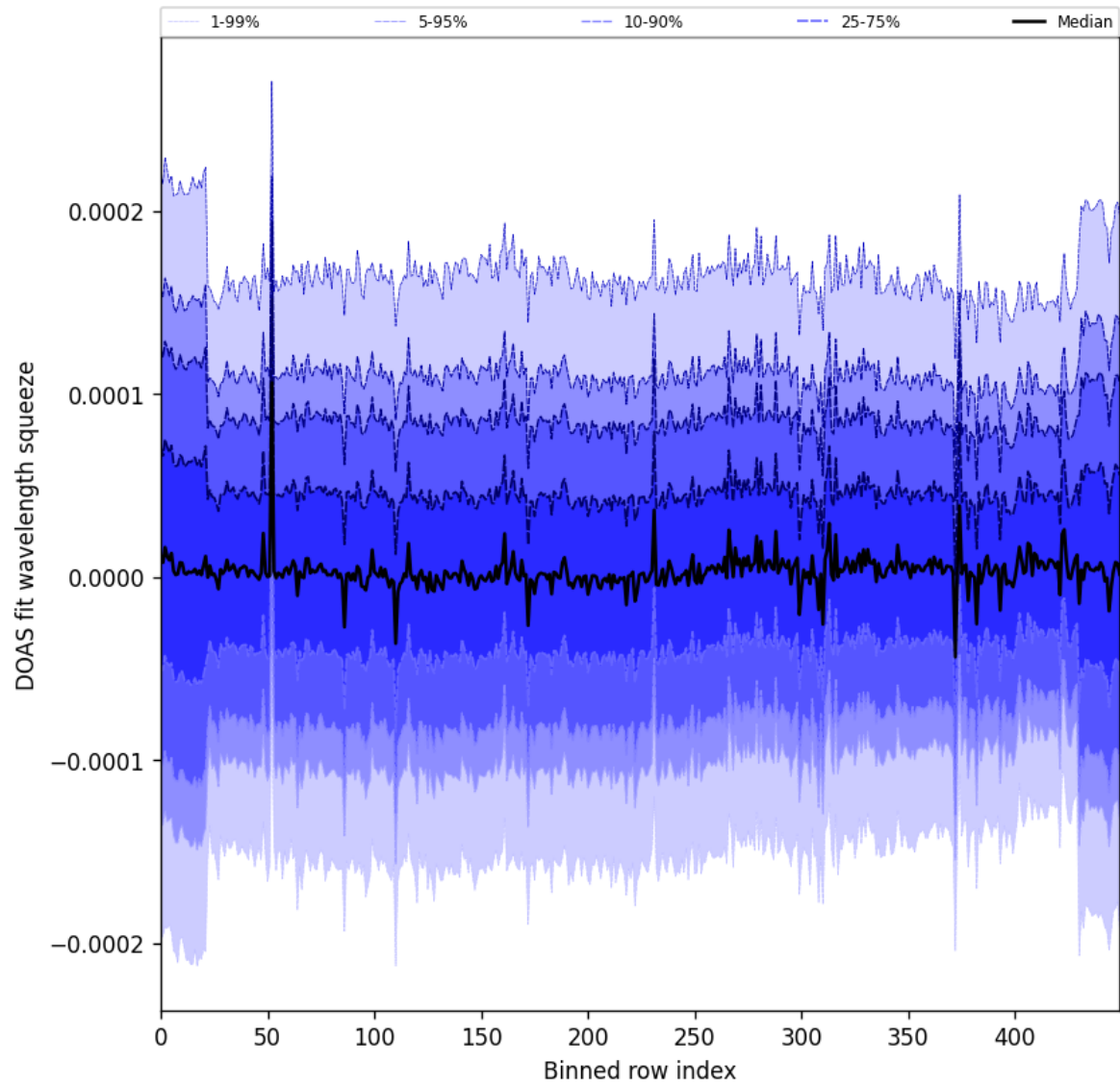
Figure 62: Along track statistics of “DOAS fit wavelength squeeze” for 2025-11-19 to 2025-11-21
