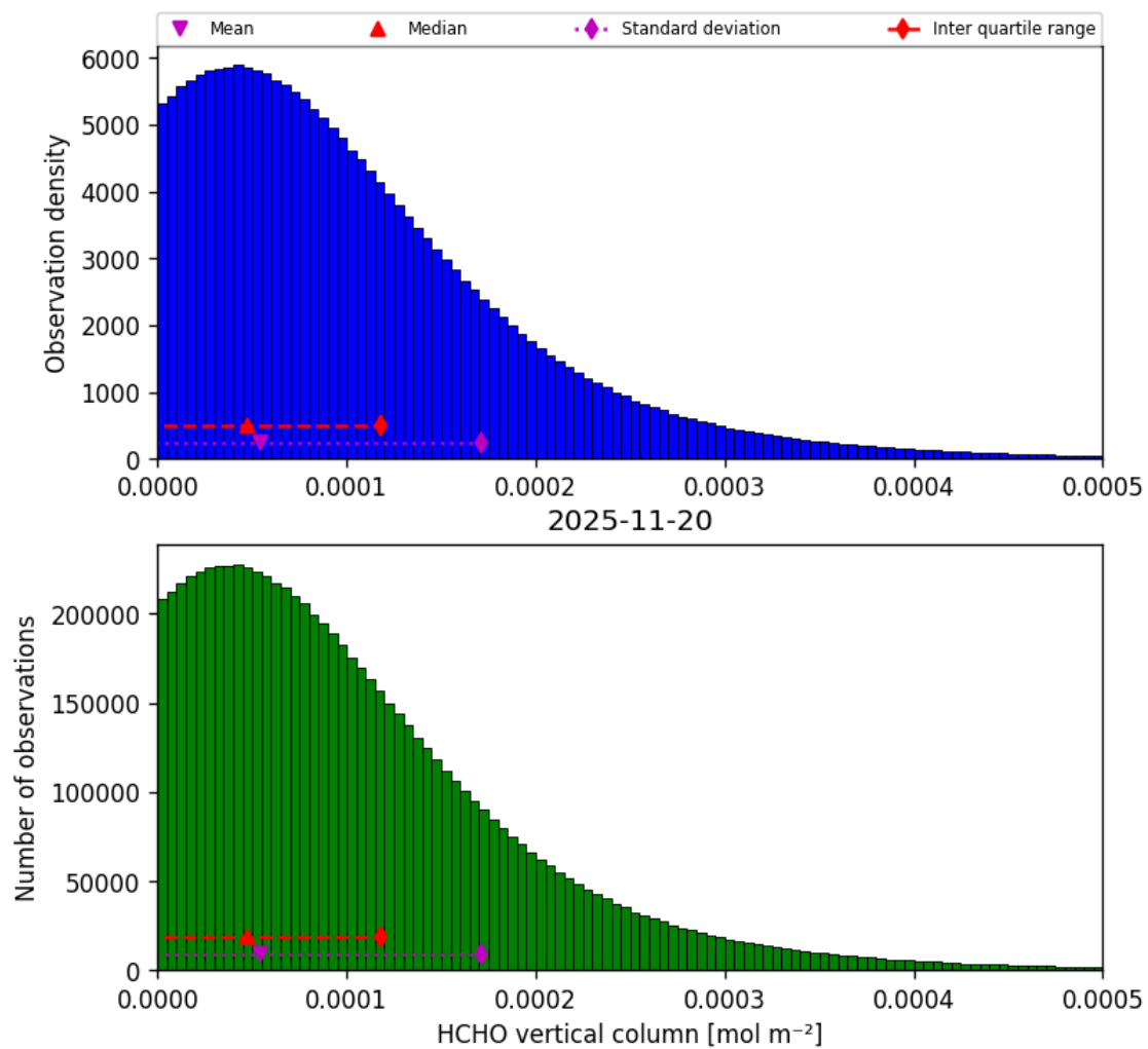
Figure 37: Histogram of “HCHO vertical column” for 2025-11-19 to 2025-11-21
