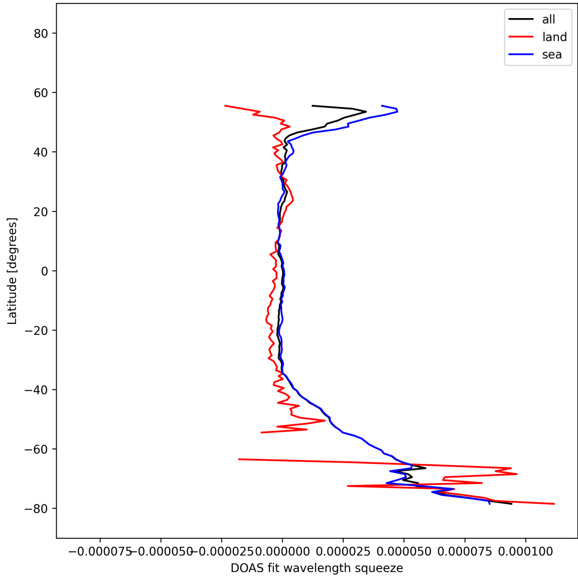
Figure 32: Zonal average of “DOAS fit wavelength squeeze” for 2025-11-19 to 2025-11-21.
