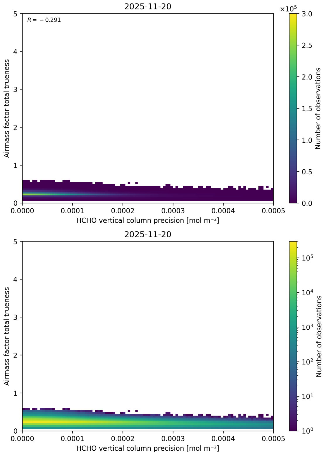
Figure 161: Scatter density plot of “HCHO vertical column precision” against “Airmass factor total trueneess” for 2025-11-19 to 2025-11-21.
