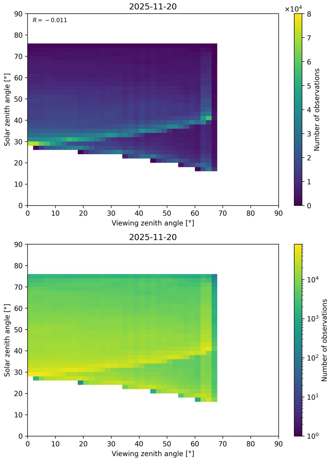
Figure 218: Scatter density plot of “Viewing zenith angle” against “Solar zenith angle” for 2025-11-19 to 2025-11-21.
