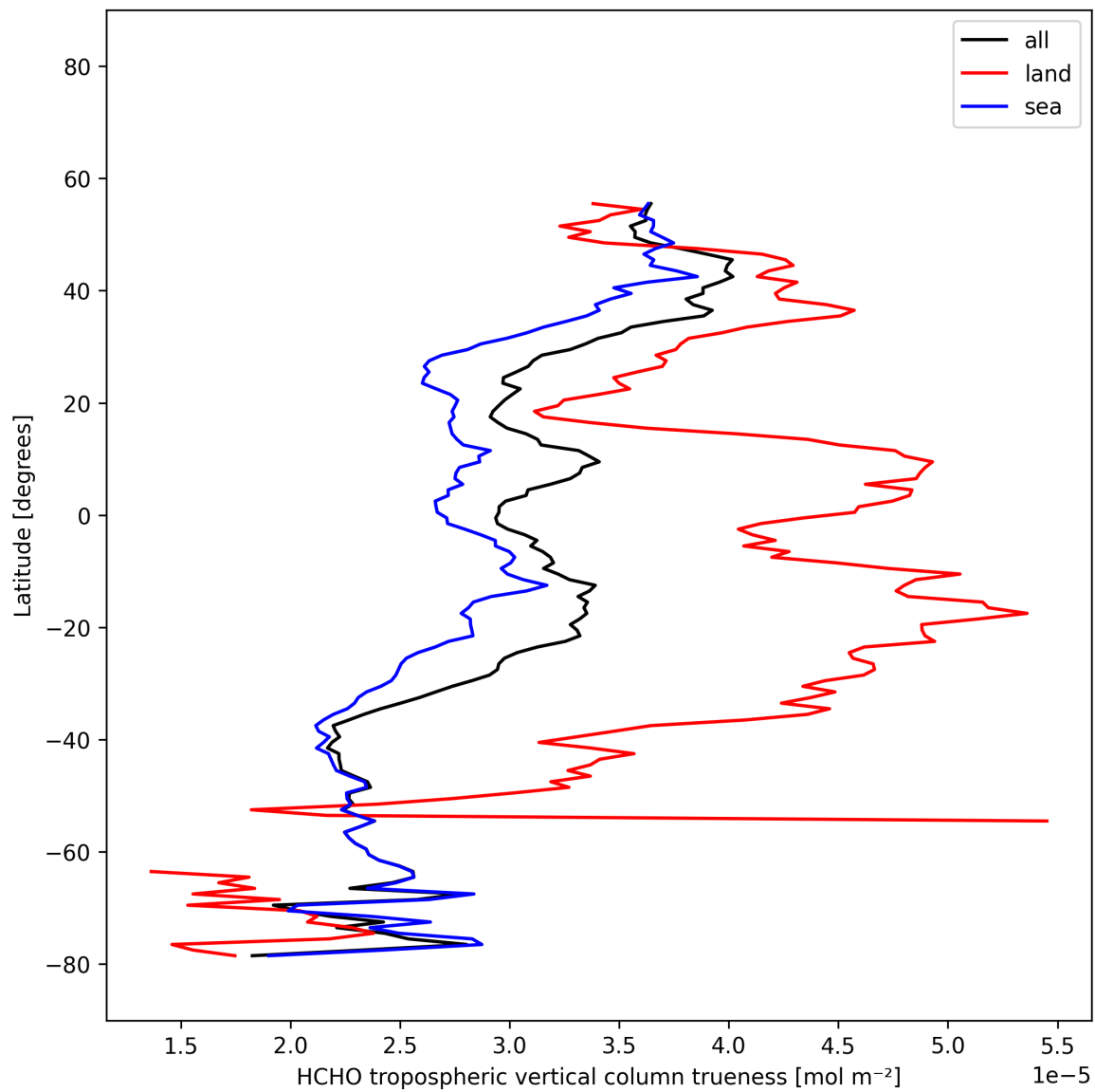
Figure 35: Zonal average of “HCHO tropospheric vertical column trueness” for 2025-11-19 to 2025-11-21.
