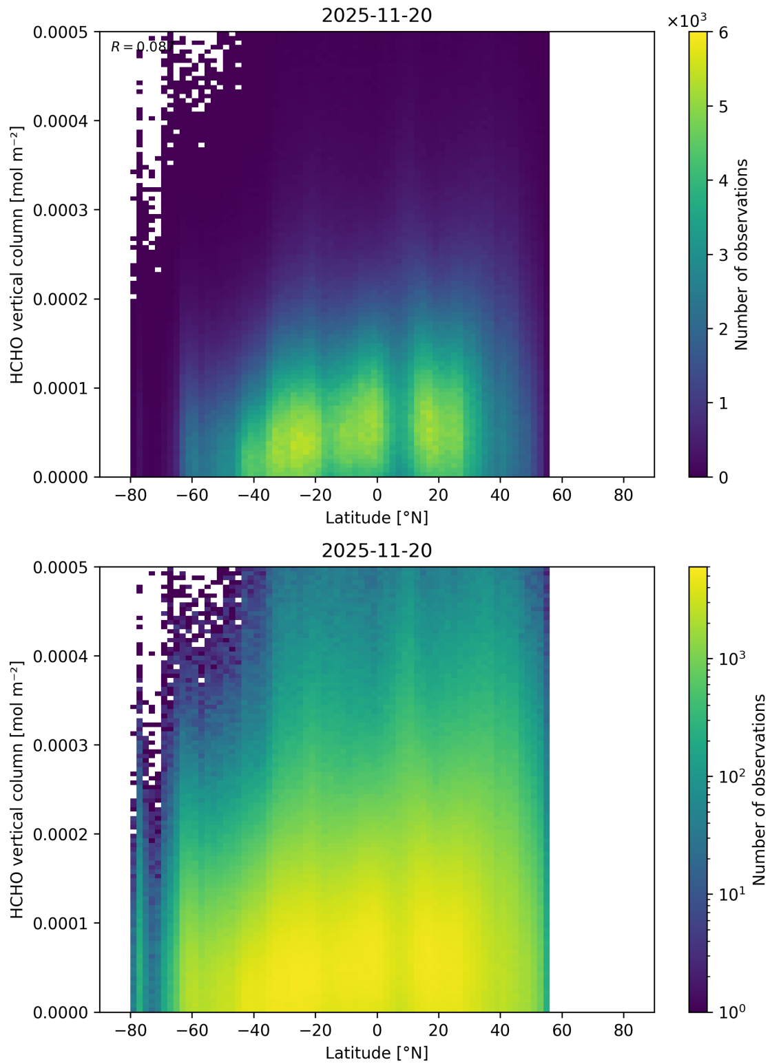
Figure 181: Scatter density plot of “Latitude” against “HCHO vertical column” for 2025-11-19 to 2025-11-21.
