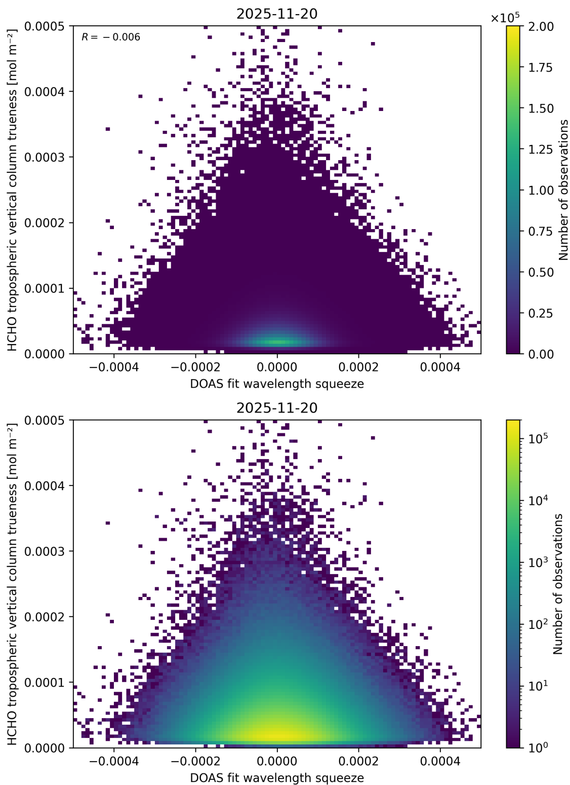
Figure 77: Scatter density plot of “DOAS fit wavelength squeeze” against “HCHO tropospheric vertical column trueness” for 2025-11-19 to 2025-11-21.
