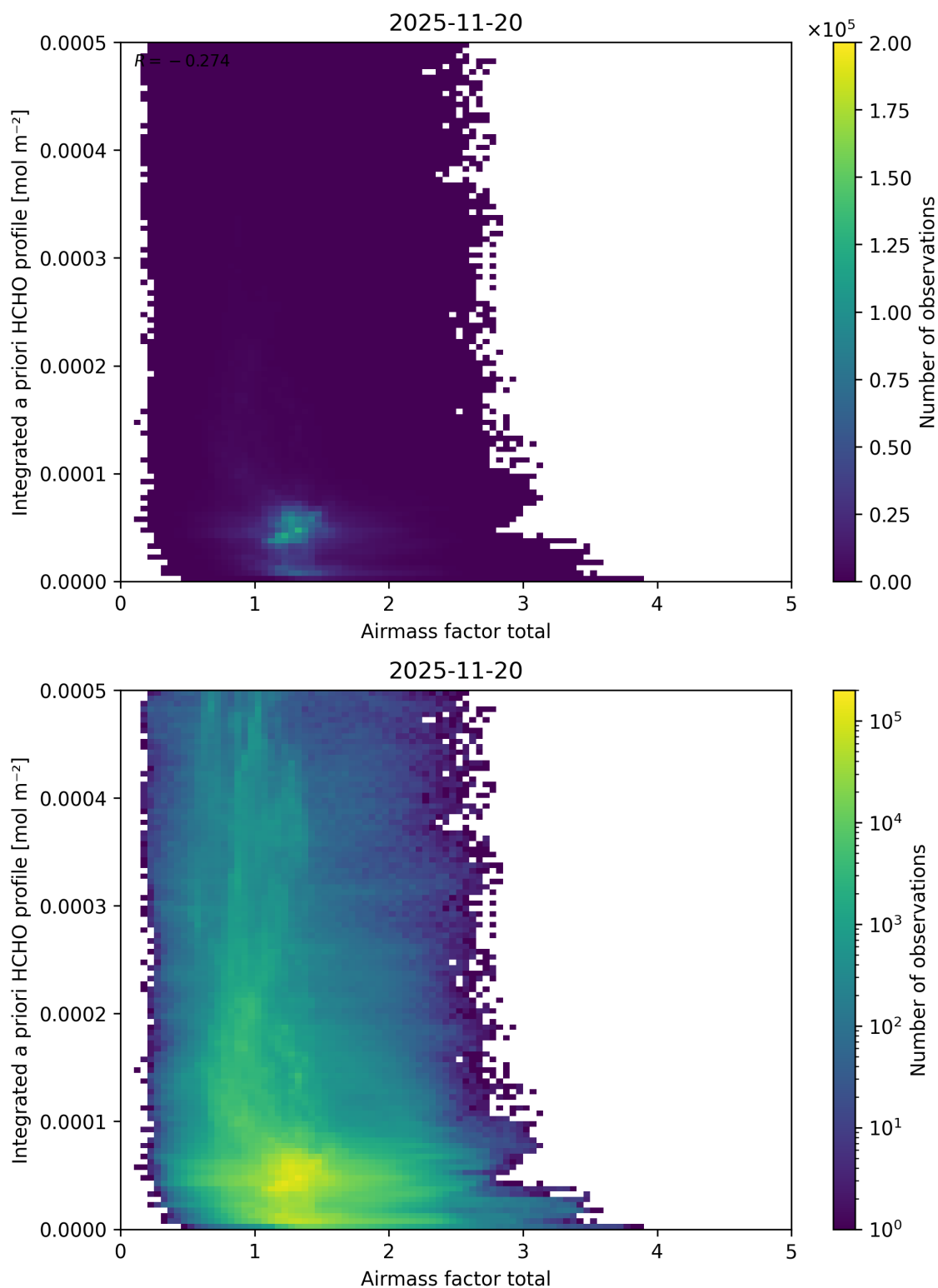
Figure 117: Scatter density plot of “Airmass factor total” against “Integrated a priori HCHO profile” for 2025-11-19 to 2025-11-21.
