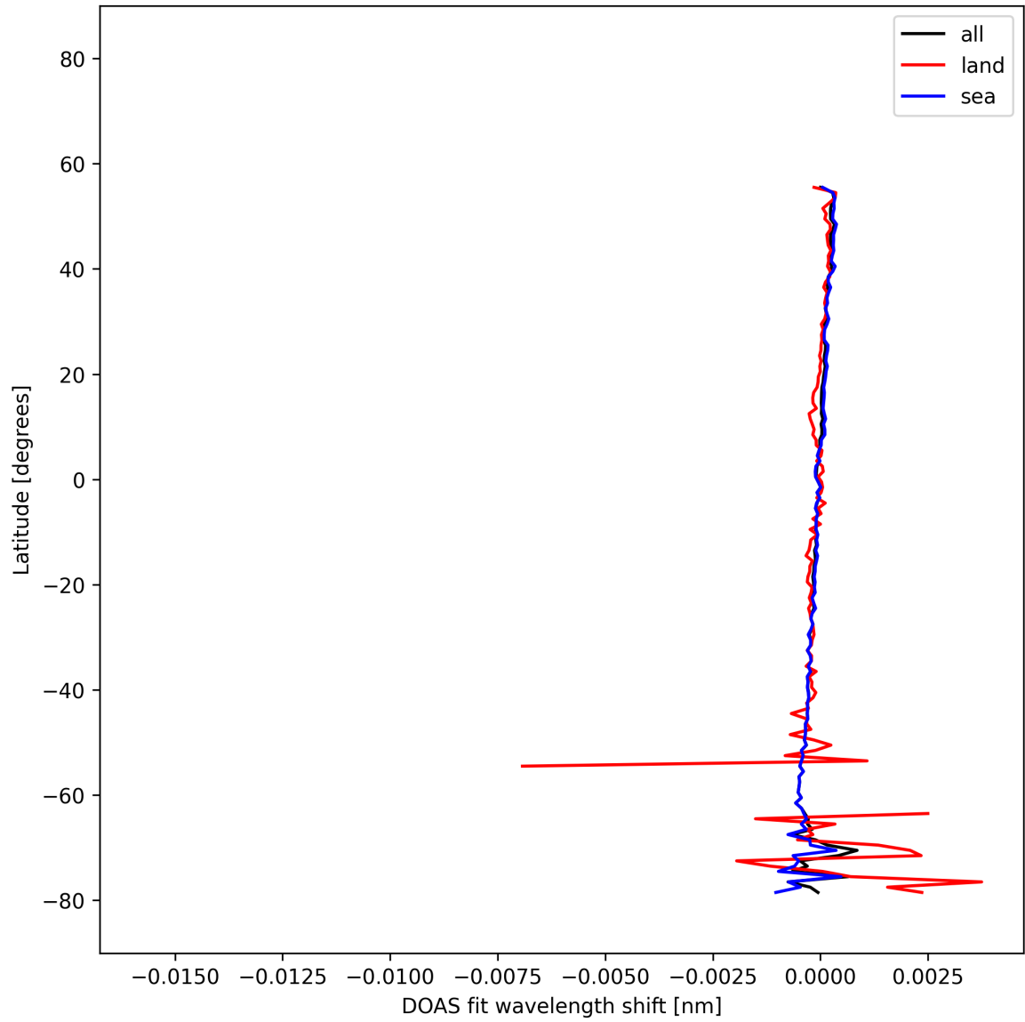
Figure 31: Zonal average of “DOAS fit wavelength shift” for 2025-11-19 to 2025-11-21.
