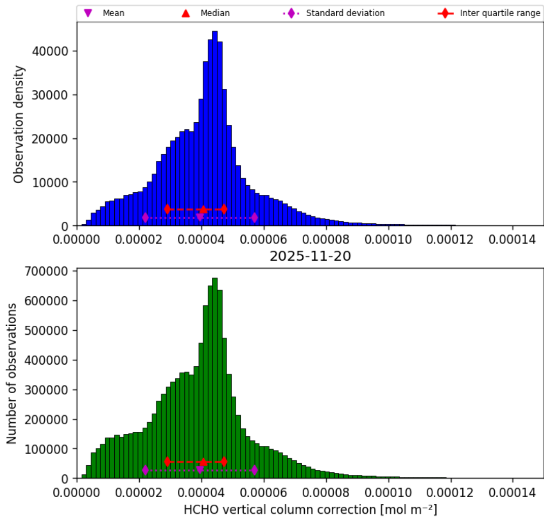
Figure 39: Histogram of “HCHO vertical column correction” for 2025-11-19 to 2025-11-21
