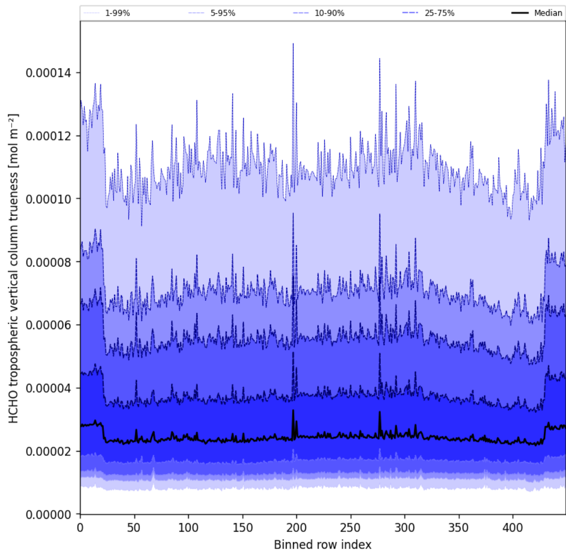
Figure 65: Along track statistics of “HCHO tropospheric vertical column trueness” for 2025-11-19 to 2025-11-21
