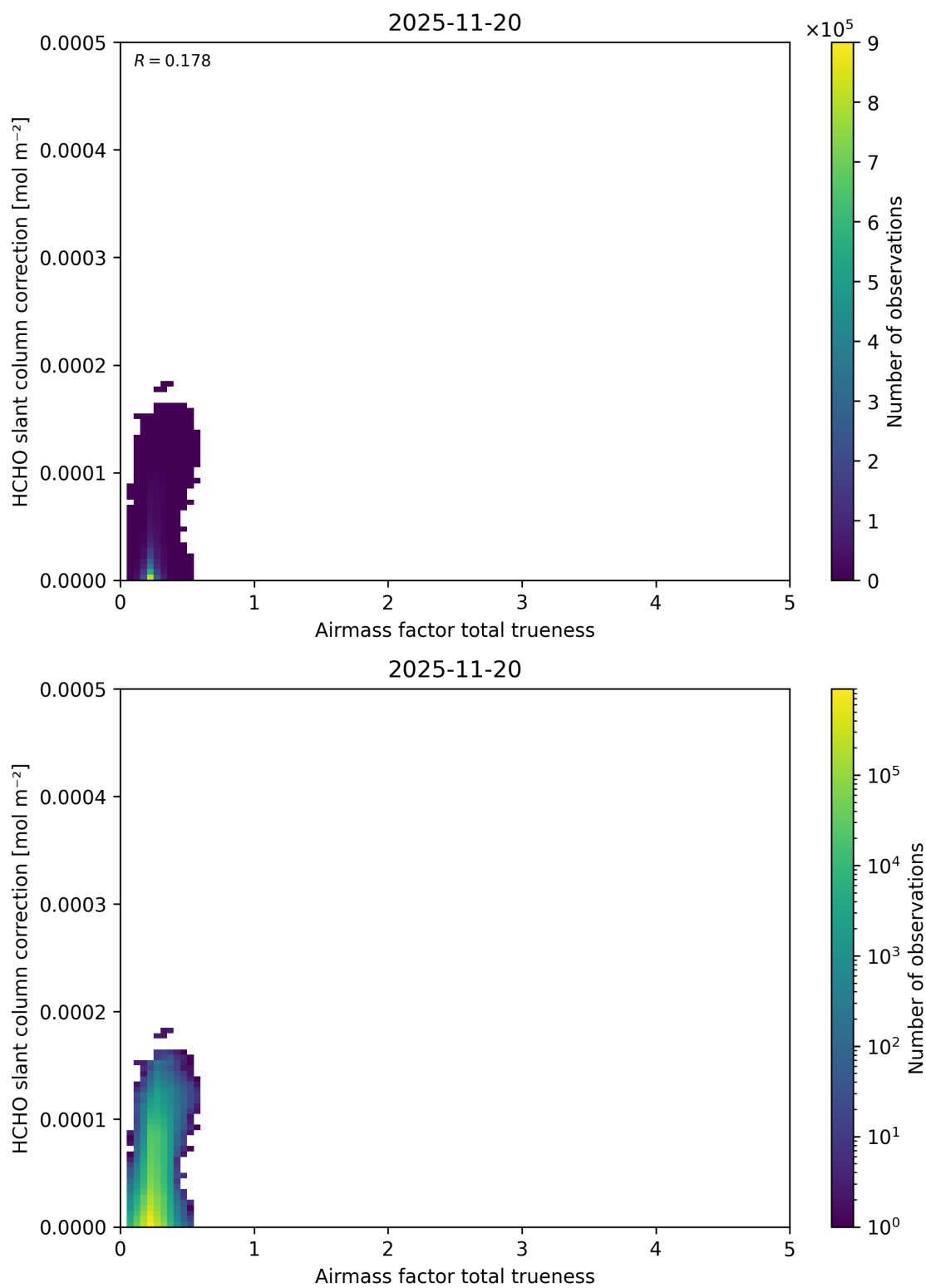
Figure 123: Scatter density plot of “Airmass factor total truiness” against “HCHO slant column correction” for 2025-11-19 to 2025-11-21.
