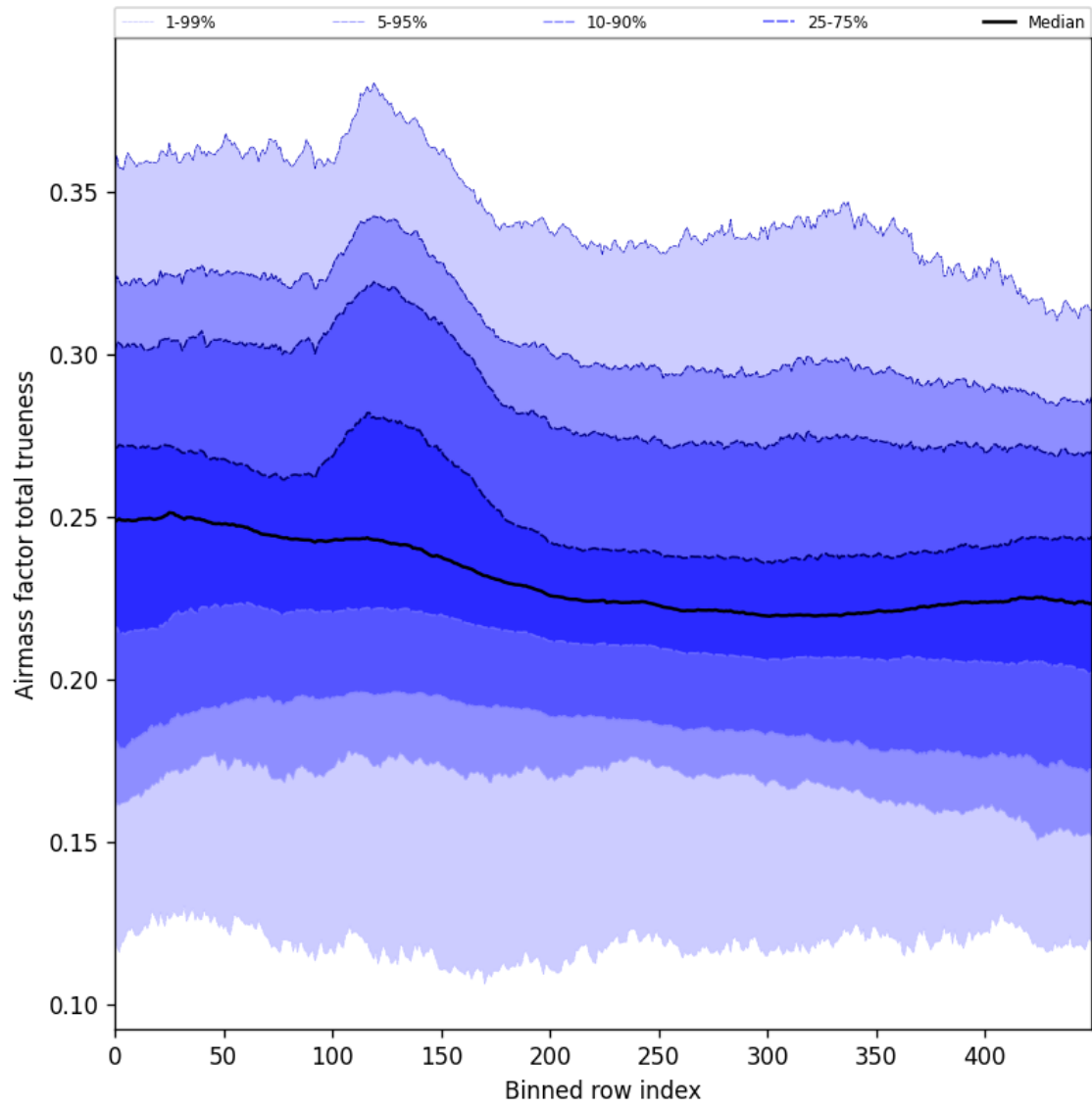
Figure 58: Along track statistics of “Airmass factor total trueness” for 2025-11-19 to 2025-11-21
