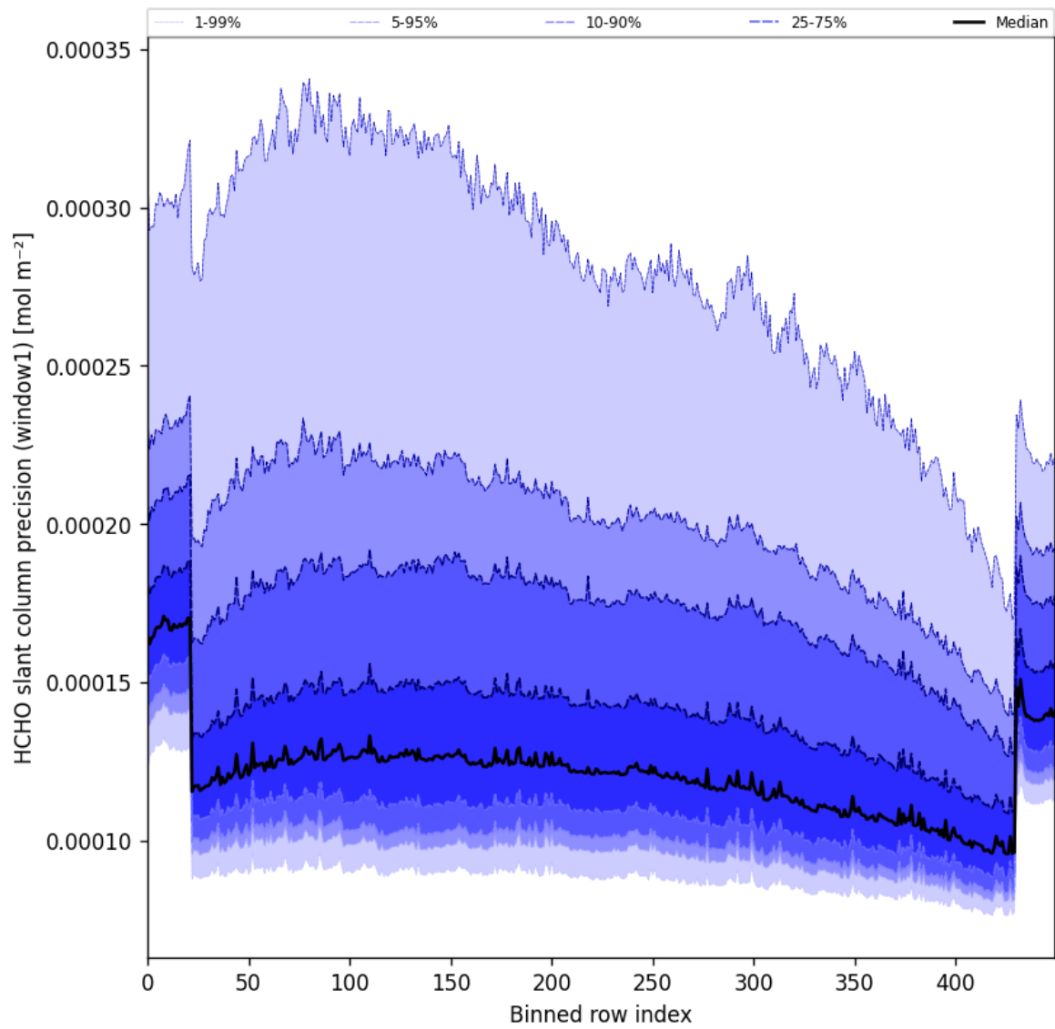
Figure 56: Along track statistics of “HCHO slant column precision (window1)” for 2025-11-19 to 2025-11-21
