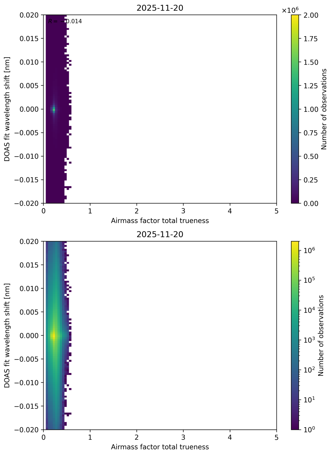
Figure 119: Scatter density plot of “Airmass factor total trueness” against “DOAS fit wavelength shift” for 2025-11-19 to 2025-11-21.
