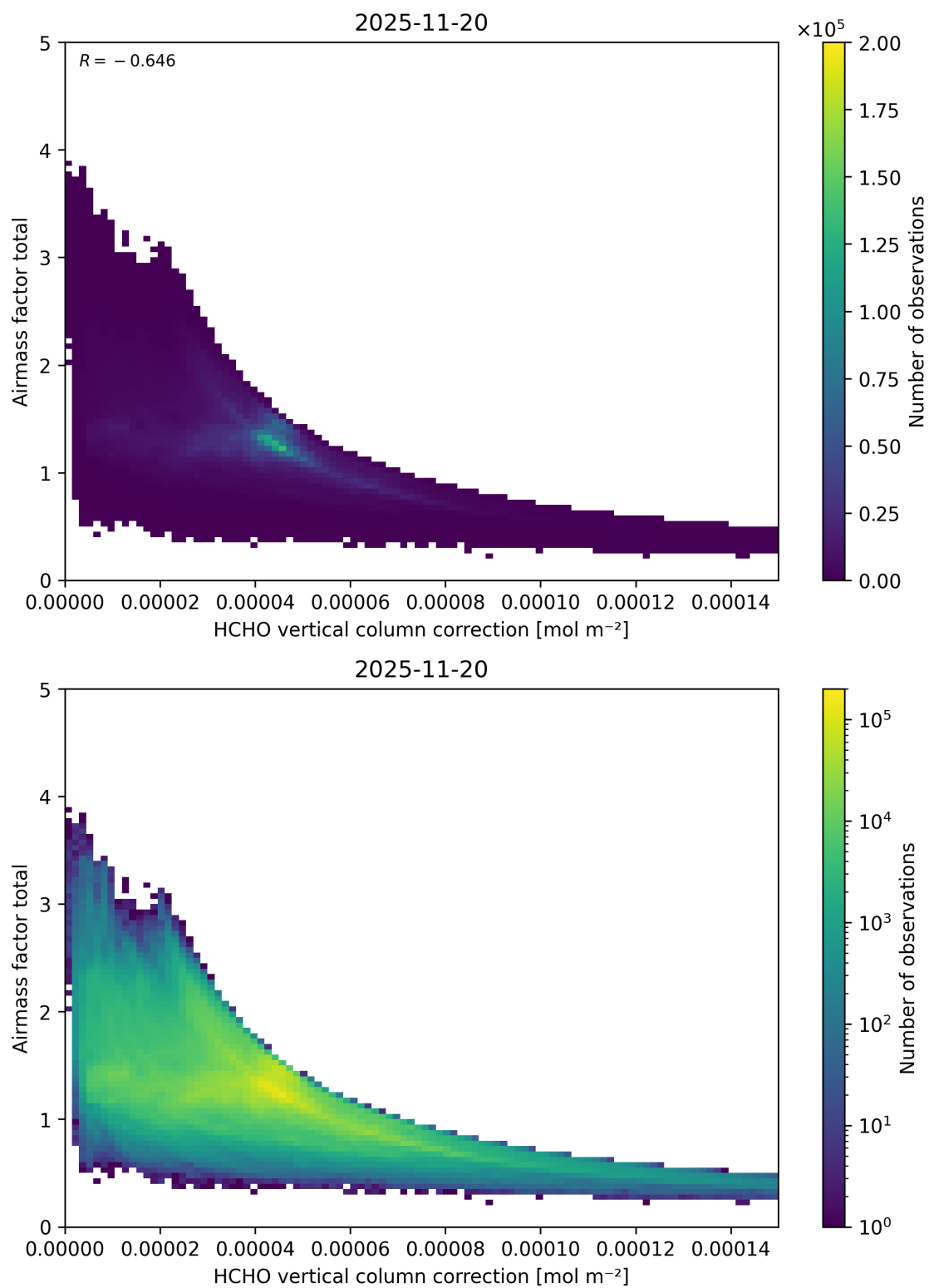
Figure 134: Scatter density plot of “HCHO vertical column correction” against “Airmass factor total” for 2025-11-19 to 2025-11-21.
