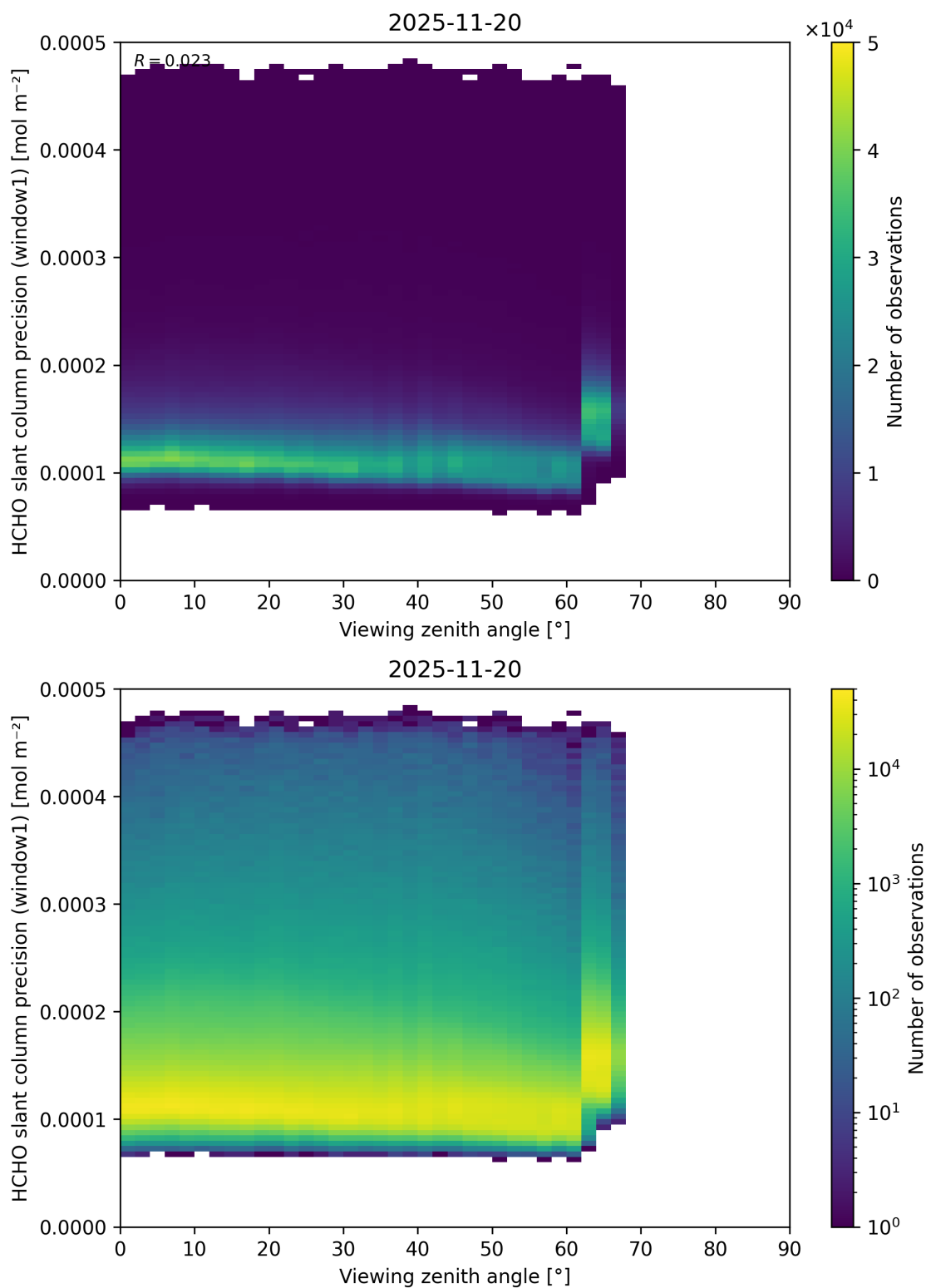
Figure 209: Scatter density plot of “Viewing zenith angle” against “HCHO slant column precision (window1)” for 2025-11-19 to 2025-11-21.
