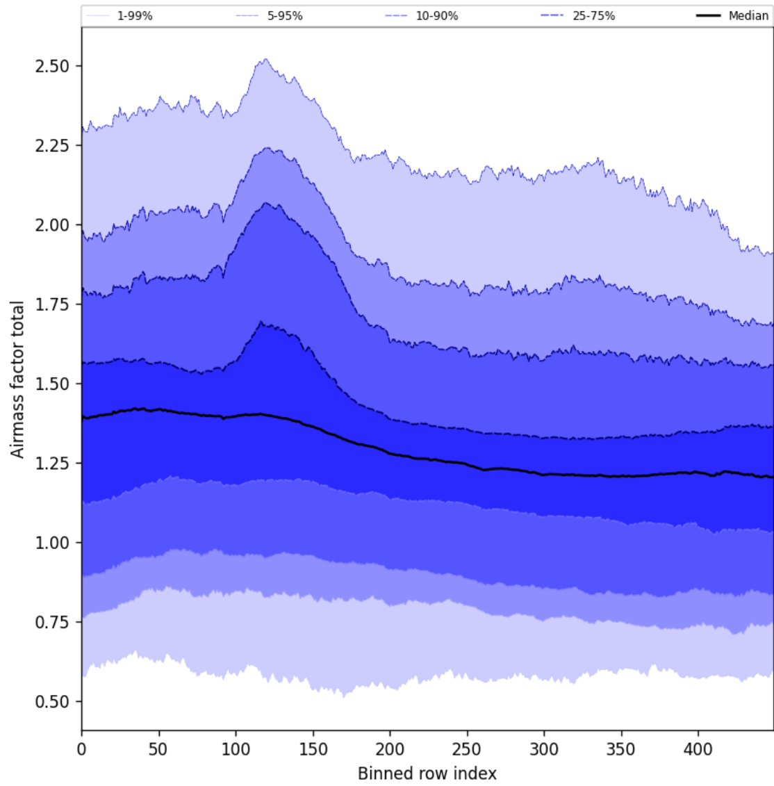
Figure 57: Along track statistics of “Airmass factor total” for 2025-11-19 to 2025-11-21
