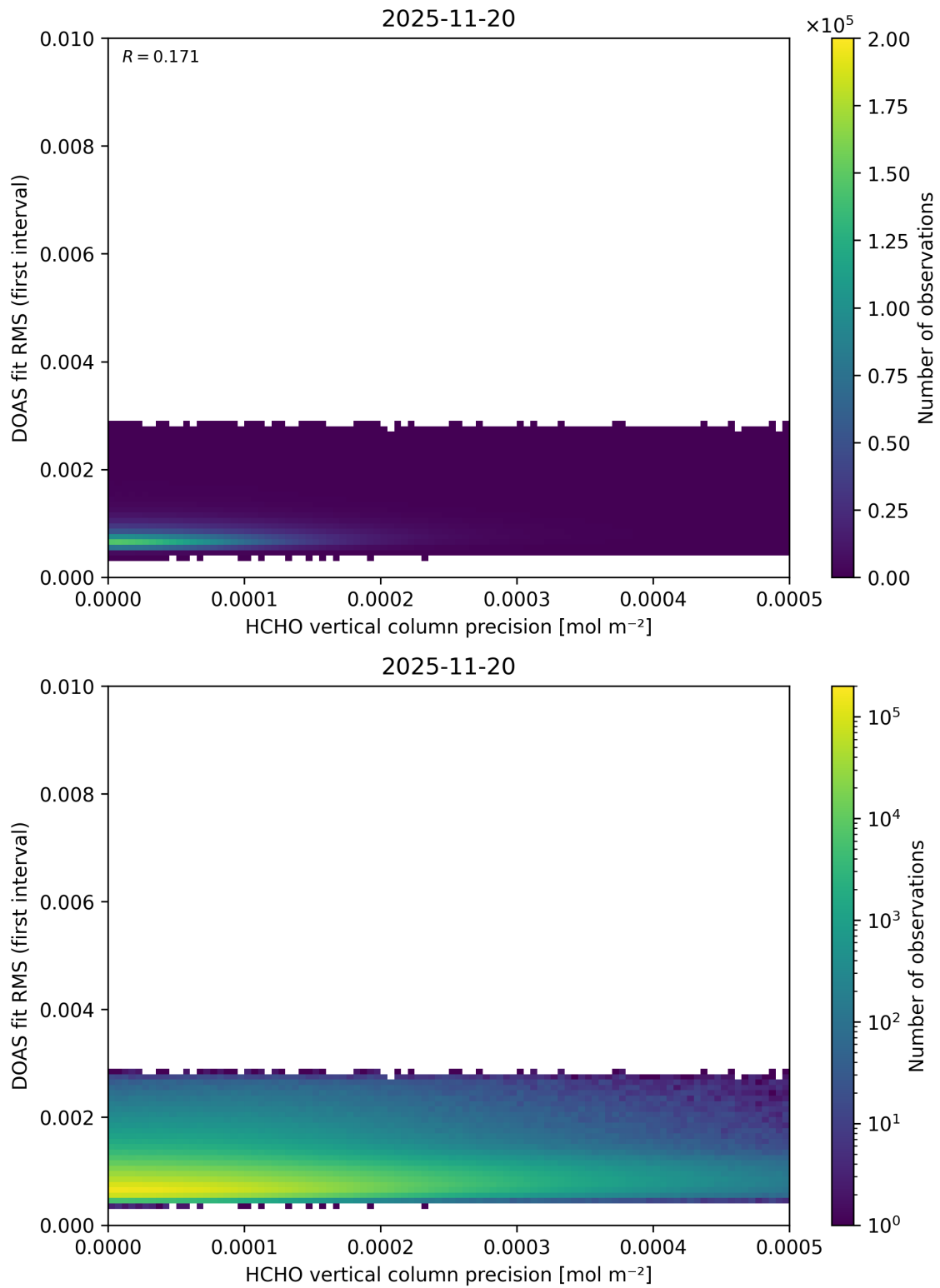
Figure 152: Scatter density plot of “HCHO vertical column precision” against “DOAS fit RMS (first interval)” for 2025-11-19 to 2025-11-21.
