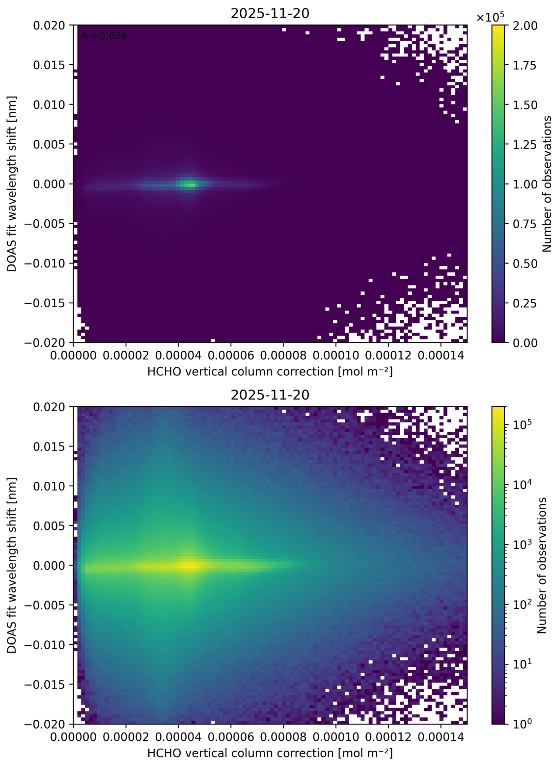
Figure 127: Scatter density plot of “HCHO vertical column correction” against “DOAS fit wavelength shift” for 2025-11-19 to 2025-11-21.
