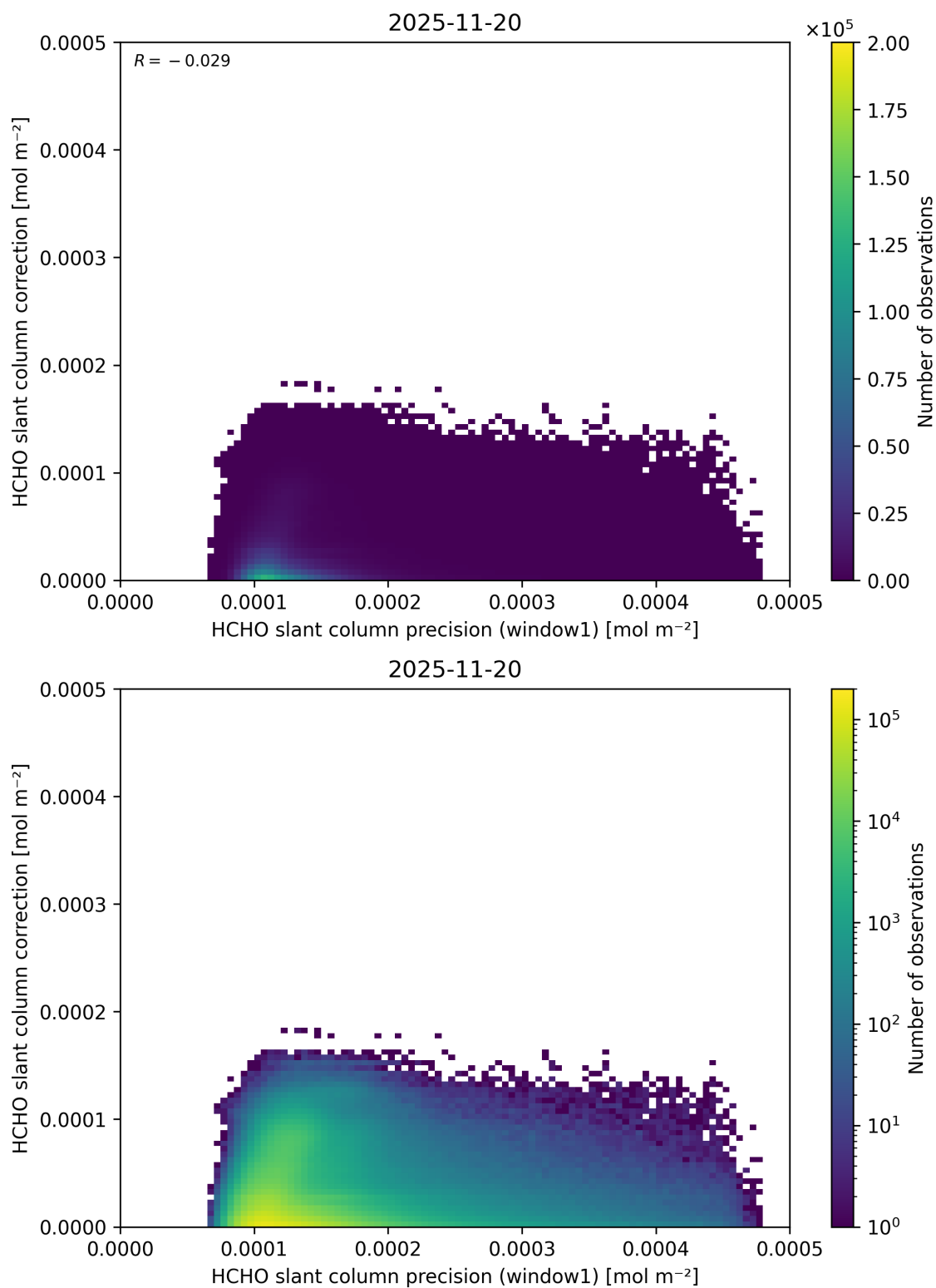
Figure 104: Scatter density plot of “HCHO slant column precision (window1)” against “HCHO slant column correction” for 2025-11-19 to 2025-11-21.
