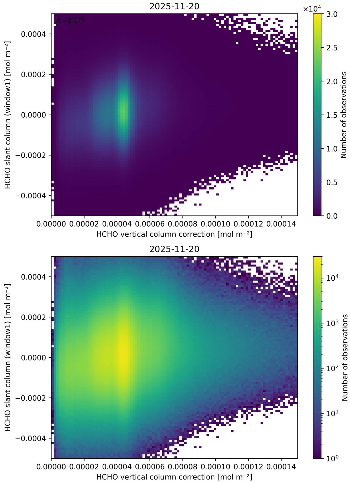
Figure 132: Scatter density plot of “HCHO vertical column correction” against “HCHO slant column (window1)” for 2025-11-19 to 2025-11-21.
