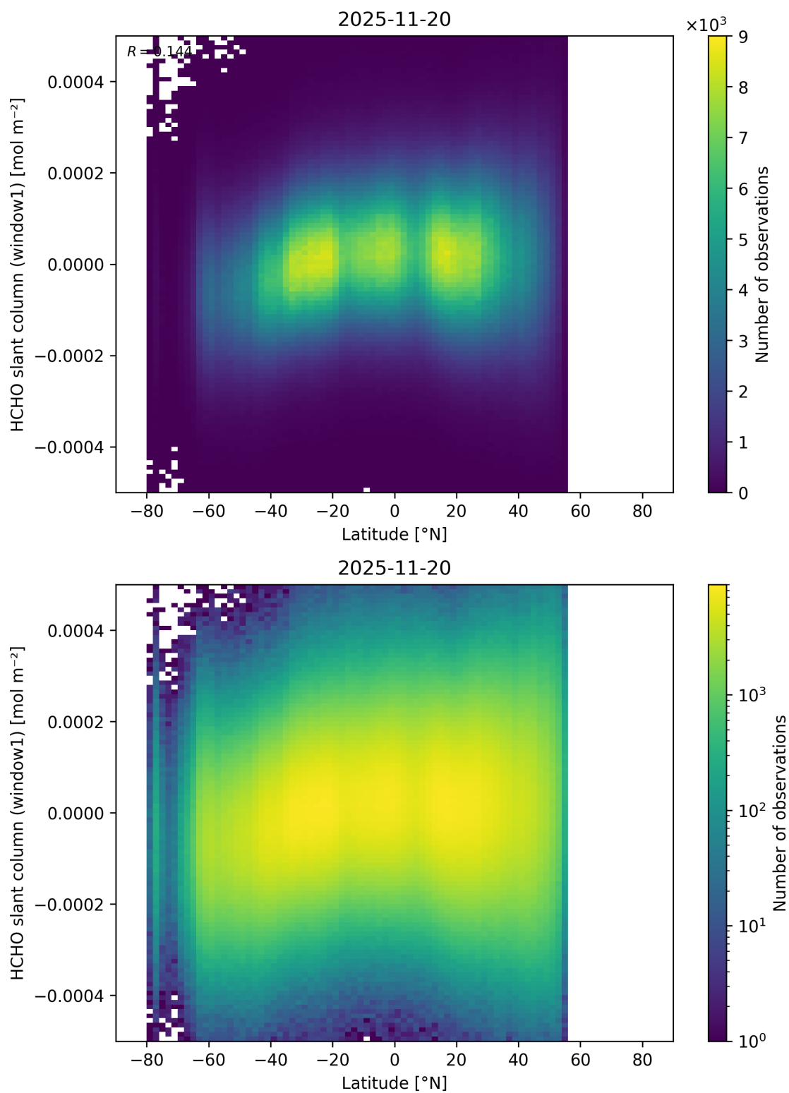
Figure 177: Scatter density plot of “Latitude” against “HCHO slant column (window1)” for 2025-11-19 to 2025-11-21.
