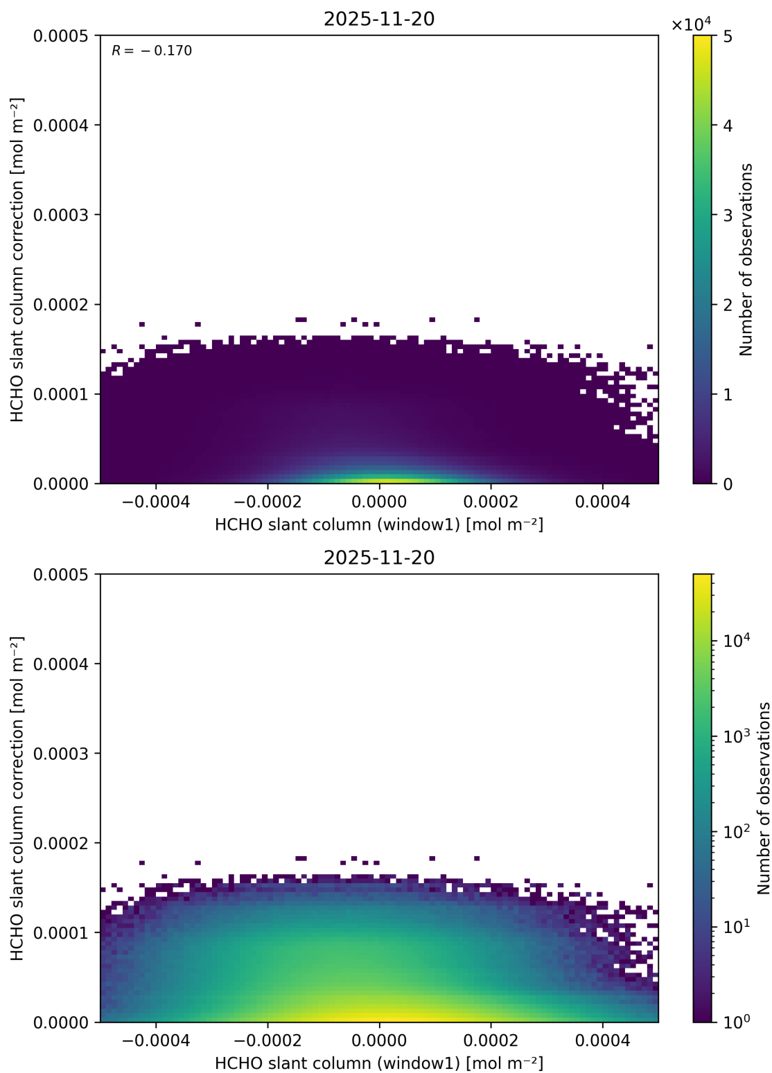
Figure 93: Scatter density plot of “HCHO slant column (window1)” against “HCHO slant column correction” for 2025-11-19 to 2025-11-21.
