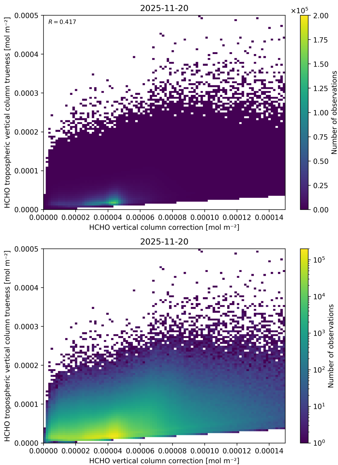
Figure 136: Scatter density plot of “HCHO vertical column correction” against “HCHO tropospheric vertical column true-ness” for 2025-11-19 to 2025-11-21.
