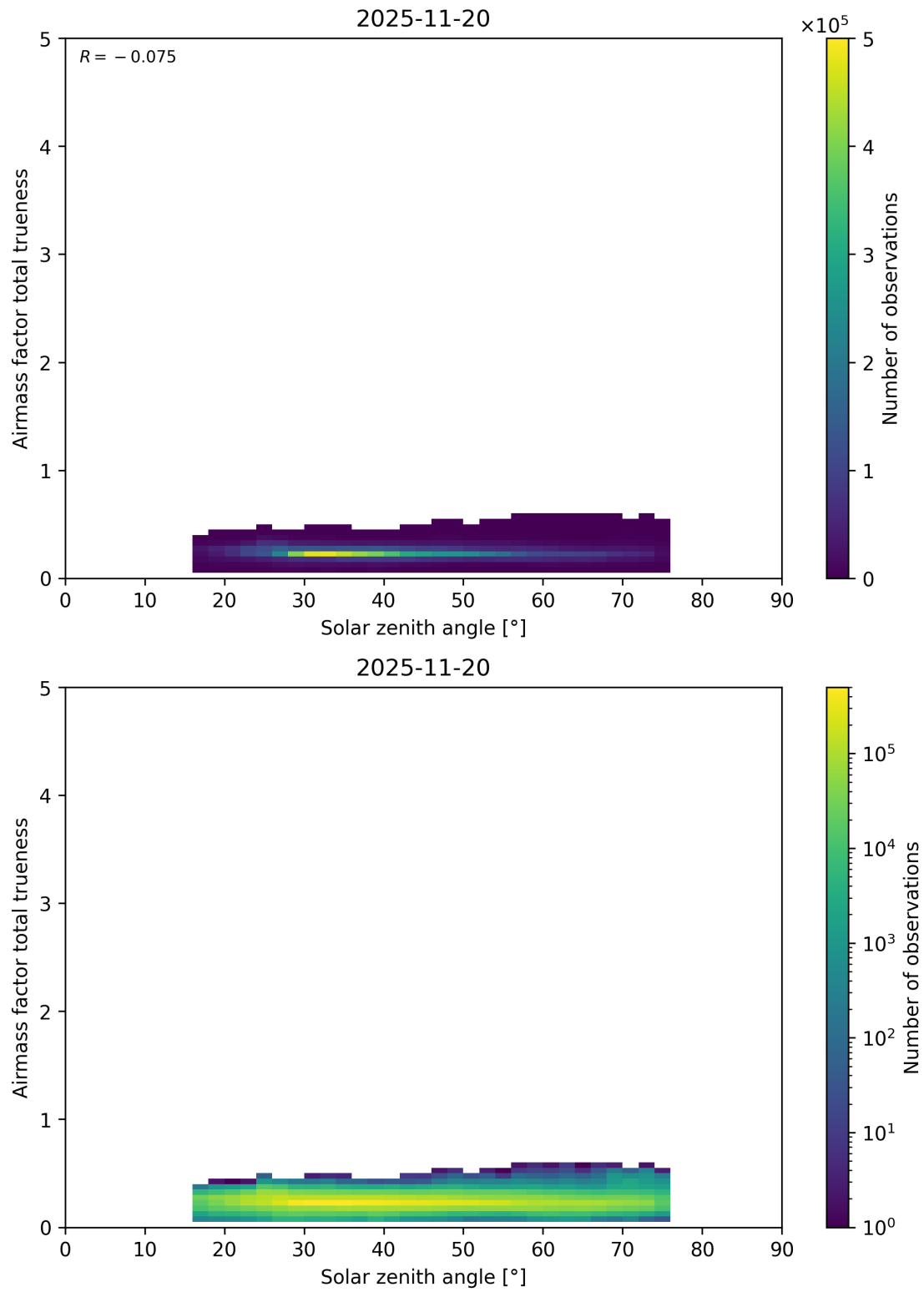
Figure 195: Scatter density plot of “Solar zenith angle” against “Airmass factor total trueneess” for 2025-11-19 to 2025-11-21.
