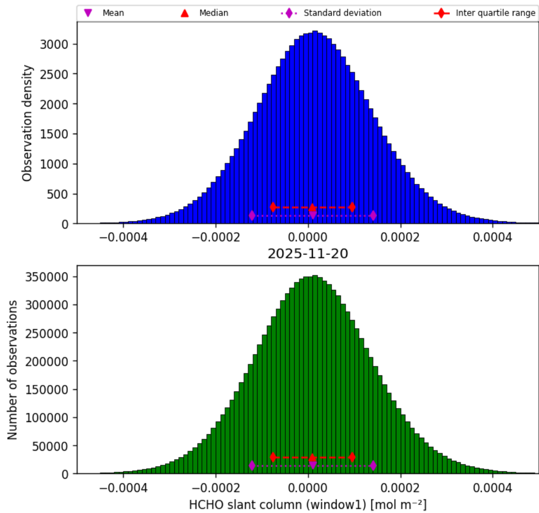
Figure 40: Histogram of “HCHO slant column (window1)” for 2025-11-19 to 2025-11-21
