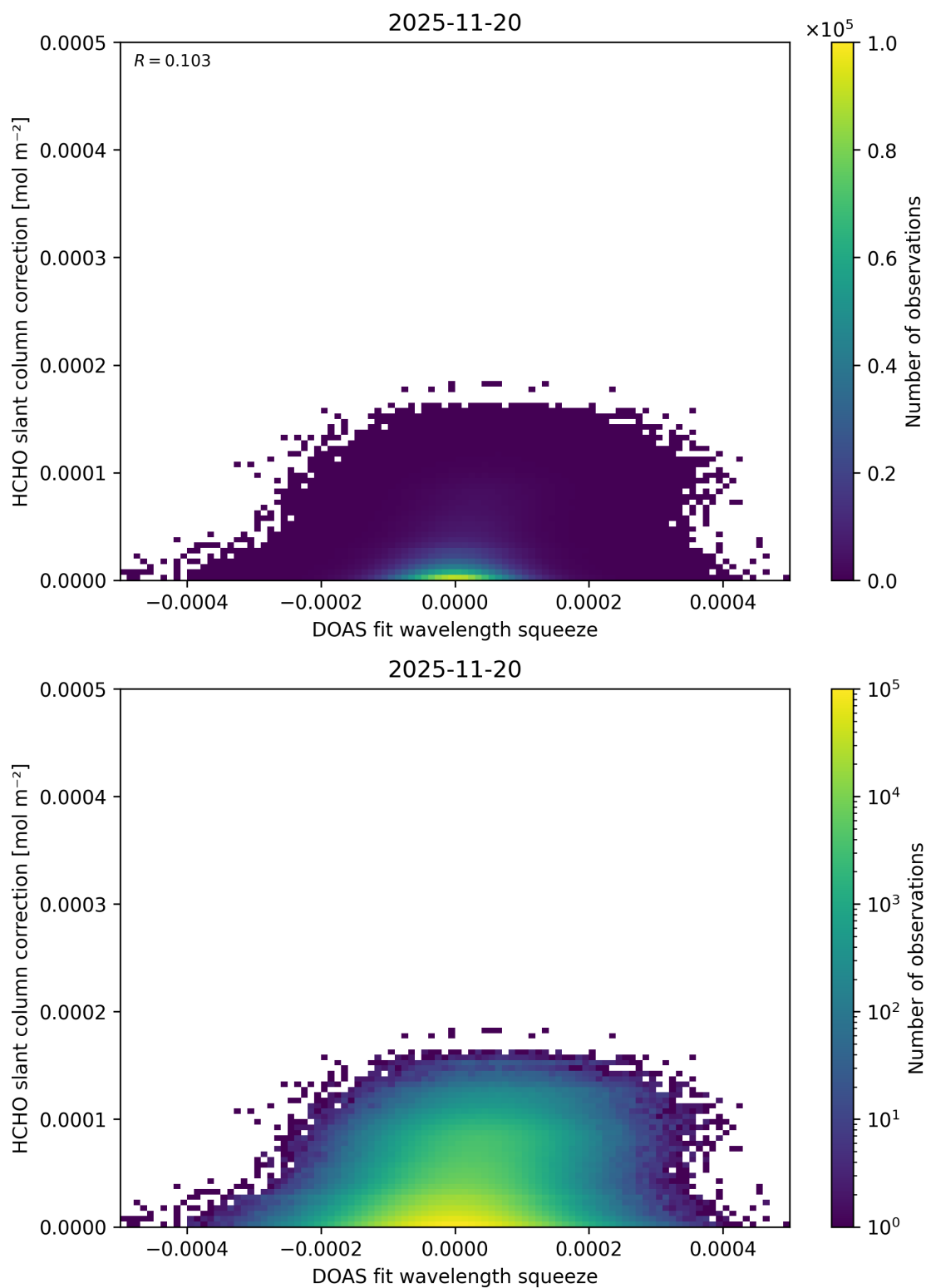
Figure 76: Scatter density plot of “DOAS fit wavelength squeeze” against “HCHO slant column correction” for 2025-11-19 to 2025-11-21.
