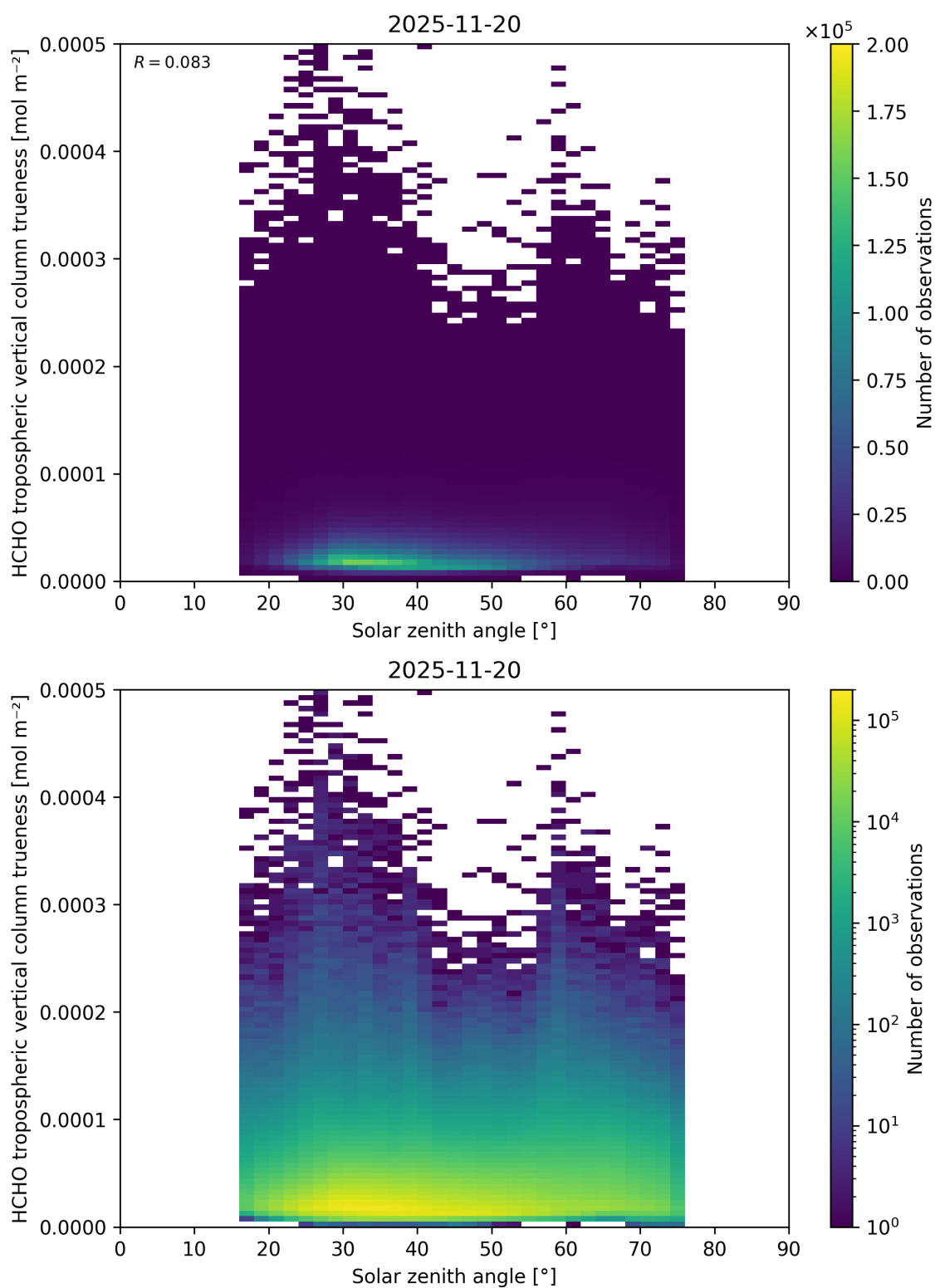
Figure 199: Scatter density plot of “Solar zenith angle” against “HCHO tropospheric vertical column trueness” for 2025-11-19 to 2025-11-21.
