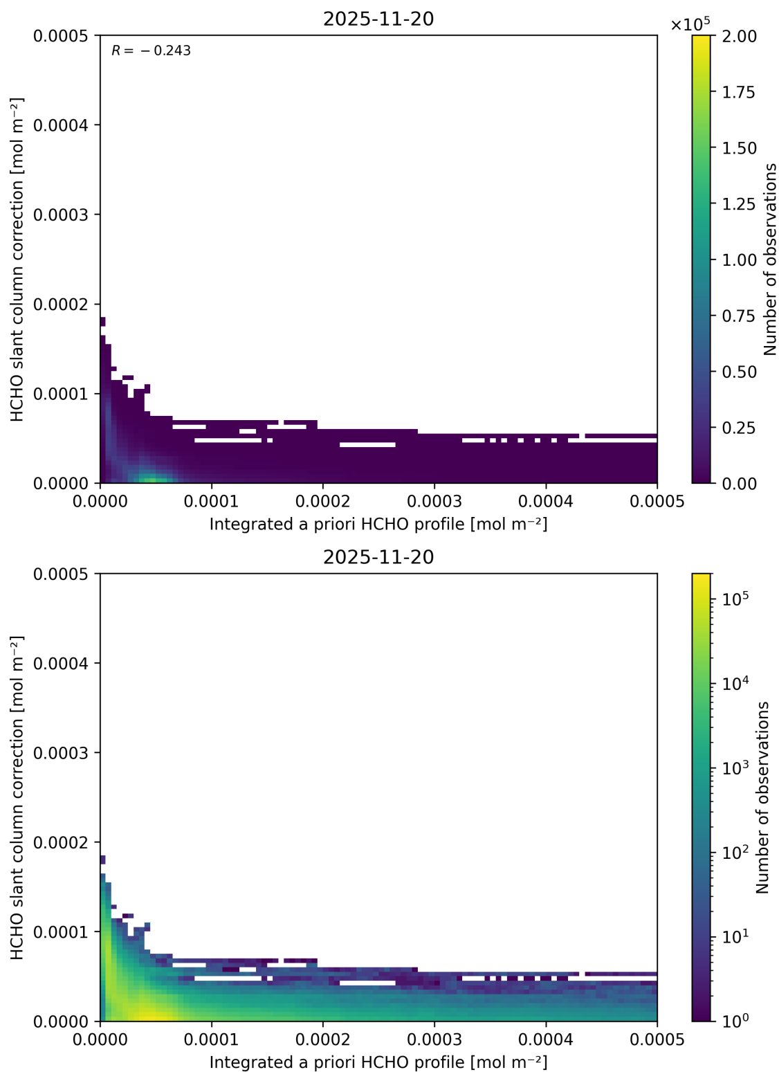
Figure 169: Scatter density plot of “Integrated a priori HCHO profile” against “HCHO slant column correction” for 2025-11-19 to 2025-11-21.
