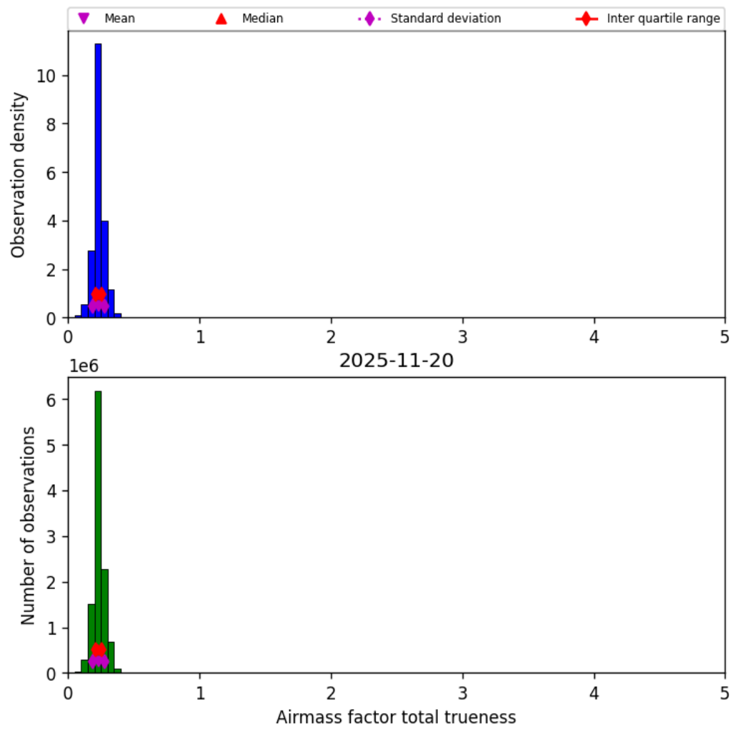
Figure 43: Histogram of “Airmass factor total trueness” for 2025-11-19 to 2025-11-21
