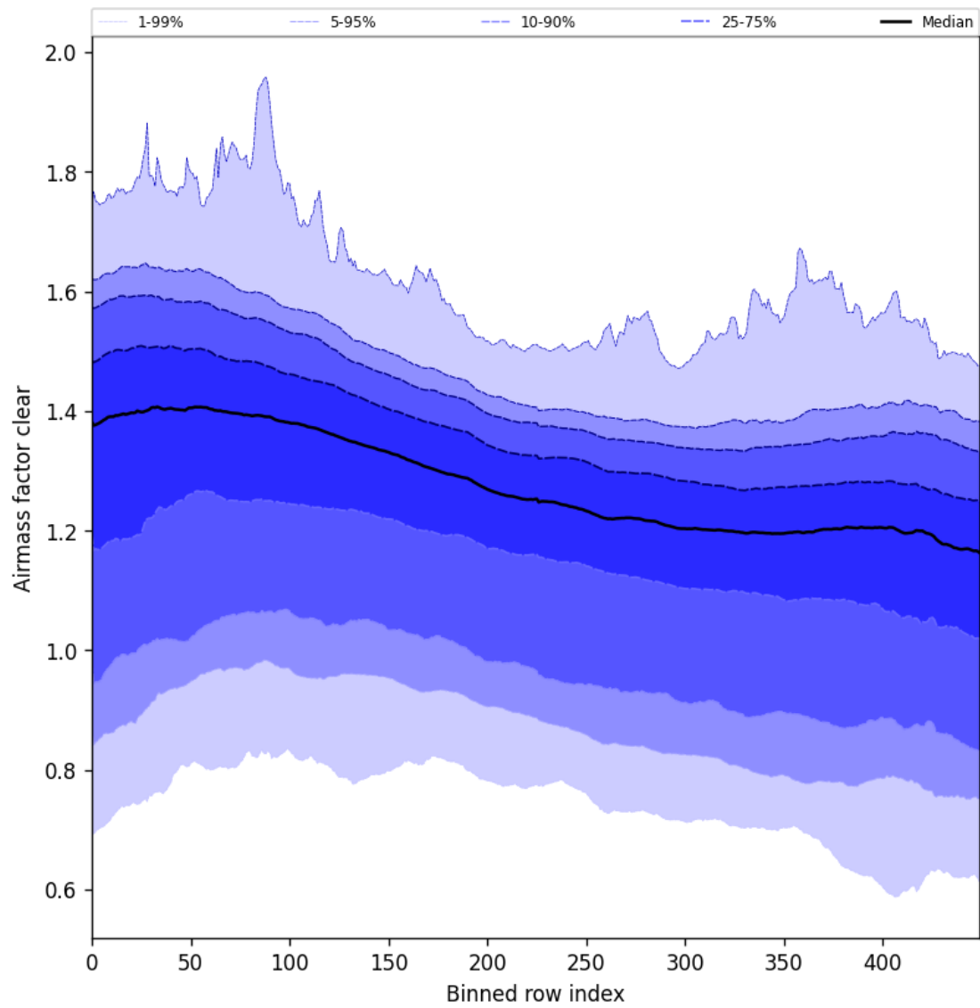
Figure 59: Along track statistics of “Airmass factor clear” for 2025-11-19 to 2025-11-21
