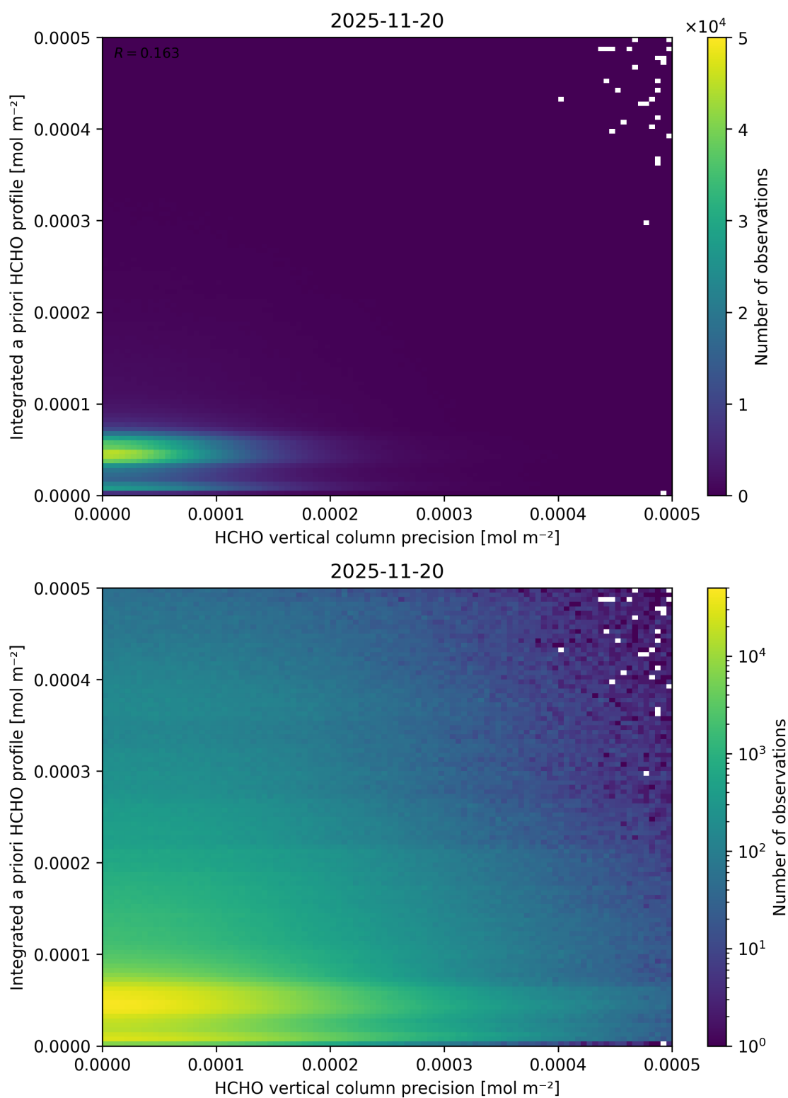
Figure 164: Scatter density plot of “HCHO vertical column precision” against “Integrated a priori HCHO profile” for 2025-11-19 to 2025-11-21.
