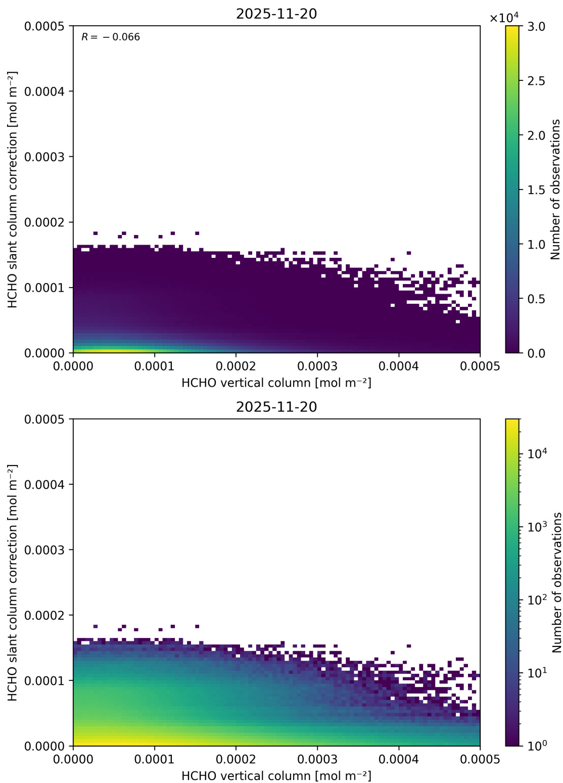
Figure 143: Scatter density plot of “HCHO vertical column” against “HCHO slant column correction” for 2025-11-19 to 2025-11-21.
