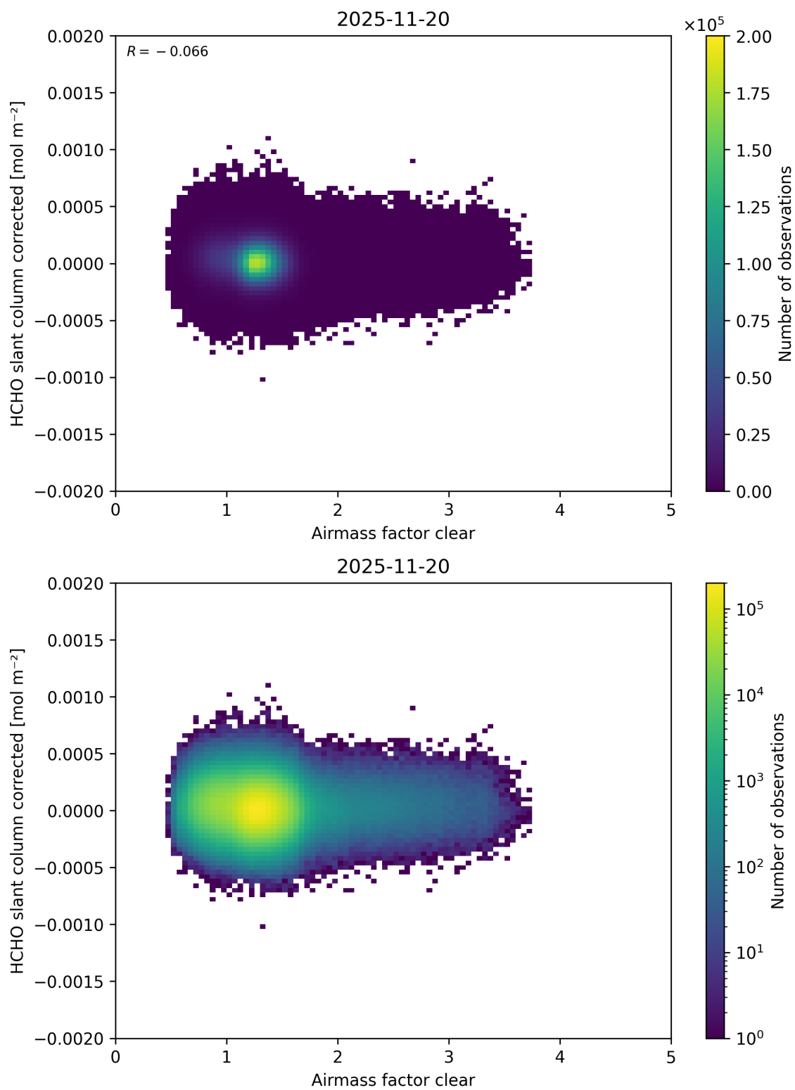
Figure 81: Scatter density plot of “Airmass factor clear” against “HCHO slant column corrected” for 2025-11-19 to 2025-11-21.
