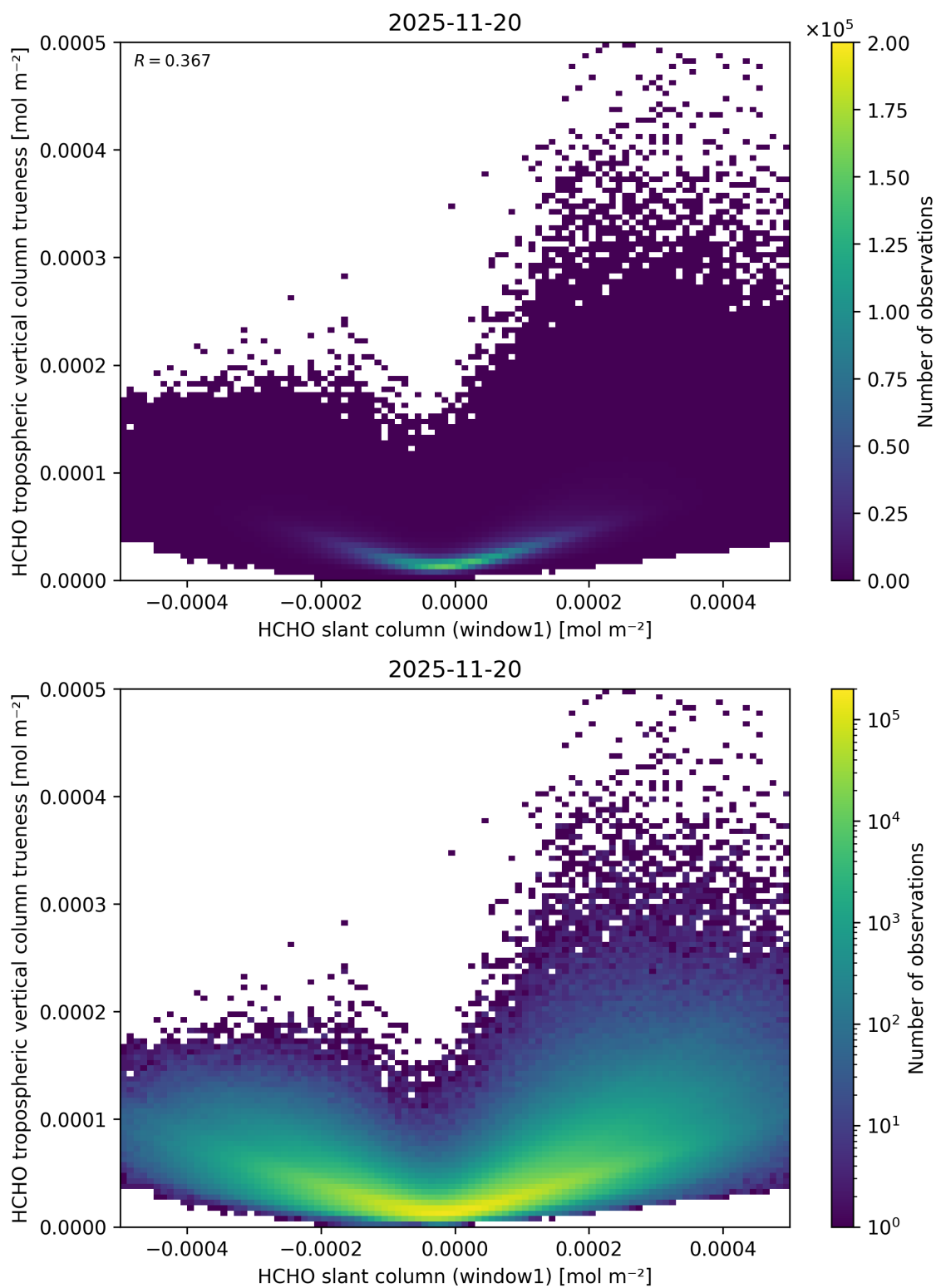
Figure 97: Scatter density plot of “HCHO slant column (window1)” against “HCHO tropospheric vertical column trueness” for 2025-11-19 to 2025-11-21.
