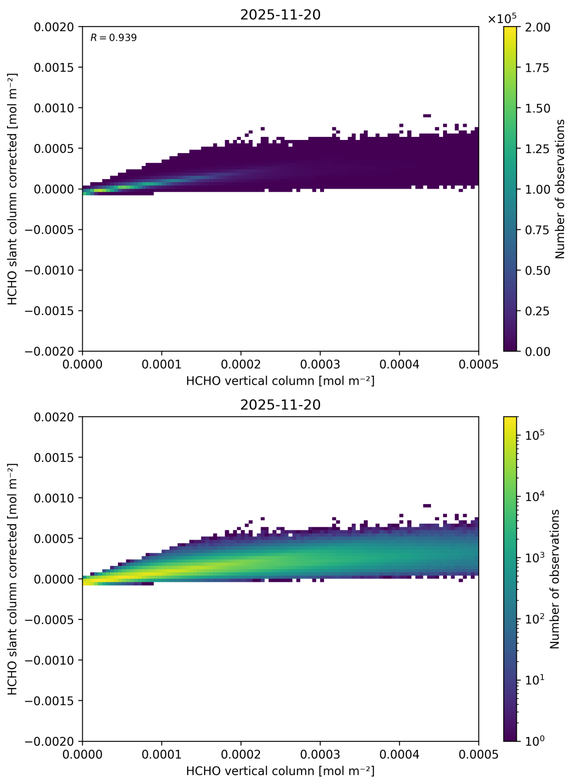
Figure 142: Scatter density plot of “HCHO vertical column” against “HCHO slant column corrected” for 2025-11-19 to 2025-11-21.
