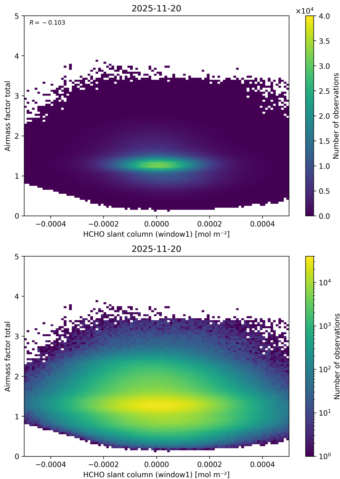
Figure 95: Scatter density plot of “HCHO slant column (window1)” against “Airmass factor total” for 2025-11-19 to 2025-11-21.
