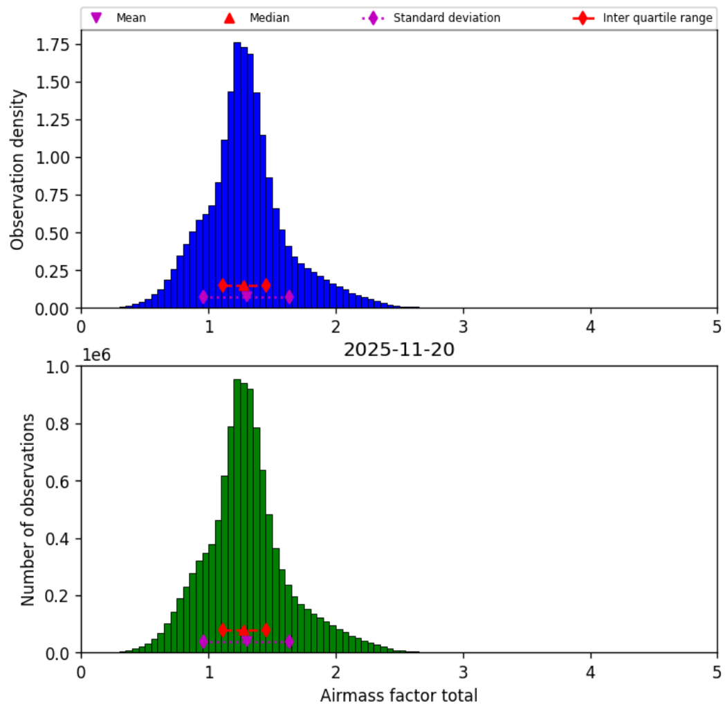
Figure 42: Histogram of “Airmass factor total” for 2025-11-19 to 2025-11-21
