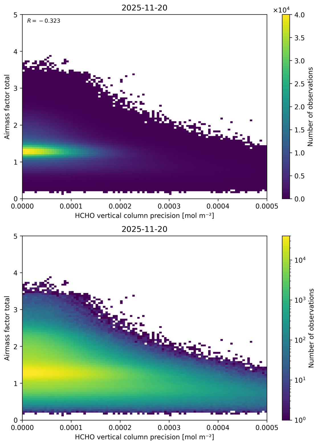
Figure 160: Scatter density plot of “HCHO vertical column precision” against “Airmass factor total” for 2025-11-19 to 2025-11-21.
