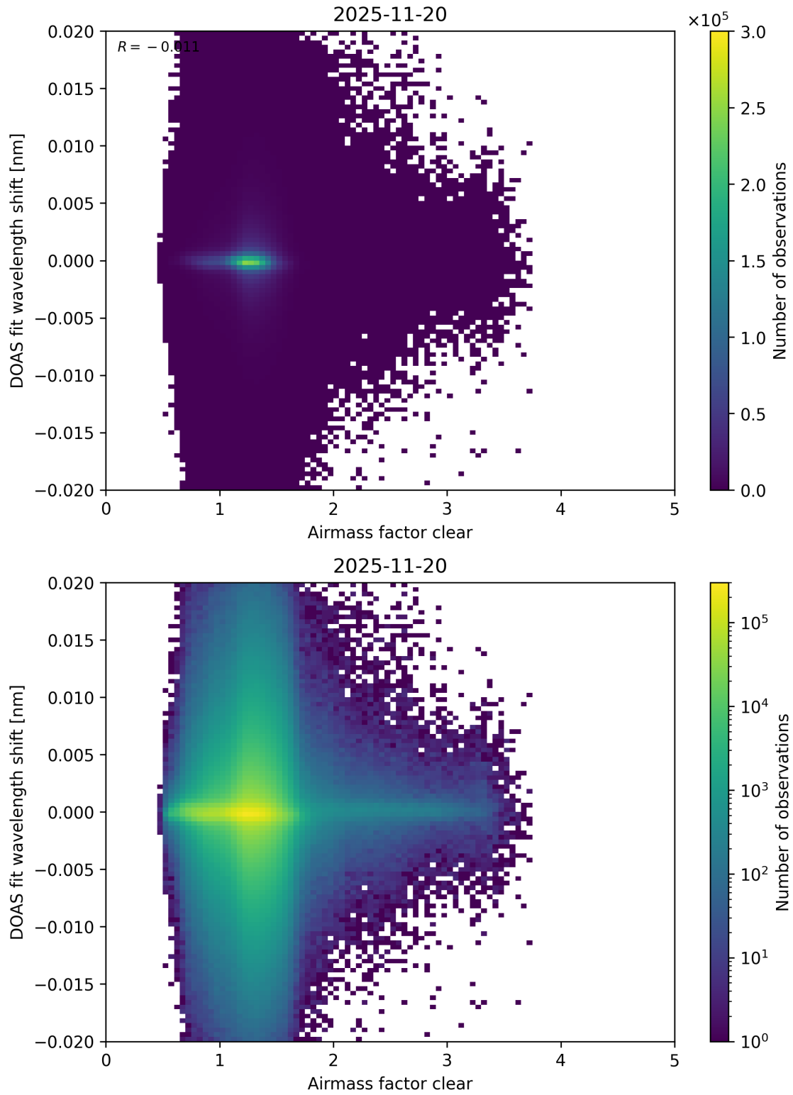
Figure 79: Scatter density plot of “Airmass factor clear” against “DOAS fit wavelength shift” for 2025-11-19 to 2025-11-21.
