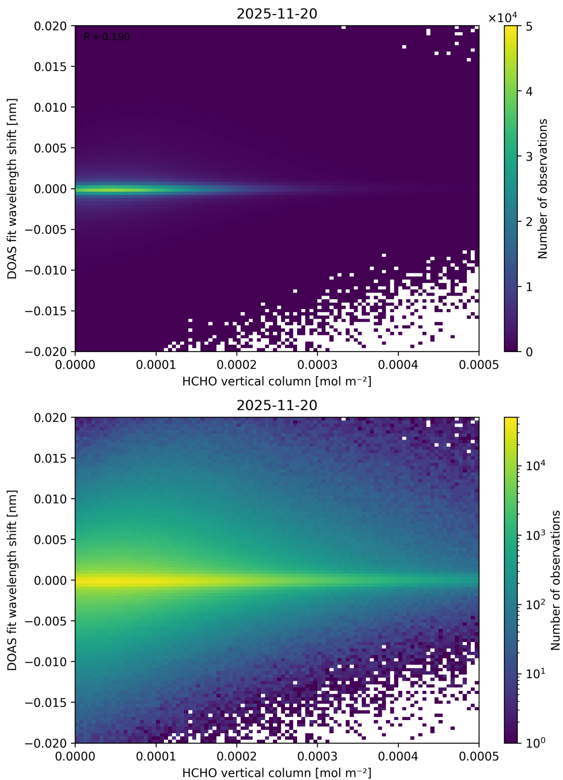
Figure 139: Scatter density plot of “HCHO vertical column” against “DOAS fit wavelength shift” for 2025-11-19 to 2025-11-21.
