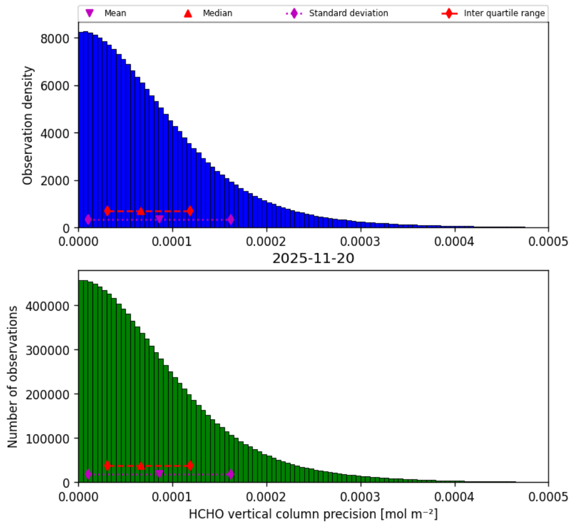
Figure 38: Histogram of “HCHO vertical column precision” for 2025-11-19 to 2025-11-21
