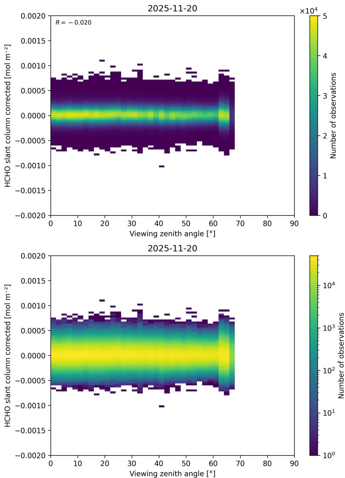
Figure 206: Scatter density plot of “Viewing zenith angle” against “HCHO slant column corrected” for 2025-11-19 to 2025-11-21.
