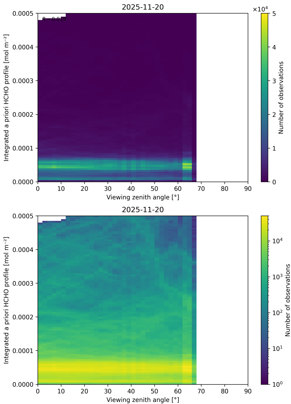
Figure 216: Scatter density plot of “Viewing zenith angle” against “Integrated a priori HCHO profile” for 2025-11-19 to 2025-11-21.
