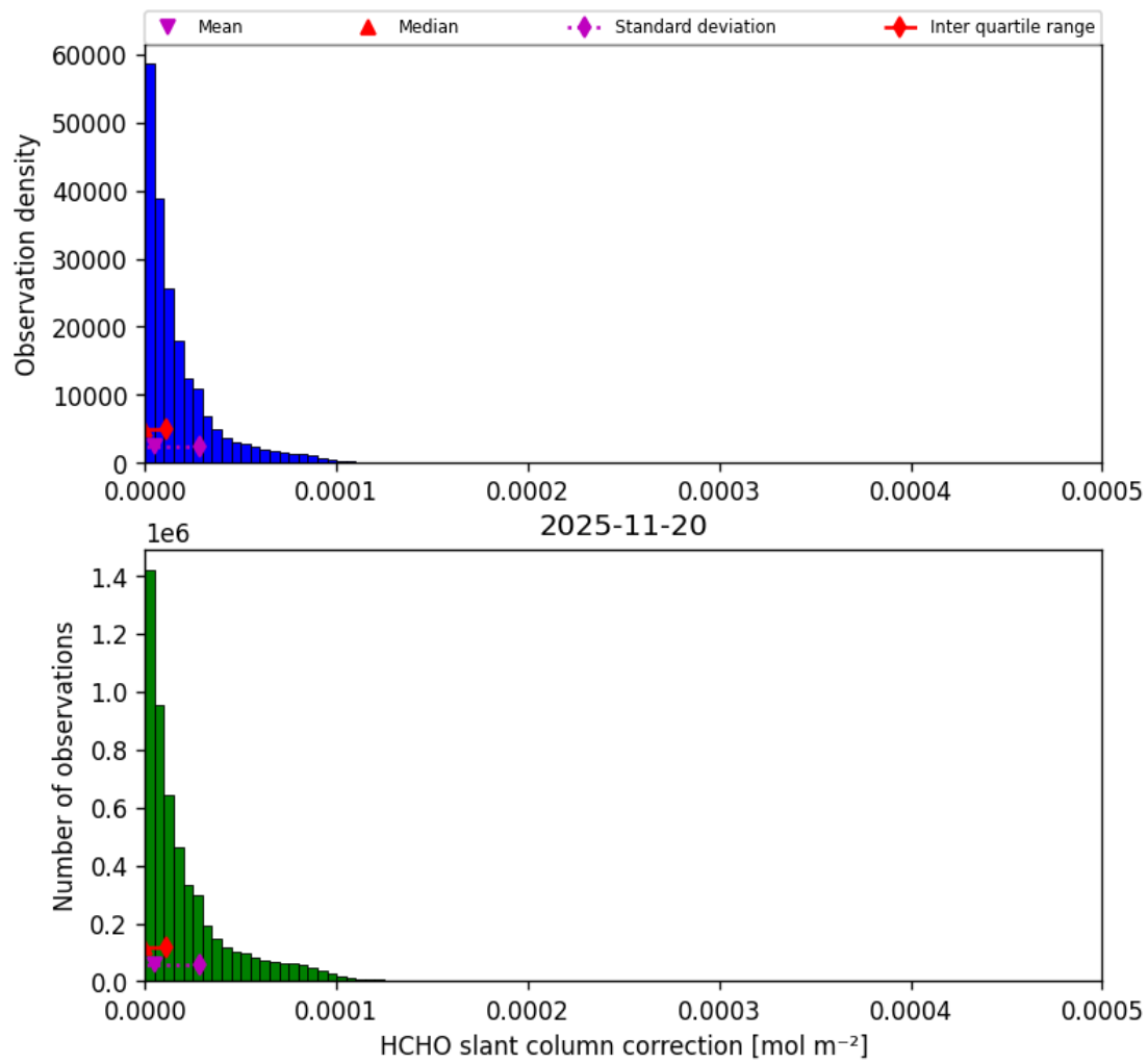
Figure 49: Histogram of “HCHO slant column correction” for 2025-11-19 to 2025-11-21
