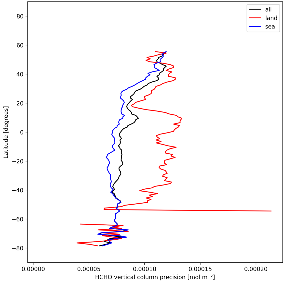
Figure 23: Zonal average of “HCHO vertical column precision” for 2025-11-19 to 2025-11-21.
