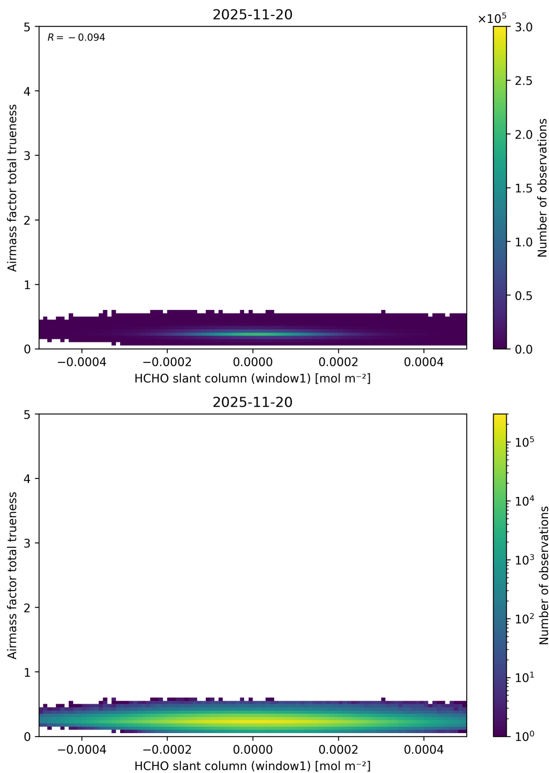
Figure 96: Scatter density plot of “HCHO slant column (window1)” against “Airmass factor total trueneess” for 2025-11-19 to 2025-11-21.
