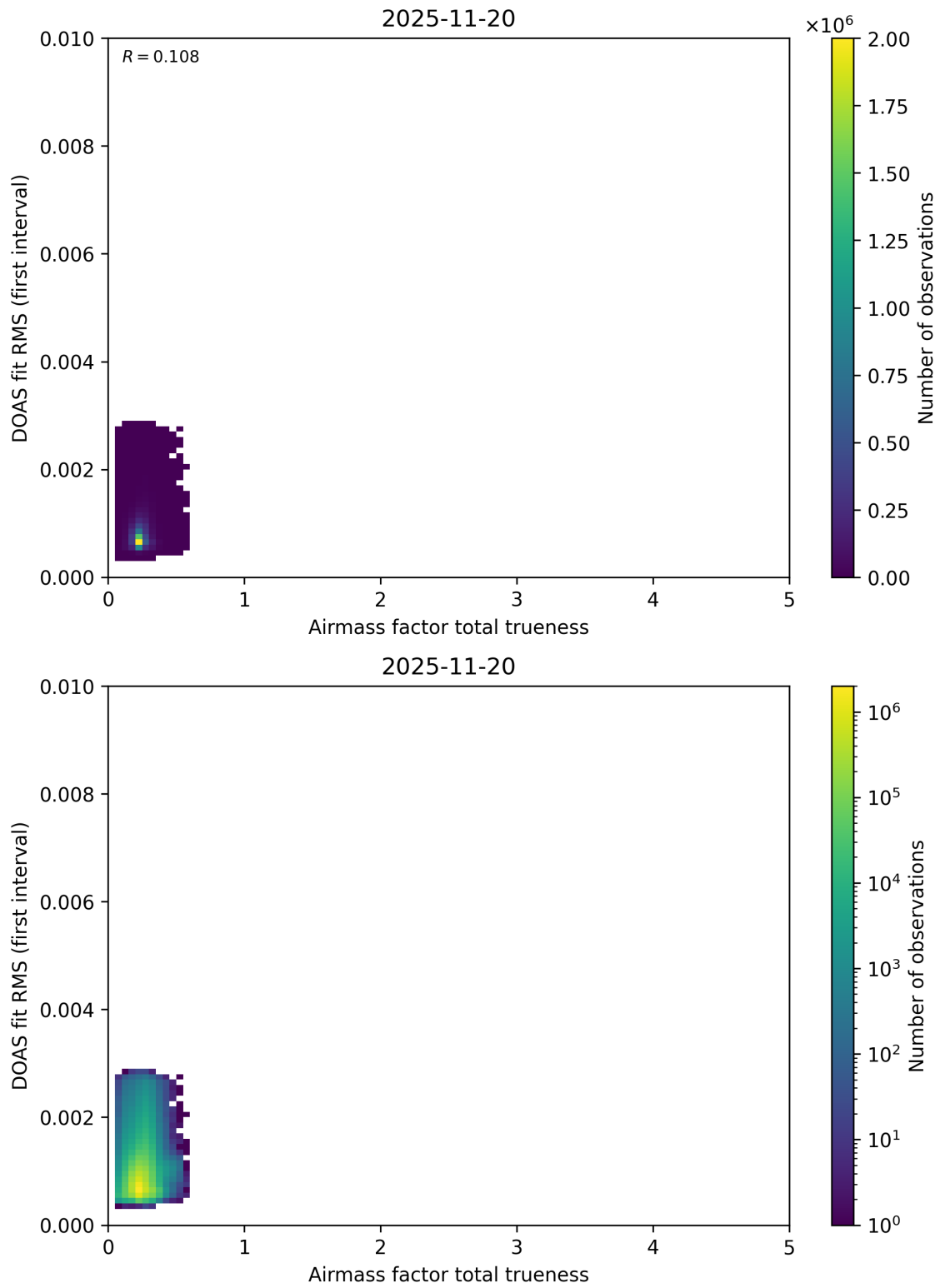
Figure 118: Scatter density plot of “Airmass factor total trueness” against “DOAS fit RMS (first interval)” for 2025-11-19 to 2025-11-21.
