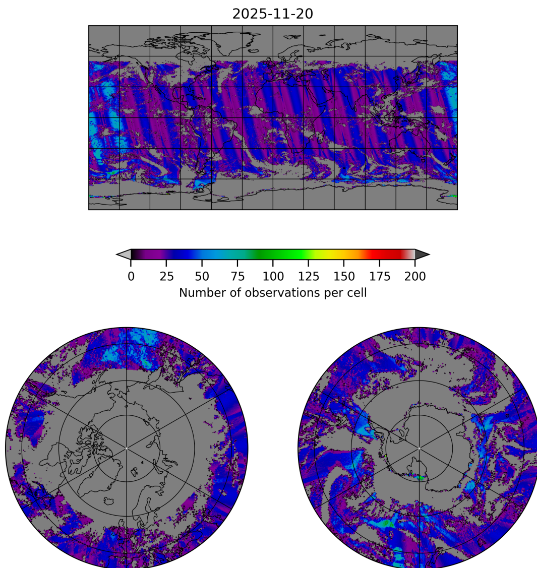
Figure 20: Map of the number of observations for 2025-11-19 to 2025-11-21
