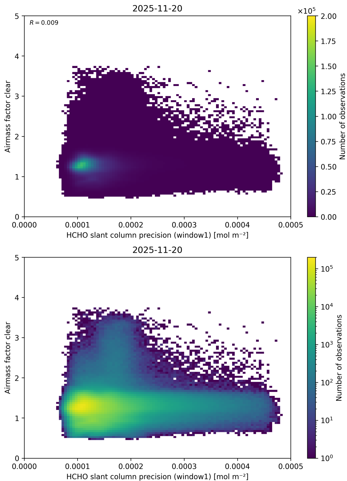
Figure 102: Scatter density plot of “HCHO slant column precision (window1)” against “Airmass factor clear” for 2025-11-19 to 2025-11-21.
