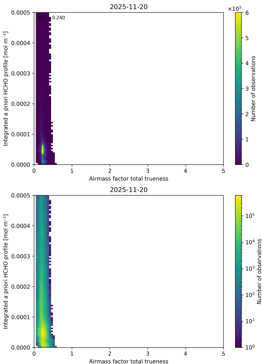
Figure 125: Scatter density plot of “Airmass factor total trueness” against “Integrated a priori HCHO profile” for 2025-11-19 to 2025-11-21.
