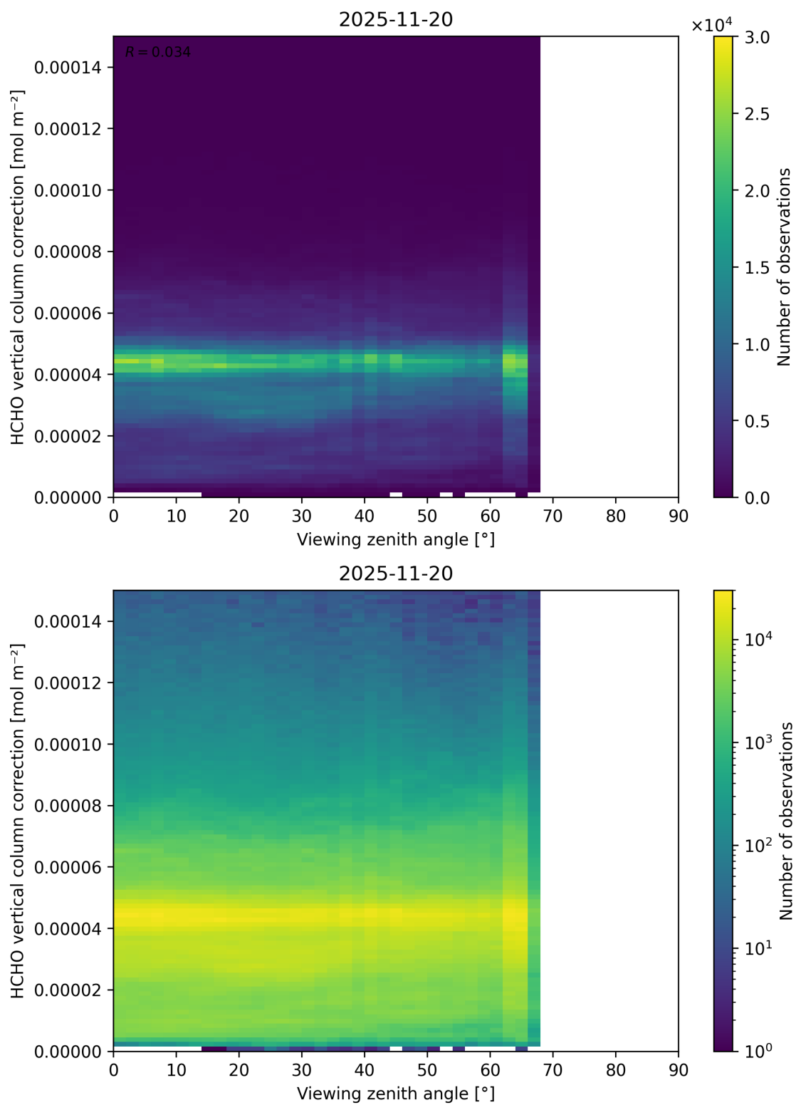
Figure 213: Scatter density plot of “Viewing zenith angle” against “HCHO vertical column correction” for 2025-11-19 to 2025-11-21.
