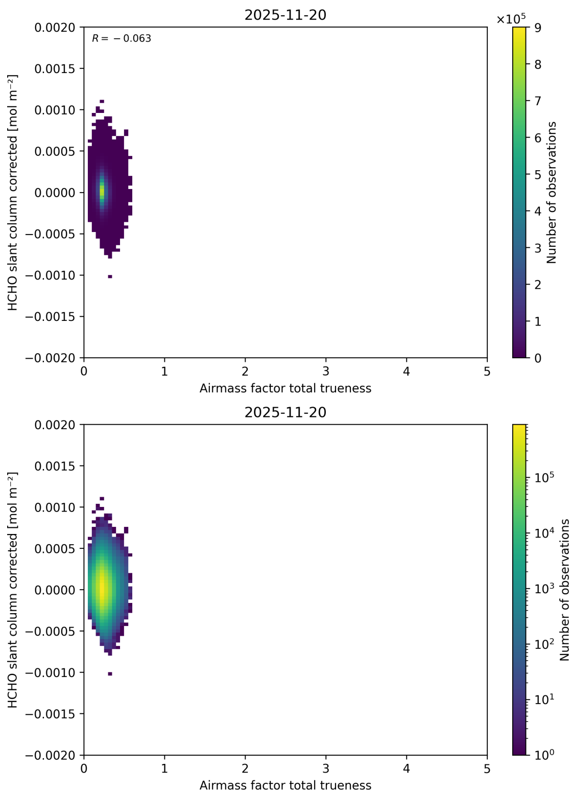
Figure 122: Scatter density plot of “Airmass factor total trueness” against “HCHO slant column corrected” for 2025-11-19 to 2025-11-21.
