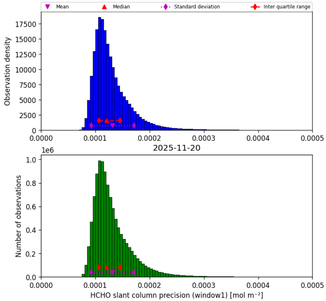
Figure 41: Histogram of “HCHO slant column precision (window1)” for 2025-11-19 to 2025-11-21
