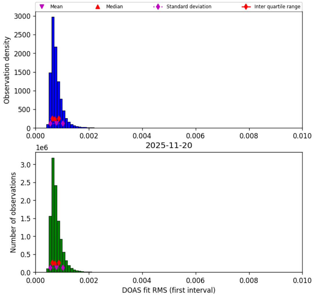
Figure 48: Histogram of “DOAS fit RMS (first interval)” for 2025-11-19 to 2025-11-21
