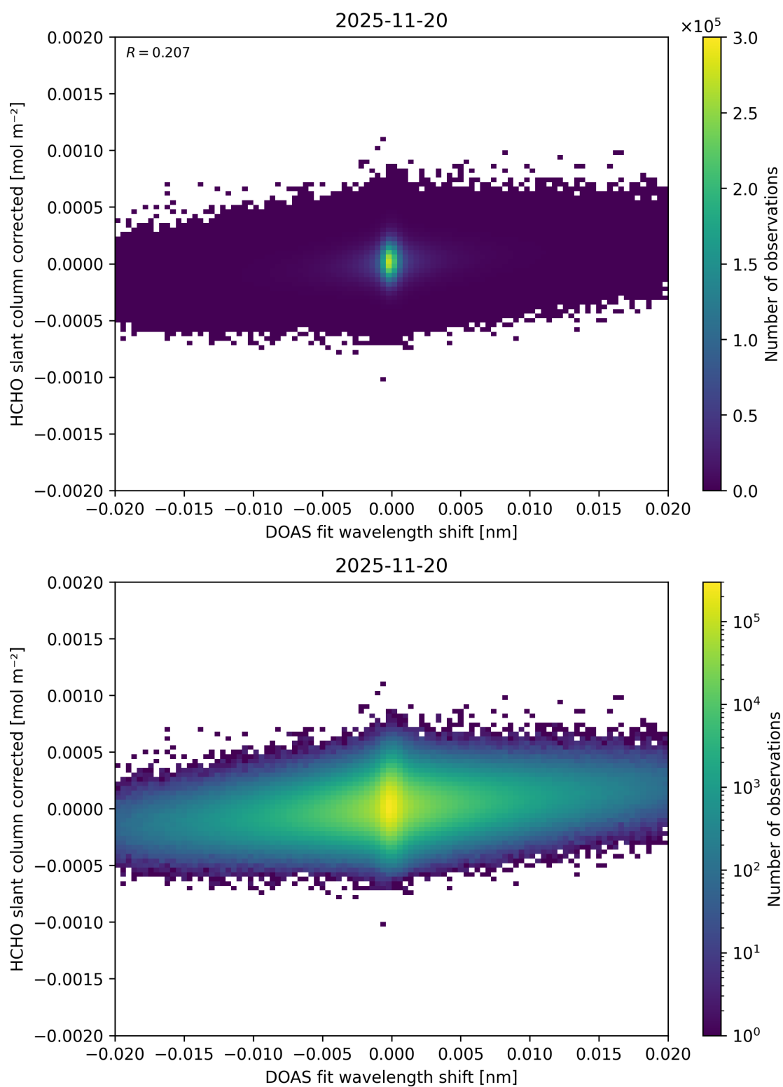
Figure 71: Scatter density plot of “DOAS fit wavelength shift” against “HCHO slant column corrected” for 2025-11-19 to 2025-11-21.
