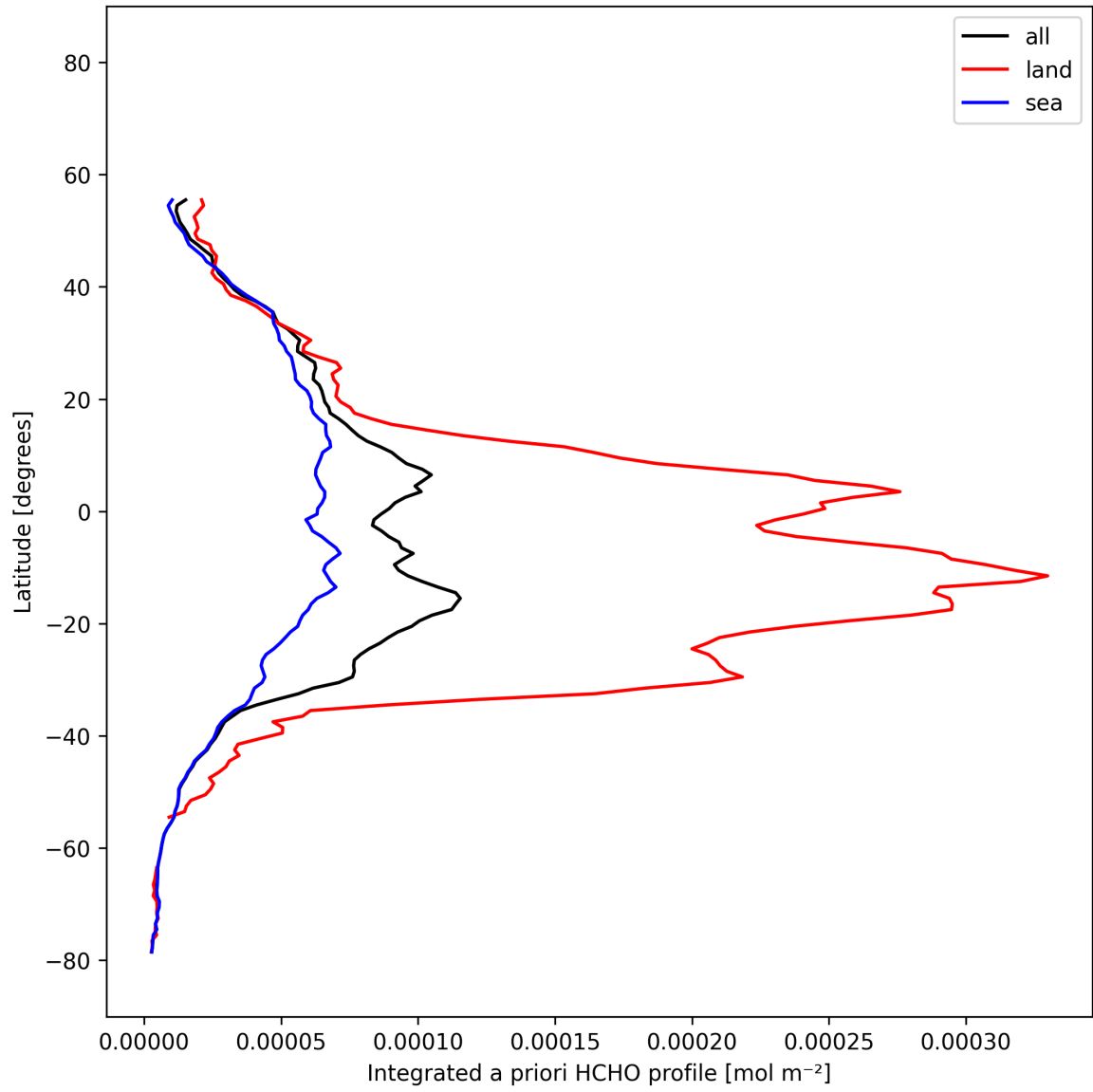
Figure 30: Zonal average of “Integrated a priori HCHO profile” for 2025-11-19 to 2025-11-21.
