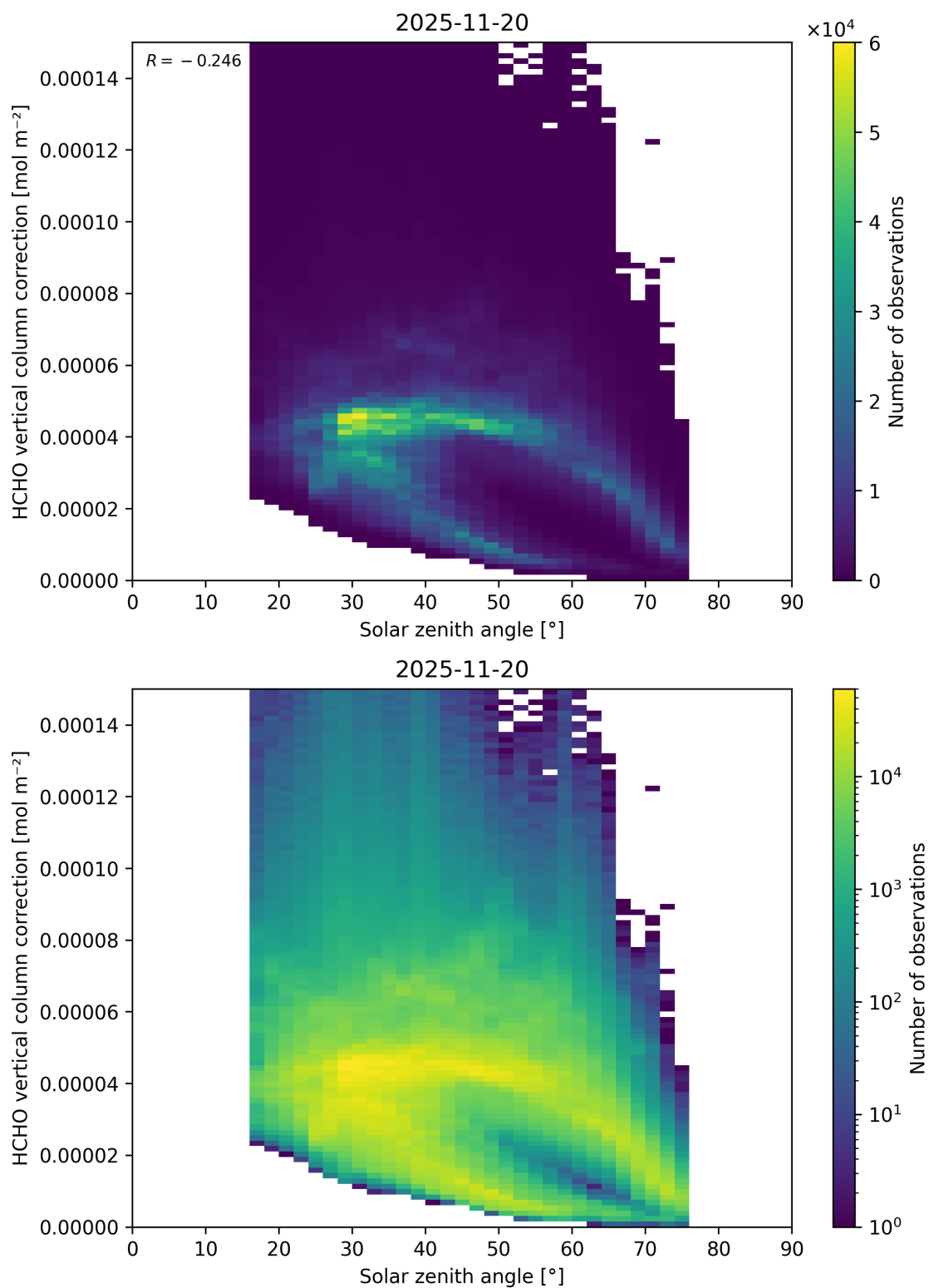
Figure 197: Scatter density plot of “Solar zenith angle” against “HCHO vertical column correction” for 2025-11-19 to 2025-11-21.
