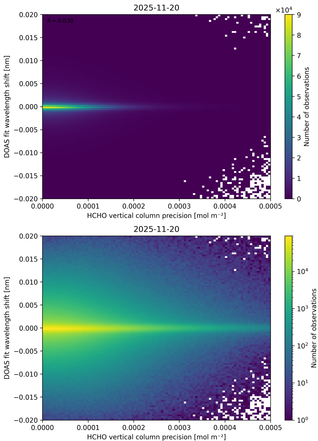
Figure 153: Scatter density plot of “HCHO vertical column precision” against “DOAS fit wavelength shift” for 2025-11-19 to 2025-11-21.
