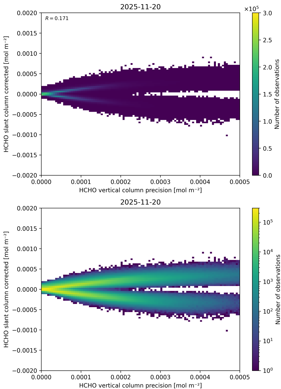
Figure 156: Scatter density plot of “HCHO vertical column precision” against “HCHO slant column corrected” for 2025-11-19 to 2025-11-21.
