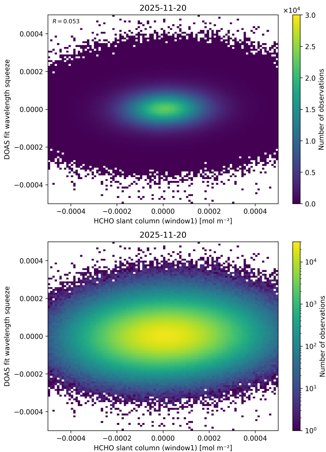
Figure 90: Scatter density plot of “HCHO slant column (window1)” against “DOAS fit wavelength squeeze” for 2025-11-19 to 2025-11-21.
