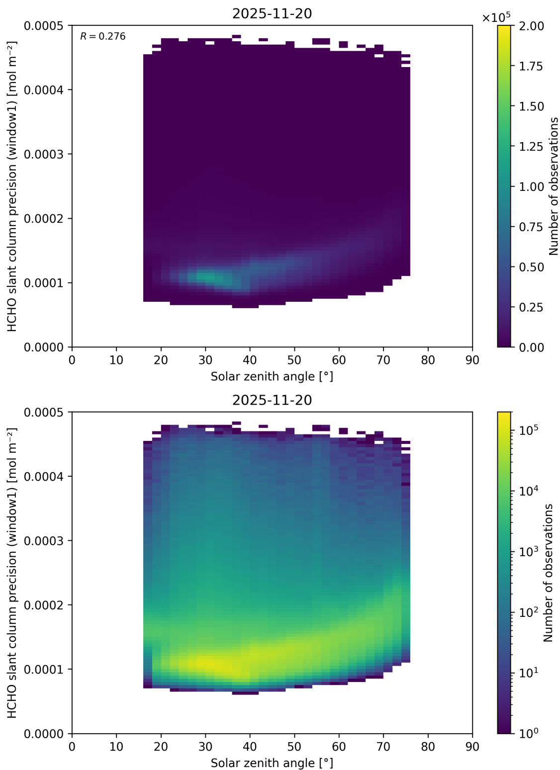
Figure 193: Scatter density plot of “Solar zenith angle” against “HCHO slant column precision (window1)” for 2025-11-19 to 2025-11-21.
