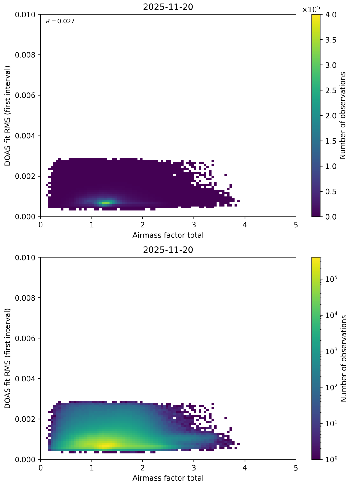
Figure 109: Scatter density plot of “Airmass factor total” against “DOAS fit RMS (first interval)” for 2025-11-19 to 2025-11-21.
