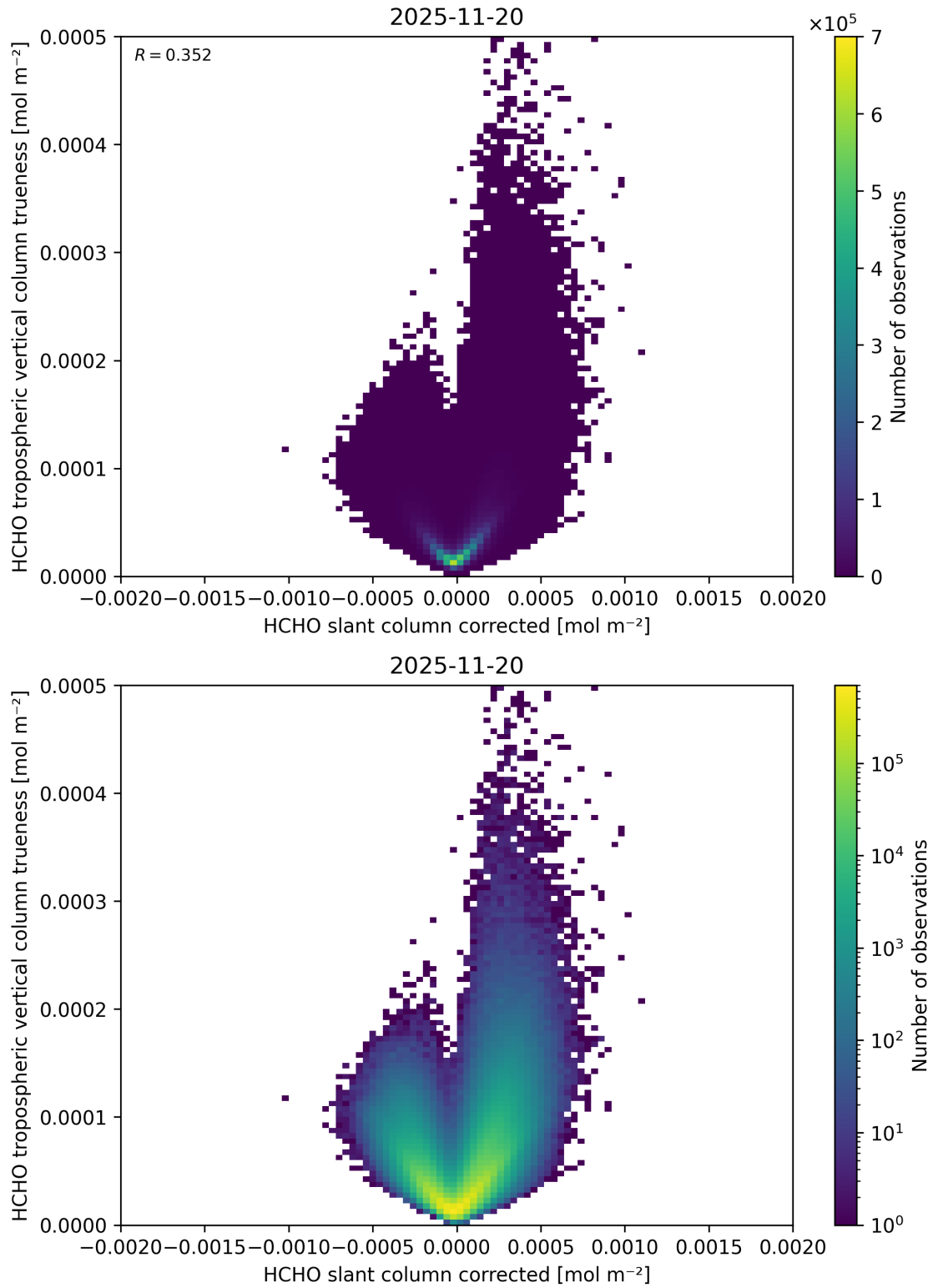
Figure 86: Scatter density plot of “HCHO slant column corrected” against “HCHO tropospheric vertical column trueness” for 2025-11-19 to 2025-11-21.
