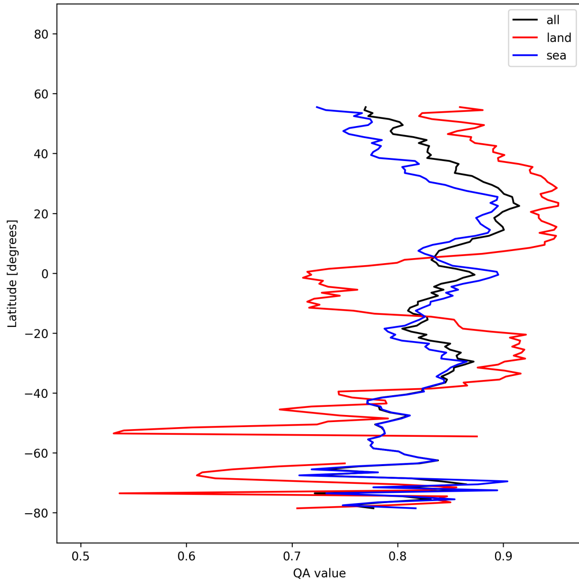
Figure 21: Zonal average of “QA value” for 2025-11-19 to 2025-11-21.
