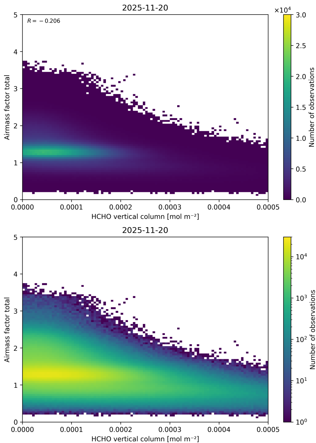
Figure 146: Scatter density plot of “HCHO vertical column” against “Airmass factor total” for 2025-11-19 to 2025-11-21.
