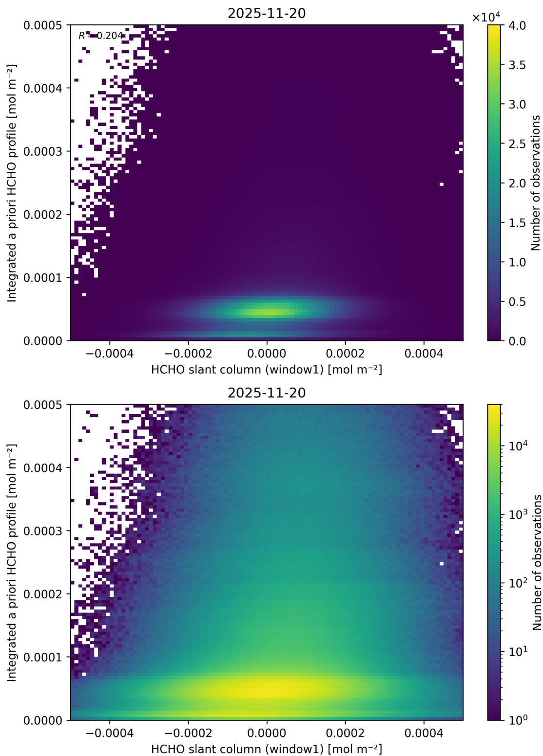
Figure 98: Scatter density plot of “HCHO slant column (window1)” against “Integrated a priori HCHO profile” for 2025-11-19 to 2025-11-21.
