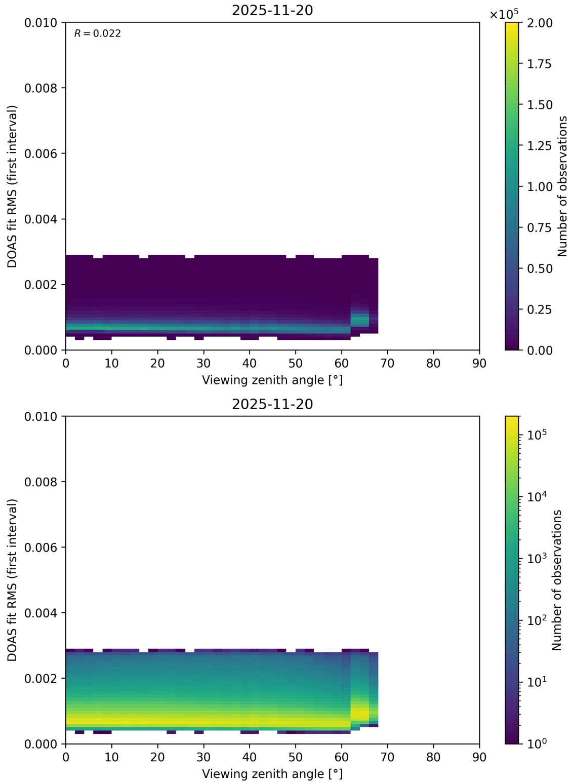
Figure 202: Scatter density plot of “Viewing zenith angle” against “DOAS fit RMS (first interval)” for 2025-11-19 to 2025-11-21.
