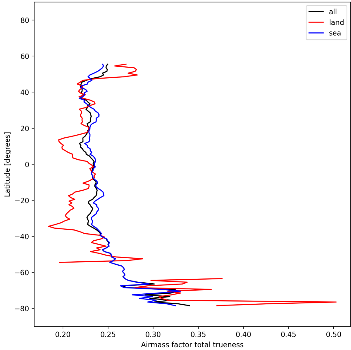
Figure 28: Zonal average of “Airmass factor total trueness” for 2025-11-19 to 2025-11-21.
