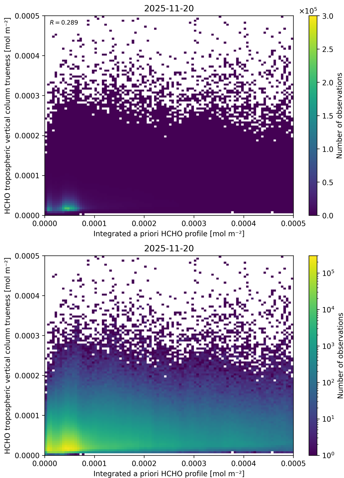
Figure 170: Scatter density plot of “Integrated a priori HCHO profile” against “HCHO tropospheric vertical column trueness” for 2025-11-19 to 2025-11-21.
