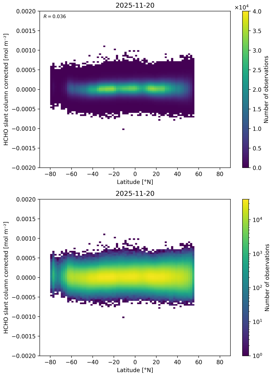
Figure 175: Scatter density plot of “Latitude” against “HCHO slant column corrected” for 2025-11-19 to 2025-11-21.
