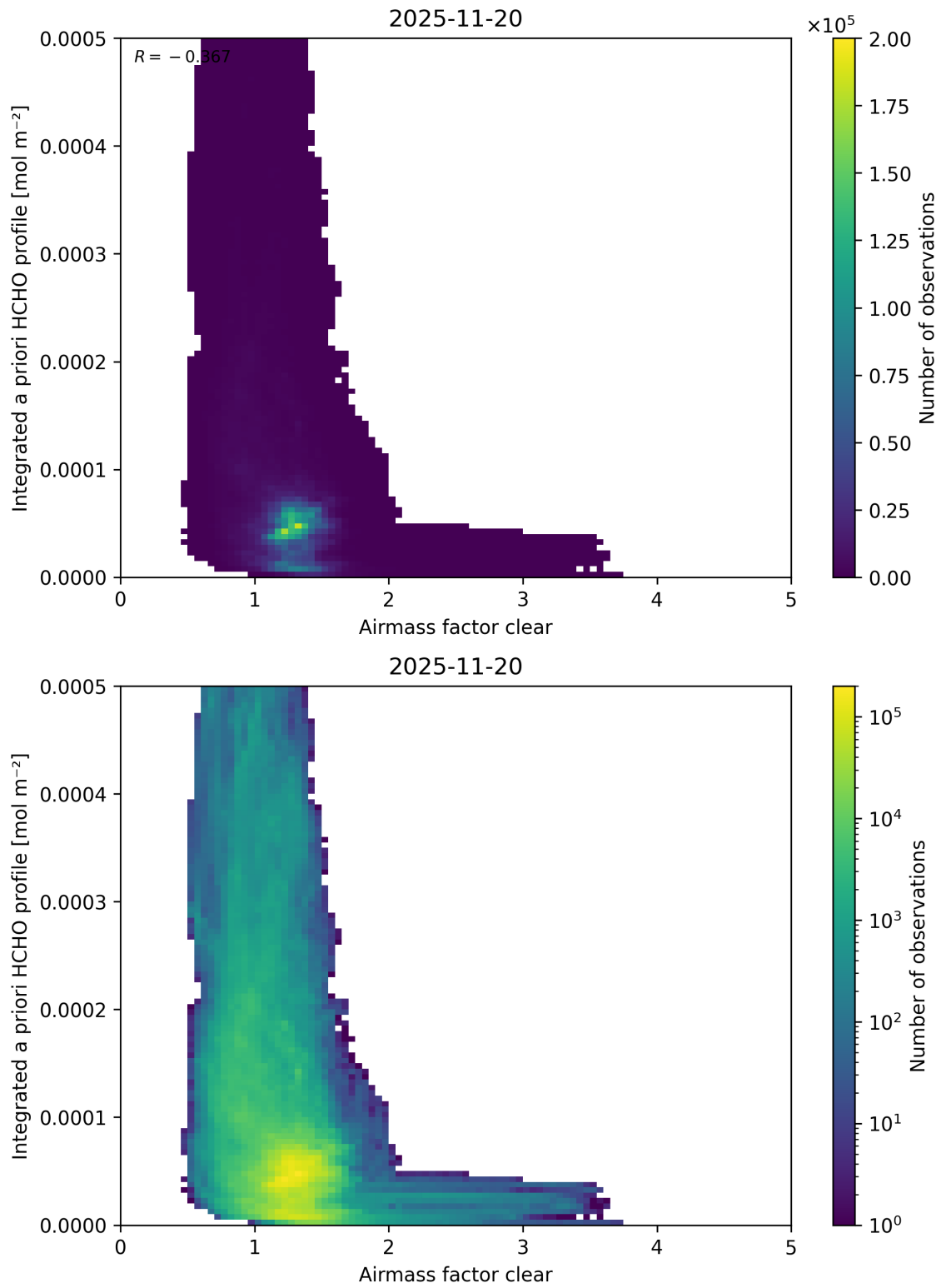
Figure 84: Scatter density plot of “Airmass factor clear” against “Integrated a priori HCHO profile” for 2025-11-19 to 2025-11-21.
