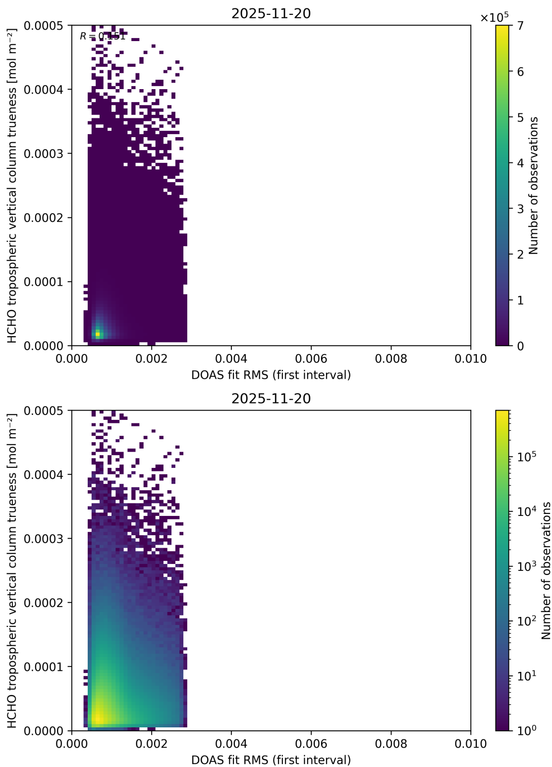
Figure 68: Scatter density plot of “DOAS fit RMS (first interval)” against “HCHO tropospheric vertical column trueness” for 2025-11-19 to 2025-11-21.
