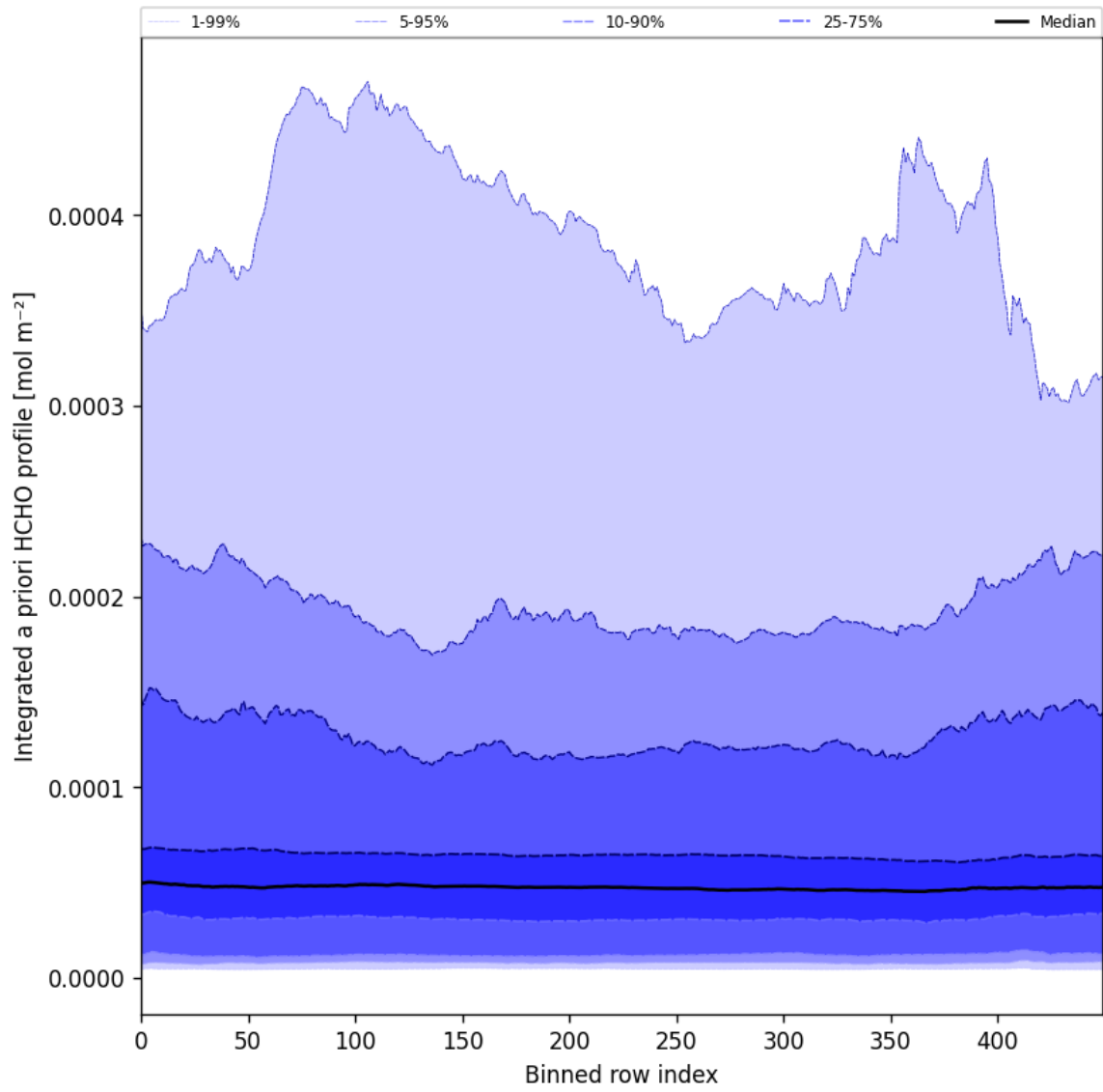
Figure 60: Along track statistics of “Integrated a priori HCHO profile” for 2025-11-19 to 2025-11-21
