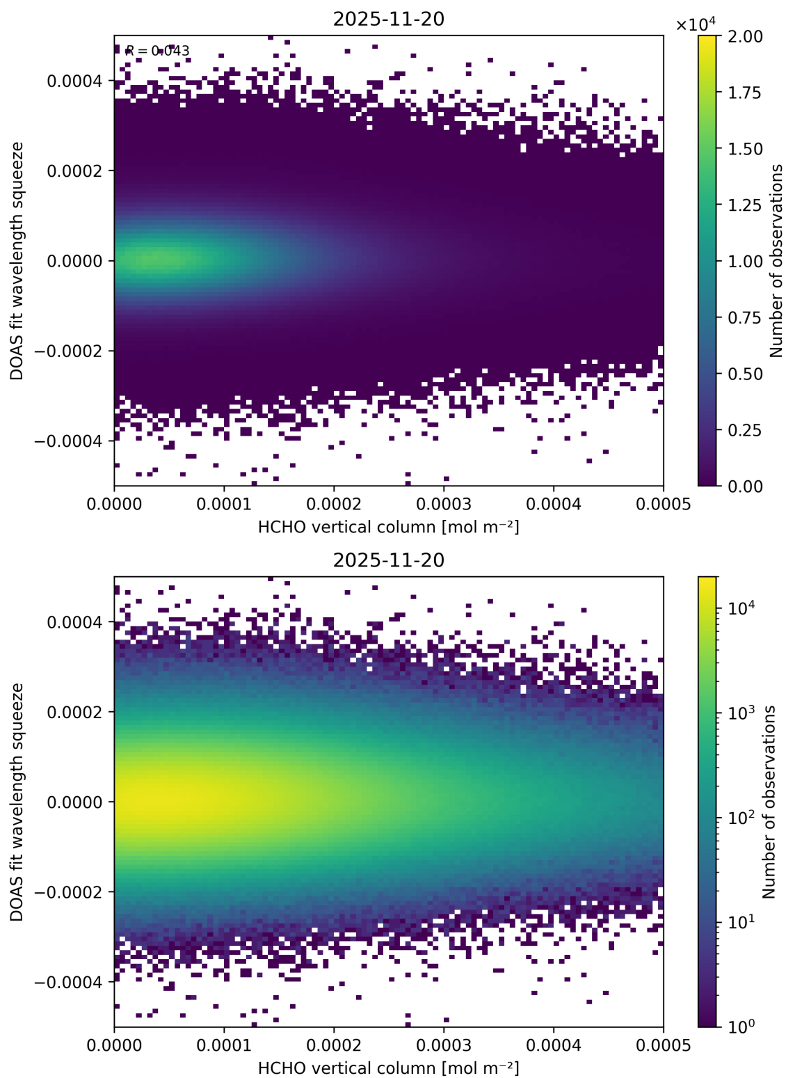
Figure 140: Scatter density plot of “HCHO vertical column” against “DOAS fit wavelength squeeze” for 2025-11-19 to 2025-11-21.
