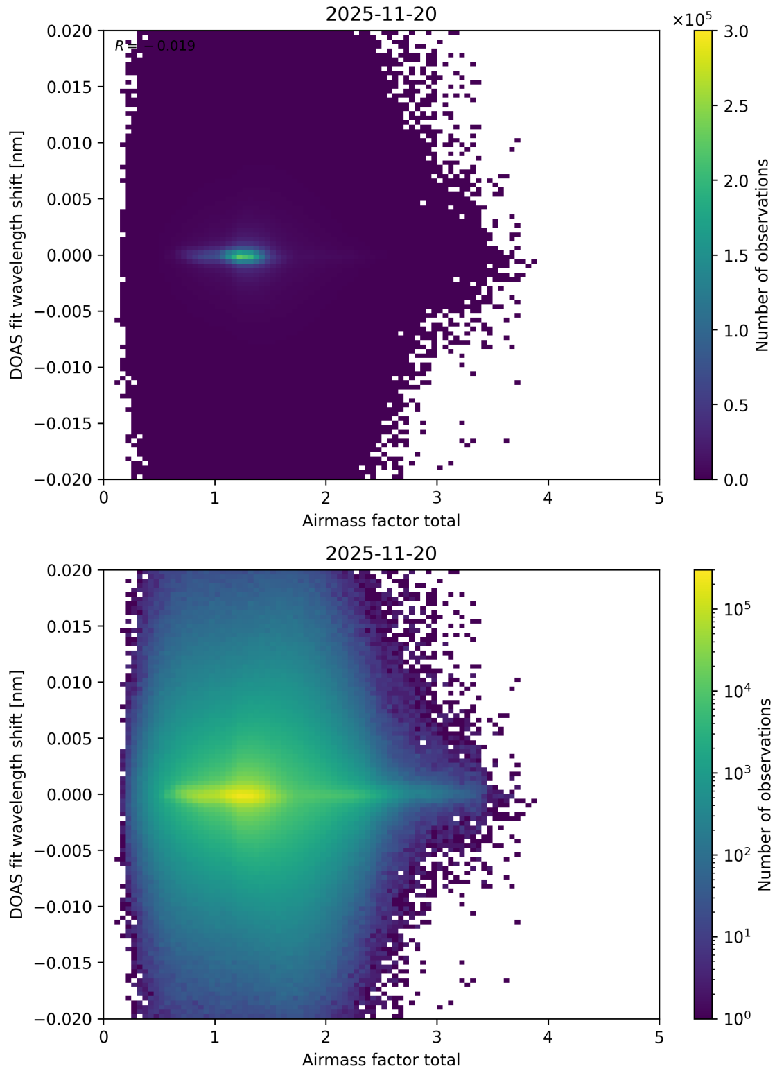
Figure 110: Scatter density plot of “Airmass factor total” against “DOAS fit wavelength shift” for 2025-11-19 to 2025-11-21.
