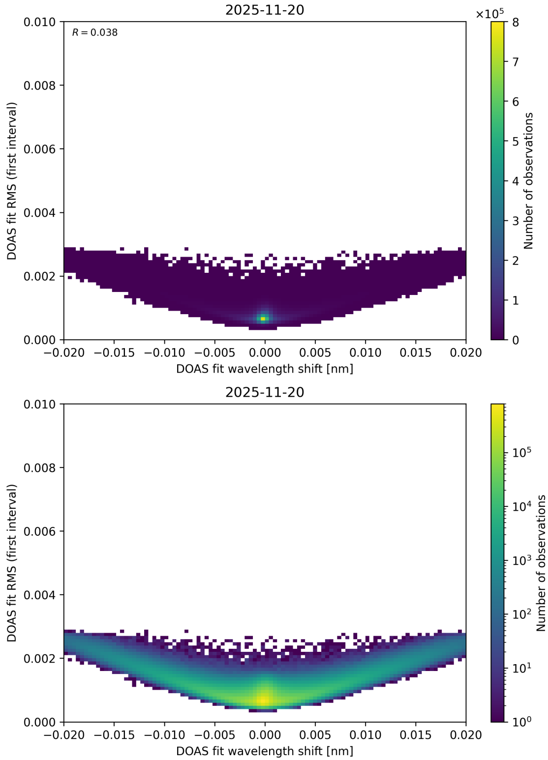
Figure 69: Scatter density plot of “DOAS fit wavelength shift” against “DOAS fit RMS (first interval)” for 2025-11-19 to 2025-11-21.
