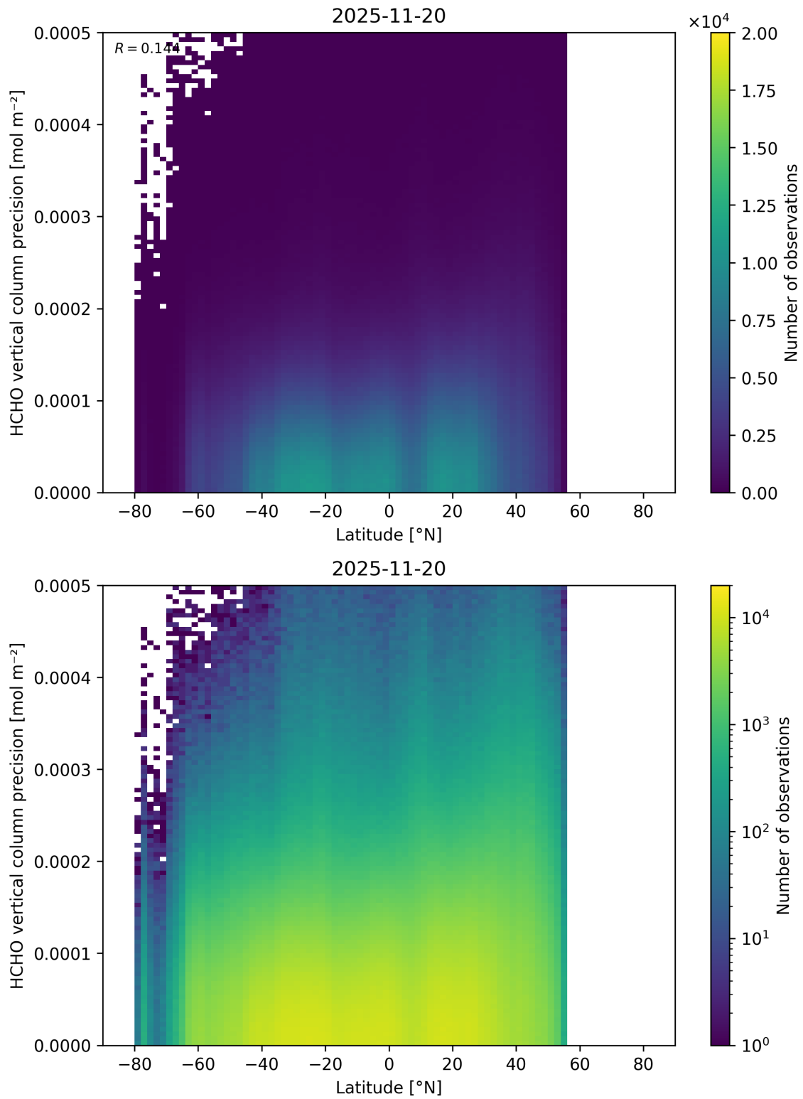
Figure 183: Scatter density plot of “Latitude” against “HCHO vertical column precision” for 2025-11-19 to 2025-11-21.
