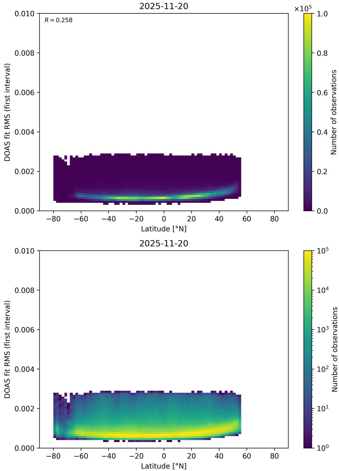
Figure 171: Scatter density plot of “Latitude” against “DOAS fit RMS (first interval)” for 2025-11-19 to 2025-11-21.
