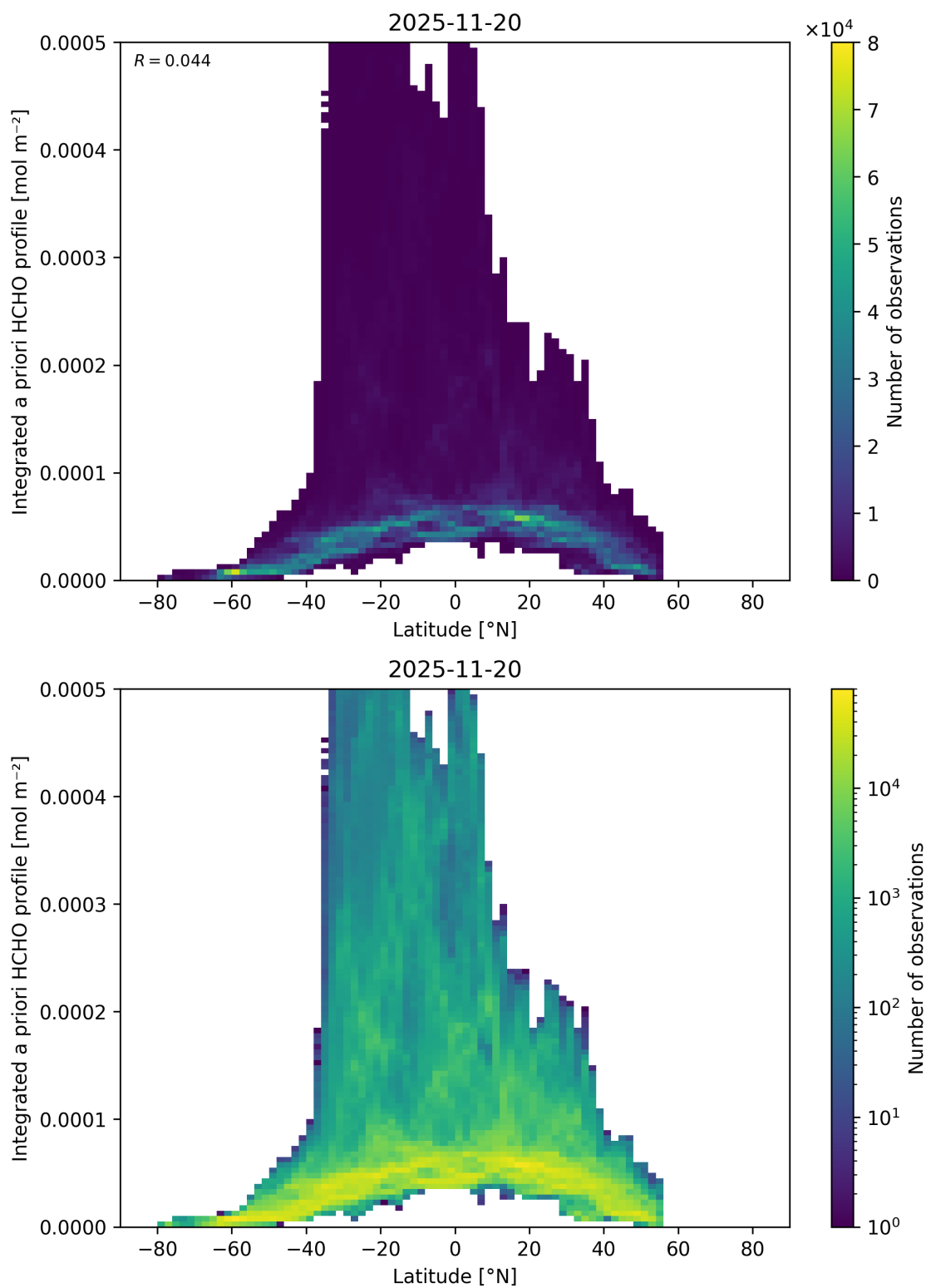
Figure 185: Scatter density plot of “Latitude” against “Integrated a priori HCHO profile” for 2025-11-19 to 2025-11-21.
