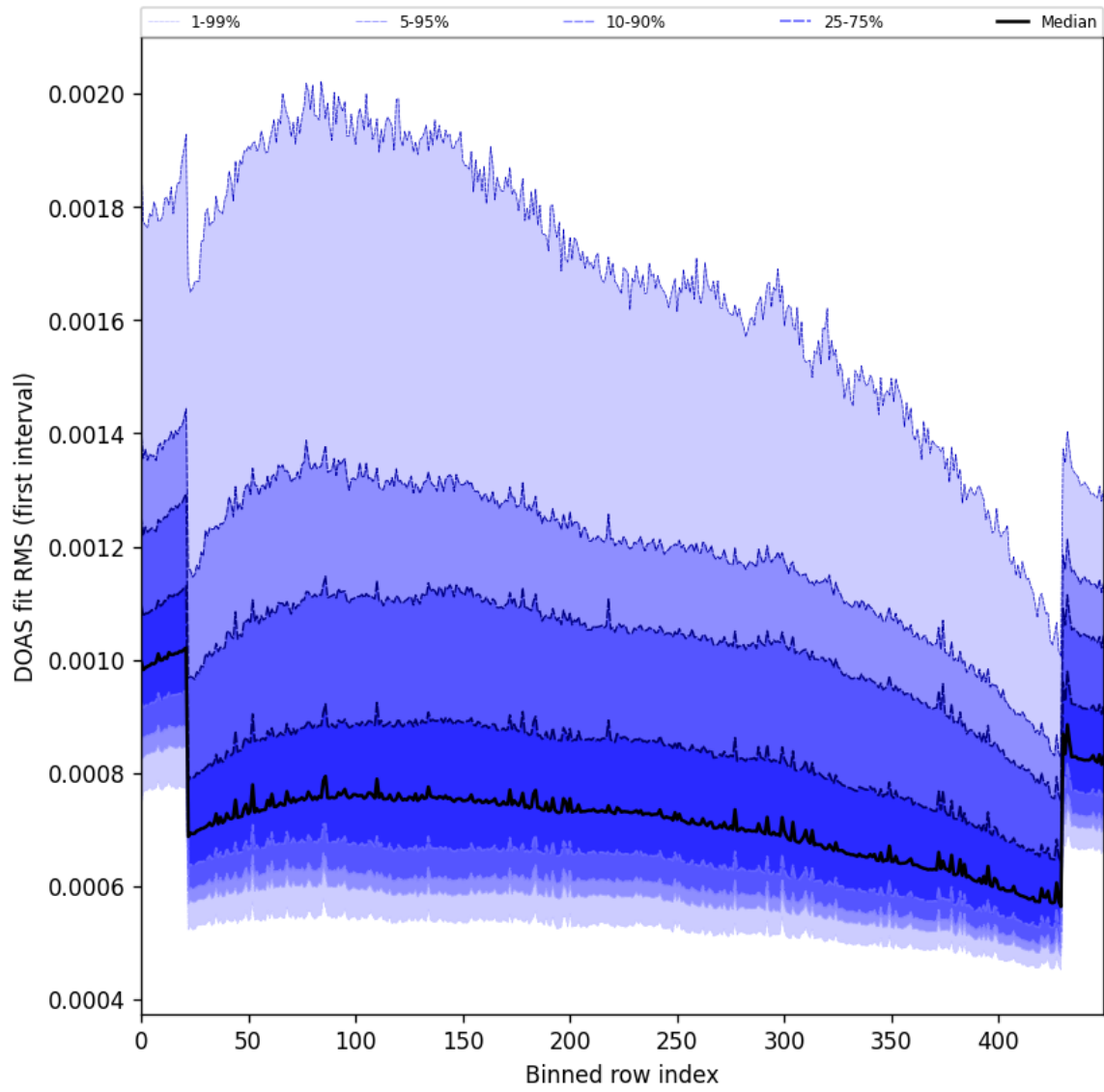
Figure 63: Along track statistics of “DOAS fit RMS (first interval)” for 2025-11-19 to 2025-11-21
