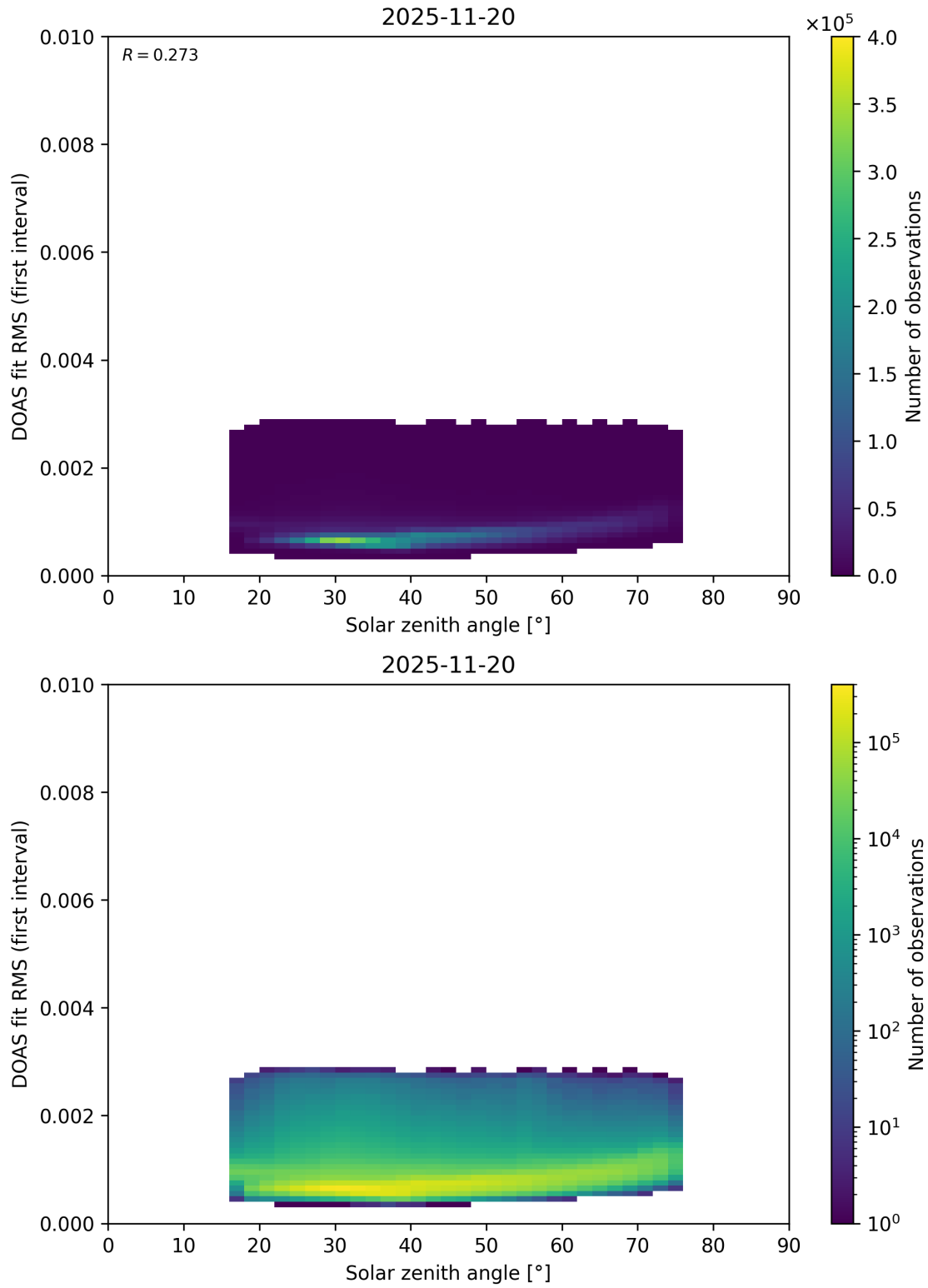
Figure 186: Scatter density plot of “Solar zenith angle” against “DOAS fit RMS (first interval)” for 2025-11-19 to 2025-11-21.
