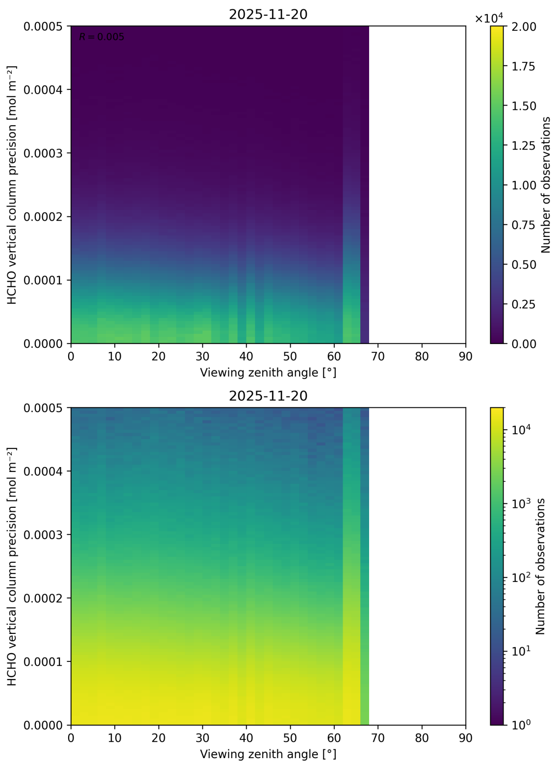
Figure 214: Scatter density plot of “Viewing zenith angle” against “HCHO vertical column precision” for 2025-11-19 to 2025-11-21.
