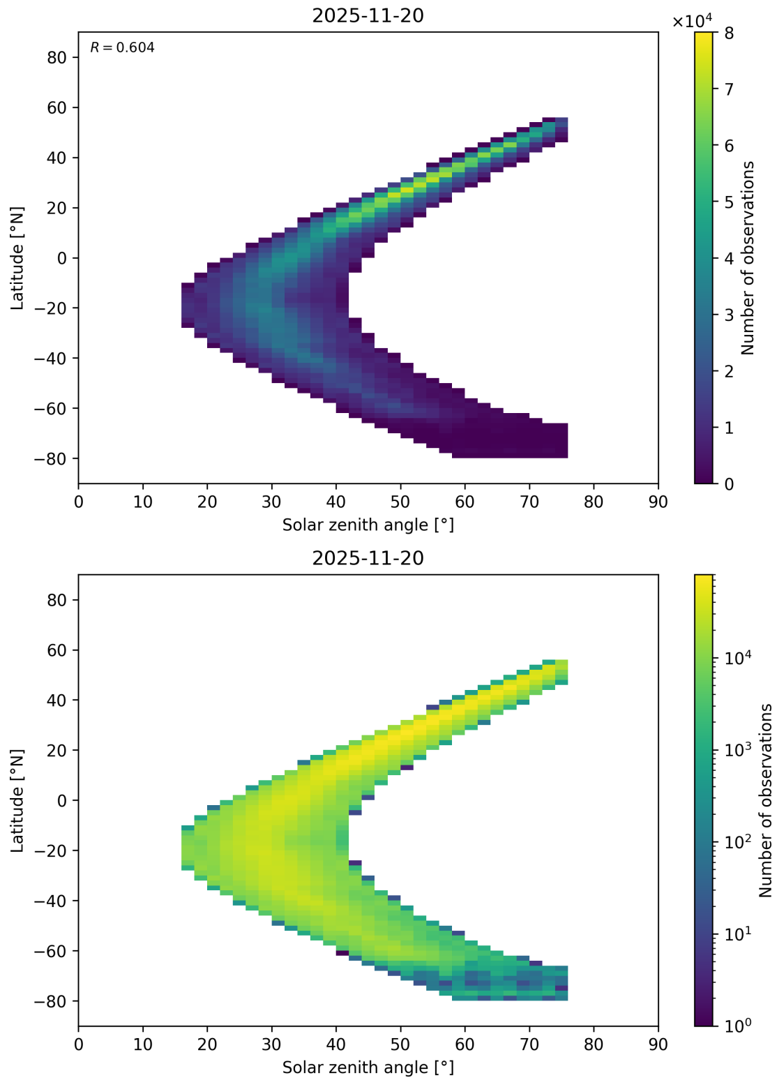
Figure 201: Scatter density plot of “Solar zenith angle” against “Latitude” for 2025-11-19 to 2025-11-21.
