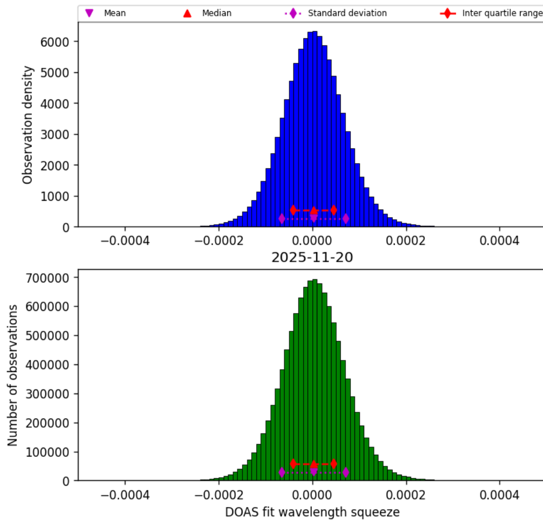
Figure 47: Histogram of “DOAS fit wavelength squeeze” for 2025-11-19 to 2025-11-21
