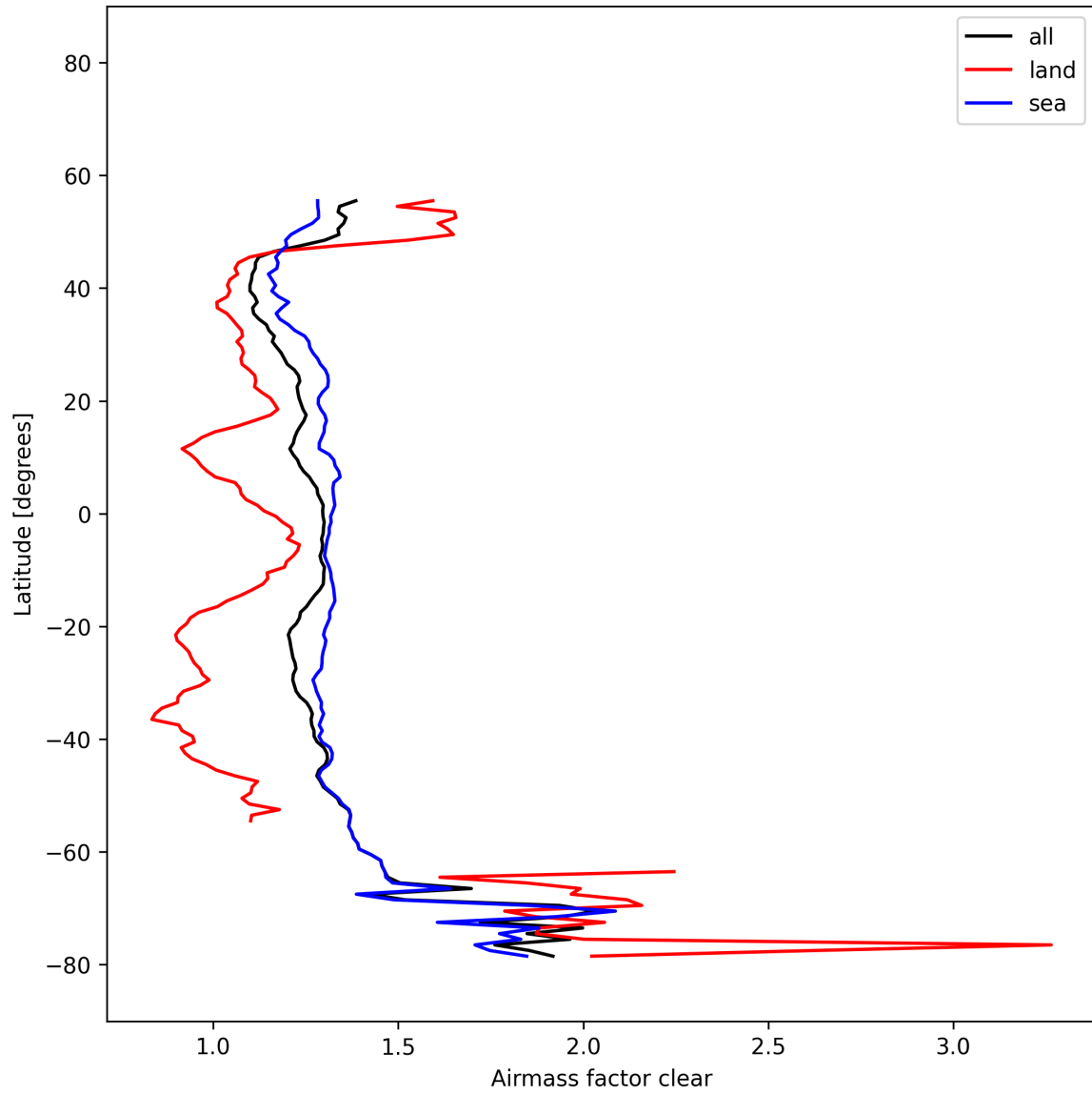
Figure 29: Zonal average of “Airmass factor clear” for 2025-11-19 to 2025-11-21.
