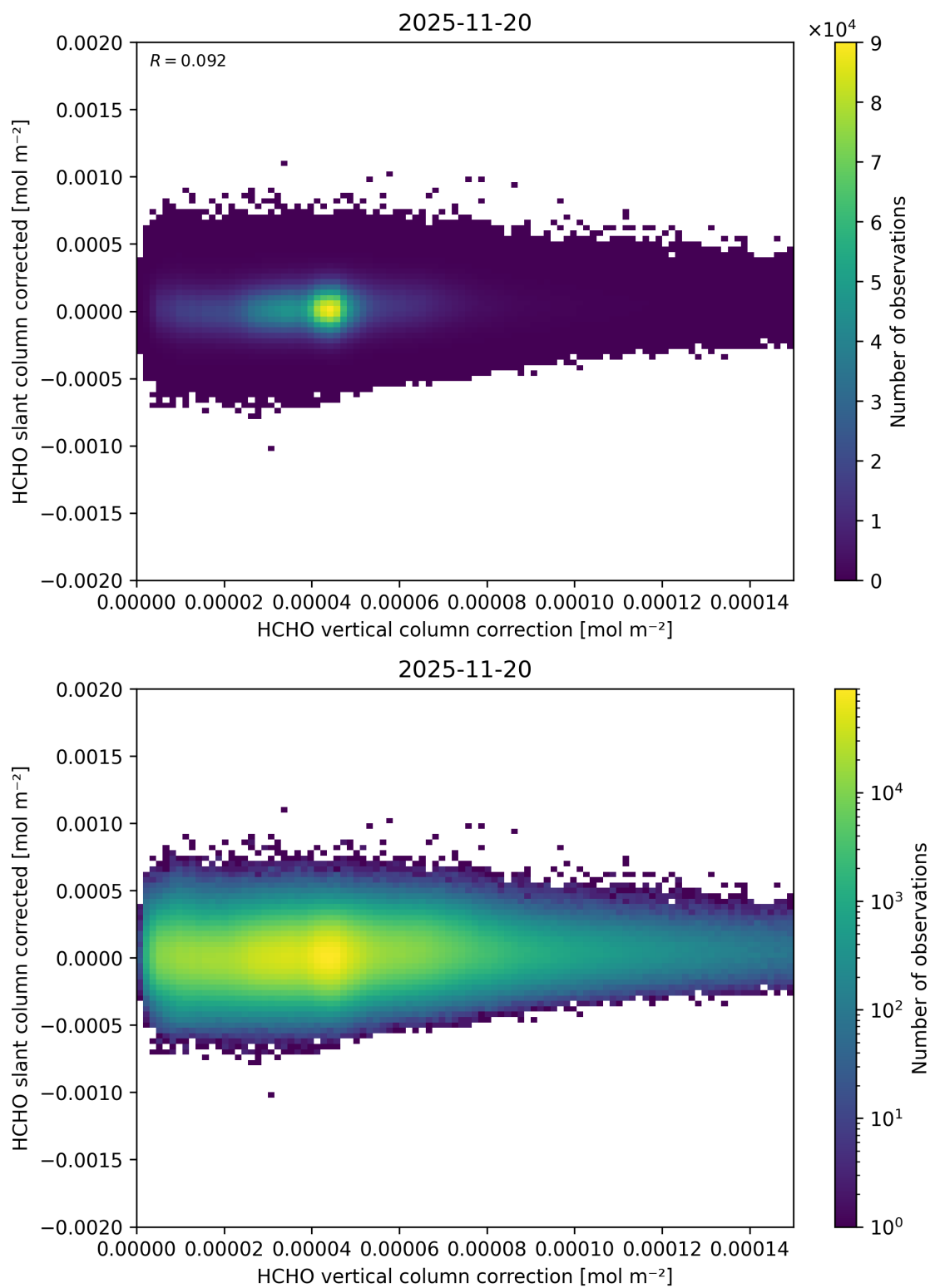
Figure 130: Scatter density plot of “HCHO vertical column correction” against “HCHO slant column corrected” for 2025-11-19 to 2025-11-21.
