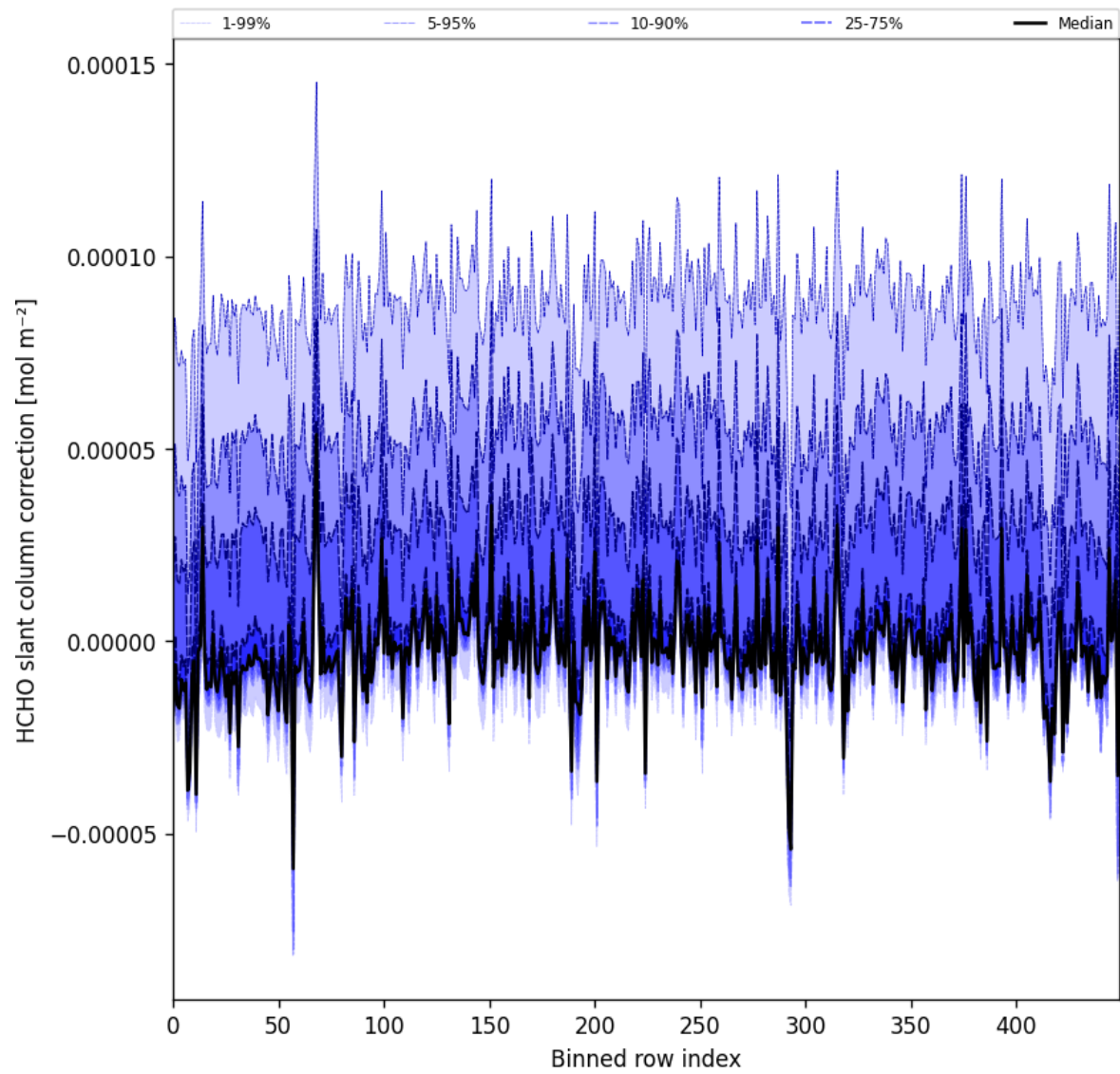
Figure 64: Along track statistics of “HCHO slant column correction” for 2025-11-19 to 2025-11-21
