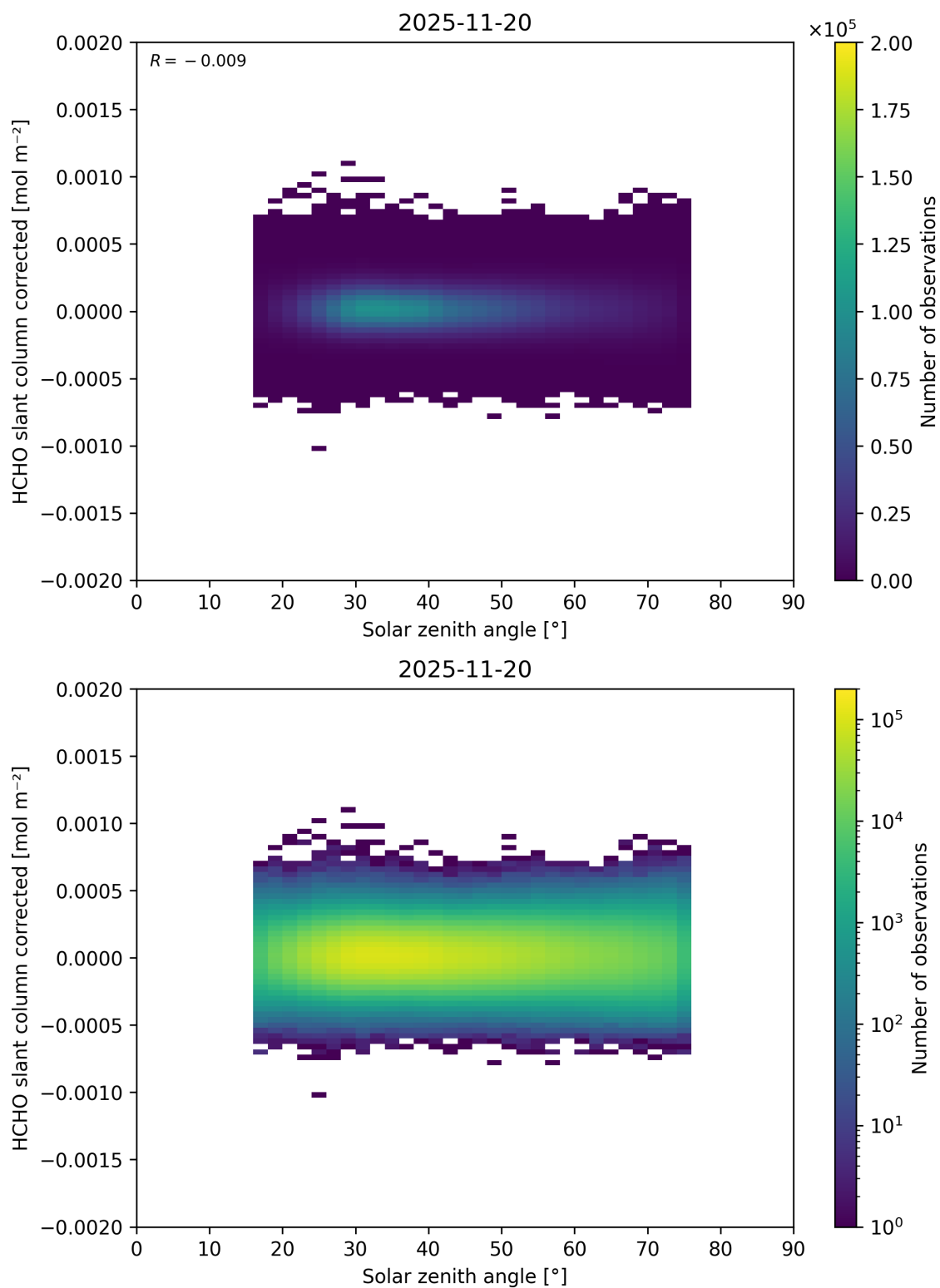
Figure 190: Scatter density plot of “Solar zenith angle” against “HCHO slant column corrected” for 2025-11-19 to 2025-11-21.
