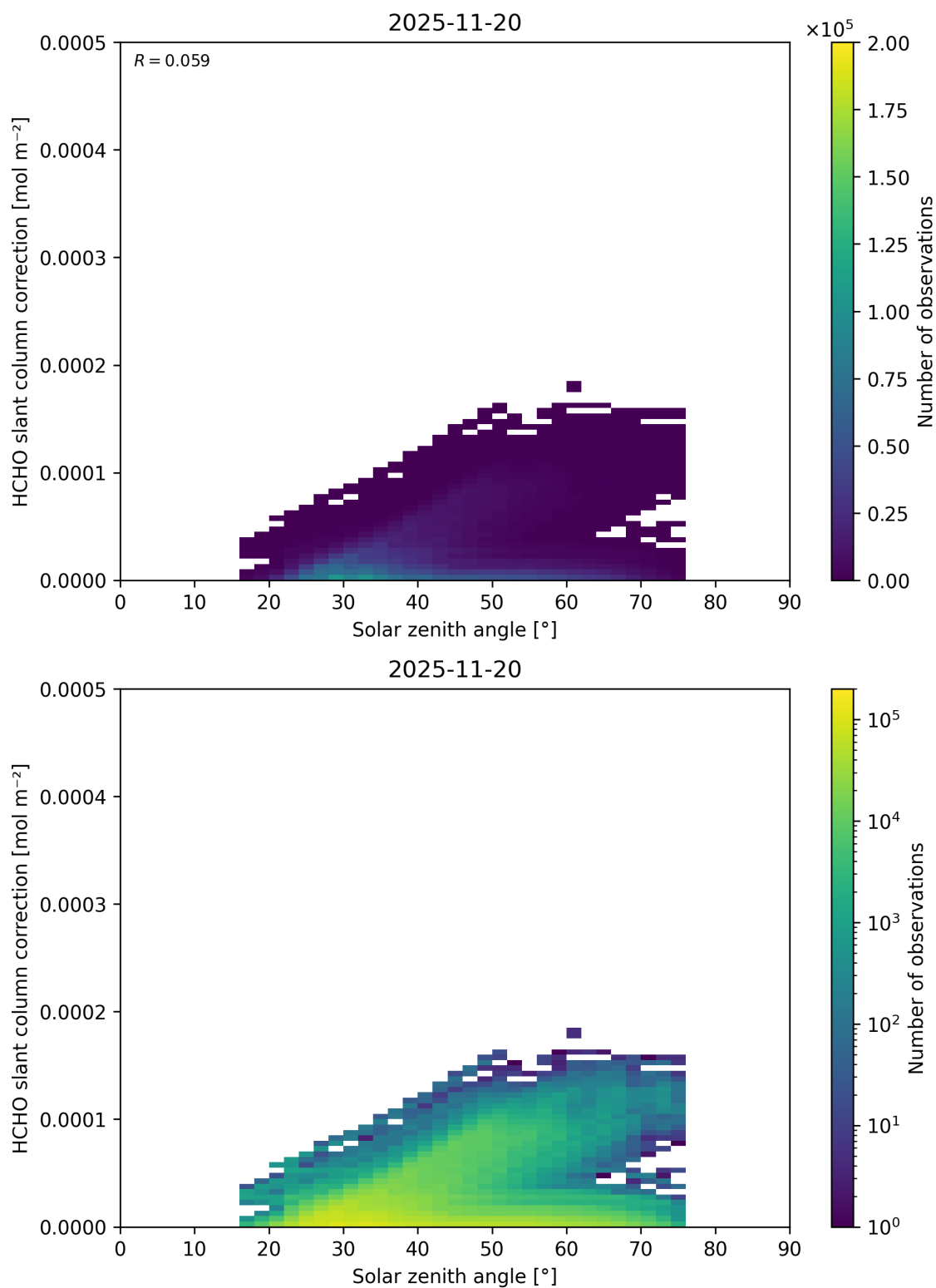
Figure 191: Scatter density plot of “Solar zenith angle” against “HCHO slant column correction” for 2025-11-19 to 2025-11-21.
