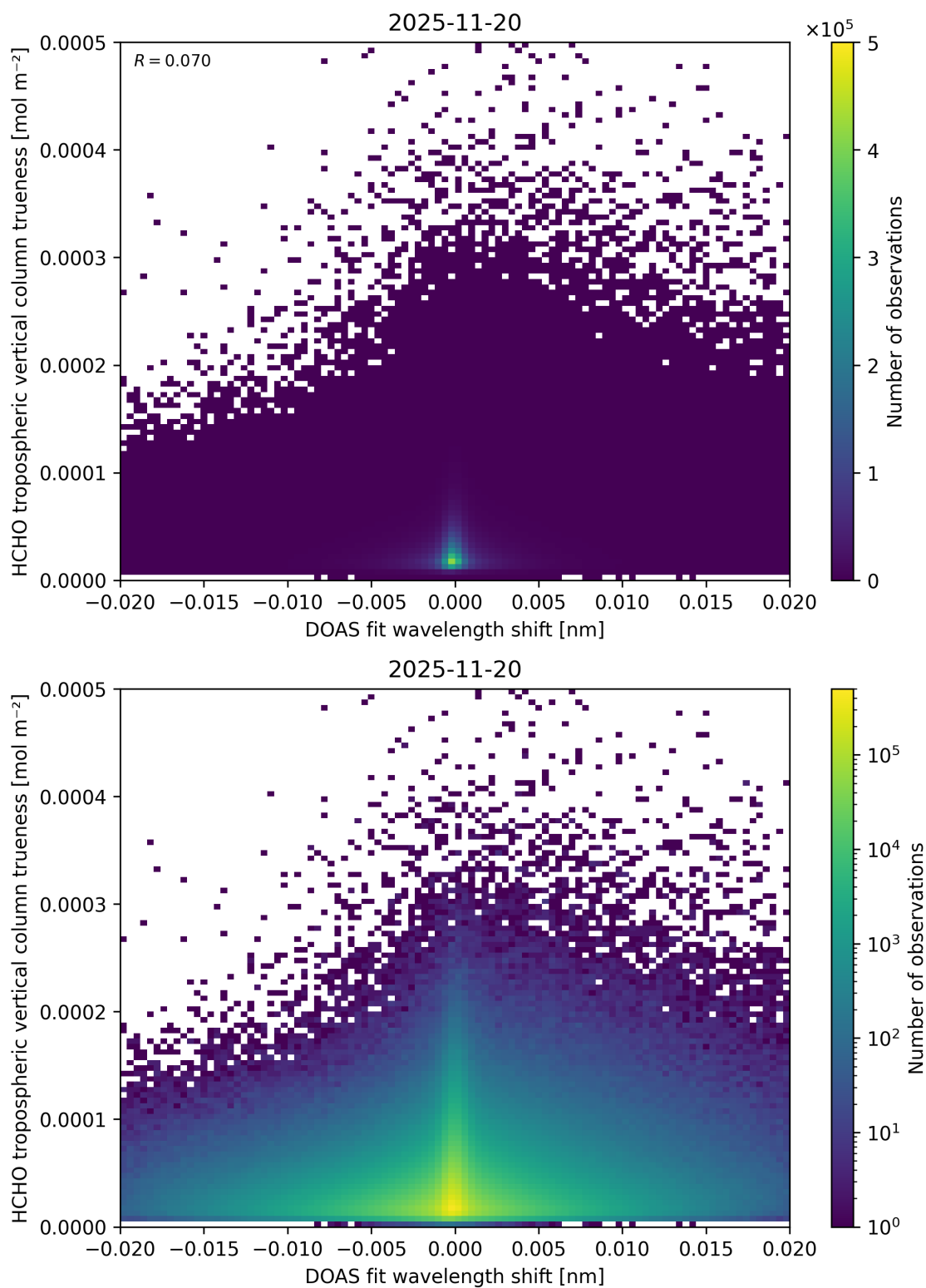
Figure 73: Scatter density plot of “DOAS fit wavelength shift” against “HCHO tropospheric vertical column trueness” for 2025-11-19 to 2025-11-21.
