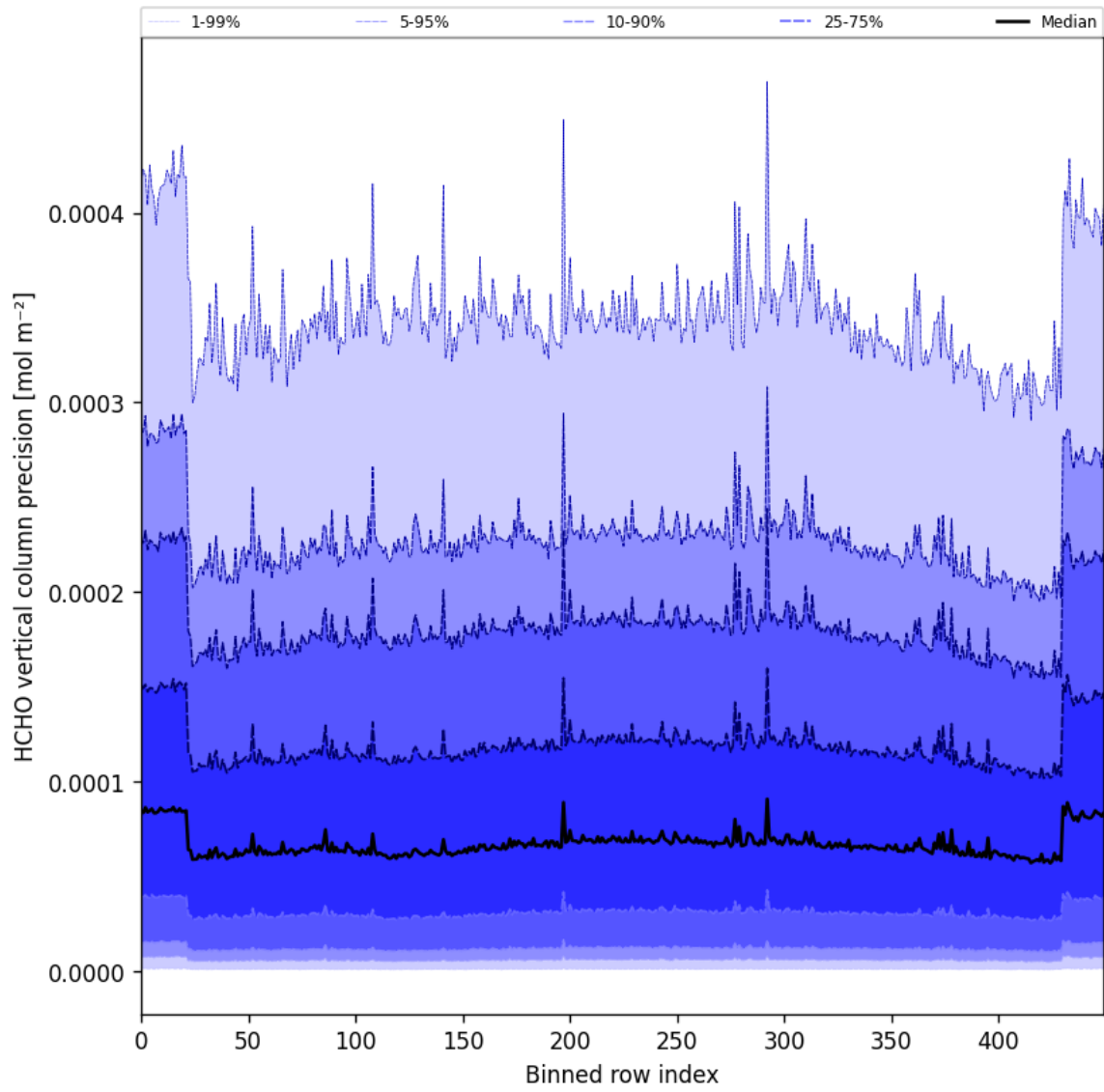
Figure 53: Along track statistics of “HCHO vertical column precision” for 2025-11-19 to 2025-11-21
