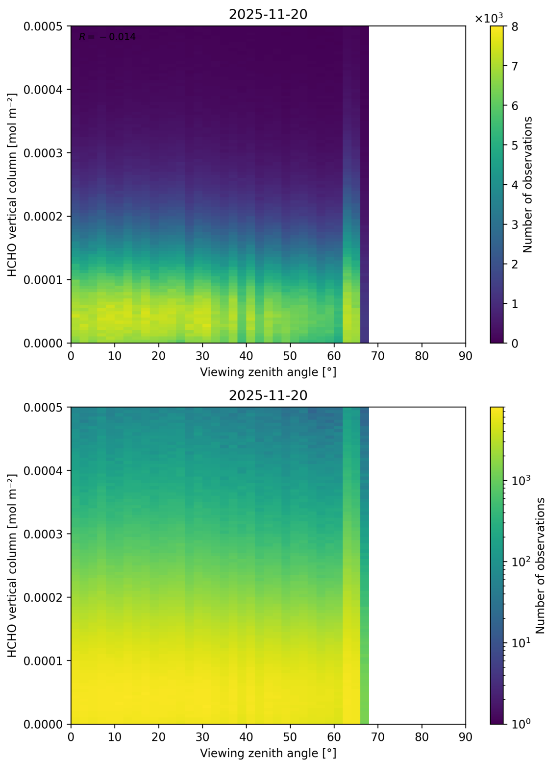
Figure 212: Scatter density plot of “Viewing zenith angle” against “HCHO vertical column” for 2025-11-19 to 2025-11-21.
