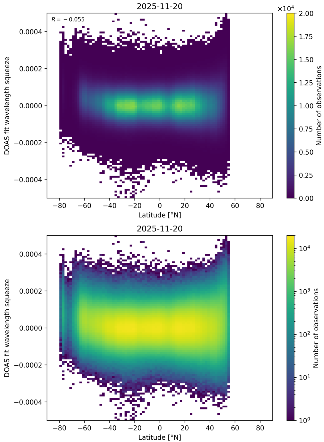
Figure 173: Scatter density plot of “Latitude” against “DOAS fit wavelength squeeze” for 2025-11-19 to 2025-11-21.
