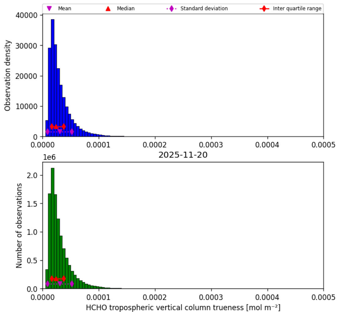
Figure 50: Histogram of “HCHO tropospheric vertical column trueness” for 2025-11-19 to 2025-11-21
