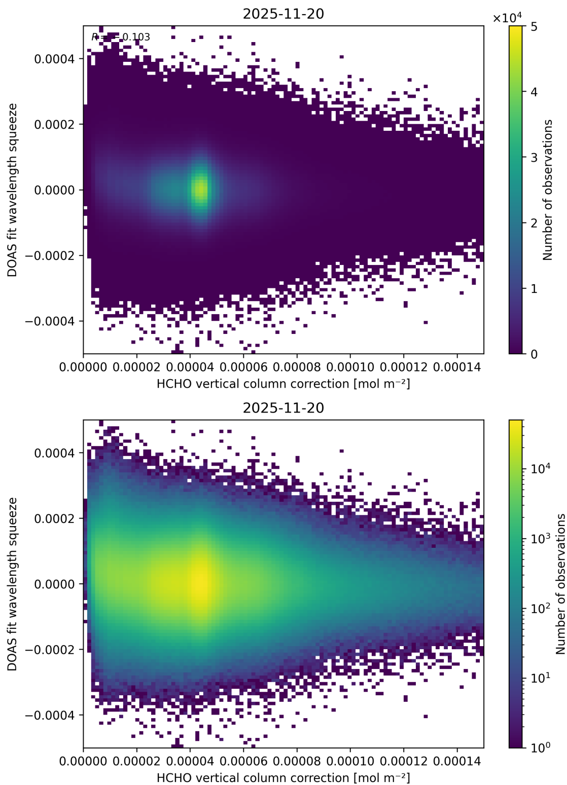
Figure 128: Scatter density plot of “HCHO vertical column correction” against “DOAS fit wavelength squeeze” for 2025-11-19 to 2025-11-21.
