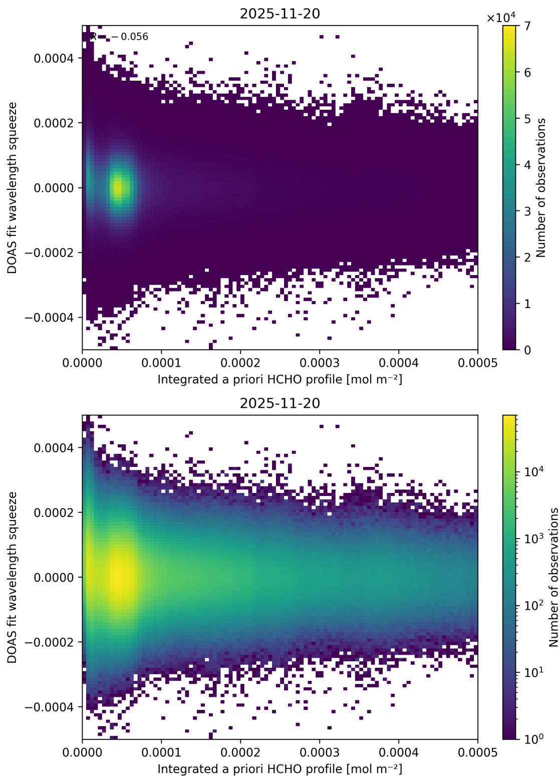
Figure 167: Scatter density plot of “Integrated a priori HCHO profile” against “DOAS fit wavelength squeeze” for 2025-11-19 to 2025-11-21.
