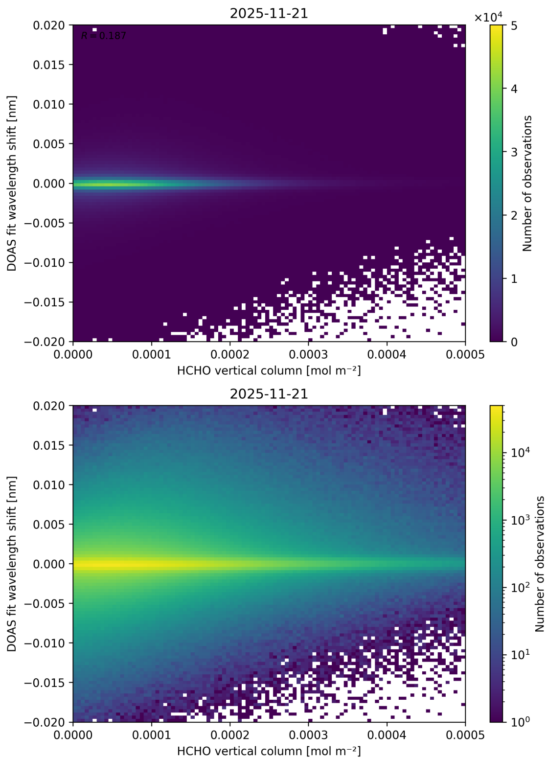
Figure 139: Scatter density plot of “HCHO vertical column” against “DOAS fit wavelength shift” for 2025-11-20 to 2025-11-22.
