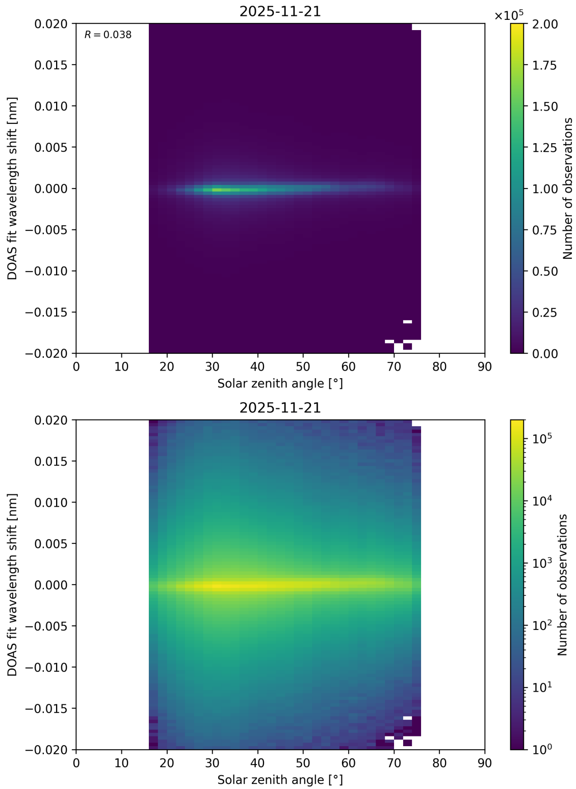
Figure 187: Scatter density plot of “Solar zenith angle” against “DOAS fit wavelength shift” for 2025-11-20 to 2025-11-22.
