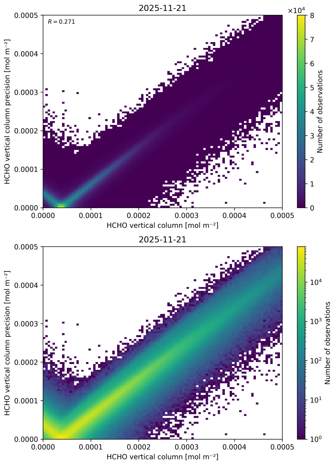
Figure 149: Scatter density plot of “HCHO vertical column” against “HCHO vertical column precision” for 2025-11-20 to 2025-11-22.
