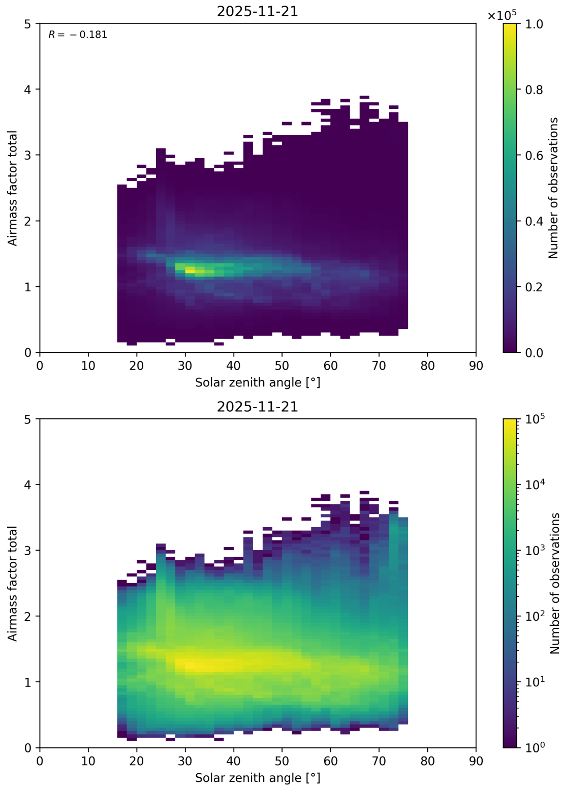
Figure 194: Scatter density plot of “Solar zenith angle” against “Airmass factor total” for 2025-11-20 to 2025-11-22.
