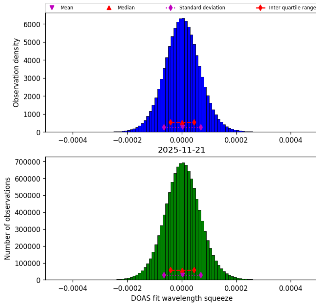
Figure 47: Histogram of “DOAS fit wavelength squeeze” for 2025-11-20 to 2025-11-22
