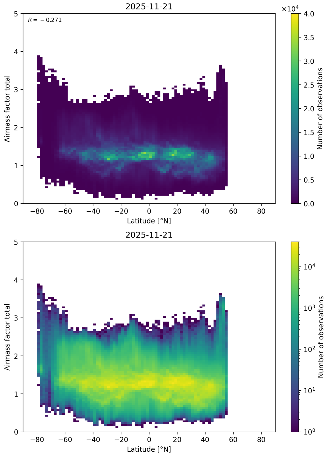
Figure 179: Scatter density plot of “Latitude” against “Airmass factor total” for 2025-11-20 to 2025-11-22.
