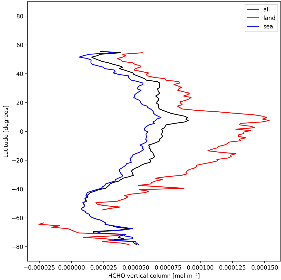
Figure 22: Zonal average of “HCHO vertical column” for 2025-11-20 to 2025-11-22.
