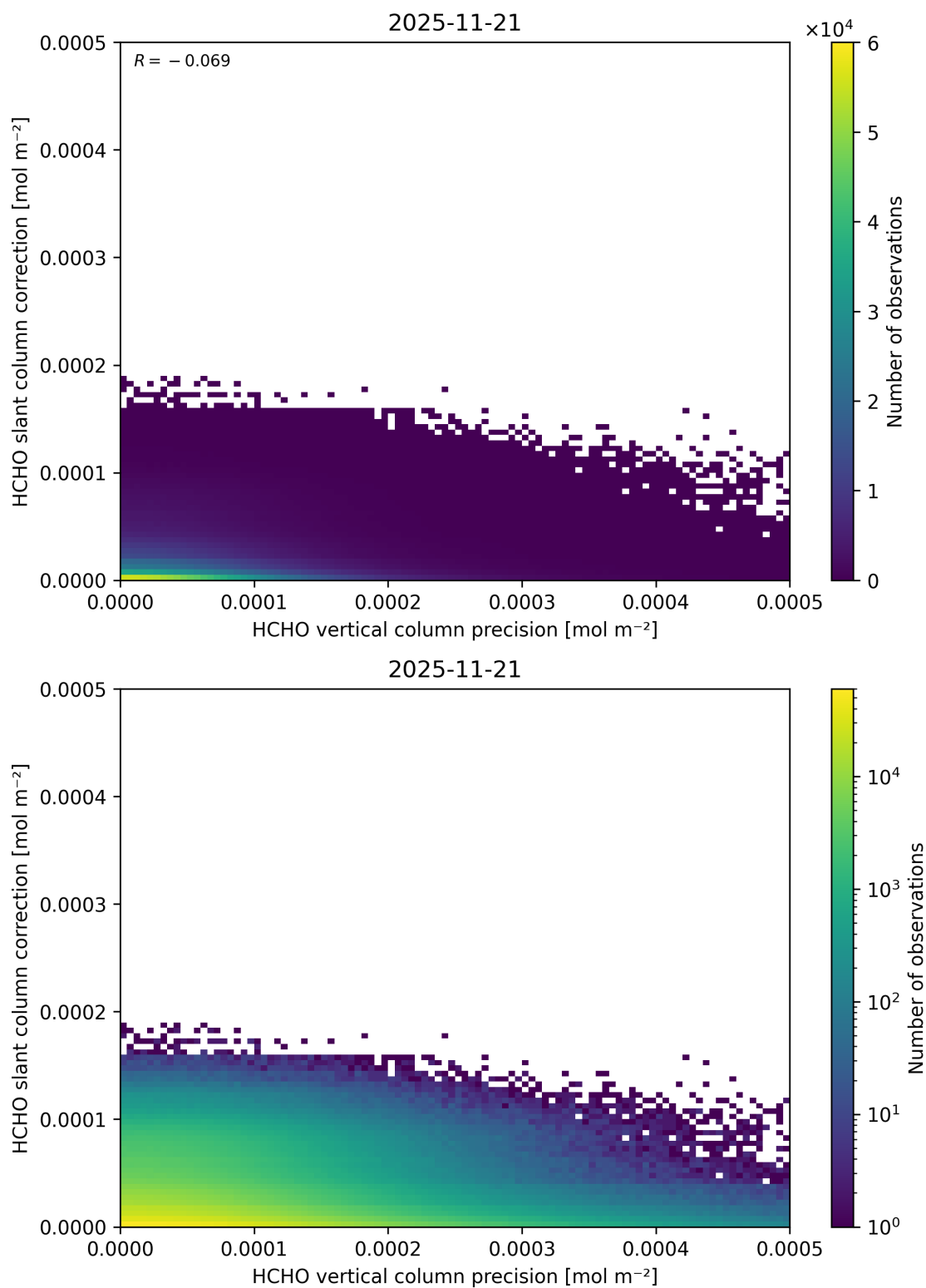
Figure 157: Scatter density plot of “HCHO vertical column precision” against “HCHO slant column correction” for 2025-11-20 to 2025-11-22.
