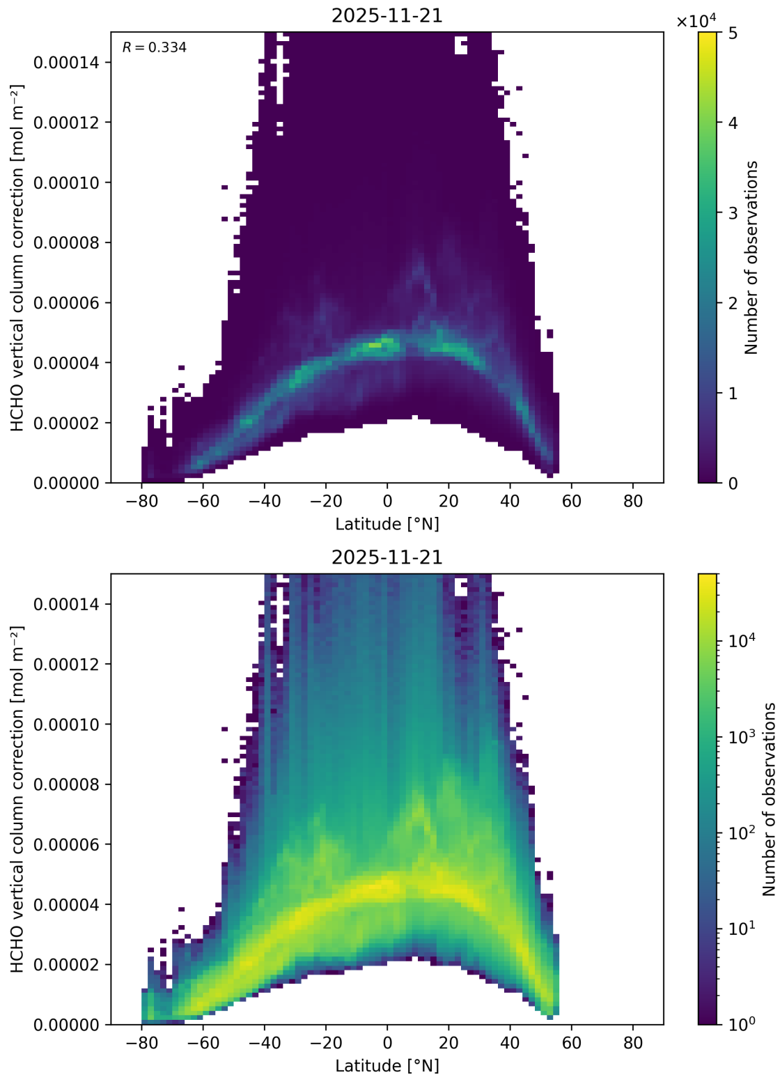
Figure 182: Scatter density plot of “Latitude” against “HCHO vertical column correction” for 2025-11-20 to 2025-11-22.
