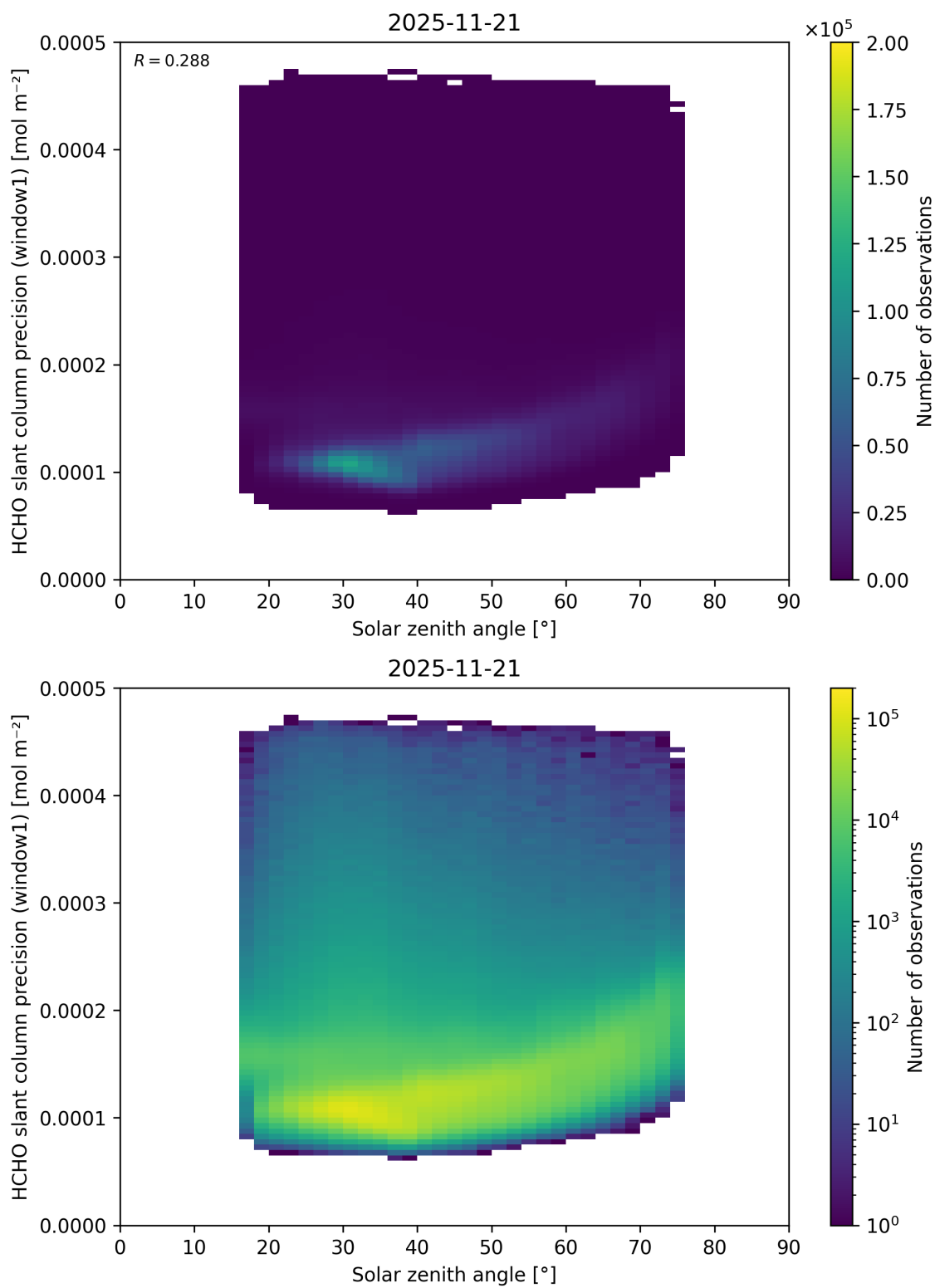
Figure 193: Scatter density plot of “Solar zenith angle” against “HCHO slant column precision (window1)” for 2025-11-20 to 2025-11-22.
