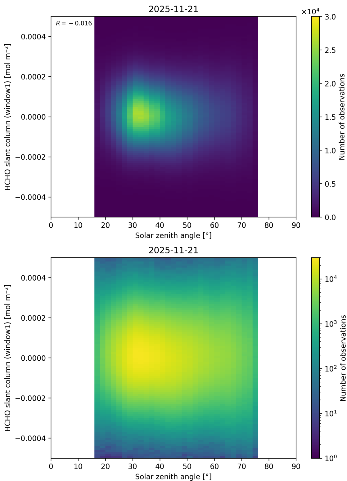
Figure 192: Scatter density plot of “Solar zenith angle” against “HCHO slant column (window1)” for 2025-11-20 to 2025-11-22.
