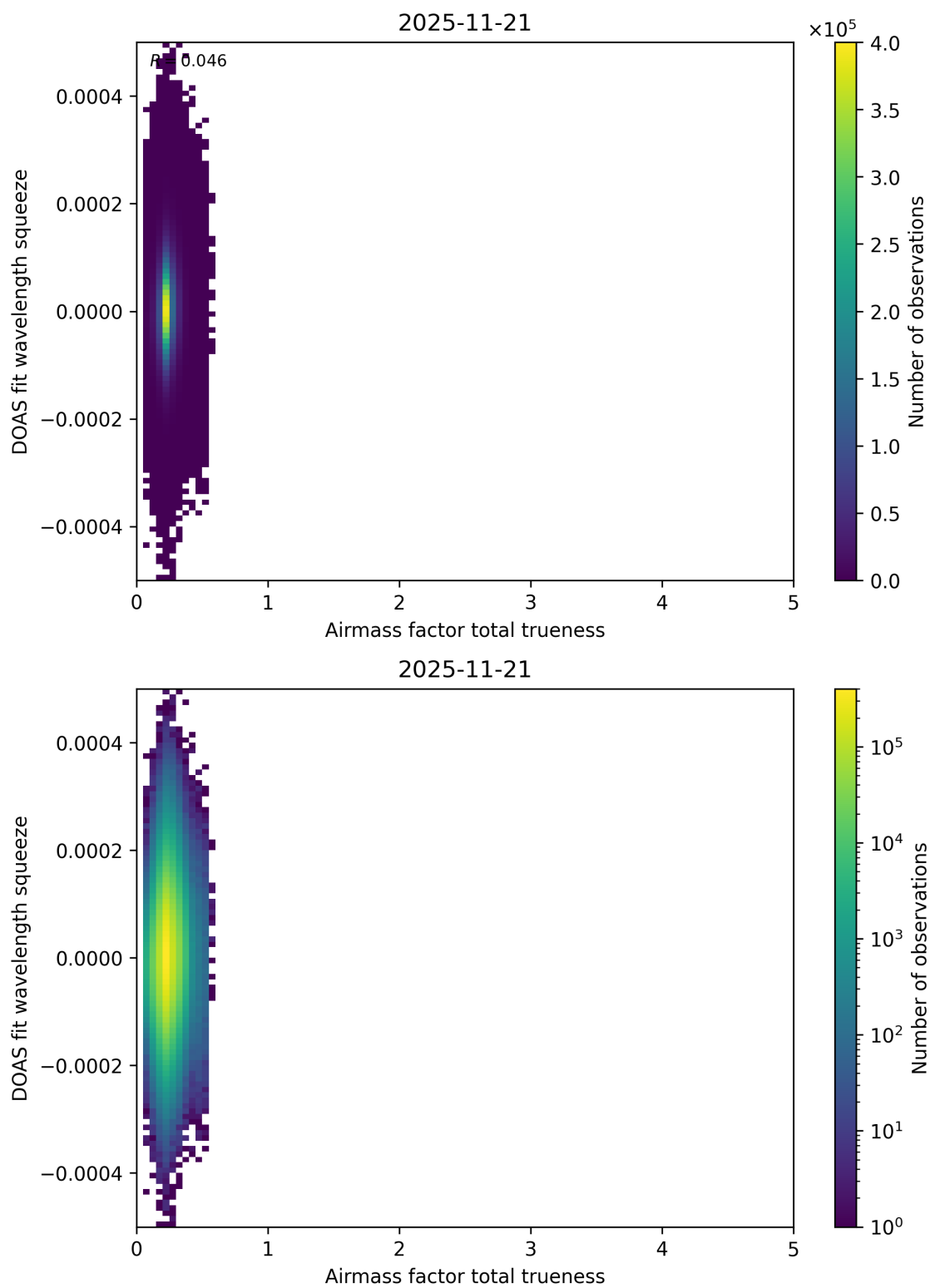
Figure 120: Scatter density plot of “Airmass factor total trueness” against “DOAS fit wavelength squeeze” for 2025-11-20 to 2025-11-22.
