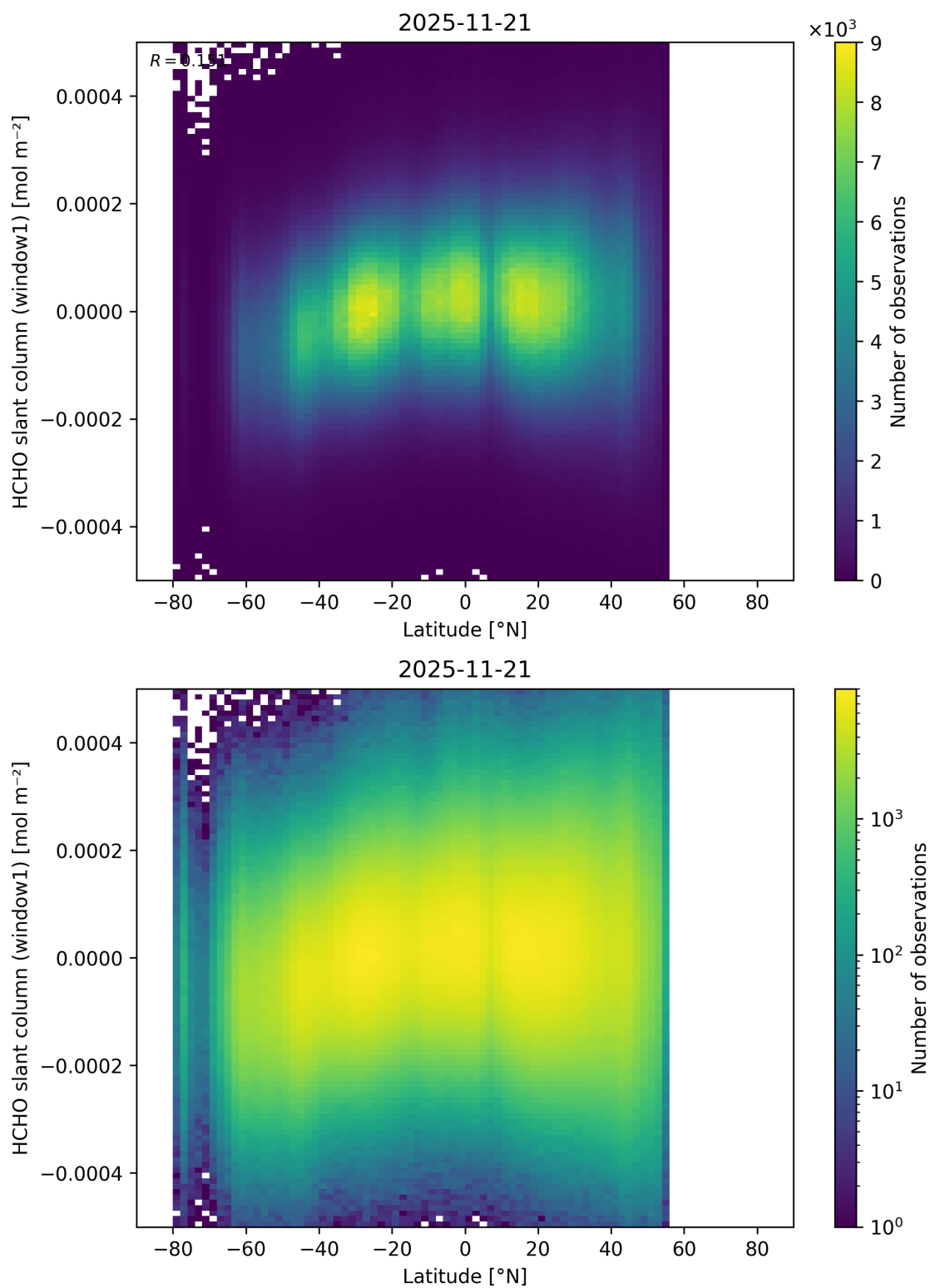
Figure 177: Scatter density plot of “Latitude” against “HCHO slant column (window1)” for 2025-11-20 to 2025-11-22.
