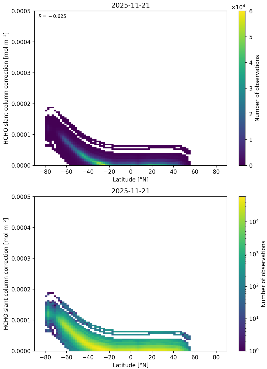
Figure 176: Scatter density plot of “Latitude” against “HCHO slant column correction” for 2025-11-20 to 2025-11-22.
