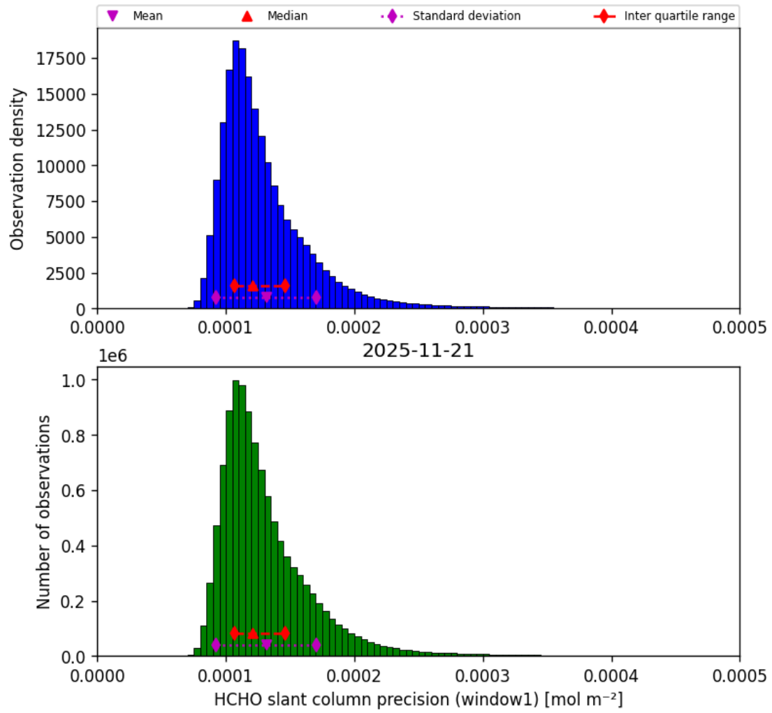
Figure 41: Histogram of “HCHO slant column precision (window1)” for 2025-11-20 to 2025-11-22
