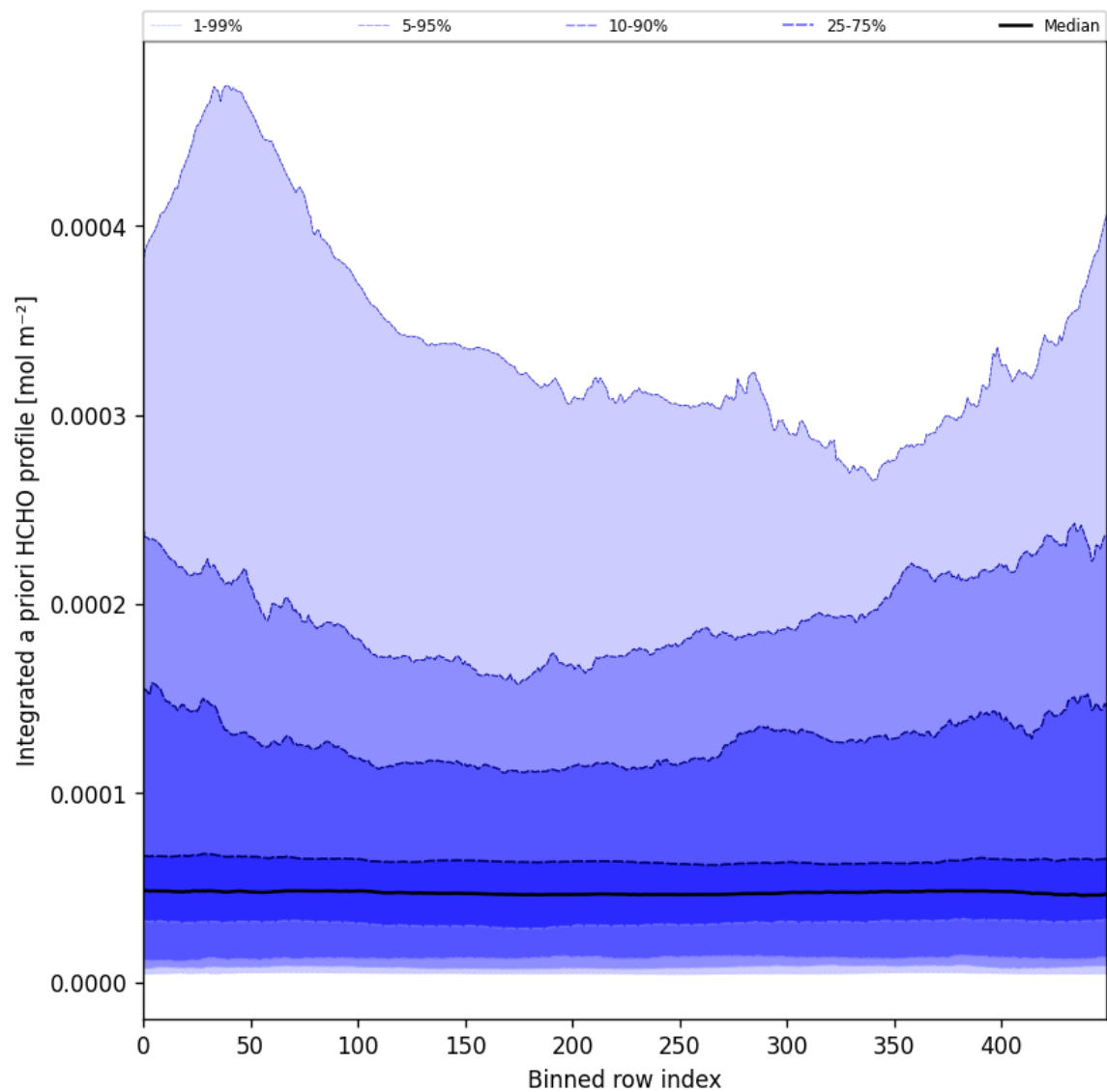
Figure 60: Along track statistics of “Integrated a priori HCHO profile” for 2025-11-20 to 2025-11-22
