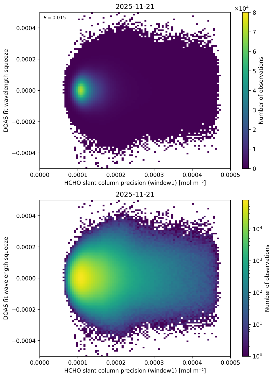
Figure 101: Scatter density plot of “HCHO slant column precision (window1)” against “DOAS fit wavelength squeeze” for 2025-11-20 to 2025-11-22.
