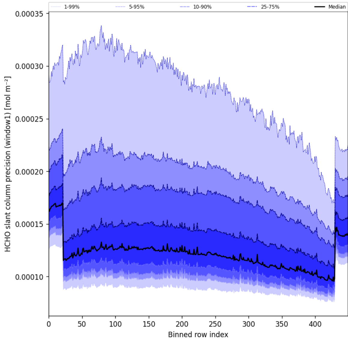
Figure 56: Along track statistics of “HCHO slant column precision (window1)” for 2025-11-20 to 2025-11-22
