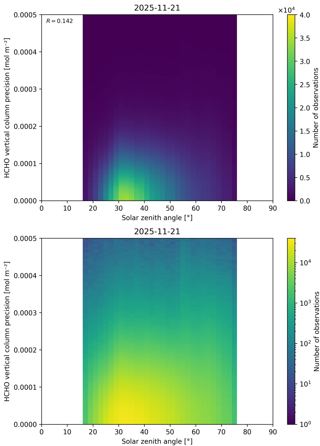
Figure 198: Scatter density plot of “Solar zenith angle” against “HCHO vertical column precision” for 2025-11-20 to 2025-11-22.
