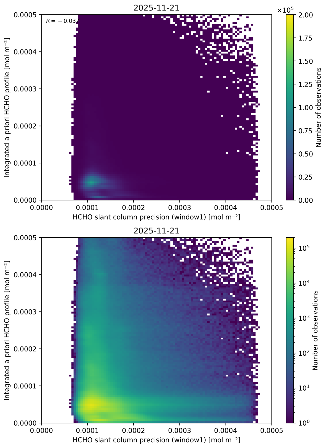
Figure 108: Scatter density plot of “HCHO slant column precision (window1)” against “Integrated a priori HCHO profile” for 2025-11-20 to 2025-11-22.
