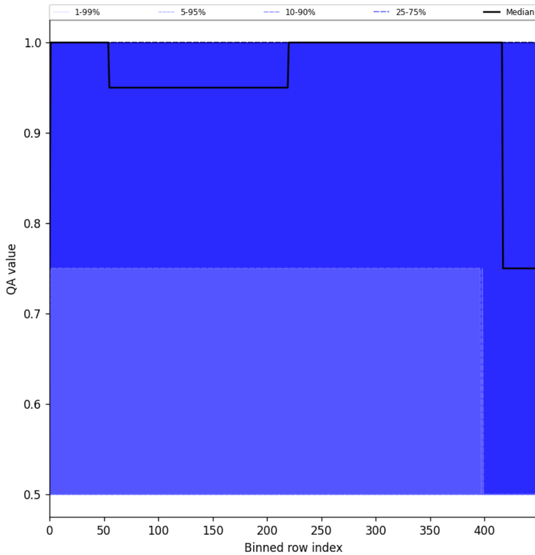
Figure 51: Along track statistics of “QA value” for 2025-11-20 to 2025-11-22
