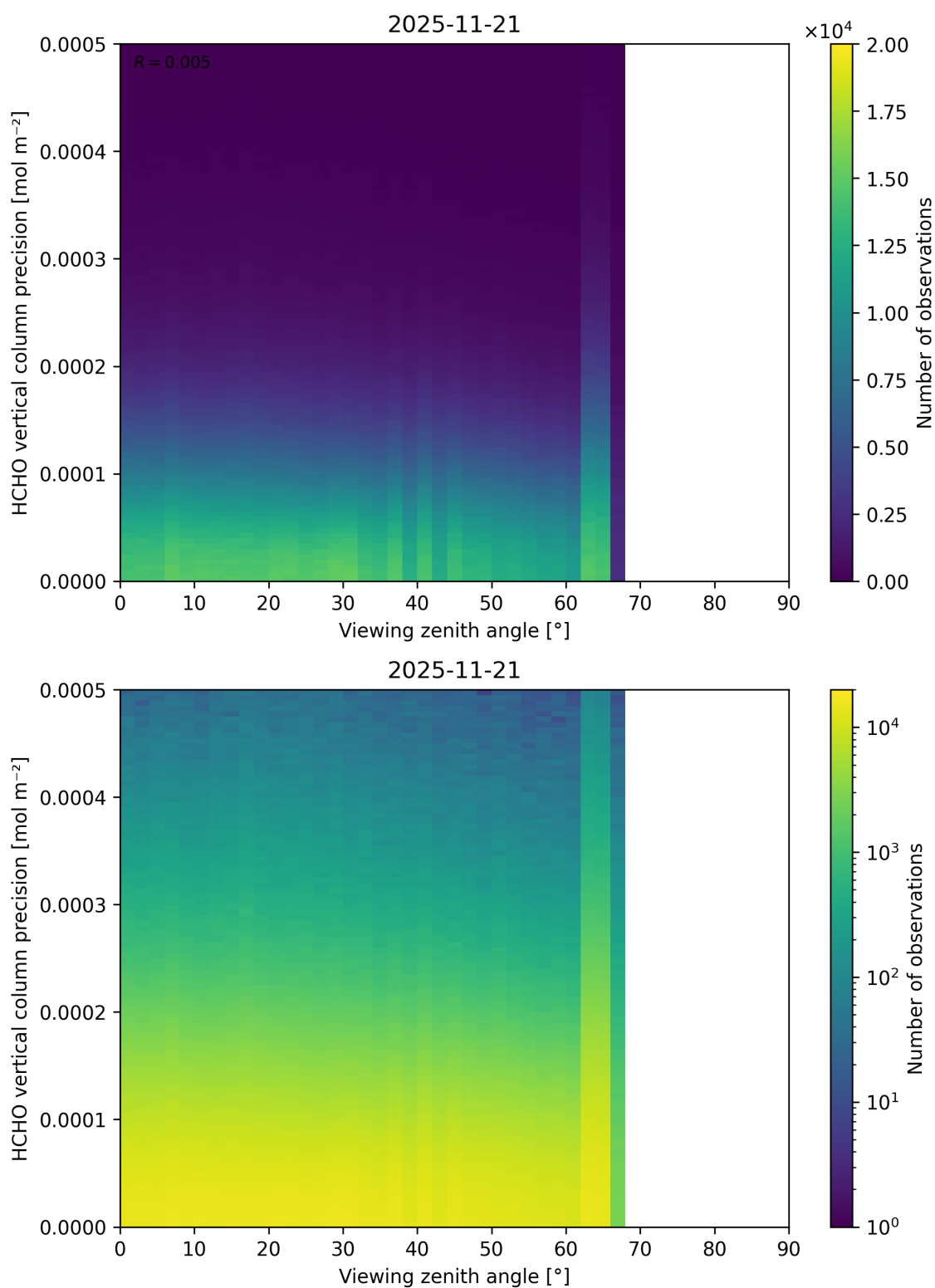
Figure 214: Scatter density plot of “Viewing zenith angle” against “HCHO vertical column precision” for 2025-11-20 to 2025-11-22.
