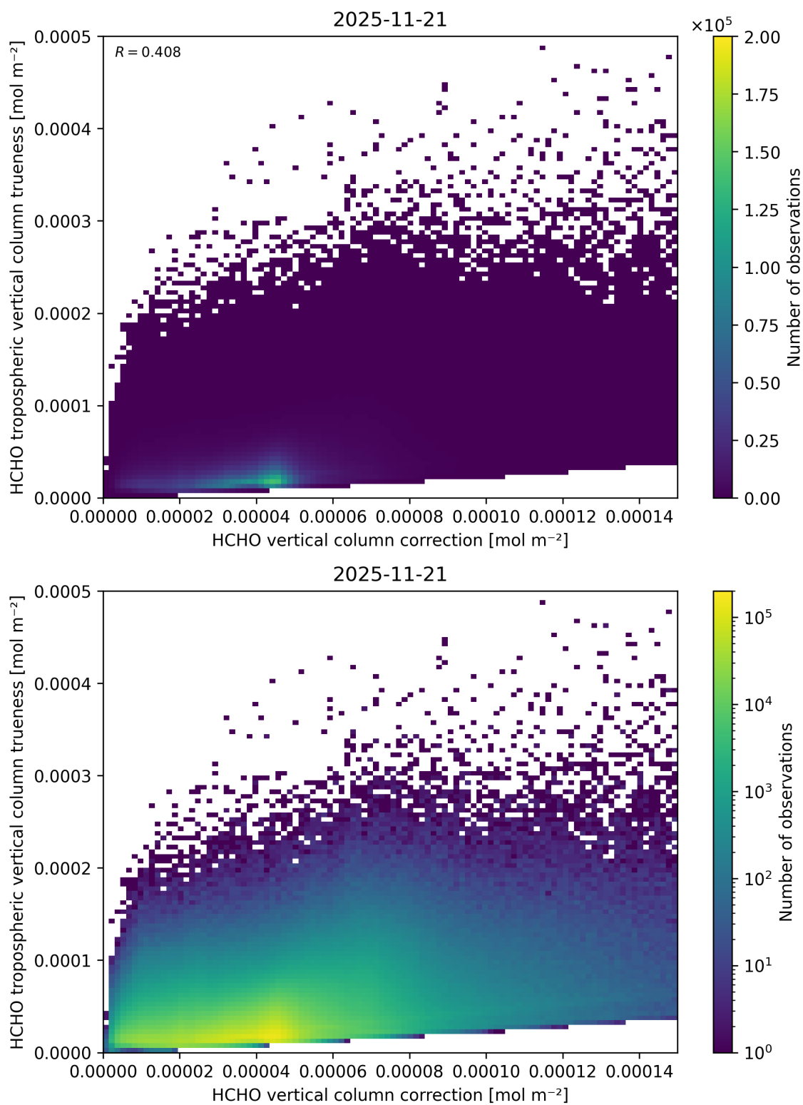
Figure 136: Scatter density plot of “HCHO vertical column correction” against “HCHO tropospheric vertical column true-ness” for 2025-11-20 to 2025-11-22.
