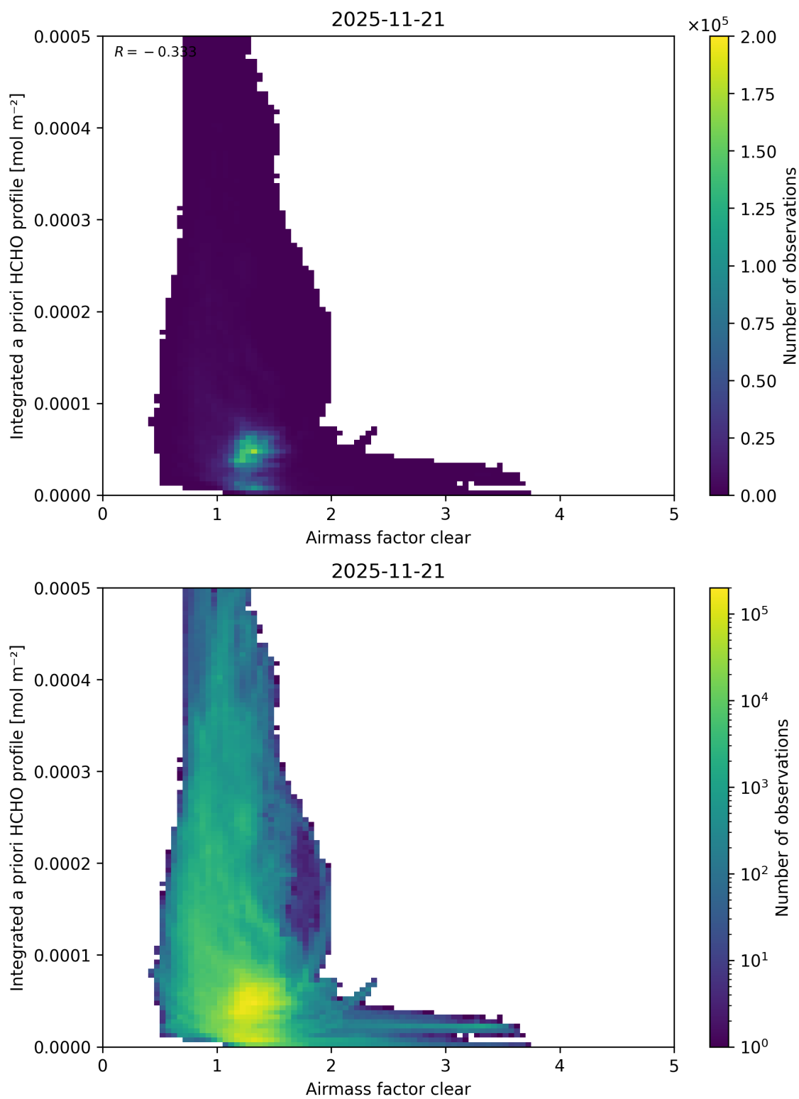
Figure 84: Scatter density plot of “Airmass factor clear” against “Integrated a priori HCHO profile” for 2025-11-20 to 2025-11-22.
