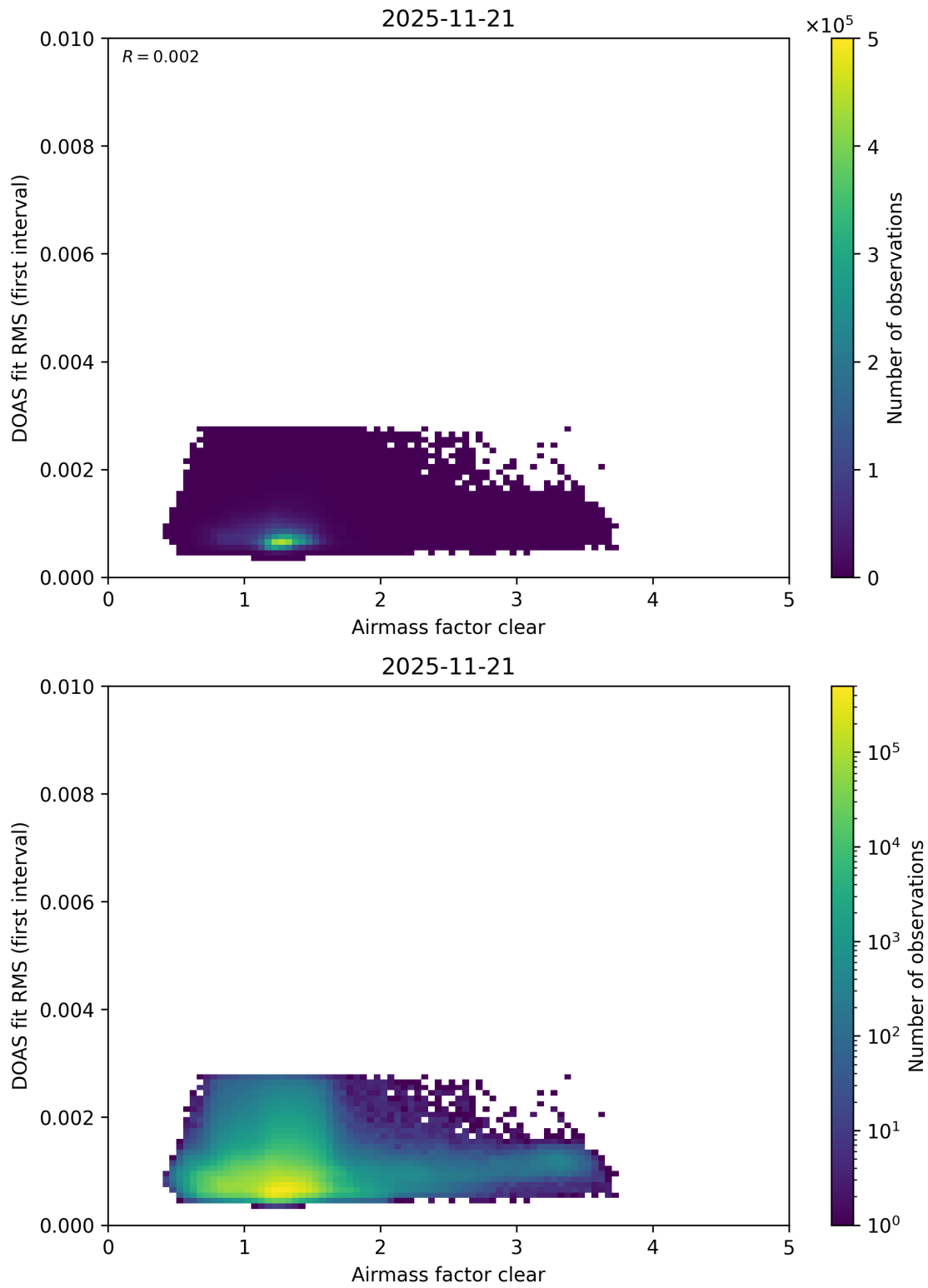
Figure 78: Scatter density plot of “Airmass factor clear” against “DOAS fit RMS (first interval)” for 2025-11-20 to 2025-11-22.
