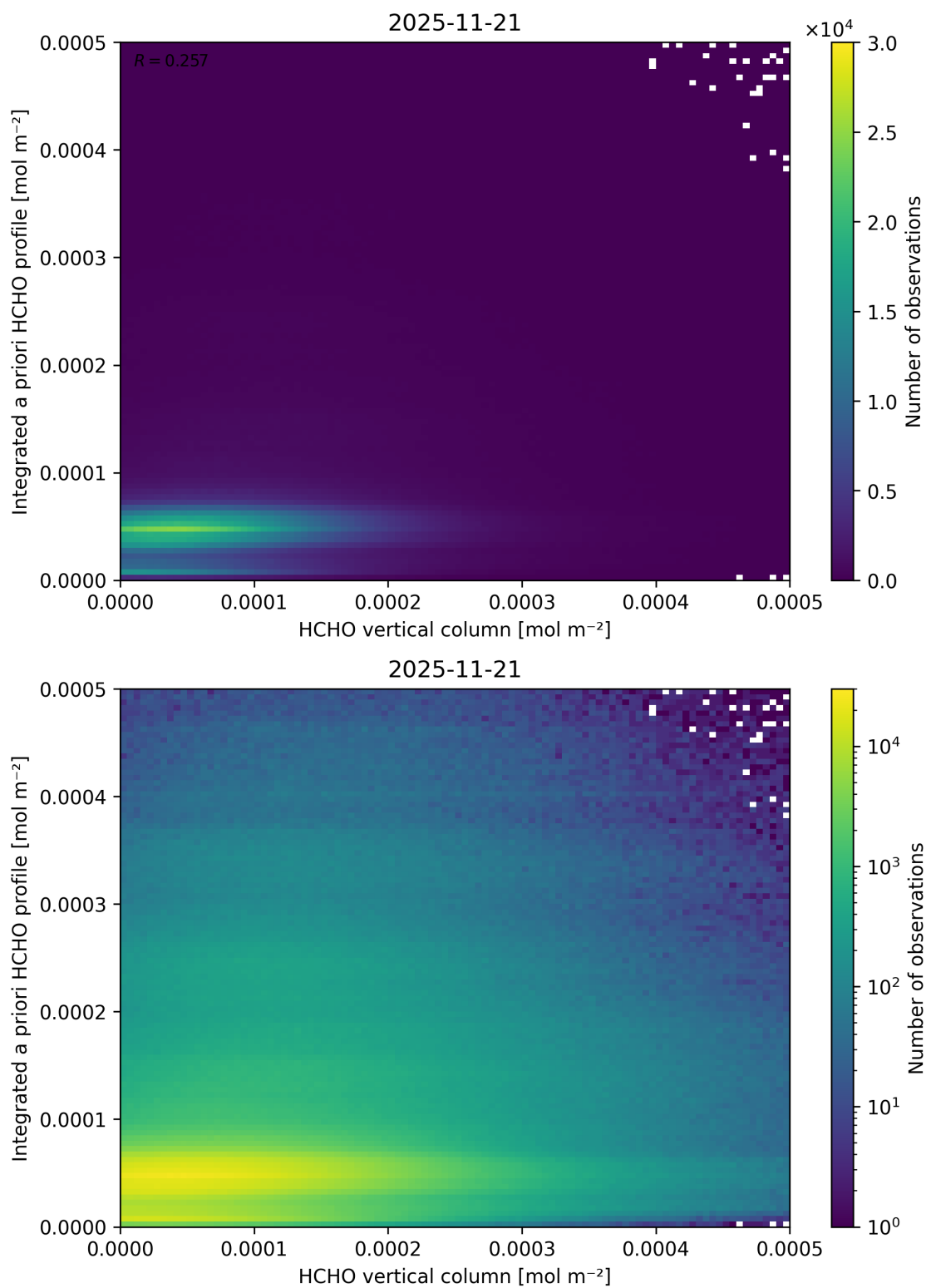
Figure 151: Scatter density plot of “HCHO vertical column” against “Integrated a priori HCHO profile” for 2025-11-20 to 2025-11-22.
