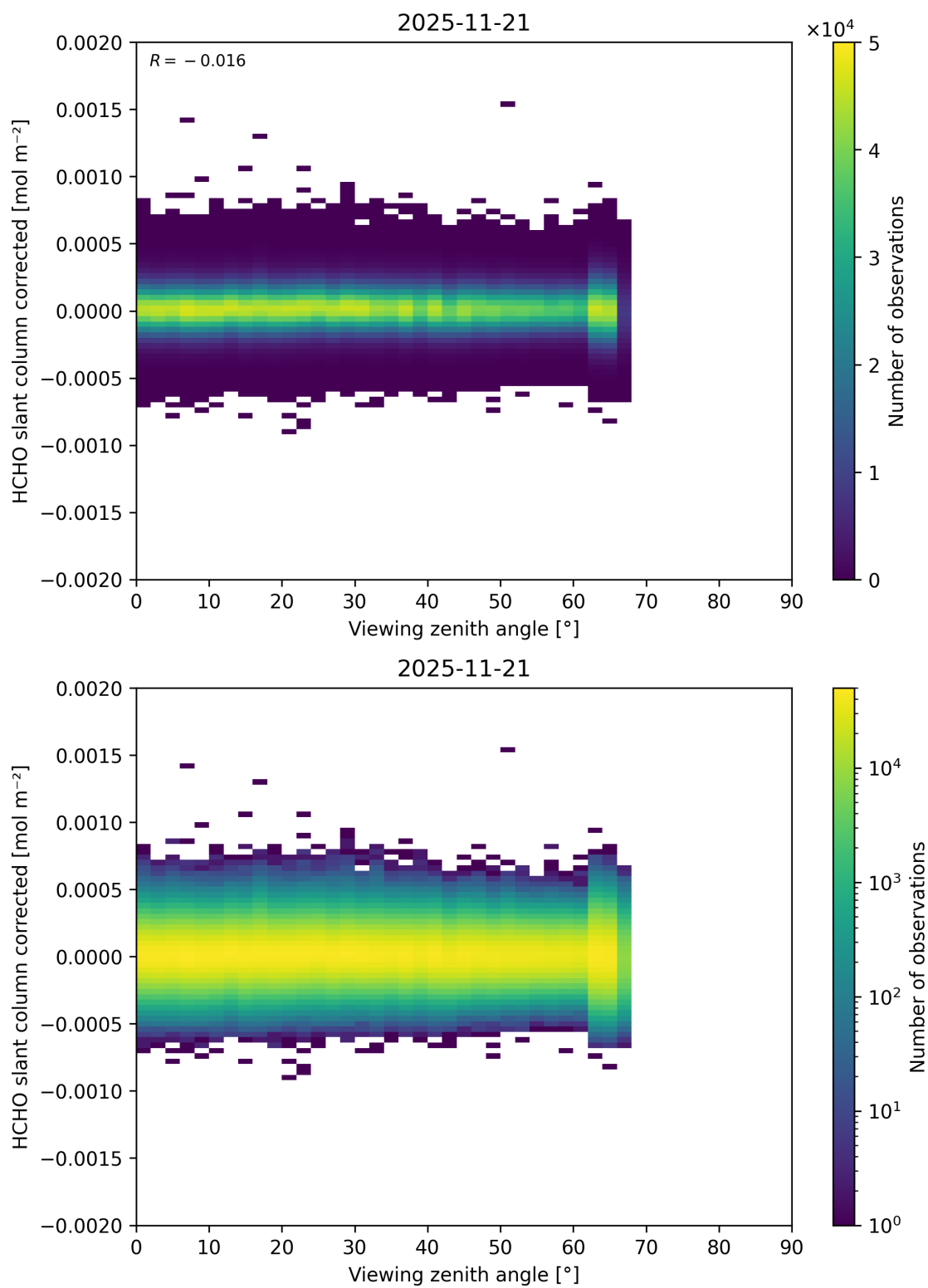
Figure 206: Scatter density plot of “Viewing zenith angle” against “HCHO slant column corrected” for 2025-11-20 to 2025-11-22.
