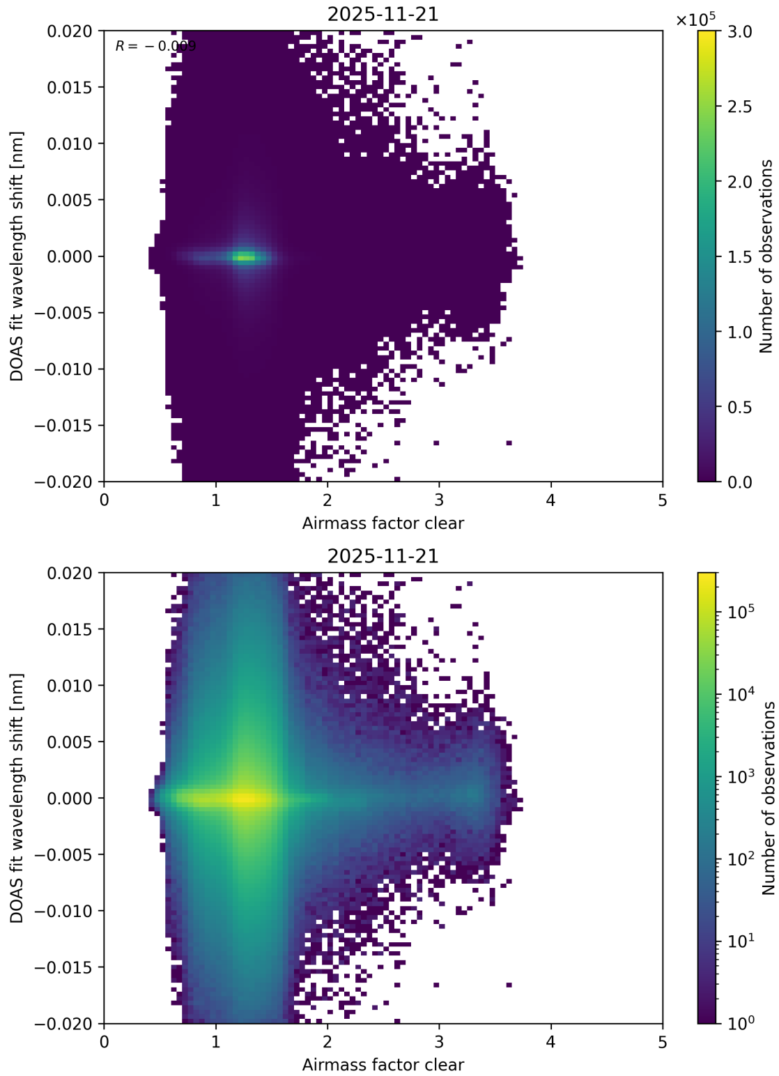
Figure 79: Scatter density plot of “Airmass factor clear” against “DOAS fit wavelength shift” for 2025-11-20 to 2025-11-22.
