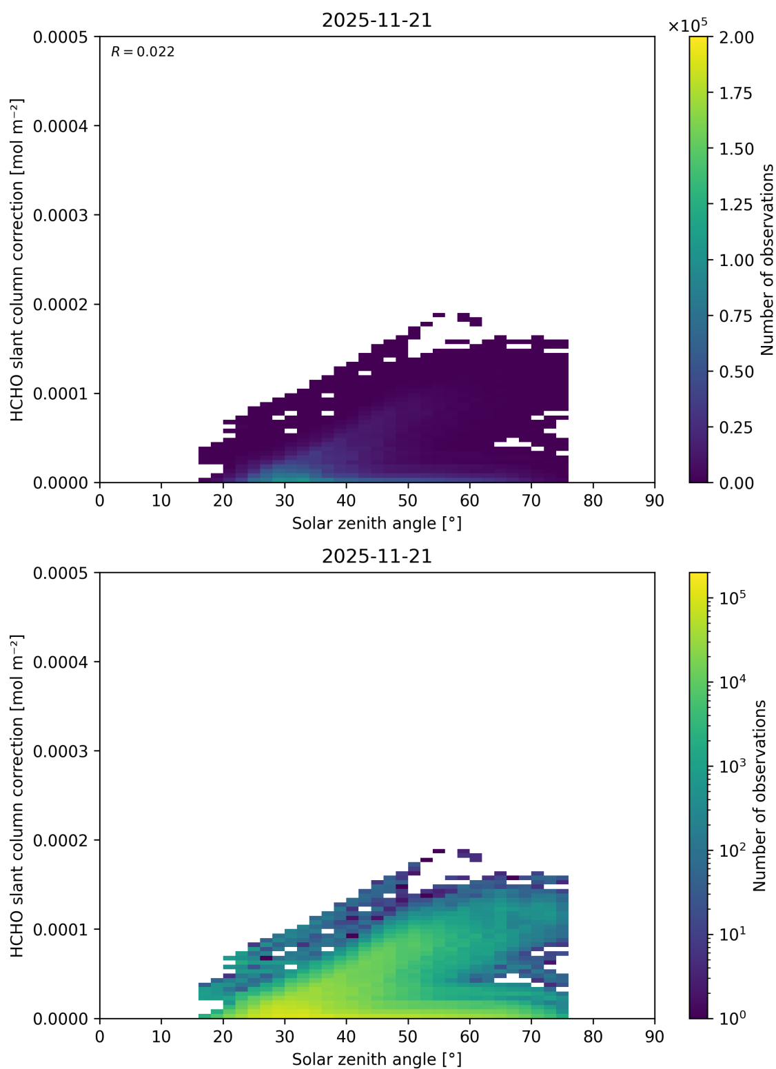
Figure 191: Scatter density plot of “Solar zenith angle” against “HCHO slant column correction” for 2025-11-20 to 2025-11-22.
