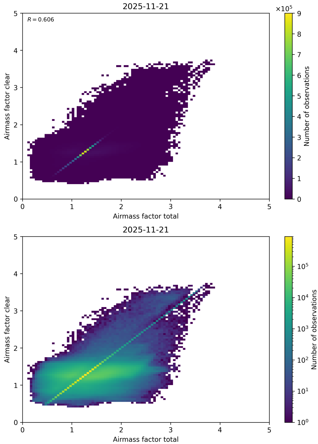
Figure 112: Scatter density plot of “Airmass factor total” against “Airmass factor clear” for 2025-11-20 to 2025-11-22.
