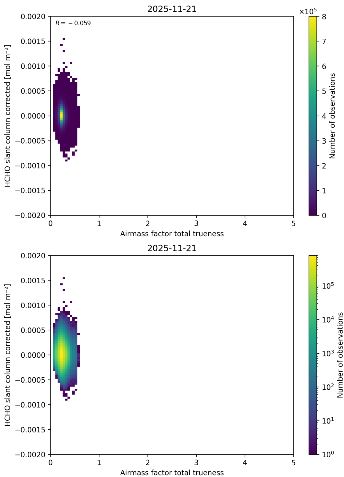
Figure 122: Scatter density plot of “Airmass factor total trueness” against “HCHO slant column corrected” for 2025-11-20 to 2025-11-22.
