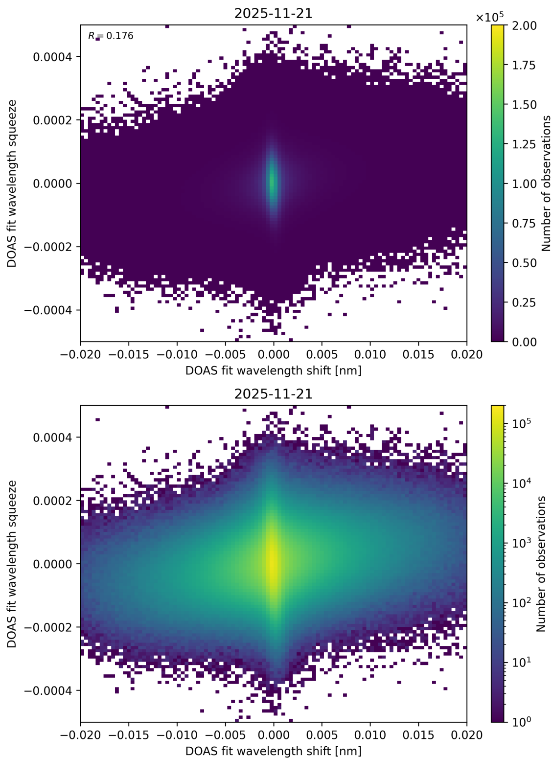
Figure 70: Scatter density plot of “DOAS fit wavelength shift” against “DOAS fit wavelength squeeze” for 2025-11-20 to 2025-11-22.
