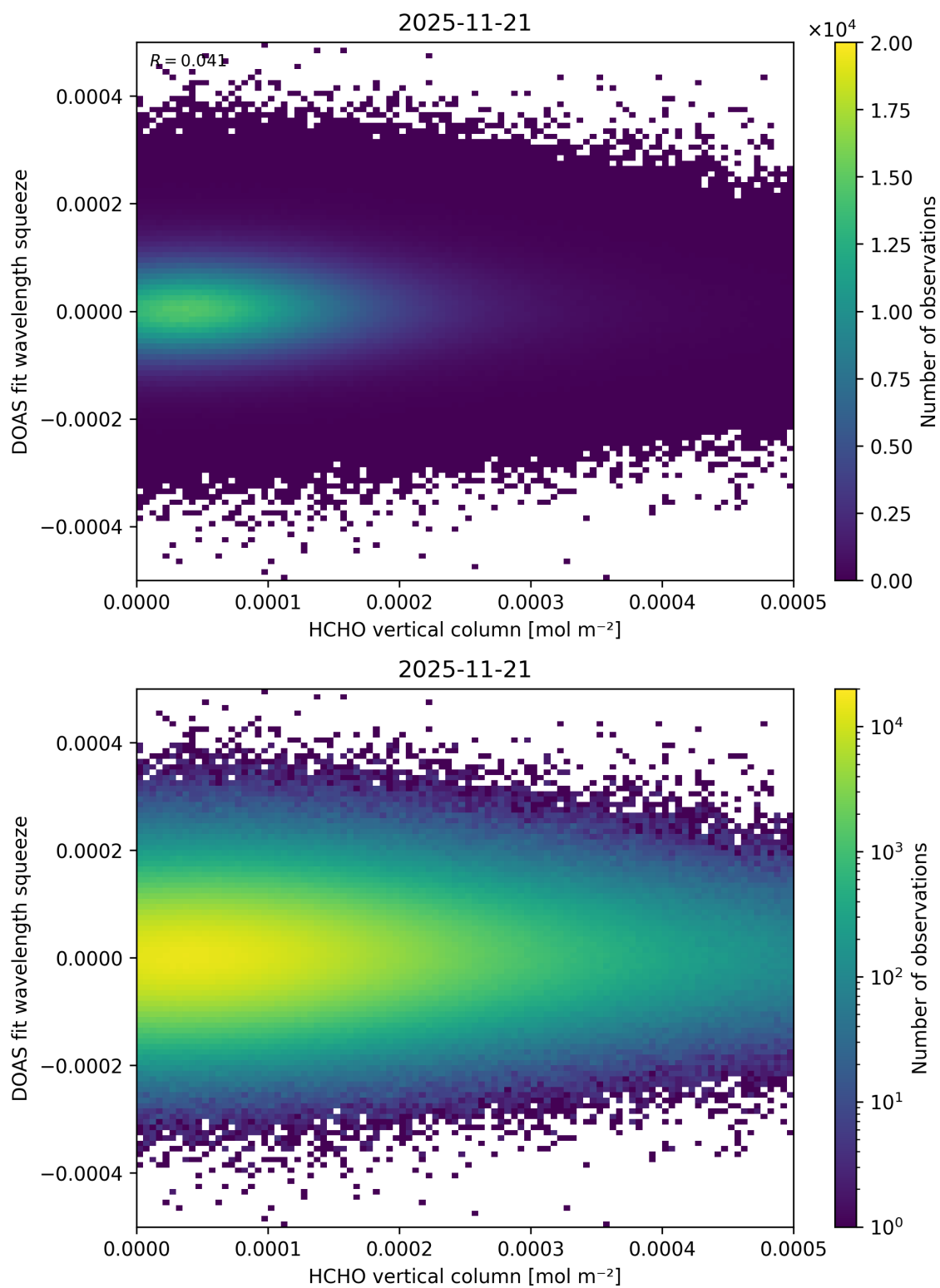
Figure 140: Scatter density plot of “HCHO vertical column” against “DOAS fit wavelength squeeze” for 2025-11-20 to 2025-11-22.
