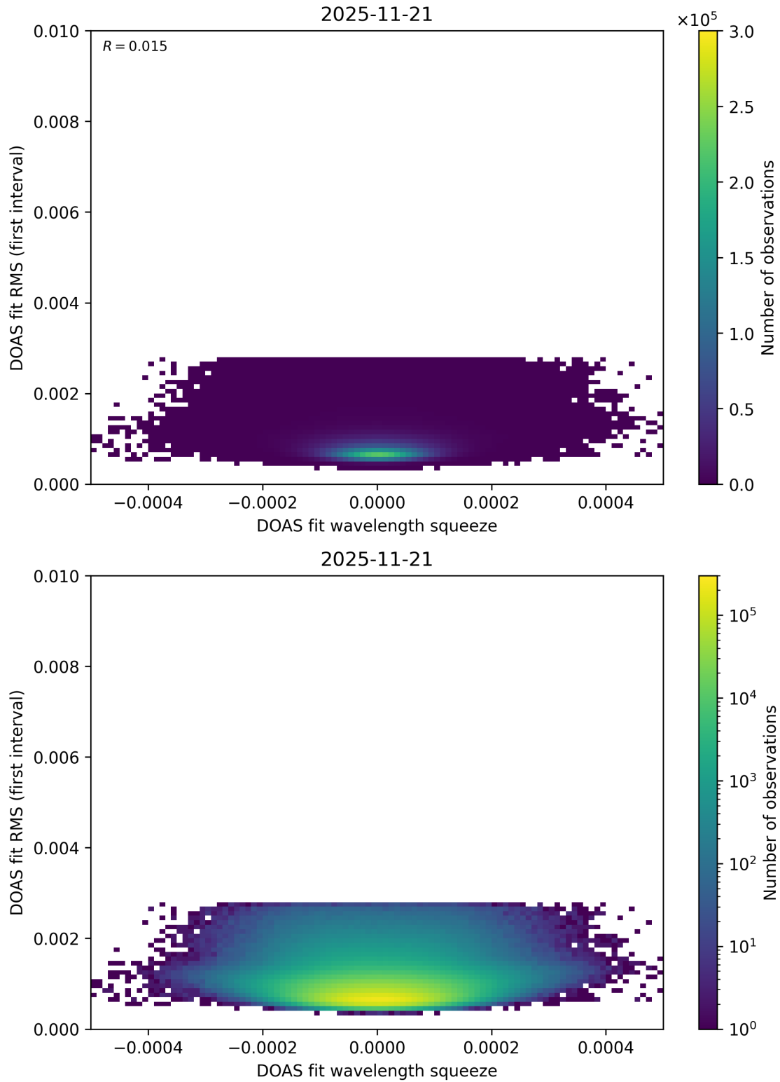
Figure 74: Scatter density plot of “DOAS fit wavelength squeeze” against “DOAS fit RMS (first interval)” for 2025-11-20 to 2025-11-22.
