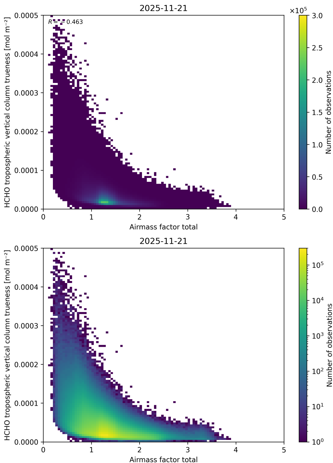
Figure 116: Scatter density plot of “Air mass factor total” against “HCHO tropospheric vertical column trueiness” for 2025-11-20 to 2025-11-22.
