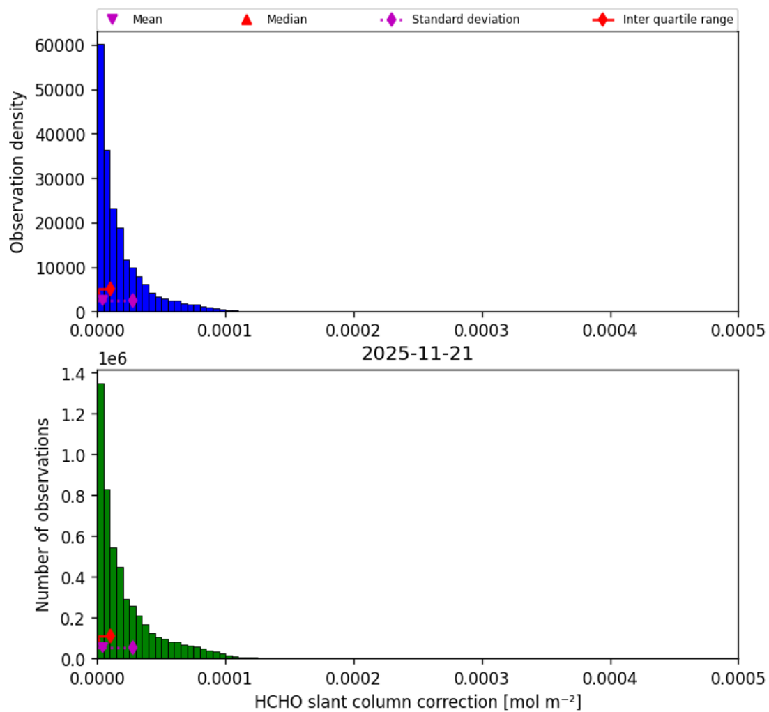
Figure 49: Histogram of “HCHO slant column correction” for 2025-11-20 to 2025-11-22
