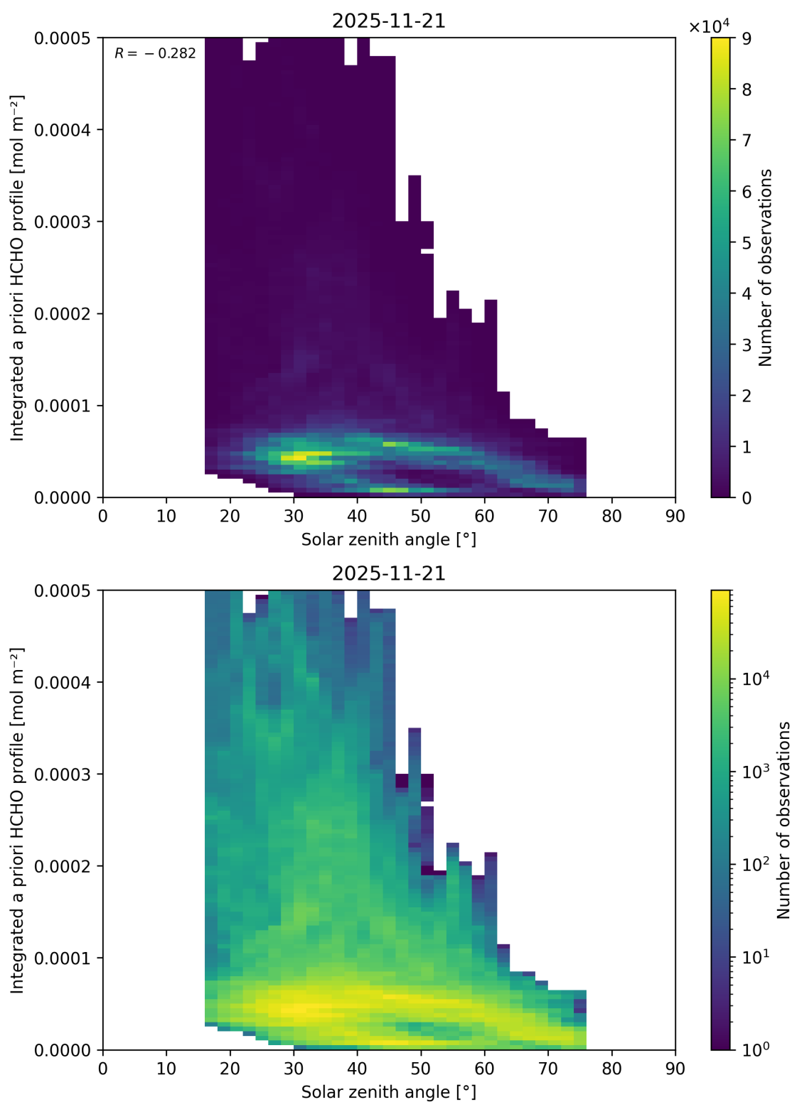
Figure 200: Scatter density plot of “Solar zenith angle” against “Integrated a priori HCHO profile” for 2025-11-20 to 2025-11-22.
