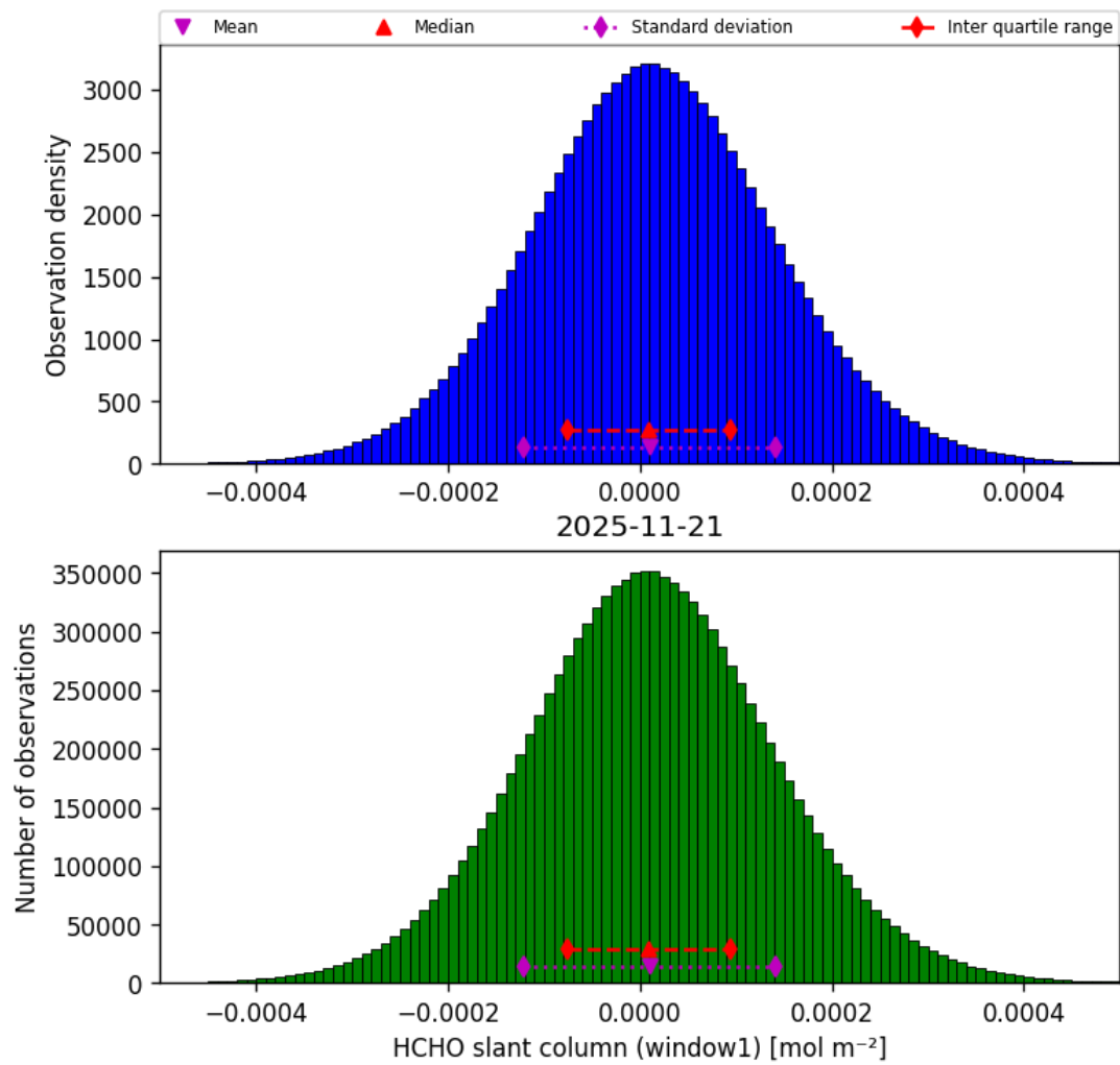
Figure 40: Histogram of “HCHO slant column (window1)” for 2025-11-20 to 2025-11-22
