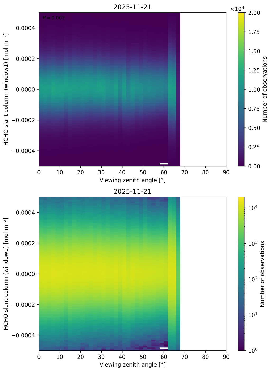
Figure 208: Scatter density plot of “Viewing zenith angle” against “HCHO slant column (window1)” for 2025-11-20 to 2025-11-22.
