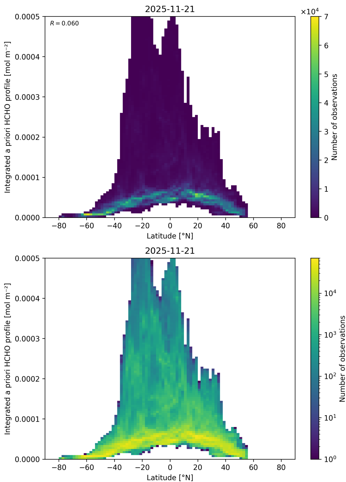
Figure 185: Scatter density plot of “Latitude” against “Integrated a priori HCHO profile” for 2025-11-20 to 2025-11-22.
