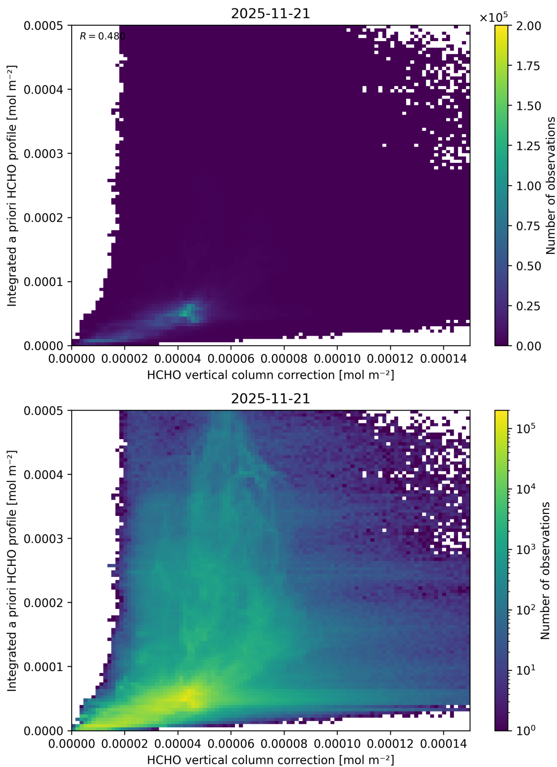
Figure 137: Scatter density plot of “HCHO vertical column correction” against “Integrated a priori HCHO profile” for 2025-11-20 to 2025-11-22.
