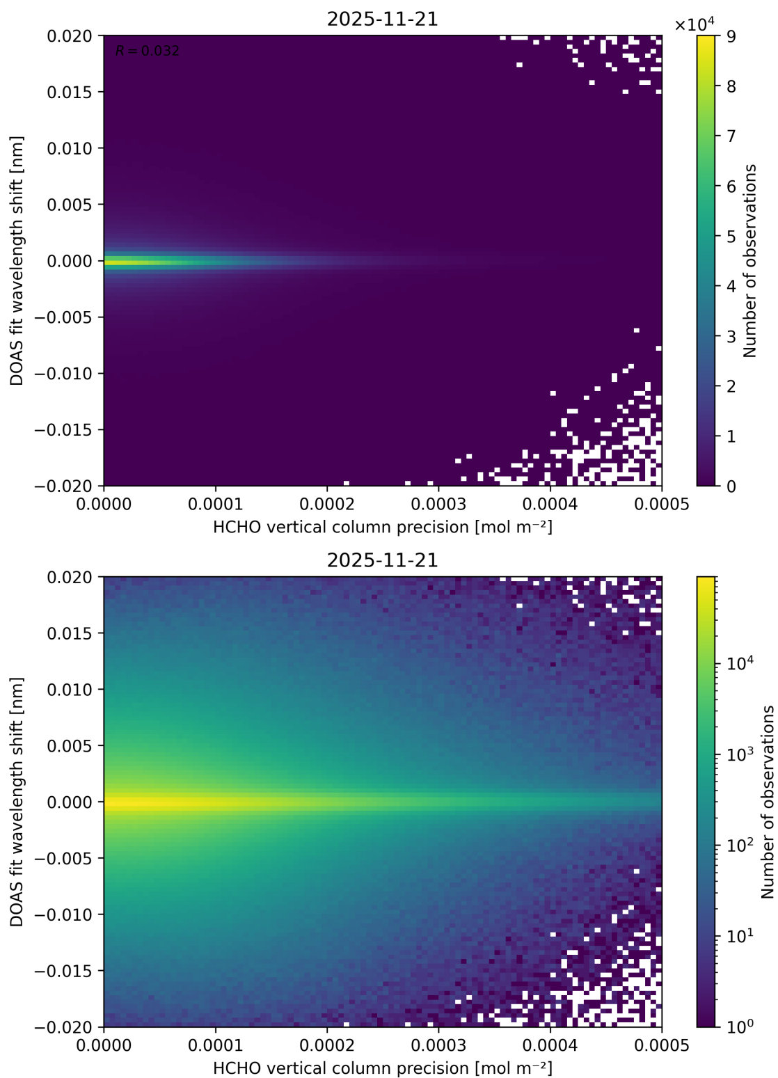
Figure 153: Scatter density plot of “HCHO vertical column precision” against “DOAS fit wavelength shift” for 2025-11-20 to 2025-11-22.
