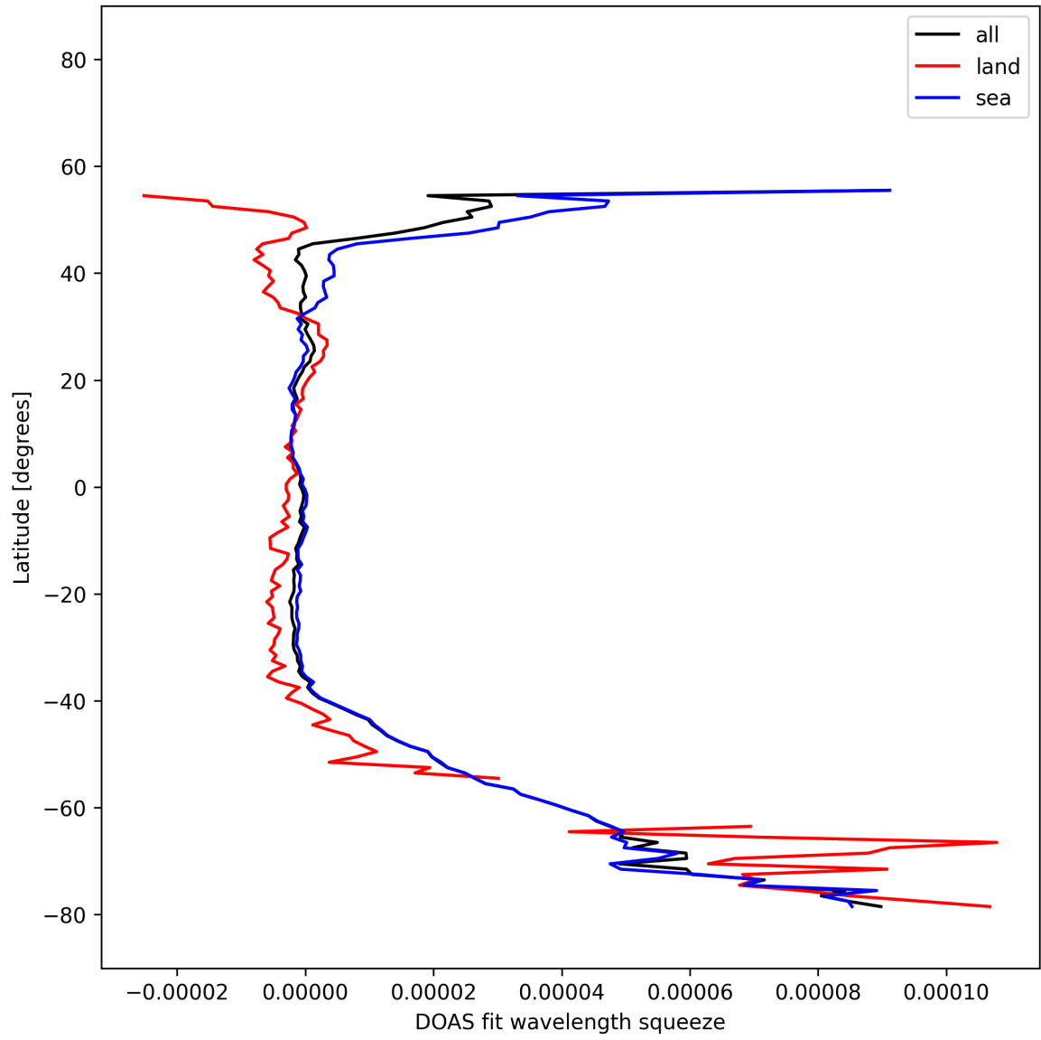
Figure 32: Zonal average of “DOAS fit wavelength squeeze” for 2025-11-20 to 2025-11-22.
