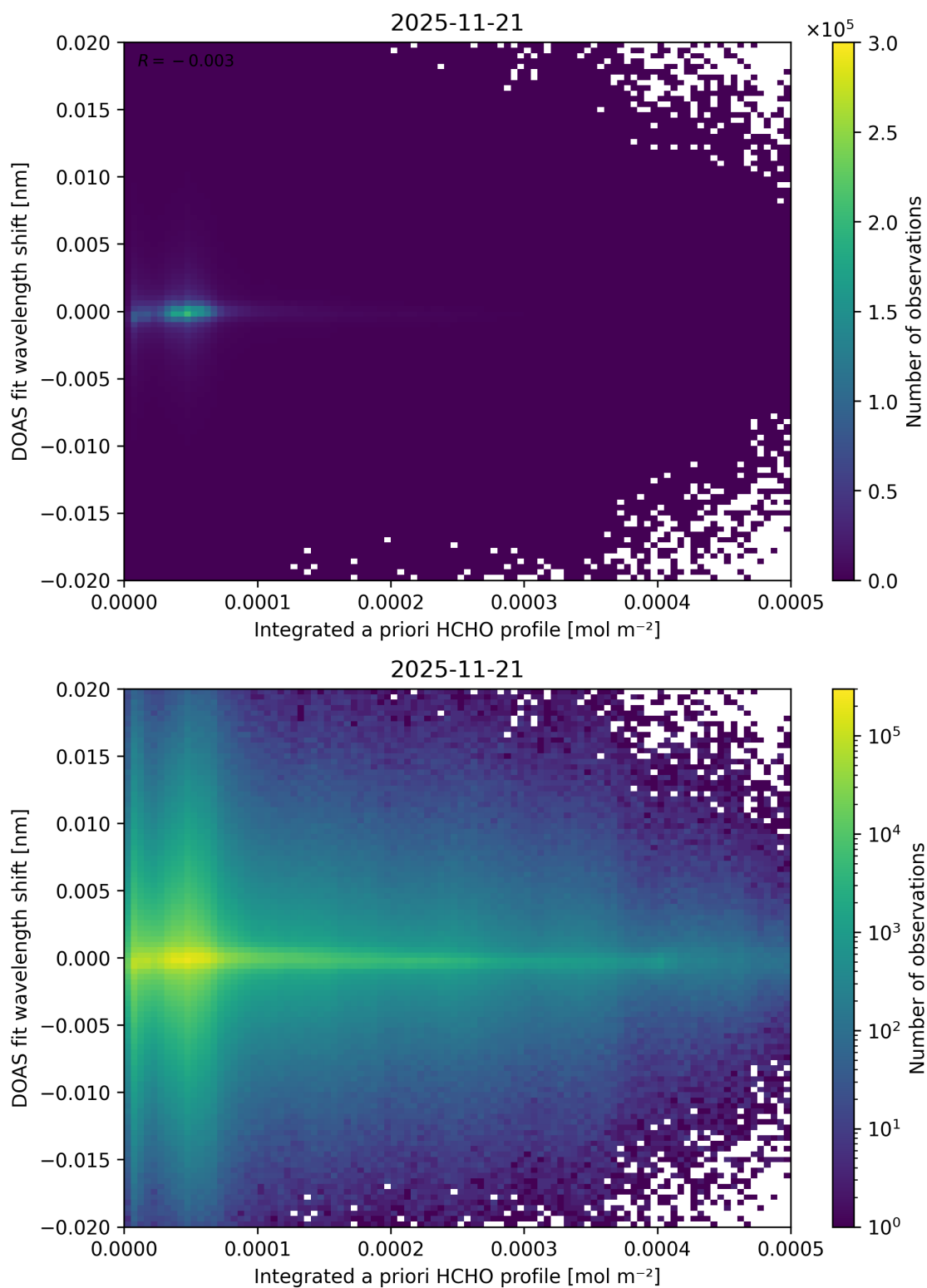
Figure 166: Scatter density plot of “Integrated a priori HCHO profile” against “DOAS fit wavelength shift” for 2025-11-20 to 2025-11-22.
