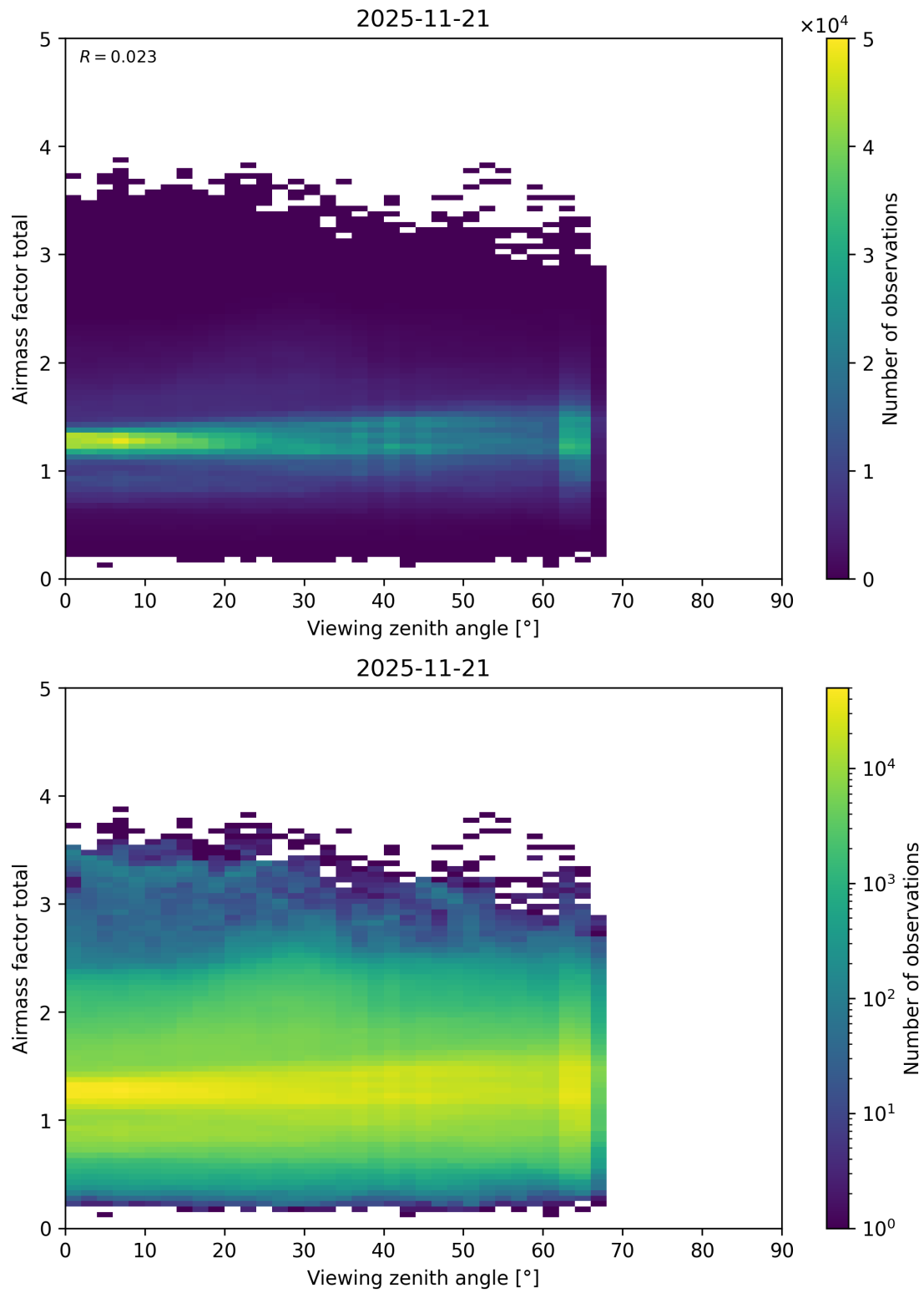
Figure 210: Scatter density plot of “Viewing zenith angle” against “Airmass factor total” for 2025-11-20 to 2025-11-22.
