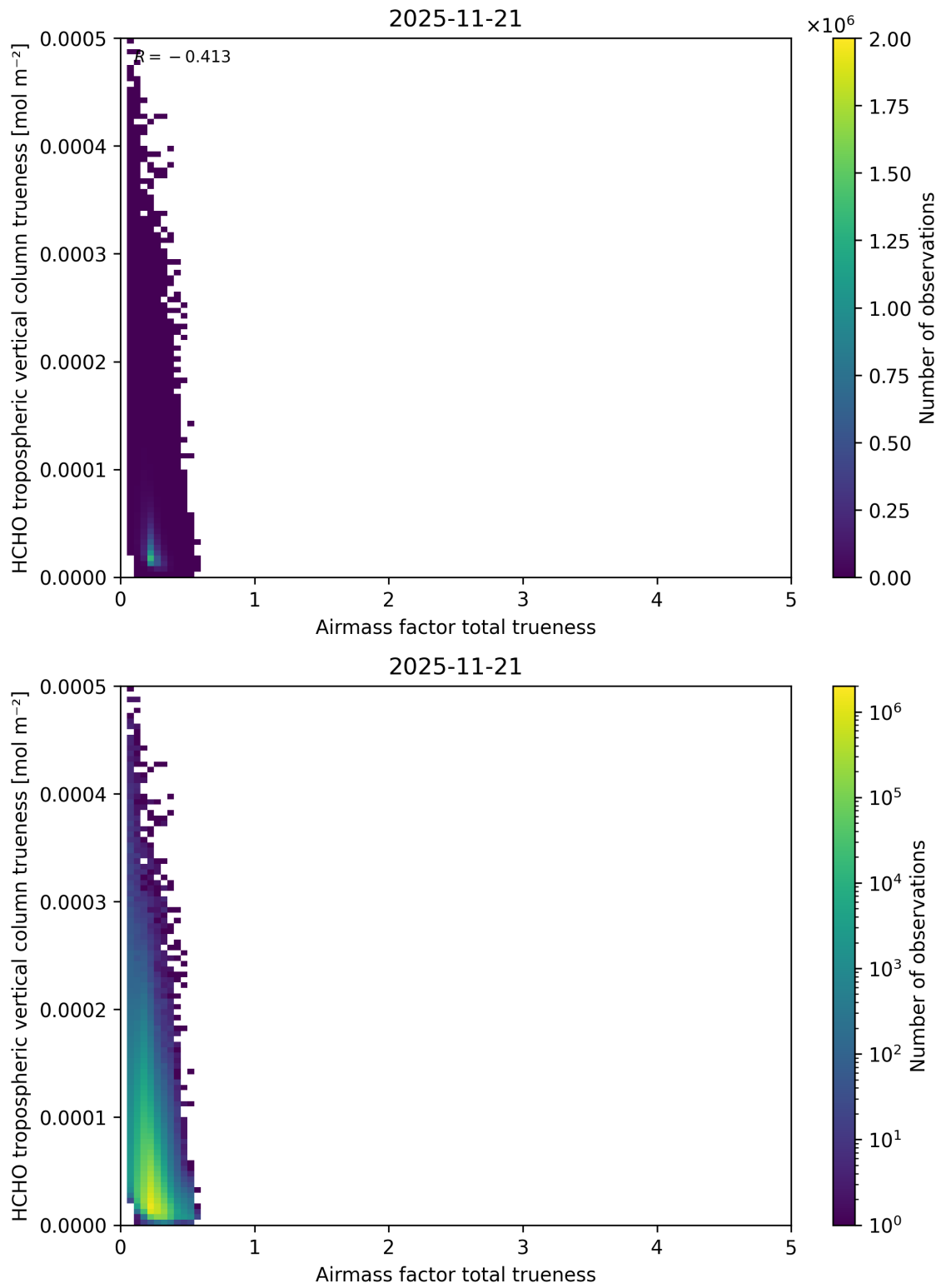
Figure 124: Scatter density plot of “Airmass factor total trueness” against “HCHO tropospheric vertical column trueness” for 2025-11-20 to 2025-11-22.
