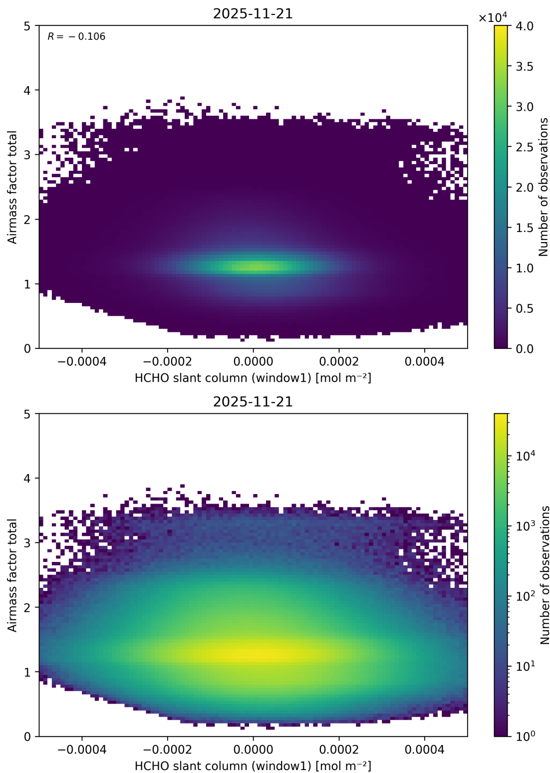
Figure 95: Scatter density plot of “HCHO slant column (window1)” against “Airmass factor total” for 2025-11-20 to 2025-11-22.
