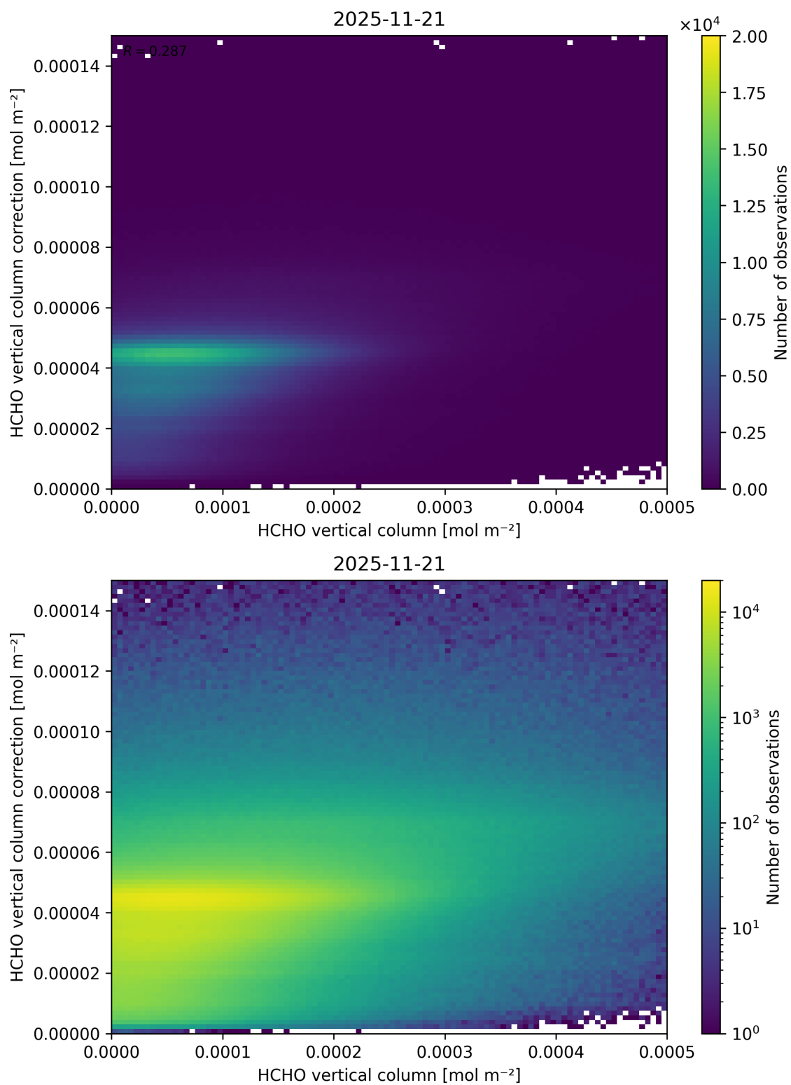
Figure 148: Scatter density plot of “HCHO vertical column” against “HCHO vertical column correction” for 2025-11-20 to 2025-11-22.
