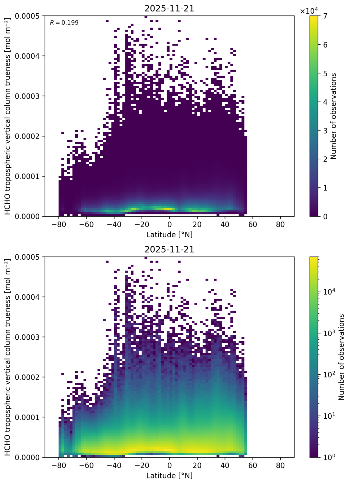
Figure 184: Scatter density plot of “Latitude” against “HCHO tropospheric vertical column trueness” for 2025-11-20 to 2025-11-22.
