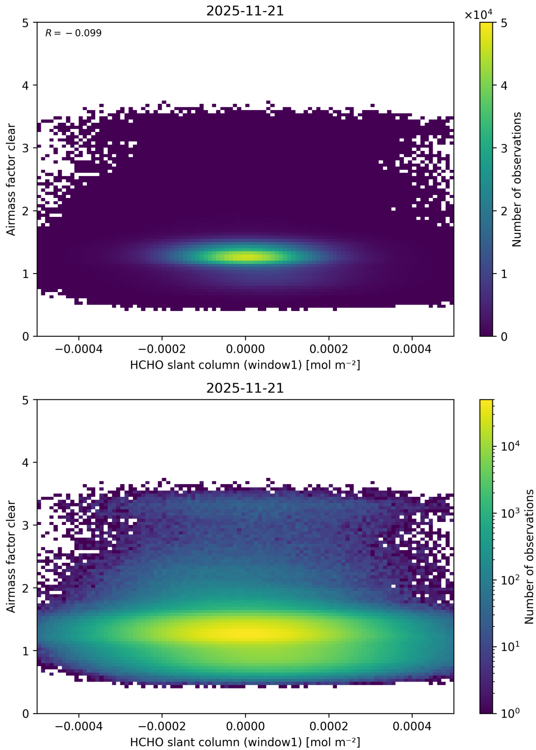
Figure 91: Scatter density plot of “HCHO slant column (window1)” against “Airmass factor clear” for 2025-11-20 to 2025-11-22.
