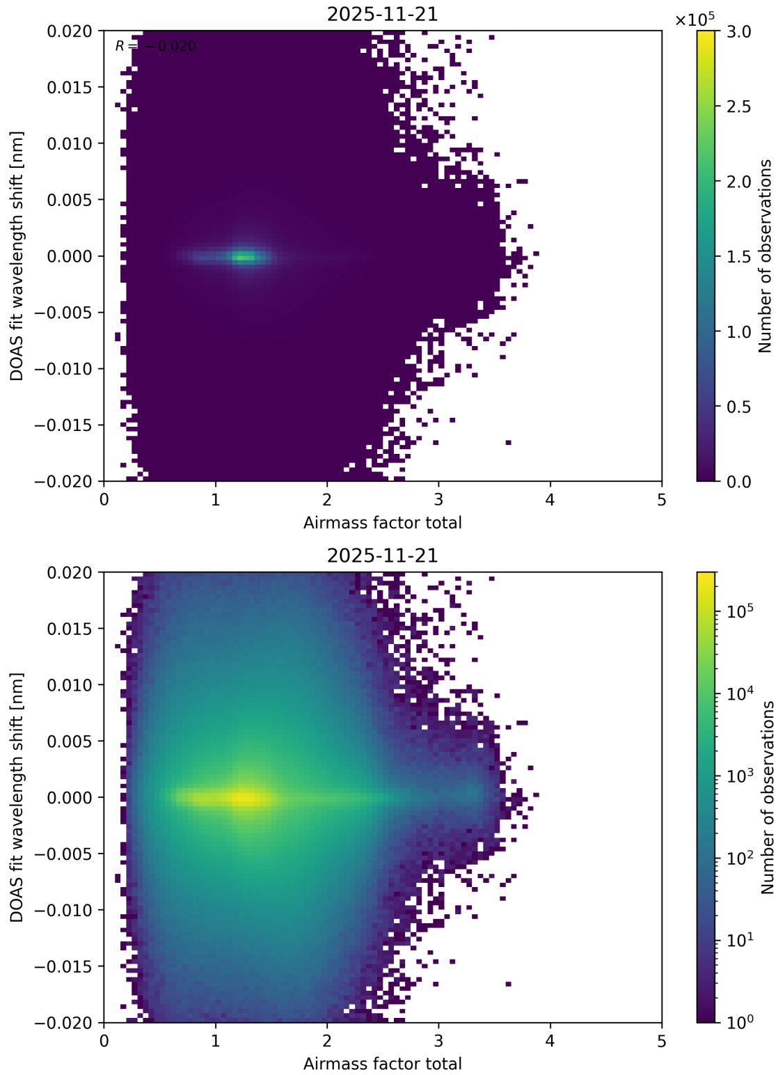
Figure 110: Scatter density plot of “Airmass factor total” against “DOAS fit wavelength shift” for 2025-11-20 to 2025-11-22.
