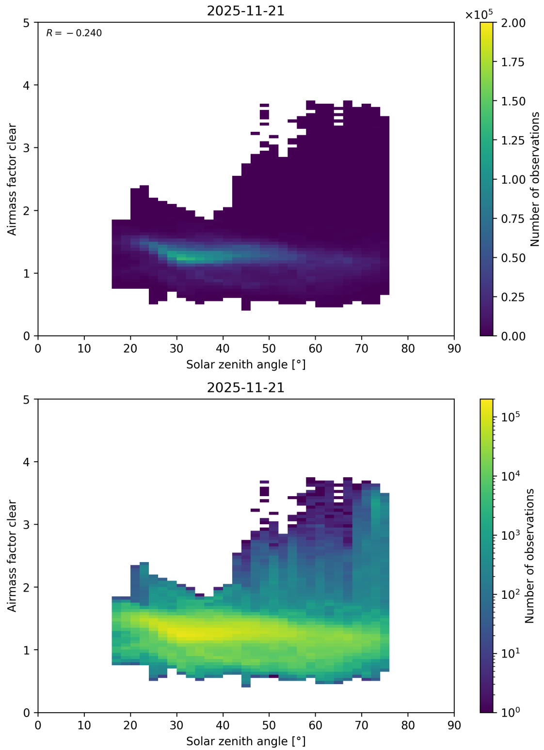
Figure 189: Scatter density plot of “Solar zenith angle” against “Airmass factor clear” for 2025-11-20 to 2025-11-22.
