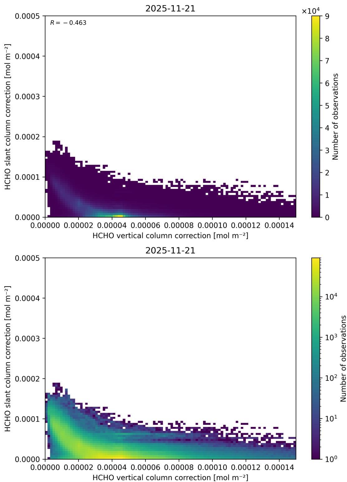
Figure 131: Scatter density plot of “HCHO vertical column correction” against “HCHO slant column correction” for 2025-11-20 to 2025-11-22.
