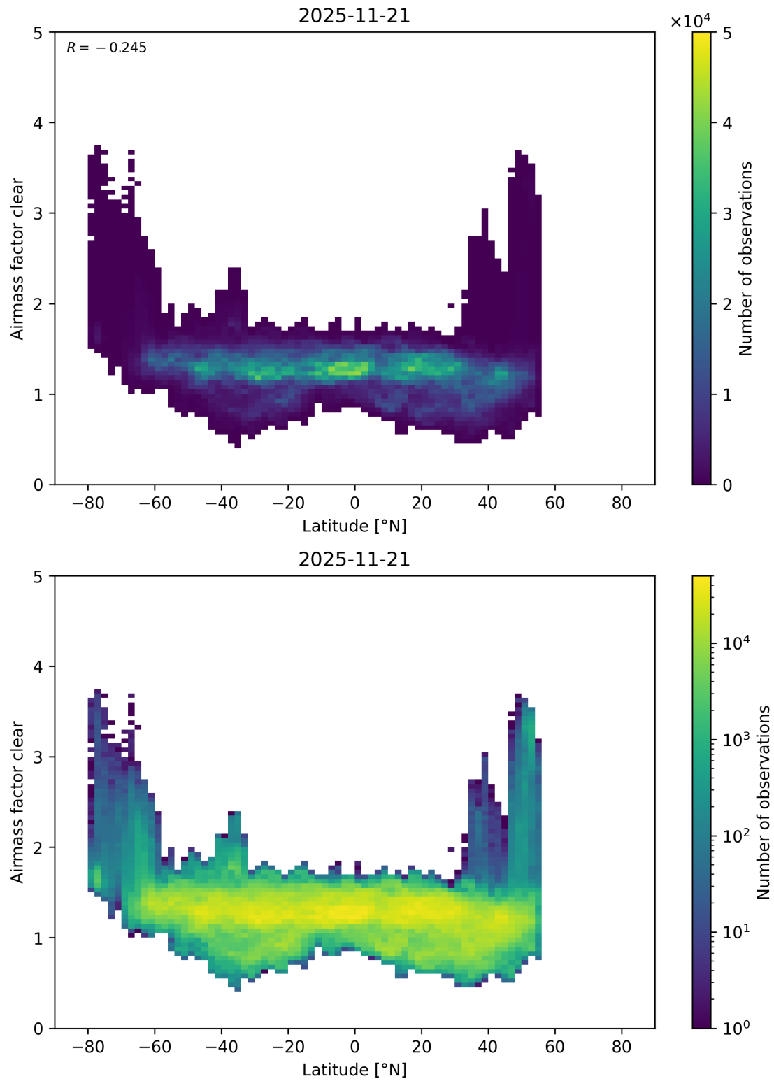
Figure 174: Scatter density plot of “Latitude” against “Airmass factor clear” for 2025-11-20 to 2025-11-22.
