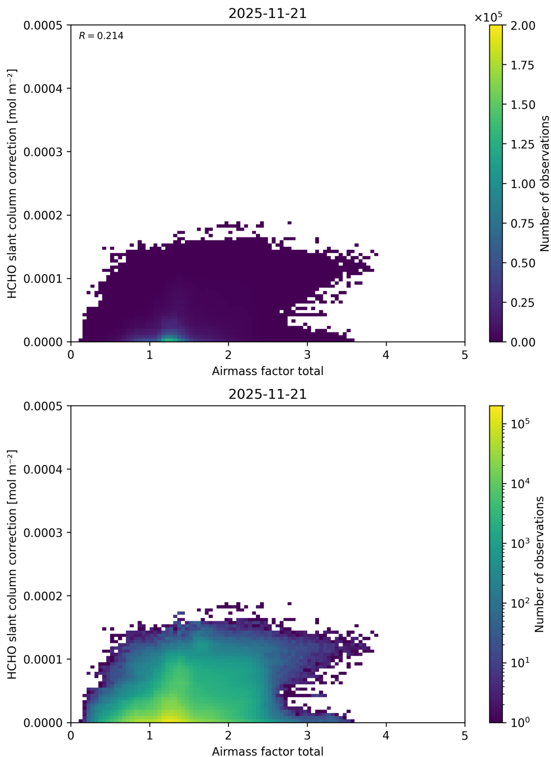
Figure 114: Scatter density plot of “Airmass factor total” against “HCHO slant column correction” for 2025-11-20 to 2025-11-22.
