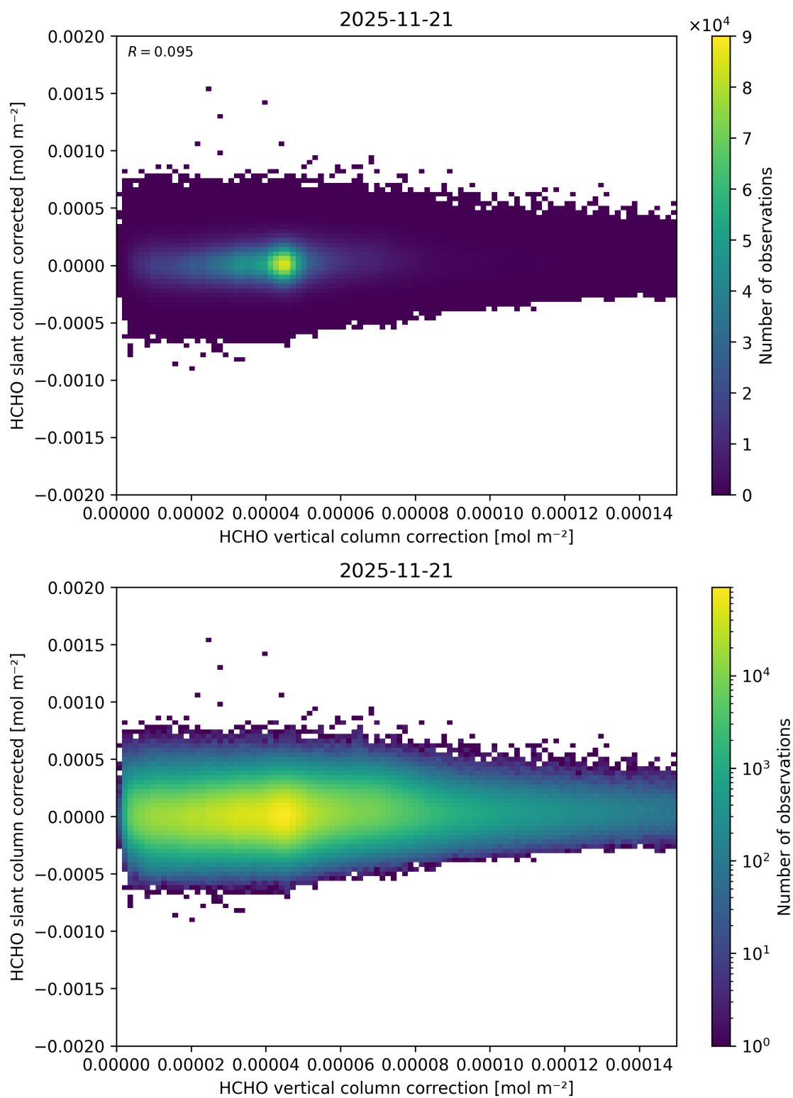
Figure 130: Scatter density plot of “HCHO vertical column correction” against “HCHO slant column corrected” for 2025-11-20 to 2025-11-22.
