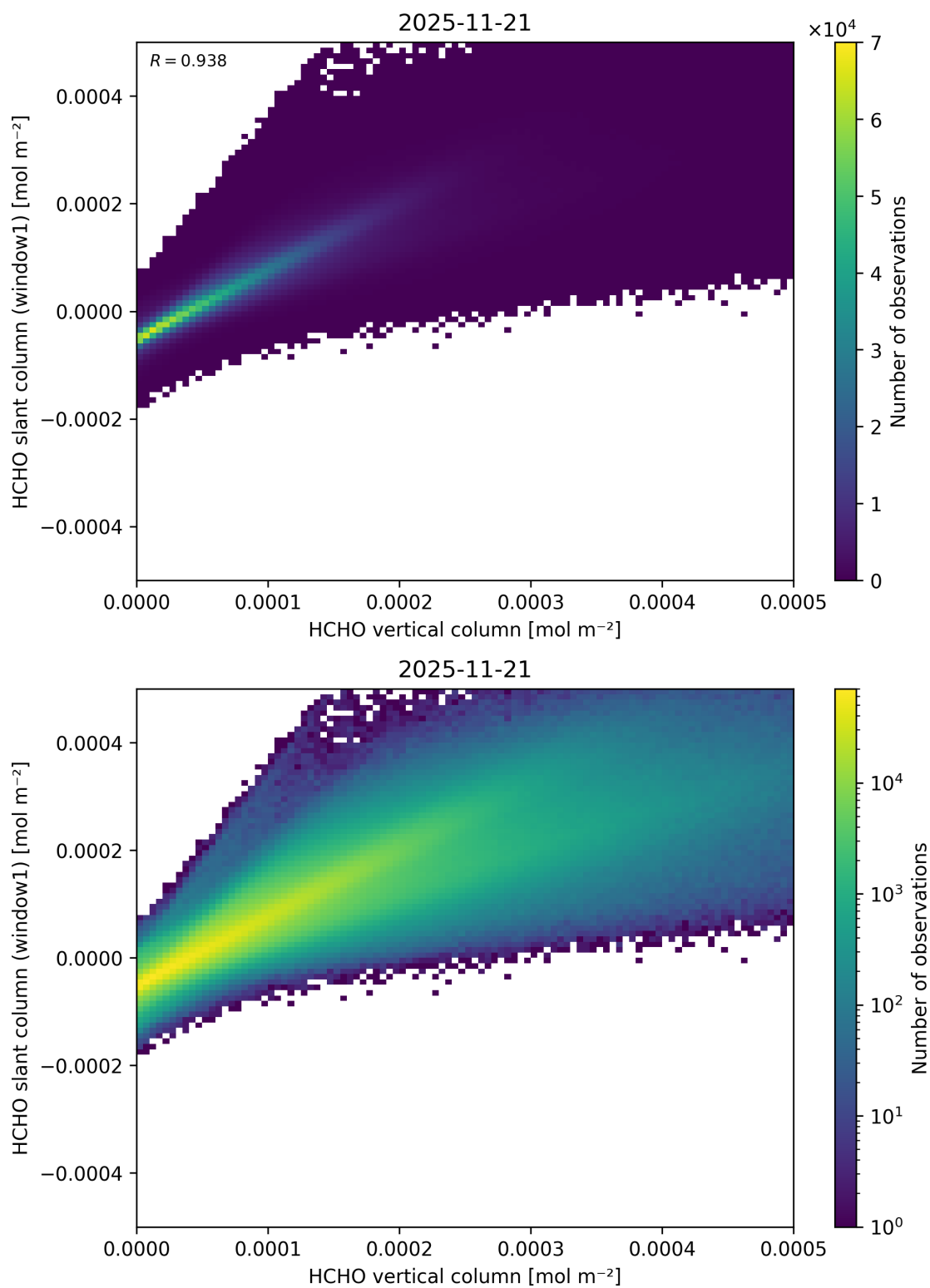
Figure 144: Scatter density plot of “HCHO vertical column” against “HCHO slant column (window1)” for 2025-11-20 to 2025-11-22.
