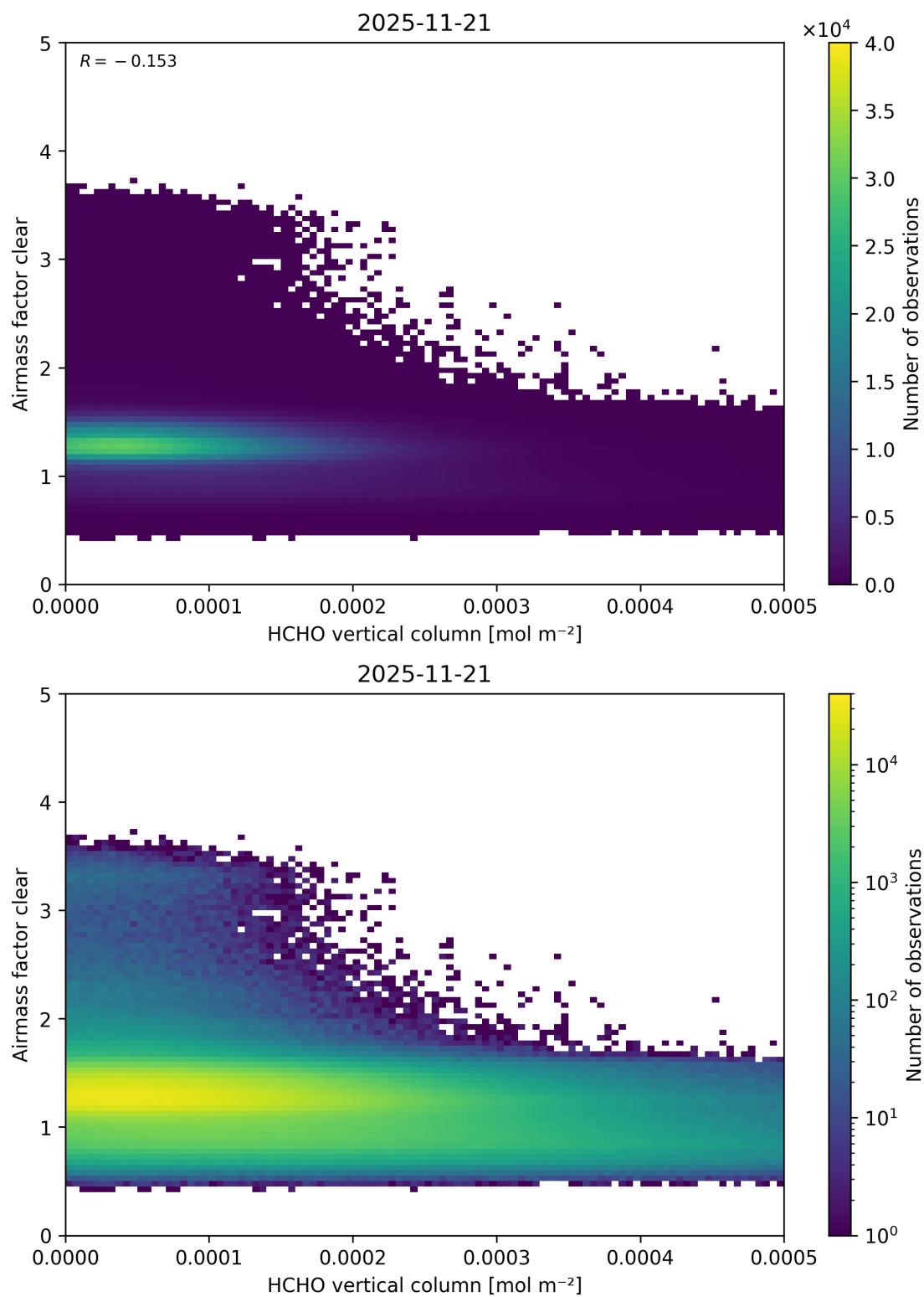
Figure 141: Scatter density plot of “HCHO vertical column” against “Airmass factor clear” for 2025-11-20 to 2025-11-22.
