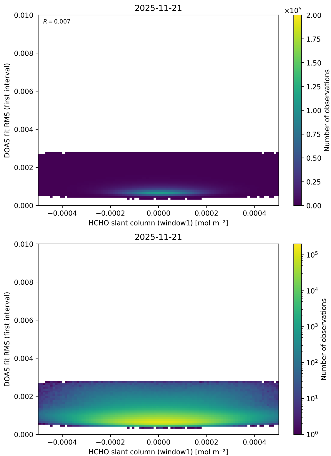
Figure 88: Scatter density plot of “HCHO slant column (window1)” against “DOAS fit RMS (first interval)” for 2025-11-20 to 2025-11-22.
