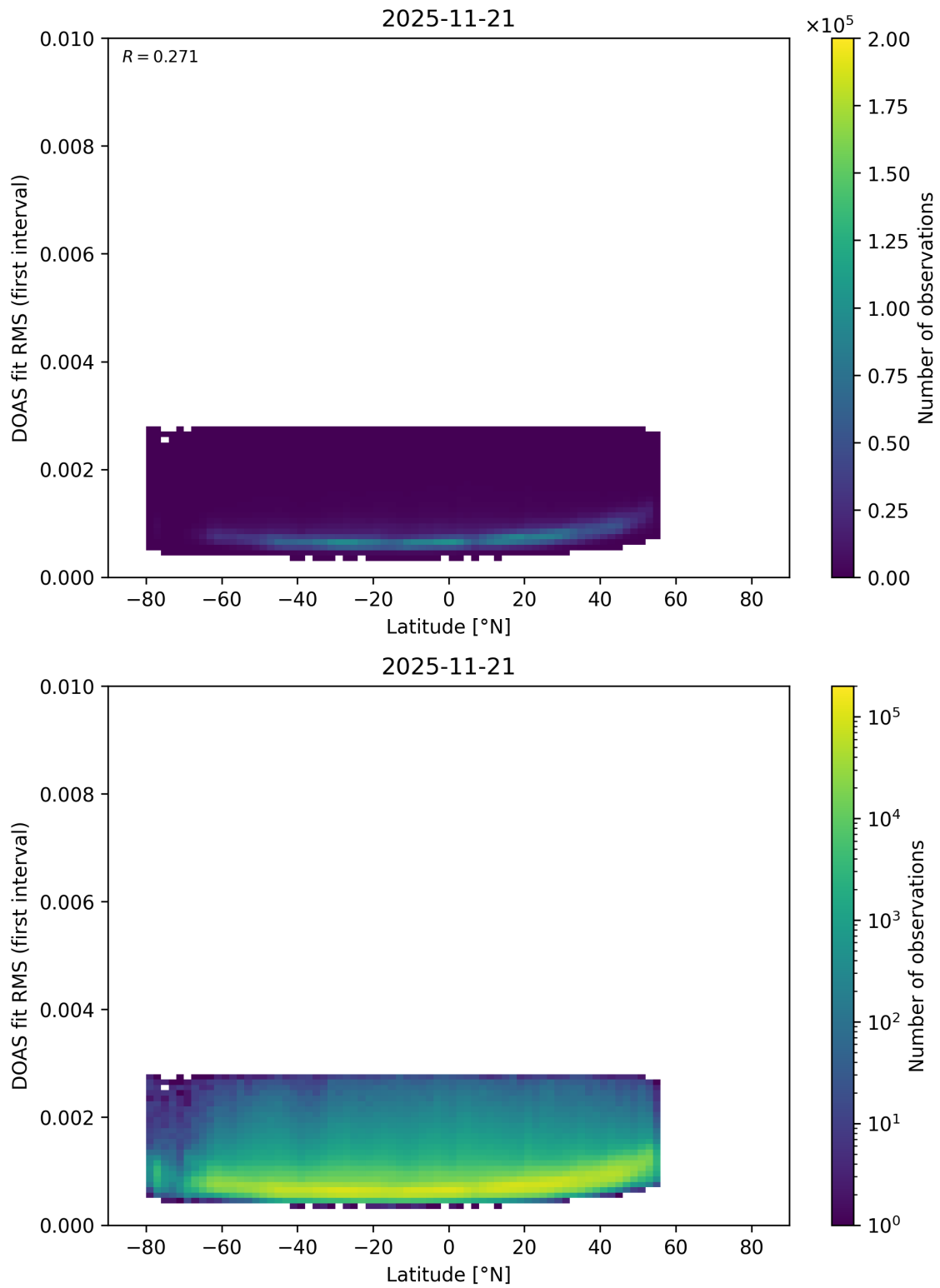
Figure 171: Scatter density plot of “Latitude” against “DOAS fit RMS (first interval)” for 2025-11-20 to 2025-11-22.
