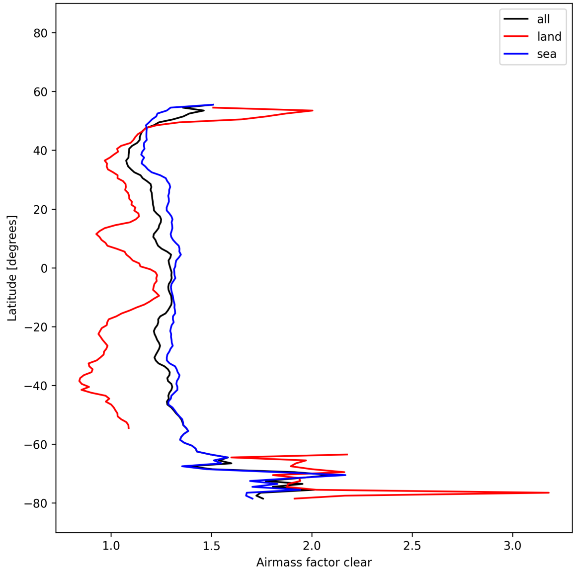
Figure 29: Zonal average of “Airmass factor clear” for 2025-11-20 to 2025-11-22.
