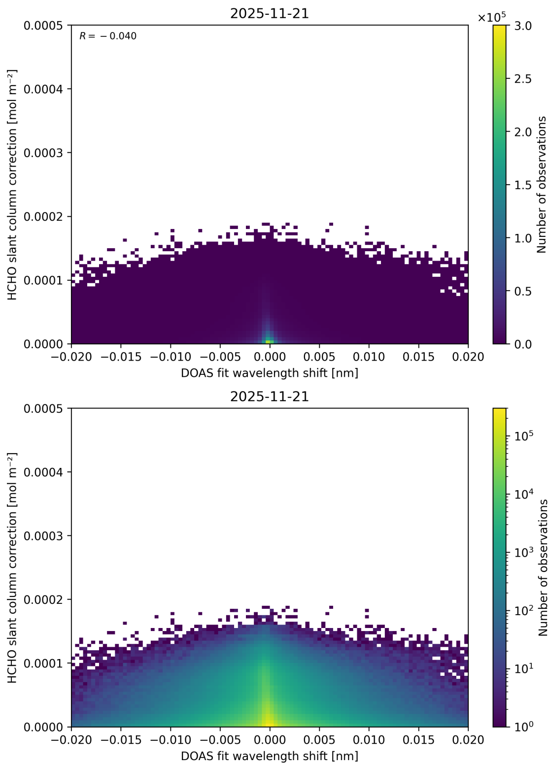
Figure 72: Scatter density plot of “DOAS fit wavelength shift” against “HCHO slant column correction” for 2025-11-20 to 2025-11-22.
