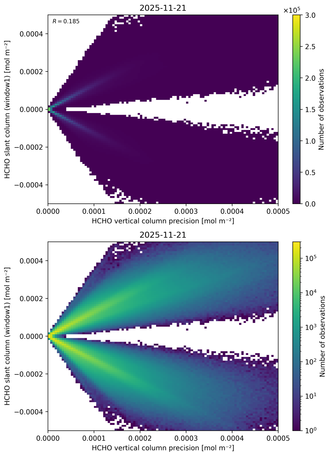
Figure 158: Scatter density plot of “HCHO vertical column precision” against “HCHO slant column (window1)” for 2025-11-20 to 2025-11-22.
