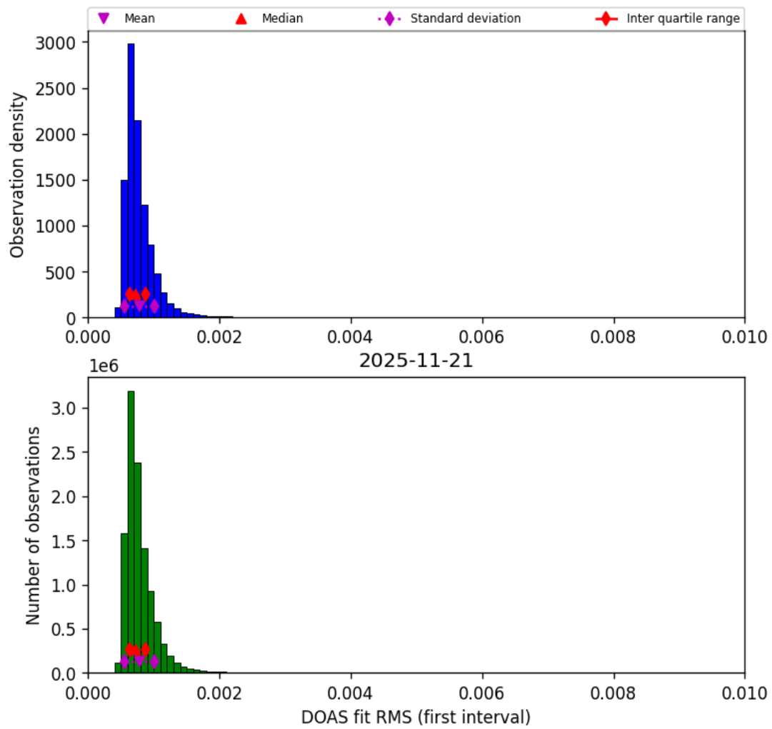
Figure 48: Histogram of “DOAS fit RMS (first interval)” for 2025-11-20 to 2025-11-22
