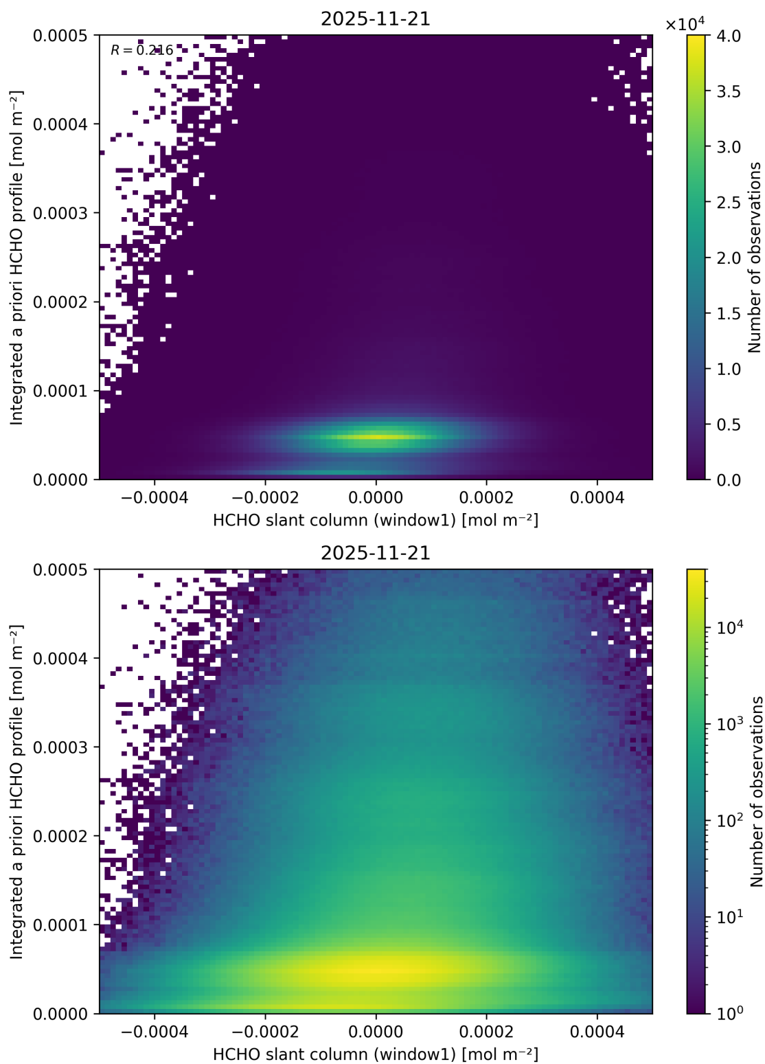
Figure 98: Scatter density plot of “HCHO slant column (window1)” against “Integrated a priori HCHO profile” for 2025-11-20 to 2025-11-22.
