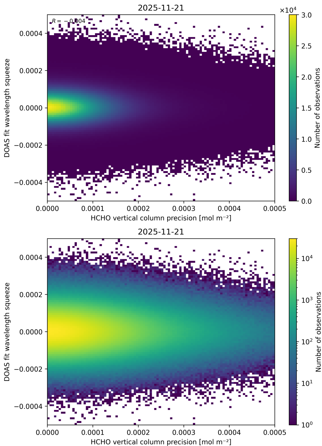
Figure 154: Scatter density plot of “HCHO vertical column precision” against “DOAS fit wavelength squeeze” for 2025-11-20 to 2025-11-22.
