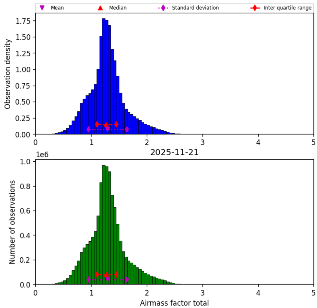
Figure 42: Histogram of “Airmass factor total” for 2025-11-20 to 2025-11-22
