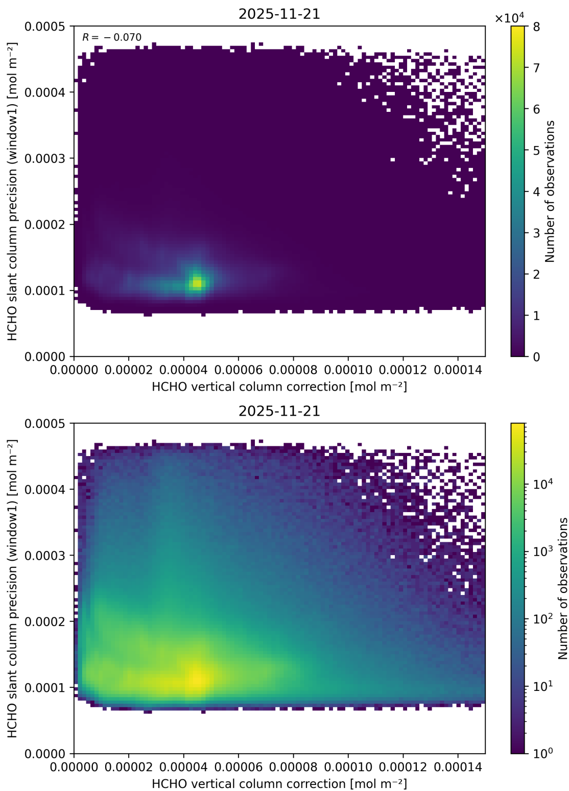
Figure 133: Scatter density plot of “HCHO vertical column correction” against “HCHO slant column precision (window1)” for 2025-11-20 to 2025-11-22.
