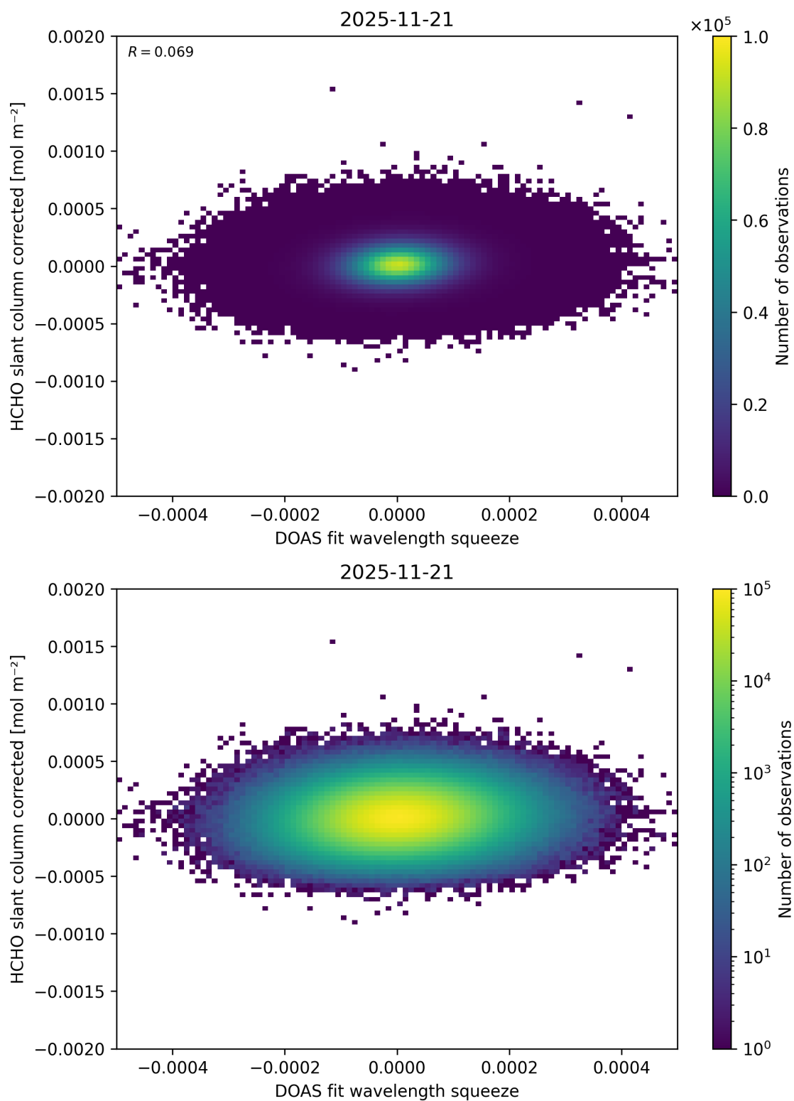
Figure 75: Scatter density plot of “DOAS fit wavelength squeeze” against “HCHO slant column corrected” for 2025-11-20 to 2025-11-22.
