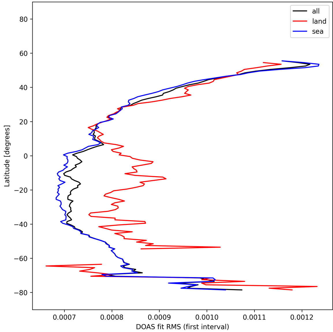
Figure 33: Zonal average of “DOAS fit RMS (first interval)” for 2025-11-20 to 2025-11-22.
