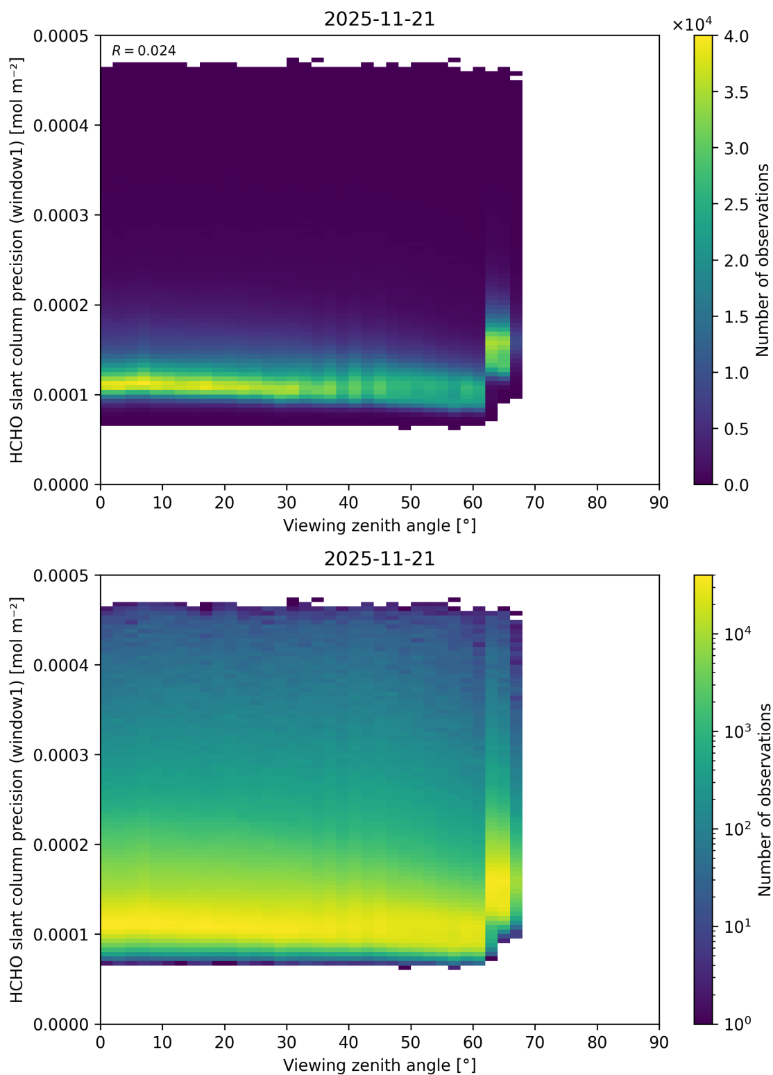
Figure 209: Scatter density plot of “Viewing zenith angle” against “HCHO slant column precision (window1)” for 2025-11-20 to 2025-11-22.
