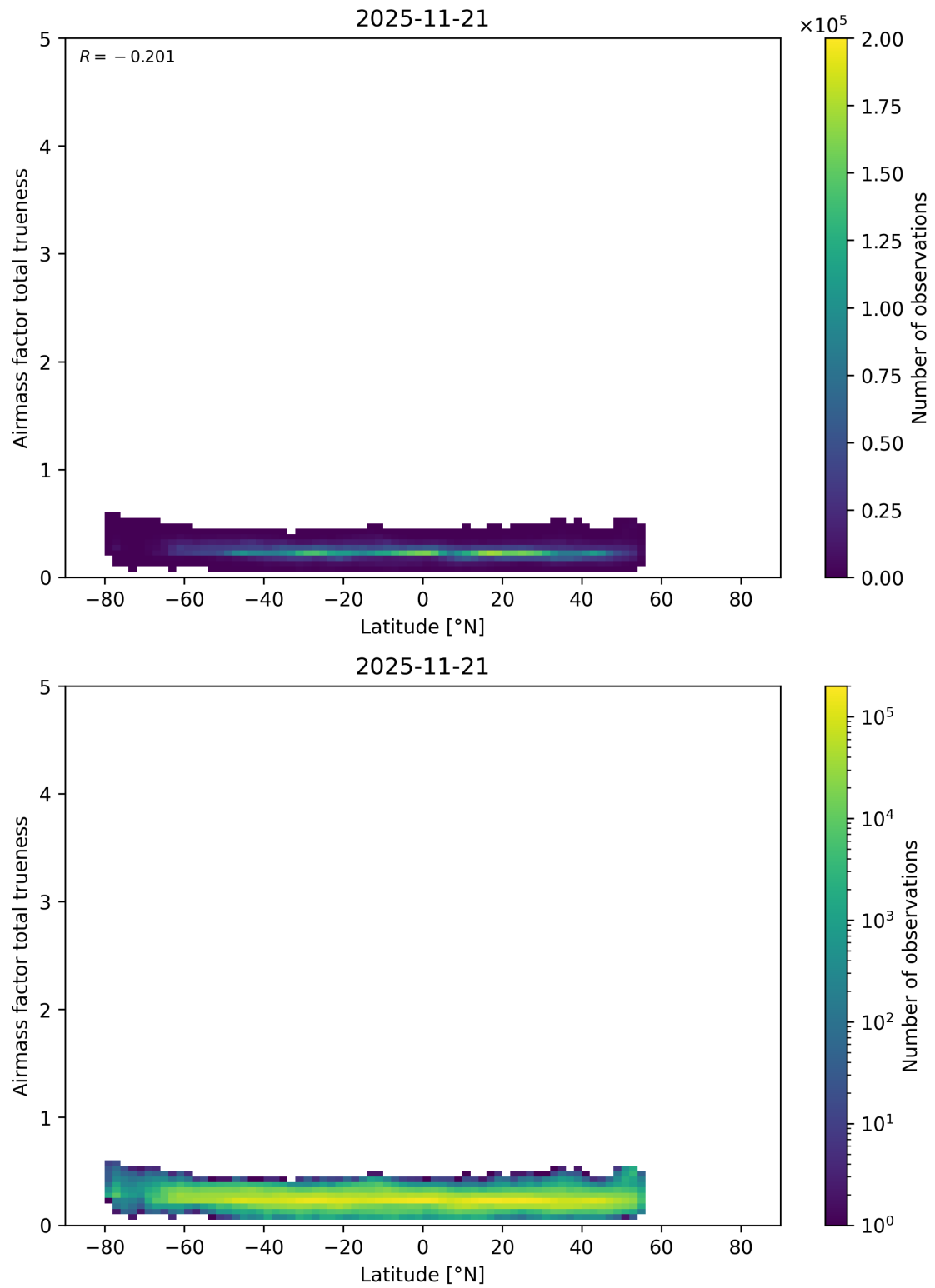
Figure 180: Scatter density plot of “Latitude” against “Airmass factor total trueneess” for 2025-11-20 to 2025-11-22.
