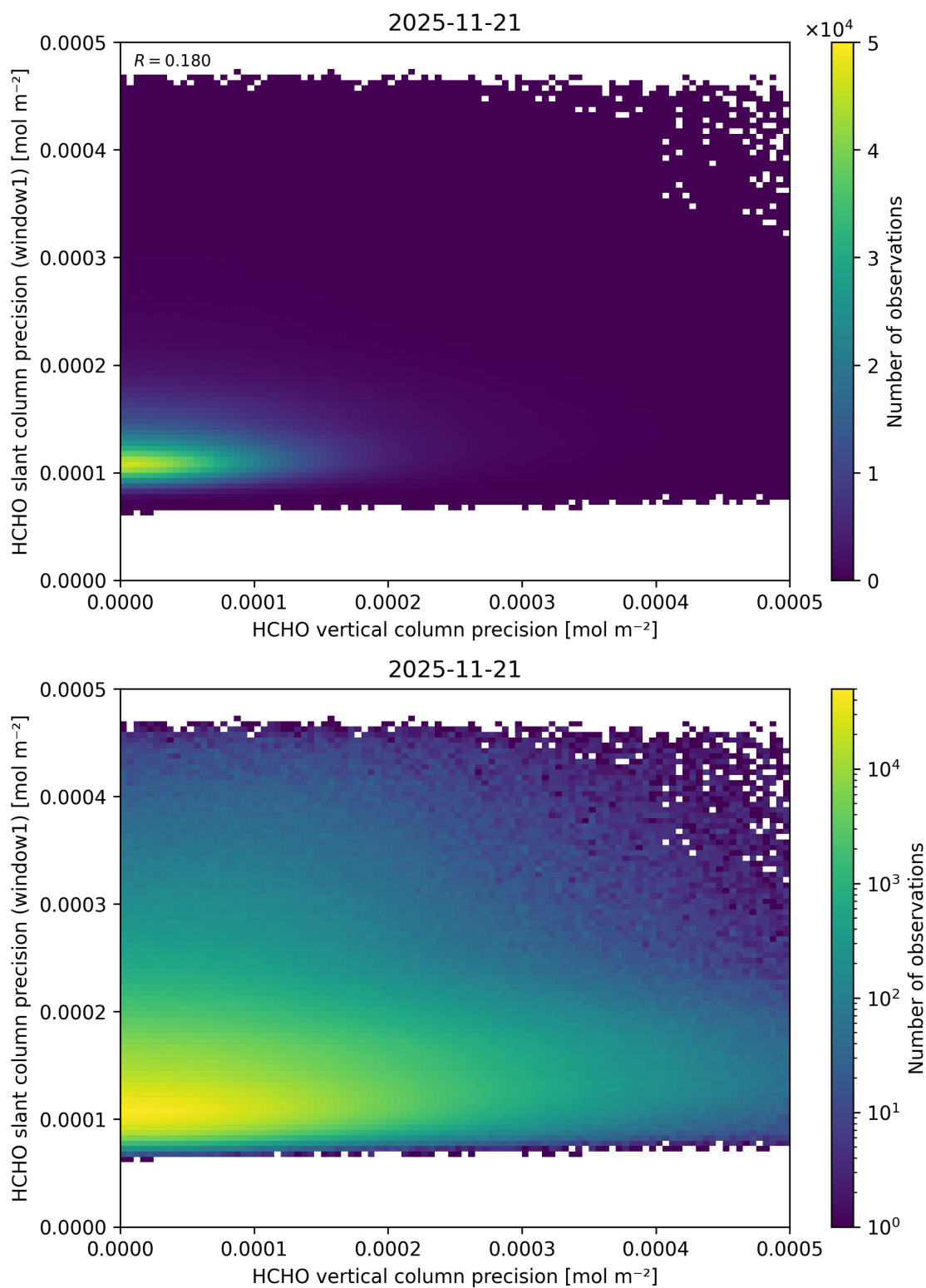
Figure 159: Scatter density plot of “HCHO vertical column precision” against “HCHO slant column precision (window1)” for 2025-11-20 to 2025-11-22.
