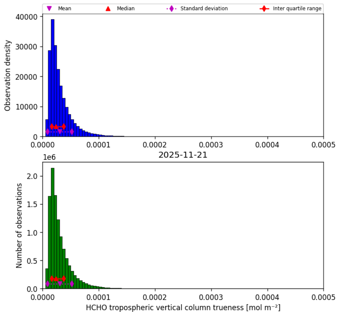
Figure 50: Histogram of “HCHO tropospheric vertical column trueness” for 2025-11-20 to 2025-11-22
