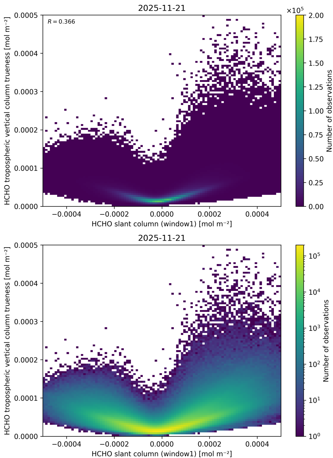
Figure 97: Scatter density plot of “HCHO slant column (window1)” against “HCHO tropospheric vertical column trueness” for 2025-11-20 to 2025-11-22.
