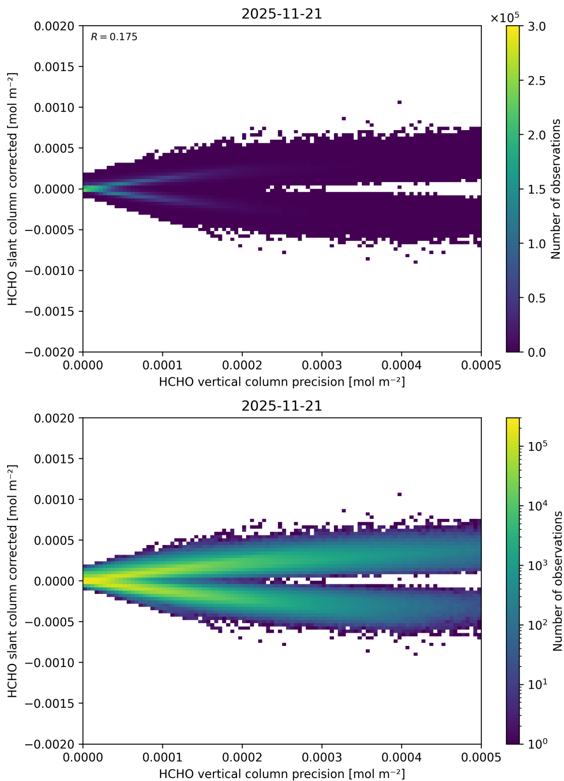
Figure 156: Scatter density plot of “HCHO vertical column precision” against “HCHO slant column corrected” for 2025-11-20 to 2025-11-22.
