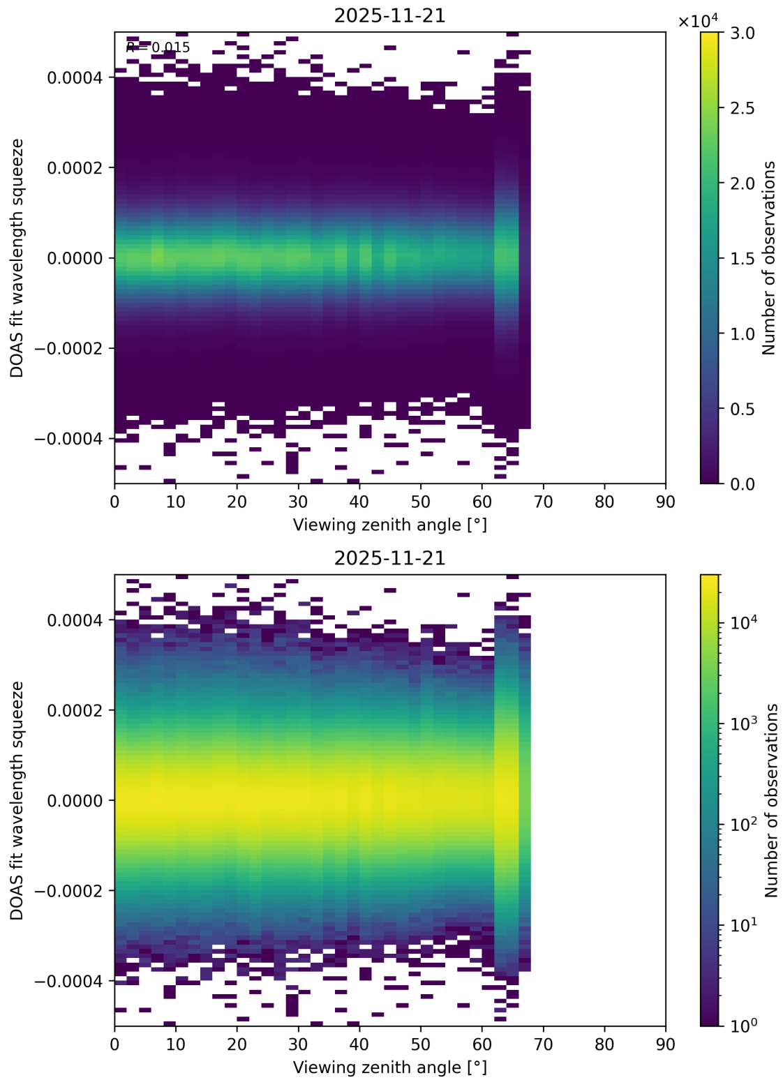
Figure 204: Scatter density plot of “Viewing zenith angle” against “DOAS fit wavelength squeeze” for 2025-11-20 to 2025-11-22.
