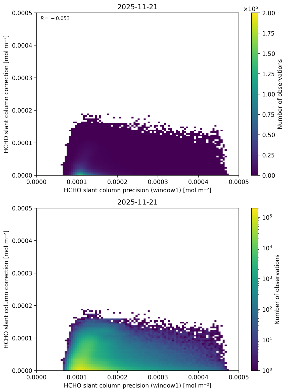
Figure 104: Scatter density plot of “HCHO slant column precision (window1)” against “HCHO slant column correction” for 2025-11-20 to 2025-11-22.
