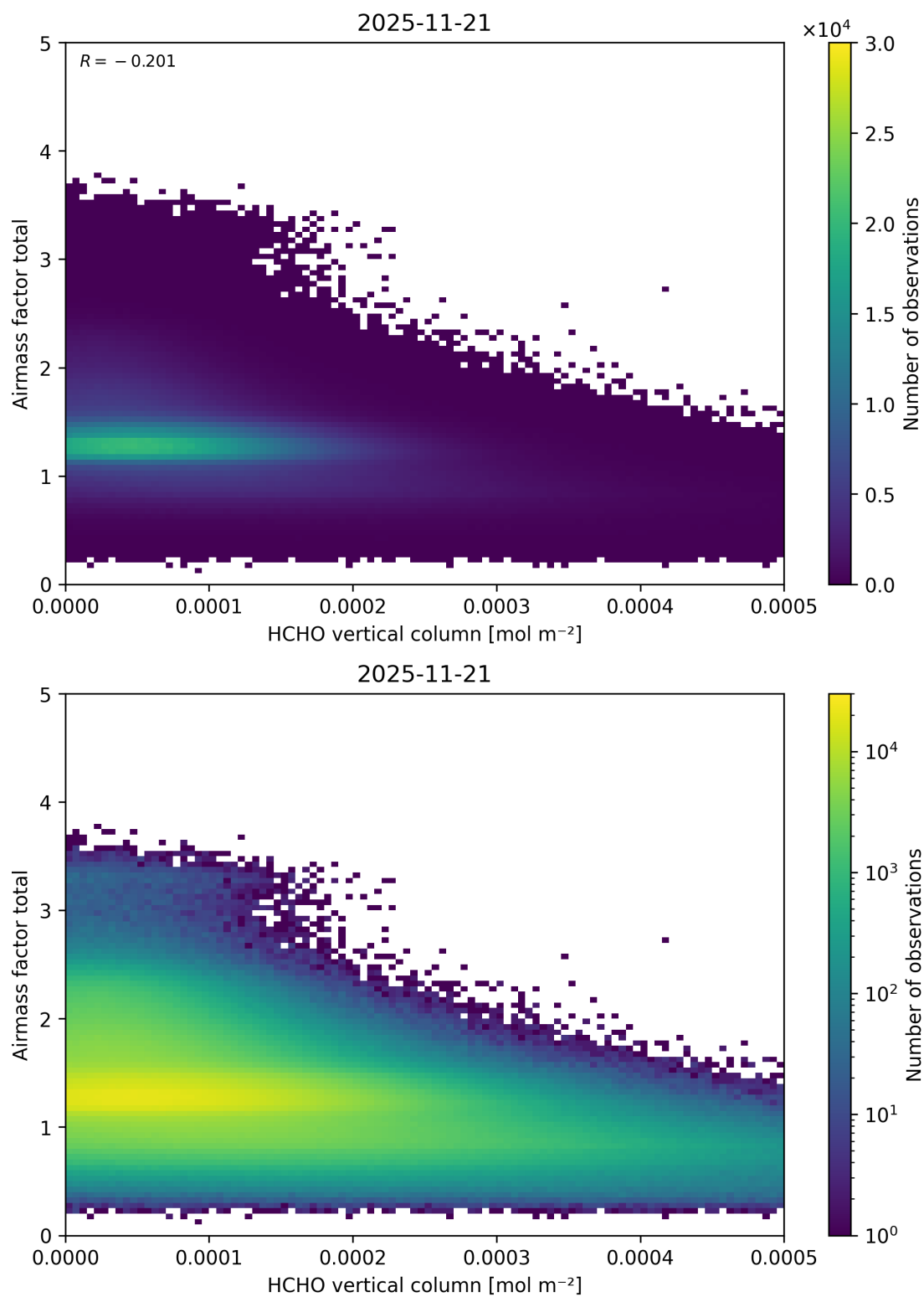
Figure 146: Scatter density plot of “HCHO vertical column” against “Airmass factor total” for 2025-11-20 to 2025-11-22.
