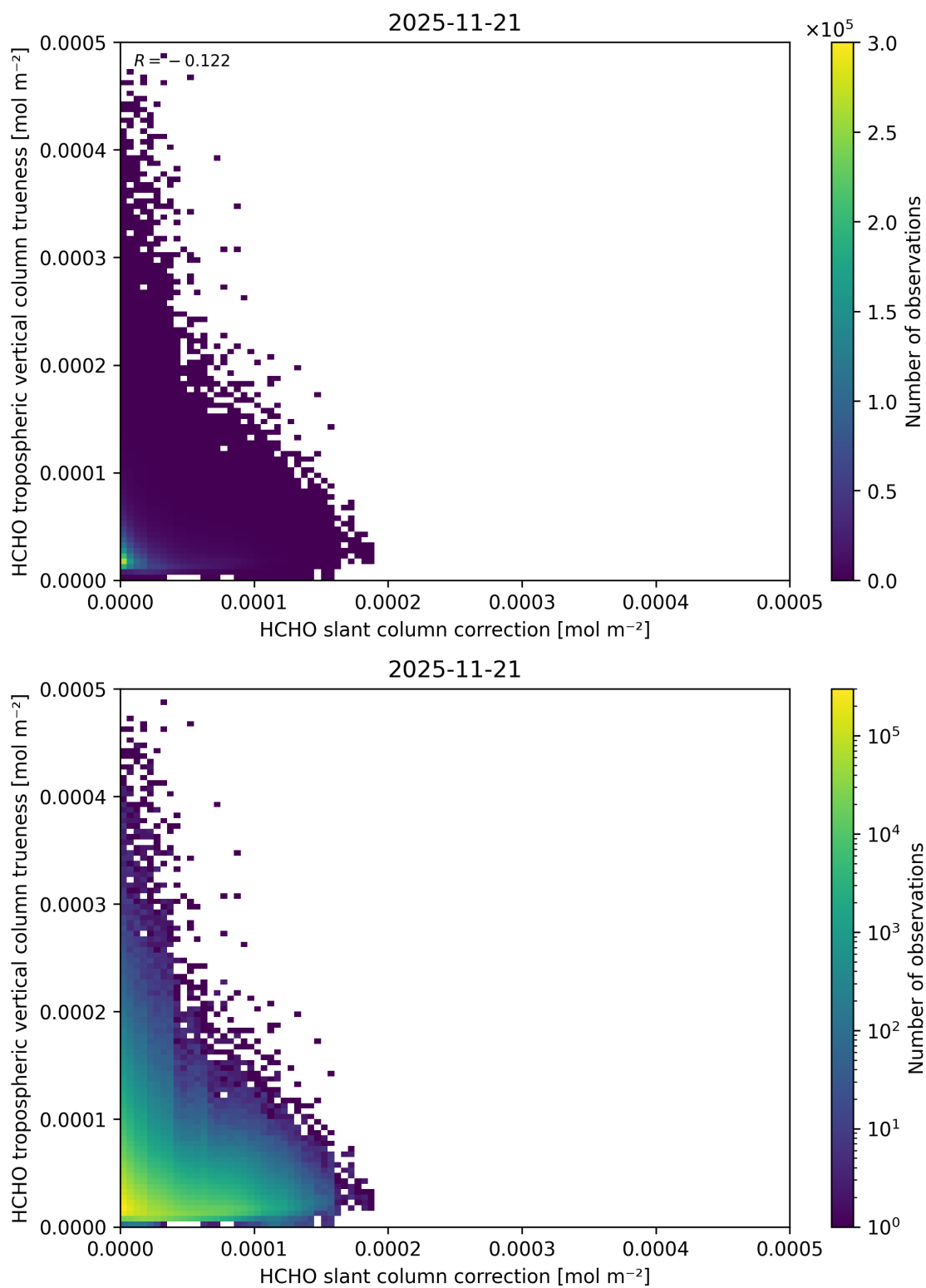
Figure 87: Scatter density plot of “HCHO slant column correction” against “HCHO tropospheric vertical column trueness” for 2025-11-20 to 2025-11-22.
