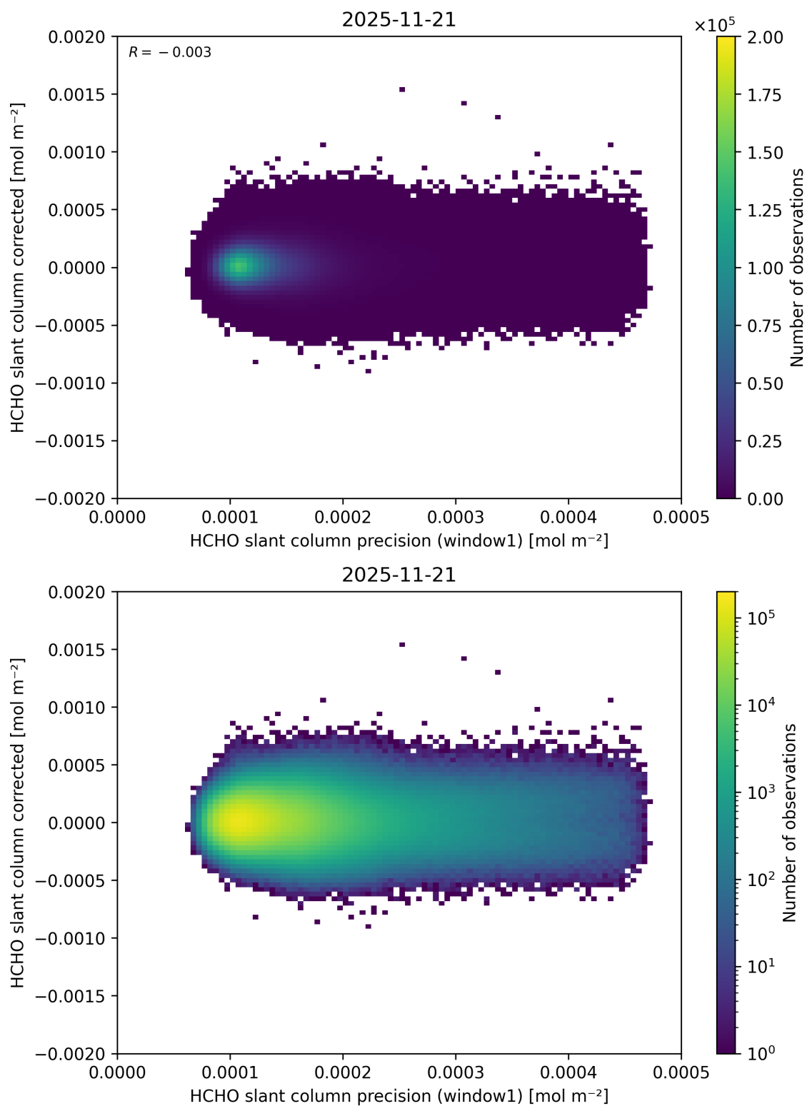
Figure 103: Scatter density plot of “HCHO slant column precision (window1)” against “HCHO slant column corrected” for 2025-11-20 to 2025-11-22.
