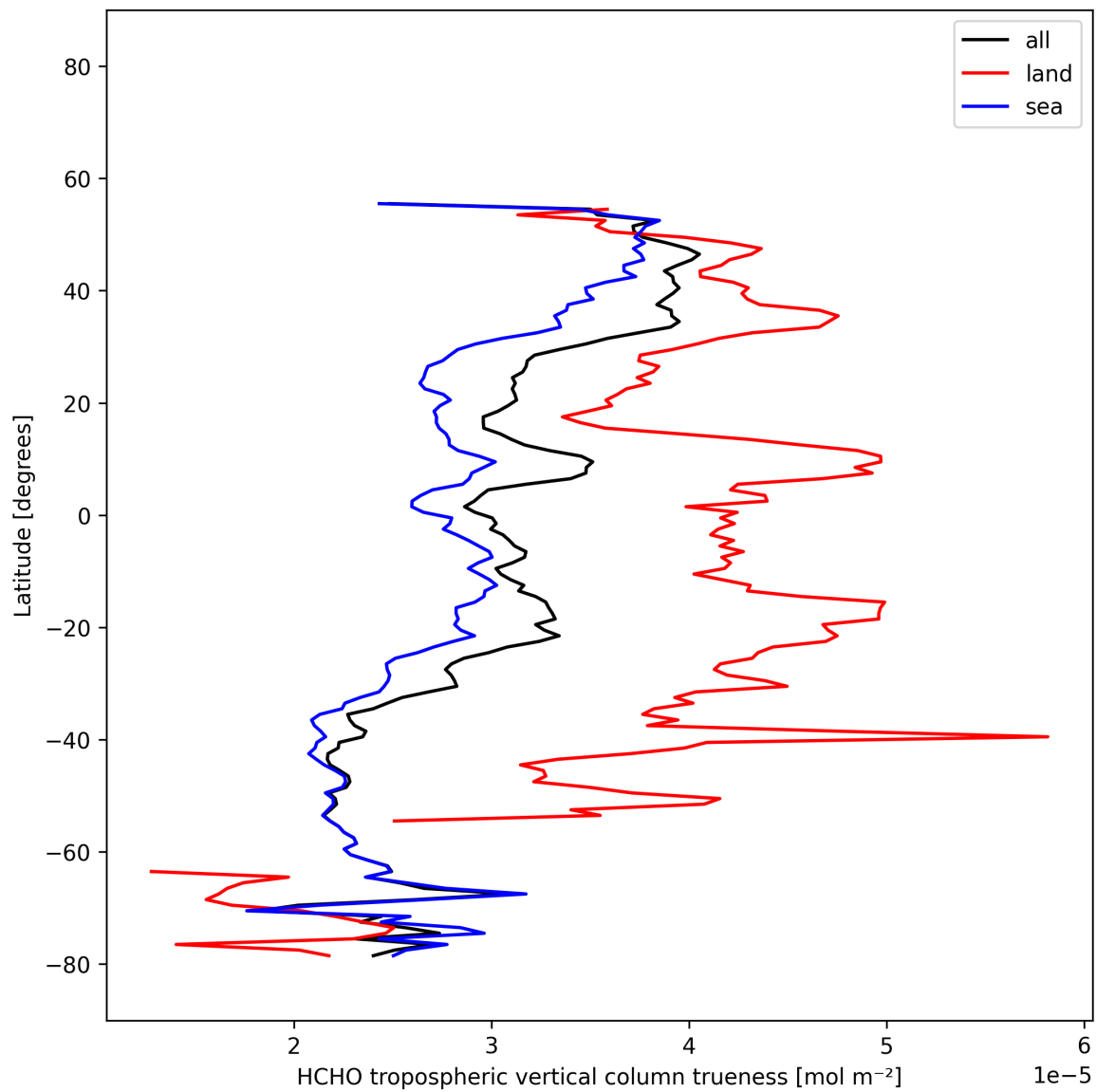
Figure 35: Zonal average of “HCHO tropospheric vertical column trueness” for 2025-11-20 to 2025-11-22.
