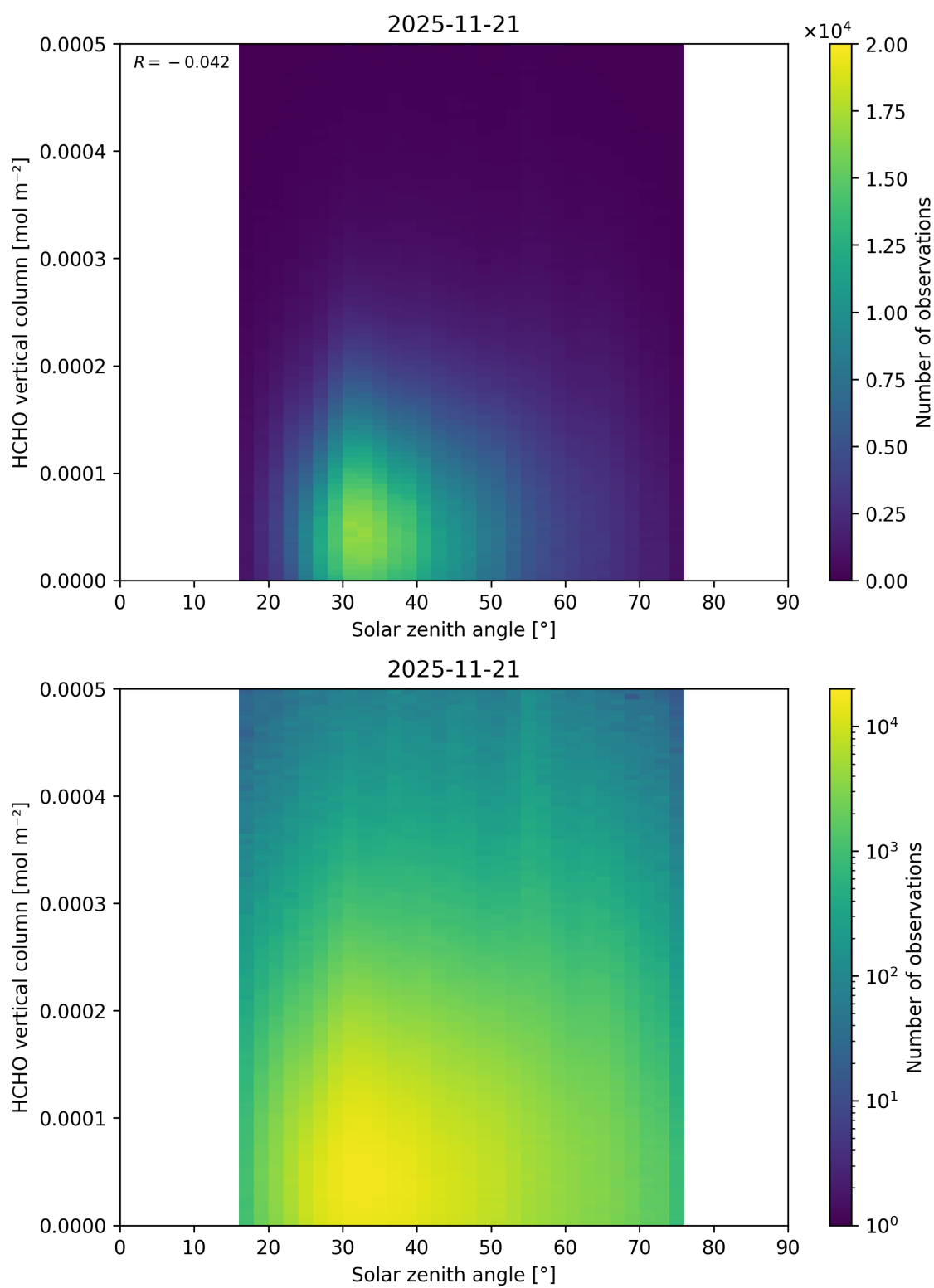
Figure 196: Scatter density plot of “Solar zenith angle” against “HCHO vertical column” for 2025-11-20 to 2025-11-22.
