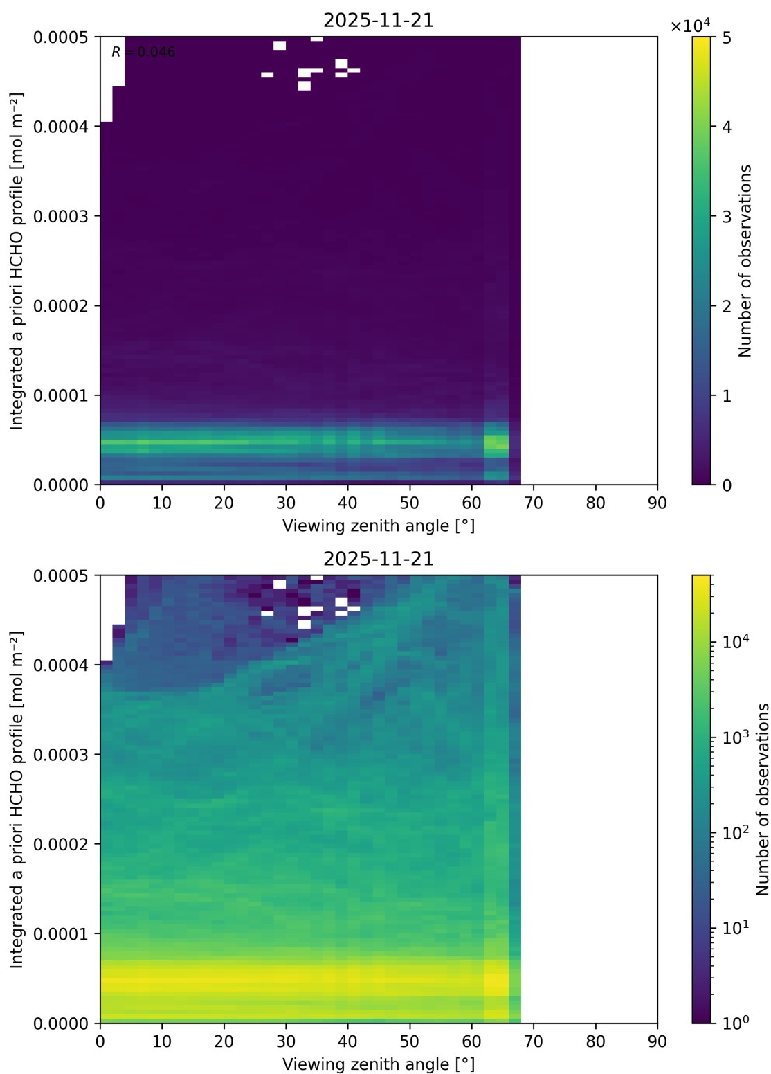
Figure 216: Scatter density plot of “Viewing zenith angle” against “Integrated a priori HCHO profile” for 2025-11-20 to 2025-11-22.
