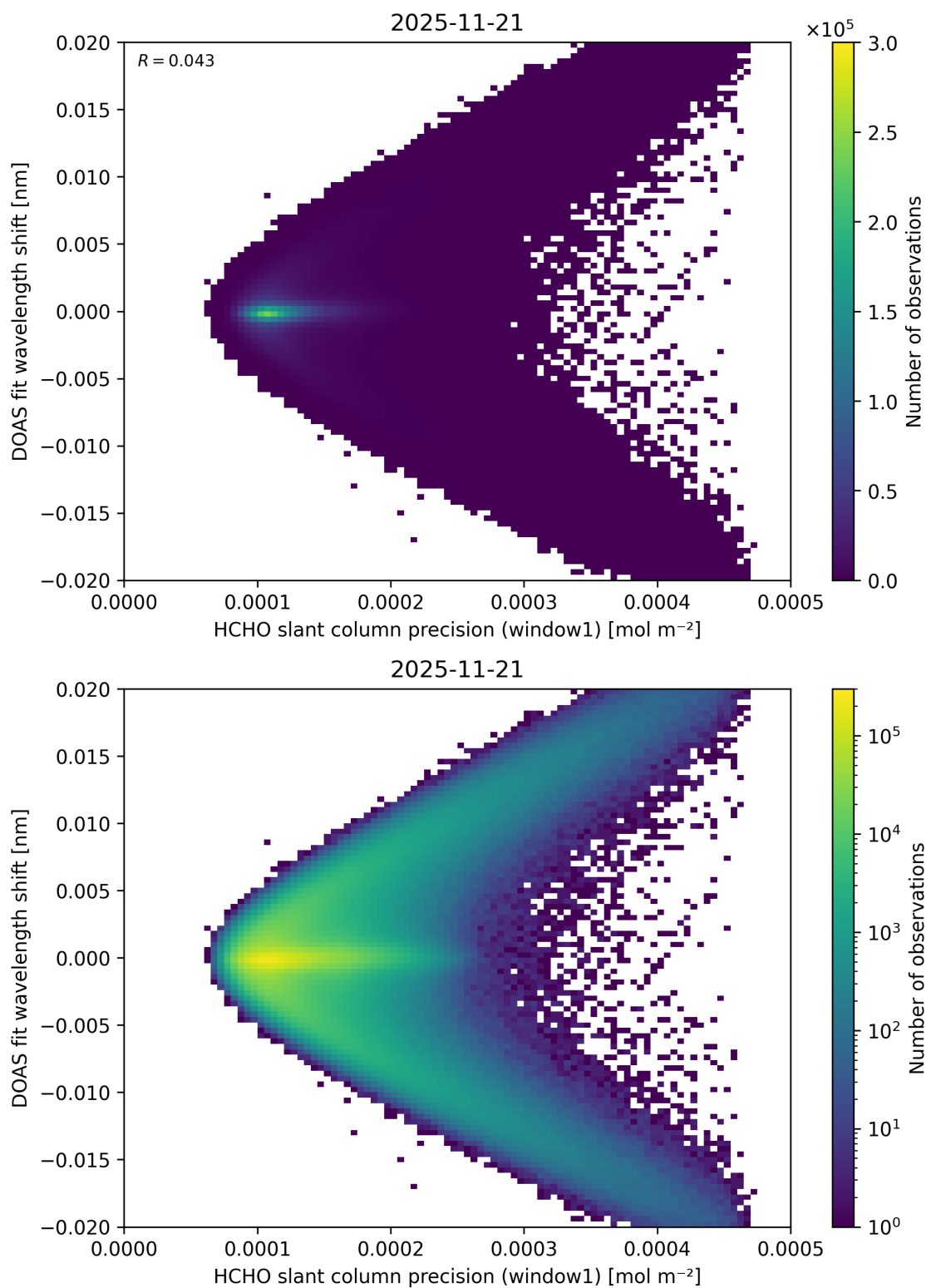
Figure 100: Scatter density plot of “HCHO slant column precision (window1)” against “DOAS fit wavelength shift” for 2025-11-20 to 2025-11-22.
