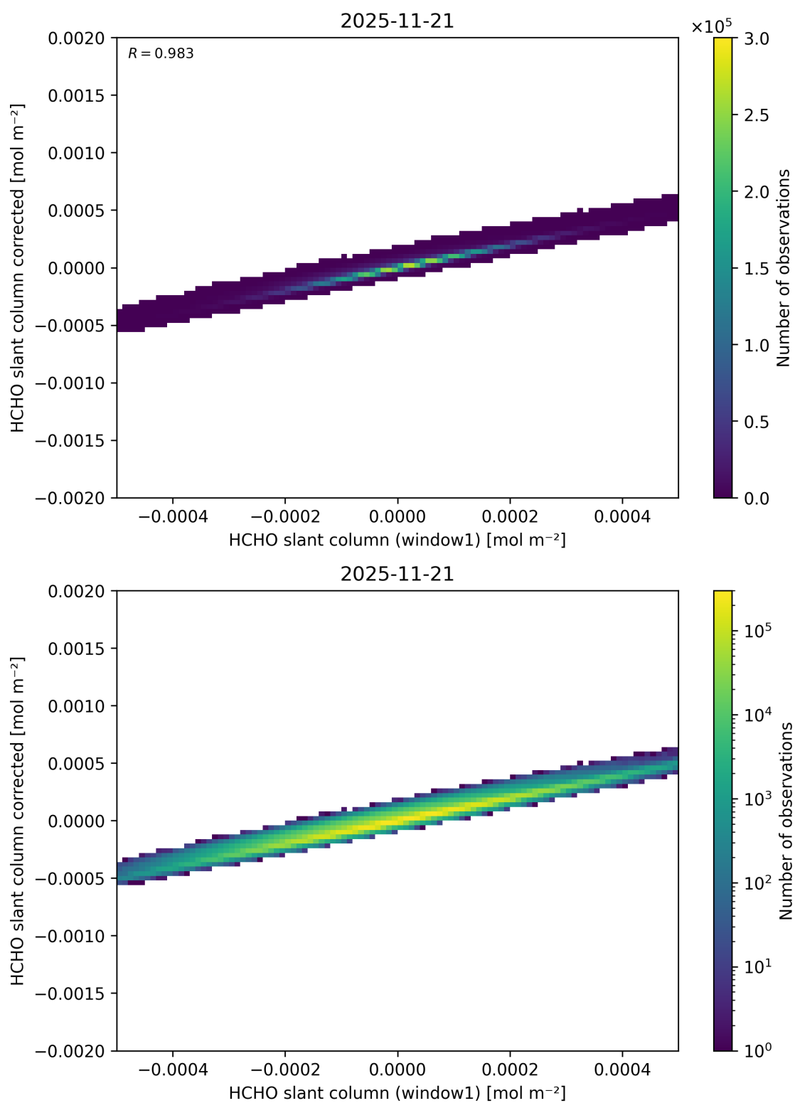
Figure 92: Scatter density plot of “HCHO slant column (window1)” against “HCHO slant column corrected” for 2025-11-20 to 2025-11-22.
