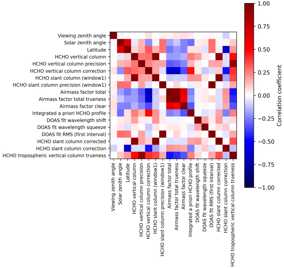
Figure 2: Map of correlation matrix for 2025-11-20 to 2025-11-22.
