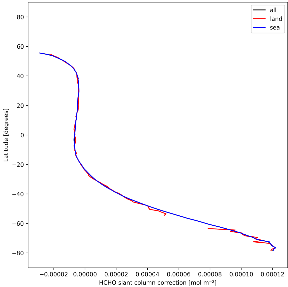
Figure 34: Zonal average of “HCHO slant column correction” for 2025-11-20 to 2025-11-22.
