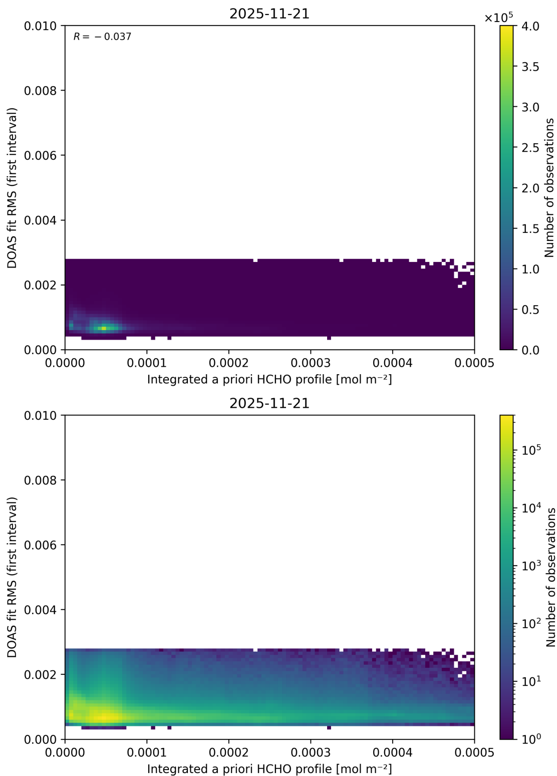
Figure 165: Scatter density plot of “Integrated a priori HCHO profile” against “DOAS fit RMS (first interval)” for 2025-11-20 to 2025-11-22.
