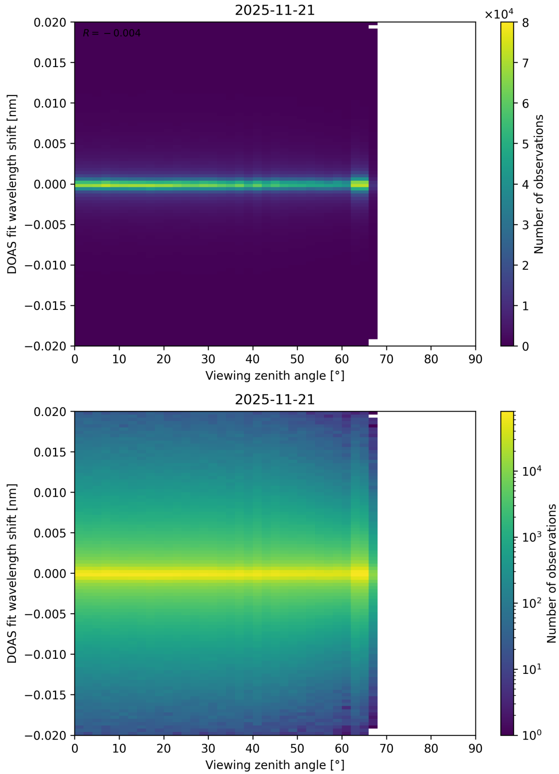
Figure 203: Scatter density plot of “Viewing zenith angle” against “DOAS fit wavelength shift” for 2025-11-20 to 2025-11-22.
