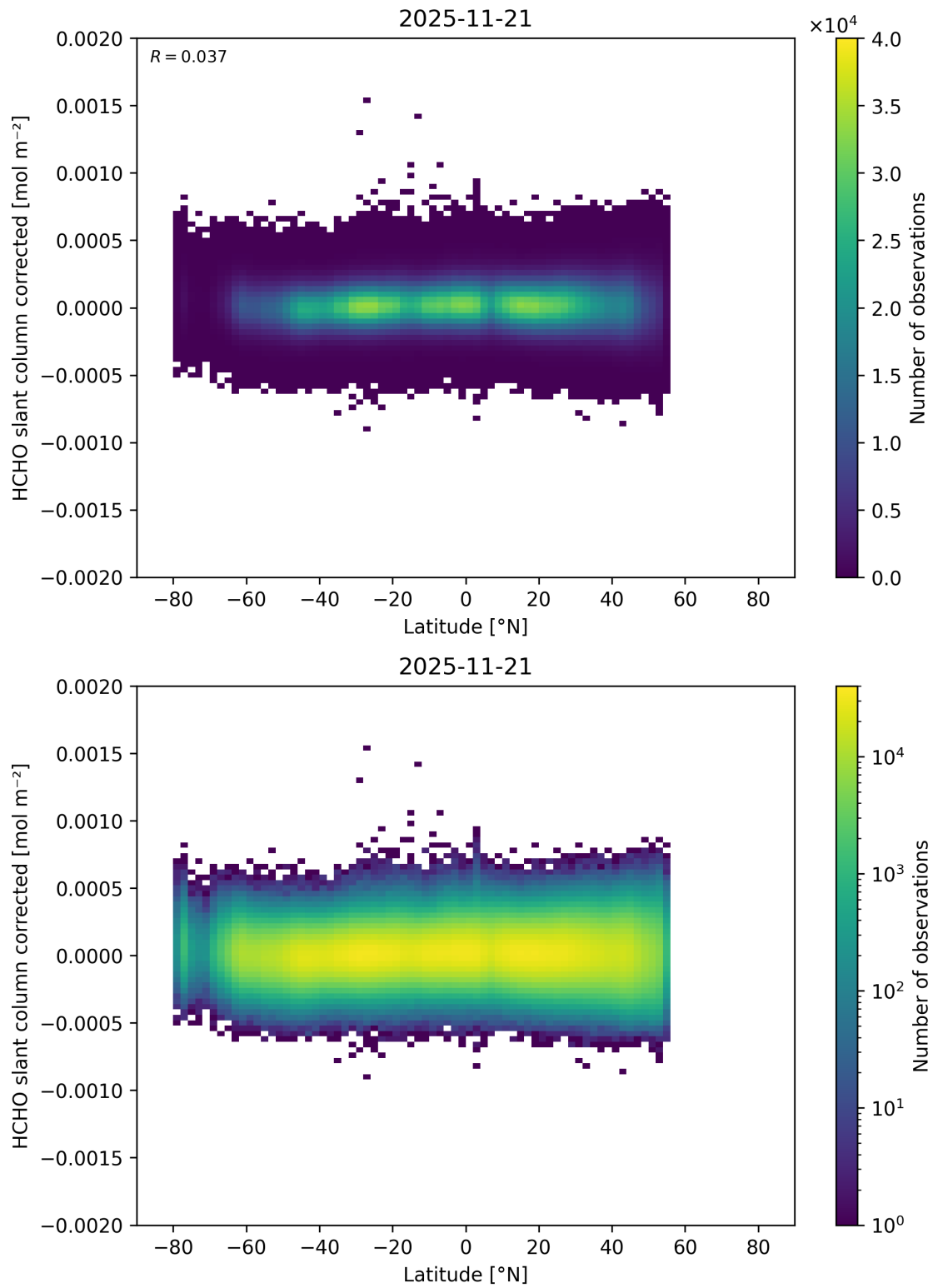
Figure 175: Scatter density plot of “Latitude” against “HCHO slant column corrected” for 2025-11-20 to 2025-11-22.
