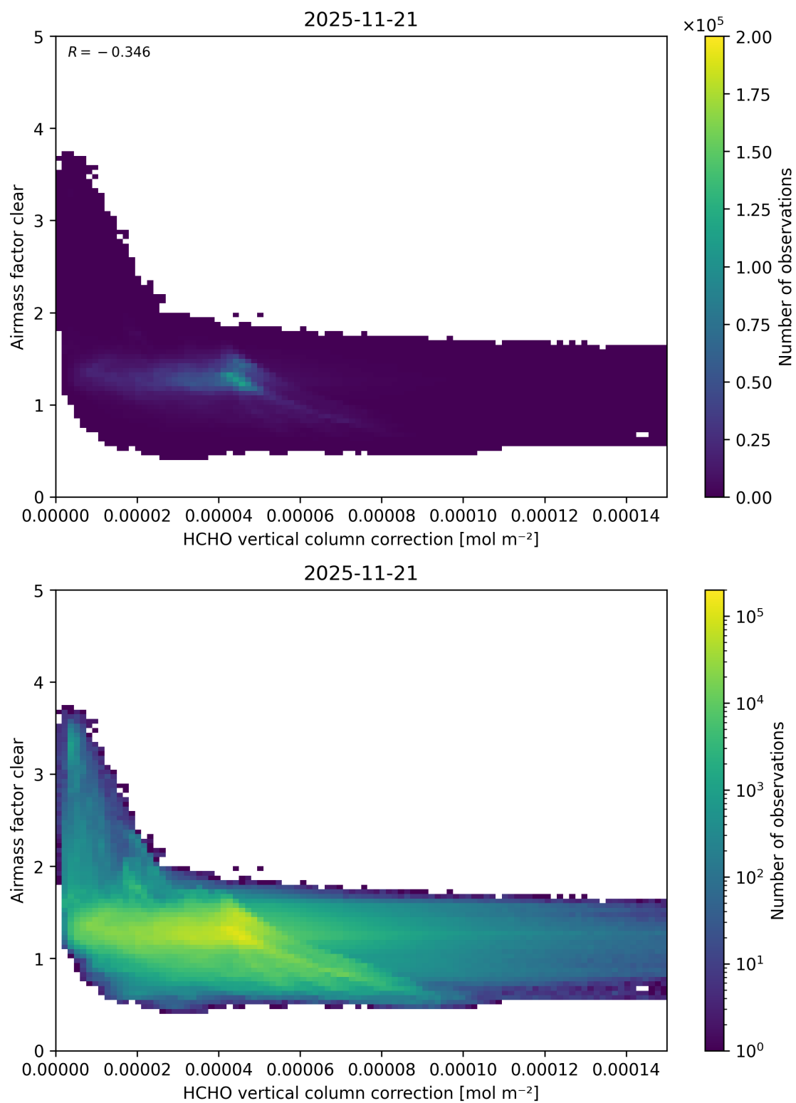
Figure 129: Scatter density plot of “HCHO vertical column correction” against “Airmass factor clear” for 2025-11-20 to 2025-11-22.
