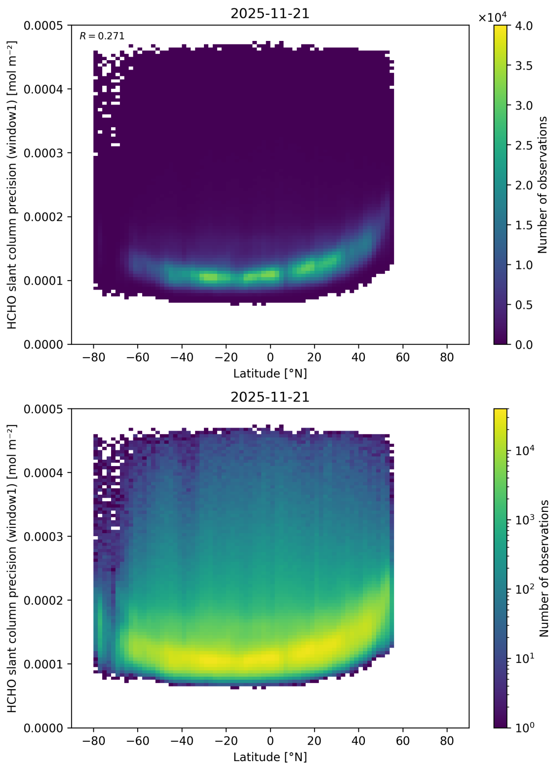
Figure 178: Scatter density plot of “Latitude” against “HCHO slant column precision (window1)” for 2025-11-20 to 2025-11-22.
