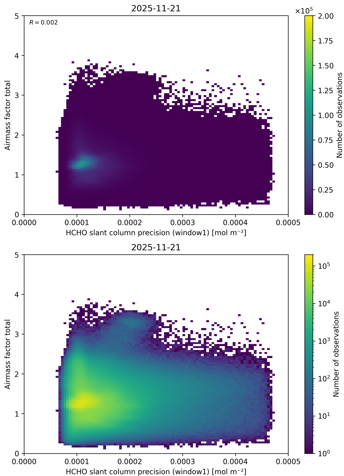
Figure 105: Scatter density plot of “HCHO slant column precision (window1)” against “Airmass factor total” for 2025-11-20 to 2025-11-22.
