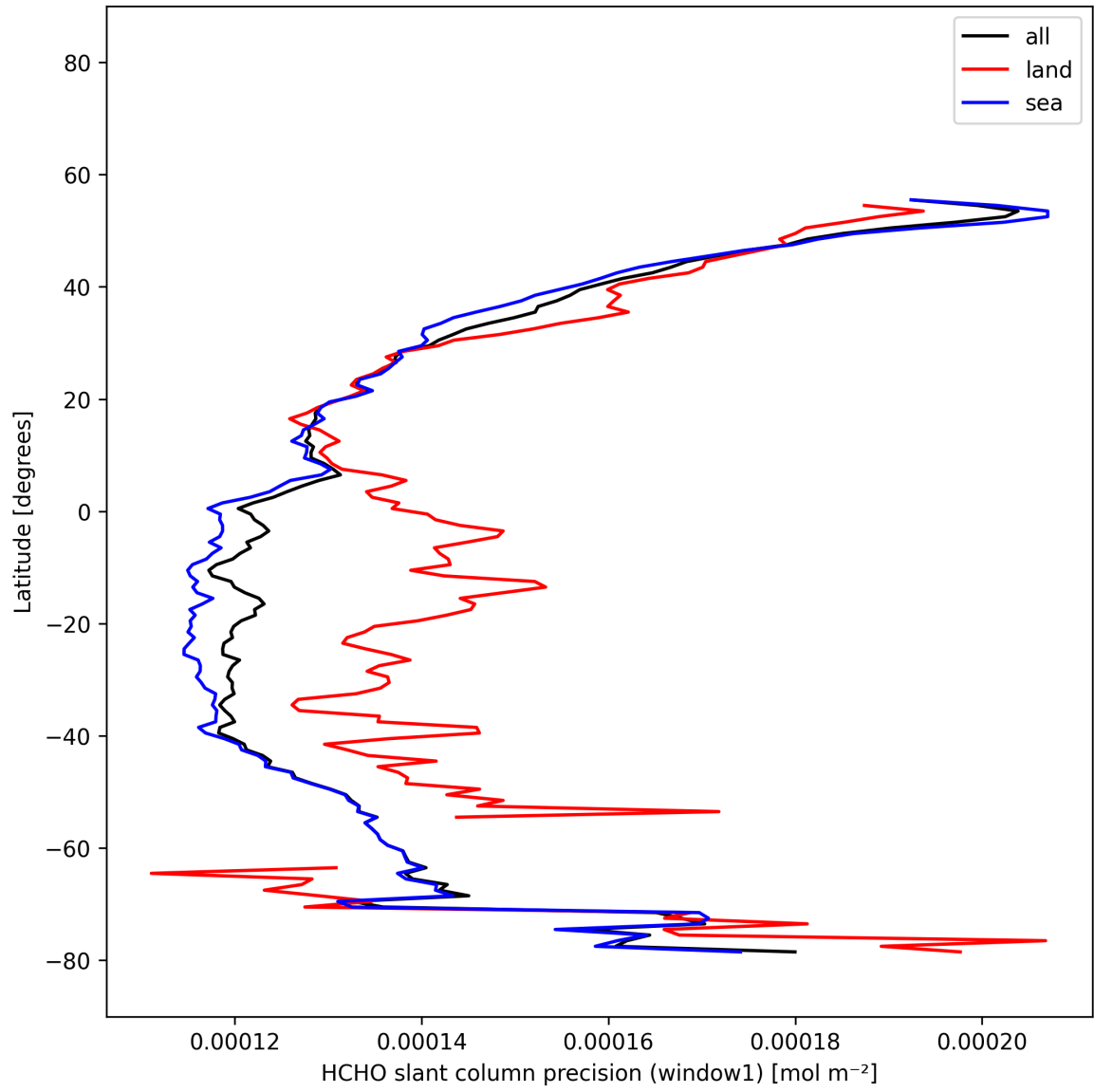
Figure 26: Zonal average of “HCHO slant column precision (window1)” for 2025-11-20 to 2025-11-22.
