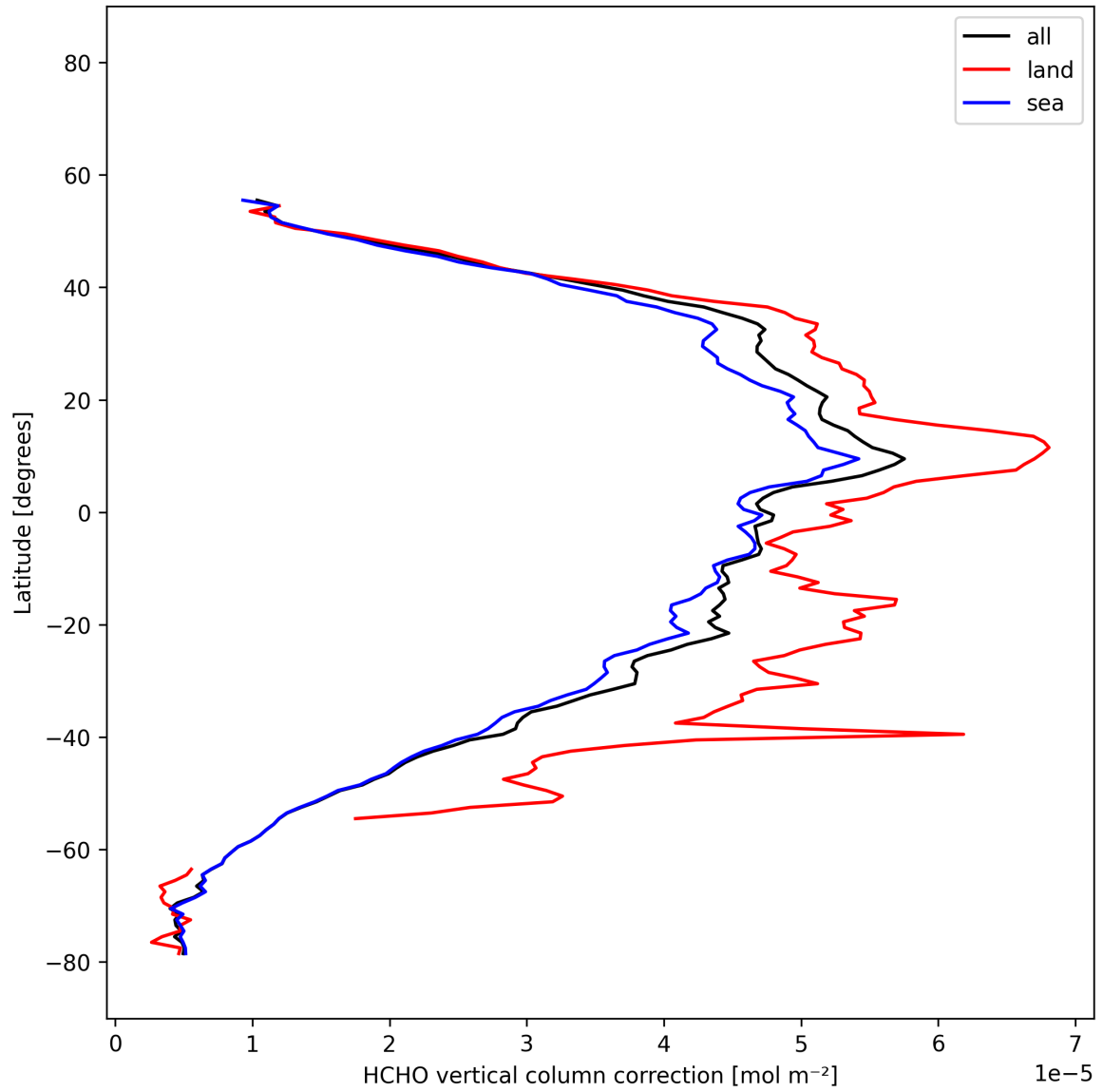
Figure 24: Zonal average of “HCHO vertical column correction” for 2025-11-20 to 2025-11-22.
