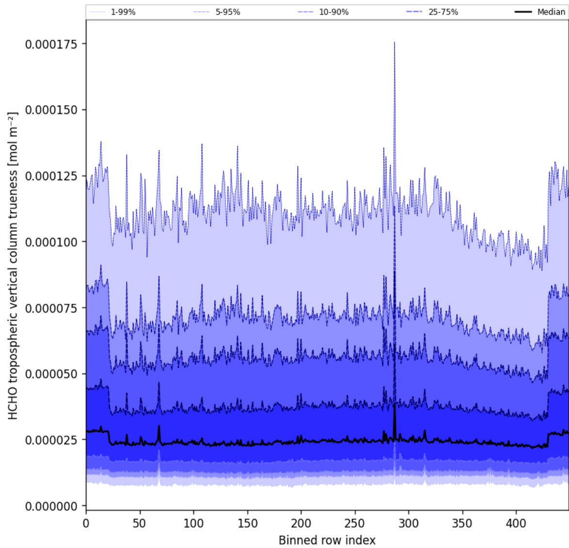
Figure 65: Along track statistics of “HCHO tropospheric vertical column trueness” for 2025-11-20 to 2025-11-22
