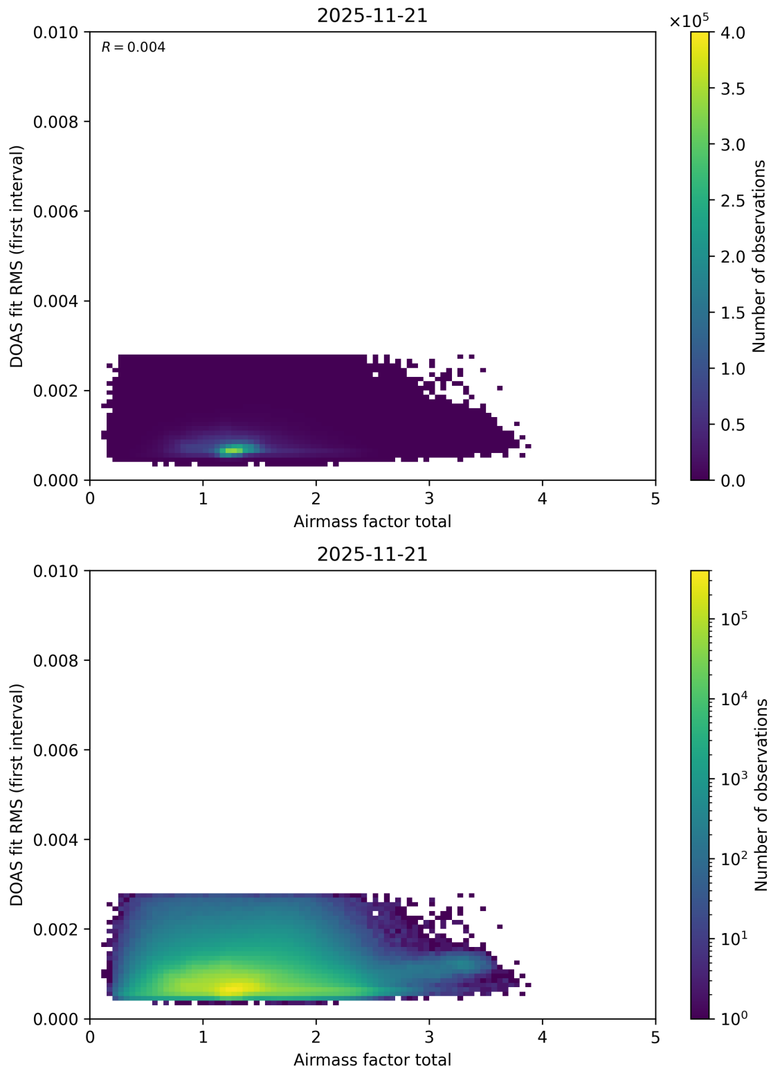
Figure 109: Scatter density plot of “Airmass factor total” against “DOAS fit RMS (first interval)” for 2025-11-20 to 2025-11-22.
