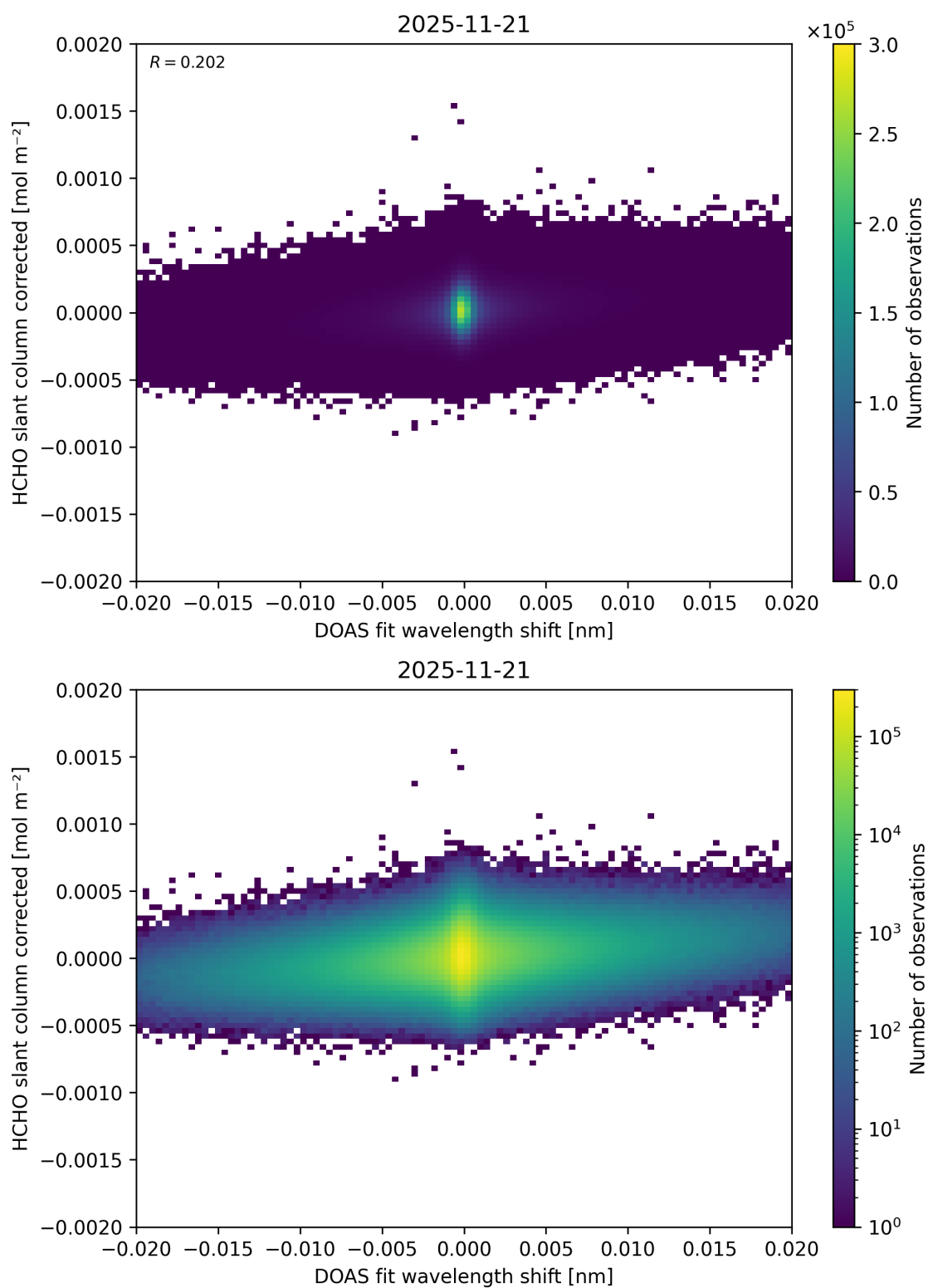
Figure 71: Scatter density plot of “DOAS fit wavelength shift” against “HCHO slant column corrected” for 2025-11-20 to 2025-11-22.
