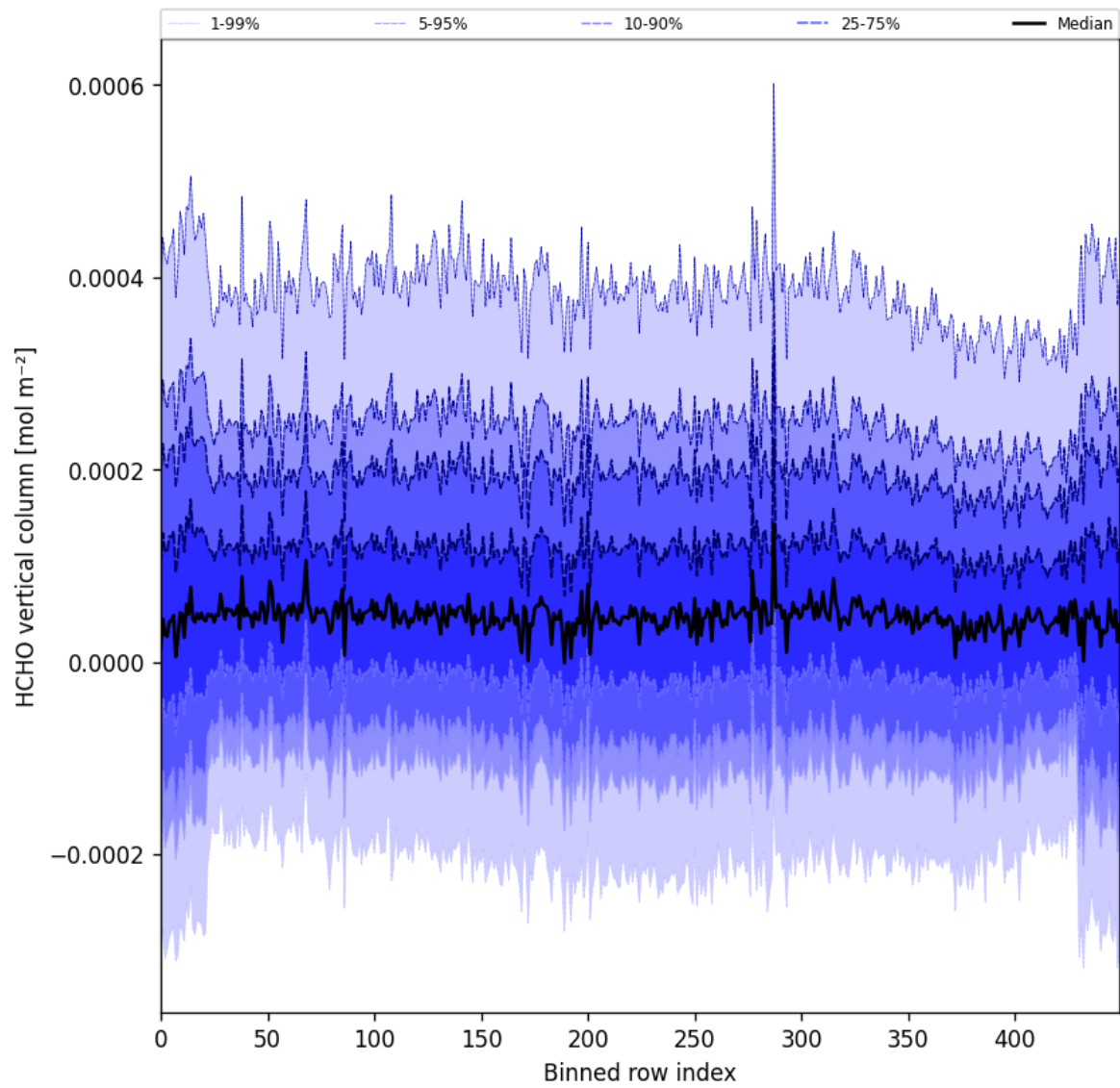
Figure 52: Along track statistics of “HCHO vertical column” for 2025-11-20 to 2025-11-22
