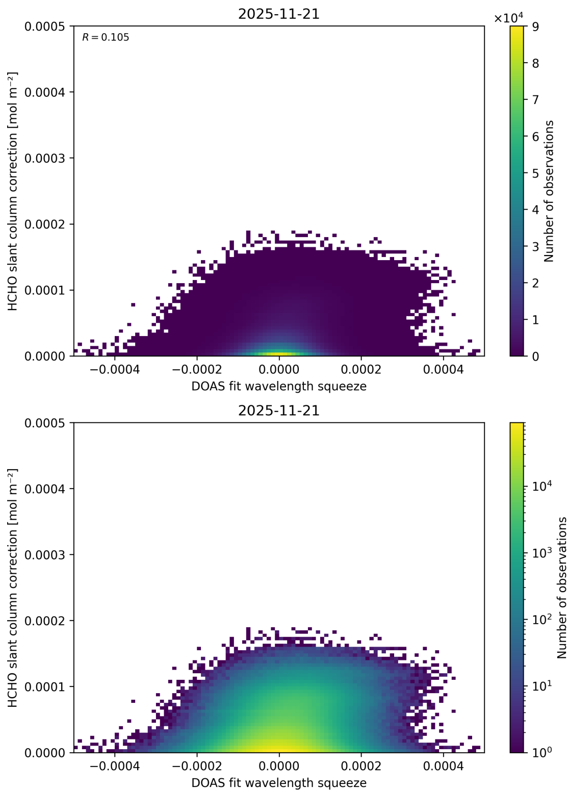
Figure 76: Scatter density plot of “DOAS fit wavelength squeeze” against “HCHO slant column correction” for 2025-11-20 to 2025-11-22.
