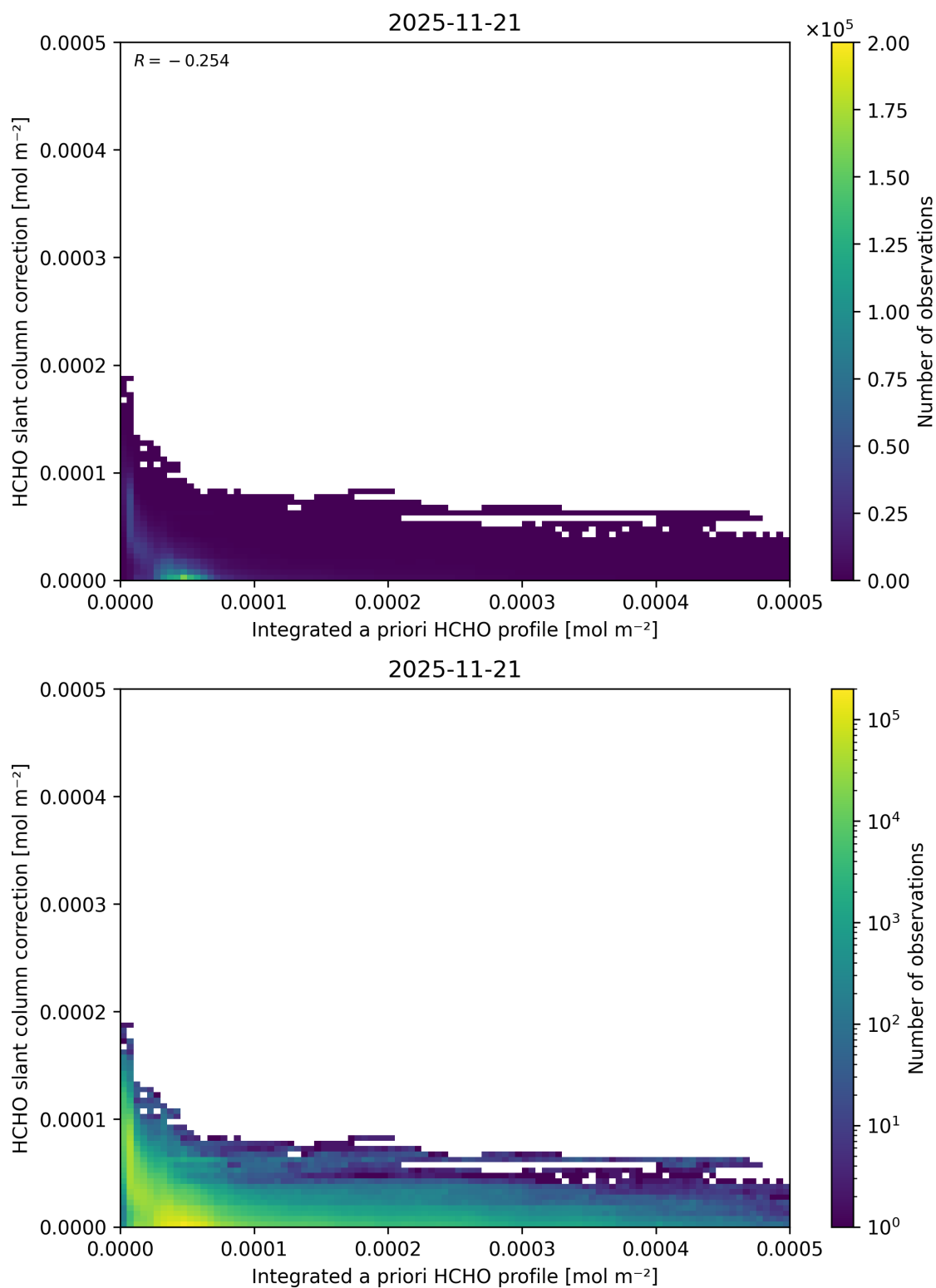
Figure 169: Scatter density plot of “Integrated a priori HCHO profile” against “HCHO slant column correction” for 2025-11-20 to 2025-11-22.
