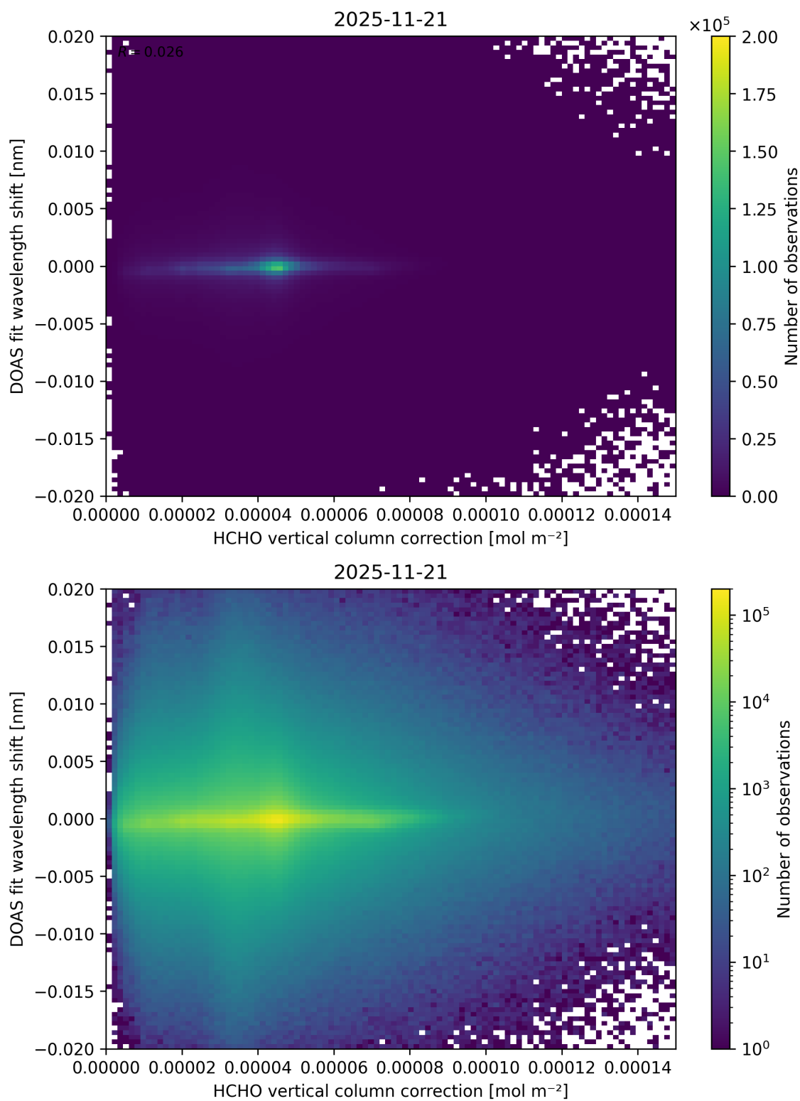
Figure 127: Scatter density plot of “HCHO vertical column correction” against “DOAS fit wavelength shift” for 2025-11-20 to 2025-11-22.
