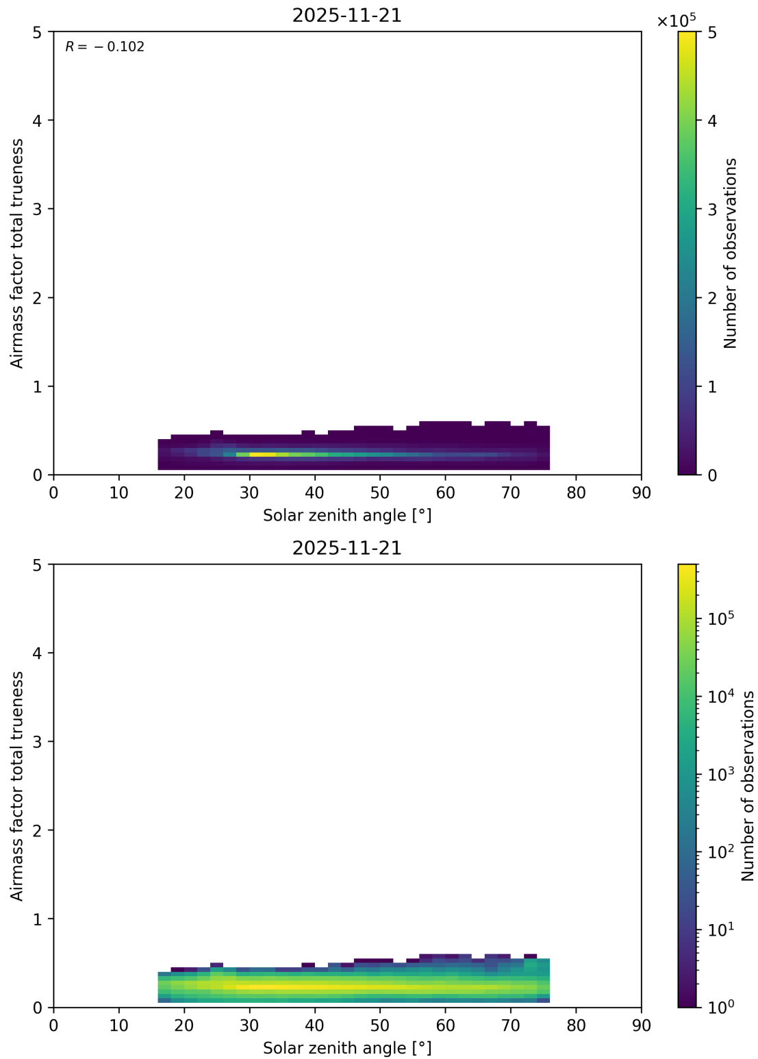
Figure 195: Scatter density plot of “Solar zenith angle” against “Airmass factor total trueneess” for 2025-11-20 to 2025-11-22.
