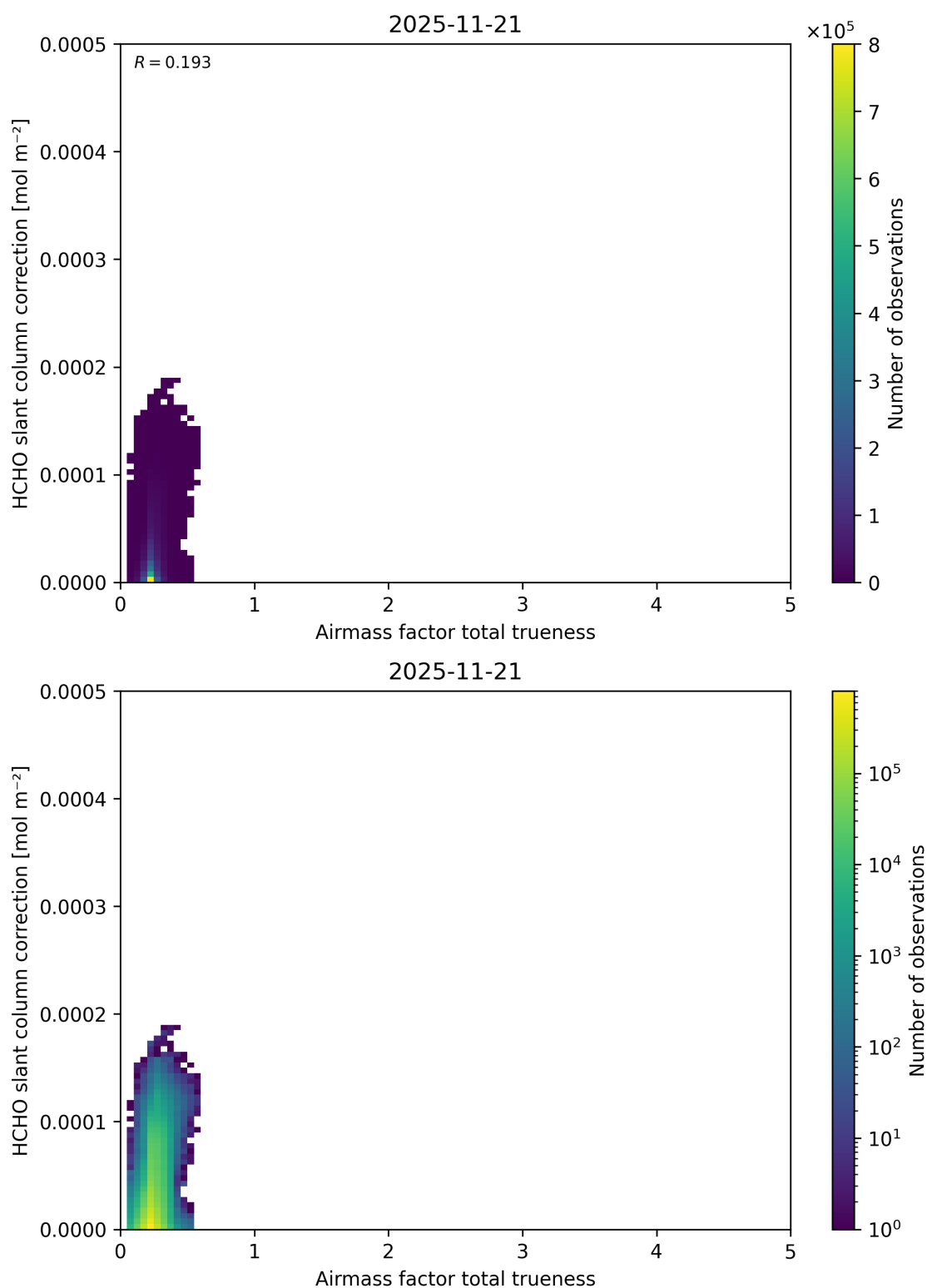
Figure 123: Scatter density plot of “Airmass factor total truiness” against “HCHO slant column correction” for 2025-11-20 to 2025-11-22.
