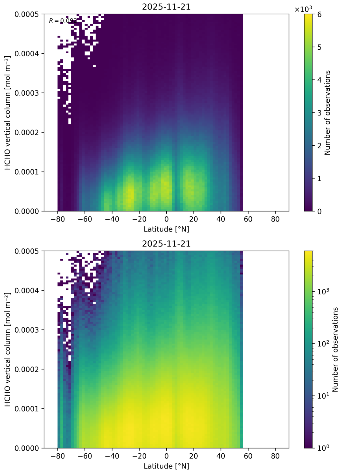
Figure 181: Scatter density plot of “Latitude” against “HCHO vertical column” for 2025-11-20 to 2025-11-22.
