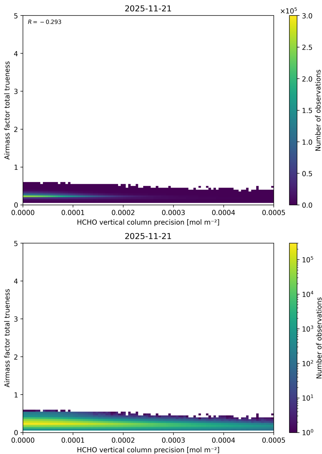
Figure 161: Scatter density plot of “HCHO vertical column precision” against “Airmass factor total trueness” for 2025-11-20 to 2025-11-22.
