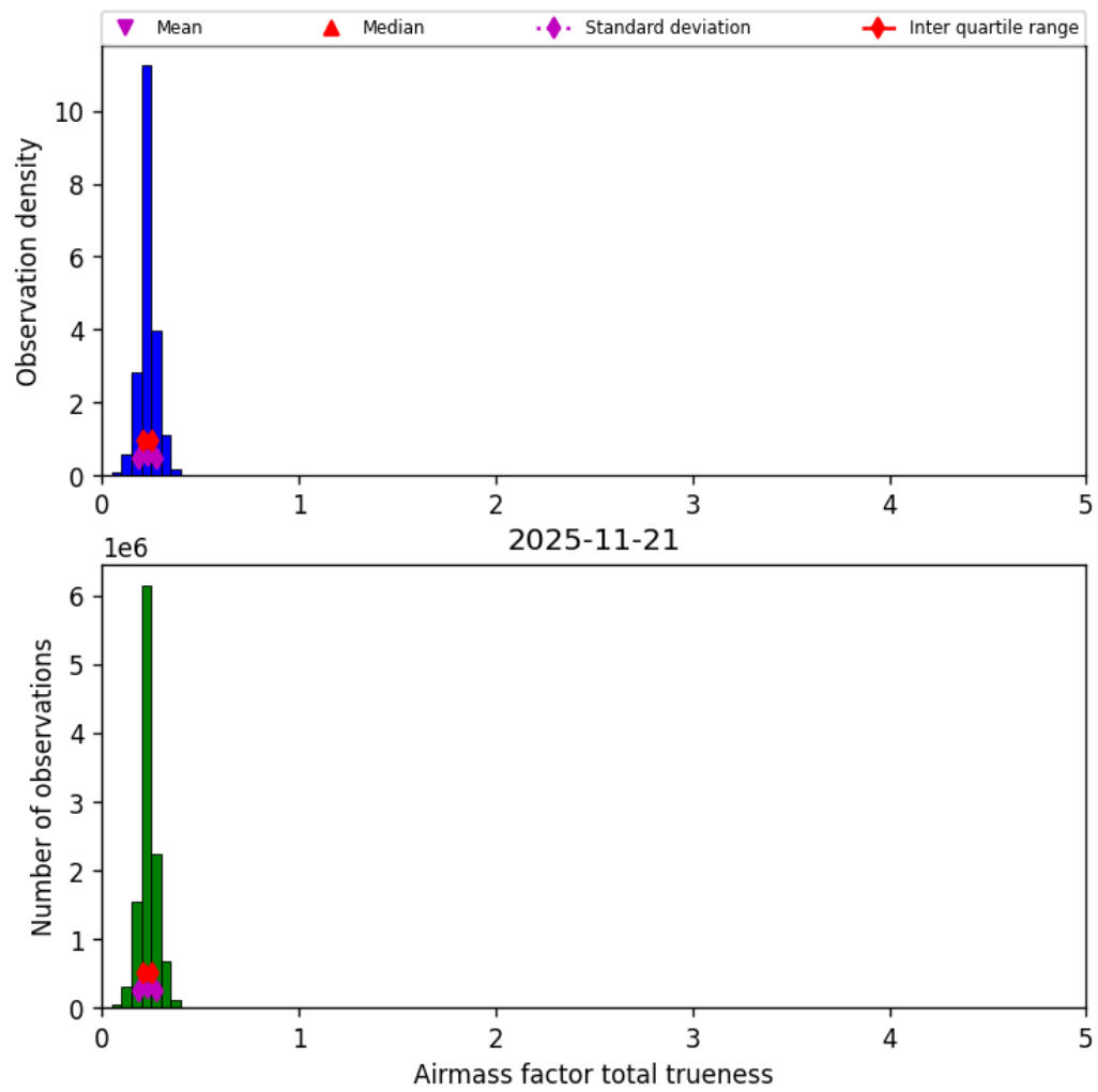
Figure 43: Histogram of “Airmass factor total trueness” for 2025-11-20 to 2025-11-22
