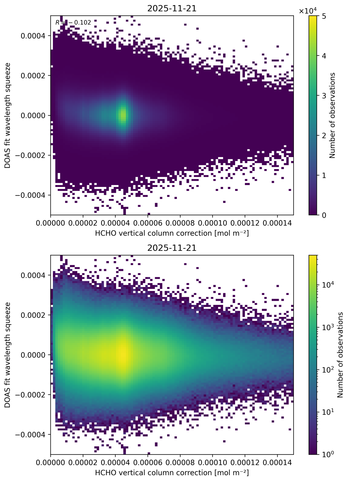
Figure 128: Scatter density plot of “HCHO vertical column correction” against “DOAS fit wavelength squeeze” for 2025-11-20 to 2025-11-22.
