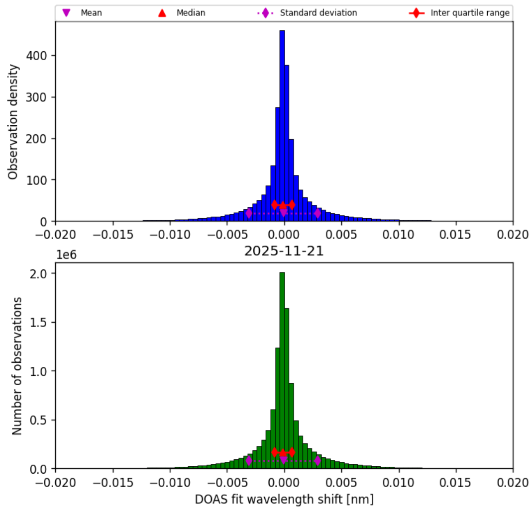
Figure 46: Histogram of “DOAS fit wavelength shift” for 2025-11-20 to 2025-11-22
