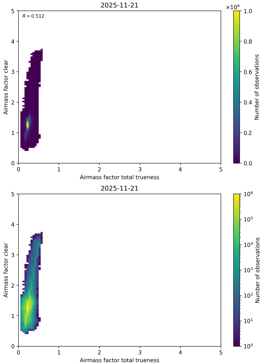
Figure 121: Scatter density plot of “Airmass factor total trueness” against “Airmass factor clear” for 2025-11-20 to 2025-11-22.
