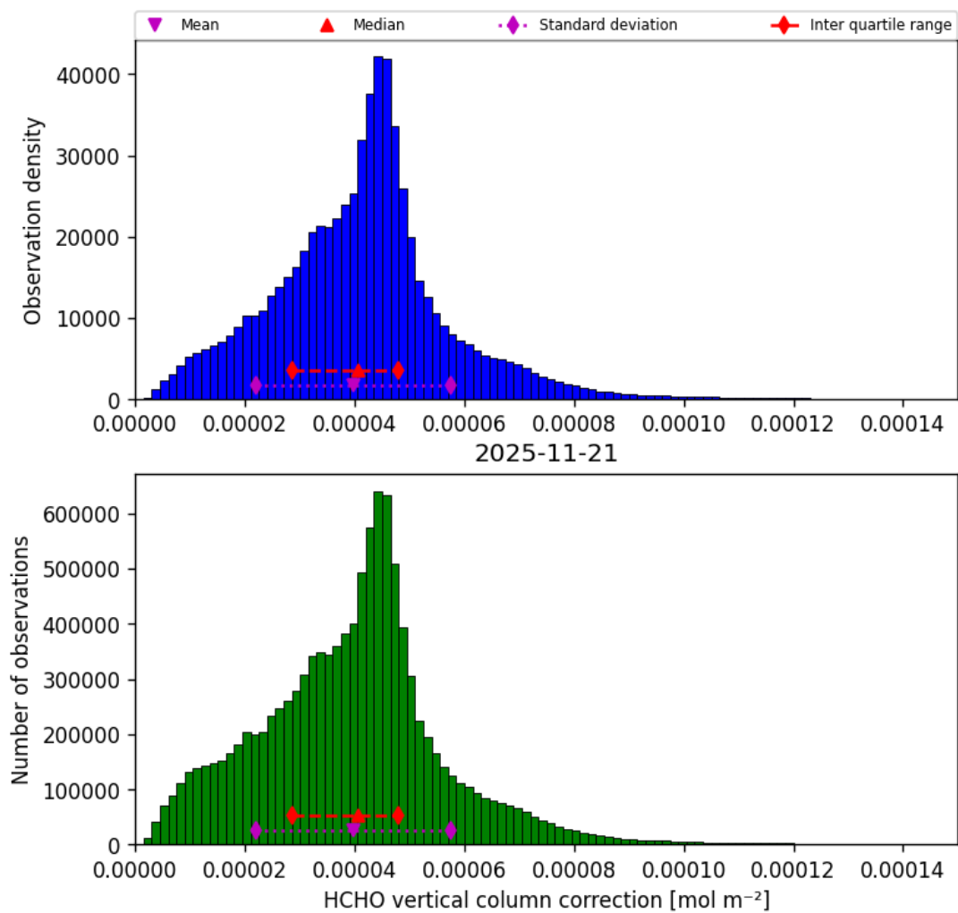
Figure 39: Histogram of “HCHO vertical column correction” for 2025-11-20 to 2025-11-22
