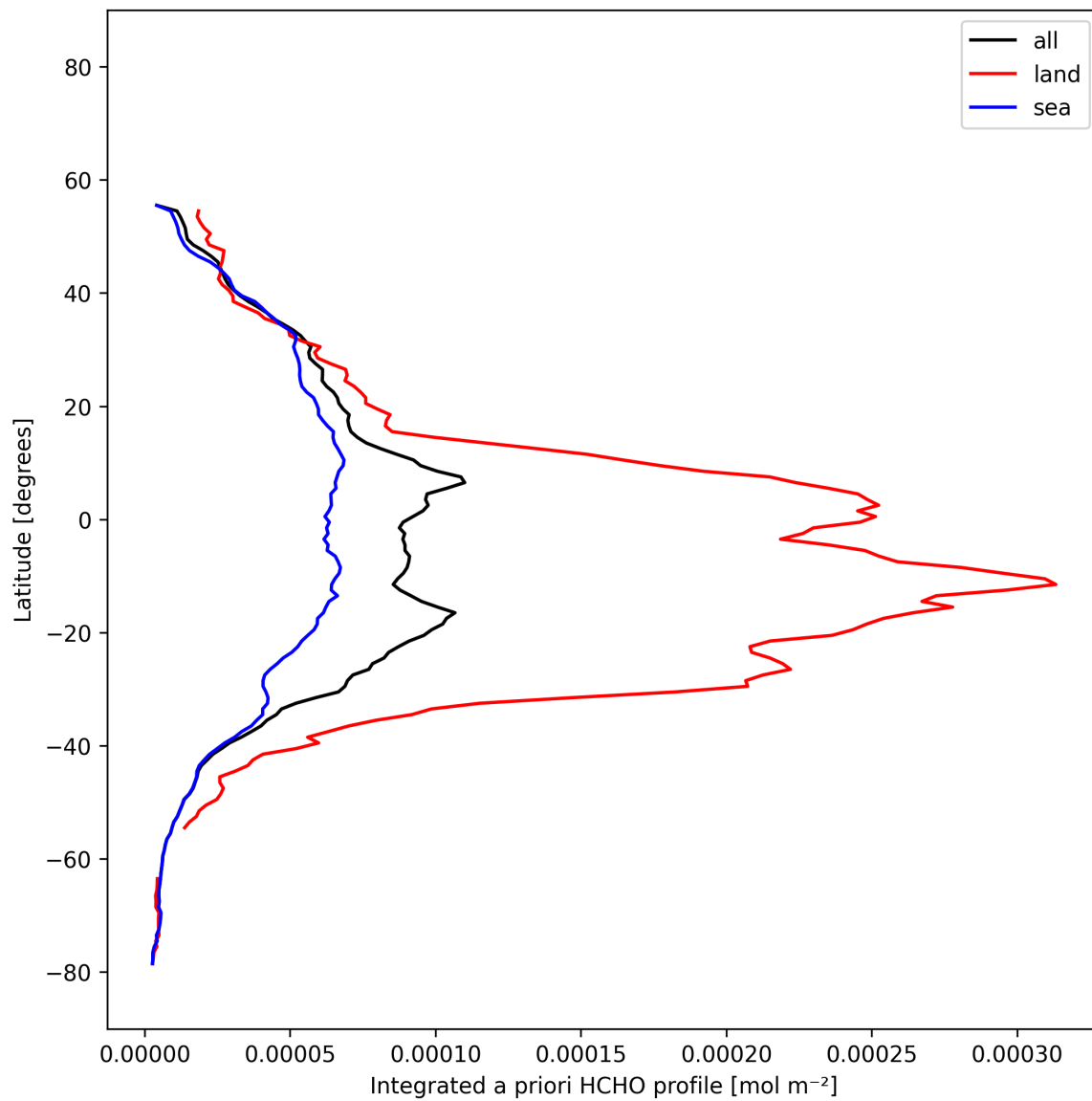
Figure 30: Zonal average of “Integrated a priori HCHO profile” for 2025-11-20 to 2025-11-22.
