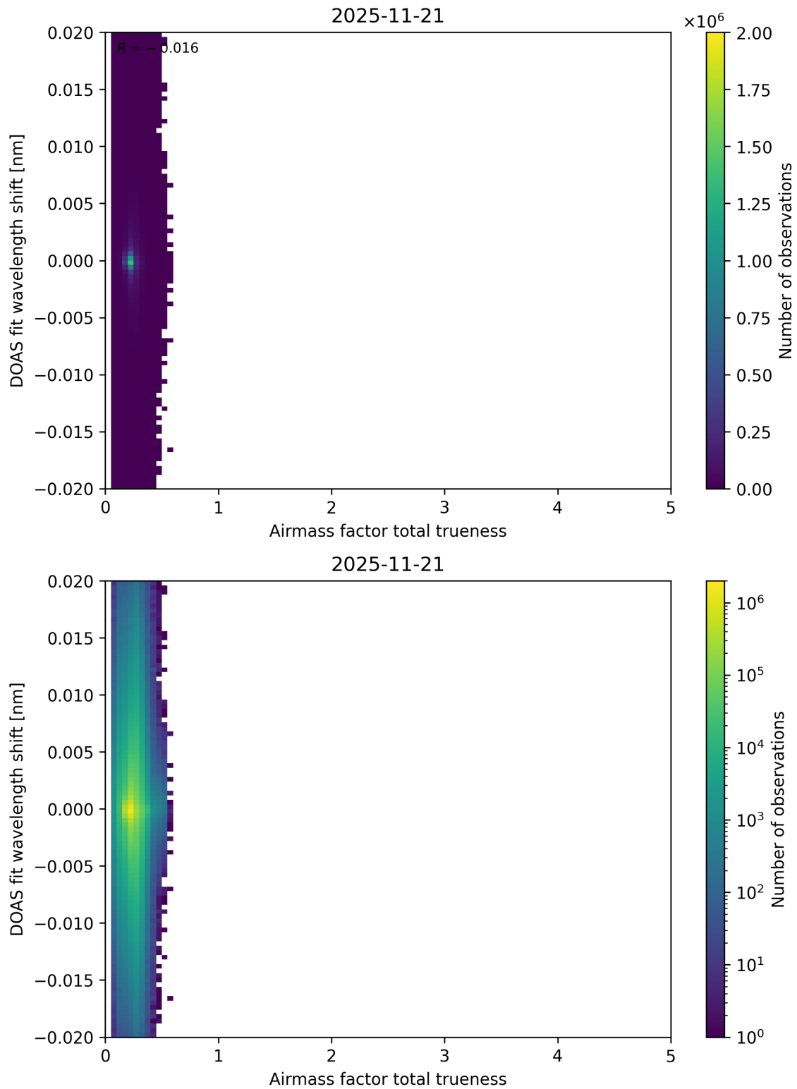
Figure 119: Scatter density plot of “Airmass factor total trueness” against “DOAS fit wavelength shift” for 2025-11-20 to 2025-11-22.
