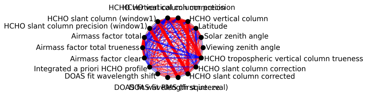
Figure 1: Map of correlation graph for 2025-11-20 to 2025-11-22.
