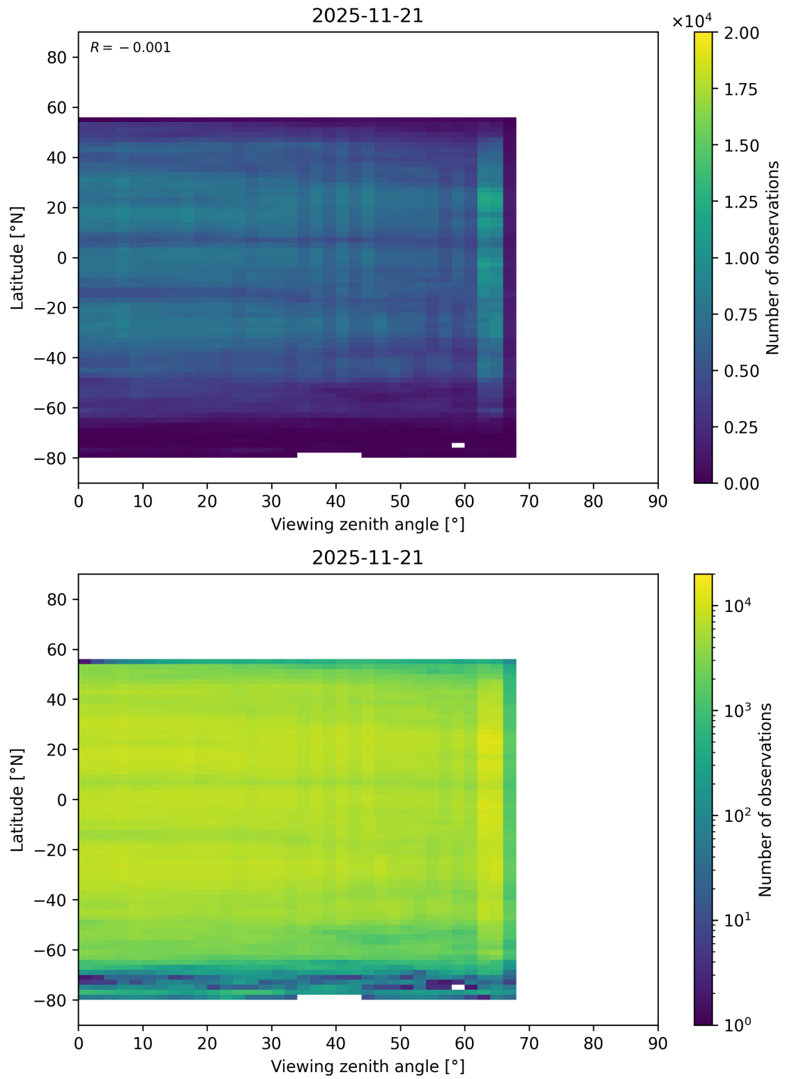
Figure 217: Scatter density plot of “Viewing zenith angle” against “Latitude” for 2025-11-20 to 2025-11-22.
