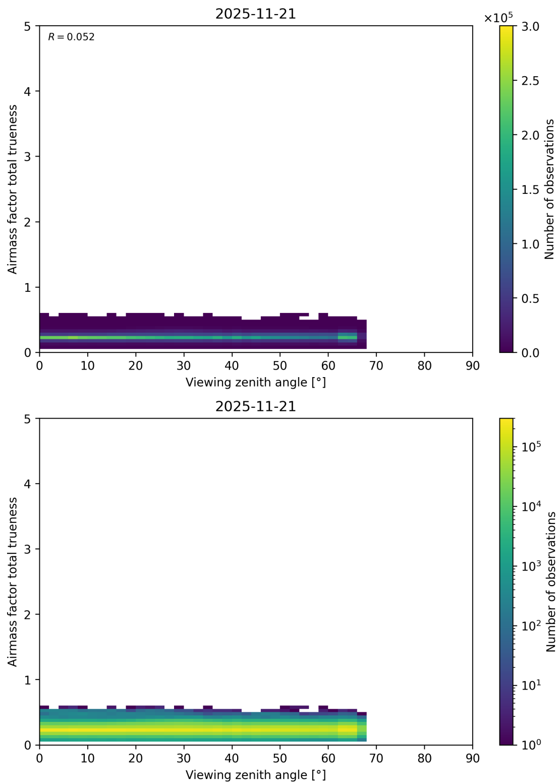
Figure 211: Scatter density plot of “Viewing zenith angle” against “Airmass factor total trueness” for 2025-11-20 to 2025-11-22.
