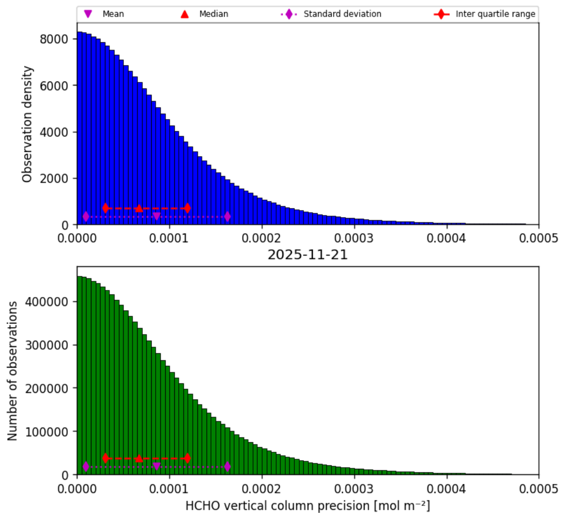
Figure 38: Histogram of “HCHO vertical column precision” for 2025-11-20 to 2025-11-22
