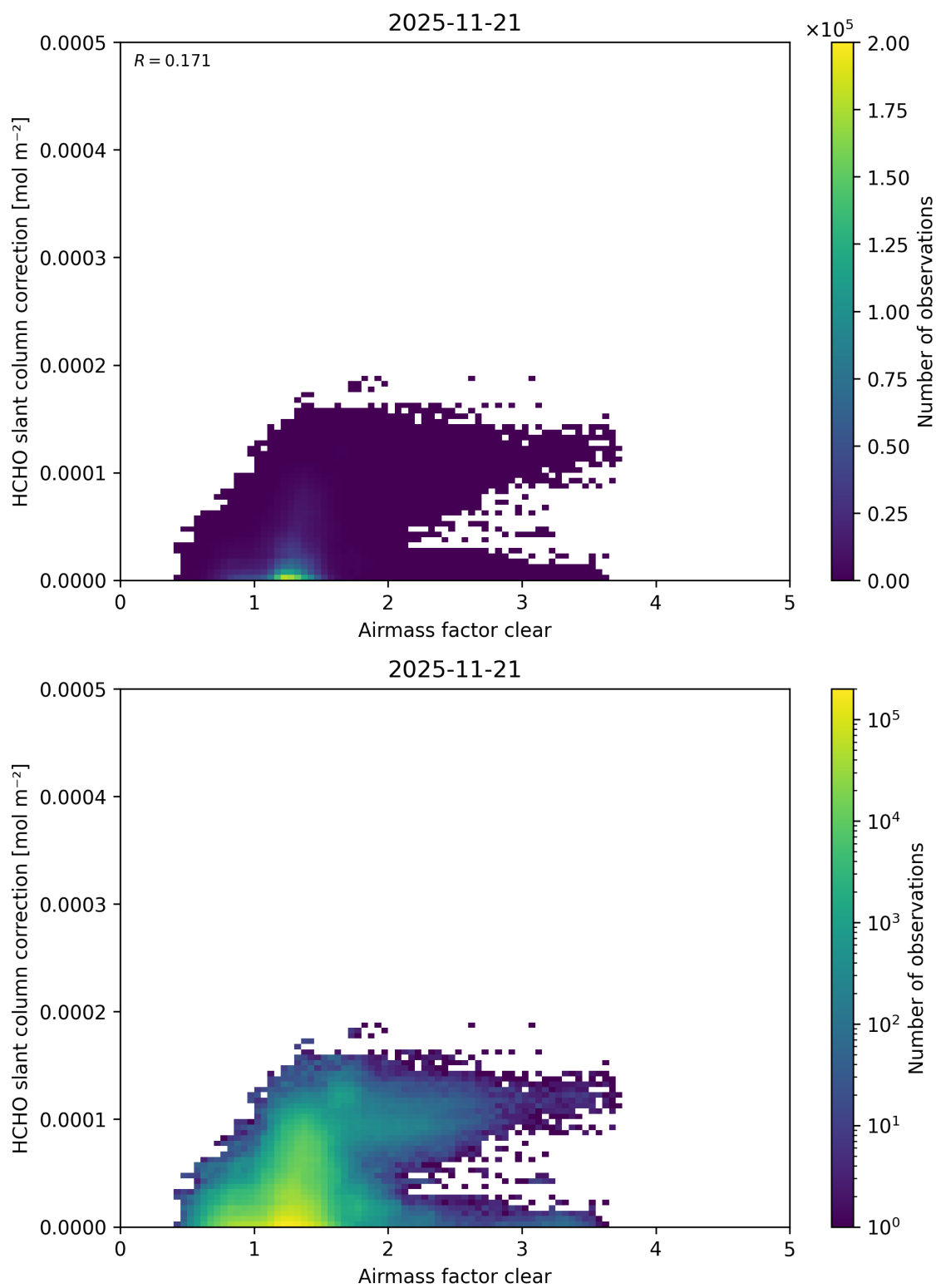
Figure 82: Scatter density plot of “Airmass factor clear” against “HCHO slant column correction” for 2025-11-20 to 2025-11-22.
