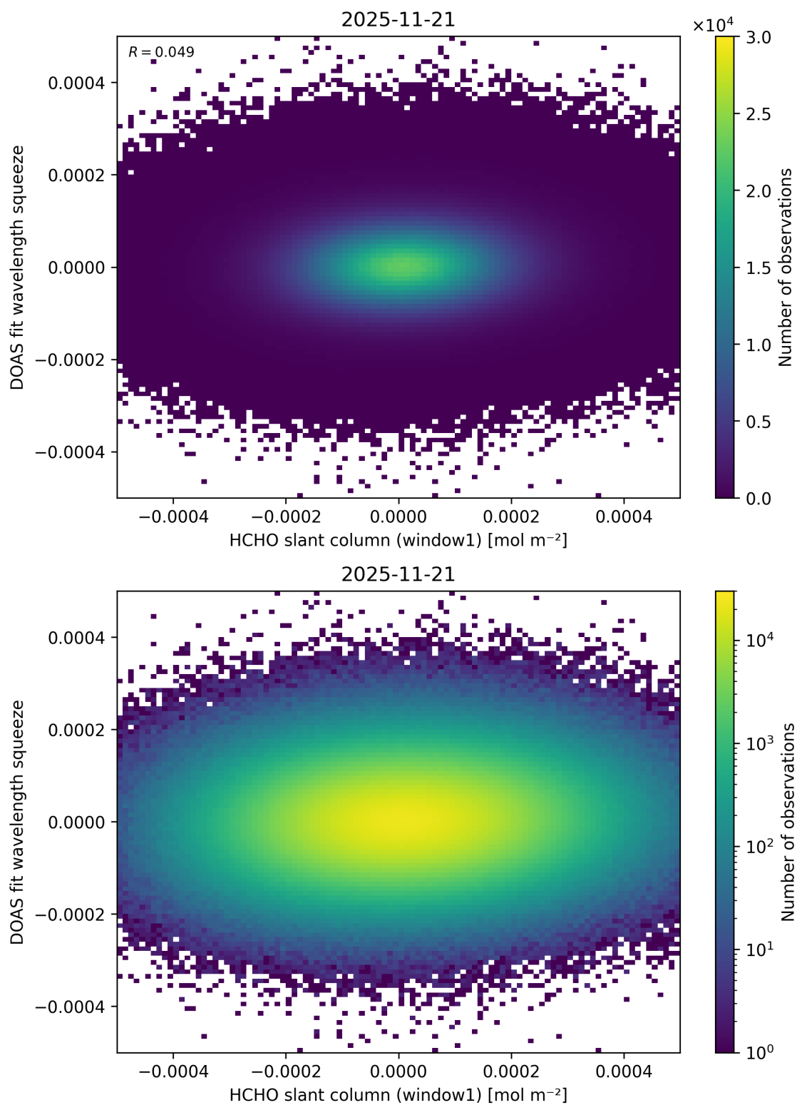
Figure 90: Scatter density plot of “HCHO slant column (window1)” against “DOAS fit wavelength squeeze” for 2025-11-20 to 2025-11-22.
