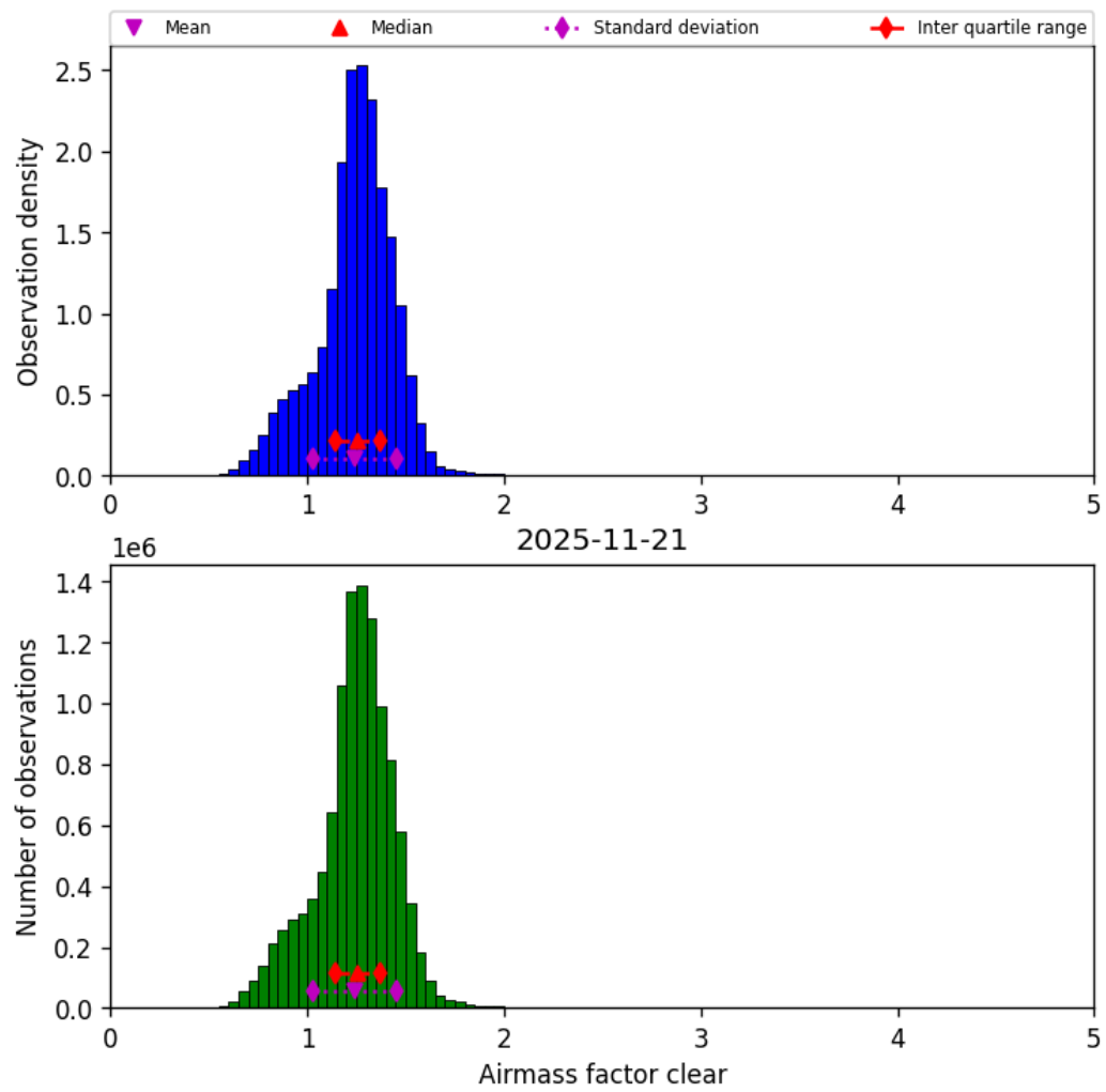
Figure 44: Histogram of “Airmass factor clear” for 2025-11-20 to 2025-11-22
