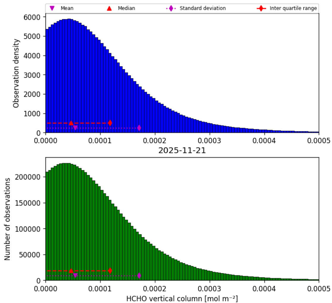
Figure 37: Histogram of “HCHO vertical column” for 2025-11-20 to 2025-11-22
