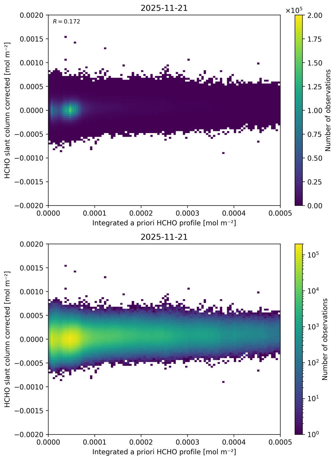
Figure 168: Scatter density plot of “Integrated a priori HCHO profile” against “HCHO slant column corrected” for 2025-11-20 to 2025-11-22.
