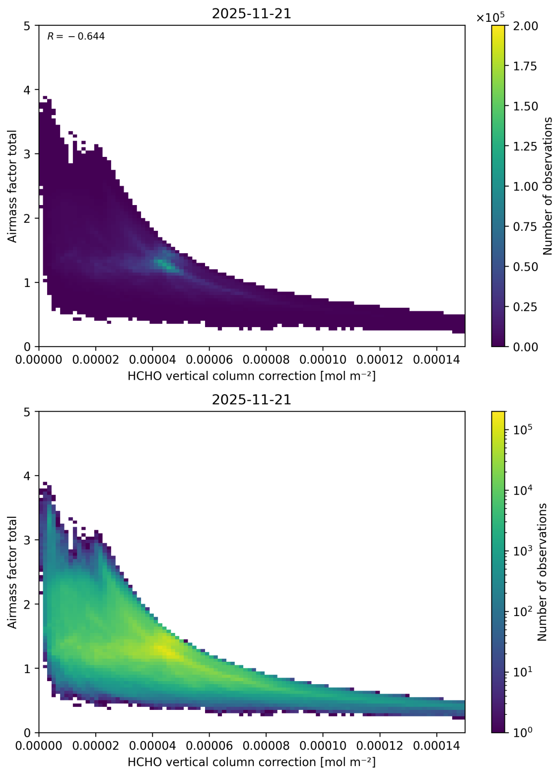
Figure 134: Scatter density plot of “HCHO vertical column correction” against “Airmass factor total” for 2025-11-20 to 2025-11-22.
