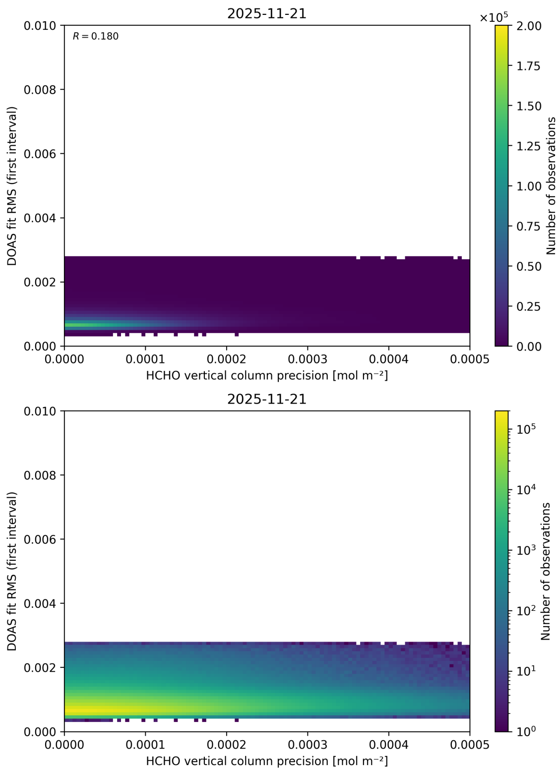
Figure 152: Scatter density plot of “HCHO vertical column precision” against “DOAS fit RMS (first interval)” for 2025-11-20 to 2025-11-22.
