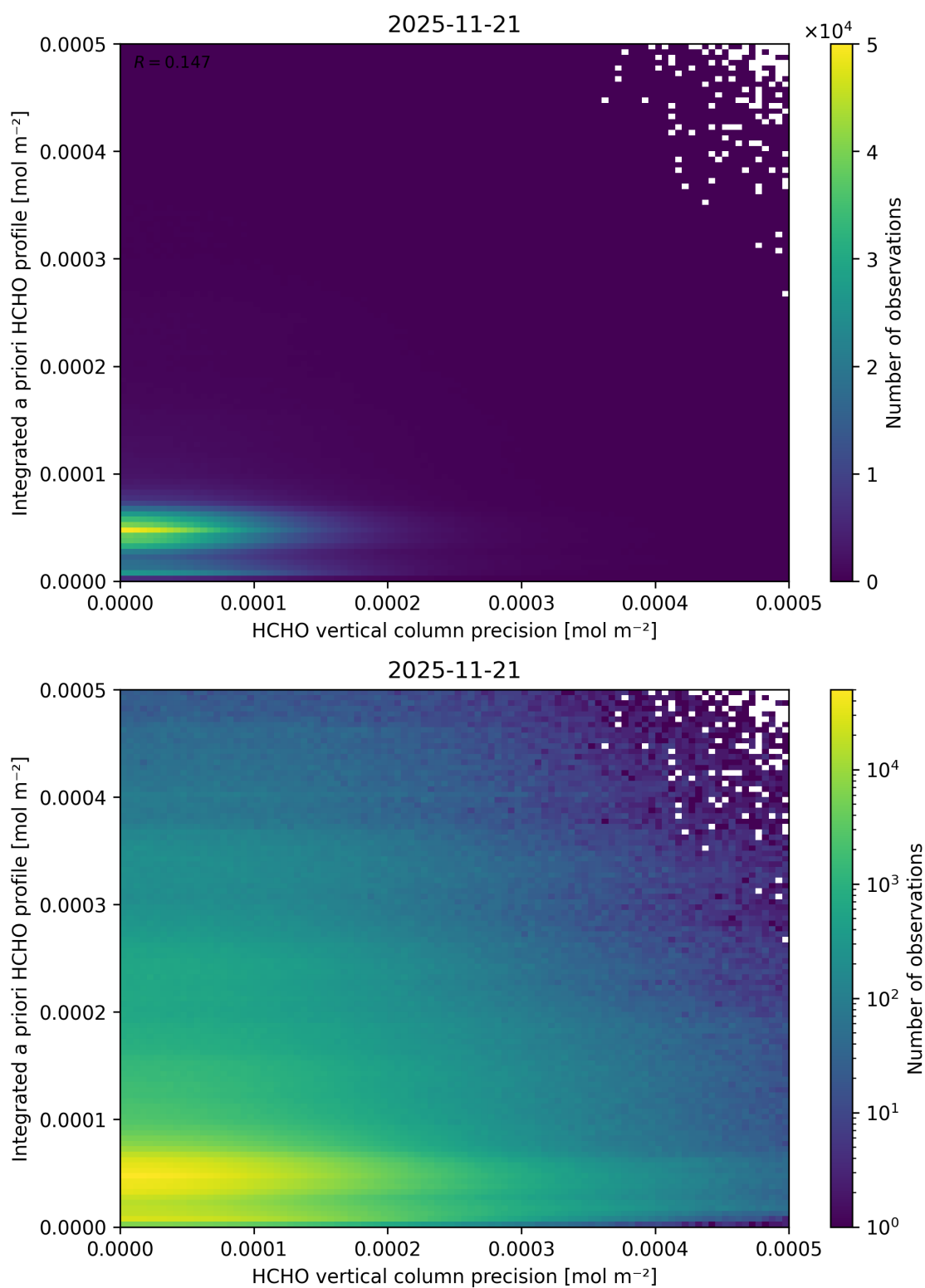
Figure 164: Scatter density plot of “HCHO vertical column precision” against “Integrated a priori HCHO profile” for 2025-11-20 to 2025-11-22.
