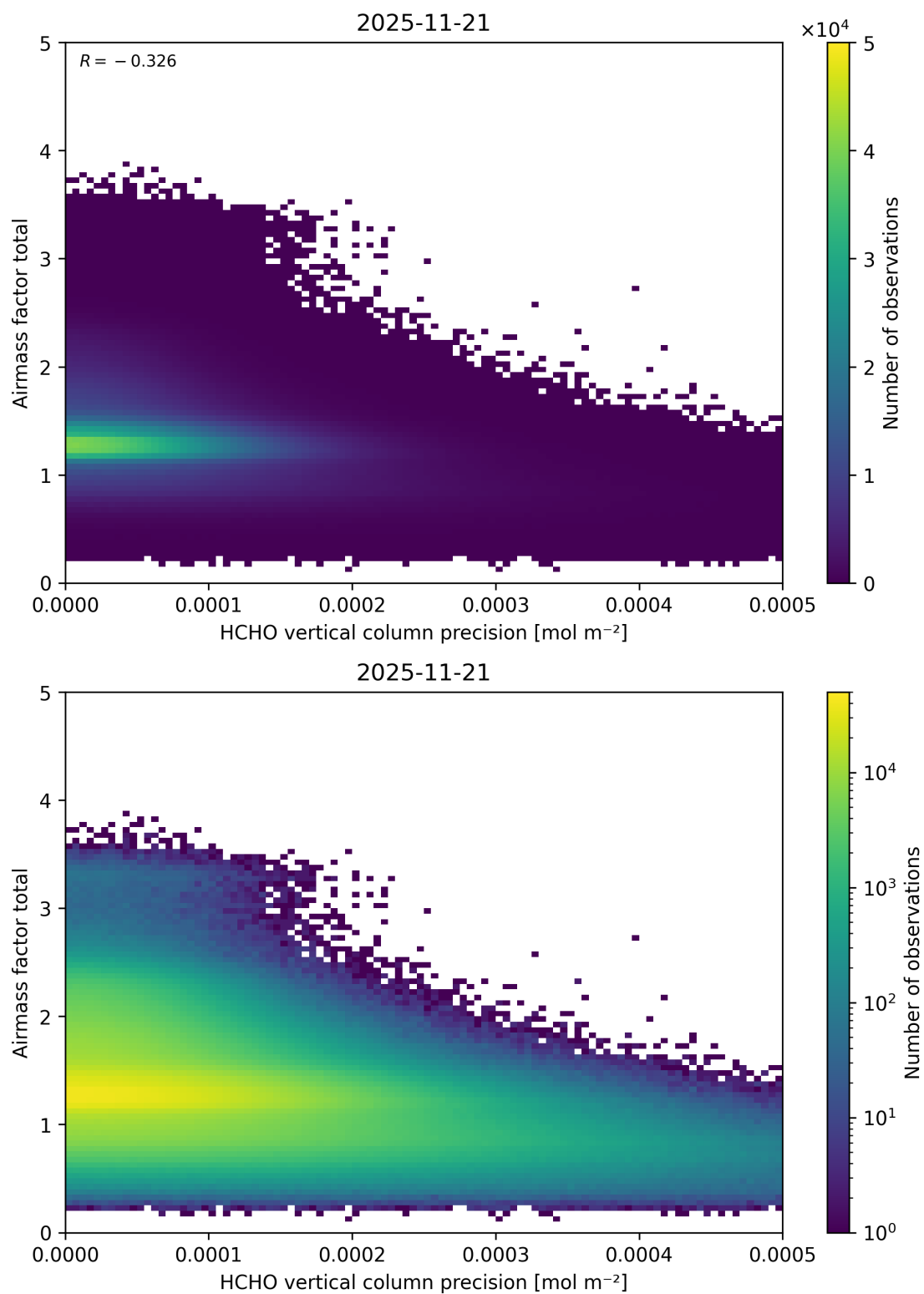
Figure 160: Scatter density plot of “HCHO vertical column precision” against “Airmass factor total” for 2025-11-20 to 2025-11-22.
