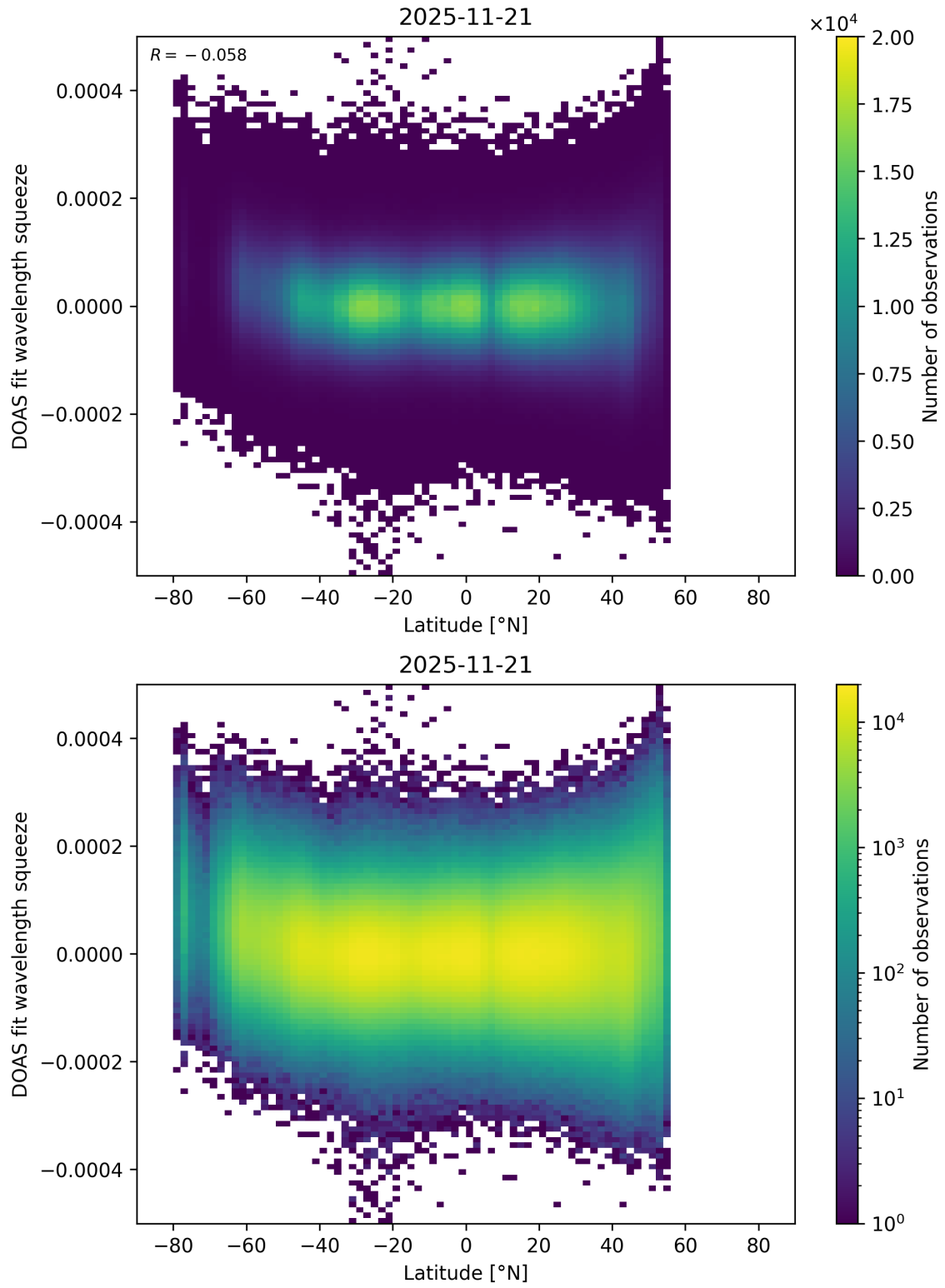
Figure 173: Scatter density plot of “Latitude” against “DOAS fit wavelength squeeze” for 2025-11-20 to 2025-11-22.
