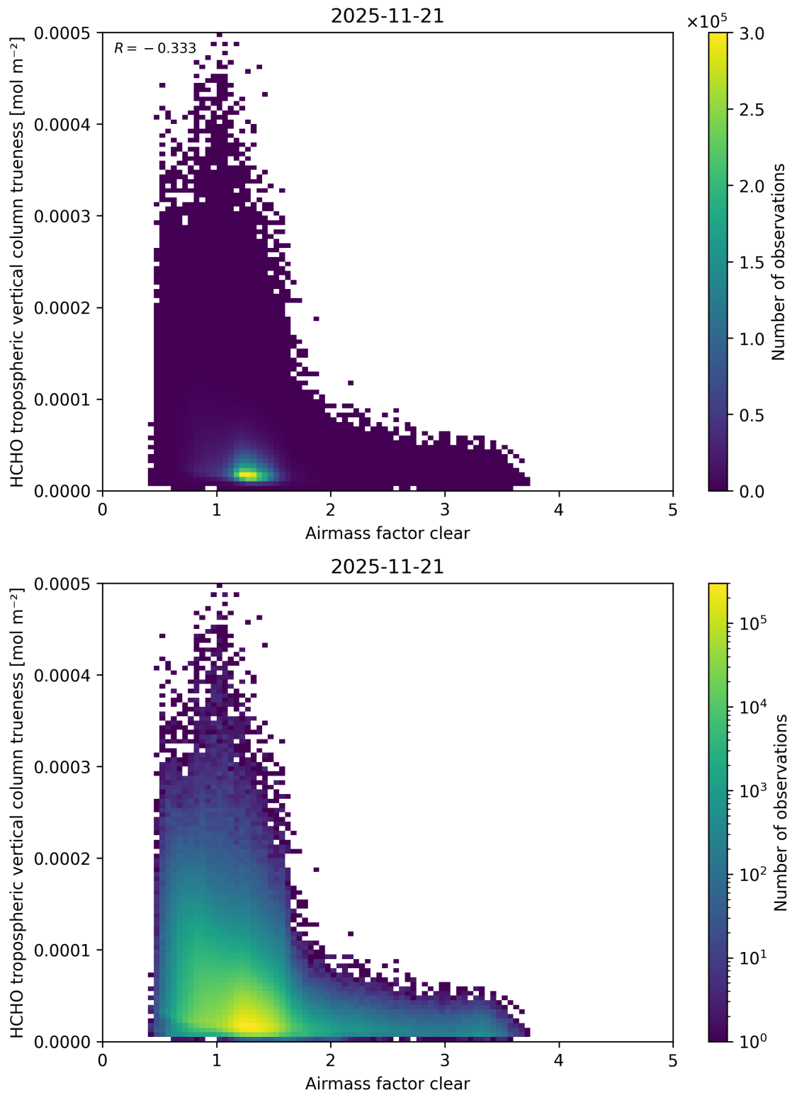
Figure 83: Scatter density plot of “Airmass factor clear” against “HCHO tropospheric vertical column trueness” for 2025-11-20 to 2025-11-22.
