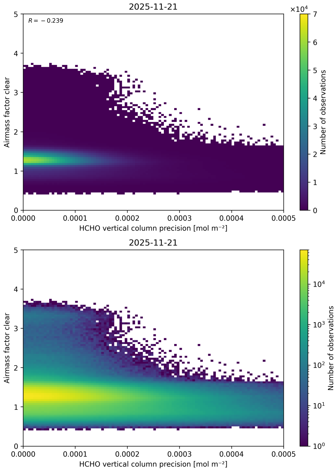
Figure 155: Scatter density plot of “HCHO vertical column precision” against “Airmass factor clear” for 2025-11-20 to 2025-11-22.
