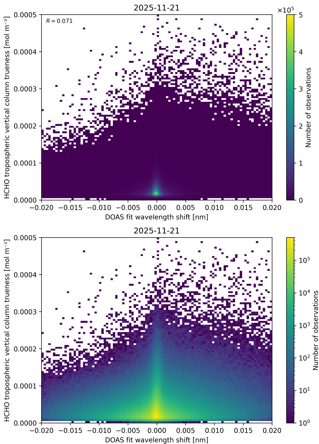
Figure 73: Scatter density plot of “DOAS fit wavelength shift” against “HCHO tropospheric vertical column trueness” for 2025-11-20 to 2025-11-22.
