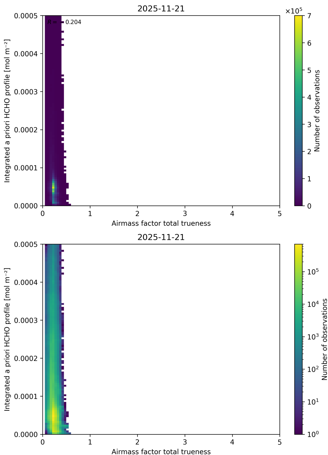
Figure 125: Scatter density plot of “Airmass factor total trueness” against “Integrated a priori HCHO profile” for 2025-11-20 to 2025-11-22.
