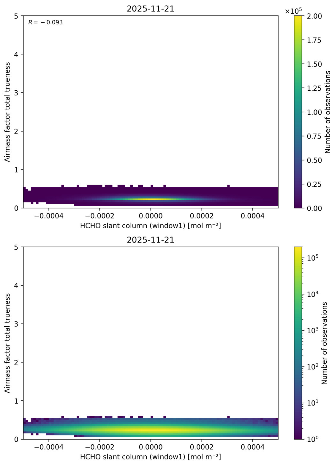
Figure 96: Scatter density plot of “HCHO slant column (window1)” against “Airmass factor total trueneess” for 2025-11-20 to 2025-11-22.
