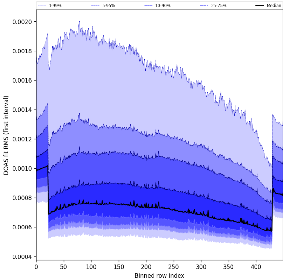
Figure 63: Along track statistics of “DOAS fit RMS (first interval)” for 2025-11-20 to 2025-11-22
