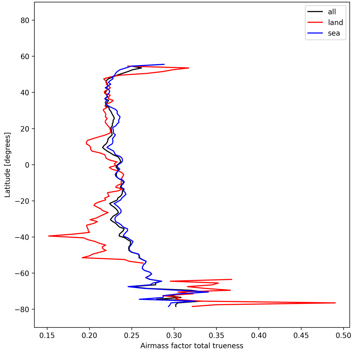
Figure 28: Zonal average of “Airmass factor total trueness” for 2025-11-20 to 2025-11-22.
