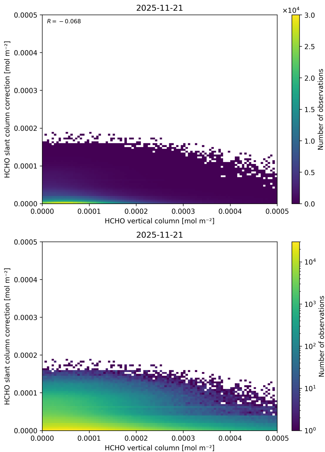
Figure 143: Scatter density plot of “HCHO vertical column” against “HCHO slant column correction” for 2025-11-20 to 2025-11-22.
