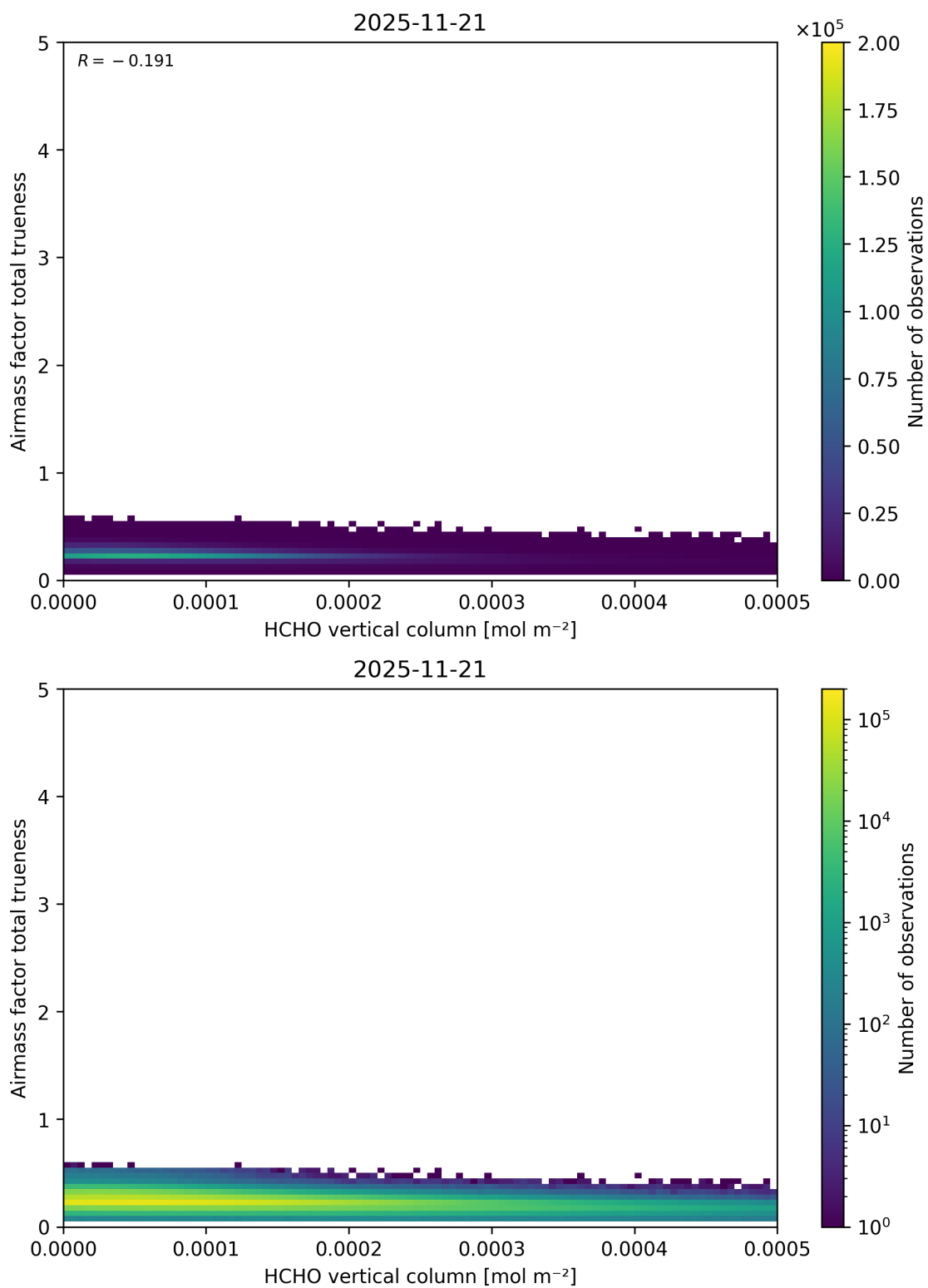
Figure 147: Scatter density plot of “HCHO vertical column” against “Airmass factor total truiness” for 2025-11-20 to 2025-11-22.
