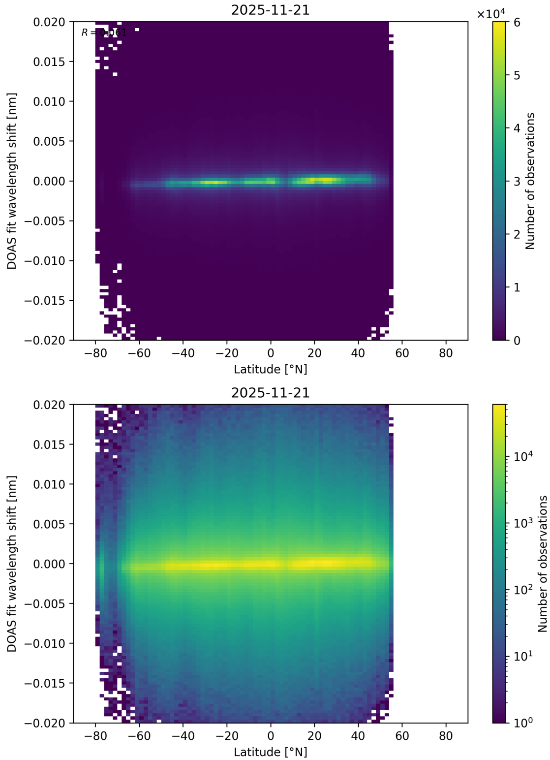
Figure 172: Scatter density plot of “Latitude” against “DOAS fit wavelength shift” for 2025-11-20 to 2025-11-22.
