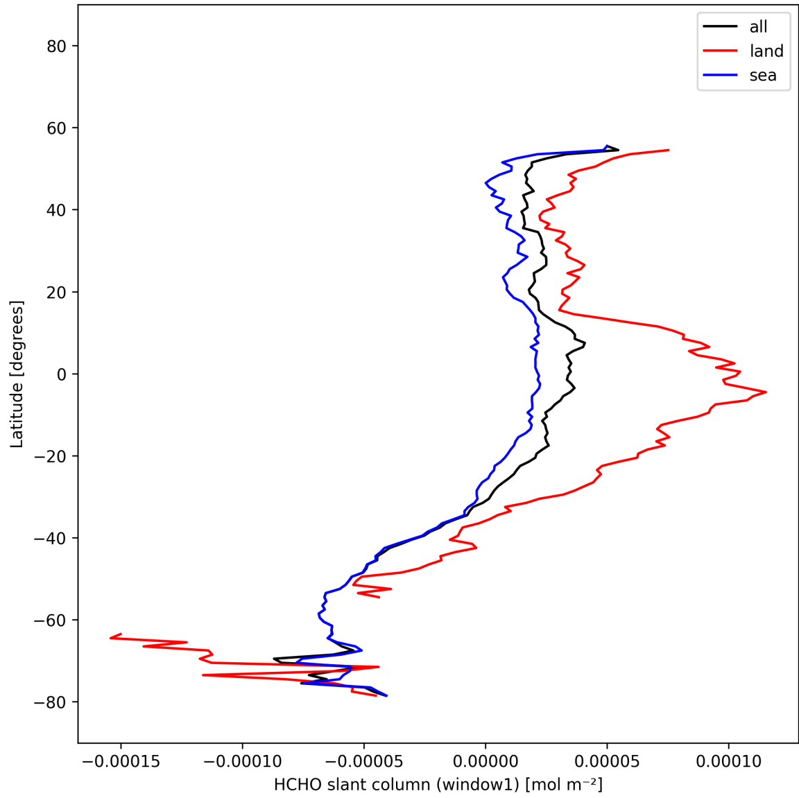
Figure 25: Zonal average of “HCHO slant column (window1)” for 2025-11-20 to 2025-11-22.
