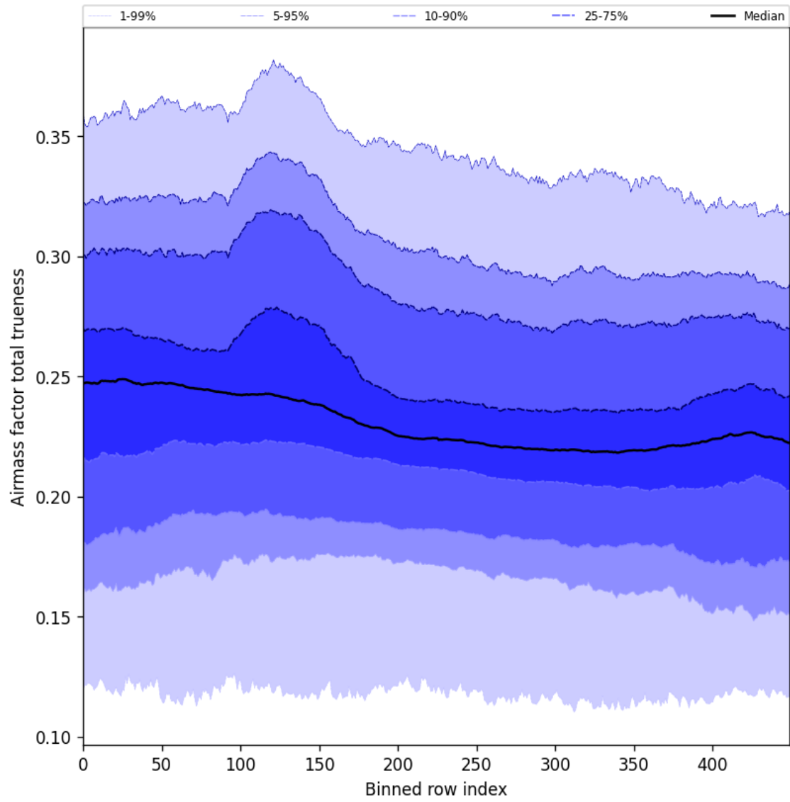
Figure 58: Along track statistics of “Airmass factor total trueness” for 2025-11-20 to 2025-11-22
