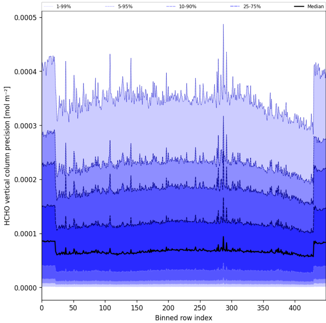
Figure 53: Along track statistics of "HCHO vertical column precision" for 2025-11-20 to 2025-11-22
