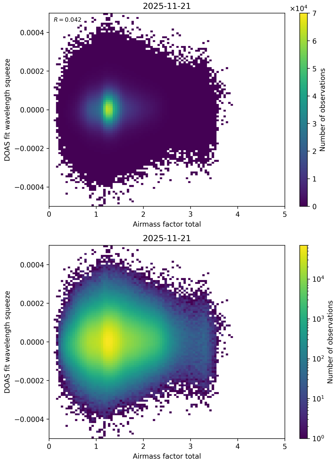
Figure 111: Scatter density plot of “Airmass factor total” against “DOAS fit wavelength squeeze” for 2025-11-20 to 2025-11-22.
