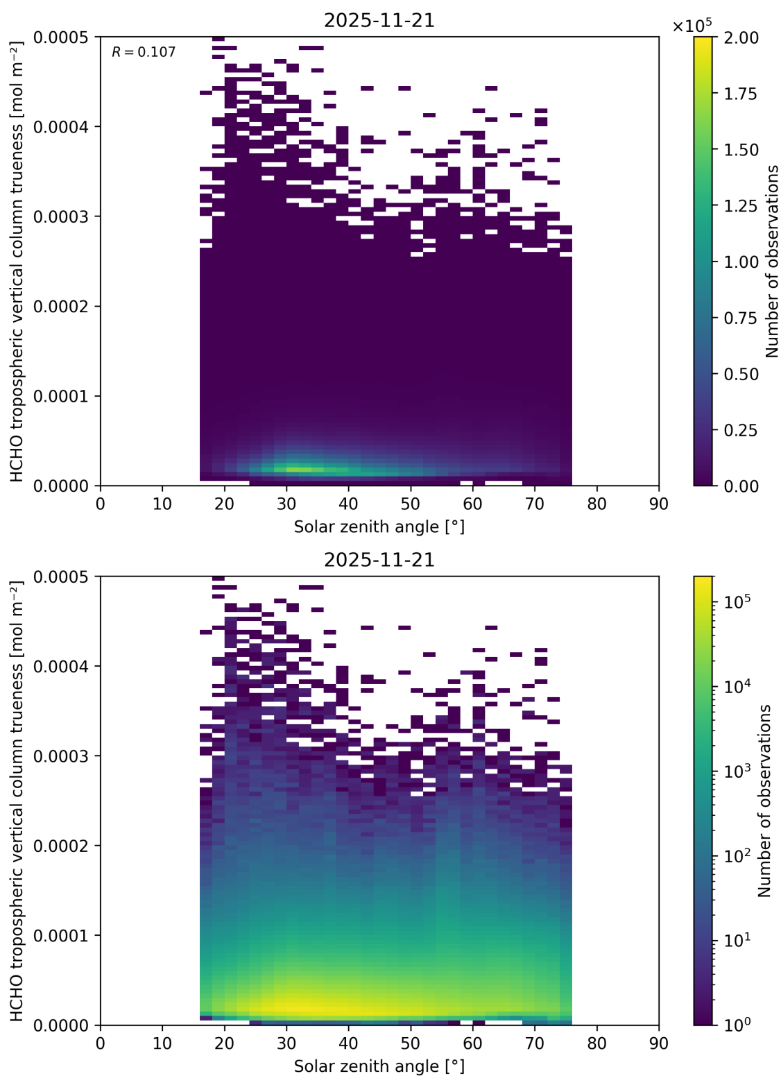
Figure 199: Scatter density plot of “Solar zenith angle” against “HCHO tropospheric vertical column trueness” for 2025-11-20 to 2025-11-22.
