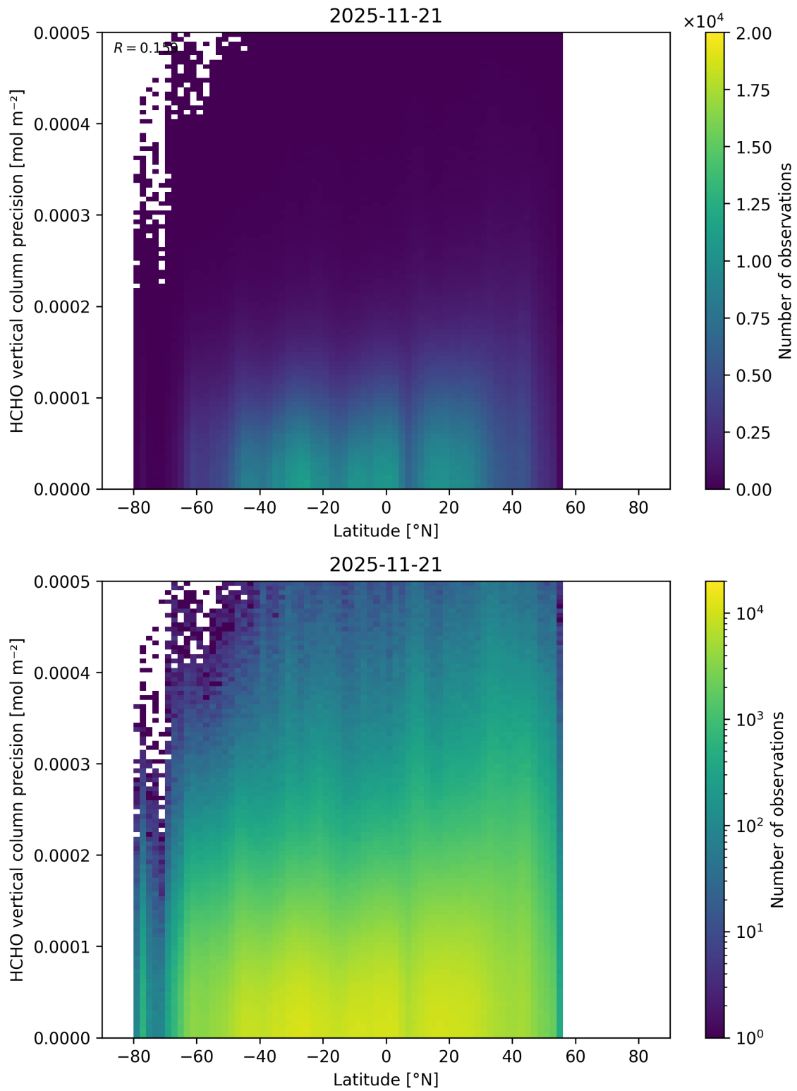
Figure 183: Scatter density plot of “Latitude” against “HCHO vertical column precision” for 2025-11-20 to 2025-11-22.
