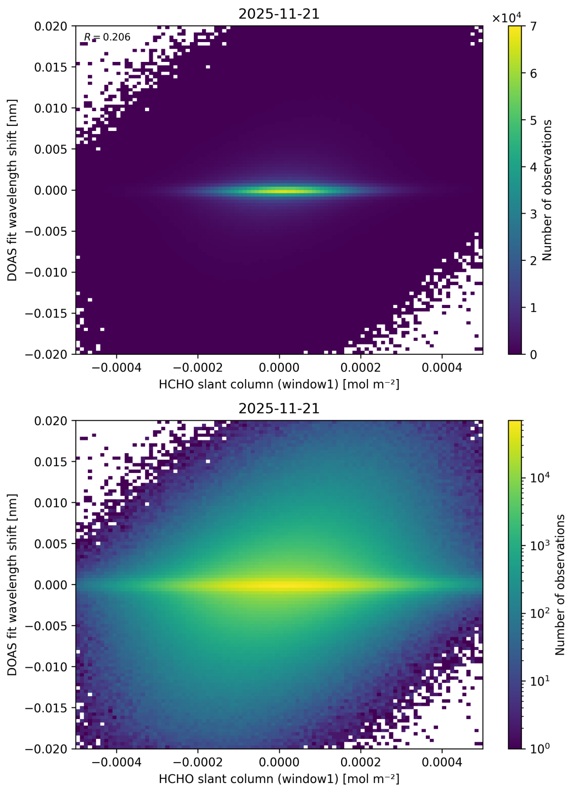
Figure 89: Scatter density plot of “HCHO slant column (window1)” against “DOAS fit wavelength shift” for 2025-11-20 to 2025-11-22.
