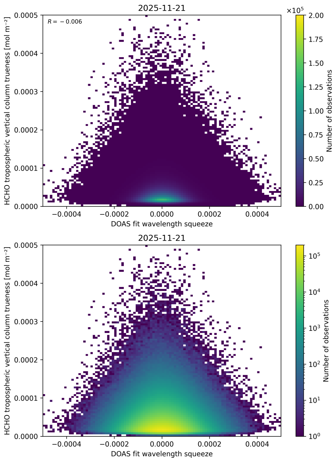
Figure 77: Scatter density plot of “DOAS fit wavelength squeeze” against “HCHO tropospheric vertical column trueness” for 2025-11-20 to 2025-11-22.
