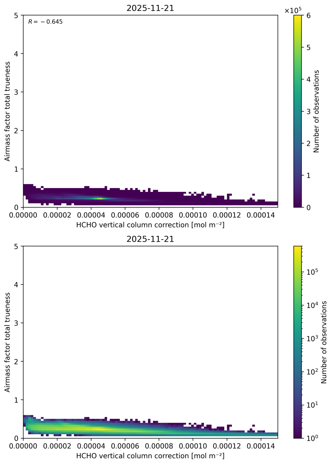
Figure 135: Scatter density plot of “HCHO vertical column correction” against “Airmass factor total trueness” for 2025-11-20 to 2025-11-22.
