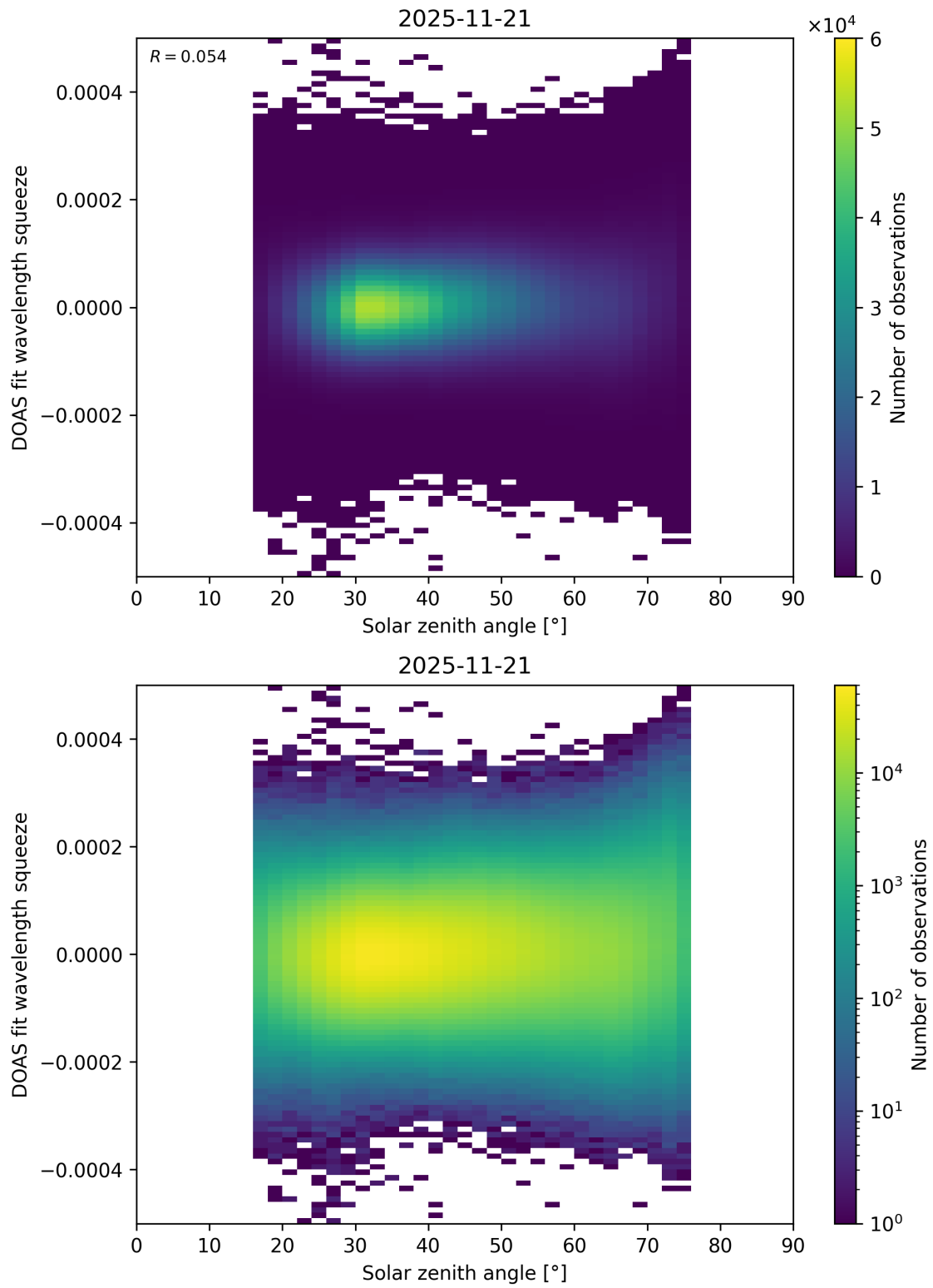
Figure 188: Scatter density plot of “Solar zenith angle” against “DOAS fit wavelength squeeze” for 2025-11-20 to 2025-11-22.
