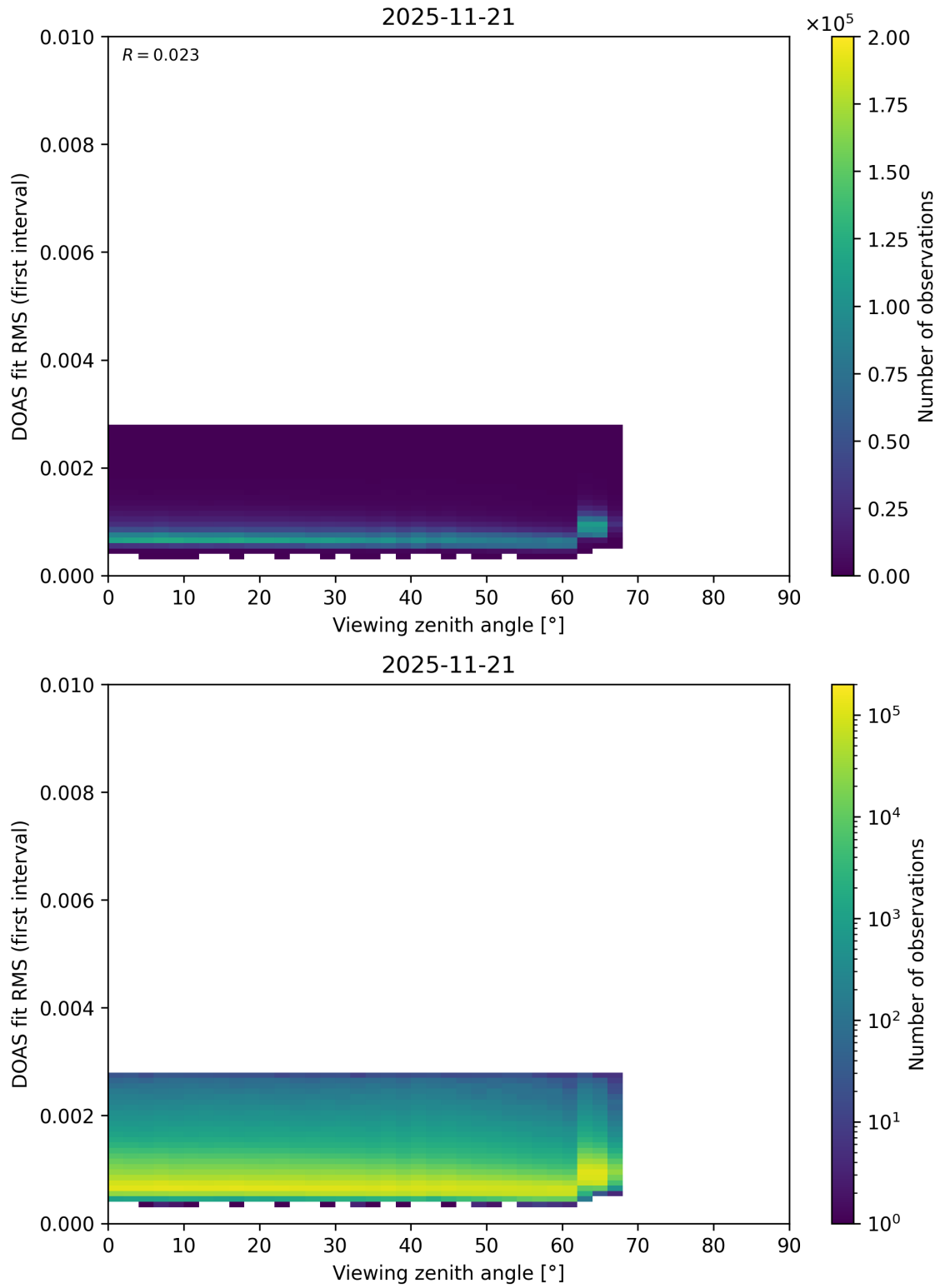
Figure 202: Scatter density plot of “Viewing zenith angle” against “DOAS fit RMS (first interval)” for 2025-11-20 to 2025-11-22.
