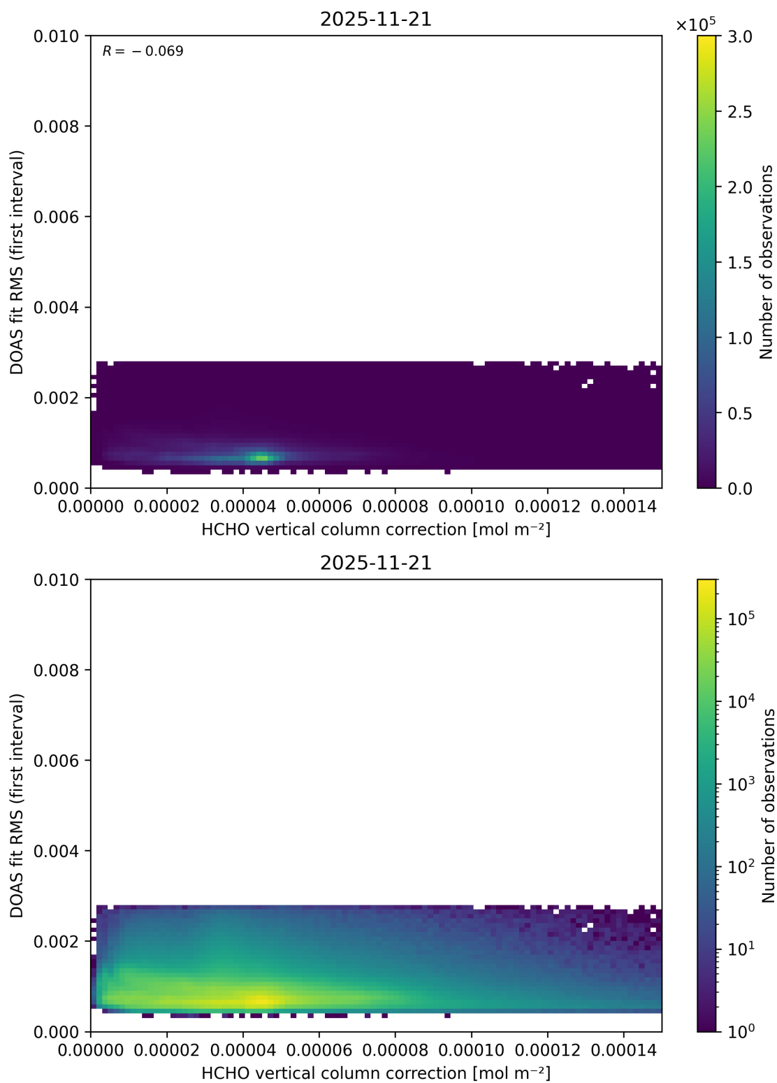
Figure 126: Scatter density plot of “HCHO vertical column correction” against “DOAS fit RMS (first interval)” for 2025-11-20 to 2025-11-22.
