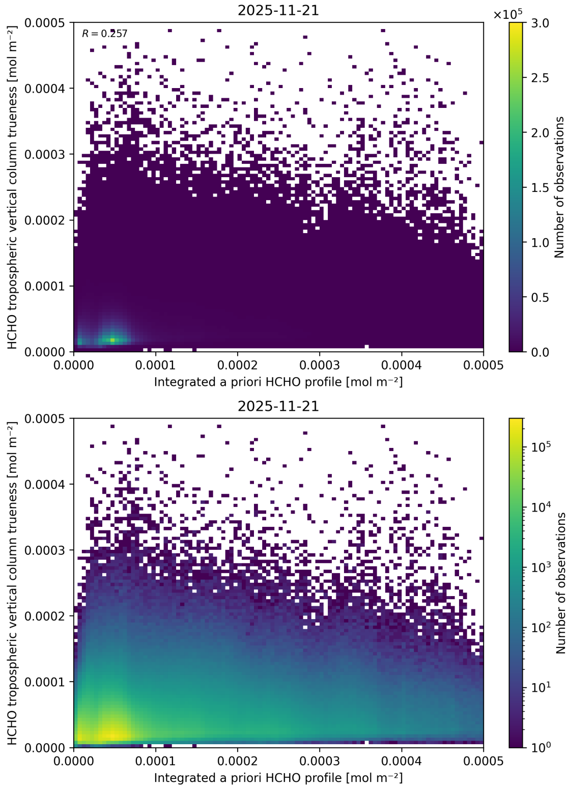
Figure 170: Scatter density plot of “Integrated a priori HCHO profile” against “HCHO tropospheric vertical column trueness” for 2025-11-20 to 2025-11-22.
