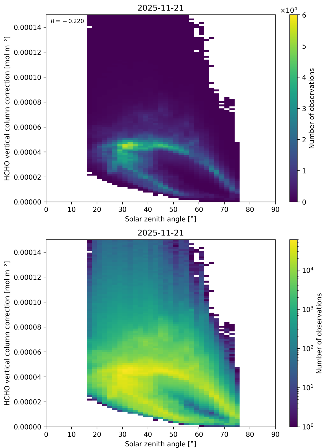
Figure 197: Scatter density plot of “Solar zenith angle” against “HCHO vertical column correction” for 2025-11-20 to 2025-11-22.
