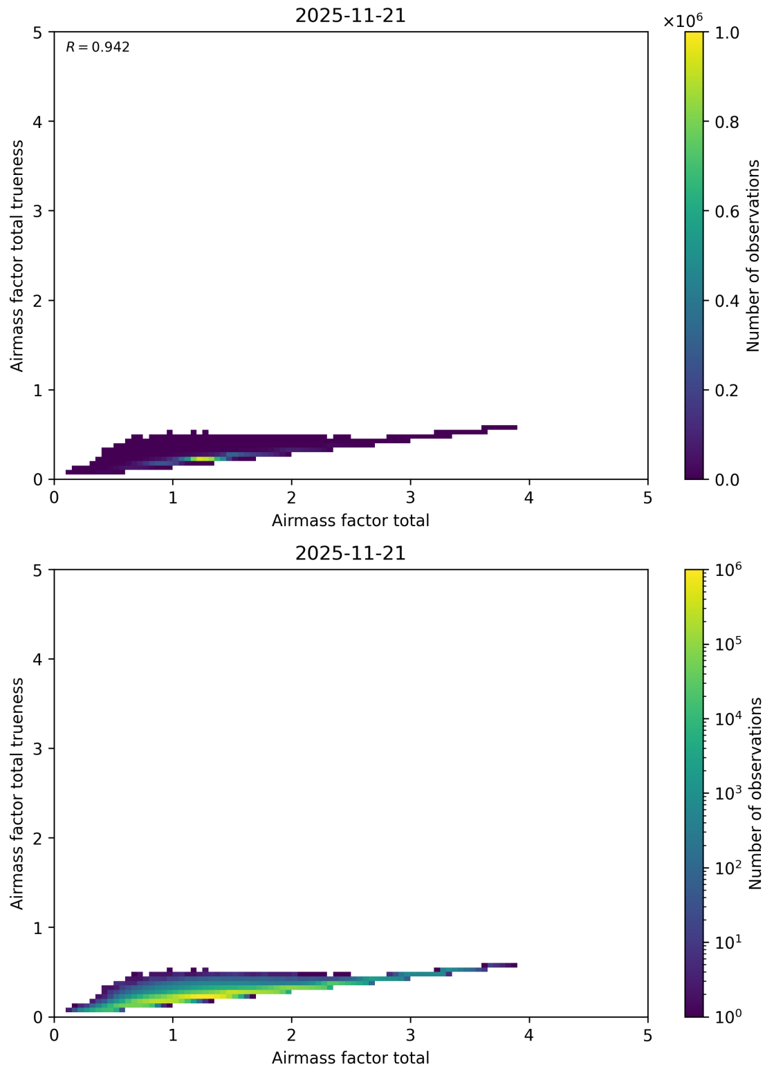
Figure 115: Scatter density plot of “Airmass factor total” against “Airmass factor total trueness” for 2025-11-20 to 2025-11-22.
