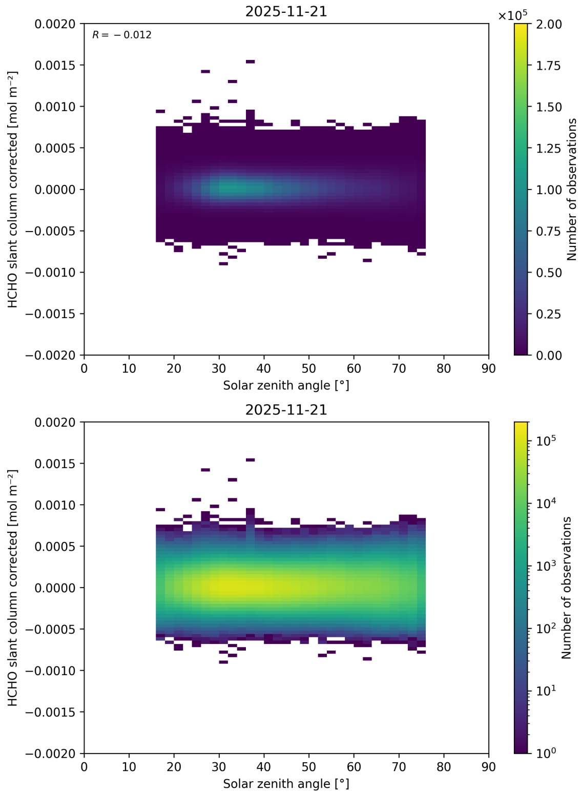
Figure 190: Scatter density plot of “Solar zenith angle” against “HCHO slant column corrected” for 2025-11-20 to 2025-11-22.
