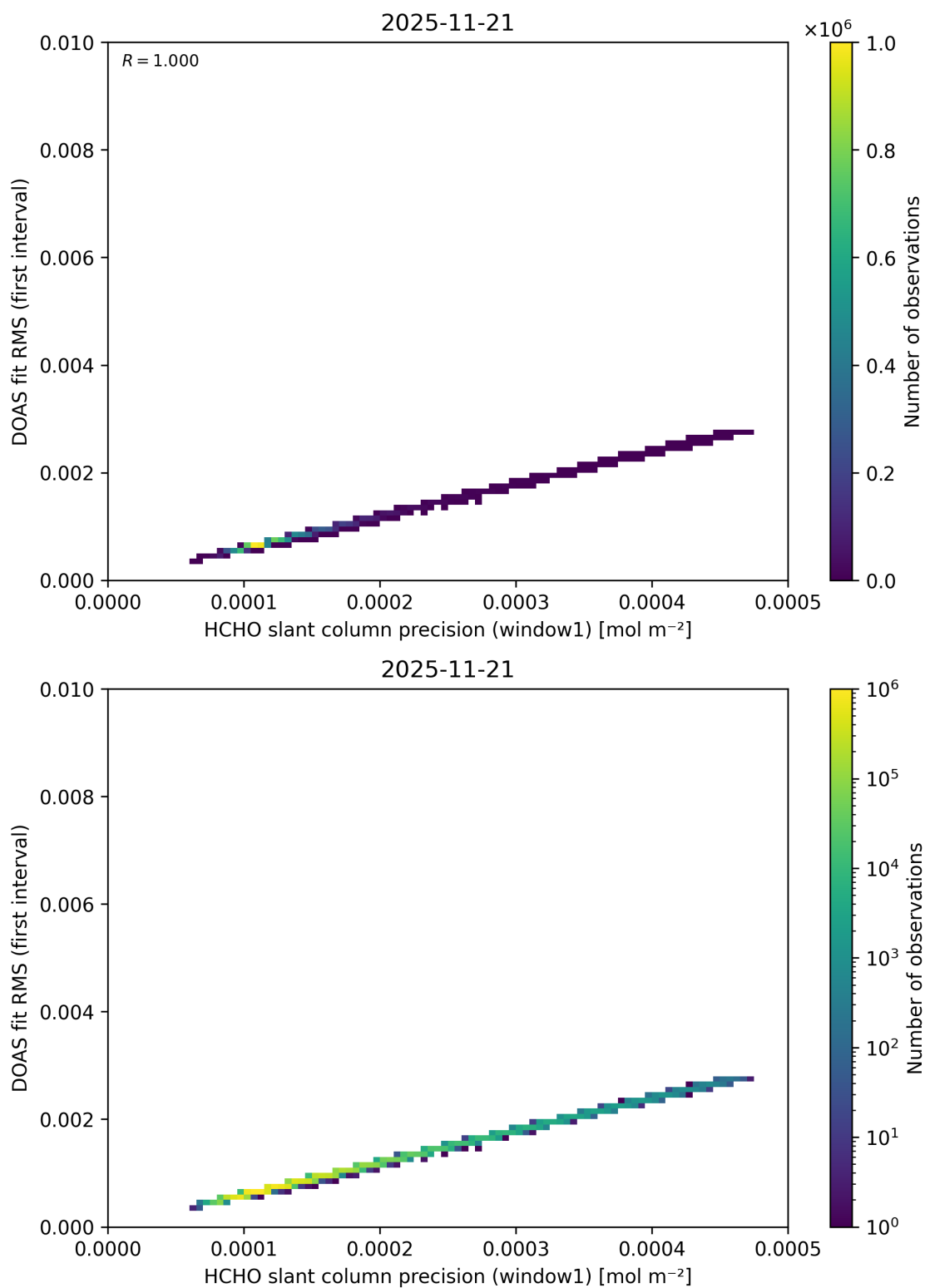
Figure 99: Scatter density plot of “HCHO slant column precision (window1)” against “DOAS fit RMS (first interval)” for 2025-11-20 to 2025-11-22.
