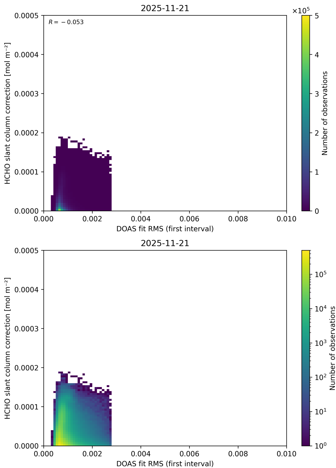
Figure 67: Scatter density plot of “DOAS fit RMS (first interval)” against “HCHO slant column correction” for 2025-11-20 to 2025-11-22.
