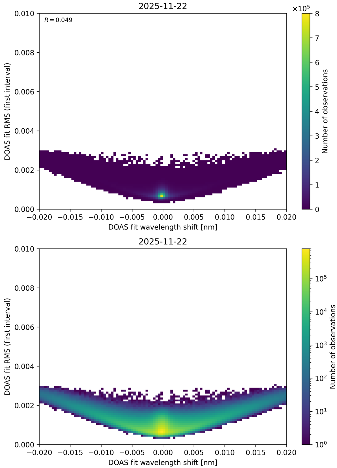
Figure 69: Scatter density plot of “DOAS fit wavelength shift” against “DOAS fit RMS (first interval)” for 2025-11-21 to 2025-11-23.
