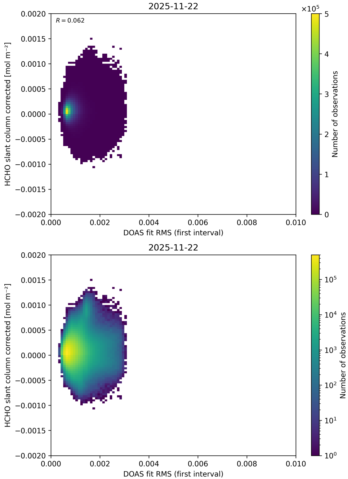
Figure 66: Scatter density plot of “DOAS fit RMS (first interval)” against “HCHO slant column corrected” for 2025-11-21 to 2025-11-23.
