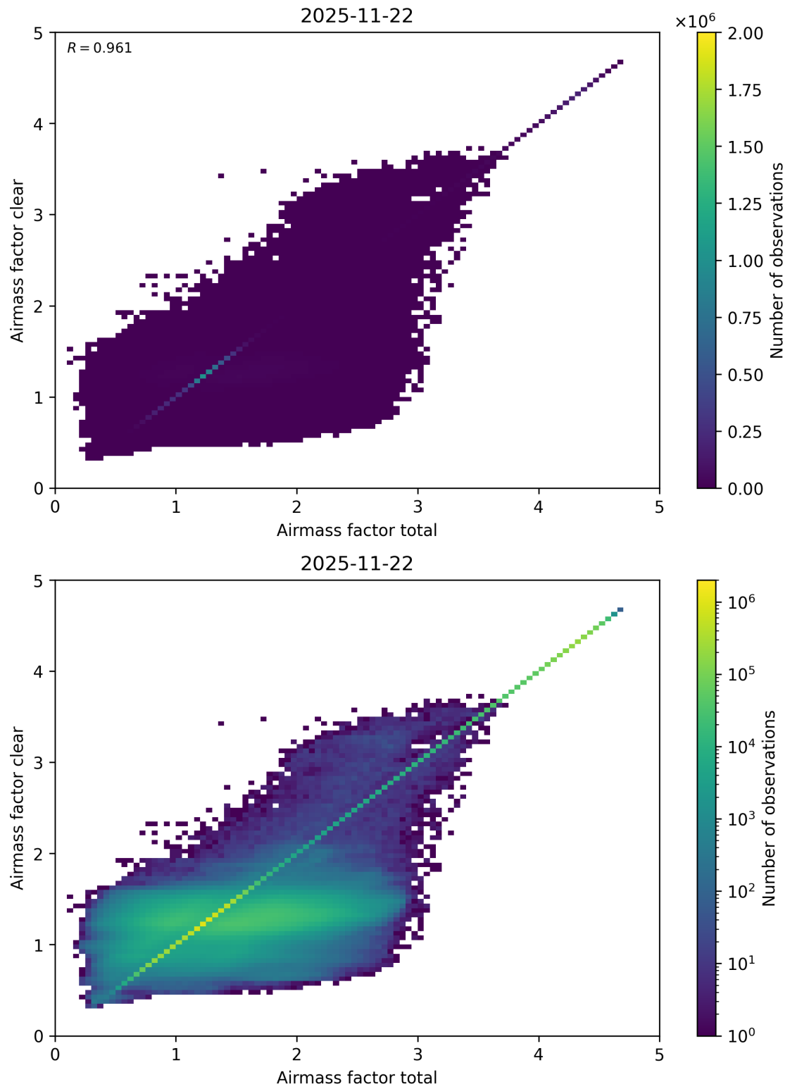
Figure 112: Scatter density plot of “Airmass factor total” against “Airmass factor clear” for 2025-11-21 to 2025-11-23.
