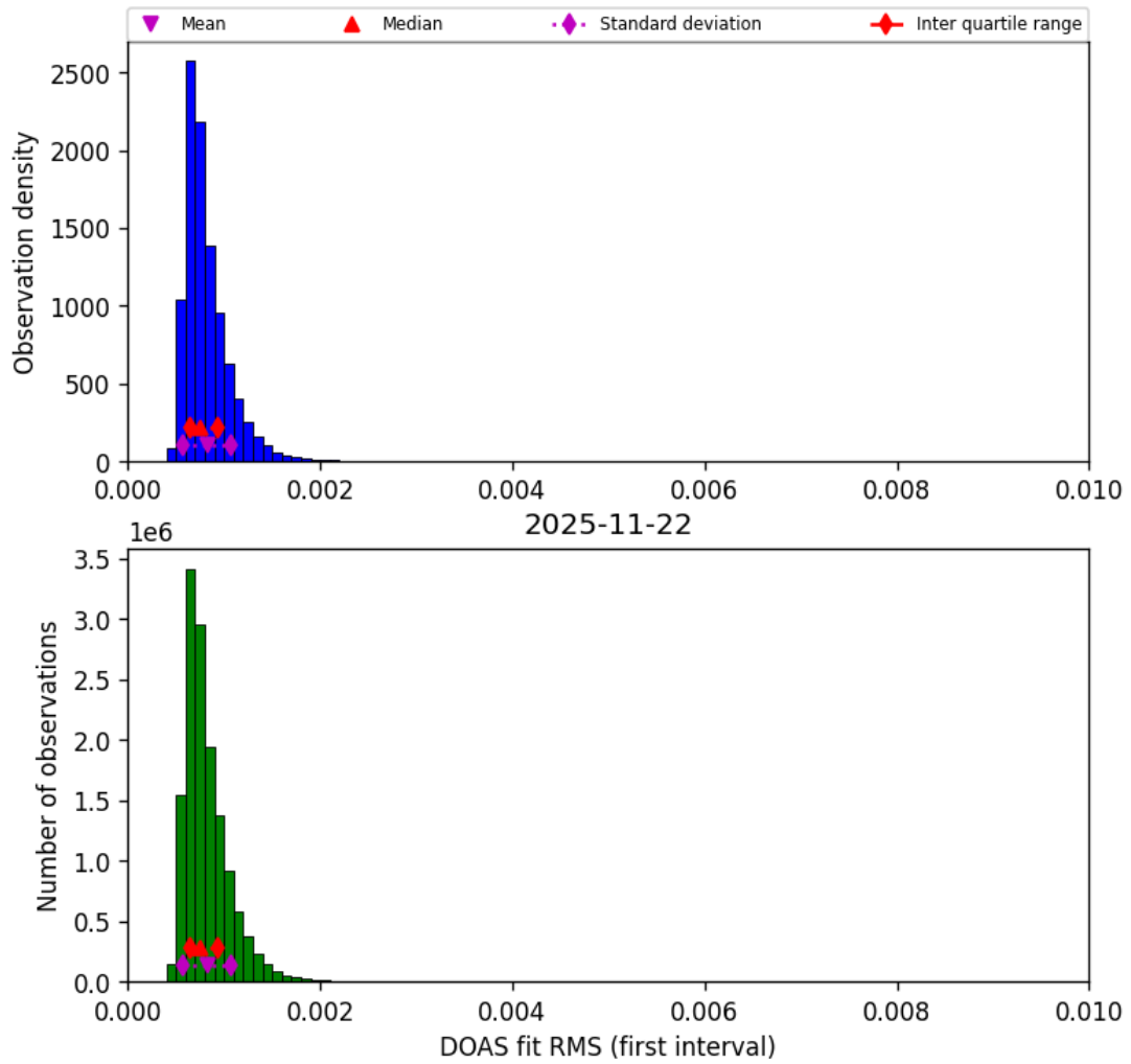
Figure 48: Histogram of “DOAS fit RMS (first interval)” for 2025-11-21 to 2025-11-23
