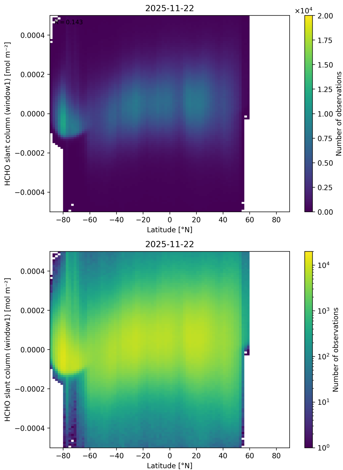
Figure 177: Scatter density plot of “Latitude” against “HCHO slant column (window1)” for 2025-11-21 to 2025-11-23.
