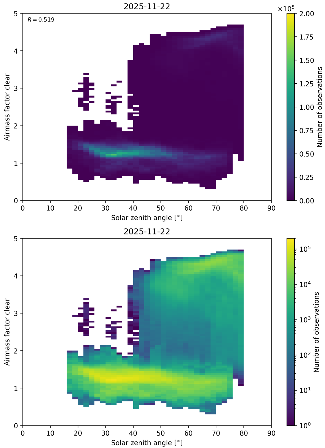
Figure 189: Scatter density plot of “Solar zenith angle” against “Airmass factor clear” for 2025-11-21 to 2025-11-23.
