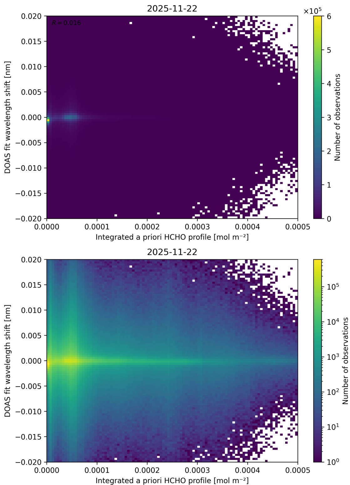
Figure 166: Scatter density plot of “Integrated a priori HCHO profile” against “DOAS fit wavelength shift” for 2025-11-21 to 2025-11-23.
