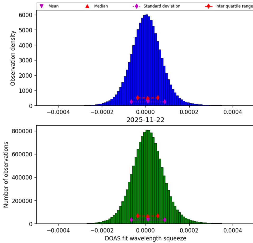
Figure 47: Histogram of “DOAS fit wavelength squeeze” for 2025-11-21 to 2025-11-23
