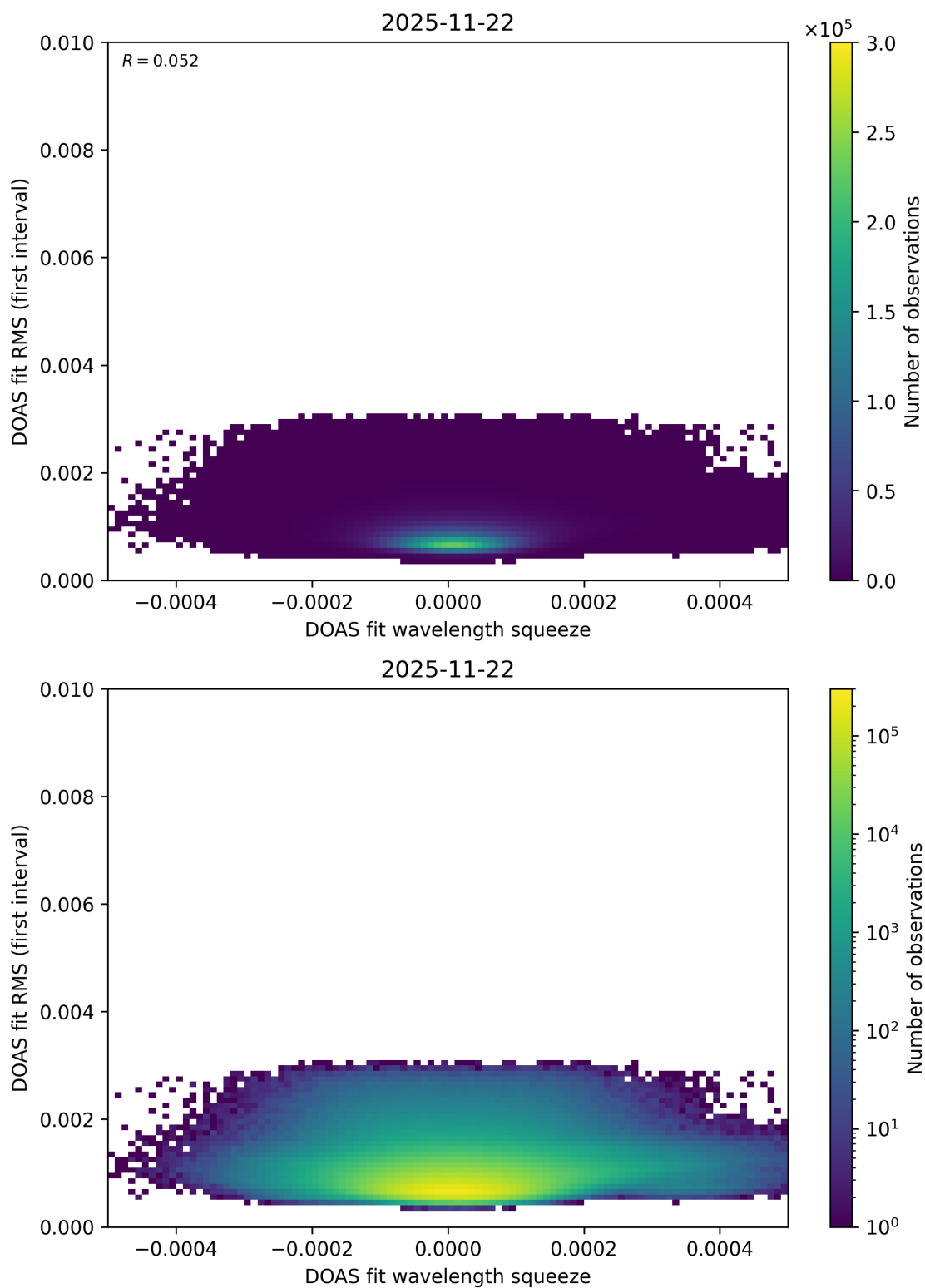
Figure 74: Scatter density plot of “DOAS fit wavelength squeeze” against “DOAS fit RMS (first interval)” for 2025-11-21 to 2025-11-23.
