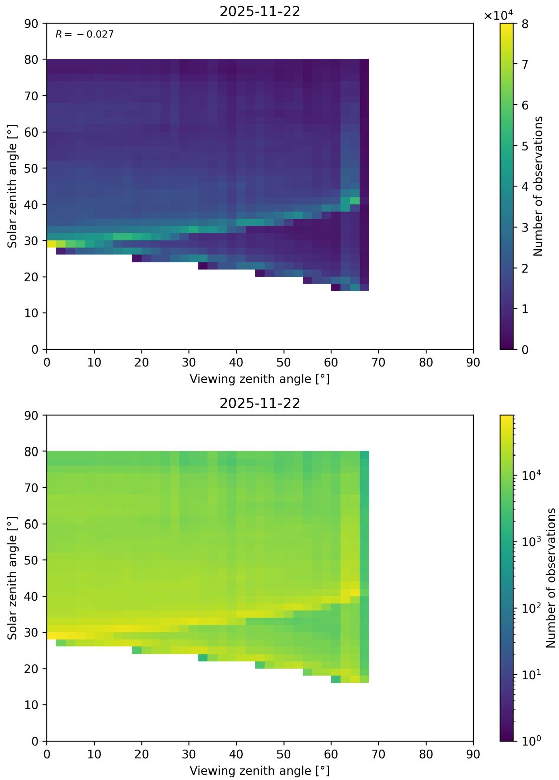
Figure 218: Scatter density plot of “Viewing zenith angle” against “Solar zenith angle” for 2025-11-21 to 2025-11-23.
