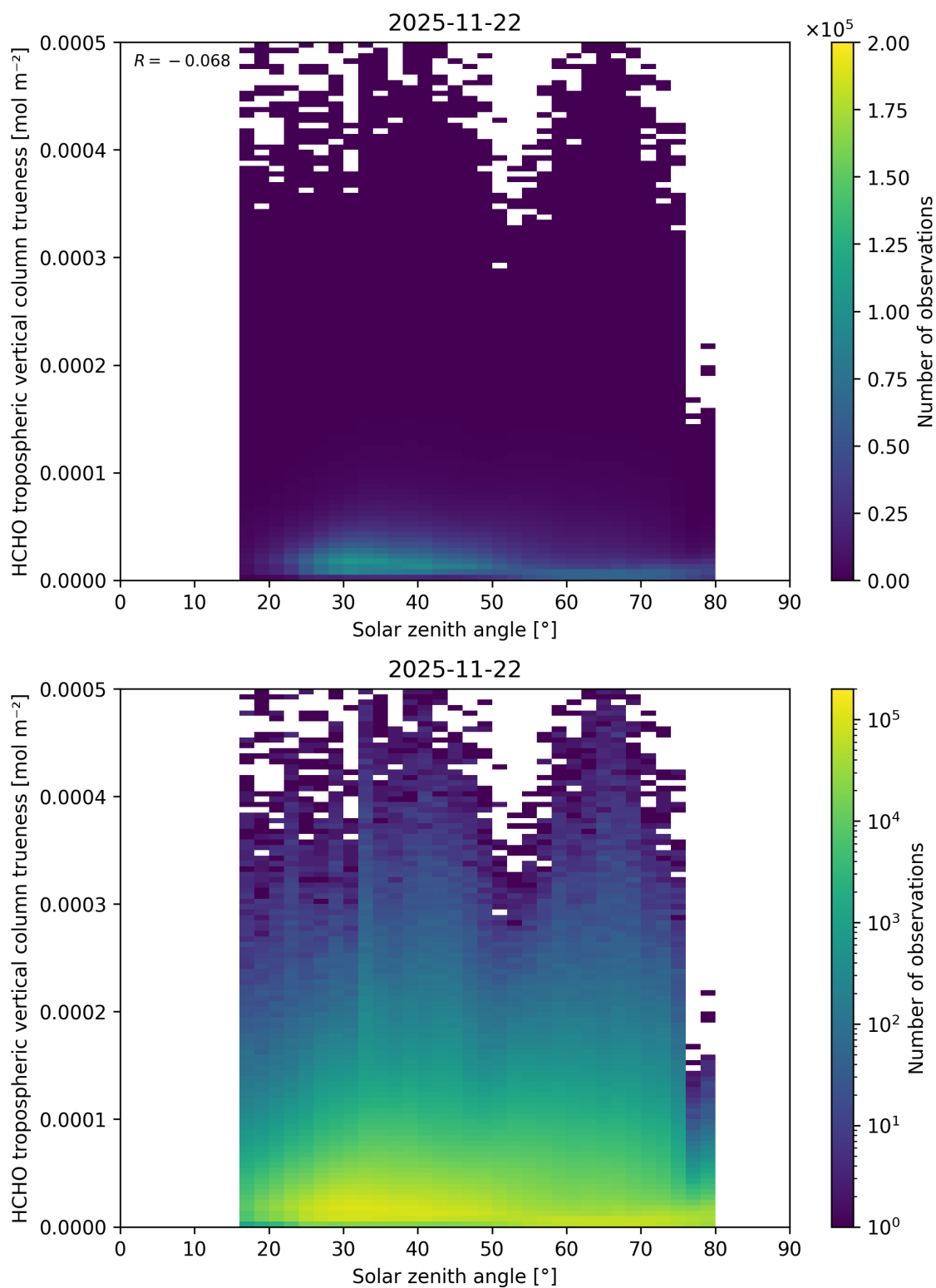
Figure 199: Scatter density plot of “Solar zenith angle” against “HCHO tropospheric vertical column trueness” for 2025-11-21 to 2025-11-23.
