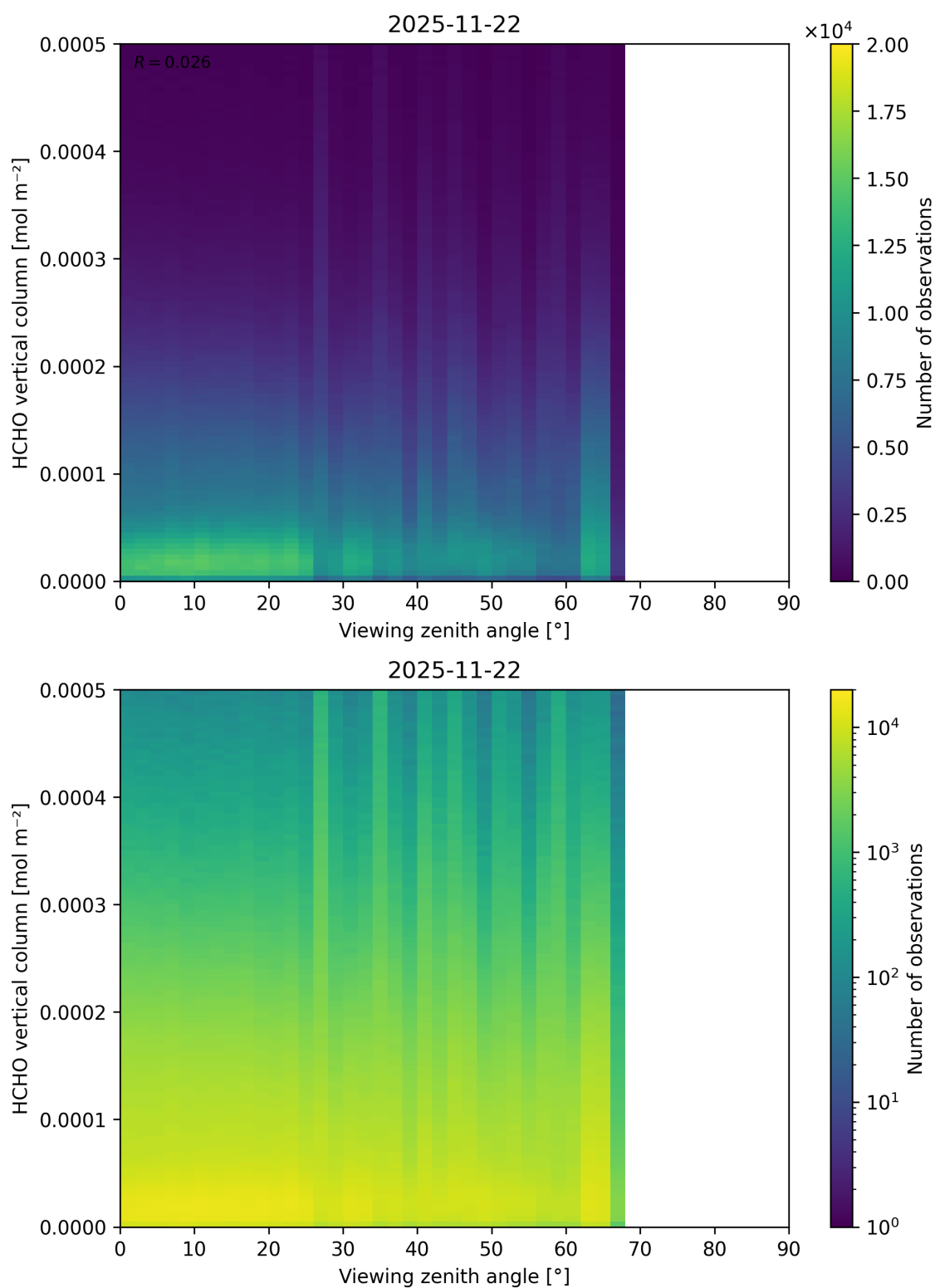
Figure 212: Scatter density plot of “Viewing zenith angle” against “HCHO vertical column” for 2025-11-21 to 2025-11-23.
