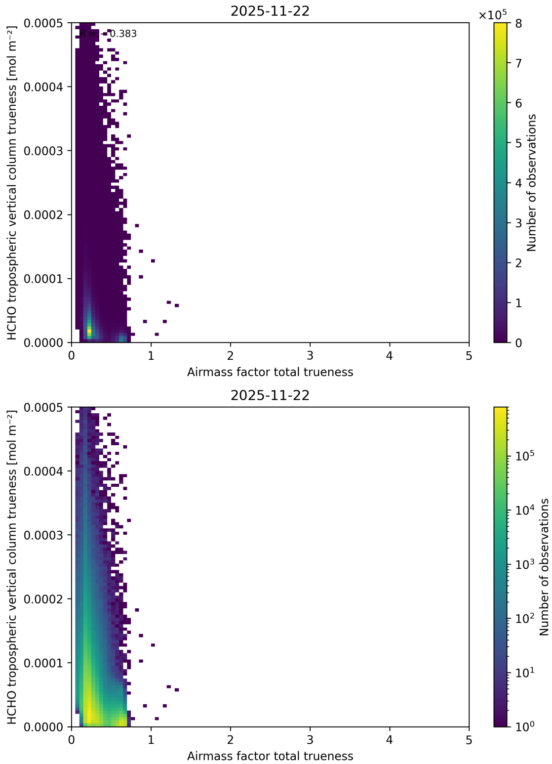
Figure 124: Scatter density plot of “Airmass factor total trueness” against “HCHO tropospheric vertical column trueness” for 2025-11-21 to 2025-11-23.
