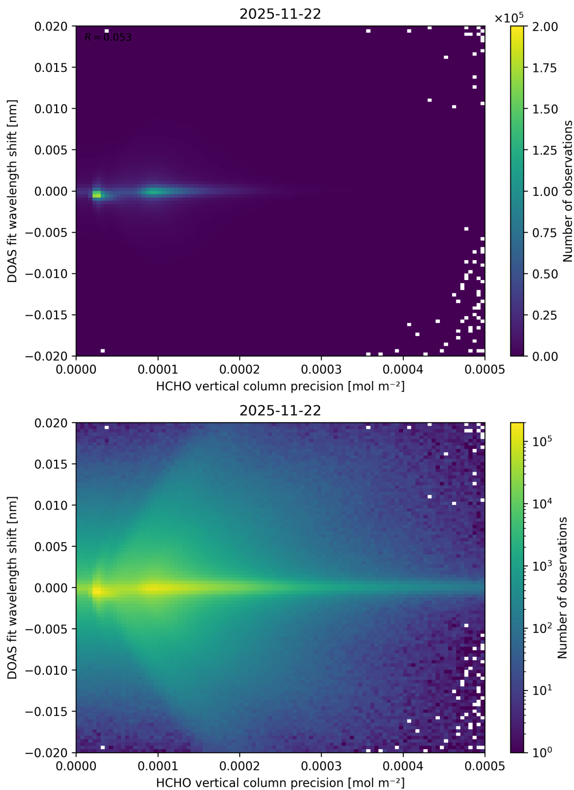
Figure 153: Scatter density plot of “HCHO vertical column precision” against “DOAS fit wavelength shift” for 2025-11-21 to 2025-11-23.
