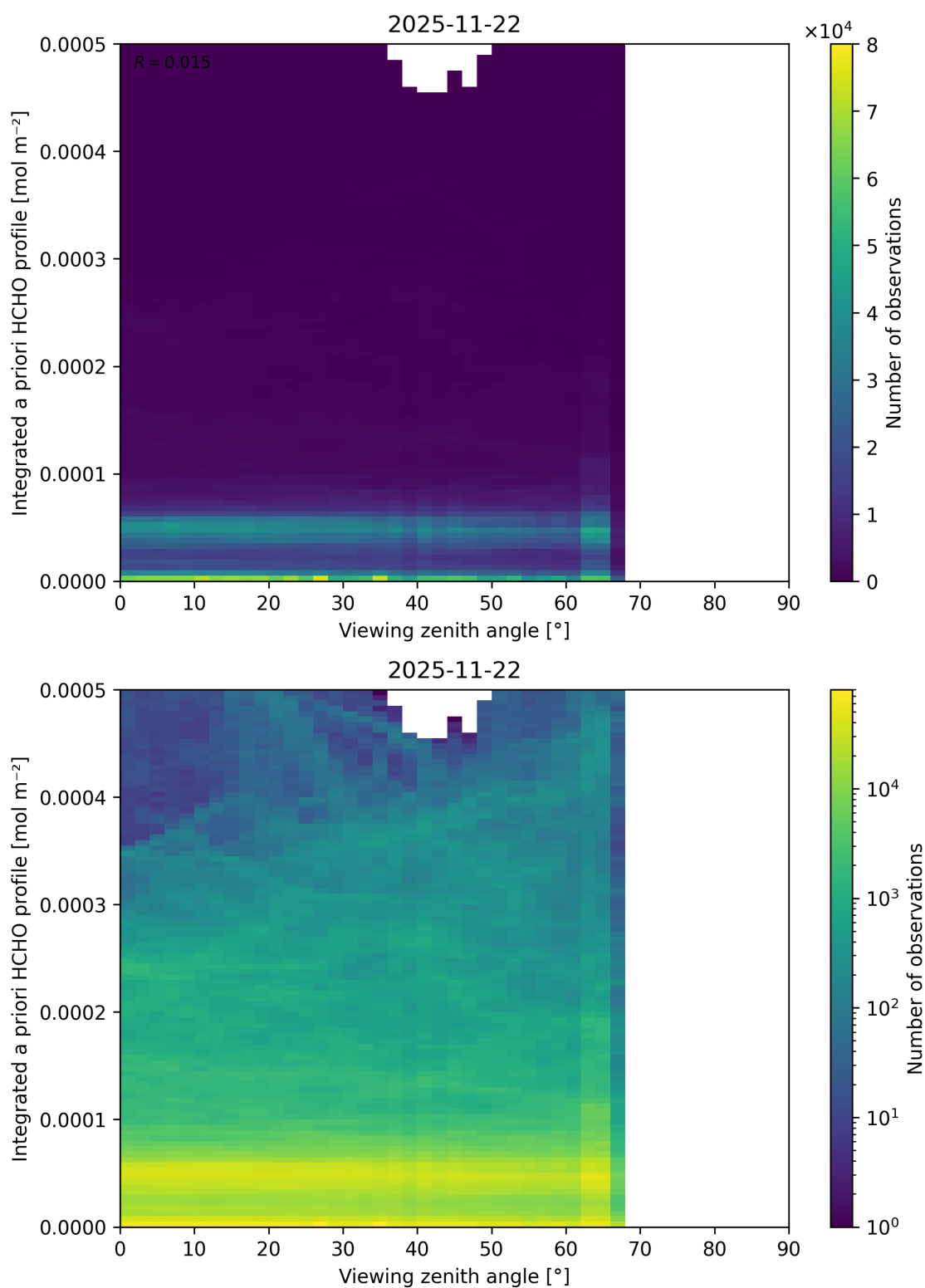
Figure 216: Scatter density plot of “Viewing zenith angle” against “Integrated a priori HCHO profile” for 2025-11-21 to 2025-11-23.
