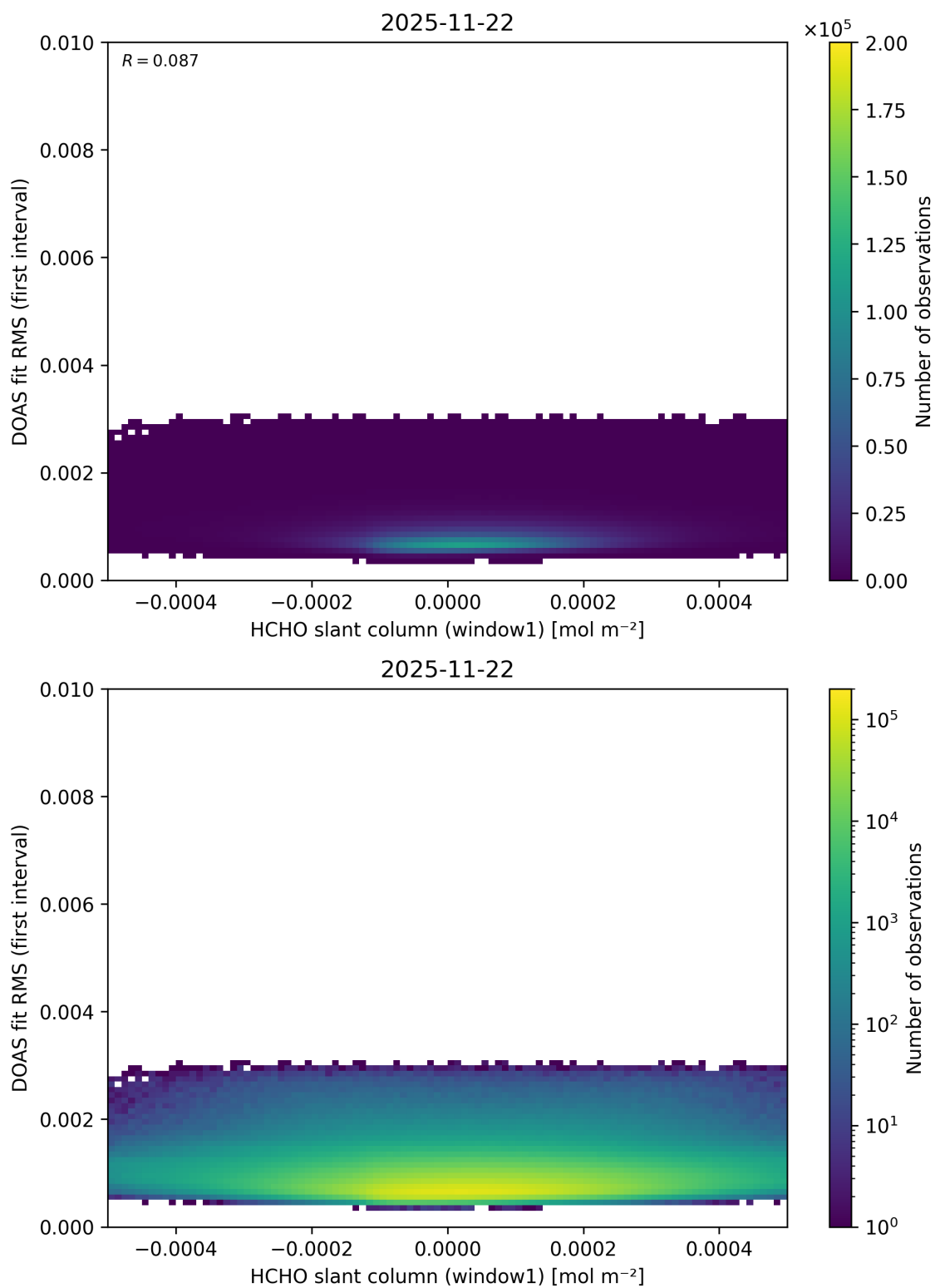
Figure 88: Scatter density plot of “HCHO slant column (window1)” against “DOAS fit RMS (first interval)” for 2025-11-21 to 2025-11-23.
