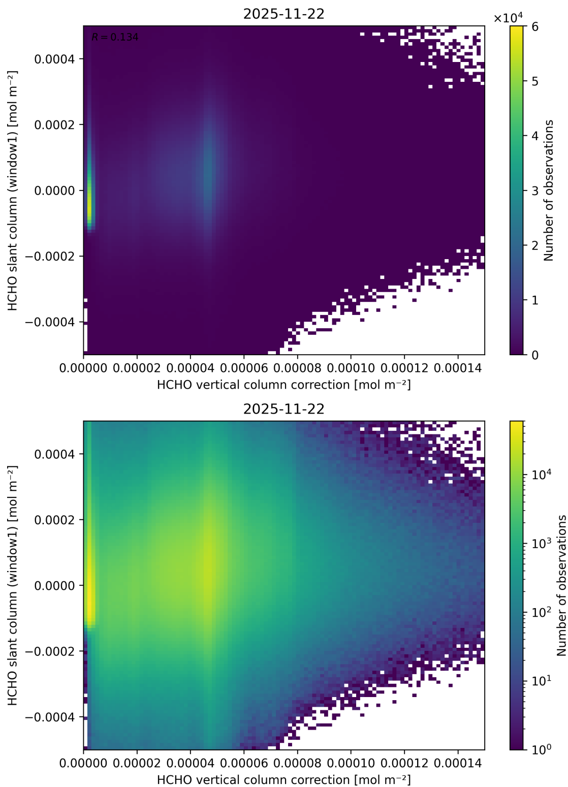
Figure 132: Scatter density plot of “HCHO vertical column correction” against “HCHO slant column (window1)” for 2025-11-21 to 2025-11-23.
