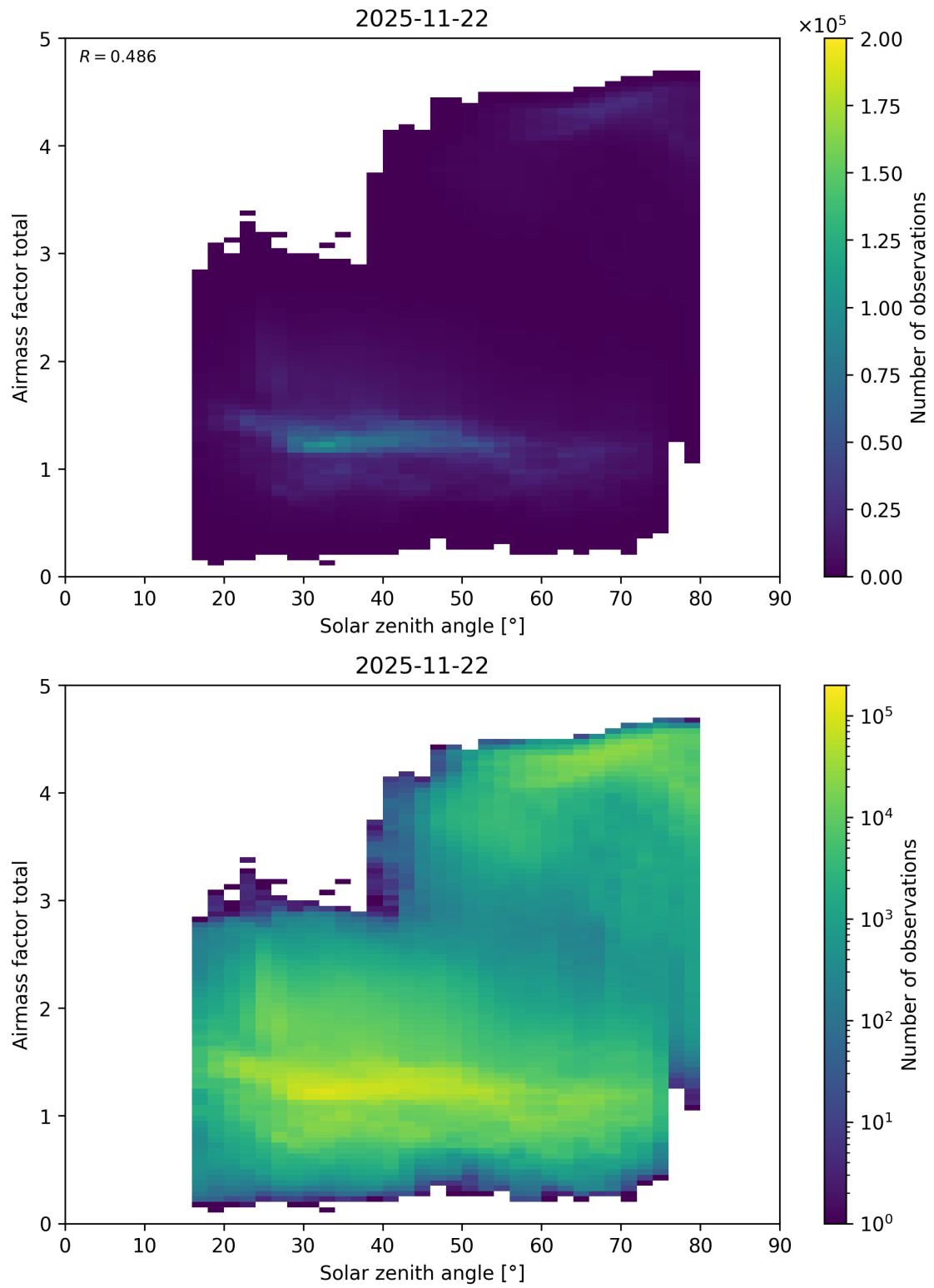
Figure 194: Scatter density plot of “Solar zenith angle” against “Airmass factor total” for 2025-11-21 to 2025-11-23.
