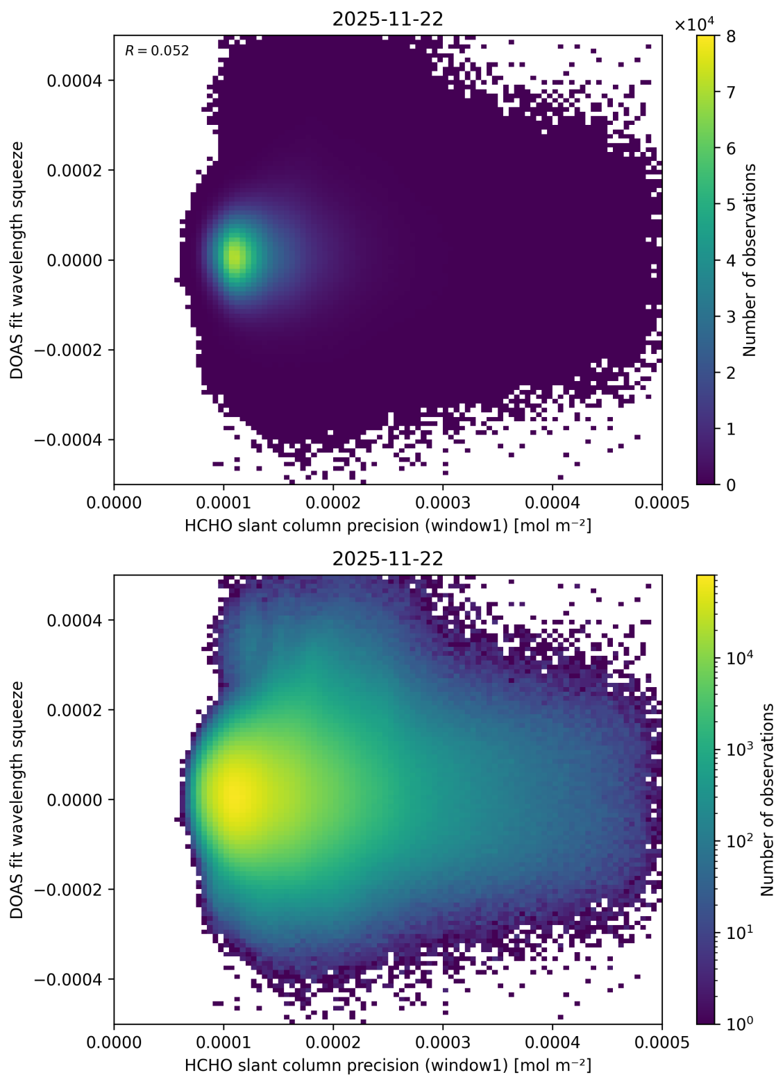
Figure 101: Scatter density plot of “HCHO slant column precision (window1)” against “DOAS fit wavelength squeeze” for 2025-11-21 to 2025-11-23.
