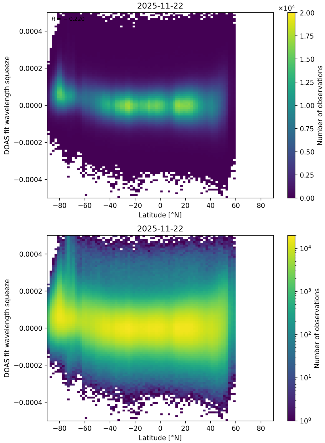
Figure 173: Scatter density plot of “Latitude” against “DOAS fit wavelength squeeze” for 2025-11-21 to 2025-11-23.
