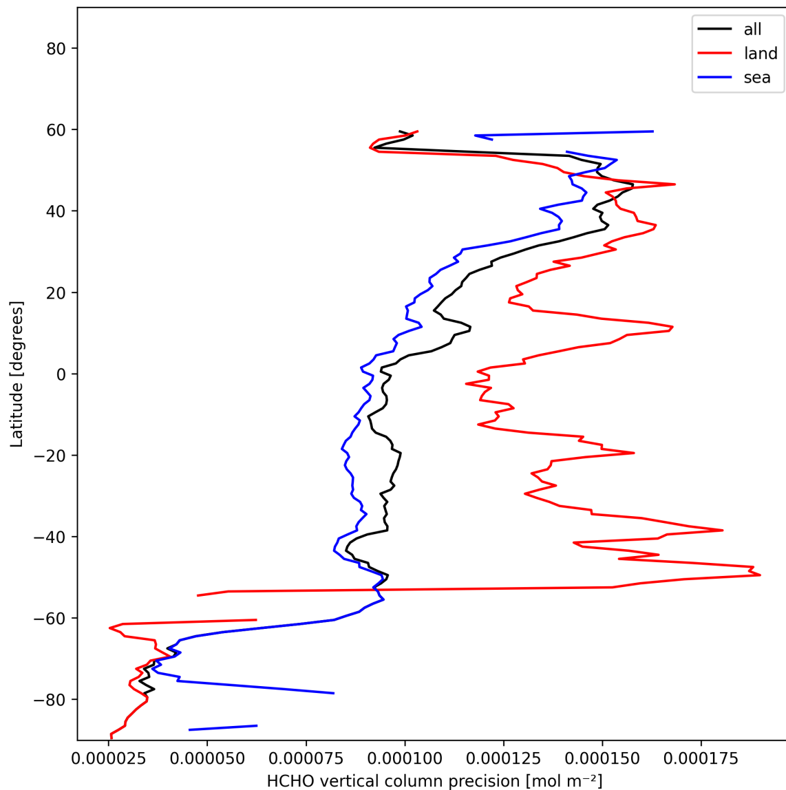
Figure 23: Zonal average of “HCHO vertical column precision” for 2025-11-21 to 2025-11-23.
