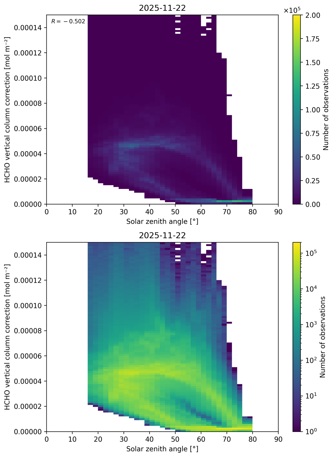
Figure 197: Scatter density plot of “Solar zenith angle” against “HCHO vertical column correction” for 2025-11-21 to 2025-11-23.
