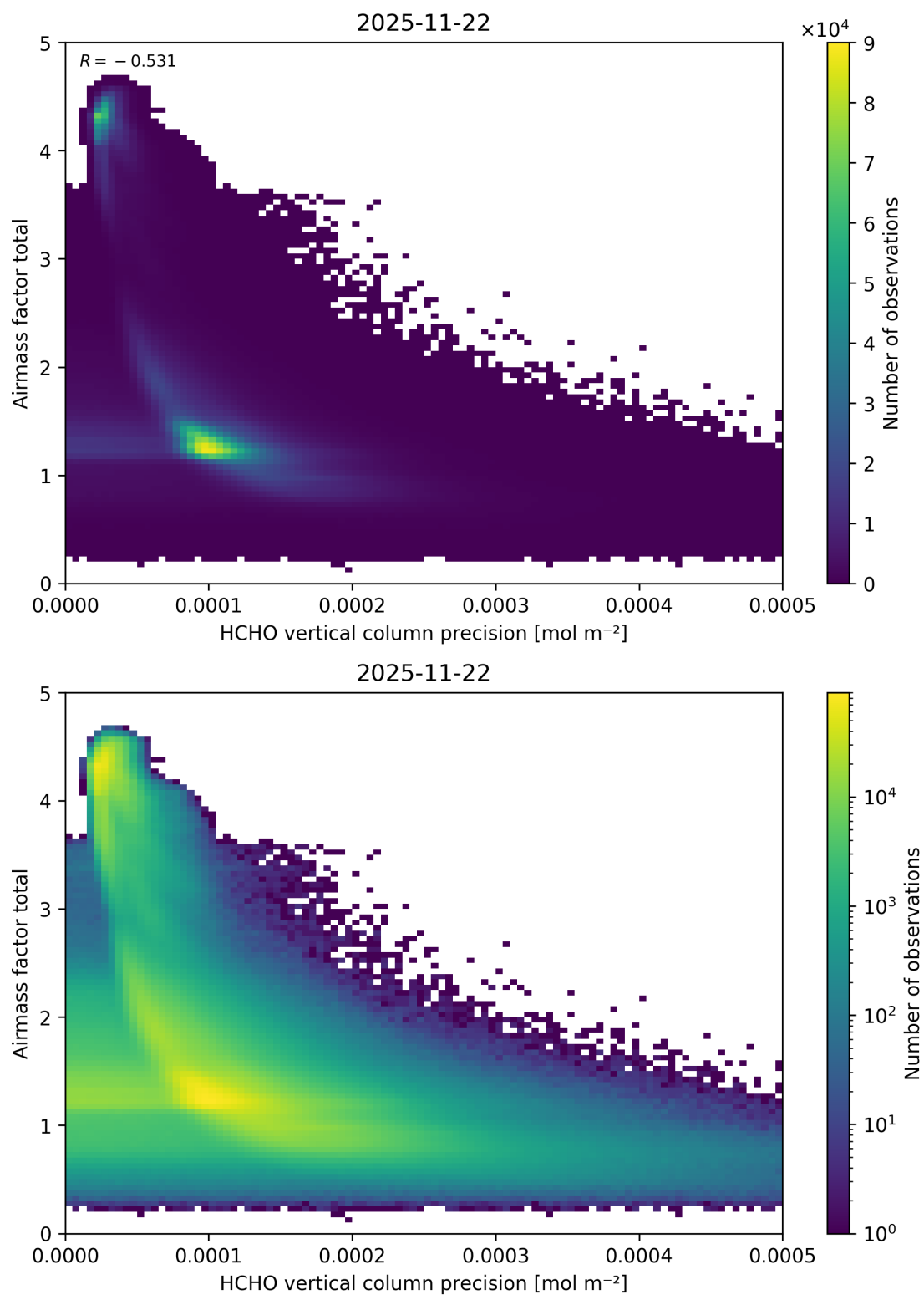
Figure 160: Scatter density plot of “HCHO vertical column precision” against “Airmass factor total” for 2025-11-21 to 2025-11-23.
