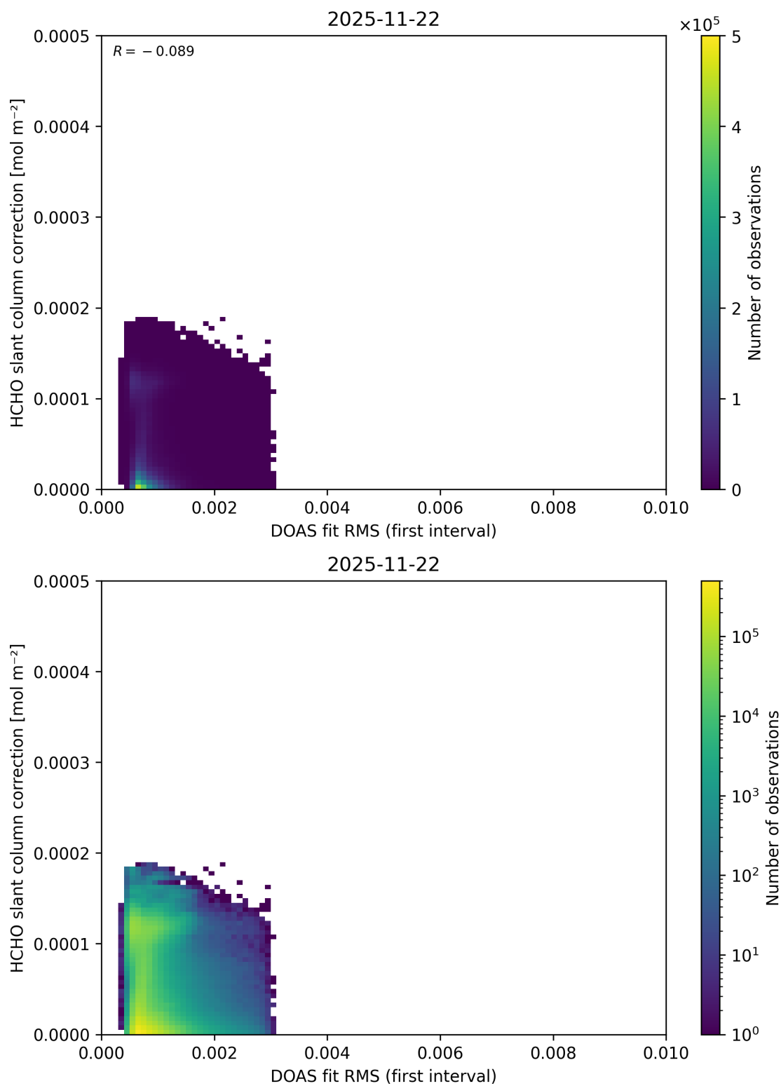
Figure 67: Scatter density plot of “DOAS fit RMS (first interval)” against “HCHO slant column correction” for 2025-11-21 to 2025-11-23.
