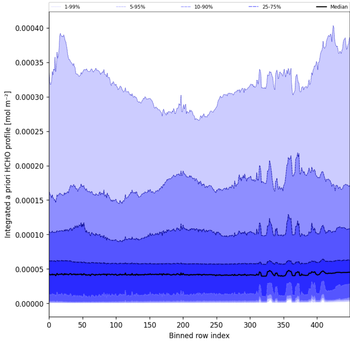
Figure 60: Along track statistics of “Integrated a priori HCHO profile” for 2025-11-21 to 2025-11-23
