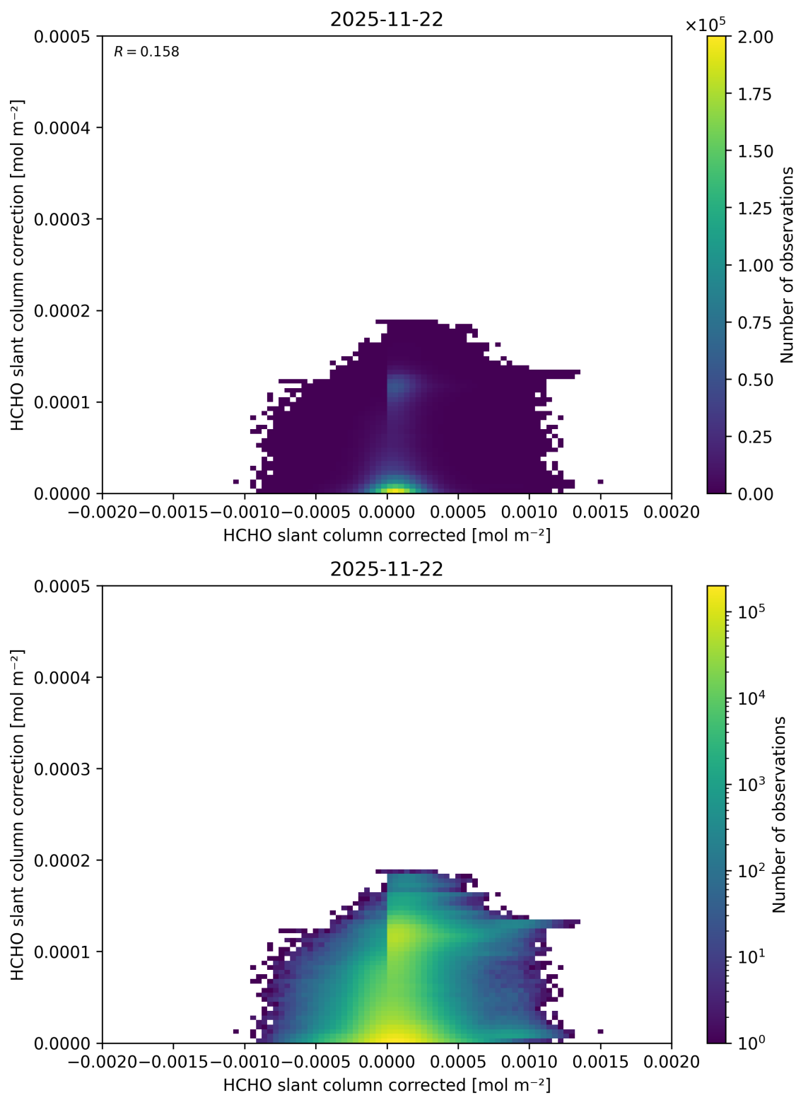
Figure 85: Scatter density plot of “HCHO slant column corrected” against “HCHO slant column correction” for 2025-11-21 to 2025-11-23.
