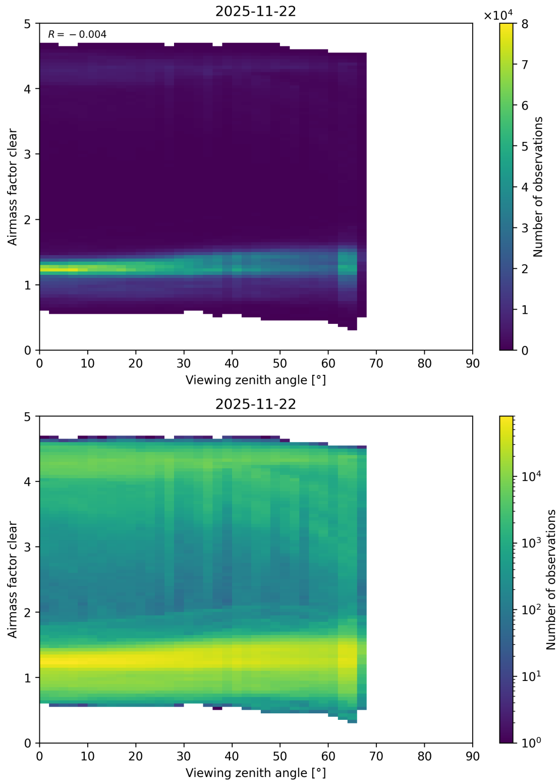
Figure 205: Scatter density plot of “Viewing zenith angle” against “Airmass factor clear” for 2025-11-21 to 2025-11-23.
