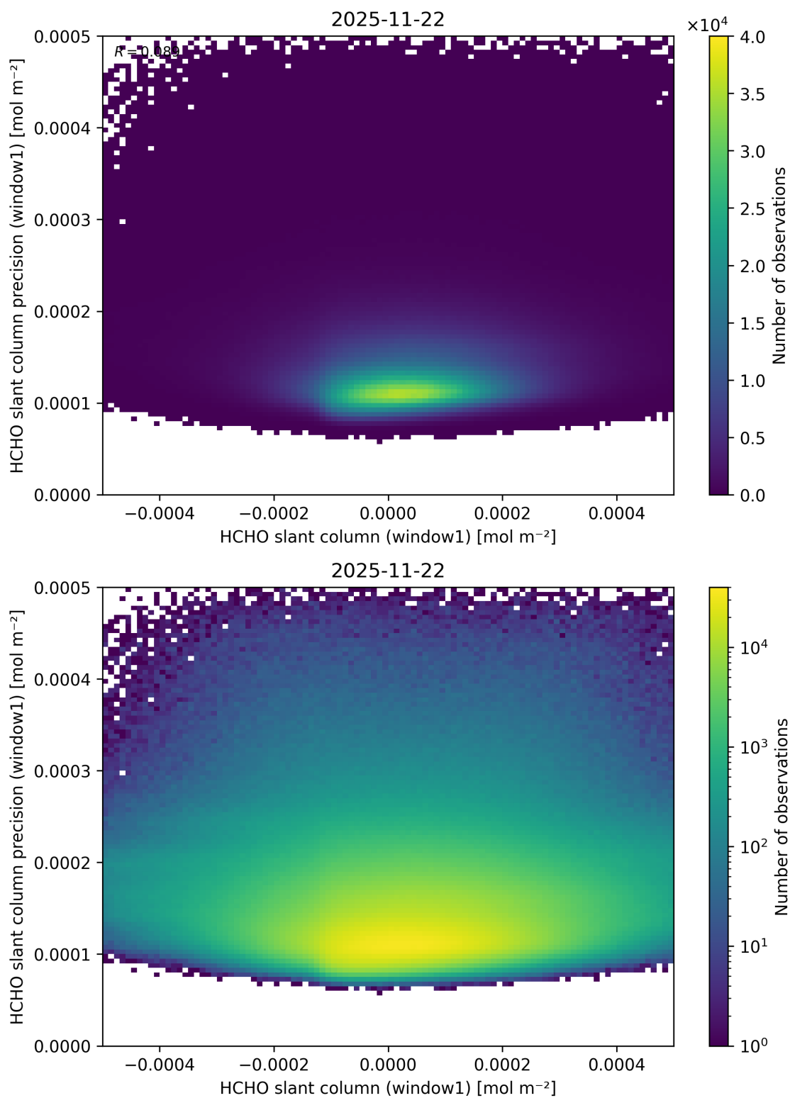
Figure 94: Scatter density plot of “HCHO slant column (window1)” against “HCHO slant column precision (window1)” for 2025-11-21 to 2025-11-23.
