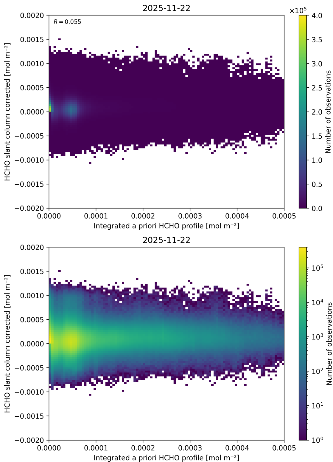
Figure 168: Scatter density plot of “Integrated a priori HCHO profile” against “HCHO slant column corrected” for 2025-11-21 to 2025-11-23.
