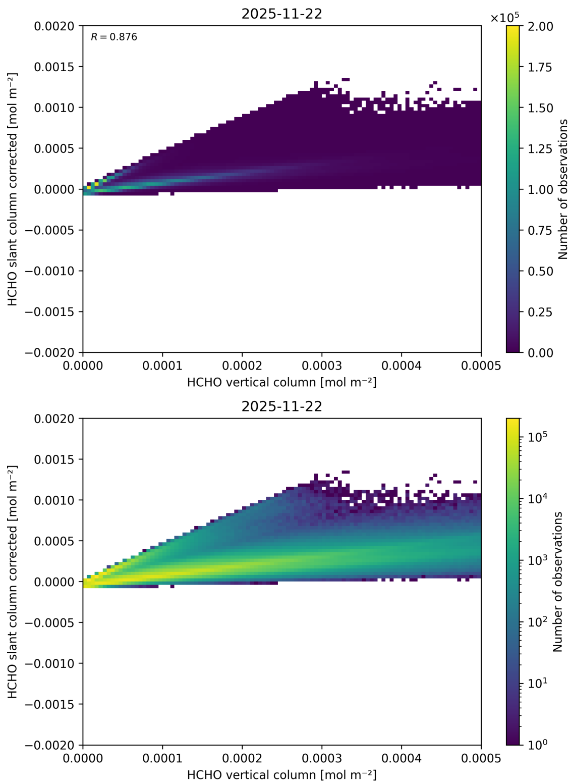
Figure 142: Scatter density plot of “HCHO vertical column” against “HCHO slant column corrected” for 2025-11-21 to 2025-11-23.
