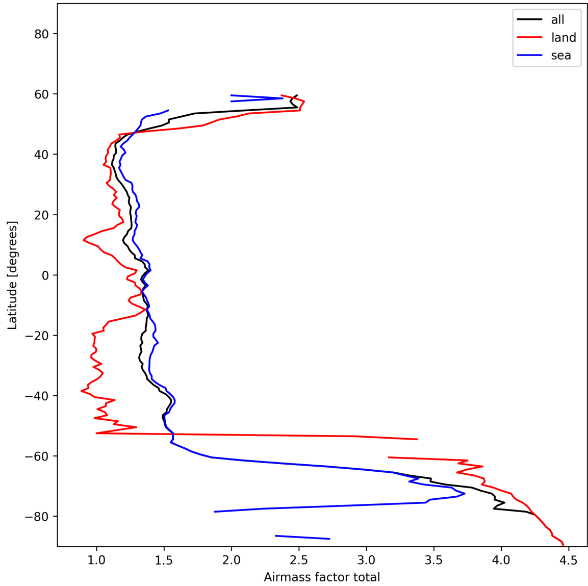
Figure 27: Zonal average of “Airmass factor total” for 2025-11-21 to 2025-11-23.
