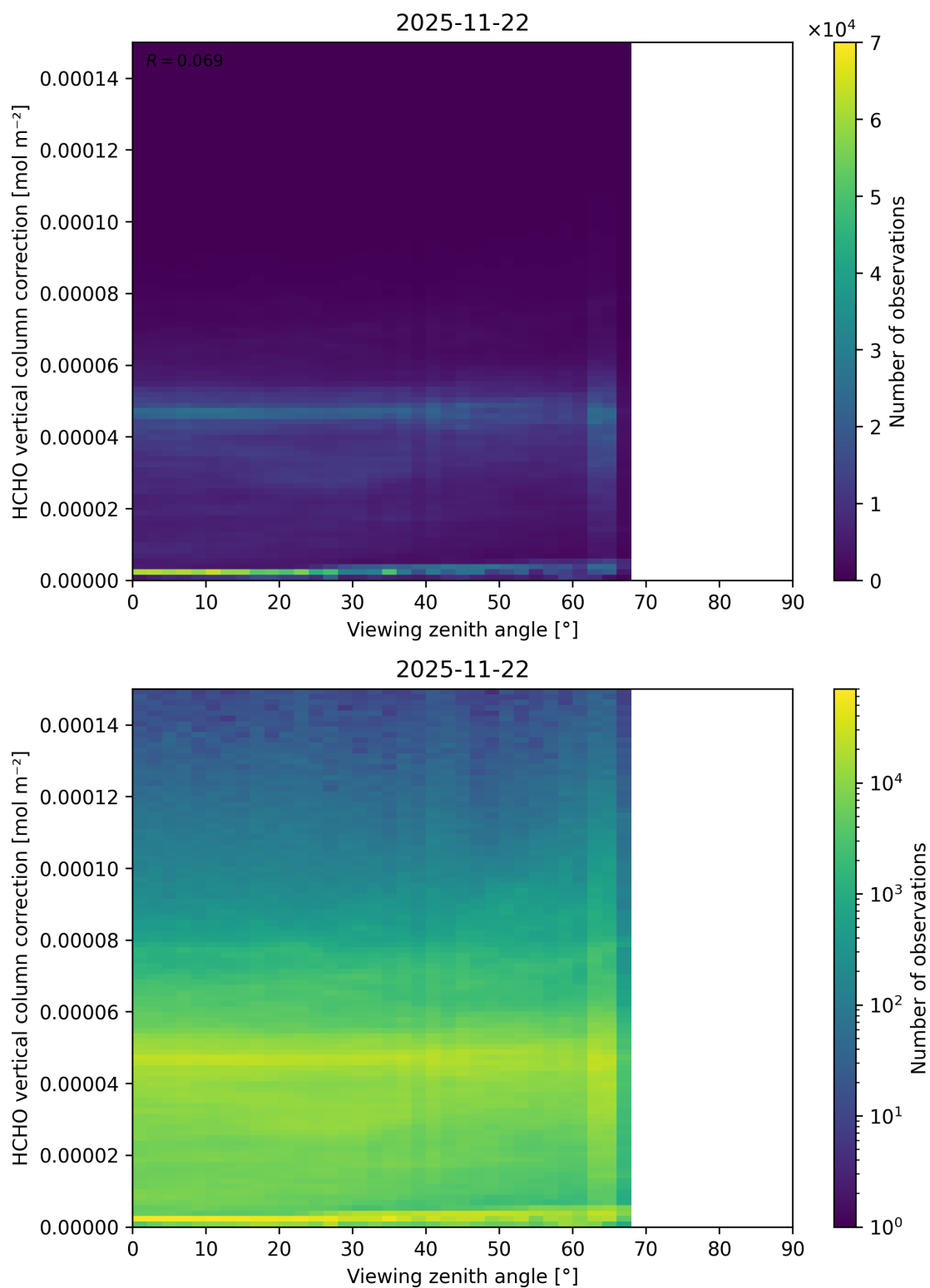
Figure 213: Scatter density plot of “Viewing zenith angle” against “HCHO vertical column correction” for 2025-11-21 to 2025-11-23.
