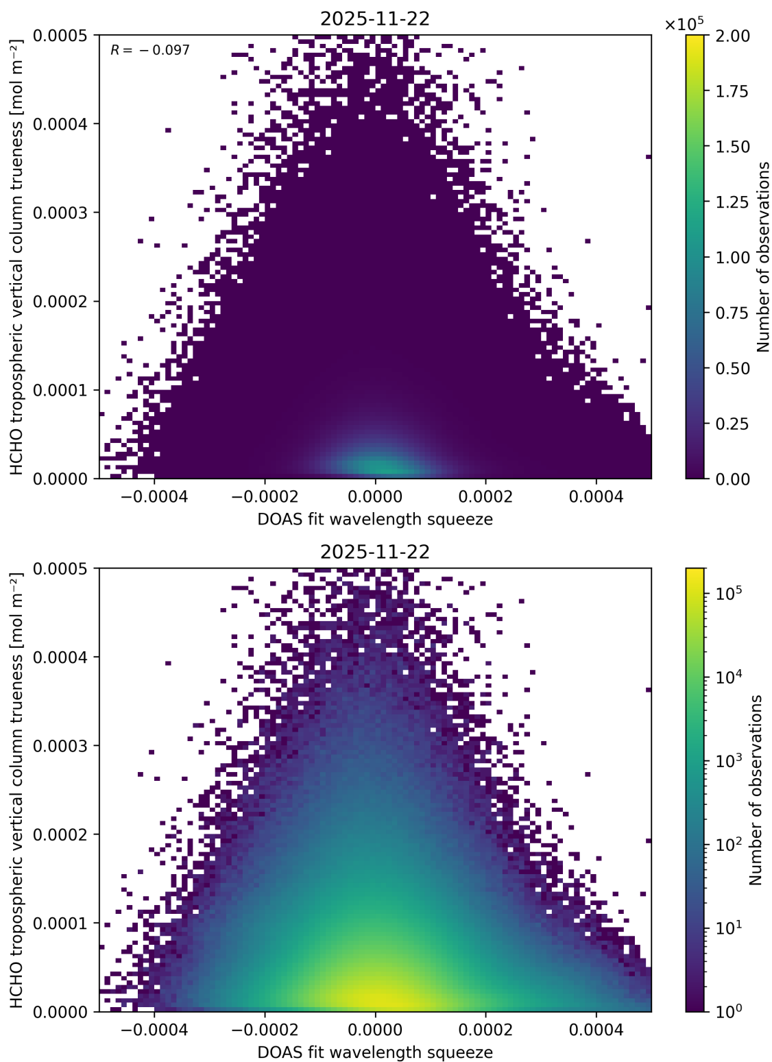
Figure 77: Scatter density plot of “DOAS fit wavelength squeeze” against “HCHO tropospheric vertical column trueness” for 2025-11-21 to 2025-11-23.
