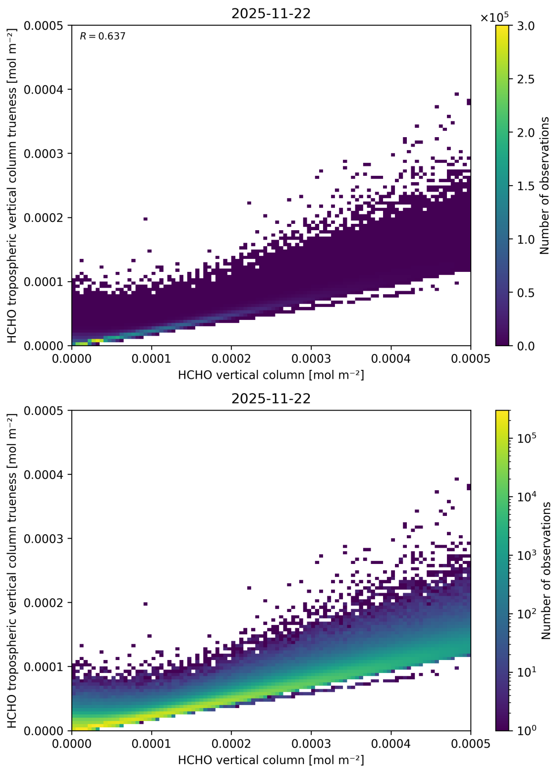
Figure 150: Scatter density plot of “HCHO vertical column” against “HCHO tropospheric vertical column trueness” for 2025-11-21 to 2025-11-23.
