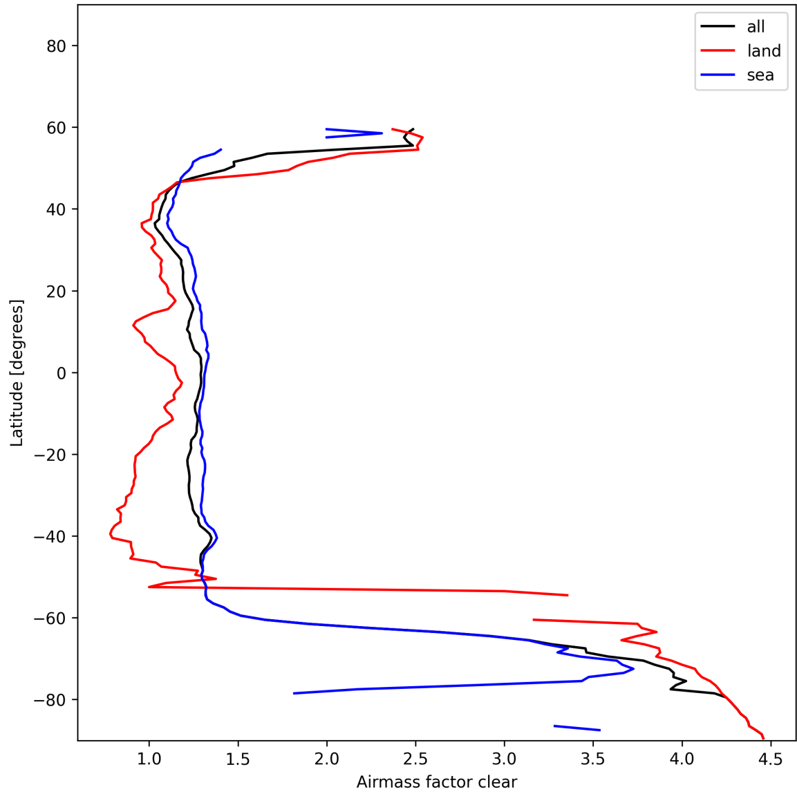
Figure 29: Zonal average of “Airmass factor clear” for 2025-11-21 to 2025-11-23.
