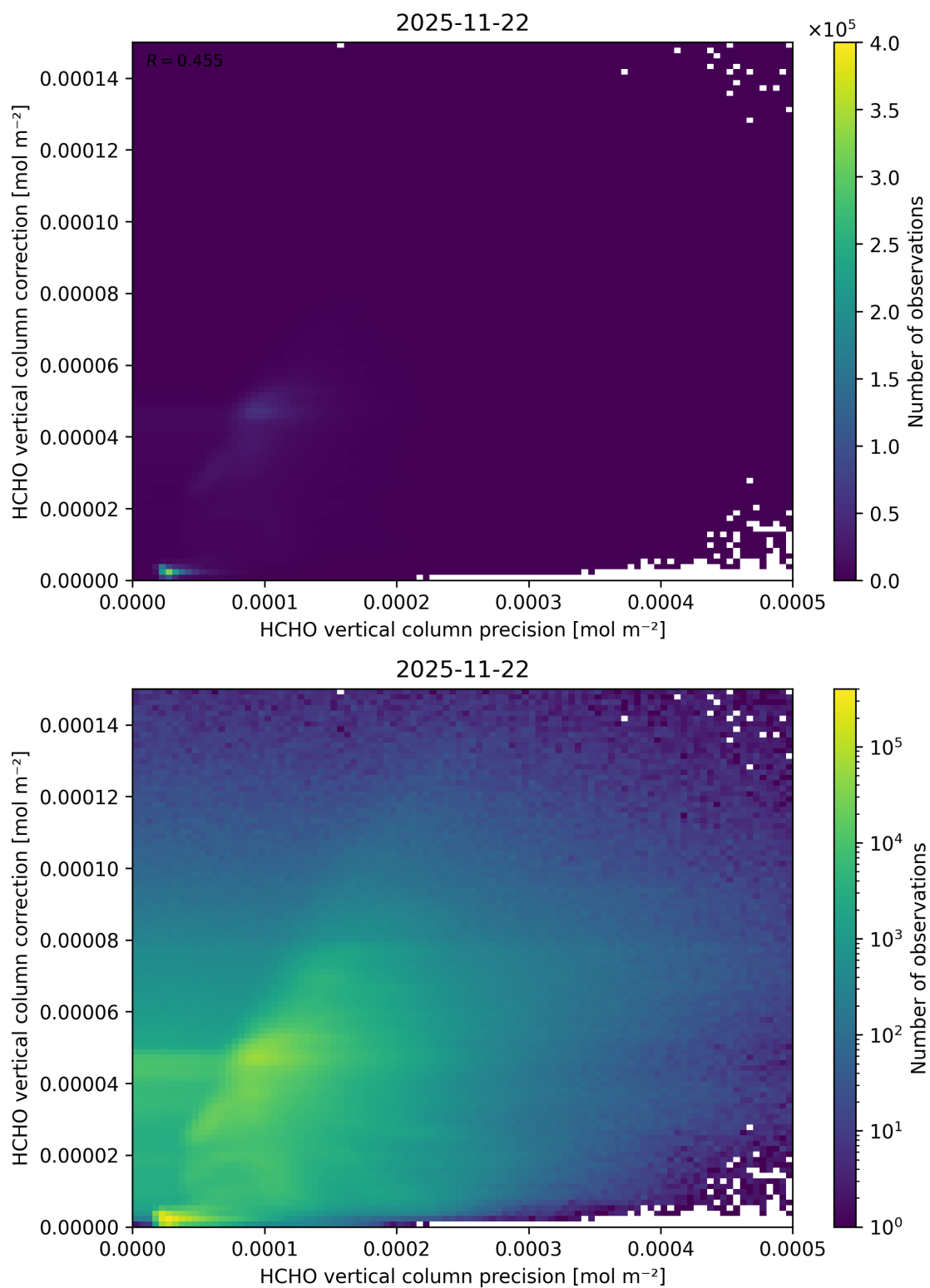
Figure 162: Scatter density plot of “HCHO vertical column precision” against “HCHO vertical column correction” for 2025-11-21 to 2025-11-23.
