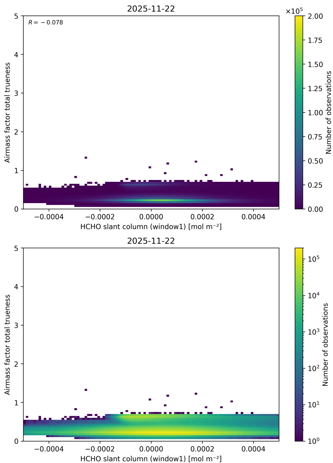
Figure 96: Scatter density plot of “HCHO slant column (window1)” against “Airmass factor total trueneess” for 2025-11-21 to 2025-11-23.
