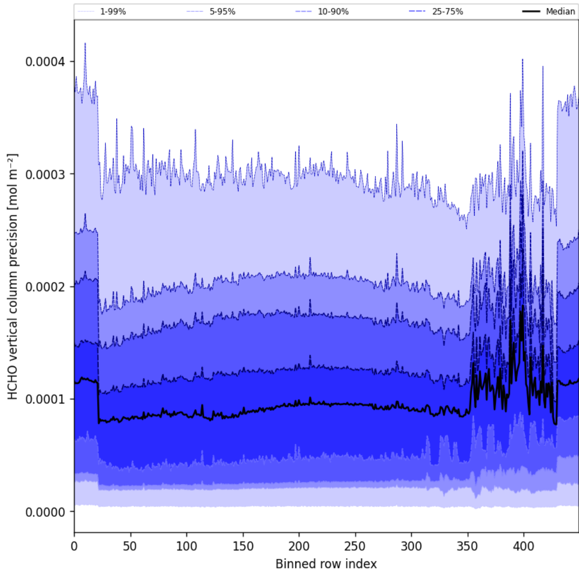
Figure 53: Along track statistics of “HCHO vertical column precision” for 2025-11-21 to 2025-11-23
