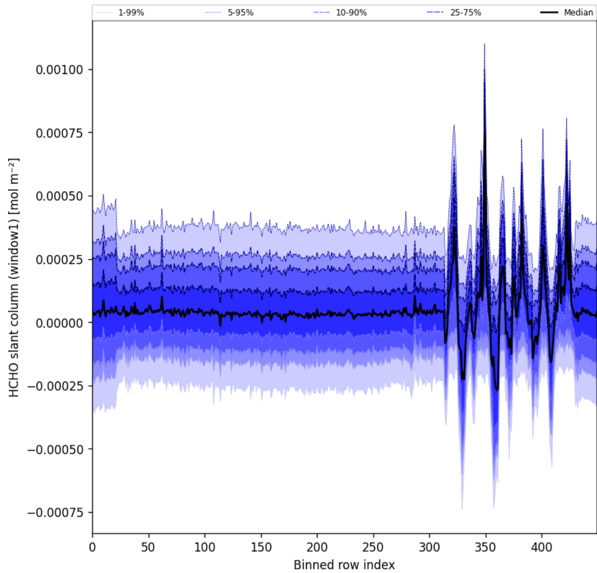
Figure 55: Along track statistics of "HCHO slant column (window1)" for 2025-11-21 to 2025-11-23
