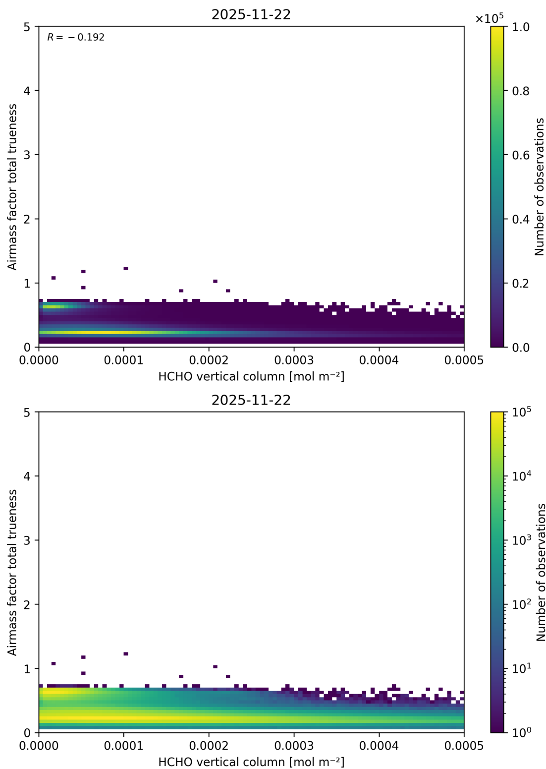
Figure 147: Scatter density plot of “HCHO vertical column” against “Airmass factor total trueneess” for 2025-11-21 to 2025-11-23.
