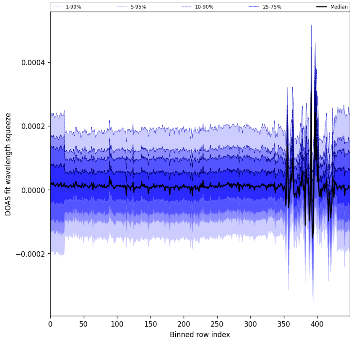
Figure 62: Along track statistics of “DOAS fit wavelength squeeze” for 2025-11-21 to 2025-11-23
