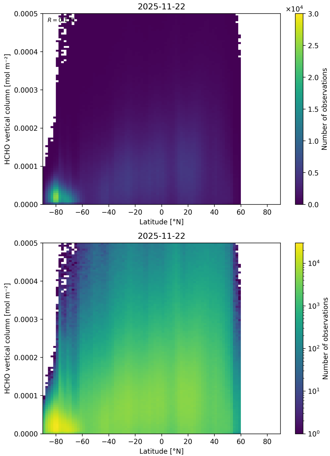
Figure 181: Scatter density plot of “Latitude” against “HCHO vertical column” for 2025-11-21 to 2025-11-23.
