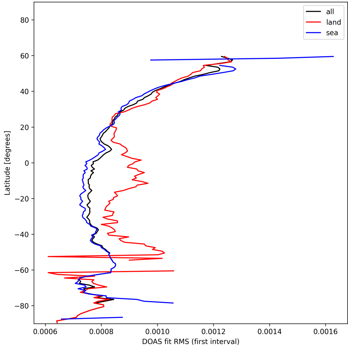
Figure 33: Zonal average of "DOAS fit RMS (first interval)" for 2025-11-21 to 2025-11-23.
