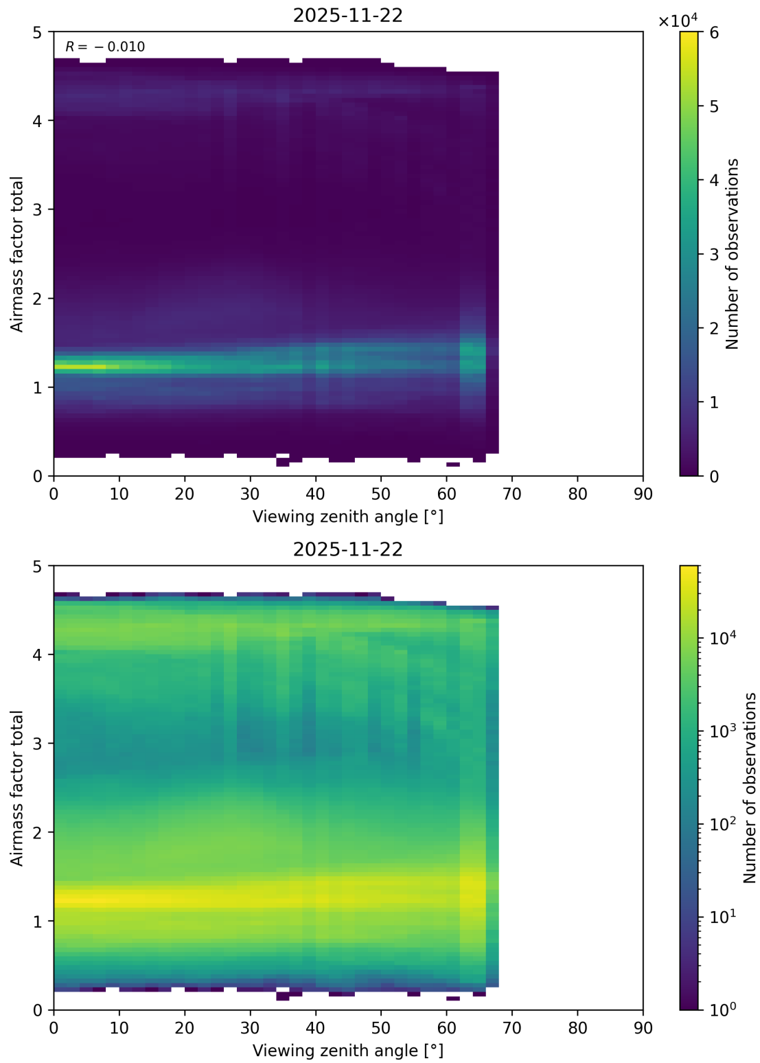
Figure 210: Scatter density plot of “Viewing zenith angle” against “Airmass factor total” for 2025-11-21 to 2025-11-23.
