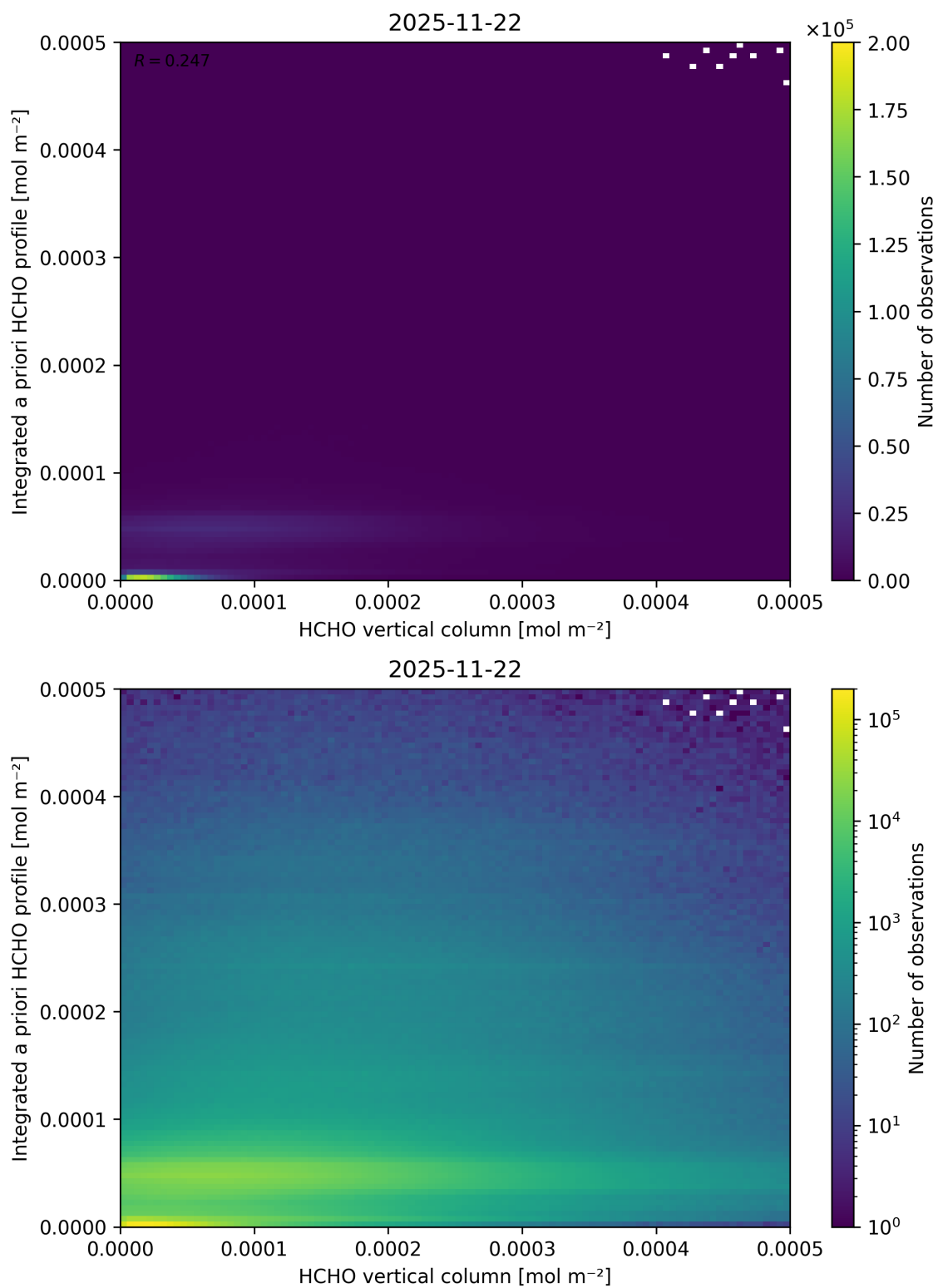
Figure 151: Scatter density plot of “HCHO vertical column” against “Integrated a priori HCHO profile” for 2025-11-21 to 2025-11-23.
