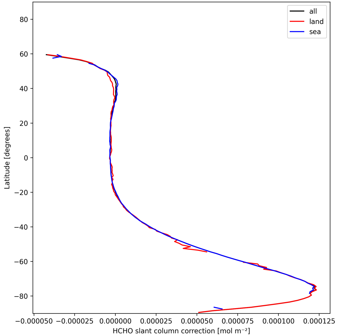
Figure 34: Zonal average of “HCHO slant column correction” for 2025-11-21 to 2025-11-23.
