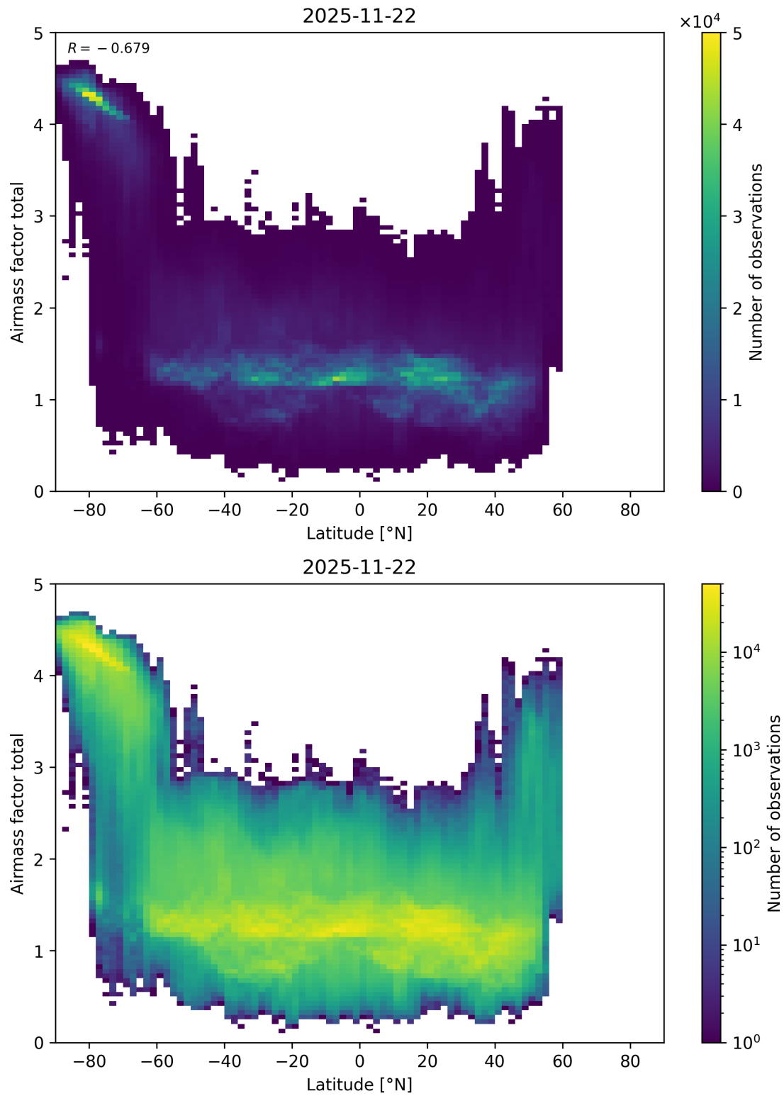
Figure 179: Scatter density plot of “Latitude” against “Airmass factor total” for 2025-11-21 to 2025-11-23.
