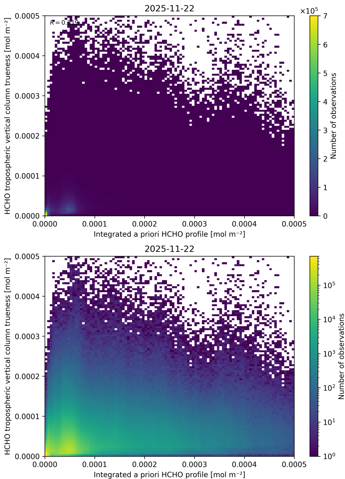
Figure 170: Scatter density plot of “Integrated a priori HCHO profile” against “HCHO tropospheric vertical column trueness” for 2025-11-21 to 2025-11-23.
