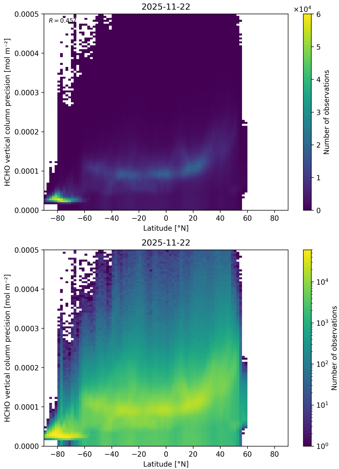
Figure 183: Scatter density plot of “Latitude” against “HCHO vertical column precision” for 2025-11-21 to 2025-11-23.
