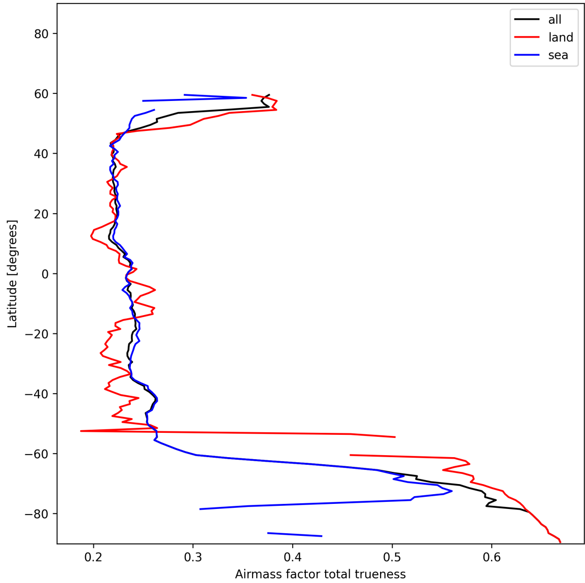
Figure 28: Zonal average of “Airmass factor total trueness” for 2025-11-21 to 2025-11-23.
