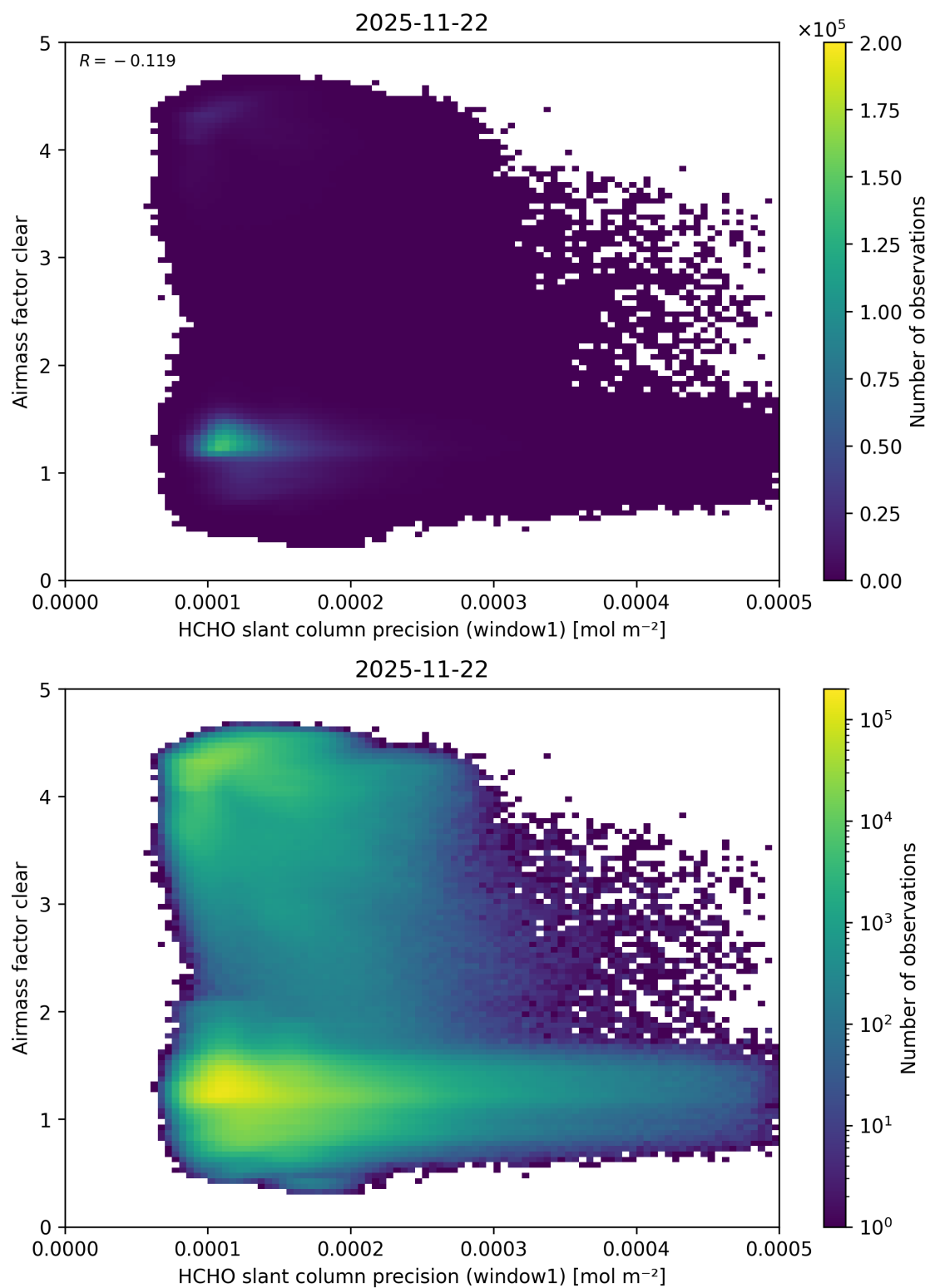
Figure 102: Scatter density plot of “HCHO slant column precision (window1)” against “Airmass factor clear” for 2025-11-21 to 2025-11-23.
