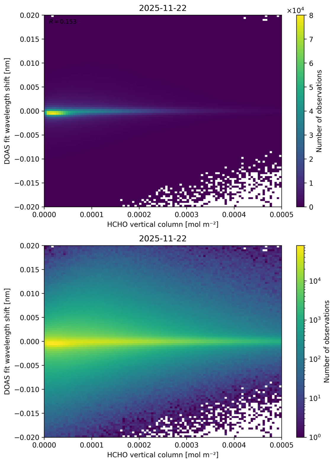
Figure 139: Scatter density plot of “HCHO vertical column” against “DOAS fit wavelength shift” for 2025-11-21 to 2025-11-23.
