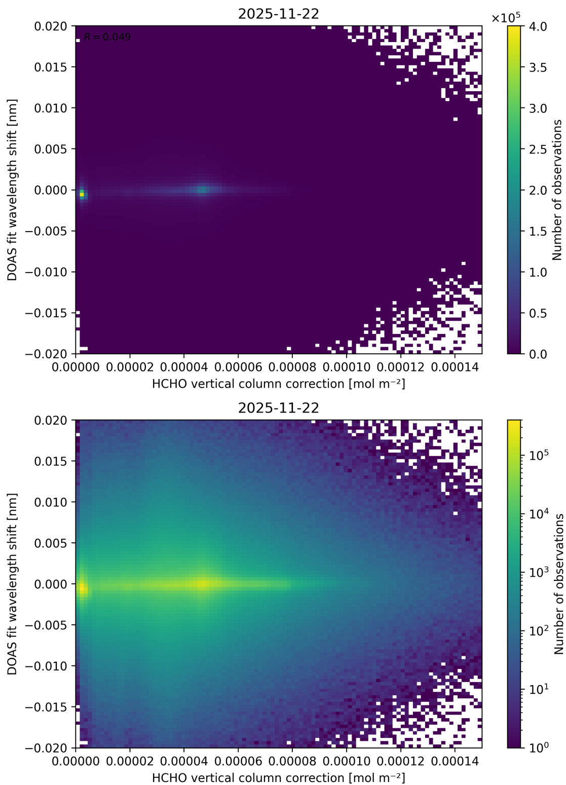
Figure 127: Scatter density plot of “HCHO vertical column correction” against “DOAS fit wavelength shift” for 2025-11-21 to 2025-11-23.
