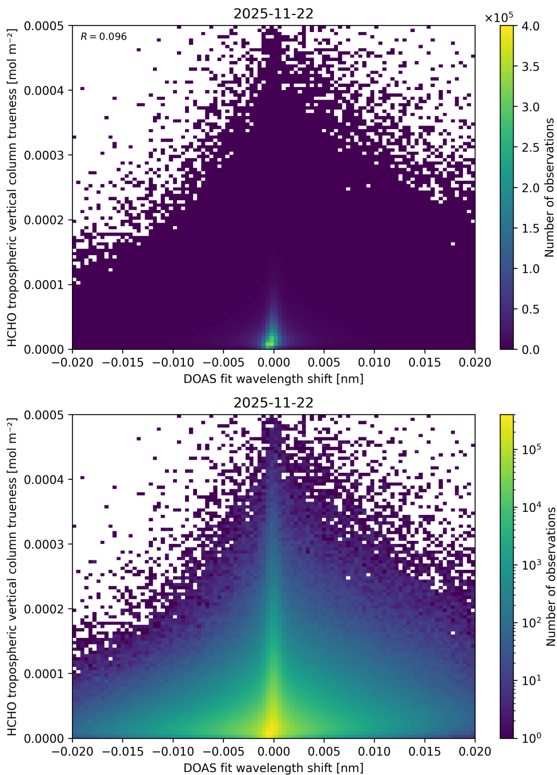
Figure 73: Scatter density plot of “DOAS fit wavelength shift” against “HCHO tropospheric vertical column trueness” for 2025-11-21 to 2025-11-23.
