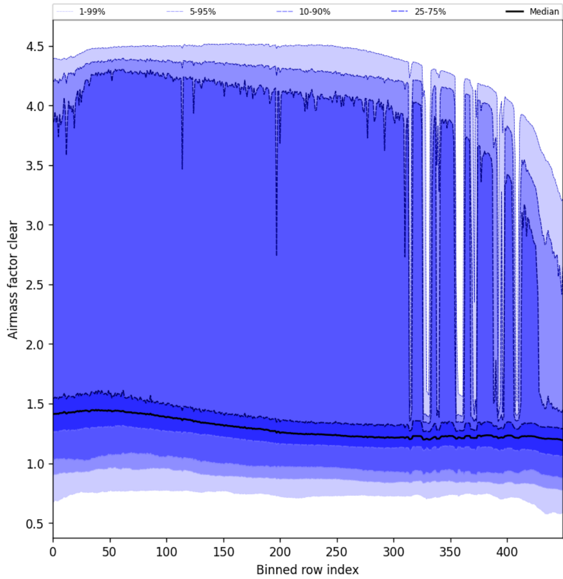
Figure 59: Along track statistics of “Air mass factor clear” for 2025-11-21 to 2025-11-23
