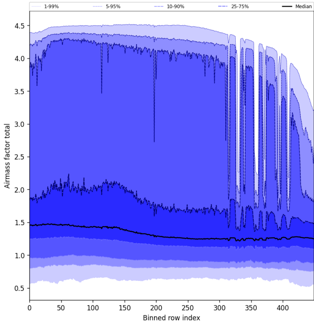
Figure 57: Along track statistics of “Airmass factor total” for 2025-11-21 to 2025-11-23
