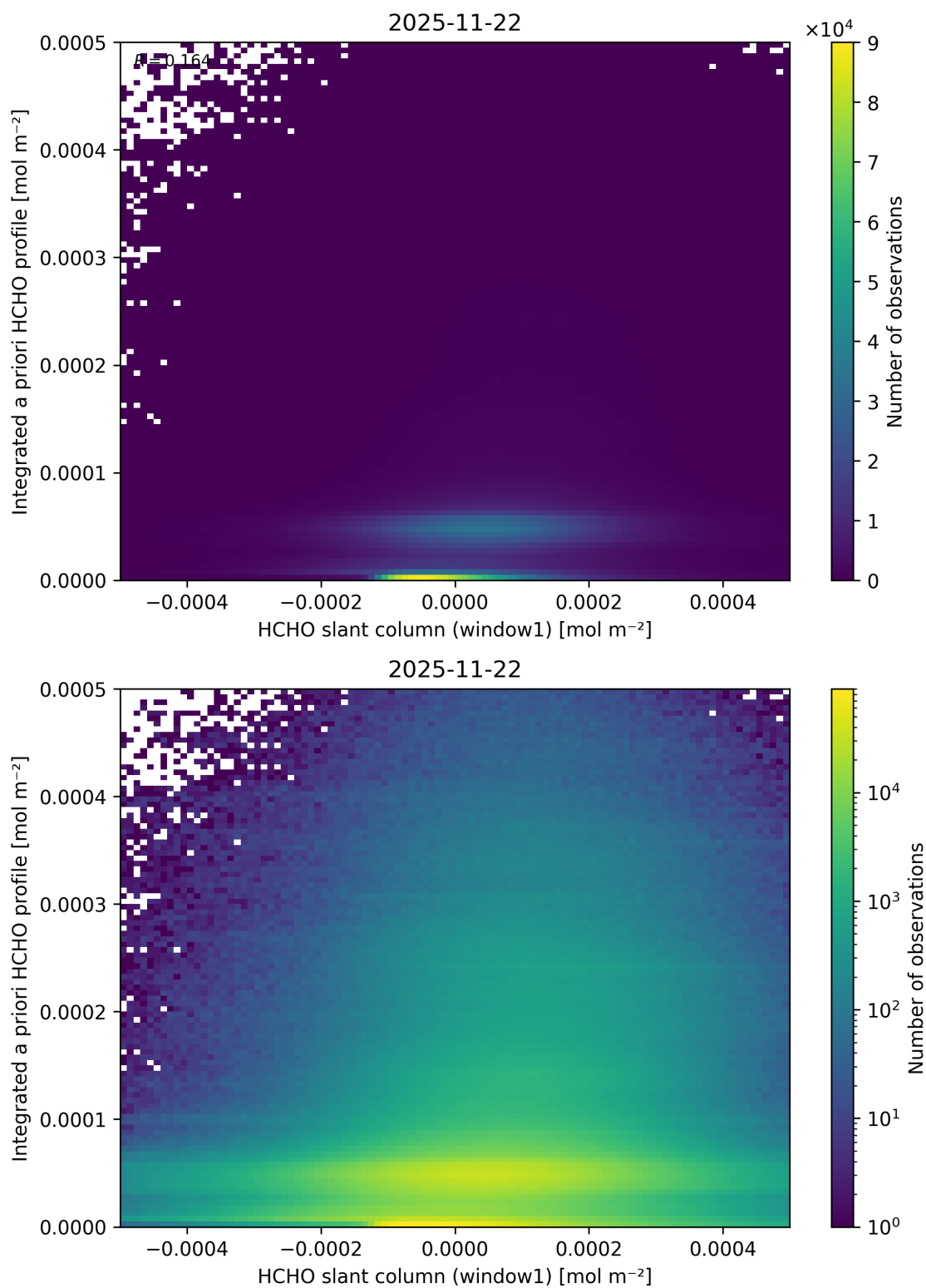
Figure 98: Scatter density plot of “HCHO slant column (window1)” against “Integrated a priori HCHO profile” for 2025-11-21 to 2025-11-23.
