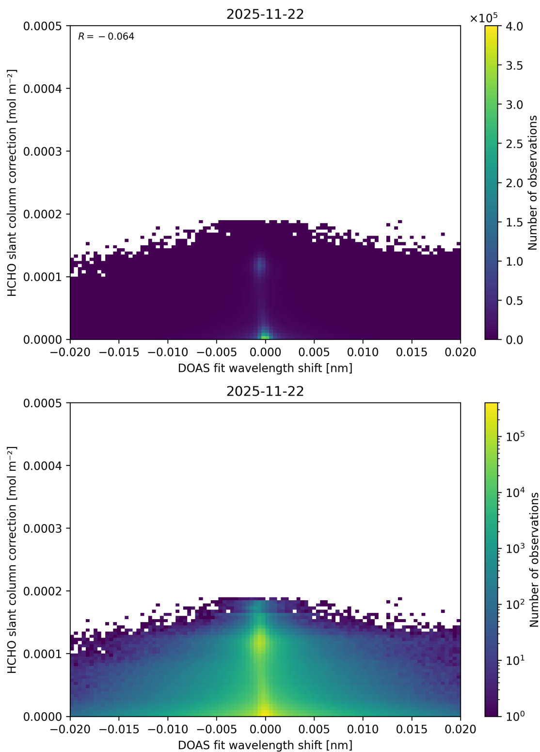
Figure 72: Scatter density plot of “DOAS fit wavelength shift” against “HCHO slant column correction” for 2025-11-21 to 2025-11-23.
