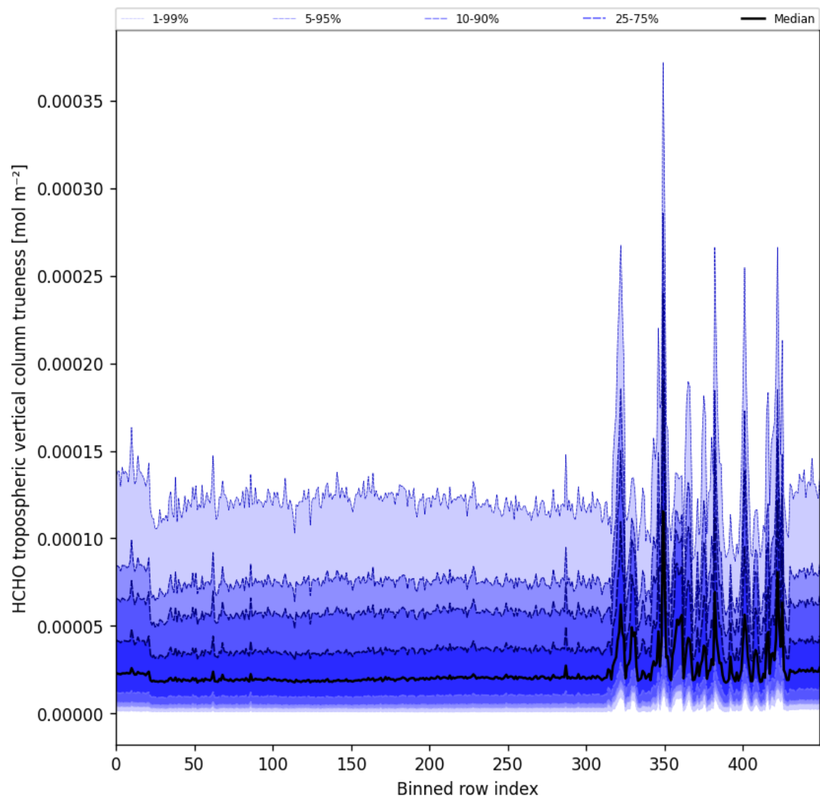
Figure 65: Along track statistics of “HCHO tropospheric vertical column trueness” for 2025-11-21 to 2025-11-23
