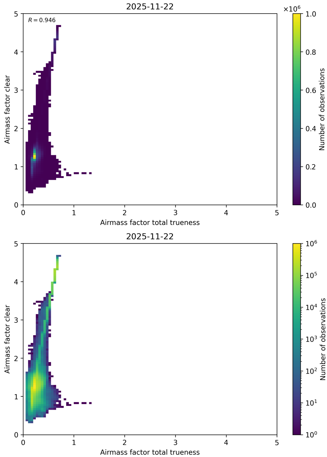
Figure 121: Scatter density plot of “Airmass factor total trueness” against “Airmass factor clear” for 2025-11-21 to 2025-11-23.
