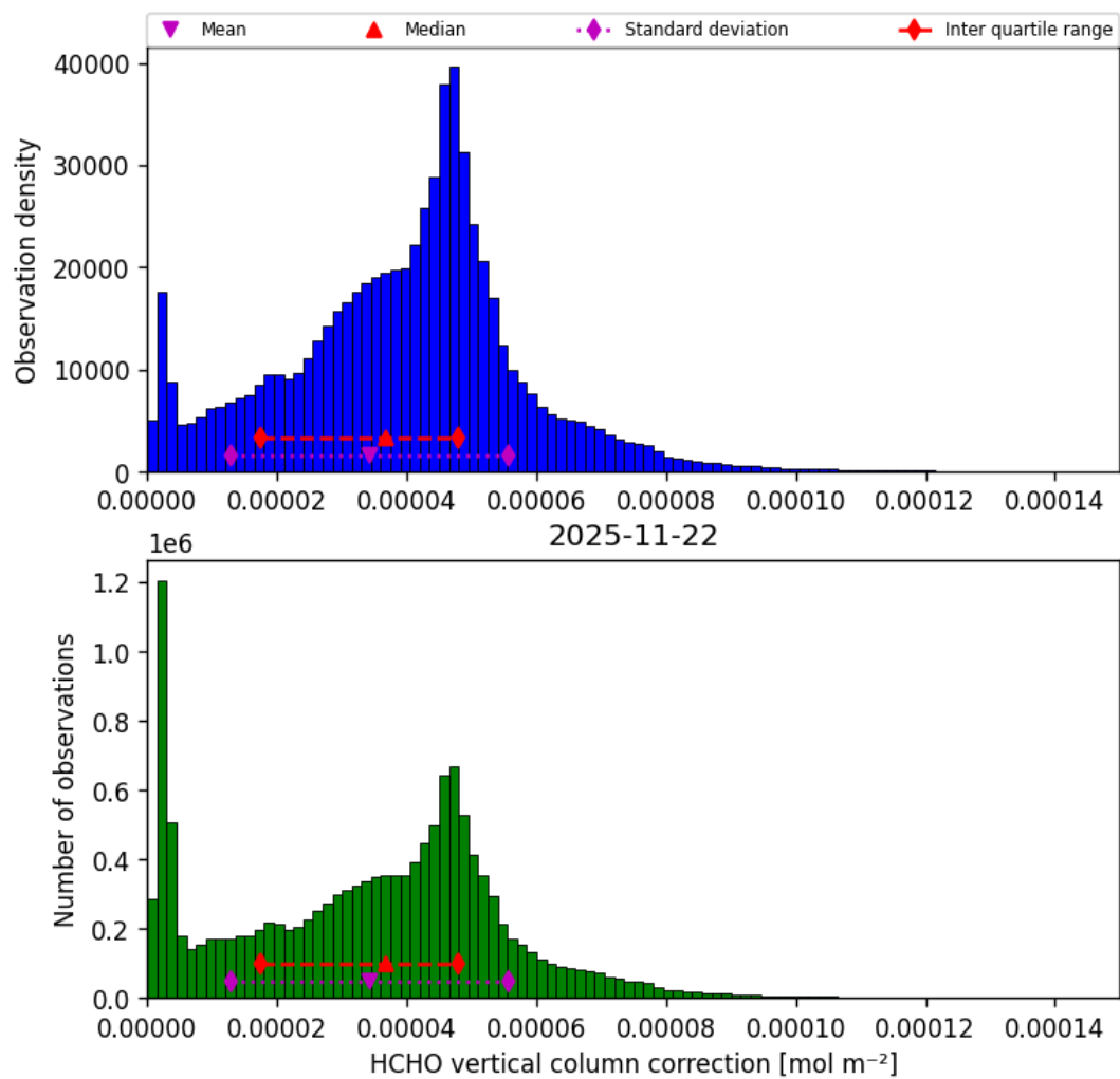
Figure 39: Histogram of “HCHO vertical column correction” for 2025-11-21 to 2025-11-23
