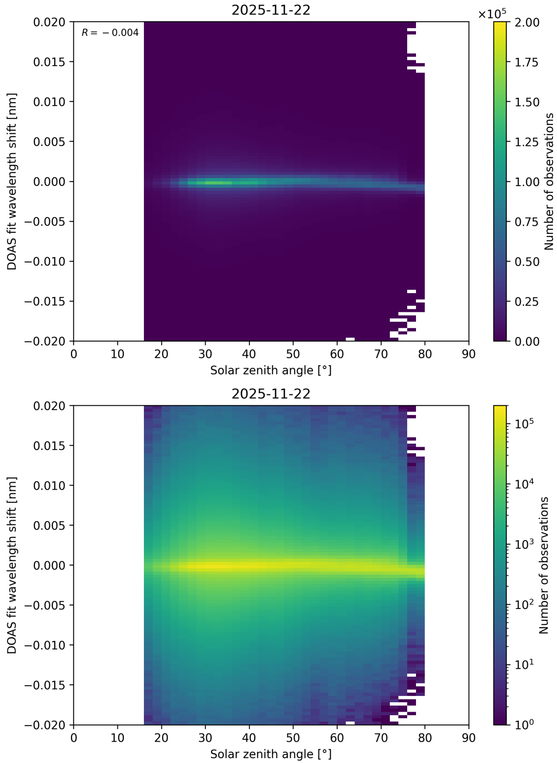
Figure 187: Scatter density plot of “Solar zenith angle” against “DOAS fit wavelength shift” for 2025-11-21 to 2025-11-23.
