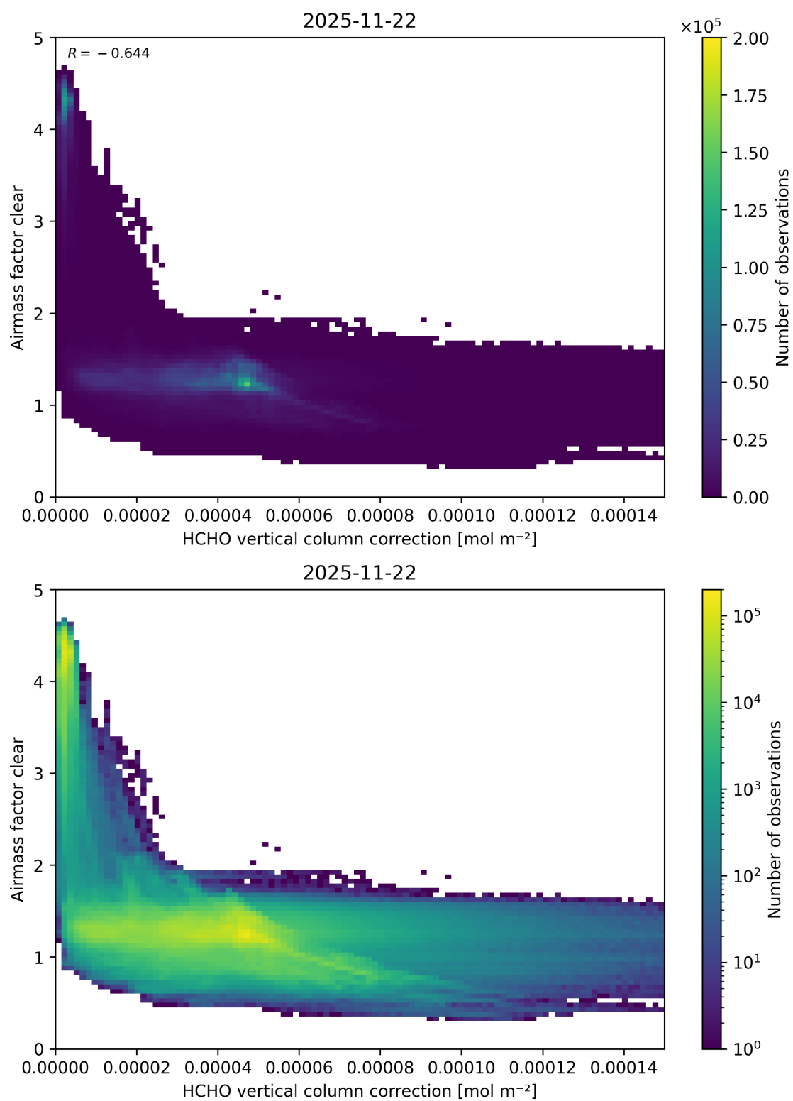
Figure 129: Scatter density plot of “HCHO vertical column correction” against “Airmass factor clear” for 2025-11-21 to 2025-11-23.
