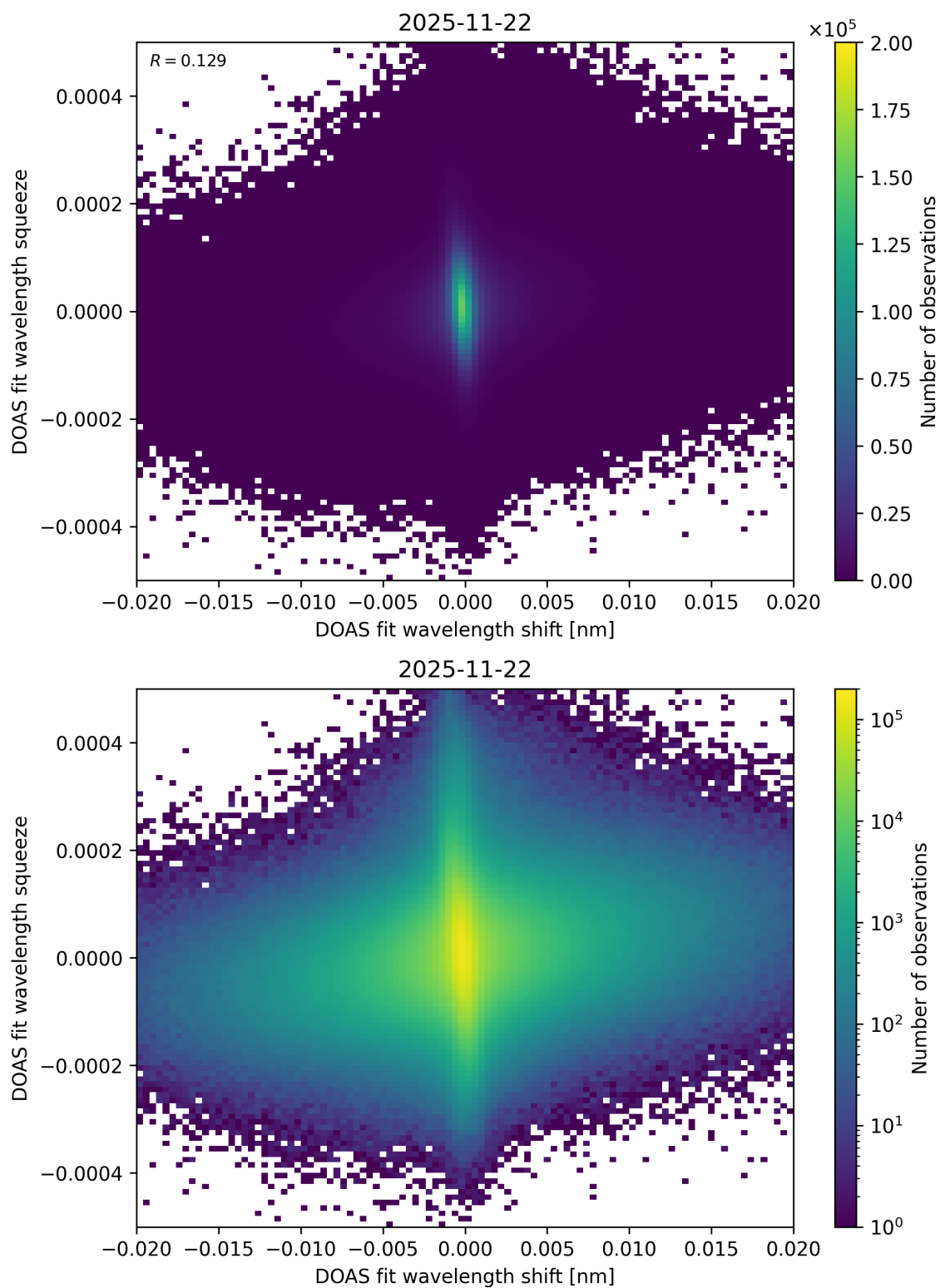
Figure 70: Scatter density plot of “DOAS fit wavelength shift” against “DOAS fit wavelength squeeze” for 2025-11-21 to 2025-11-23.
