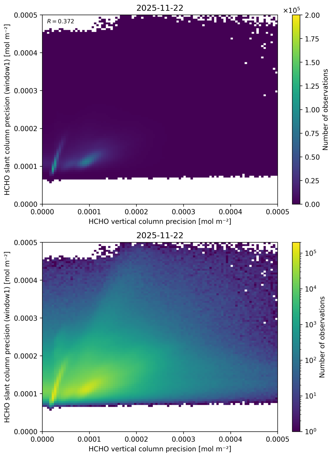
Figure 159: Scatter density plot of “HCHO vertical column precision” against “HCHO slant column precision (window1)” for 2025-11-21 to 2025-11-23.
