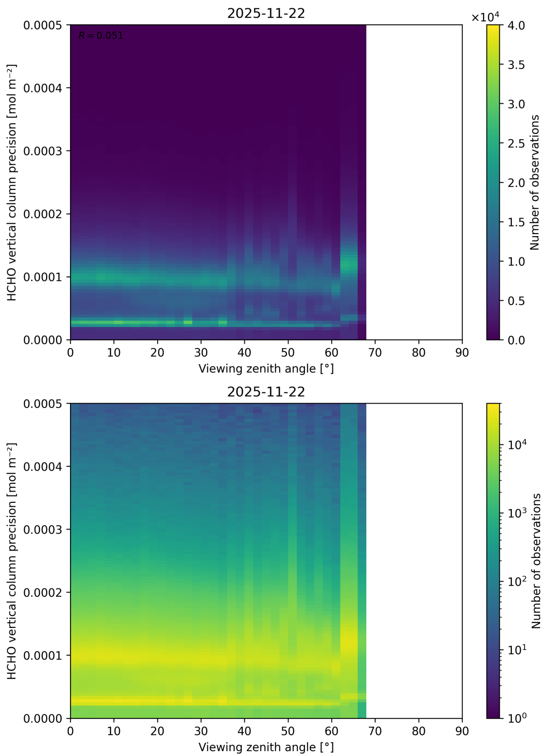
Figure 214: Scatter density plot of “Viewing zenith angle” against “HCHO vertical column precision” for 2025-11-21 to 2025-11-23.
