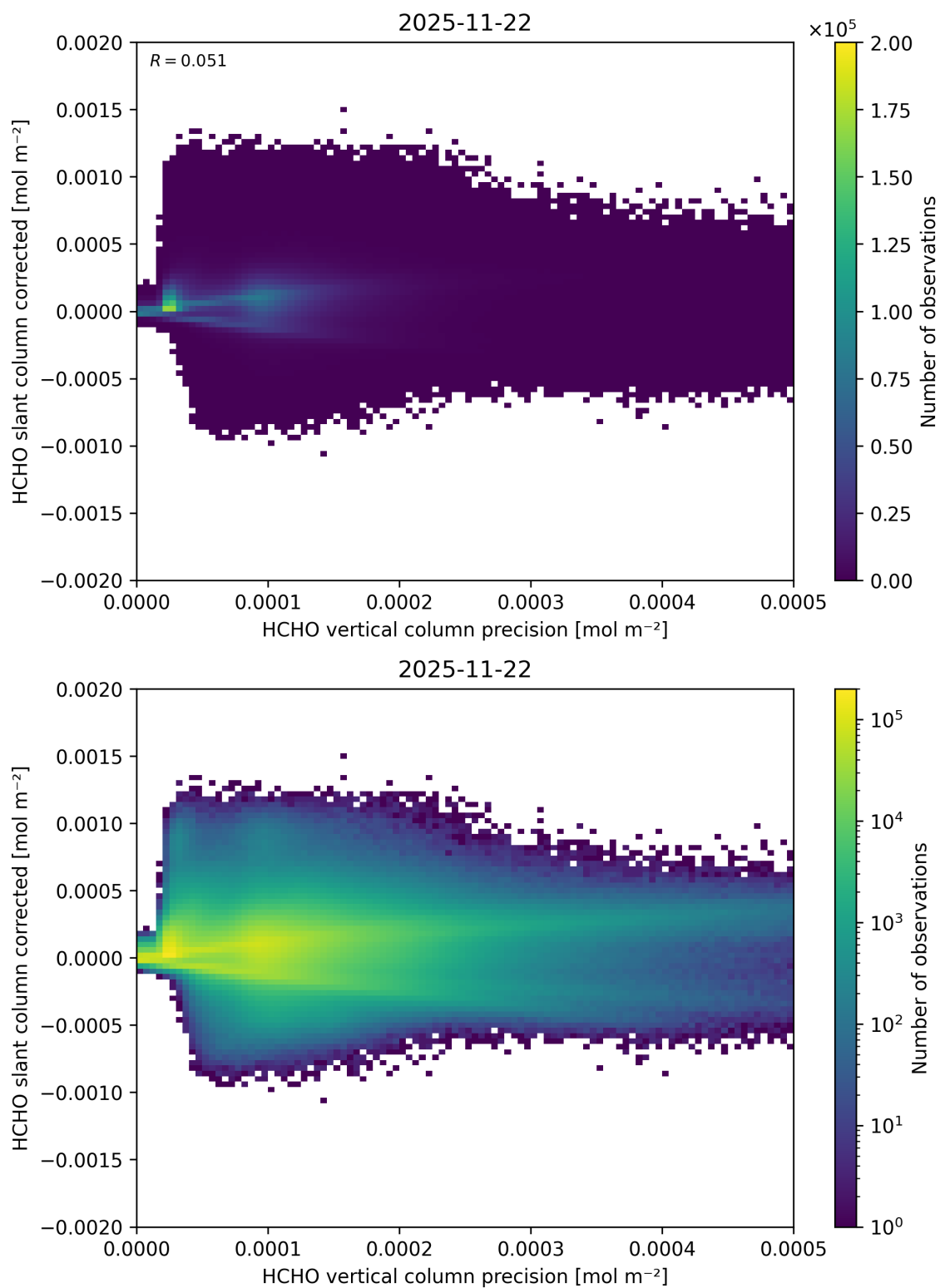
Figure 156: Scatter density plot of “HCHO vertical column precision” against “HCHO slant column corrected” for 2025-11-21 to 2025-11-23.
