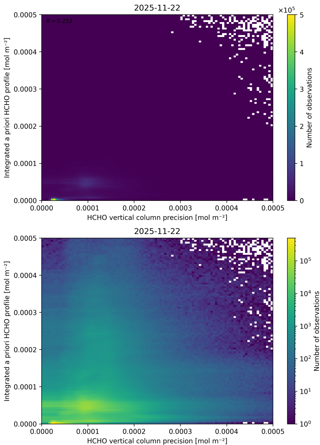
Figure 164: Scatter density plot of “HCHO vertical column precision” against “Integrated a priori HCHO profile” for 2025-11-21 to 2025-11-23.
