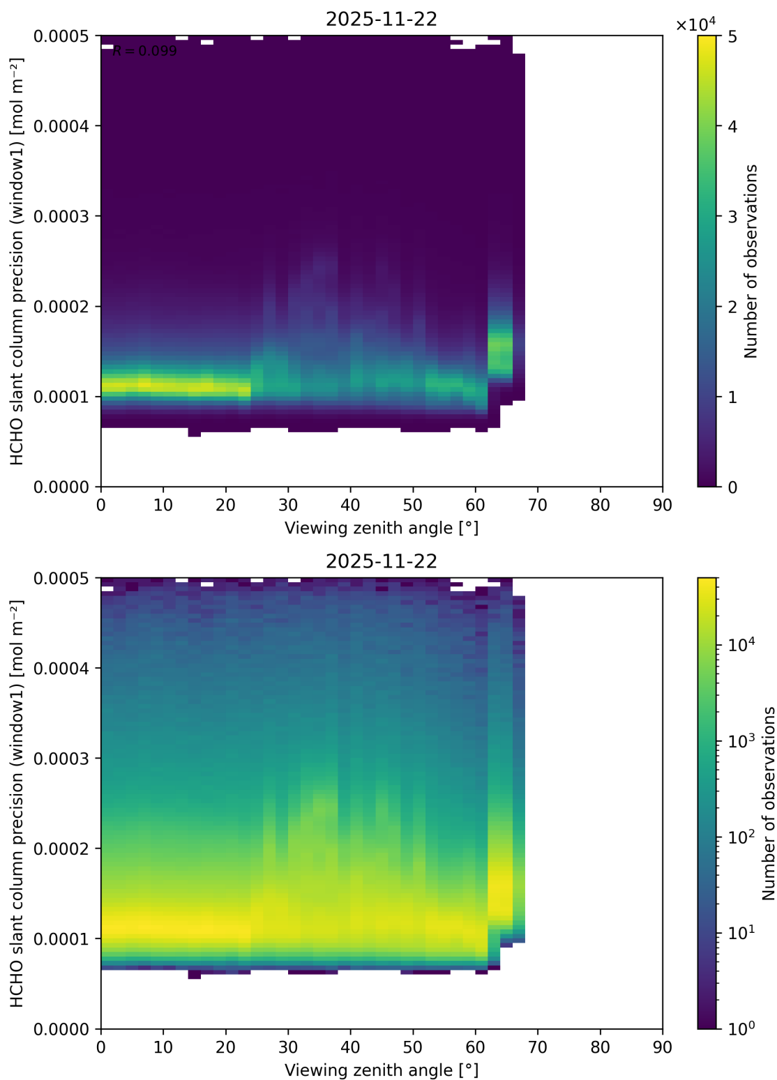
Figure 209: Scatter density plot of “Viewing zenith angle” against “HCHO slant column precision (window1)” for 2025-11-21 to 2025-11-23.
