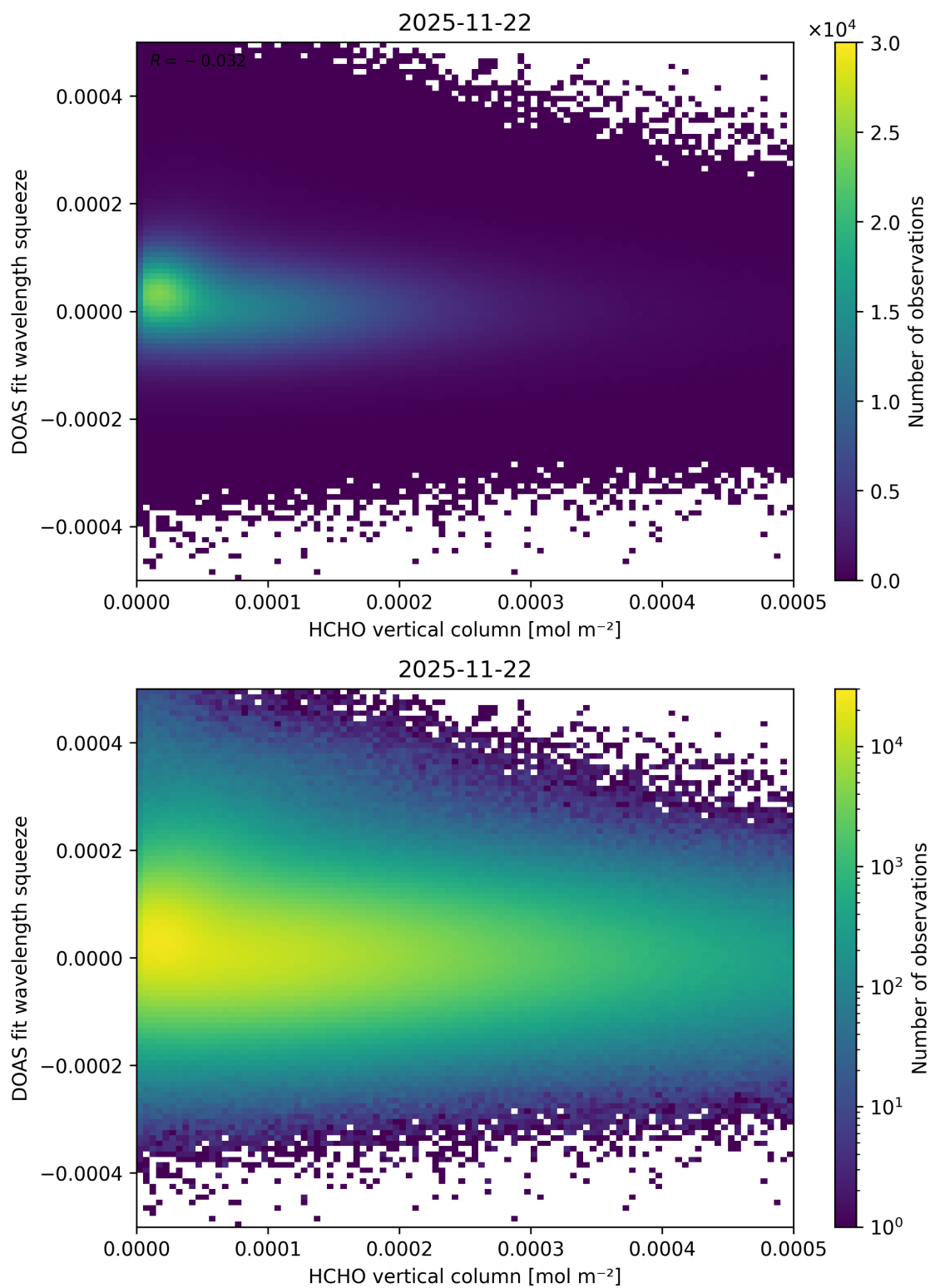
Figure 140: Scatter density plot of “HCHO vertical column” against “DOAS fit wavelength squeeze” for 2025-11-21 to 2025-11-23.
