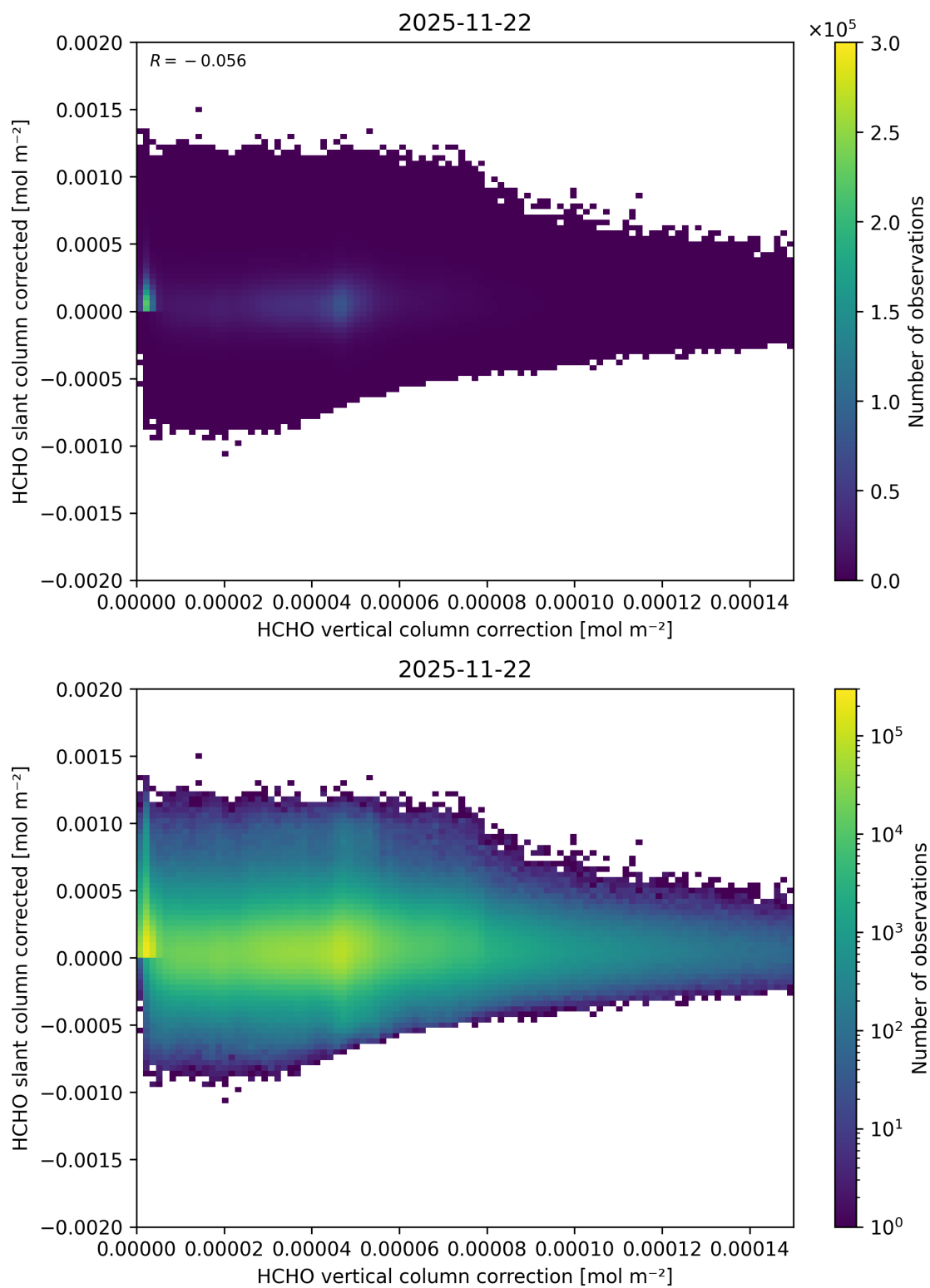
Figure 130: Scatter density plot of “HCHO vertical column correction” against “HCHO slant column corrected” for 2025-11-21 to 2025-11-23.
