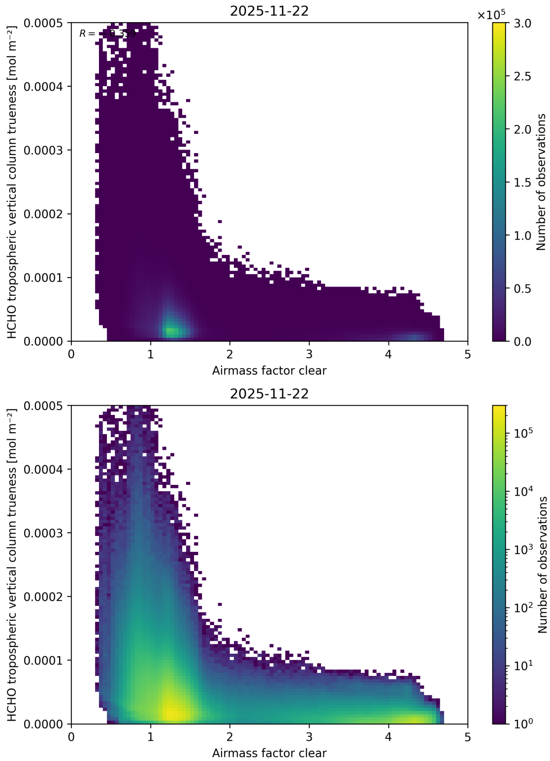
Figure 83: Scatter density plot of “Airmass factor clear” against “HCHO tropospheric vertical column truiness” for 2025-11-21 to 2025-11-23.
