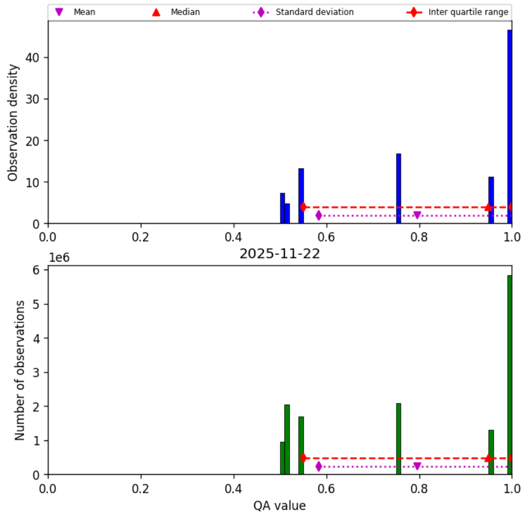
Figure 36: Histogram of “QA value” for 2025-11-21 to 2025-11-23
