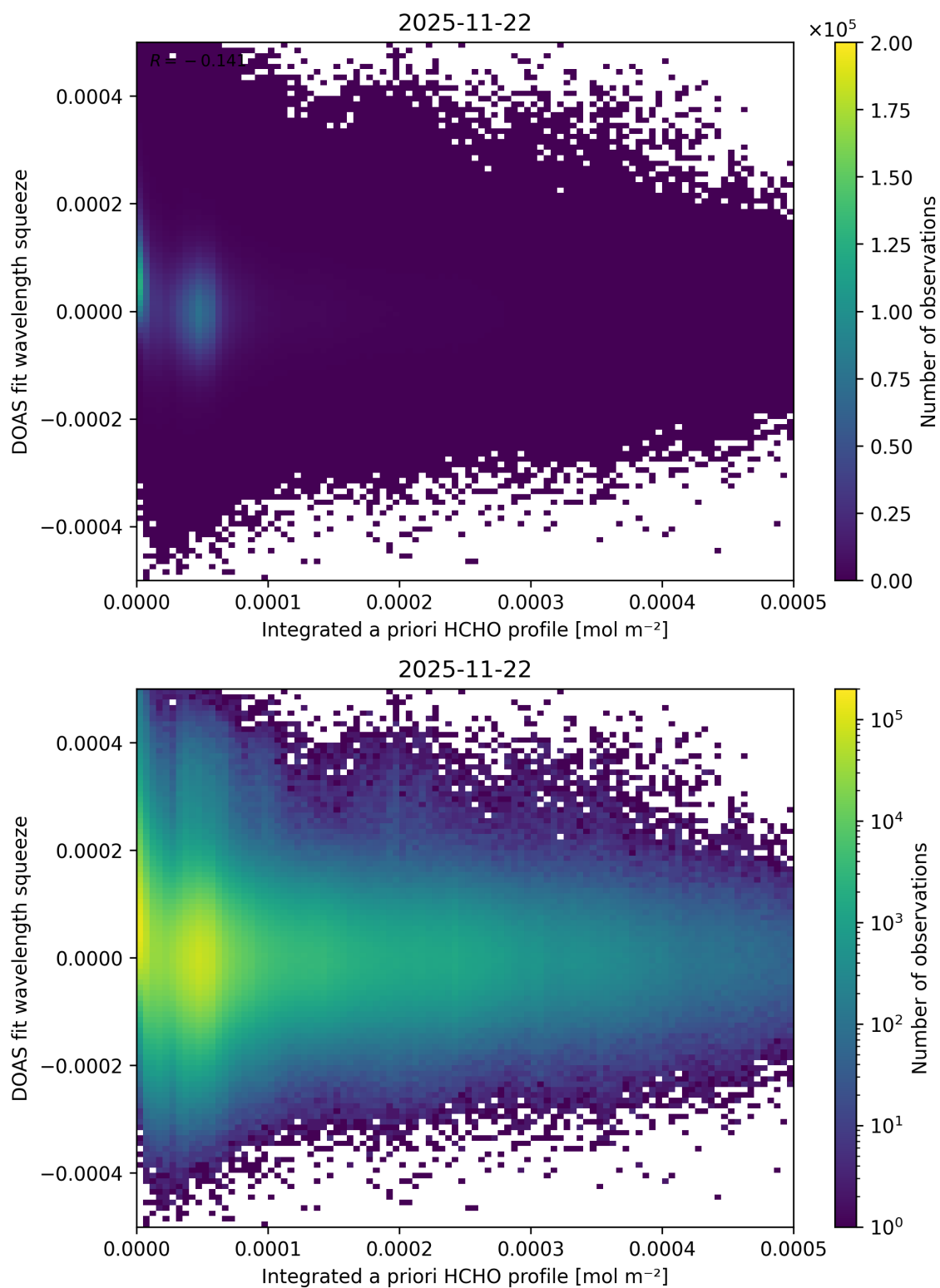
Figure 167: Scatter density plot of “Integrated a priori HCHO profile” against “DOAS fit wavelength squeeze” for 2025-11-21 to 2025-11-23.
