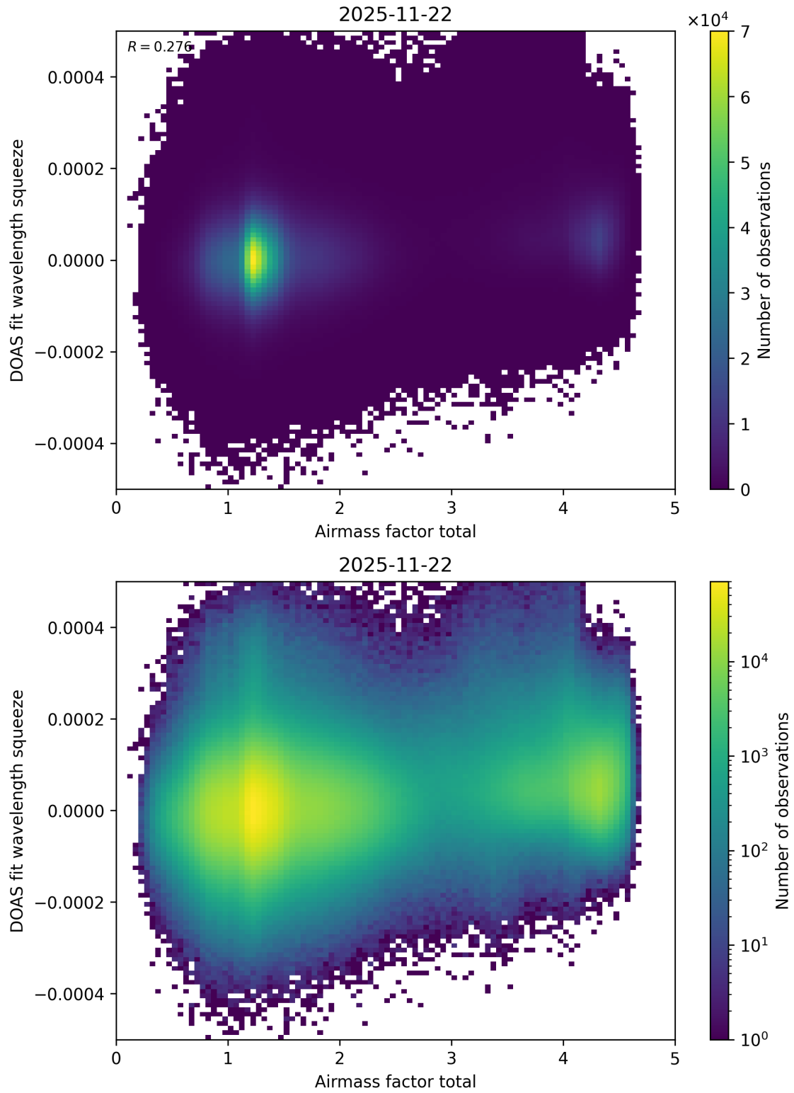
Figure 111: Scatter density plot of “Airmass factor total” against “DOAS fit wavelength squeeze” for 2025-11-21 to 2025-11-23.
