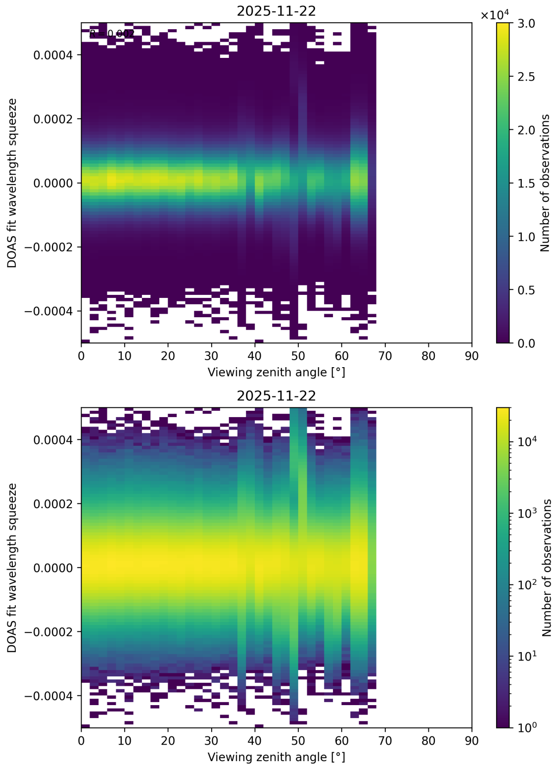
Figure 204: Scatter density plot of “Viewing zenith angle” against “DOAS fit wavelength squeeze” for 2025-11-21 to 2025-11-23.
