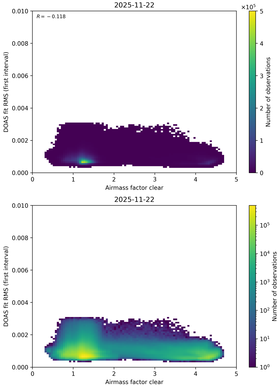
Figure 78: Scatter density plot of “Airmass factor clear” against “DOAS fit RMS (first interval)” for 2025-11-21 to 2025-11-23.
