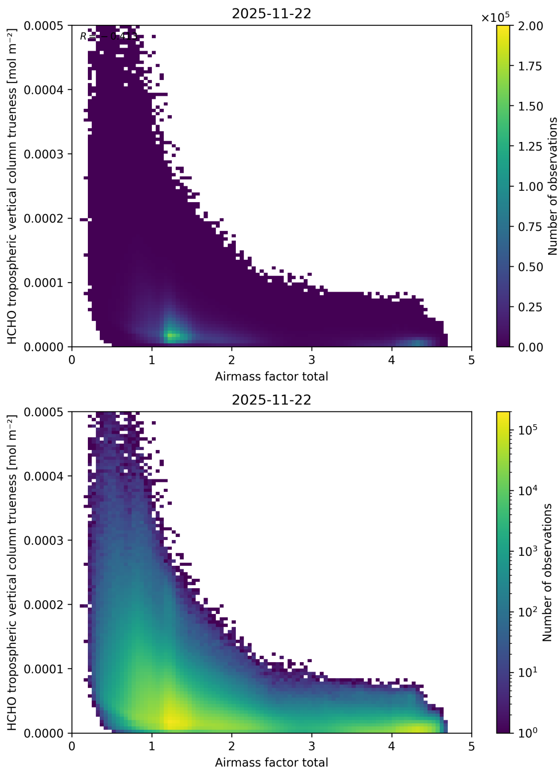
Figure 116: Scatter density plot of “Airmass factor total” against “HCHO tropospheric vertical column truiness” for 2025-11-21 to 2025-11-23.
