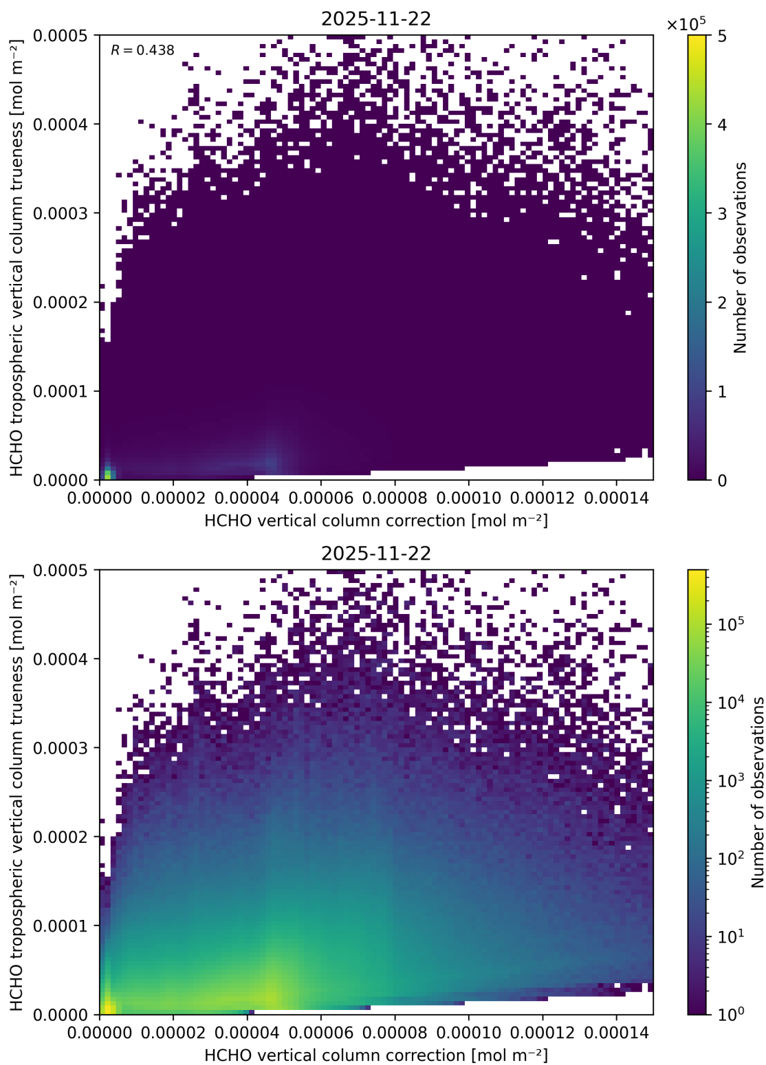
Figure 136: Scatter density plot of “HCHO vertical column correction” against “HCHO tropospheric vertical column true-ness” for 2025-11-21 to 2025-11-23.
