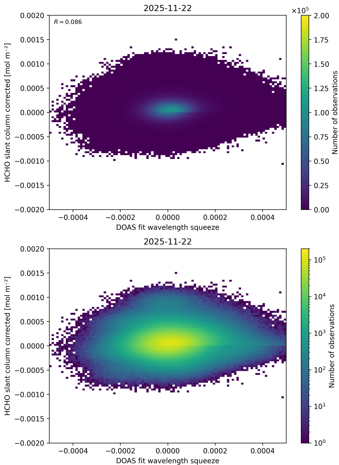
Figure 75: Scatter density plot of “DOAS fit wavelength squeeze” against “HCHO slant column corrected” for 2025-11-21 to 2025-11-23.
