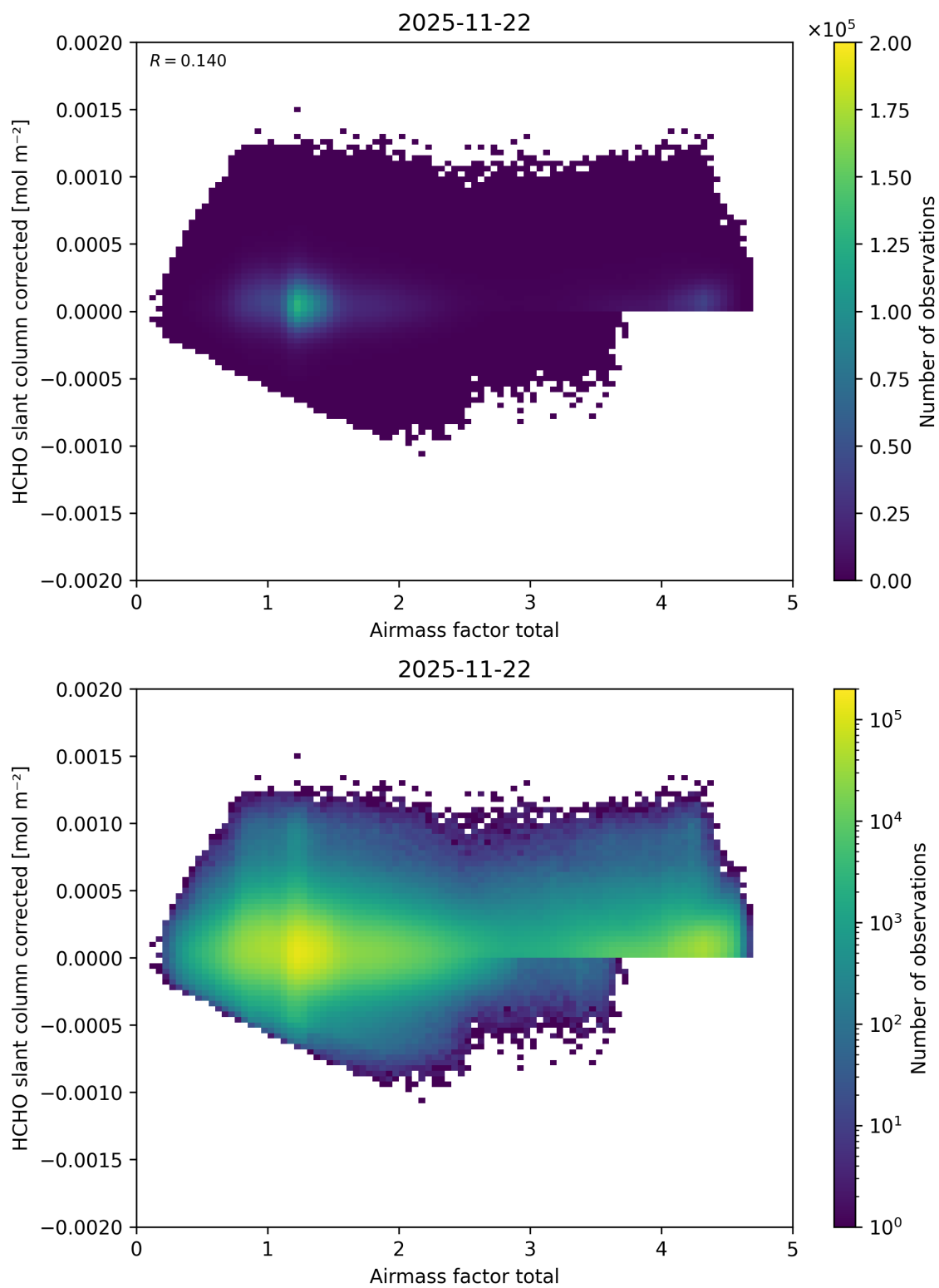
Figure 113: Scatter density plot of “Airmass factor total” against “HCHO slant column corrected” for 2025-11-21 to 2025-11-23.
