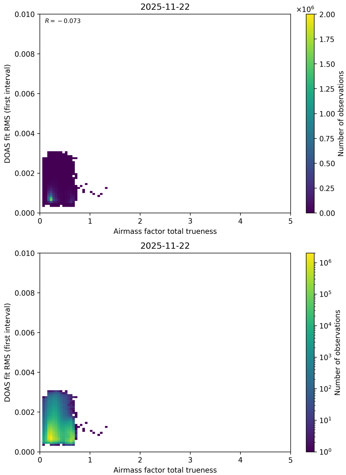
Figure 118: Scatter density plot of “Airmass factor total trueness” against “DOAS fit RMS (first interval)” for 2025-11-21 to 2025-11-23.
