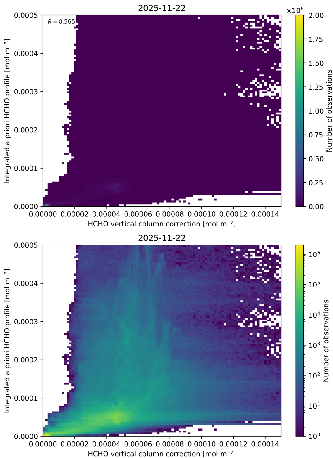
Figure 137: Scatter density plot of “HCHO vertical column correction” against “Integrated a priori HCHO profile” for 2025-11-21 to 2025-11-23.
