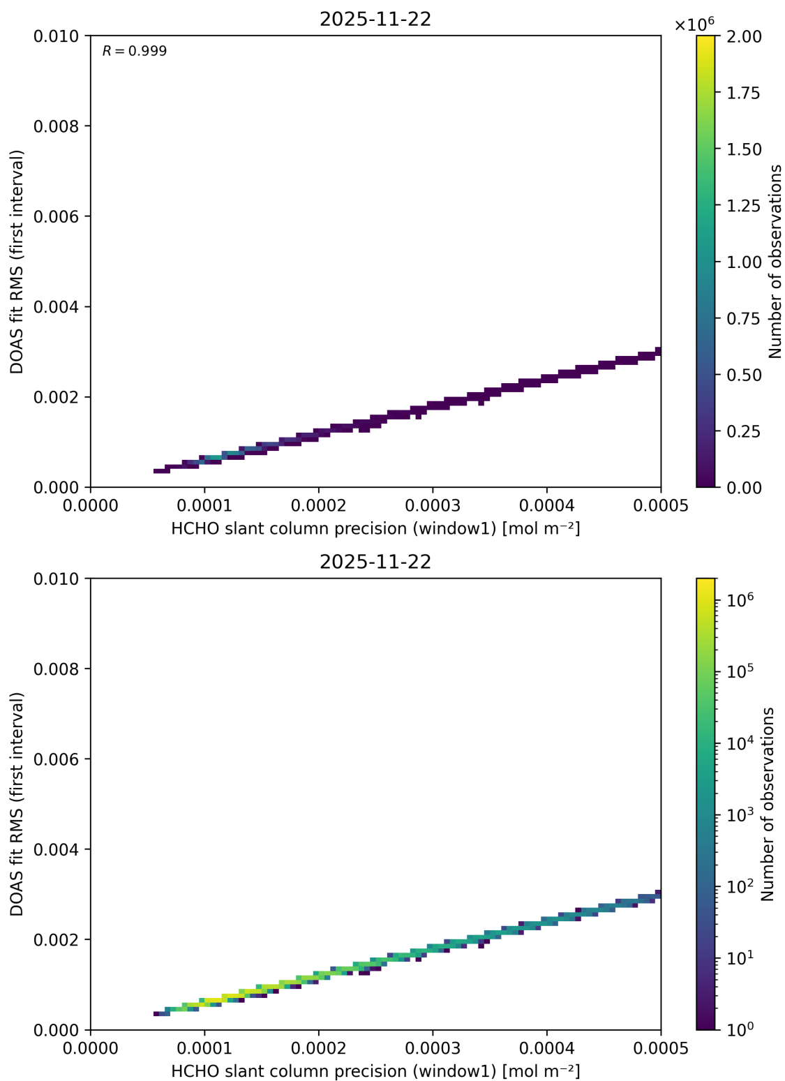
Figure 99: Scatter density plot of “HCHO slant column precision (window1)” against “DOAS fit RMS (first interval)” for 2025-11-21 to 2025-11-23.
