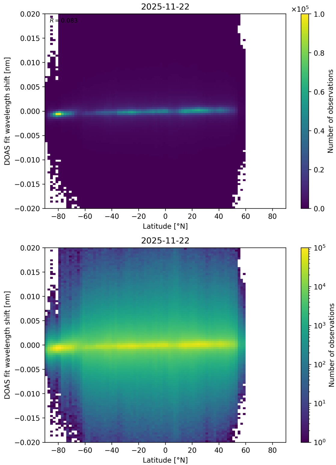
Figure 172: Scatter density plot of “Latitude” against “DOAS fit wavelength shift” for 2025-11-21 to 2025-11-23.
