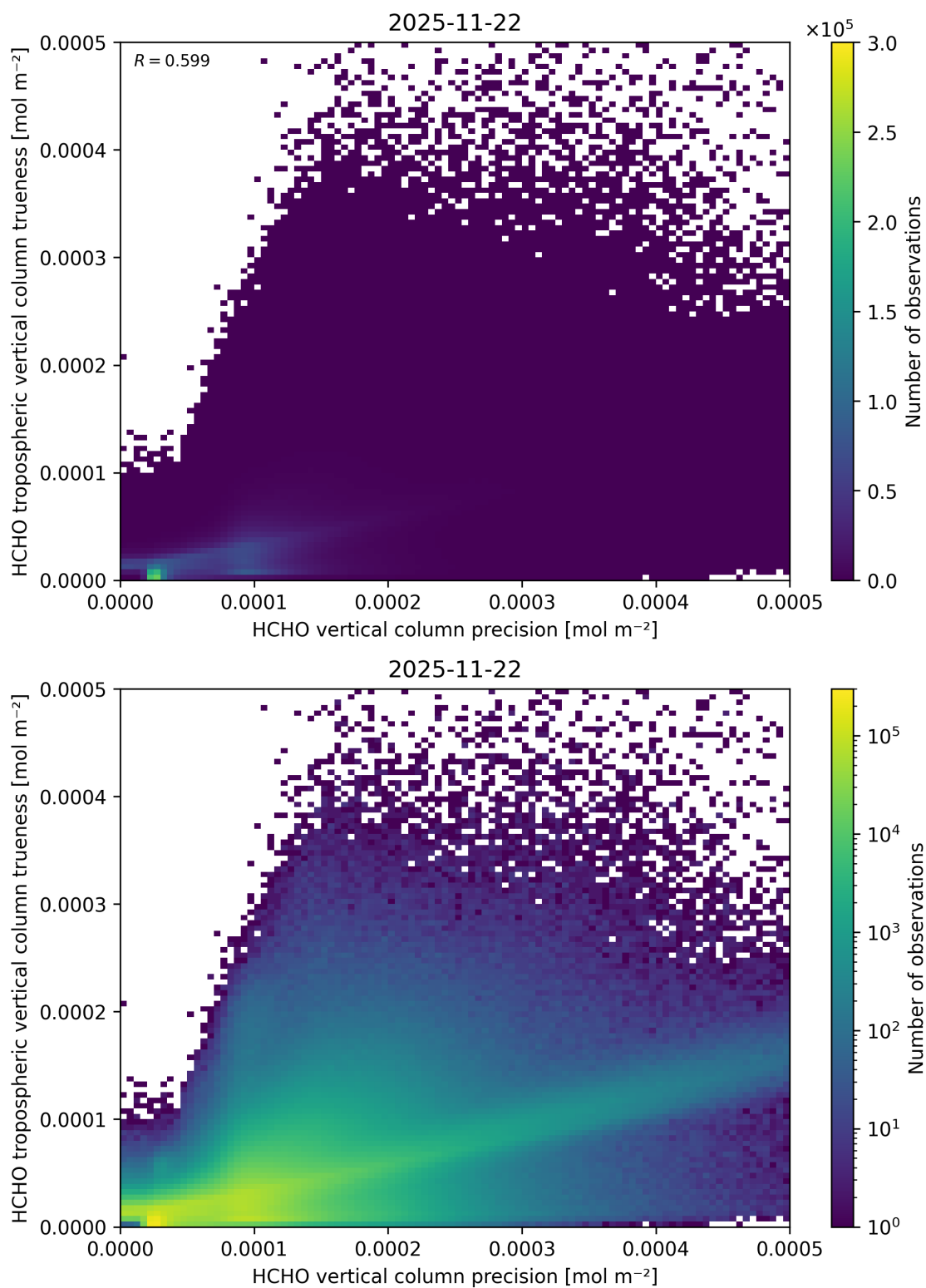
Figure 163: Scatter density plot of “HCHO vertical column precision” against “HCHO tropospheric vertical column true-ness” for 2025-11-21 to 2025-11-23.
