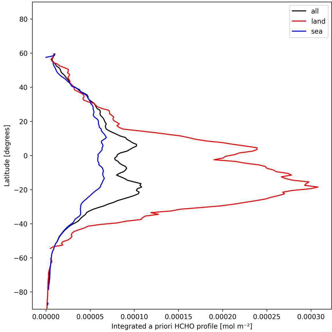
Figure 30: Zonal average of “Integrated a priori HCHO profile” for 2025-11-21 to 2025-11-23.
