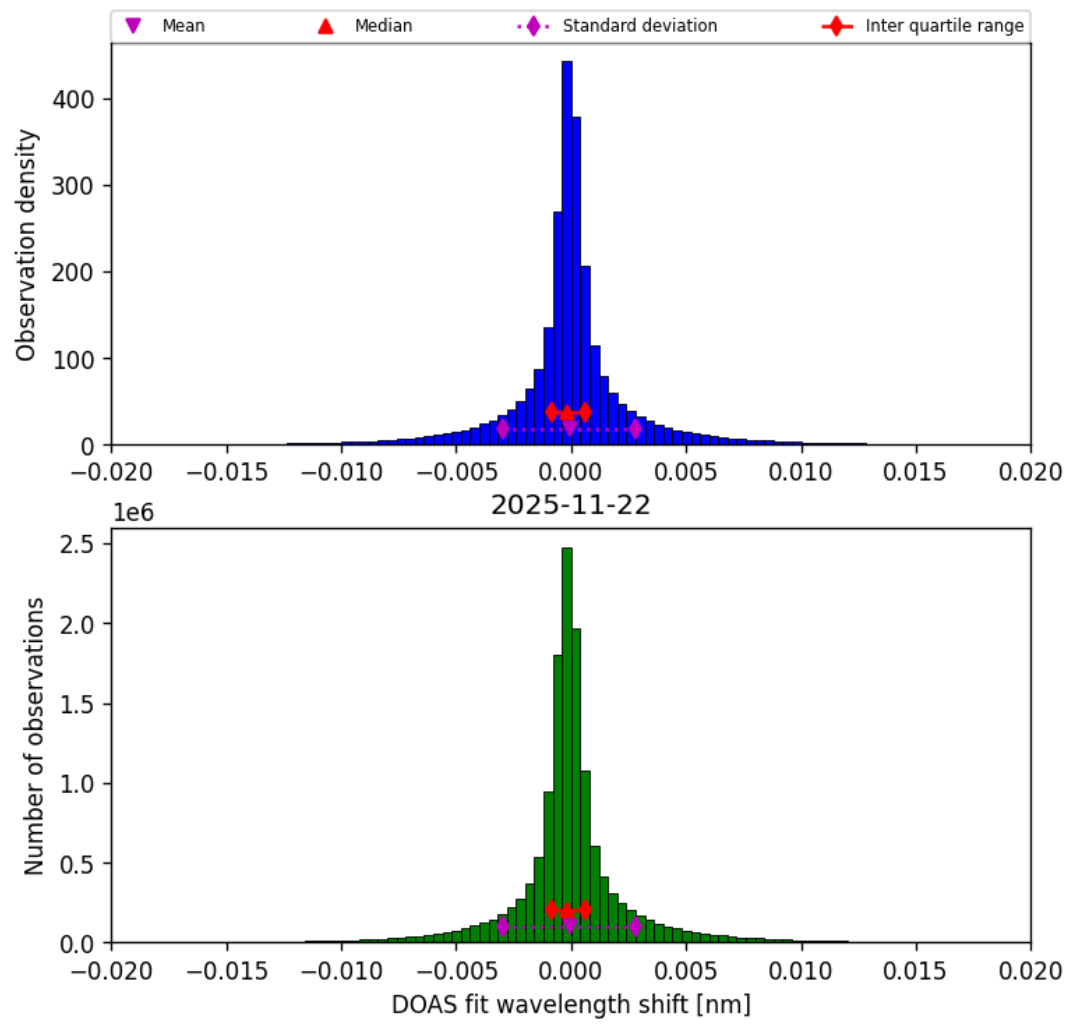
Figure 46: Histogram of “DOAS fit wavelength shift” for 2025-11-21 to 2025-11-23
