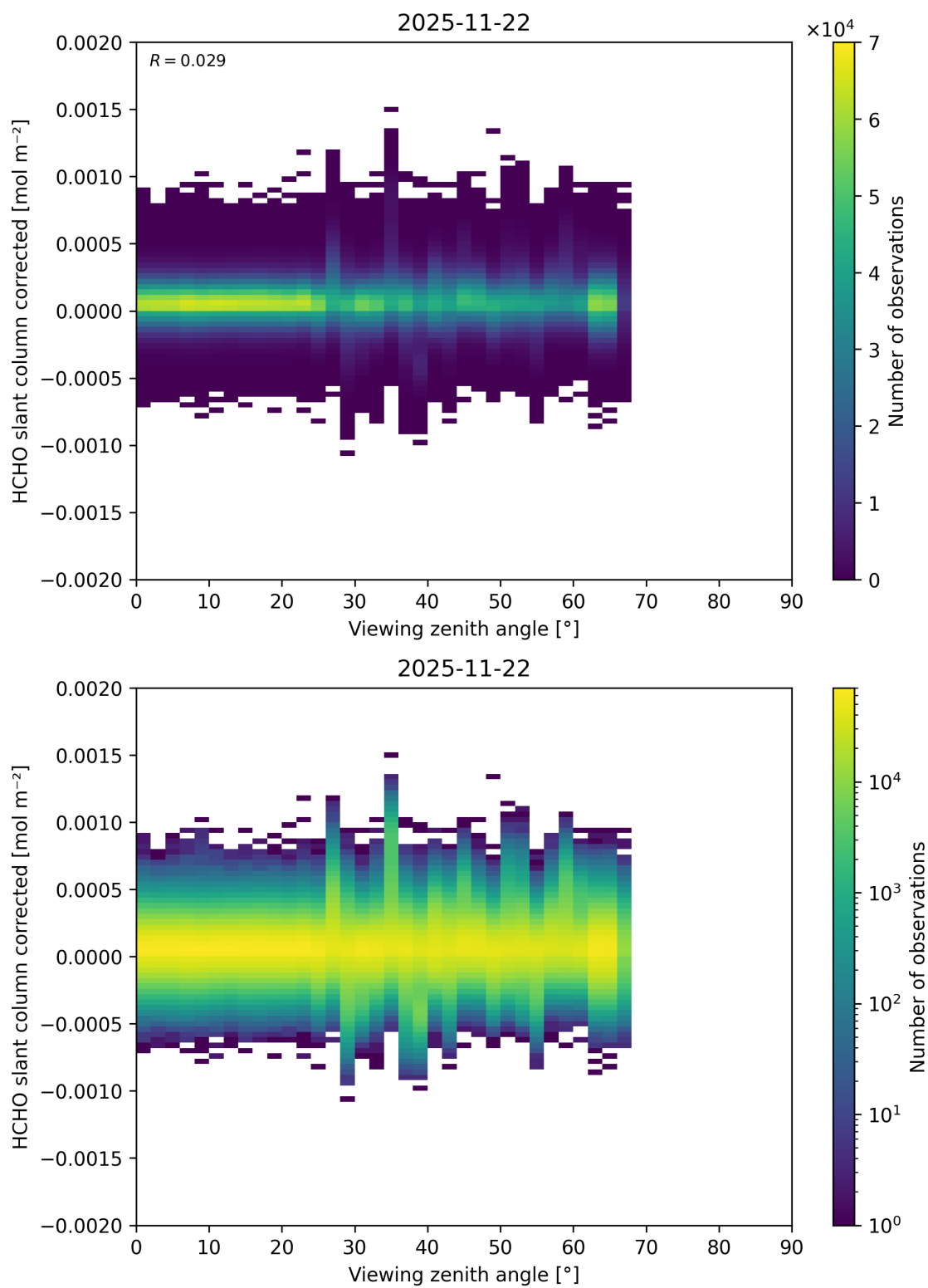
Figure 206: Scatter density plot of “Viewing zenith angle” against “HCHO slant column corrected” for 2025-11-21 to 2025-11-23.
