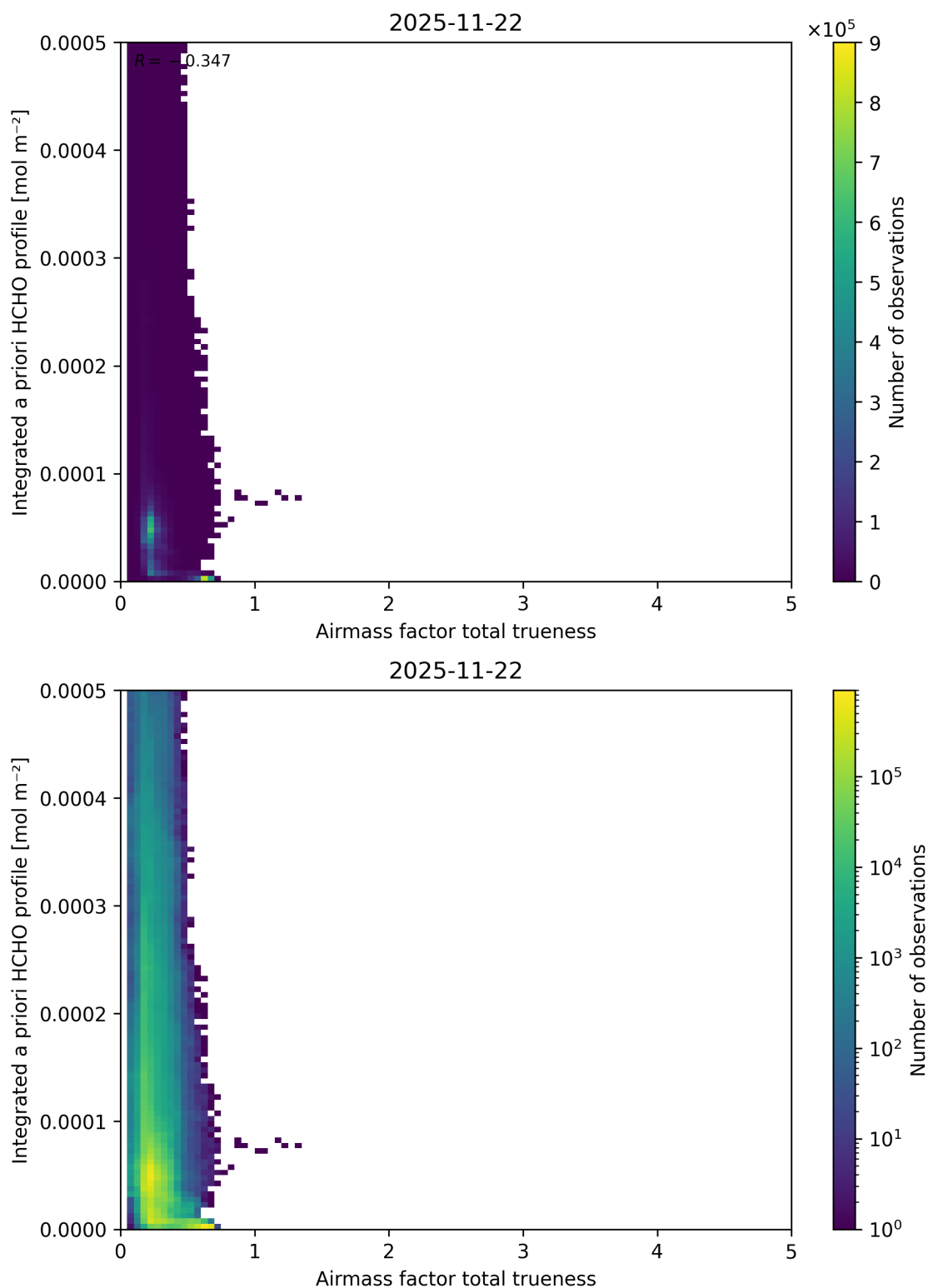
Figure 125: Scatter density plot of “Airmass factor total truiness” against “Integrated a priori HCHO profile” for 2025-11-21 to 2025-11-23.
