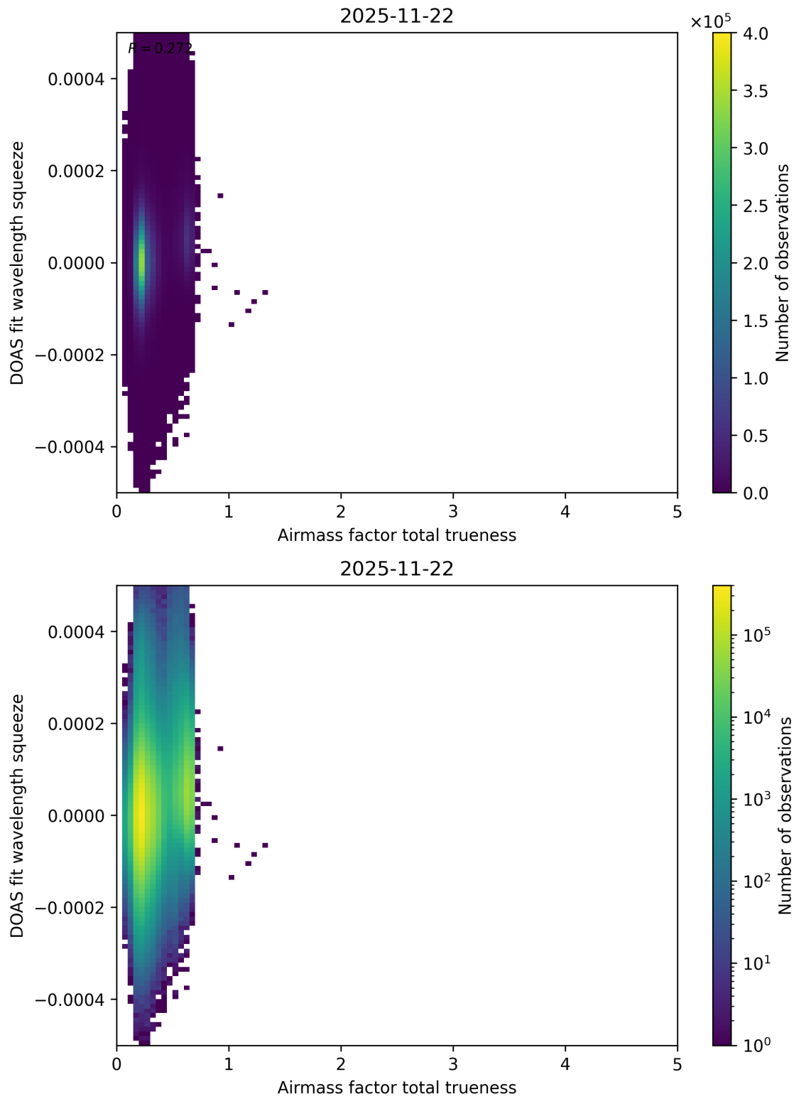
Figure 120: Scatter density plot of “Airmass factor total trueness” against “DOAS fit wavelength squeeze” for 2025-11-21 to 2025-11-23.
