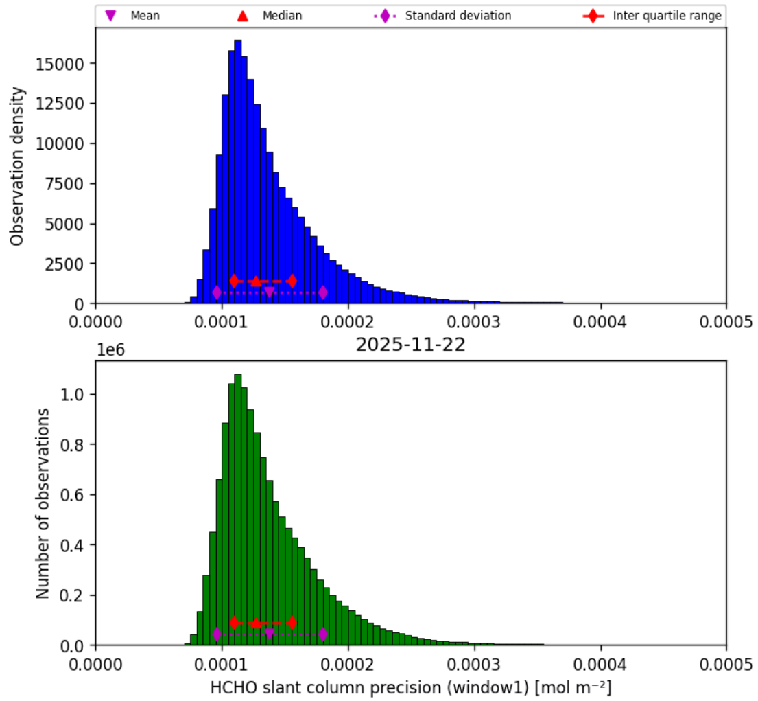
Figure 41: Histogram of “HCHO slant column precision (window1)” for 2025-11-21 to 2025-11-23
