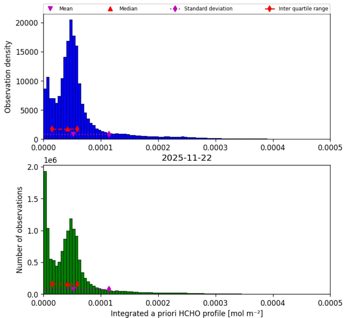
Figure 45: Histogram of “Integrated a priori HCHO profile” for 2025-11-21 to 2025-11-23
