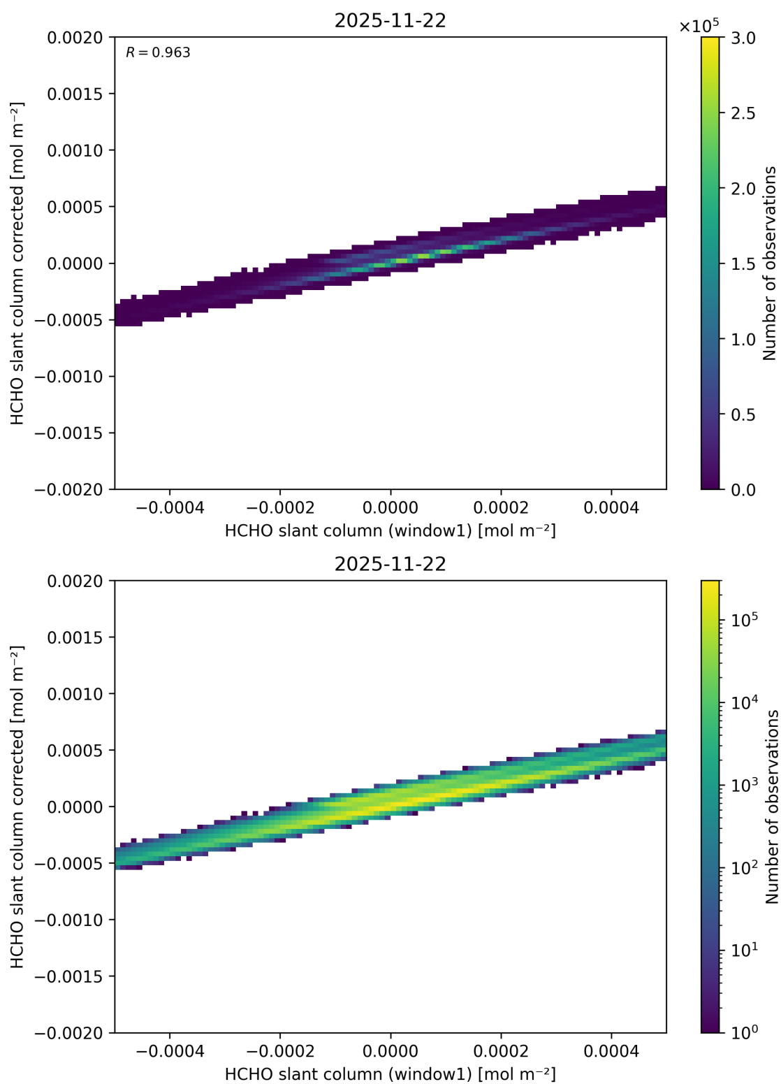
Figure 92: Scatter density plot of “HCHO slant column (window1)” against “HCHO slant column corrected” for 2025-11-21 to 2025-11-23.
