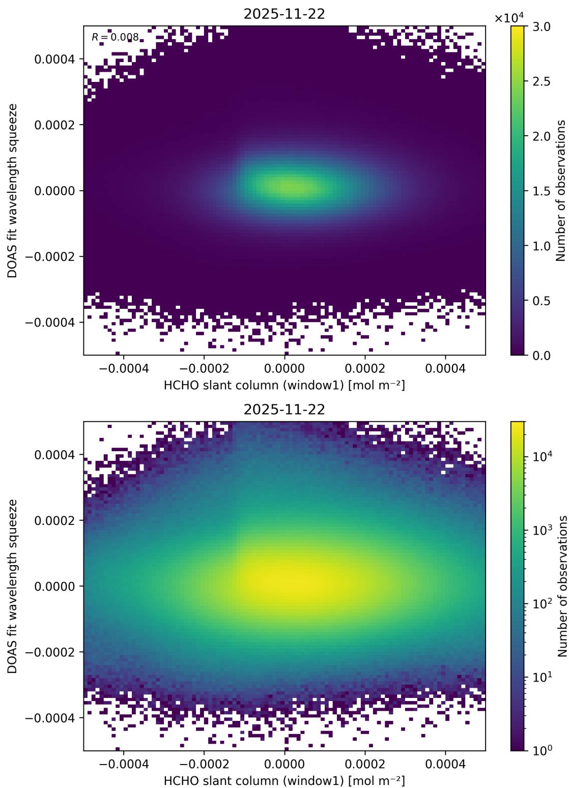
Figure 90: Scatter density plot of “HCHO slant column (window1)” against “DOAS fit wavelength squeeze” for 2025-11-21 to 2025-11-23.
