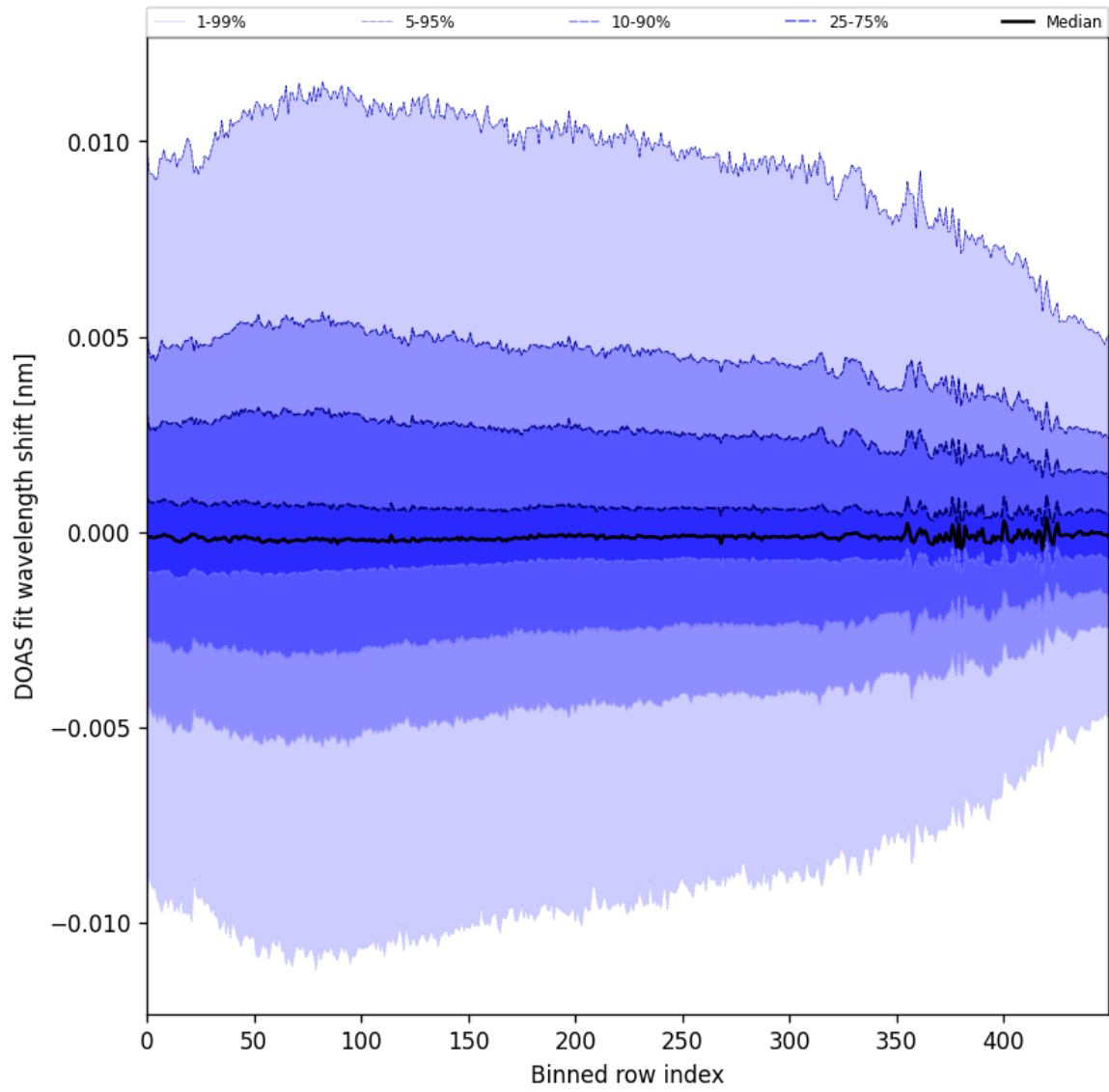
Figure 61: Along track statistics of “DOAS fit wavelength shift” for 2025-11-21 to 2025-11-23
