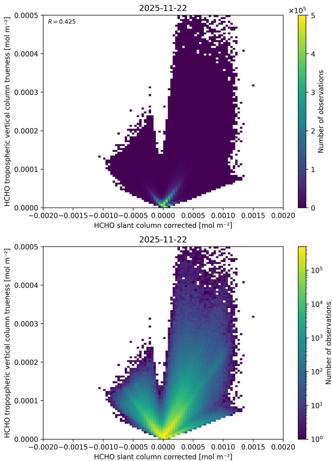
Figure 86: Scatter density plot of “HCHO slant column corrected” against “HCHO tropospheric vertical column trueness” for 2025-11-21 to 2025-11-23.
