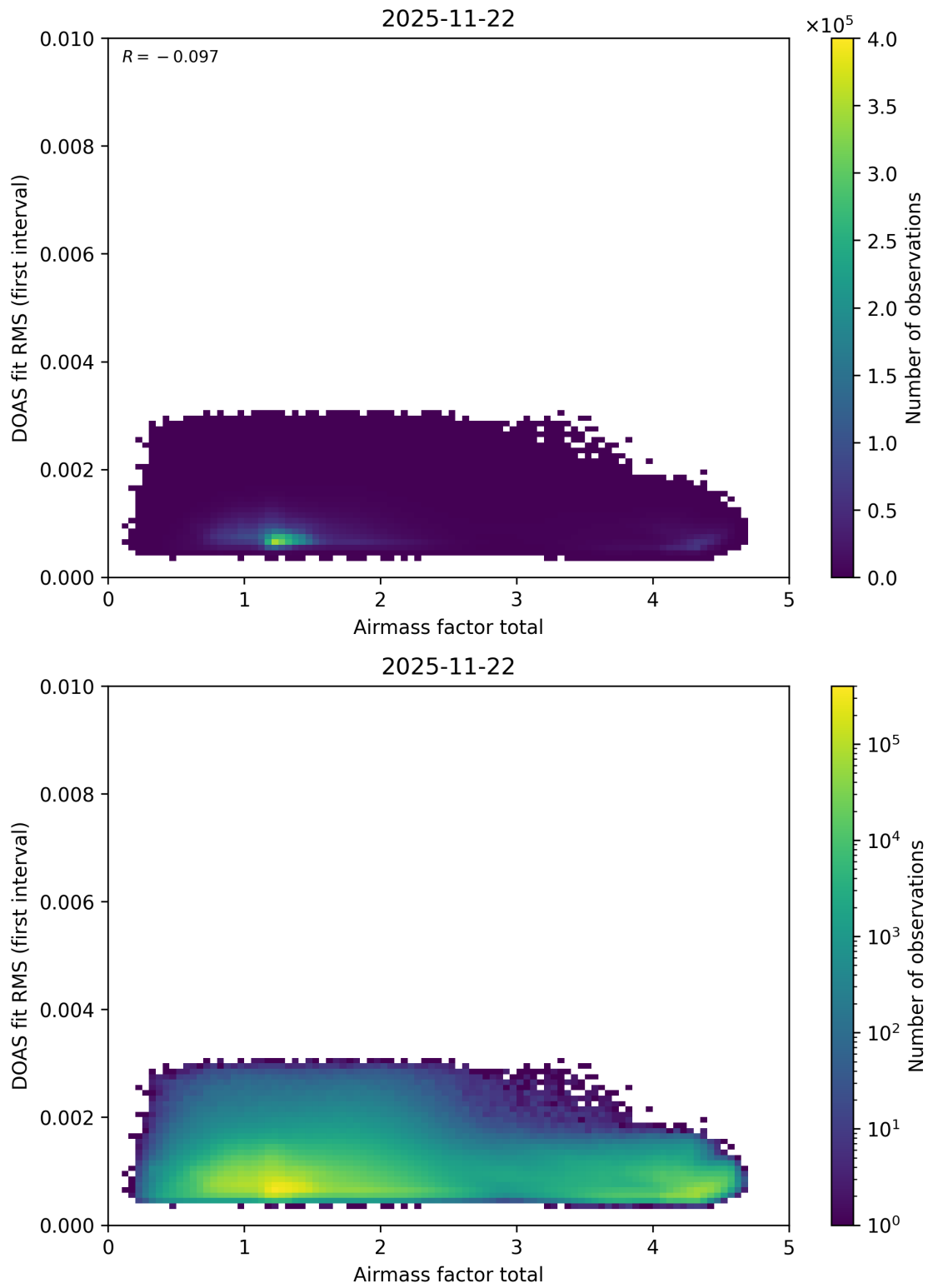
Figure 109: Scatter density plot of “Airmass factor total” against “DOAS fit RMS (first interval)” for 2025-11-21 to 2025-11-23.
