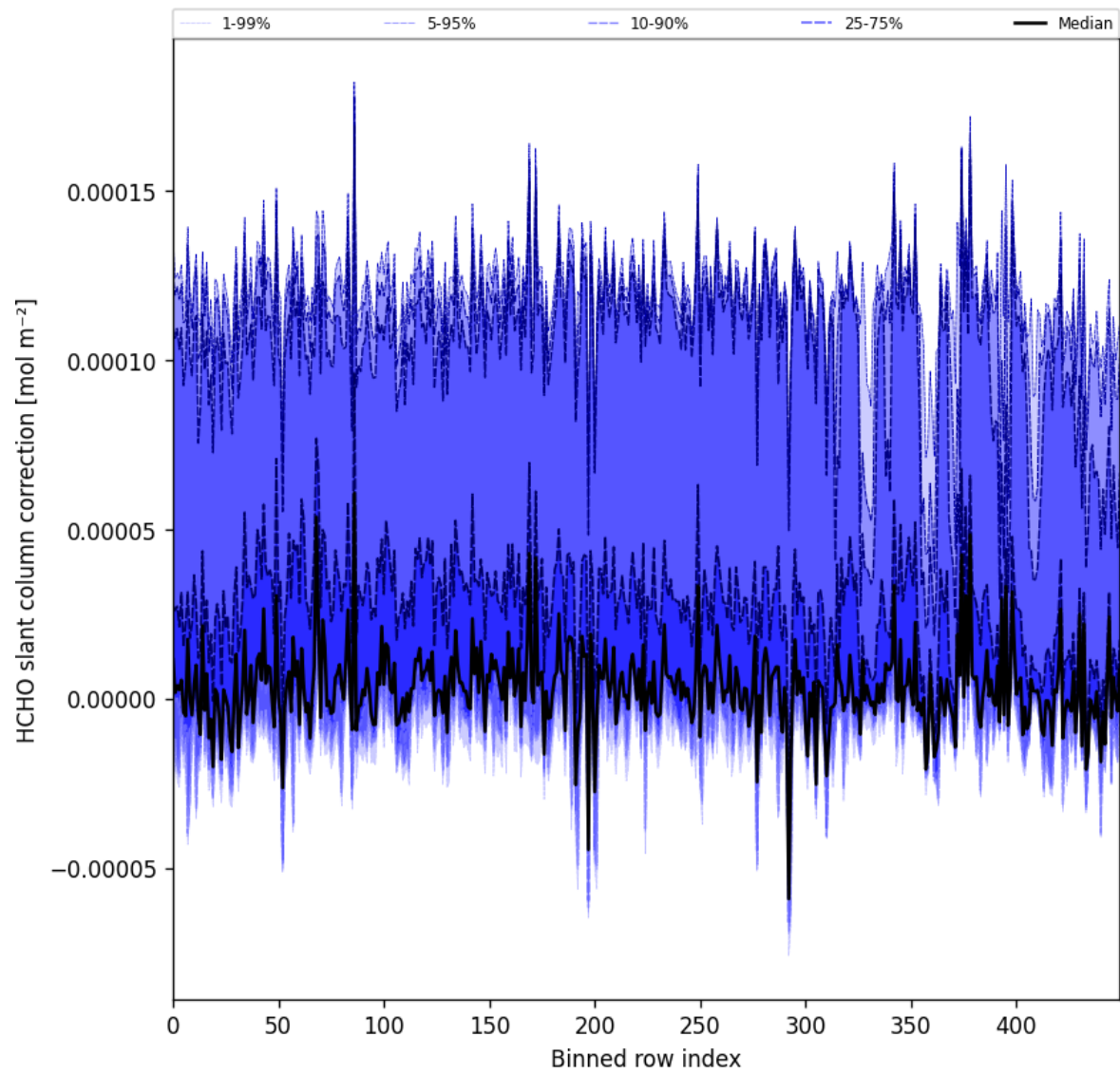
Figure 64: Along track statistics of “HCHO slant column correction” for 2025-11-21 to 2025-11-23
