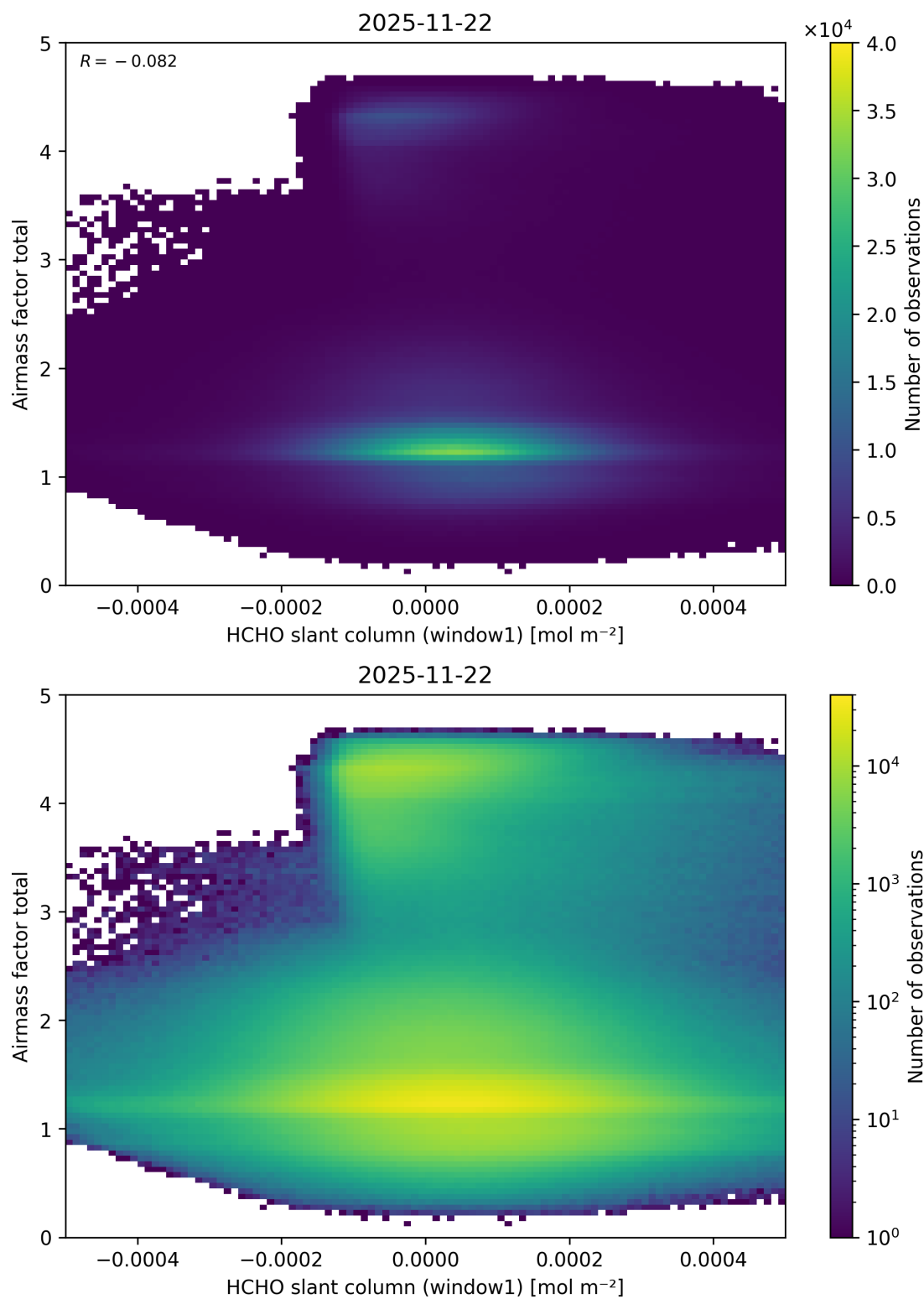
Figure 95: Scatter density plot of “HCHO slant column (window1)” against “Airmass factor total” for 2025-11-21 to 2025-11-23.
