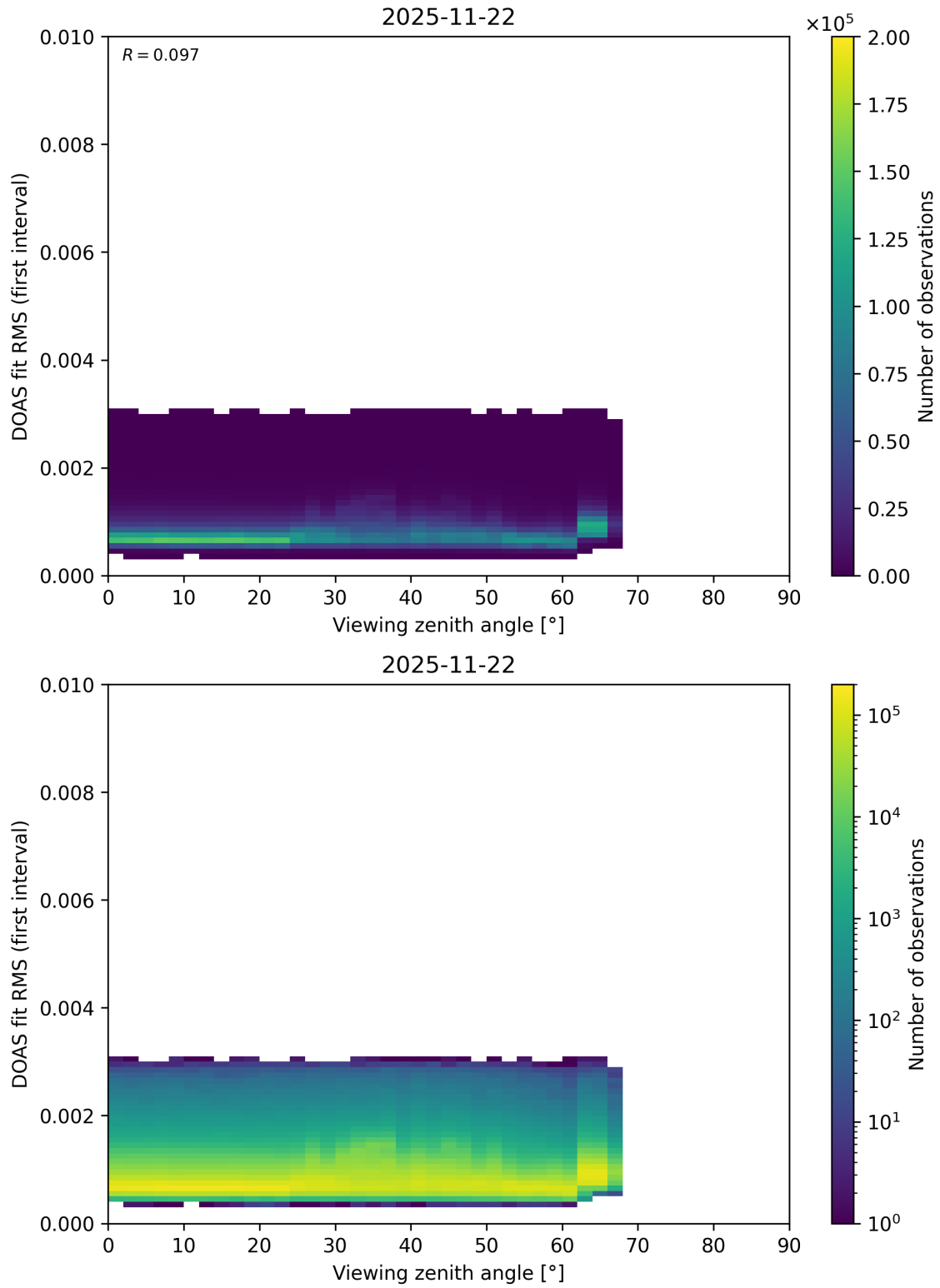
Figure 202: Scatter density plot of “Viewing zenith angle” against “DOAS fit RMS (first interval)” for 2025-11-21 to 2025-11-23.
