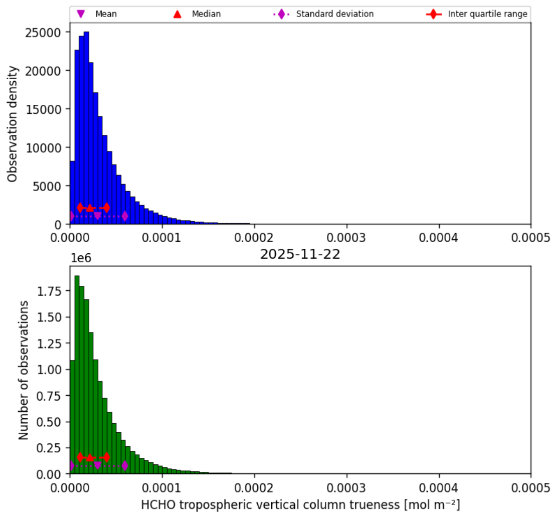
Figure 50: Histogram of “HCHO tropospheric vertical column trueness” for 2025-11-21 to 2025-11-23
