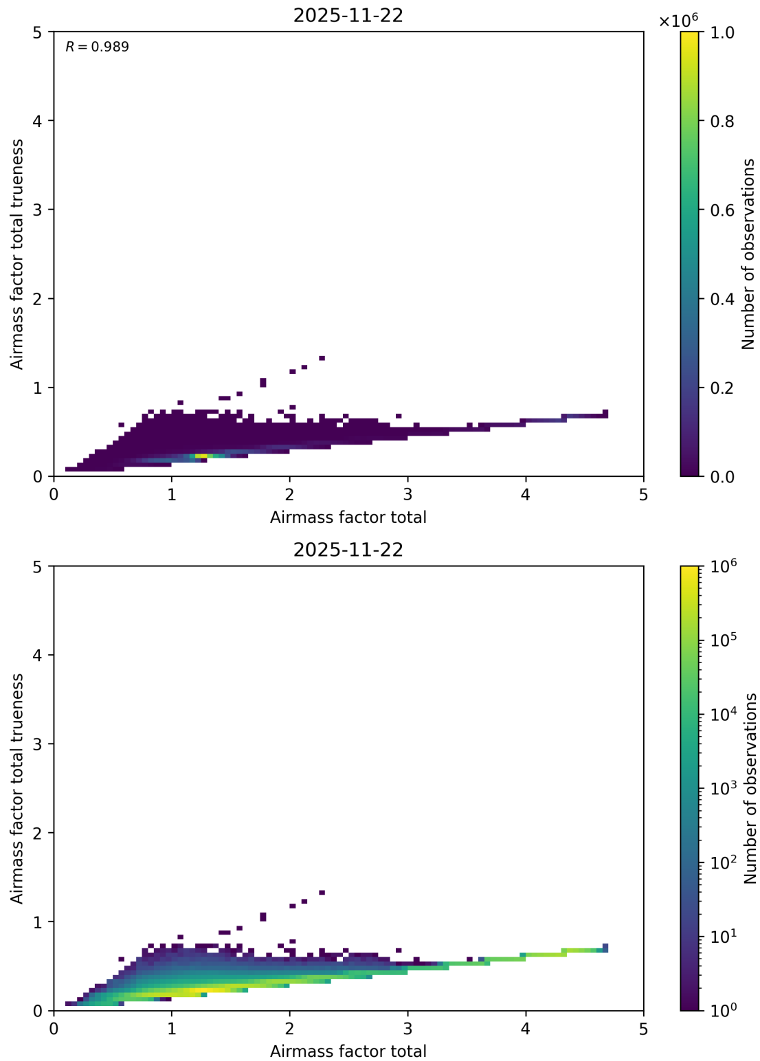
Figure 115: Scatter density plot of “Airmass factor total” against “Airmass factor total trueness” for 2025-11-21 to 2025-11-23.
