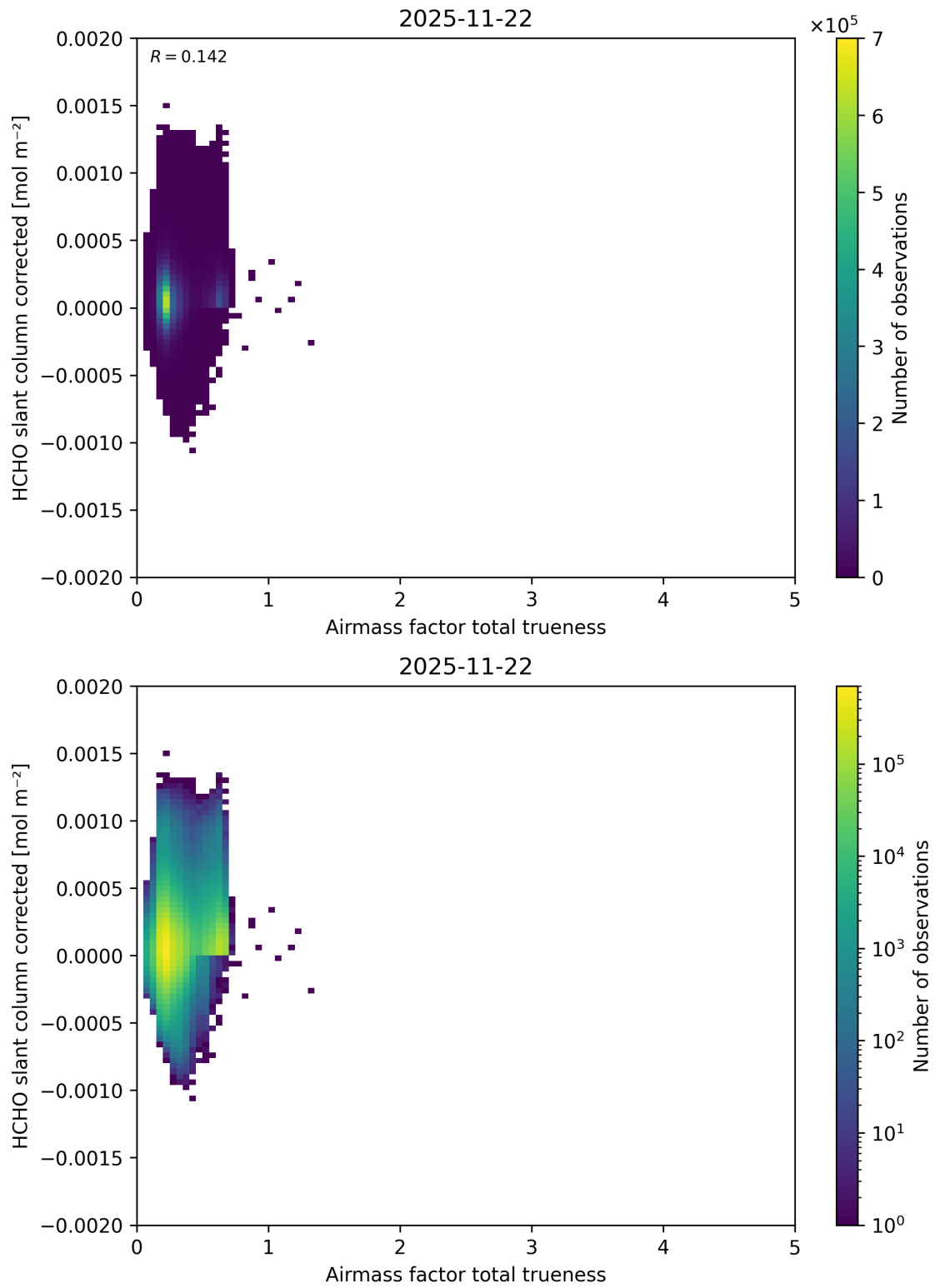
Figure 122: Scatter density plot of “Airmass factor total trueness” against “HCHO slant column corrected” for 2025-11-21 to 2025-11-23.
