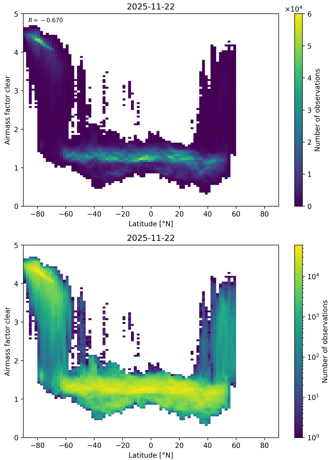
Figure 174: Scatter density plot of “Latitude” against “Airmass factor clear” for 2025-11-21 to 2025-11-23.
