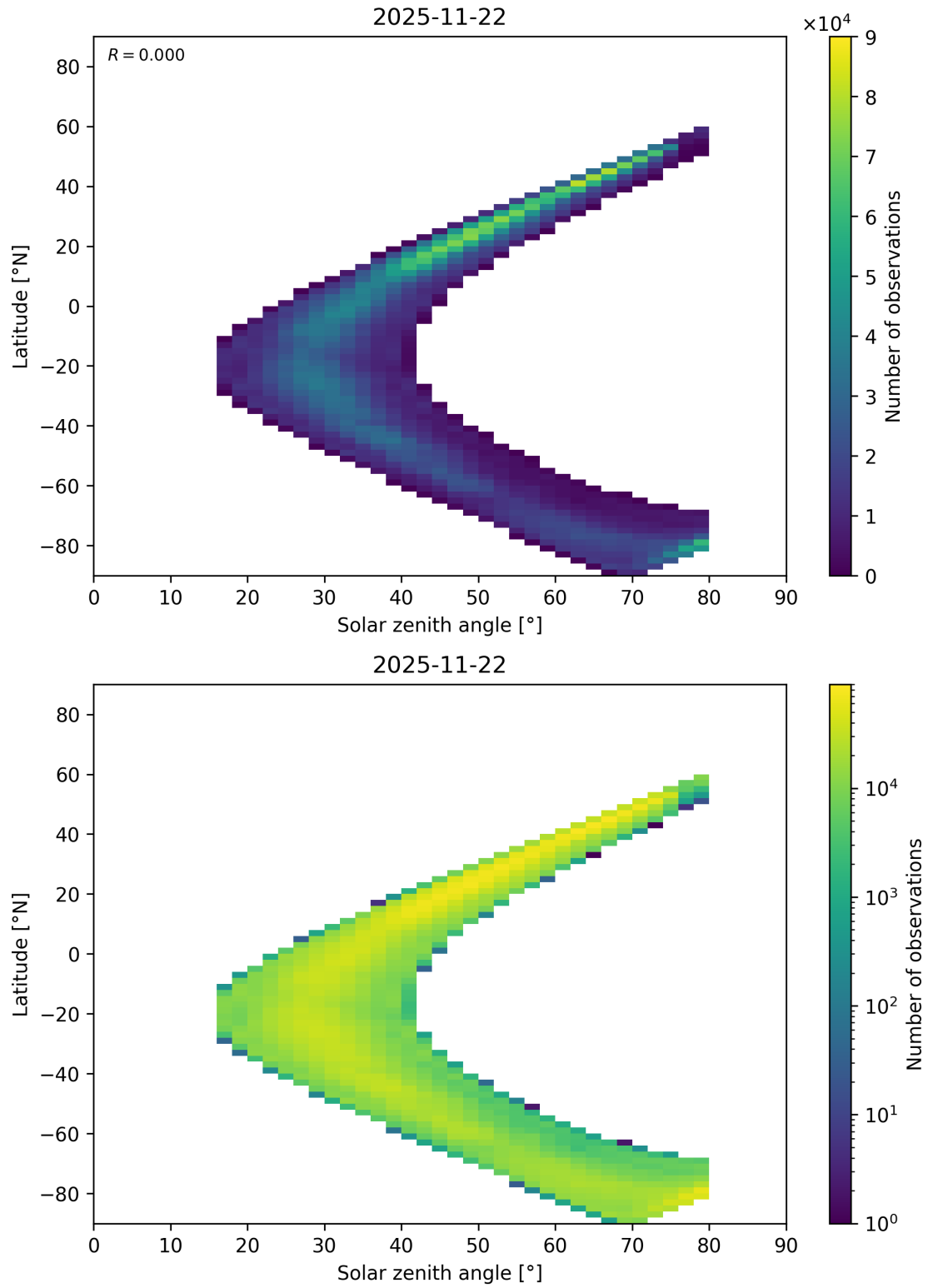
Figure 201: Scatter density plot of “Solar zenith angle” against “Latitude” for 2025-11-21 to 2025-11-23.
