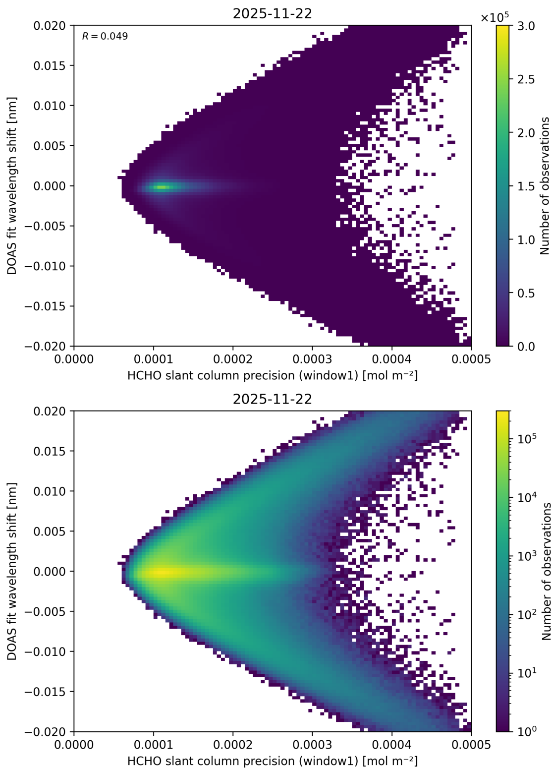
Figure 100: Scatter density plot of “HCHO slant column precision (window1)” against “DOAS fit wavelength shift” for 2025-11-21 to 2025-11-23.
