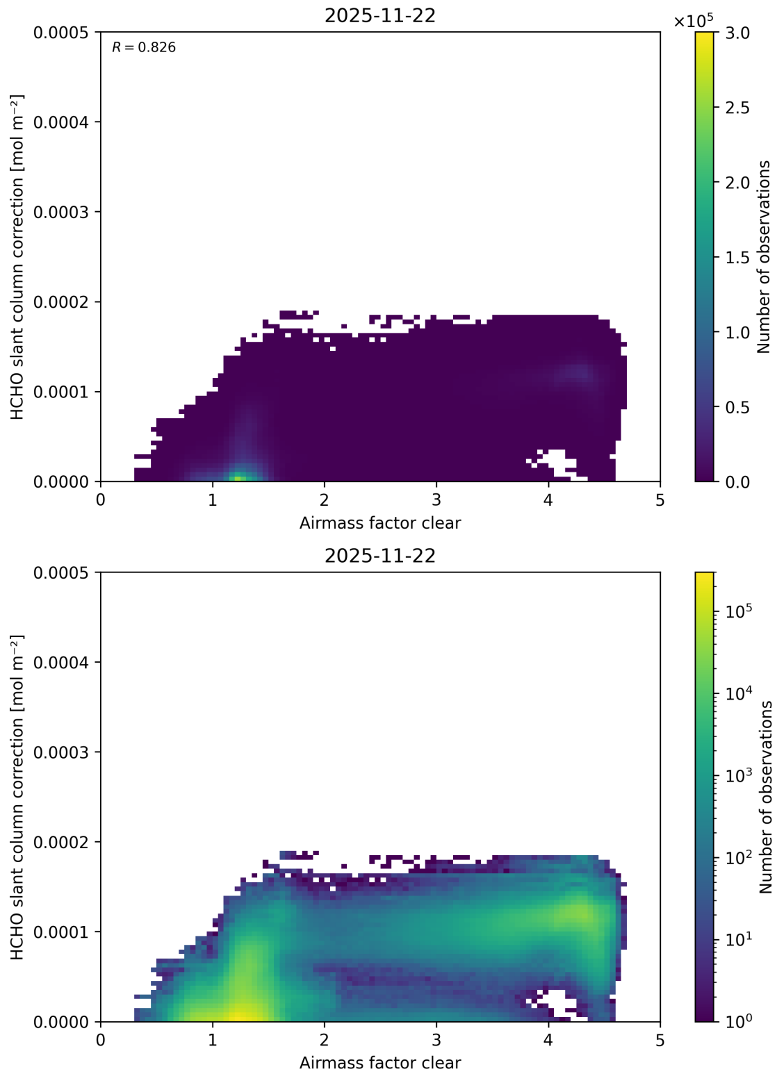
Figure 82: Scatter density plot of “Airmass factor clear” against “HCHO slant column correction” for 2025-11-21 to 2025-11-23.
