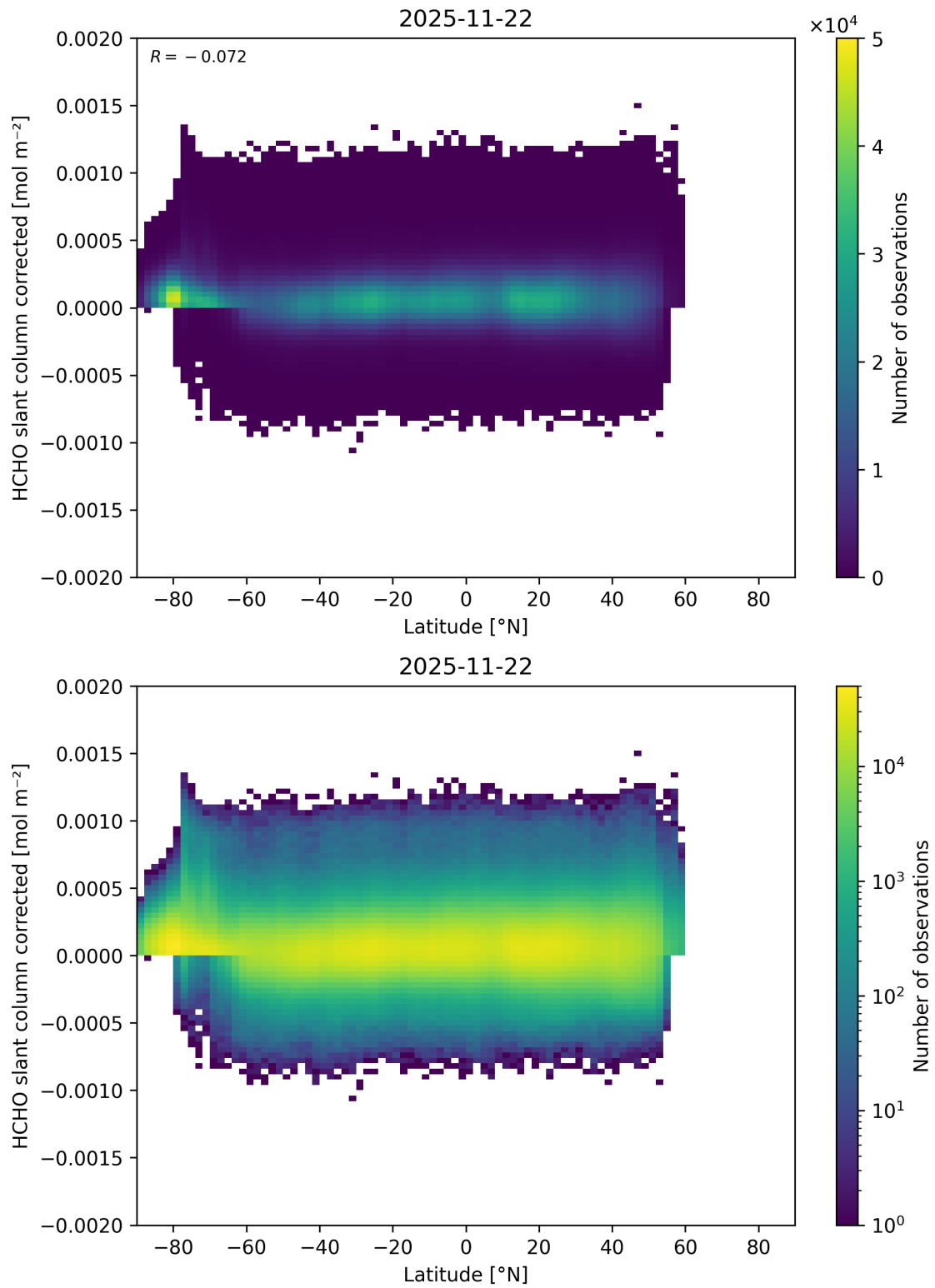
Figure 175: Scatter density plot of “Latitude” against “HCHO slant column corrected” for 2025-11-21 to 2025-11-23.
