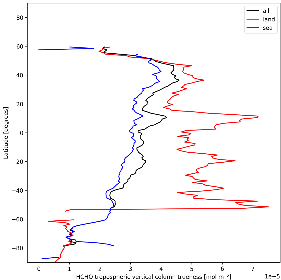
Figure 35: Zonal average of “HCHO tropospheric vertical column trueness” for 2025-11-21 to 2025-11-23.
