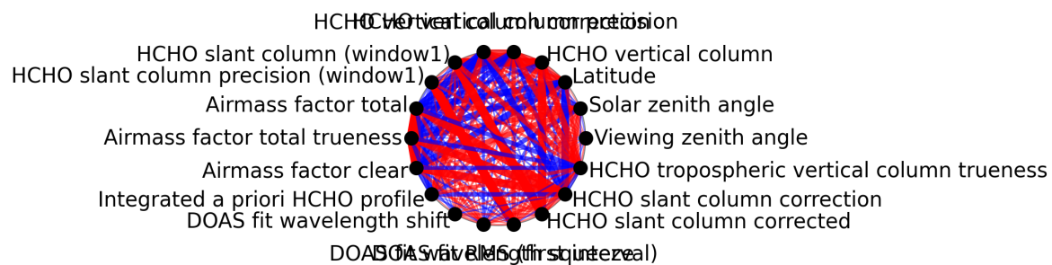
Figure 1: Map of correlation graph for 2025-11-21 to 2025-11-23.
