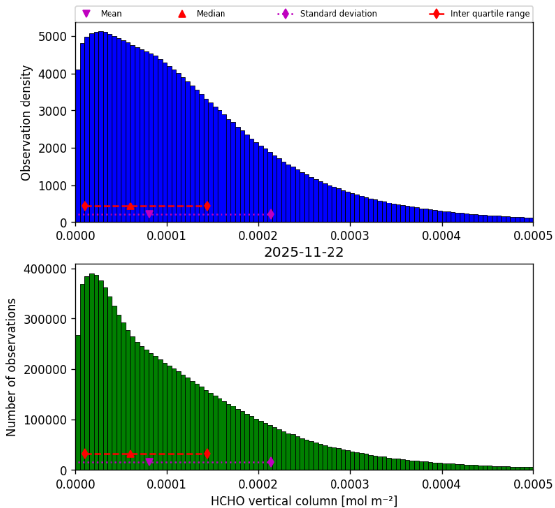
Figure 37: Histogram of “HCHO vertical column” for 2025-11-21 to 2025-11-23
