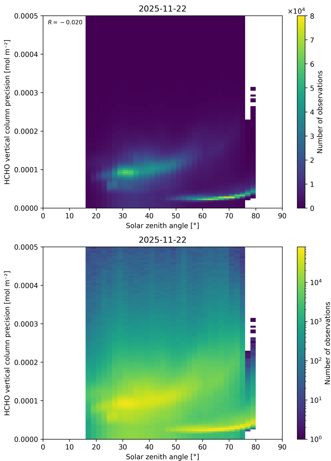
Figure 198: Scatter density plot of “Solar zenith angle” against “HCHO vertical column precision” for 2025-11-21 to 2025-11-23.
