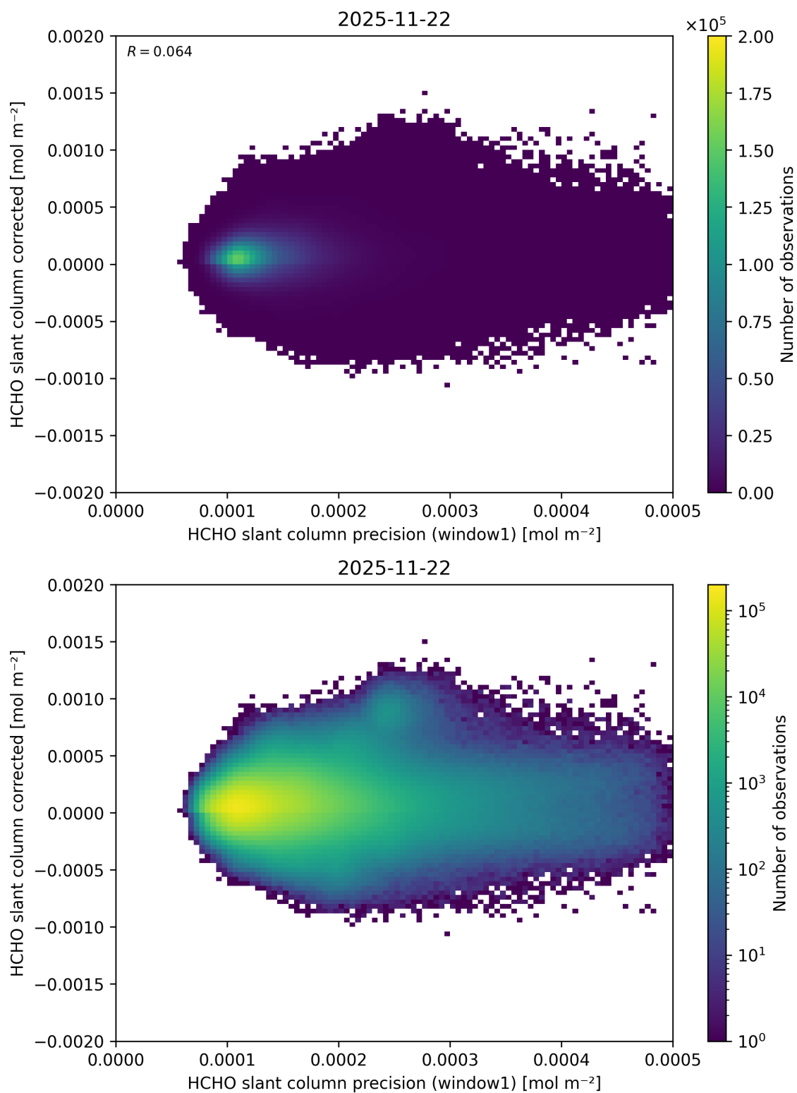
Figure 103: Scatter density plot of “HCHO slant column precision (window1)” against “HCHO slant column corrected” for 2025-11-21 to 2025-11-23.
