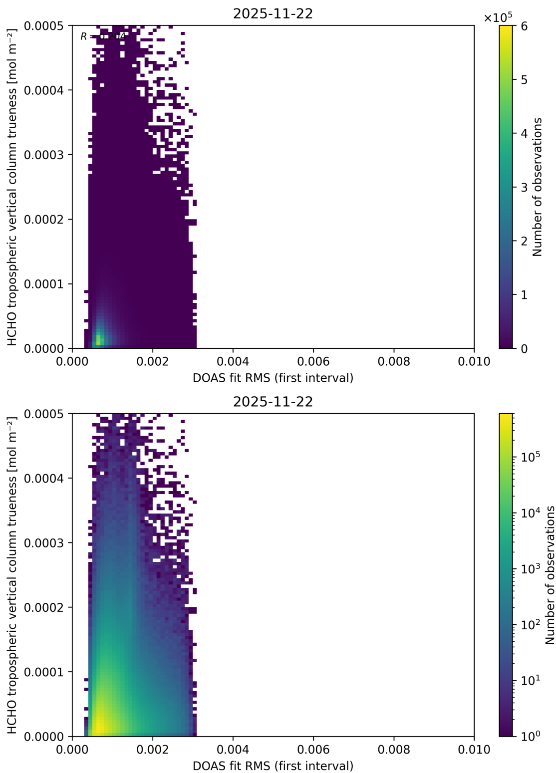
Figure 68: Scatter density plot of “DOAS fit RMS (first interval)” against “HCHO tropospheric vertical column trueness” for 2025-11-21 to 2025-11-23.
