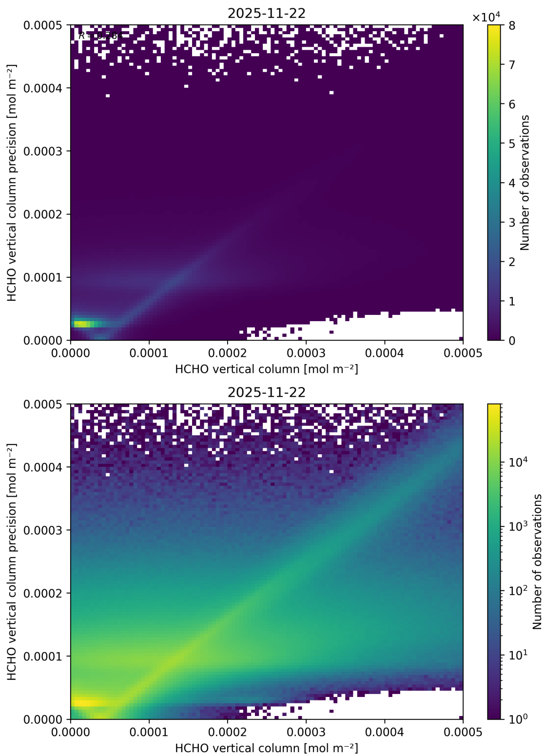
Figure 149: Scatter density plot of “HCHO vertical column” against “HCHO vertical column precision” for 2025-11-21 to 2025-11-23.
