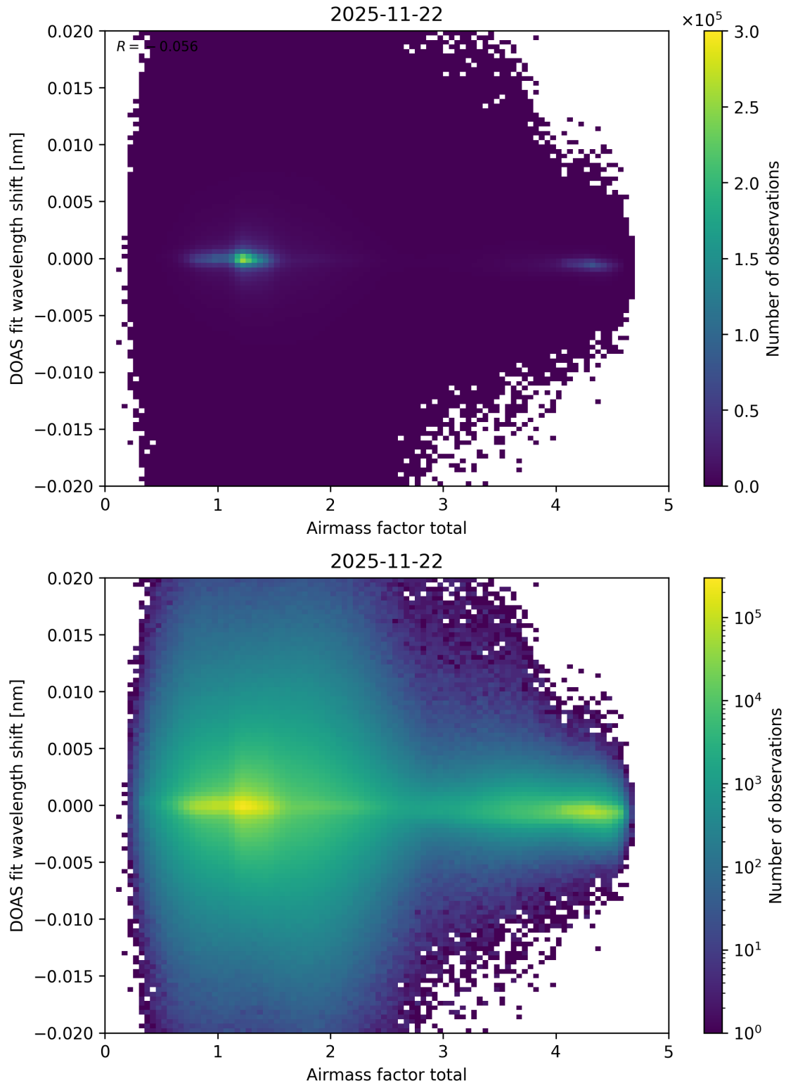
Figure 110: Scatter density plot of “Airmass factor total” against “DOAS fit wavelength shift” for 2025-11-21 to 2025-11-23.
