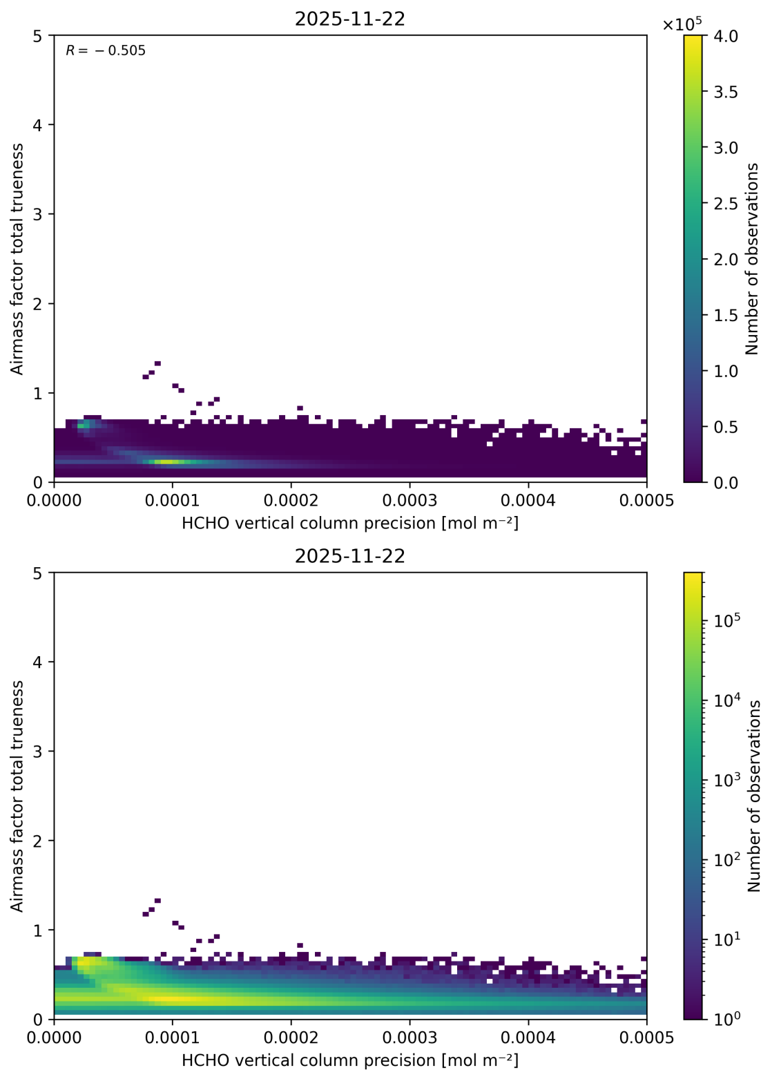
Figure 161: Scatter density plot of “HCHO vertical column precision” against “Airmass factor total trueness” for 2025-11-21 to 2025-11-23.
