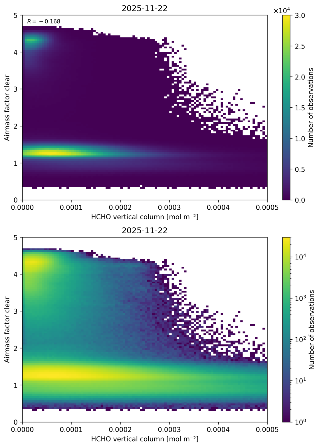
Figure 141: Scatter density plot of “HCHO vertical column” against “Airmass factor clear” for 2025-11-21 to 2025-11-23.
