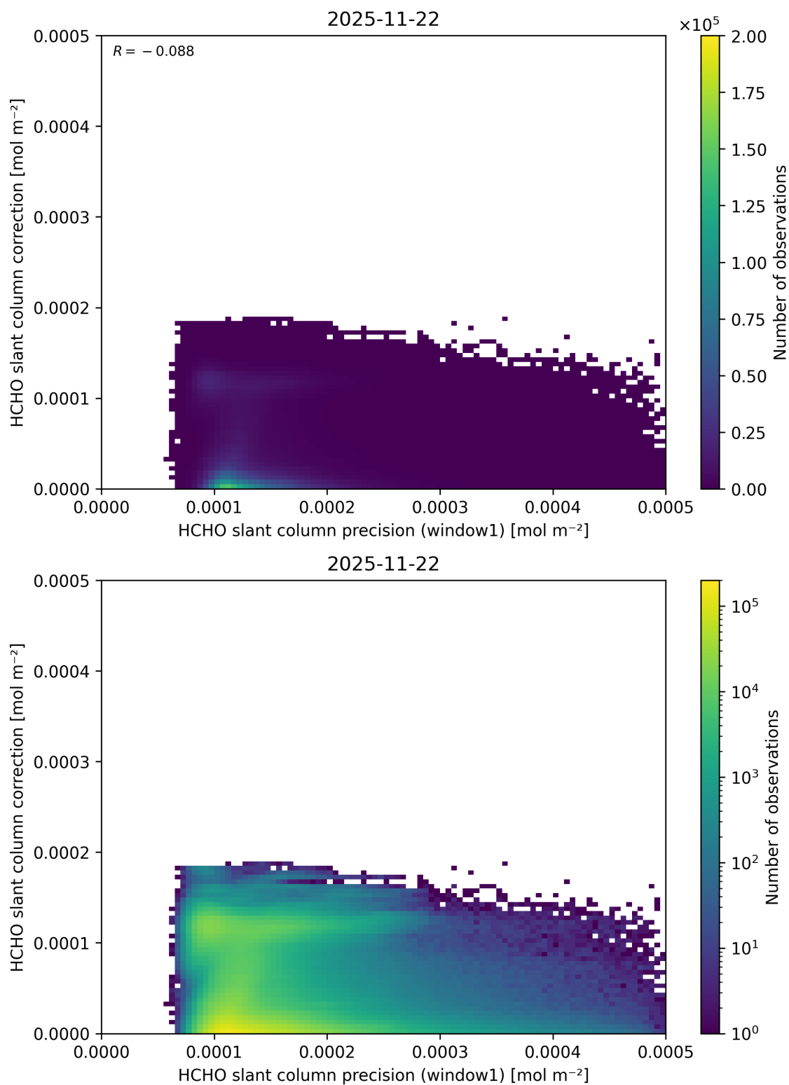
Figure 104: Scatter density plot of “HCHO slant column precision (window1)” against “HCHO slant column correction” for 2025-11-21 to 2025-11-23.
