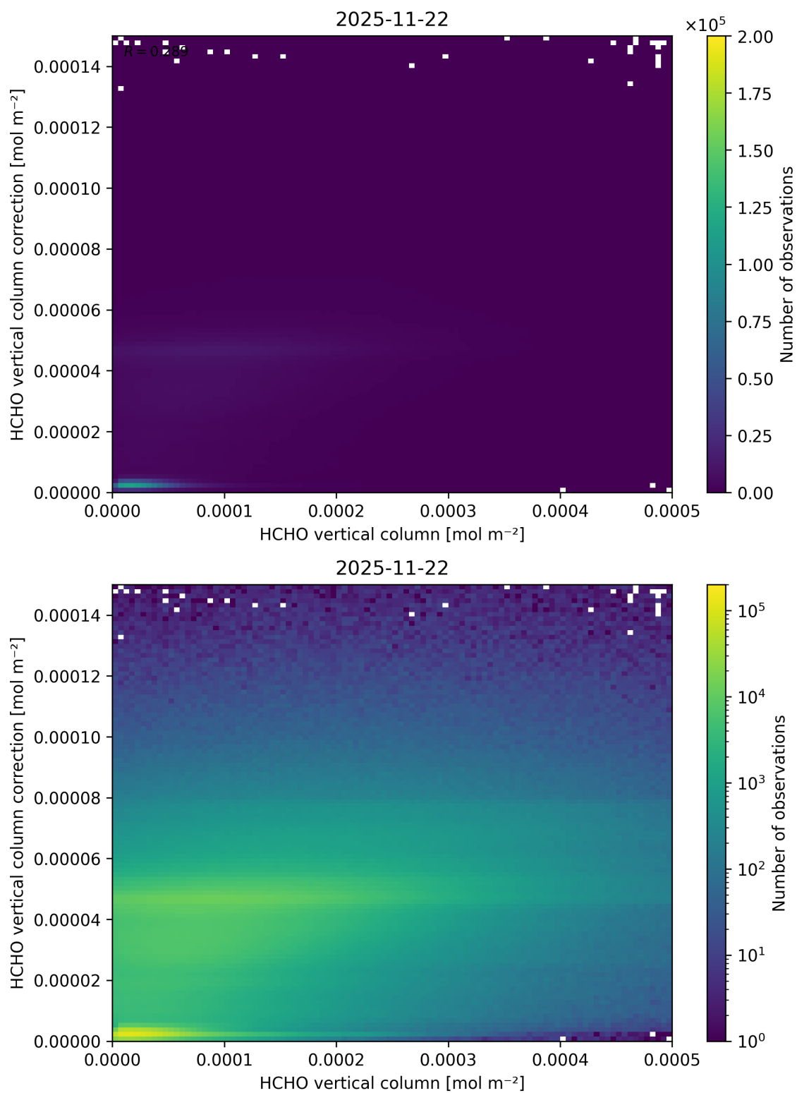
Figure 148: Scatter density plot of “HCHO vertical column” against “HCHO vertical column correction” for 2025-11-21 to 2025-11-23.
