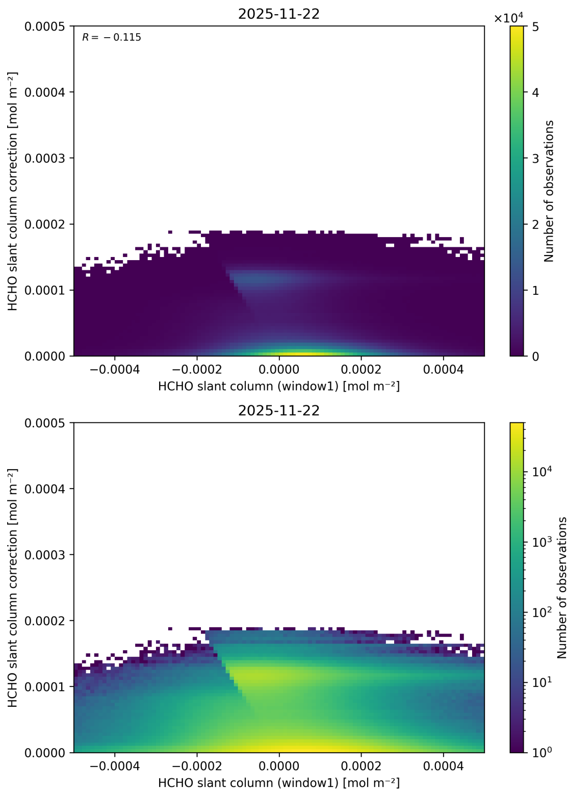
Figure 93: Scatter density plot of “HCHO slant column (window1)” against “HCHO slant column correction” for 2025-11-21 to 2025-11-23.
