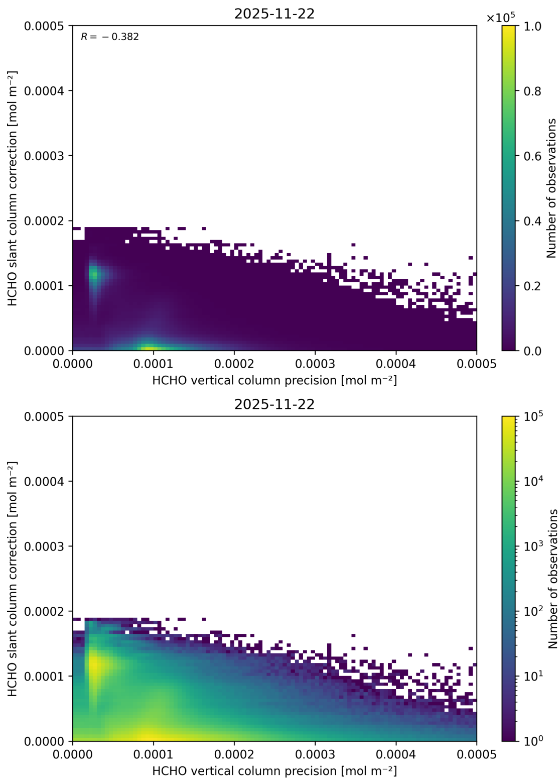
Figure 157: Scatter density plot of “HCHO vertical column precision” against “HCHO slant column correction” for 2025-11-21 to 2025-11-23.
