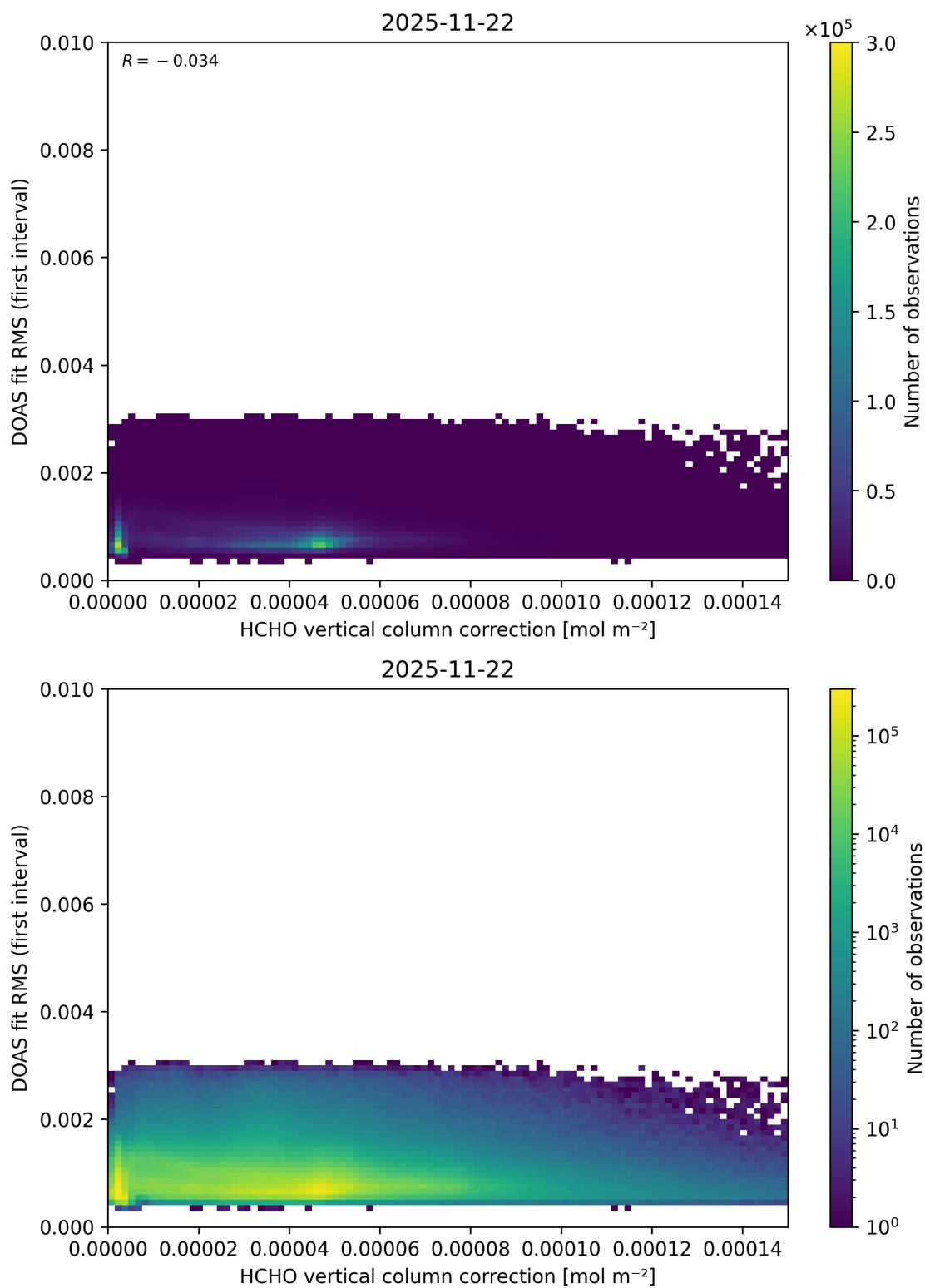
Figure 126: Scatter density plot of “HCHO vertical column correction” against “DOAS fit RMS (first interval)” for 2025-11-21 to 2025-11-23.
