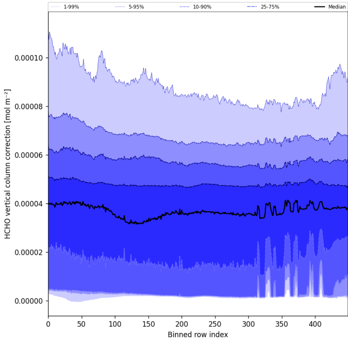
Figure 54: Along track statistics of “HCHO vertical column correction” for 2025-11-21 to 2025-11-23
