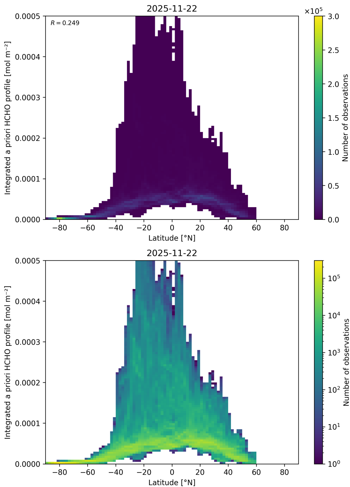
Figure 185: Scatter density plot of “Latitude” against “Integrated a priori HCHO profile” for 2025-11-21 to 2025-11-23.
