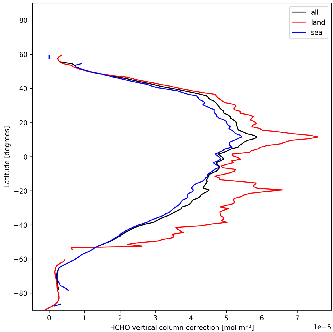
Figure 24: Zonal average of “HCHO vertical column correction” for 2025-11-21 to 2025-11-23.
