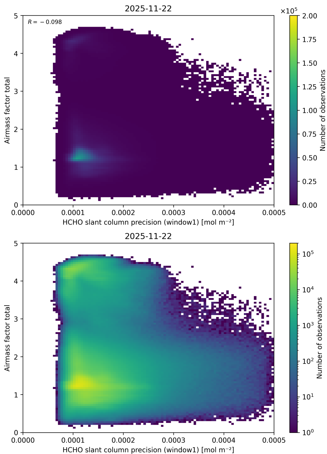
Figure 105: Scatter density plot of “HCHO slant column precision (window1)” against “Airmass factor total” for 2025-11-21 to 2025-11-23.
