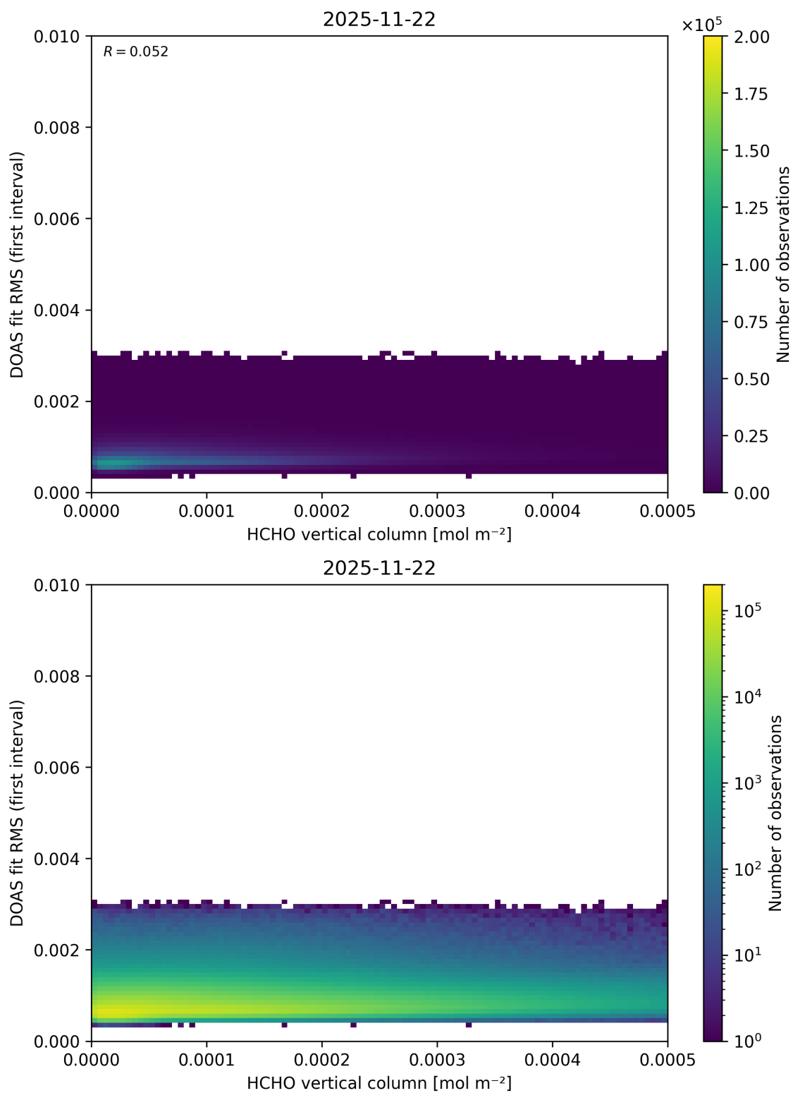
Figure 138: Scatter density plot of “HCHO vertical column” against “DOAS fit RMS (first interval)” for 2025-11-21 to 2025-11-23.
