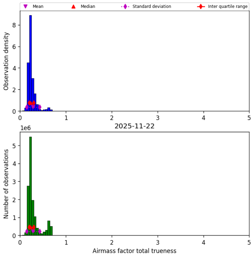
Figure 43: Histogram of “Airmass factor total trueness” for 2025-11-21 to 2025-11-23
