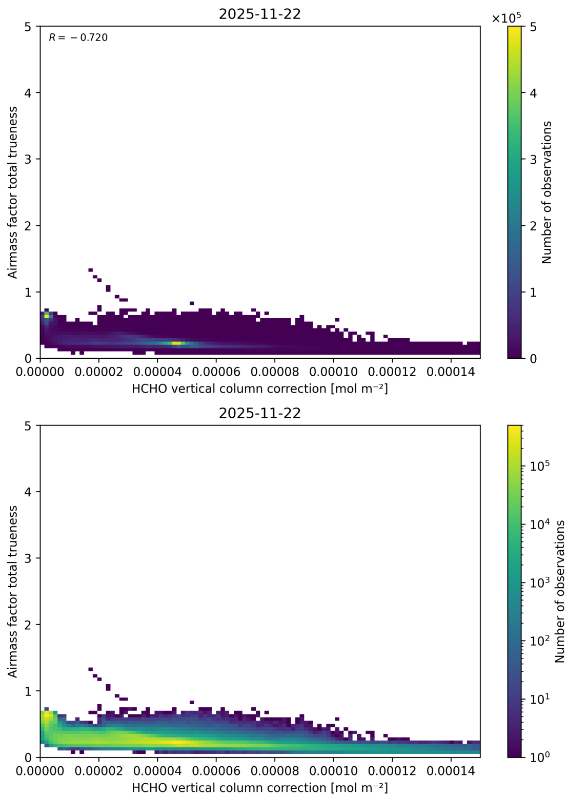
Figure 135: Scatter density plot of “HCHO vertical column correction” against “Airmass factor total truiness” for 2025-11-21 to 2025-11-23.
