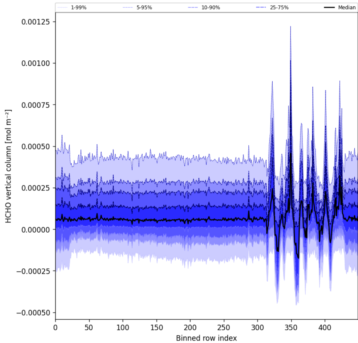
Figure 52: Along track statistics of "HCHO vertical column" for 2025-11-21 to 2025-11-23
