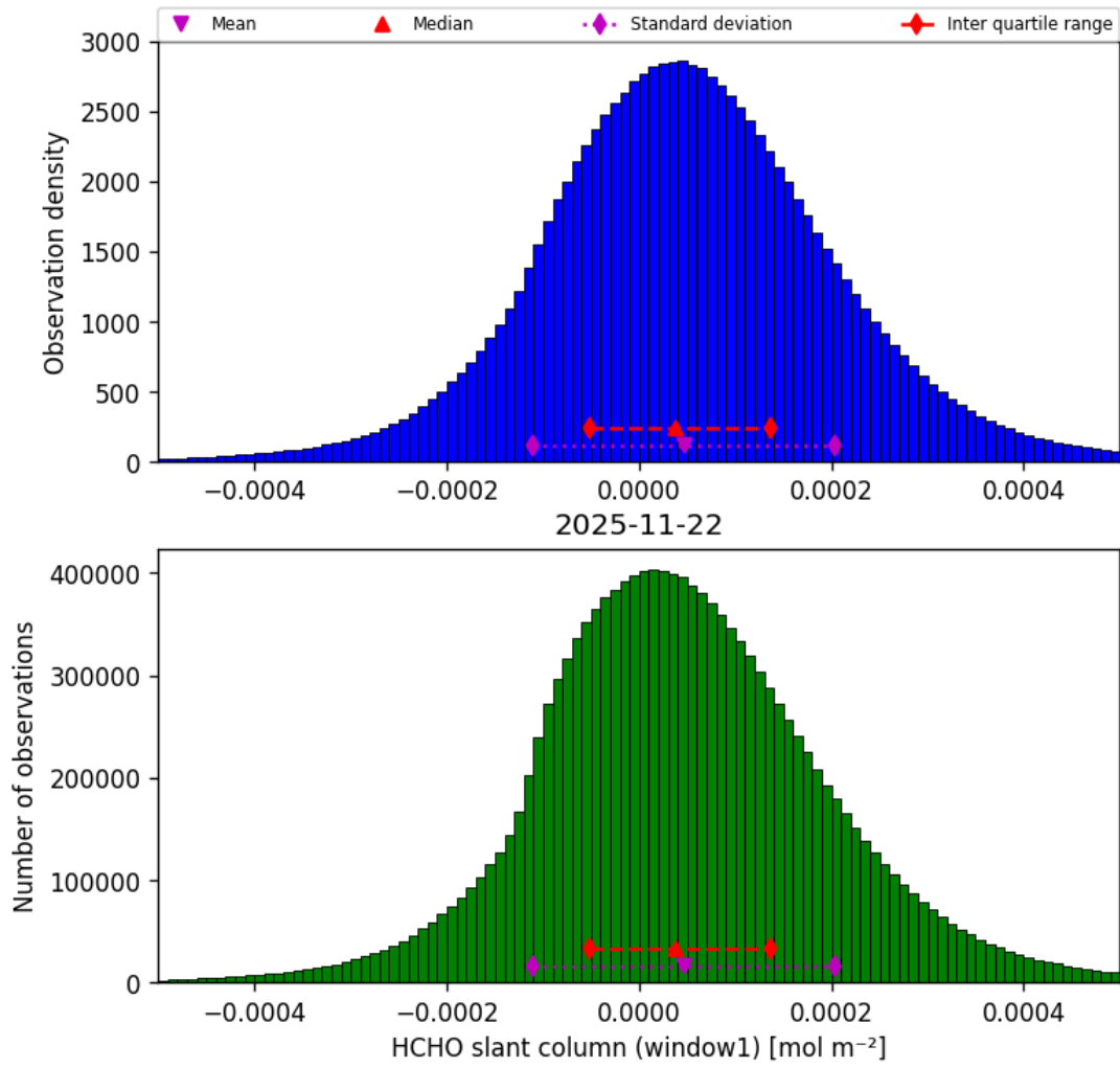
Figure 40: Histogram of “HCHO slant column (window1)” for 2025-11-21 to 2025-11-23
