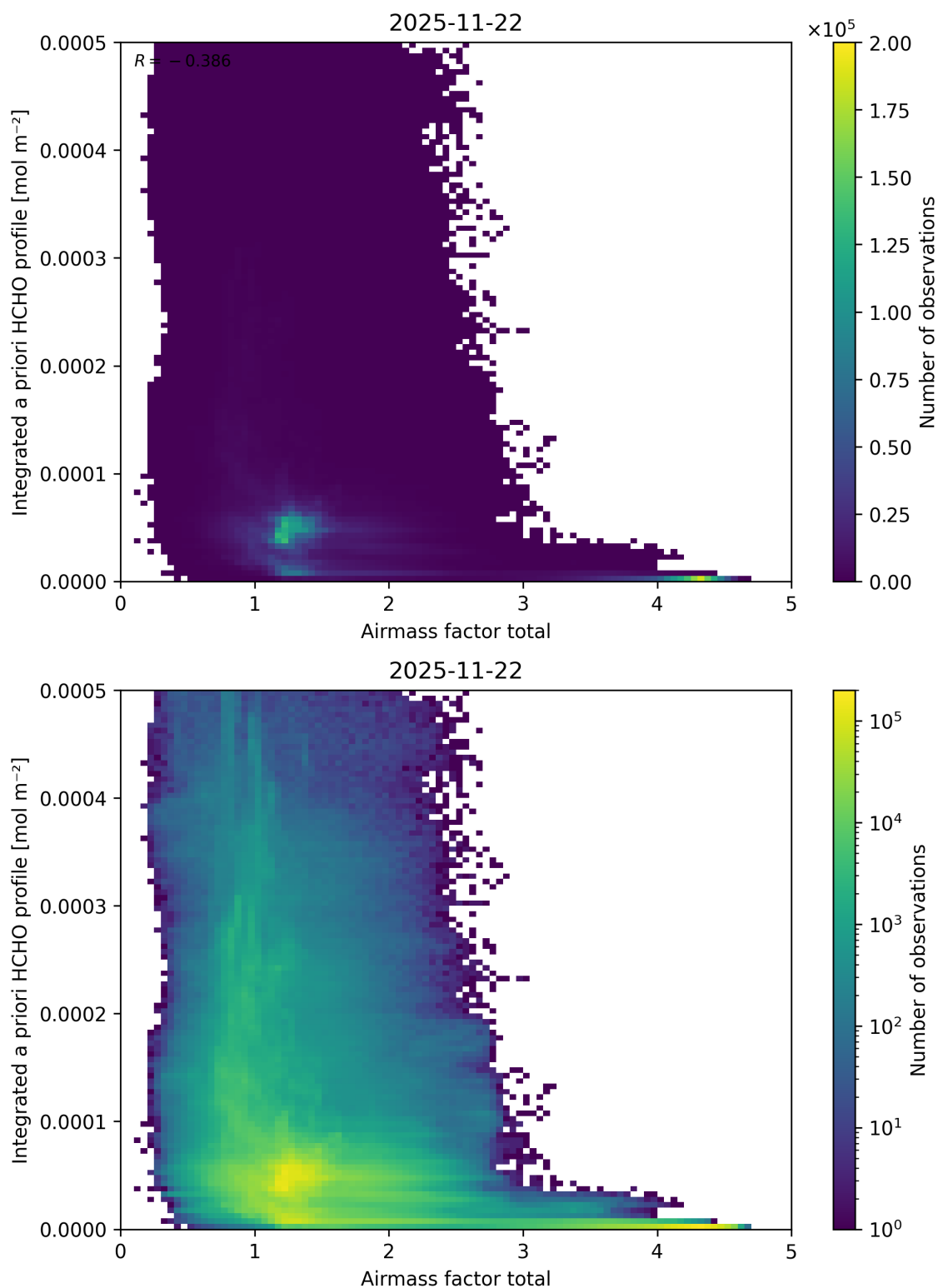
Figure 117: Scatter density plot of “Airmass factor total” against “Integrated a priori HCHO profile” for 2025-11-21 to 2025-11-23.
