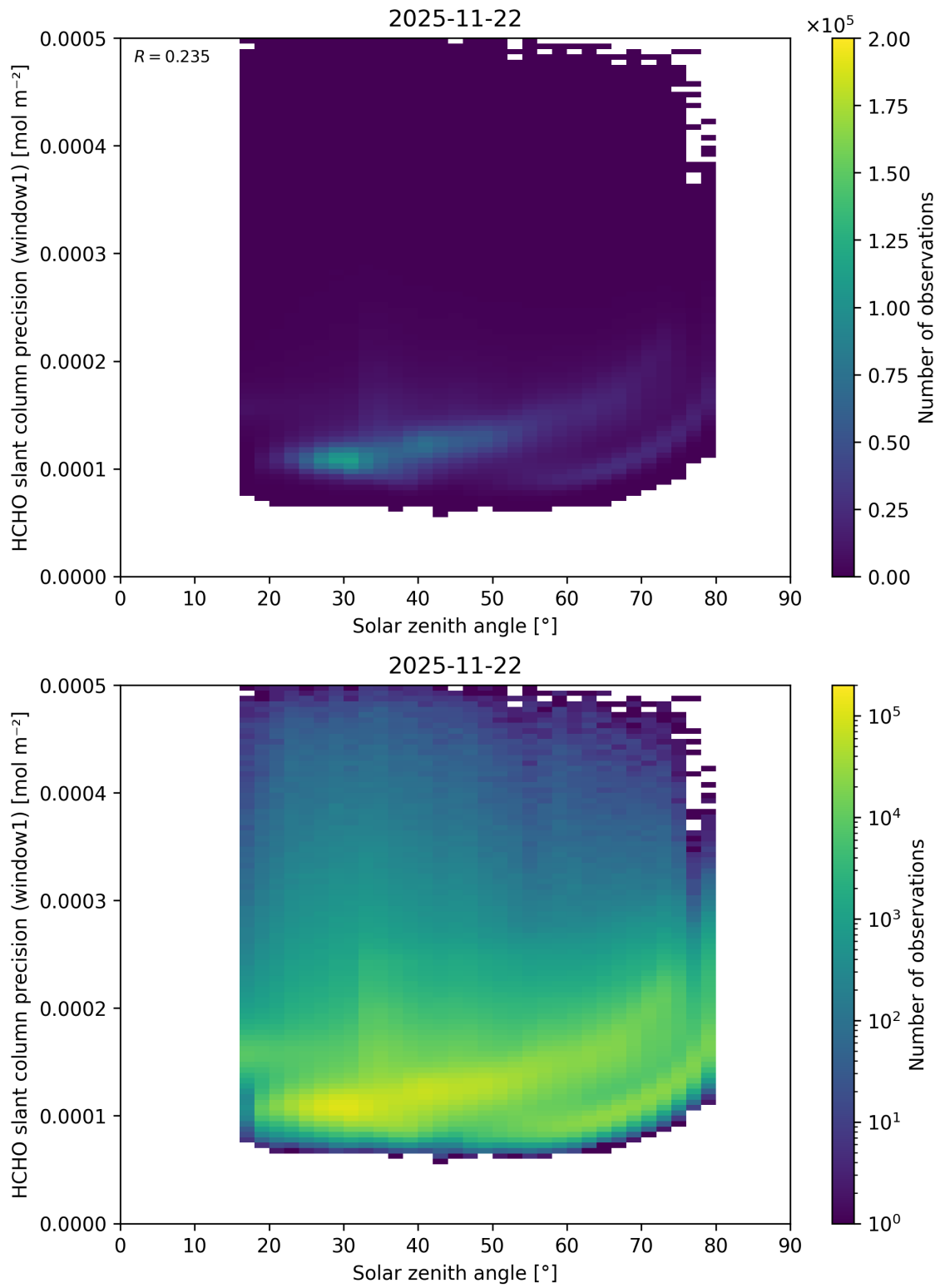
Figure 193: Scatter density plot of “Solar zenith angle” against “HCHO slant column precision (window1)” for 2025-11-21 to 2025-11-23.
