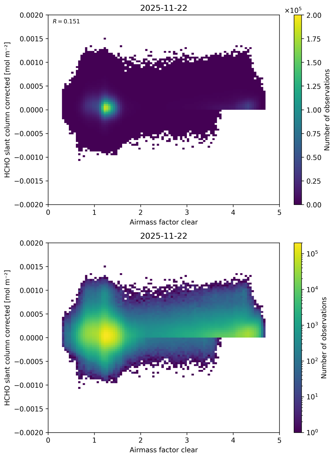
Figure 81: Scatter density plot of “Airmass factor clear” against “HCHO slant column corrected” for 2025-11-21 to 2025-11-23.
