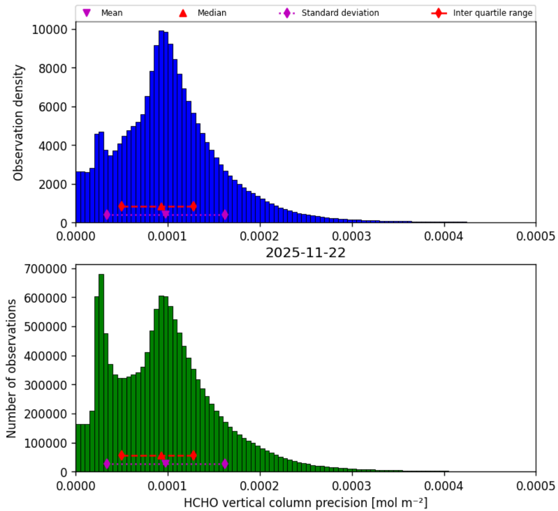
Figure 38: Histogram of “HCHO vertical column precision” for 2025-11-21 to 2025-11-23
