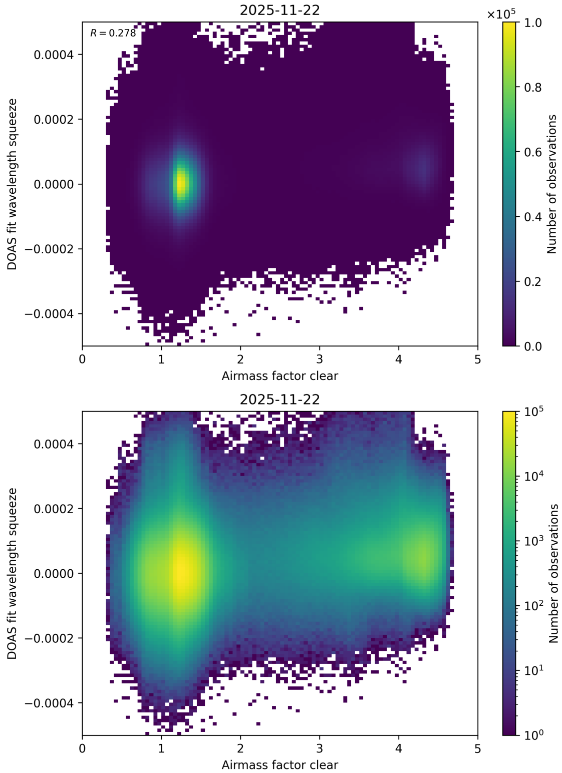
Figure 80: Scatter density plot of “Airmass factor clear” against “DOAS fit wavelength squeeze” for 2025-11-21 to 2025-11-23.
