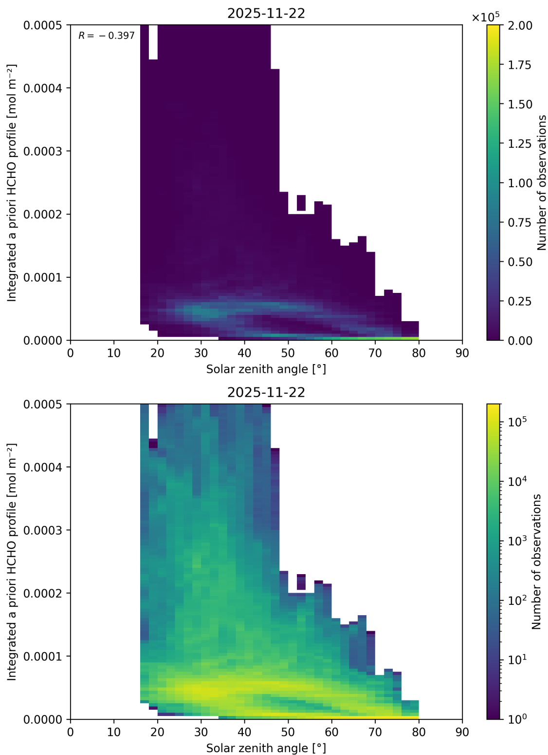
Figure 200: Scatter density plot of “Solar zenith angle” against “Integrated a priori HCHO profile” for 2025-11-21 to 2025-11-23.
