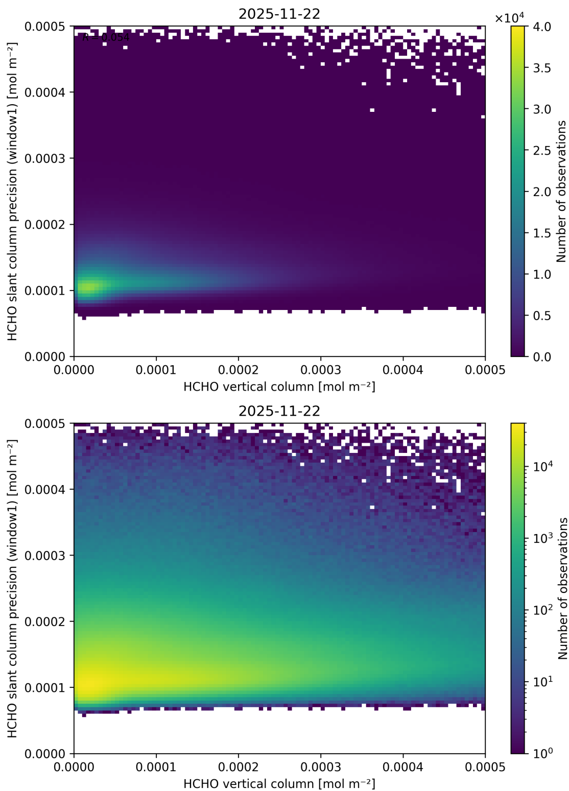
Figure 145: Scatter density plot of “HCHO vertical column” against “HCHO slant column precision (window1)” for 2025-11-21 to 2025-11-23.
