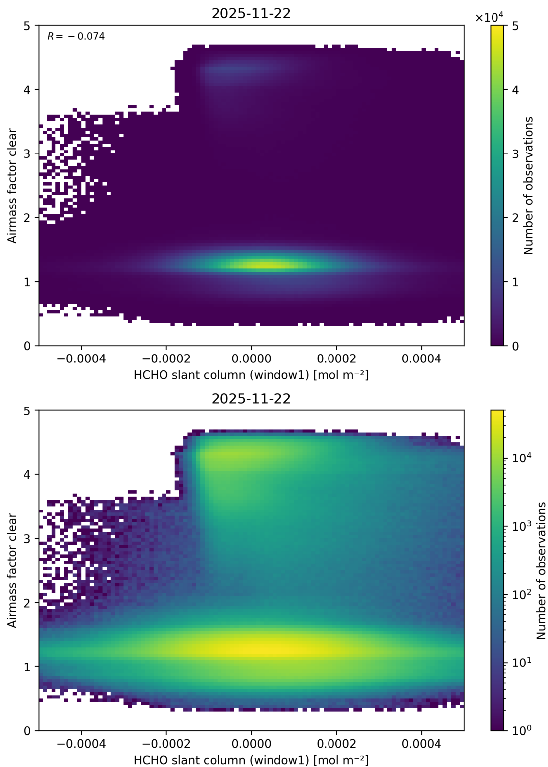
Figure 91: Scatter density plot of “HCHO slant column (window1)” against “Airmass factor clear” for 2025-11-21 to 2025-11-23.
