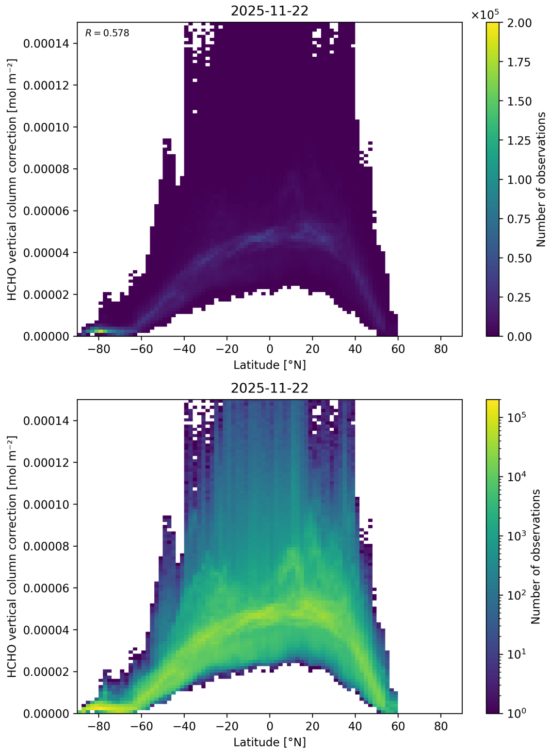
Figure 182: Scatter density plot of “Latitude” against “HCHO vertical column correction” for 2025-11-21 to 2025-11-23.
