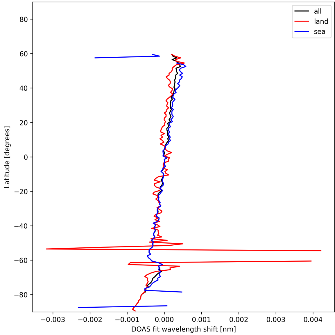
Figure 31: Zonal average of “DOAS fit wavelength shift” for 2025-11-21 to 2025-11-23.
