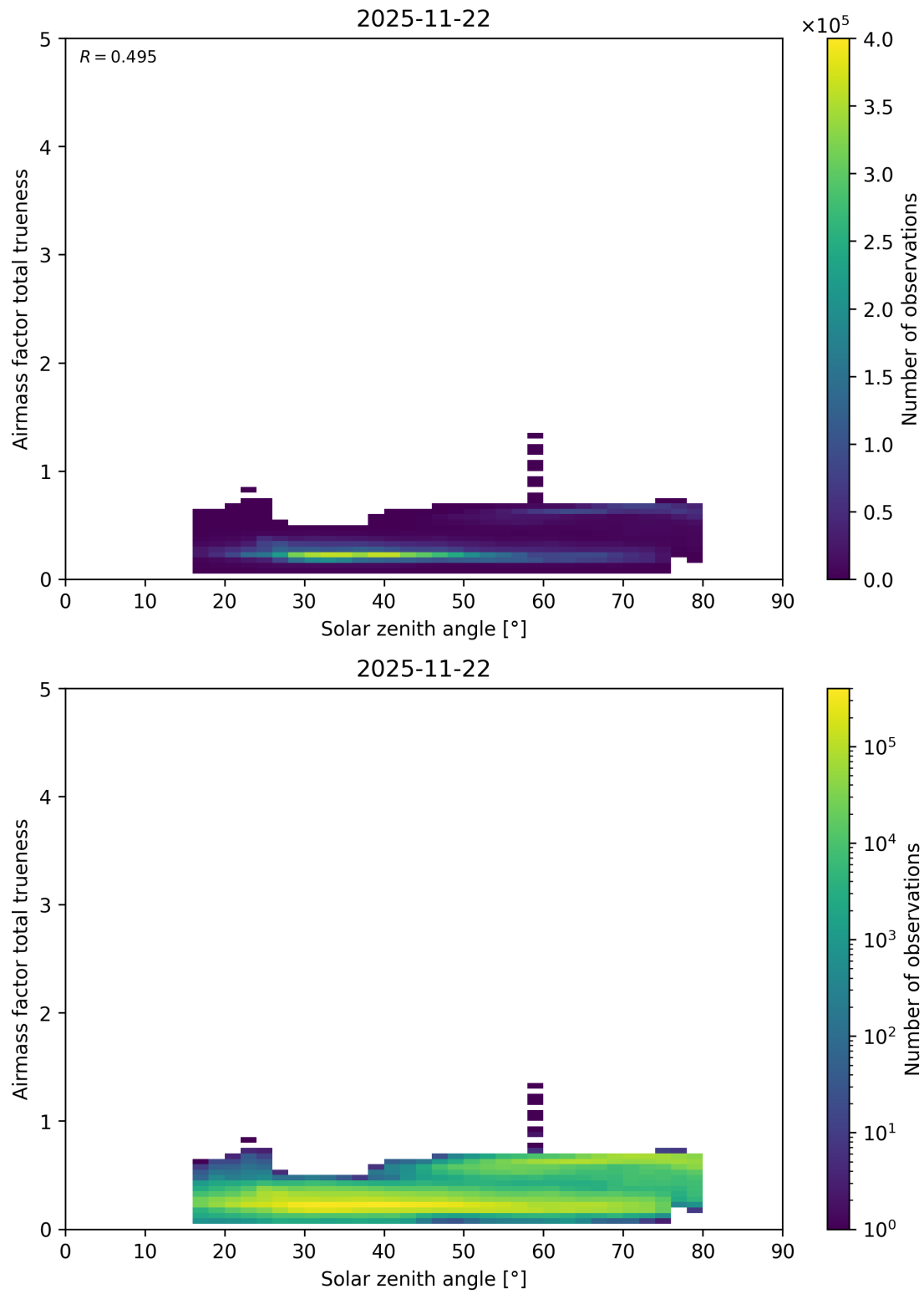
Figure 195: Scatter density plot of “Solar zenith angle” against “Airmass factor total trueness” for 2025-11-21 to 2025-11-23.
