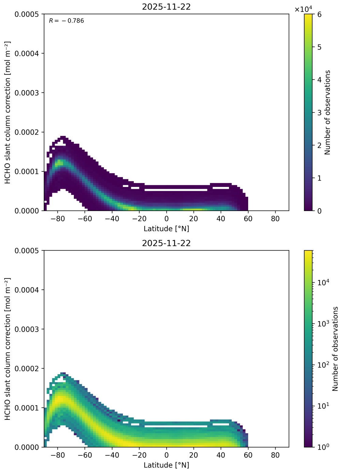
Figure 176: Scatter density plot of “Latitude” against “HCHO slant column correction” for 2025-11-21 to 2025-11-23.
