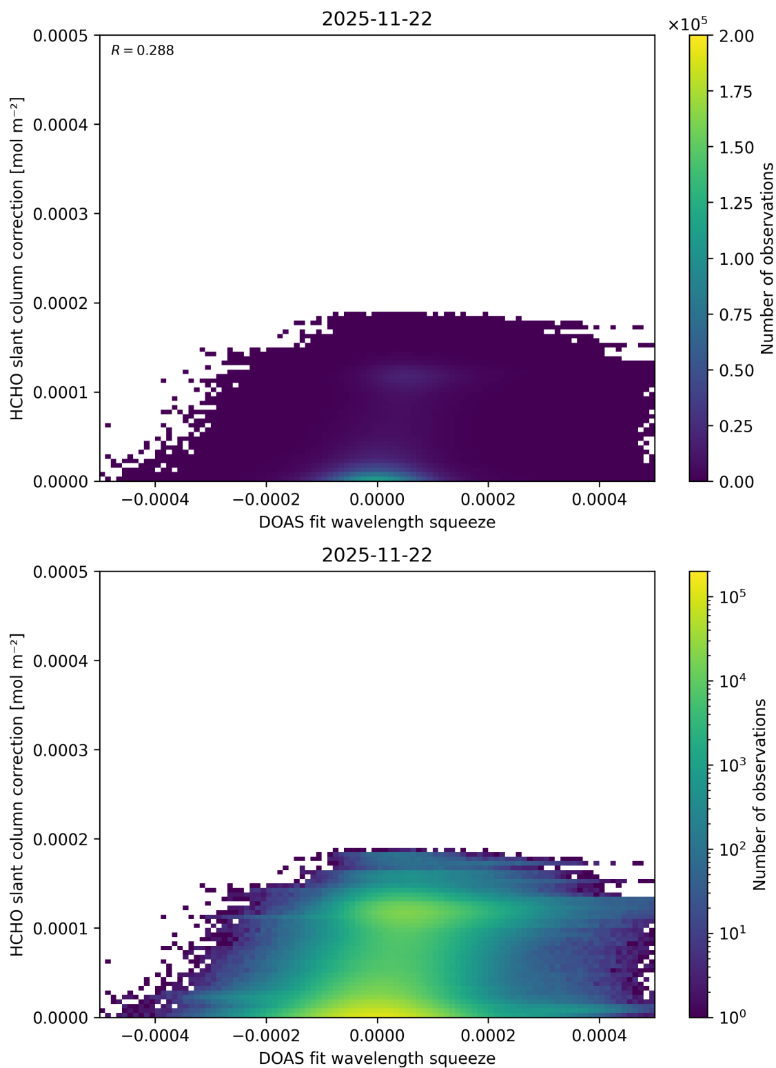
Figure 76: Scatter density plot of “DOAS fit wavelength squeeze” against “HCHO slant column correction” for 2025-11-21 to 2025-11-23.
