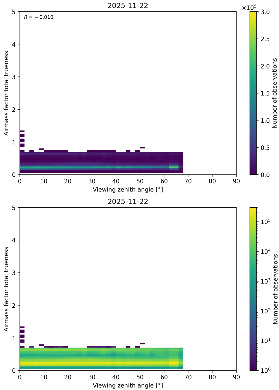
Figure 211: Scatter density plot of “Viewing zenith angle” against “Airmass factor total trueness” for 2025-11-21 to 2025-11-23.
