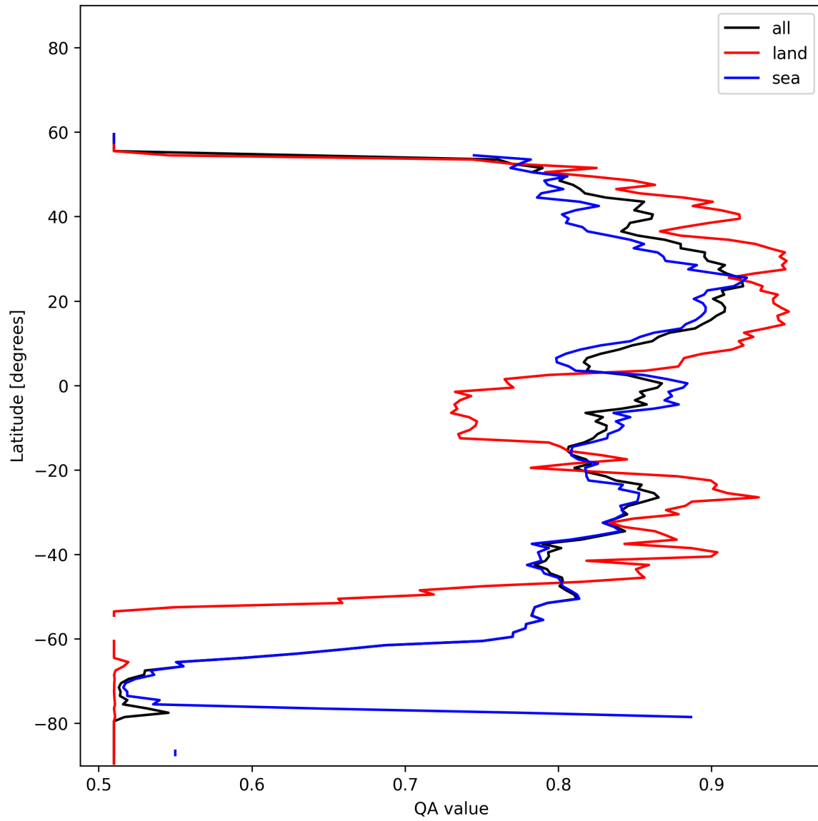
Figure 21: Zonal average of “QA value” for 2025-11-21 to 2025-11-23.
