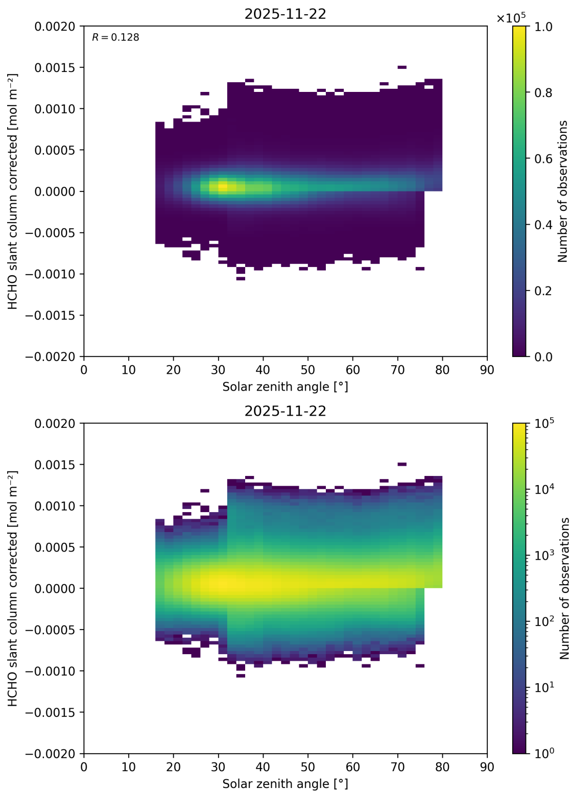
Figure 190: Scatter density plot of “Solar zenith angle” against “HCHO slant column corrected” for 2025-11-21 to 2025-11-23.
