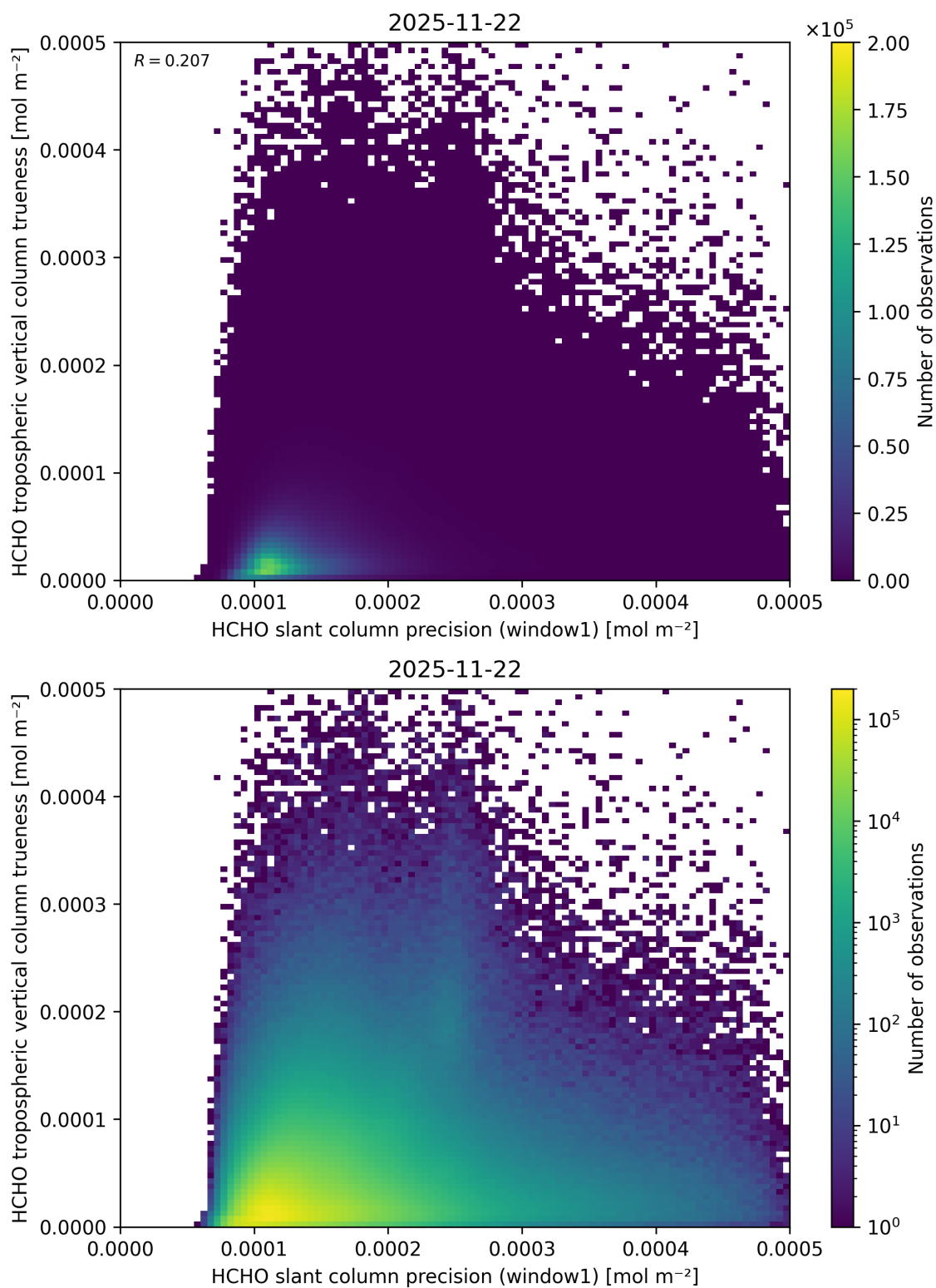
Figure 107: Scatter density plot of “HCHO slant column precision (window1)” against “HCHO tropospheric vertical column trueness” for 2025-11-21 to 2025-11-23.
