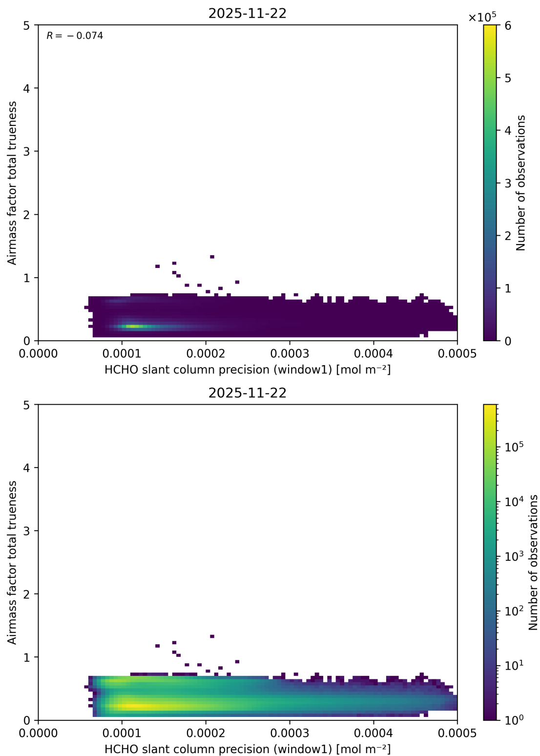
Figure 106: Scatter density plot of “HCHO slant column precision (window1)” against “Airmass factor total trueness” for 2025-11-21 to 2025-11-23.
