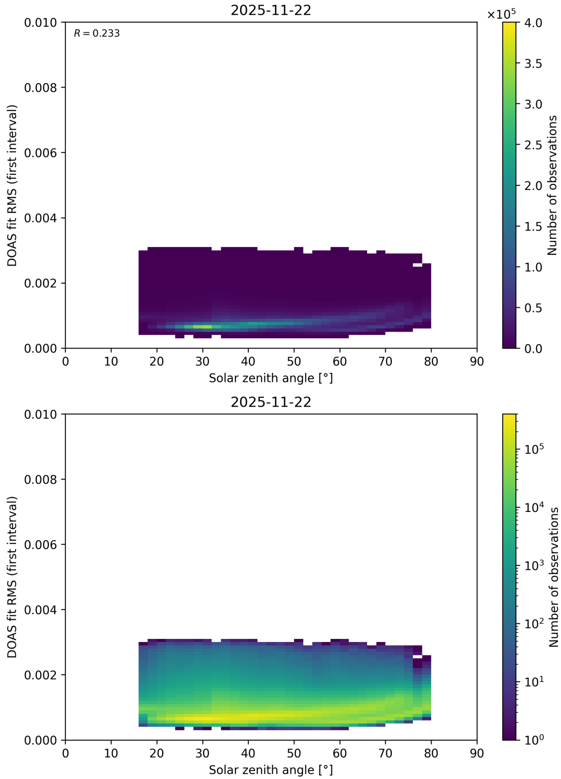
Figure 186: Scatter density plot of “Solar zenith angle” against “DOAS fit RMS (first interval)” for 2025-11-21 to 2025-11-23.
