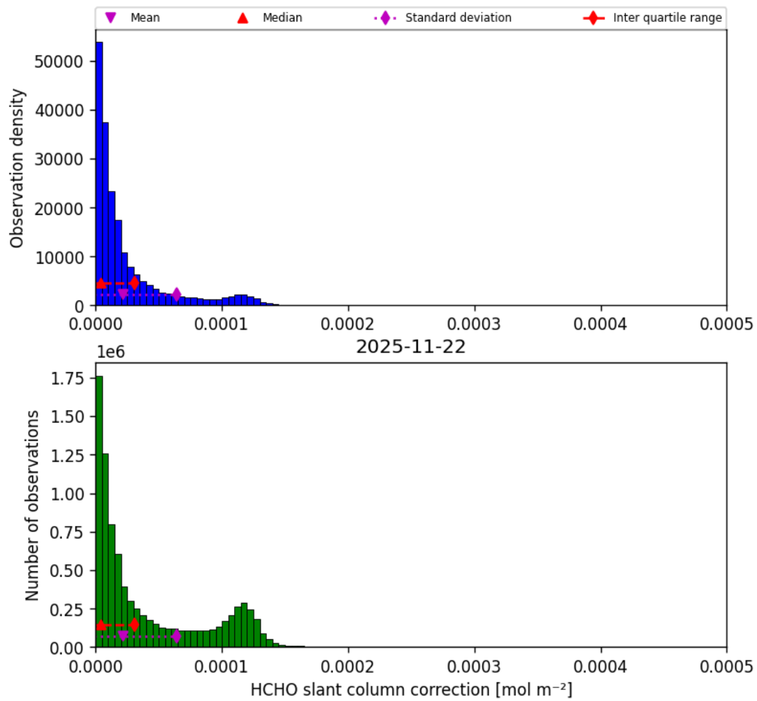
Figure 49: Histogram of “HCHO slant column correction” for 2025-11-21 to 2025-11-23
