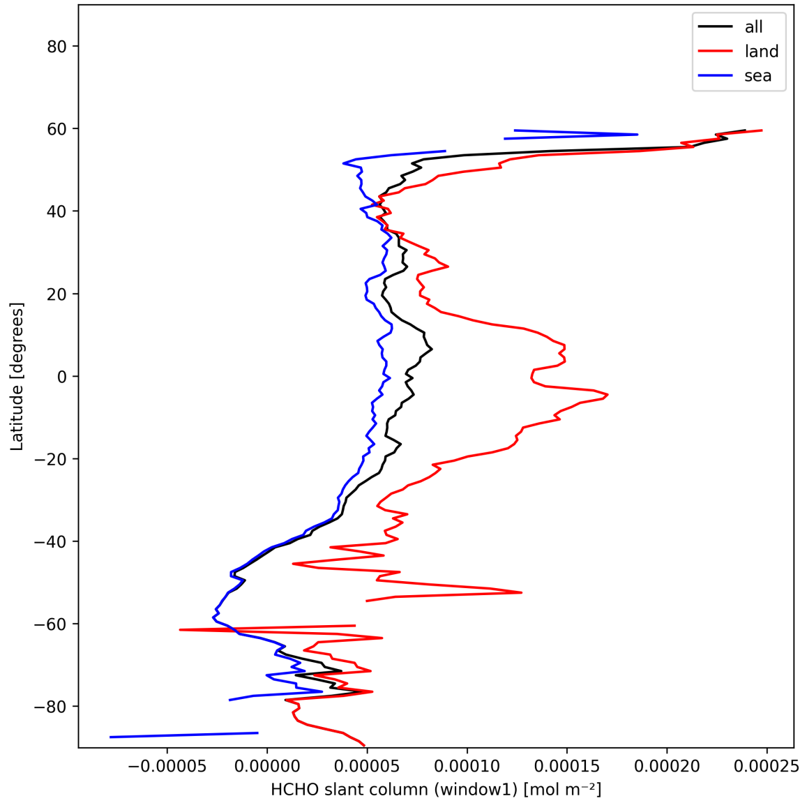
Figure 25: Zonal average of “HCHO slant column (window1)” for 2025-11-21 to 2025-11-23.
