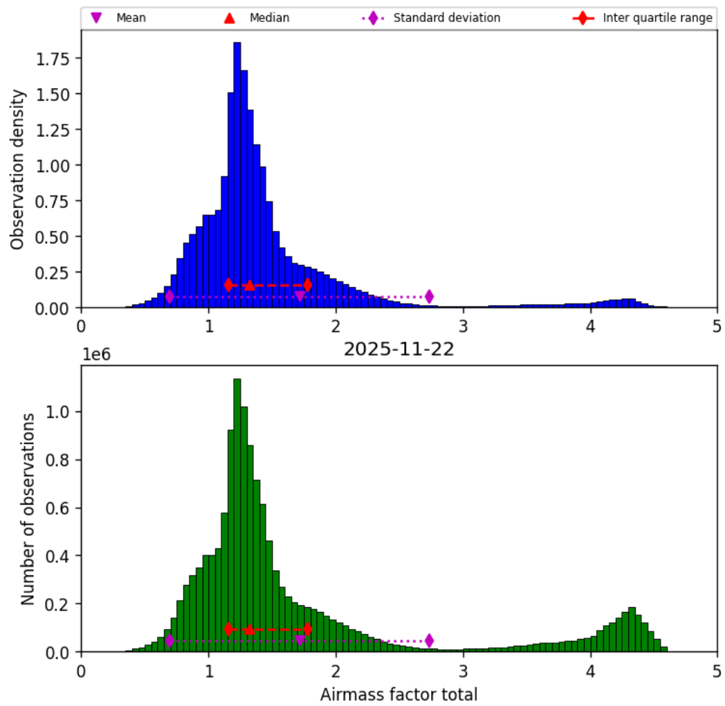
Figure 42: Histogram of “Airmass factor total” for 2025-11-21 to 2025-11-23
