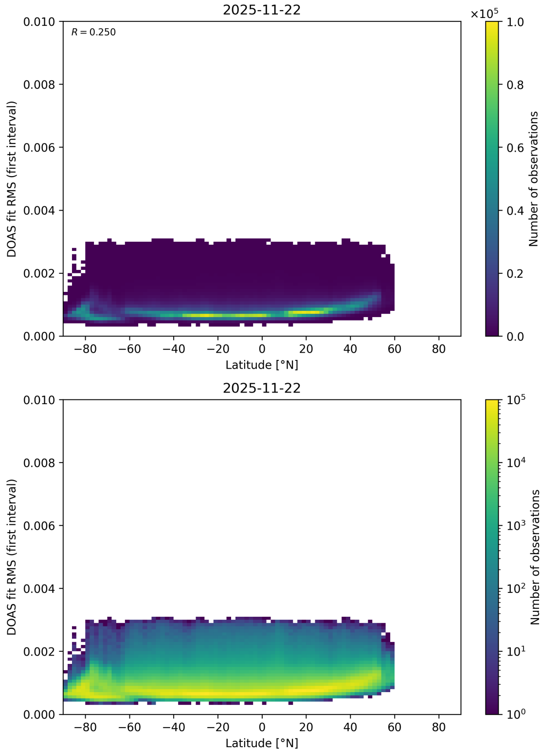
Figure 171: Scatter density plot of “Latitude” against “DOAS fit RMS (first interval)” for 2025-11-21 to 2025-11-23.
