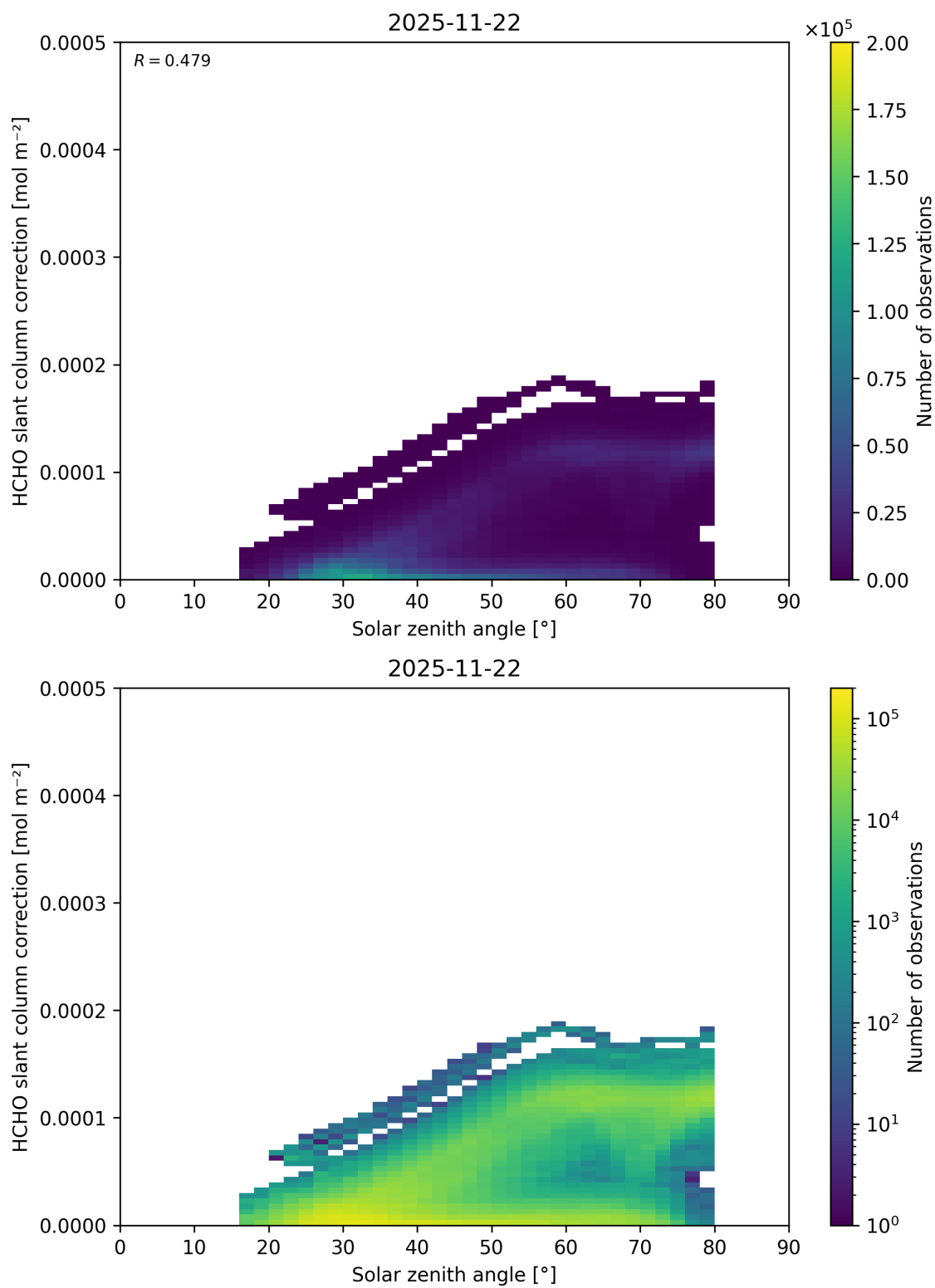
Figure 191: Scatter density plot of “Solar zenith angle” against “HCHO slant column correction” for 2025-11-21 to 2025-11-23.
