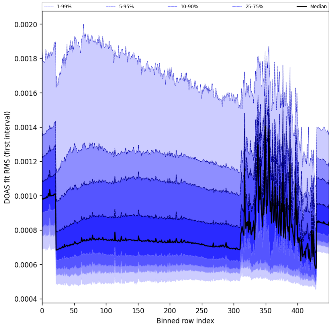
Figure 63: Along track statistics of “DOAS fit RMS (first interval)” for 2025-11-21 to 2025-11-23
