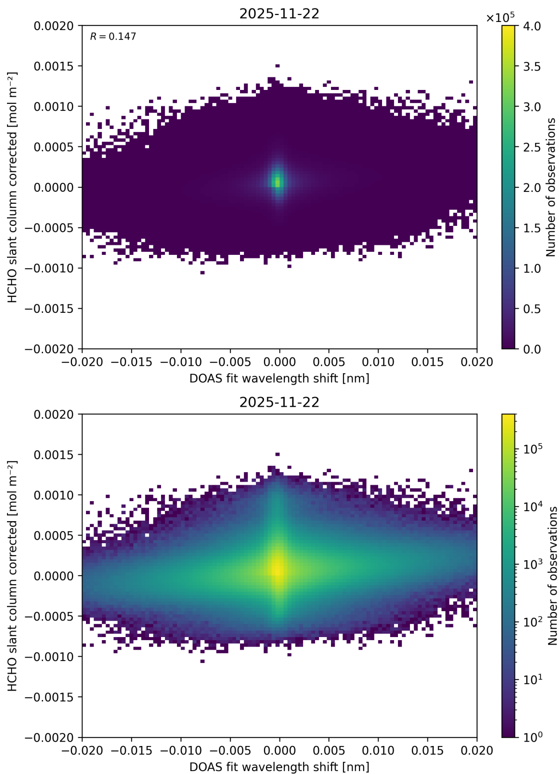
Figure 71: Scatter density plot of “DOAS fit wavelength shift” against “HCHO slant column corrected” for 2025-11-21 to 2025-11-23.
