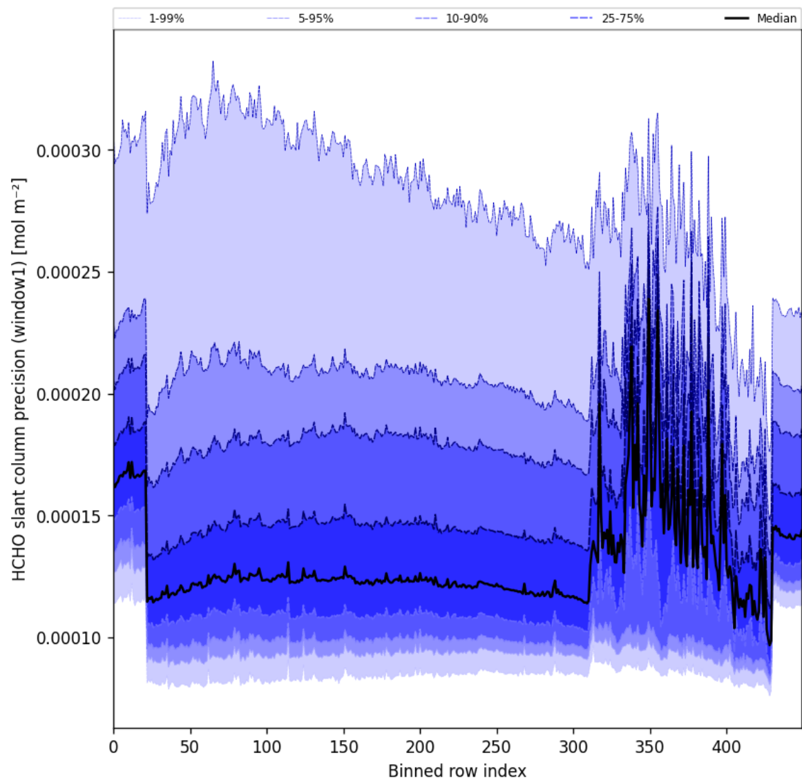
Figure 56: Along track statistics of “HCHO slant column precision (window1)” for 2025-11-21 to 2025-11-23
