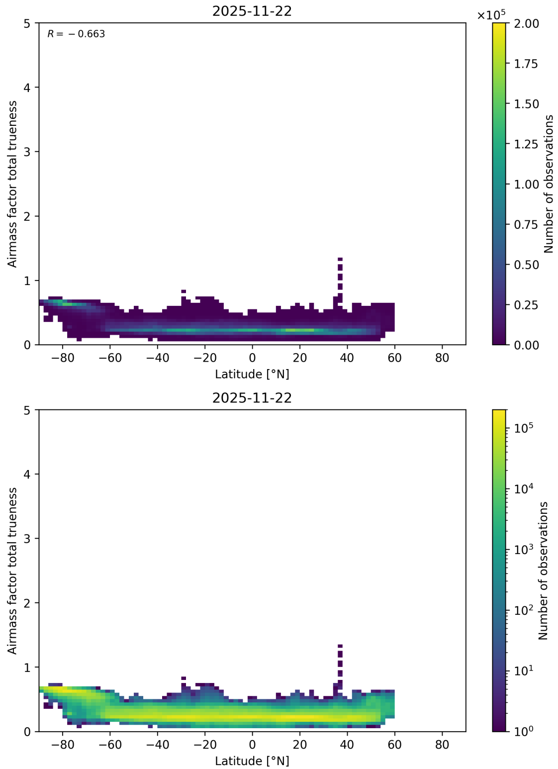
Figure 180: Scatter density plot of “Latitude” against “Airmass factor total trueness” for 2025-11-21 to 2025-11-23.
