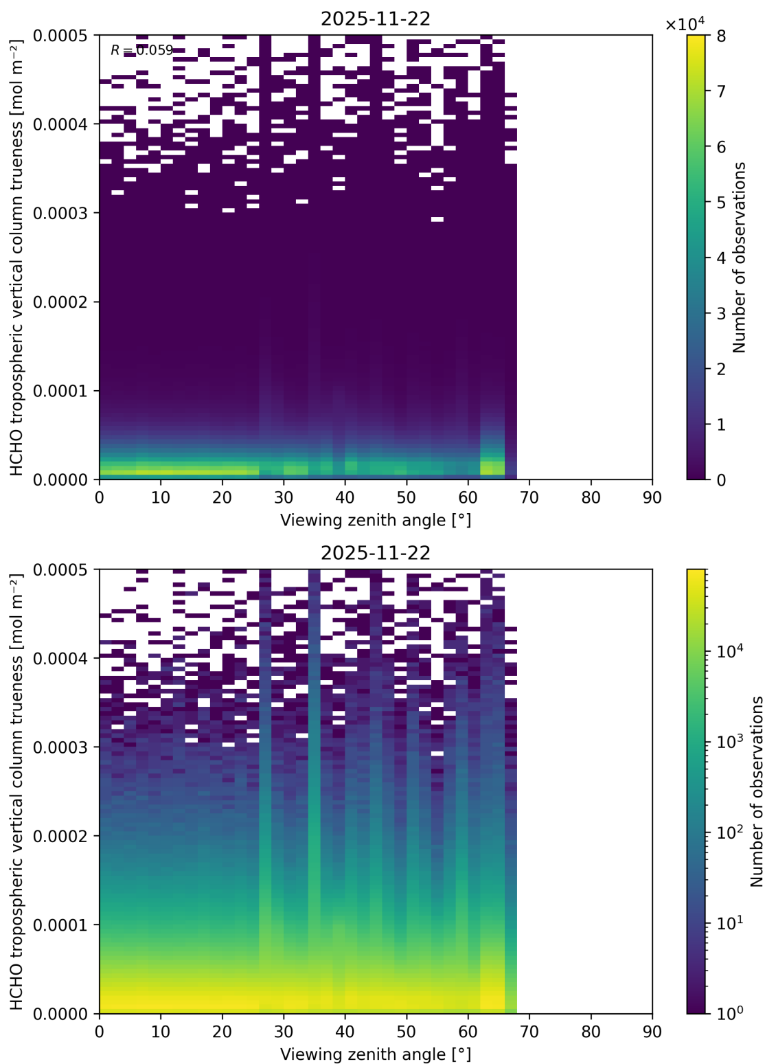
Figure 215: Scatter density plot of “Viewing zenith angle” against “HCHO tropospheric vertical column trueness” for 2025-11-21 to 2025-11-23.
