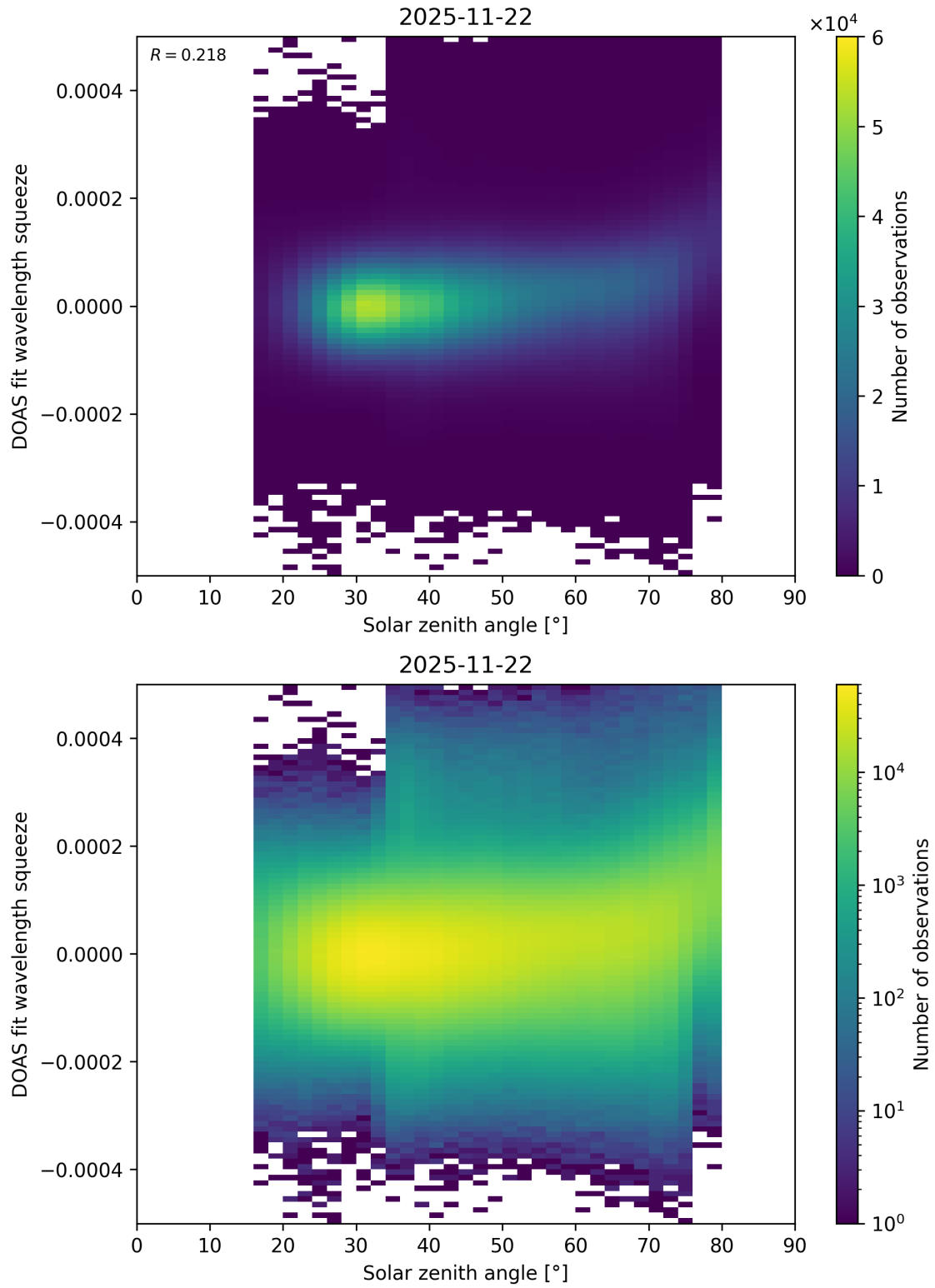
Figure 188: Scatter density plot of “Solar zenith angle” against “DOAS fit wavelength squeeze” for 2025-11-21 to 2025-11-23.
