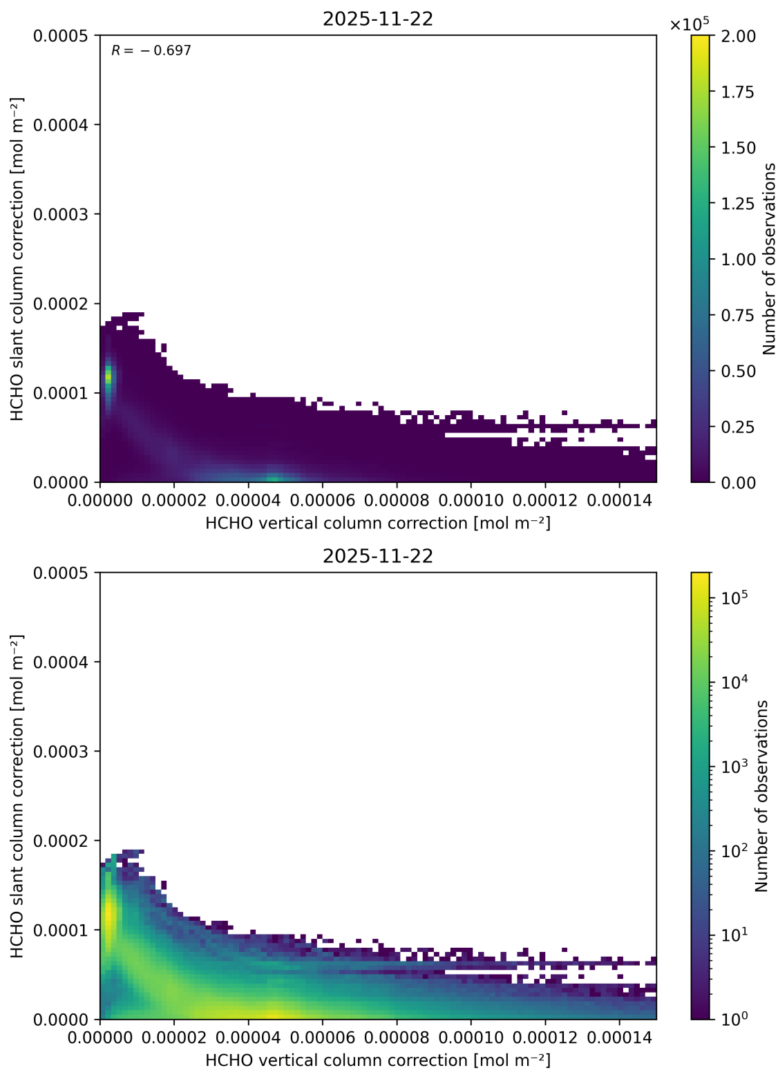
Figure 131: Scatter density plot of “HCHO vertical column correction” against “HCHO slant column correction” for 2025-11-21 to 2025-11-23.
