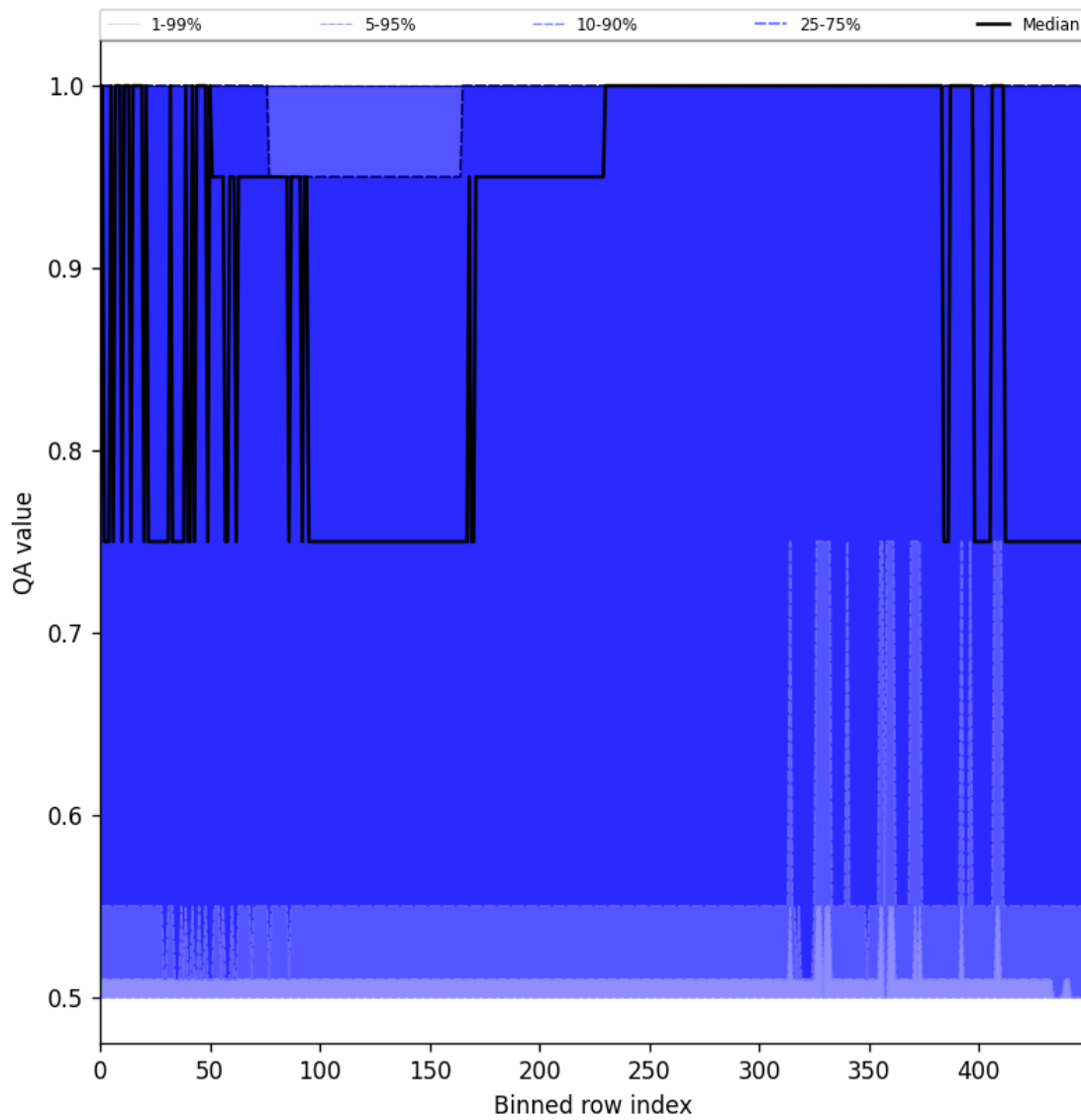
Figure 51: Along track statistics of “QA value” for 2025-11-21 to 2025-11-23
