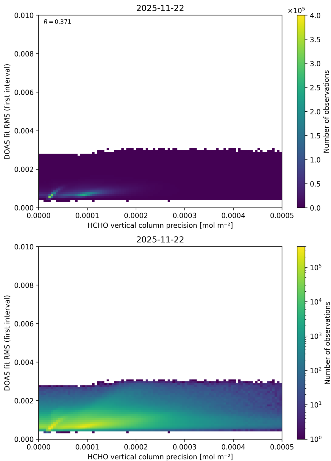
Figure 152: Scatter density plot of “HCHO vertical column precision” against “DOAS fit RMS (first interval)” for 2025-11-21 to 2025-11-23.
