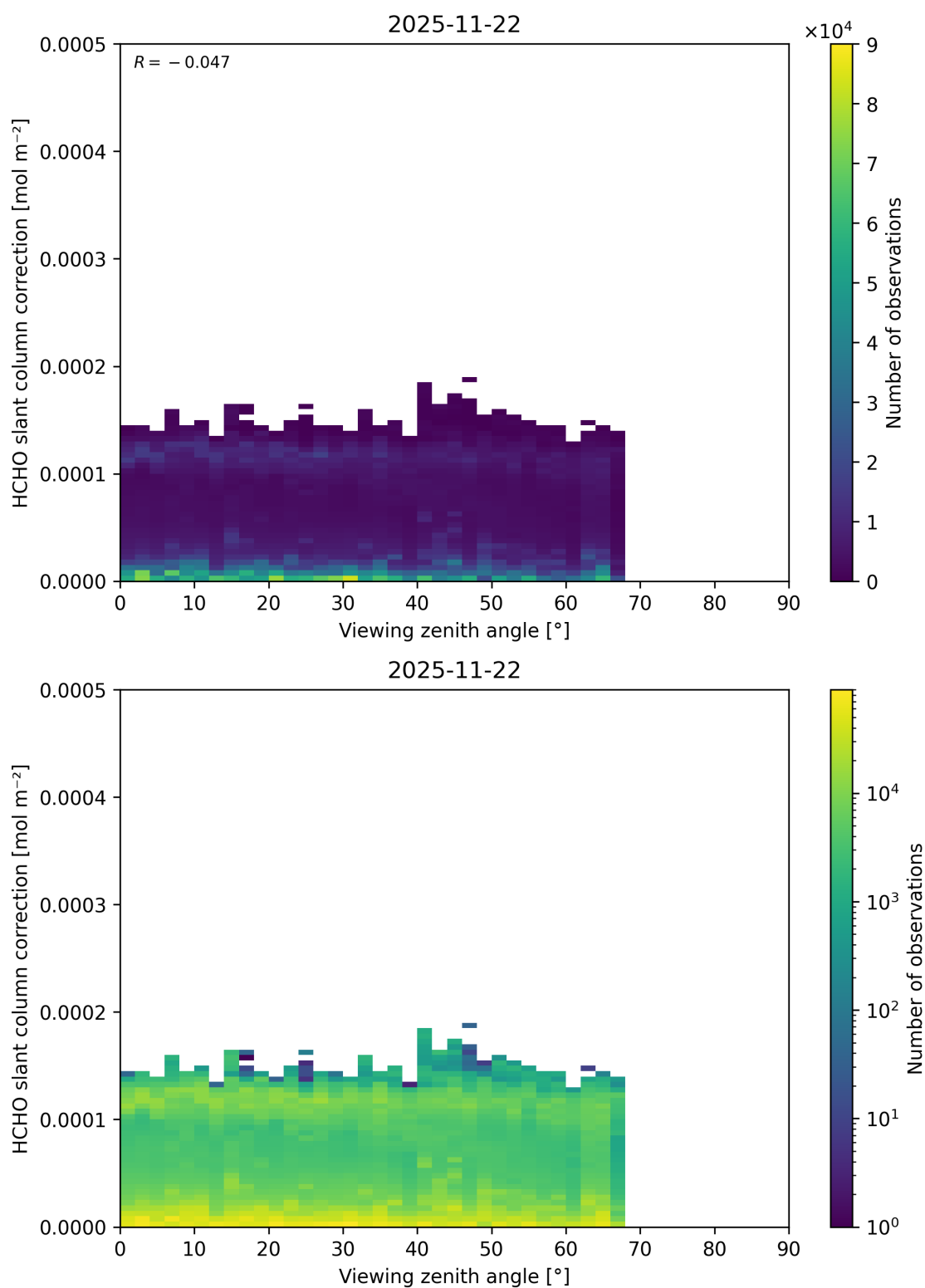
Figure 207: Scatter density plot of “Viewing zenith angle” against “HCHO slant column correction” for 2025-11-21 to 2025-11-23.
