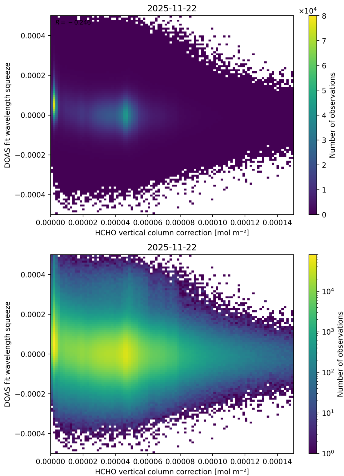
Figure 128: Scatter density plot of “HCHO vertical column correction” against “DOAS fit wavelength squeeze” for 2025-11-21 to 2025-11-23.
