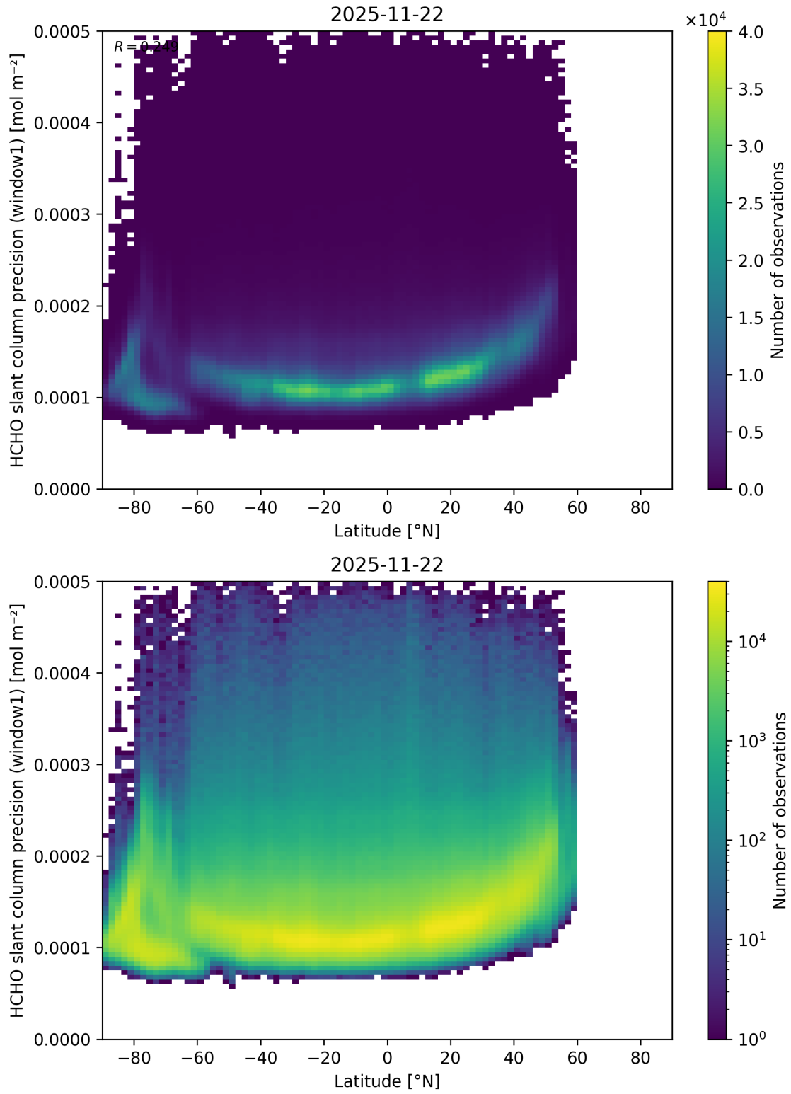
Figure 178: Scatter density plot of “Latitude” against “HCHO slant column precision (window1)” for 2025-11-21 to 2025-11-23.
