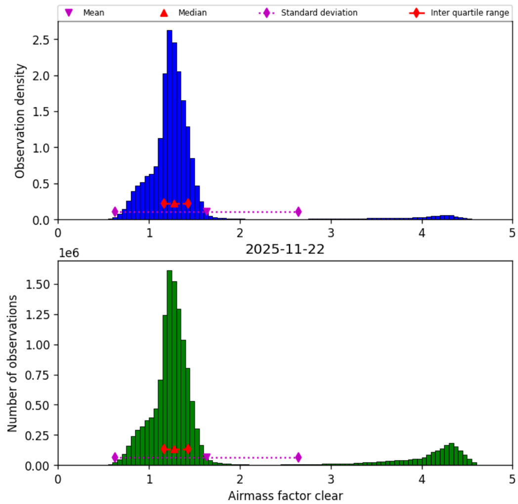
Figure 44: Histogram of “Airmass factor clear” for 2025-11-21 to 2025-11-23
