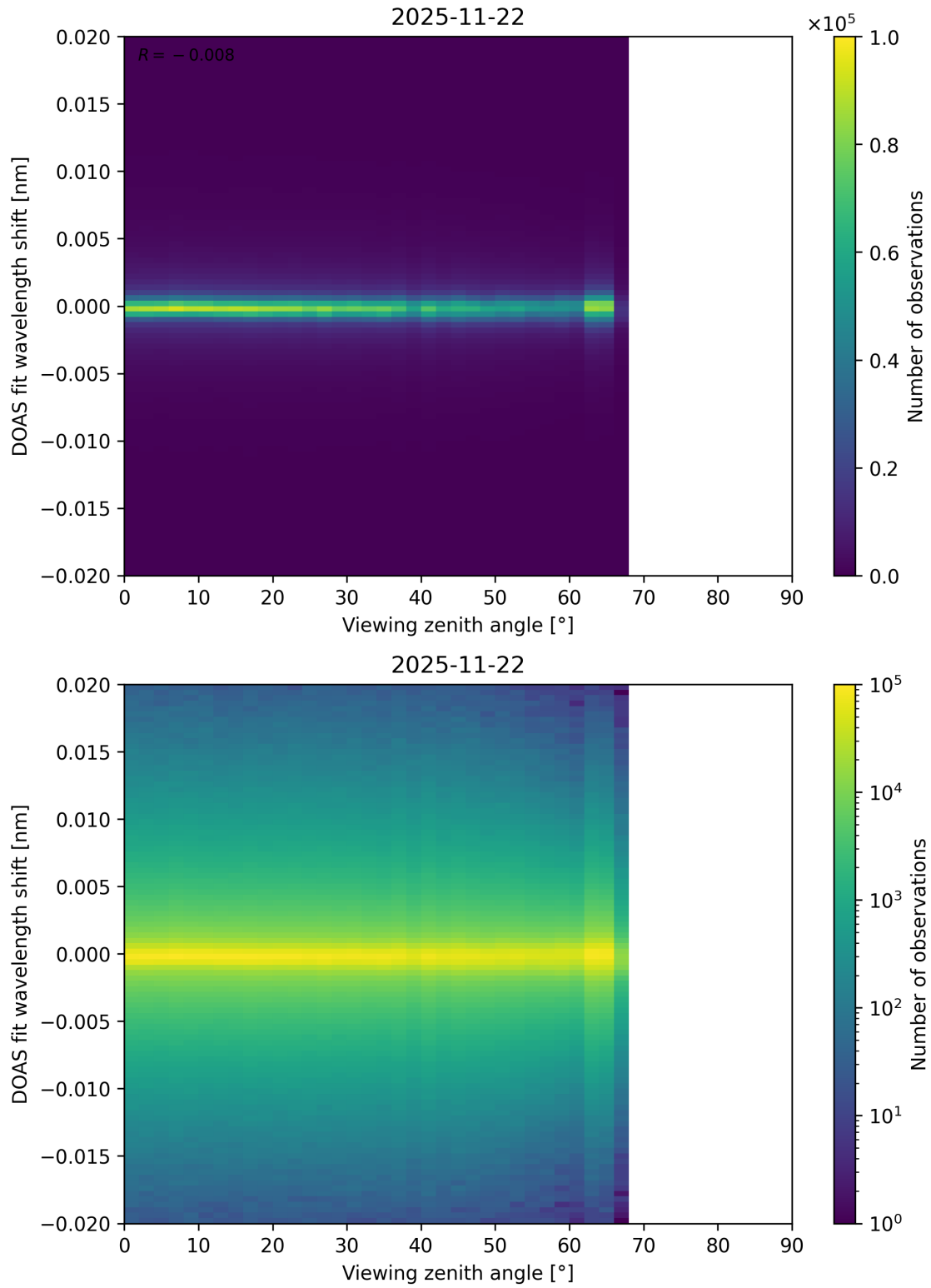
Figure 203: Scatter density plot of “Viewing zenith angle” against “DOAS fit wavelength shift” for 2025-11-21 to 2025-11-23.
