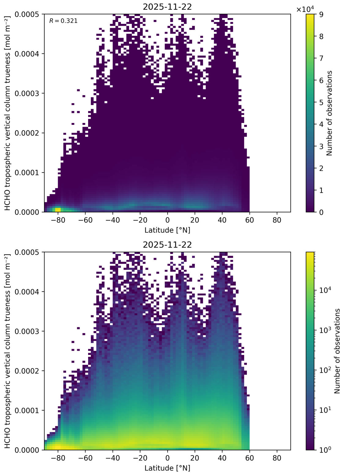
Figure 184: Scatter density plot of “Latitude” against “HCHO tropospheric vertical column trueeness” for 2025-11-21 to 2025-11-23.
