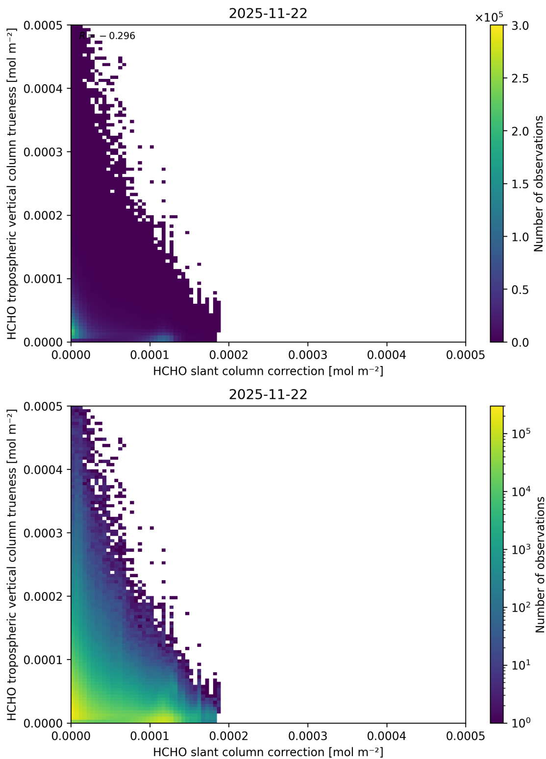
Figure 87: Scatter density plot of “HCHO slant column correction” against “HCHO tropospheric vertical column trueness” for 2025-11-21 to 2025-11-23.
