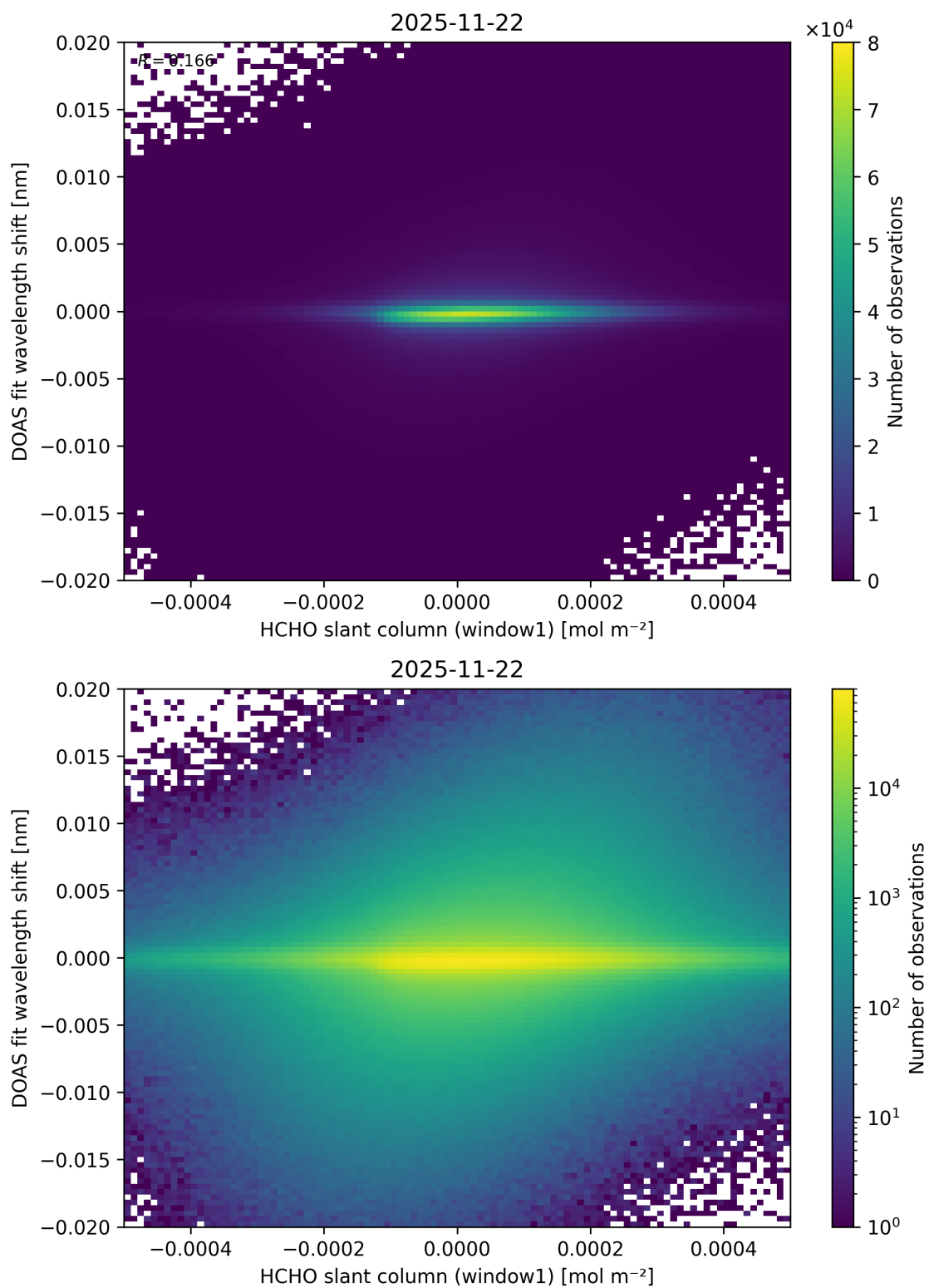
Figure 89: Scatter density plot of “HCHO slant column (window1)” against “DOAS fit wavelength shift” for 2025-11-21 to 2025-11-23.
