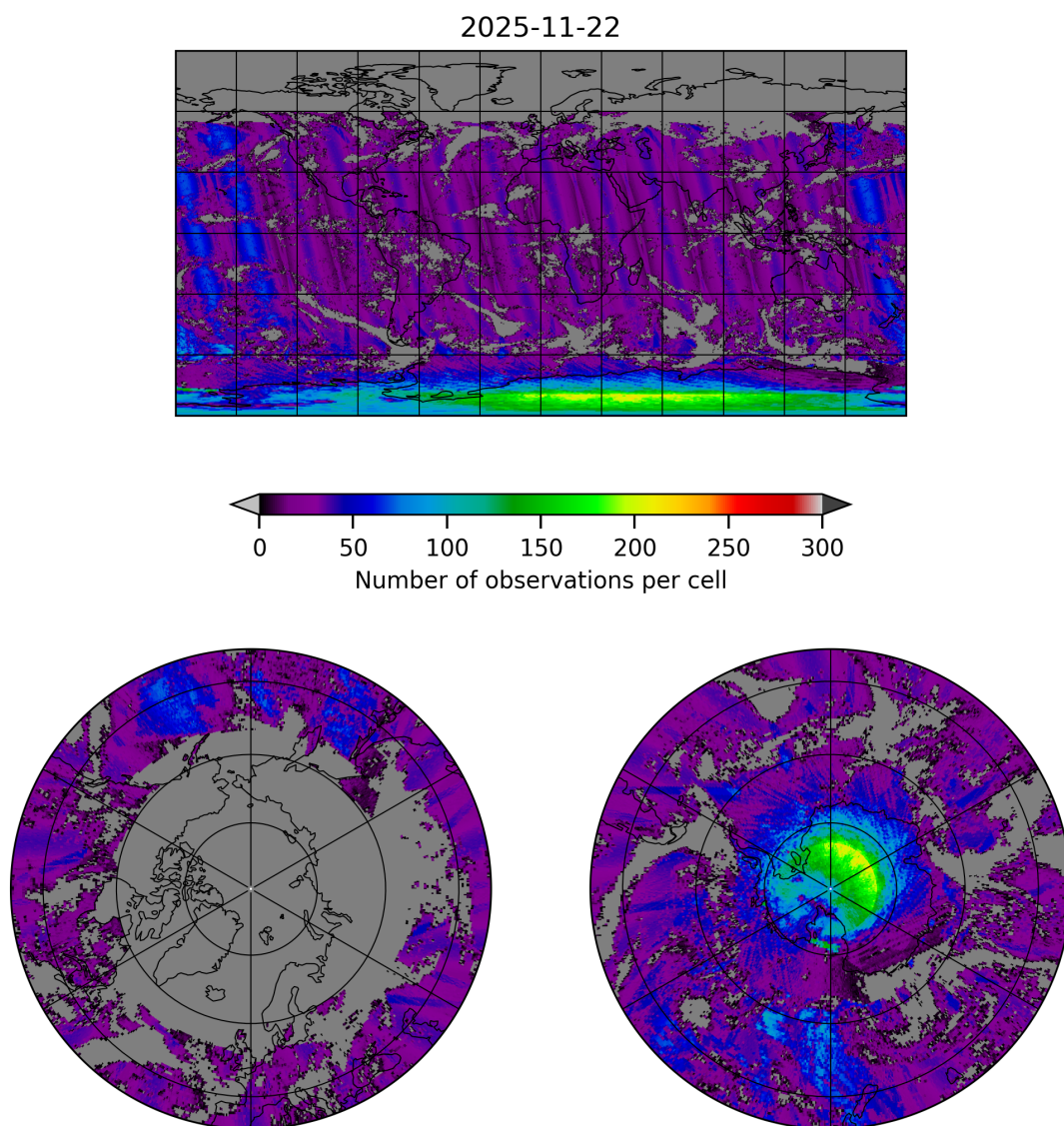
Figure 20: Map of the number of observations for 2025-11-21 to 2025-11-23
