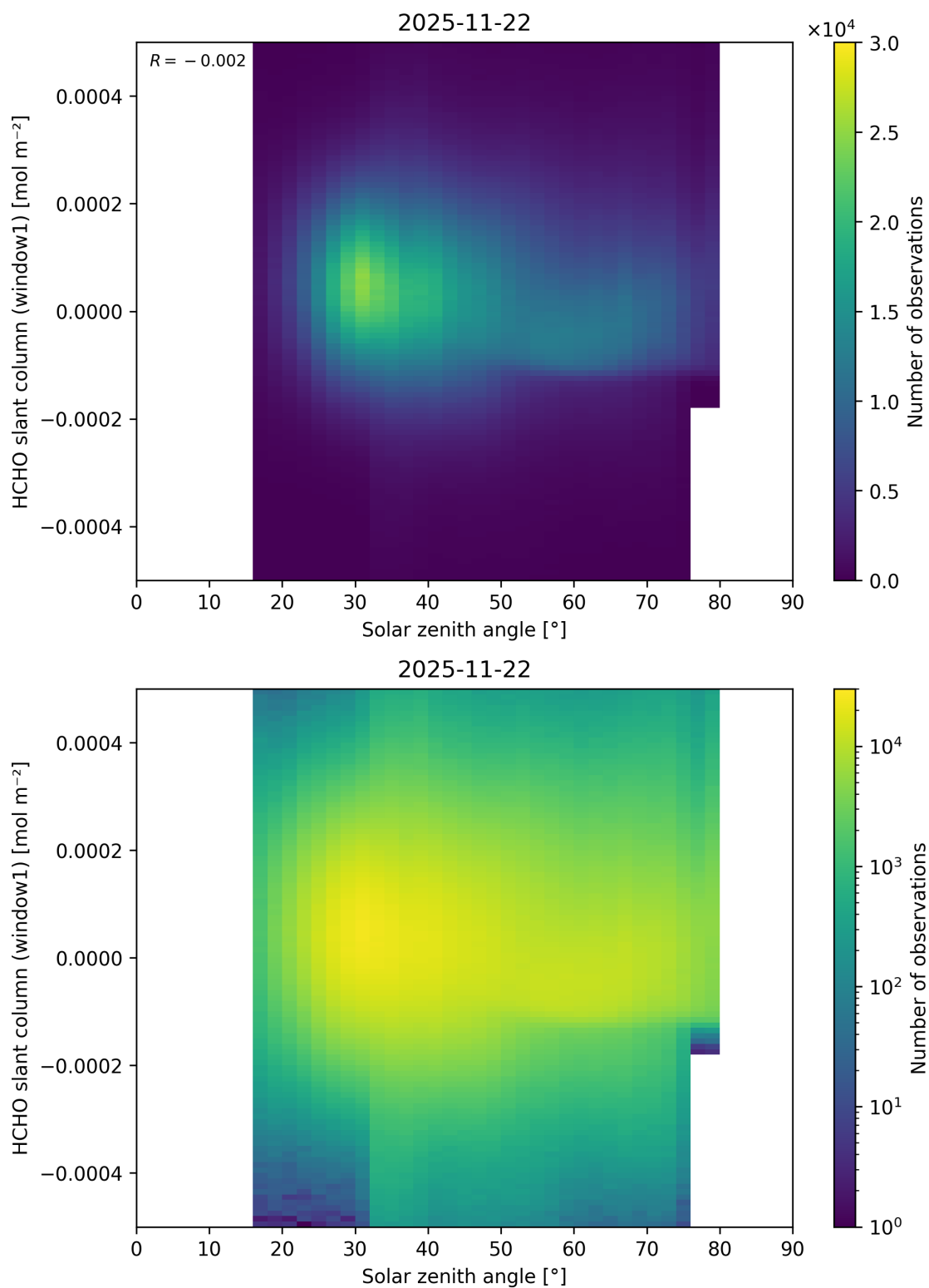
Figure 192: Scatter density plot of “Solar zenith angle” against “HCHO slant column (window1)” for 2025-11-21 to 2025-11-23.
