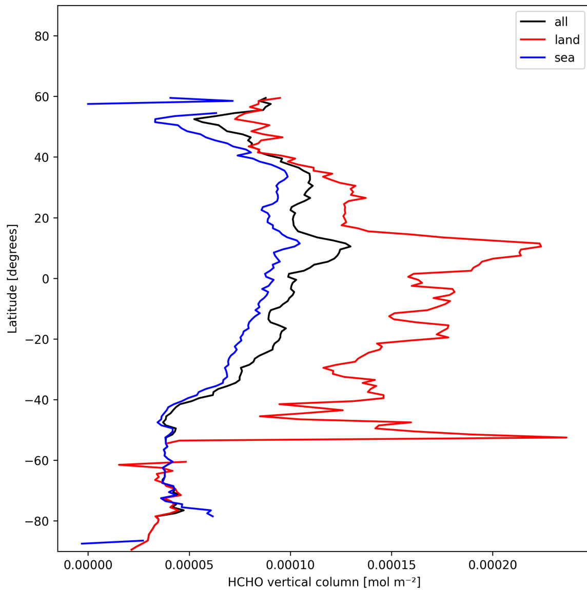
Figure 22: Zonal average of “HCHO vertical column” for 2025-11-21 to 2025-11-23.
