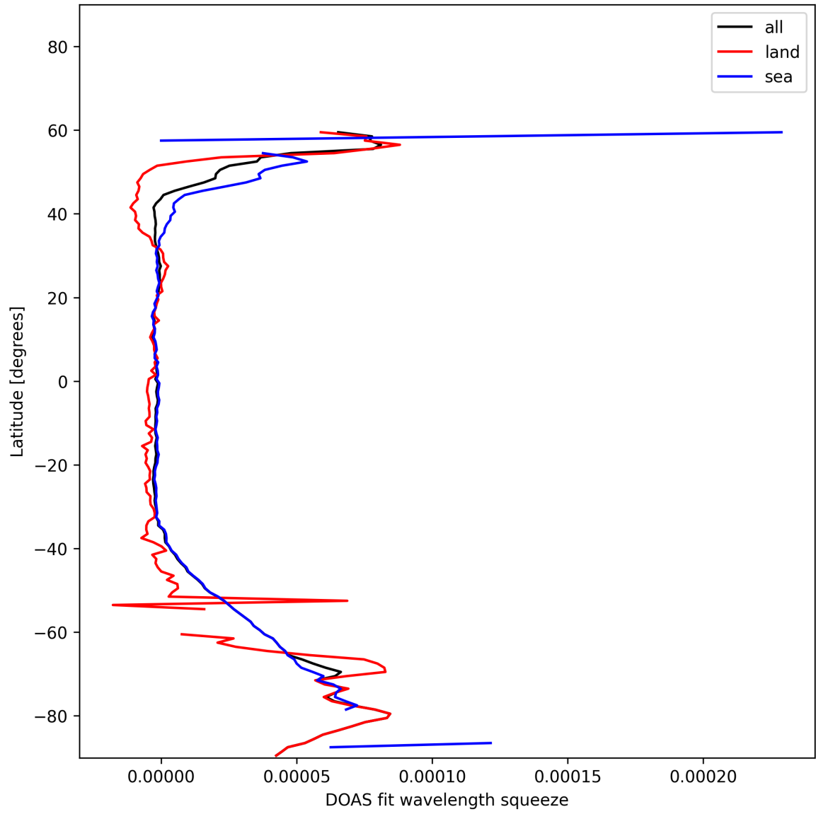
Figure 32: Zonal average of “DOAS fit wavelength squeeze” for 2025-11-21 to 2025-11-23.
