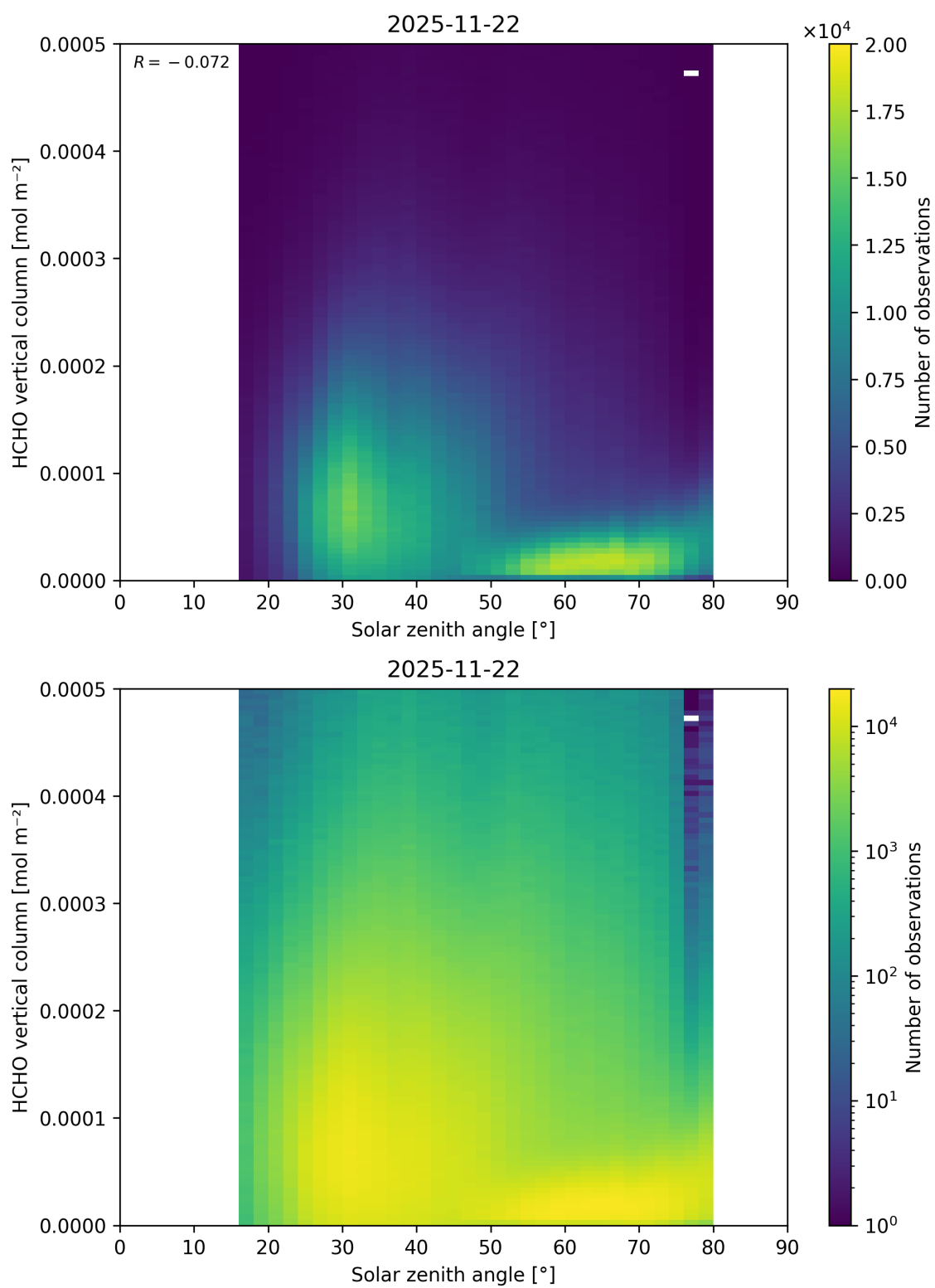
Figure 196: Scatter density plot of “Solar zenith angle” against “HCHO vertical column” for 2025-11-21 to 2025-11-23.
