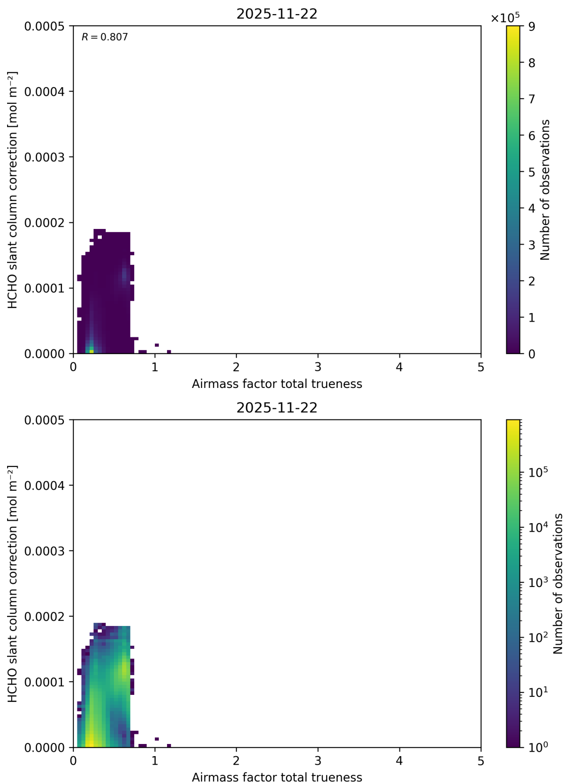
Figure 123: Scatter density plot of “Airmass factor total truiness” against “HCHO slant column correction” for 2025-11-21 to 2025-11-23.
