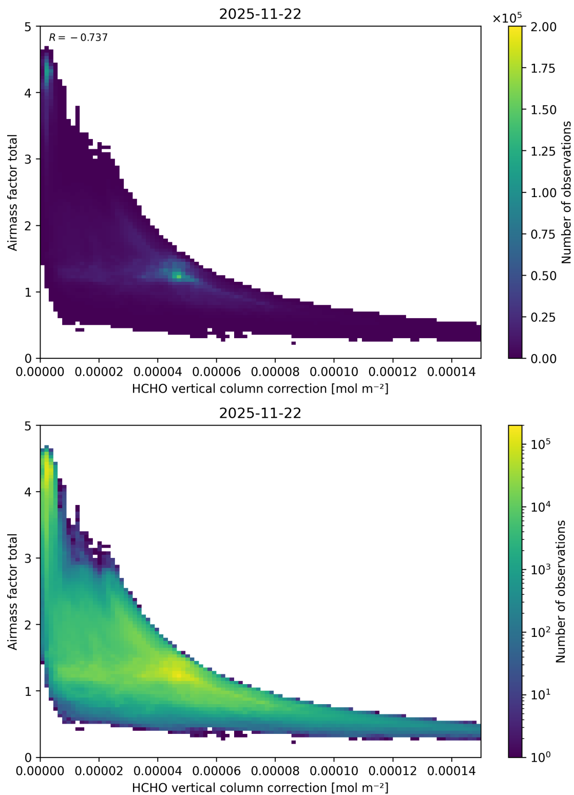
Figure 134: Scatter density plot of “HCHO vertical column correction” against “Airmass factor total” for 2025-11-21 to 2025-11-23.
