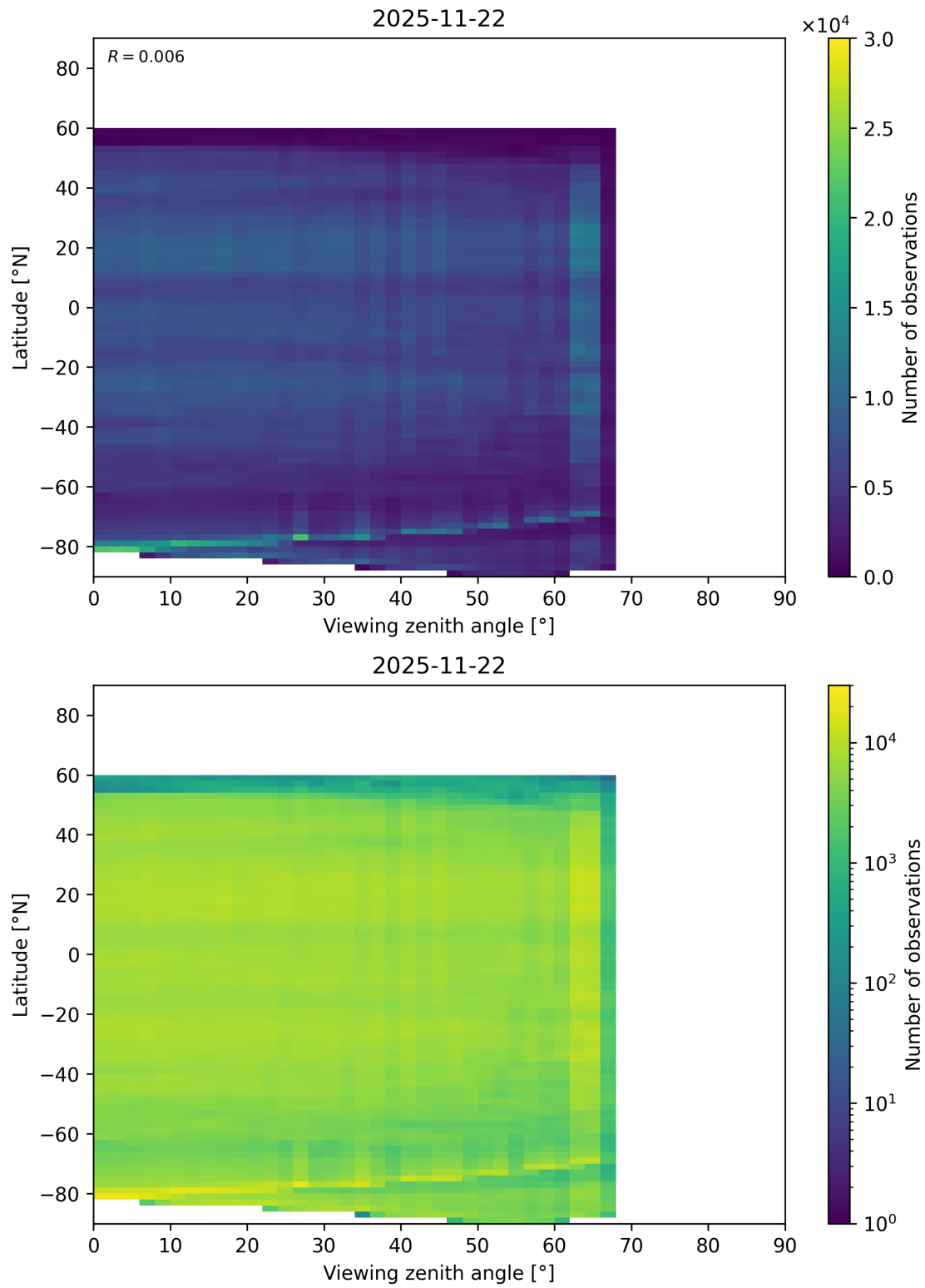
Figure 217: Scatter density plot of “Viewing zenith angle” against “Latitude” for 2025-11-21 to 2025-11-23.
