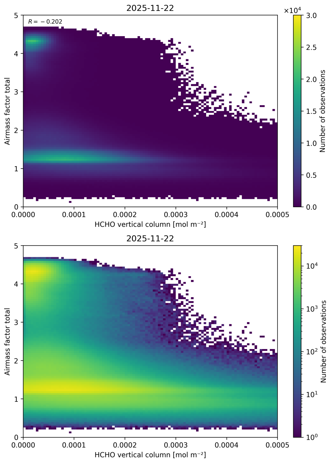
Figure 146: Scatter density plot of “HCHO vertical column” against “Airmass factor total” for 2025-11-21 to 2025-11-23.
