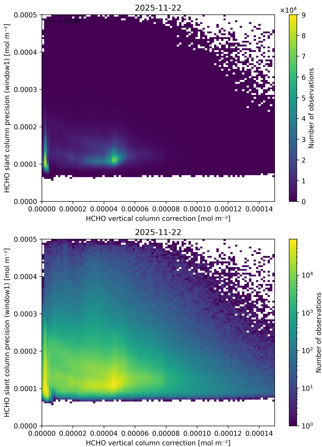
Figure 133: Scatter density plot of “HCHO vertical column correction” against “HCHO slant column precision (window1)” for 2025-11-21 to 2025-11-23.
