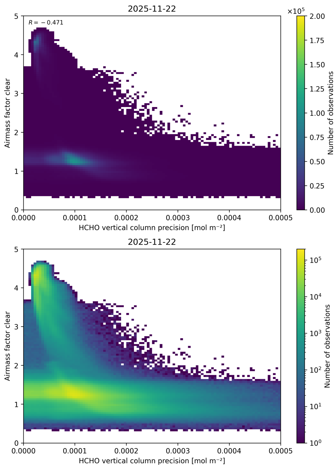
Figure 155: Scatter density plot of “HCHO vertical column precision” against “Airmass factor clear” for 2025-11-21 to 2025-11-23.
