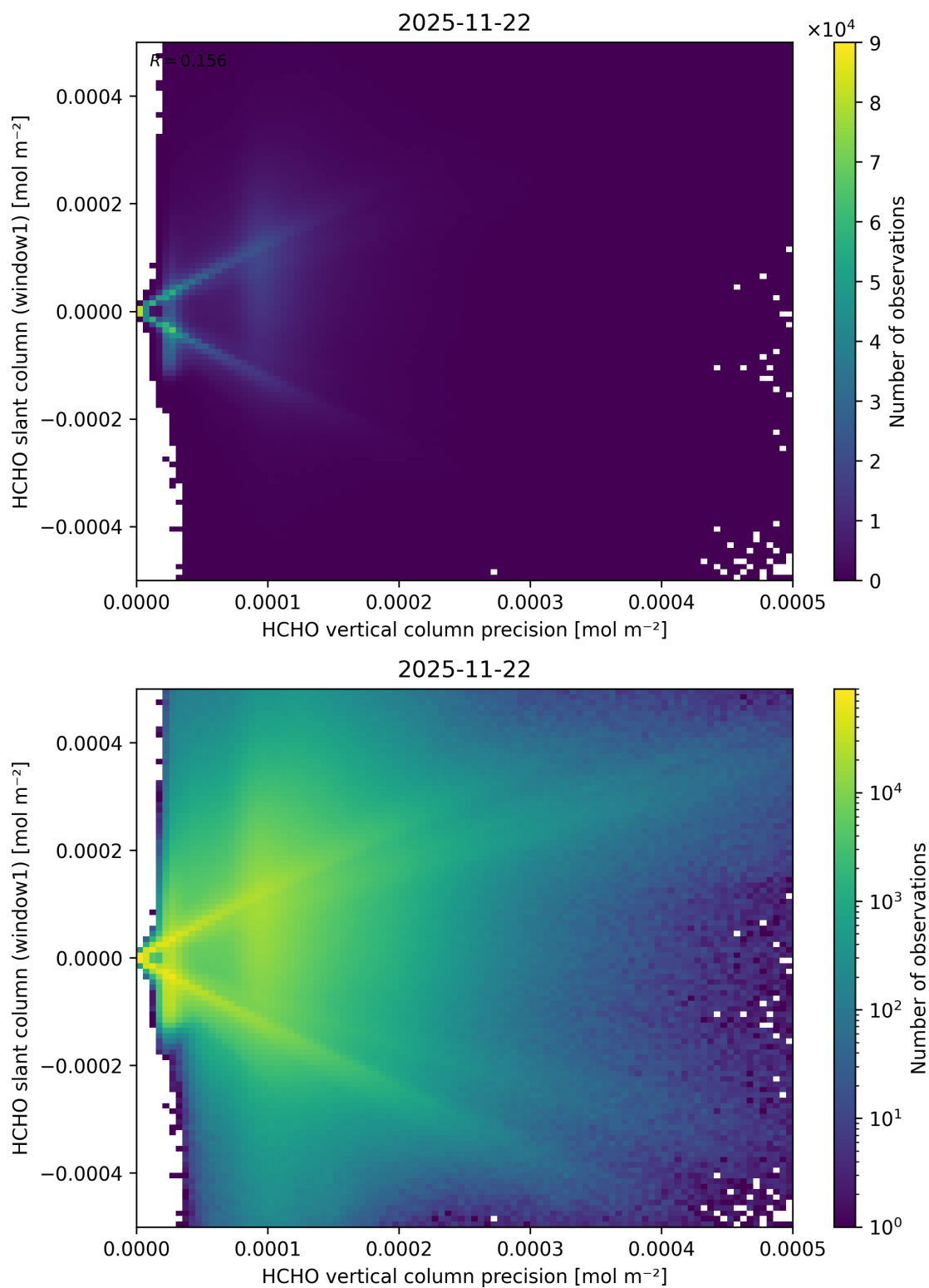
Figure 158: Scatter density plot of “HCHO vertical column precision” against “HCHO slant column (window1)” for 2025-11-21 to 2025-11-23.
