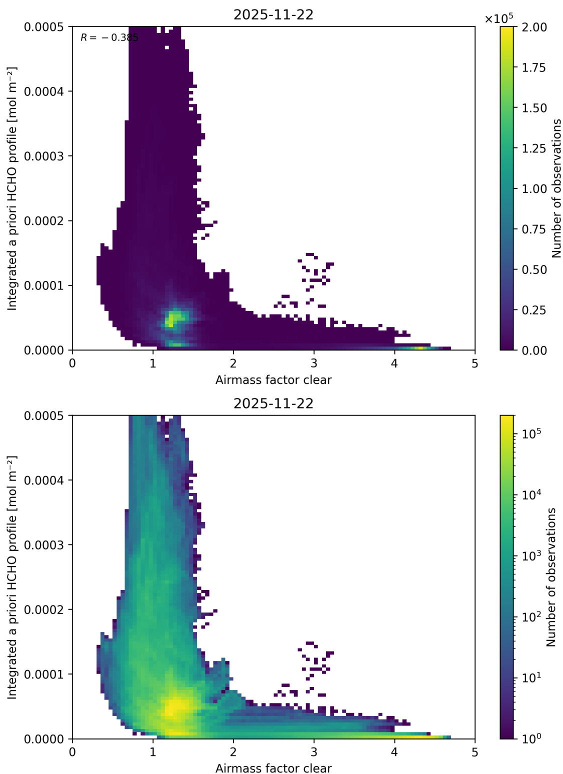
Figure 84: Scatter density plot of “Airmass factor clear” against “Integrated a priori HCHO profile” for 2025-11-21 to 2025-11-23.
