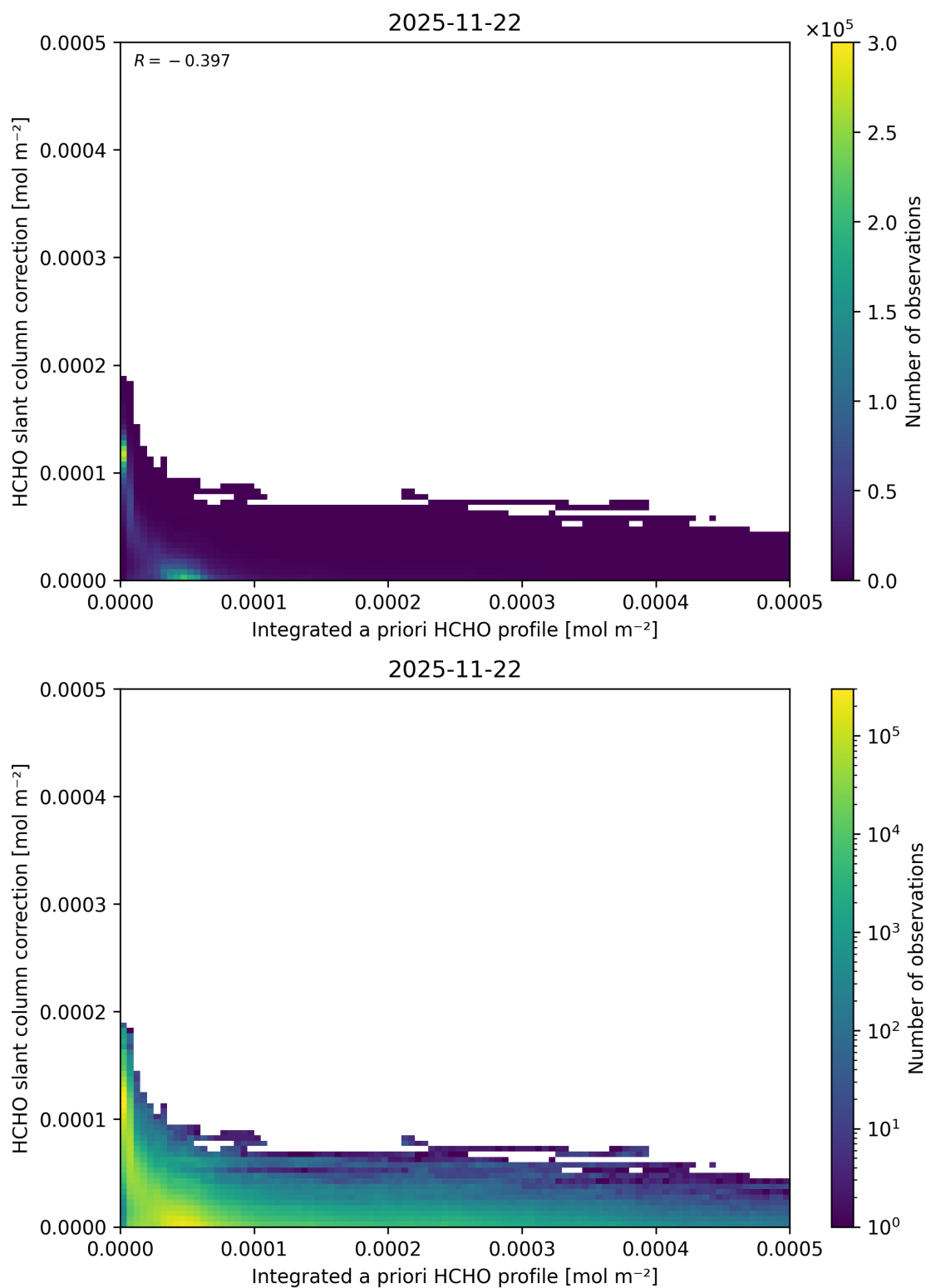
Figure 169: Scatter density plot of “Integrated a priori HCHO profile” against “HCHO slant column correction” for 2025-11-21 to 2025-11-23.
