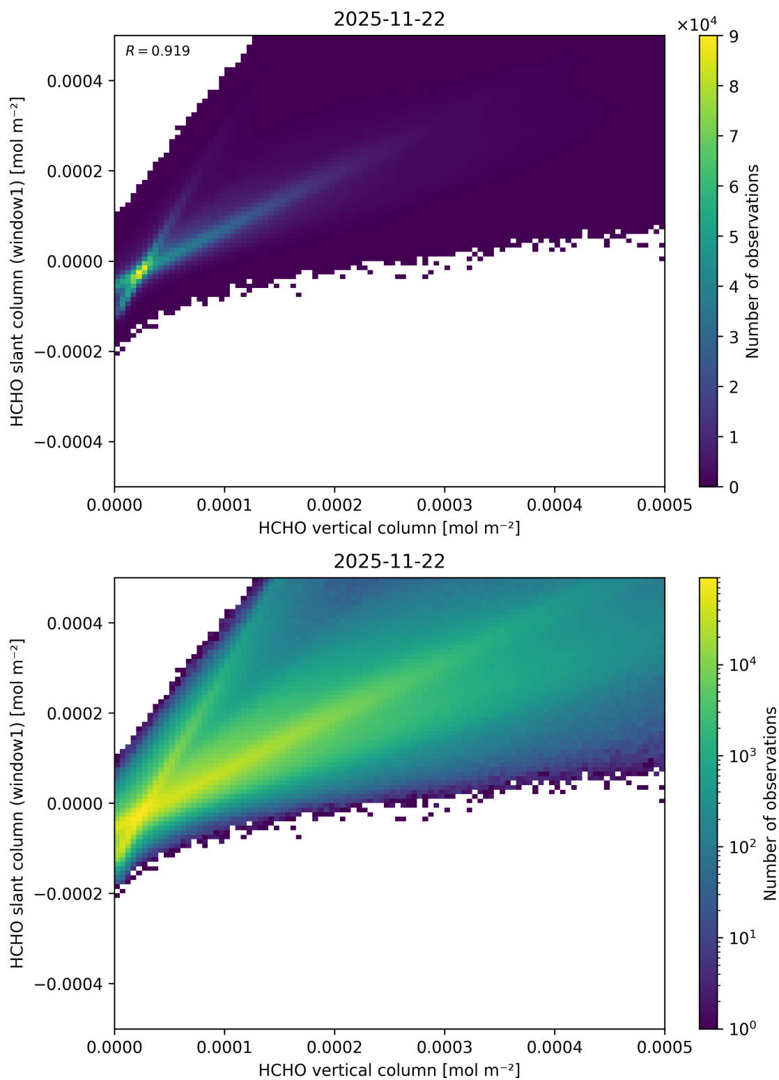
Figure 144: Scatter density plot of “HCHO vertical column” against “HCHO slant column (window1)” for 2025-11-21 to 2025-11-23.
