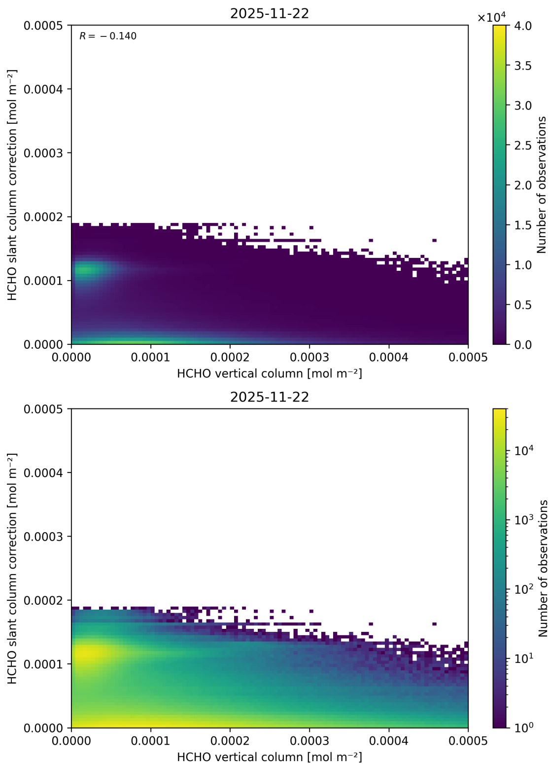
Figure 143: Scatter density plot of “HCHO vertical column” against “HCHO slant column correction” for 2025-11-21 to 2025-11-23.
