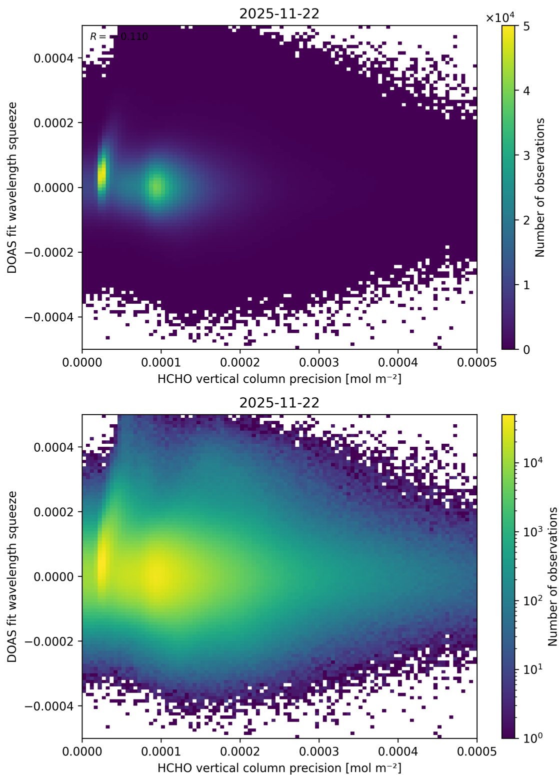
Figure 154: Scatter density plot of “HCHO vertical column precision” against “DOAS fit wavelength squeeze” for 2025-11-21 to 2025-11-23.
