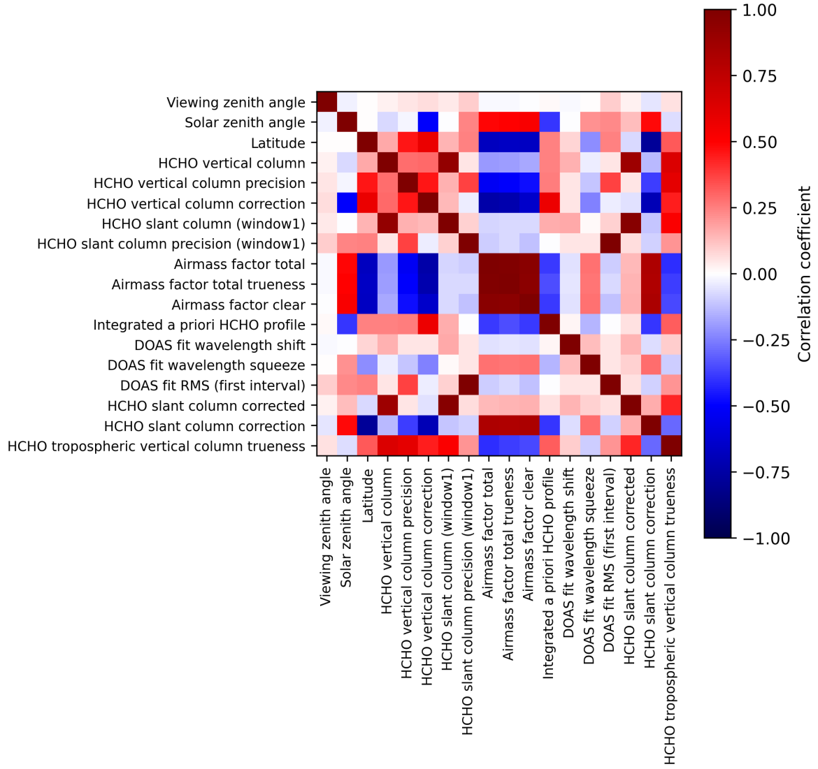
Figure 2: Map of correlation matrix for 2025-11-21 to 2025-11-23.
