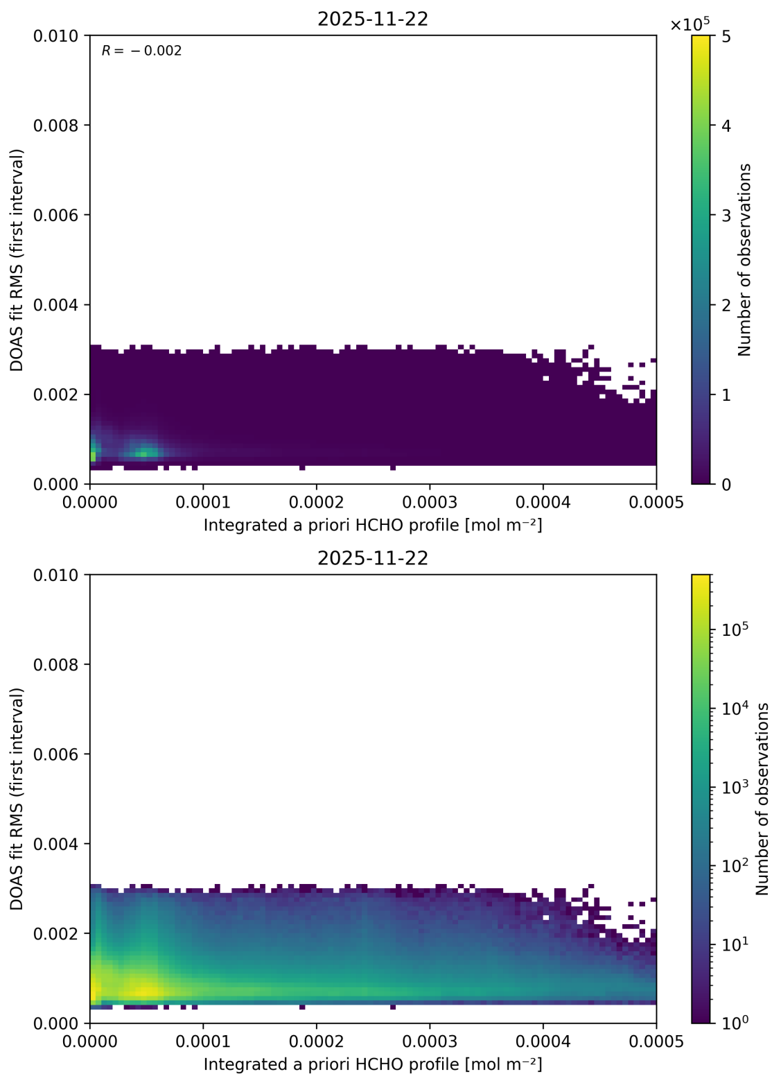
Figure 165: Scatter density plot of “Integrated a priori HCHO profile” against “DOAS fit RMS (first interval)” for 2025-11-21 to 2025-11-23.
