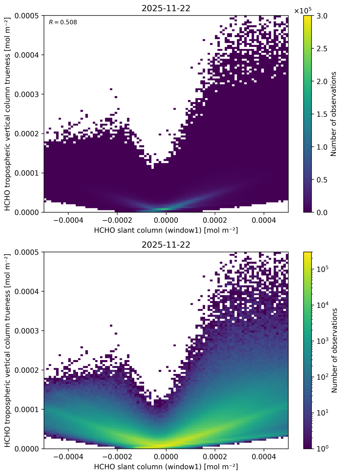
Figure 97: Scatter density plot of “HCHO slant column (window1)” against “HCHO tropospheric vertical column trueness” for 2025-11-21 to 2025-11-23.
