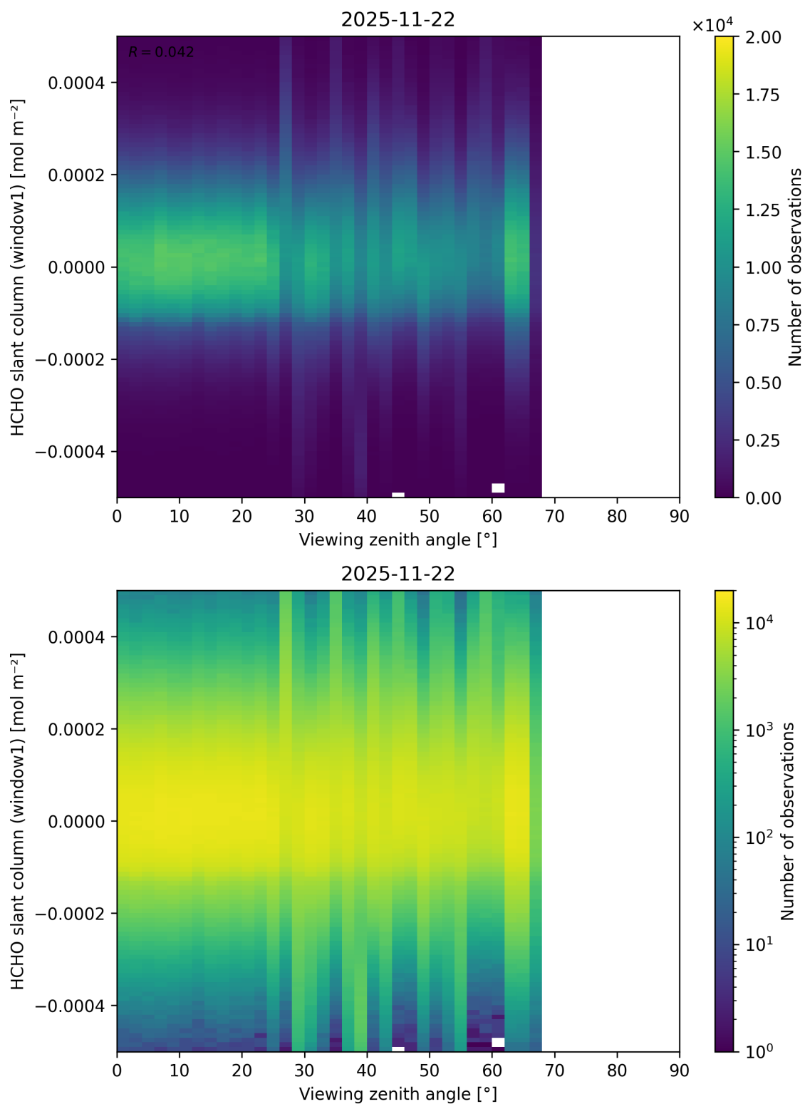
Figure 208: Scatter density plot of “Viewing zenith angle” against “HCHO slant column (window1)” for 2025-11-21 to 2025-11-23.
