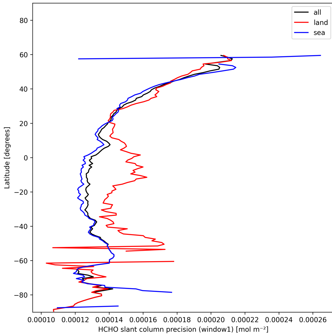
Figure 26: Zonal average of “HCHO slant column precision (window1)” for 2025-11-21 to 2025-11-23.
