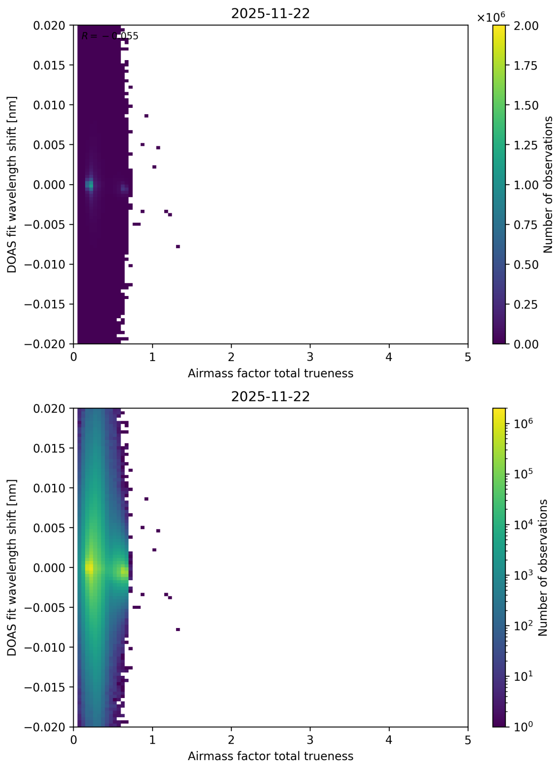
Figure 119: Scatter density plot of “Airmass factor total trueness” against “DOAS fit wavelength shift” for 2025-11-21 to 2025-11-23.
