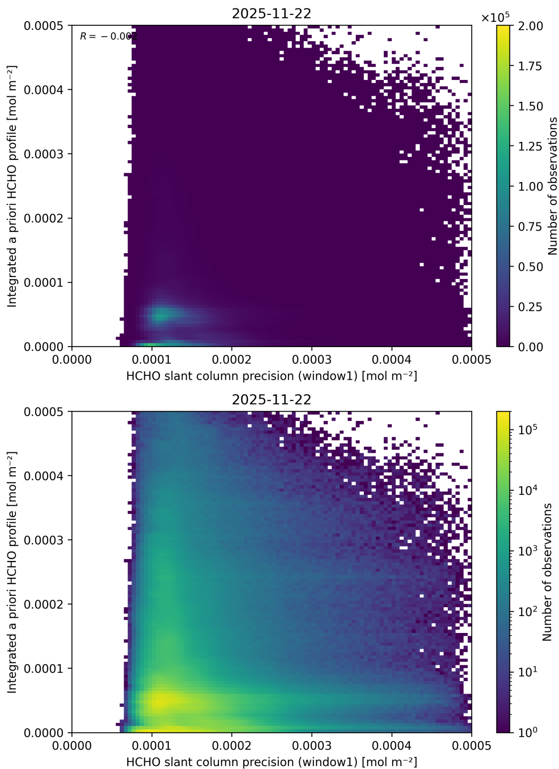
Figure 108: Scatter density plot of “HCHO slant column precision (window1)” against “Integrated a priori HCHO profile” for 2025-11-21 to 2025-11-23.
