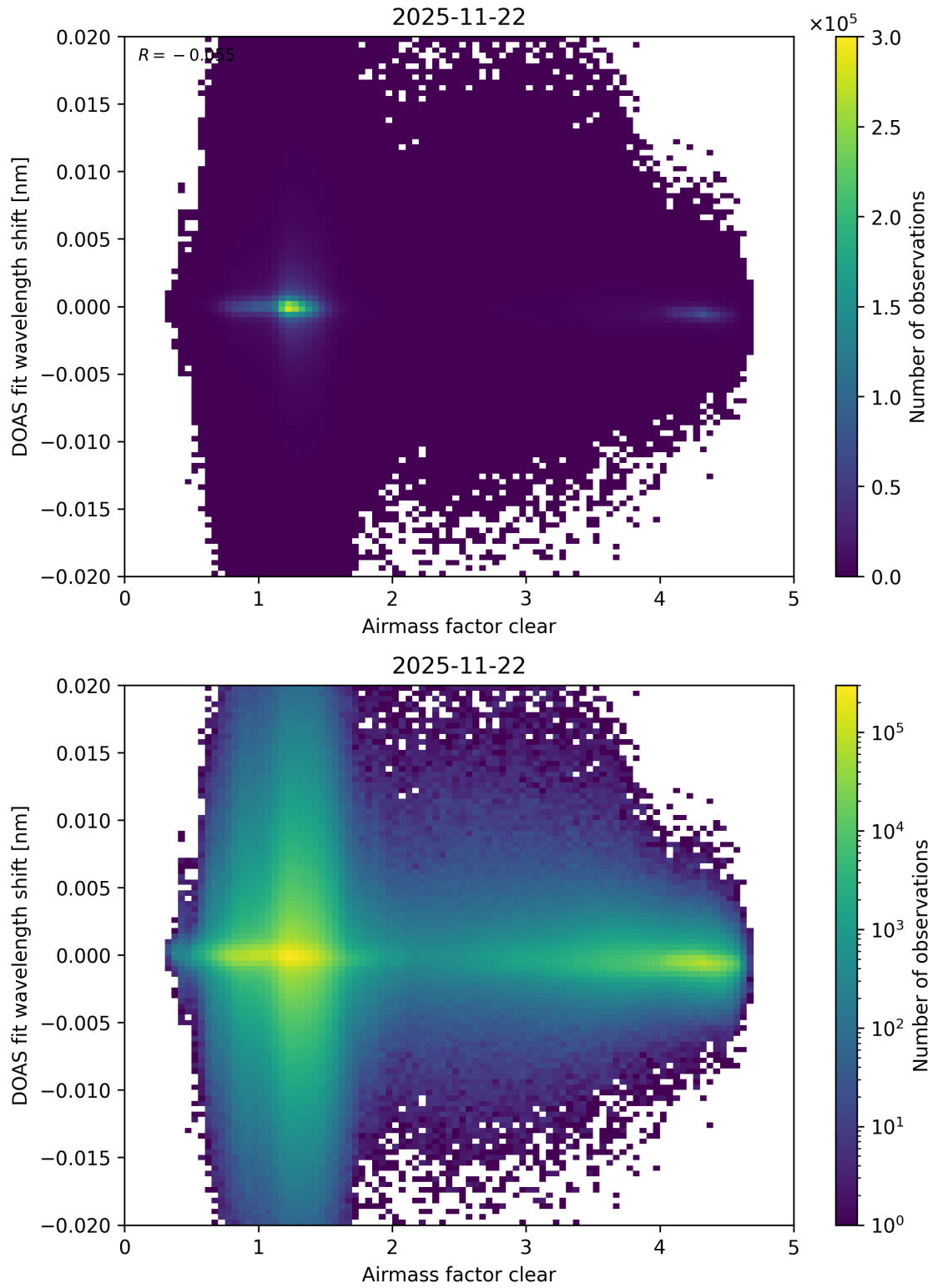
Figure 79: Scatter density plot of “Airmass factor clear” against “DOAS fit wavelength shift” for 2025-11-21 to 2025-11-23.
