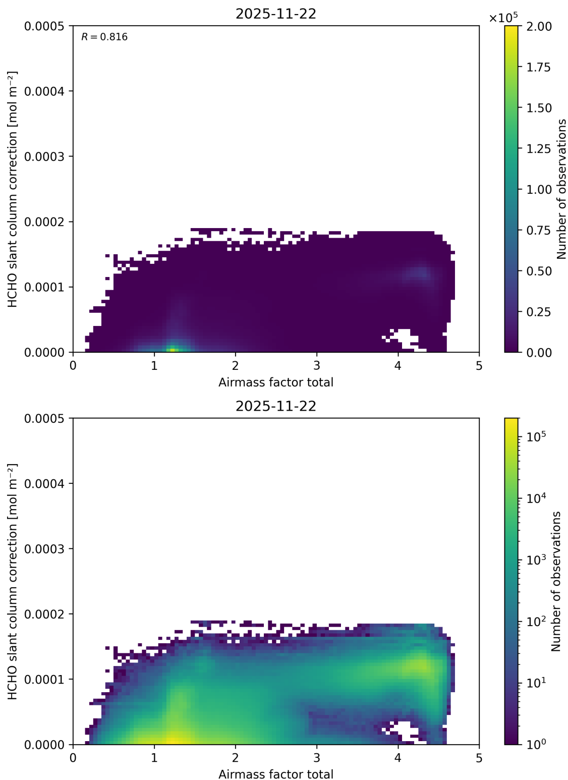
Figure 114: Scatter density plot of “Airmass factor total” against “HCHO slant column correction” for 2025-11-21 to 2025-11-23.
