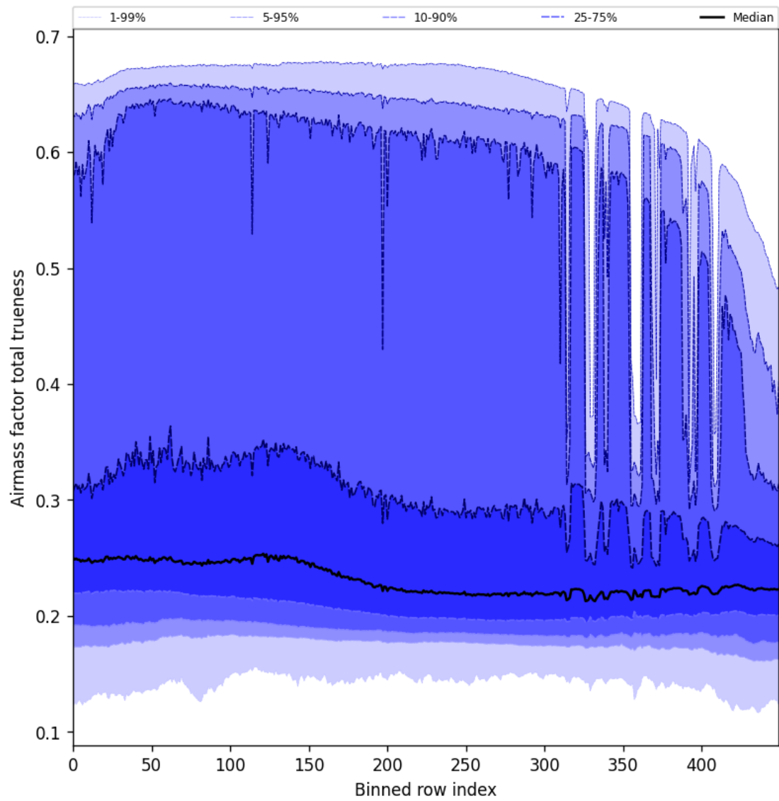
Figure 58: Along track statistics of “Airmass factor total trueness” for 2025-11-21 to 2025-11-23
