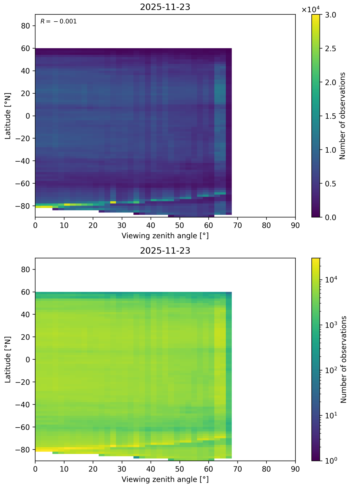
Figure 217: Scatter density plot of “Viewing zenith angle” against “Latitude” for 2025-11-23 to 2025-11-24.
