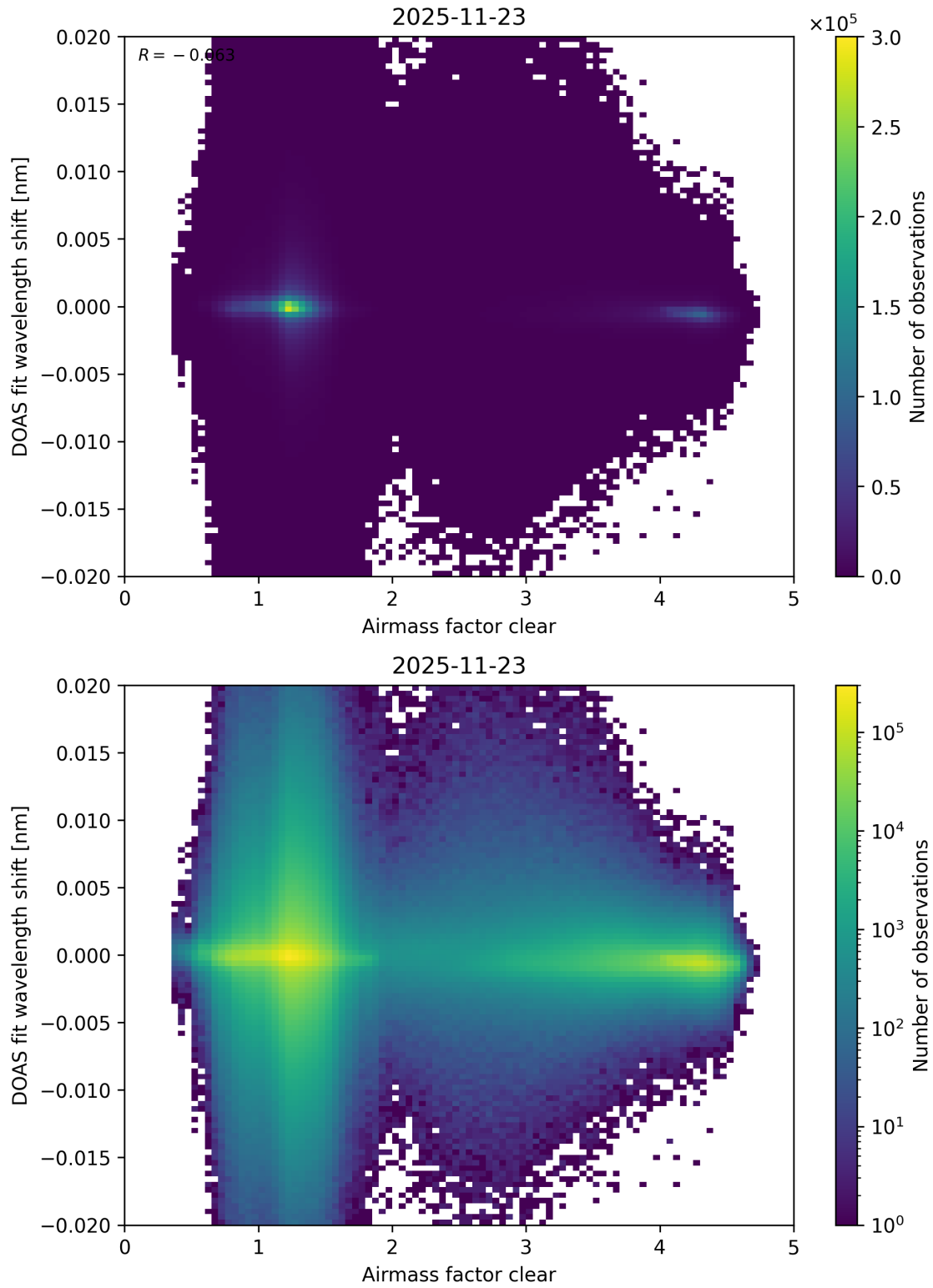
Figure 79: Scatter density plot of “Airmass factor clear” against “DOAS fit wavelength shift” for 2025-11-23 to 2025-11-24.
