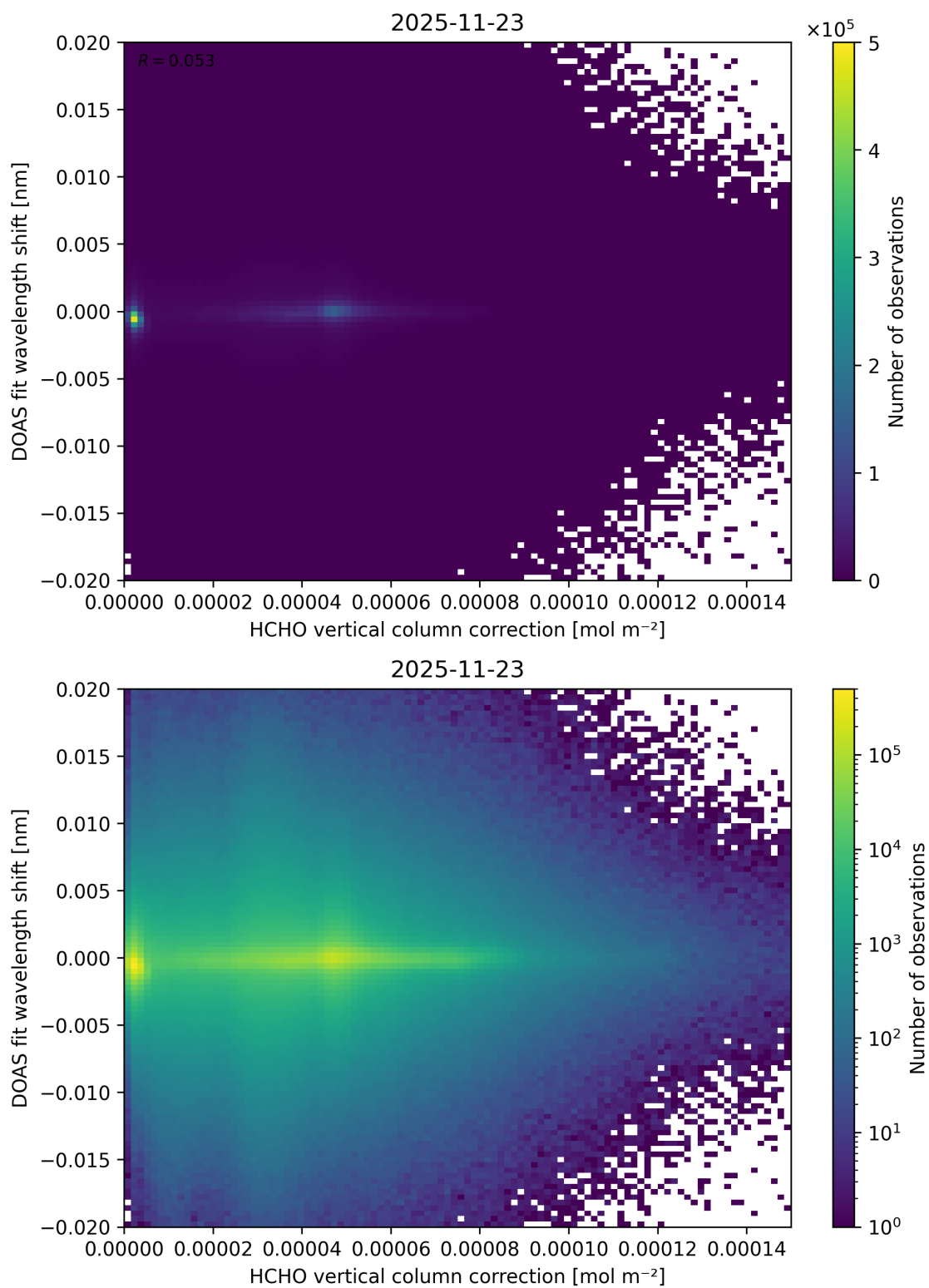
Figure 127: Scatter density plot of “HCHO vertical column correction” against “DOAS fit wavelength shift” for 2025-11-23 to 2025-11-24.
