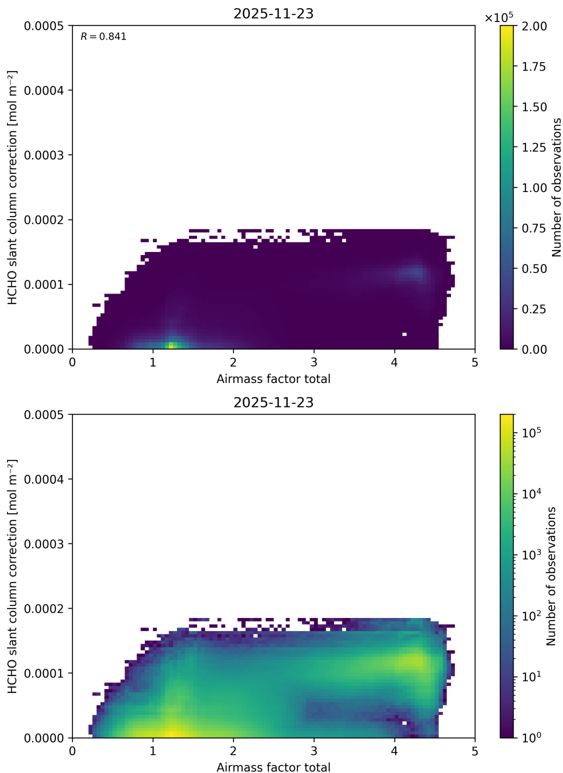
Figure 114: Scatter density plot of “Airmass factor total” against “HCHO slant column correction” for 2025-11-23 to 2025-11-24.
