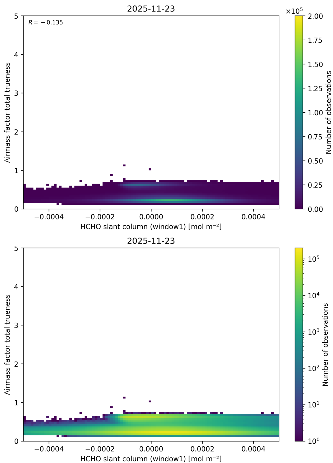
Figure 96: Scatter density plot of “HCHO slant column (window1)” against “Airmass factor total trueneess” for 2025-11-23 to 2025-11-24.
