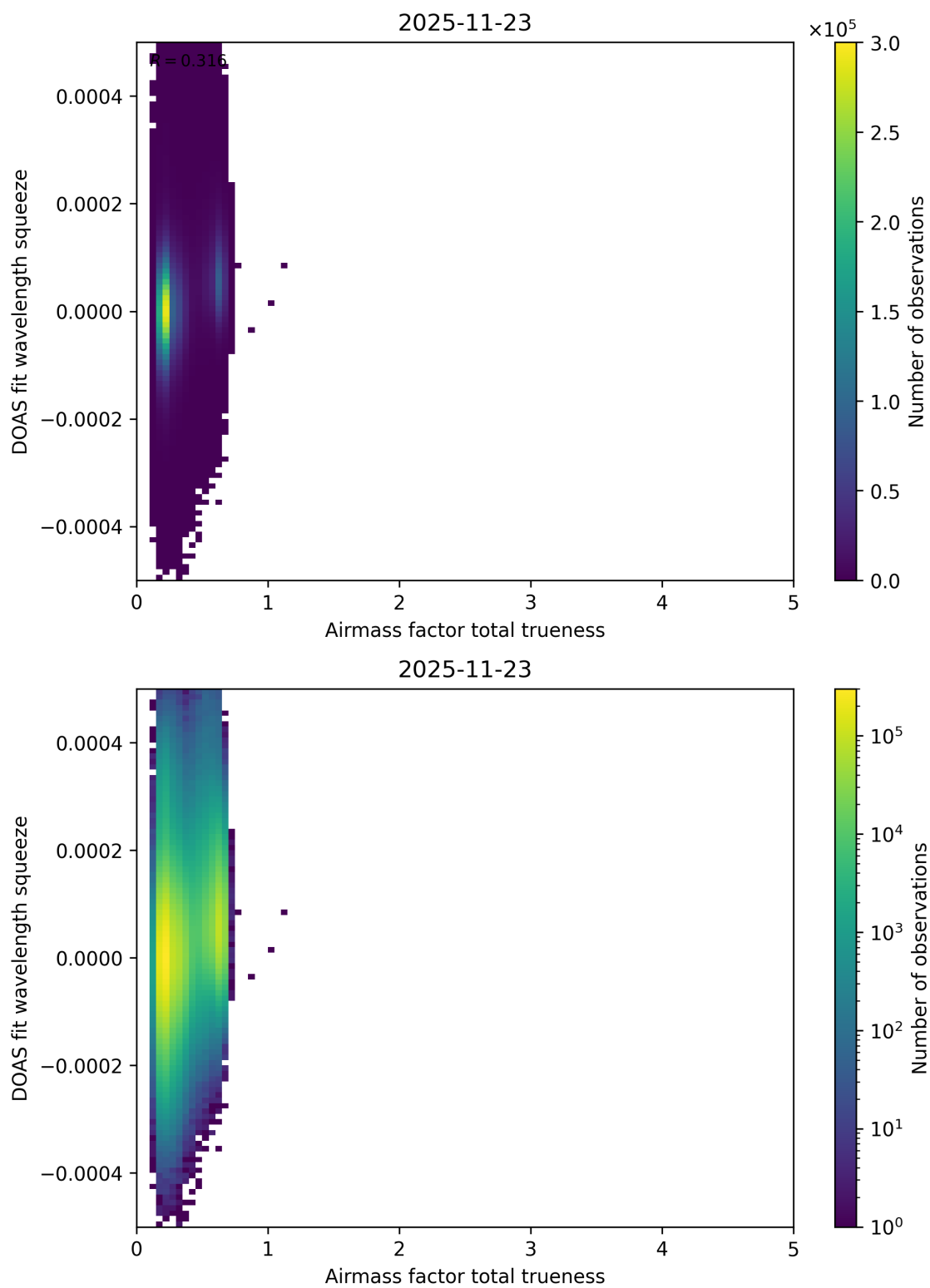
Figure 120: Scatter density plot of “Airmass factor total trueness” against “DOAS fit wavelength squeeze” for 2025-11-23 to 2025-11-24.
