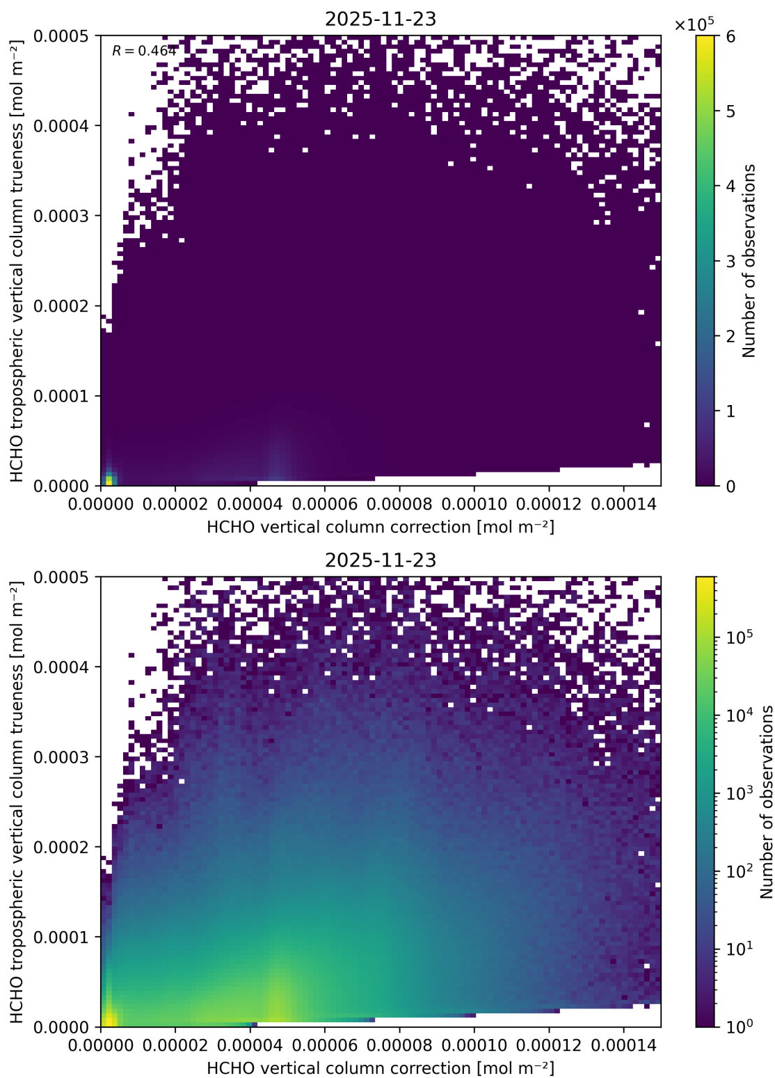
Figure 136: Scatter density plot of “HCHO vertical column correction” against “HCHO tropospheric vertical column true-ness” for 2025-11-23 to 2025-11-24.
