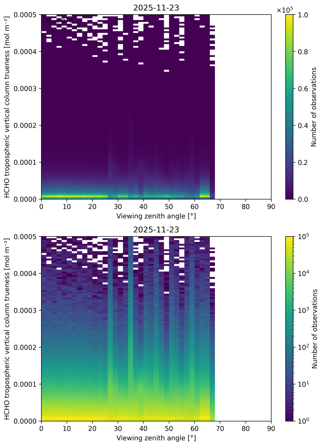
Figure 215: Scatter density plot of “Viewing zenith angle” against “HCHO tropospheric vertical column truthness” for 2025-11-23 to 2025-11-24.
