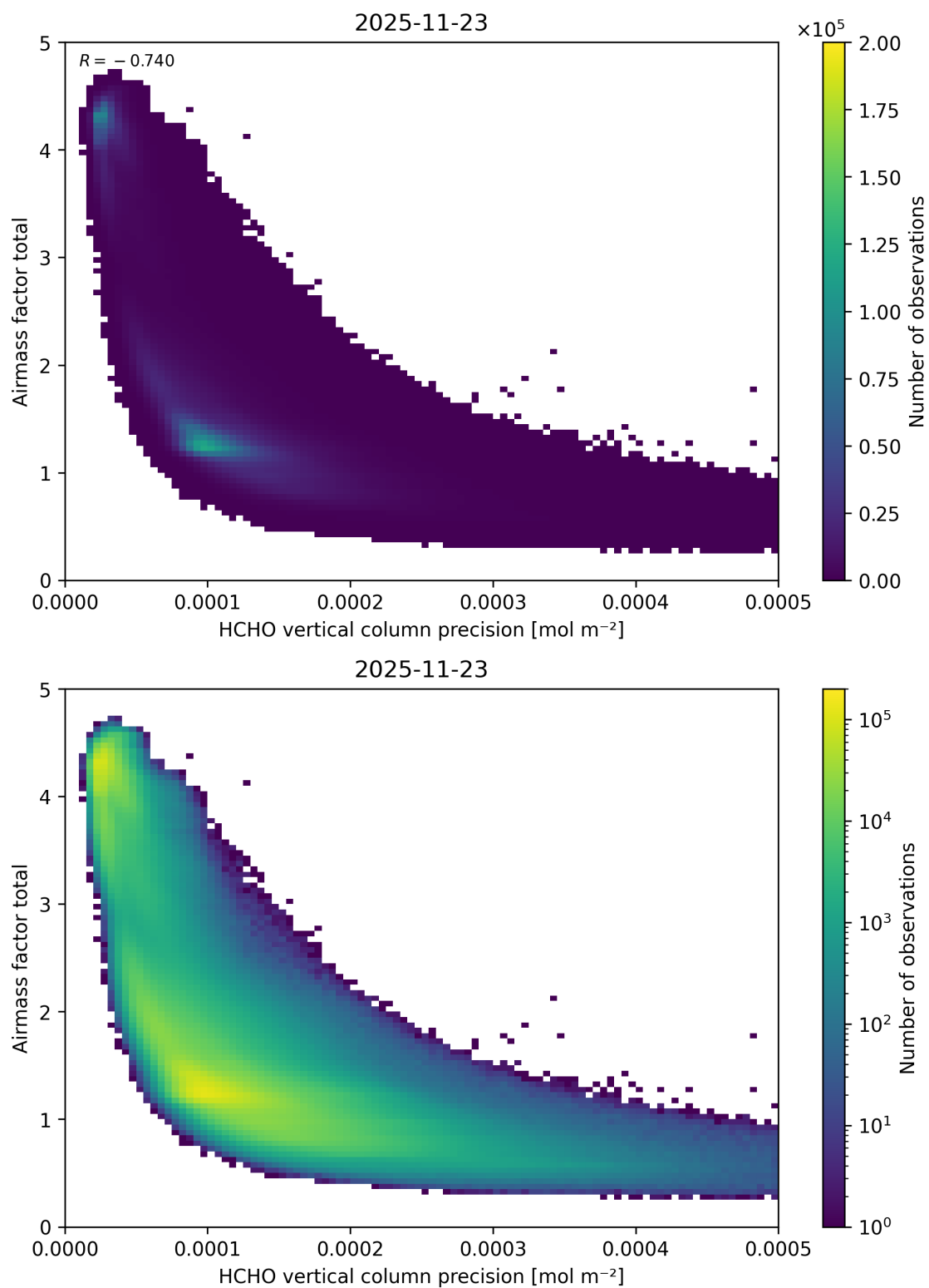
Figure 160: Scatter density plot of “HCHO vertical column precision” against “Airmass factor total” for 2025-11-23 to 2025-11-24.
