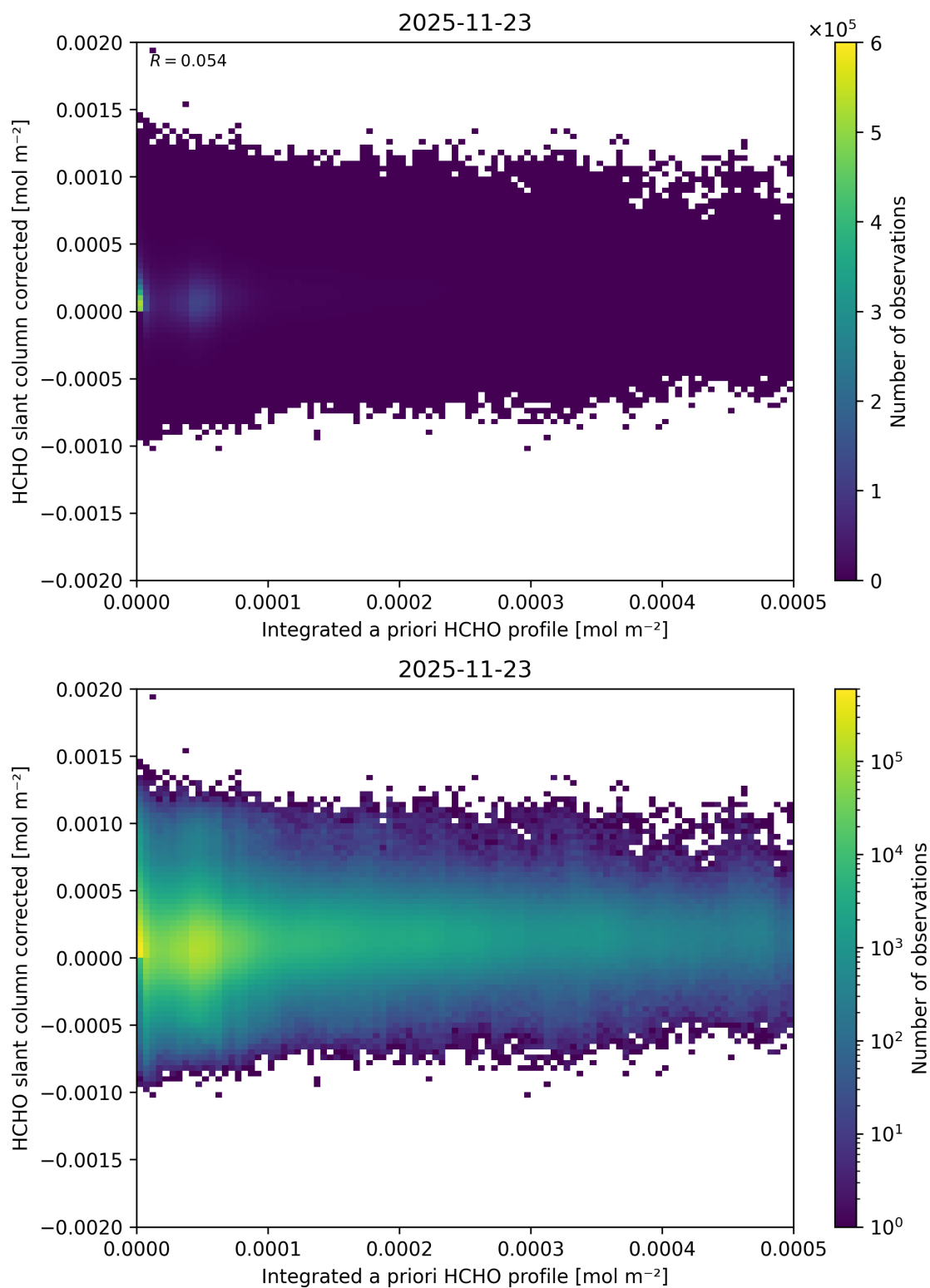
Figure 168: Scatter density plot of “Integrated a priori HCHO profile” against “HCHO slant column corrected” for 2025-11-23 to 2025-11-24.
