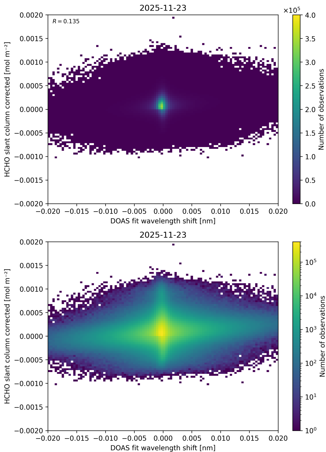
Figure 71: Scatter density plot of “DOAS fit wavelength shift” against “HCHO slant column corrected” for 2025-11-23 to 2025-11-24.
