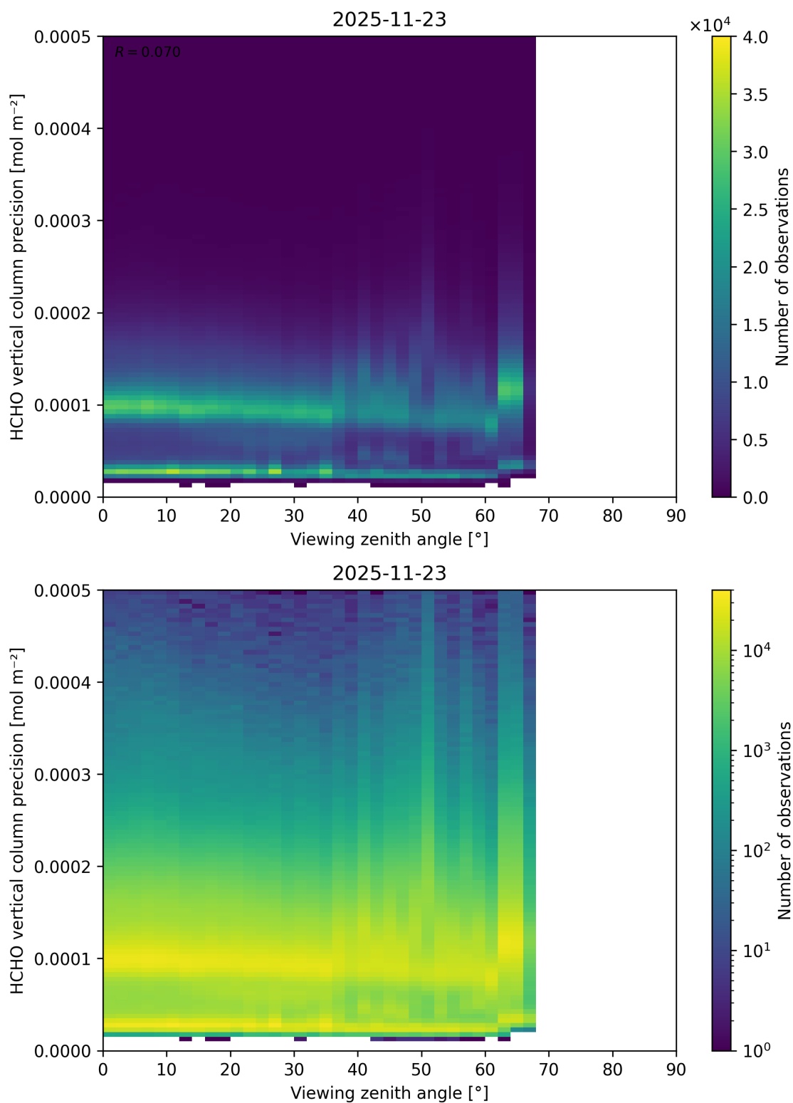
Figure 214: Scatter density plot of “Viewing zenith angle” against “HCHO vertical column precision” for 2025-11-23 to 2025-11-24.
