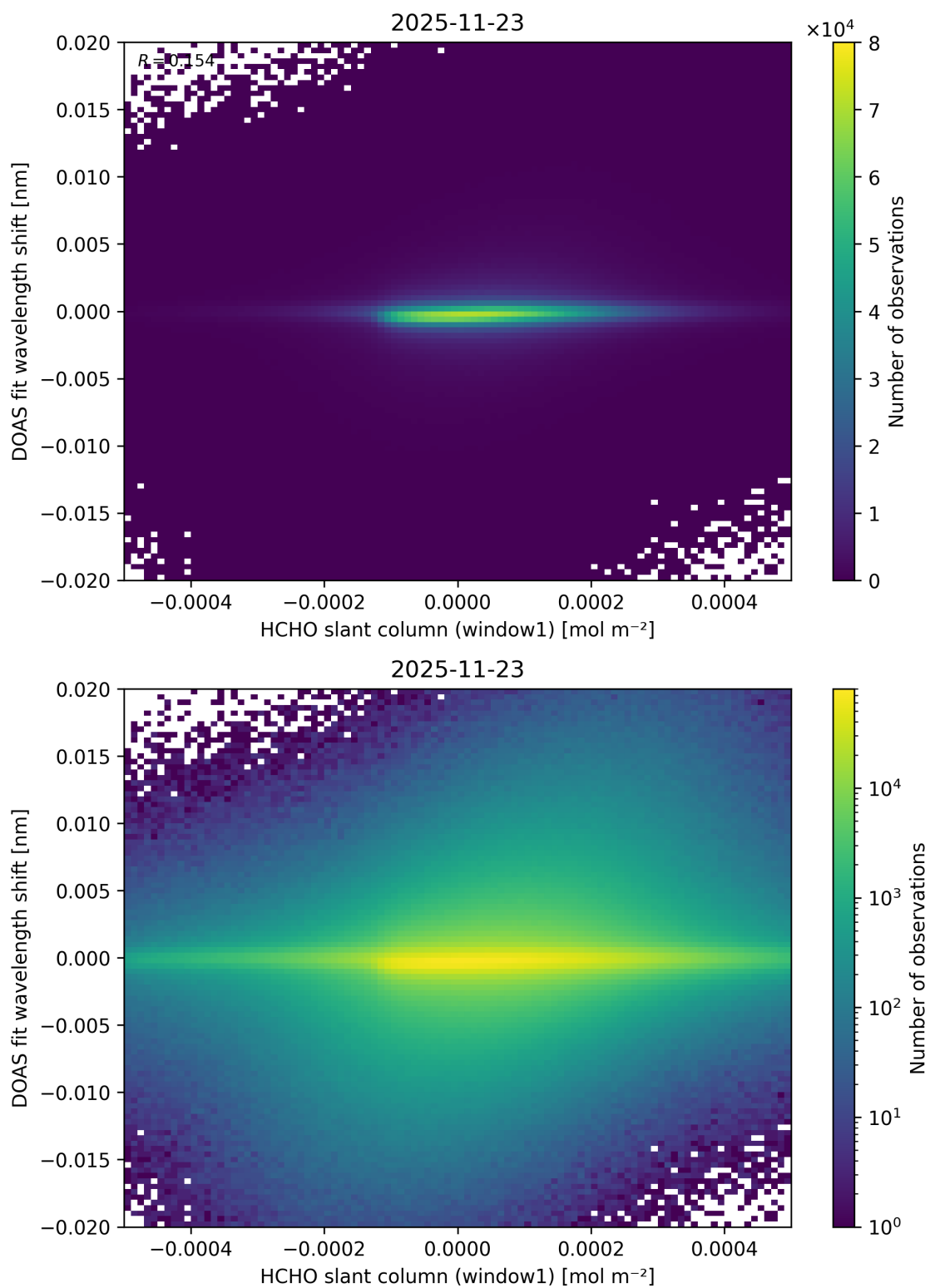
Figure 89: Scatter density plot of “HCHO slant column (window1)” against “DOAS fit wavelength shift” for 2025-11-23 to 2025-11-24.
