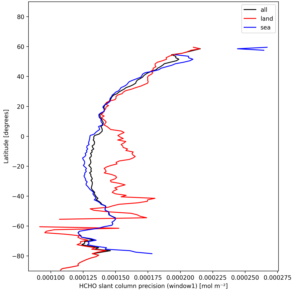
Figure 26: Zonal average of “HCHO slant column precision (window1)” for 2025-11-23 to 2025-11-24.
