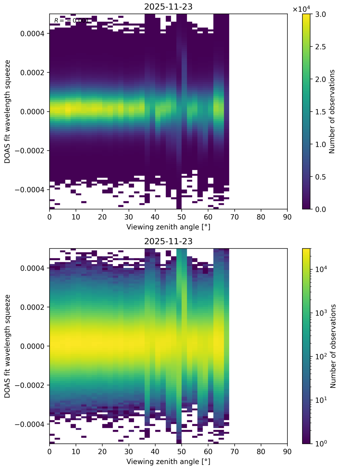
Figure 204: Scatter density plot of “Viewing zenith angle” against “DOAS fit wavelength squeeze” for 2025-11-23 to 2025-11-24.
