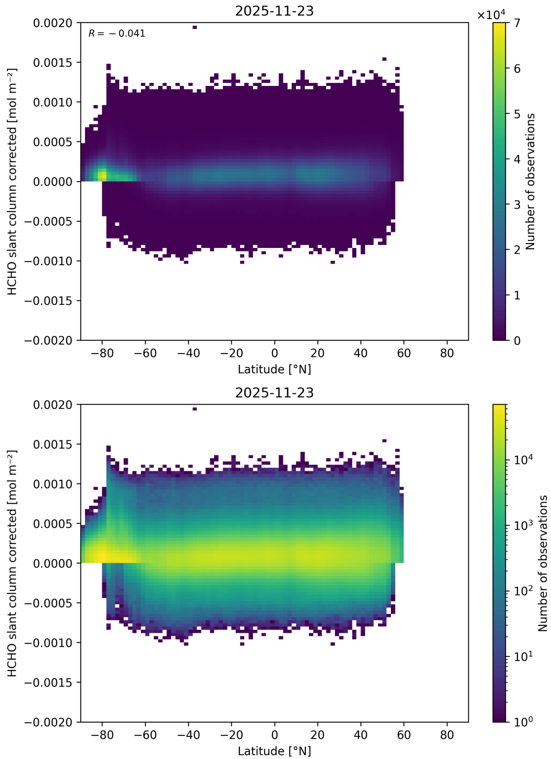
Figure 175: Scatter density plot of “Latitude” against “HCHO slant column corrected” for 2025-11-23 to 2025-11-24.
