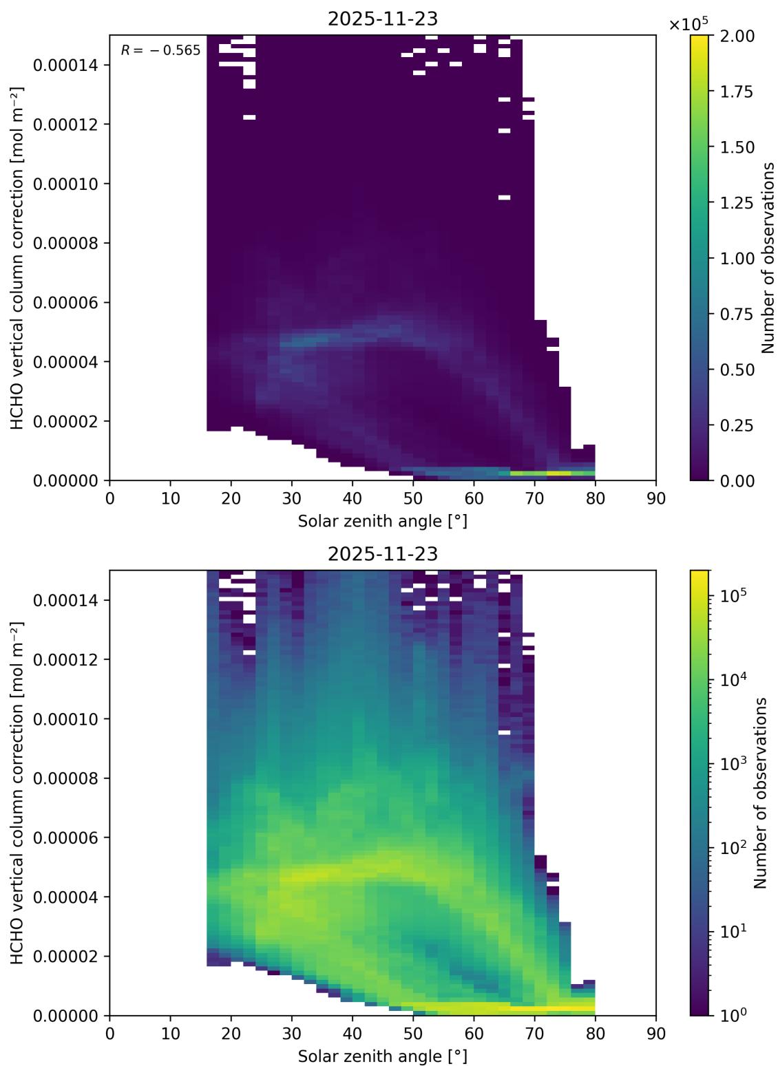
Figure 197: Scatter density plot of “Solar zenith angle” against “HCHO vertical column correction” for 2025-11-23 to 2025-11-24.
