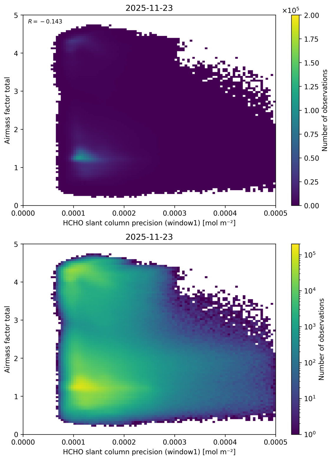
Figure 105: Scatter density plot of “HCHO slant column precision (window1)” against “Airmass factor total” for 2025-11-23 to 2025-11-24.
