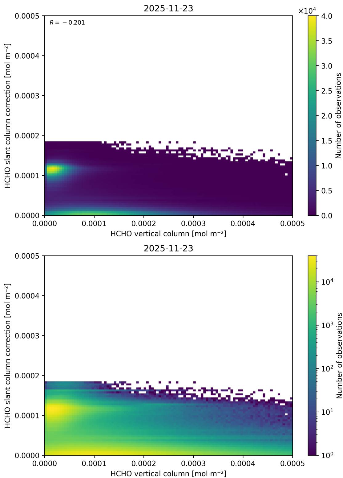
Figure 143: Scatter density plot of “HCHO vertical column” against “HCHO slant column correction” for 2025-11-23 to 2025-11-24.
