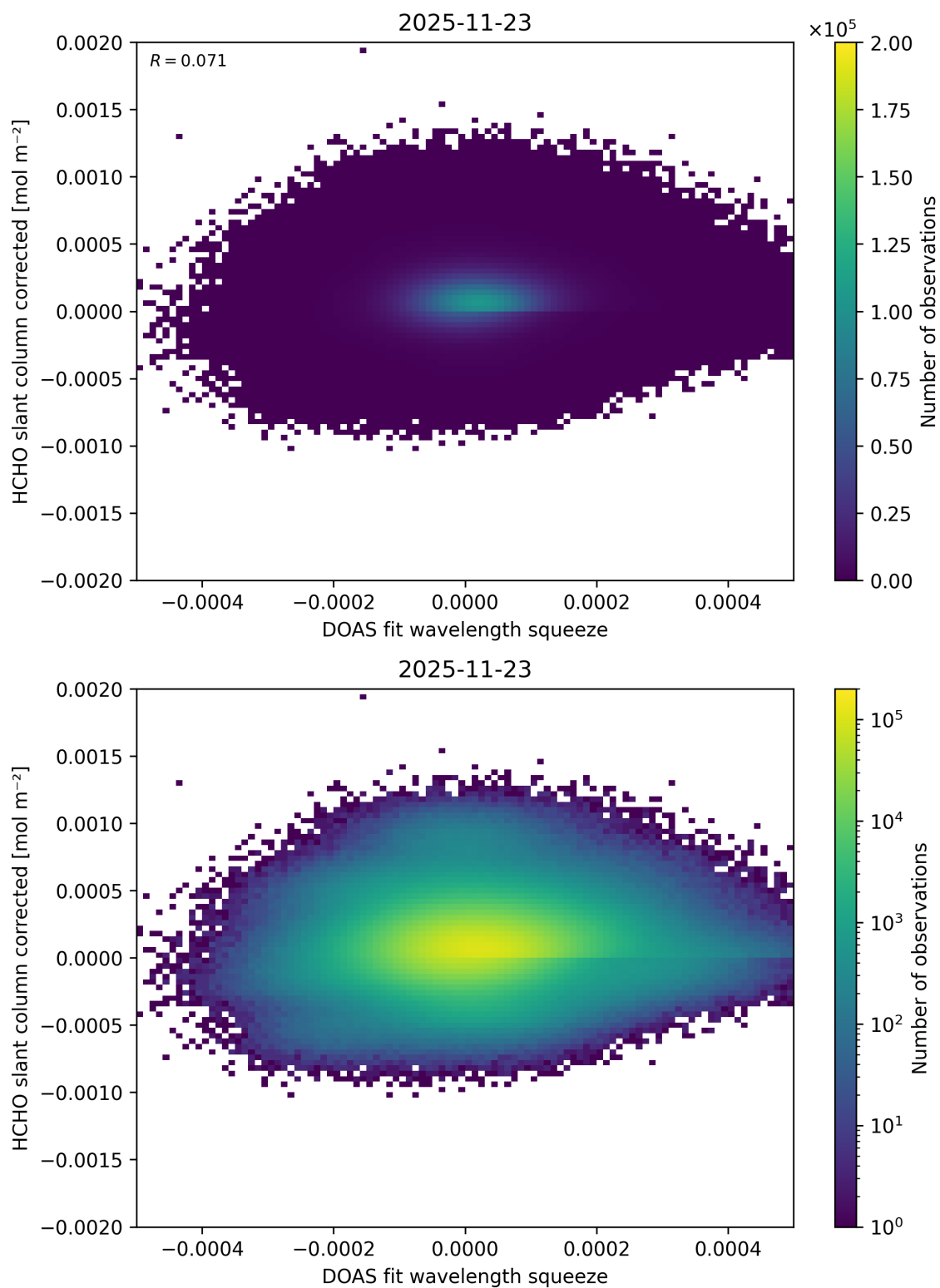
Figure 75: Scatter density plot of “DOAS fit wavelength squeeze” against “HCHO slant column corrected” for 2025-11-23 to 2025-11-24.
