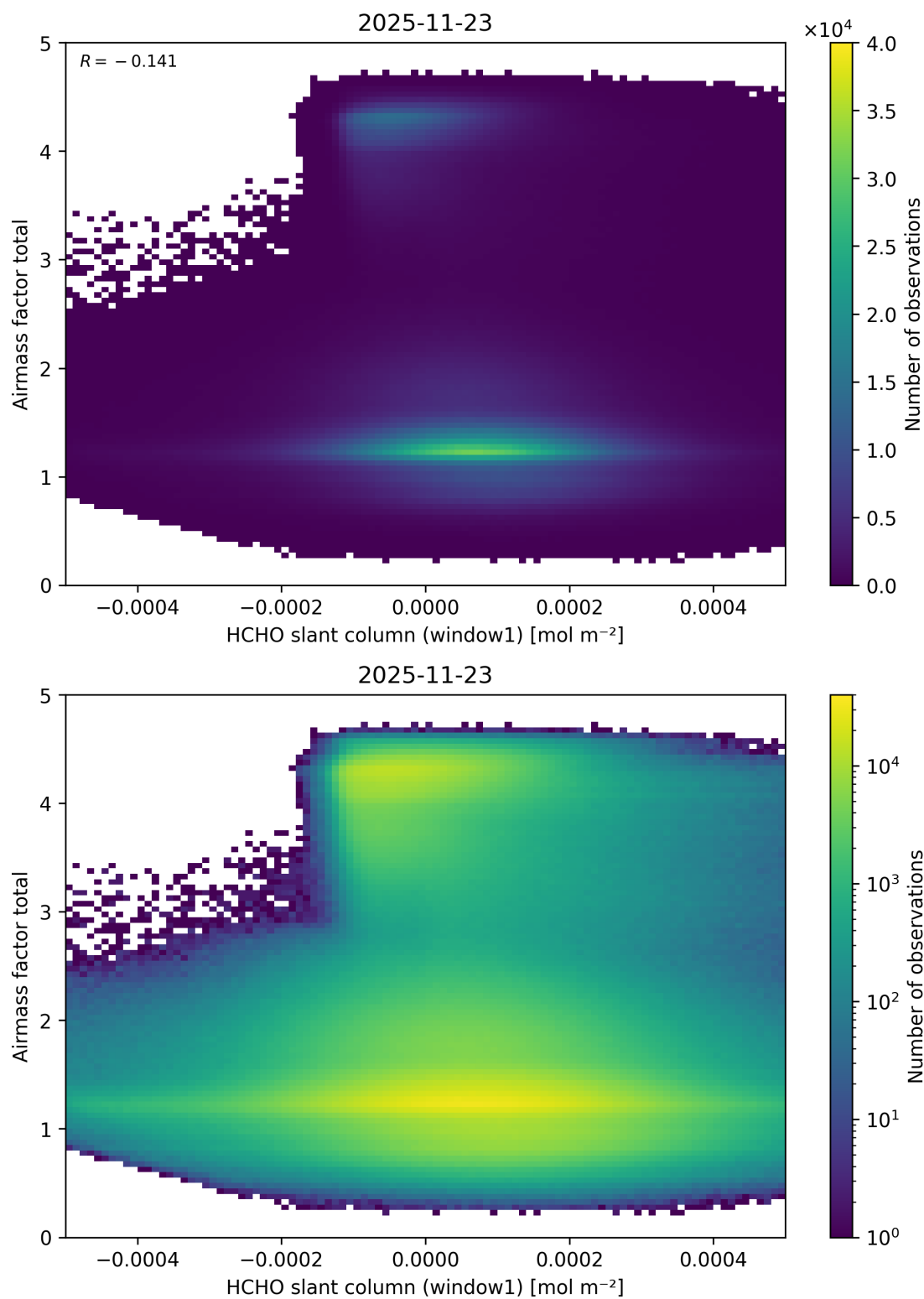
Figure 95: Scatter density plot of “HCHO slant column (window1)” against “Airmass factor total” for 2025-11-23 to 2025-11-24.
