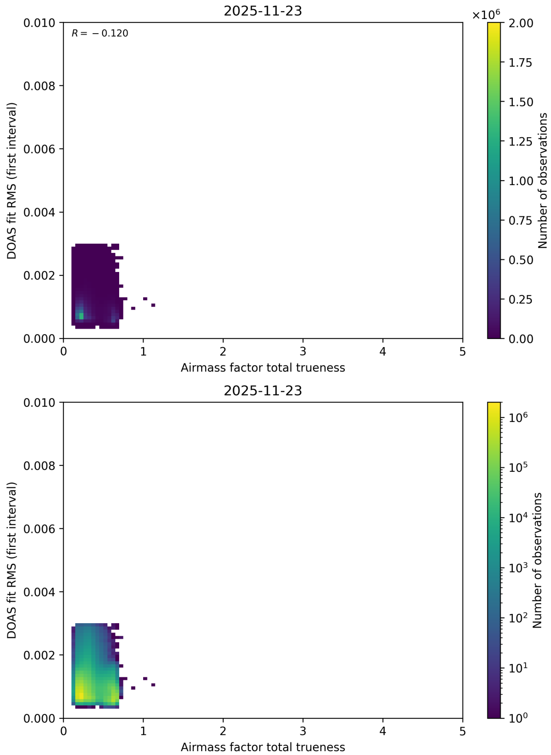
Figure 118: Scatter density plot of “Airmass factor total trueness” against “DOAS fit RMS (first interval)” for 2025-11-23 to 2025-11-24.
