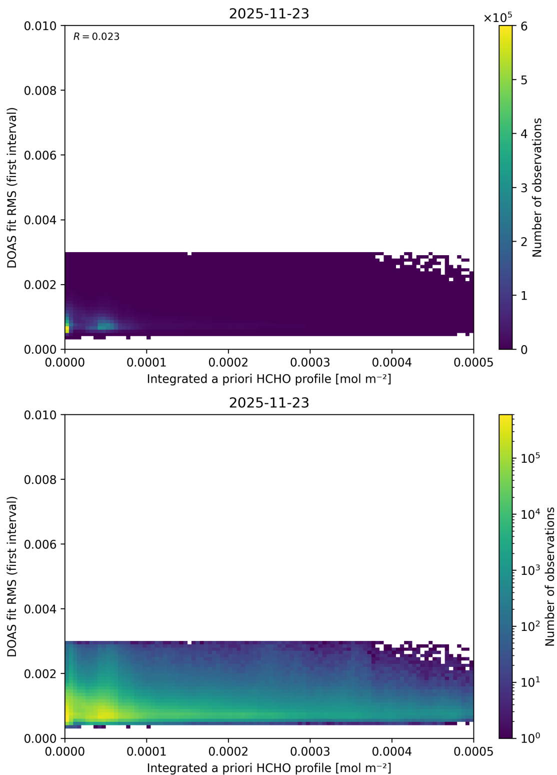
Figure 165: Scatter density plot of “Integrated a priori HCHO profile” against “DOAS fit RMS (first interval)” for 2025-11-23 to 2025-11-24.
