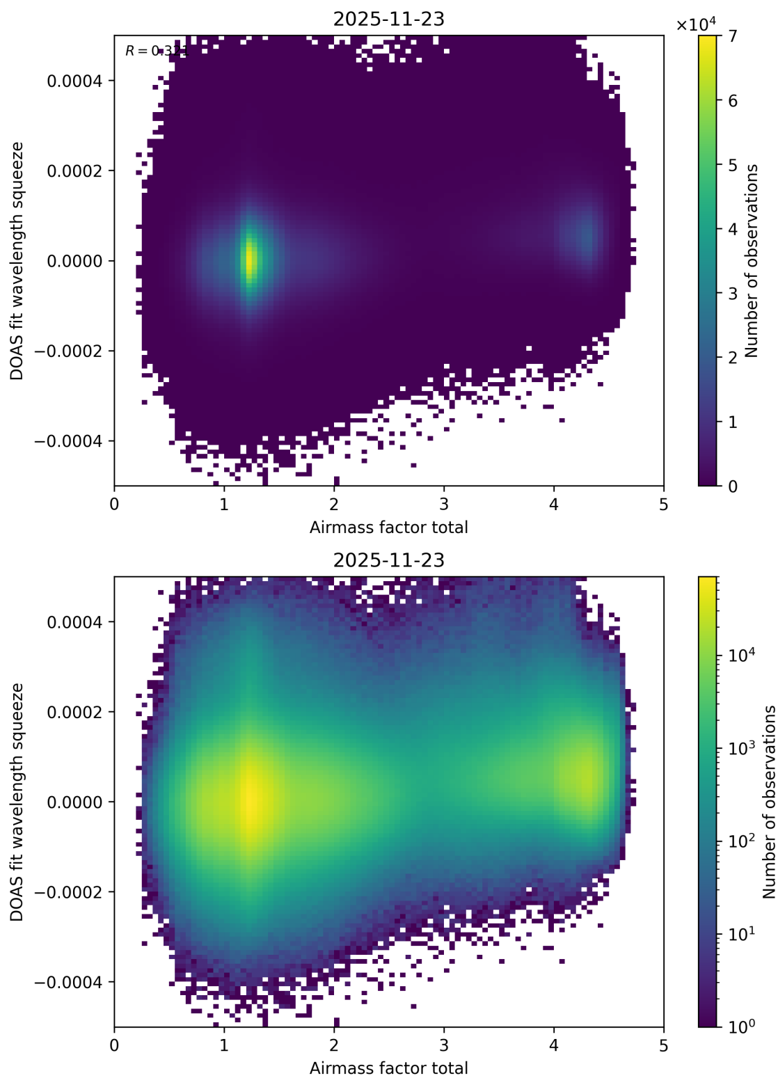
Figure 111: Scatter density plot of “Airmass factor total” against “DOAS fit wavelength squeeze” for 2025-11-23 to 2025-11-24.
