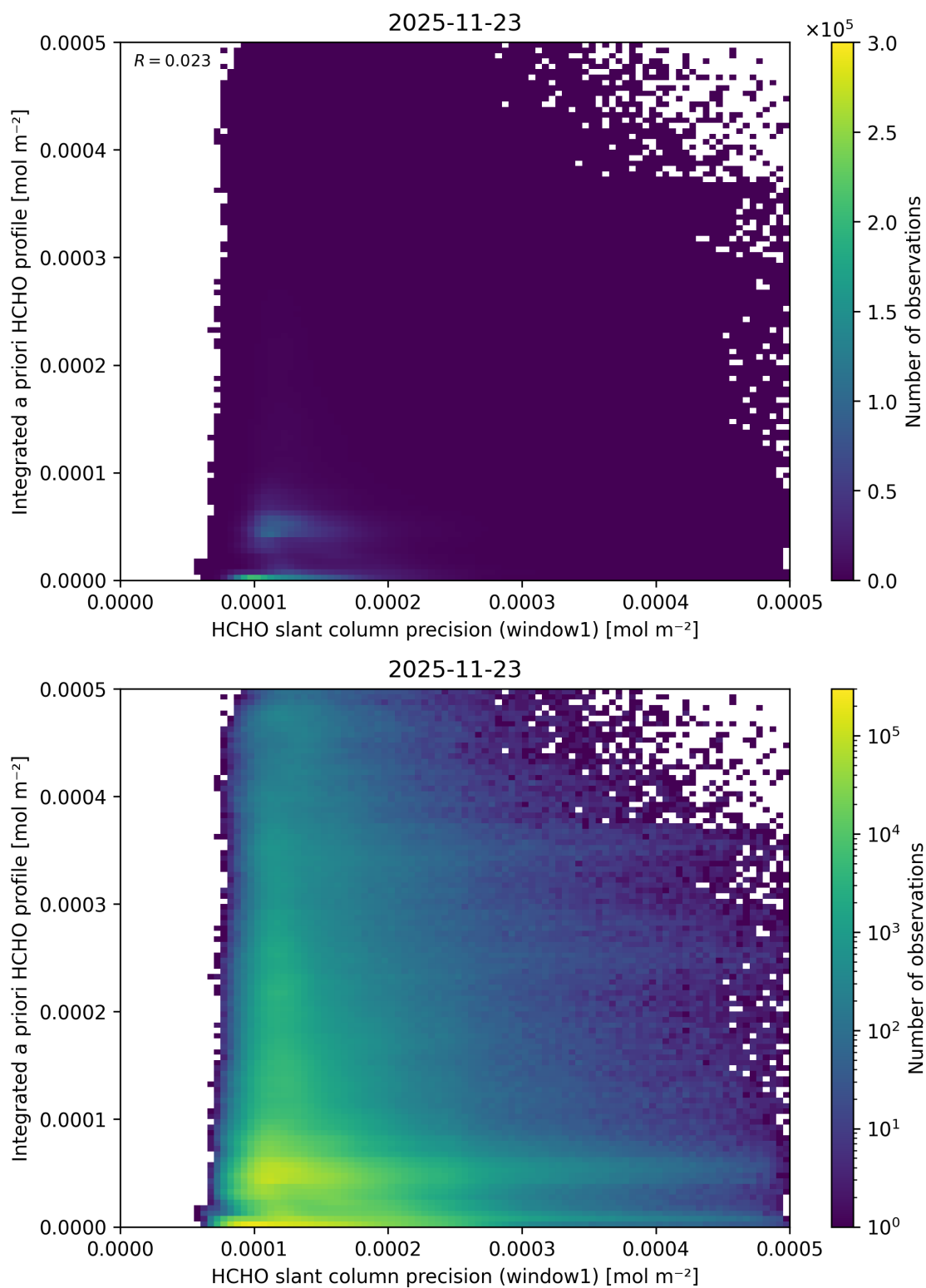
Figure 108: Scatter density plot of “HCHO slant column precision (window1)” against “Integrated a priori HCHO profile” for 2025-11-23 to 2025-11-24.
