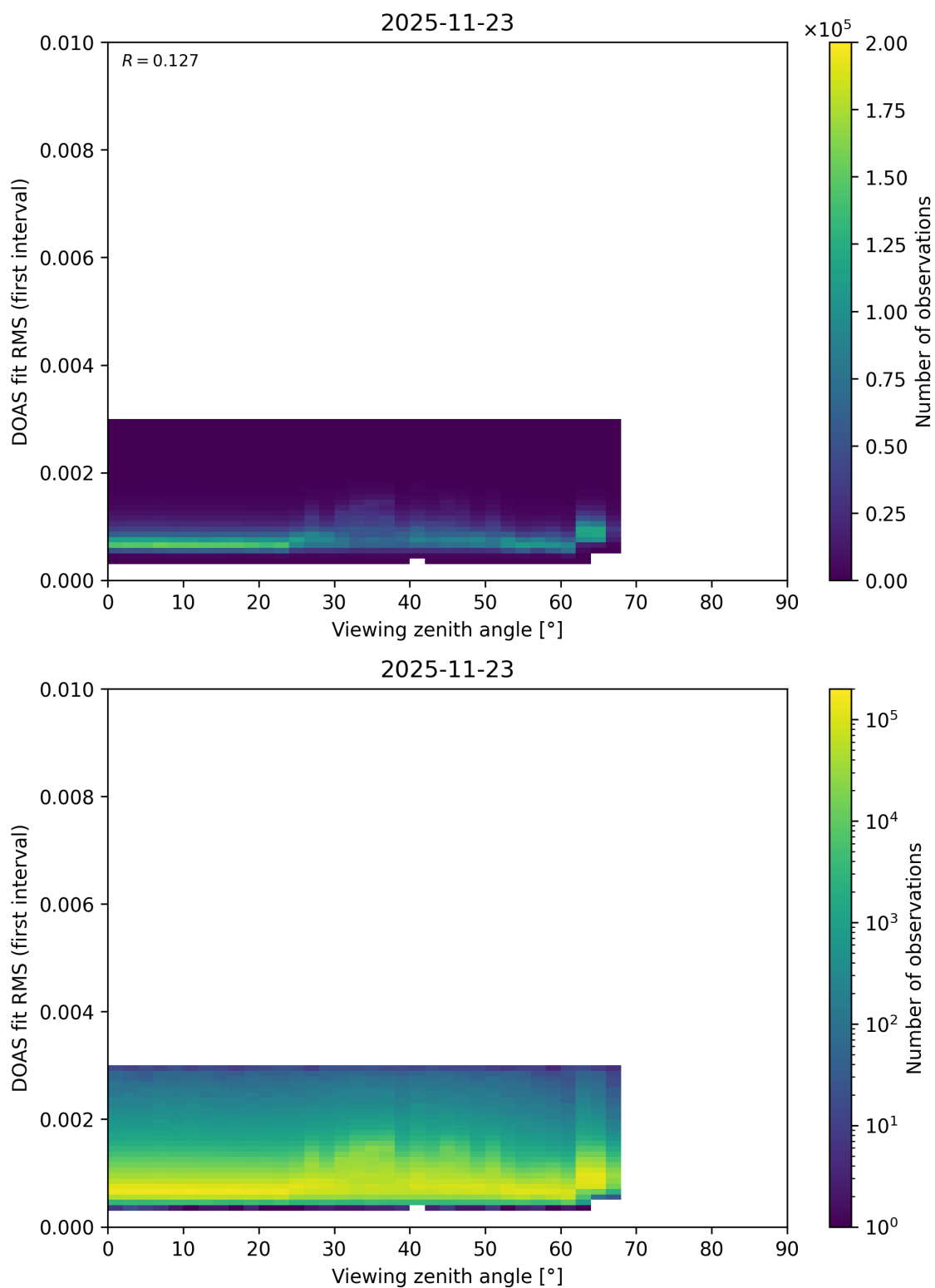
Figure 202: Scatter density plot of “Viewing zenith angle” against “DOAS fit RMS (first interval)” for 2025-11-23 to 2025-11-24.
