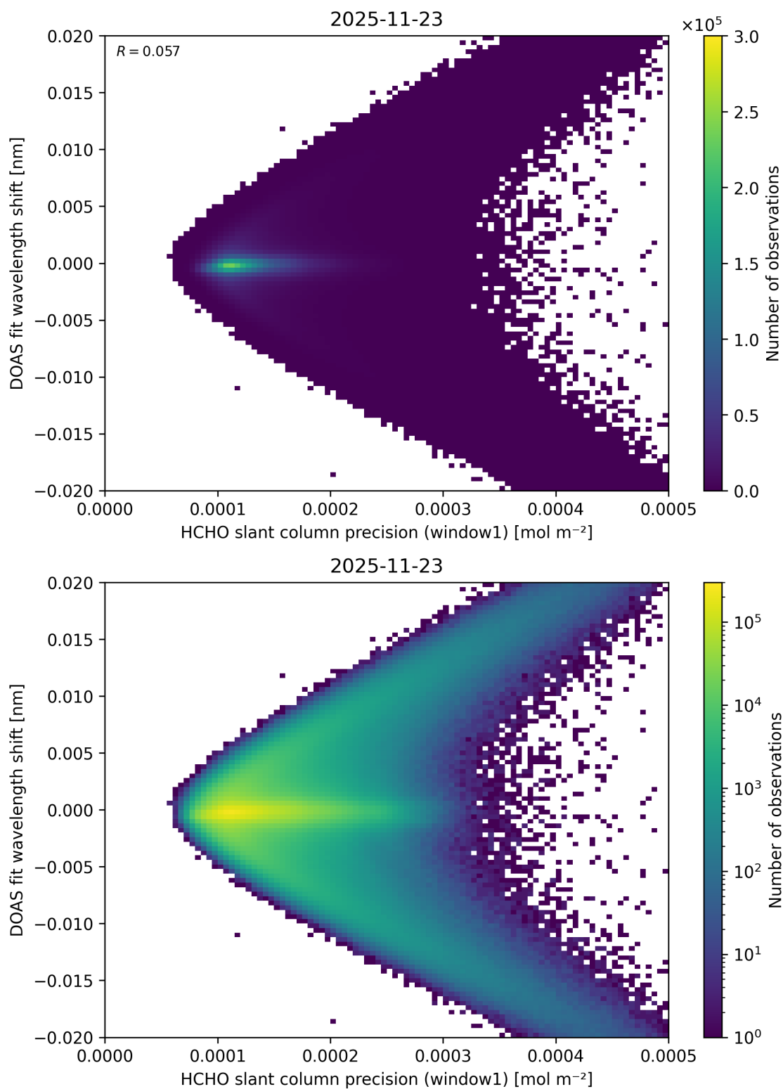
Figure 100: Scatter density plot of “HCHO slant column precision (window1)” against “DOAS fit wavelength shift” for 2025-11-23 to 2025-11-24.
