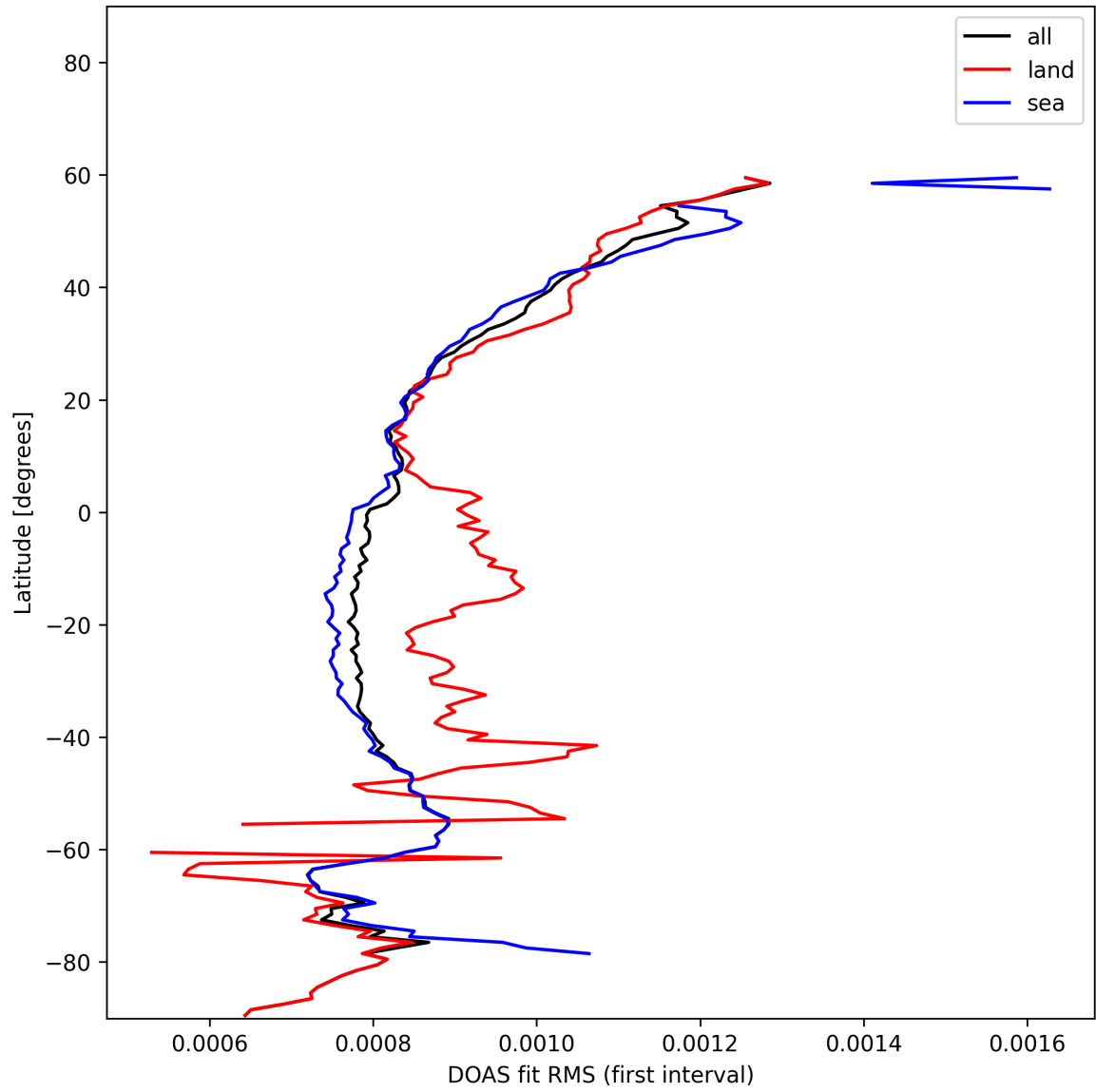
Figure 33: Zonal average of “DOAS fit RMS (first interval)” for 2025-11-23 to 2025-11-24.
