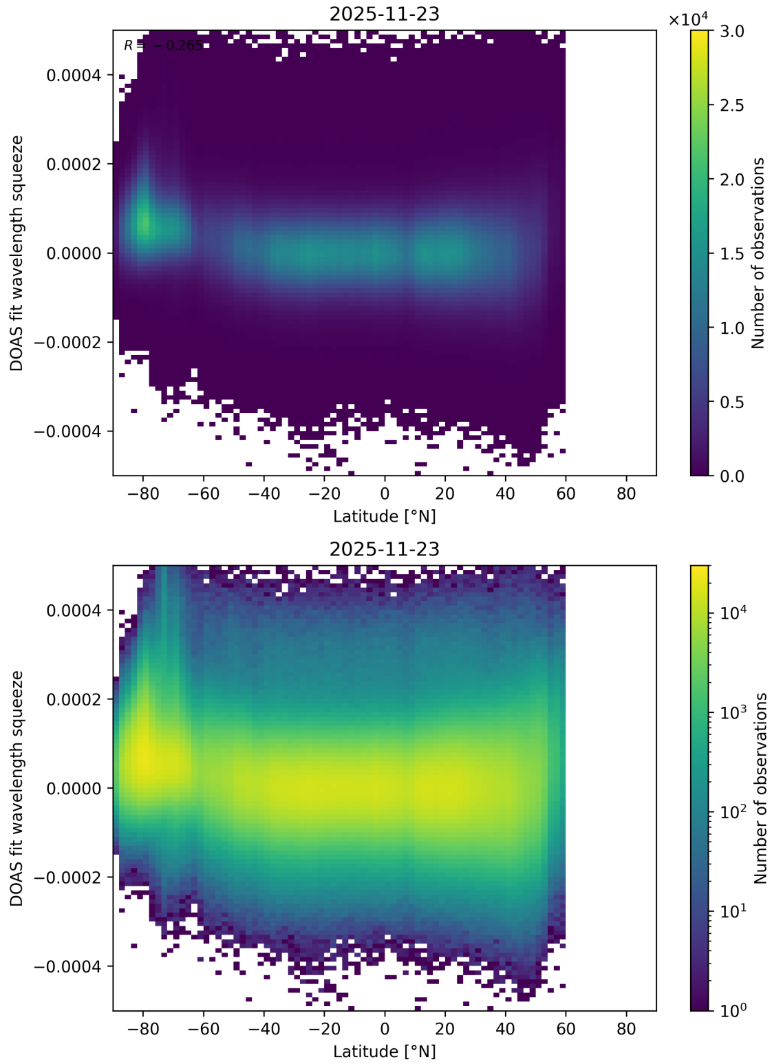
Figure 173: Scatter density plot of “Latitude” against “DOAS fit wavelength squeeze” for 2025-11-23 to 2025-11-24.
