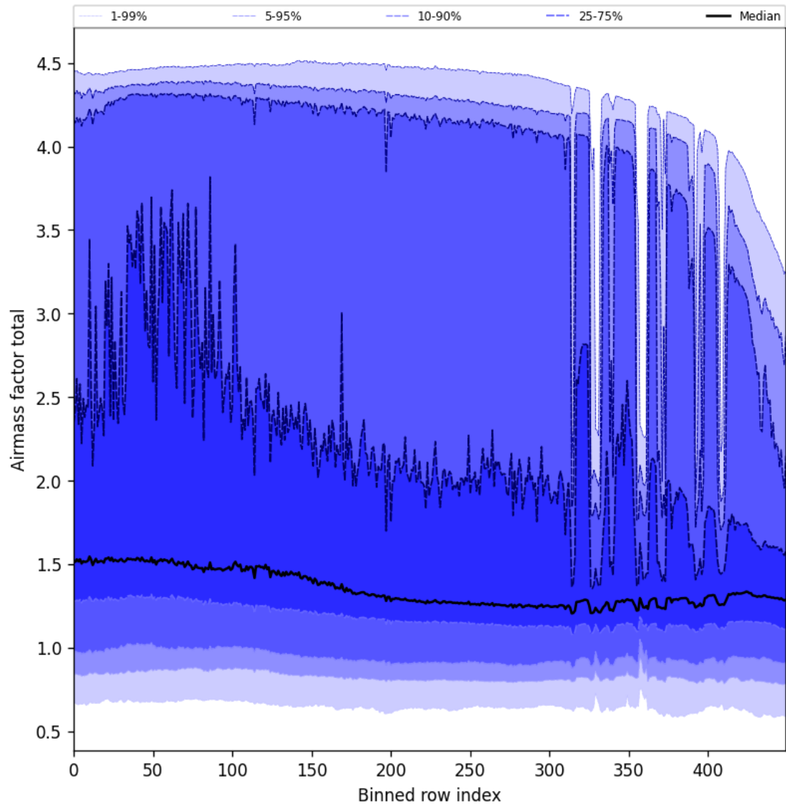
Figure 57: Along track statistics of “Airmass factor total” for 2025-11-23 to 2025-11-24
