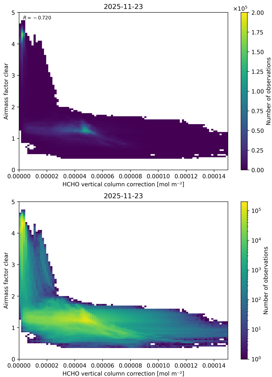
Figure 129: Scatter density plot of “HCHO vertical column correction” against “Airmass factor clear” for 2025-11-23 to 2025-11-24.
