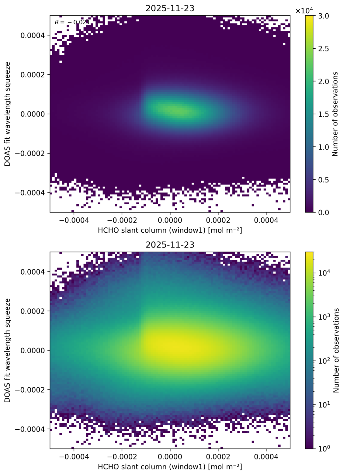
Figure 90: Scatter density plot of “HCHO slant column (window1)” against “DOAS fit wavelength squeeze” for 2025-11-23 to 2025-11-24.
