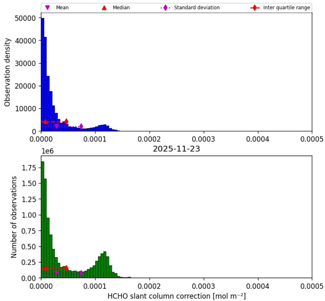
Figure 49: Histogram of “HCHO slant column correction” for 2025-11-23 to 2025-11-24
