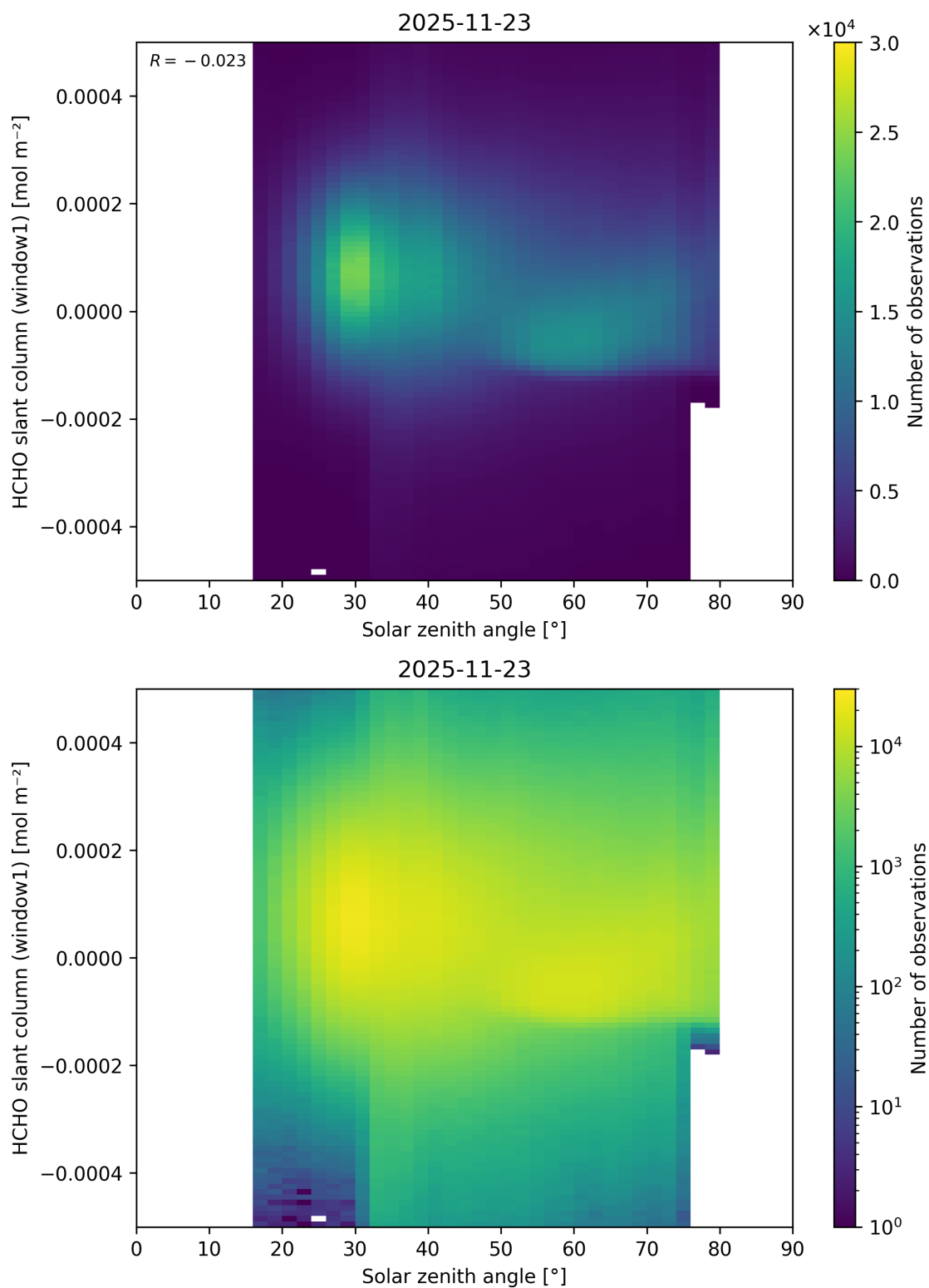
Figure 192: Scatter density plot of “Solar zenith angle” against “HCHO slant column (window1)” for 2025-11-23 to 2025-11-24.
