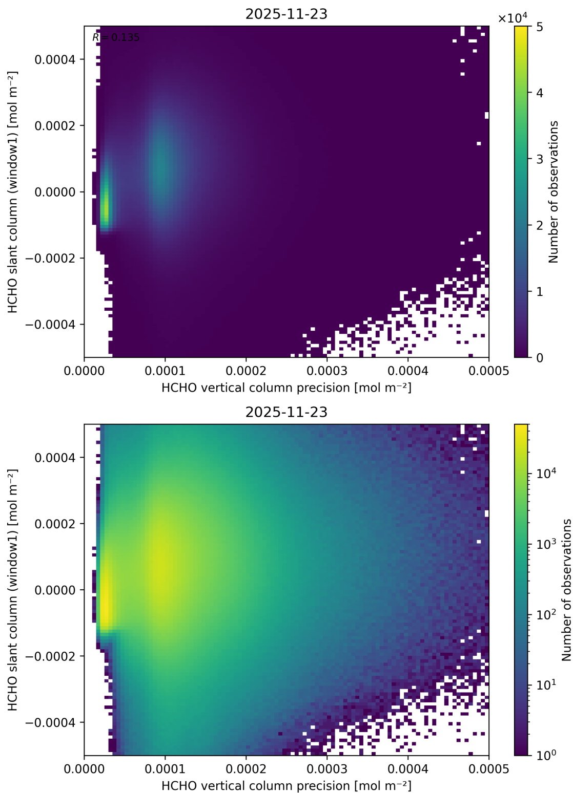
Figure 158: Scatter density plot of “HCHO vertical column precision” against “HCHO slant column (window1)” for 2025-11-23 to 2025-11-24.
