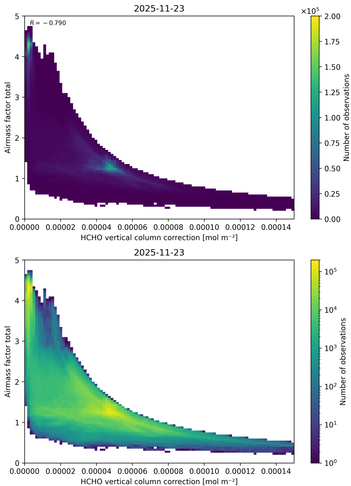
Figure 134: Scatter density plot of “HCHO vertical column correction” against “Airmass factor total” for 2025-11-23 to 2025-11-24.
