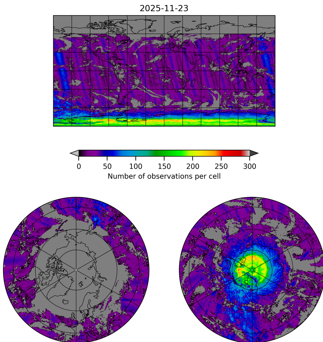
Figure 20: Map of the number of observations for 2025-11-23 to 2025-11-24
