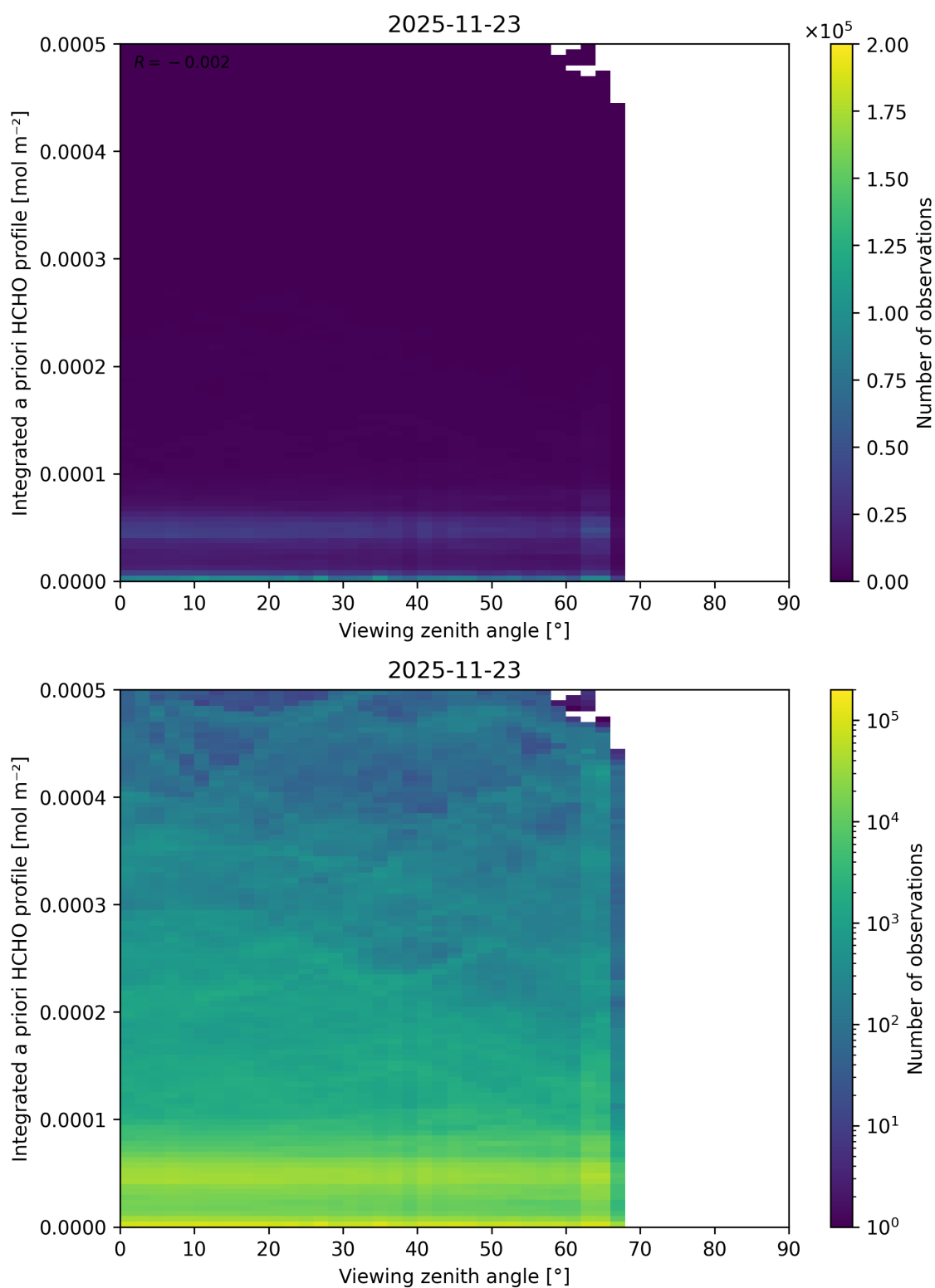
Figure 216: Scatter density plot of “Viewing zenith angle” against “Integrated a priori HCHO profile” for 2025-11-23 to 2025-11-24.
