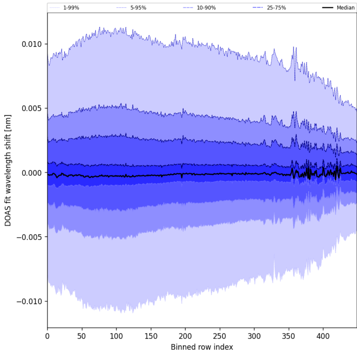
Figure 61: Along track statistics of “DOAS fit wavelength shift” for 2025-11-23 to 2025-11-24
