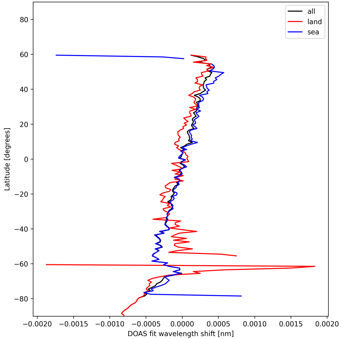
Figure 31: Zonal average of "DOAS fit wavelength shift" for 2025-11-23 to 2025-11-24.
