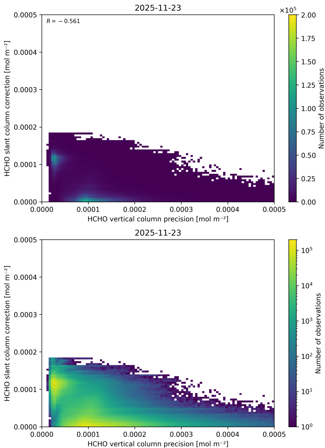
Figure 157: Scatter density plot of “HCHO vertical column precision” against “HCHO slant column correction” for 2025-11-23 to 2025-11-24.
