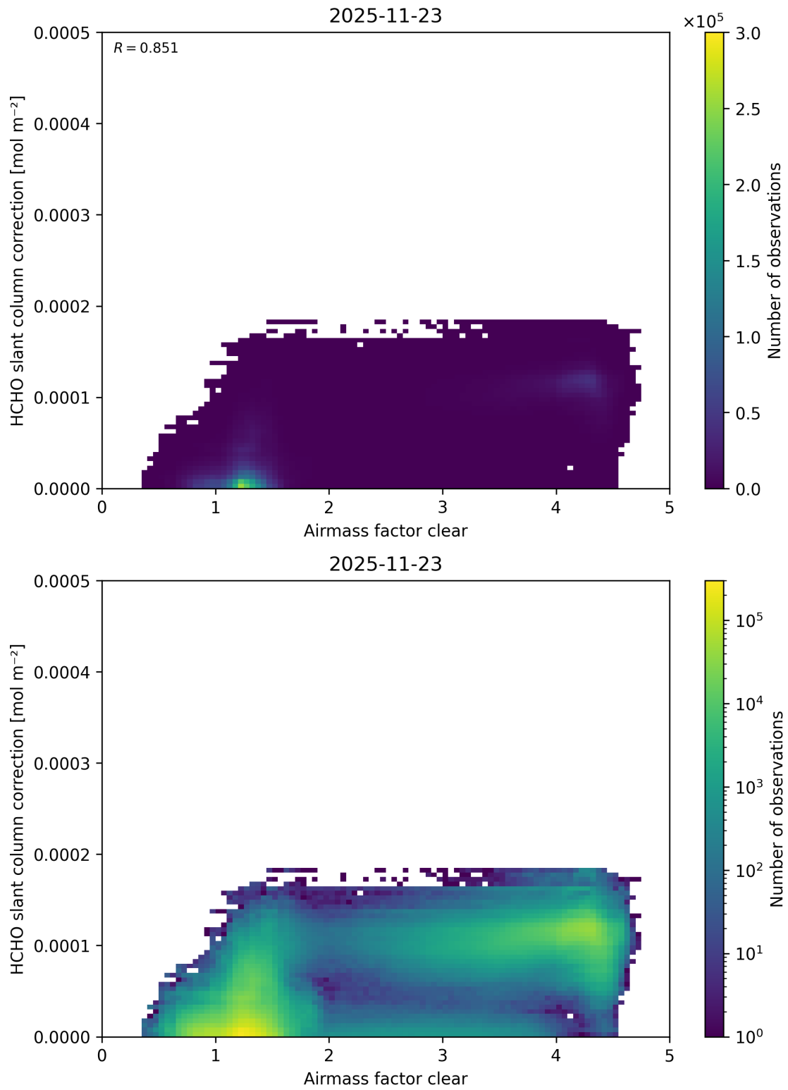
Figure 82: Scatter density plot of “Airmass factor clear” against “HCHO slant column correction” for 2025-11-23 to 2025-11-24.
