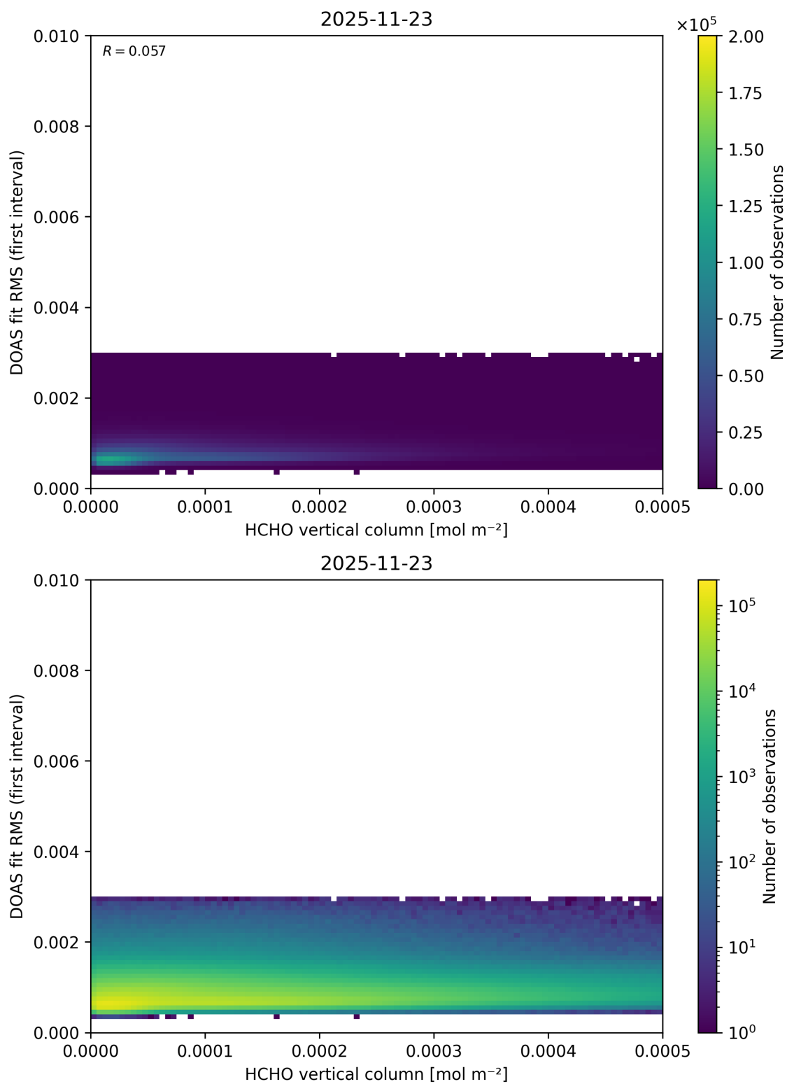
Figure 138: Scatter density plot of “HCHO vertical column” against “DOAS fit RMS (first interval)” for 2025-11-23 to 2025-11-24.
