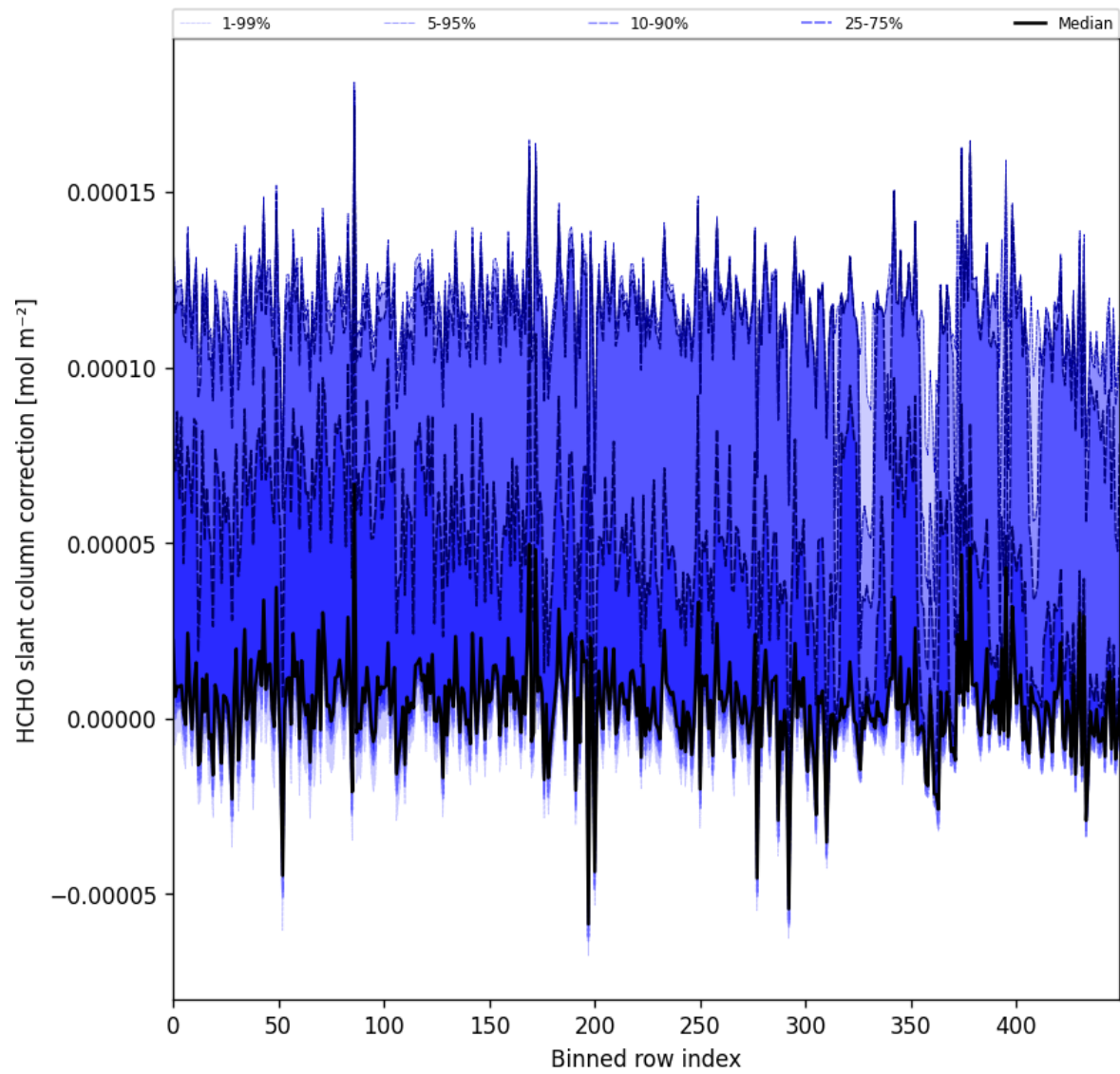
Figure 64: Along track statistics of “HCHO slant column correction” for 2025-11-23 to 2025-11-24
