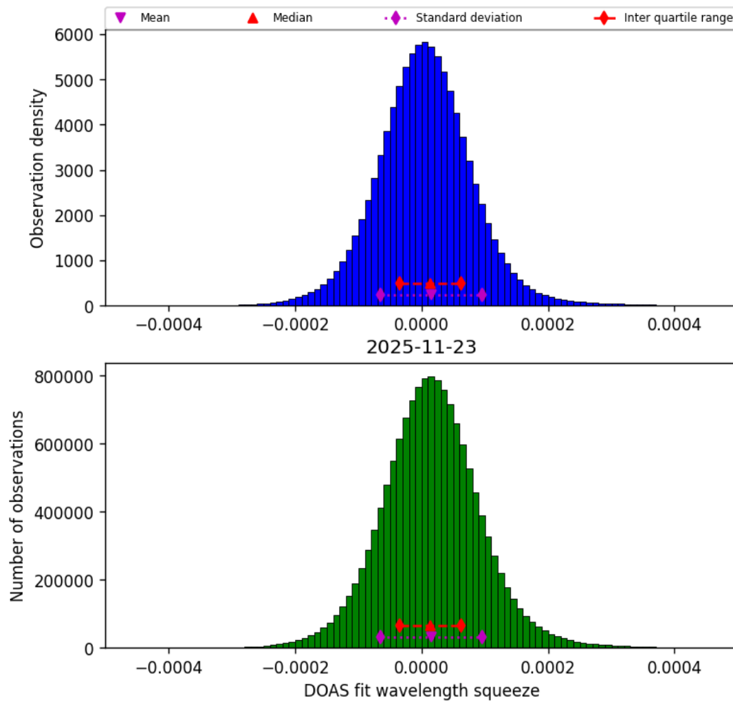
Figure 47: Histogram of “DOAS fit wavelength squeeze” for 2025-11-23 to 2025-11-24
