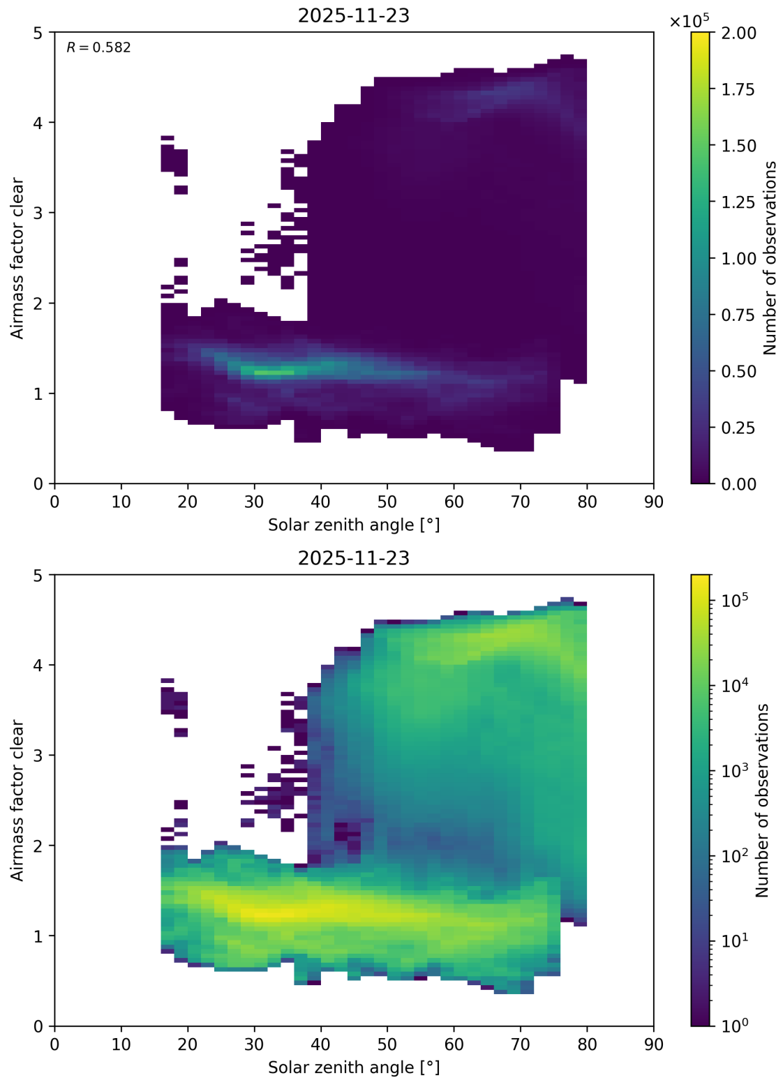
Figure 189: Scatter density plot of “Solar zenith angle” against “Airmass factor clear” for 2025-11-23 to 2025-11-24.
