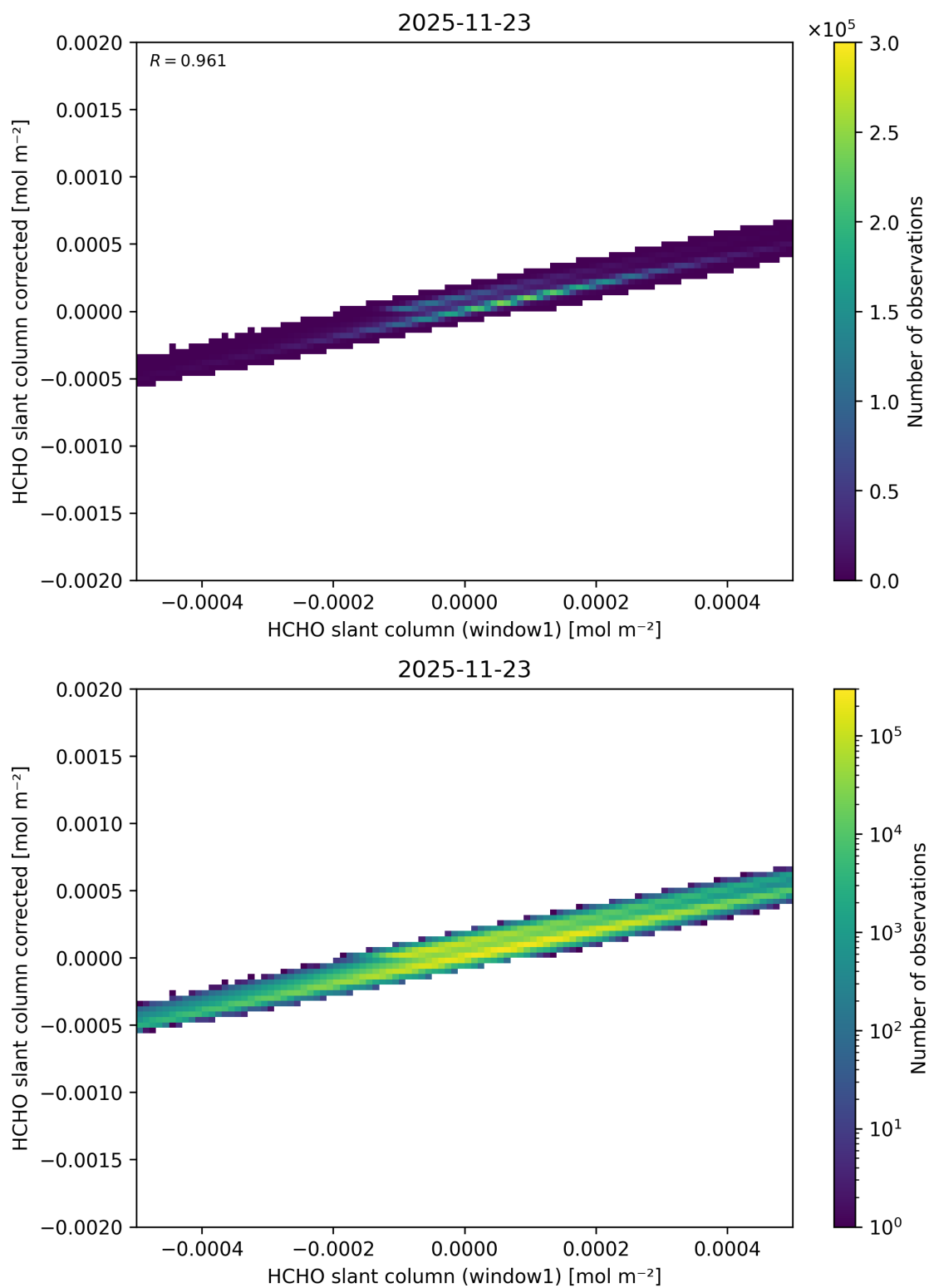
Figure 92: Scatter density plot of “HCHO slant column (window1)” against “HCHO slant column corrected” for 2025-11-23 to 2025-11-24.
