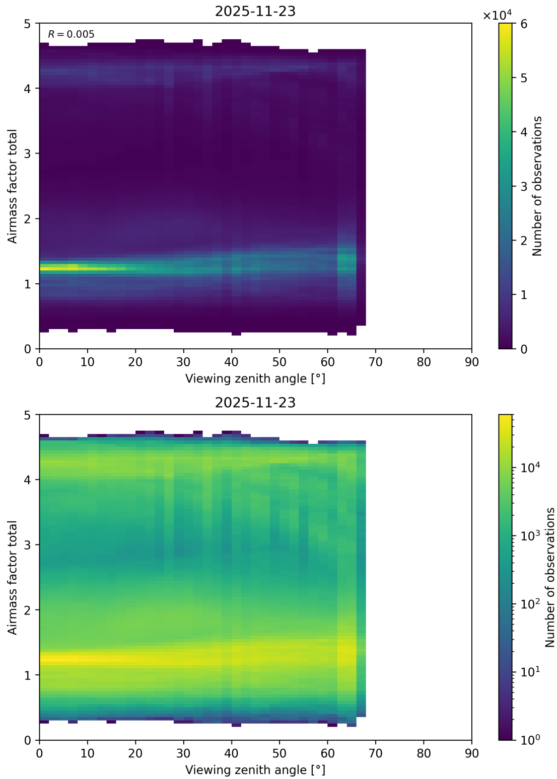
Figure 210: Scatter density plot of “Viewing zenith angle” against “Airmass factor total” for 2025-11-23 to 2025-11-24.
