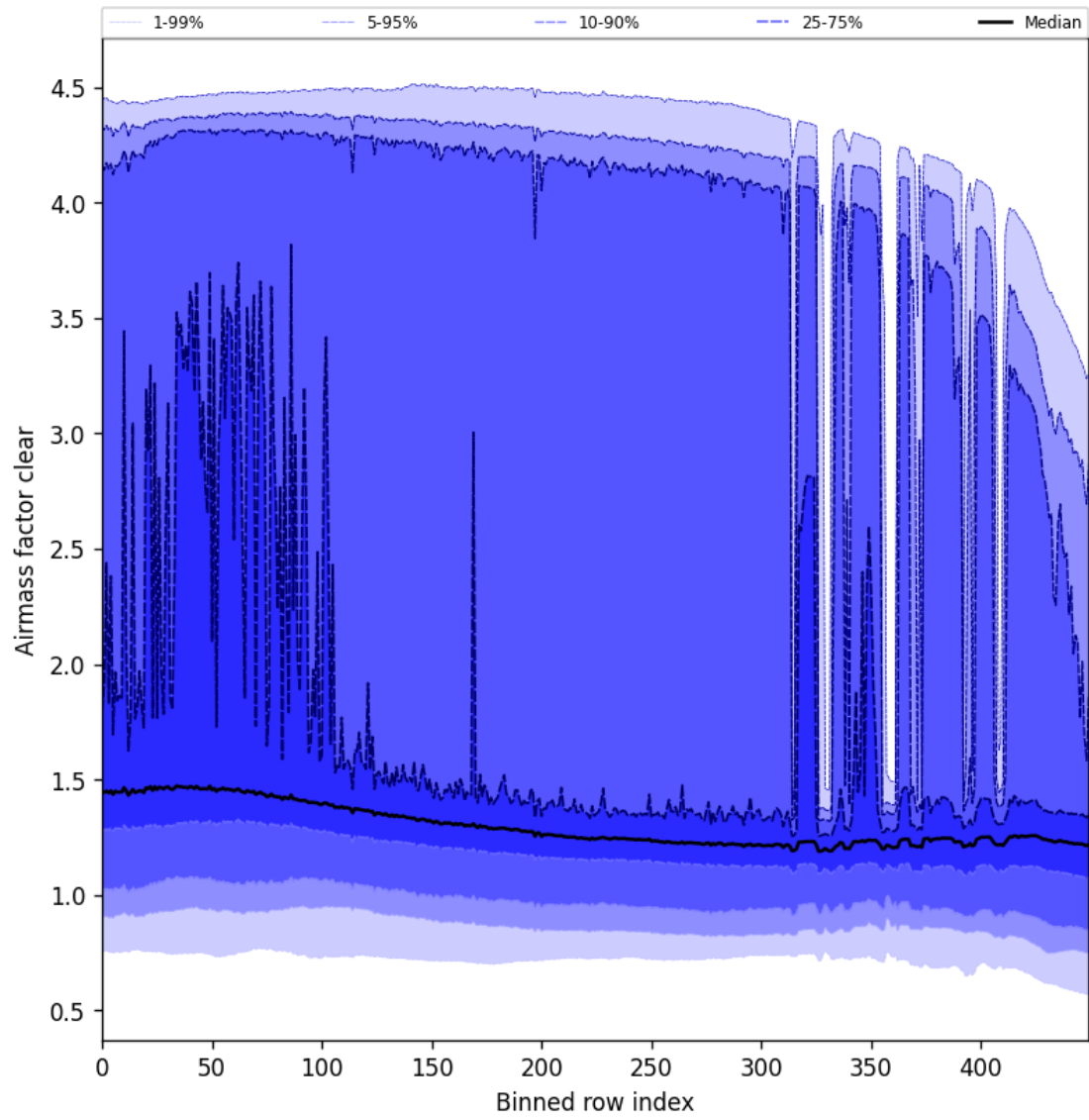
Figure 59: Along track statistics of “Air mass factor clear” for 2025-11-23 to 2025-11-24
