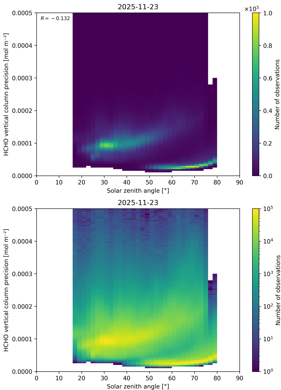
Figure 198: Scatter density plot of “Solar zenith angle” against “HCHO vertical column precision” for 2025-11-23 to 2025-11-24.
