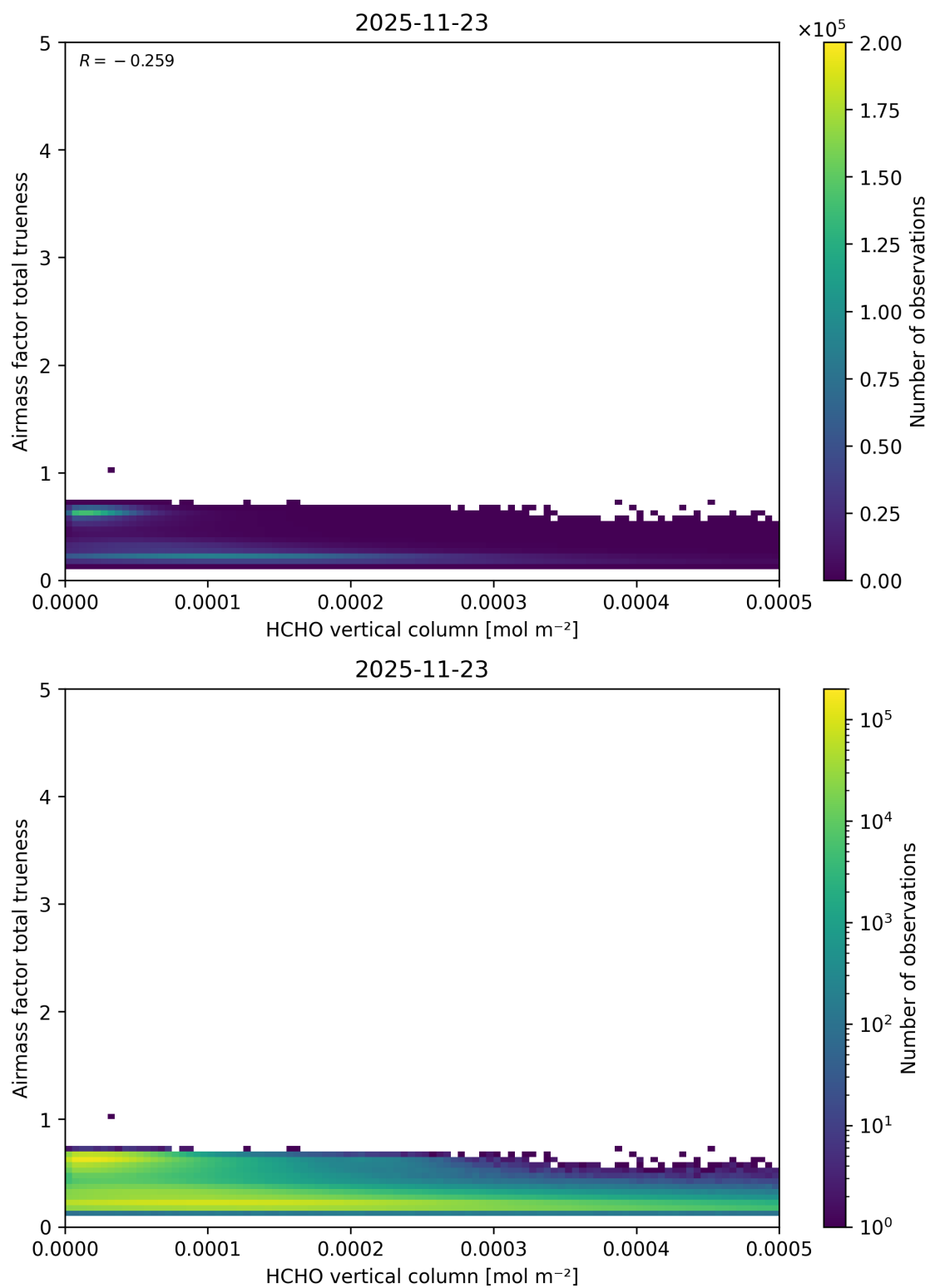
Figure 147: Scatter density plot of “HCHO vertical column” against “Airmass factor total trueneess” for 2025-11-23 to 2025-11-24.
