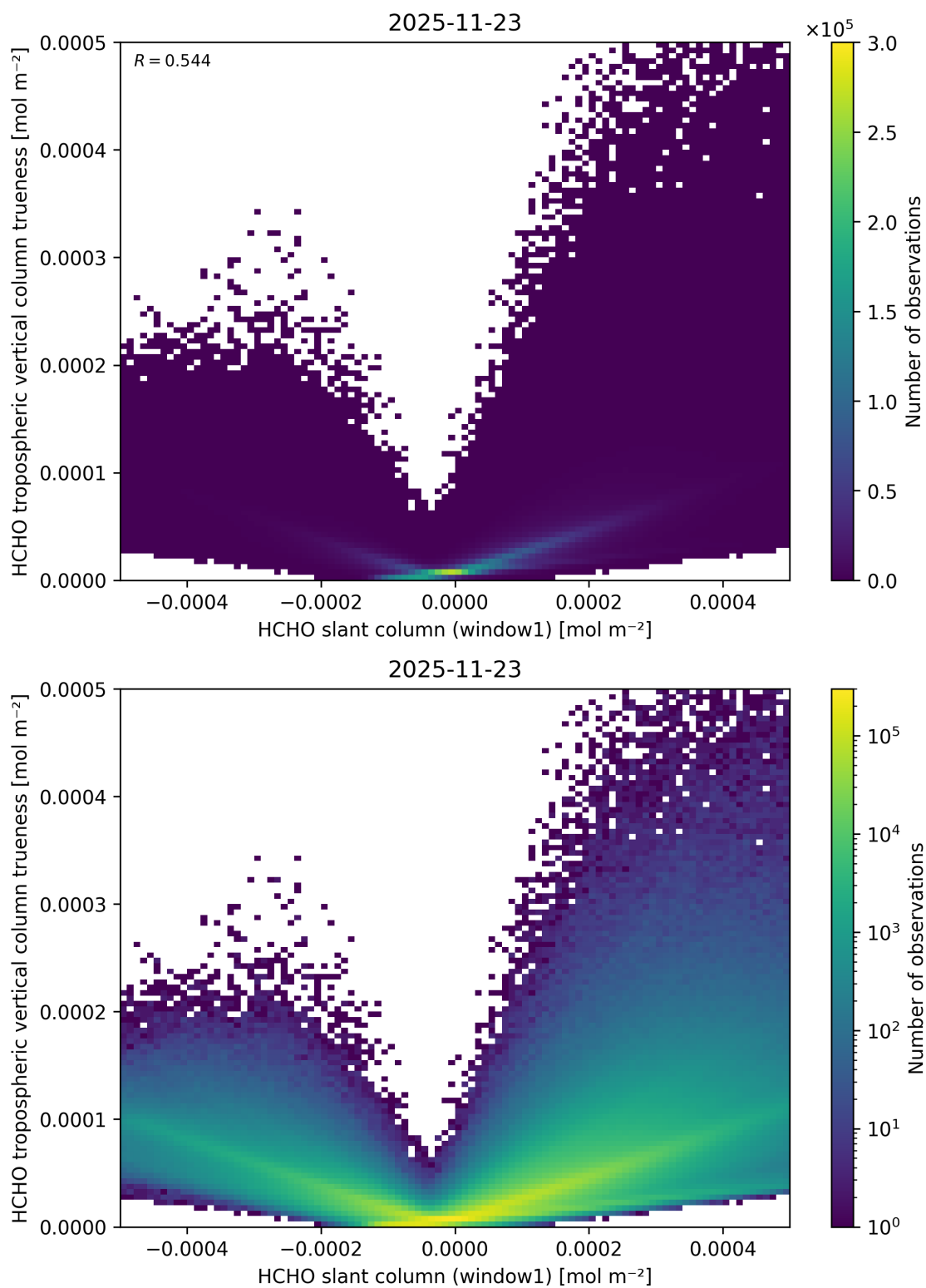
Figure 97: Scatter density plot of “HCHO slant column (window1)” against “HCHO tropospheric vertical column trueness” for 2025-11-23 to 2025-11-24.
