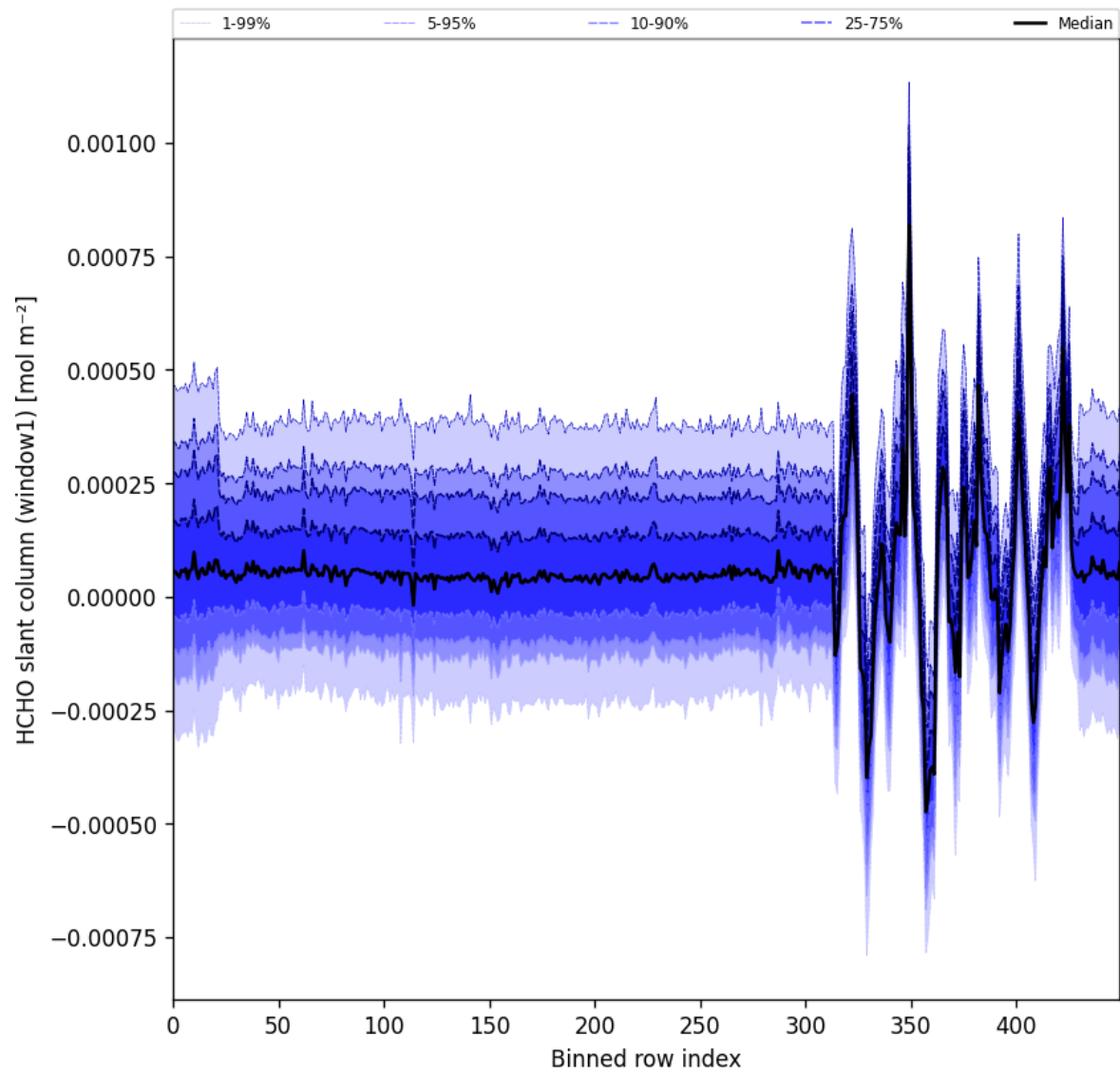
Figure 55: Along track statistics of “HCHO slant column (window1)” for 2025-11-23 to 2025-11-24
