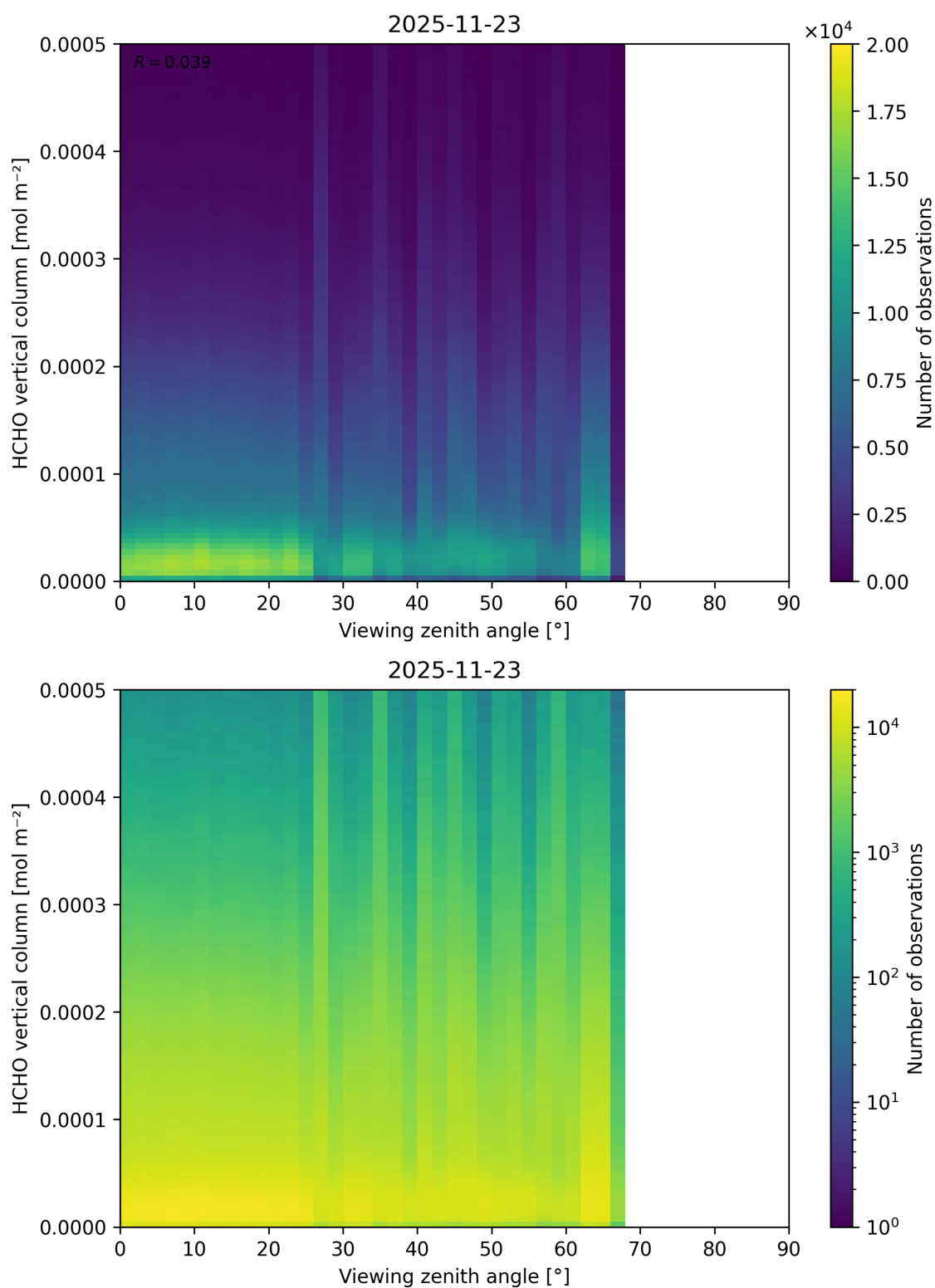
Figure 212: Scatter density plot of “Viewing zenith angle” against “HCHO vertical column” for 2025-11-23 to 2025-11-24.
