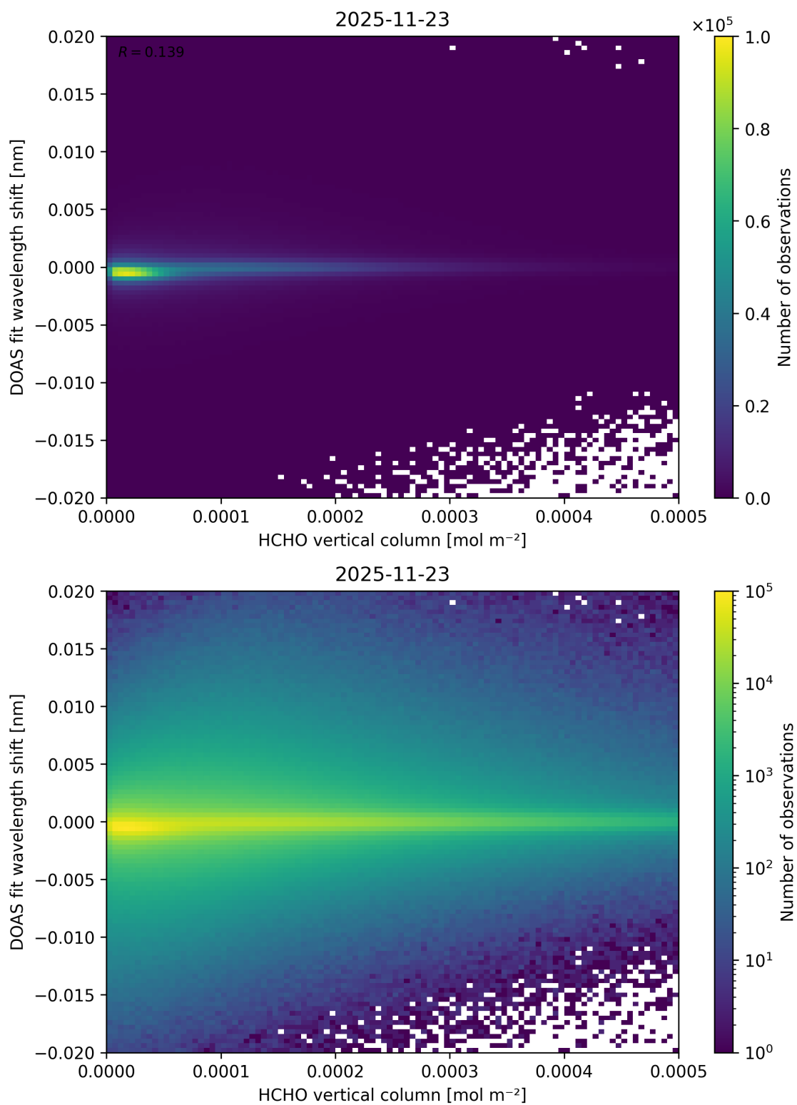
Figure 139: Scatter density plot of “HCHO vertical column” against “DOAS fit wavelength shift” for 2025-11-23 to 2025-11-24.
