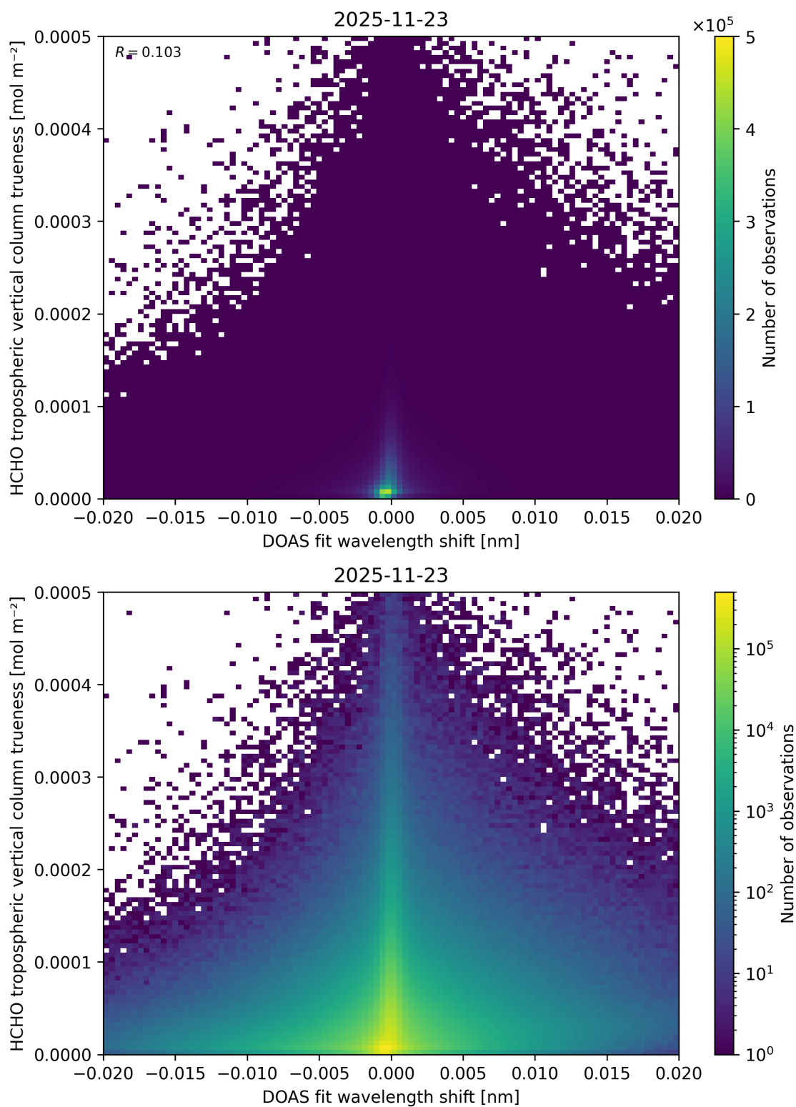
Figure 73: Scatter density plot of “DOAS fit wavelength shift” against “HCHO tropospheric vertical column trueness” for 2025-11-23 to 2025-11-24.
