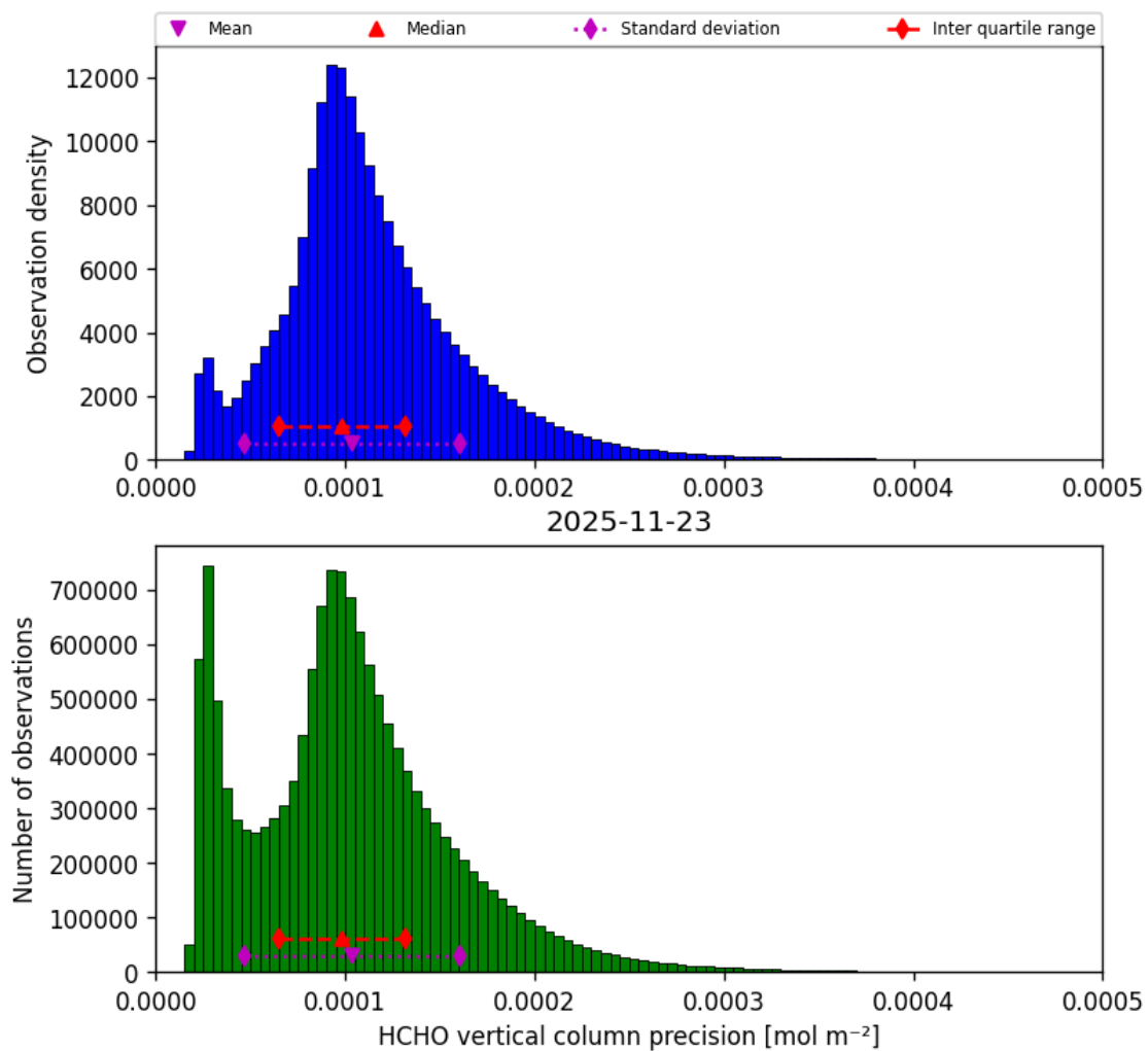
Figure 38: Histogram of “HCHO vertical column precision” for 2025-11-23 to 2025-11-24
