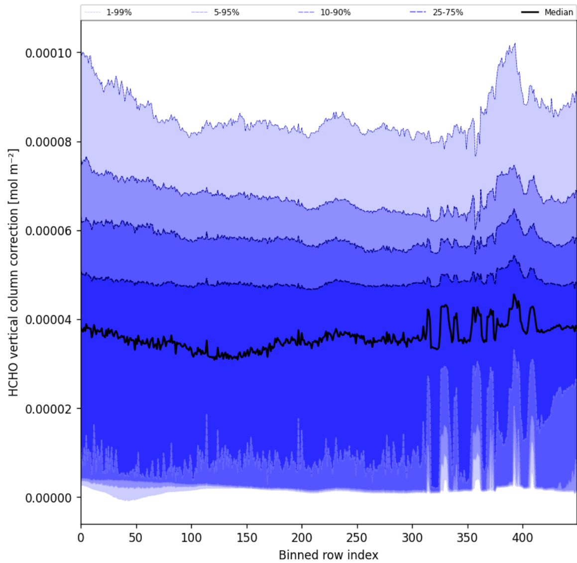
Figure 54: Along track statistics of “HCHO vertical column correction” for 2025-11-23 to 2025-11-24
