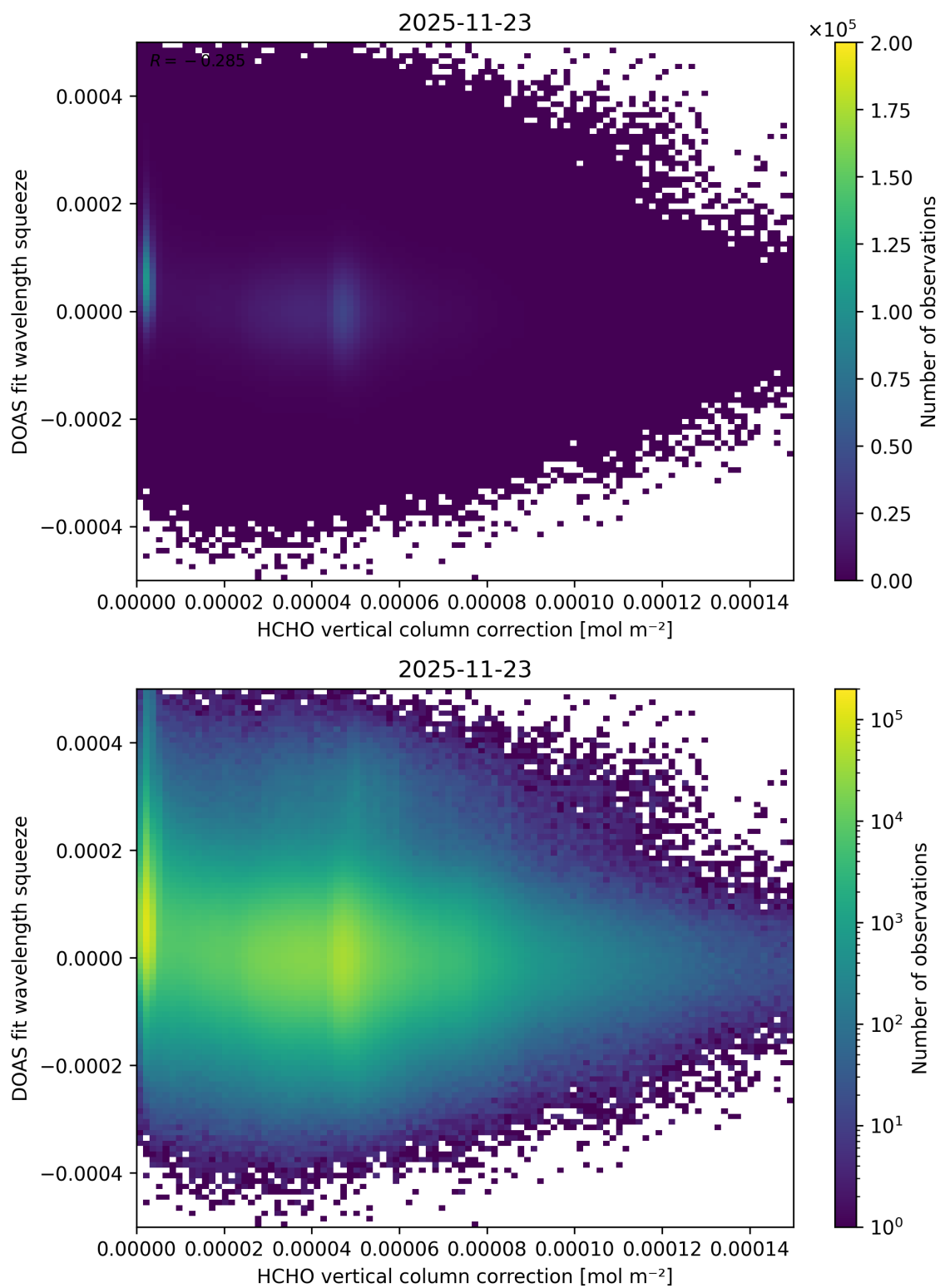
Figure 128: Scatter density plot of “HCHO vertical column correction” against “DOAS fit wavelength squeeze” for 2025-11-23 to 2025-11-24.
