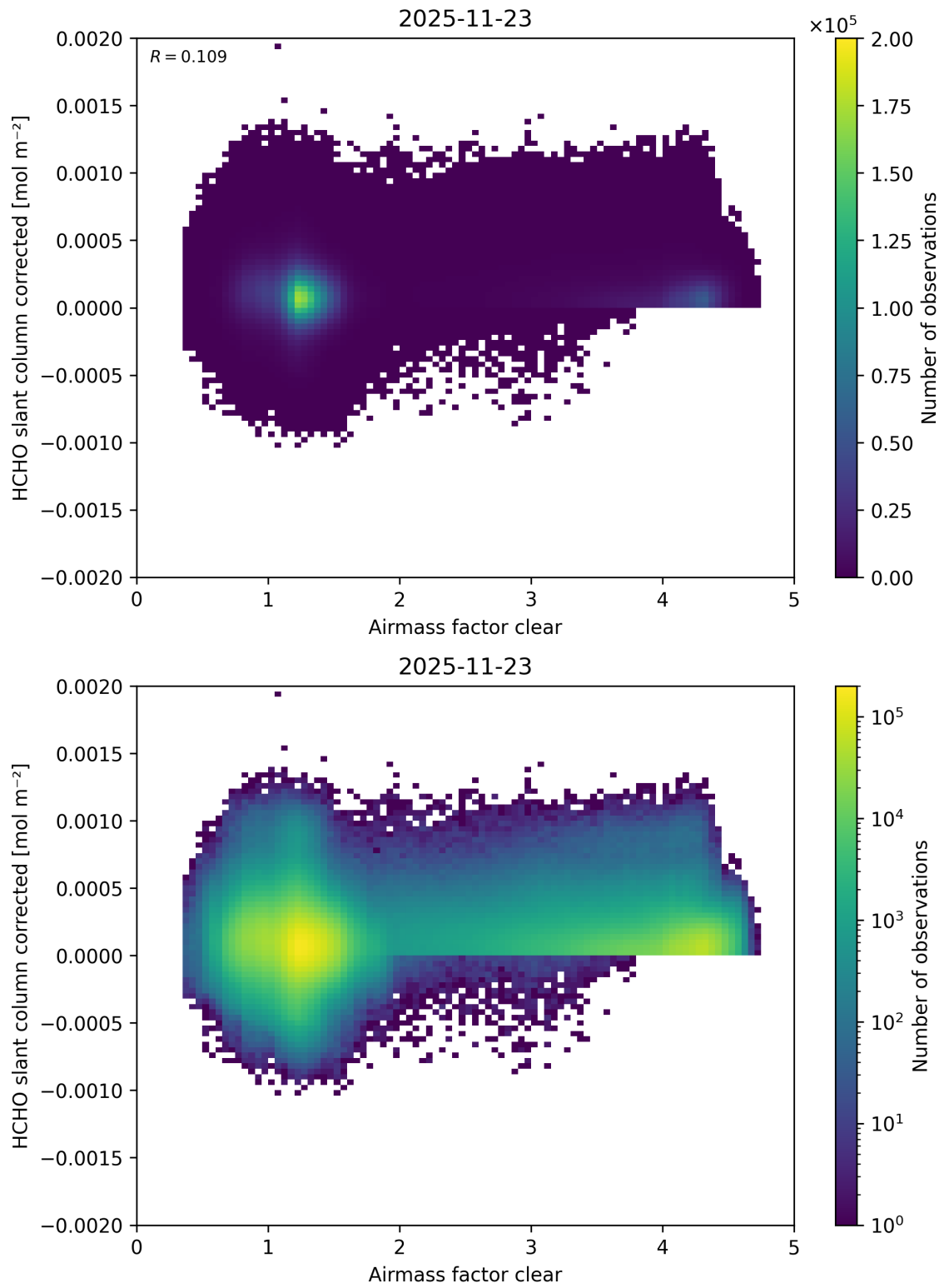
Figure 81: Scatter density plot of “Airmass factor clear” against “HCHO slant column corrected” for 2025-11-23 to 2025-11-24.
