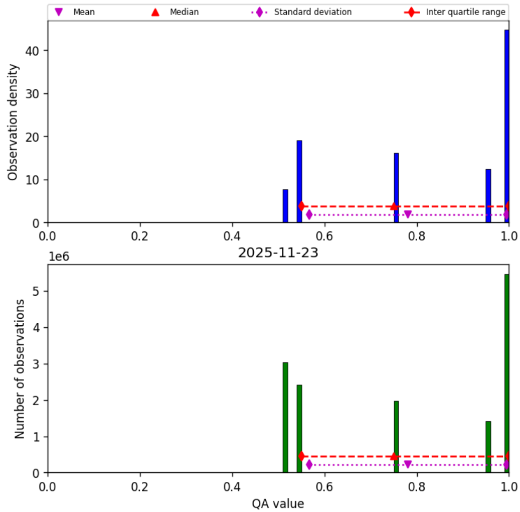
Figure 36: Histogram of “QA value” for 2025-11-23 to 2025-11-24
