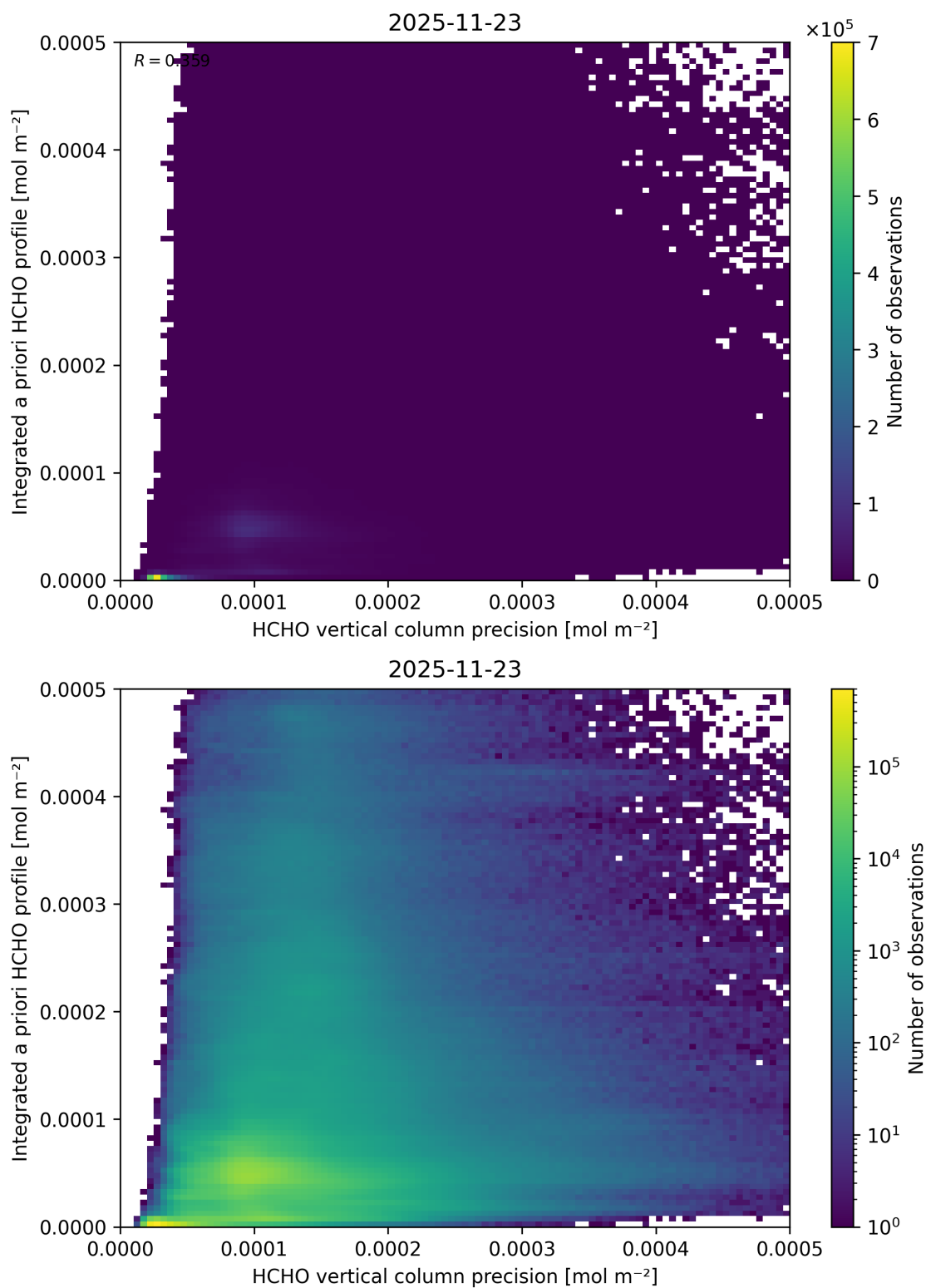
Figure 164: Scatter density plot of “HCHO vertical column precision” against “Integrated a priori HCHO profile” for 2025-11-23 to 2025-11-24.
