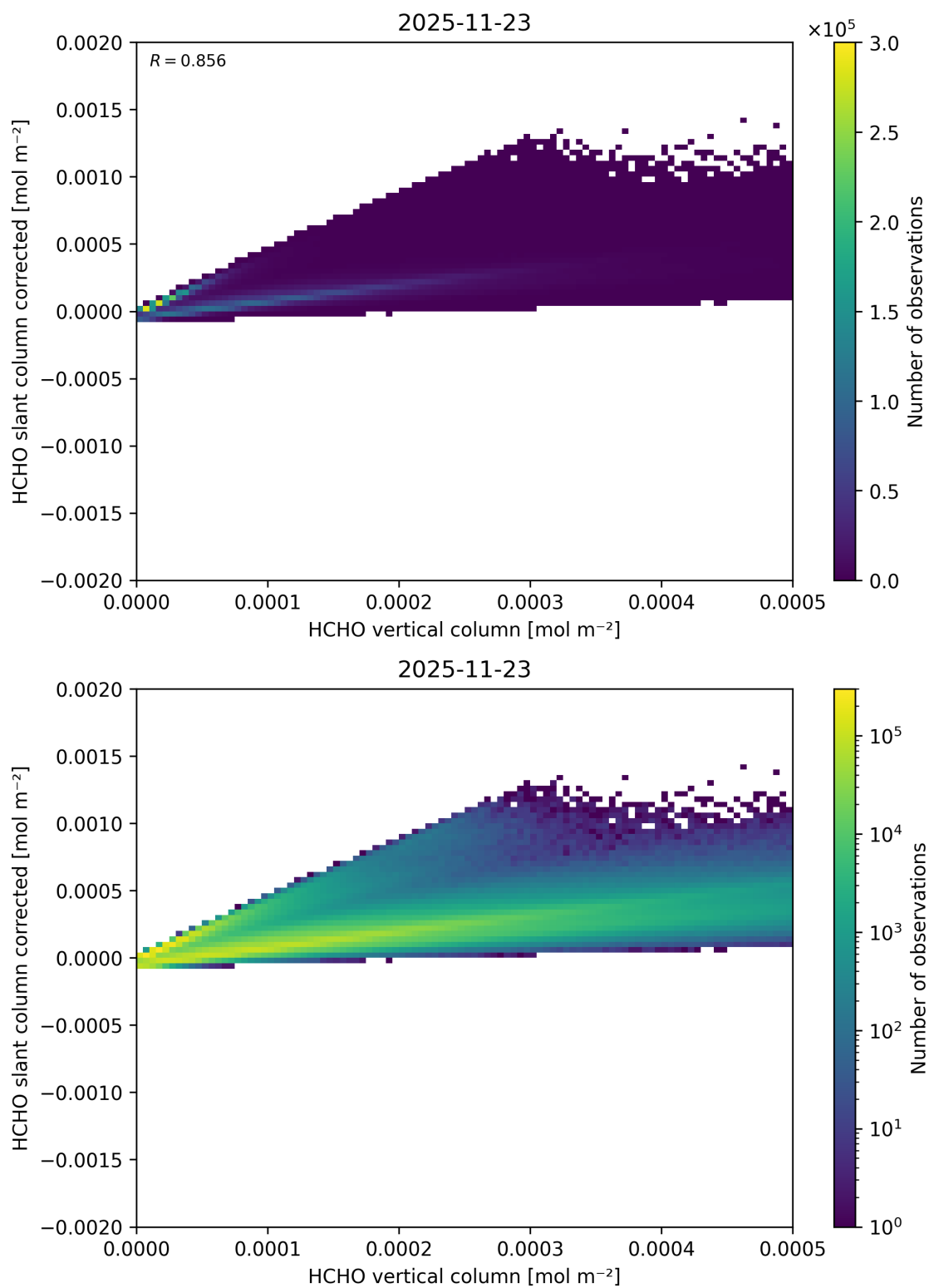
Figure 142: Scatter density plot of “HCHO vertical column” against “HCHO slant column corrected” for 2025-11-23 to 2025-11-24.
