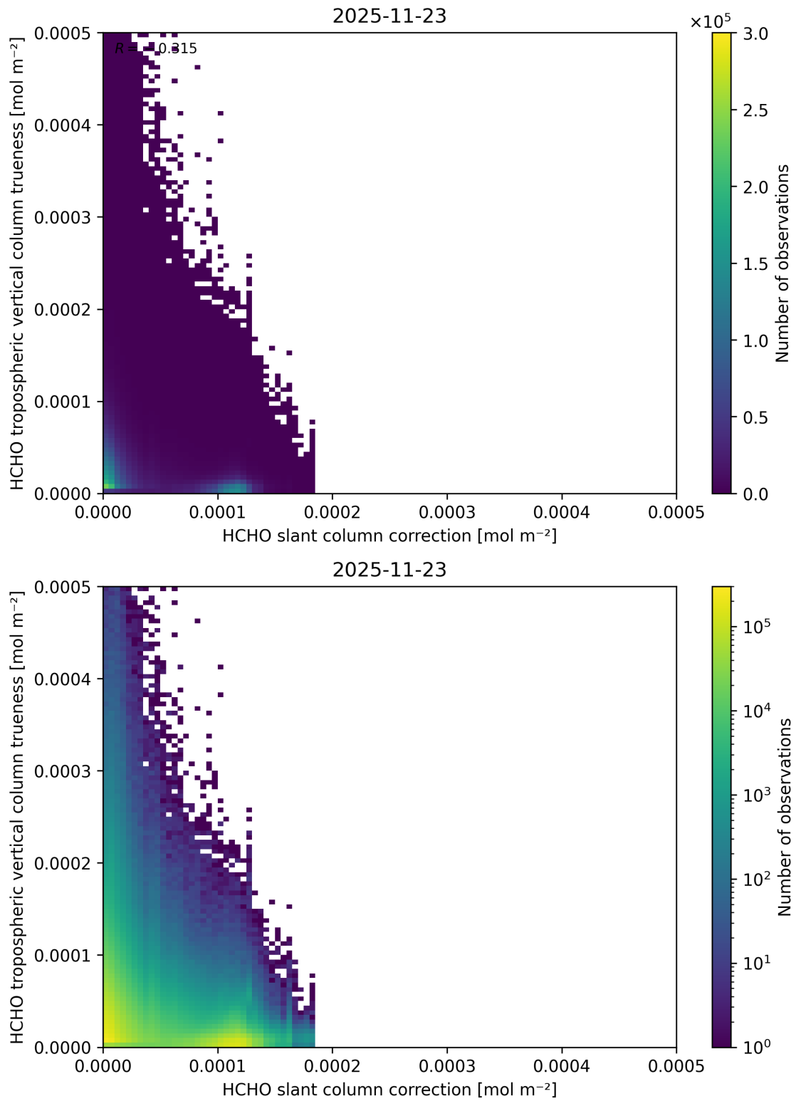
Figure 87: Scatter density plot of “HCHO slant column correction” against “HCHO tropospheric vertical column trueness” for 2025-11-23 to 2025-11-24.
