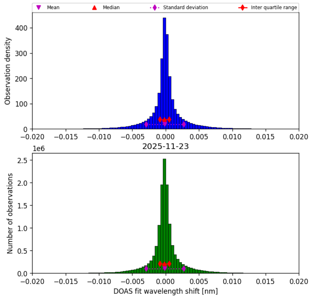
Figure 46: Histogram of “DOAS fit wavelength shift” for 2025-11-23 to 2025-11-24
