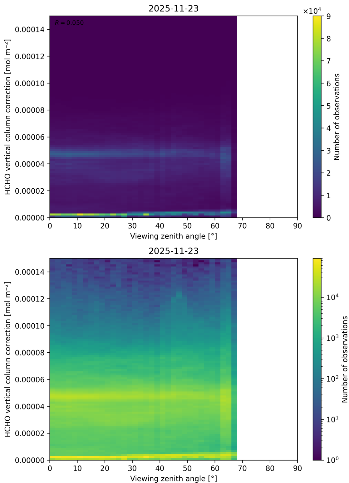
Figure 213: Scatter density plot of “Viewing zenith angle” against “HCHO vertical column correction” for 2025-11-23 to 2025-11-24.
