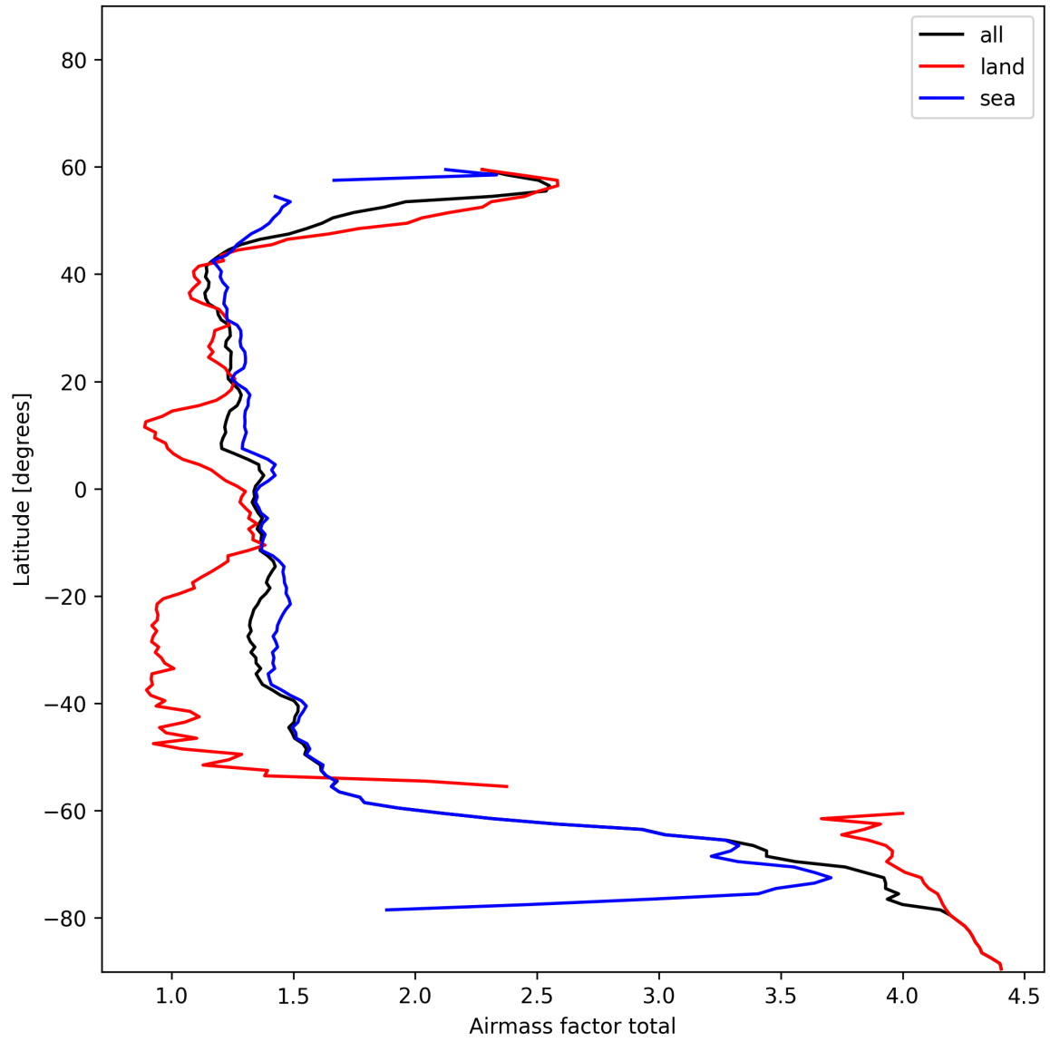
Figure 27: Zonal average of “Airmass factor total” for 2025-11-23 to 2025-11-24.
