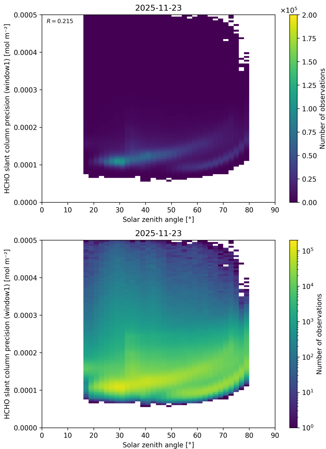
Figure 193: Scatter density plot of “Solar zenith angle” against “HCHO slant column precision (window1)” for 2025-11-23 to 2025-11-24.
