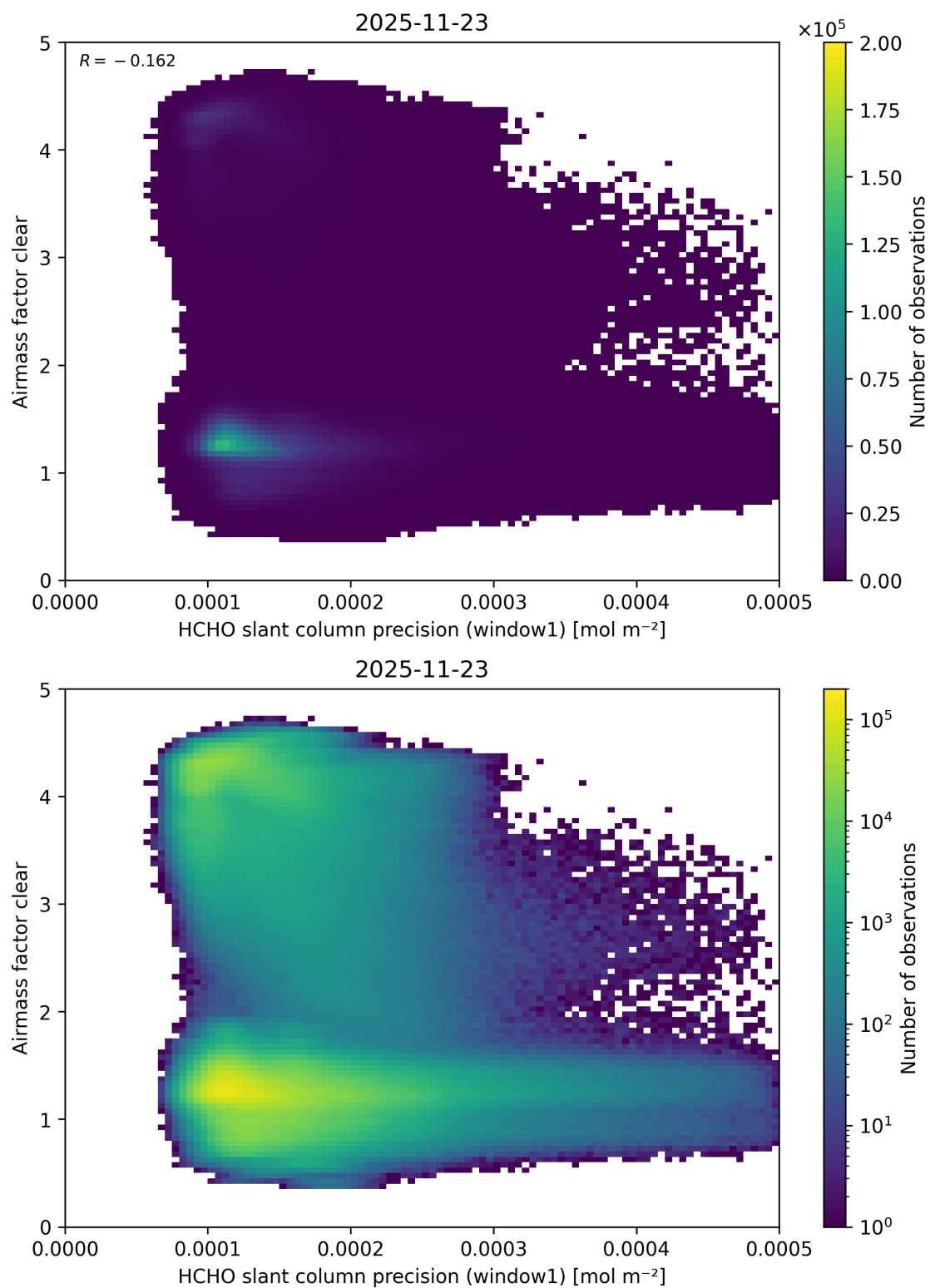
Figure 102: Scatter density plot of “HCHO slant column precision (window1)” against “Airmass factor clear” for 2025-11-23 to 2025-11-24.
