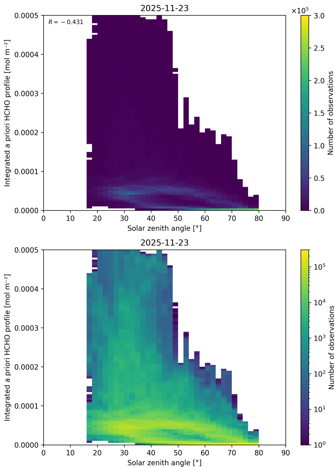
Figure 200: Scatter density plot of “Solar zenith angle” against “Integrated a priori HCHO profile” for 2025-11-23 to 2025-11-24.
