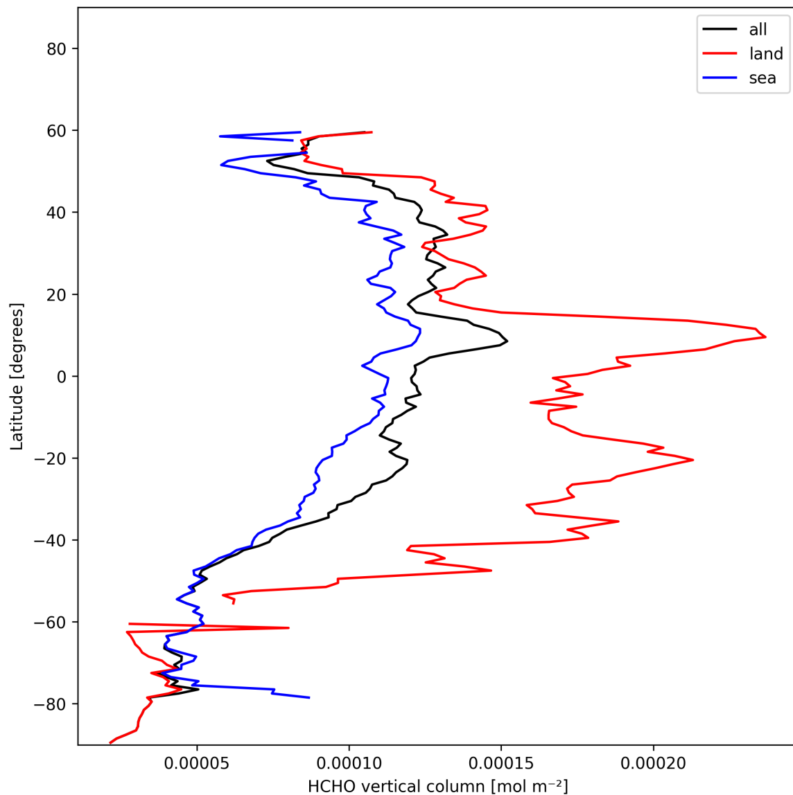
Figure 22: Zonal average of “HCHO vertical column” for 2025-11-23 to 2025-11-24.
