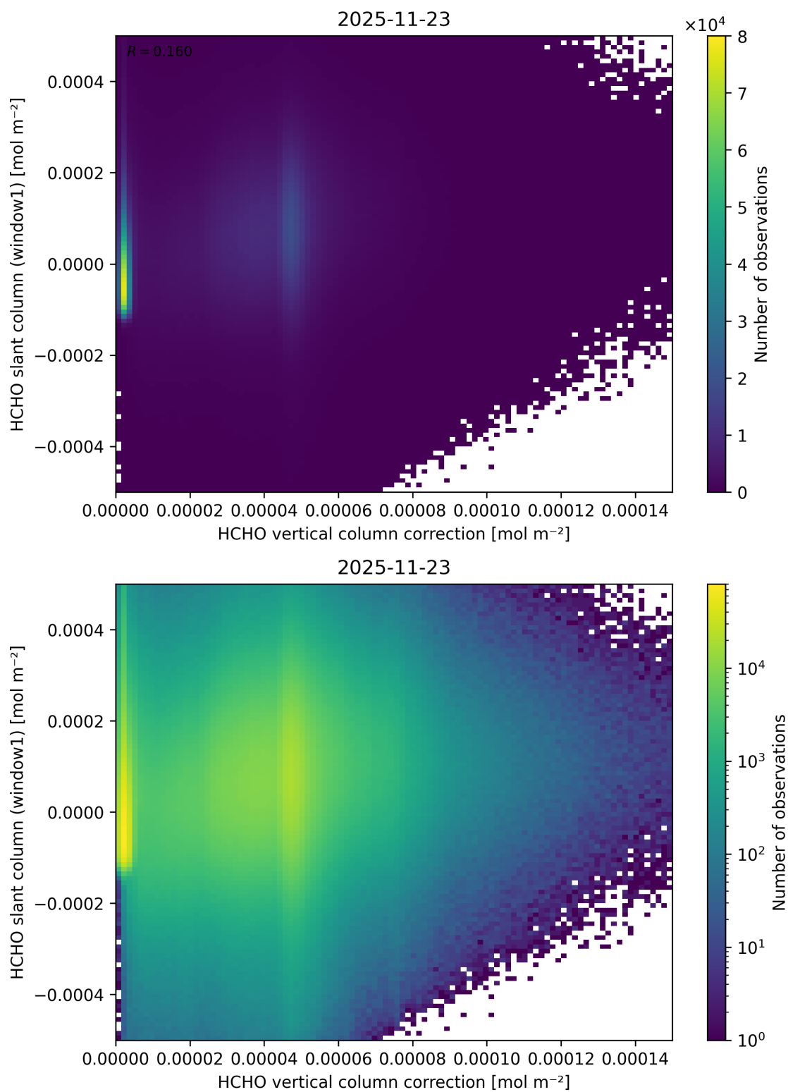
Figure 132: Scatter density plot of “HCHO vertical column correction” against “HCHO slant column (window1)” for 2025-11-23 to 2025-11-24.
