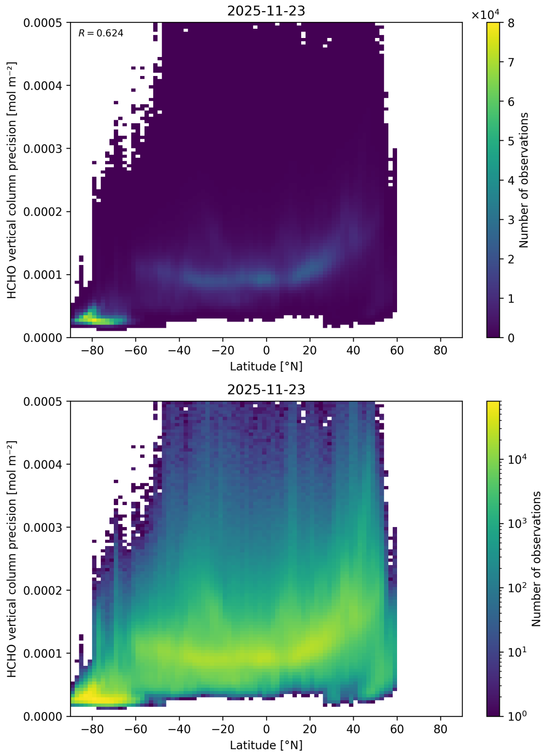
Figure 183: Scatter density plot of “Latitude” against “HCHO vertical column precision” for 2025-11-23 to 2025-11-24.
