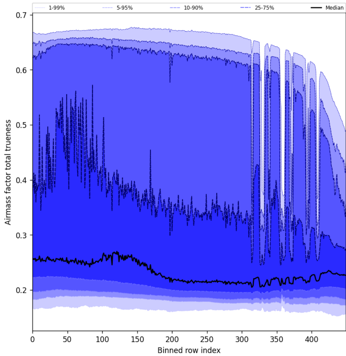
Figure 58: Along track statistics of “Airmass factor total trueness” for 2025-11-23 to 2025-11-24
