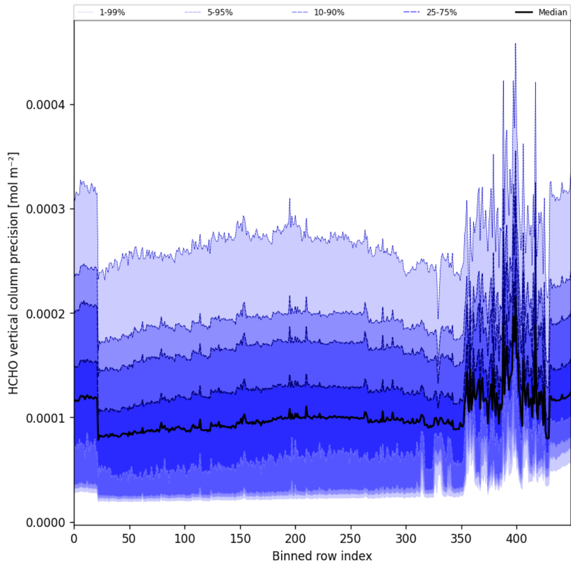
Figure 53: Along track statistics of “HCHO vertical column precision” for 2025-11-23 to 2025-11-24
