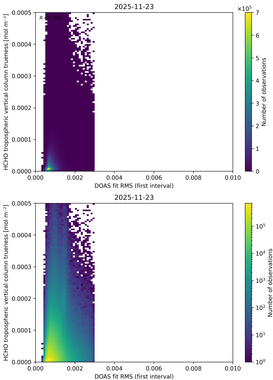
Figure 68: Scatter density plot of “DOAS fit RMS (first interval)” against “HCHO tropospheric vertical column trueness” for 2025-11-23 to 2025-11-24.
