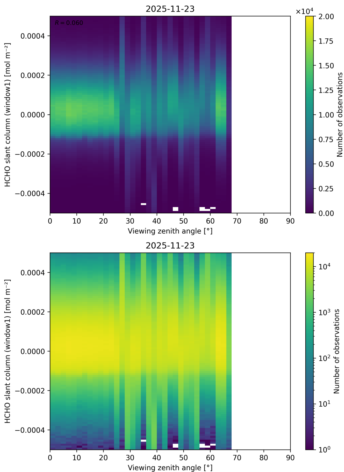
Figure 208: Scatter density plot of “Viewing zenith angle” against “HCHO slant column (window1)” for 2025-11-23 to 2025-11-24.
