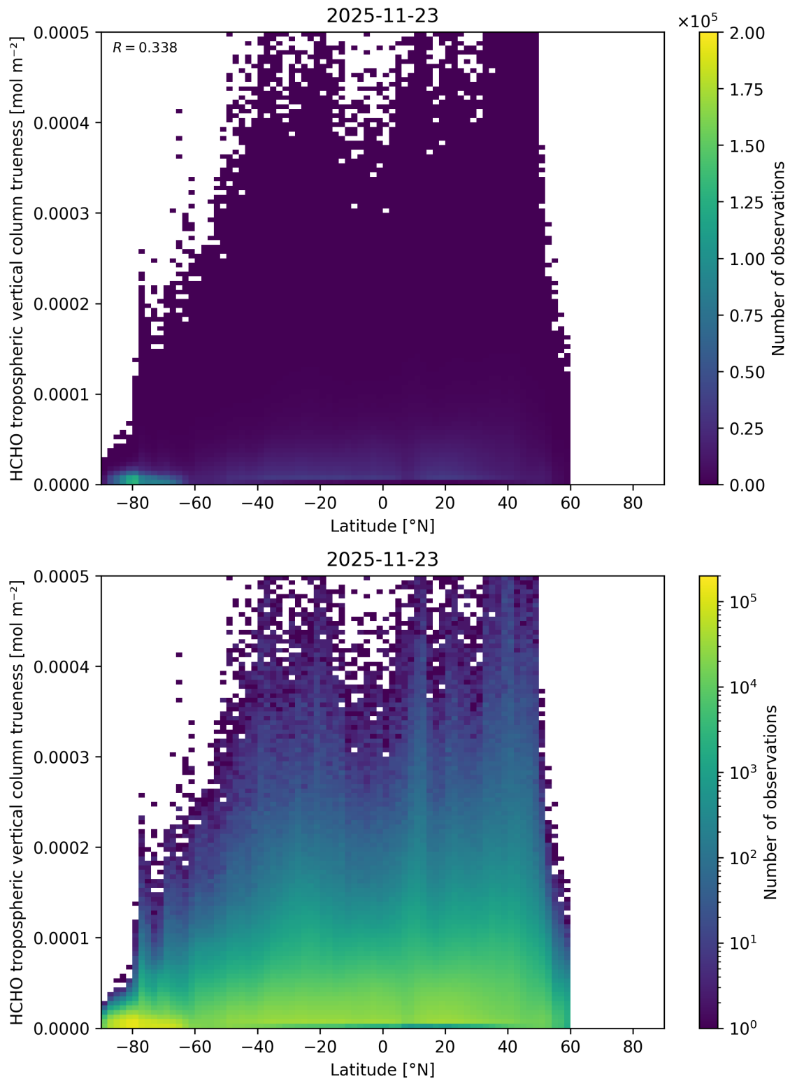
Figure 184: Scatter density plot of “Latitude” against “HCHO tropospheric vertical column trueeness” for 2025-11-23 to 2025-11-24.
