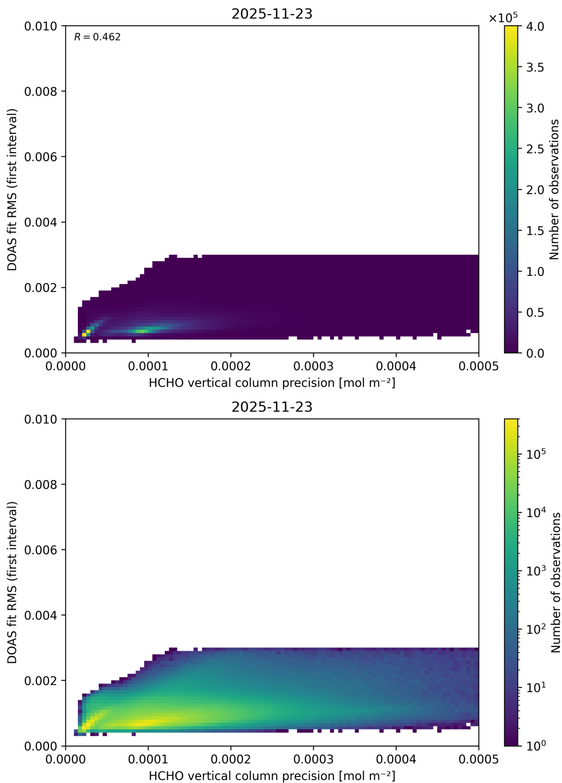
Figure 152: Scatter density plot of “HCHO vertical column precision” against “DOAS fit RMS (first interval)” for 2025-11-23 to 2025-11-24.
