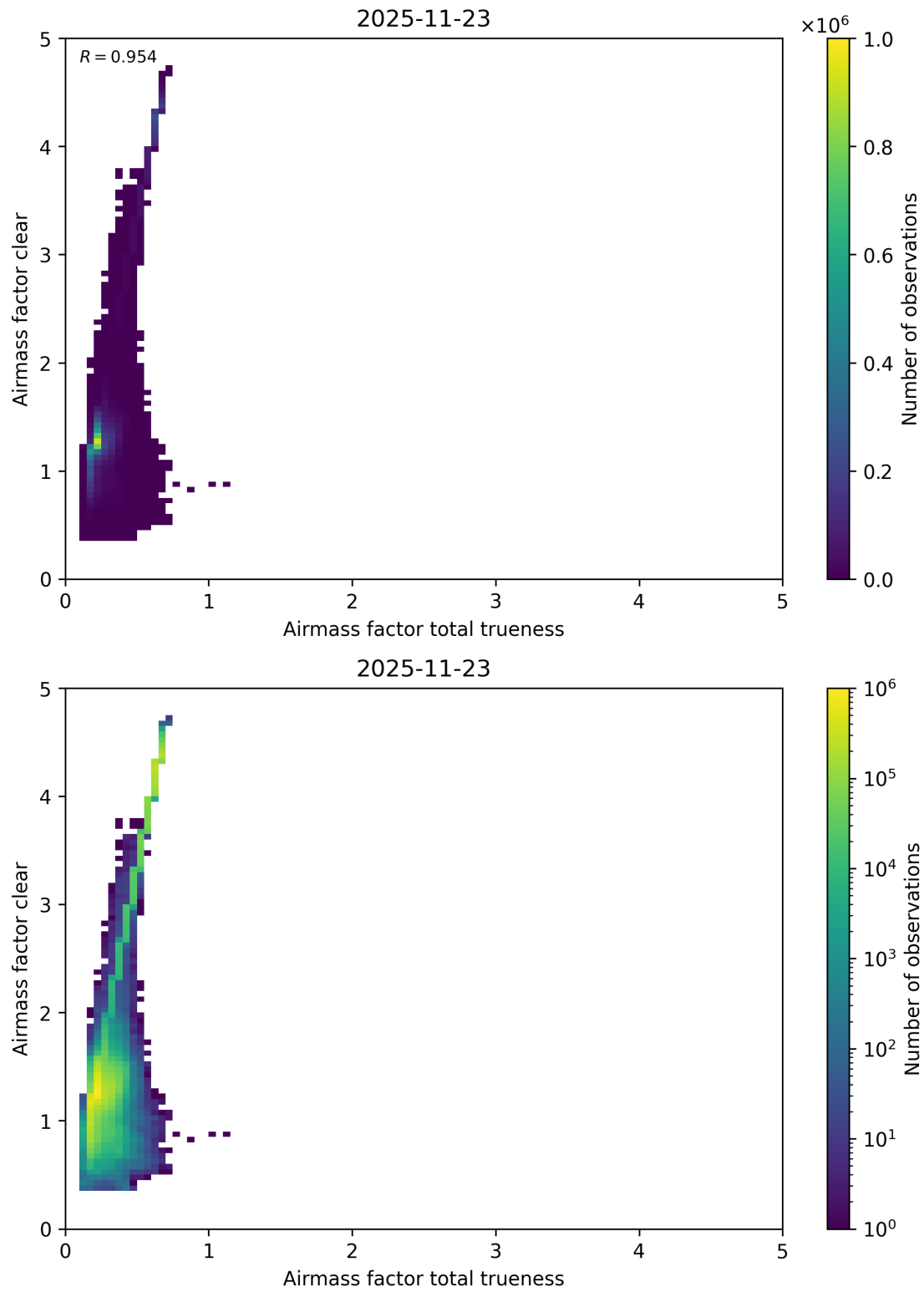
Figure 121: Scatter density plot of “Airmass factor total trueness” against “Airmass factor clear” for 2025-11-23 to 2025-11-24.
