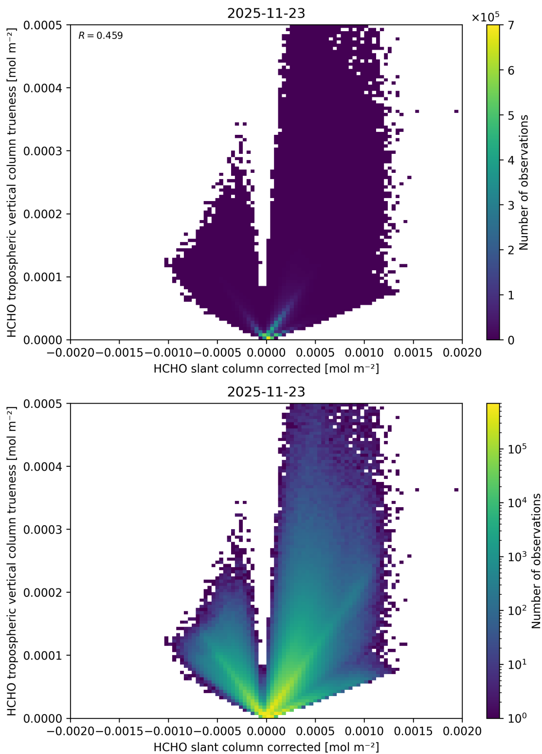
Figure 86: Scatter density plot of “HCHO slant column corrected” against “HCHO tropospheric vertical column trueness” for 2025-11-23 to 2025-11-24.
