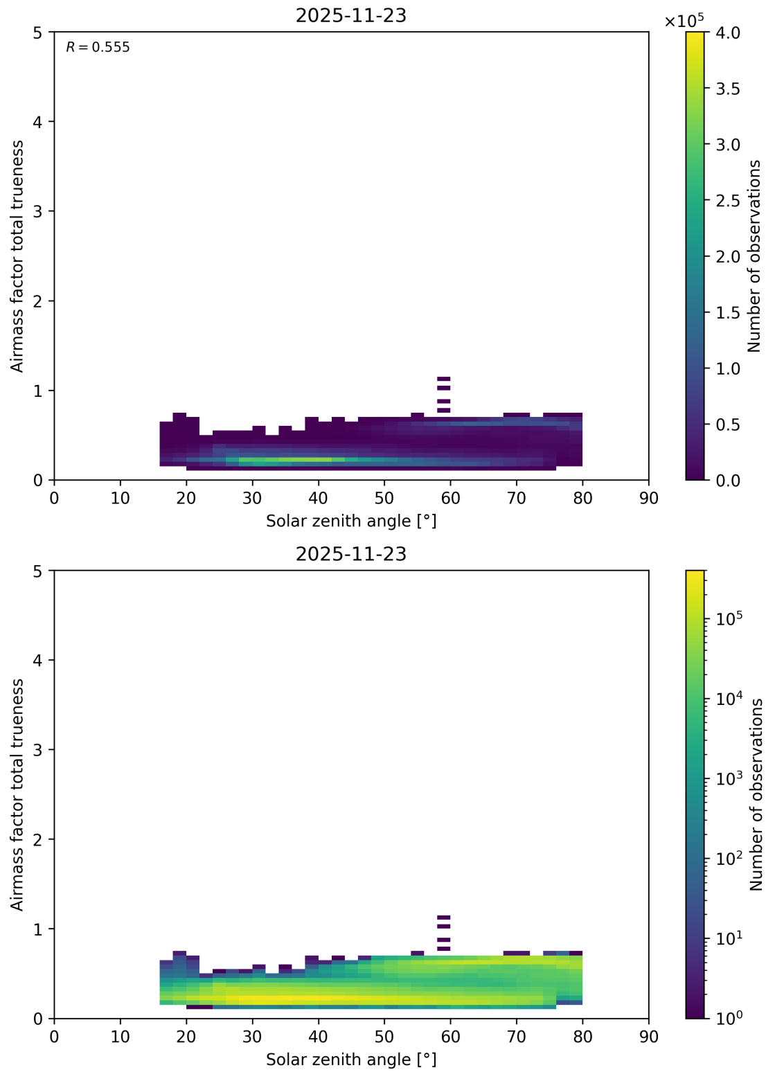
Figure 195: Scatter density plot of “Solar zenith angle” against “Airmass factor total trueness” for 2025-11-23 to 2025-11-24.
