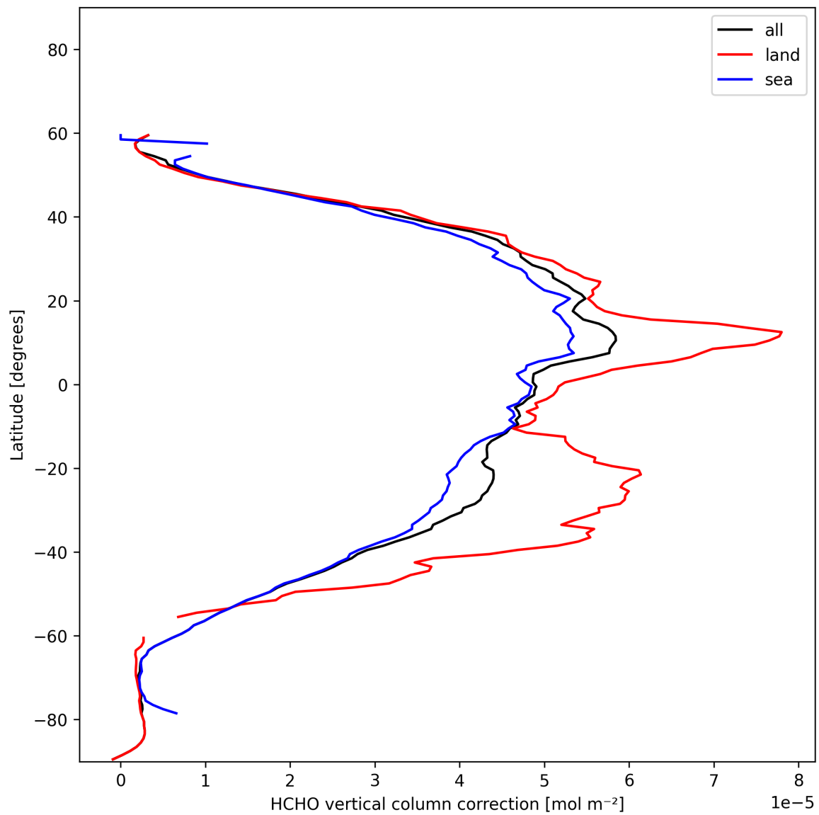
Figure 24: Zonal average of “HCHO vertical column correction” for 2025-11-23 to 2025-11-24.
