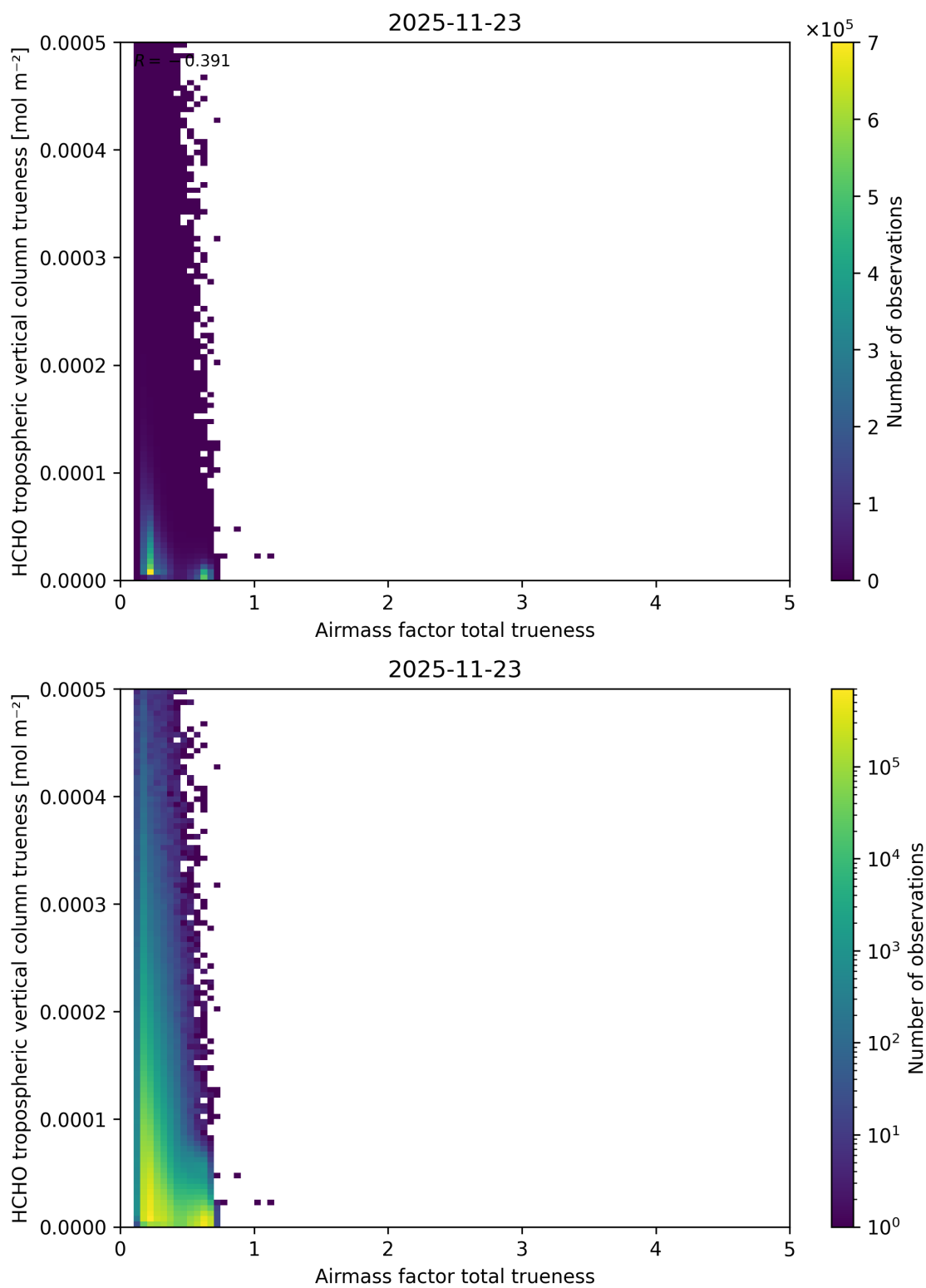
Figure 124: Scatter density plot of “Airmass factor total trueness” against “HCHO tropospheric vertical column trueness” for 2025-11-23 to 2025-11-24.
