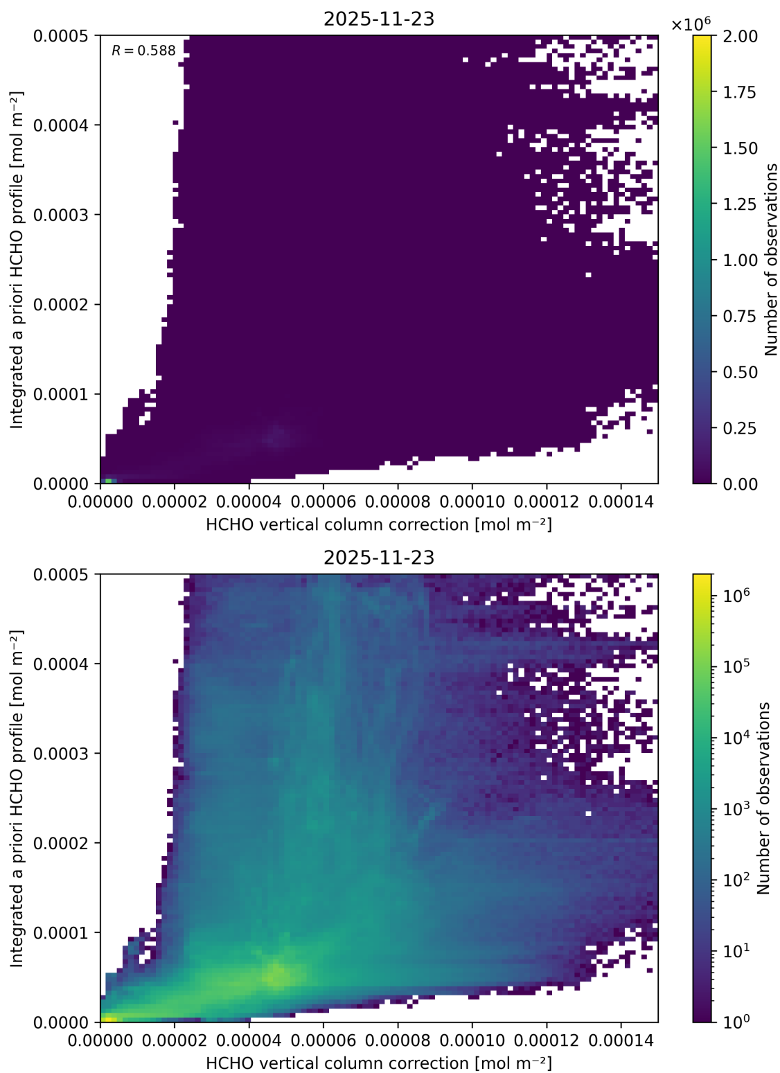
Figure 137: Scatter density plot of “HCHO vertical column correction” against “Integrated a priori HCHO profile” for 2025-11-23 to 2025-11-24.
