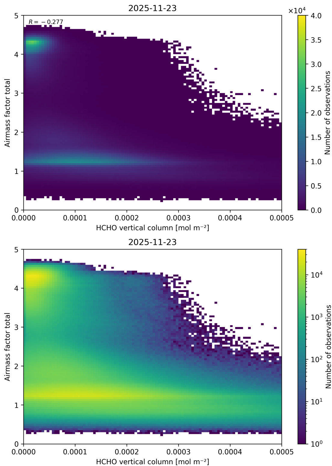
Figure 146: Scatter density plot of “HCHO vertical column” against “Airmass factor total” for 2025-11-23 to 2025-11-24.
