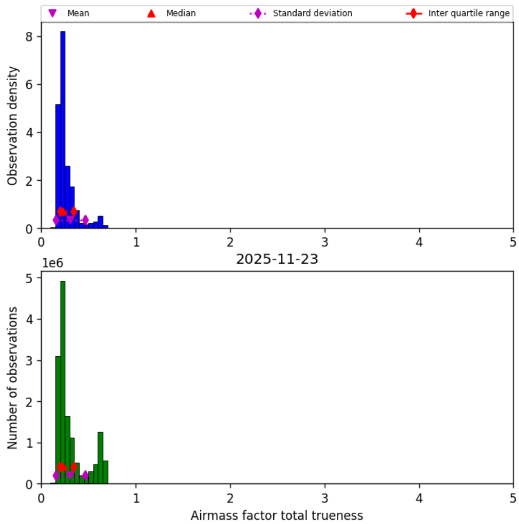
Figure 43: Histogram of “Airmass factor total trueness” for 2025-11-23 to 2025-11-24
