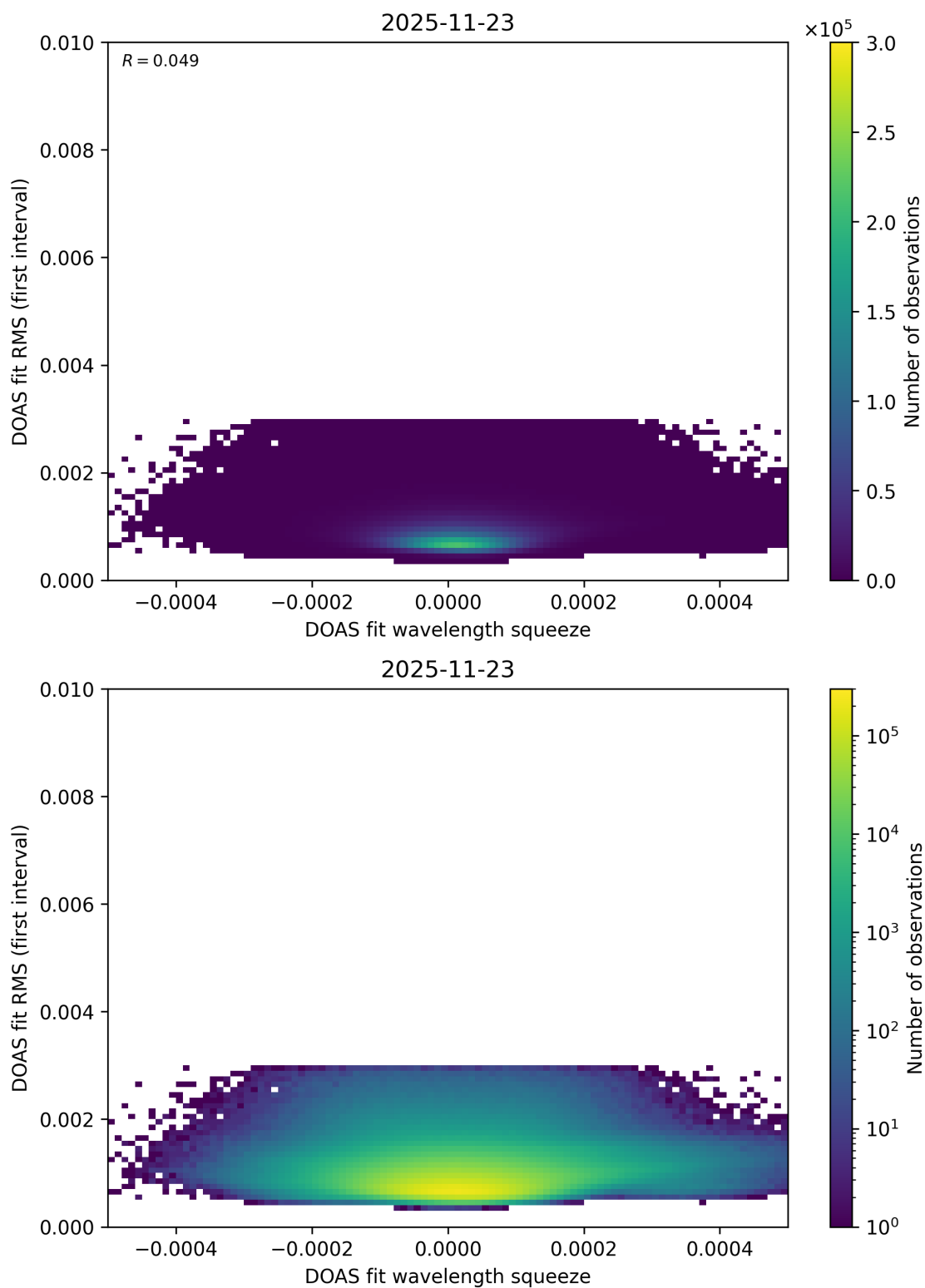
Figure 74: Scatter density plot of “DOAS fit wavelength squeeze” against “DOAS fit RMS (first interval)” for 2025-11-23 to 2025-11-24.
