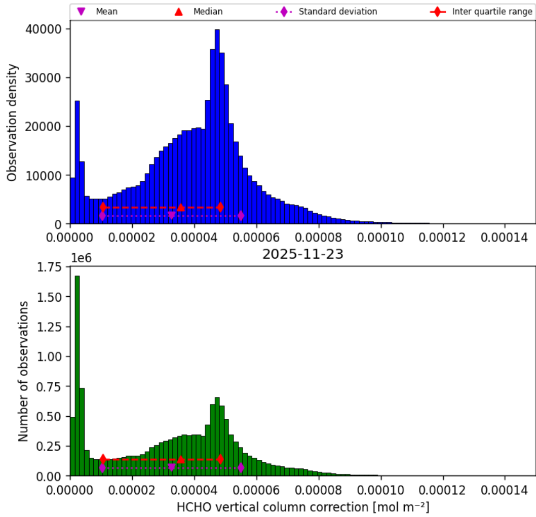
Figure 39: Histogram of “HCHO vertical column correction” for 2025-11-23 to 2025-11-24
