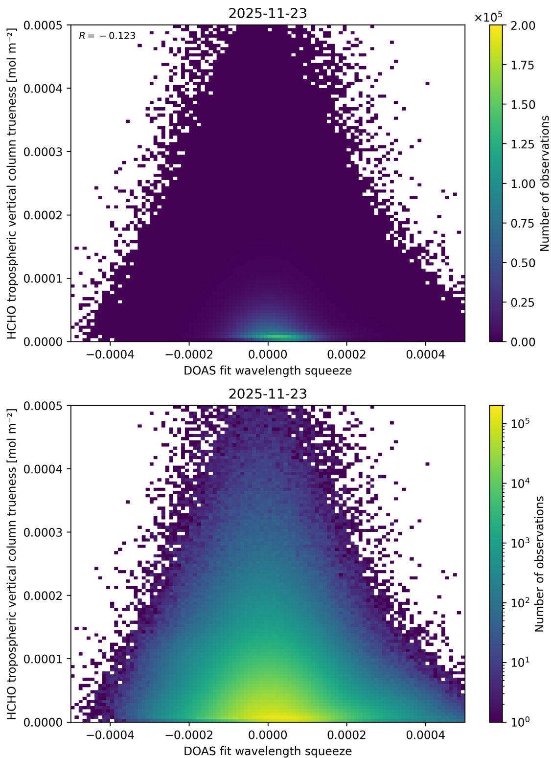
Figure 77: Scatter density plot of “DOAS fit wavelength squeeze” against “HCHO tropospheric vertical column trueness” for 2025-11-23 to 2025-11-24.
