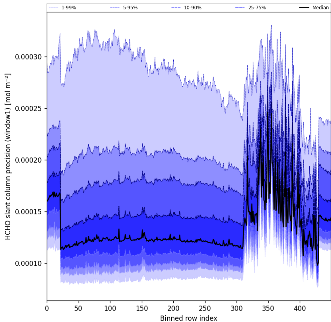
Figure 56: Along track statistics of “HCHO slant column precision (window1)” for 2025-11-23 to 2025-11-24
