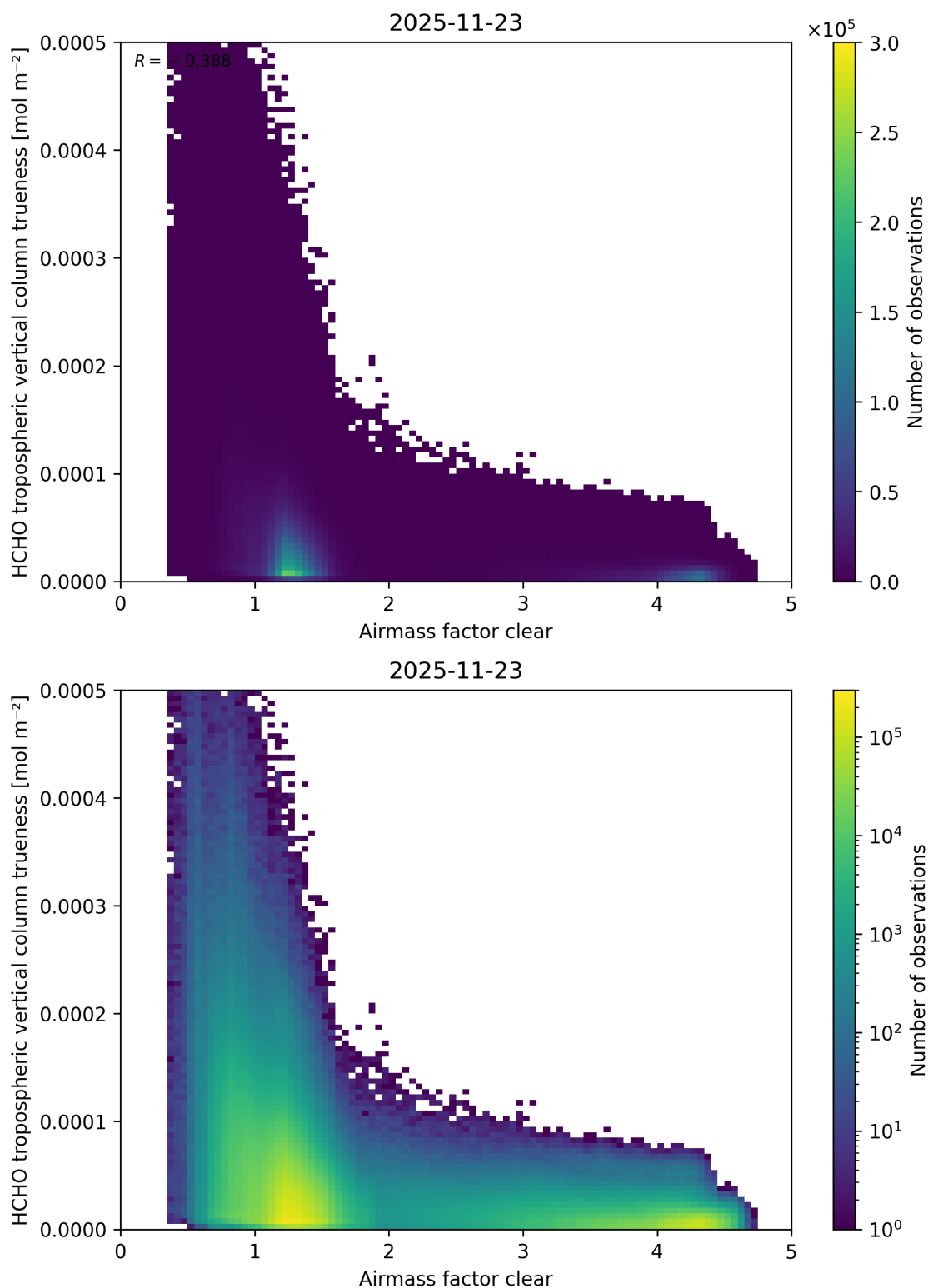
Figure 83: Scatter density plot of “Airmass factor clear” against “HCHO tropospheric vertical column trueness” for 2025-11-23 to 2025-11-24.
