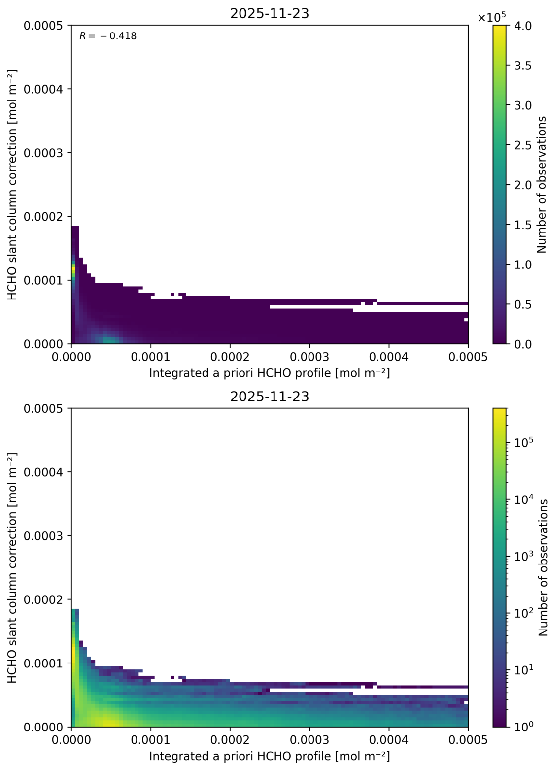
Figure 169: Scatter density plot of “Integrated a priori HCHO profile” against “HCHO slant column correction” for 2025-11-23 to 2025-11-24.
