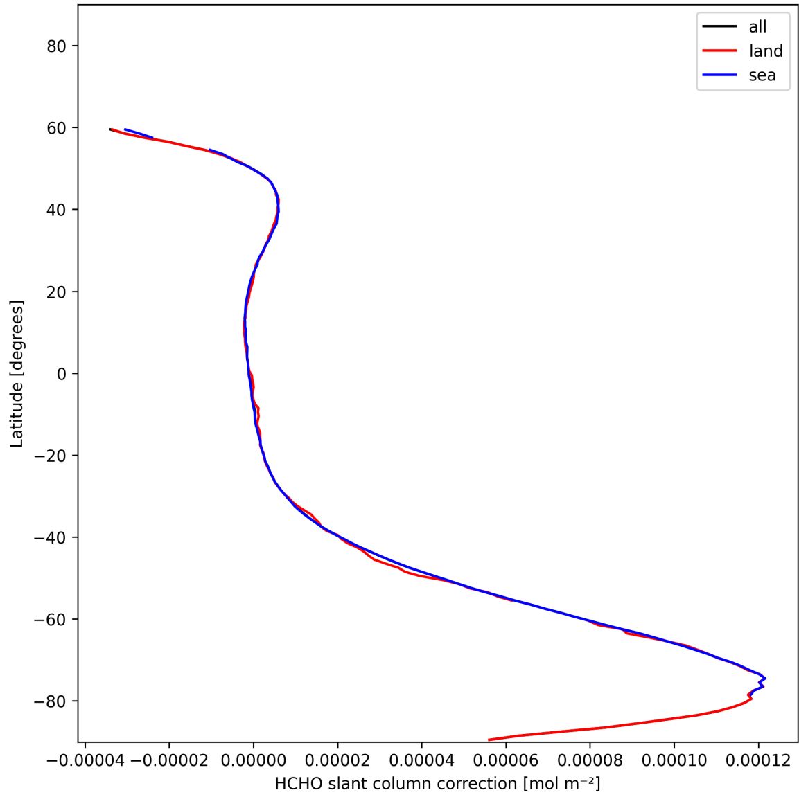
Figure 34: Zonal average of “HCHO slant column correction” for 2025-11-23 to 2025-11-24.
