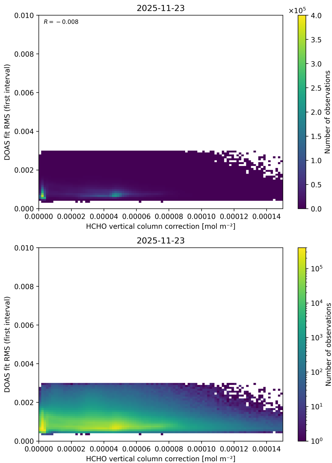
Figure 126: Scatter density plot of “HCHO vertical column correction” against “DOAS fit RMS (first interval)” for 2025-11-23 to 2025-11-24.
