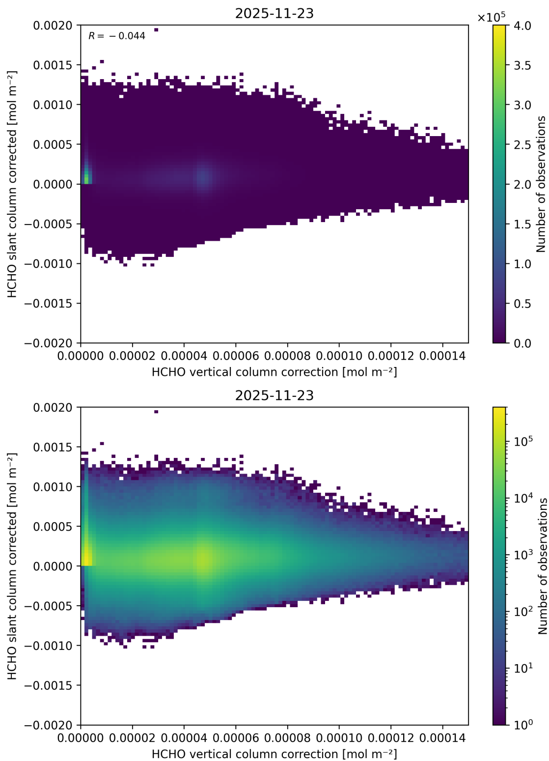
Figure 130: Scatter density plot of “HCHO vertical column correction” against “HCHO slant column corrected” for 2025-11-23 to 2025-11-24.
