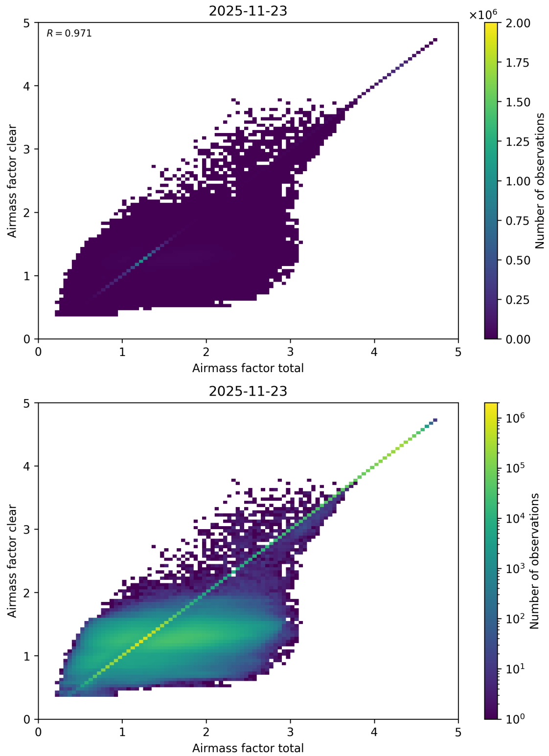
Figure 112: Scatter density plot of “Airmass factor total” against “Airmass factor clear” for 2025-11-23 to 2025-11-24.
