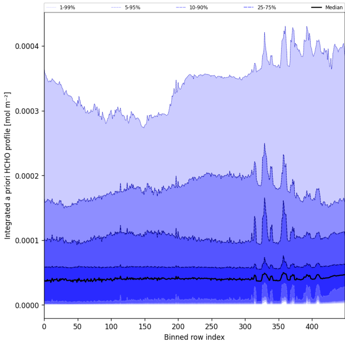
Figure 60: Along track statistics of "Integrated a priori HCHO profile" for 2025-11-23 to 2025-11-24
