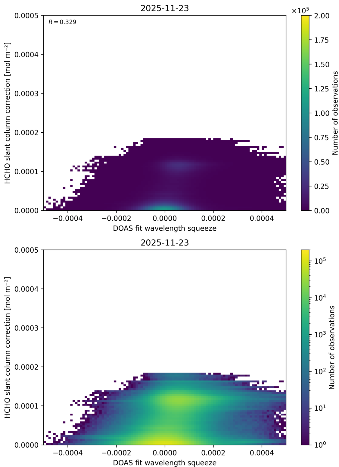
Figure 76: Scatter density plot of “DOAS fit wavelength squeeze” against “HCHO slant column correction” for 2025-11-23 to 2025-11-24.
