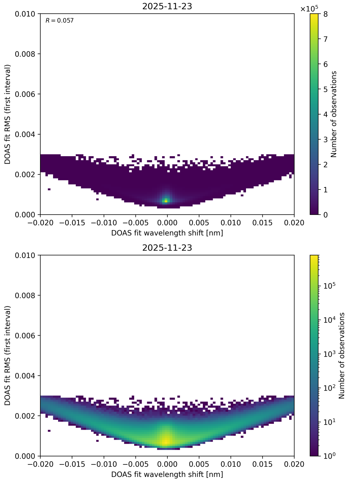
Figure 69: Scatter density plot of “DOAS fit wavelength shift” against “DOAS fit RMS (first interval)” for 2025-11-23 to 2025-11-24.
