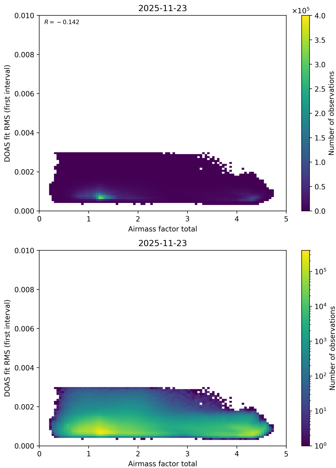
Figure 109: Scatter density plot of “Airmass factor total” against “DOAS fit RMS (first interval)” for 2025-11-23 to 2025-11-24.
