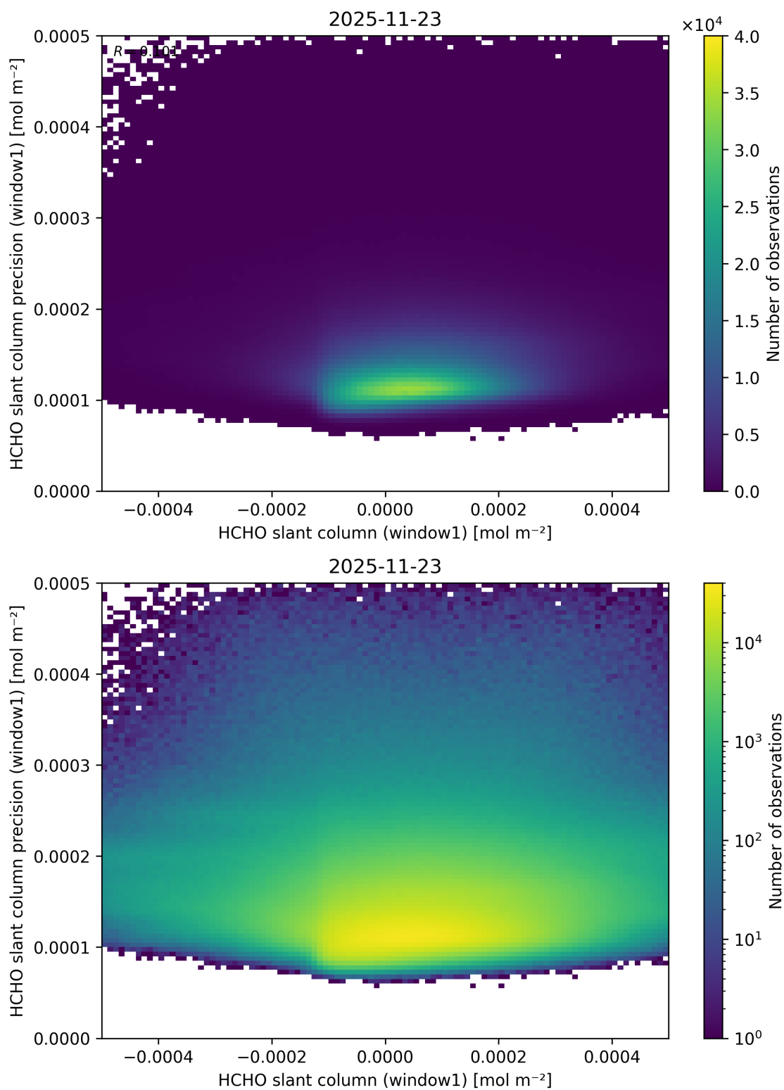
Figure 94: Scatter density plot of “HCHO slant column (window1)” against “HCHO slant column precision (window1)” for 2025-11-23 to 2025-11-24.
