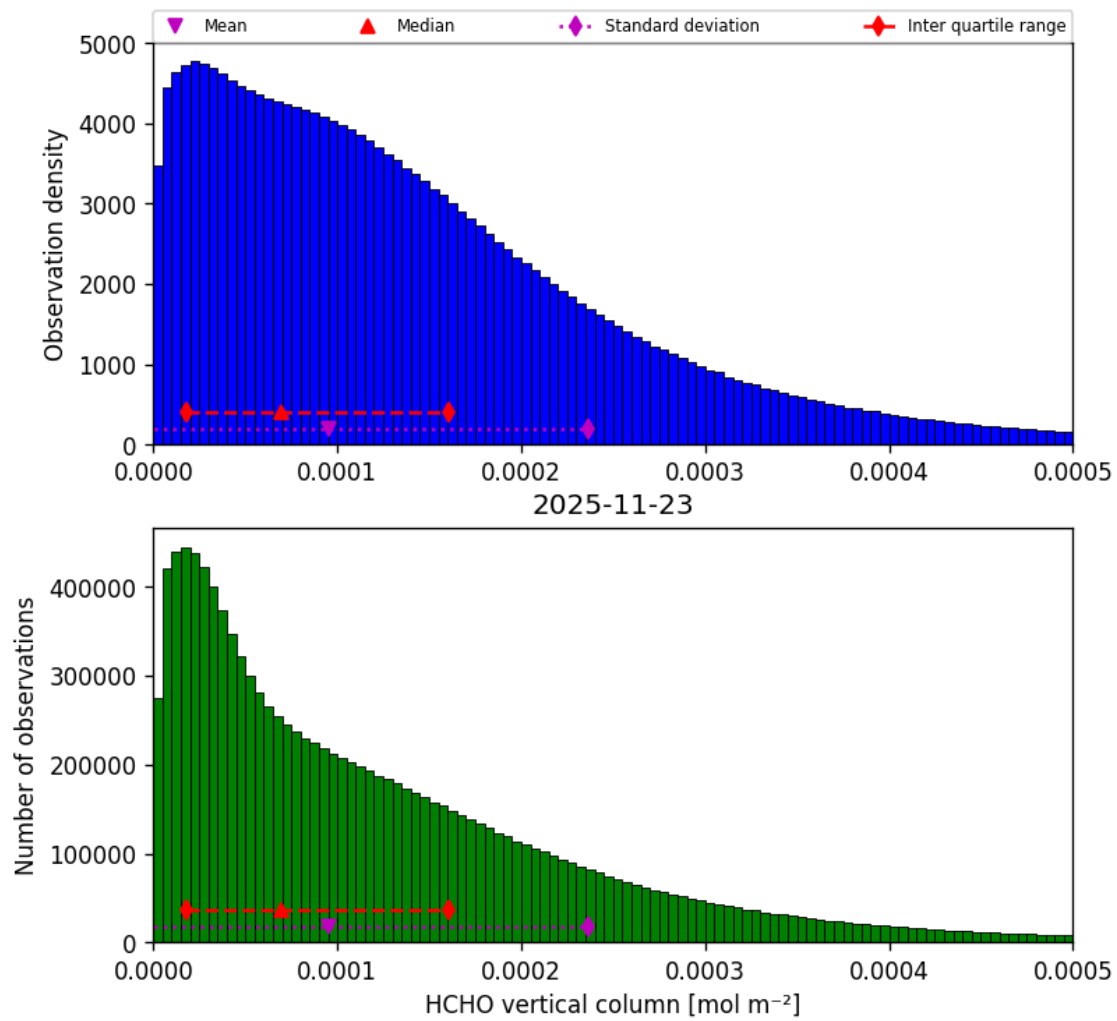
Figure 37: Histogram of “HCHO vertical column” for 2025-11-23 to 2025-11-24
