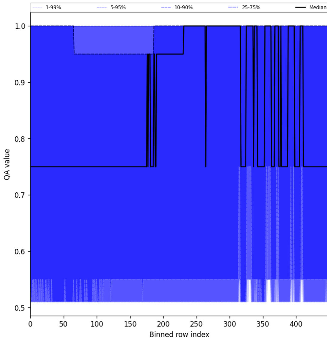
Figure 51: Along track statistics of “QA value” for 2025-11-23 to 2025-11-24
