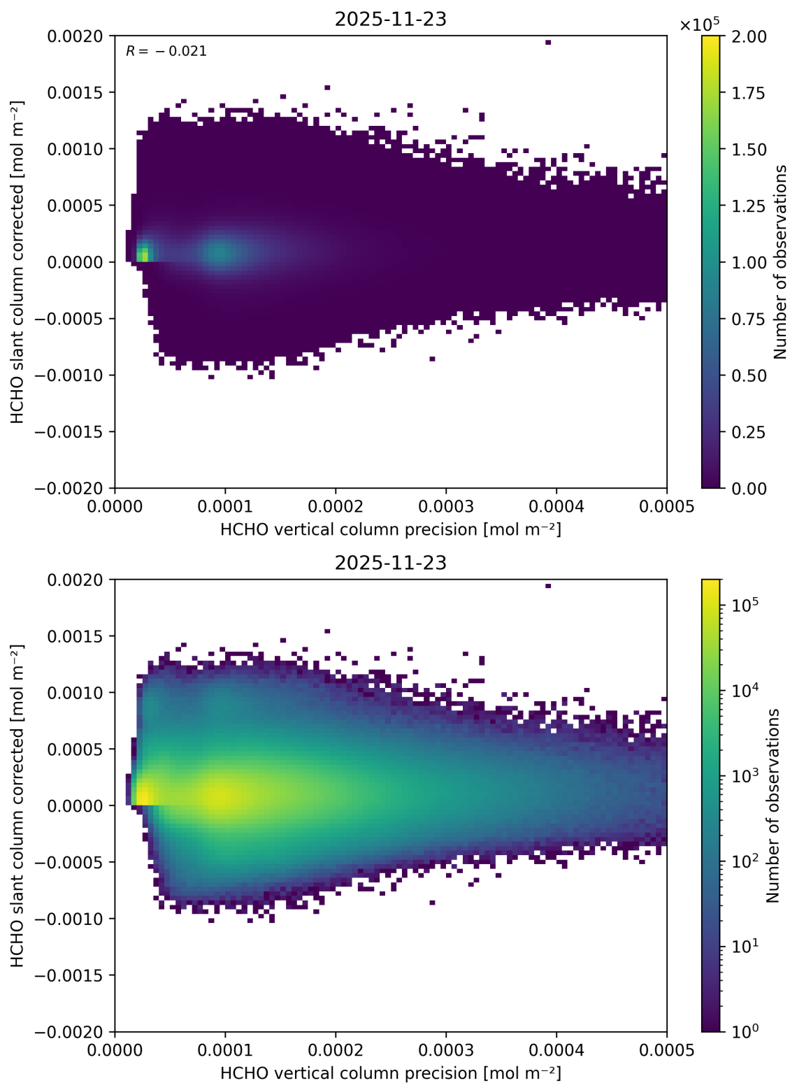
Figure 156: Scatter density plot of “HCHO vertical column precision” against “HCHO slant column corrected” for 2025-11-23 to 2025-11-24.
