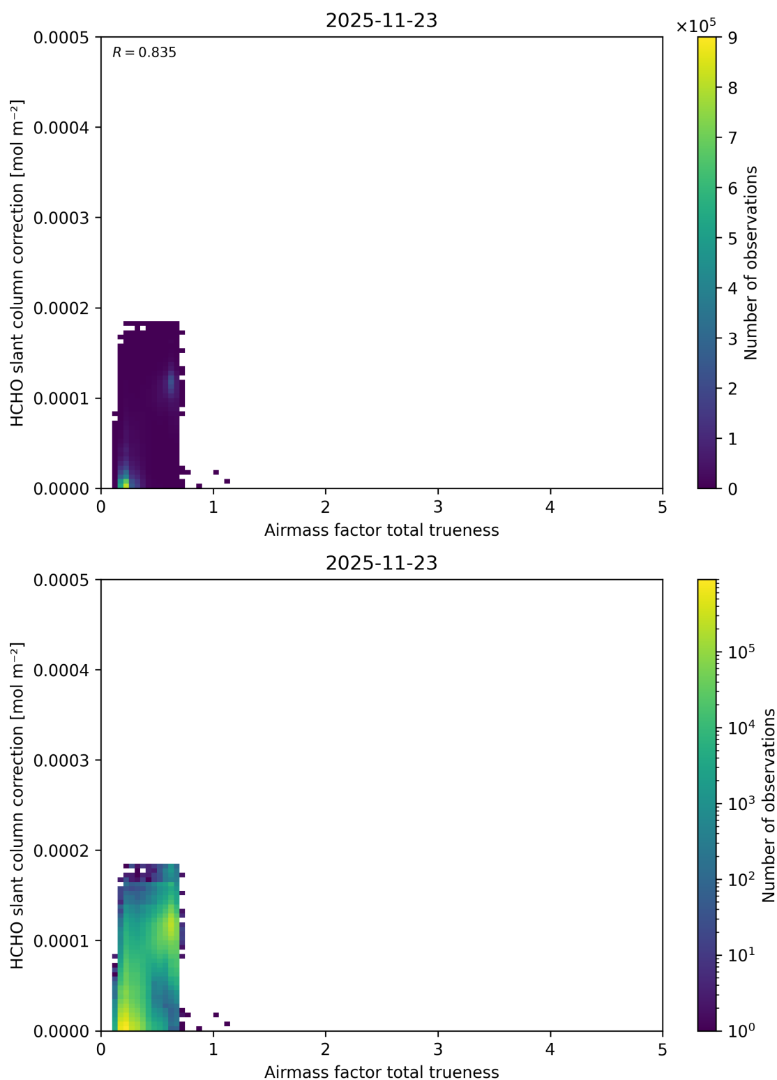
Figure 123: Scatter density plot of “Airmass factor total truiness” against “HCHO slant column correction” for 2025-11-23 to 2025-11-24.
