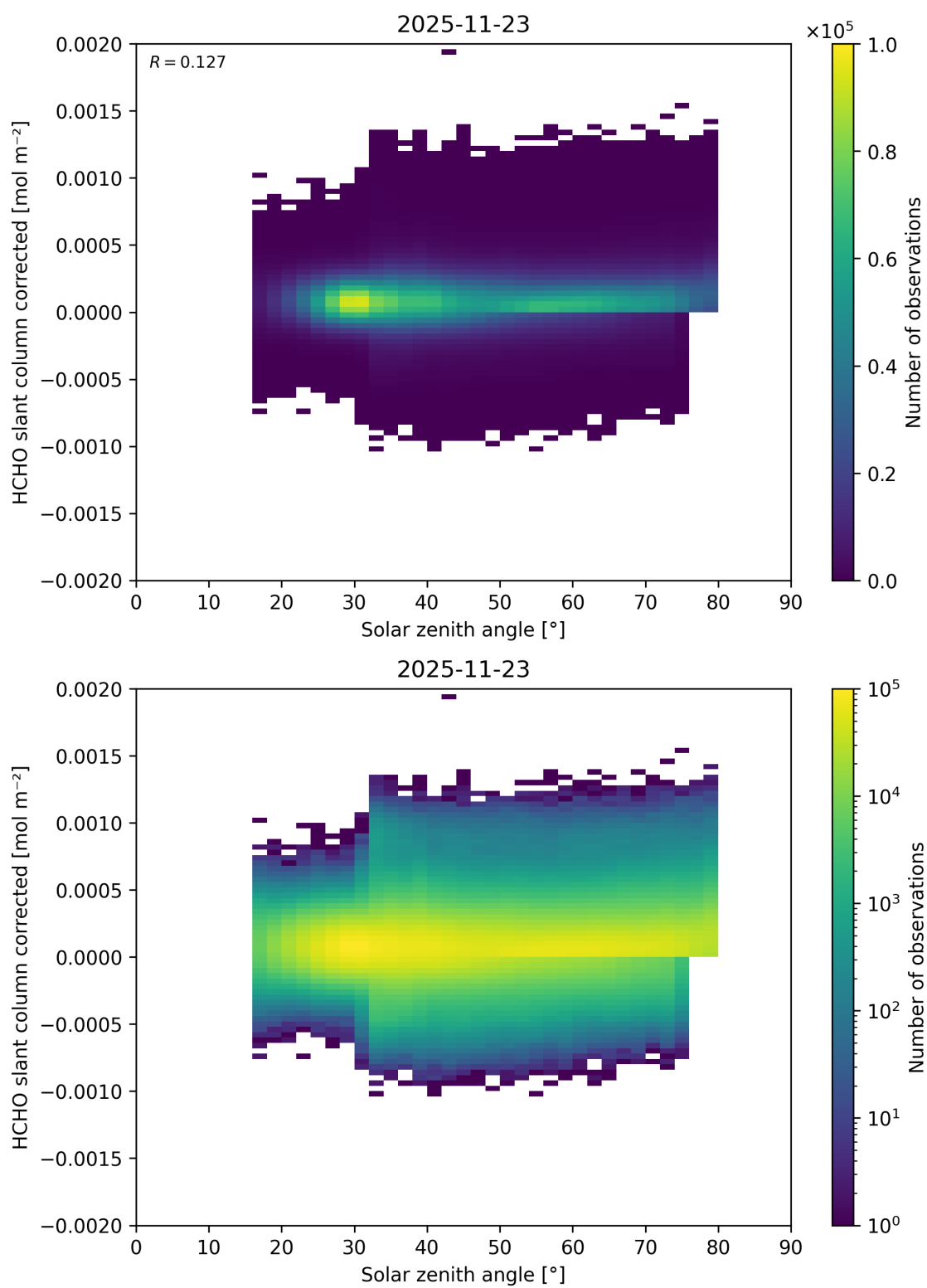
Figure 190: Scatter density plot of “Solar zenith angle” against “HCHO slant column corrected” for 2025-11-23 to 2025-11-24.
