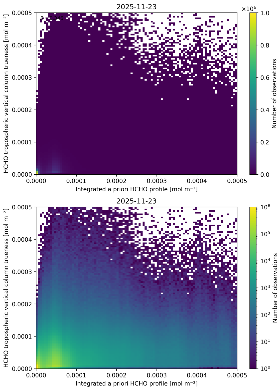
Figure 170: Scatter density plot of “Integrated a priori HCHO profile” against “HCHO tropospheric vertical column trueness” for 2025-11-23 to 2025-11-24.
