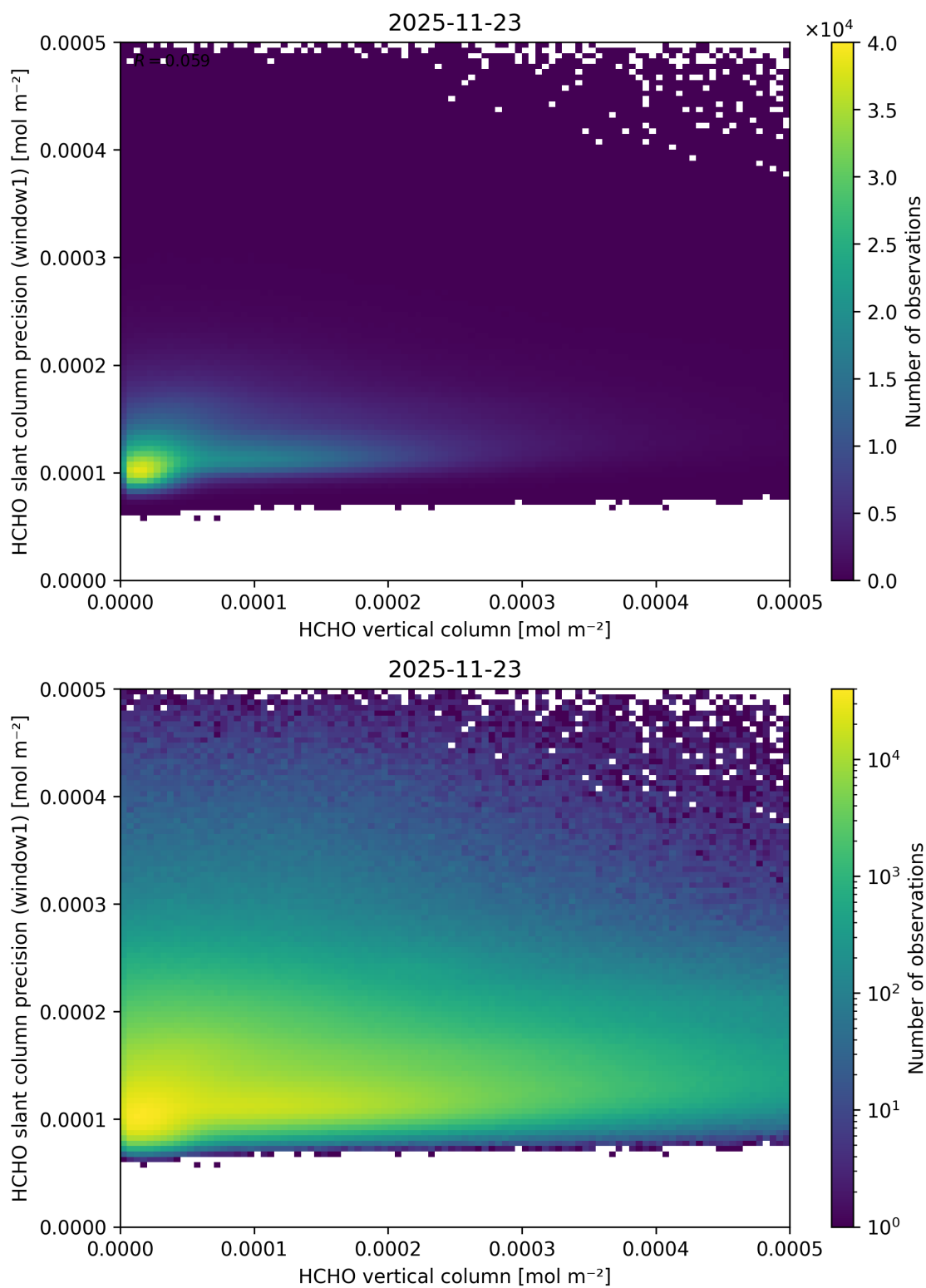
Figure 145: Scatter density plot of “HCHO vertical column” against “HCHO slant column precision (window1)” for 2025-11-23 to 2025-11-24.
