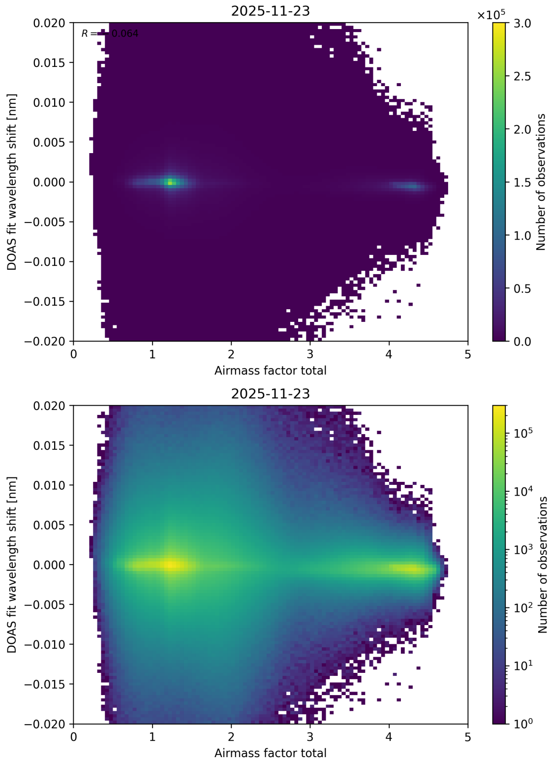
Figure 110: Scatter density plot of “Airmass factor total” against “DOAS fit wavelength shift” for 2025-11-23 to 2025-11-24.
