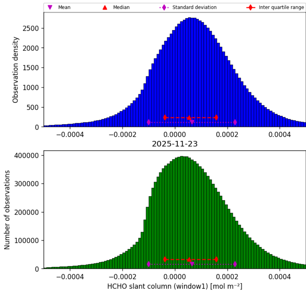
Figure 40: Histogram of “HCHO slant column (window1)” for 2025-11-23 to 2025-11-24
