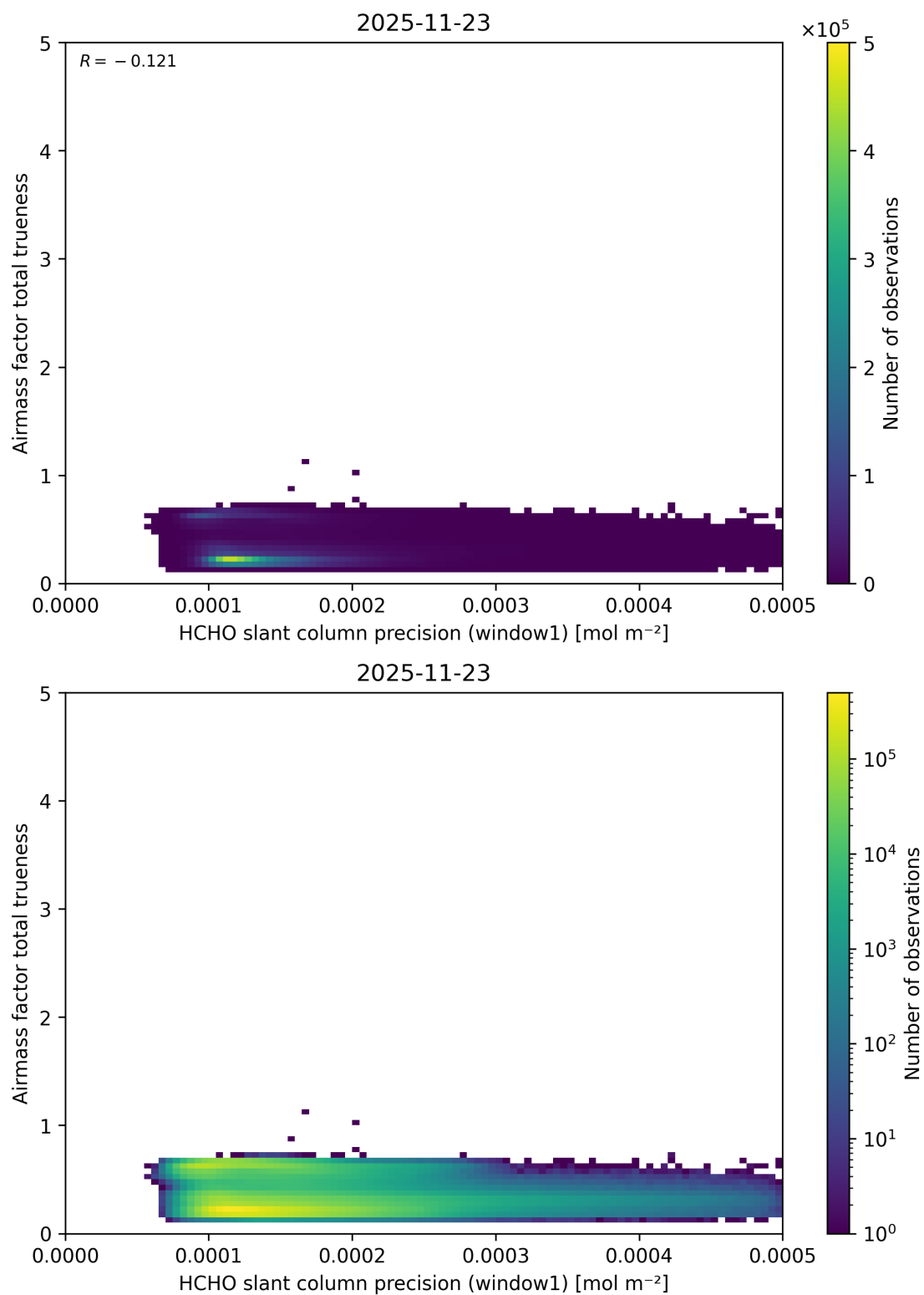
Figure 106: Scatter density plot of “HCHO slant column precision (window1)” against “Airmass factor total trueness” for 2025-11-23 to 2025-11-24.
