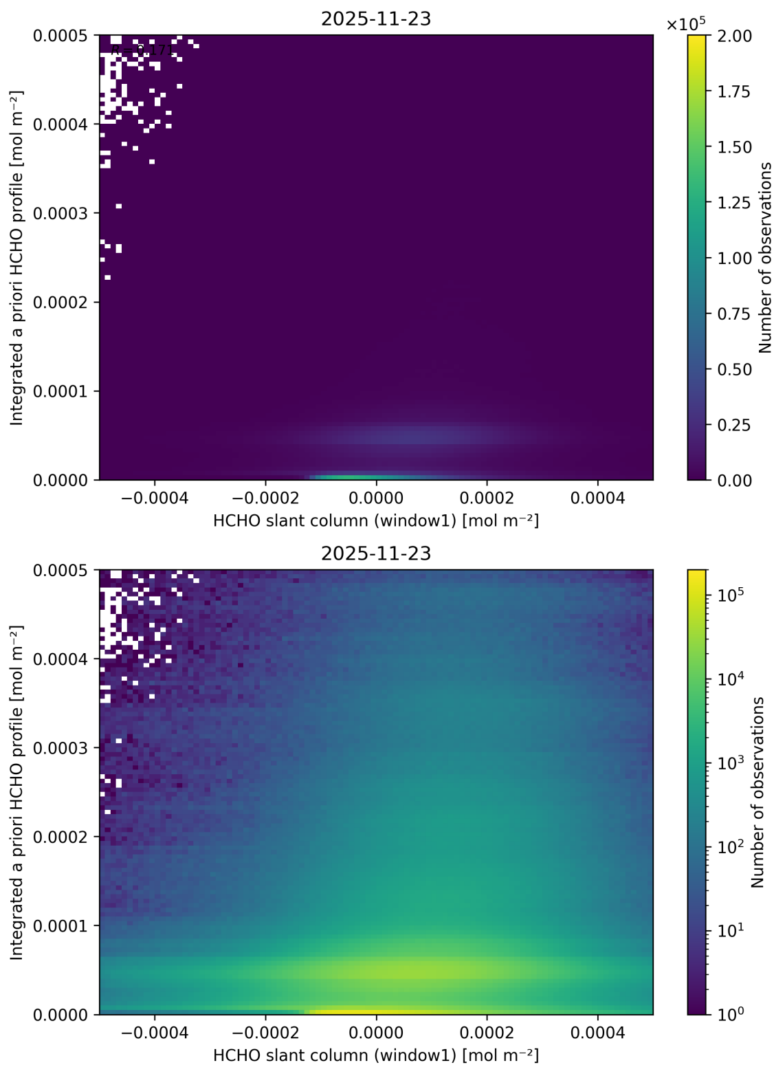
Figure 98: Scatter density plot of “HCHO slant column (window1)” against “Integrated a priori HCHO profile” for 2025-11-23 to 2025-11-24.
