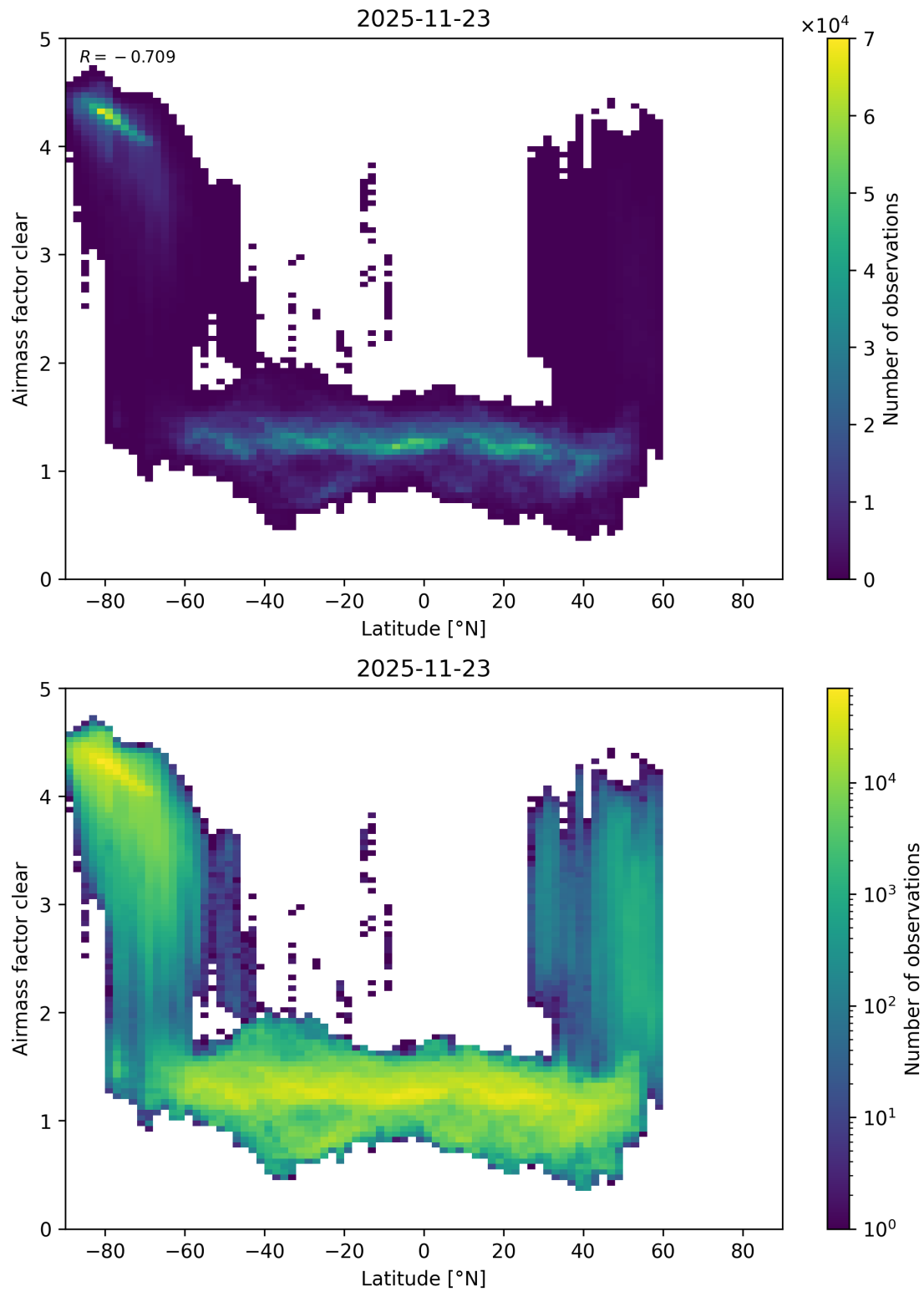
Figure 174: Scatter density plot of “Latitude” against “Airmass factor clear” for 2025-11-23 to 2025-11-24.
