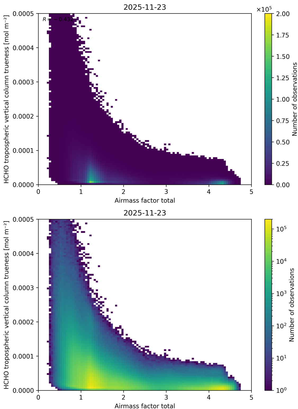
Figure 116: Scatter density plot of “Airmass factor total” against “HCHO tropospheric vertical column trueeness” for 2025-11-23 to 2025-11-24.
