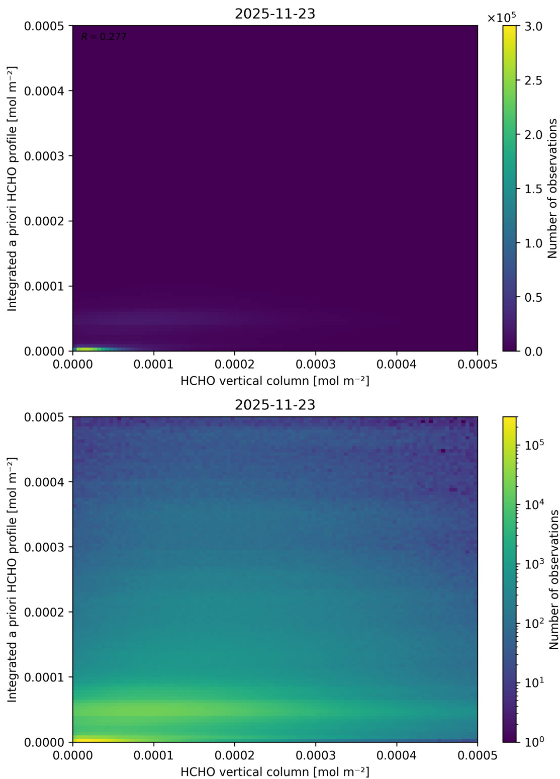
Figure 151: Scatter density plot of “HCHO vertical column” against “Integrated a priori HCHO profile” for 2025-11-23 to 2025-11-24.
