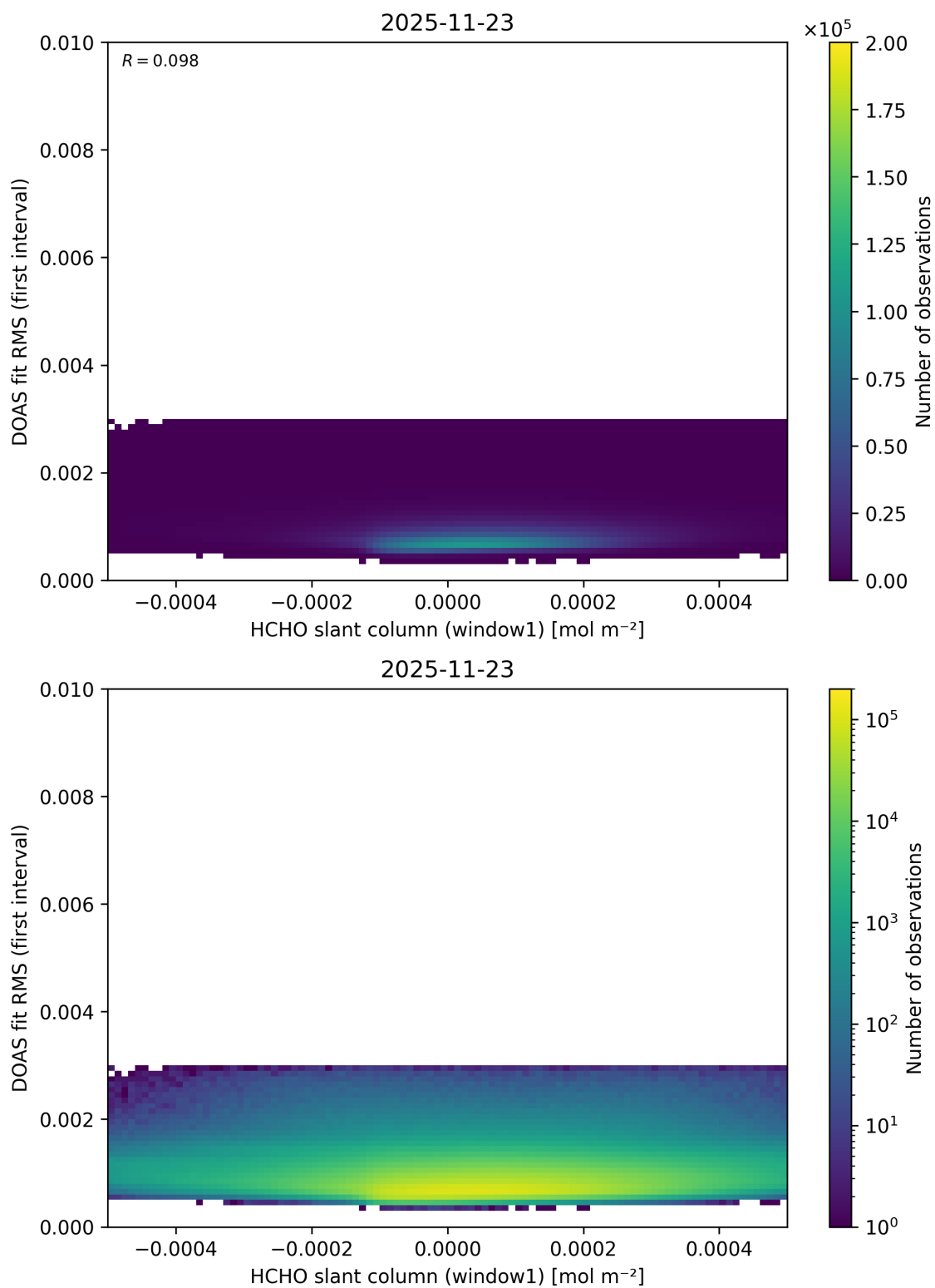
Figure 88: Scatter density plot of “HCHO slant column (window1)” against “DOAS fit RMS (first interval)” for 2025-11-23 to 2025-11-24.
