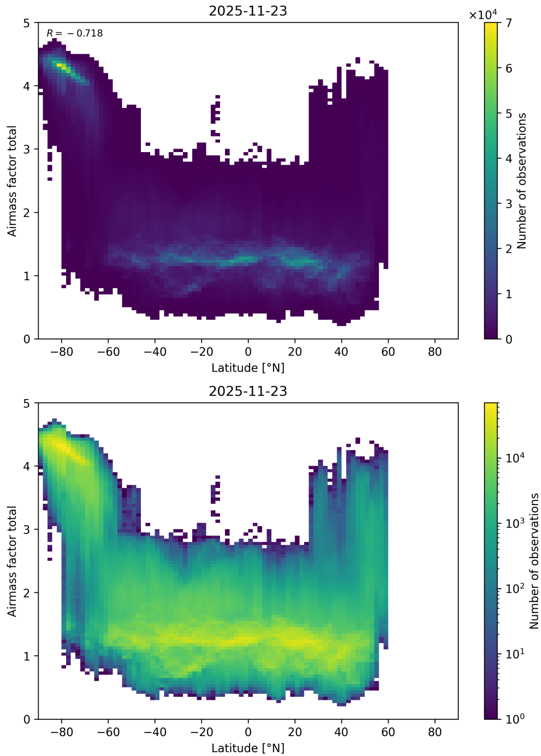
Figure 179: Scatter density plot of “Latitude” against “Airmass factor total” for 2025-11-23 to 2025-11-24.
