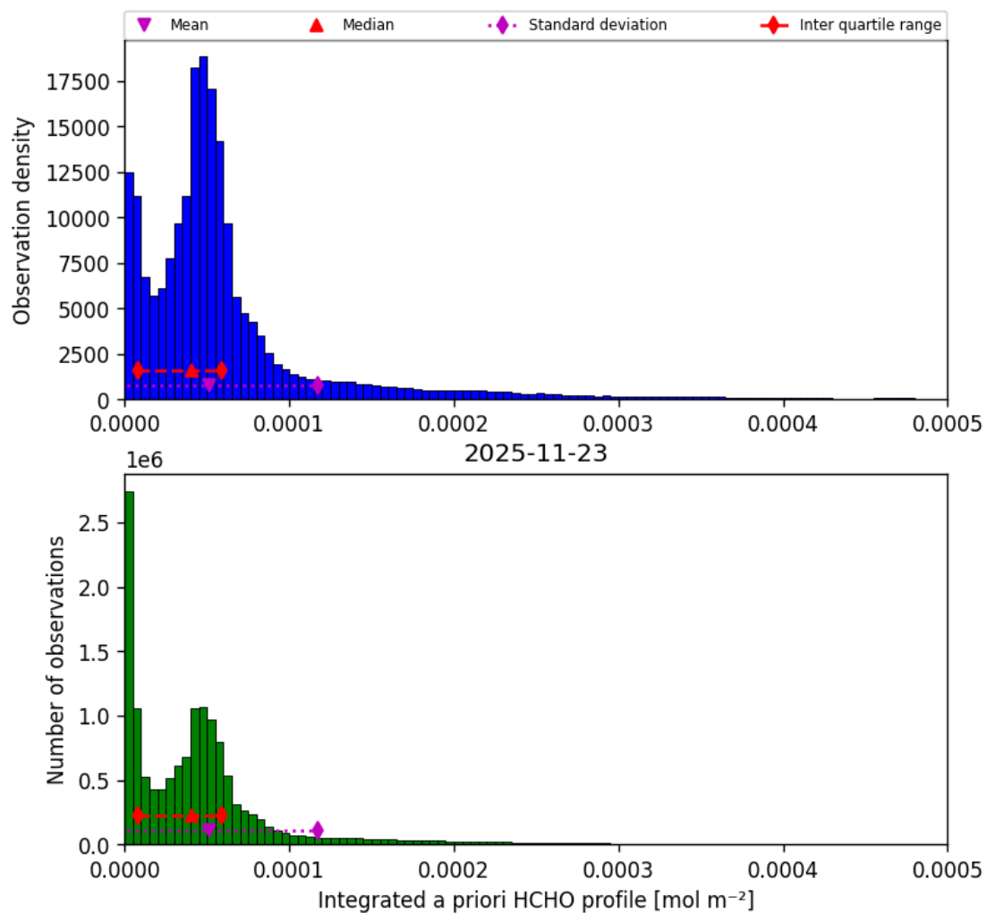
Figure 45: Histogram of “Integrated a priori HCHO profile” for 2025-11-23 to 2025-11-24
