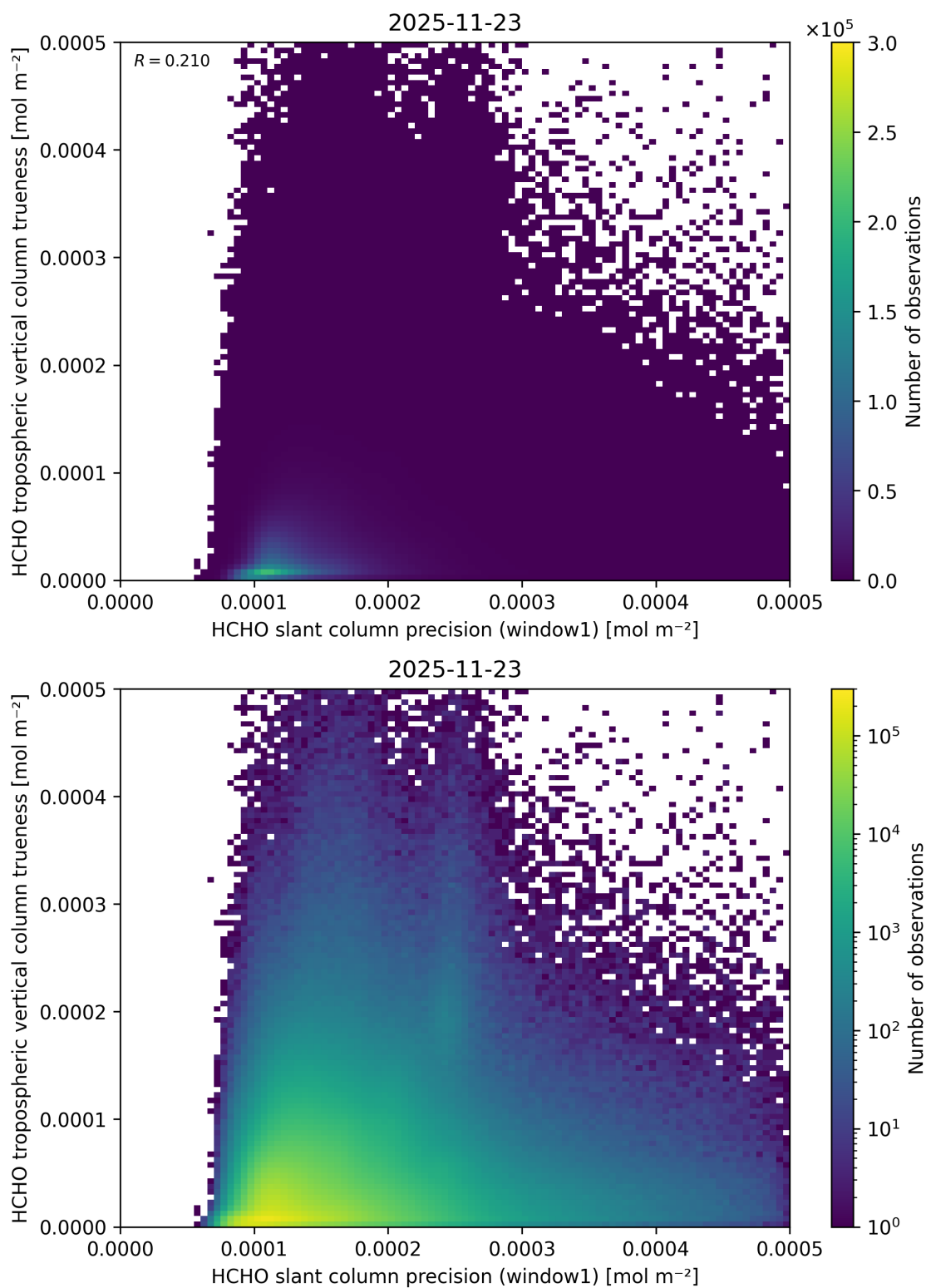
Figure 107: Scatter density plot of “HCHO slant column precision (window1)” against “HCHO tropospheric vertical column trueness” for 2025-11-23 to 2025-11-24.
