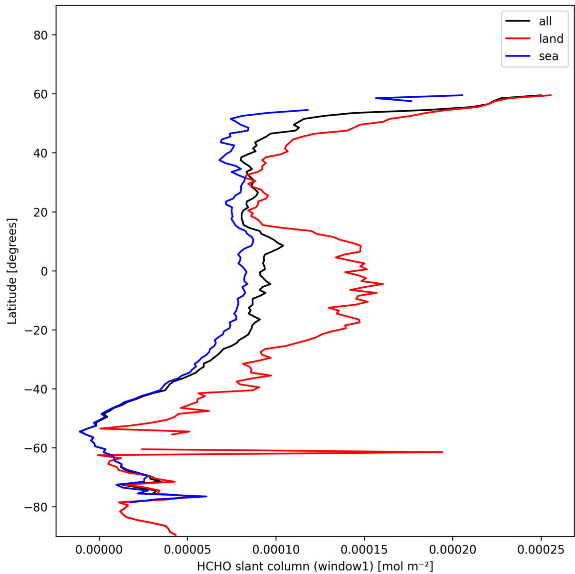
Figure 25: Zonal average of “HCHO slant column (window1)” for 2025-11-23 to 2025-11-24.
