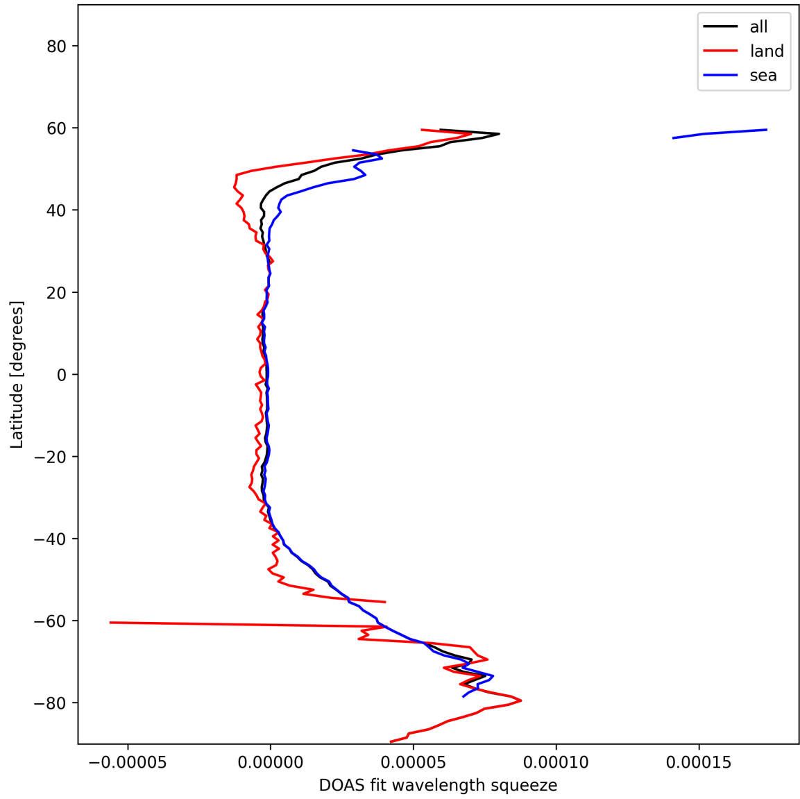
Figure 32: Zonal average of “DOAS fit wavelength squeeze” for 2025-11-23 to 2025-11-24.
