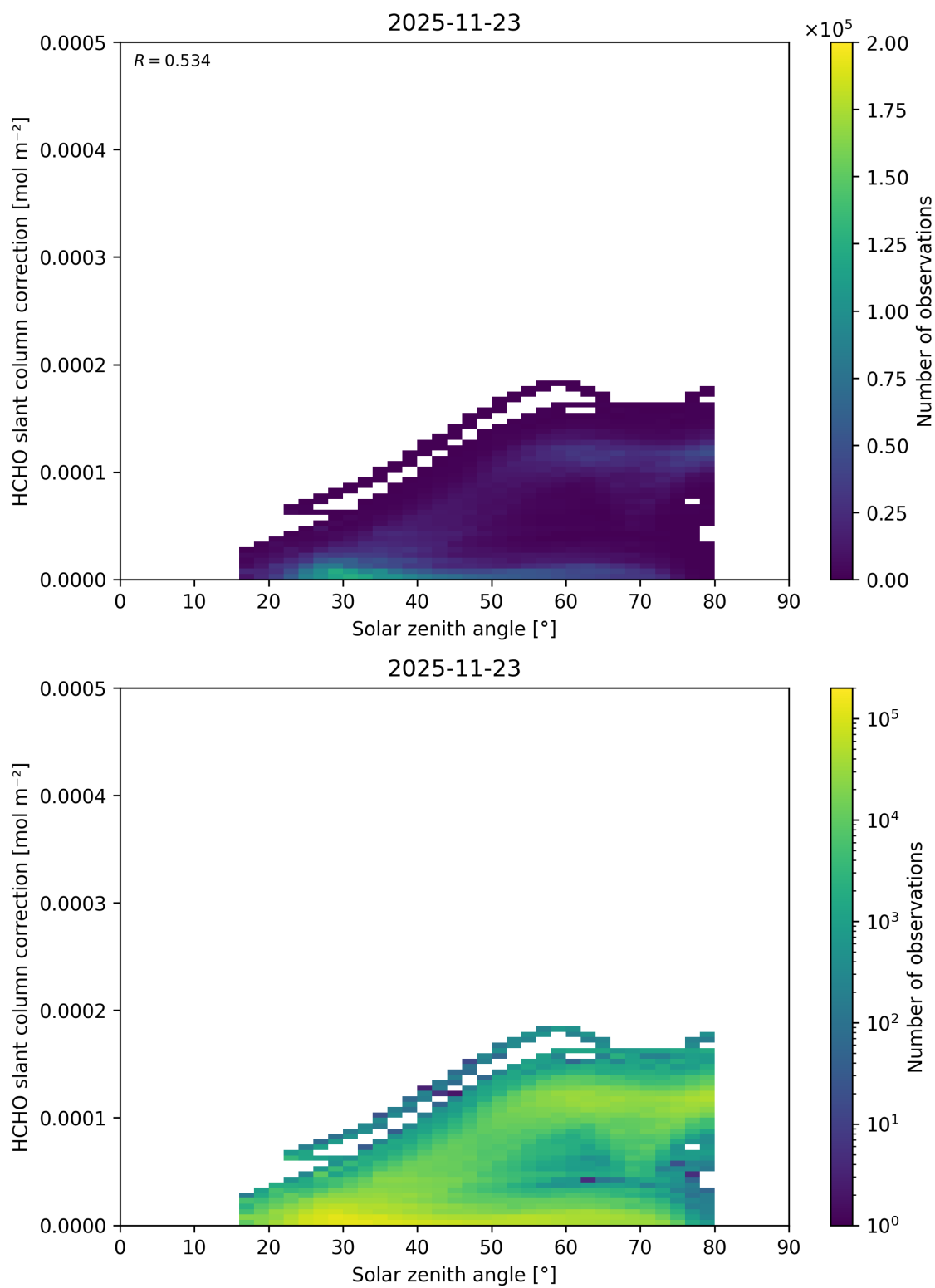
Figure 191: Scatter density plot of “Solar zenith angle” against “HCHO slant column correction” for 2025-11-23 to 2025-11-24.
