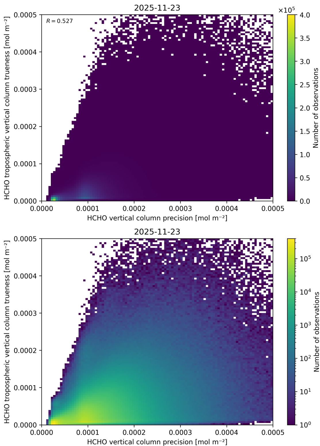
Figure 163: Scatter density plot of “HCHO vertical column precision” against “HCHO tropospheric vertical column truthness” for 2025-11-23 to 2025-11-24.
