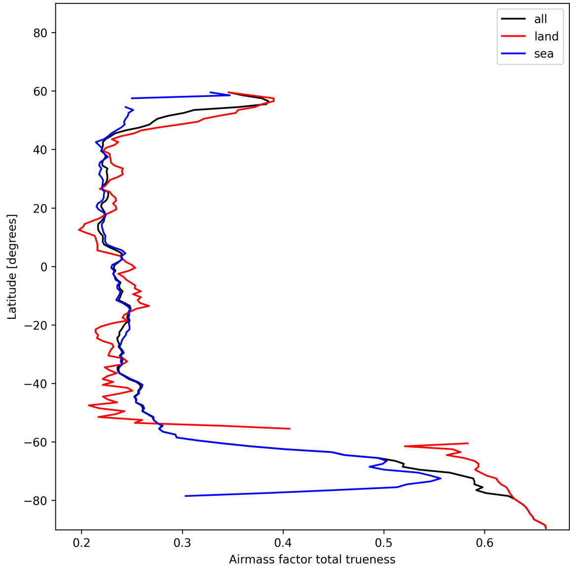
Figure 28: Zonal average of “Airmass factor total trueness” for 2025-11-23 to 2025-11-24.
