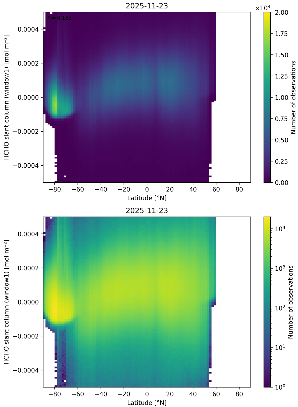
Figure 177: Scatter density plot of “Latitude” against “HCHO slant column (window1)” for 2025-11-23 to 2025-11-24.
