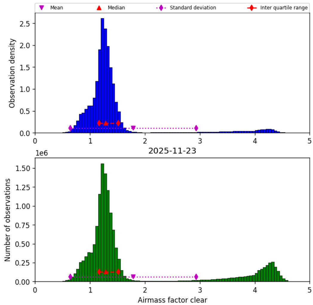
Figure 44: Histogram of “Airmass factor clear” for 2025-11-23 to 2025-11-24
