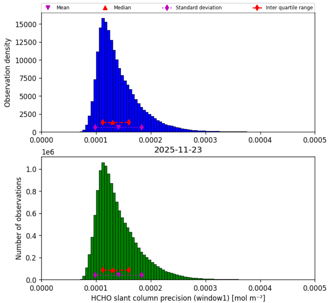
Figure 41: Histogram of “HCHO slant column precision (window1)” for 2025-11-23 to 2025-11-24
