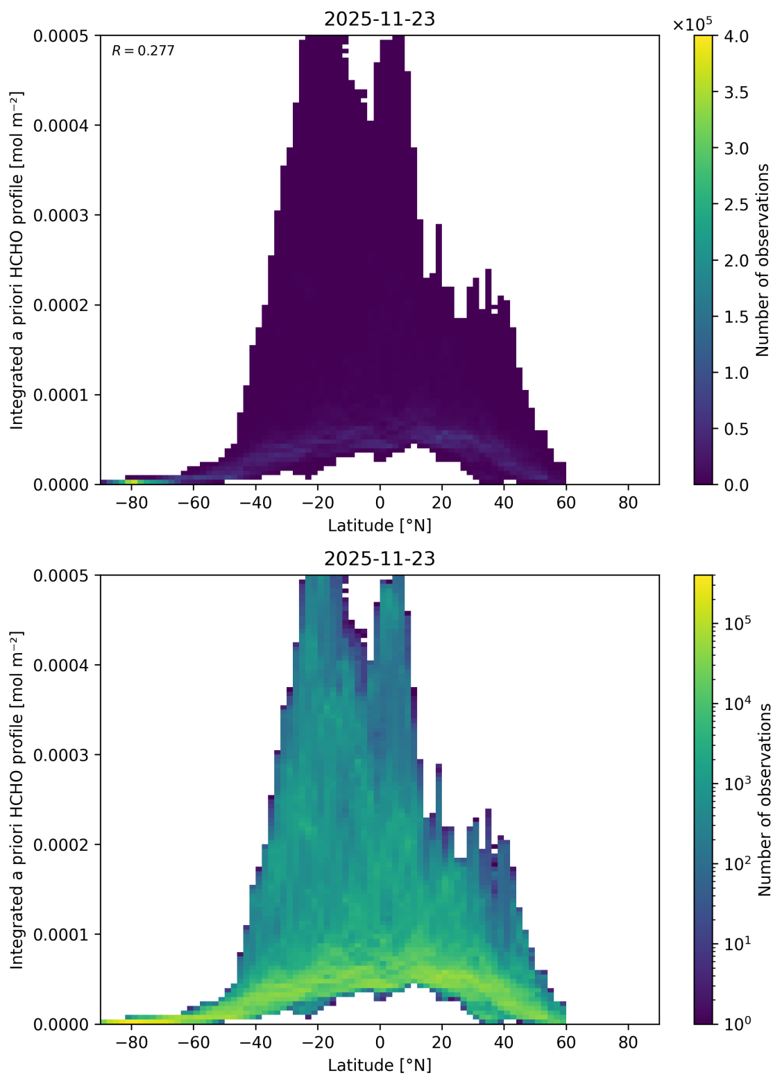
Figure 185: Scatter density plot of “Latitude” against “Integrated a priori HCHO profile” for 2025-11-23 to 2025-11-24.
