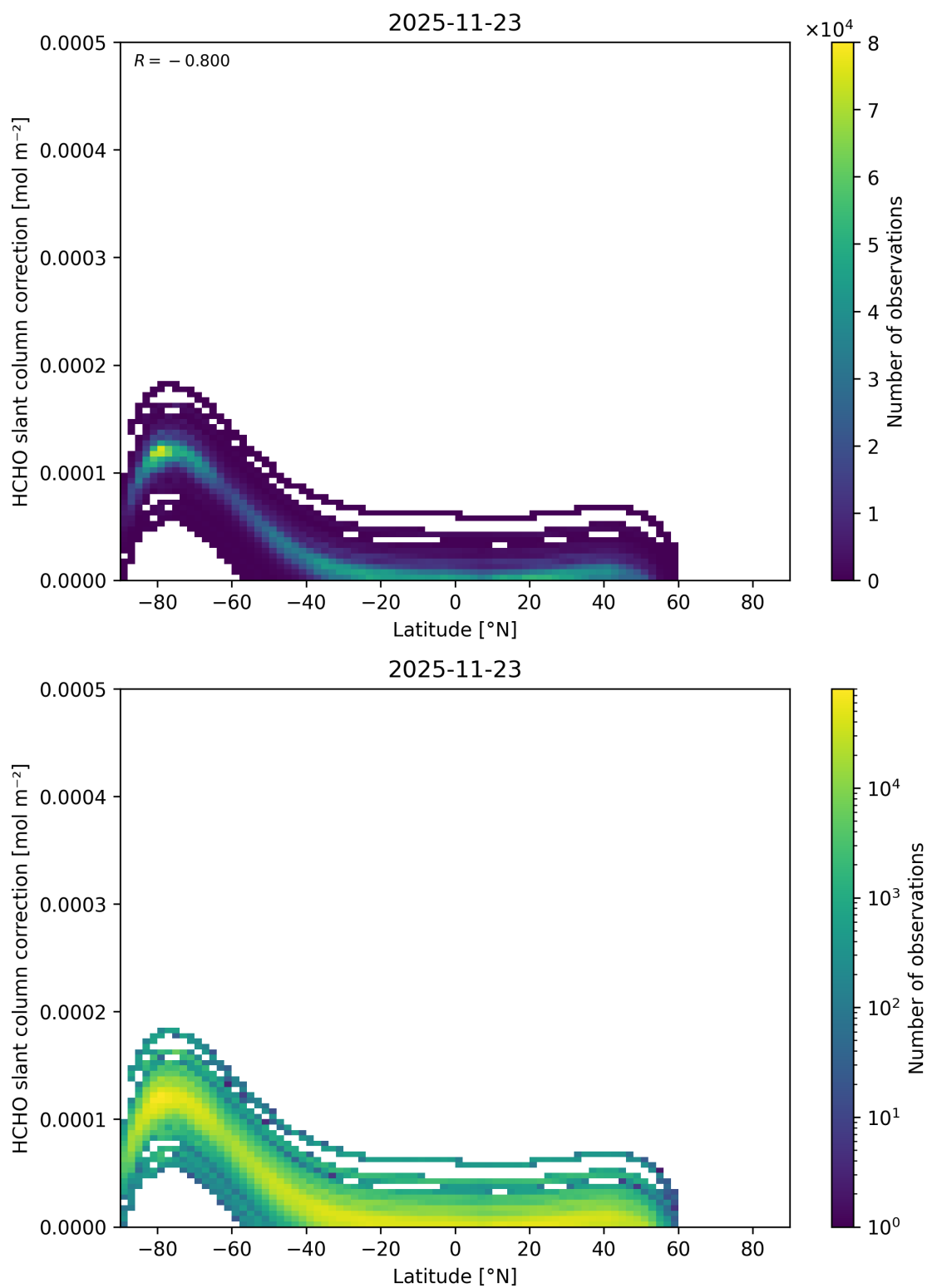
Figure 176: Scatter density plot of “Latitude” against “HCHO slant column correction” for 2025-11-23 to 2025-11-24.
