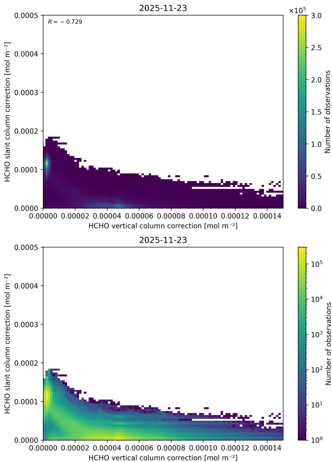
Figure 131: Scatter density plot of “HCHO vertical column correction” against “HCHO slant column correction” for 2025-11-23 to 2025-11-24.
