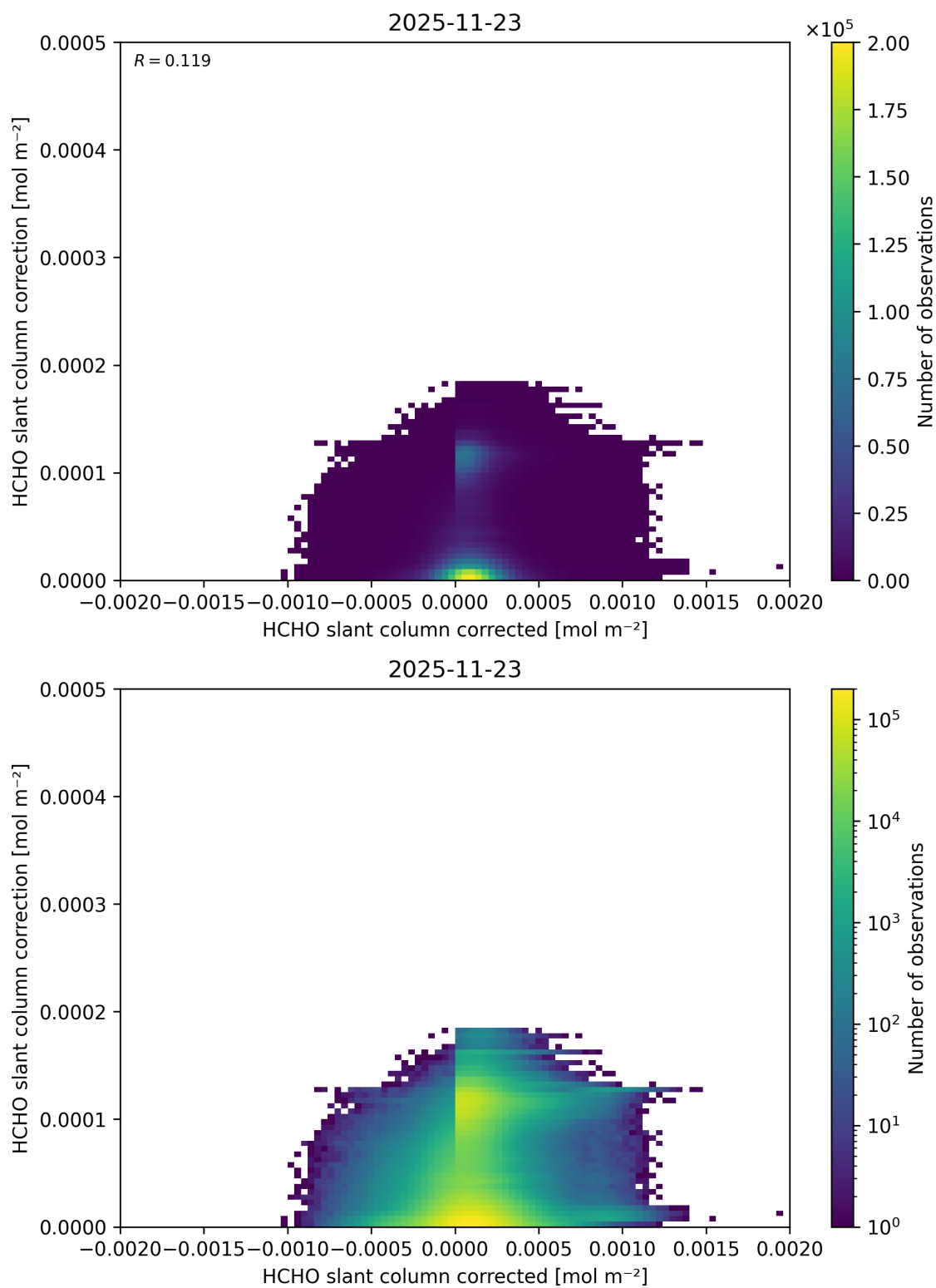
Figure 85: Scatter density plot of “HCHO slant column corrected” against “HCHO slant column correction” for 2025-11-23 to 2025-11-24.
