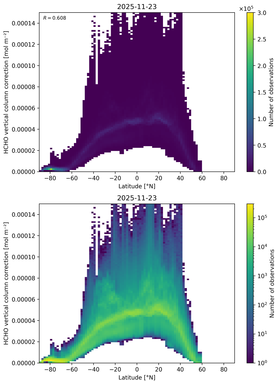
Figure 182: Scatter density plot of “Latitude” against “HCHO vertical column correction” for 2025-11-23 to 2025-11-24.
