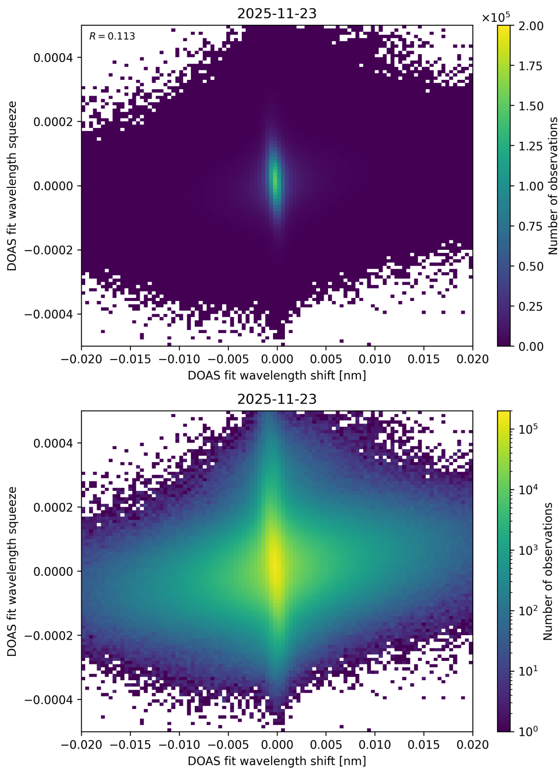
Figure 70: Scatter density plot of “DOAS fit wavelength shift” against “DOAS fit wavelength squeeze” for 2025-11-23 to 2025-11-24.
