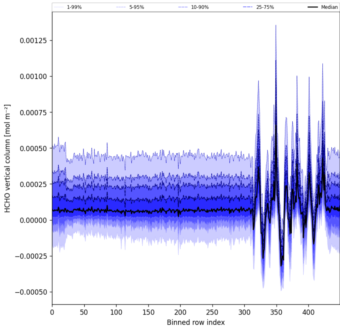
Figure 52: Along track statistics of “HCHO vertical column” for 2025-11-23 to 2025-11-24
