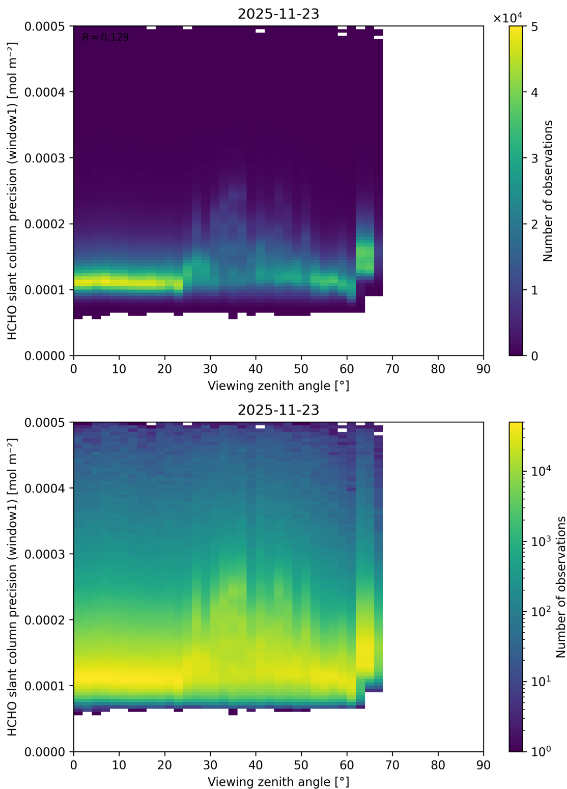
Figure 209: Scatter density plot of “Viewing zenith angle” against “HCHO slant column precision (window1)” for 2025-11-23 to 2025-11-24.
