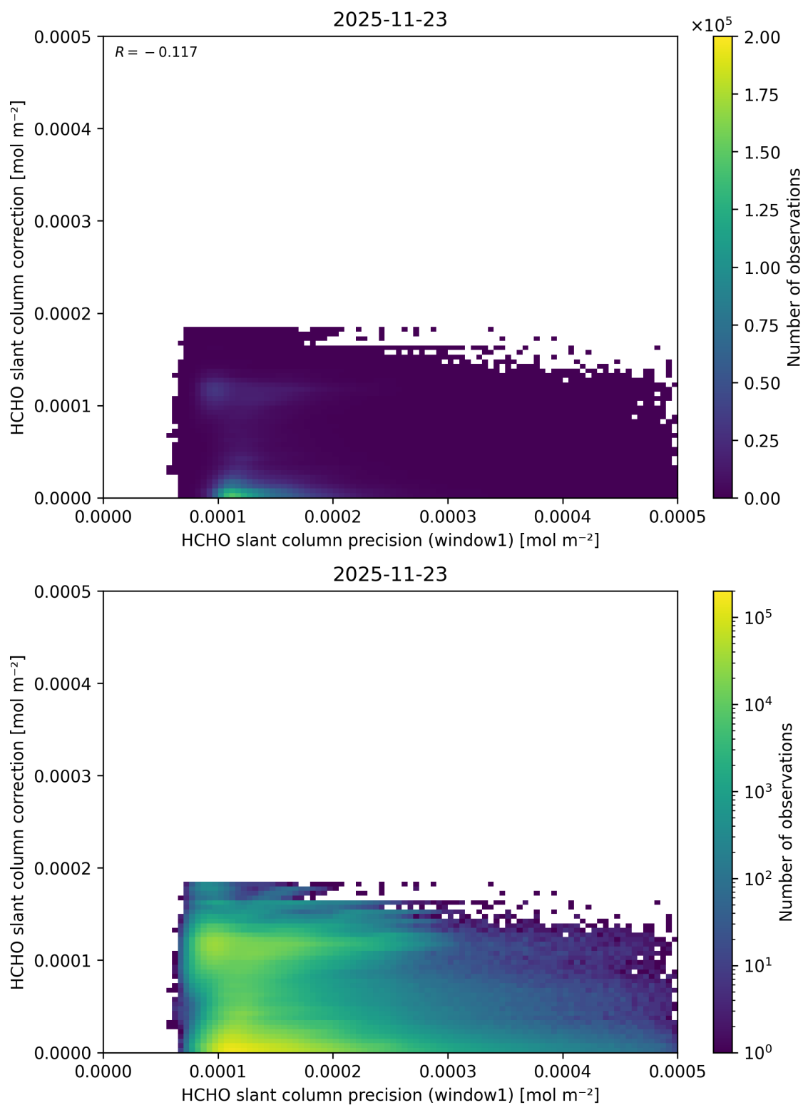
Figure 104: Scatter density plot of “HCHO slant column precision (window1)” against “HCHO slant column correction” for 2025-11-23 to 2025-11-24.
