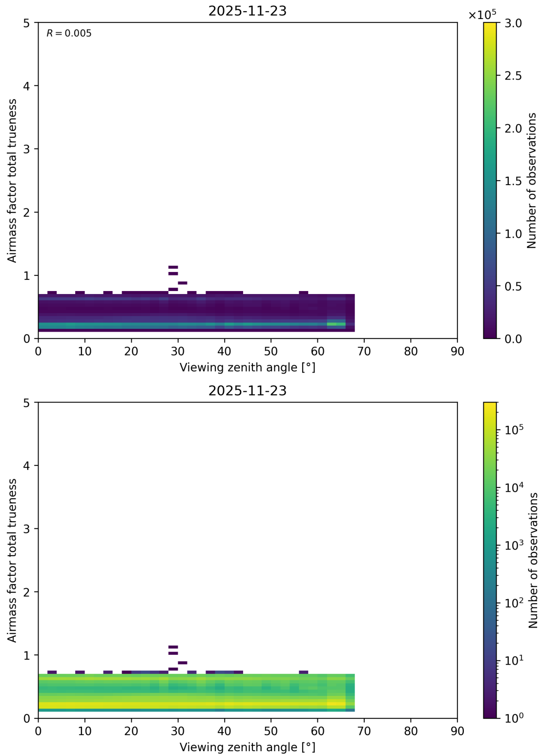
Figure 211: Scatter density plot of “Viewing zenith angle” against “Airmass factor total trueness” for 2025-11-23 to 2025-11-24.
