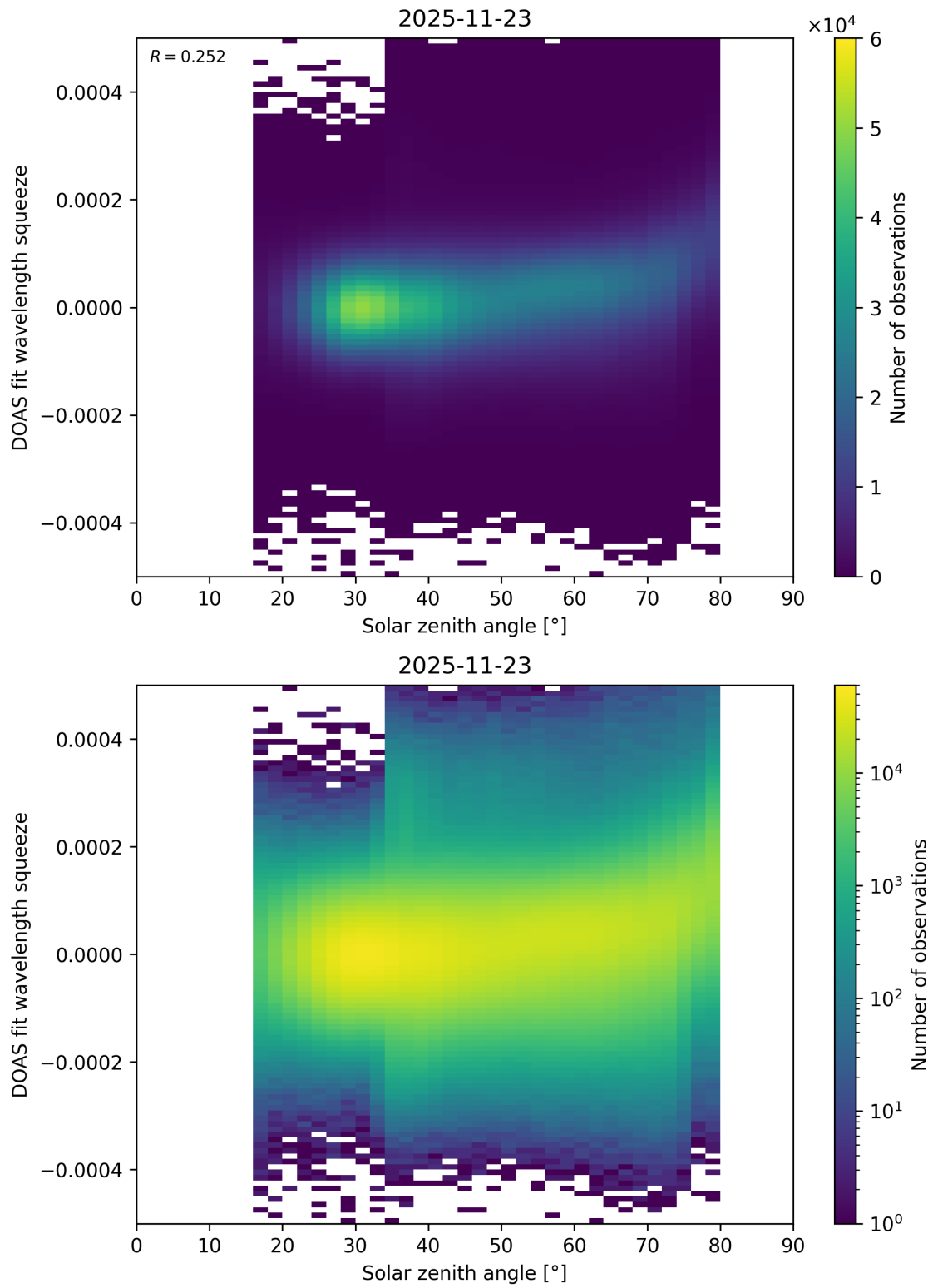
Figure 188: Scatter density plot of “Solar zenith angle” against “DOAS fit wavelength squeeze” for 2025-11-23 to 2025-11-24.
