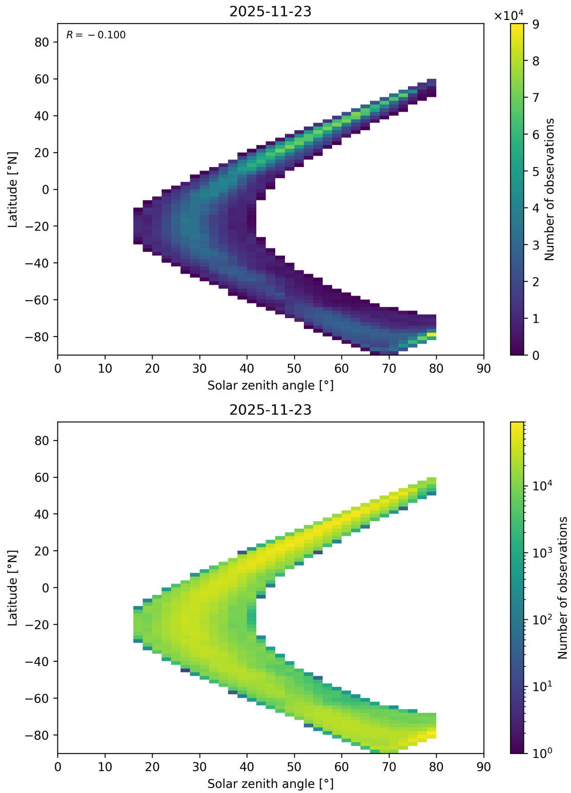
Figure 201: Scatter density plot of “Solar zenith angle” against “Latitude” for 2025-11-23 to 2025-11-24.
