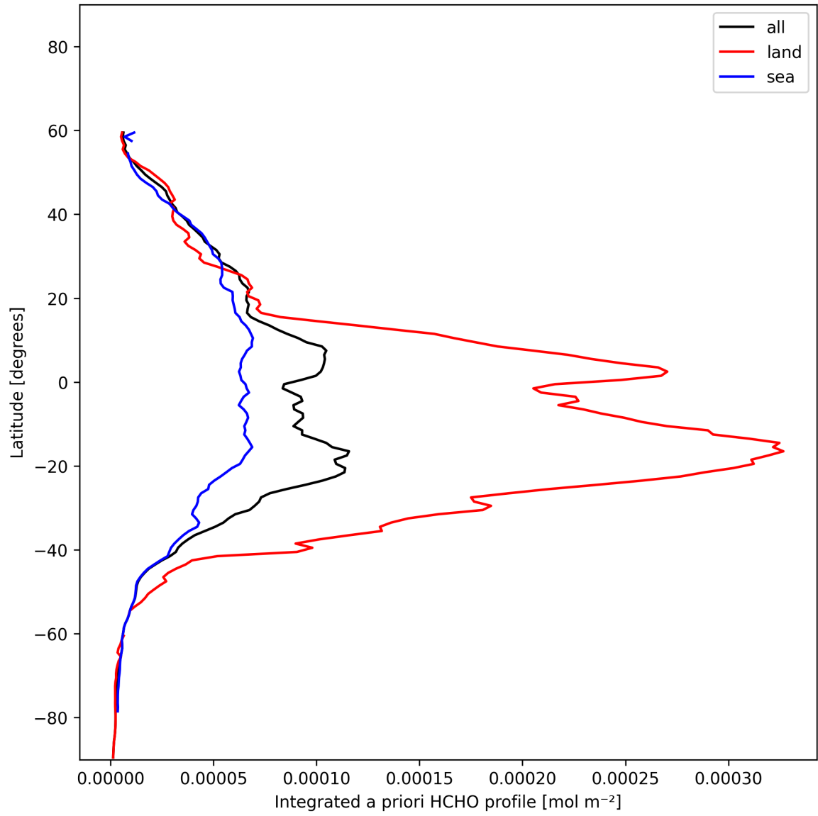
Figure 30: Zonal average of “Integrated a priori HCHO profile” for 2025-11-23 to 2025-11-24.
