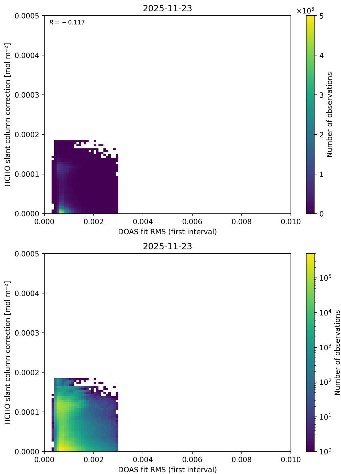
Figure 67: Scatter density plot of “DOAS fit RMS (first interval)” against “HCHO slant column correction” for 2025-11-23 to 2025-11-24.
