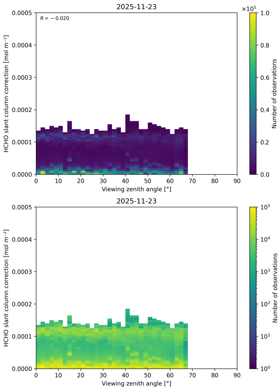
Figure 207: Scatter density plot of “Viewing zenith angle” against “HCHO slant column correction” for 2025-11-23 to 2025-11-24.
