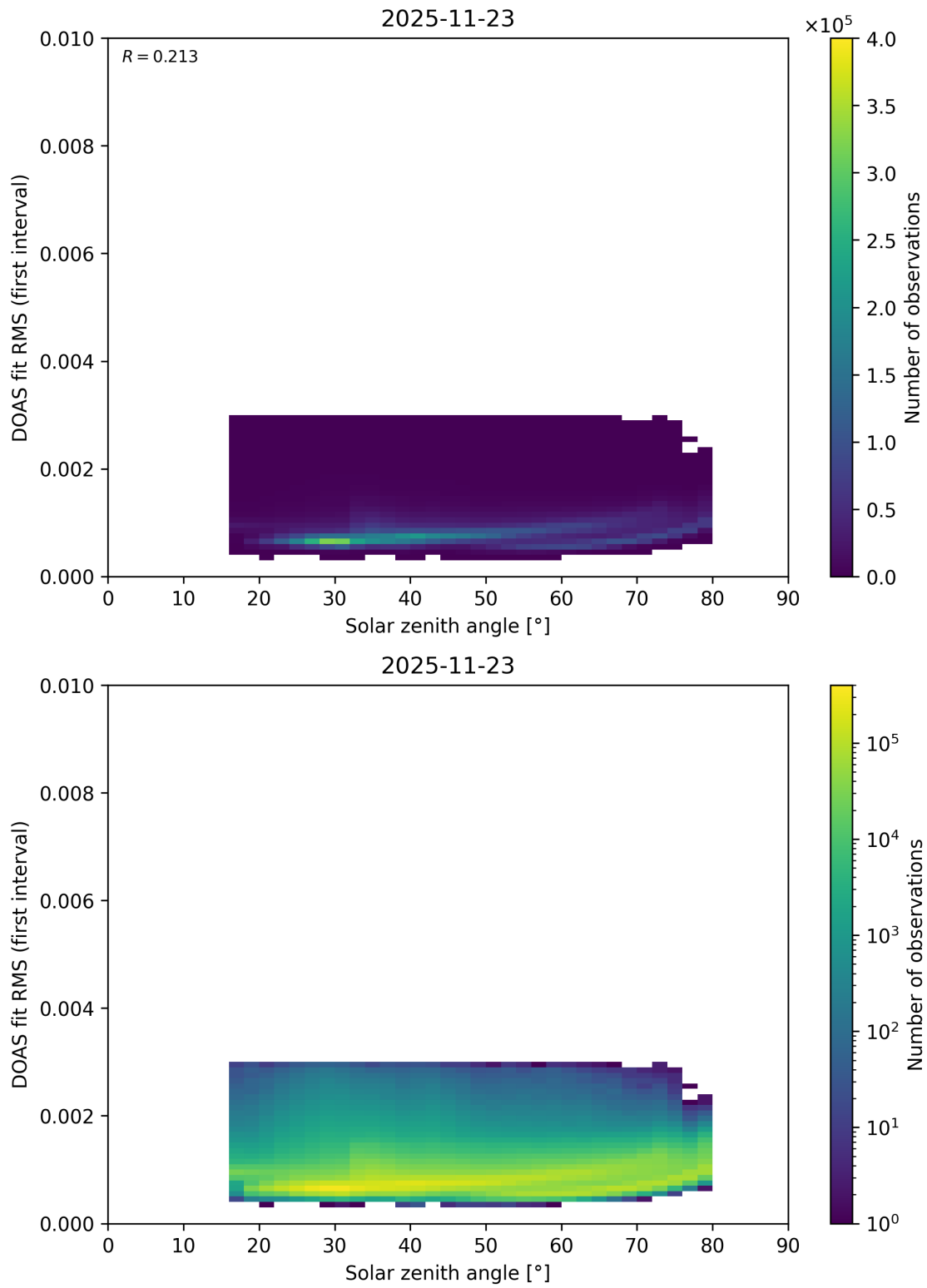
Figure 186: Scatter density plot of “Solar zenith angle” against “DOAS fit RMS (first interval)” for 2025-11-23 to 2025-11-24.
