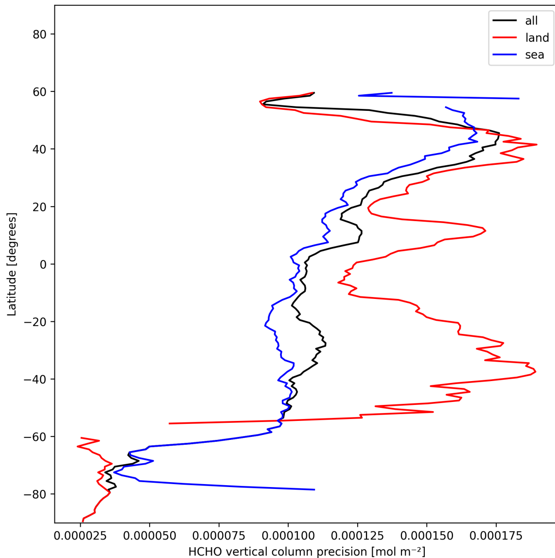
Figure 23: Zonal average of “HCHO vertical column precision” for 2025-11-23 to 2025-11-24.
