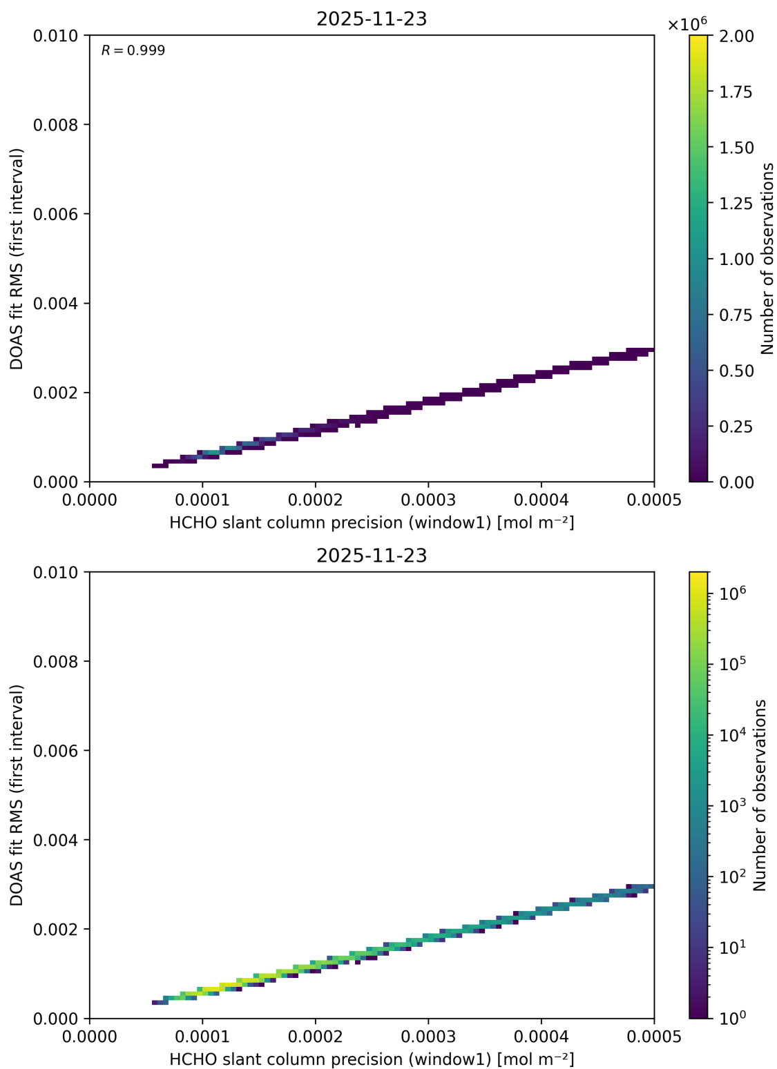
Figure 99: Scatter density plot of “HCHO slant column precision (window1)” against “DOAS fit RMS (first interval)” for 2025-11-23 to 2025-11-24.
