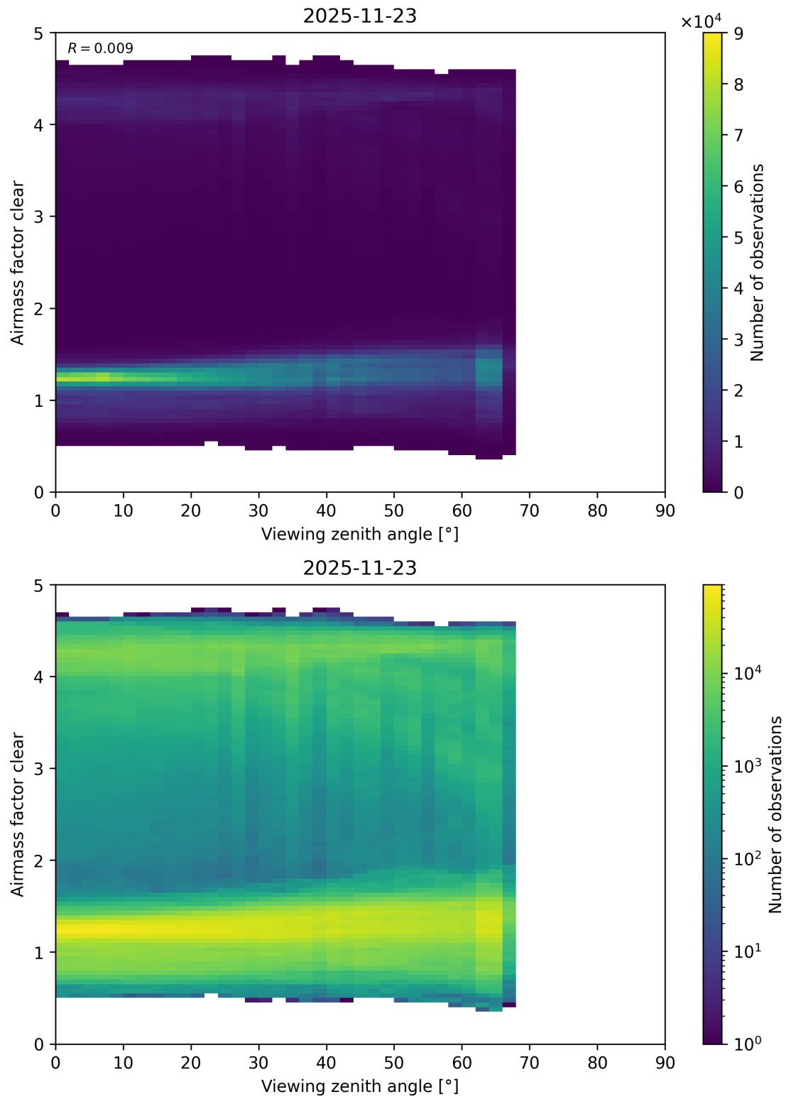
Figure 205: Scatter density plot of “Viewing zenith angle” against “Airmass factor clear” for 2025-11-23 to 2025-11-24.
