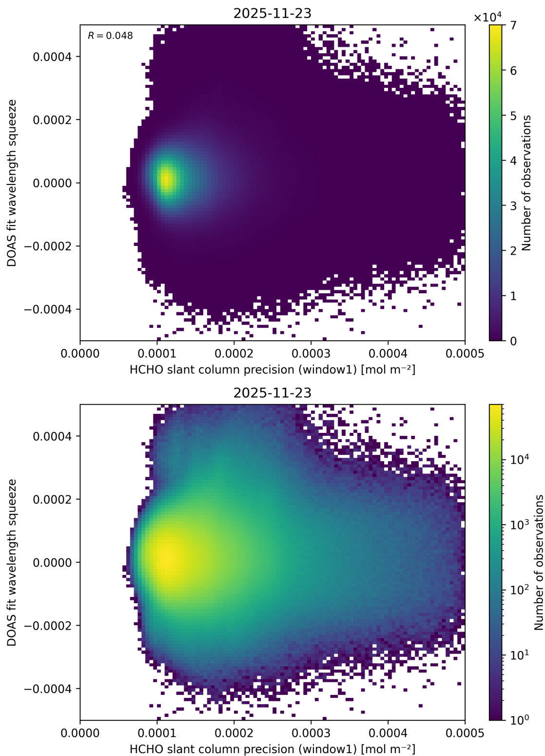
Figure 101: Scatter density plot of “HCHO slant column precision (window1)” against “DOAS fit wavelength squeeze” for 2025-11-23 to 2025-11-24.
