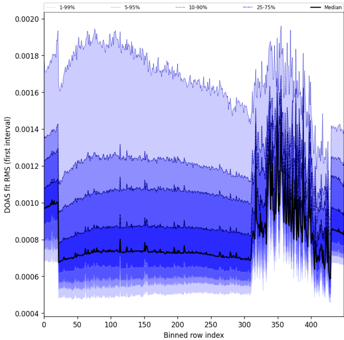
Figure 63: Along track statistics of “DOAS fit RMS (first interval)” for 2025-11-23 to 2025-11-24
