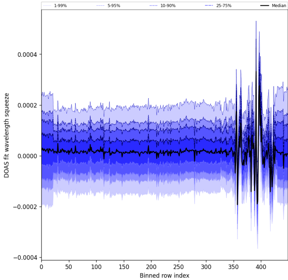
Figure 62: Along track statistics of “DOAS fit wavelength squeeze” for 2025-11-23 to 2025-11-24
