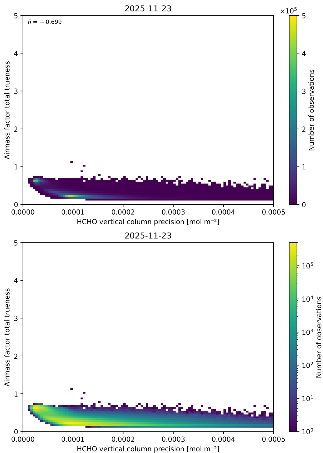
Figure 161: Scatter density plot of “HCHO vertical column precision” against “Airmass factor total trueness” for 2025-11-23 to 2025-11-24.
