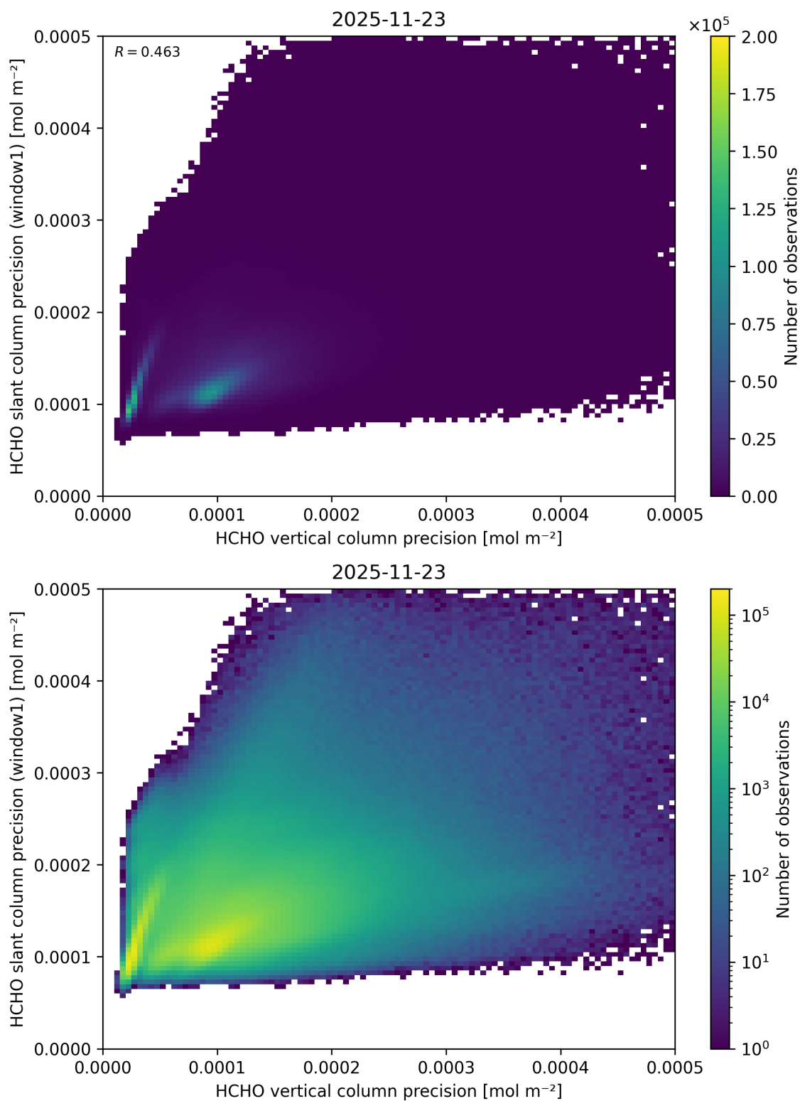
Figure 159: Scatter density plot of “HCHO vertical column precision” against “HCHO slant column precision (window1)” for 2025-11-23 to 2025-11-24.
