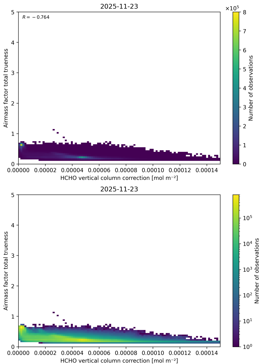
Figure 135: Scatter density plot of “HCHO vertical column correction” against “Airmass factor total truiness” for 2025-11-23 to 2025-11-24.
