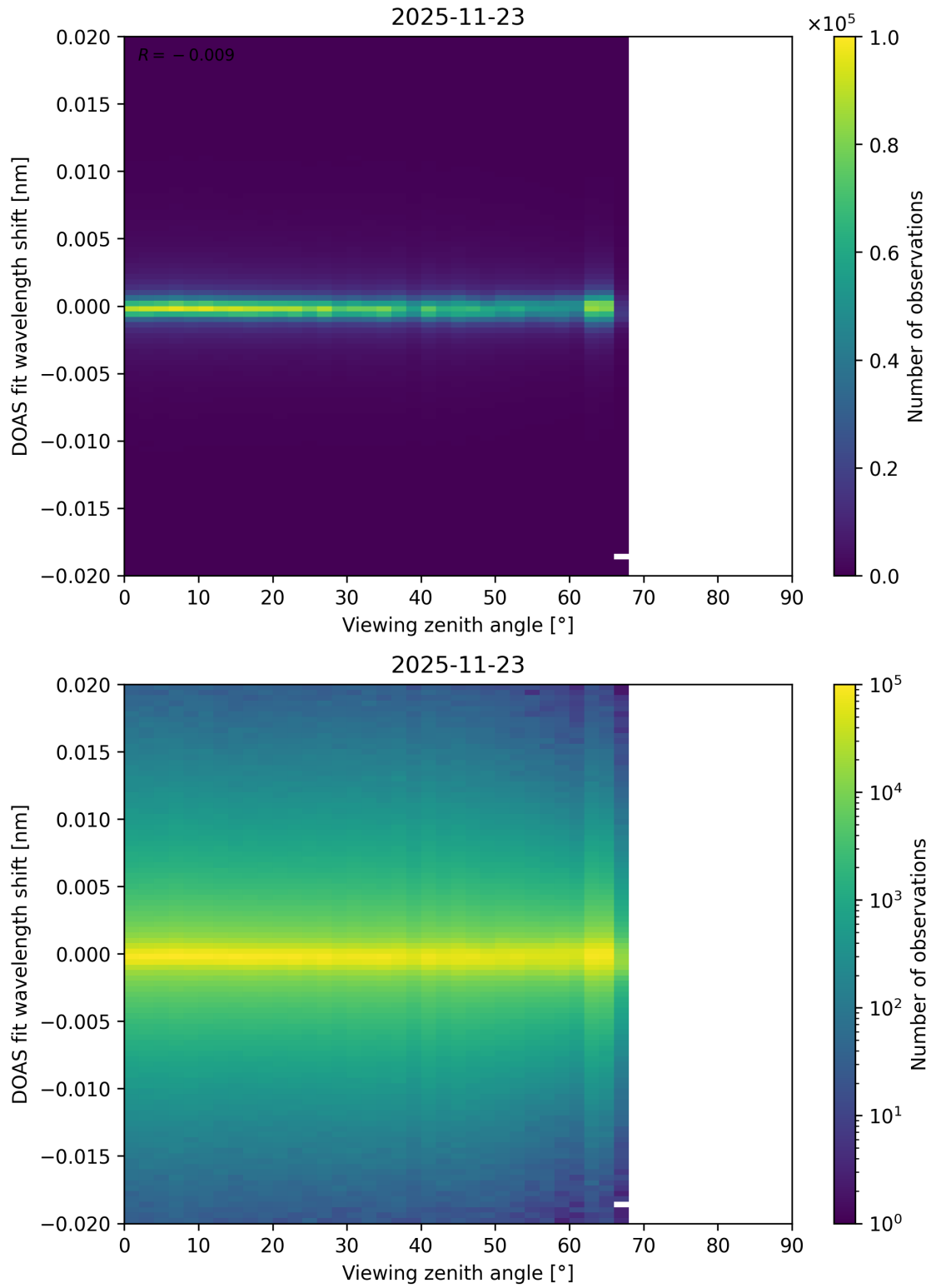
Figure 203: Scatter density plot of “Viewing zenith angle” against “DOAS fit wavelength shift” for 2025-11-23 to 2025-11-24.
