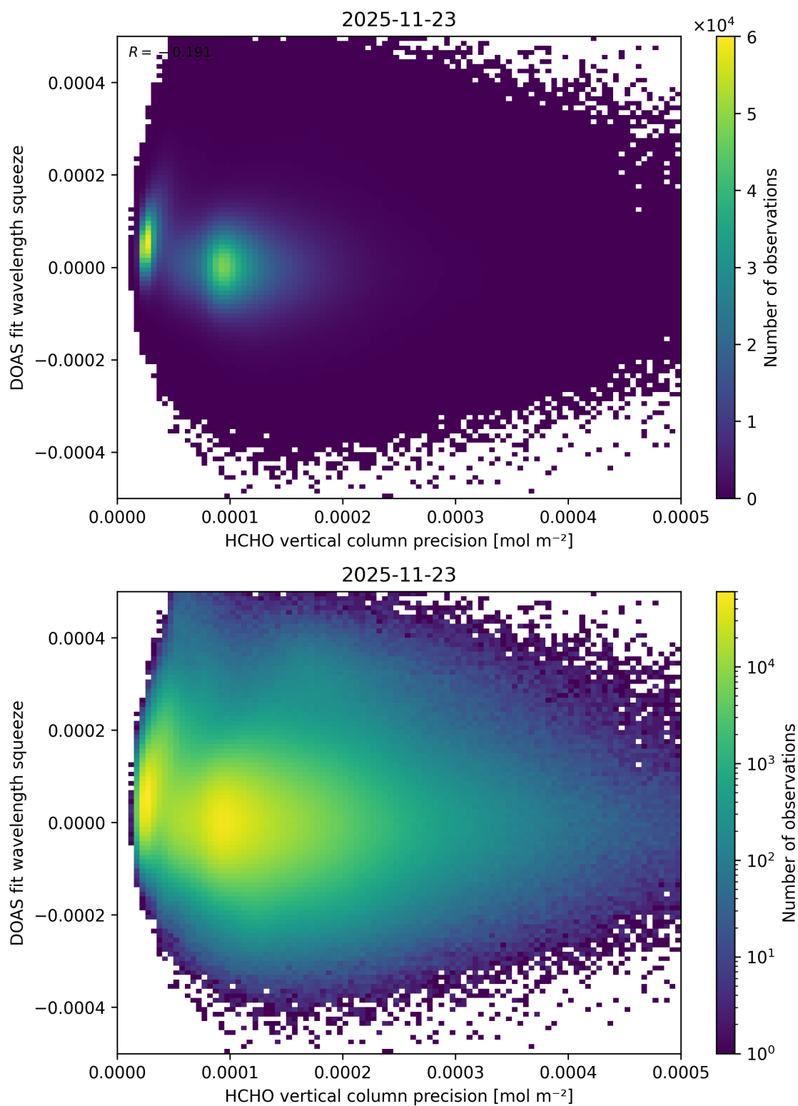
Figure 154: Scatter density plot of “HCHO vertical column precision” against “DOAS fit wavelength squeeze” for 2025-11-23 to 2025-11-24.
