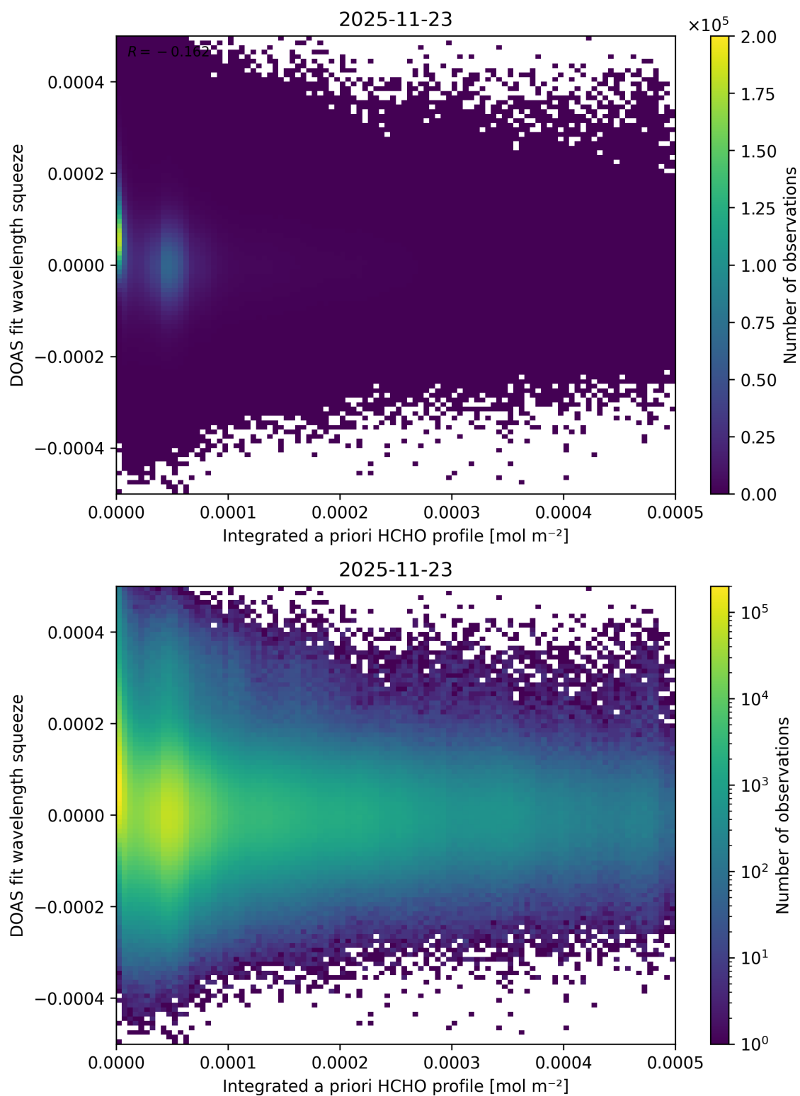
Figure 167: Scatter density plot of “Integrated a priori HCHO profile” against “DOAS fit wavelength squeeze” for 2025-11-23 to 2025-11-24.
