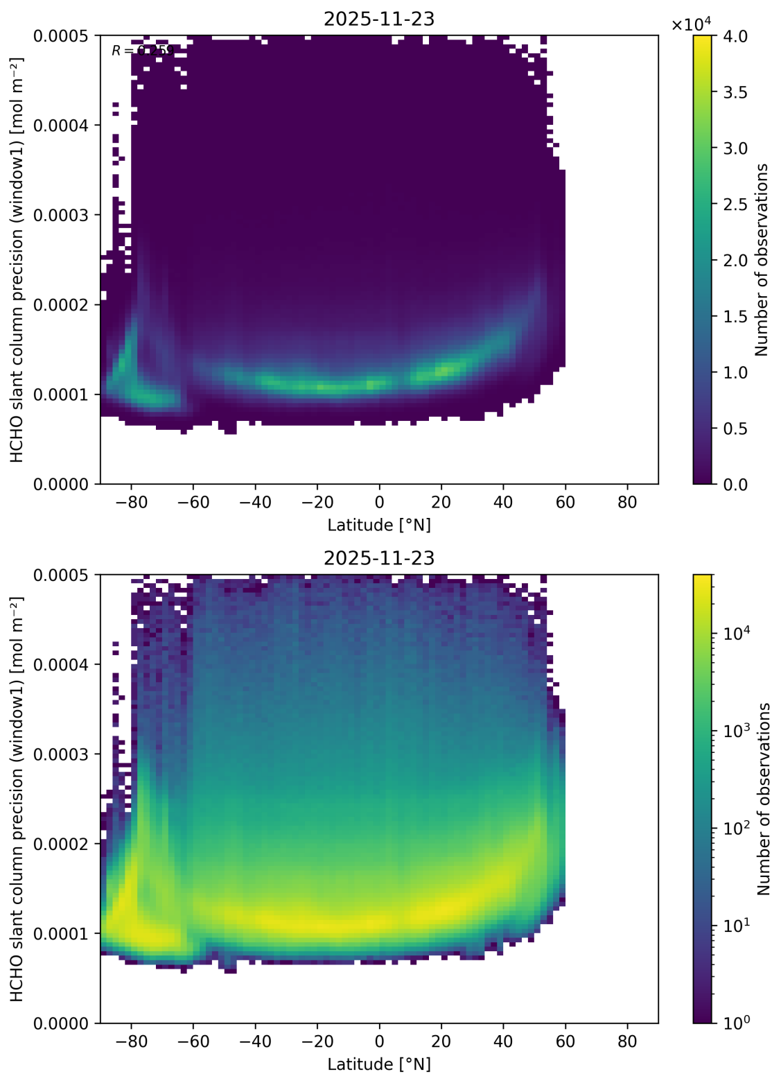
Figure 178: Scatter density plot of “Latitude” against “HCHO slant column precision (window1)” for 2025-11-23 to 2025-11-24.
