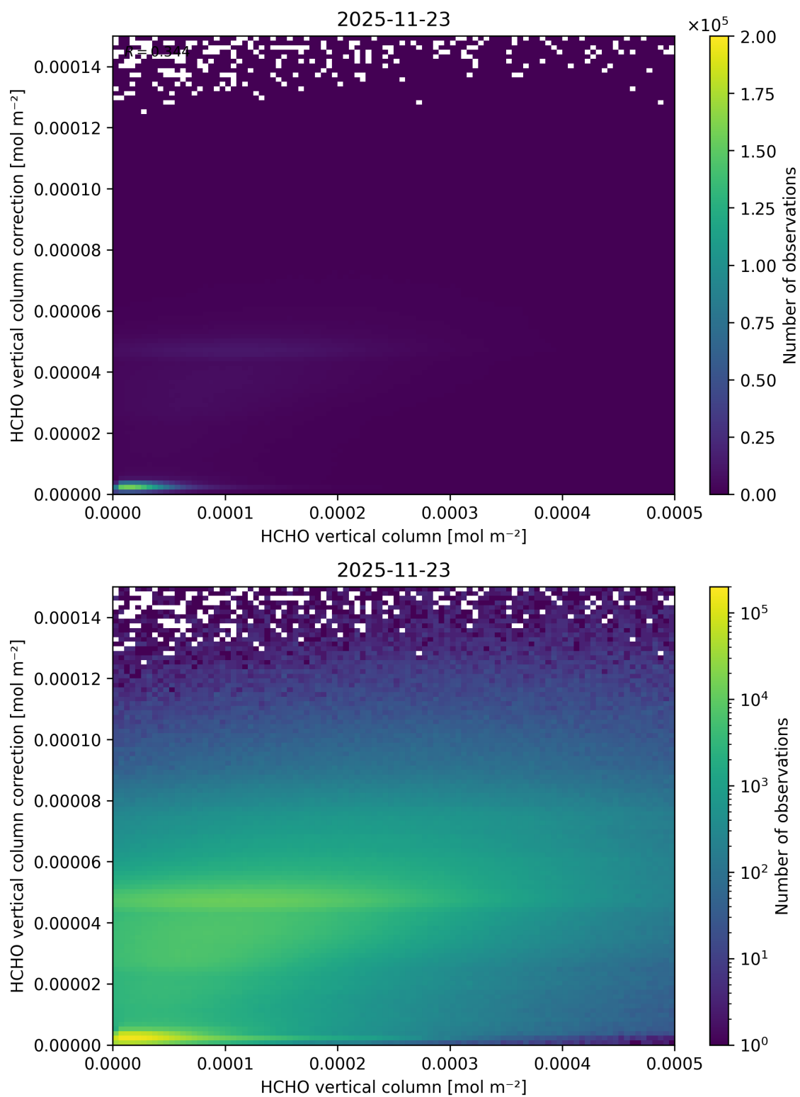
Figure 148: Scatter density plot of “HCHO vertical column” against “HCHO vertical column correction” for 2025-11-23 to 2025-11-24.
