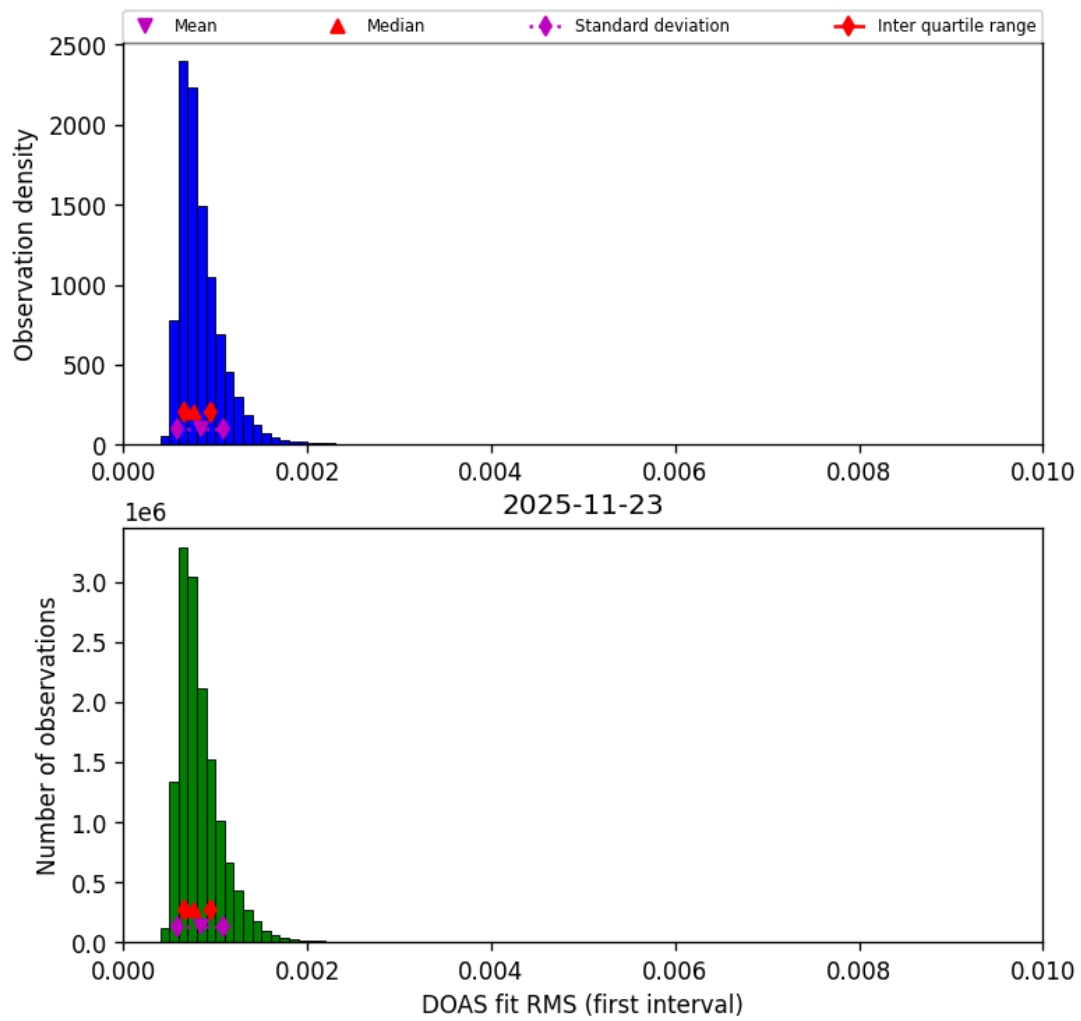
Figure 48: Histogram of “DOAS fit RMS (first interval)” for 2025-11-23 to 2025-11-24
