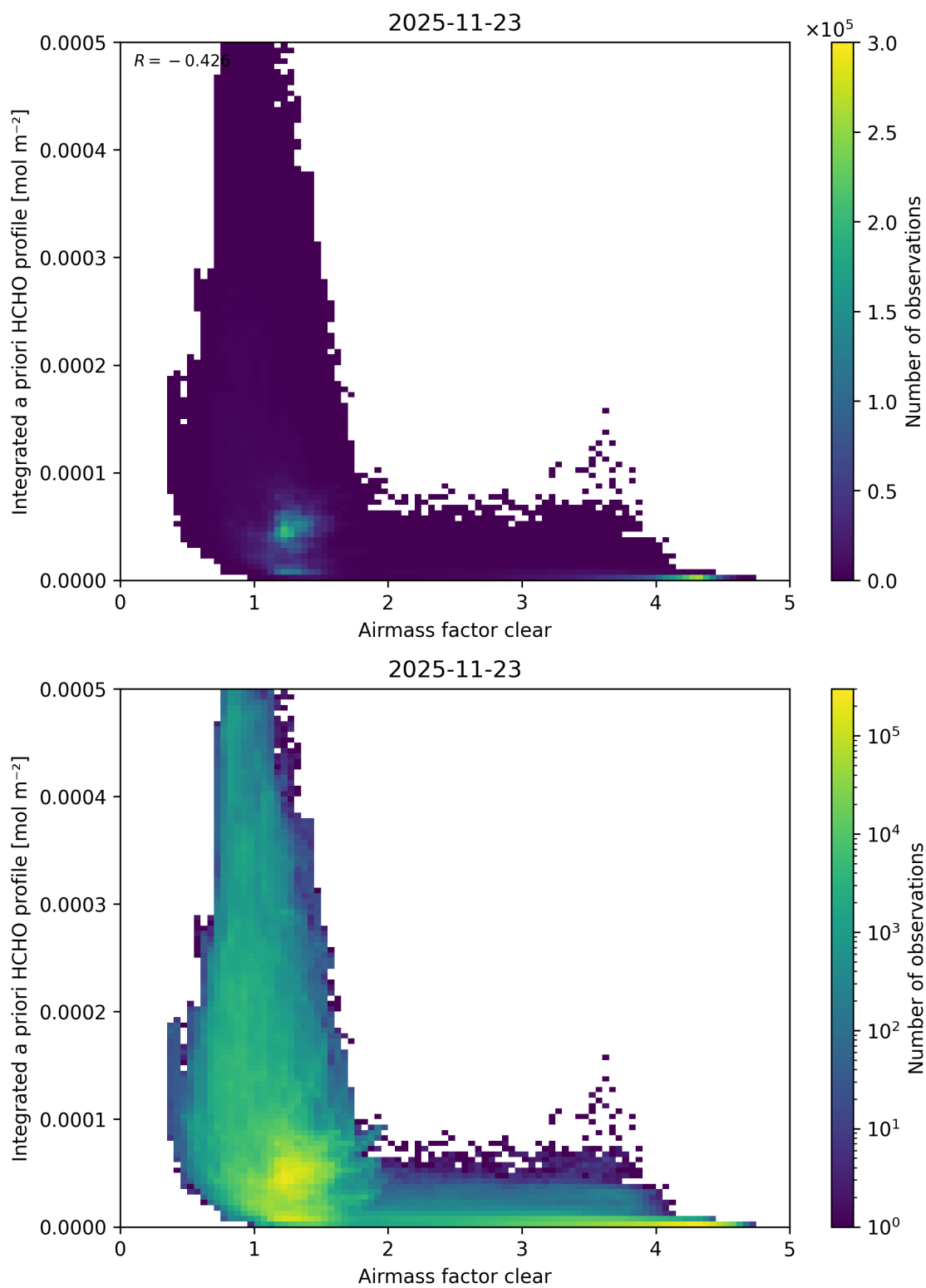
Figure 84: Scatter density plot of “Airmass factor clear” against “Integrated a priori HCHO profile” for 2025-11-23 to 2025-11-24.
