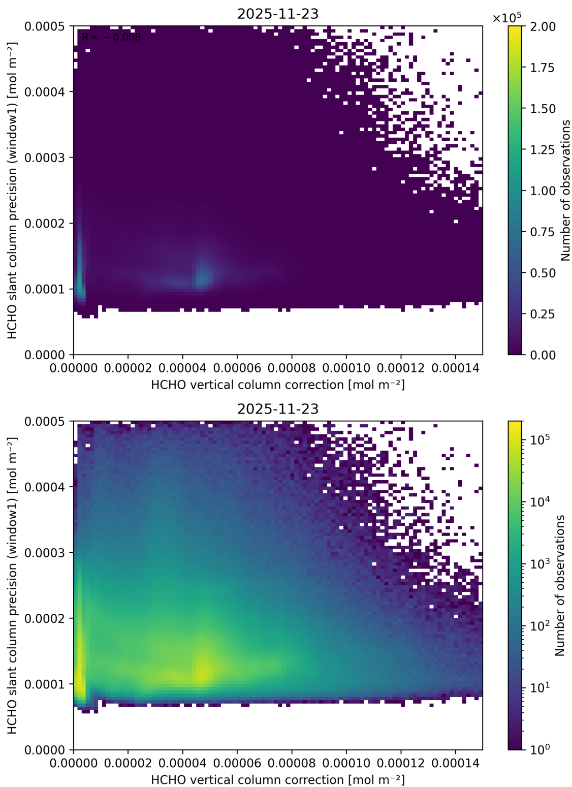
Figure 133: Scatter density plot of “HCHO vertical column correction” against “HCHO slant column precision (window1)” for 2025-11-23 to 2025-11-24.
