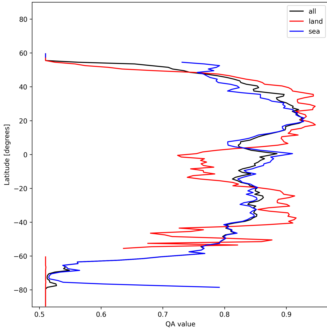
Figure 21: Zonal average of “QA value” for 2025-11-23 to 2025-11-24.
