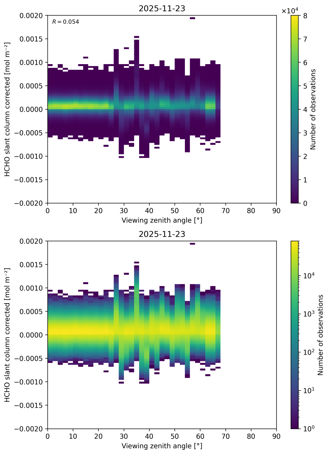
Figure 206: Scatter density plot of “Viewing zenith angle” against “HCHO slant column corrected” for 2025-11-23 to 2025-11-24.
