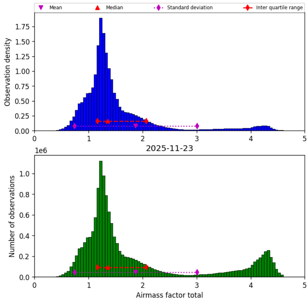
Figure 42: Histogram of “Airmass factor total” for 2025-11-23 to 2025-11-24
