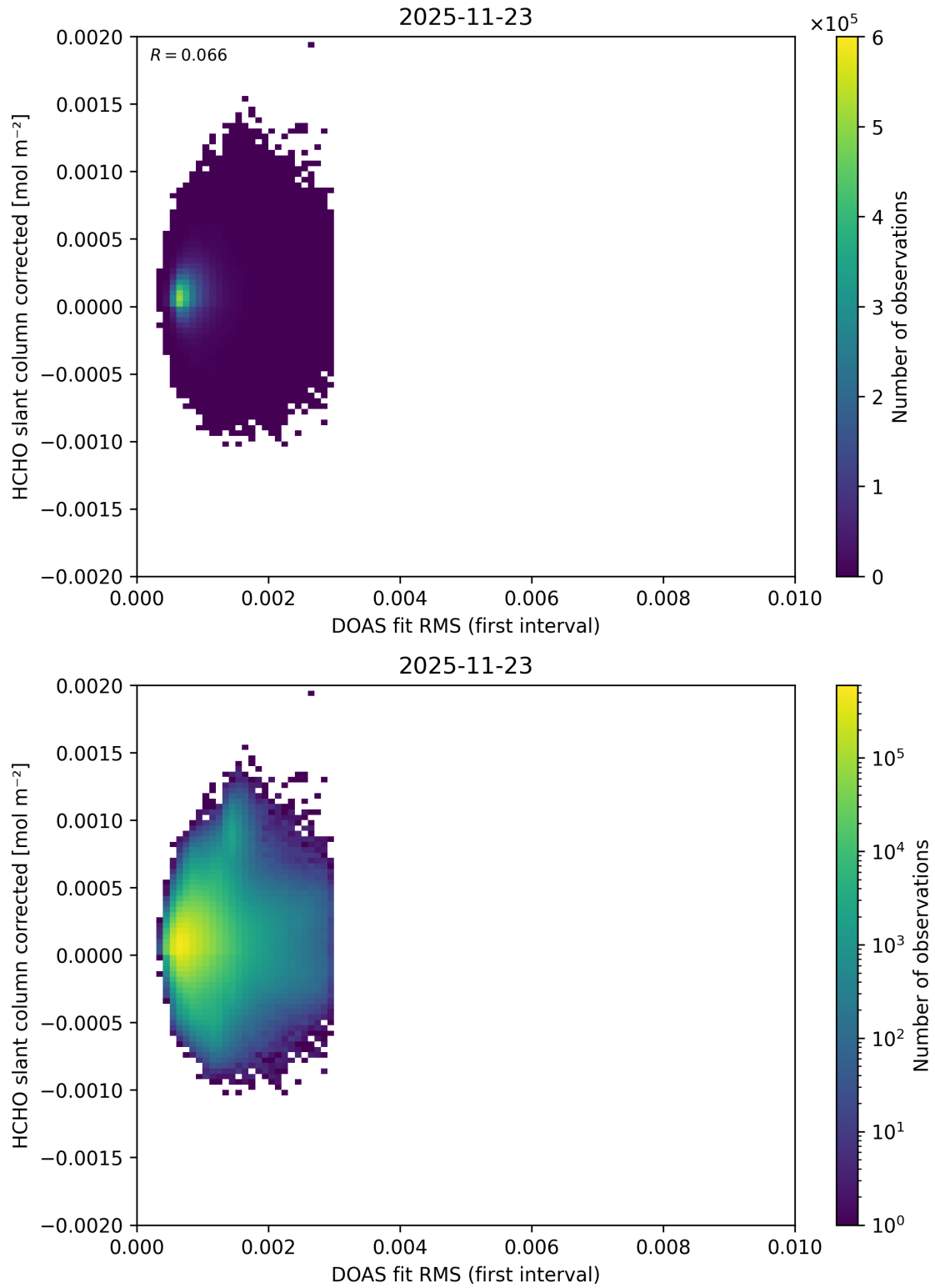
Figure 66: Scatter density plot of “DOAS fit RMS (first interval)” against “HCHO slant column corrected” for 2025-11-23 to 2025-11-24.
