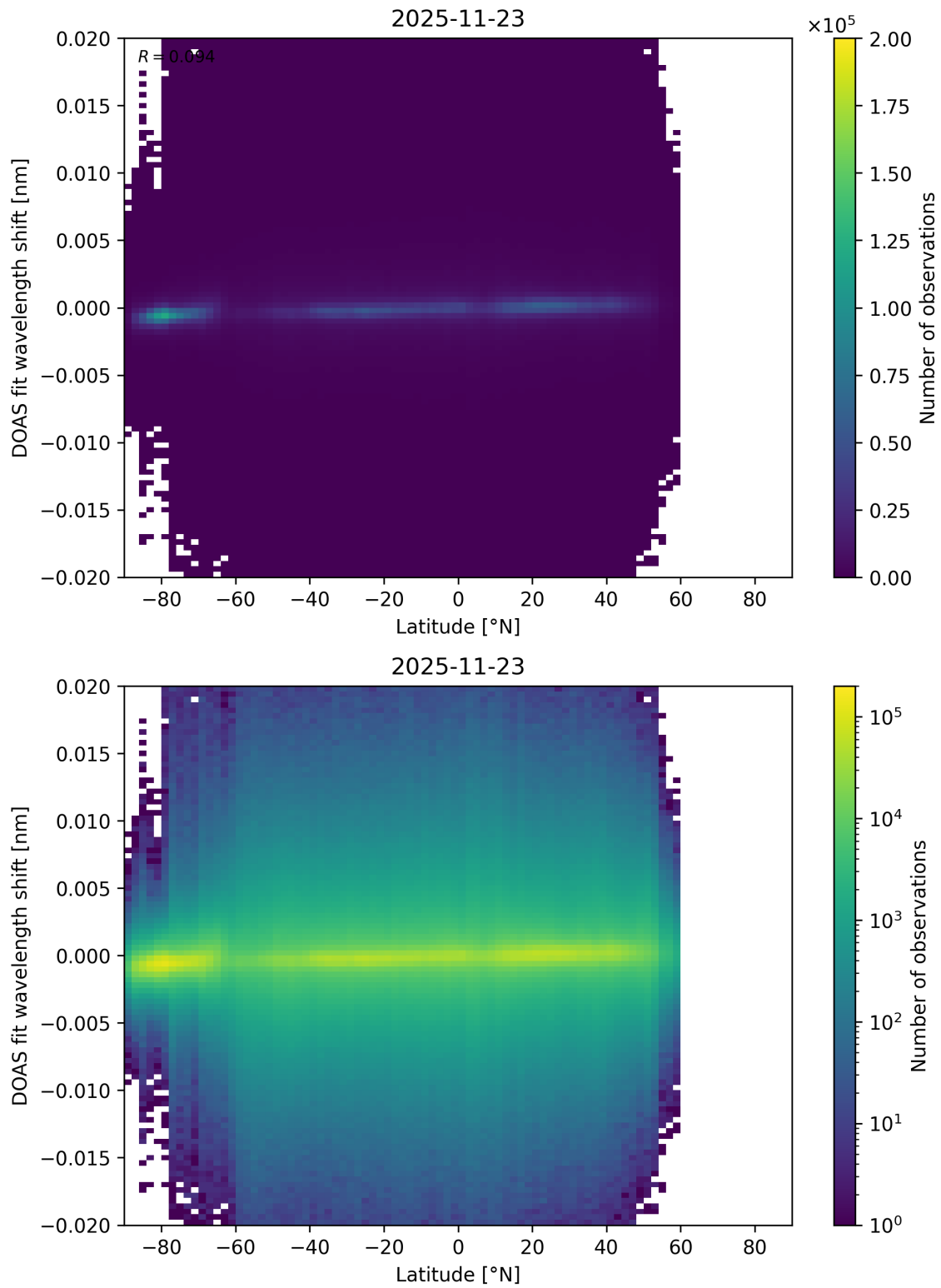
Figure 172: Scatter density plot of “Latitude” against “DOAS fit wavelength shift” for 2025-11-23 to 2025-11-24.
