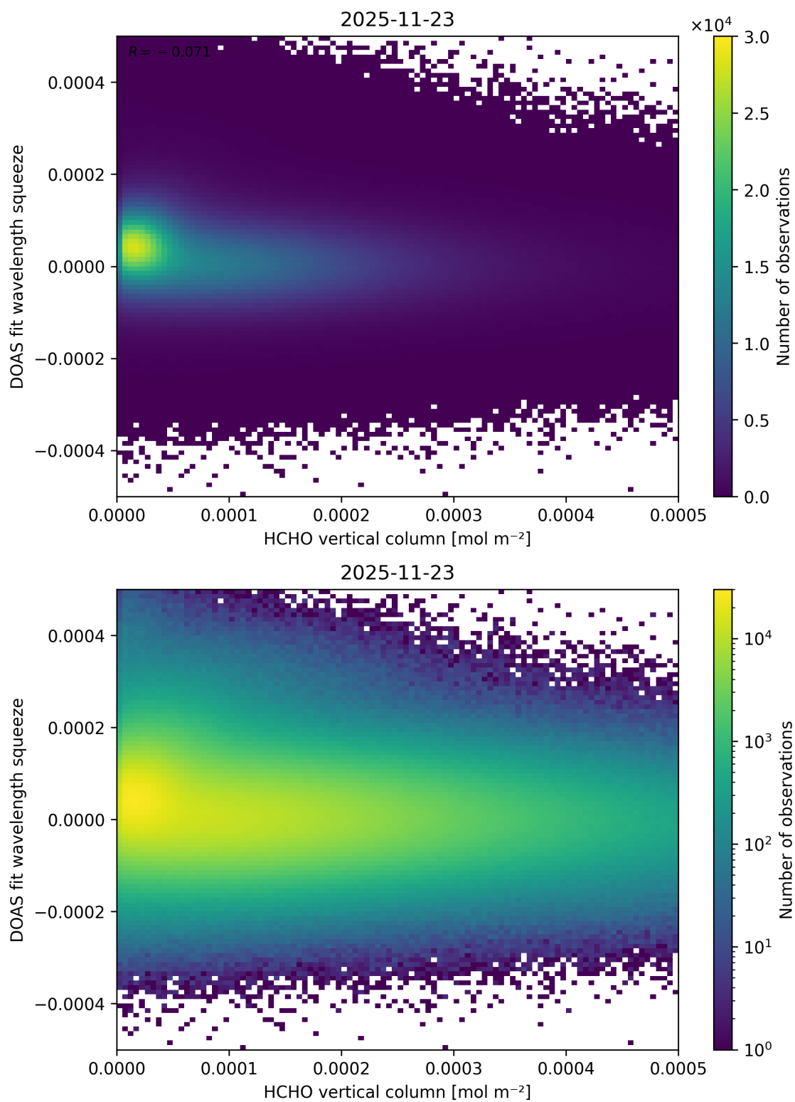
Figure 140: Scatter density plot of “HCHO vertical column” against “DOAS fit wavelength squeeze” for 2025-11-23 to 2025-11-24.
