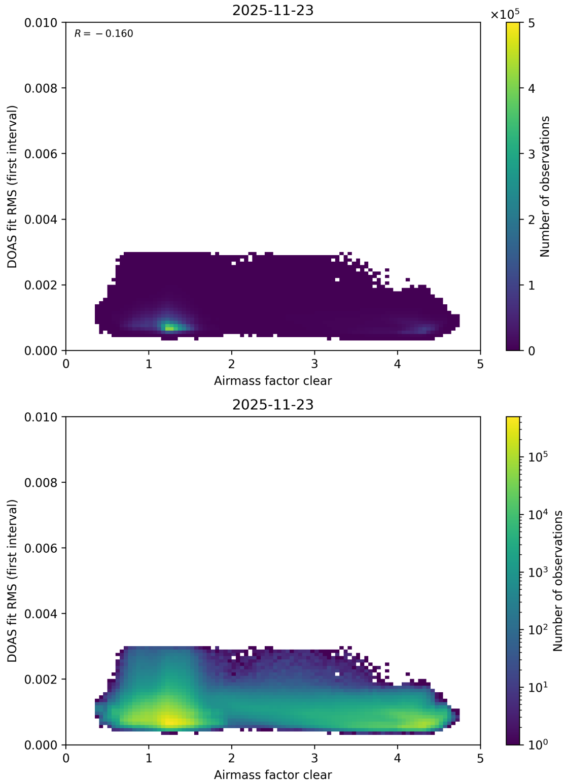
Figure 78: Scatter density plot of “Airmass factor clear” against “DOAS fit RMS (first interval)” for 2025-11-23 to 2025-11-24.
