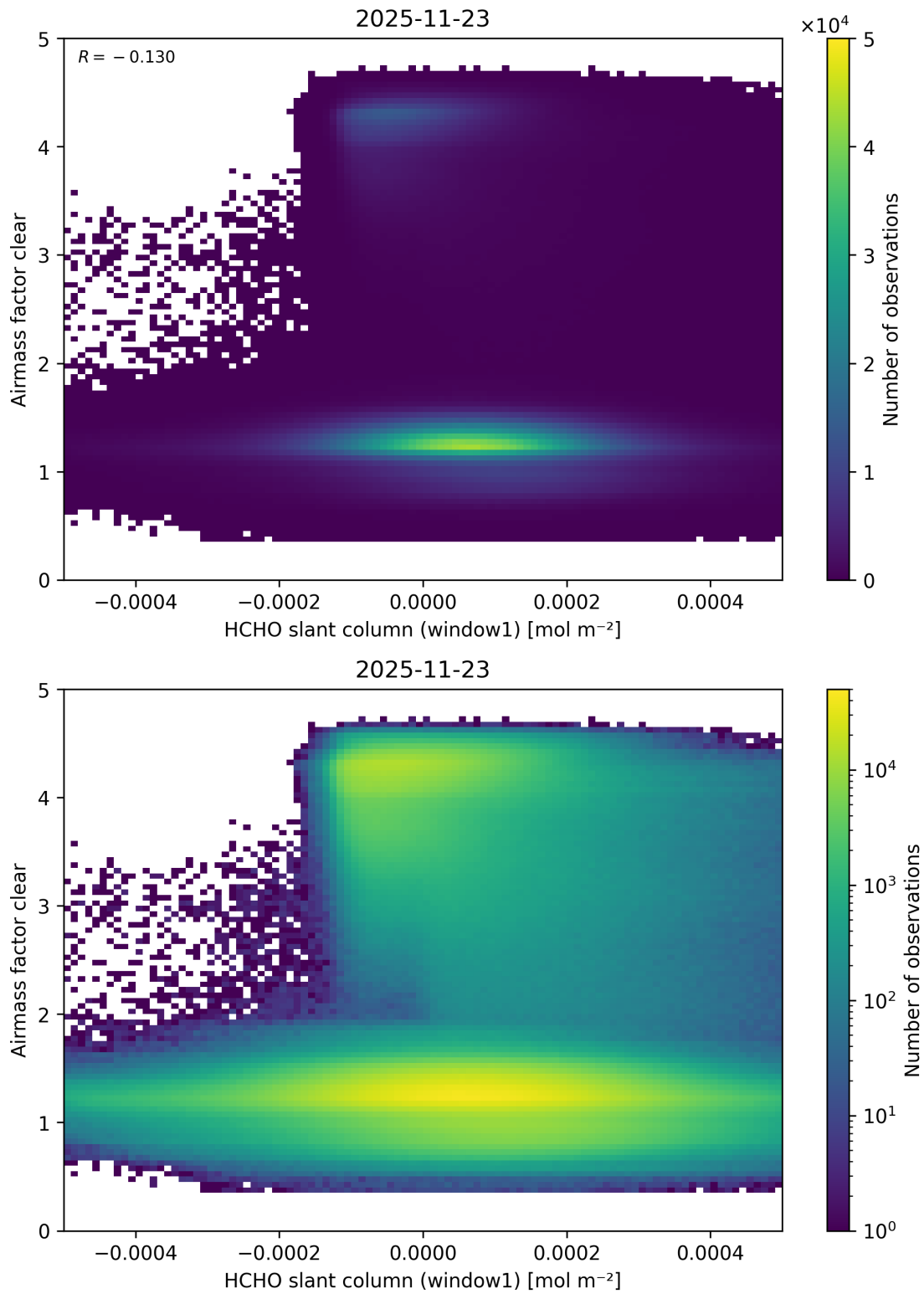
Figure 91: Scatter density plot of “HCHO slant column (window1)” against “Airmass factor clear” for 2025-11-23 to 2025-11-24.
