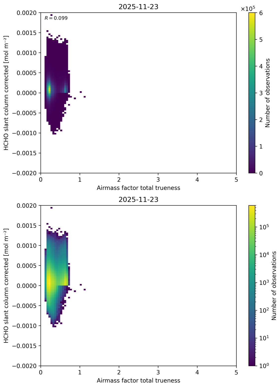
Figure 122: Scatter density plot of “Airmass factor total trueness” against “HCHO slant column corrected” for 2025-11-23 to 2025-11-24.
