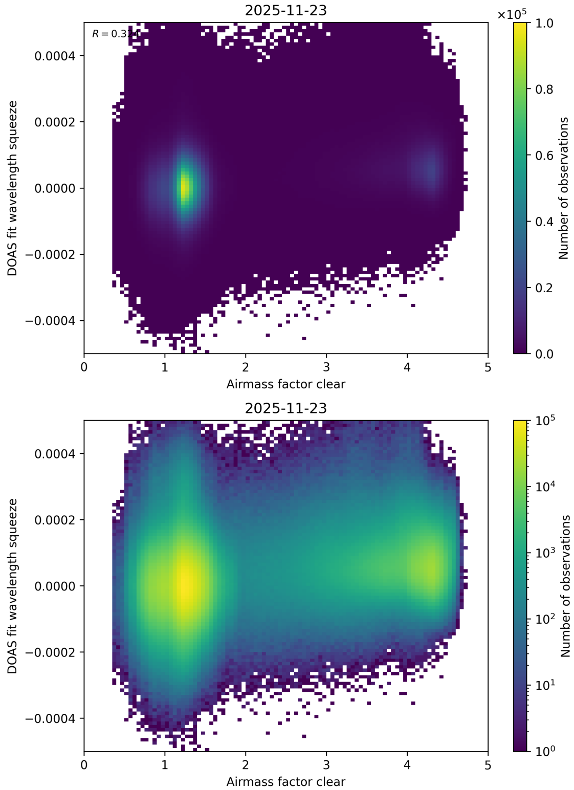
Figure 80: Scatter density plot of “Airmass factor clear” against “DOAS fit wavelength squeeze” for 2025-11-23 to 2025-11-24.
