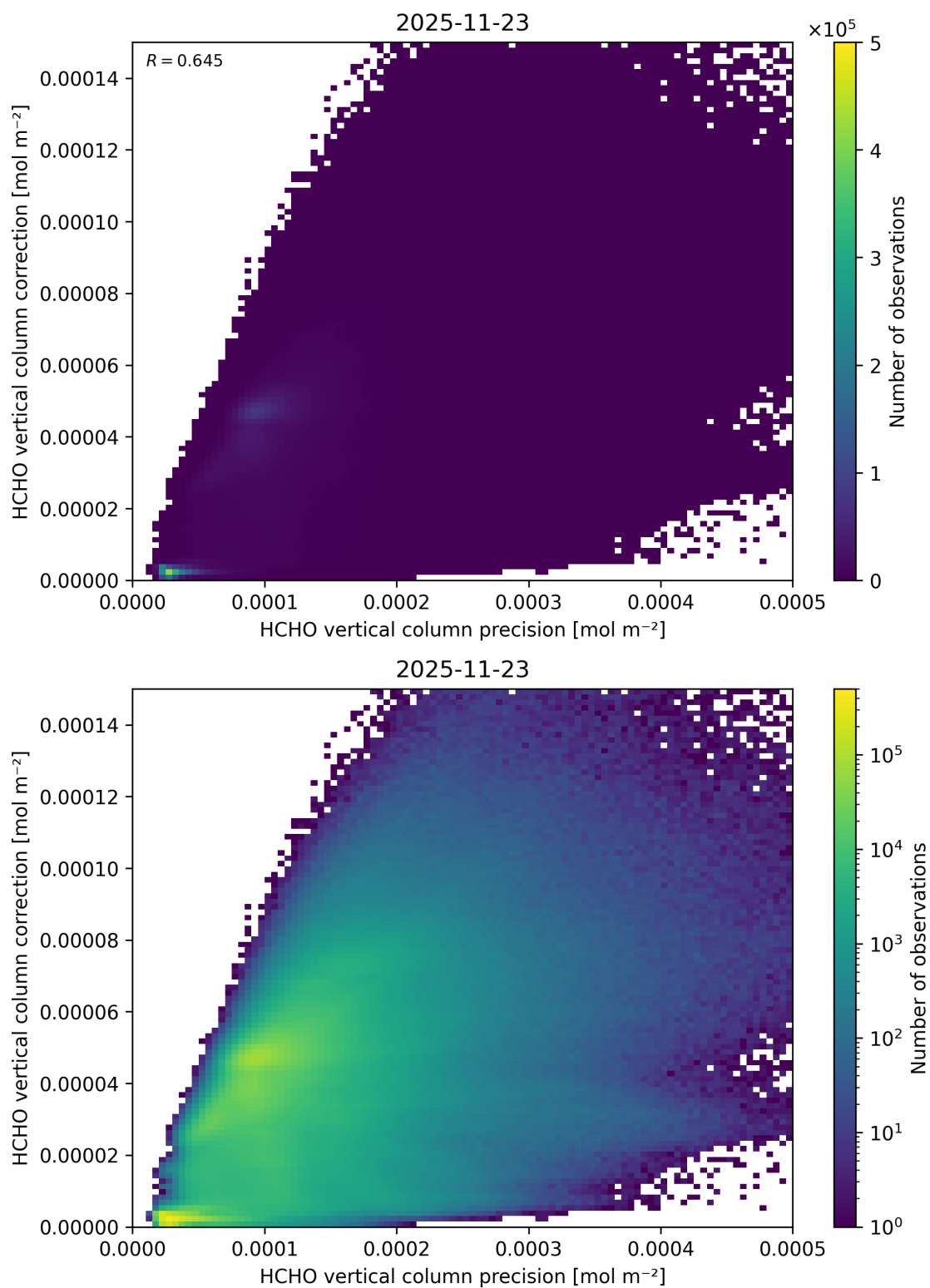
Figure 162: Scatter density plot of “HCHO vertical column precision” against “HCHO vertical column correction” for 2025-11-23 to 2025-11-24.
