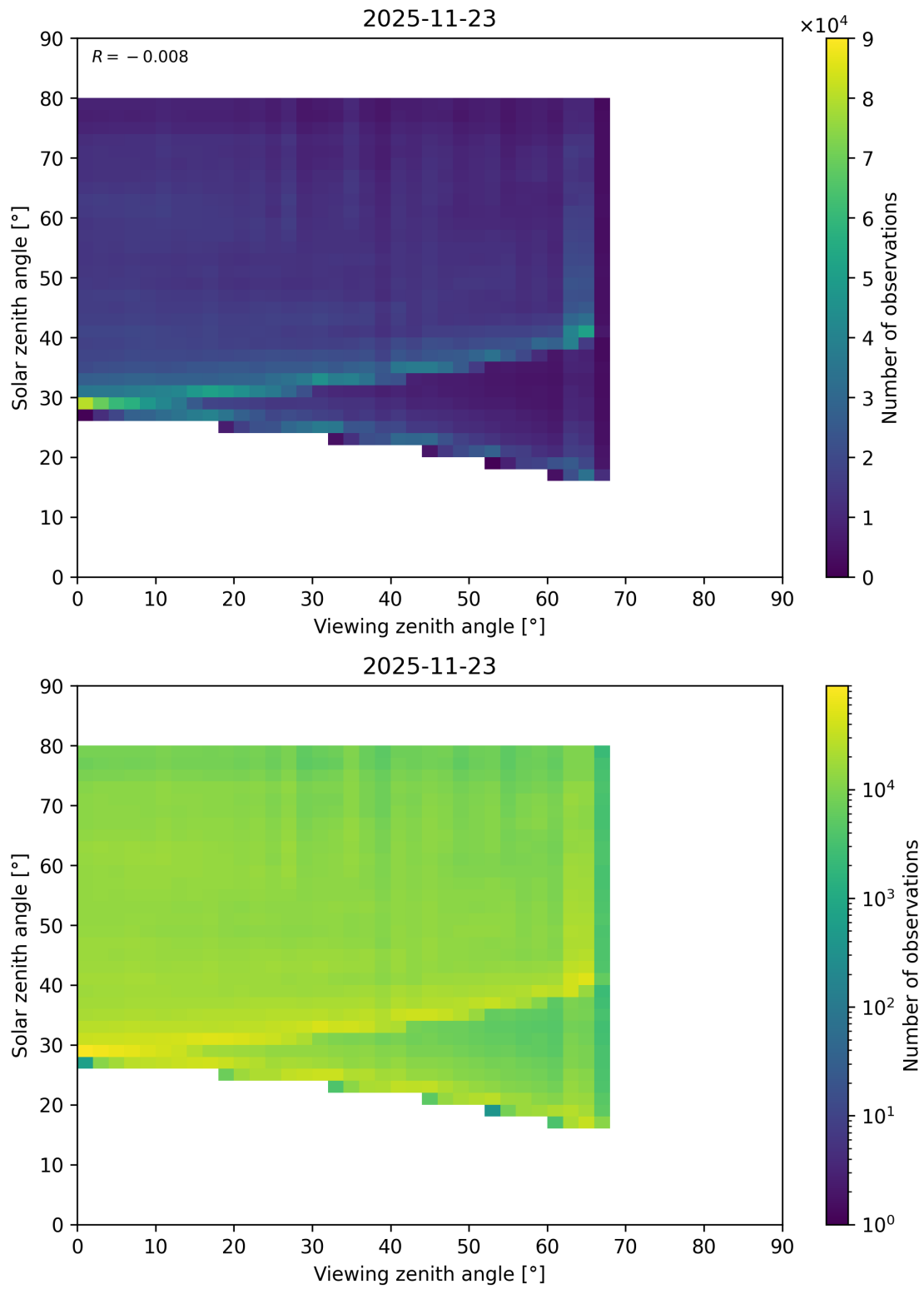
Figure 218: Scatter density plot of “Viewing zenith angle” against “Solar zenith angle” for 2025-11-23 to 2025-11-24.
