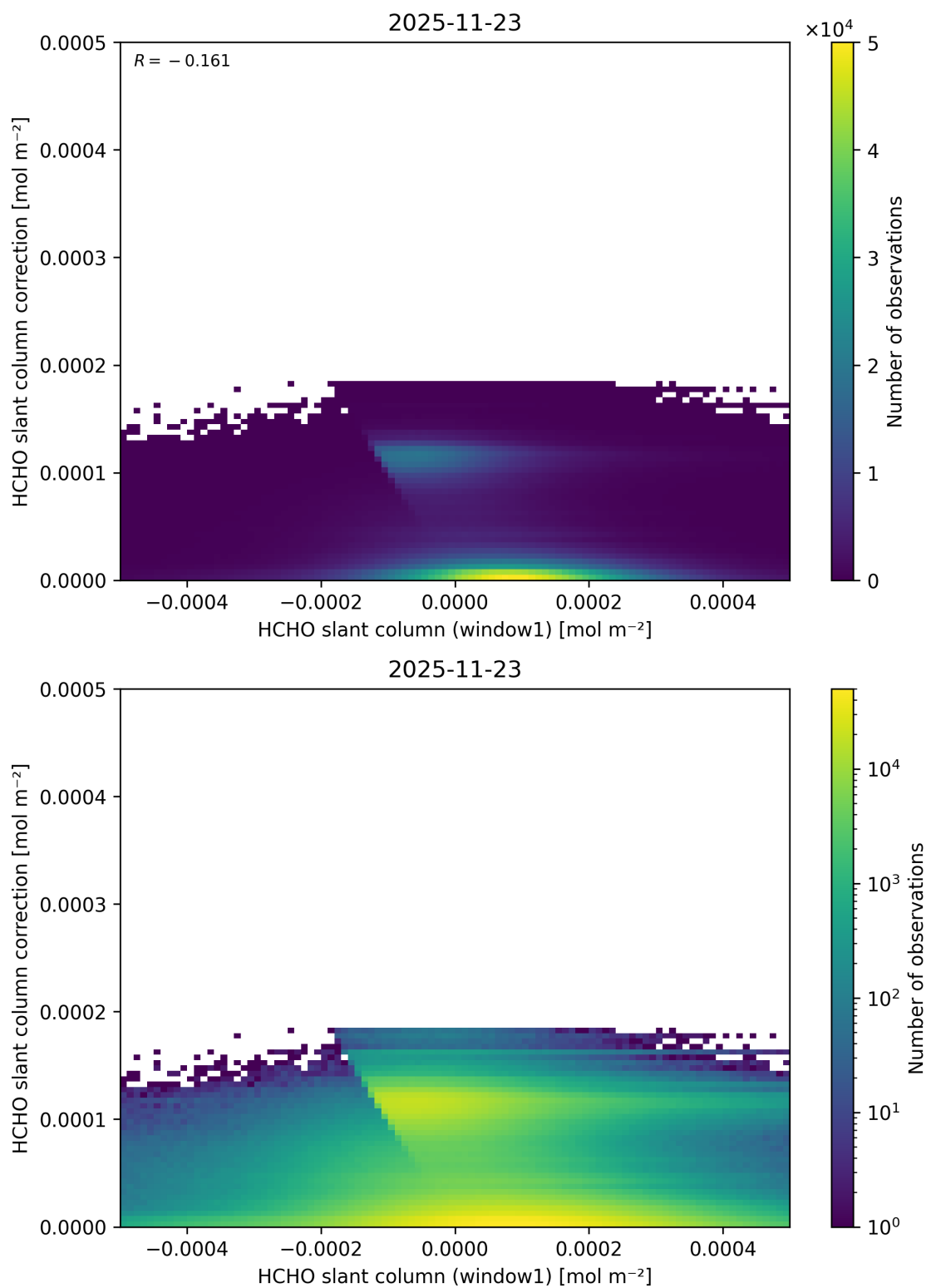
Figure 93: Scatter density plot of “HCHO slant column (window1)” against “HCHO slant column correction” for 2025-11-23 to 2025-11-24.
