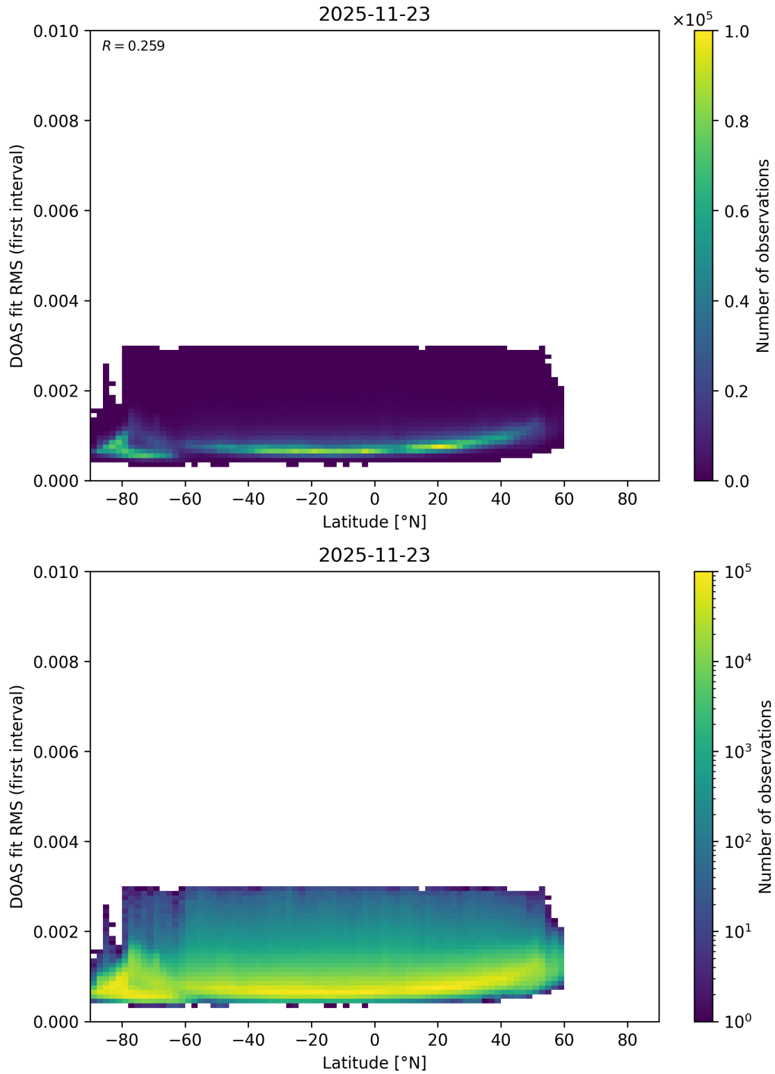
Figure 171: Scatter density plot of “Latitude” against “DOAS fit RMS (first interval)” for 2025-11-23 to 2025-11-24.
