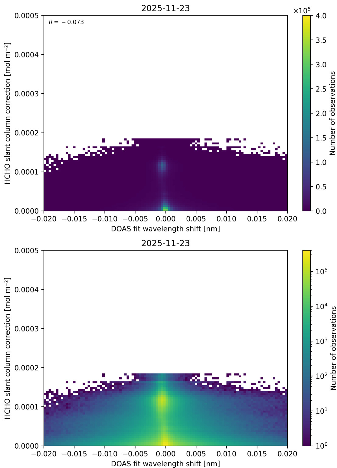
Figure 72: Scatter density plot of “DOAS fit wavelength shift” against “HCHO slant column correction” for 2025-11-23 to 2025-11-24.
