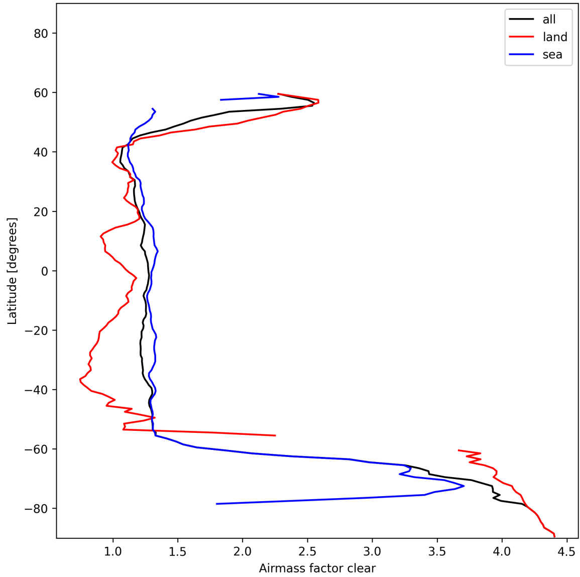
Figure 29: Zonal average of “Airmass factor clear” for 2025-11-23 to 2025-11-24.
