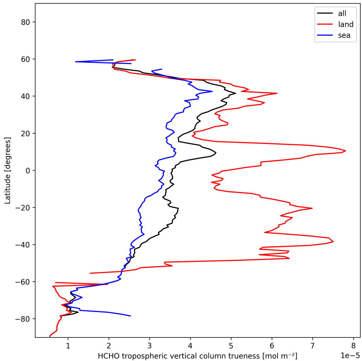
Figure 35: Zonal average of “HCHO tropospheric vertical column trueness” for 2025-11-23 to 2025-11-24.
