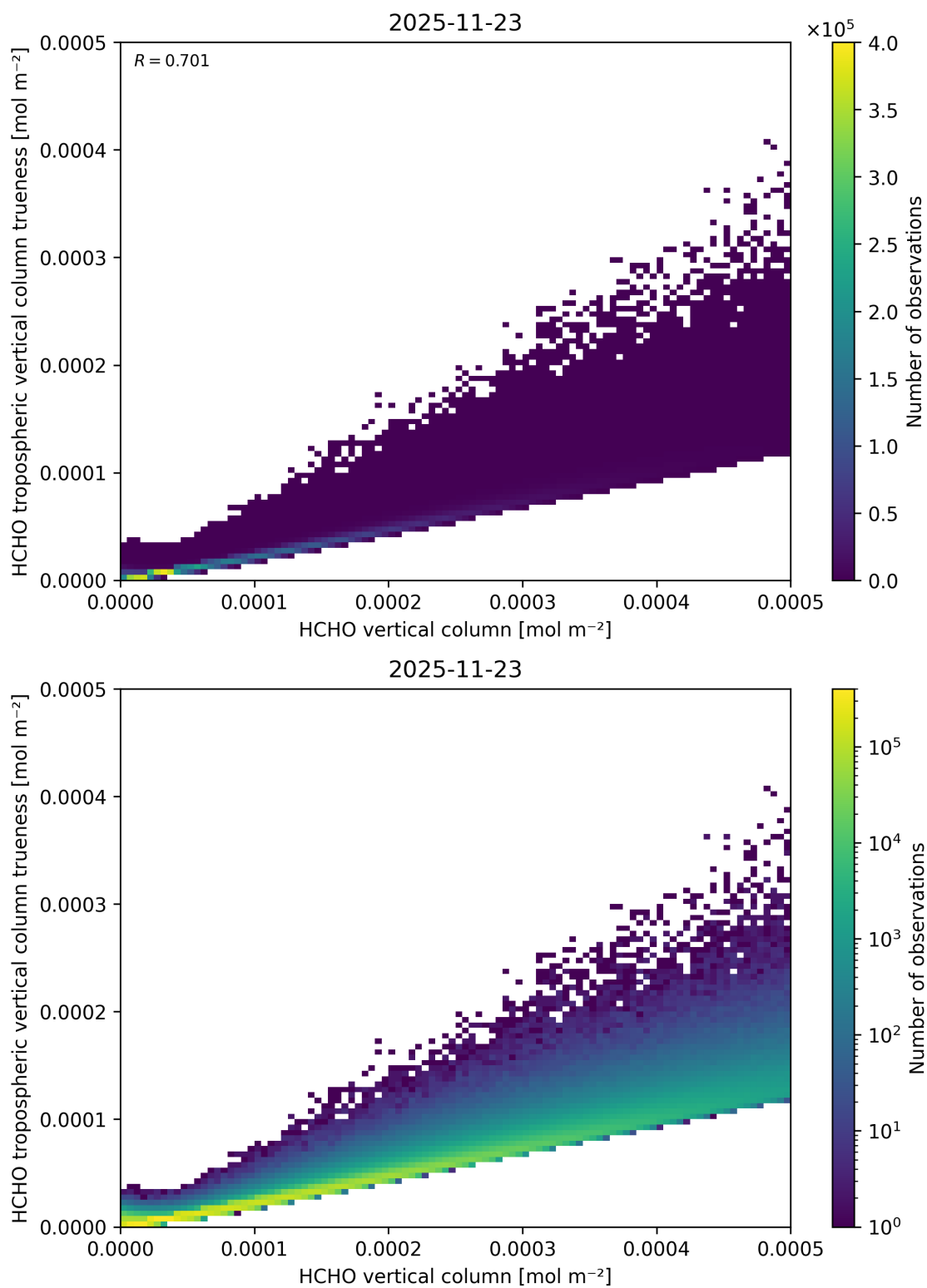
Figure 150: Scatter density plot of “HCHO vertical column” against “HCHO tropospheric vertical column trueness” for 2025-11-23 to 2025-11-24.
