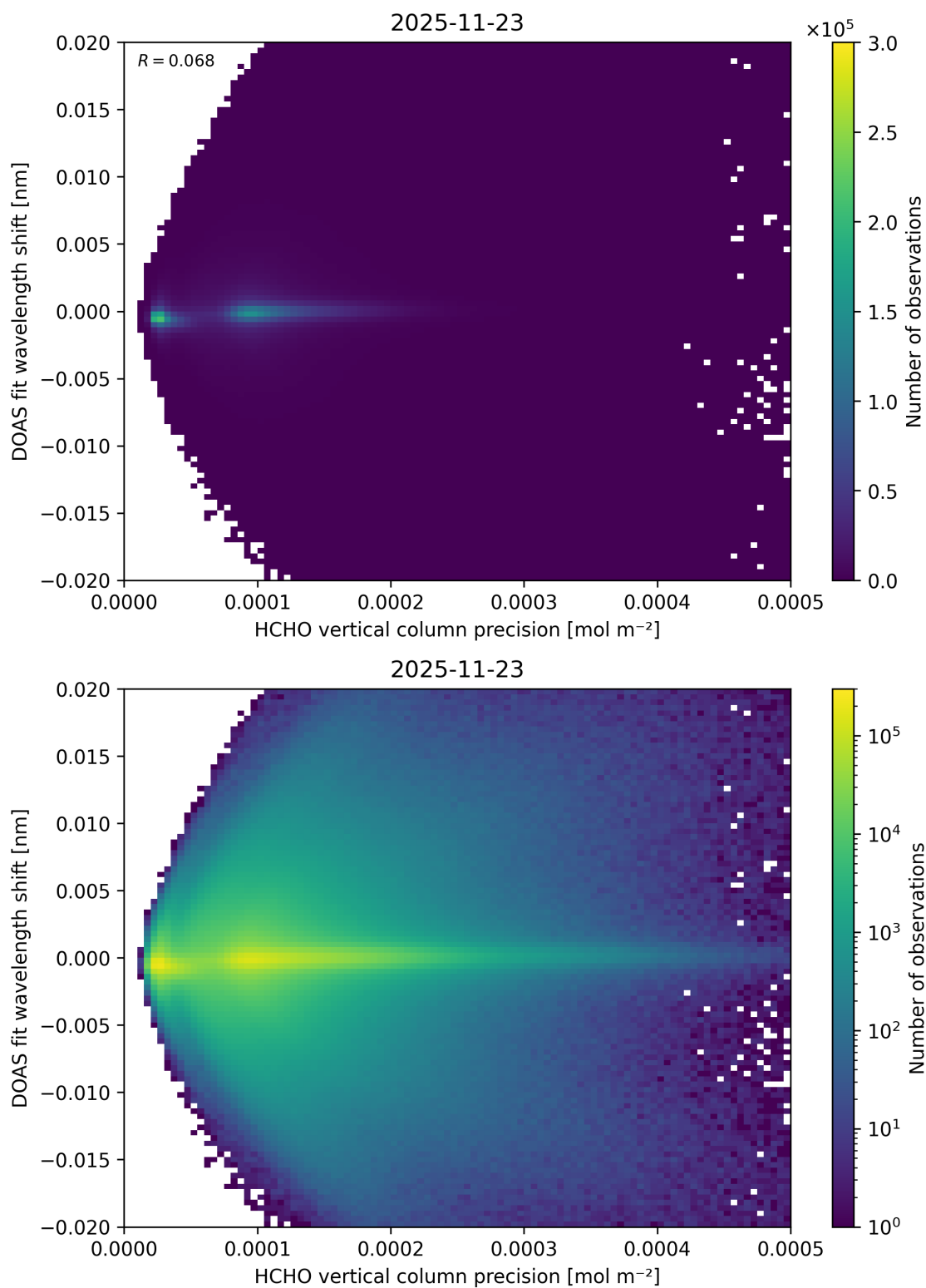
Figure 153: Scatter density plot of “HCHO vertical column precision” against “DOAS fit wavelength shift” for 2025-11-23 to 2025-11-24.
