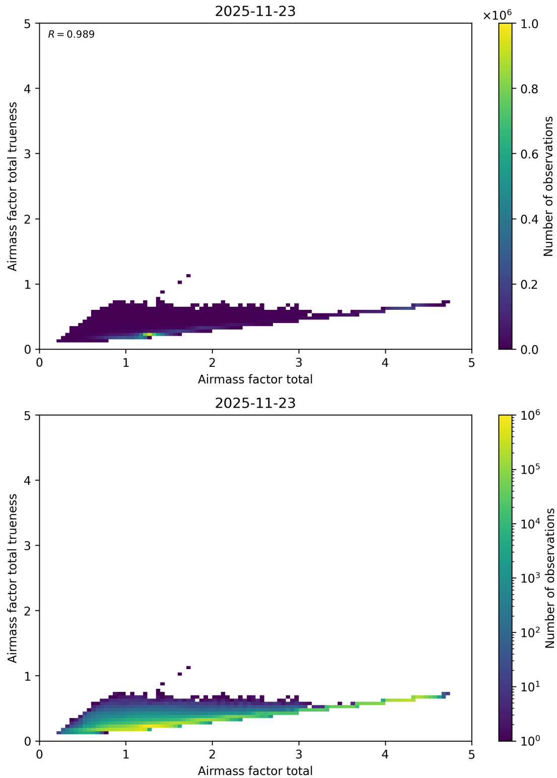
Figure 115: Scatter density plot of “Airmass factor total” against “Airmass factor total trueness” for 2025-11-23 to 2025-11-24.
