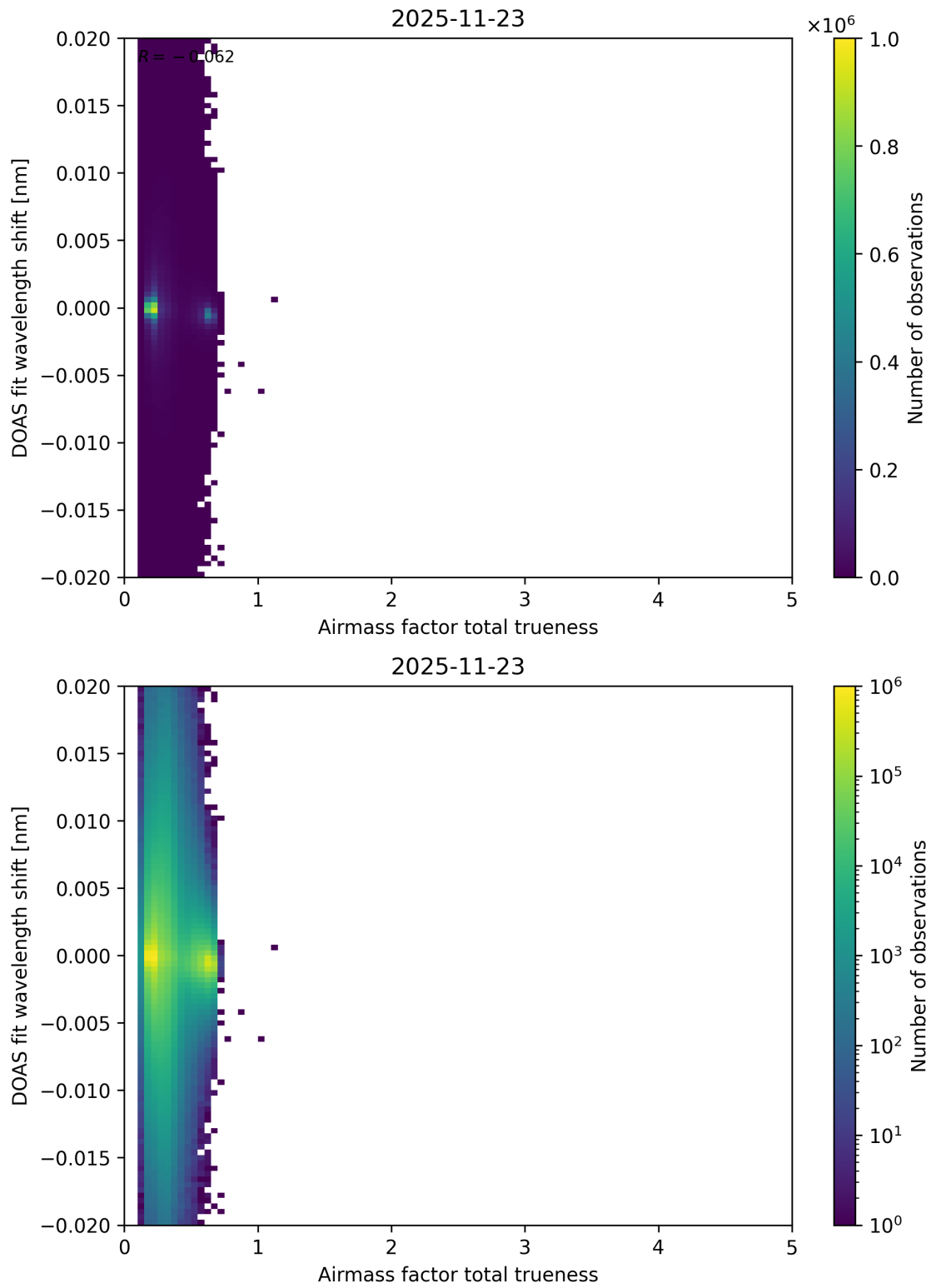
Figure 119: Scatter density plot of “Airmass factor total trueness” against “DOAS fit wavelength shift” for 2025-11-23 to 2025-11-24.
