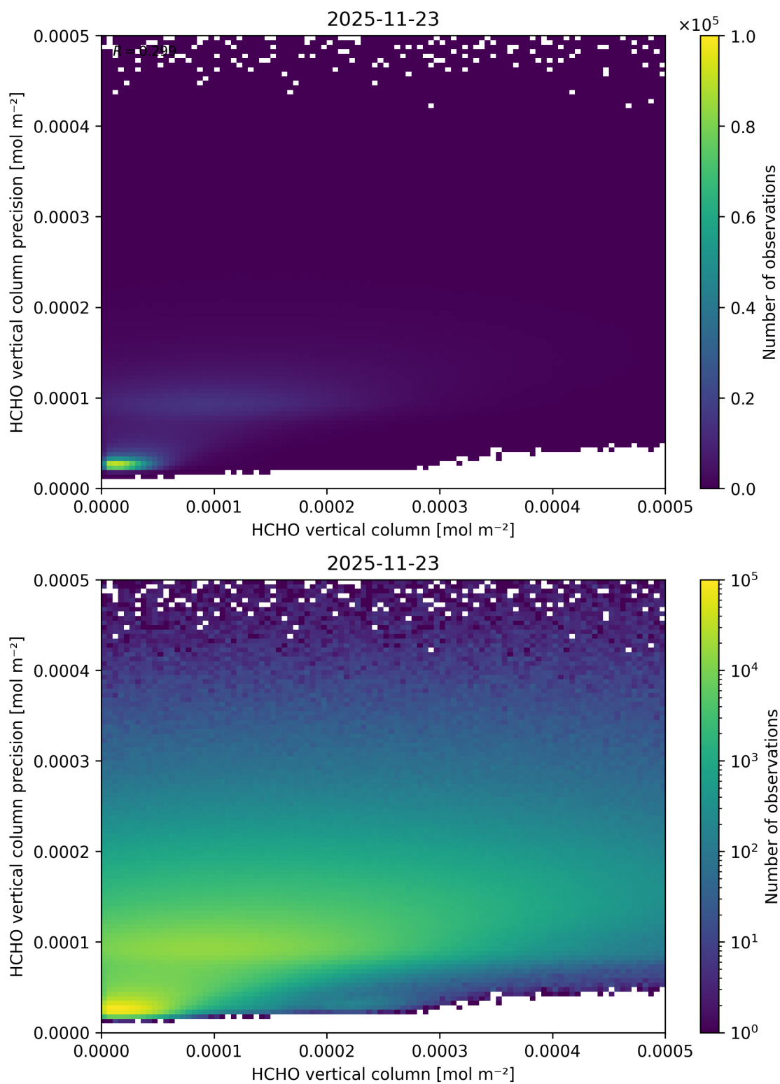
Figure 149: Scatter density plot of “HCHO vertical column” against “HCHO vertical column precision” for 2025-11-23 to 2025-11-24.
