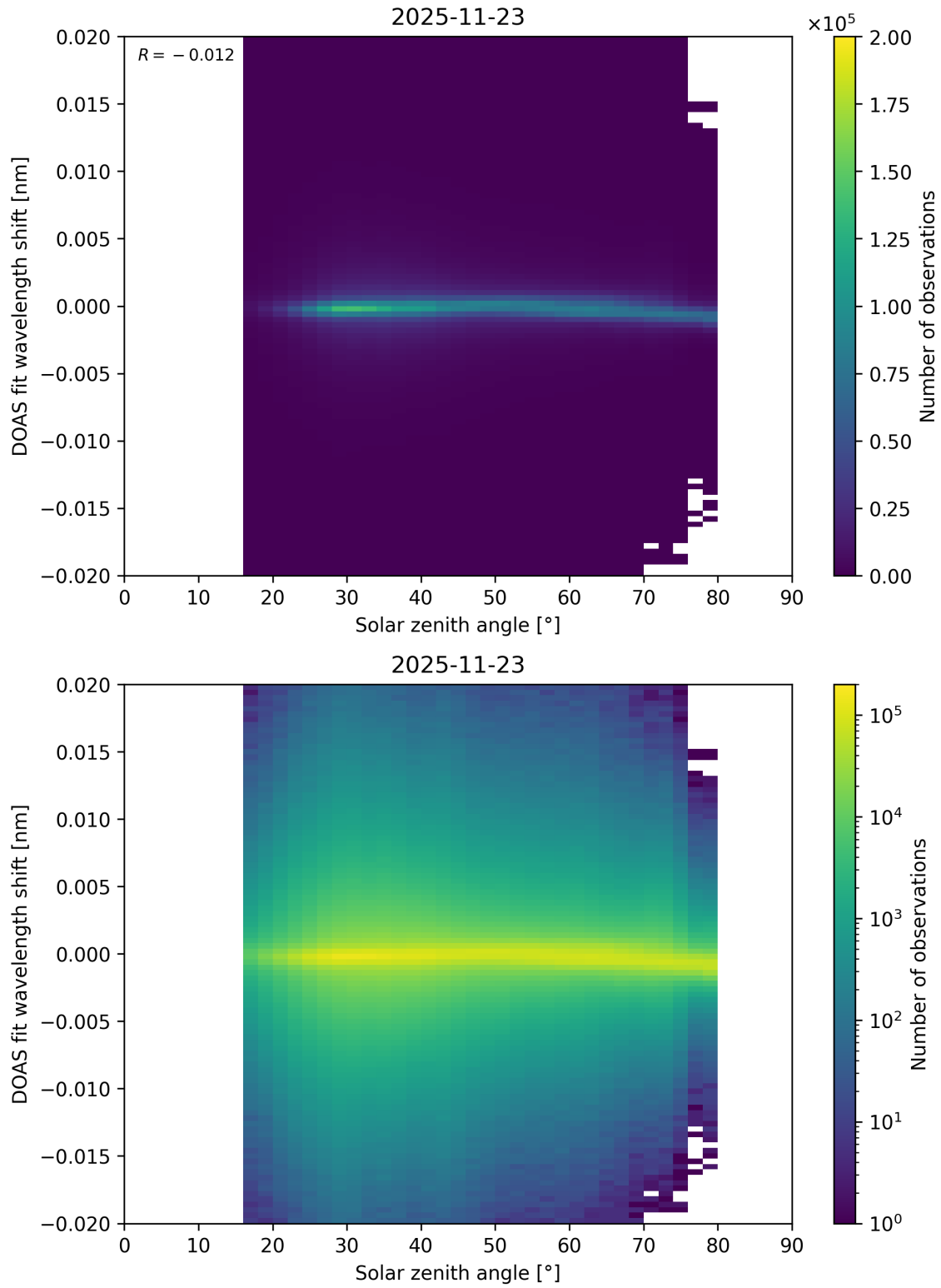
Figure 187: Scatter density plot of “Solar zenith angle” against “DOAS fit wavelength shift” for 2025-11-23 to 2025-11-24.
