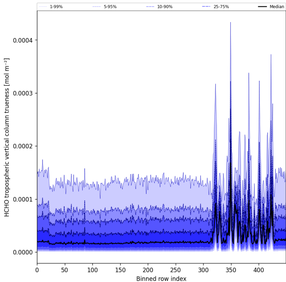
Figure 65: Along track statistics of “HCHO tropospheric vertical column trueness” for 2025-11-23 to 2025-11-24
