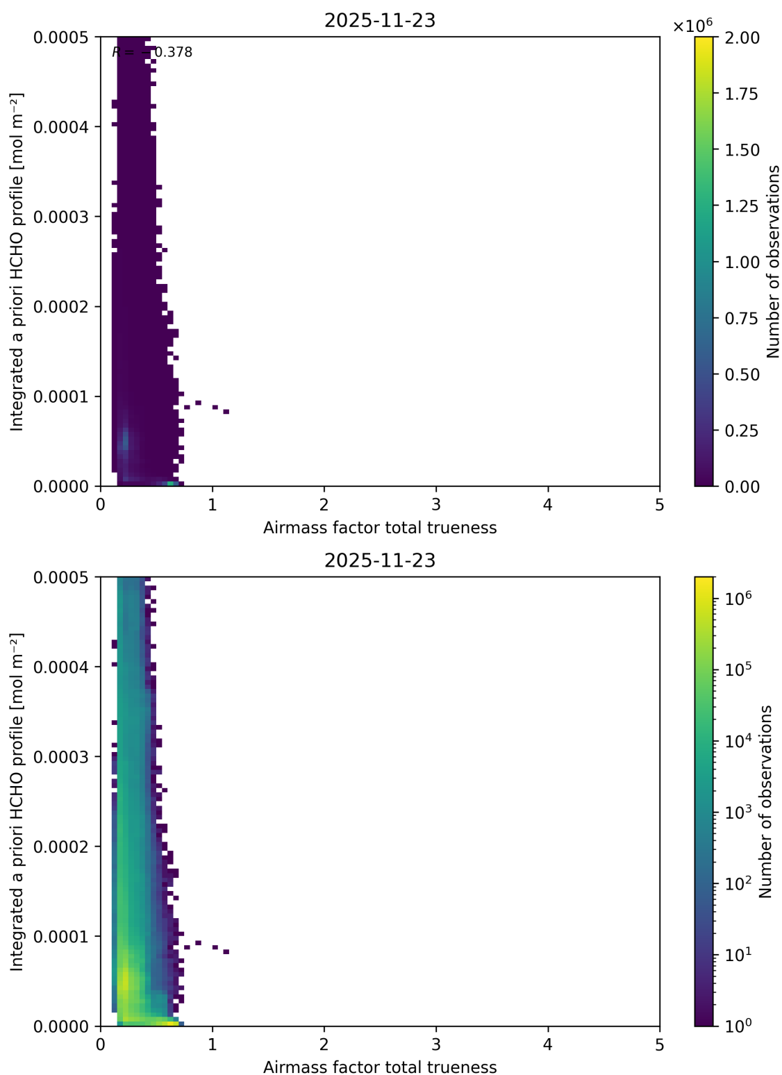
Figure 125: Scatter density plot of “Airmass factor total truiness” against “Integrated a priori HCHO profile” for 2025-11-23 to 2025-11-24.
