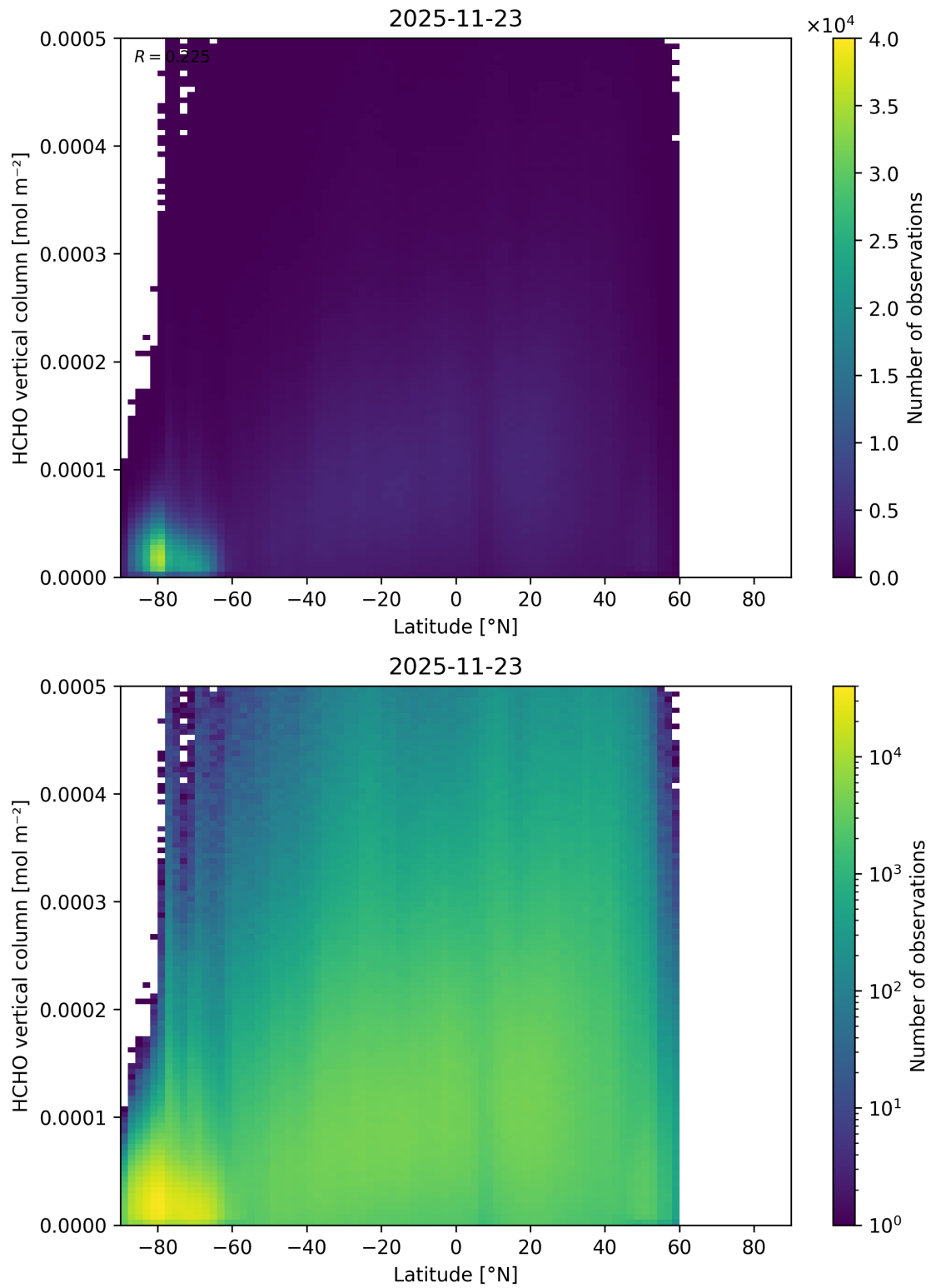
Figure 181: Scatter density plot of “Latitude” against “HCHO vertical column” for 2025-11-23 to 2025-11-24.
