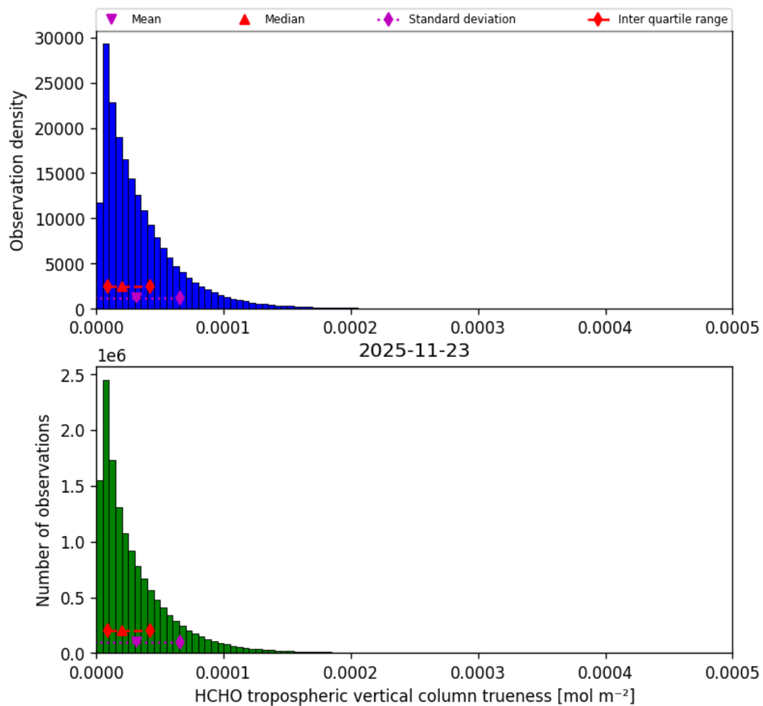
Figure 50: Histogram of “HCHO tropospheric vertical column trueness” for 2025-11-23 to 2025-11-24
