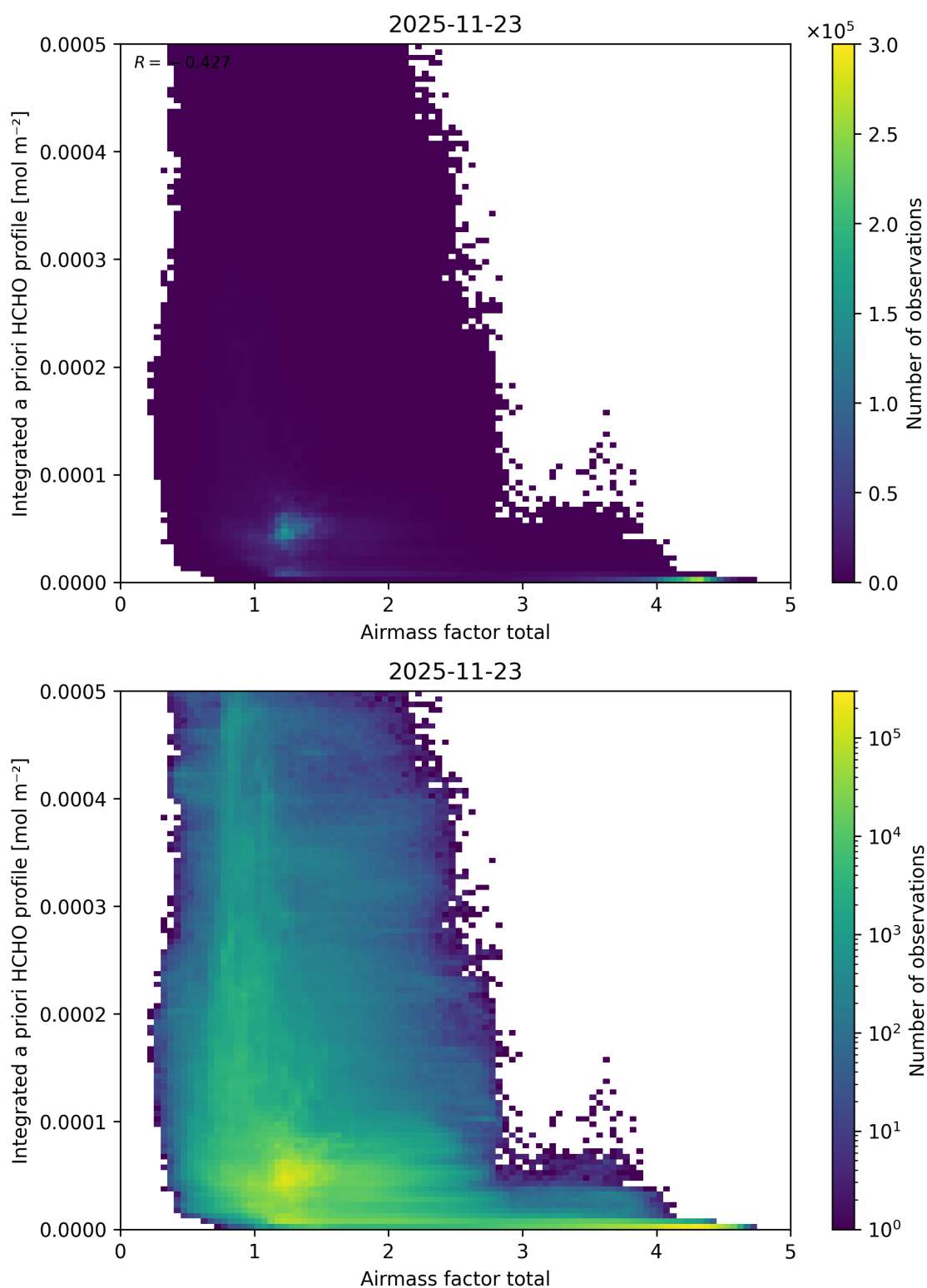
Figure 117: Scatter density plot of “Airmass factor total” against “Integrated a priori HCHO profile” for 2025-11-23 to 2025-11-24.
