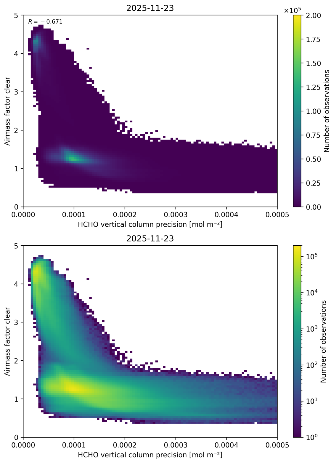
Figure 155: Scatter density plot of “HCHO vertical column precision” against “Airmass factor clear” for 2025-11-23 to 2025-11-24.
