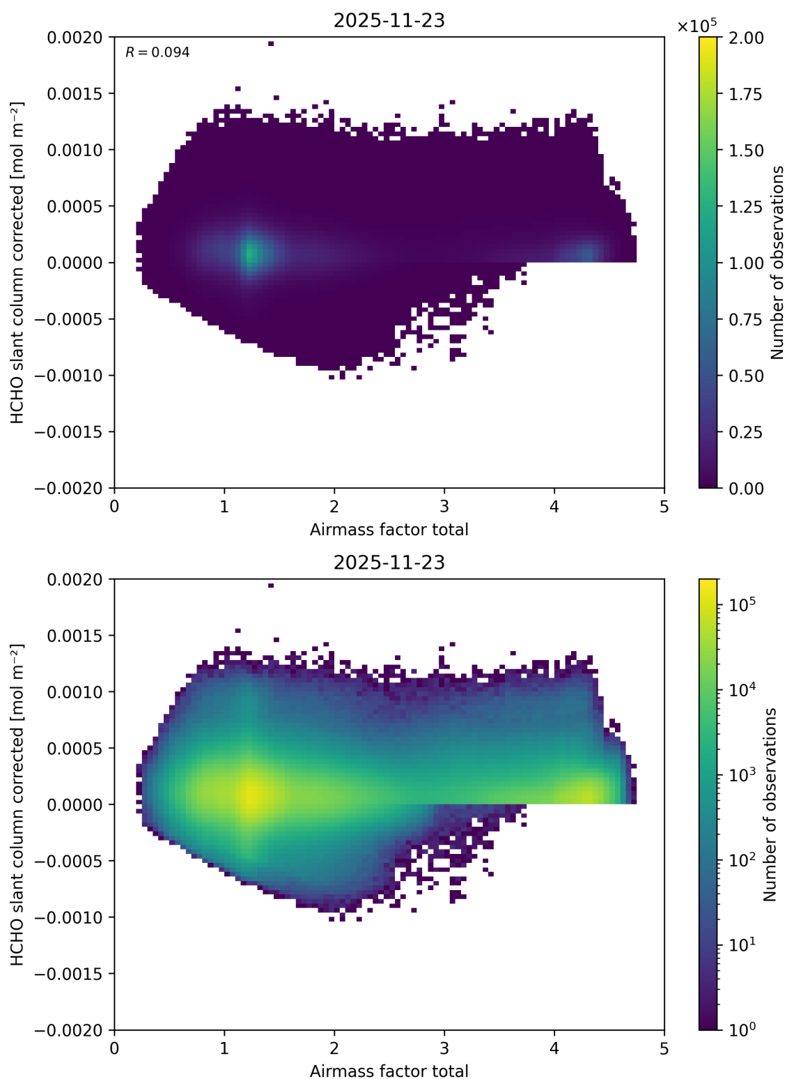
Figure 113: Scatter density plot of “Airmass factor total” against “HCHO slant column corrected” for 2025-11-23 to 2025-11-24.
