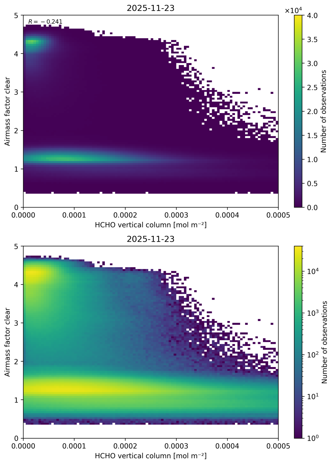
Figure 141: Scatter density plot of “HCHO vertical column” against “Airmass factor clear” for 2025-11-23 to 2025-11-24.
