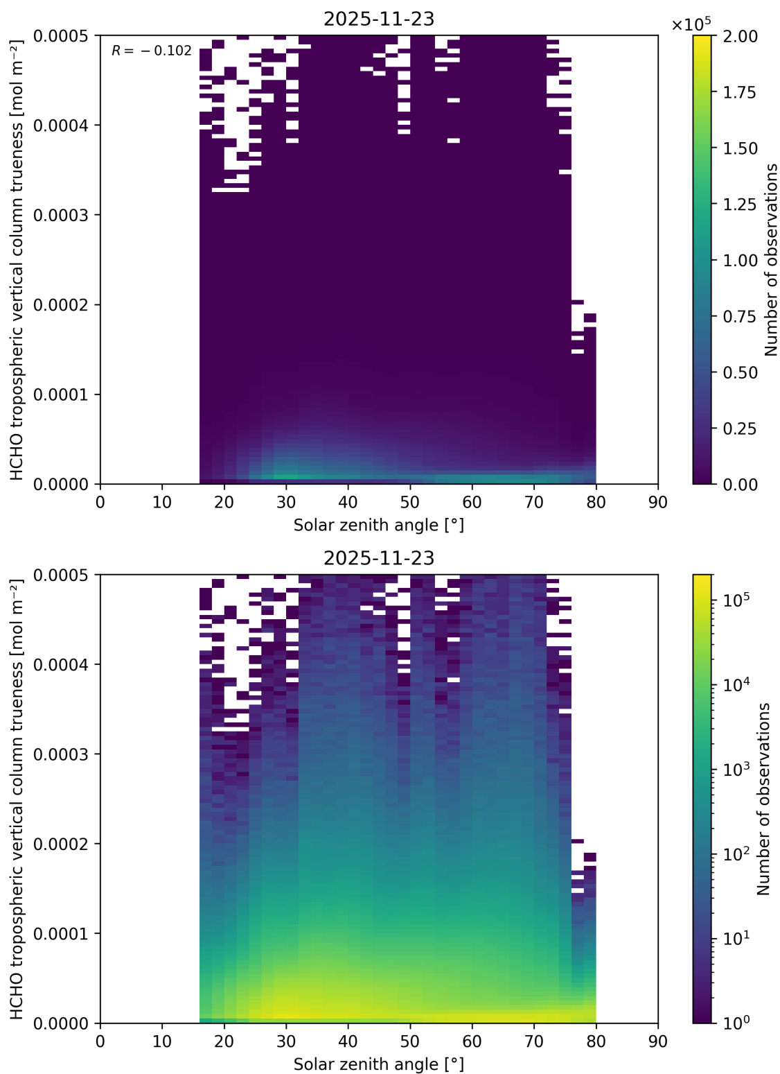
Figure 199: Scatter density plot of “Solar zenith angle” against “HCHO tropospheric vertical column trueness” for 2025-11-23 to 2025-11-24.
