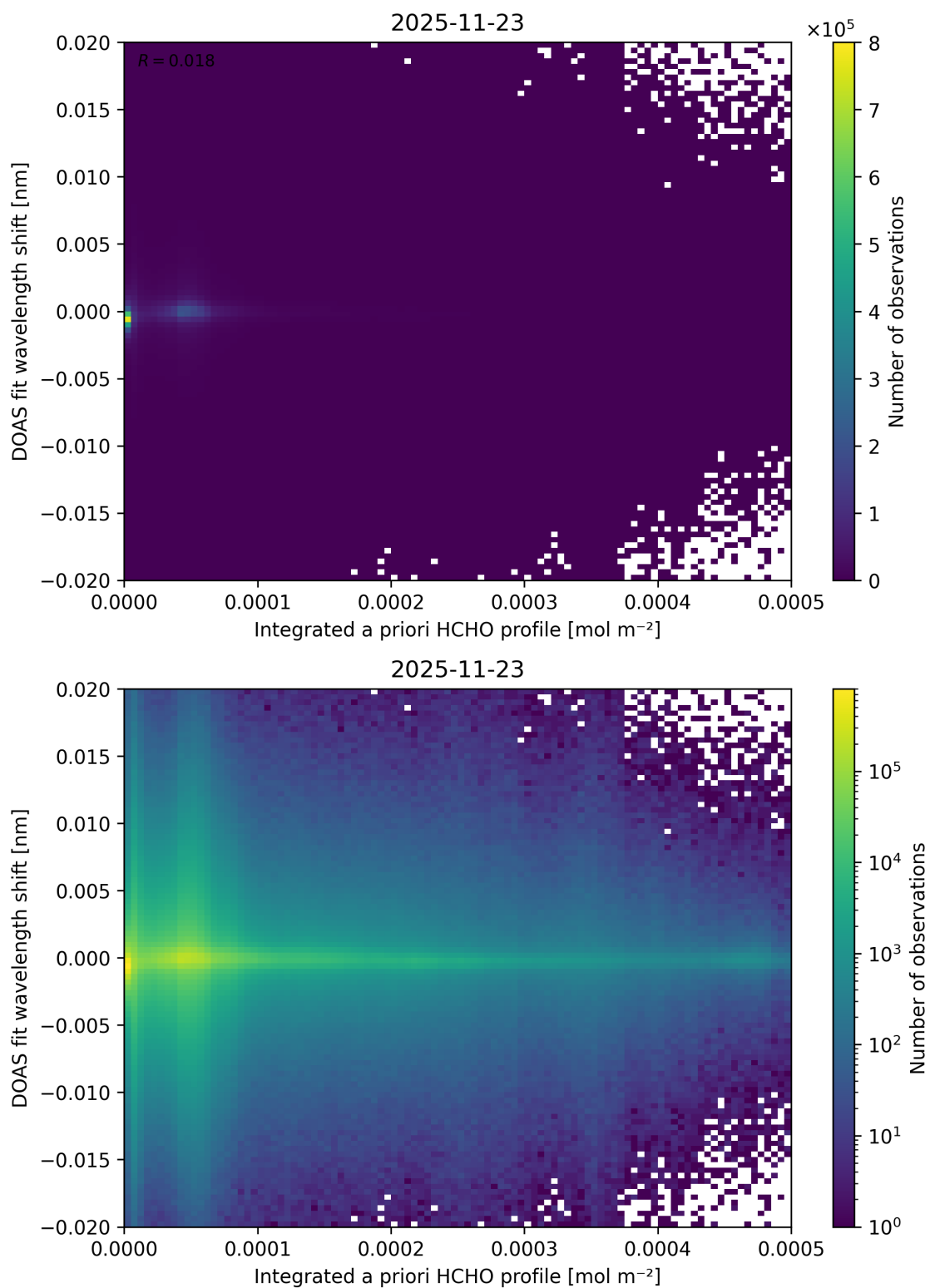
Figure 166: Scatter density plot of “Integrated a priori HCHO profile” against “DOAS fit wavelength shift” for 2025-11-23 to 2025-11-24.
