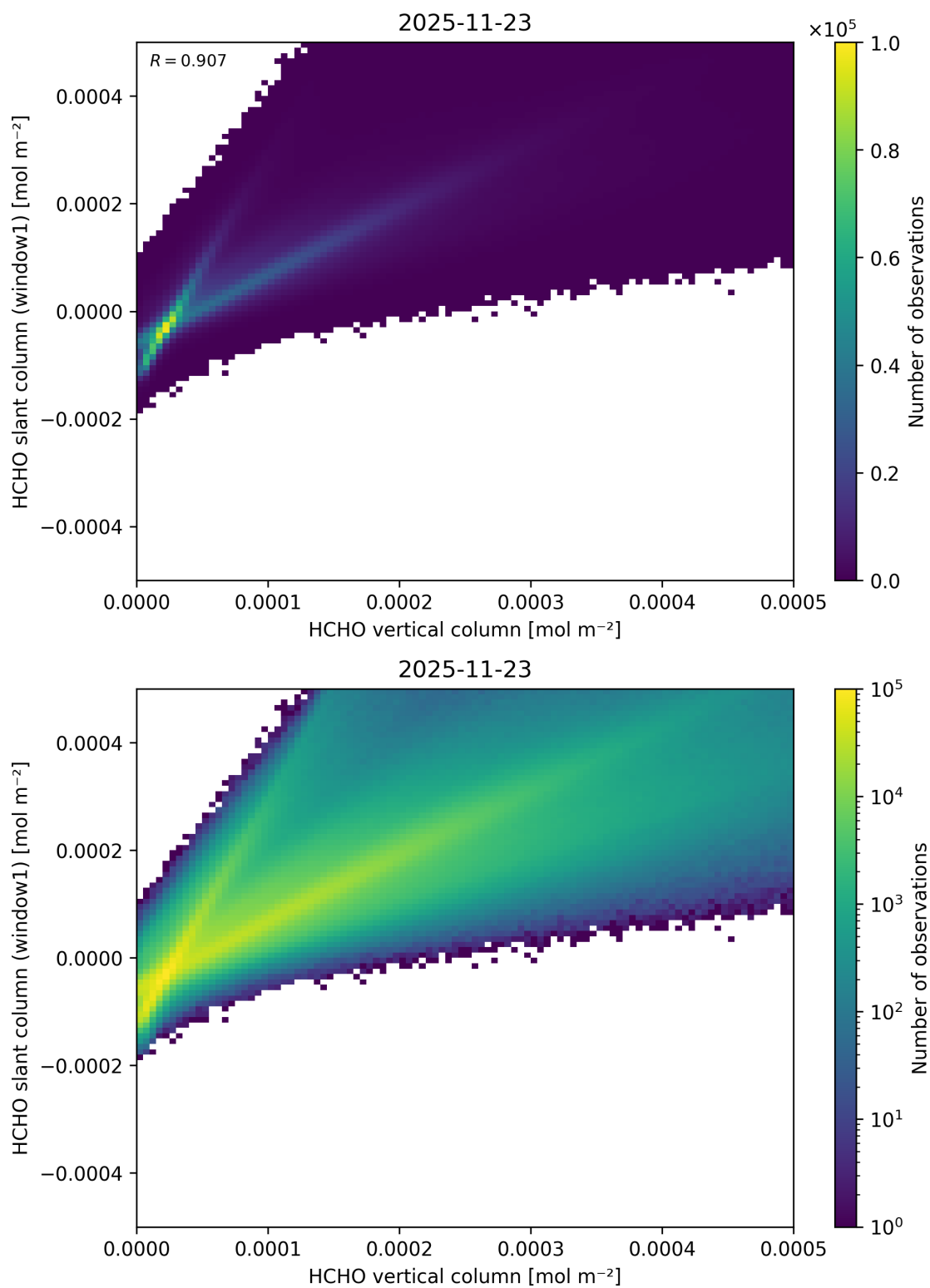
Figure 144: Scatter density plot of “HCHO vertical column” against “HCHO slant column (window1)” for 2025-11-23 to 2025-11-24.
