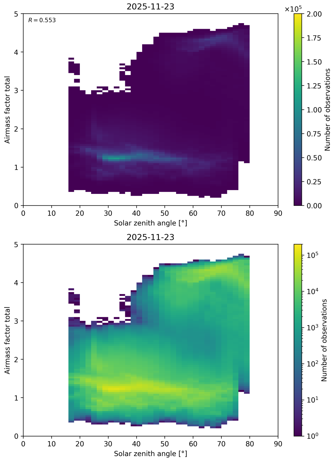
Figure 194: Scatter density plot of “Solar zenith angle” against “Airmass factor total” for 2025-11-23 to 2025-11-24.
