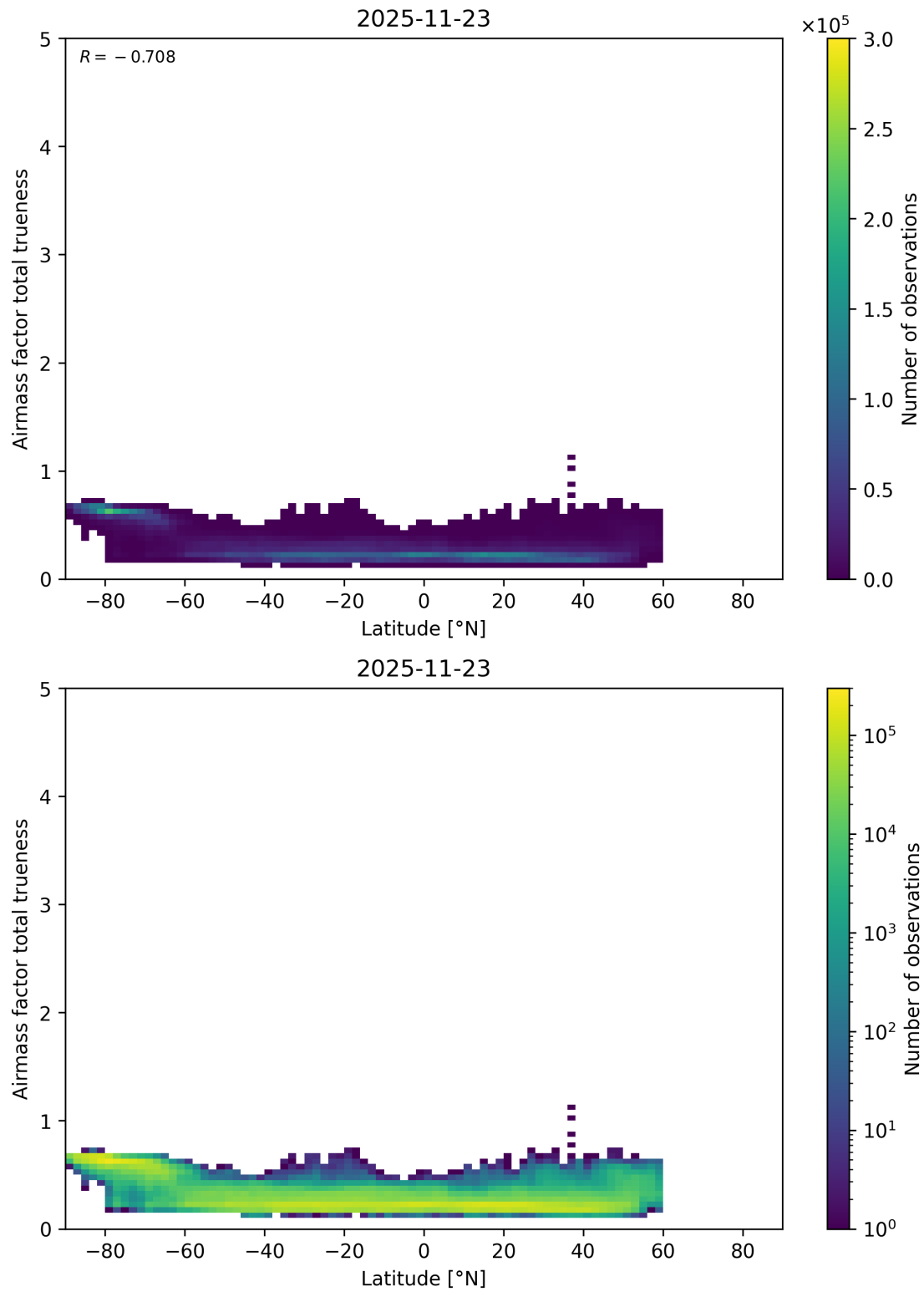
Figure 180: Scatter density plot of “Latitude” against “Airmass factor total trueness” for 2025-11-23 to 2025-11-24.
