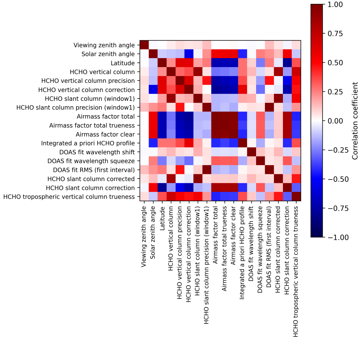
Figure 2: Map of correlation matrix for 2025-11-23 to 2025-11-24.
