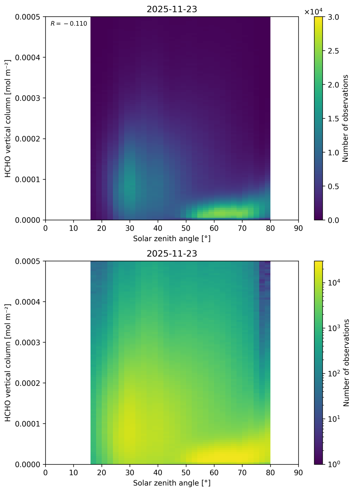
Figure 196: Scatter density plot of “Solar zenith angle” against “HCHO vertical column” for 2025-11-23 to 2025-11-24.
