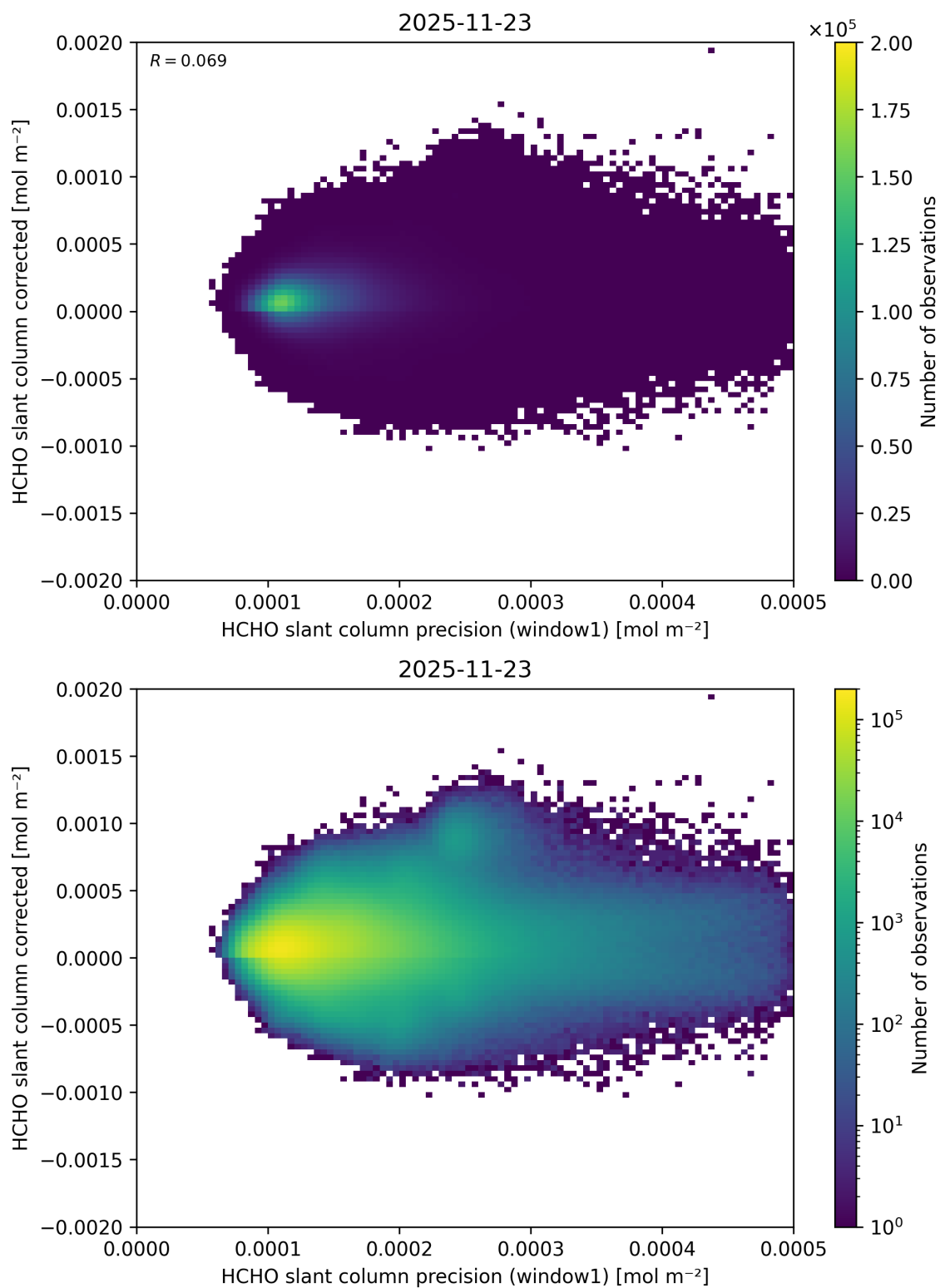
Figure 103: Scatter density plot of “HCHO slant column precision (window1)” against “HCHO slant column corrected” for 2025-11-23 to 2025-11-24.
