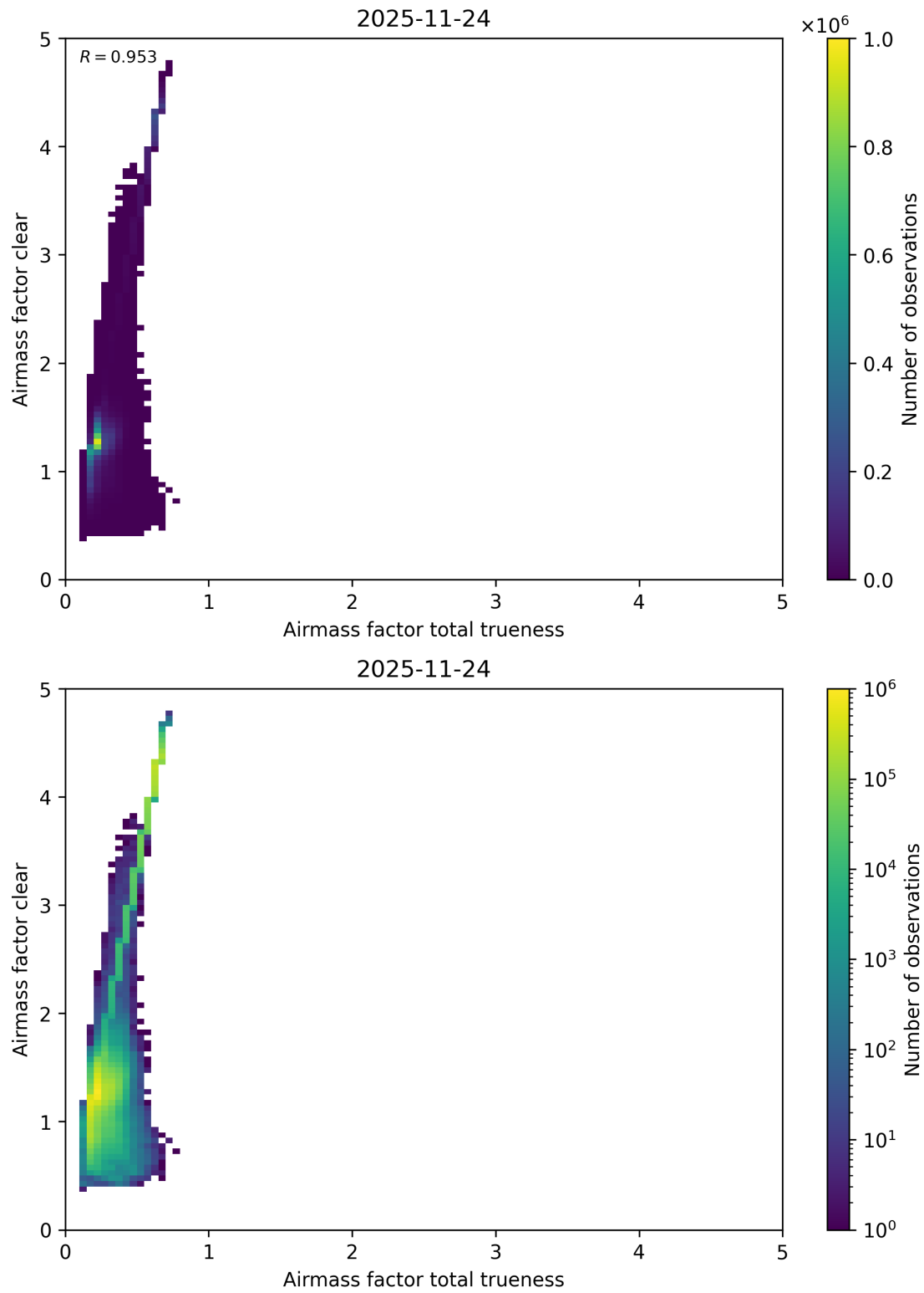
Figure 121: Scatter density plot of “Airmass factor total trueness” against “Airmass factor clear” for 2025-11-23 to 2025-11-25.
