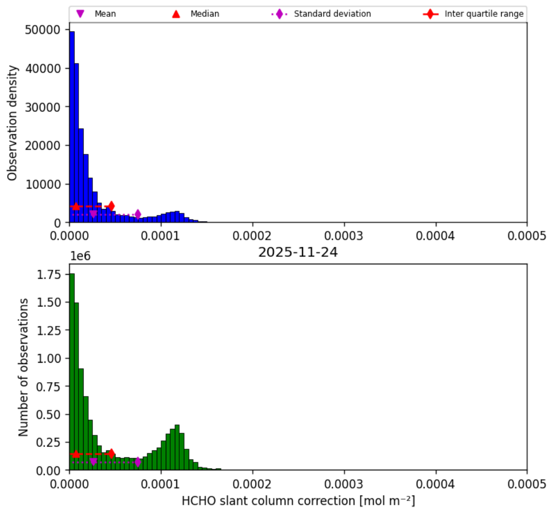
Figure 49: Histogram of “HCHO slant column correction” for 2025-11-23 to 2025-11-25
