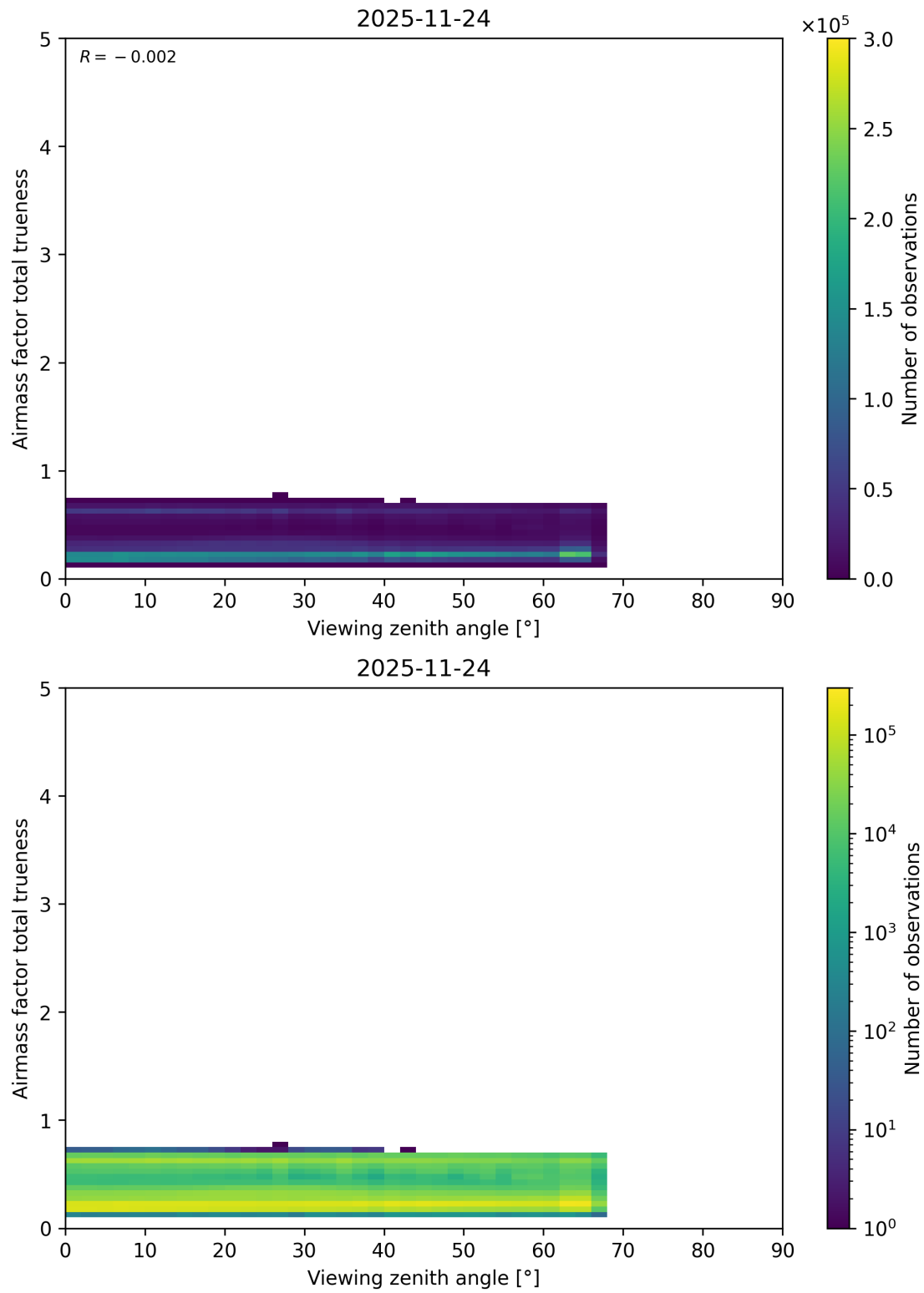
Figure 211: Scatter density plot of “Viewing zenith angle” against “Airmass factor total trueness” for 2025-11-23 to 2025-11-25.
