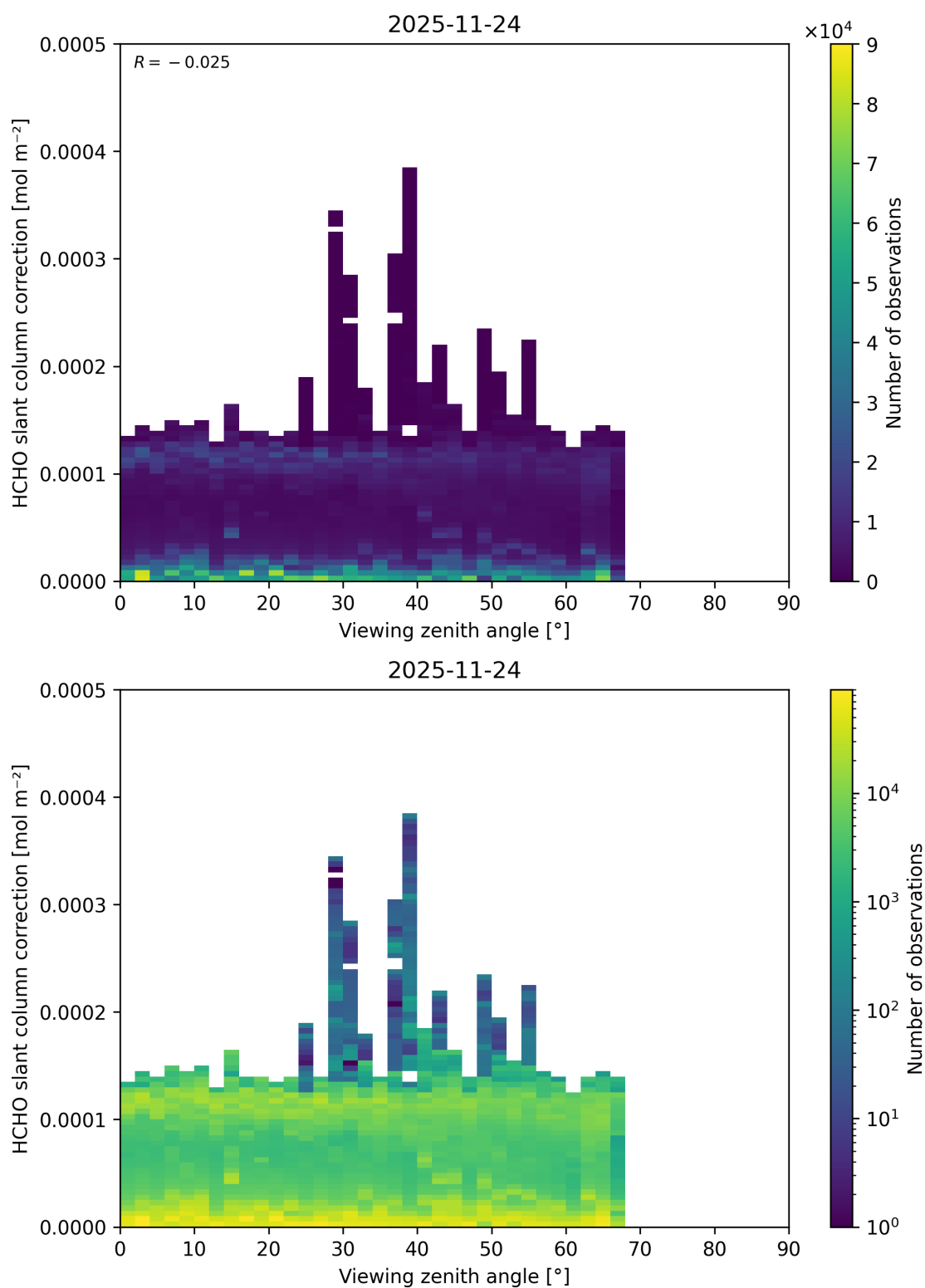
Figure 207: Scatter density plot of “Viewing zenith angle” against “HCHO slant column correction” for 2025-11-23 to 2025-11-25.
