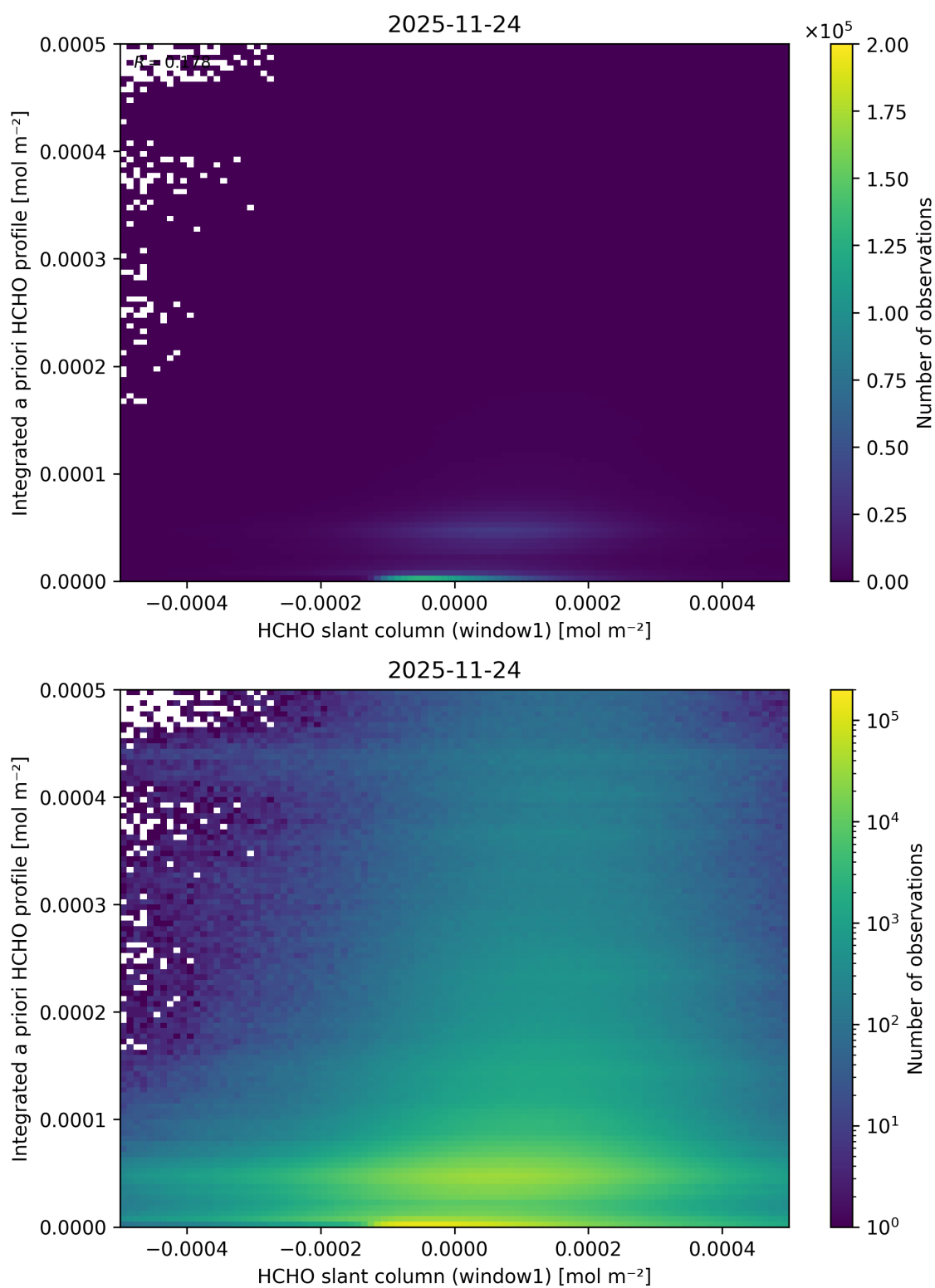
Figure 98: Scatter density plot of “HCHO slant column (window1)” against “Integrated a priori HCHO profile” for 2025-11-23 to 2025-11-25.
