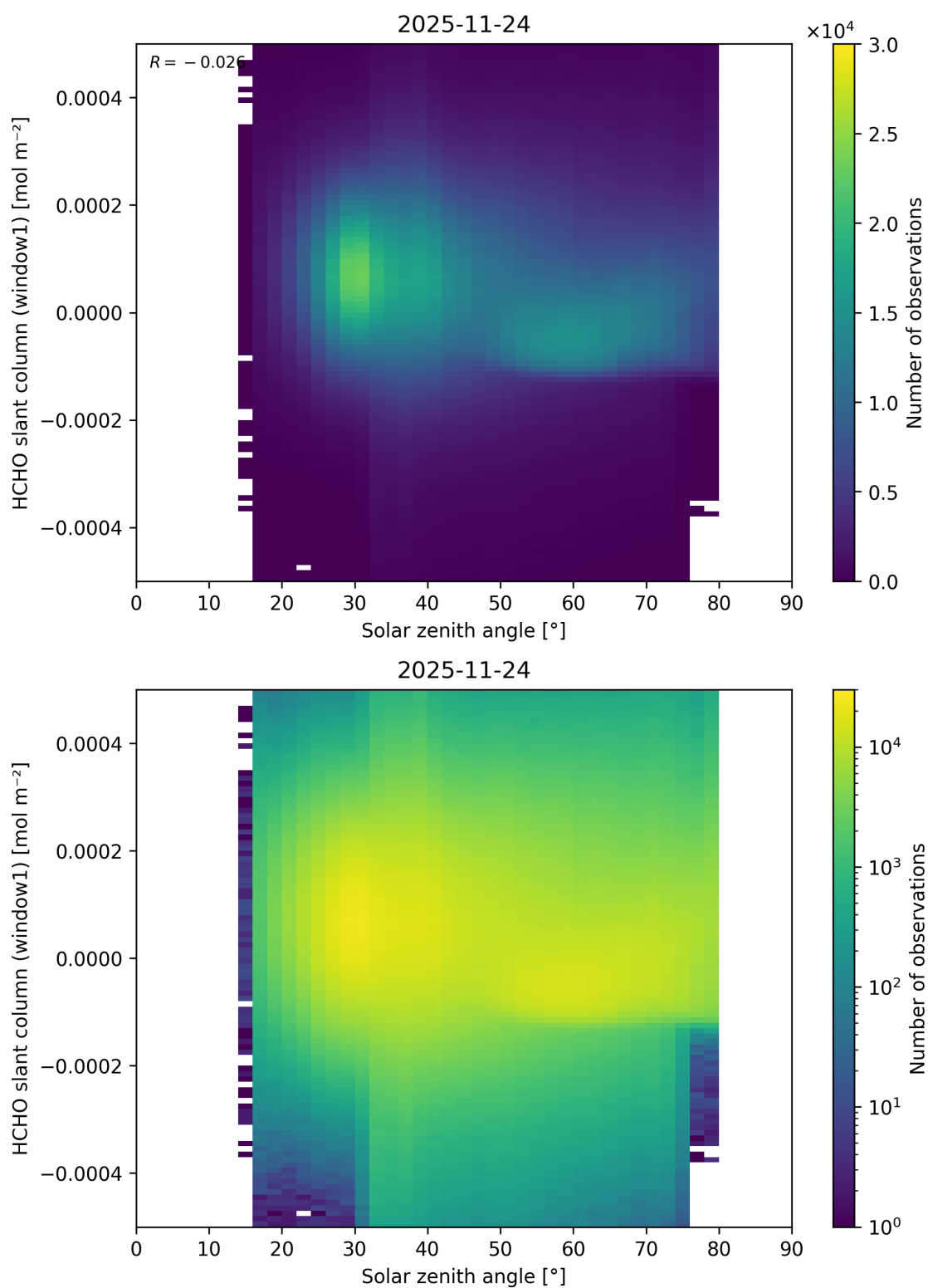
Figure 192: Scatter density plot of “Solar zenith angle” against “HCHO slant column (window1)” for 2025-11-23 to 2025-11-25.
