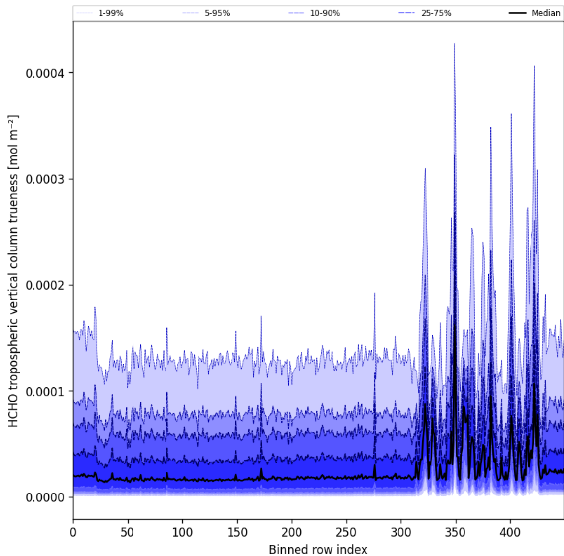
Figure 65: Along track statistics of "HCHO tropospheric vertical column trueness" for 2025-11-23 to 2025-11-25
