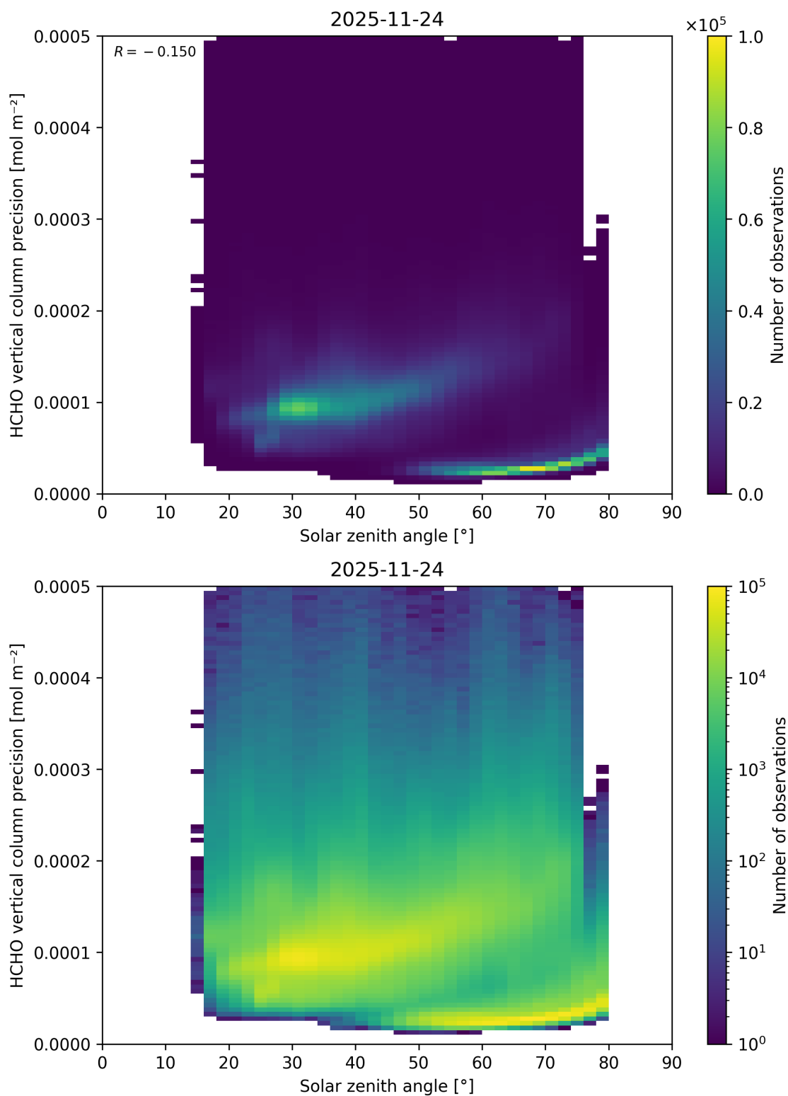
Figure 198: Scatter density plot of “Solar zenith angle” against “HCHO vertical column precision” for 2025-11-23 to 2025-11-25.
