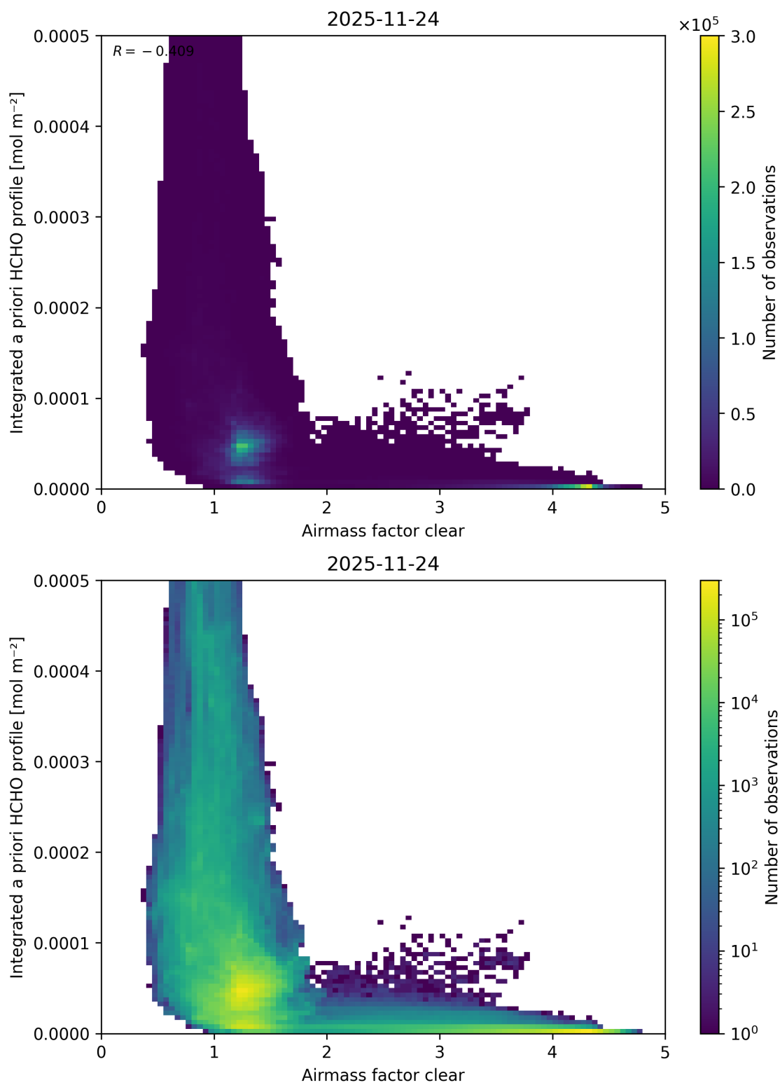
Figure 84: Scatter density plot of “Airmass factor clear” against “Integrated a priori HCHO profile” for 2025-11-23 to 2025-11-25.
