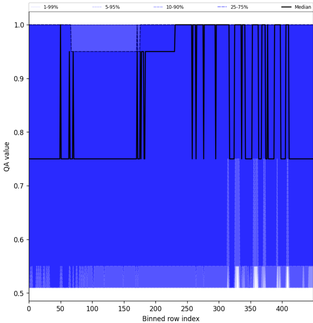
Figure 51: Along track statistics of “QA value” for 2025-11-23 to 2025-11-25
