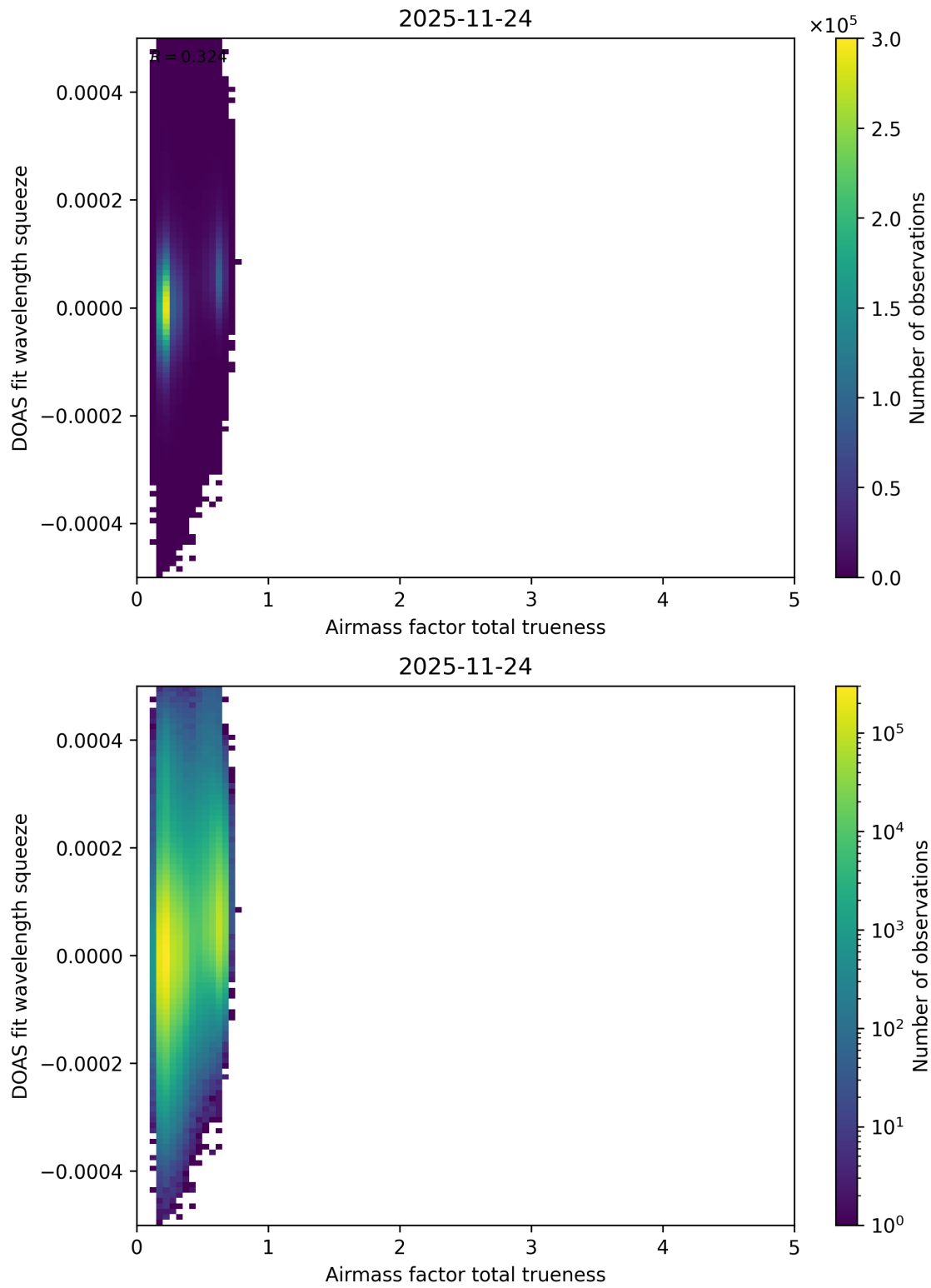
Figure 120: Scatter density plot of “Airmass factor total trueness” against “DOAS fit wavelength squeeze” for 2025-11-23 to 2025-11-25.
