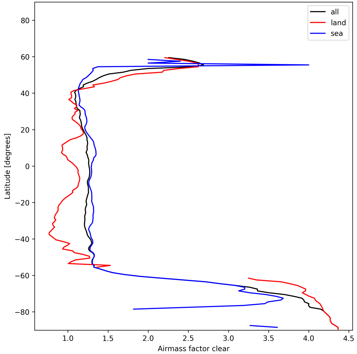
Figure 29: Zonal average of “Airmass factor clear” for 2025-11-23 to 2025-11-25.
