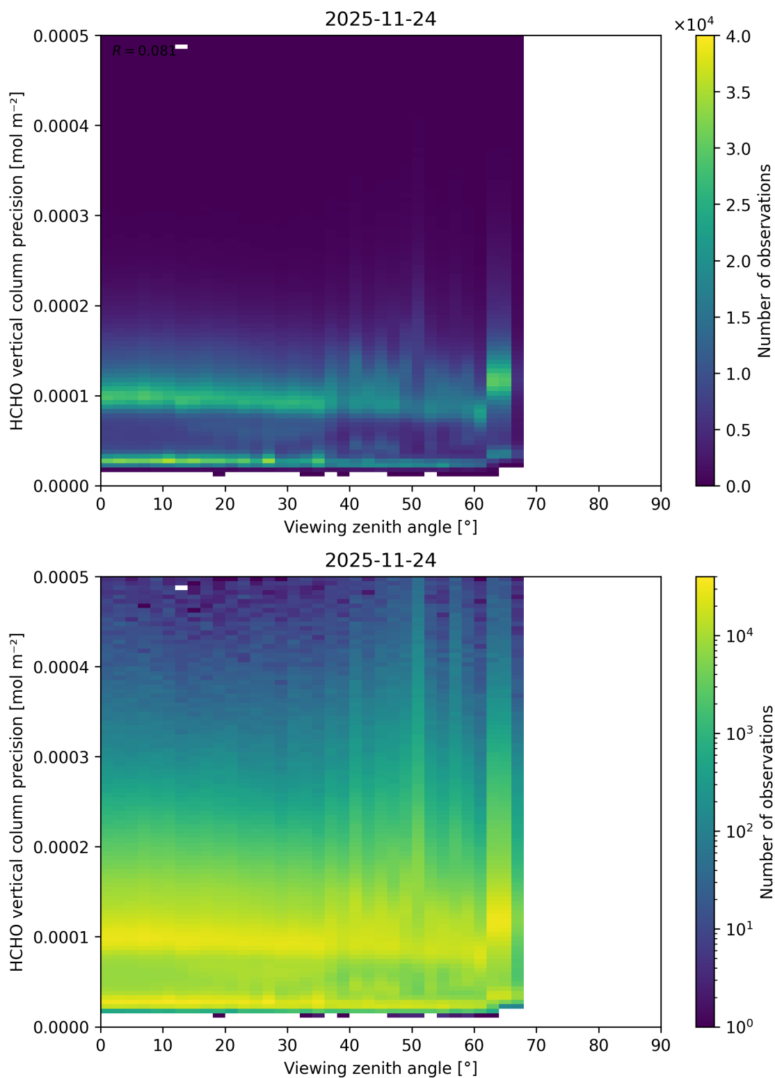
Figure 214: Scatter density plot of “Viewing zenith angle” against “HCHO vertical column precision” for 2025-11-23 to 2025-11-25.
