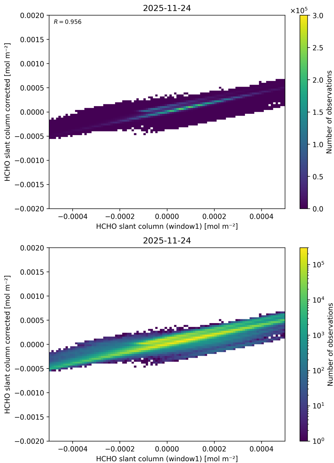
Figure 92: Scatter density plot of “HCHO slant column (window1)” against “HCHO slant column corrected” for 2025-11-23 to 2025-11-25.
