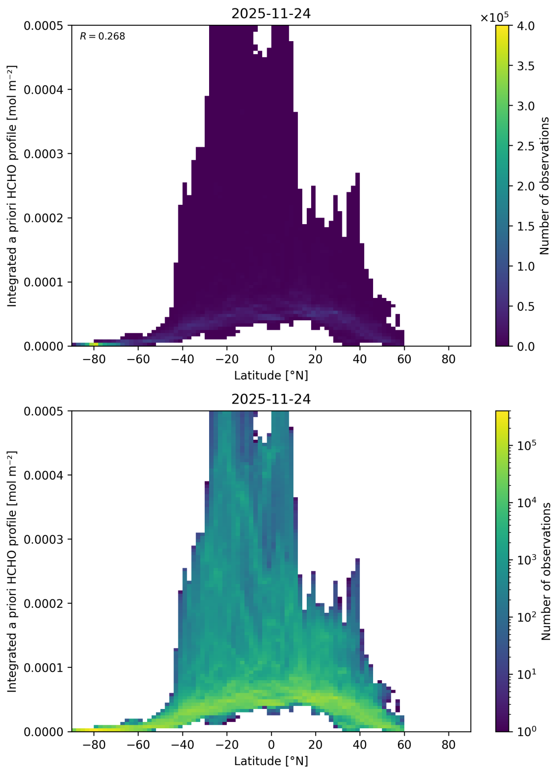
Figure 185: Scatter density plot of “Latitude” against “Integrated a priori HCHO profile” for 2025-11-23 to 2025-11-25.
