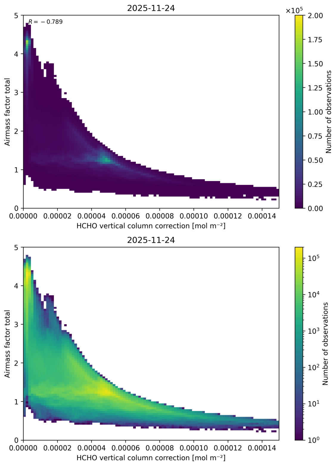
Figure 134: Scatter density plot of “HCHO vertical column correction” against “Airmass factor total” for 2025-11-23 to 2025-11-25.
