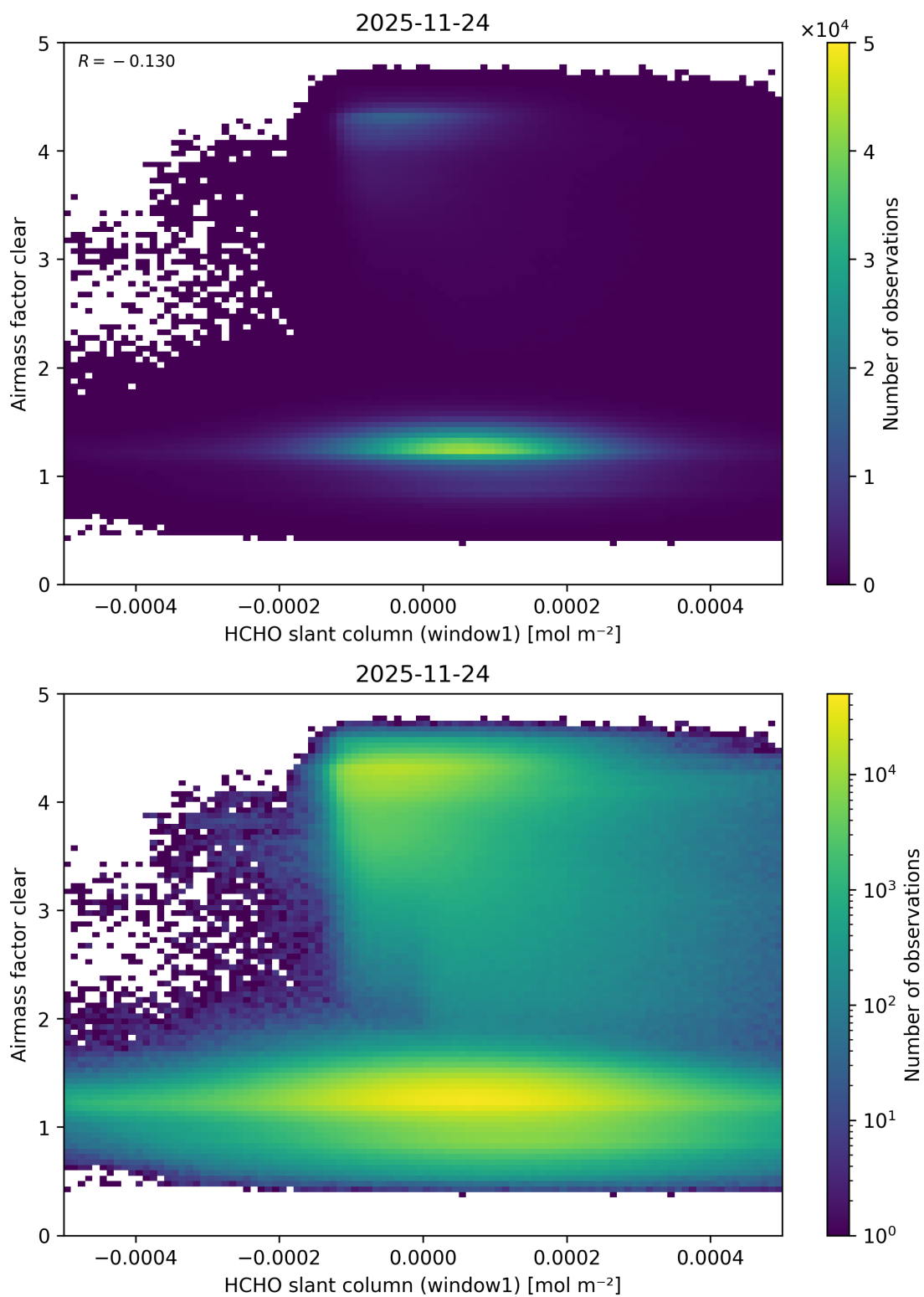
Figure 91: Scatter density plot of “HCHO slant column (window1)” against “Airmass factor clear” for 2025-11-23 to 2025-11-25.
