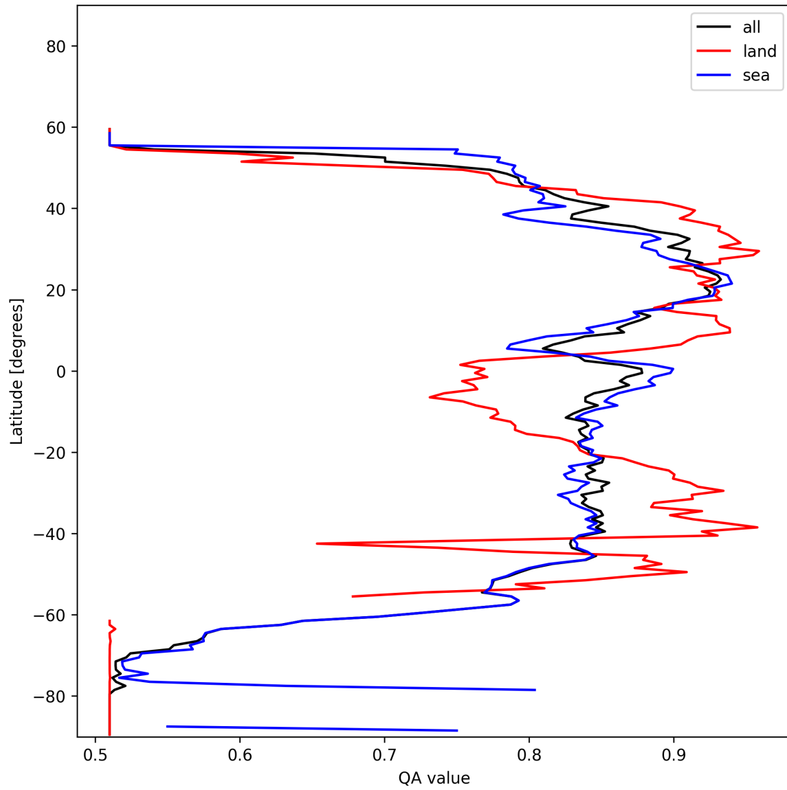
Figure 21: Zonal average of "QA value" for 2025-11-23 to 2025-11-25.
