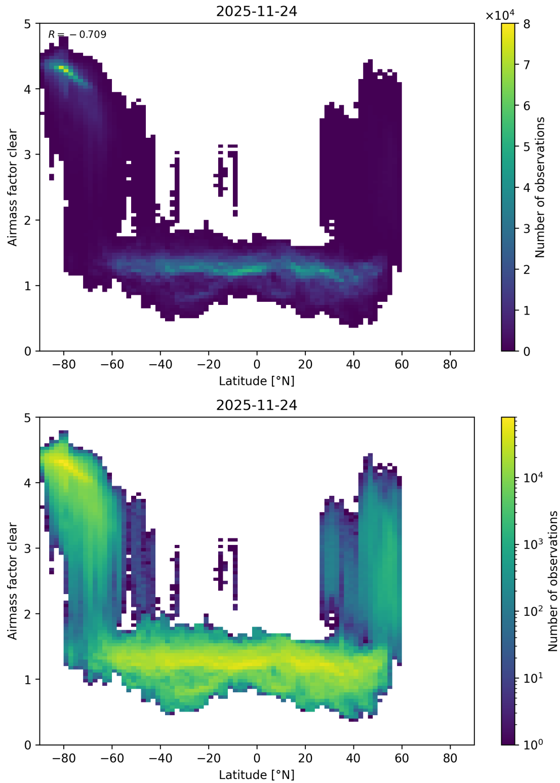
Figure 174: Scatter density plot of “Latitude” against “Airmass factor clear” for 2025-11-23 to 2025-11-25.
