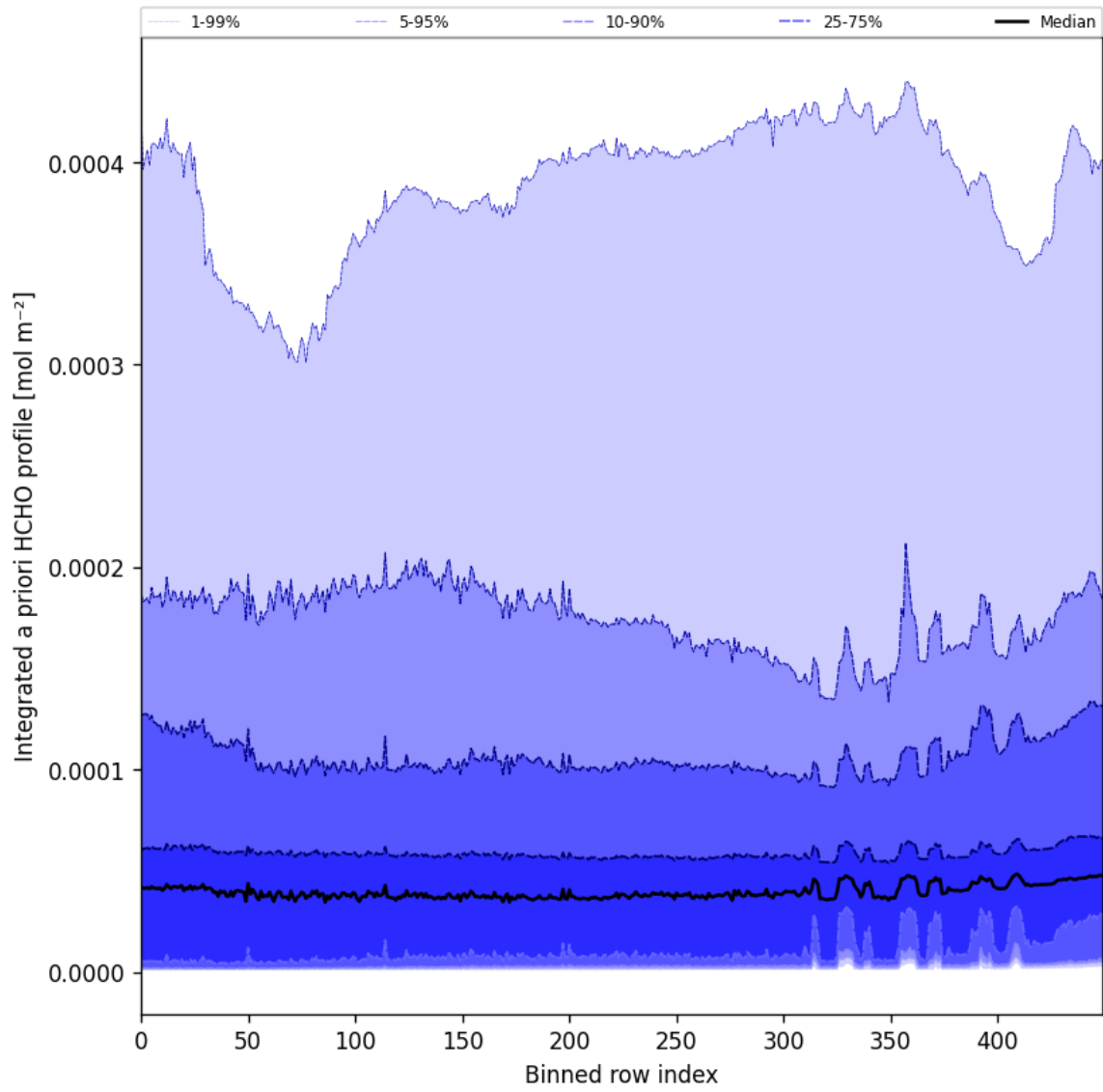
Figure 60: Along track statistics of "Integrated a priori HCHO profile" for 2025-11-23 to 2025-11-25
