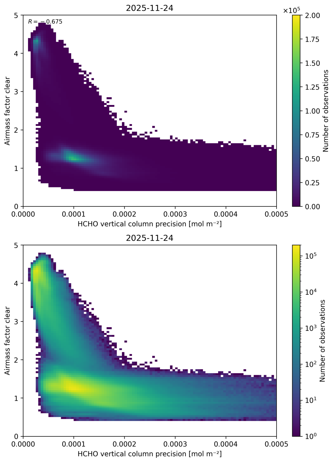
Figure 155: Scatter density plot of “HCHO vertical column precision” against “Airmass factor clear” for 2025-11-23 to 2025-11-25.
