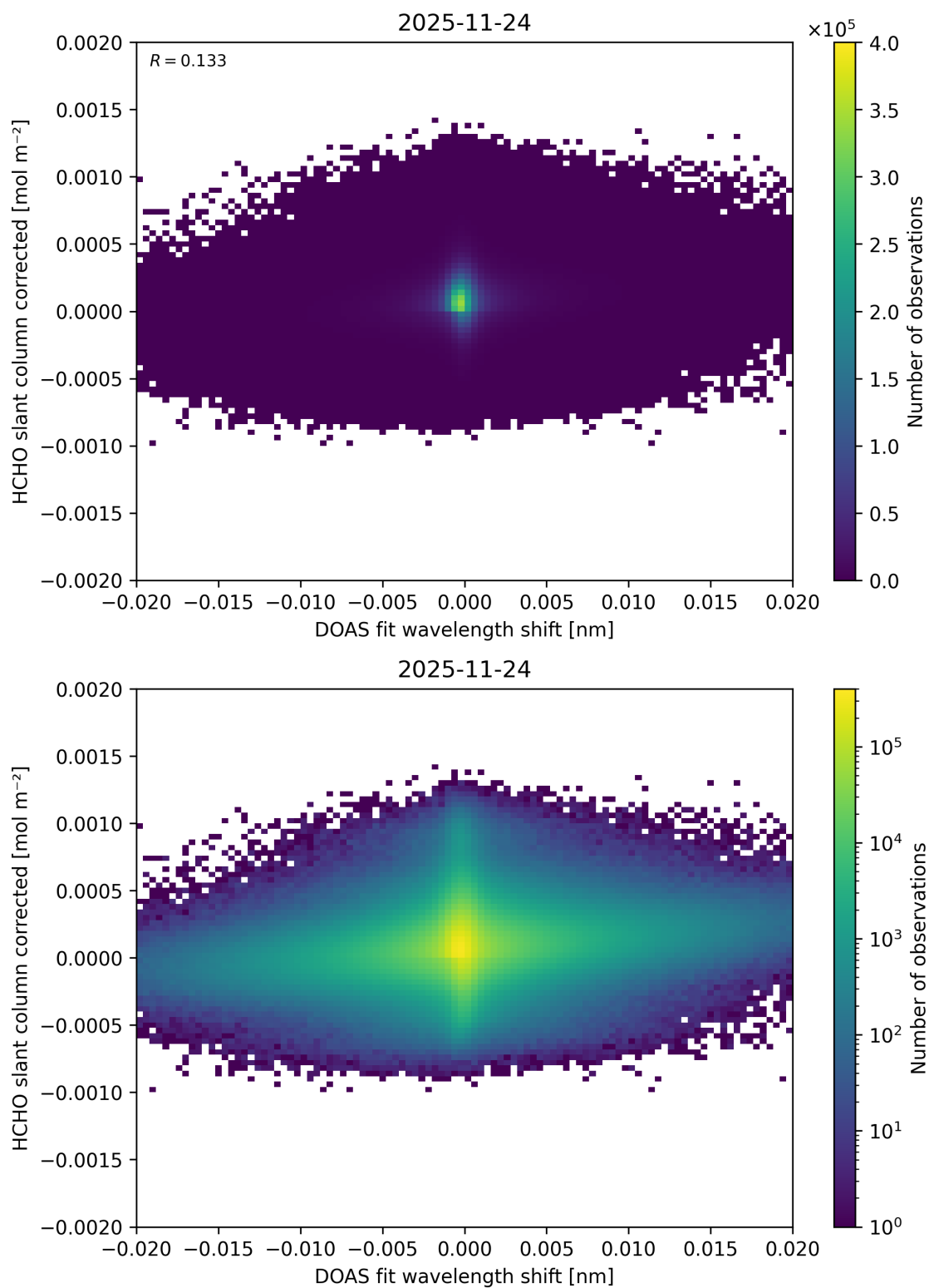
Figure 71: Scatter density plot of “DOAS fit wavelength shift” against “HCHO slant column corrected” for 2025-11-23 to 2025-11-25.
