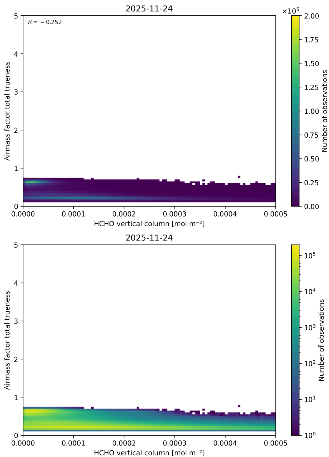
Figure 147: Scatter density plot of “HCHO vertical column” against “Airmass factor total trueneess” for 2025-11-23 to 2025-11-25.
