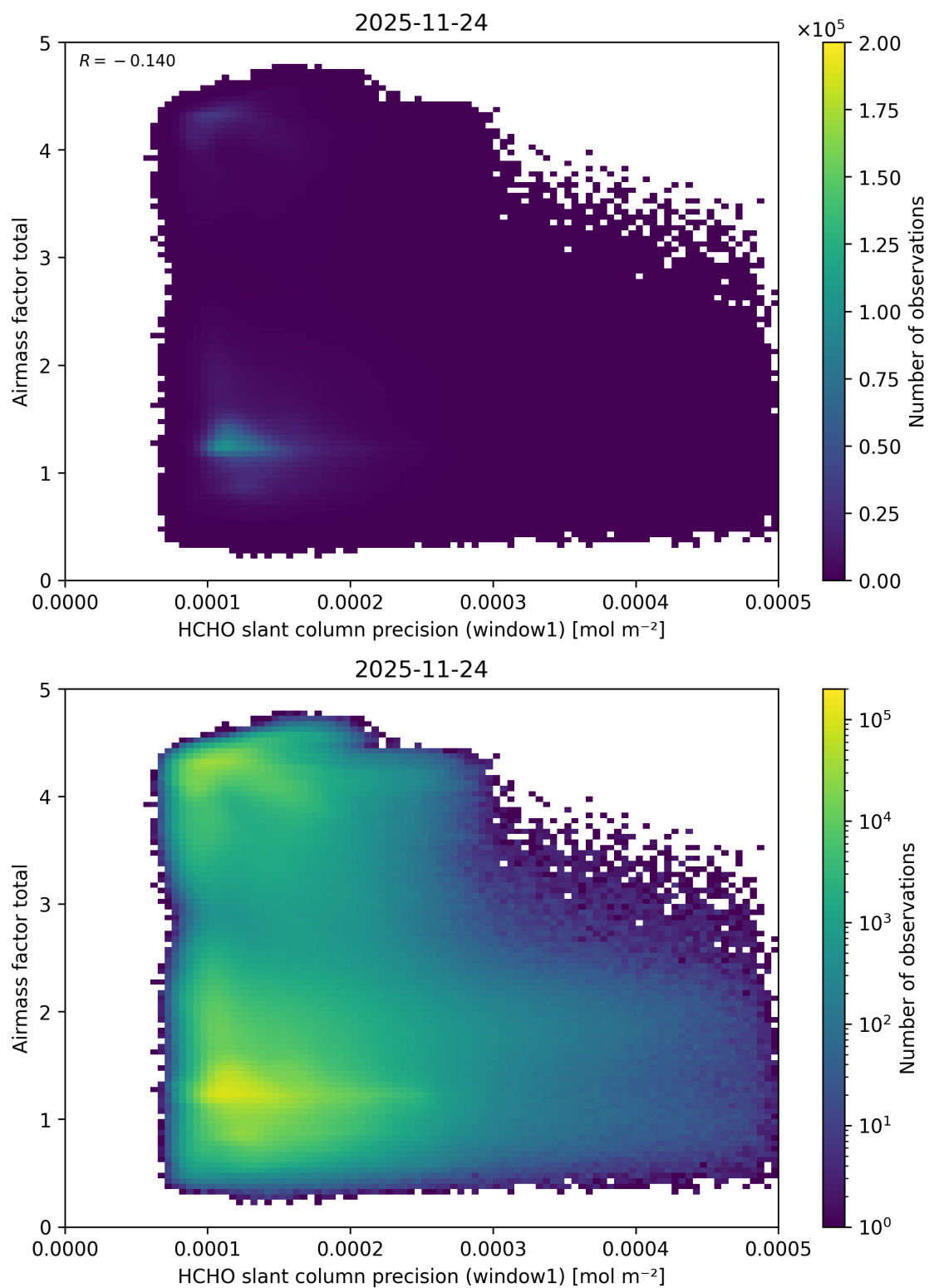
Figure 105: Scatter density plot of “HCHO slant column precision (window1)” against “Airmass factor total” for 2025-11-23 to 2025-11-25.
