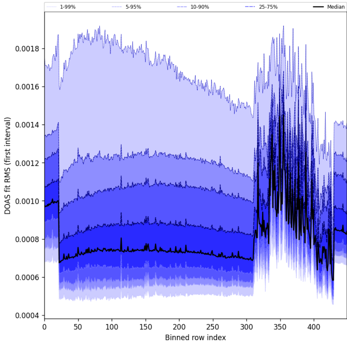
Figure 63: Along track statistics of “DOAS fit RMS (first interval)” for 2025-11-23 to 2025-11-25
