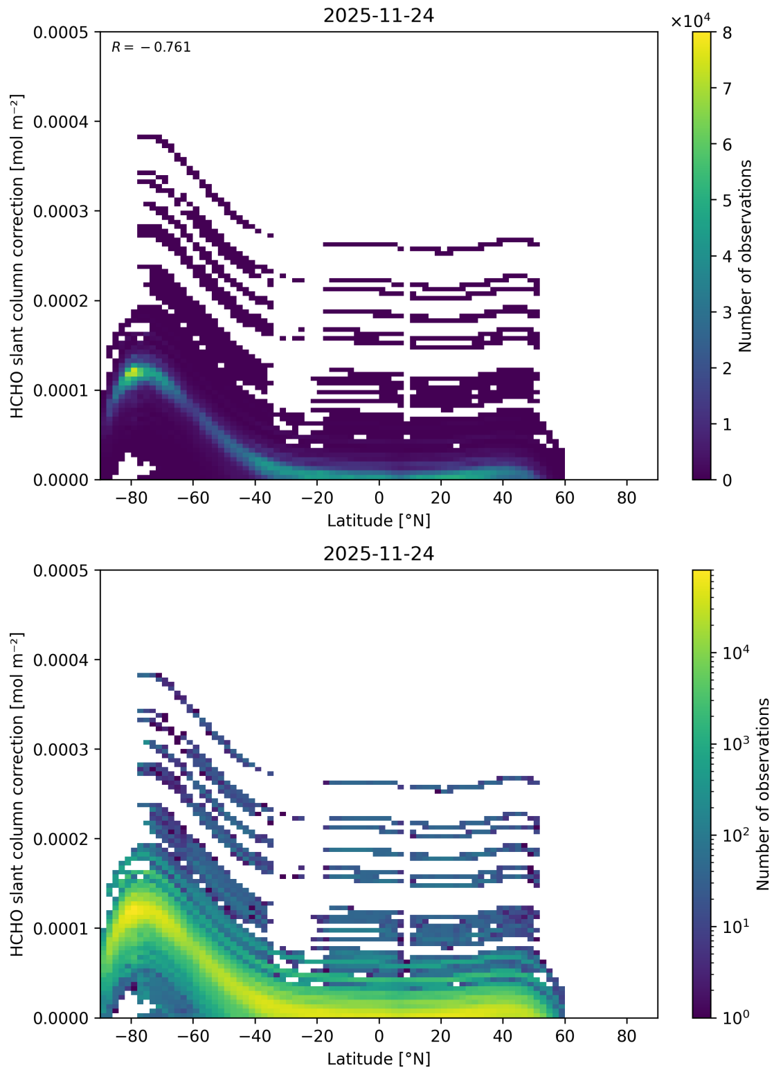
Figure 176: Scatter density plot of “Latitude” against “HCHO slant column correction” for 2025-11-23 to 2025-11-25.
