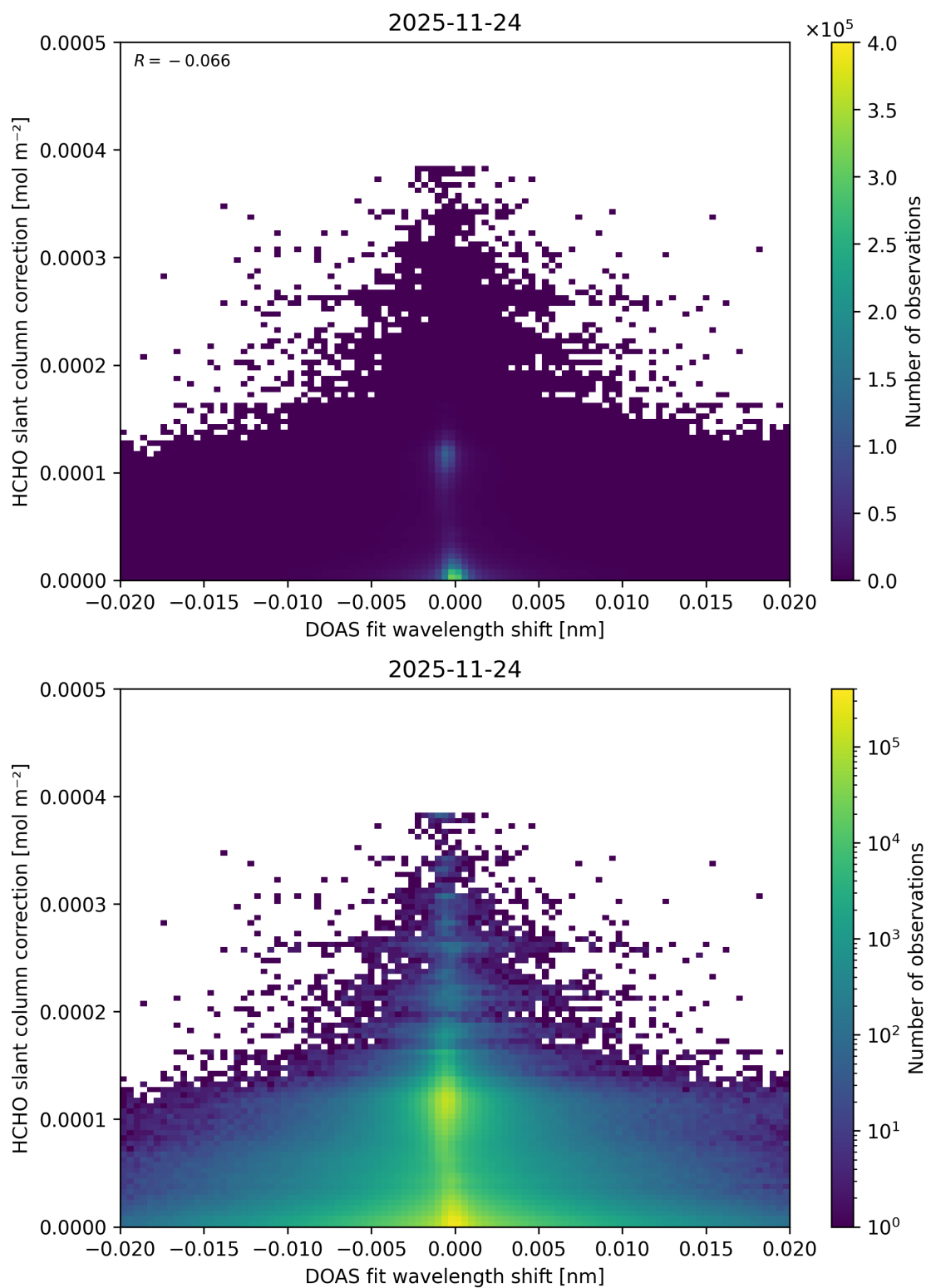
Figure 72: Scatter density plot of “DOAS fit wavelength shift” against “HCHO slant column correction” for 2025-11-23 to 2025-11-25.
