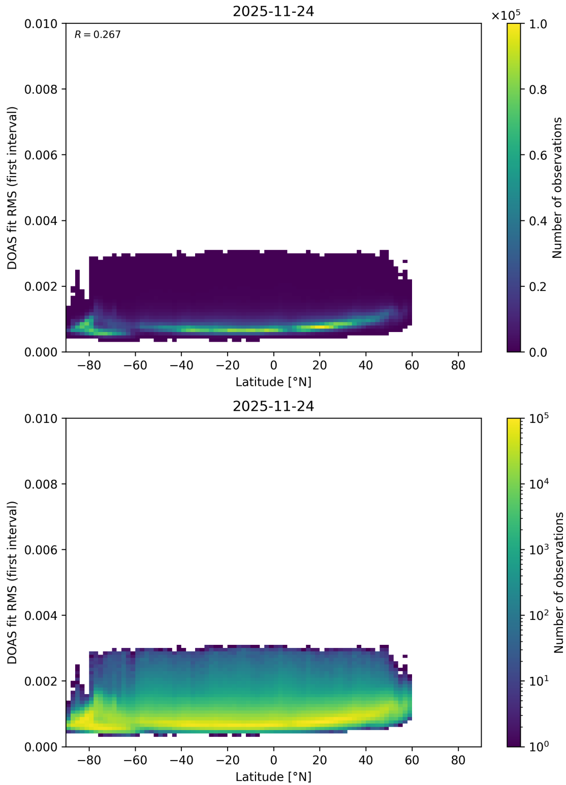
Figure 171: Scatter density plot of “Latitude” against “DOAS fit RMS (first interval)” for 2025-11-23 to 2025-11-25.
