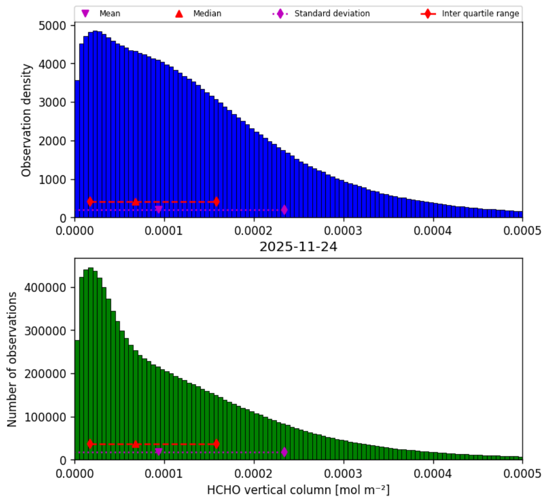
Figure 37: Histogram of “HCHO vertical column” for 2025-11-23 to 2025-11-25
