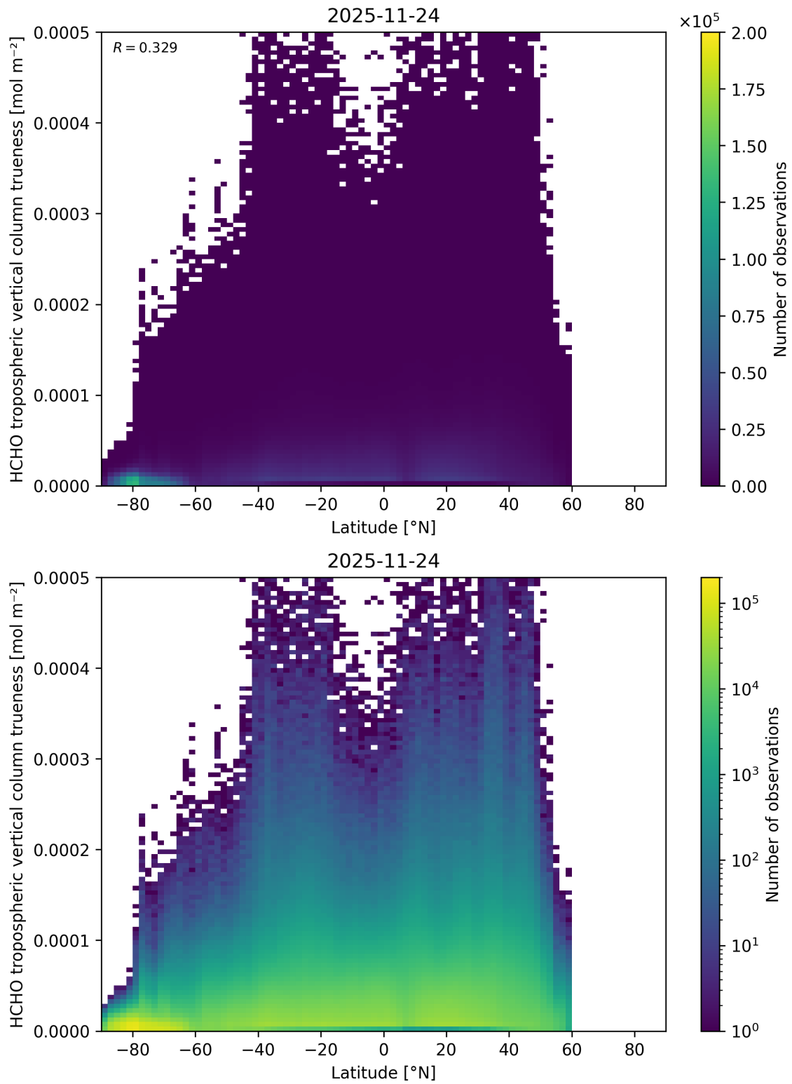
Figure 184: Scatter density plot of “Latitude” against “HCHO tropospheric vertical column trueeness” for 2025-11-23 to 2025-11-25.
