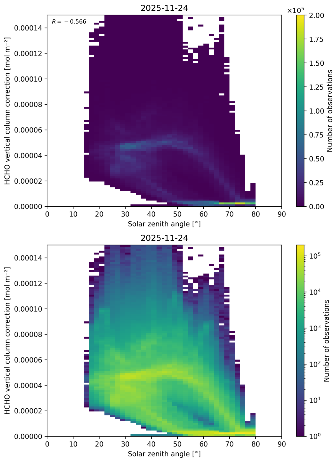
Figure 197: Scatter density plot of “Solar zenith angle” against “HCHO vertical column correction” for 2025-11-23 to 2025-11-25.
