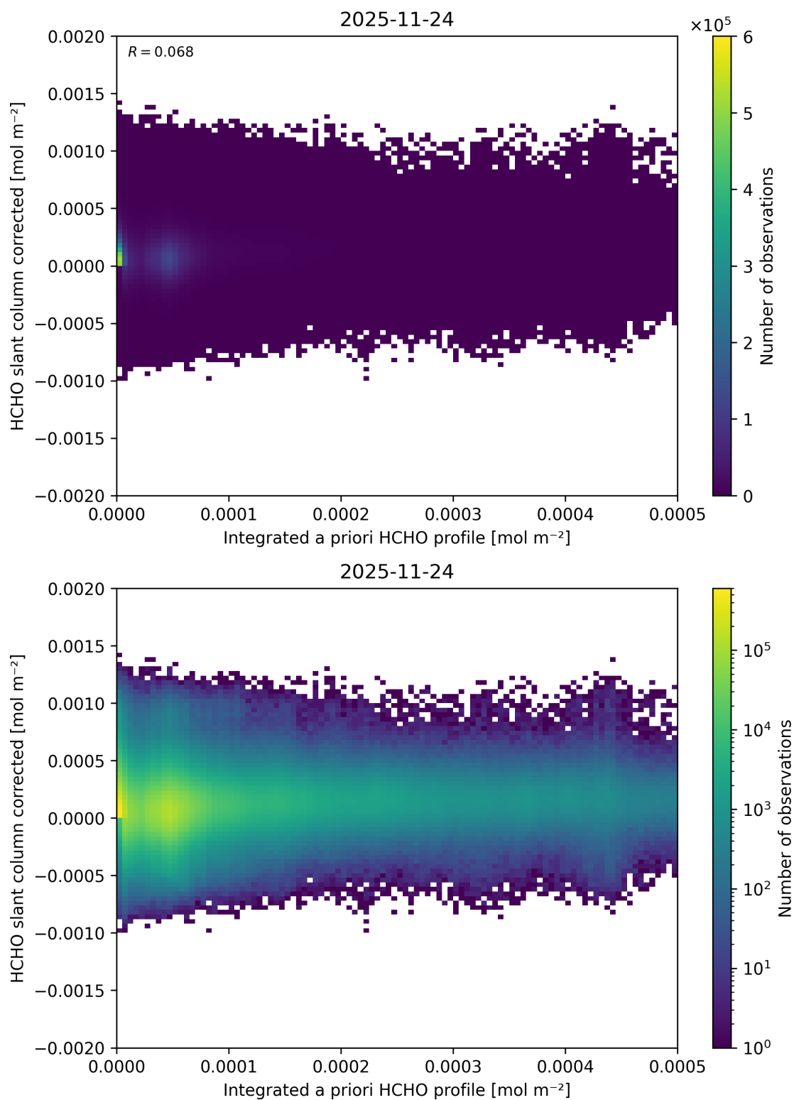
Figure 168: Scatter density plot of “Integrated a priori HCHO profile” against “HCHO slant column corrected” for 2025-11-23 to 2025-11-25.
