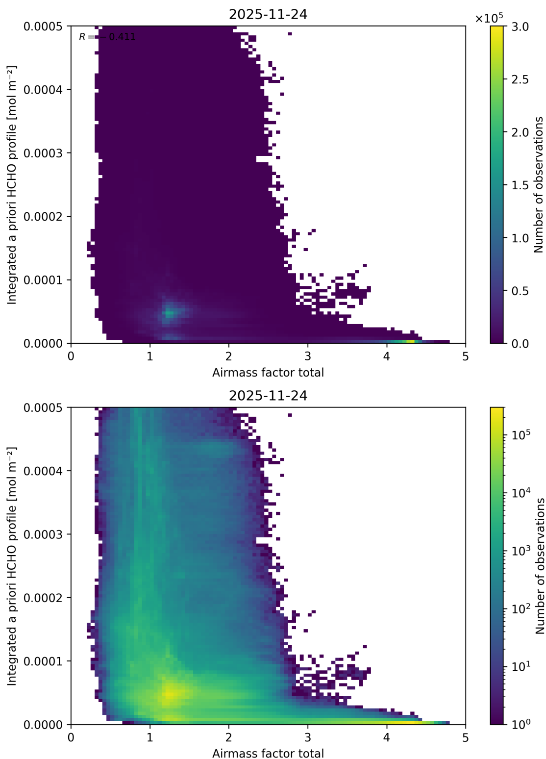
Figure 117: Scatter density plot of “Airmass factor total” against “Integrated a priori HCHO profile” for 2025-11-23 to 2025-11-25.
