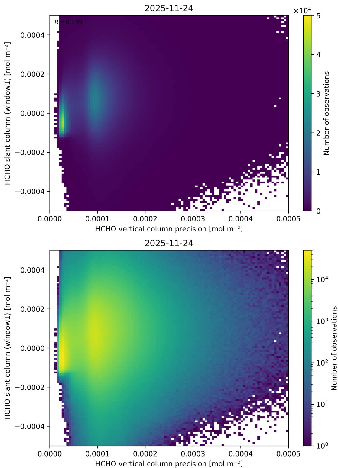
Figure 158: Scatter density plot of “HCHO vertical column precision” against “HCHO slant column (window1)” for 2025-11-23 to 2025-11-25.
