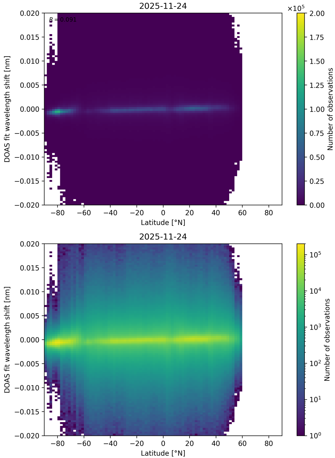
Figure 172: Scatter density plot of “Latitude” against “DOAS fit wavelength shift” for 2025-11-23 to 2025-11-25.
