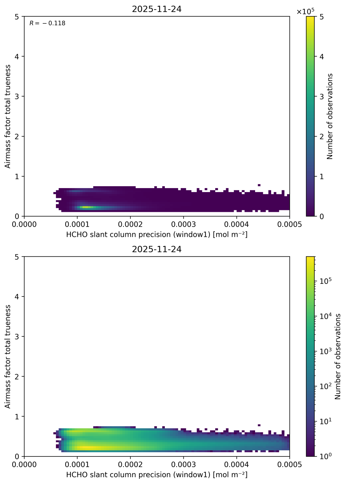
Figure 106: Scatter density plot of “HCHO slant column precision (window1)” against “Airmass factor total trueness” for 2025-11-23 to 2025-11-25.
