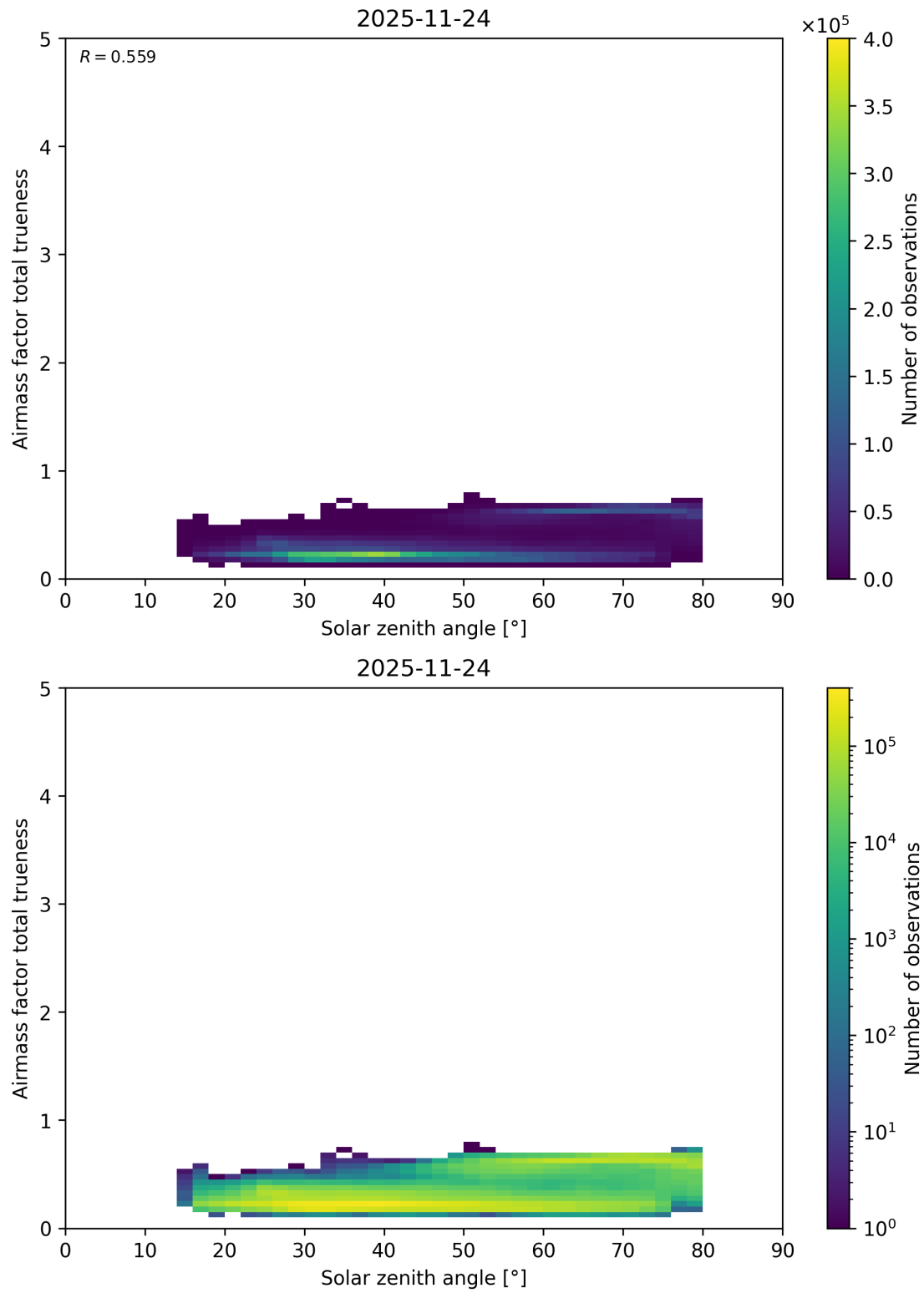
Figure 195: Scatter density plot of “Solar zenith angle” against “Airmass factor total trueness” for 2025-11-23 to 2025-11-25.
