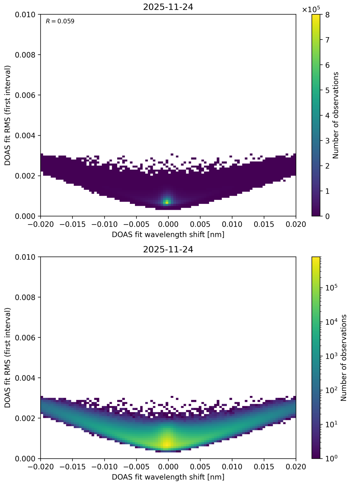
Figure 69: Scatter density plot of “DOAS fit wavelength shift” against “DOAS fit RMS (first interval)” for 2025-11-23 to 2025-11-25.
