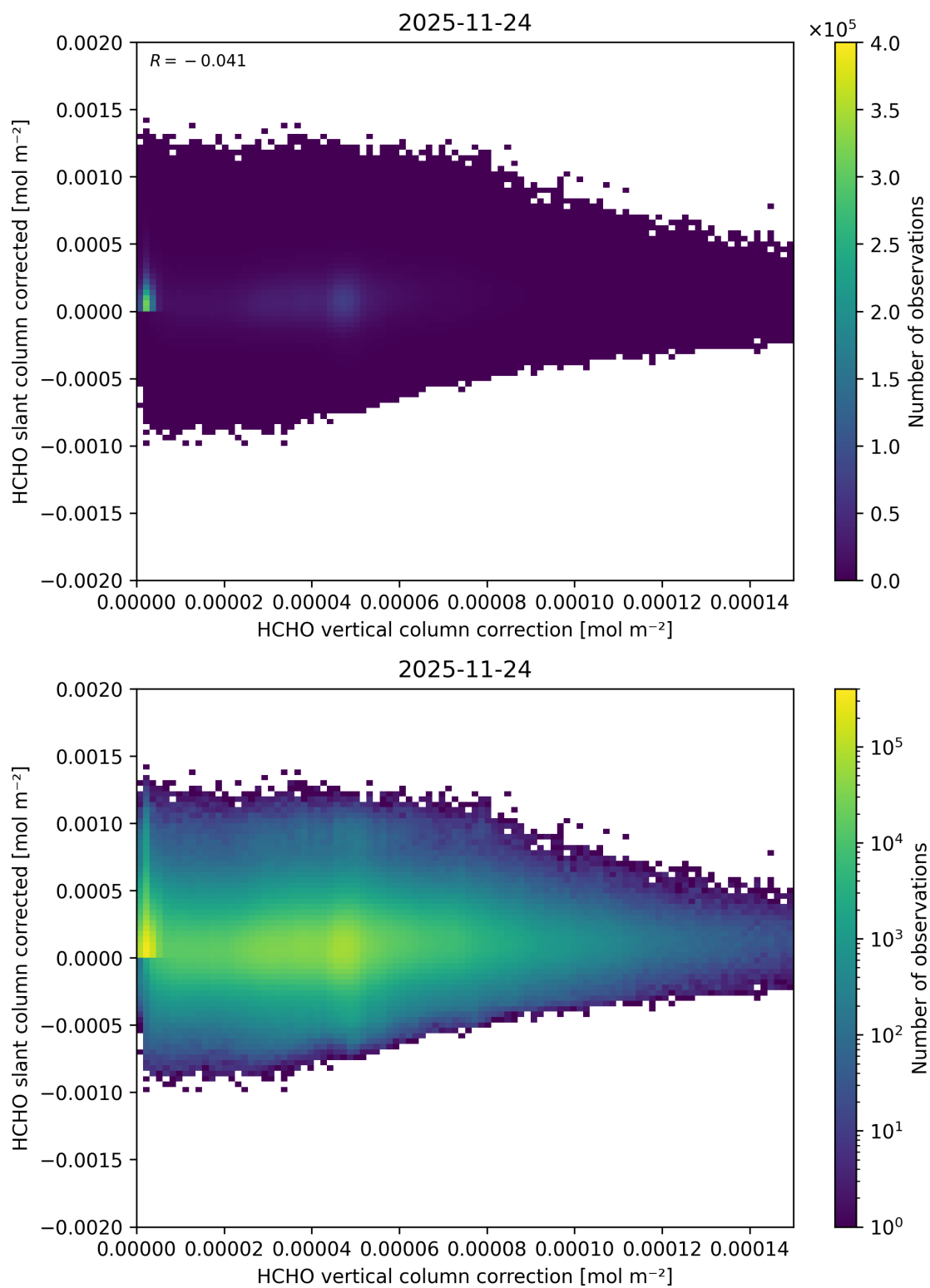
Figure 130: Scatter density plot of “HCHO vertical column correction” against “HCHO slant column corrected” for 2025-11-23 to 2025-11-25.
