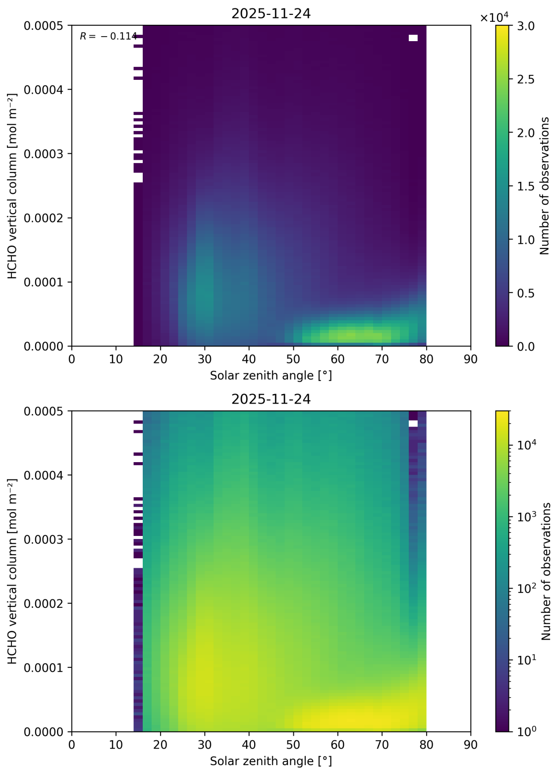
Figure 196: Scatter density plot of “Solar zenith angle” against “HCHO vertical column” for 2025-11-23 to 2025-11-25.
