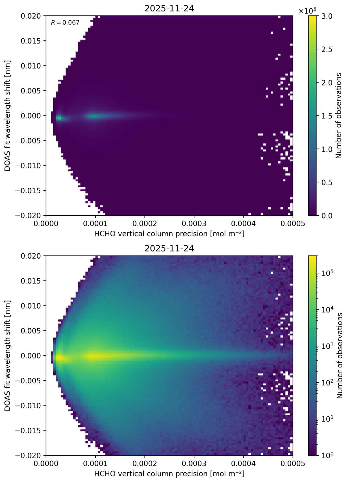
Figure 153: Scatter density plot of “HCHO vertical column precision” against “DOAS fit wavelength shift” for 2025-11-23 to 2025-11-25.
