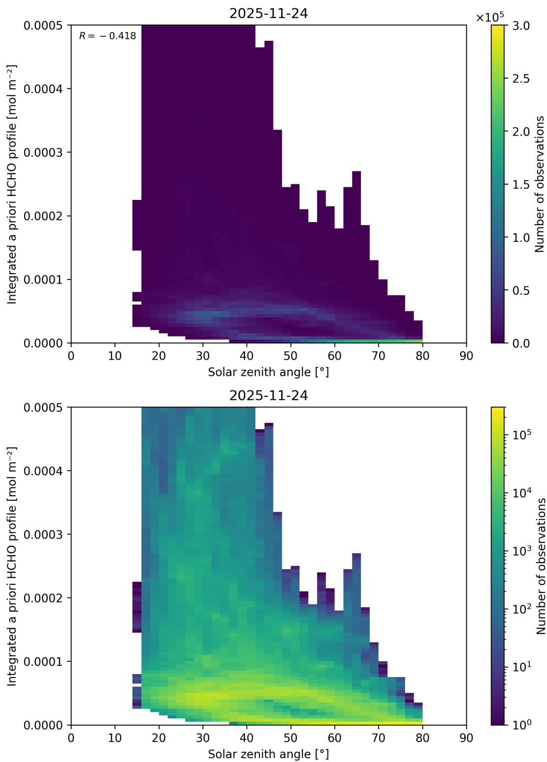
Figure 200: Scatter density plot of “Solar zenith angle” against “Integrated a priori HCHO profile” for 2025-11-23 to 2025-11-25.
