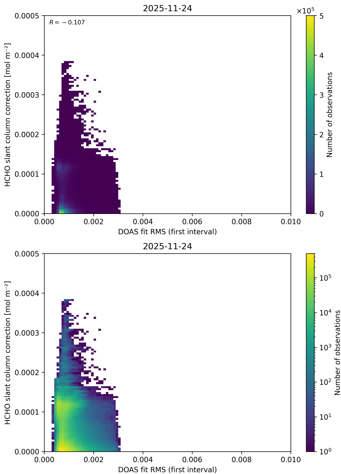
Figure 67: Scatter density plot of “DOAS fit RMS (first interval)” against “HCHO slant column correction” for 2025-11-23 to 2025-11-25.
