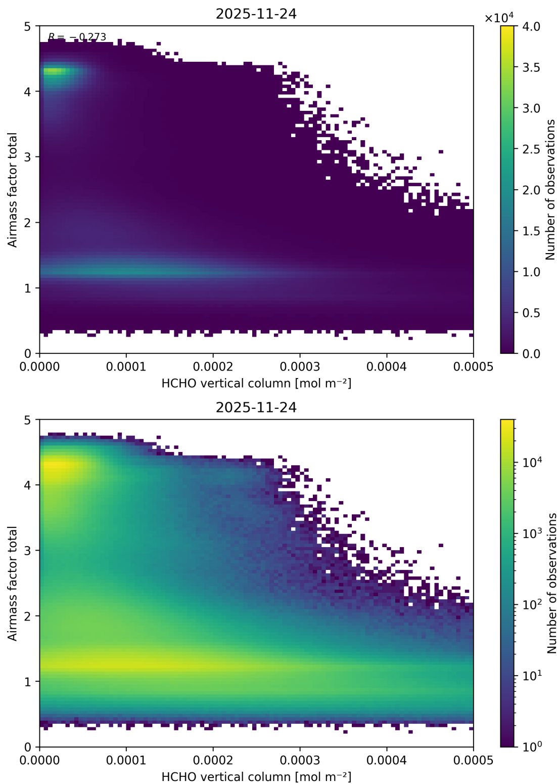
Figure 146: Scatter density plot of “HCHO vertical column” against “Airmass factor total” for 2025-11-23 to 2025-11-25.
