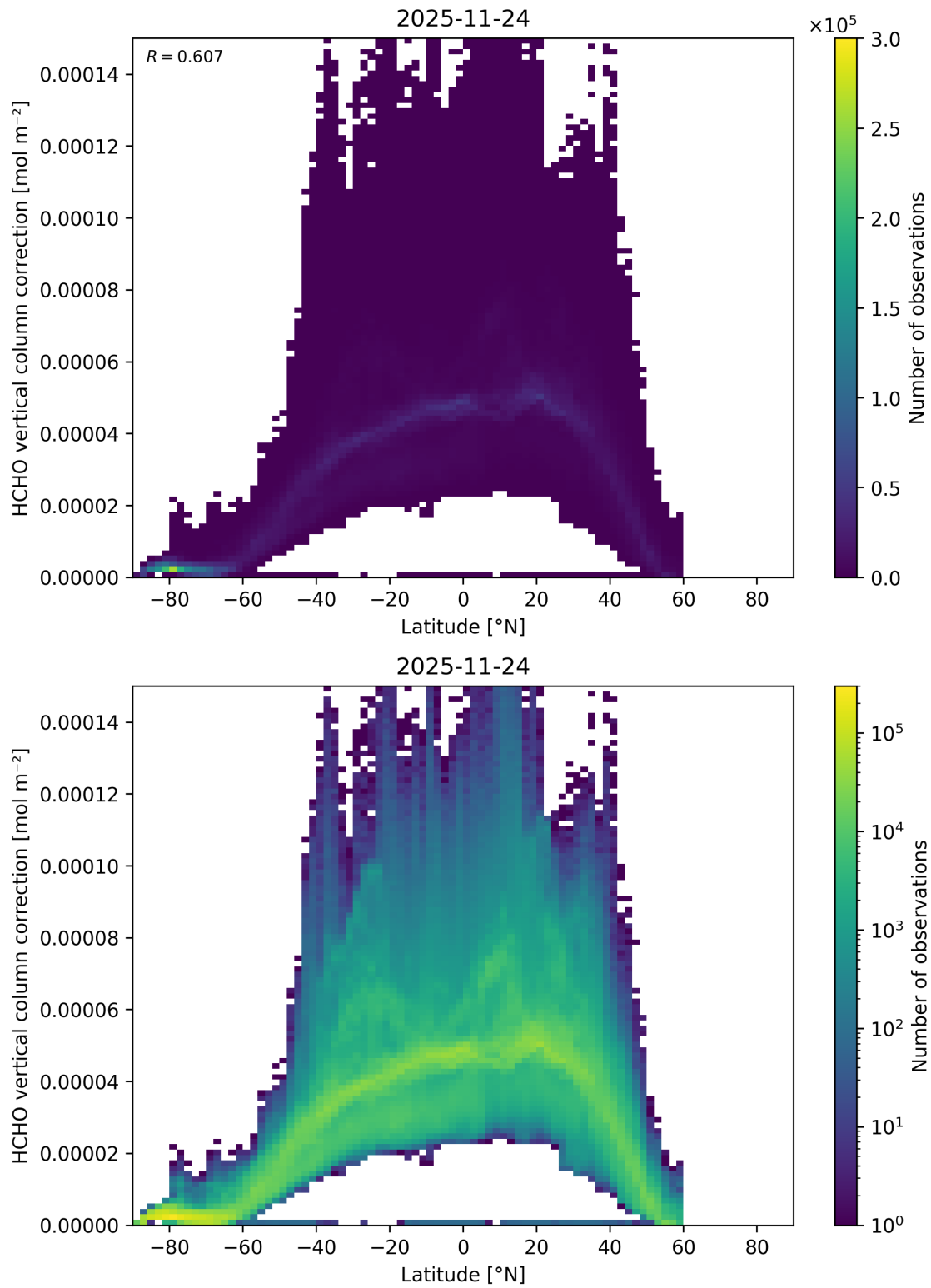
Figure 182: Scatter density plot of “Latitude” against “HCHO vertical column correction” for 2025-11-23 to 2025-11-25.
