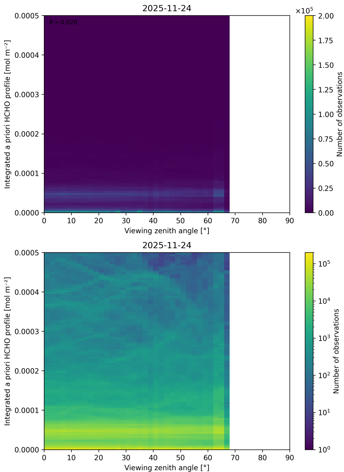
Figure 216: Scatter density plot of “Viewing zenith angle” against “Integrated a priori HCHO profile” for 2025-11-23 to 2025-11-25.
