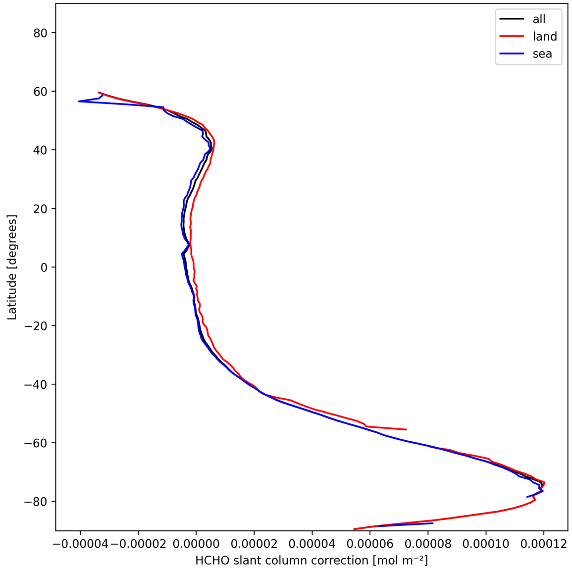
Figure 34: Zonal average of “HCHO slant column correction” for 2025-11-23 to 2025-11-25.
