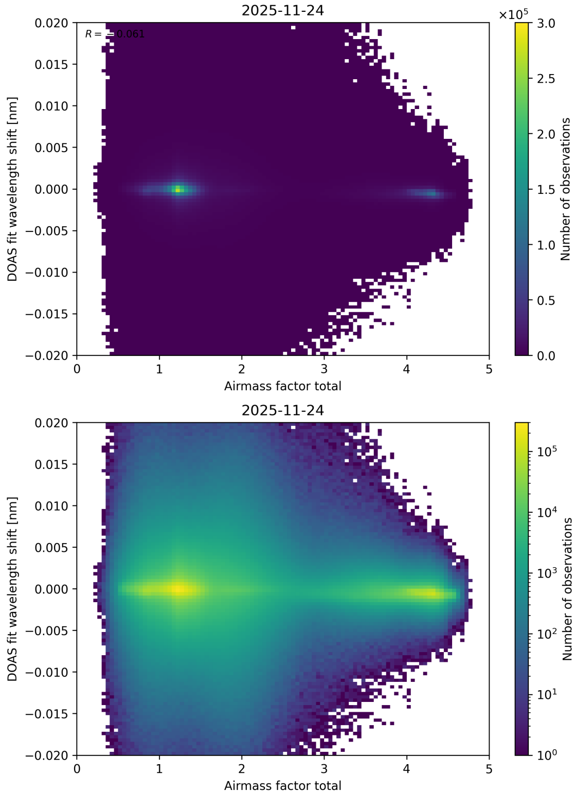
Figure 110: Scatter density plot of “Airmass factor total” against “DOAS fit wavelength shift” for 2025-11-23 to 2025-11-25.
