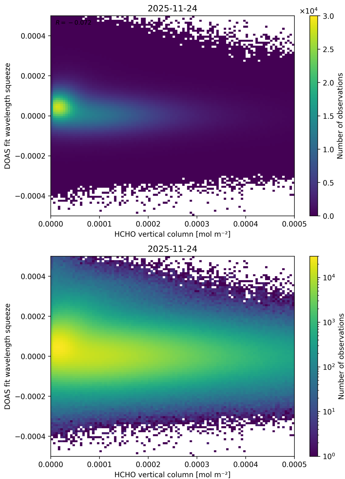
Figure 140: Scatter density plot of “HCHO vertical column” against “DOAS fit wavelength squeeze” for 2025-11-23 to 2025-11-25.
