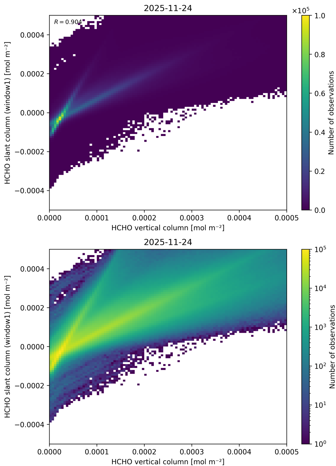
Figure 144: Scatter density plot of “HCHO vertical column” against “HCHO slant column (window1)” for 2025-11-23 to 2025-11-25.
