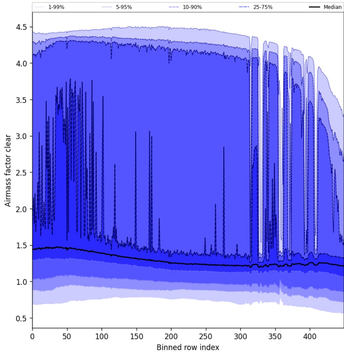
Figure 59: Along track statistics of “Airmass factor clear” for 2025-11-23 to 2025-11-25
