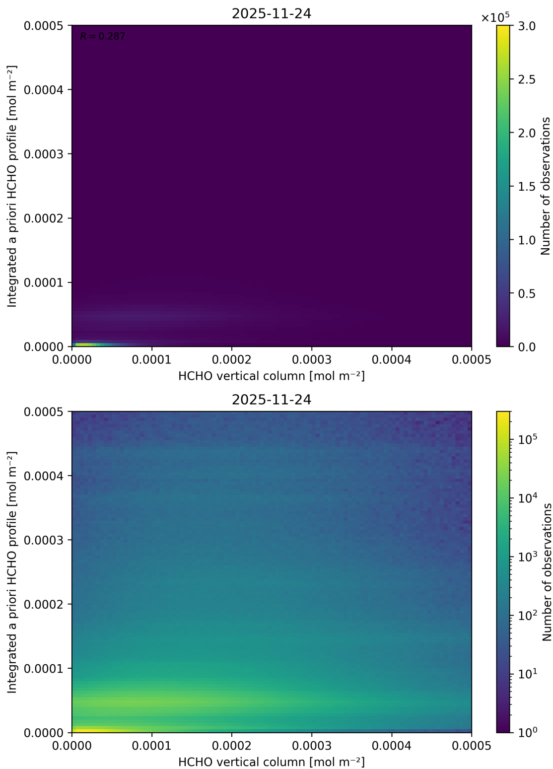
Figure 151: Scatter density plot of “HCHO vertical column” against “Integrated a priori HCHO profile” for 2025-11-23 to 2025-11-25.
