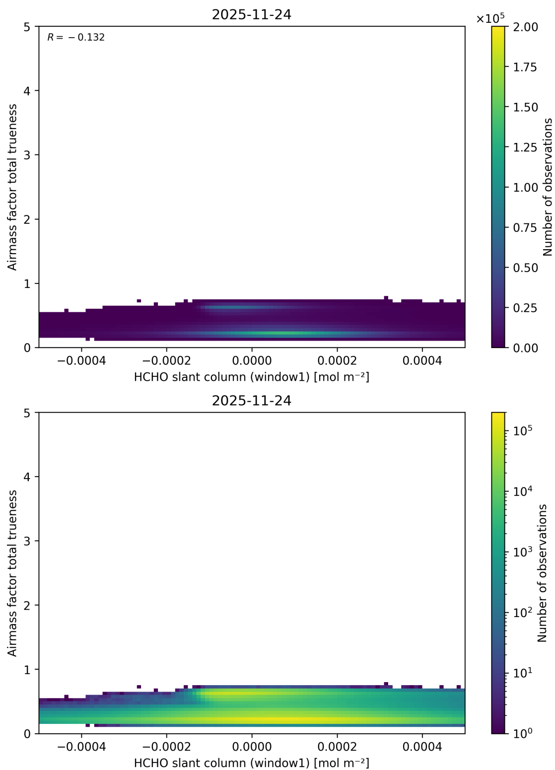
Figure 96: Scatter density plot of “HCHO slant column (window1)” against “Airmass factor total trueneess” for 2025-11-23 to 2025-11-25.
