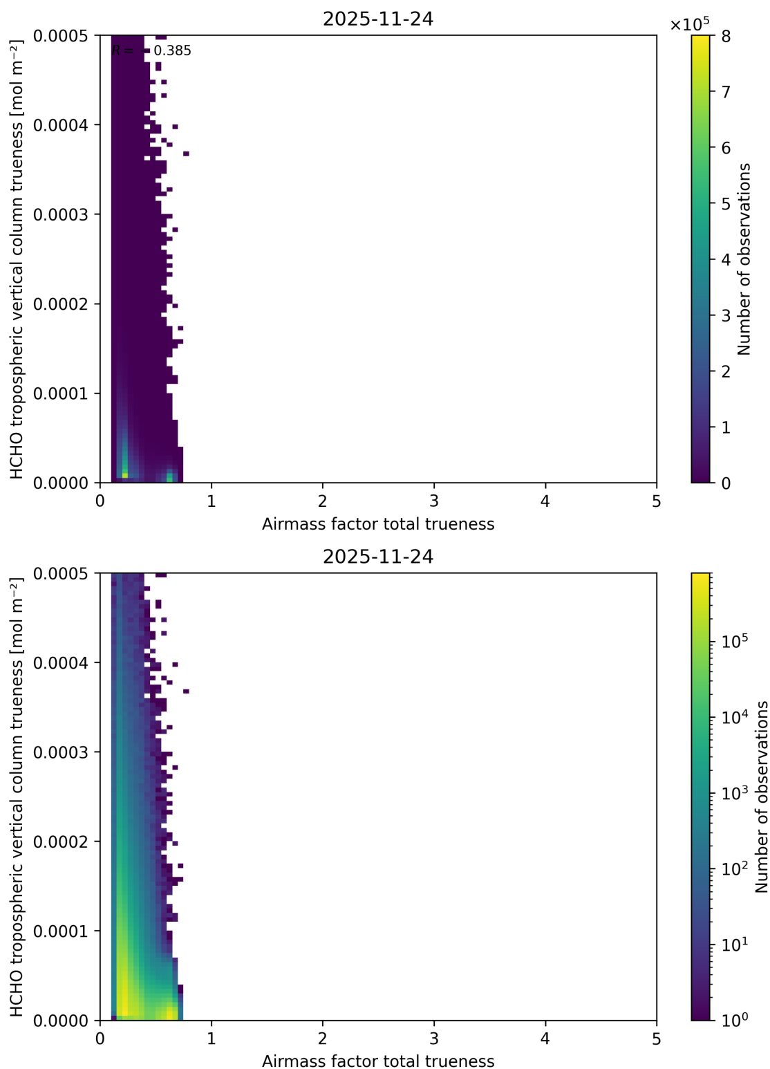
Figure 124: Scatter density plot of “Airmass factor total trueness” against “HCHO tropospheric vertical column trueness” for 2025-11-23 to 2025-11-25.
