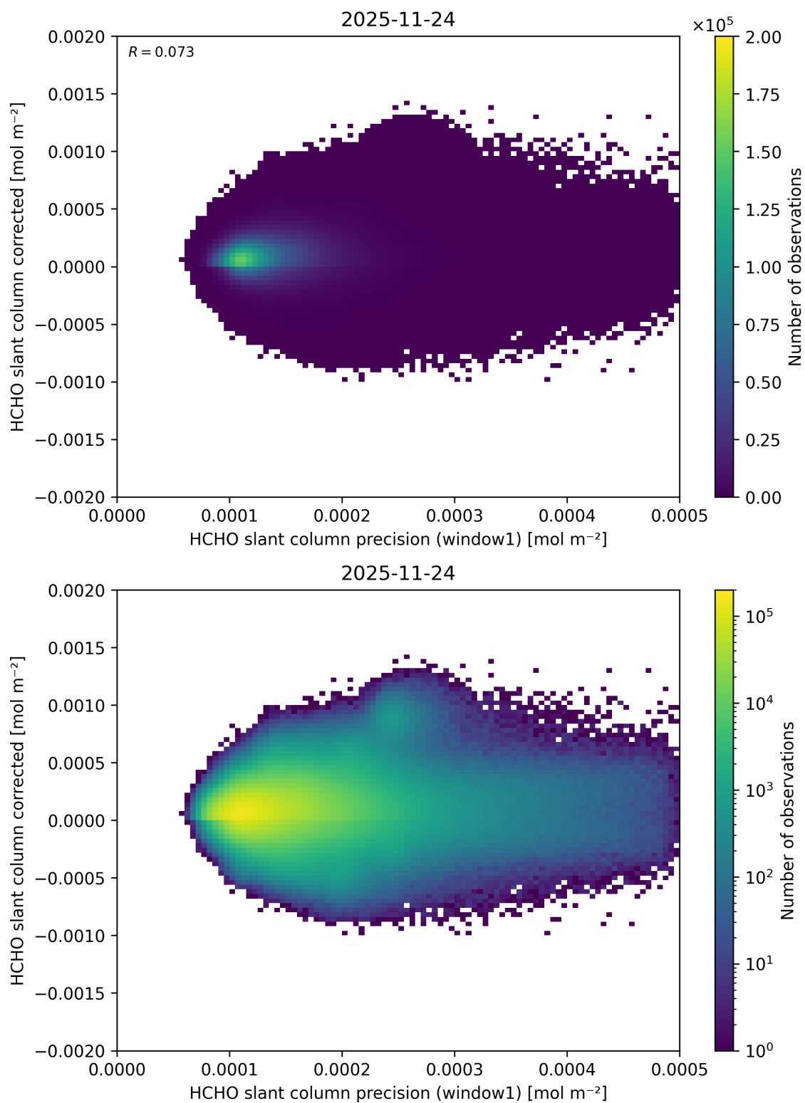
Figure 103: Scatter density plot of “HCHO slant column precision (window1)” against “HCHO slant column corrected” for 2025-11-23 to 2025-11-25.
