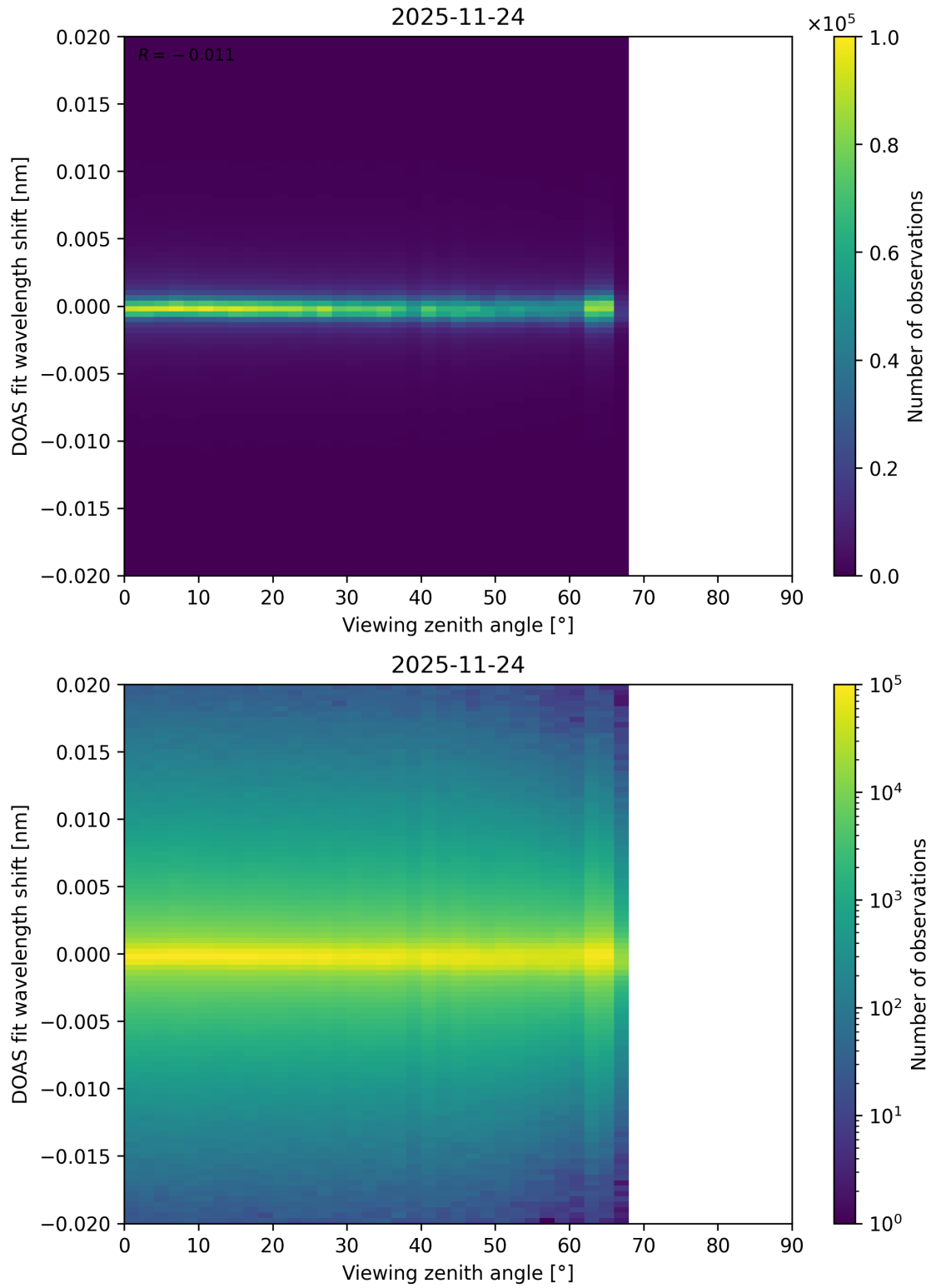
Figure 203: Scatter density plot of “Viewing zenith angle” against “DOAS fit wavelength shift” for 2025-11-23 to 2025-11-25.
