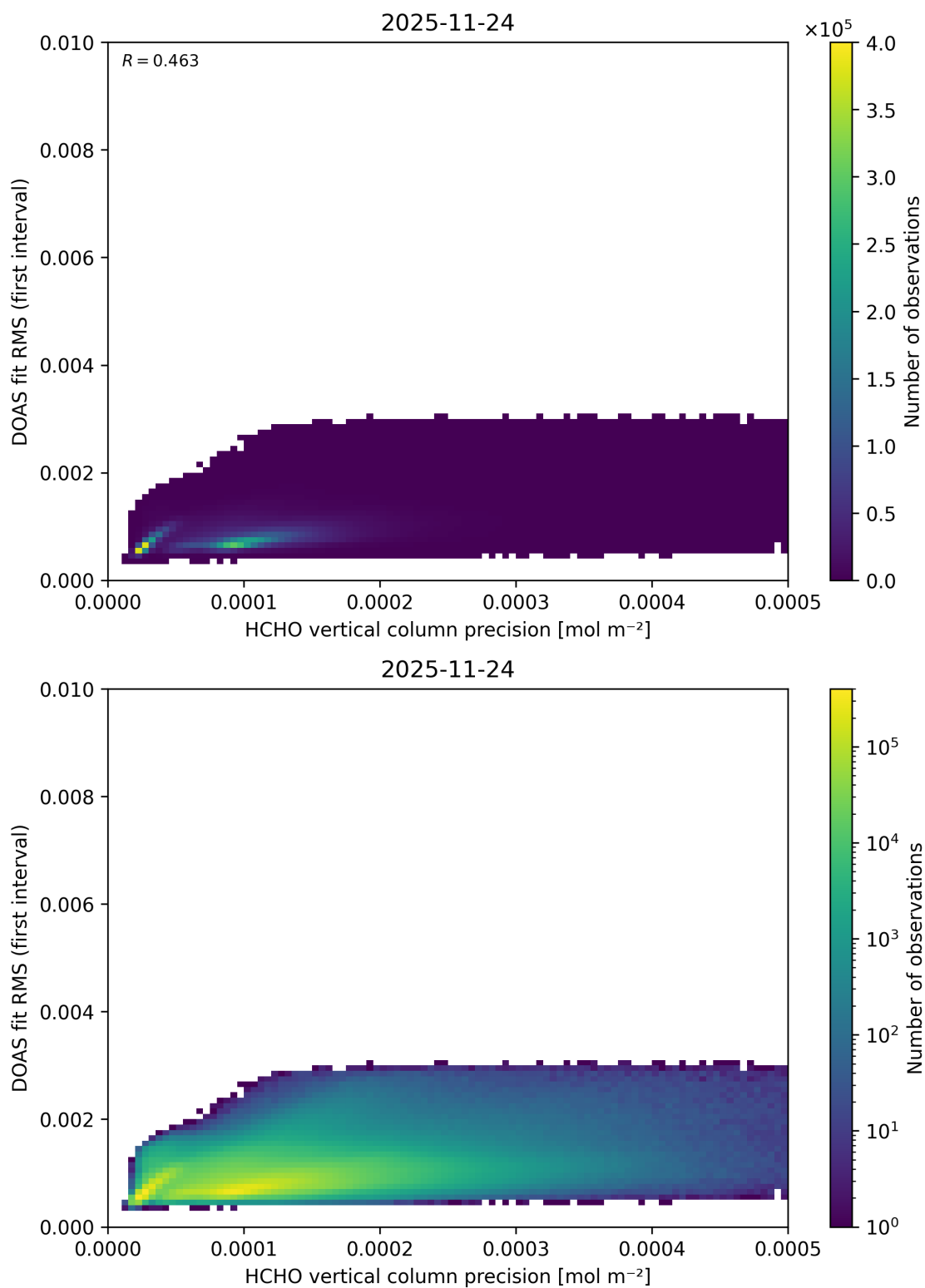
Figure 152: Scatter density plot of “HCHO vertical column precision” against “DOAS fit RMS (first interval)” for 2025-11-23 to 2025-11-25.
