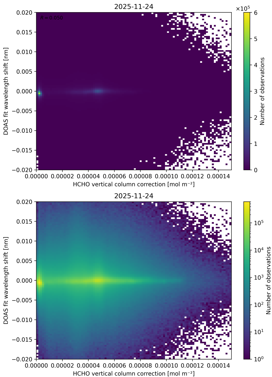
Figure 127: Scatter density plot of “HCHO vertical column correction” against “DOAS fit wavelength shift” for 2025-11-23 to 2025-11-25.
