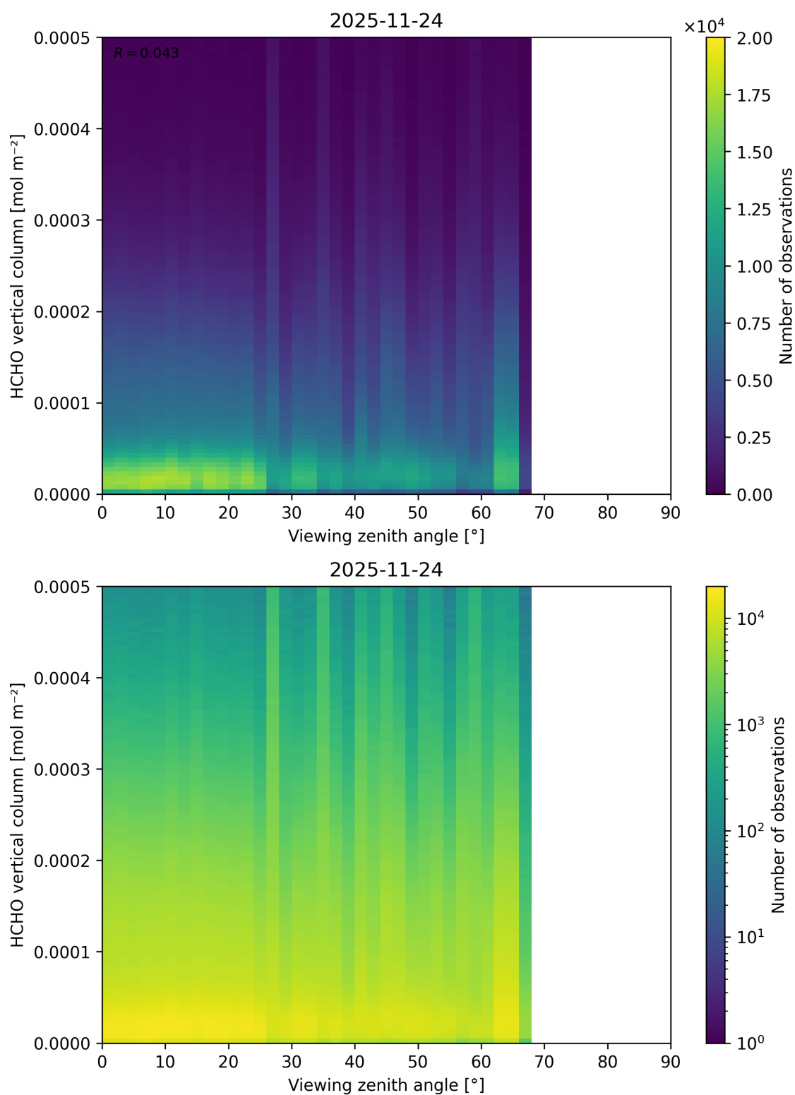
Figure 212: Scatter density plot of “Viewing zenith angle” against “HCHO vertical column” for 2025-11-23 to 2025-11-25.
