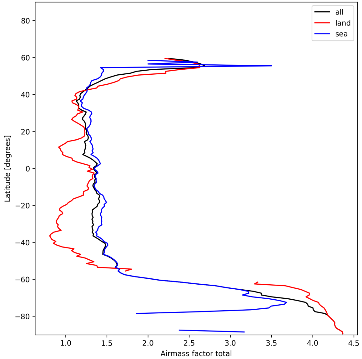
Figure 27: Zonal average of “Airmass factor total” for 2025-11-23 to 2025-11-25.
