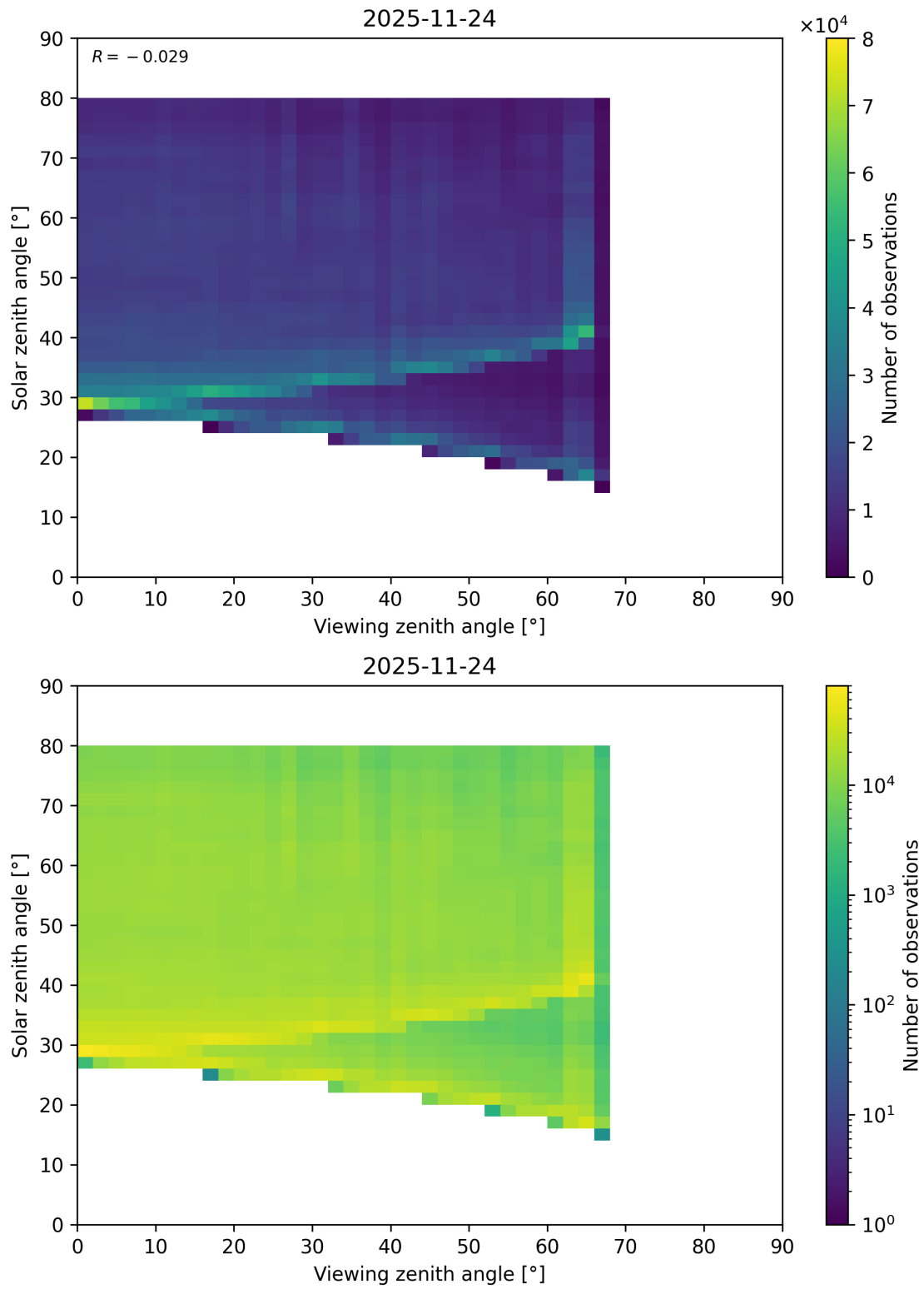
Figure 218: Scatter density plot of “Viewing zenith angle” against “Solar zenith angle” for 2025-11-23 to 2025-11-25.
