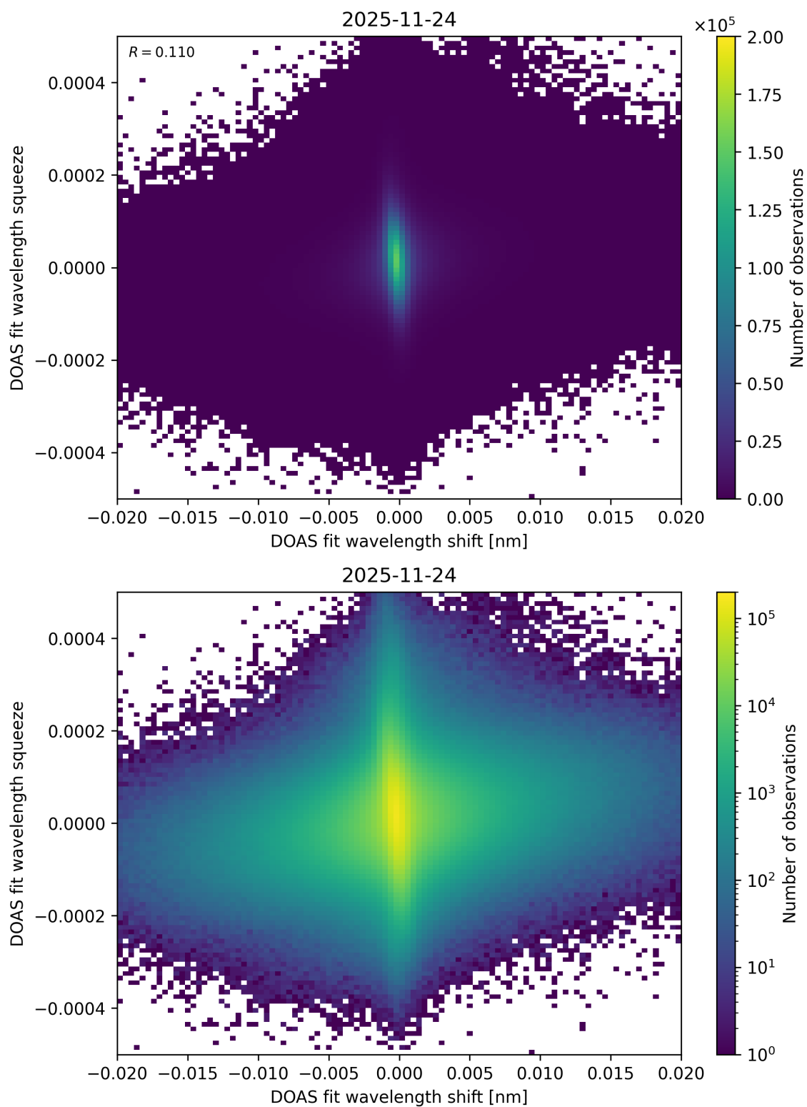
Figure 70: Scatter density plot of “DOAS fit wavelength shift” against “DOAS fit wavelength squeeze” for 2025-11-23 to 2025-11-25.
