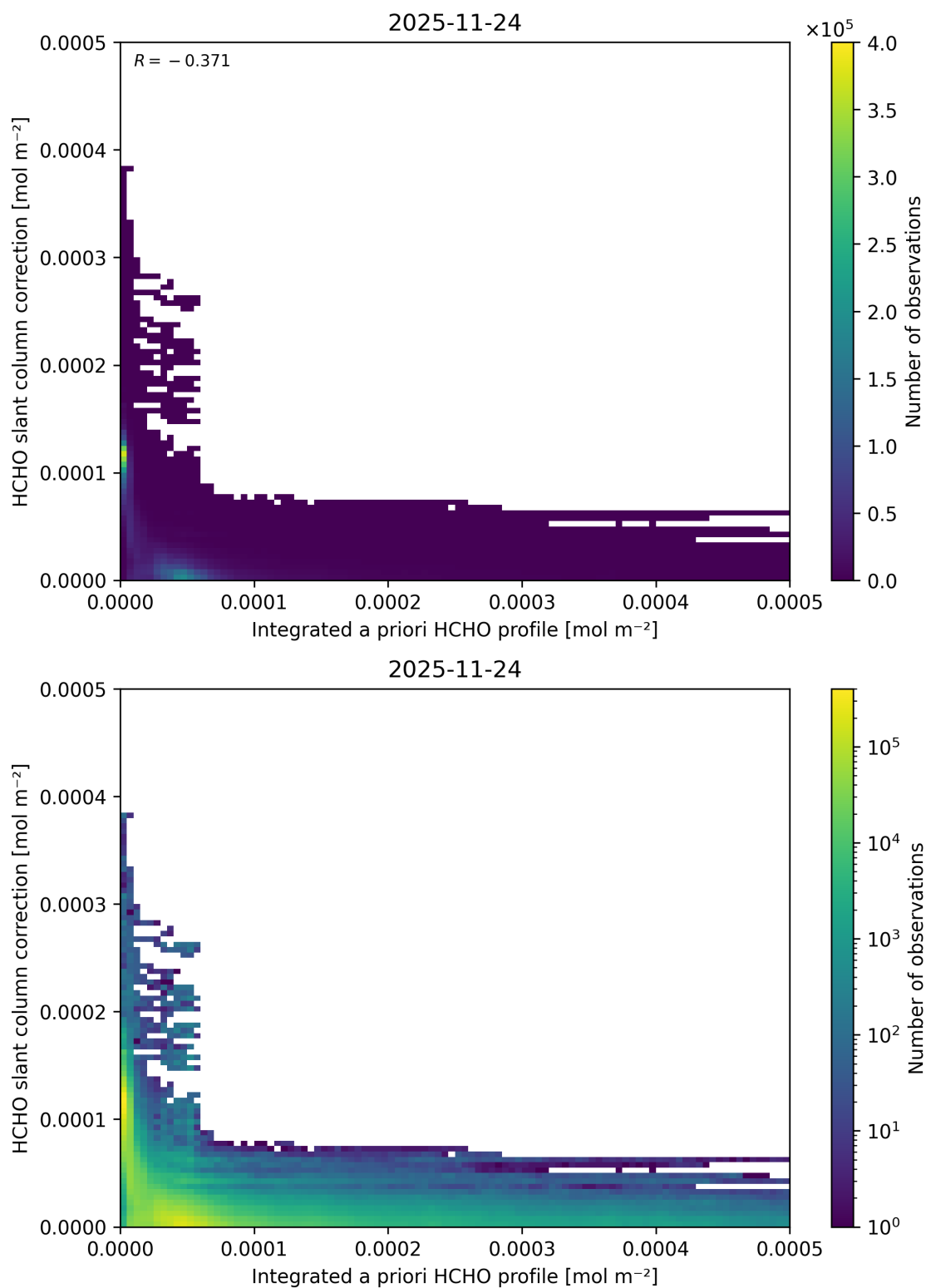
Figure 169: Scatter density plot of “Integrated a priori HCHO profile” against “HCHO slant column correction” for 2025-11-23 to 2025-11-25.
