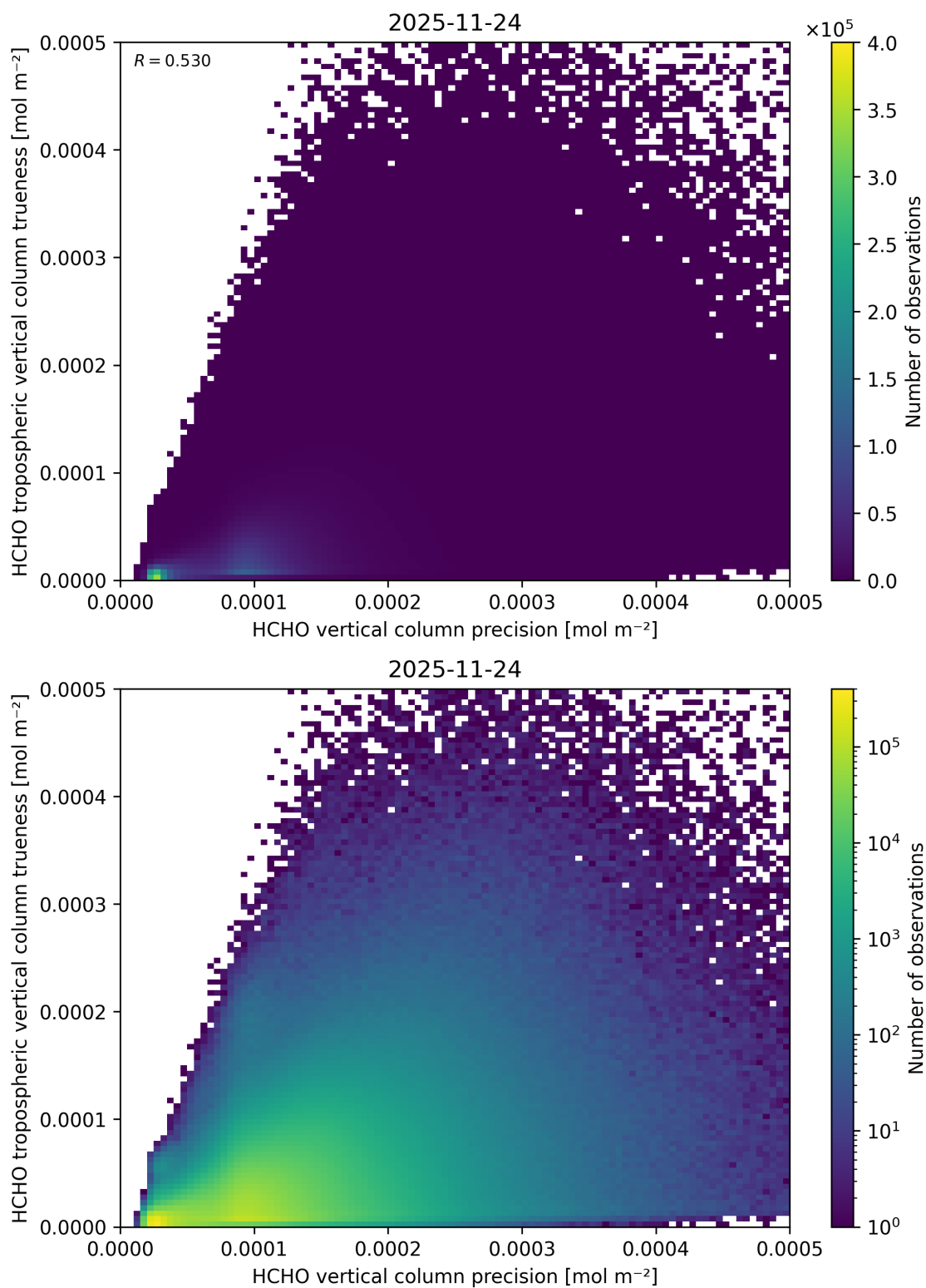
Figure 163: Scatter density plot of “HCHO vertical column precision” against “HCHO tropospheric vertical column trueness” for 2025-11-23 to 2025-11-25.
