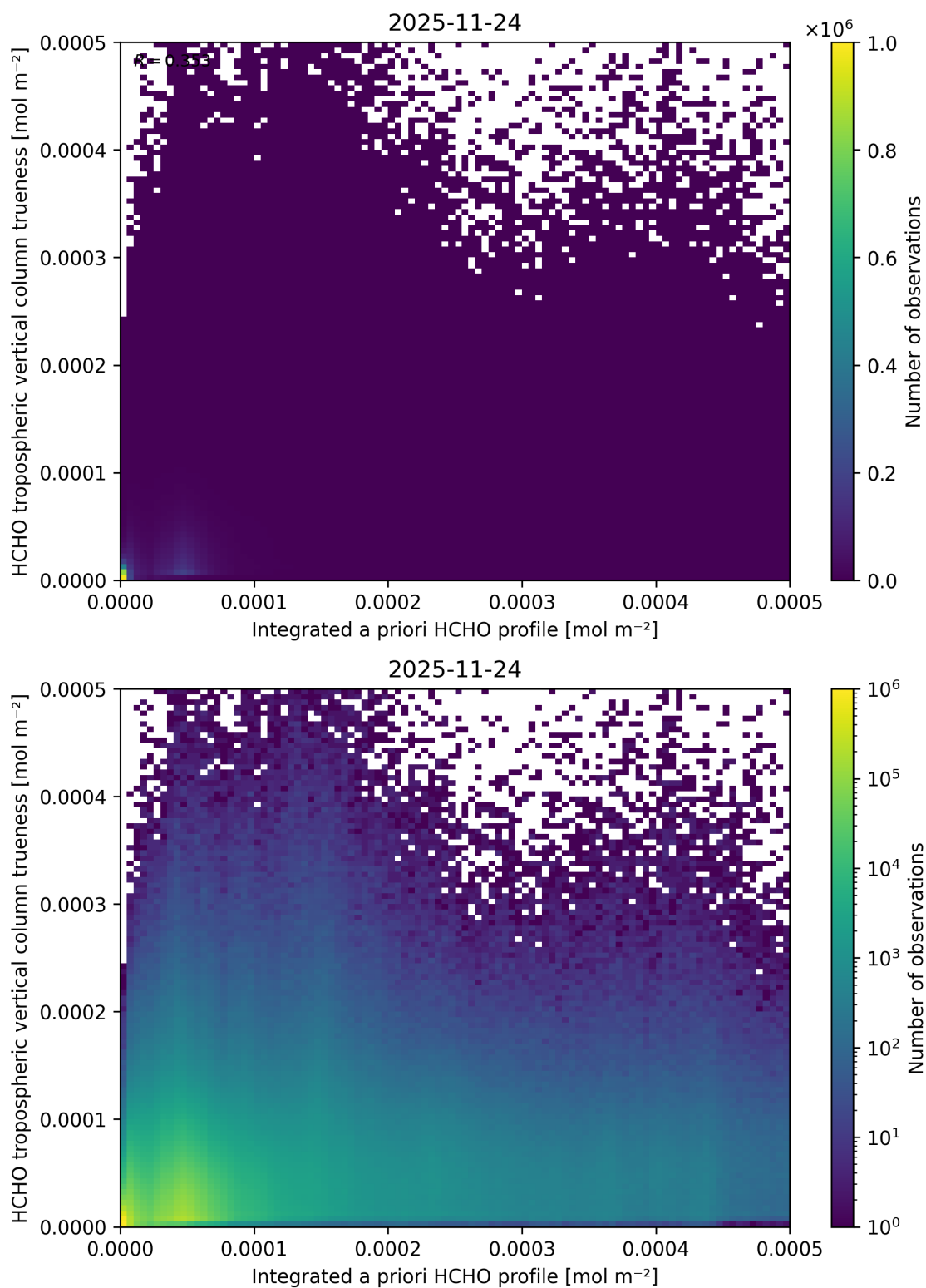
Figure 170: Scatter density plot of “Integrated a priori HCHO profile” against “HCHO tropospheric vertical column trueness” for 2025-11-23 to 2025-11-25.
