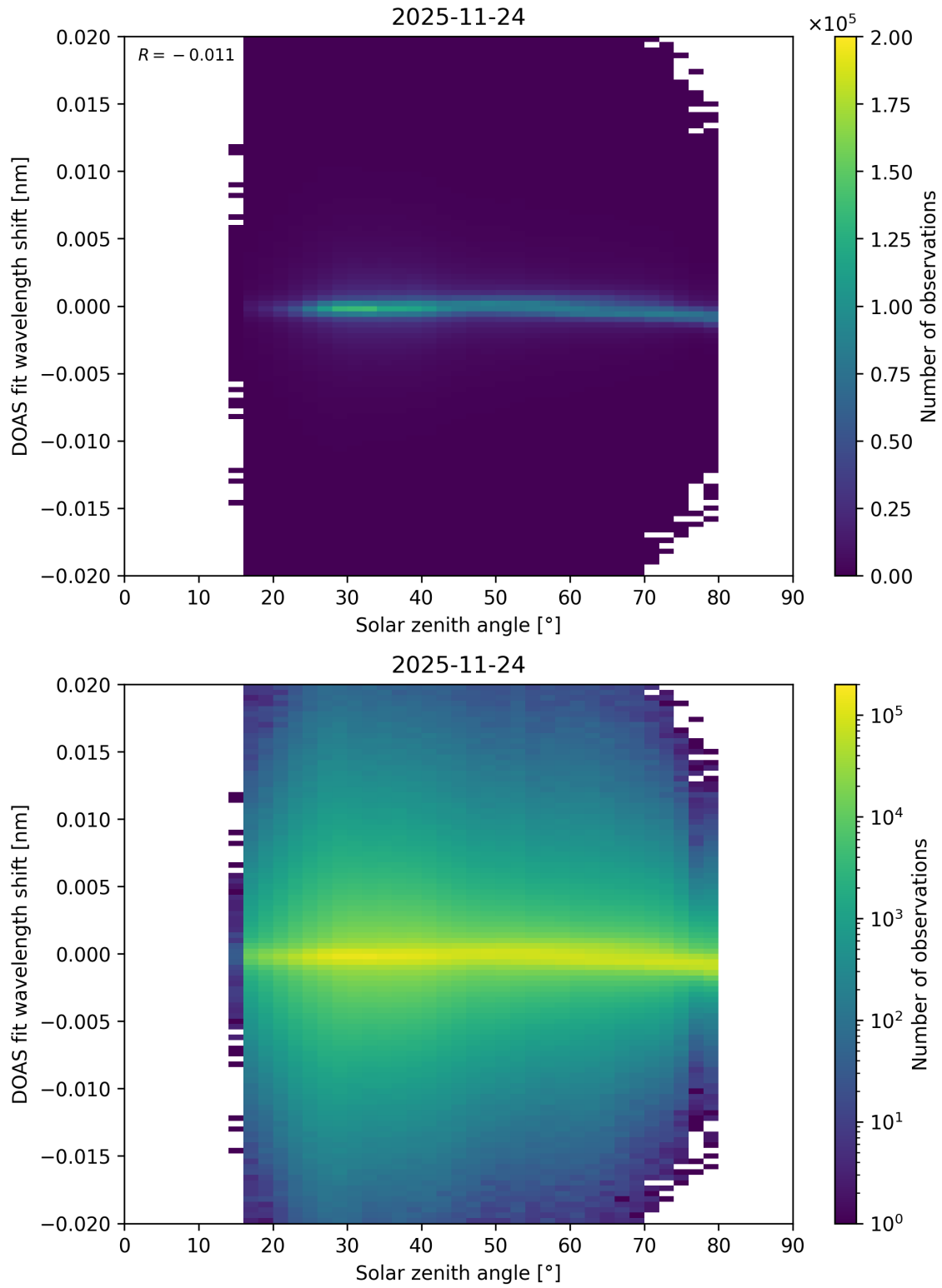
Figure 187: Scatter density plot of “Solar zenith angle” against “DOAS fit wavelength shift” for 2025-11-23 to 2025-11-25.
