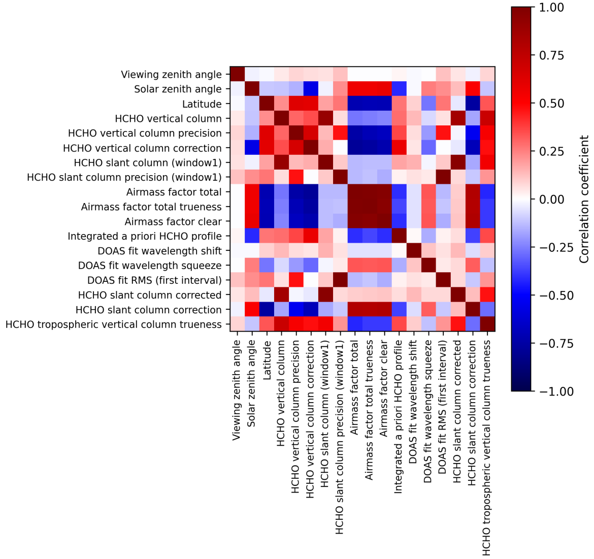
Figure 2: Map of correlation matrix for 2025-11-23 to 2025-11-25.
