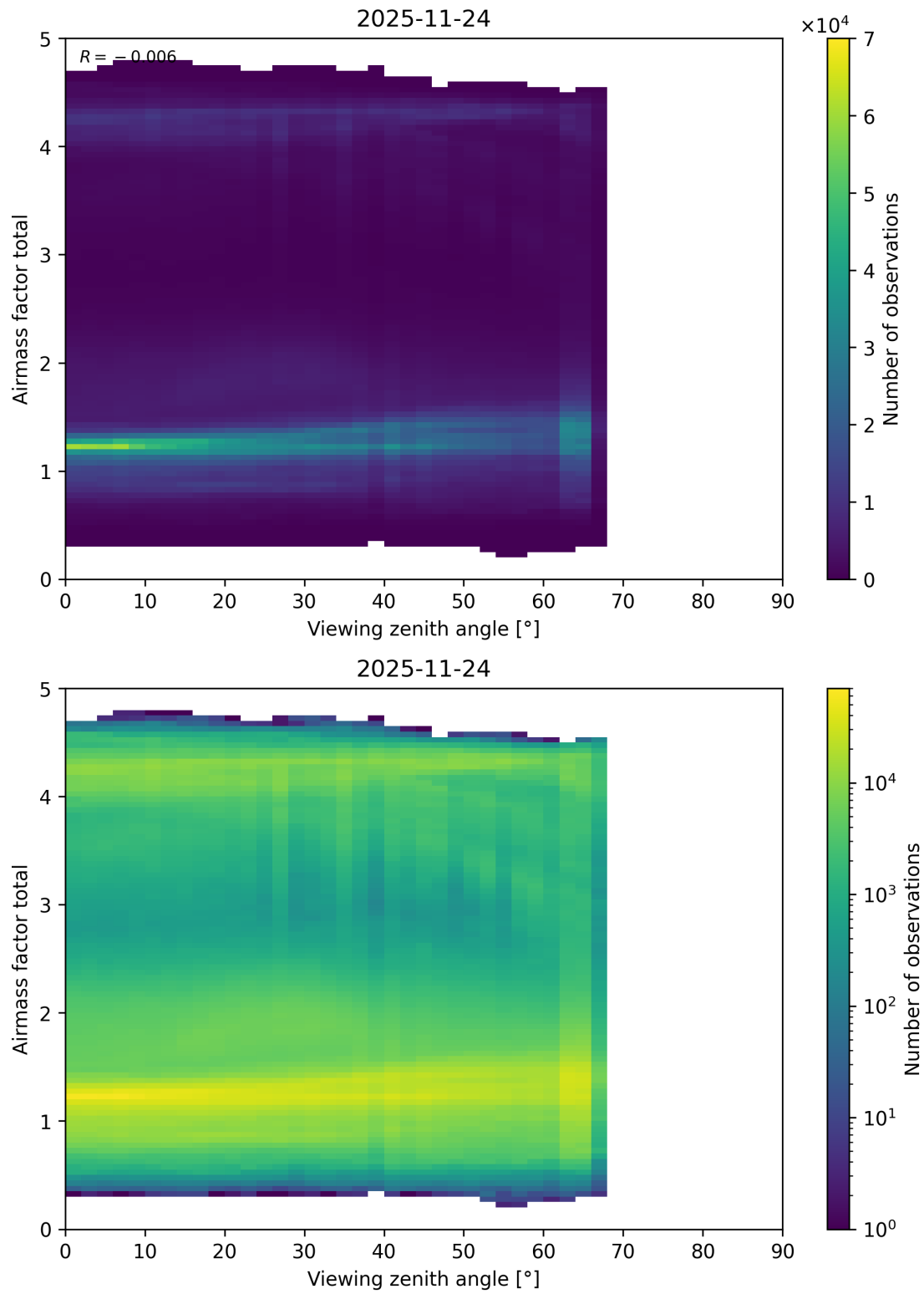
Figure 210: Scatter density plot of “Viewing zenith angle” against “Airmass factor total” for 2025-11-23 to 2025-11-25.
