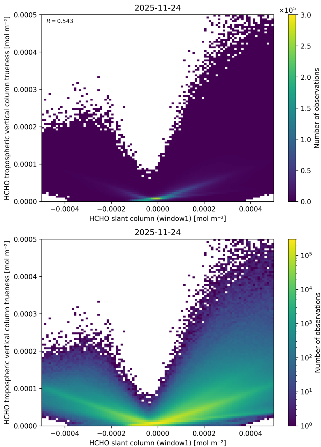
Figure 97: Scatter density plot of “HCHO slant column (window1)” against “HCHO tropospheric vertical column trueness” for 2025-11-23 to 2025-11-25.
