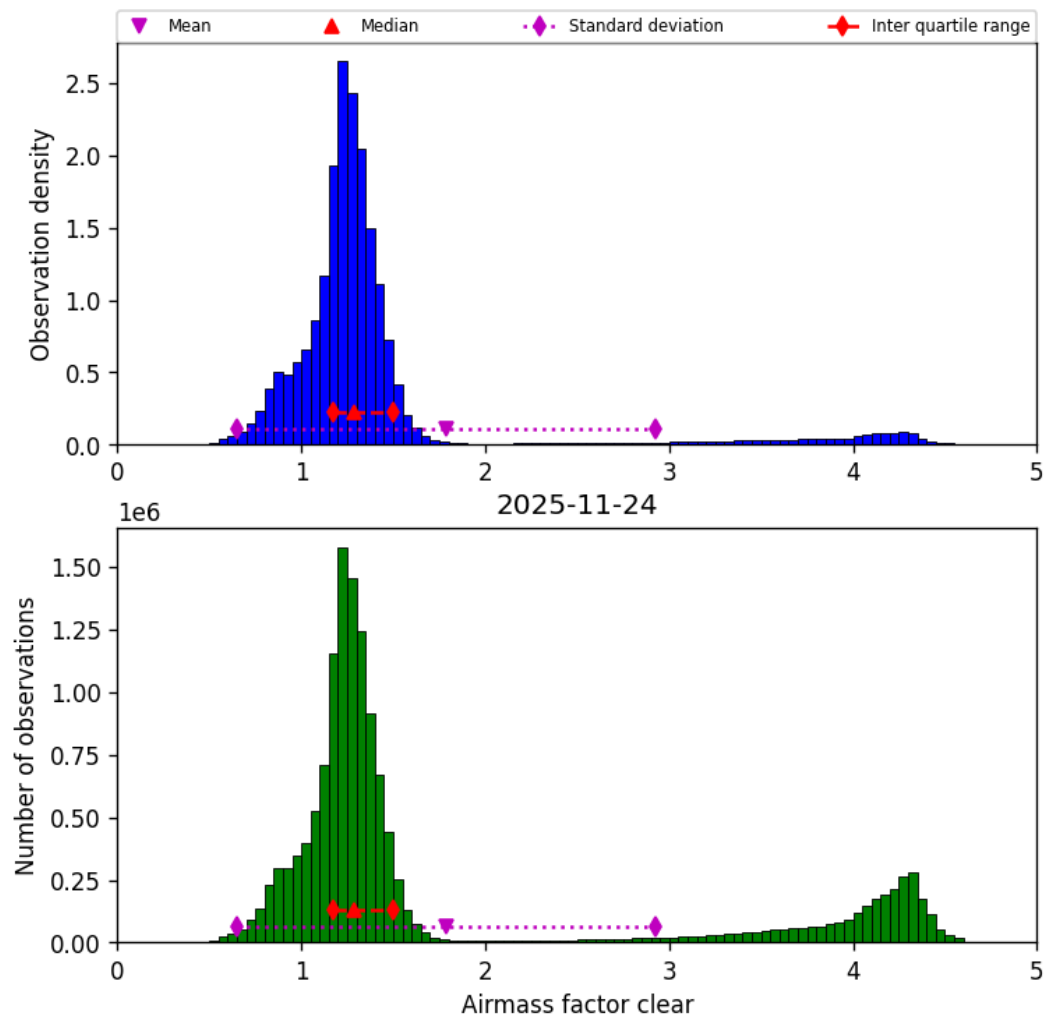
Figure 44: Histogram of “Airmass factor clear” for 2025-11-23 to 2025-11-25
