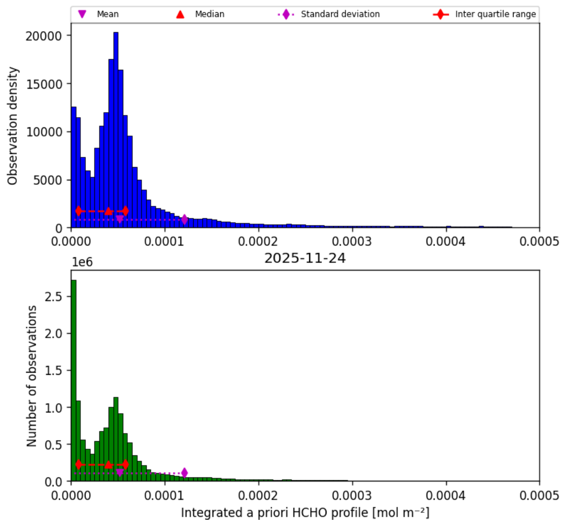
Figure 45: Histogram of “Integrated a priori HCHO profile” for 2025-11-23 to 2025-11-25
