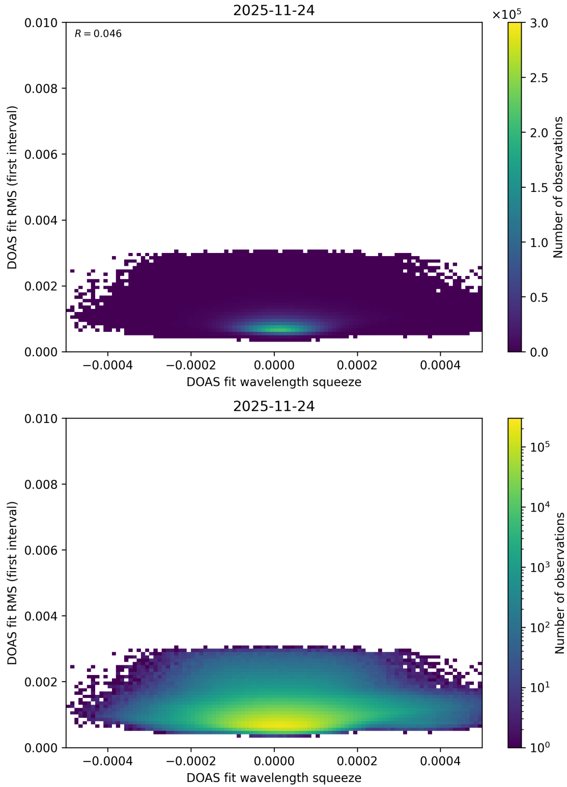
Figure 74: Scatter density plot of “DOAS fit wavelength squeeze” against “DOAS fit RMS (first interval)” for 2025-11-23 to 2025-11-25.
