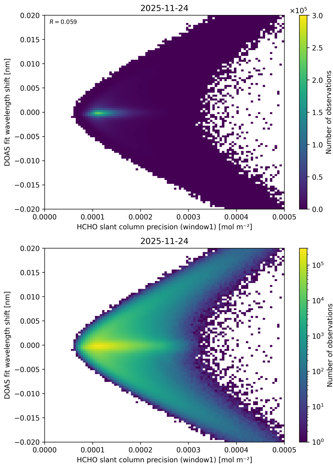
Figure 100: Scatter density plot of “HCHO slant column precision (window1)” against “DOAS fit wavelength shift” for 2025-11-23 to 2025-11-25.
