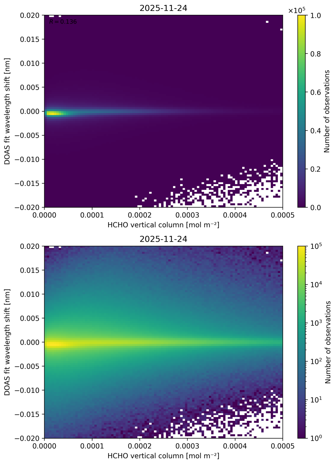
Figure 139: Scatter density plot of “HCHO vertical column” against “DOAS fit wavelength shift” for 2025-11-23 to 2025-11-25.
