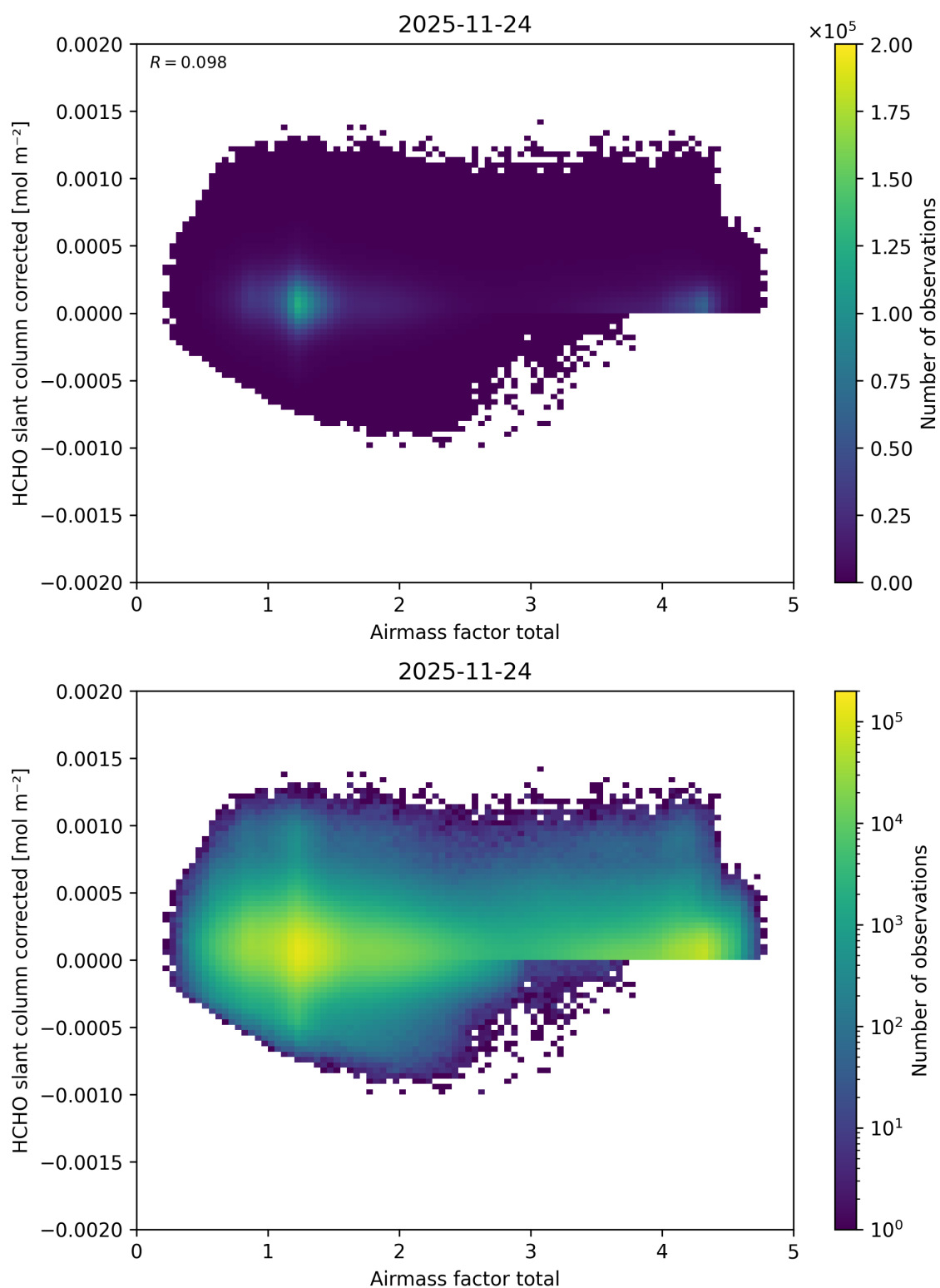
Figure 113: Scatter density plot of “Airmass factor total” against “HCHO slant column corrected” for 2025-11-23 to 2025-11-25.
