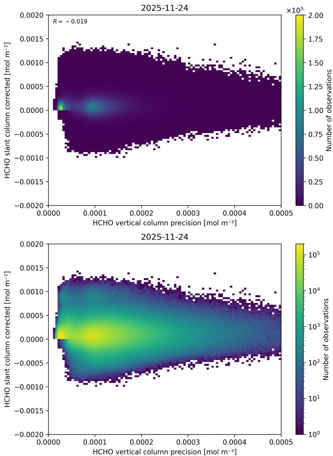
Figure 156: Scatter density plot of “HCHO vertical column precision” against “HCHO slant column corrected” for 2025-11-23 to 2025-11-25.
