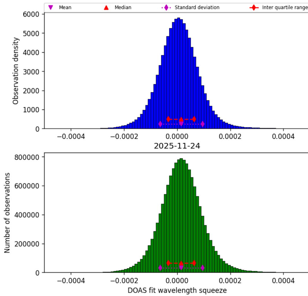
Figure 47: Histogram of “DOAS fit wavelength squeeze” for 2025-11-23 to 2025-11-25
