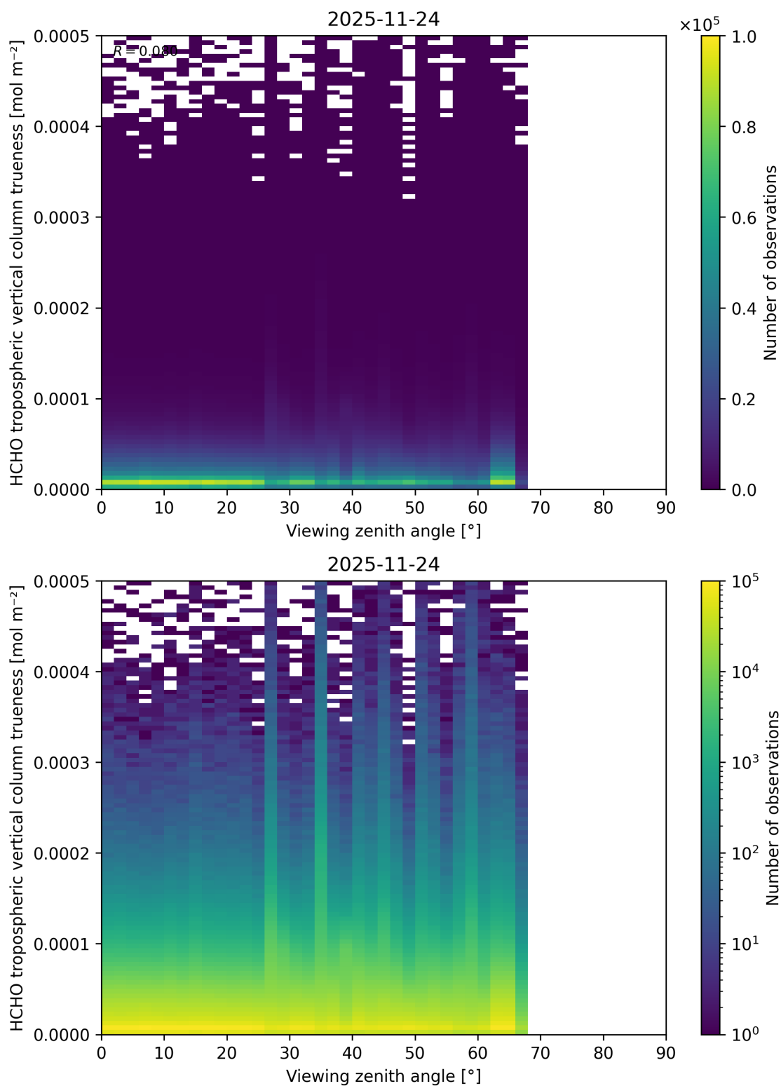
Figure 215: Scatter density plot of “Viewing zenith angle” against “HCHO tropospheric vertical column truthness” for 2025-11-23 to 2025-11-25.
