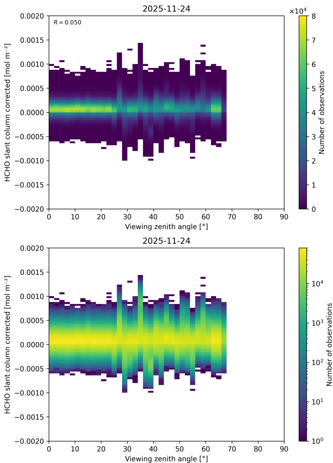
Figure 206: Scatter density plot of “Viewing zenith angle” against “HCHO slant column corrected” for 2025-11-23 to 2025-11-25.
