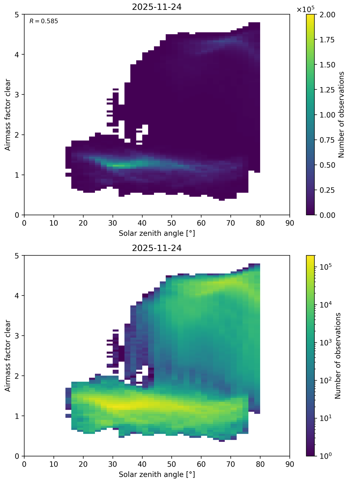
Figure 189: Scatter density plot of “Solar zenith angle” against “Airmass factor clear” for 2025-11-23 to 2025-11-25.
