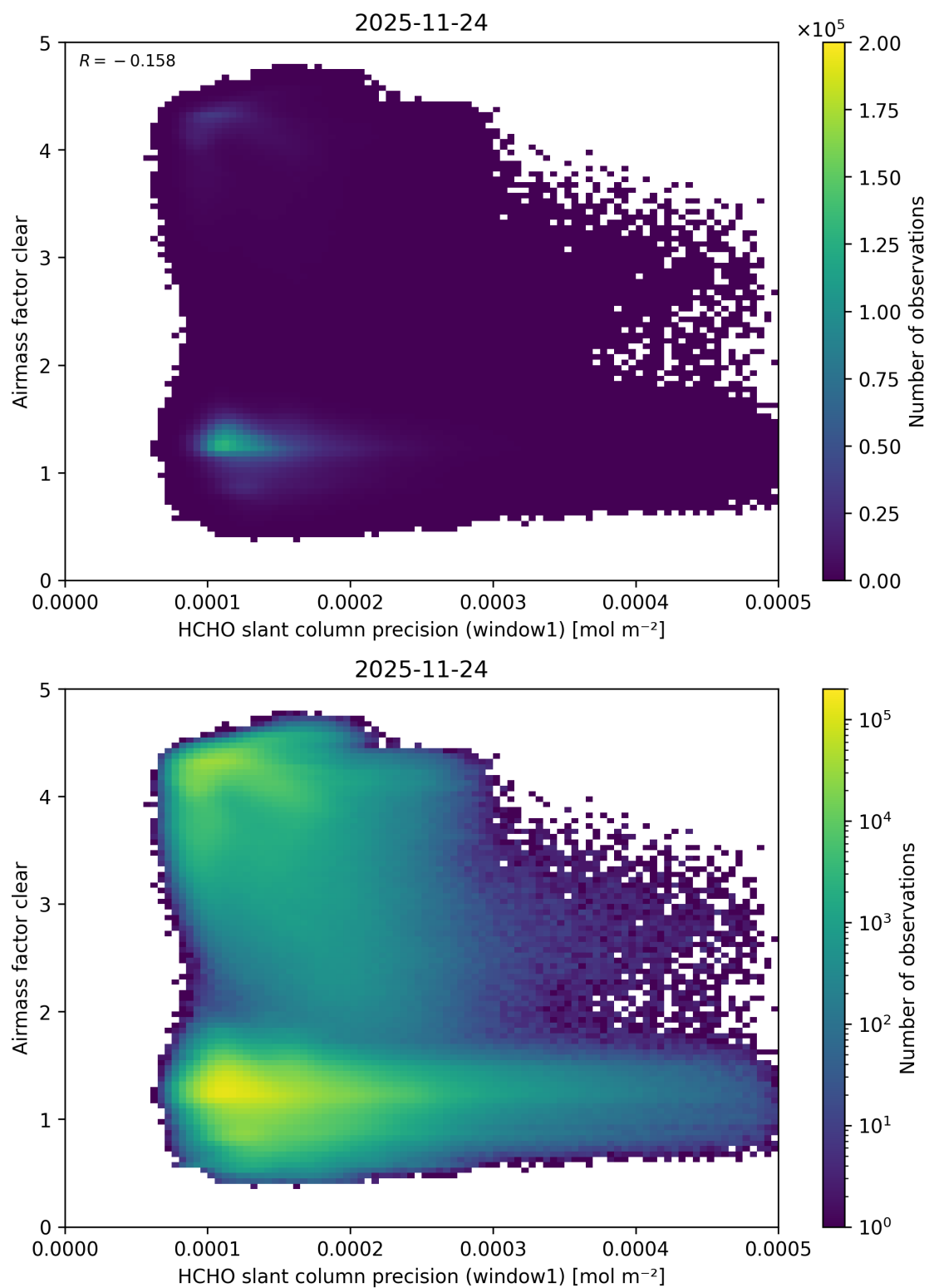
Figure 102: Scatter density plot of “HCHO slant column precision (window1)” against “Airmass factor clear” for 2025-11-23 to 2025-11-25.
