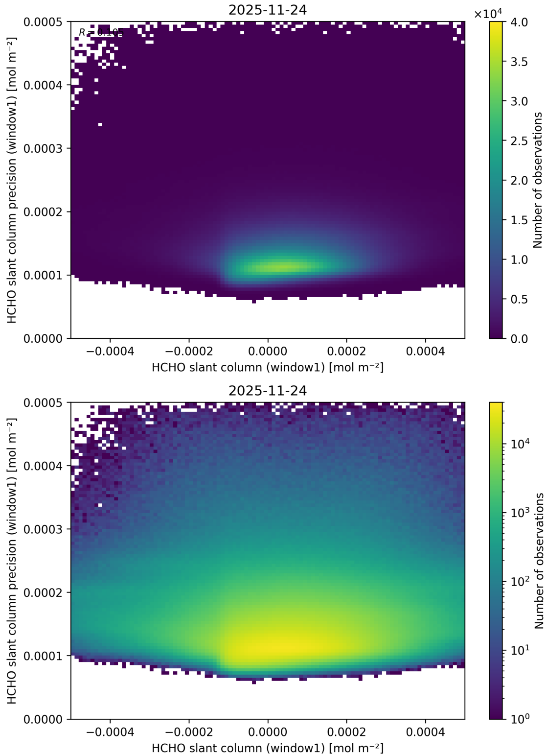
Figure 94: Scatter density plot of “HCHO slant column (window1)” against “HCHO slant column precision (window1)” for 2025-11-23 to 2025-11-25.
