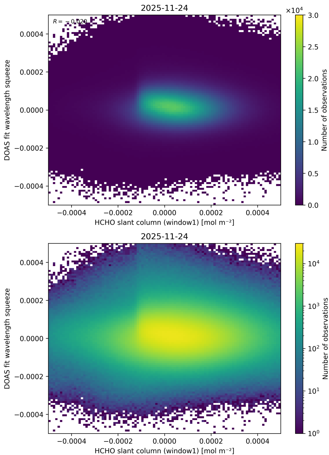
Figure 90: Scatter density plot of “HCHO slant column (window1)” against “DOAS fit wavelength squeeze” for 2025-11-23 to 2025-11-25.
