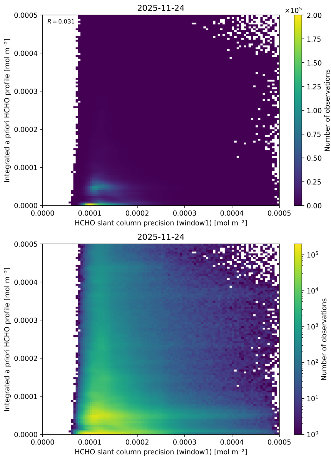
Figure 108: Scatter density plot of “HCHO slant column precision (window1)” against “Integrated a priori HCHO profile” for 2025-11-23 to 2025-11-25.
