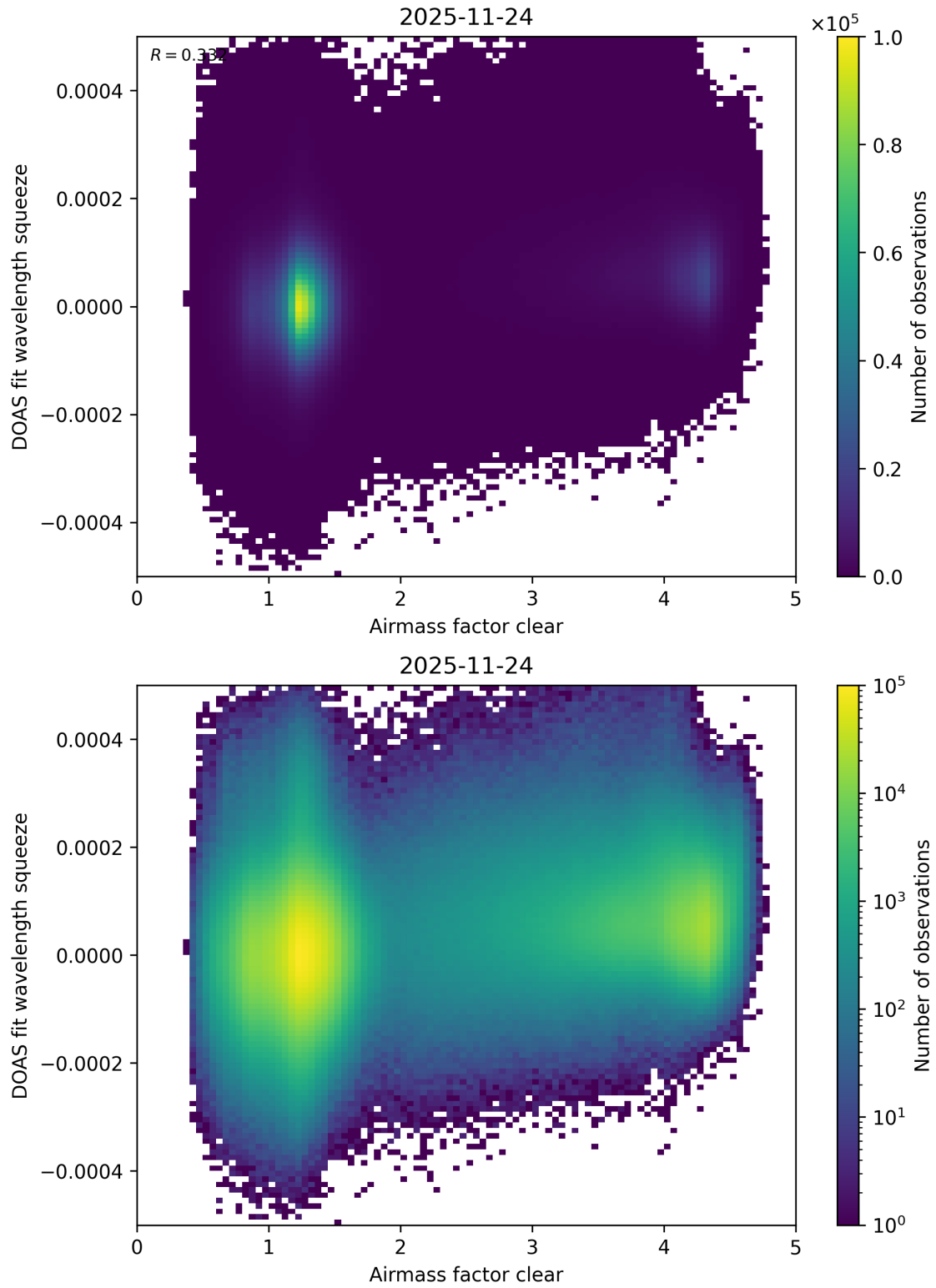
Figure 80: Scatter density plot of “Airmass factor clear” against “DOAS fit wavelength squeeze” for 2025-11-23 to 2025-11-25.
