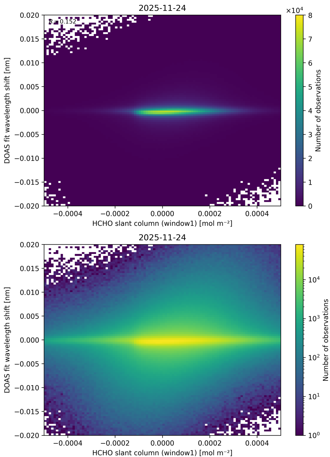
Figure 89: Scatter density plot of “HCHO slant column (window1)” against “DOAS fit wavelength shift” for 2025-11-23 to 2025-11-25.
