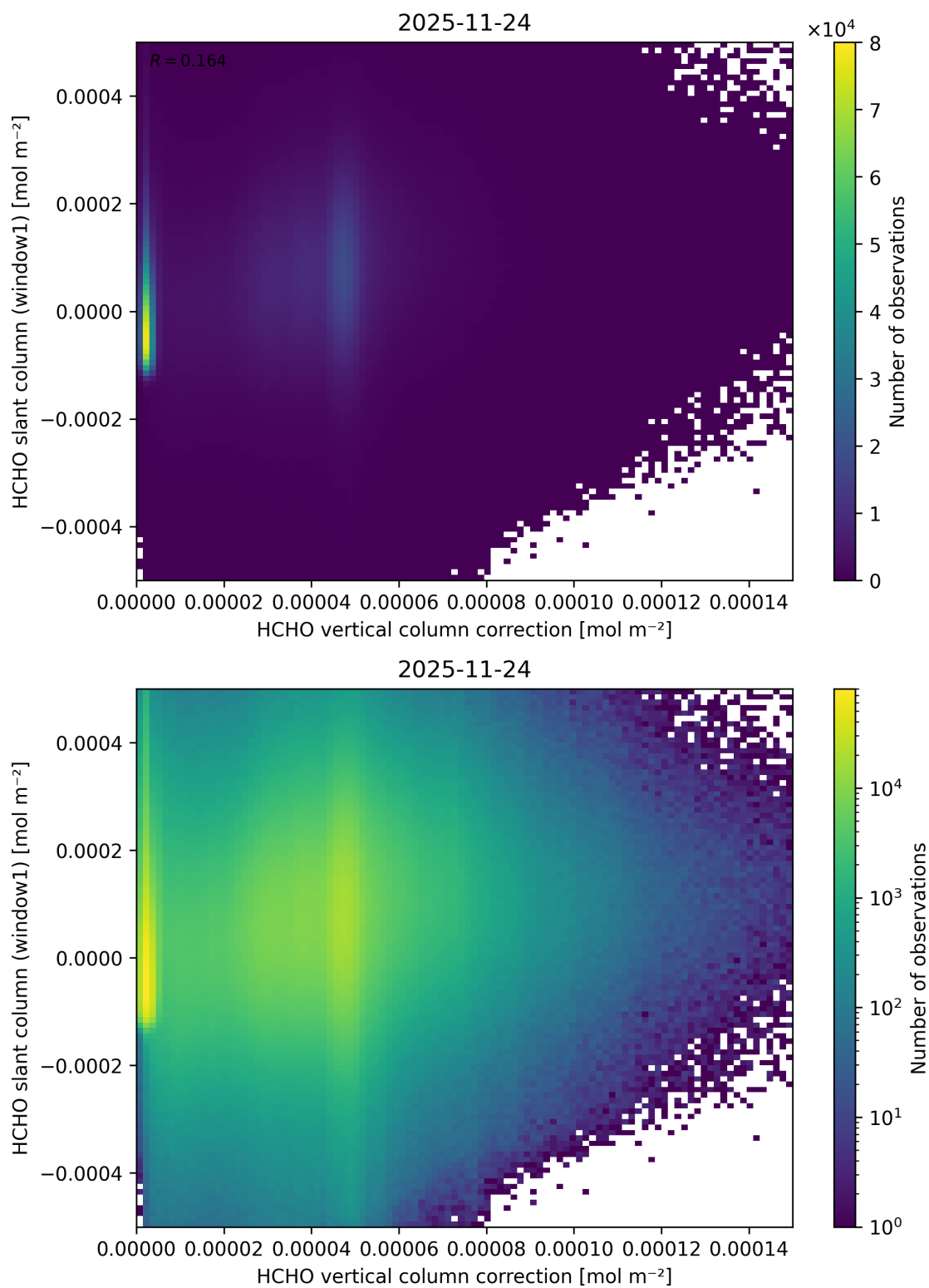
Figure 132: Scatter density plot of “HCHO vertical column correction” against “HCHO slant column (window1)” for 2025-11-23 to 2025-11-25.
