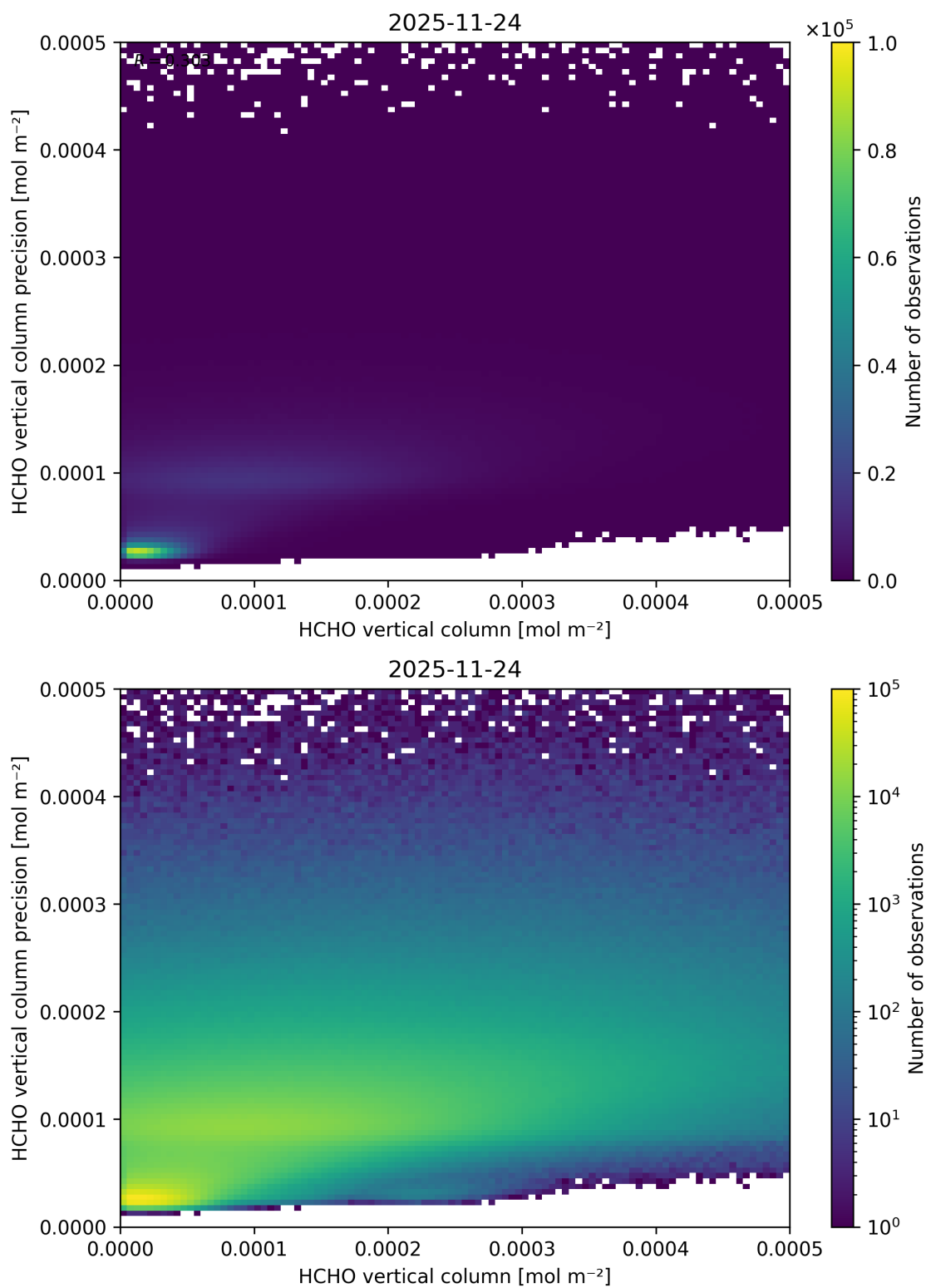
Figure 149: Scatter density plot of “HCHO vertical column” against “HCHO vertical column precision” for 2025-11-23 to 2025-11-25.
