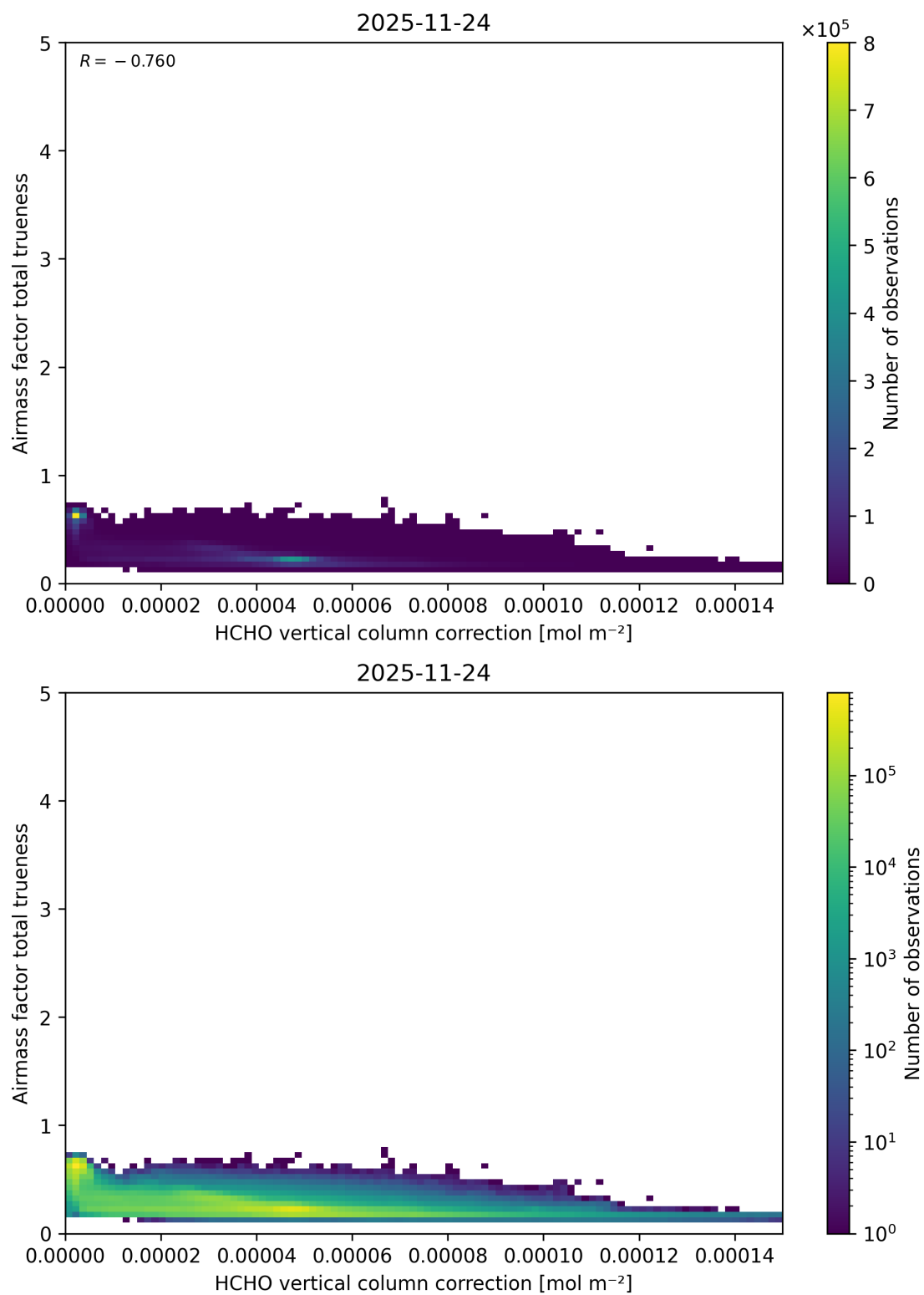
Figure 135: Scatter density plot of “HCHO vertical column correction” against “Airmass factor total trueness” for 2025-11-23 to 2025-11-25.
