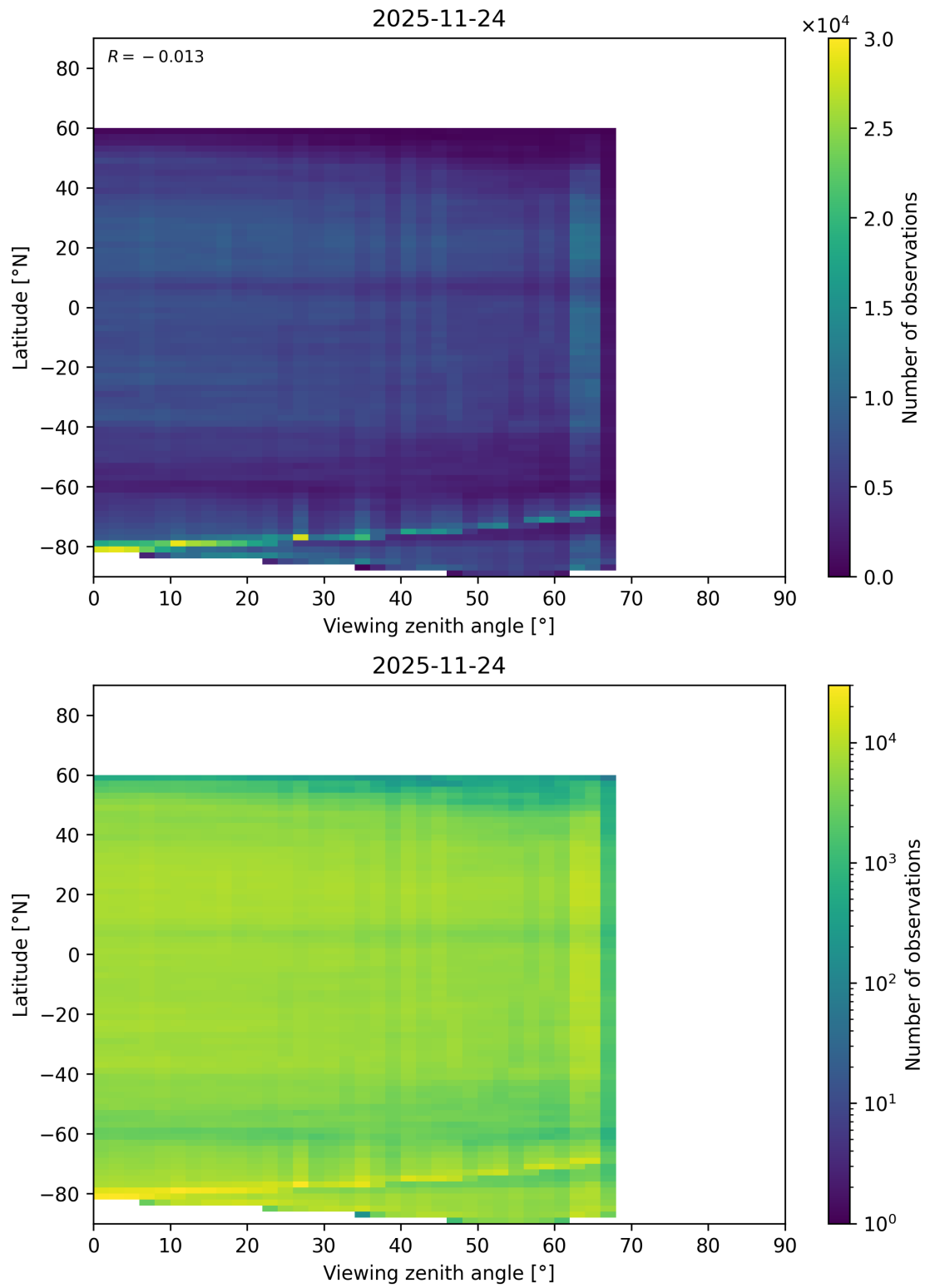
Figure 217: Scatter density plot of “Viewing zenith angle” against “Latitude” for 2025-11-23 to 2025-11-25.
