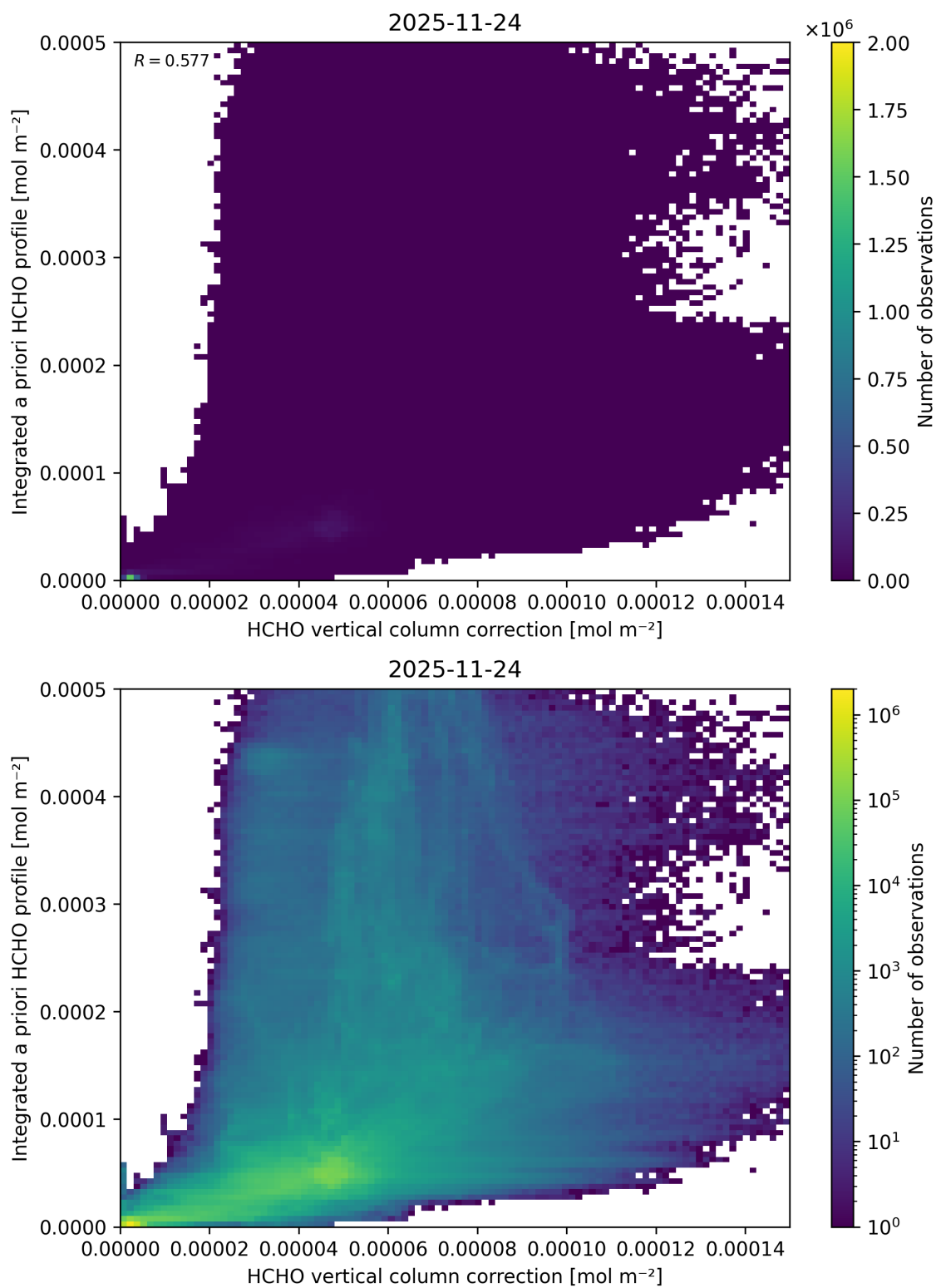
Figure 137: Scatter density plot of “HCHO vertical column correction” against “Integrated a priori HCHO profile” for 2025-11-23 to 2025-11-25.
