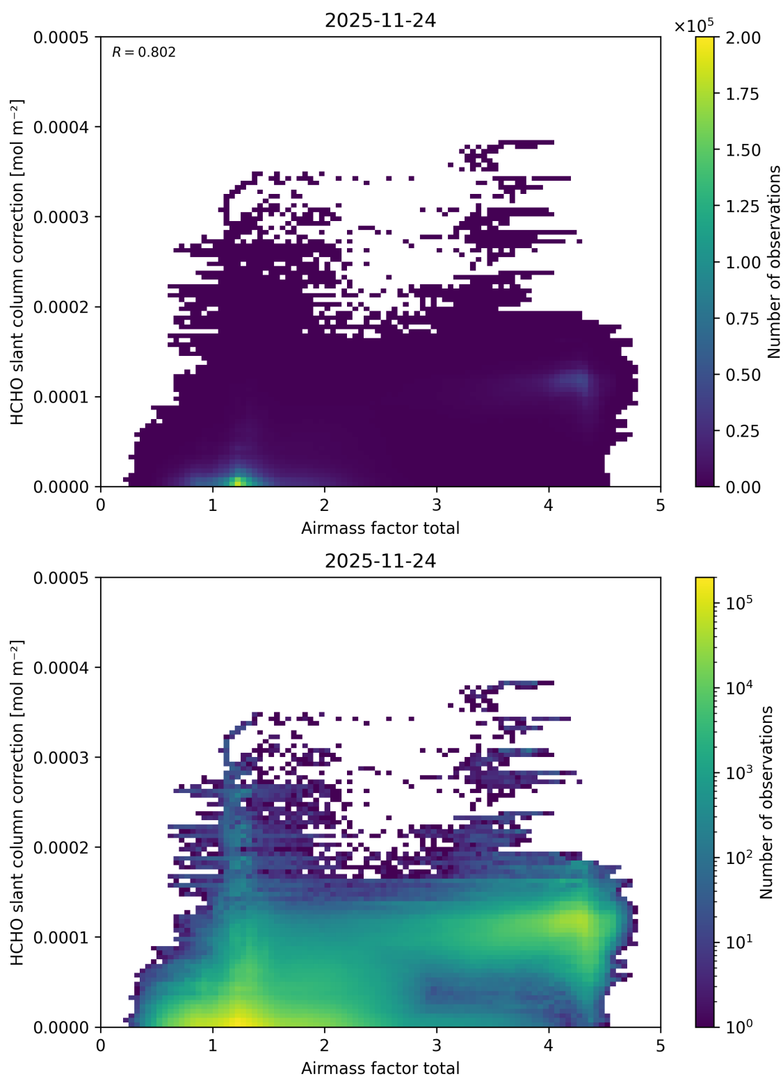
Figure 114: Scatter density plot of “Airmass factor total” against “HCHO slant column correction” for 2025-11-23 to 2025-11-25.
