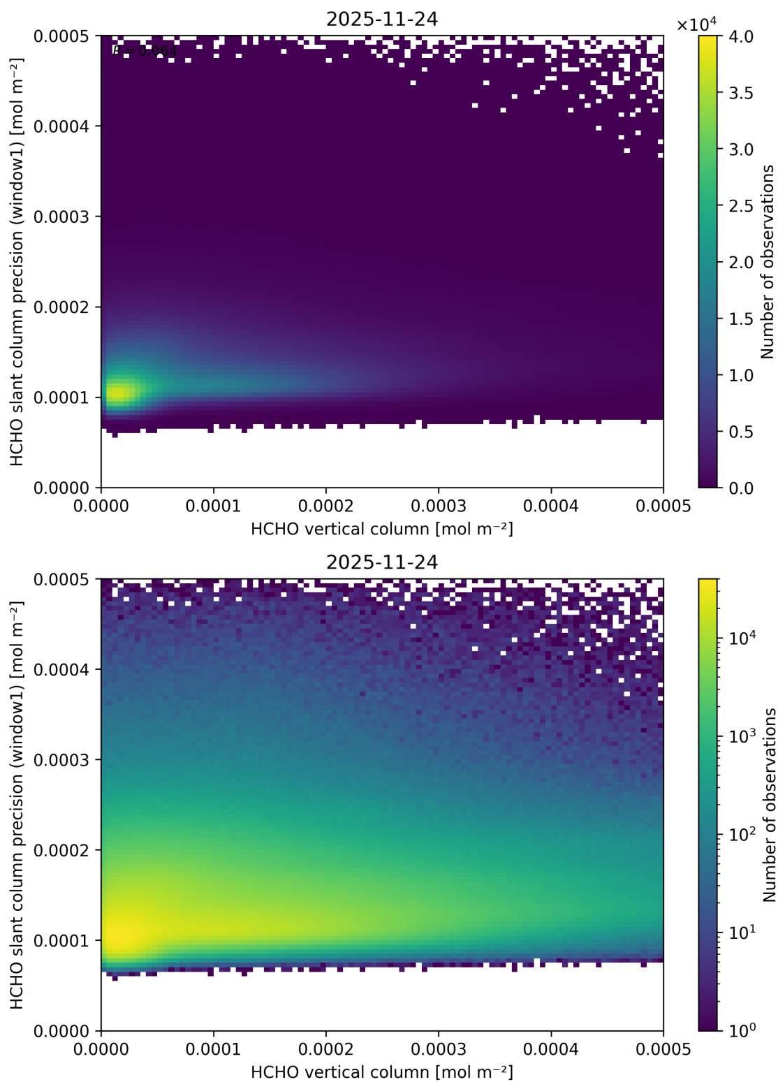
Figure 145: Scatter density plot of “HCHO vertical column” against “HCHO slant column precision (window1)” for 2025-11-23 to 2025-11-25.
