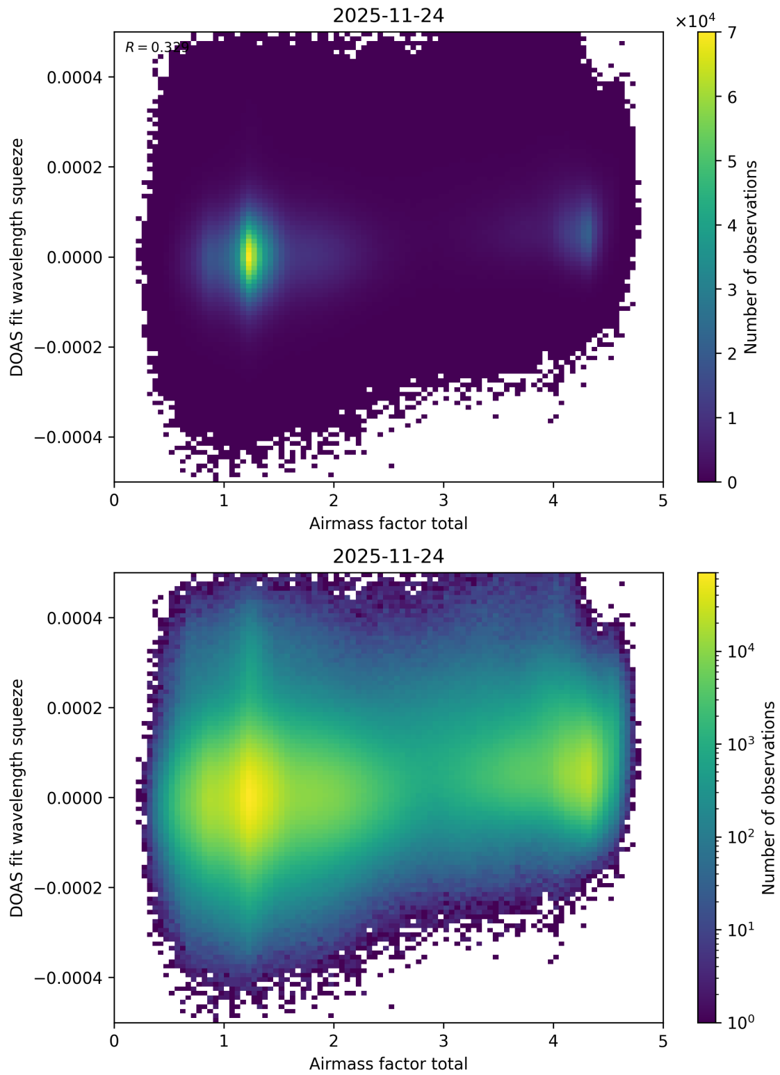
Figure 111: Scatter density plot of “Airmass factor total” against “DOAS fit wavelength squeeze” for 2025-11-23 to 2025-11-25.
