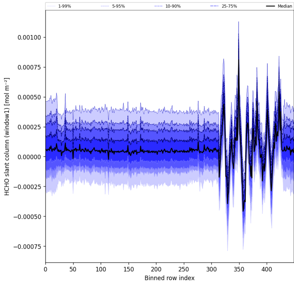
Figure 55: Along track statistics of “HCHO slant column (window1)” for 2025-11-23 to 2025-11-25
