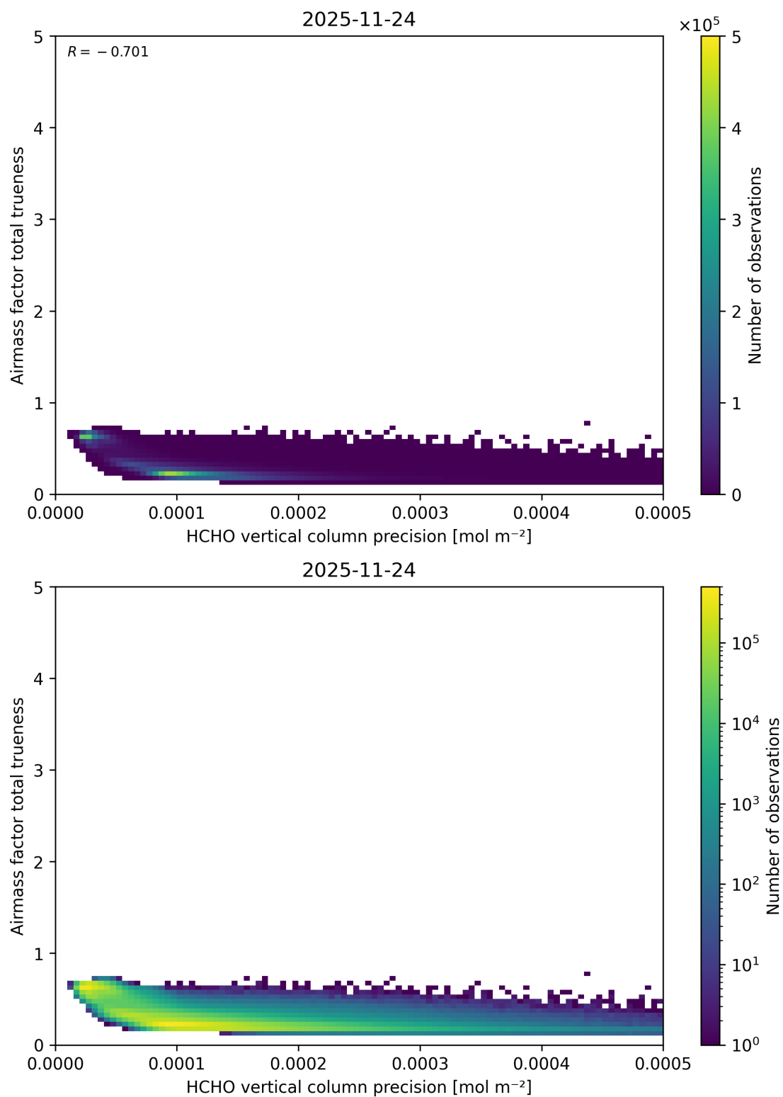
Figure 161: Scatter density plot of “HCHO vertical column precision” against “Airmass factor total trueness” for 2025-11-23 to 2025-11-25.
