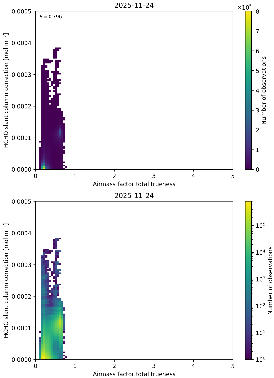
Figure 123: Scatter density plot of “Airmass factor total truiness” against “HCHO slant column correction” for 2025-11-23 to 2025-11-25.
