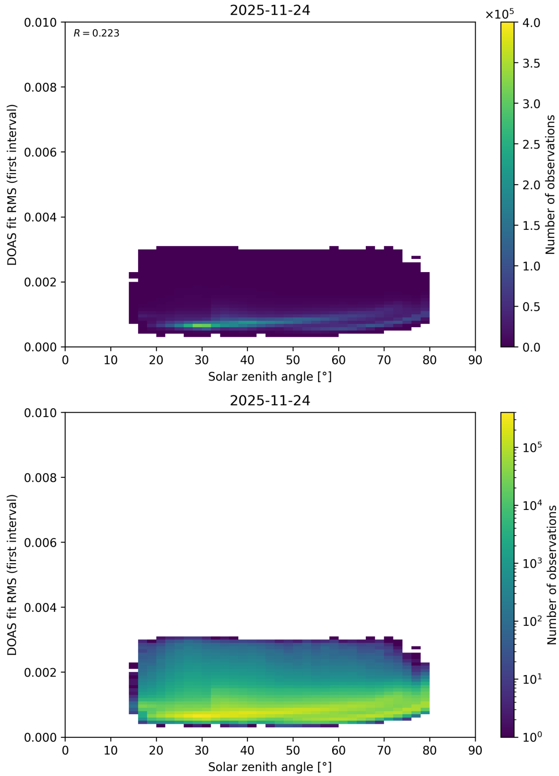
Figure 186: Scatter density plot of “Solar zenith angle” against “DOAS fit RMS (first interval)” for 2025-11-23 to 2025-11-25.
