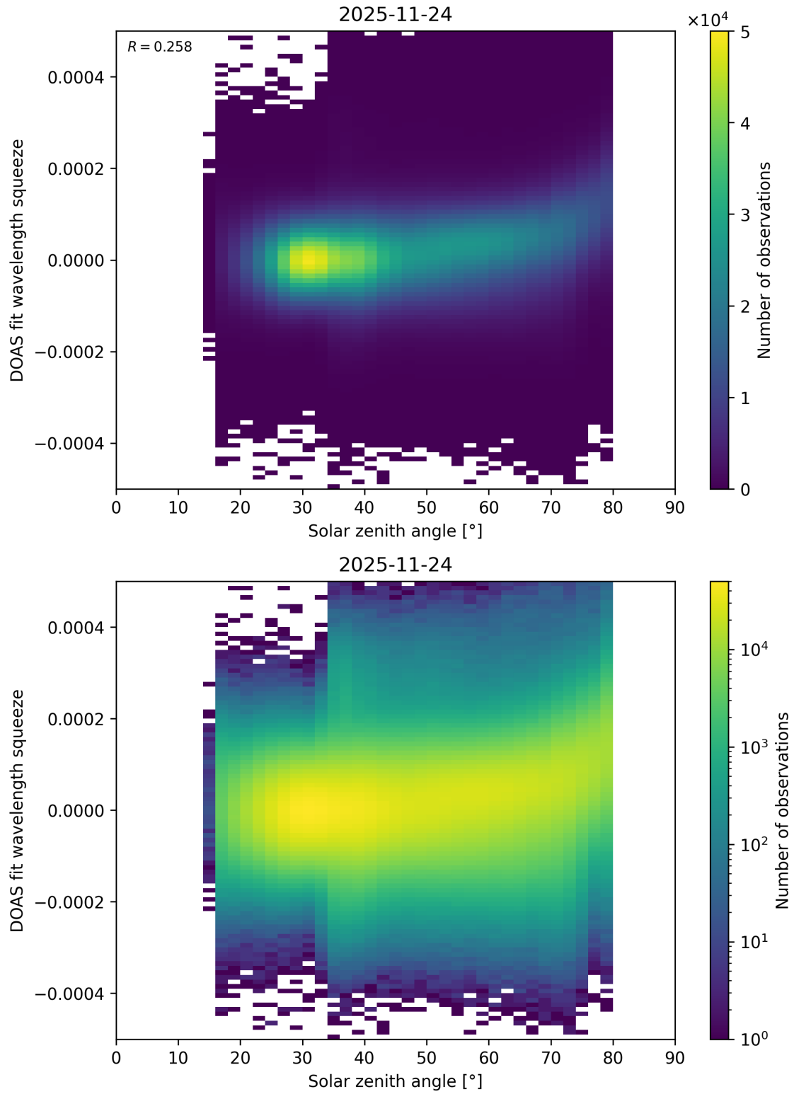
Figure 188: Scatter density plot of “Solar zenith angle” against “DOAS fit wavelength squeeze” for 2025-11-23 to 2025-11-25.
