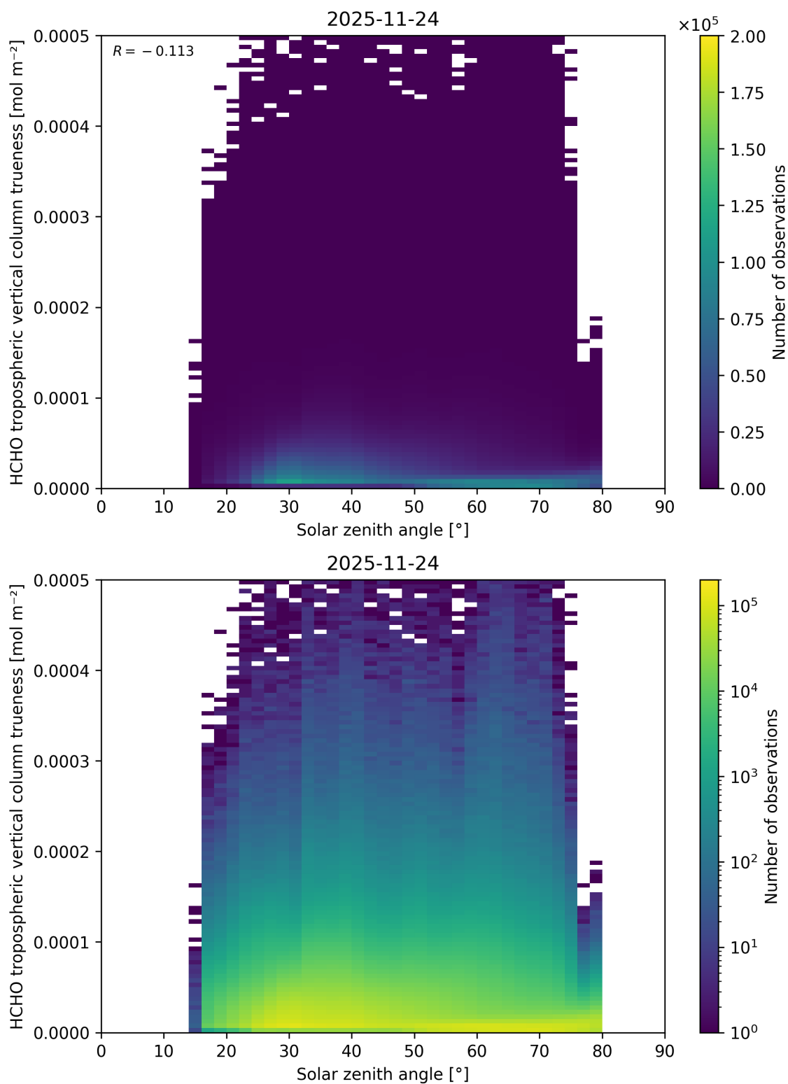
Figure 199: Scatter density plot of “Solar zenith angle” against “HCHO tropospheric vertical column trueness” for 2025-11-23 to 2025-11-25.
