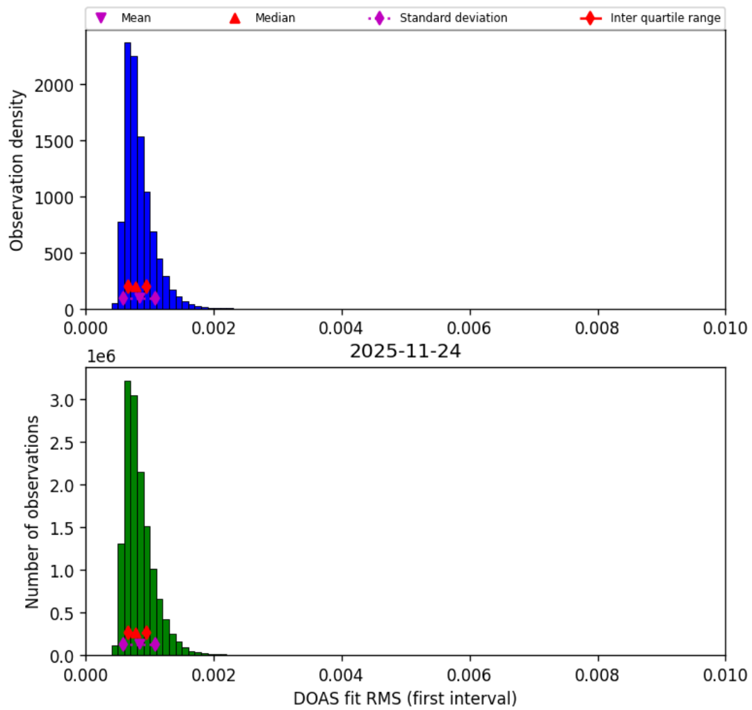
Figure 48: Histogram of “DOAS fit RMS (first interval)” for 2025-11-23 to 2025-11-25
