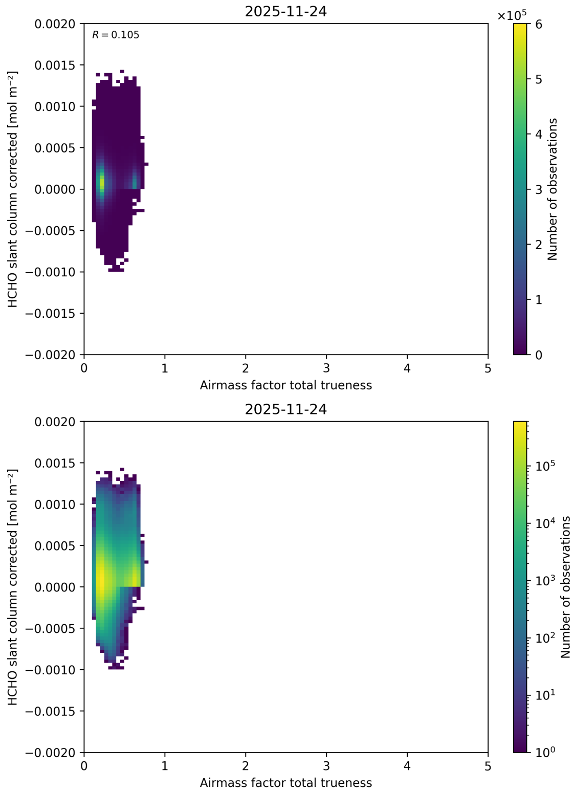
Figure 122: Scatter density plot of “Airmass factor total trueness” against “HCHO slant column corrected” for 2025-11-23 to 2025-11-25.
