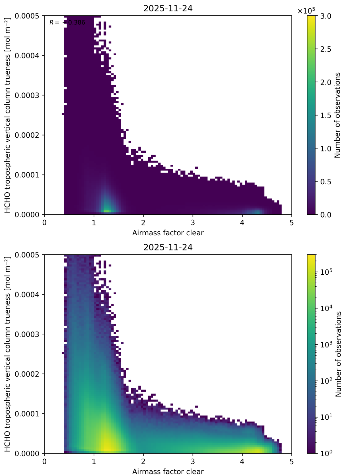
Figure 83: Scatter density plot of “Airmass factor clear” against “HCHO tropospheric vertical column trueness” for 2025-11-23 to 2025-11-25.
