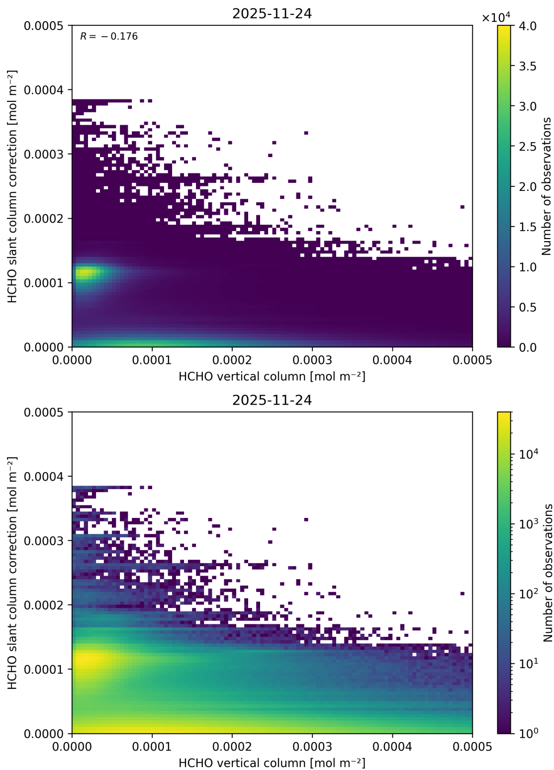
Figure 143: Scatter density plot of “HCHO vertical column” against “HCHO slant column correction” for 2025-11-23 to 2025-11-25.
