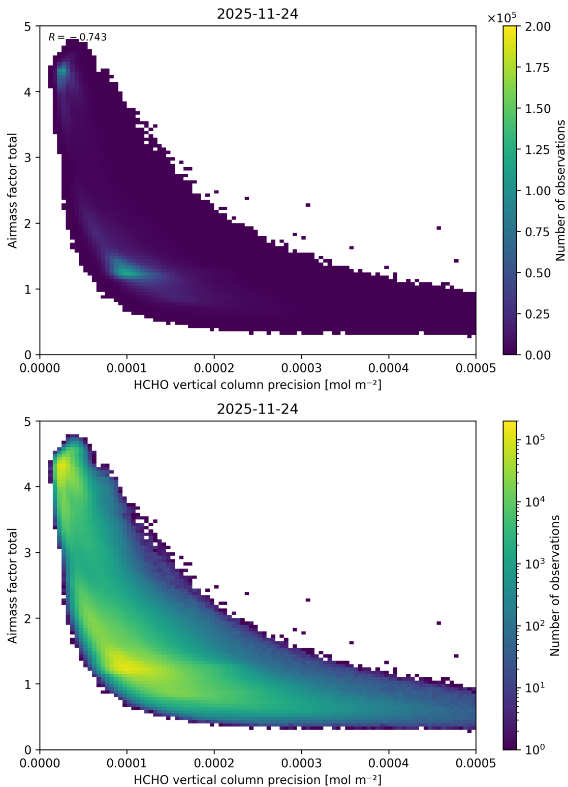
Figure 160: Scatter density plot of “HCHO vertical column precision” against “Airmass factor total” for 2025-11-23 to 2025-11-25.
