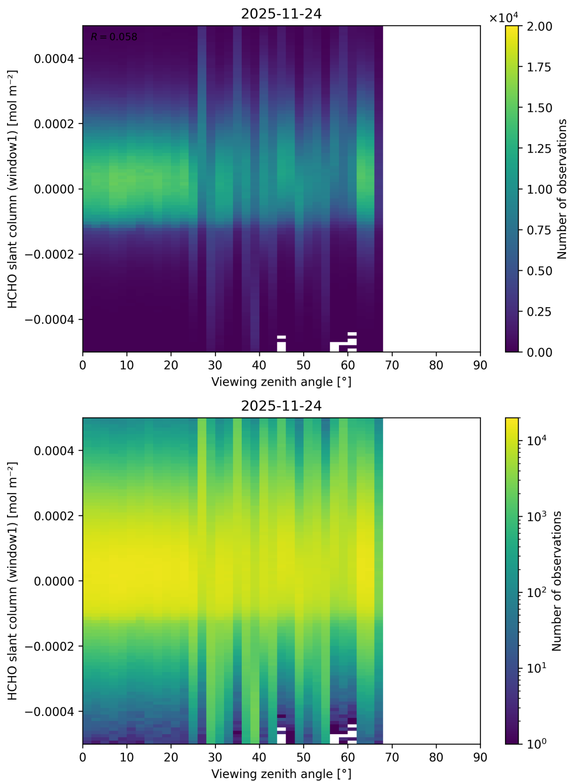
Figure 208: Scatter density plot of “Viewing zenith angle” against “HCHO slant column (window1)” for 2025-11-23 to 2025-11-25.
