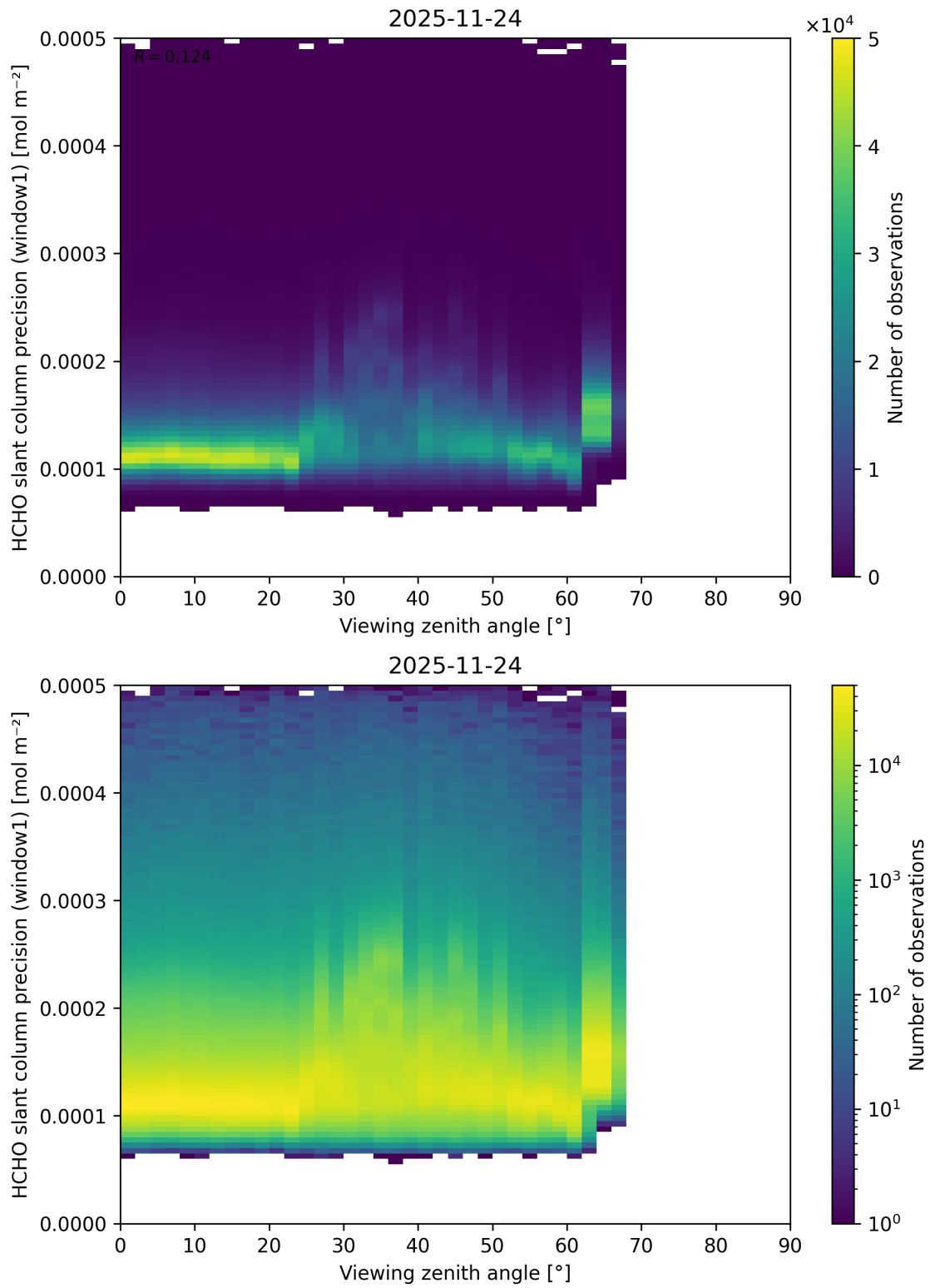
Figure 209: Scatter density plot of “Viewing zenith angle” against “HCHO slant column precision (window1)” for 2025-11-23 to 2025-11-25.
