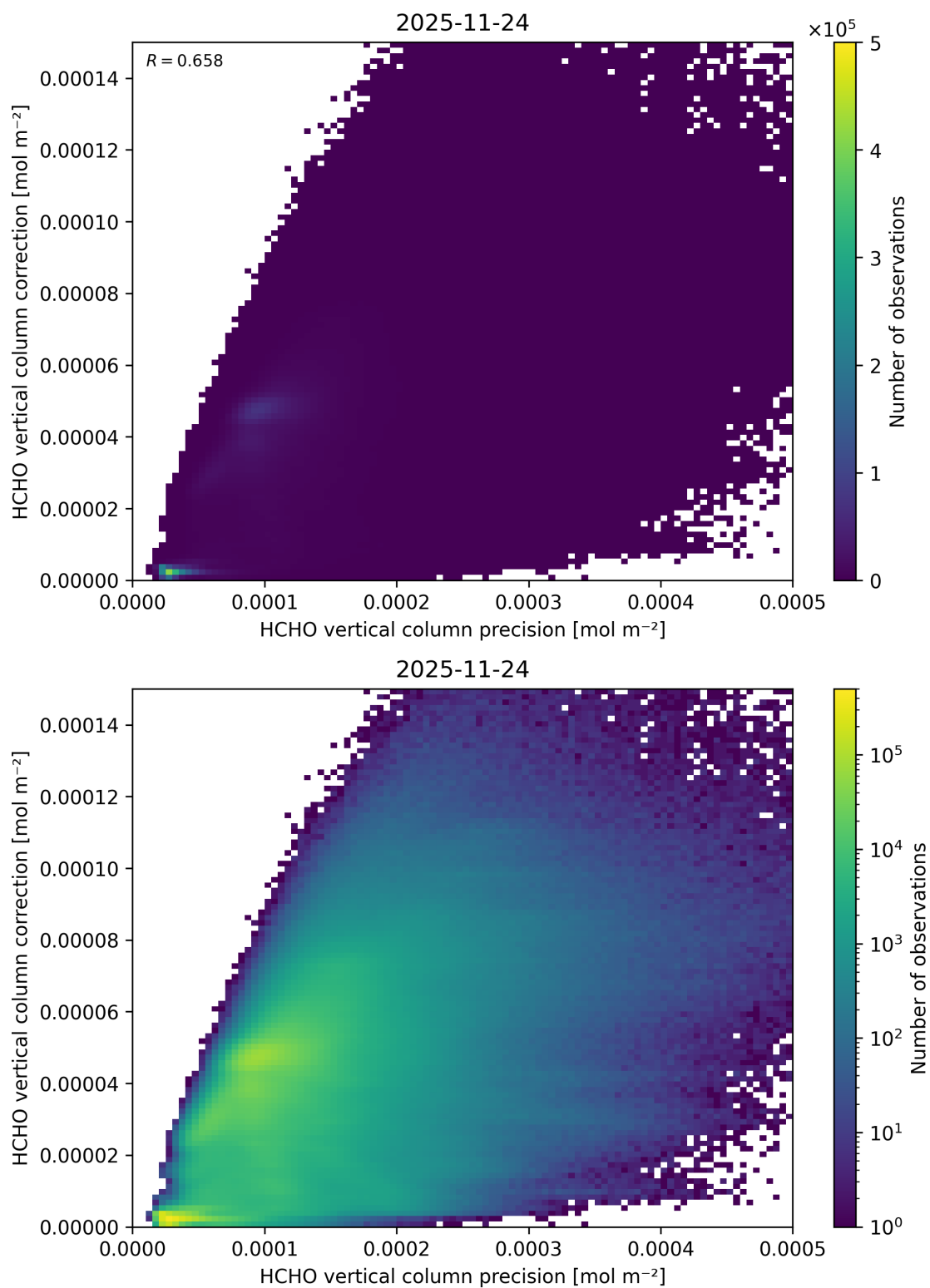
Figure 162: Scatter density plot of “HCHO vertical column precision” against “HCHO vertical column correction” for 2025-11-23 to 2025-11-25.
