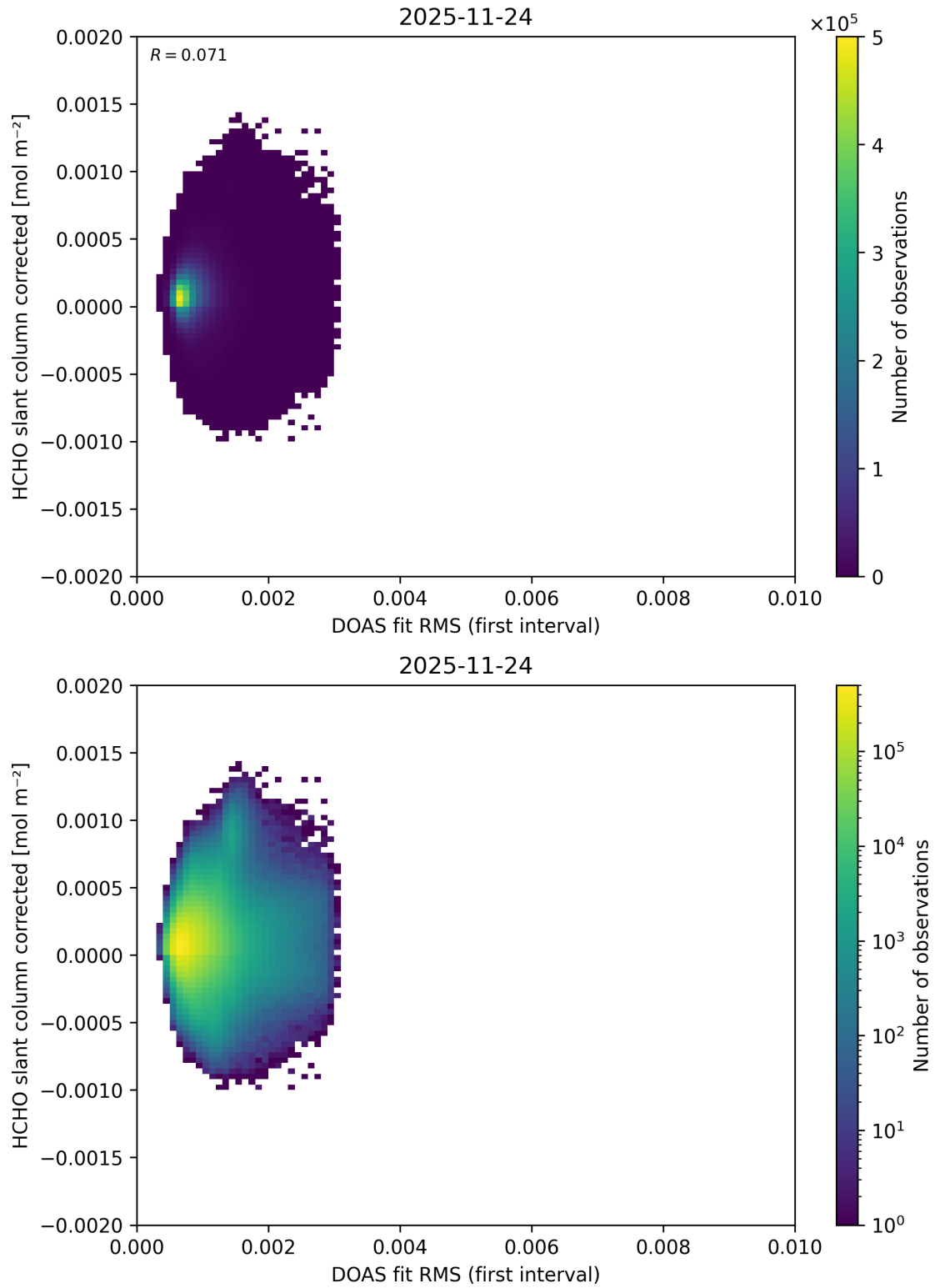
Figure 66: Scatter density plot of “DOAS fit RMS (first interval)” against “HCHO slant column corrected” for 2025-11-23 to 2025-11-25.
