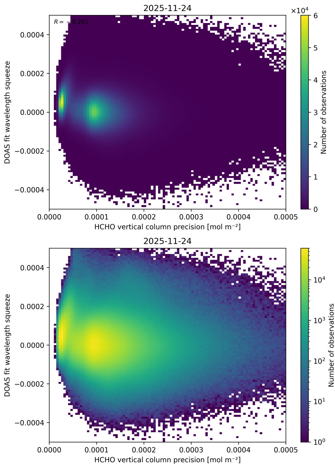
Figure 154: Scatter density plot of “HCHO vertical column precision” against “DOAS fit wavelength squeeze” for 2025-11-23 to 2025-11-25.
