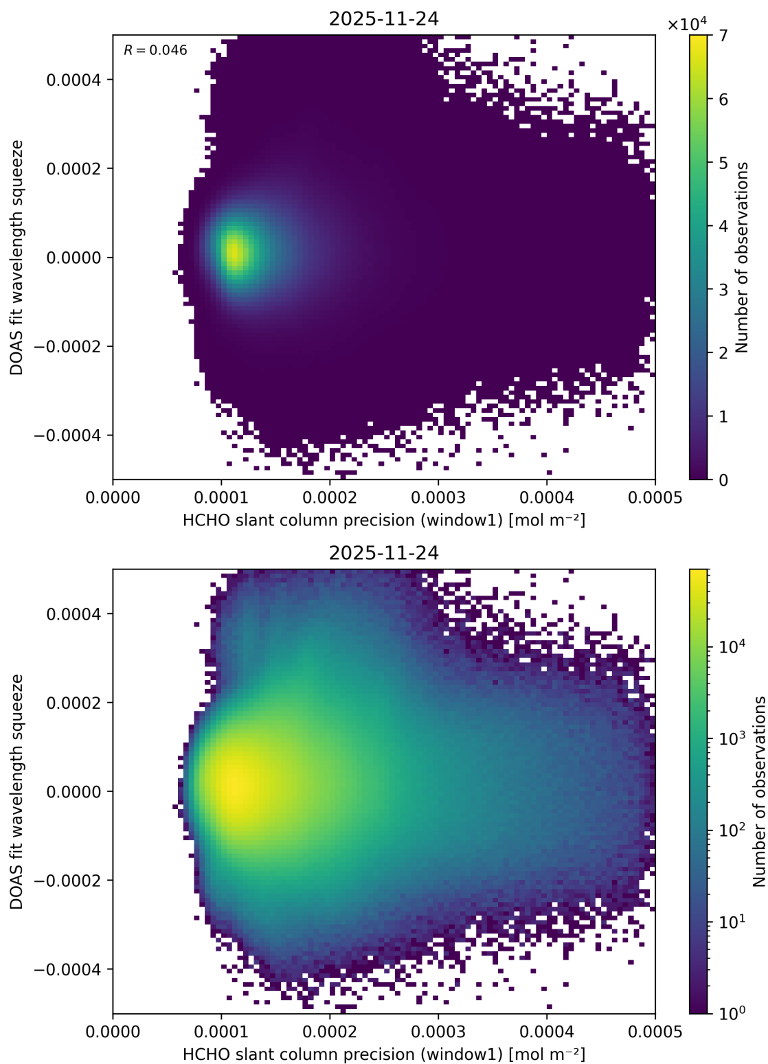
Figure 101: Scatter density plot of “HCHO slant column precision (window1)” against “DOAS fit wavelength squeeze” for 2025-11-23 to 2025-11-25.
