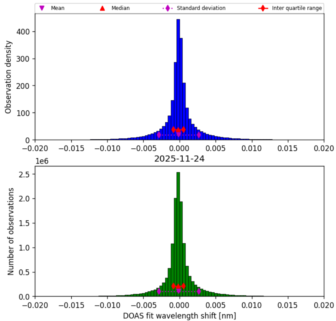
Figure 46: Histogram of “DOAS fit wavelength shift” for 2025-11-23 to 2025-11-25
