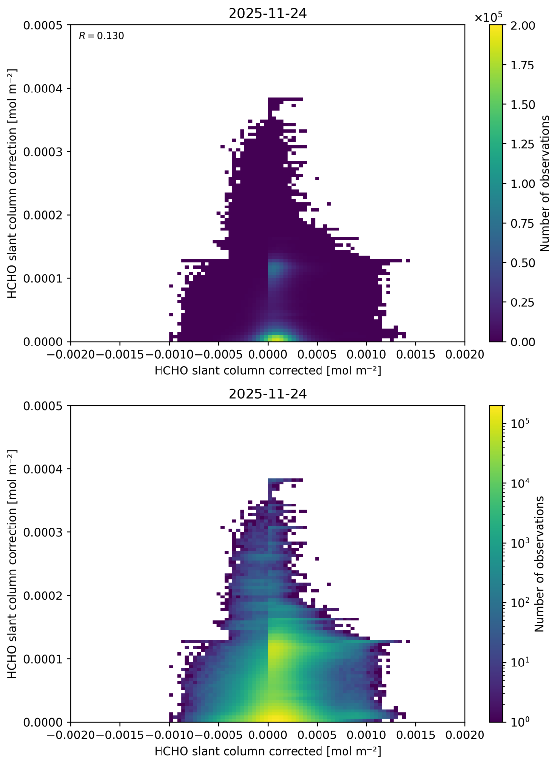
Figure 85: Scatter density plot of “HCHO slant column corrected” against “HCHO slant column correction” for 2025-11-23 to 2025-11-25.
