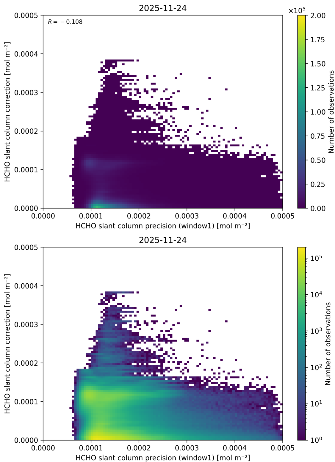
Figure 104: Scatter density plot of “HCHO slant column precision (window1)” against “HCHO slant column correction” for 2025-11-23 to 2025-11-25.
