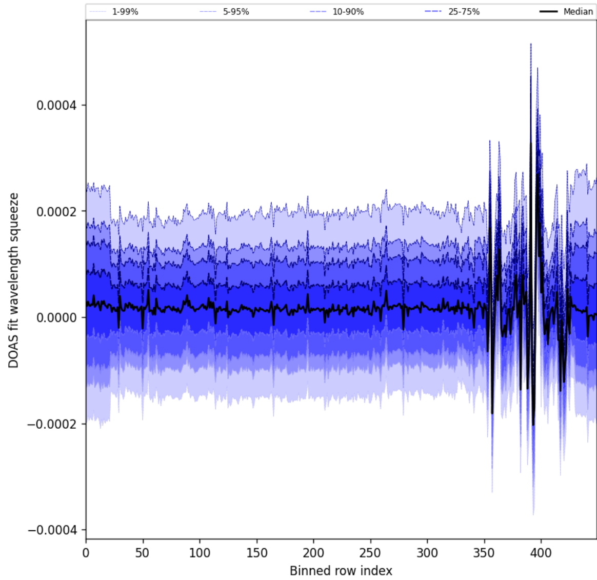
Figure 62: Along track statistics of “DOAS fit wavelength squeeze” for 2025-11-23 to 2025-11-25
