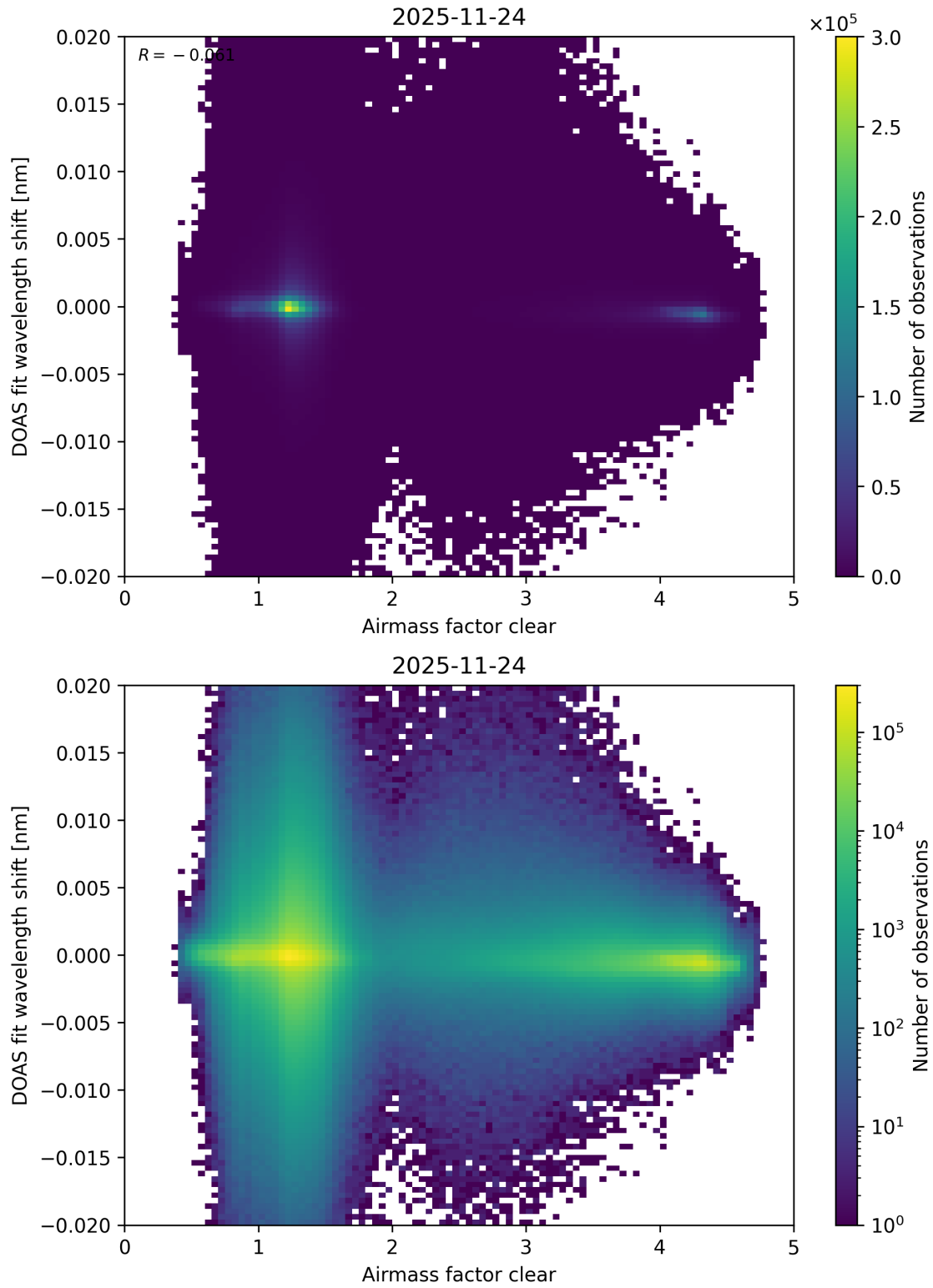
Figure 79: Scatter density plot of “Airmass factor clear” against “DOAS fit wavelength shift” for 2025-11-23 to 2025-11-25.
