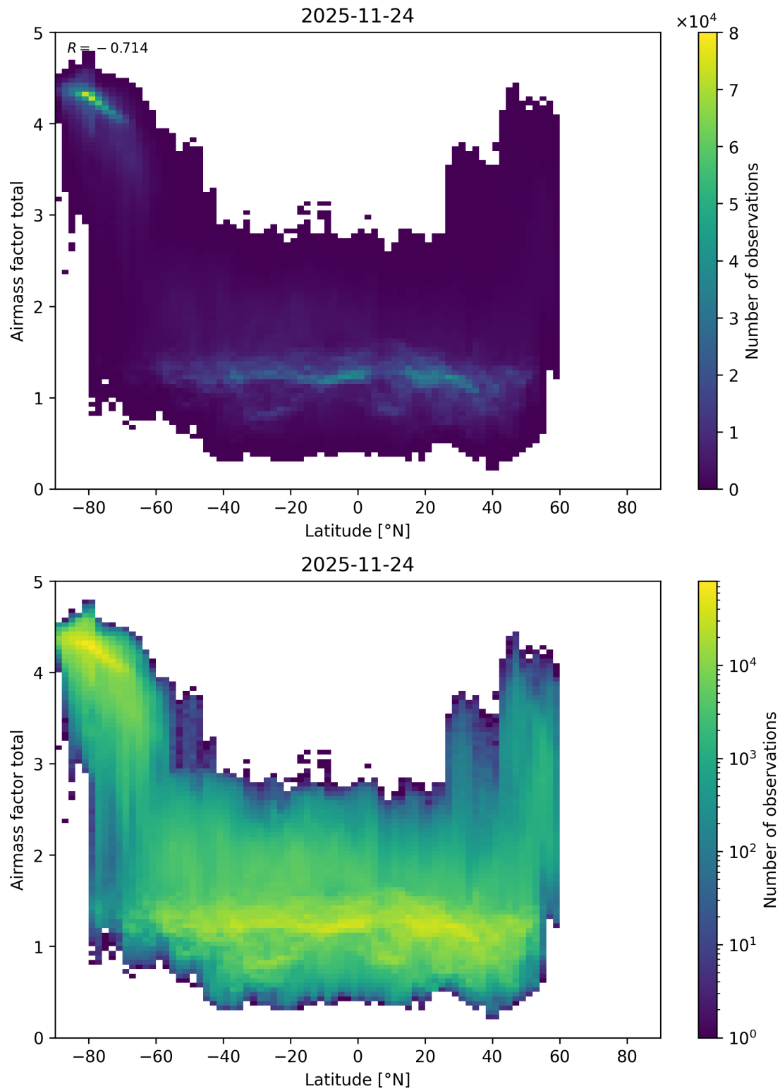
Figure 179: Scatter density plot of “Latitude” against “Airmass factor total” for 2025-11-23 to 2025-11-25.
