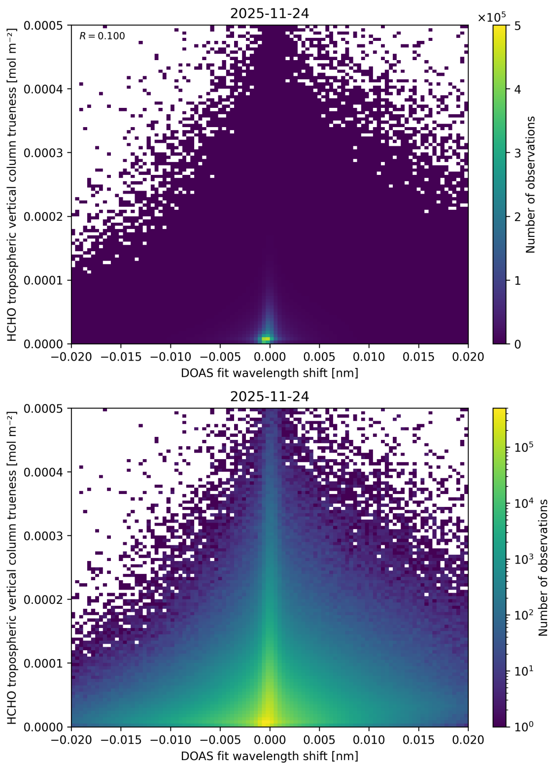
Figure 73: Scatter density plot of “DOAS fit wavelength shift” against “HCHO tropospheric vertical column trueness” for 2025-11-23 to 2025-11-25.
