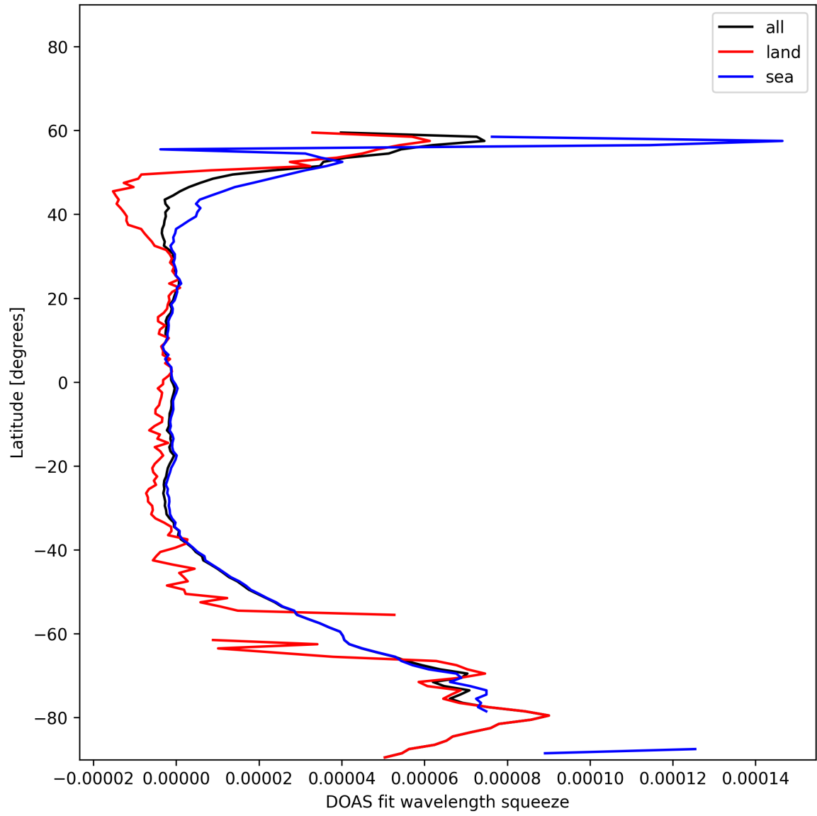
Figure 32: Zonal average of “DOAS fit wavelength squeeze” for 2025-11-23 to 2025-11-25.
