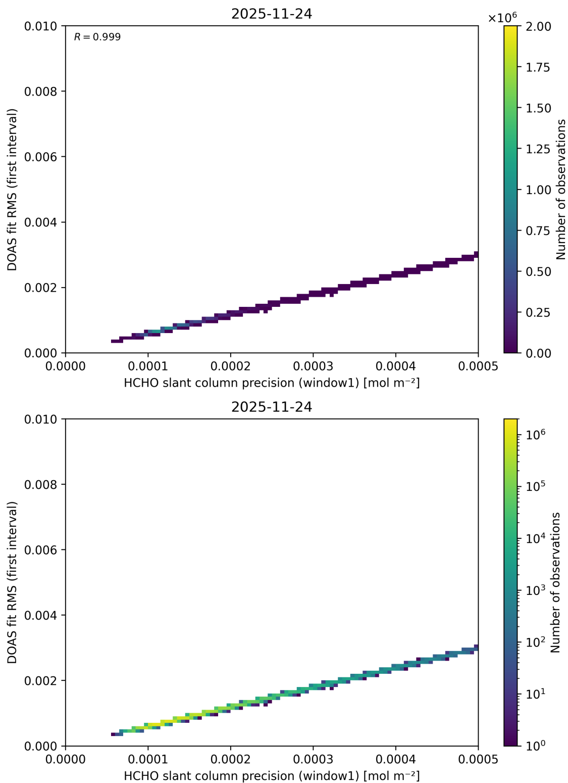
Figure 99: Scatter density plot of “HCHO slant column precision (window1)” against “DOAS fit RMS (first interval)” for 2025-11-23 to 2025-11-25.
