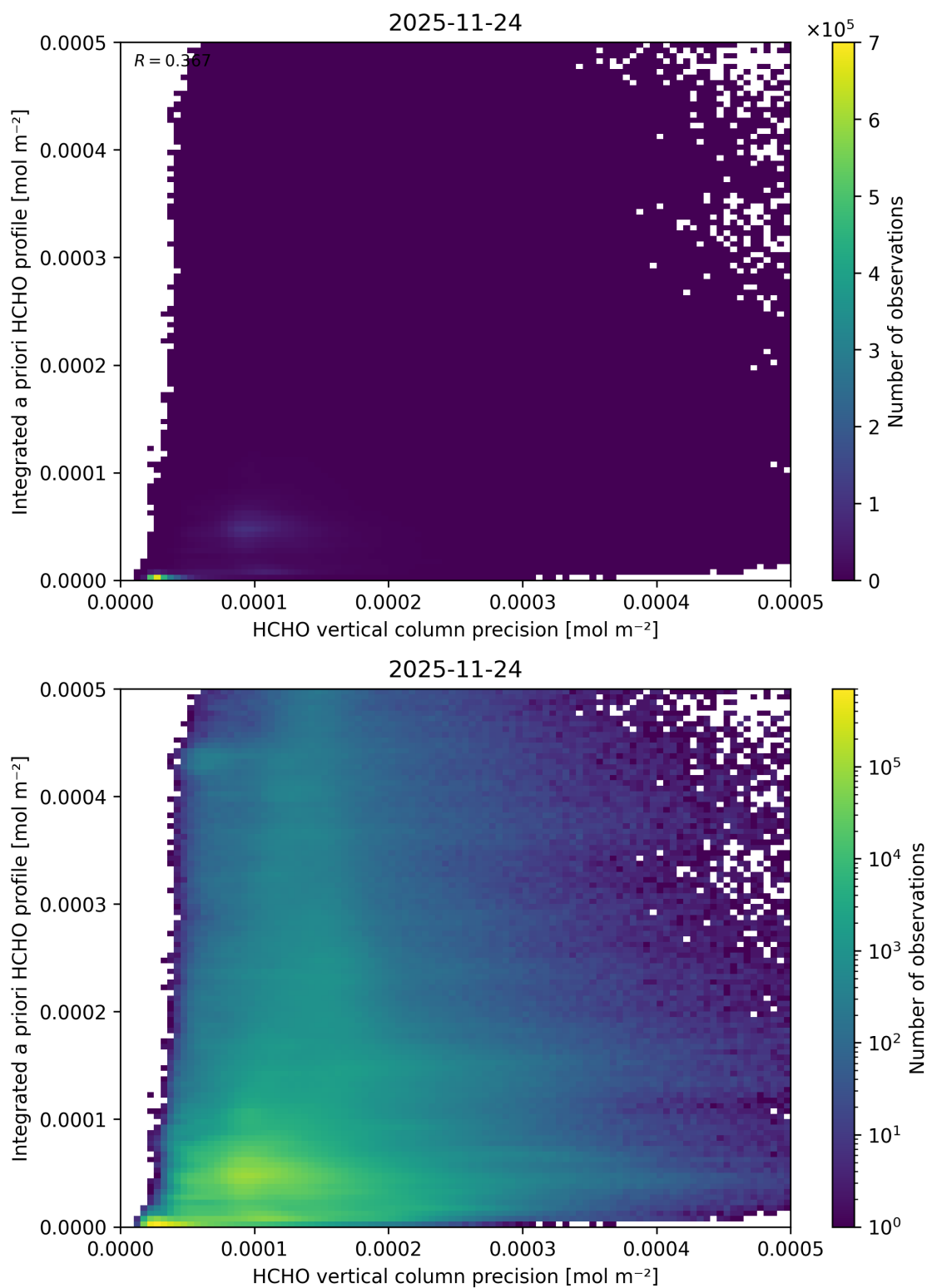
Figure 164: Scatter density plot of “HCHO vertical column precision” against “Integrated a priori HCHO profile” for 2025-11-23 to 2025-11-25.
