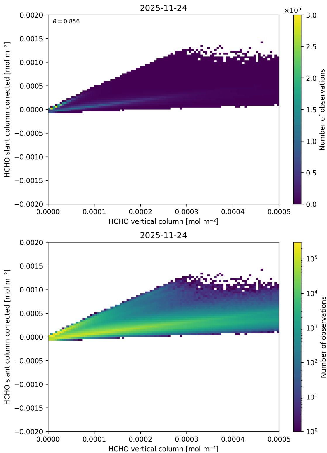
Figure 142: Scatter density plot of “HCHO vertical column” against “HCHO slant column corrected” for 2025-11-23 to 2025-11-25.
