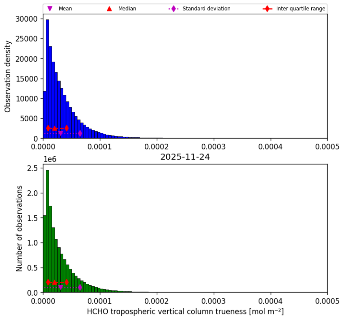
Figure 50: Histogram of “HCHO tropospheric vertical column trueness” for 2025-11-23 to 2025-11-25
