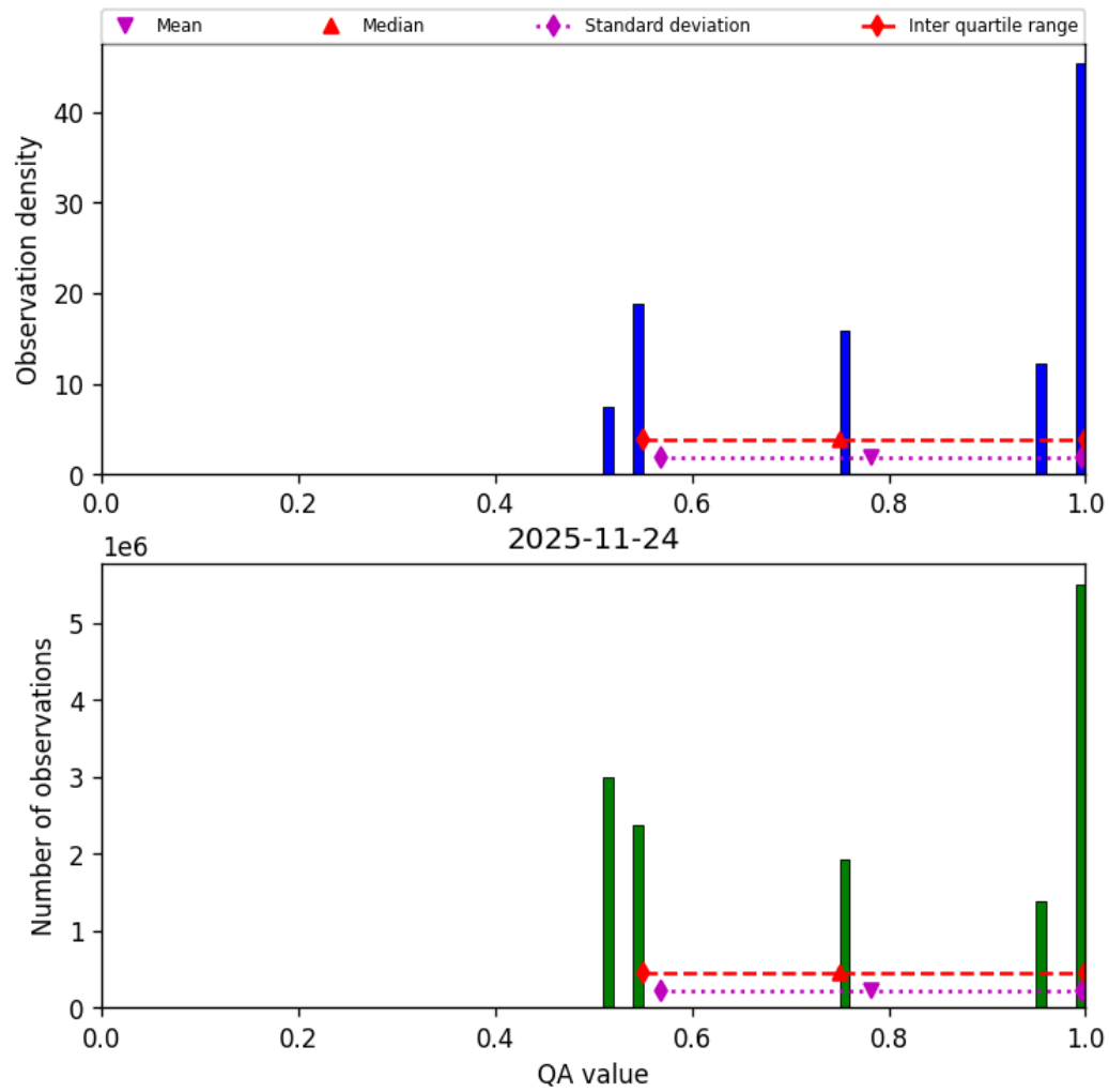
Figure 36: Histogram of “QA value” for 2025-11-23 to 2025-11-25
