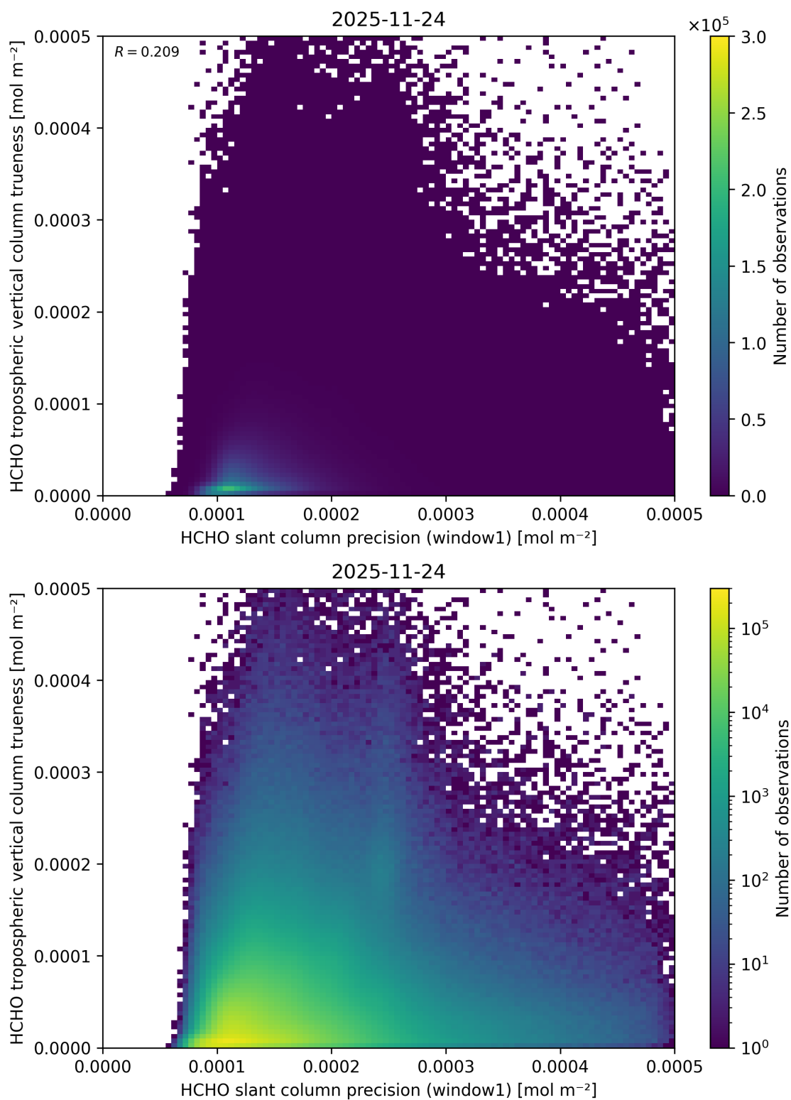
Figure 107: Scatter density plot of “HCHO slant column precision (window1)” against “HCHO tropospheric vertical column trueness” for 2025-11-23 to 2025-11-25.
