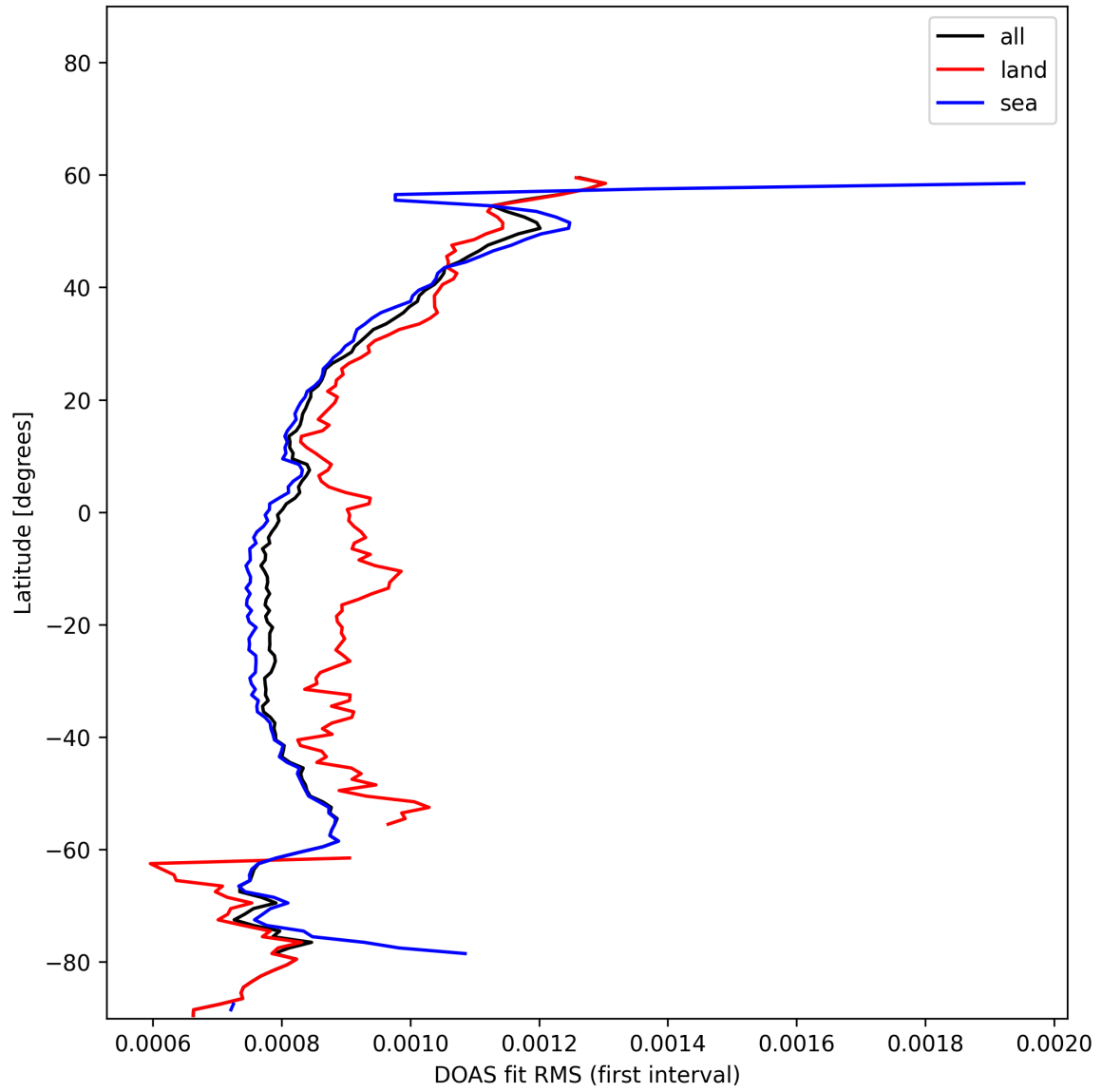
Figure 33: Zonal average of "DOAS fit RMS (first interval)" for 2025-11-23 to 2025-11-25.
