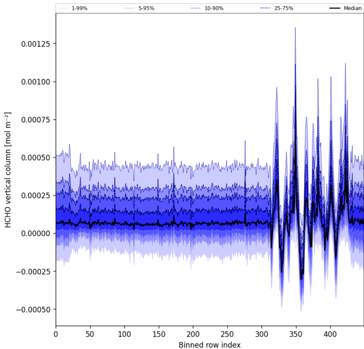
Figure 52: Along track statistics of “HCHO vertical column” for 2025-11-23 to 2025-11-25
