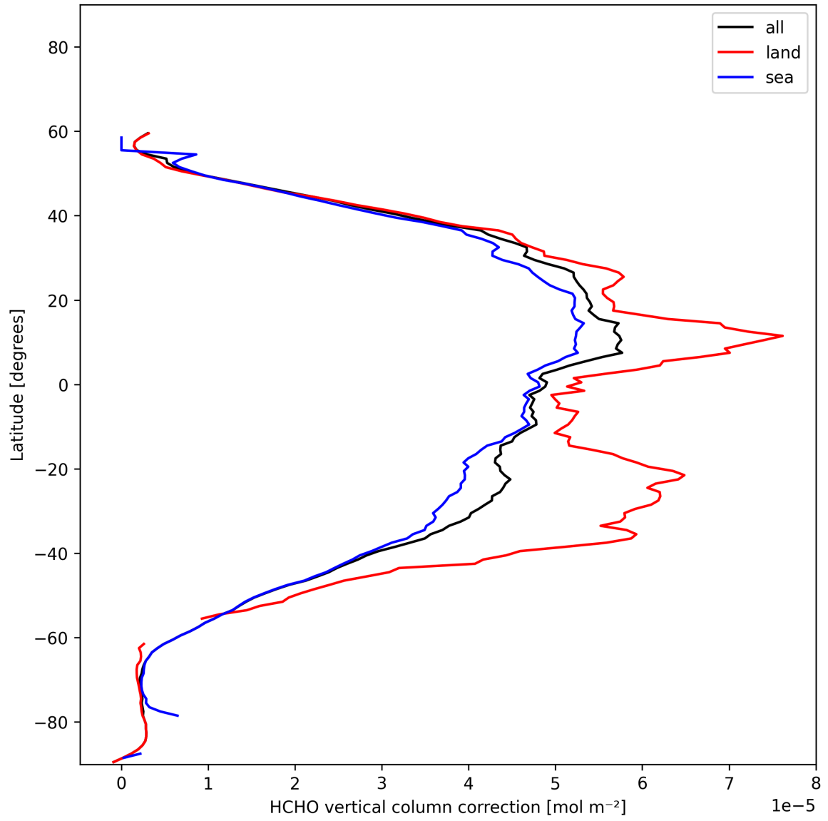
Figure 24: Zonal average of “HCHO vertical column correction” for 2025-11-23 to 2025-11-25.
