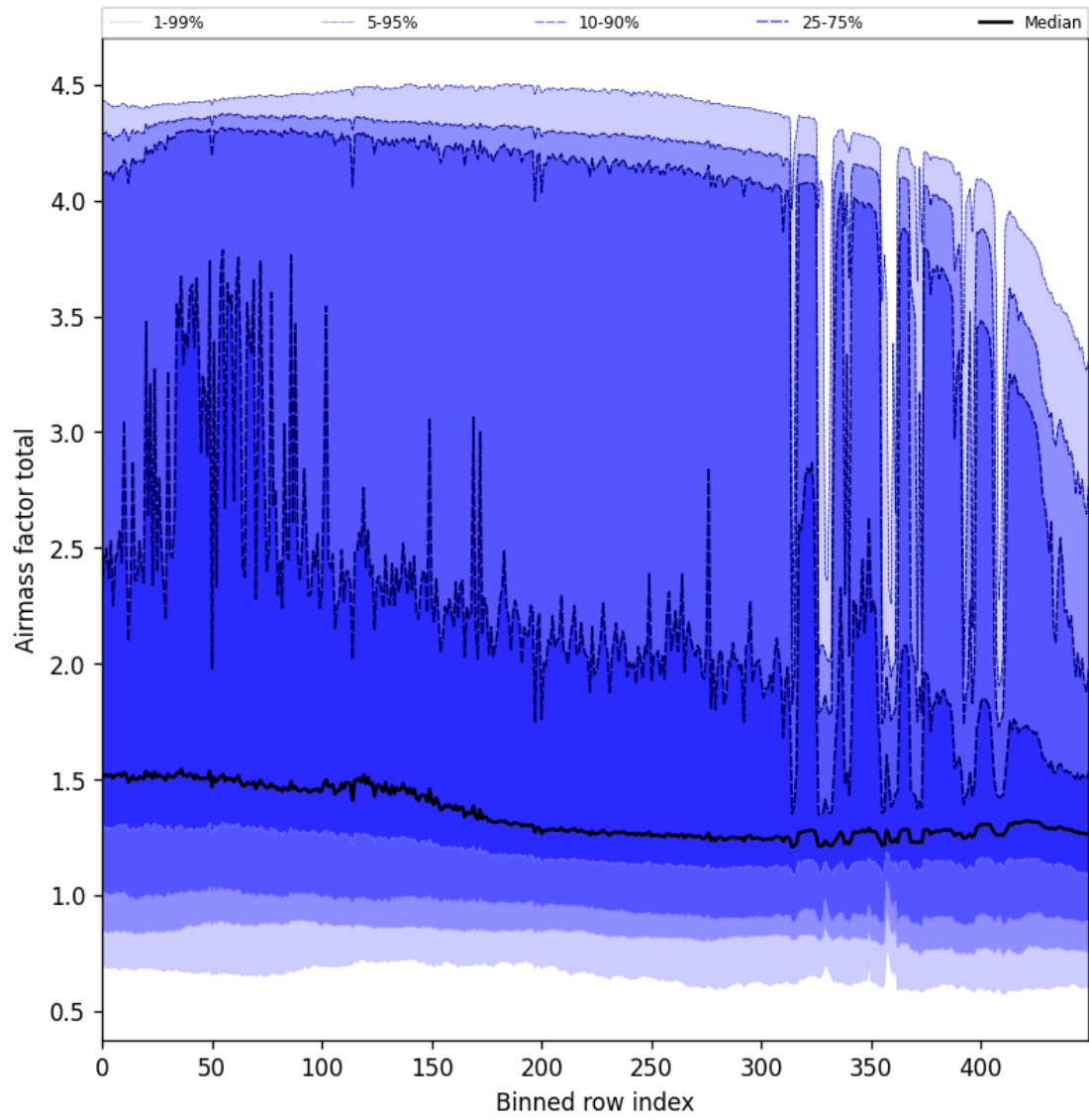
Figure 57: Along track statistics of “Airmass factor total” for 2025-11-23 to 2025-11-25
