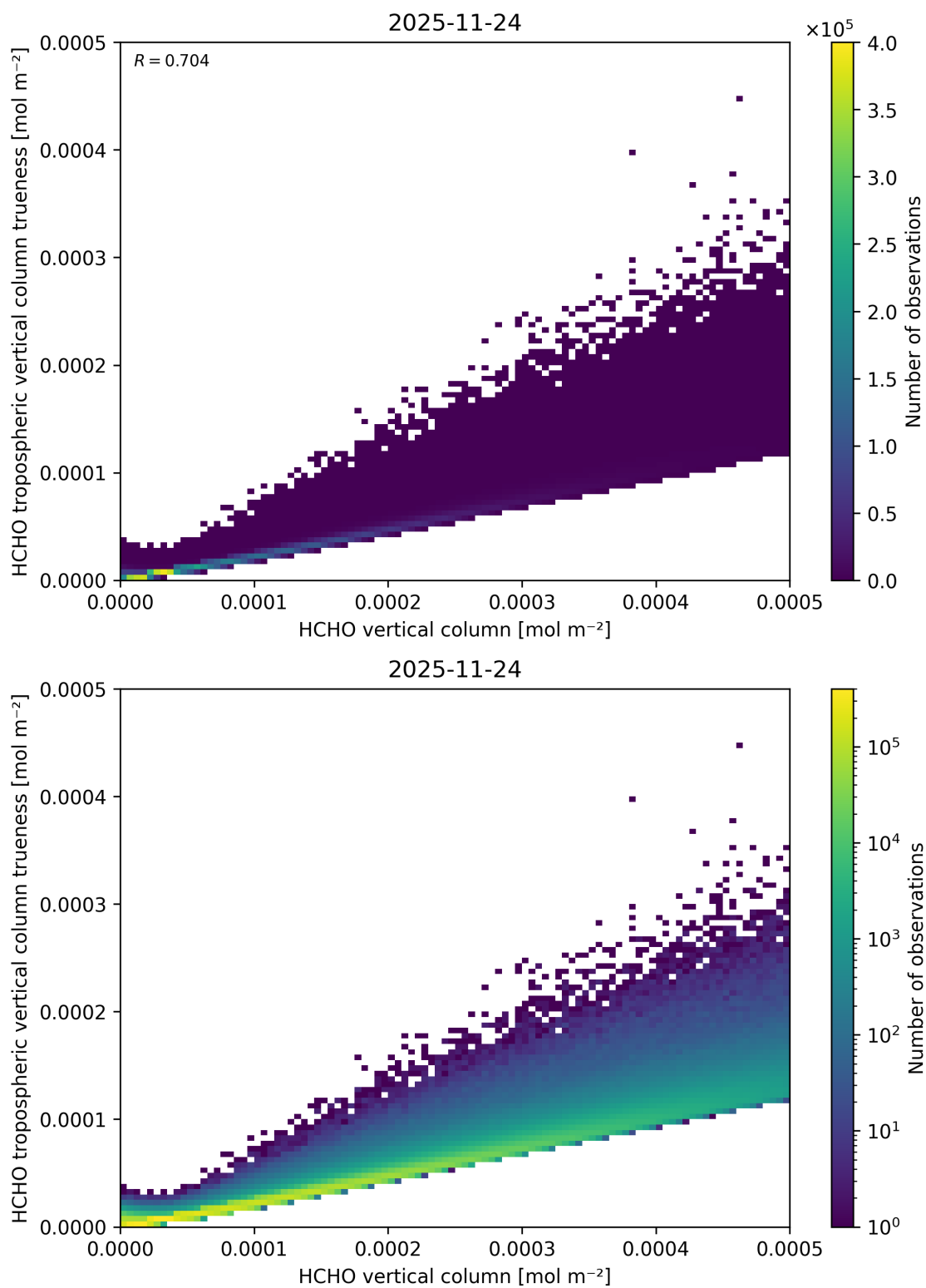
Figure 150: Scatter density plot of “HCHO vertical column” against “HCHO tropospheric vertical column trueness” for 2025-11-23 to 2025-11-25.
