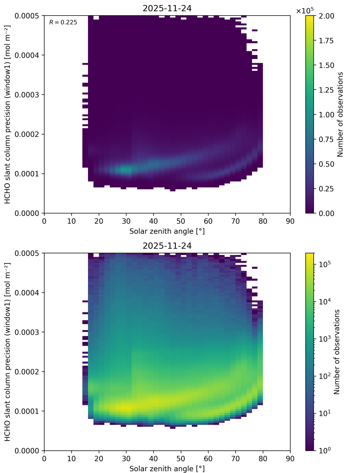
Figure 193: Scatter density plot of “Solar zenith angle” against “HCHO slant column precision (window1)” for 2025-11-23 to 2025-11-25.
