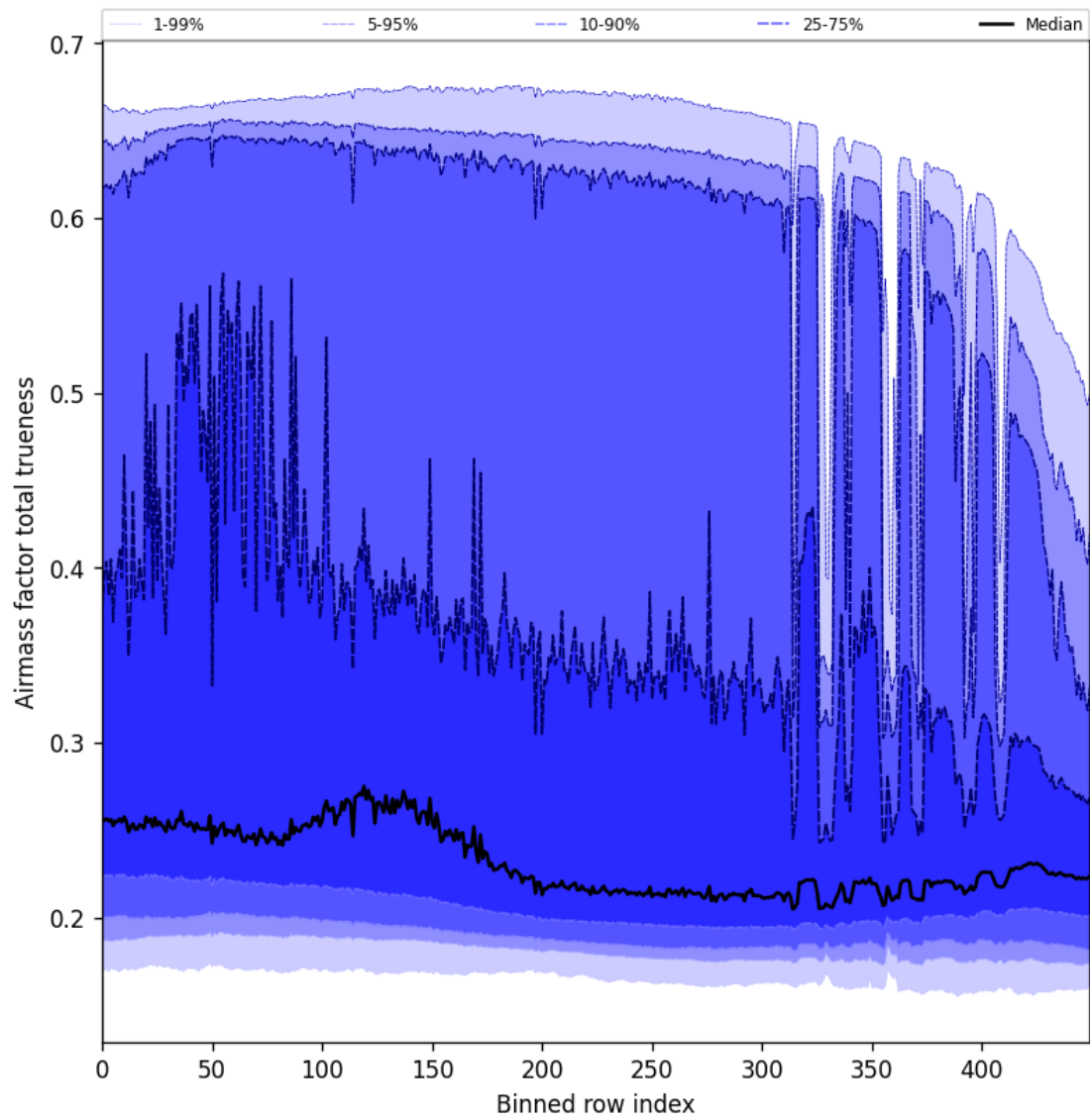
Figure 58: Along track statistics of “Airmass factor total trueness” for 2025-11-23 to 2025-11-25
