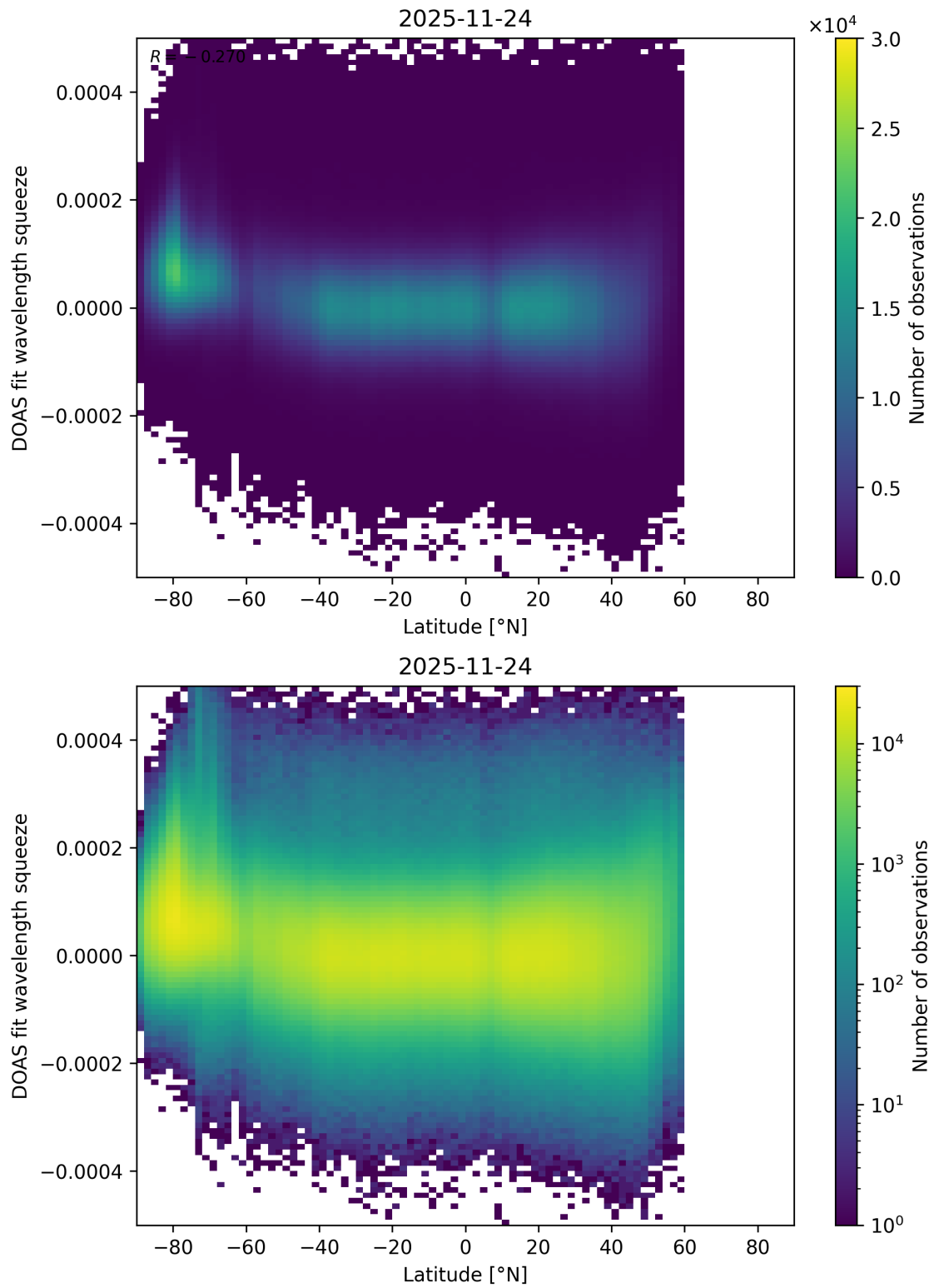
Figure 173: Scatter density plot of “Latitude” against “DOAS fit wavelength squeeze” for 2025-11-23 to 2025-11-25.
