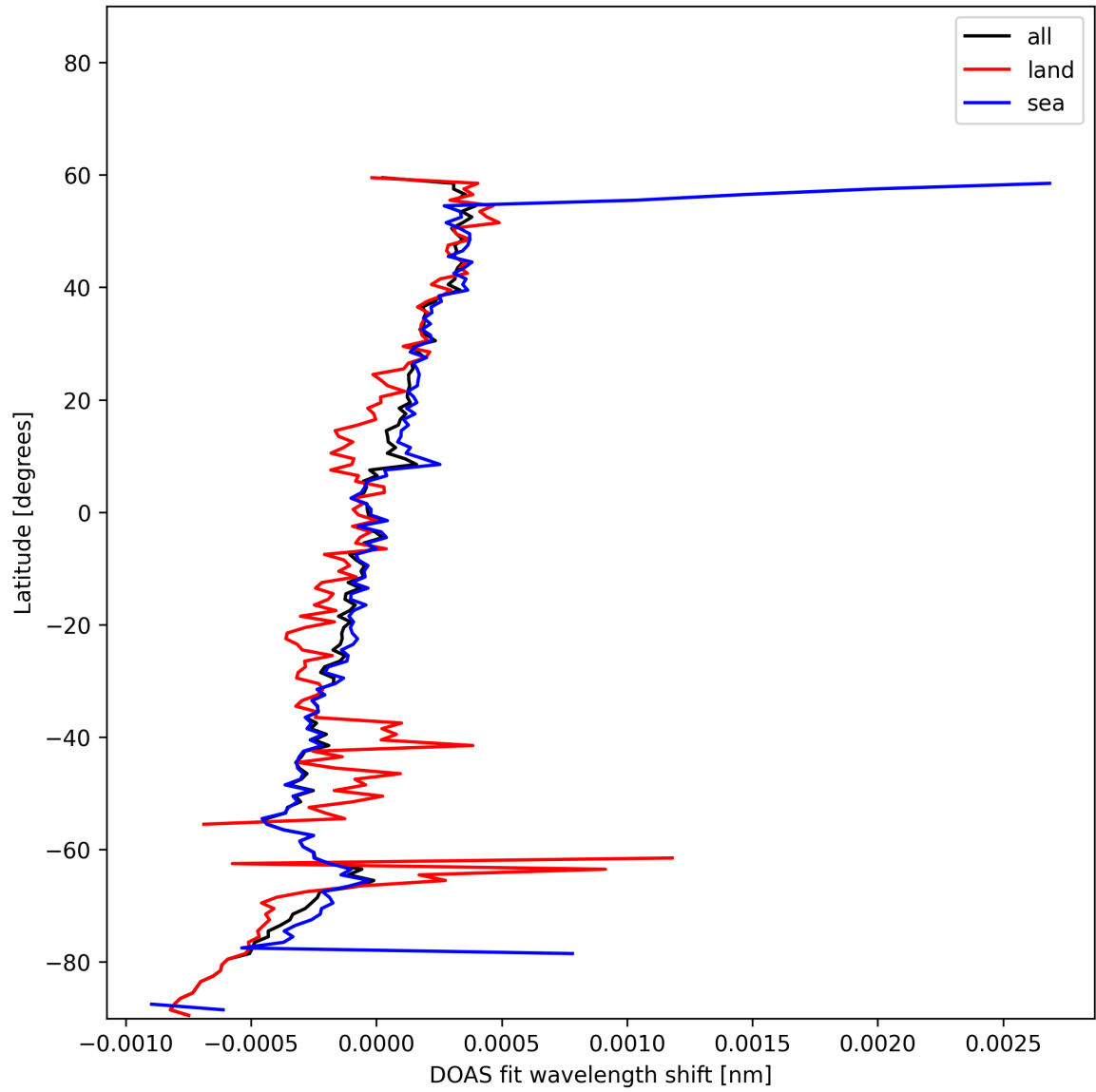
Figure 31: Zonal average of "DOAS fit wavelength shift" for 2025-11-23 to 2025-11-25.
