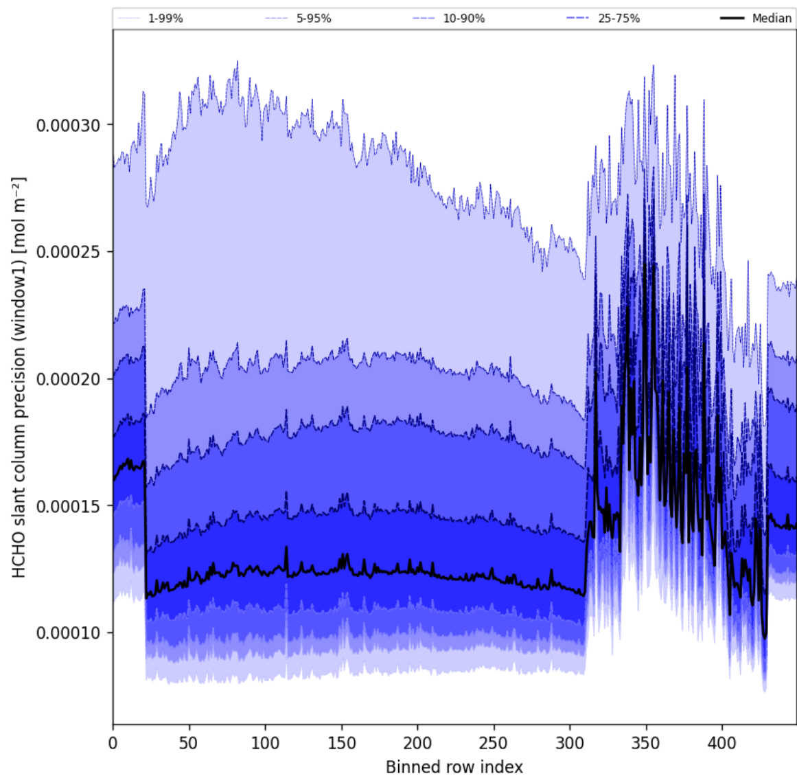
Figure 56: Along track statistics of “HCHO slant column precision (window1)” for 2025-11-23 to 2025-11-25
