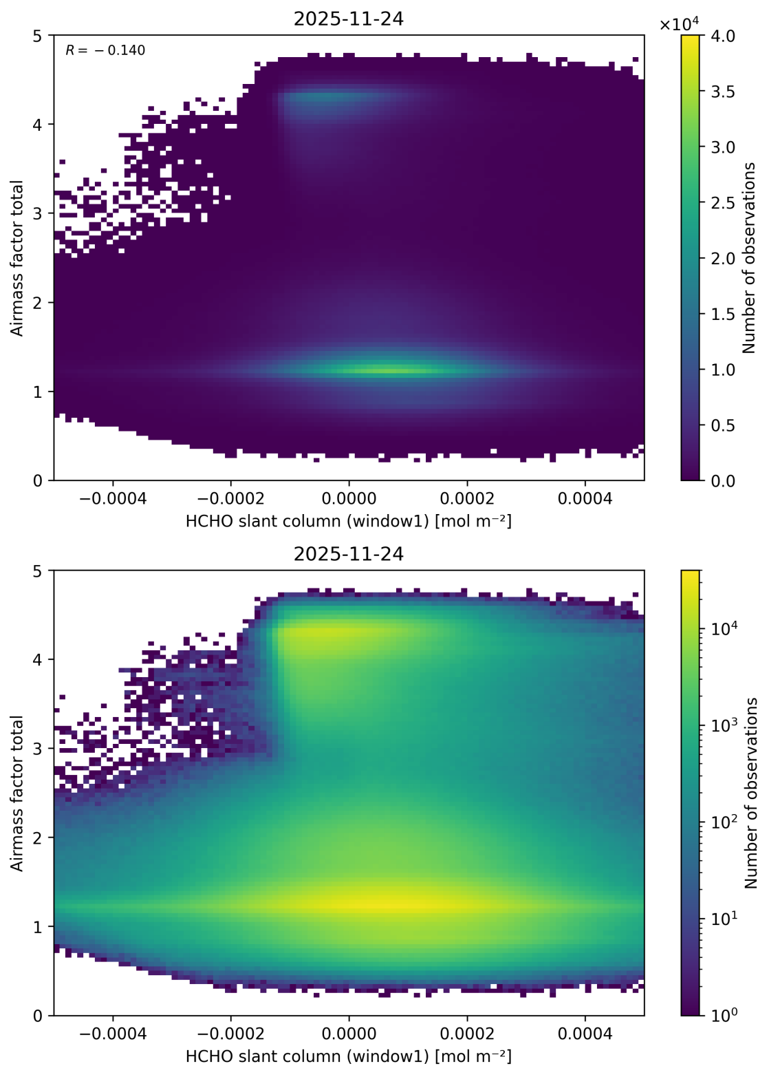
Figure 95: Scatter density plot of “HCHO slant column (window1)” against “Airmass factor total” for 2025-11-23 to 2025-11-25.
