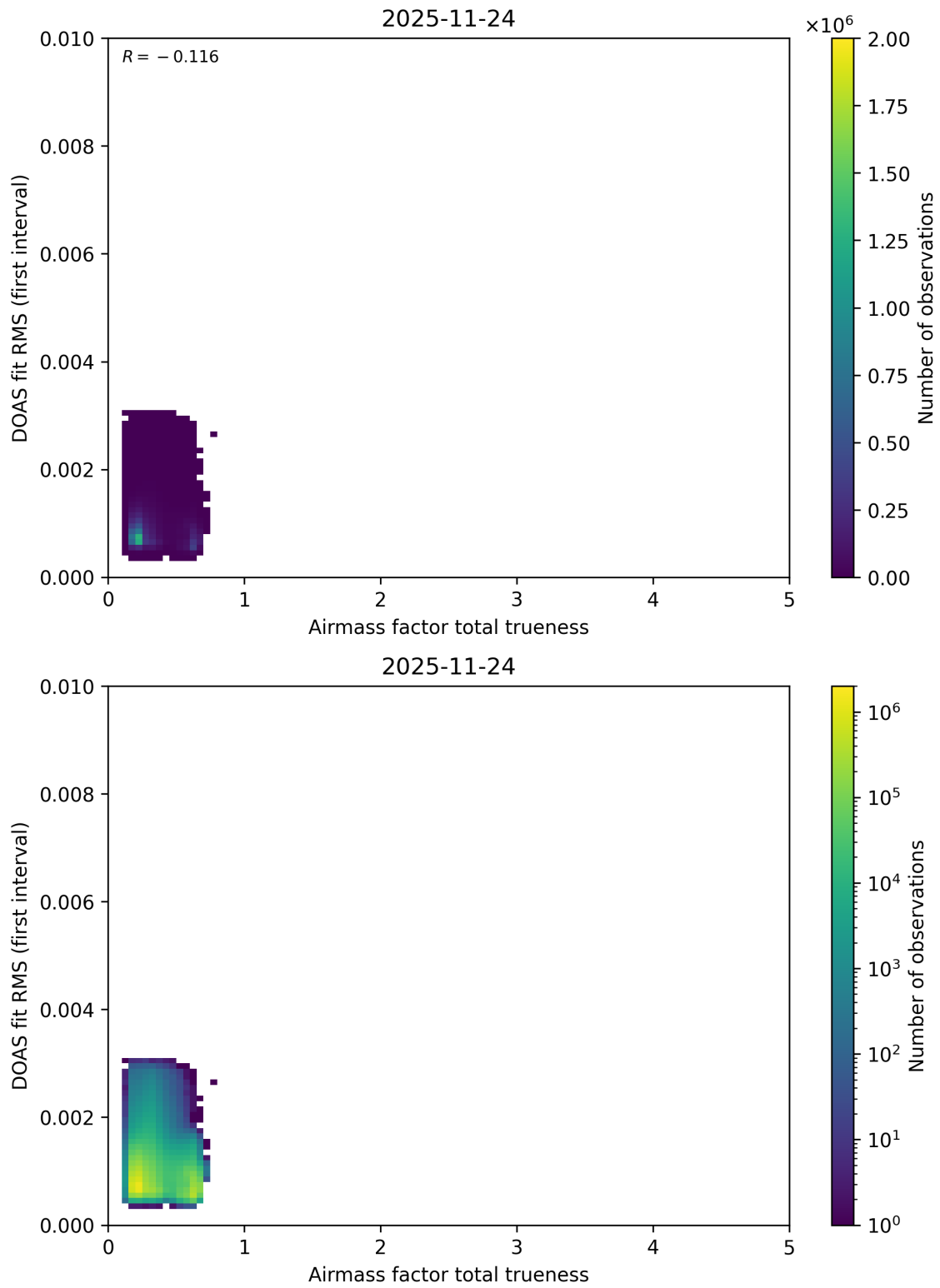
Figure 118: Scatter density plot of “Airmass factor total trueness” against “DOAS fit RMS (first interval)” for 2025-11-23 to 2025-11-25.
