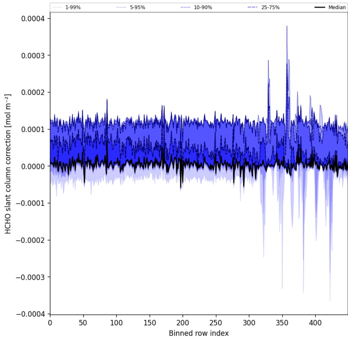
Figure 64: Along track statistics of “HCHO slant column correction” for 2025-11-23 to 2025-11-25
