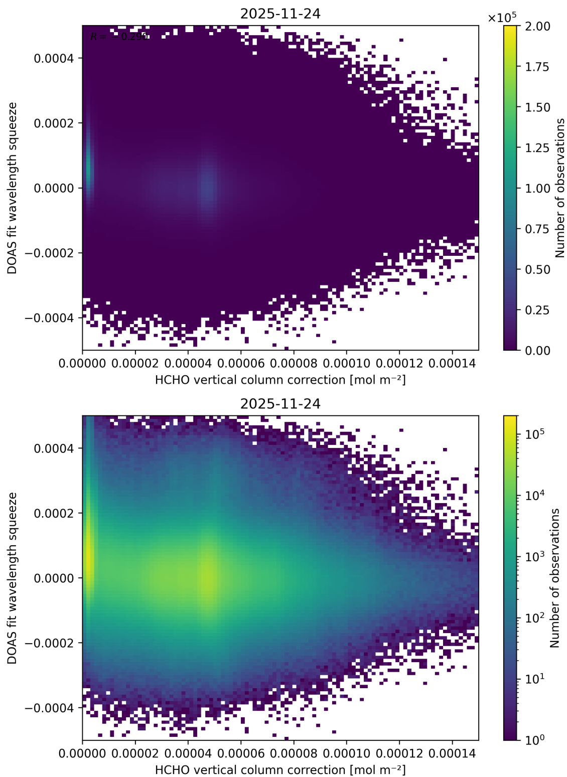
Figure 128: Scatter density plot of “HCHO vertical column correction” against “DOAS fit wavelength squeeze” for 2025-11-23 to 2025-11-25.
