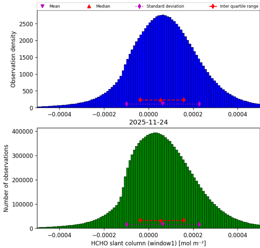
Figure 40: Histogram of “HCHO slant column (window1)” for 2025-11-23 to 2025-11-25
