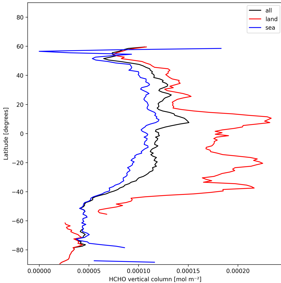
Figure 22: Zonal average of “HCHO vertical column” for 2025-11-23 to 2025-11-25.
