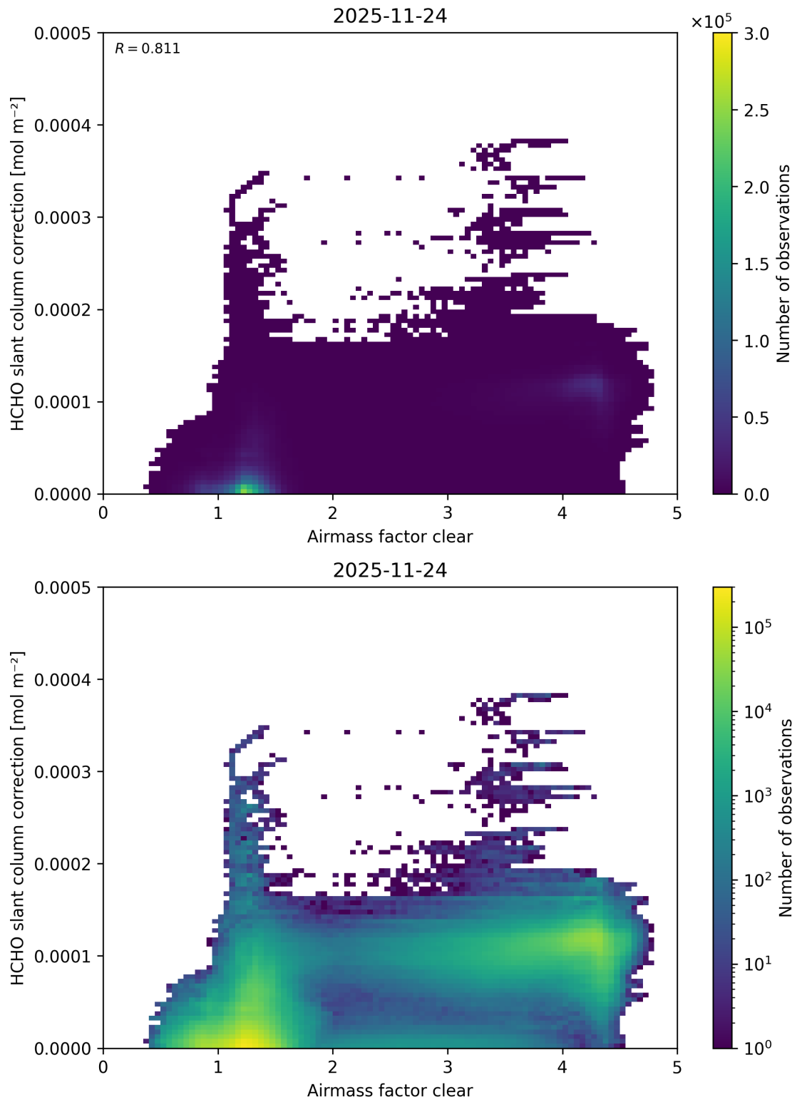
Figure 82: Scatter density plot of “Airmass factor clear” against “HCHO slant column correction” for 2025-11-23 to 2025-11-25.
