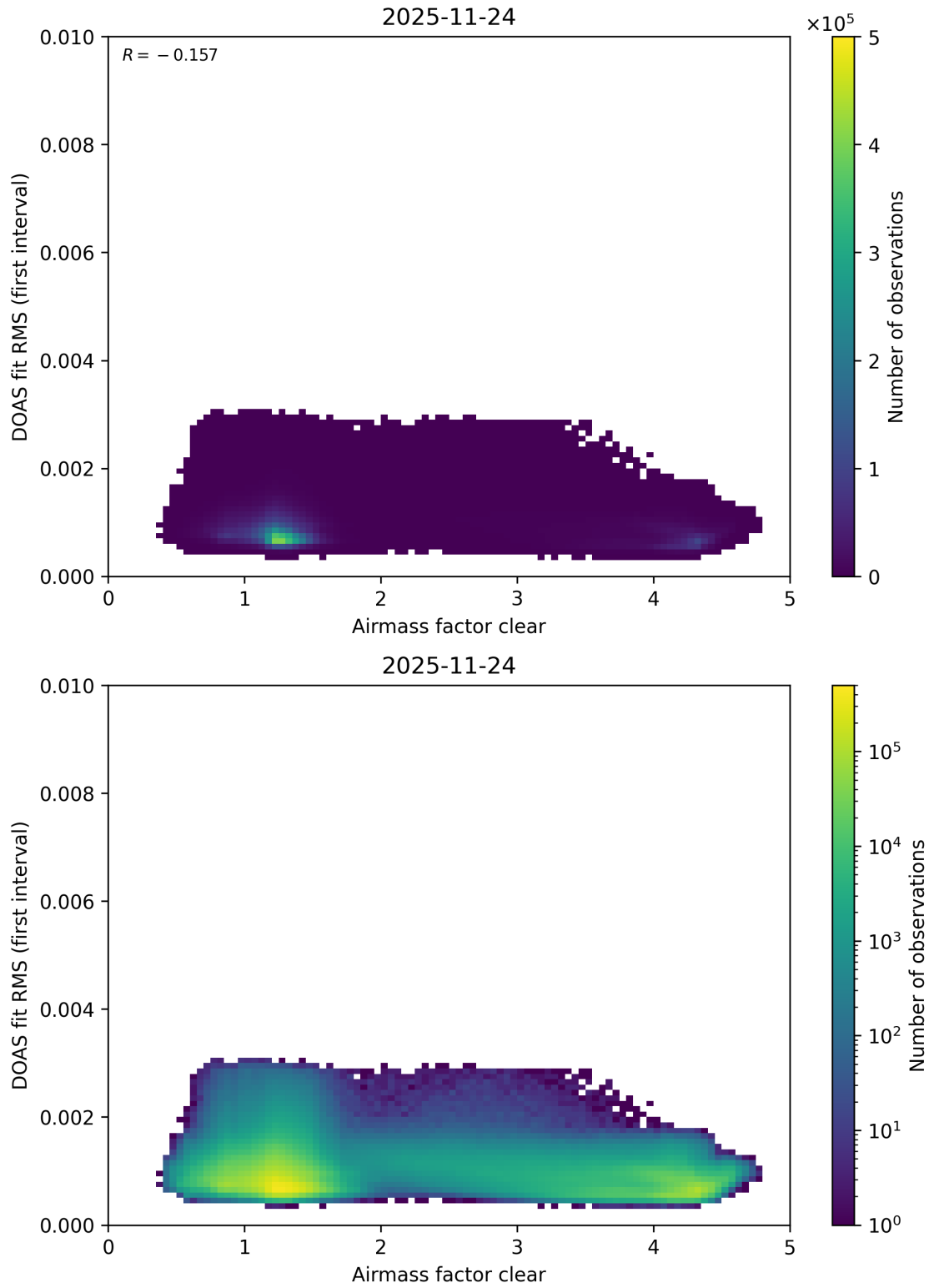
Figure 78: Scatter density plot of “Airmass factor clear” against “DOAS fit RMS (first interval)” for 2025-11-23 to 2025-11-25.
