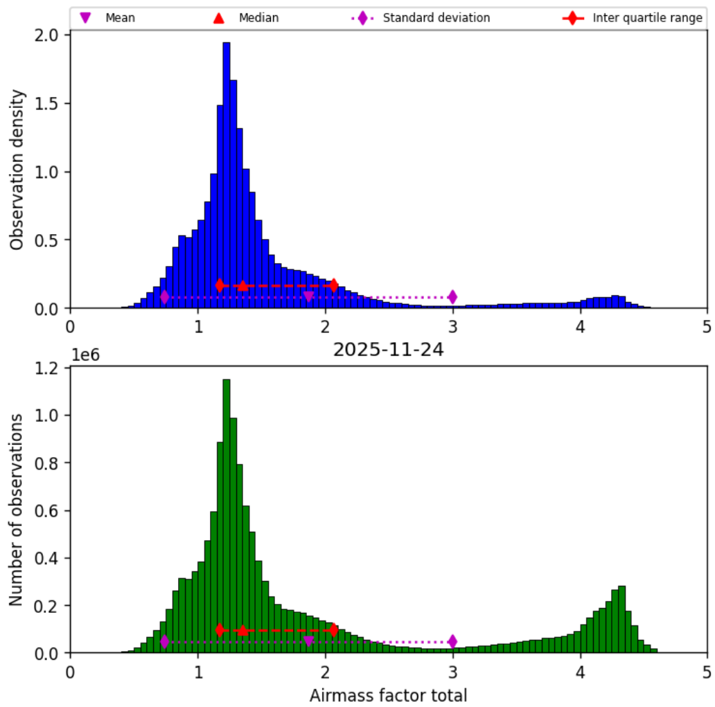
Figure 42: Histogram of “Airmass factor total” for 2025-11-23 to 2025-11-25
