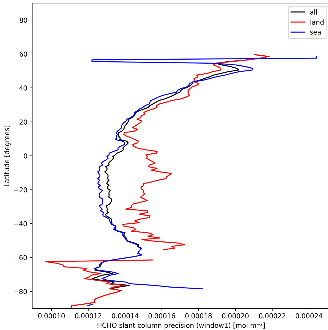
Figure 26: Zonal average of “HCHO slant column precision (window1)” for 2025-11-23 to 2025-11-25.
