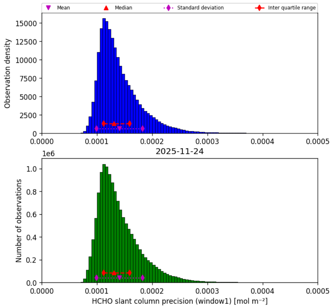
Figure 41: Histogram of “HCHO slant column precision (window1)” for 2025-11-23 to 2025-11-25
