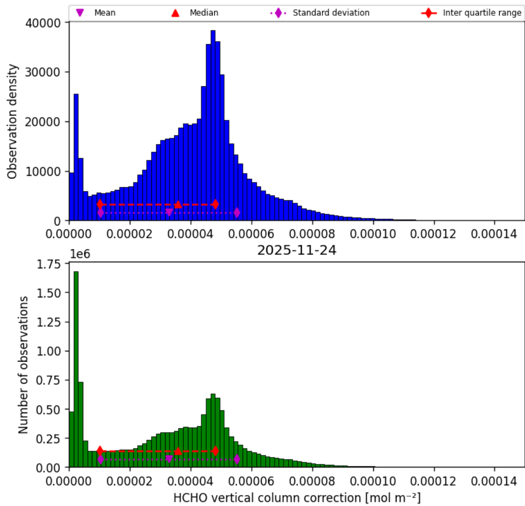
Figure 39: Histogram of “HCHO vertical column correction” for 2025-11-23 to 2025-11-25
