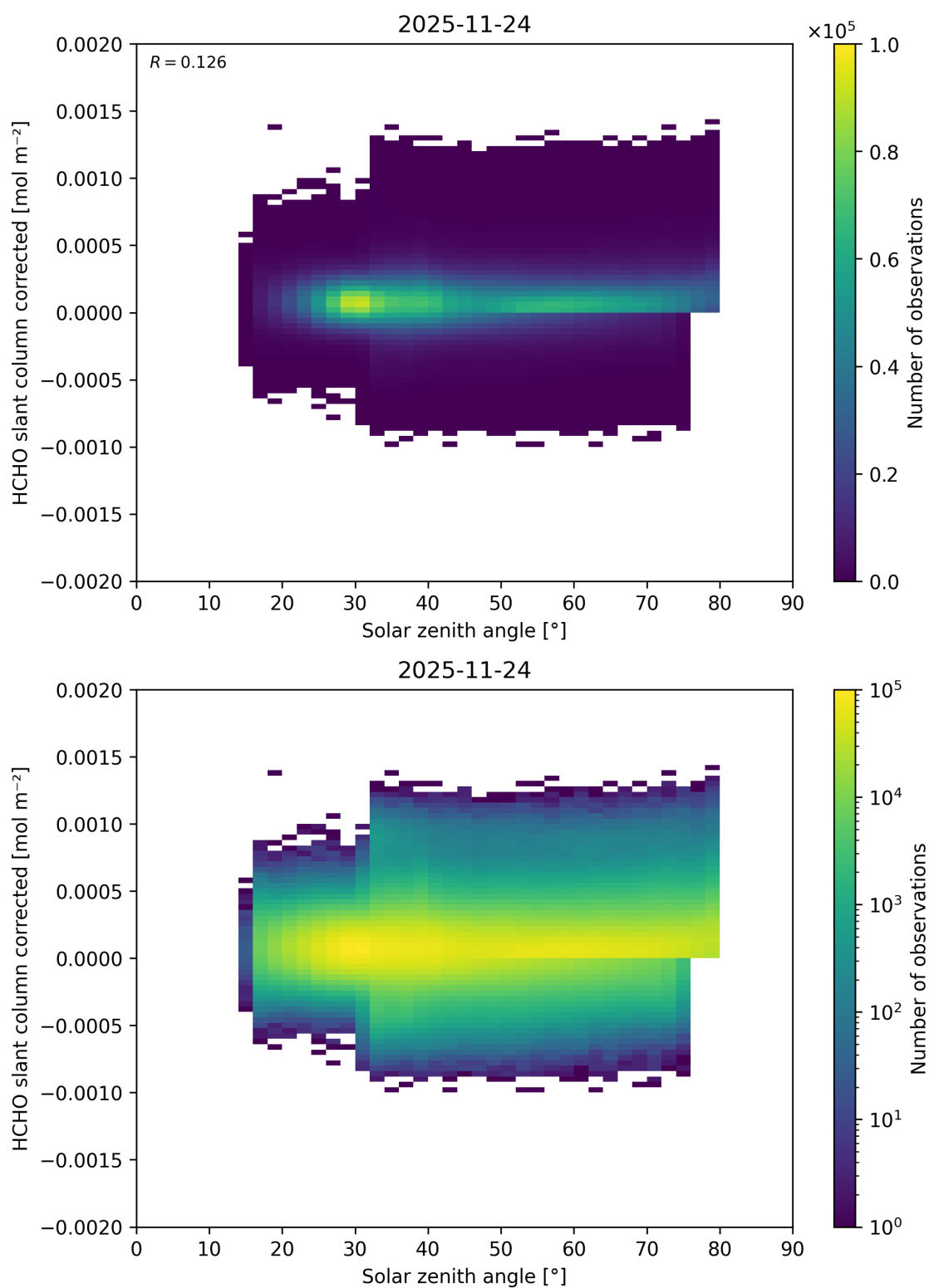
Figure 190: Scatter density plot of “Solar zenith angle” against “HCHO slant column corrected” for 2025-11-23 to 2025-11-25.
