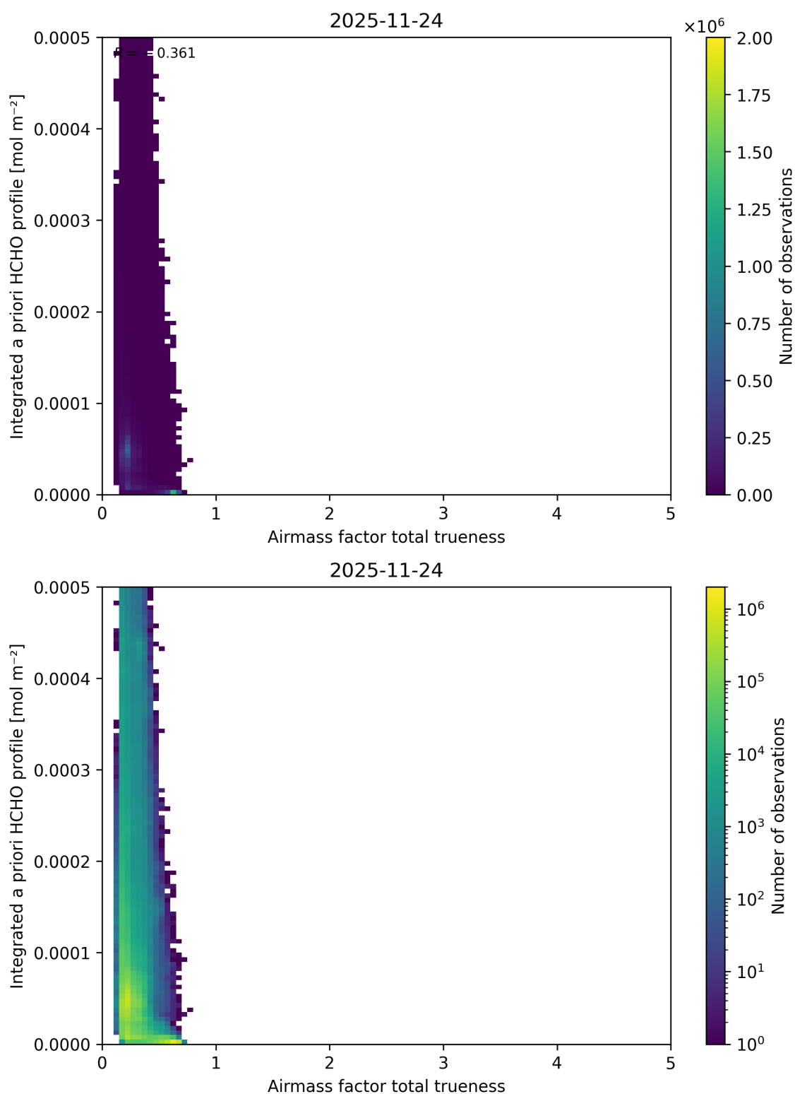
Figure 125: Scatter density plot of “Airmass factor total trueness” against “Integrated a priori HCHO profile” for 2025-11-23 to 2025-11-25.
