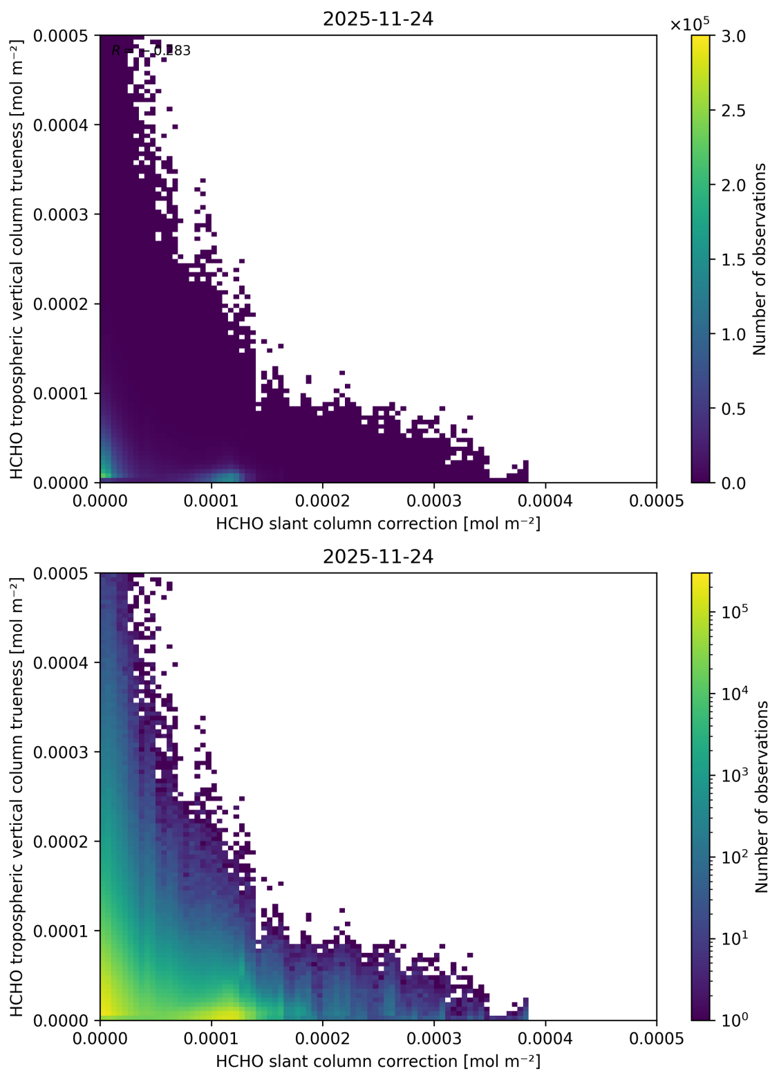
Figure 87: Scatter density plot of “HCHO slant column correction” against “HCHO tropospheric vertical column trueness” for 2025-11-23 to 2025-11-25.
