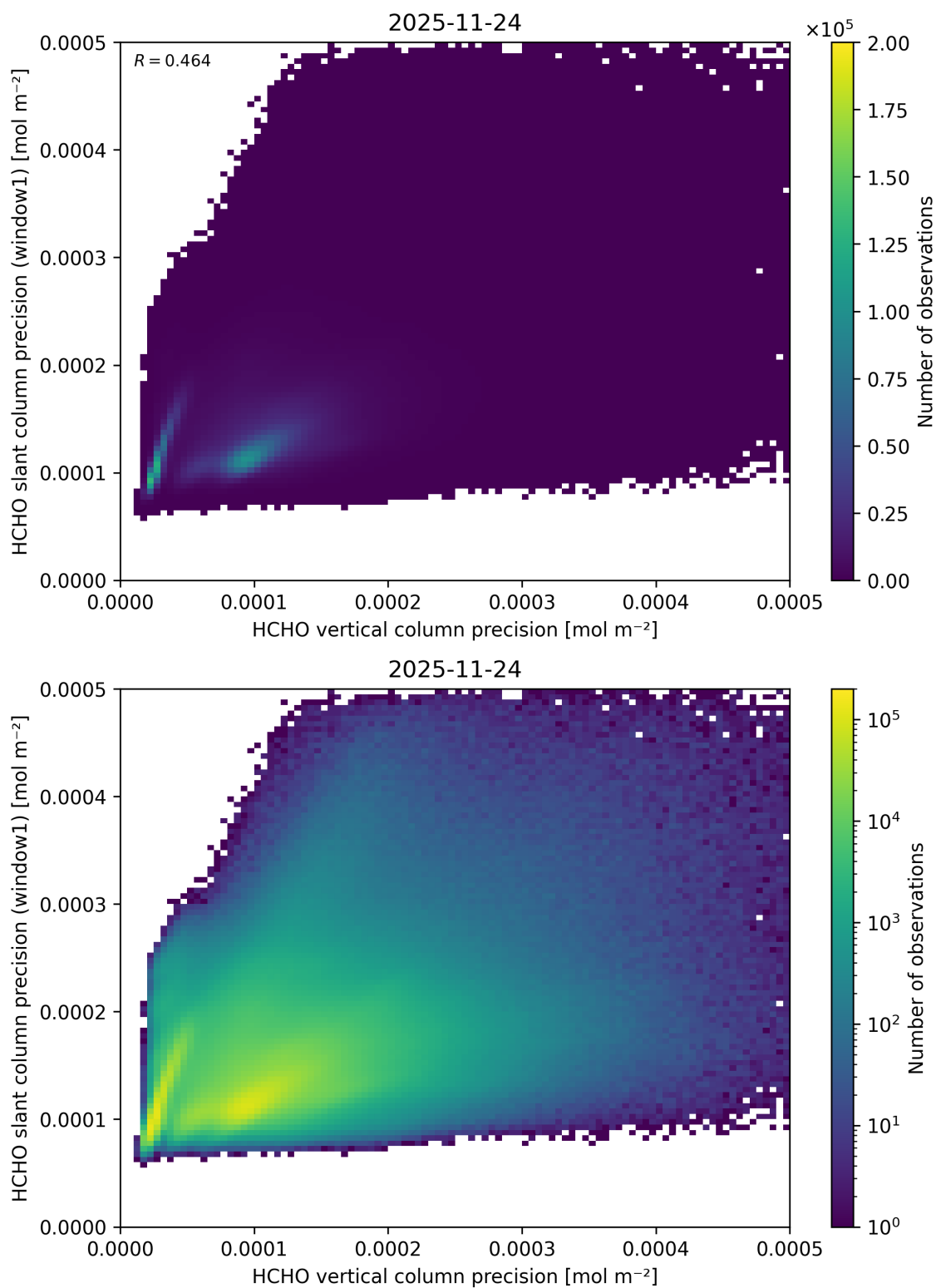
Figure 159: Scatter density plot of “HCHO vertical column precision” against “HCHO slant column precision (window1)” for 2025-11-23 to 2025-11-25.
