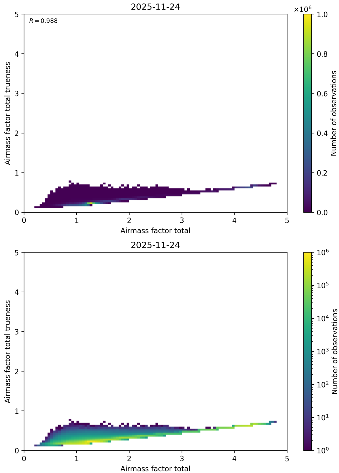
Figure 115: Scatter density plot of “Airmass factor total” against “Airmass factor total trueness” for 2025-11-23 to 2025-11-25.
