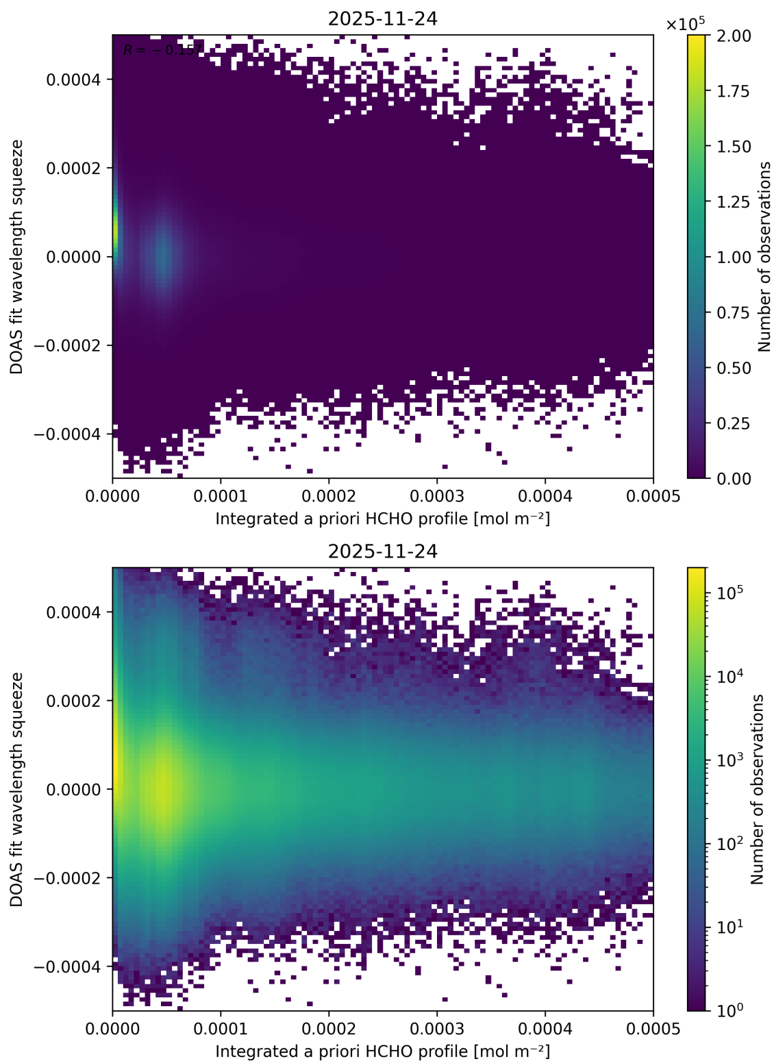
Figure 167: Scatter density plot of “Integrated a priori HCHO profile” against “DOAS fit wavelength squeeze” for 2025-11-23 to 2025-11-25.
