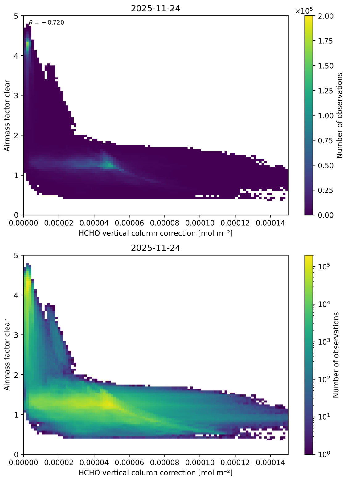
Figure 129: Scatter density plot of “HCHO vertical column correction” against “Airmass factor clear” for 2025-11-23 to 2025-11-25.
