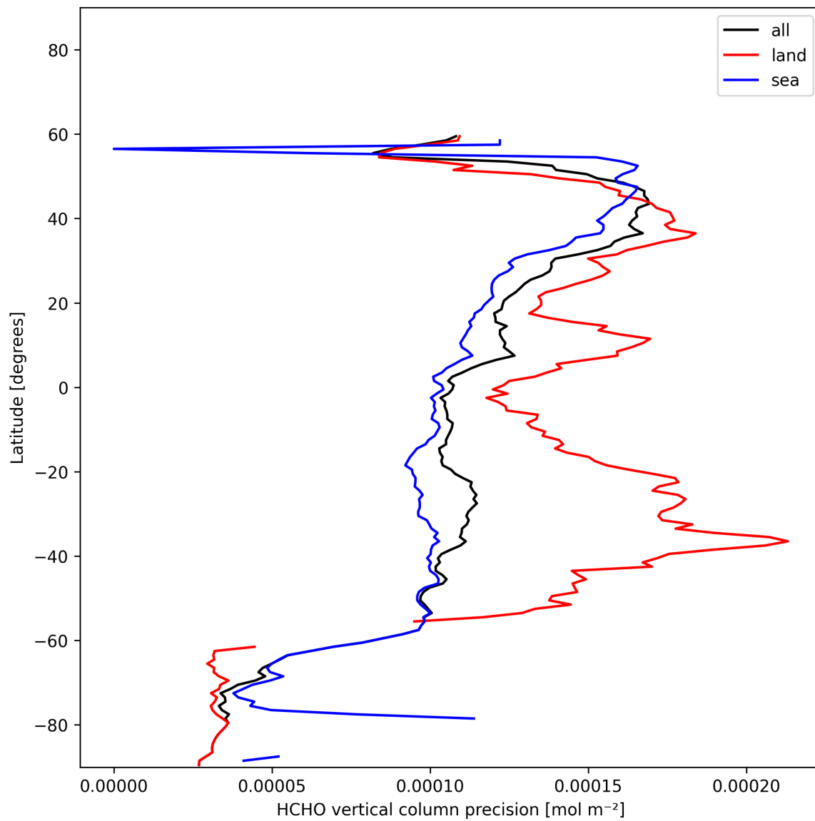
Figure 23: Zonal average of “HCHO vertical column precision” for 2025-11-23 to 2025-11-25.
