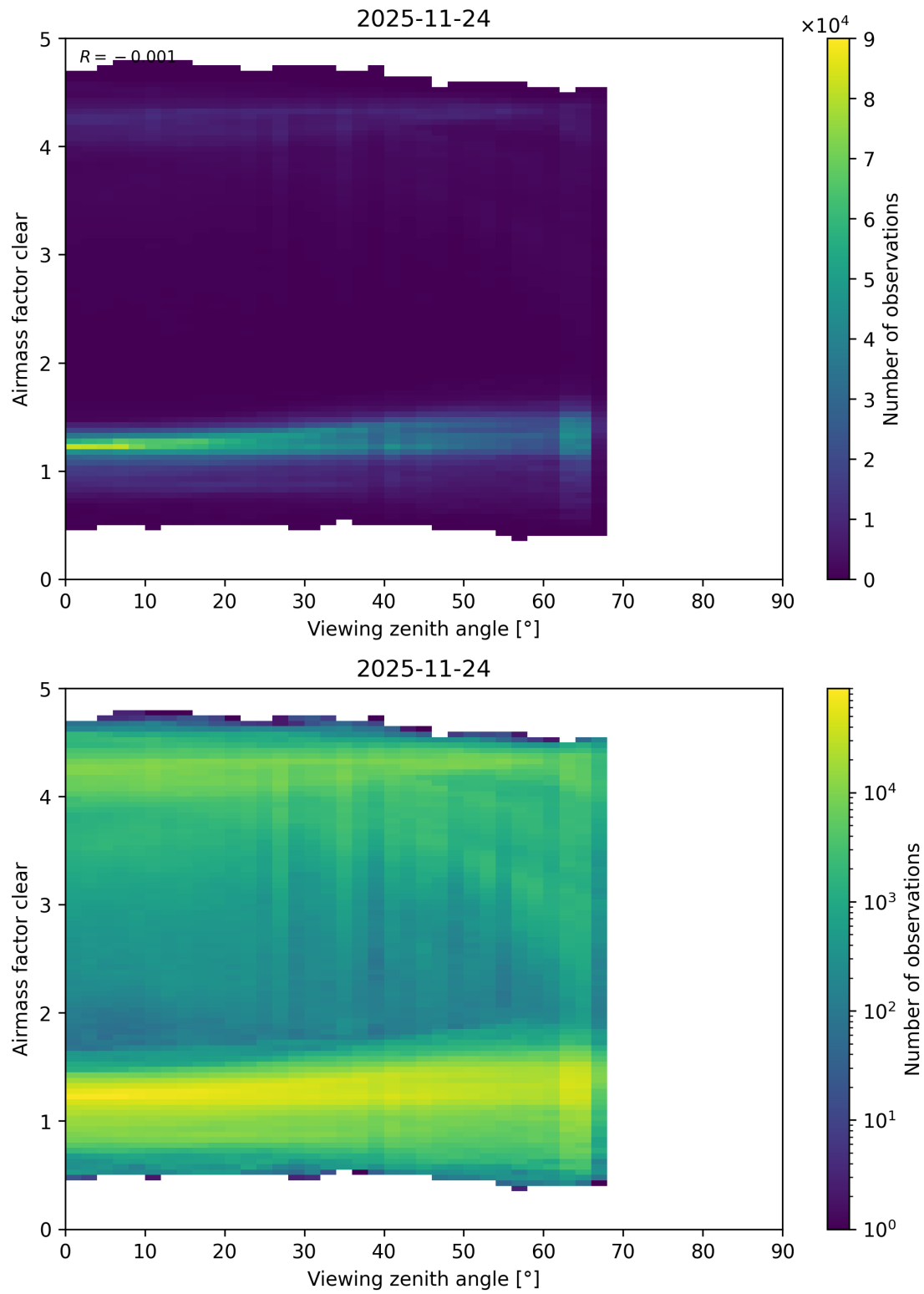
Figure 205: Scatter density plot of “Viewing zenith angle” against “Airmass factor clear” for 2025-11-23 to 2025-11-25.
