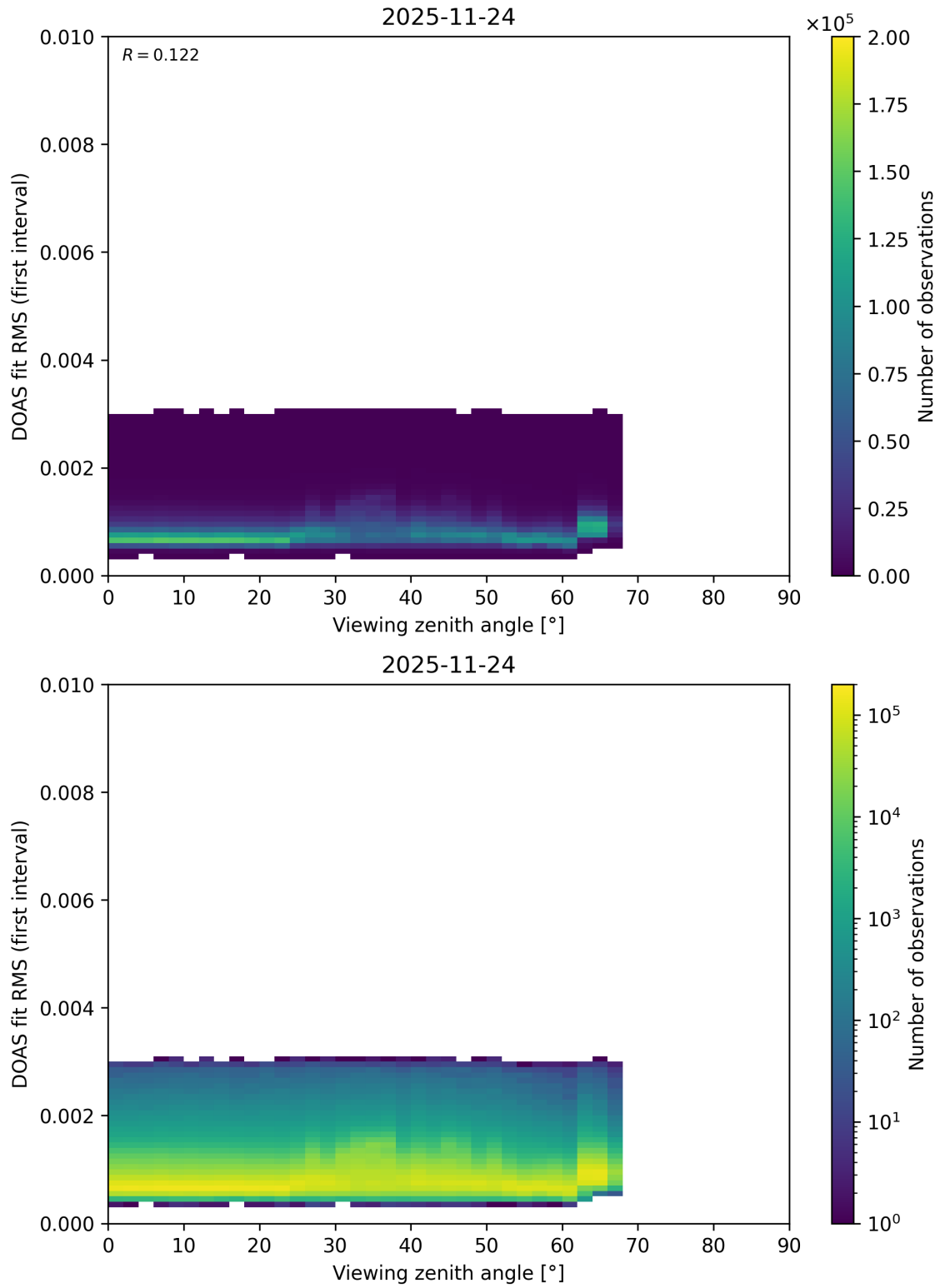
Figure 202: Scatter density plot of “Viewing zenith angle” against “DOAS fit RMS (first interval)” for 2025-11-23 to 2025-11-25.
