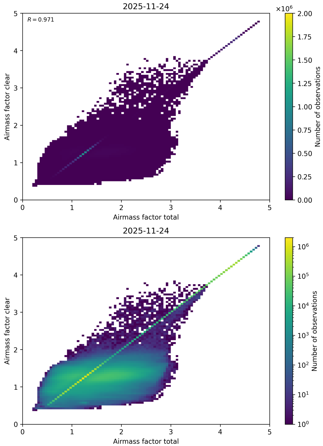
Figure 112: Scatter density plot of “Airmass factor total” against “Airmass factor clear” for 2025-11-23 to 2025-11-25.
