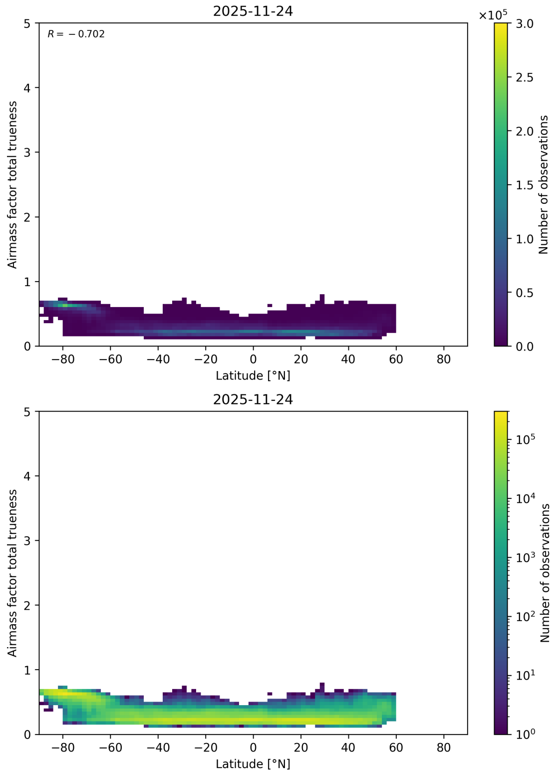
Figure 180: Scatter density plot of “Latitude” against “Airmass factor total trueneess” for 2025-11-23 to 2025-11-25.
