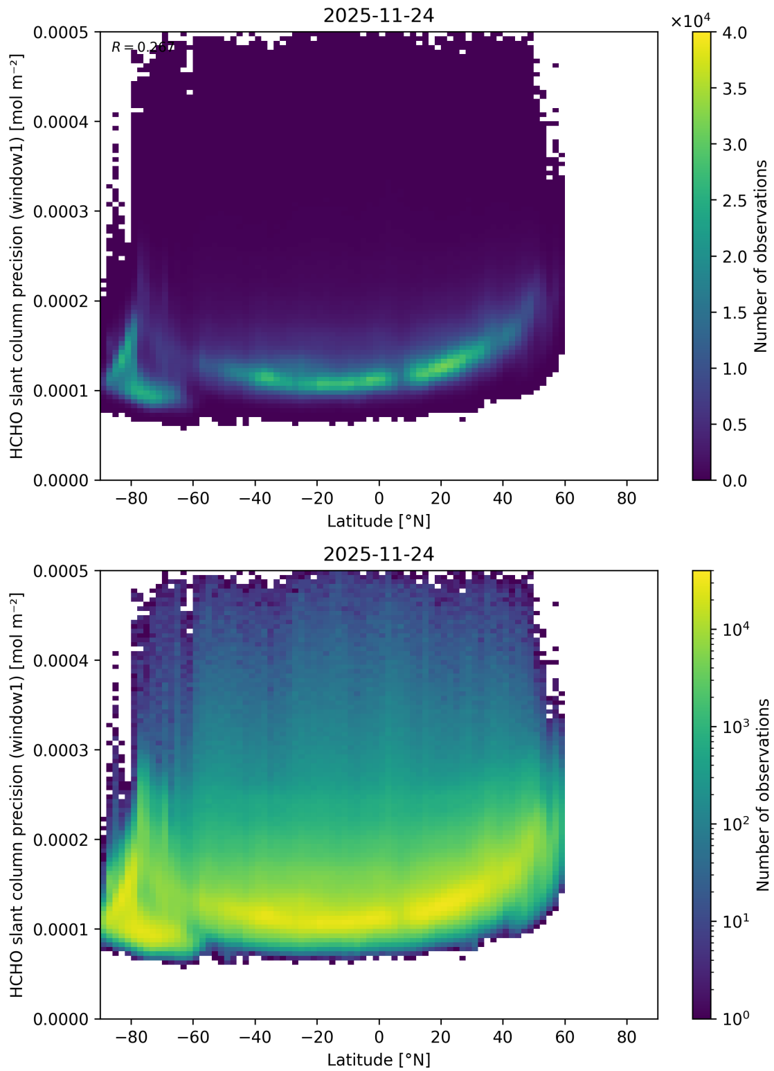
Figure 178: Scatter density plot of “Latitude” against “HCHO slant column precision (window1)” for 2025-11-23 to 2025-11-25.
