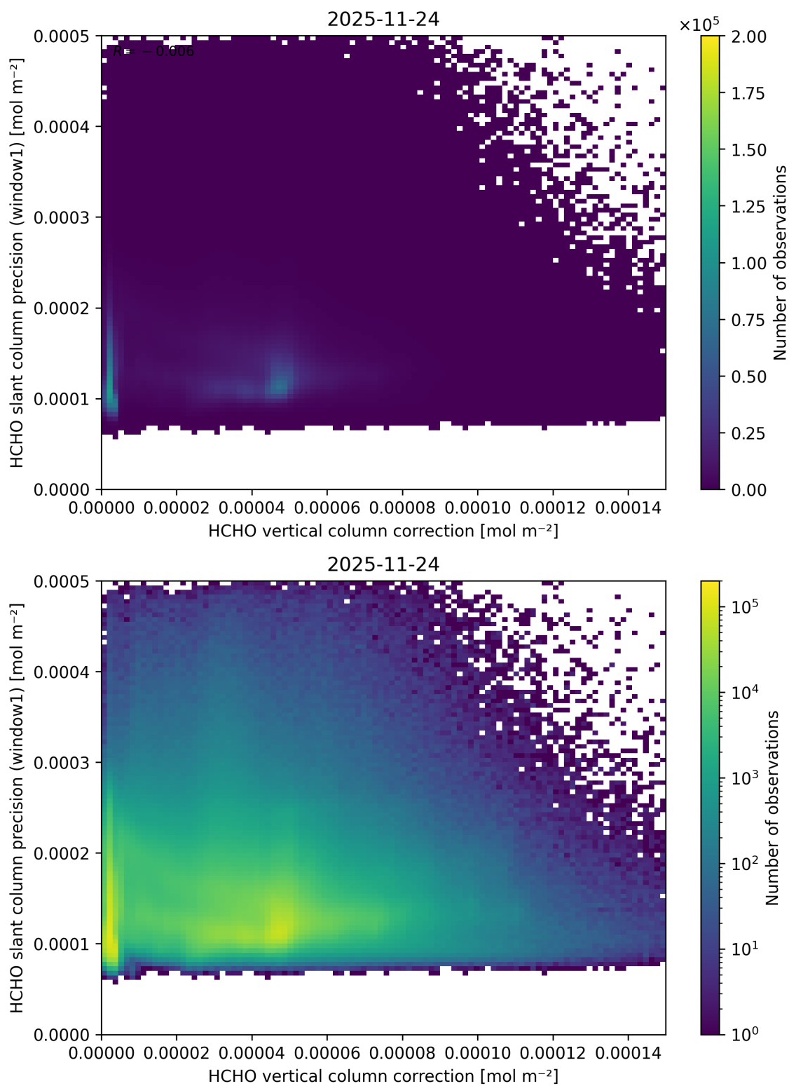
Figure 133: Scatter density plot of “HCHO vertical column correction” against “HCHO slant column precision (window1)” for 2025-11-23 to 2025-11-25.
