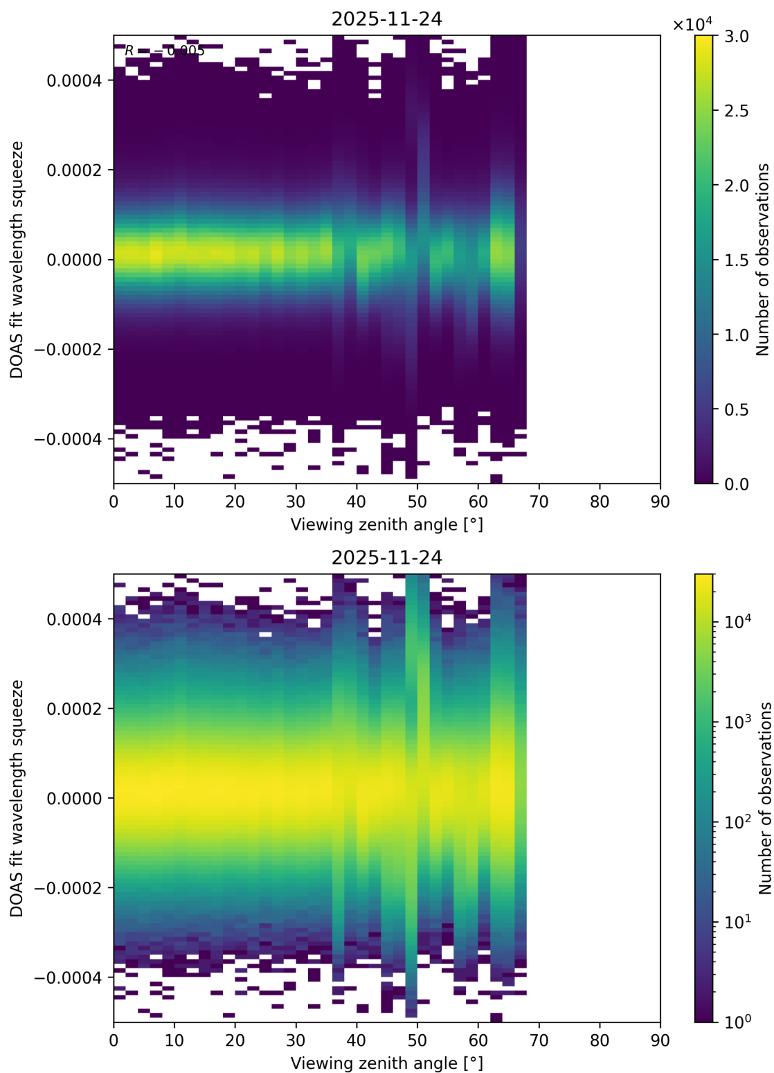
Figure 204: Scatter density plot of “Viewing zenith angle” against “DOAS fit wavelength squeeze” for 2025-11-23 to 2025-11-25.
