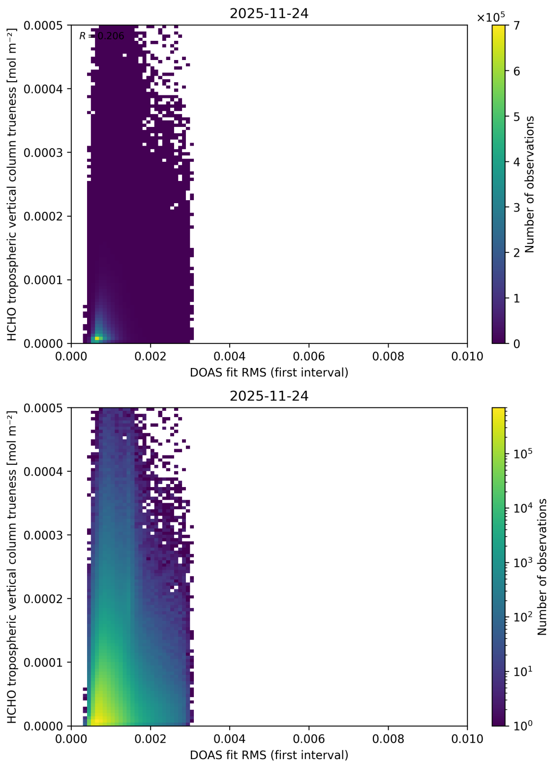
Figure 68: Scatter density plot of “DOAS fit RMS (first interval)” against “HCHO tropospheric vertical column trueness” for 2025-11-23 to 2025-11-25.
