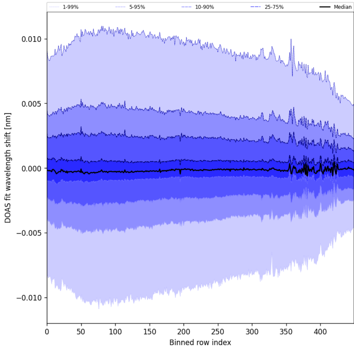
Figure 61: Along track statistics of “DOAS fit wavelength shift” for 2025-11-23 to 2025-11-25
