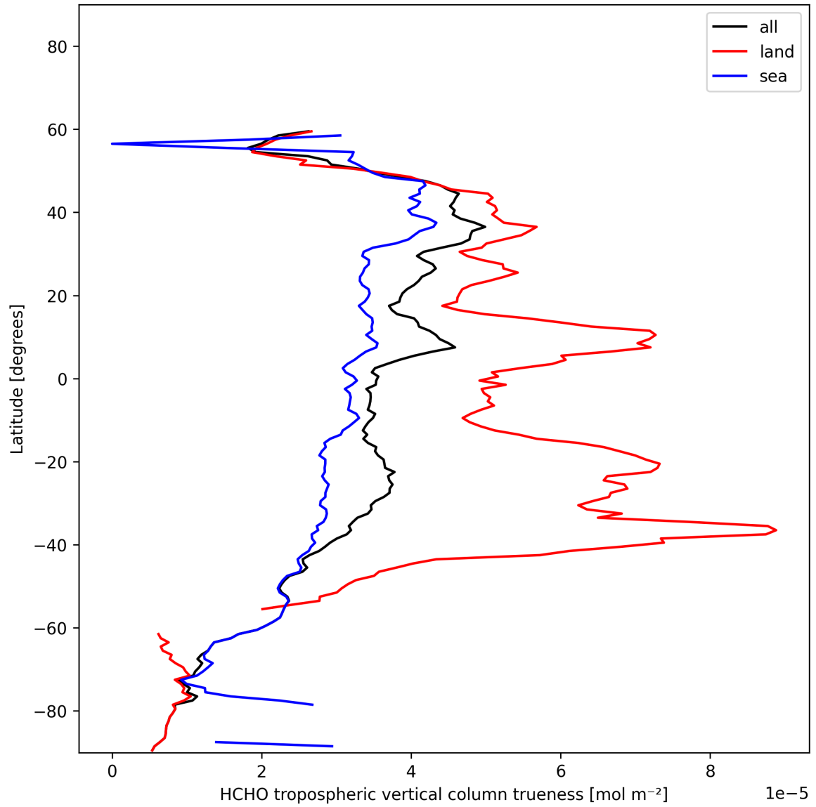
Figure 35: Zonal average of “HCHO tropospheric vertical column trueness” for 2025-11-23 to 2025-11-25.
