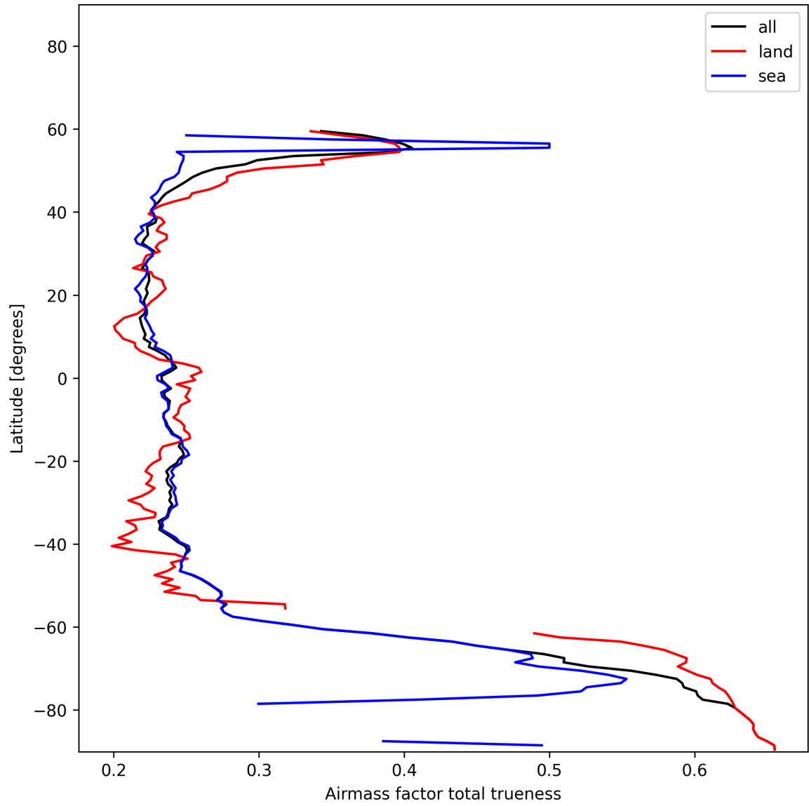
Figure 28: Zonal average of “Airmass factor total trueness” for 2025-11-23 to 2025-11-25.
