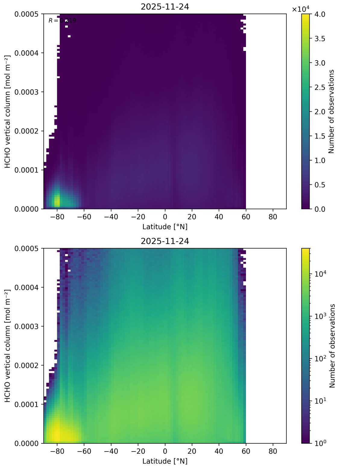
Figure 181: Scatter density plot of “Latitude” against “HCHO vertical column” for 2025-11-23 to 2025-11-25.
