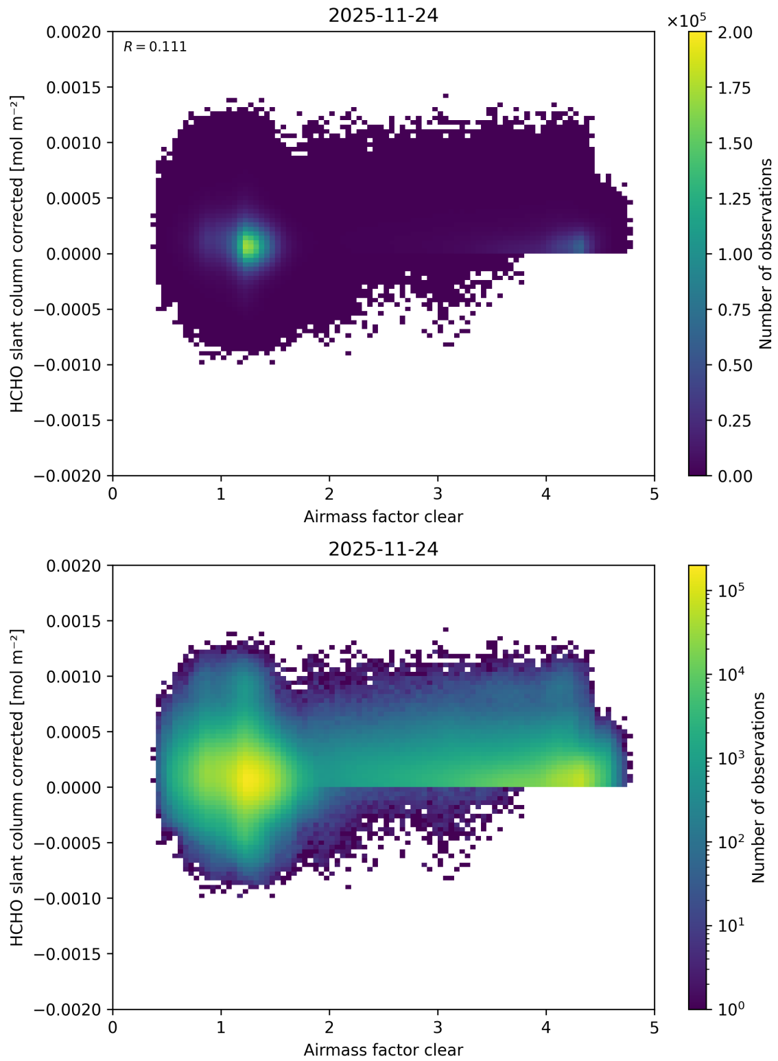
Figure 81: Scatter density plot of “Airmass factor clear” against “HCHO slant column corrected” for 2025-11-23 to 2025-11-25.
