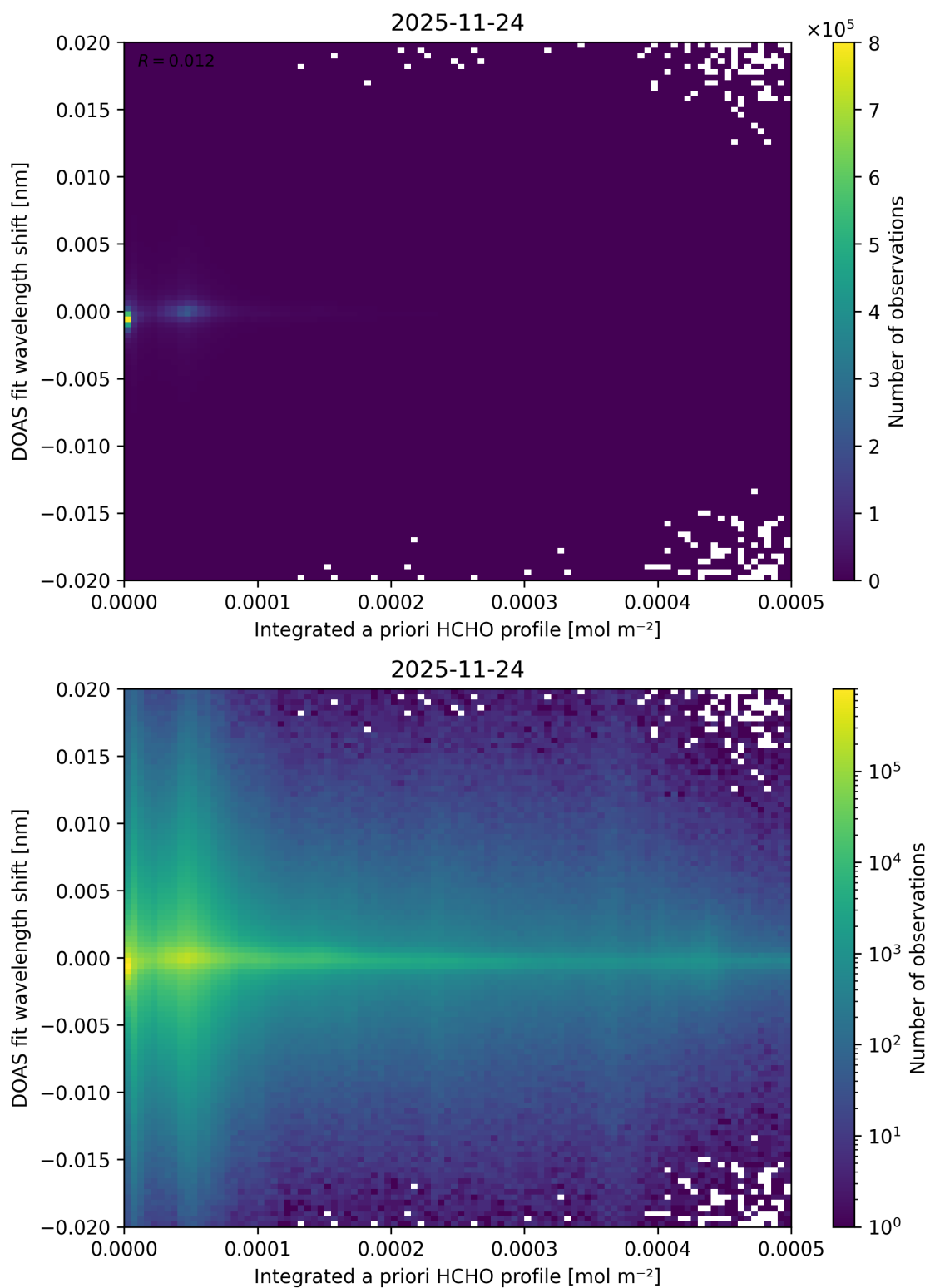
Figure 166: Scatter density plot of “Integrated a priori HCHO profile” against “DOAS fit wavelength shift” for 2025-11-23 to 2025-11-25.
