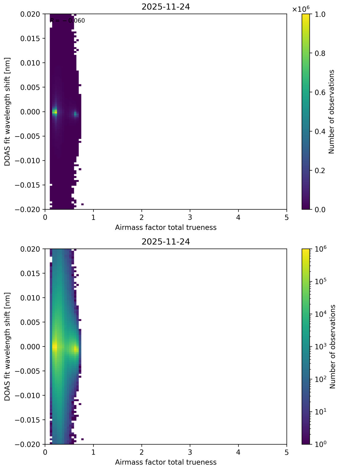
Figure 119: Scatter density plot of “Airmass factor total trueness” against “DOAS fit wavelength shift” for 2025-11-23 to 2025-11-25.
