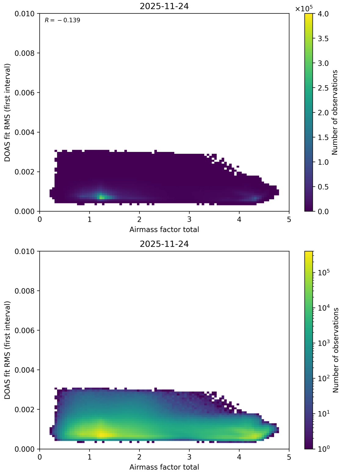
Figure 109: Scatter density plot of “Airmass factor total” against “DOAS fit RMS (first interval)” for 2025-11-23 to 2025-11-25.
