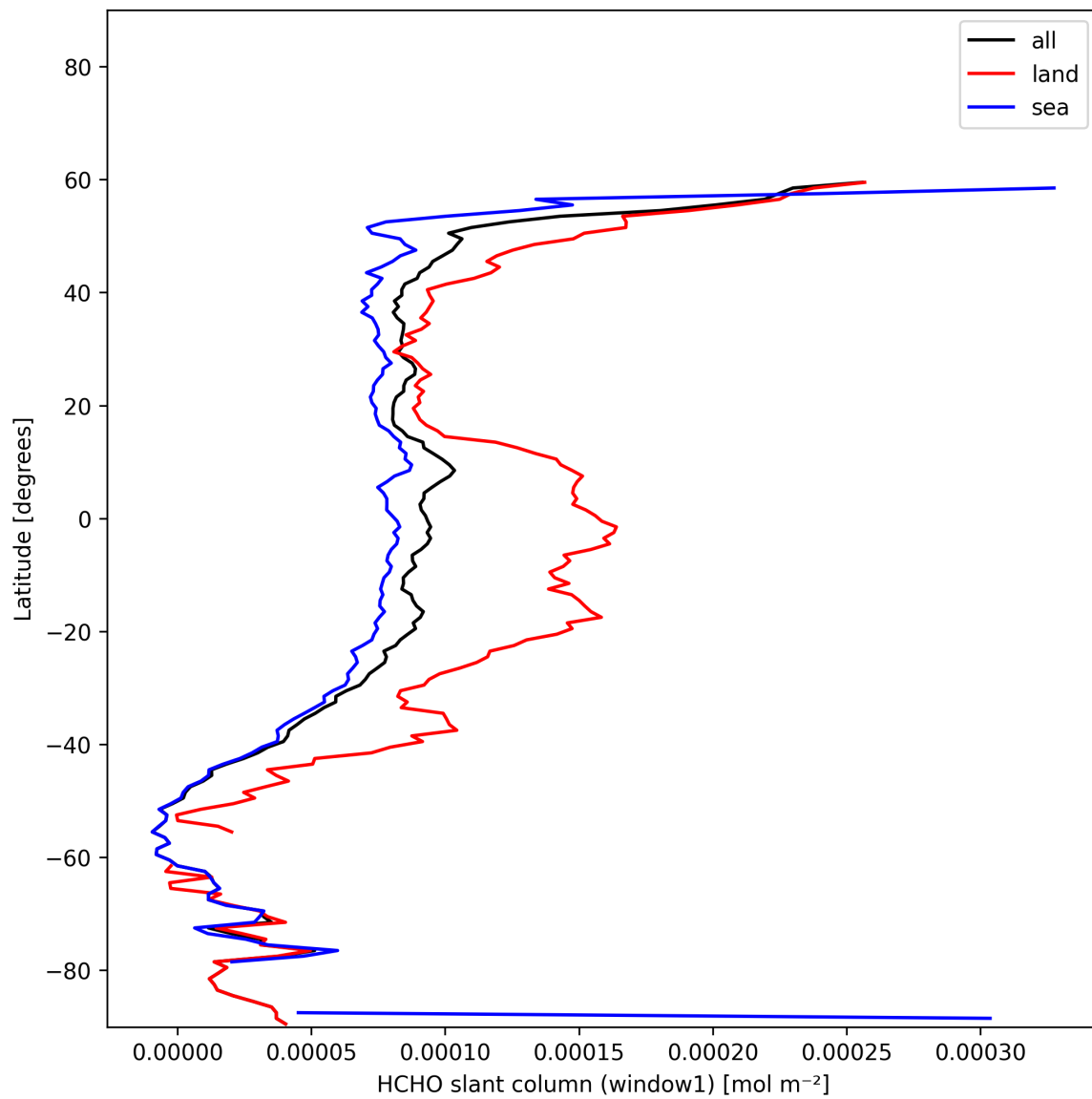
Figure 25: Zonal average of “HCHO slant column (window1)” for 2025-11-23 to 2025-11-25.
