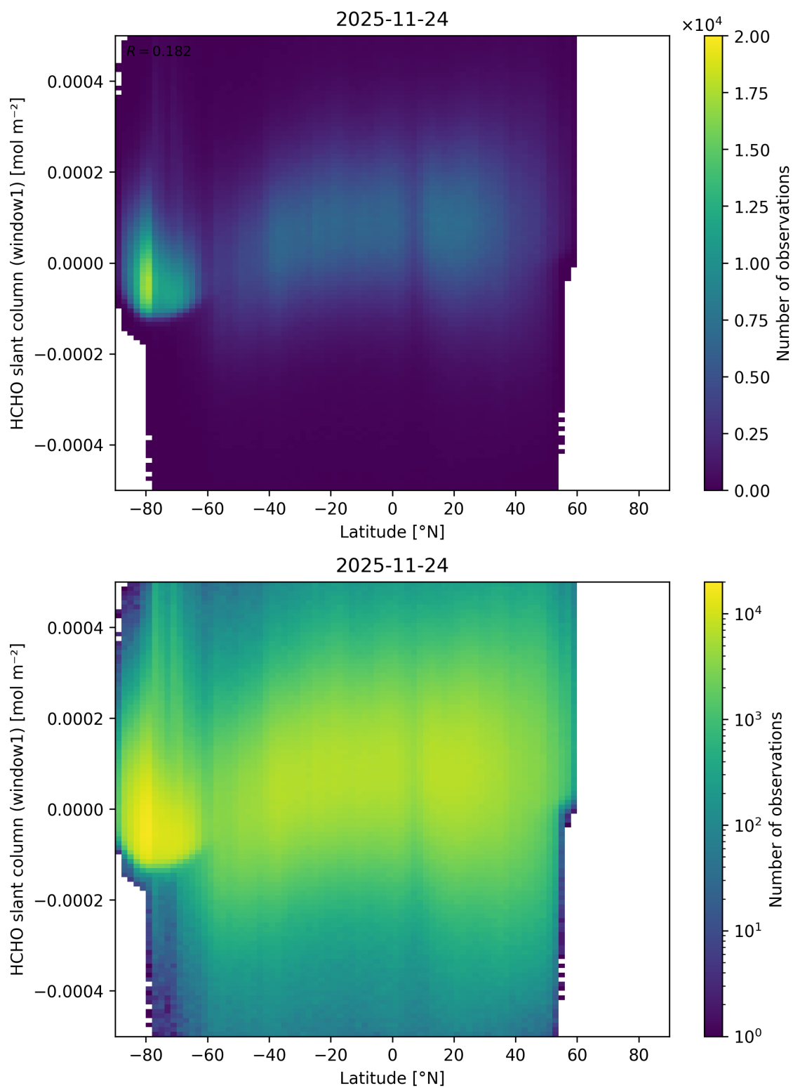
Figure 177: Scatter density plot of “Latitude” against “HCHO slant column (window1)” for 2025-11-23 to 2025-11-25.
