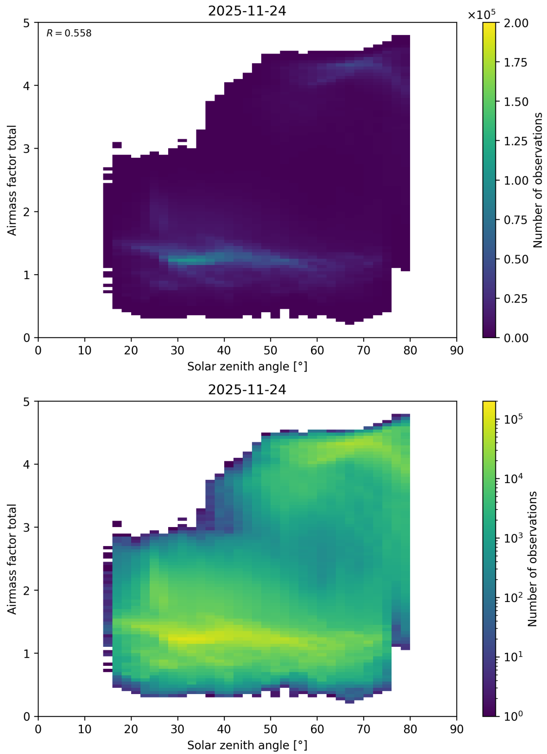
Figure 194: Scatter density plot of “Solar zenith angle” against “Airmass factor total” for 2025-11-23 to 2025-11-25.
