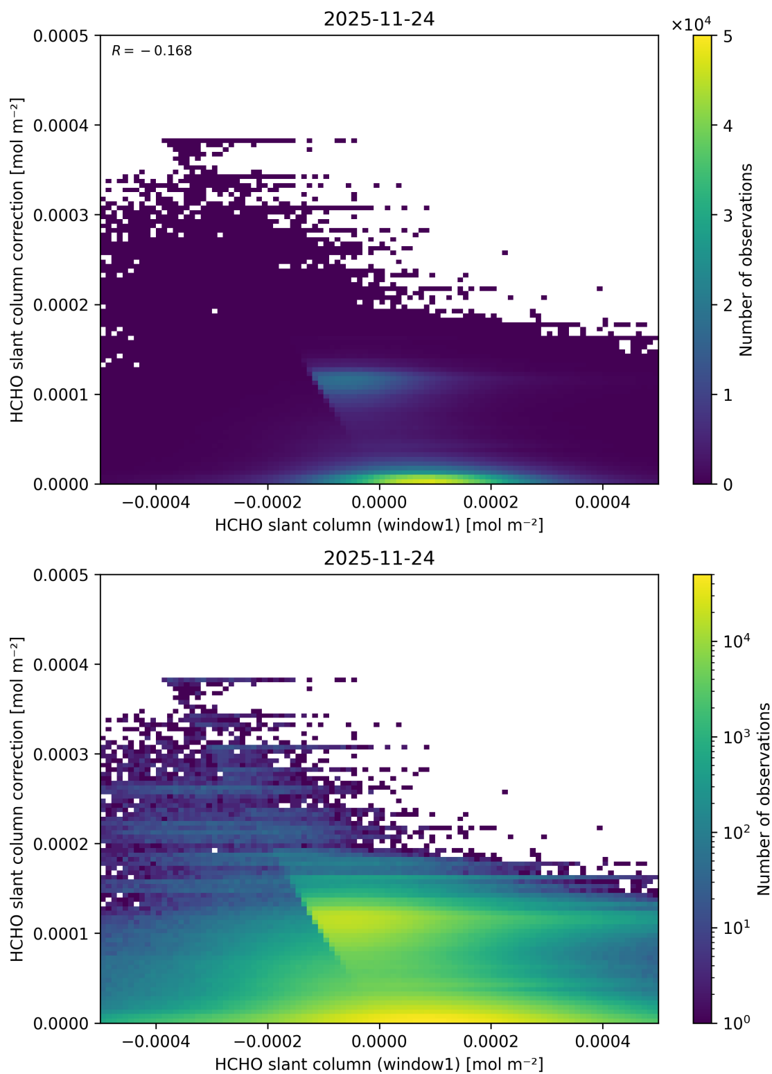
Figure 93: Scatter density plot of “HCHO slant column (window1)” against “HCHO slant column correction” for 2025-11-23 to 2025-11-25.
