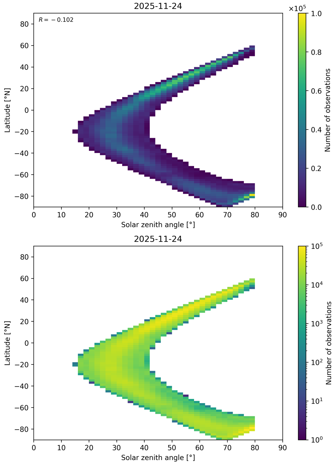
Figure 201: Scatter density plot of “Solar zenith angle” against “Latitude” for 2025-11-23 to 2025-11-25.
