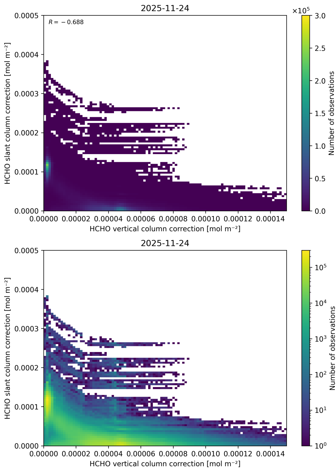
Figure 131: Scatter density plot of “HCHO vertical column correction” against “HCHO slant column correction” for 2025-11-23 to 2025-11-25.
