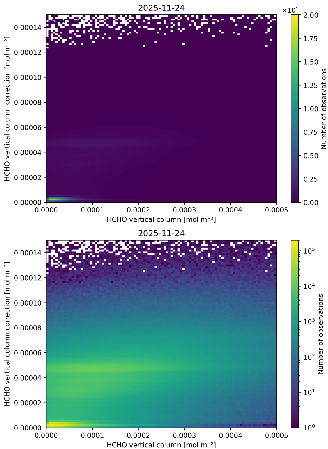
Figure 148: Scatter density plot of “HCHO vertical column” against “HCHO vertical column correction” for 2025-11-23 to 2025-11-25.
