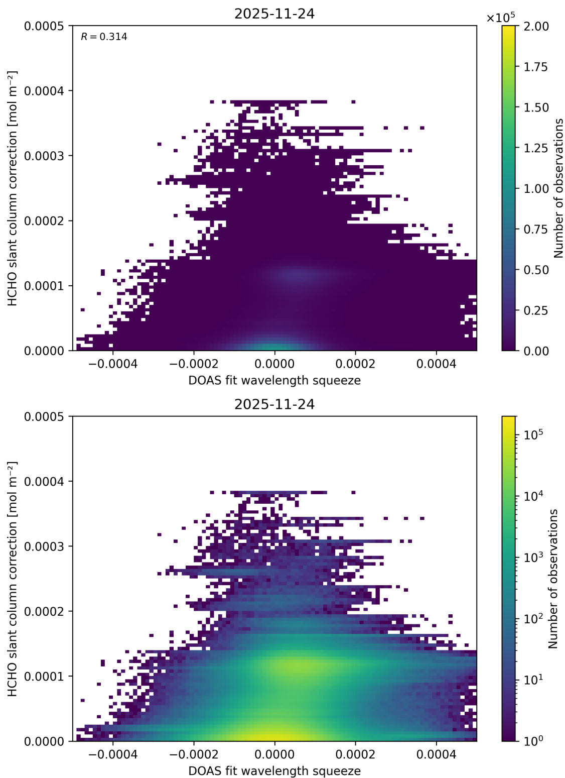
Figure 76: Scatter density plot of “DOAS fit wavelength squeeze” against “HCHO slant column correction” for 2025-11-23 to 2025-11-25.
