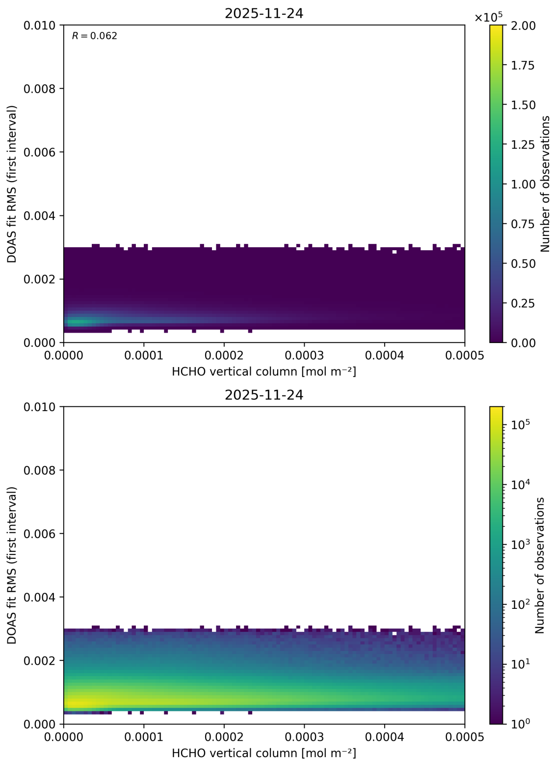
Figure 138: Scatter density plot of “HCHO vertical column” against “DOAS fit RMS (first interval)” for 2025-11-23 to 2025-11-25.
