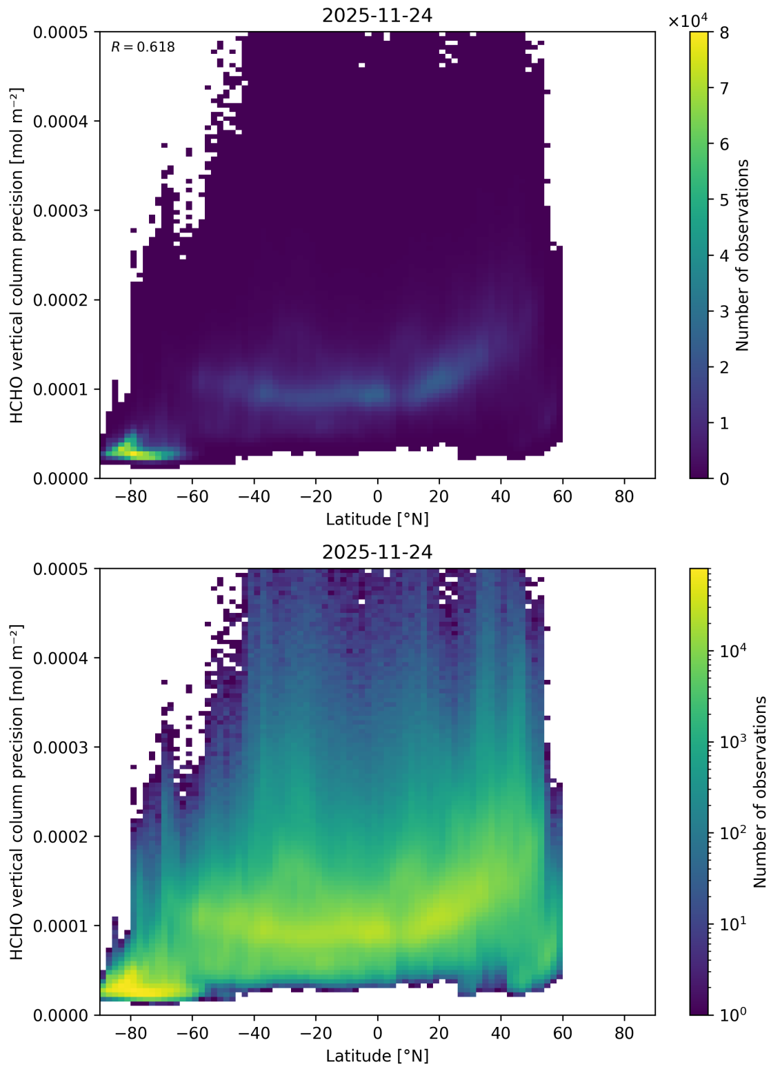
Figure 183: Scatter density plot of “Latitude” against “HCHO vertical column precision” for 2025-11-23 to 2025-11-25.
