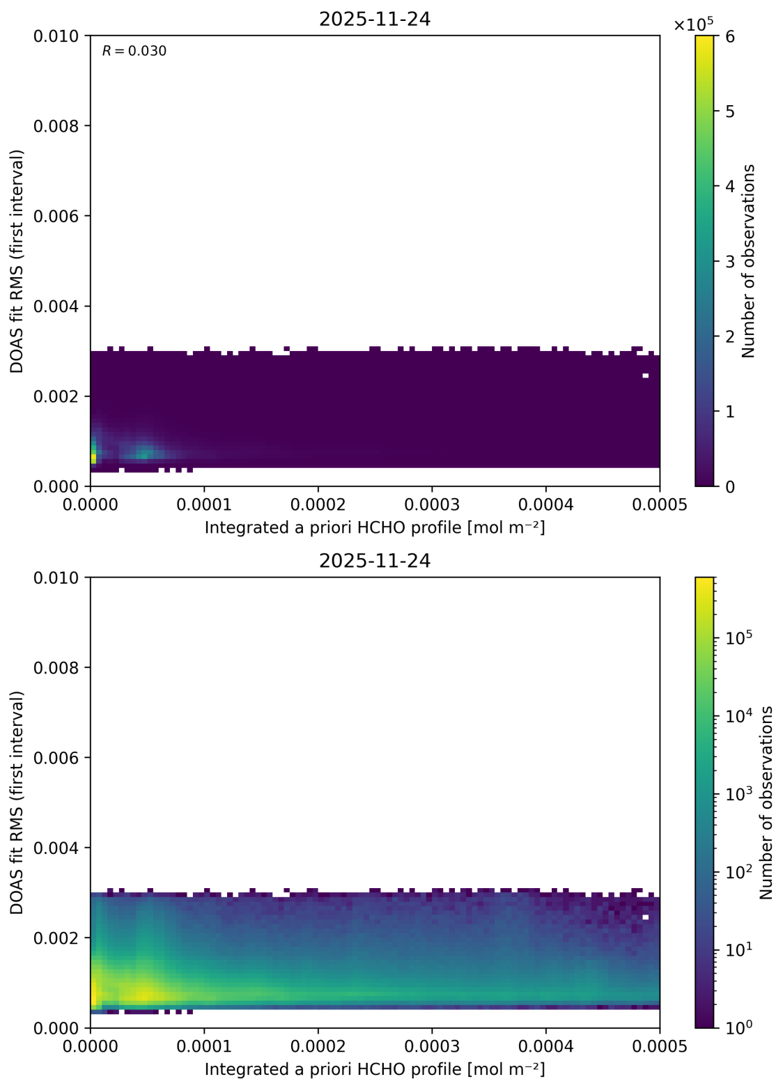
Figure 165: Scatter density plot of “Integrated a priori HCHO profile” against “DOAS fit RMS (first interval)” for 2025-11-23 to 2025-11-25.
