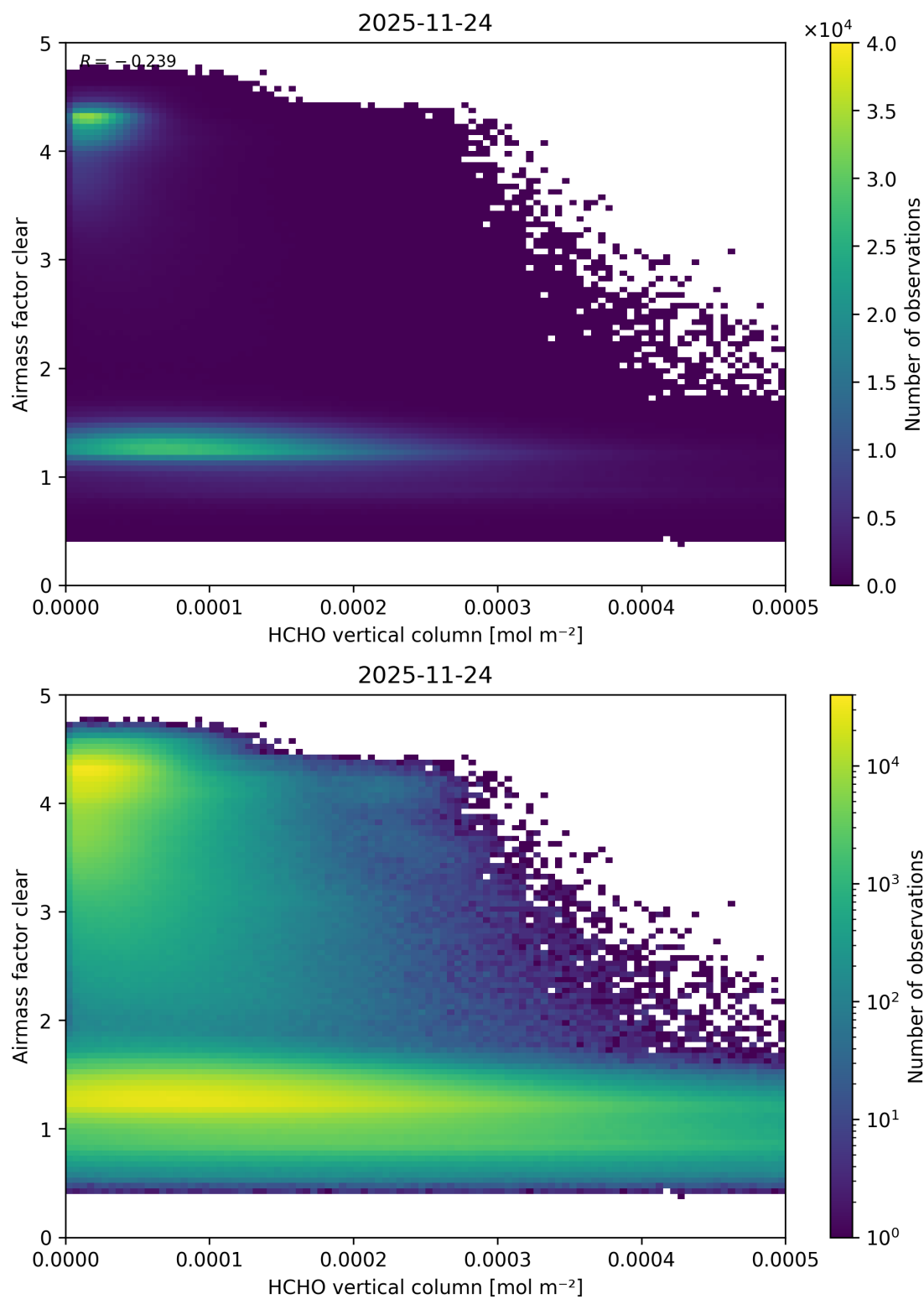
Figure 141: Scatter density plot of “HCHO vertical column” against “Airmass factor clear” for 2025-11-23 to 2025-11-25.
