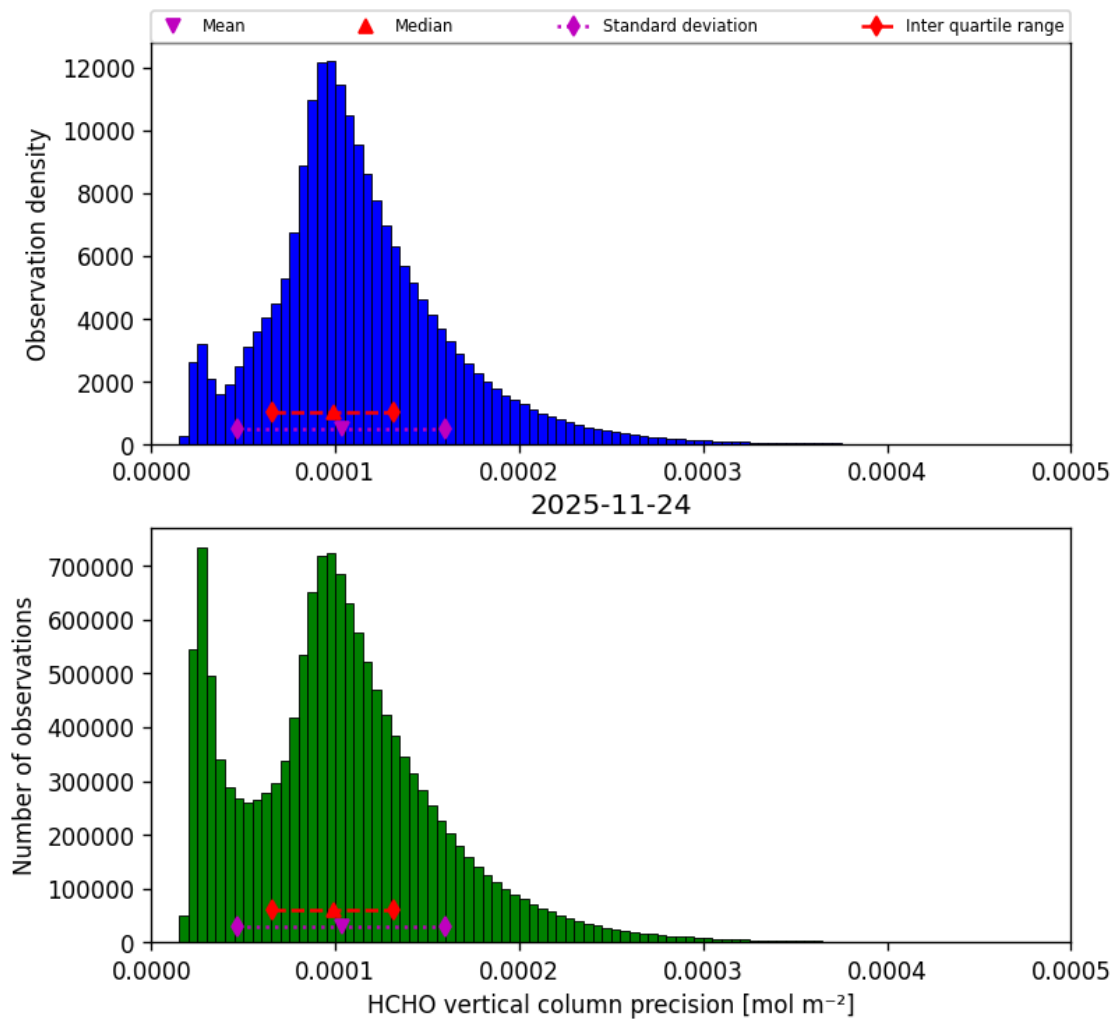
Figure 38: Histogram of “HCHO vertical column precision” for 2025-11-23 to 2025-11-25
