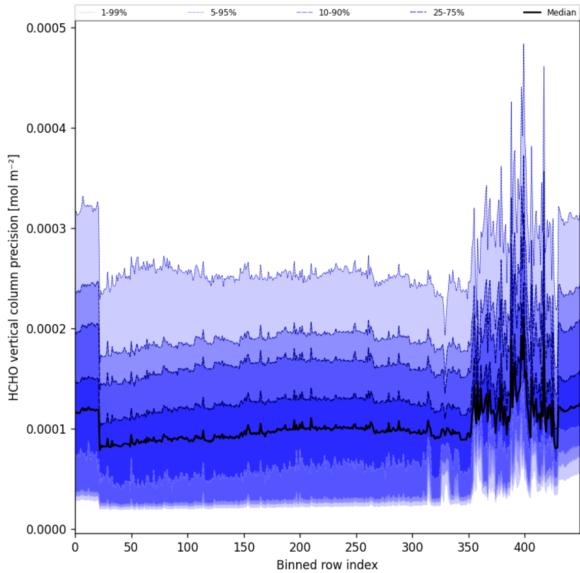
Figure 53: Along track statistics of “HCHO vertical column precision” for 2025-11-23 to 2025-11-25
