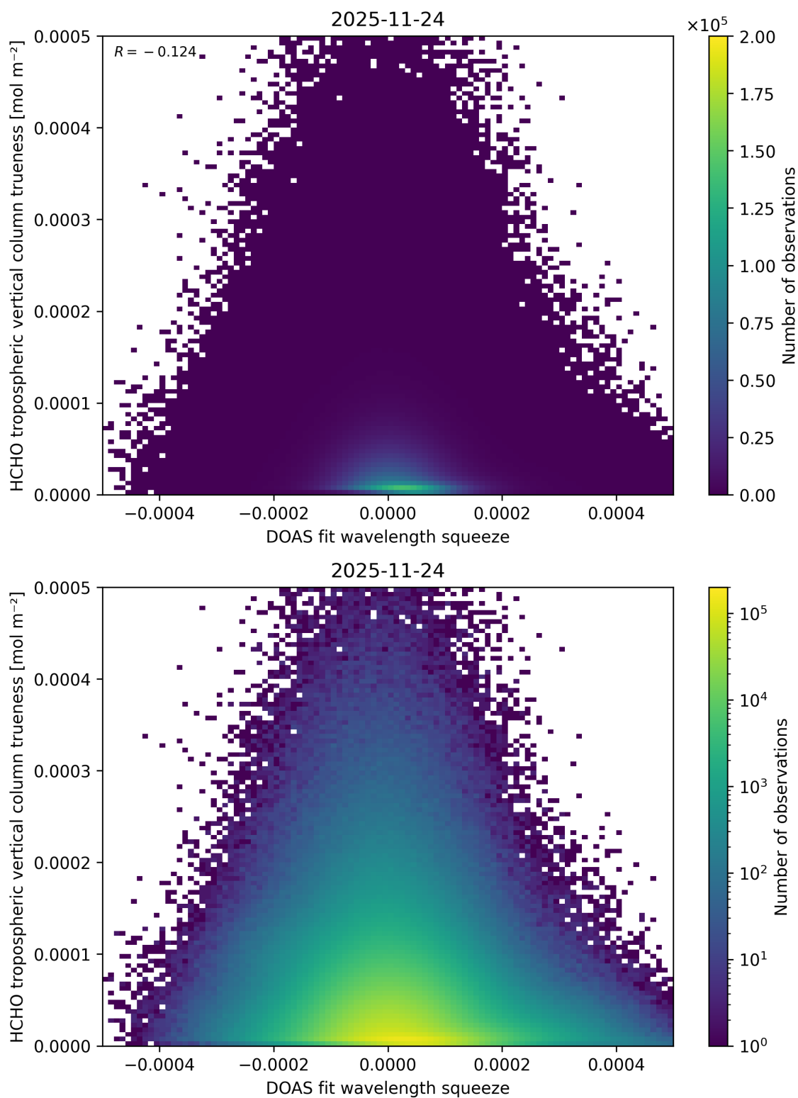
Figure 77: Scatter density plot of “DOAS fit wavelength squeeze” against “HCHO tropospheric vertical column trueness” for 2025-11-23 to 2025-11-25.
