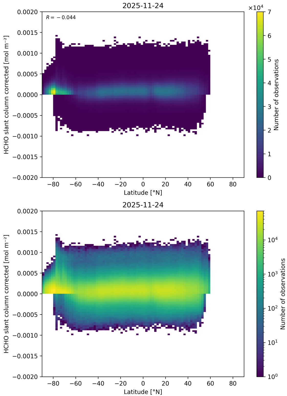
Figure 175: Scatter density plot of “Latitude” against “HCHO slant column corrected” for 2025-11-23 to 2025-11-25.
