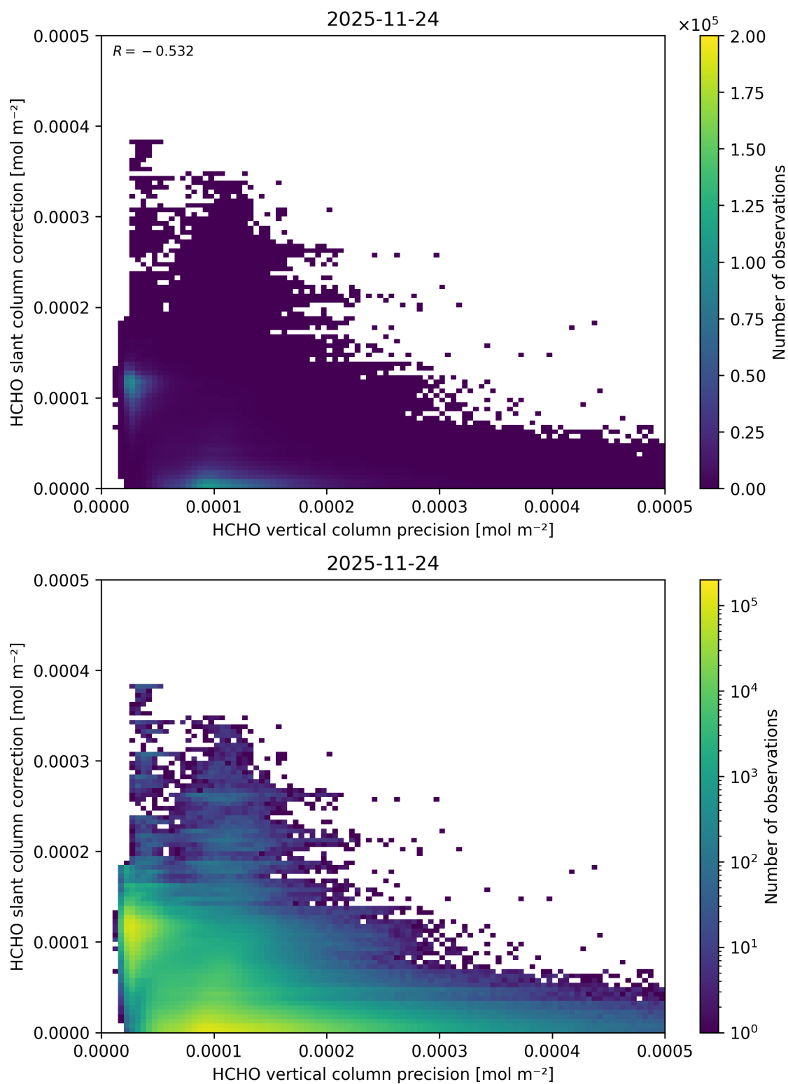
Figure 157: Scatter density plot of “HCHO vertical column precision” against “HCHO slant column correction” for 2025-11-23 to 2025-11-25.
