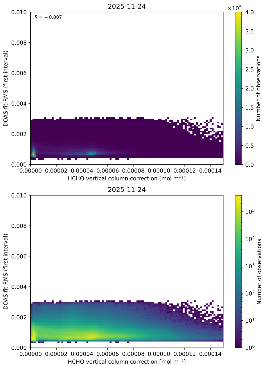
Figure 126: Scatter density plot of “HCHO vertical column correction” against “DOAS fit RMS (first interval)” for 2025-11-23 to 2025-11-25.
