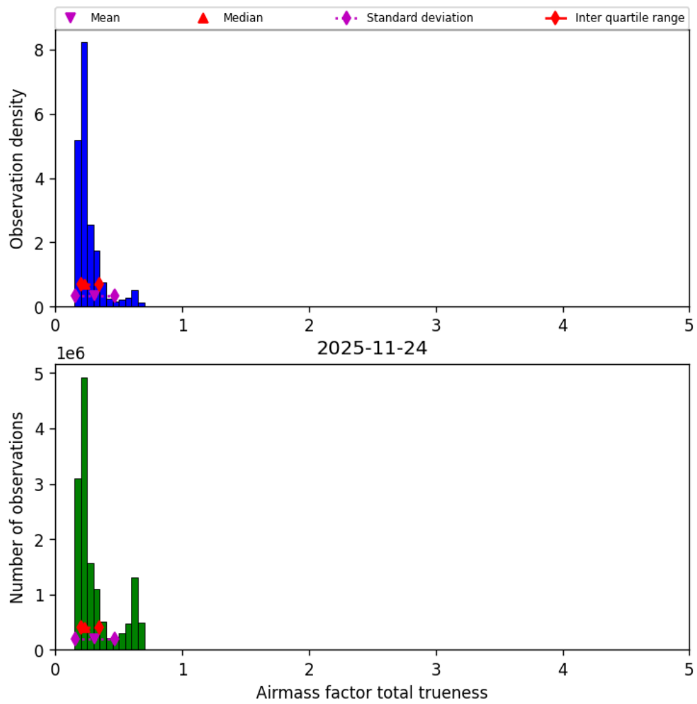
Figure 43: Histogram of “Airmass factor total trueness” for 2025-11-23 to 2025-11-25
