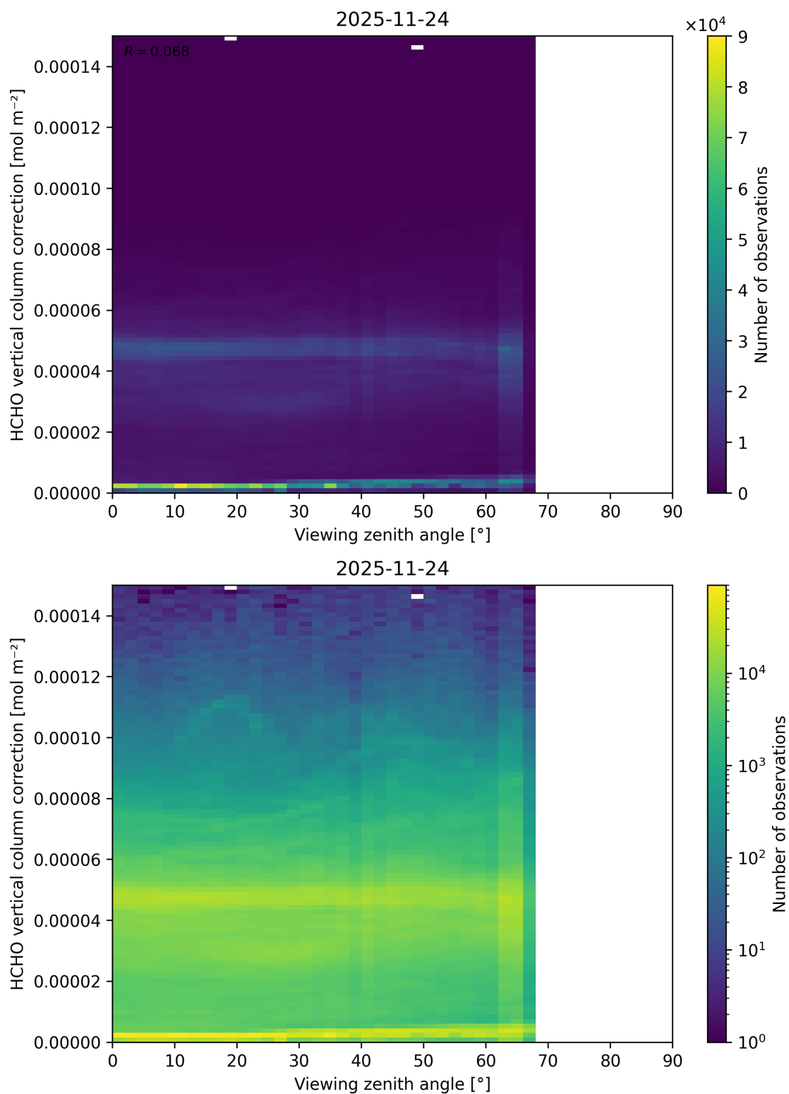
Figure 213: Scatter density plot of “Viewing zenith angle” against “HCHO vertical column correction” for 2025-11-23 to 2025-11-25.
