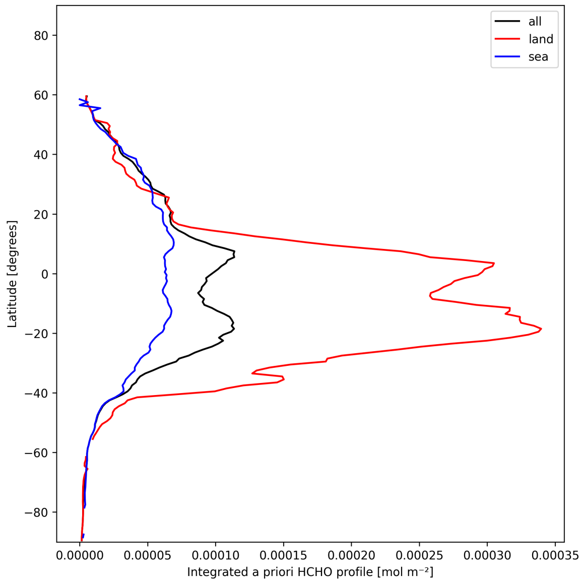
Figure 30: Zonal average of “Integrated a priori HCHO profile” for 2025-11-23 to 2025-11-25.
