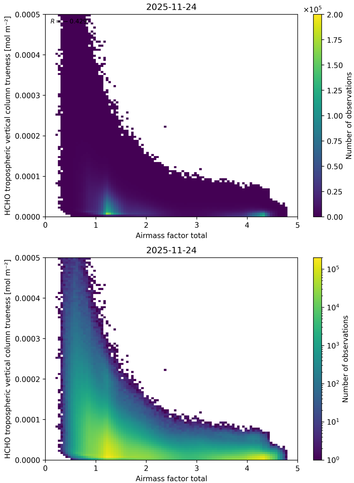
Figure 116: Scatter density plot of “Airmass factor total” against “HCHO tropospheric vertical column truiness” for 2025-11-23 to 2025-11-25.
