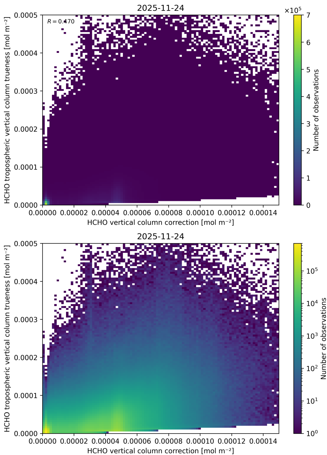
Figure 136: Scatter density plot of “HCHO vertical column correction” against “HCHO tropospheric vertical column true-ness” for 2025-11-23 to 2025-11-25.
