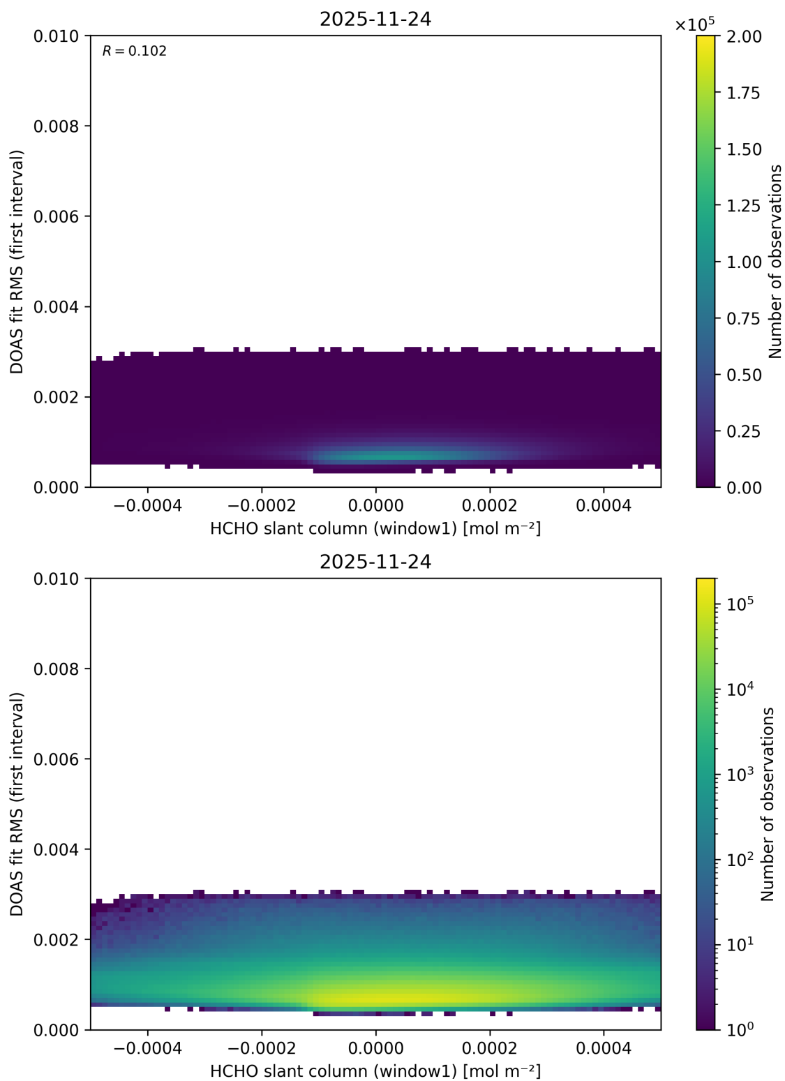
Figure 88: Scatter density plot of “HCHO slant column (window1)” against “DOAS fit RMS (first interval)” for 2025-11-23 to 2025-11-25.
