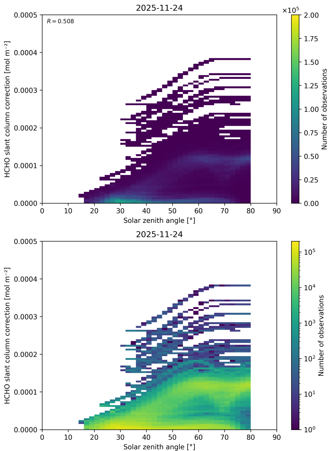
Figure 191: Scatter density plot of “Solar zenith angle” against “HCHO slant column correction” for 2025-11-23 to 2025-11-25.
