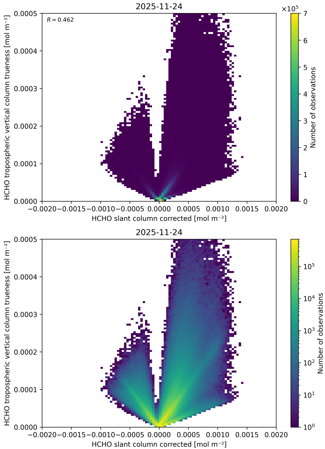
Figure 86: Scatter density plot of “HCHO slant column corrected” against “HCHO tropospheric vertical column trueness” for 2025-11-23 to 2025-11-25.
