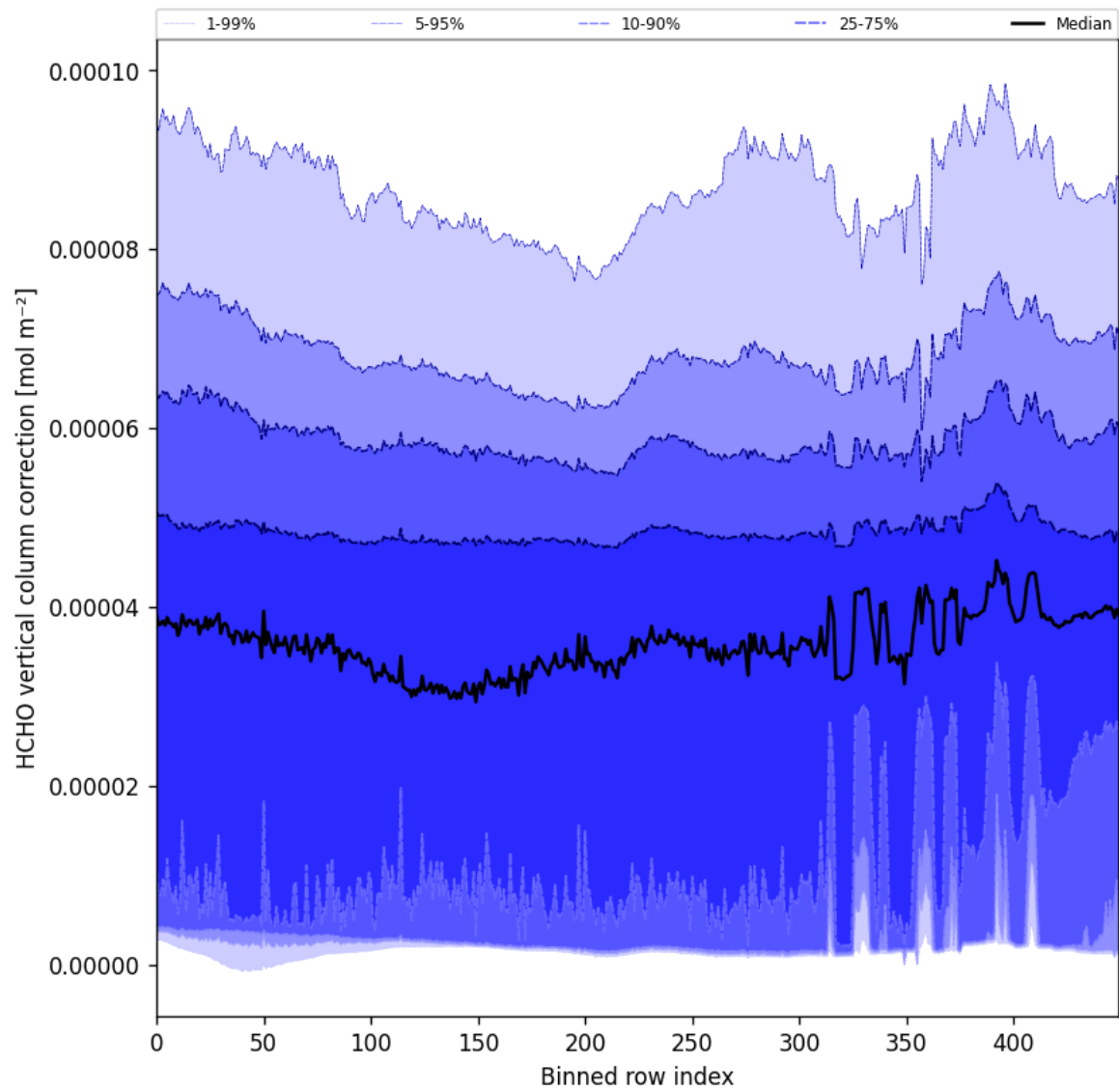
Figure 54: Along track statistics of “HCHO vertical column correction” for 2025-11-23 to 2025-11-25
