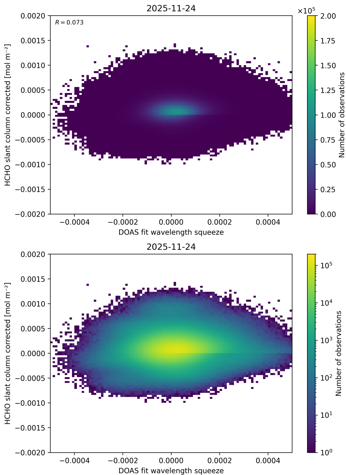
Figure 75: Scatter density plot of “DOAS fit wavelength squeeze” against “HCHO slant column corrected” for 2025-11-23 to 2025-11-25.
