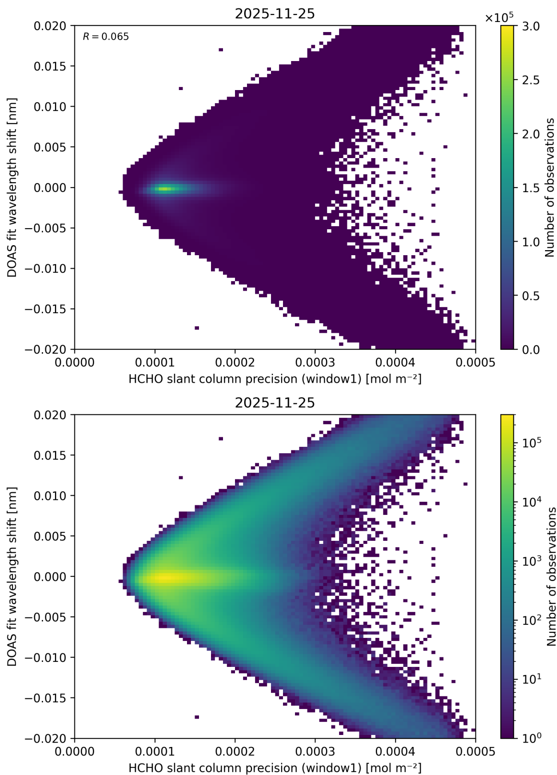
Figure 100: Scatter density plot of “HCHO slant column precision (window1)” against “DOAS fit wavelength shift” for 2025-11-24 to 2025-11-26.
