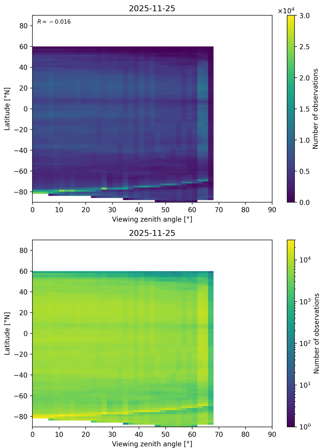
Figure 217: Scatter density plot of “Viewing zenith angle” against “Latitude” for 2025-11-24 to 2025-11-26.
