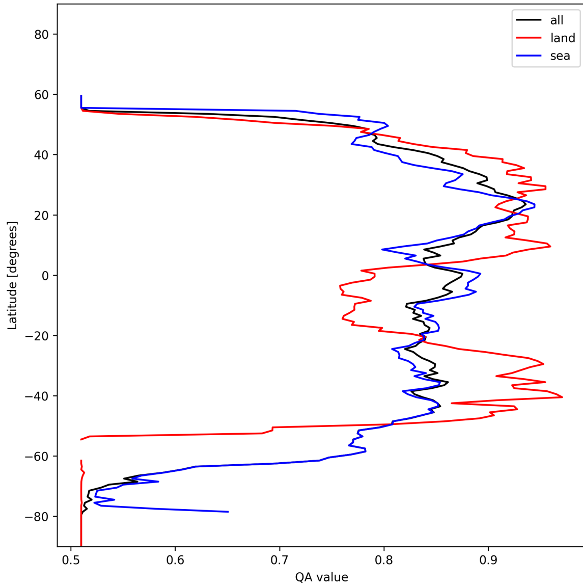
Figure 21: Zonal average of “QA value” for 2025-11-24 to 2025-11-26.
