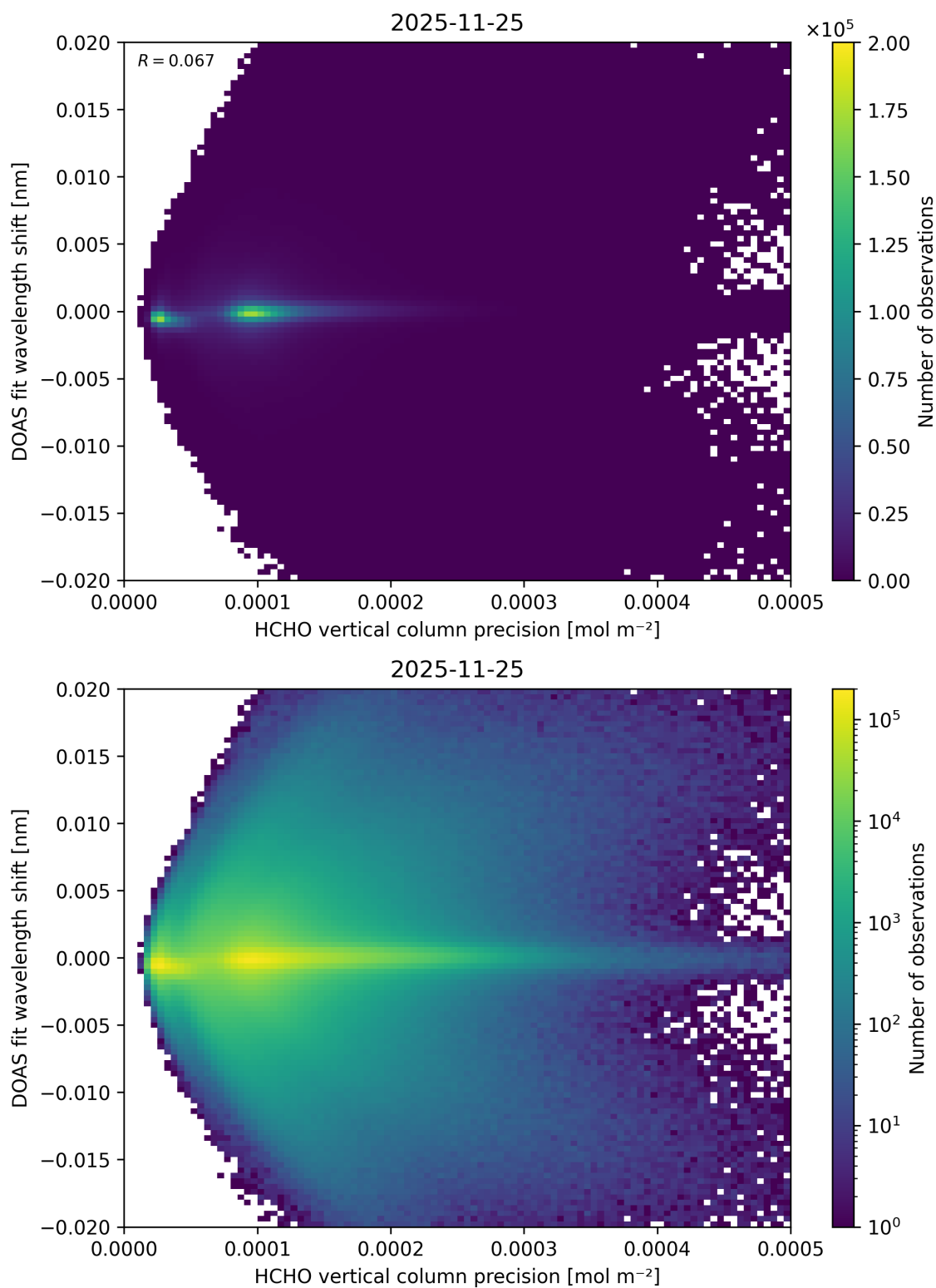
Figure 153: Scatter density plot of “HCHO vertical column precision” against “DOAS fit wavelength shift” for 2025-11-24 to 2025-11-26.
