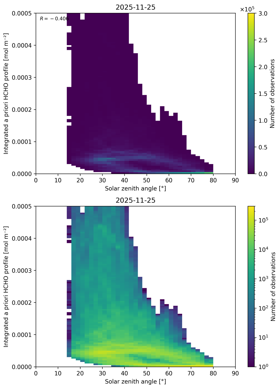
Figure 200: Scatter density plot of “Solar zenith angle” against “Integrated a priori HCHO profile” for 2025-11-24 to 2025-11-26.
