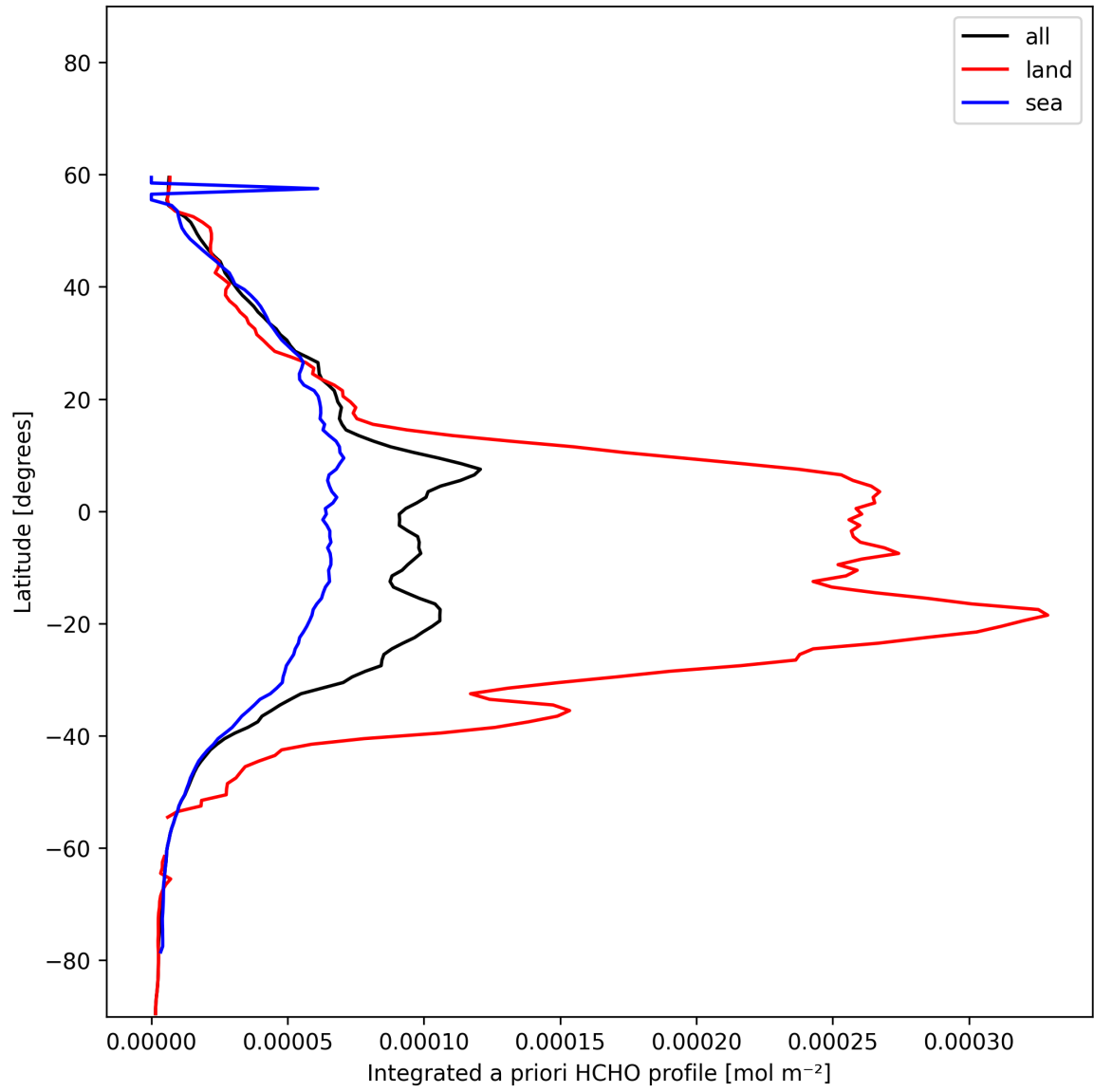
Figure 30: Zonal average of “Integrated a priori HCHO profile” for 2025-11-24 to 2025-11-26.
