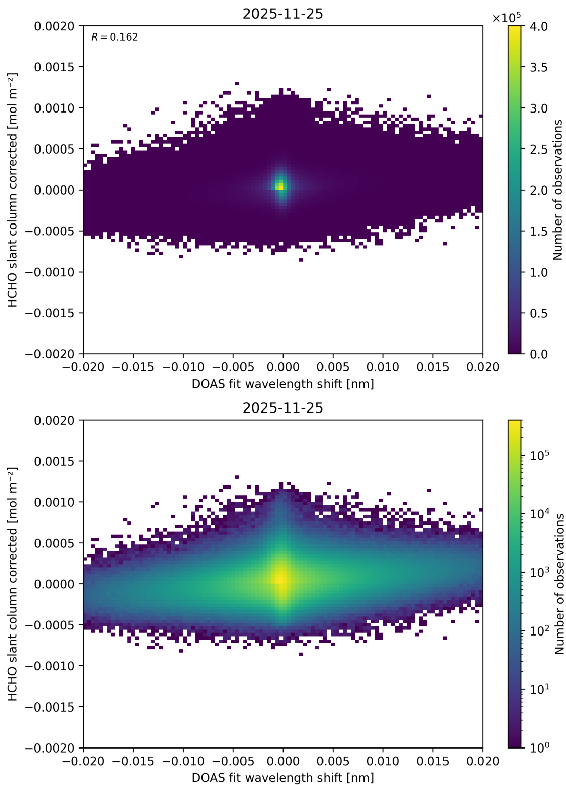
Figure 71: Scatter density plot of “DOAS fit wavelength shift” against “HCHO slant column corrected” for 2025-11-24 to 2025-11-26.
