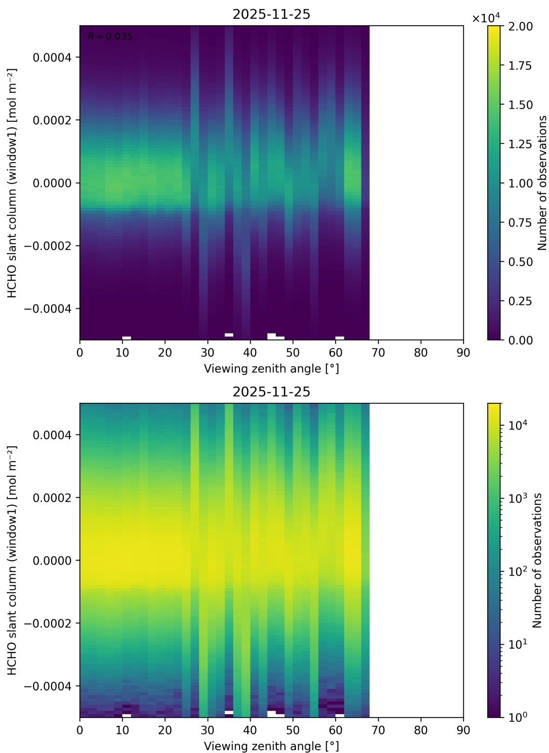
Figure 208: Scatter density plot of “Viewing zenith angle” against “HCHO slant column (window1)” for 2025-11-24 to 2025-11-26.
