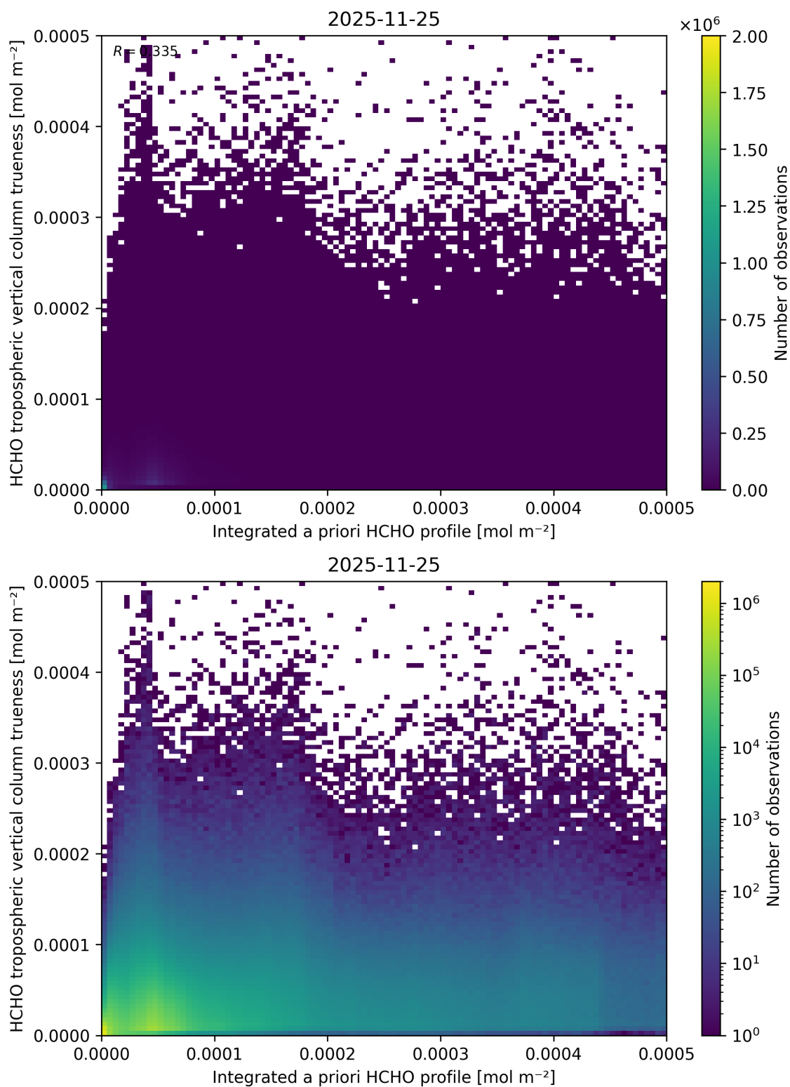
Figure 170: Scatter density plot of “Integrated a priori HCHO profile” against “HCHO tropospheric vertical column truthness” for 2025-11-24 to 2025-11-26.
