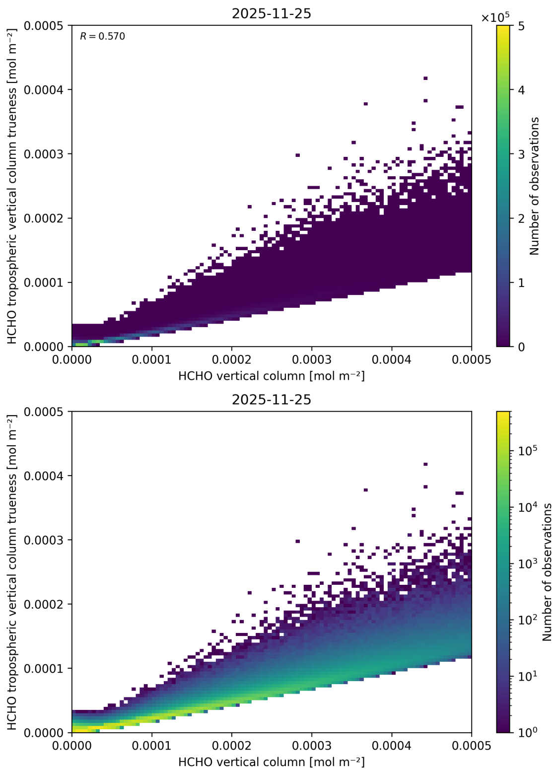
Figure 150: Scatter density plot of “HCHO vertical column” against “HCHO tropospheric vertical column trueness” for 2025-11-24 to 2025-11-26.
