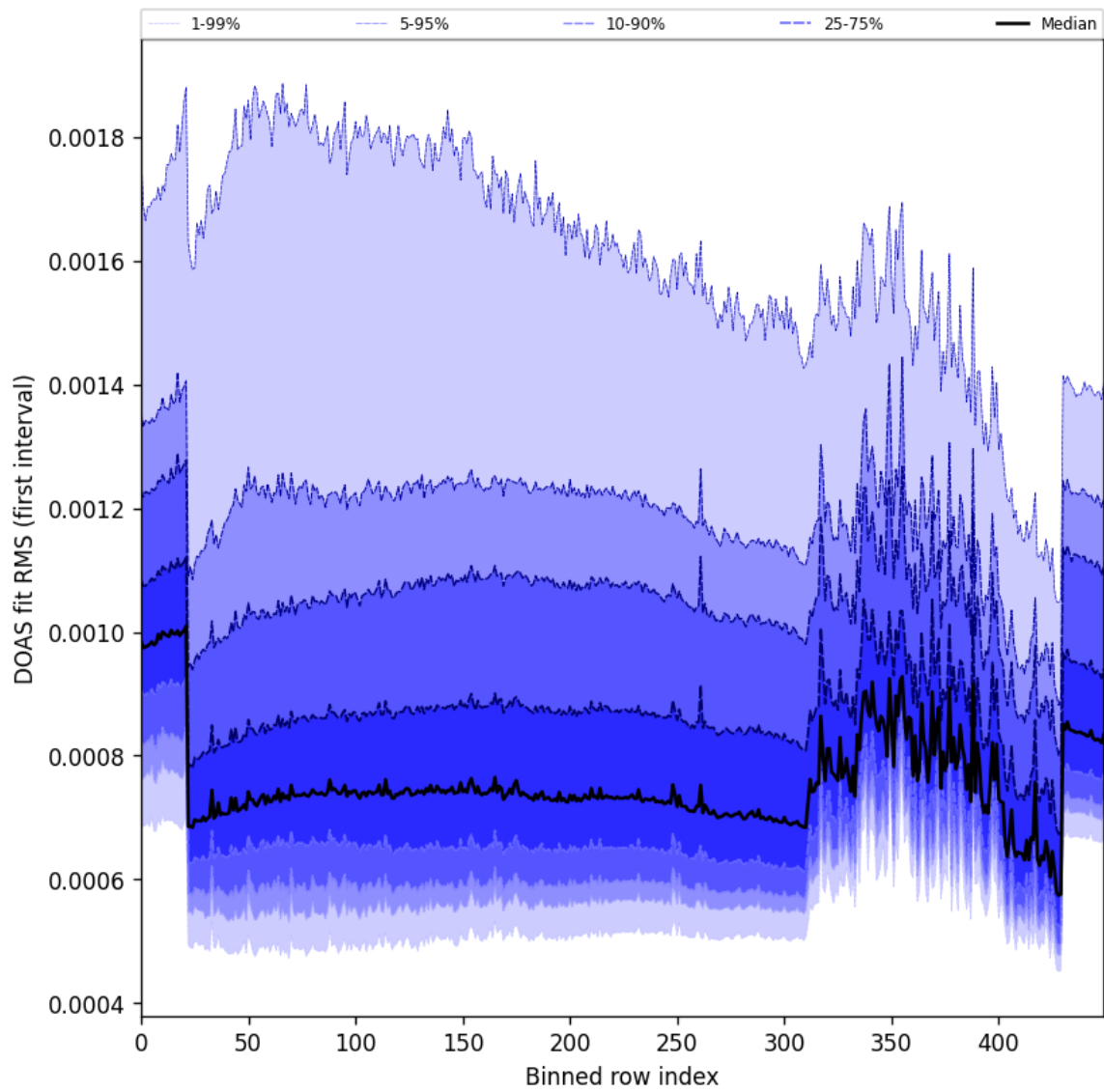
Figure 63: Along track statistics of “DOAS fit RMS (first interval)” for 2025-11-24 to 2025-11-26
