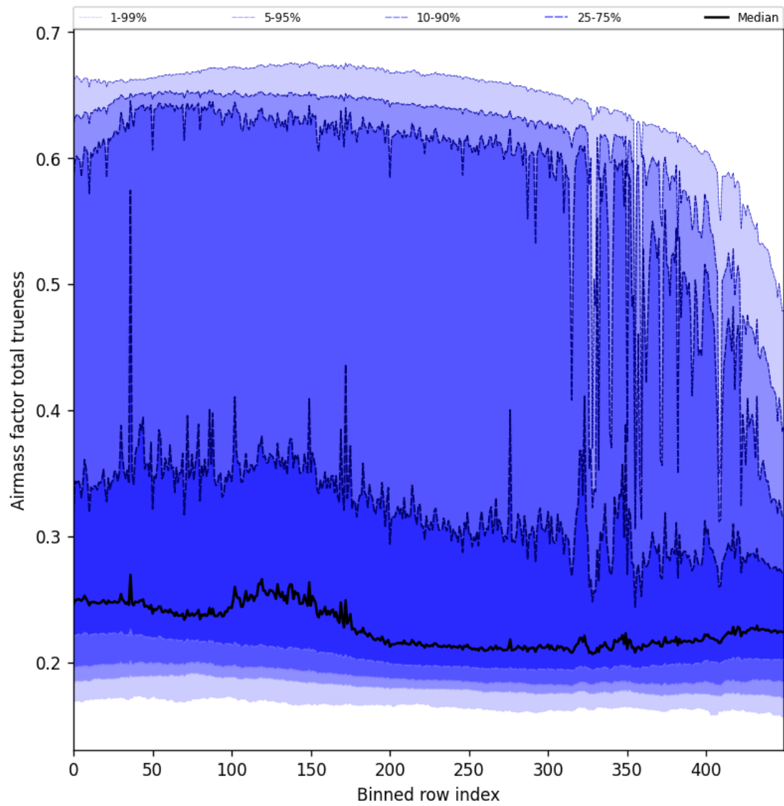
Figure 58: Along track statistics of “Airmass factor total trueness” for 2025-11-24 to 2025-11-26
