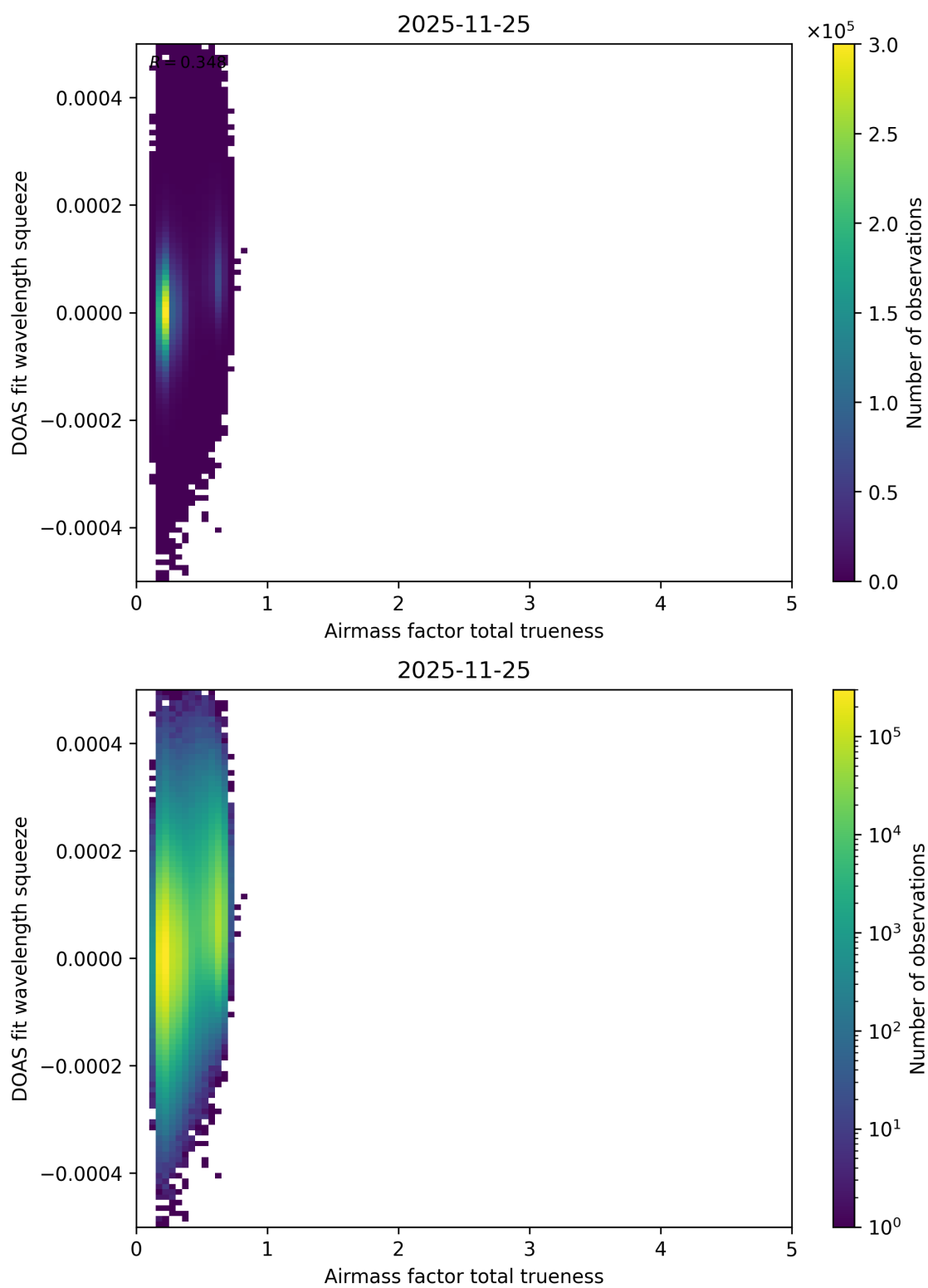
Figure 120: Scatter density plot of “Airmass factor total trueness” against “DOAS fit wavelength squeeze” for 2025-11-24 to 2025-11-26.
