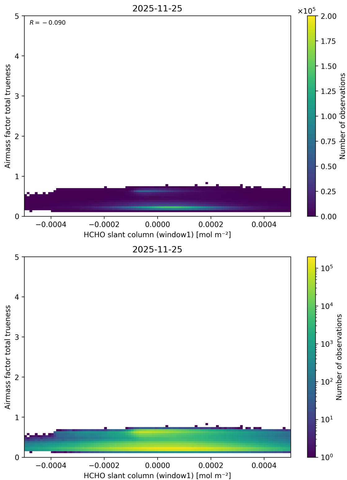
Figure 96: Scatter density plot of “HCHO slant column (window1)” against “Airmass factor total trueneess” for 2025-11-24 to 2025-11-26.
