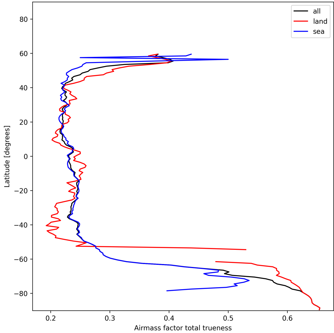
Figure 28: Zonal average of “Airmass factor total trueness” for 2025-11-24 to 2025-11-26.
