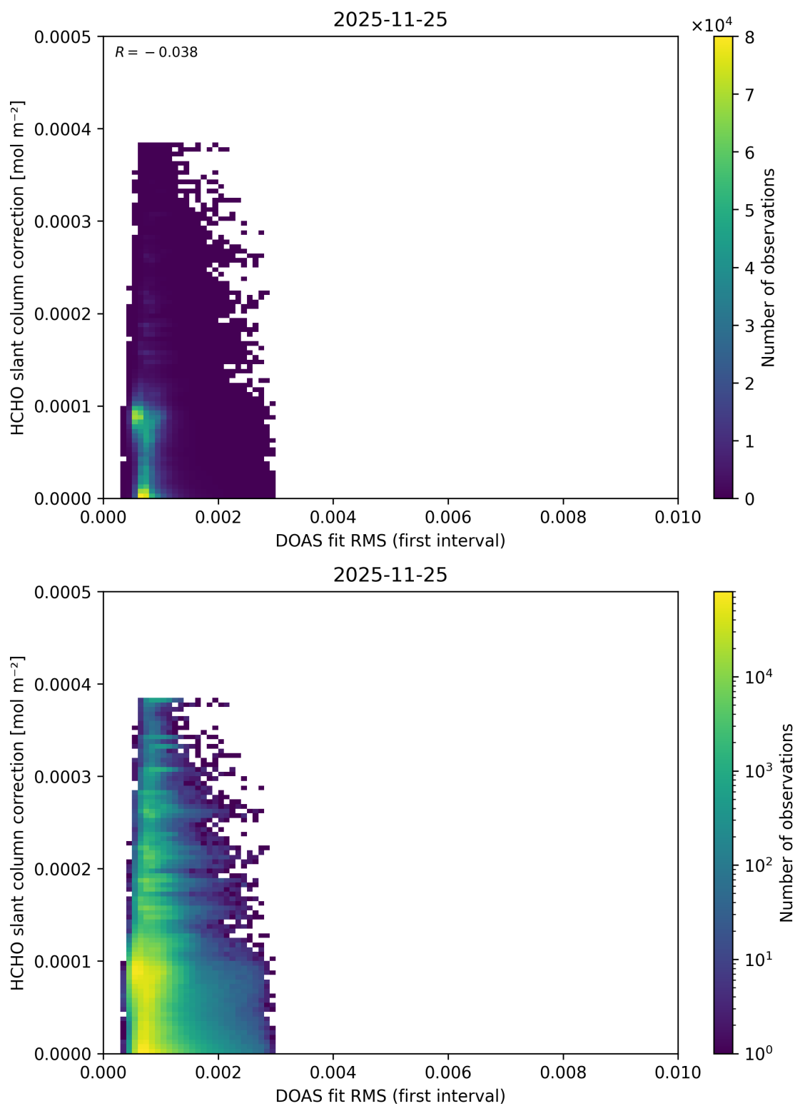
Figure 67: Scatter density plot of “DOAS fit RMS (first interval)” against “HCHO slant column correction” for 2025-11-24 to 2025-11-26.
