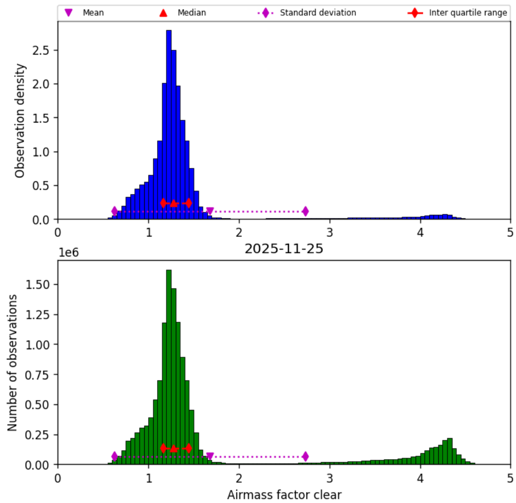
Figure 44: Histogram of “Airmass factor clear” for 2025-11-24 to 2025-11-26
