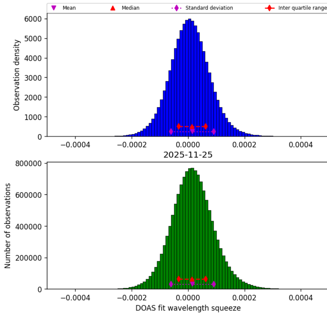
Figure 47: Histogram of “DOAS fit wavelength squeeze” for 2025-11-24 to 2025-11-26
