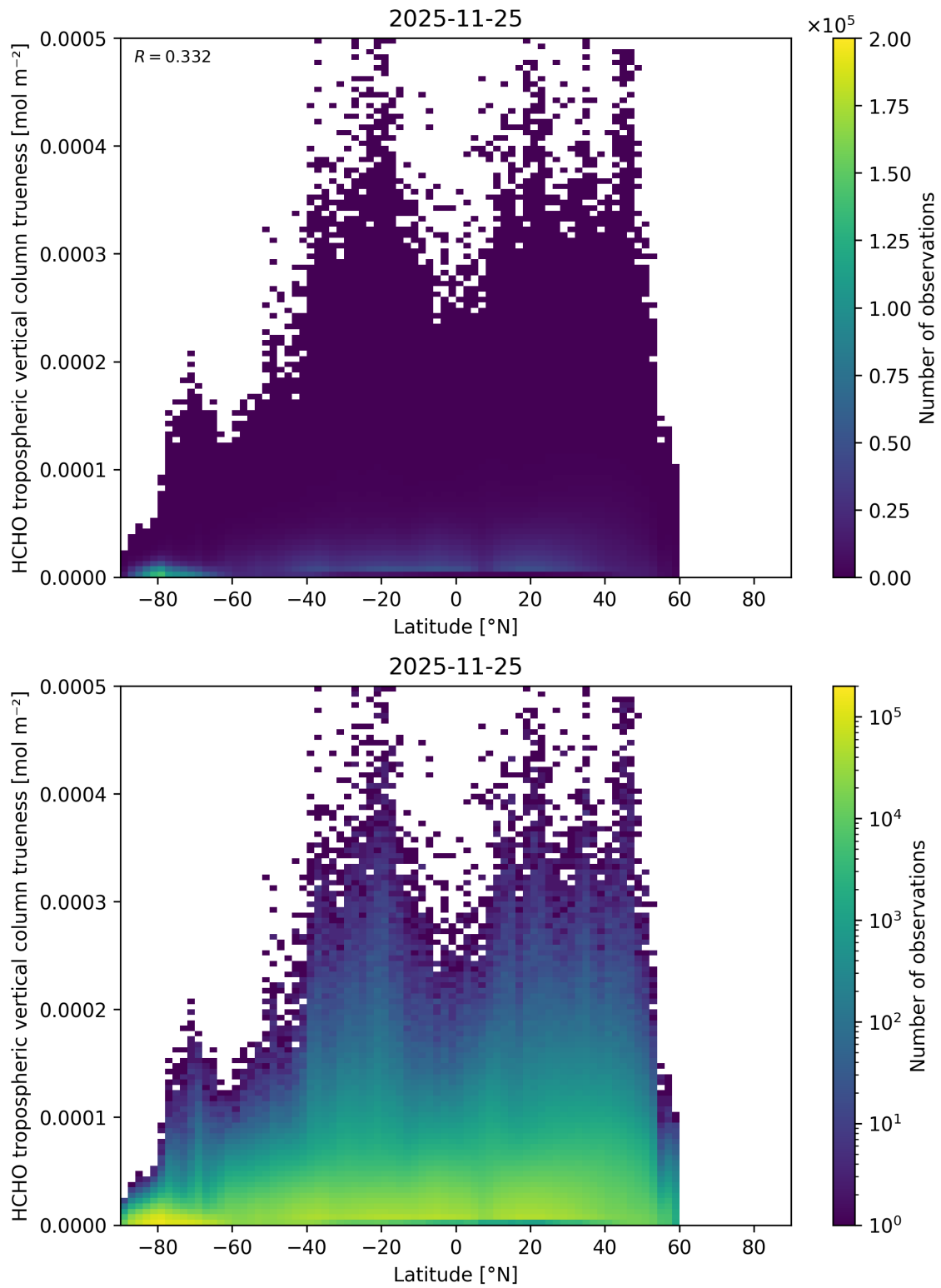
Figure 184: Scatter density plot of “Latitude” against “HCHO tropospheric vertical column trueeness” for 2025-11-24 to 2025-11-26.
