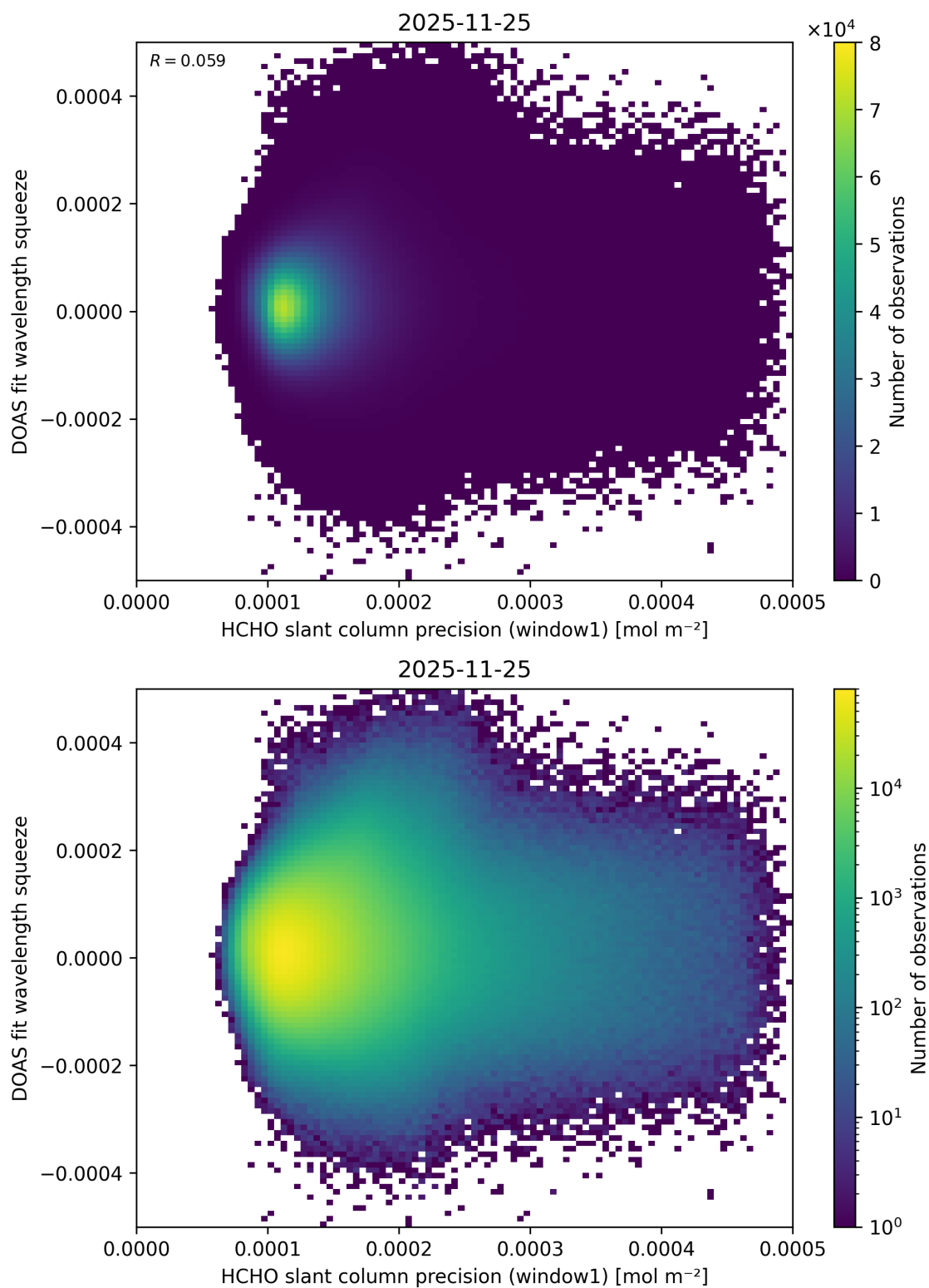
Figure 101: Scatter density plot of “HCHO slant column precision (window1)” against “DOAS fit wavelength squeeze” for 2025-11-24 to 2025-11-26.
