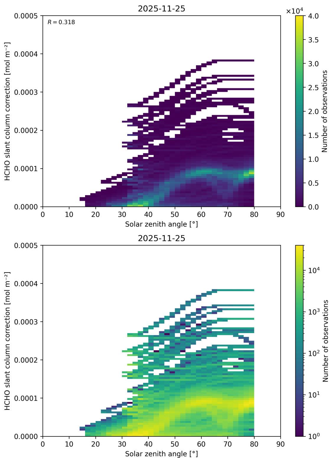
Figure 191: Scatter density plot of “Solar zenith angle” against “HCHO slant column correction” for 2025-11-24 to 2025-11-26.
