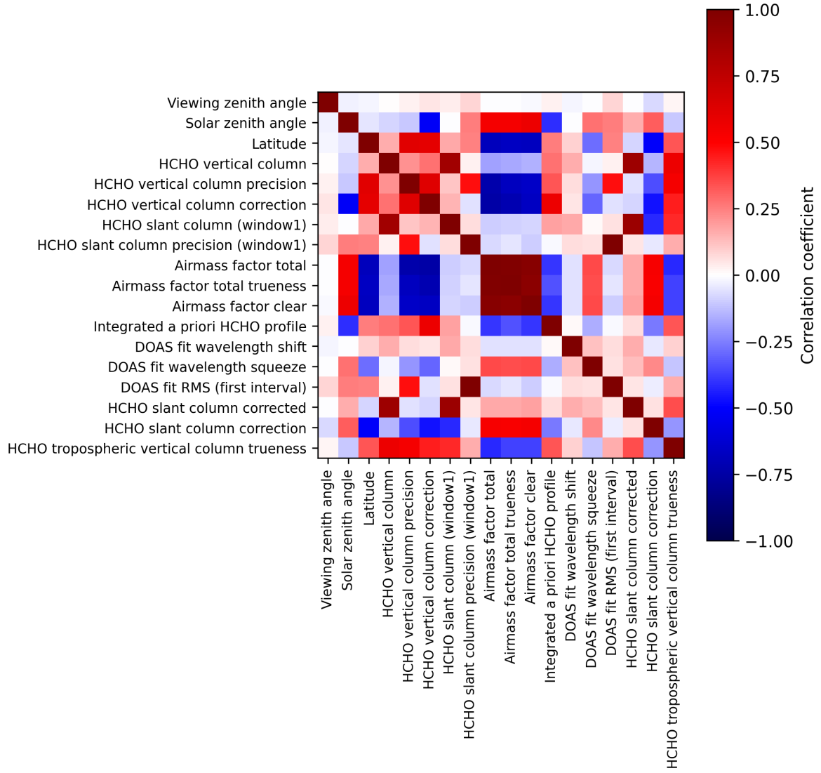
Figure 2: Map of correlation matrix for 2025-11-24 to 2025-11-26.
