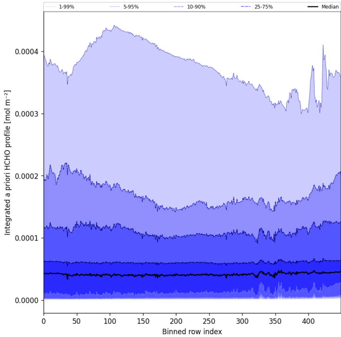
Figure 60: Along track statistics of “Integrated a priori HCHO profile” for 2025-11-24 to 2025-11-26
