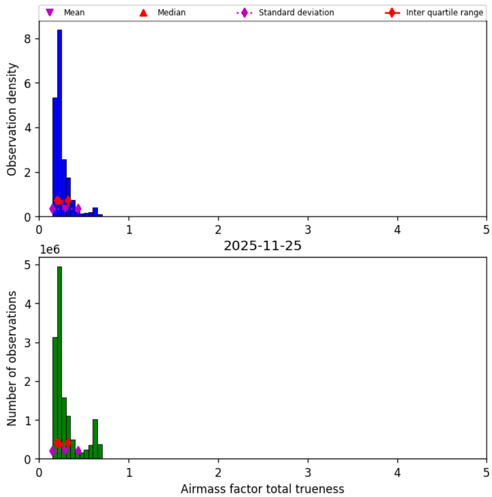
Figure 43: Histogram of “Airmass factor total trueness” for 2025-11-24 to 2025-11-26
