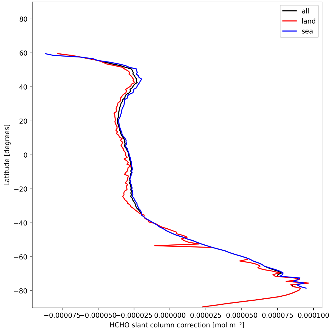
Figure 34: Zonal average of “HCHO slant column correction” for 2025-11-24 to 2025-11-26.
