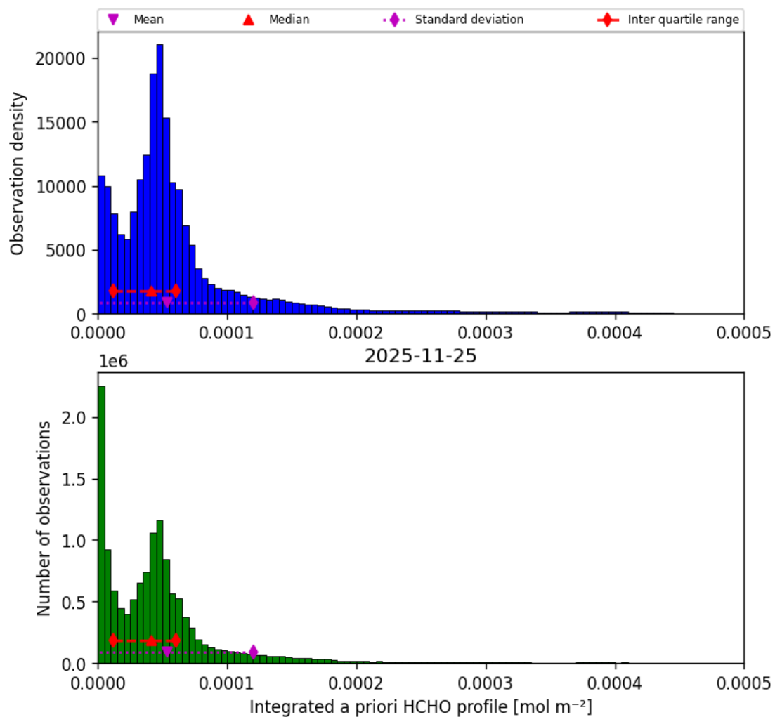
Figure 45: Histogram of “Integrated a priori HCHO profile” for 2025-11-24 to 2025-11-26
