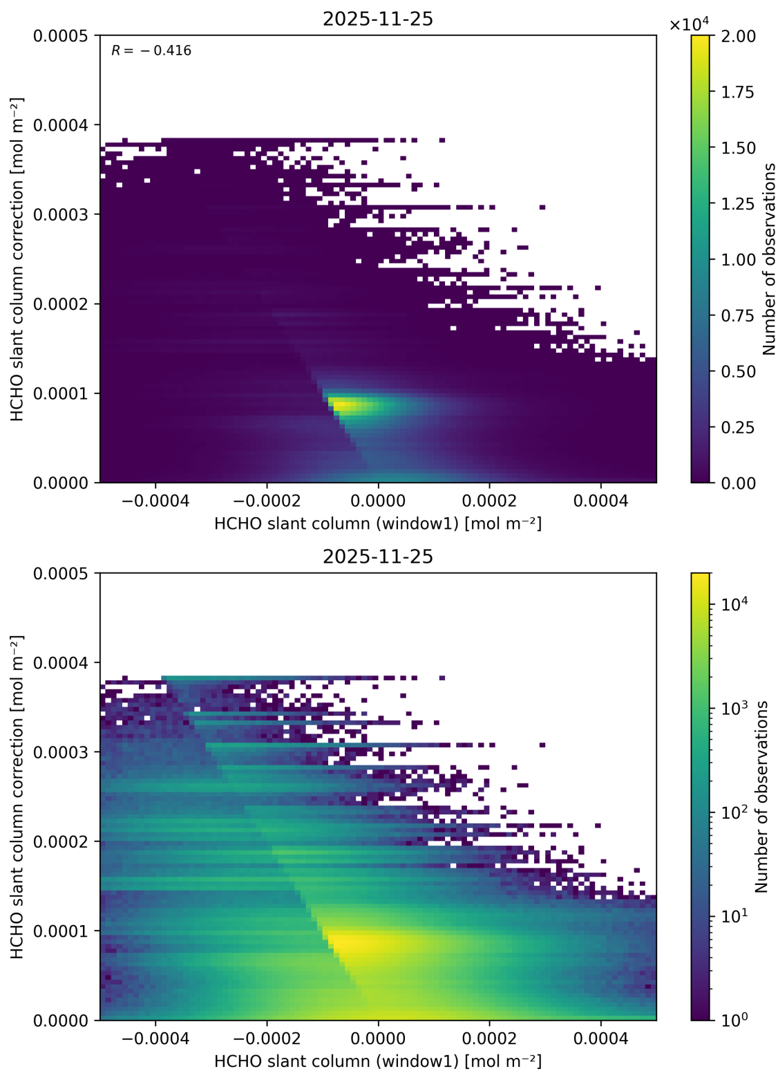
Figure 93: Scatter density plot of “HCHO slant column (window1)” against “HCHO slant column correction” for 2025-11-24 to 2025-11-26.
