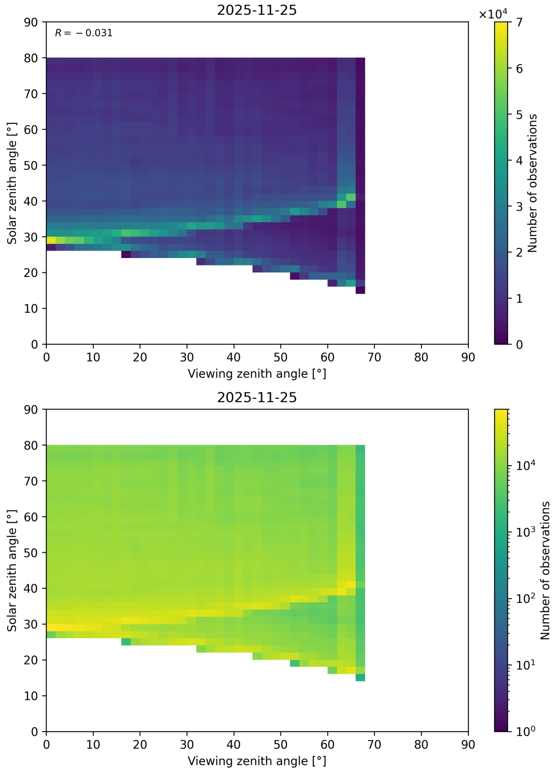
Figure 218: Scatter density plot of “Viewing zenith angle” against “Solar zenith angle” for 2025-11-24 to 2025-11-26.
