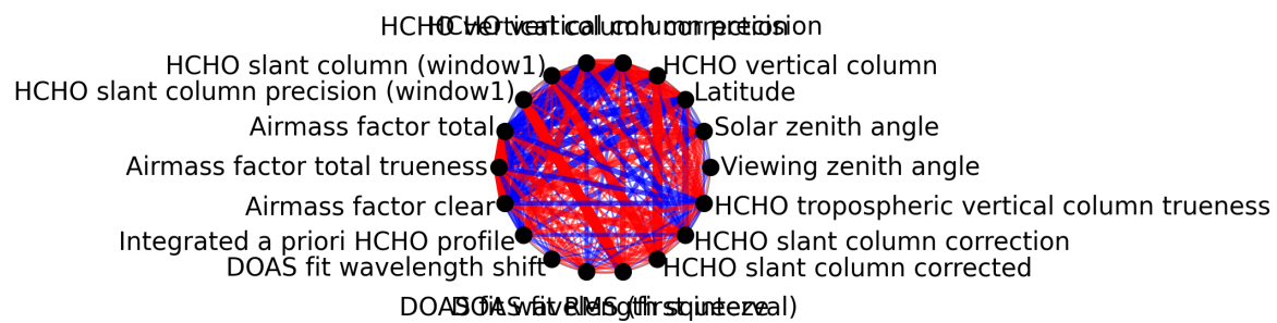
Figure 1: Map of correlation graph for 2025-11-24 to 2025-11-26.
