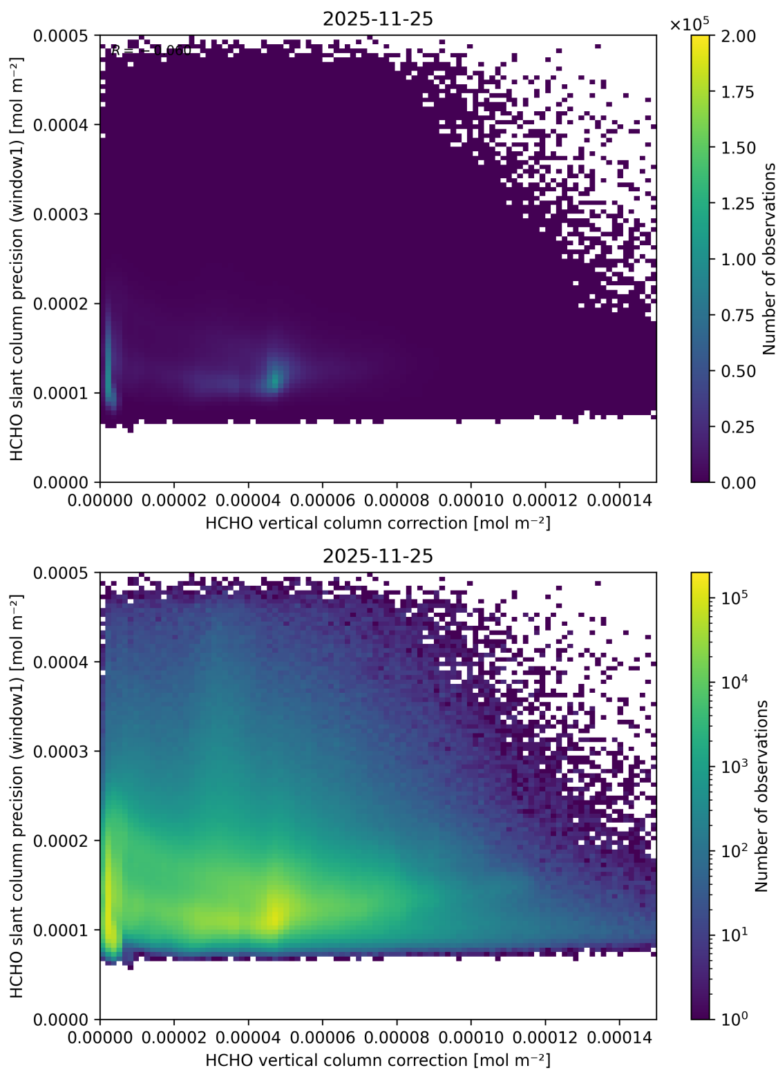
Figure 133: Scatter density plot of “HCHO vertical column correction” against “HCHO slant column precision (window1)” for 2025-11-24 to 2025-11-26.
