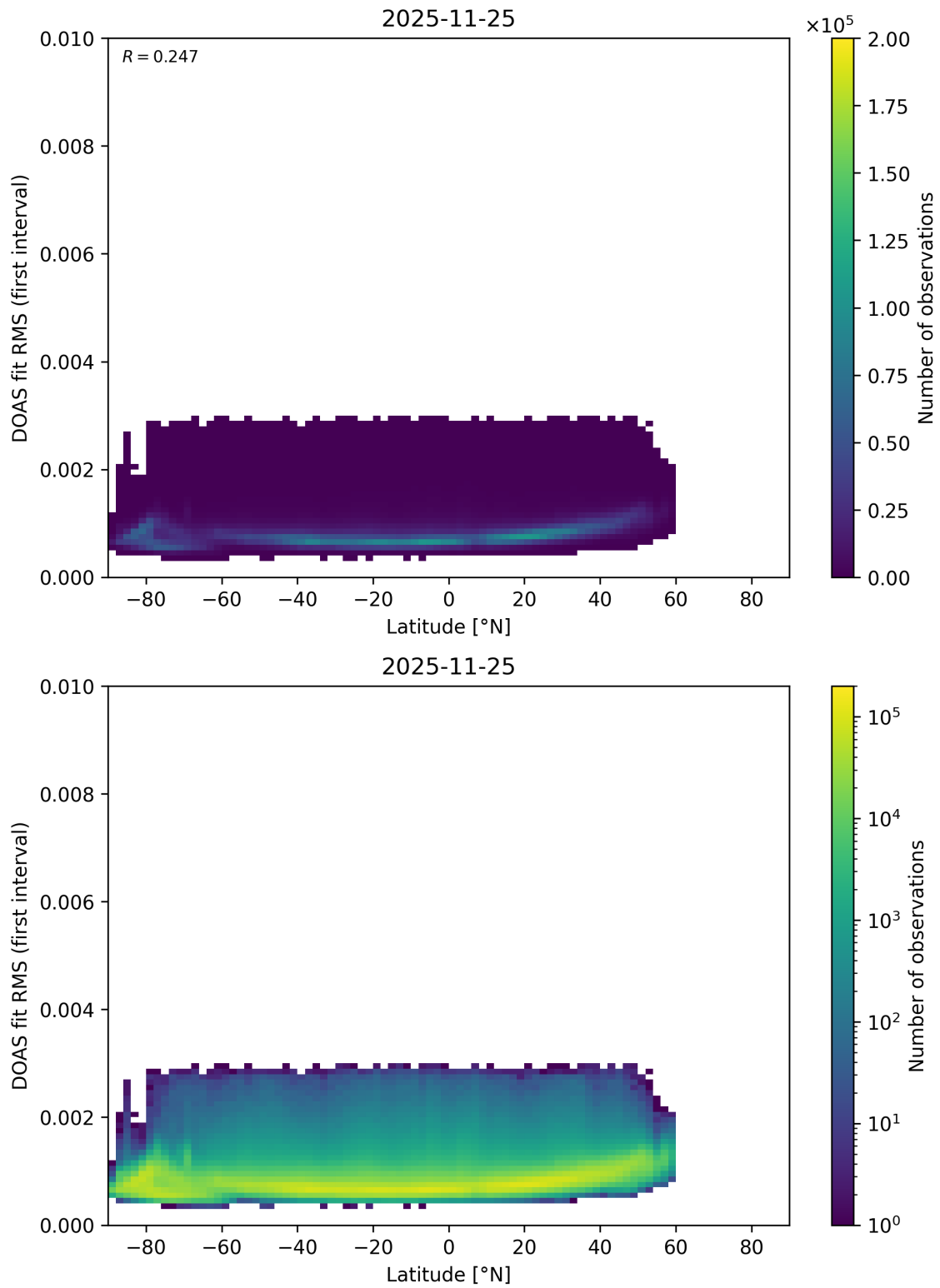
Figure 171: Scatter density plot of “Latitude” against “DOAS fit RMS (first interval)” for 2025-11-24 to 2025-11-26.
