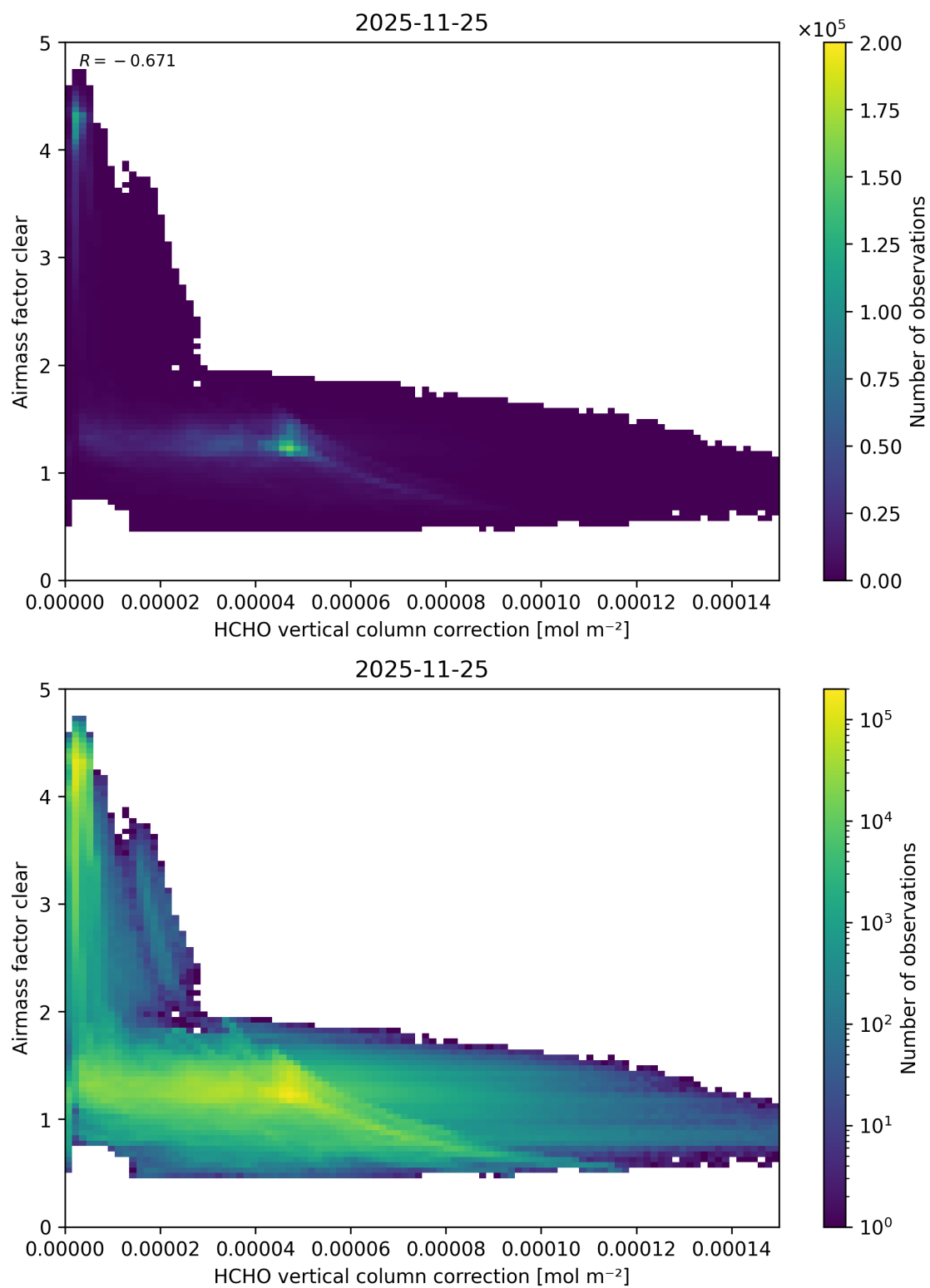
Figure 129: Scatter density plot of “HCHO vertical column correction” against “Airmass factor clear” for 2025-11-24 to 2025-11-26.
