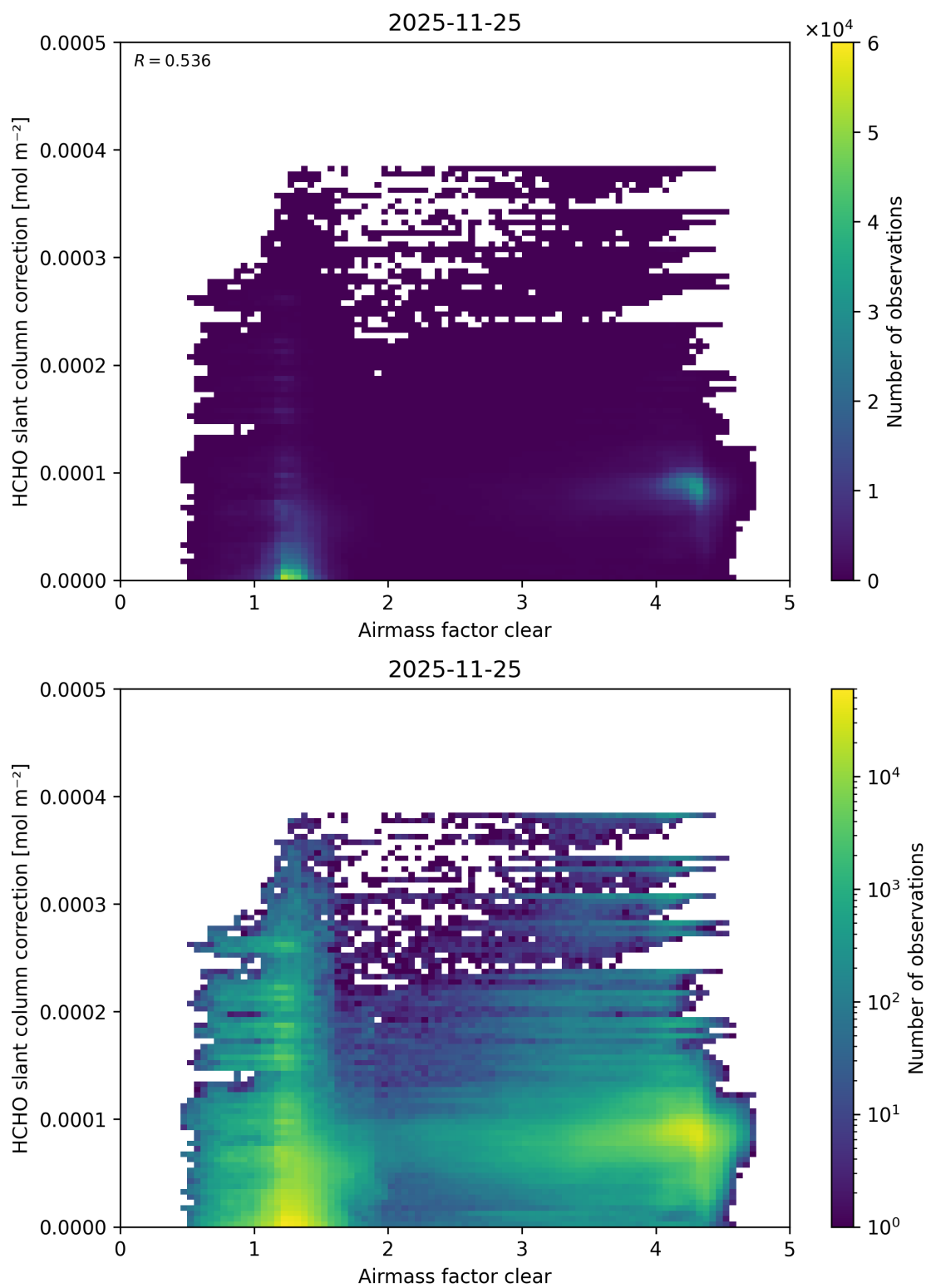
Figure 82: Scatter density plot of “Airmass factor clear” against “HCHO slant column correction” for 2025-11-24 to 2025-11-26.
