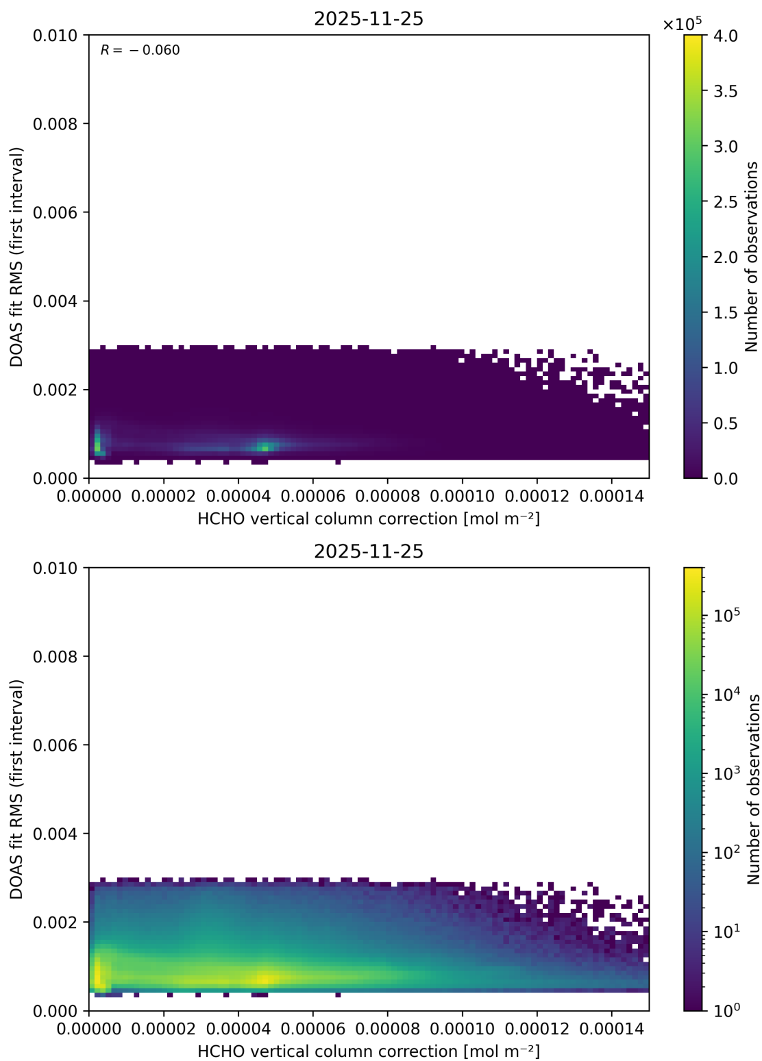
Figure 126: Scatter density plot of “HCHO vertical column correction” against “DOAS fit RMS (first interval)” for 2025-11-24 to 2025-11-26.
