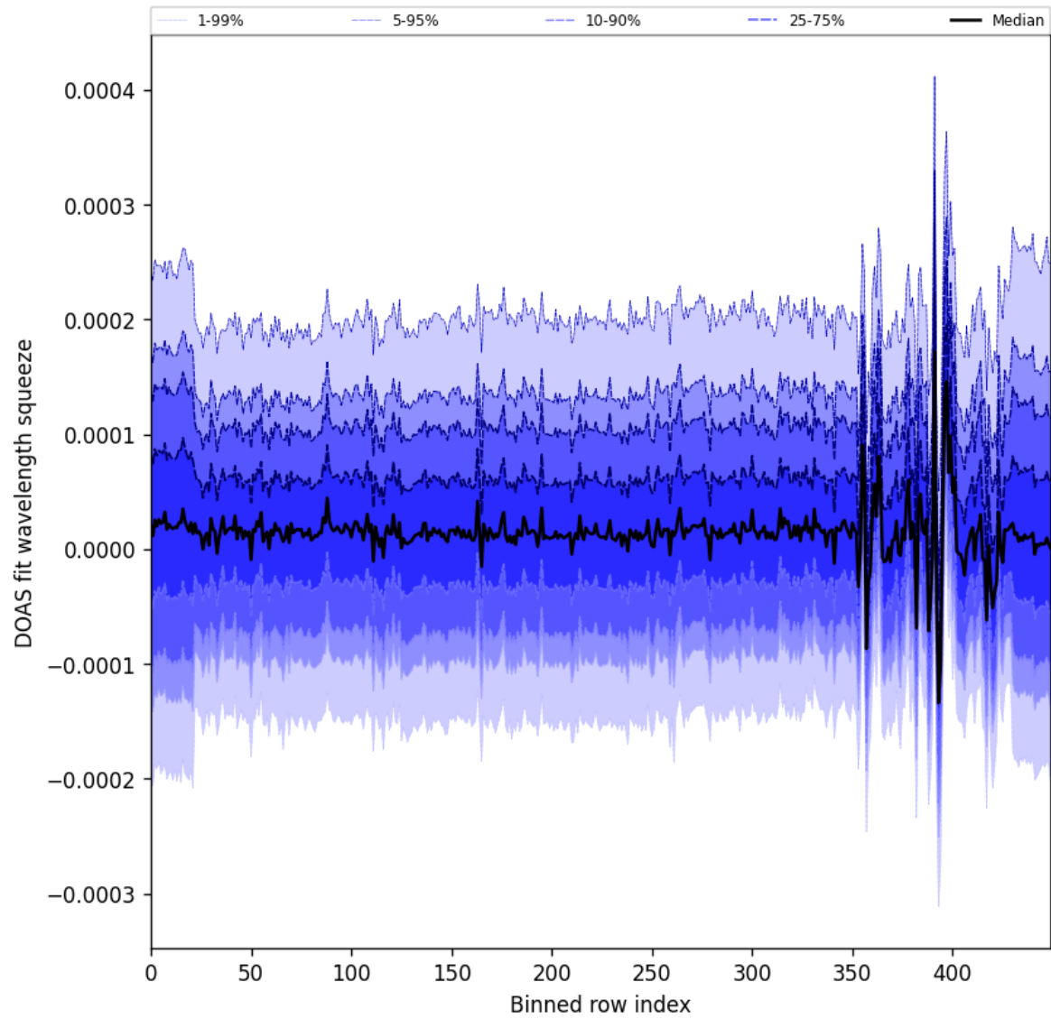
Figure 62: Along track statistics of “DOAS fit wavelength squeeze” for 2025-11-24 to 2025-11-26
