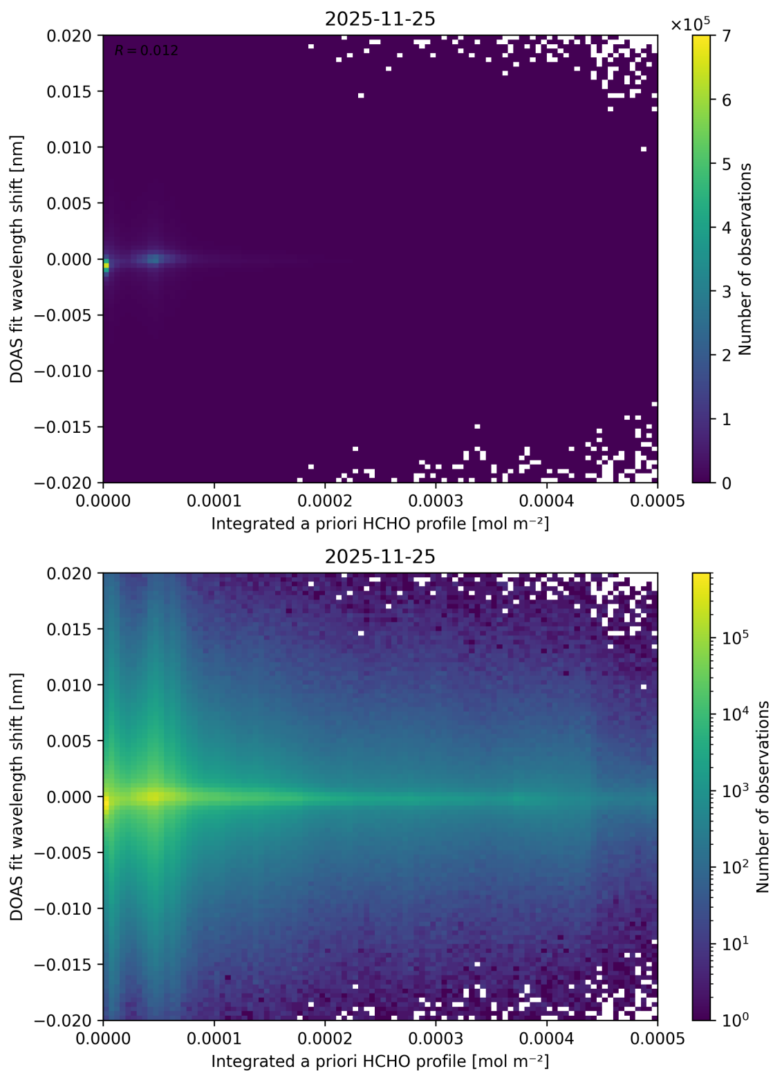
Figure 166: Scatter density plot of “Integrated a priori HCHO profile” against “DOAS fit wavelength shift” for 2025-11-24 to 2025-11-26.
