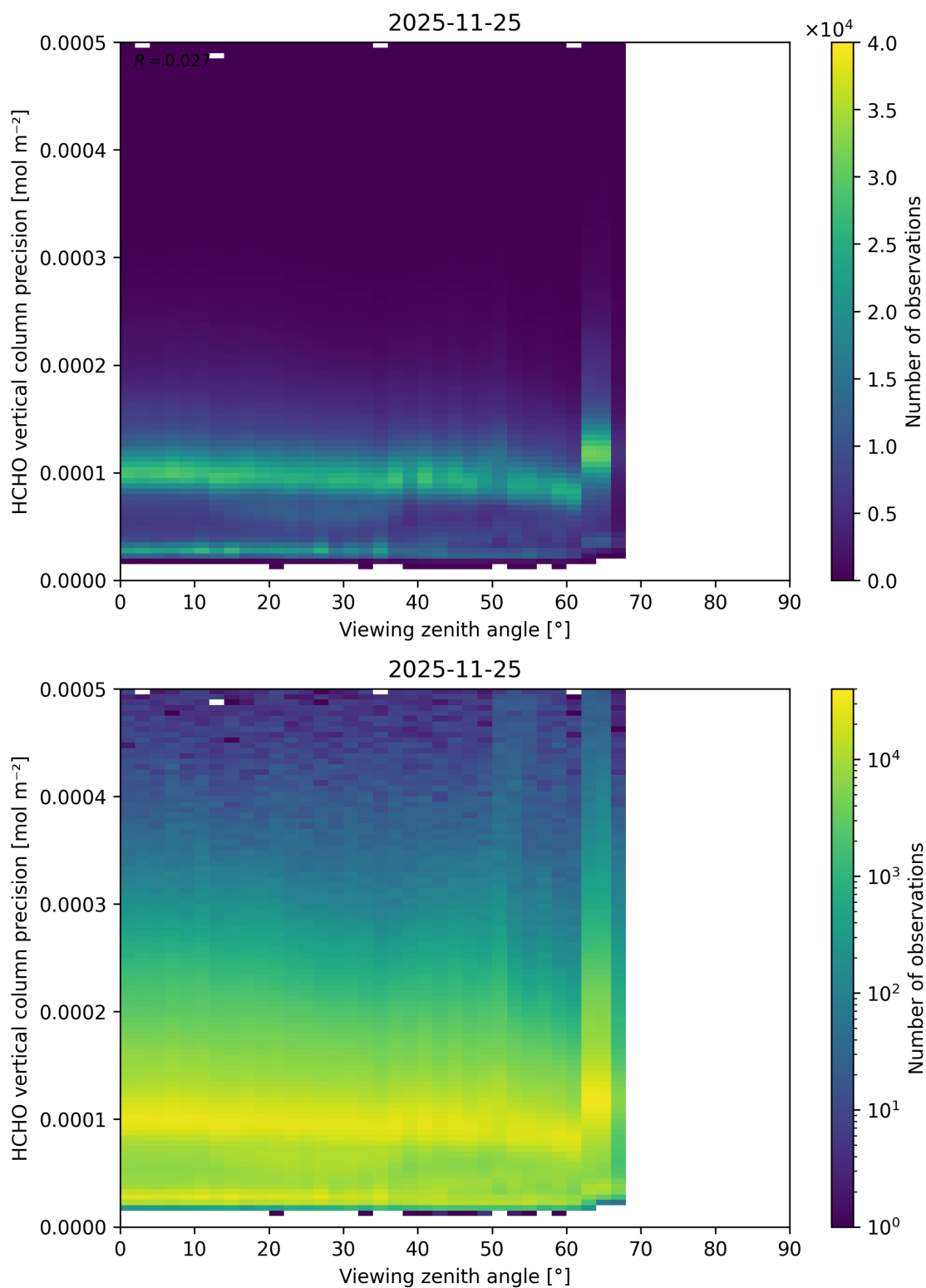
Figure 214: Scatter density plot of “Viewing zenith angle” against “HCHO vertical column precision” for 2025-11-24 to 2025-11-26.
