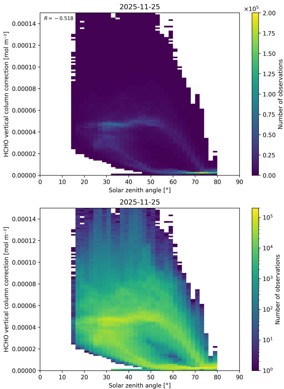
Figure 197: Scatter density plot of “Solar zenith angle” against “HCHO vertical column correction” for 2025-11-24 to 2025-11-26.
