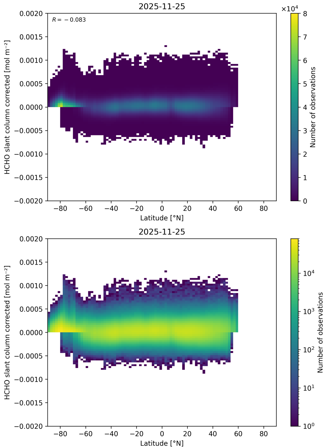
Figure 175: Scatter density plot of “Latitude” against “HCHO slant column corrected” for 2025-11-24 to 2025-11-26.
