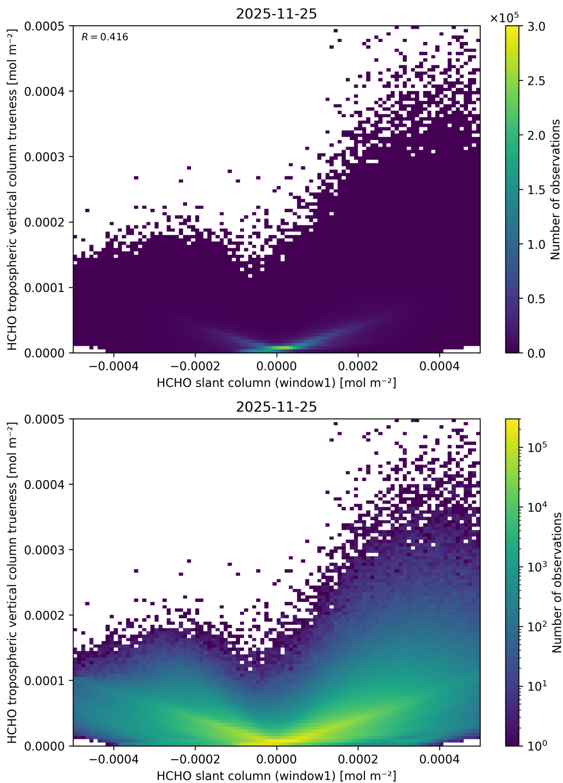
Figure 97: Scatter density plot of “HCHO slant column (window1)” against “HCHO tropospheric vertical column trueness” for 2025-11-24 to 2025-11-26.
