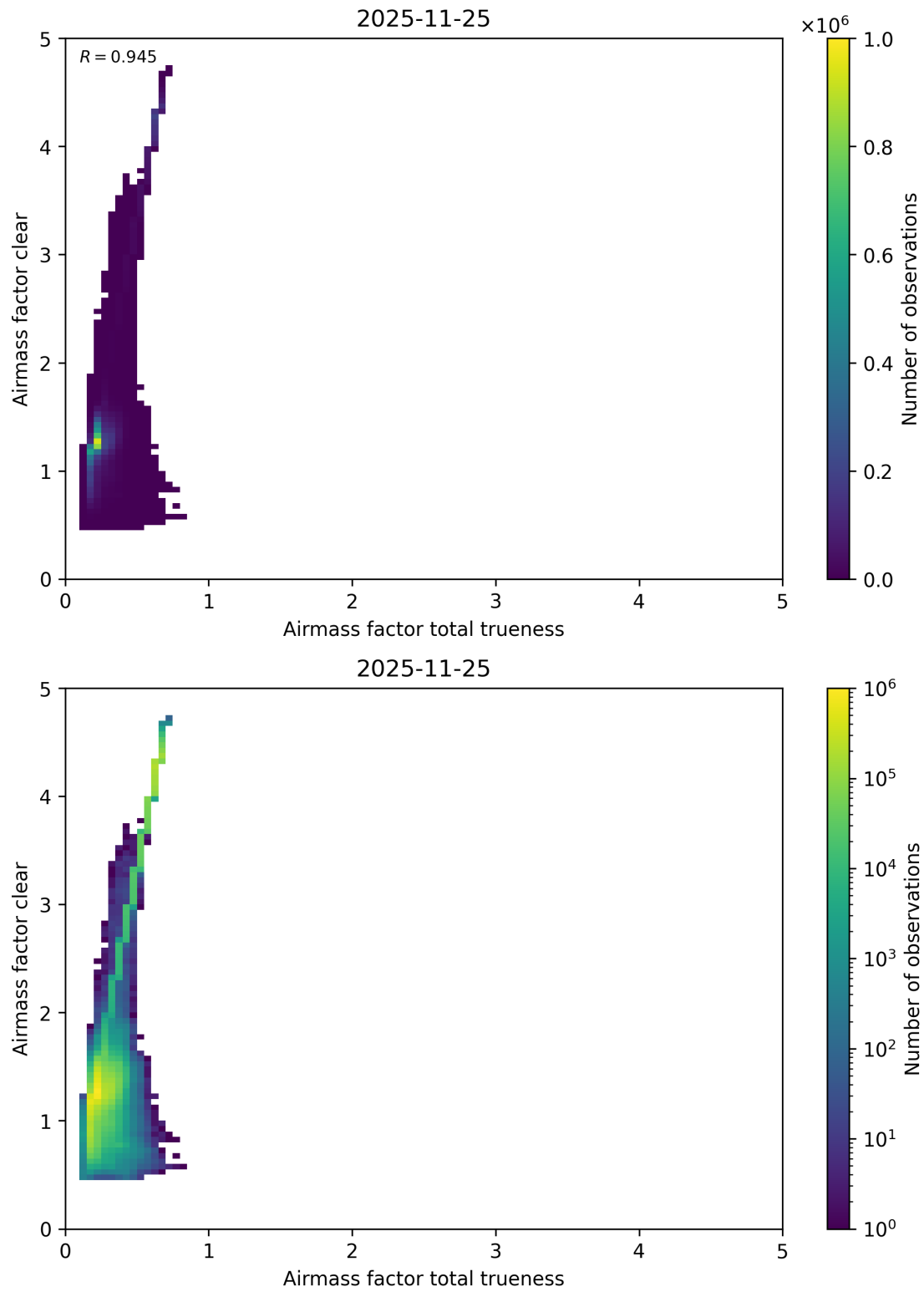
Figure 121: Scatter density plot of “Airmass factor total trueness” against “Airmass factor clear” for 2025-11-24 to 2025-11-26.
