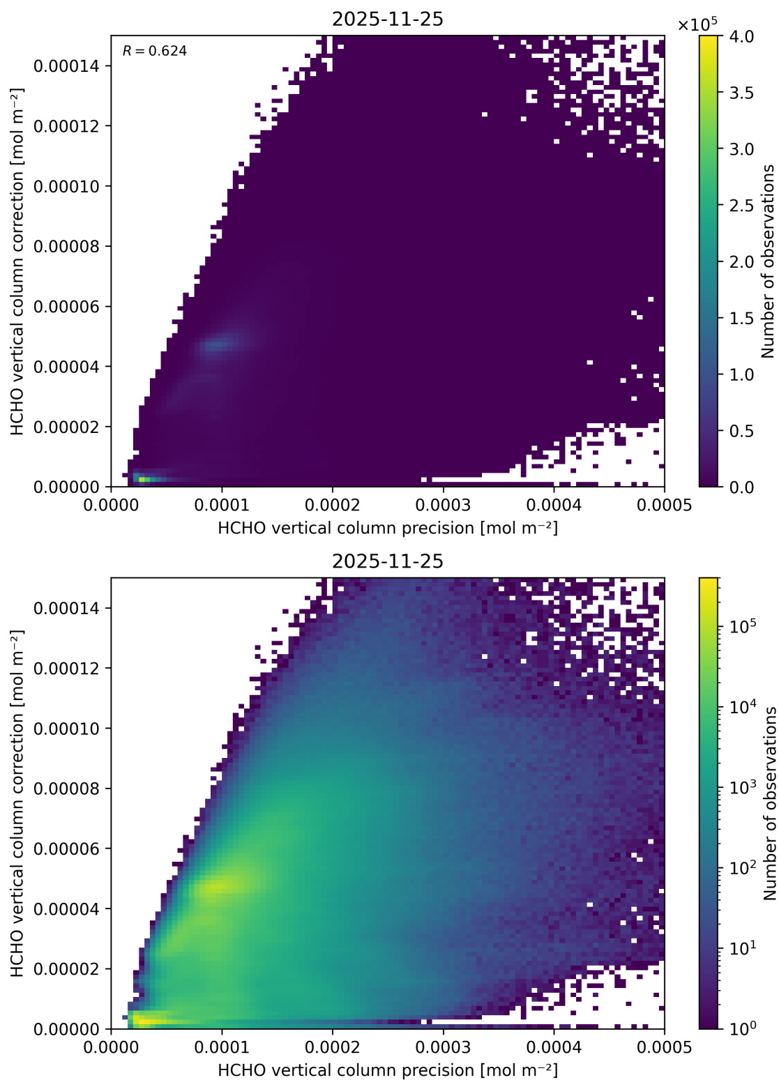
Figure 162: Scatter density plot of “HCHO vertical column precision” against “HCHO vertical column correction” for 2025-11-24 to 2025-11-26.
