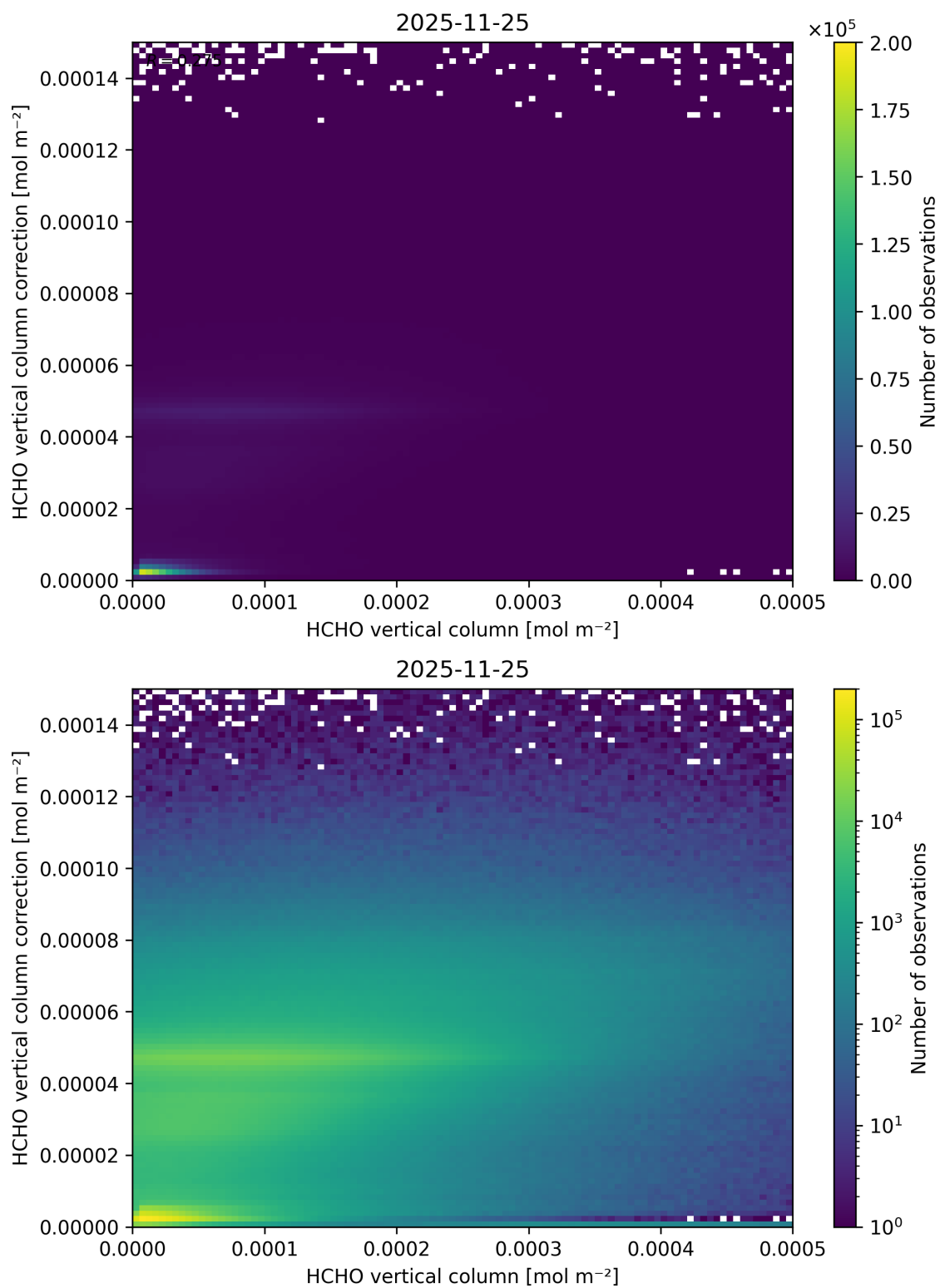
Figure 148: Scatter density plot of “HCHO vertical column” against “HCHO vertical column correction” for 2025-11-24 to 2025-11-26.
