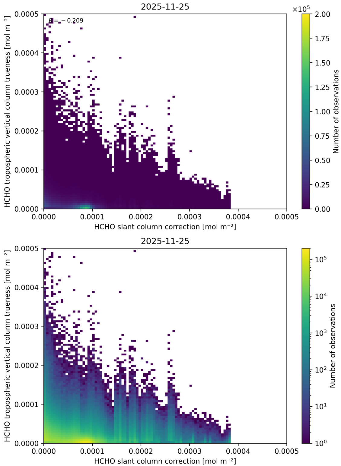
Figure 87: Scatter density plot of “HCHO slant column correction” against “HCHO tropospheric vertical column trueness” for 2025-11-24 to 2025-11-26.
