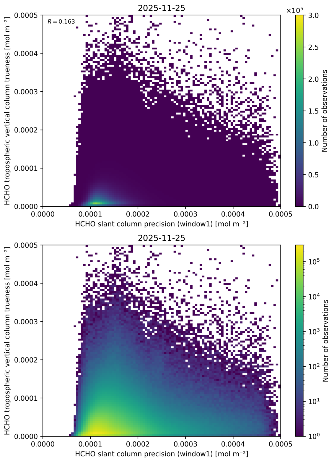
Figure 107: Scatter density plot of “HCHO slant column precision (window1)” against “HCHO tropospheric vertical column trueness” for 2025-11-24 to 2025-11-26.
