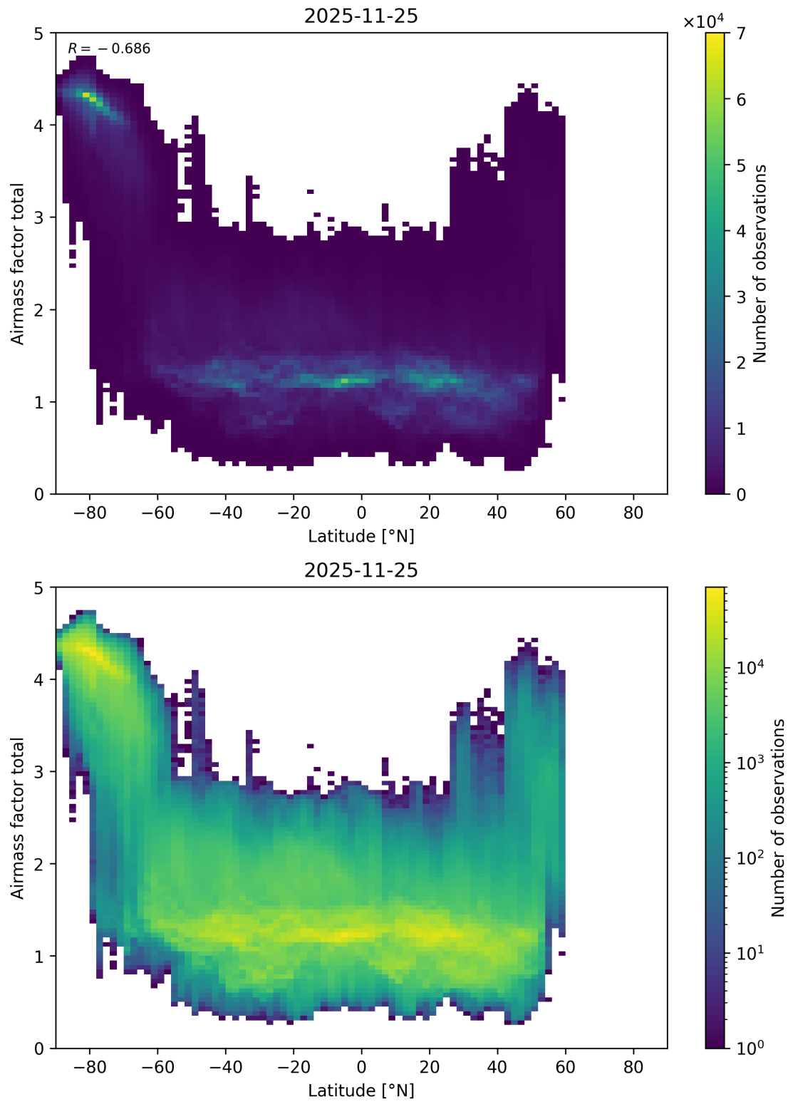
Figure 179: Scatter density plot of “Latitude” against “Airmass factor total” for 2025-11-24 to 2025-11-26.
