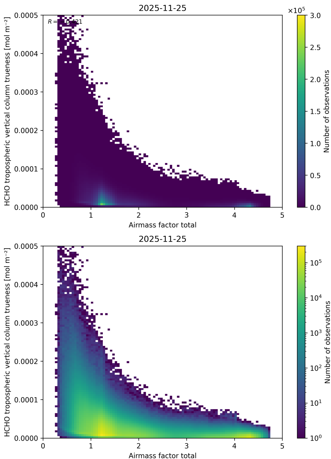
Figure 116: Scatter density plot of “Airmass factor total” against “HCHO tropospheric vertical column trueeness” for 2025-11-24 to 2025-11-26.
