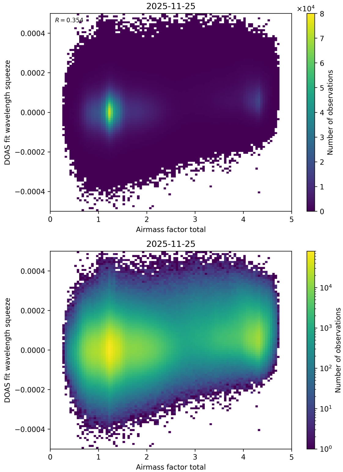
Figure 111: Scatter density plot of “Airmass factor total” against “DOAS fit wavelength squeeze” for 2025-11-24 to 2025-11-26.
