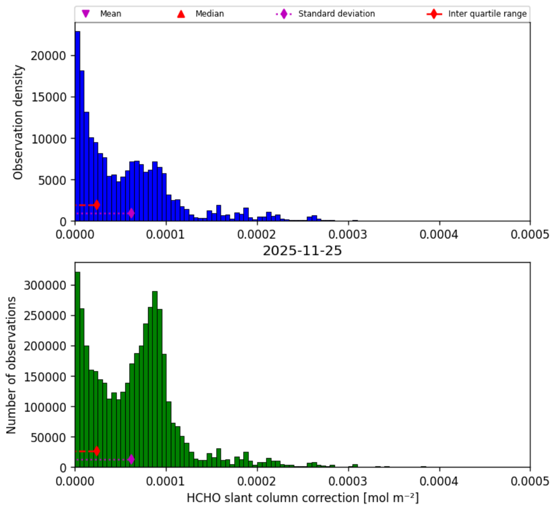
Figure 49: Histogram of “HCHO slant column correction” for 2025-11-24 to 2025-11-26
