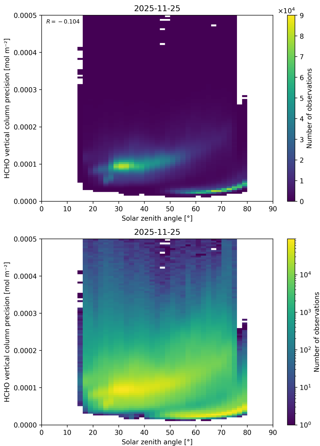
Figure 198: Scatter density plot of “Solar zenith angle” against “HCHO vertical column precision” for 2025-11-24 to 2025-11-26.
