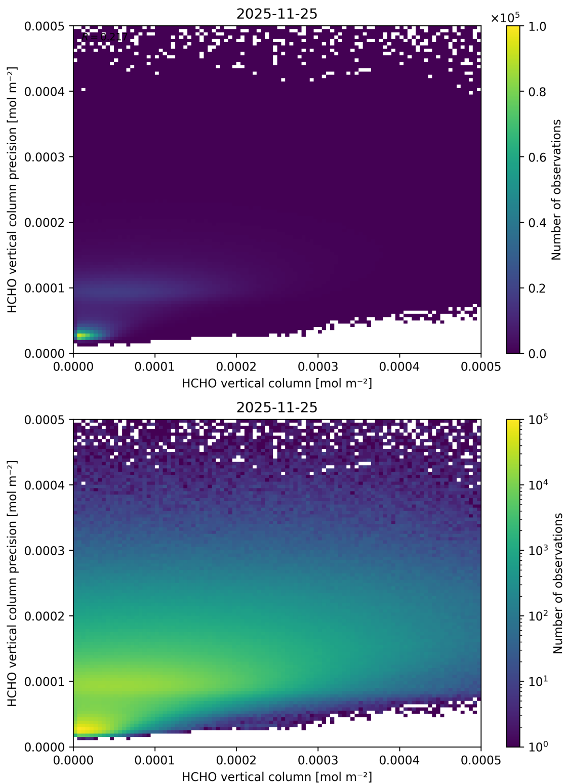
Figure 149: Scatter density plot of “HCHO vertical column” against “HCHO vertical column precision” for 2025-11-24 to 2025-11-26.
