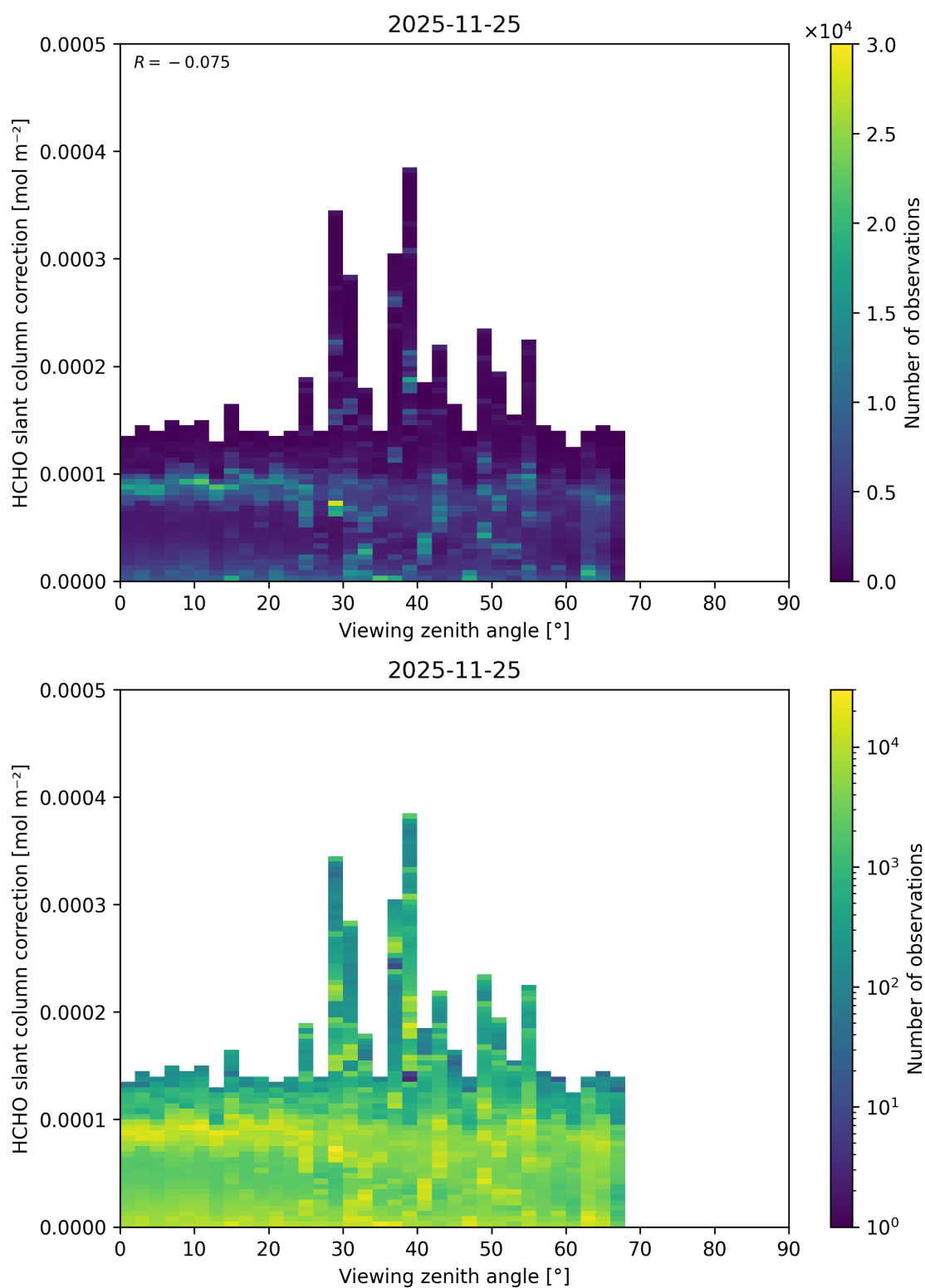
Figure 207: Scatter density plot of “Viewing zenith angle” against “HCHO slant column correction” for 2025-11-24 to 2025-11-26.
