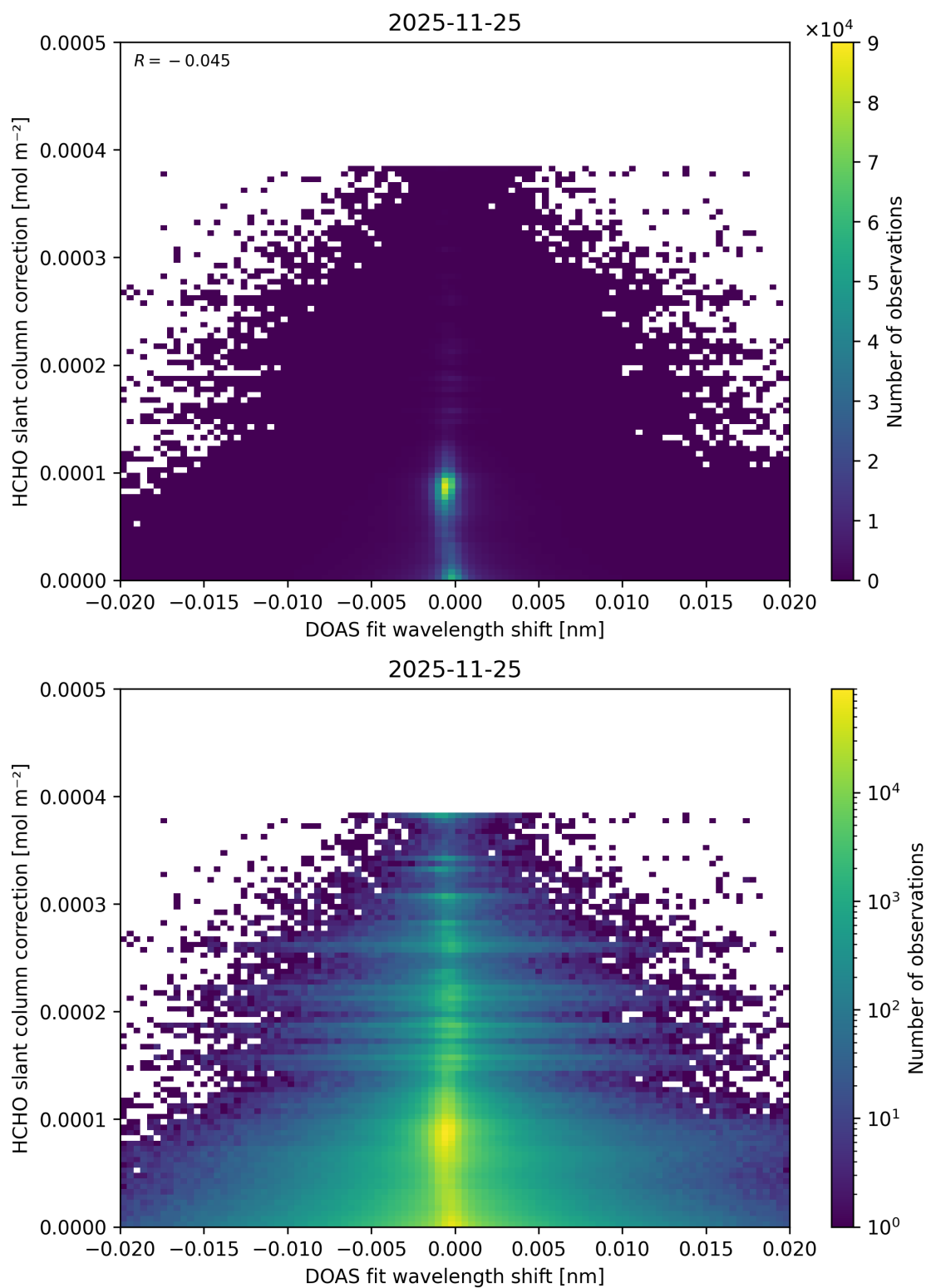
Figure 72: Scatter density plot of “DOAS fit wavelength shift” against “HCHO slant column correction” for 2025-11-24 to 2025-11-26.
