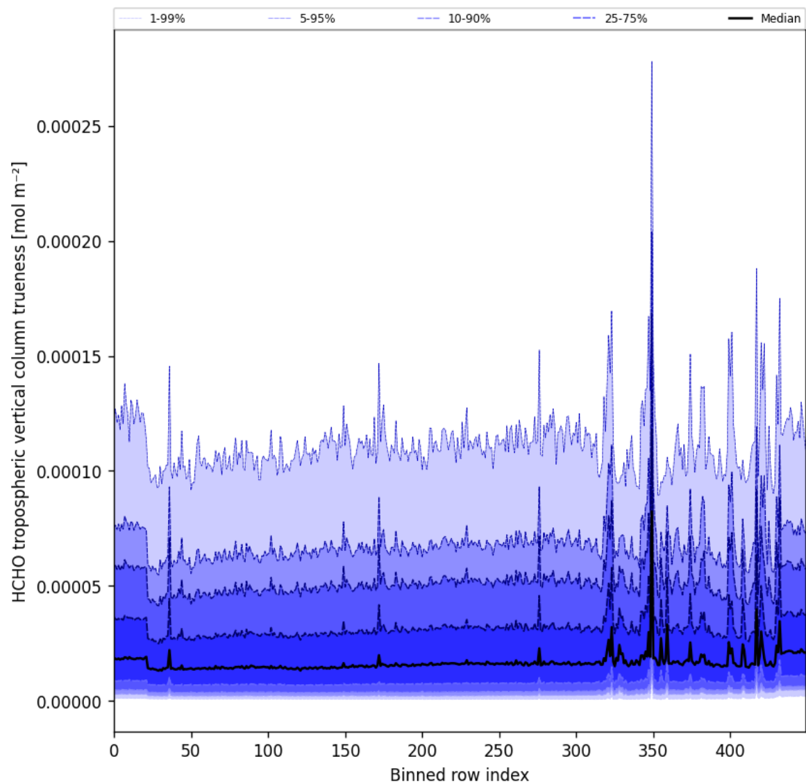
Figure 65: Along track statistics of “HCHO tropospheric vertical column trueness” for 2025-11-24 to 2025-11-26
