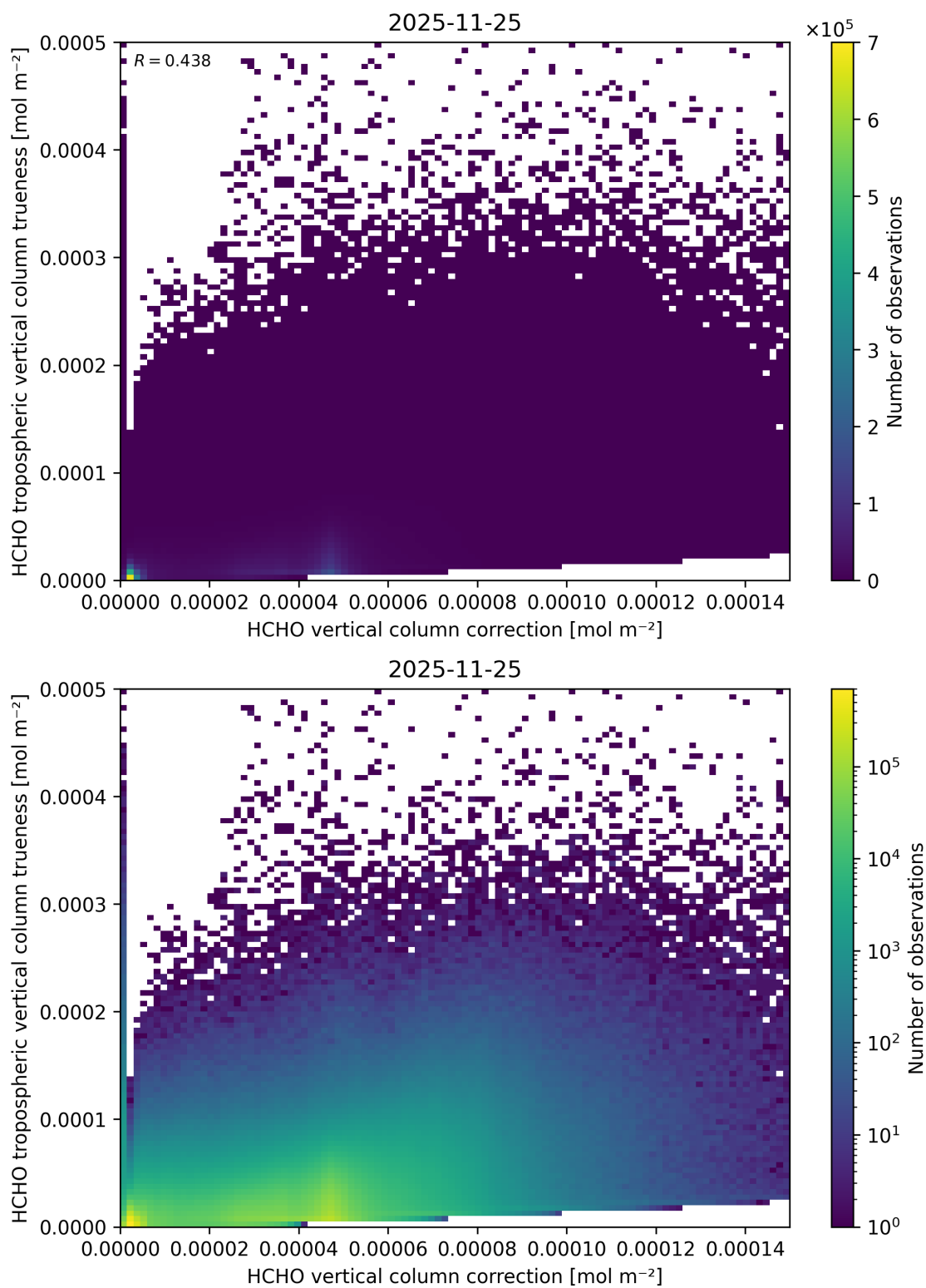
Figure 136: Scatter density plot of “HCHO vertical column correction” against “HCHO tropospheric vertical column true-ness” for 2025-11-24 to 2025-11-26.
