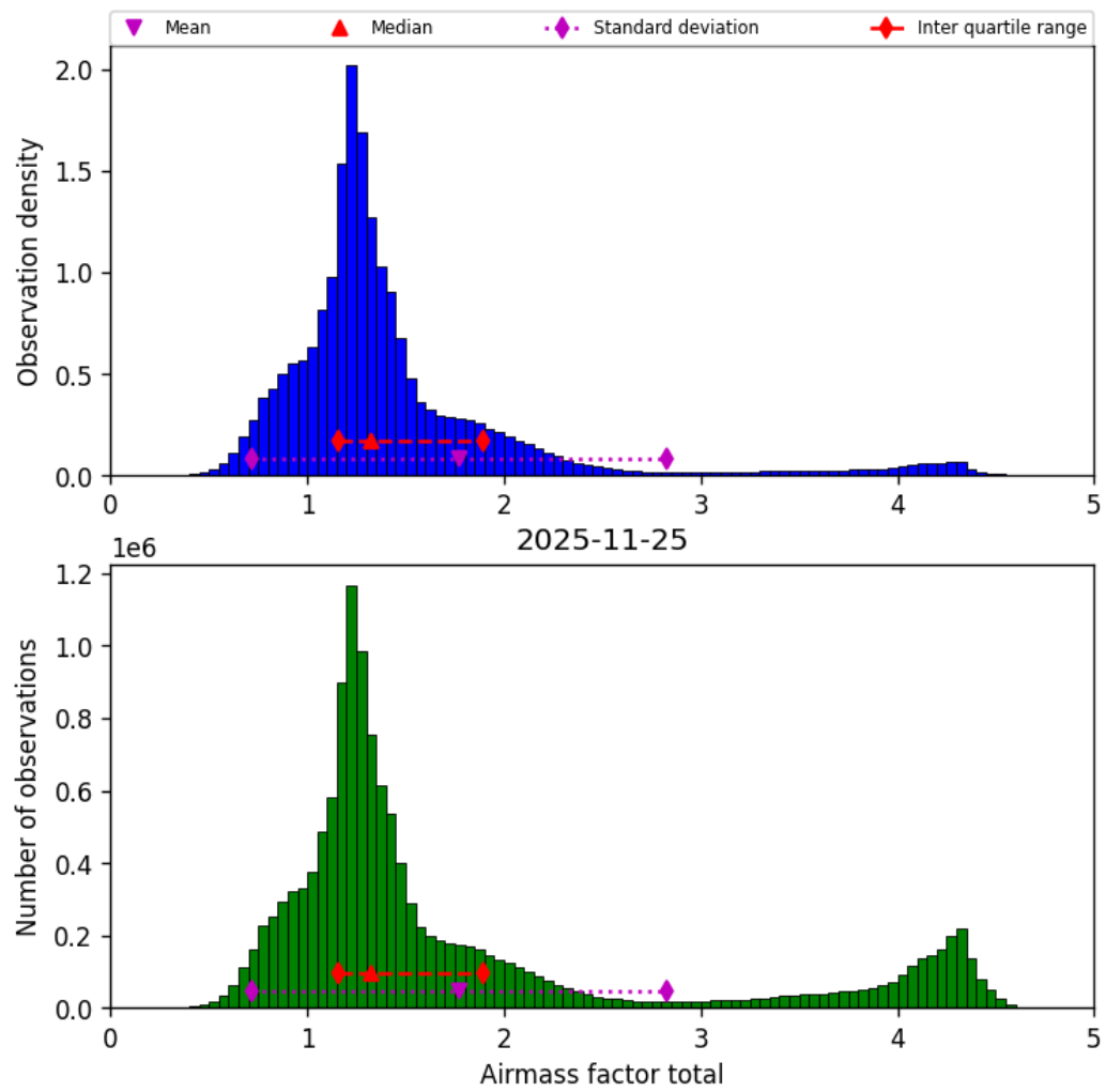
Figure 42: Histogram of “Airmass factor total” for 2025-11-24 to 2025-11-26
