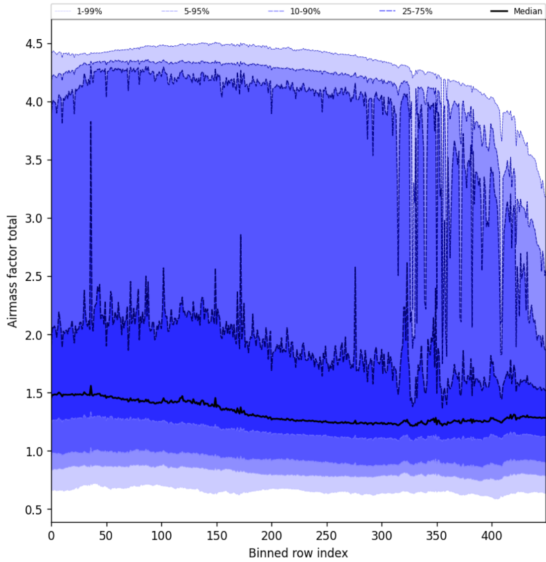
Figure 57: Along track statistics of “Airmass factor total” for 2025-11-24 to 2025-11-26
