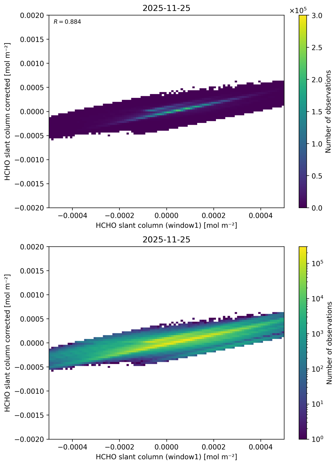
Figure 92: Scatter density plot of “HCHO slant column (window1)” against “HCHO slant column corrected” for 2025-11-24 to 2025-11-26.
