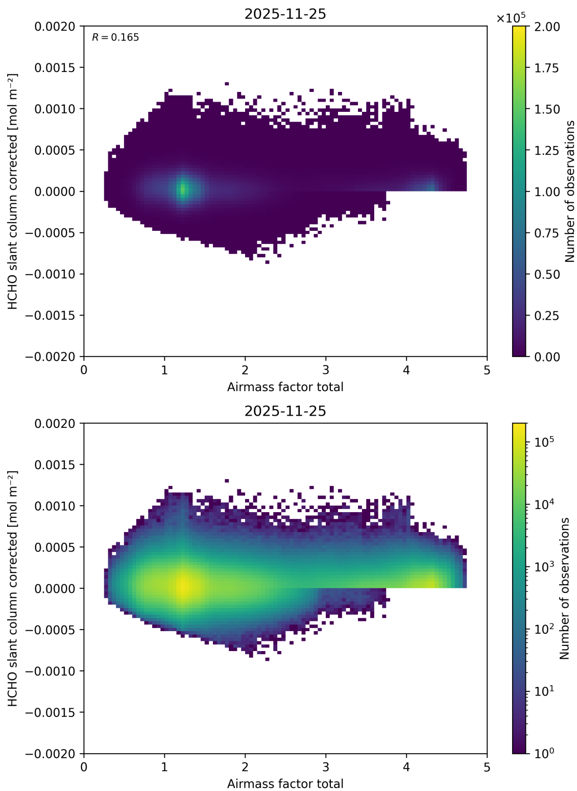
Figure 113: Scatter density plot of “Airmass factor total” against “HCHO slant column corrected” for 2025-11-24 to 2025-11-26.
