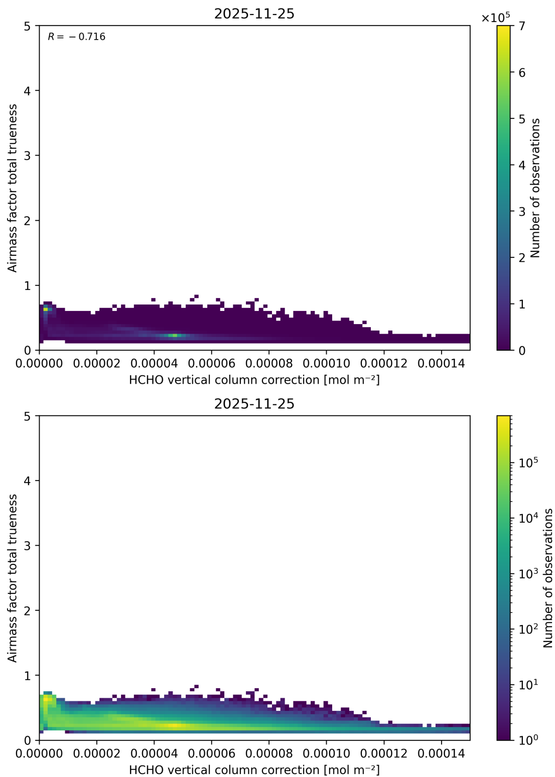
Figure 135: Scatter density plot of “HCHO vertical column correction” against “Airmass factor total truiness” for 2025-11-24 to 2025-11-26.
