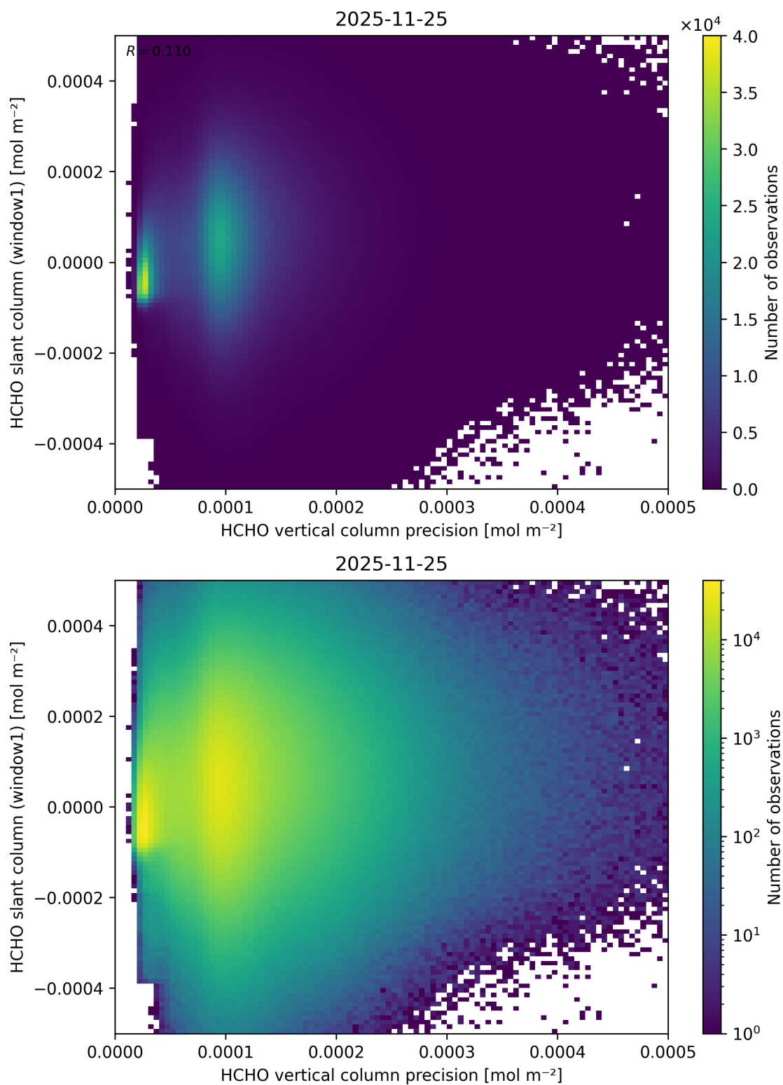
Figure 158: Scatter density plot of “HCHO vertical column precision” against “HCHO slant column (window1)” for 2025-11-24 to 2025-11-26.
