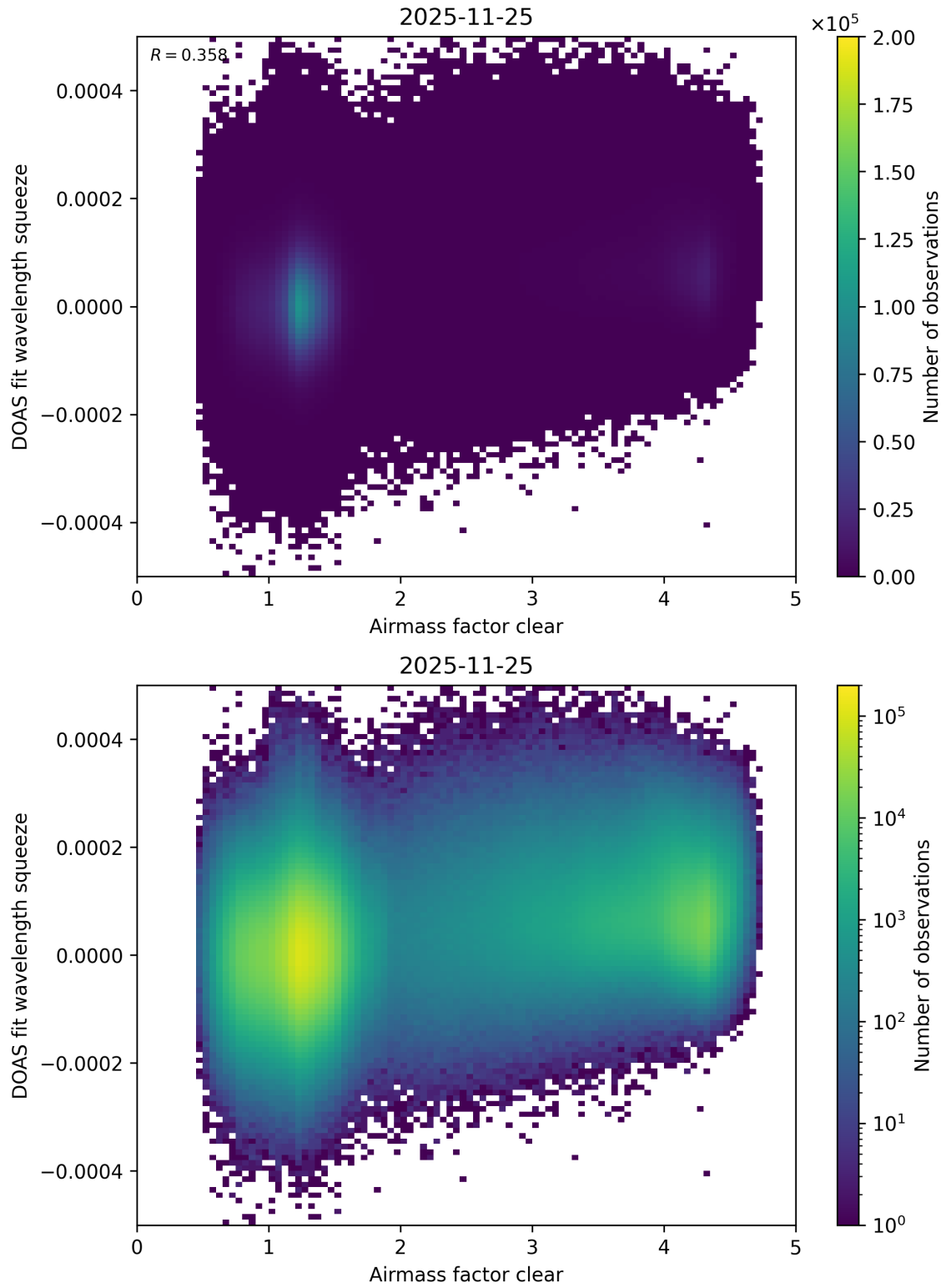
Figure 80: Scatter density plot of “Airmass factor clear” against “DOAS fit wavelength squeeze” for 2025-11-24 to 2025-11-26.
