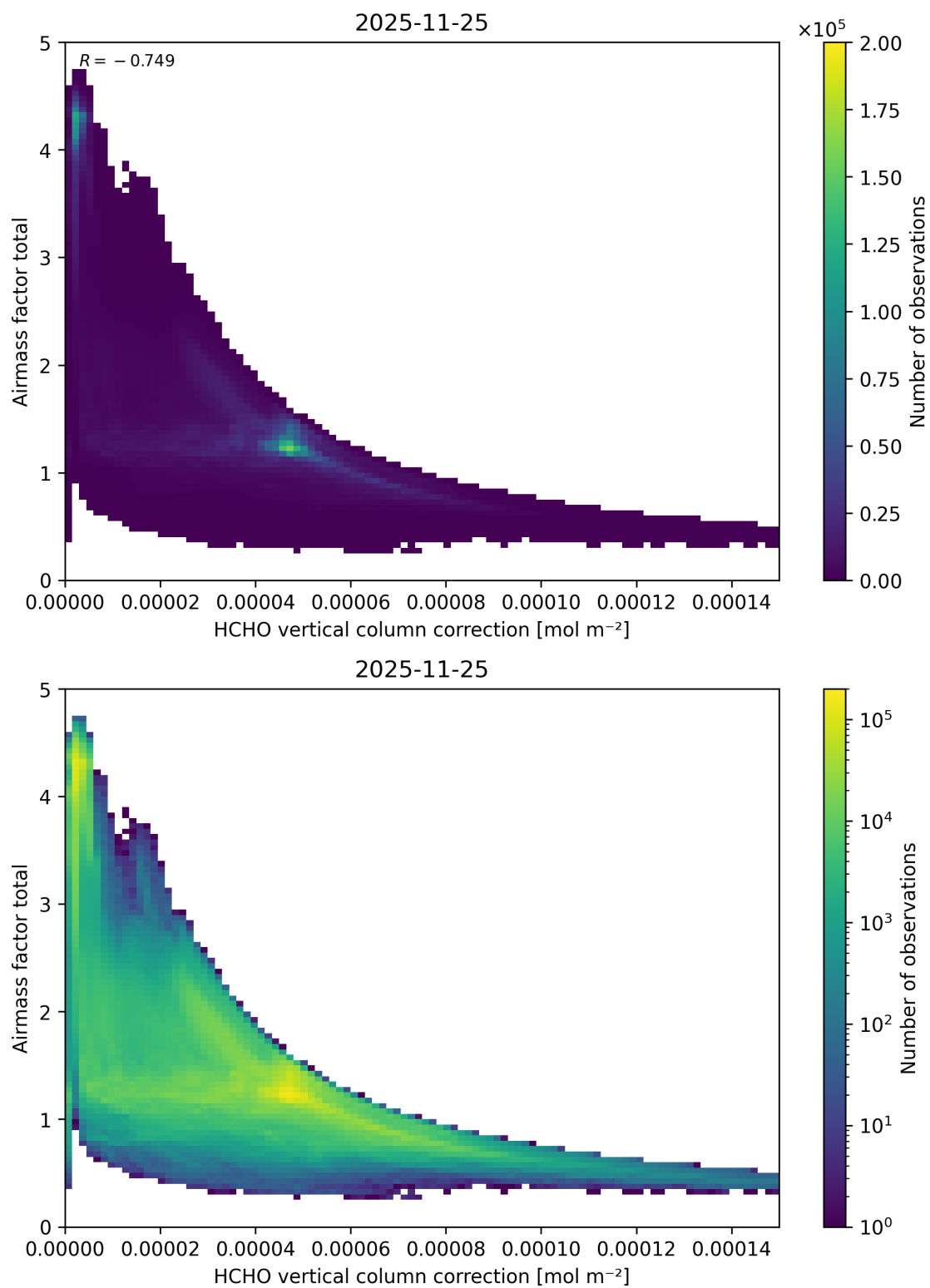
Figure 134: Scatter density plot of “HCHO vertical column correction” against “Airmass factor total” for 2025-11-24 to 2025-11-26.
