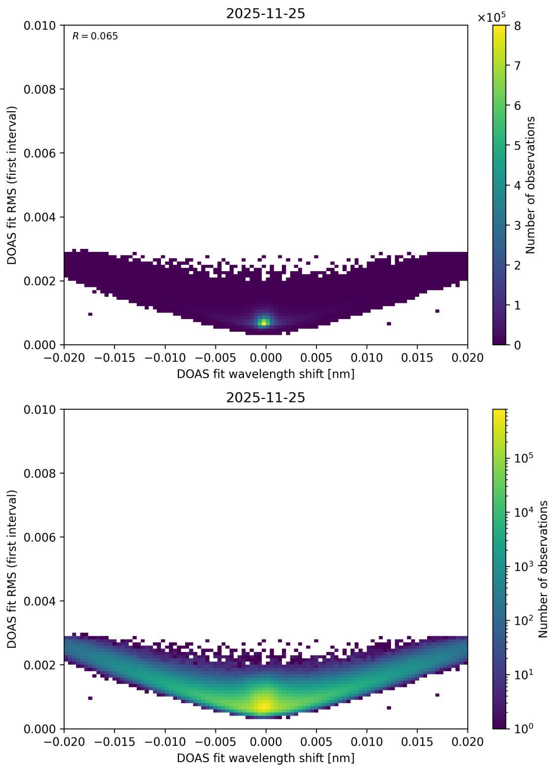
Figure 69: Scatter density plot of “DOAS fit wavelength shift” against “DOAS fit RMS (first interval)” for 2025-11-24 to 2025-11-26.
