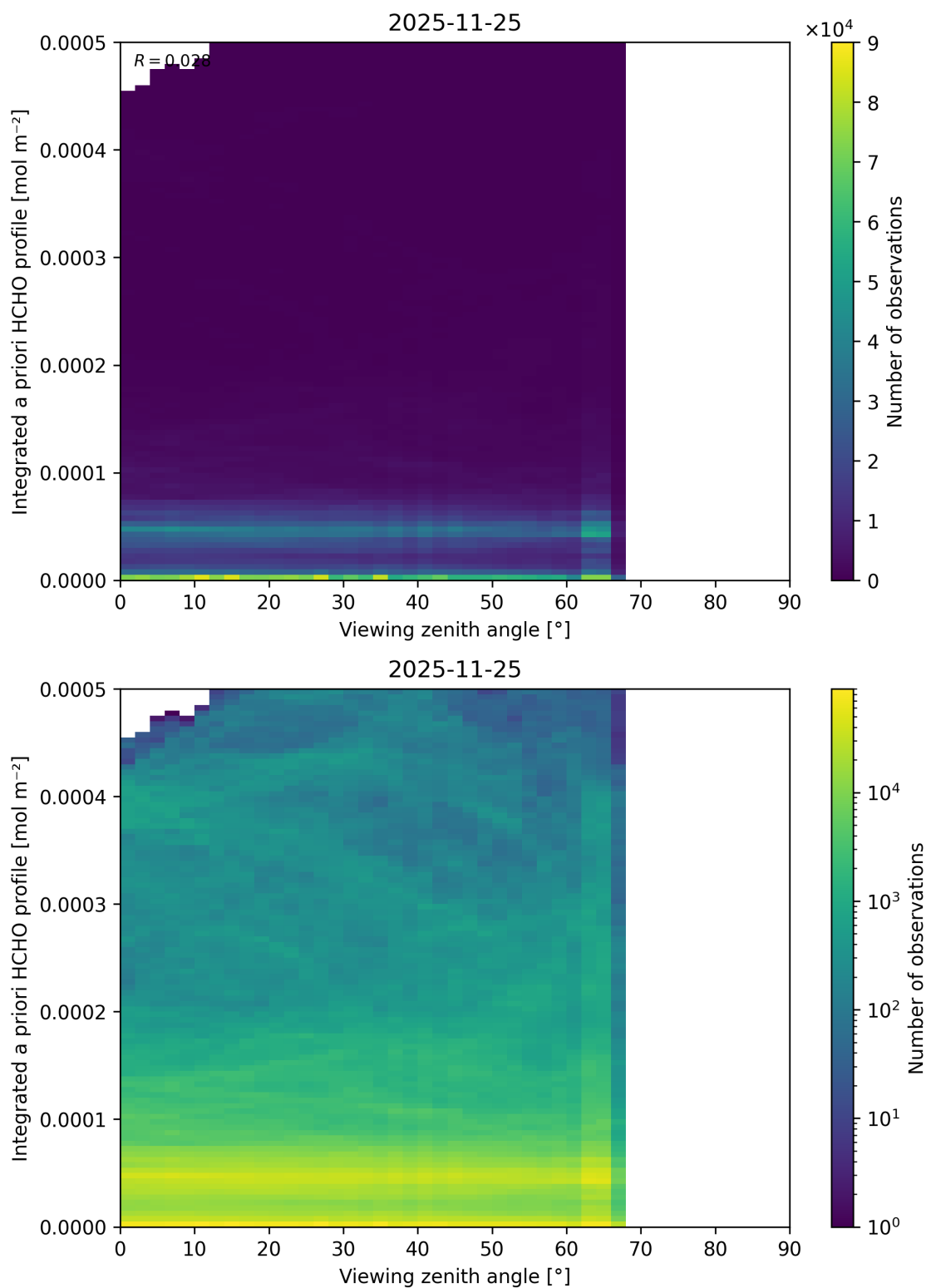
Figure 216: Scatter density plot of “Viewing zenith angle” against “Integrated a priori HCHO profile” for 2025-11-24 to 2025-11-26.
