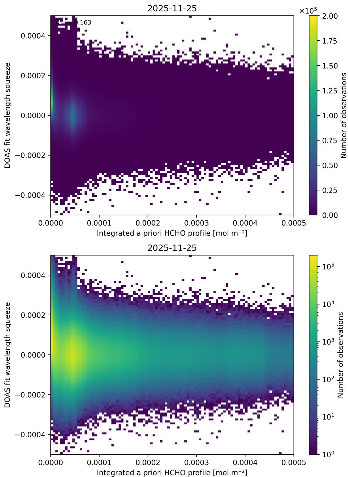
Figure 167: Scatter density plot of “Integrated a priori HCHO profile” against “DOAS fit wavelength squeeze” for 2025-11-24 to 2025-11-26.
