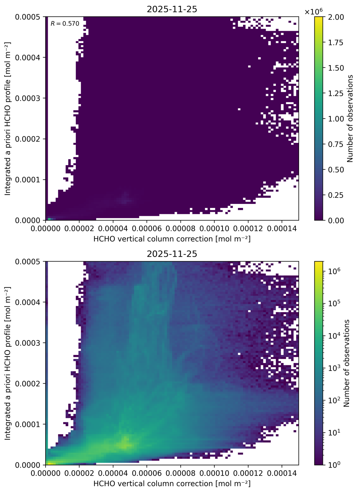
Figure 137: Scatter density plot of “HCHO vertical column correction” against “Integrated a priori HCHO profile” for 2025-11-24 to 2025-11-26.
