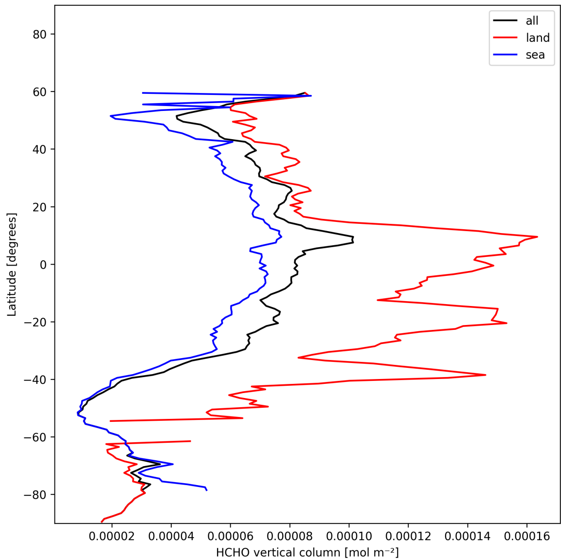
Figure 22: Zonal average of “HCHO vertical column” for 2025-11-24 to 2025-11-26.
