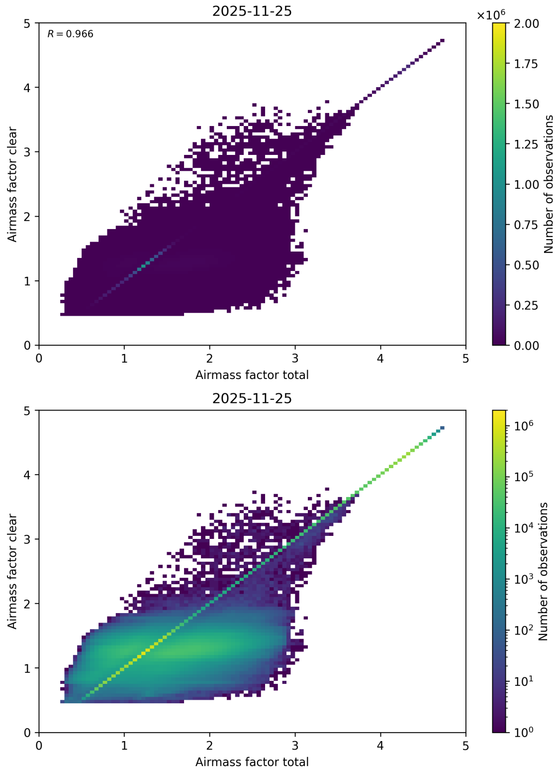
Figure 112: Scatter density plot of “Airmass factor total” against “Airmass factor clear” for 2025-11-24 to 2025-11-26.
