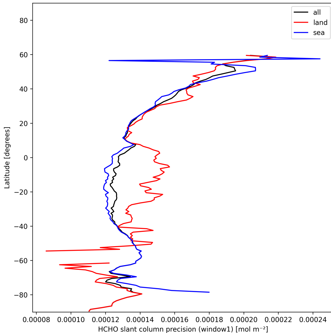
Figure 26: Zonal average of “HCHO slant column precision (window1)” for 2025-11-24 to 2025-11-26.
