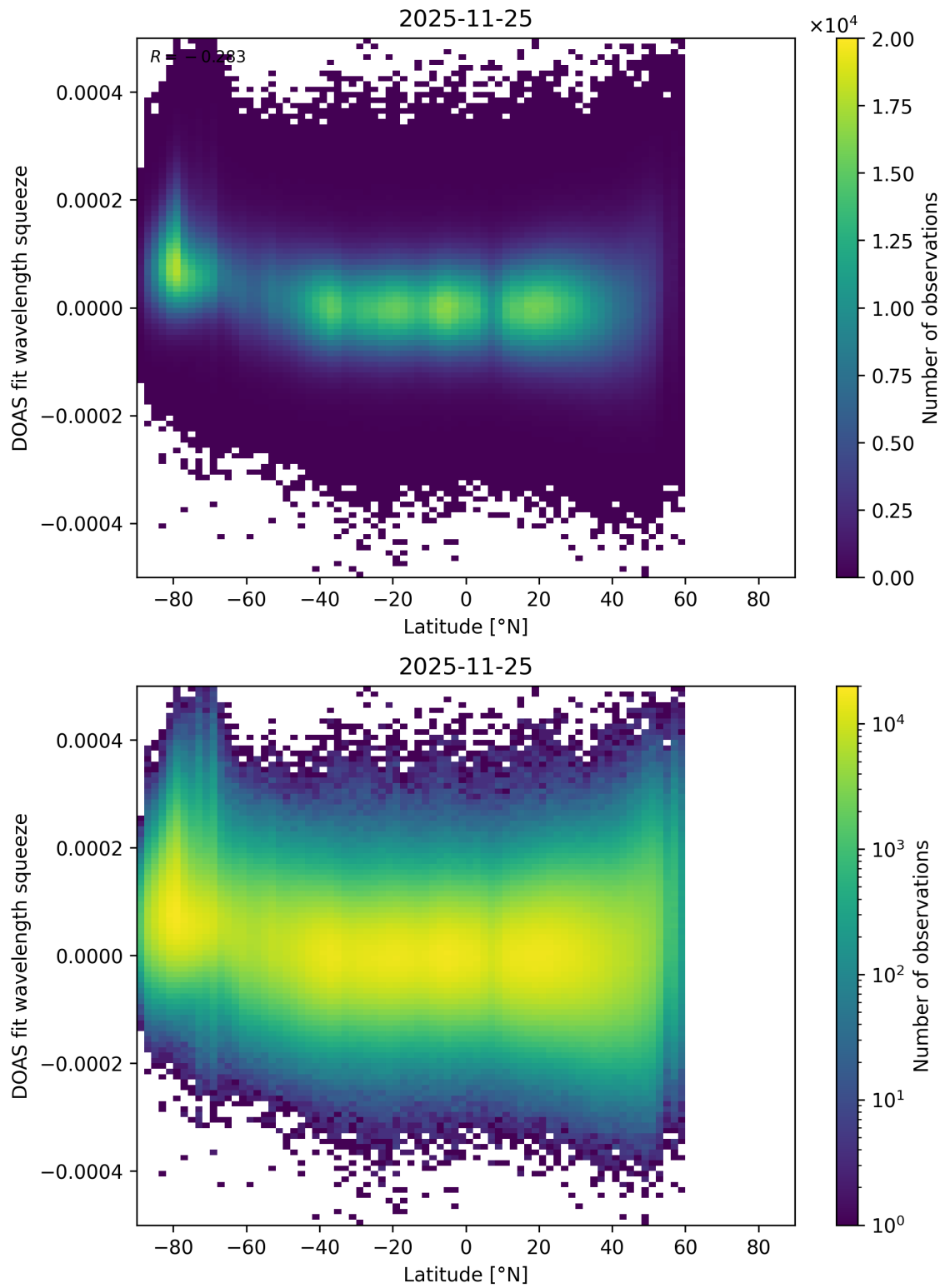
Figure 173: Scatter density plot of “Latitude” against “DOAS fit wavelength squeeze” for 2025-11-24 to 2025-11-26.
