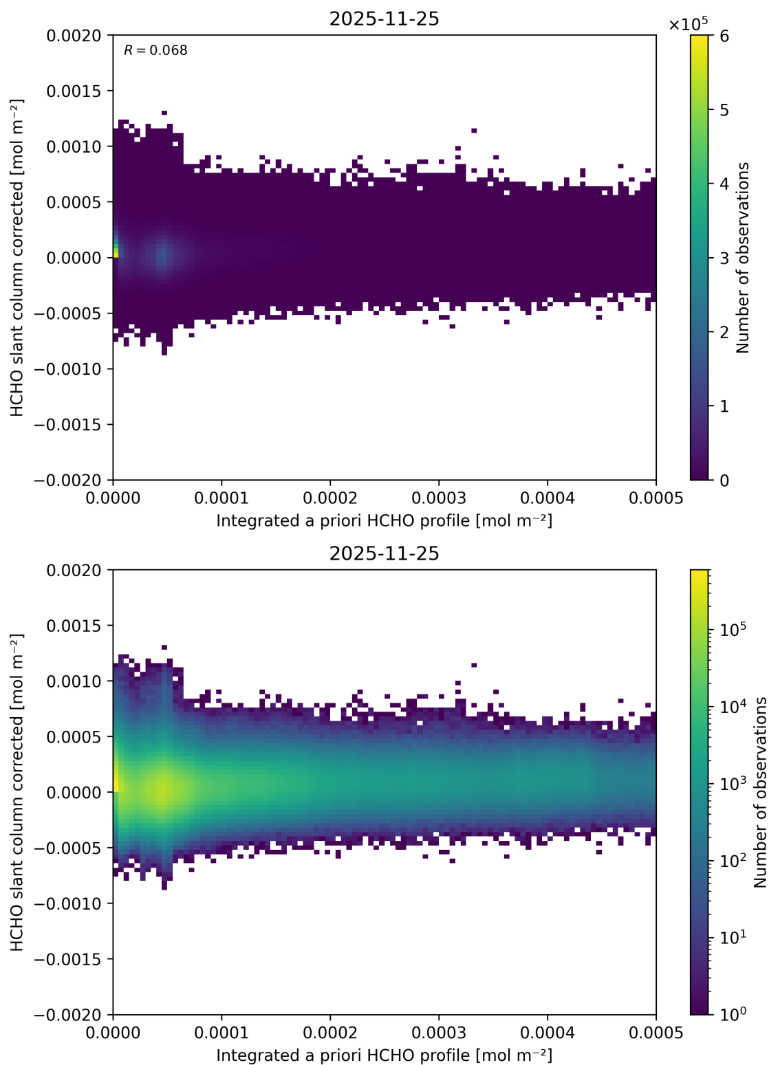
Figure 168: Scatter density plot of “Integrated a priori HCHO profile” against “HCHO slant column corrected” for 2025-11-24 to 2025-11-26.
