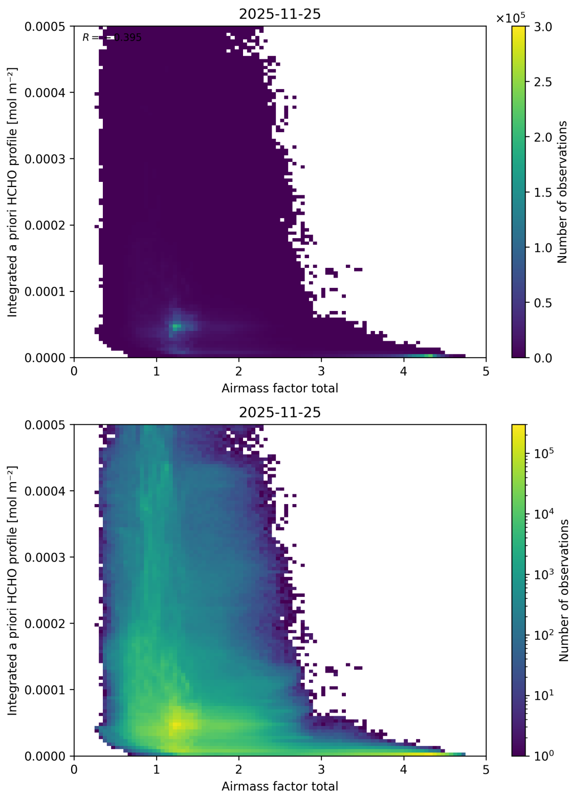
Figure 117: Scatter density plot of “Airmass factor total” against “Integrated a priori HCHO profile” for 2025-11-24 to 2025-11-26.
