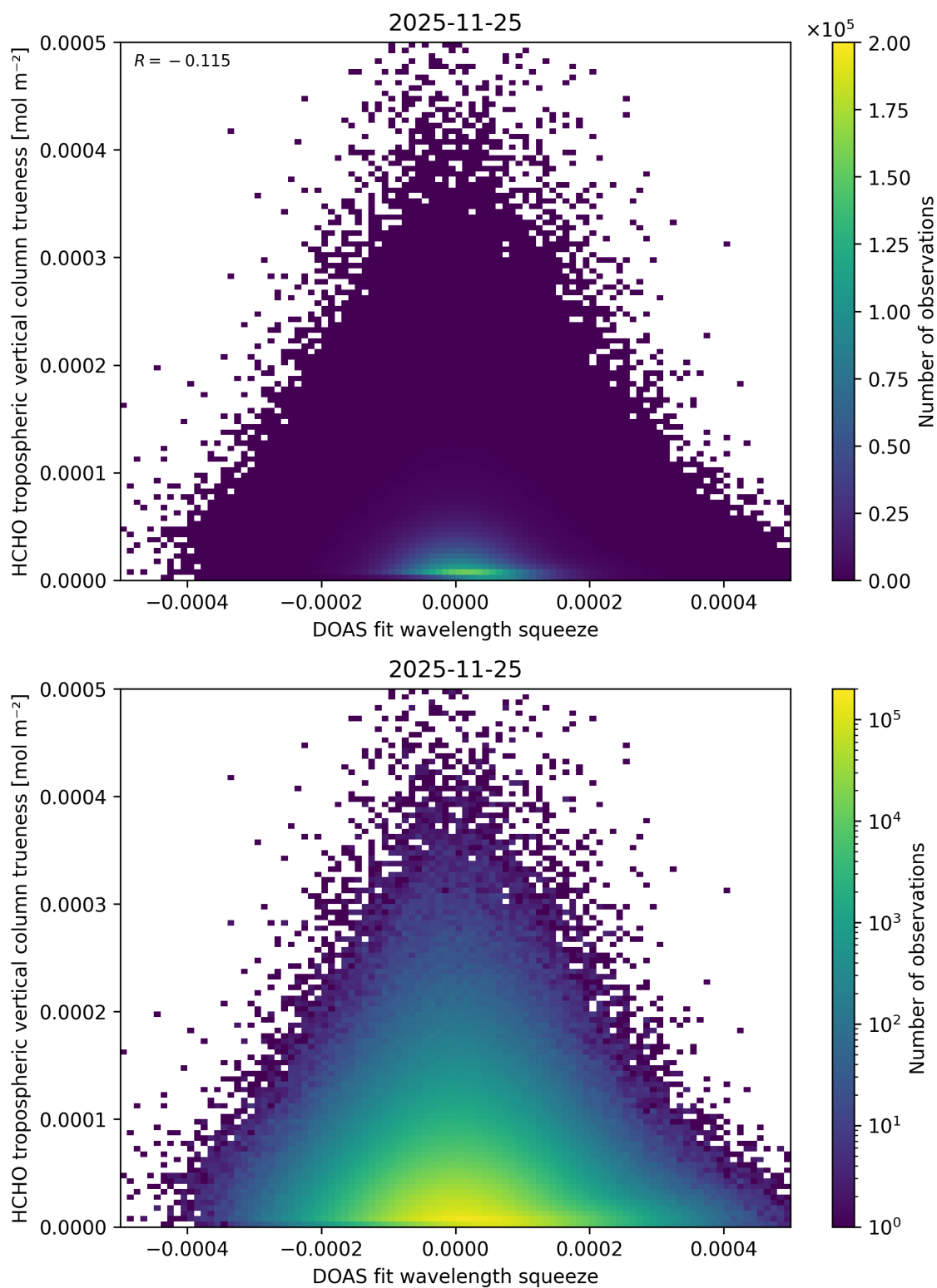
Figure 77: Scatter density plot of “DOAS fit wavelength squeeze” against “HCHO tropospheric vertical column trueness” for 2025-11-24 to 2025-11-26.
