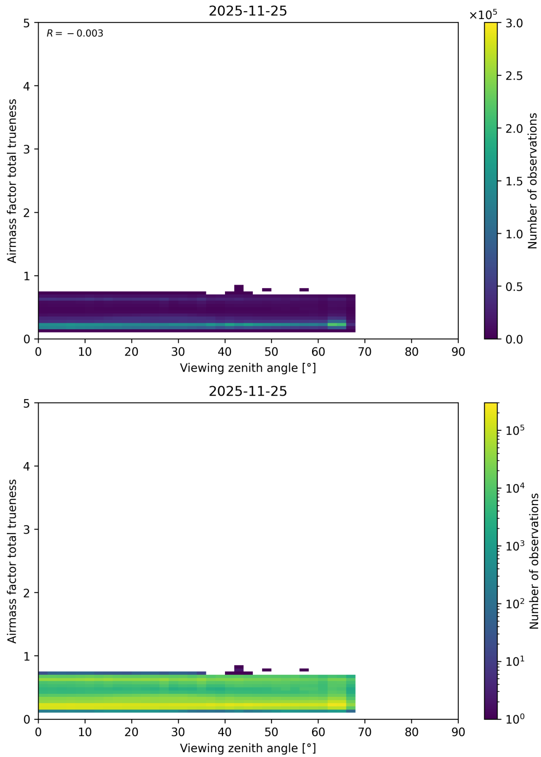
Figure 211: Scatter density plot of “Viewing zenith angle” against “Airmass factor total trueness” for 2025-11-24 to 2025-11-26.
