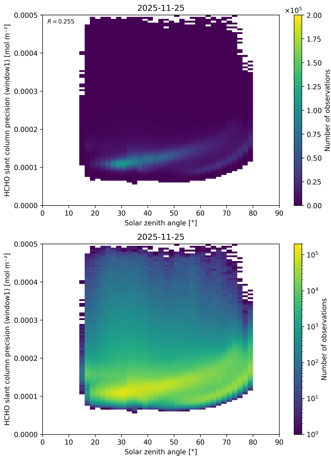
Figure 193: Scatter density plot of “Solar zenith angle” against “HCHO slant column precision (window1)” for 2025-11-24 to 2025-11-26.
