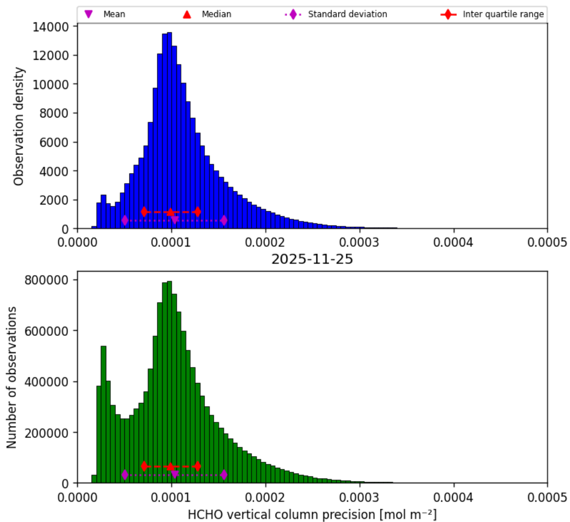
Figure 38: Histogram of “HCHO vertical column precision” for 2025-11-24 to 2025-11-26
