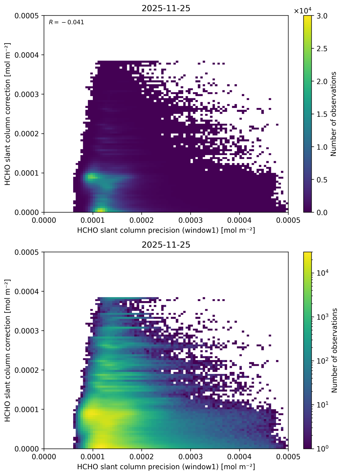
Figure 104: Scatter density plot of “HCHO slant column precision (window1)” against “HCHO slant column correction” for 2025-11-24 to 2025-11-26.
