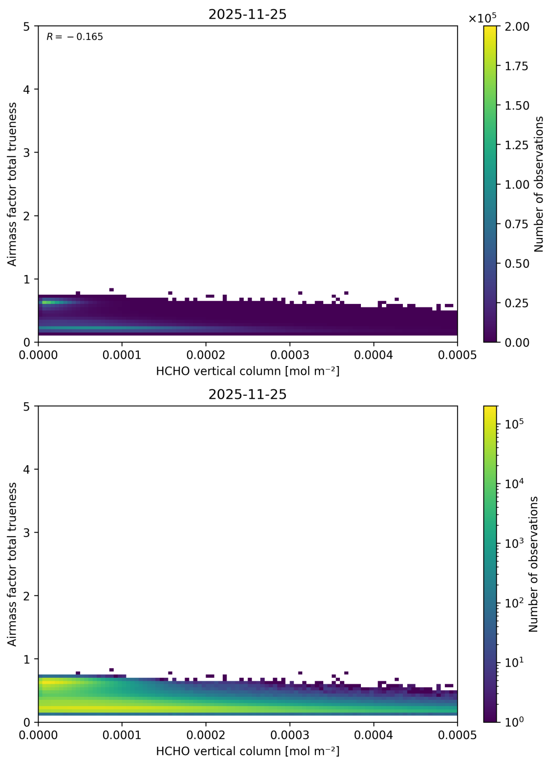
Figure 147: Scatter density plot of “HCHO vertical column” against “Airmass factor total truiness” for 2025-11-24 to 2025-11-26.
