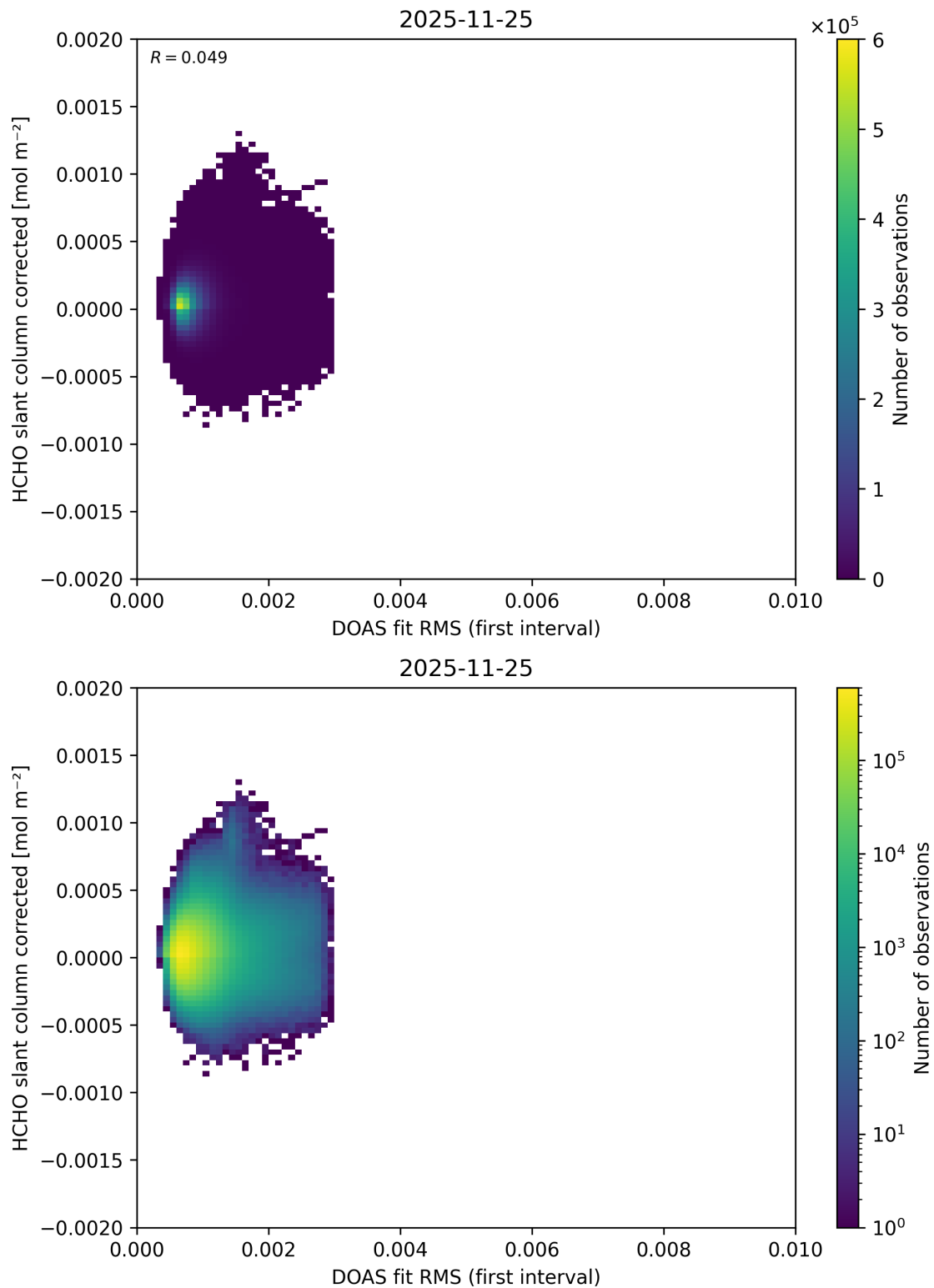
Figure 66: Scatter density plot of “DOAS fit RMS (first interval)” against “HCHO slant column corrected” for 2025-11-24 to 2025-11-26.
