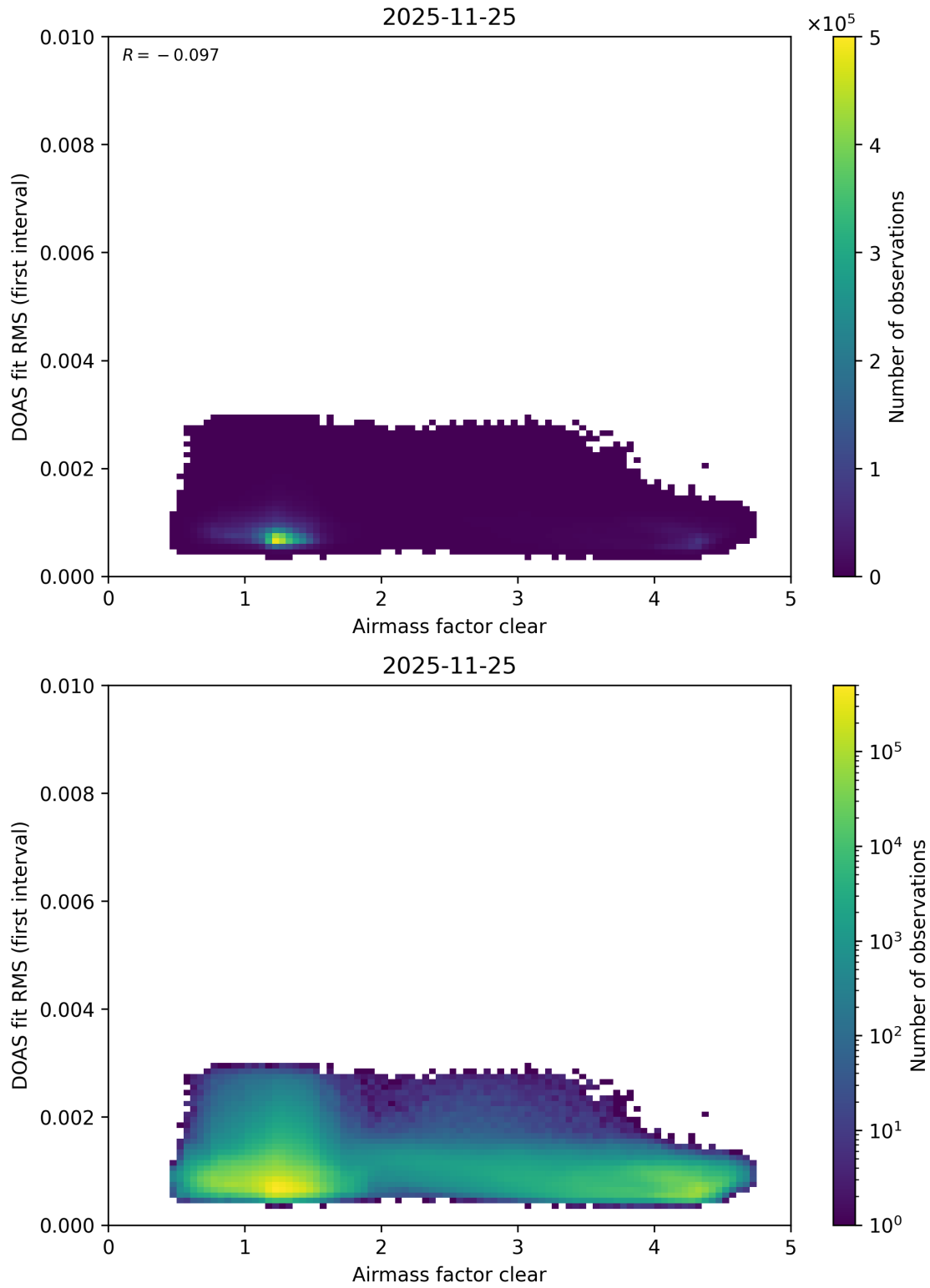
Figure 78: Scatter density plot of “Airmass factor clear” against “DOAS fit RMS (first interval)” for 2025-11-24 to 2025-11-26.
