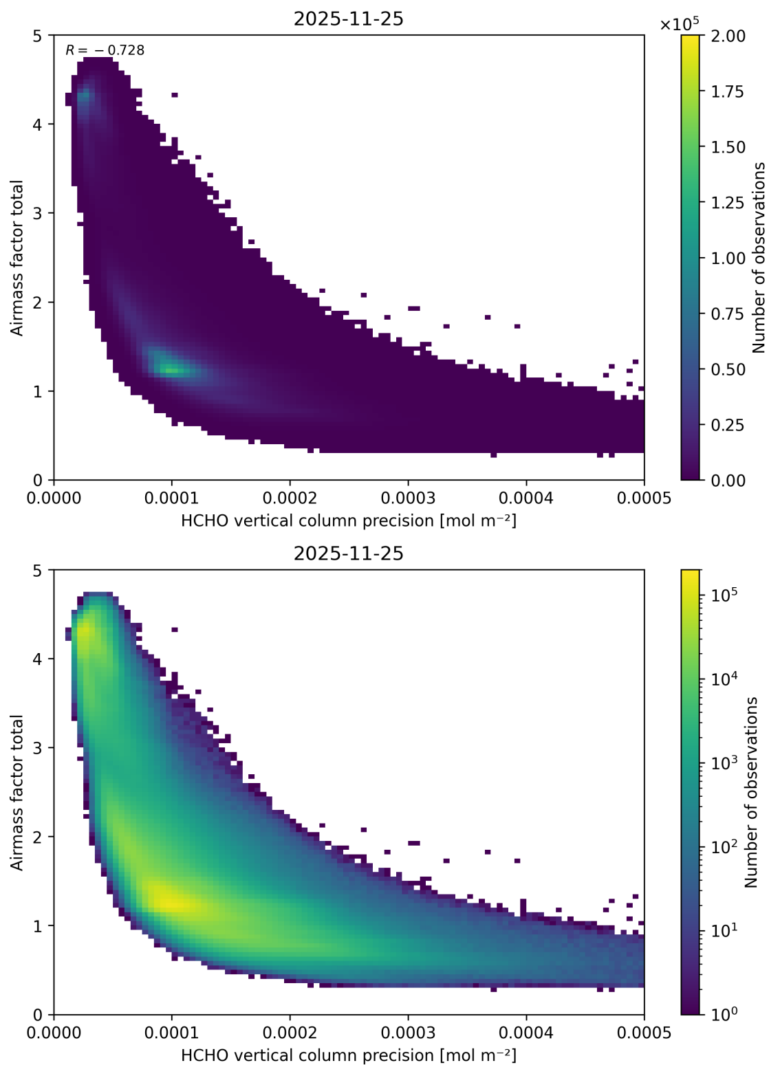
Figure 160: Scatter density plot of “HCHO vertical column precision” against “Airmass factor total” for 2025-11-24 to 2025-11-26.
