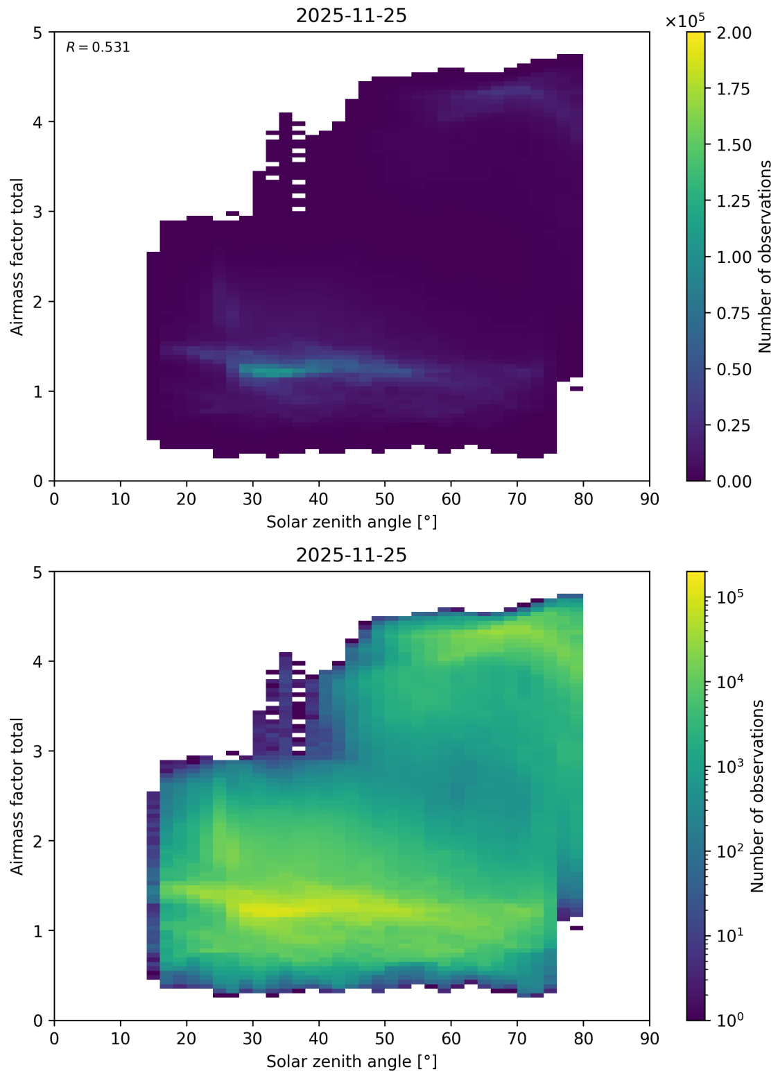
Figure 194: Scatter density plot of “Solar zenith angle” against “Airmass factor total” for 2025-11-24 to 2025-11-26.
