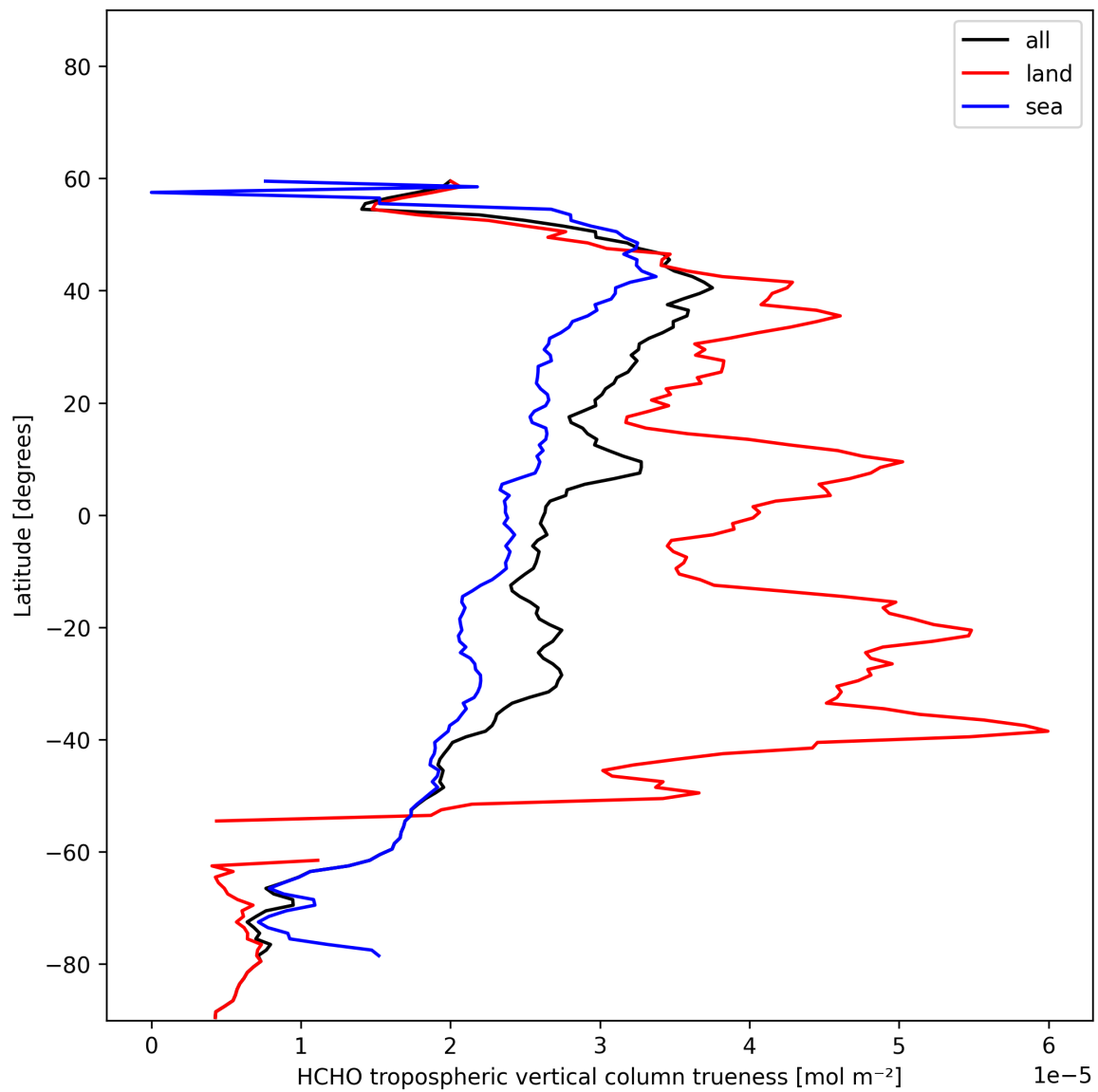
Figure 35: Zonal average of “HCHO tropospheric vertical column trueness” for 2025-11-24 to 2025-11-26.
