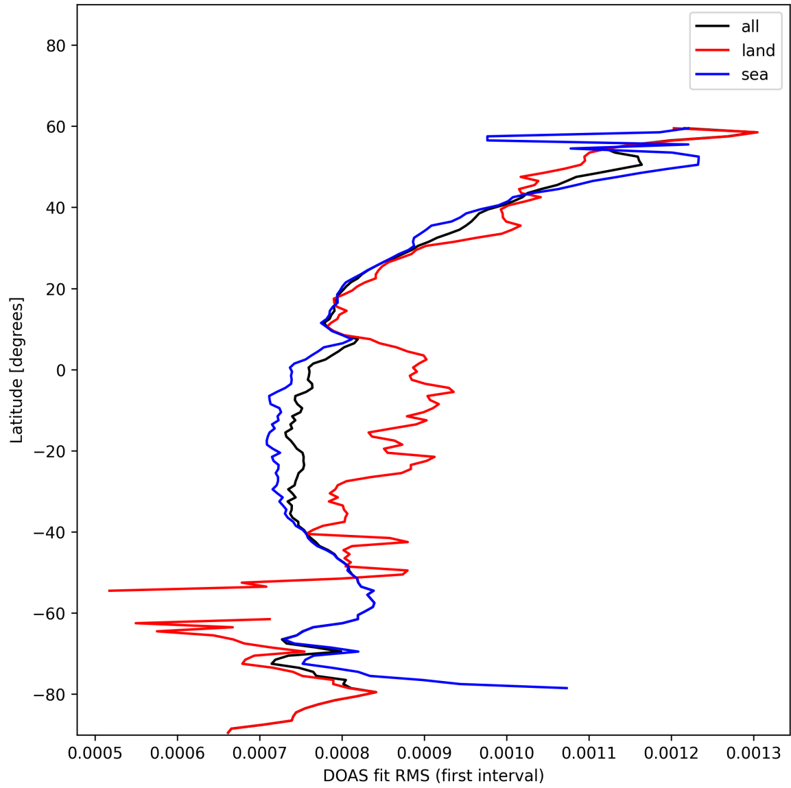
Figure 33: Zonal average of “DOAS fit RMS (first interval)” for 2025-11-24 to 2025-11-26.
