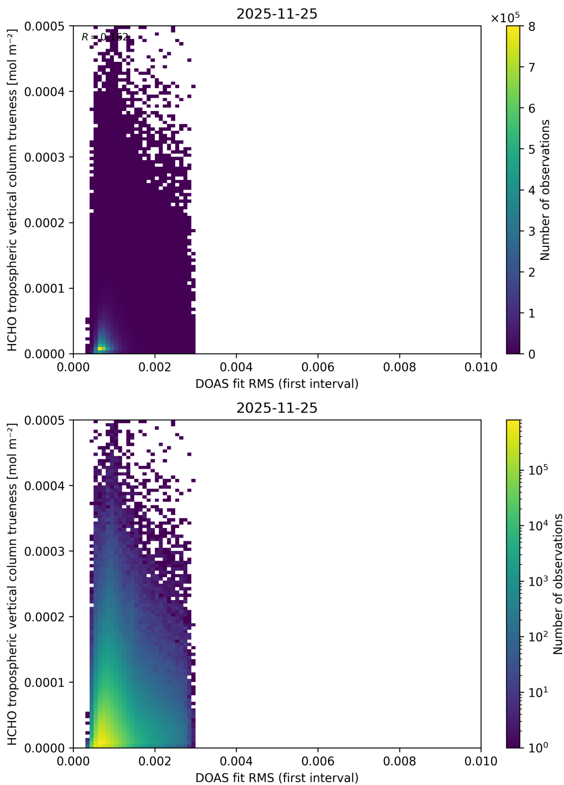
Figure 68: Scatter density plot of “DOAS fit RMS (first interval)” against “HCHO tropospheric vertical column trueness” for 2025-11-24 to 2025-11-26.
