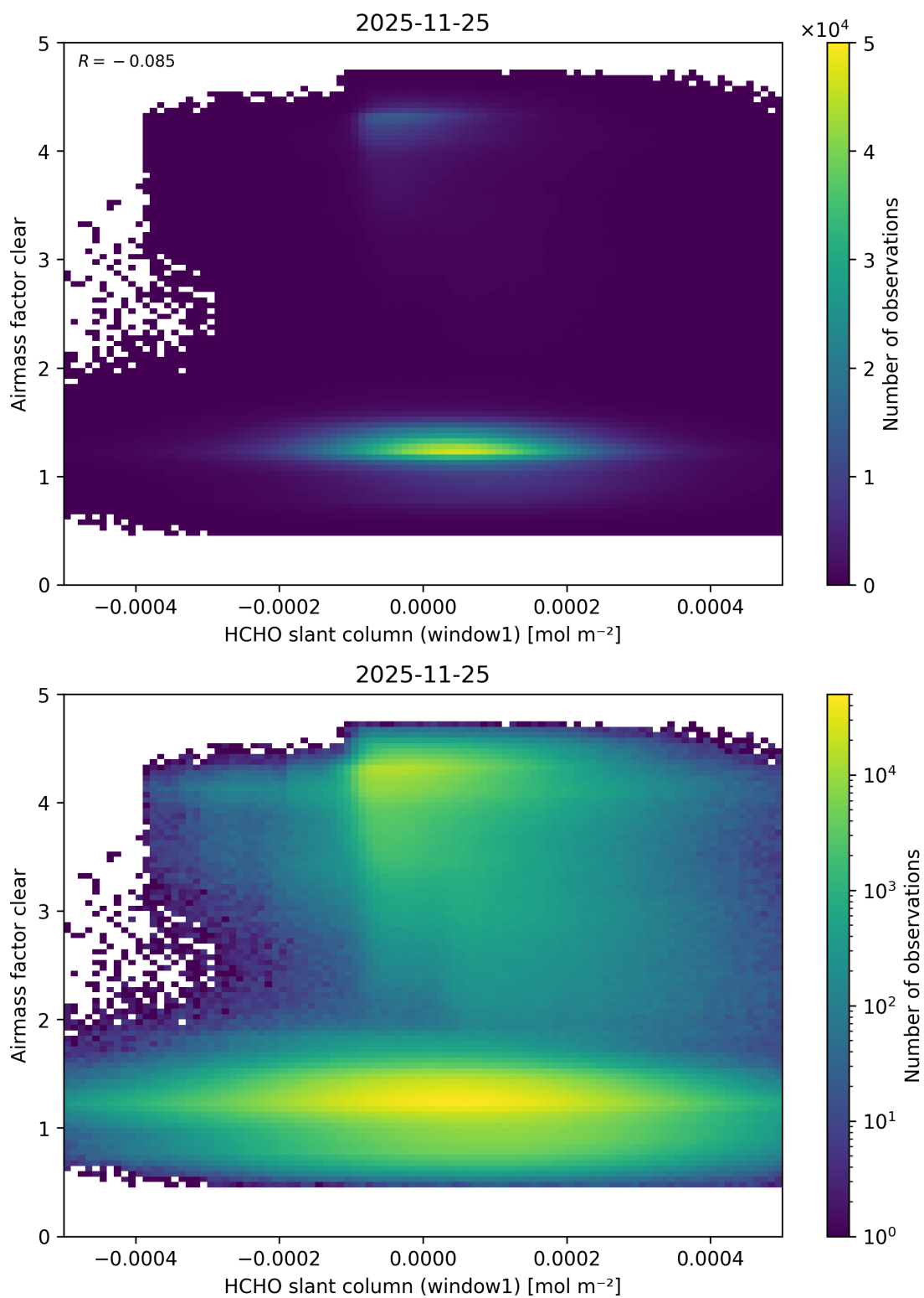
Figure 91: Scatter density plot of “HCHO slant column (window1)” against “Airmass factor clear” for 2025-11-24 to 2025-11-26.
