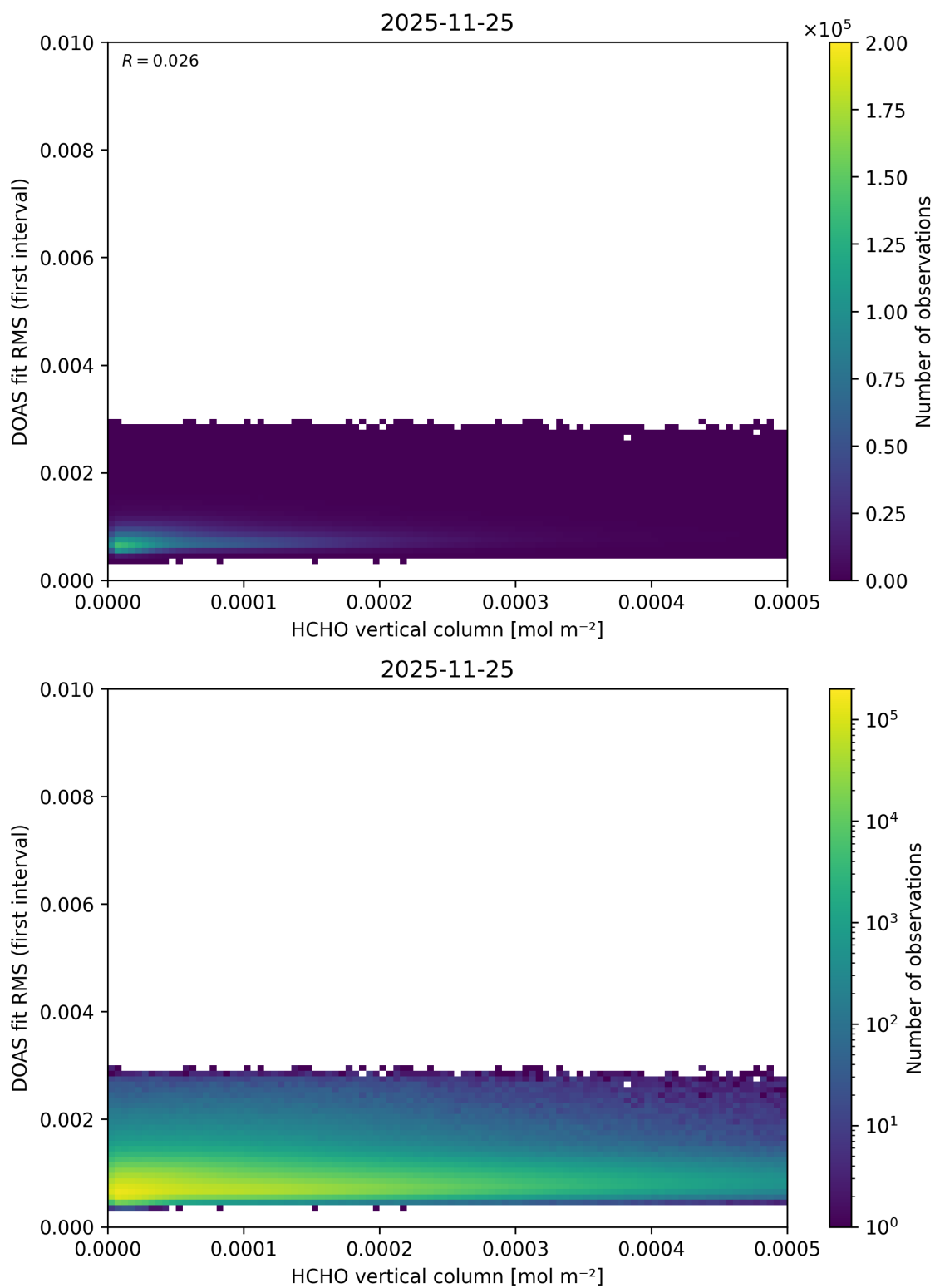
Figure 138: Scatter density plot of “HCHO vertical column” against “DOAS fit RMS (first interval)” for 2025-11-24 to 2025-11-26.
