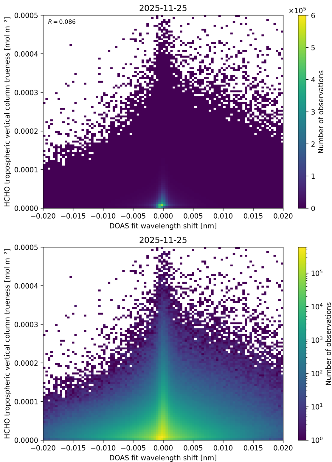
Figure 73: Scatter density plot of “DOAS fit wavelength shift” against “HCHO tropospheric vertical column trueness” for 2025-11-24 to 2025-11-26.
