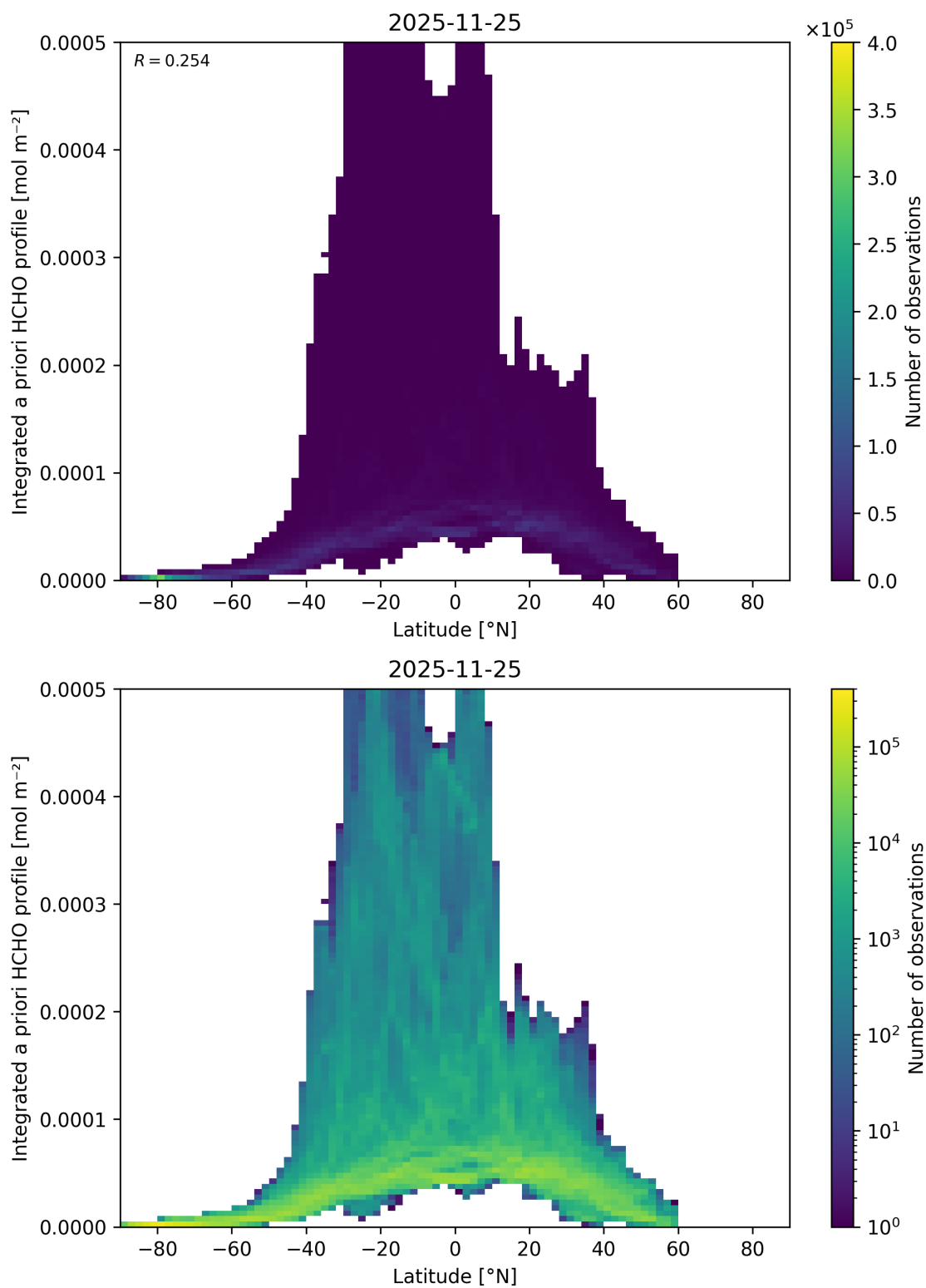
Figure 185: Scatter density plot of “Latitude” against “Integrated a priori HCHO profile” for 2025-11-24 to 2025-11-26.
