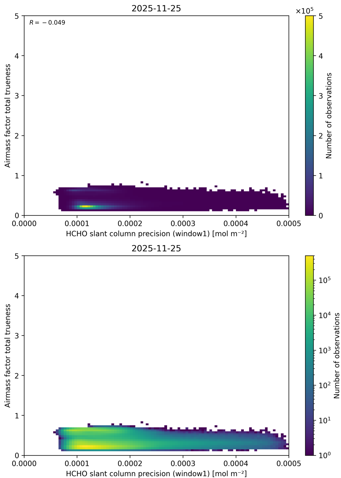
Figure 106: Scatter density plot of “HCHO slant column precision (window1)” against “Airmass factor total trueness” for 2025-11-24 to 2025-11-26.
