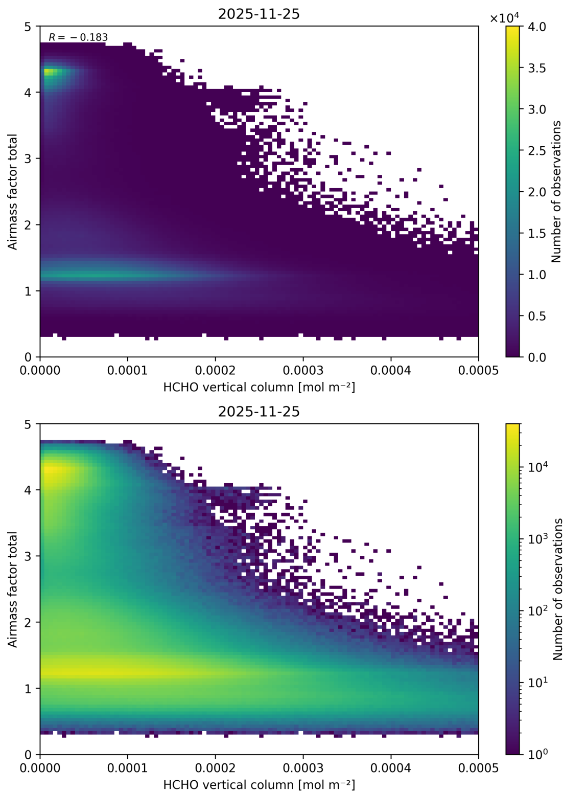
Figure 146: Scatter density plot of “HCHO vertical column” against “Airmass factor total” for 2025-11-24 to 2025-11-26.
