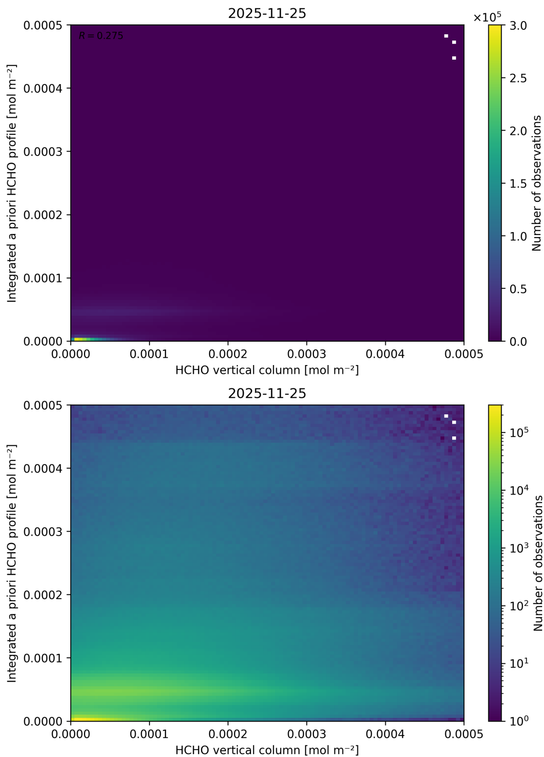
Figure 151: Scatter density plot of “HCHO vertical column” against “Integrated a priori HCHO profile” for 2025-11-24 to 2025-11-26.
