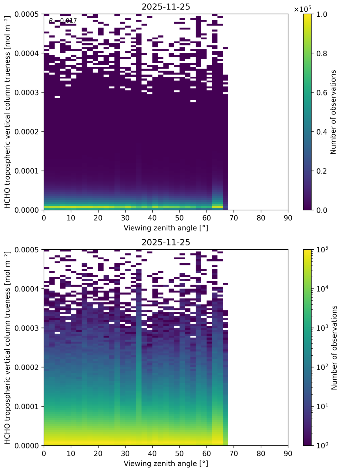
Figure 215: Scatter density plot of “Viewing zenith angle” against “HCHO tropospheric vertical column trueness” for 2025-11-24 to 2025-11-26.
