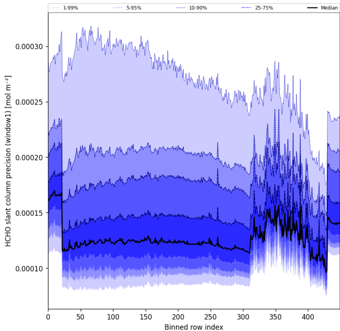
Figure 56: Along track statistics of “HCHO slant column precision (window1)” for 2025-11-24 to 2025-11-26
