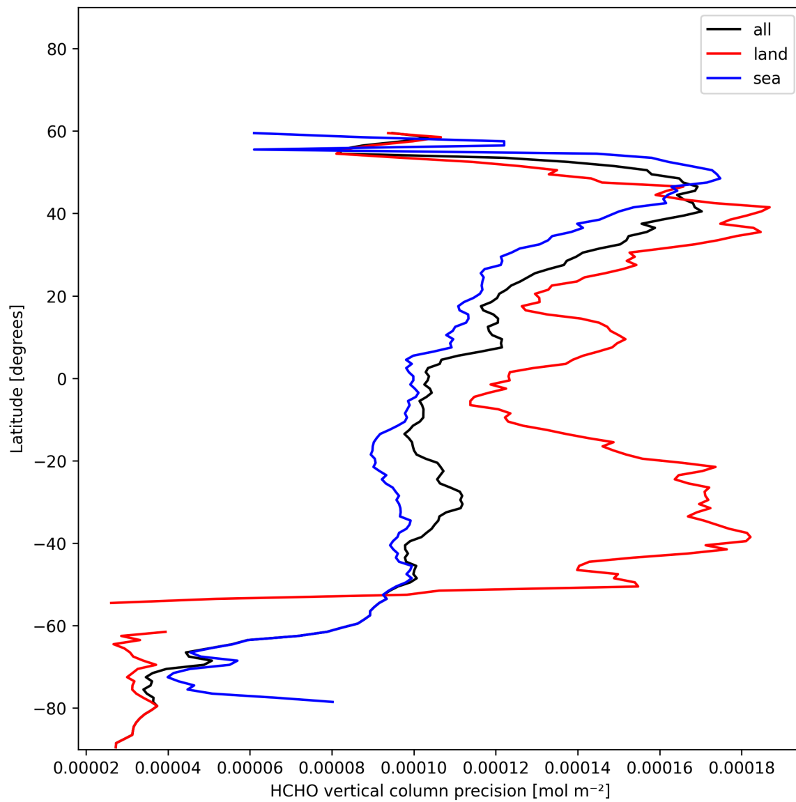
Figure 23: Zonal average of “HCHO vertical column precision” for 2025-11-24 to 2025-11-26.
