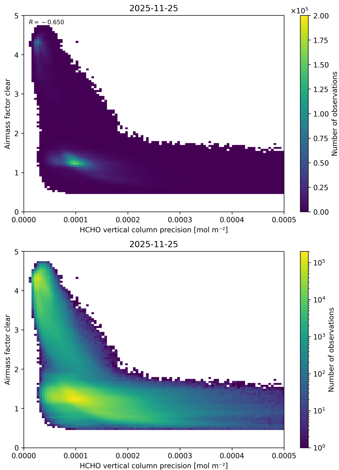
Figure 155: Scatter density plot of “HCHO vertical column precision” against “Airmass factor clear” for 2025-11-24 to 2025-11-26.
