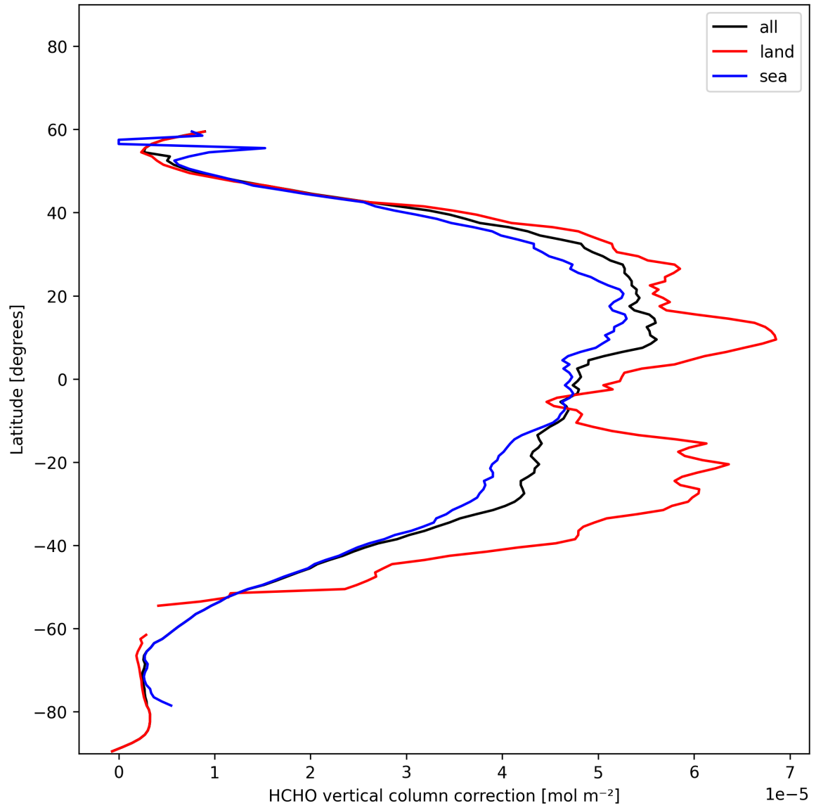
Figure 24: Zonal average of “HCHO vertical column correction” for 2025-11-24 to 2025-11-26.
