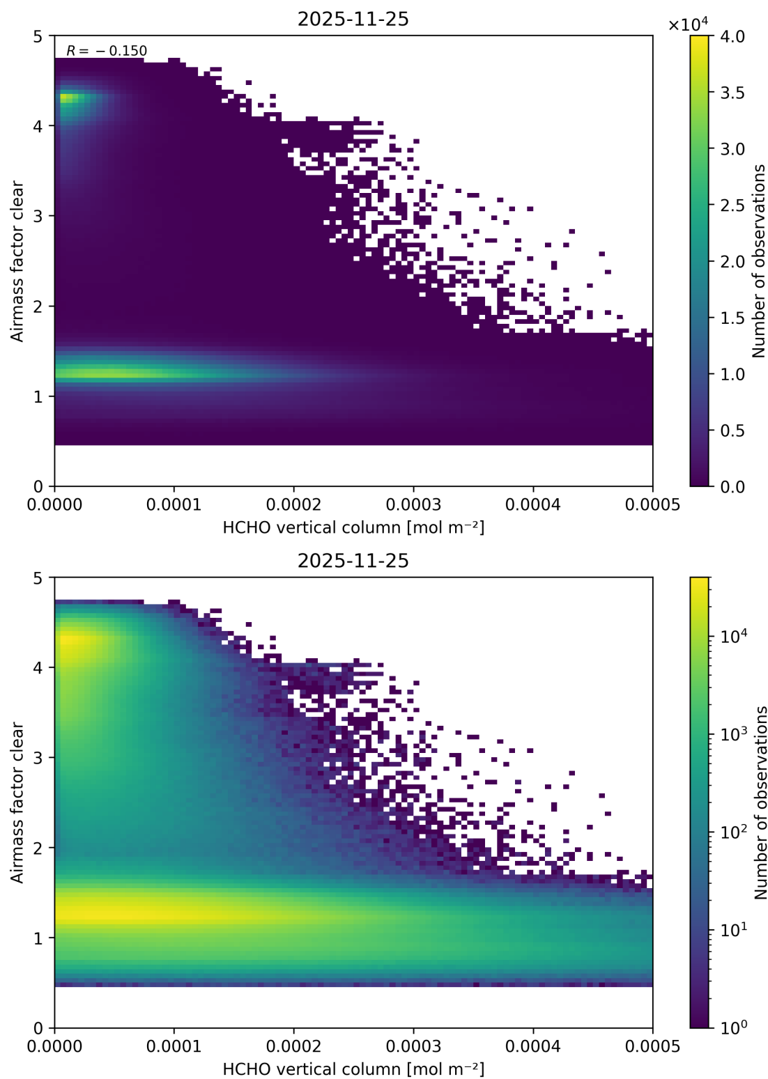
Figure 141: Scatter density plot of “HCHO vertical column” against “Airmass factor clear” for 2025-11-24 to 2025-11-26.
