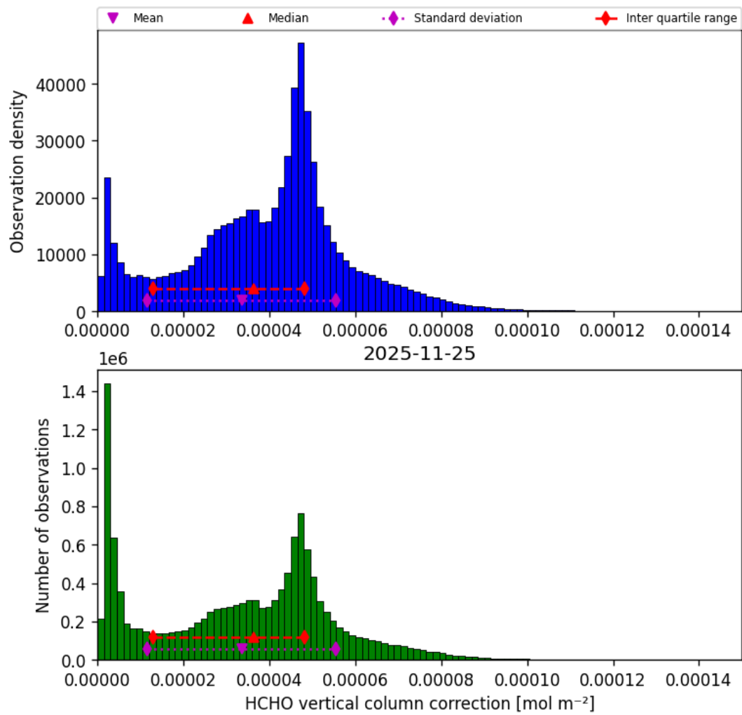
Figure 39: Histogram of “HCHO vertical column correction” for 2025-11-24 to 2025-11-26
