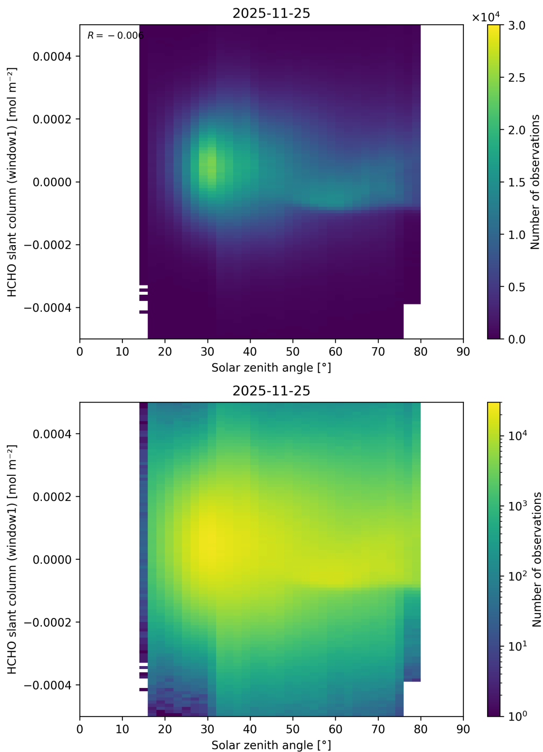
Figure 192: Scatter density plot of “Solar zenith angle” against “HCHO slant column (window1)” for 2025-11-24 to 2025-11-26.
