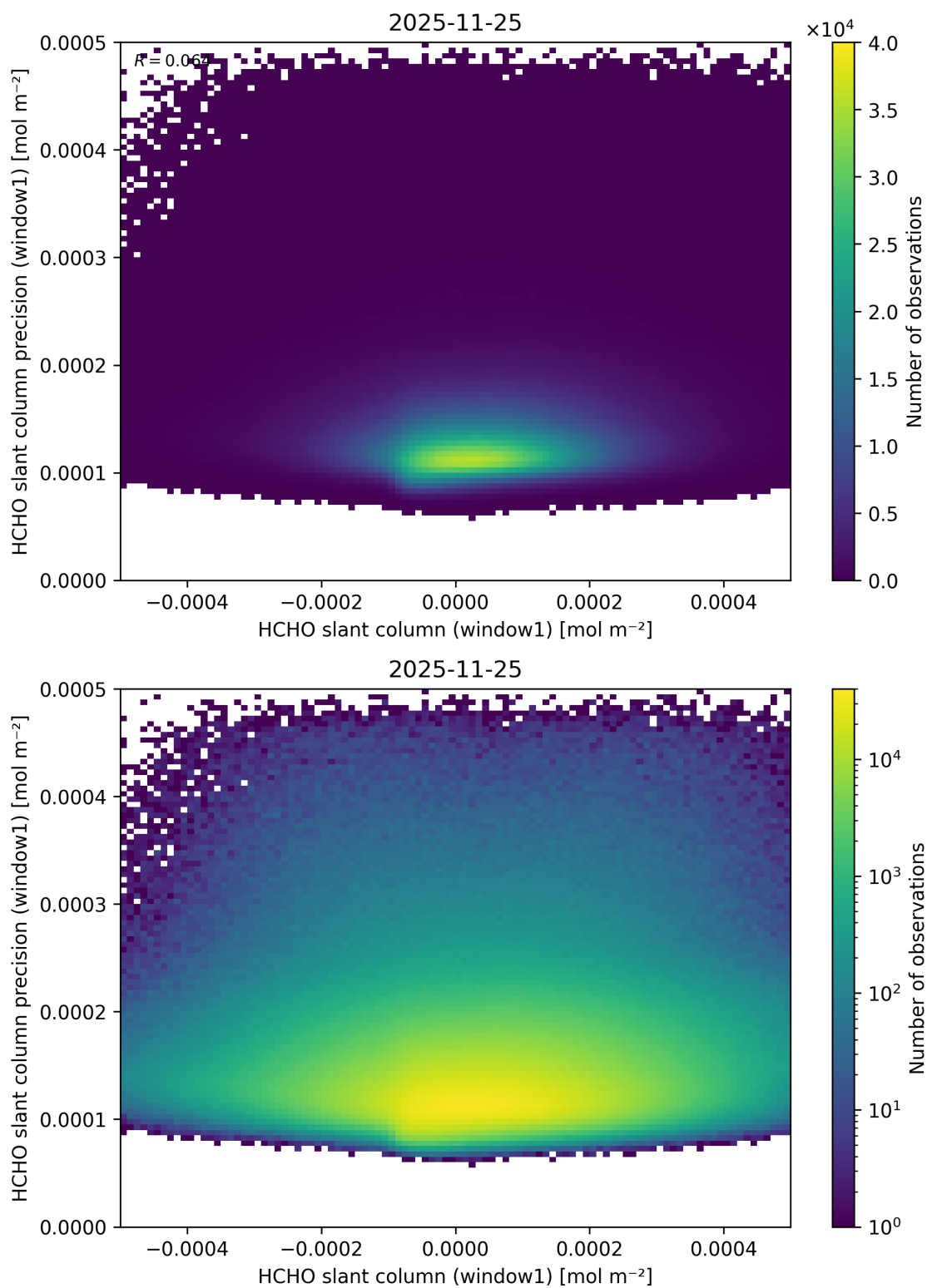
Figure 94: Scatter density plot of “HCHO slant column (window1)” against “HCHO slant column precision (window1)” for 2025-11-24 to 2025-11-26.
