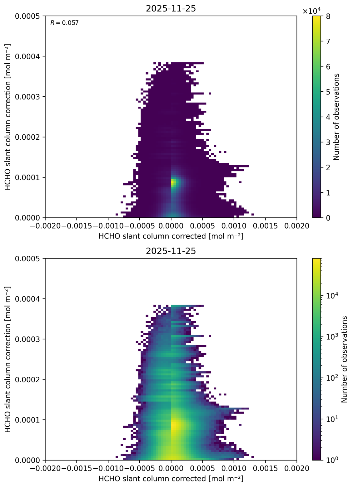
Figure 85: Scatter density plot of “HCHO slant column corrected” against “HCHO slant column correction” for 2025-11-24 to 2025-11-26.
