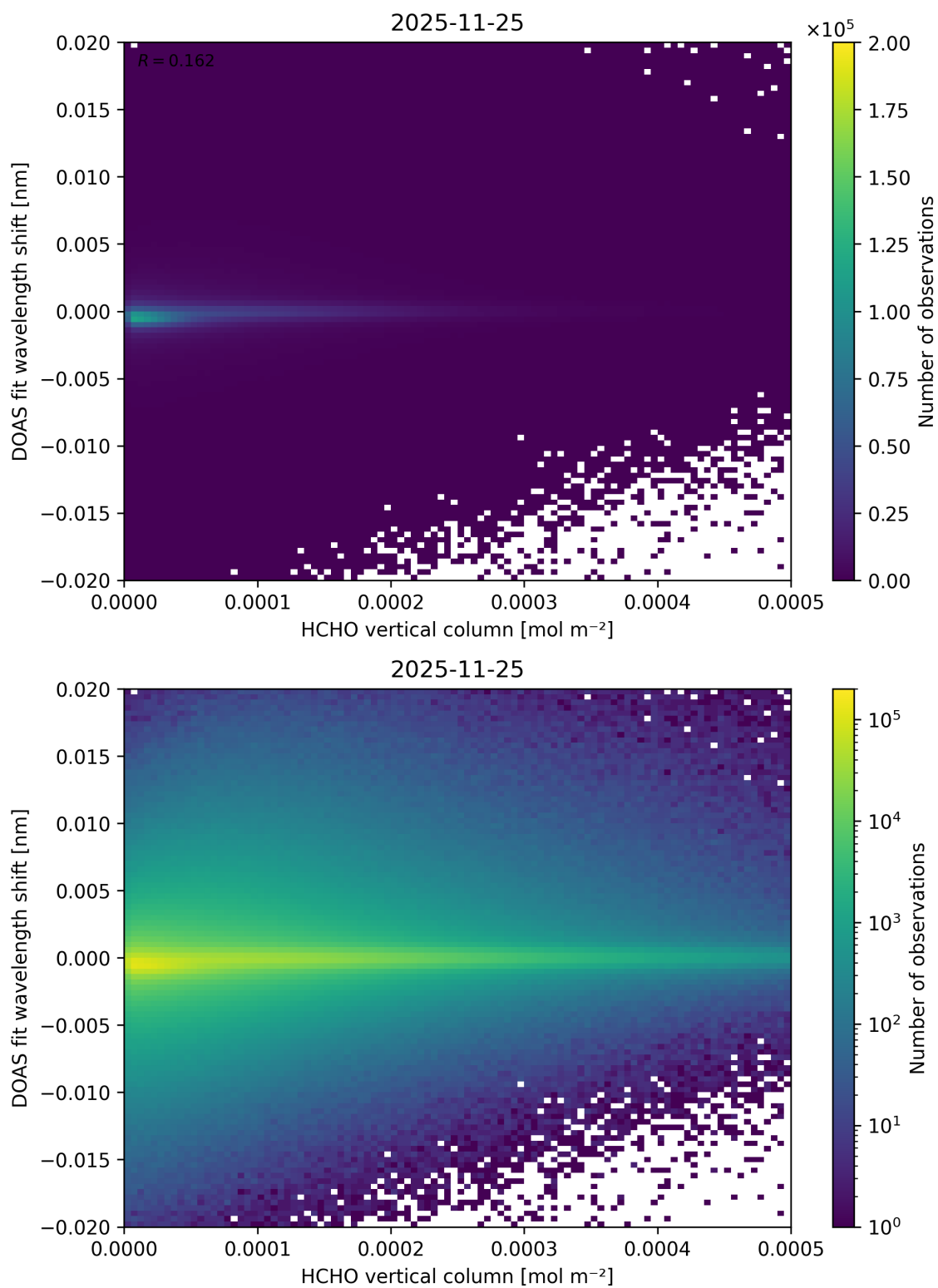
Figure 139: Scatter density plot of “HCHO vertical column” against “DOAS fit wavelength shift” for 2025-11-24 to 2025-11-26.
