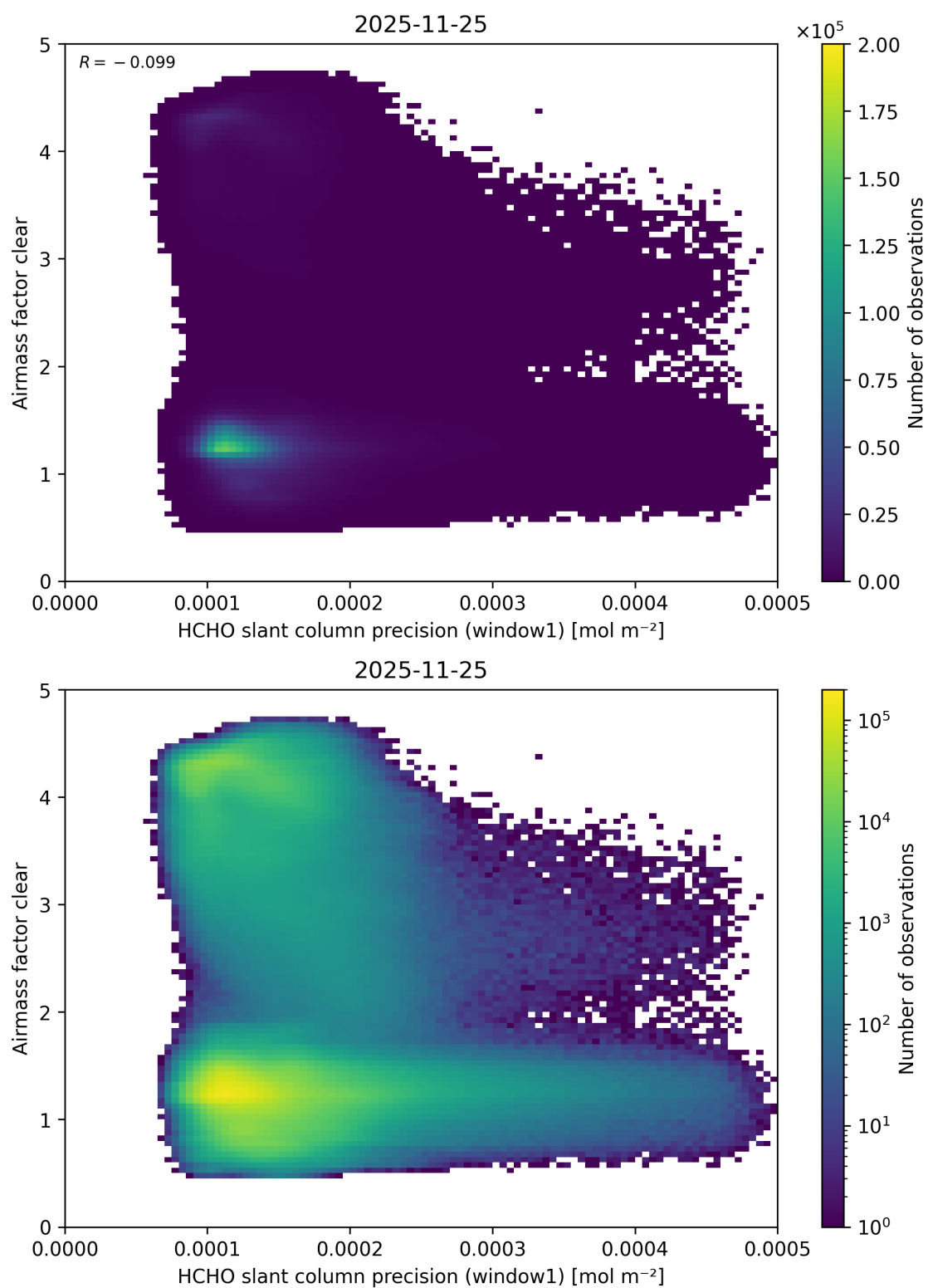
Figure 102: Scatter density plot of “HCHO slant column precision (window1)” against “Airmass factor clear” for 2025-11-24 to 2025-11-26.
