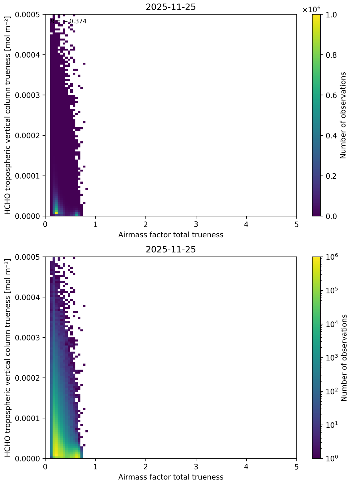
Figure 124: Scatter density plot of “Airmass factor total trueness” against “HCHO tropospheric vertical column trueness” for 2025-11-24 to 2025-11-26.
