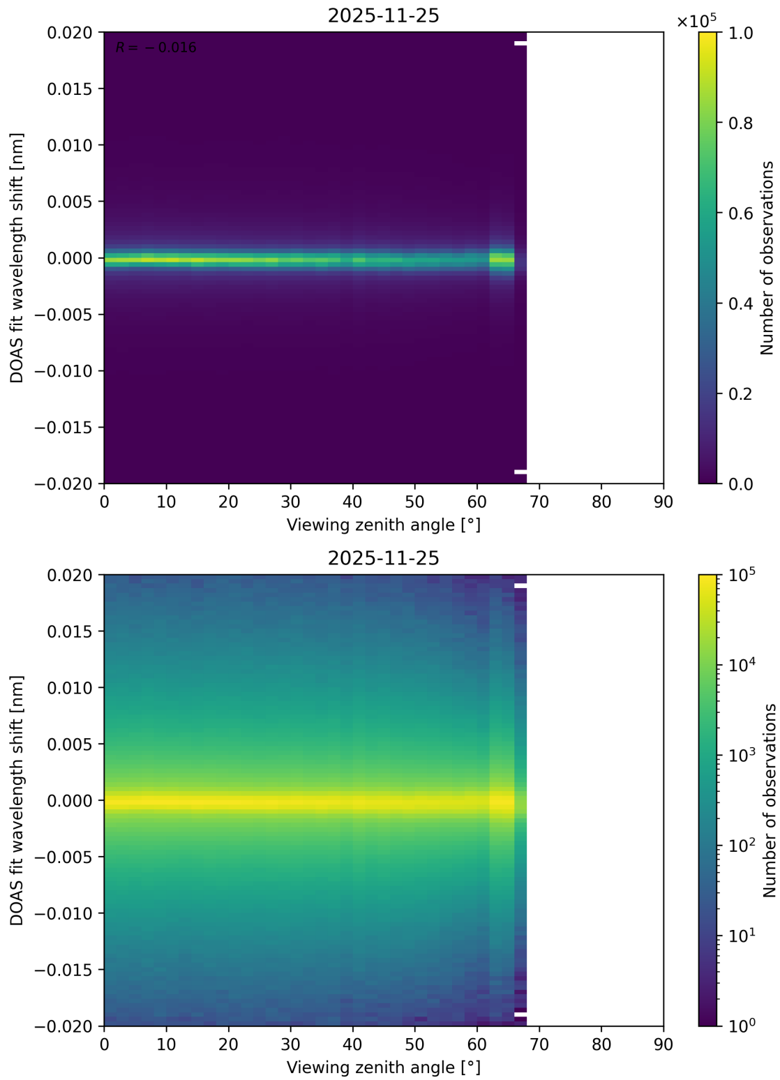
Figure 203: Scatter density plot of “Viewing zenith angle” against “DOAS fit wavelength shift” for 2025-11-24 to 2025-11-26.
