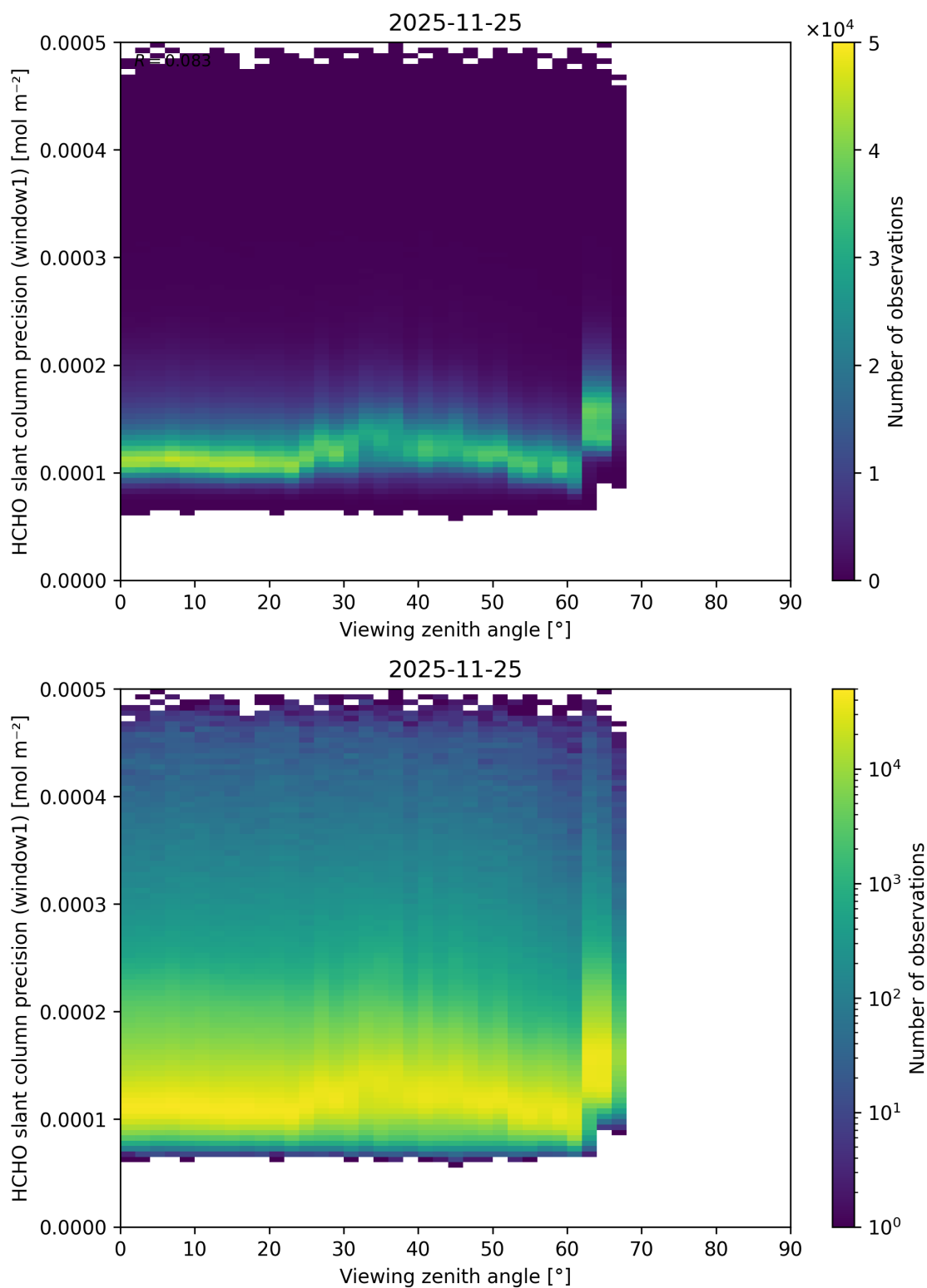
Figure 209: Scatter density plot of “Viewing zenith angle” against “HCHO slant column precision (window1)” for 2025-11-24 to 2025-11-26.
