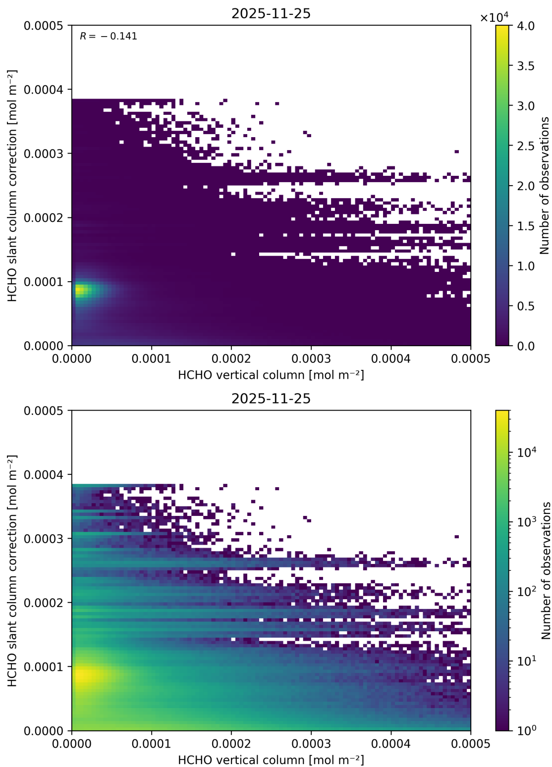
Figure 143: Scatter density plot of “HCHO vertical column” against “HCHO slant column correction” for 2025-11-24 to 2025-11-26.
