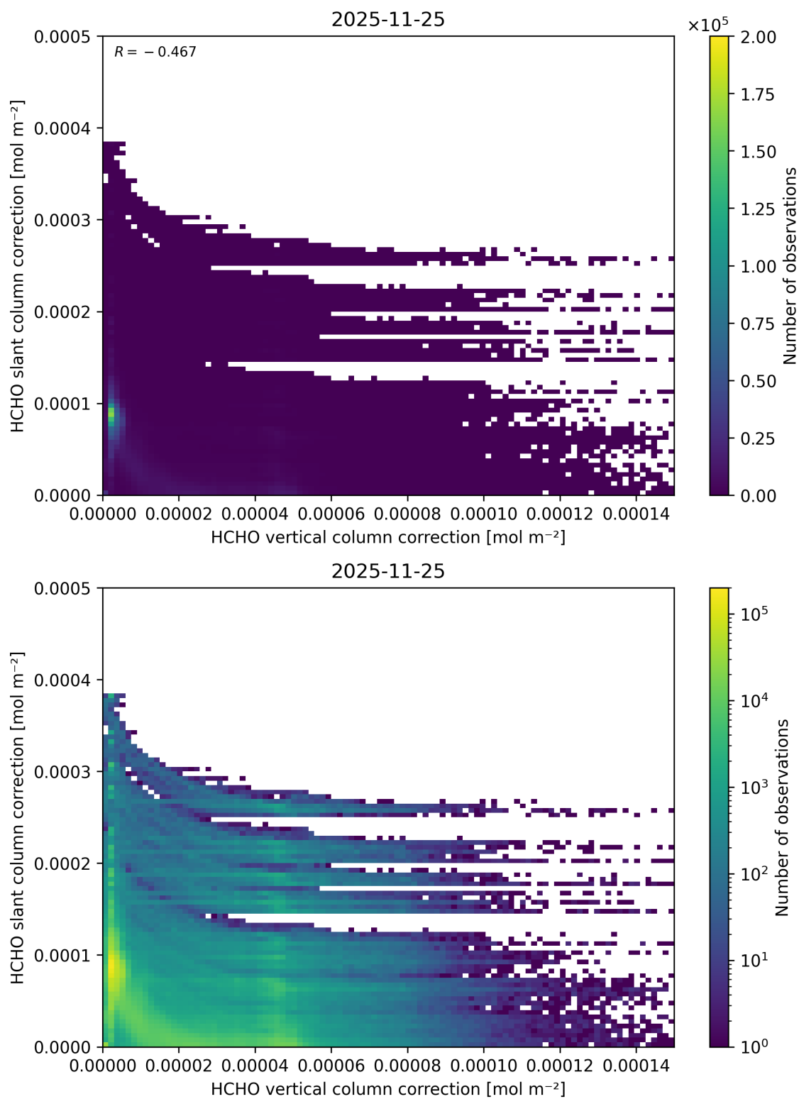
Figure 131: Scatter density plot of “HCHO vertical column correction” against “HCHO slant column correction” for 2025-11-24 to 2025-11-26.
