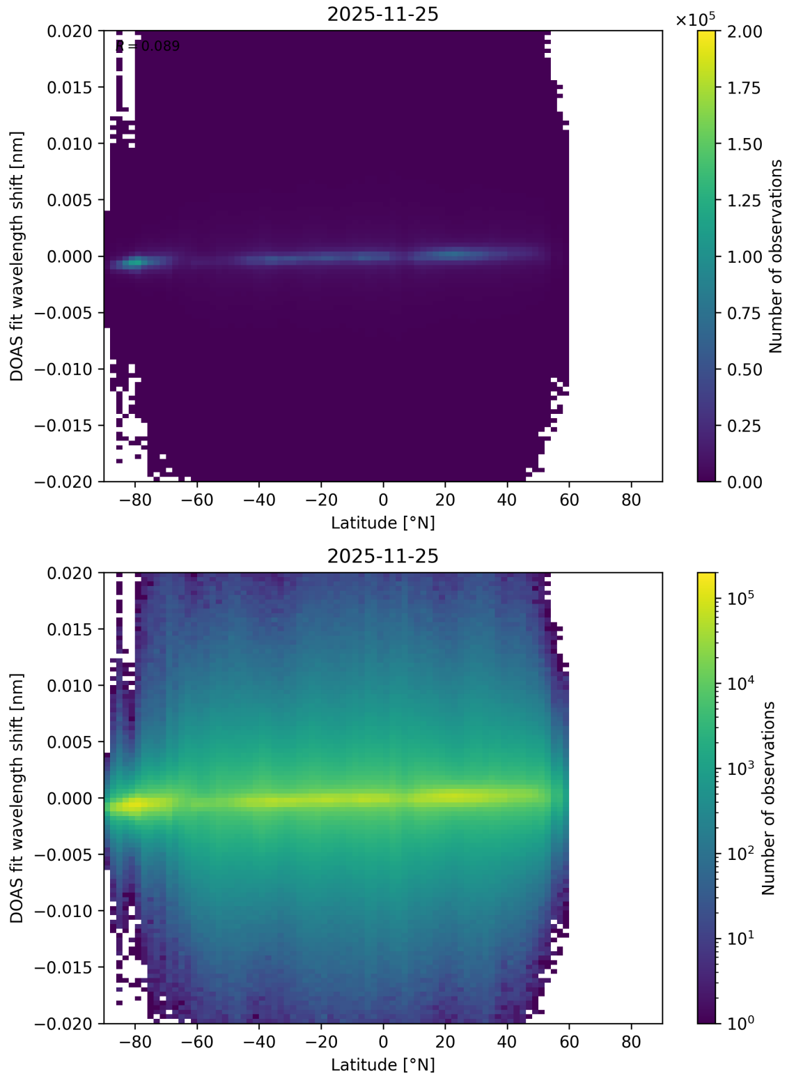
Figure 172: Scatter density plot of “Latitude” against “DOAS fit wavelength shift” for 2025-11-24 to 2025-11-26.
