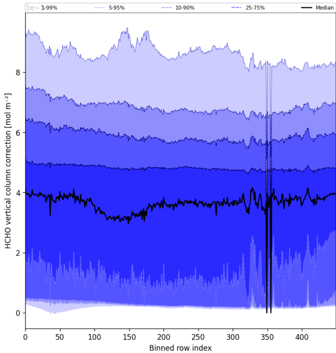
Figure 54: Along track statistics of "HCHO vertical column correction" for 2025-11-24 to 2025-11-26
