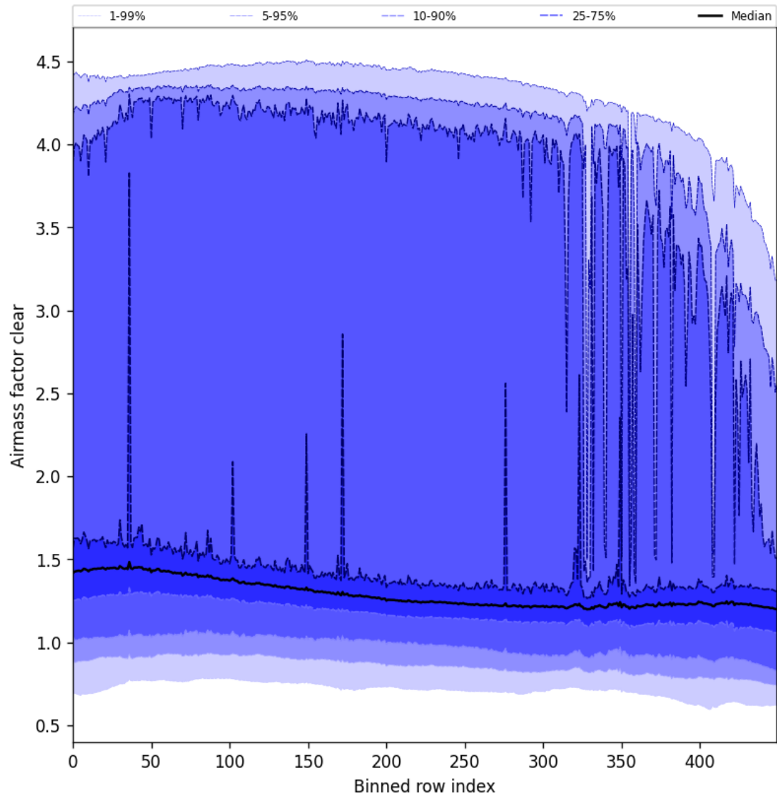
Figure 59: Along track statistics of “Airmass factor clear” for 2025-11-24 to 2025-11-26
