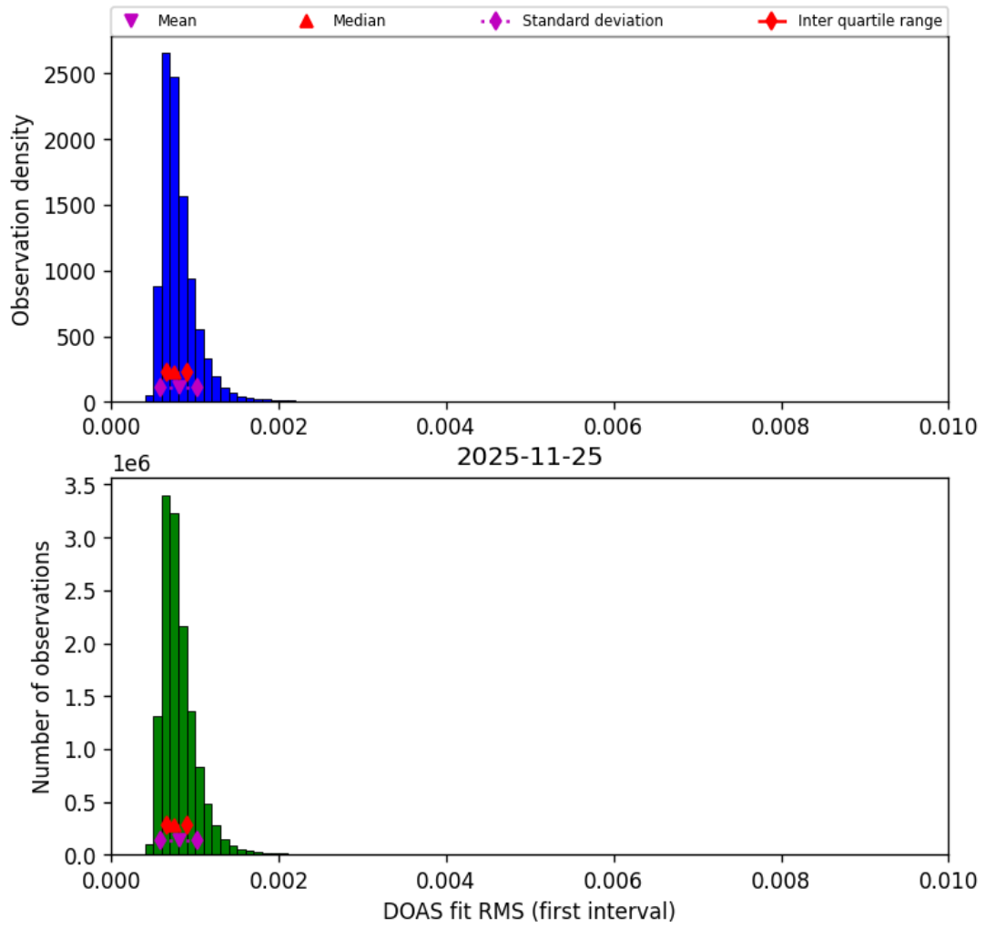
Figure 48: Histogram of “DOAS fit RMS (first interval)” for 2025-11-24 to 2025-11-26
