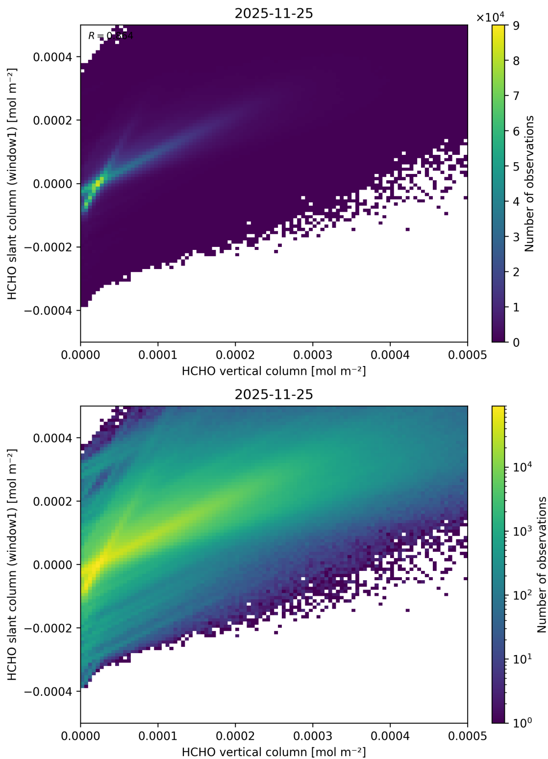
Figure 144: Scatter density plot of “HCHO vertical column” against “HCHO slant column (window1)” for 2025-11-24 to 2025-11-26.
