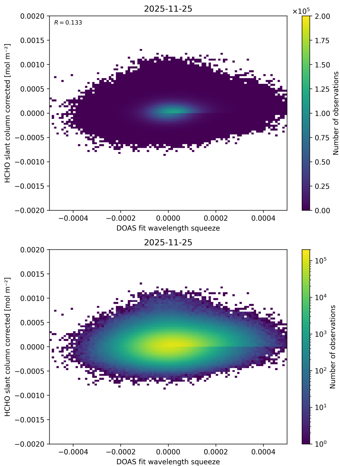
Figure 75: Scatter density plot of “DOAS fit wavelength squeeze” against “HCHO slant column corrected” for 2025-11-24 to 2025-11-26.
