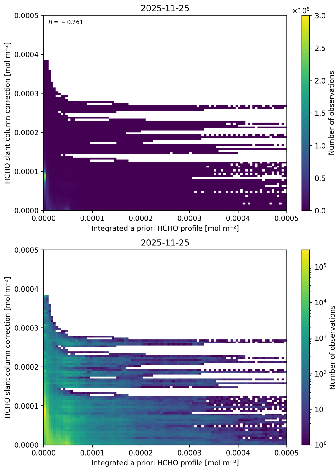
Figure 169: Scatter density plot of “Integrated a priori HCHO profile” against “HCHO slant column correction” for 2025-11-24 to 2025-11-26.
