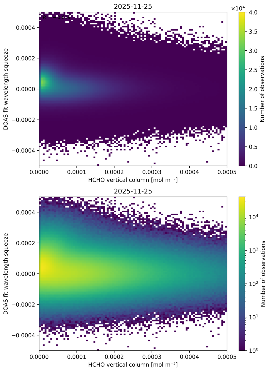
Figure 140: Scatter density plot of “HCHO vertical column” against “DOAS fit wavelength squeeze” for 2025-11-24 to 2025-11-26.
