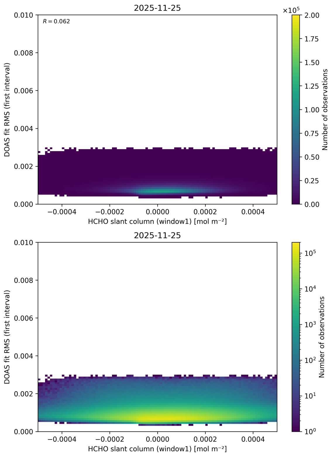
Figure 88: Scatter density plot of “HCHO slant column (window1)” against “DOAS fit RMS (first interval)” for 2025-11-24 to 2025-11-26.
