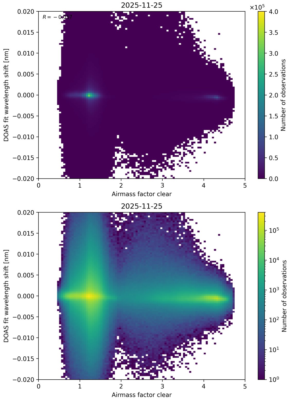
Figure 79: Scatter density plot of “Airmass factor clear” against “DOAS fit wavelength shift” for 2025-11-24 to 2025-11-26.
