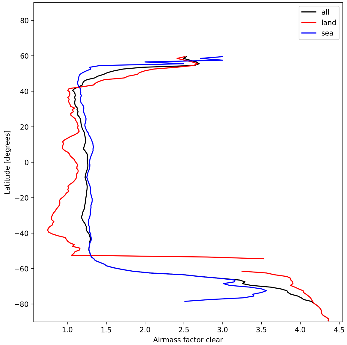
Figure 29: Zonal average of “Airmass factor clear” for 2025-11-24 to 2025-11-26.
