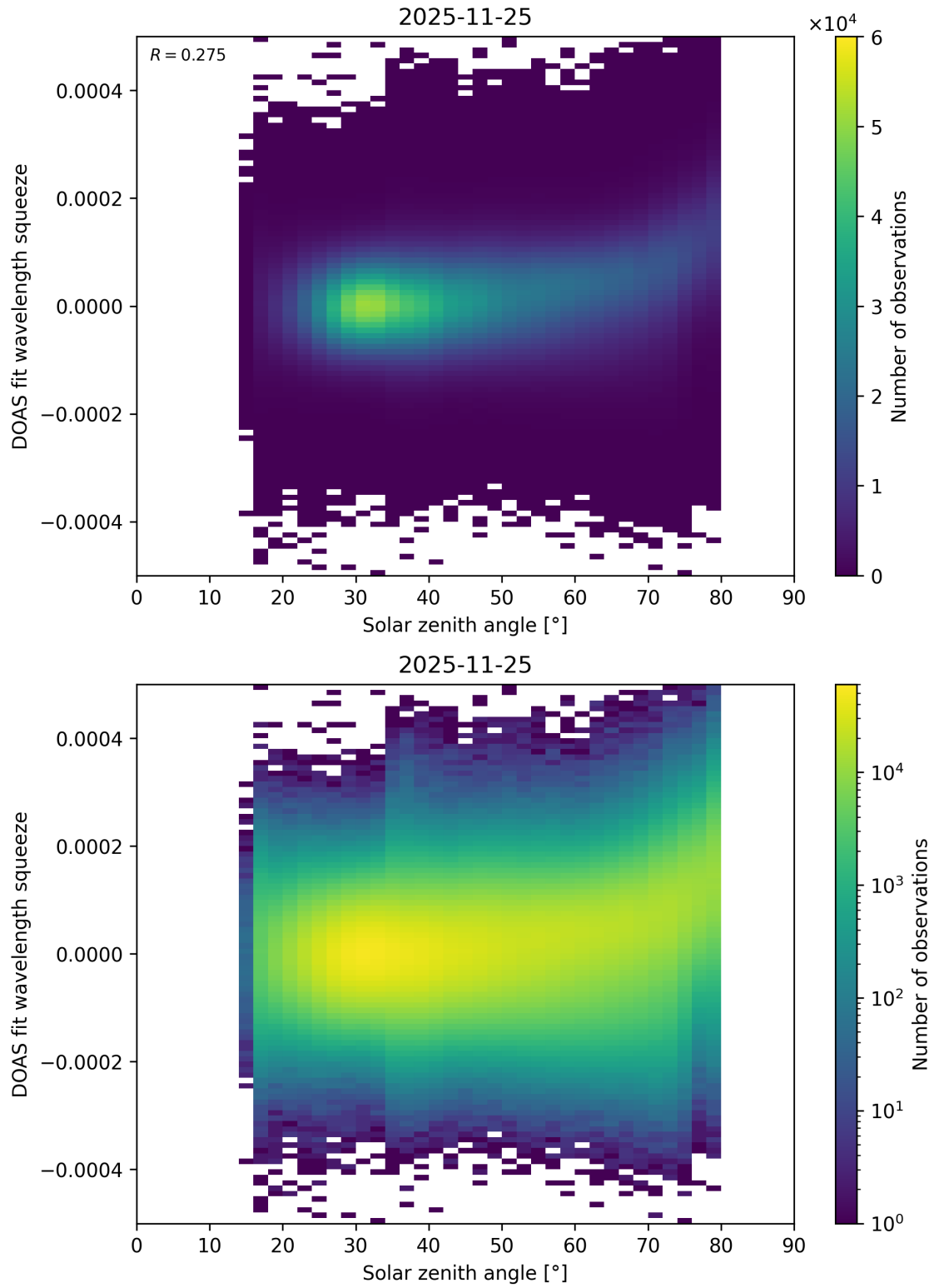
Figure 188: Scatter density plot of “Solar zenith angle” against “DOAS fit wavelength squeeze” for 2025-11-24 to 2025-11-26.
