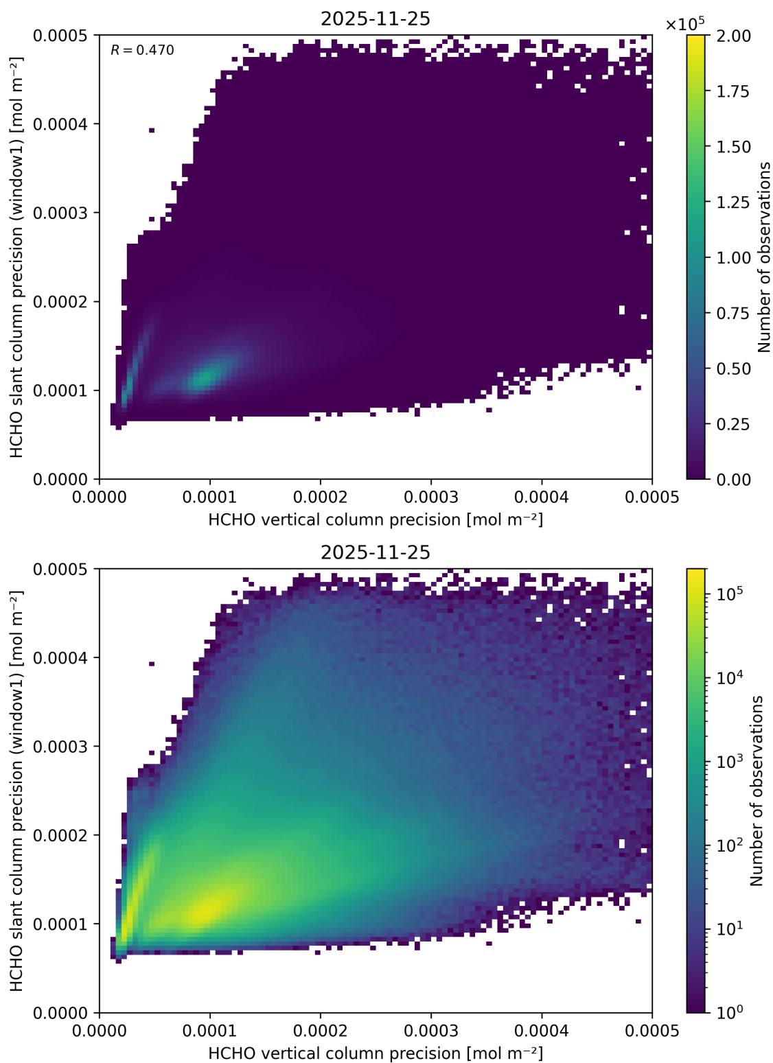
Figure 159: Scatter density plot of “HCHO vertical column precision” against “HCHO slant column precision (window1)” for 2025-11-24 to 2025-11-26.
