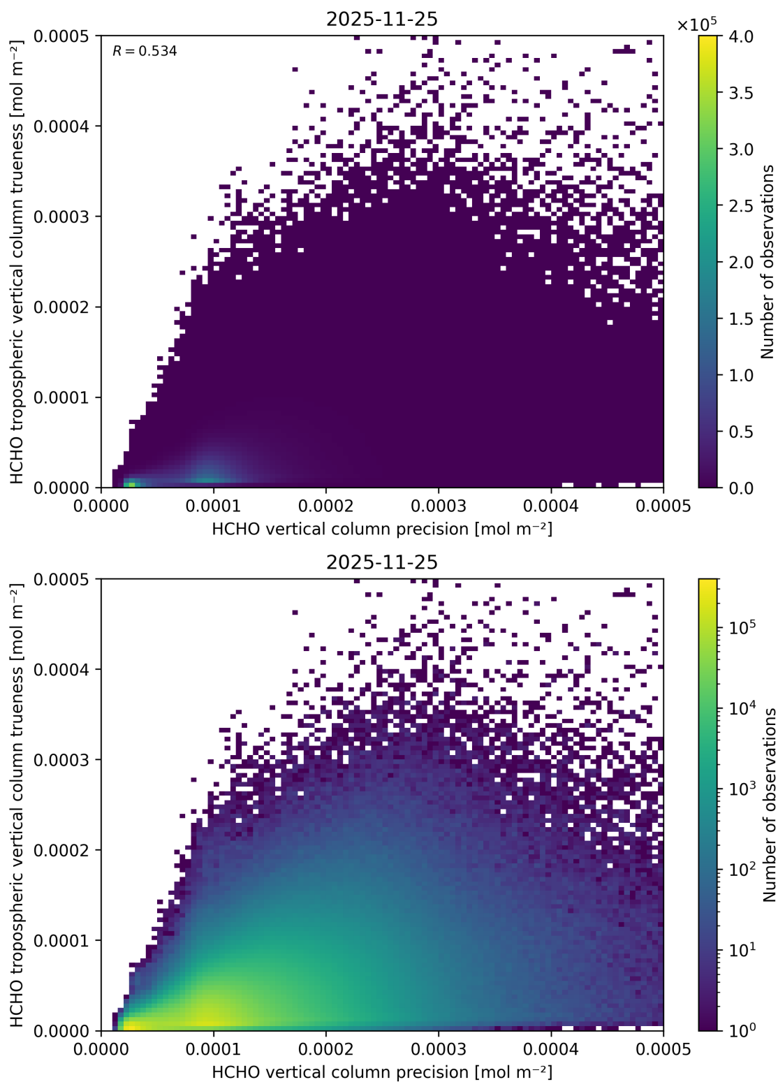
Figure 163: Scatter density plot of “HCHO vertical column precision” against “HCHO tropospheric vertical column true-ness” for 2025-11-24 to 2025-11-26.
