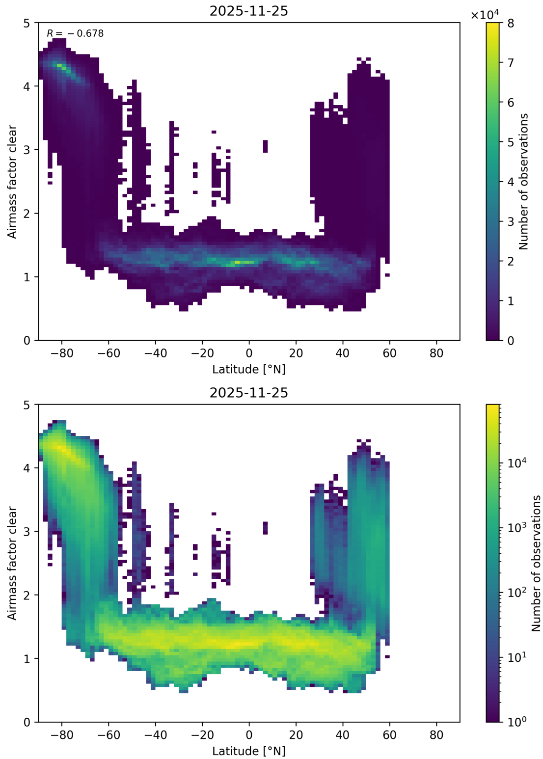
Figure 174: Scatter density plot of “Latitude” against “Airmass factor clear” for 2025-11-24 to 2025-11-26.
