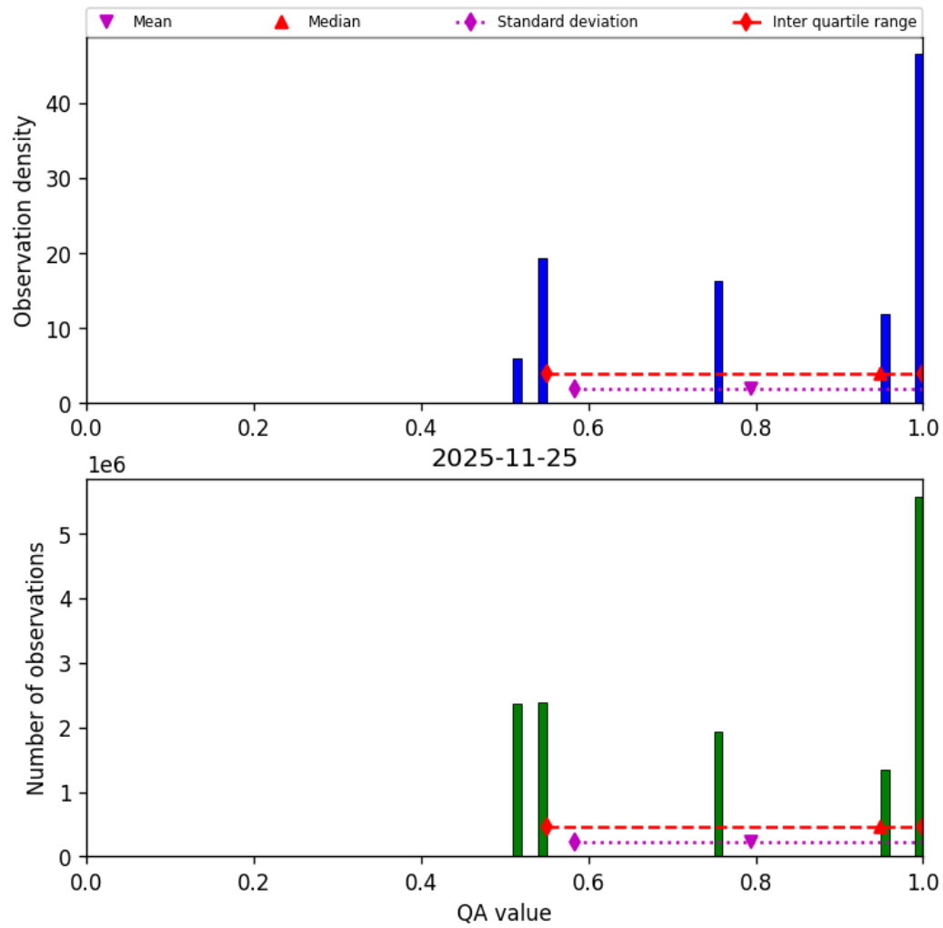
Figure 36: Histogram of “QA value” for 2025-11-24 to 2025-11-26
