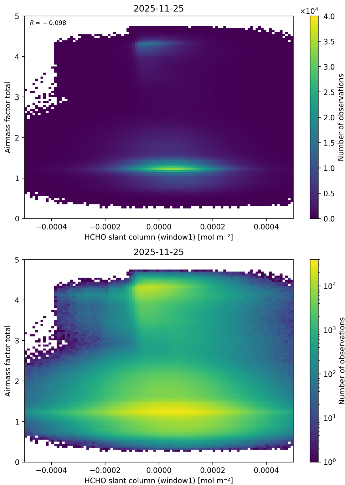
Figure 95: Scatter density plot of “HCHO slant column (window1)” against “Airmass factor total” for 2025-11-24 to 2025-11-26.
