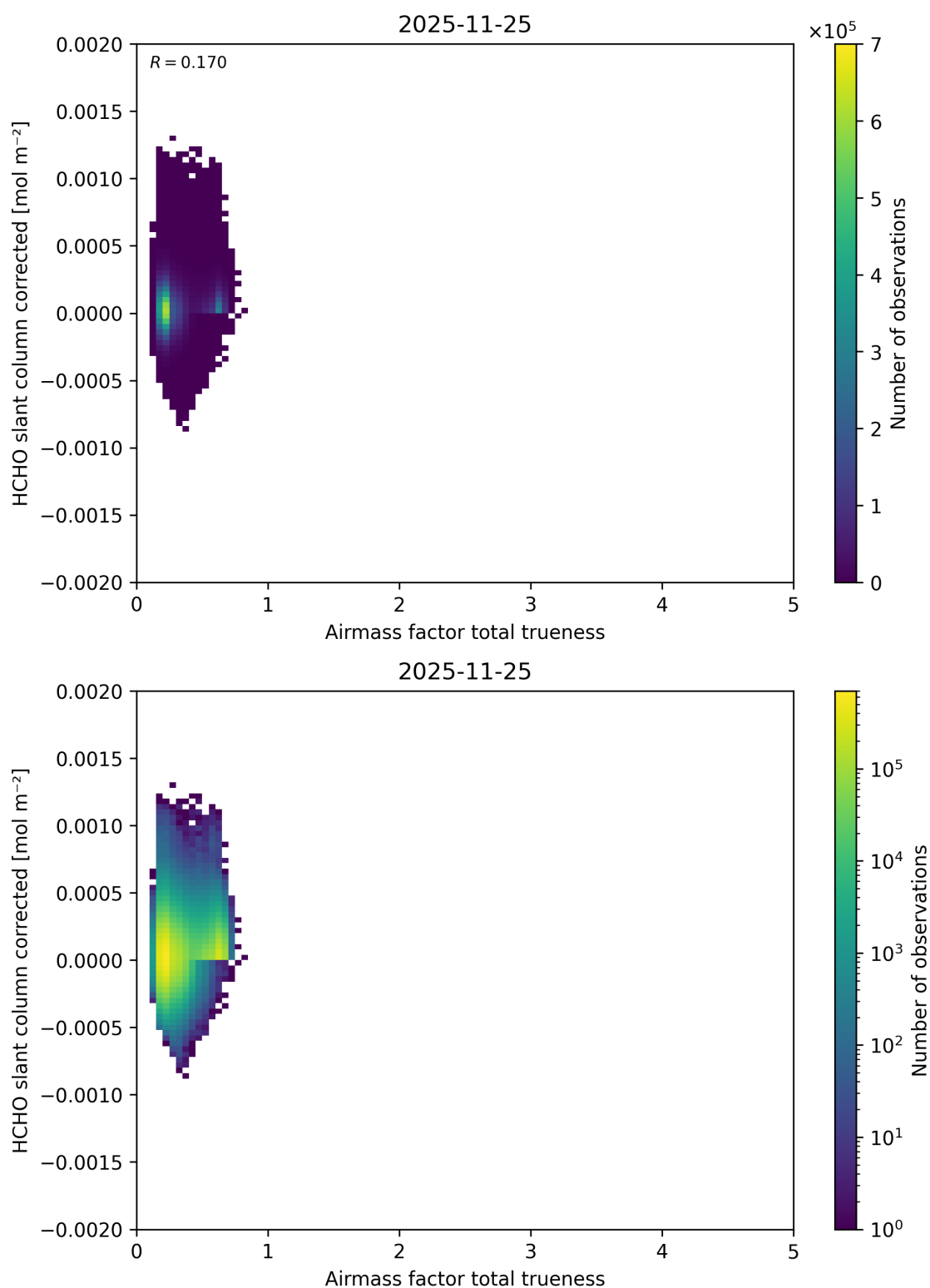
Figure 122: Scatter density plot of “Airmass factor total trueness” against “HCHO slant column corrected” for 2025-11-24 to 2025-11-26.
