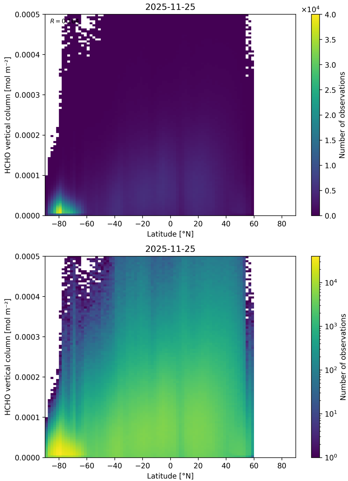
Figure 181: Scatter density plot of “Latitude” against “HCHO vertical column” for 2025-11-24 to 2025-11-26.
