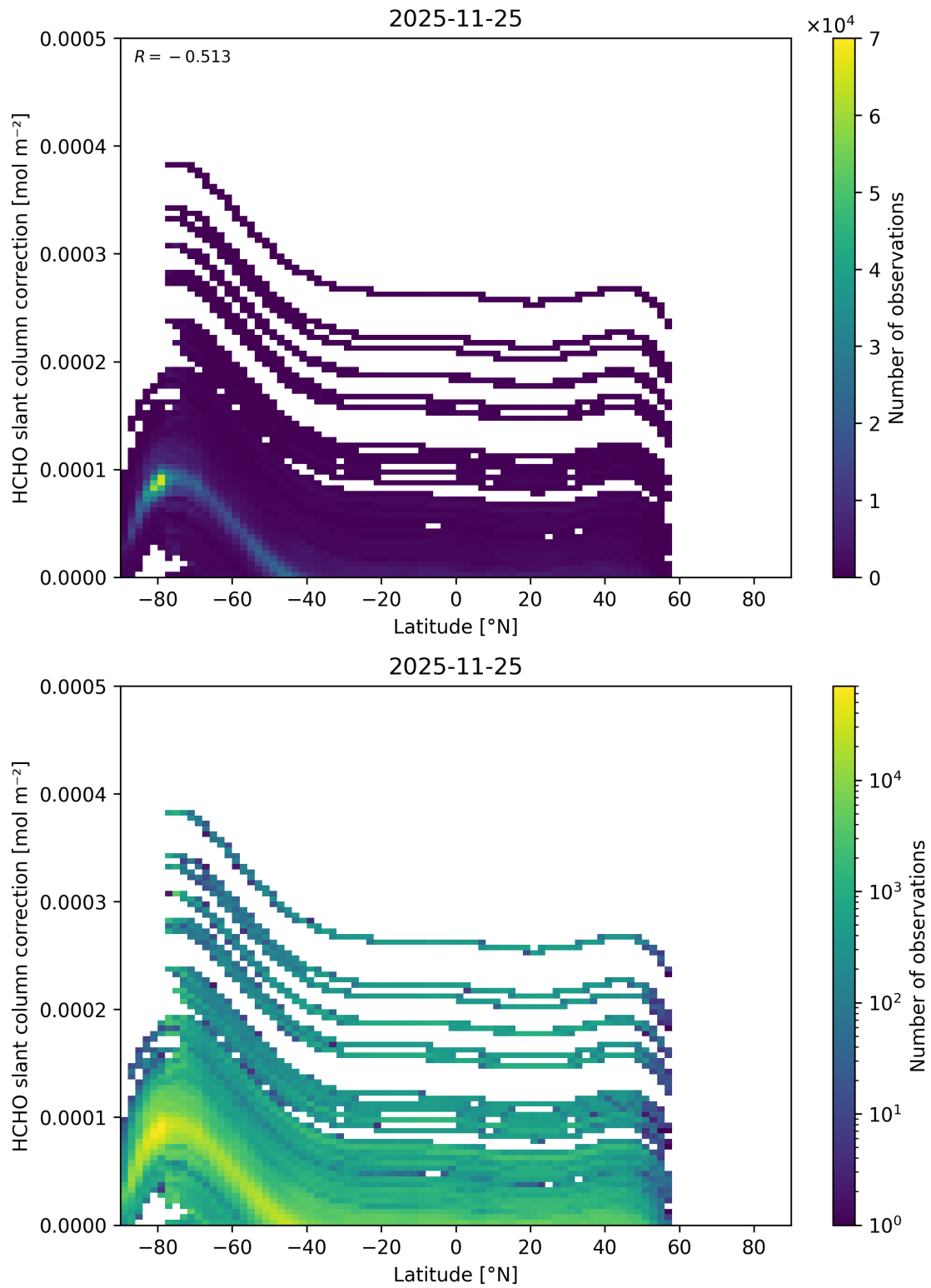
Figure 176: Scatter density plot of “Latitude” against “HCHO slant column correction” for 2025-11-24 to 2025-11-26.
