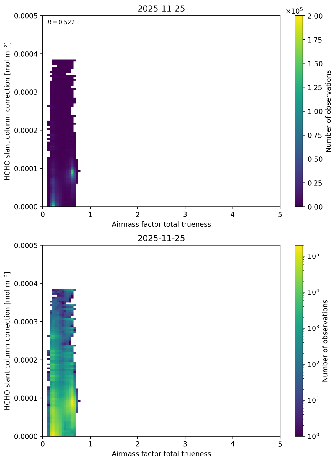
Figure 123: Scatter density plot of “Airmass factor total truiness” against “HCHO slant column correction” for 2025-11-24 to 2025-11-26.
