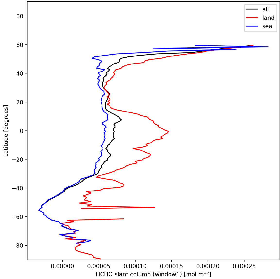
Figure 25: Zonal average of “HCHO slant column (window1)” for 2025-11-24 to 2025-11-26.
