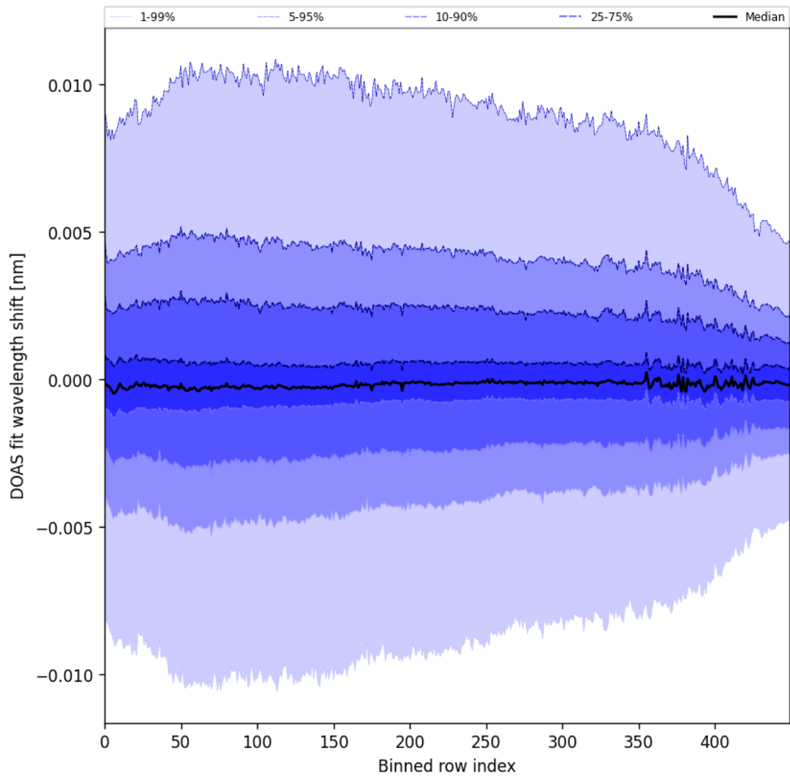
Figure 61: Along track statistics of “DOAS fit wavelength shift” for 2025-11-24 to 2025-11-26
