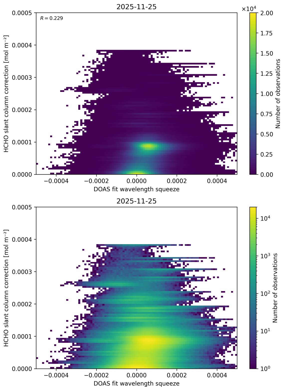
Figure 76: Scatter density plot of “DOAS fit wavelength squeeze” against “HCHO slant column correction” for 2025-11-24 to 2025-11-26.
