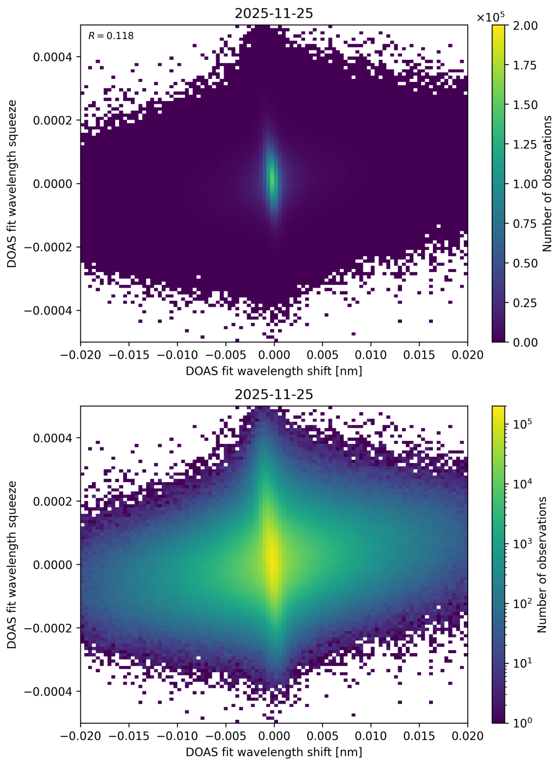
Figure 70: Scatter density plot of “DOAS fit wavelength shift” against “DOAS fit wavelength squeeze” for 2025-11-24 to 2025-11-26.
