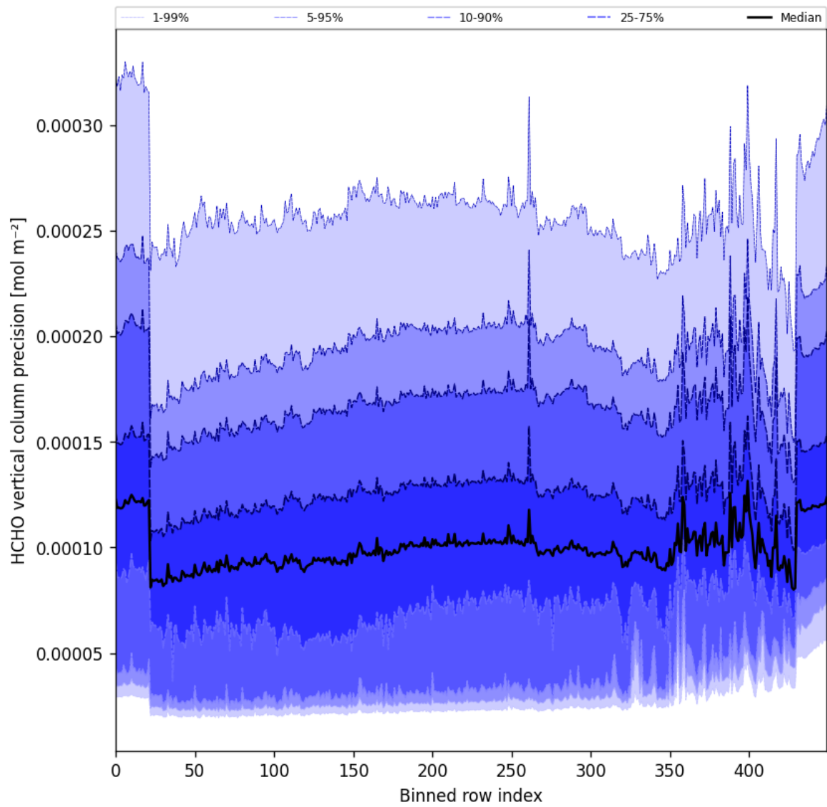
Figure 53: Along track statistics of “HCHO vertical column precision” for 2025-11-24 to 2025-11-26
