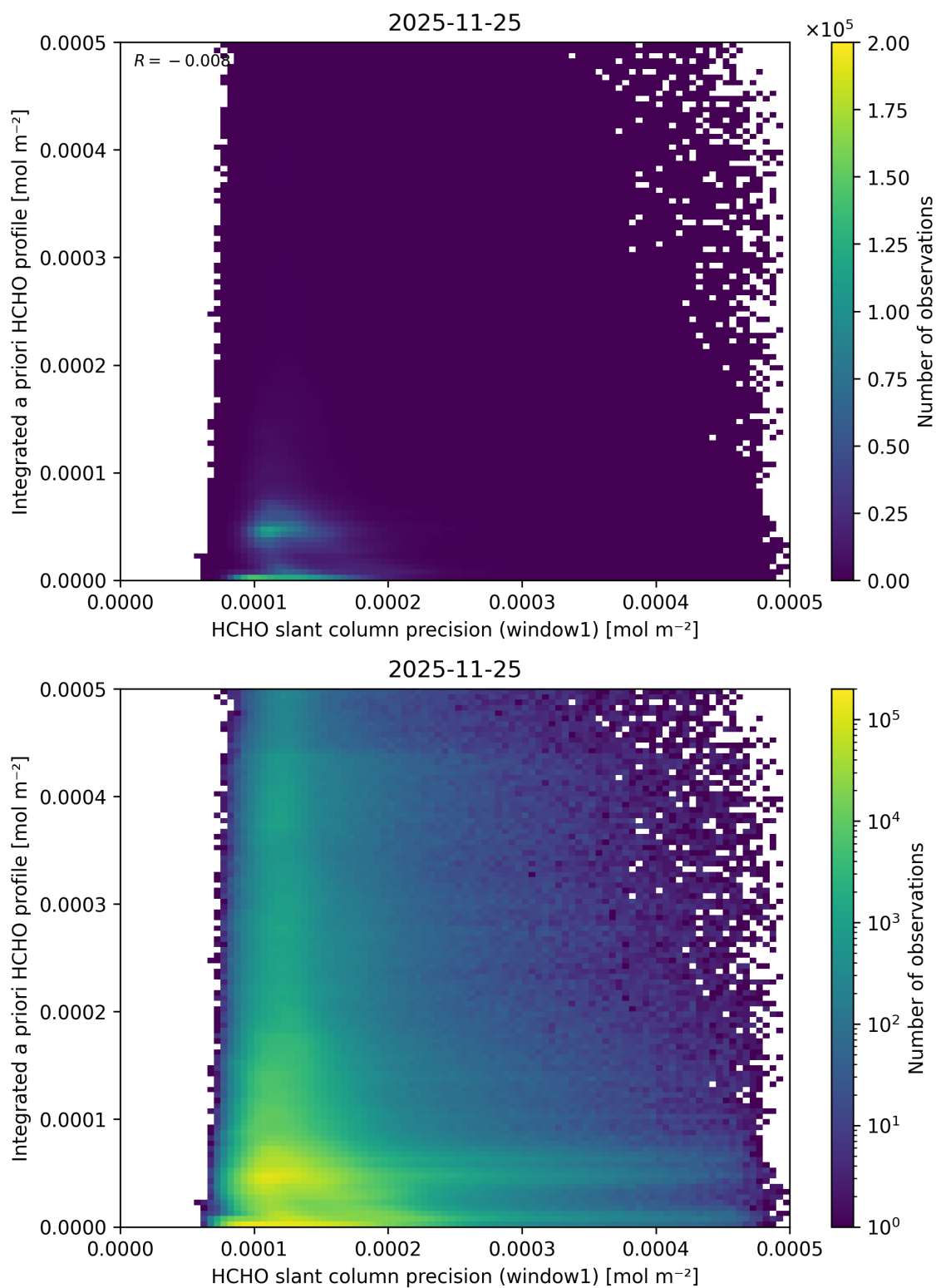
Figure 108: Scatter density plot of “HCHO slant column precision (window1)” against “Integrated a priori HCHO profile” for 2025-11-24 to 2025-11-26.
