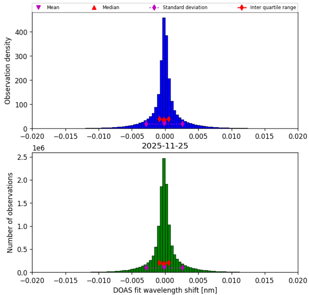
Figure 46: Histogram of “DOAS fit wavelength shift” for 2025-11-24 to 2025-11-26
