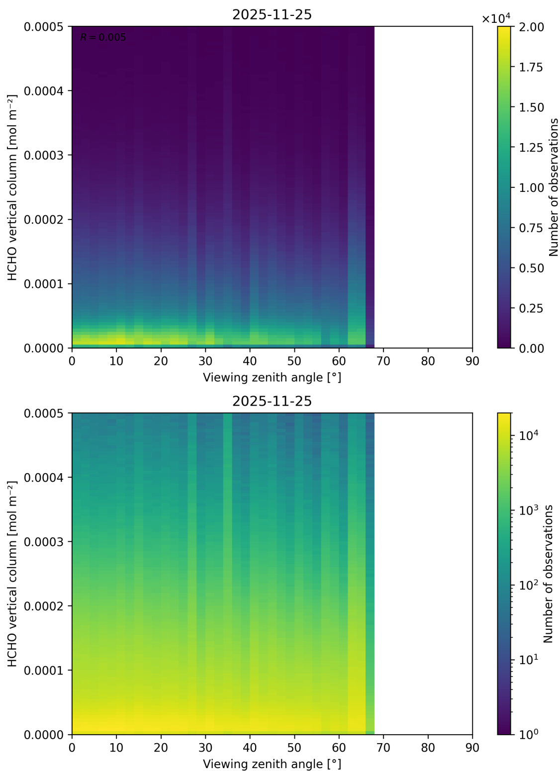
Figure 212: Scatter density plot of “Viewing zenith angle” against “HCHO vertical column” for 2025-11-24 to 2025-11-26.
