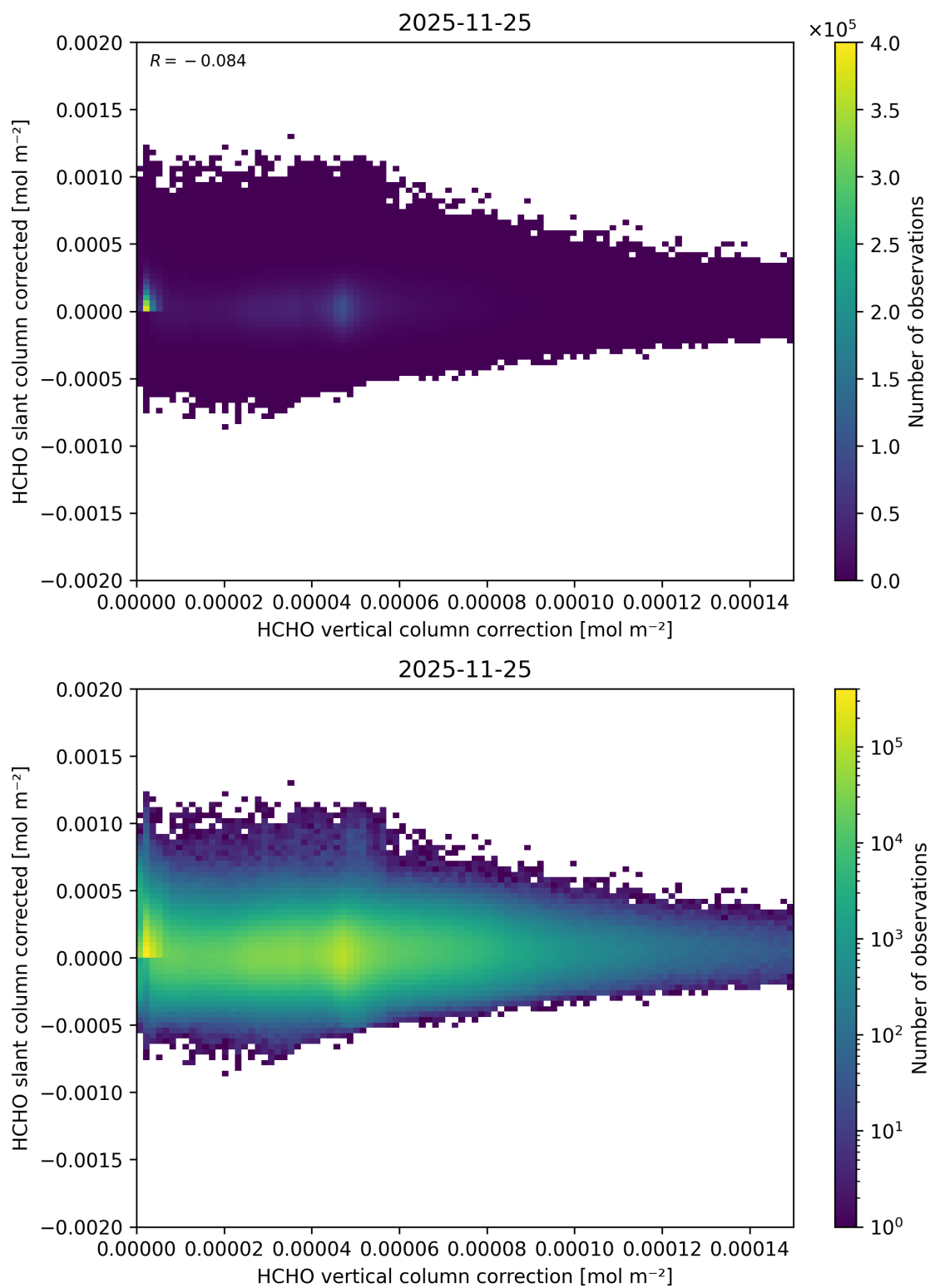
Figure 130: Scatter density plot of “HCHO vertical column correction” against “HCHO slant column corrected” for 2025-11-24 to 2025-11-26.
