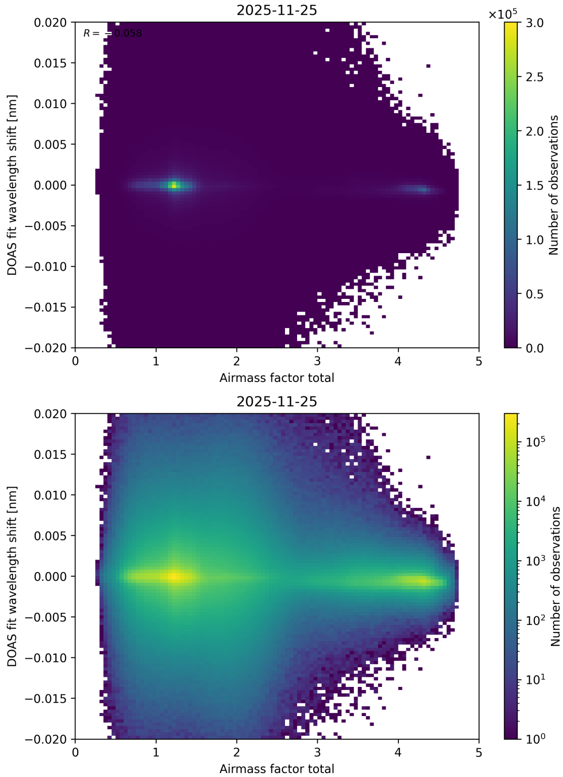
Figure 110: Scatter density plot of “Airmass factor total” against “DOAS fit wavelength shift” for 2025-11-24 to 2025-11-26.
