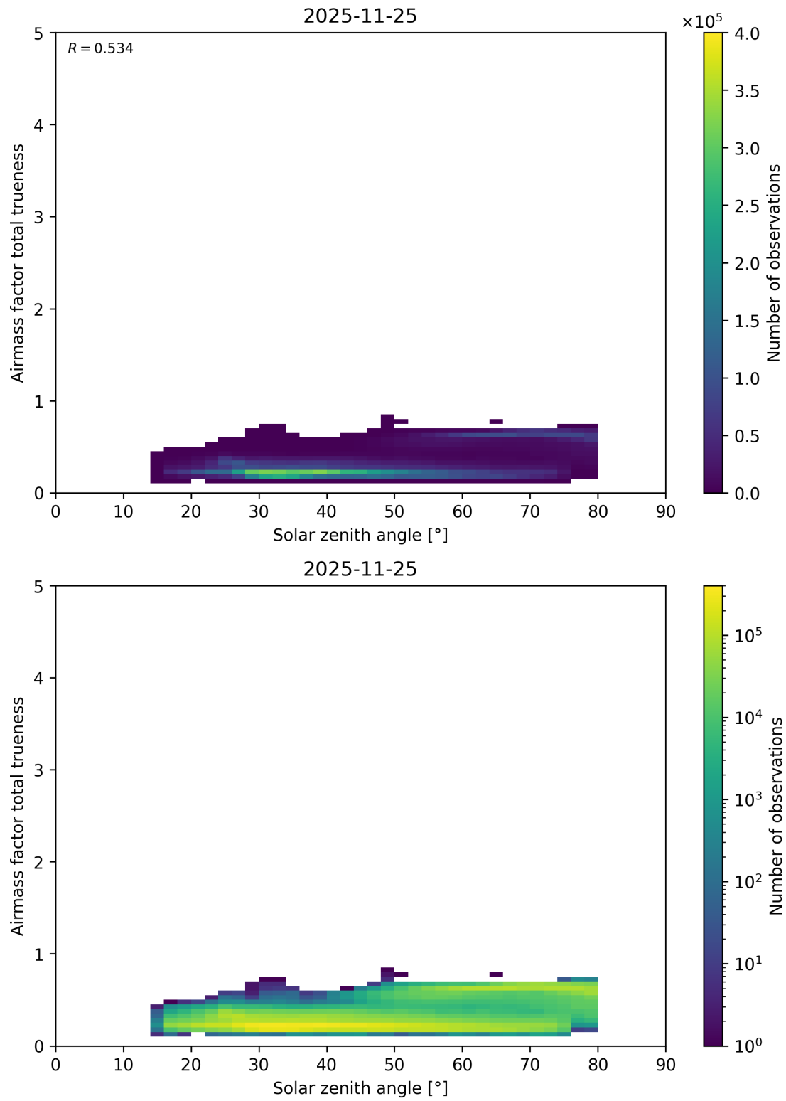
Figure 195: Scatter density plot of “Solar zenith angle” against “Airmass factor total trueneess” for 2025-11-24 to 2025-11-26.
