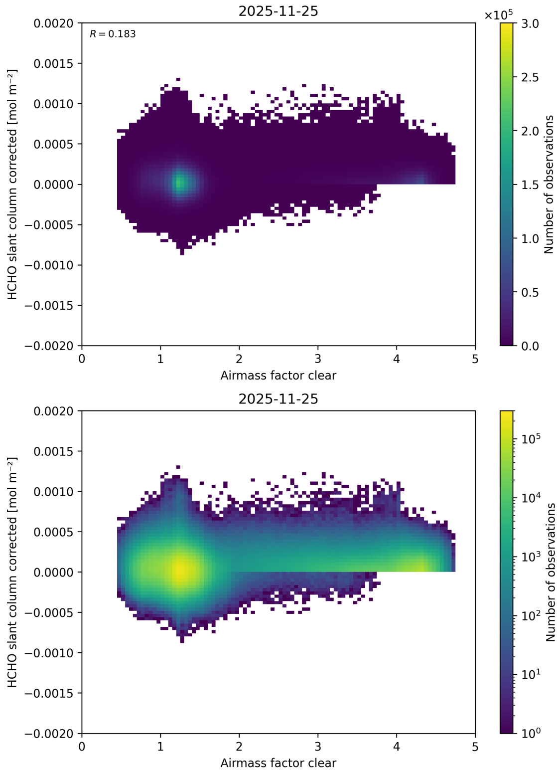
Figure 81: Scatter density plot of “Airmass factor clear” against “HCHO slant column corrected” for 2025-11-24 to 2025-11-26.
