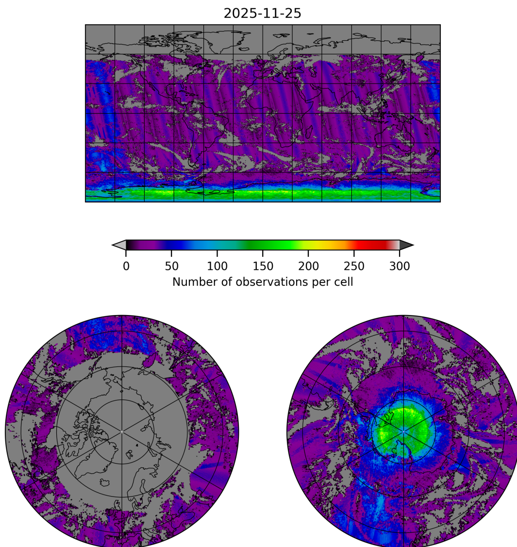
Figure 20: Map of the number of observations for 2025-11-24 to 2025-11-26
