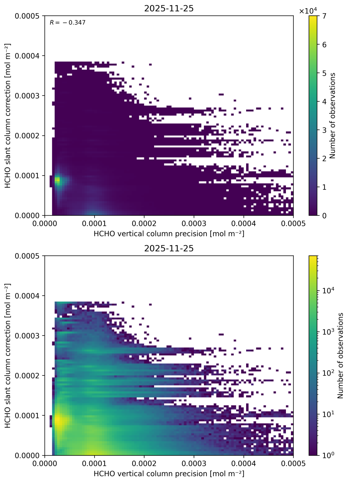
Figure 157: Scatter density plot of “HCHO vertical column precision” against “HCHO slant column correction” for 2025-11-24 to 2025-11-26.
