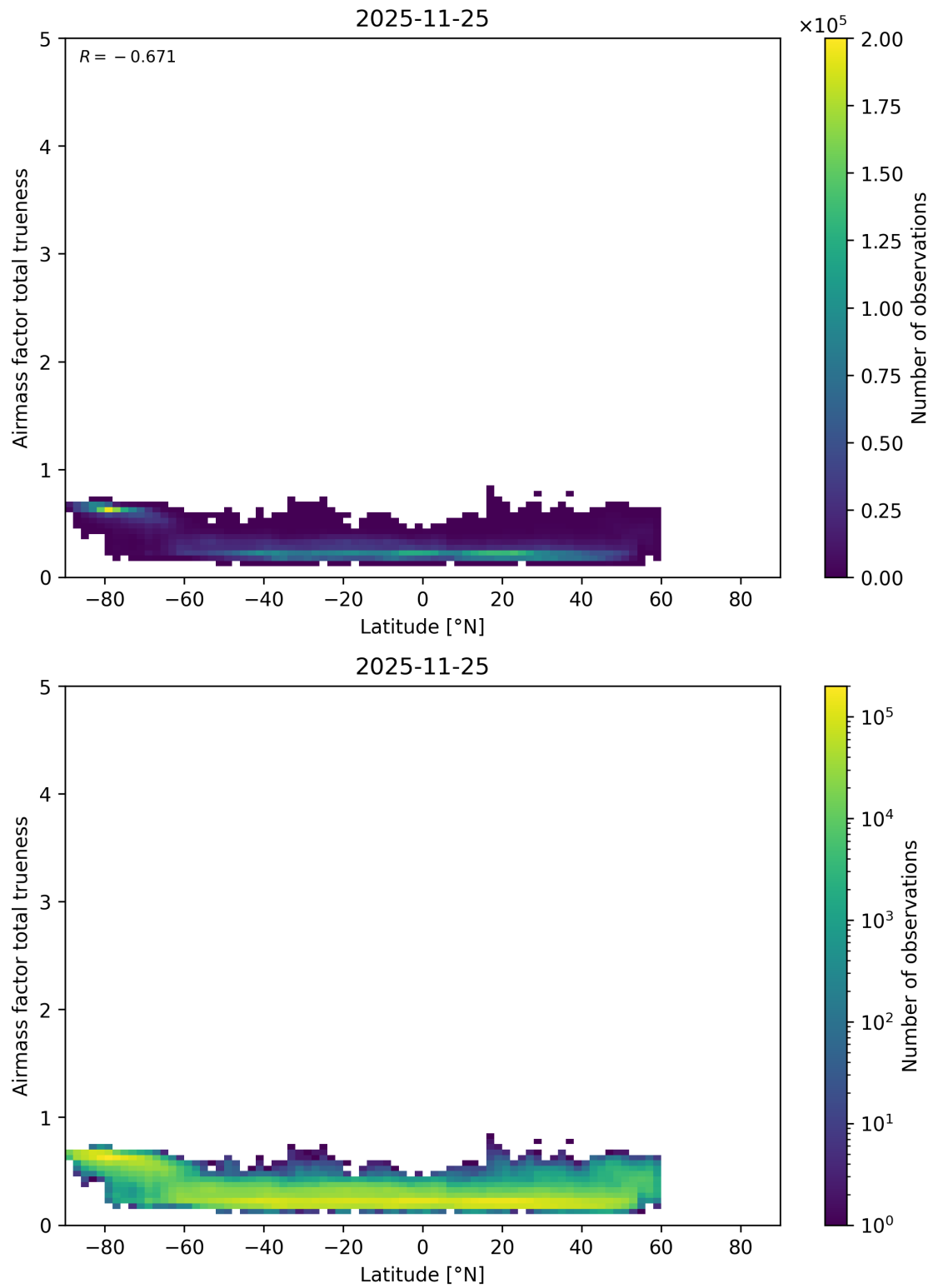
Figure 180: Scatter density plot of “Latitude” against “Airmass factor total trueness” for 2025-11-24 to 2025-11-26.
