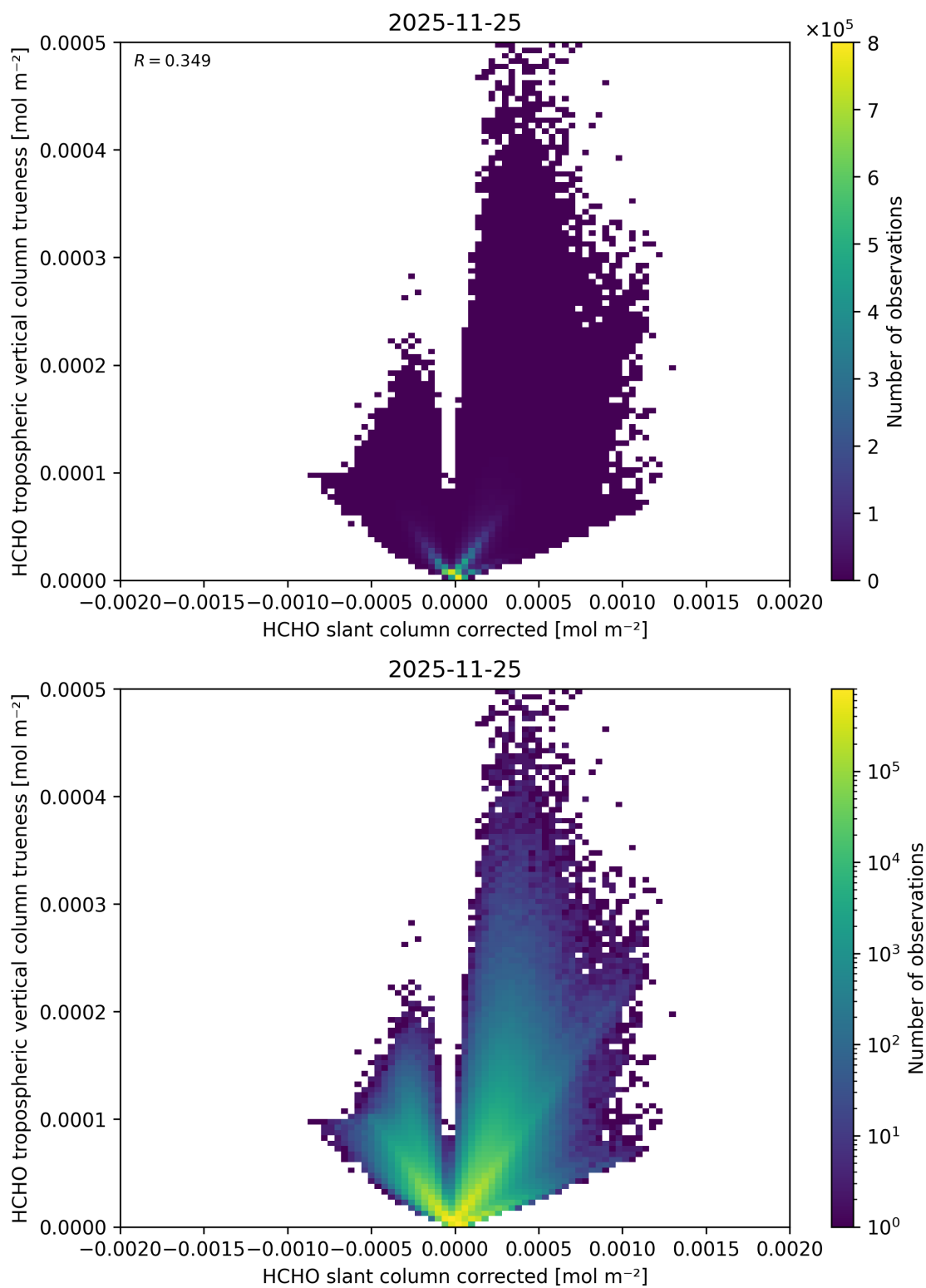
Figure 86: Scatter density plot of “HCHO slant column corrected” against “HCHO tropospheric vertical column trueness” for 2025-11-24 to 2025-11-26.
