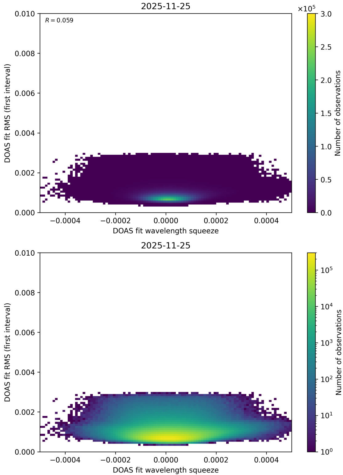
Figure 74: Scatter density plot of “DOAS fit wavelength squeeze” against “DOAS fit RMS (first interval)” for 2025-11-24 to 2025-11-26.
