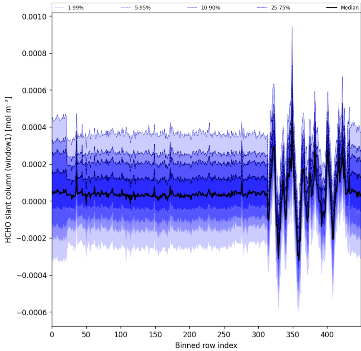
Figure 55: Along track statistics of “HCHO slant column (window1)” for 2025-11-24 to 2025-11-26
