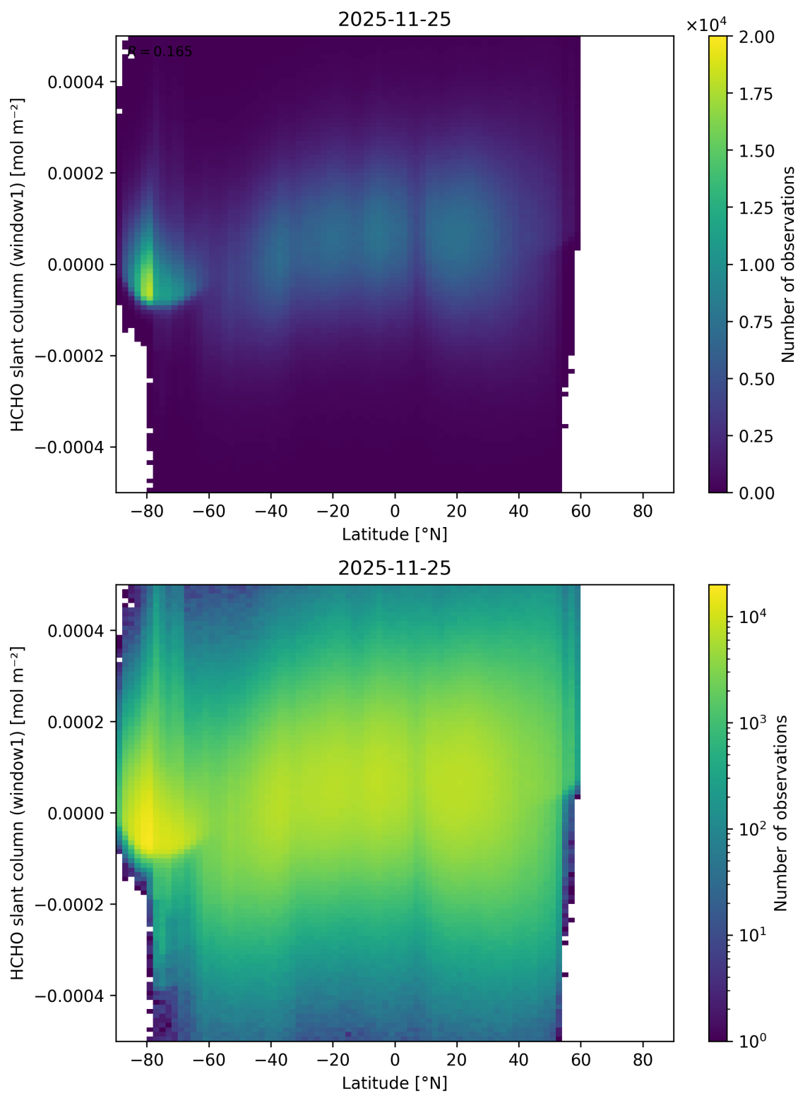
Figure 177: Scatter density plot of “Latitude” against “HCHO slant column (window1)” for 2025-11-24 to 2025-11-26.
