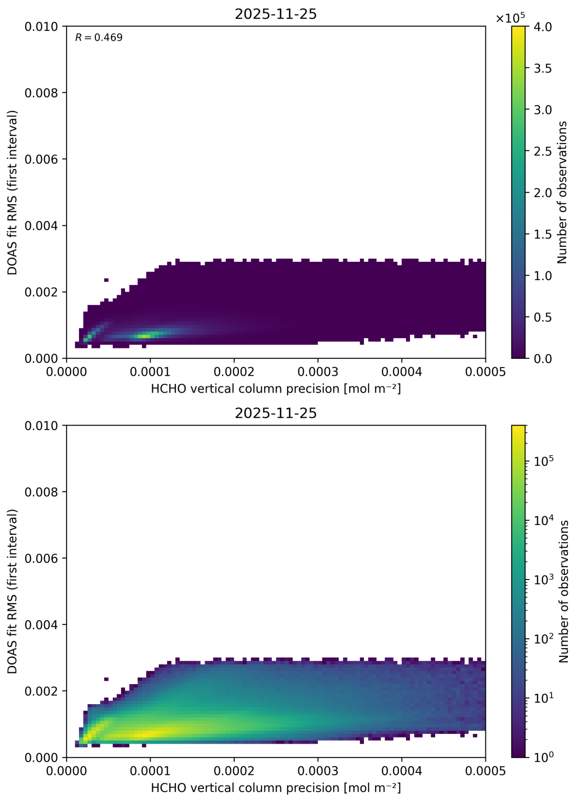
Figure 152: Scatter density plot of “HCHO vertical column precision” against “DOAS fit RMS (first interval)” for 2025-11-24 to 2025-11-26.
