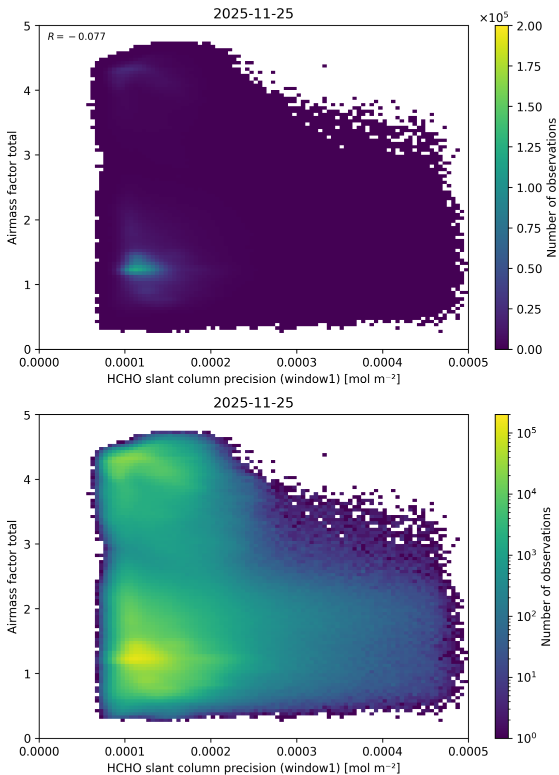
Figure 105: Scatter density plot of “HCHO slant column precision (window1)” against “Airmass factor total” for 2025-11-24 to 2025-11-26.
