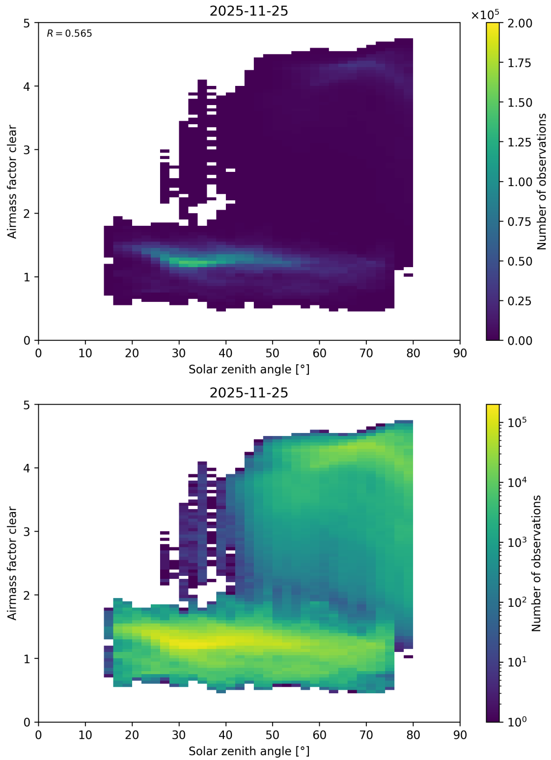
Figure 189: Scatter density plot of “Solar zenith angle” against “Airmass factor clear” for 2025-11-24 to 2025-11-26.
