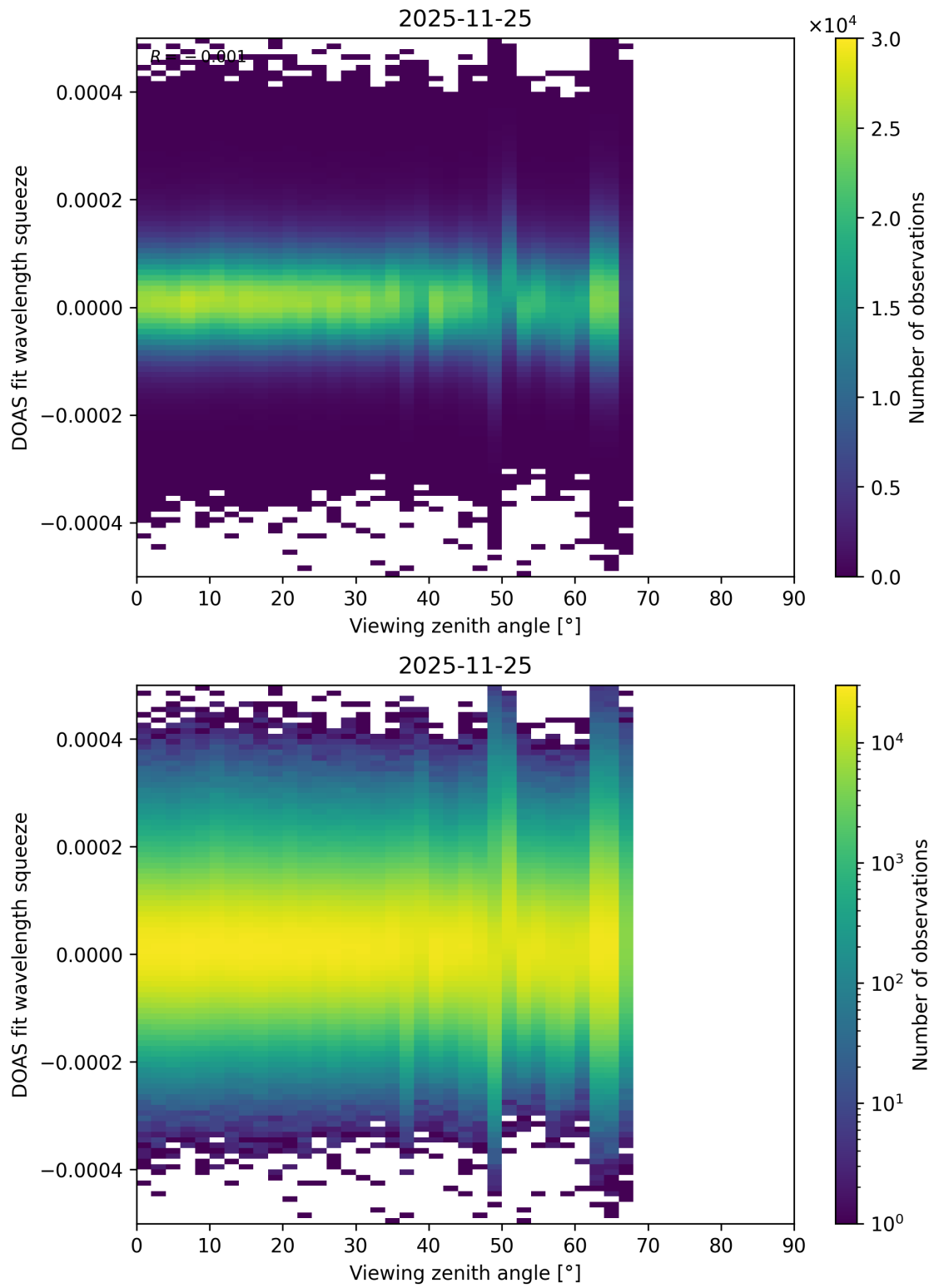
Figure 204: Scatter density plot of “Viewing zenith angle” against “DOAS fit wavelength squeeze” for 2025-11-24 to 2025-11-26.
