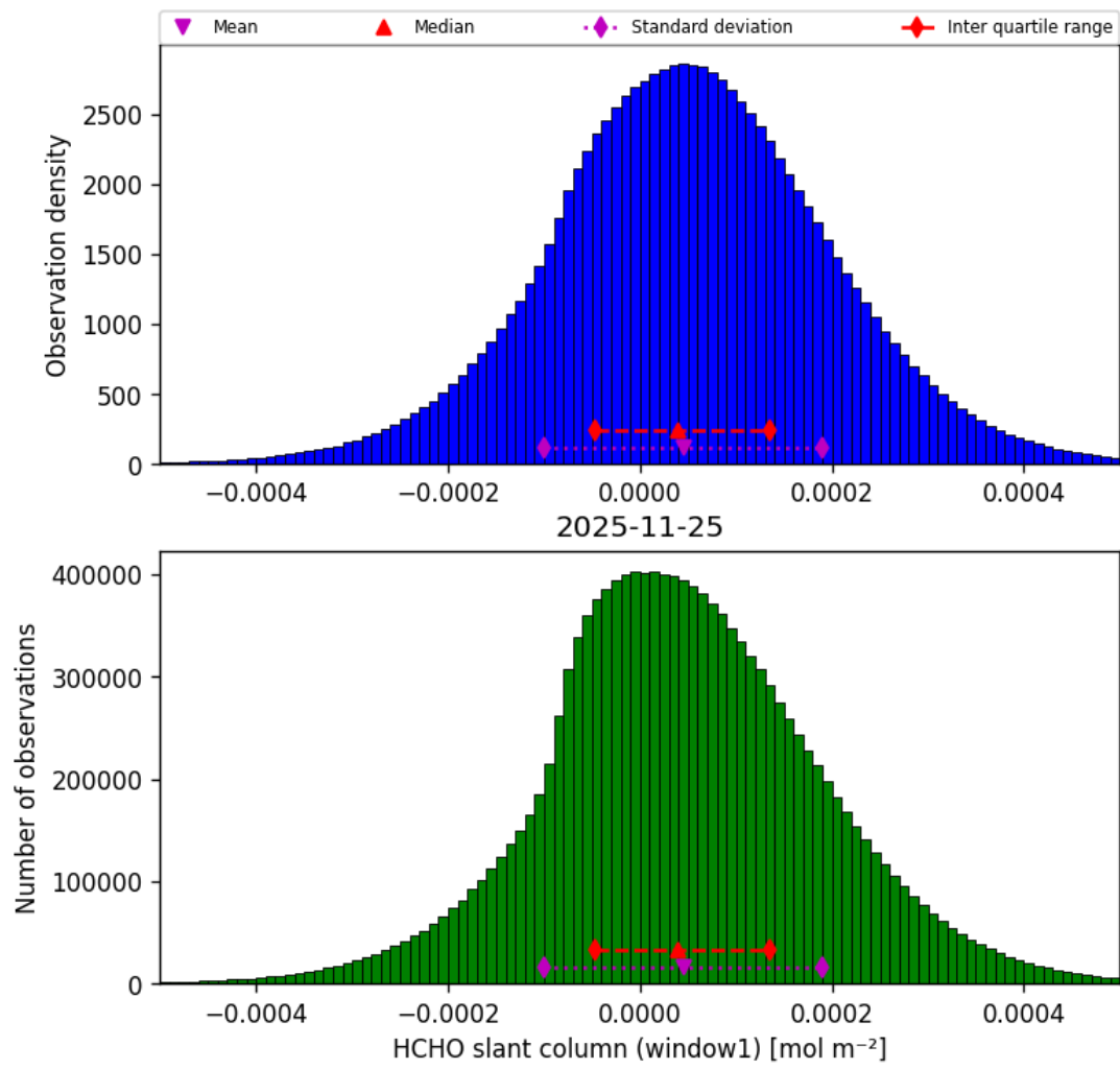
Figure 40: Histogram of “HCHO slant column (window1)” for 2025-11-24 to 2025-11-26
