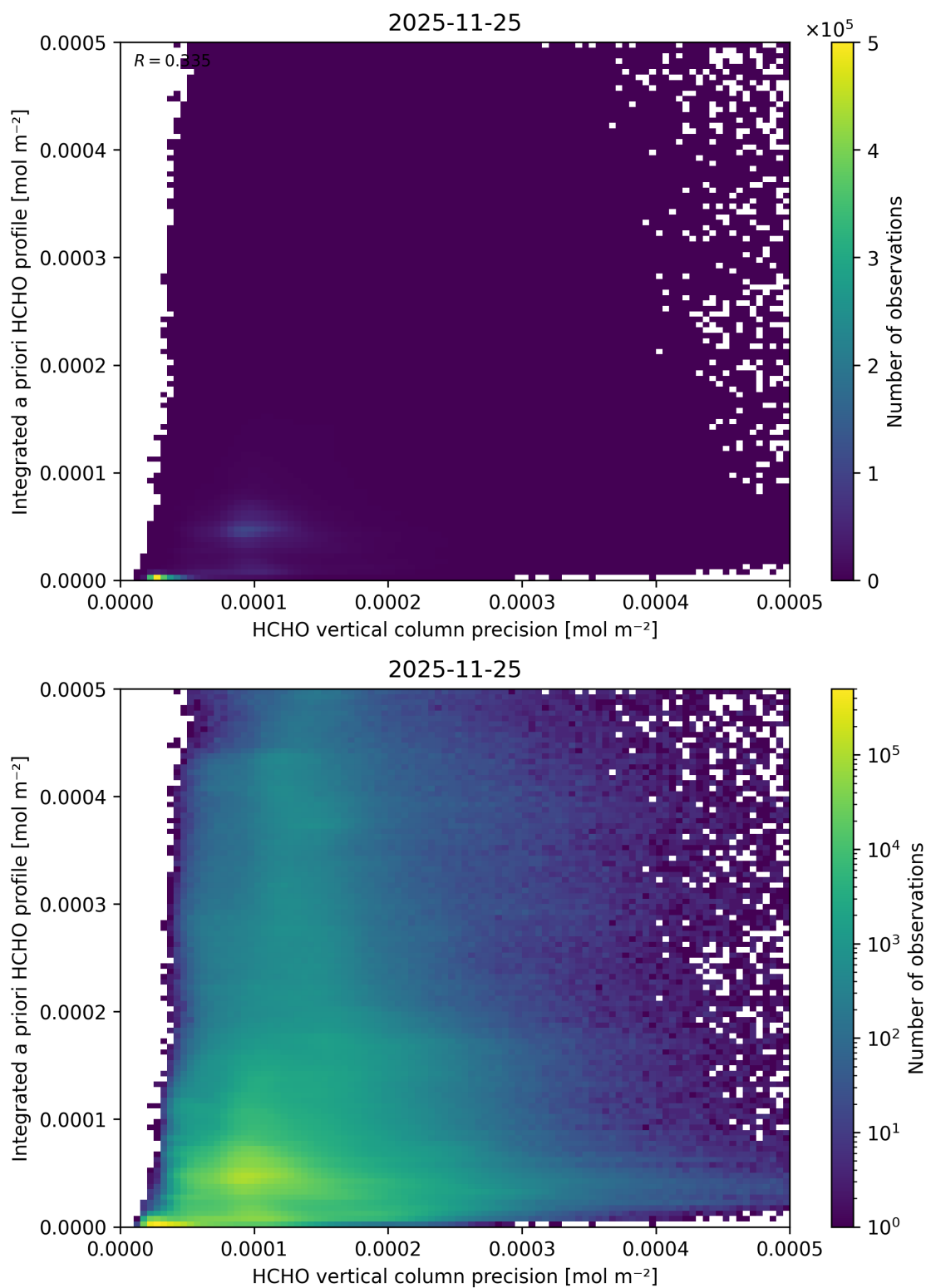
Figure 164: Scatter density plot of “HCHO vertical column precision” against “Integrated a priori HCHO profile” for 2025-11-24 to 2025-11-26.
