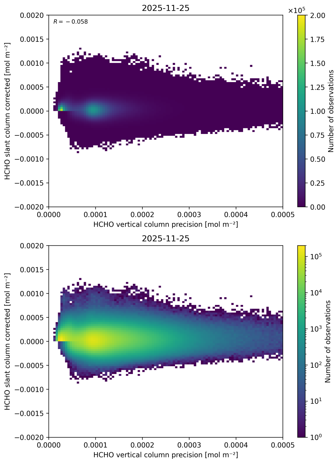
Figure 156: Scatter density plot of “HCHO vertical column precision” against “HCHO slant column corrected” for 2025-11-24 to 2025-11-26.
