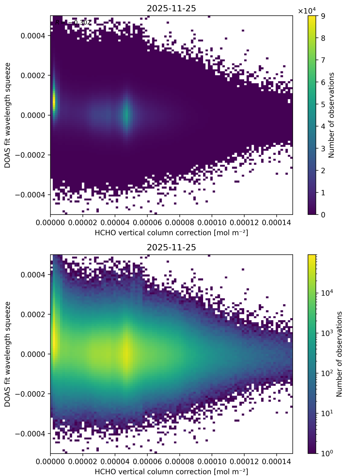
Figure 128: Scatter density plot of “HCHO vertical column correction” against “DOAS fit wavelength squeeze” for 2025-11-24 to 2025-11-26.
