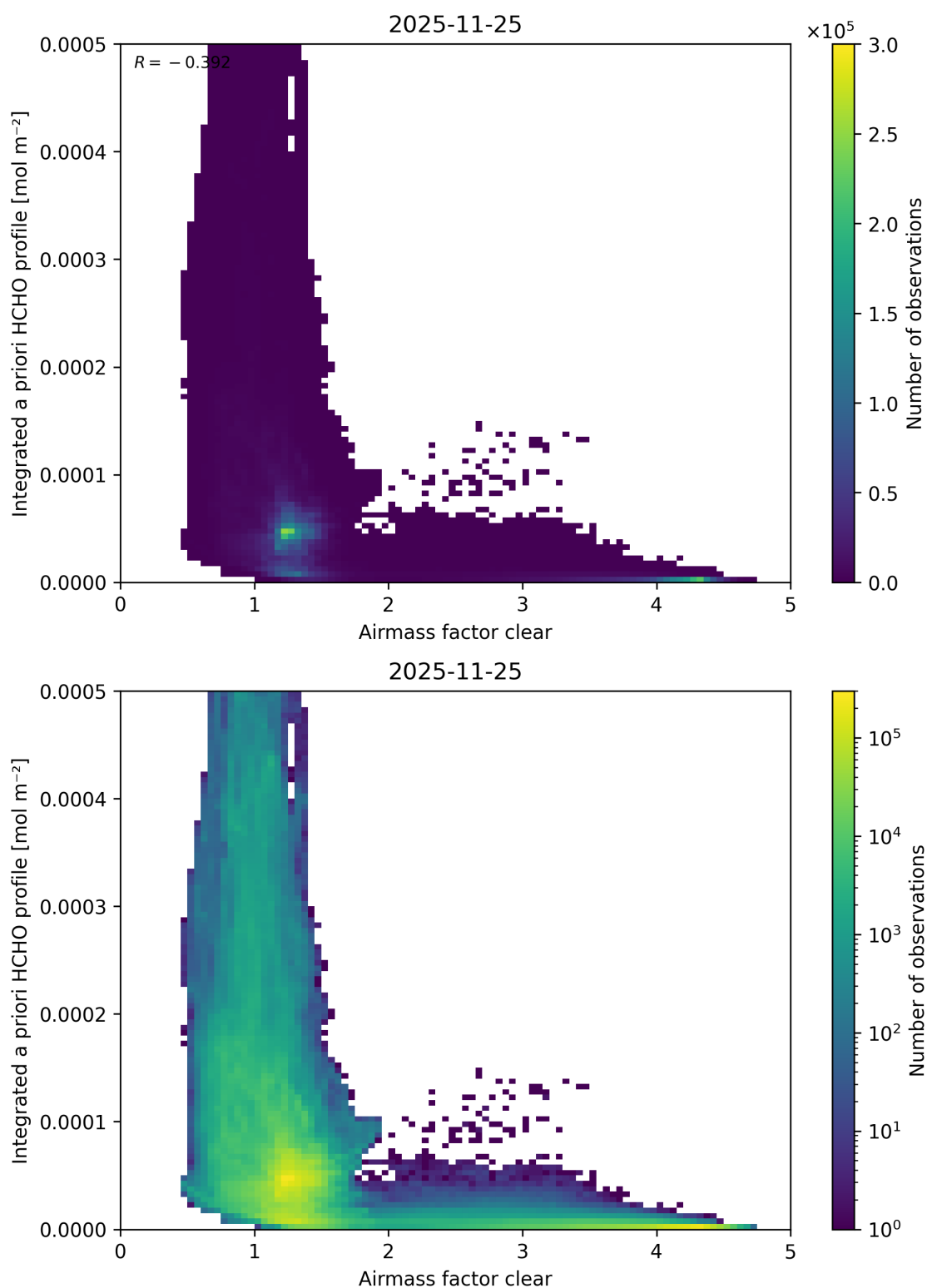
Figure 84: Scatter density plot of “Airmass factor clear” against “Integrated a priori HCHO profile” for 2025-11-24 to 2025-11-26.
