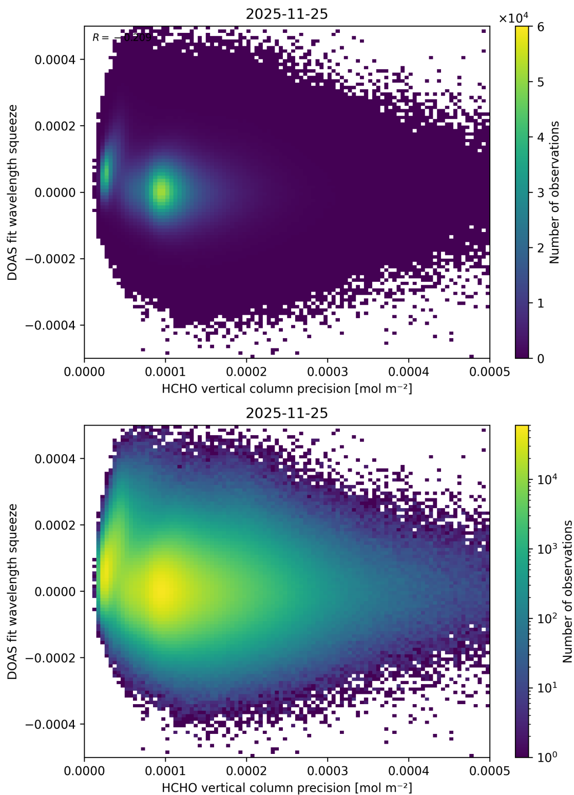
Figure 154: Scatter density plot of “HCHO vertical column precision” against “DOAS fit wavelength squeeze” for 2025-11-24 to 2025-11-26.
