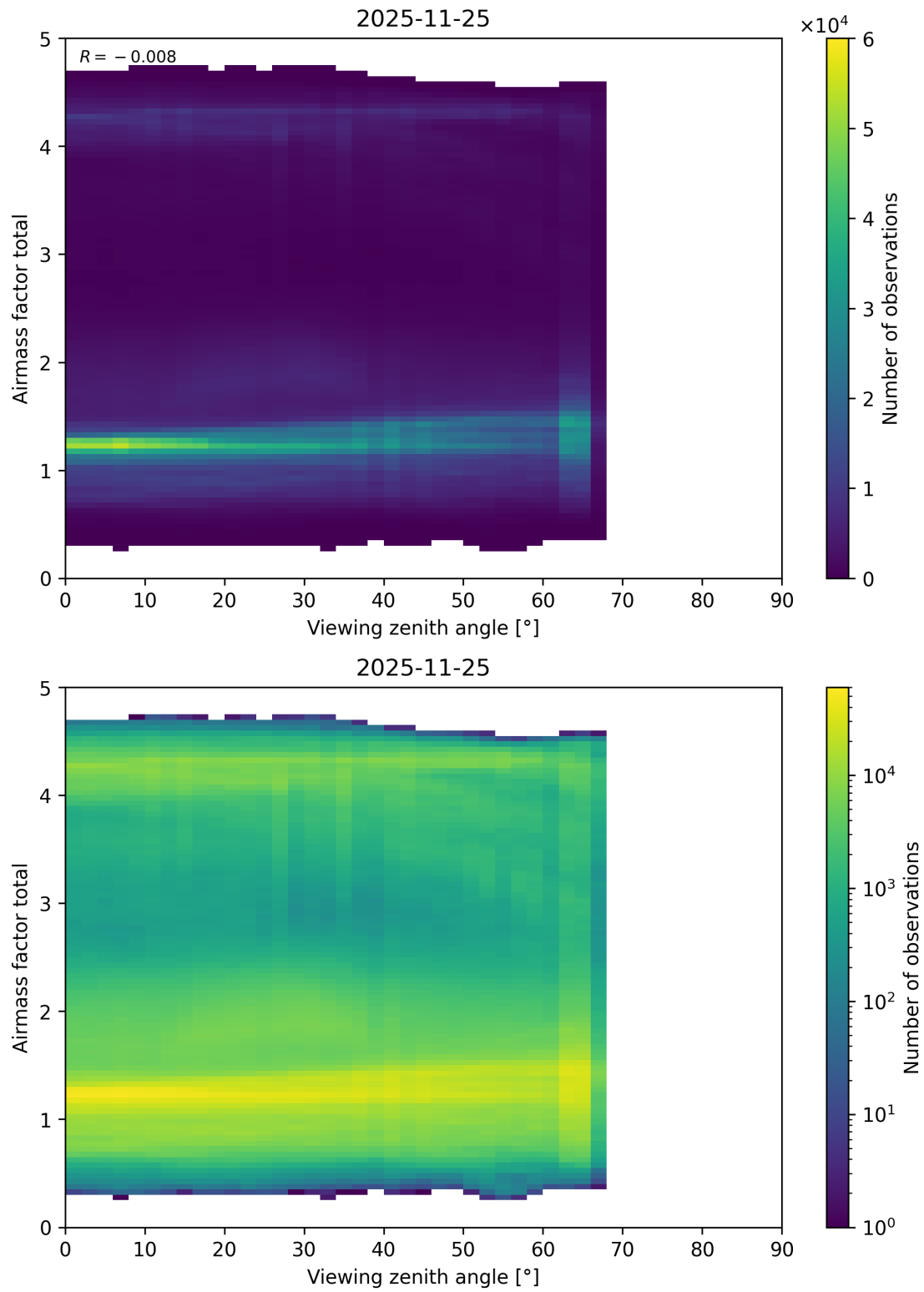
Figure 210: Scatter density plot of “Viewing zenith angle” against “Airmass factor total” for 2025-11-24 to 2025-11-26.
