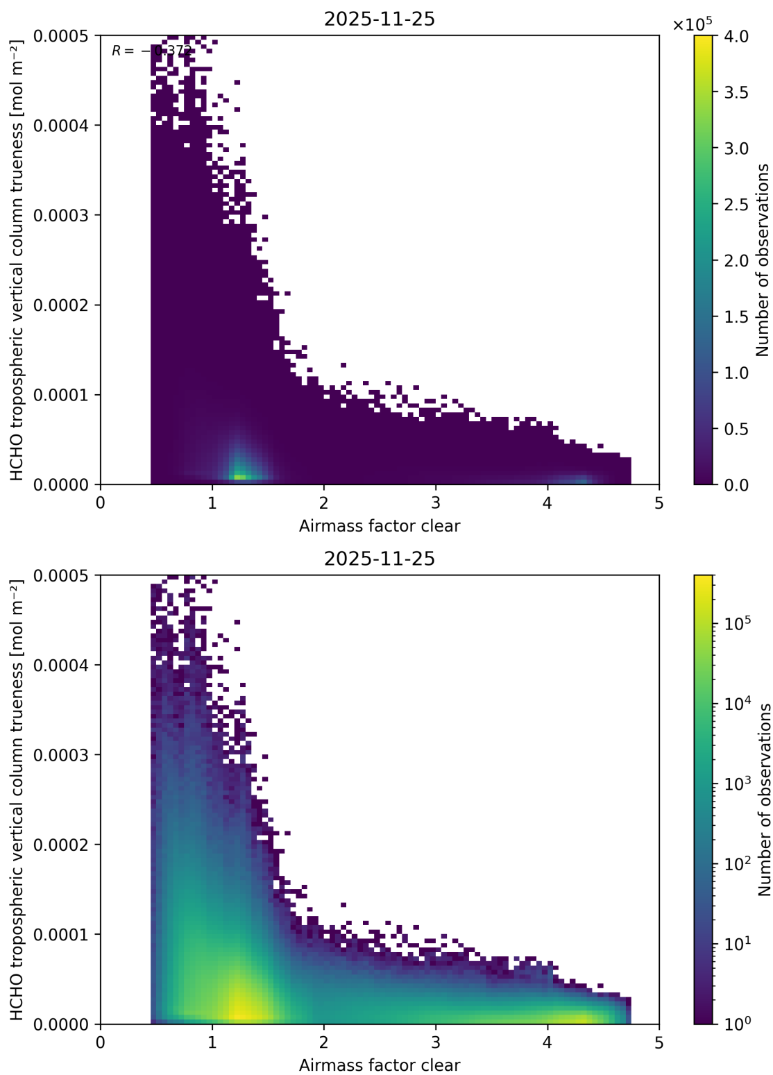
Figure 83: Scatter density plot of “Airmass factor clear” against “HCHO tropospheric vertical column truthness” for 2025-11-24 to 2025-11-26.
