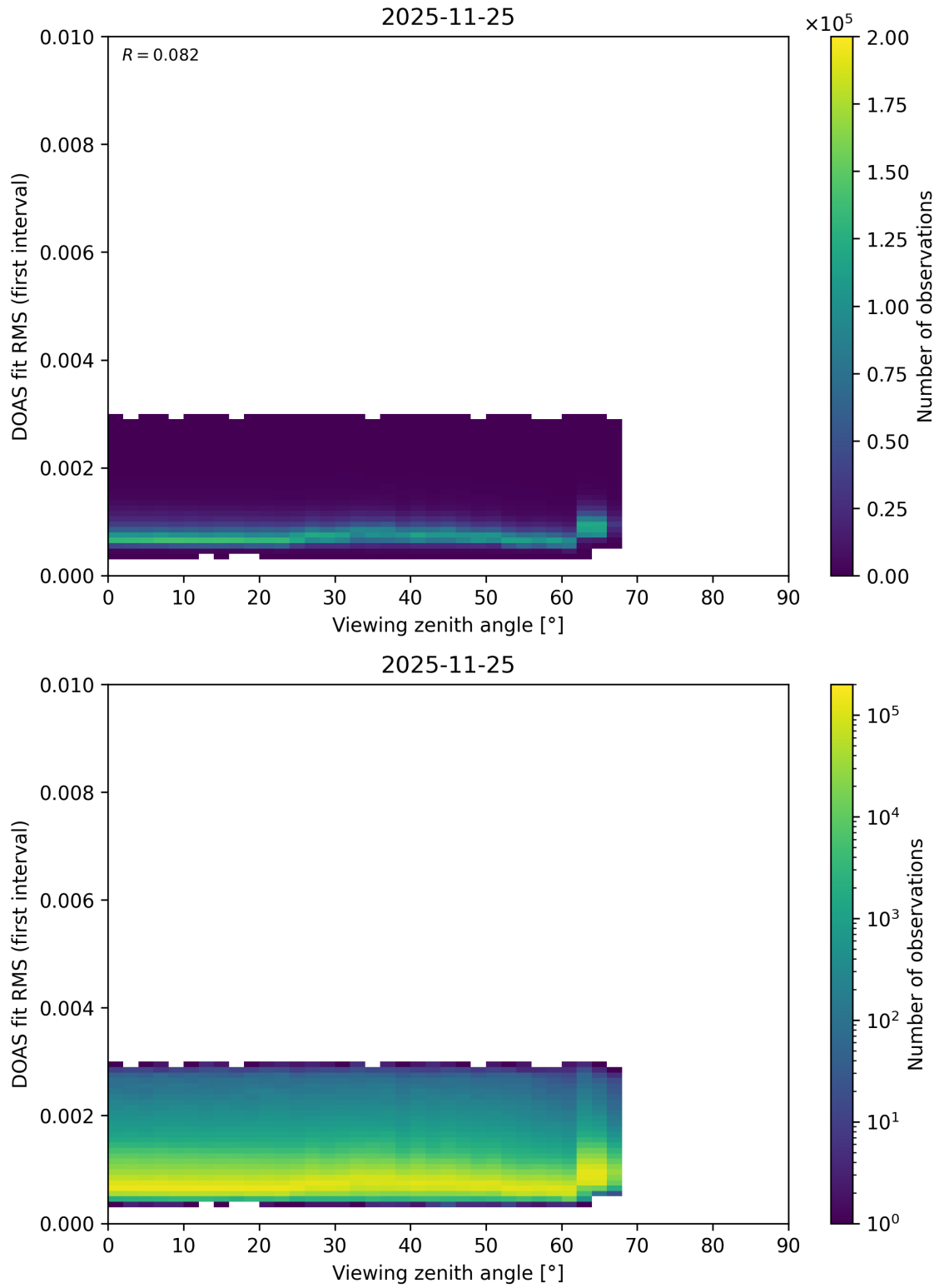
Figure 202: Scatter density plot of “Viewing zenith angle” against “DOAS fit RMS (first interval)” for 2025-11-24 to 2025-11-26.
