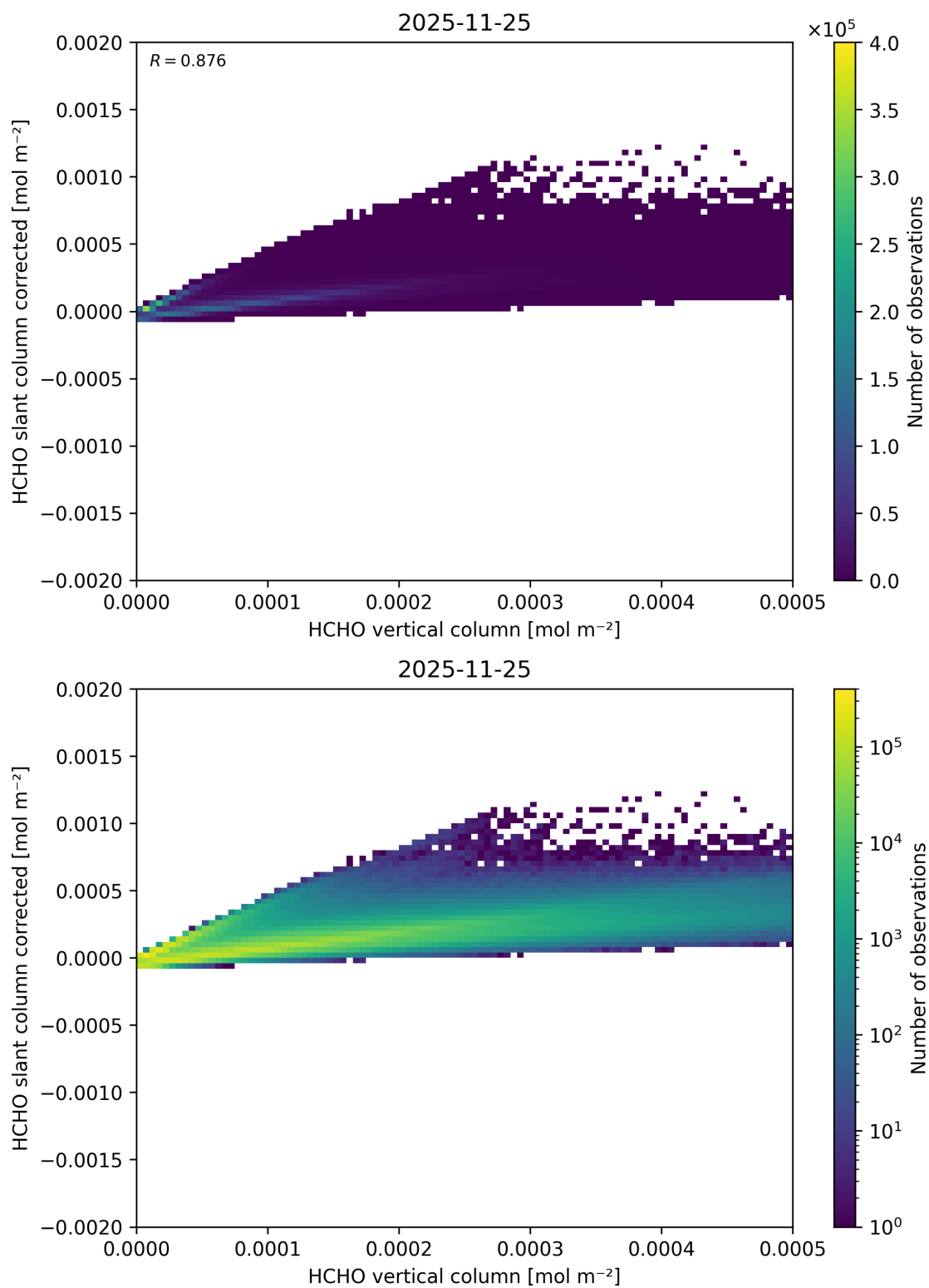
Figure 142: Scatter density plot of “HCHO vertical column” against “HCHO slant column corrected” for 2025-11-24 to 2025-11-26.
