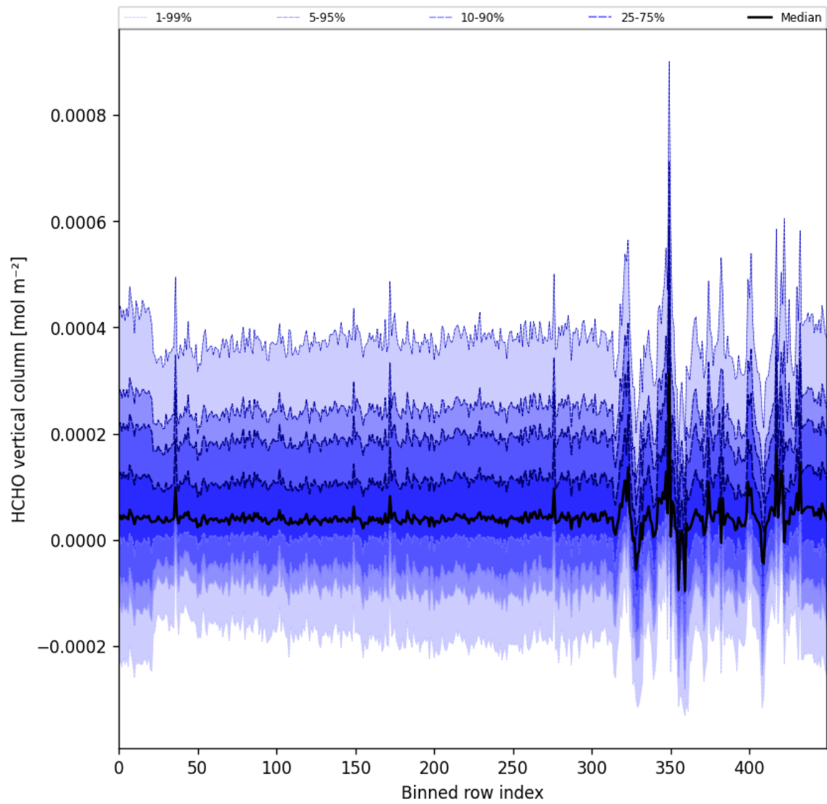
Figure 52: Along track statistics of “HCHO vertical column” for 2025-11-24 to 2025-11-26
