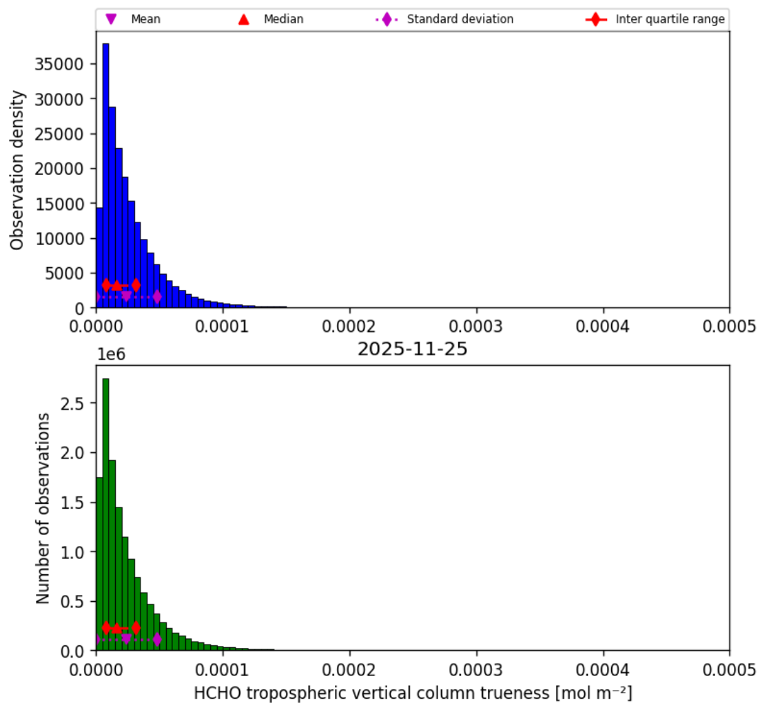
Figure 50: Histogram of “HCHO tropospheric vertical column trueness” for 2025-11-24 to 2025-11-26
