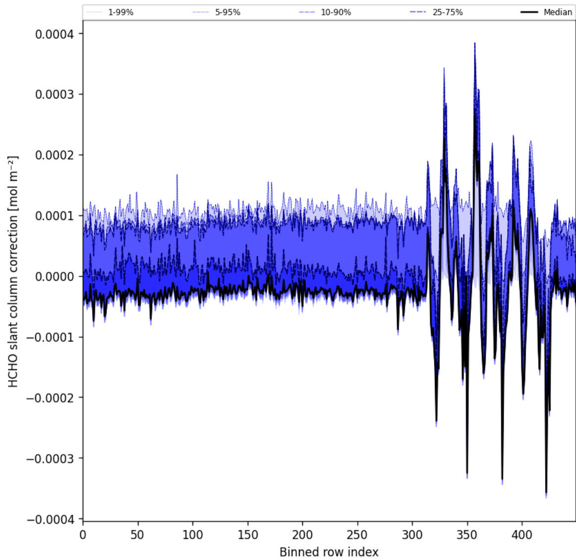
Figure 64: Along track statistics of “HCHO slant column correction” for 2025-11-24 to 2025-11-26
