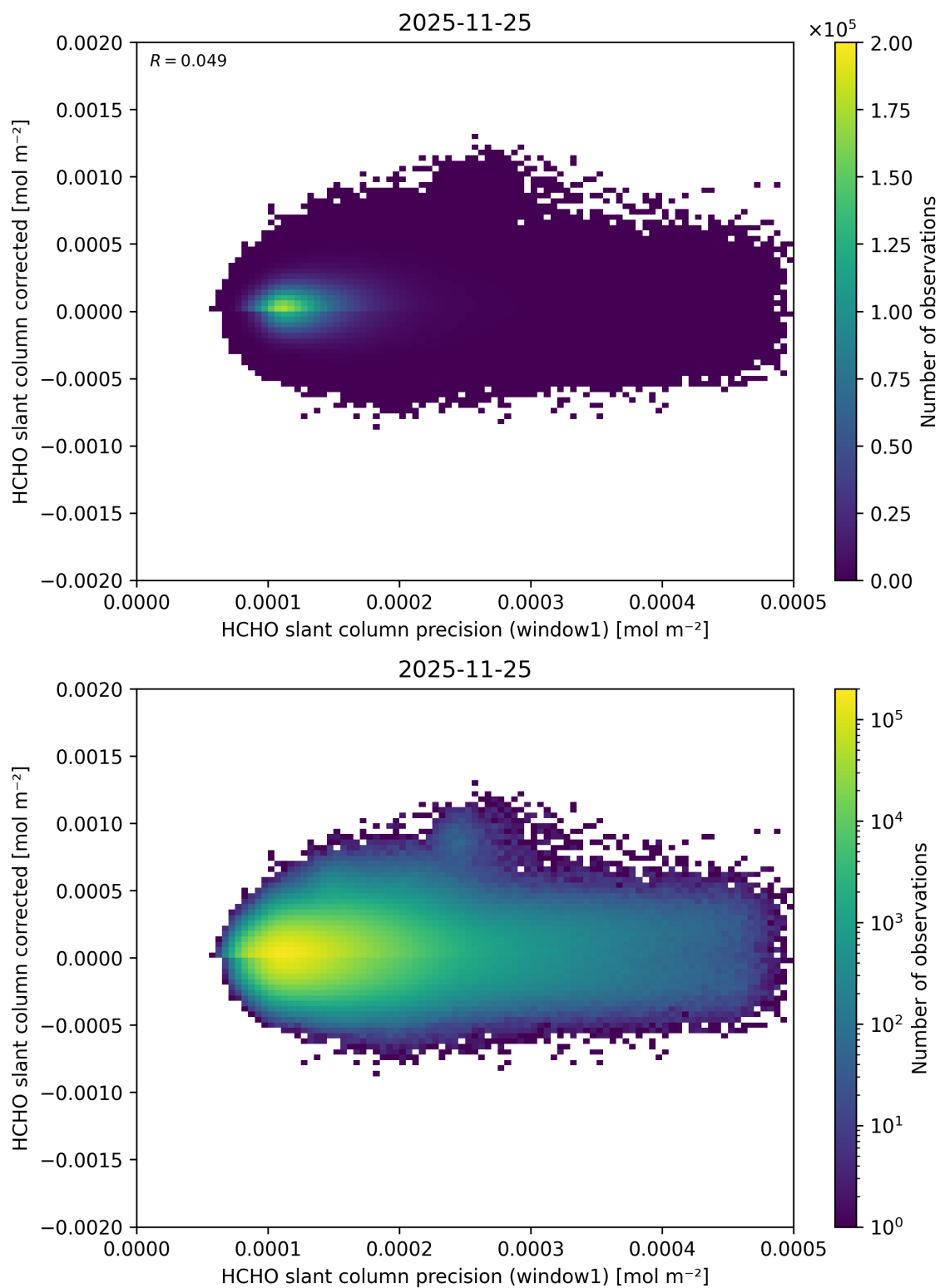
Figure 103: Scatter density plot of “HCHO slant column precision (window1)” against “HCHO slant column corrected” for 2025-11-24 to 2025-11-26.
