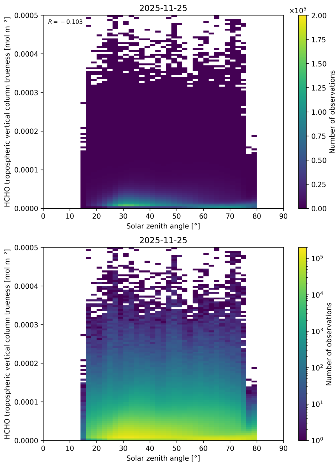
Figure 199: Scatter density plot of “Solar zenith angle” against “HCHO tropospheric vertical column trueness” for 2025-11-24 to 2025-11-26.
