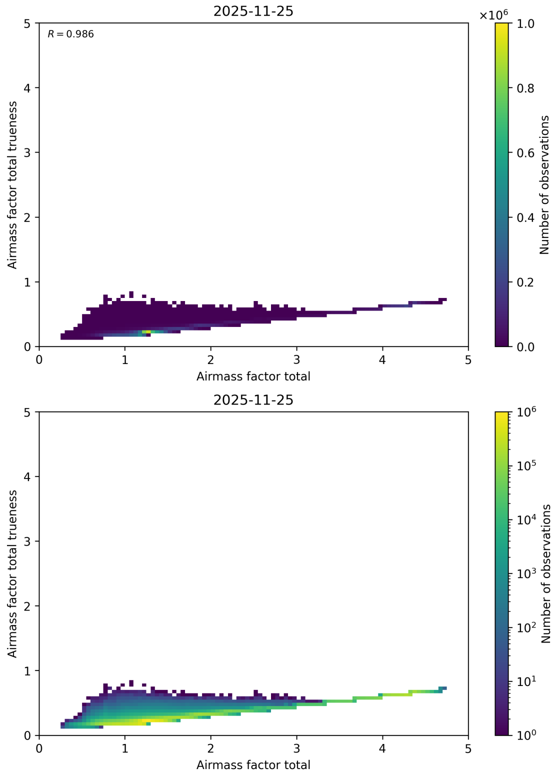
Figure 115: Scatter density plot of “Airmass factor total” against “Airmass factor total trueness” for 2025-11-24 to 2025-11-26.
