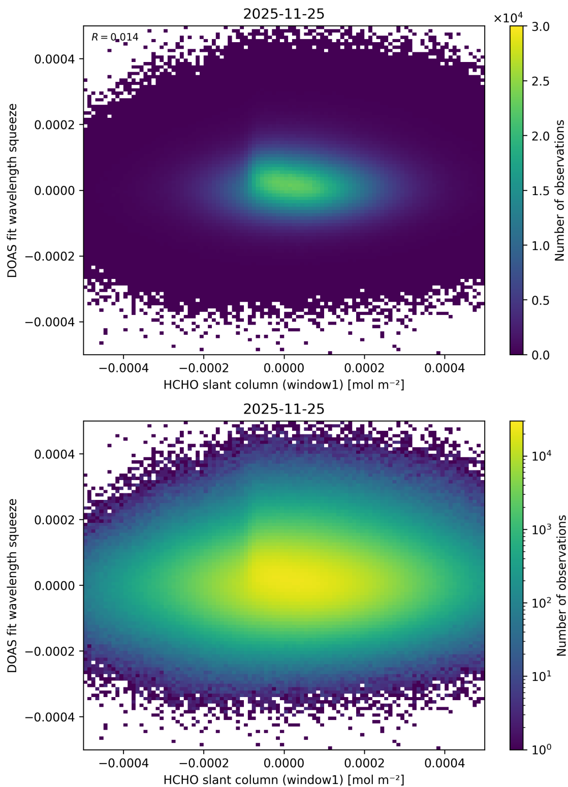
Figure 90: Scatter density plot of “HCHO slant column (window1)” against “DOAS fit wavelength squeeze” for 2025-11-24 to 2025-11-26.
