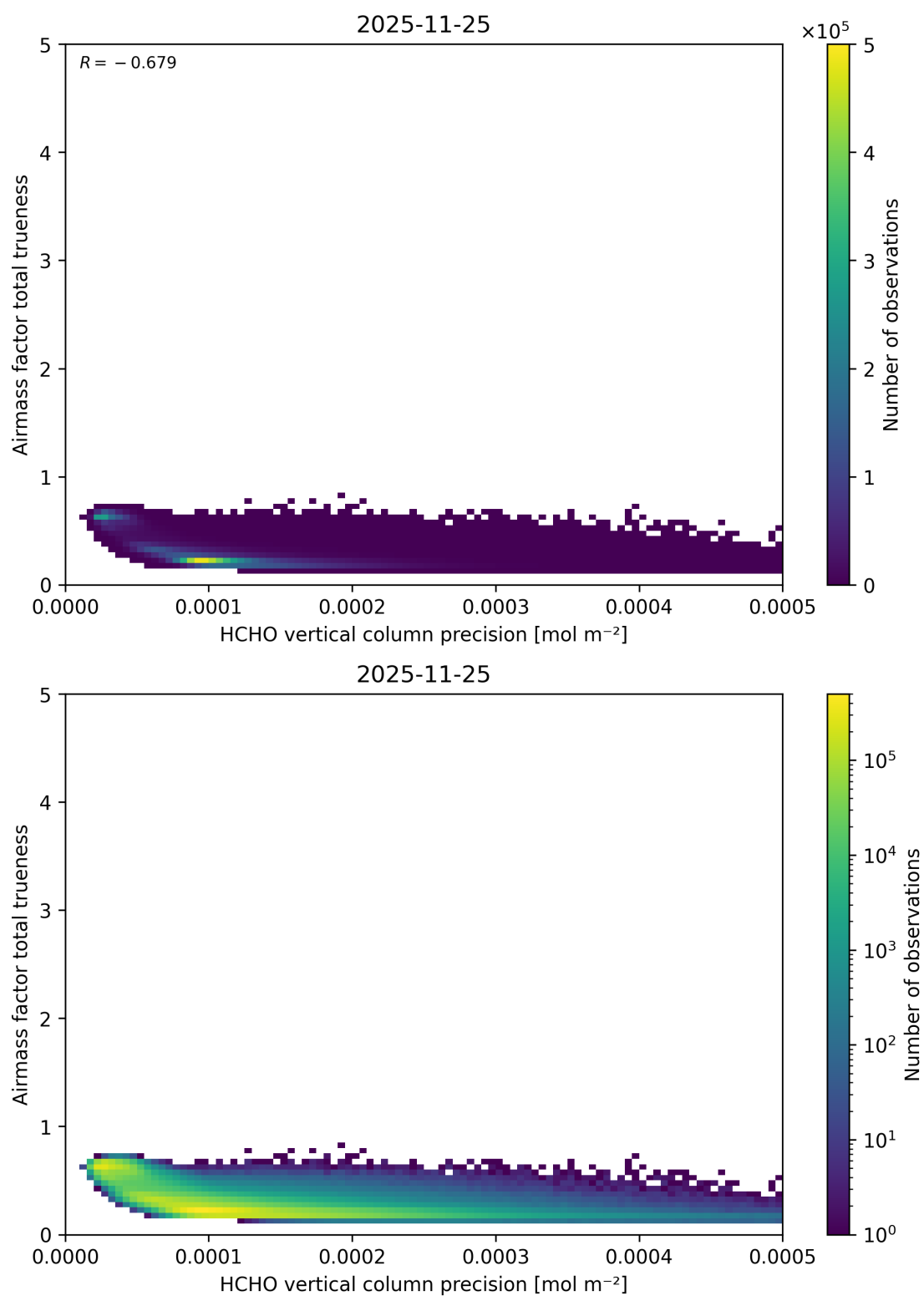
Figure 161: Scatter density plot of “HCHO vertical column precision” against “Airmass factor total trueness” for 2025-11-24 to 2025-11-26.
