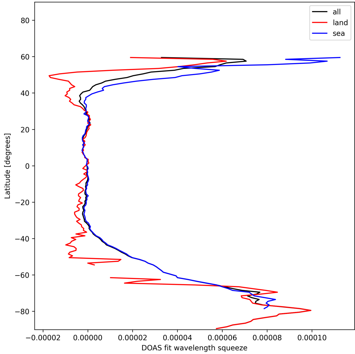
Figure 32: Zonal average of “DOAS fit wavelength squeeze” for 2025-11-24 to 2025-11-26.
