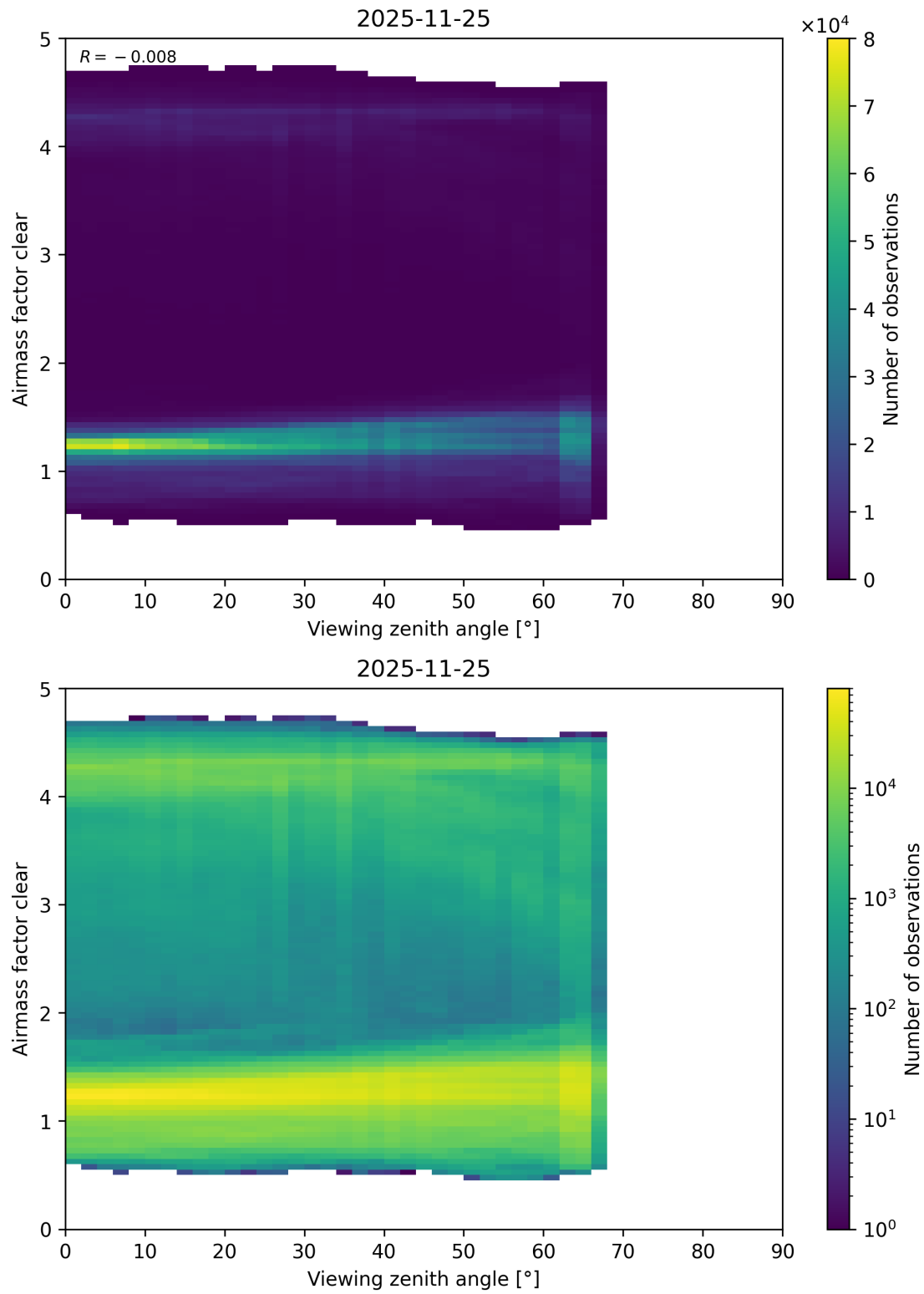
Figure 205: Scatter density plot of “Viewing zenith angle” against “Airmass factor clear” for 2025-11-24 to 2025-11-26.
