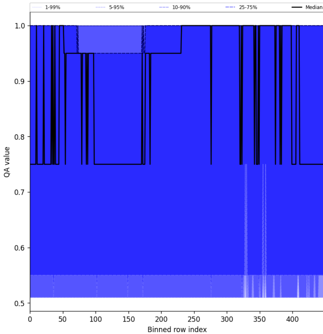
Figure 51: Along track statistics of “QA value” for 2025-11-24 to 2025-11-26
