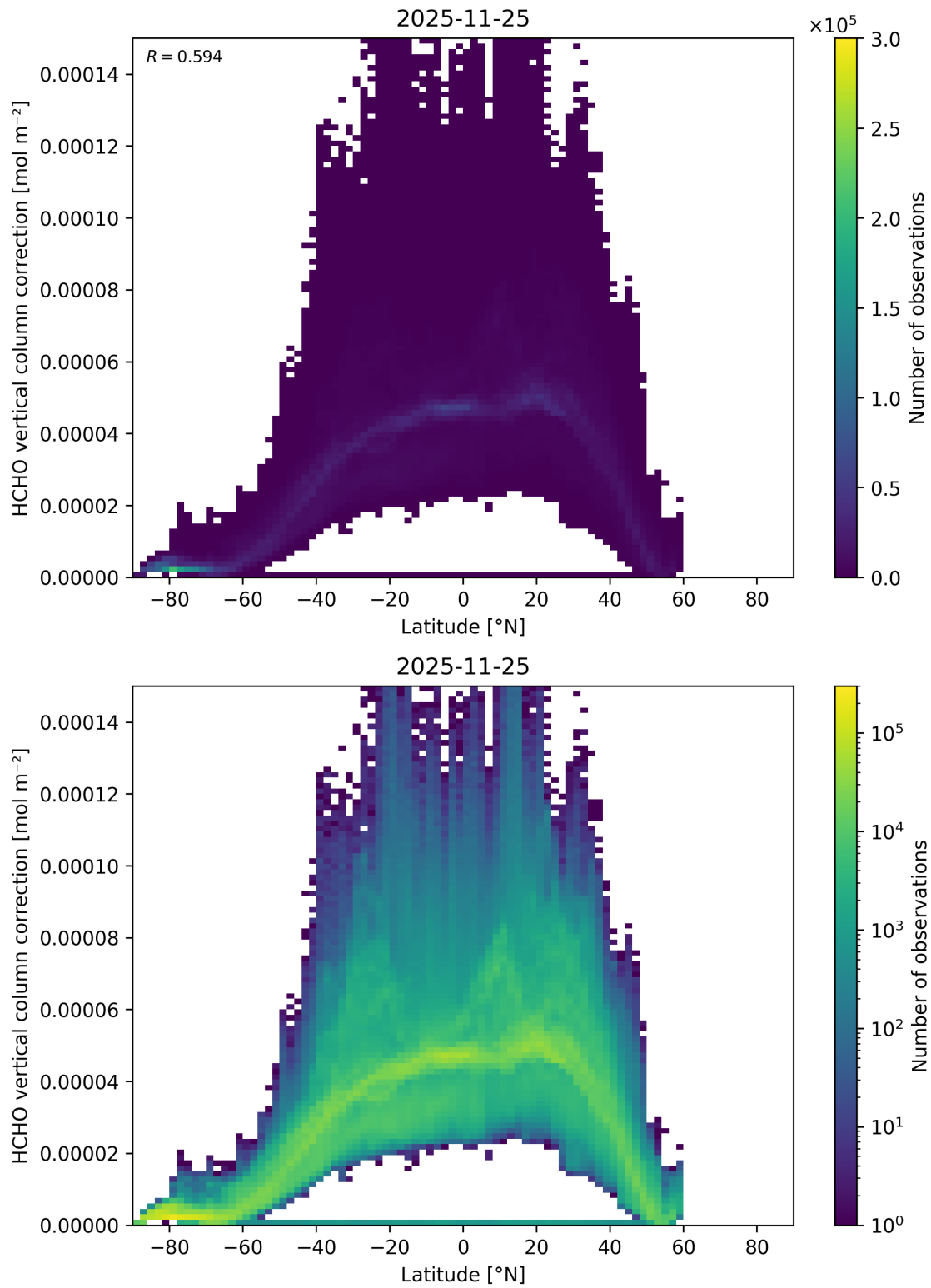
Figure 182: Scatter density plot of “Latitude” against “HCHO vertical column correction” for 2025-11-24 to 2025-11-26.
