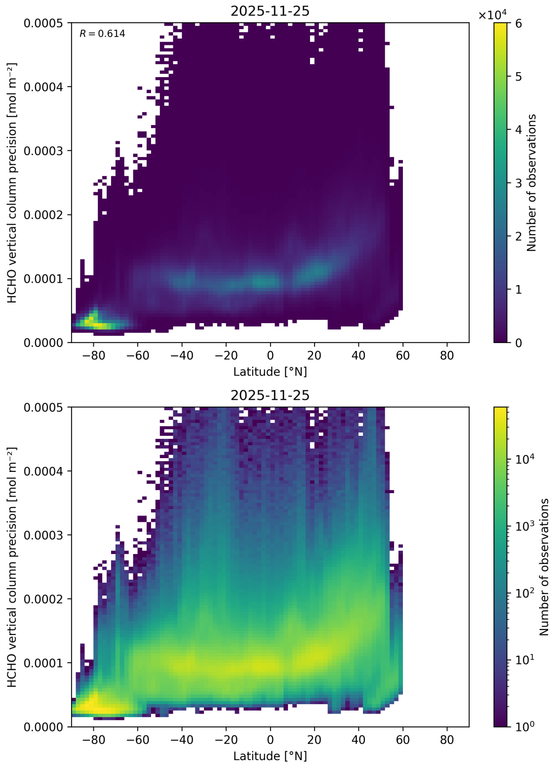
Figure 183: Scatter density plot of “Latitude” against “HCHO vertical column precision” for 2025-11-24 to 2025-11-26.
