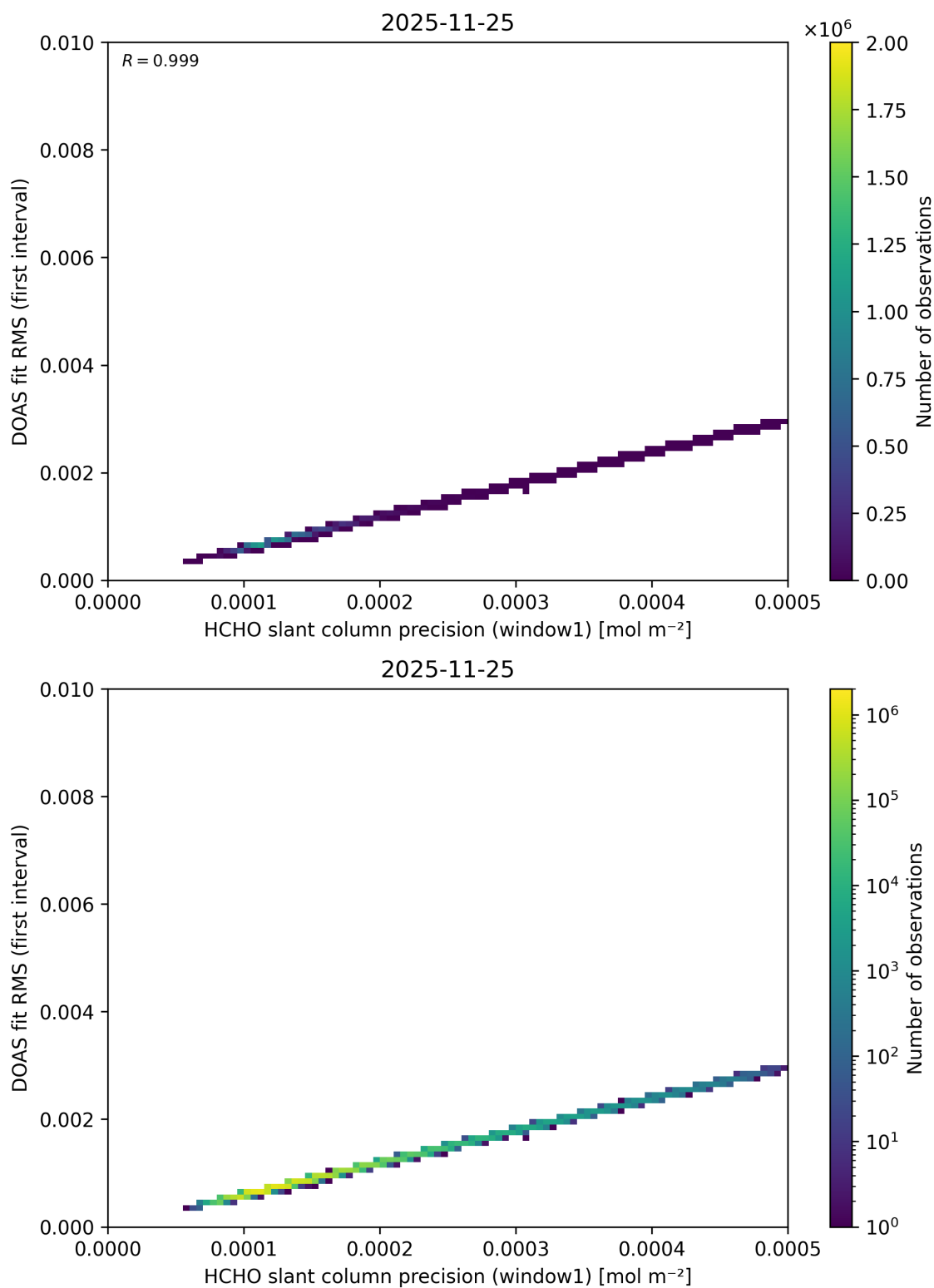
Figure 99: Scatter density plot of “HCHO slant column precision (window1)” against “DOAS fit RMS (first interval)” for 2025-11-24 to 2025-11-26.
