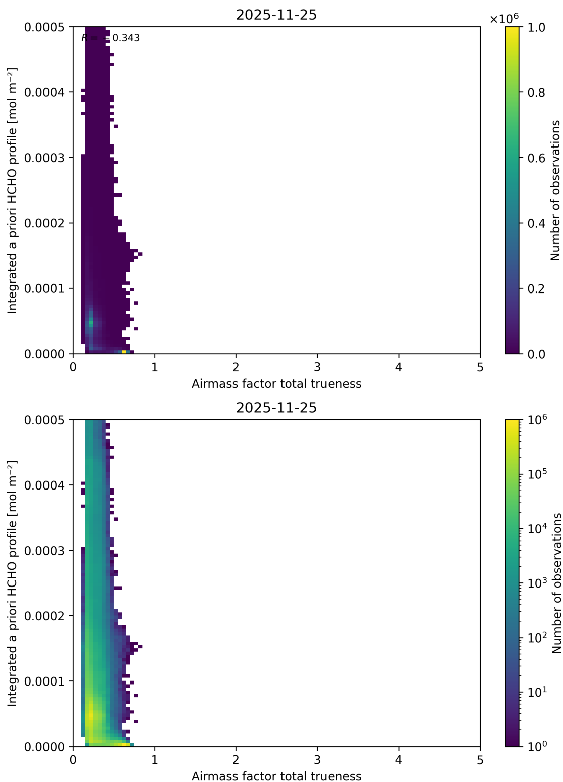
Figure 125: Scatter density plot of “Airmass factor total truiness” against “Integrated a priori HCHO profile” for 2025-11-24 to 2025-11-26.
