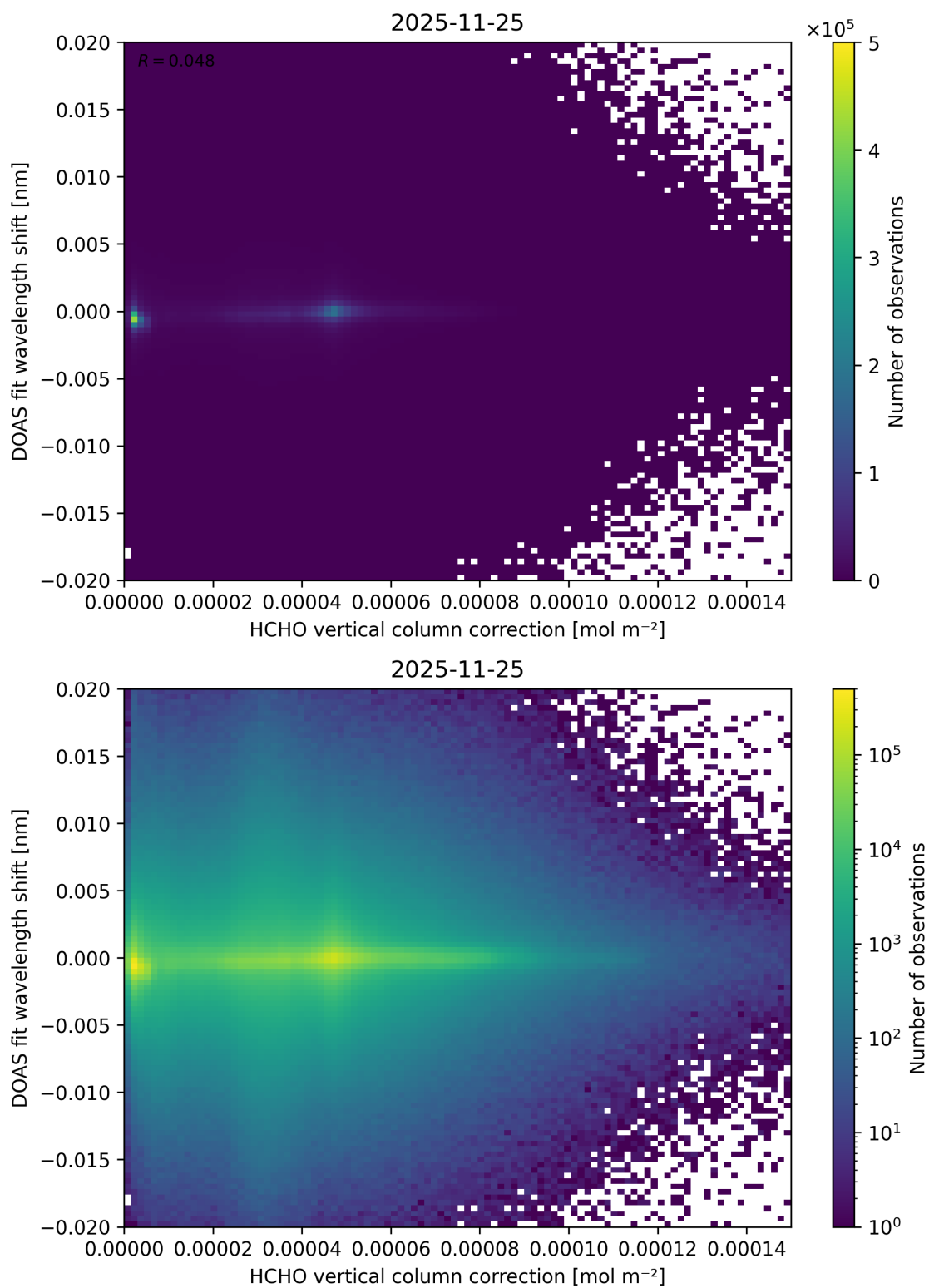
Figure 127: Scatter density plot of “HCHO vertical column correction” against “DOAS fit wavelength shift” for 2025-11-24 to 2025-11-26.
