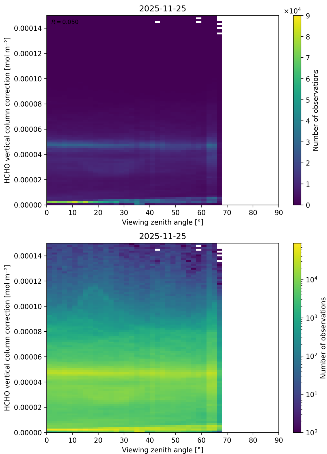
Figure 213: Scatter density plot of “Viewing zenith angle” against “HCHO vertical column correction” for 2025-11-24 to 2025-11-26.
