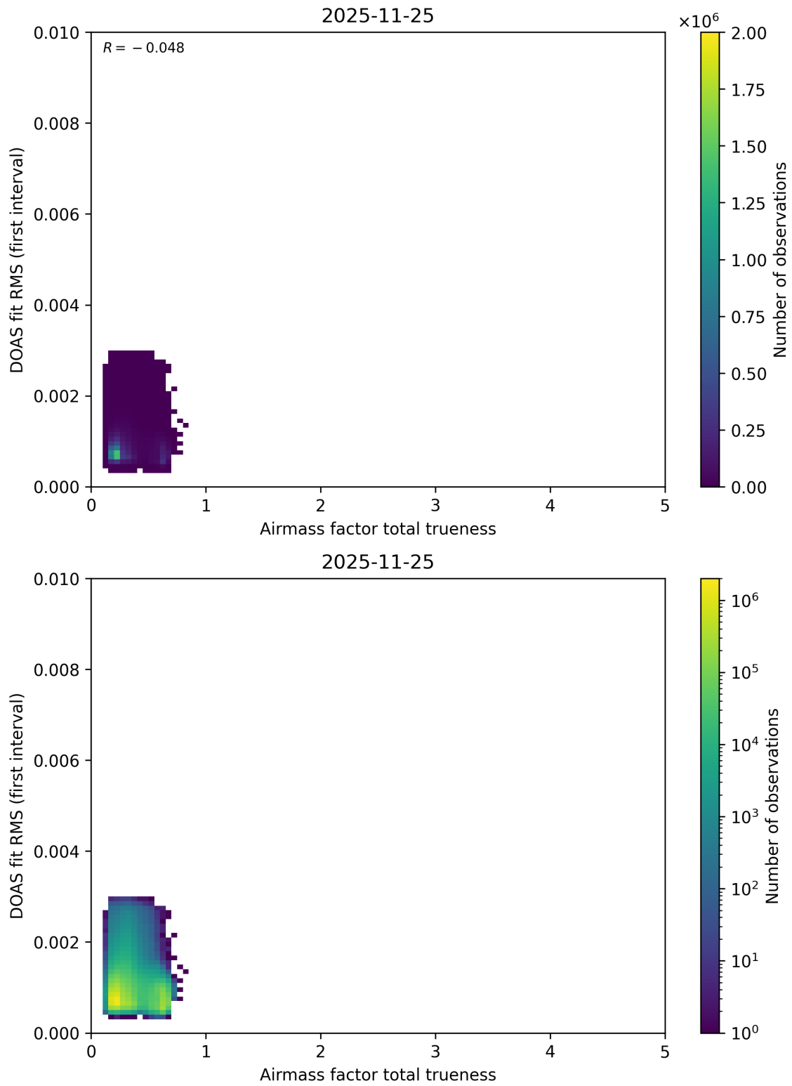
Figure 118: Scatter density plot of “Airmass factor total trueness” against “DOAS fit RMS (first interval)” for 2025-11-24 to 2025-11-26.
