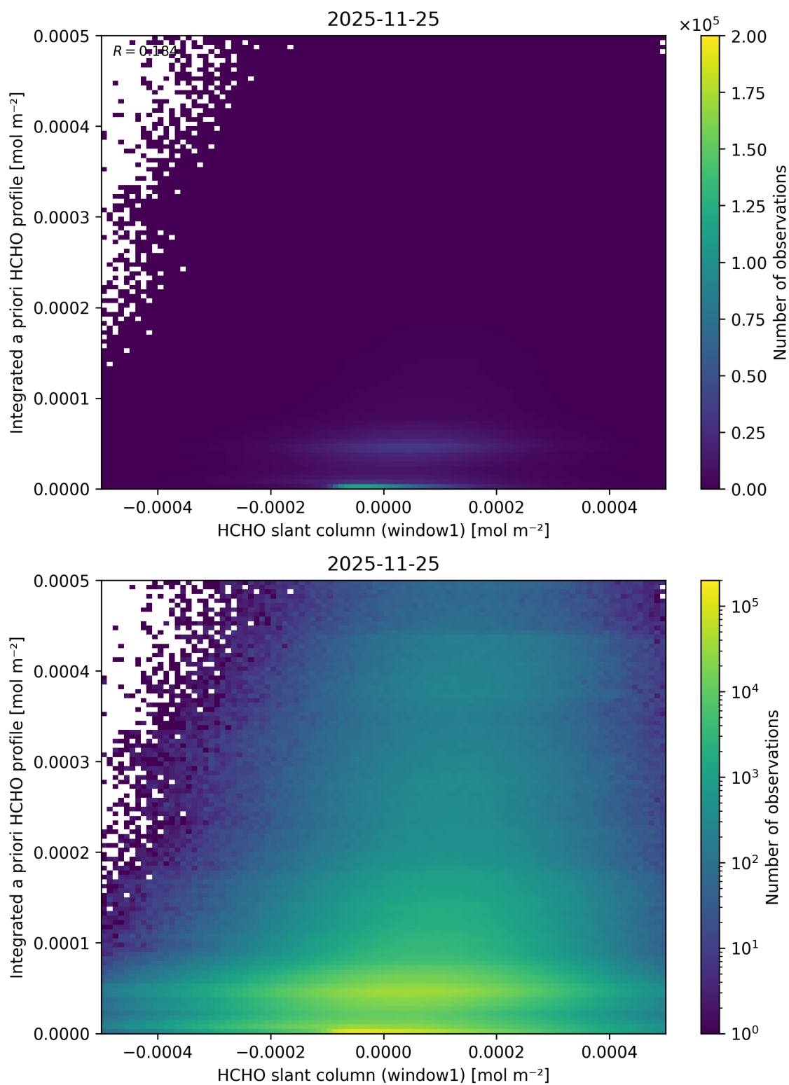
Figure 98: Scatter density plot of “HCHO slant column (window1)” against “Integrated a priori HCHO profile” for 2025-11-24 to 2025-11-26.
