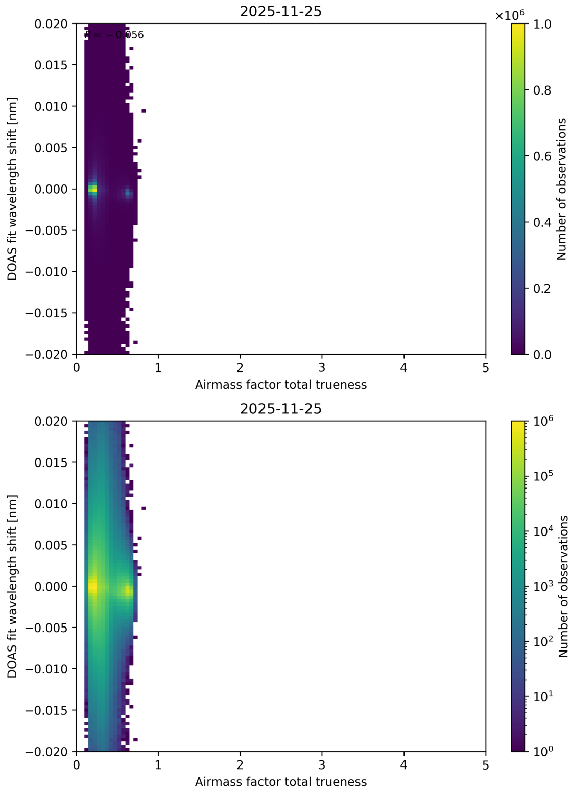
Figure 119: Scatter density plot of “Airmass factor total trueness” against “DOAS fit wavelength shift” for 2025-11-24 to 2025-11-26.
