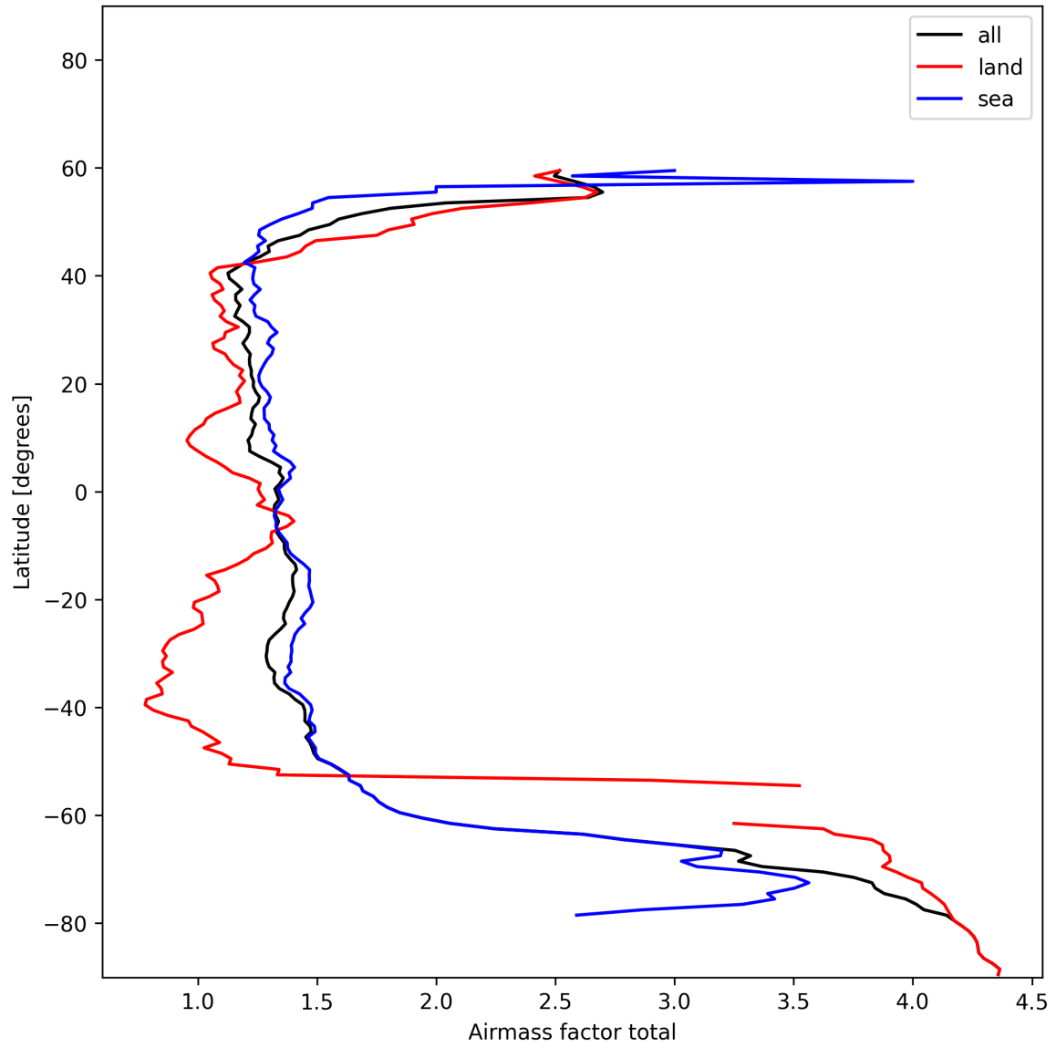
Figure 27: Zonal average of “Airmass factor total” for 2025-11-24 to 2025-11-26.
