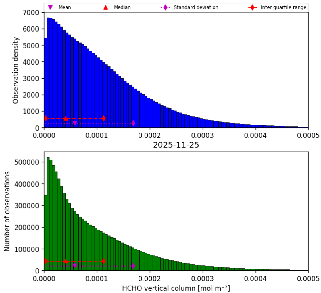
Figure 37: Histogram of “HCHO vertical column” for 2025-11-24 to 2025-11-26
