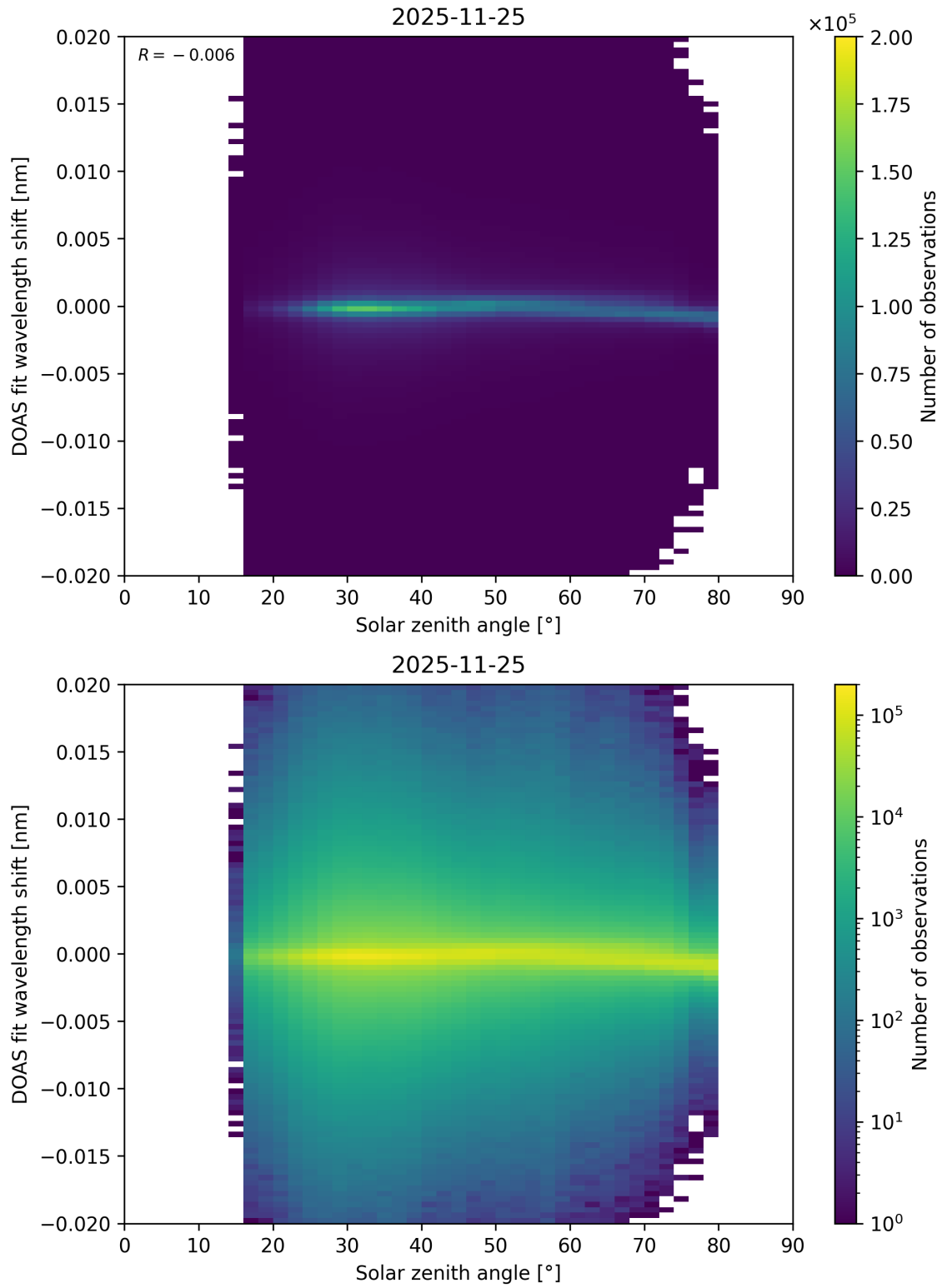
Figure 187: Scatter density plot of “Solar zenith angle” against “DOAS fit wavelength shift” for 2025-11-24 to 2025-11-26.
