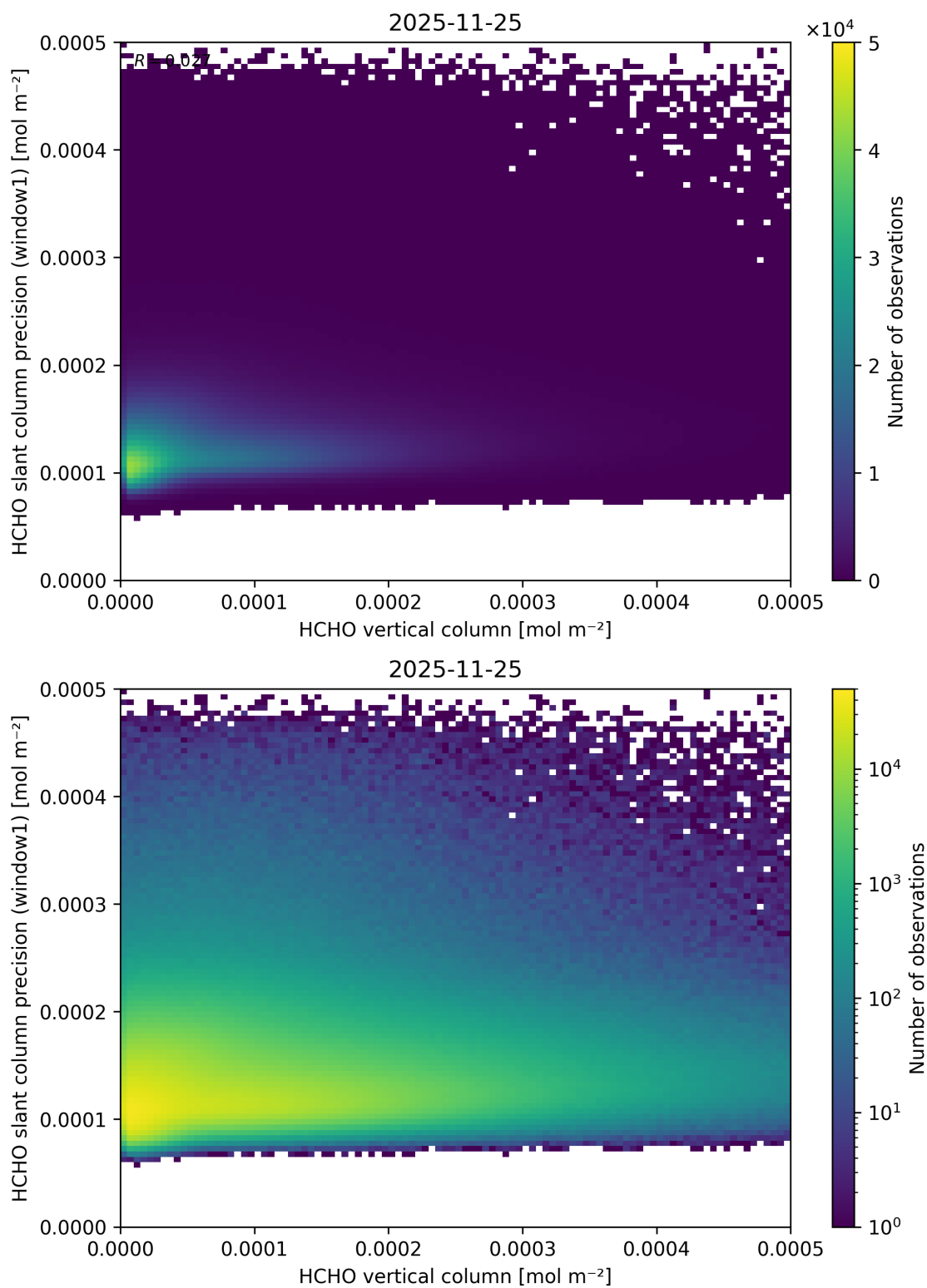
Figure 145: Scatter density plot of “HCHO vertical column” against “HCHO slant column precision (window1)” for 2025-11-24 to 2025-11-26.
