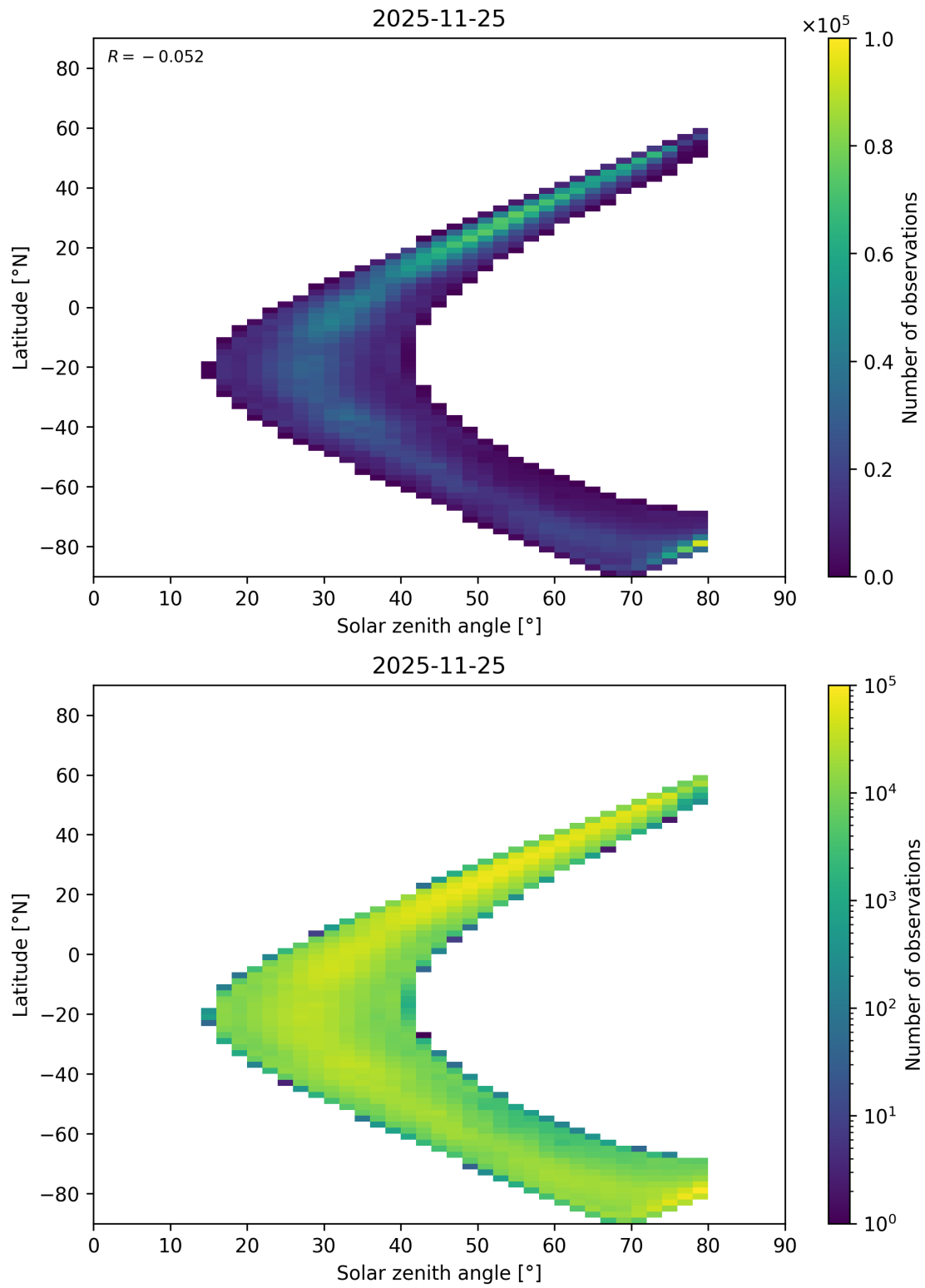
Figure 201: Scatter density plot of “Solar zenith angle” against “Latitude” for 2025-11-24 to 2025-11-26.
