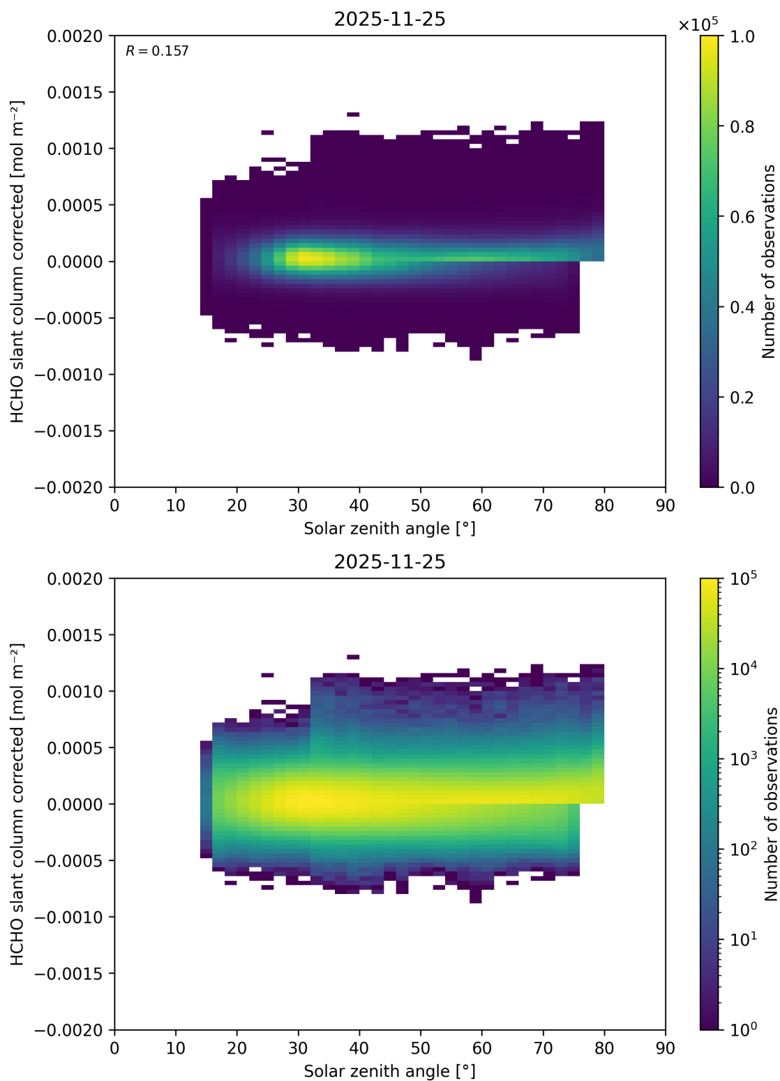
Figure 190: Scatter density plot of “Solar zenith angle” against “HCHO slant column corrected” for 2025-11-24 to 2025-11-26.
