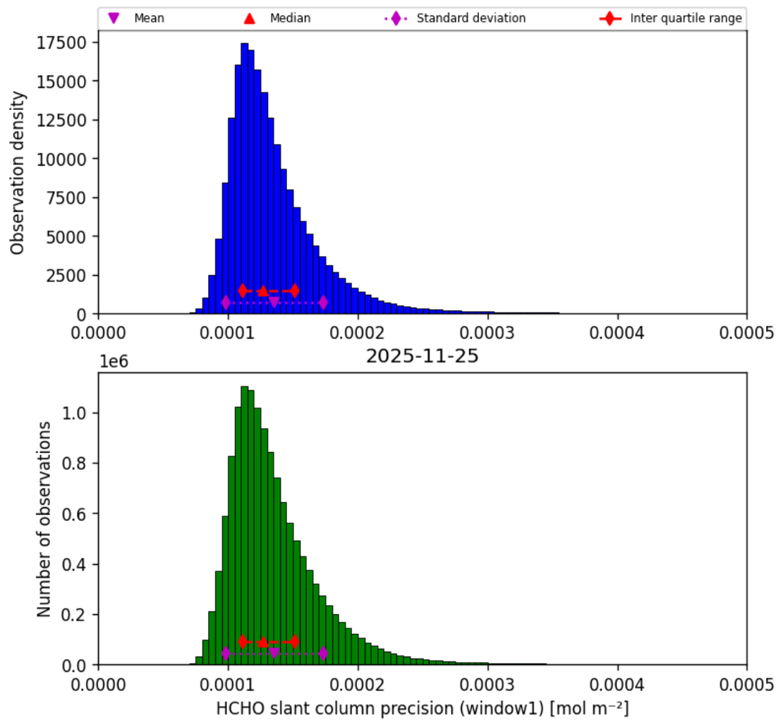
Figure 41: Histogram of “HCHO slant column precision (window1)” for 2025-11-24 to 2025-11-26
