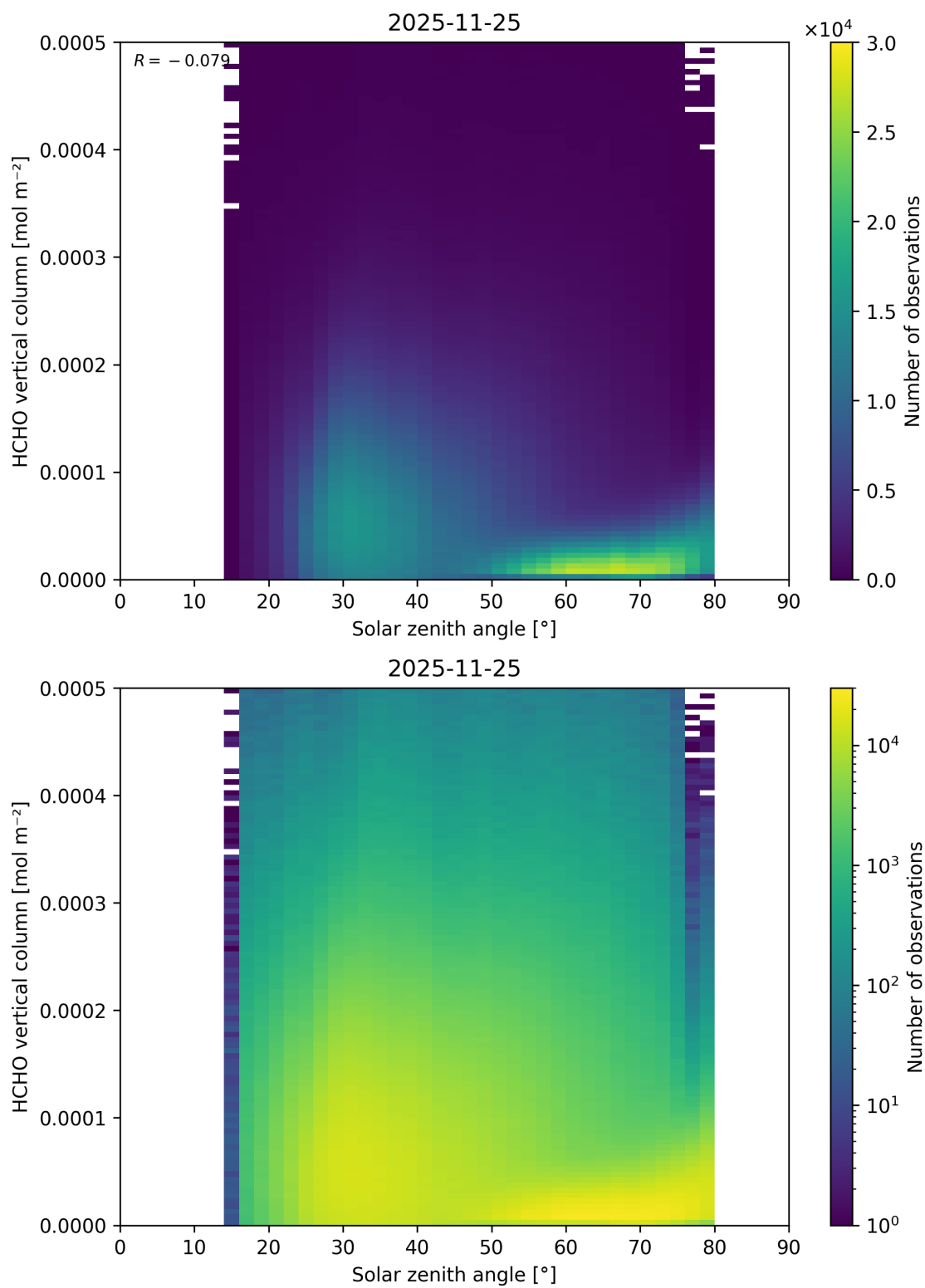
Figure 196: Scatter density plot of “Solar zenith angle” against “HCHO vertical column” for 2025-11-24 to 2025-11-26.
