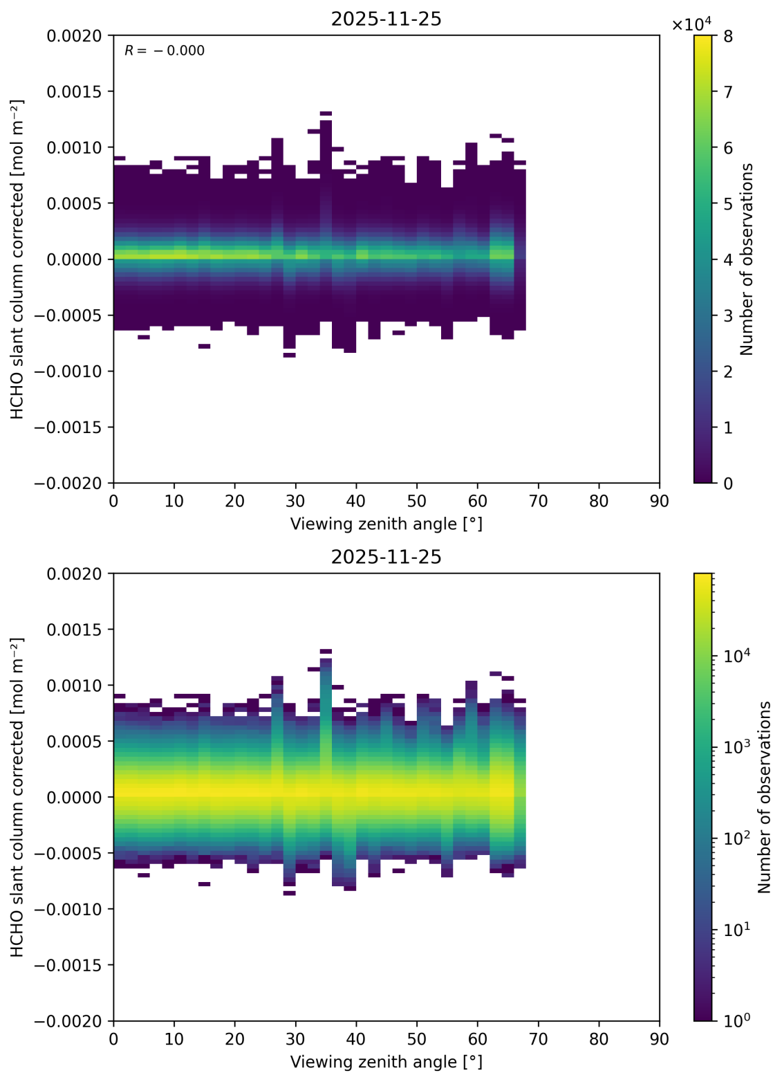
Figure 206: Scatter density plot of “Viewing zenith angle” against “HCHO slant column corrected” for 2025-11-24 to 2025-11-26.
