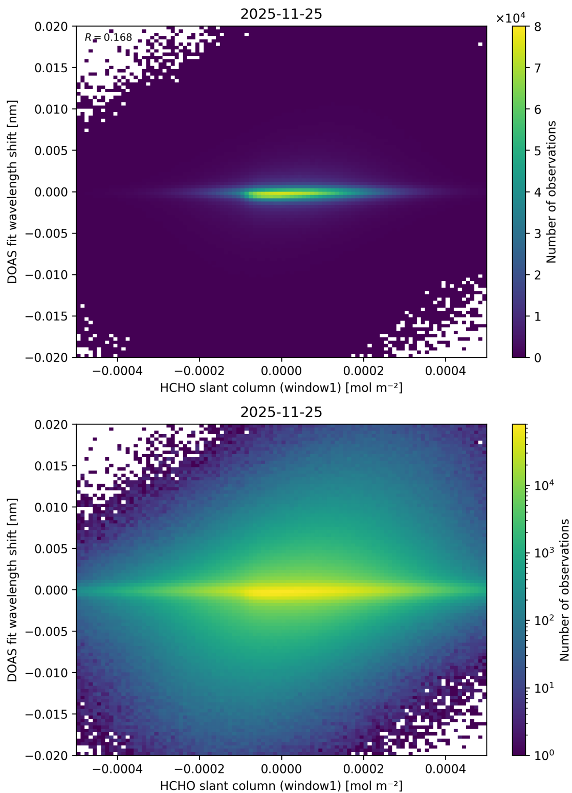
Figure 89: Scatter density plot of “HCHO slant column (window1)” against “DOAS fit wavelength shift” for 2025-11-24 to 2025-11-26.
