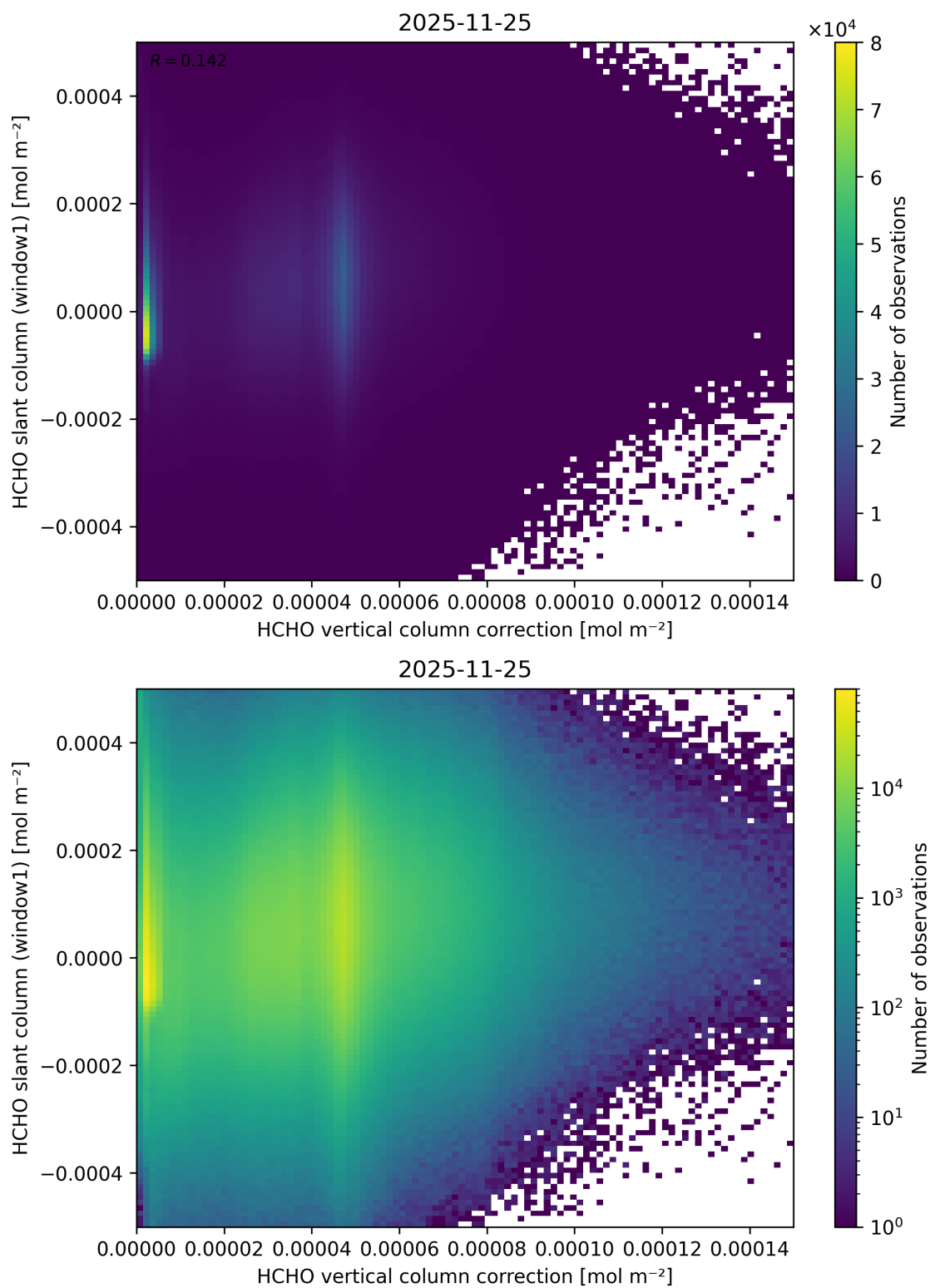
Figure 132: Scatter density plot of “HCHO vertical column correction” against “HCHO slant column (window1)” for 2025-11-24 to 2025-11-26.
