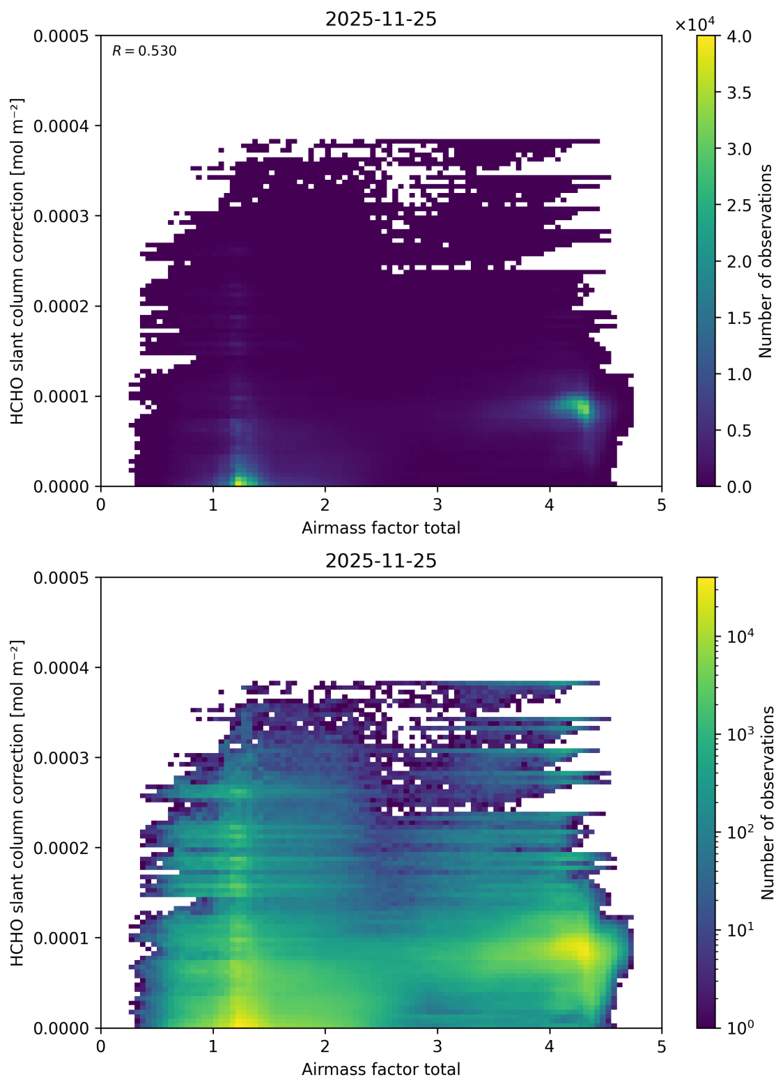
Figure 114: Scatter density plot of “Airmass factor total” against “HCHO slant column correction” for 2025-11-24 to 2025-11-26.
