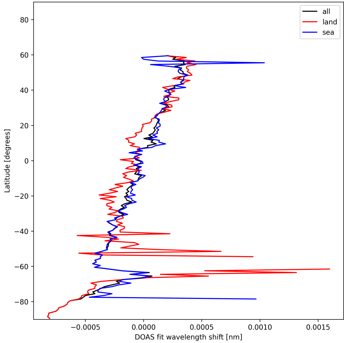
Figure 31: Zonal average of "DOAS fit wavelength shift" for 2025-11-24 to 2025-11-26.
