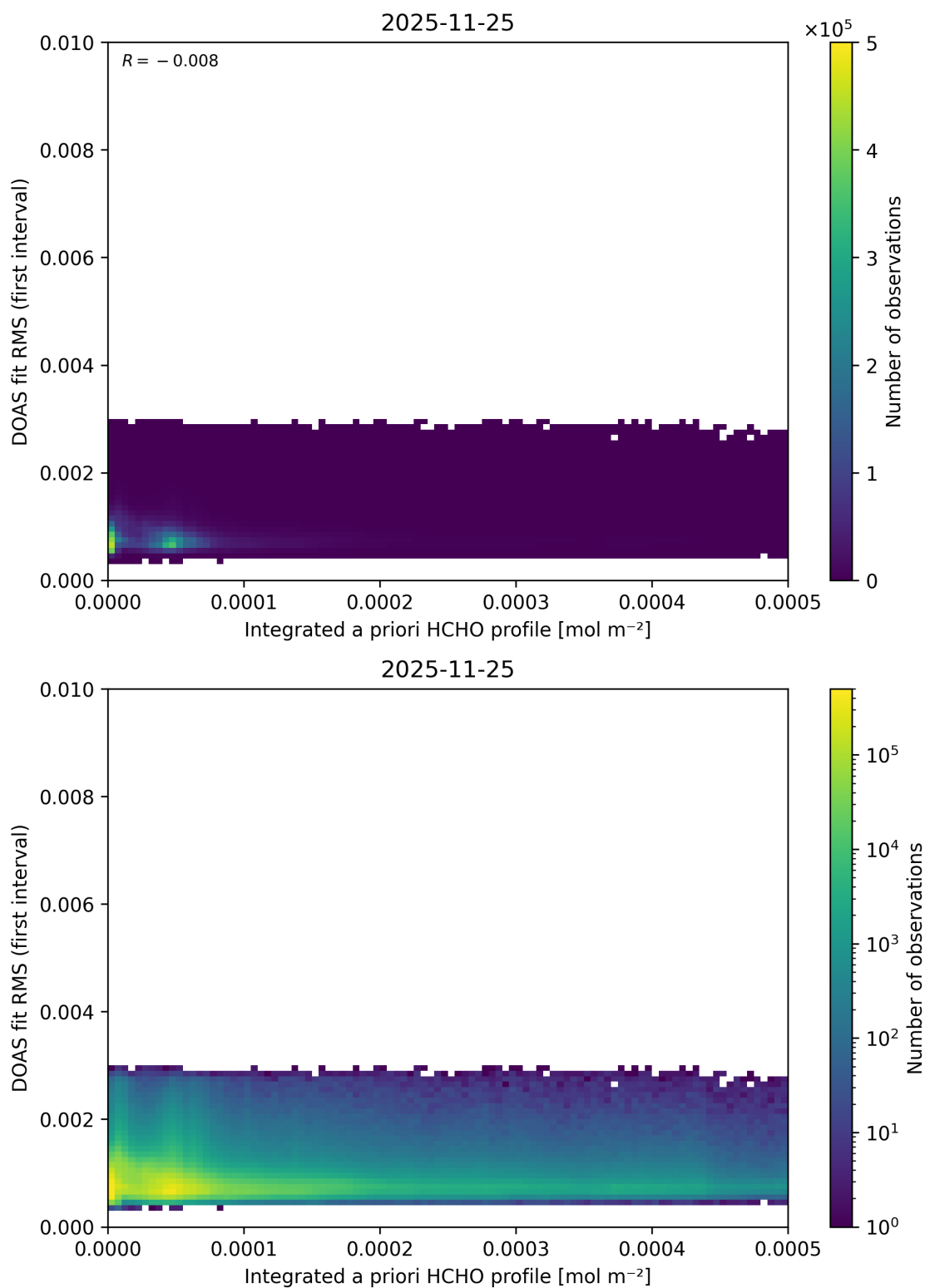
Figure 165: Scatter density plot of “Integrated a priori HCHO profile” against “DOAS fit RMS (first interval)” for 2025-11-24 to 2025-11-26.
