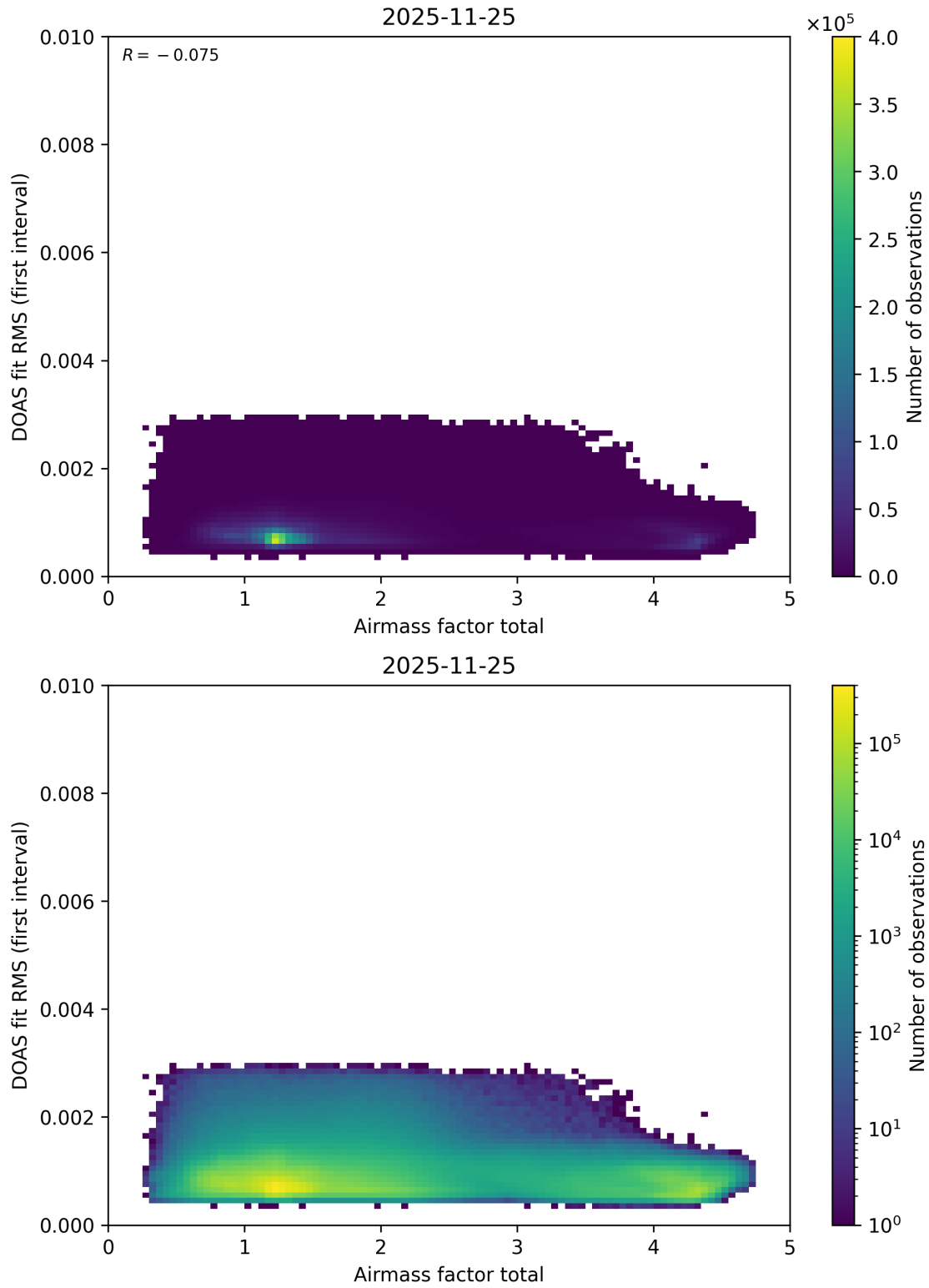
Figure 109: Scatter density plot of “Airmass factor total” against “DOAS fit RMS (first interval)” for 2025-11-24 to 2025-11-26.
