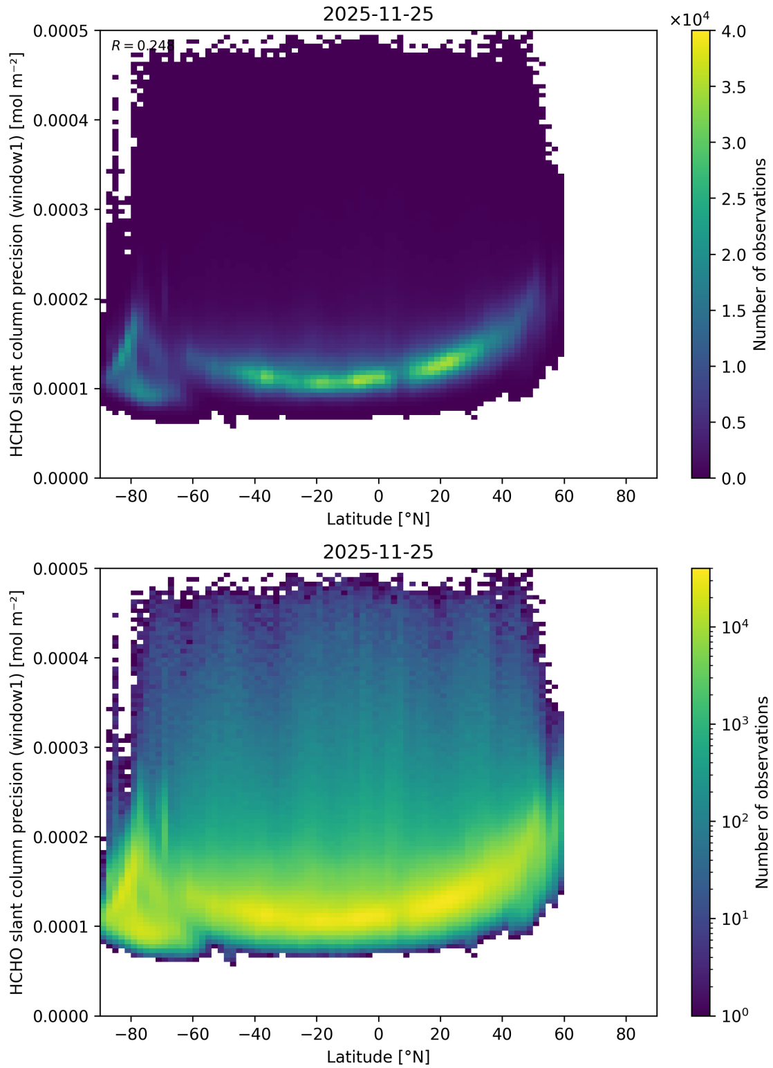
Figure 178: Scatter density plot of “Latitude” against “HCHO slant column precision (window1)” for 2025-11-24 to 2025-11-26.
