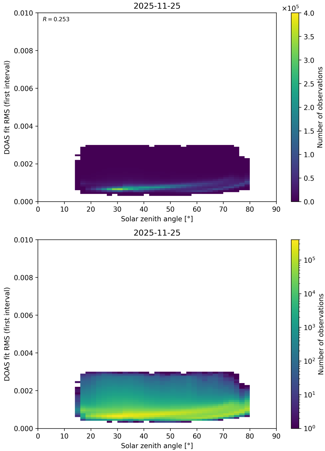
Figure 186: Scatter density plot of “Solar zenith angle” against “DOAS fit RMS (first interval)” for 2025-11-24 to 2025-11-26.
