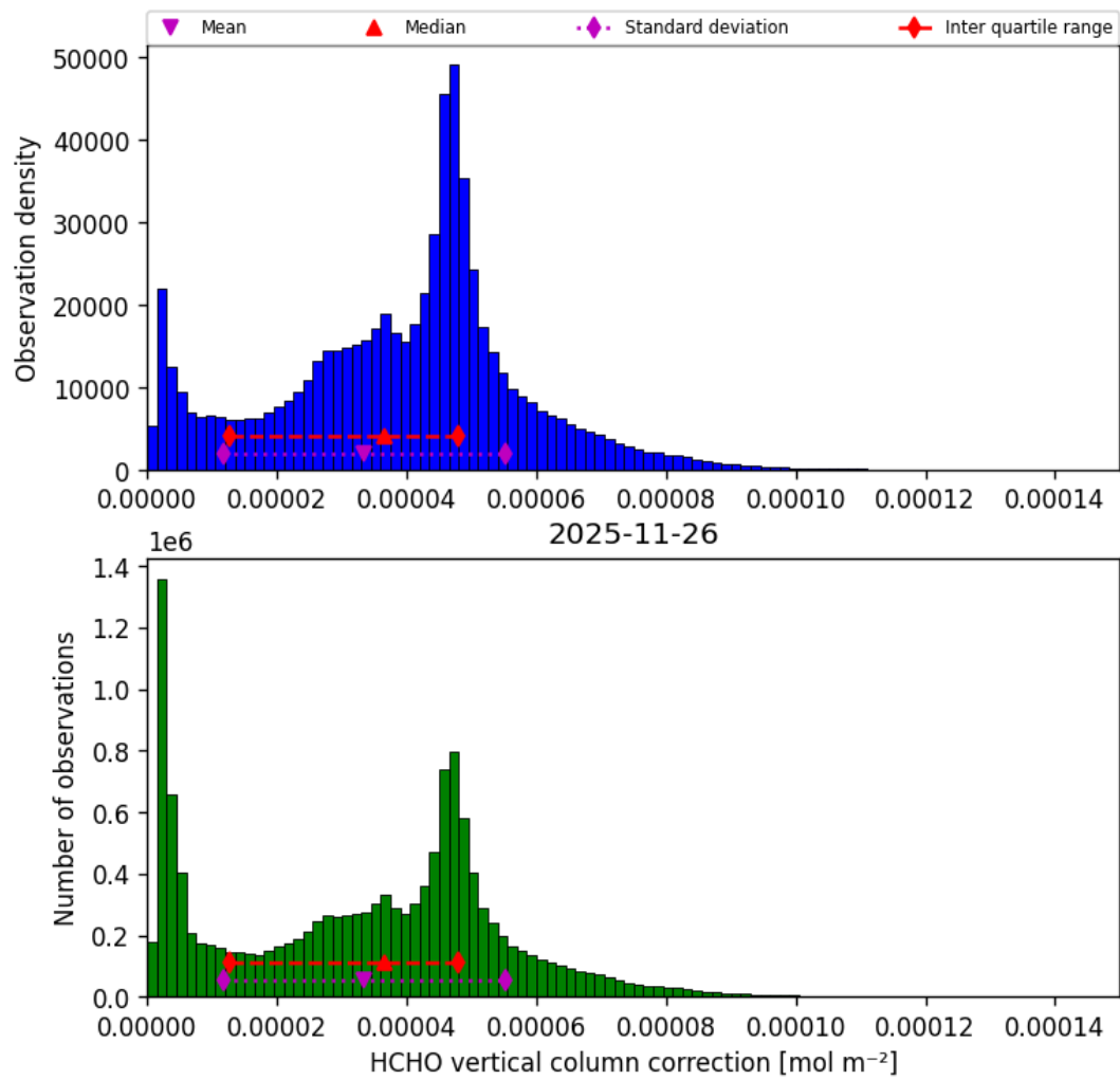
Figure 39: Histogram of “HCHO vertical column correction” for 2025-11-25 to 2025-11-27
