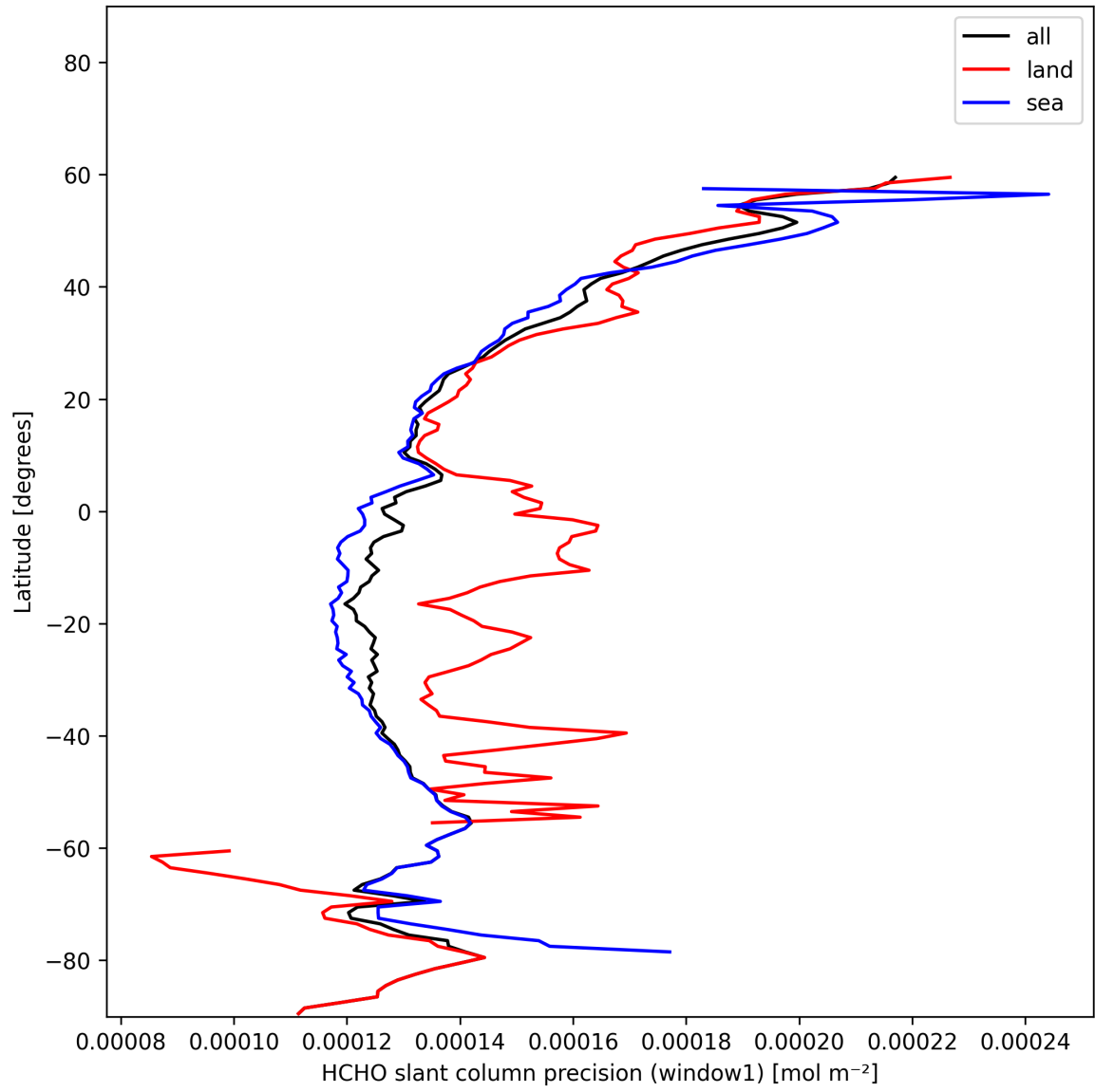
Figure 26: Zonal average of “HCHO slant column precision (window1)” for 2025-11-25 to 2025-11-27.
