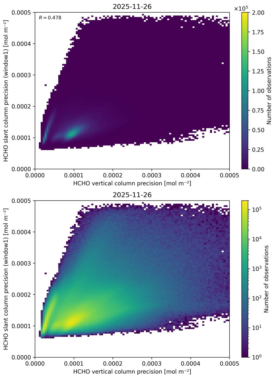
Figure 159: Scatter density plot of “HCHO vertical column precision” against “HCHO slant column precision (window1)” for 2025-11-25 to 2025-11-27.
