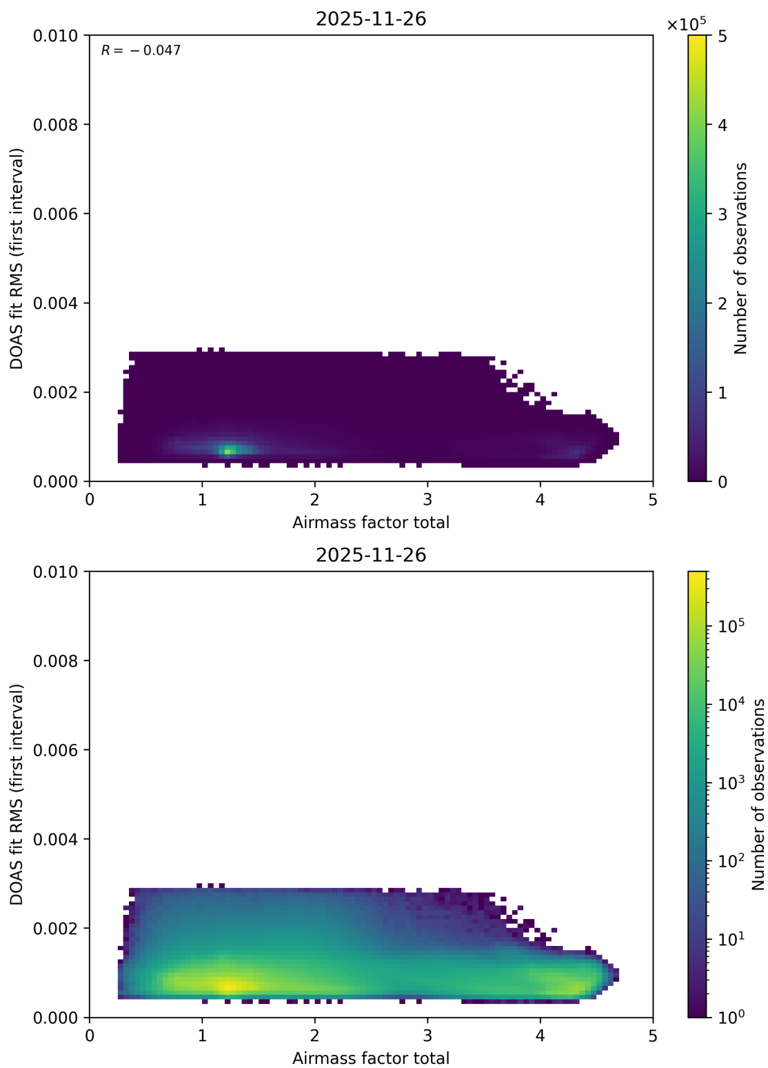
Figure 109: Scatter density plot of “Airmass factor total” against “DOAS fit RMS (first interval)” for 2025-11-25 to 2025-11-27.
