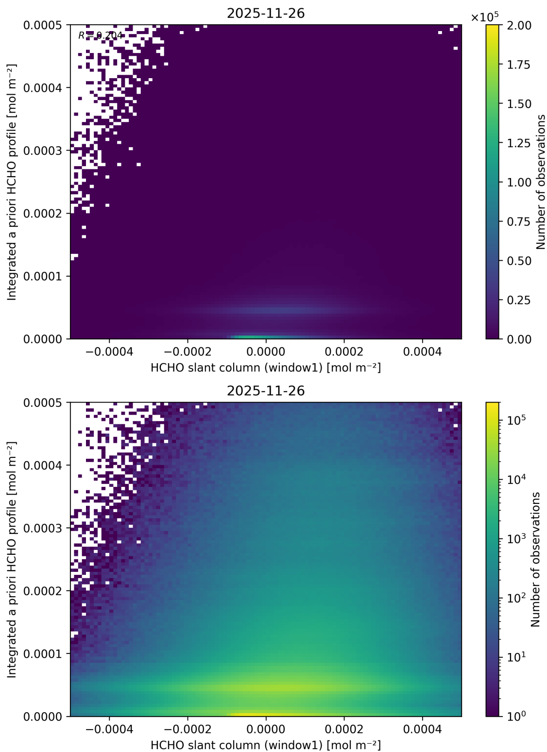
Figure 98: Scatter density plot of “HCHO slant column (window1)” against “Integrated a priori HCHO profile” for 2025-11-25 to 2025-11-27.
