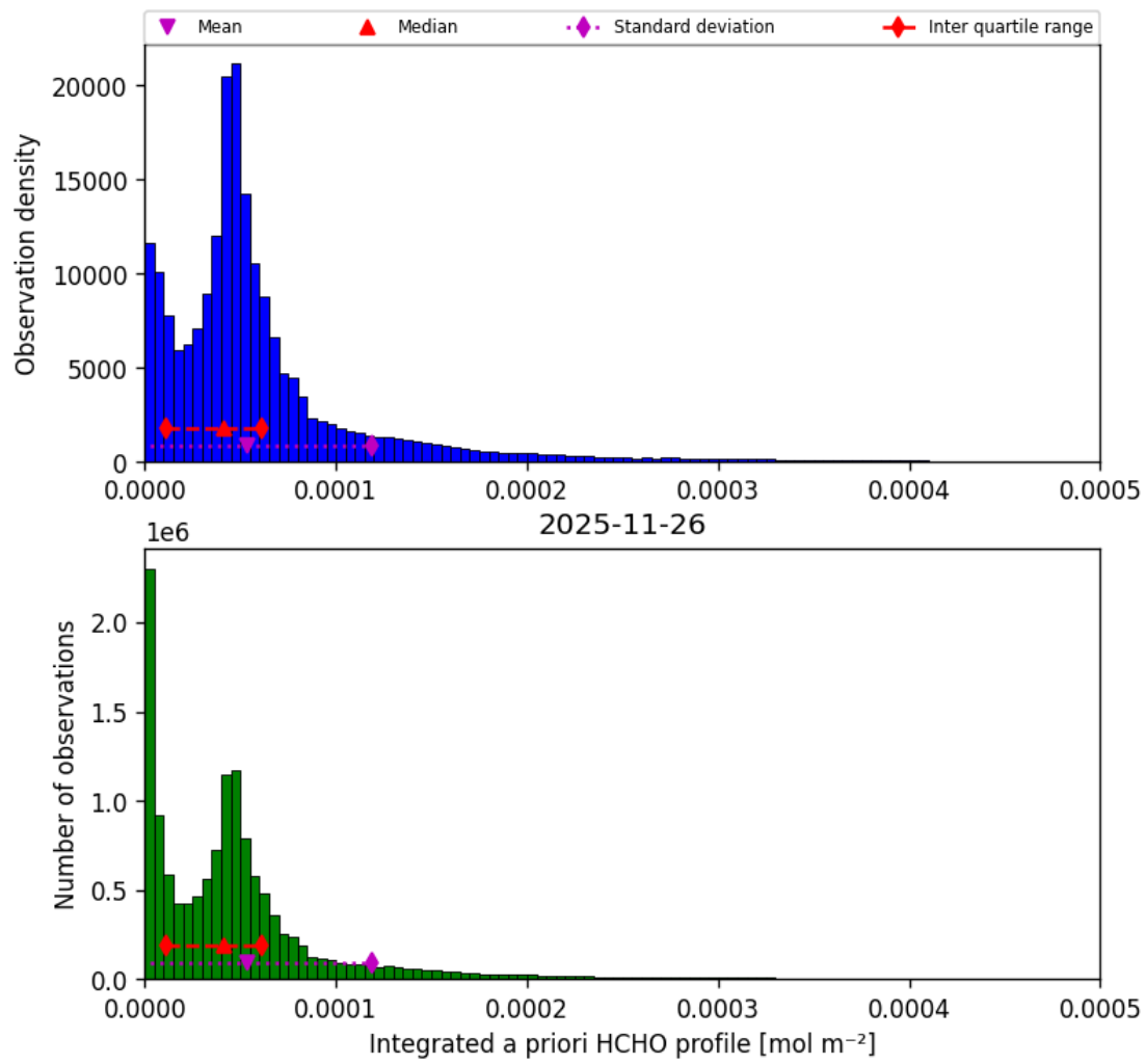
Figure 45: Histogram of “Integrated a priori HCHO profile” for 2025-11-25 to 2025-11-27
