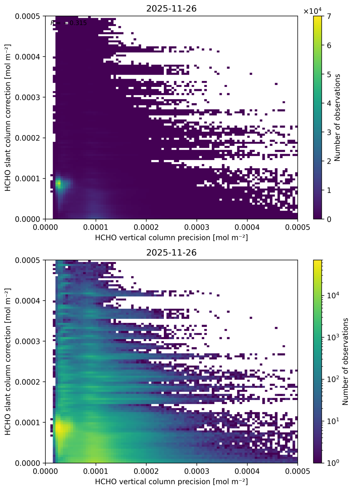
Figure 157: Scatter density plot of “HCHO vertical column precision” against “HCHO slant column correction” for 2025-11-25 to 2025-11-27.
