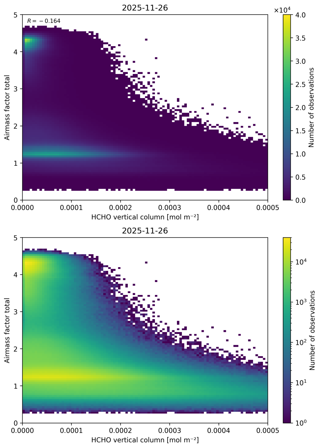
Figure 146: Scatter density plot of “HCHO vertical column” against “Airmass factor total” for 2025-11-25 to 2025-11-27.
