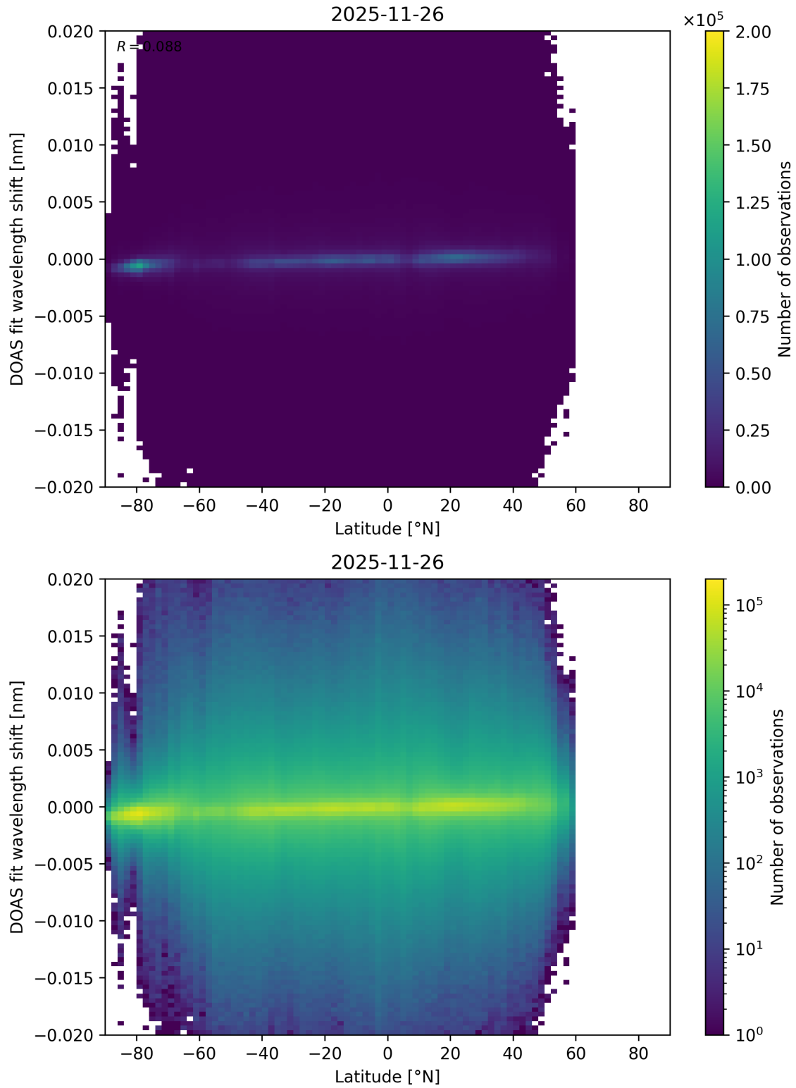
Figure 172: Scatter density plot of “Latitude” against “DOAS fit wavelength shift” for 2025-11-25 to 2025-11-27.
