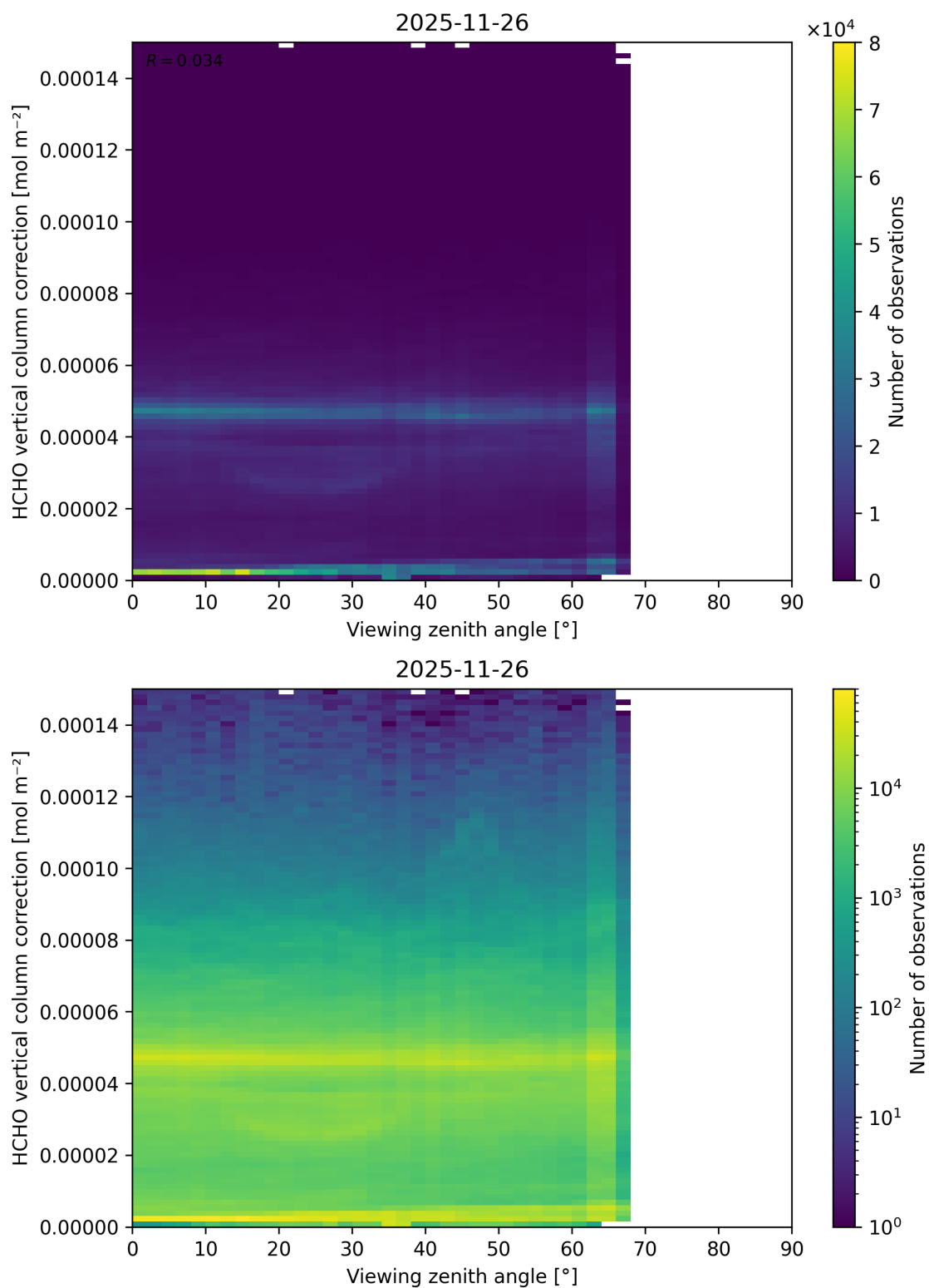
Figure 213: Scatter density plot of “Viewing zenith angle” against “HCHO vertical column correction” for 2025-11-25 to 2025-11-27.
