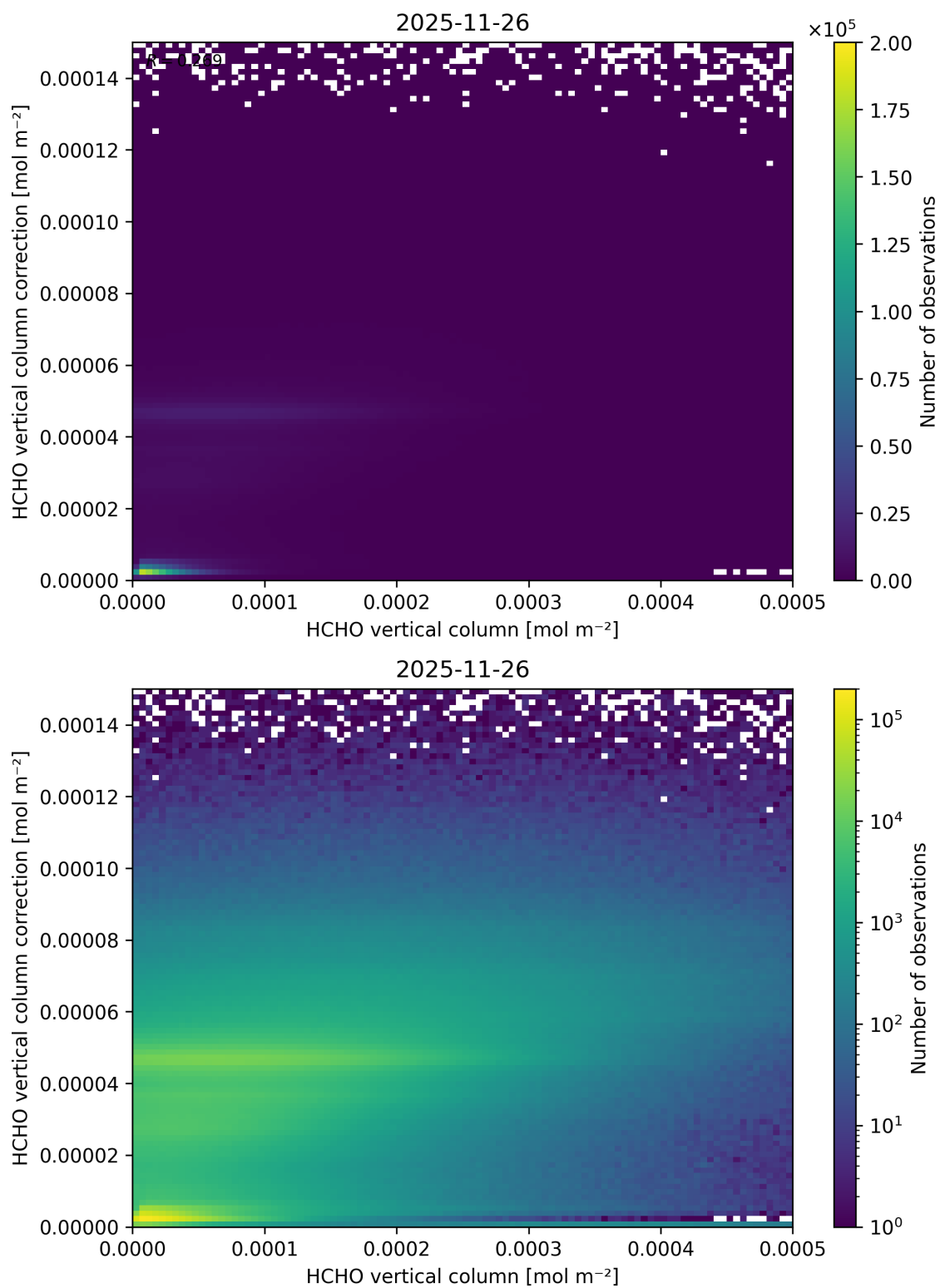
Figure 148: Scatter density plot of “HCHO vertical column” against “HCHO vertical column correction” for 2025-11-25 to 2025-11-27.
