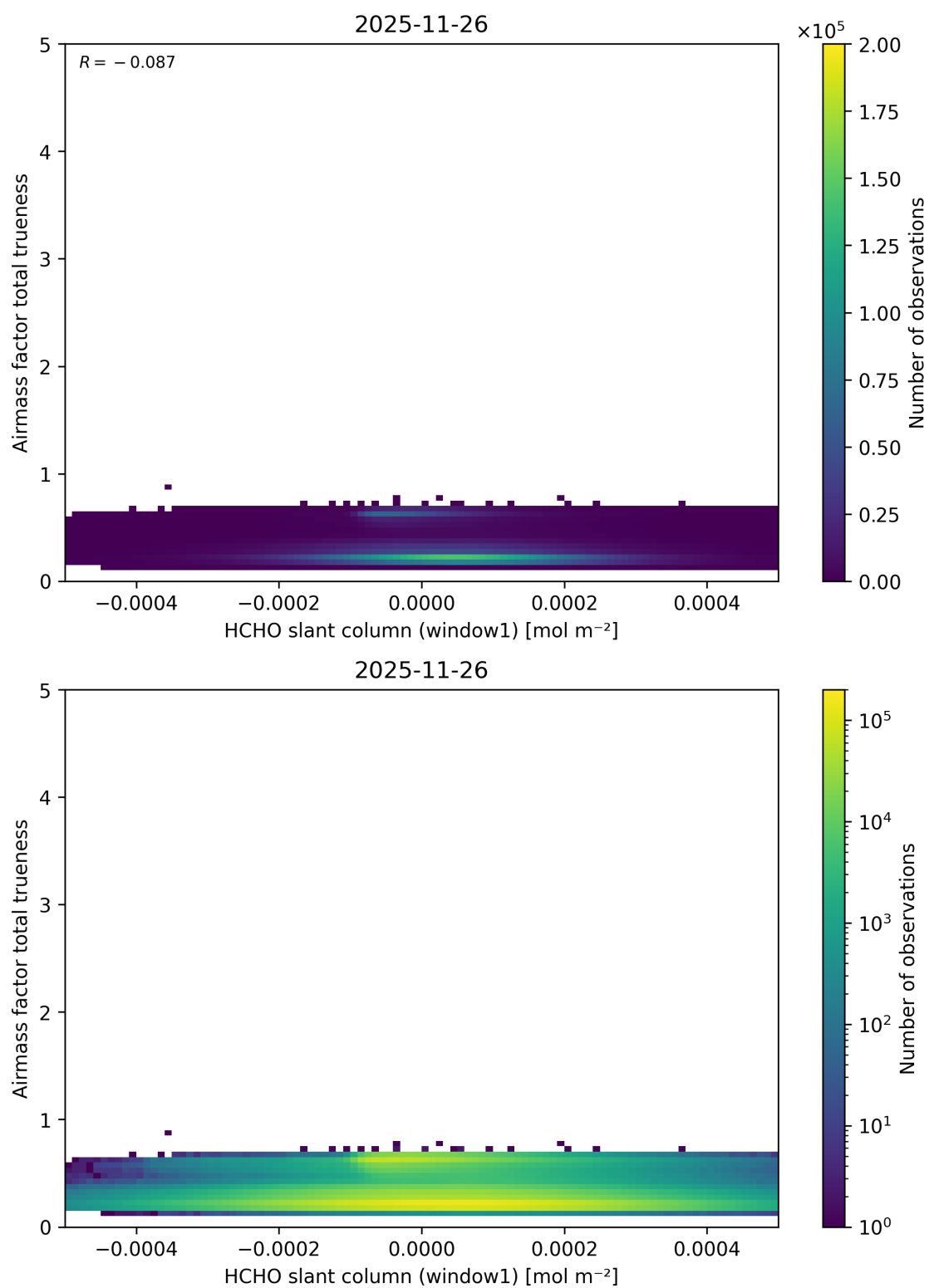
Figure 96: Scatter density plot of “HCHO slant column (window1)” against “Airmass factor total trueneess” for 2025-11-25 to 2025-11-27.
