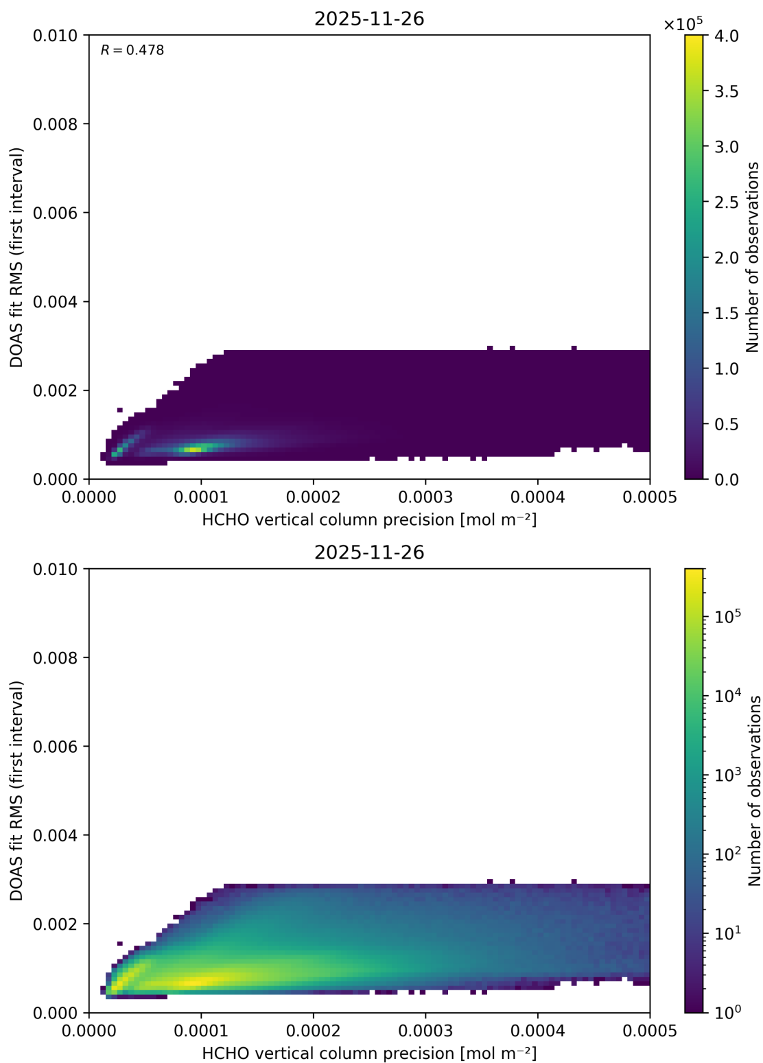
Figure 152: Scatter density plot of “HCHO vertical column precision” against “DOAS fit RMS (first interval)” for 2025-11-25 to 2025-11-27.
