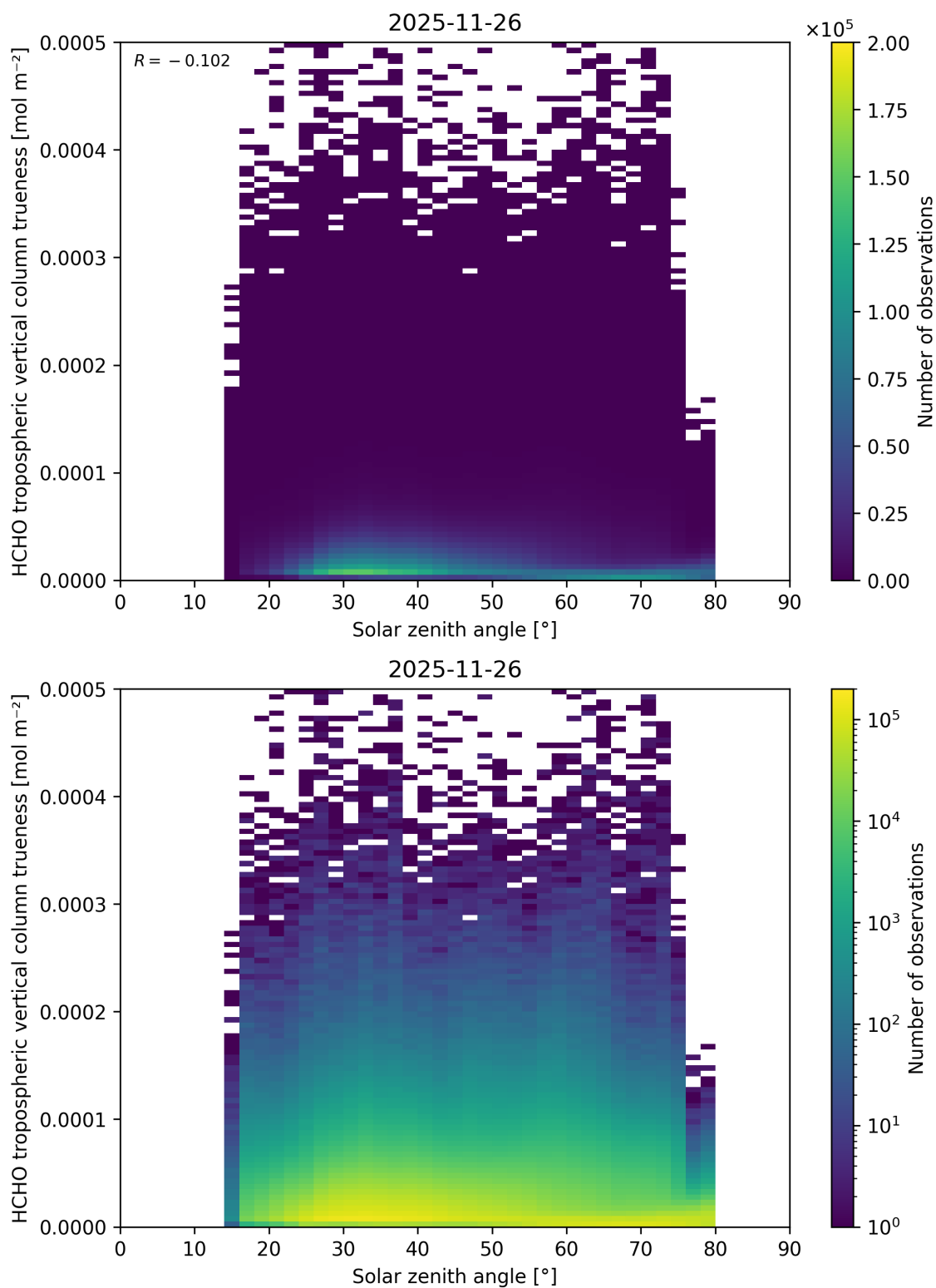
Figure 199: Scatter density plot of “Solar zenith angle” against “HCHO tropospheric vertical column trueness” for 2025-11-25 to 2025-11-27.
