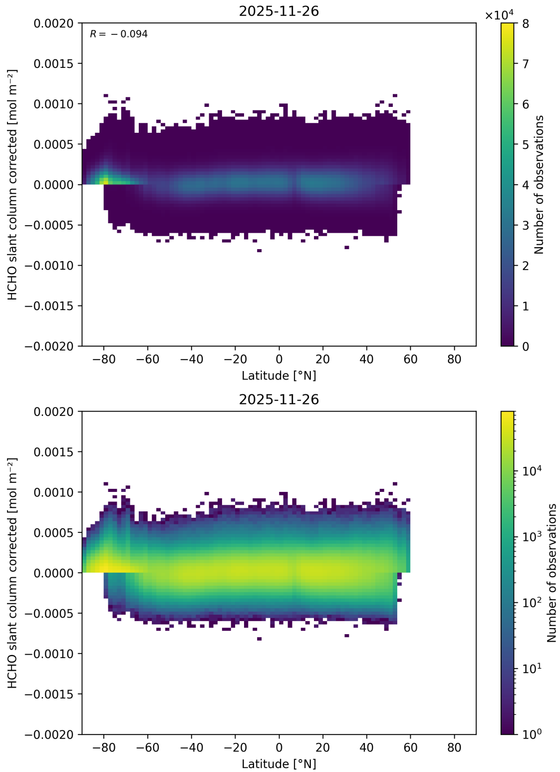
Figure 175: Scatter density plot of “Latitude” against “HCHO slant column corrected” for 2025-11-25 to 2025-11-27.
