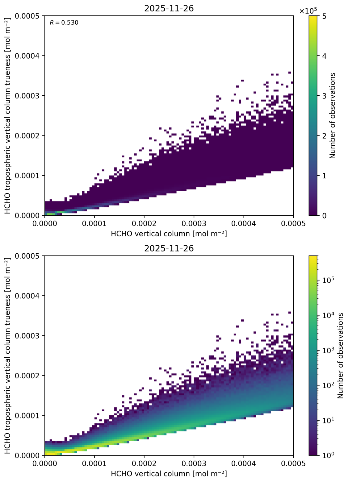
Figure 150: Scatter density plot of “HCHO vertical column” against “HCHO tropospheric vertical column trueness” for 2025-11-25 to 2025-11-27.
