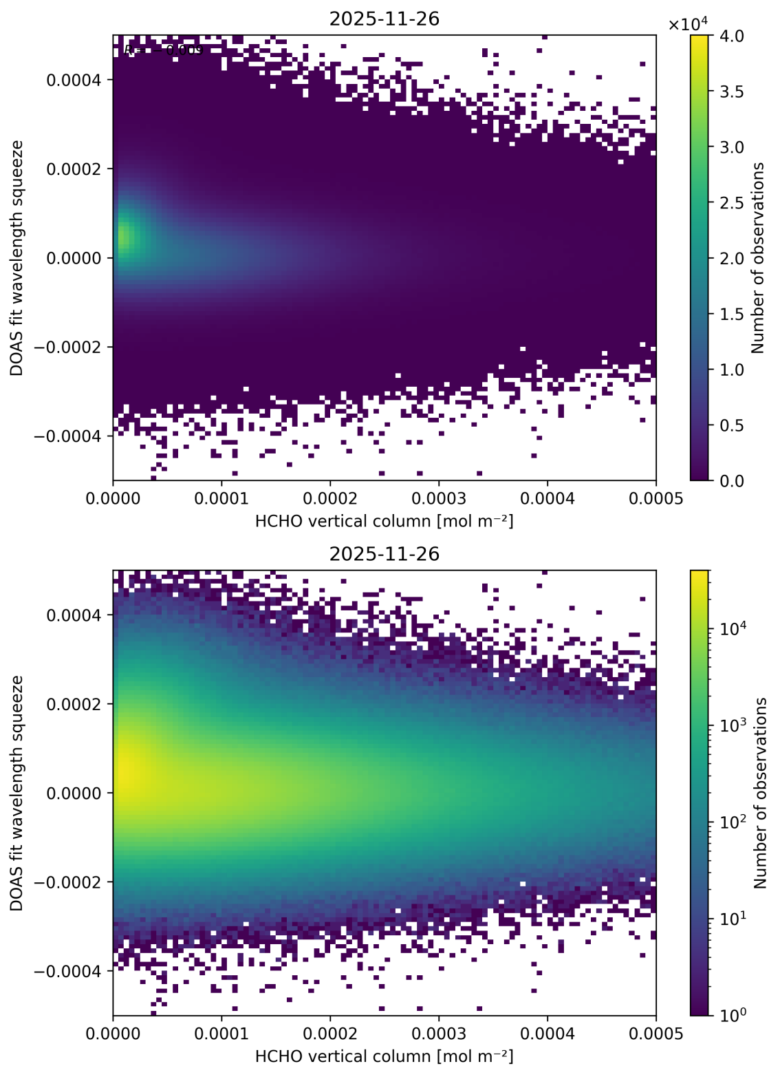
Figure 140: Scatter density plot of “HCHO vertical column” against “DOAS fit wavelength squeeze” for 2025-11-25 to 2025-11-27.
