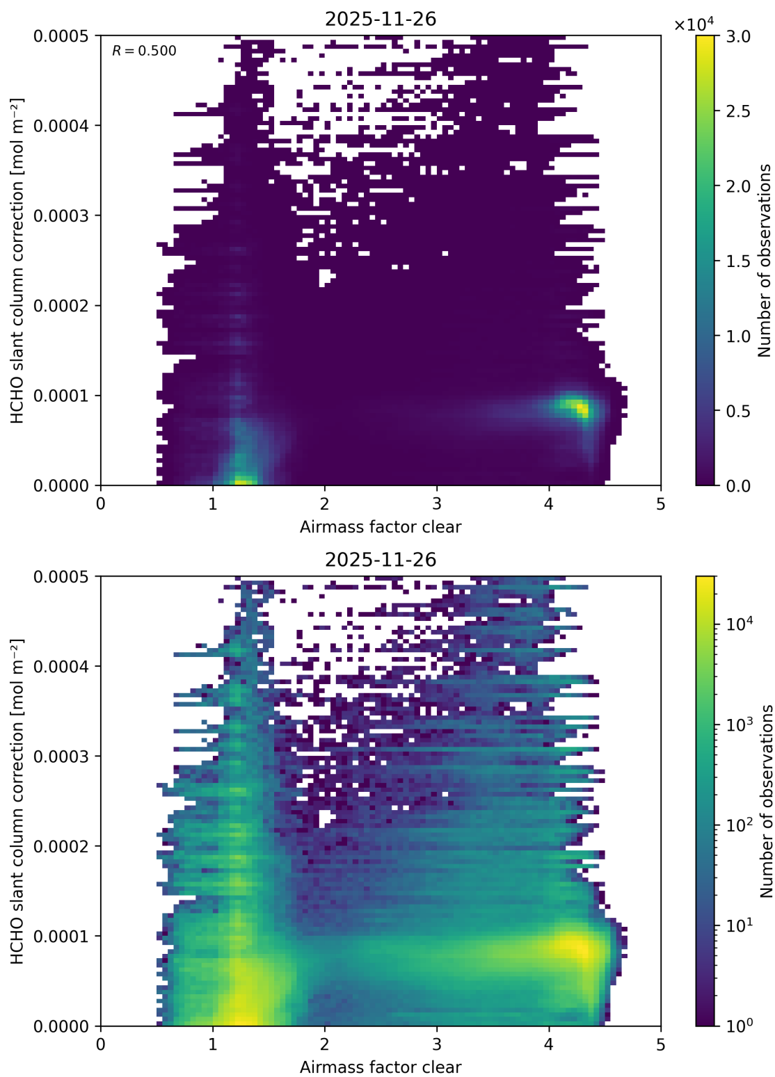
Figure 82: Scatter density plot of “Airmass factor clear” against “HCHO slant column correction” for 2025-11-25 to 2025-11-27.
