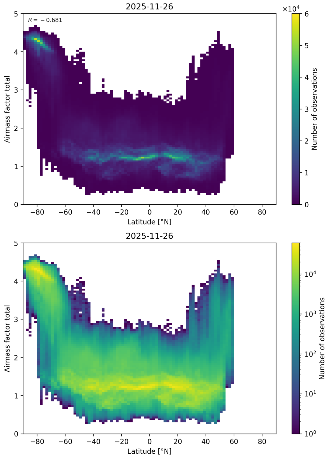
Figure 179: Scatter density plot of “Latitude” against “Airmass factor total” for 2025-11-25 to 2025-11-27.
