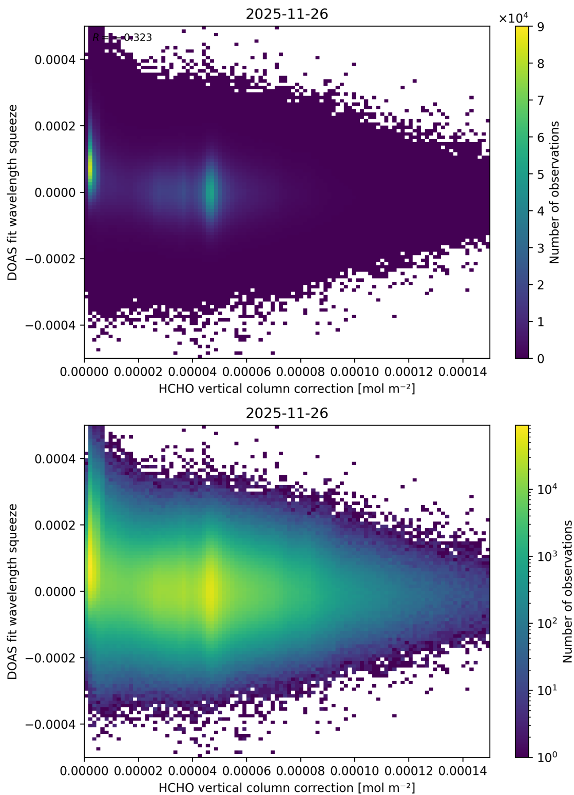
Figure 128: Scatter density plot of “HCHO vertical column correction” against “DOAS fit wavelength squeeze” for 2025-11-25 to 2025-11-27.
