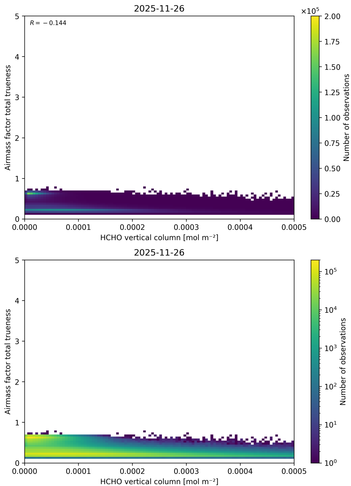
Figure 147: Scatter density plot of “HCHO vertical column” against “Airmass factor total trueneess” for 2025-11-25 to 2025-11-27.
