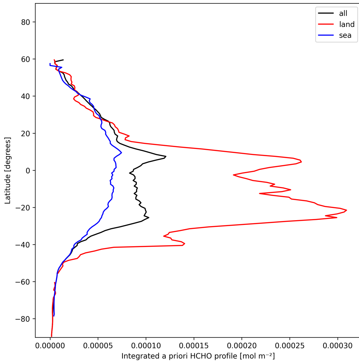
Figure 30: Zonal average of “Integrated a priori HCHO profile” for 2025-11-25 to 2025-11-27.
