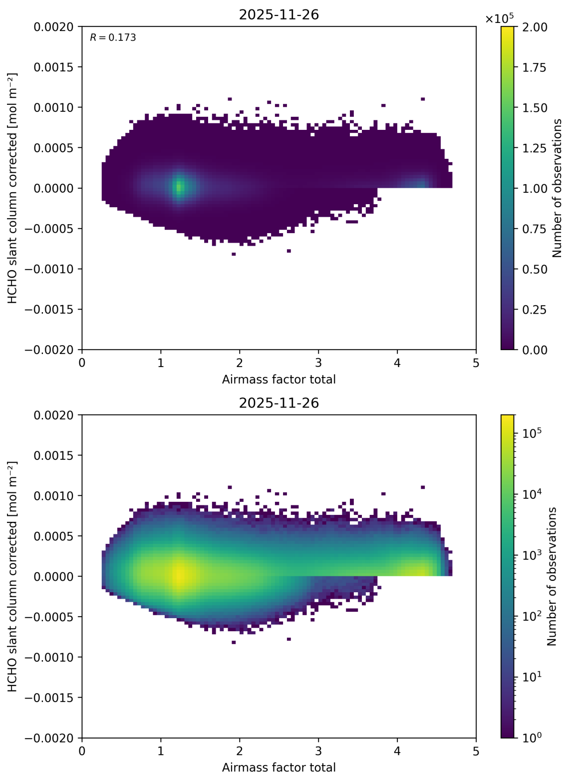
Figure 113: Scatter density plot of “Airmass factor total” against “HCHO slant column corrected” for 2025-11-25 to 2025-11-27.
