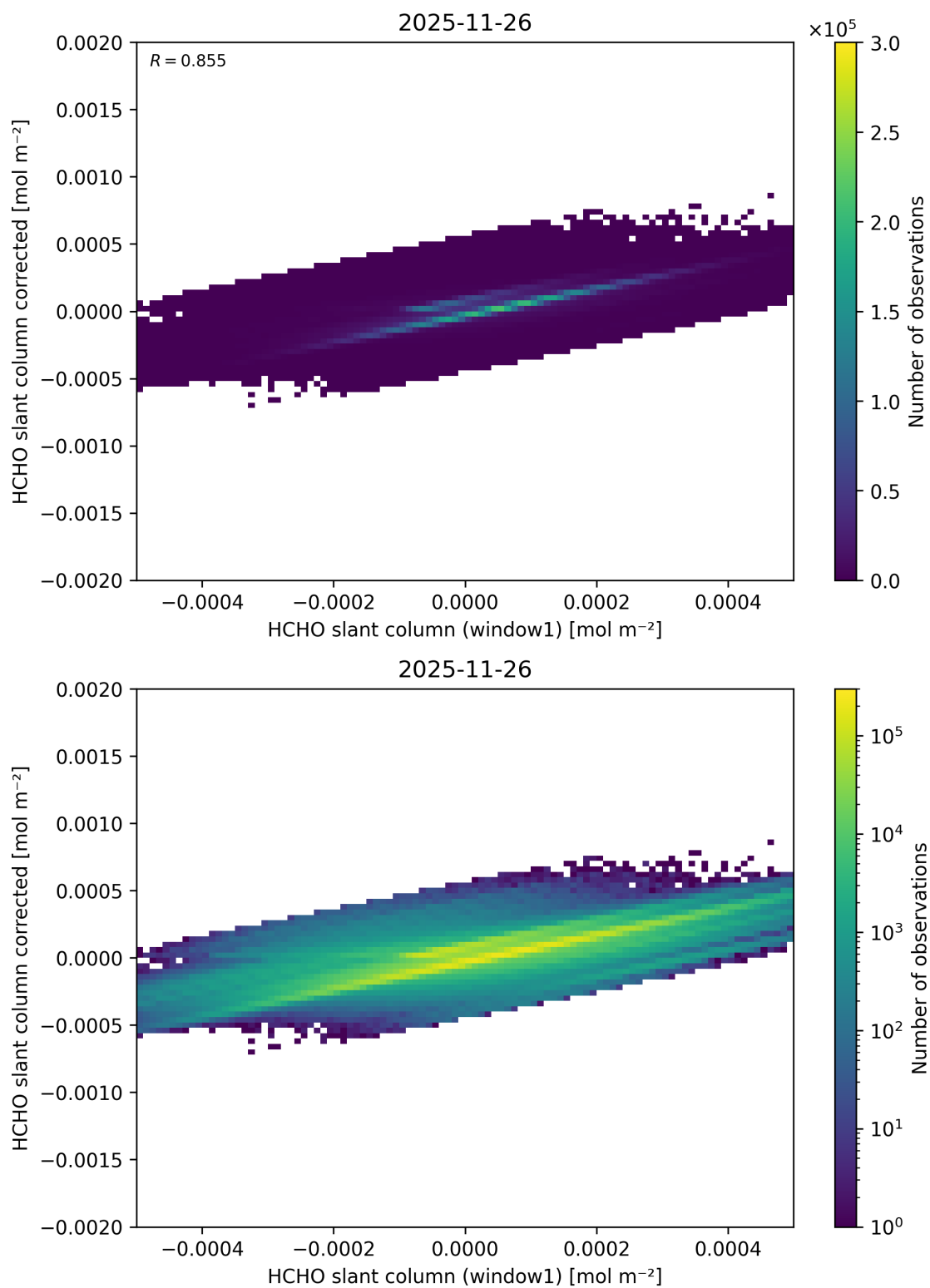
Figure 92: Scatter density plot of “HCHO slant column (window1)” against “HCHO slant column corrected” for 2025-11-25 to 2025-11-27.
