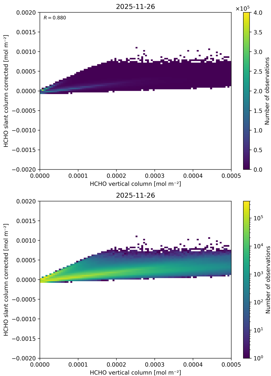
Figure 142: Scatter density plot of “HCHO vertical column” against “HCHO slant column corrected” for 2025-11-25 to 2025-11-27.
