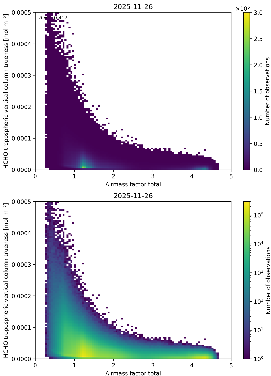
Figure 116: Scatter density plot of “Air mass factor total” against “HCHO tropospheric vertical column trueeness” for 2025-11-25 to 2025-11-27.
