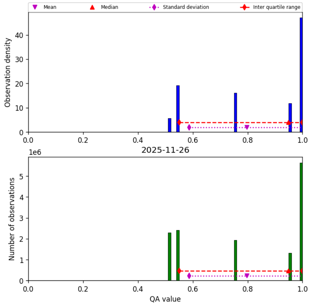
Figure 36: Histogram of “QA value” for 2025-11-25 to 2025-11-27
