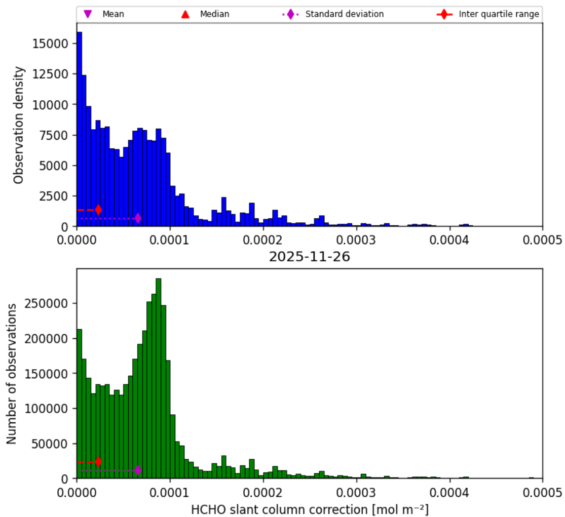
Figure 49: Histogram of “HCHO slant column correction” for 2025-11-25 to 2025-11-27
