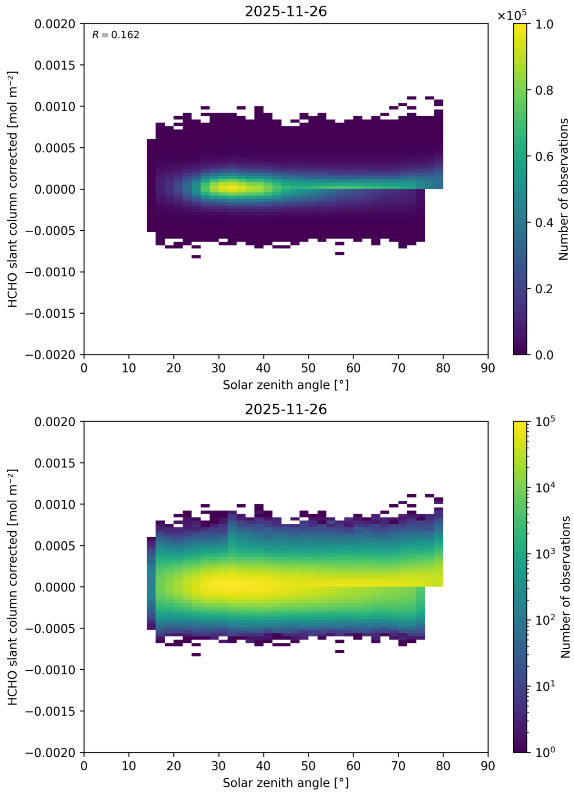
Figure 190: Scatter density plot of “Solar zenith angle” against “HCHO slant column corrected” for 2025-11-25 to 2025-11-27.
