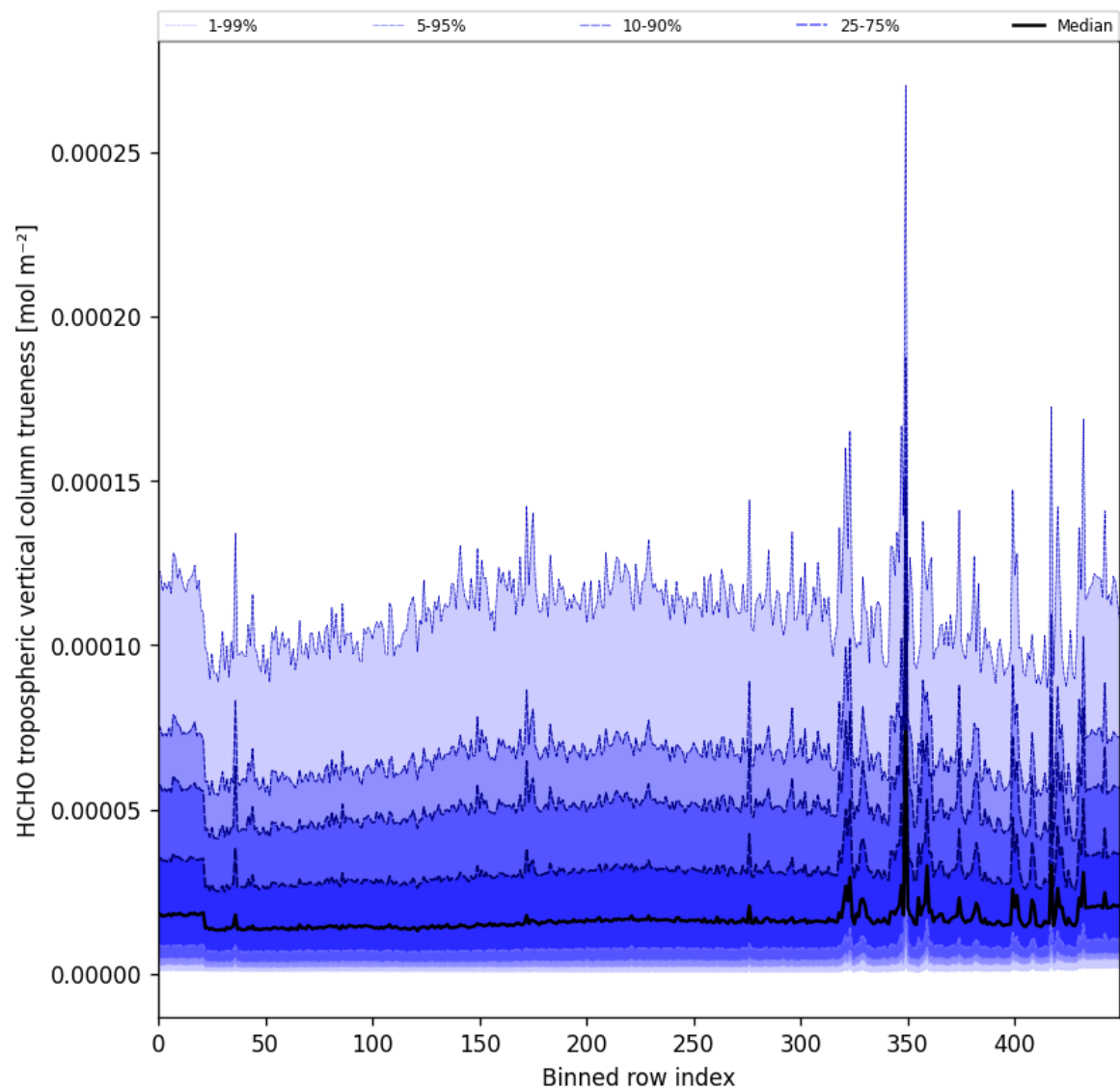
Figure 65: Along track statistics of “HCHO tropospheric vertical column trueness” for 2025-11-25 to 2025-11-27
