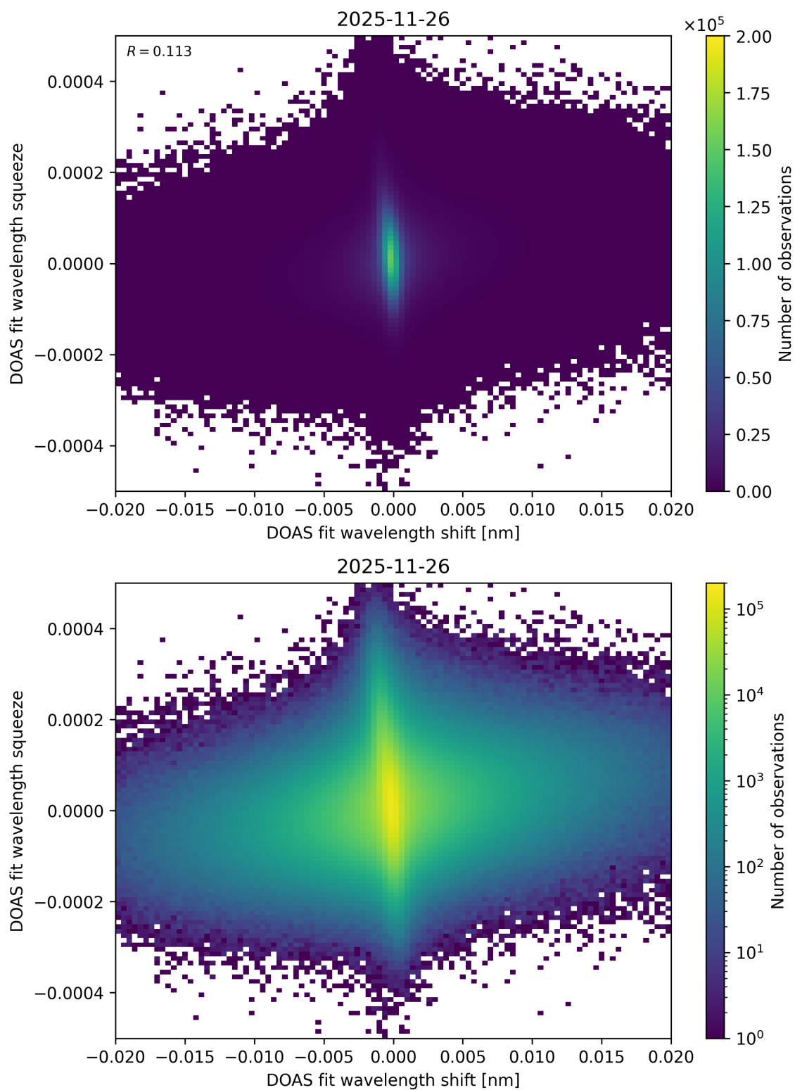
Figure 70: Scatter density plot of “DOAS fit wavelength shift” against “DOAS fit wavelength squeeze” for 2025-11-25 to 2025-11-27.
