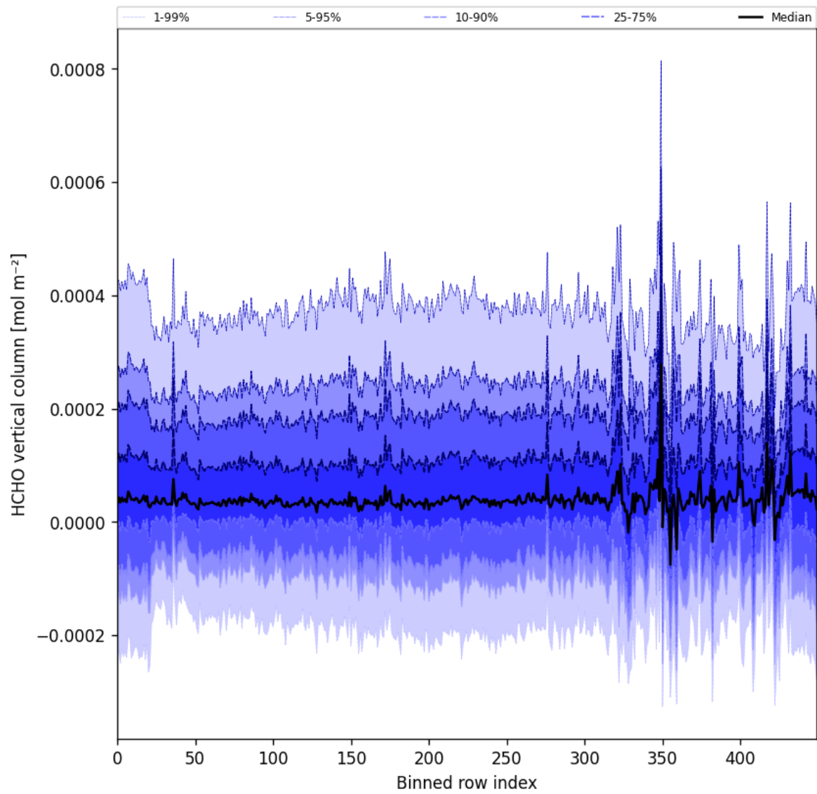
Figure 52: Along track statistics of “HCHO vertical column” for 2025-11-25 to 2025-11-27
