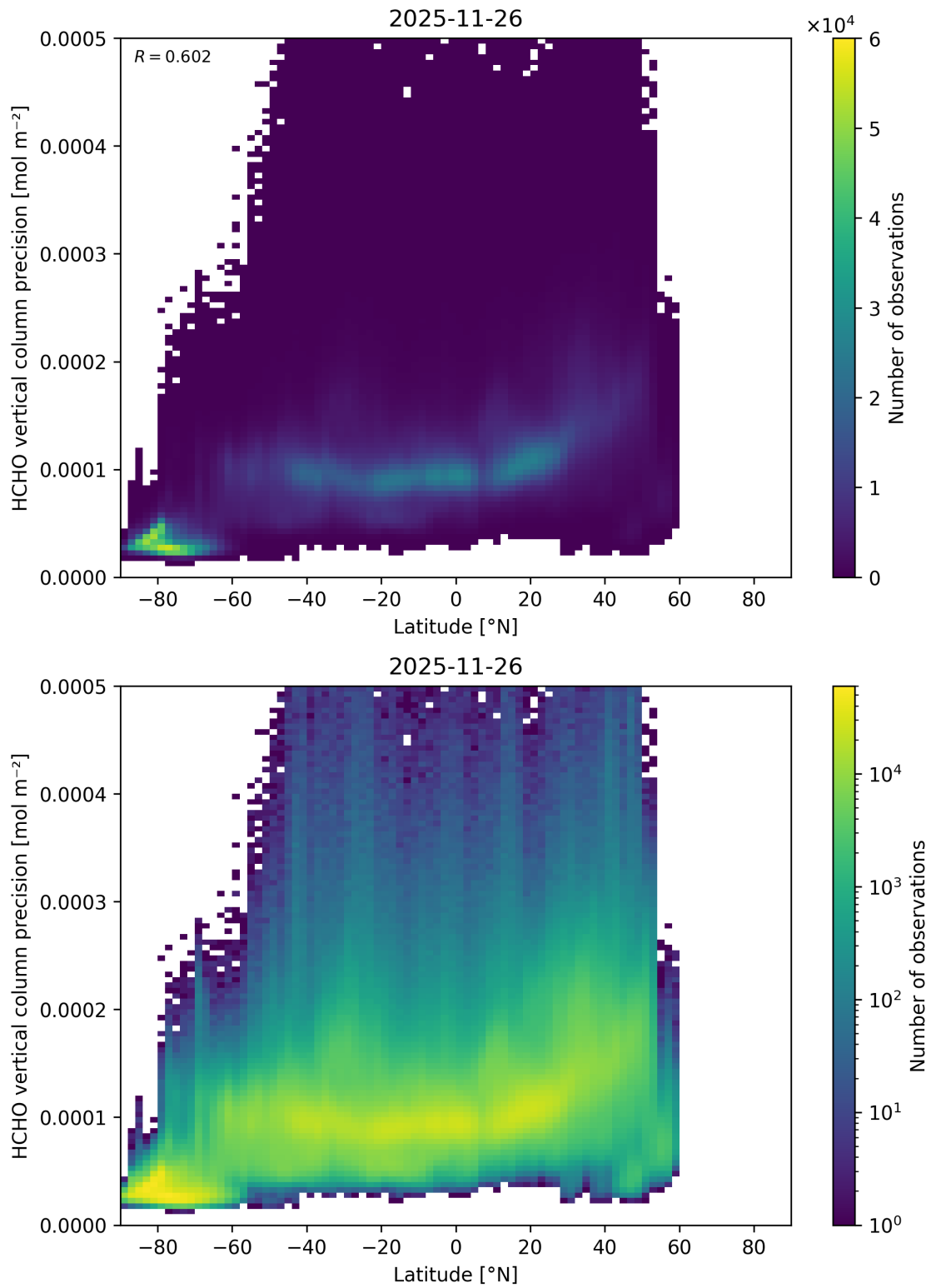
Figure 183: Scatter density plot of “Latitude” against “HCHO vertical column precision” for 2025-11-25 to 2025-11-27.
