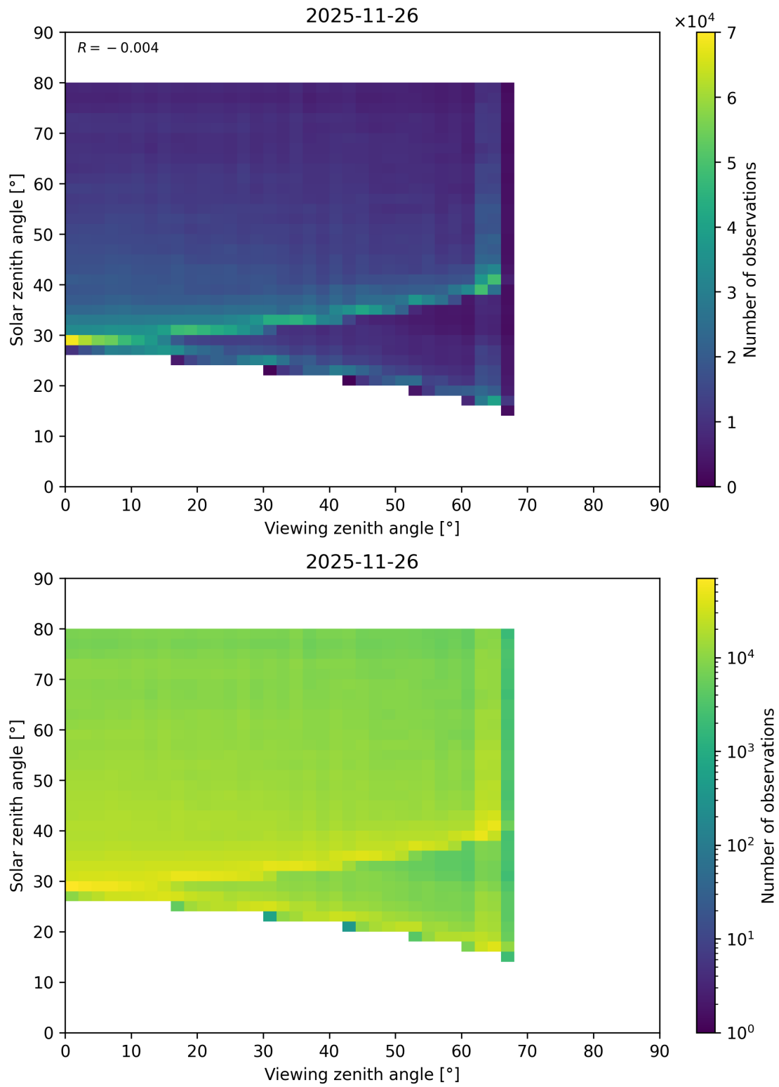
Figure 218: Scatter density plot of “Viewing zenith angle” against “Solar zenith angle” for 2025-11-25 to 2025-11-27.
