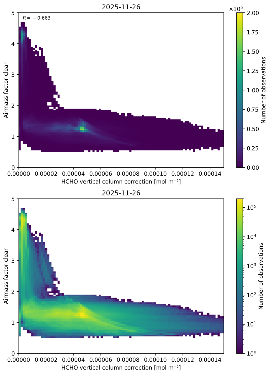
Figure 129: Scatter density plot of “HCHO vertical column correction” against “Airmass factor clear” for 2025-11-25 to 2025-11-27.
