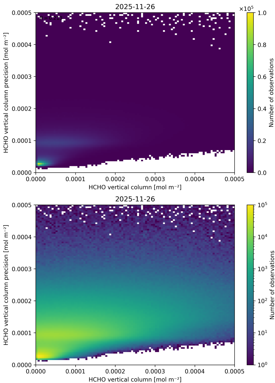
Figure 149: Scatter density plot of “HCHO vertical column” against “HCHO vertical column precision” for 2025-11-25 to 2025-11-27.
