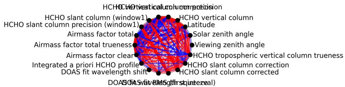
Figure 1: Map of correlation graph for 2025-11-25 to 2025-11-27.
