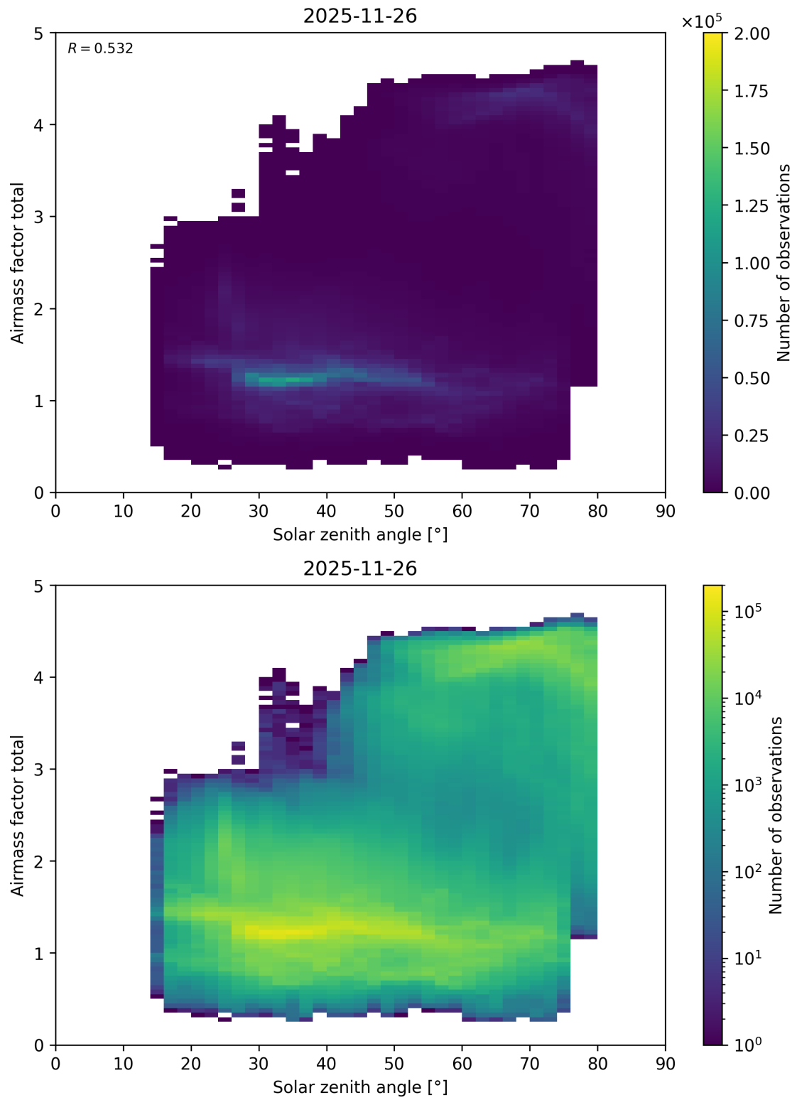
Figure 194: Scatter density plot of “Solar zenith angle” against “Airmass factor total” for 2025-11-25 to 2025-11-27.
