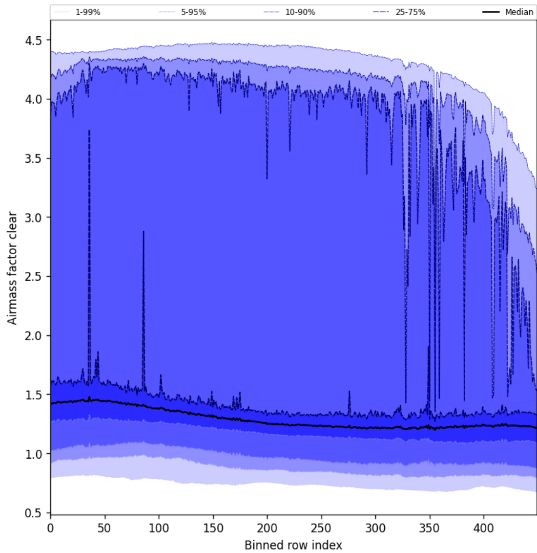
Figure 59: Along track statistics of “Airmass factor clear” for 2025-11-25 to 2025-11-27
