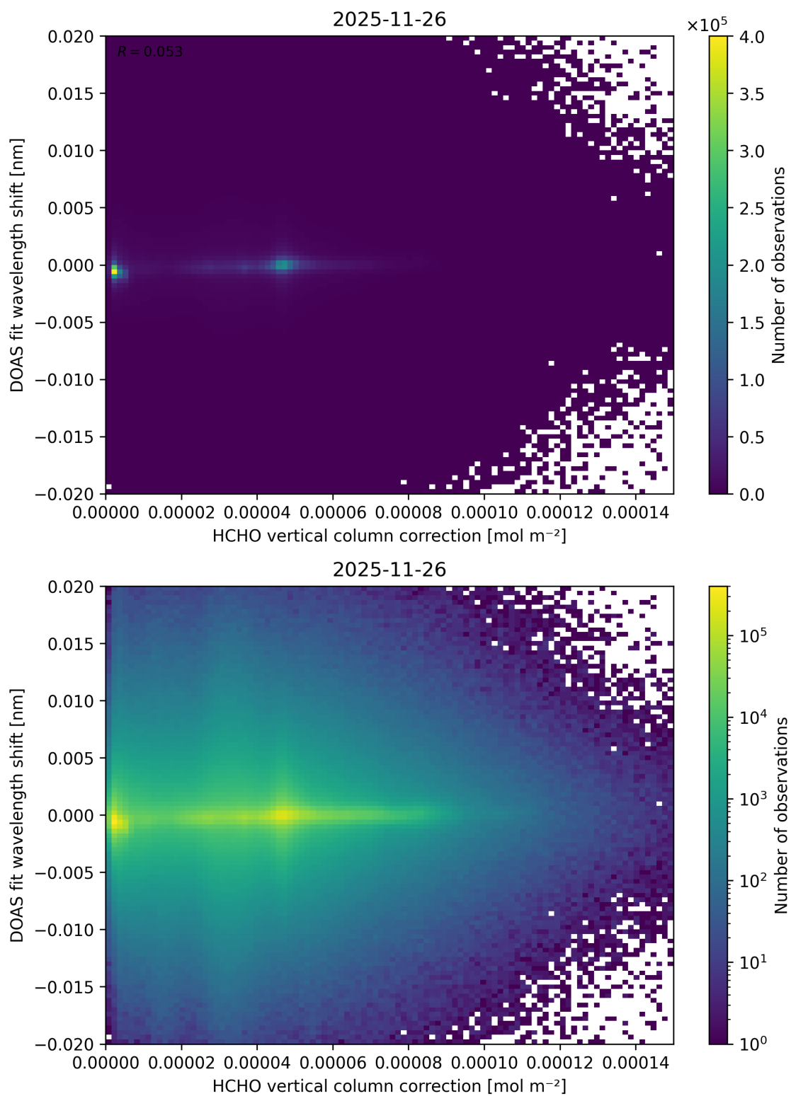
Figure 127: Scatter density plot of “HCHO vertical column correction” against “DOAS fit wavelength shift” for 2025-11-25 to 2025-11-27.
