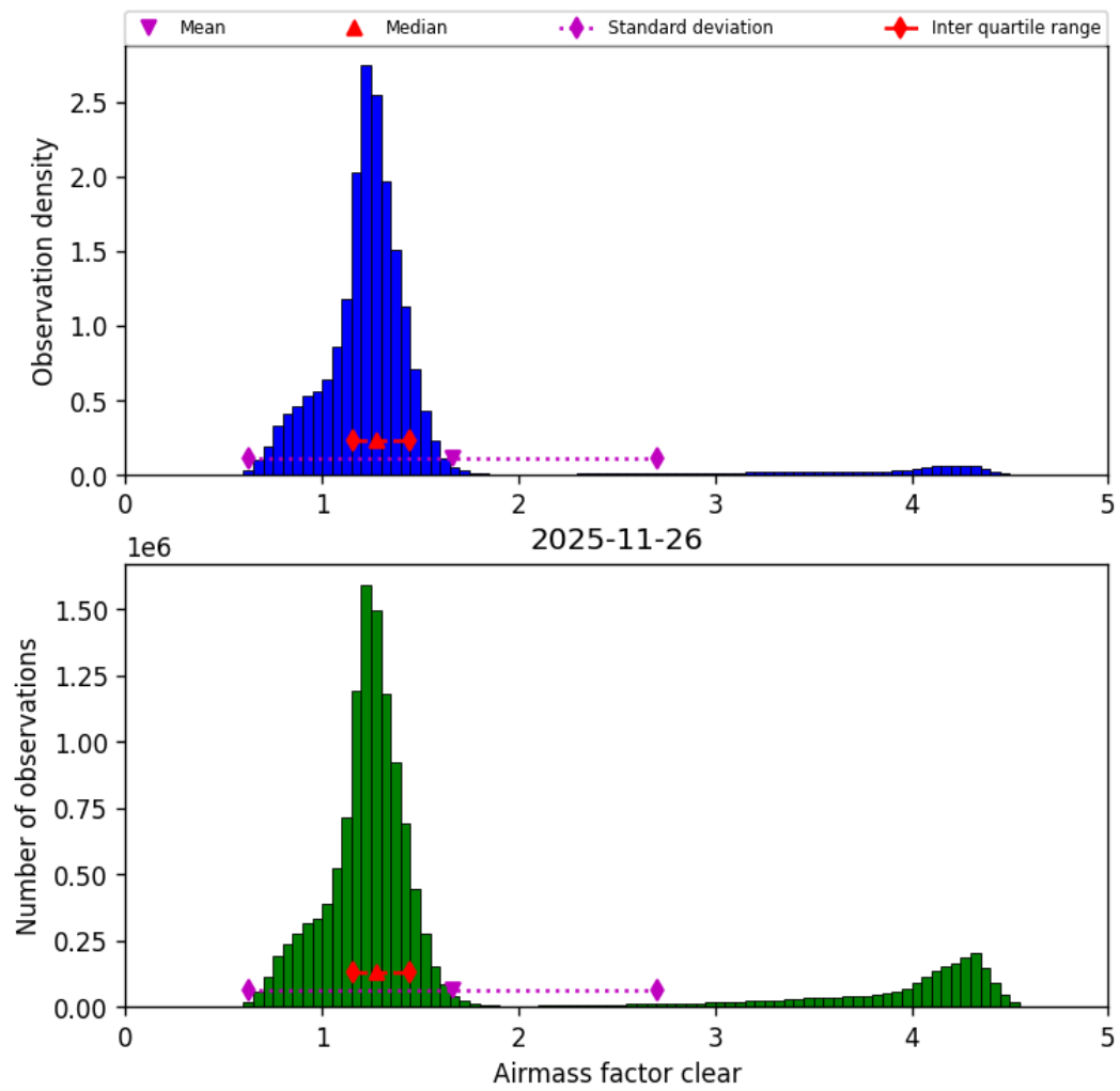
Figure 44: Histogram of “Airmass factor clear” for 2025-11-25 to 2025-11-27
