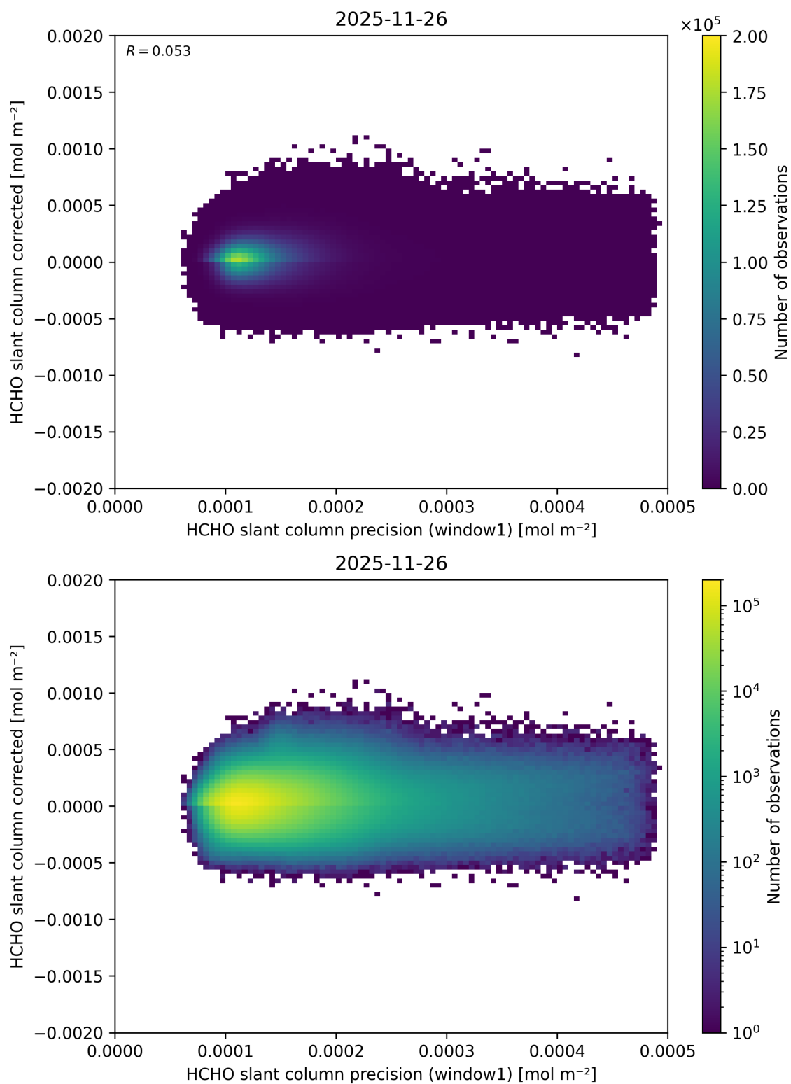
Figure 103: Scatter density plot of “HCHO slant column precision (window1)” against “HCHO slant column corrected” for 2025-11-25 to 2025-11-27.
