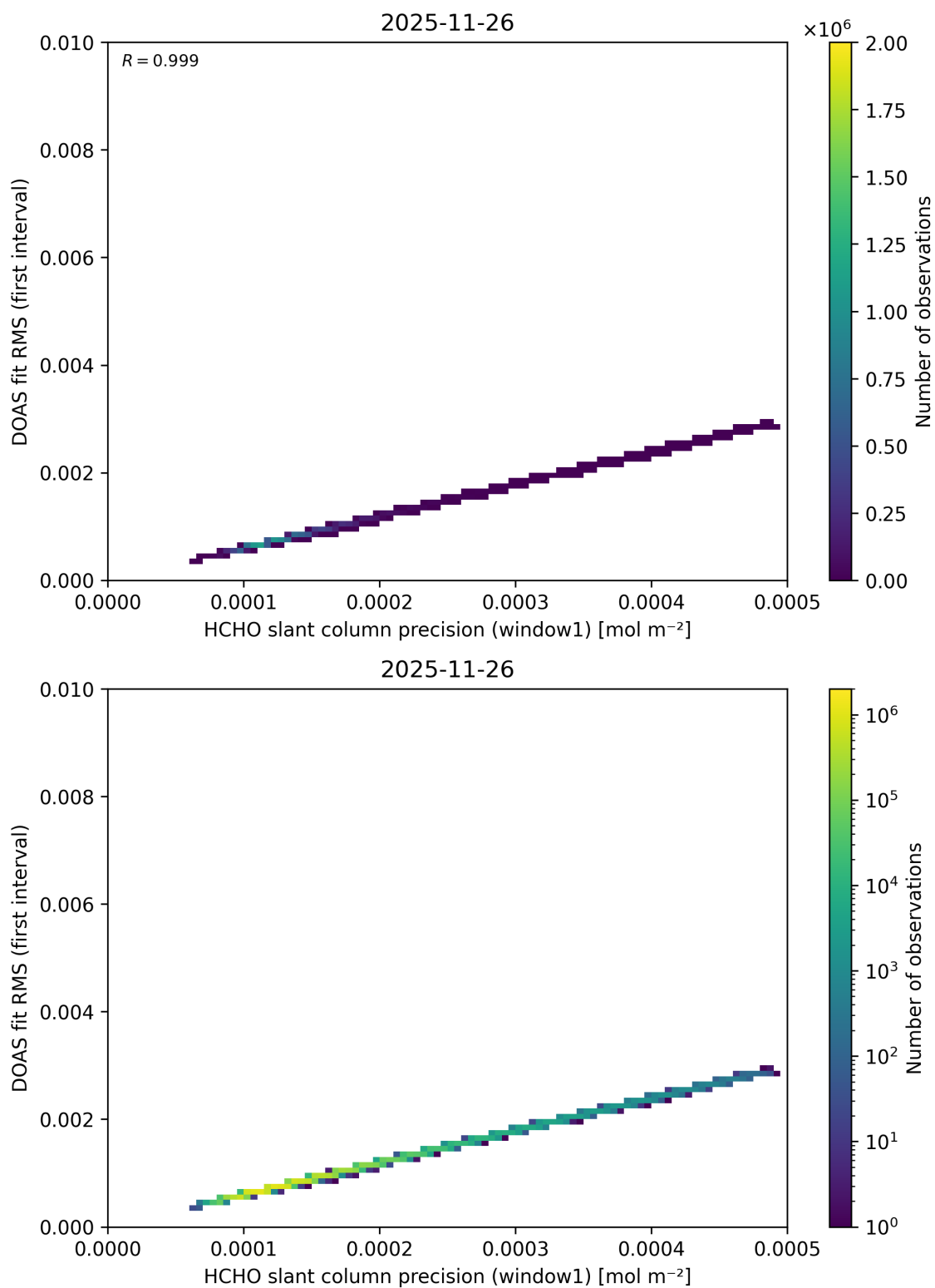
Figure 99: Scatter density plot of “HCHO slant column precision (window1)” against “DOAS fit RMS (first interval)” for 2025-11-25 to 2025-11-27.
