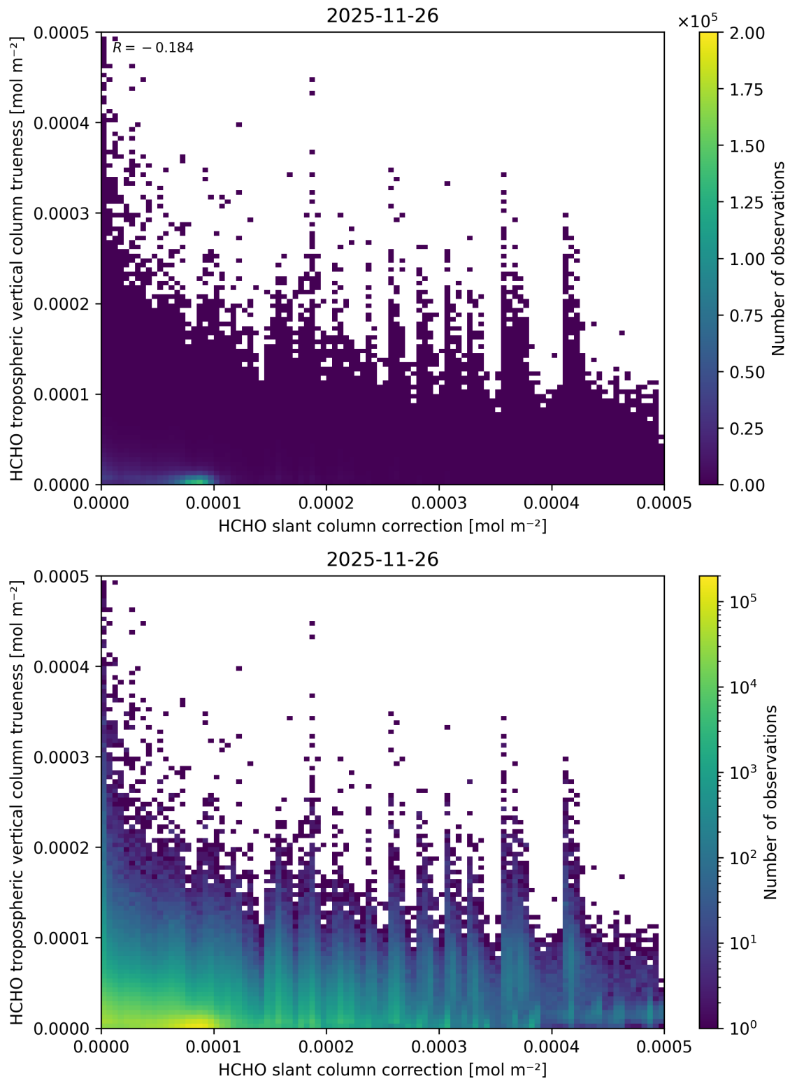
Figure 87: Scatter density plot of “HCHO slant column correction” against “HCHO tropospheric vertical column trueness” for 2025-11-25 to 2025-11-27.
