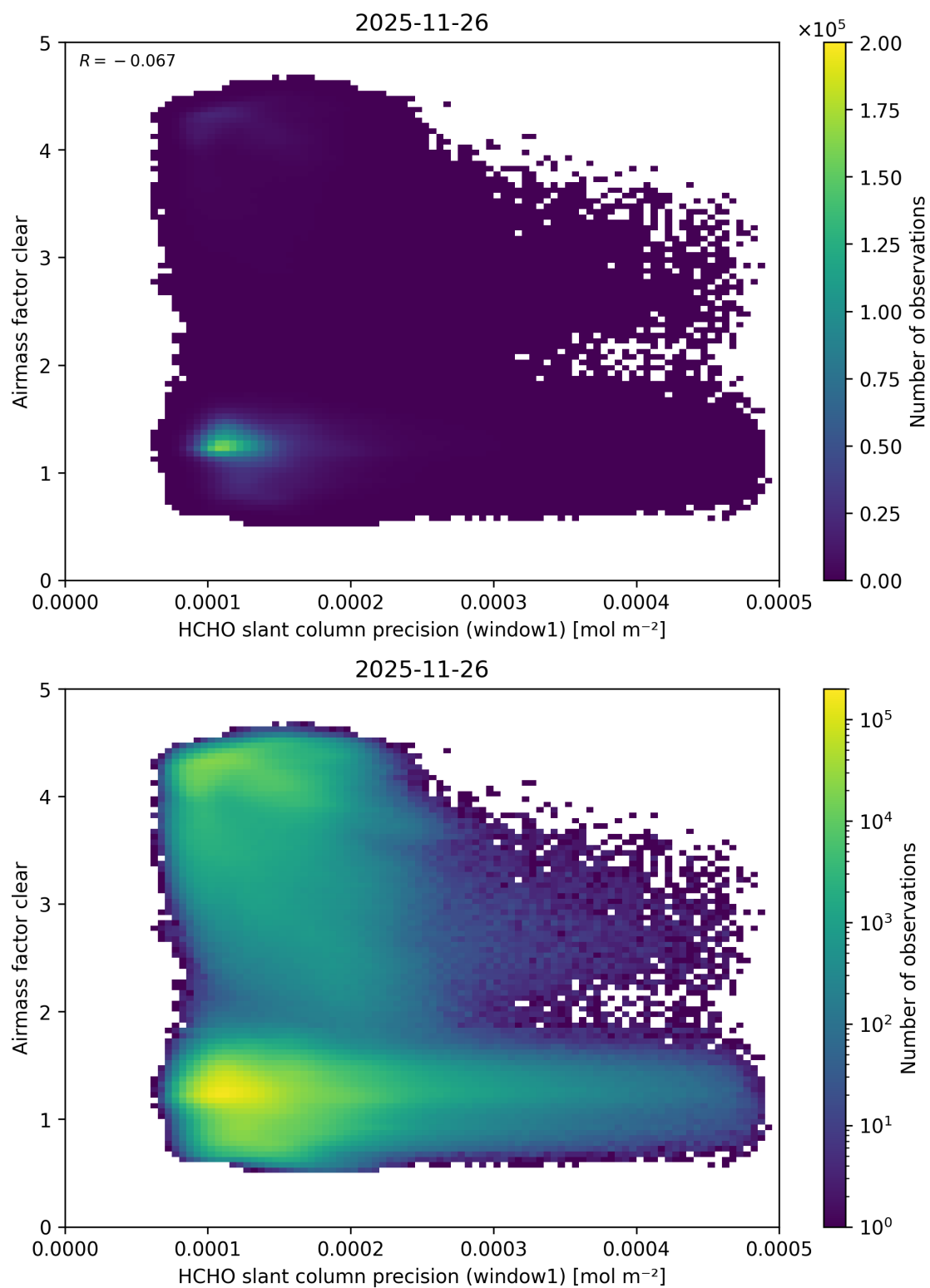
Figure 102: Scatter density plot of “HCHO slant column precision (window1)” against “Airmass factor clear” for 2025-11-25 to 2025-11-27.
