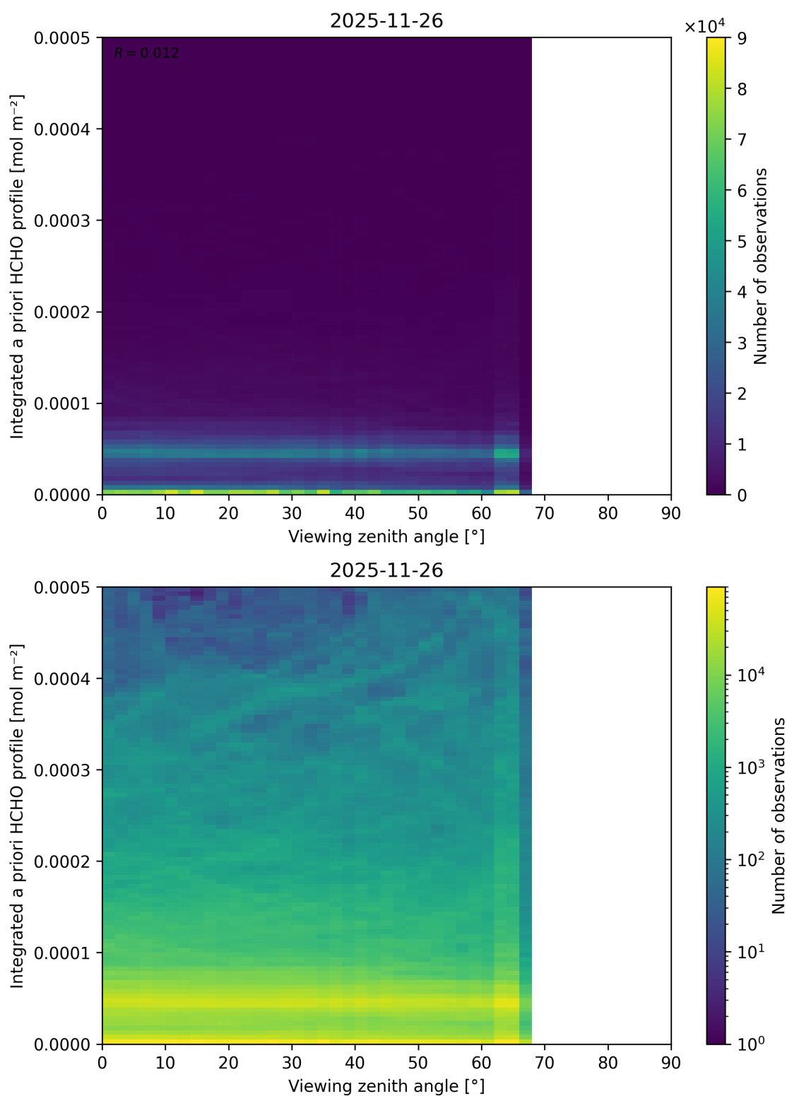
Figure 216: Scatter density plot of “Viewing zenith angle” against “Integrated a priori HCHO profile” for 2025-11-25 to 2025-11-27.
