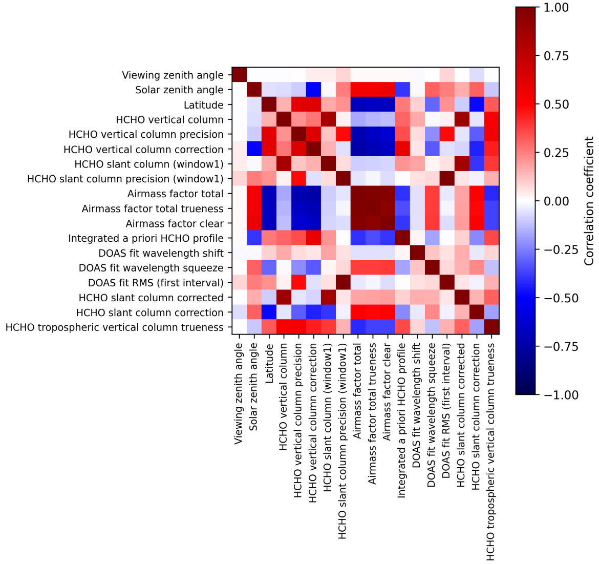
Figure 2: Map of correlation matrix for 2025-11-25 to 2025-11-27.
