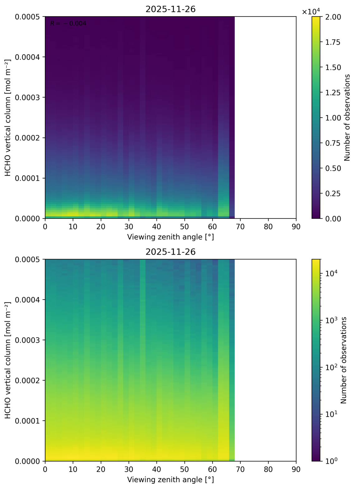
Figure 212: Scatter density plot of “Viewing zenith angle” against “HCHO vertical column” for 2025-11-25 to 2025-11-27.
