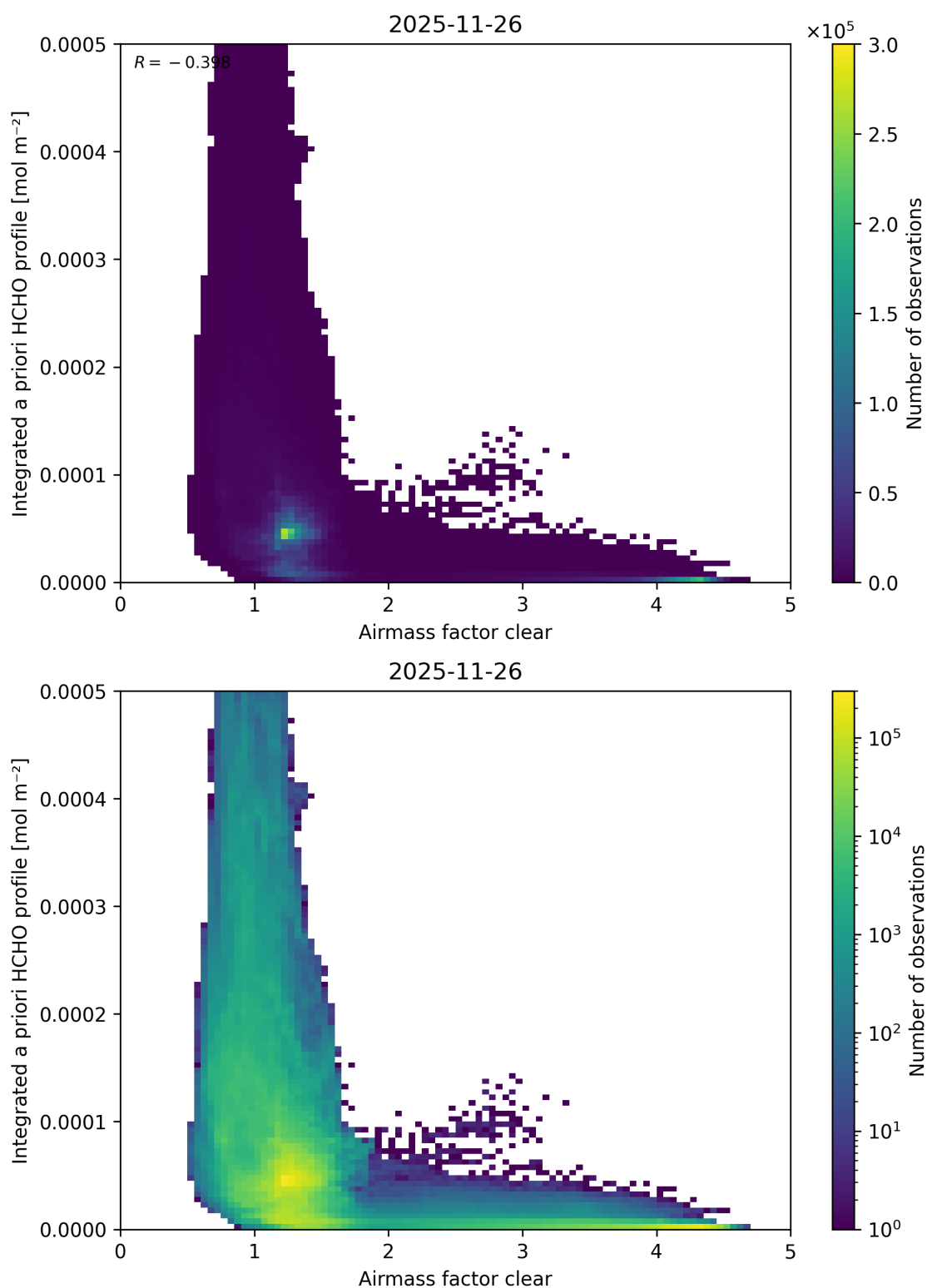
Figure 84: Scatter density plot of “Airmass factor clear” against “Integrated a priori HCHO profile” for 2025-11-25 to 2025-11-27.
