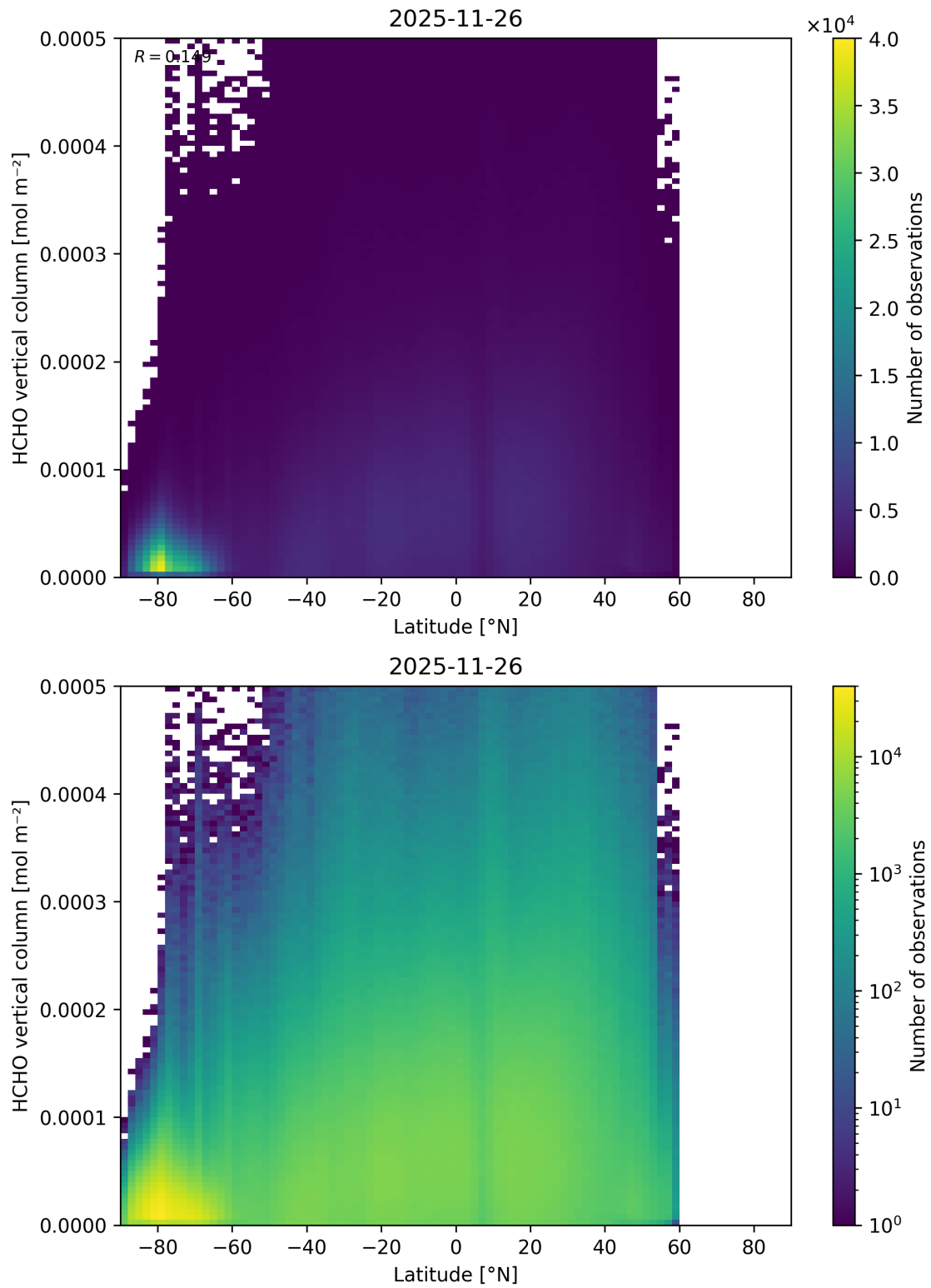
Figure 181: Scatter density plot of “Latitude” against “HCHO vertical column” for 2025-11-25 to 2025-11-27.
