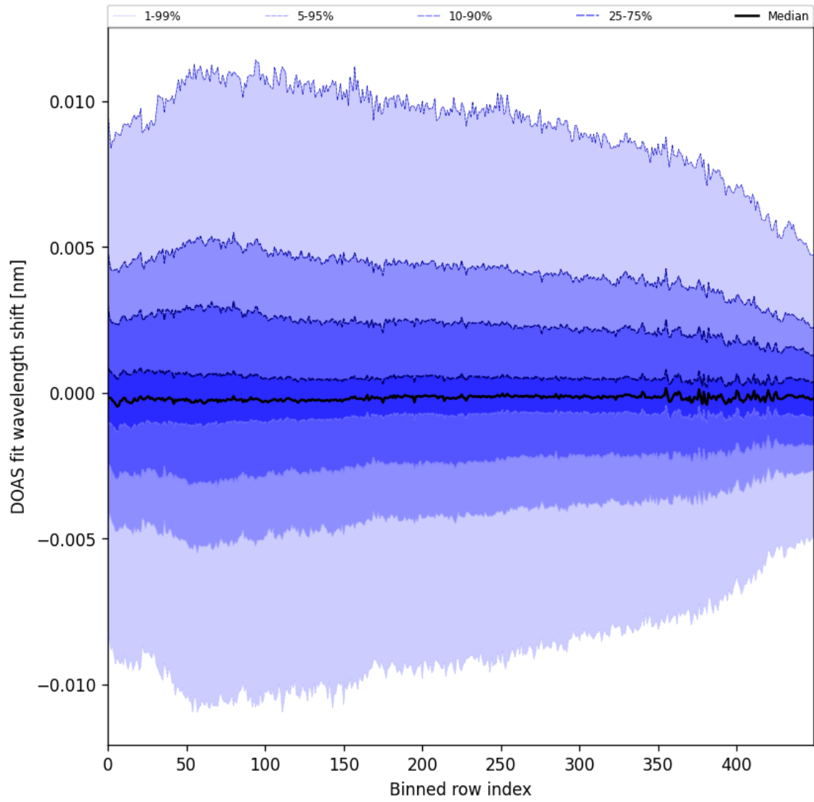
Figure 61: Along track statistics of “DOAS fit wavelength shift” for 2025-11-25 to 2025-11-27
