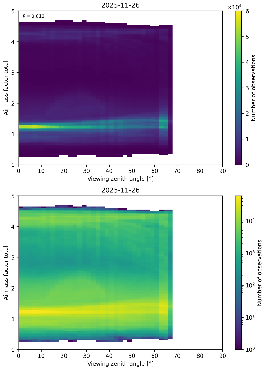
Figure 210: Scatter density plot of “Viewing zenith angle” against “Airmass factor total” for 2025-11-25 to 2025-11-27.
