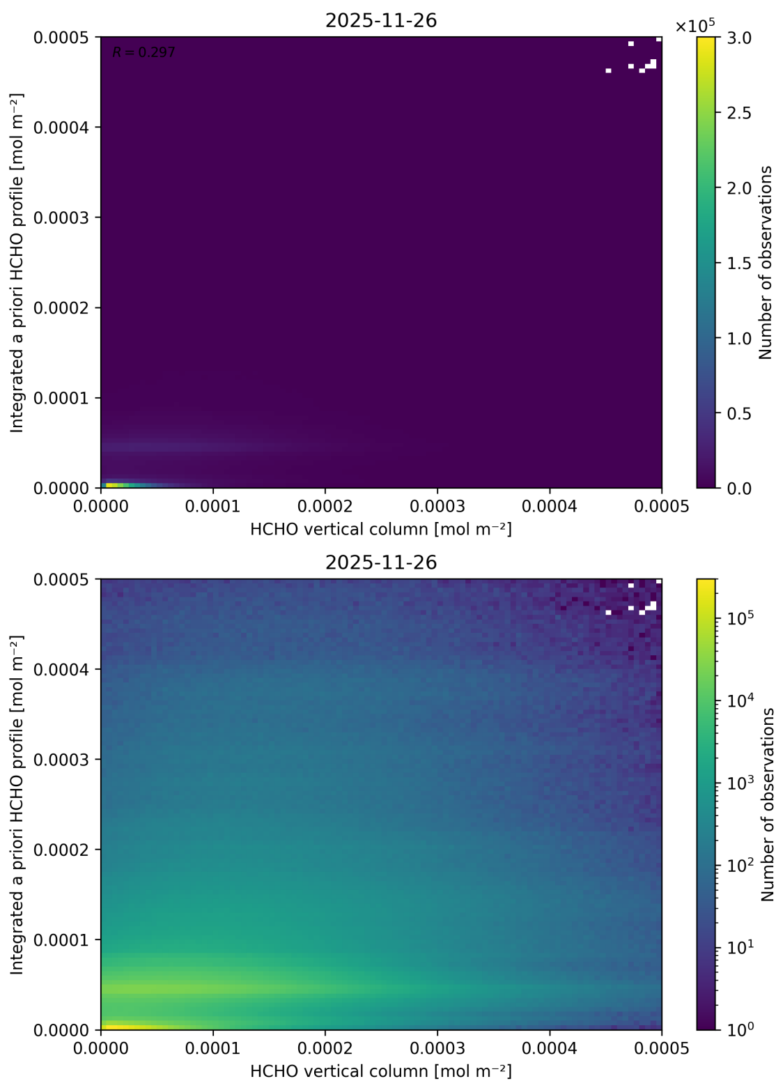
Figure 151: Scatter density plot of “HCHO vertical column” against “Integrated a priori HCHO profile” for 2025-11-25 to 2025-11-27.
