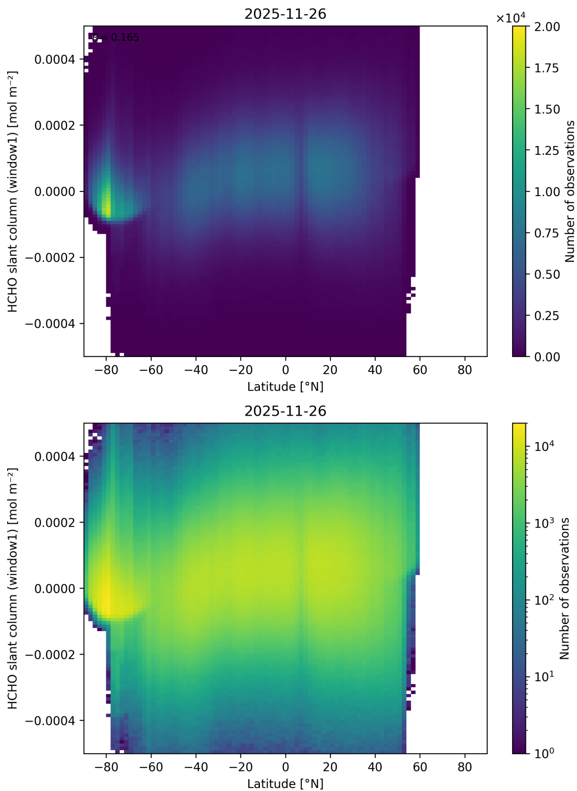
Figure 177: Scatter density plot of “Latitude” against “HCHO slant column (window1)” for 2025-11-25 to 2025-11-27.
