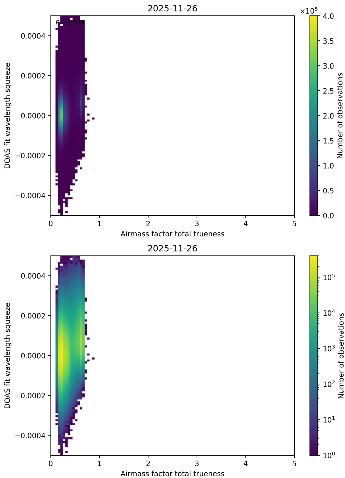
Figure 120: Scatter density plot of “Airmass factor total trueness” against “DOAS fit wavelength squeeze” for 2025-11-25 to 2025-11-27.
