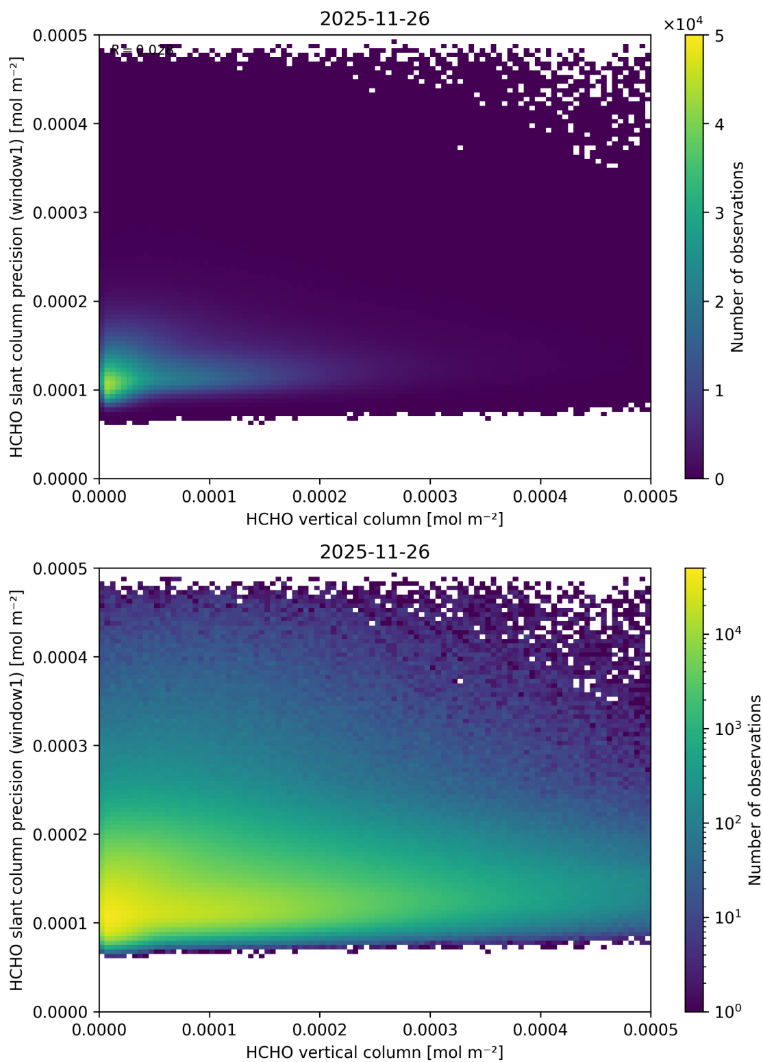
Figure 145: Scatter density plot of “HCHO vertical column” against “HCHO slant column precision (window1)” for 2025-11-25 to 2025-11-27.
