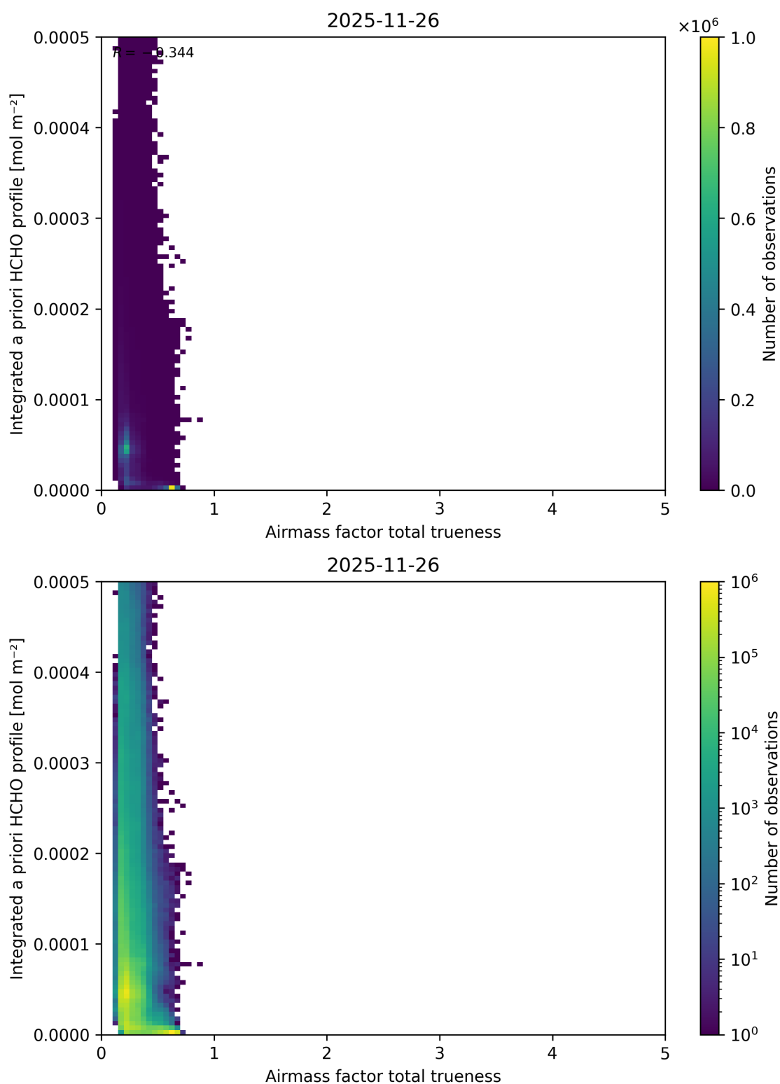
Figure 125: Scatter density plot of “Airmass factor total trueness” against “Integrated a priori HCHO profile” for 2025-11-25 to 2025-11-27.
