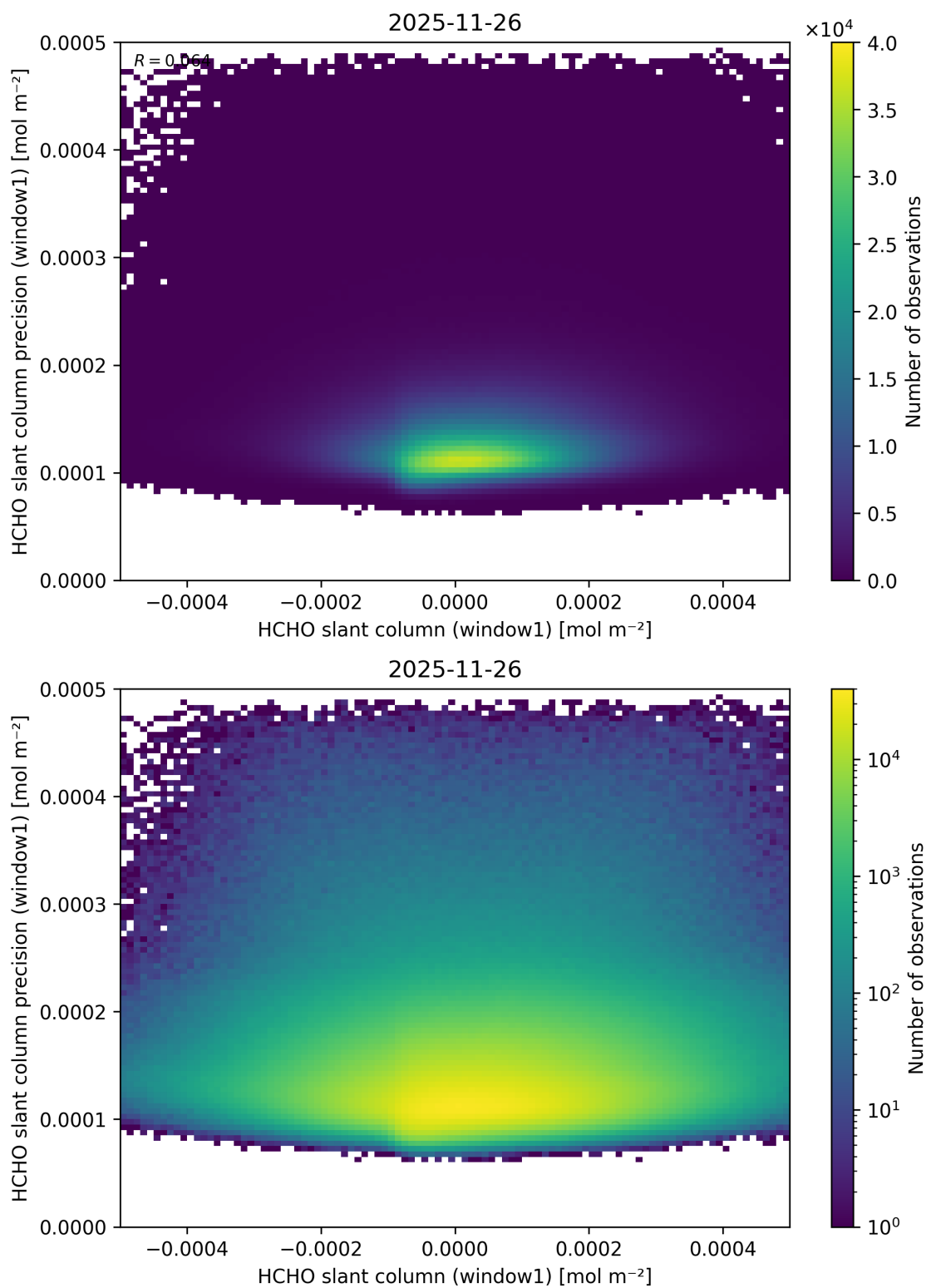
Figure 94: Scatter density plot of “HCHO slant column (window1)” against “HCHO slant column precision (window1)” for 2025-11-25 to 2025-11-27.
