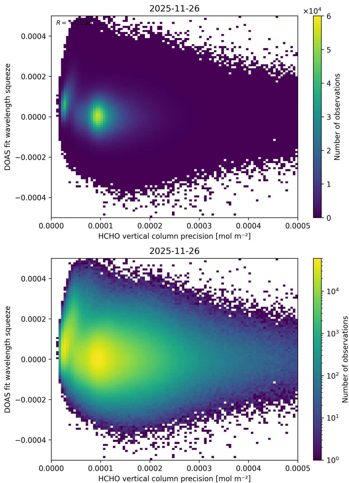
Figure 154: Scatter density plot of “HCHO vertical column precision” against “DOAS fit wavelength squeeze” for 2025-11-25 to 2025-11-27.
