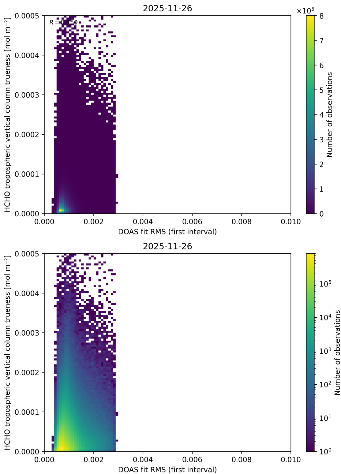
Figure 68: Scatter density plot of “DOAS fit RMS (first interval)” against “HCHO tropospheric vertical column trueness” for 2025-11-25 to 2025-11-27.
