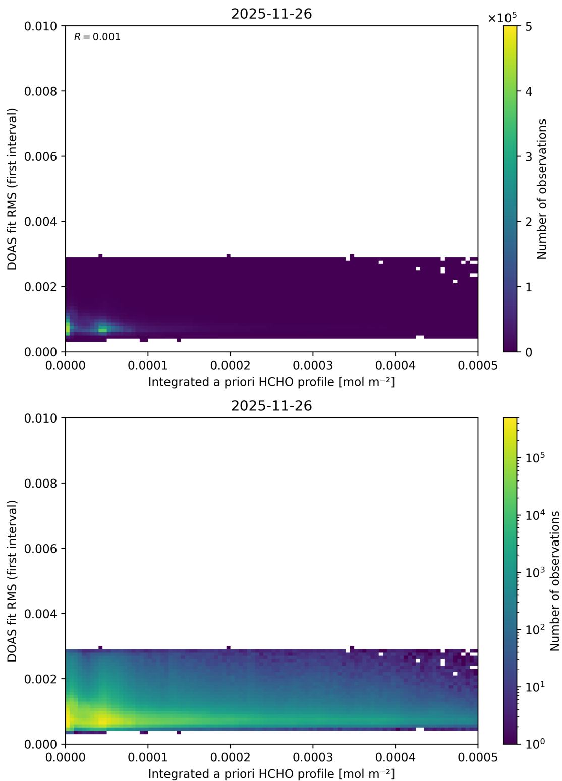
Figure 165: Scatter density plot of “Integrated a priori HCHO profile” against “DOAS fit RMS (first interval)” for 2025-11-25 to 2025-11-27.
