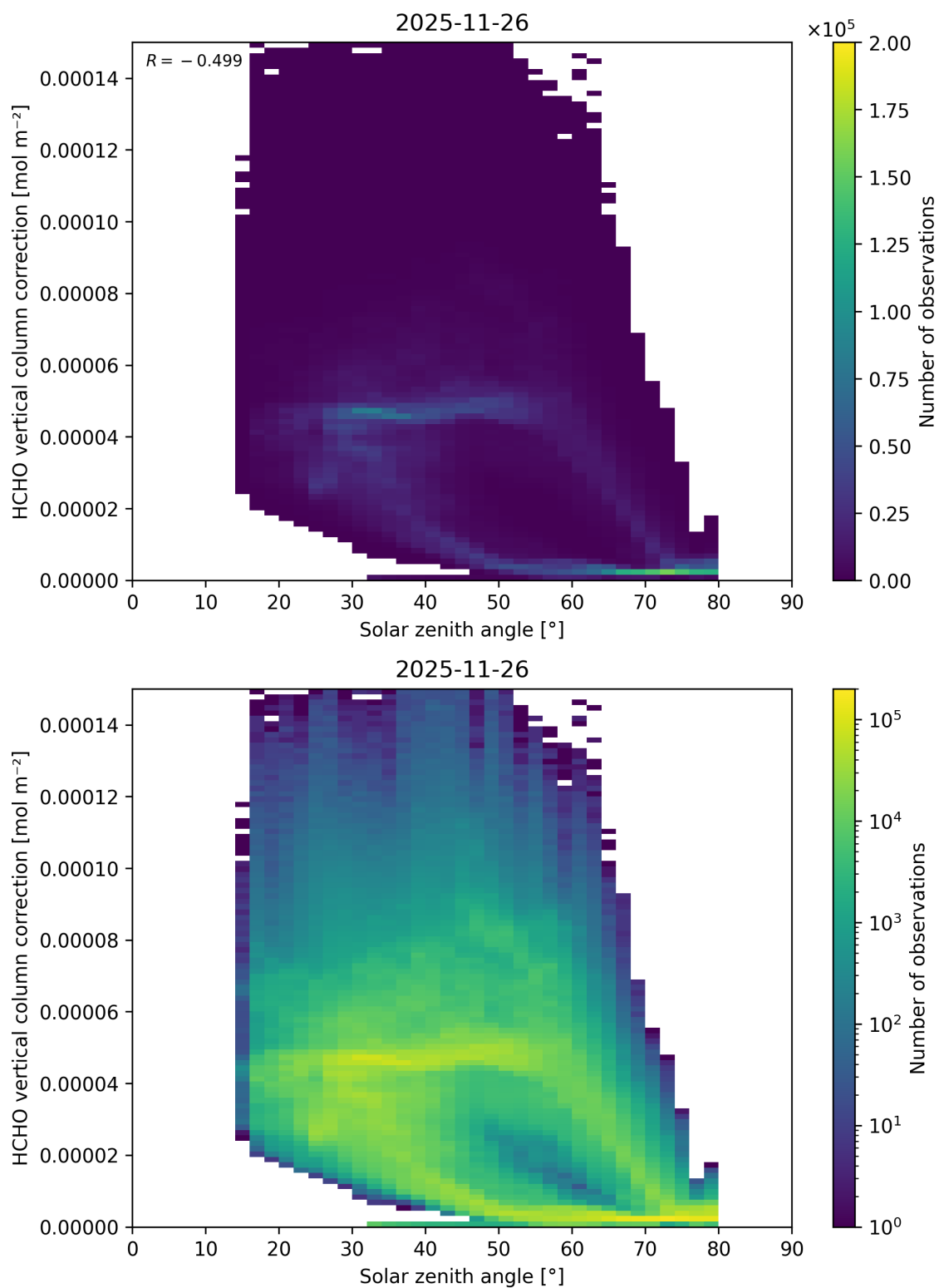
Figure 197: Scatter density plot of “Solar zenith angle” against “HCHO vertical column correction” for 2025-11-25 to 2025-11-27.
