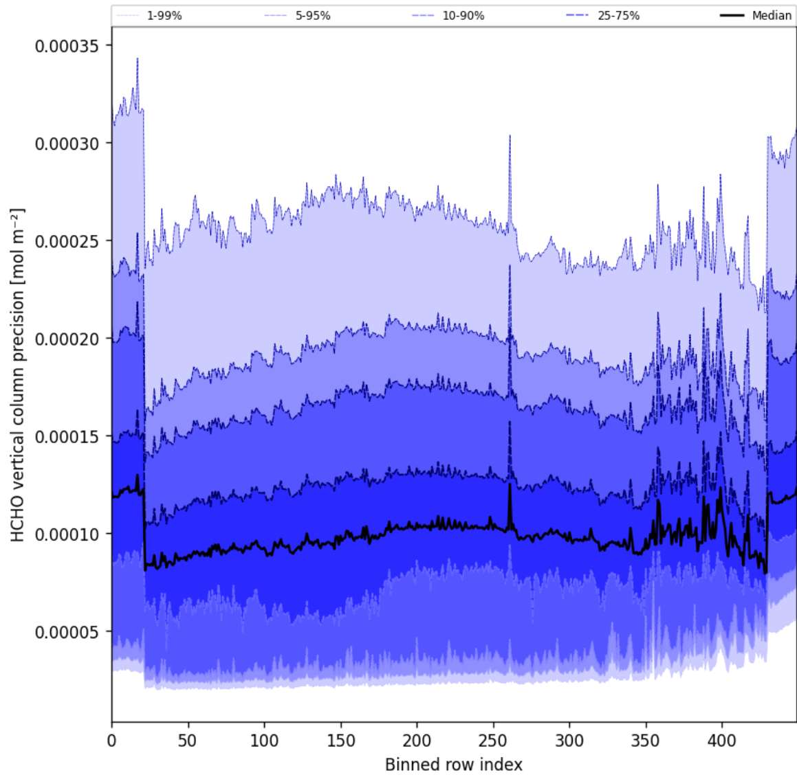
Figure 53: Along track statistics of “HCHO vertical column precision” for 2025-11-25 to 2025-11-27
