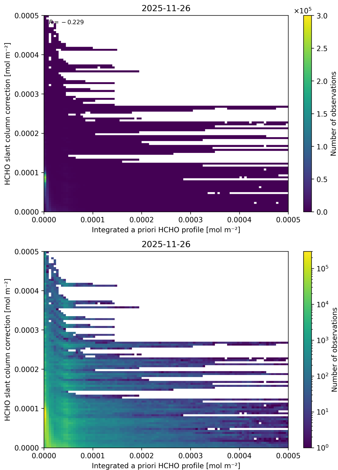
Figure 169: Scatter density plot of “Integrated a priori HCHO profile” against “HCHO slant column correction” for 2025-11-25 to 2025-11-27.
