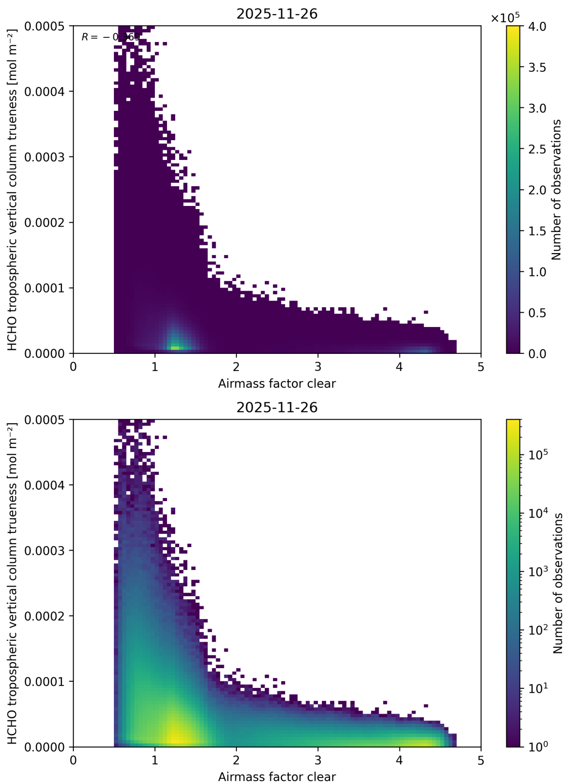
Figure 83: Scatter density plot of “Airmass factor clear” against “HCHO tropospheric vertical column trueeness” for 2025-11-25 to 2025-11-27.
