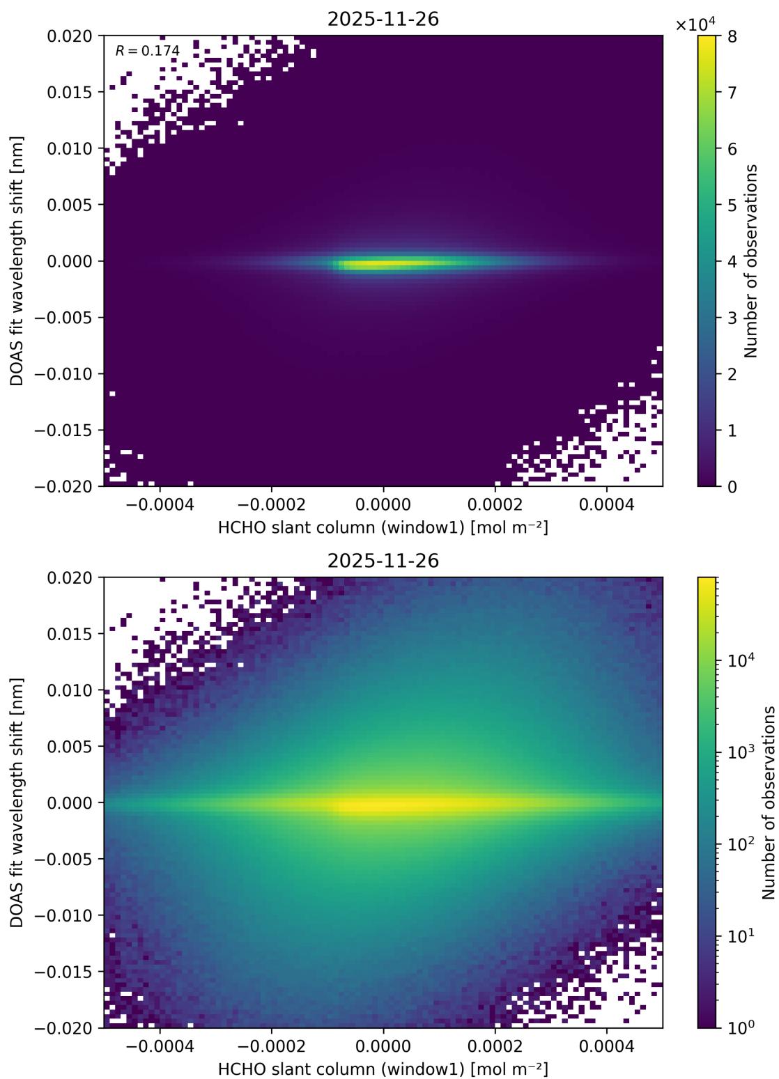
Figure 89: Scatter density plot of “HCHO slant column (window1)” against “DOAS fit wavelength shift” for 2025-11-25 to 2025-11-27.
