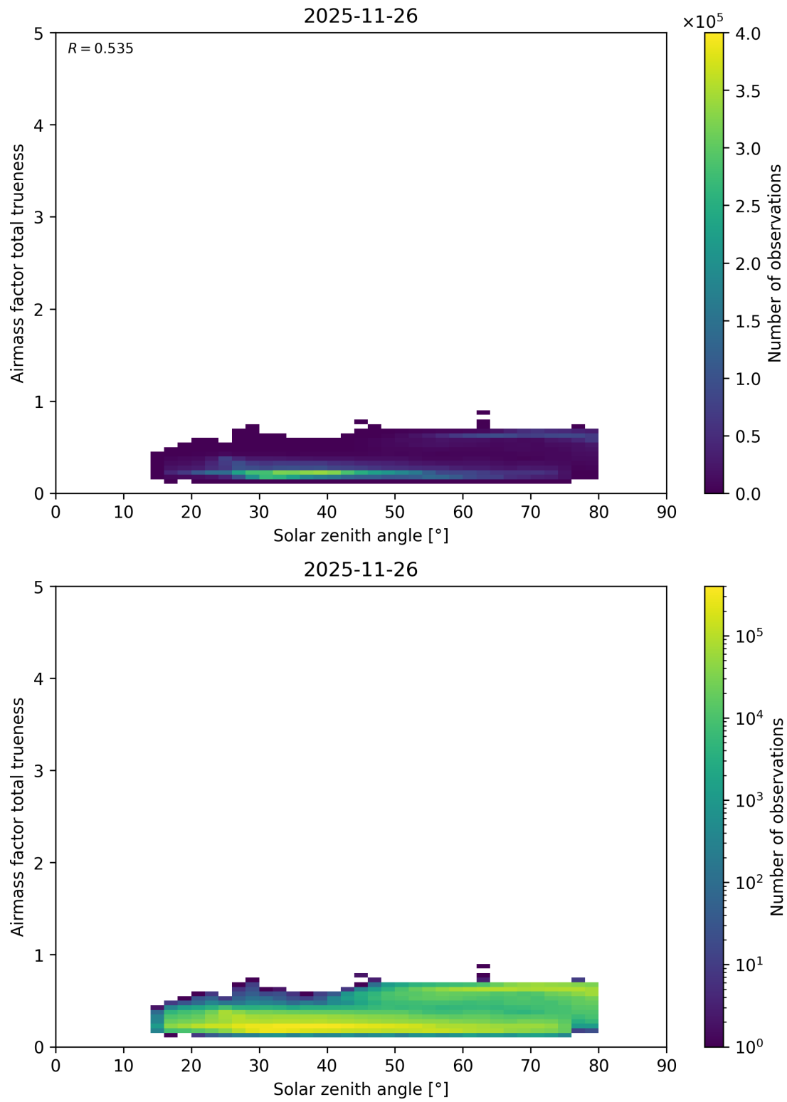
Figure 195: Scatter density plot of “Solar zenith angle” against “Airmass factor total trueneess” for 2025-11-25 to 2025-11-27.
