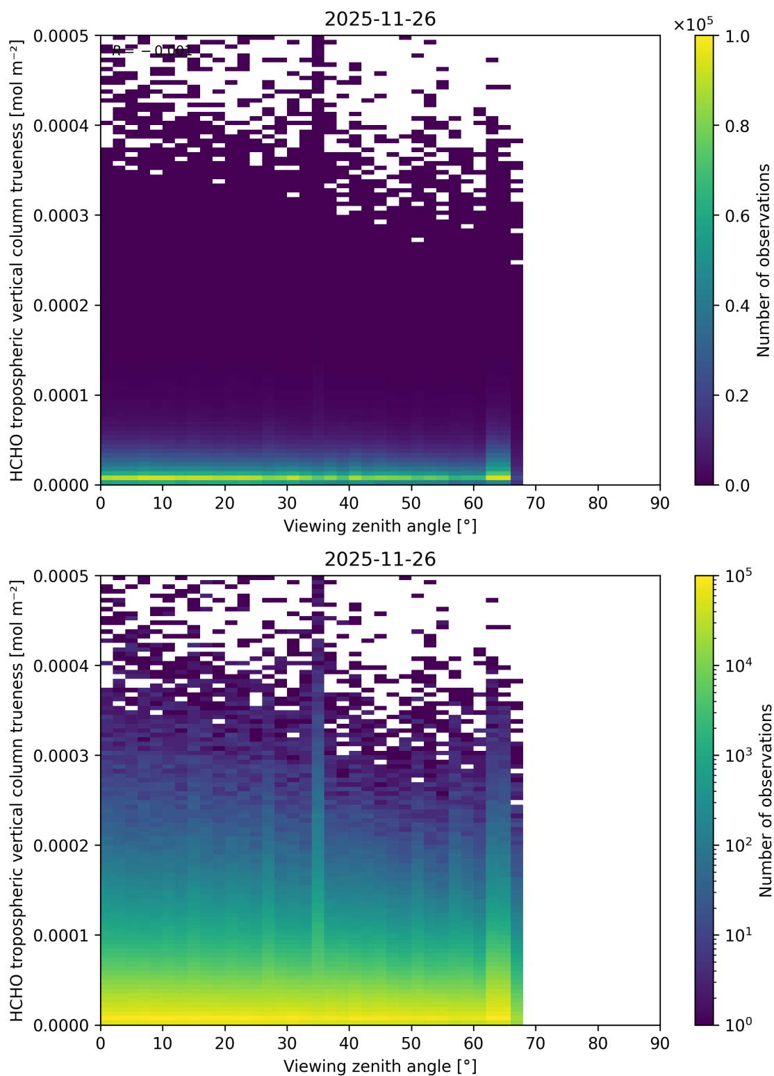
Figure 215: Scatter density plot of “Viewing zenith angle” against “HCHO tropospheric vertical column trueness” for 2025-11-25 to 2025-11-27.
