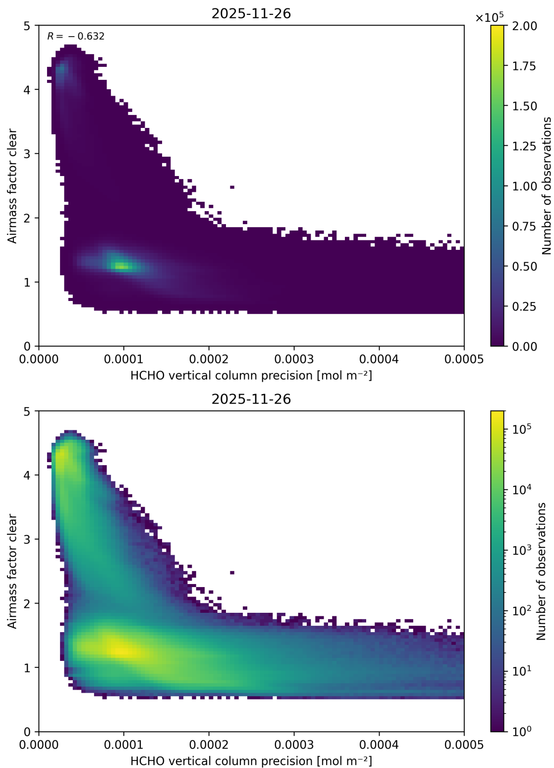
Figure 155: Scatter density plot of “HCHO vertical column precision” against “Airmass factor clear” for 2025-11-25 to 2025-11-27.
