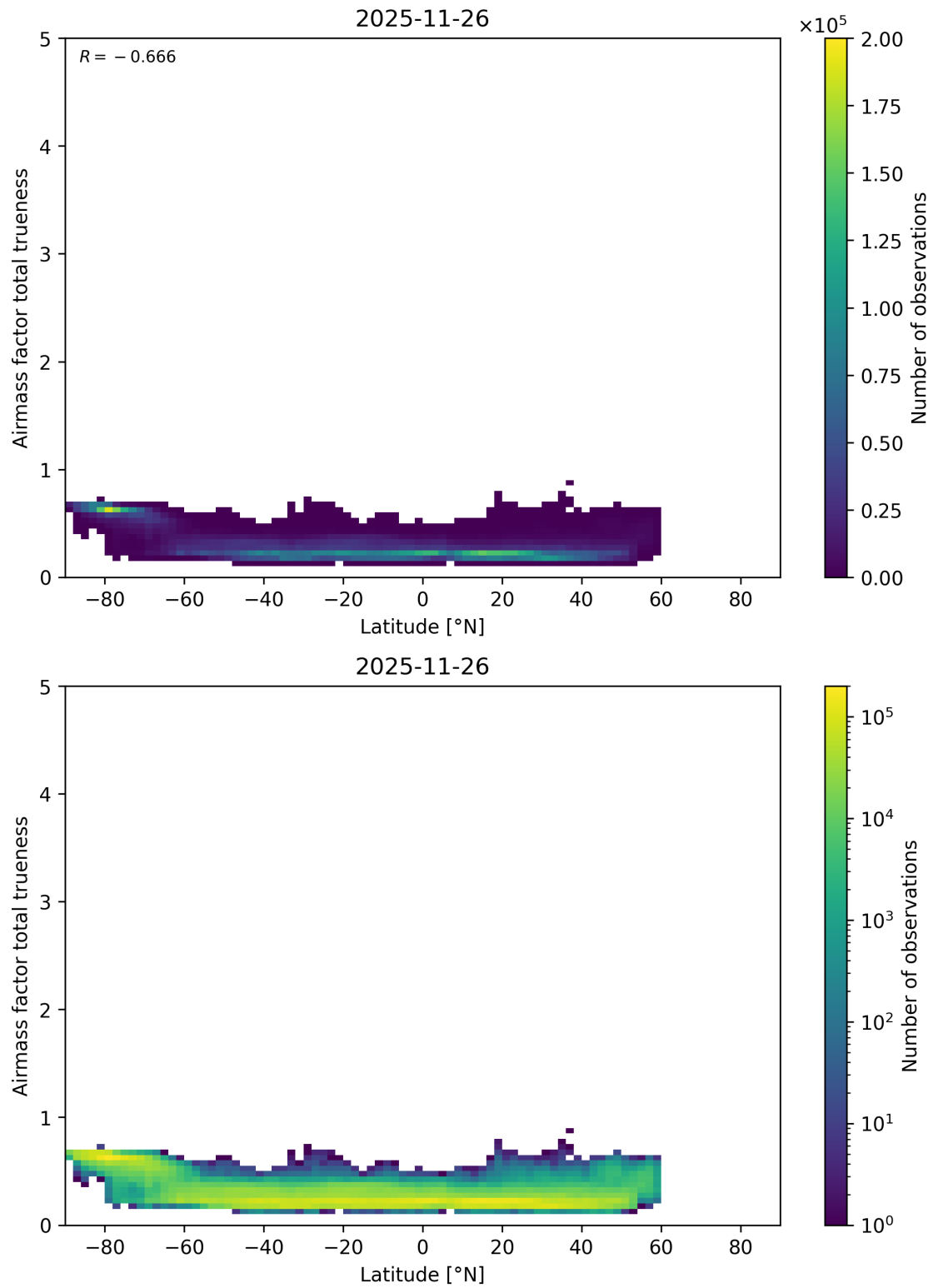
Figure 180: Scatter density plot of “Latitude” against “Airmass factor total trueness” for 2025-11-25 to 2025-11-27.
