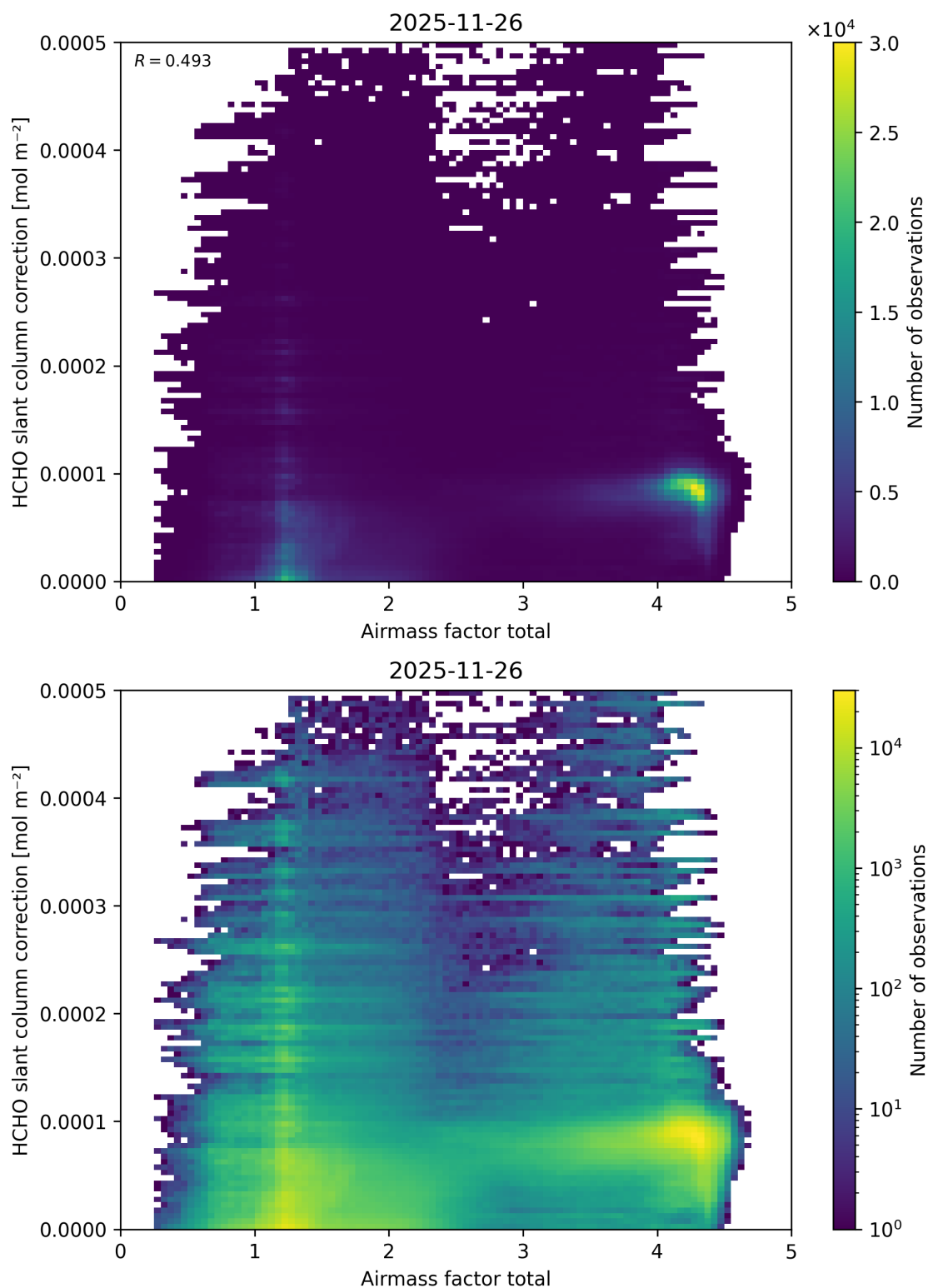
Figure 114: Scatter density plot of “Airmass factor total” against “HCHO slant column correction” for 2025-11-25 to 2025-11-27.
