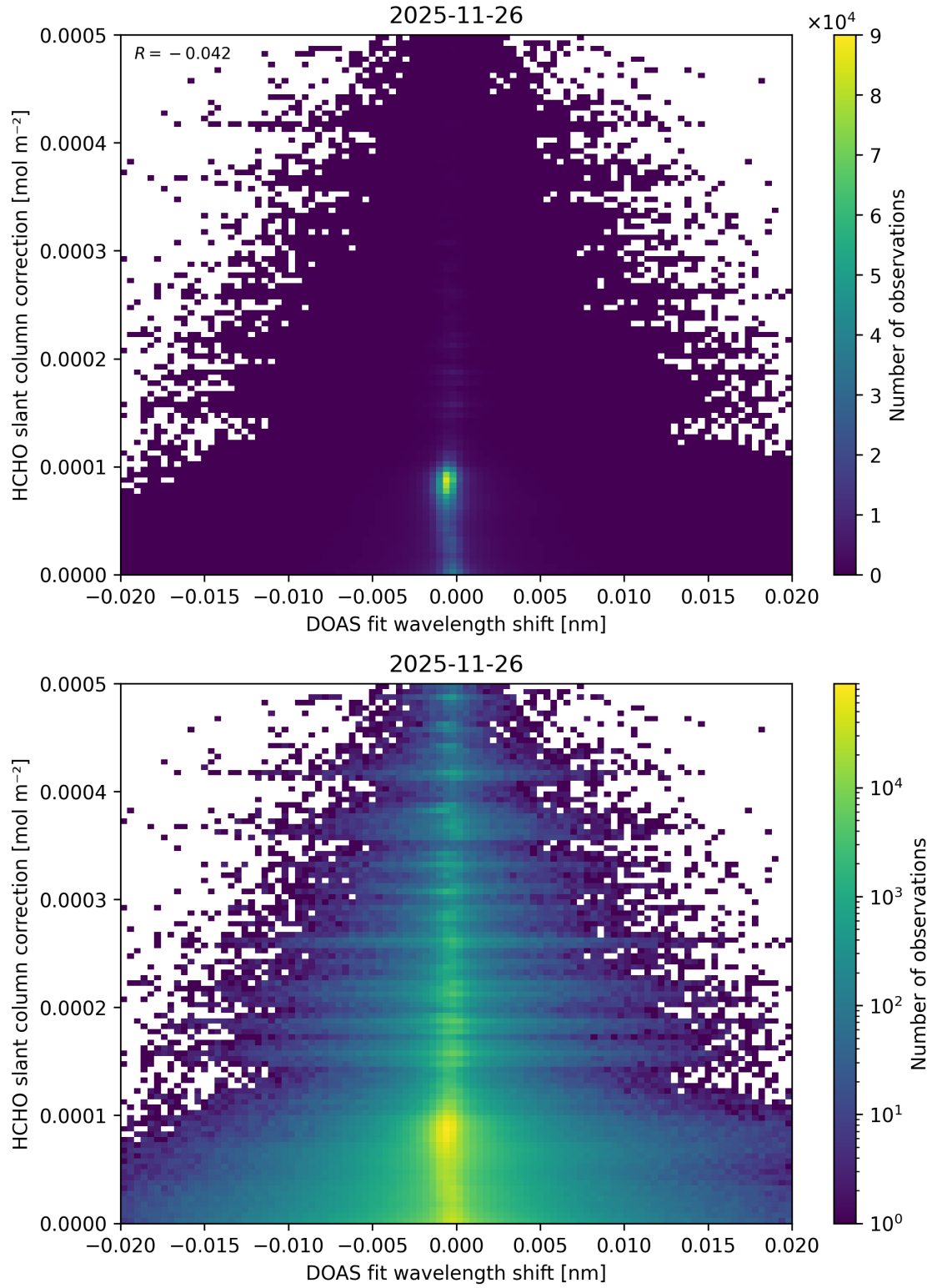
Figure 72: Scatter density plot of “DOAS fit wavelength shift” against “HCHO slant column correction” for 2025-11-25 to 2025-11-27.
