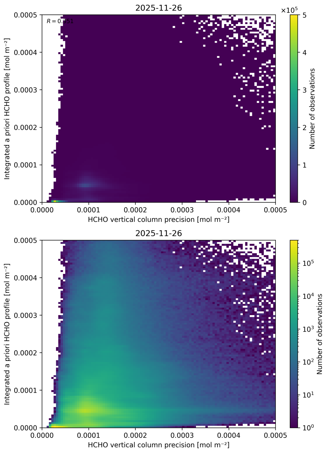
Figure 164: Scatter density plot of “HCHO vertical column precision” against “Integrated a priori HCHO profile” for 2025-11-25 to 2025-11-27.
