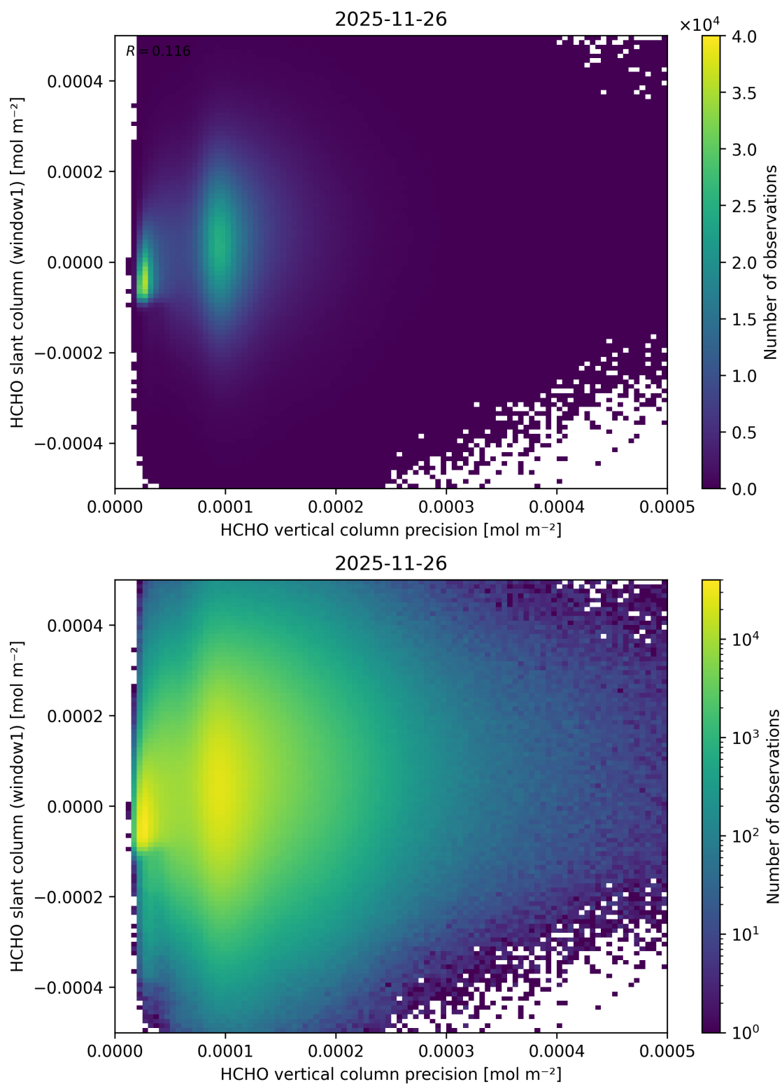
Figure 158: Scatter density plot of “HCHO vertical column precision” against “HCHO slant column (window1)” for 2025-11-25 to 2025-11-27.
