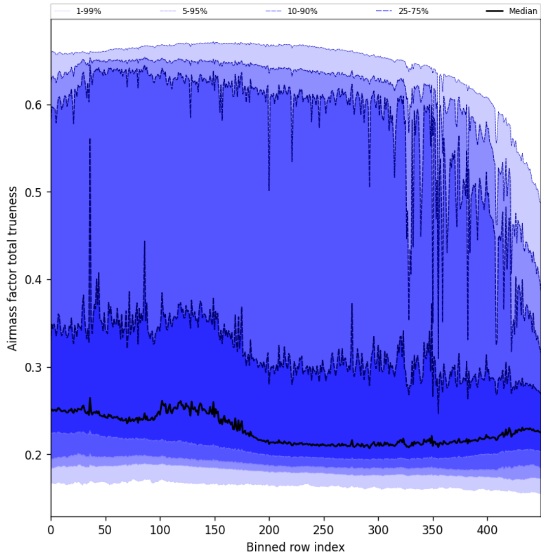
Figure 58: Along track statistics of “Airmass factor total trueness” for 2025-11-25 to 2025-11-27
