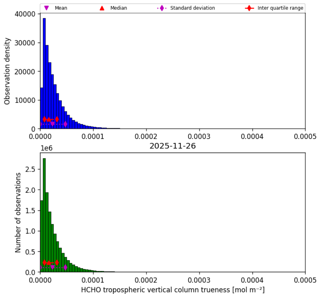
Figure 50: Histogram of “HCHO tropospheric vertical column trueness” for 2025-11-25 to 2025-11-27
