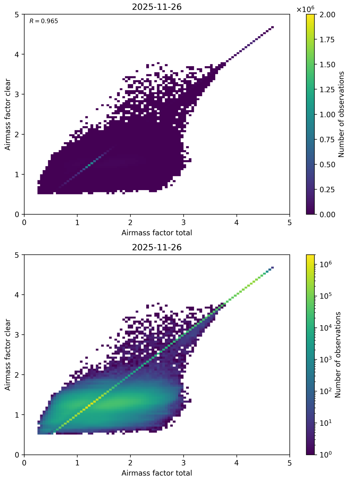
Figure 112: Scatter density plot of “Airmass factor total” against “Airmass factor clear” for 2025-11-25 to 2025-11-27.
