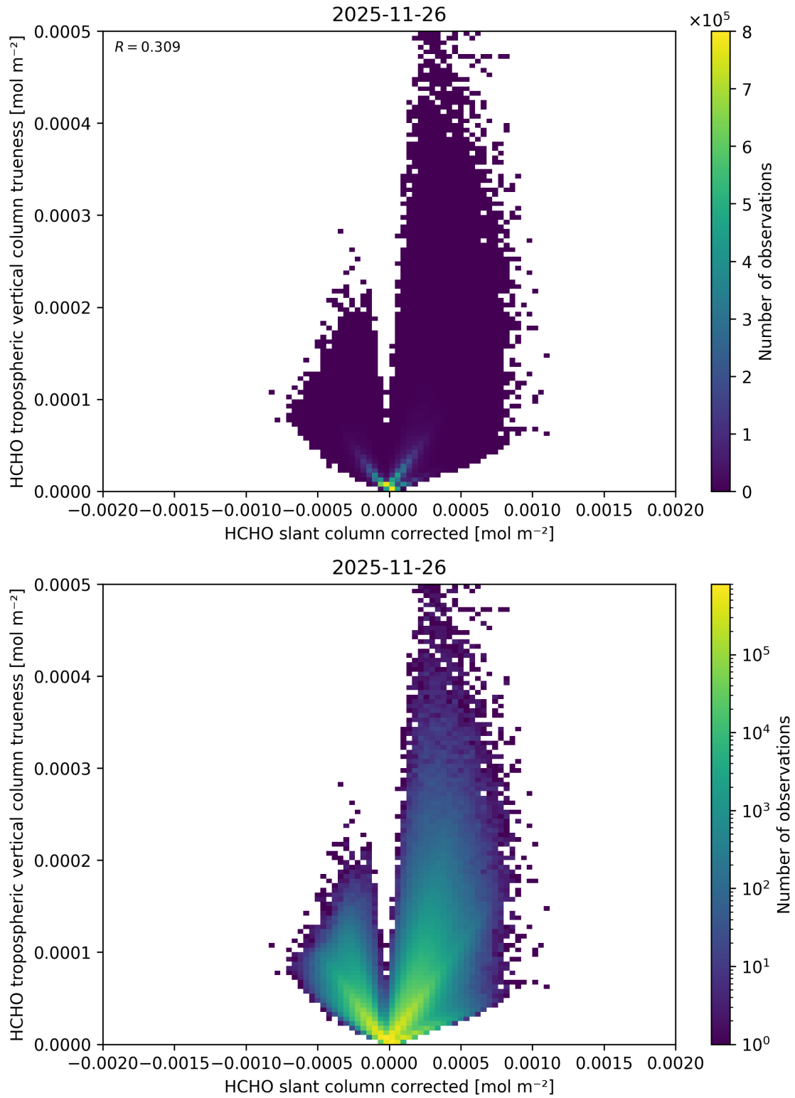
Figure 86: Scatter density plot of “HCHO slant column corrected” against “HCHO tropospheric vertical column trueness” for 2025-11-25 to 2025-11-27.
