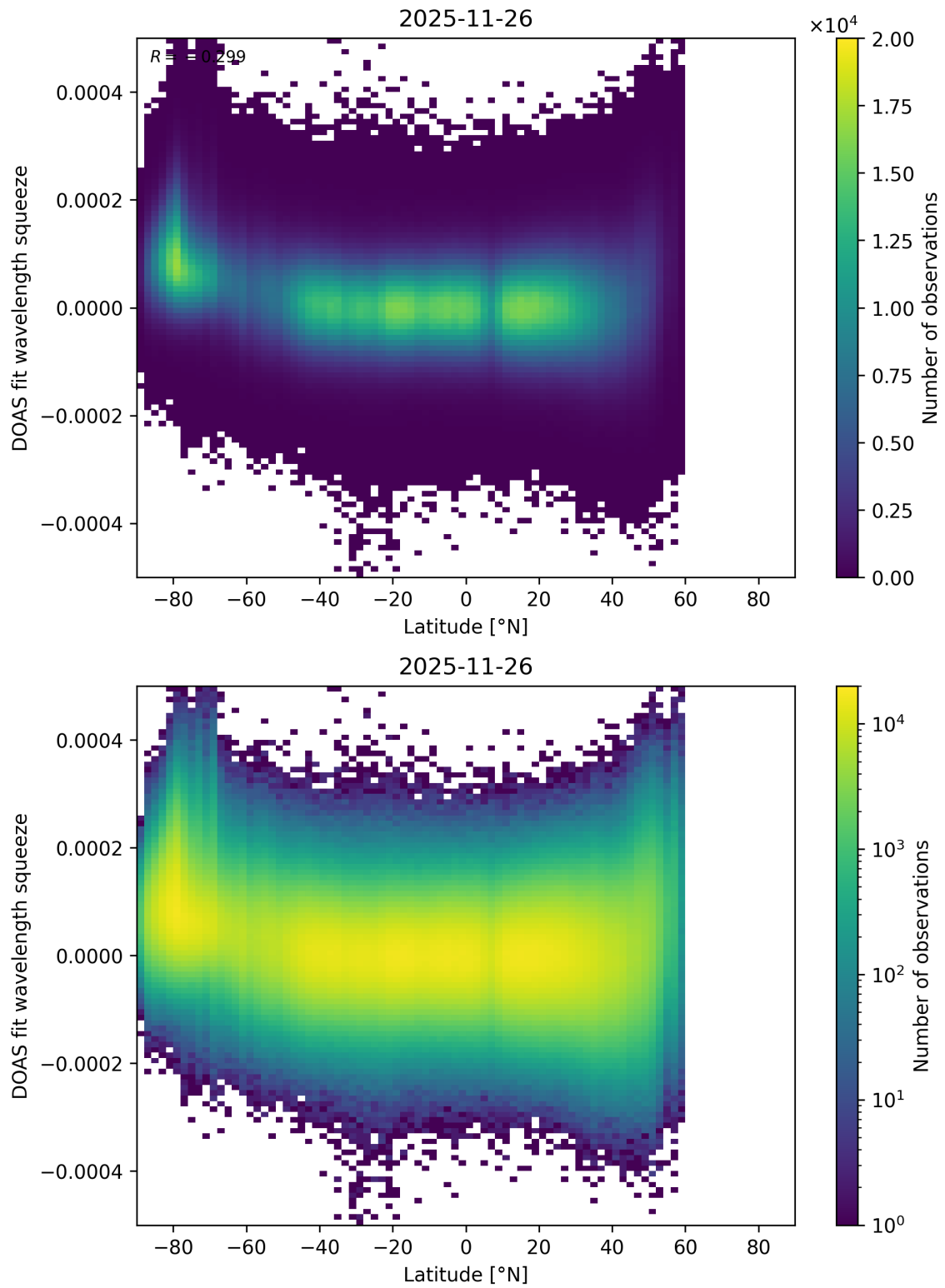
Figure 173: Scatter density plot of “Latitude” against “DOAS fit wavelength squeeze” for 2025-11-25 to 2025-11-27.
