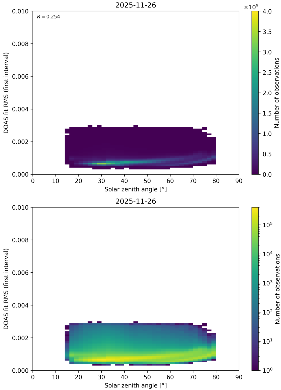
Figure 186: Scatter density plot of “Solar zenith angle” against “DOAS fit RMS (first interval)” for 2025-11-25 to 2025-11-27.
