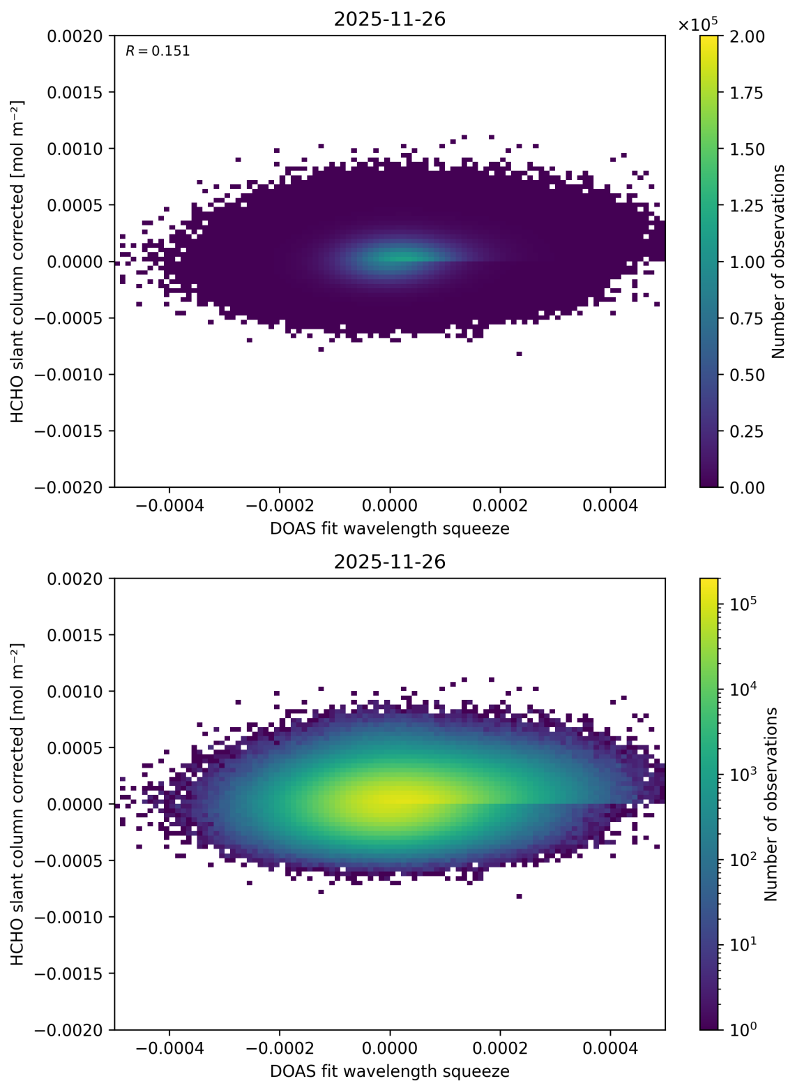
Figure 75: Scatter density plot of “DOAS fit wavelength squeeze” against “HCHO slant column corrected” for 2025-11-25 to 2025-11-27.
