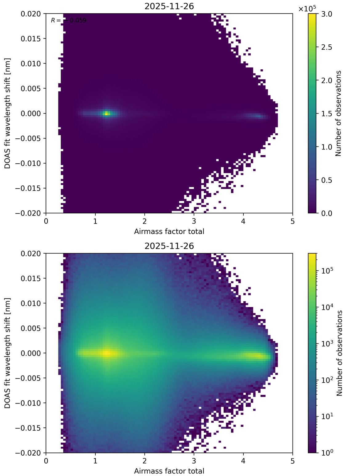
Figure 110: Scatter density plot of “Airmass factor total” against “DOAS fit wavelength shift” for 2025-11-25 to 2025-11-27.
