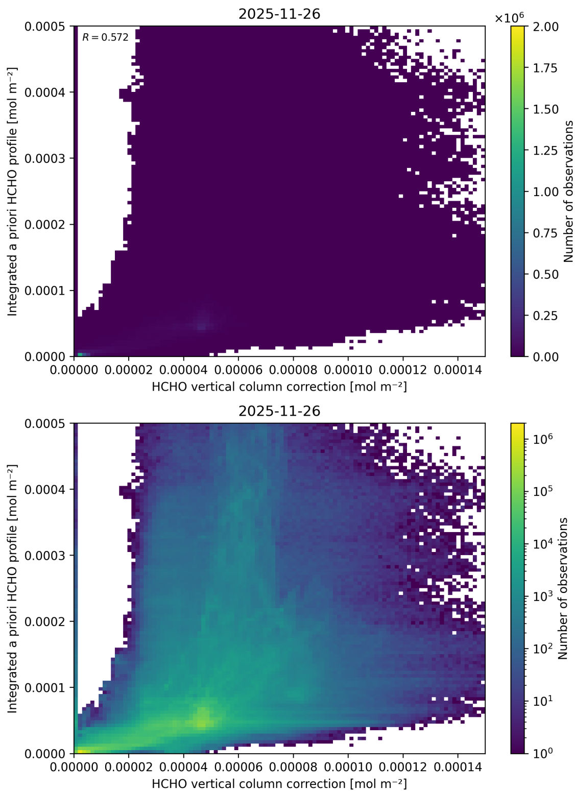
Figure 137: Scatter density plot of “HCHO vertical column correction” against “Integrated a priori HCHO profile” for 2025-11-25 to 2025-11-27.
