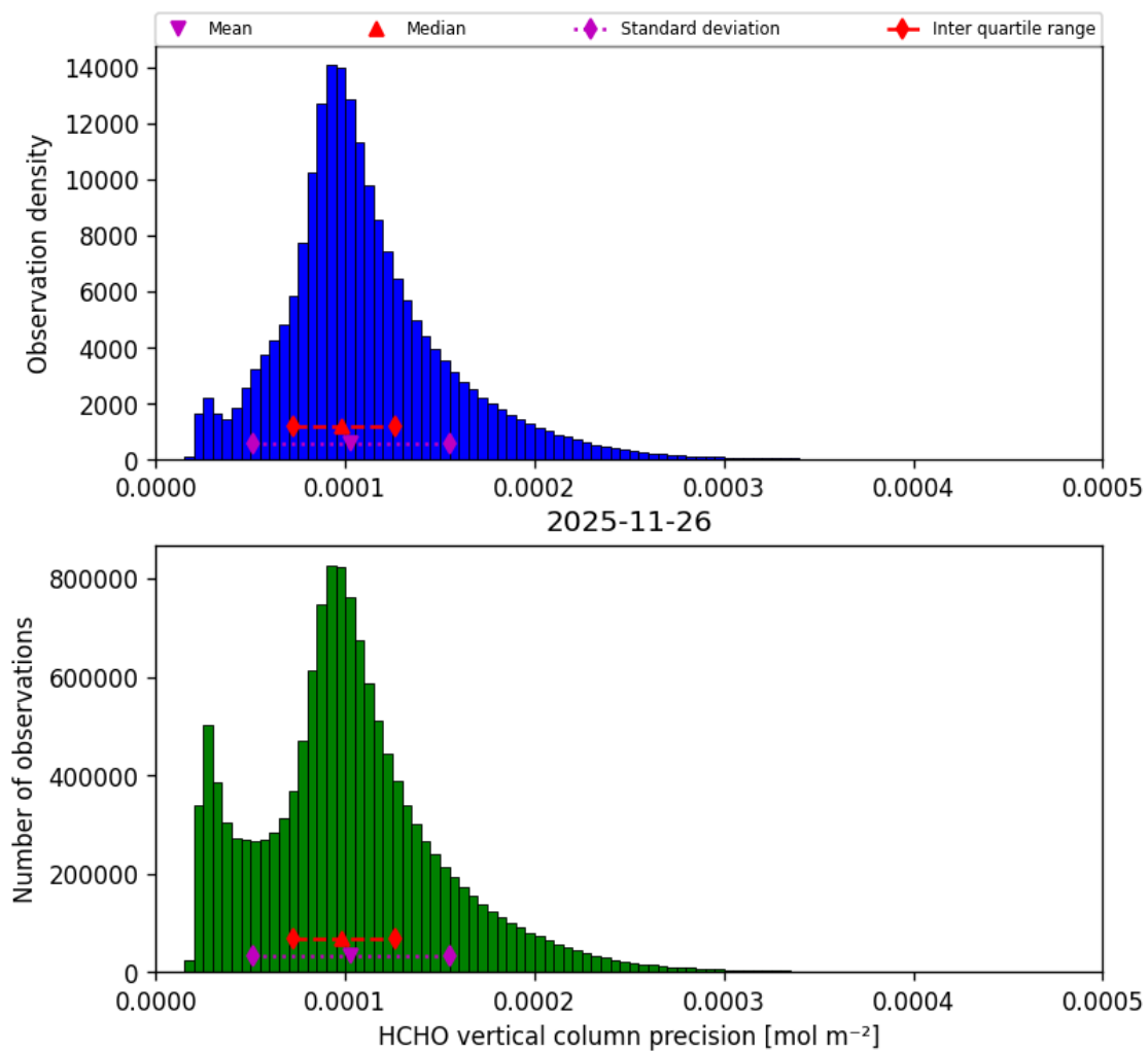
Figure 38: Histogram of “HCHO vertical column precision” for 2025-11-25 to 2025-11-27
