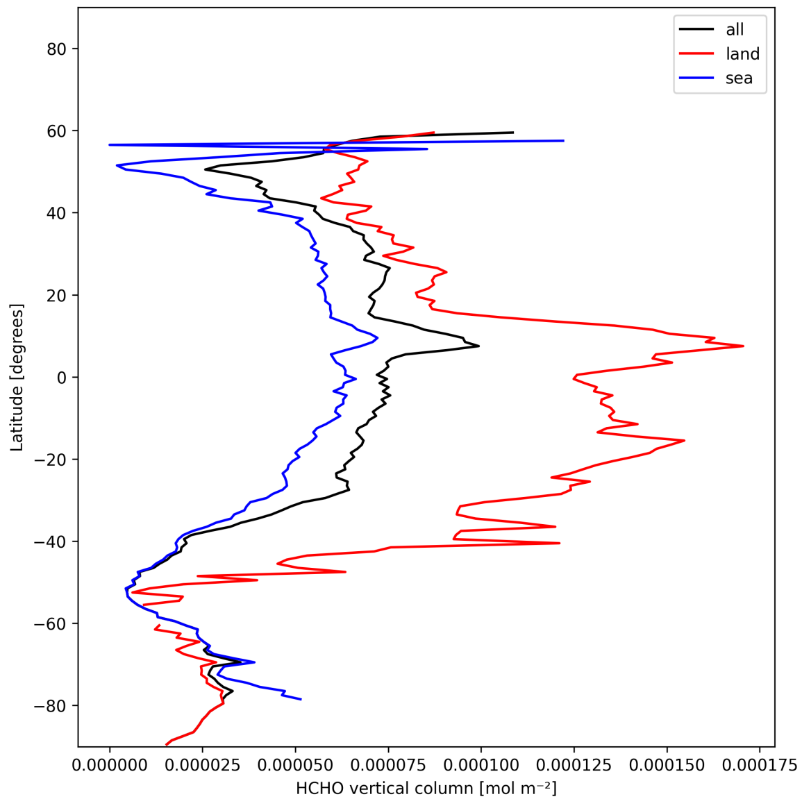
Figure 22: Zonal average of “HCHO vertical column” for 2025-11-25 to 2025-11-27.
