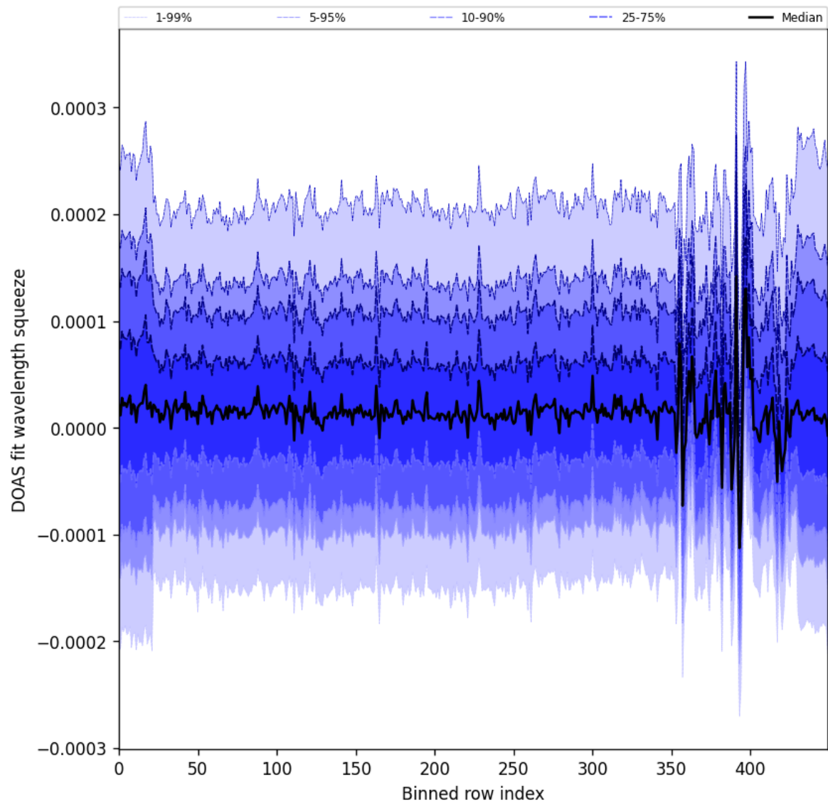
Figure 62: Along track statistics of “DOAS fit wavelength squeeze” for 2025-11-25 to 2025-11-27
