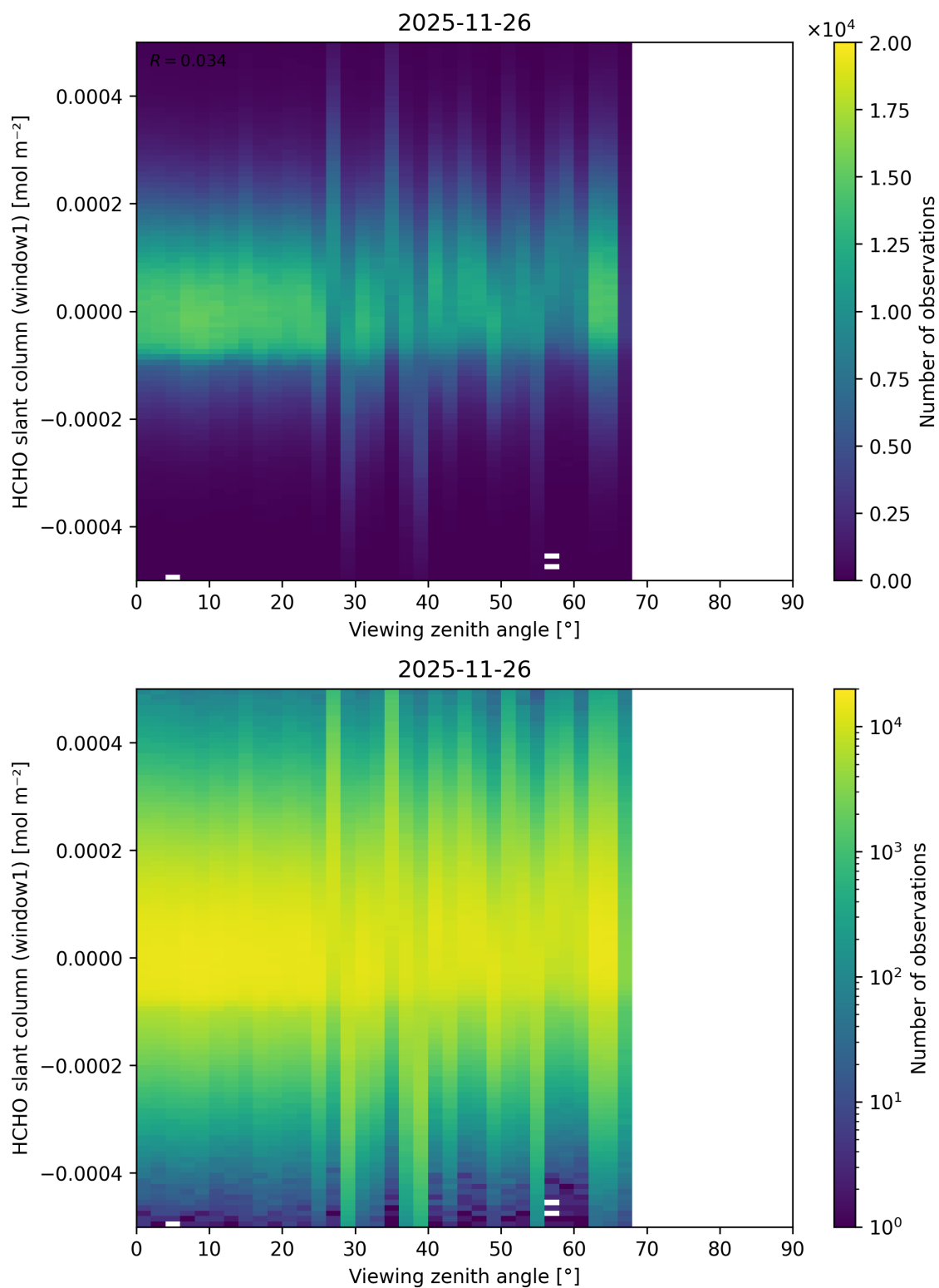
Figure 208: Scatter density plot of “Viewing zenith angle” against “HCHO slant column (window1)” for 2025-11-25 to 2025-11-27.
