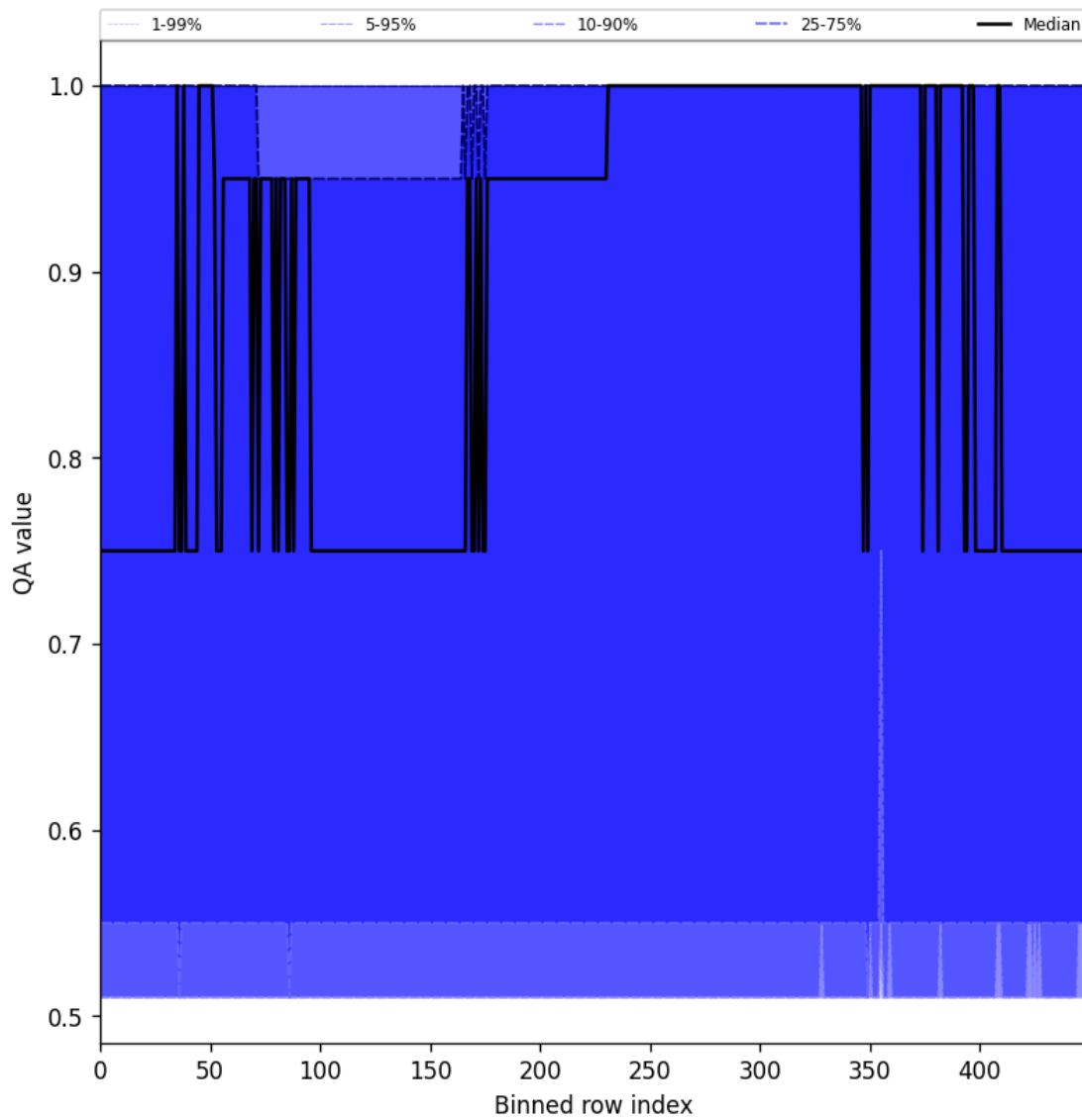
Figure 51: Along track statistics of “QA value” for 2025-11-25 to 2025-11-27
