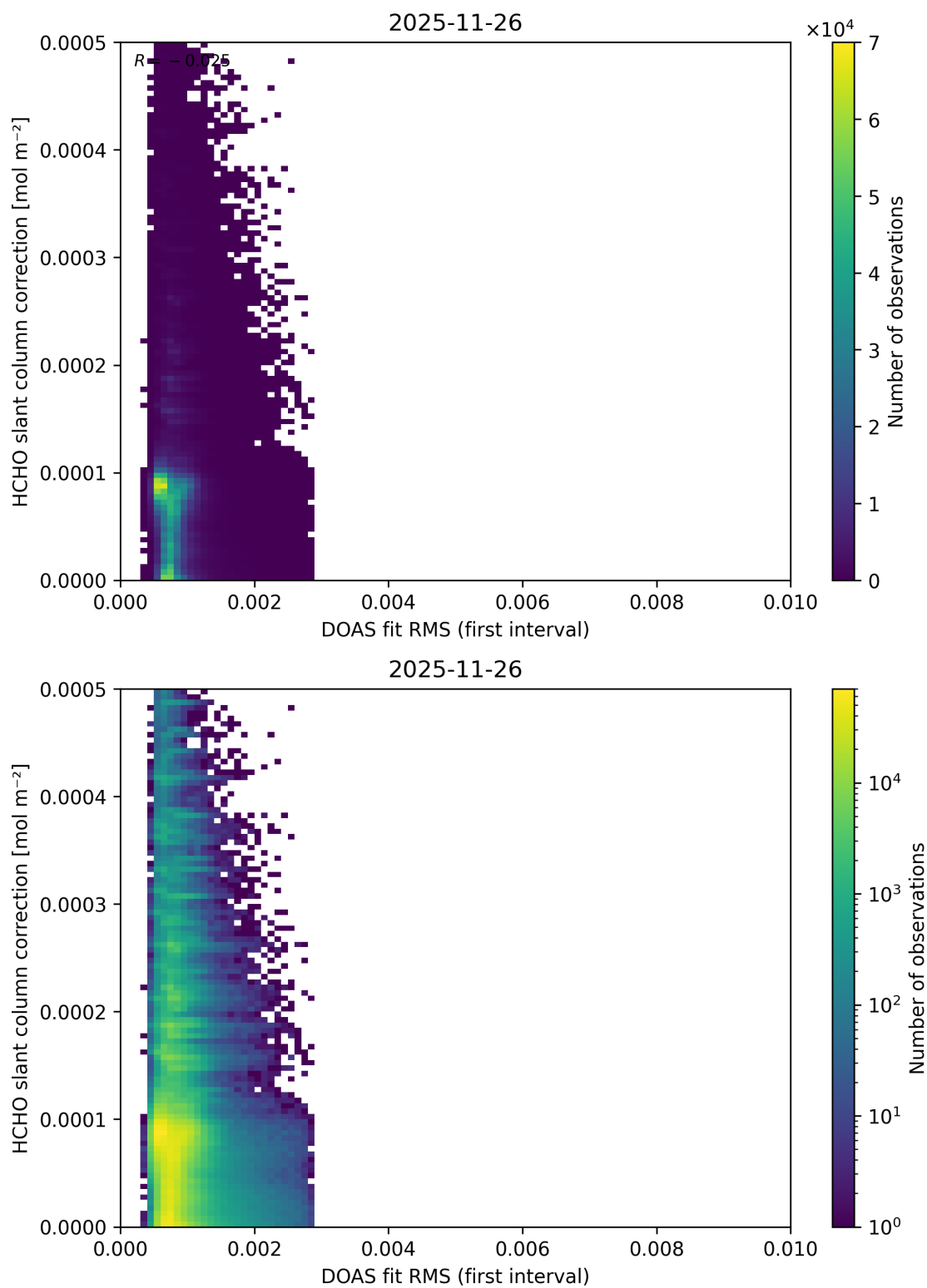
Figure 67: Scatter density plot of “DOAS fit RMS (first interval)” against “HCHO slant column correction” for 2025-11-25 to 2025-11-27.
