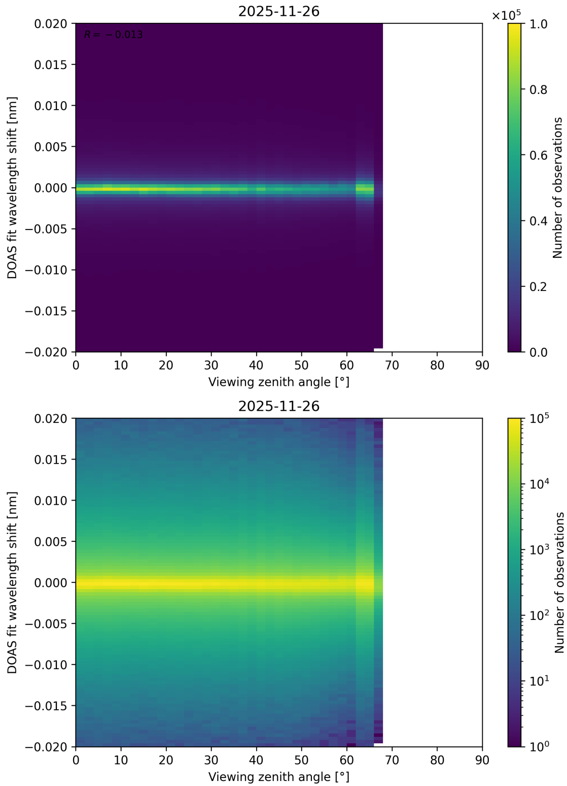
Figure 203: Scatter density plot of “Viewing zenith angle” against “DOAS fit wavelength shift” for 2025-11-25 to 2025-11-27.
