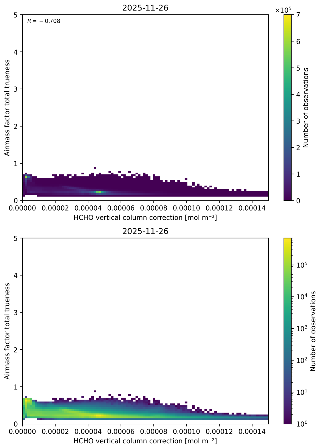
Figure 135: Scatter density plot of “HCHO vertical column correction” against “Airmass factor total trueneess” for 2025-11-25 to 2025-11-27.
