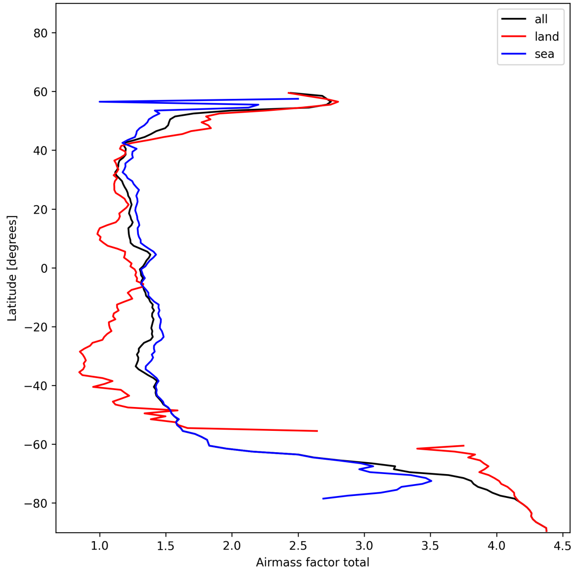
Figure 27: Zonal average of “Airmass factor total” for 2025-11-25 to 2025-11-27.
