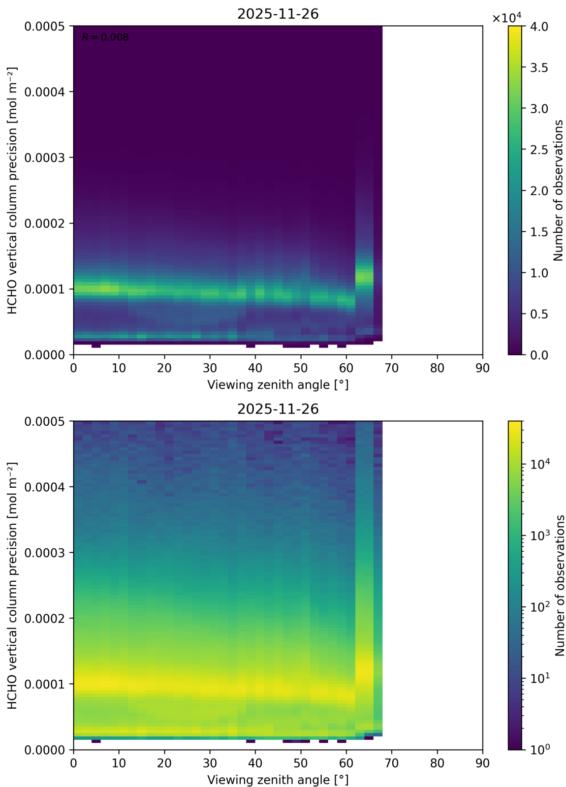
Figure 214: Scatter density plot of “Viewing zenith angle” against “HCHO vertical column precision” for 2025-11-25 to 2025-11-27.
