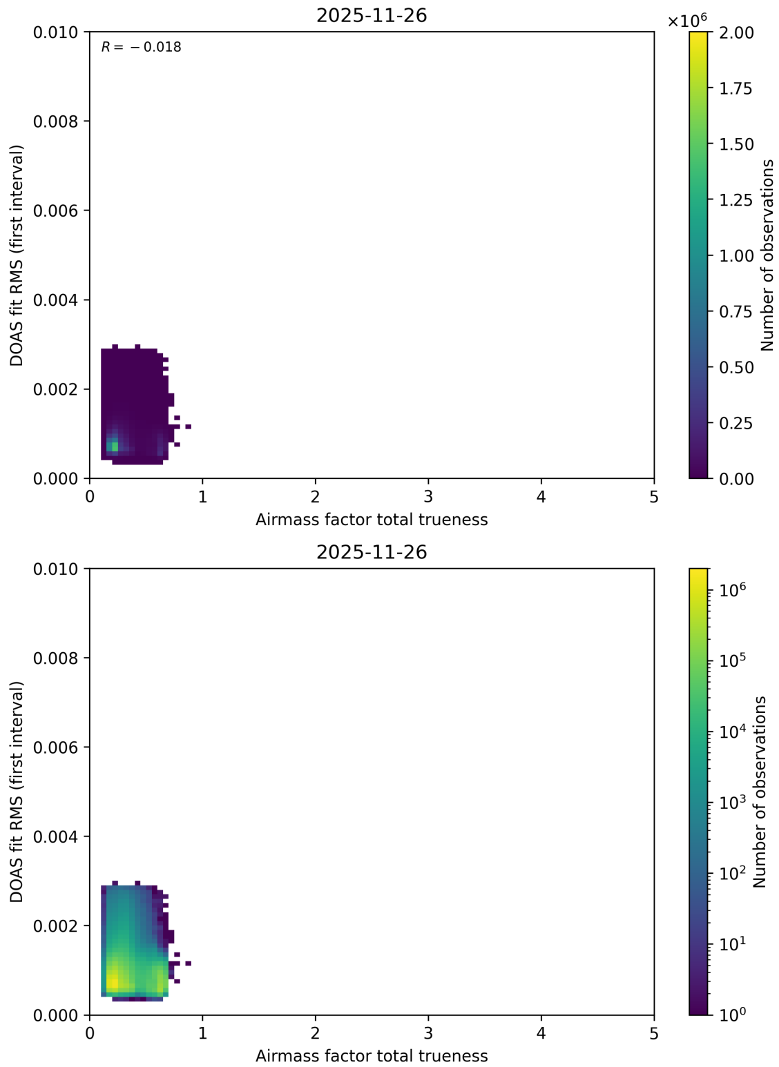
Figure 118: Scatter density plot of “Airmass factor total trueness” against “DOAS fit RMS (first interval)” for 2025-11-25 to 2025-11-27.
