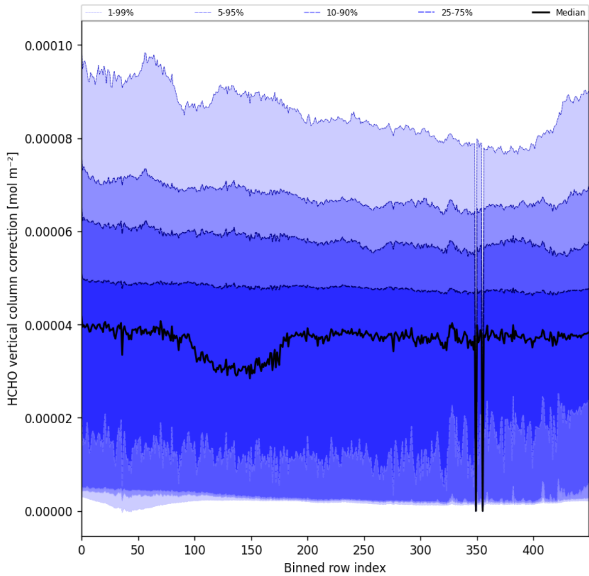
Figure 54: Along track statistics of “HCHO vertical column correction” for 2025-11-25 to 2025-11-27
