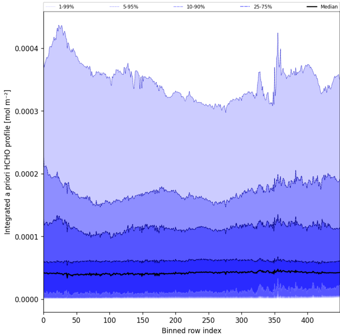
Figure 60: Along track statistics of “Integrated a priori HCHO profile” for 2025-11-25 to 2025-11-27
