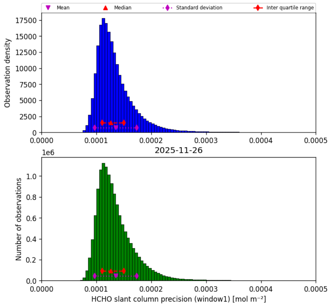
Figure 41: Histogram of “HCHO slant column precision (window1)” for 2025-11-25 to 2025-11-27
