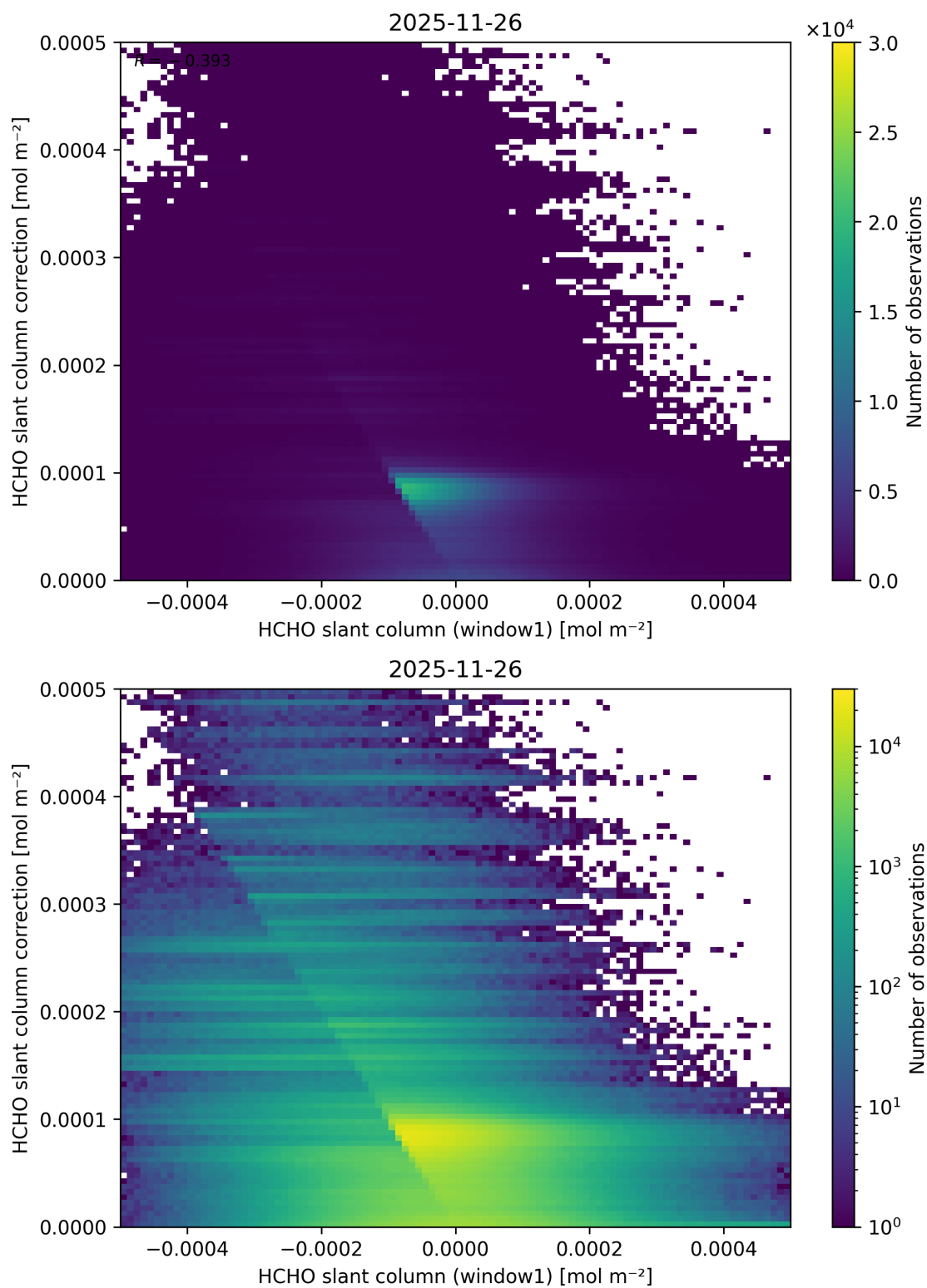
Figure 93: Scatter density plot of “HCHO slant column (window1)” against “HCHO slant column correction” for 2025-11-25 to 2025-11-27.
