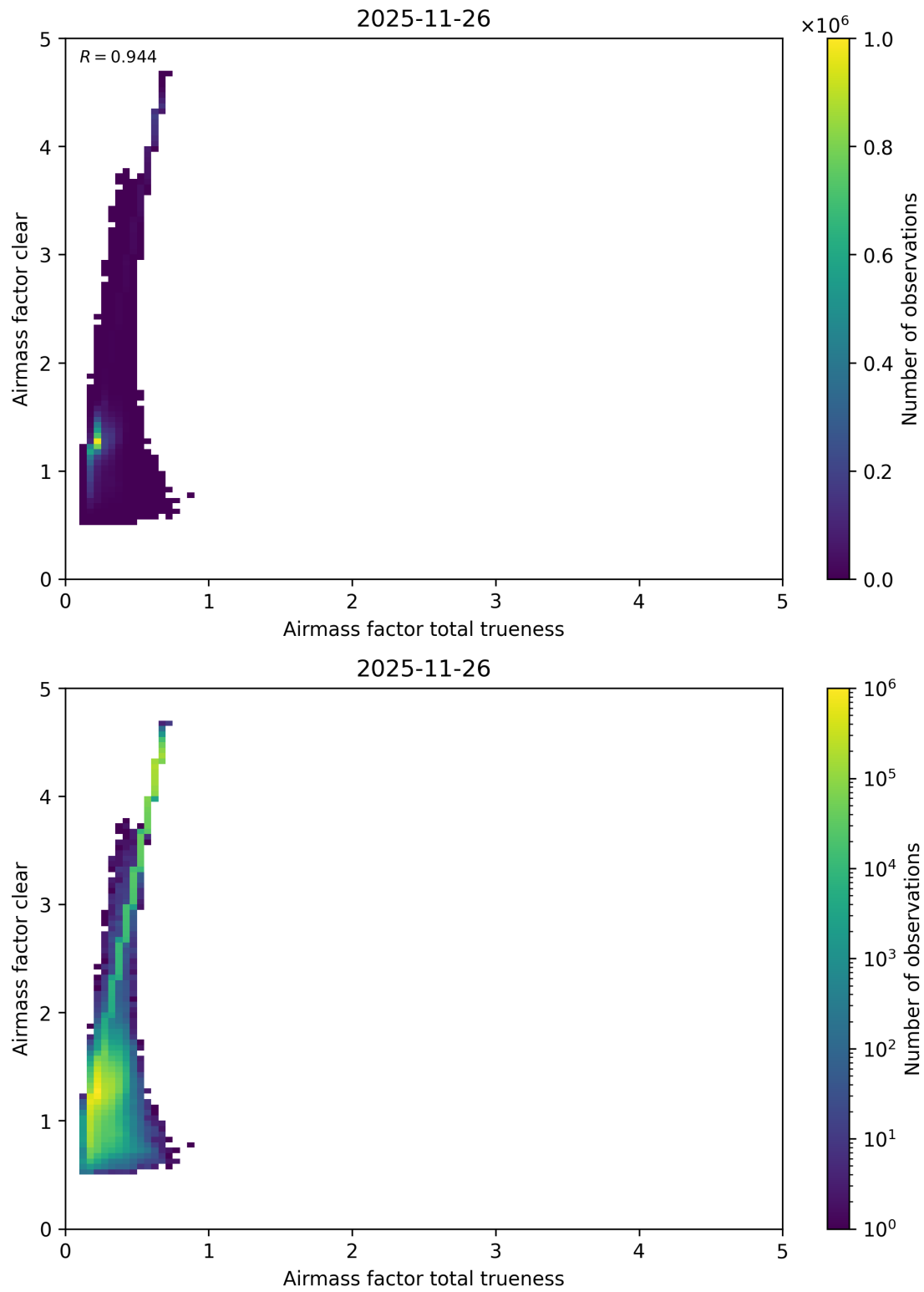
Figure 121: Scatter density plot of “Airmass factor total trueness” against “Airmass factor clear” for 2025-11-25 to 2025-11-27.
