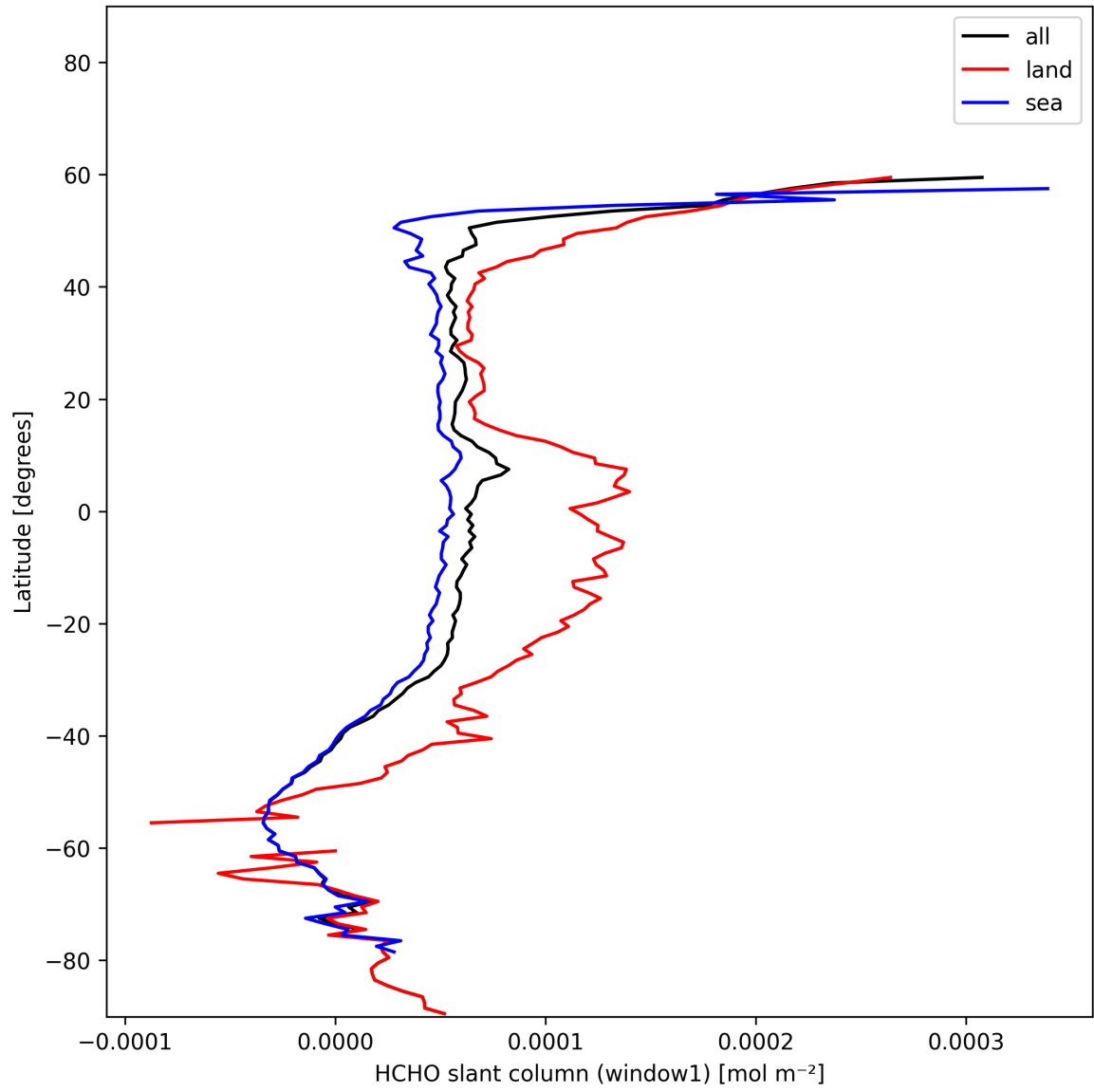
Figure 25: Zonal average of “HCHO slant column (window1)” for 2025-11-25 to 2025-11-27.
