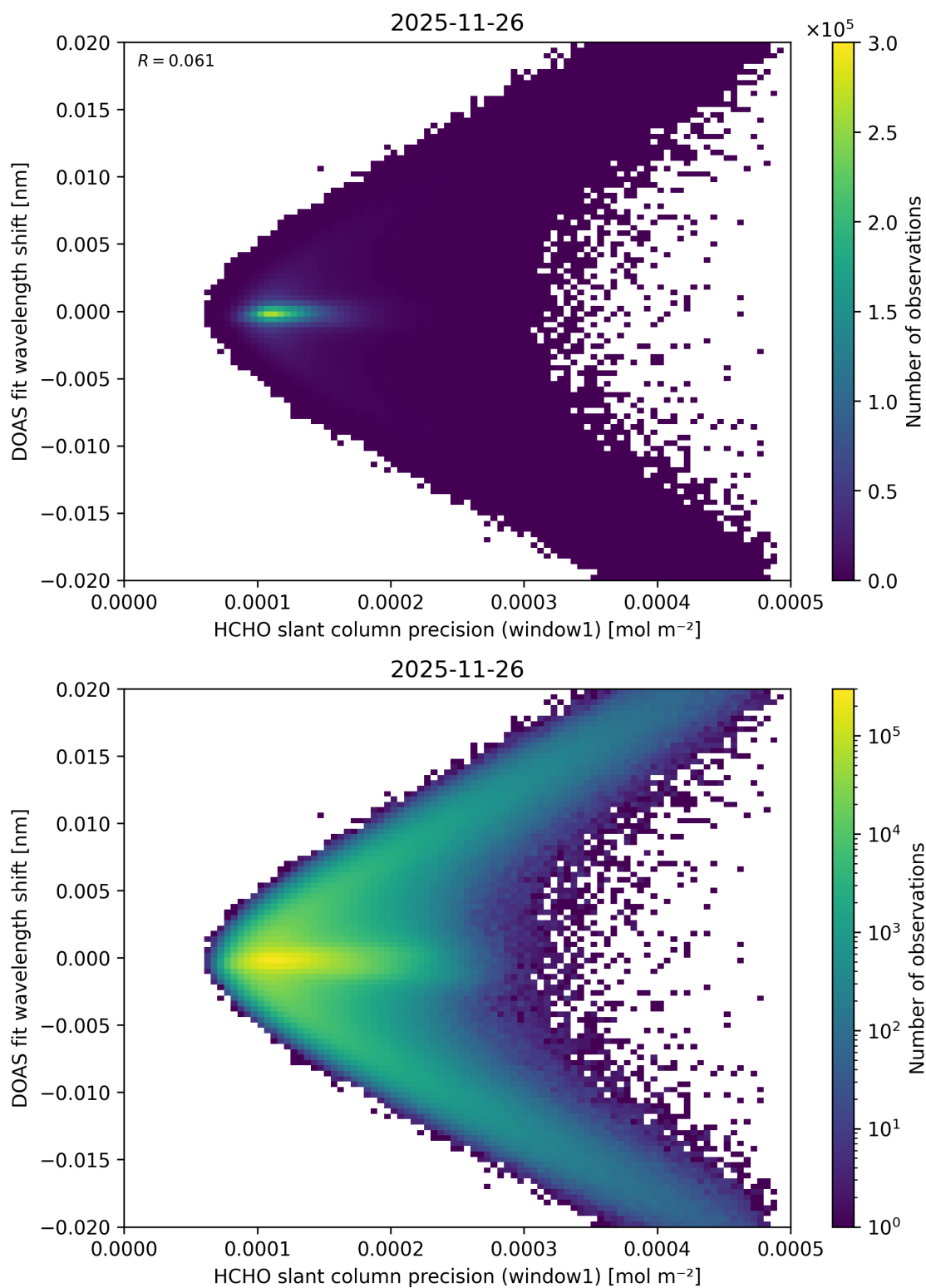
Figure 100: Scatter density plot of “HCHO slant column precision (window1)” against “DOAS fit wavelength shift” for 2025-11-25 to 2025-11-27.
