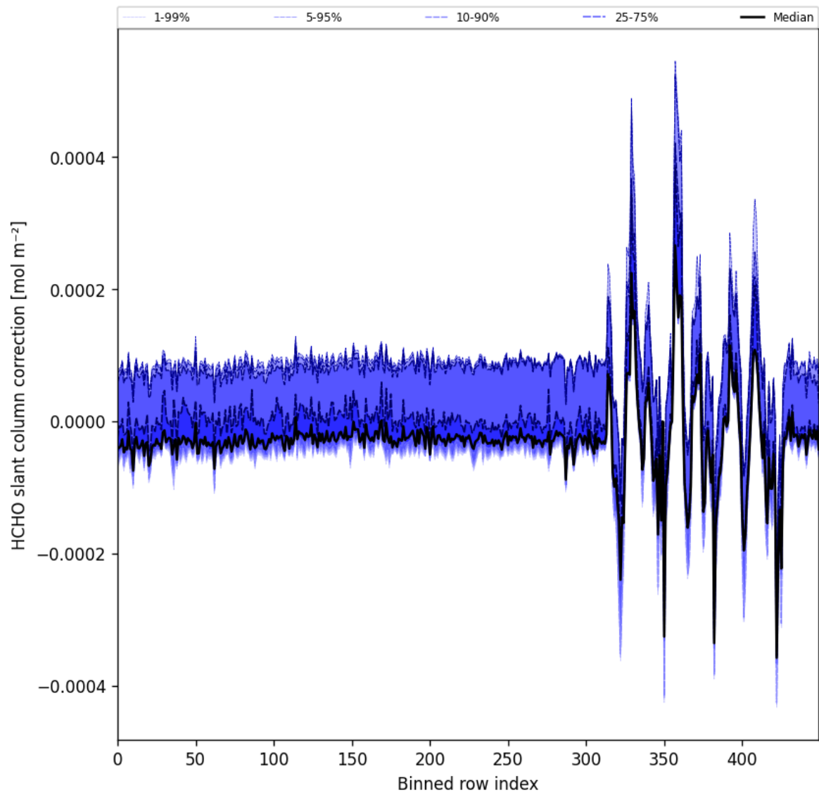
Figure 64: Along track statistics of “HCHO slant column correction” for 2025-11-25 to 2025-11-27
