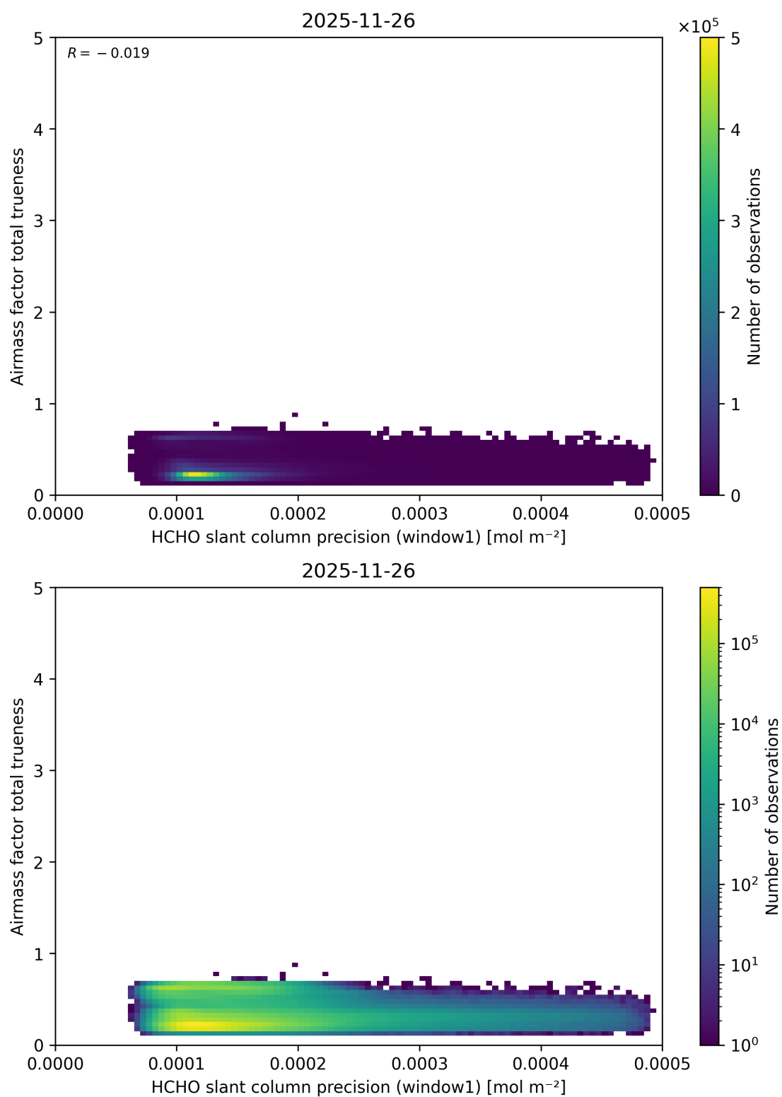
Figure 106: Scatter density plot of “HCHO slant column precision (window1)” against “Airmass factor total trueness” for 2025-11-25 to 2025-11-27.
