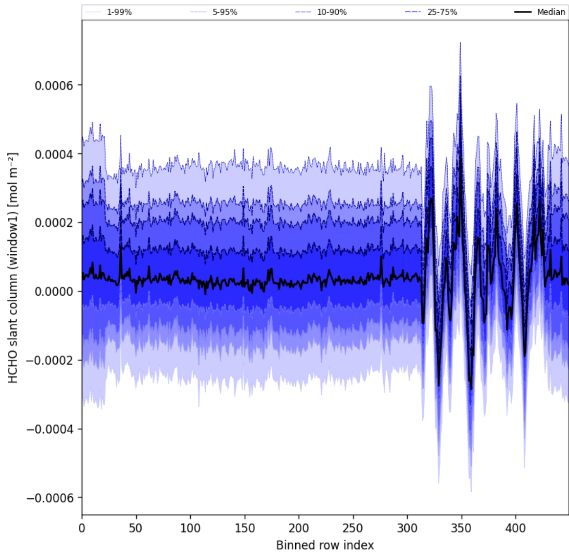
Figure 55: Along track statistics of “HCHO slant column (window1)” for 2025-11-25 to 2025-11-27
