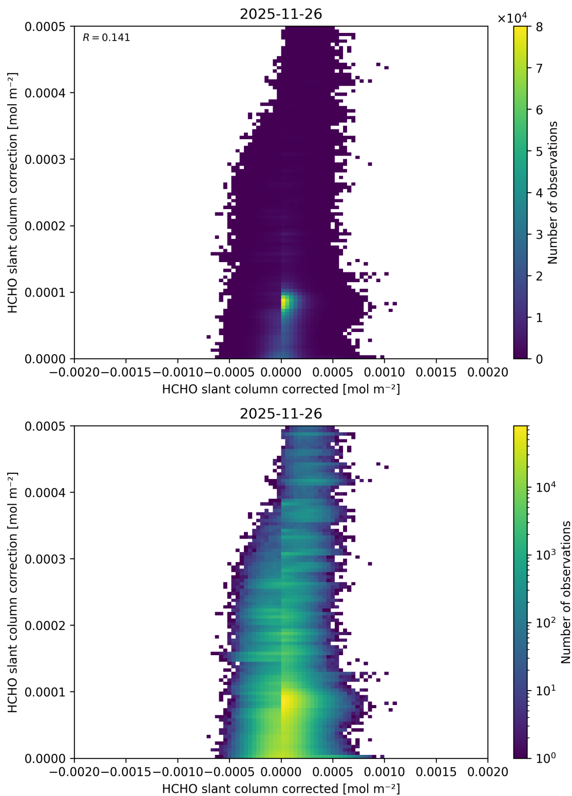
Figure 85: Scatter density plot of “HCHO slant column corrected” against “HCHO slant column correction” for 2025-11-25 to 2025-11-27.
