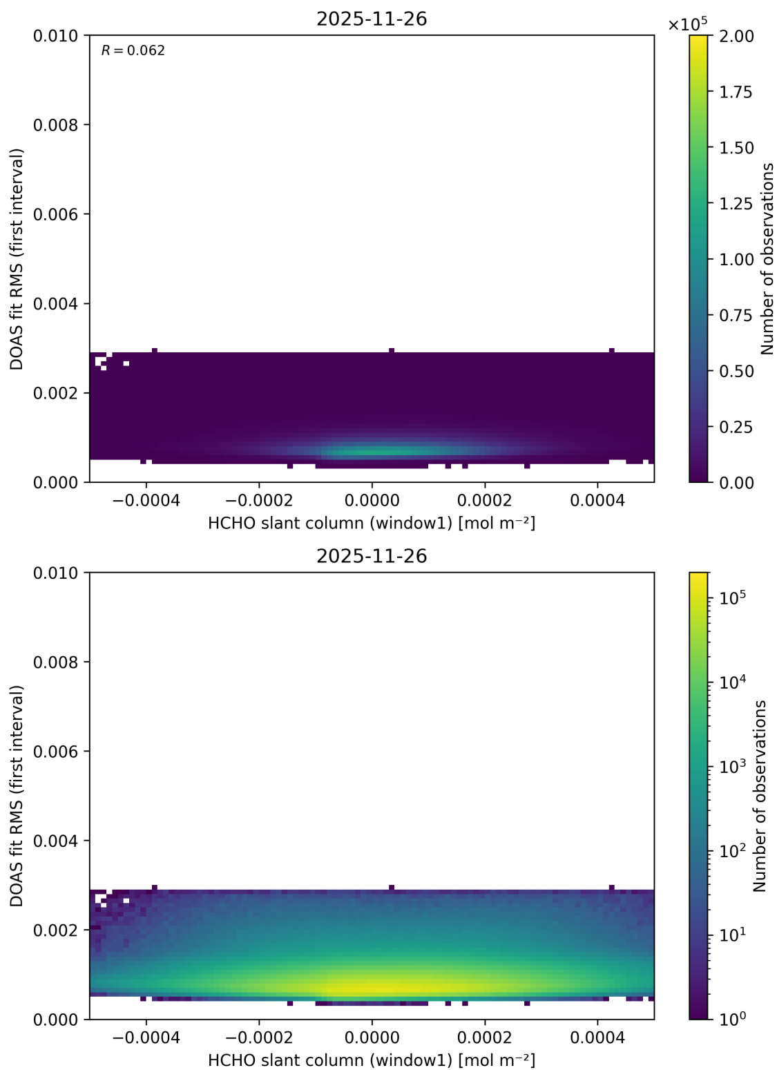
Figure 88: Scatter density plot of “HCHO slant column (window1)” against “DOAS fit RMS (first interval)” for 2025-11-25 to 2025-11-27.
