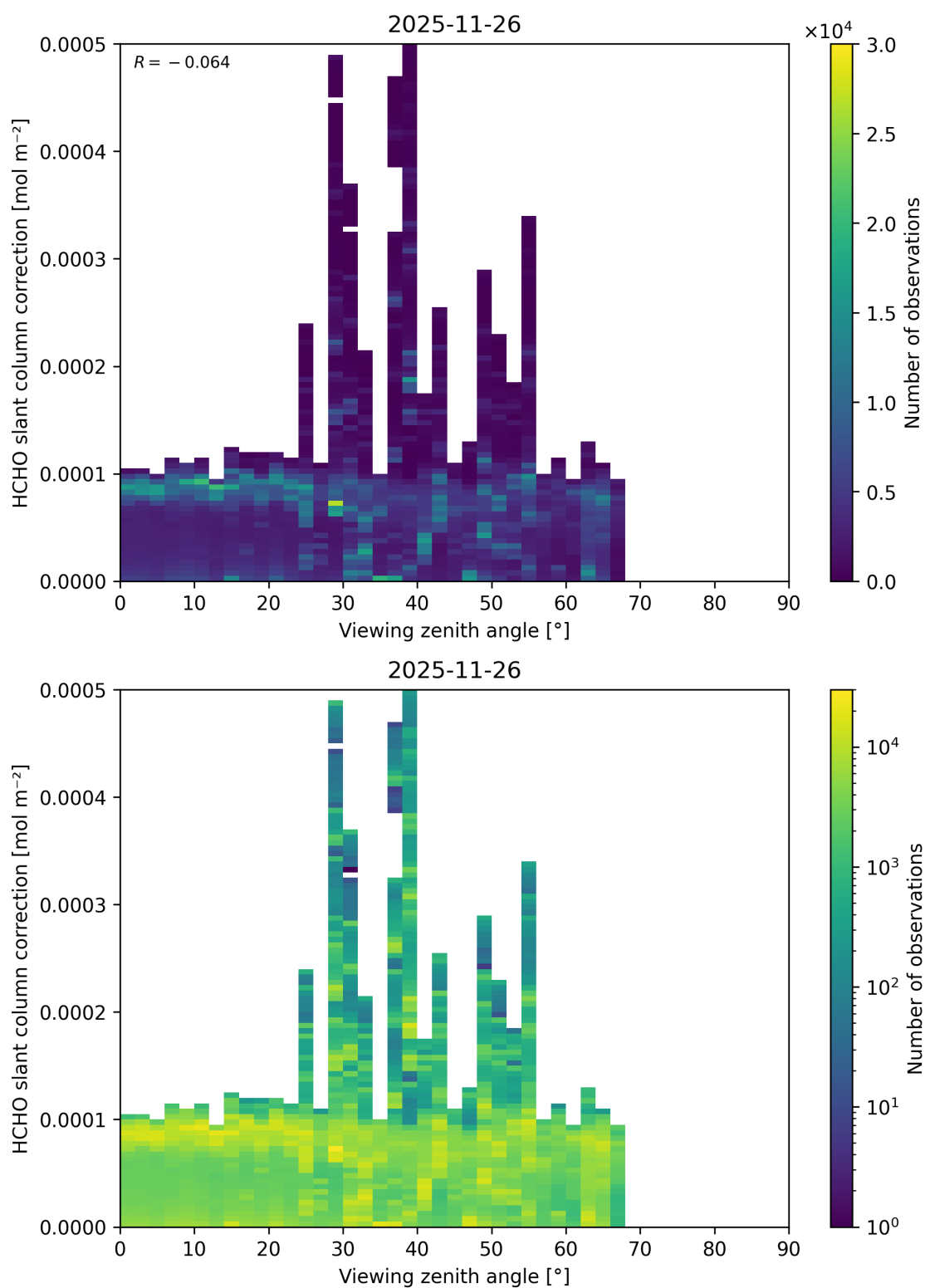
Figure 207: Scatter density plot of “Viewing zenith angle” against “HCHO slant column correction” for 2025-11-25 to 2025-11-27.
