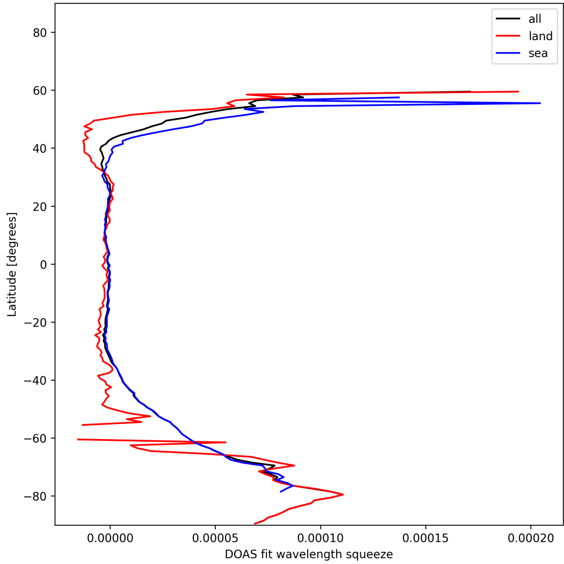
Figure 32: Zonal average of “DOAS fit wavelength squeeze” for 2025-11-25 to 2025-11-27.
