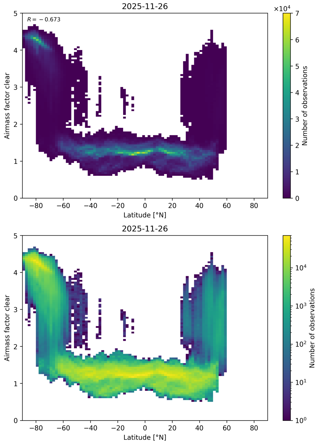
Figure 174: Scatter density plot of “Latitude” against “Airmass factor clear” for 2025-11-25 to 2025-11-27.
