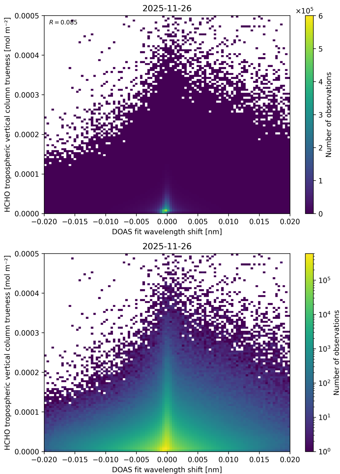
Figure 73: Scatter density plot of “DOAS fit wavelength shift” against “HCHO tropospheric vertical column trueness” for 2025-11-25 to 2025-11-27.
