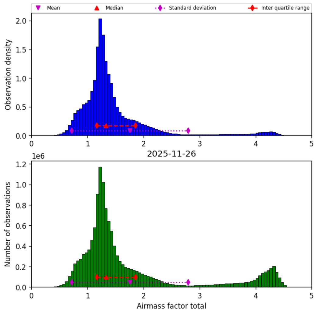
Figure 42: Histogram of “Airmass factor total” for 2025-11-25 to 2025-11-27
