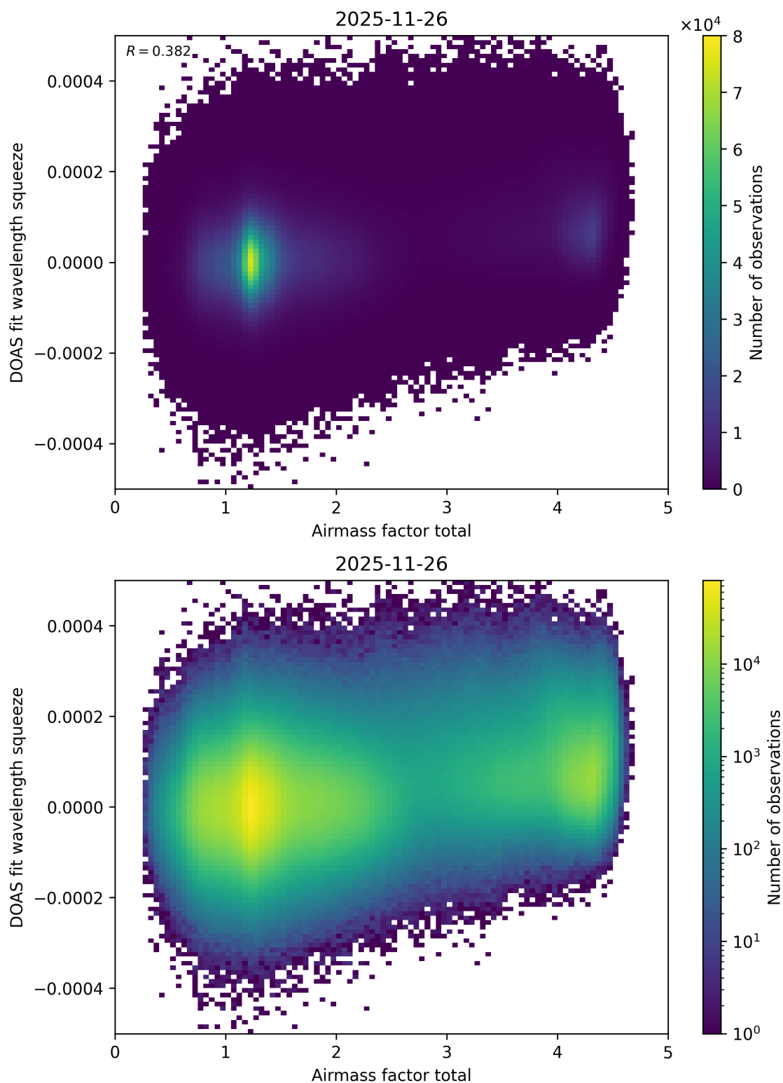
Figure 111: Scatter density plot of “Airmass factor total” against “DOAS fit wavelength squeeze” for 2025-11-25 to 2025-11-27.
