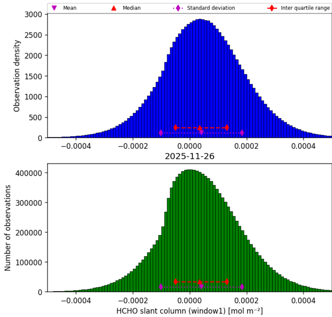
Figure 40: Histogram of “HCHO slant column (window1)” for 2025-11-25 to 2025-11-27
