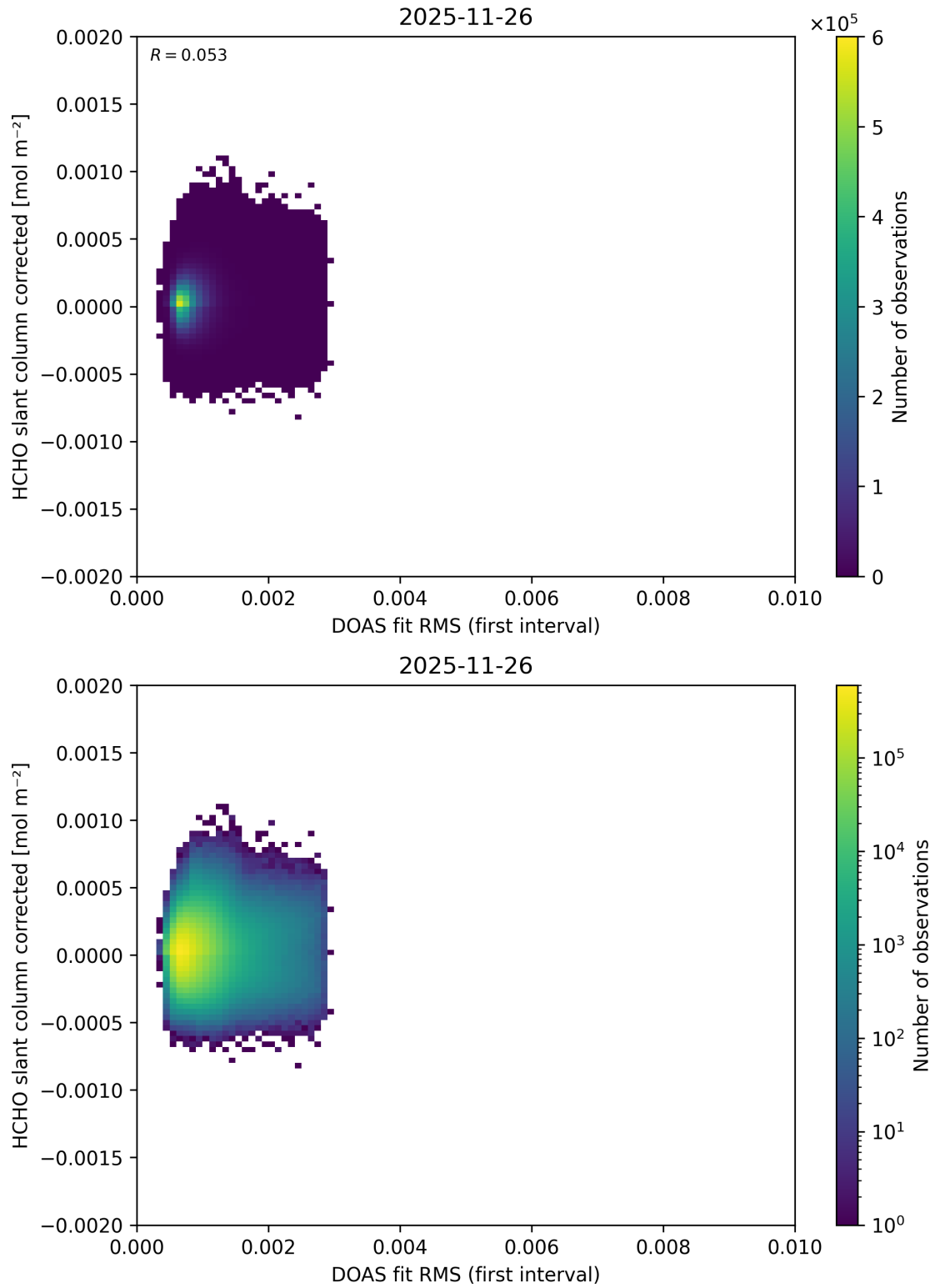
Figure 66: Scatter density plot of “DOAS fit RMS (first interval)” against “HCHO slant column corrected” for 2025-11-25 to 2025-11-27.
