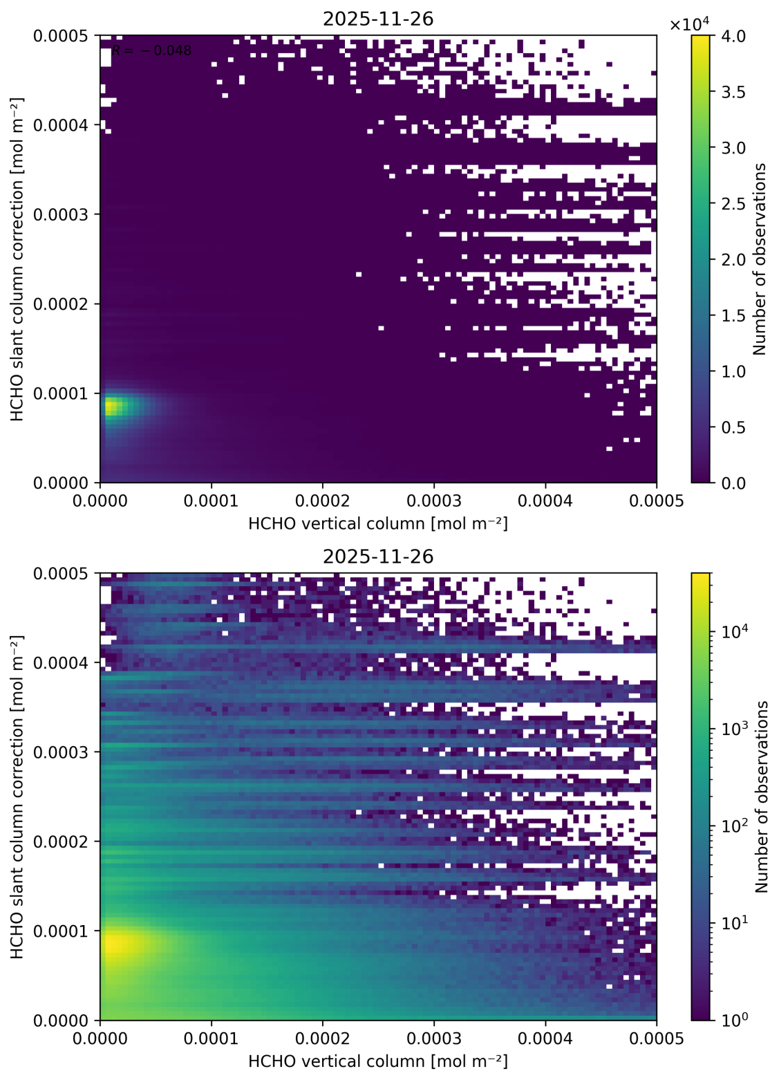
Figure 143: Scatter density plot of “HCHO vertical column” against “HCHO slant column correction” for 2025-11-25 to 2025-11-27.
