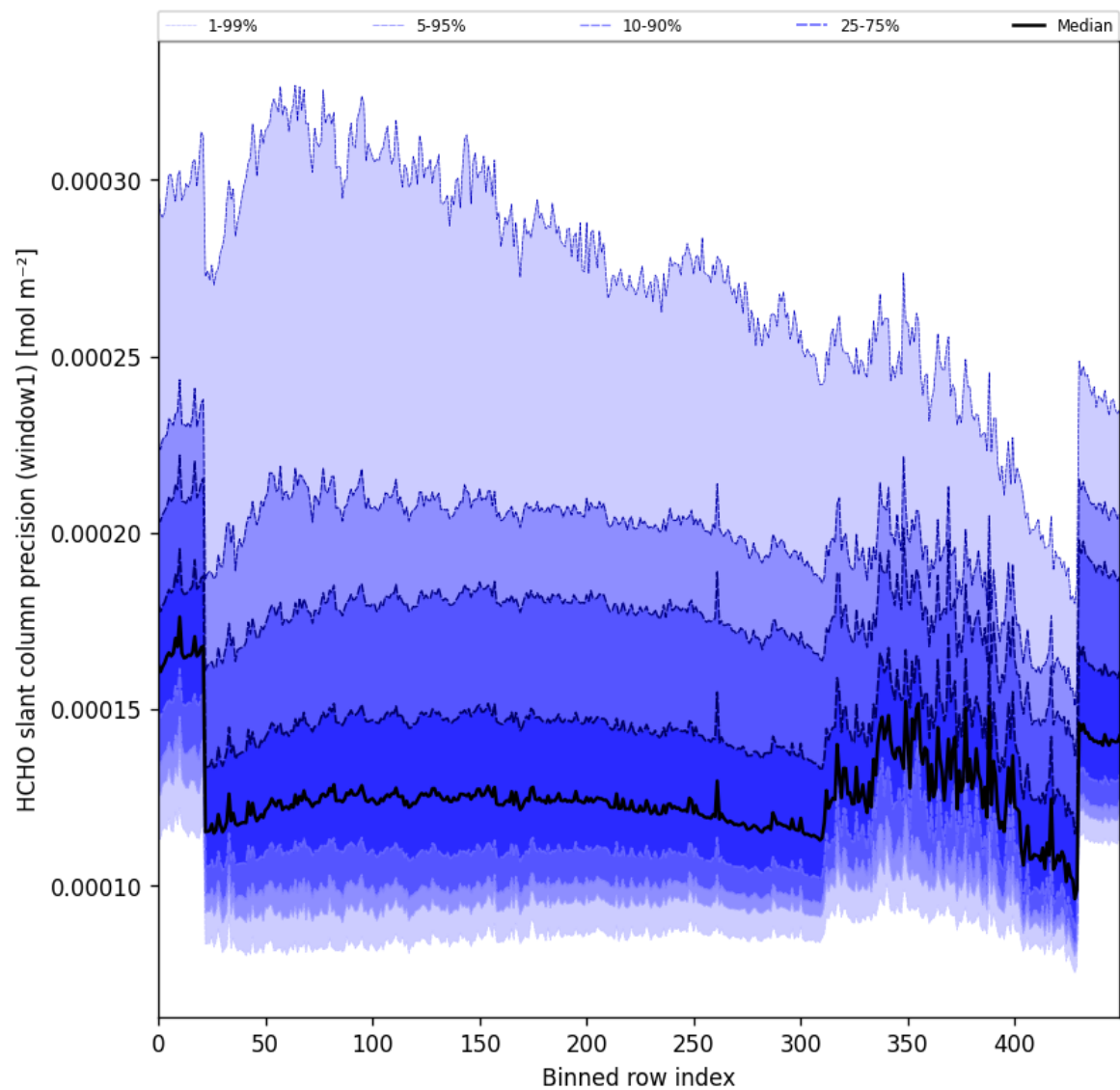
Figure 56: Along track statistics of “HCHO slant column precision (window1)” for 2025-11-25 to 2025-11-27
