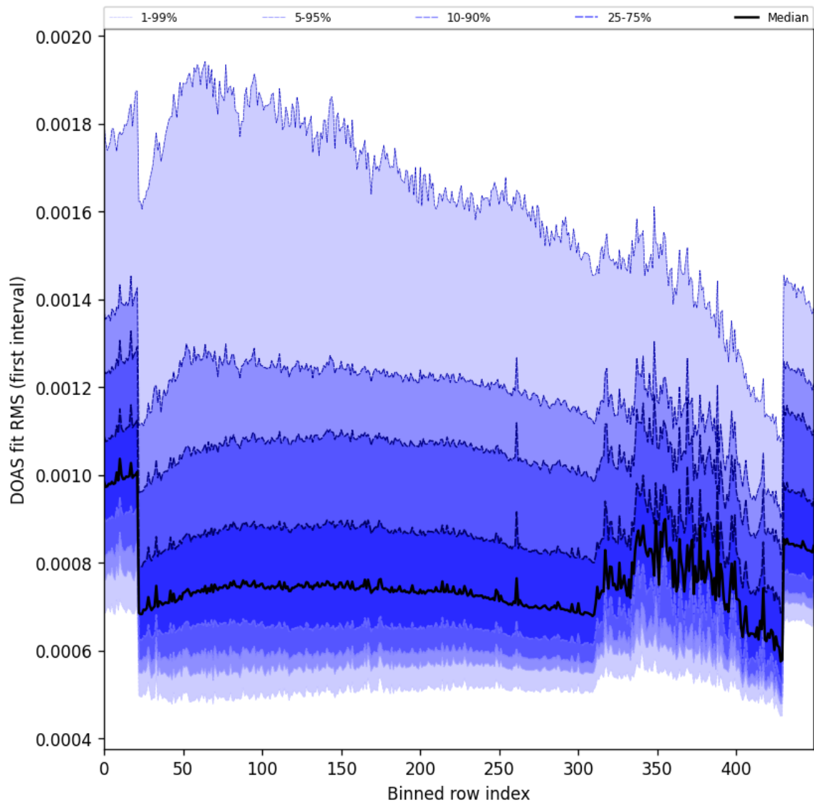
Figure 63: Along track statistics of “DOAS fit RMS (first interval)” for 2025-11-25 to 2025-11-27
