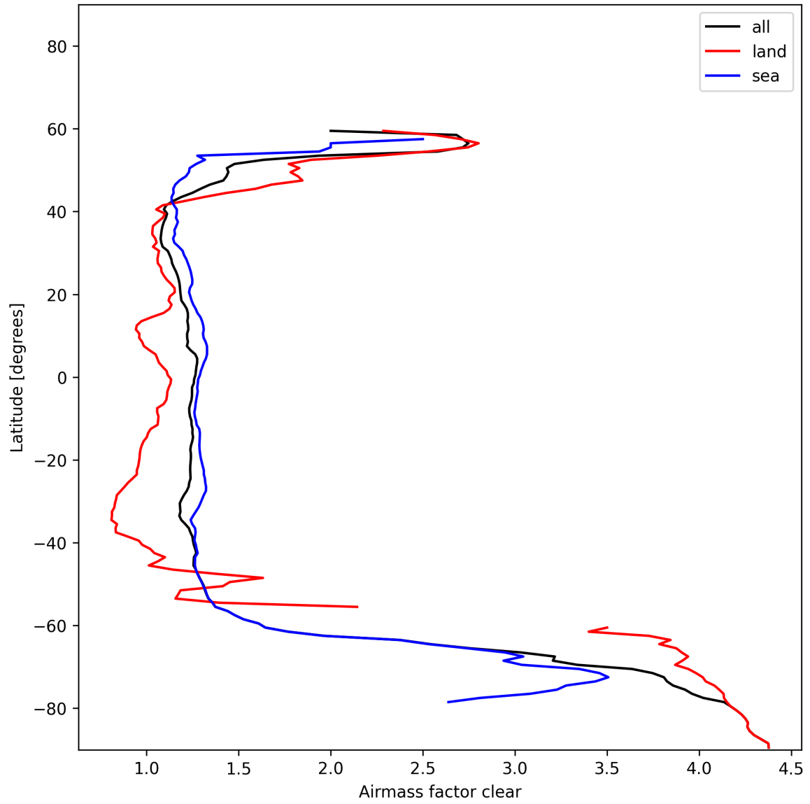
Figure 29: Zonal average of “Airmass factor clear” for 2025-11-25 to 2025-11-27.
