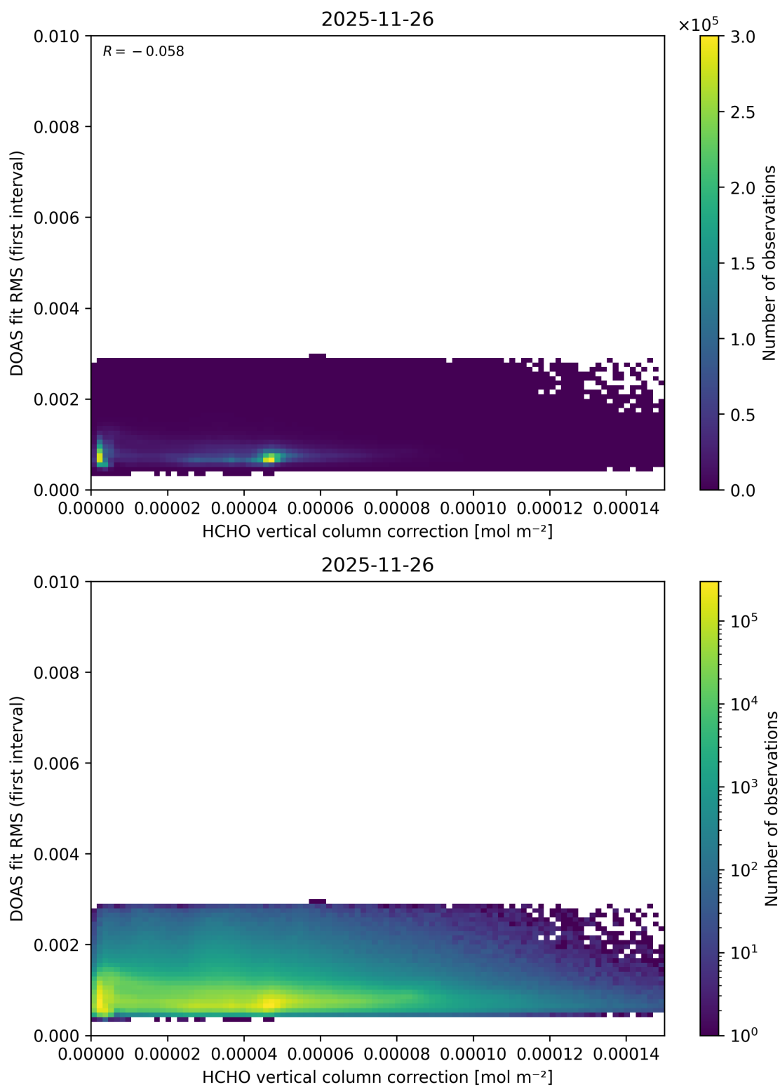
Figure 126: Scatter density plot of “HCHO vertical column correction” against “DOAS fit RMS (first interval)” for 2025-11-25 to 2025-11-27.
