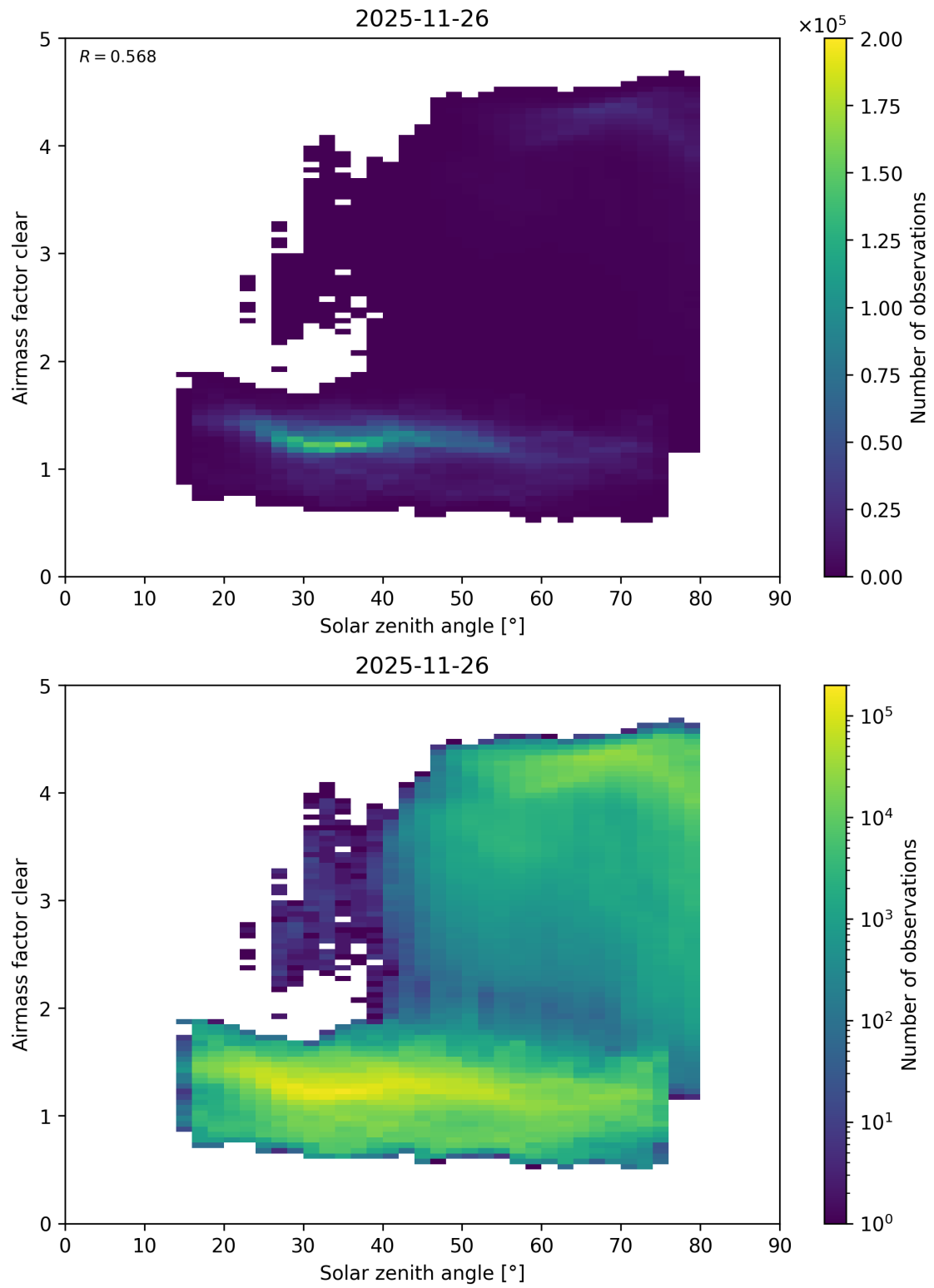
Figure 189: Scatter density plot of “Solar zenith angle” against “Airmass factor clear” for 2025-11-25 to 2025-11-27.
