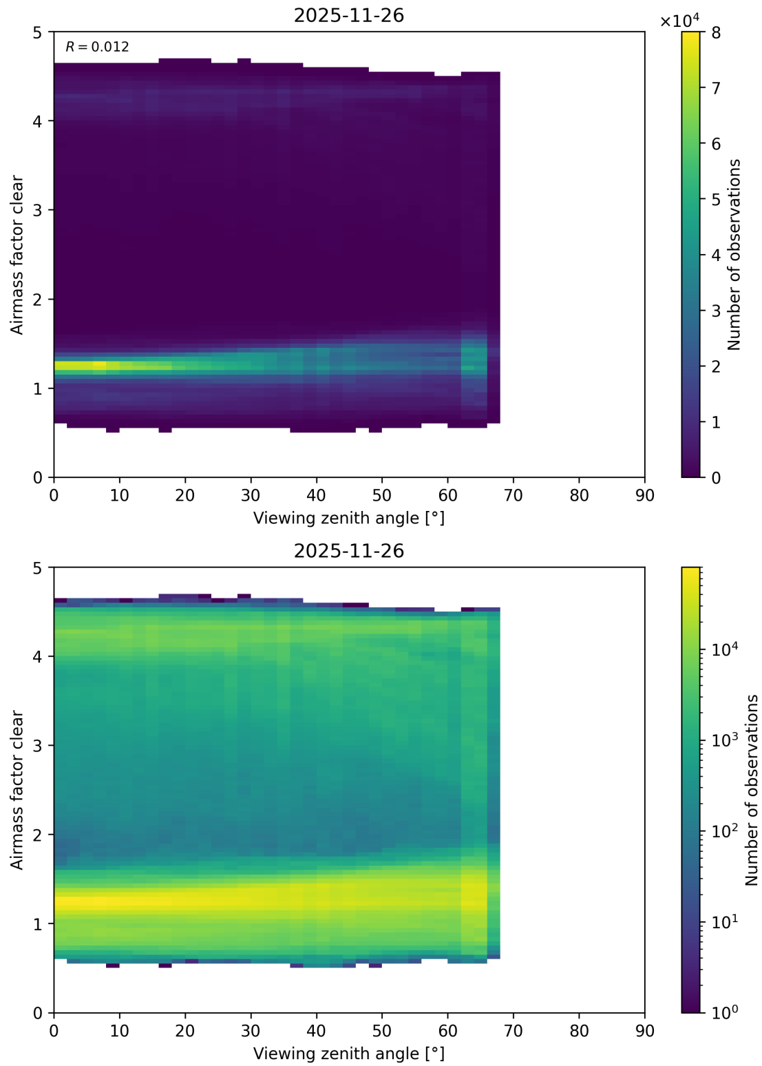
Figure 205: Scatter density plot of “Viewing zenith angle” against “Airmass factor clear” for 2025-11-25 to 2025-11-27.
