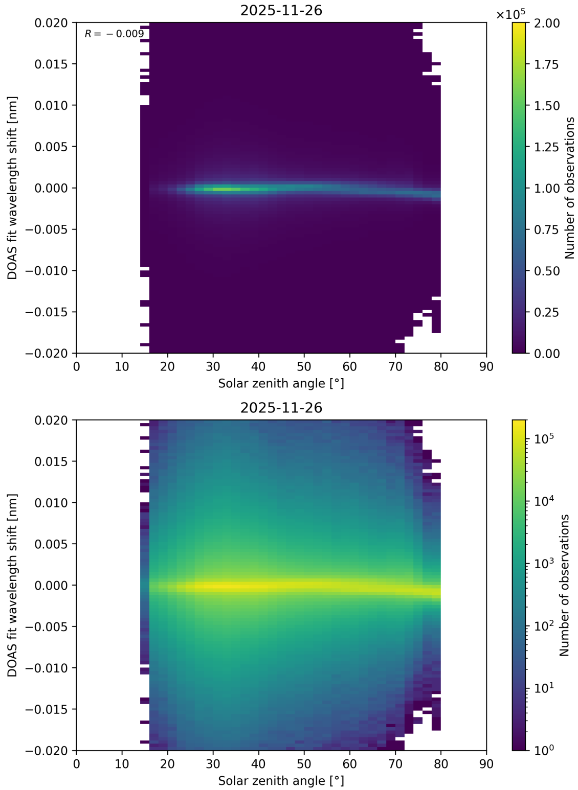
Figure 187: Scatter density plot of “Solar zenith angle” against “DOAS fit wavelength shift” for 2025-11-25 to 2025-11-27.
