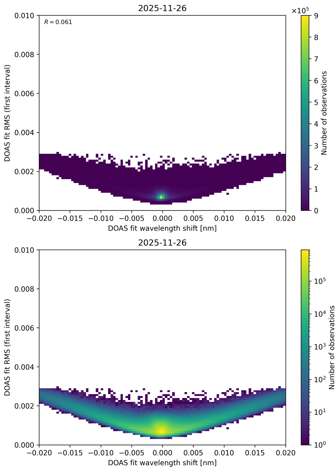
Figure 69: Scatter density plot of “DOAS fit wavelength shift” against “DOAS fit RMS (first interval)” for 2025-11-25 to 2025-11-27.
