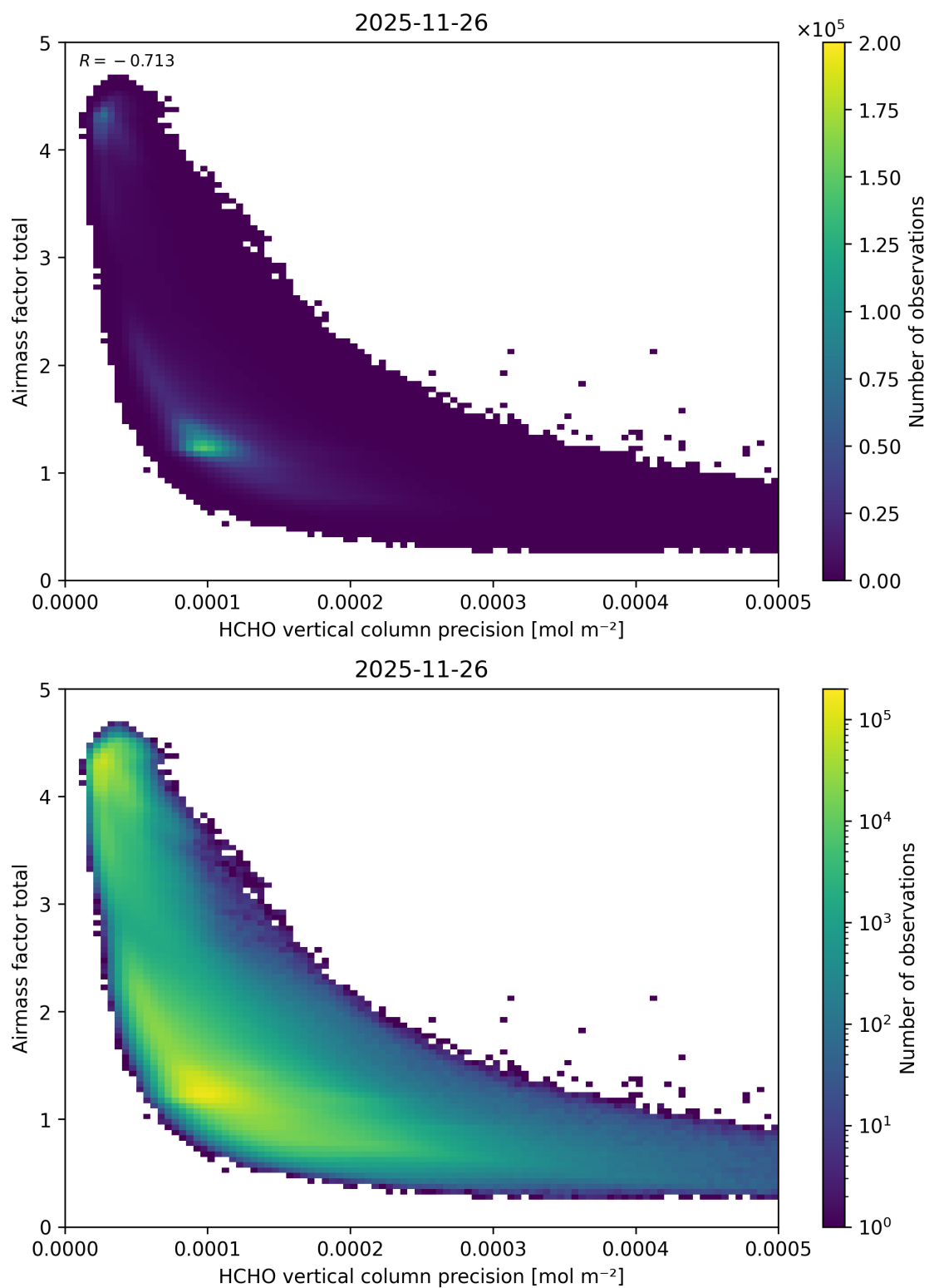
Figure 160: Scatter density plot of “HCHO vertical column precision” against “Airmass factor total” for 2025-11-25 to 2025-11-27.
