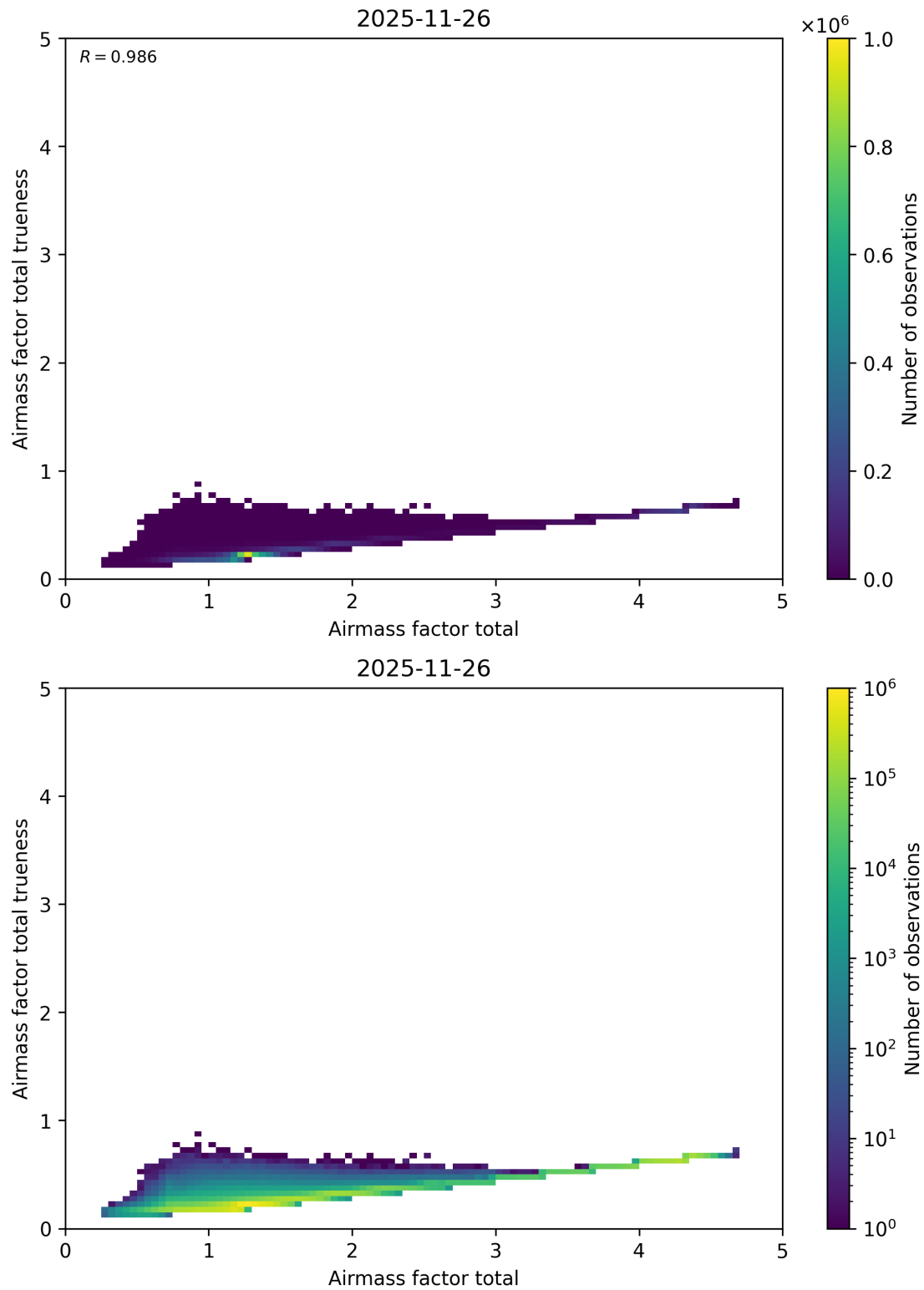
Figure 115: Scatter density plot of “Airmass factor total” against “Airmass factor total trueness” for 2025-11-25 to 2025-11-27.
