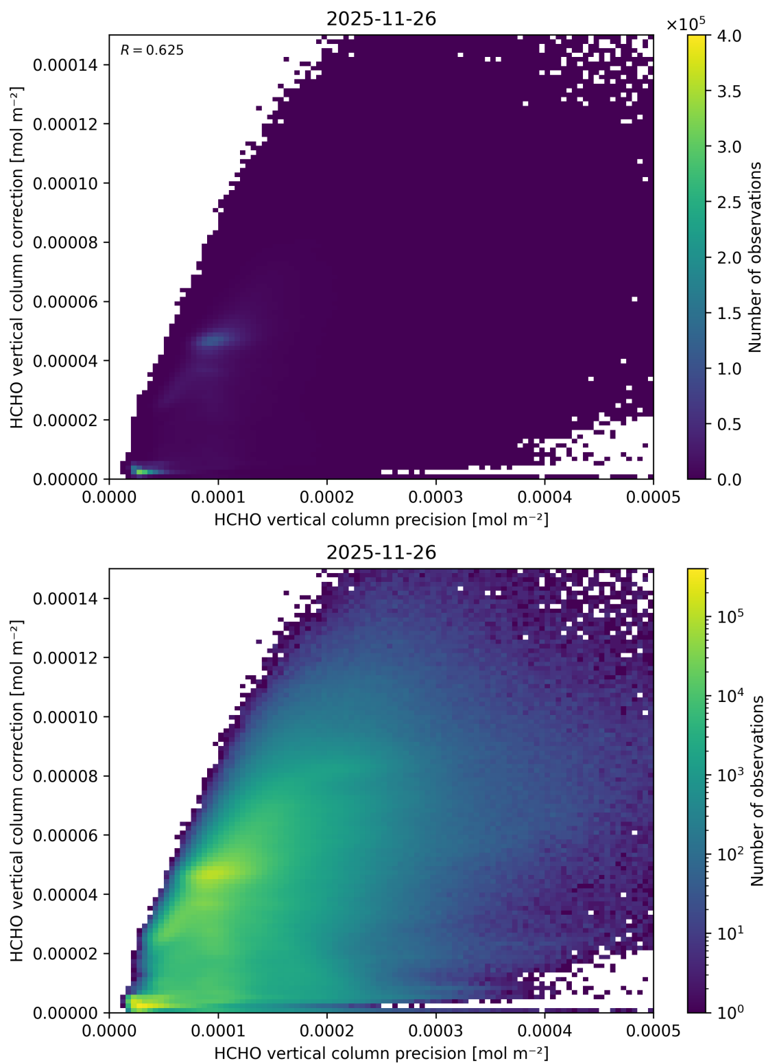
Figure 162: Scatter density plot of “HCHO vertical column precision” against “HCHO vertical column correction” for 2025-11-25 to 2025-11-27.
