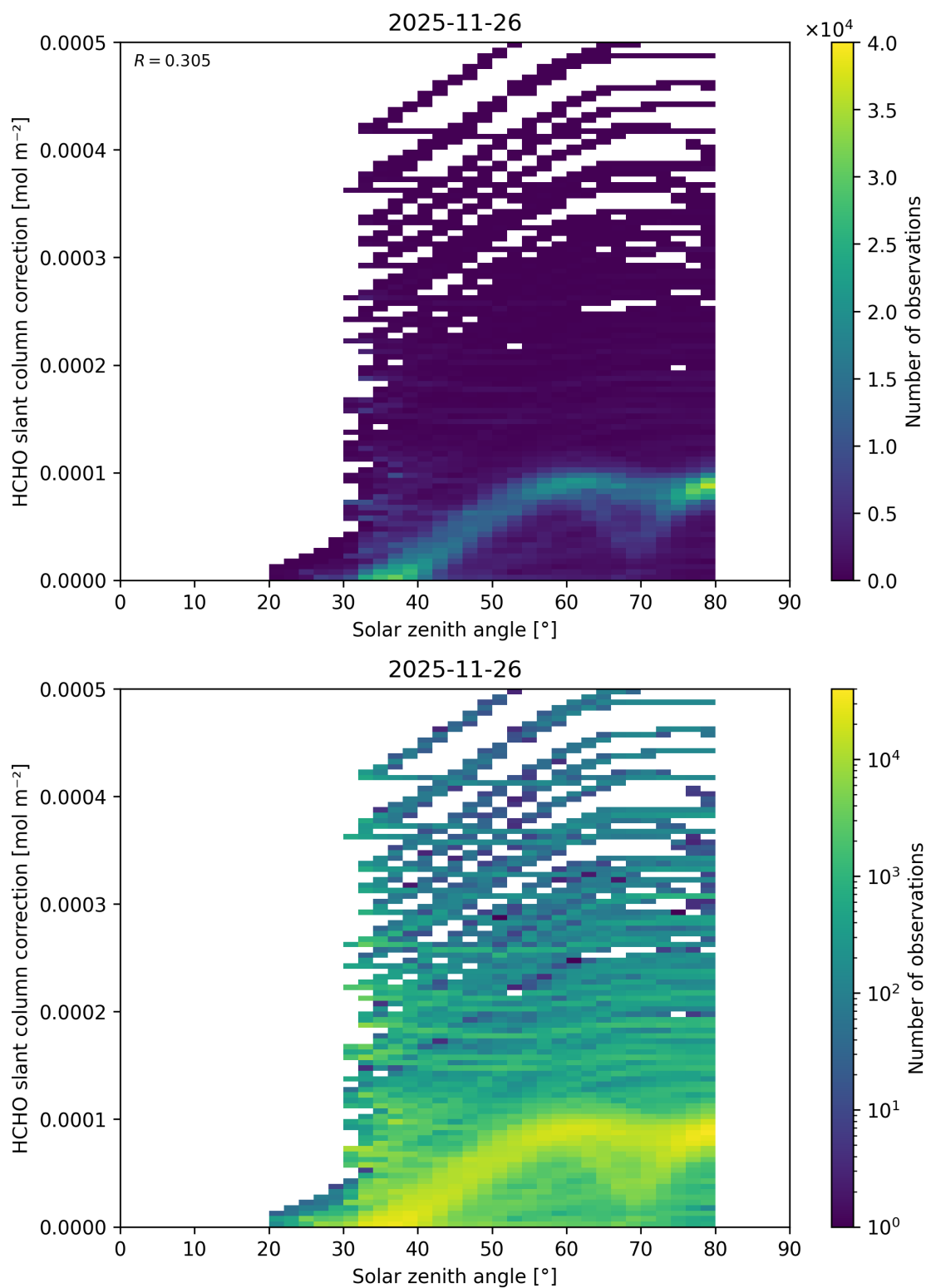
Figure 191: Scatter density plot of “Solar zenith angle” against “HCHO slant column correction” for 2025-11-25 to 2025-11-27.
