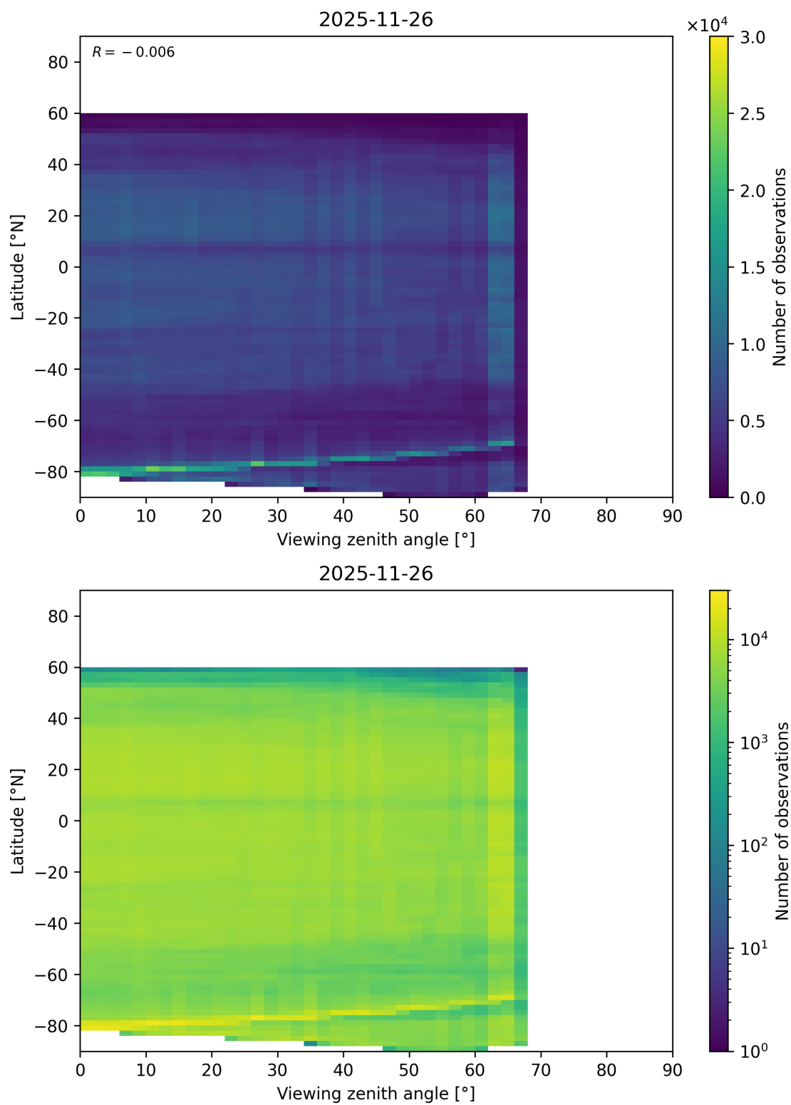
Figure 217: Scatter density plot of “Viewing zenith angle” against “Latitude” for 2025-11-25 to 2025-11-27.
