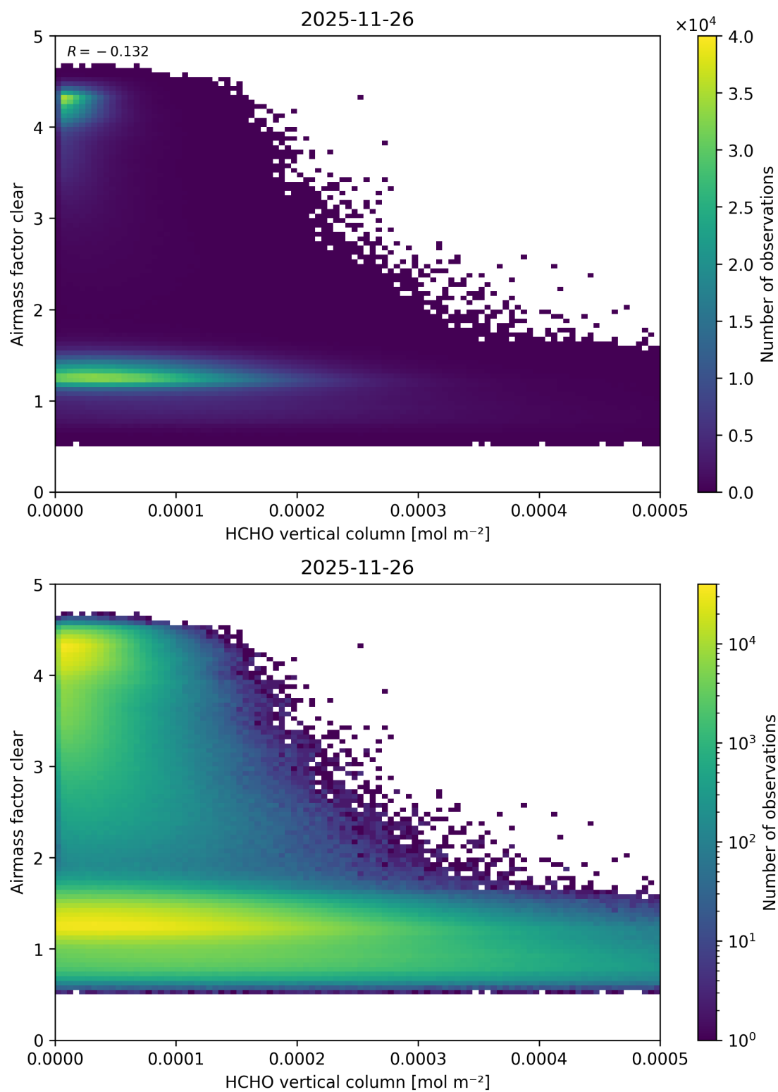
Figure 141: Scatter density plot of “HCHO vertical column” against “Airmass factor clear” for 2025-11-25 to 2025-11-27.
