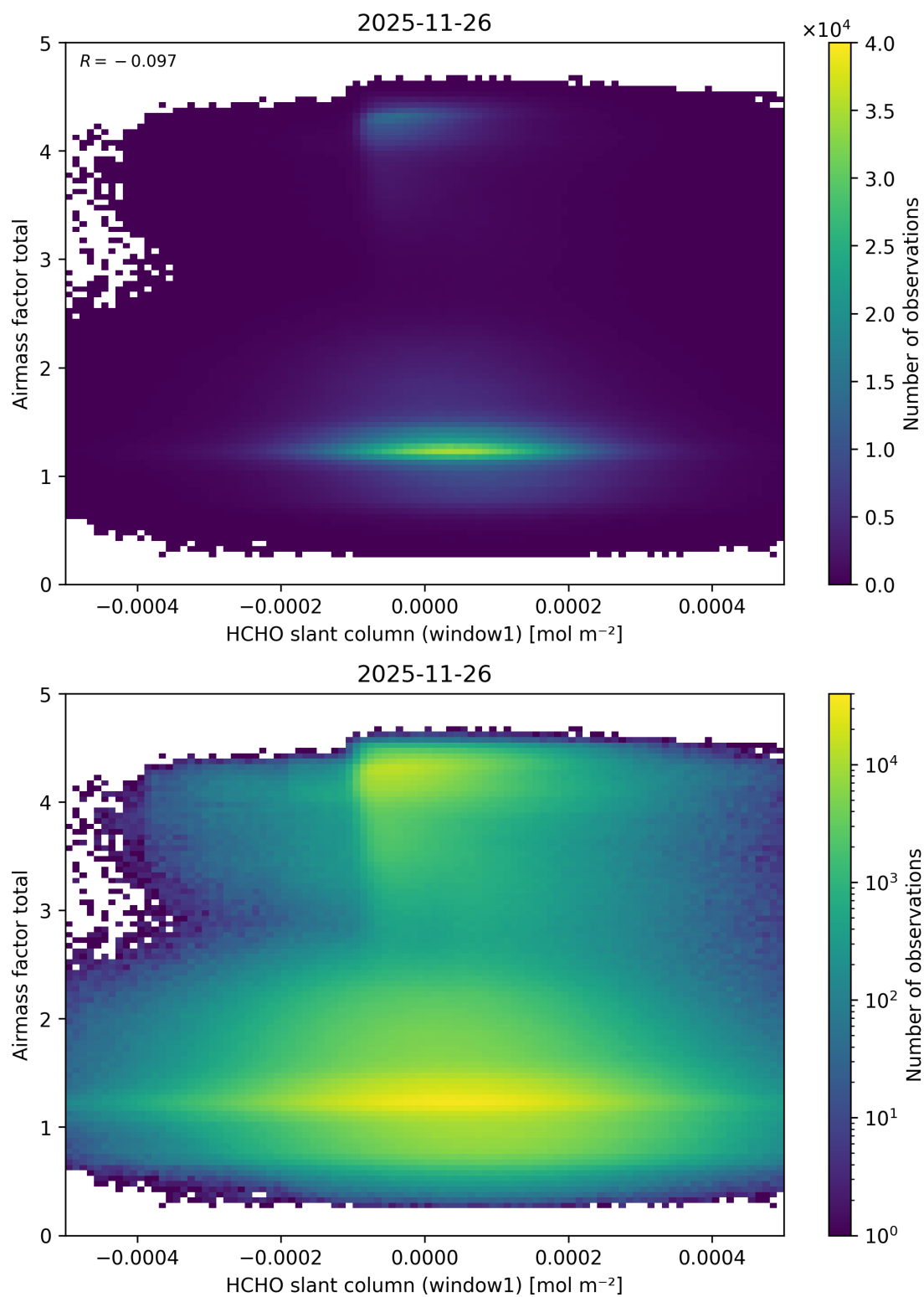
Figure 95: Scatter density plot of “HCHO slant column (window1)” against “Airmass factor total” for 2025-11-25 to 2025-11-27.
