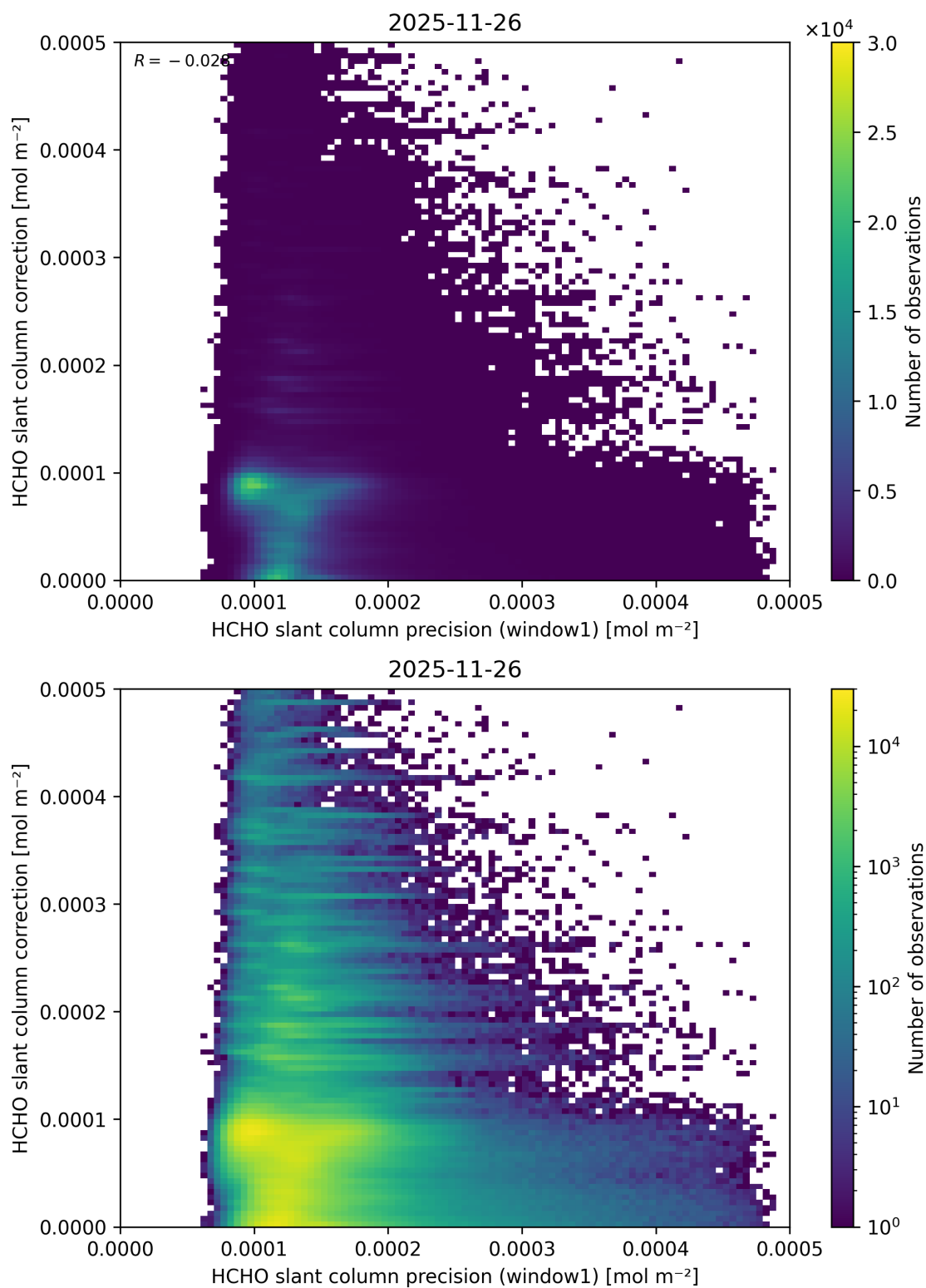
Figure 104: Scatter density plot of “HCHO slant column precision (window1)” against “HCHO slant column correction” for 2025-11-25 to 2025-11-27.
