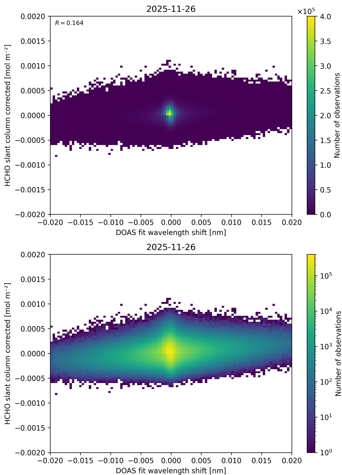
Figure 71: Scatter density plot of “DOAS fit wavelength shift” against “HCHO slant column corrected” for 2025-11-25 to 2025-11-27.
