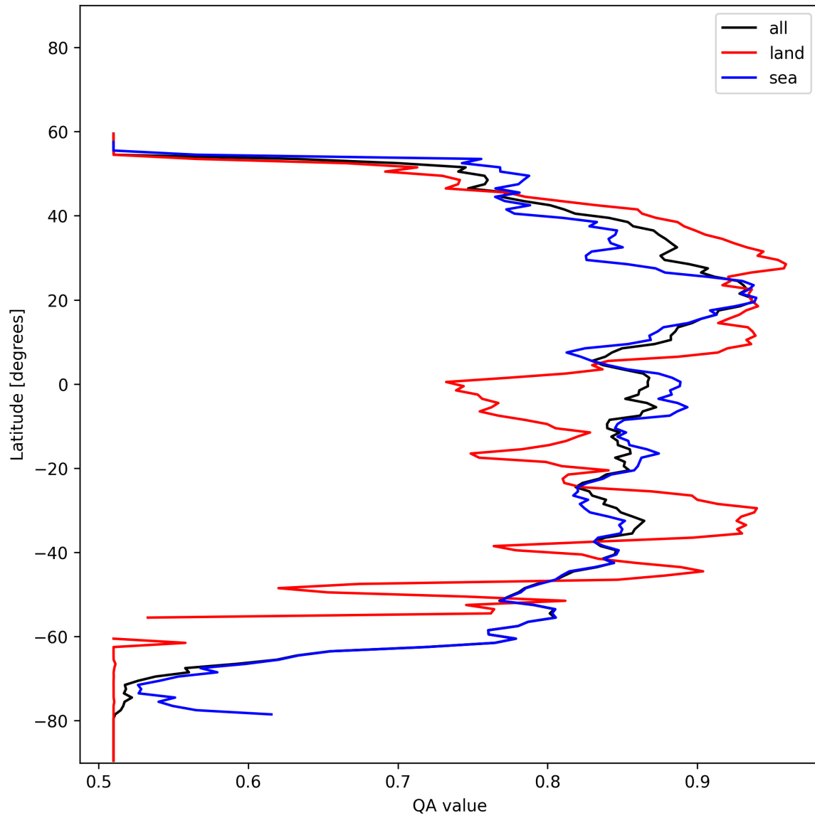
Figure 21: Zonal average of “QA value” for 2025-11-25 to 2025-11-27.
