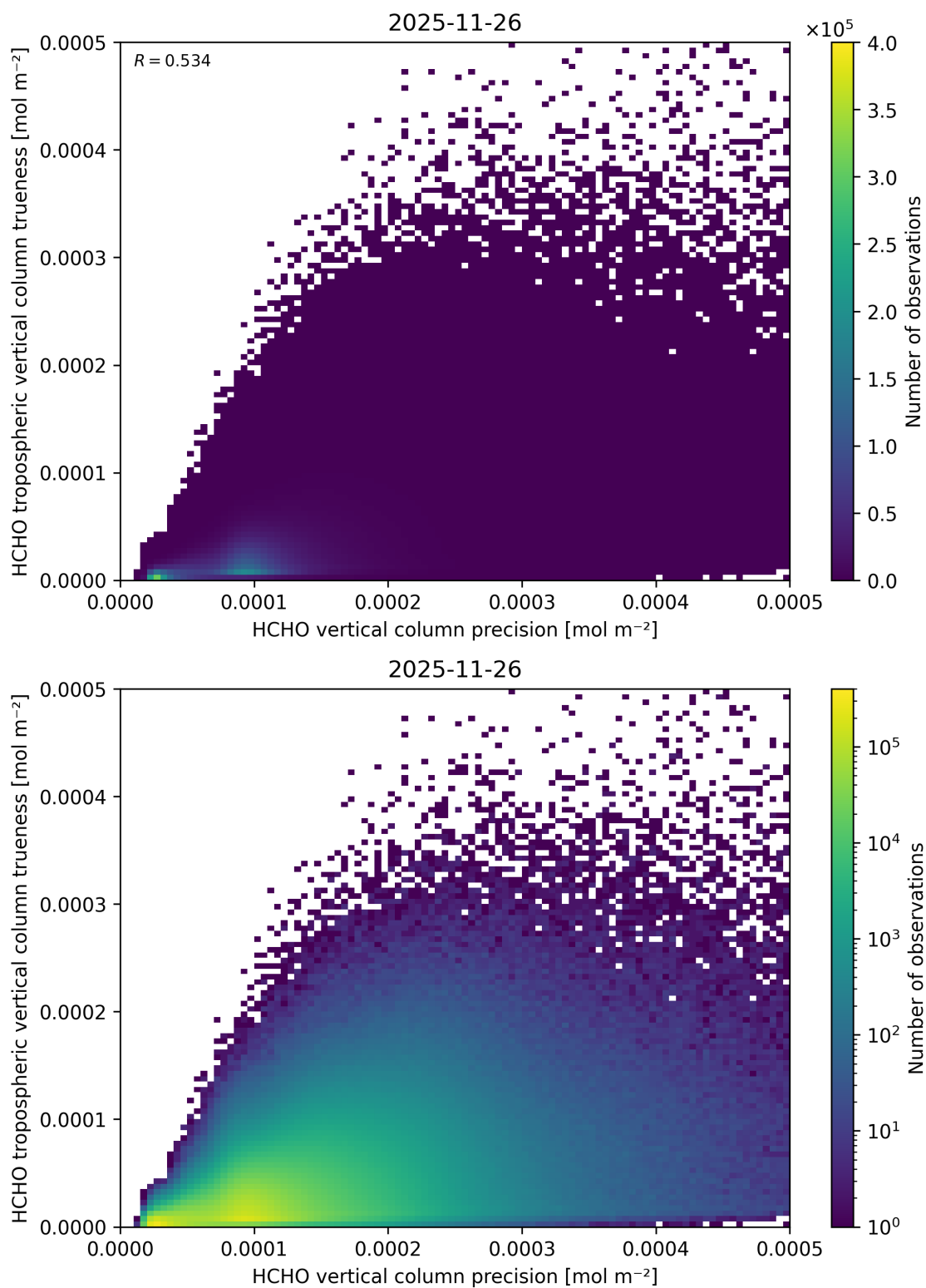
Figure 163: Scatter density plot of “HCHO vertical column precision” against “HCHO tropospheric vertical column truthness” for 2025-11-25 to 2025-11-27.
