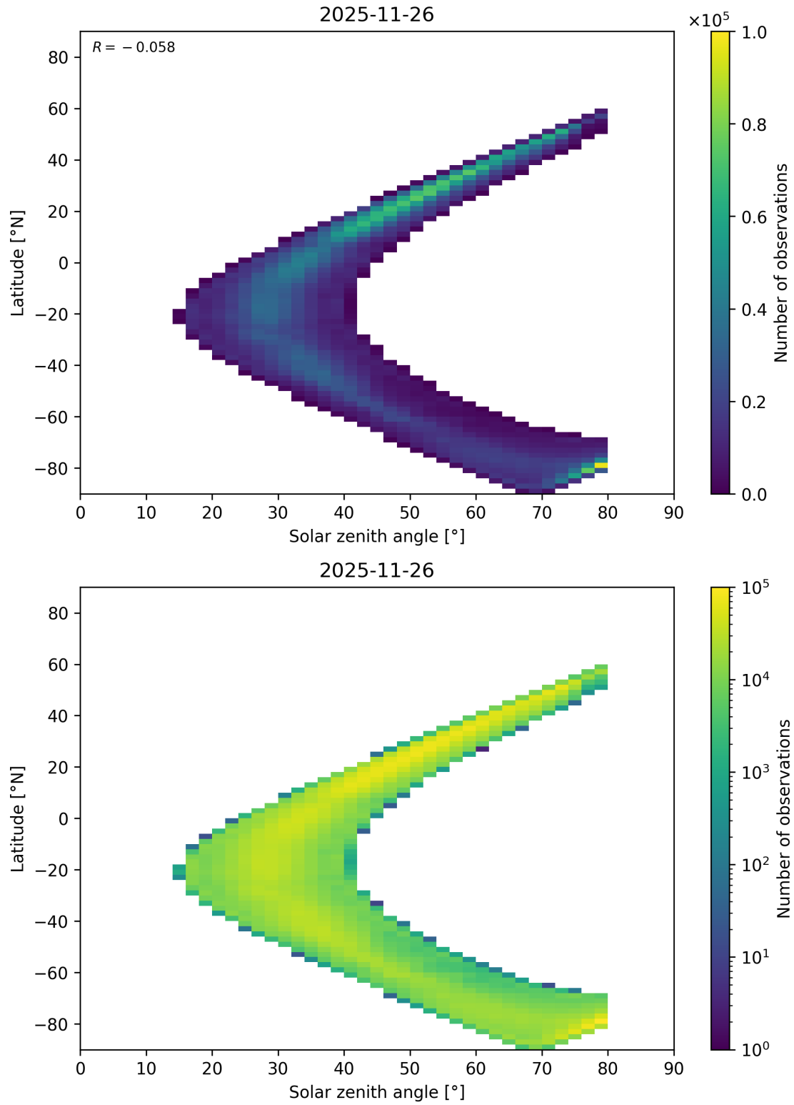
Figure 201: Scatter density plot of “Solar zenith angle” against “Latitude” for 2025-11-25 to 2025-11-27.
