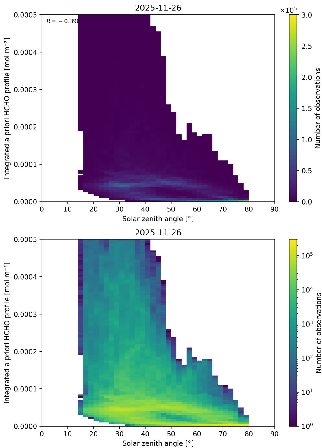
Figure 200: Scatter density plot of “Solar zenith angle” against “Integrated a priori HCHO profile” for 2025-11-25 to 2025-11-27.
