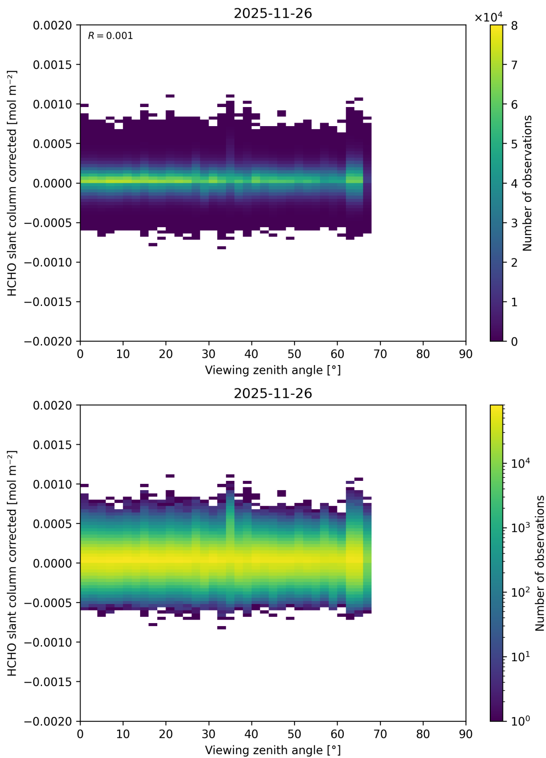
Figure 206: Scatter density plot of “Viewing zenith angle” against “HCHO slant column corrected” for 2025-11-25 to 2025-11-27.
