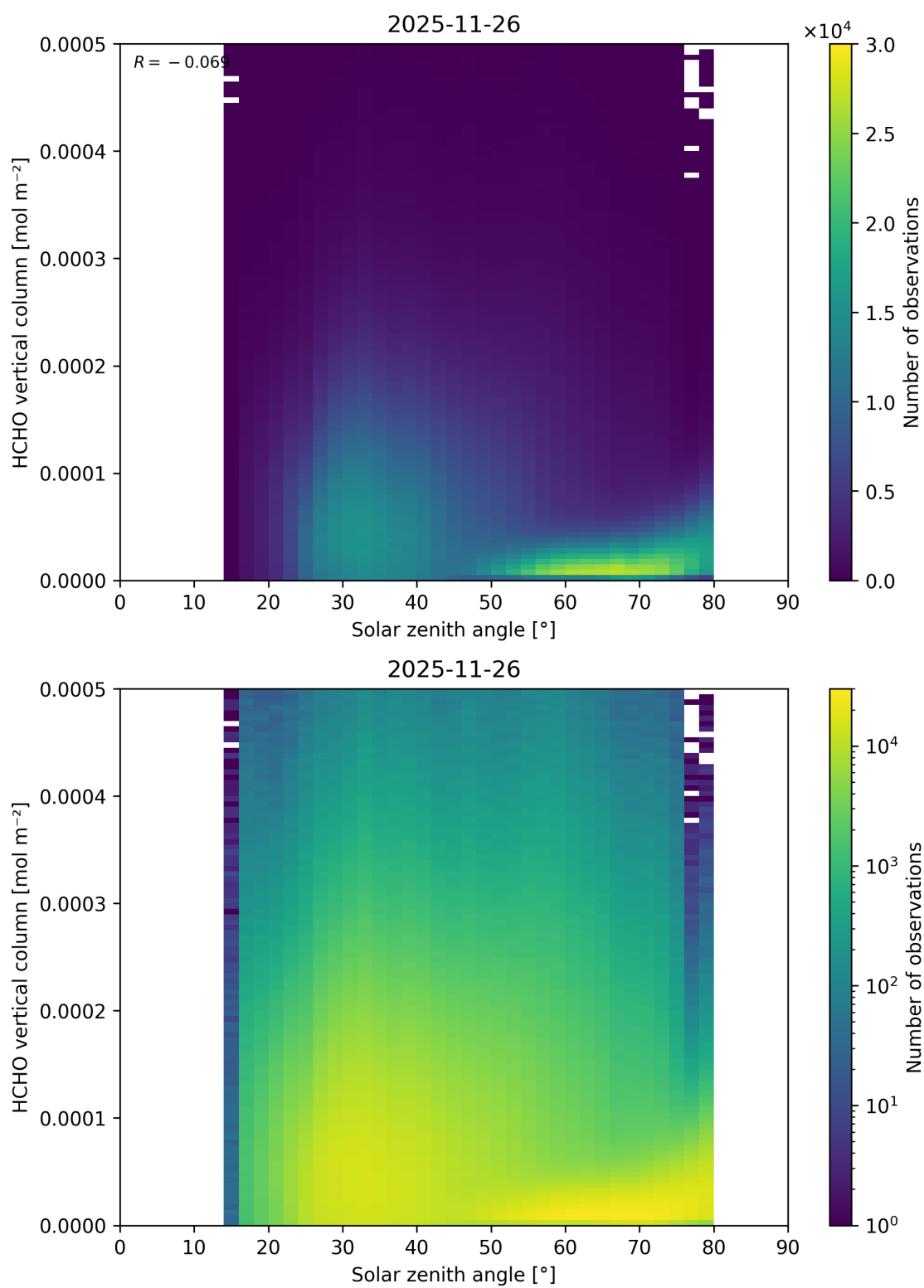
Figure 196: Scatter density plot of “Solar zenith angle” against “HCHO vertical column” for 2025-11-25 to 2025-11-27.
