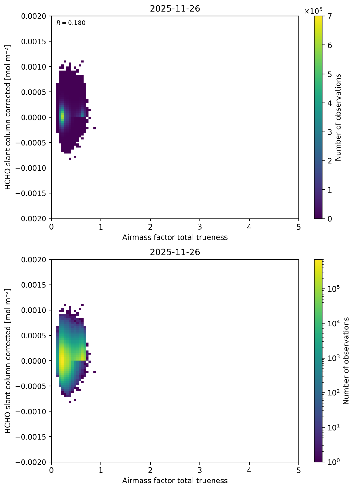
Figure 122: Scatter density plot of “Airmass factor total trueness” against “HCHO slant column corrected” for 2025-11-25 to 2025-11-27.
