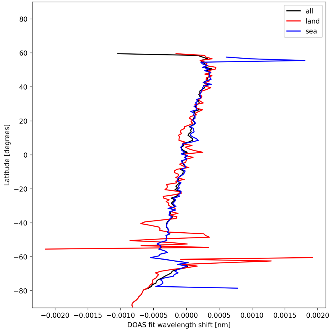
Figure 31: Zonal average of “DOAS fit wavelength shift” for 2025-11-25 to 2025-11-27.
