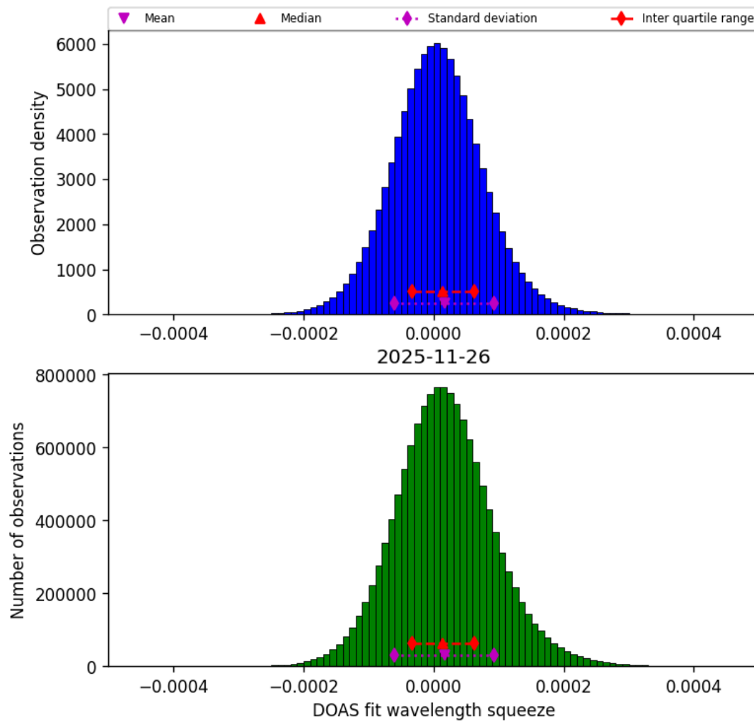
Figure 47: Histogram of “DOAS fit wavelength squeeze” for 2025-11-25 to 2025-11-27
