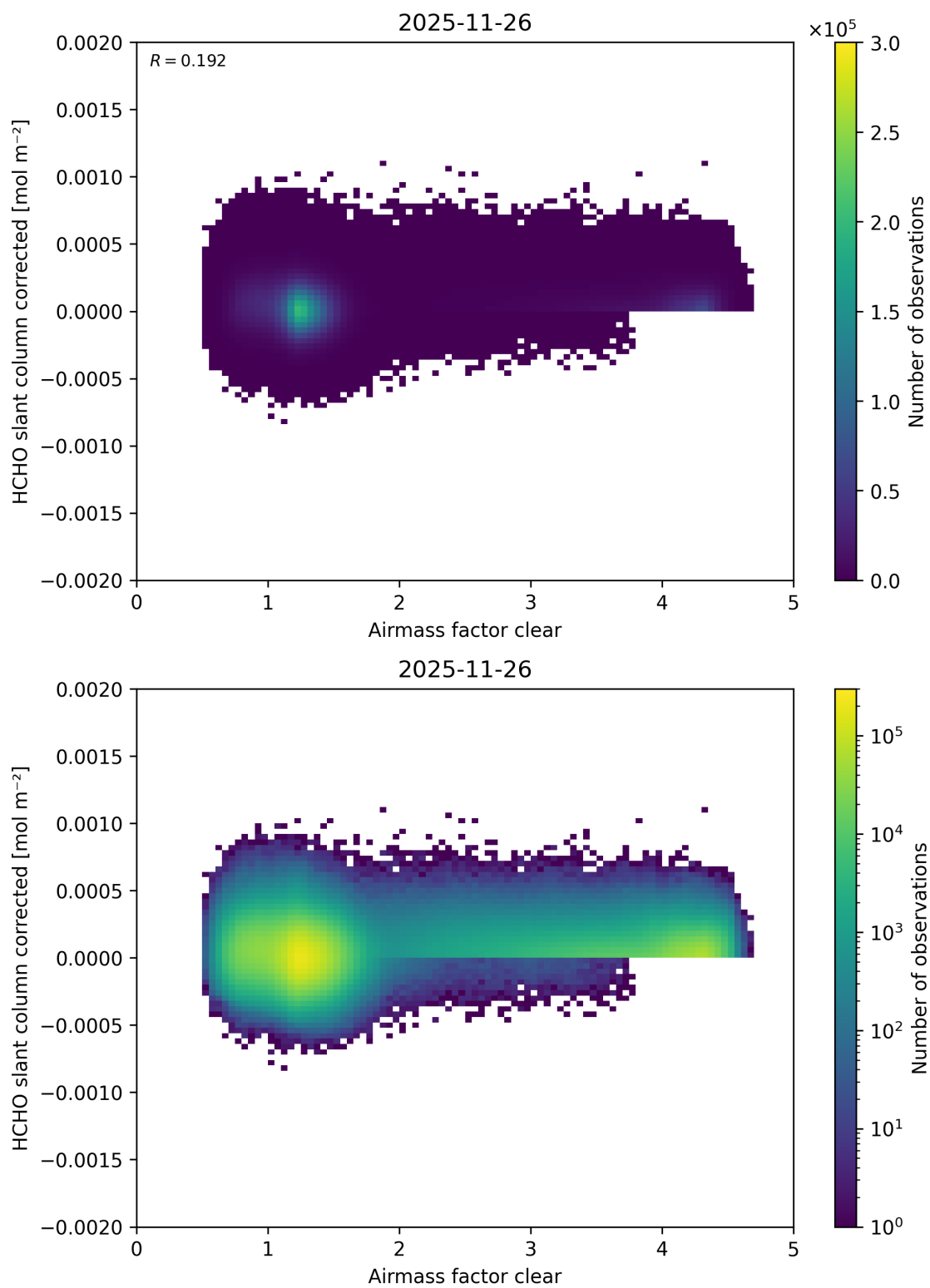
Figure 81: Scatter density plot of “Airmass factor clear” against “HCHO slant column corrected” for 2025-11-25 to 2025-11-27.
