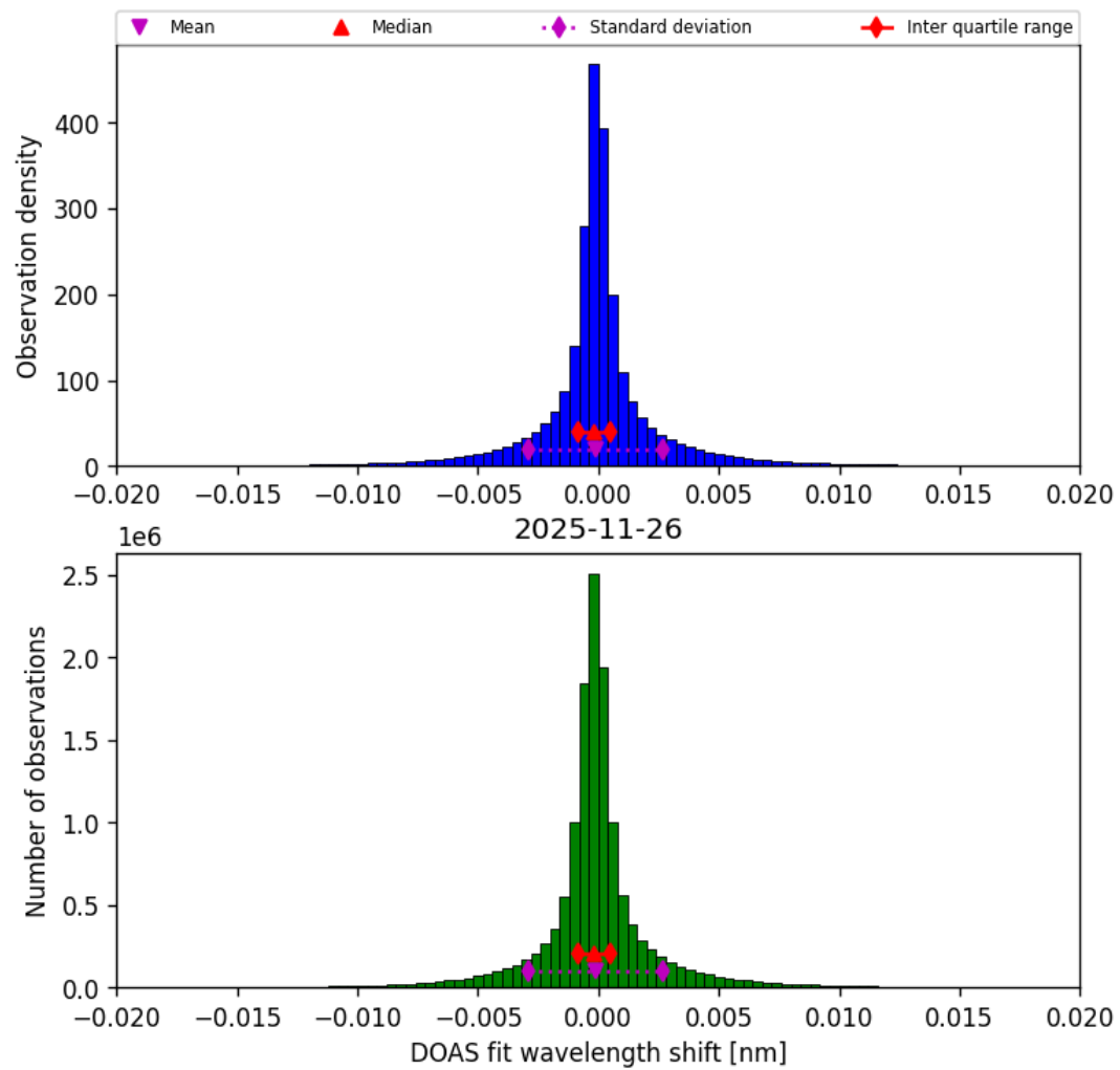
Figure 46: Histogram of “DOAS fit wavelength shift” for 2025-11-25 to 2025-11-27
