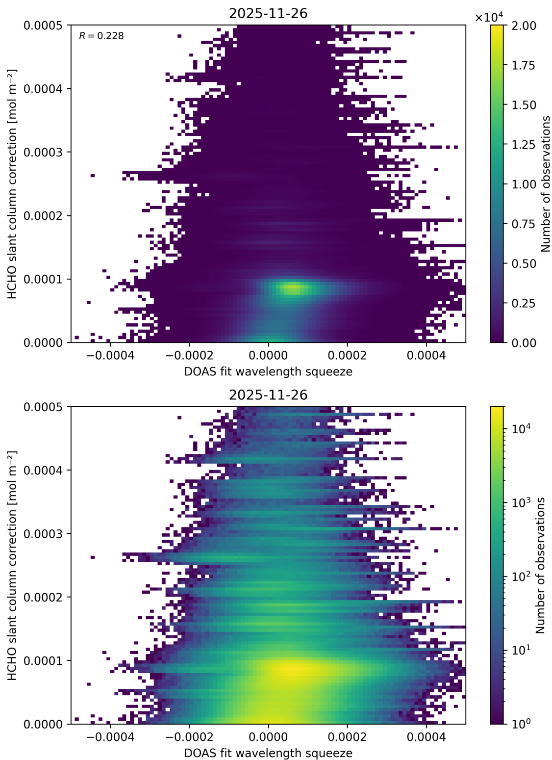
Figure 76: Scatter density plot of “DOAS fit wavelength squeeze” against “HCHO slant column correction” for 2025-11-25 to 2025-11-27.
