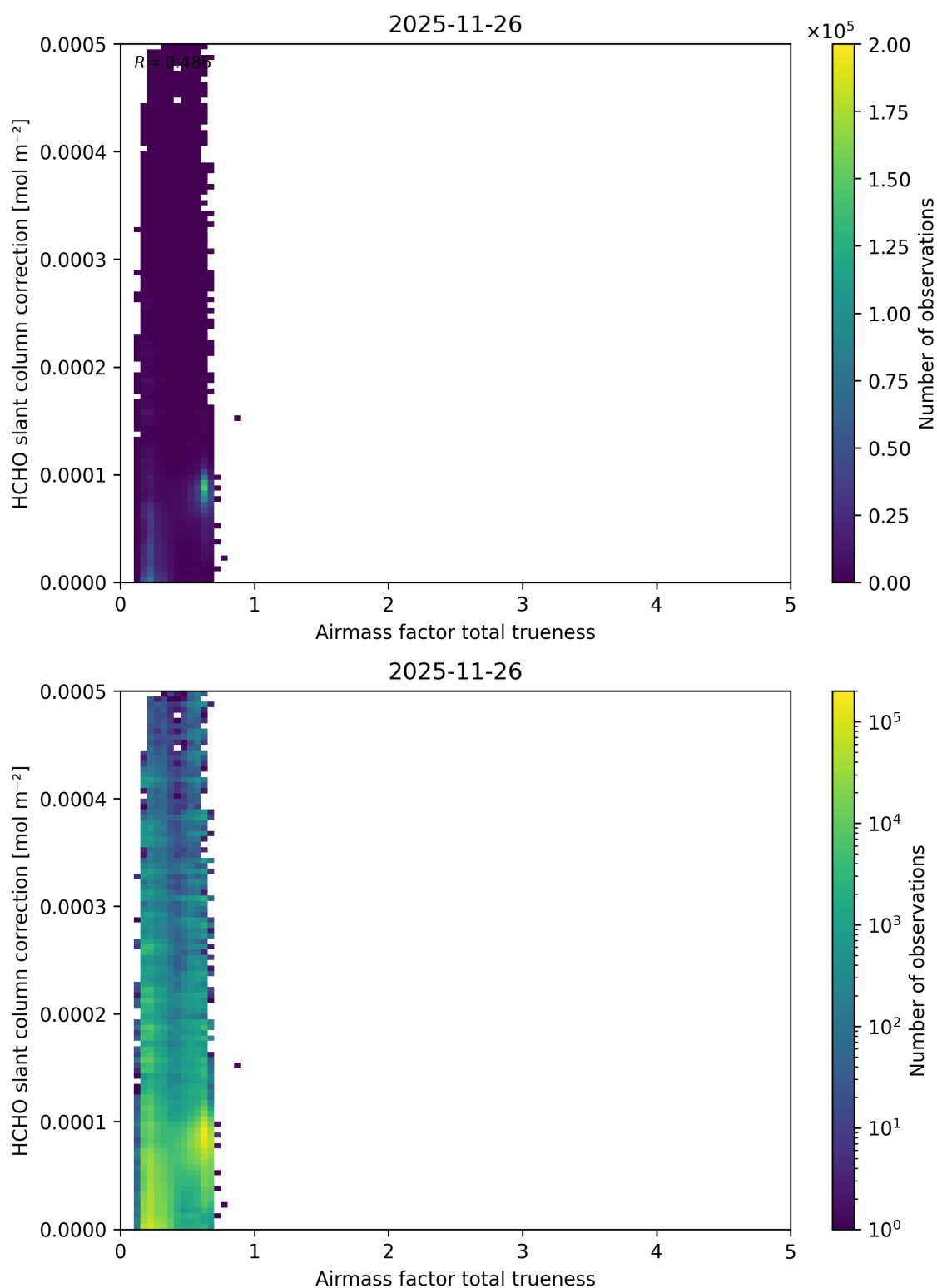
Figure 123: Scatter density plot of “Airmass factor total trueness” against “HCHO slant column correction” for 2025-11-25 to 2025-11-27.
