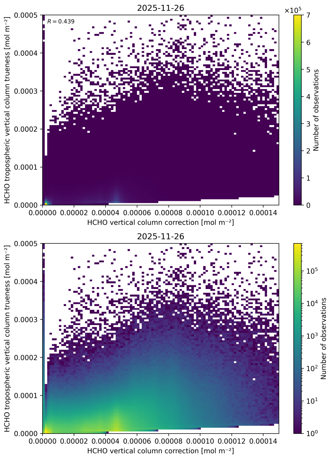
Figure 136: Scatter density plot of “HCHO vertical column correction” against “HCHO tropospheric vertical column true-ness” for 2025-11-25 to 2025-11-27.
