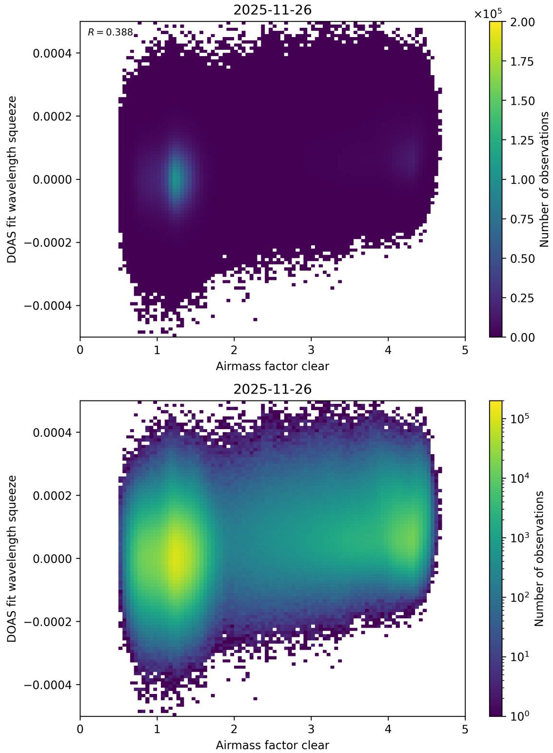
Figure 80: Scatter density plot of “Airmass factor clear” against “DOAS fit wavelength squeeze” for 2025-11-25 to 2025-11-27.
