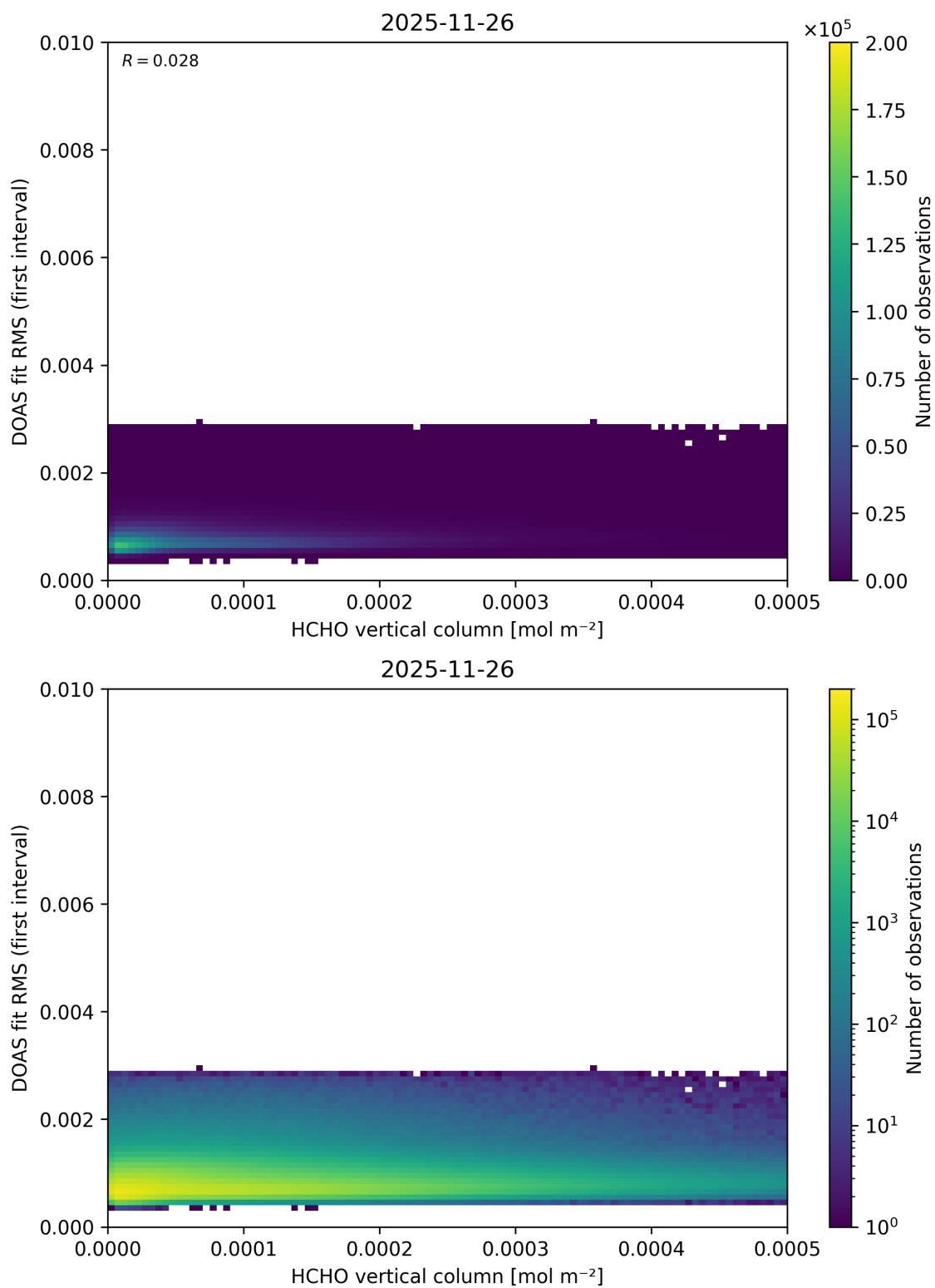
Figure 138: Scatter density plot of “HCHO vertical column” against “DOAS fit RMS (first interval)” for 2025-11-25 to 2025-11-27.
