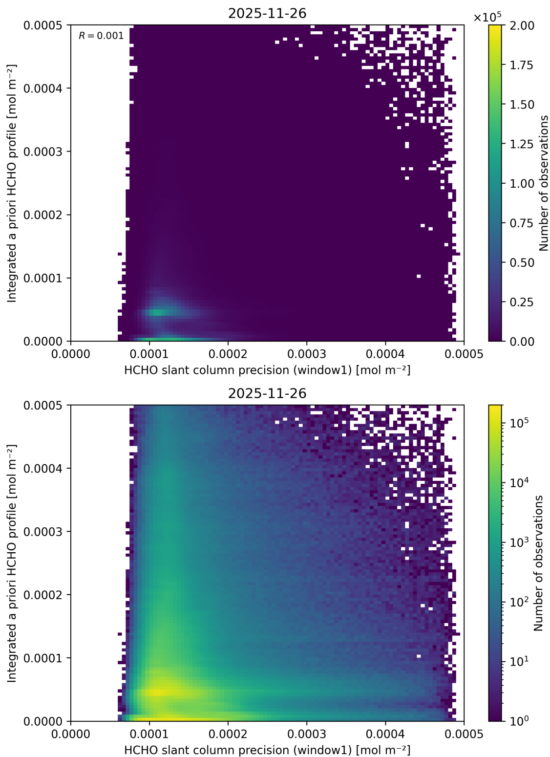
Figure 108: Scatter density plot of “HCHO slant column precision (window1)” against “Integrated a priori HCHO profile” for 2025-11-25 to 2025-11-27.
