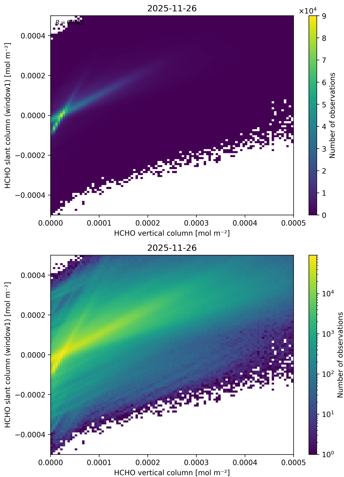
Figure 144: Scatter density plot of “HCHO vertical column” against “HCHO slant column (window1)” for 2025-11-25 to 2025-11-27.
