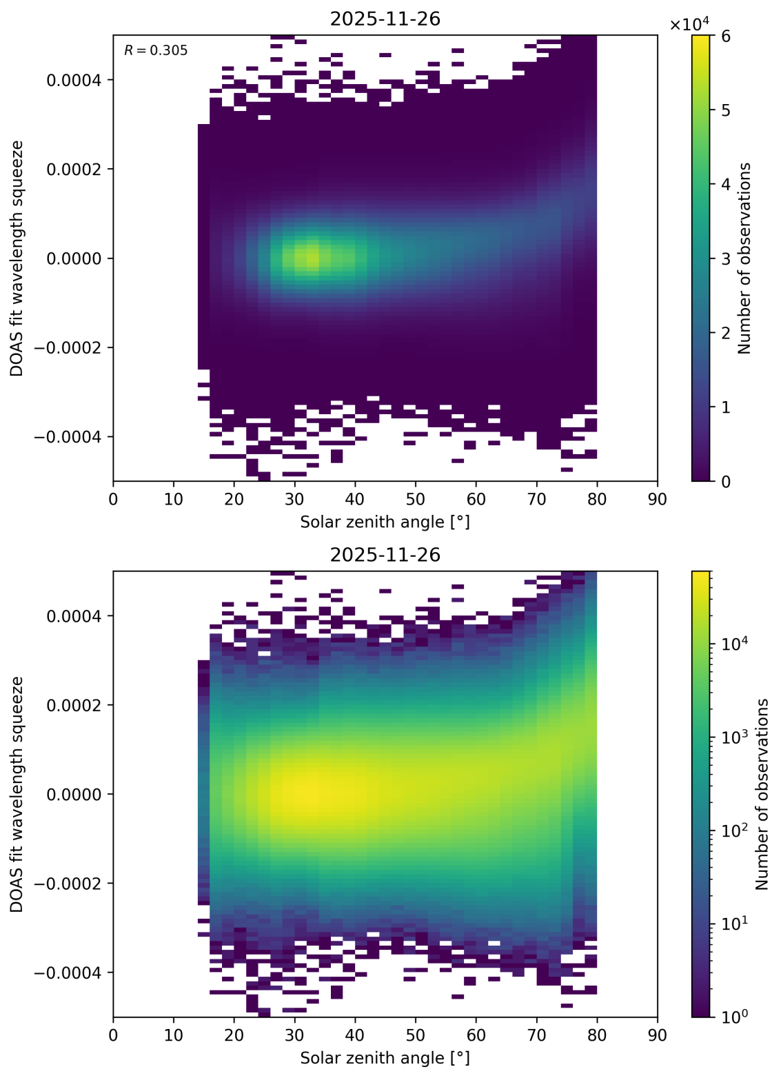
Figure 188: Scatter density plot of “Solar zenith angle” against “DOAS fit wavelength squeeze” for 2025-11-25 to 2025-11-27.
