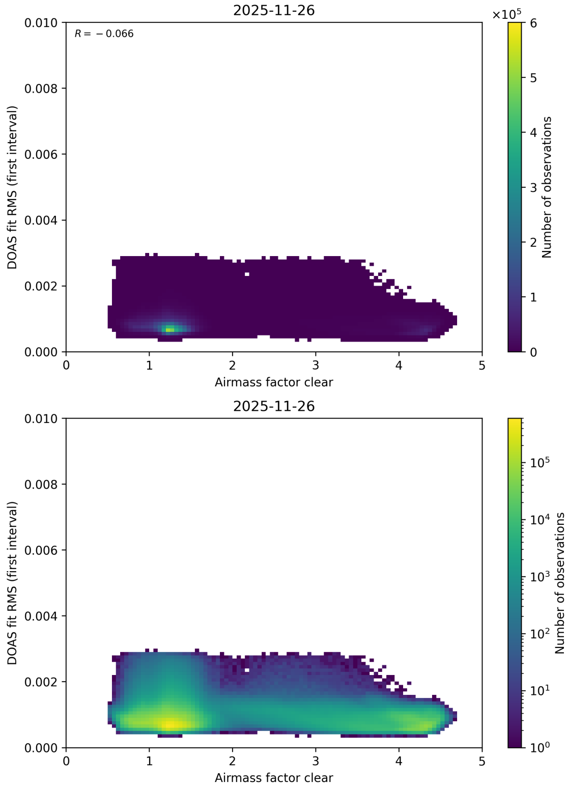
Figure 78: Scatter density plot of “Airmass factor clear” against “DOAS fit RMS (first interval)” for 2025-11-25 to 2025-11-27.
