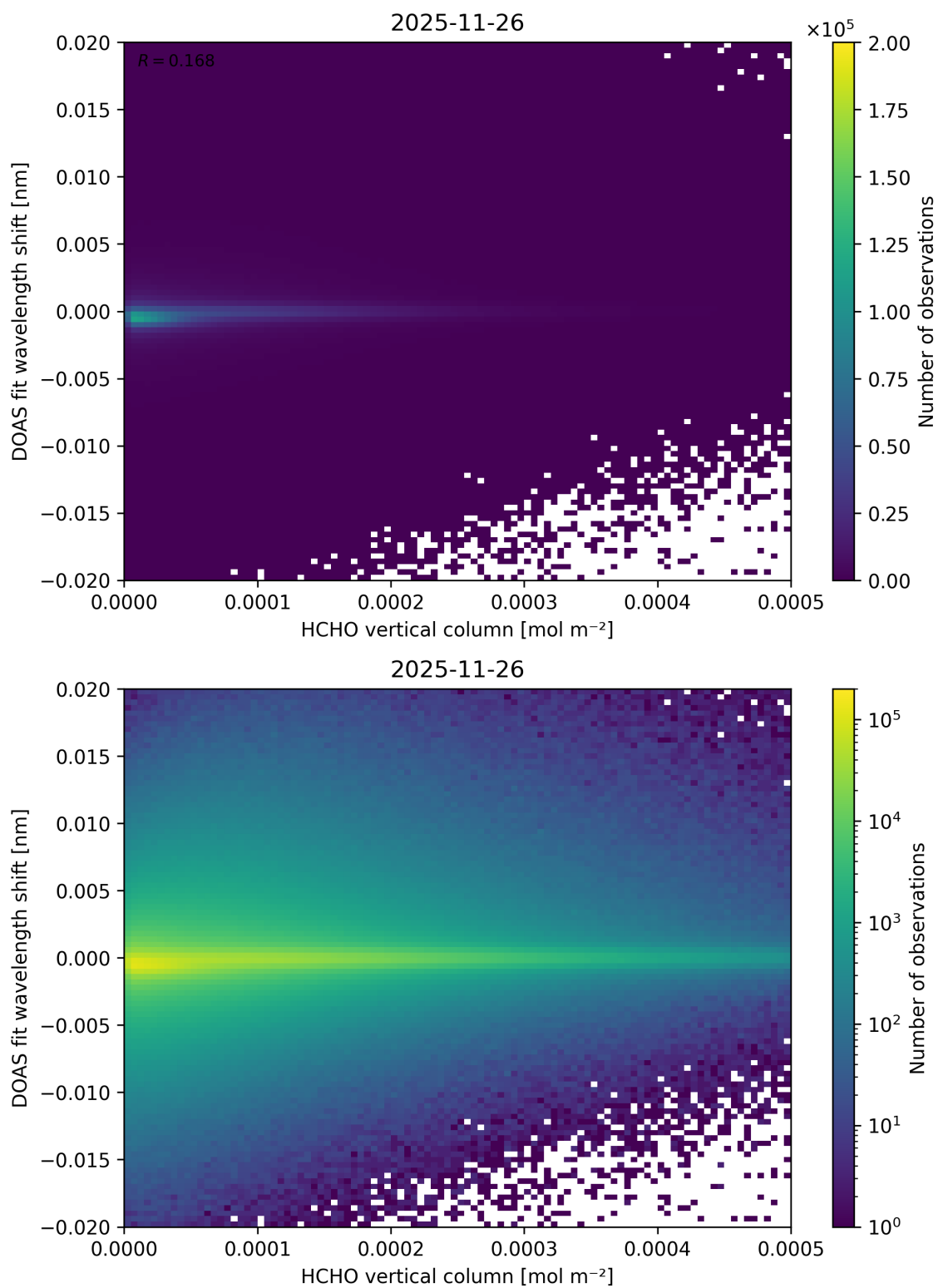
Figure 139: Scatter density plot of “HCHO vertical column” against “DOAS fit wavelength shift” for 2025-11-25 to 2025-11-27.
