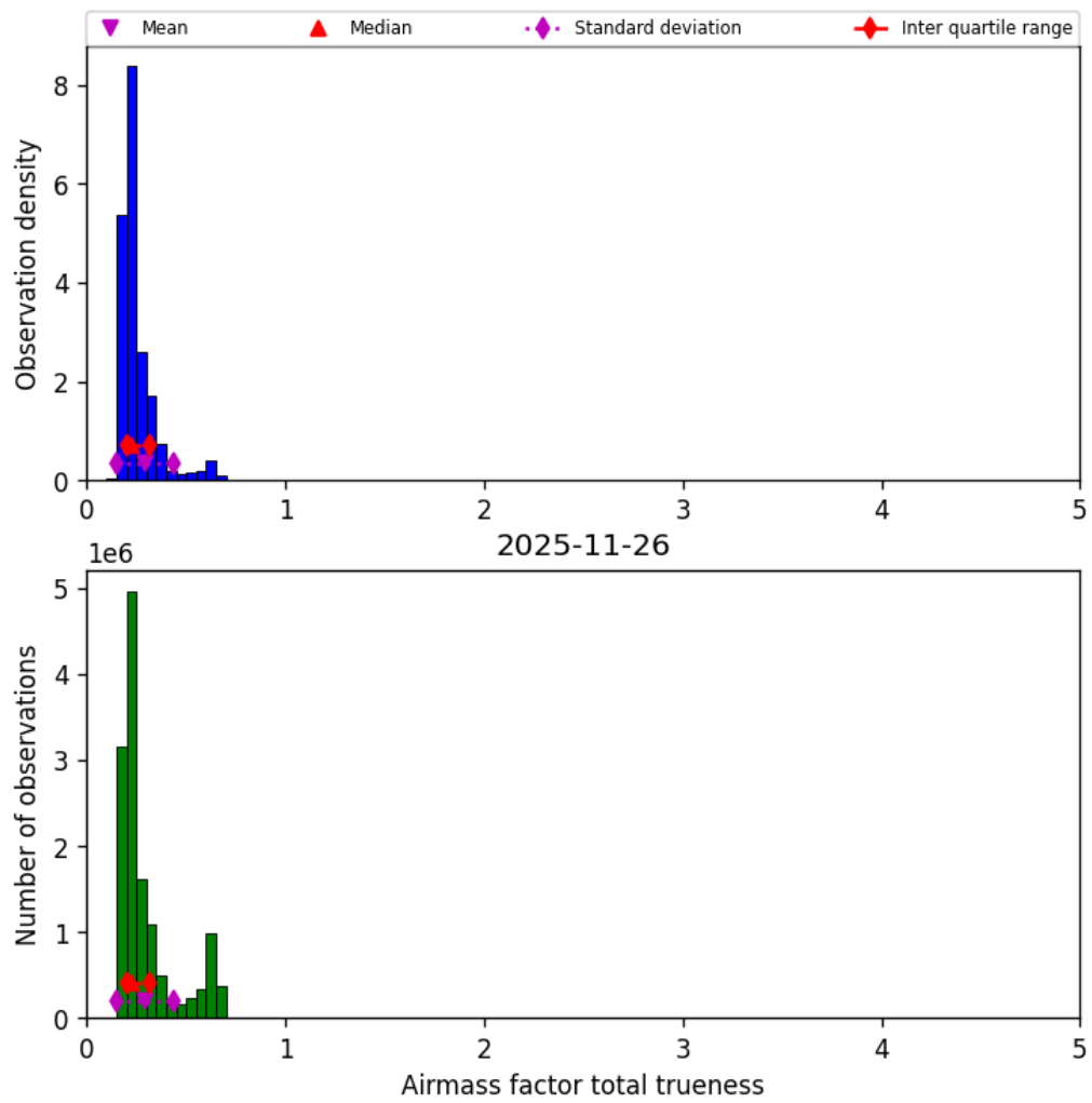
Figure 43: Histogram of “Airmass factor total trueness” for 2025-11-25 to 2025-11-27
