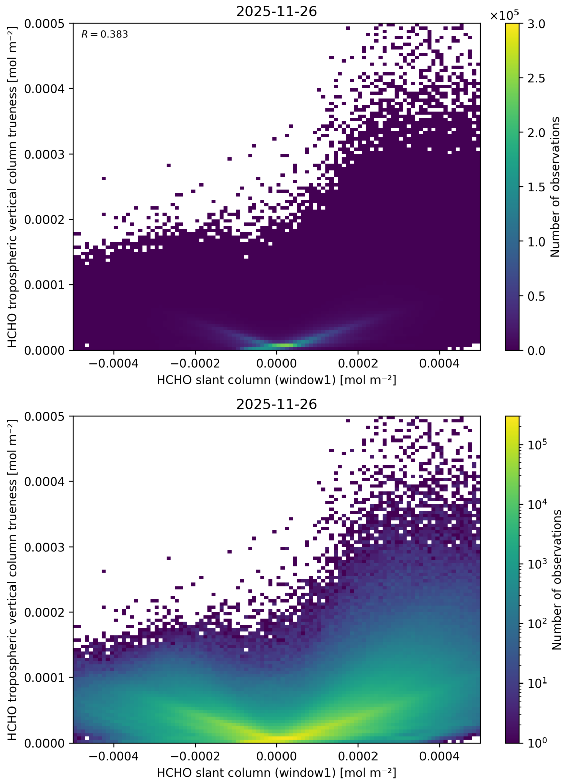
Figure 97: Scatter density plot of “HCHO slant column (window1)” against “HCHO tropospheric vertical column trueness” for 2025-11-25 to 2025-11-27.
