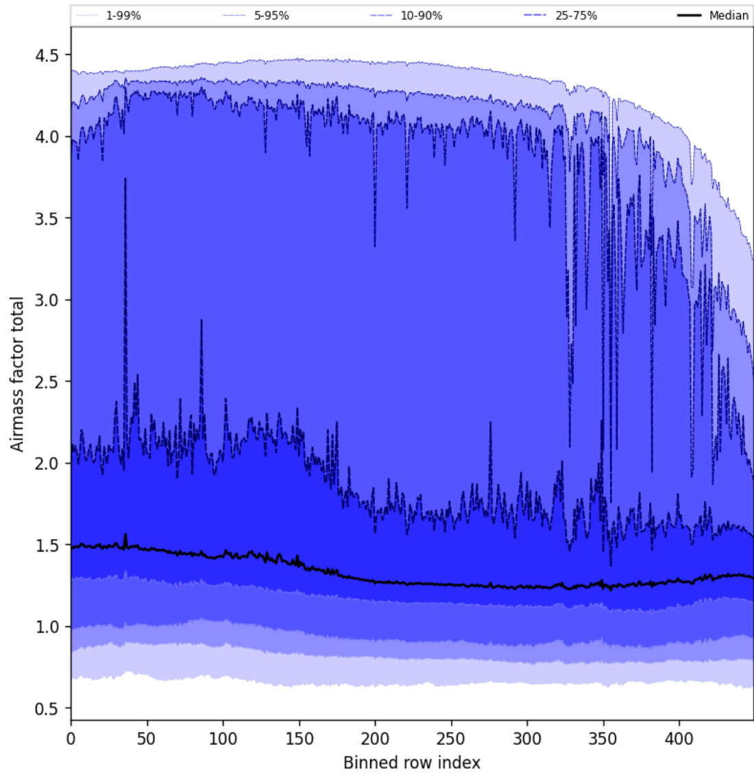
Figure 57: Along track statistics of “Airmass factor total” for 2025-11-25 to 2025-11-27
