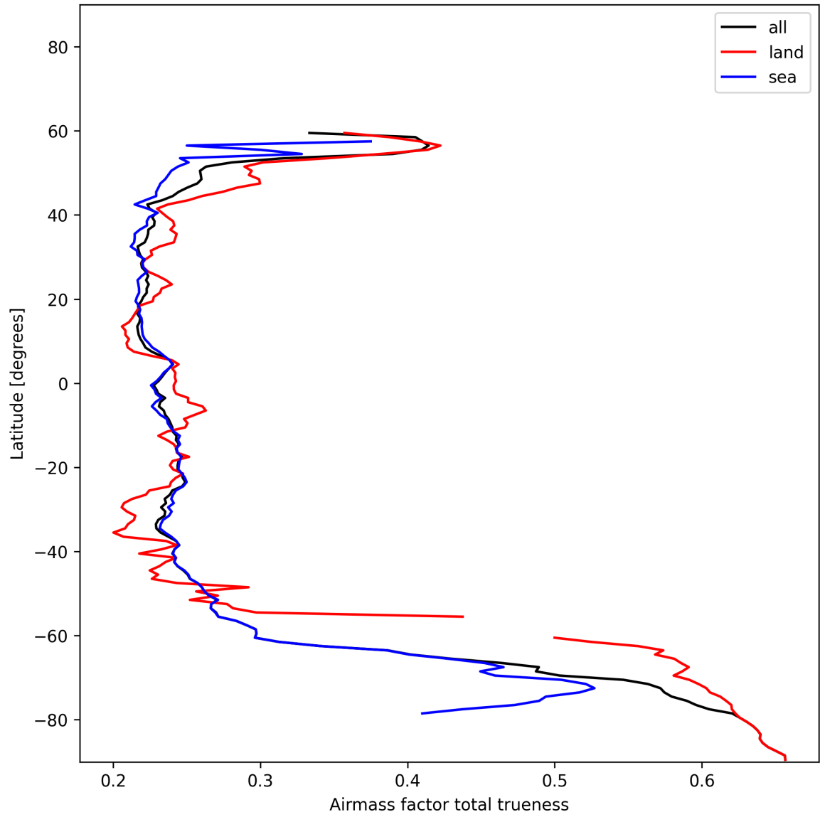
Figure 28: Zonal average of “Airmass factor total trueness” for 2025-11-25 to 2025-11-27.
