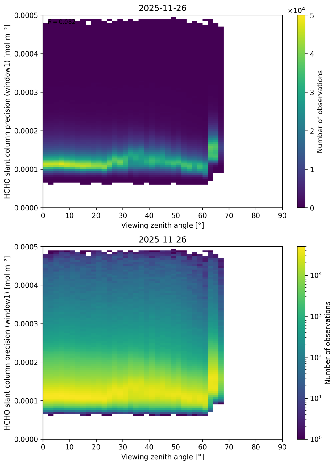
Figure 209: Scatter density plot of “Viewing zenith angle” against “HCHO slant column precision (window1)” for 2025-11-25 to 2025-11-27.
