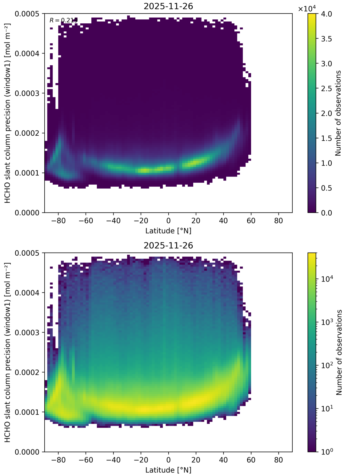
Figure 178: Scatter density plot of “Latitude” against “HCHO slant column precision (window1)” for 2025-11-25 to 2025-11-27.
