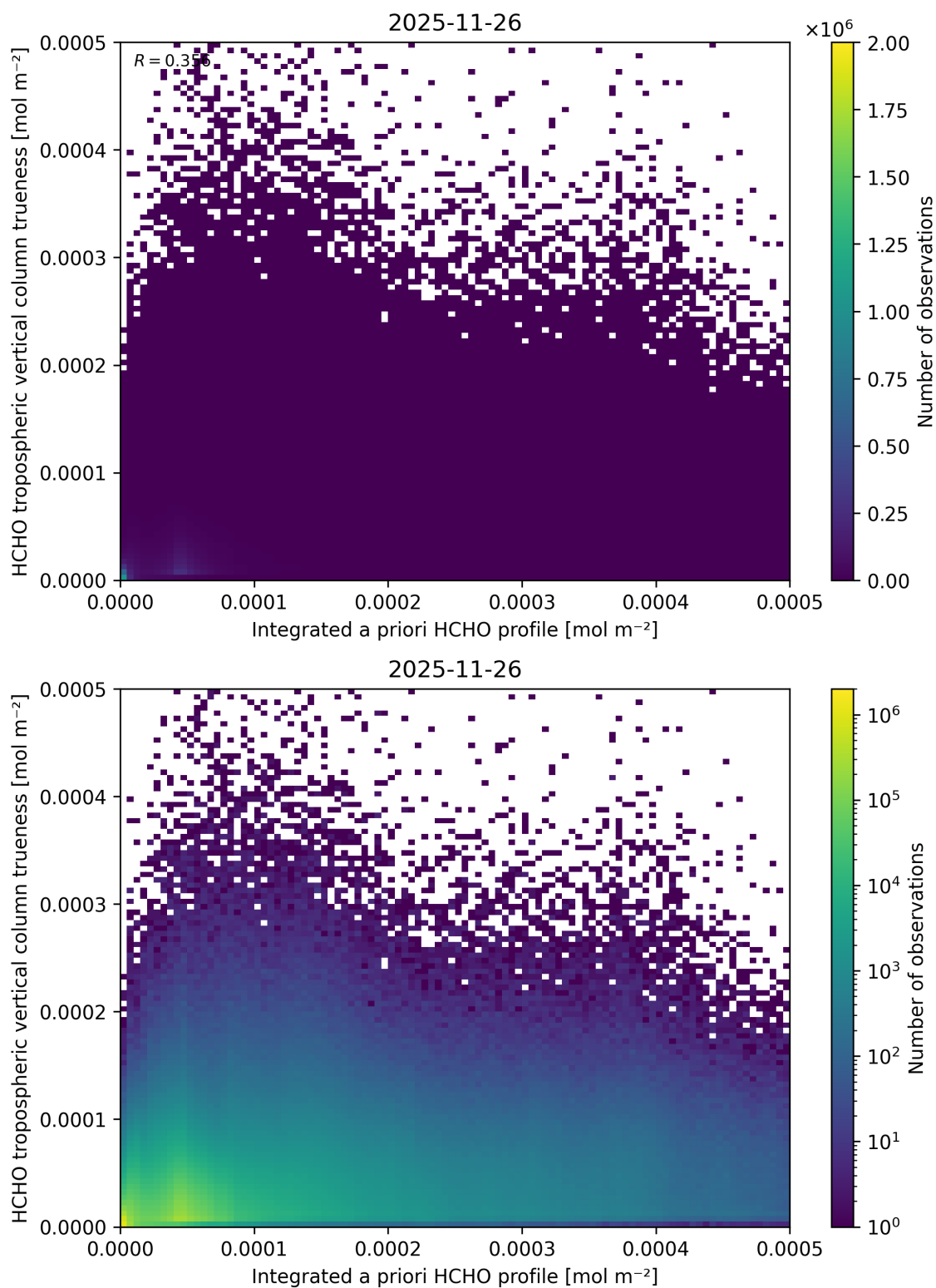
Figure 170: Scatter density plot of “Integrated a priori HCHO profile” against “HCHO tropospheric vertical column trueness” for 2025-11-25 to 2025-11-27.
