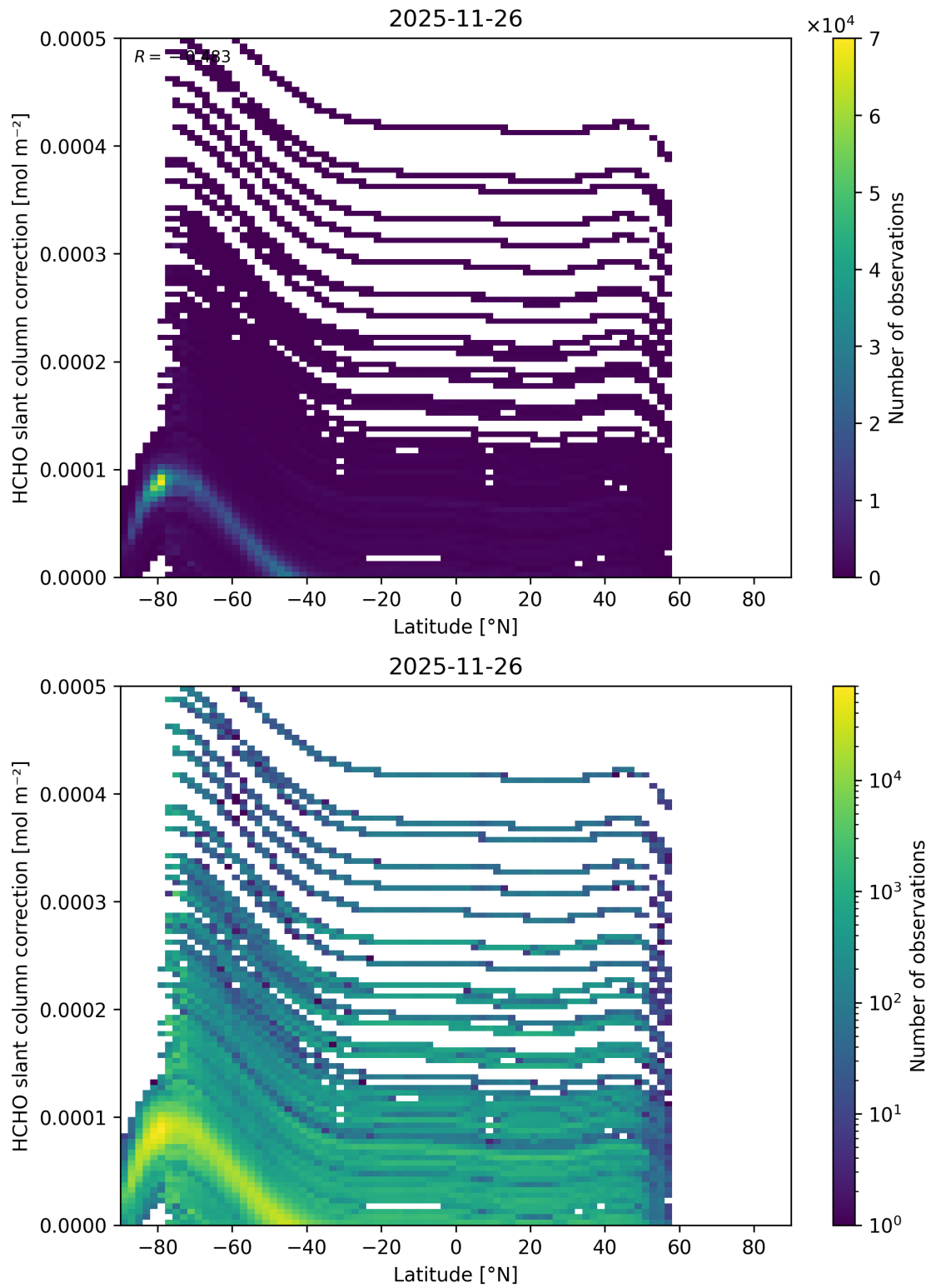
Figure 176: Scatter density plot of “Latitude” against “HCHO slant column correction” for 2025-11-25 to 2025-11-27.
