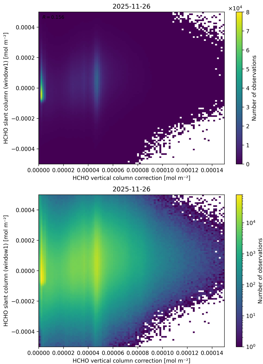
Figure 132: Scatter density plot of “HCHO vertical column correction” against “HCHO slant column (window1)” for 2025-11-25 to 2025-11-27.
