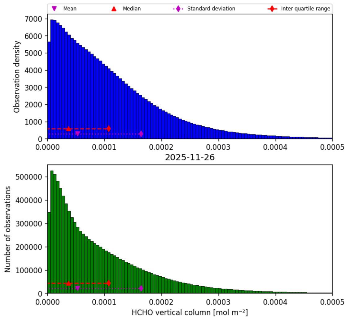
Figure 37: Histogram of “HCHO vertical column” for 2025-11-25 to 2025-11-27
