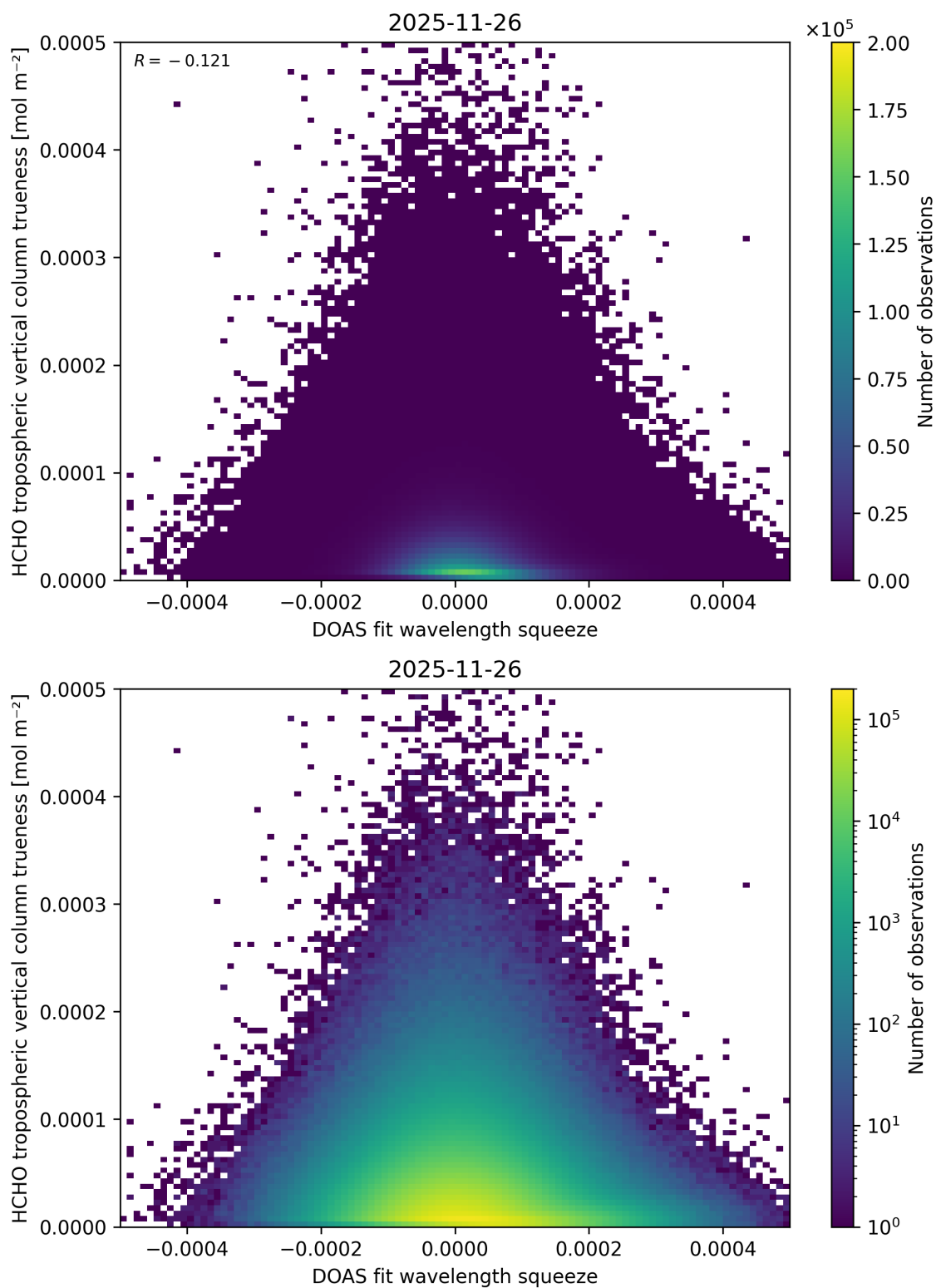
Figure 77: Scatter density plot of “DOAS fit wavelength squeeze” against “HCHO tropospheric vertical column trueness” for 2025-11-25 to 2025-11-27.
