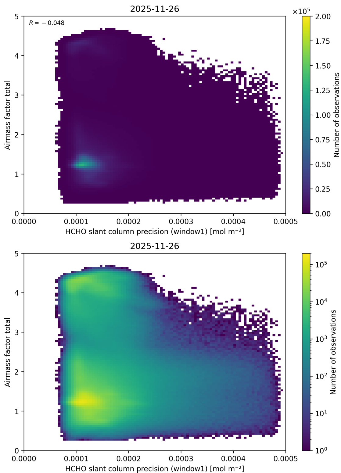
Figure 105: Scatter density plot of “HCHO slant column precision (window1)” against “Airmass factor total” for 2025-11-25 to 2025-11-27.
