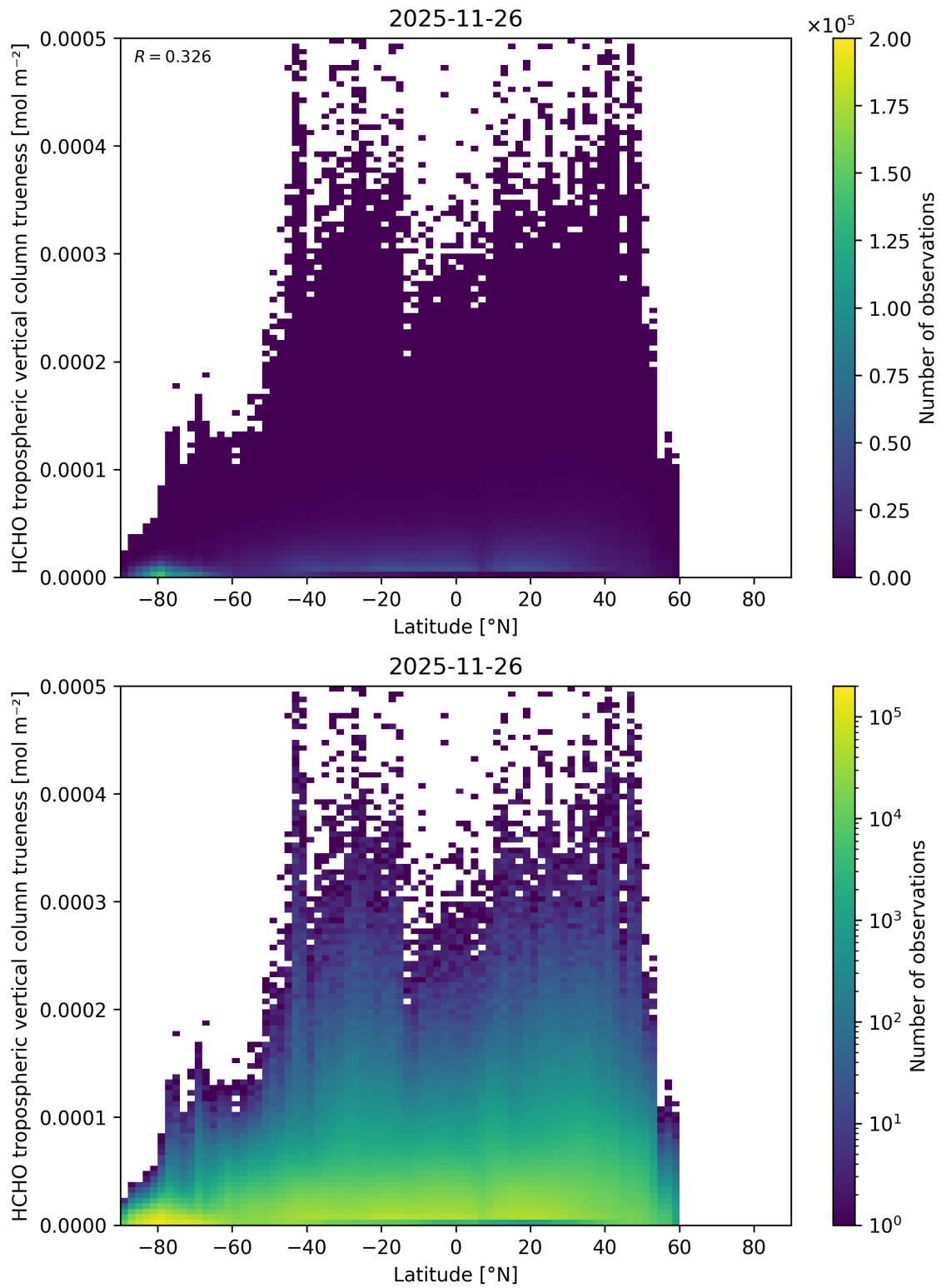
Figure 184: Scatter density plot of “Latitude” against “HCHO tropospheric vertical column trueness” for 2025-11-25 to 2025-11-27.
