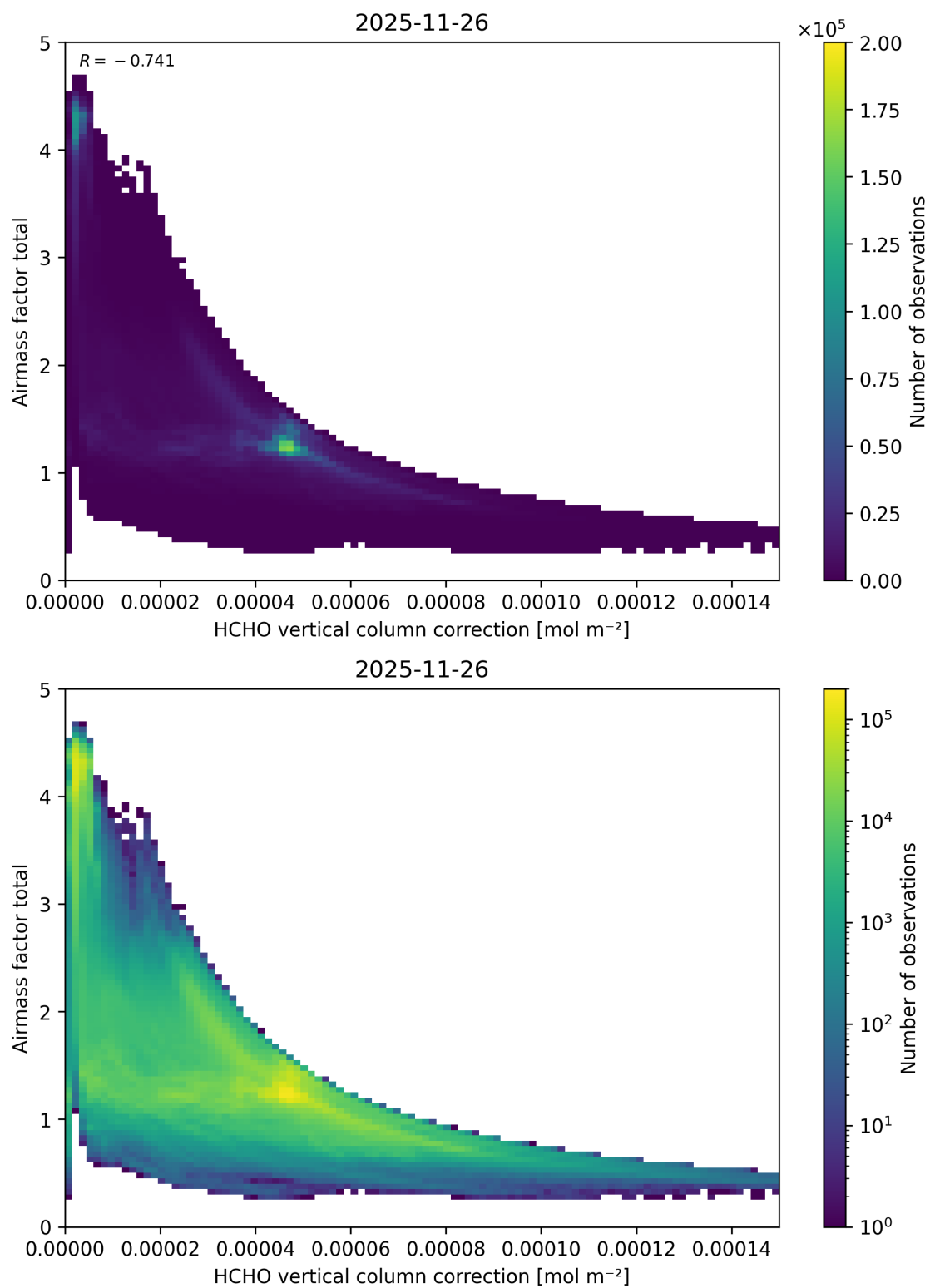
Figure 134: Scatter density plot of “HCHO vertical column correction” against “Airmass factor total” for 2025-11-25 to 2025-11-27.
