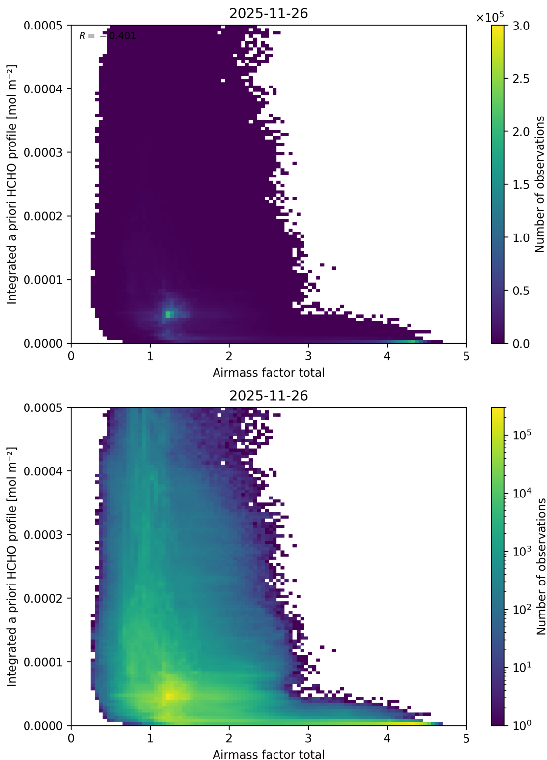
Figure 117: Scatter density plot of “Airmass factor total” against “Integrated a priori HCHO profile” for 2025-11-25 to 2025-11-27.
