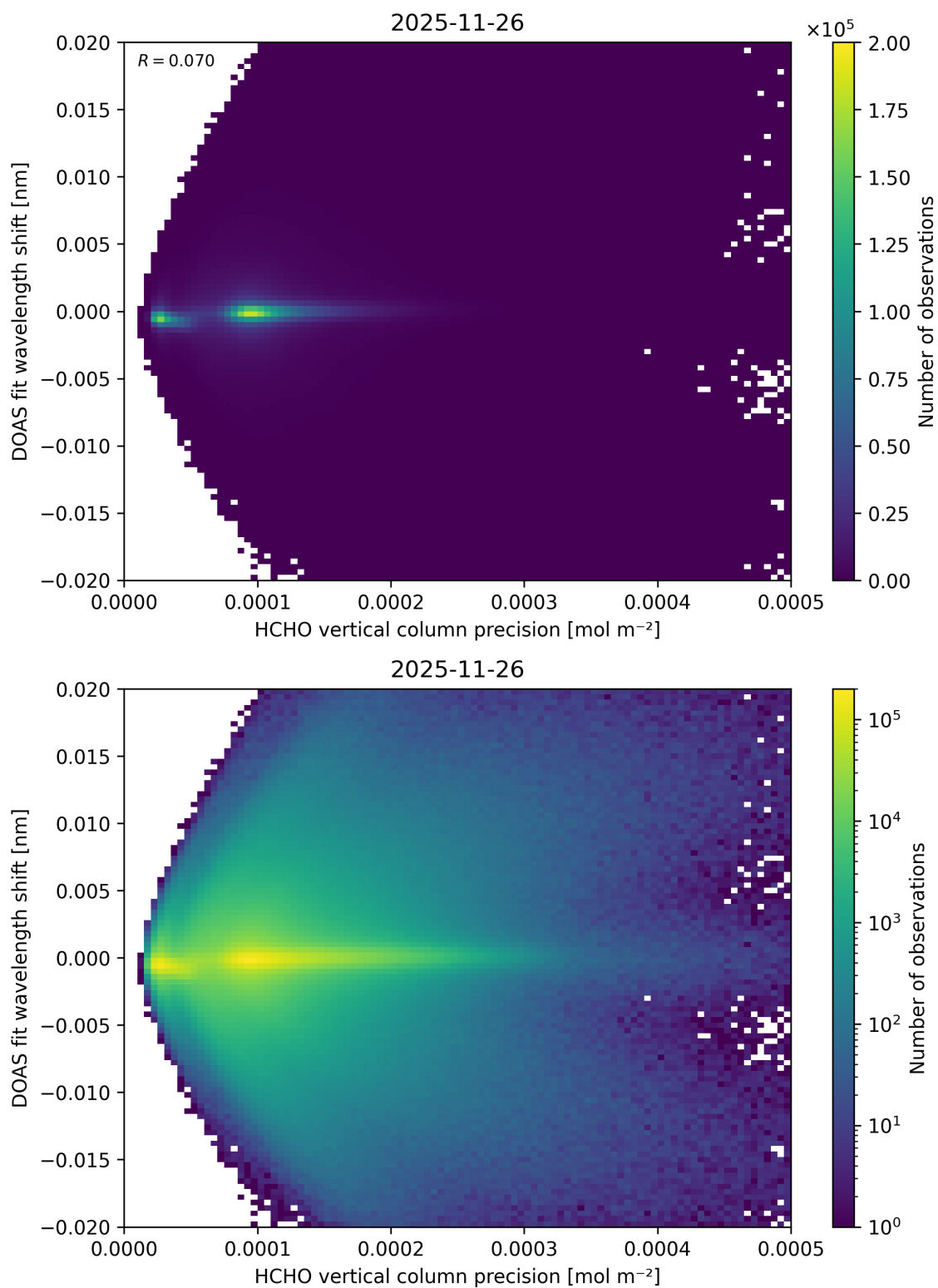
Figure 153: Scatter density plot of “HCHO vertical column precision” against “DOAS fit wavelength shift” for 2025-11-25 to 2025-11-27.
