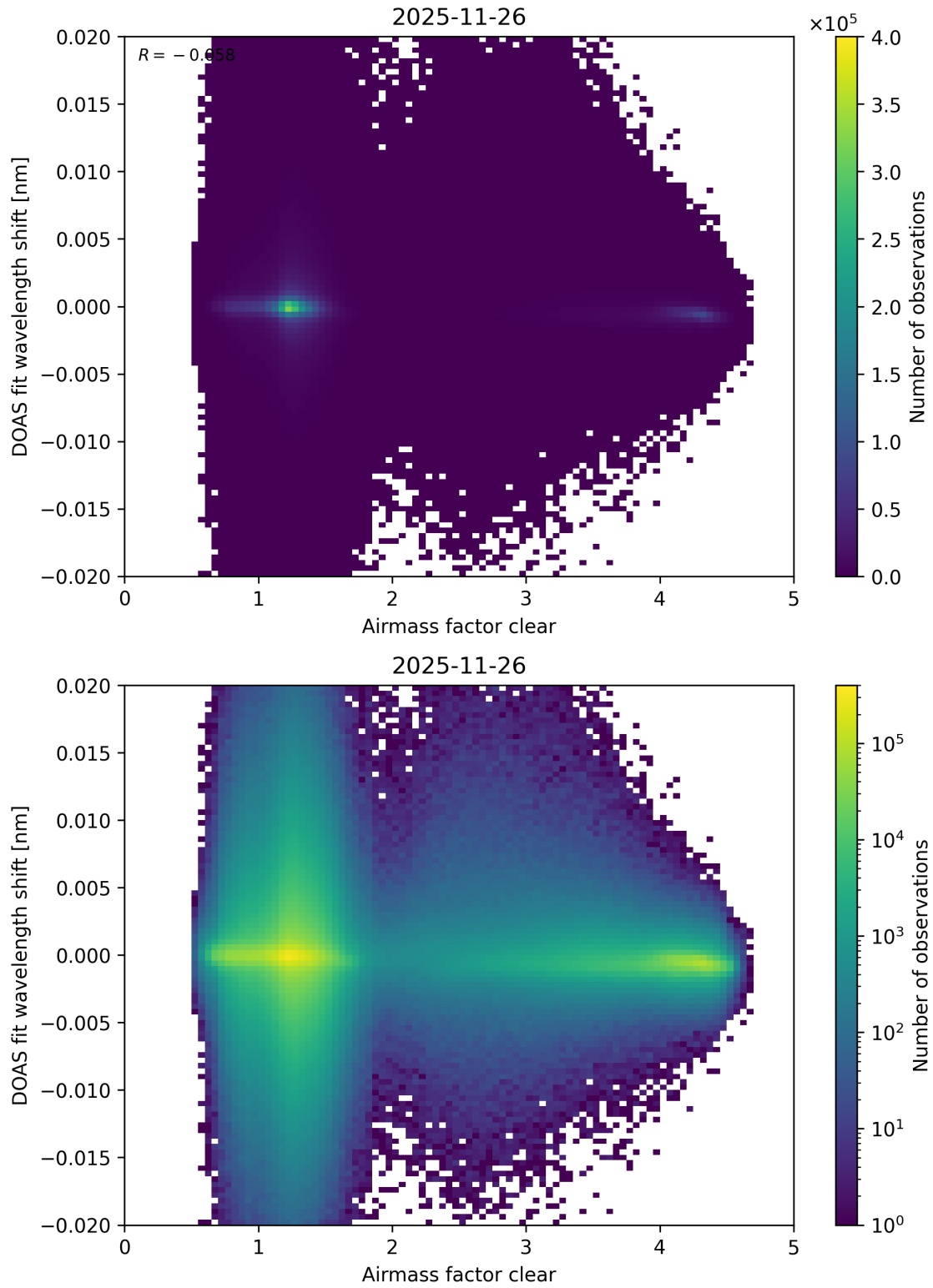
Figure 79: Scatter density plot of “Airmass factor clear” against “DOAS fit wavelength shift” for 2025-11-25 to 2025-11-27.
