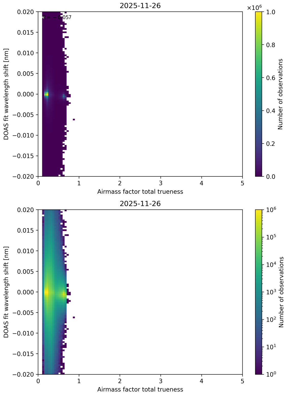
Figure 119: Scatter density plot of “Airmass factor total trueness” against “DOAS fit wavelength shift” for 2025-11-25 to 2025-11-27.
