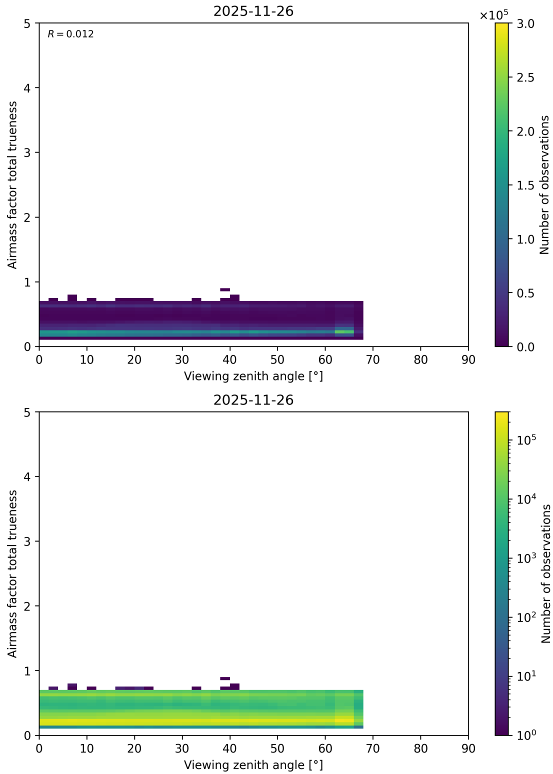
Figure 211: Scatter density plot of “Viewing zenith angle” against “Airmass factor total trueness” for 2025-11-25 to 2025-11-27.
