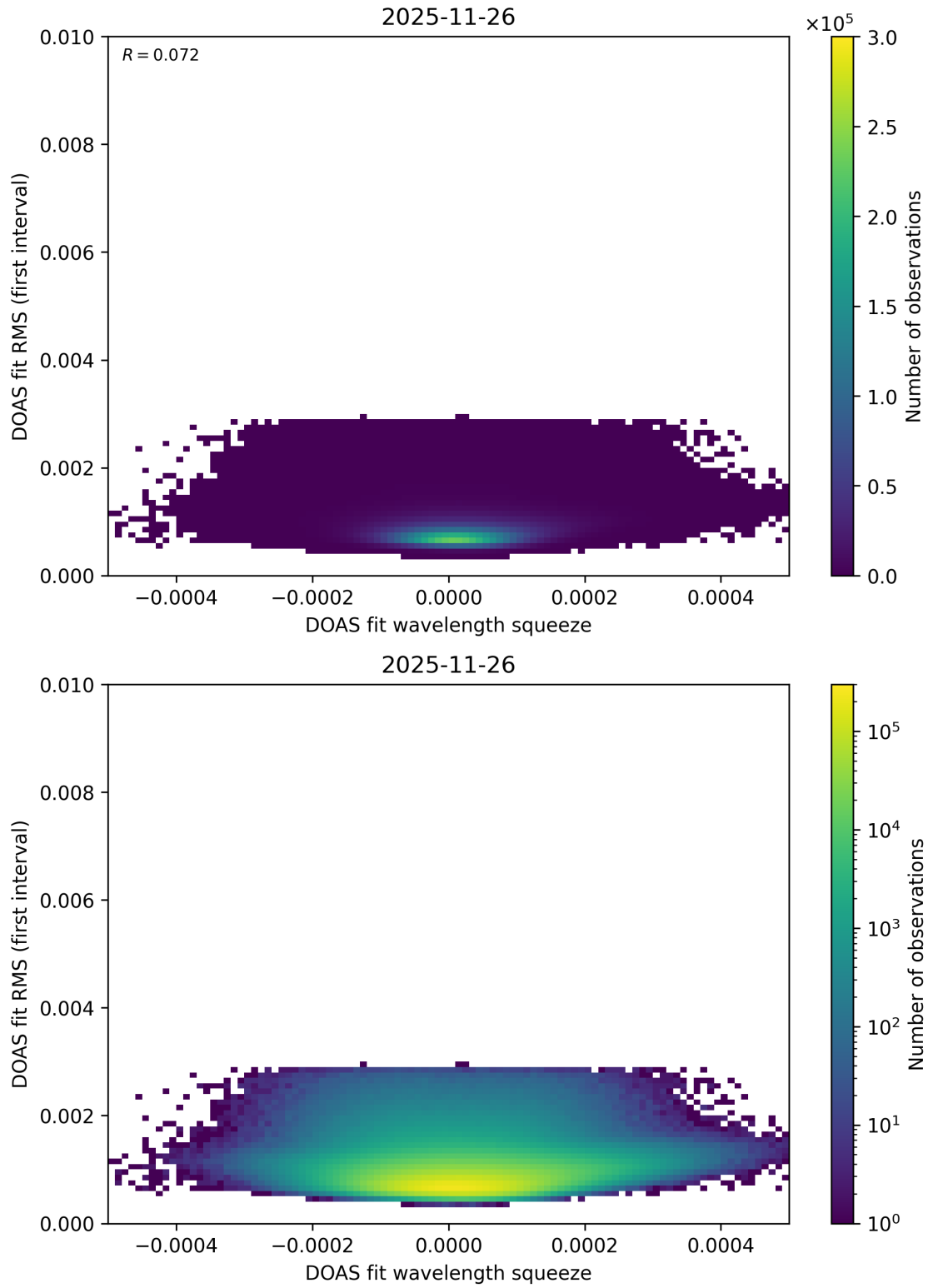
Figure 74: Scatter density plot of “DOAS fit wavelength squeeze” against “DOAS fit RMS (first interval)” for 2025-11-25 to 2025-11-27.
