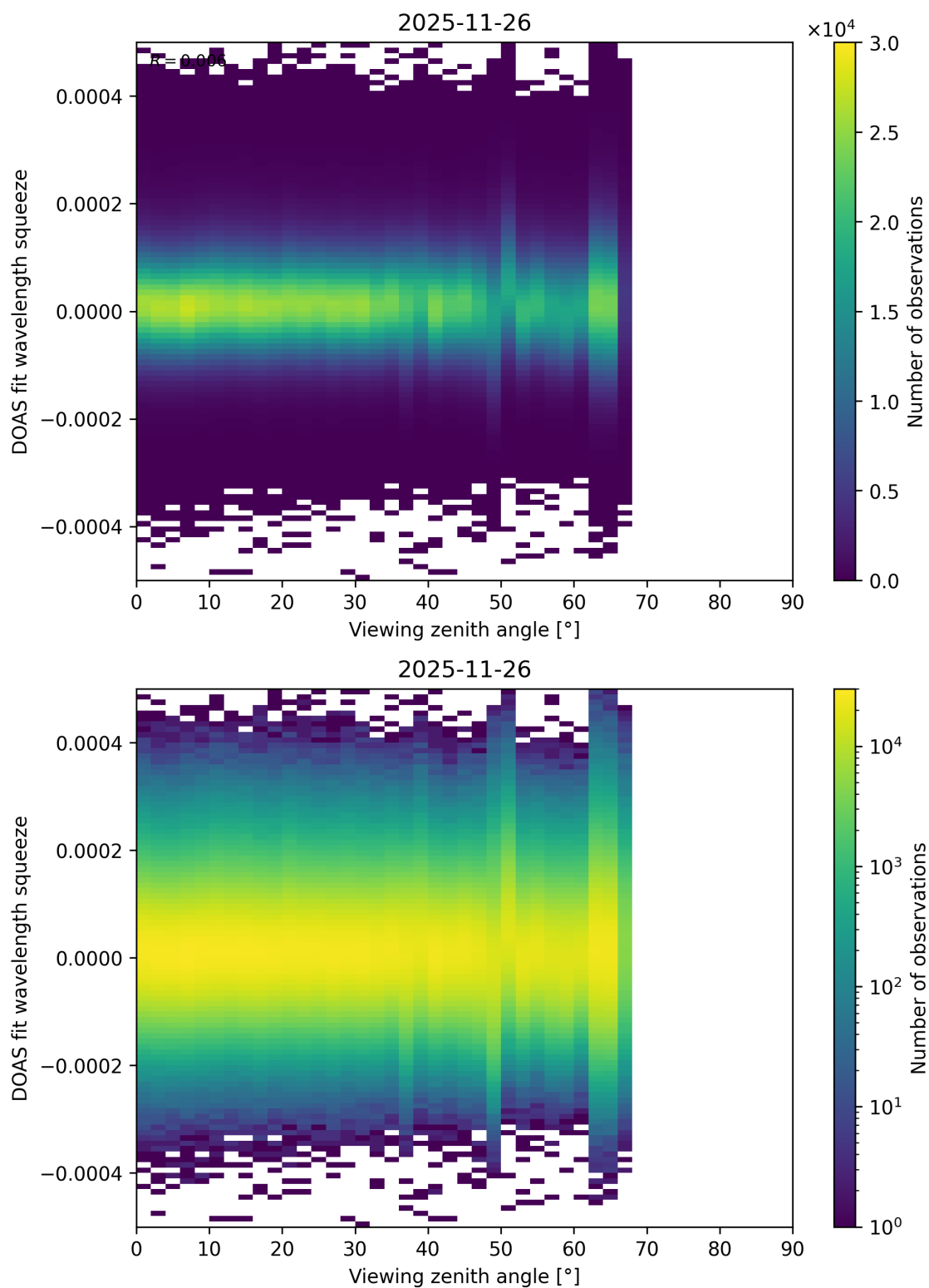
Figure 204: Scatter density plot of “Viewing zenith angle” against “DOAS fit wavelength squeeze” for 2025-11-25 to 2025-11-27.
