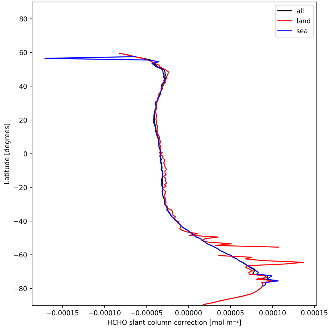
Figure 34: Zonal average of “HCHO slant column correction” for 2025-11-25 to 2025-11-27.
