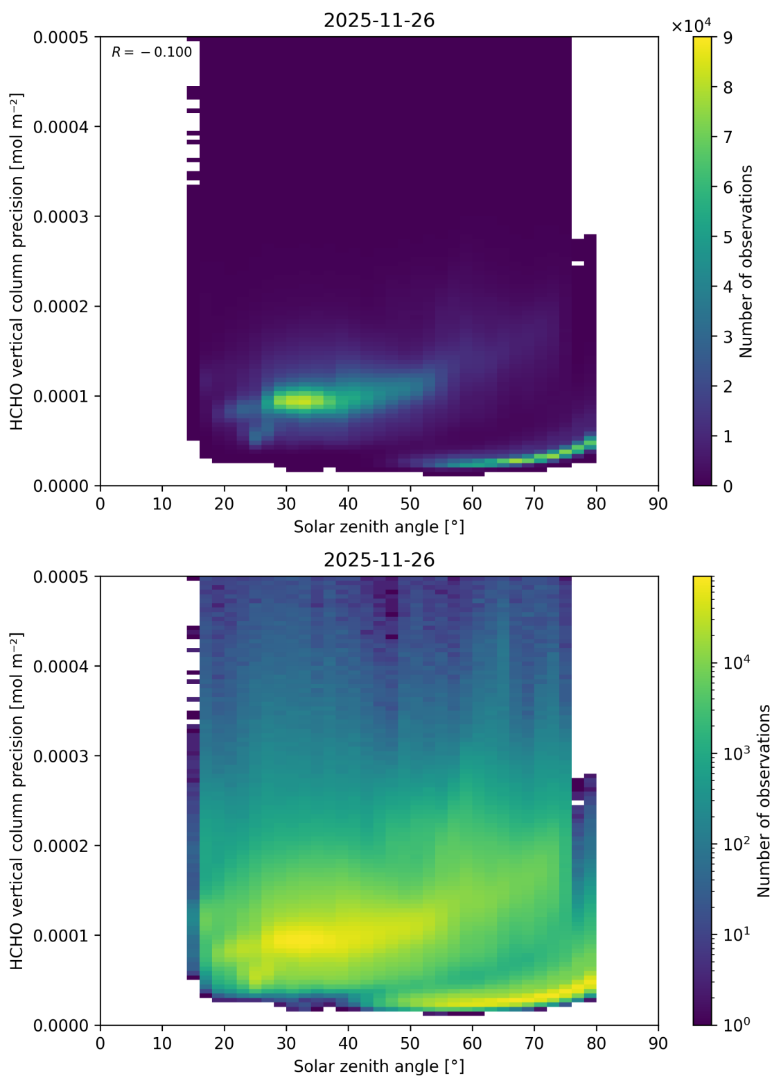
Figure 198: Scatter density plot of “Solar zenith angle” against “HCHO vertical column precision” for 2025-11-25 to 2025-11-27.
