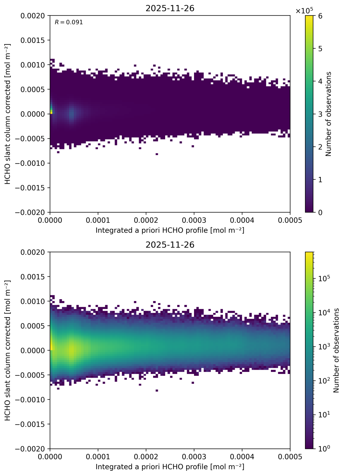
Figure 168: Scatter density plot of “Integrated a priori HCHO profile” against “HCHO slant column corrected” for 2025-11-25 to 2025-11-27.
