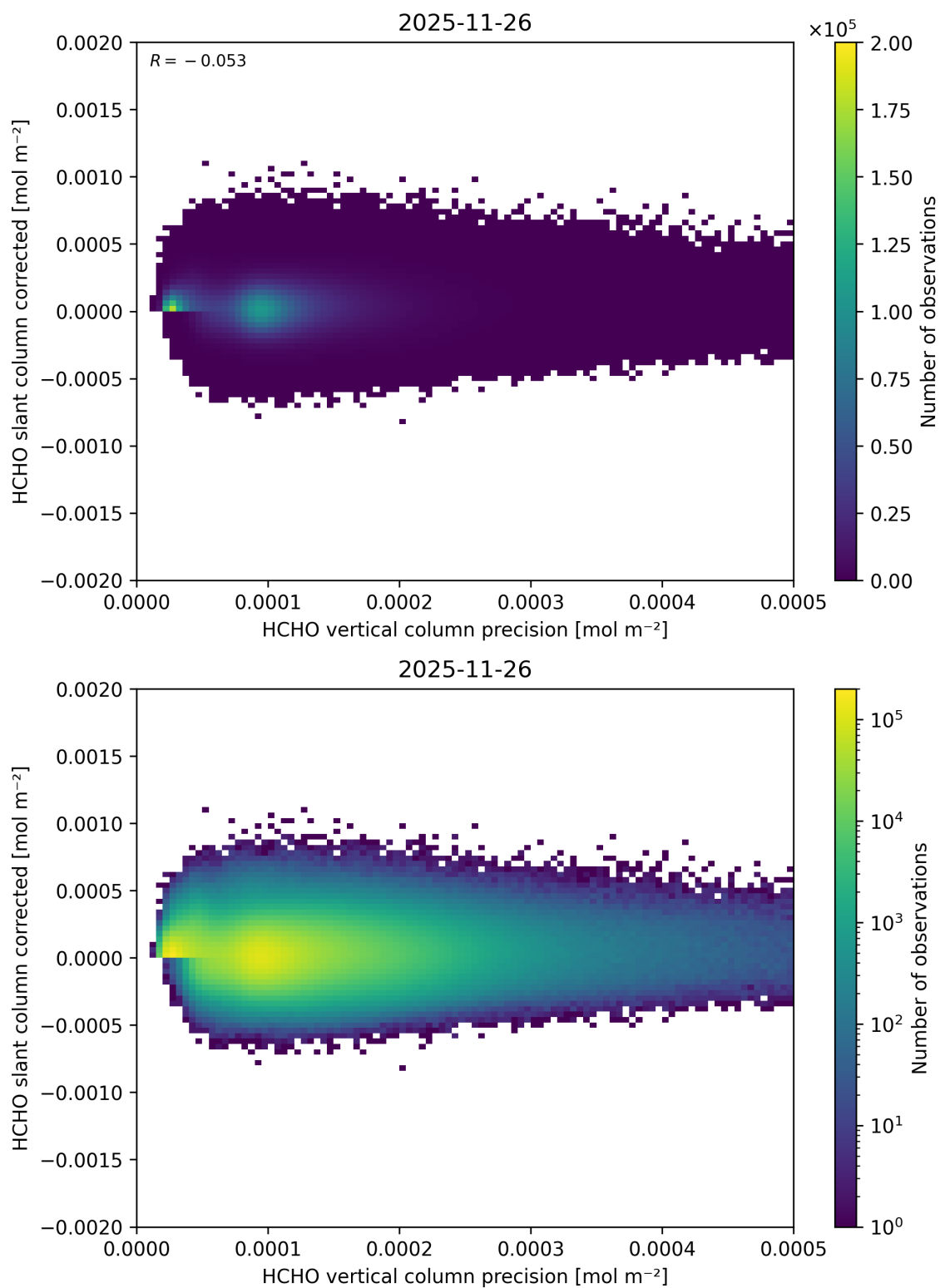
Figure 156: Scatter density plot of “HCHO vertical column precision” against “HCHO slant column corrected” for 2025-11-25 to 2025-11-27.
