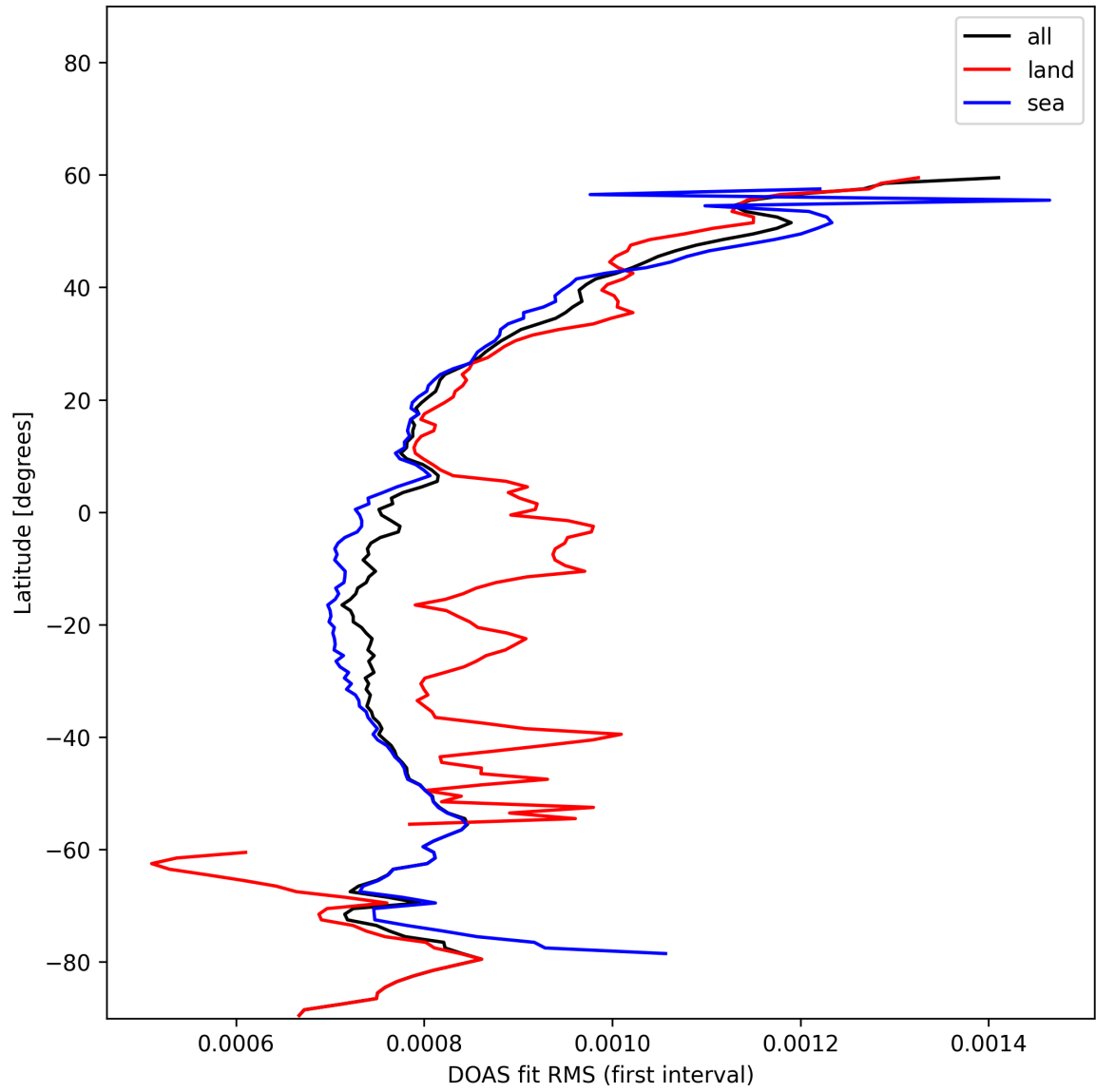
Figure 33: Zonal average of “DOAS fit RMS (first interval)” for 2025-11-25 to 2025-11-27.
