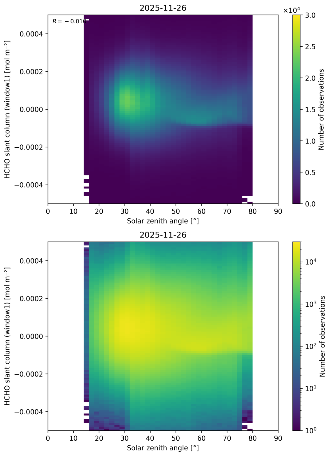
Figure 192: Scatter density plot of “Solar zenith angle” against “HCHO slant column (window1)” for 2025-11-25 to 2025-11-27.
