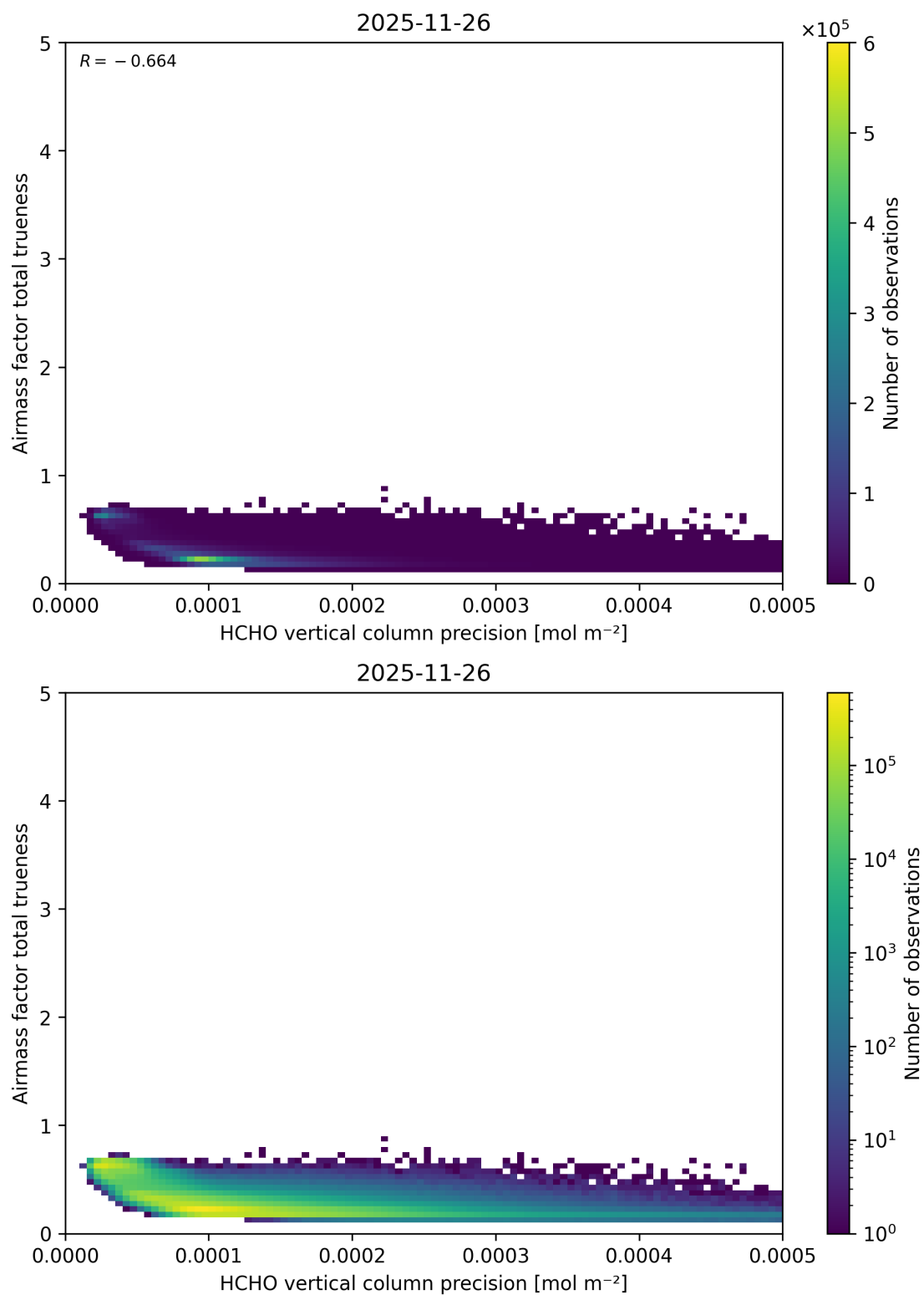
Figure 161: Scatter density plot of “HCHO vertical column precision” against “Airmass factor total trueness” for 2025-11-25 to 2025-11-27.
