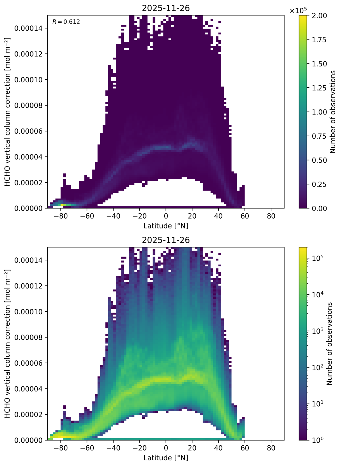
Figure 182: Scatter density plot of “Latitude” against “HCHO vertical column correction” for 2025-11-25 to 2025-11-27.
