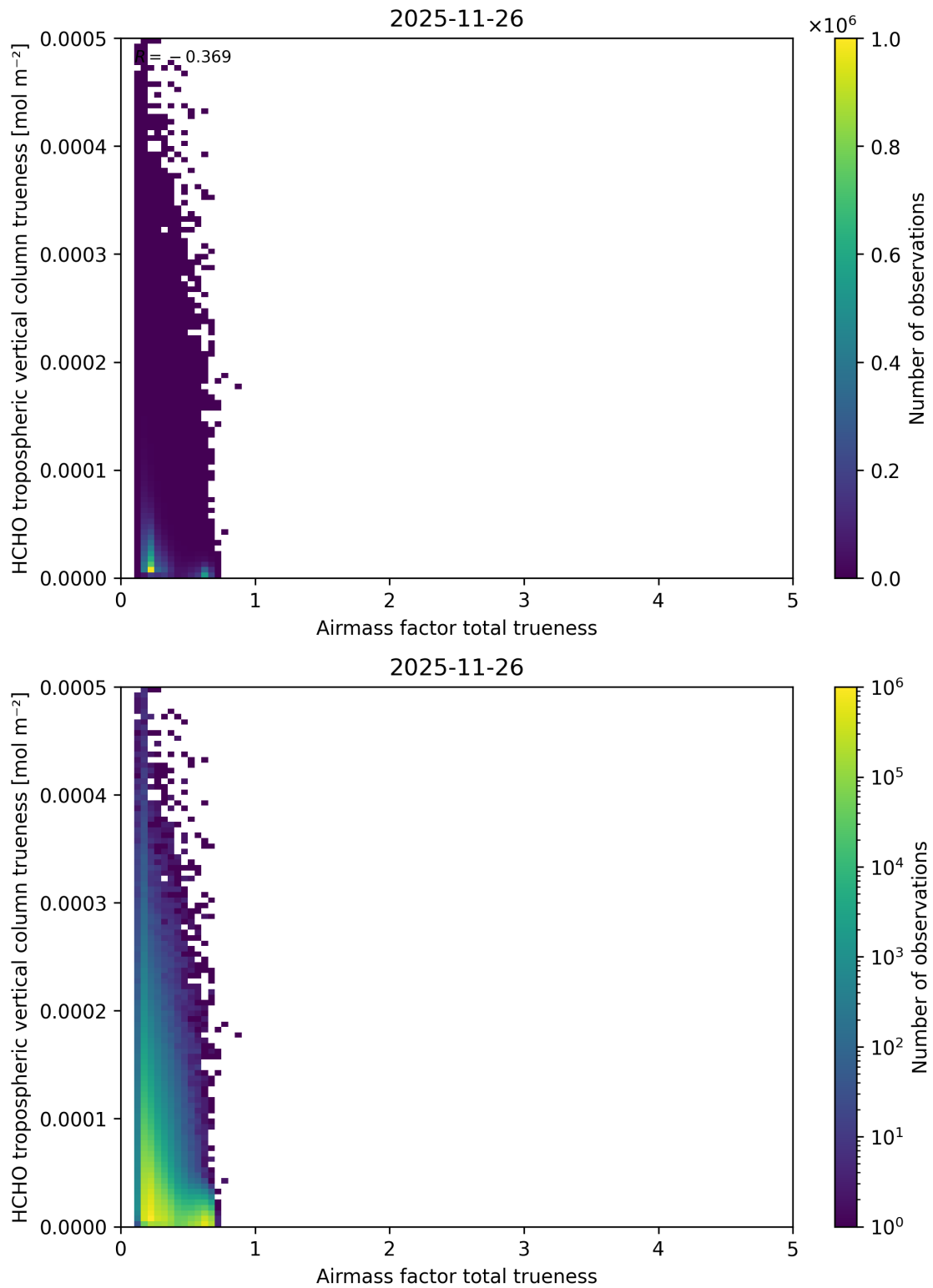
Figure 124: Scatter density plot of “Airmass factor total trueness” against “HCHO tropospheric vertical column trueness” for 2025-11-25 to 2025-11-27.
