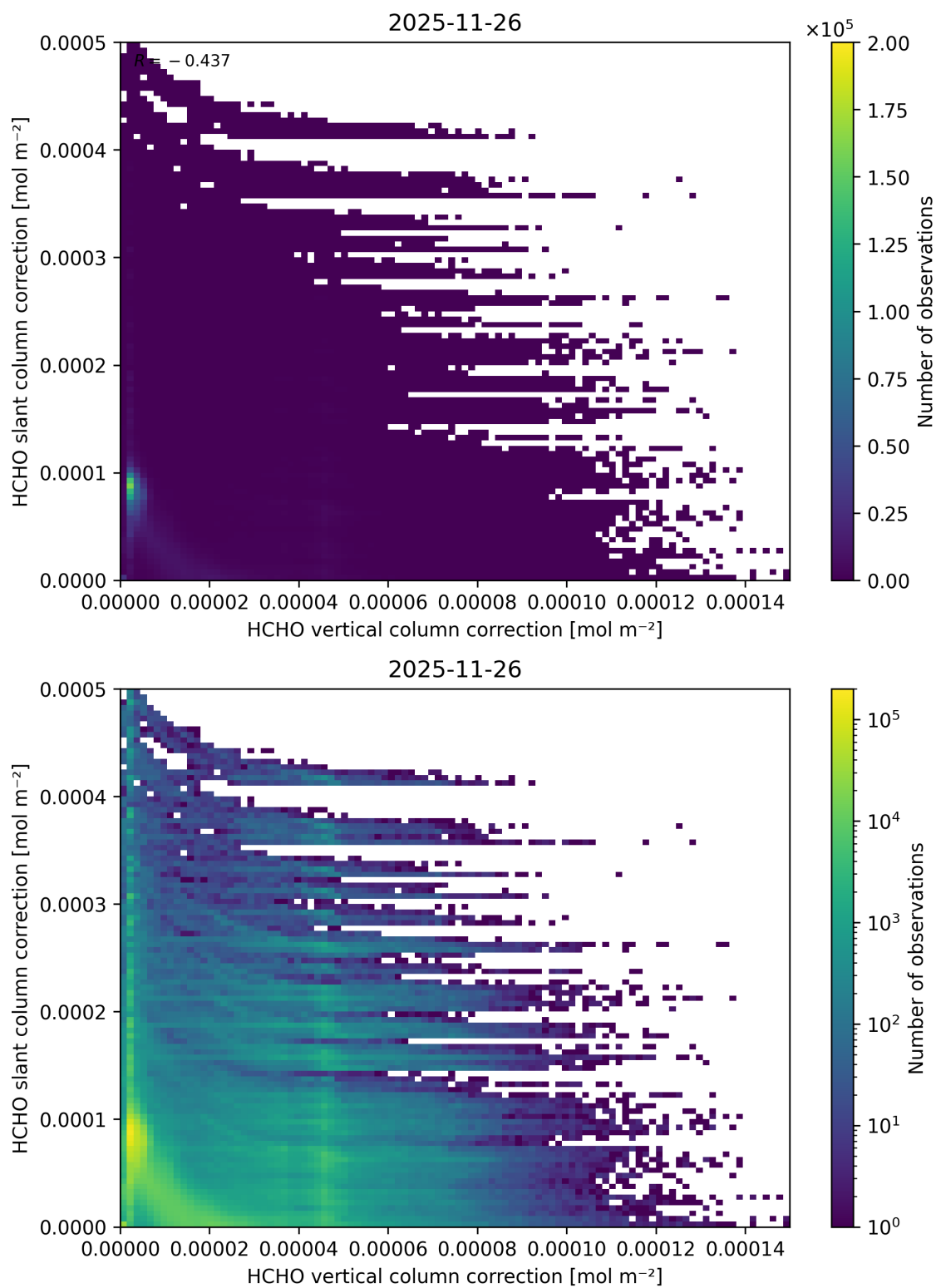
Figure 131: Scatter density plot of “HCHO vertical column correction” against “HCHO slant column correction” for 2025-11-25 to 2025-11-27.
