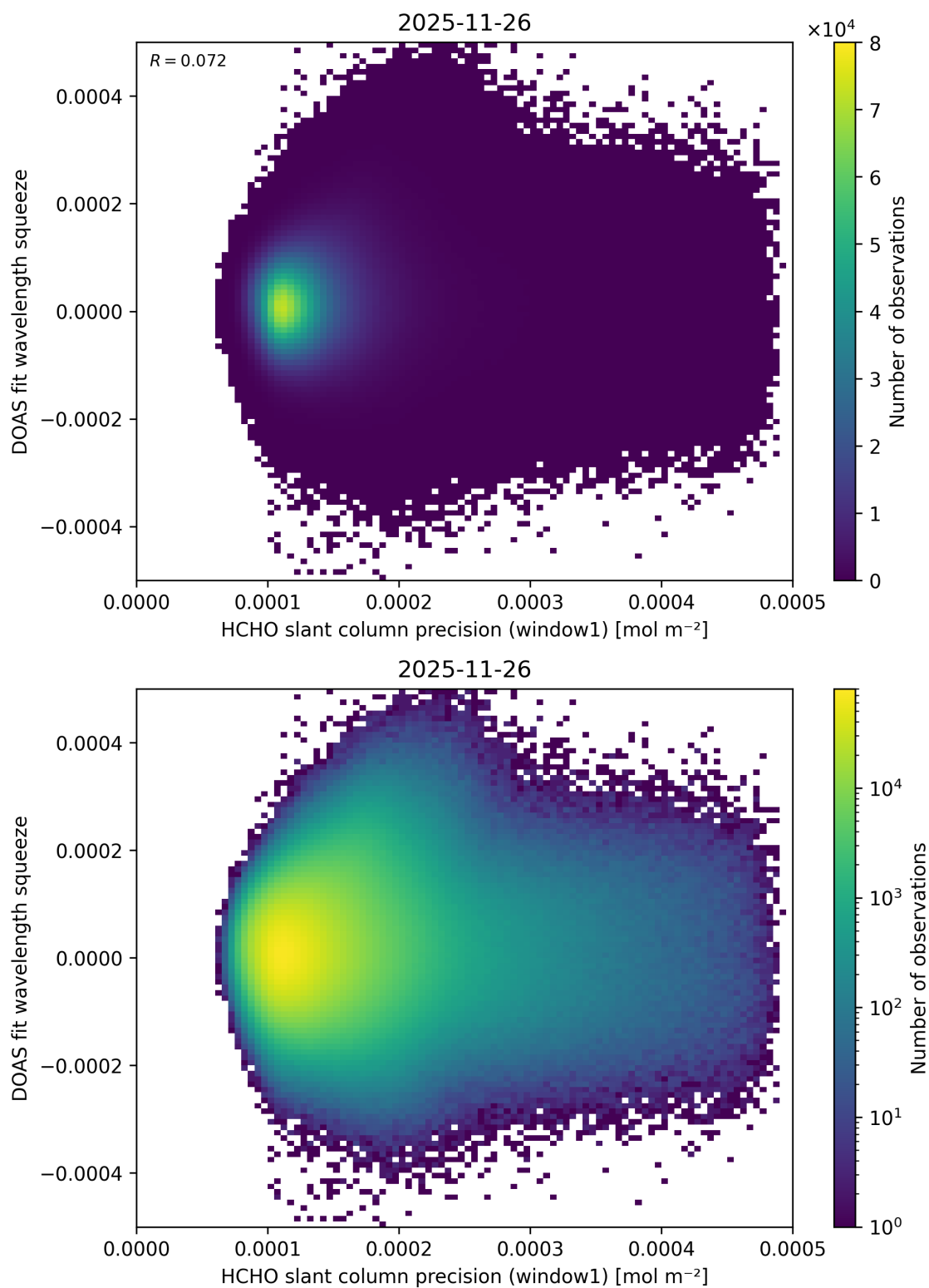
Figure 101: Scatter density plot of “HCHO slant column precision (window1)” against “DOAS fit wavelength squeeze” for 2025-11-25 to 2025-11-27.
