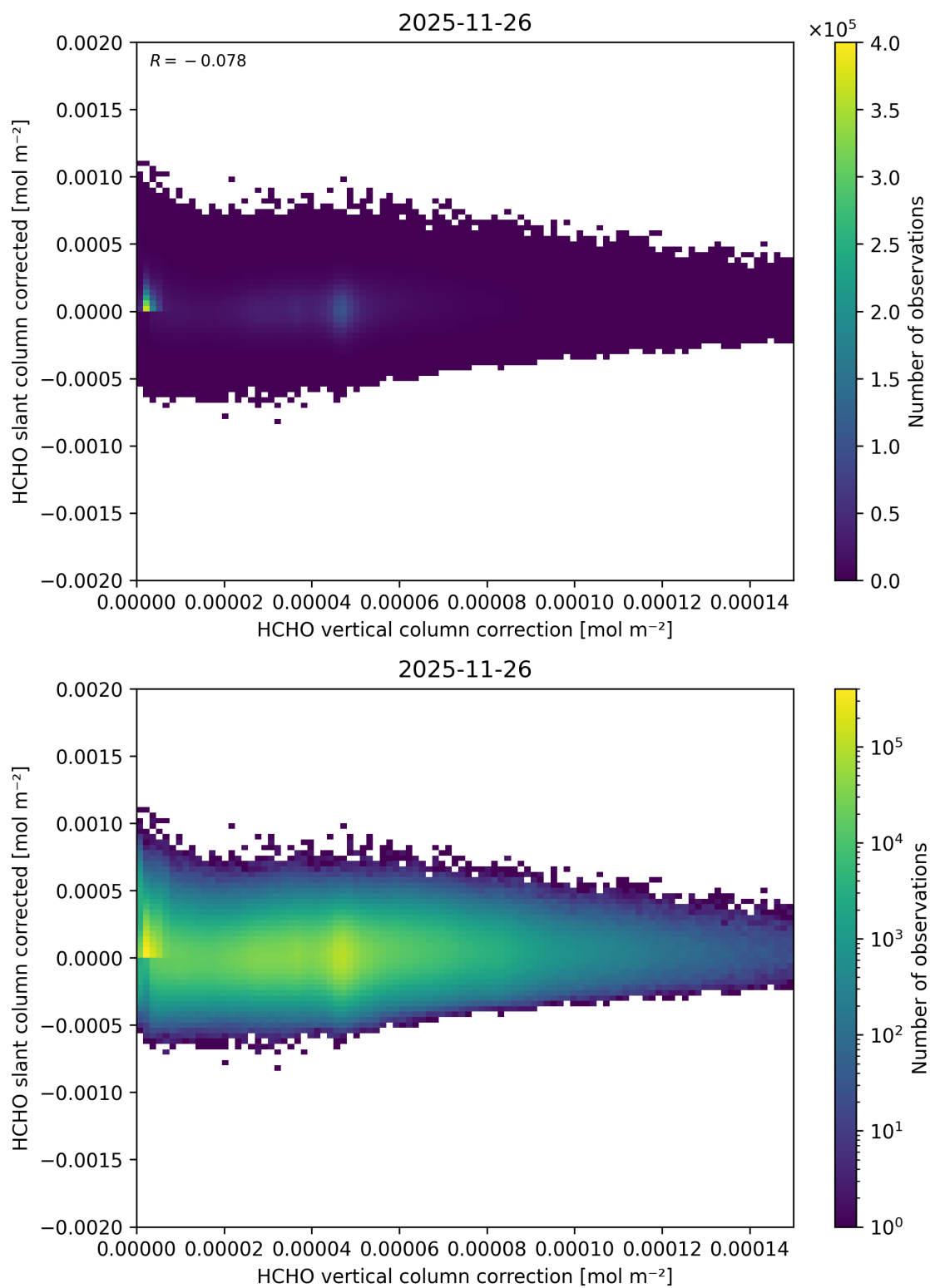
Figure 130: Scatter density plot of “HCHO vertical column correction” against “HCHO slant column corrected” for 2025-11-25 to 2025-11-27.
