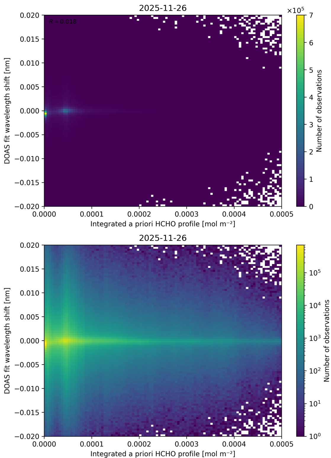
Figure 166: Scatter density plot of “Integrated a priori HCHO profile” against “DOAS fit wavelength shift” for 2025-11-25 to 2025-11-27.
