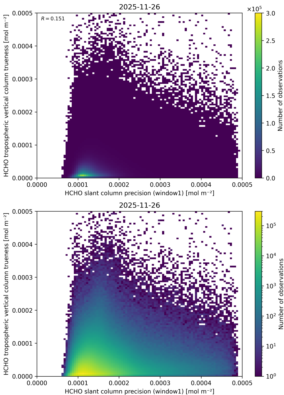
Figure 107: Scatter density plot of “HCHO slant column precision (window1)” against “HCHO tropospheric vertical column trueness” for 2025-11-25 to 2025-11-27.
