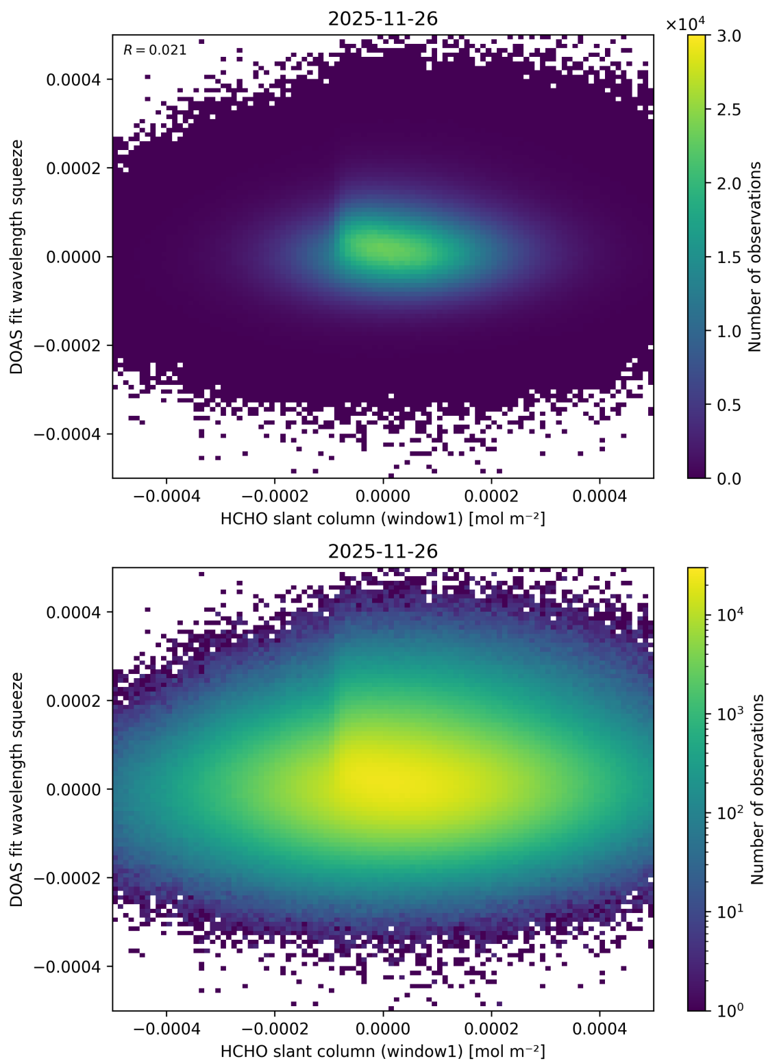
Figure 90: Scatter density plot of “HCHO slant column (window1)” against “DOAS fit wavelength squeeze” for 2025-11-25 to 2025-11-27.
