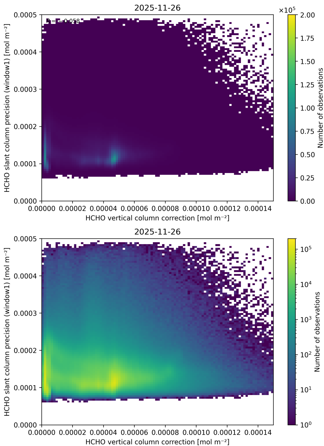
Figure 133: Scatter density plot of “HCHO vertical column correction” against “HCHO slant column precision (window1)” for 2025-11-25 to 2025-11-27.
