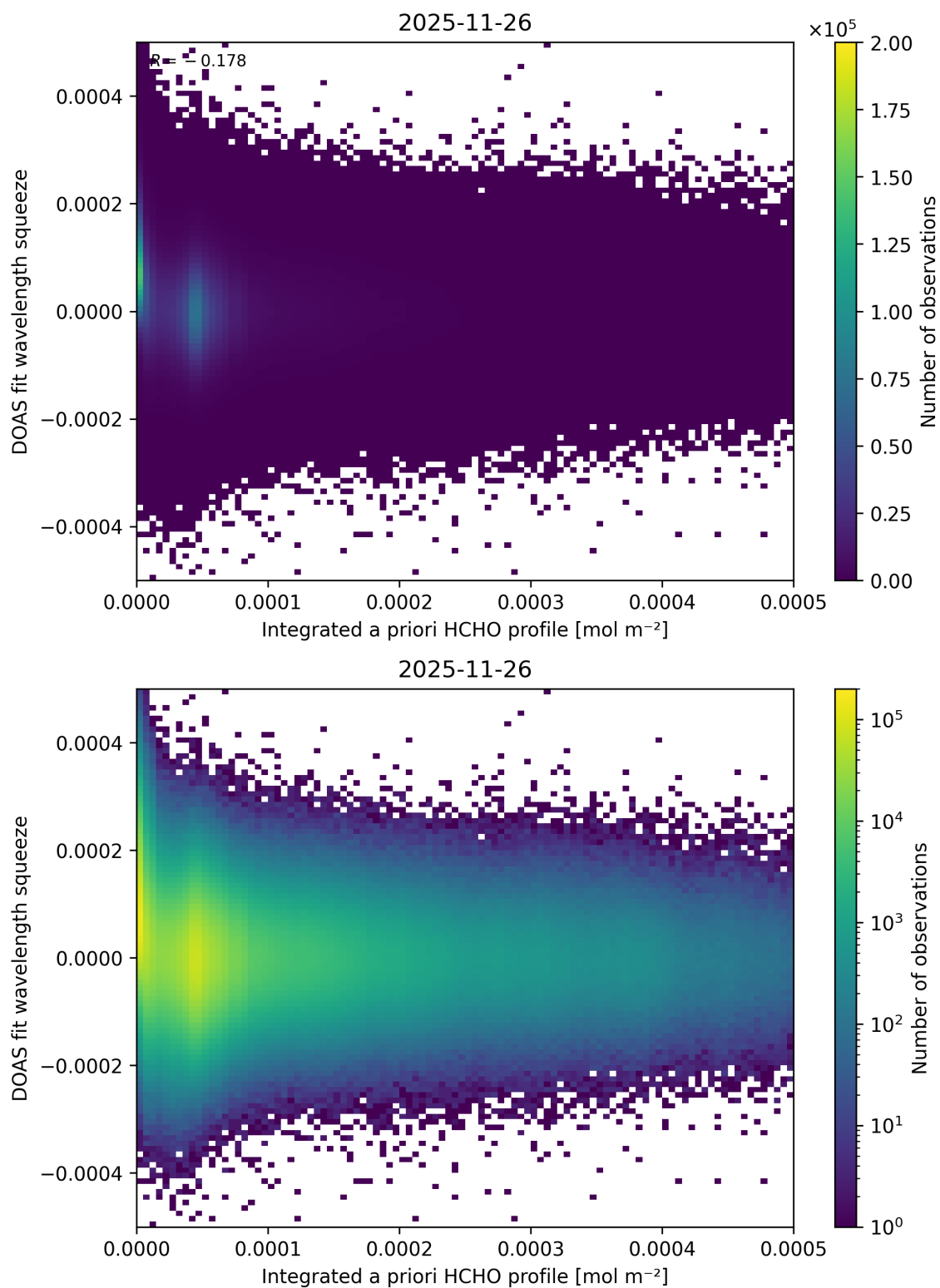
Figure 167: Scatter density plot of “Integrated a priori HCHO profile” against “DOAS fit wavelength squeeze” for 2025-11-25 to 2025-11-27.
