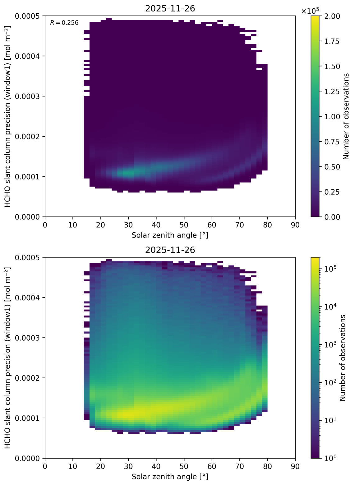
Figure 193: Scatter density plot of “Solar zenith angle” against “HCHO slant column precision (window1)” for 2025-11-25 to 2025-11-27.
