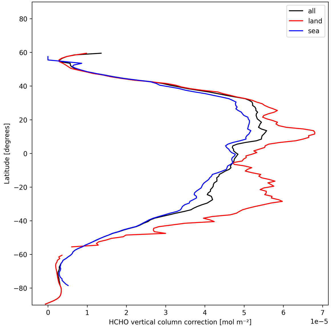
Figure 24: Zonal average of “HCHO vertical column correction” for 2025-11-25 to 2025-11-27.
