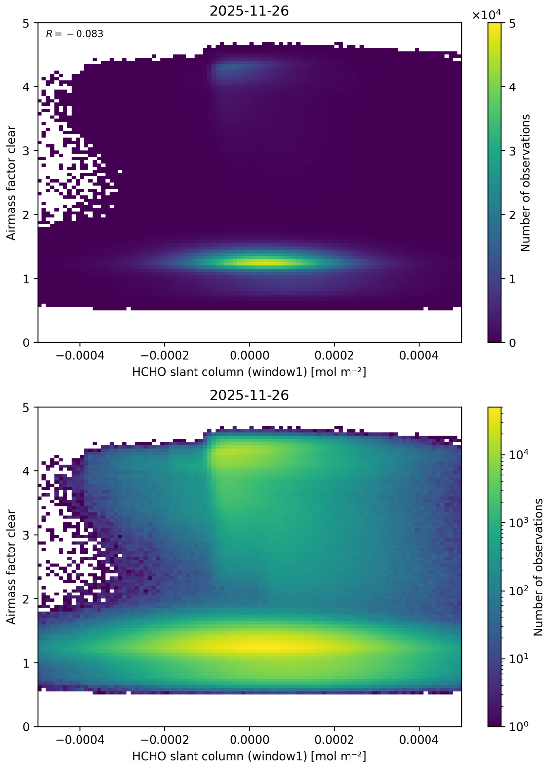
Figure 91: Scatter density plot of “HCHO slant column (window1)” against “Airmass factor clear” for 2025-11-25 to 2025-11-27.
