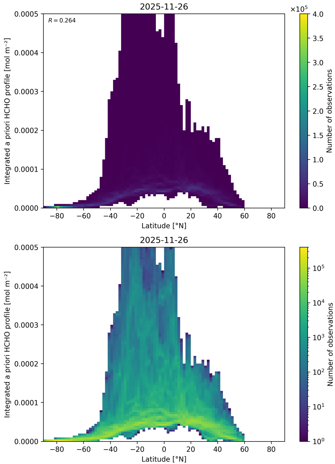
Figure 185: Scatter density plot of “Latitude” against “Integrated a priori HCHO profile” for 2025-11-25 to 2025-11-27.
