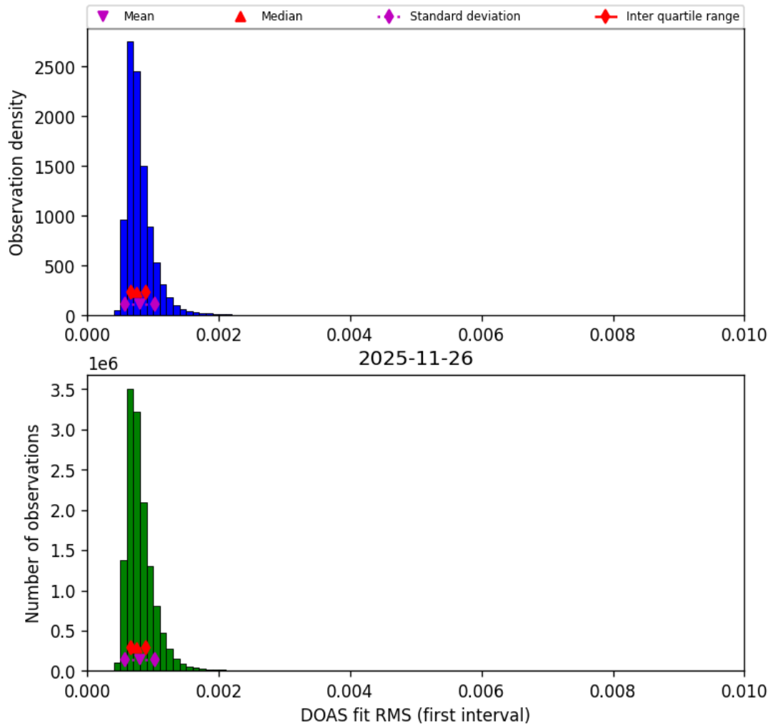
Figure 48: Histogram of “DOAS fit RMS (first interval)” for 2025-11-25 to 2025-11-27
