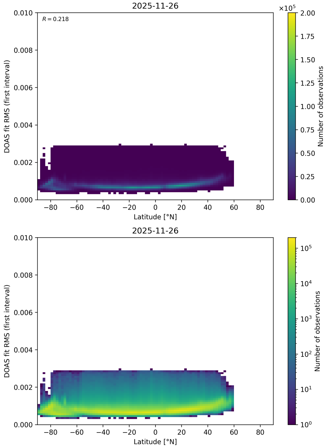
Figure 171: Scatter density plot of “Latitude” against “DOAS fit RMS (first interval)” for 2025-11-25 to 2025-11-27.
