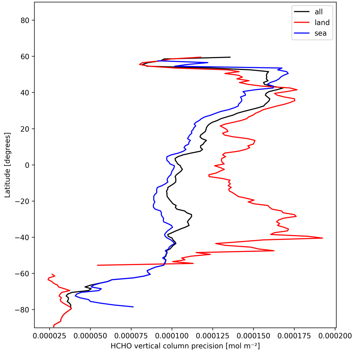
Figure 23: Zonal average of "HCHO vertical column precision" for 2025-11-25 to 2025-11-27.
