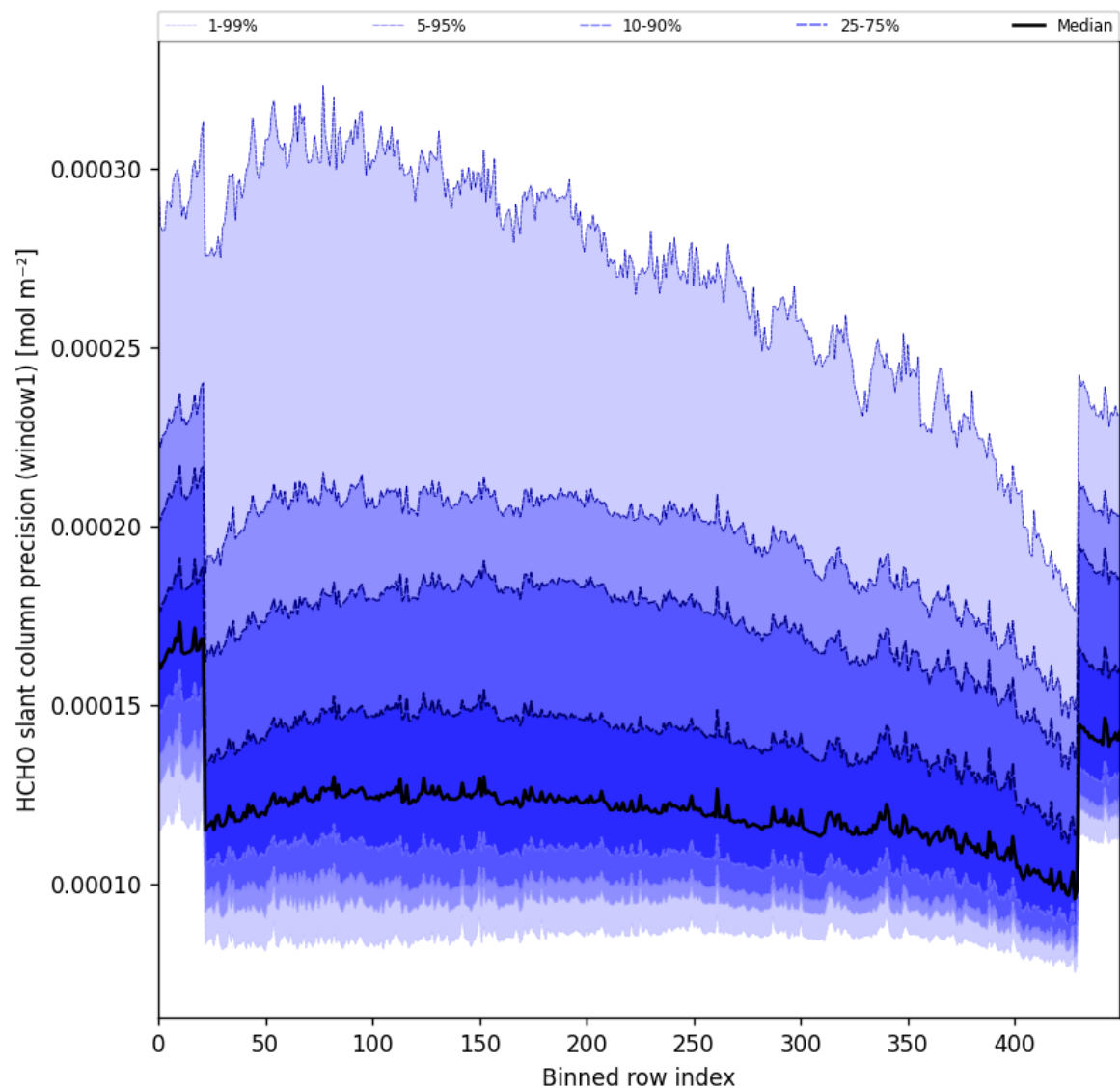
Figure 56: Along track statistics of “HCHO slant column precision (window1)” for 2025-11-26 to 2025-11-28
