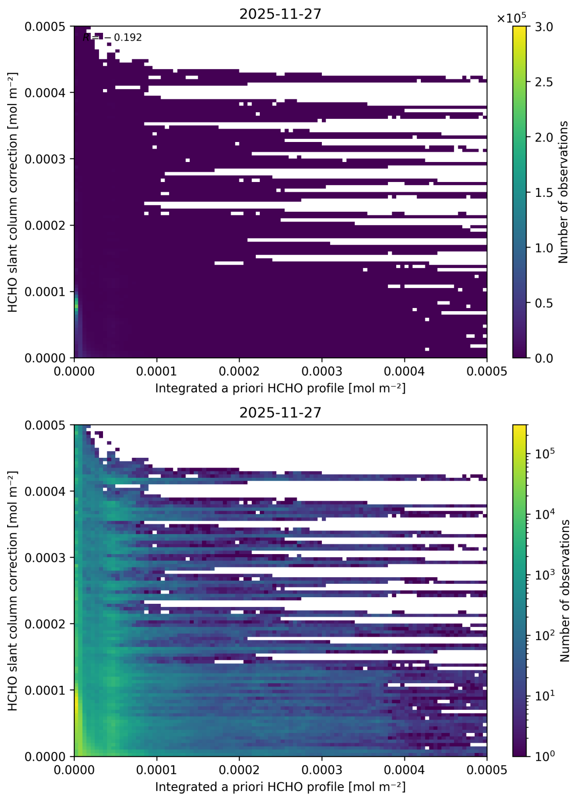
Figure 169: Scatter density plot of “Integrated a priori HCHO profile” against “HCHO slant column correction” for 2025-11-26 to 2025-11-28.
