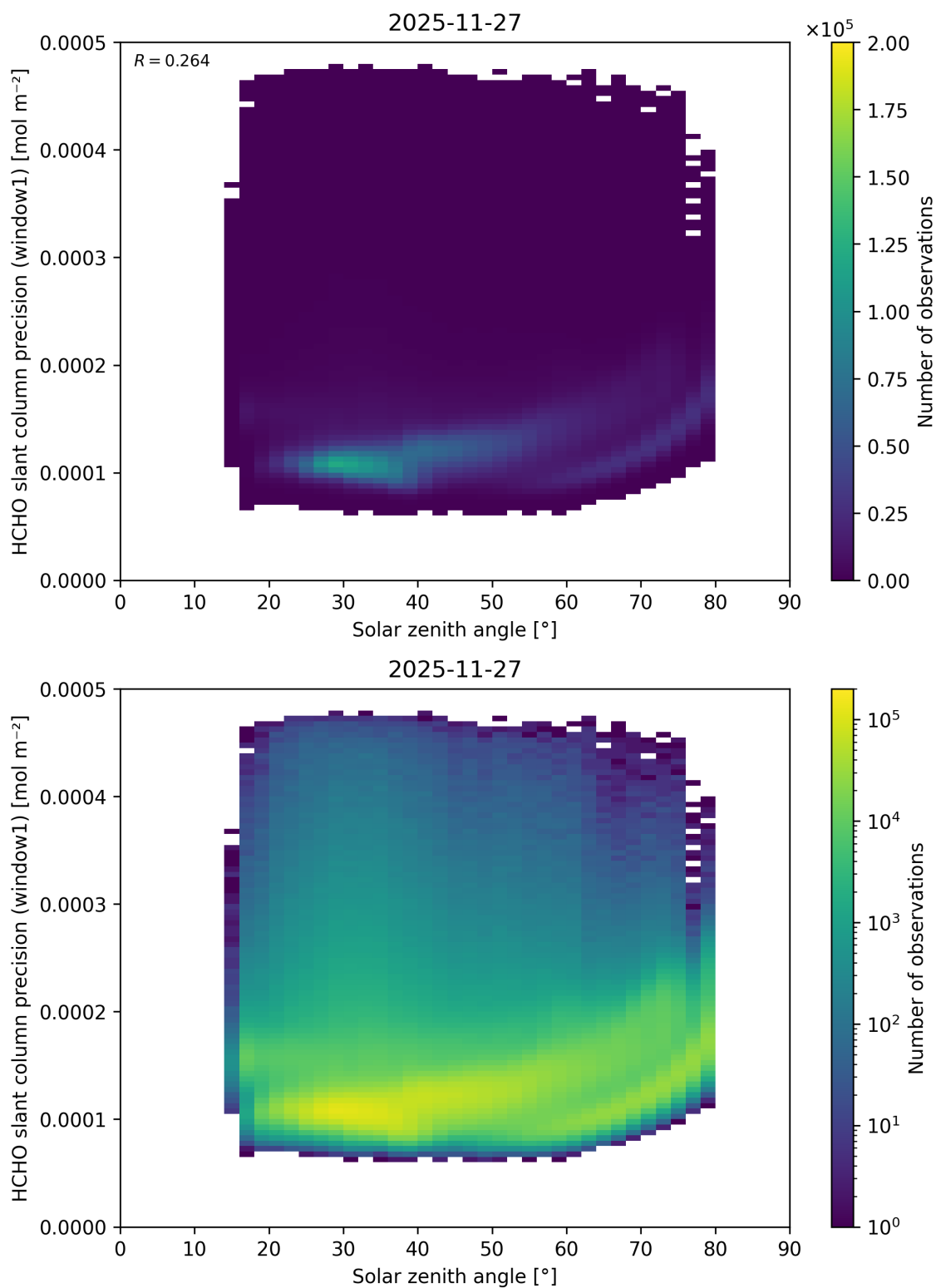
Figure 193: Scatter density plot of “Solar zenith angle” against “HCHO slant column precision (window1)” for 2025-11-26 to 2025-11-28.
