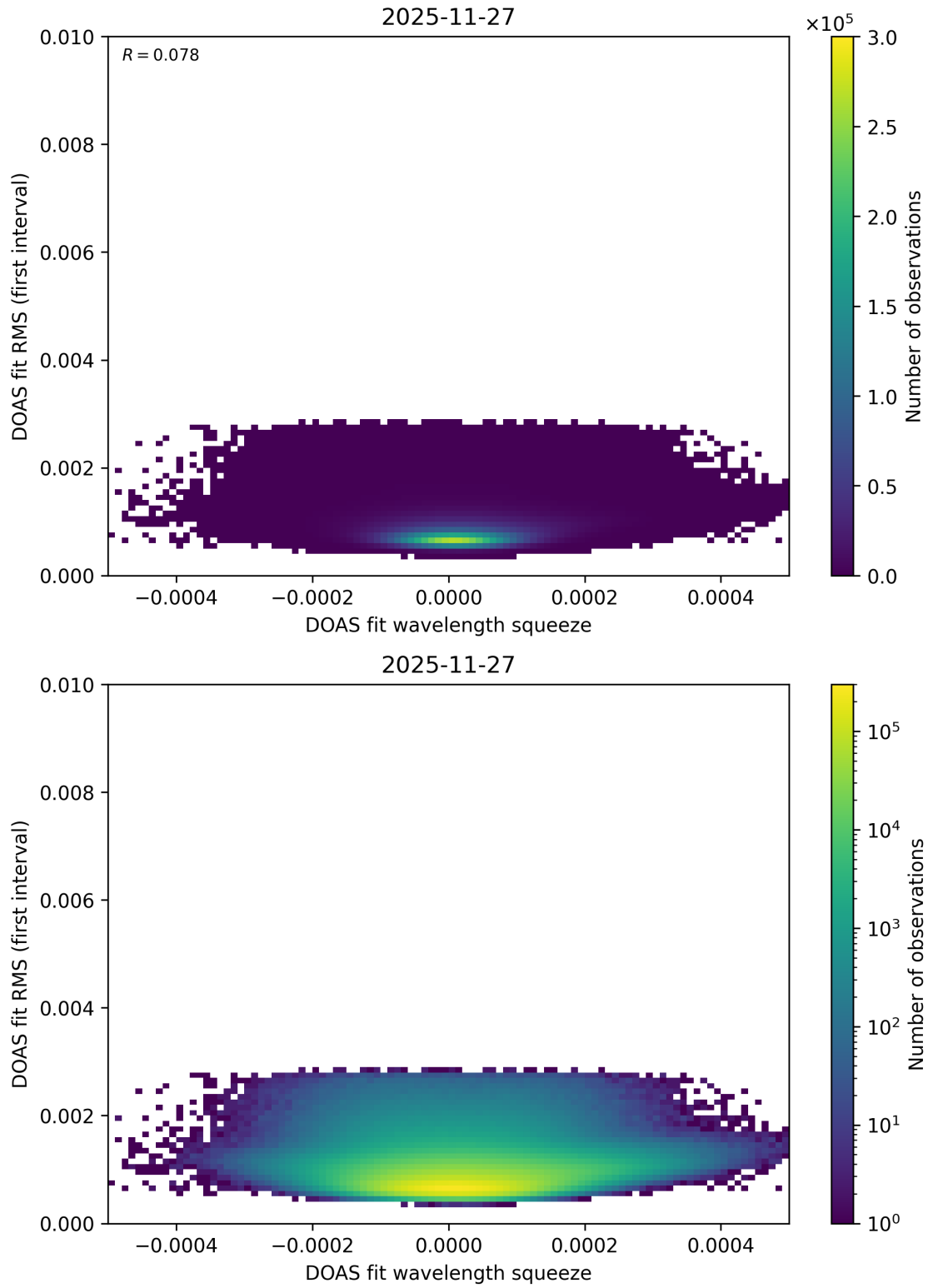
Figure 74: Scatter density plot of “DOAS fit wavelength squeeze” against “DOAS fit RMS (first interval)” for 2025-11-26 to 2025-11-28.
