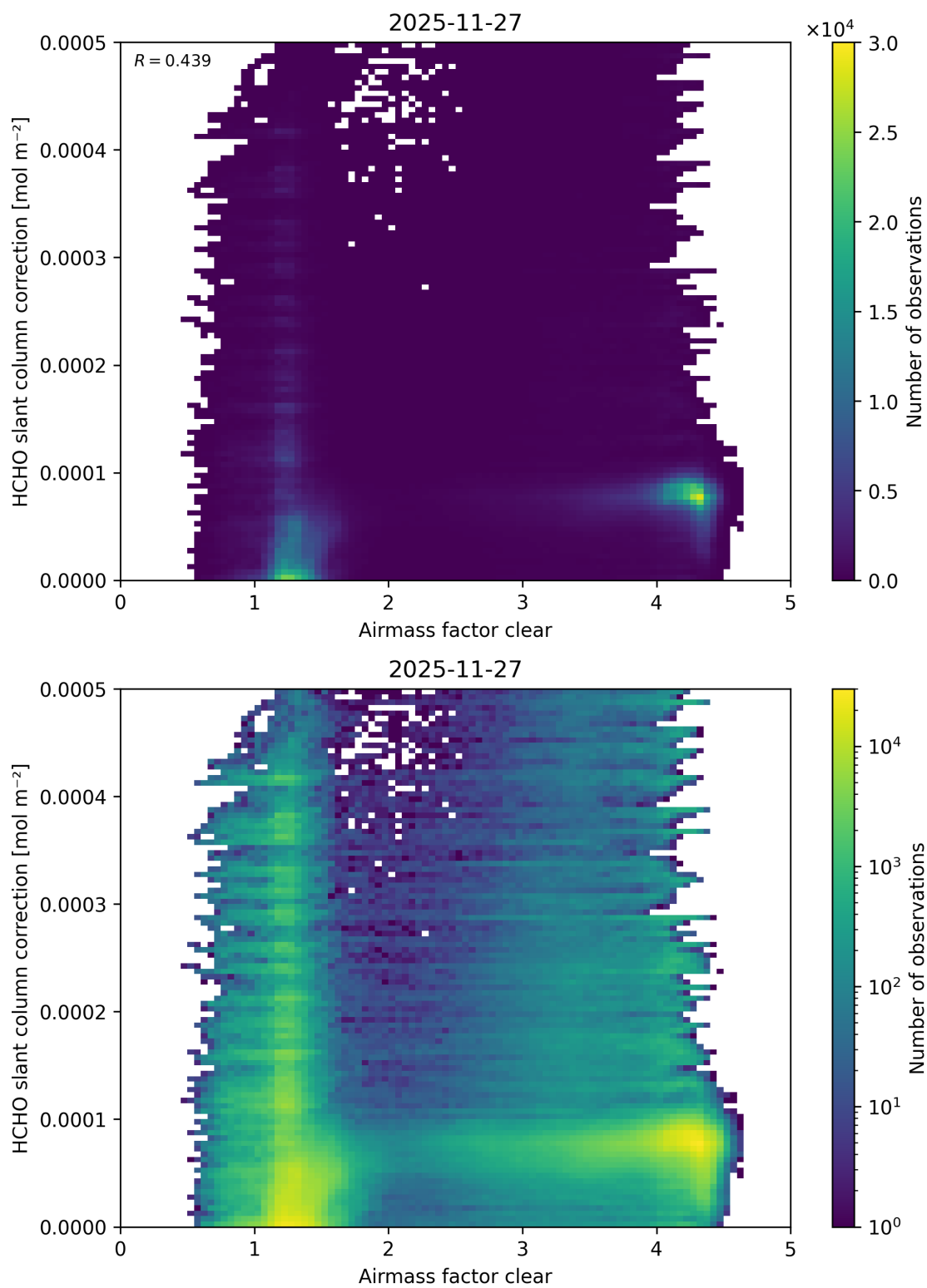
Figure 82: Scatter density plot of “Airmass factor clear” against “HCHO slant column correction” for 2025-11-26 to 2025-11-28.
