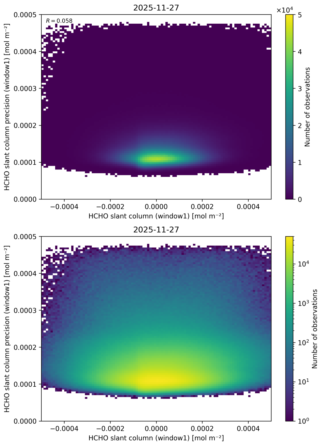
Figure 94: Scatter density plot of “HCHO slant column (window1)” against “HCHO slant column precision (window1)” for 2025-11-26 to 2025-11-28.
