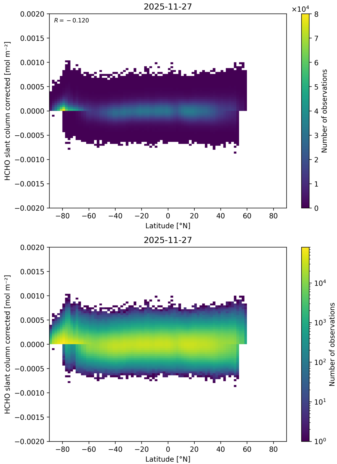
Figure 175: Scatter density plot of “Latitude” against “HCHO slant column corrected” for 2025-11-26 to 2025-11-28.
