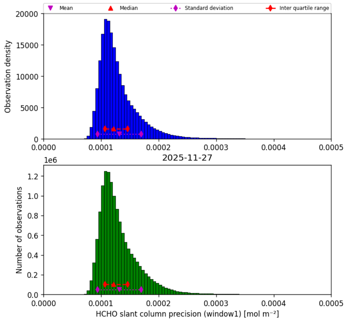
Figure 41: Histogram of “HCHO slant column precision (window1)” for 2025-11-26 to 2025-11-28
