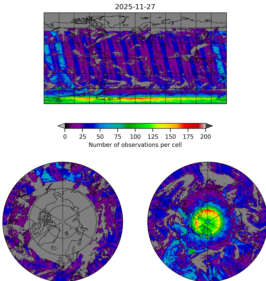
Figure 20: Map of the number of observations for 2025-11-26 to 2025-11-28
