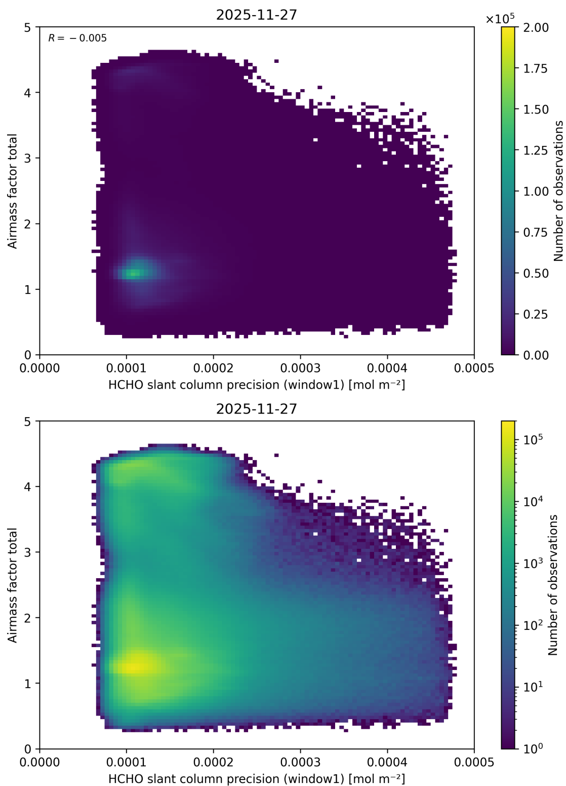
Figure 105: Scatter density plot of “HCHO slant column precision (window1)” against “Airmass factor total” for 2025-11-26 to 2025-11-28.
