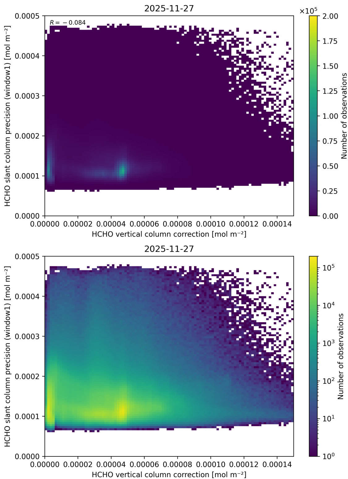
Figure 133: Scatter density plot of “HCHO vertical column correction” against “HCHO slant column precision (window1)” for 2025-11-26 to 2025-11-28.
