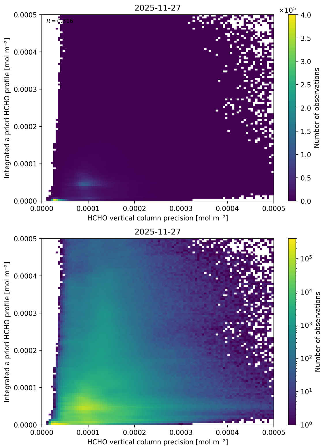
Figure 164: Scatter density plot of “HCHO vertical column precision” against “Integrated a priori HCHO profile” for 2025-11-26 to 2025-11-28.
