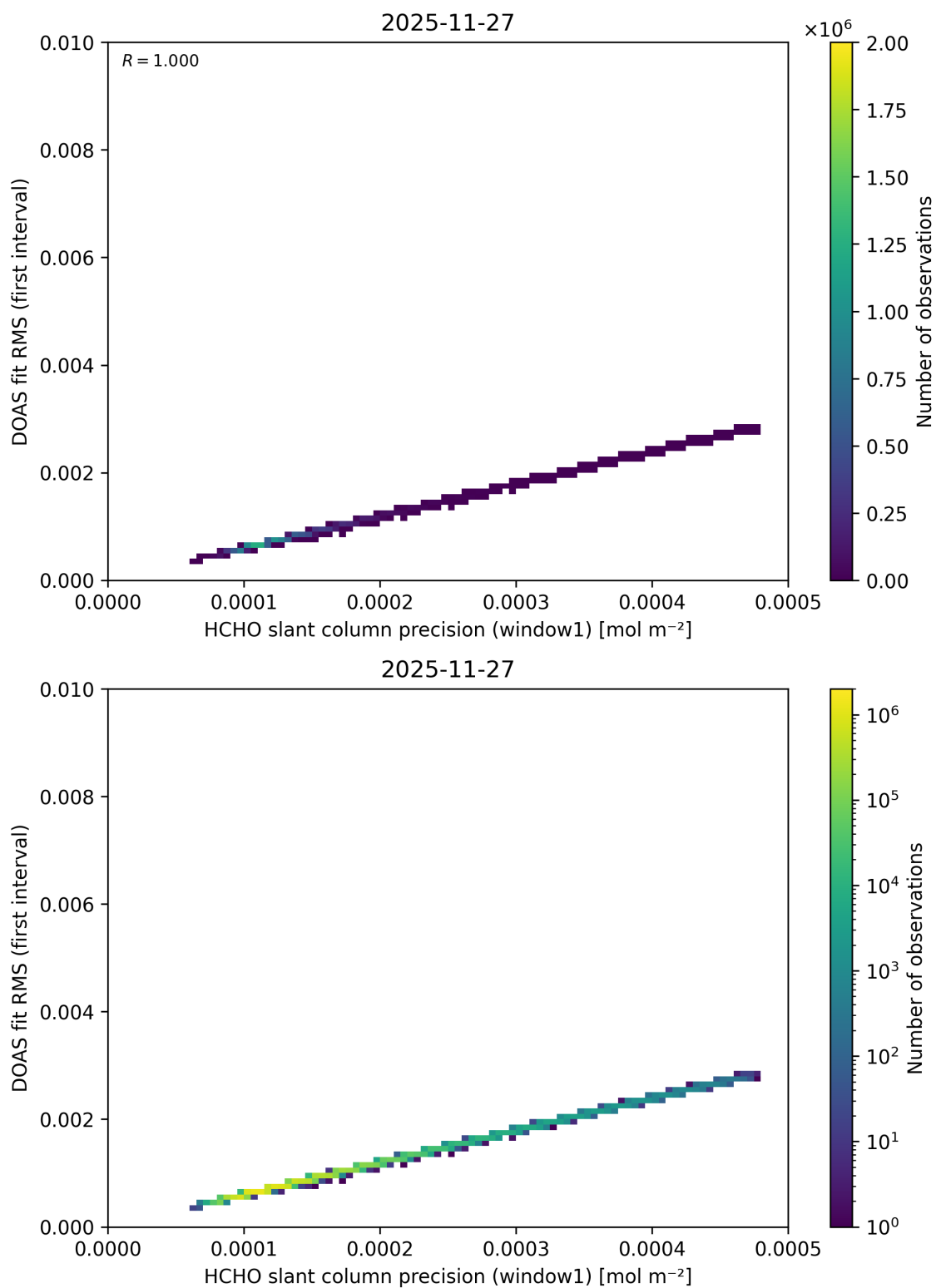
Figure 99: Scatter density plot of “HCHO slant column precision (window1)” against “DOAS fit RMS (first interval)” for 2025-11-26 to 2025-11-28.
