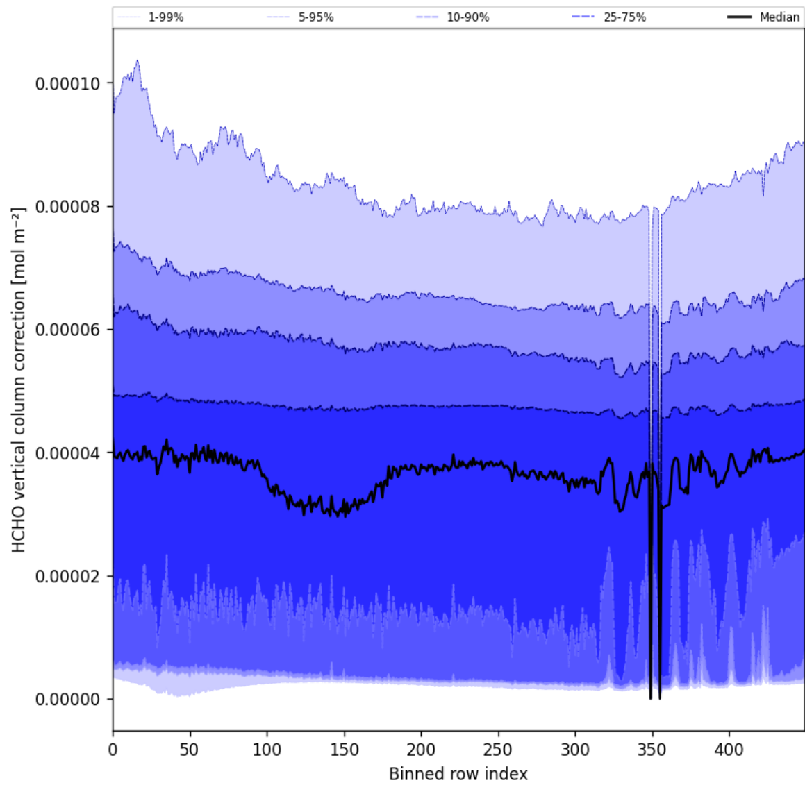
Figure 54: Along track statistics of “HCHO vertical column correction” for 2025-11-26 to 2025-11-28
