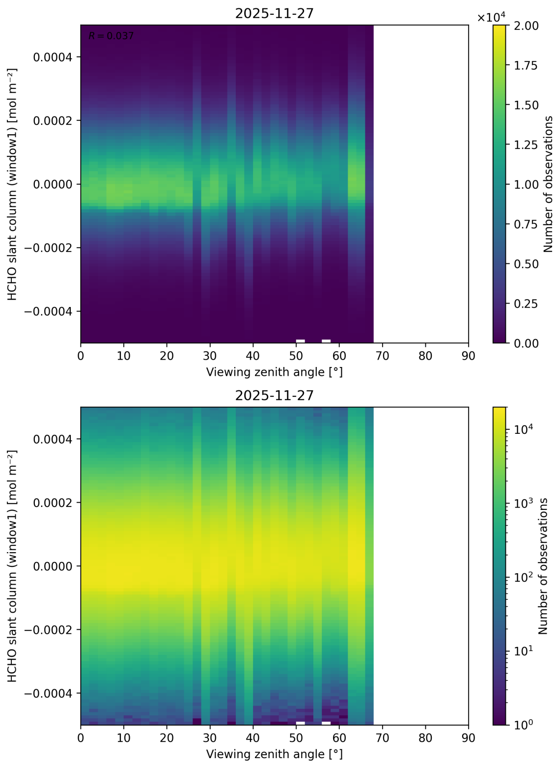
Figure 208: Scatter density plot of “Viewing zenith angle” against “HCHO slant column (window1)” for 2025-11-26 to 2025-11-28.
