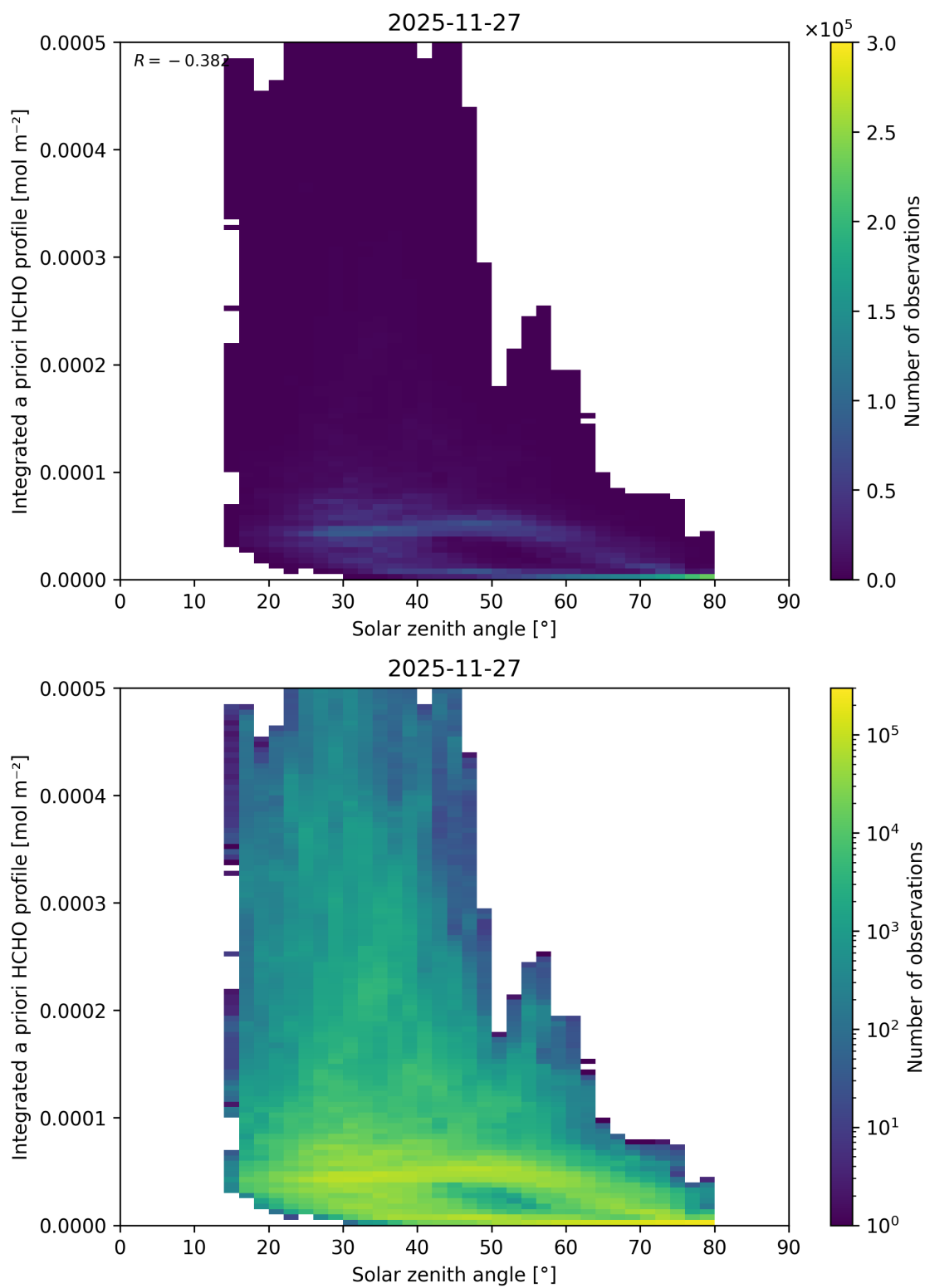
Figure 200: Scatter density plot of “Solar zenith angle” against “Integrated a priori HCHO profile” for 2025-11-26 to 2025-11-28.
