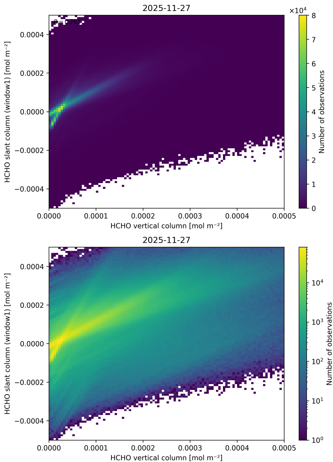
Figure 144: Scatter density plot of “HCHO vertical column” against “HCHO slant column (window1)” for 2025-11-26 to 2025-11-28.
