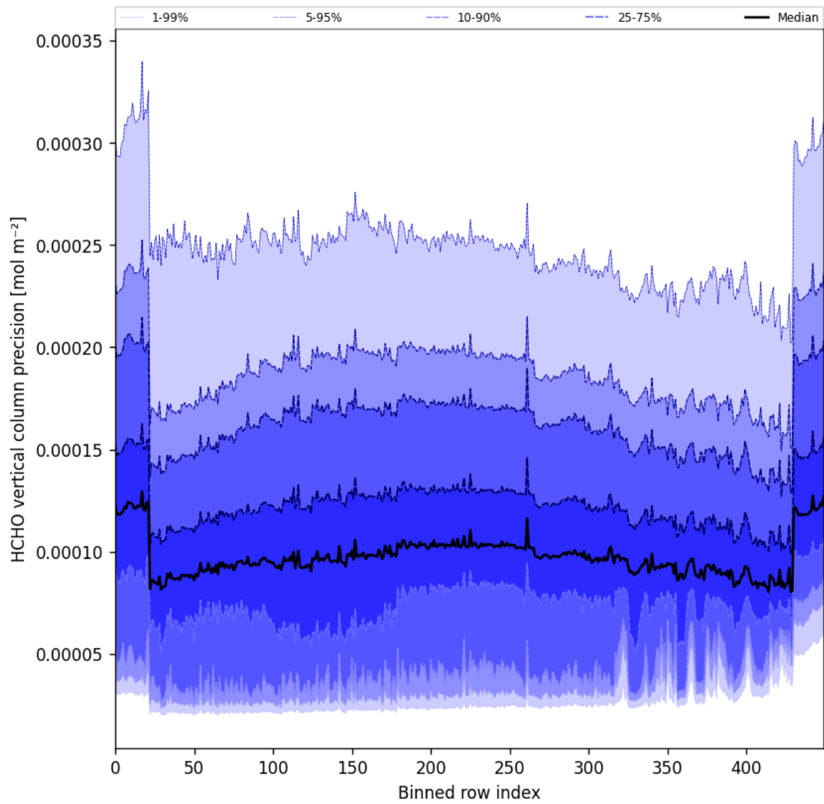
Figure 53: Along track statistics of “HCHO vertical column precision” for 2025-11-26 to 2025-11-28
