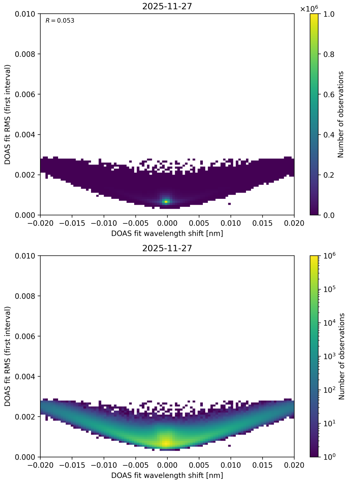
Figure 69: Scatter density plot of “DOAS fit wavelength shift” against “DOAS fit RMS (first interval)” for 2025-11-26 to 2025-11-28.
