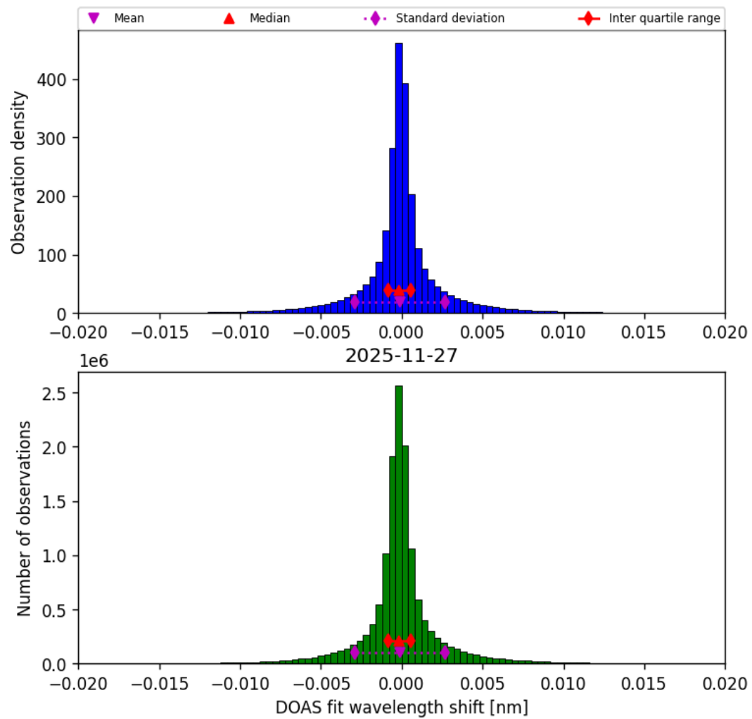
Figure 46: Histogram of “DOAS fit wavelength shift” for 2025-11-26 to 2025-11-28
