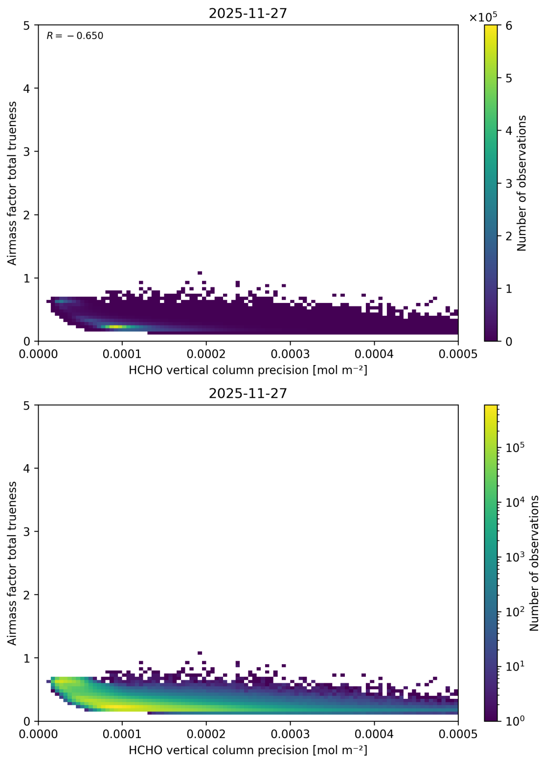
Figure 161: Scatter density plot of “HCHO vertical column precision” against “Airmass factor total trueness” for 2025-11-26 to 2025-11-28.
