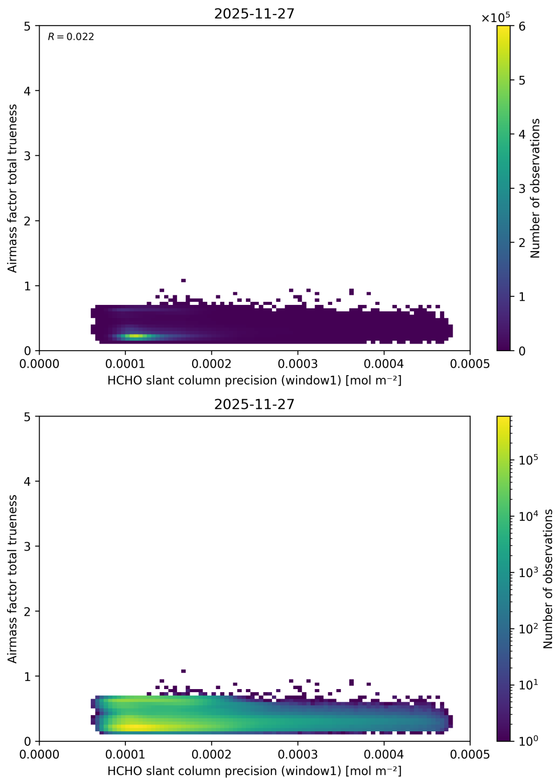
Figure 106: Scatter density plot of “HCHO slant column precision (window1)” against “Airmass factor total trueness” for 2025-11-26 to 2025-11-28.
