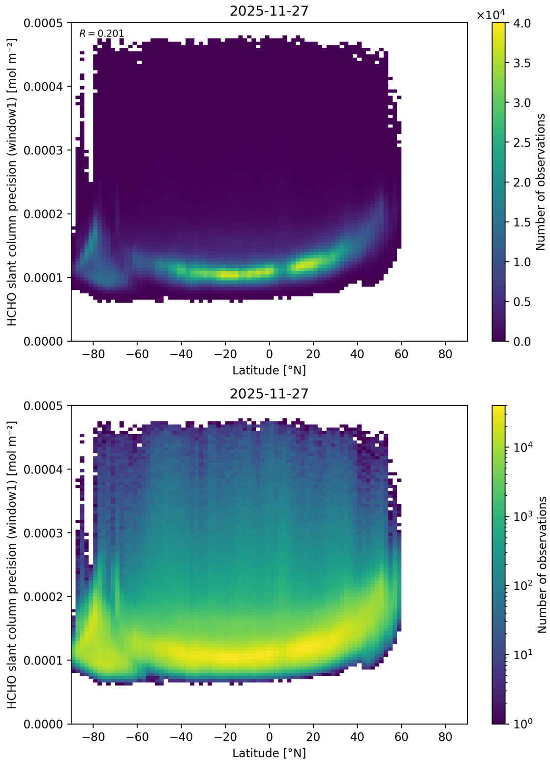
Figure 178: Scatter density plot of “Latitude” against “HCHO slant column precision (window1)” for 2025-11-26 to 2025-11-28.
