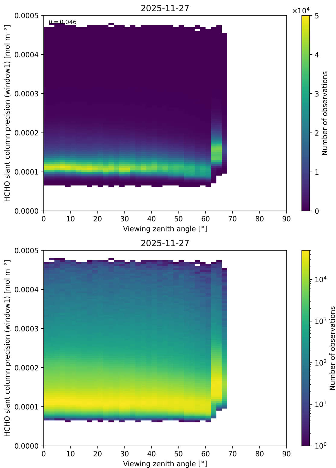
Figure 209: Scatter density plot of “Viewing zenith angle” against “HCHO slant column precision (window1)” for 2025-11-26 to 2025-11-28.
