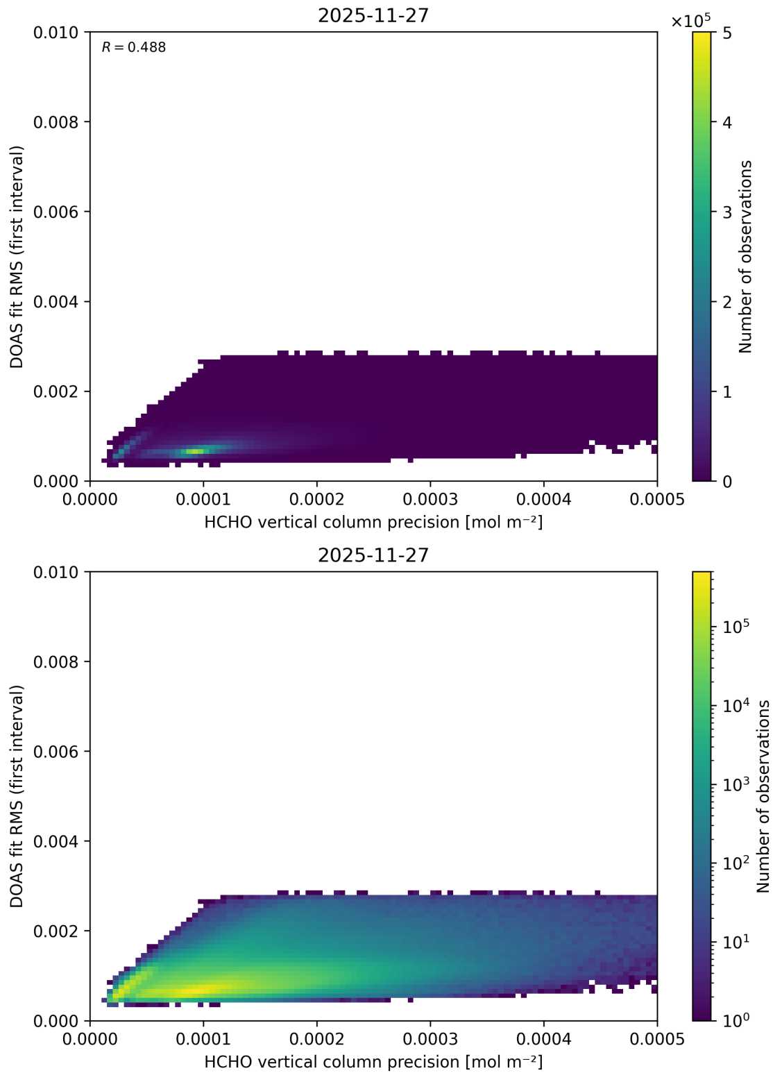
Figure 152: Scatter density plot of “HCHO vertical column precision” against “DOAS fit RMS (first interval)” for 2025-11-26 to 2025-11-28.
