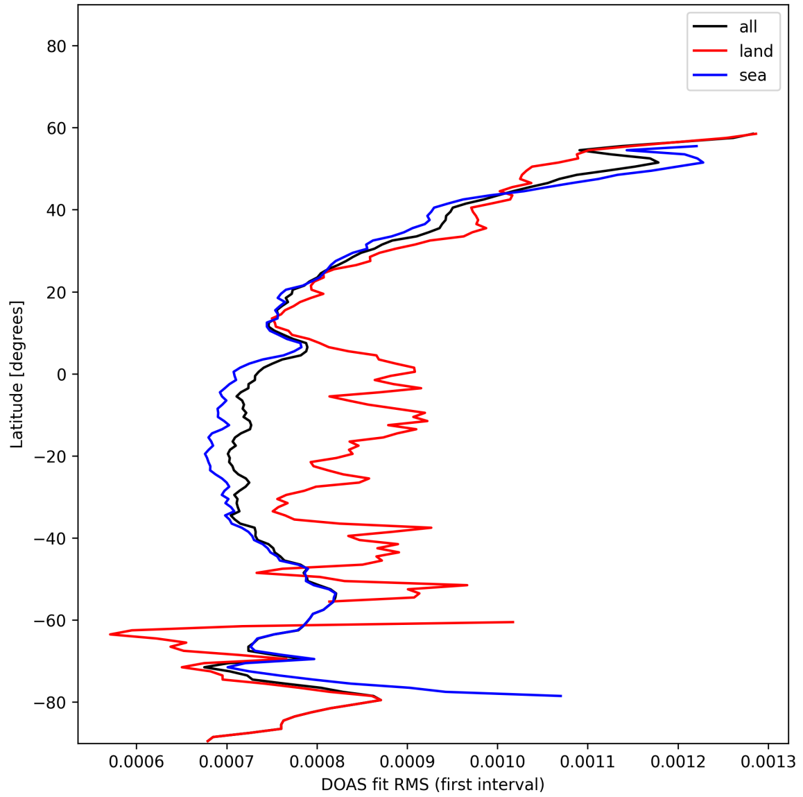
Figure 33: Zonal average of “DOAS fit RMS (first interval)” for 2025-11-26 to 2025-11-28.
