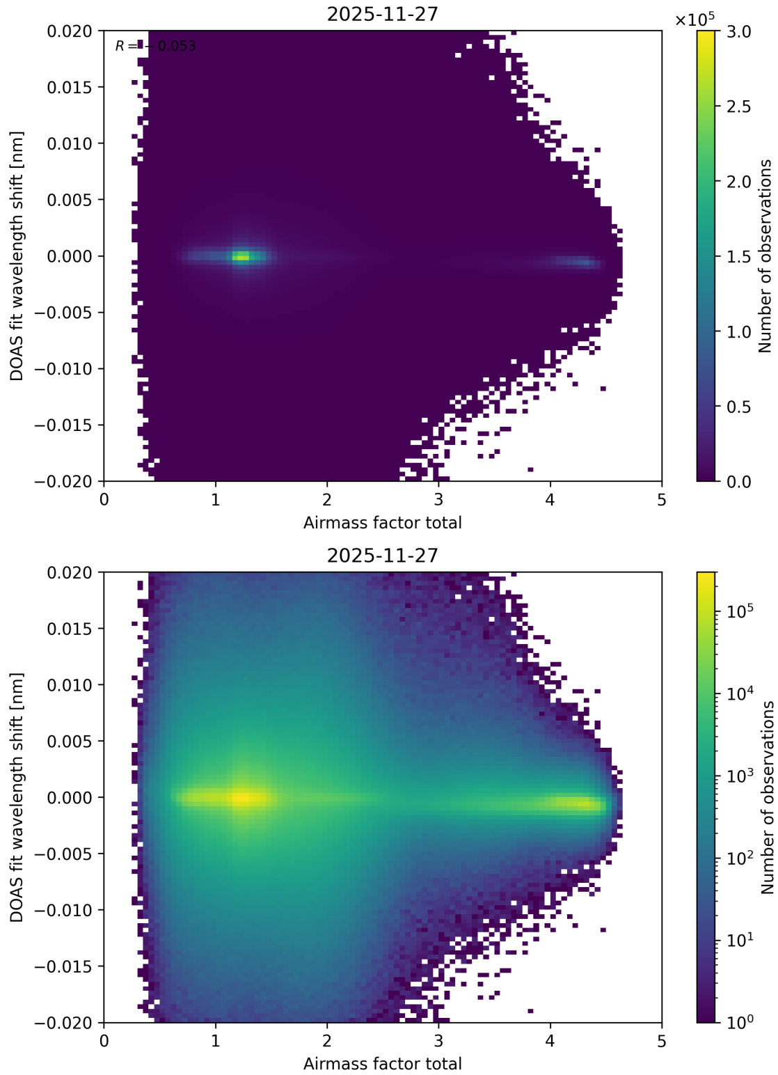
Figure 110: Scatter density plot of “Airmass factor total” against “DOAS fit wavelength shift” for 2025-11-26 to 2025-11-28.
