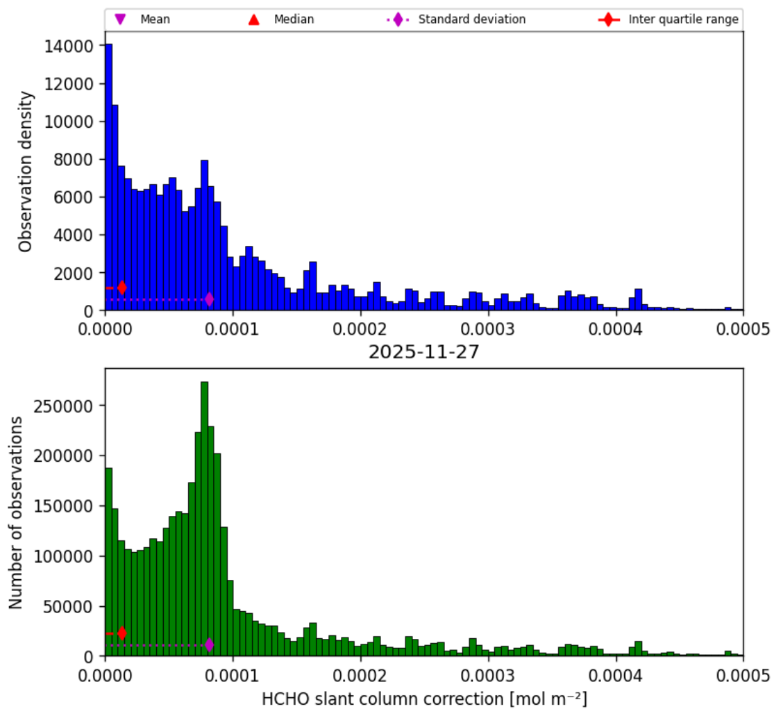
Figure 49: Histogram of “HCHO slant column correction” for 2025-11-26 to 2025-11-28
