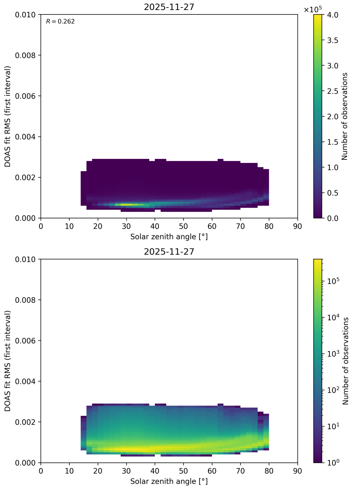
Figure 186: Scatter density plot of “Solar zenith angle” against “DOAS fit RMS (first interval)” for 2025-11-26 to 2025-11-28.
