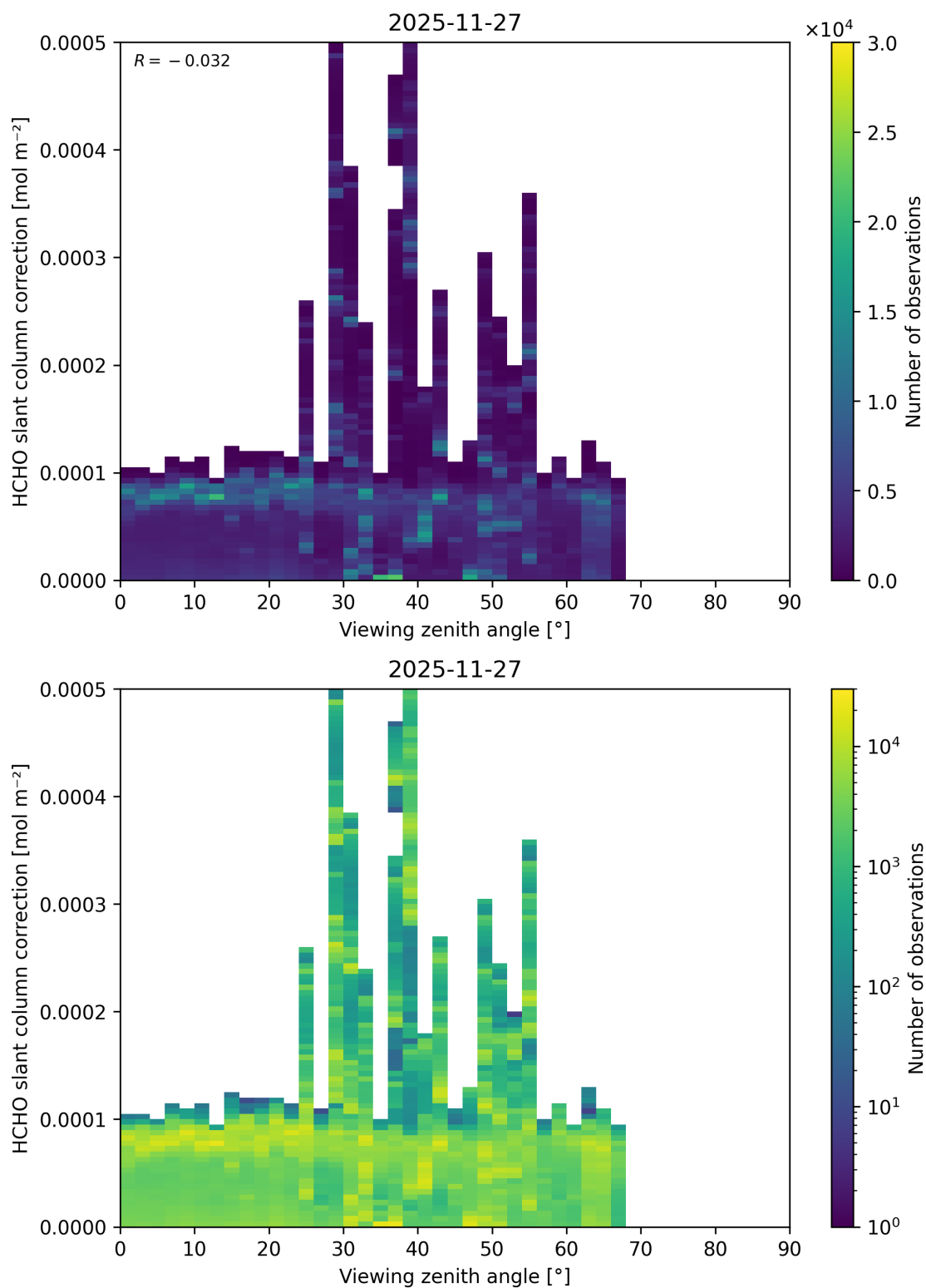
Figure 207: Scatter density plot of “Viewing zenith angle” against “HCHO slant column correction” for 2025-11-26 to 2025-11-28.
