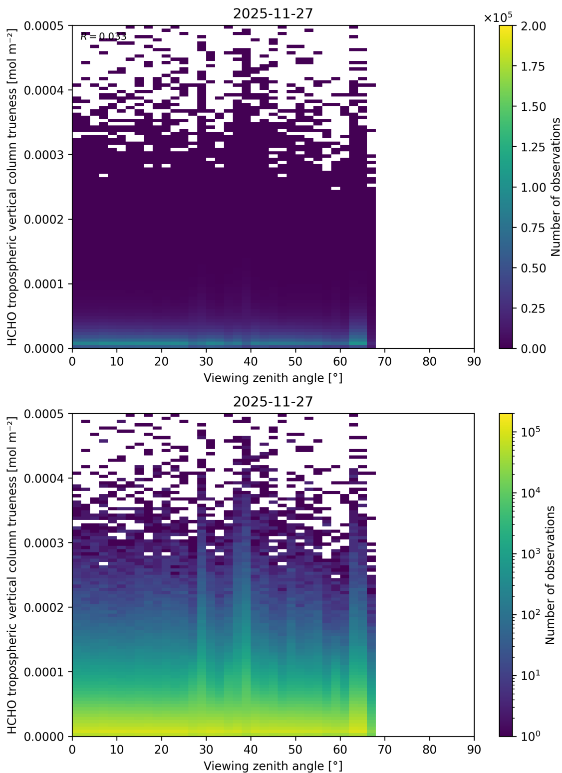
Figure 215: Scatter density plot of “Viewing zenith angle” against “HCHO tropospheric vertical column trueness” for 2025-11-26 to 2025-11-28.
