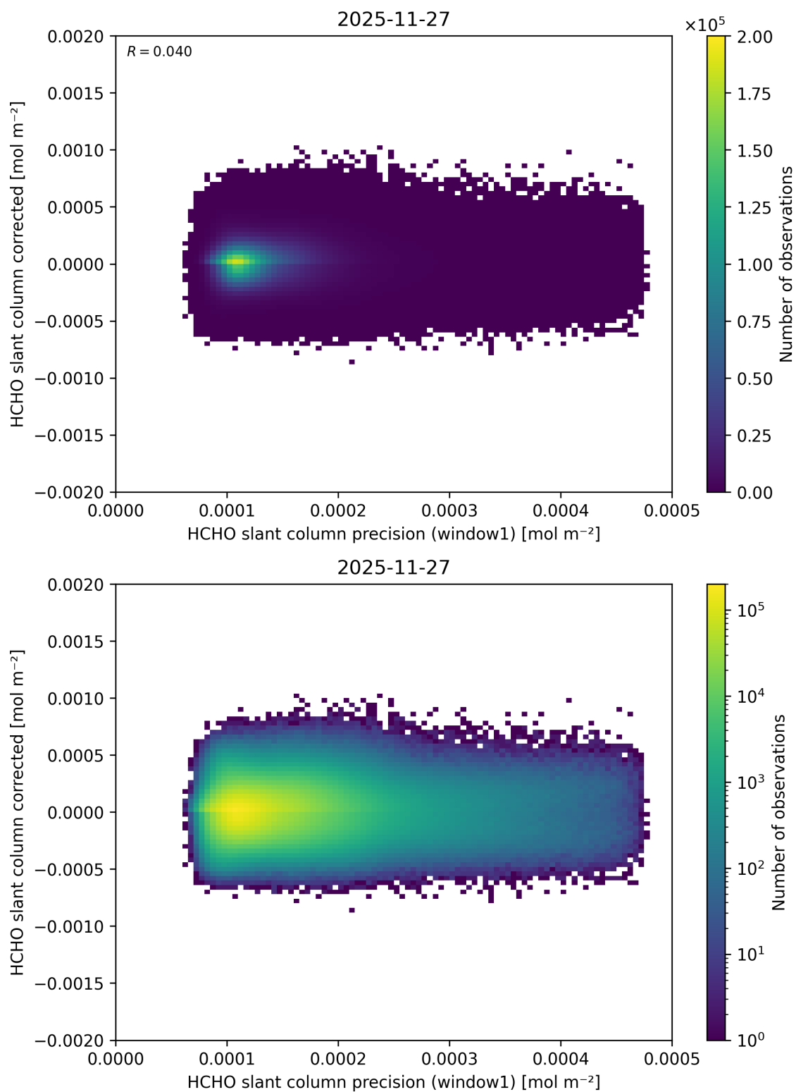
Figure 103: Scatter density plot of “HCHO slant column precision (window1)” against “HCHO slant column corrected” for 2025-11-26 to 2025-11-28.
