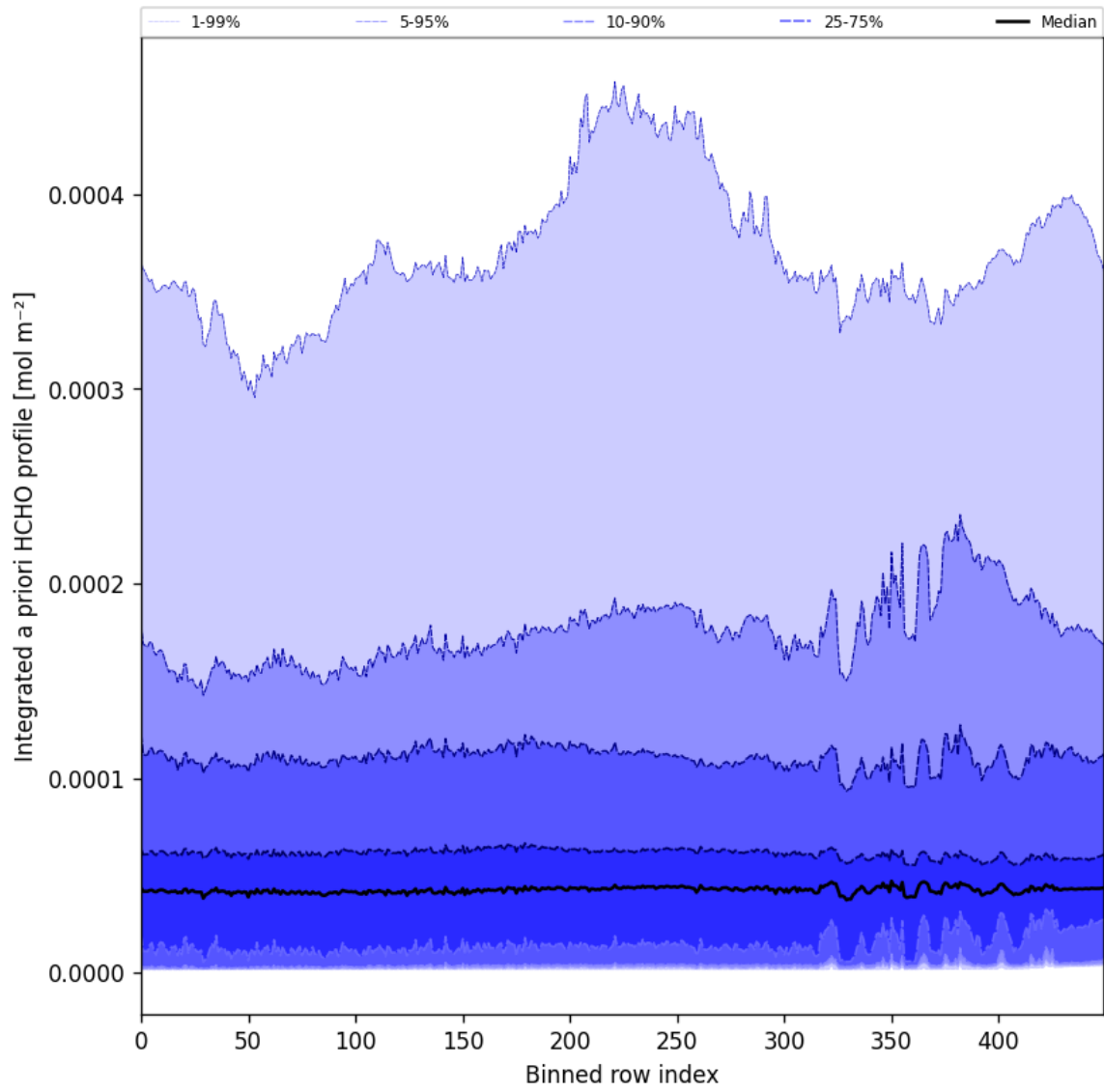
Figure 60: Along track statistics of “Integrated a priori HCHO profile” for 2025-11-26 to 2025-11-28
