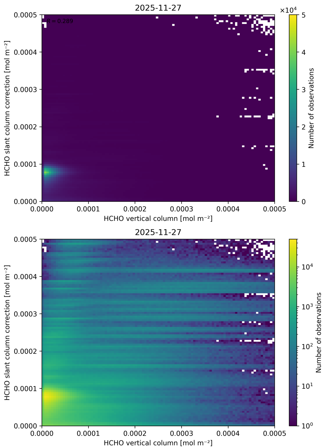
Figure 143: Scatter density plot of “HCHO vertical column” against “HCHO slant column correction” for 2025-11-26 to 2025-11-28.
