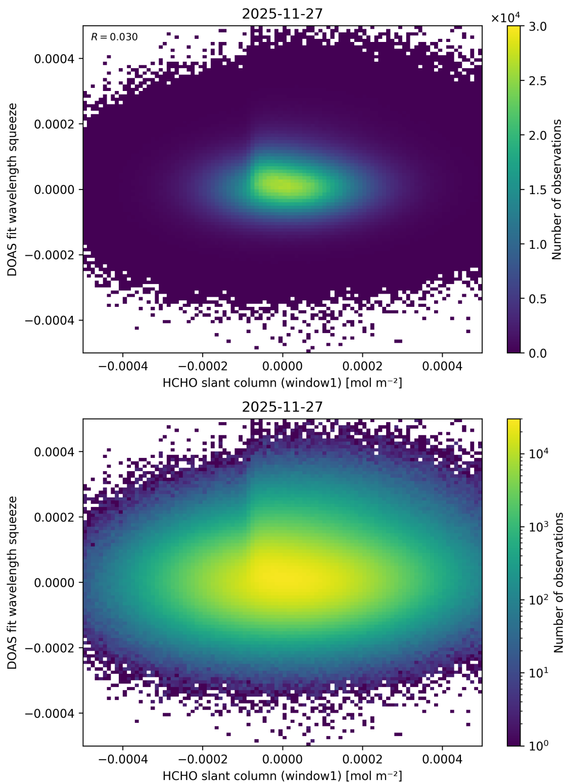
Figure 90: Scatter density plot of “HCHO slant column (window1)” against “DOAS fit wavelength squeeze” for 2025-11-26 to 2025-11-28.
