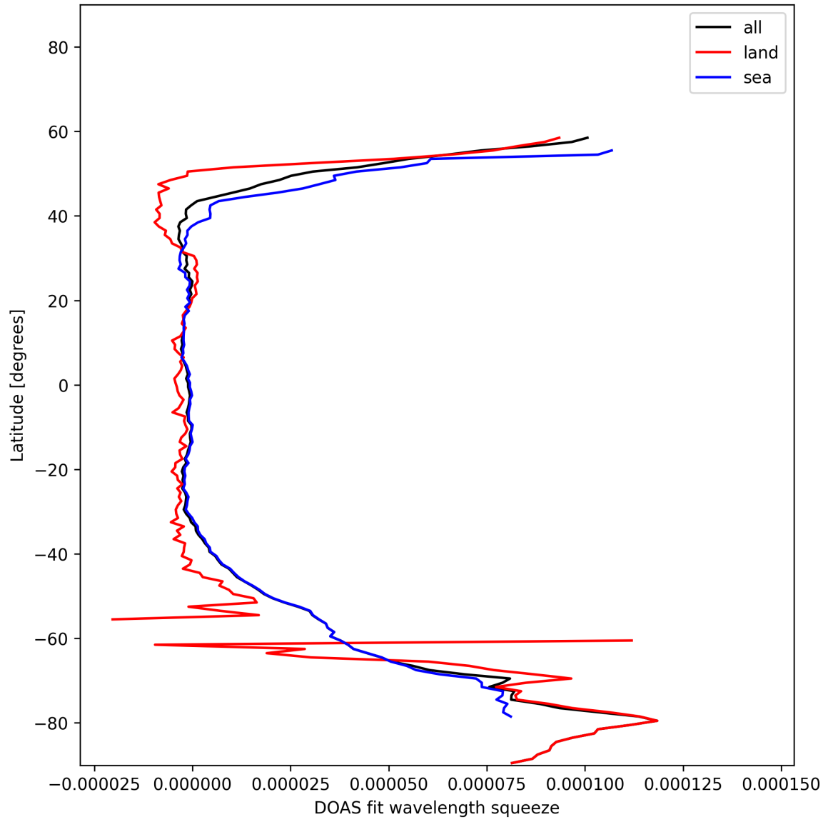
Figure 32: Zonal average of “DOAS fit wavelength squeeze” for 2025-11-26 to 2025-11-28.
