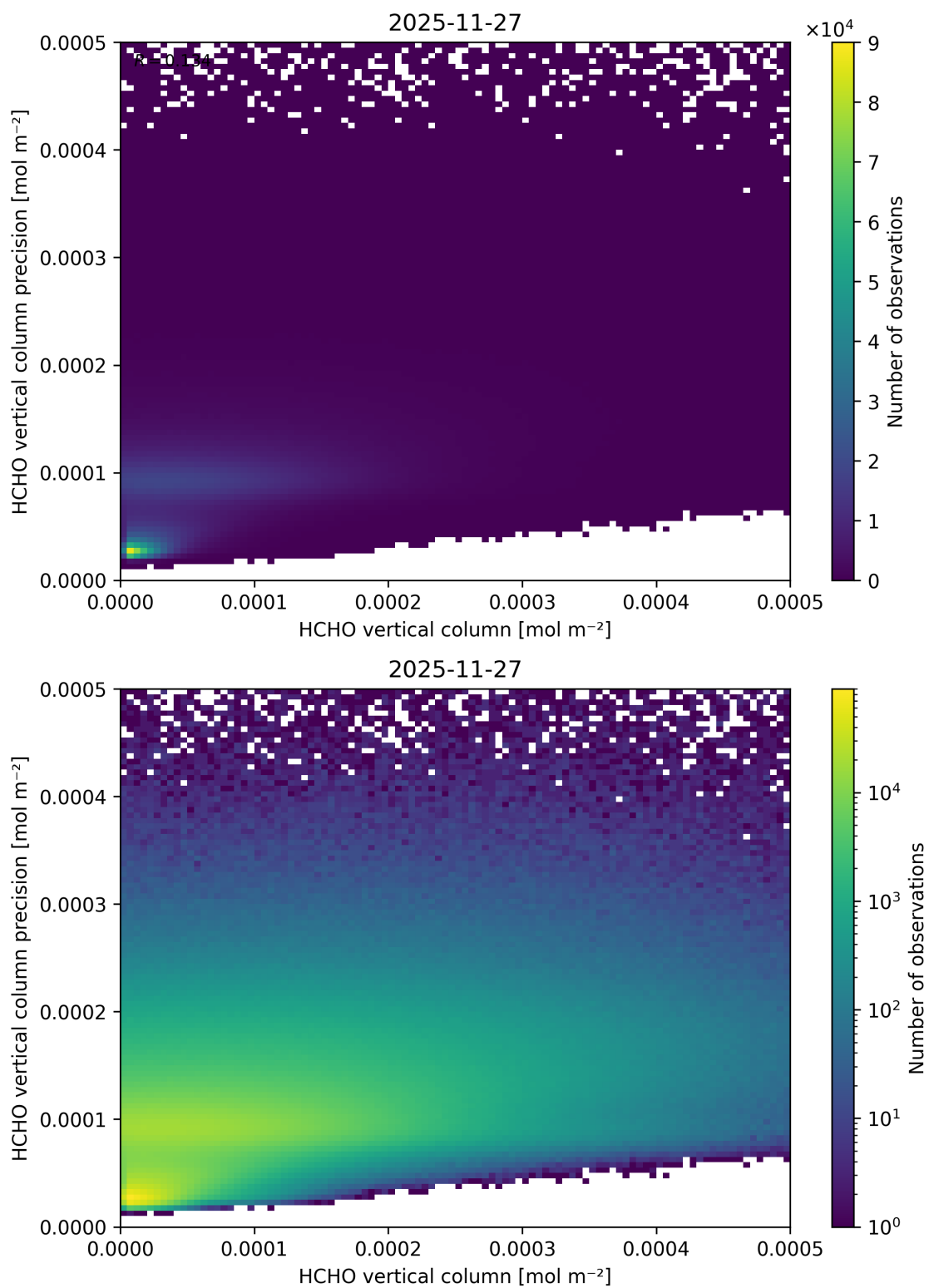
Figure 149: Scatter density plot of “HCHO vertical column” against “HCHO vertical column precision” for 2025-11-26 to 2025-11-28.
