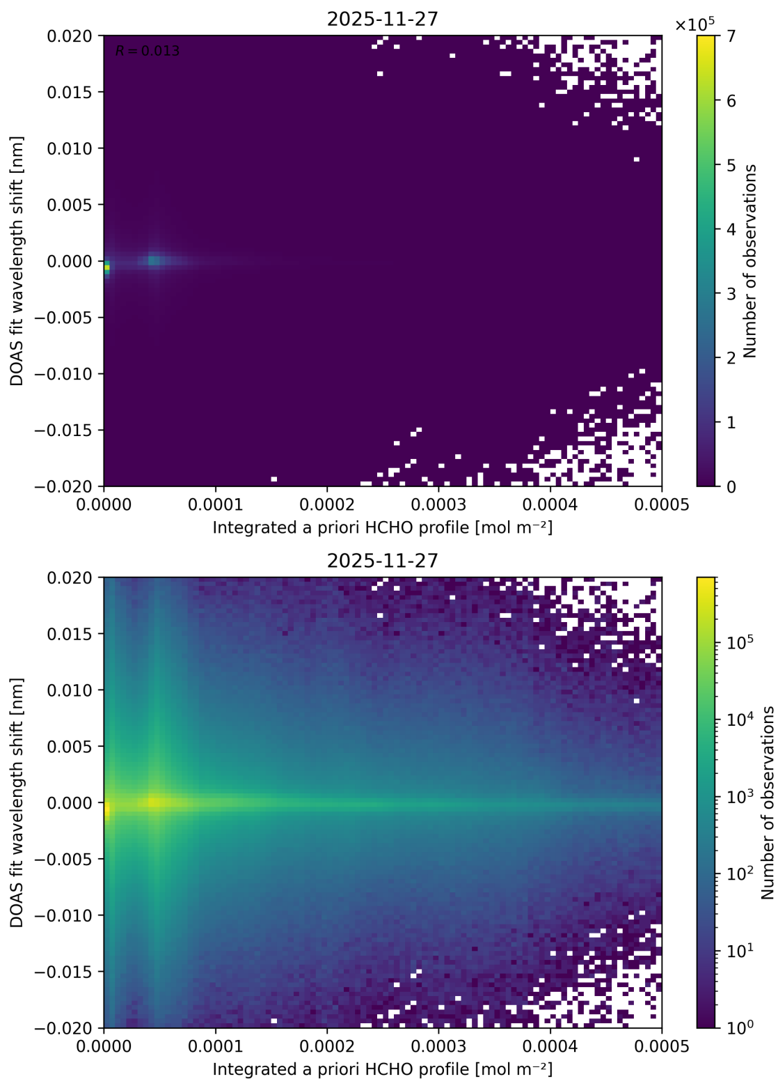
Figure 166: Scatter density plot of “Integrated a priori HCHO profile” against “DOAS fit wavelength shift” for 2025-11-26 to 2025-11-28.
