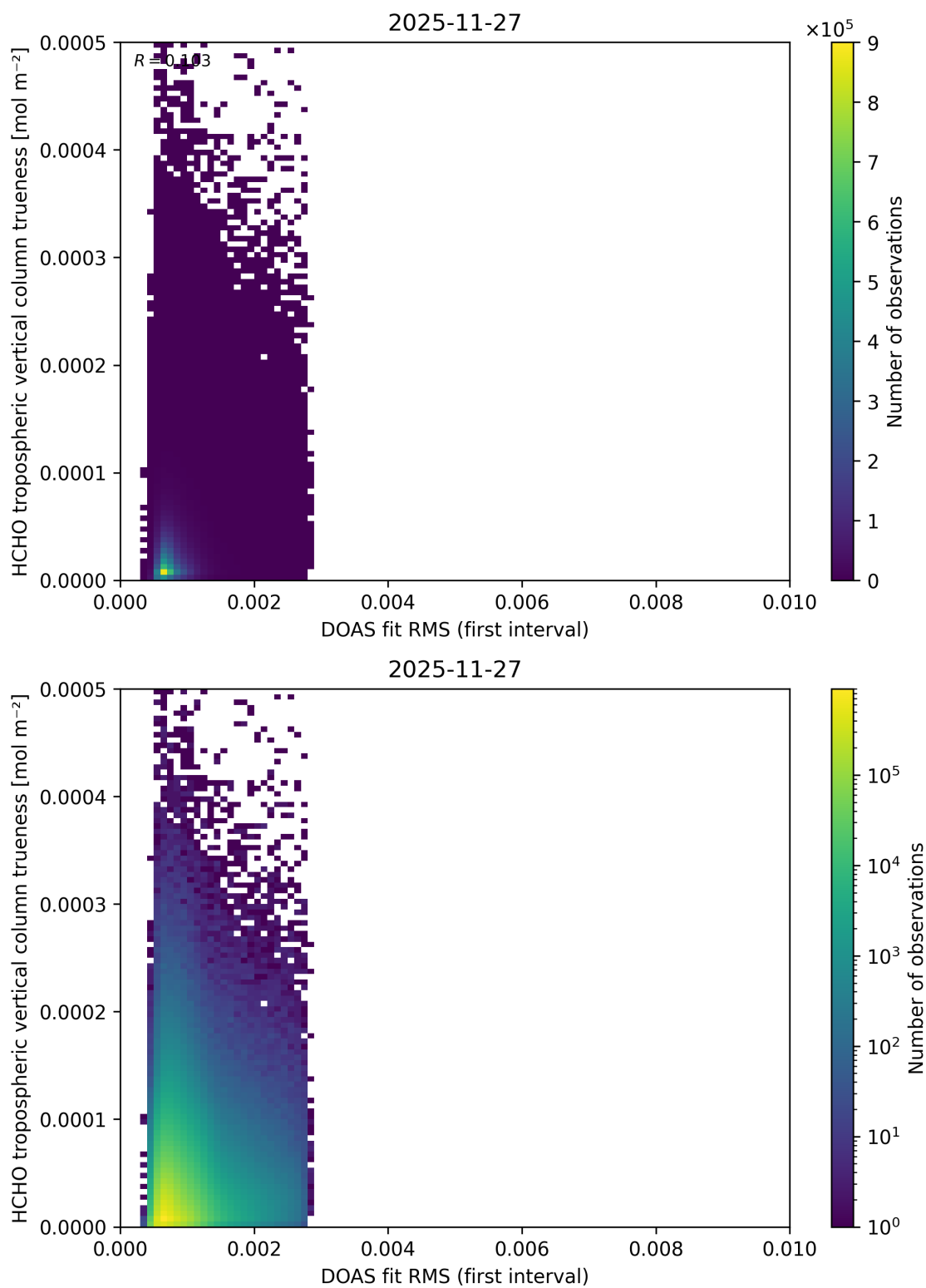
Figure 68: Scatter density plot of “DOAS fit RMS (first interval)” against “HCHO tropospheric vertical column trueness” for 2025-11-26 to 2025-11-28.
