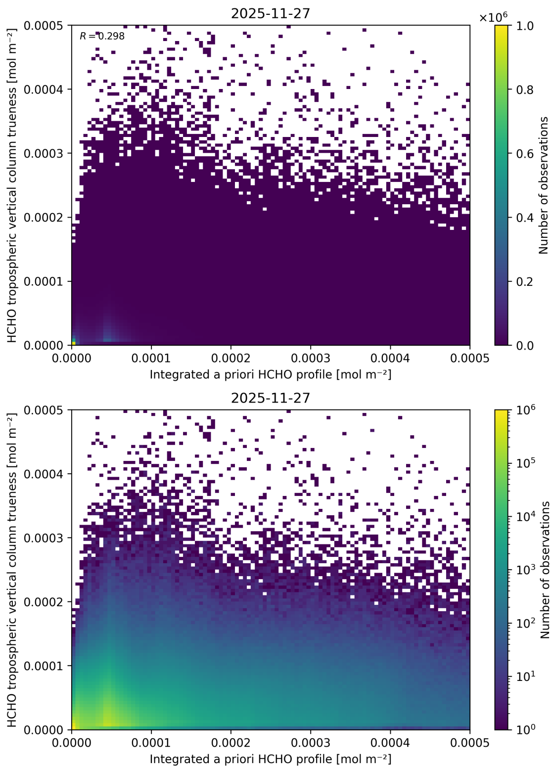
Figure 170: Scatter density plot of “Integrated a priori HCHO profile” against “HCHO tropospheric vertical column truthness” for 2025-11-26 to 2025-11-28.
