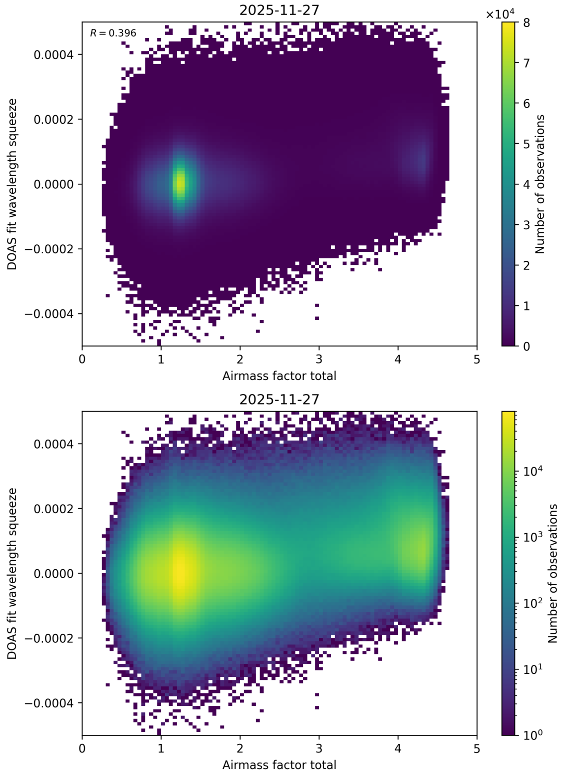
Figure 111: Scatter density plot of “Airmass factor total” against “DOAS fit wavelength squeeze” for 2025-11-26 to 2025-11-28.
