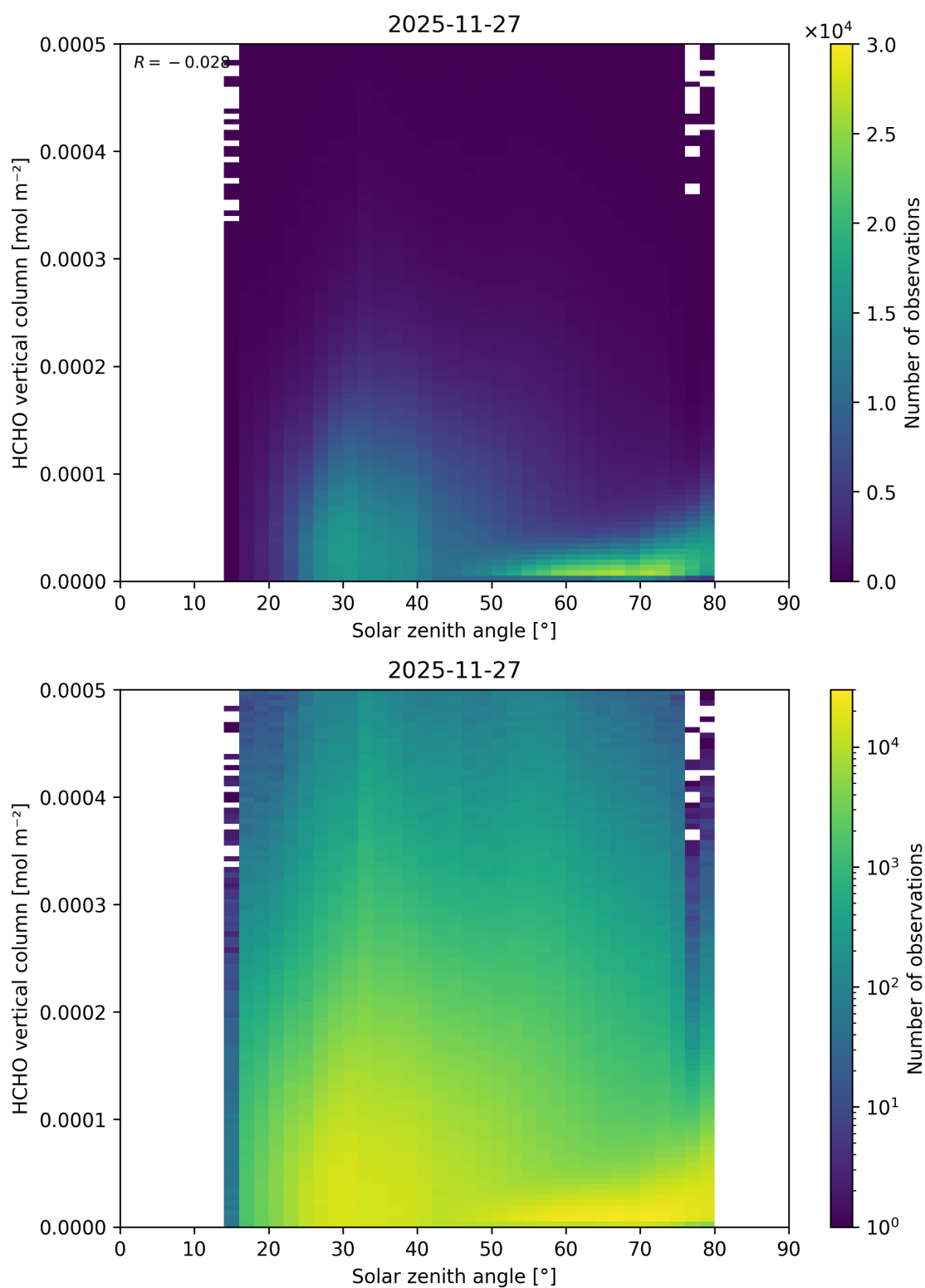
Figure 196: Scatter density plot of “Solar zenith angle” against “HCHO vertical column” for 2025-11-26 to 2025-11-28.
