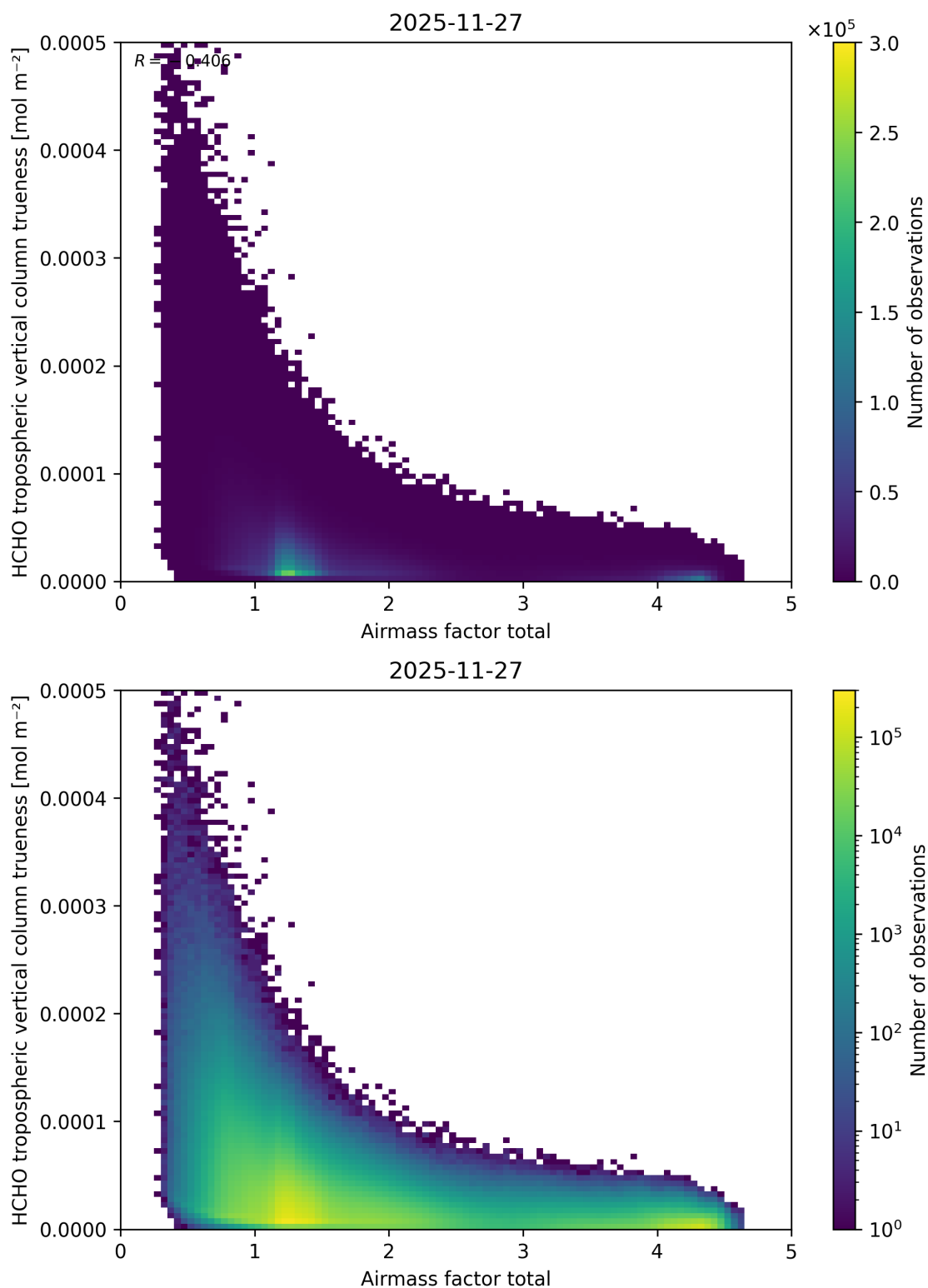
Figure 116: Scatter density plot of “Airmass factor total” against “HCHO tropospheric vertical column trueeness” for 2025-11-26 to 2025-11-28.
