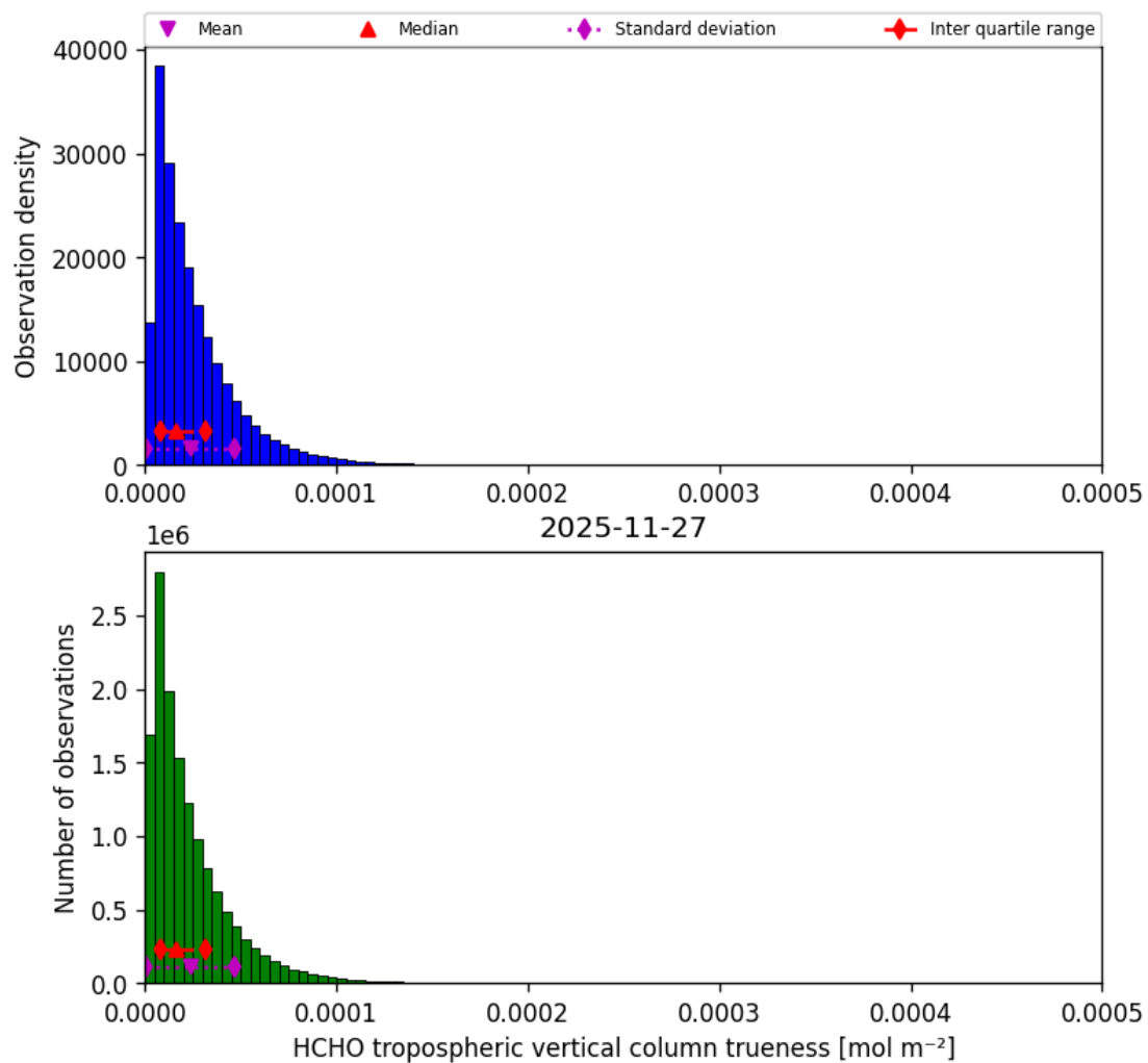
Figure 50: Histogram of “HCHO tropospheric vertical column trueness” for 2025-11-26 to 2025-11-28
