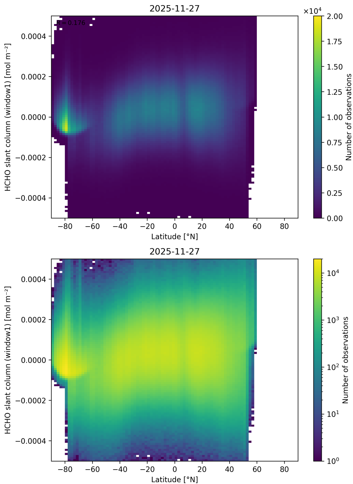
Figure 177: Scatter density plot of “Latitude” against “HCHO slant column (window1)” for 2025-11-26 to 2025-11-28.
