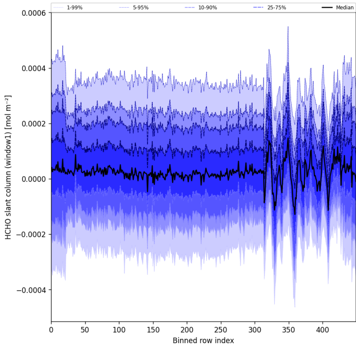
Figure 55: Along track statistics of “HCHO slant column (window1)” for 2025-11-26 to 2025-11-28
