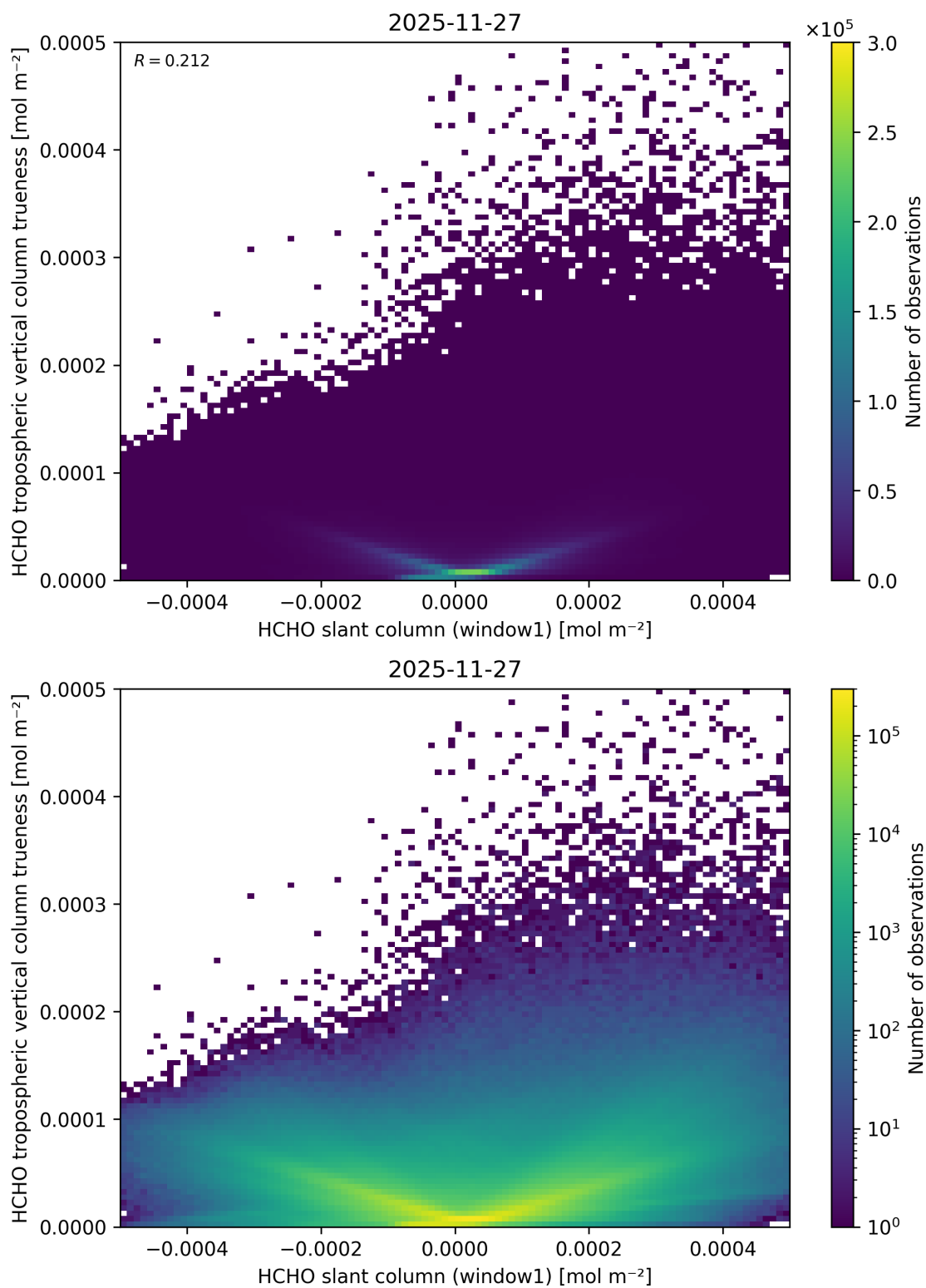
Figure 97: Scatter density plot of “HCHO slant column (window1)” against “HCHO tropospheric vertical column trueness” for 2025-11-26 to 2025-11-28.
