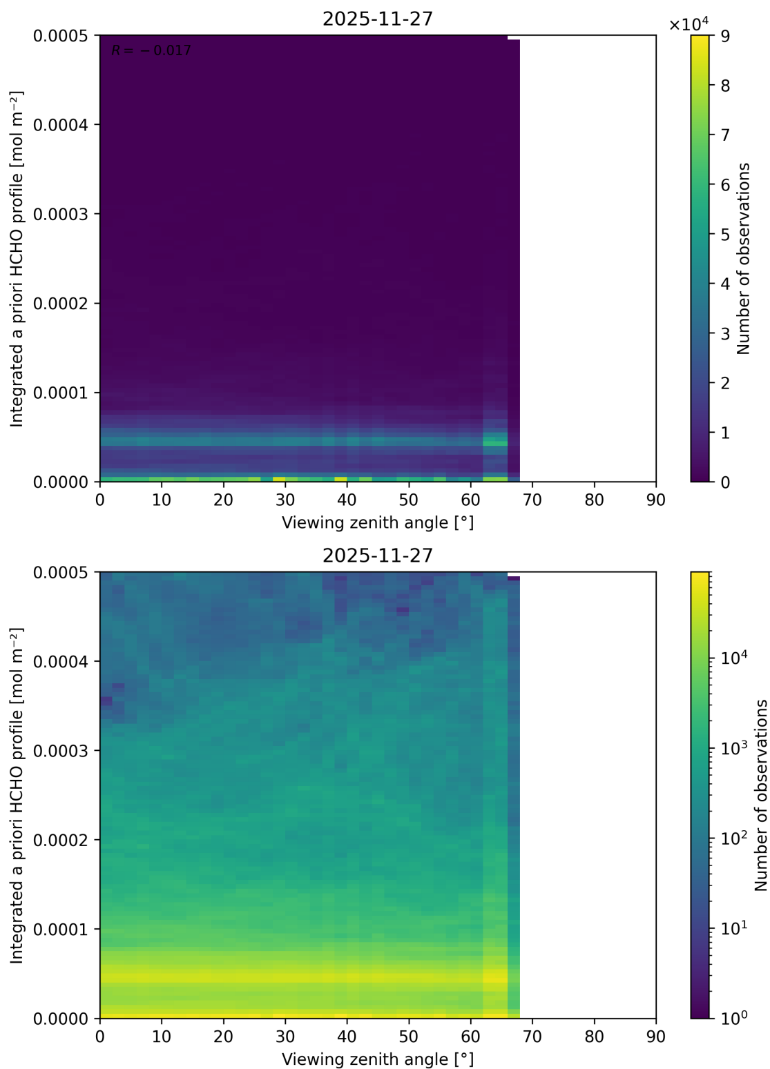
Figure 216: Scatter density plot of “Viewing zenith angle” against “Integrated a priori HCHO profile” for 2025-11-26 to 2025-11-28.
