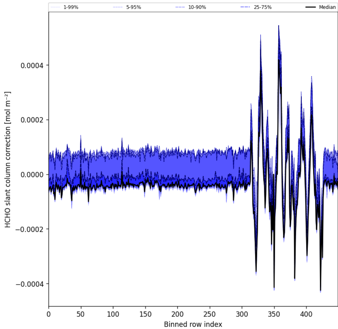
Figure 64: Along track statistics of “HCHO slant column correction” for 2025-11-26 to 2025-11-28
