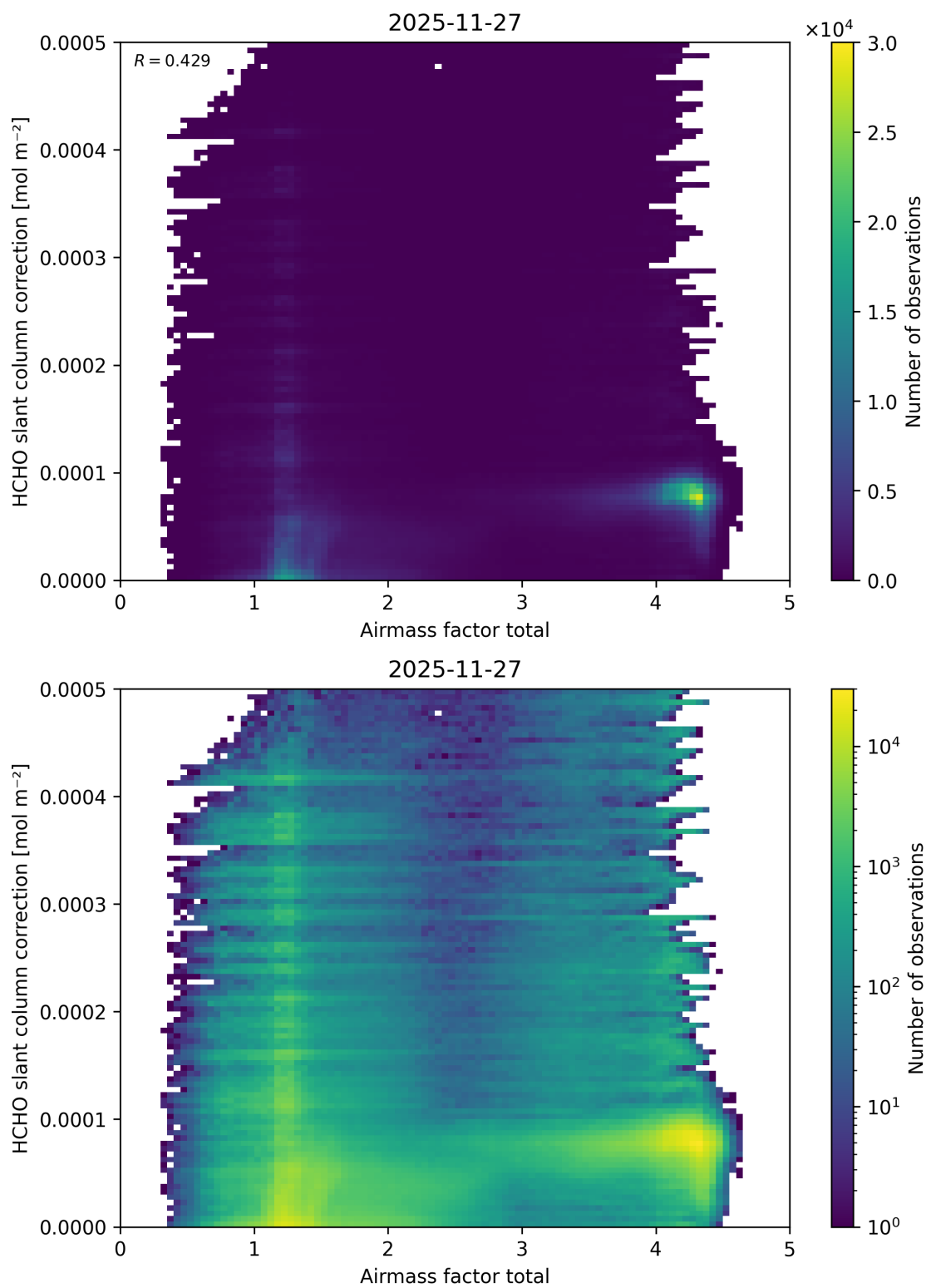
Figure 114: Scatter density plot of “Airmass factor total” against “HCHO slant column correction” for 2025-11-26 to 2025-11-28.
