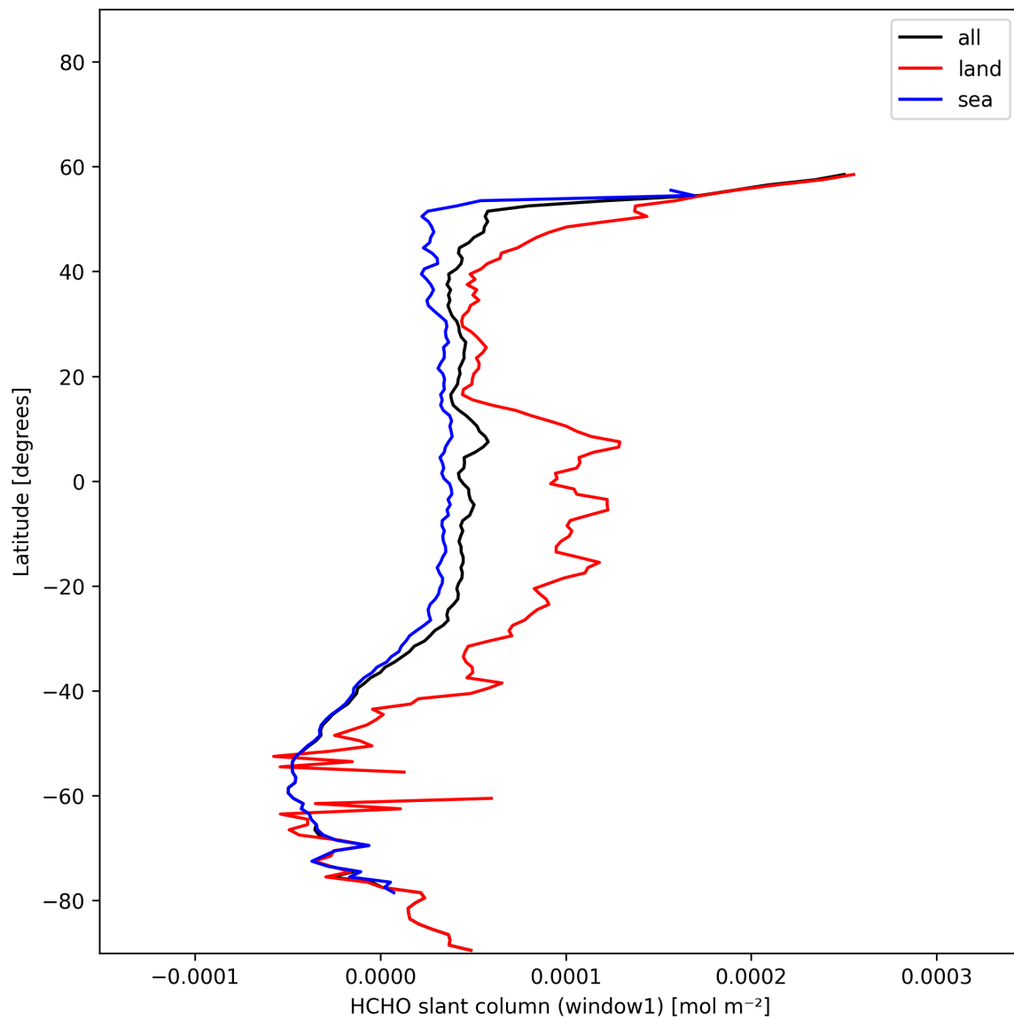
Figure 25: Zonal average of “HCHO slant column (window1)” for 2025-11-26 to 2025-11-28.
