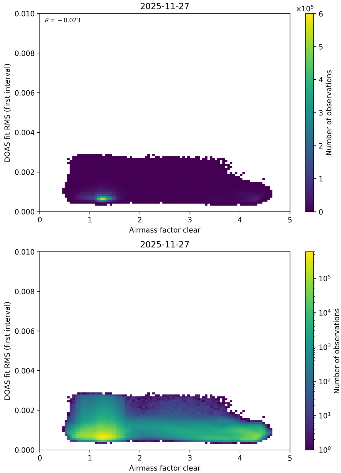
Figure 78: Scatter density plot of “Airmass factor clear” against “DOAS fit RMS (first interval)” for 2025-11-26 to 2025-11-28.
