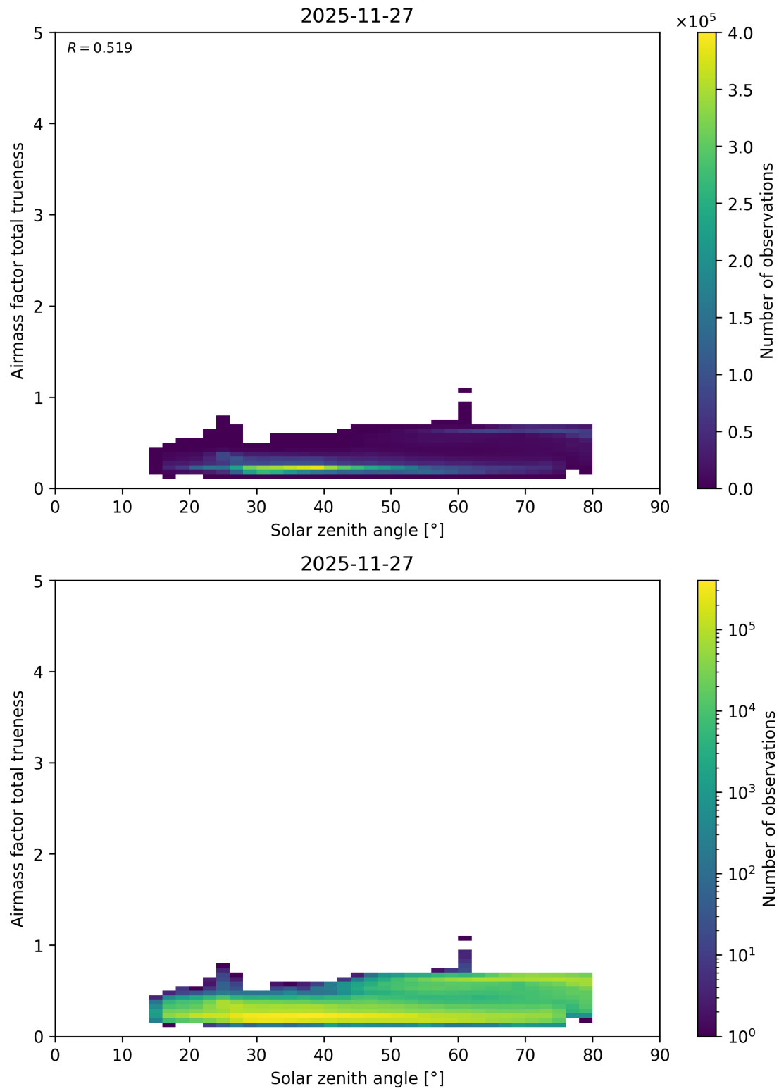
Figure 195: Scatter density plot of “Solar zenith angle” against “Airmass factor total trueness” for 2025-11-26 to 2025-11-28.
