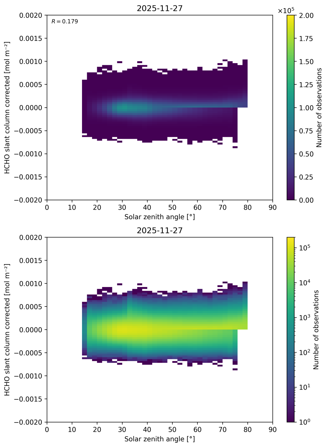
Figure 190: Scatter density plot of “Solar zenith angle” against “HCHO slant column corrected” for 2025-11-26 to 2025-11-28.
