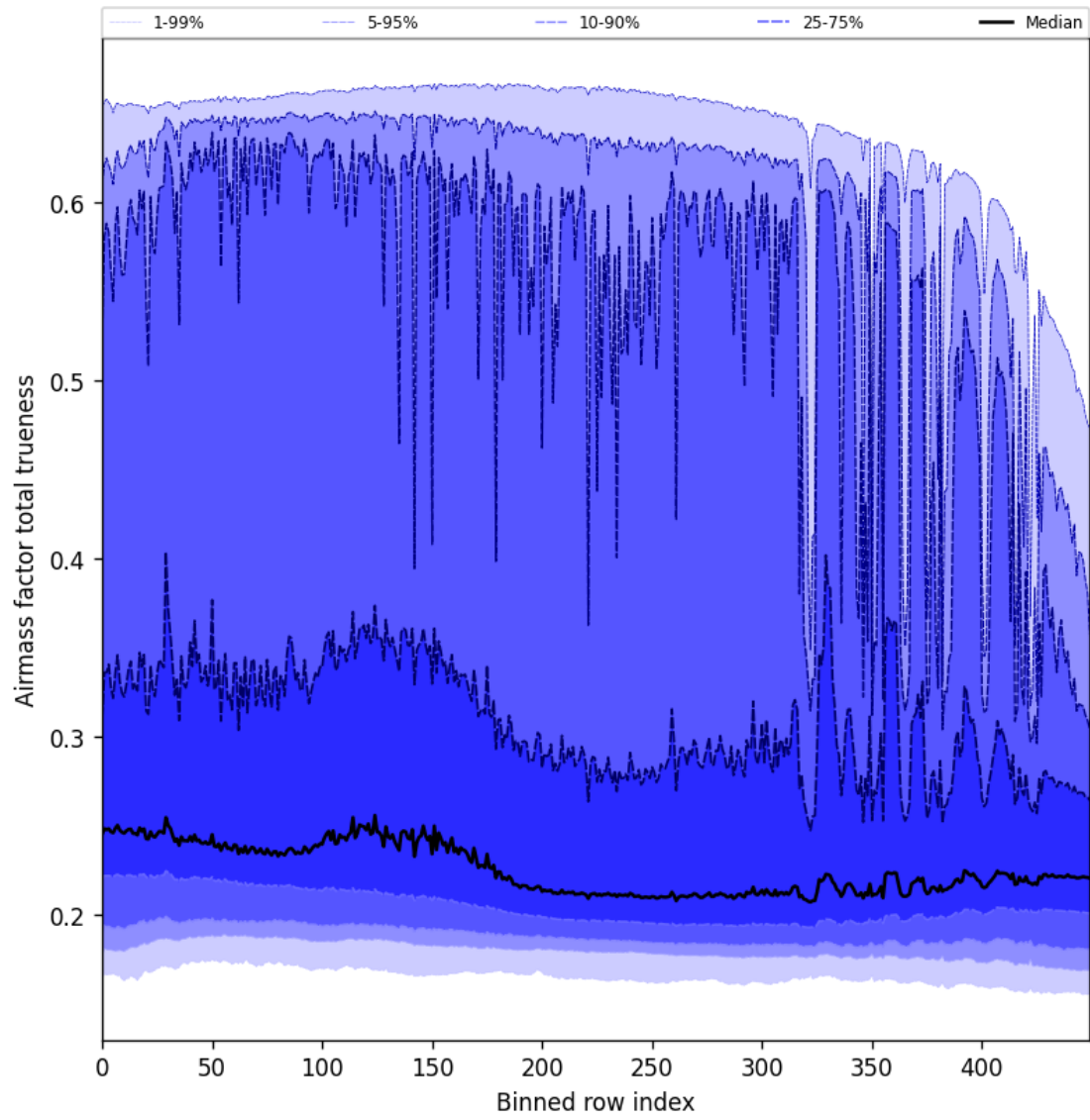
Figure 58: Along track statistics of “Airmass factor total trueness” for 2025-11-26 to 2025-11-28
