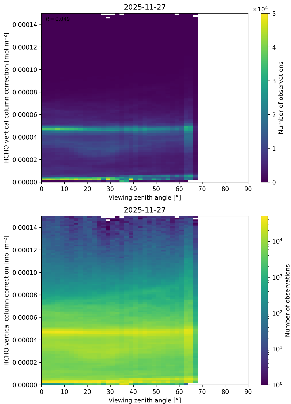
Figure 213: Scatter density plot of “Viewing zenith angle” against “HCHO vertical column correction” for 2025-11-26 to 2025-11-28.
