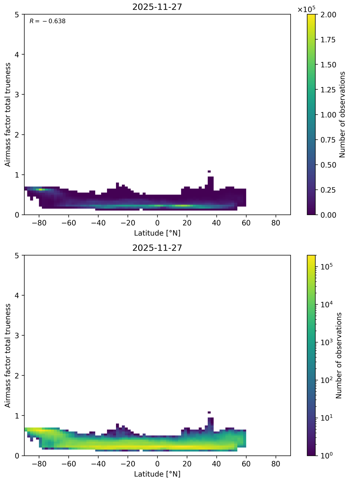
Figure 180: Scatter density plot of “Latitude” against “Airmass factor total trueness” for 2025-11-26 to 2025-11-28.
