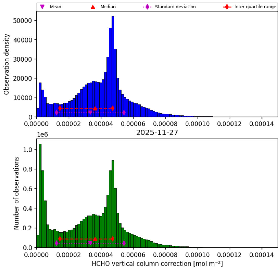
Figure 39: Histogram of “HCHO vertical column correction” for 2025-11-26 to 2025-11-28
