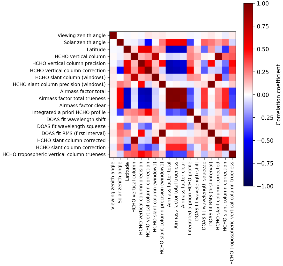
Figure 2: Map of correlation matrix for 2025-11-26 to 2025-11-28.
