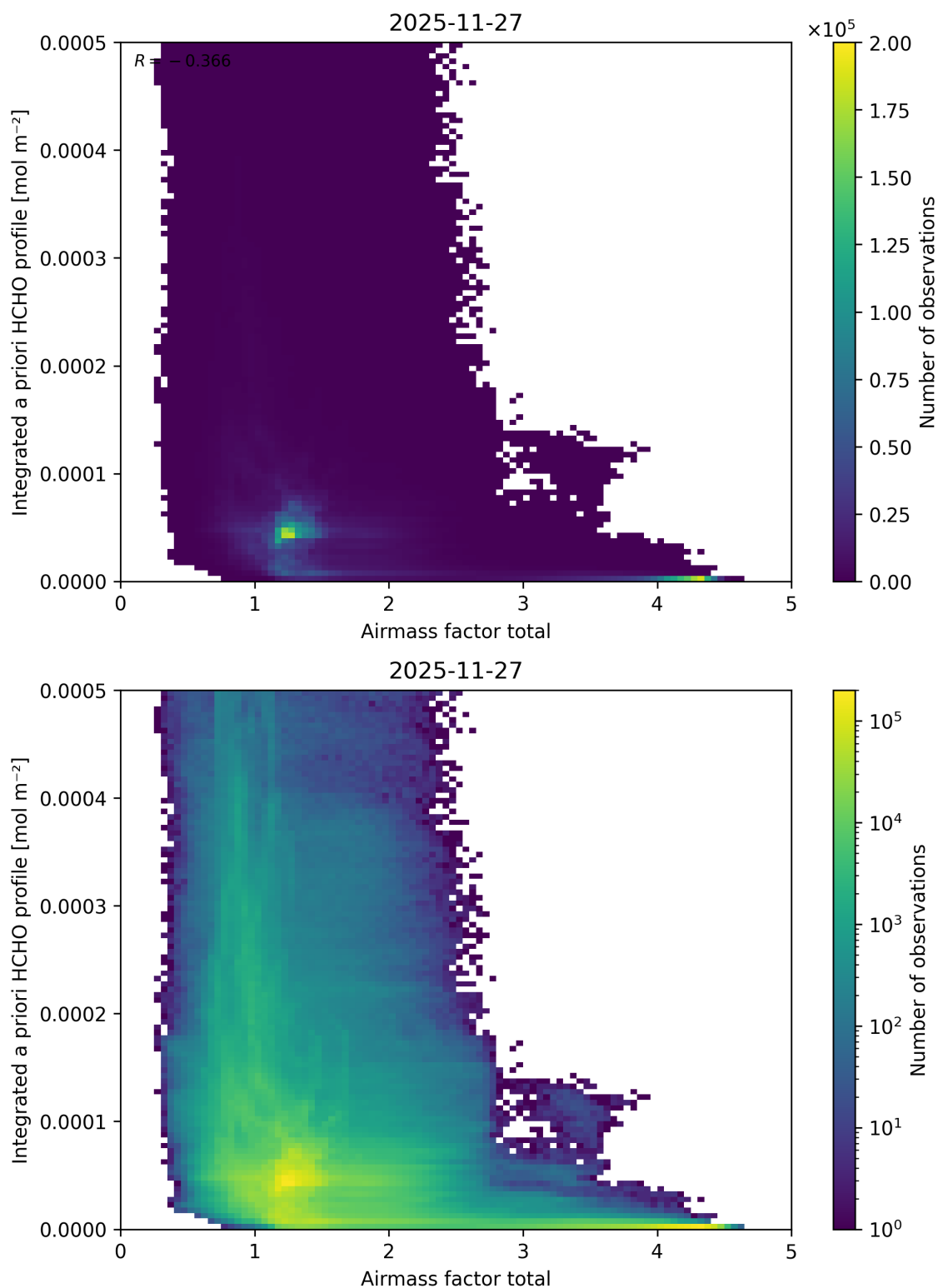
Figure 117: Scatter density plot of “Airmass factor total” against “Integrated a priori HCHO profile” for 2025-11-26 to 2025-11-28.
