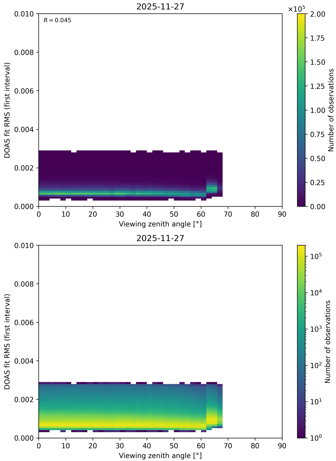
Figure 202: Scatter density plot of “Viewing zenith angle” against “DOAS fit RMS (first interval)” for 2025-11-26 to 2025-11-28.
