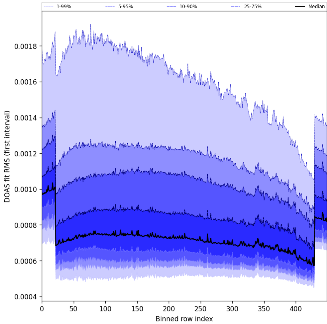
Figure 63: Along track statistics of “DOAS fit RMS (first interval)” for 2025-11-26 to 2025-11-28
