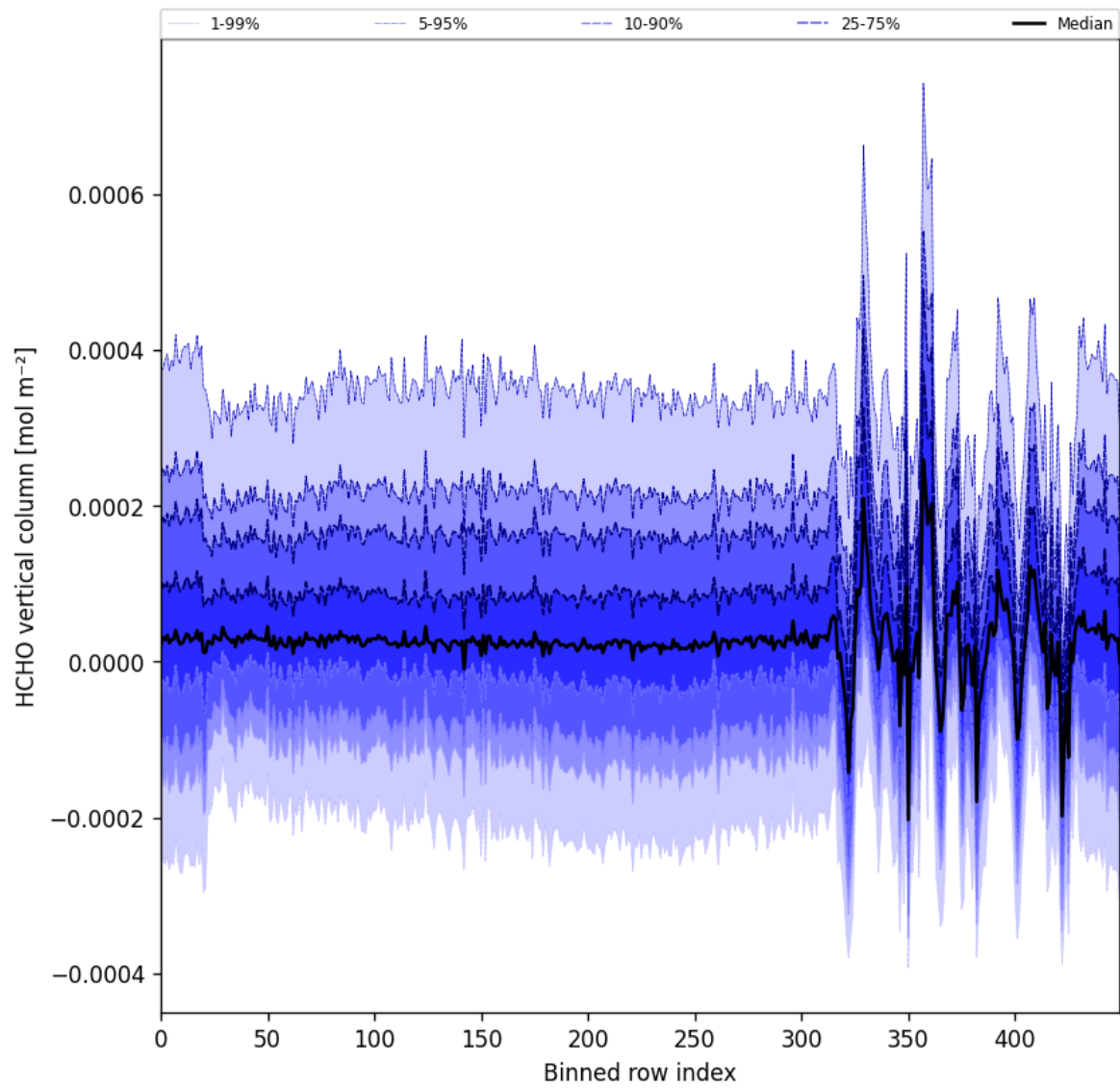
Figure 52: Along track statistics of “HCHO vertical column” for 2025-11-26 to 2025-11-28
