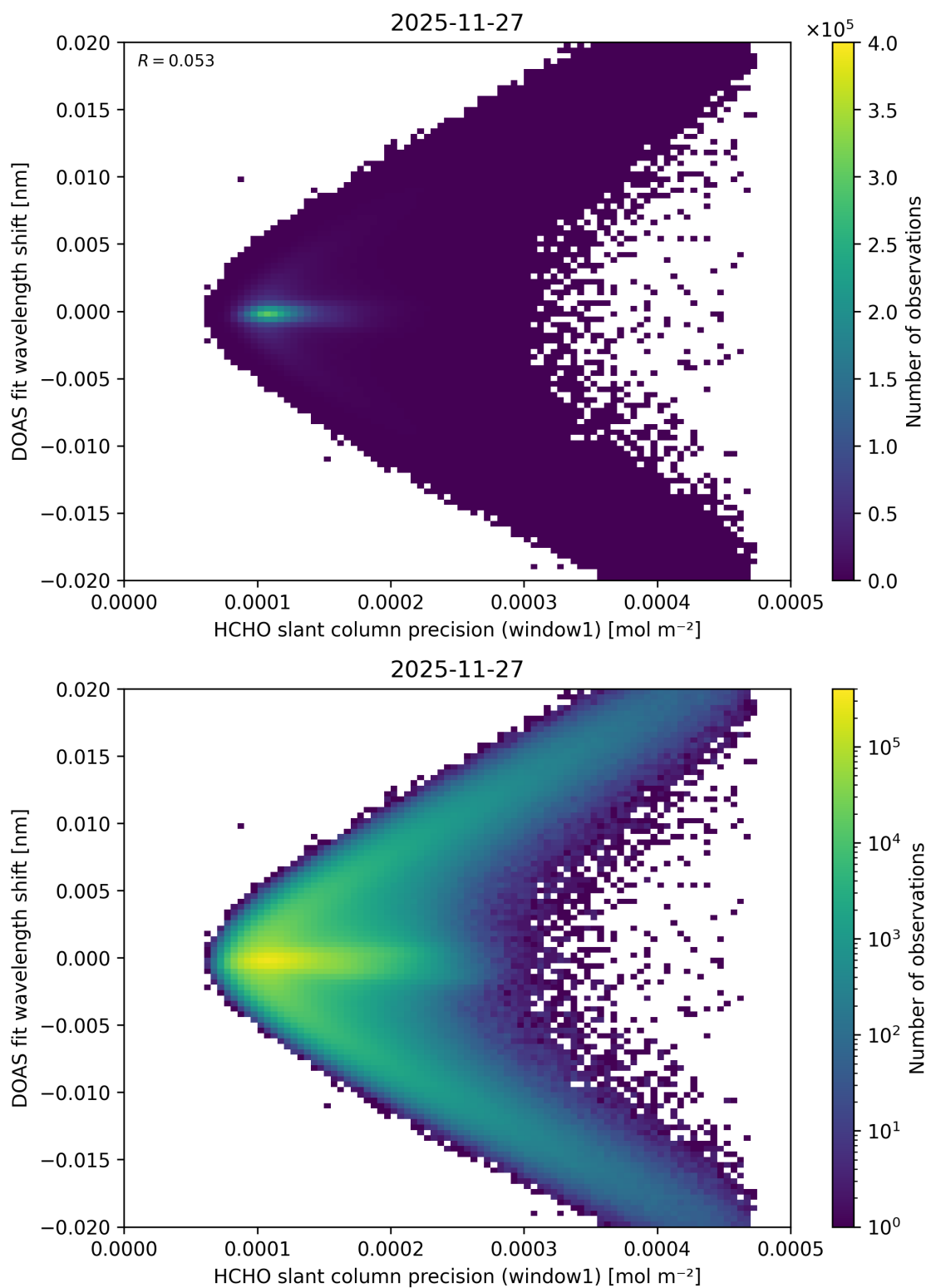
Figure 100: Scatter density plot of “HCHO slant column precision (window1)” against “DOAS fit wavelength shift” for 2025-11-26 to 2025-11-28.
