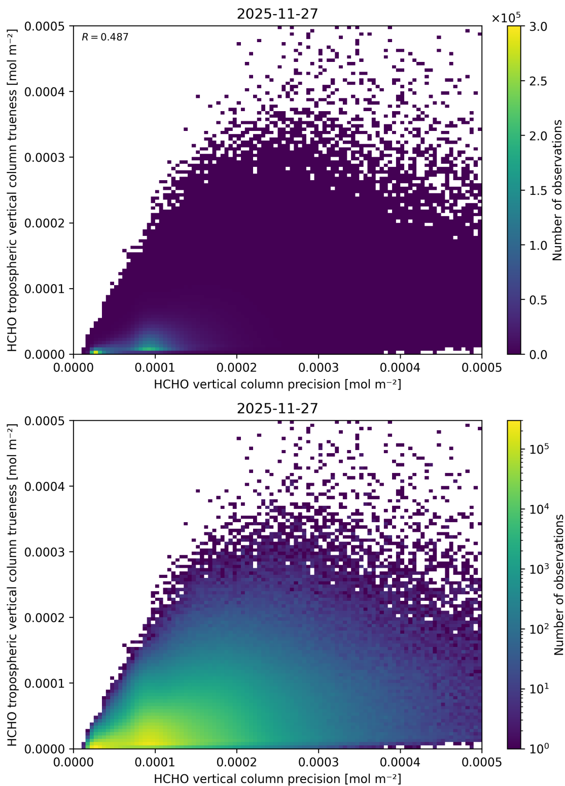
Figure 163: Scatter density plot of “HCHO vertical column precision” against “HCHO tropospheric vertical column truthness” for 2025-11-26 to 2025-11-28.
