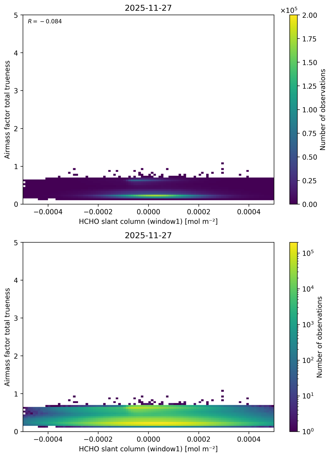
Figure 96: Scatter density plot of “HCHO slant column (window1)” against “Airmass factor total trueness” for 2025-11-26 to 2025-11-28.
