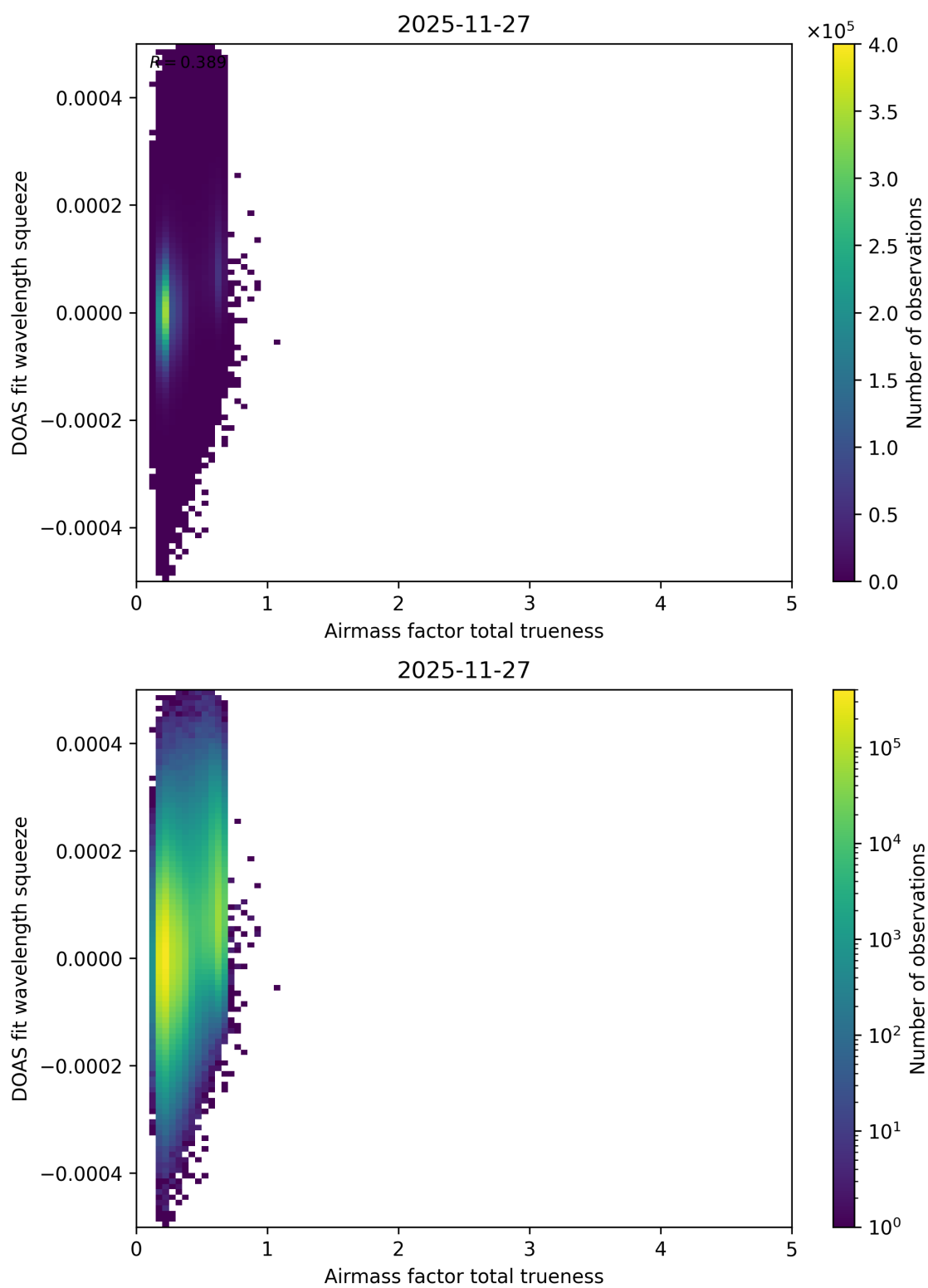
Figure 120: Scatter density plot of “Airmass factor total trueness” against “DOAS fit wavelength squeeze” for 2025-11-26 to 2025-11-28.
