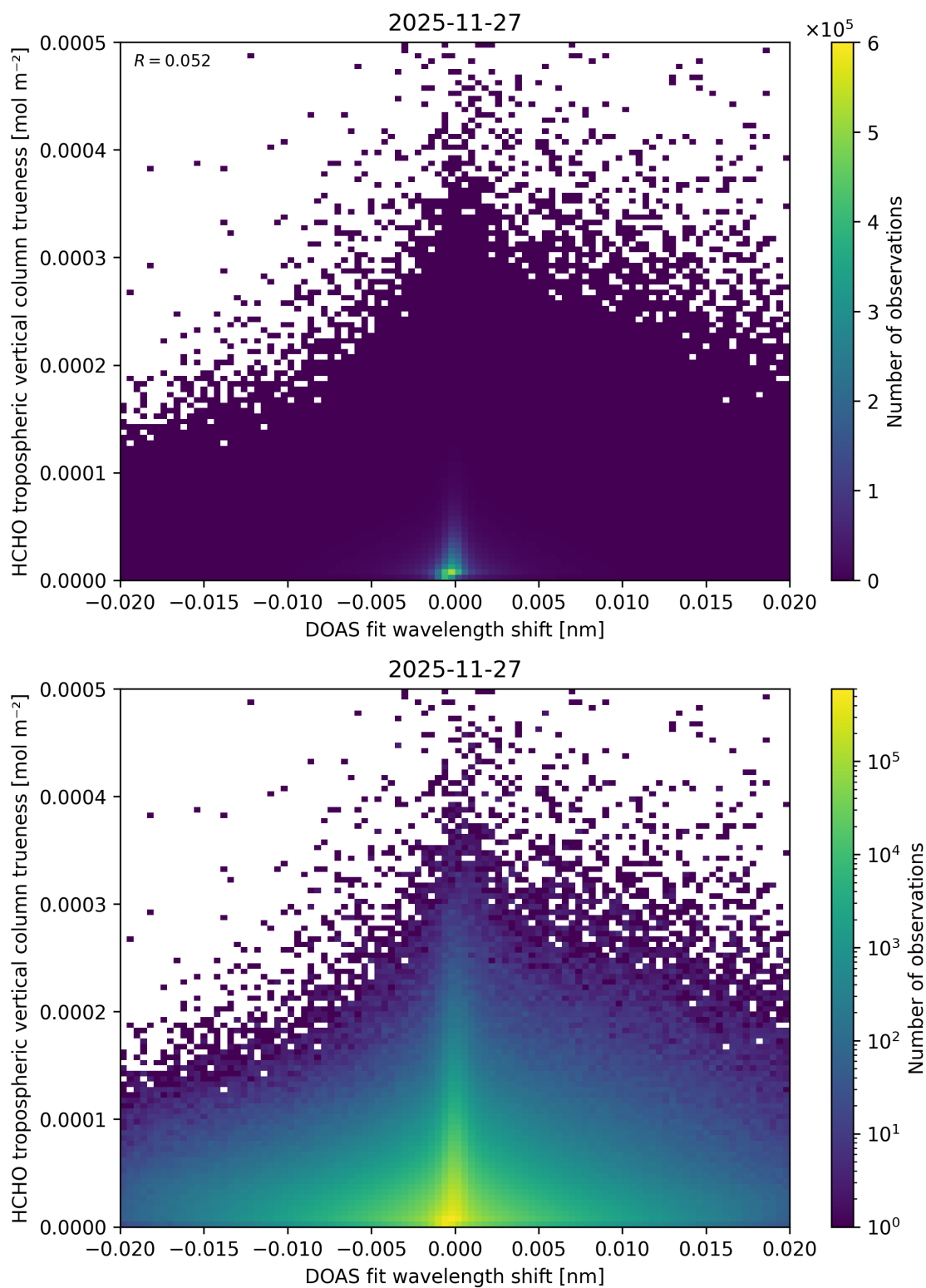
Figure 73: Scatter density plot of “DOAS fit wavelength shift” against “HCHO tropospheric vertical column trueness” for 2025-11-26 to 2025-11-28.
