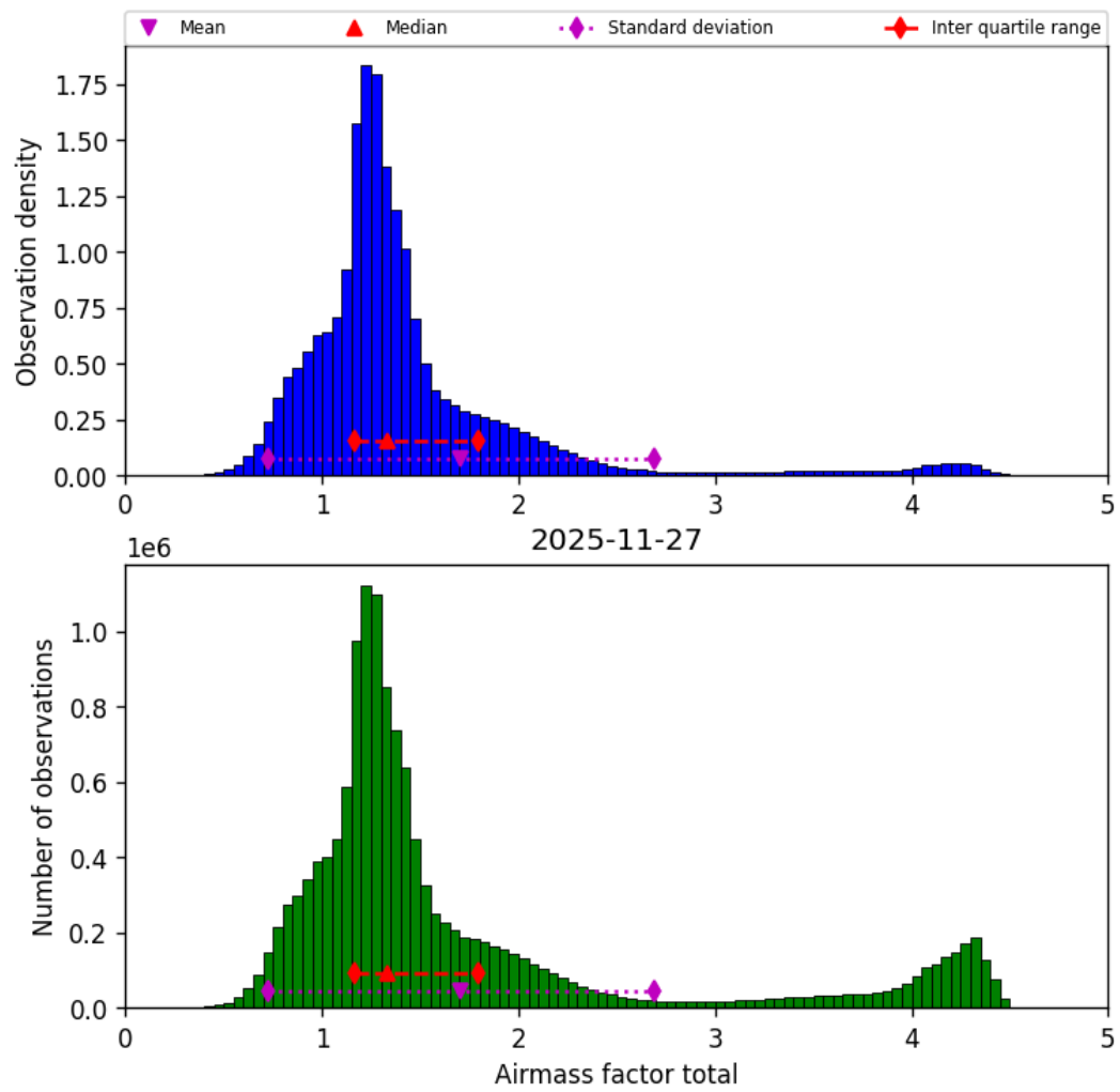
Figure 42: Histogram of “Airmass factor total” for 2025-11-26 to 2025-11-28
