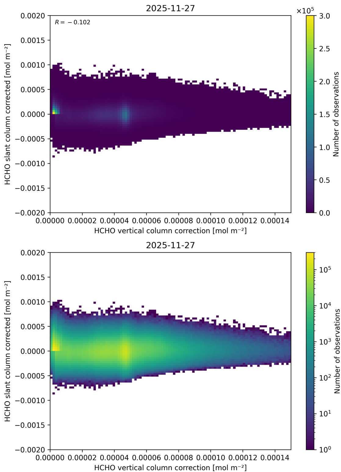
Figure 130: Scatter density plot of “HCHO vertical column correction” against “HCHO slant column corrected” for 2025-11-26 to 2025-11-28.
