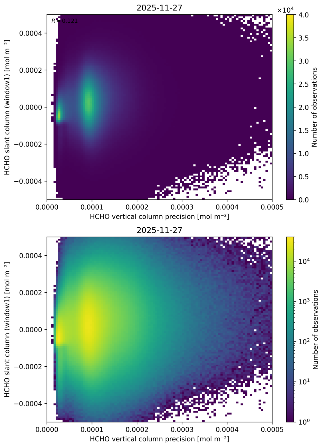
Figure 158: Scatter density plot of “HCHO vertical column precision” against “HCHO slant column (window1)” for 2025-11-26 to 2025-11-28.
