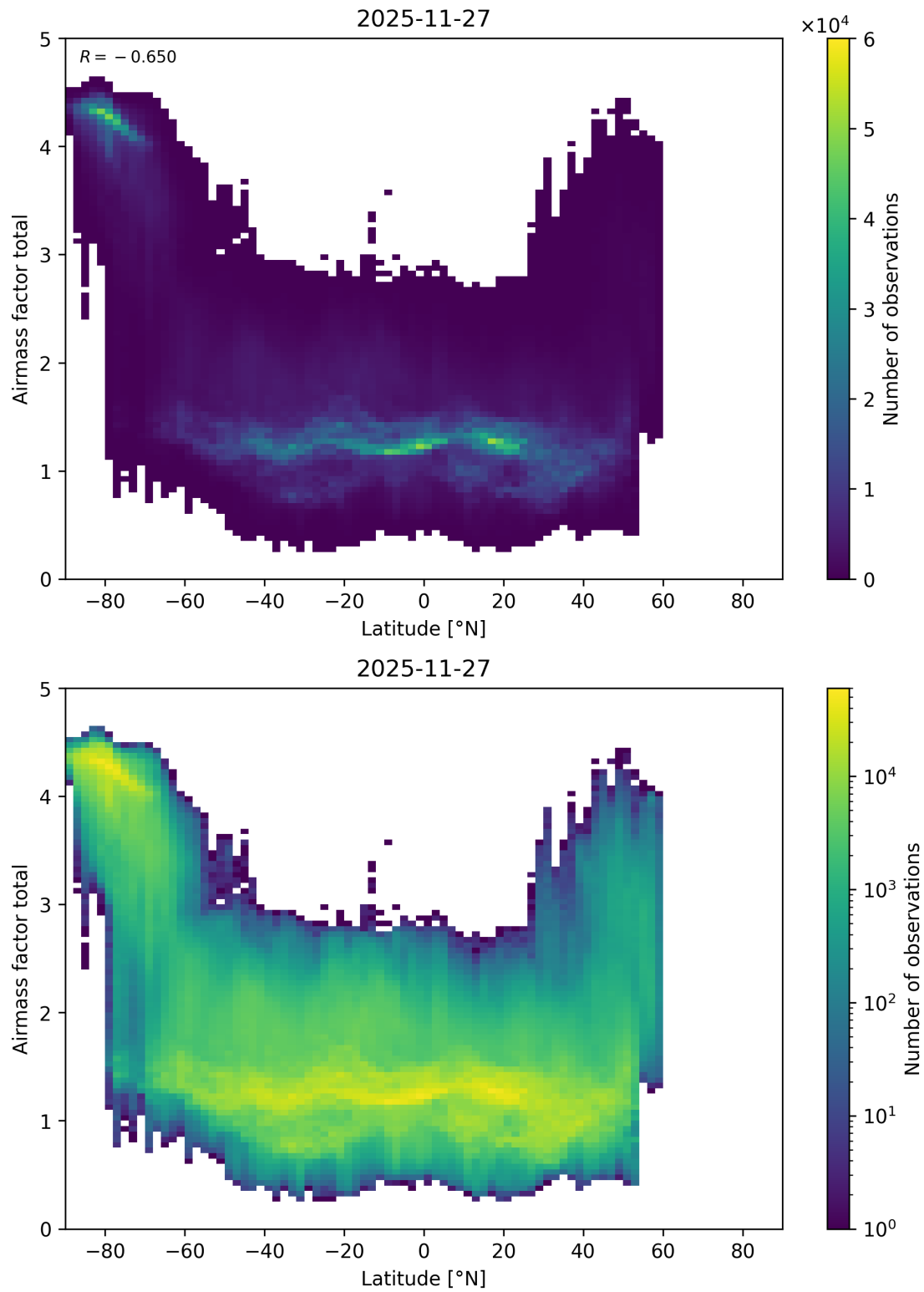
Figure 179: Scatter density plot of “Latitude” against “Airmass factor total” for 2025-11-26 to 2025-11-28.
