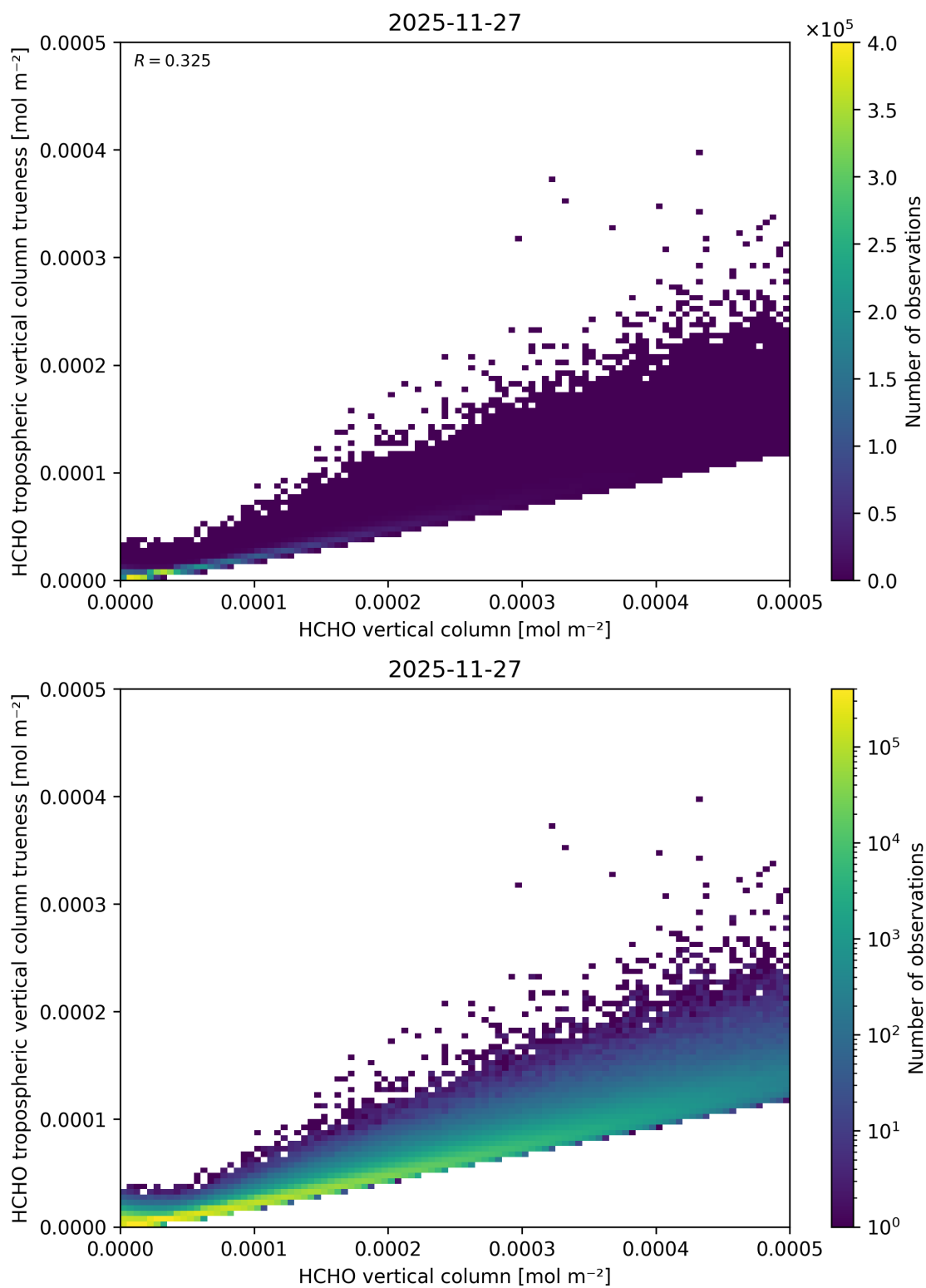
Figure 150: Scatter density plot of “HCHO vertical column” against “HCHO tropospheric vertical column trueness” for 2025-11-26 to 2025-11-28.
