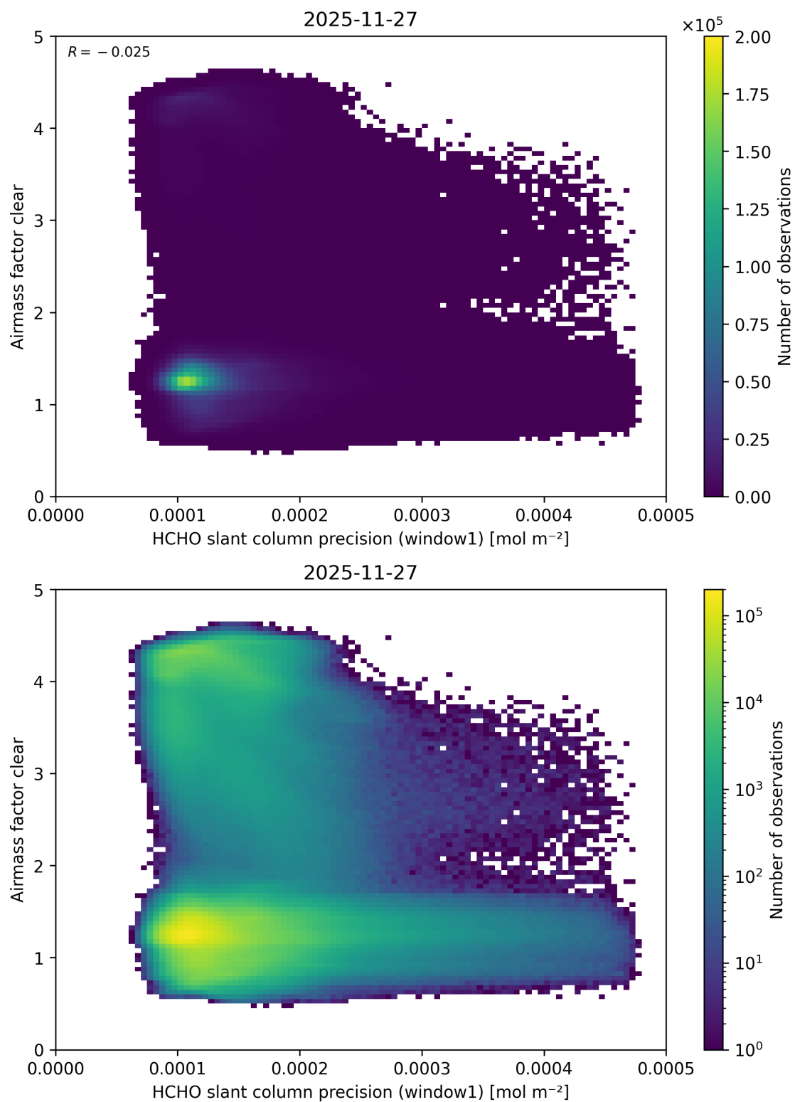
Figure 102: Scatter density plot of “HCHO slant column precision (window1)” against “Airmass factor clear” for 2025-11-26 to 2025-11-28.
