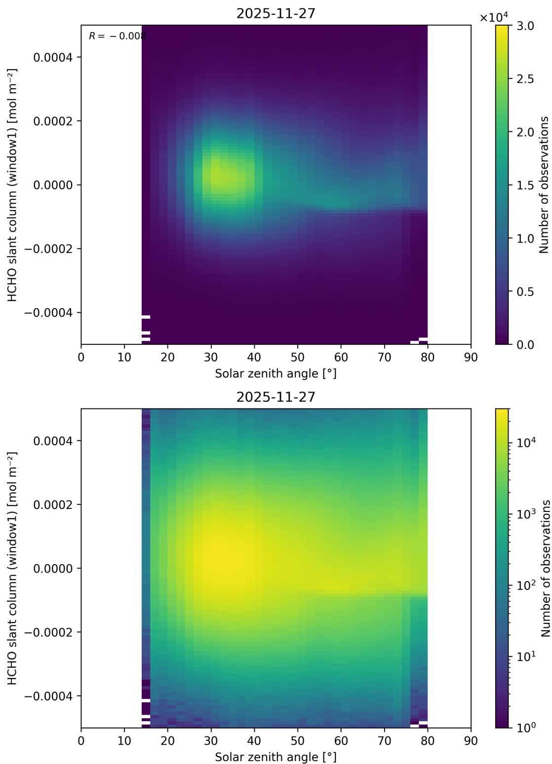
Figure 192: Scatter density plot of “Solar zenith angle” against “HCHO slant column (window1)” for 2025-11-26 to 2025-11-28.
