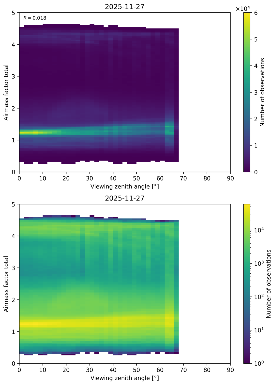
Figure 210: Scatter density plot of “Viewing zenith angle” against “Airmass factor total” for 2025-11-26 to 2025-11-28.
