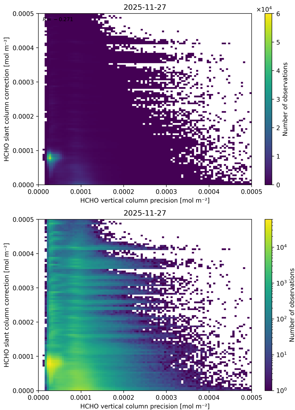
Figure 157: Scatter density plot of “HCHO vertical column precision” against “HCHO slant column correction” for 2025-11-26 to 2025-11-28.
