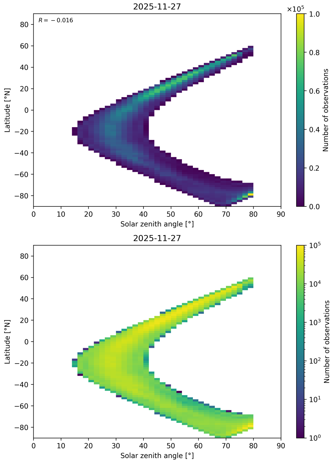
Figure 201: Scatter density plot of “Solar zenith angle” against “Latitude” for 2025-11-26 to 2025-11-28.
