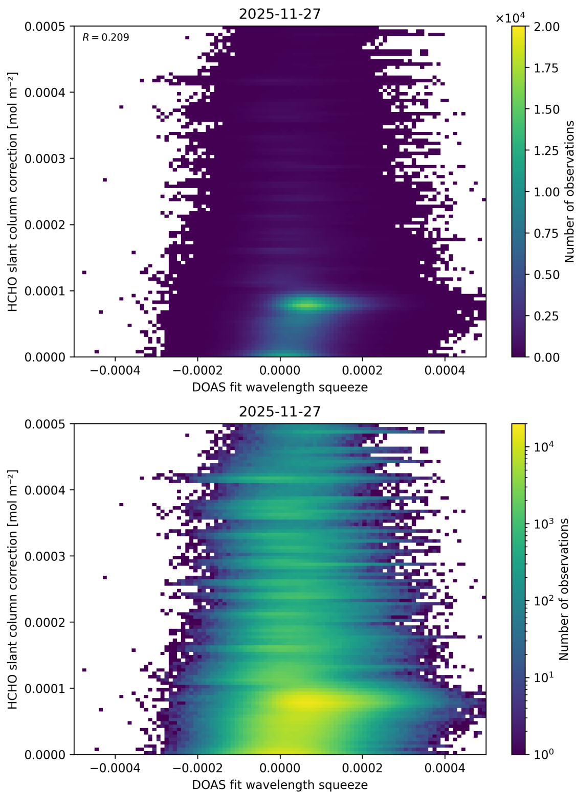
Figure 76: Scatter density plot of “DOAS fit wavelength squeeze” against “HCHO slant column correction” for 2025-11-26 to 2025-11-28.
