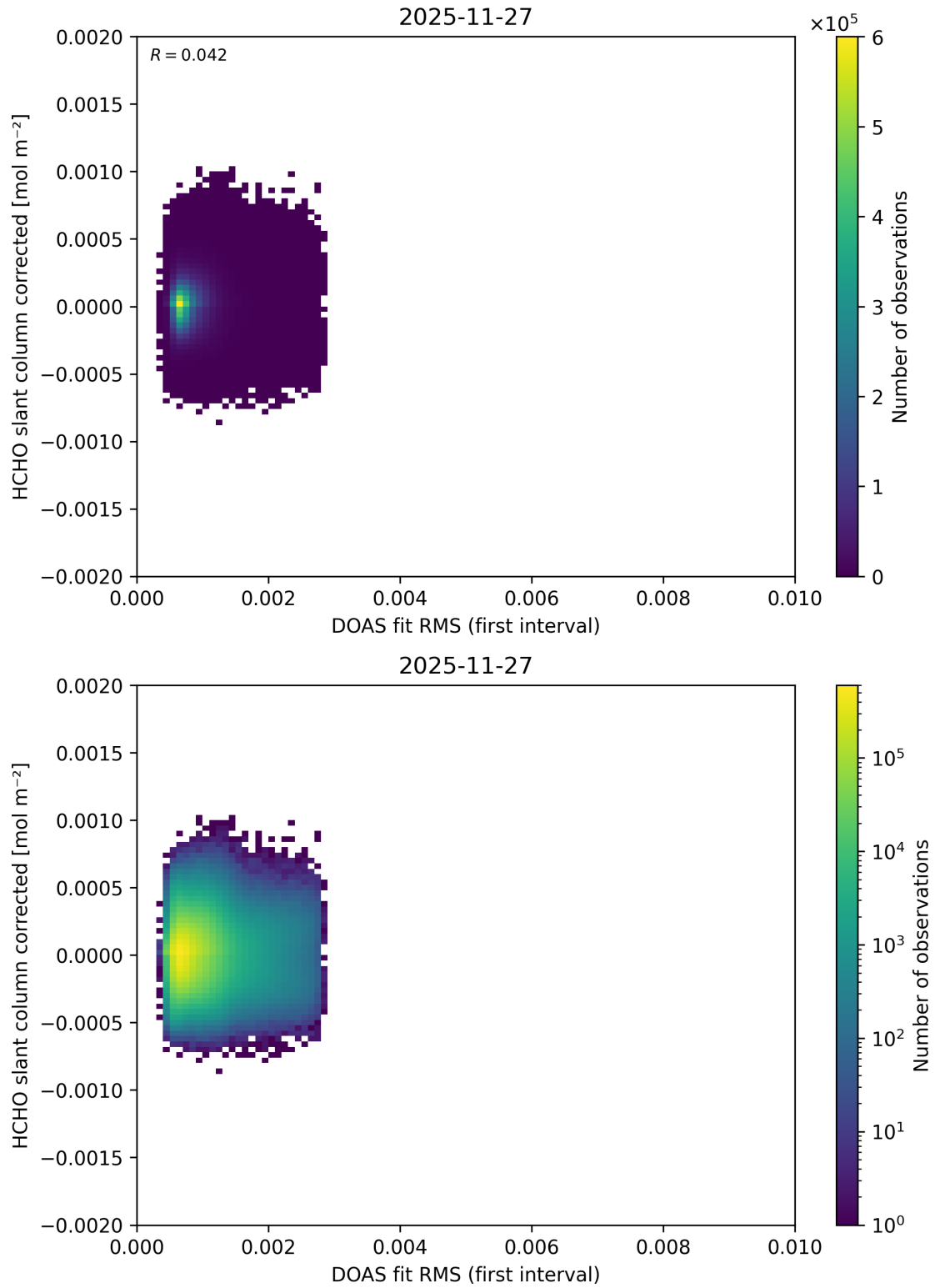
Figure 66: Scatter density plot of “DOAS fit RMS (first interval)” against “HCHO slant column corrected” for 2025-11-26 to 2025-11-28.
