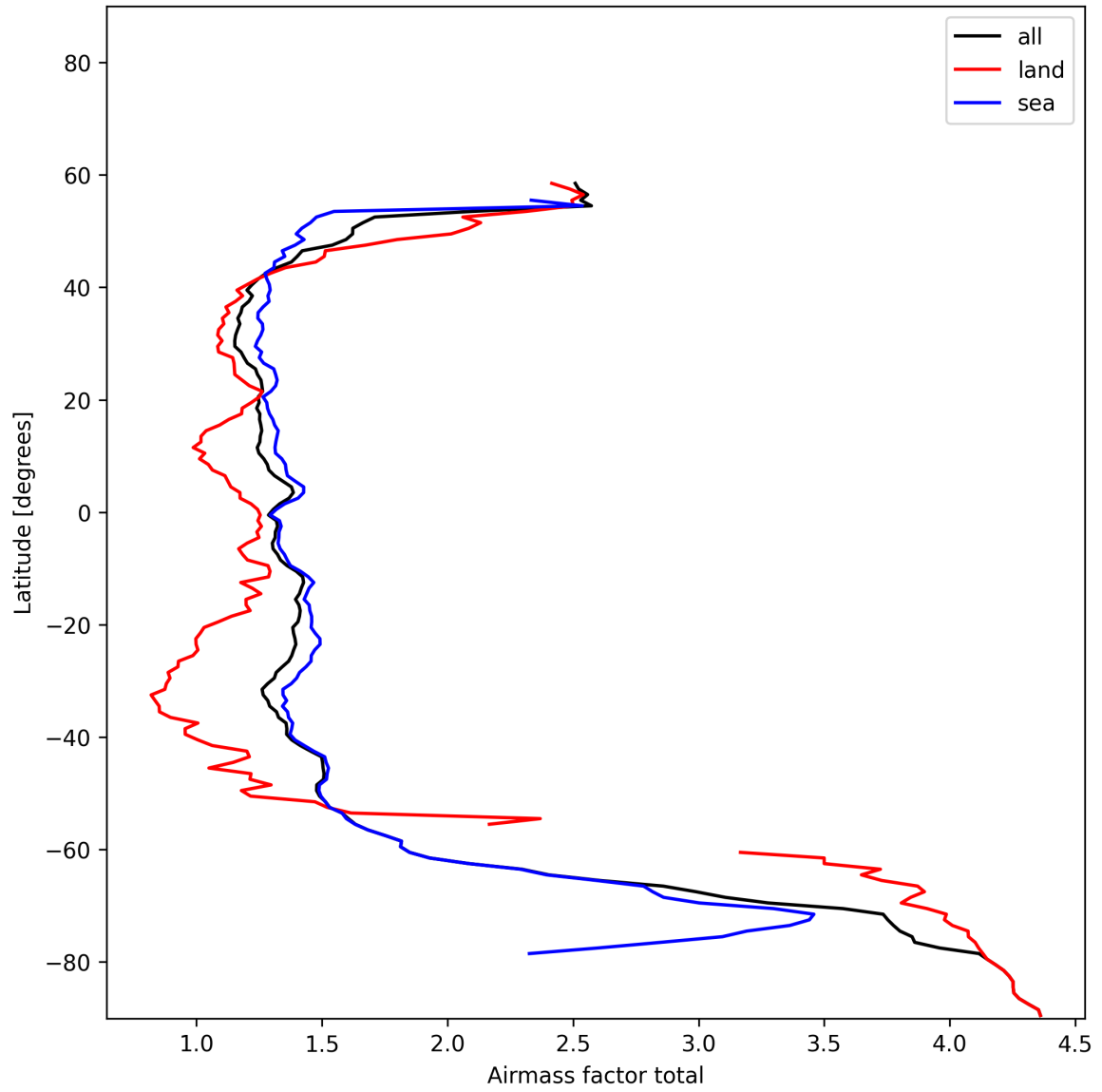
Figure 27: Zonal average of “Airmass factor total” for 2025-11-26 to 2025-11-28.
