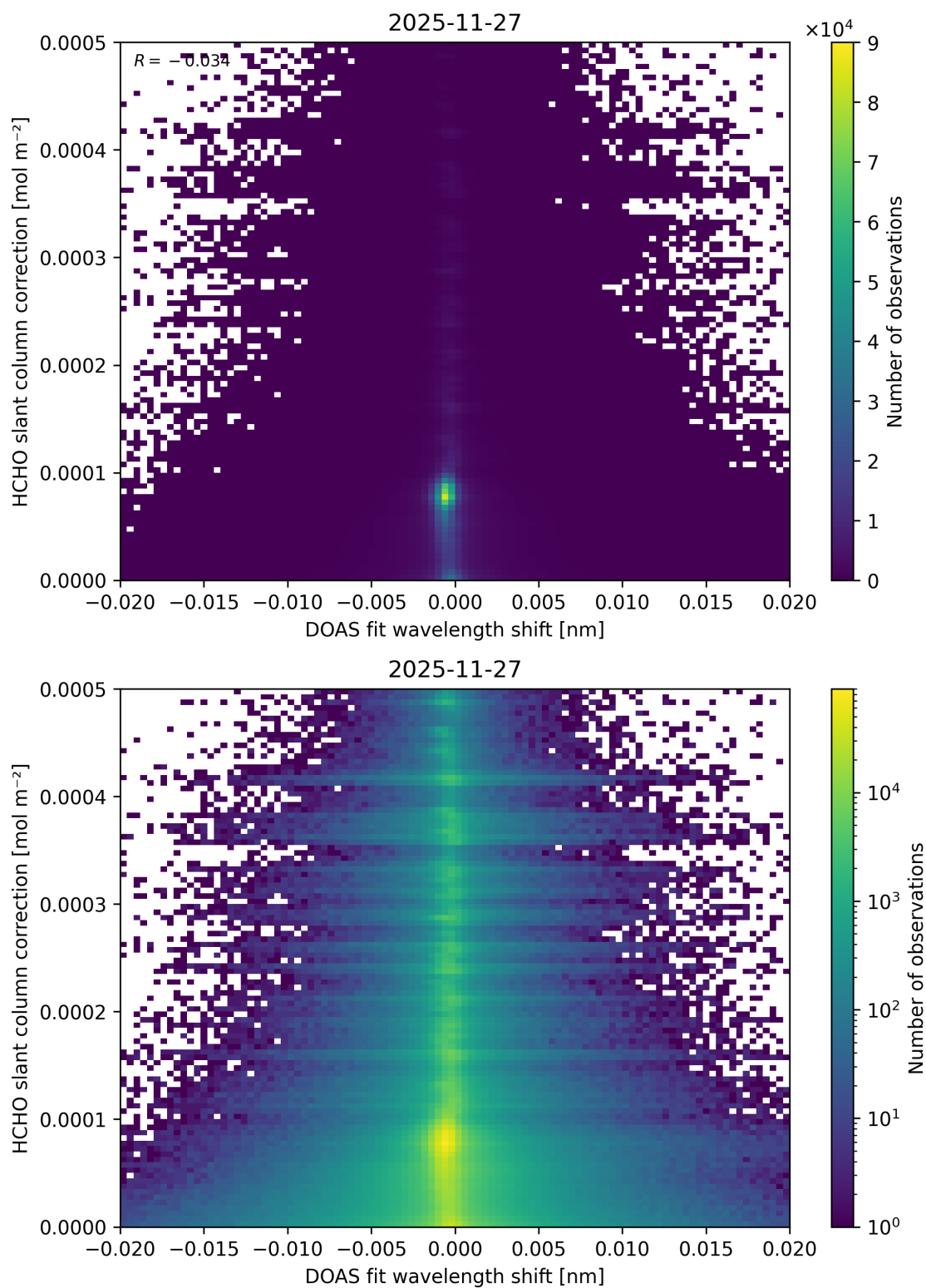
Figure 72: Scatter density plot of “DOAS fit wavelength shift” against “HCHO slant column correction” for 2025-11-26 to 2025-11-28.
