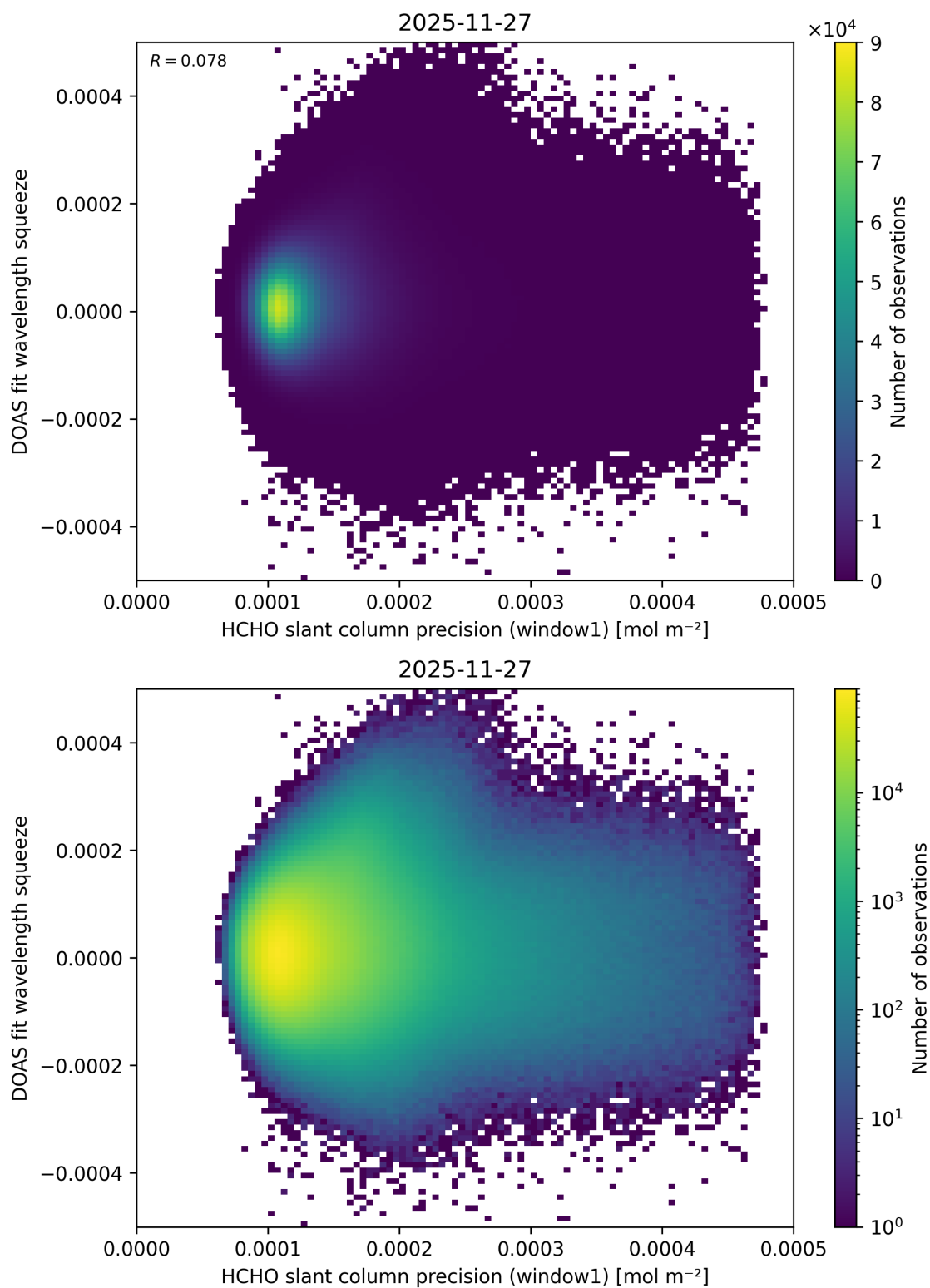
Figure 101: Scatter density plot of “HCHO slant column precision (window1)” against “DOAS fit wavelength squeeze” for 2025-11-26 to 2025-11-28.
