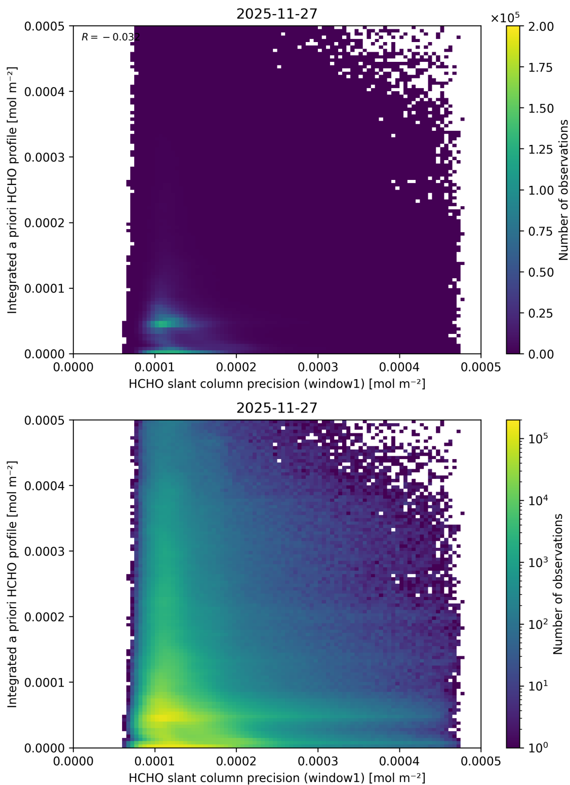
Figure 108: Scatter density plot of “HCHO slant column precision (window1)” against “Integrated a priori HCHO profile” for 2025-11-26 to 2025-11-28.
