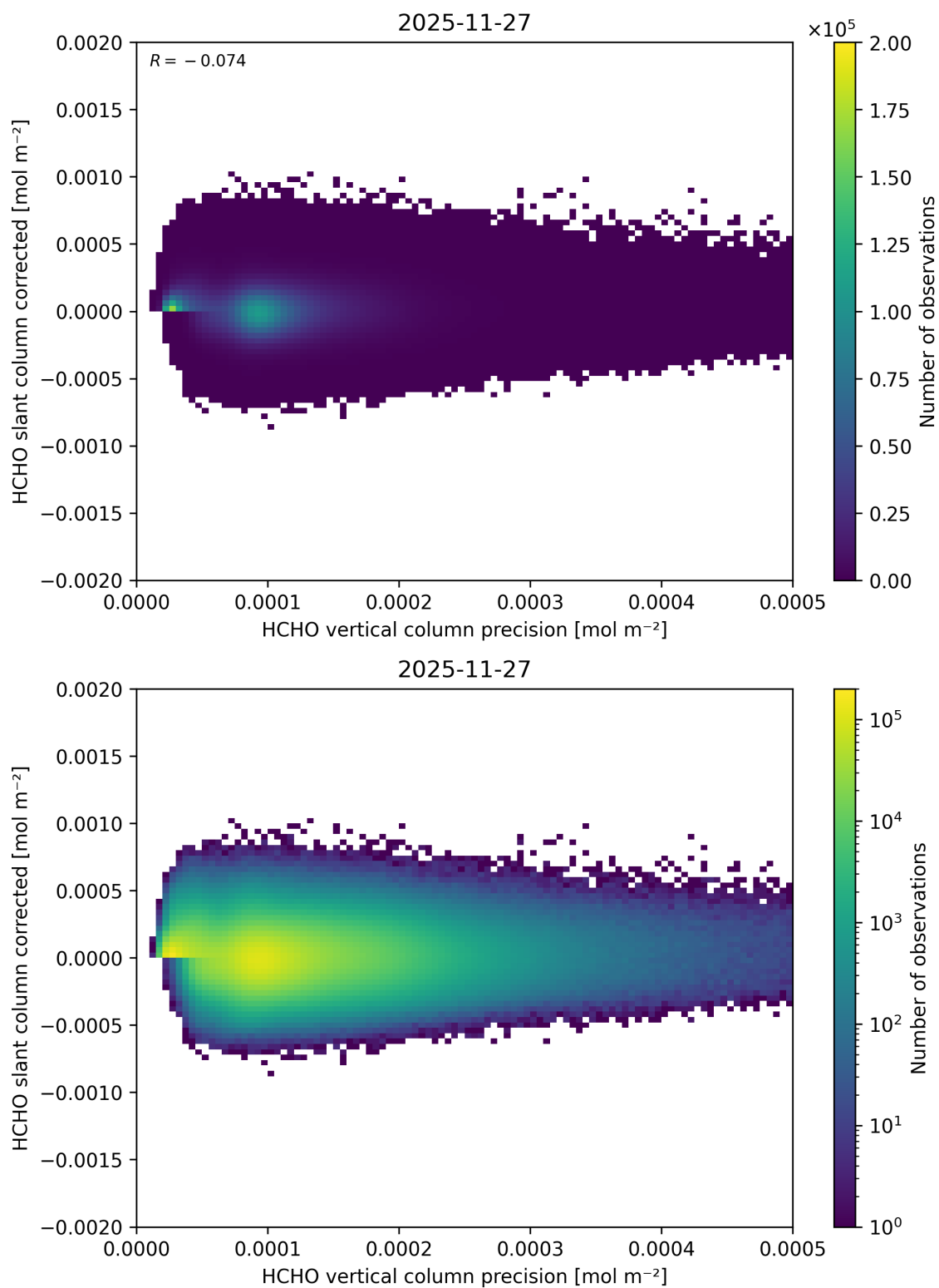
Figure 156: Scatter density plot of “HCHO vertical column precision” against “HCHO slant column corrected” for 2025-11-26 to 2025-11-28.
