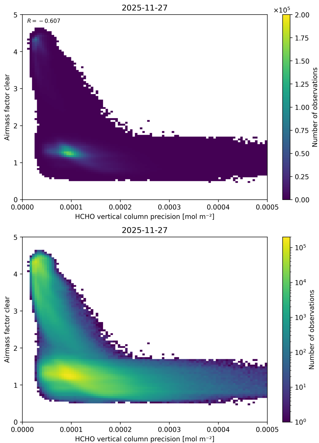
Figure 155: Scatter density plot of “HCHO vertical column precision” against “Airmass factor clear” for 2025-11-26 to 2025-11-28.
