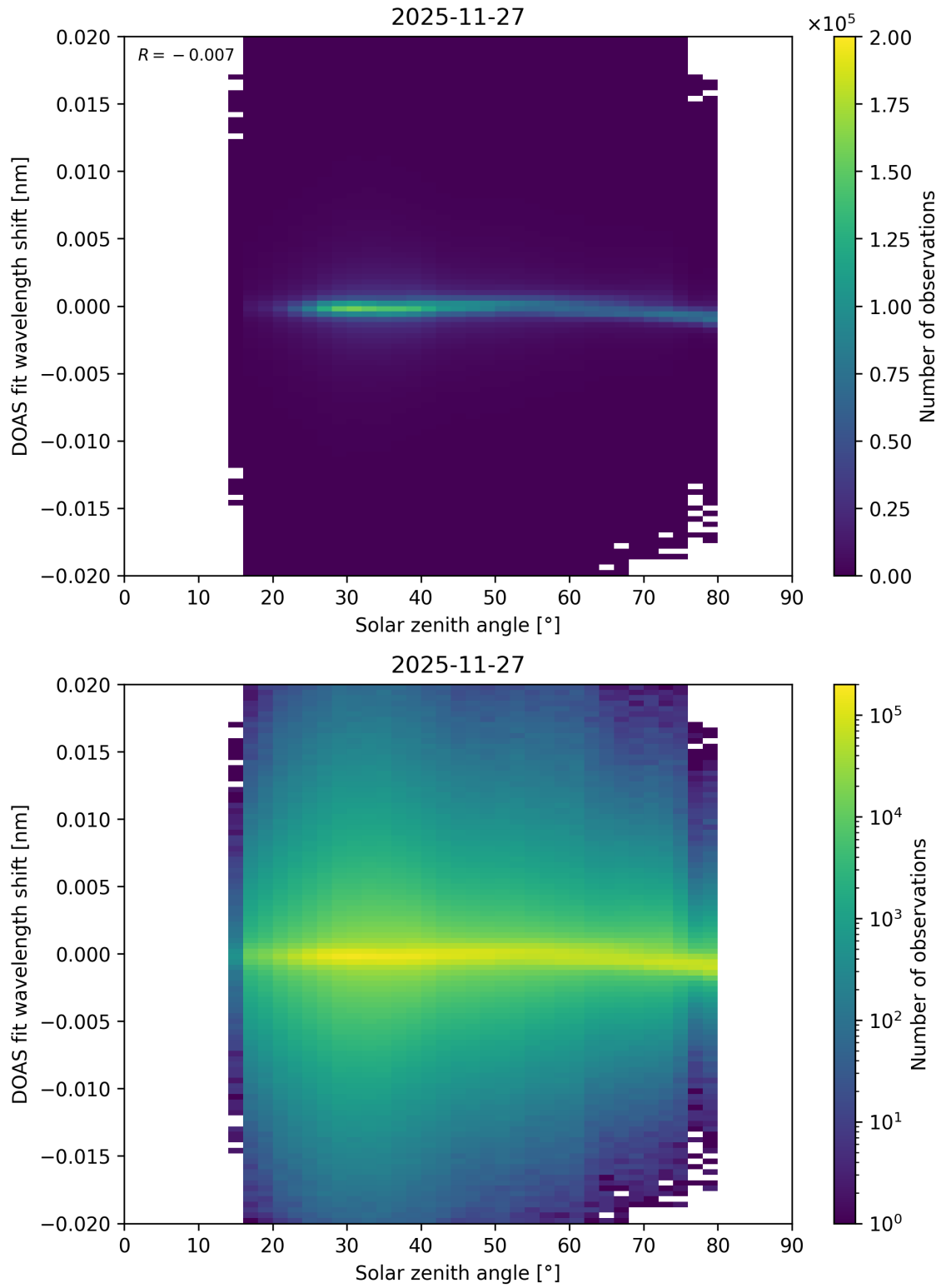
Figure 187: Scatter density plot of “Solar zenith angle” against “DOAS fit wavelength shift” for 2025-11-26 to 2025-11-28.
