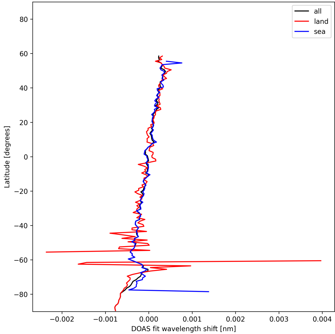
Figure 31: Zonal average of "DOAS fit wavelength shift" for 2025-11-26 to 2025-11-28.
