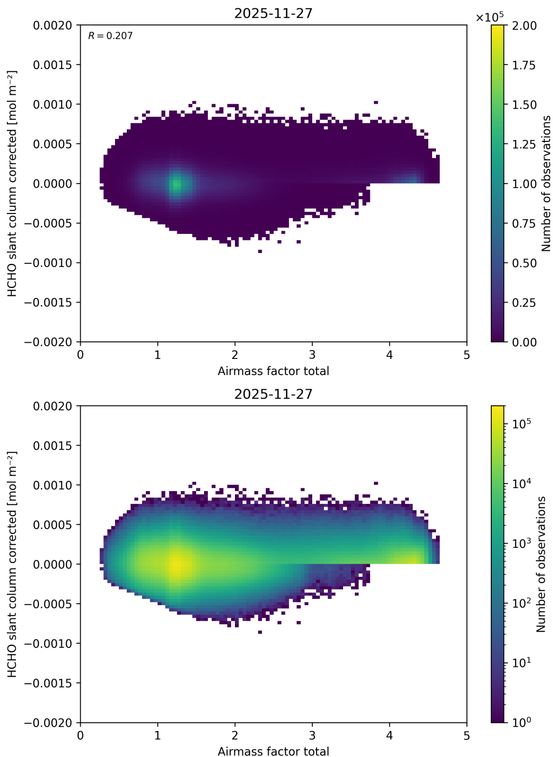
Figure 113: Scatter density plot of “Airmass factor total” against “HCHO slant column corrected” for 2025-11-26 to 2025-11-28.
