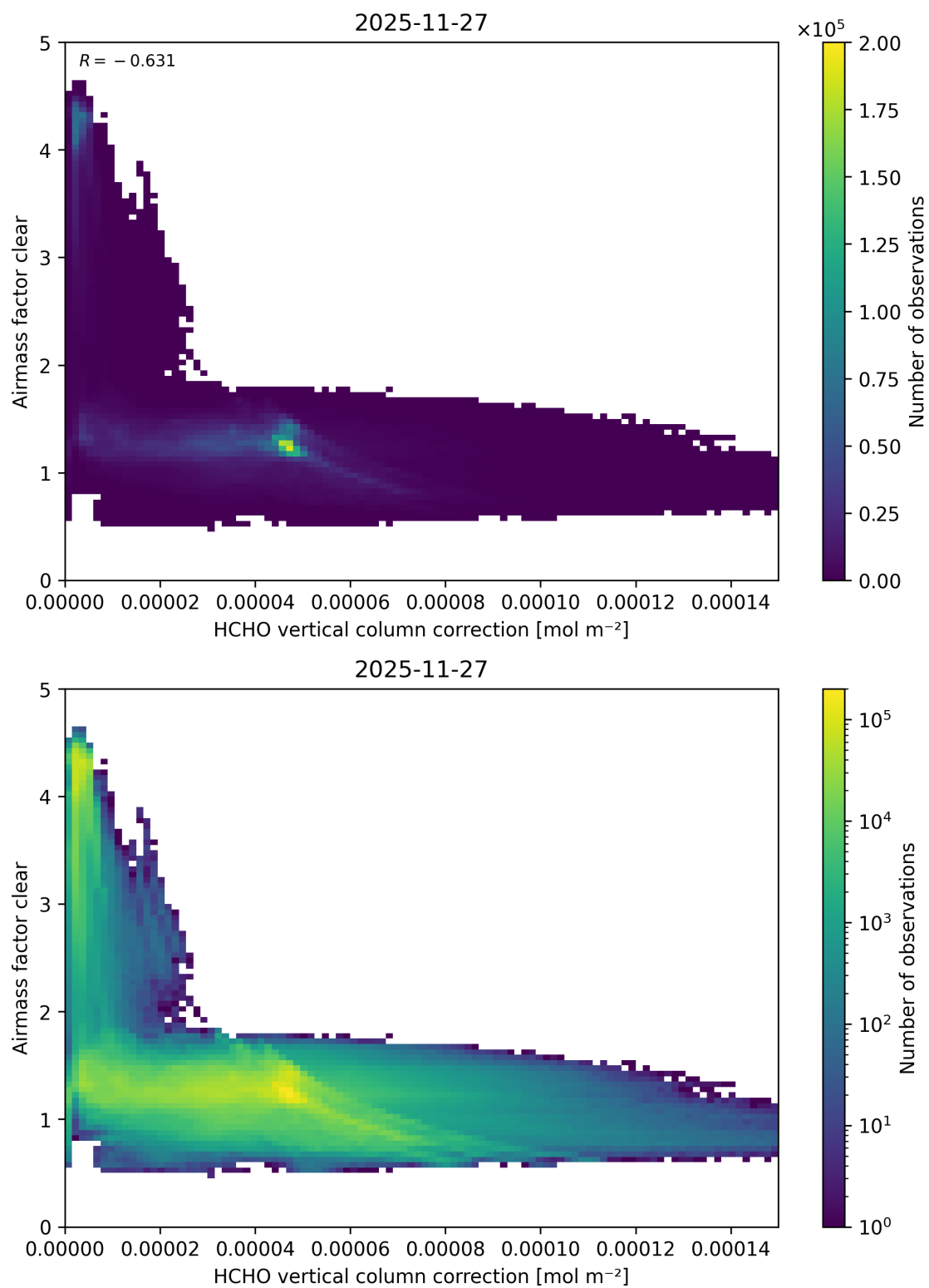
Figure 129: Scatter density plot of “HCHO vertical column correction” against “Airmass factor clear” for 2025-11-26 to 2025-11-28.
