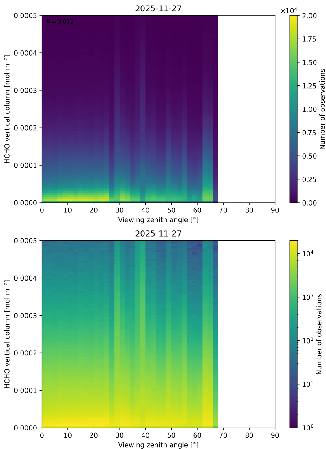
Figure 212: Scatter density plot of “Viewing zenith angle” against “HCHO vertical column” for 2025-11-26 to 2025-11-28.
