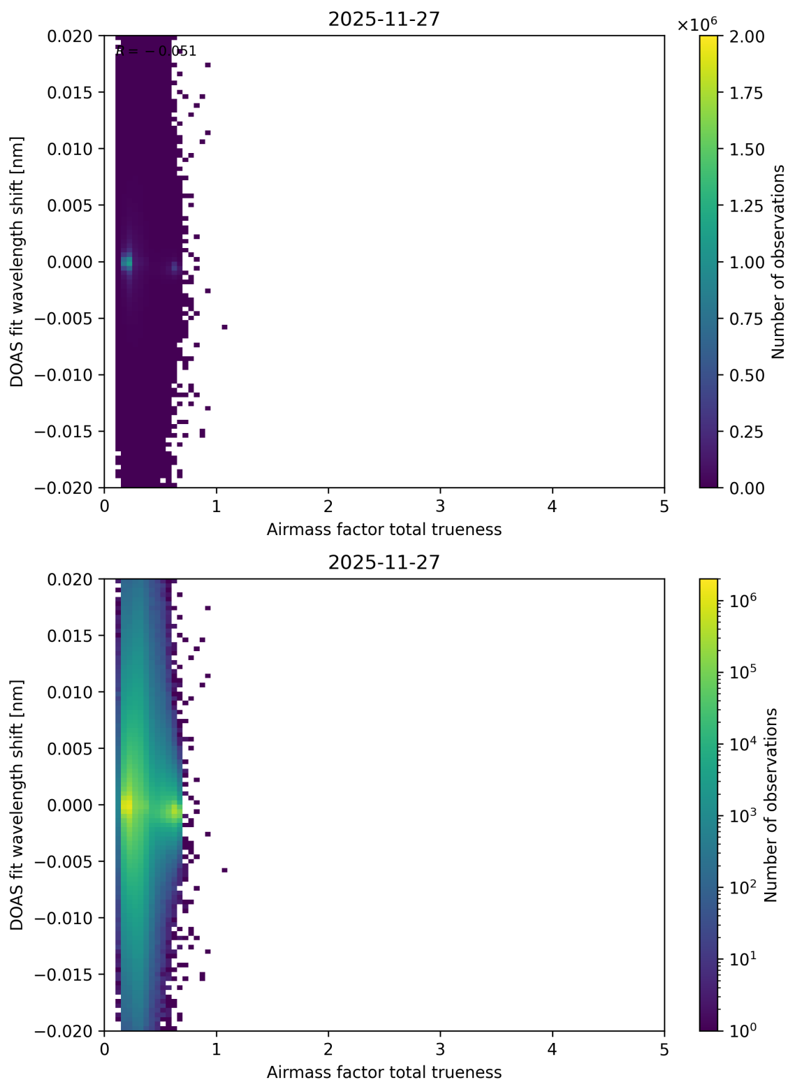
Figure 119: Scatter density plot of “Airmass factor total trueness” against “DOAS fit wavelength shift” for 2025-11-26 to 2025-11-28.
