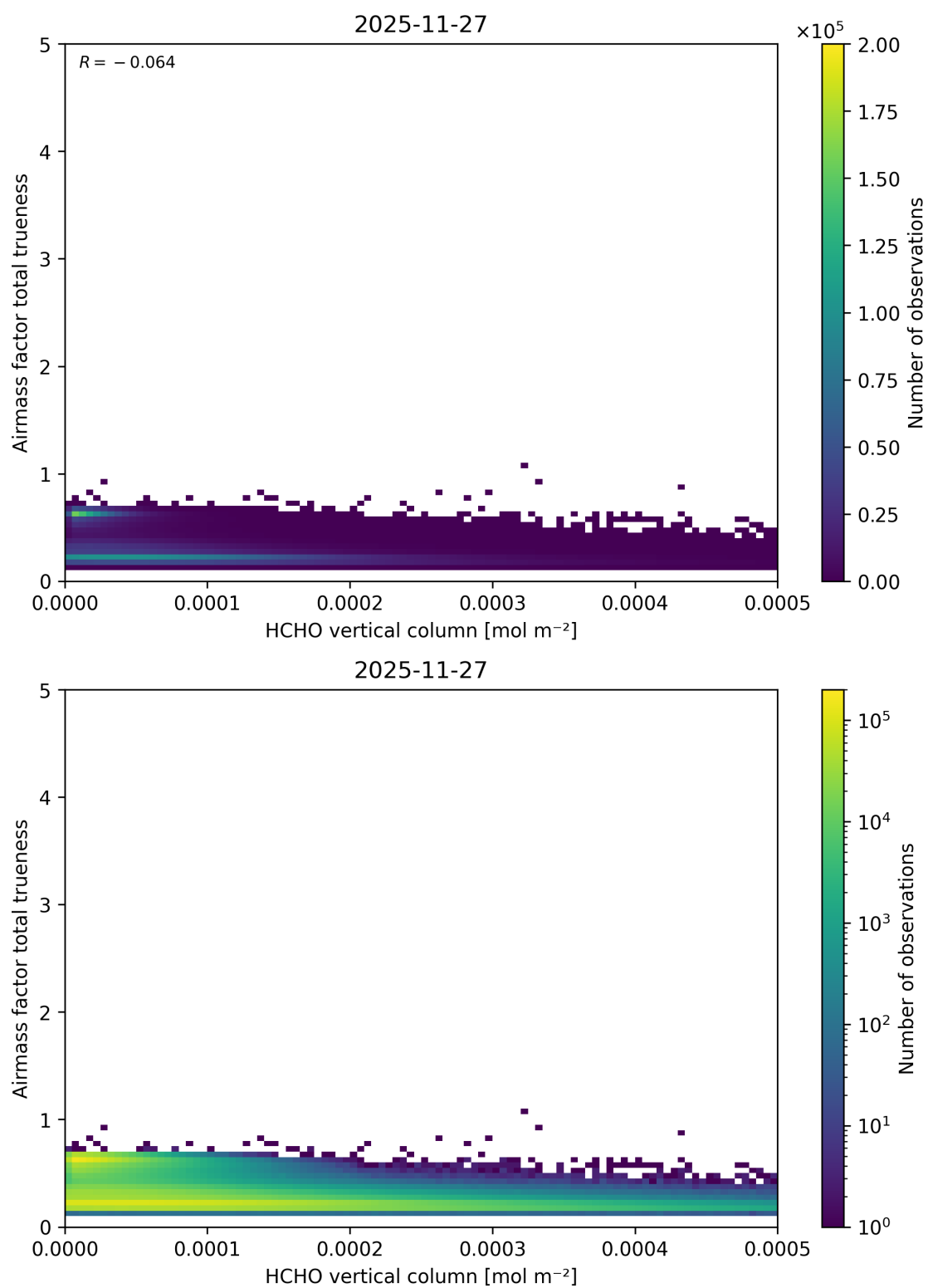
Figure 147: Scatter density plot of “HCHO vertical column” against “Airmass factor total trueneess” for 2025-11-26 to 2025-11-28.
