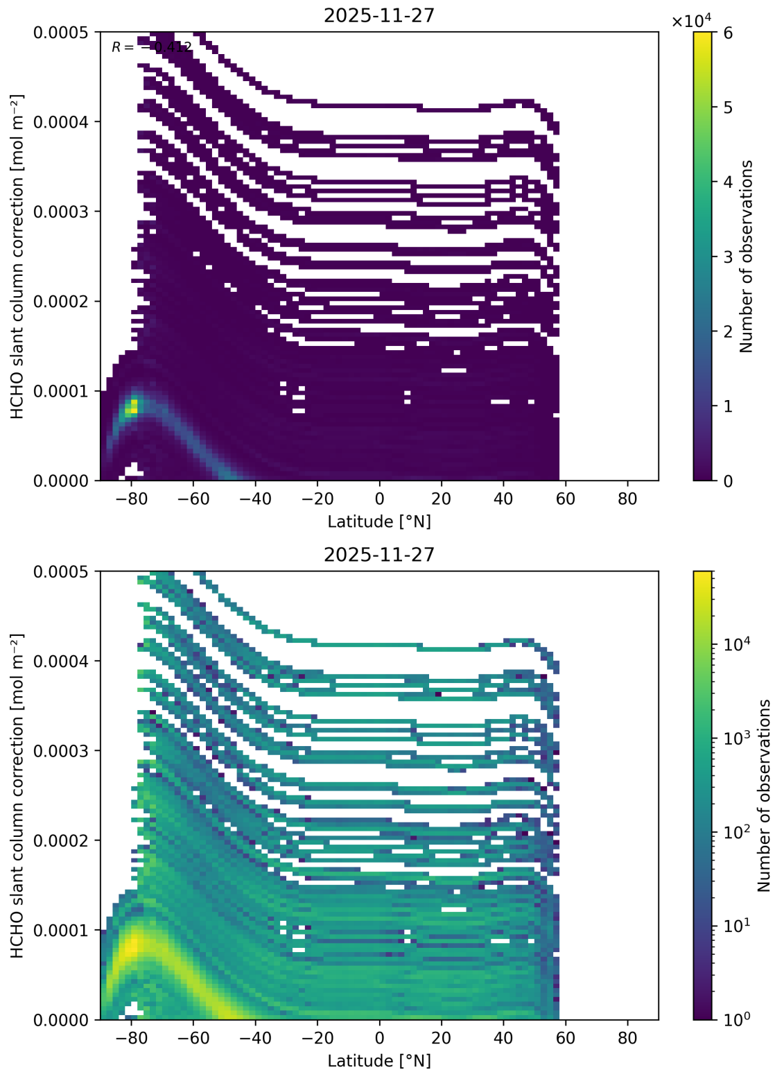
Figure 176: Scatter density plot of “Latitude” against “HCHO slant column correction” for 2025-11-26 to 2025-11-28.
