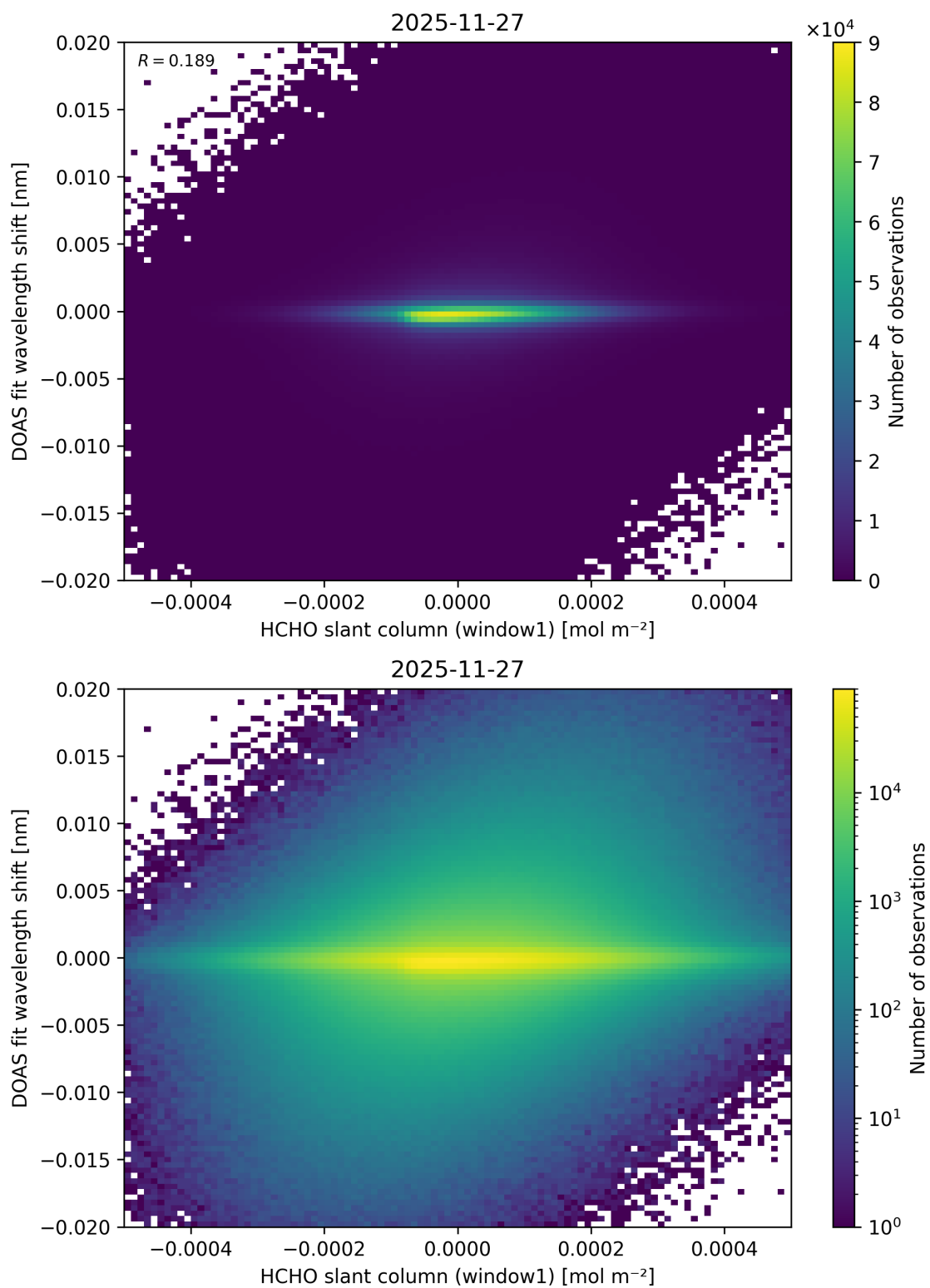
Figure 89: Scatter density plot of “HCHO slant column (window1)” against “DOAS fit wavelength shift” for 2025-11-26 to 2025-11-28.
