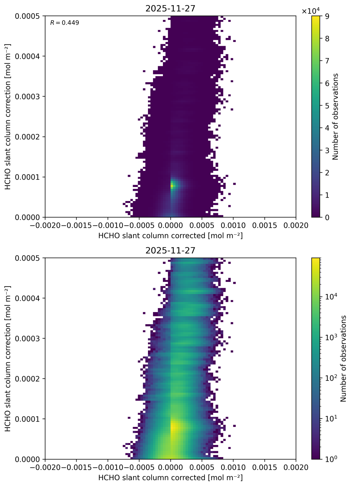
Figure 85: Scatter density plot of “HCHO slant column corrected” against “HCHO slant column correction” for 2025-11-26 to 2025-11-28.
