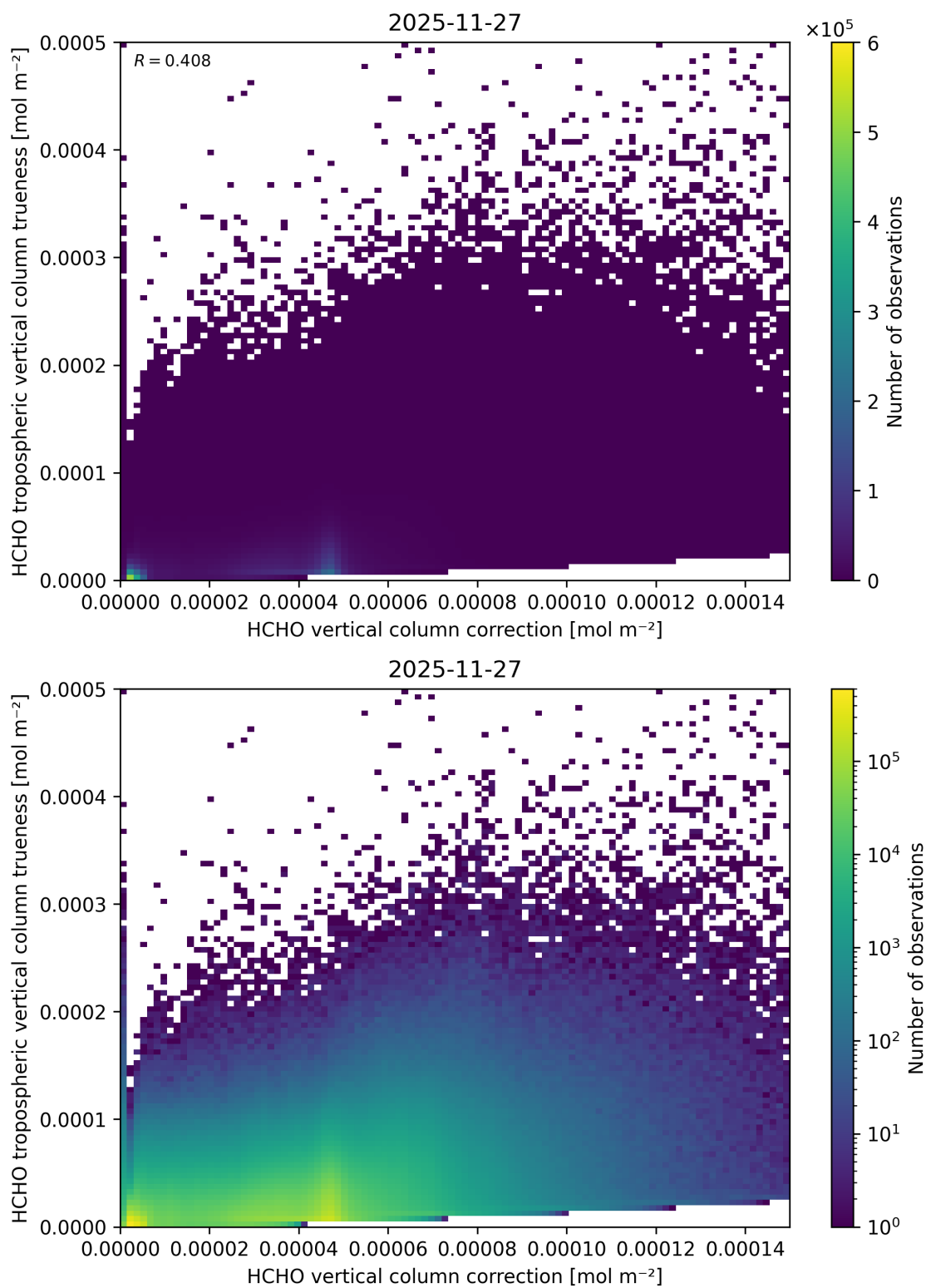
Figure 136: Scatter density plot of “HCHO vertical column correction” against “HCHO tropospheric vertical column true-ness” for 2025-11-26 to 2025-11-28.
