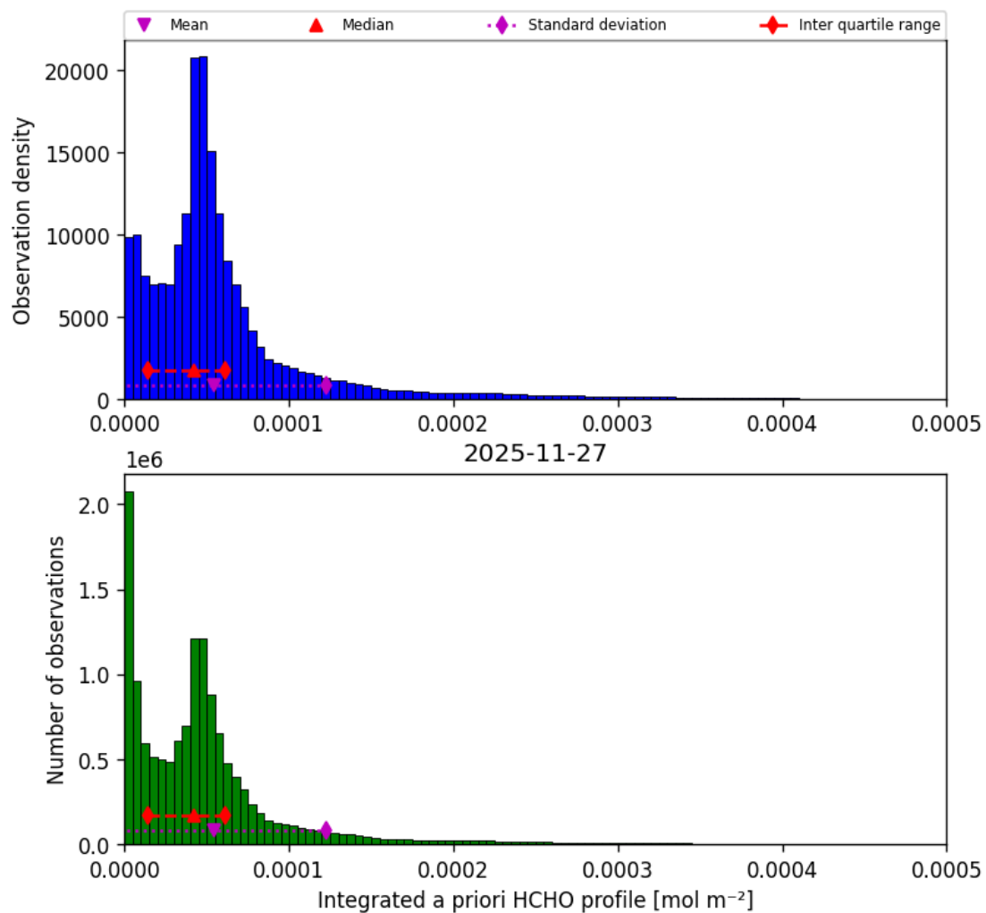
Figure 45: Histogram of “Integrated a priori HCHO profile” for 2025-11-26 to 2025-11-28
