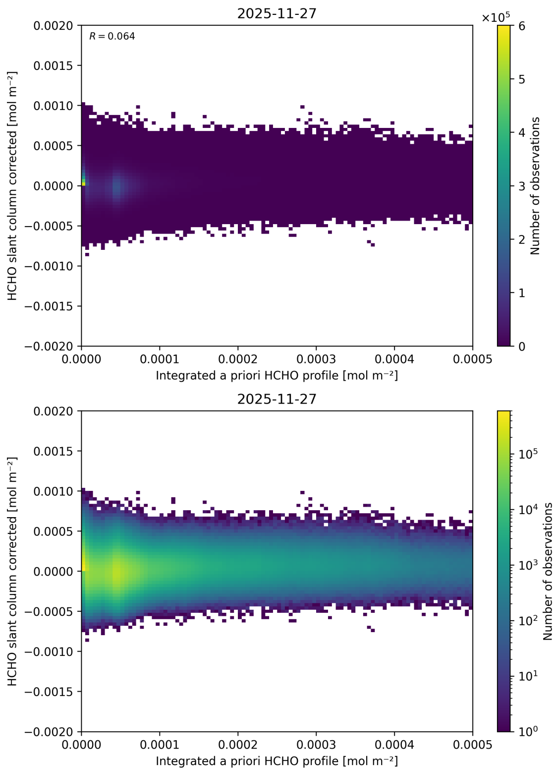
Figure 168: Scatter density plot of “Integrated a priori HCHO profile” against “HCHO slant column corrected” for 2025-11-26 to 2025-11-28.
