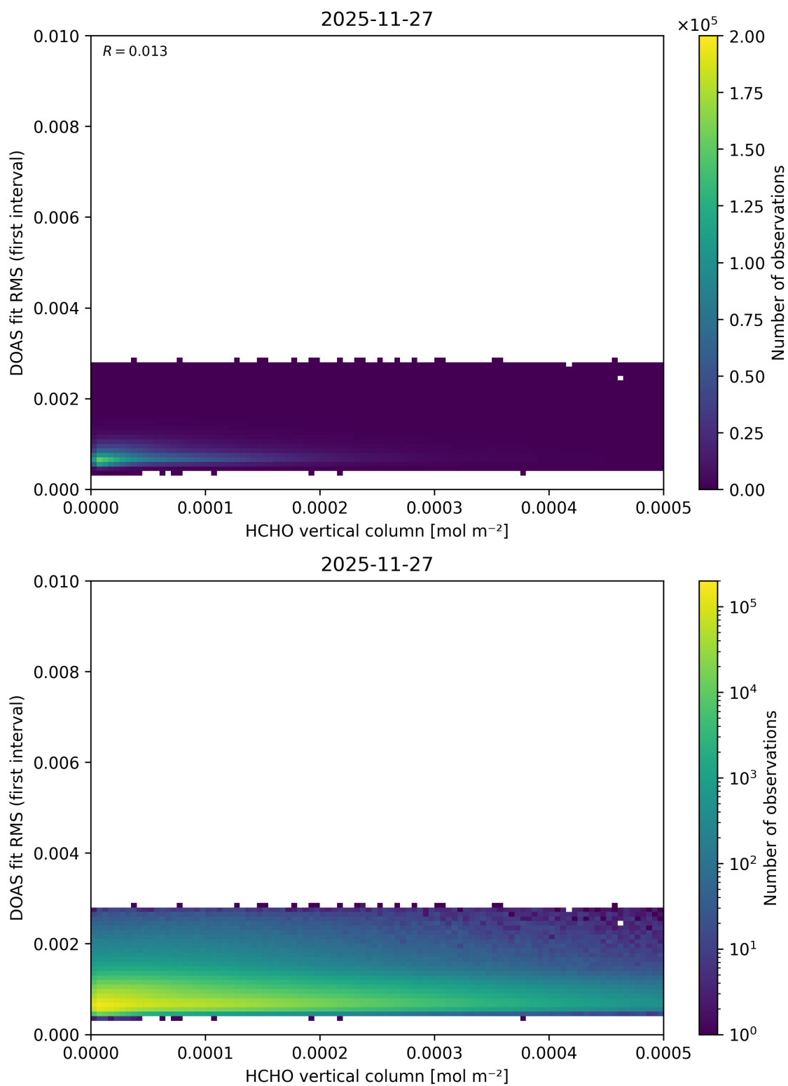
Figure 138: Scatter density plot of “HCHO vertical column” against “DOAS fit RMS (first interval)” for 2025-11-26 to 2025-11-28.
