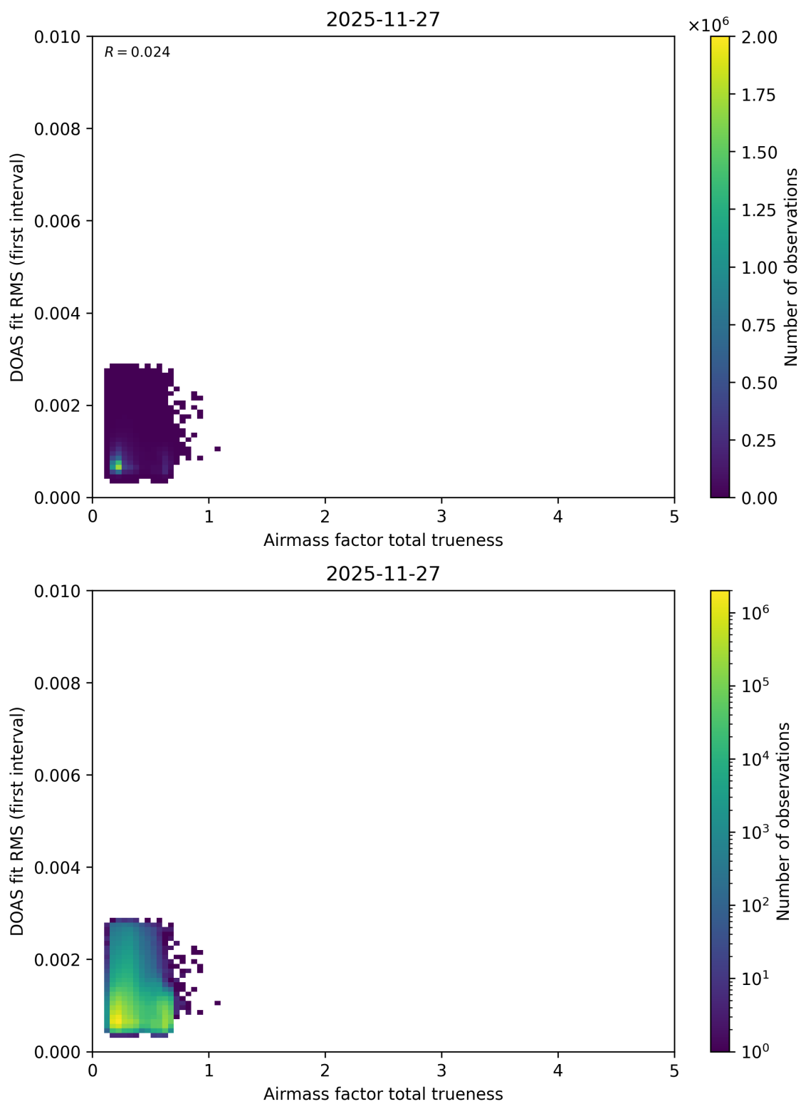
Figure 118: Scatter density plot of “Airmass factor total trueness” against “DOAS fit RMS (first interval)” for 2025-11-26 to 2025-11-28.
