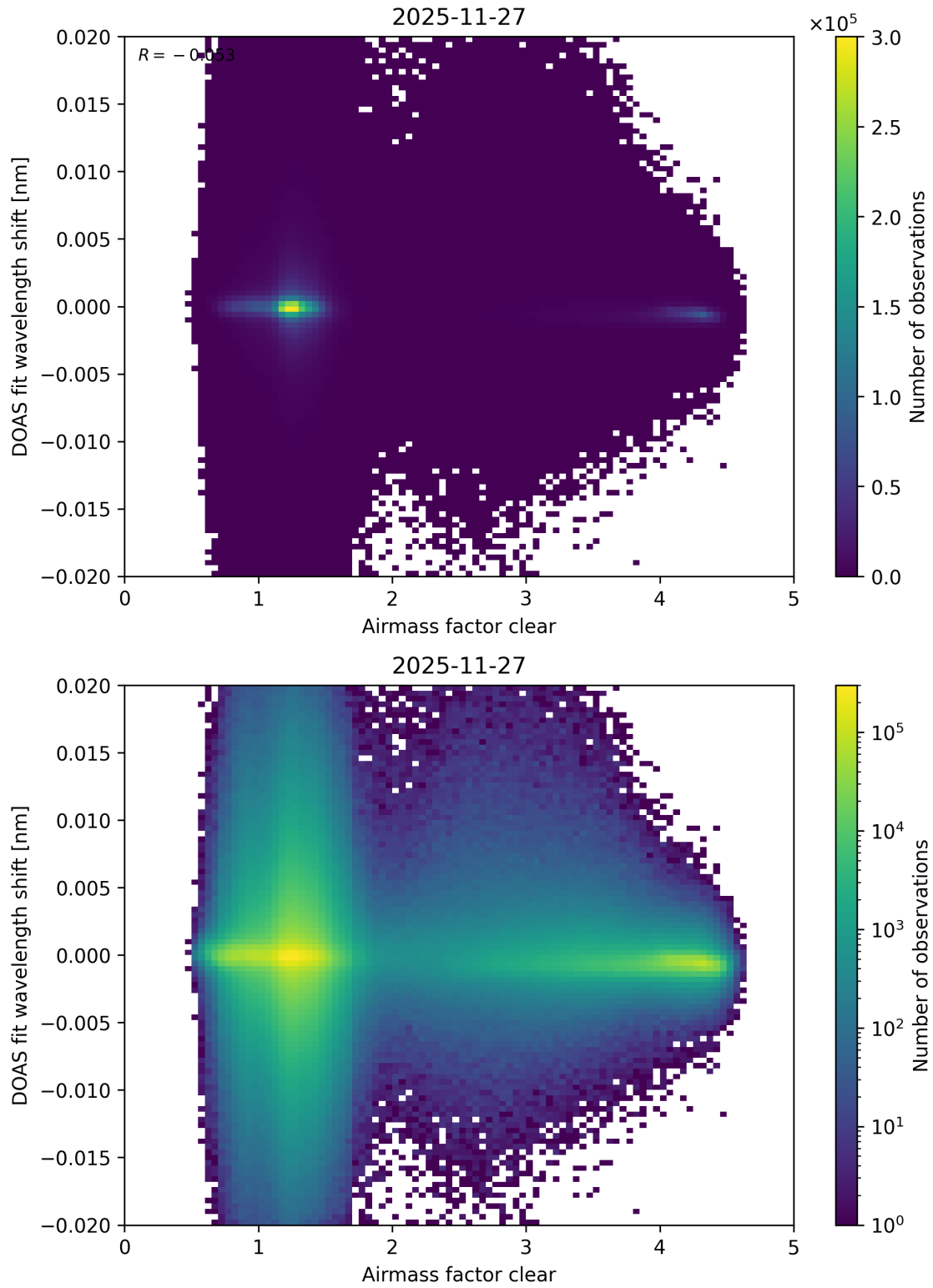
Figure 79: Scatter density plot of “Airmass factor clear” against “DOAS fit wavelength shift” for 2025-11-26 to 2025-11-28.
