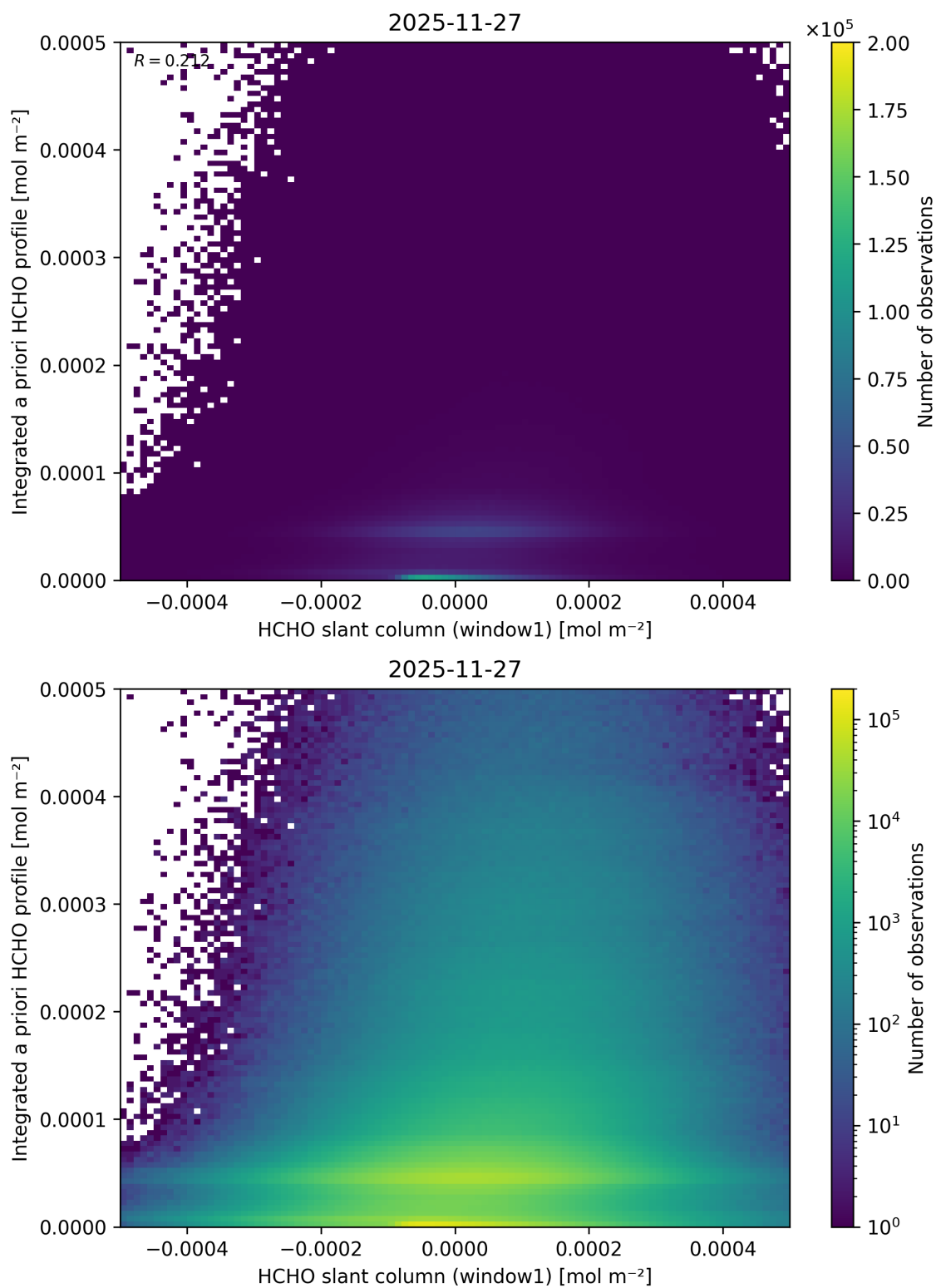
Figure 98: Scatter density plot of “HCHO slant column (window1)” against “Integrated a priori HCHO profile” for 2025-11-26 to 2025-11-28.
