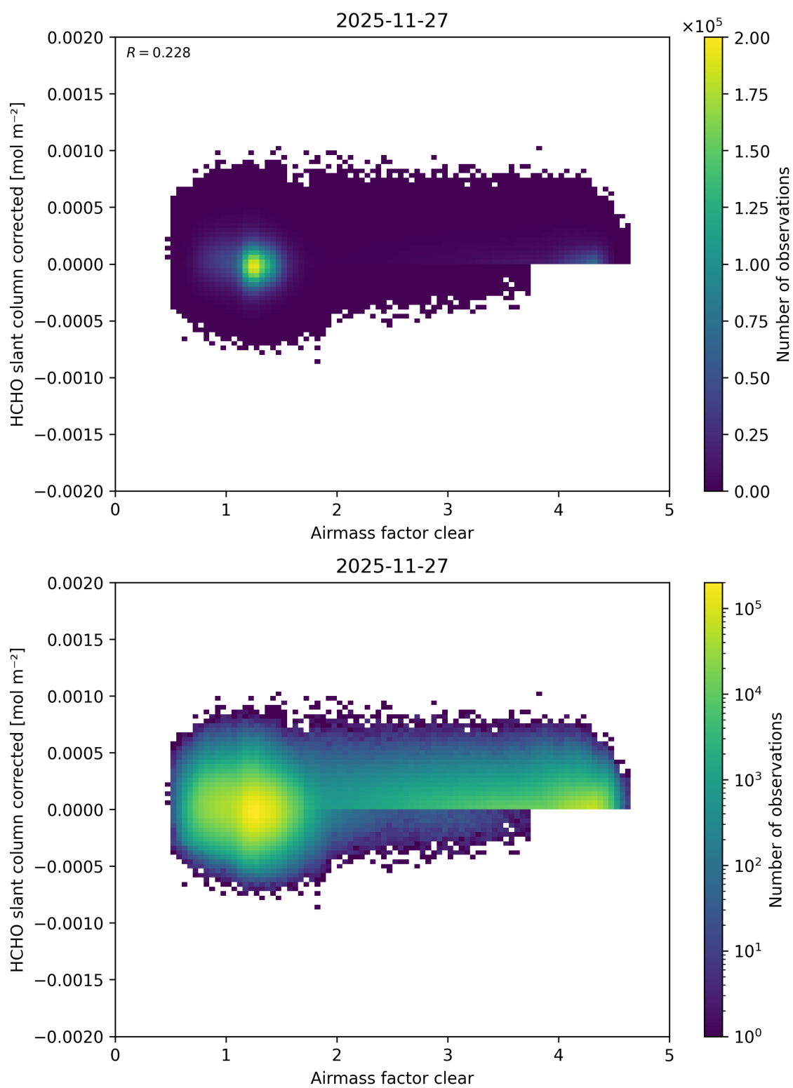
Figure 81: Scatter density plot of “Airmass factor clear” against “HCHO slant column corrected” for 2025-11-26 to 2025-11-28.
