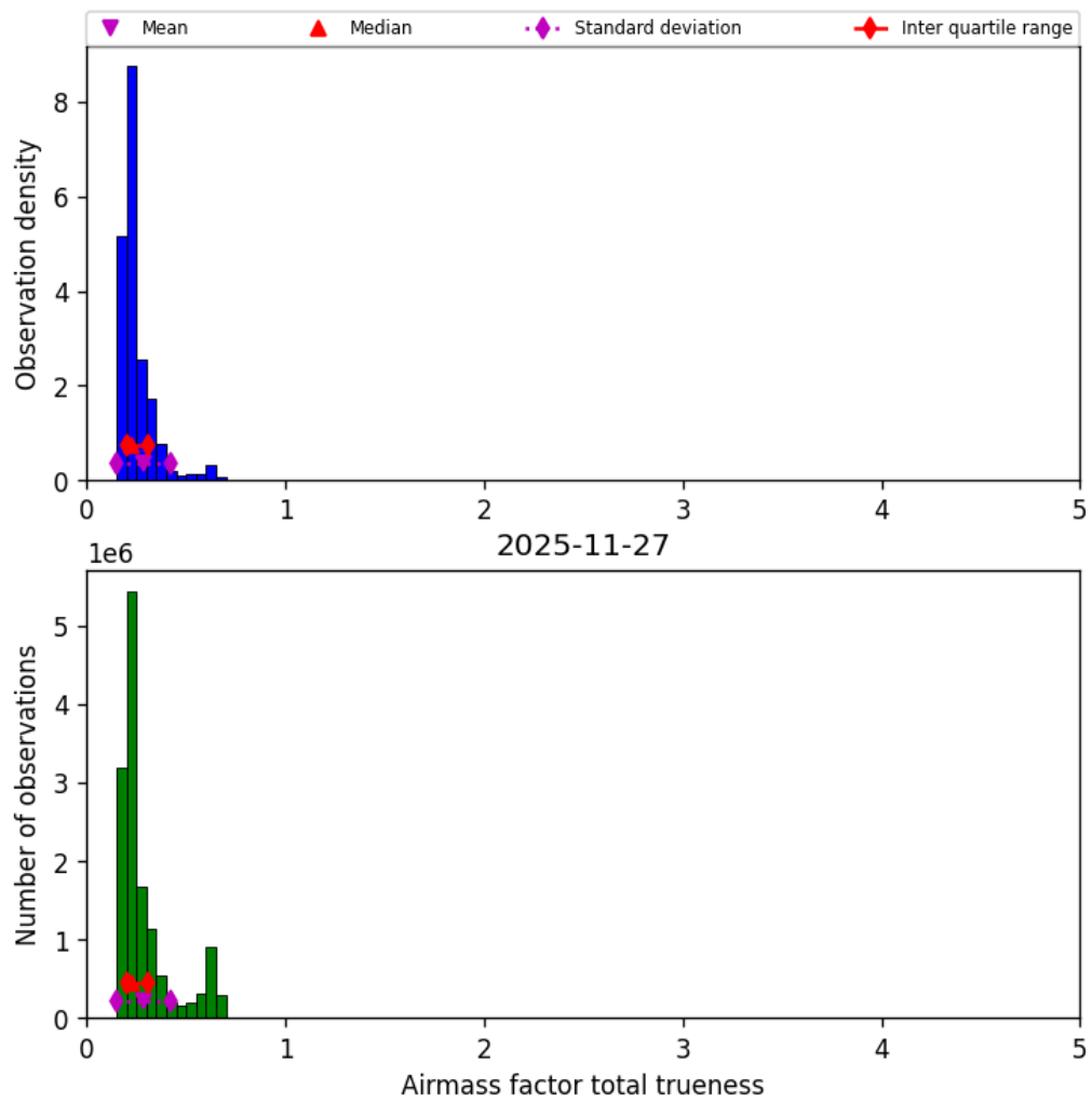
Figure 43: Histogram of “Airmass factor total trueness” for 2025-11-26 to 2025-11-28
