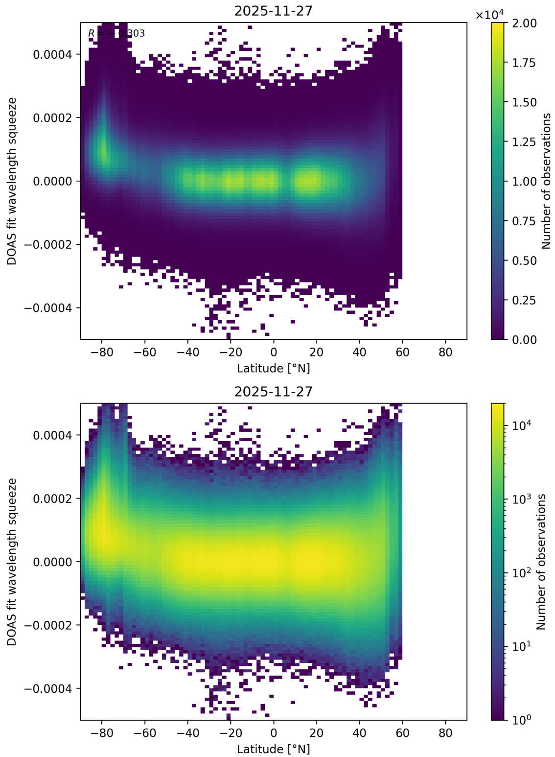
Figure 173: Scatter density plot of “Latitude” against “DOAS fit wavelength squeeze” for 2025-11-26 to 2025-11-28.
