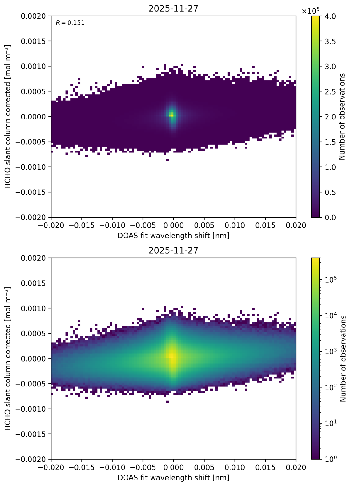
Figure 71: Scatter density plot of “DOAS fit wavelength shift” against “HCHO slant column corrected” for 2025-11-26 to 2025-11-28.
