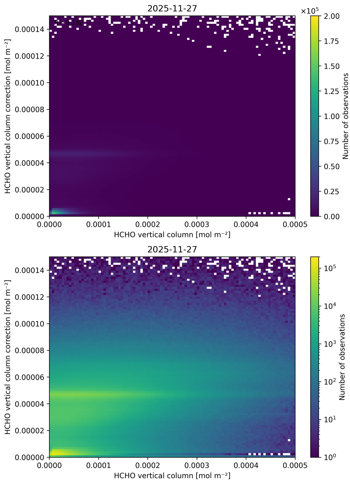
Figure 148: Scatter density plot of “HCHO vertical column” against “HCHO vertical column correction” for 2025-11-26 to 2025-11-28.
