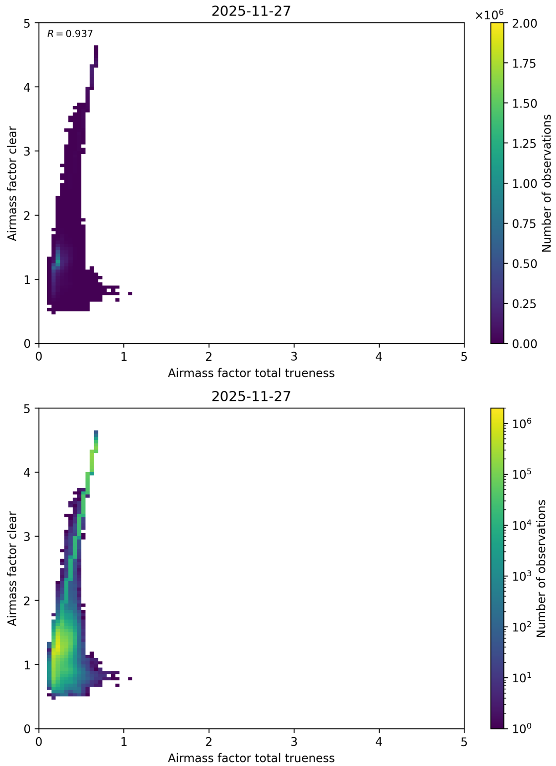
Figure 121: Scatter density plot of “Airmass factor total trueness” against “Airmass factor clear” for 2025-11-26 to 2025-11-28.
