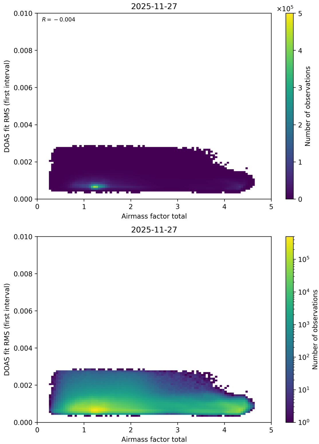
Figure 109: Scatter density plot of “Airmass factor total” against “DOAS fit RMS (first interval)” for 2025-11-26 to 2025-11-28.
