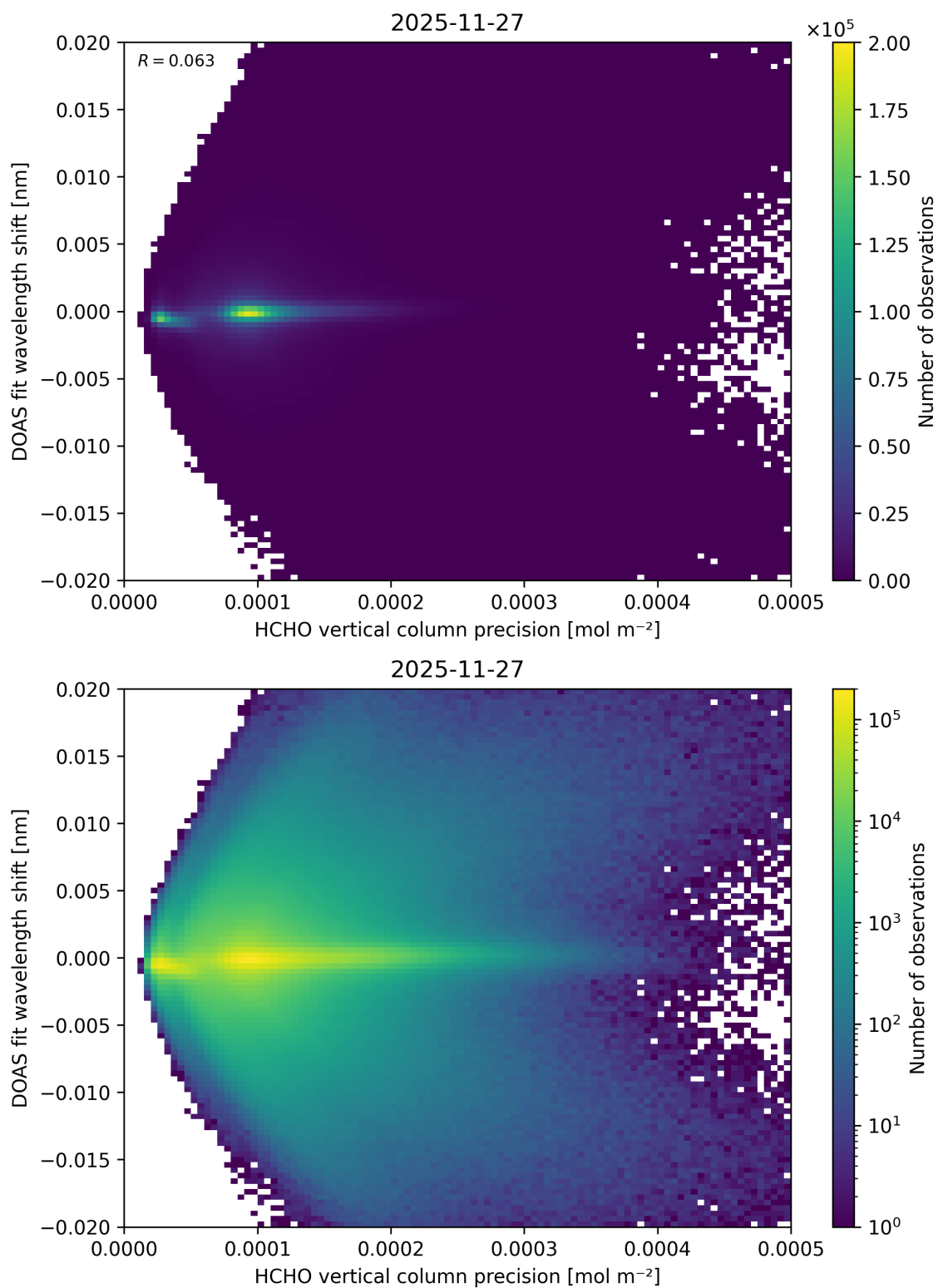
Figure 153: Scatter density plot of “HCHO vertical column precision” against “DOAS fit wavelength shift” for 2025-11-26 to 2025-11-28.
