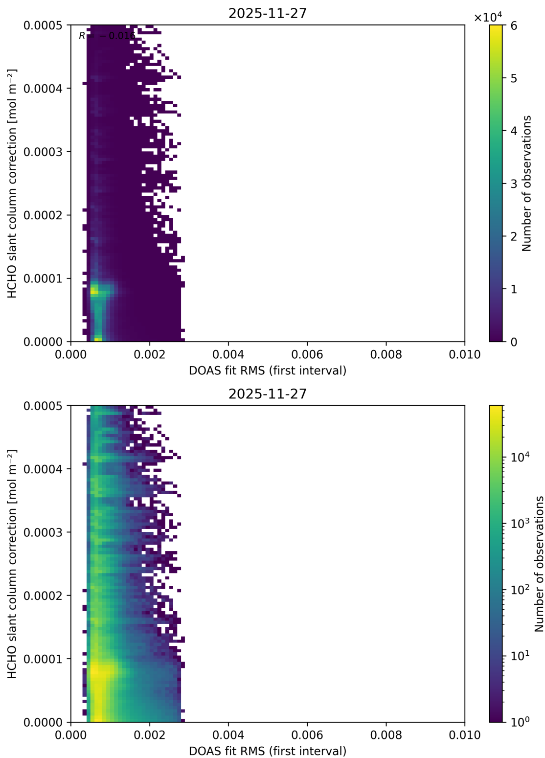
Figure 67: Scatter density plot of “DOAS fit RMS (first interval)” against “HCHO slant column correction” for 2025-11-26 to 2025-11-28.
