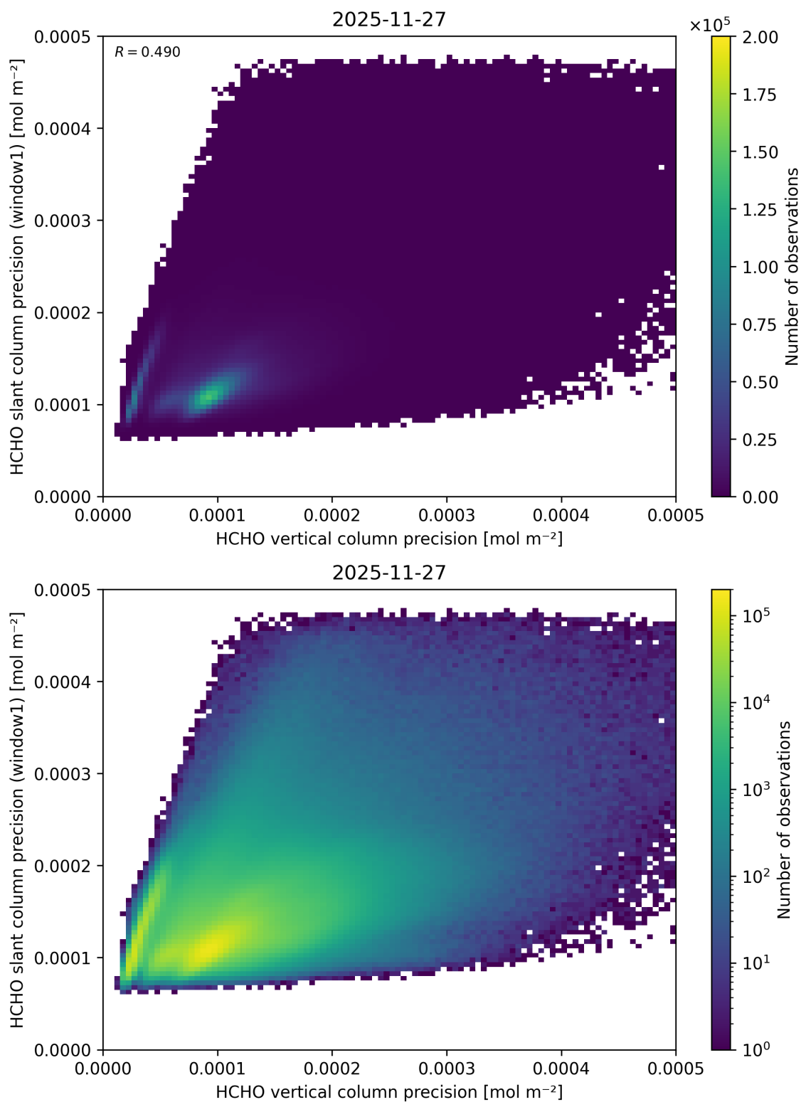
Figure 159: Scatter density plot of “HCHO vertical column precision” against “HCHO slant column precision (window1)” for 2025-11-26 to 2025-11-28.
