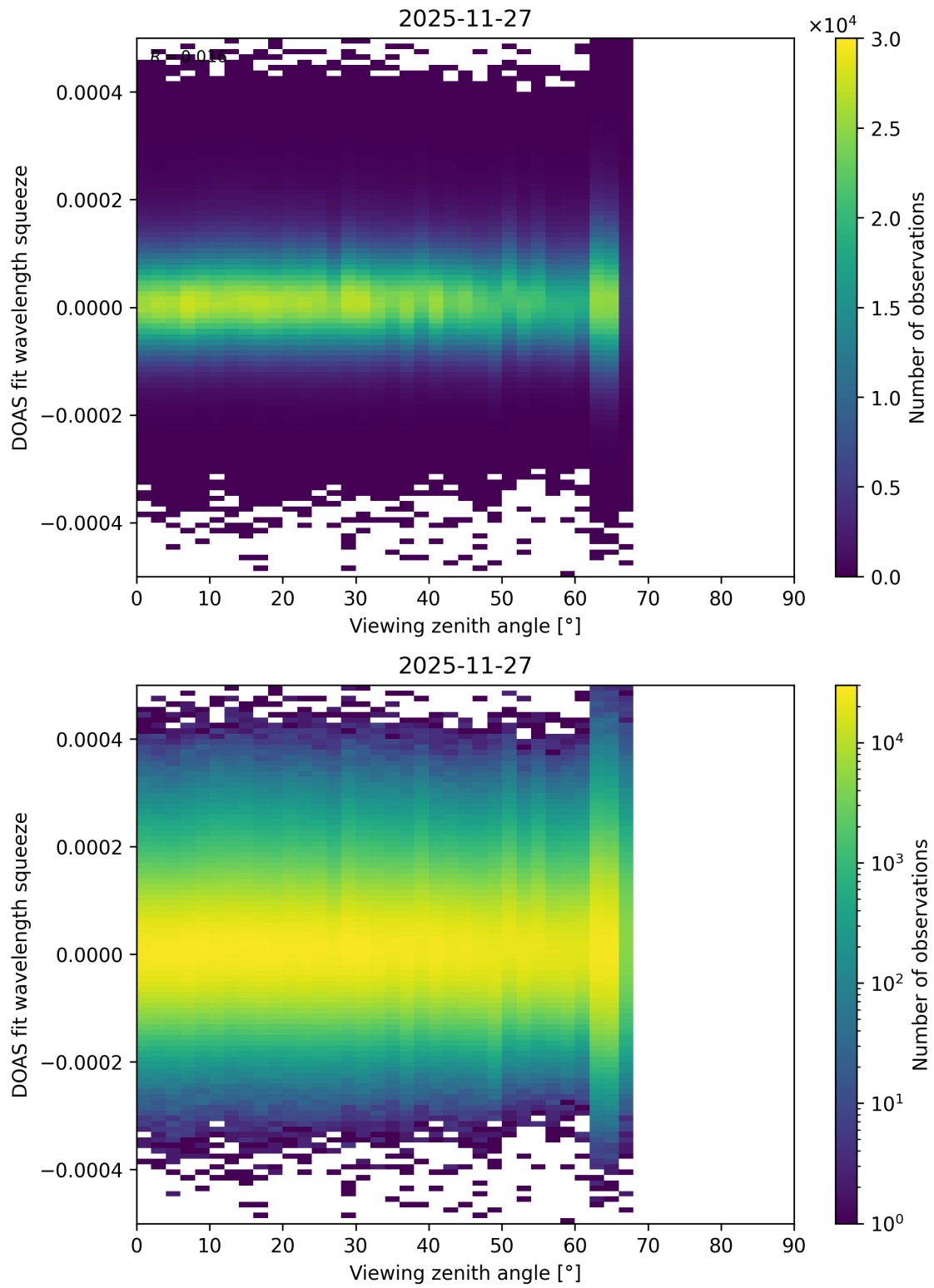
Figure 204: Scatter density plot of “Viewing zenith angle” against “DOAS fit wavelength squeeze” for 2025-11-26 to 2025-11-28.
