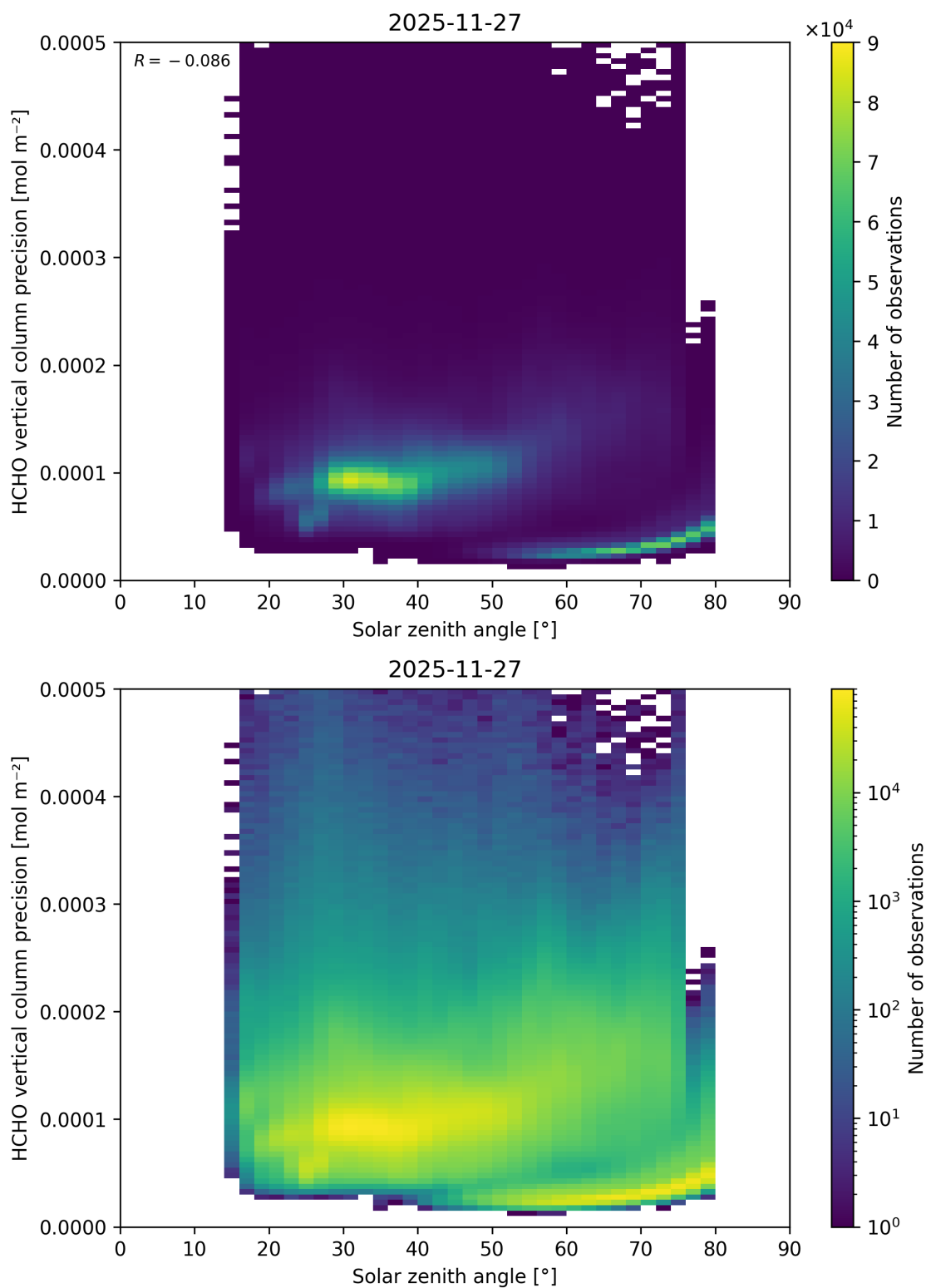
Figure 198: Scatter density plot of “Solar zenith angle” against “HCHO vertical column precision” for 2025-11-26 to 2025-11-28.
