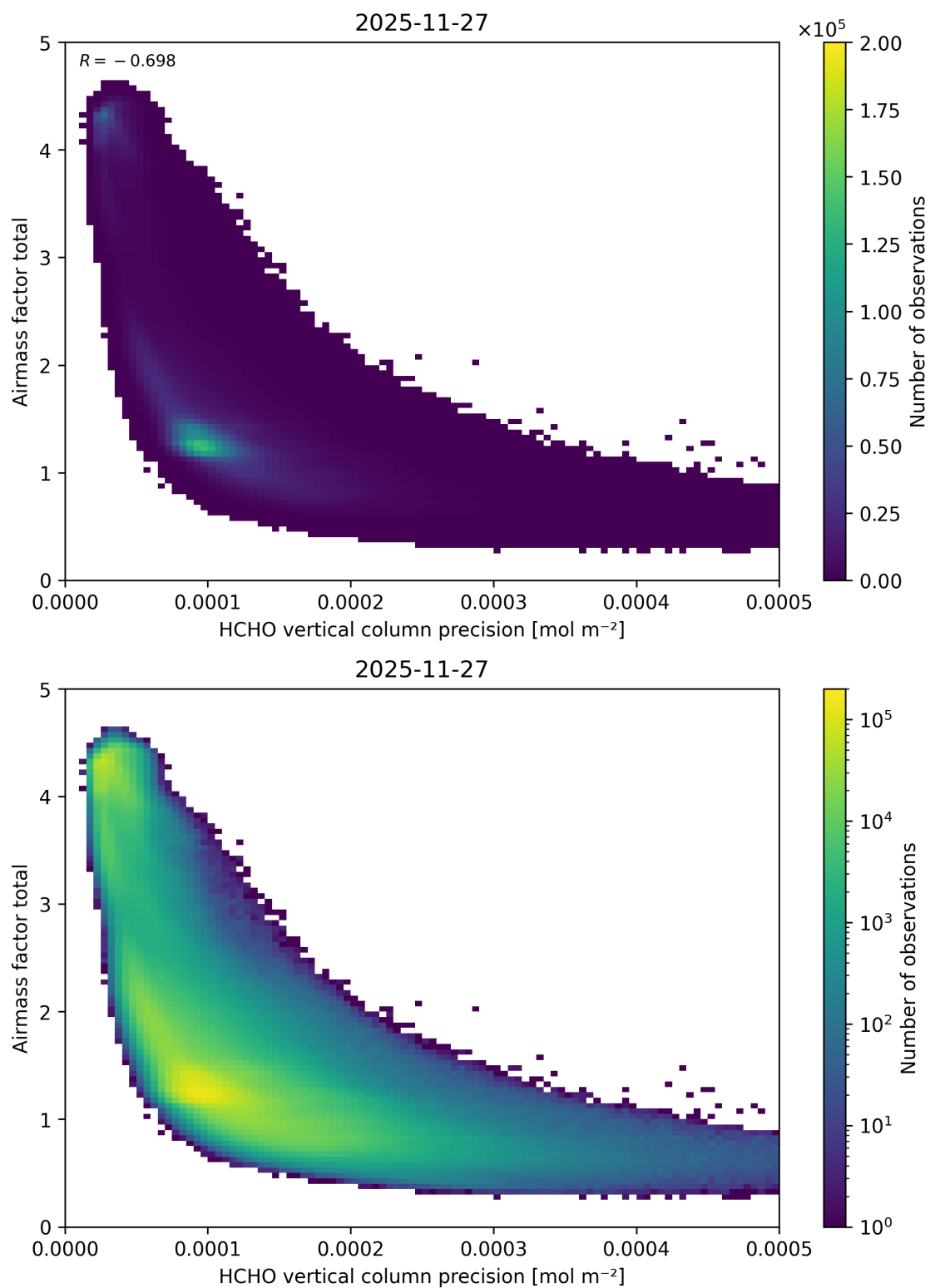
Figure 160: Scatter density plot of “HCHO vertical column precision” against “Airmass factor total” for 2025-11-26 to 2025-11-28.
