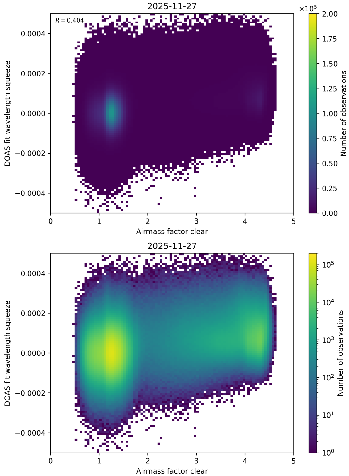
Figure 80: Scatter density plot of “Airmass factor clear” against “DOAS fit wavelength squeeze” for 2025-11-26 to 2025-11-28.
