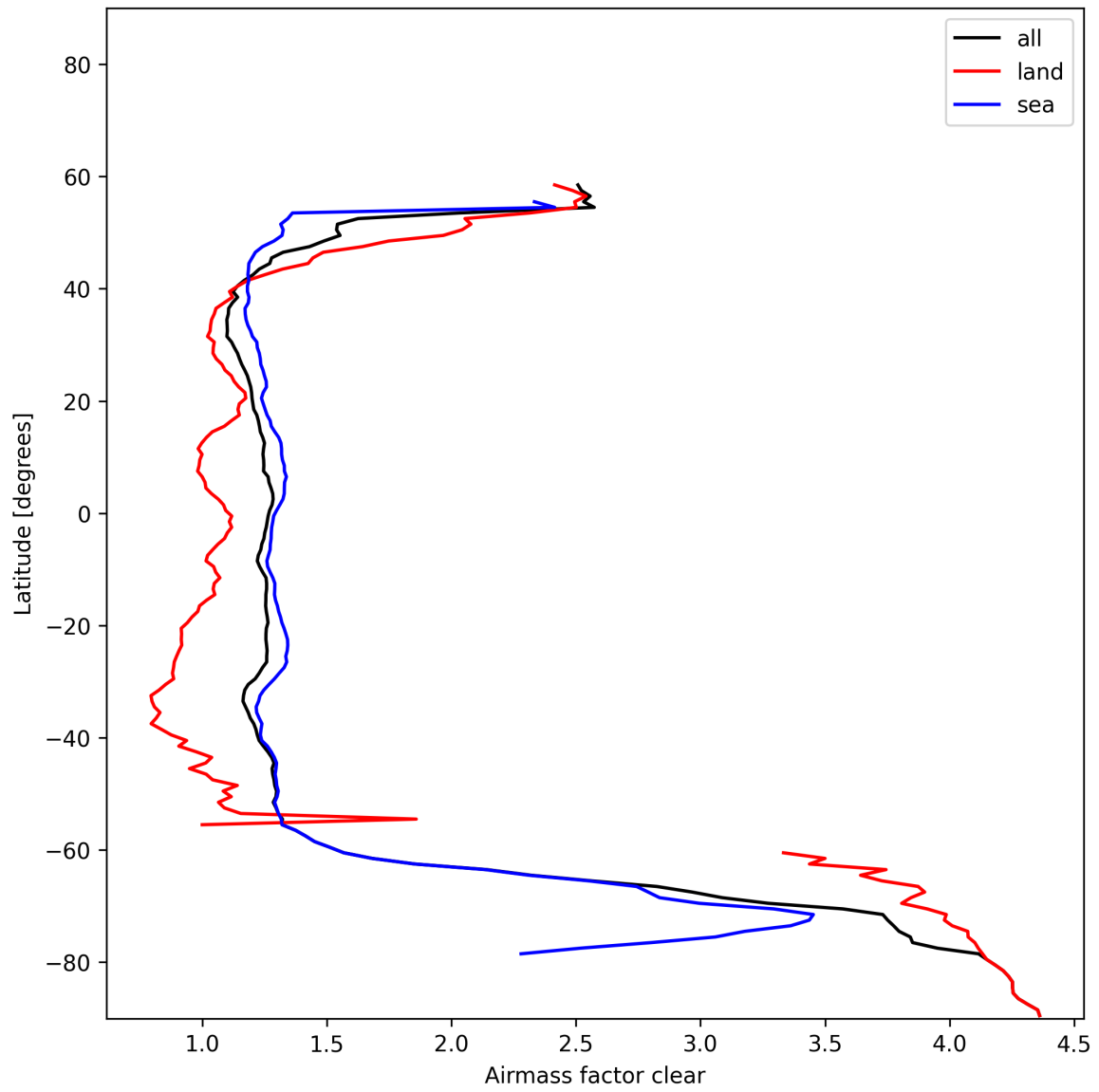
Figure 29: Zonal average of “Airmass factor clear” for 2025-11-26 to 2025-11-28.
