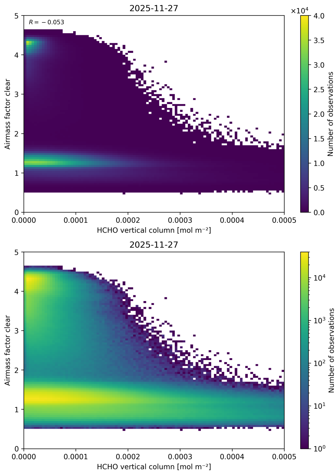
Figure 141: Scatter density plot of “HCHO vertical column” against “Airmass factor clear” for 2025-11-26 to 2025-11-28.
