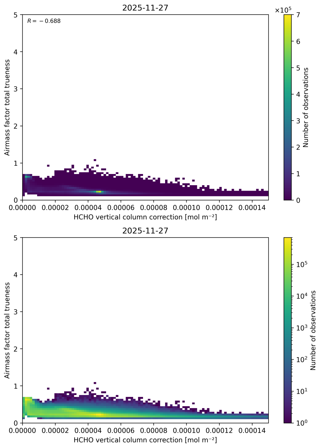
Figure 135: Scatter density plot of “HCHO vertical column correction” against “Airmass factor total truiness” for 2025-11-26 to 2025-11-28.
