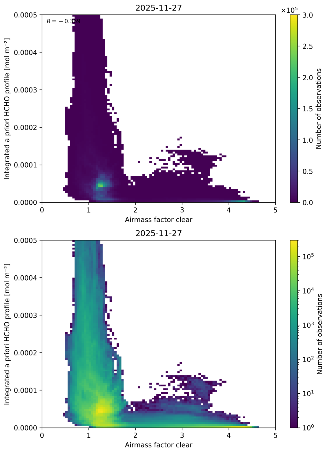
Figure 84: Scatter density plot of “Airmass factor clear” against “Integrated a priori HCHO profile” for 2025-11-26 to 2025-11-28.
