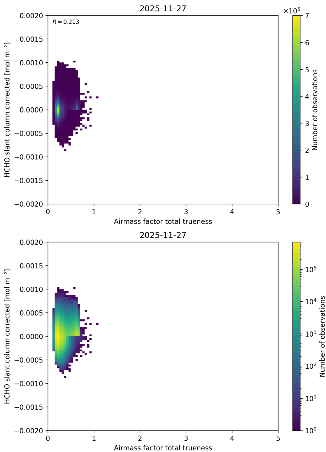
Figure 122: Scatter density plot of “Airmass factor total trueness” against “HCHO slant column corrected” for 2025-11-26 to 2025-11-28.
