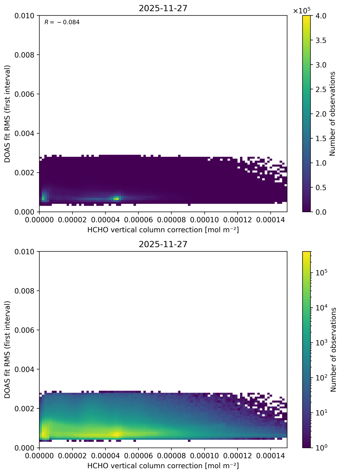
Figure 126: Scatter density plot of “HCHO vertical column correction” against “DOAS fit RMS (first interval)” for 2025-11-26 to 2025-11-28.
