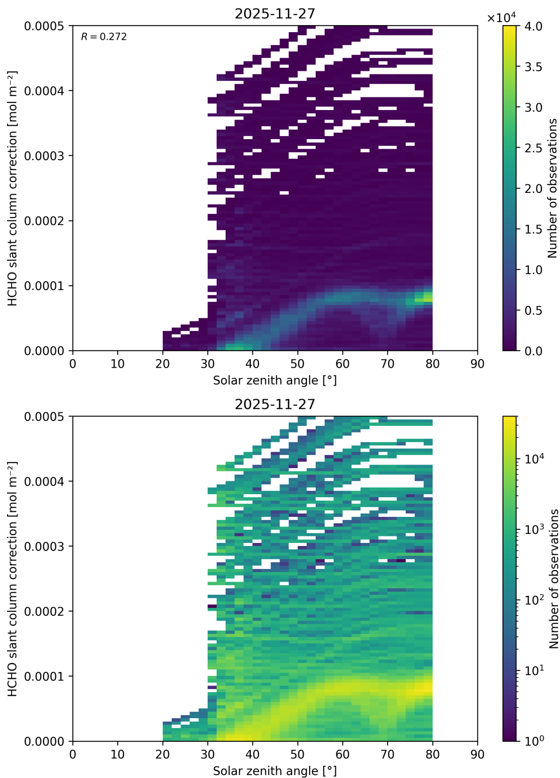
Figure 191: Scatter density plot of “Solar zenith angle” against “HCHO slant column correction” for 2025-11-26 to 2025-11-28.
