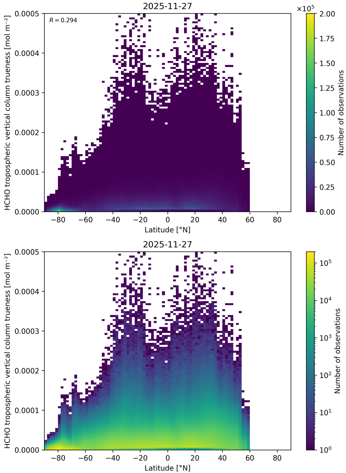
Figure 184: Scatter density plot of “Latitude” against “HCHO tropospheric vertical column trueness” for 2025-11-26 to 2025-11-28.
