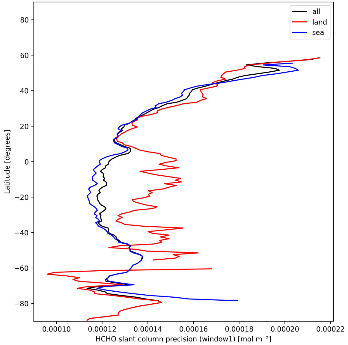
Figure 26: Zonal average of "HCHO slant column precision (window1)" for 2025-11-26 to 2025-11-28.
