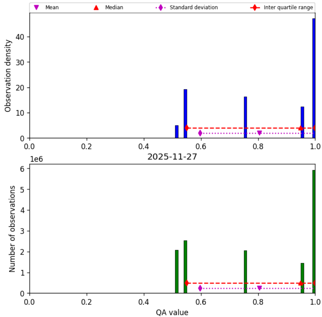
Figure 36: Histogram of “QA value” for 2025-11-26 to 2025-11-28
