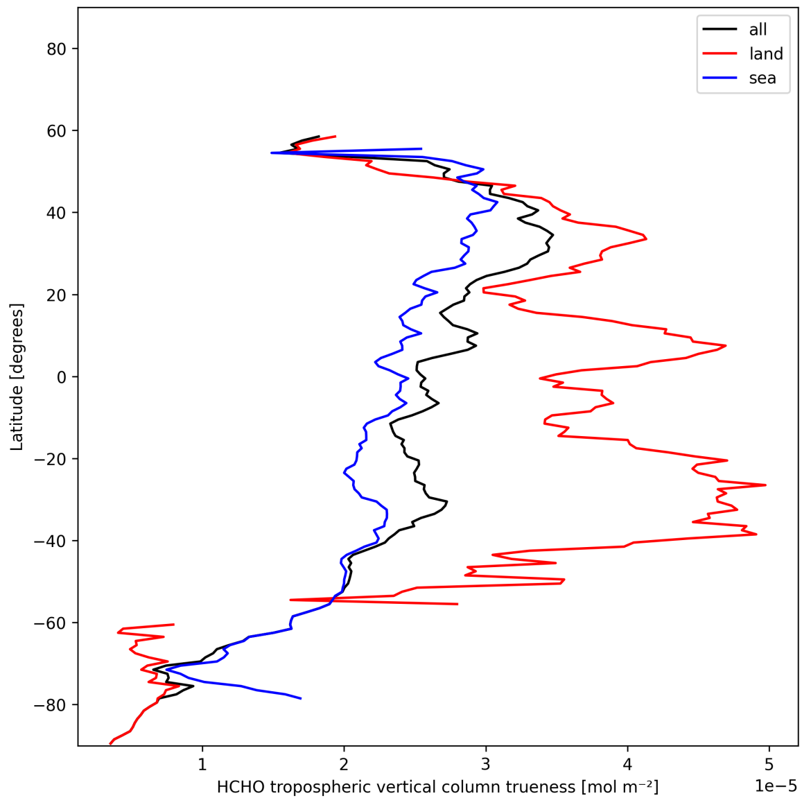
Figure 35: Zonal average of “HCHO tropospheric vertical column density” for 2025-11-26 to 2025-11-28.
