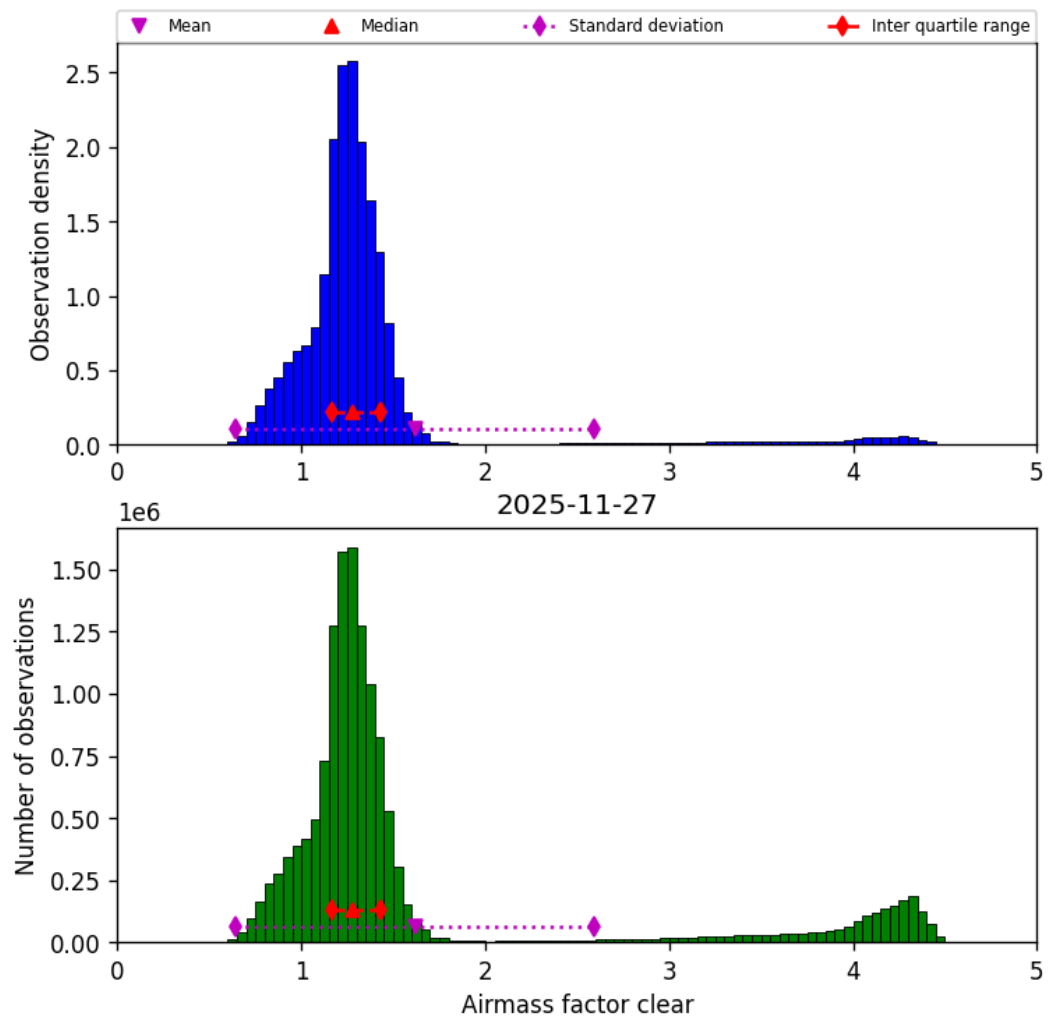
Figure 44: Histogram of “Airmass factor clear” for 2025-11-26 to 2025-11-28
