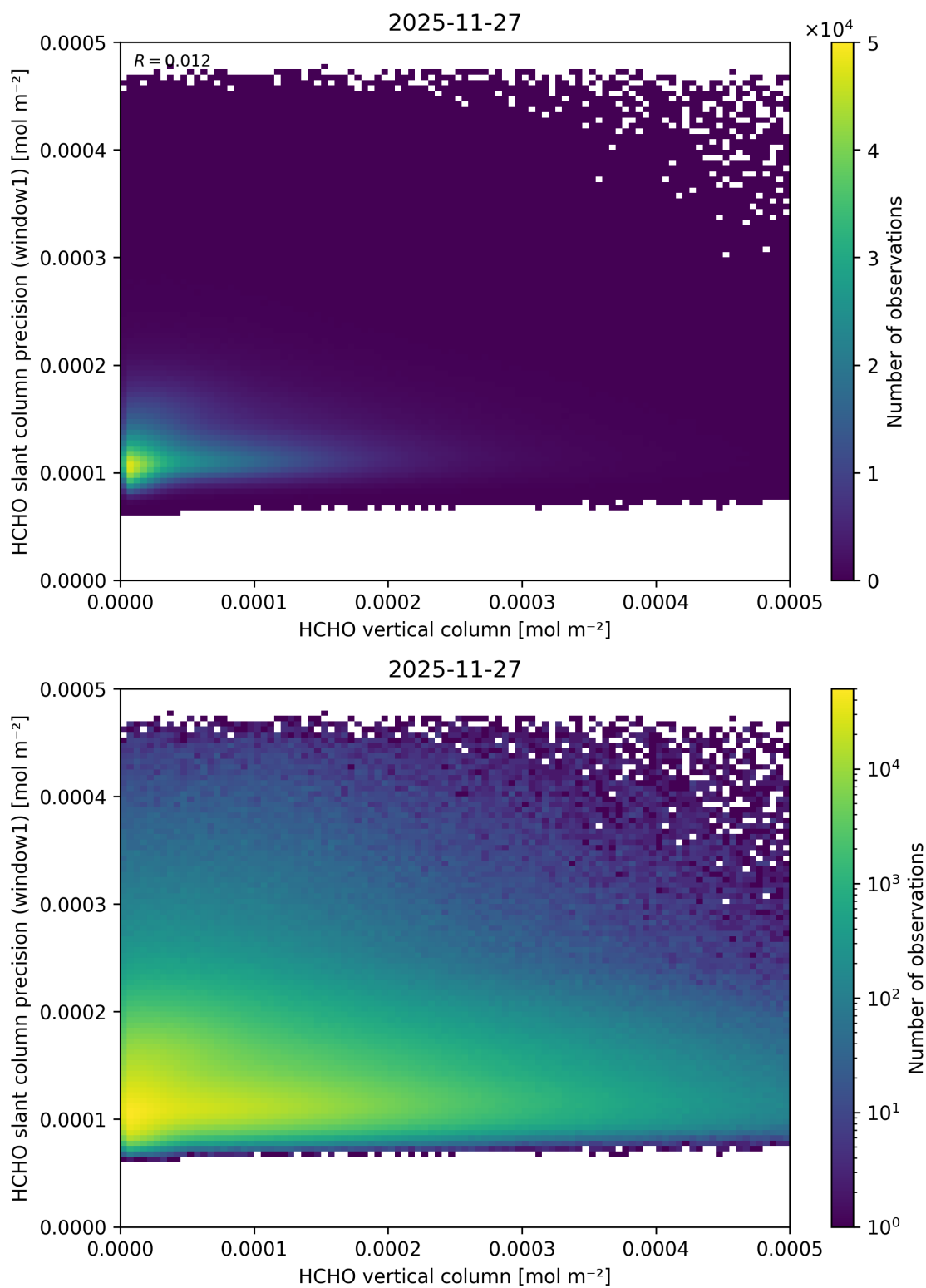
Figure 145: Scatter density plot of “HCHO vertical column” against “HCHO slant column precision (window1)” for 2025-11-26 to 2025-11-28.
