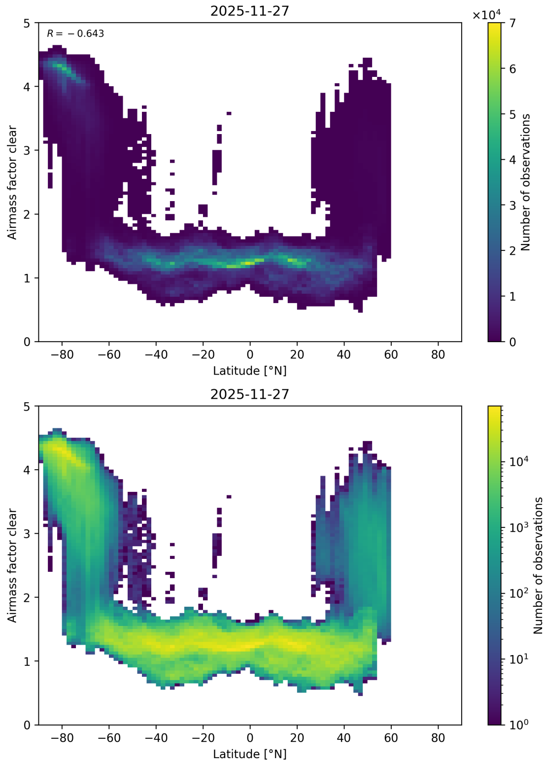
Figure 174: Scatter density plot of “Latitude” against “Airmass factor clear” for 2025-11-26 to 2025-11-28.
