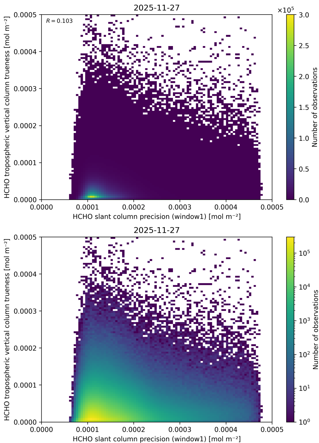
Figure 107: Scatter density plot of “HCHO slant column precision (window1)” against “HCHO tropospheric vertical column trueness” for 2025-11-26 to 2025-11-28.
