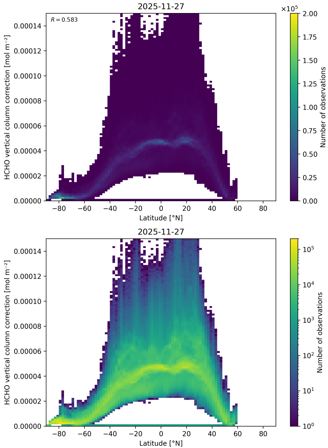
Figure 182: Scatter density plot of “Latitude” against “HCHO vertical column correction” for 2025-11-26 to 2025-11-28.
