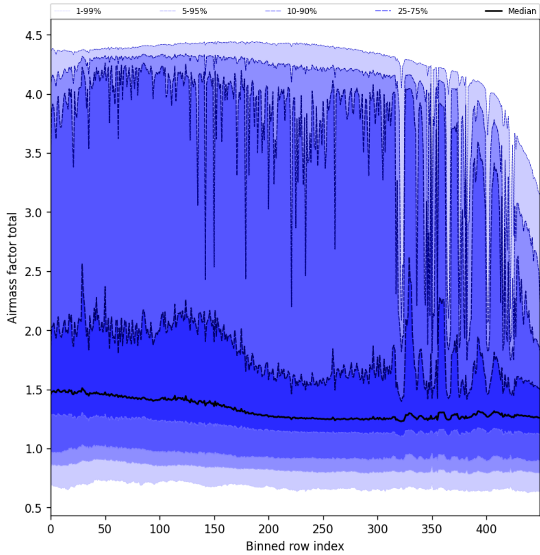
Figure 57: Along track statistics of “Airmass factor total” for 2025-11-26 to 2025-11-28
