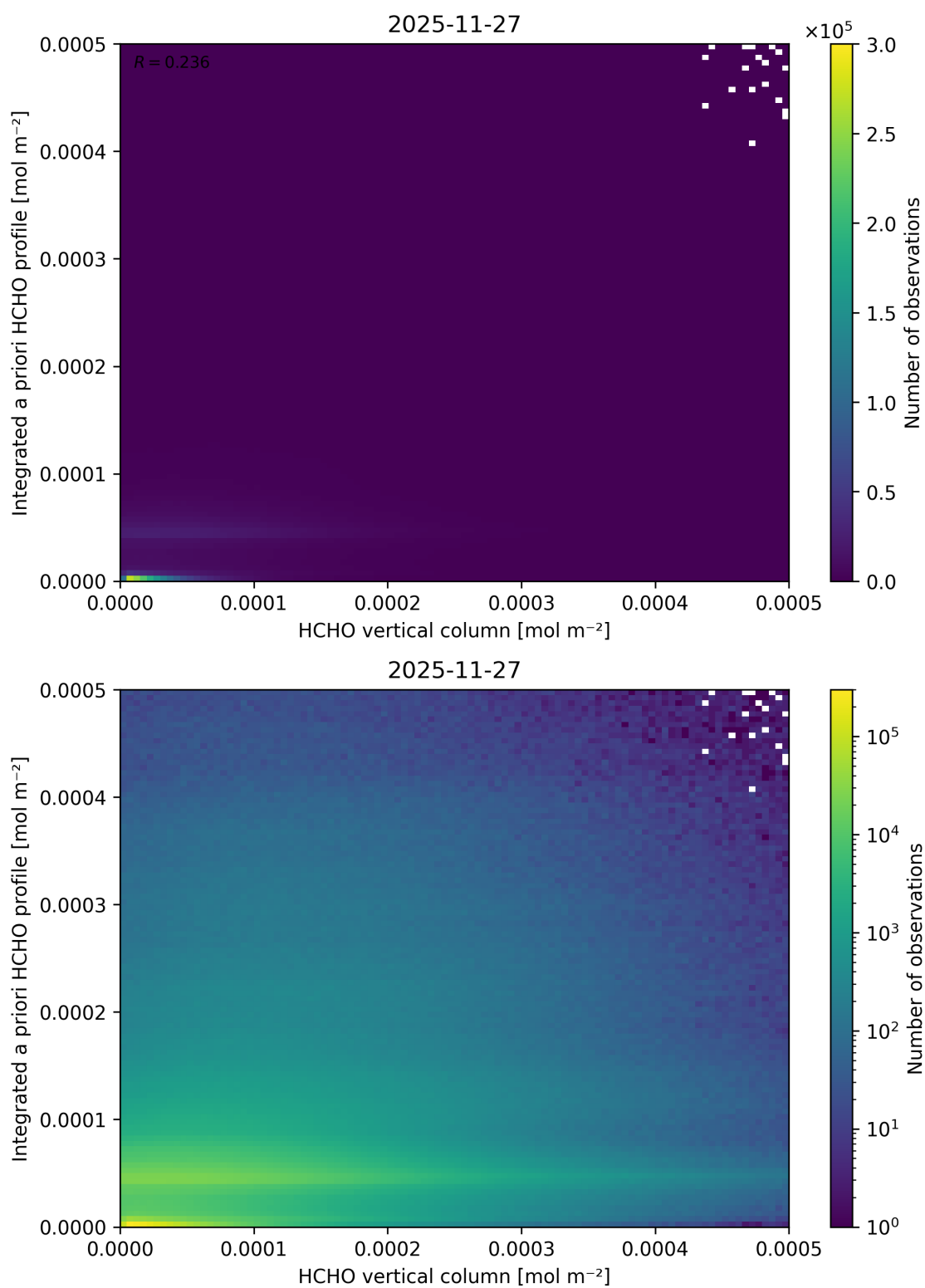
Figure 151: Scatter density plot of “HCHO vertical column” against “Integrated a priori HCHO profile” for 2025-11-26 to 2025-11-28.
