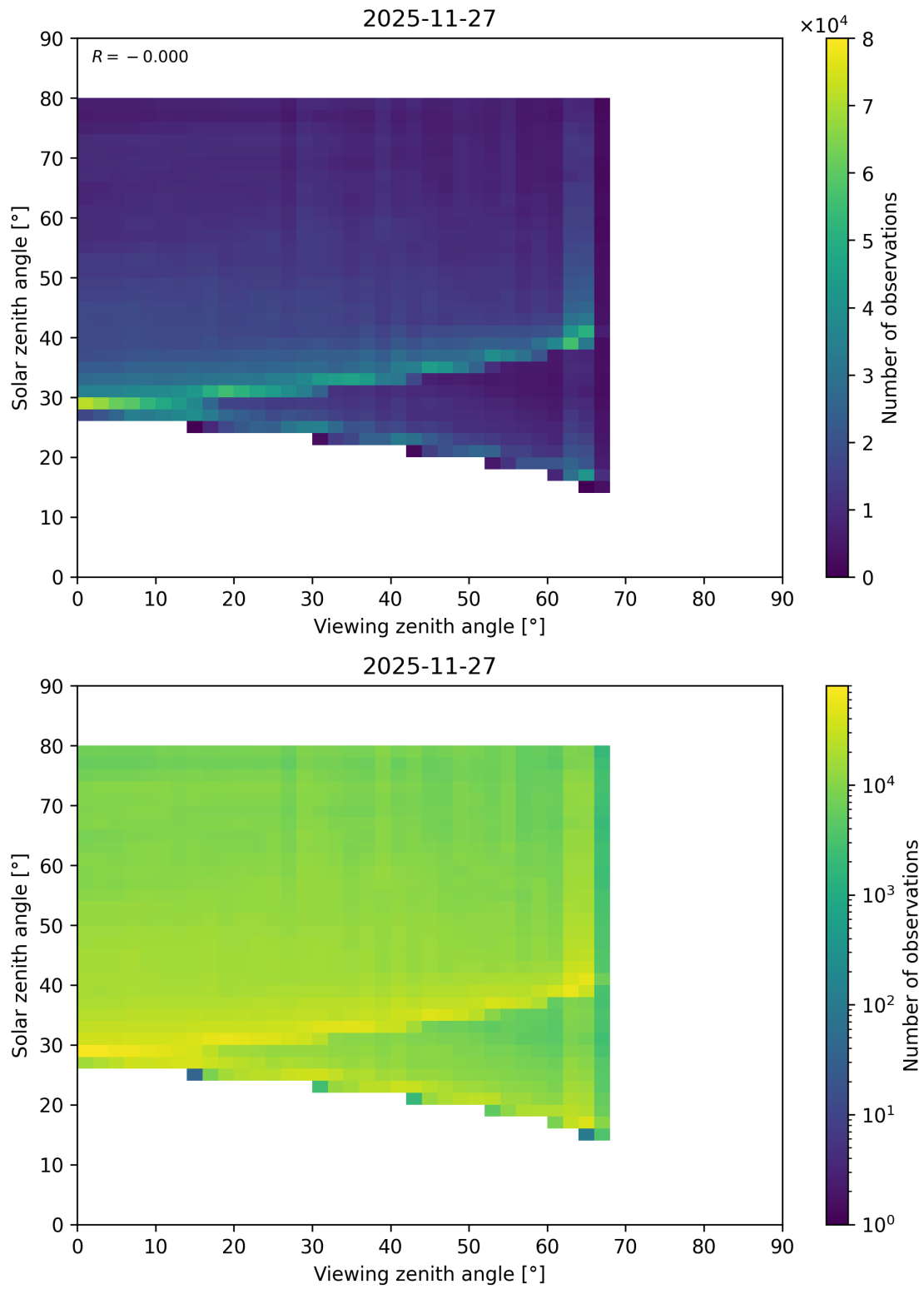
Figure 218: Scatter density plot of “Viewing zenith angle” against “Solar zenith angle” for 2025-11-26 to 2025-11-28.
