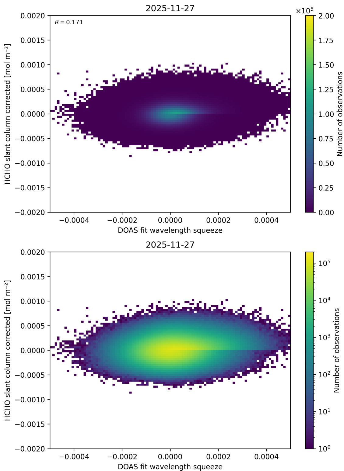
Figure 75: Scatter density plot of “DOAS fit wavelength squeeze” against “HCHO slant column corrected” for 2025-11-26 to 2025-11-28.
