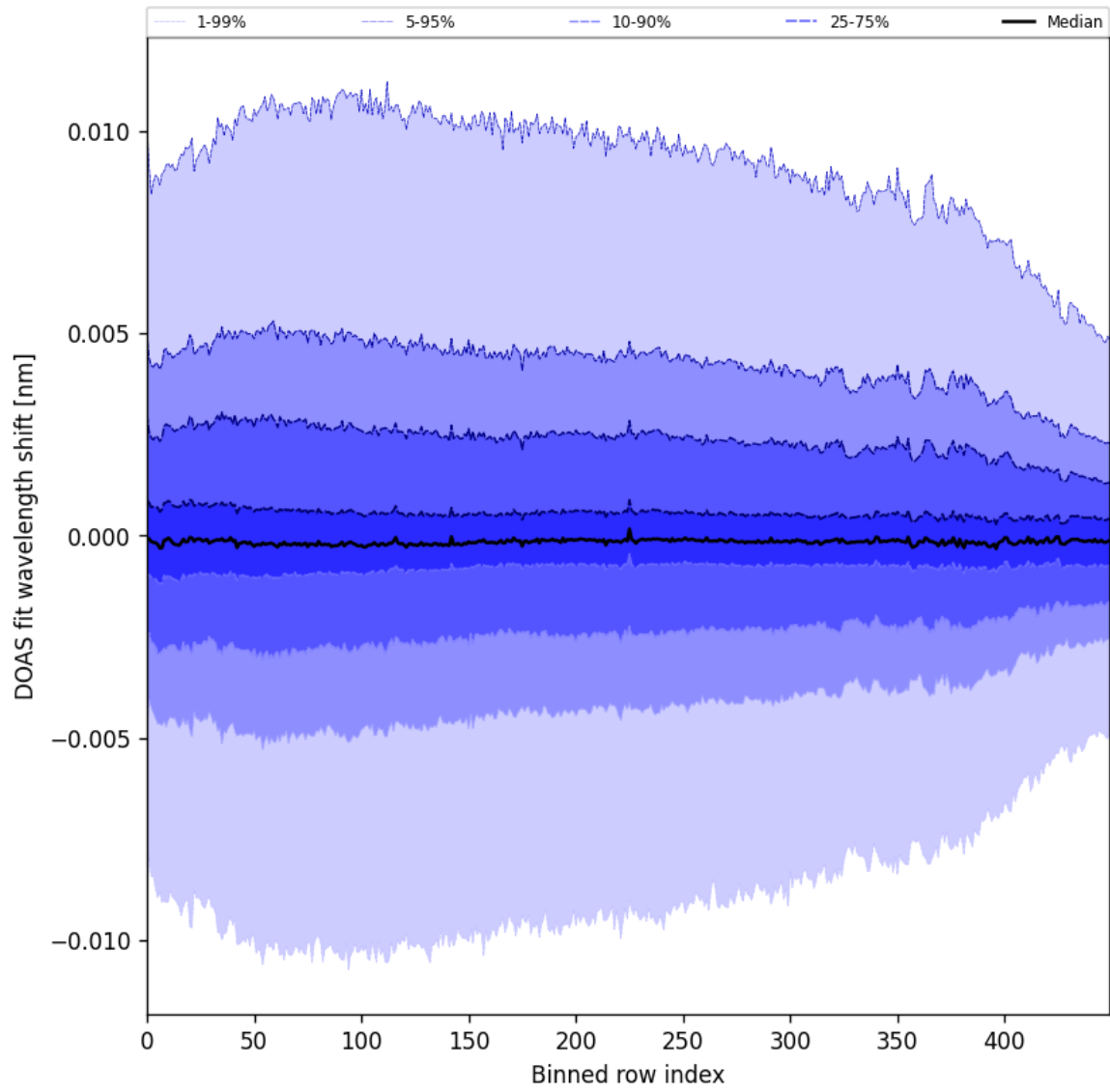
Figure 61: Along track statistics of “DOAS fit wavelength shift” for 2025-11-26 to 2025-11-28
