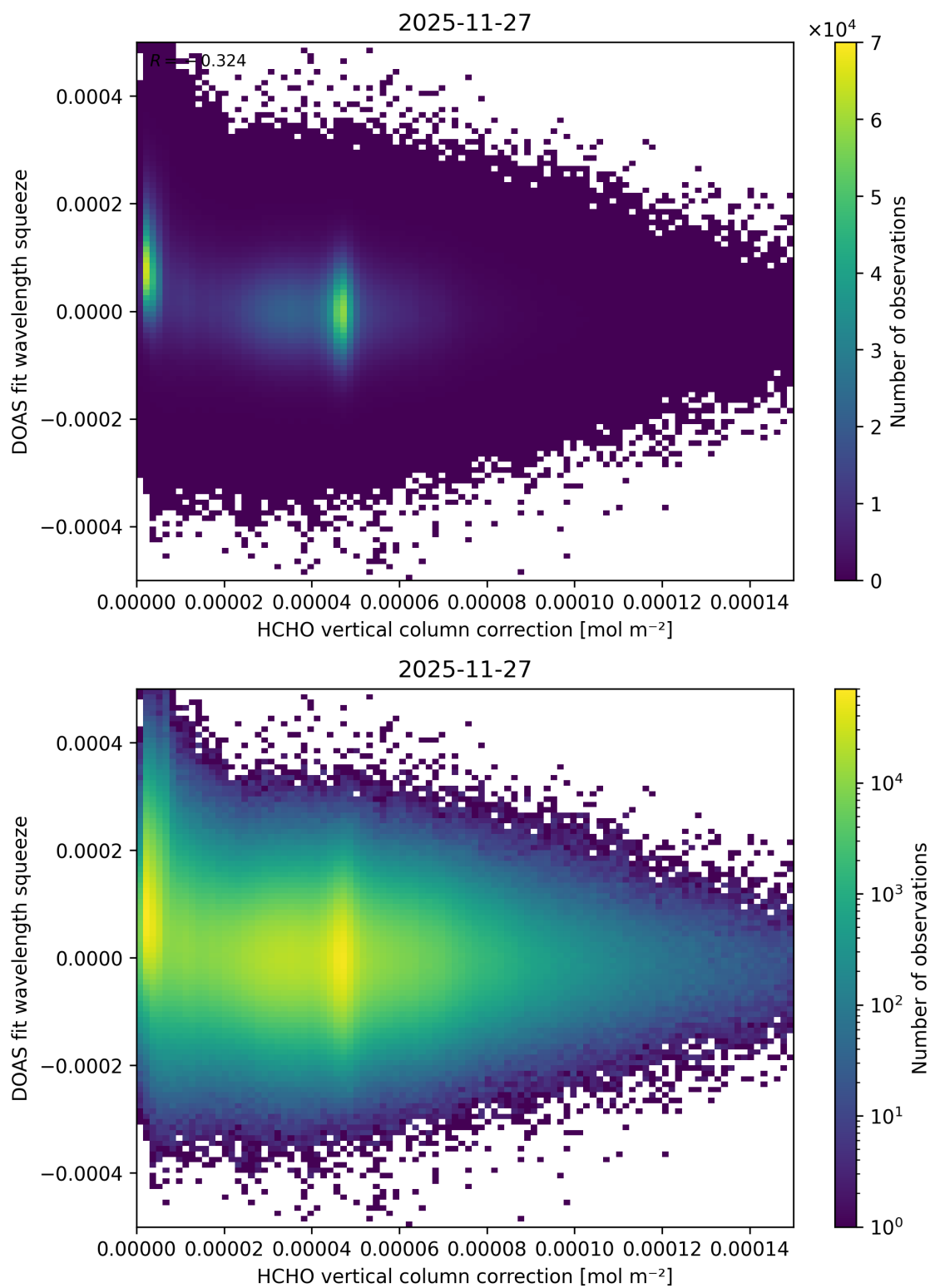
Figure 128: Scatter density plot of “HCHO vertical column correction” against “DOAS fit wavelength squeeze” for 2025-11-26 to 2025-11-28.
