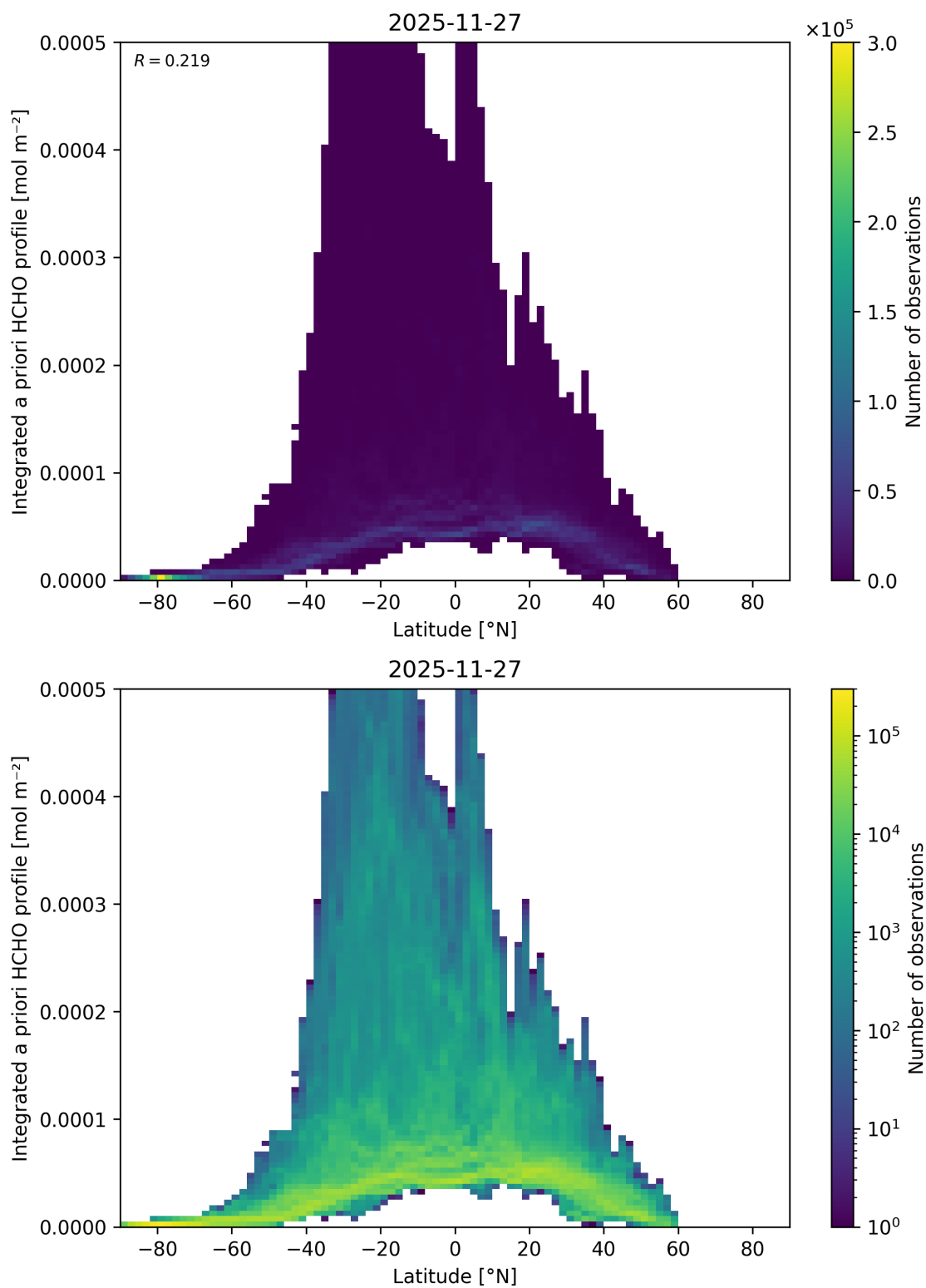
Figure 185: Scatter density plot of “Latitude” against “Integrated a priori HCHO profile” for 2025-11-26 to 2025-11-28.
