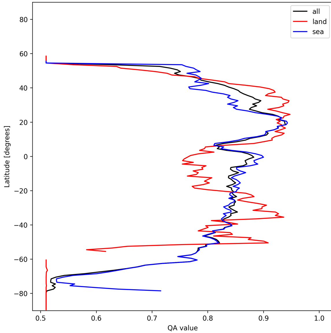
Figure 21: Zonal average of “QA value” for 2025-11-26 to 2025-11-28.
