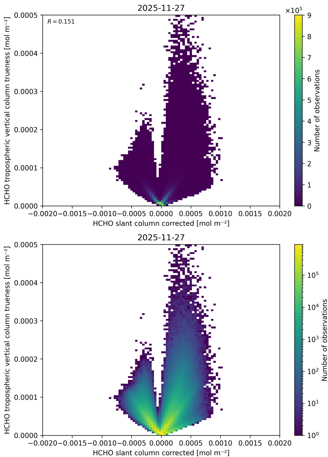
Figure 86: Scatter density plot of “HCHO slant column corrected” against “HCHO tropospheric vertical column trueness” for 2025-11-26 to 2025-11-28.
