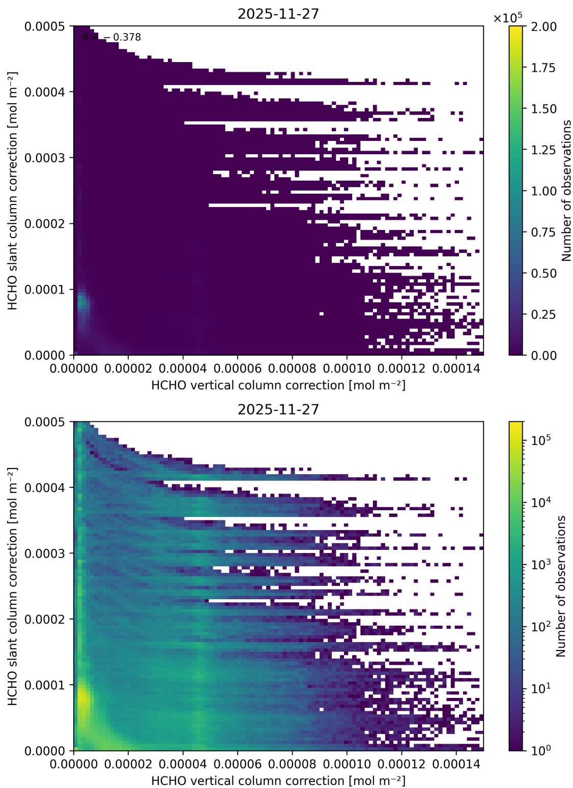
Figure 131: Scatter density plot of “HCHO vertical column correction” against “HCHO slant column correction” for 2025-11-26 to 2025-11-28.
