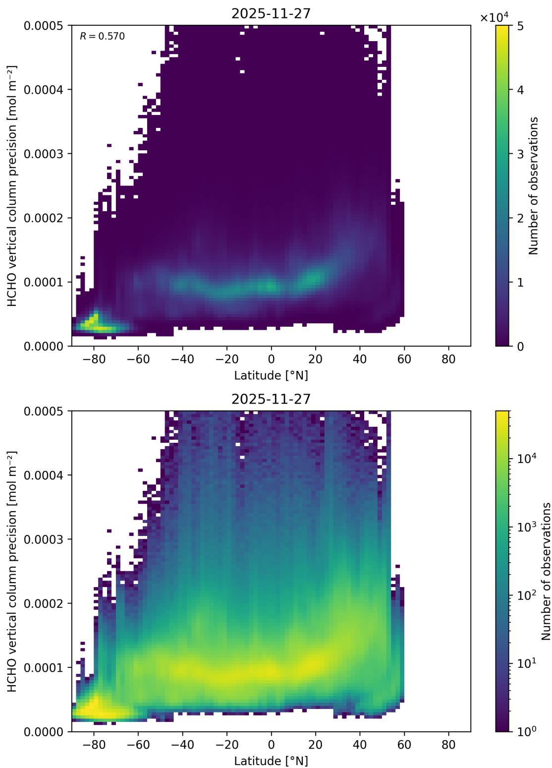
Figure 183: Scatter density plot of “Latitude” against “HCHO vertical column precision” for 2025-11-26 to 2025-11-28.
