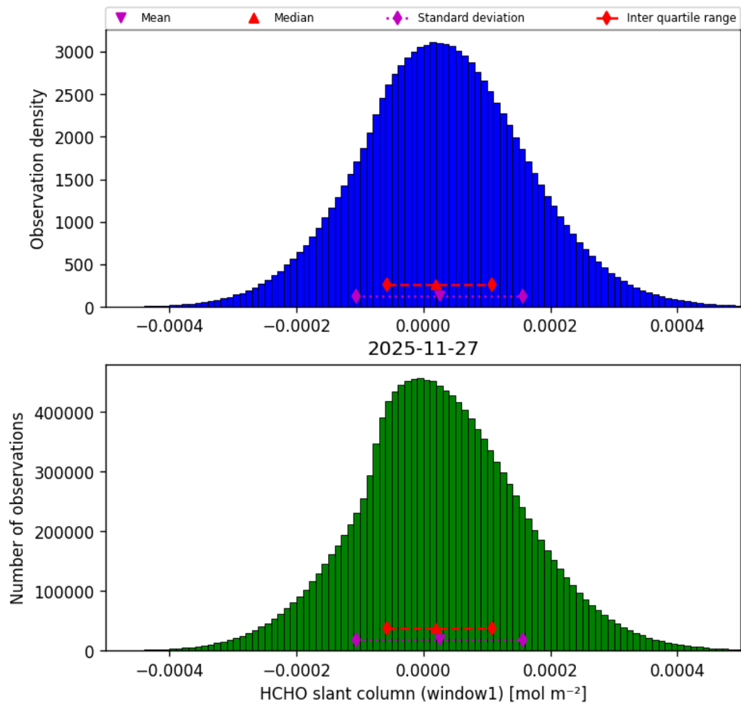
Figure 40: Histogram of “HCHO slant column (window1)” for 2025-11-26 to 2025-11-28
