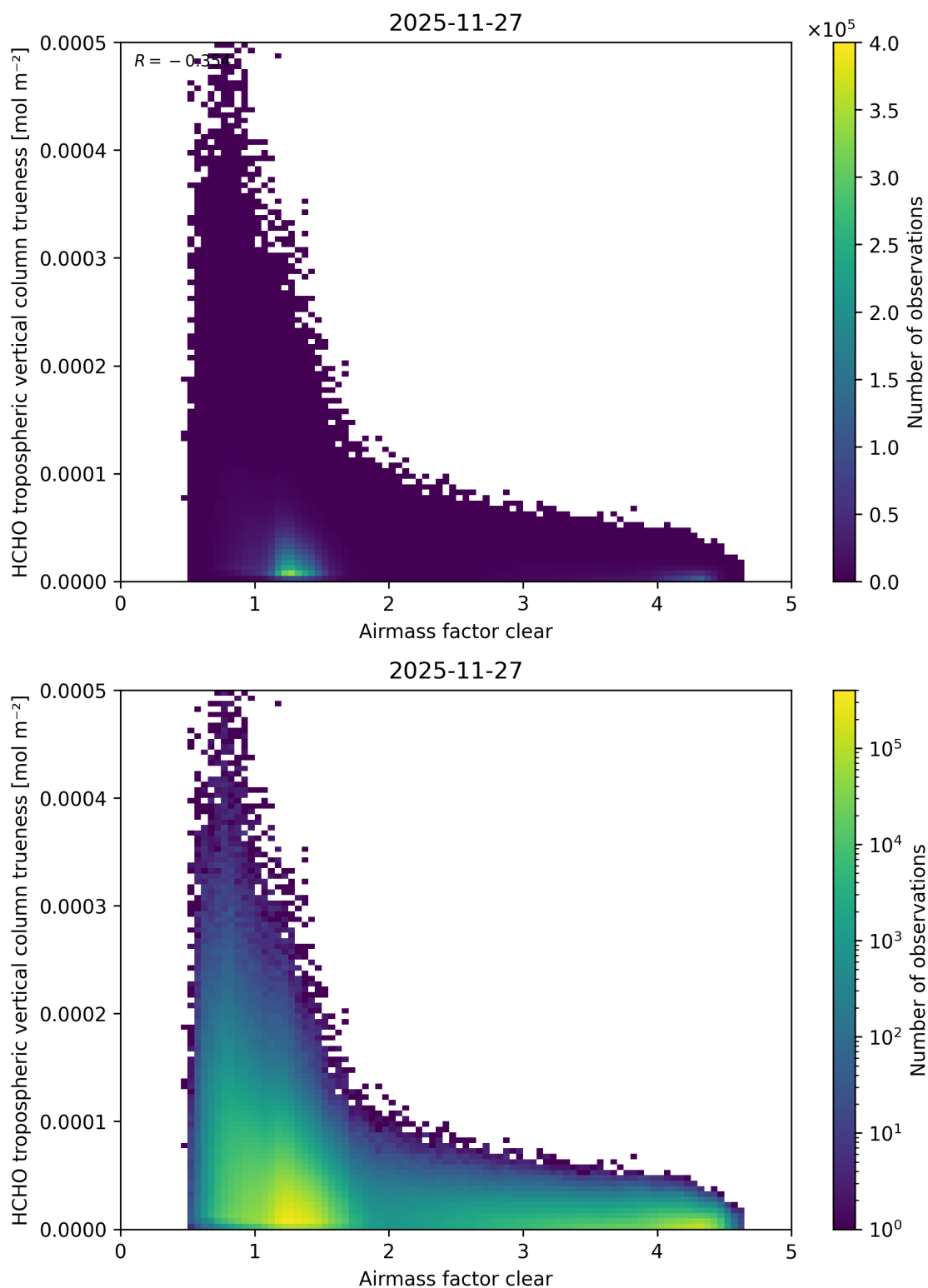
Figure 83: Scatter density plot of “Airmass factor clear” against “HCHO tropospheric vertical column trueeness” for 2025-11-26 to 2025-11-28.
