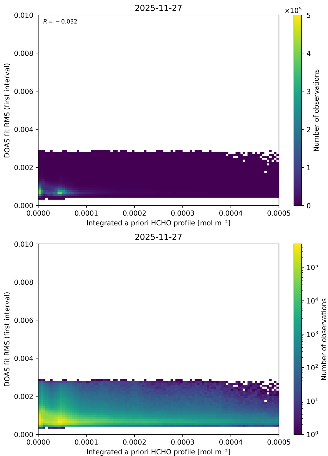
Figure 165: Scatter density plot of “Integrated a priori HCHO profile” against “DOAS fit RMS (first interval)” for 2025-11-26 to 2025-11-28.
