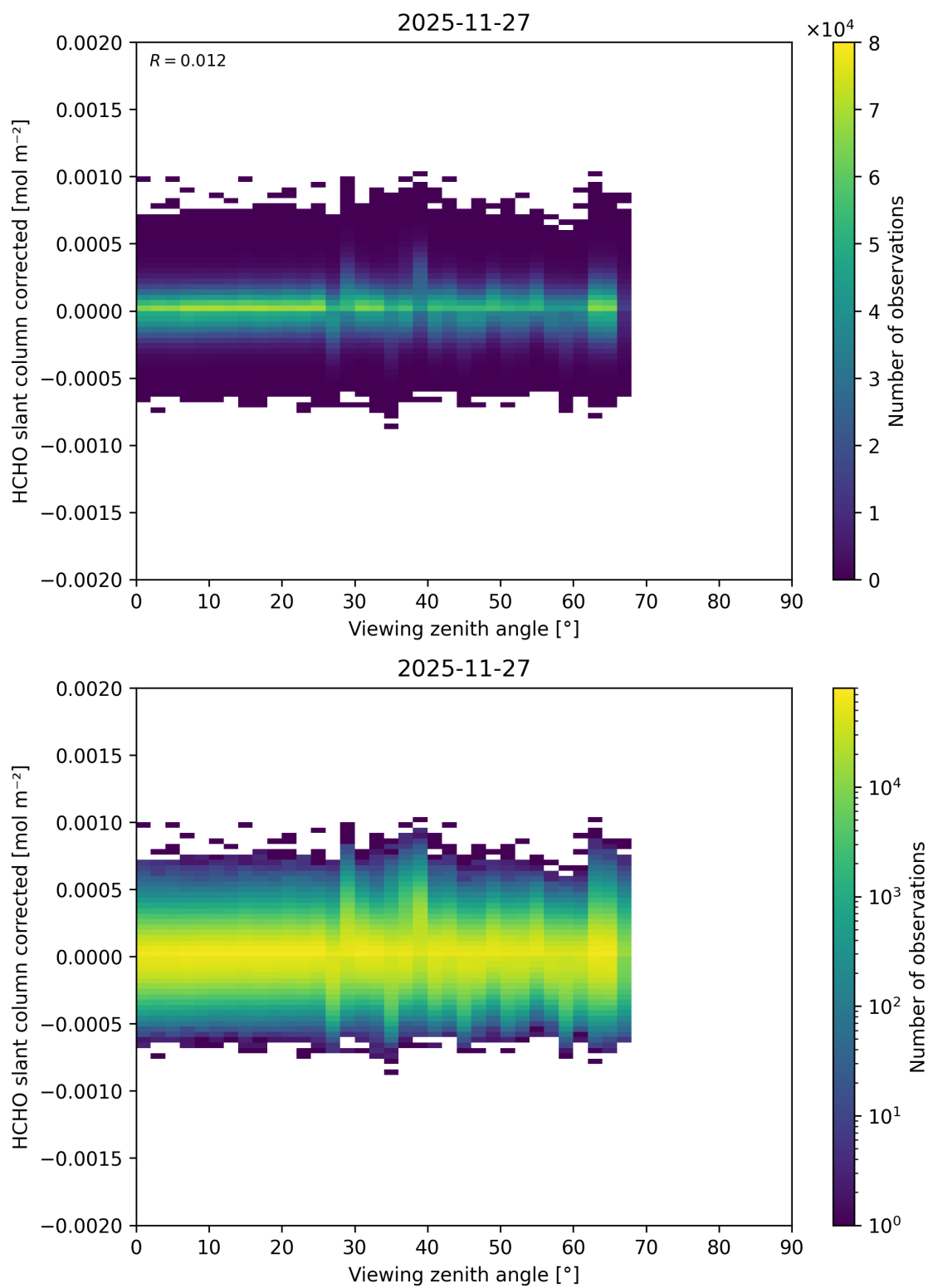
Figure 206: Scatter density plot of “Viewing zenith angle” against “HCHO slant column corrected” for 2025-11-26 to 2025-11-28.
