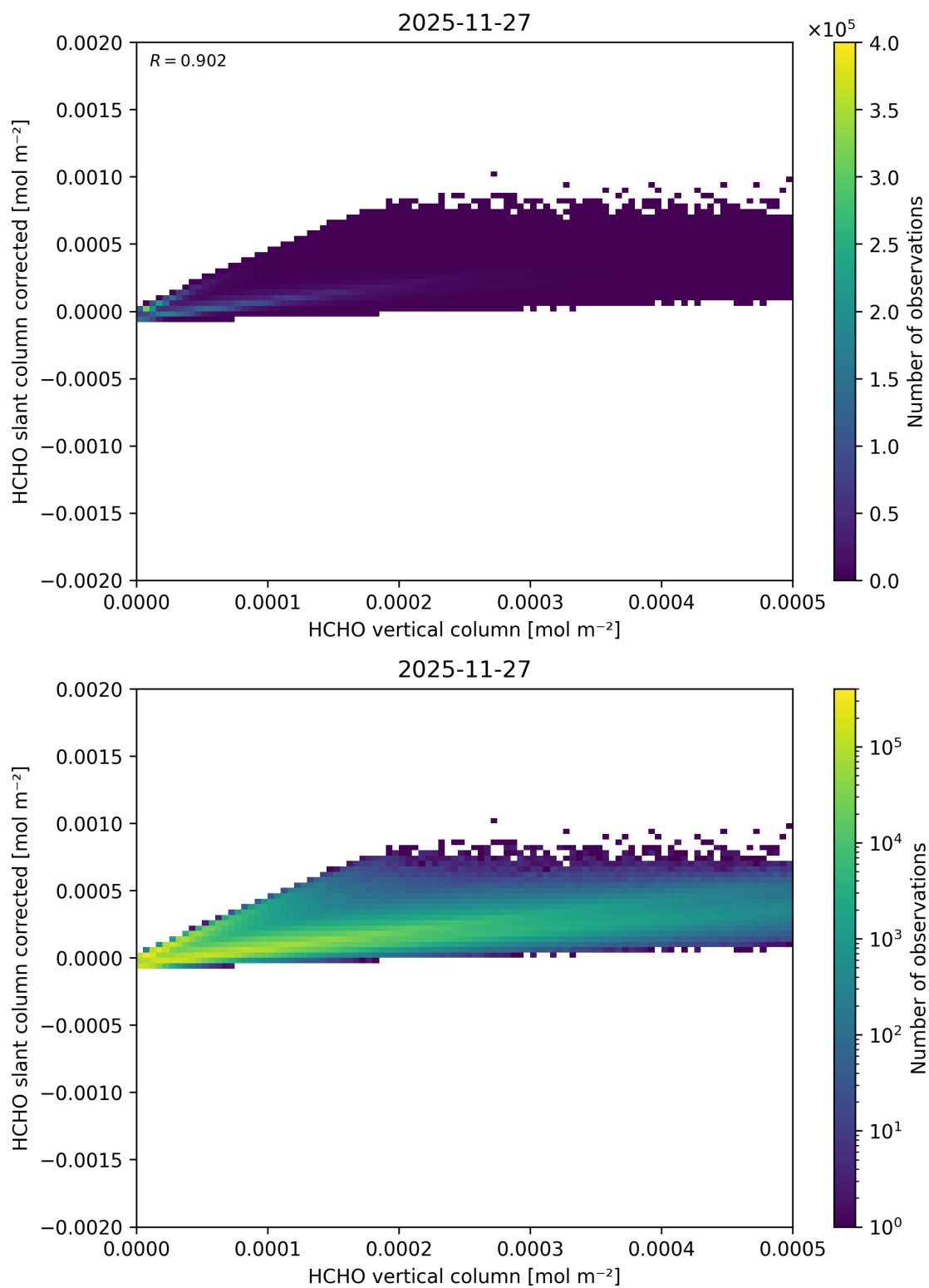
Figure 142: Scatter density plot of “HCHO vertical column” against “HCHO slant column corrected” for 2025-11-26 to 2025-11-28.
