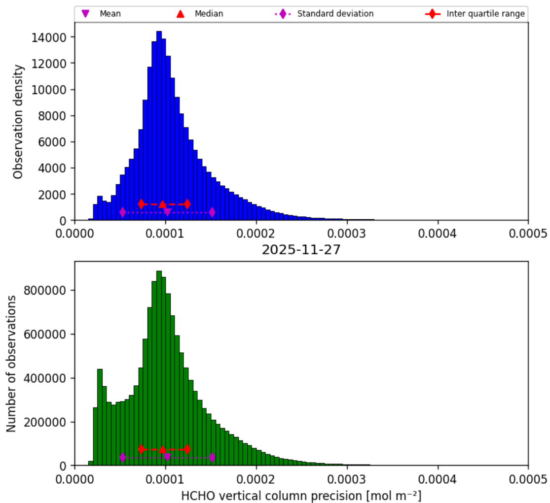
Figure 38: Histogram of “HCHO vertical column precision” for 2025-11-26 to 2025-11-28
