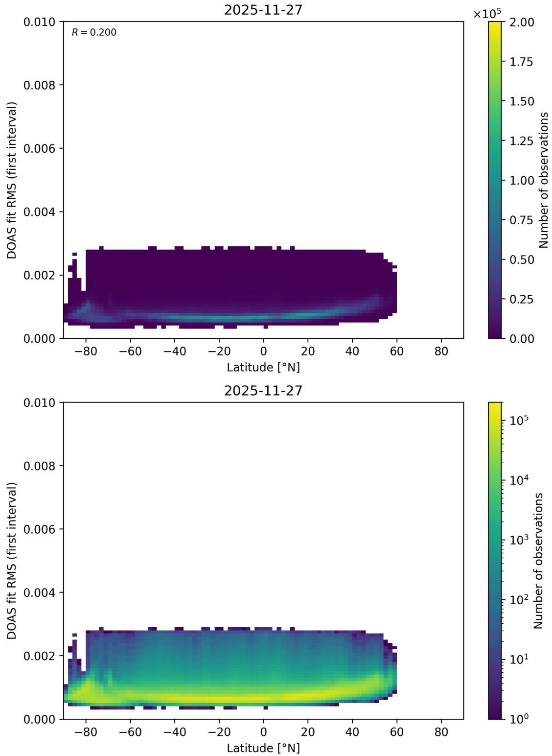
Figure 171: Scatter density plot of “Latitude” against “DOAS fit RMS (first interval)” for 2025-11-26 to 2025-11-28.
