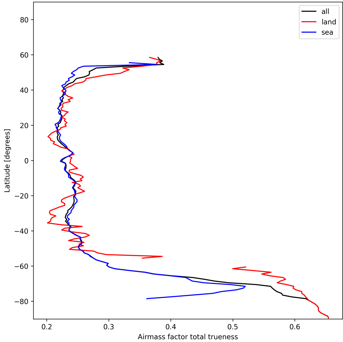
Figure 28: Zonal average of “Airmass factor total trueness” for 2025-11-26 to 2025-11-28.
