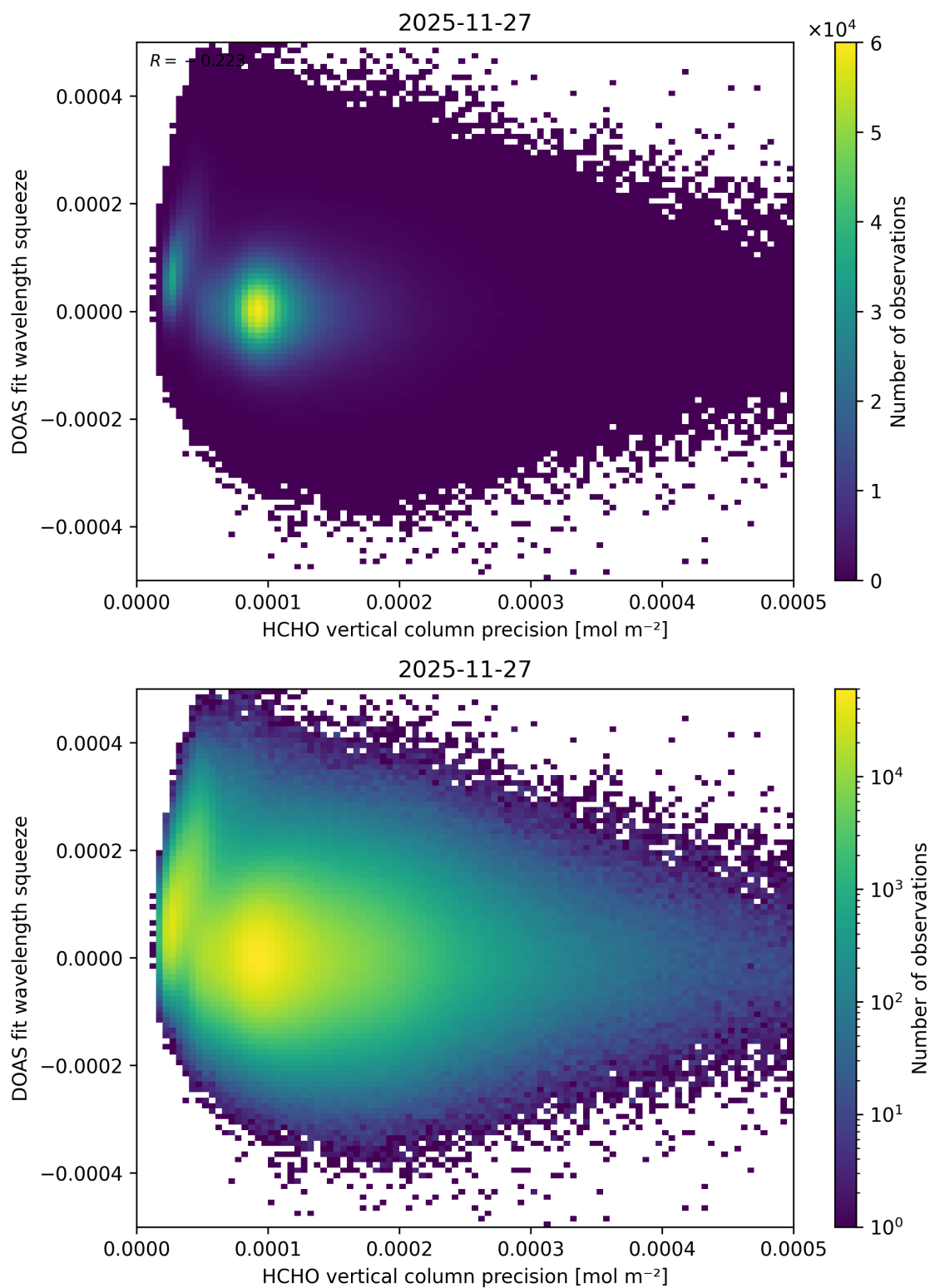
Figure 154: Scatter density plot of “HCHO vertical column precision” against “DOAS fit wavelength squeeze” for 2025-11-26 to 2025-11-28.
