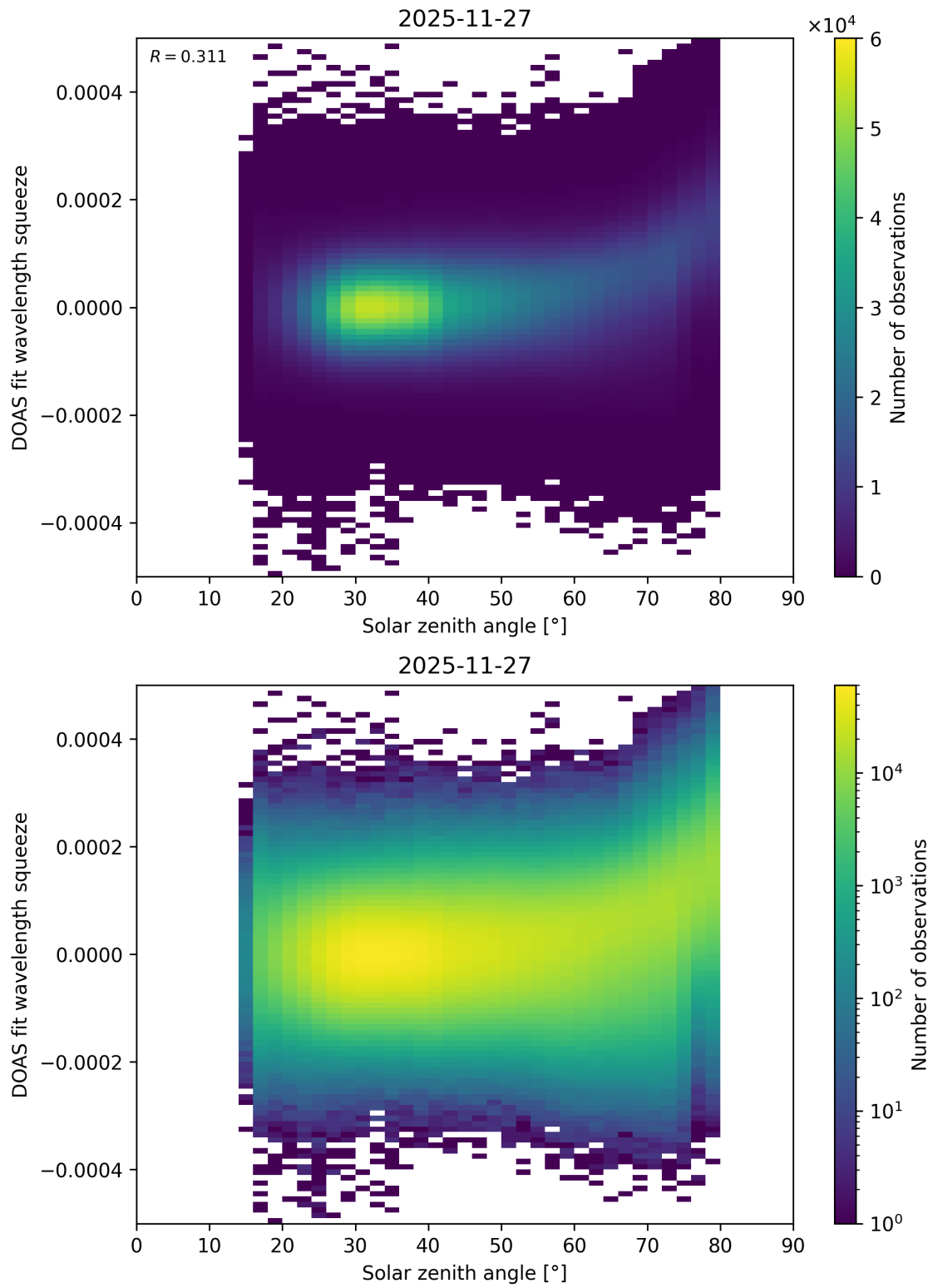
Figure 188: Scatter density plot of “Solar zenith angle” against “DOAS fit wavelength squeeze” for 2025-11-26 to 2025-11-28.
