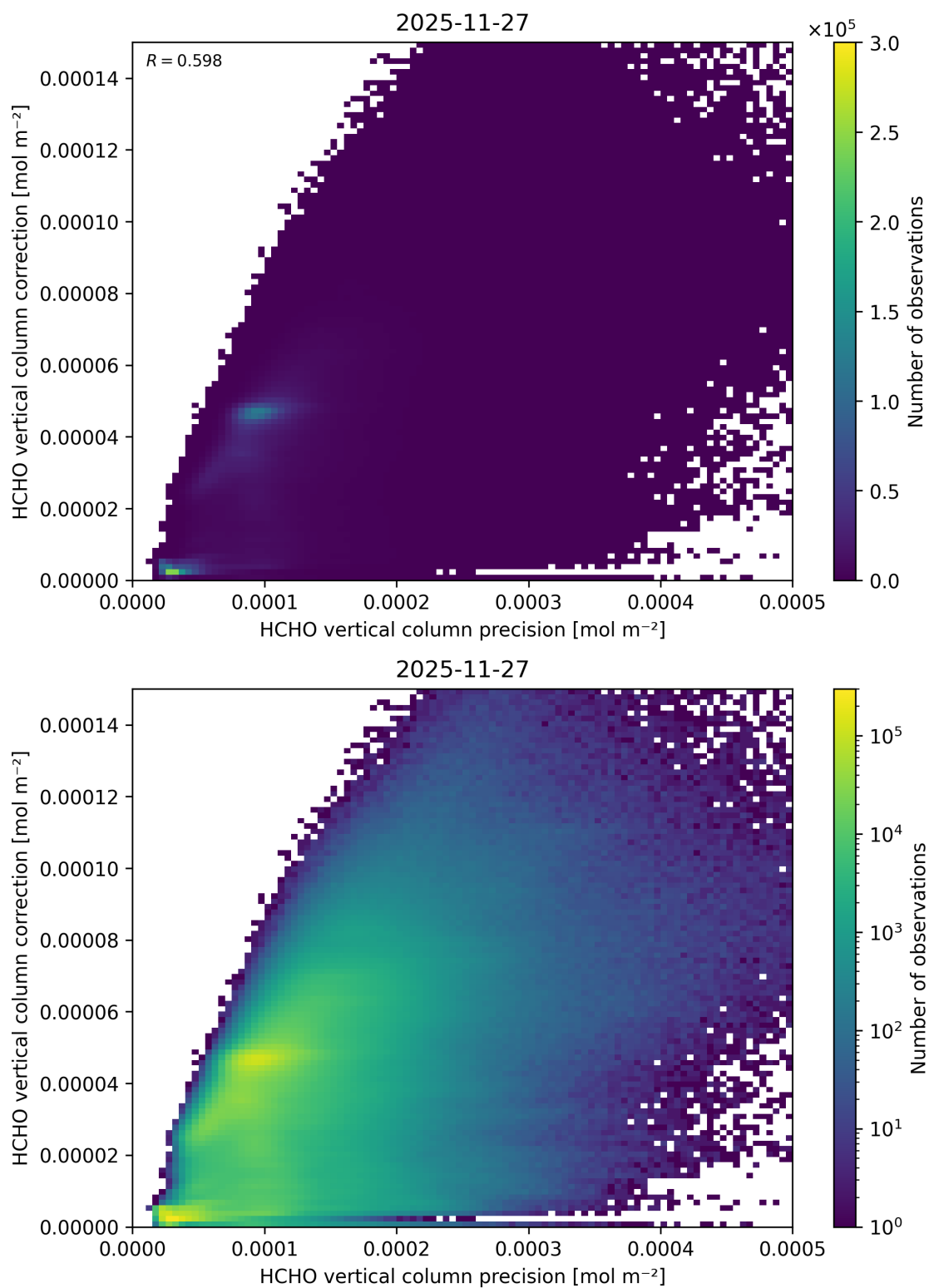
Figure 162: Scatter density plot of “HCHO vertical column precision” against “HCHO vertical column correction” for 2025-11-26 to 2025-11-28.
