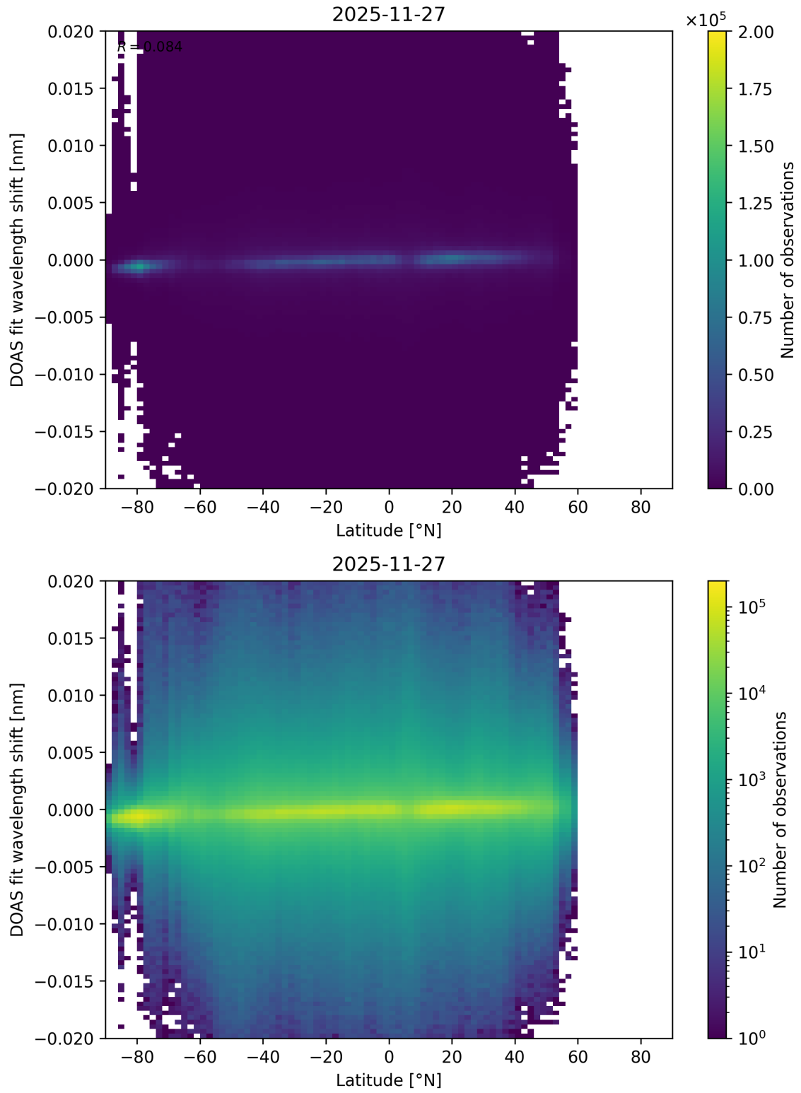
Figure 172: Scatter density plot of “Latitude” against “DOAS fit wavelength shift” for 2025-11-26 to 2025-11-28.
