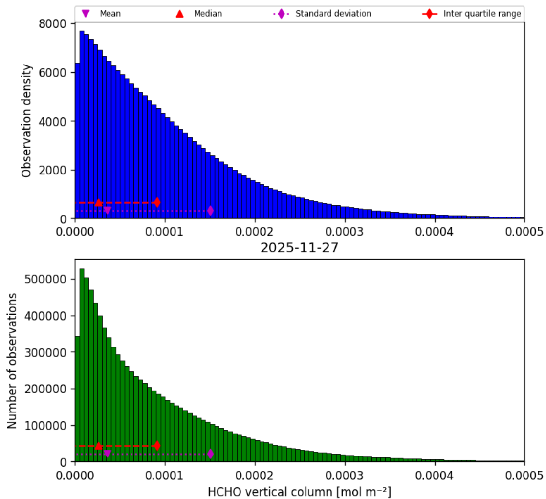
Figure 37: Histogram of “HCHO vertical column” for 2025-11-26 to 2025-11-28
