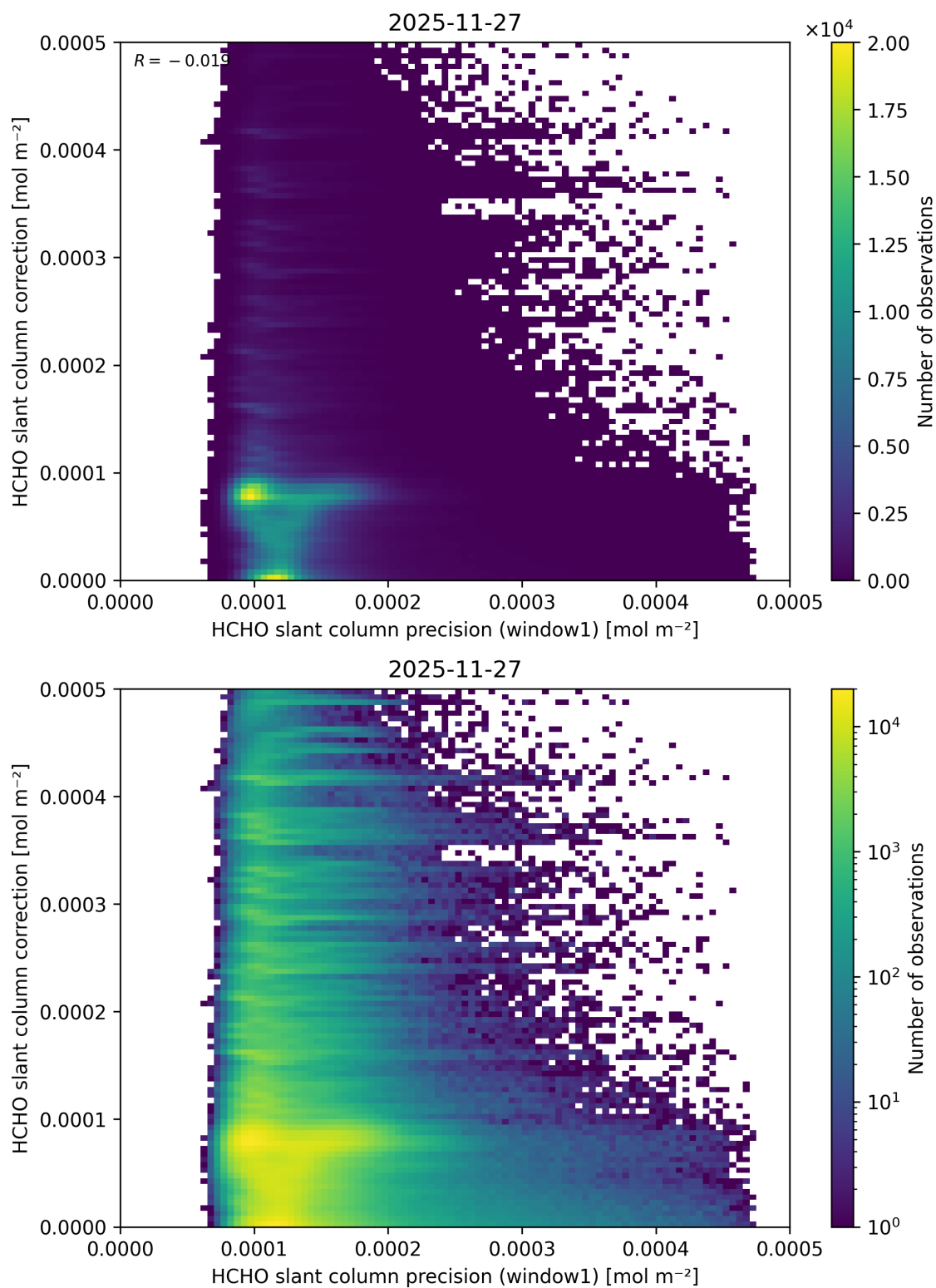
Figure 104: Scatter density plot of “HCHO slant column precision (window1)” against “HCHO slant column correction” for 2025-11-26 to 2025-11-28.
