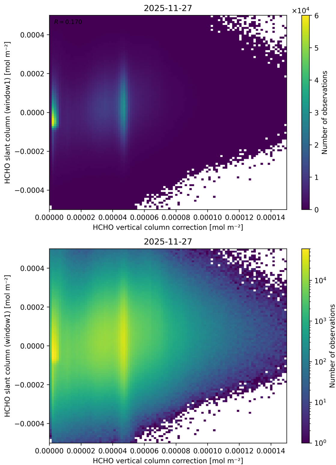
Figure 132: Scatter density plot of “HCHO vertical column correction” against “HCHO slant column (window1)” for 2025-11-26 to 2025-11-28.
