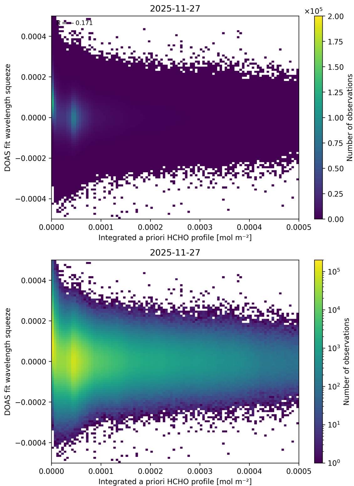
Figure 167: Scatter density plot of “Integrated a priori HCHO profile” against “DOAS fit wavelength squeeze” for 2025-11-26 to 2025-11-28.
