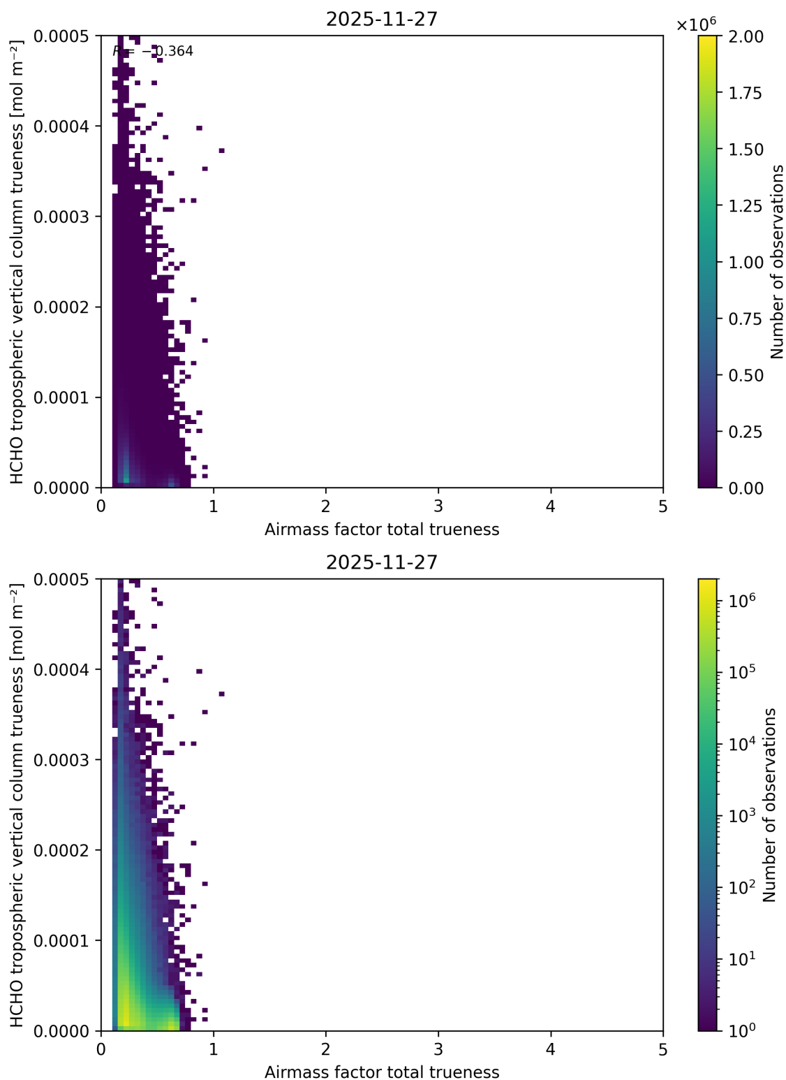
Figure 124: Scatter density plot of “Airmass factor total trueness” against “HCHO tropospheric vertical column trueness” for 2025-11-26 to 2025-11-28.
