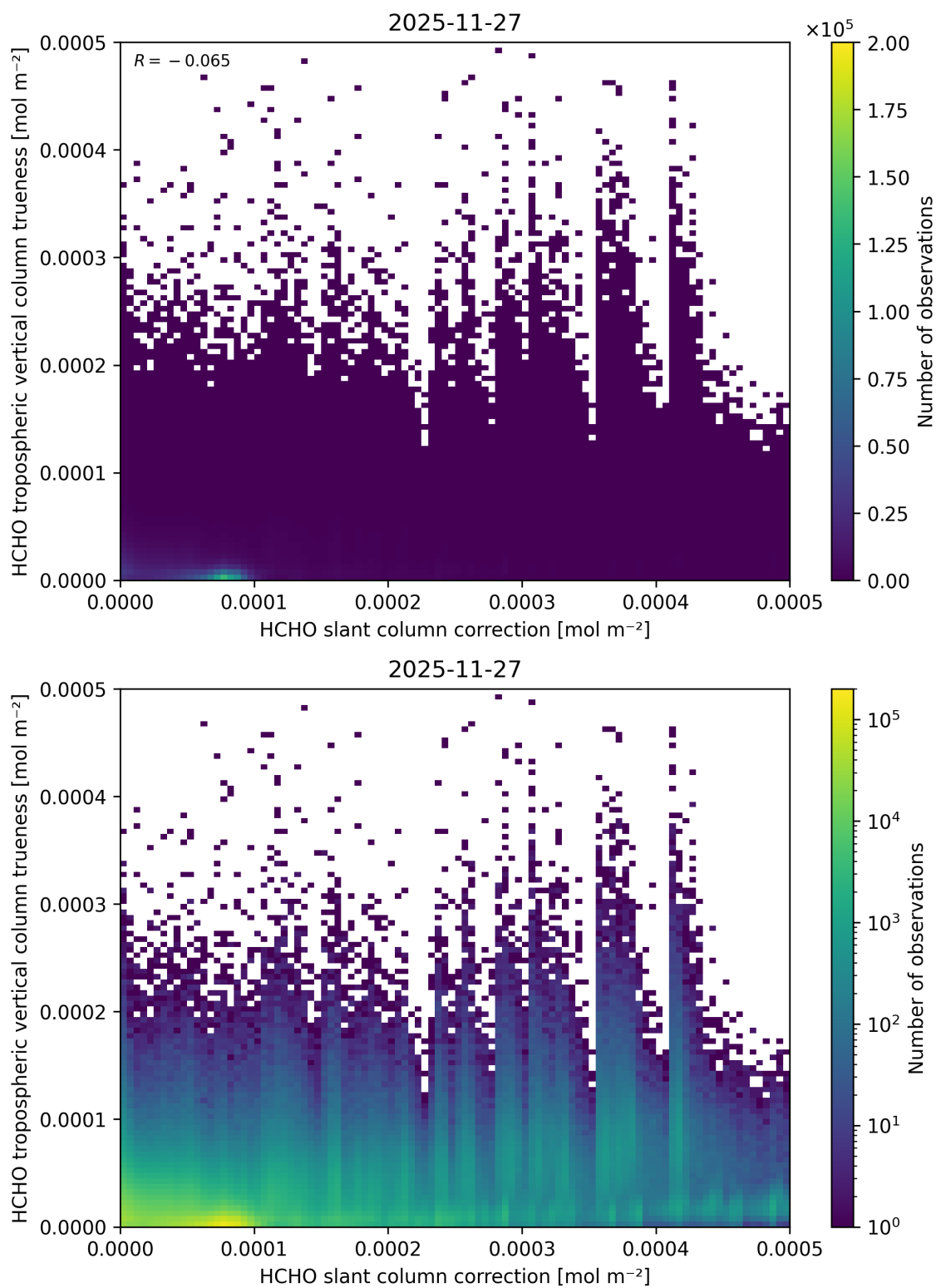
Figure 87: Scatter density plot of “HCHO slant column correction” against “HCHO tropospheric vertical column trueness” for 2025-11-26 to 2025-11-28.
