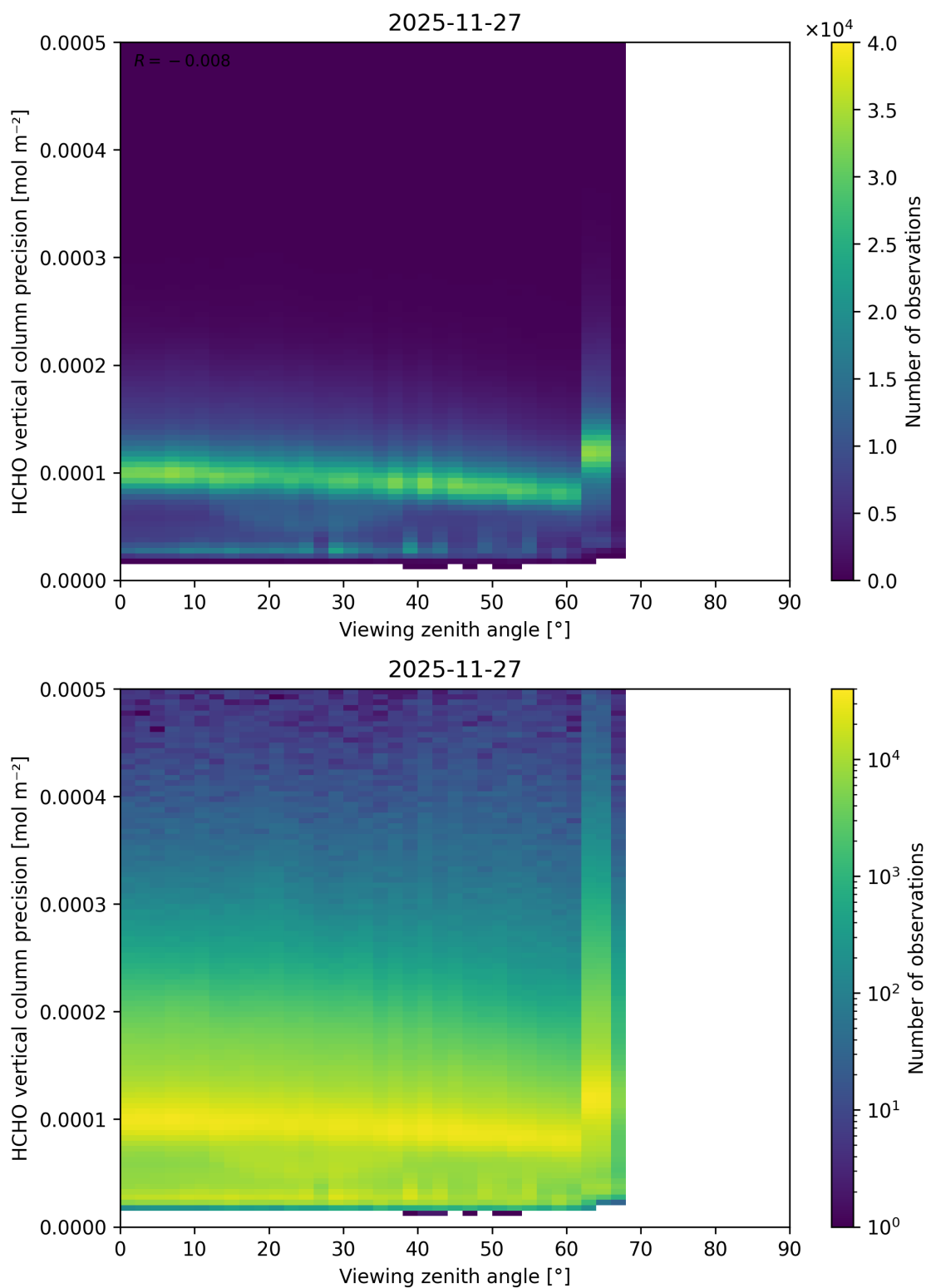
Figure 214: Scatter density plot of “Viewing zenith angle” against “HCHO vertical column precision” for 2025-11-26 to 2025-11-28.
