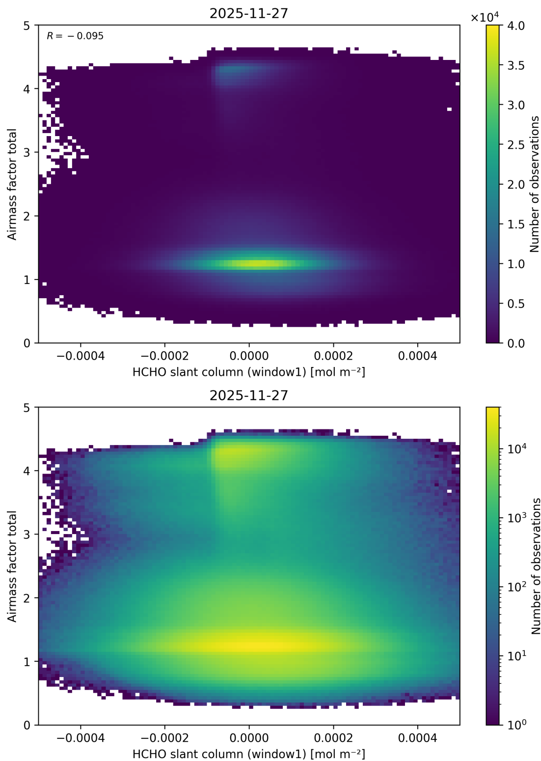
Figure 95: Scatter density plot of “HCHO slant column (window1)” against “Airmass factor total” for 2025-11-26 to 2025-11-28.
