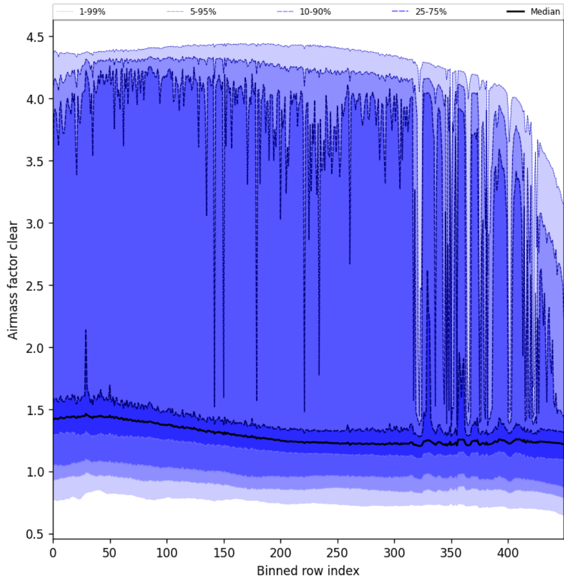
Figure 59: Along track statistics of “Airmass factor clear” for 2025-11-26 to 2025-11-28
