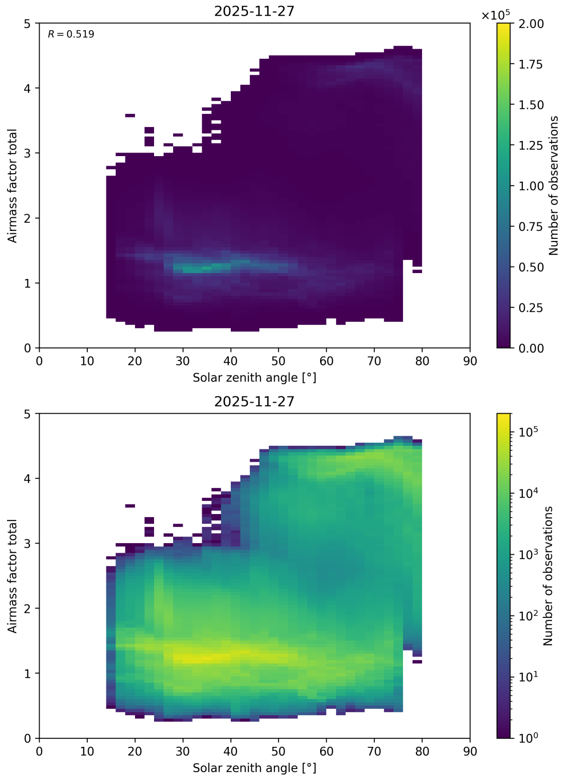
Figure 194: Scatter density plot of “Solar zenith angle” against “Airmass factor total” for 2025-11-26 to 2025-11-28.
