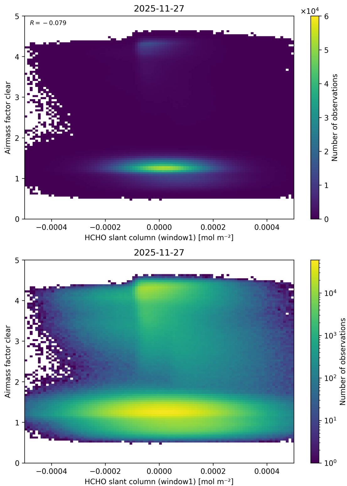
Figure 91: Scatter density plot of “HCHO slant column (window1)” against “Airmass factor clear” for 2025-11-26 to 2025-11-28.
