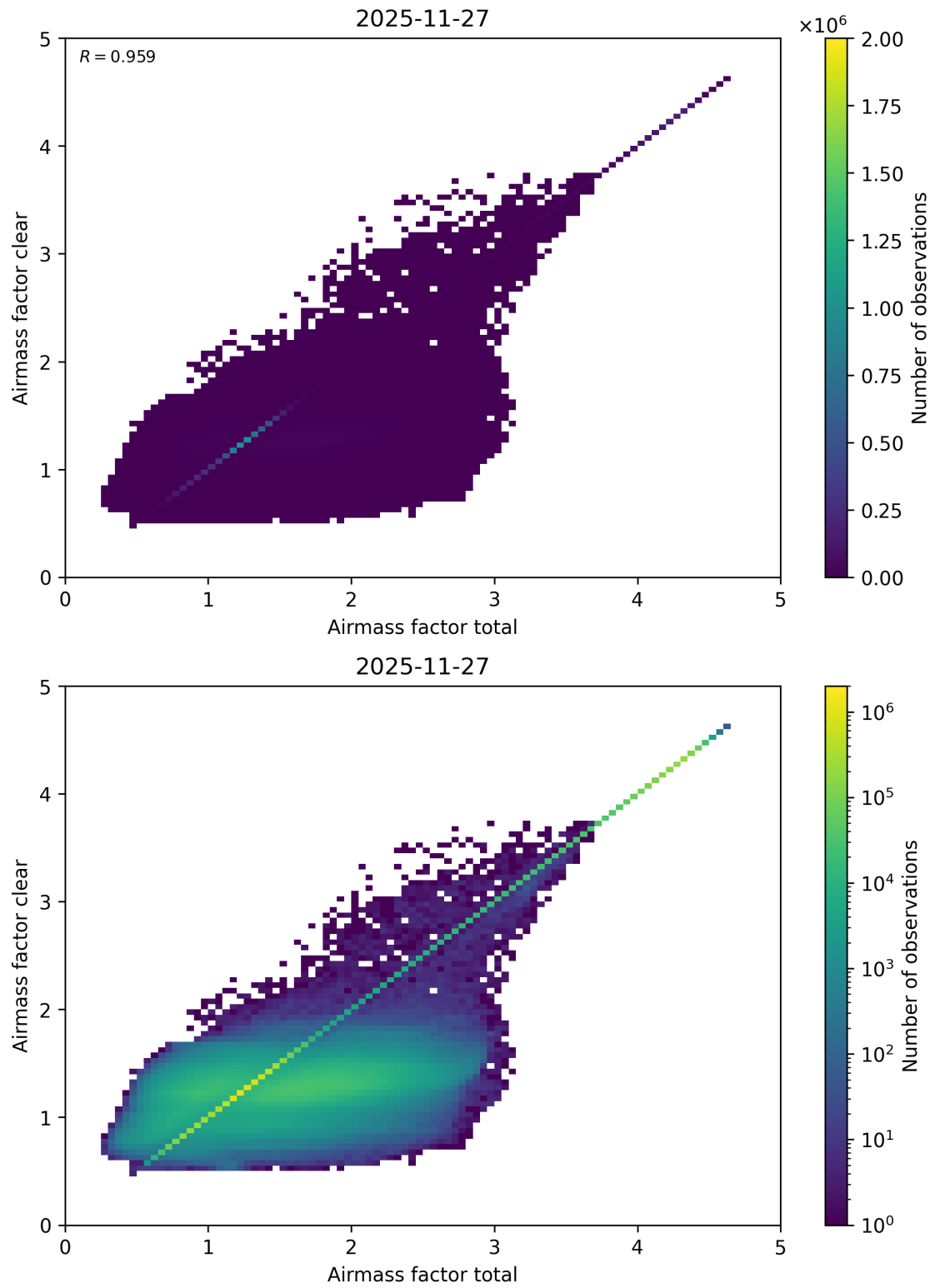
Figure 112: Scatter density plot of “Airmass factor total” against “Airmass factor clear” for 2025-11-26 to 2025-11-28.
