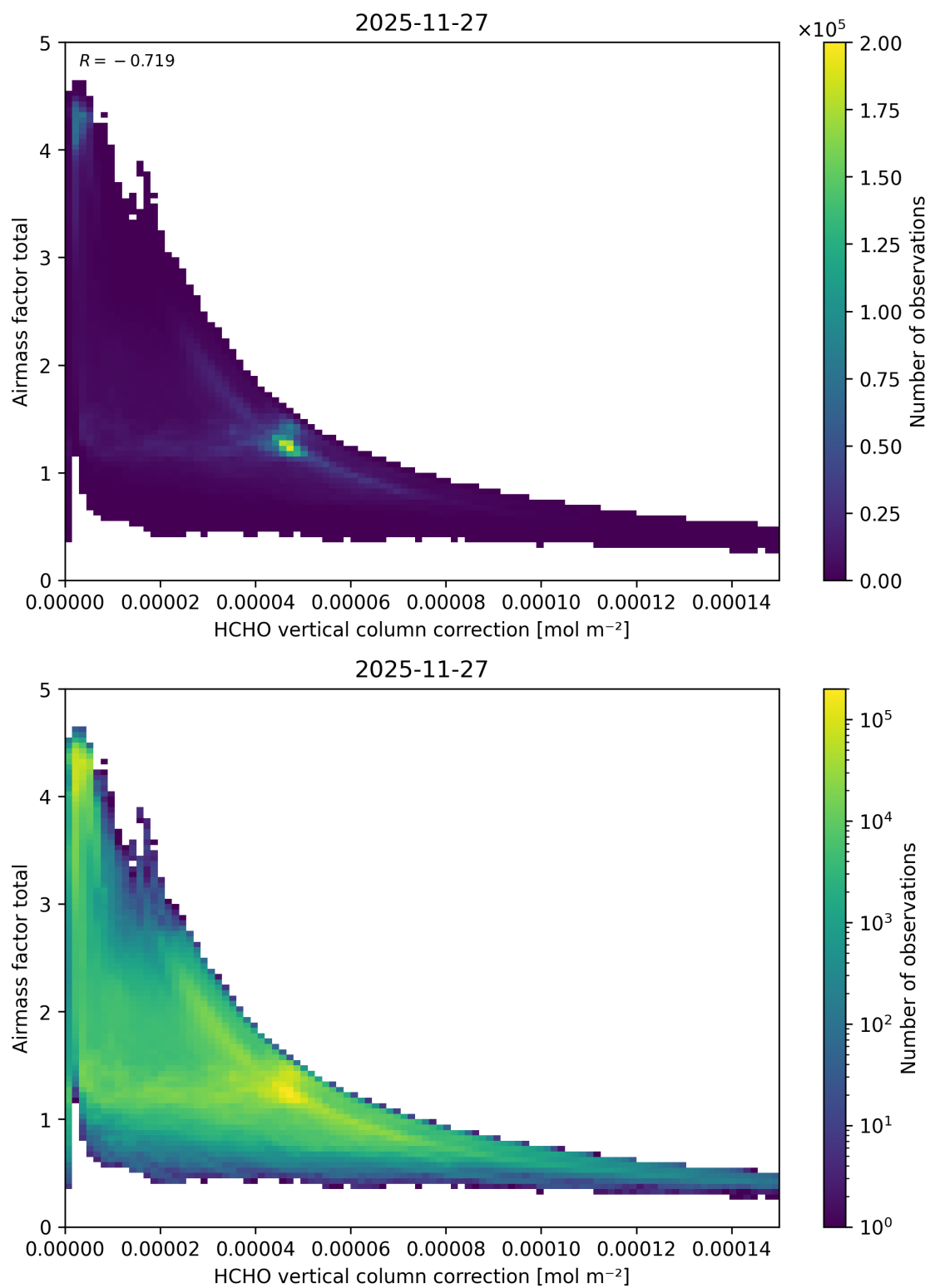
Figure 134: Scatter density plot of “HCHO vertical column correction” against “Airmass factor total” for 2025-11-26 to 2025-11-28.
