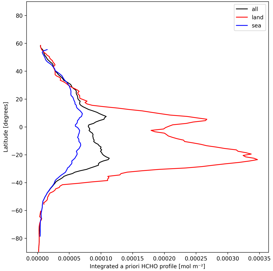
Figure 30: Zonal average of “Integrated a priori HCHO profile” for 2025-11-26 to 2025-11-28.
