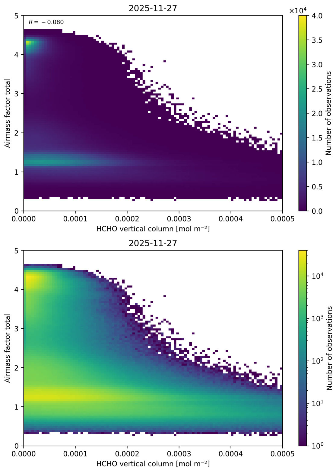
Figure 146: Scatter density plot of “HCHO vertical column” against “Airmass factor total” for 2025-11-26 to 2025-11-28.
