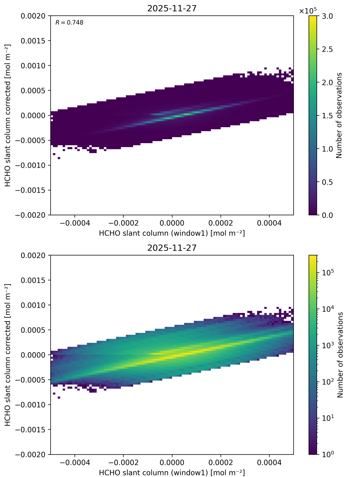
Figure 92: Scatter density plot of “HCHO slant column (window1)” against “HCHO slant column corrected” for 2025-11-26 to 2025-11-28.
