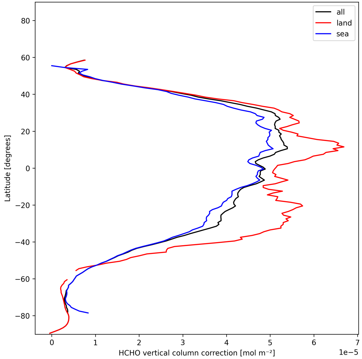
Figure 24: Zonal average of "HCHO vertical column correction" for 2025-11-26 to 2025-11-28.
