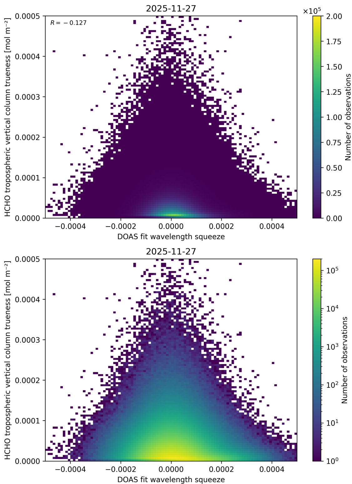
Figure 77: Scatter density plot of “DOAS fit wavelength squeeze” against “HCHO tropospheric vertical column trueness” for 2025-11-26 to 2025-11-28.
