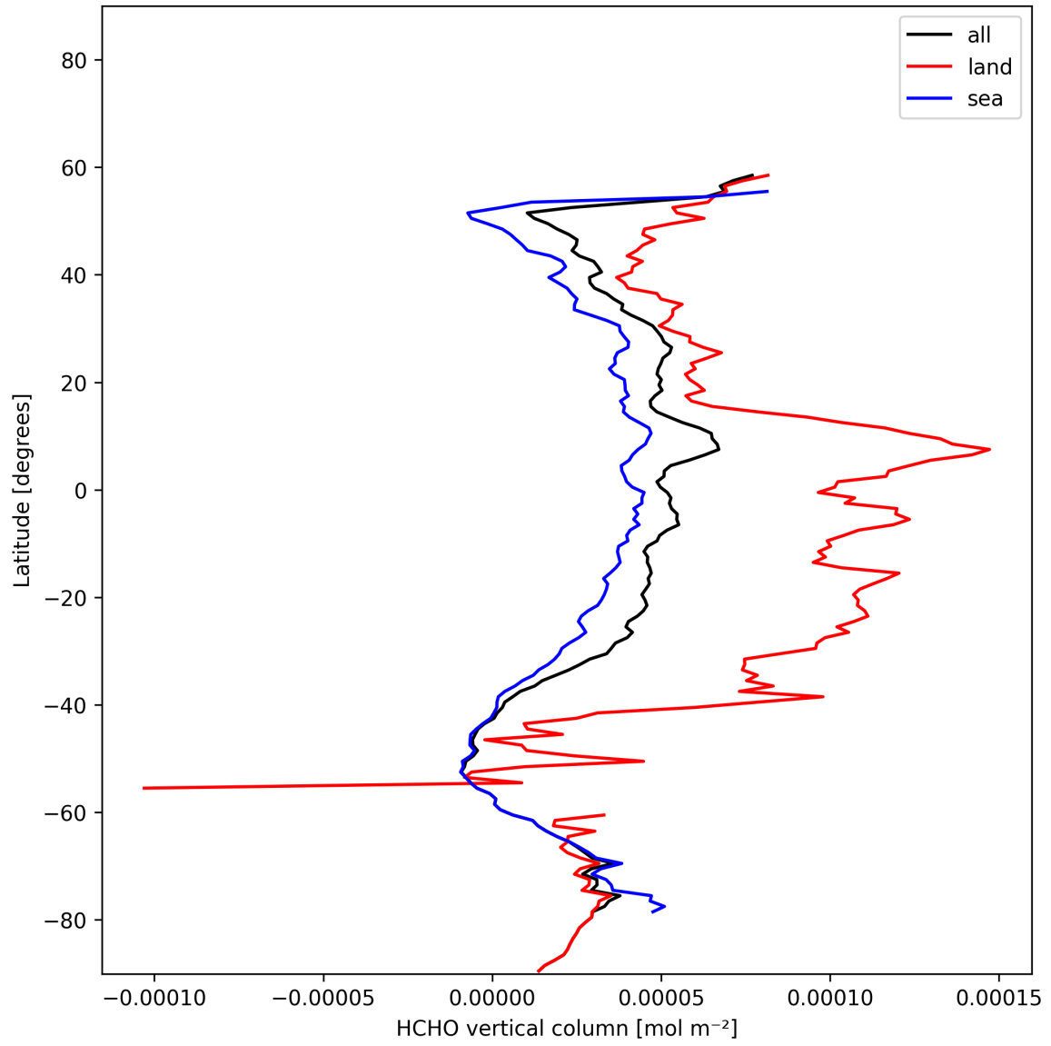
Figure 22: Zonal average of “HCHO vertical column” for 2025-11-26 to 2025-11-28.
