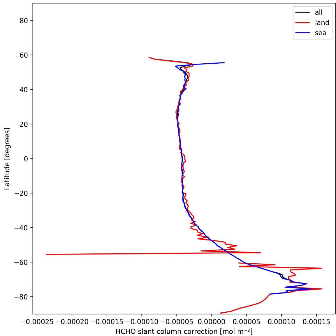
Figure 34: Zonal average of “HCHO slant column correction” for 2025-11-26 to 2025-11-28.
