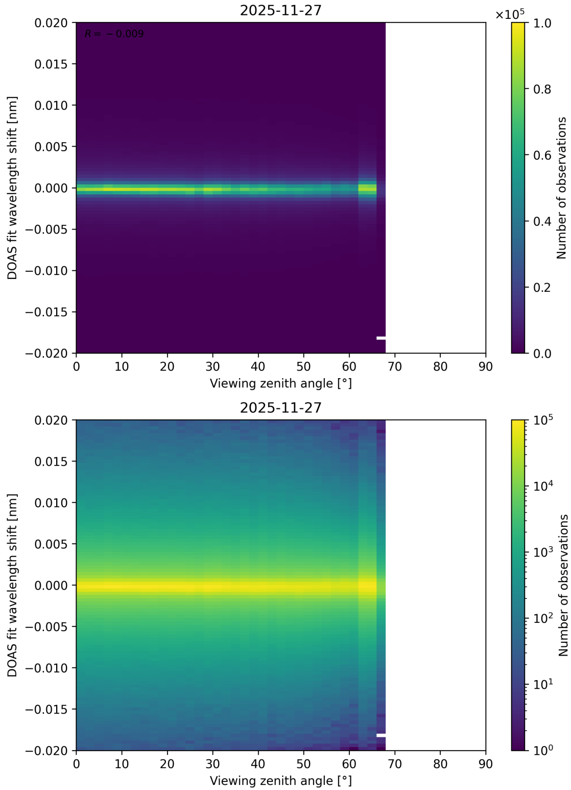
Figure 203: Scatter density plot of “Viewing zenith angle” against “DOAS fit wavelength shift” for 2025-11-26 to 2025-11-28.
