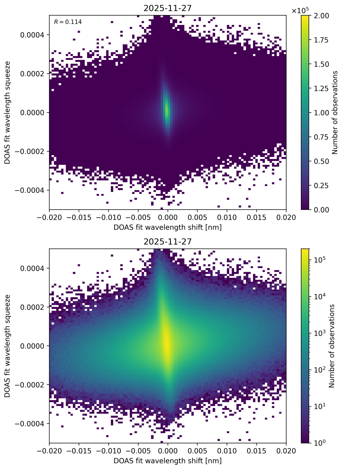
Figure 70: Scatter density plot of “DOAS fit wavelength shift” against “DOAS fit wavelength squeeze” for 2025-11-26 to 2025-11-28.
