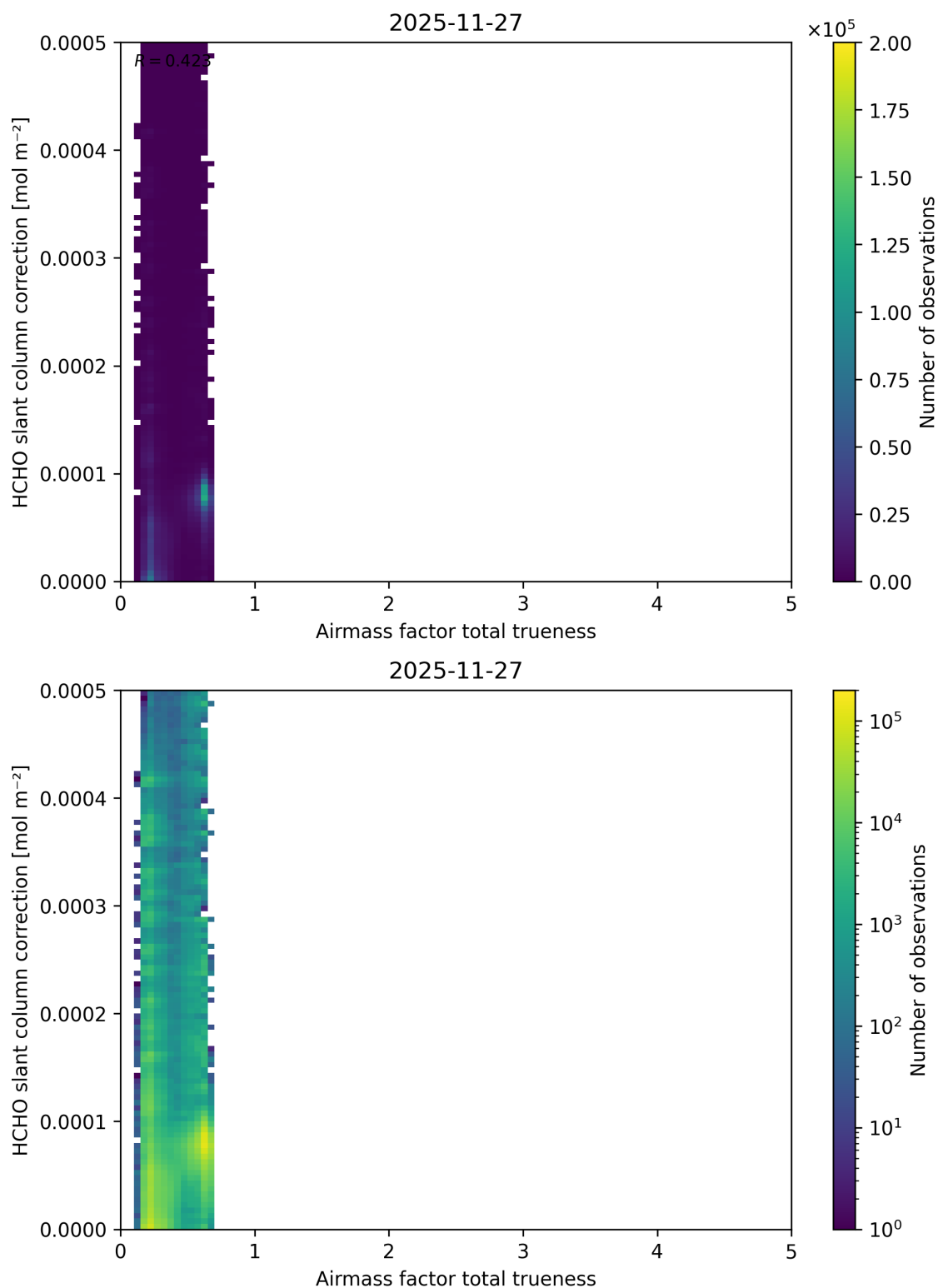
Figure 123: Scatter density plot of “Airmass factor total trueness” against “HCHO slant column correction” for 2025-11-26 to 2025-11-28.
