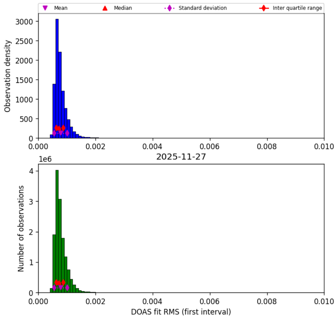
Figure 48: Histogram of “DOAS fit RMS (first interval)” for 2025-11-26 to 2025-11-28
