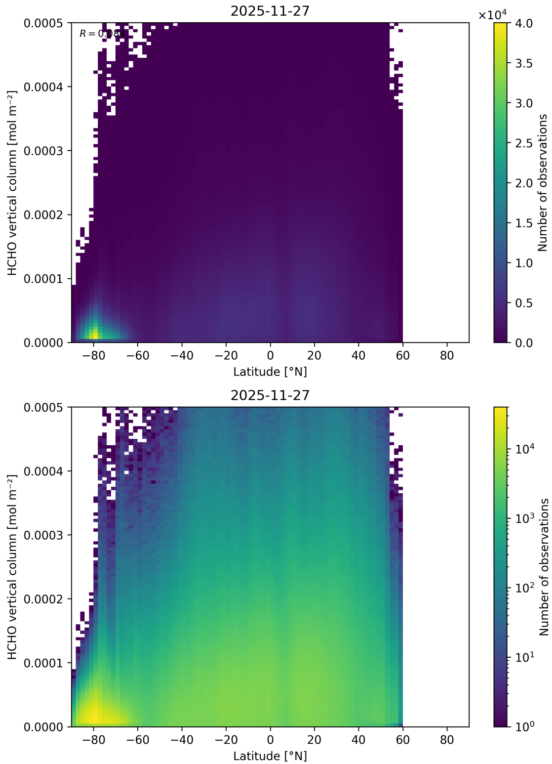
Figure 181: Scatter density plot of “Latitude” against “HCHO vertical column” for 2025-11-26 to 2025-11-28.
