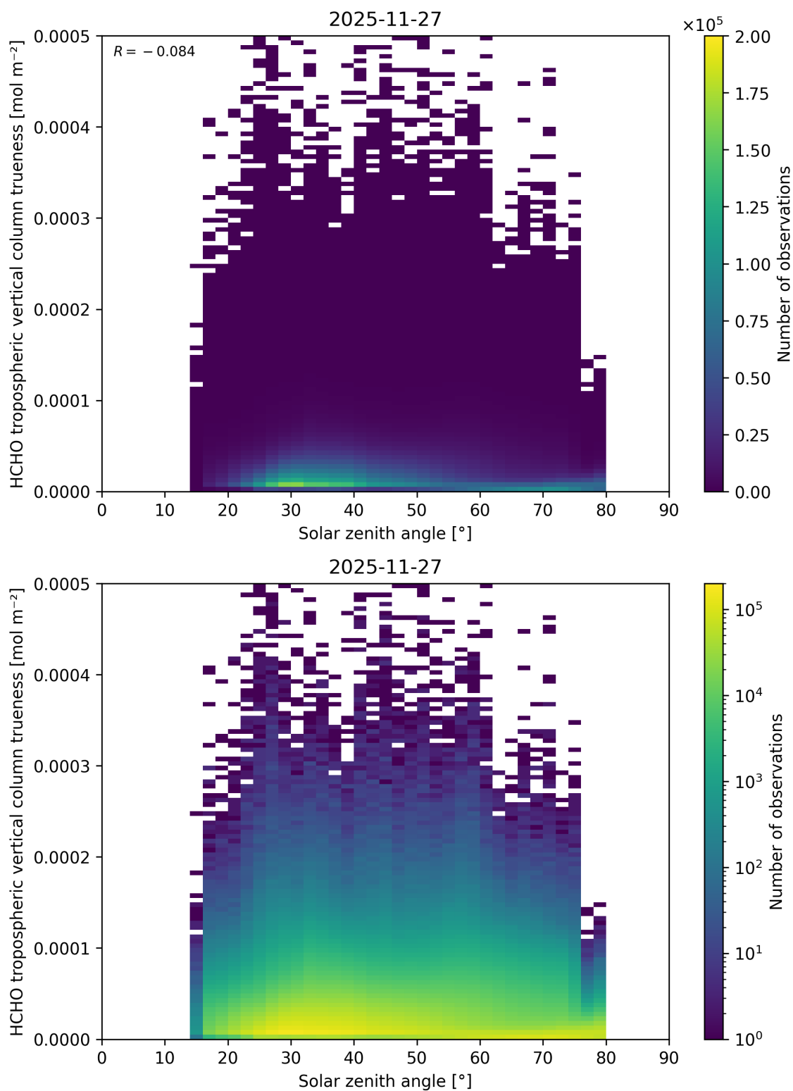
Figure 199: Scatter density plot of “Solar zenith angle” against “HCHO tropospheric vertical column trueness” for 2025-11-26 to 2025-11-28.
