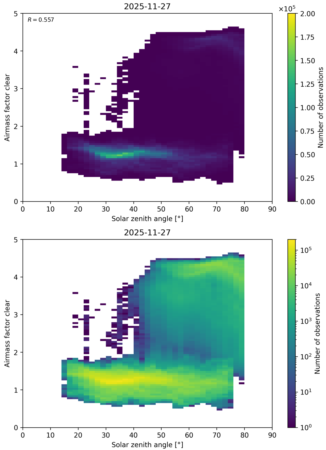
Figure 189: Scatter density plot of “Solar zenith angle” against “Airmass factor clear” for 2025-11-26 to 2025-11-28.
