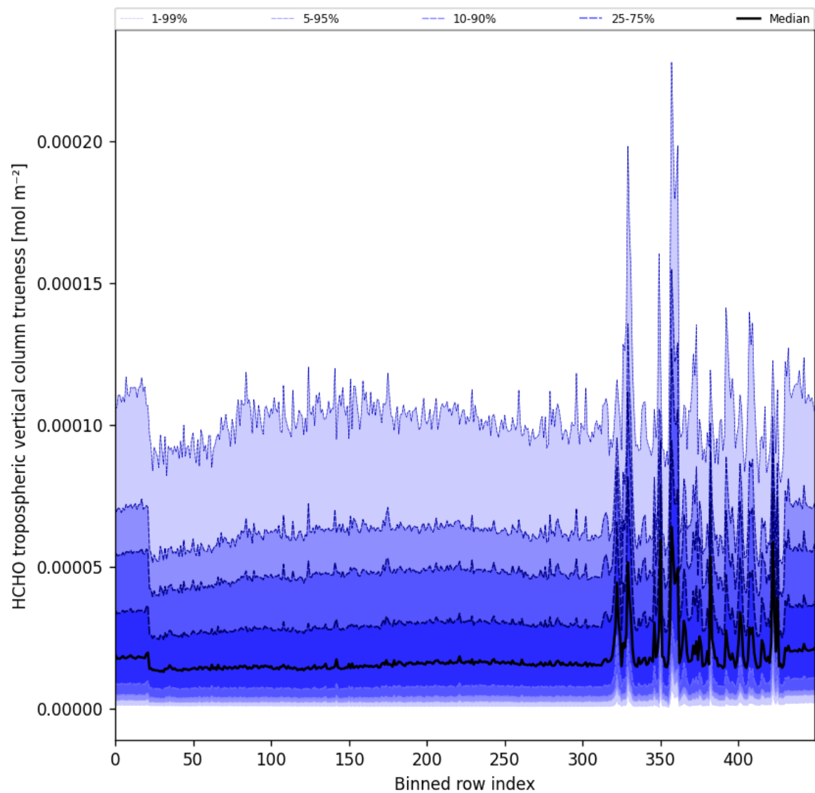
Figure 65: Along track statistics of “HCHO tropospheric vertical column trueness” for 2025-11-26 to 2025-11-28
