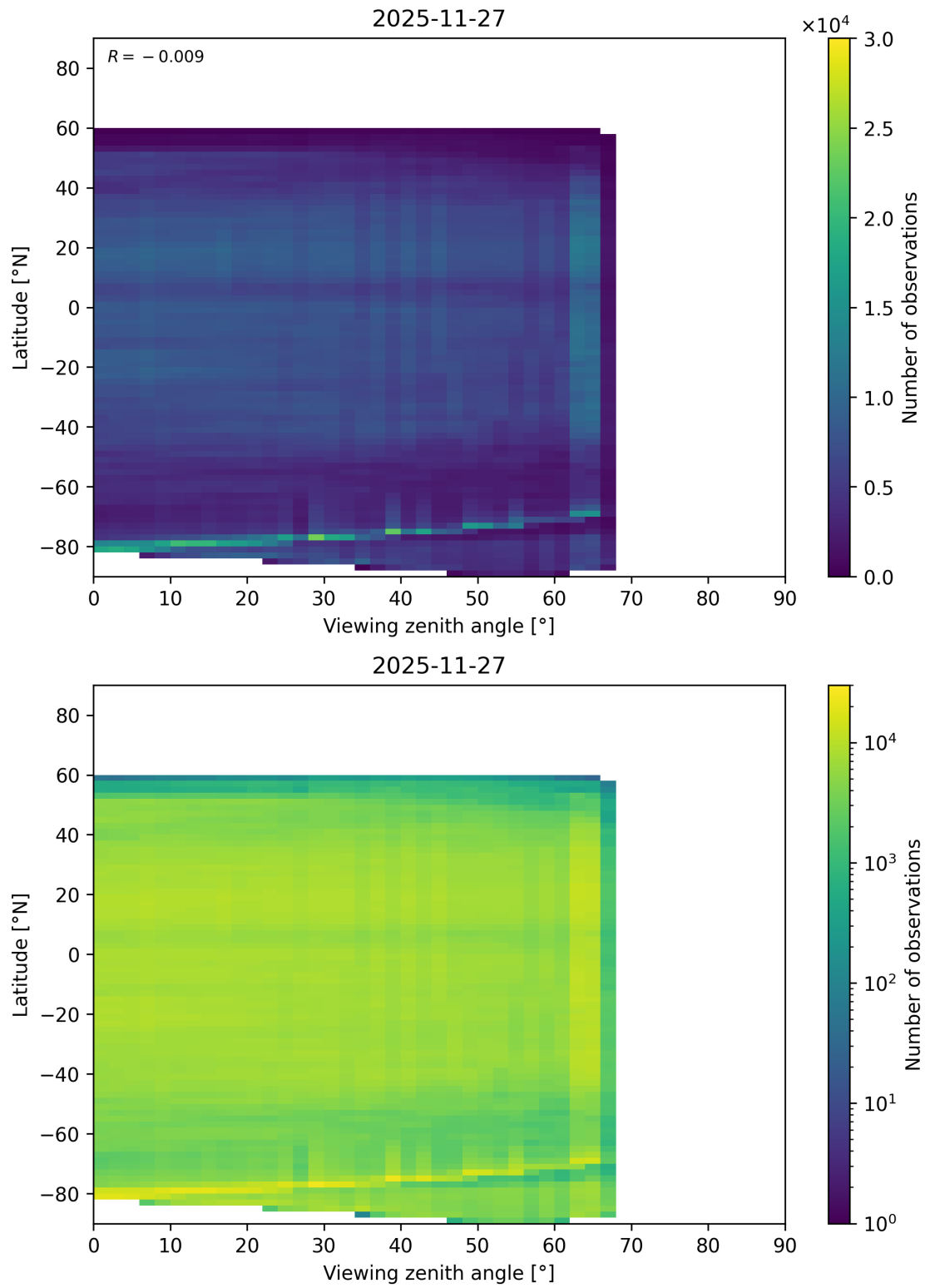
Figure 217: Scatter density plot of “Viewing zenith angle” against “Latitude” for 2025-11-26 to 2025-11-28.
