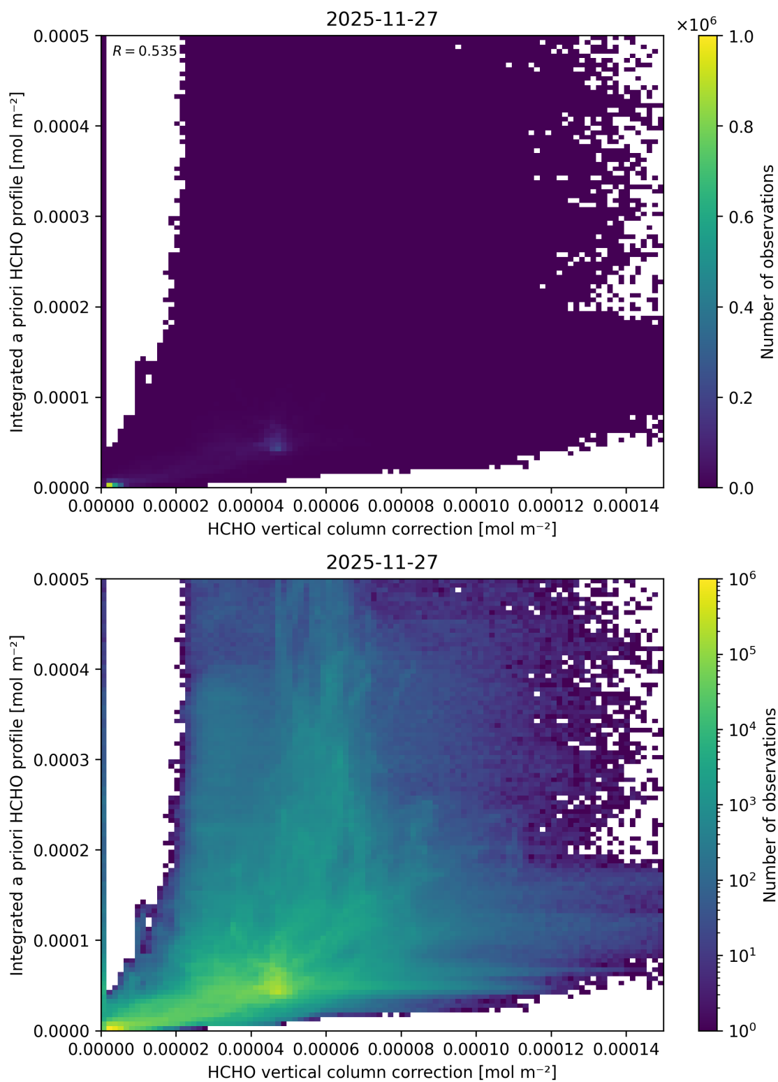
Figure 137: Scatter density plot of “HCHO vertical column correction” against “Integrated a priori HCHO profile” for 2025-11-26 to 2025-11-28.
