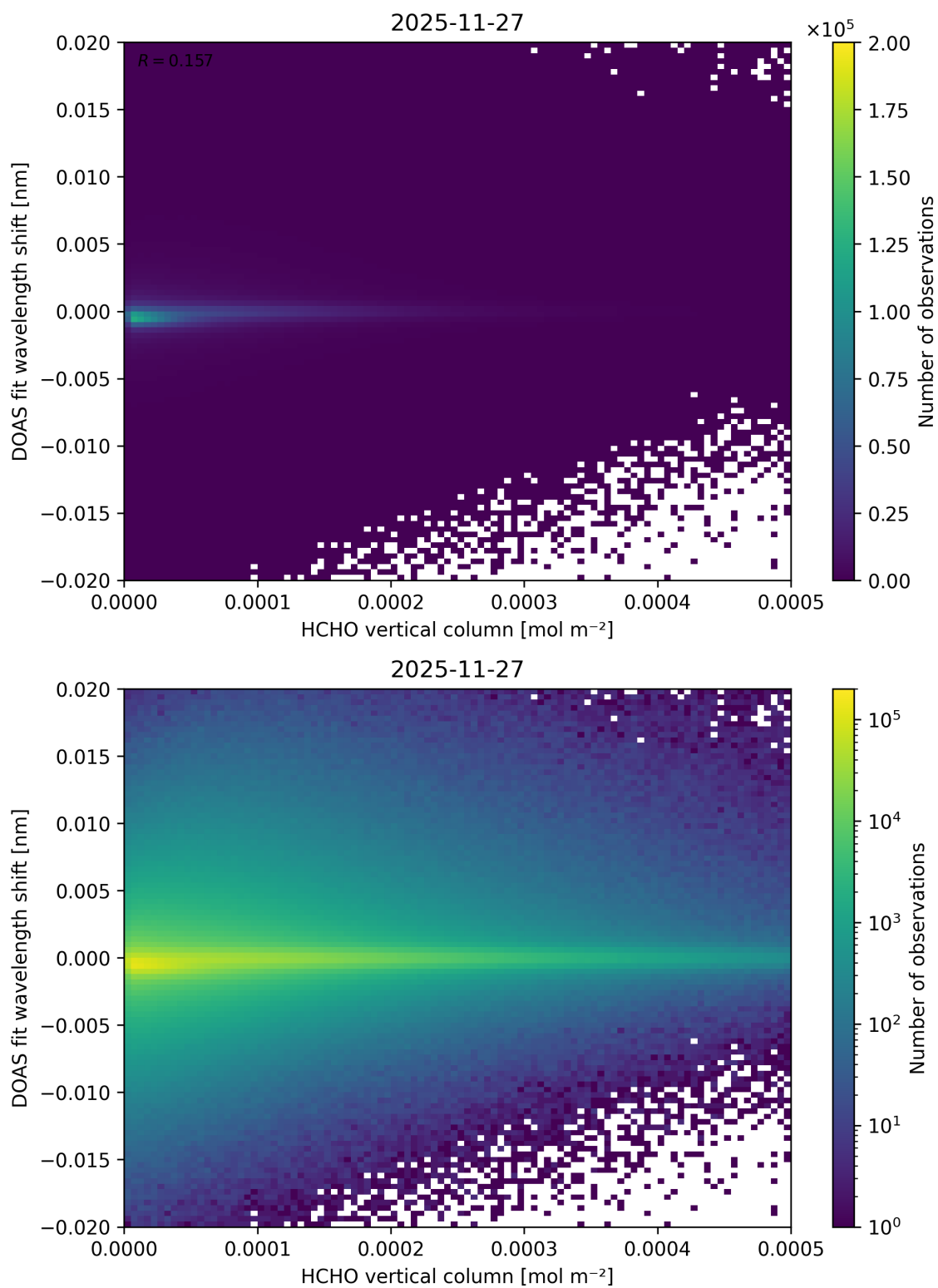
Figure 139: Scatter density plot of “HCHO vertical column” against “DOAS fit wavelength shift” for 2025-11-26 to 2025-11-28.
