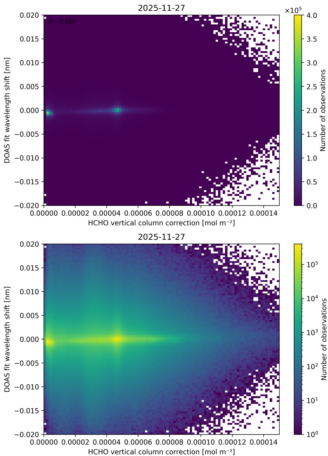
Figure 127: Scatter density plot of “HCHO vertical column correction” against “DOAS fit wavelength shift” for 2025-11-26 to 2025-11-28.
