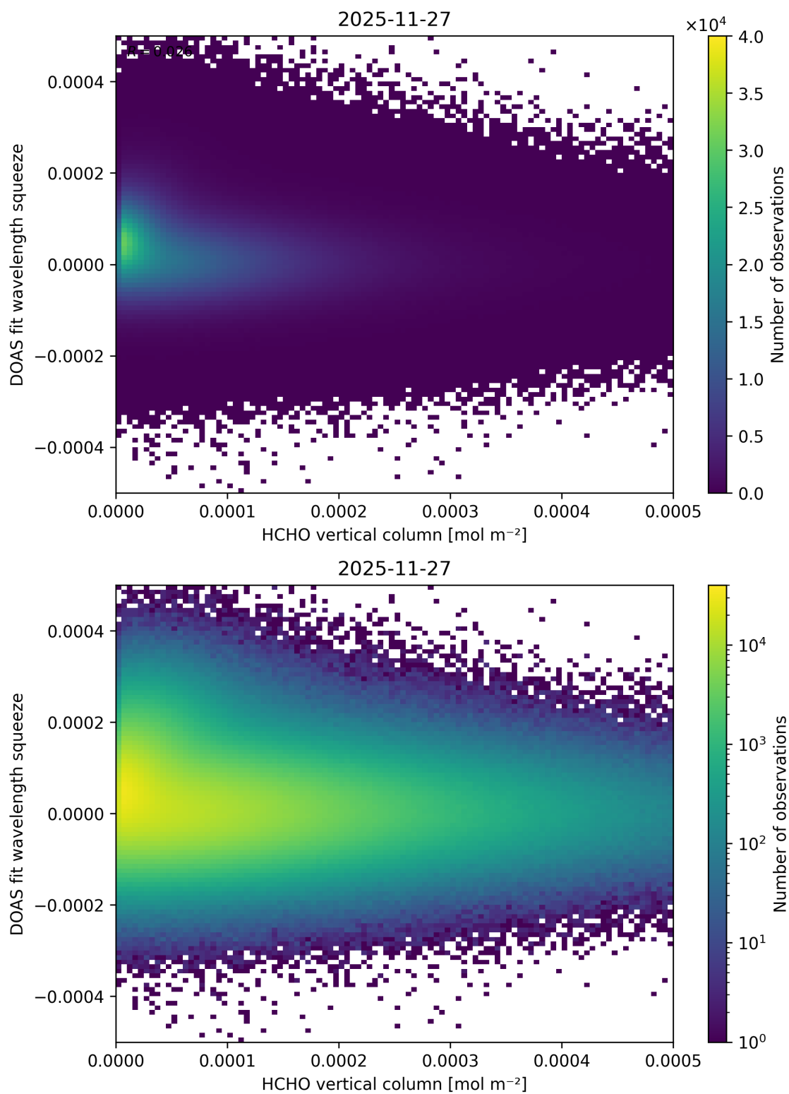
Figure 140: Scatter density plot of “HCHO vertical column” against “DOAS fit wavelength squeeze” for 2025-11-26 to 2025-11-28.
