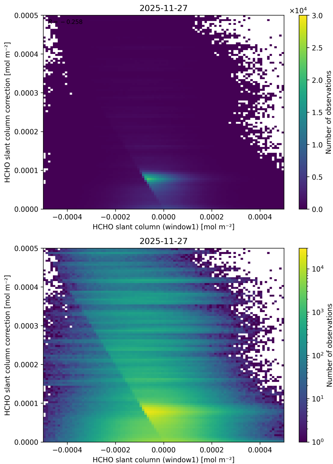
Figure 93: Scatter density plot of “HCHO slant column (window1)” against “HCHO slant column correction” for 2025-11-26 to 2025-11-28.
