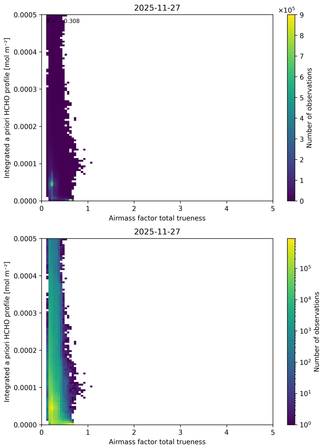
Figure 125: Scatter density plot of “Airmass factor total truiness” against “Integrated a priori HCHO profile” for 2025-11-26 to 2025-11-28.
