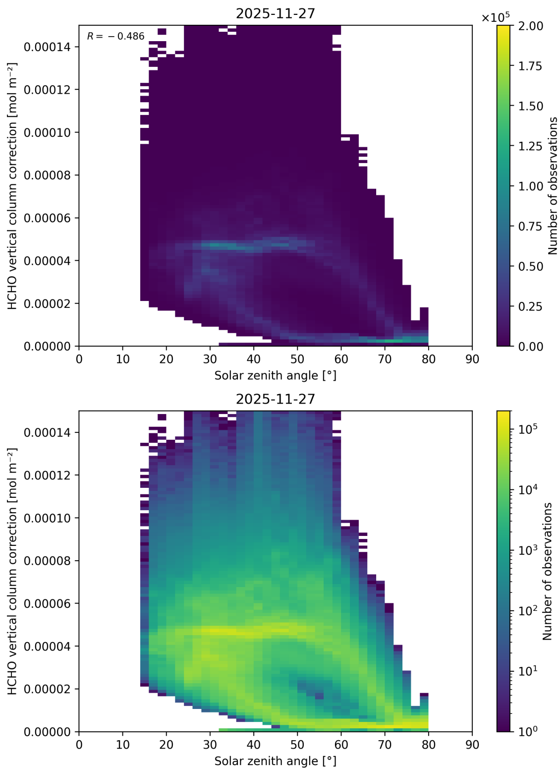
Figure 197: Scatter density plot of “Solar zenith angle” against “HCHO vertical column correction” for 2025-11-26 to 2025-11-28.
