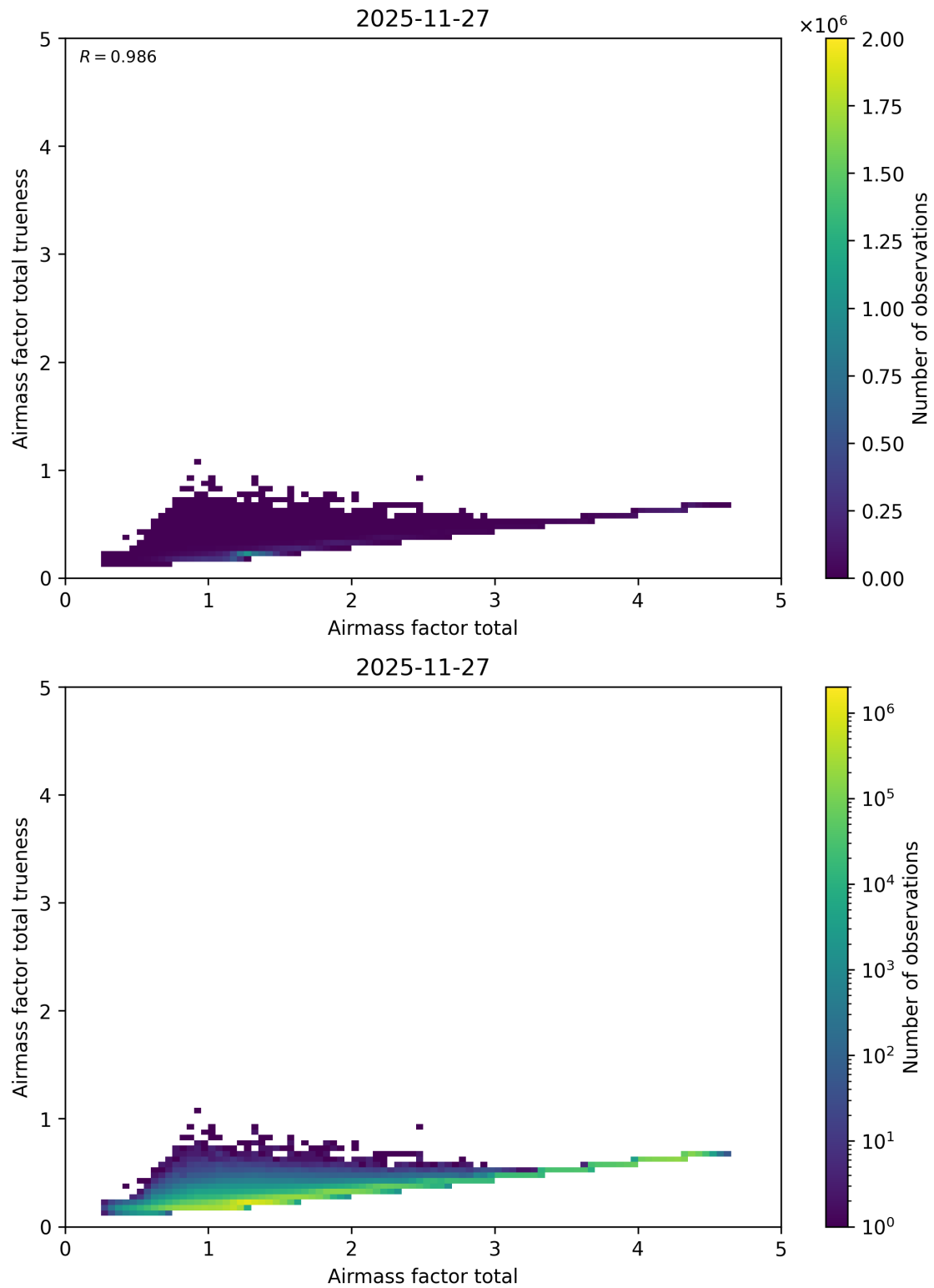
Figure 115: Scatter density plot of “Airmass factor total” against “Airmass factor total trueness” for 2025-11-26 to 2025-11-28.
