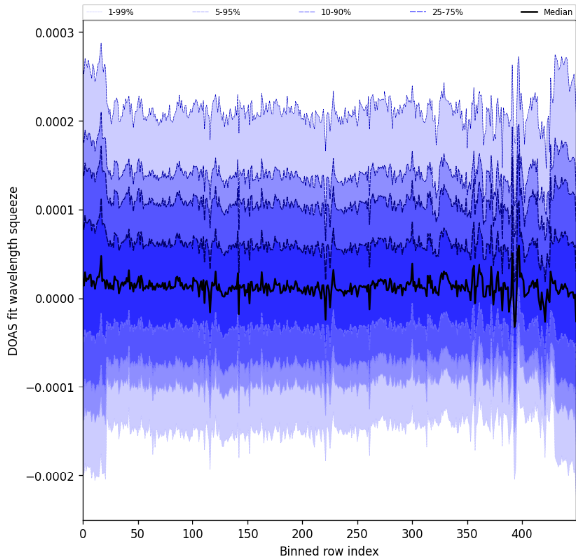
Figure 62: Along track statistics of “DOAS fit wavelength squeeze” for 2025-11-26 to 2025-11-28
