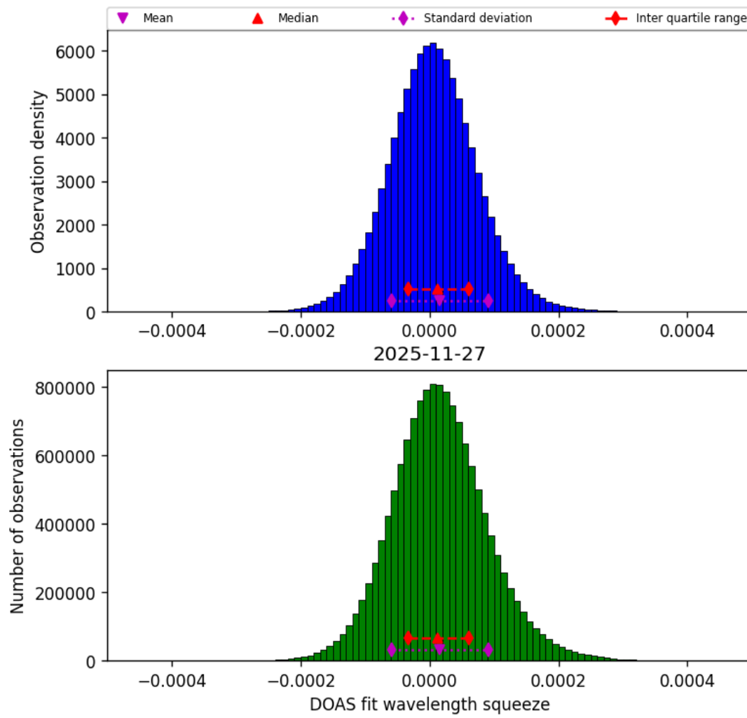
Figure 47: Histogram of “DOAS fit wavelength squeeze” for 2025-11-26 to 2025-11-28
