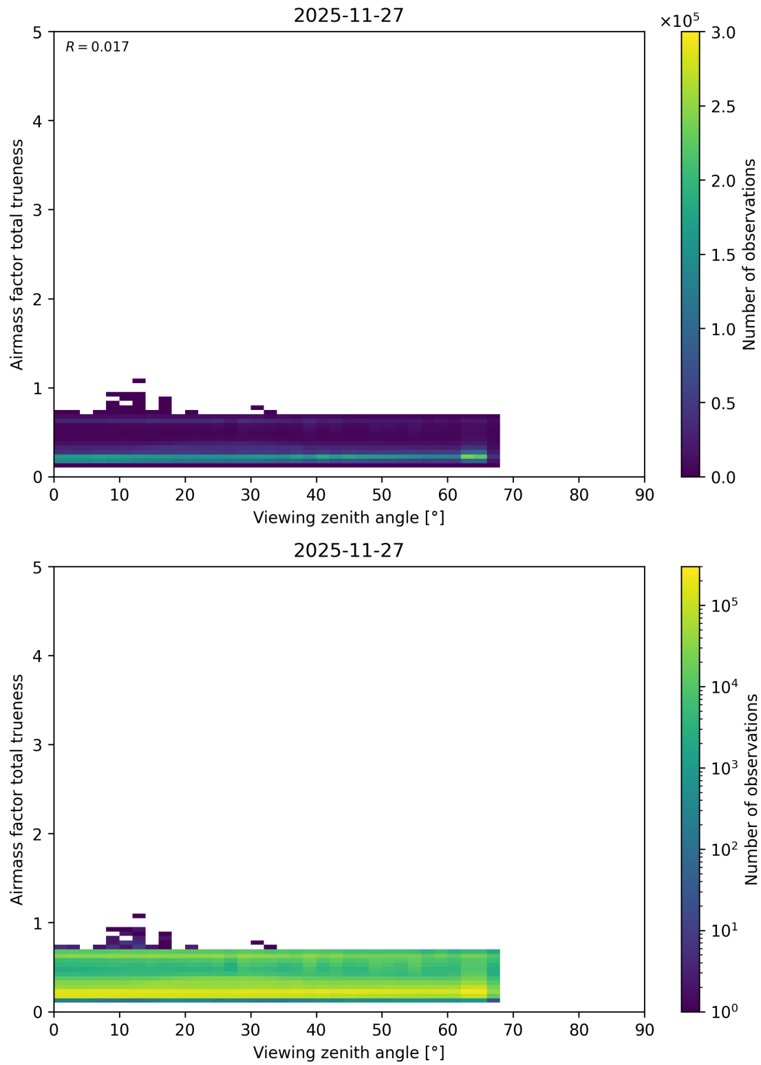
Figure 211: Scatter density plot of “Viewing zenith angle” against “Airmass factor total trueness” for 2025-11-26 to 2025-11-28.
