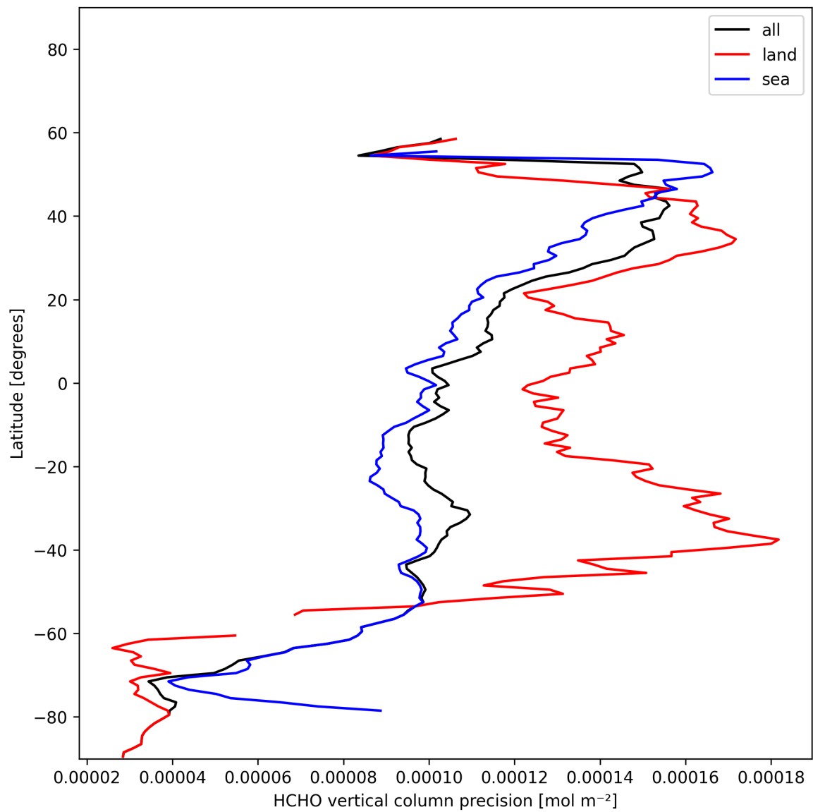
Figure 23: Zonal average of “HCHO vertical column precision” for 2025-11-26 to 2025-11-28.
