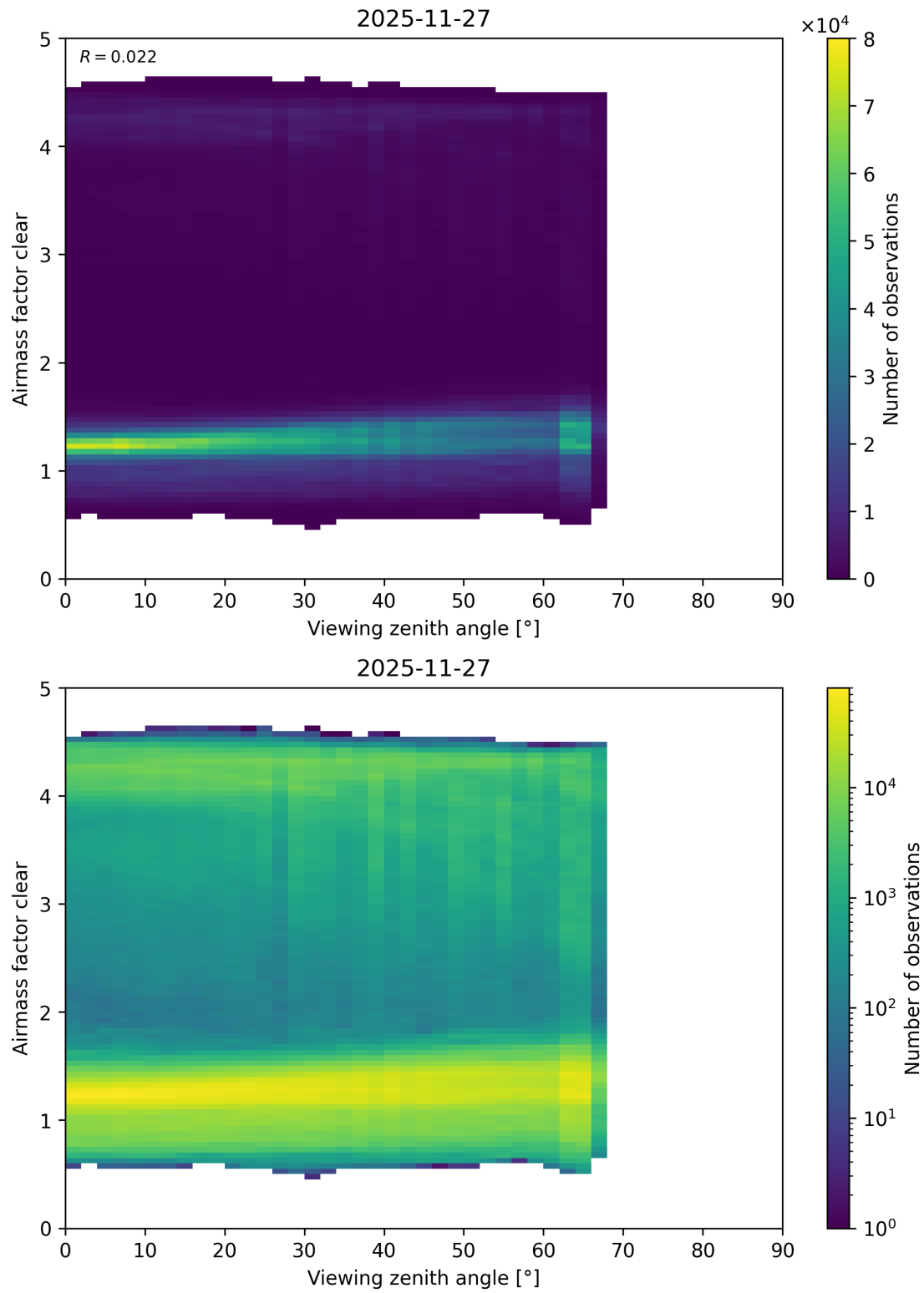
Figure 205: Scatter density plot of “Viewing zenith angle” against “Airmass factor clear” for 2025-11-26 to 2025-11-28.
