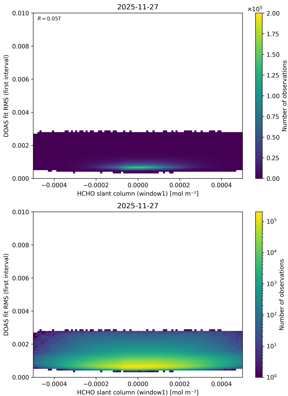
Figure 88: Scatter density plot of “HCHO slant column (window1)” against “DOAS fit RMS (first interval)” for 2025-11-26 to 2025-11-28.
