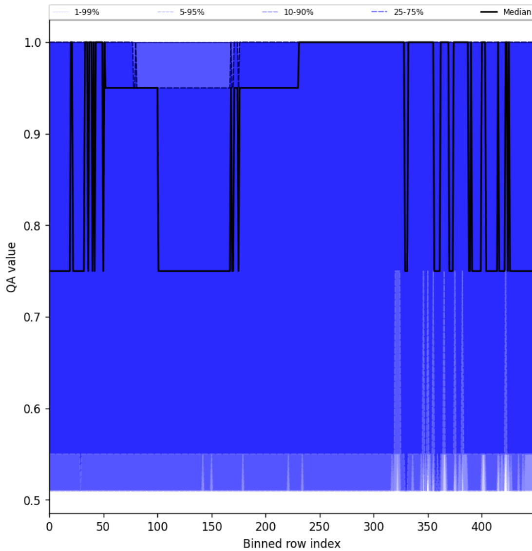
Figure 51: Along track statistics of “QA value” for 2025-11-26 to 2025-11-28
