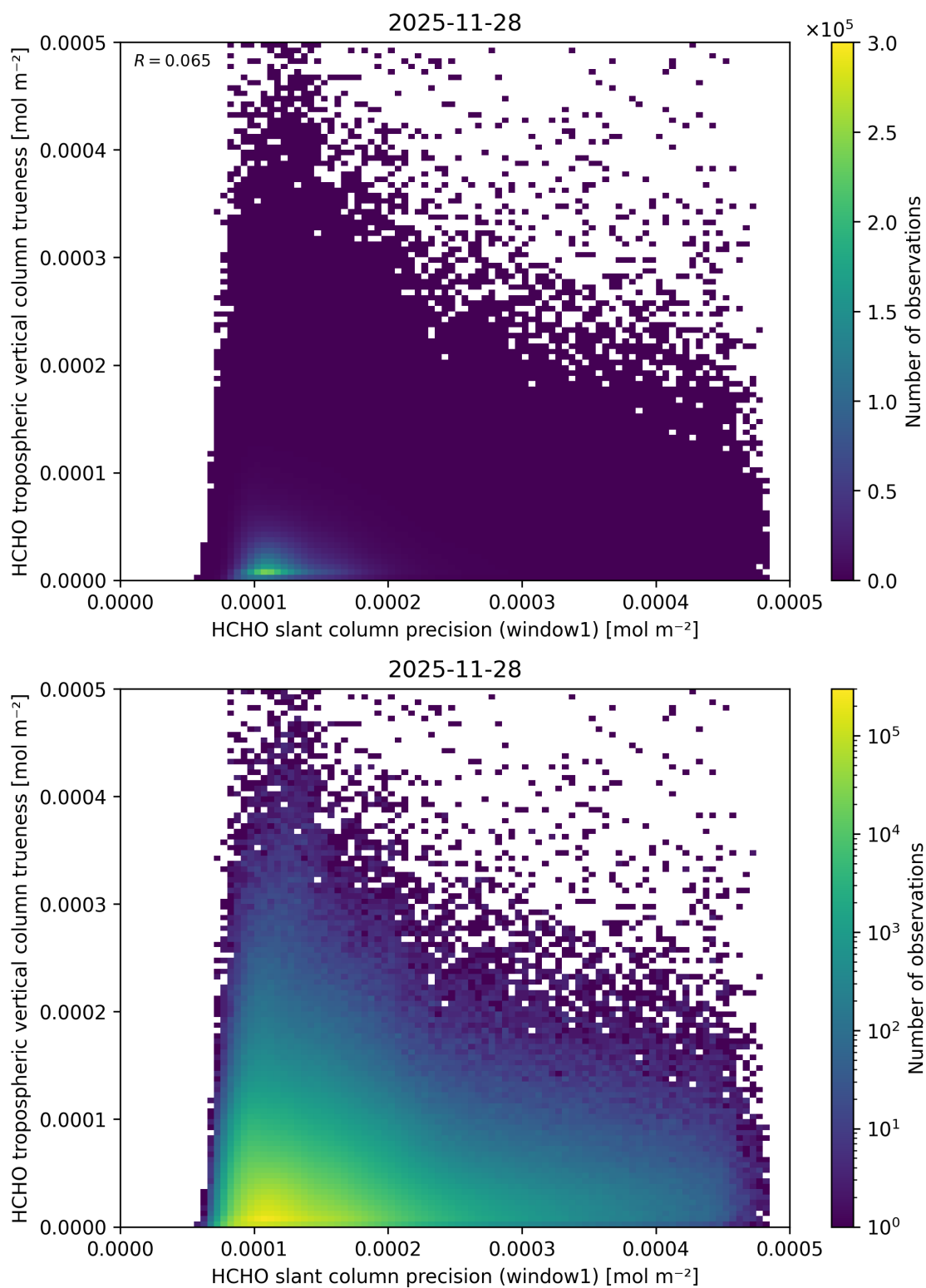
Figure 107: Scatter density plot of “HCHO slant column precision (window1)” against “HCHO tropospheric vertical column trueness” for 2025-11-28 to 2025-11-29.
