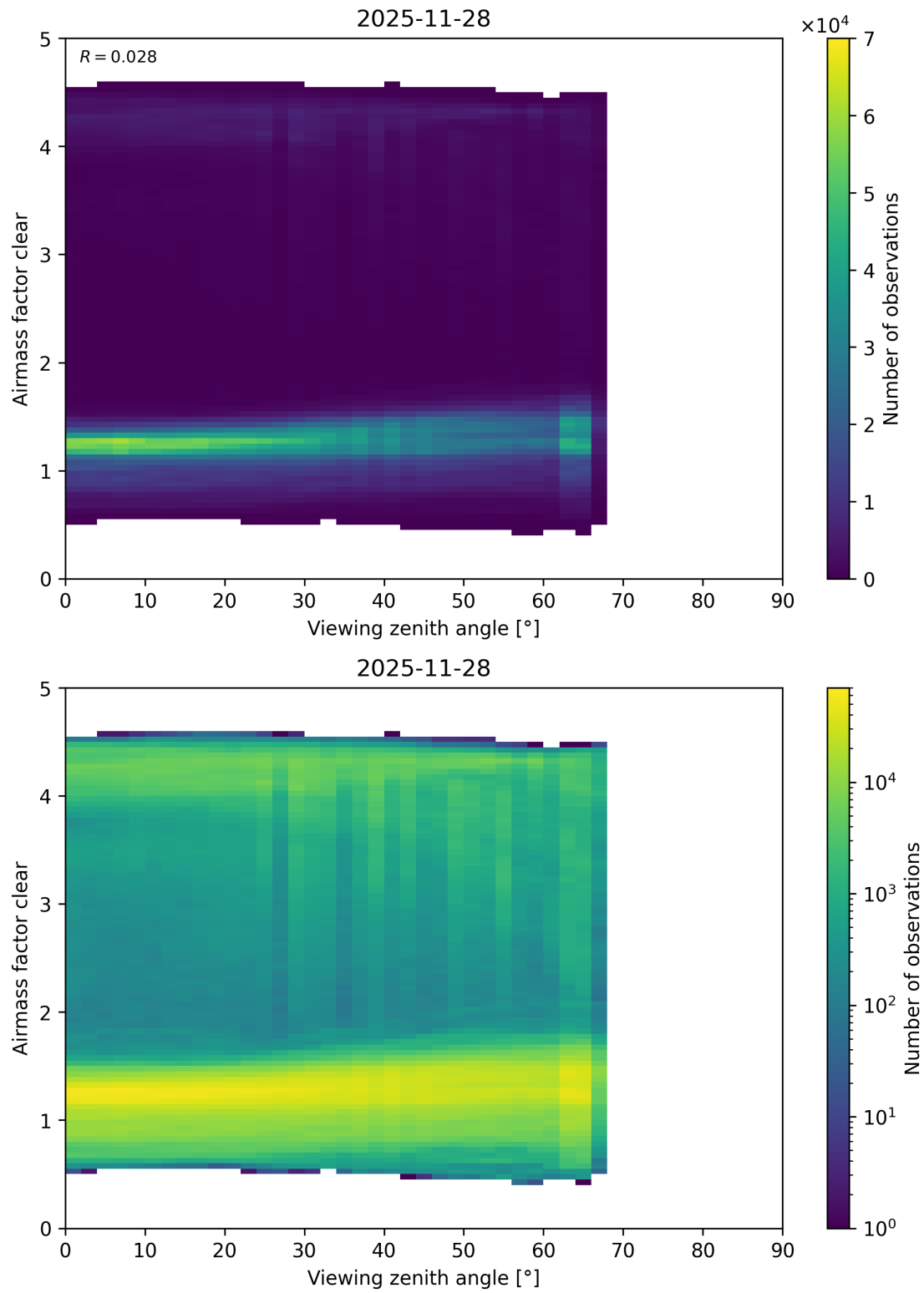
Figure 205: Scatter density plot of “Viewing zenith angle” against “Airmass factor clear” for 2025-11-28 to 2025-11-29.
