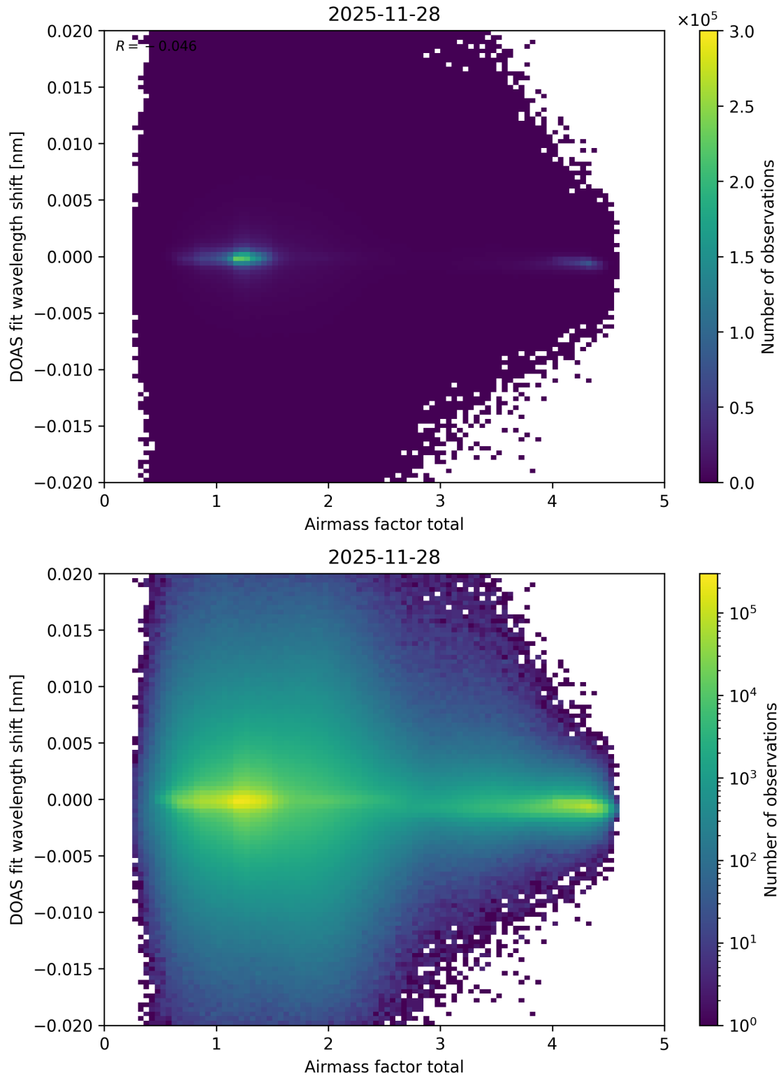
Figure 110: Scatter density plot of “Airmass factor total” against “DOAS fit wavelength shift” for 2025-11-28 to 2025-11-29.
