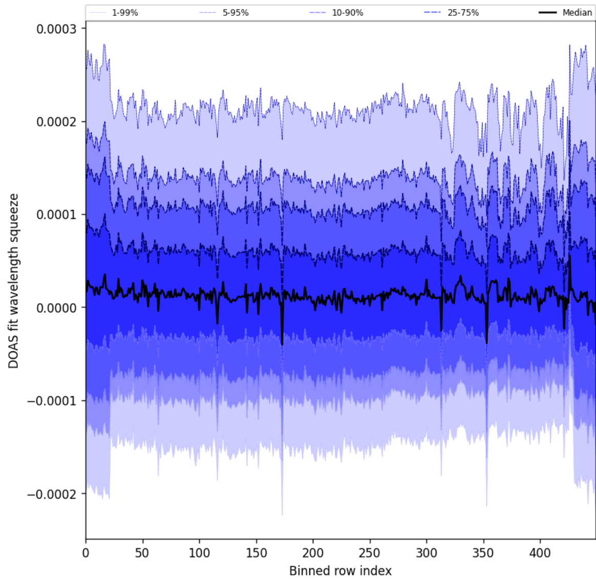
Figure 62: Along track statistics of “DOAS fit wavelength squeeze” for 2025-11-28 to 2025-11-29
