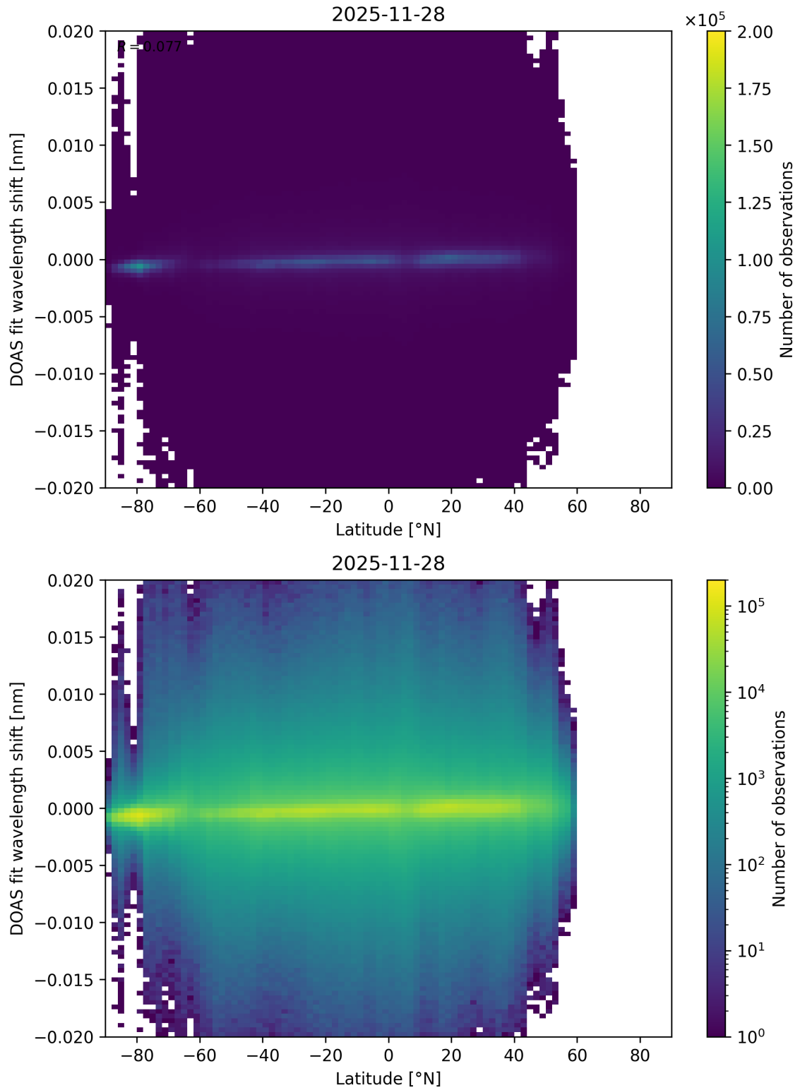
Figure 172: Scatter density plot of “Latitude” against “DOAS fit wavelength shift” for 2025-11-28 to 2025-11-29.
