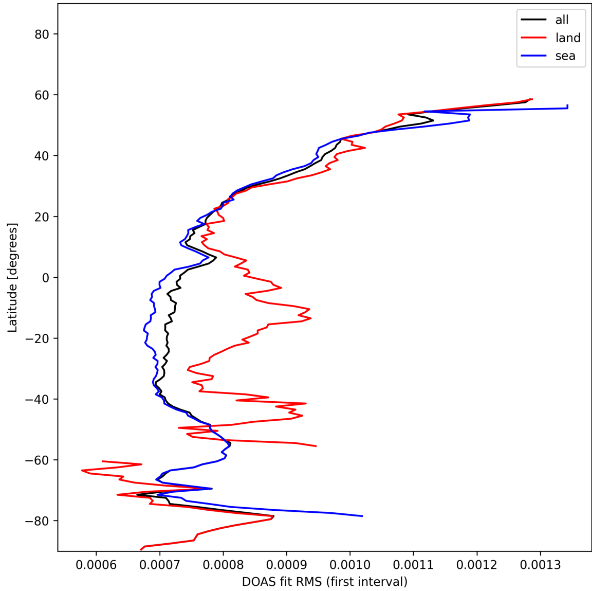
Figure 33: Zonal average of "DOAS fit RMS (first interval)" for 2025-11-28 to 2025-11-29.
