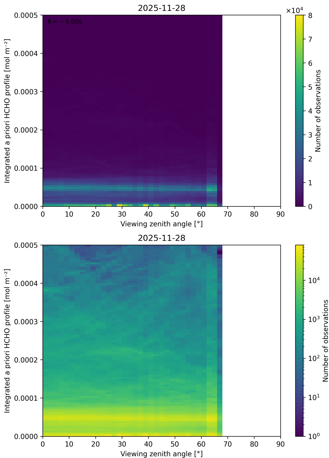
Figure 216: Scatter density plot of “Viewing zenith angle” against “Integrated a priori HCHO profile” for 2025-11-28 to 2025-11-29.
