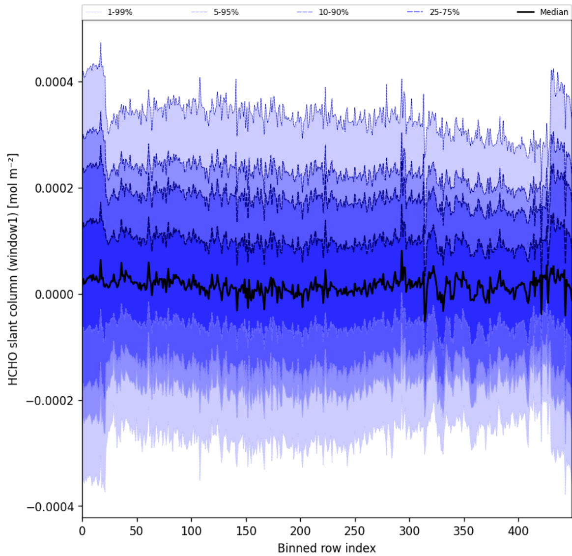
Figure 55: Along track statistics of “HCHO slant column (window1)” for 2025-11-28 to 2025-11-29
