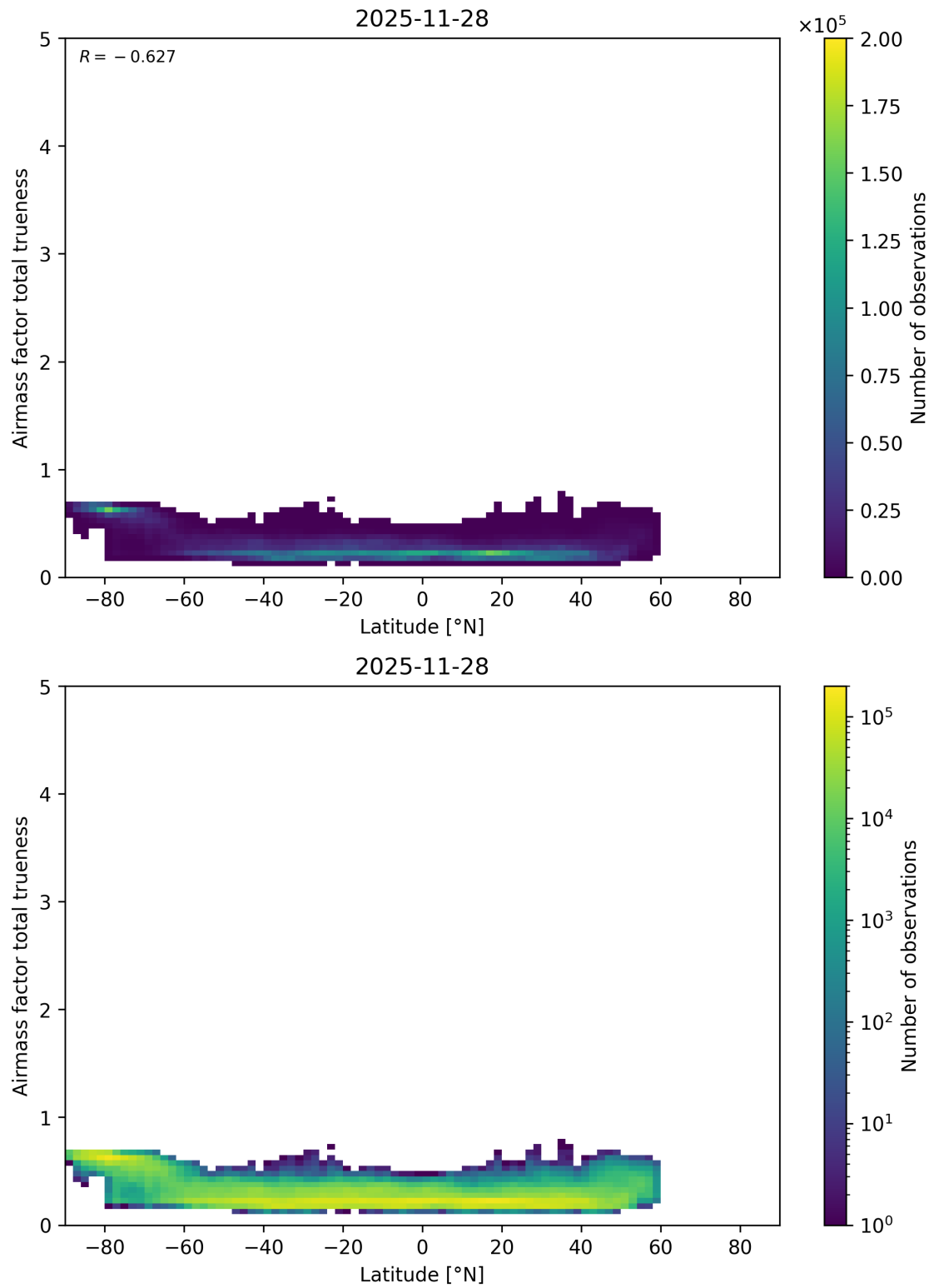
Figure 180: Scatter density plot of “Latitude” against “Airmass factor total trueneess” for 2025-11-28 to 2025-11-29.
