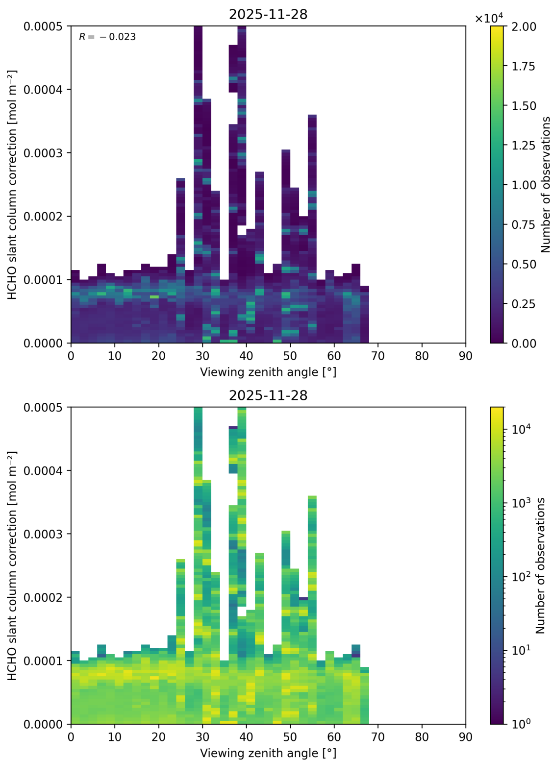
Figure 207: Scatter density plot of “Viewing zenith angle” against “HCHO slant column correction” for 2025-11-28 to 2025-11-29.
