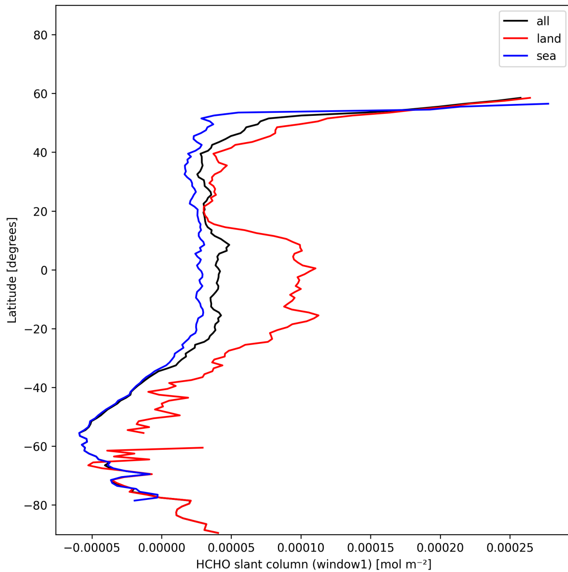
Figure 25: Zonal average of “HCHO slant column (window1)” for 2025-11-28 to 2025-11-29.
