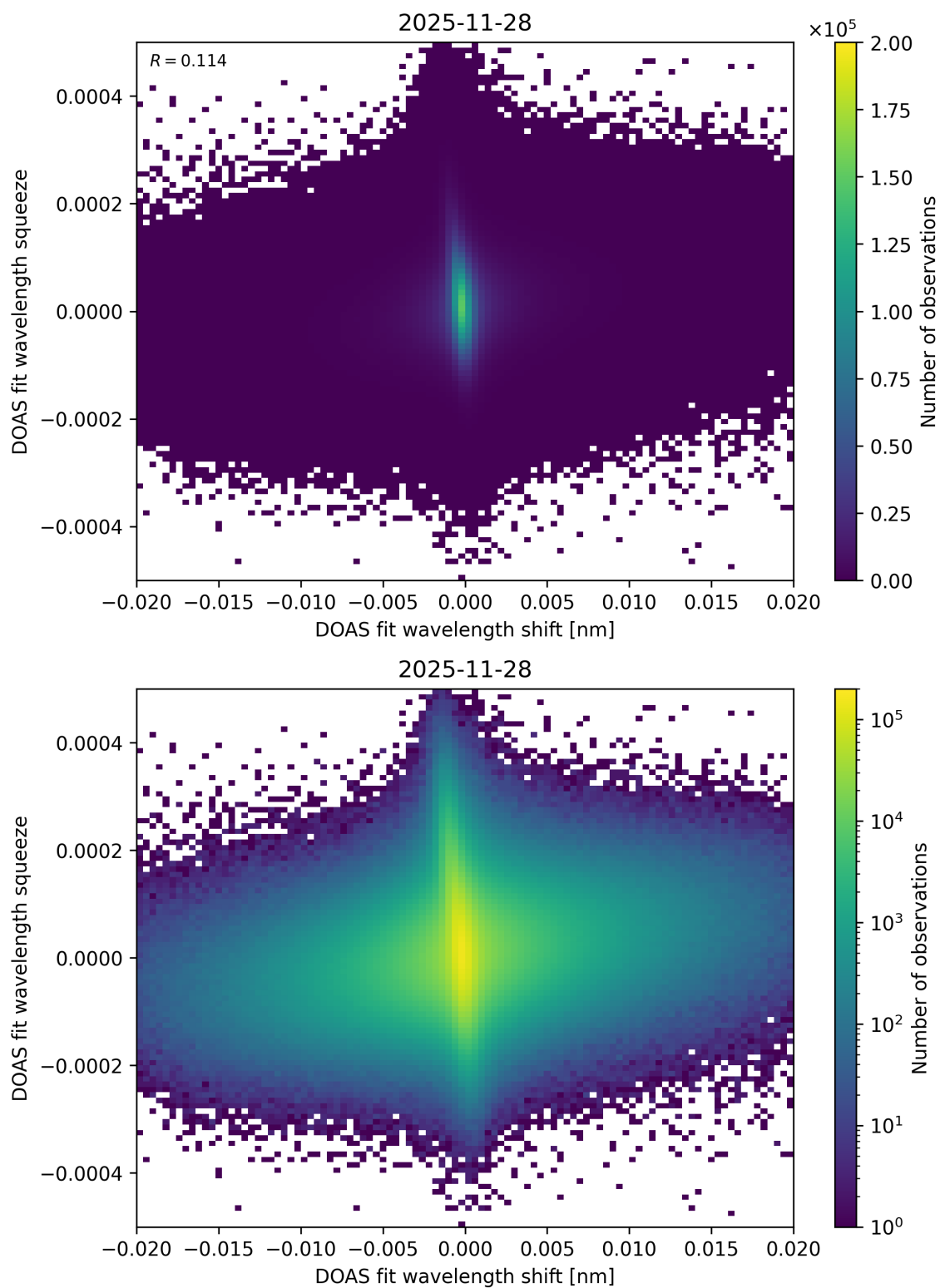
Figure 70: Scatter density plot of “DOAS fit wavelength shift” against “DOAS fit wavelength squeeze” for 2025-11-28 to 2025-11-29.
