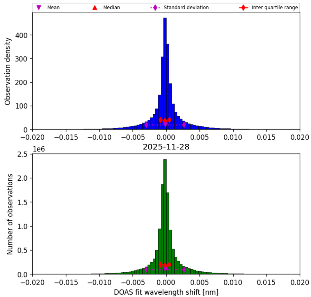
Figure 46: Histogram of “DOAS fit wavelength shift” for 2025-11-28 to 2025-11-29
