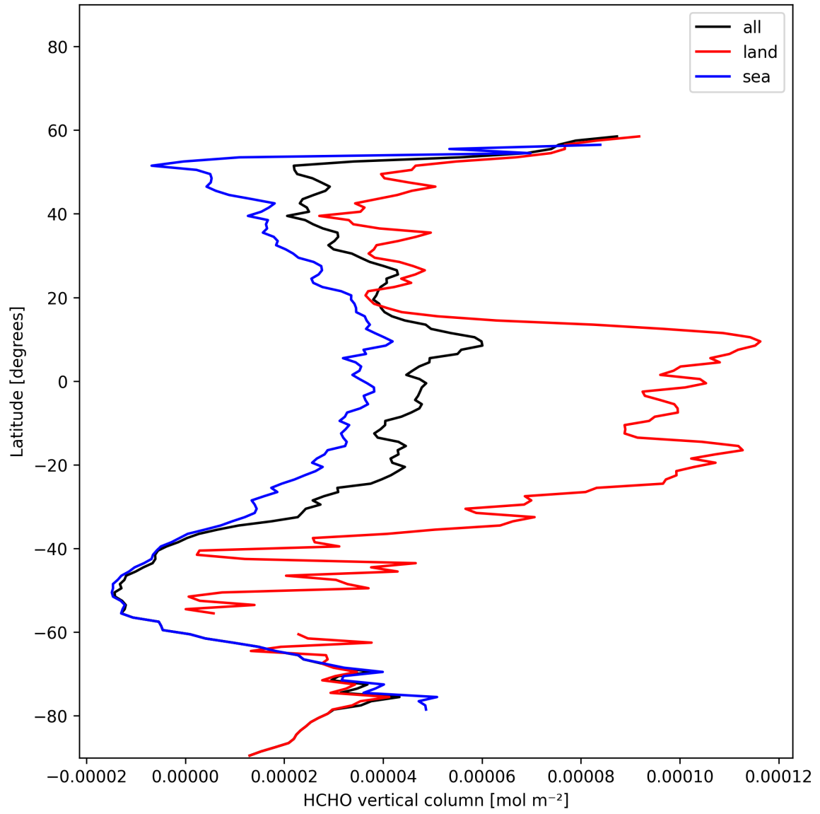
Figure 22: Zonal average of “HCHO vertical column” for 2025-11-28 to 2025-11-29.
