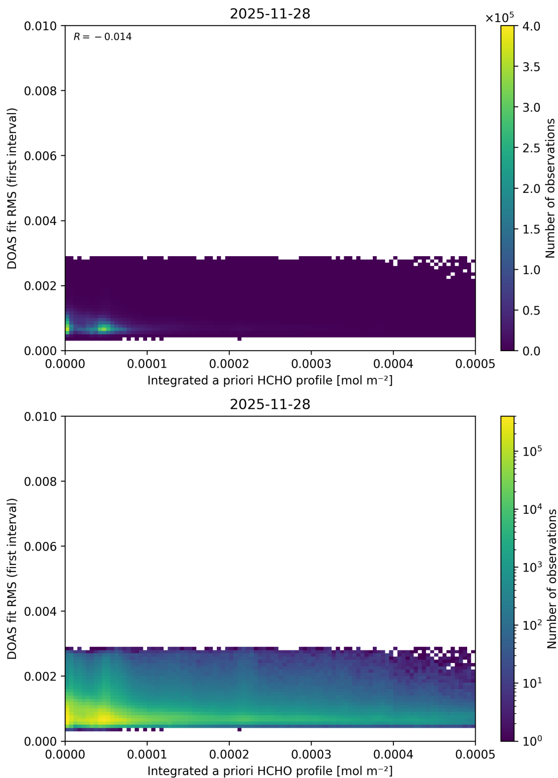
Figure 165: Scatter density plot of “Integrated a priori HCHO profile” against “DOAS fit RMS (first interval)” for 2025-11-28 to 2025-11-29.
