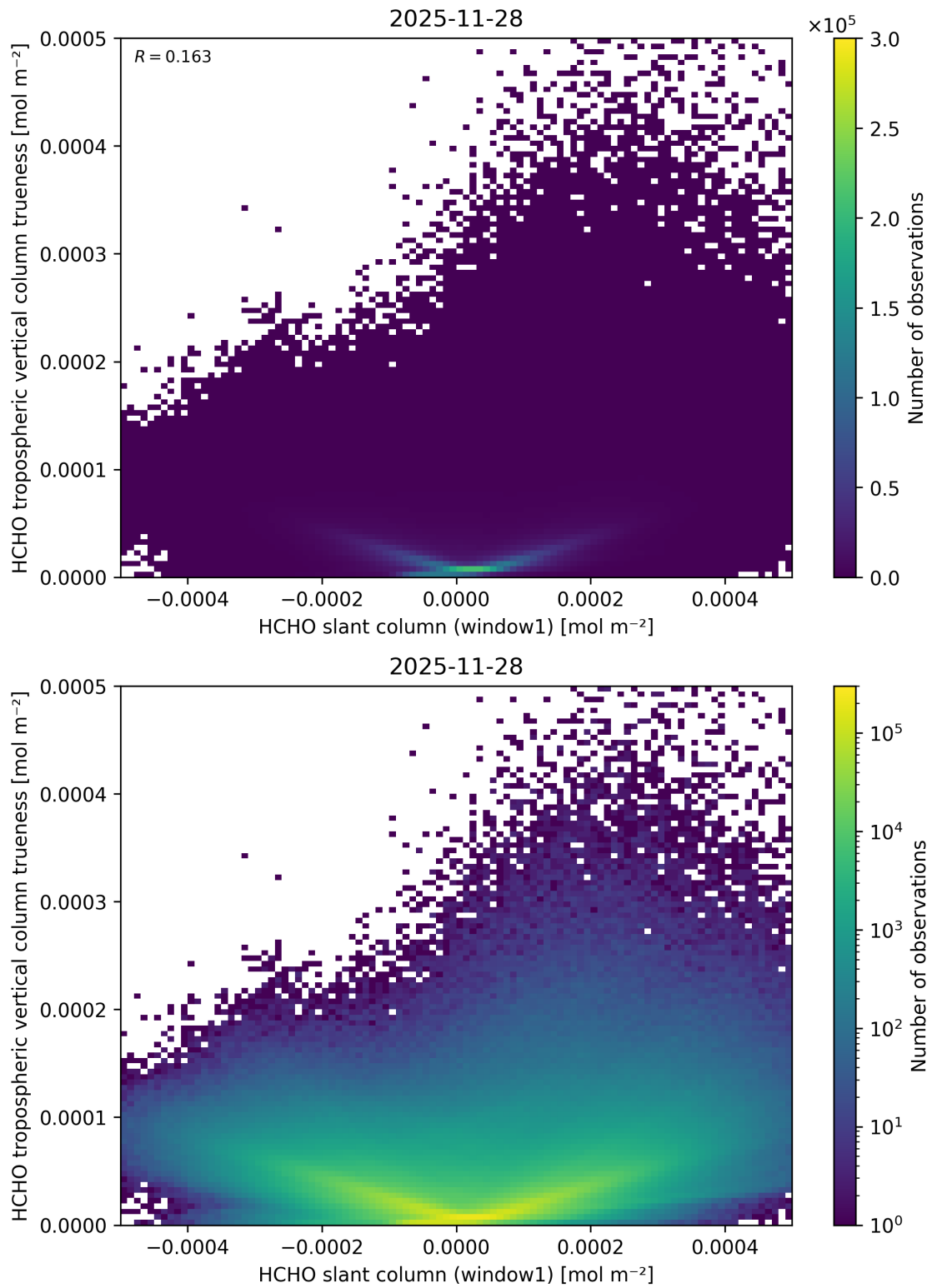
Figure 97: Scatter density plot of “HCHO slant column (window1)” against “HCHO tropospheric vertical column trueness” for 2025-11-28 to 2025-11-29.
