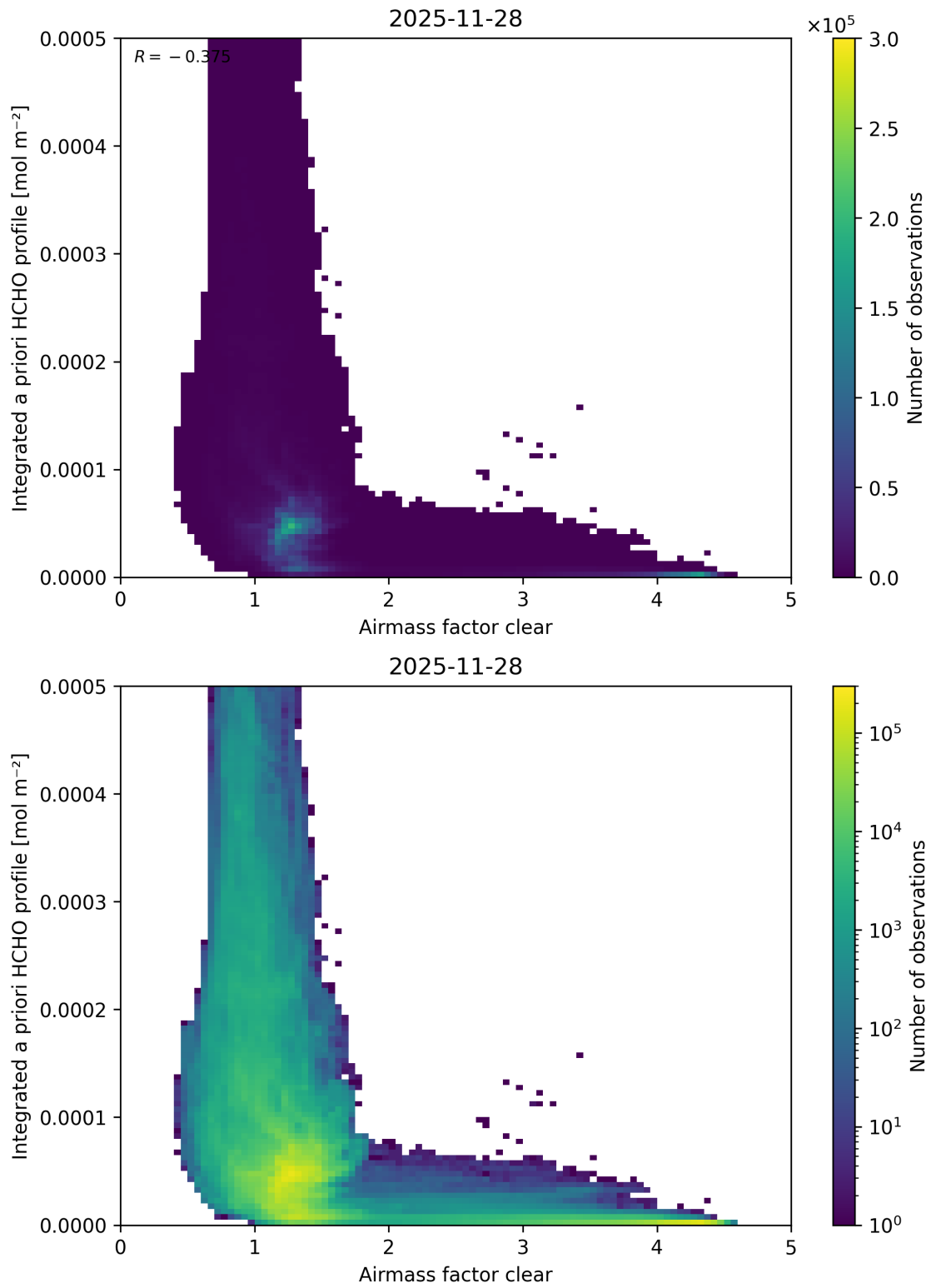
Figure 84: Scatter density plot of “Airmass factor clear” against “Integrated a priori HCHO profile” for 2025-11-28 to 2025-11-29.
