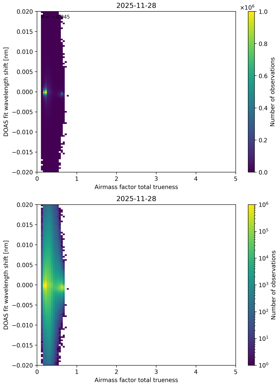
Figure 119: Scatter density plot of “Airmass factor total trueness” against “DOAS fit wavelength shift” for 2025-11-28 to 2025-11-29.
