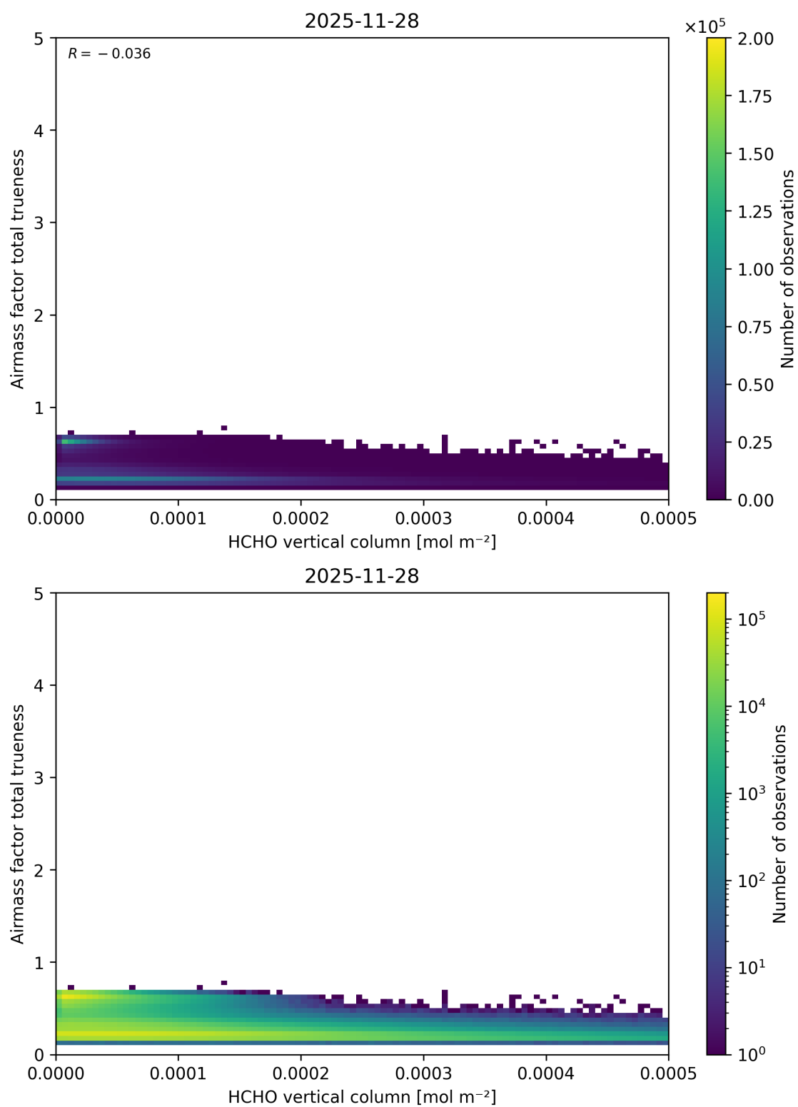
Figure 147: Scatter density plot of “HCHO vertical column” against “Airmass factor total trueneess” for 2025-11-28 to 2025-11-29.
