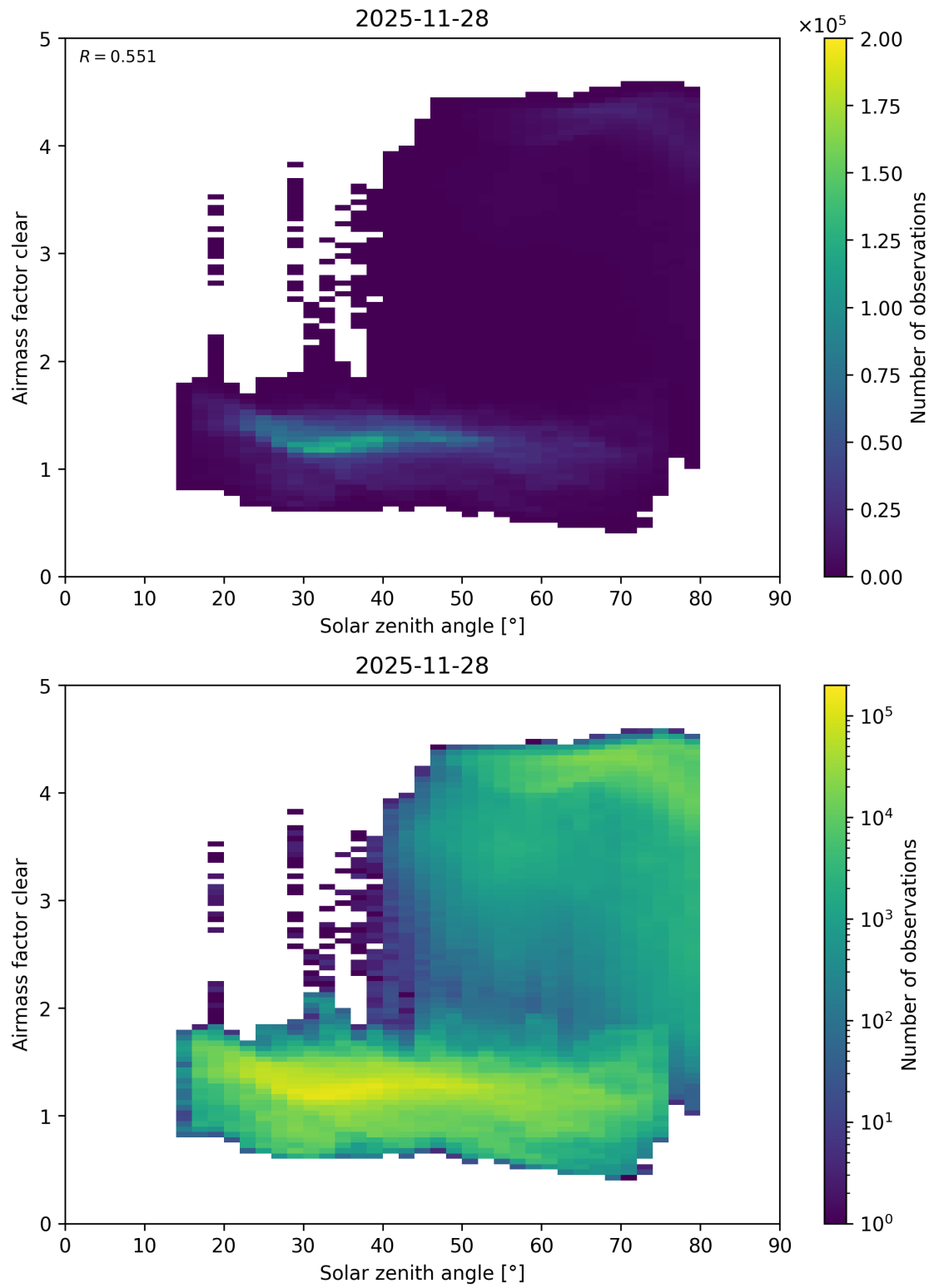
Figure 189: Scatter density plot of “Solar zenith angle” against “Airmass factor clear” for 2025-11-28 to 2025-11-29.
