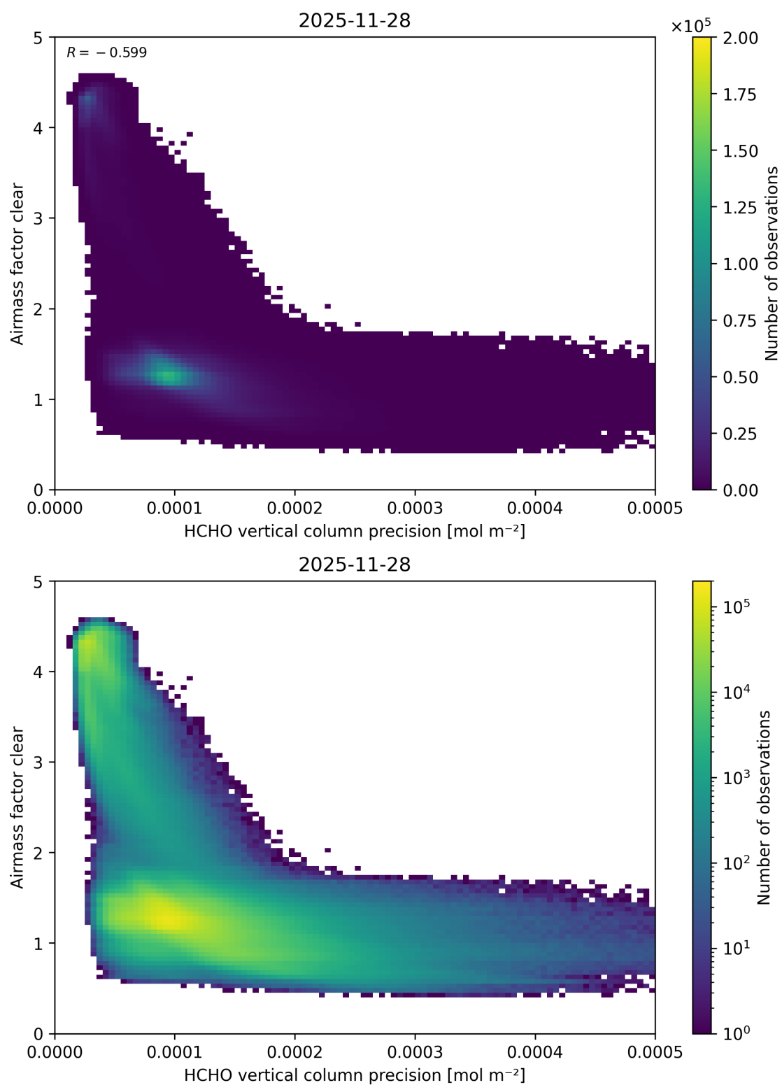
Figure 155: Scatter density plot of “HCHO vertical column precision” against “Airmass factor clear” for 2025-11-28 to 2025-11-29.
