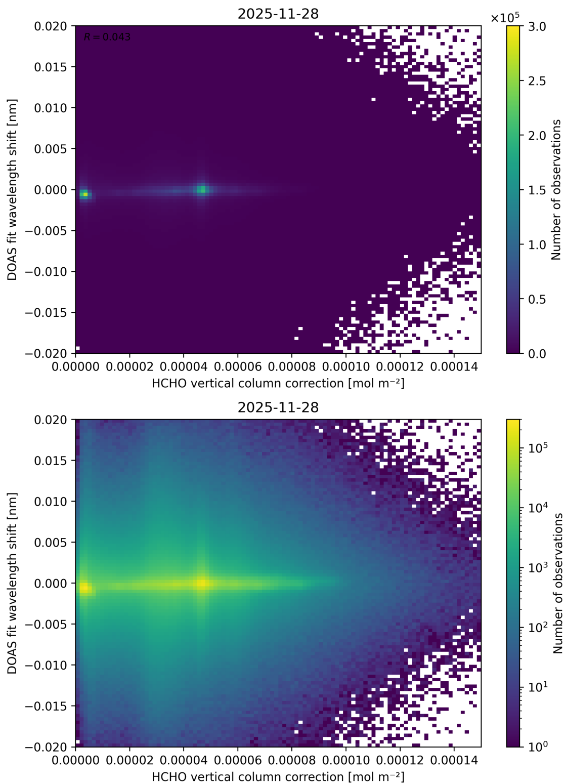
Figure 127: Scatter density plot of “HCHO vertical column correction” against “DOAS fit wavelength shift” for 2025-11-28 to 2025-11-29.
