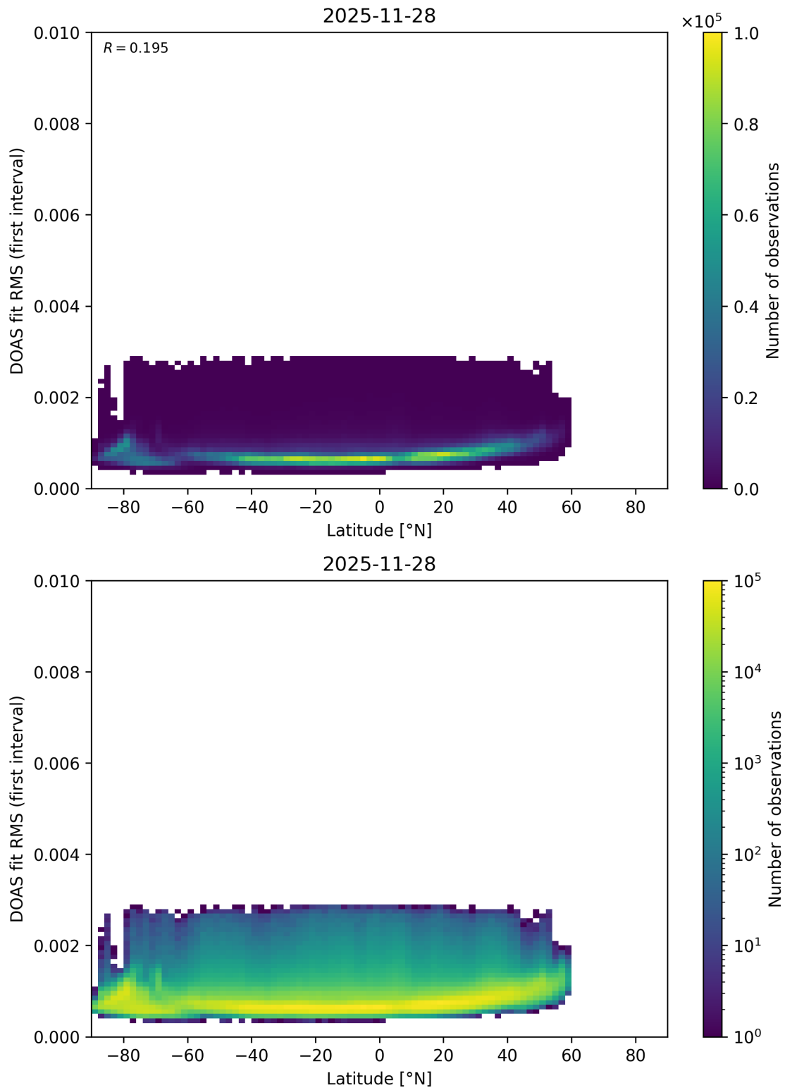
Figure 171: Scatter density plot of “Latitude” against “DOAS fit RMS (first interval)” for 2025-11-28 to 2025-11-29.
