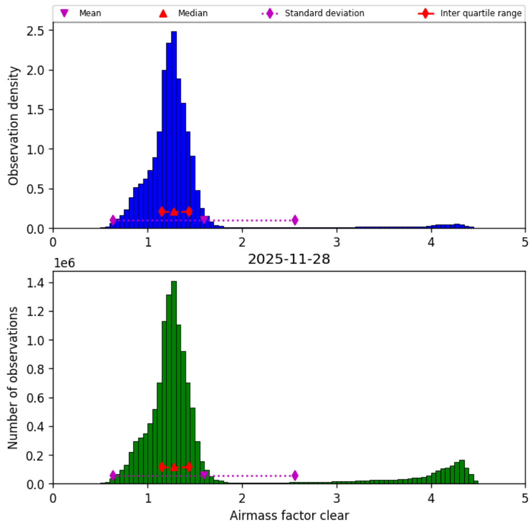
Figure 44: Histogram of “Airmass factor clear” for 2025-11-28 to 2025-11-29
