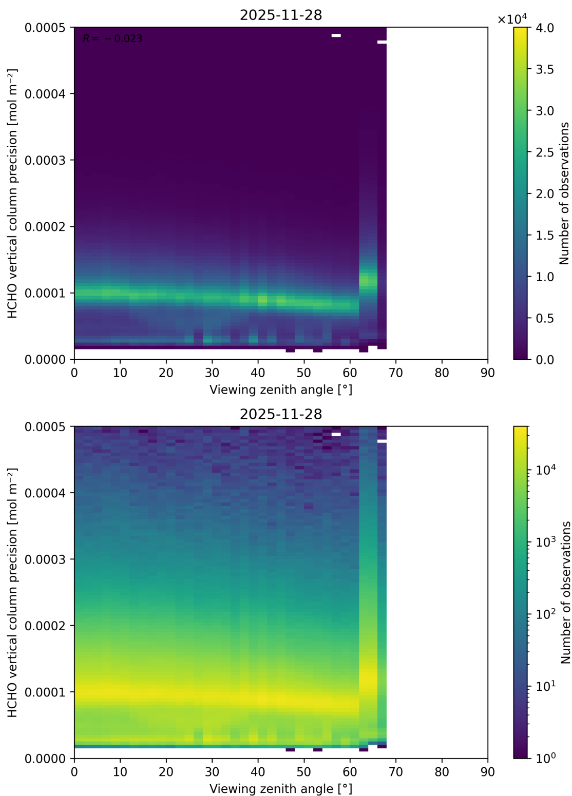
Figure 214: Scatter density plot of “Viewing zenith angle” against “HCHO vertical column precision” for 2025-11-28 to 2025-11-29.
