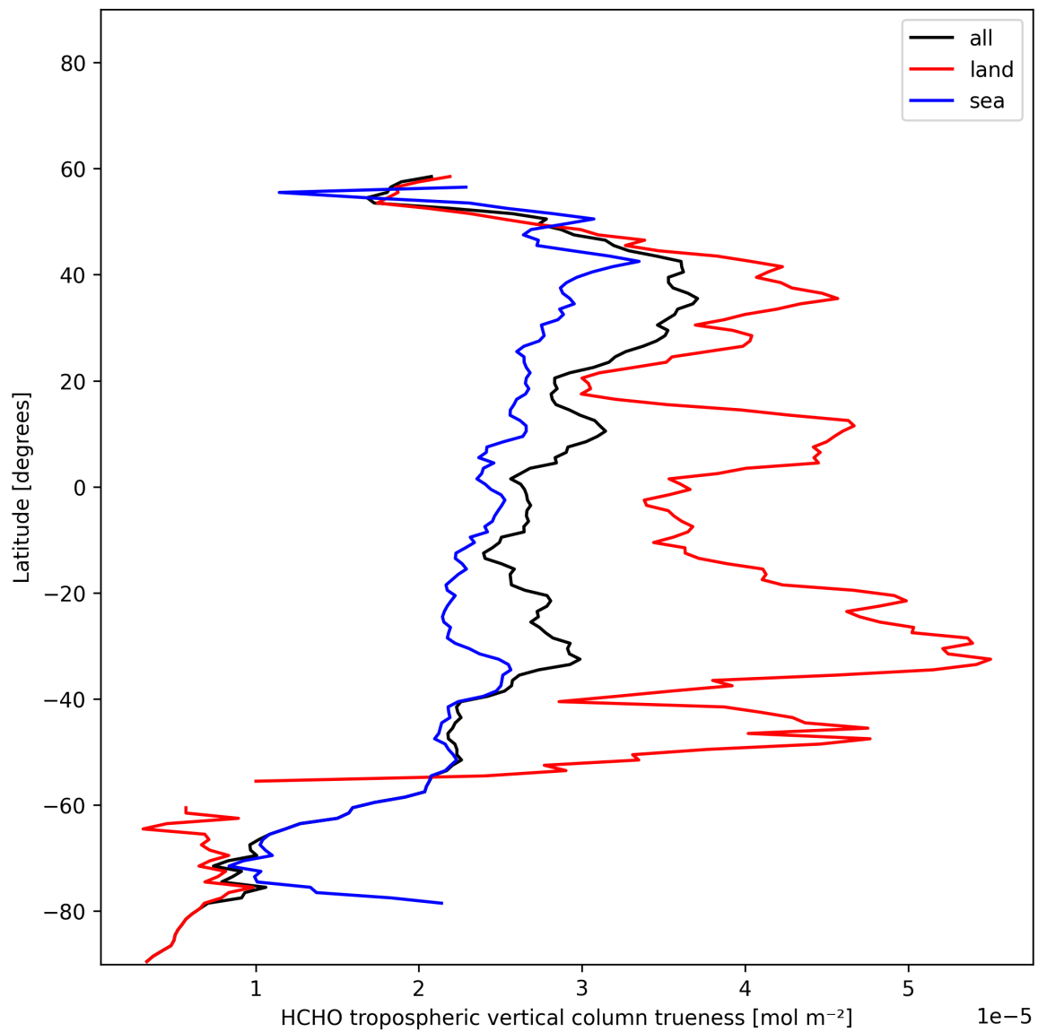
Figure 35: Zonal average of “HCHO tropospheric vertical column trueness” for 2025-11-28 to 2025-11-29.
