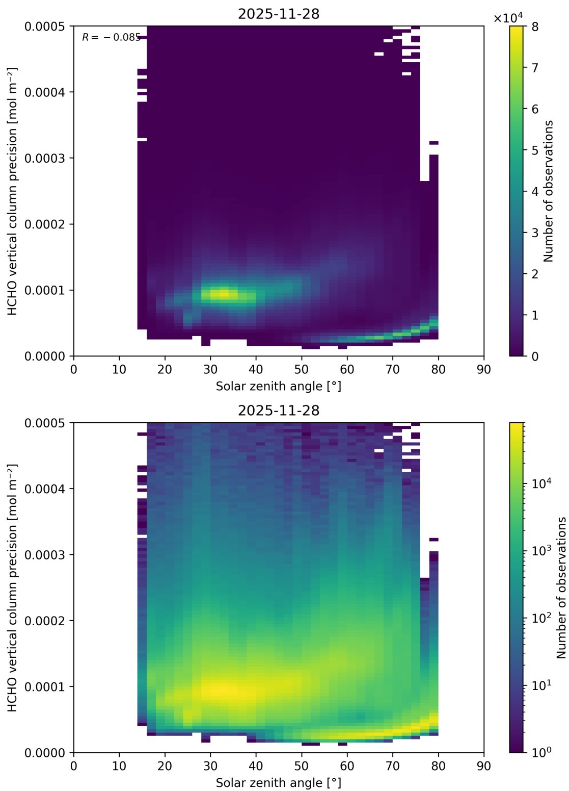
Figure 198: Scatter density plot of “Solar zenith angle” against “HCHO vertical column precision” for 2025-11-28 to 2025-11-29.
