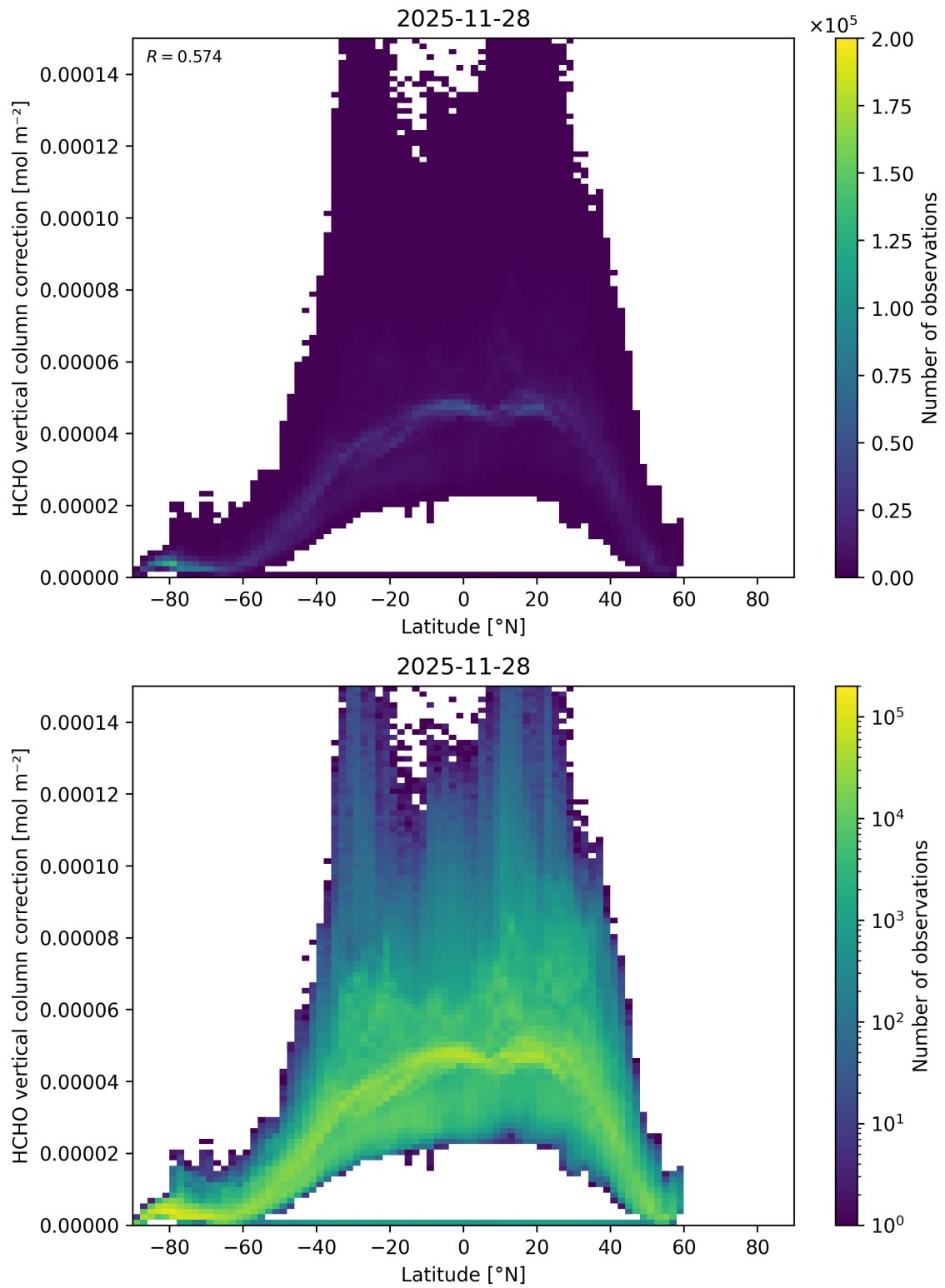
Figure 182: Scatter density plot of “Latitude” against “HCHO vertical column correction” for 2025-11-28 to 2025-11-29.
