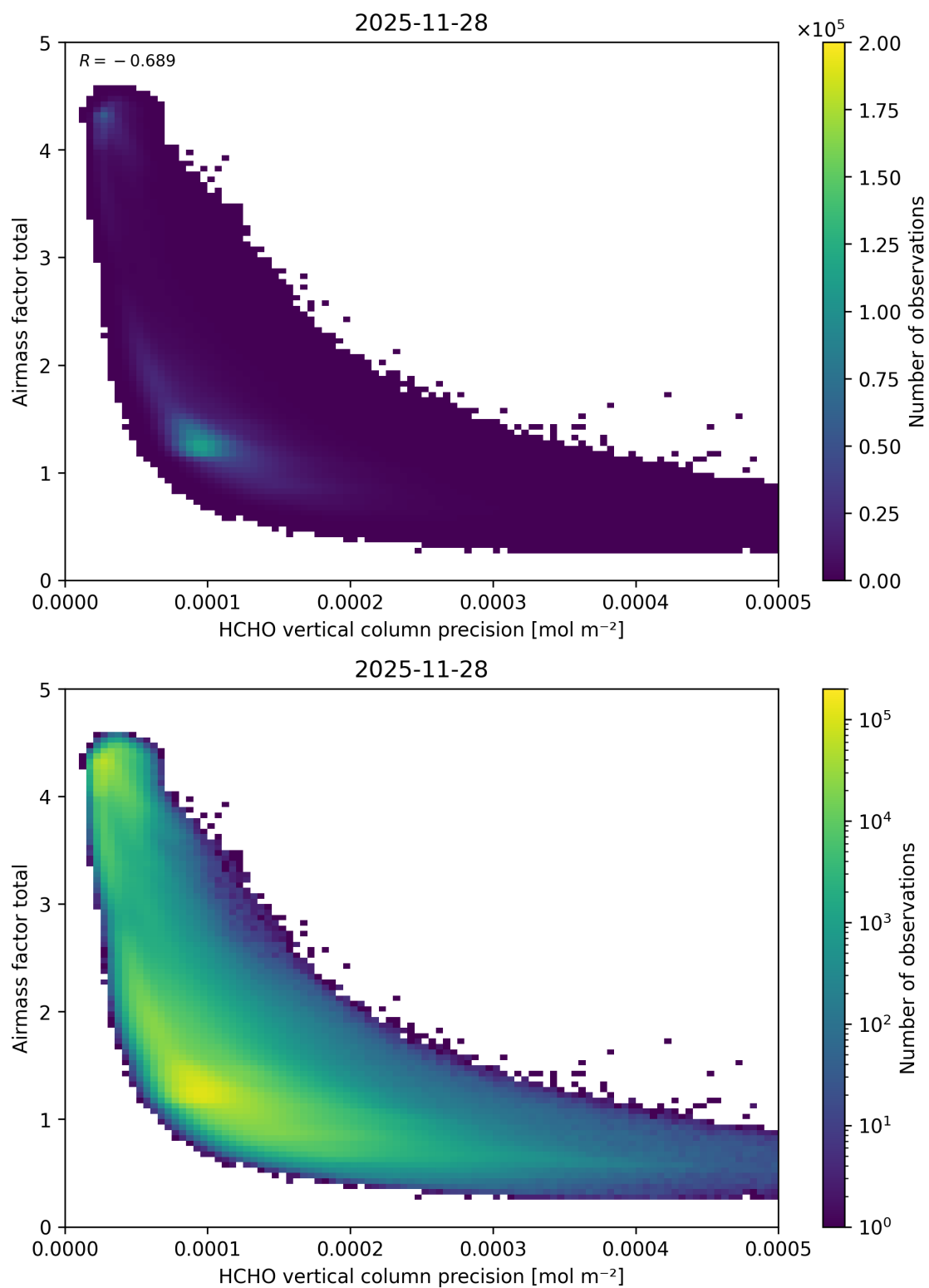
Figure 160: Scatter density plot of “HCHO vertical column precision” against “Airmass factor total” for 2025-11-28 to 2025-11-29.
