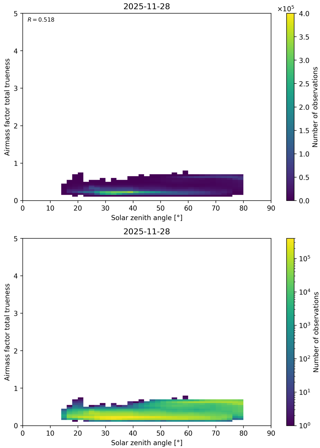
Figure 195: Scatter density plot of “Solar zenith angle” against “Airmass factor total trueness” for 2025-11-28 to 2025-11-29.
