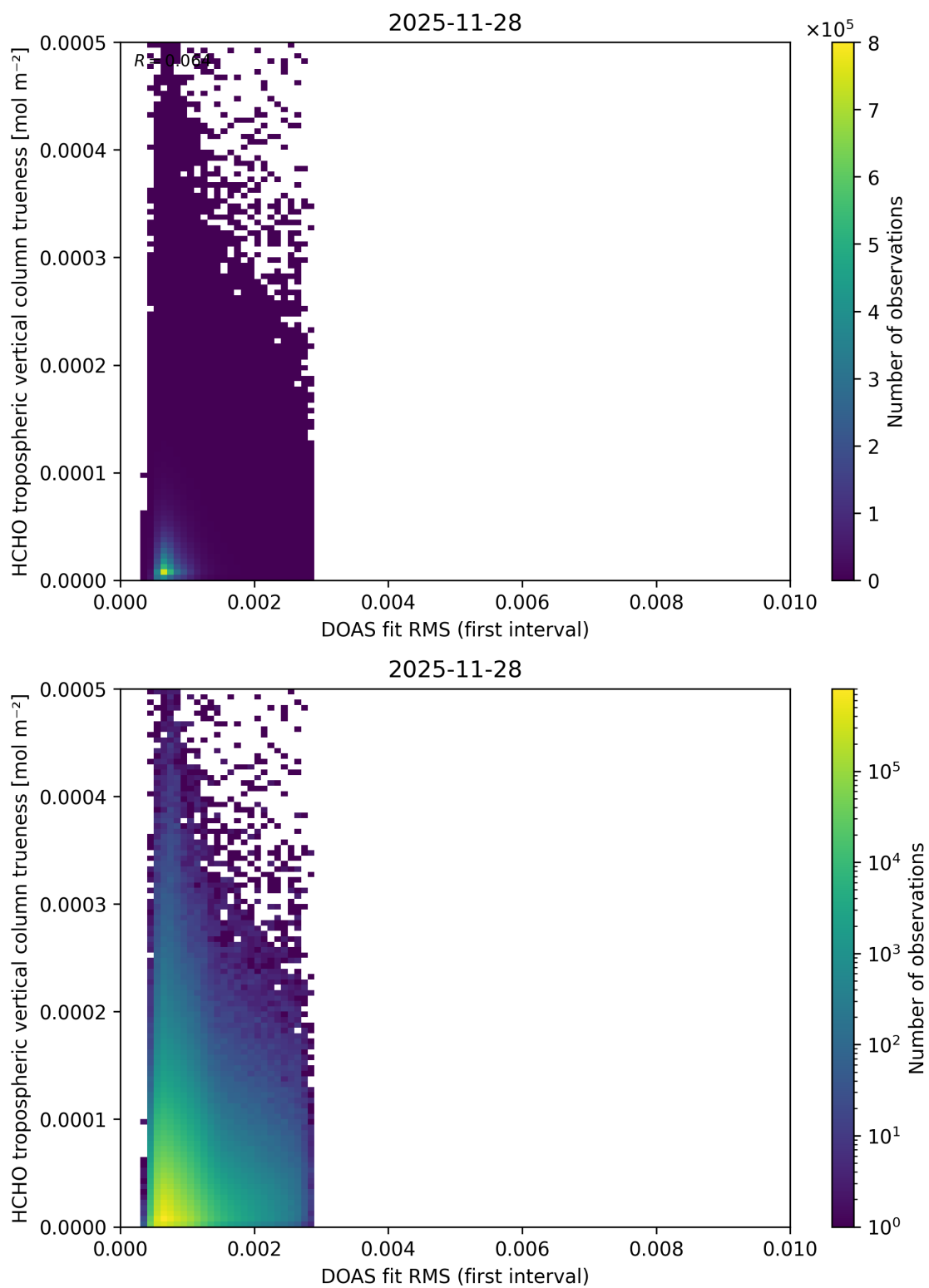
Figure 68: Scatter density plot of “DOAS fit RMS (first interval)” against “HCHO tropospheric vertical column trueness” for 2025-11-28 to 2025-11-29.
