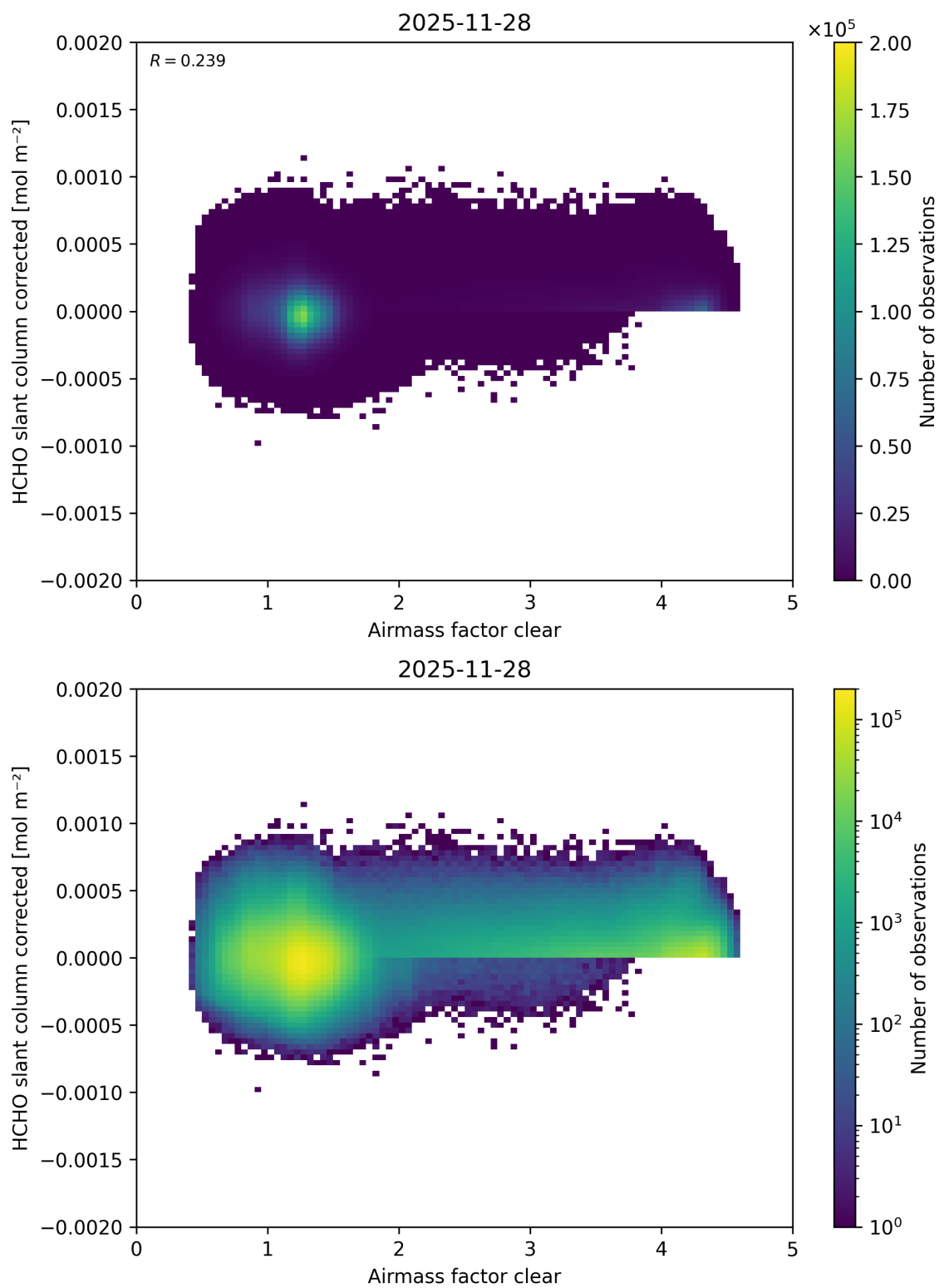
Figure 81: Scatter density plot of “Airmass factor clear” against “HCHO slant column corrected” for 2025-11-28 to 2025-11-29.
