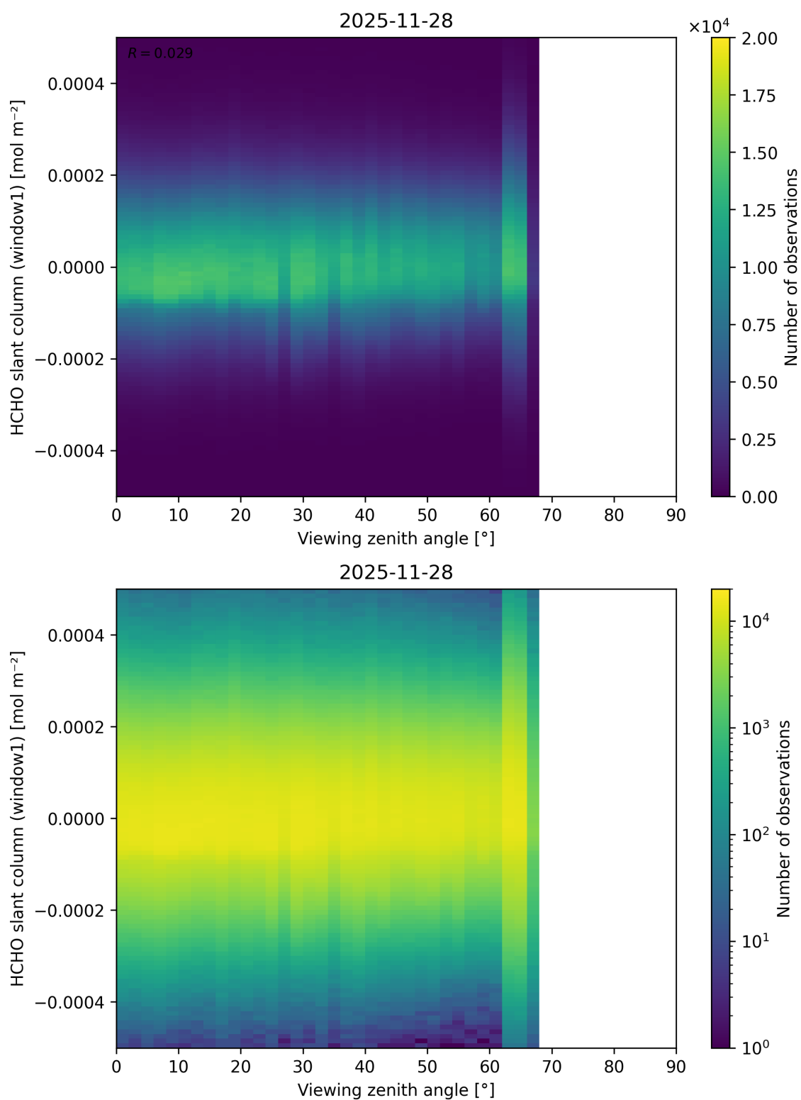
Figure 208: Scatter density plot of “Viewing zenith angle” against “HCHO slant column (window1)” for 2025-11-28 to 2025-11-29.
