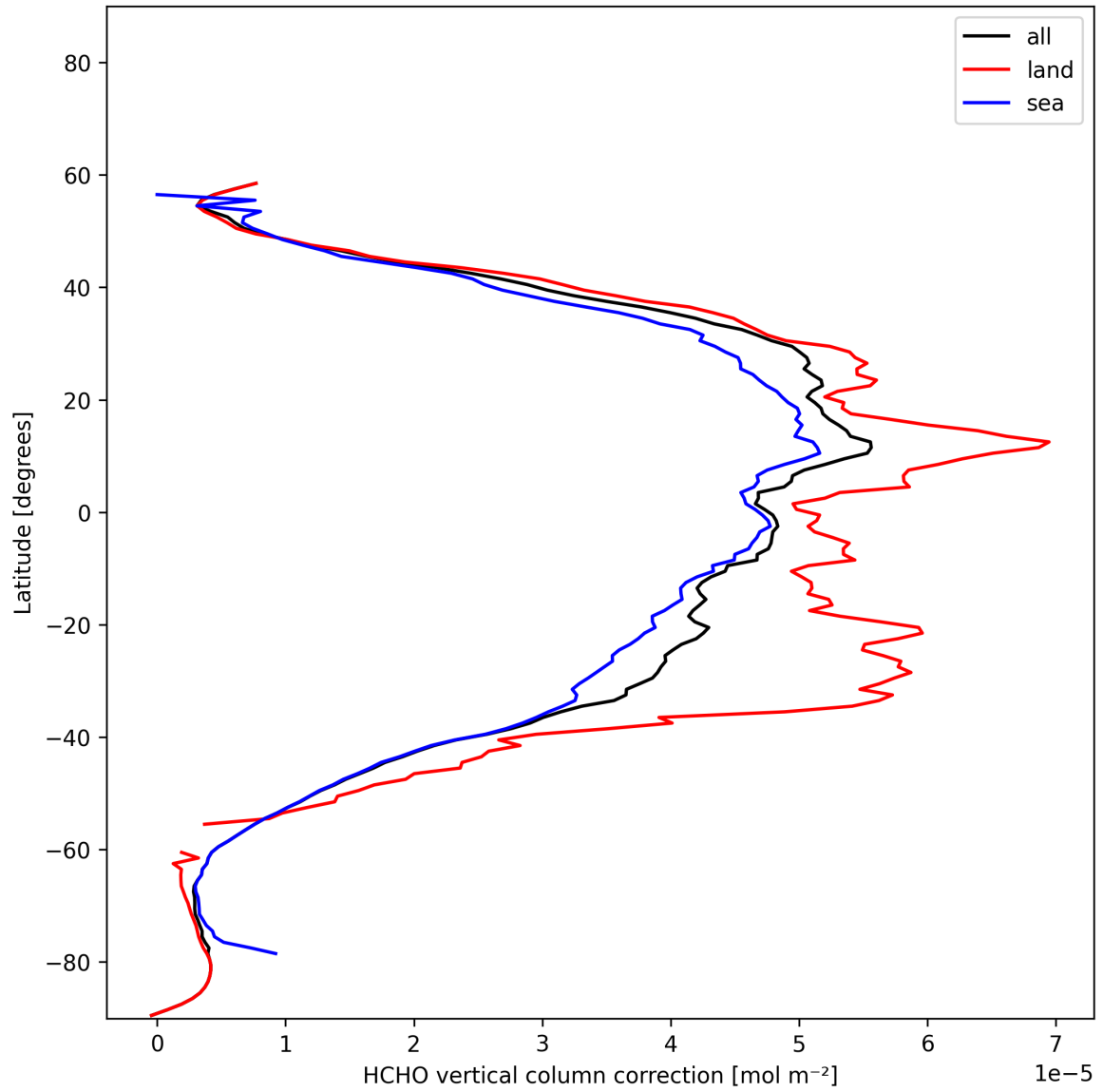
Figure 24: Zonal average of “HCHO vertical column correction” for 2025-11-28 to 2025-11-29.
