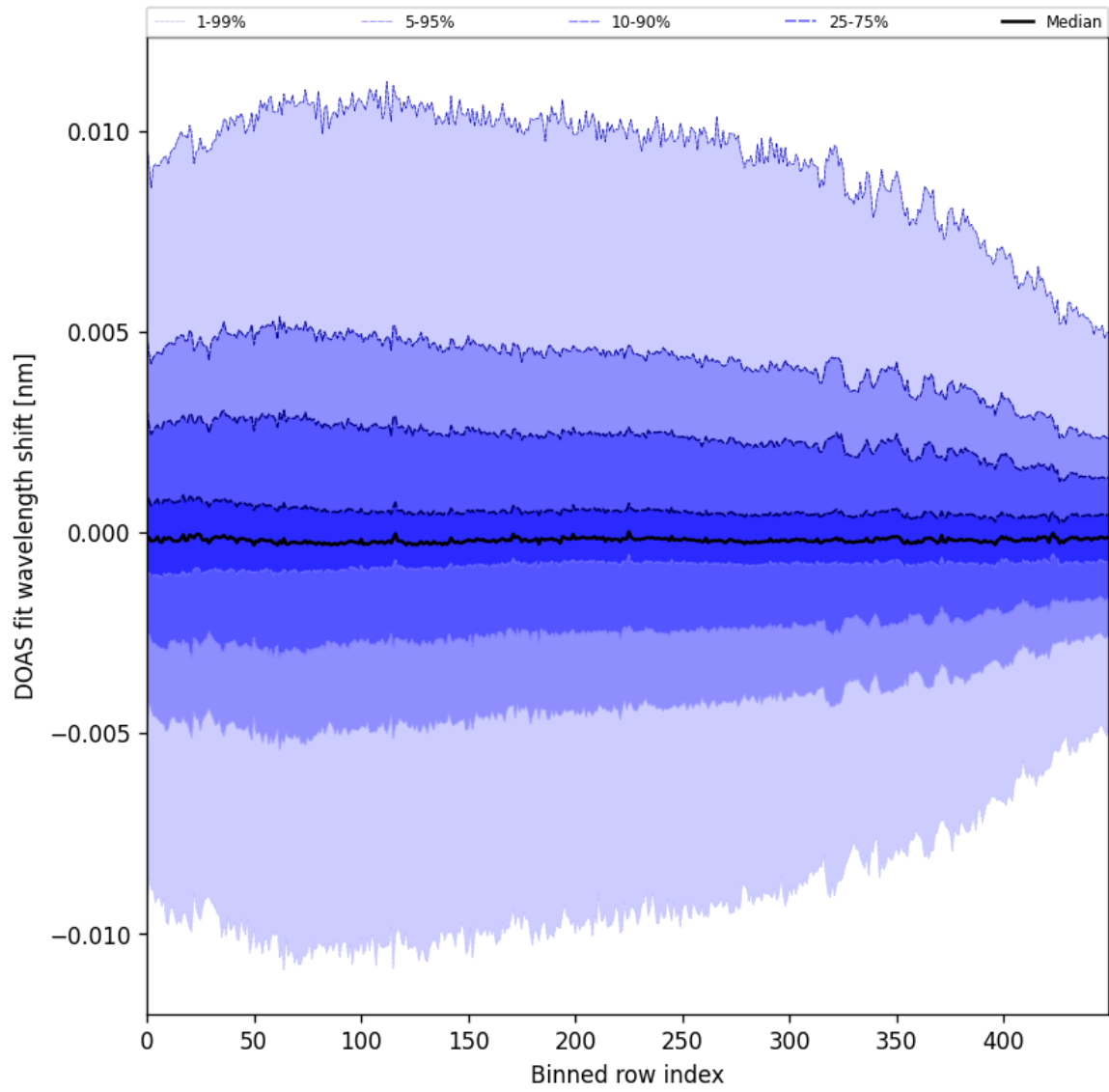
Figure 61: Along track statistics of “DOAS fit wavelength shift” for 2025-11-28 to 2025-11-29
