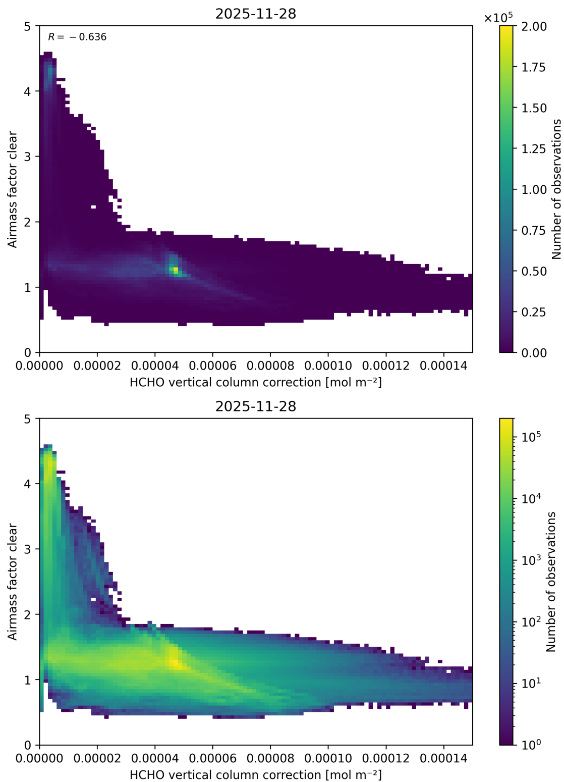
Figure 129: Scatter density plot of “HCHO vertical column correction” against “Airmass factor clear” for 2025-11-28 to 2025-11-29.
