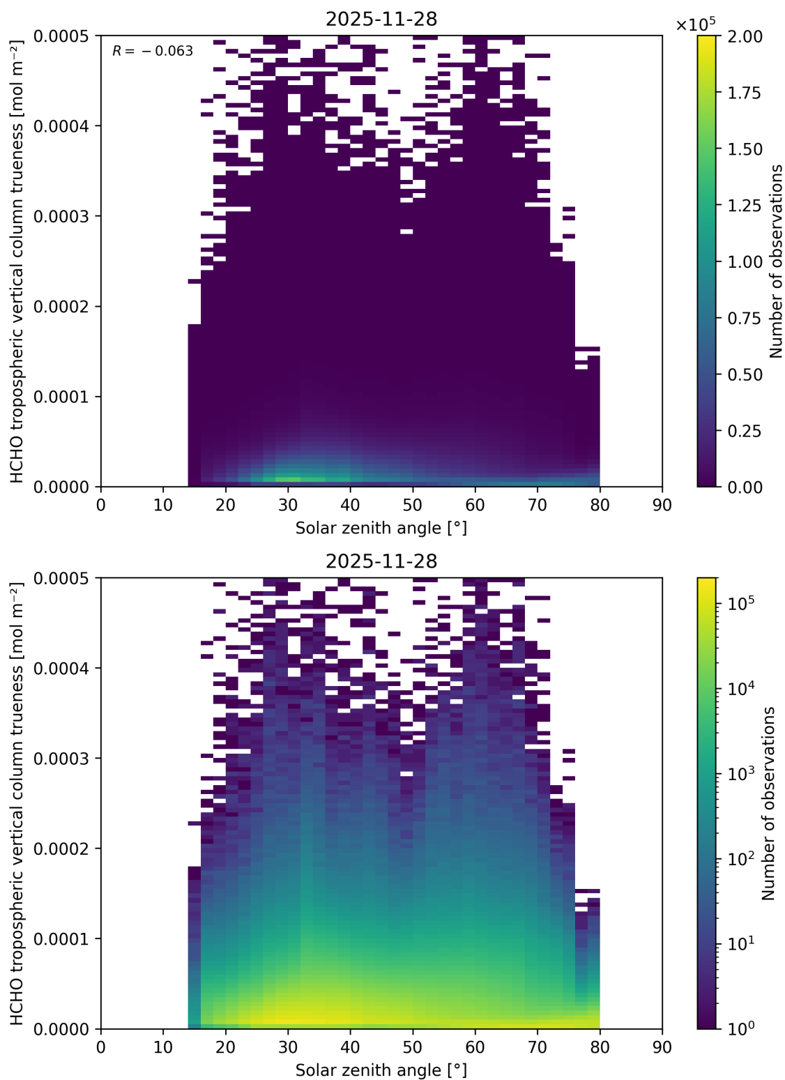
Figure 199: Scatter density plot of “Solar zenith angle” against “HCHO tropospheric vertical column trueness” for 2025-11-28 to 2025-11-29.
