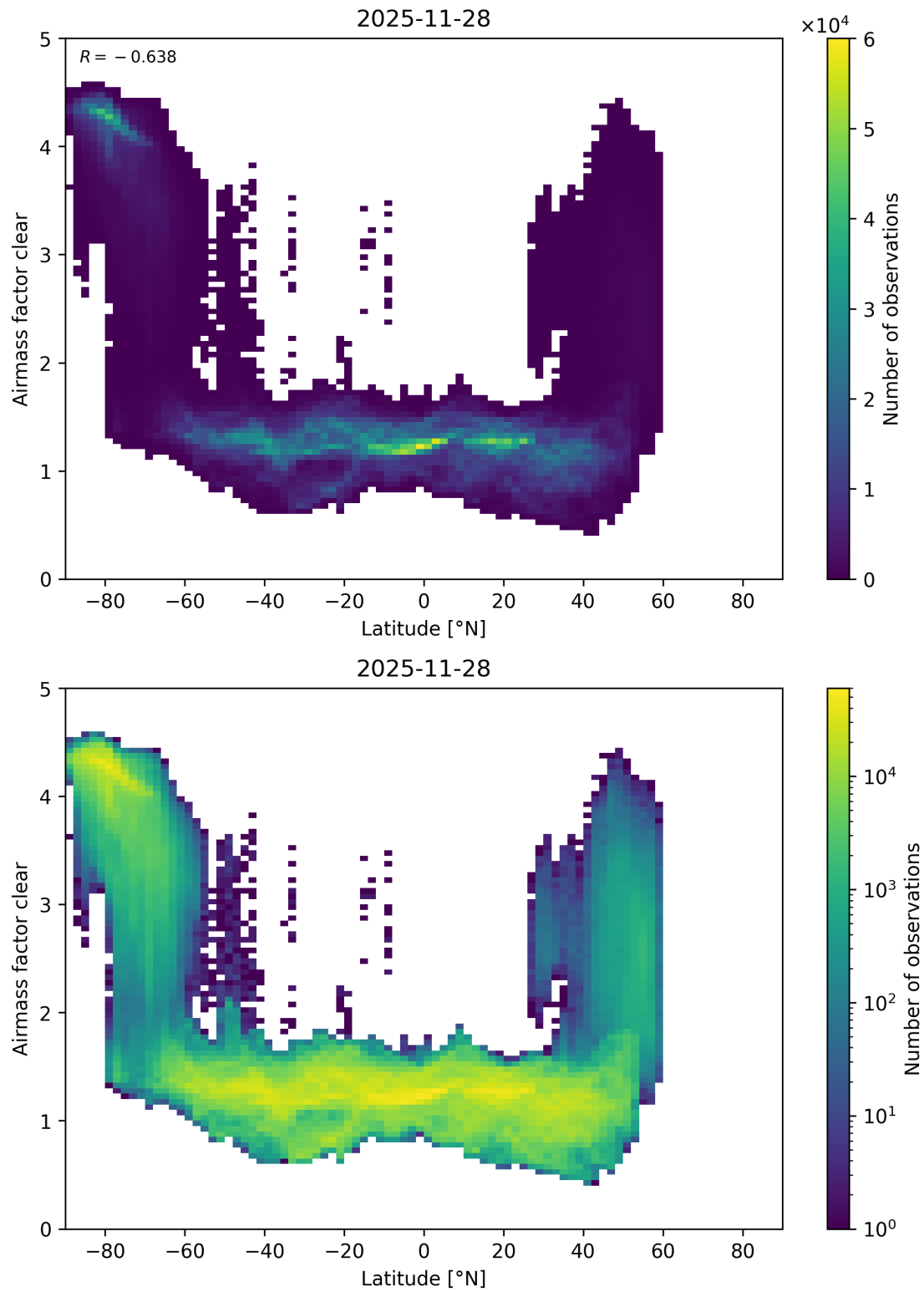
Figure 174: Scatter density plot of “Latitude” against “Airmass factor clear” for 2025-11-28 to 2025-11-29.
