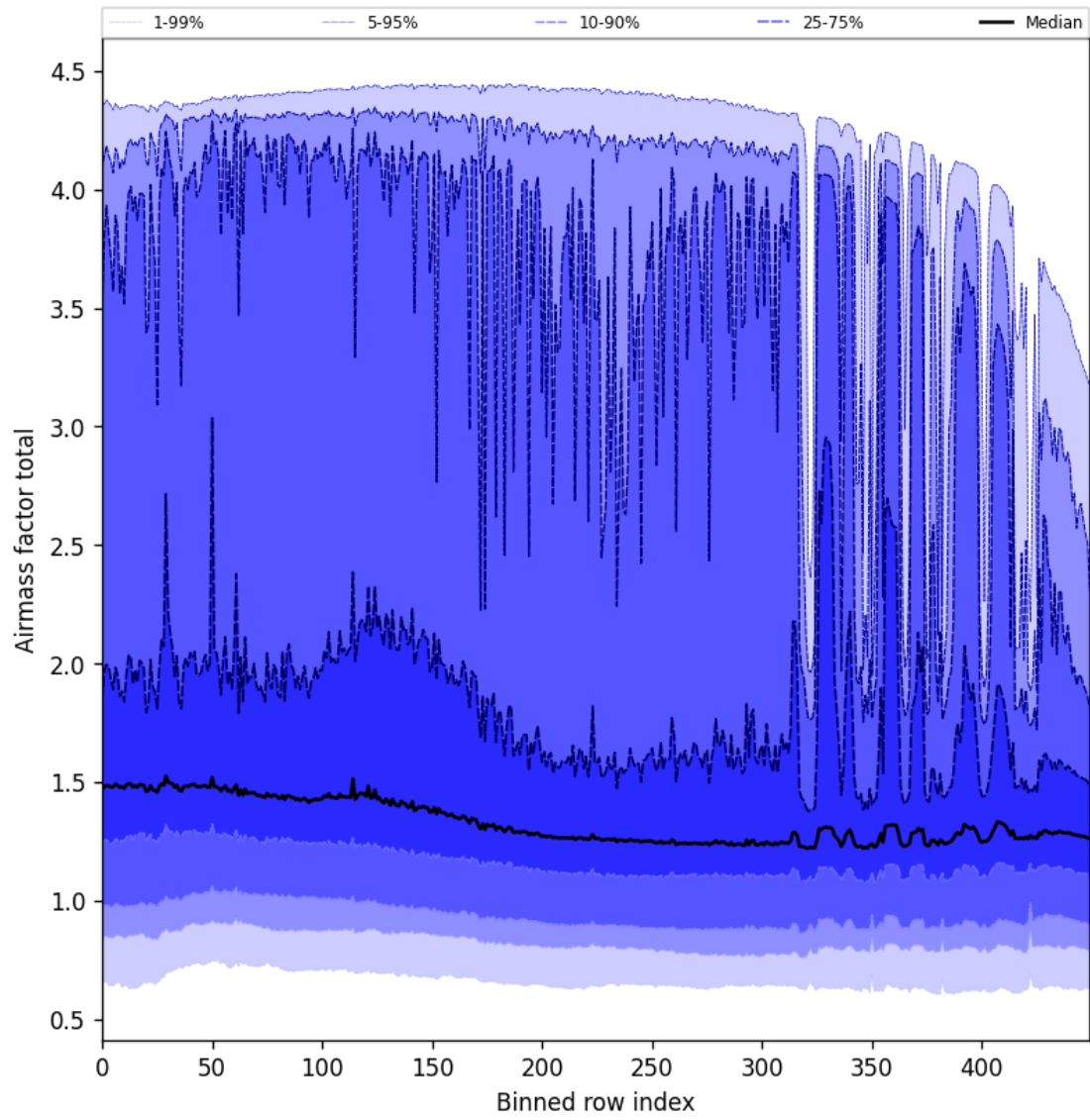
Figure 57: Along track statistics of “Airmass factor total” for 2025-11-28 to 2025-11-29
