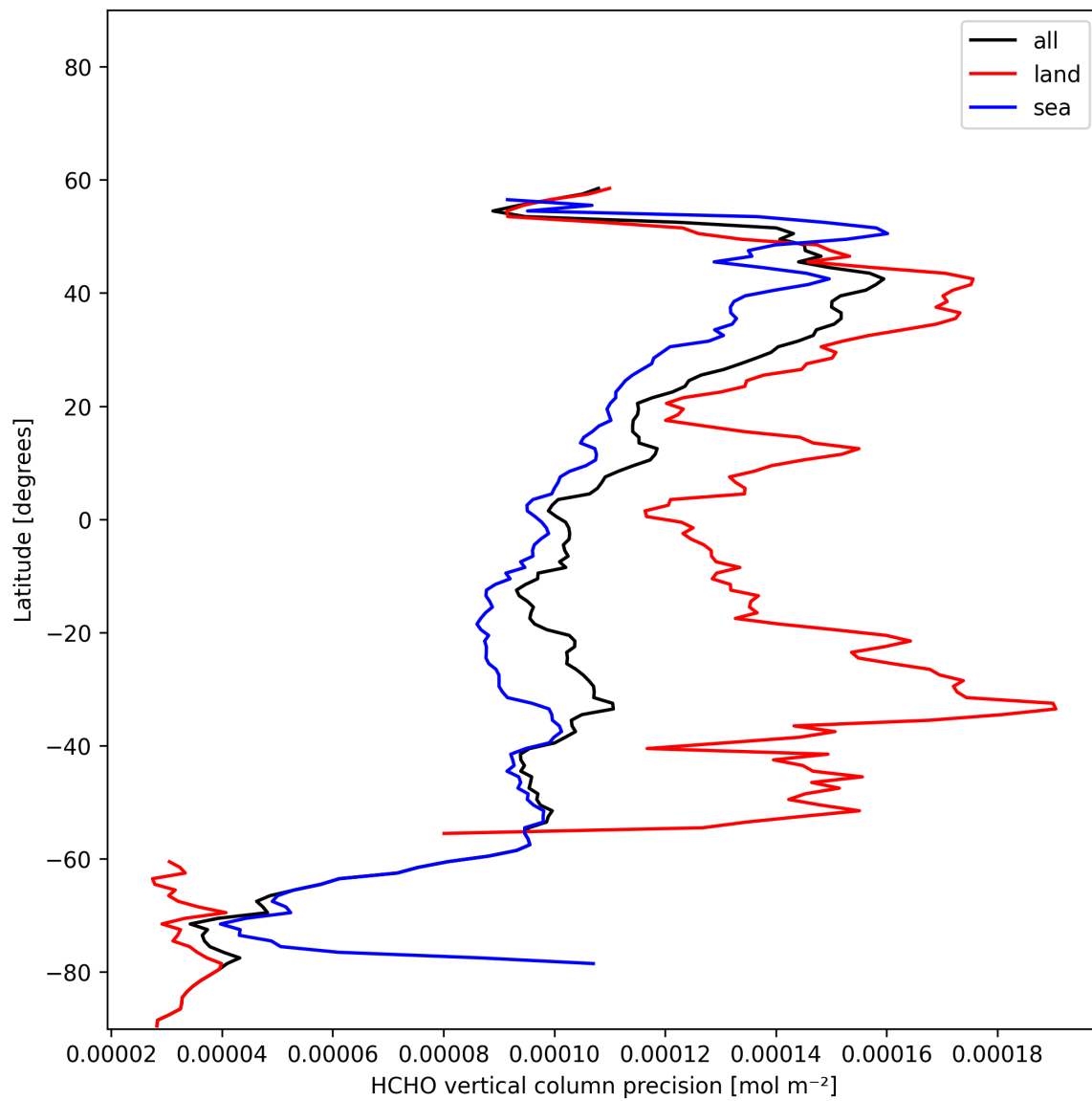
Figure 23: Zonal average of “HCHO vertical column precision” for 2025-11-28 to 2025-11-29.
