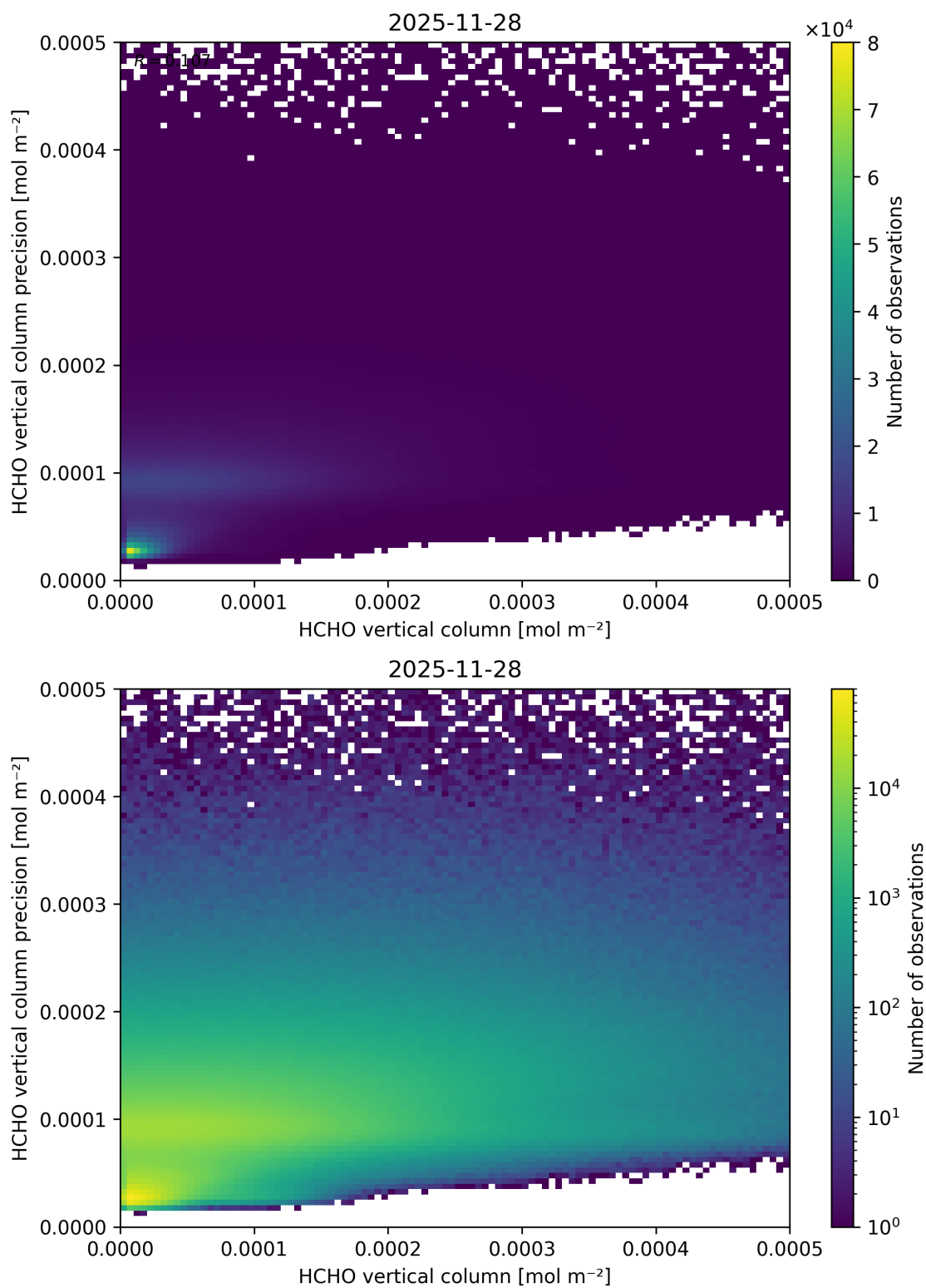
Figure 149: Scatter density plot of “HCHO vertical column” against “HCHO vertical column precision” for 2025-11-28 to 2025-11-29.
