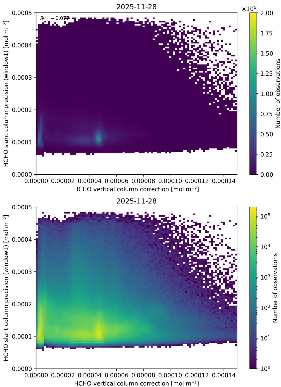
Figure 133: Scatter density plot of “HCHO vertical column correction” against “HCHO slant column precision (window1)” for 2025-11-28 to 2025-11-29.
