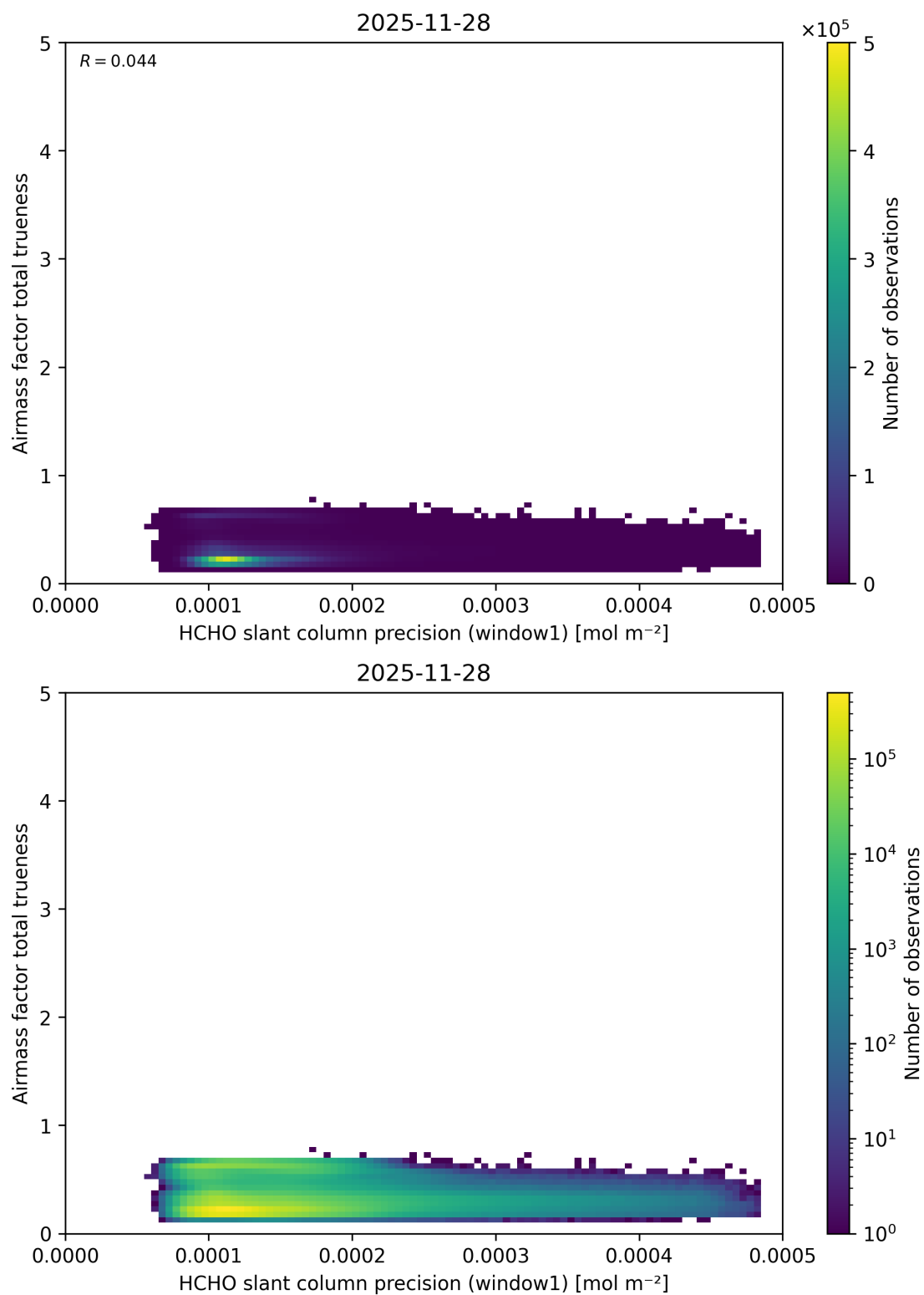
Figure 106: Scatter density plot of “HCHO slant column precision (window1)” against “Airmass factor total trueness” for 2025-11-28 to 2025-11-29.
