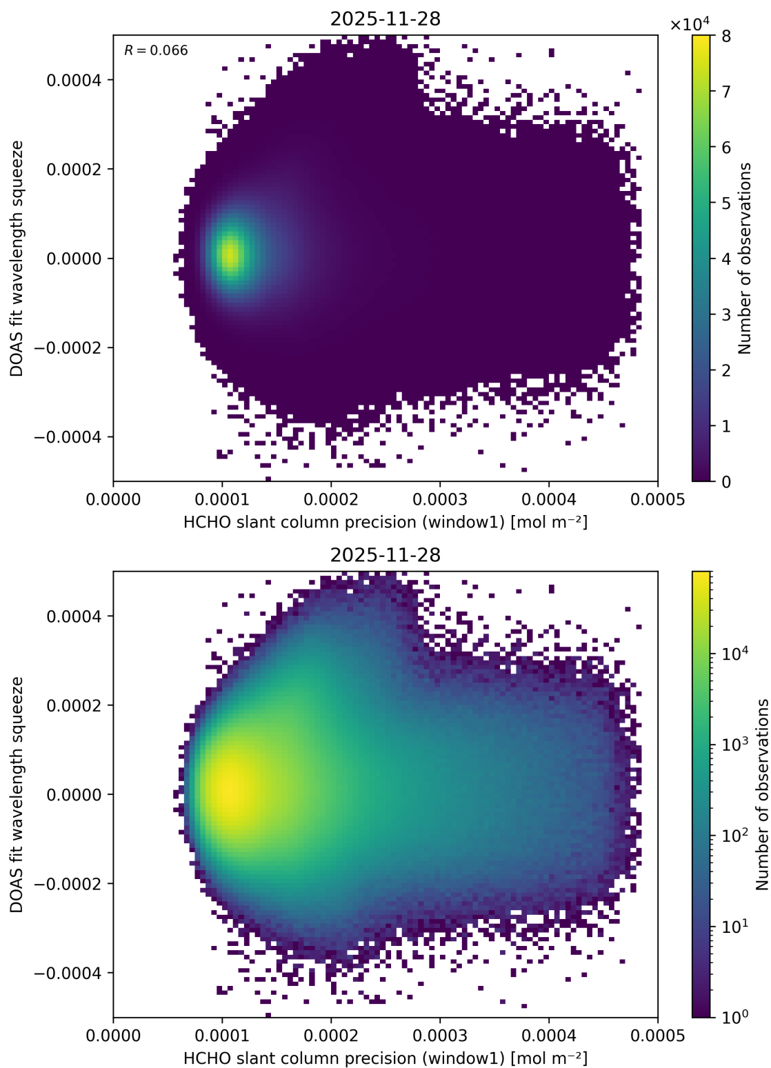
Figure 101: Scatter density plot of “HCHO slant column precision (window1)” against “DOAS fit wavelength squeeze” for 2025-11-28 to 2025-11-29.
