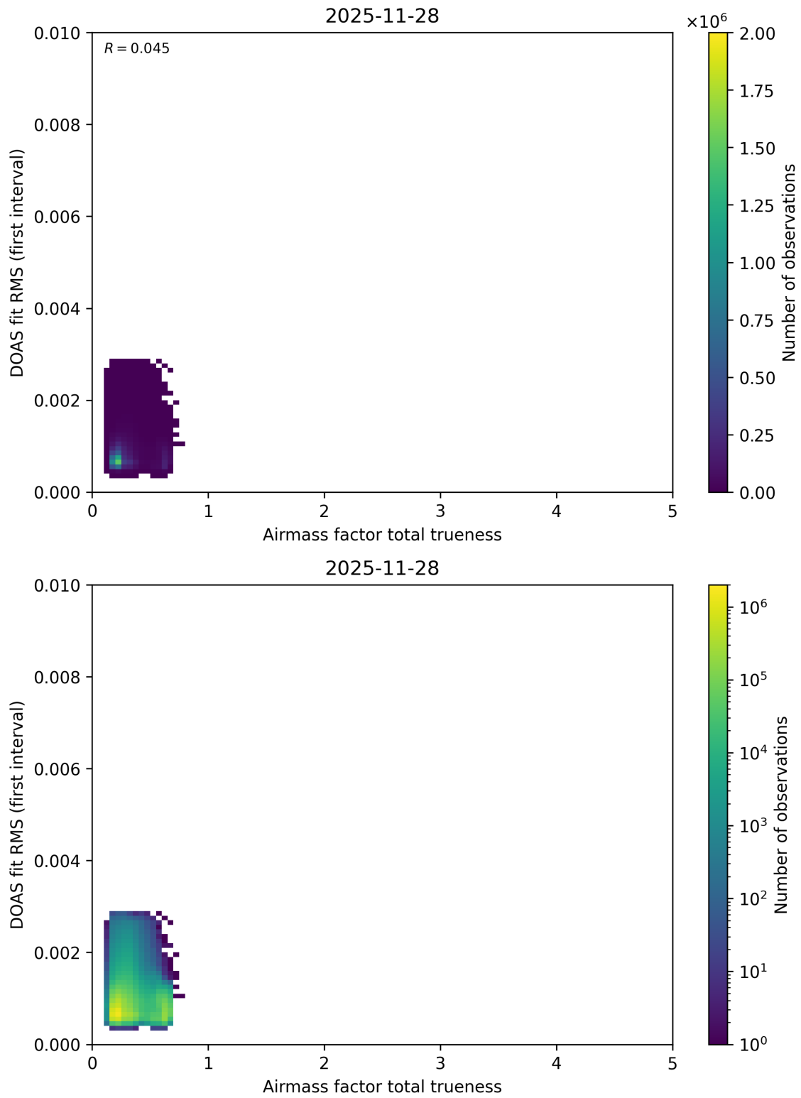
Figure 118: Scatter density plot of “Airmass factor total trueness” against “DOAS fit RMS (first interval)” for 2025-11-28 to 2025-11-29.
