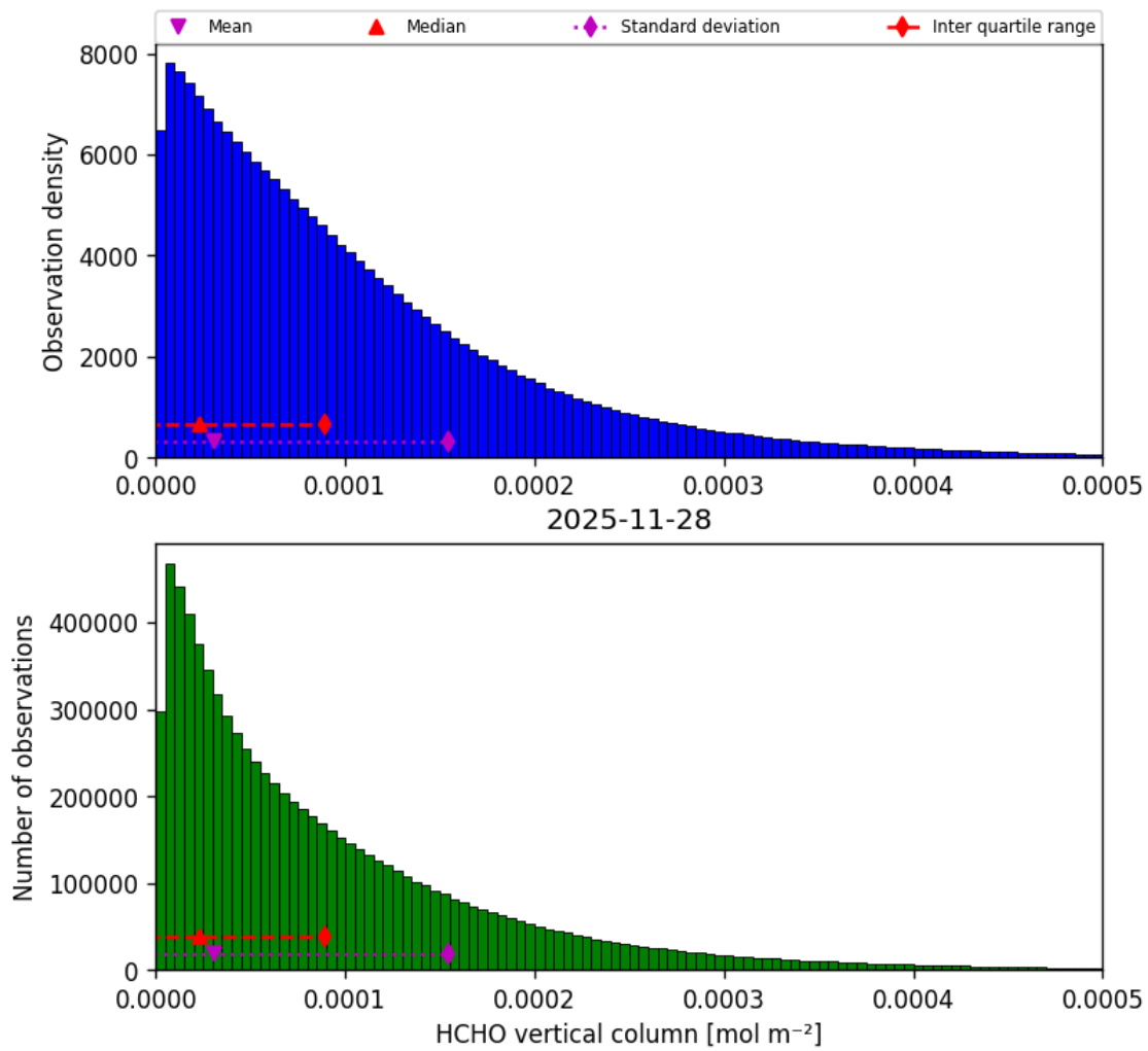
Figure 37: Histogram of “HCHO vertical column” for 2025-11-28 to 2025-11-29
