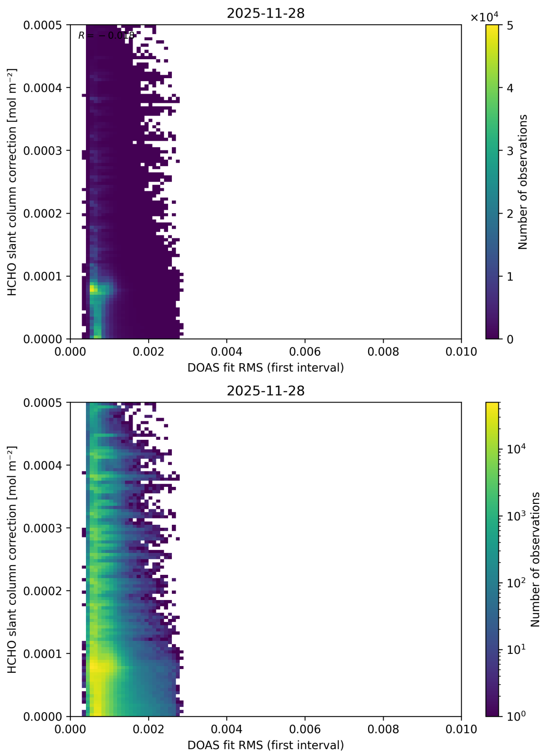
Figure 67: Scatter density plot of “DOAS fit RMS (first interval)” against “HCHO slant column correction” for 2025-11-28 to 2025-11-29.
