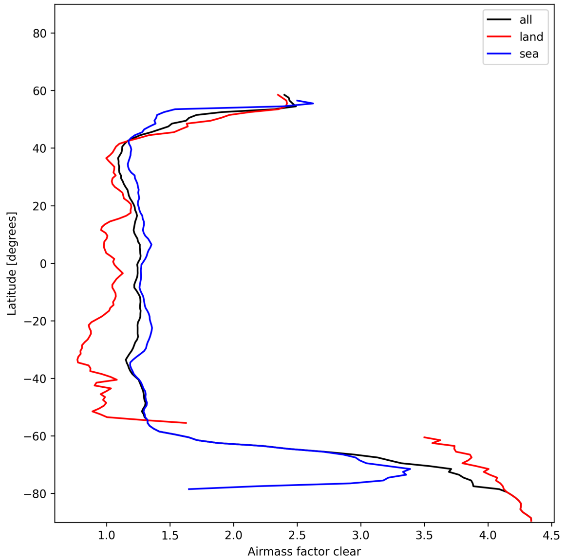
Figure 29: Zonal average of “Airmass factor clear” for 2025-11-28 to 2025-11-29.
