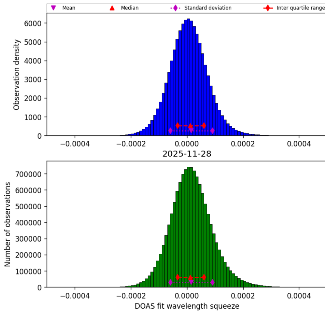
Figure 47: Histogram of “DOAS fit wavelength squeeze” for 2025-11-28 to 2025-11-29
