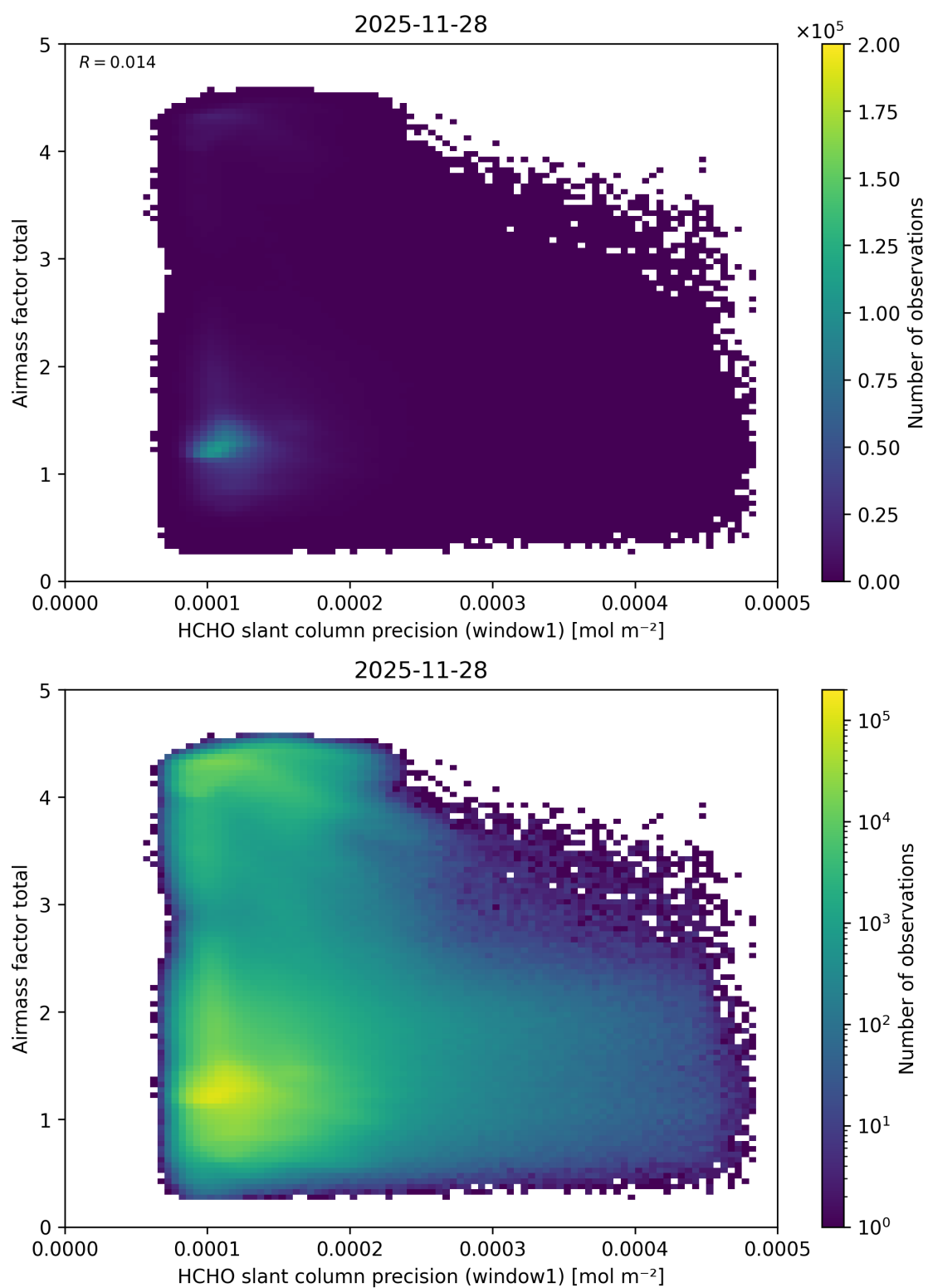
Figure 105: Scatter density plot of “HCHO slant column precision (window1)” against “Airmass factor total” for 2025-11-28 to 2025-11-29.
