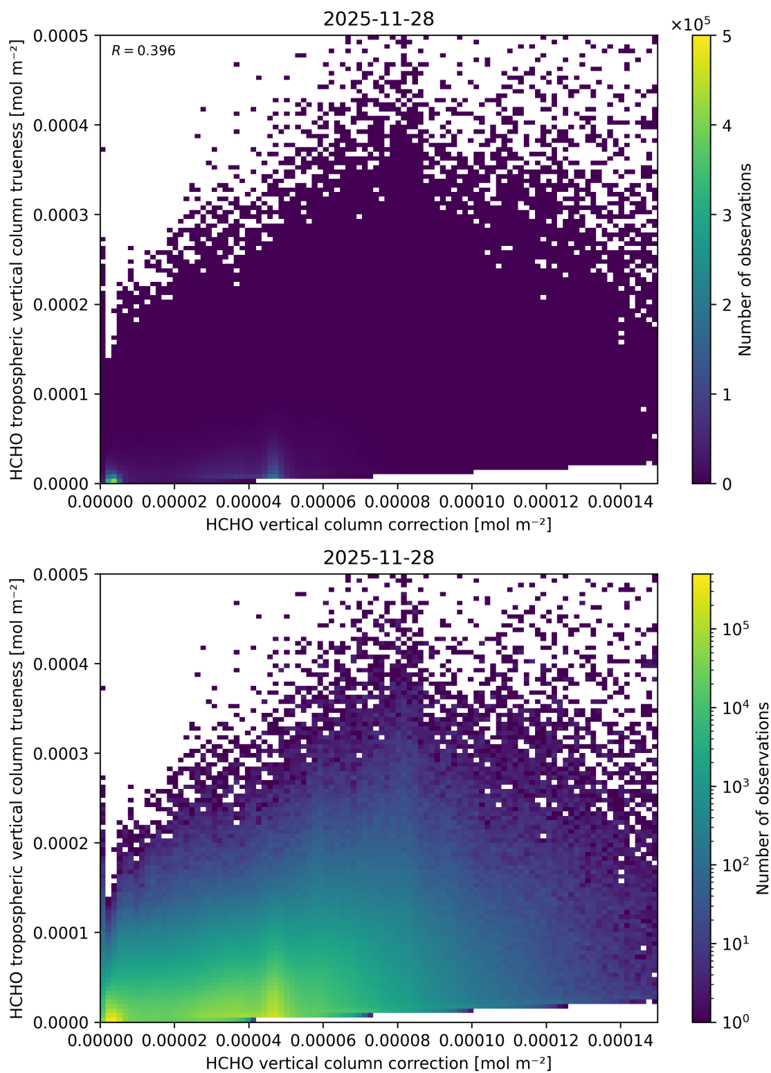
Figure 136: Scatter density plot of “HCHO vertical column correction” against “HCHO tropospheric vertical column truthness” for 2025-11-28 to 2025-11-29.
