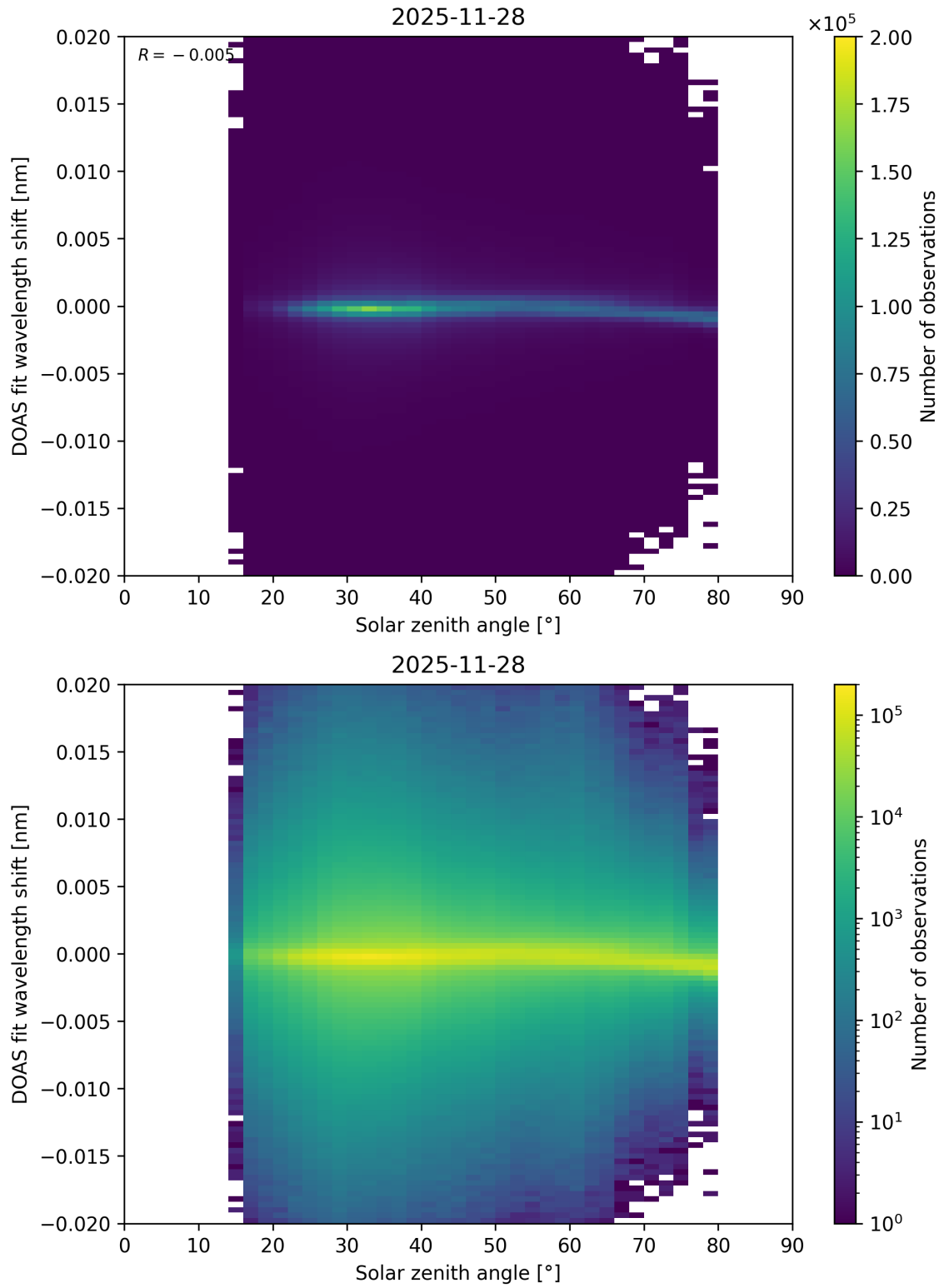
Figure 187: Scatter density plot of “Solar zenith angle” against “DOAS fit wavelength shift” for 2025-11-28 to 2025-11-29.
