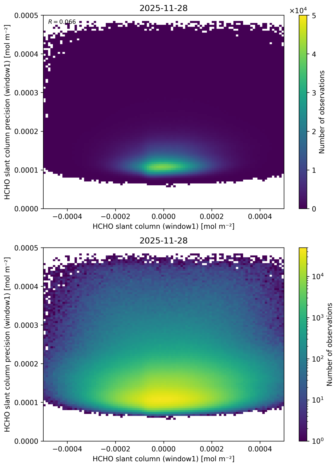
Figure 94: Scatter density plot of “HCHO slant column (window1)” against “HCHO slant column precision (window1)” for 2025-11-28 to 2025-11-29.
