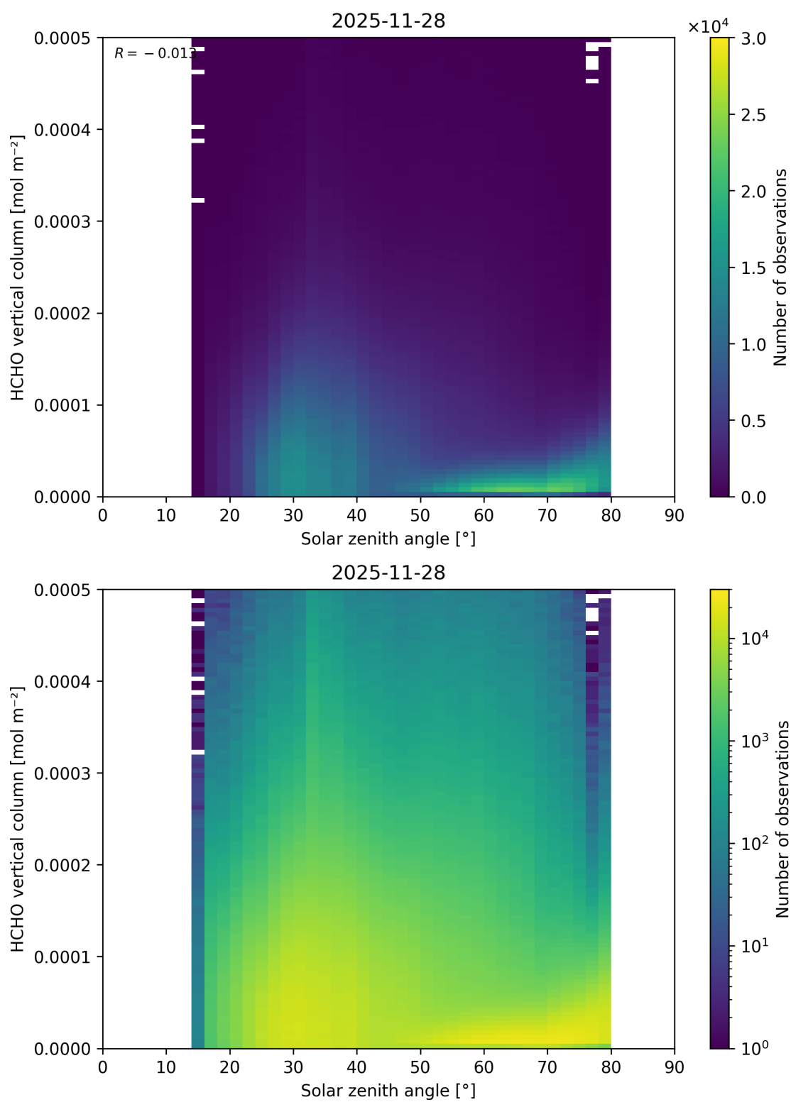
Figure 196: Scatter density plot of “Solar zenith angle” against “HCHO vertical column” for 2025-11-28 to 2025-11-29.
