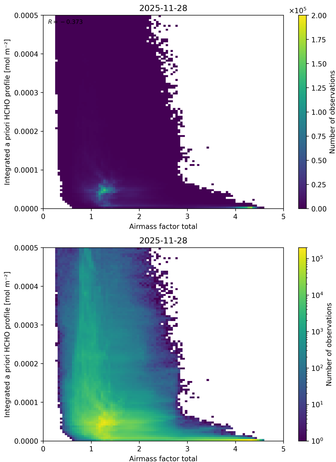
Figure 117: Scatter density plot of “Airmass factor total” against “Integrated a priori HCHO profile” for 2025-11-28 to 2025-11-29.
