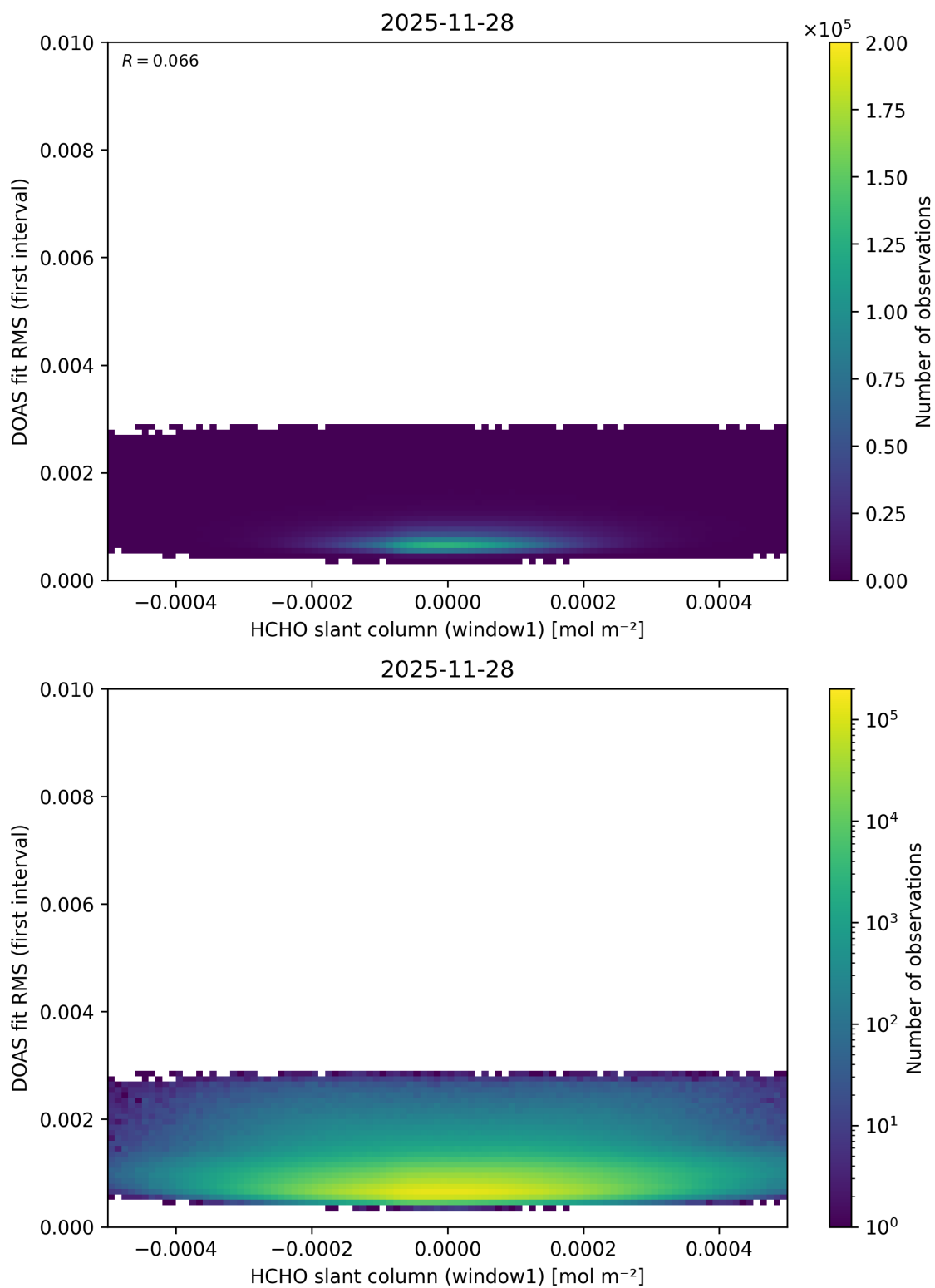
Figure 88: Scatter density plot of “HCHO slant column (window1)” against “DOAS fit RMS (first interval)” for 2025-11-28 to 2025-11-29.
