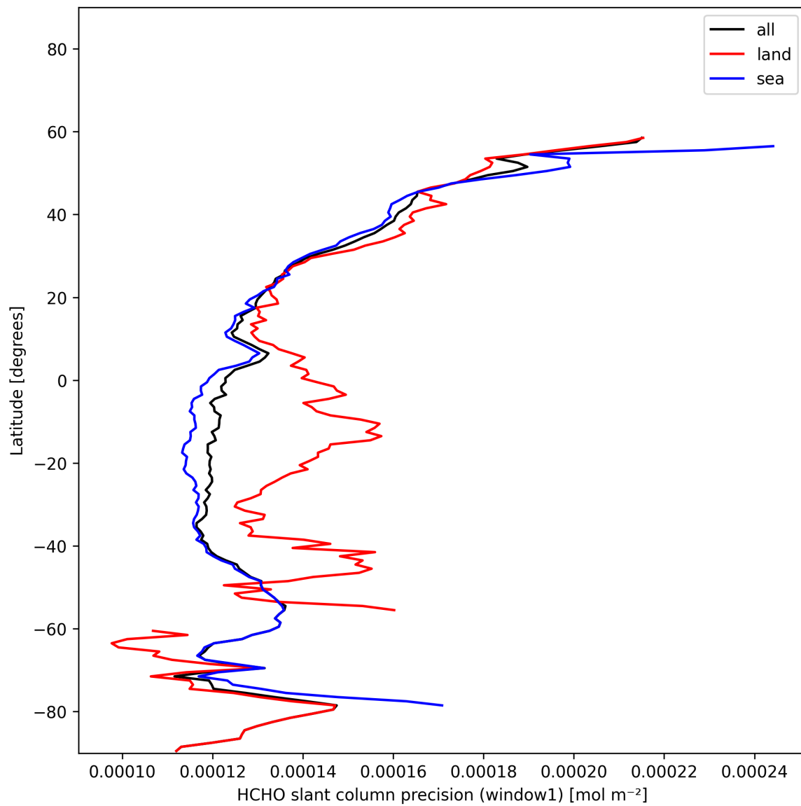
Figure 26: Zonal average of “HCHO slant column precision (window1)” for 2025-11-28 to 2025-11-29.
