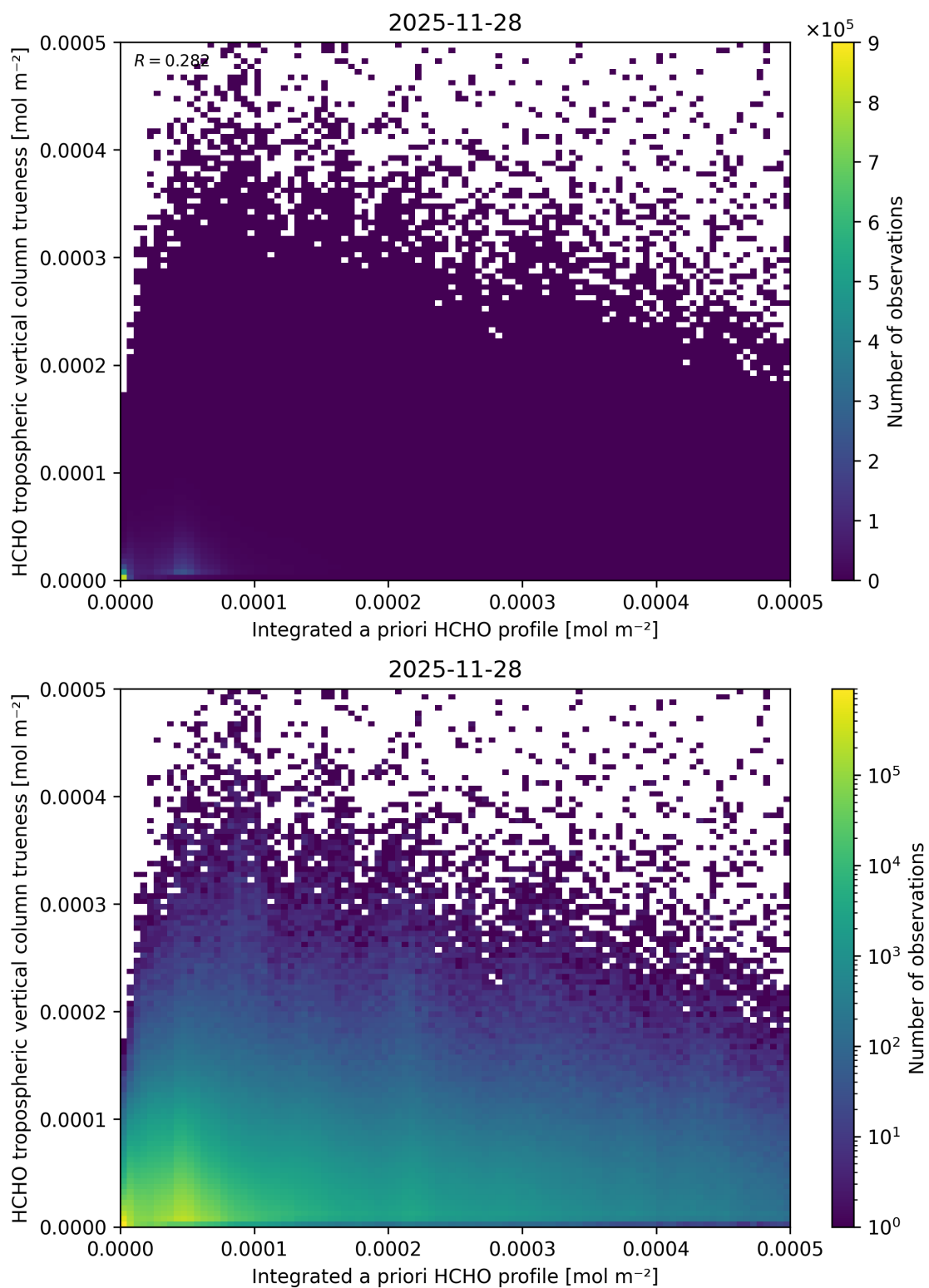
Figure 170: Scatter density plot of “Integrated a priori HCHO profile” against “HCHO tropospheric vertical column trueness” for 2025-11-28 to 2025-11-29.
