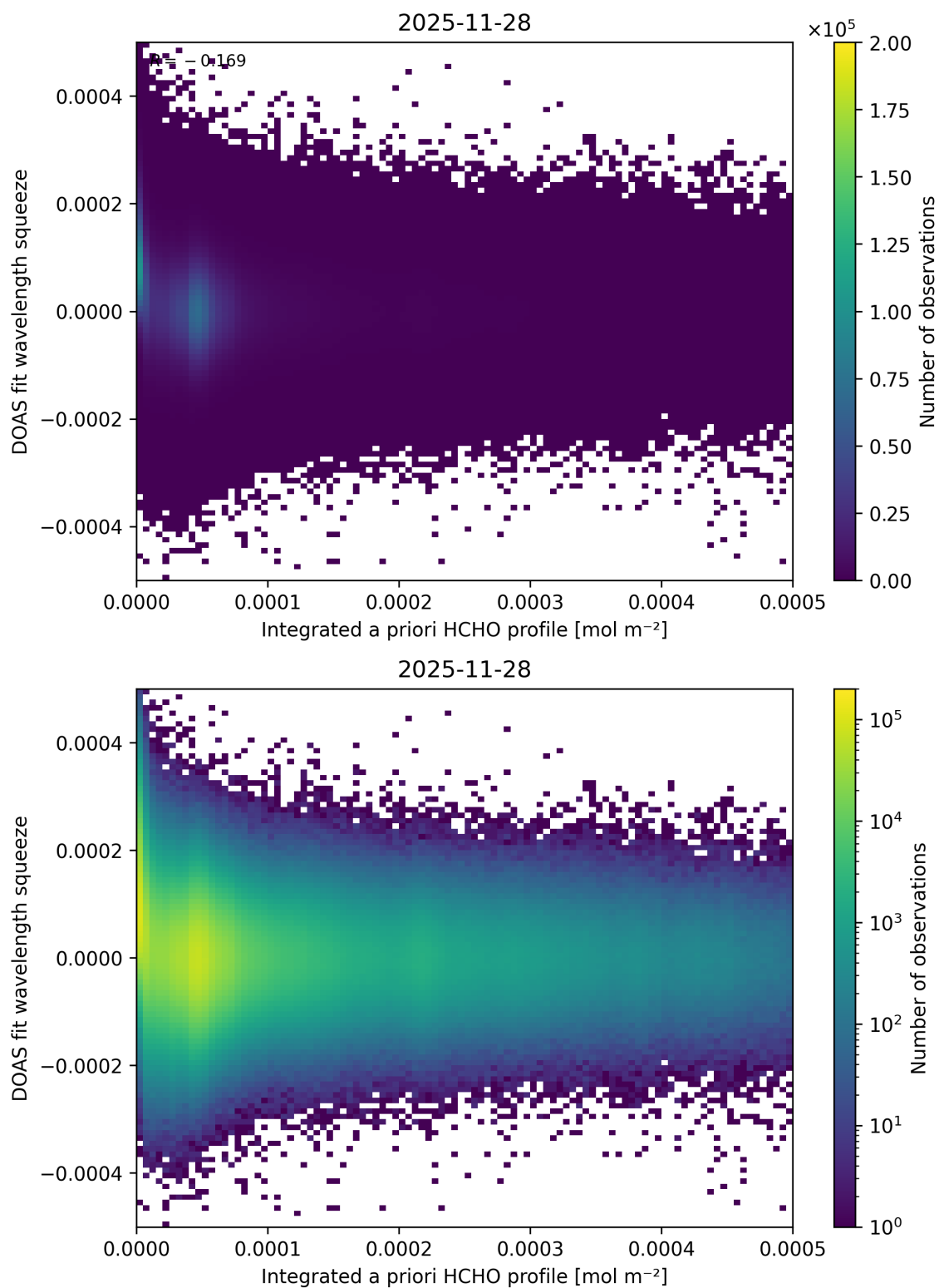
Figure 167: Scatter density plot of “Integrated a priori HCHO profile” against “DOAS fit wavelength squeeze” for 2025-11-28 to 2025-11-29.
