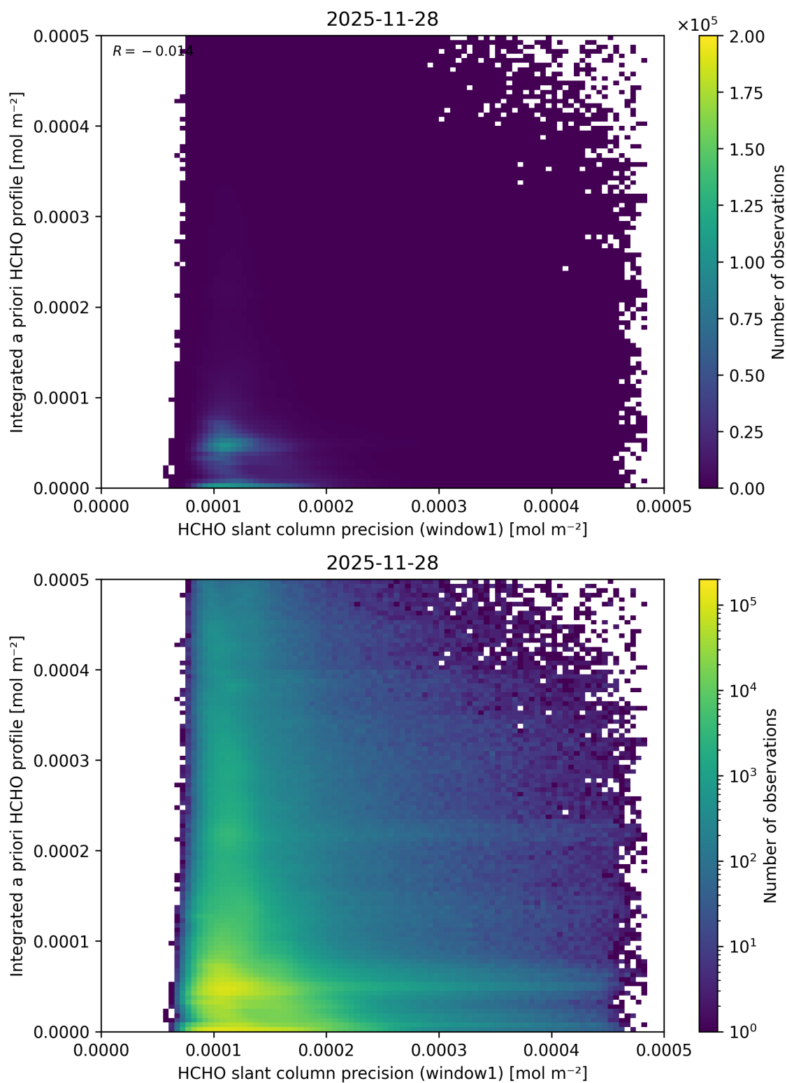
Figure 108: Scatter density plot of “HCHO slant column precision (window1)” against “Integrated a priori HCHO profile” for 2025-11-28 to 2025-11-29.
