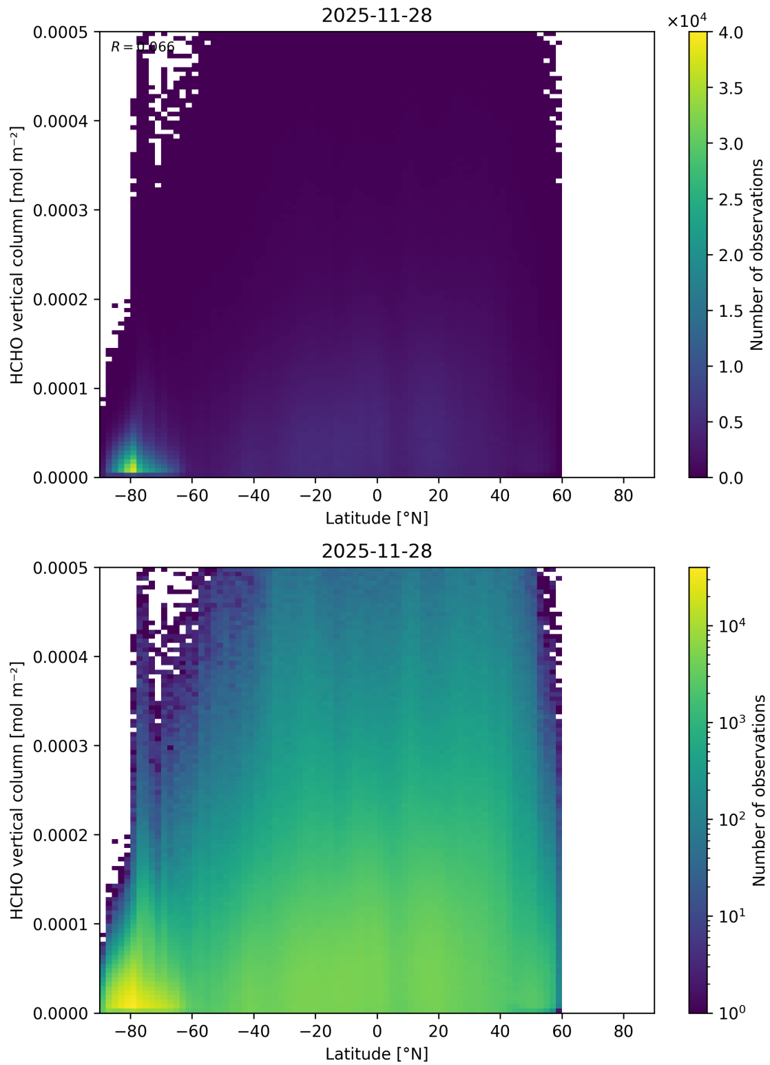
Figure 181: Scatter density plot of “Latitude” against “HCHO vertical column” for 2025-11-28 to 2025-11-29.
