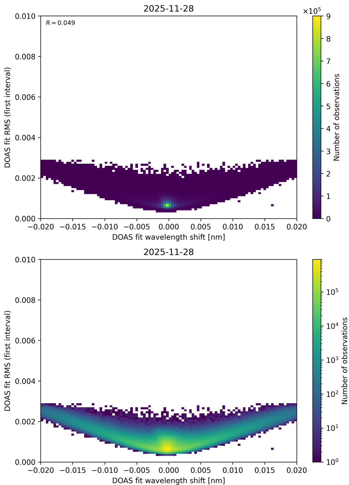
Figure 69: Scatter density plot of “DOAS fit wavelength shift” against “DOAS fit RMS (first interval)” for 2025-11-28 to 2025-11-29.
