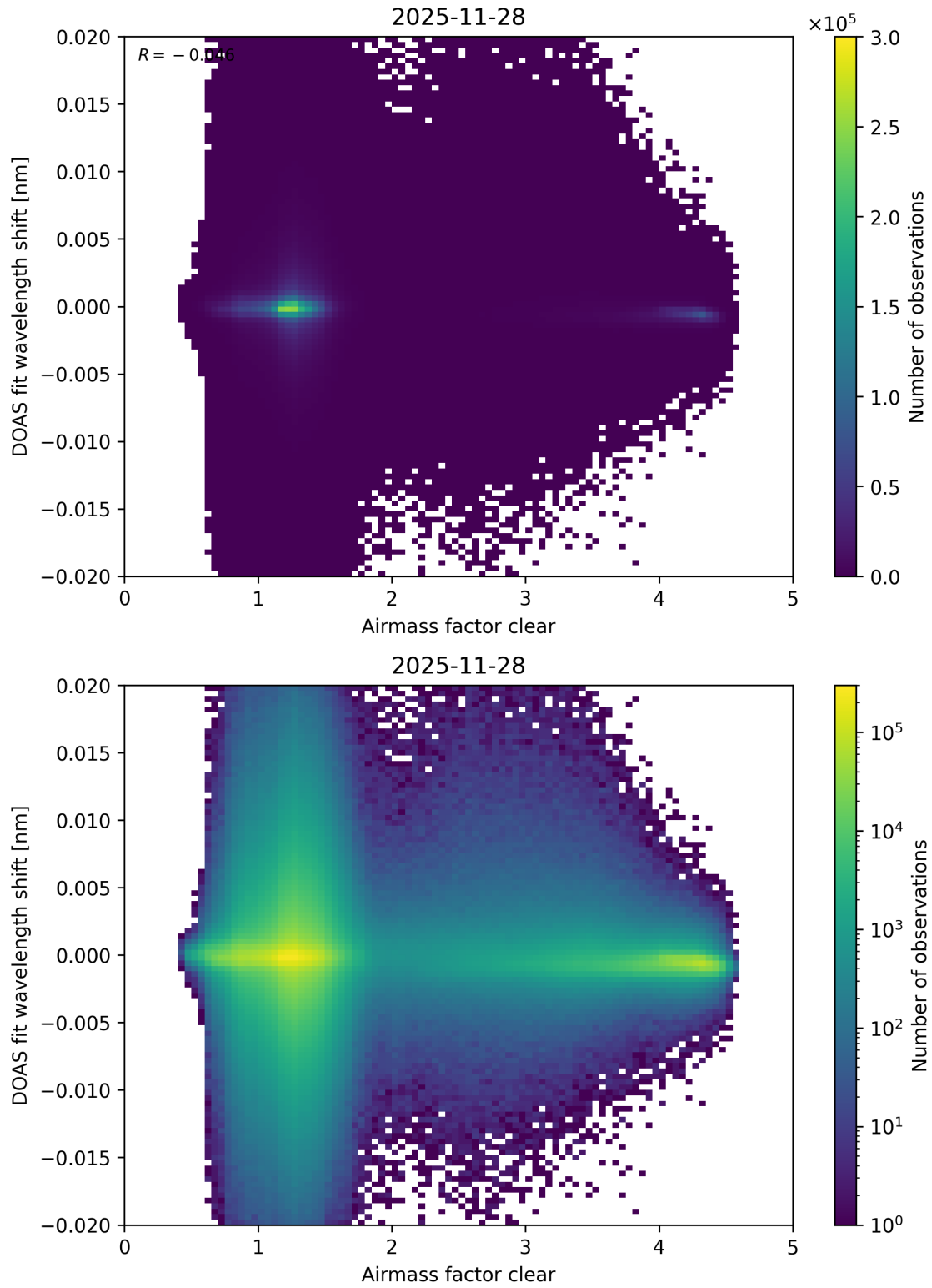
Figure 79: Scatter density plot of “Airmass factor clear” against “DOAS fit wavelength shift” for 2025-11-28 to 2025-11-29.
