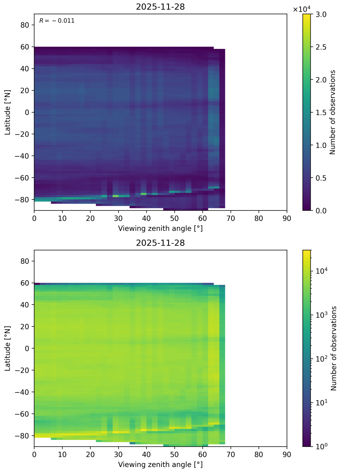
Figure 217: Scatter density plot of “Viewing zenith angle” against “Latitude” for 2025-11-28 to 2025-11-29.
