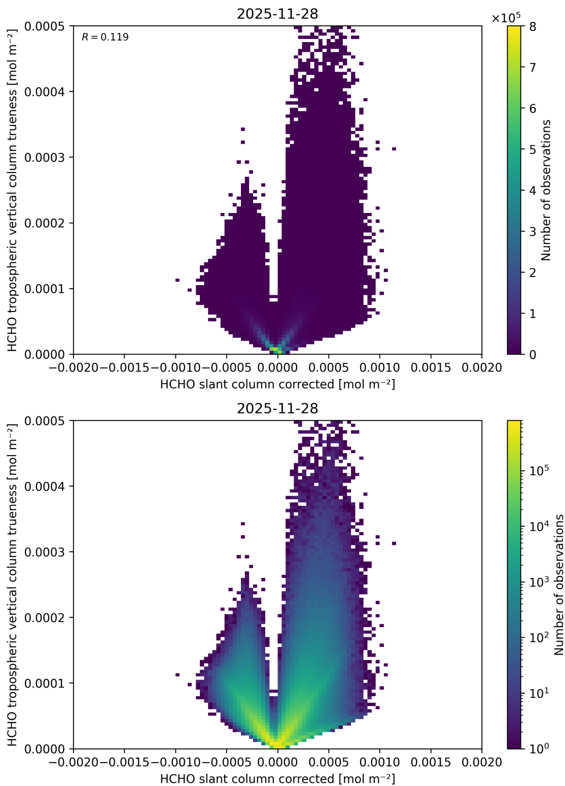
Figure 86: Scatter density plot of “HCHO slant column corrected” against “HCHO tropospheric vertical column trueness” for 2025-11-28 to 2025-11-29.
