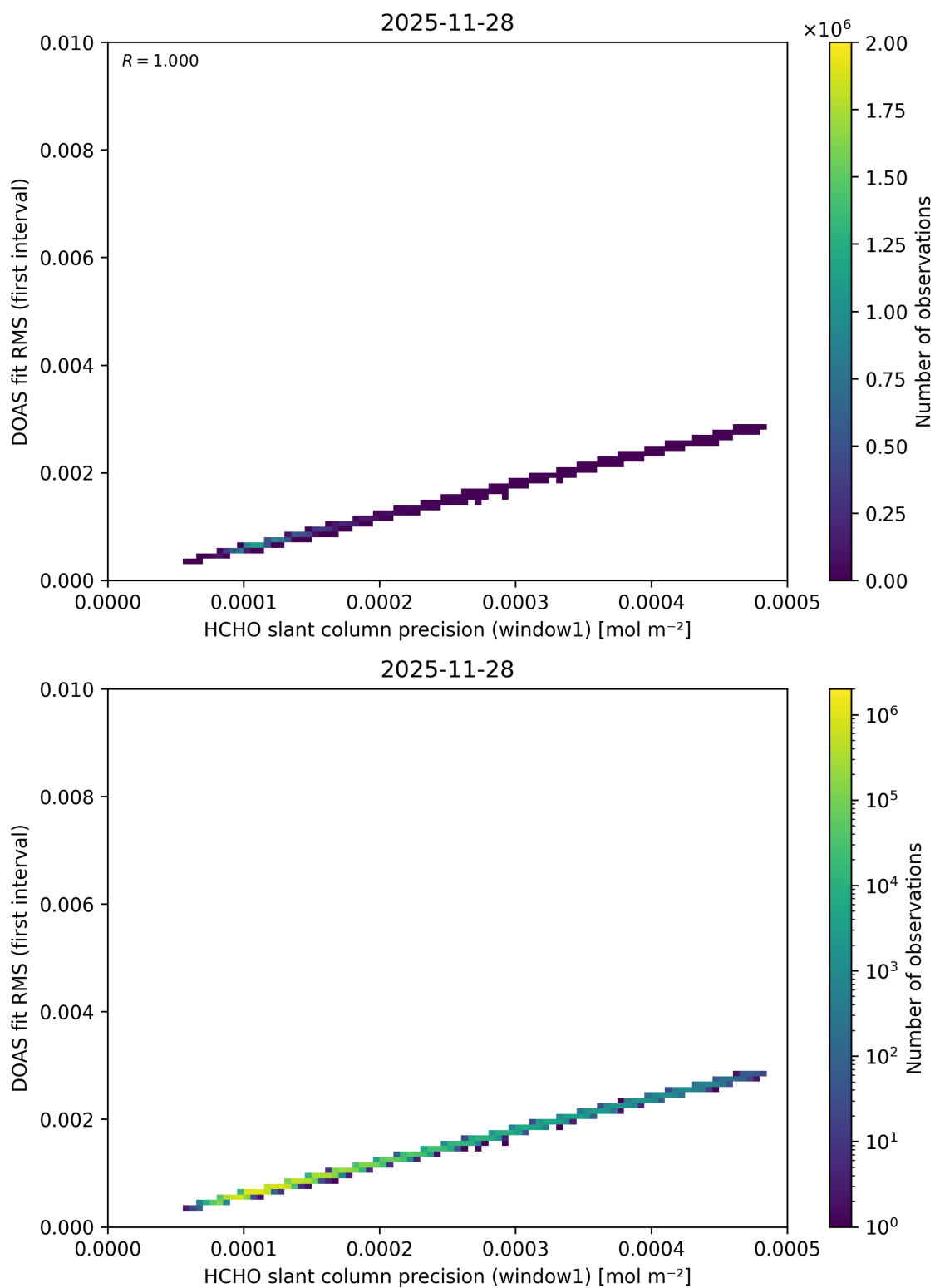
Figure 99: Scatter density plot of “HCHO slant column precision (window1)” against “DOAS fit RMS (first interval)” for 2025-11-28 to 2025-11-29.
