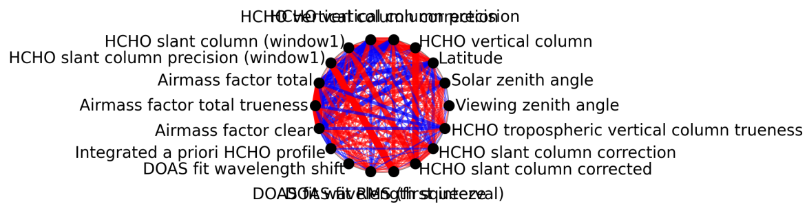
Figure 1: Map of correlation graph for 2025-11-28 to 2025-11-29.
