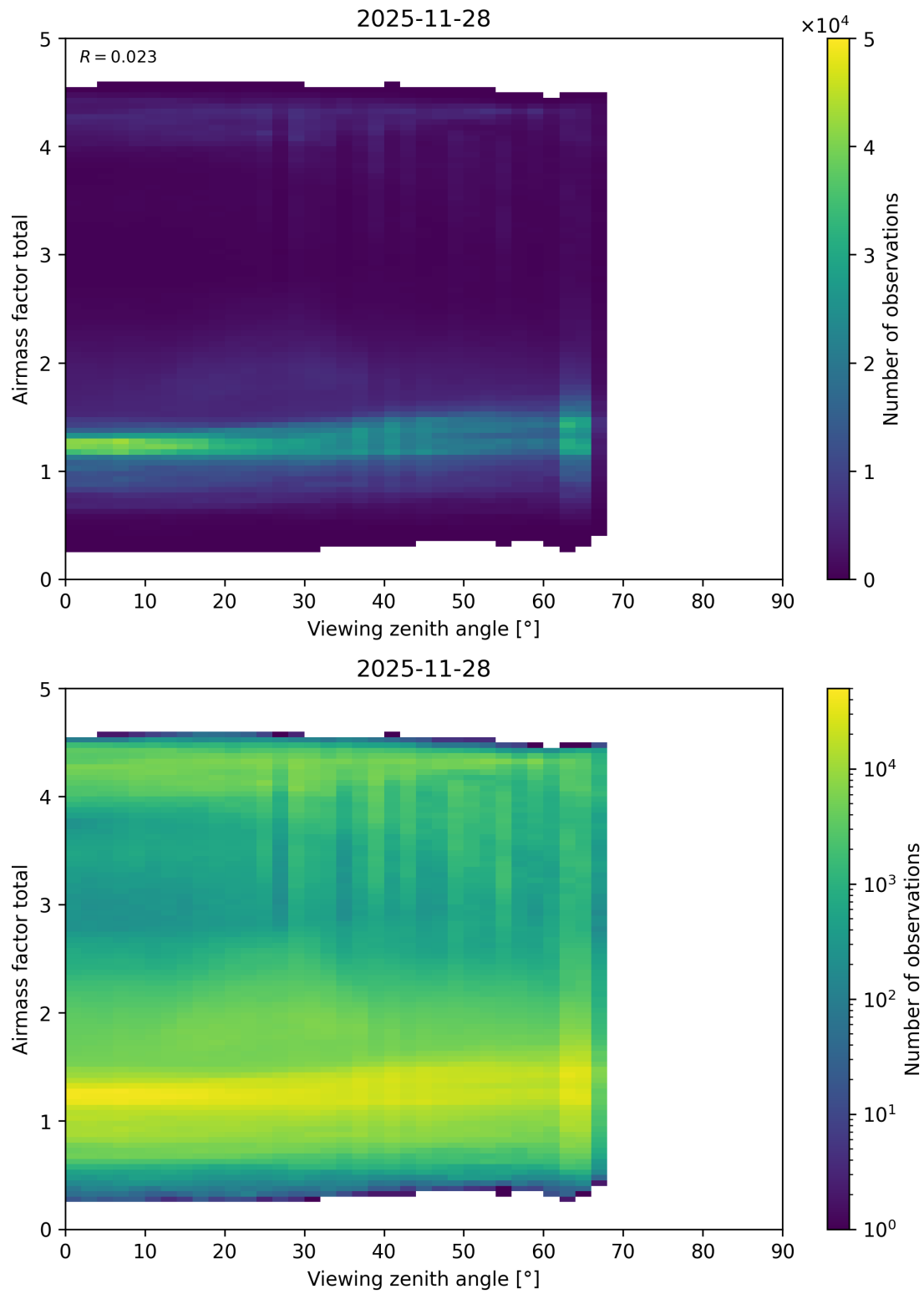
Figure 210: Scatter density plot of “Viewing zenith angle” against “Airmass factor total” for 2025-11-28 to 2025-11-29.
