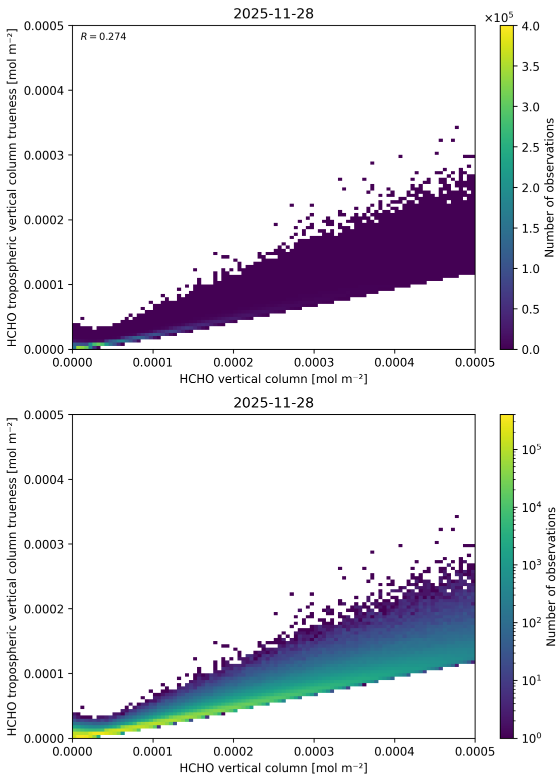
Figure 150: Scatter density plot of “HCHO vertical column” against “HCHO tropospheric vertical column trueness” for 2025-11-28 to 2025-11-29.
