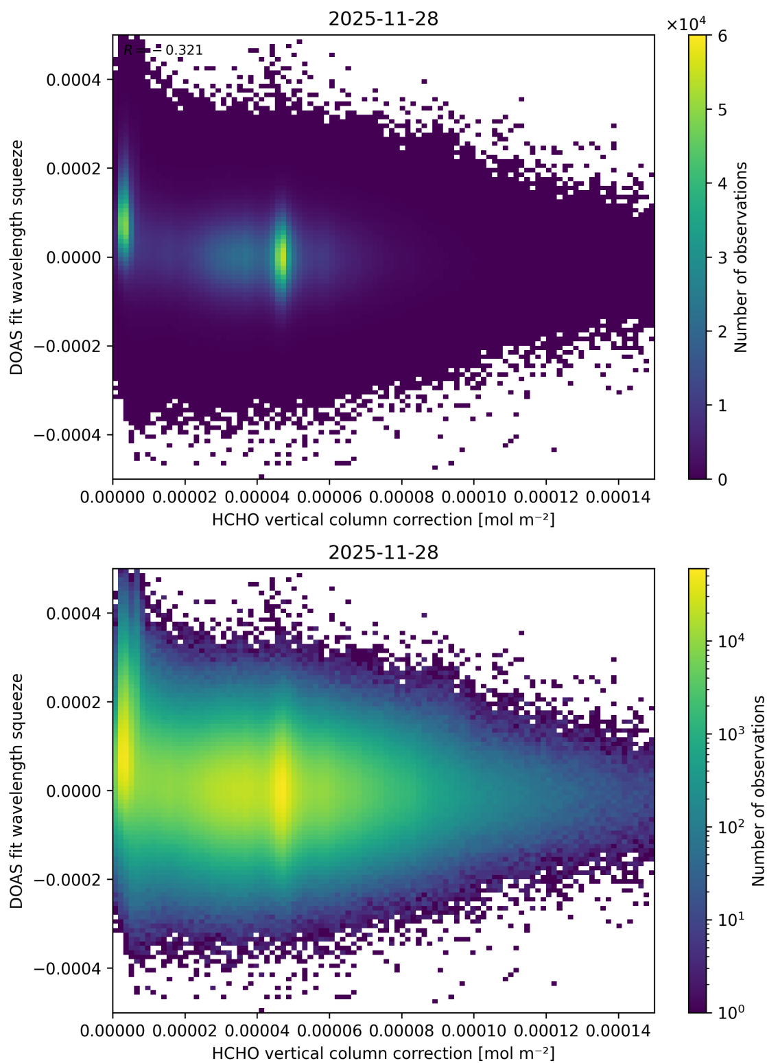
Figure 128: Scatter density plot of “HCHO vertical column correction” against “DOAS fit wavelength squeeze” for 2025-11-28 to 2025-11-29.
