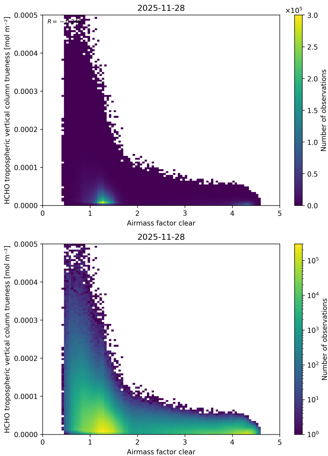
Figure 83: Scatter density plot of “Airmass factor clear” against “HCHO tropospheric vertical column trueeness” for 2025-11-28 to 2025-11-29.
