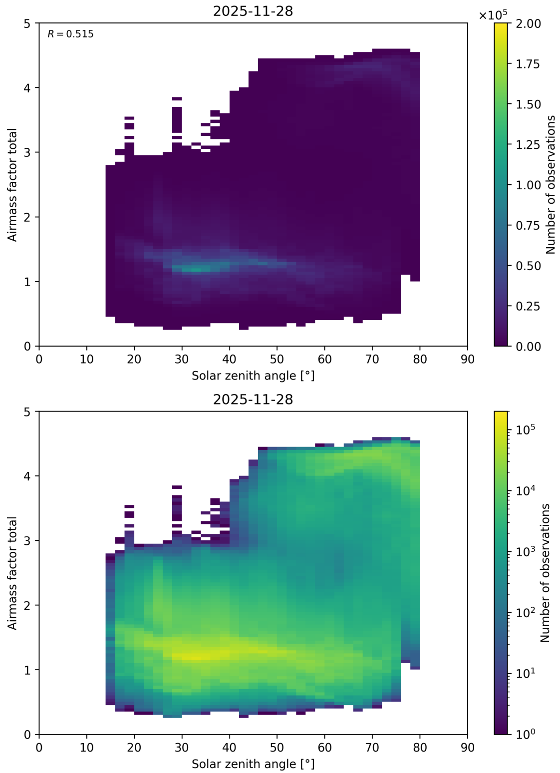
Figure 194: Scatter density plot of “Solar zenith angle” against “Airmass factor total” for 2025-11-28 to 2025-11-29.
