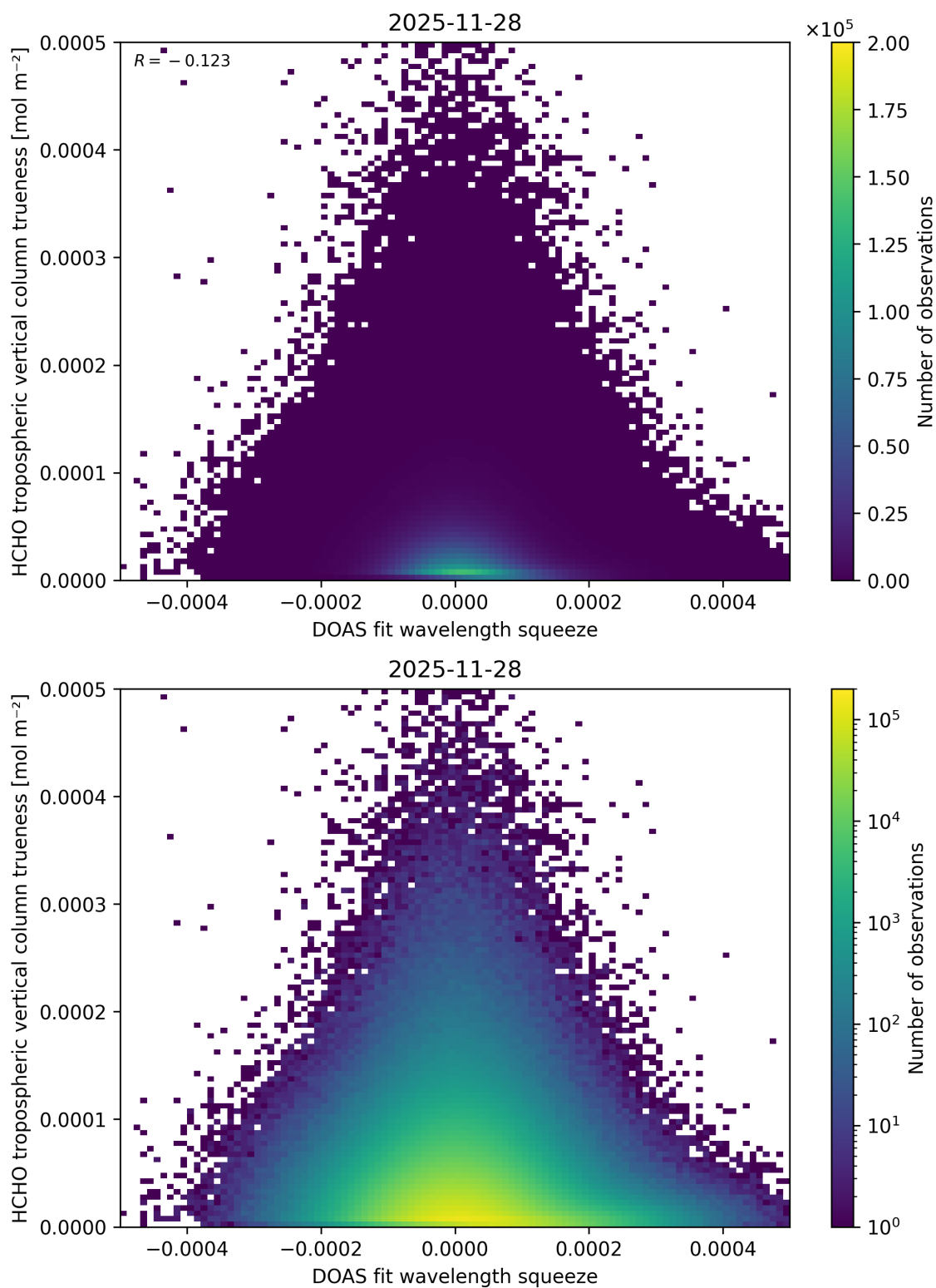
Figure 77: Scatter density plot of “DOAS fit wavelength squeeze” against “HCHO tropospheric vertical column trueness” for 2025-11-28 to 2025-11-29.
