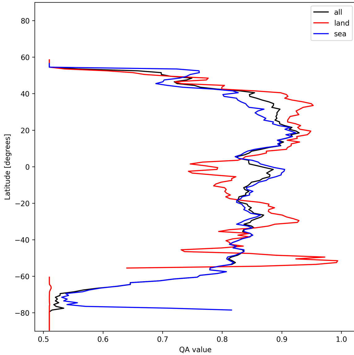
Figure 21: Zonal average of “QA value” for 2025-11-28 to 2025-11-29.
