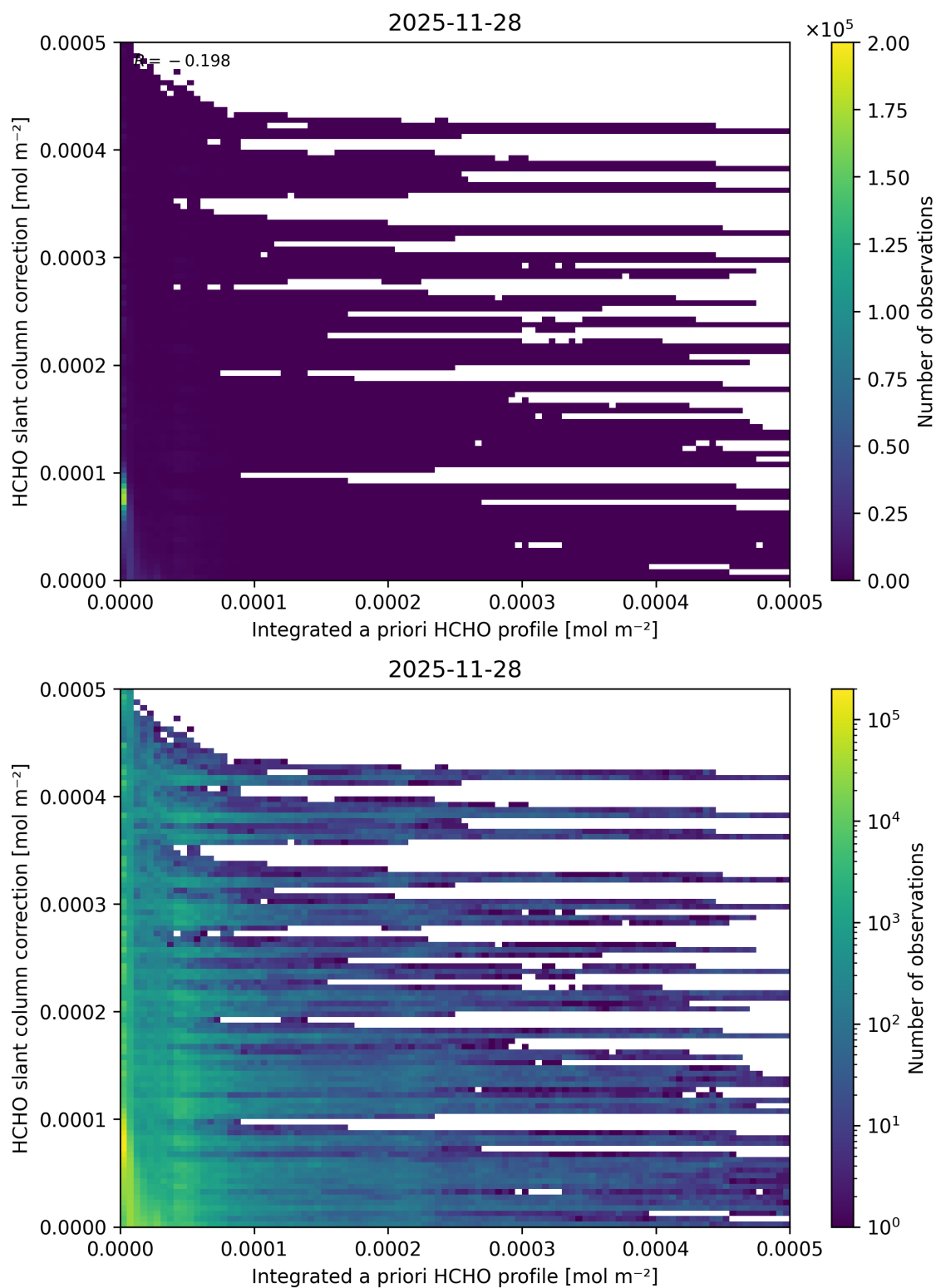
Figure 169: Scatter density plot of “Integrated a priori HCHO profile” against “HCHO slant column correction” for 2025-11-28 to 2025-11-29.
