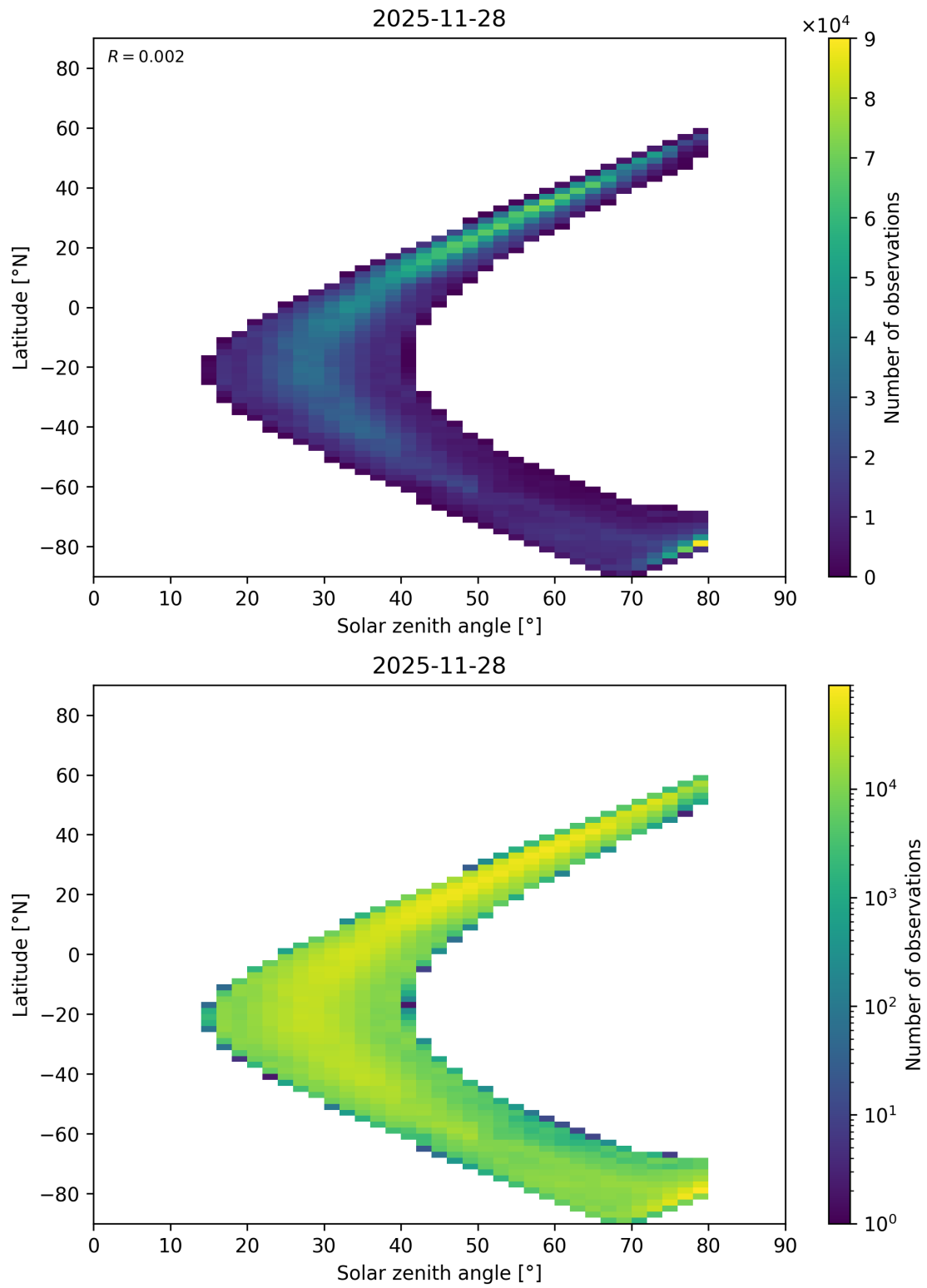
Figure 201: Scatter density plot of “Solar zenith angle” against “Latitude” for 2025-11-28 to 2025-11-29.
