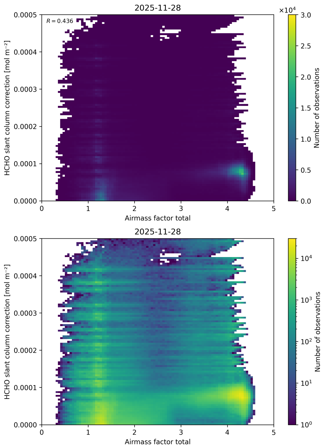
Figure 114: Scatter density plot of “Airmass factor total” against “HCHO slant column correction” for 2025-11-28 to 2025-11-29.
