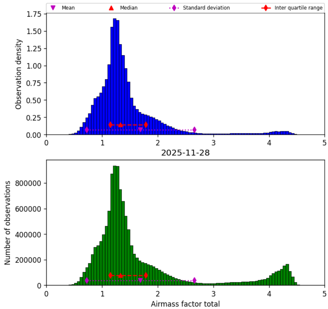
Figure 42: Histogram of “Airmass factor total” for 2025-11-28 to 2025-11-29
