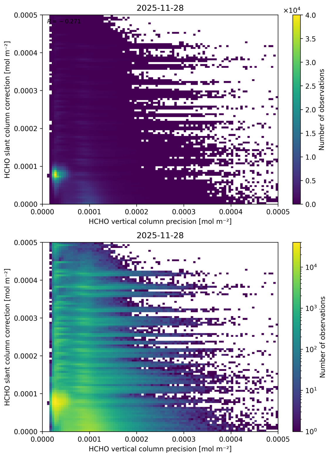
Figure 157: Scatter density plot of “HCHO vertical column precision” against “HCHO slant column correction” for 2025-11-28 to 2025-11-29.
