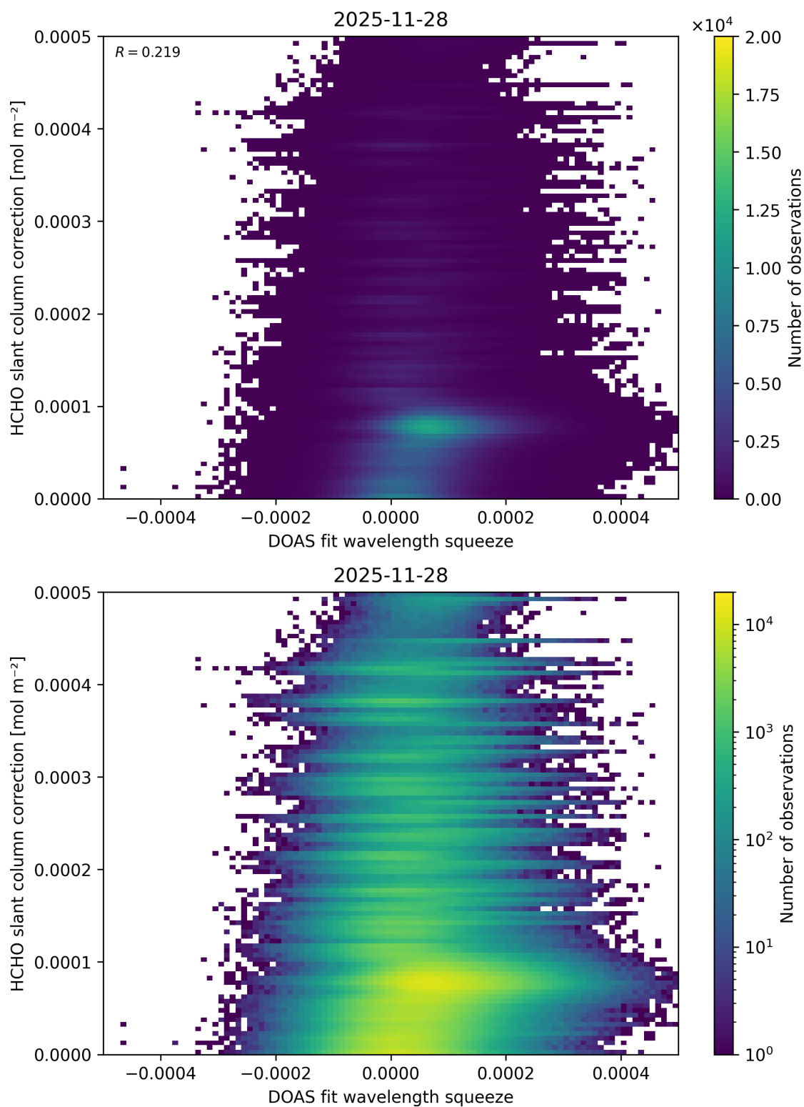
Figure 76: Scatter density plot of “DOAS fit wavelength squeeze” against “HCHO slant column correction” for 2025-11-28 to 2025-11-29.
