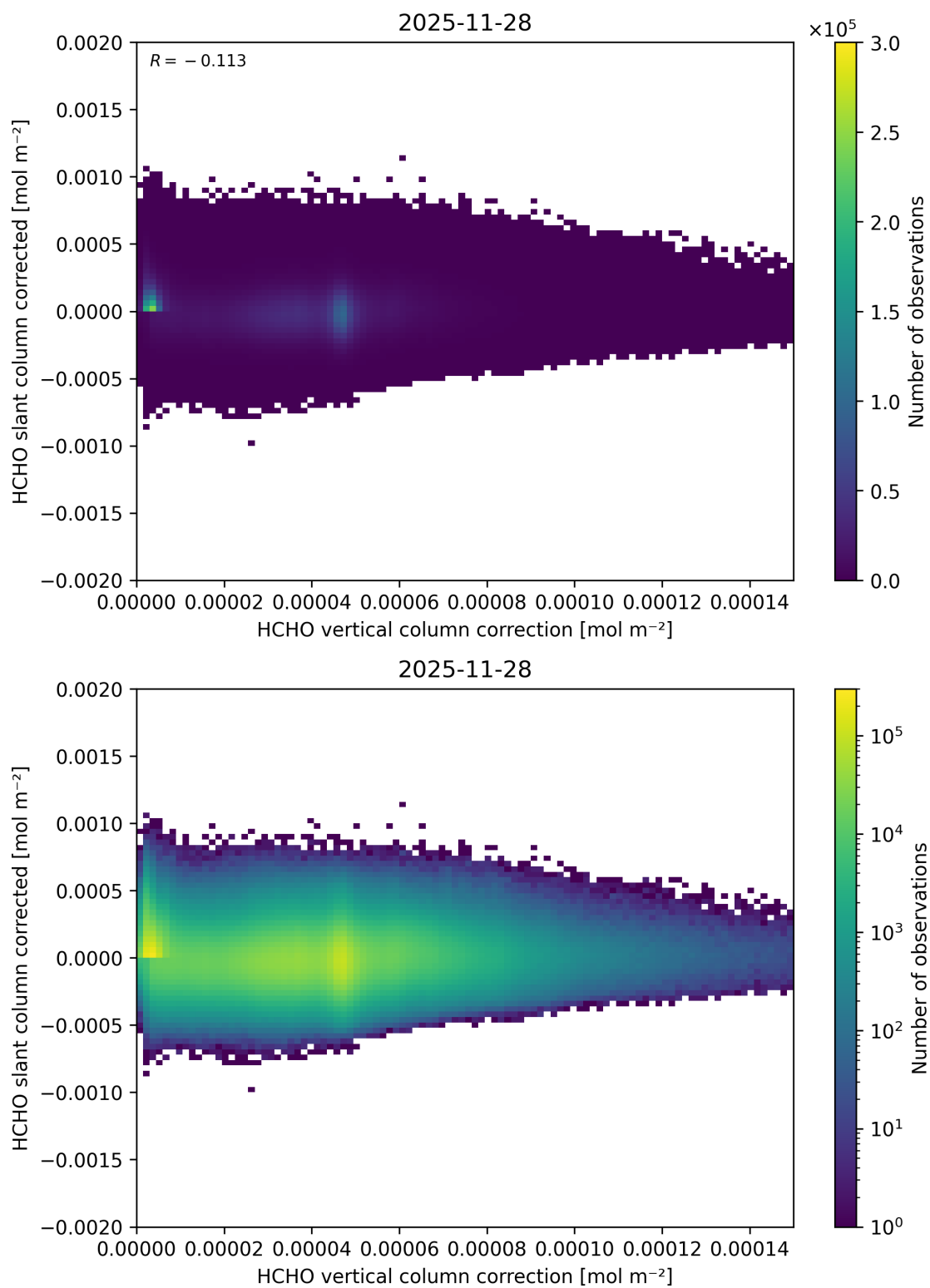
Figure 130: Scatter density plot of “HCHO vertical column correction” against “HCHO slant column corrected” for 2025-11-28 to 2025-11-29.
