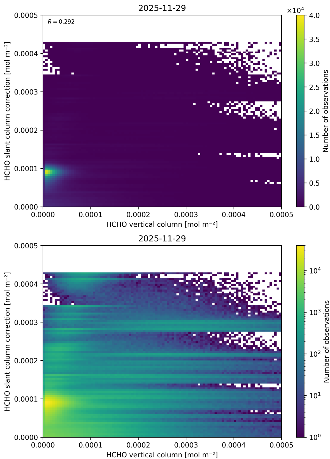
Figure 143: Scatter density plot of “HCHO vertical column” against “HCHO slant column correction” for 2025-11-28 to 2025-11-30.
