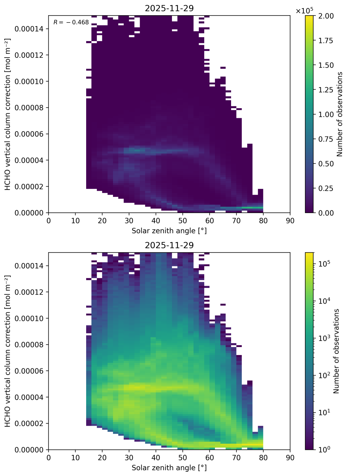
Figure 197: Scatter density plot of “Solar zenith angle” against “HCHO vertical column correction” for 2025-11-28 to 2025-11-30.
