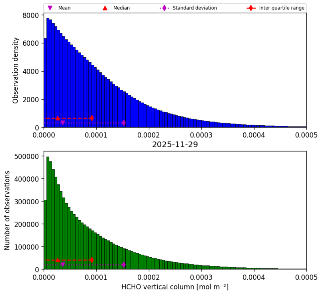
Figure 37: Histogram of “HCHO vertical column” for 2025-11-28 to 2025-11-30
