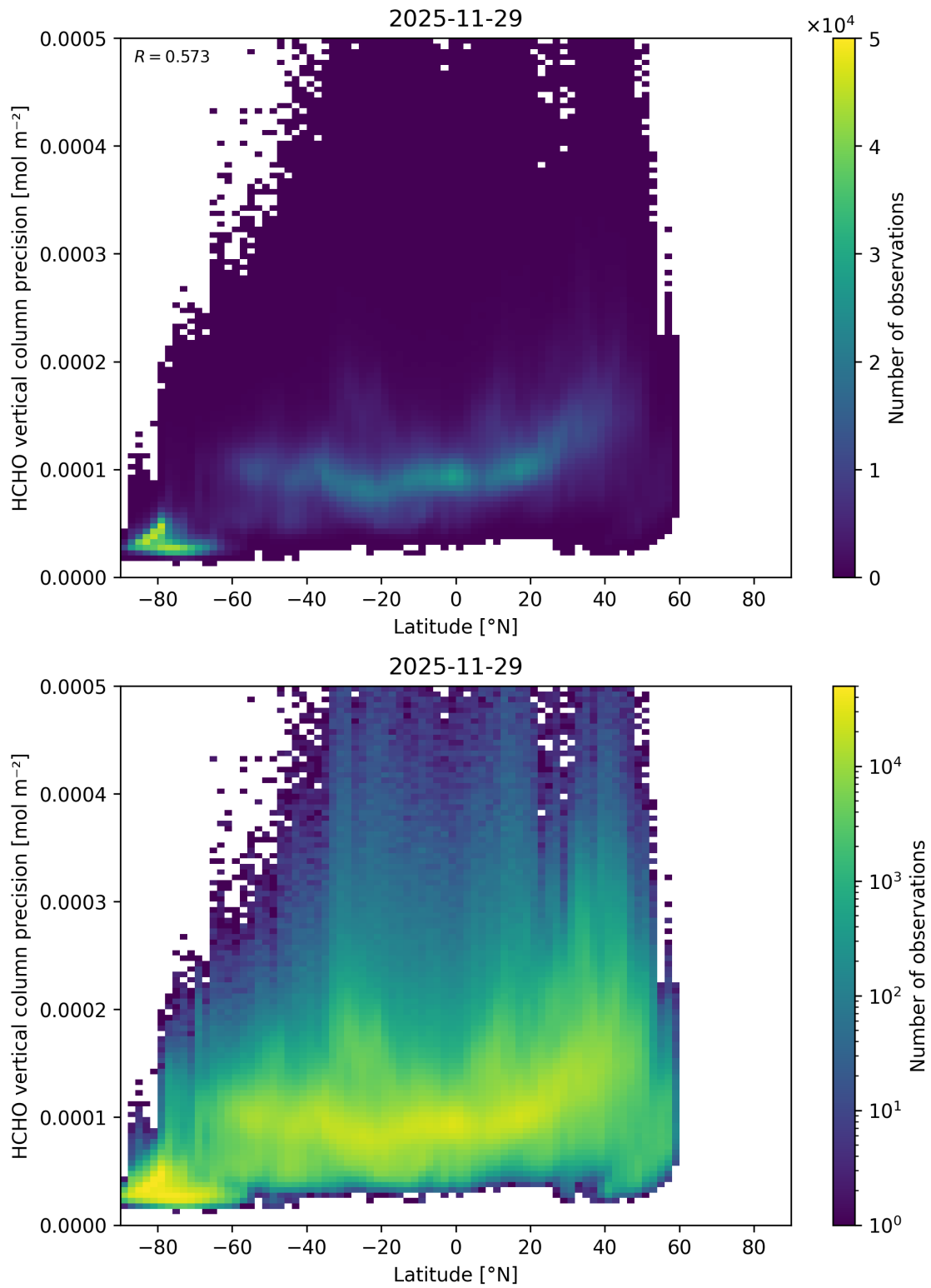
Figure 183: Scatter density plot of “Latitude” against “HCHO vertical column precision” for 2025-11-28 to 2025-11-30.
