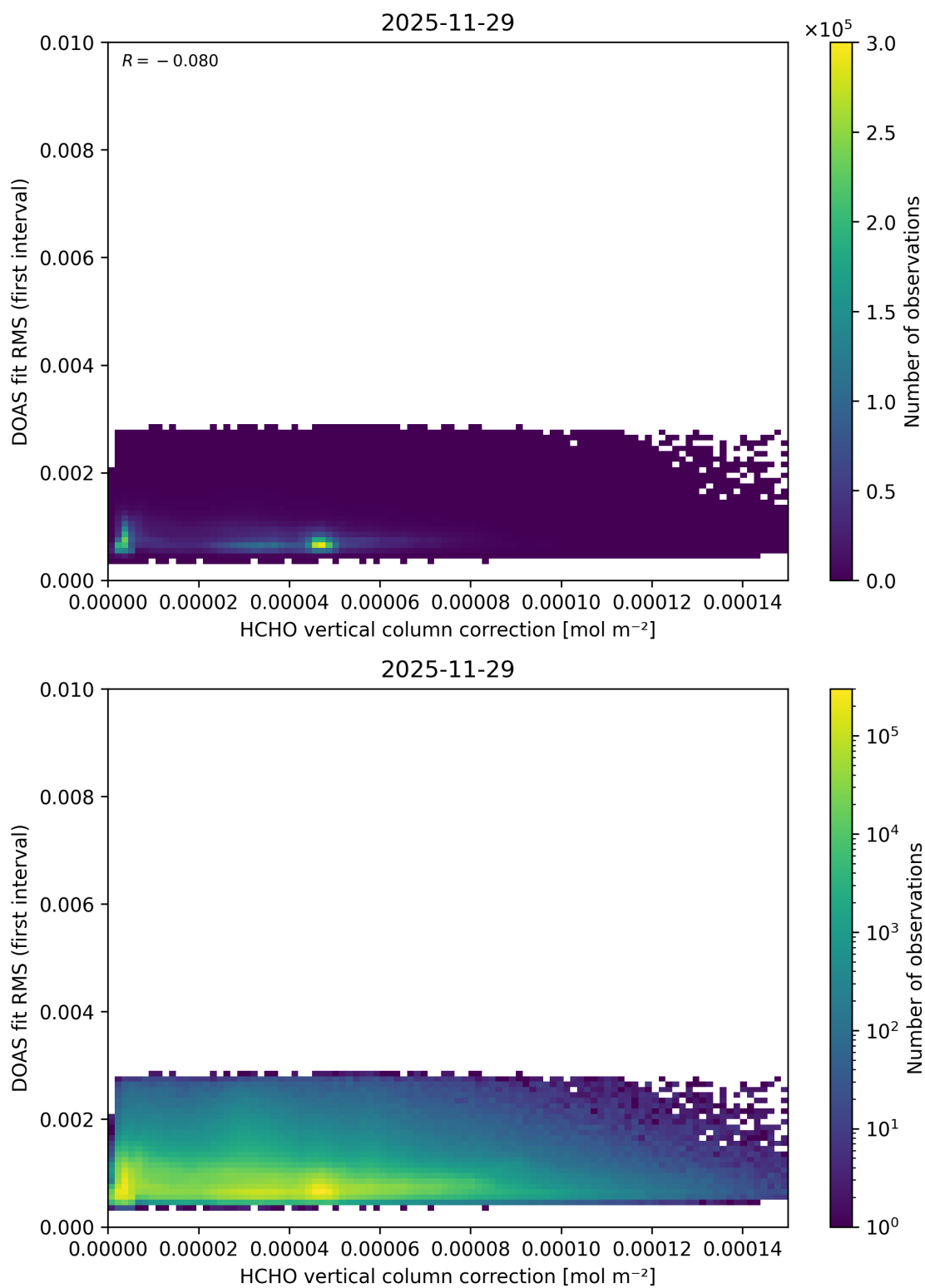
Figure 126: Scatter density plot of “HCHO vertical column correction” against “DOAS fit RMS (first interval)” for 2025-11-28 to 2025-11-30.
