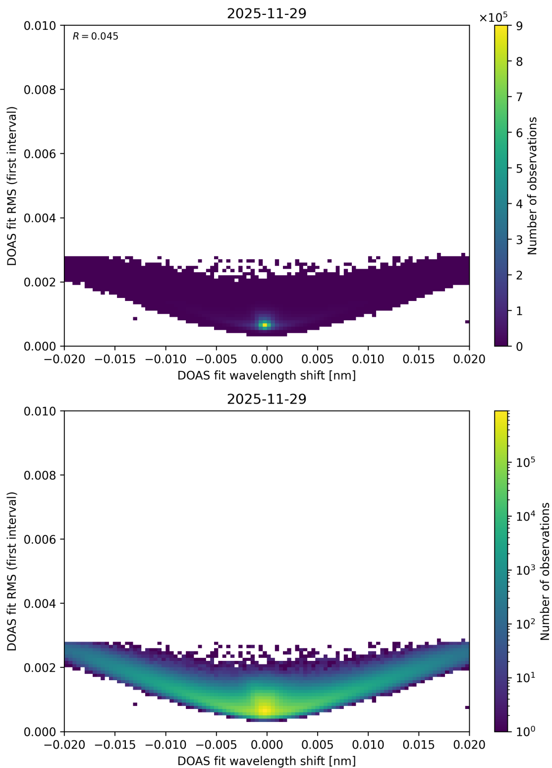
Figure 69: Scatter density plot of “DOAS fit wavelength shift” against “DOAS fit RMS (first interval)” for 2025-11-28 to 2025-11-30.
