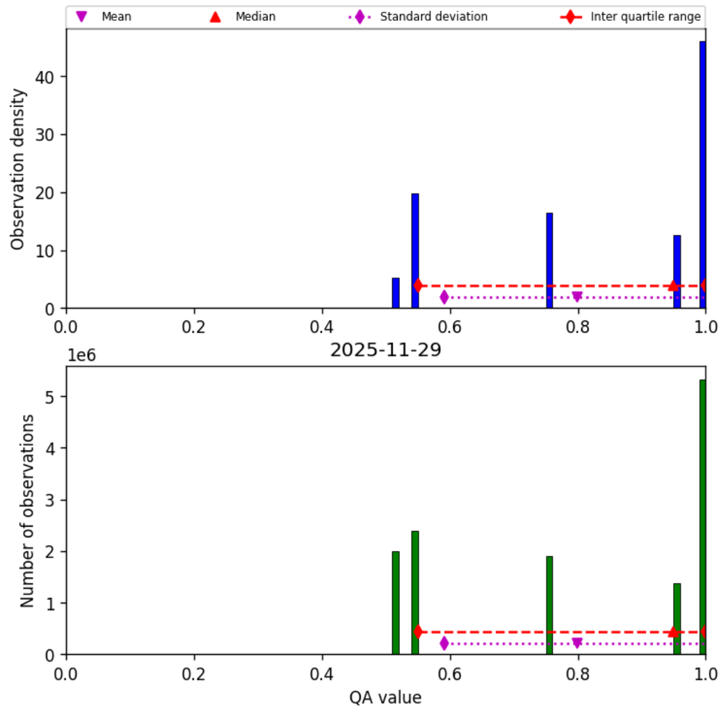
Figure 36: Histogram of “QA value” for 2025-11-28 to 2025-11-30
