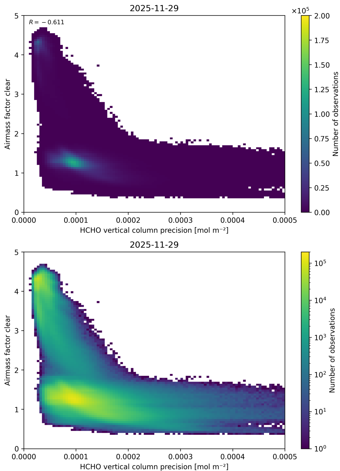
Figure 155: Scatter density plot of “HCHO vertical column precision” against “Airmass factor clear” for 2025-11-28 to 2025-11-30.
