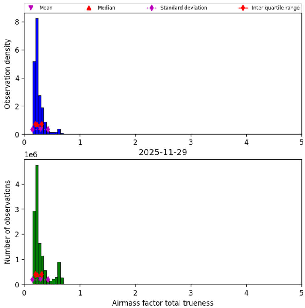
Figure 43: Histogram of “Airmass factor total trueness” for 2025-11-28 to 2025-11-30
