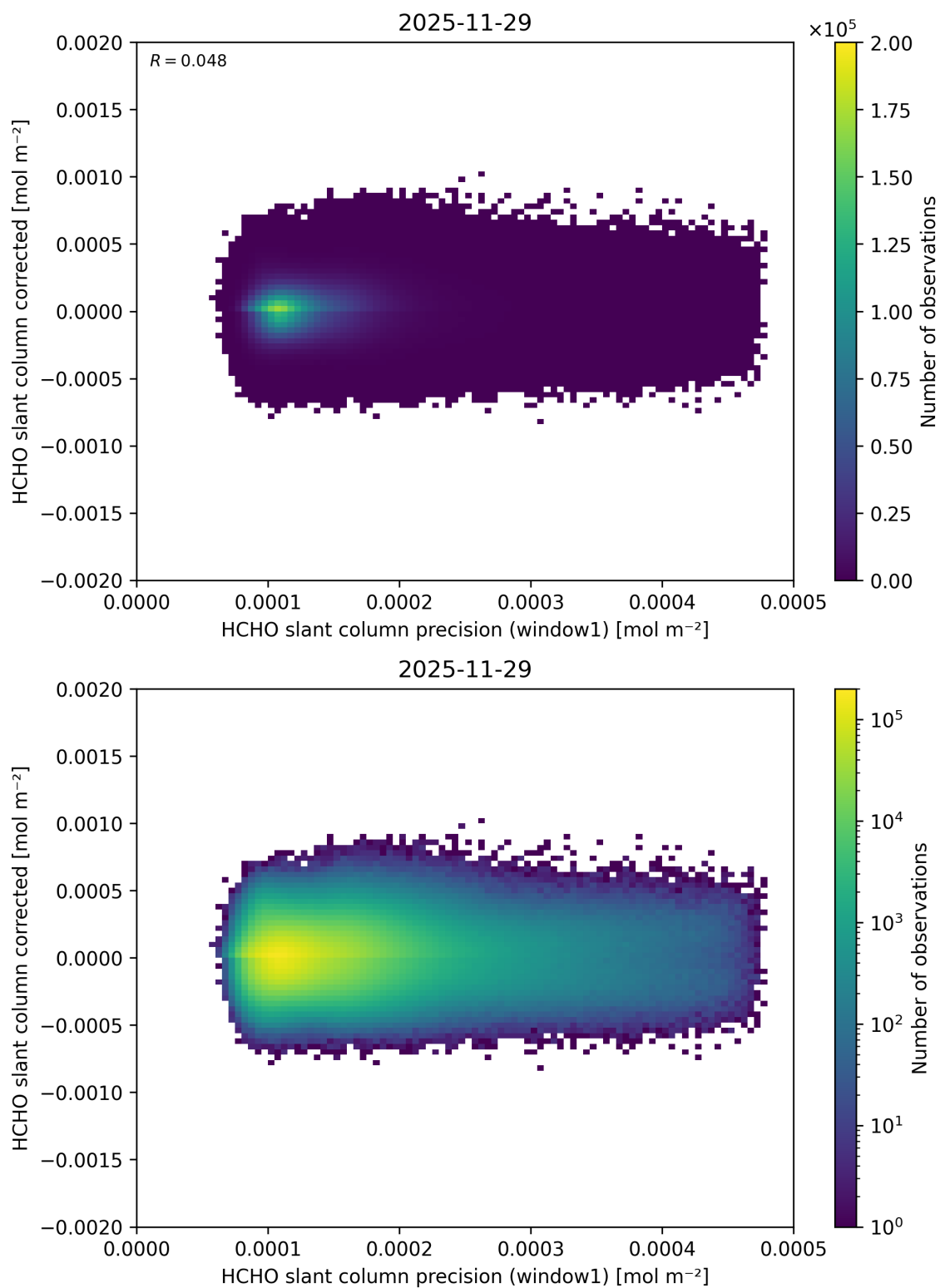
Figure 103: Scatter density plot of “HCHO slant column precision (window1)” against “HCHO slant column corrected” for 2025-11-28 to 2025-11-30.
