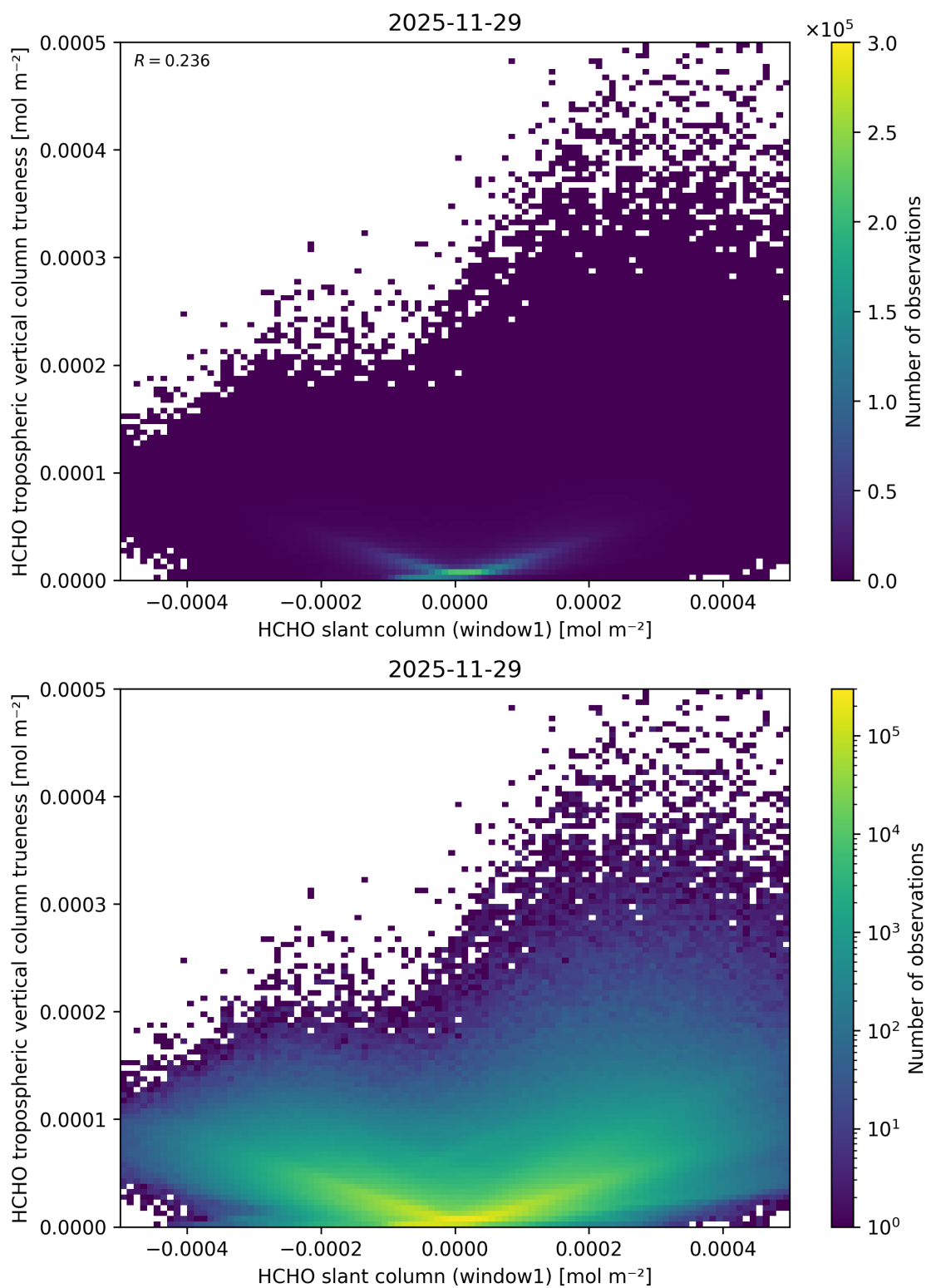
Figure 97: Scatter density plot of “HCHO slant column (window1)” against “HCHO tropospheric vertical column trueness” for 2025-11-28 to 2025-11-30.
