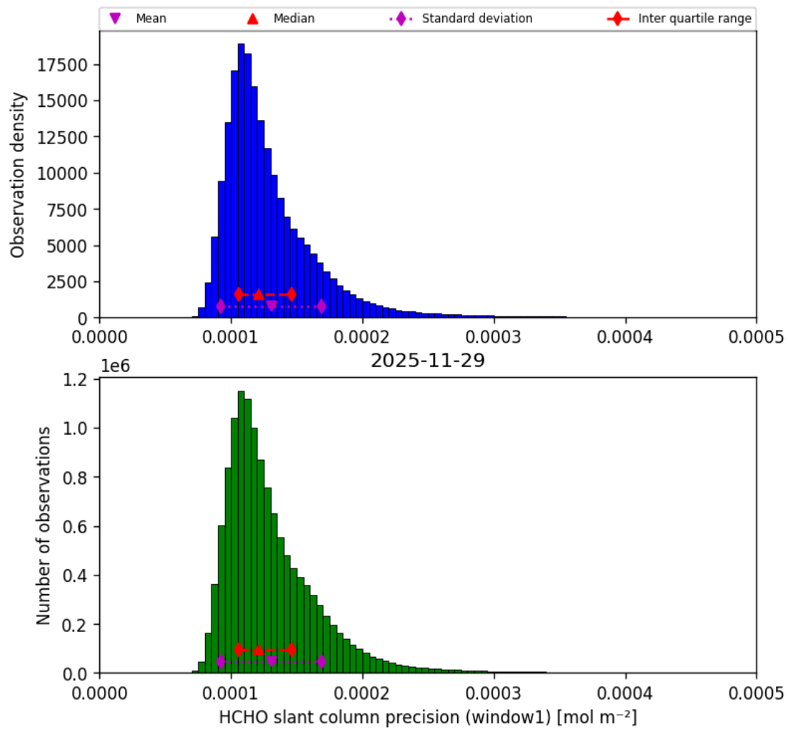
Figure 41: Histogram of “HCHO slant column precision (window1)” for 2025-11-28 to 2025-11-30
