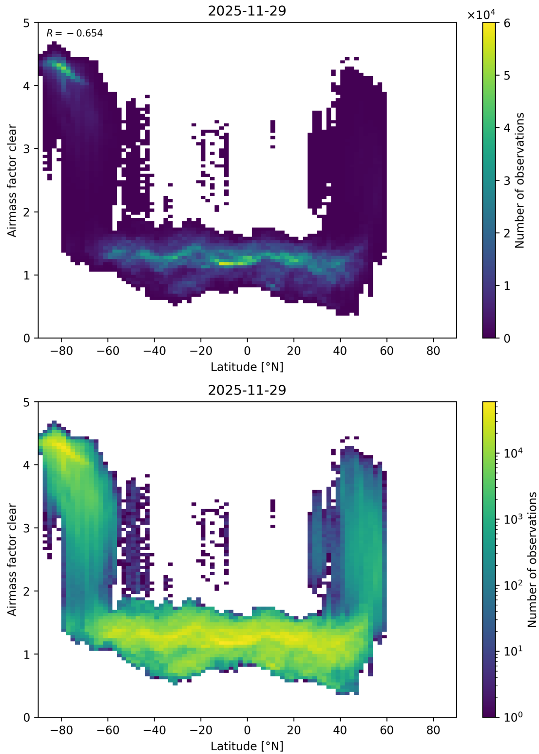
Figure 174: Scatter density plot of “Latitude” against “Airmass factor clear” for 2025-11-28 to 2025-11-30.
