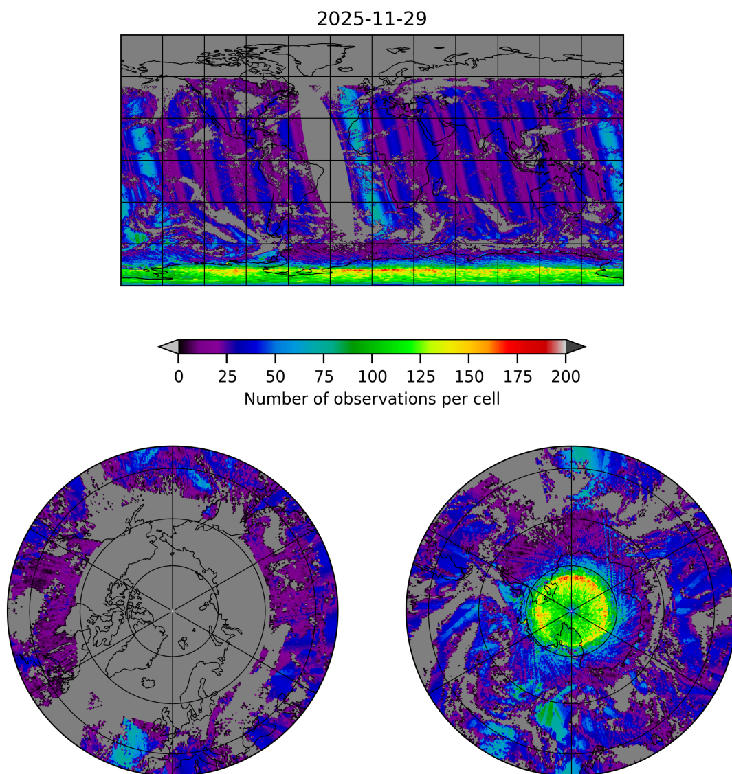
Figure 20: Map of the number of observations for 2025-11-28 to 2025-11-30
