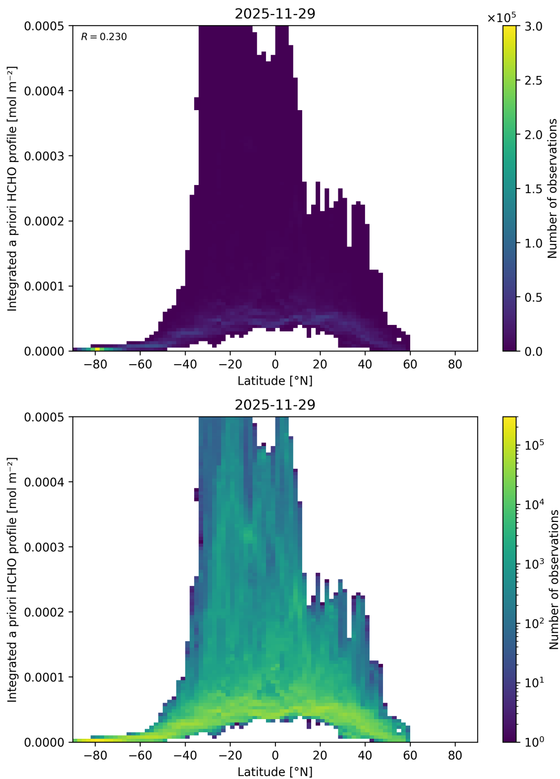
Figure 185: Scatter density plot of “Latitude” against “Integrated a priori HCHO profile” for 2025-11-28 to 2025-11-30.
