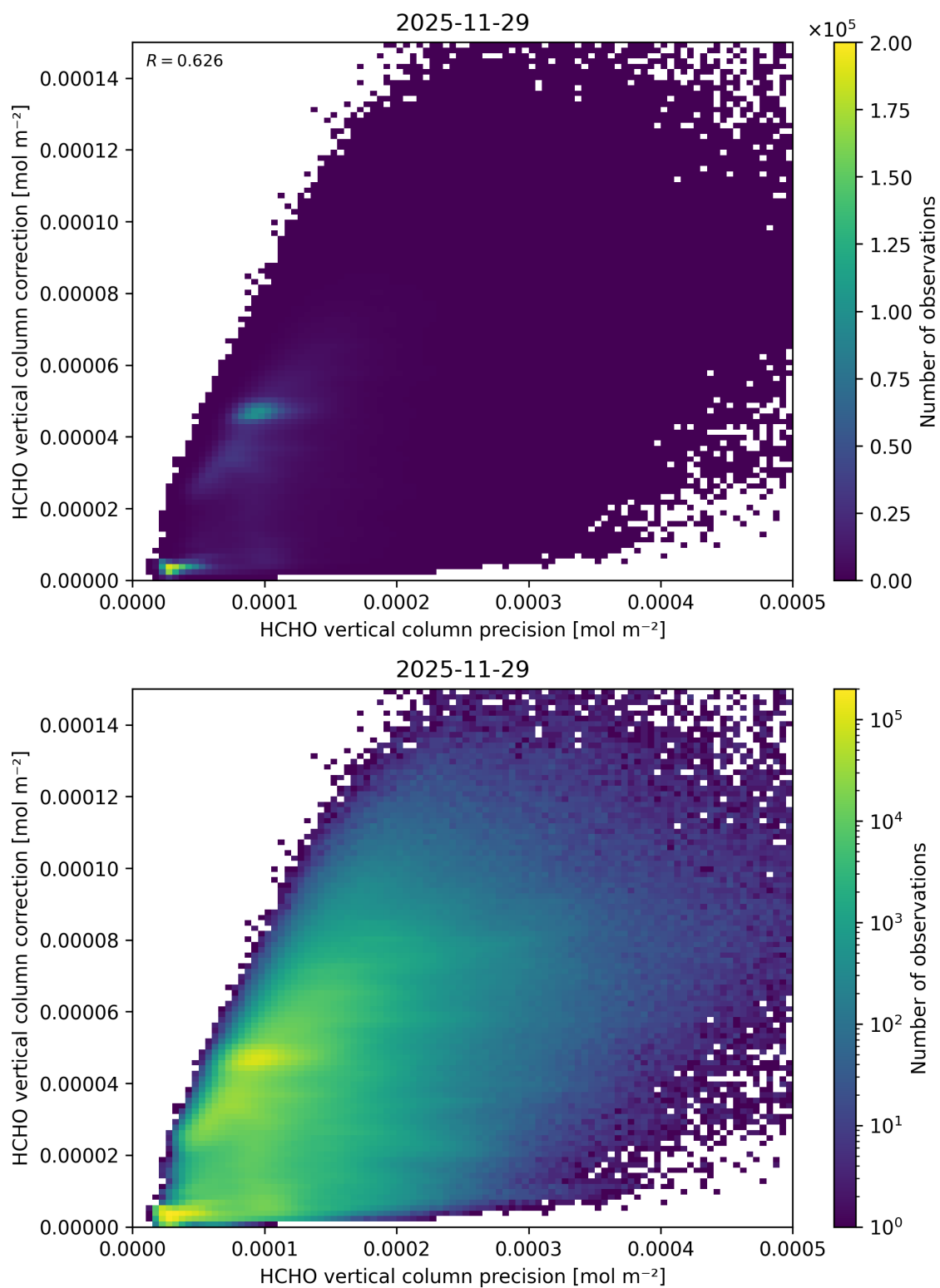
Figure 162: Scatter density plot of “HCHO vertical column precision” against “HCHO vertical column correction” for 2025-11-28 to 2025-11-30.
