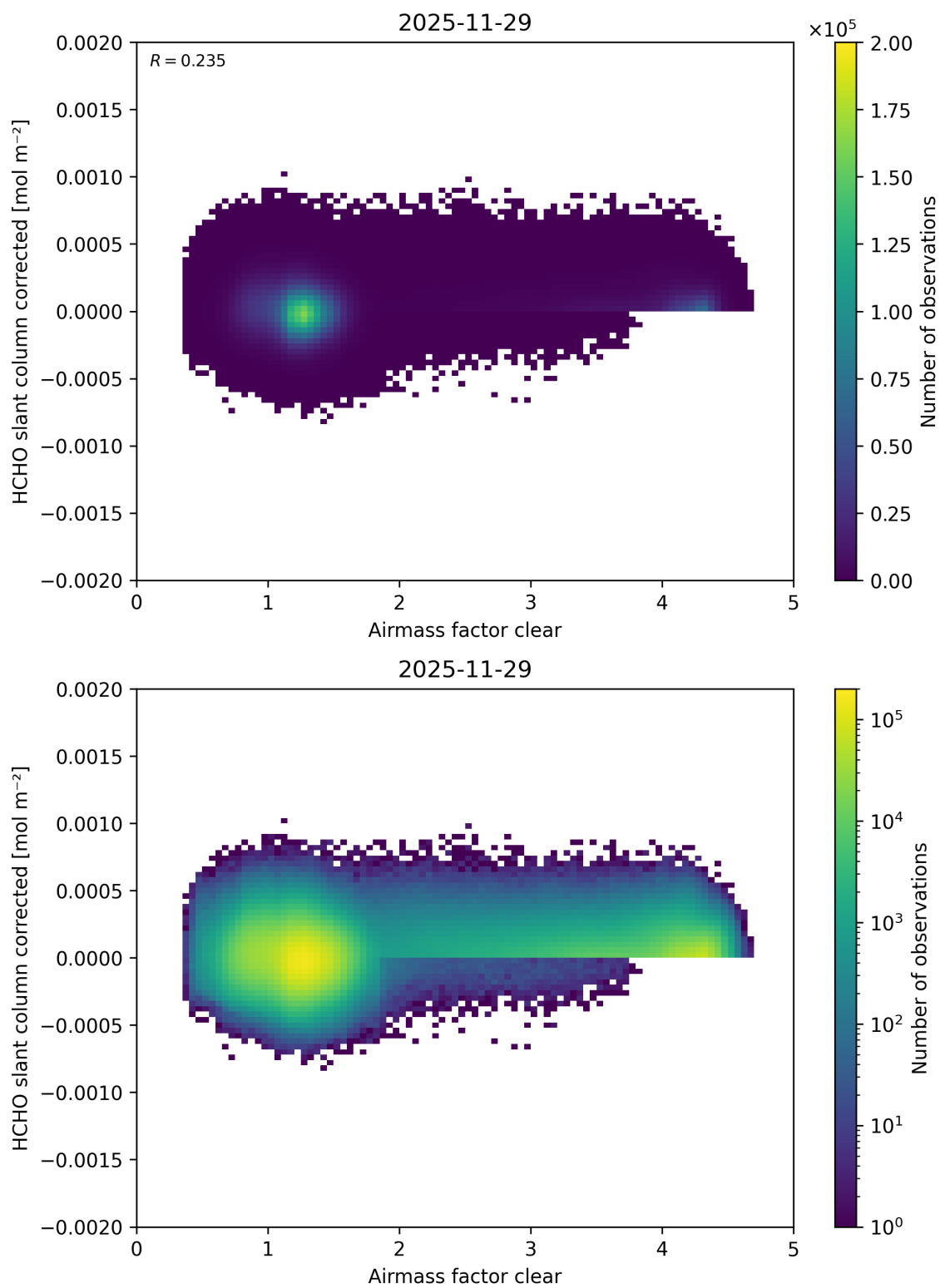
Figure 81: Scatter density plot of “Airmass factor clear” against “HCHO slant column corrected” for 2025-11-28 to 2025-11-30.
