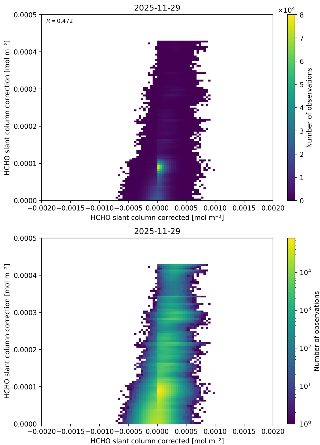
Figure 85: Scatter density plot of “HCHO slant column corrected” against “HCHO slant column correction” for 2025-11-28 to 2025-11-30.
