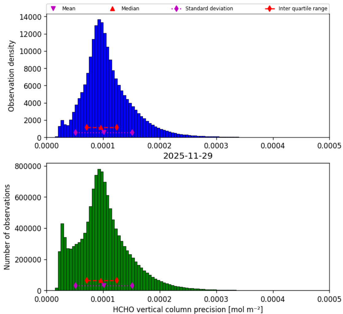
Figure 38: Histogram of “HCHO vertical column precision” for 2025-11-28 to 2025-11-30
