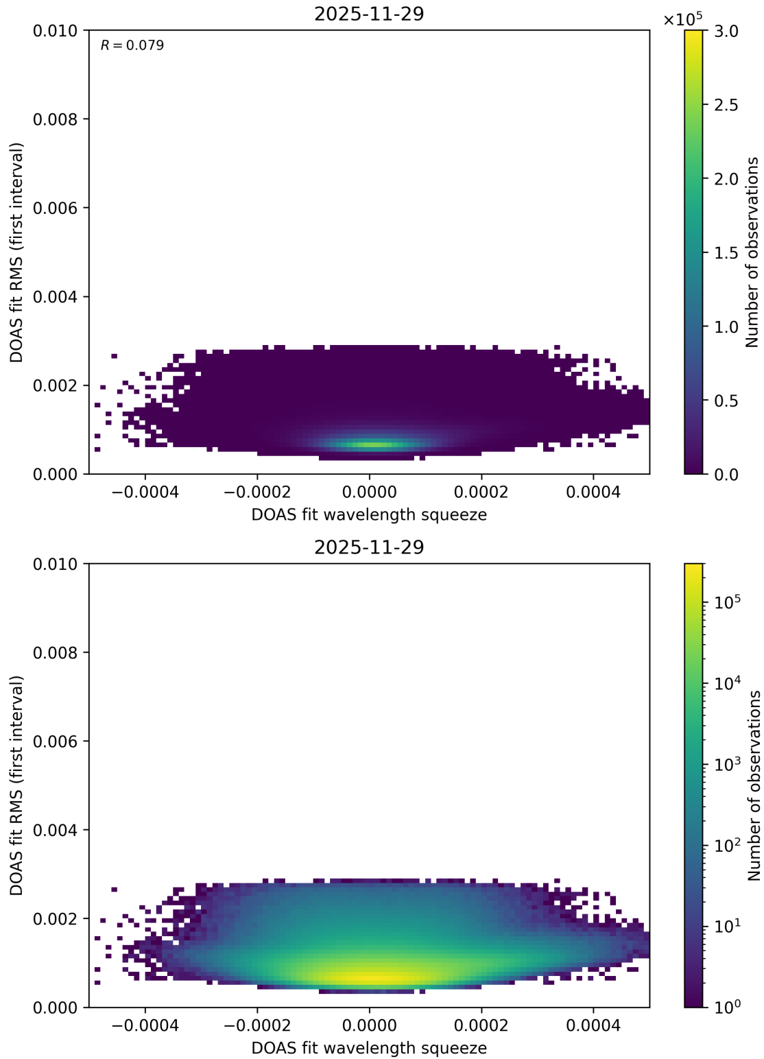
Figure 74: Scatter density plot of “DOAS fit wavelength squeeze” against “DOAS fit RMS (first interval)” for 2025-11-28 to 2025-11-30.
