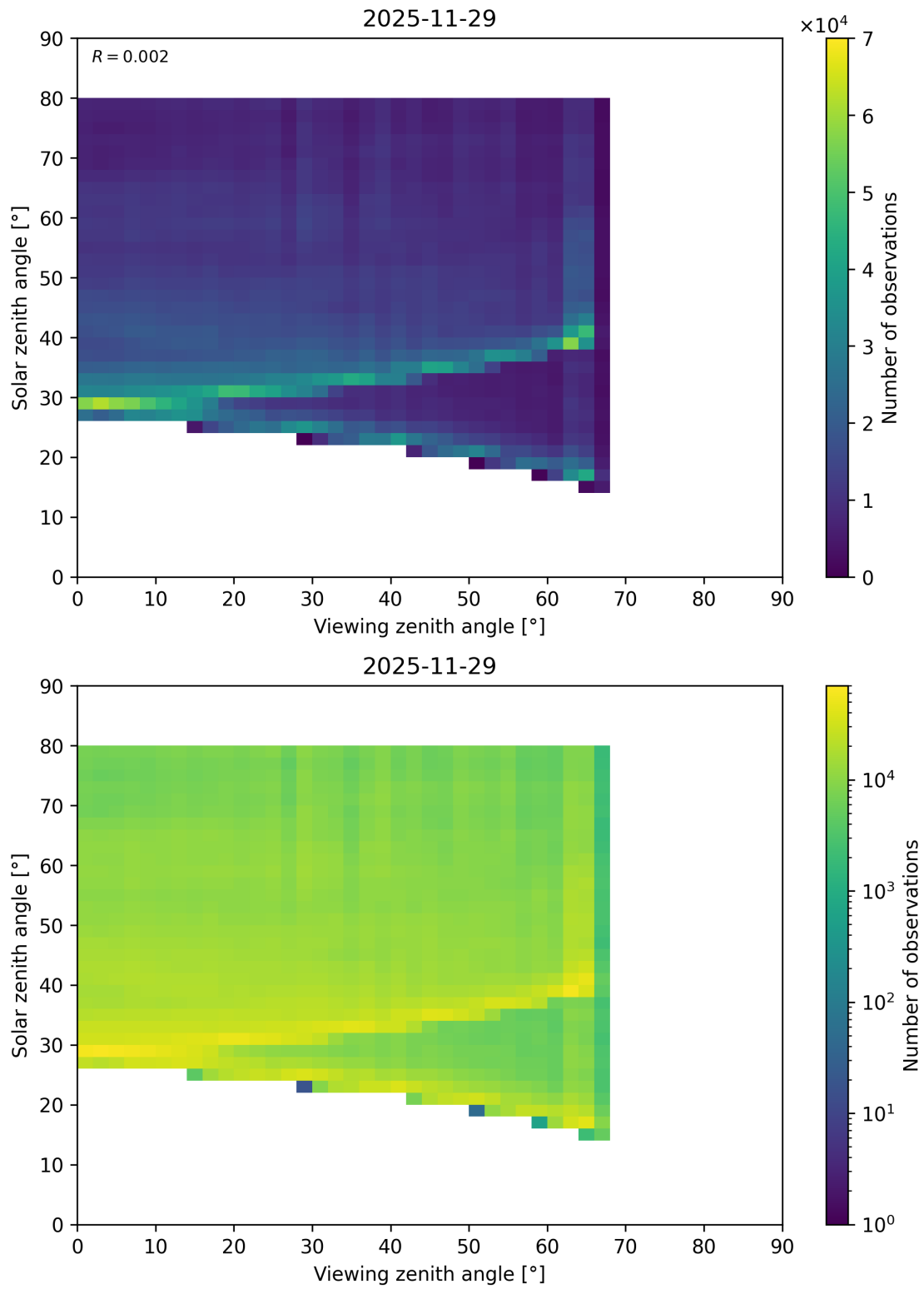
Figure 218: Scatter density plot of “Viewing zenith angle” against “Solar zenith angle” for 2025-11-28 to 2025-11-30.
