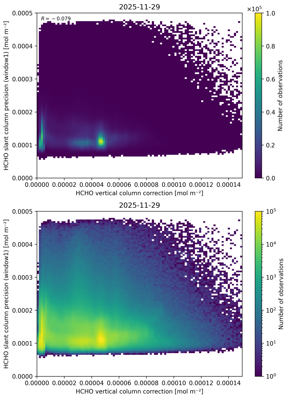
Figure 133: Scatter density plot of “HCHO vertical column correction” against “HCHO slant column precision (window1)” for 2025-11-28 to 2025-11-30.
