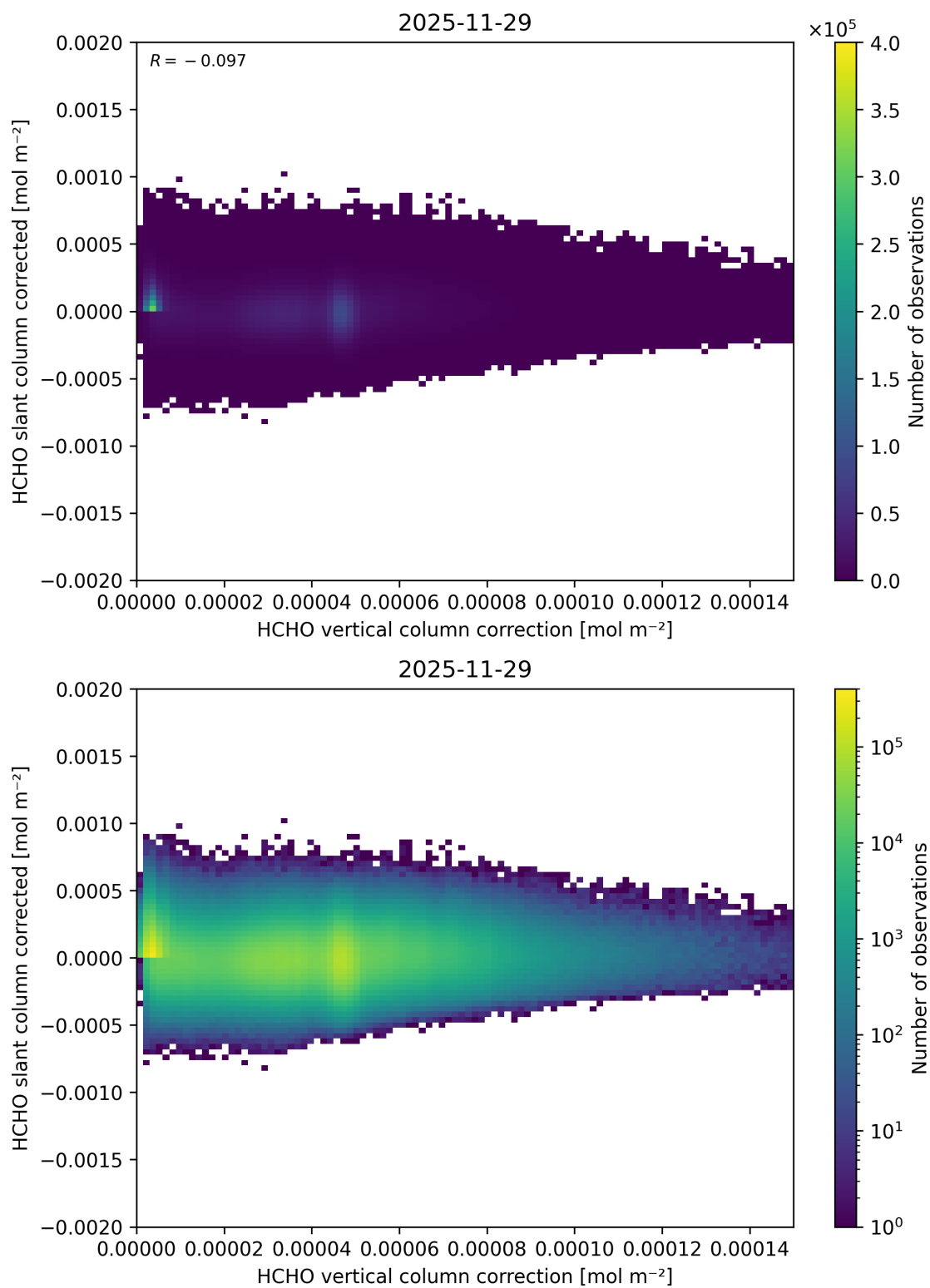
Figure 130: Scatter density plot of “HCHO vertical column correction” against “HCHO slant column corrected” for 2025-11-28 to 2025-11-30.
