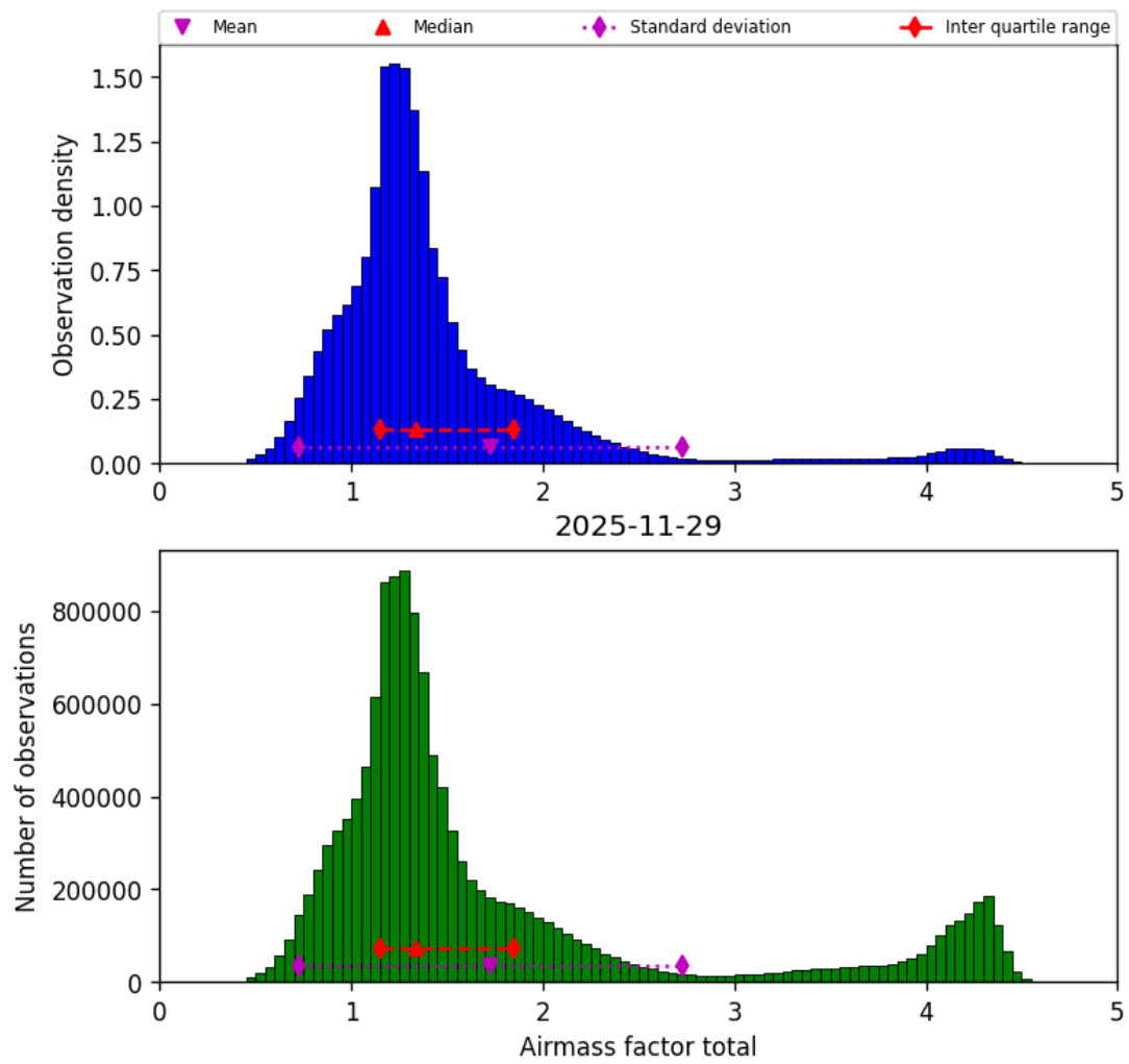
Figure 42: Histogram of “Airmass factor total” for 2025-11-28 to 2025-11-30
