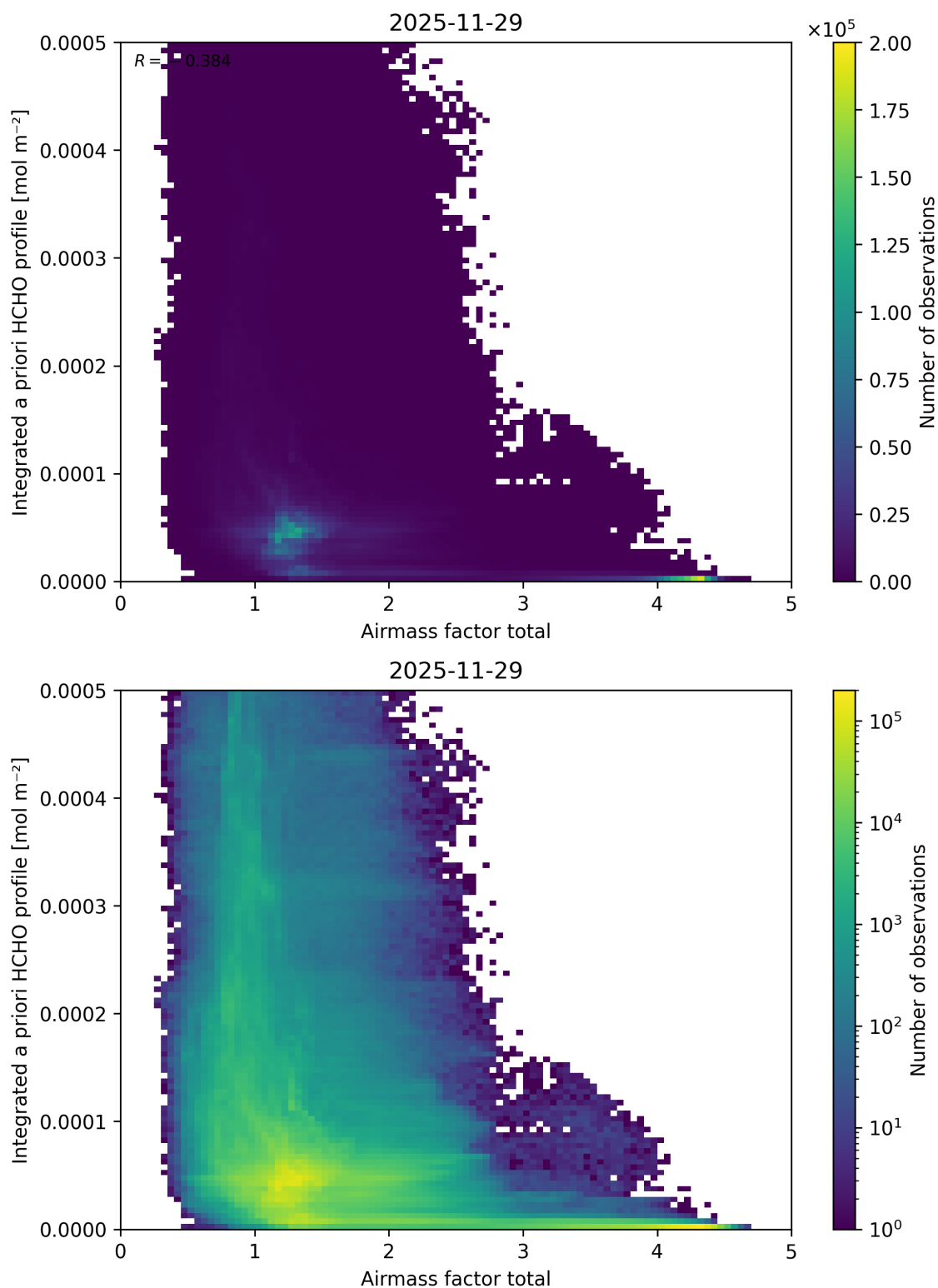
Figure 117: Scatter density plot of “Airmass factor total” against “Integrated a priori HCHO profile” for 2025-11-28 to 2025-11-30.
