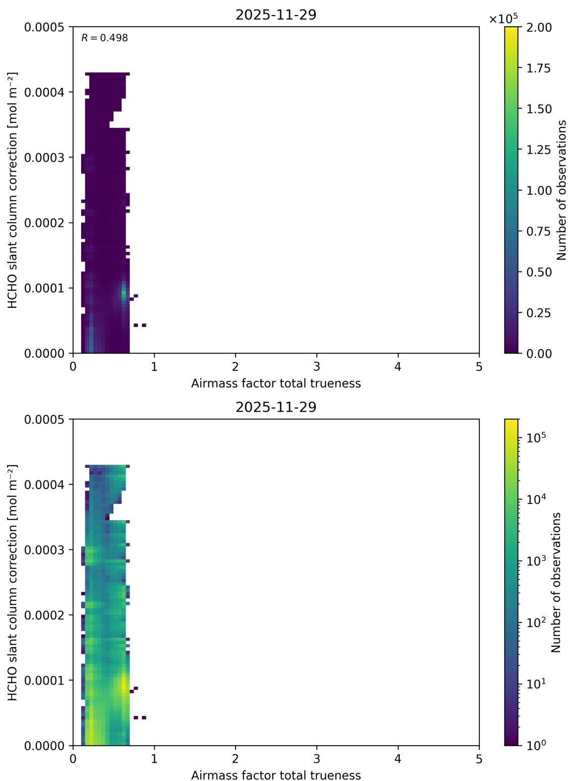
Figure 123: Scatter density plot of “Airmass factor total trueness” against “HCHO slant column correction” for 2025-11-28 to 2025-11-30.
