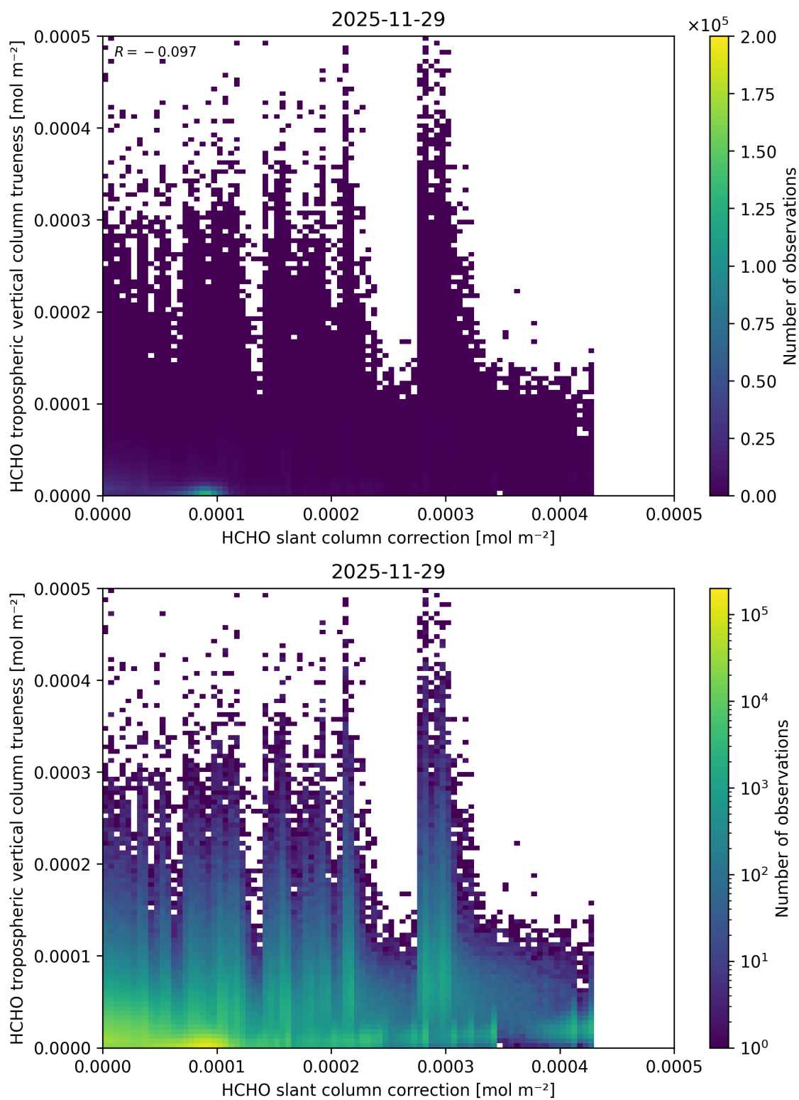
Figure 87: Scatter density plot of “HCHO slant column correction” against “HCHO tropospheric vertical column trueness” for 2025-11-28 to 2025-11-30.
