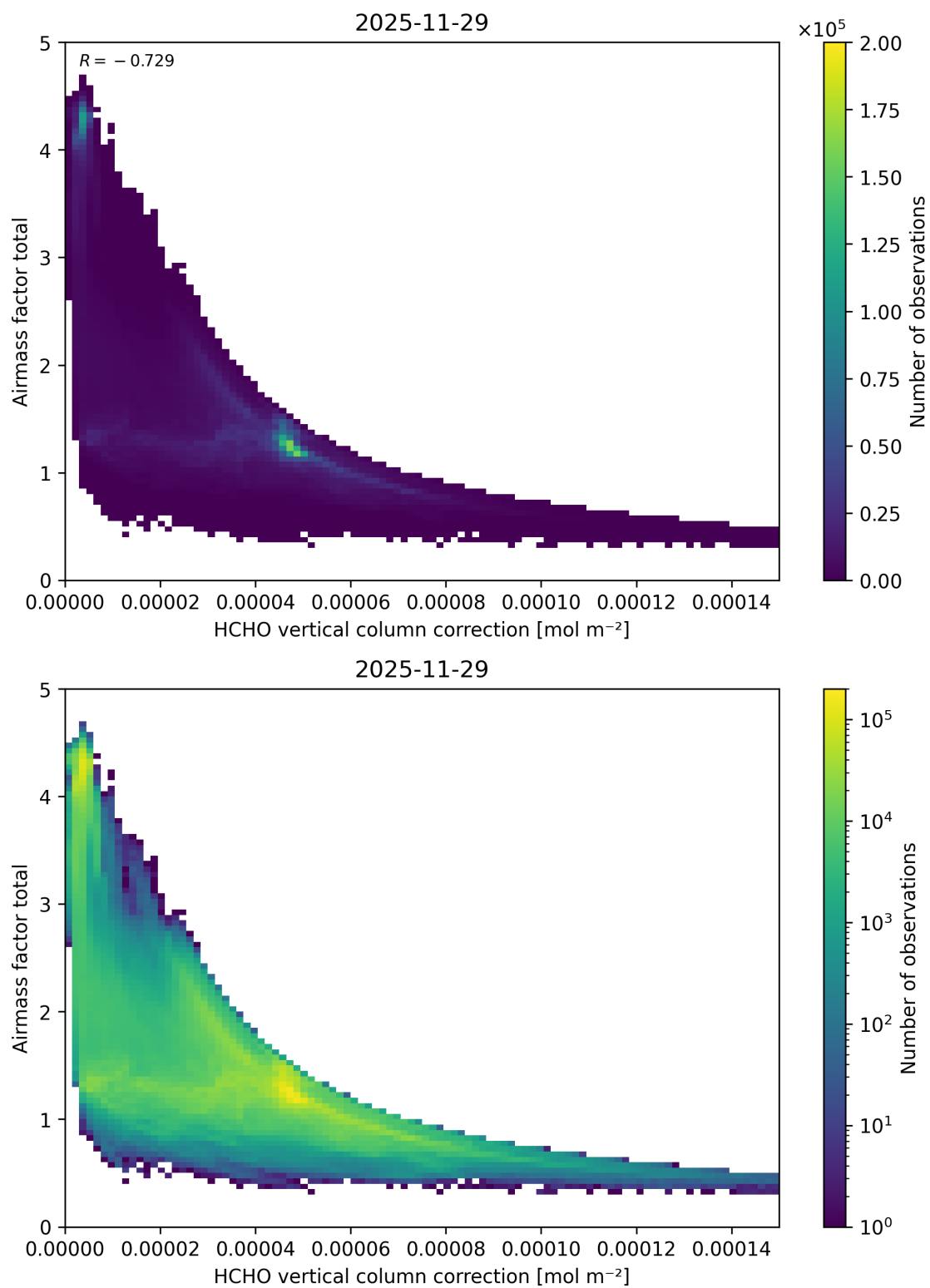
Figure 134: Scatter density plot of “HCHO vertical column correction” against “Airmass factor total” for 2025-11-28 to 2025-11-30.
