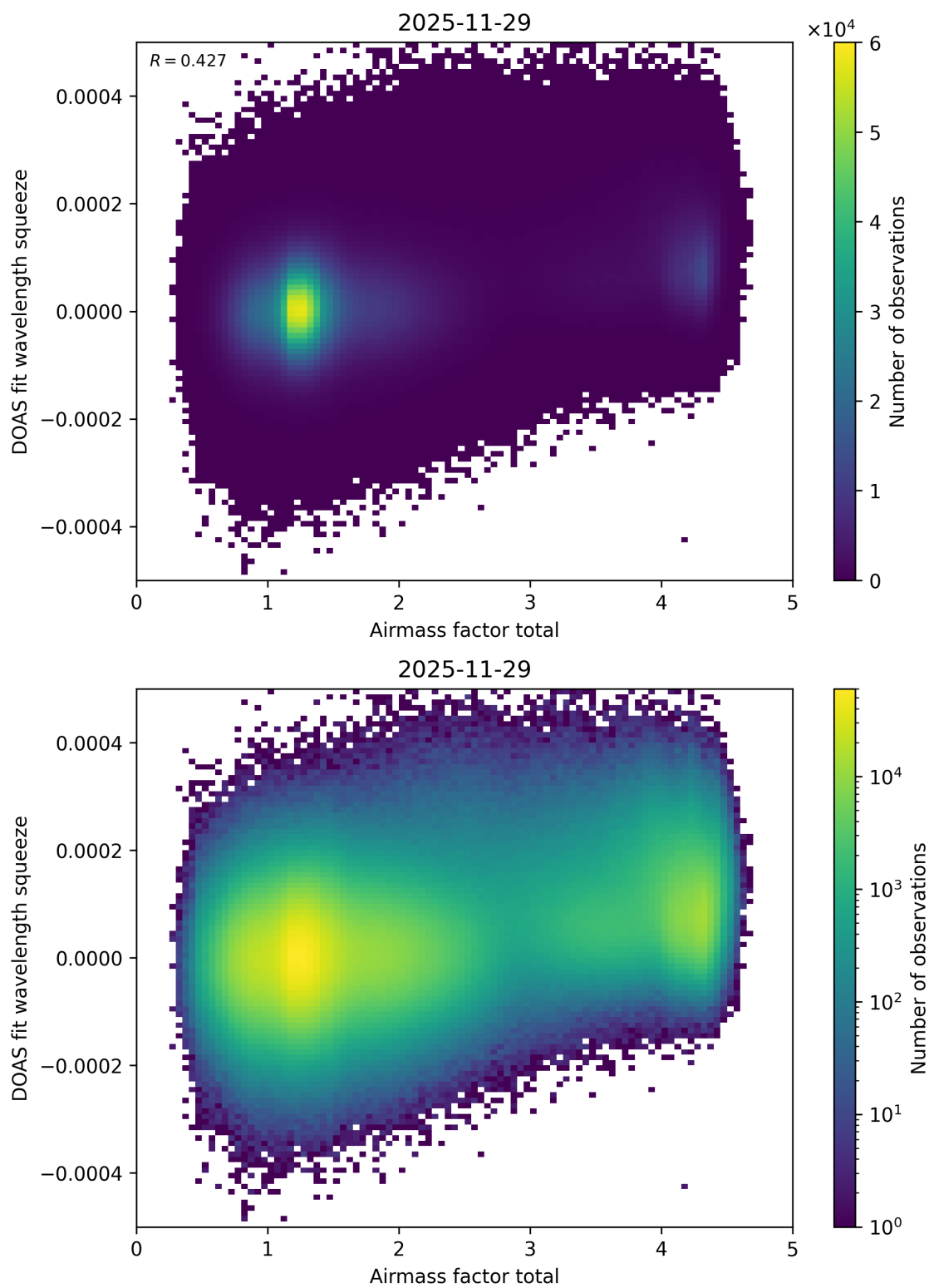
Figure 111: Scatter density plot of “Airmass factor total” against “DOAS fit wavelength squeeze” for 2025-11-28 to 2025-11-30.
