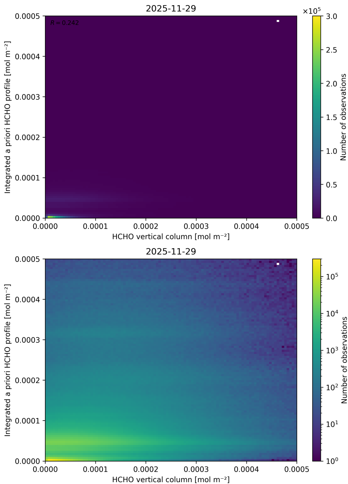
Figure 151: Scatter density plot of “HCHO vertical column” against “Integrated a priori HCHO profile” for 2025-11-28 to 2025-11-30.
