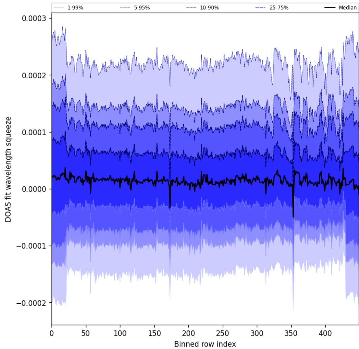
Figure 62: Along track statistics of “DOAS fit wavelength squeeze” for 2025-11-28 to 2025-11-30
