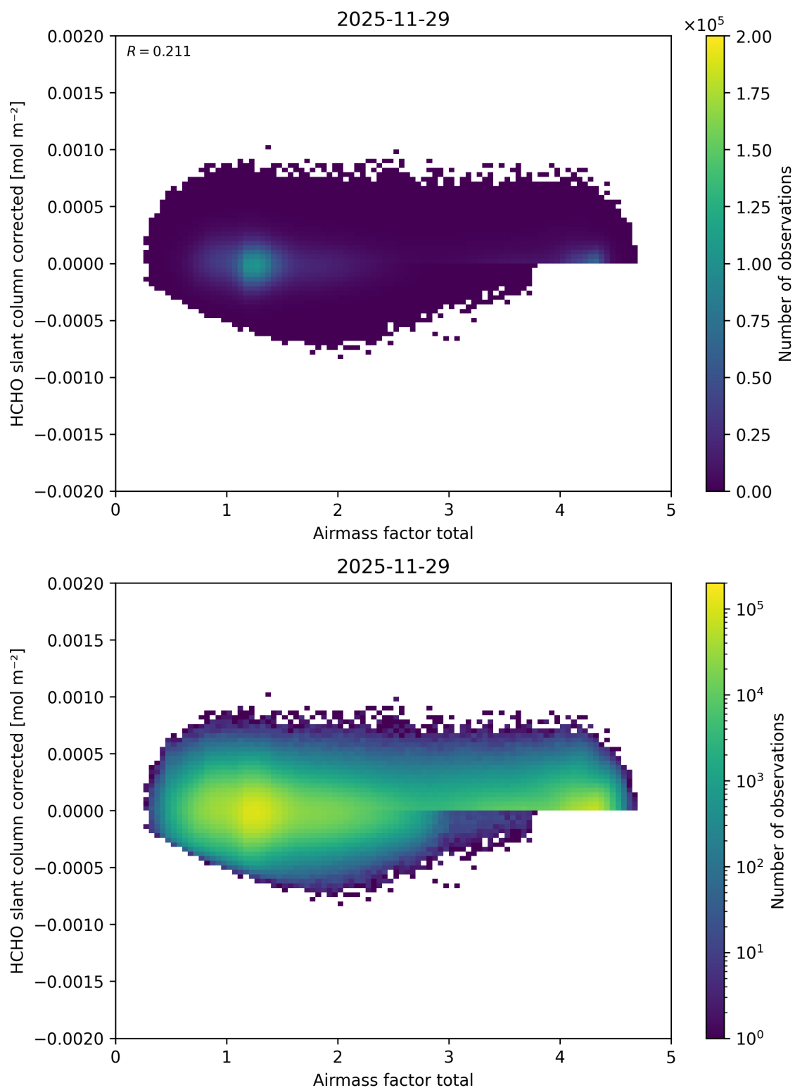
Figure 113: Scatter density plot of “Airmass factor total” against “HCHO slant column corrected” for 2025-11-28 to 2025-11-30.
