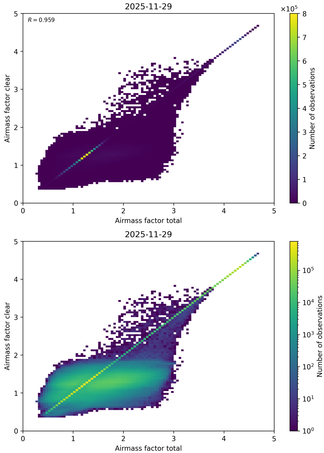
Figure 112: Scatter density plot of “Airmass factor total” against “Airmass factor clear” for 2025-11-28 to 2025-11-30.
