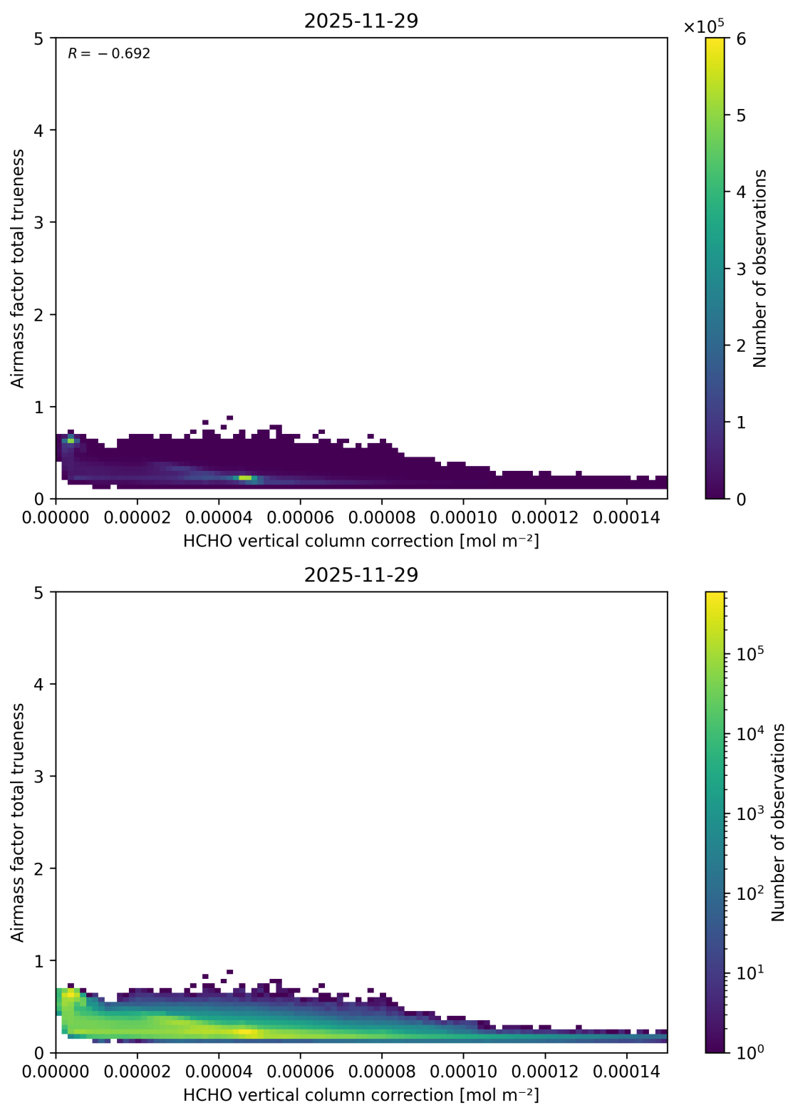
Figure 135: Scatter density plot of “HCHO vertical column correction” against “Airmass factor total trueness” for 2025-11-28 to 2025-11-30.
