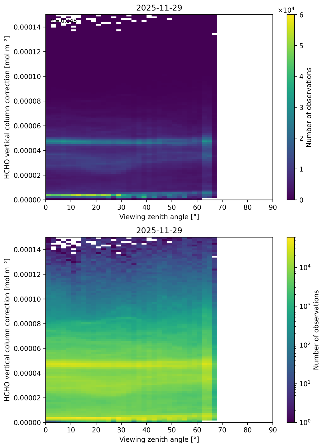
Figure 213: Scatter density plot of “Viewing zenith angle” against “HCHO vertical column correction” for 2025-11-28 to 2025-11-30.
