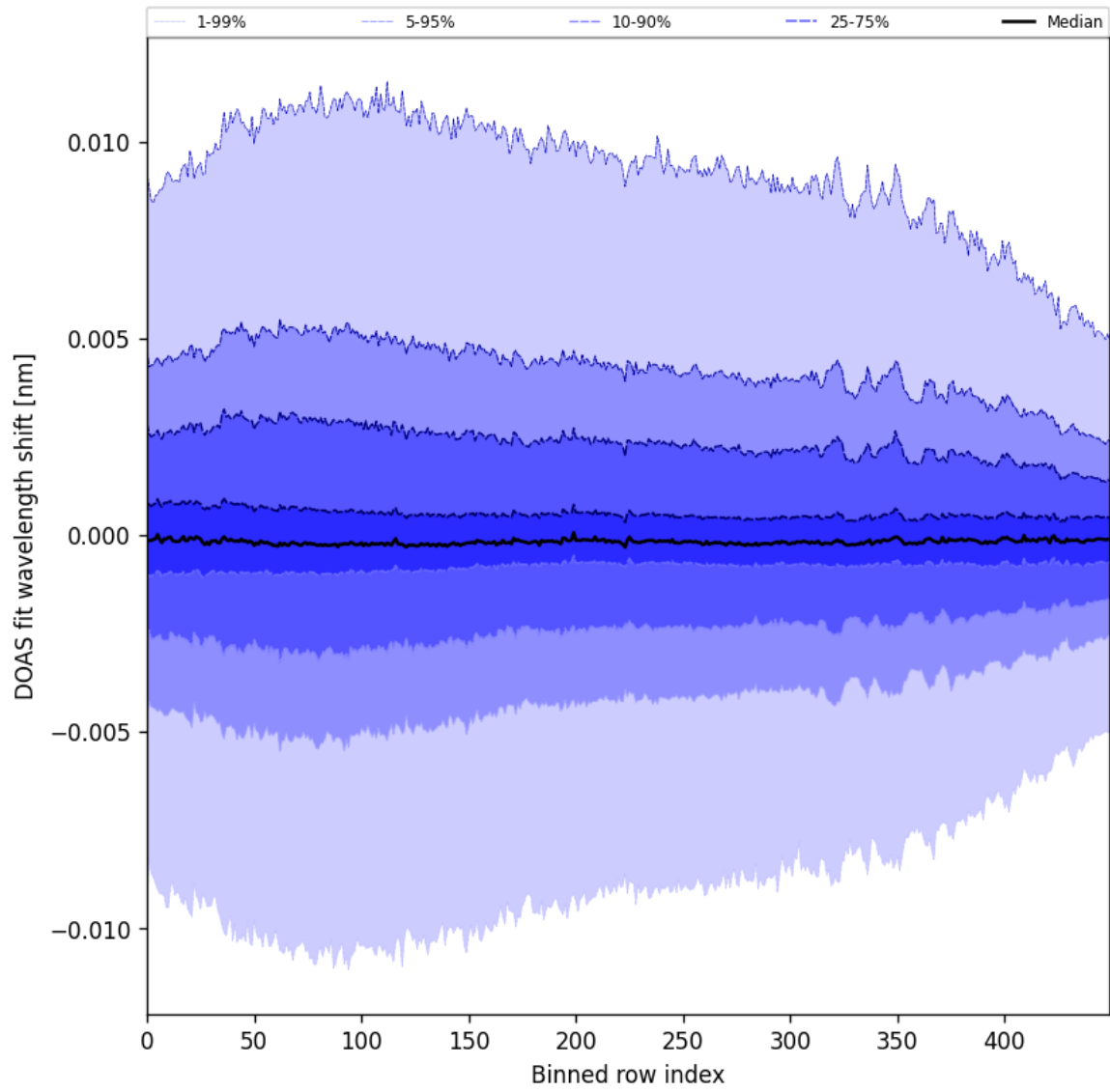
Figure 61: Along track statistics of “DOAS fit wavelength shift” for 2025-11-28 to 2025-11-30
