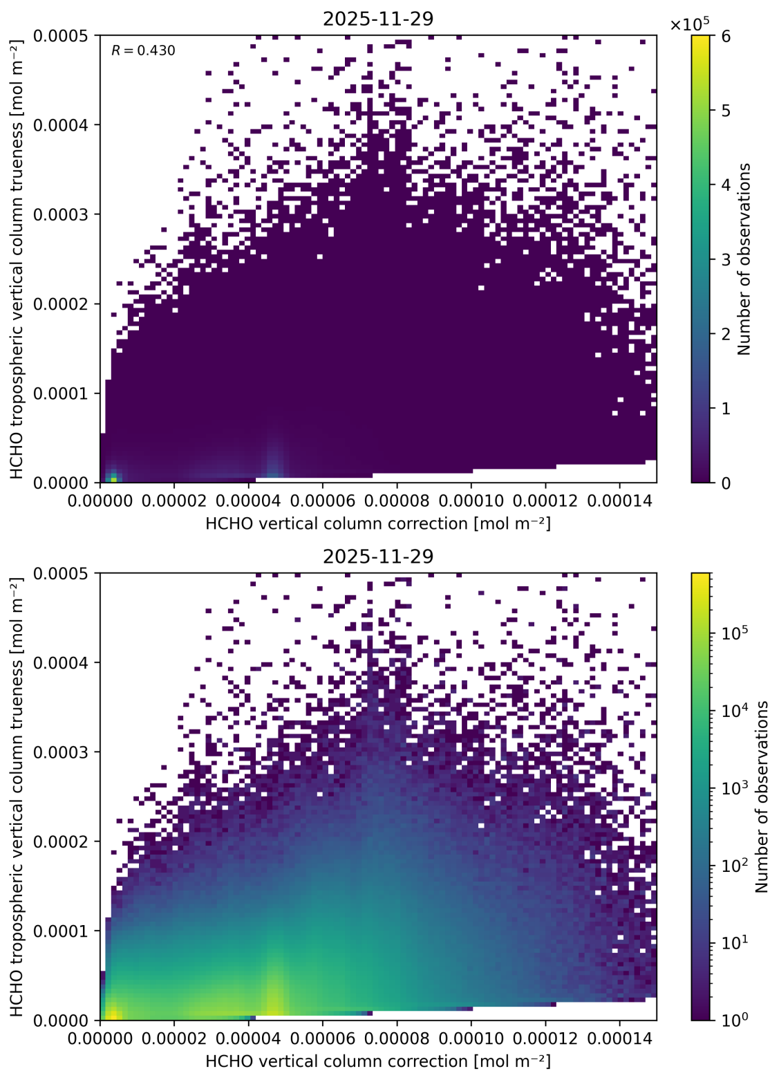
Figure 136: Scatter density plot of “HCHO vertical column correction” against “HCHO tropospheric vertical column true-ness” for 2025-11-28 to 2025-11-30.
