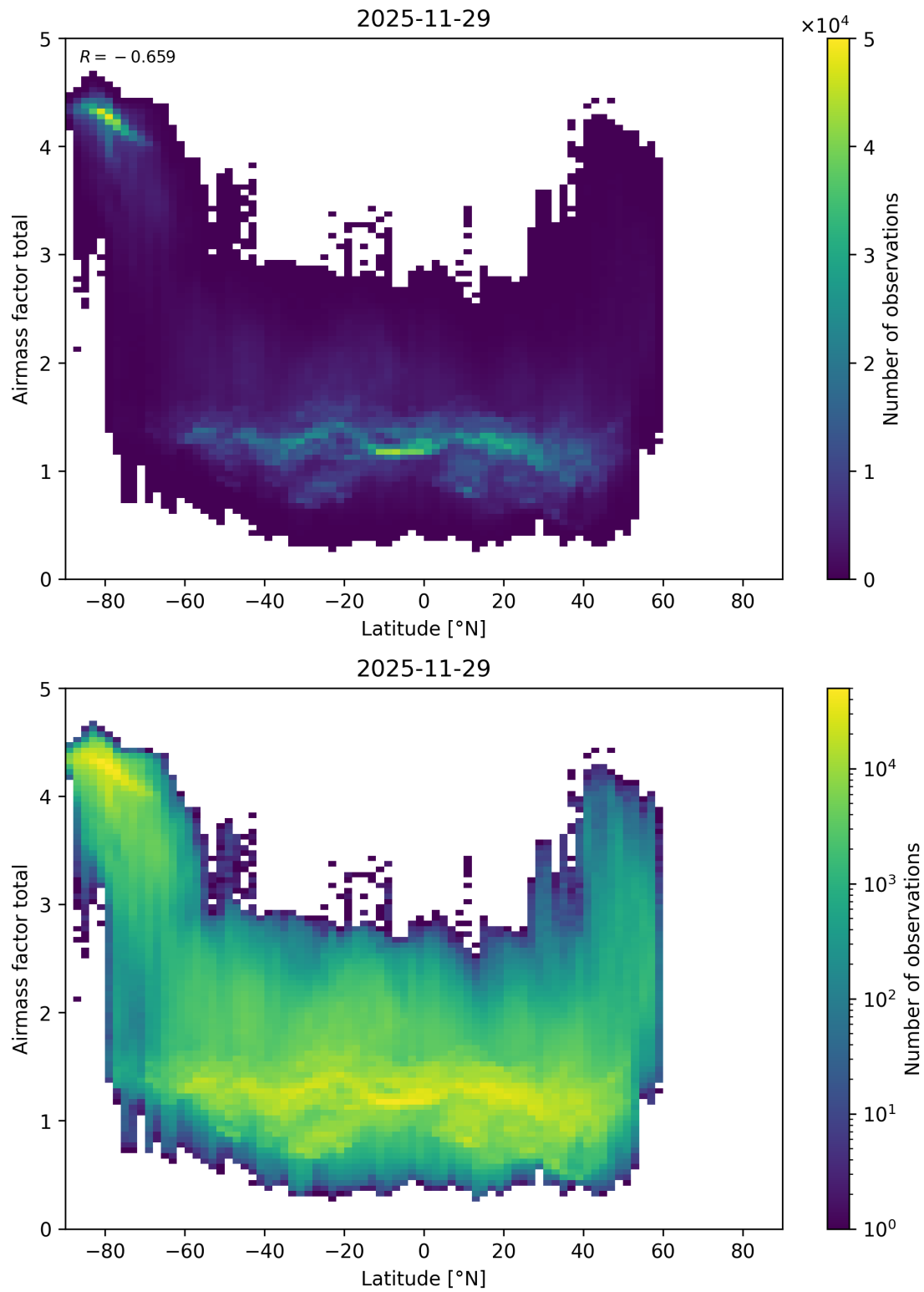
Figure 179: Scatter density plot of “Latitude” against “Airmass factor total” for 2025-11-28 to 2025-11-30.
