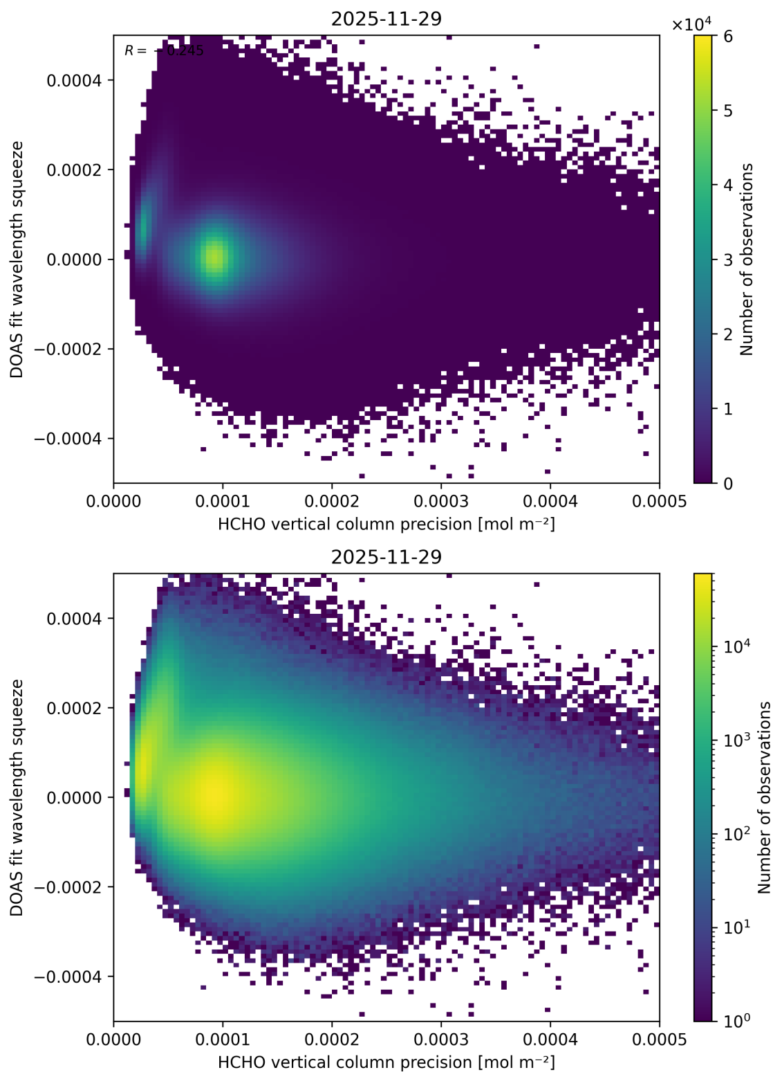
Figure 154: Scatter density plot of “HCHO vertical column precision” against “DOAS fit wavelength squeeze” for 2025-11-28 to 2025-11-30.
