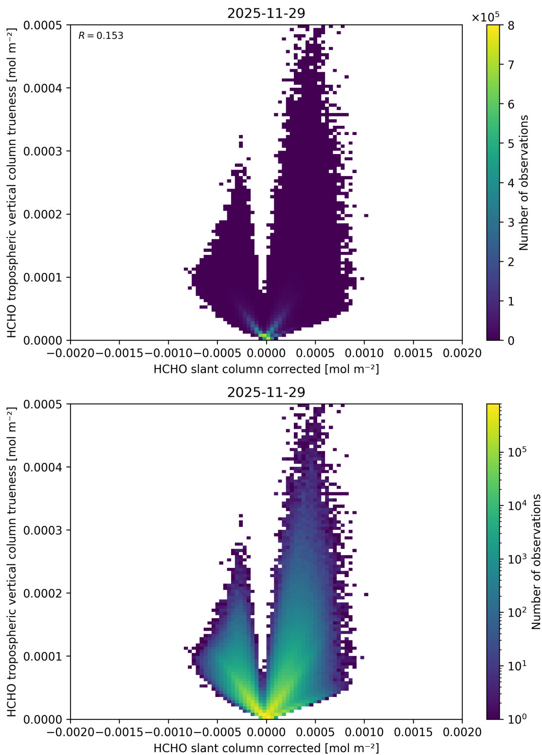
Figure 86: Scatter density plot of “HCHO slant column corrected” against “HCHO tropospheric vertical column trueness” for 2025-11-28 to 2025-11-30.
