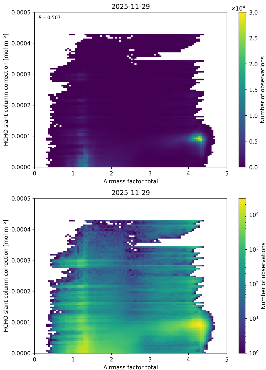
Figure 114: Scatter density plot of “Airmass factor total” against “HCHO slant column correction” for 2025-11-28 to 2025-11-30.
