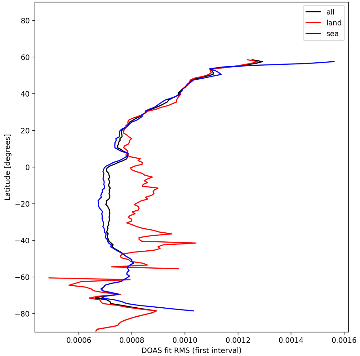
Figure 33: Zonal average of “DOAS fit RMS (first interval)” for 2025-11-28 to 2025-11-30.
