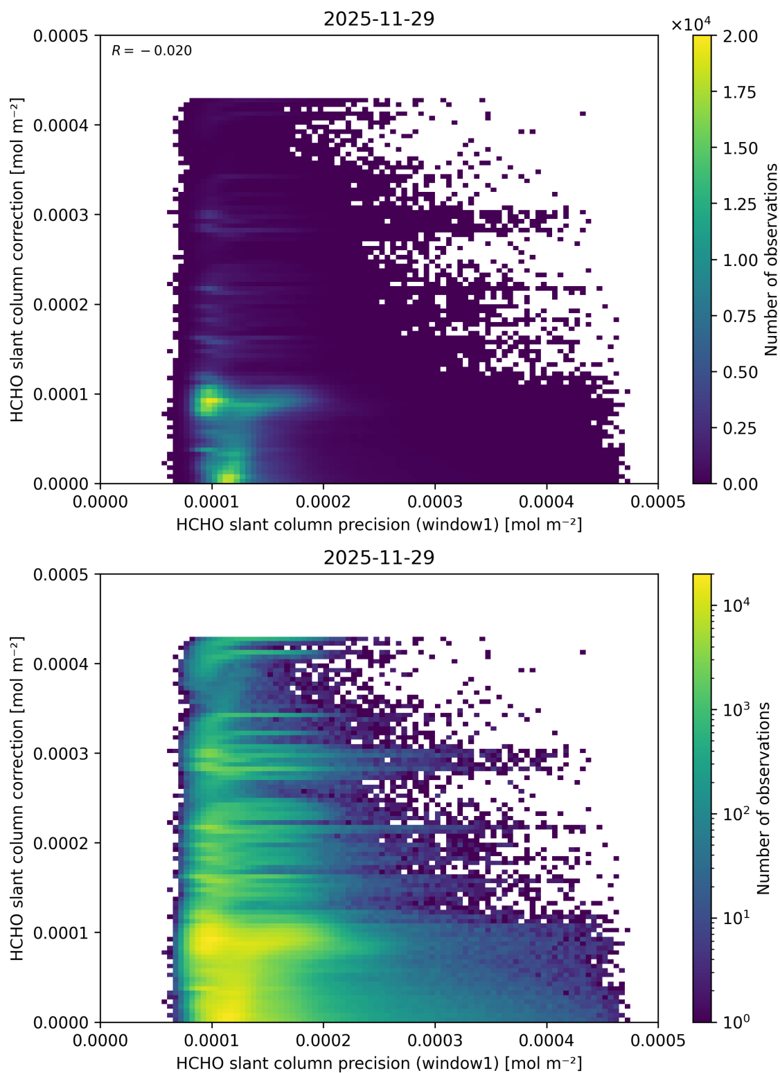
Figure 104: Scatter density plot of “HCHO slant column precision (window1)” against “HCHO slant column correction” for 2025-11-28 to 2025-11-30.
