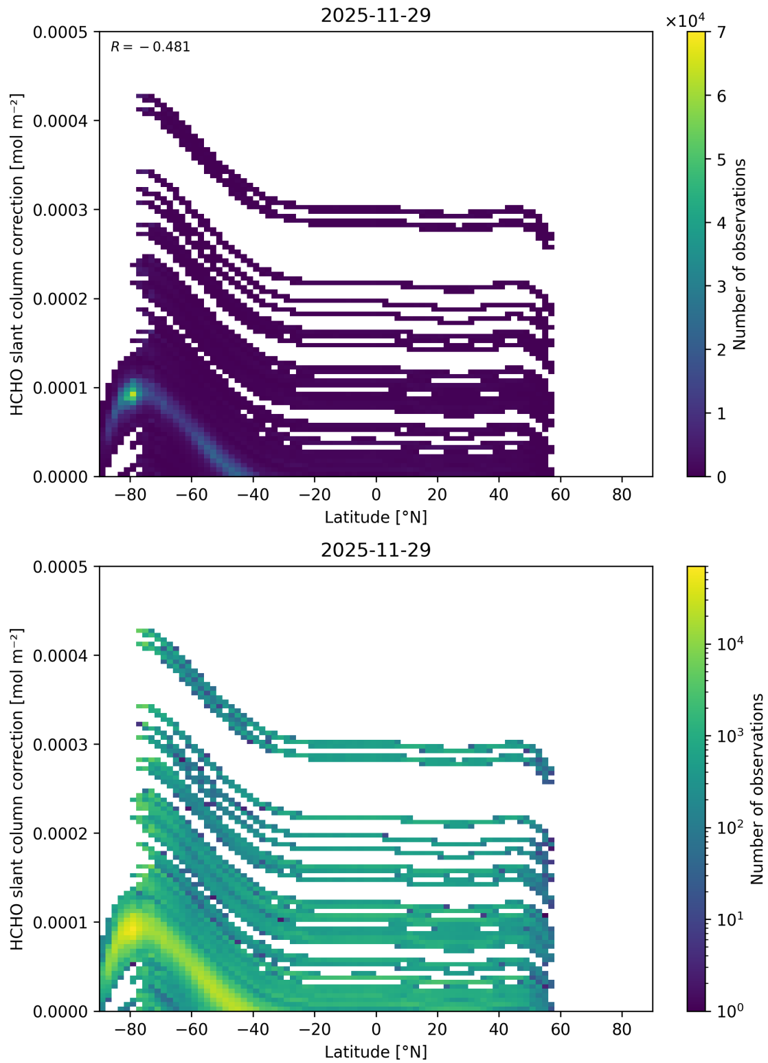
Figure 176: Scatter density plot of “Latitude” against “HCHO slant column correction” for 2025-11-28 to 2025-11-30.
