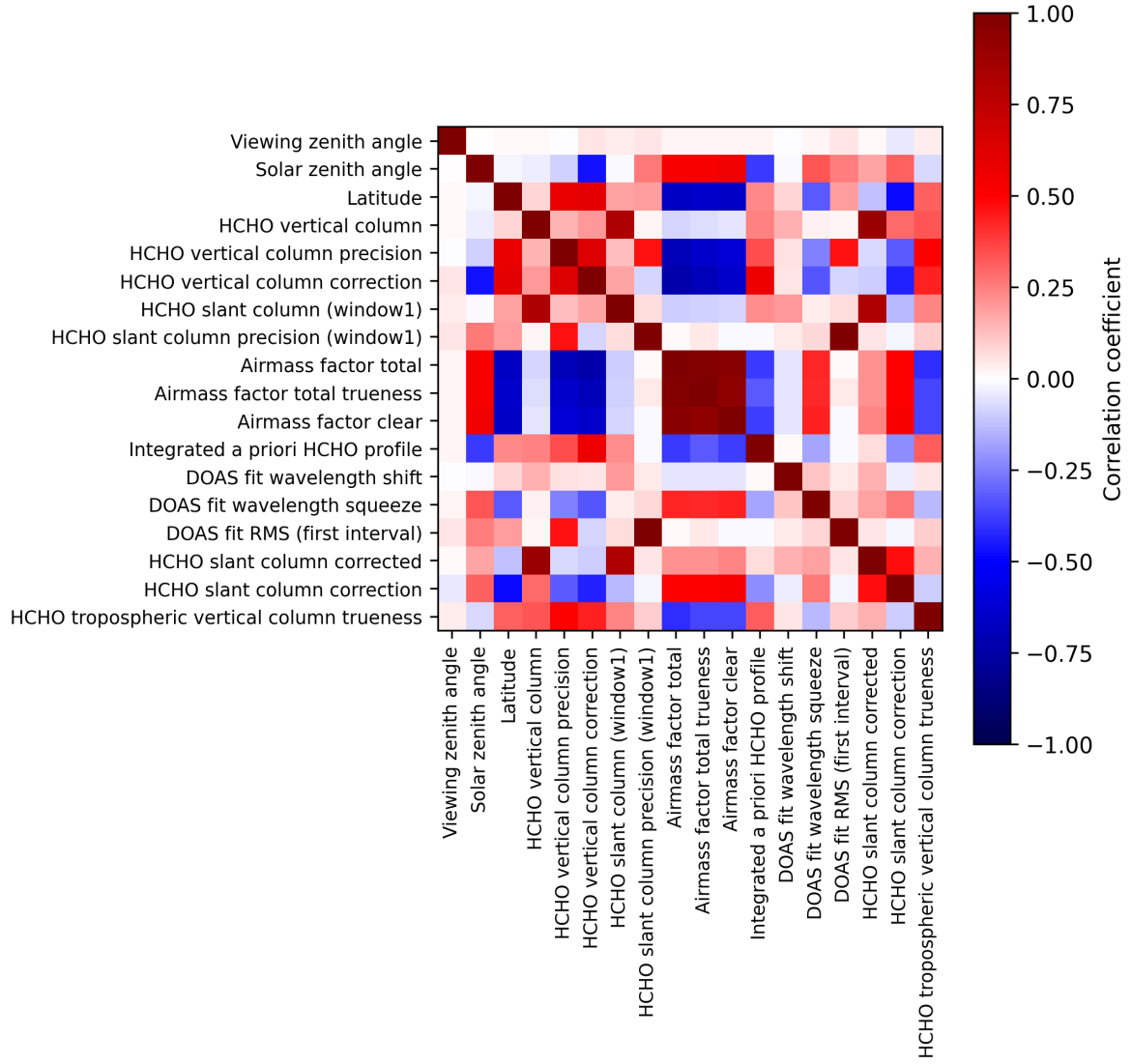
Figure 2: Map of correlation matrix for 2025-11-28 to 2025-11-30.
