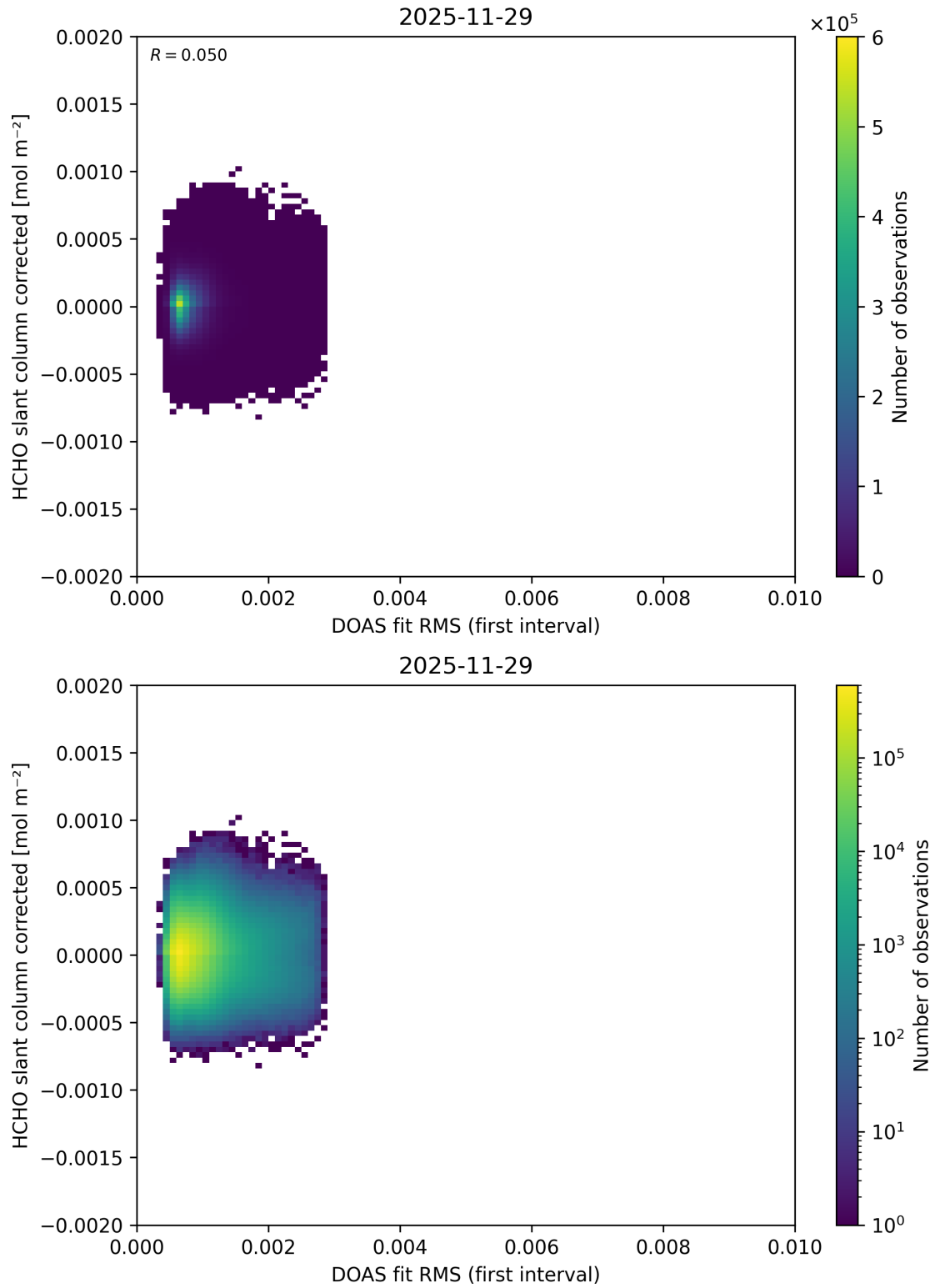
Figure 66: Scatter density plot of “DOAS fit RMS (first interval)” against “HCHO slant column corrected” for 2025-11-28 to 2025-11-30.
