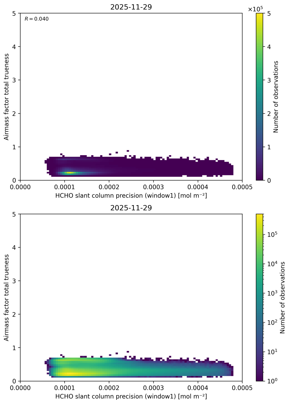
Figure 106: Scatter density plot of “HCHO slant column precision (window1)” against “Airmass factor total trueness” for 2025-11-28 to 2025-11-30.
