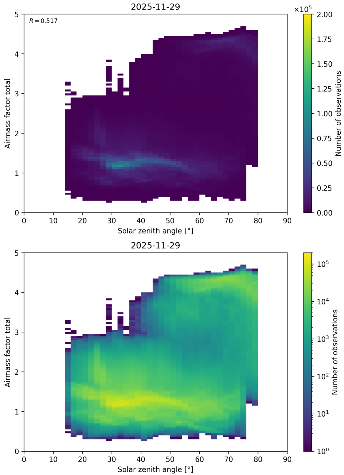
Figure 194: Scatter density plot of “Solar zenith angle” against “Airmass factor total” for 2025-11-28 to 2025-11-30.
