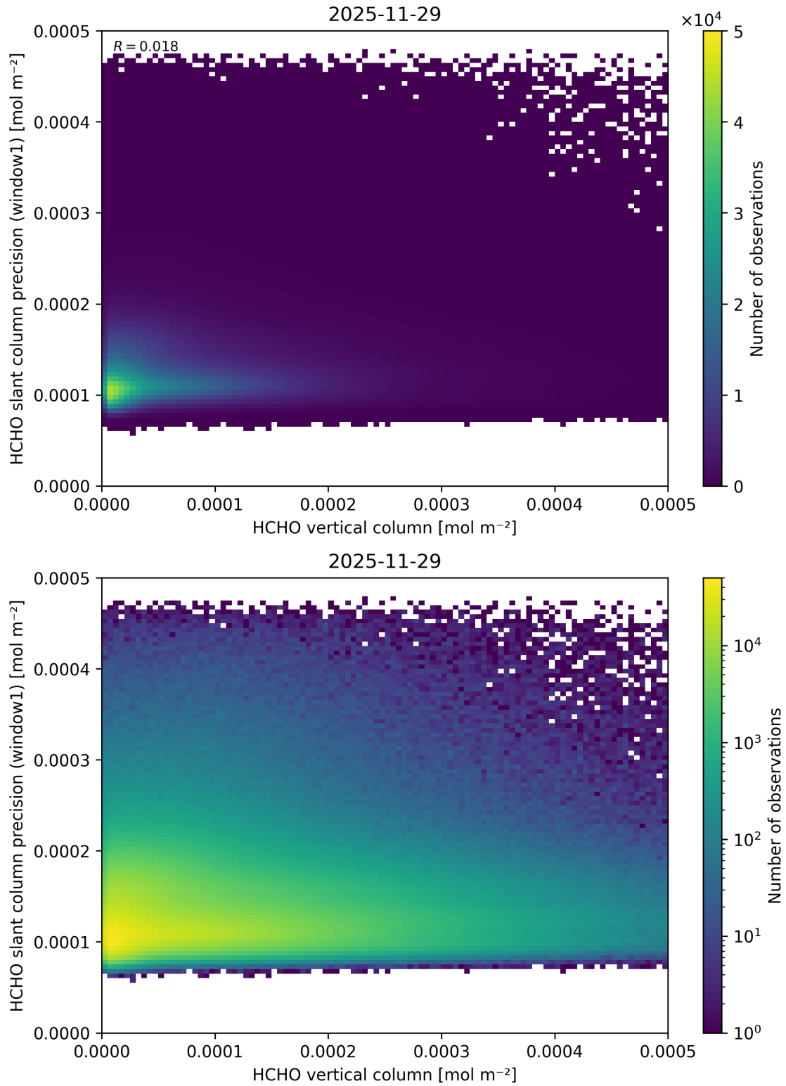
Figure 145: Scatter density plot of “HCHO vertical column” against “HCHO slant column precision (window1)” for 2025-11-28 to 2025-11-30.
