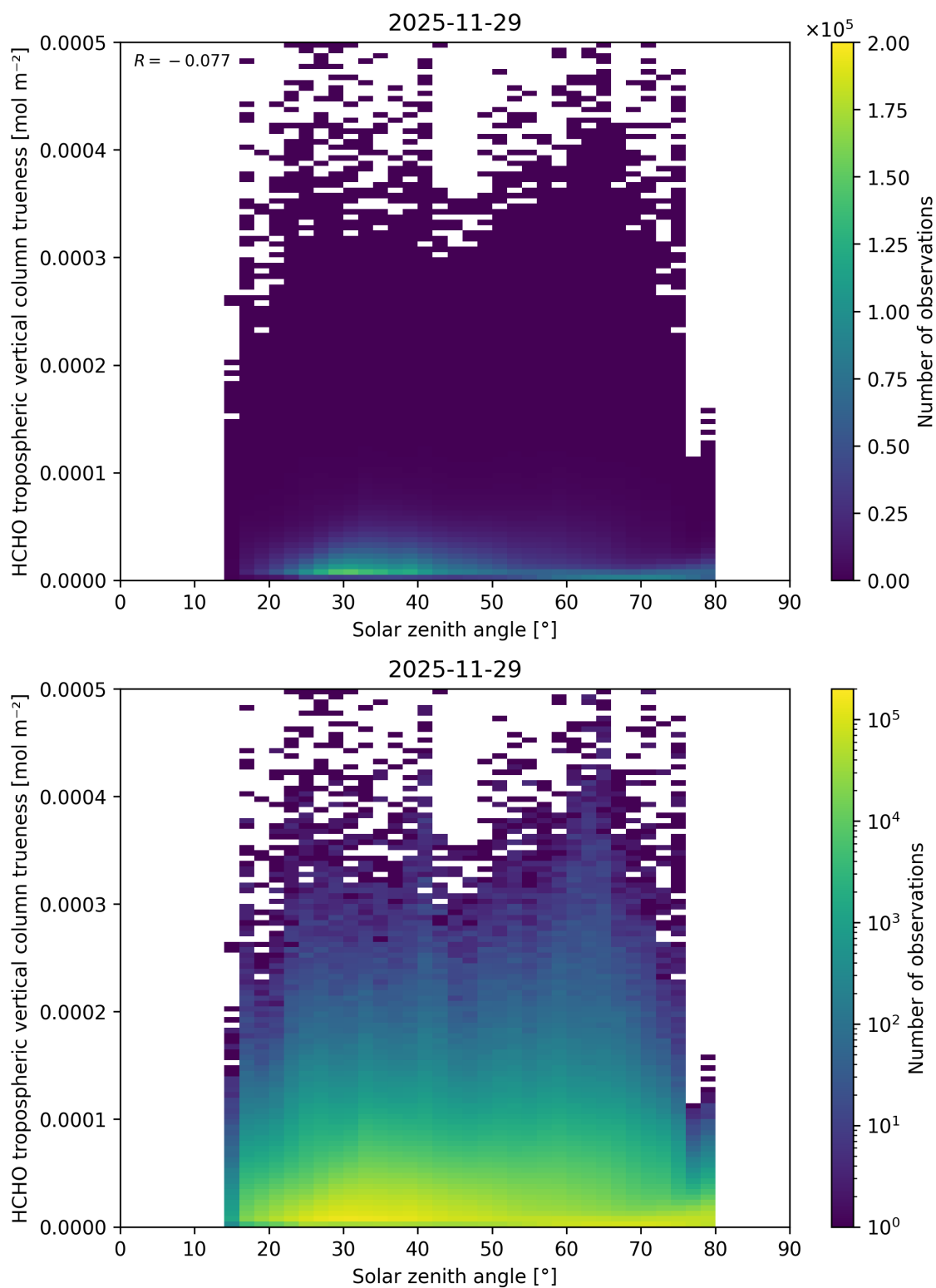
Figure 199: Scatter density plot of “Solar zenith angle” against “HCHO tropospheric vertical column trueness” for 2025-11-28 to 2025-11-30.
