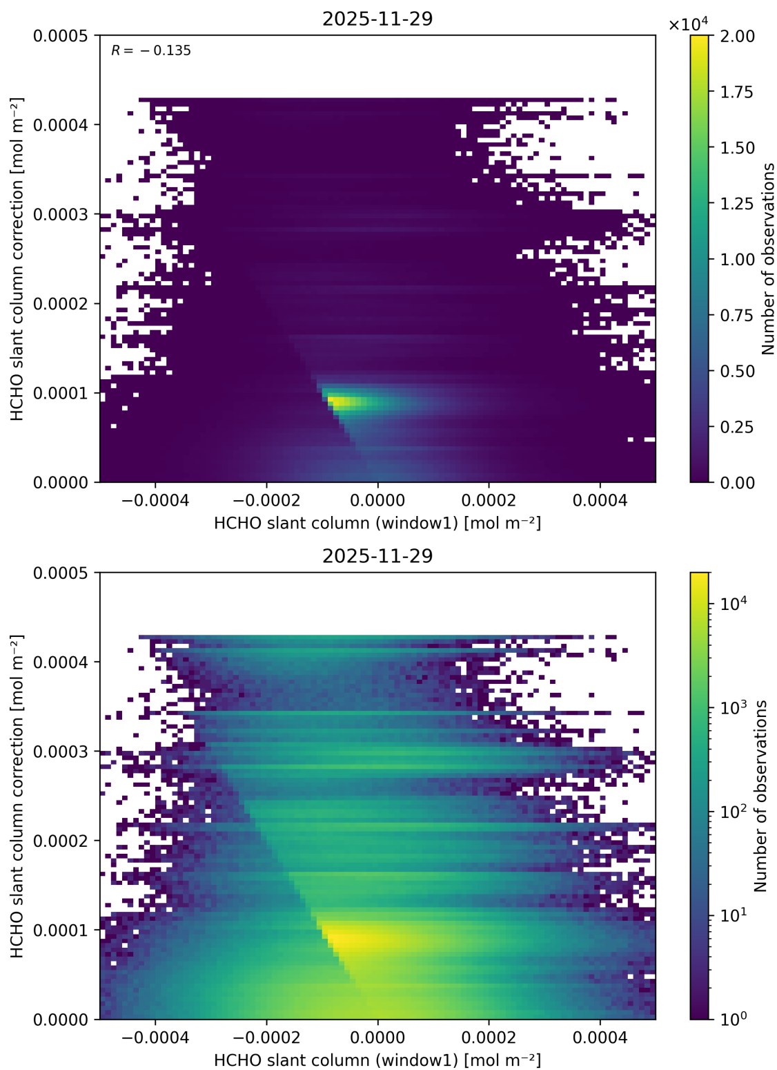
Figure 93: Scatter density plot of “HCHO slant column (window1)” against “HCHO slant column correction” for 2025-11-28 to 2025-11-30.
