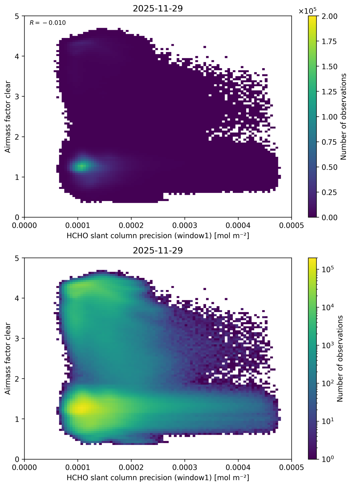
Figure 102: Scatter density plot of “HCHO slant column precision (window1)” against “Airmass factor clear” for 2025-11-28 to 2025-11-30.
