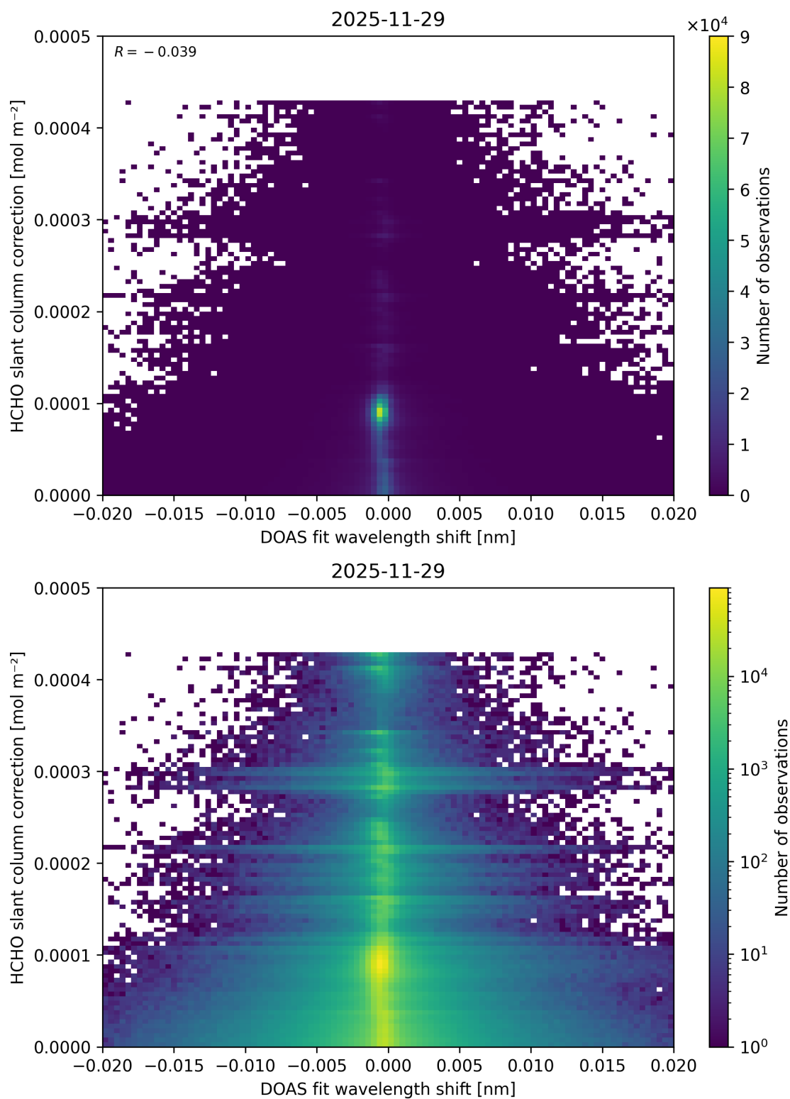
Figure 72: Scatter density plot of “DOAS fit wavelength shift” against “HCHO slant column correction” for 2025-11-28 to 2025-11-30.
