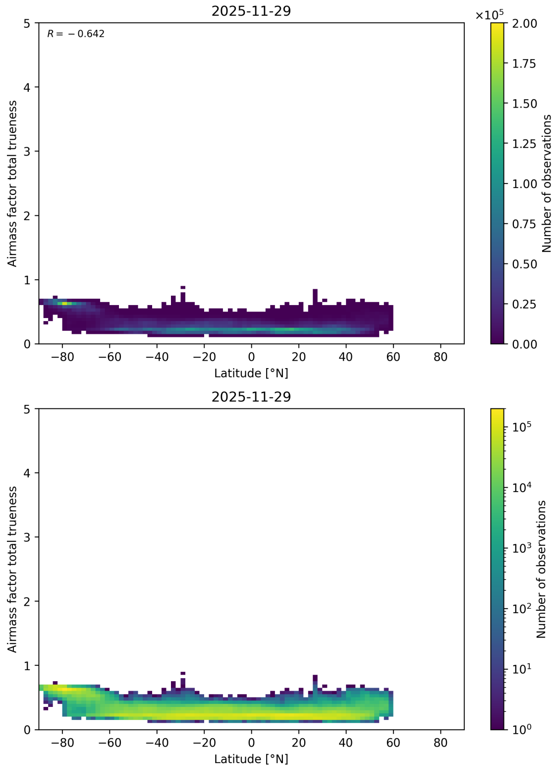
Figure 180: Scatter density plot of “Latitude” against “Airmass factor total trueness” for 2025-11-28 to 2025-11-30.
