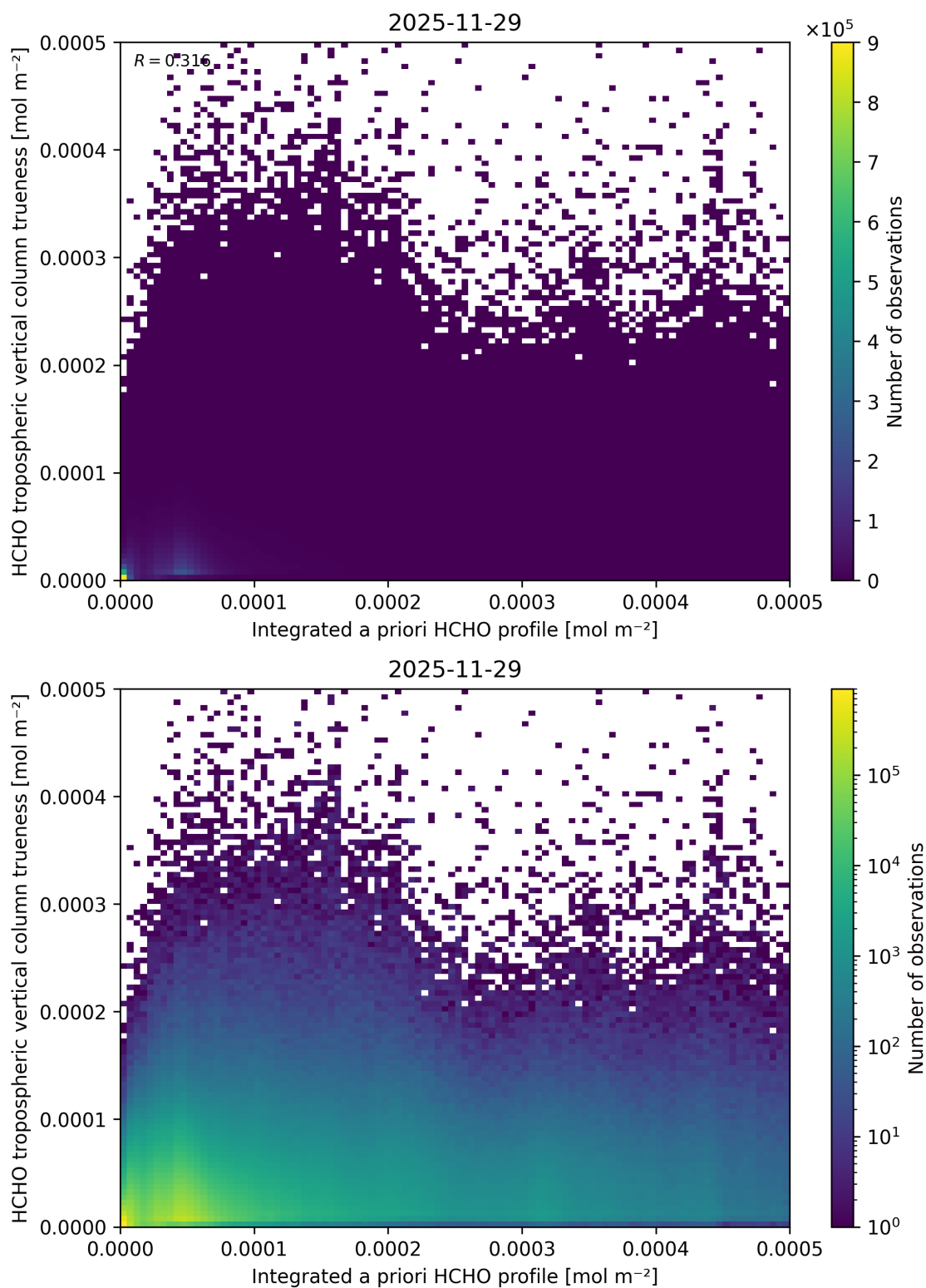
Figure 170: Scatter density plot of “Integrated a priori HCHO profile” against “HCHO tropospheric vertical column trueness” for 2025-11-28 to 2025-11-30.
