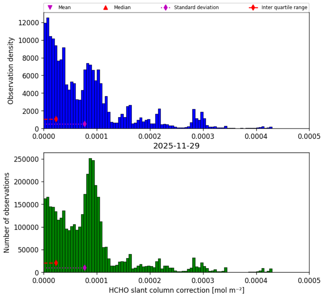
Figure 49: Histogram of “HCHO slant column correction” for 2025-11-28 to 2025-11-30
