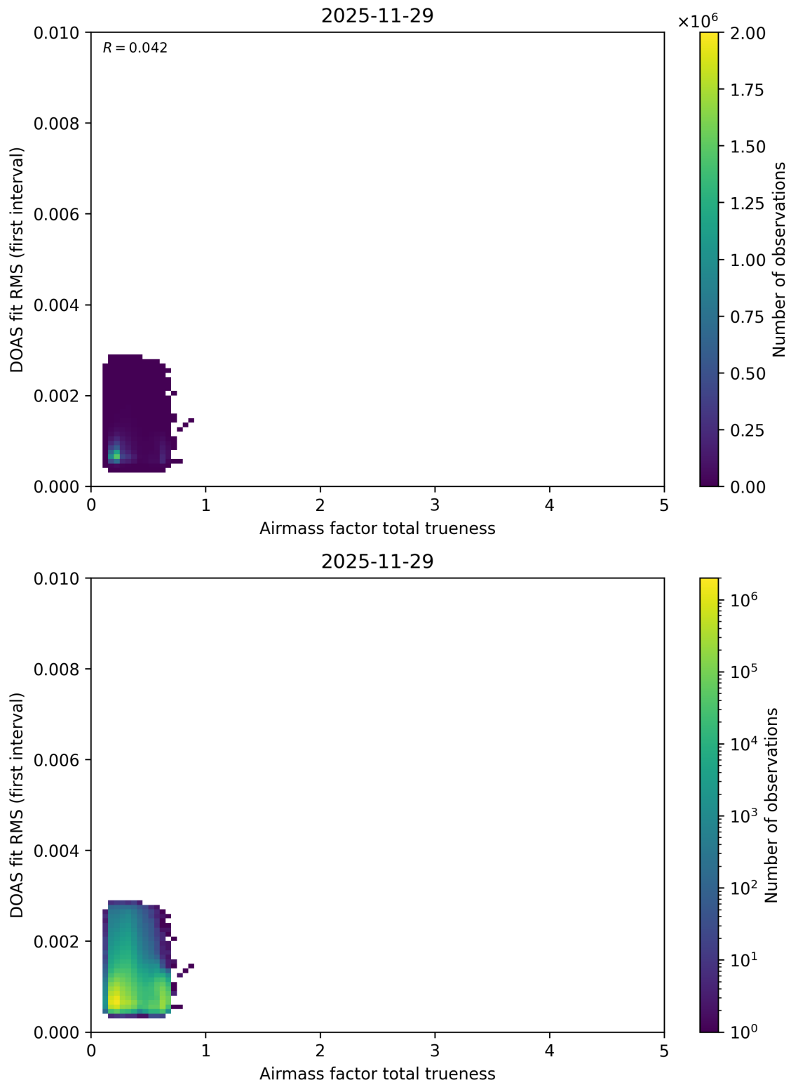
Figure 118: Scatter density plot of “Airmass factor total trueness” against “DOAS fit RMS (first interval)” for 2025-11-28 to 2025-11-30.
