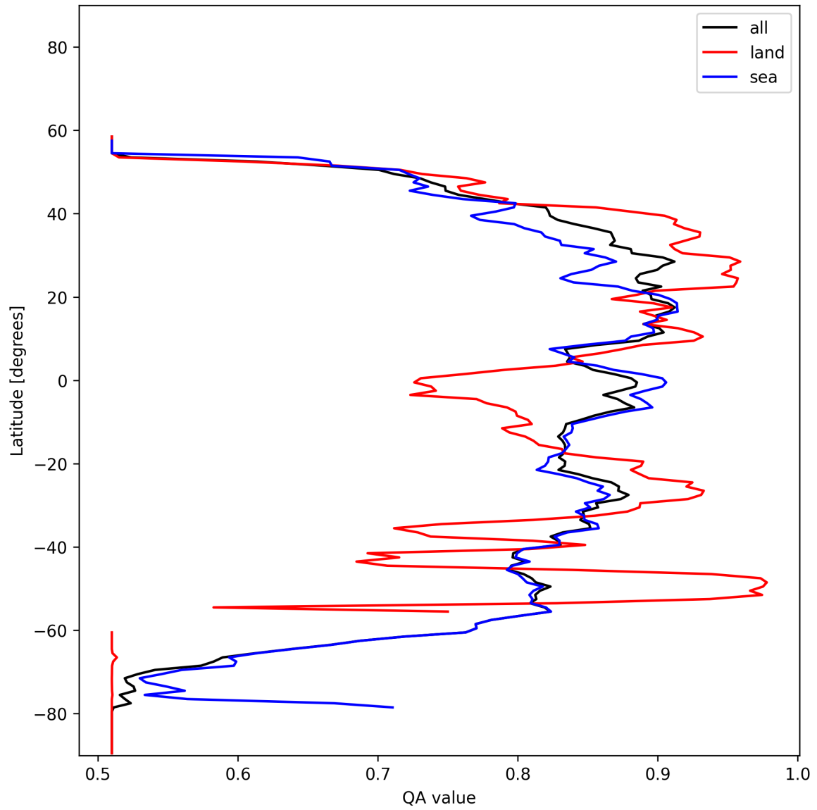
Figure 21: Zonal average of “QA value” for 2025-11-28 to 2025-11-30.
