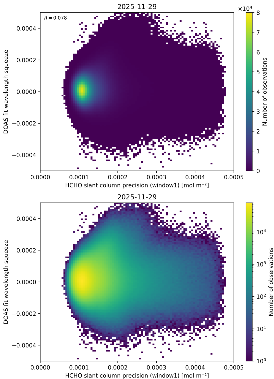
Figure 101: Scatter density plot of “HCHO slant column precision (window1)” against “DOAS fit wavelength squeeze” for 2025-11-28 to 2025-11-30.
