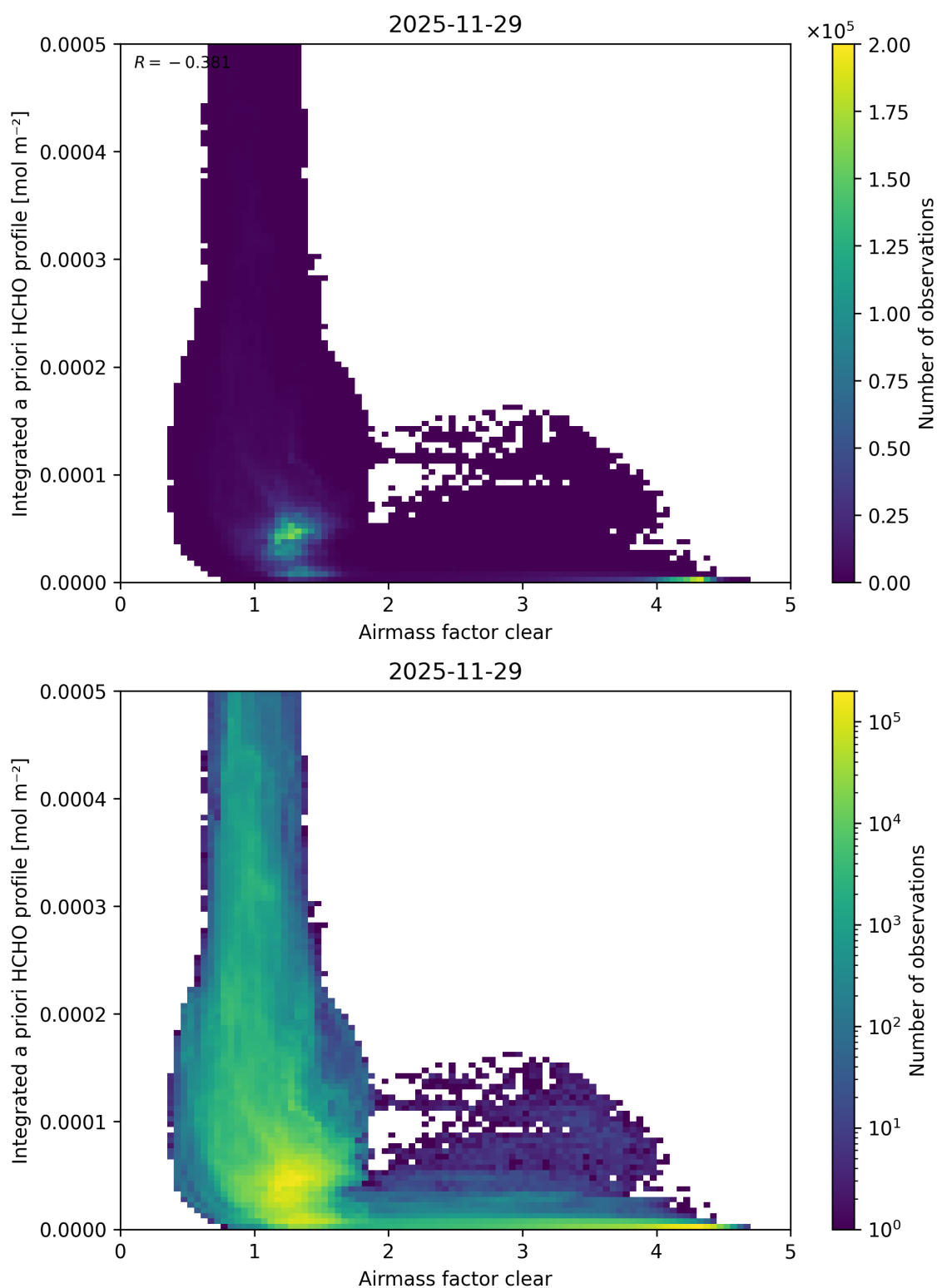
Figure 84: Scatter density plot of “Airmass factor clear” against “Integrated a priori HCHO profile” for 2025-11-28 to 2025-11-30.
