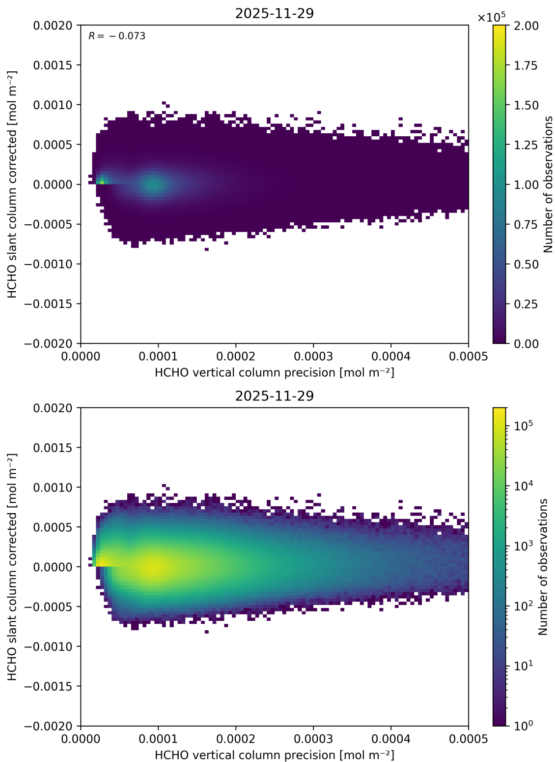
Figure 156: Scatter density plot of “HCHO vertical column precision” against “HCHO slant column corrected” for 2025-11-28 to 2025-11-30.
