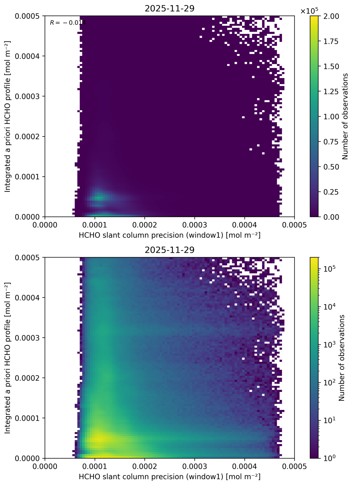
Figure 108: Scatter density plot of “HCHO slant column precision (window1)” against “Integrated a priori HCHO profile” for 2025-11-28 to 2025-11-30.
