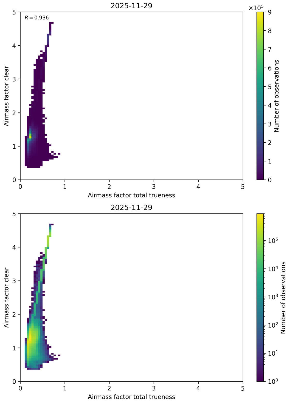
Figure 121: Scatter density plot of “Airmass factor total trueness” against “Airmass factor clear” for 2025-11-28 to 2025-11-30.
