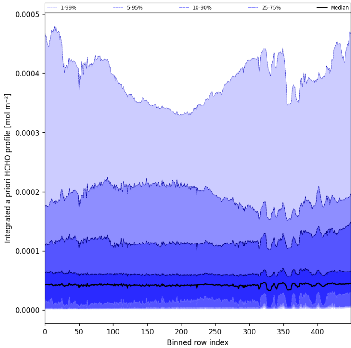
Figure 60: Along track statistics of "Integrated a priori HCHO profile" for 2025-11-28 to 2025-11-30
