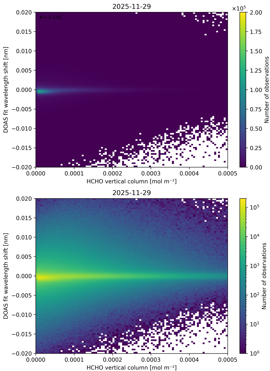
Figure 139: Scatter density plot of “HCHO vertical column” against “DOAS fit wavelength shift” for 2025-11-28 to 2025-11-30.
