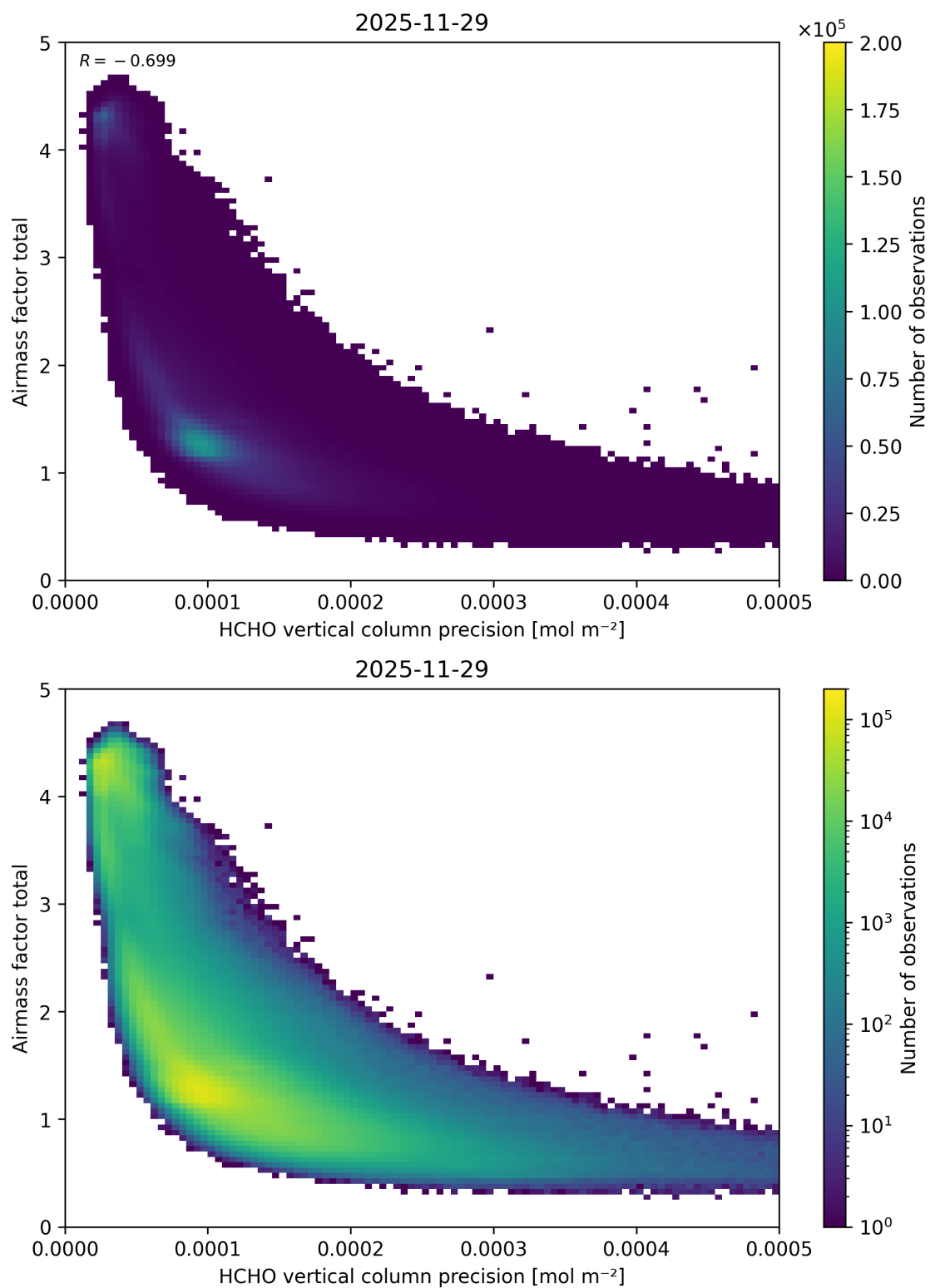
Figure 160: Scatter density plot of “HCHO vertical column precision” against “Airmass factor total” for 2025-11-28 to 2025-11-30.
