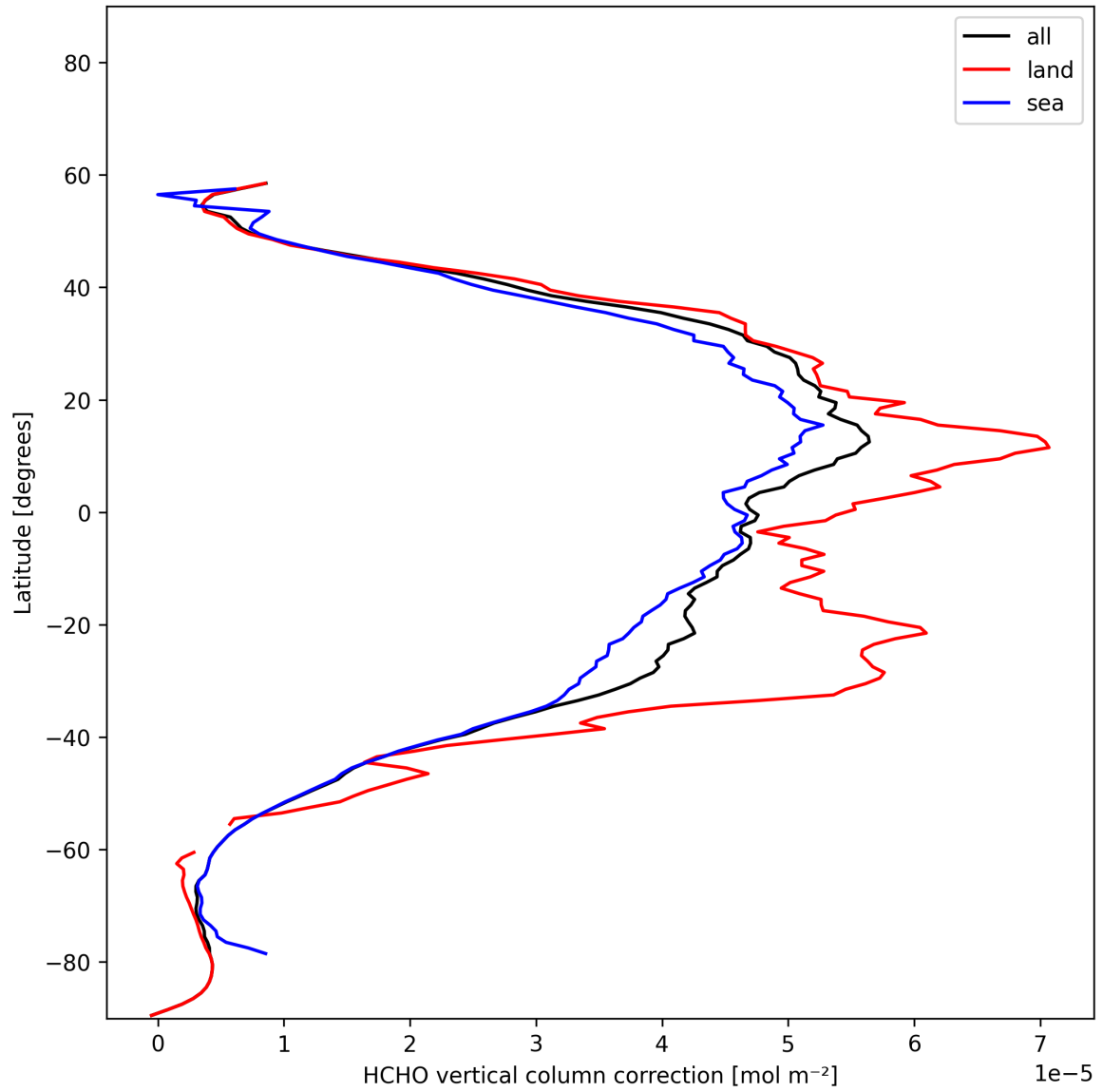
Figure 24: Zonal average of “HCHO vertical column correction” for 2025-11-28 to 2025-11-30.
