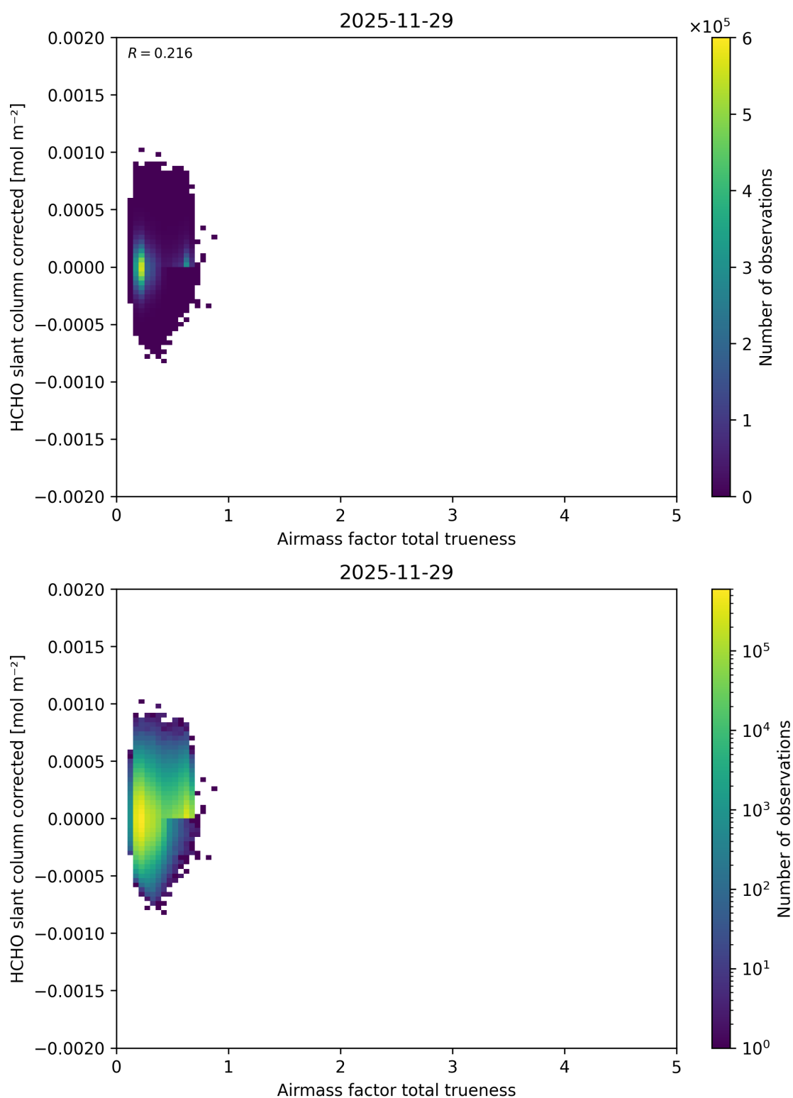
Figure 122: Scatter density plot of “Airmass factor total trueness” against “HCHO slant column corrected” for 2025-11-28 to 2025-11-30.
