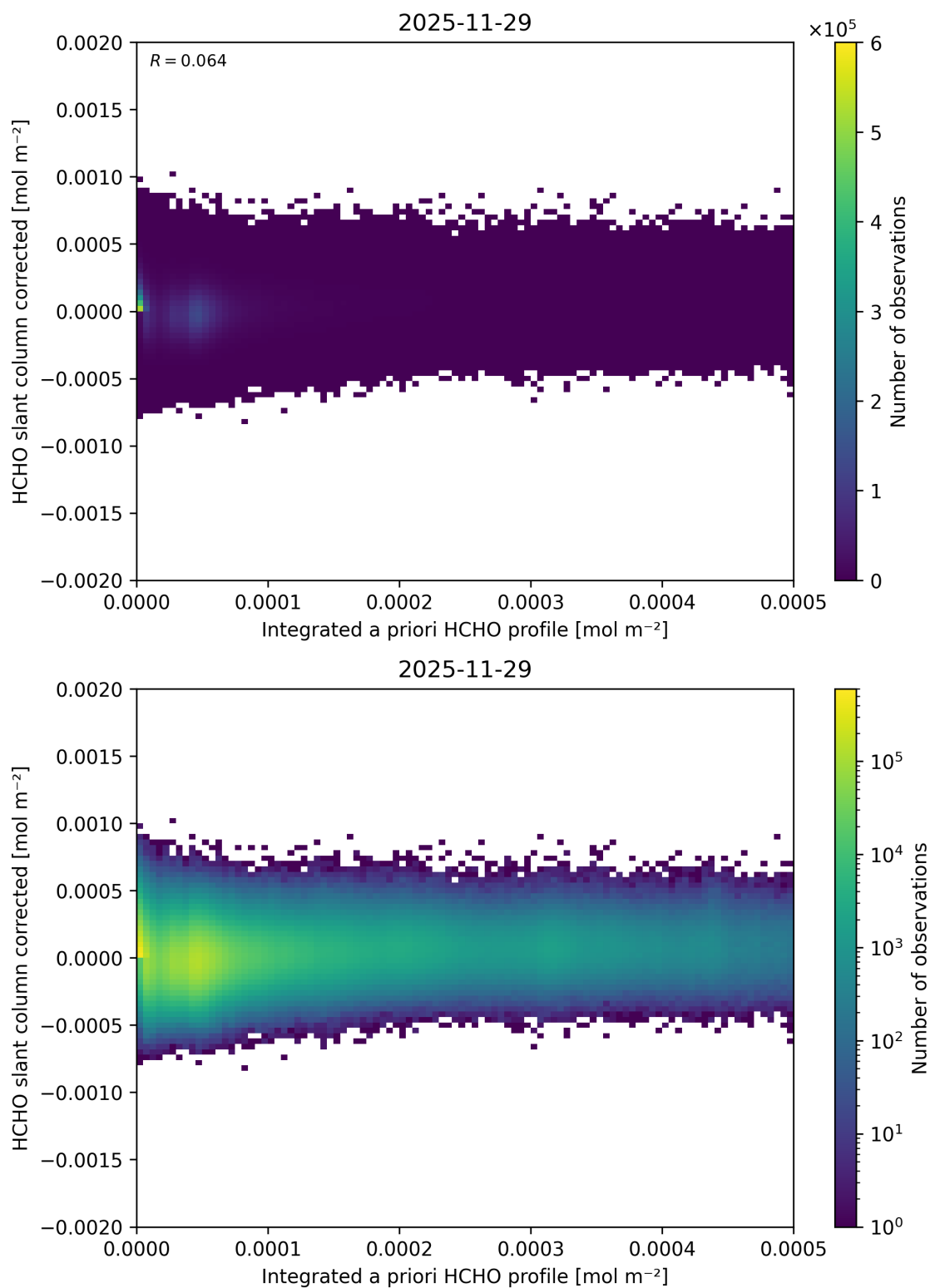
Figure 168: Scatter density plot of “Integrated a priori HCHO profile” against “HCHO slant column corrected” for 2025-11-28 to 2025-11-30.
