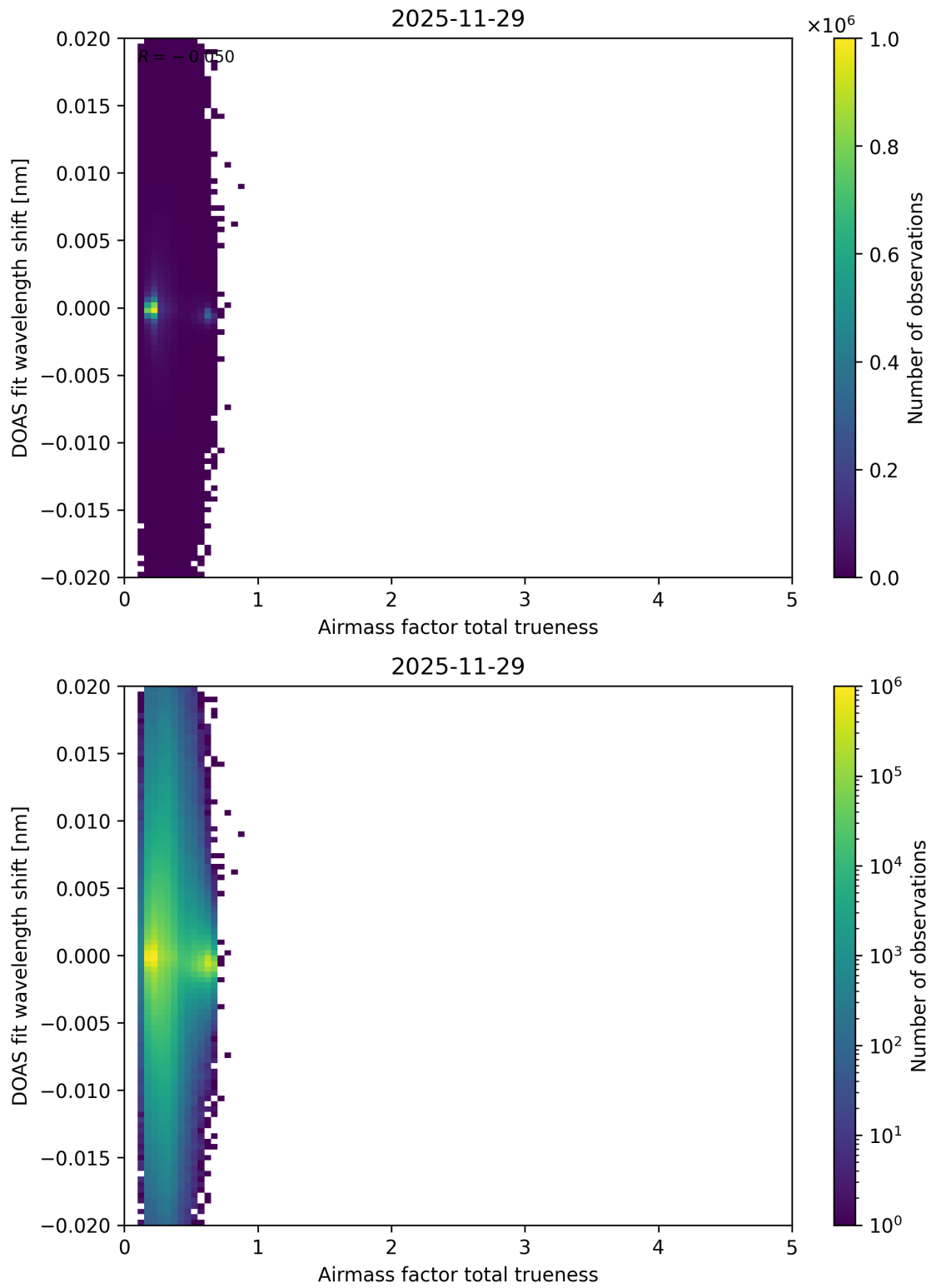
Figure 119: Scatter density plot of “Airmass factor total trueness” against “DOAS fit wavelength shift” for 2025-11-28 to 2025-11-30.
