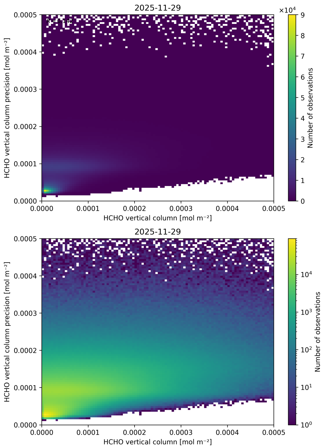
Figure 149: Scatter density plot of “HCHO vertical column” against “HCHO vertical column precision” for 2025-11-28 to 2025-11-30.
