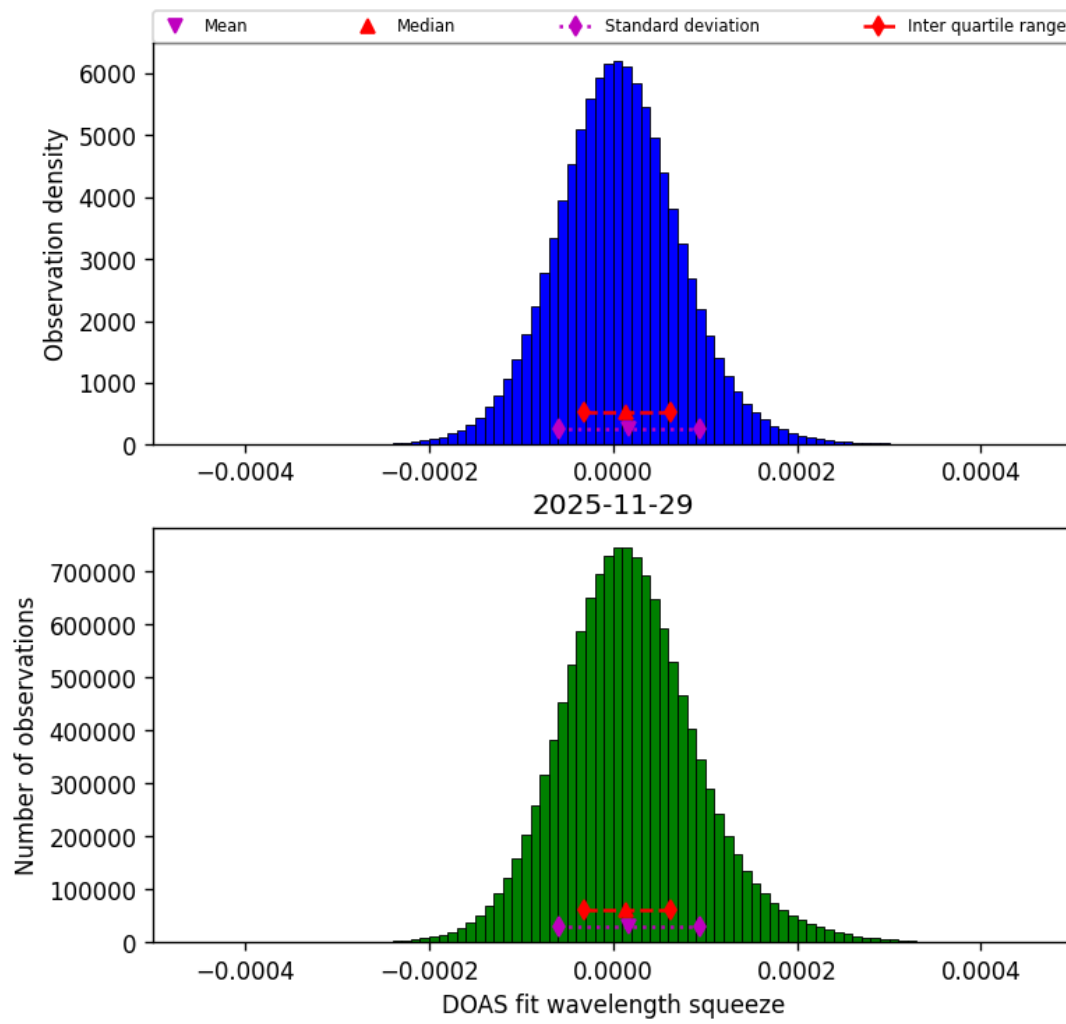
Figure 47: Histogram of “DOAS fit wavelength squeeze” for 2025-11-28 to 2025-11-30
