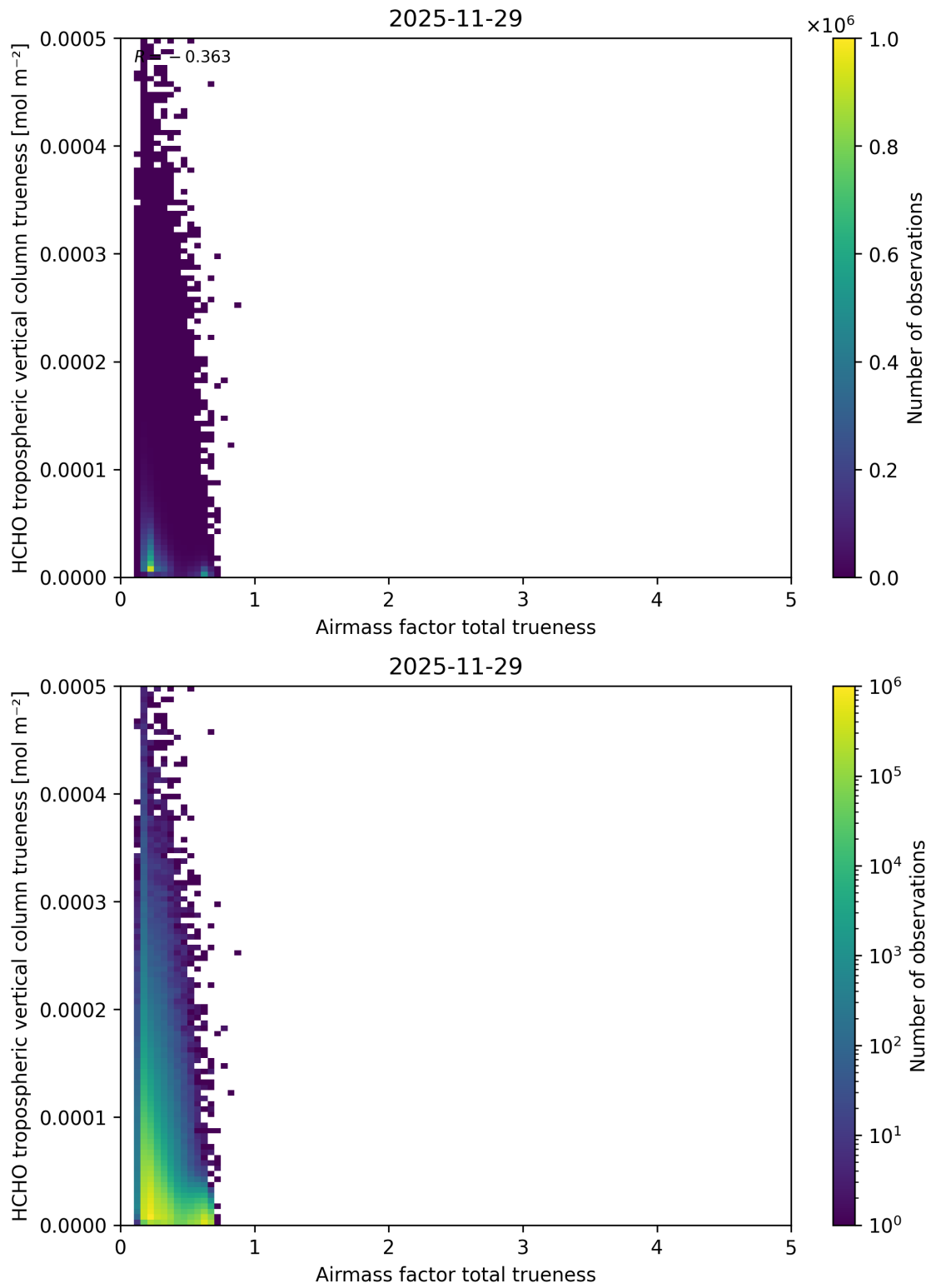
Figure 124: Scatter density plot of “Airmass factor total trueness” against “HCHO tropospheric vertical column trueness” for 2025-11-28 to 2025-11-30.
