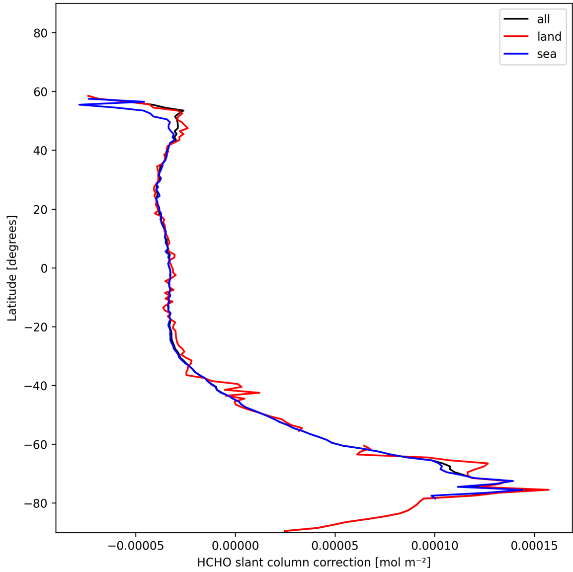
Figure 34: Zonal average of “HCHO slant column correction” for 2025-11-28 to 2025-11-30.
