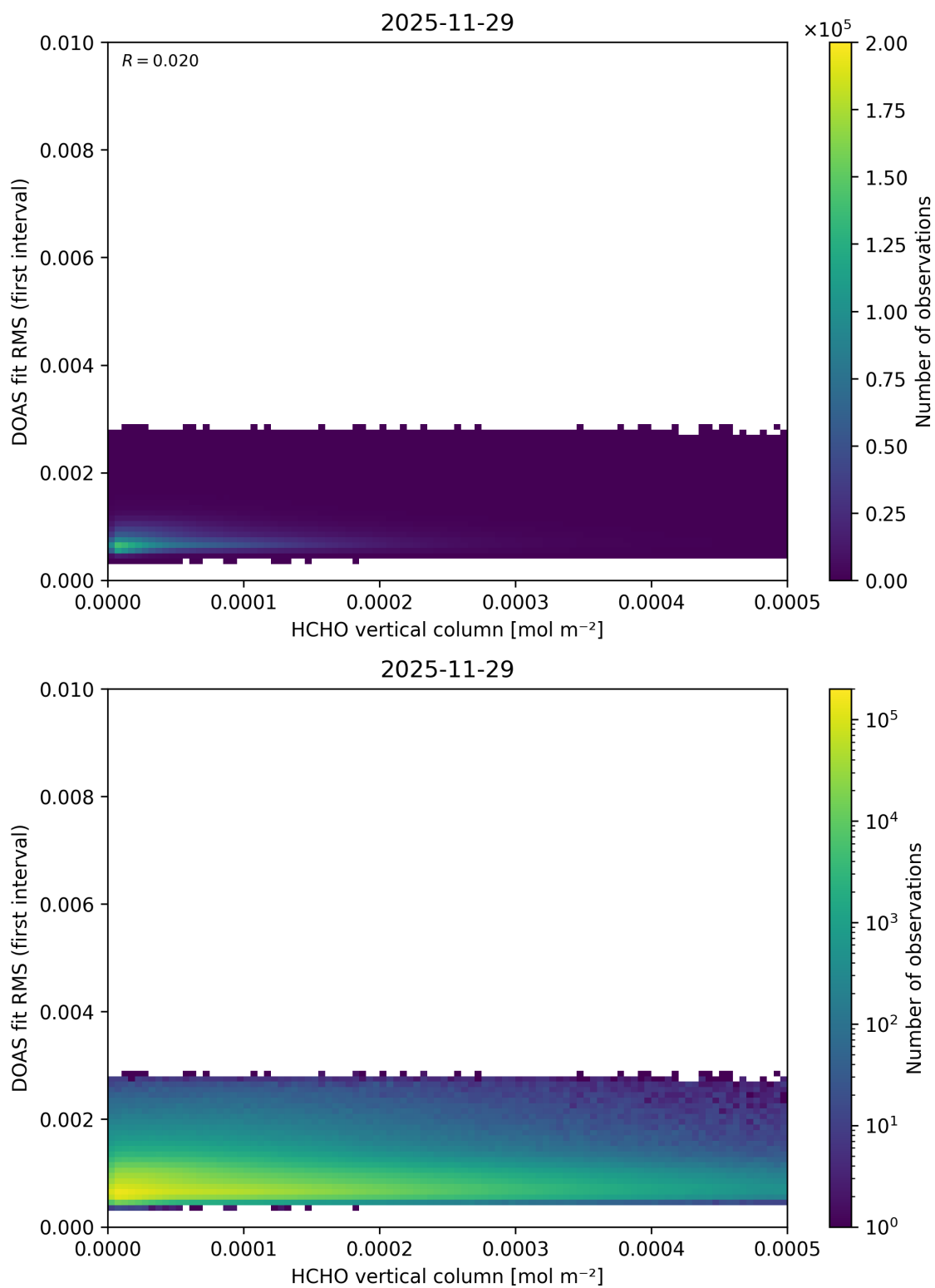
Figure 138: Scatter density plot of “HCHO vertical column” against “DOAS fit RMS (first interval)” for 2025-11-28 to 2025-11-30.
