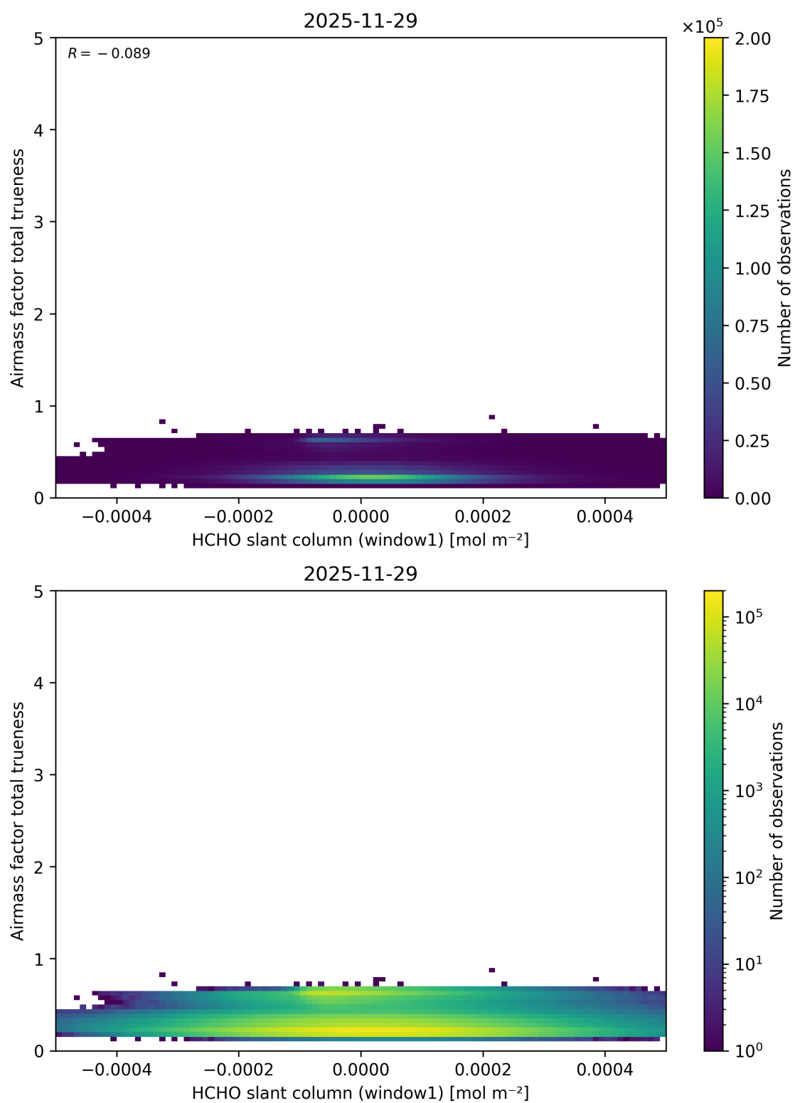
Figure 96: Scatter density plot of “HCHO slant column (window1)” against “Airmass factor total trueneess” for 2025-11-28 to 2025-11-30.
