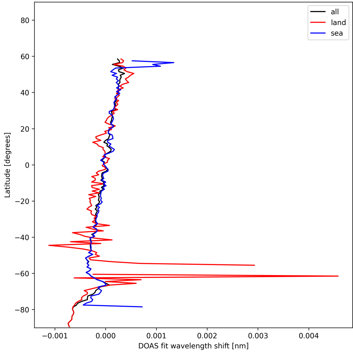
Figure 31: Zonal average of “DOAS fit wavelength shift” for 2025-11-28 to 2025-11-30.
