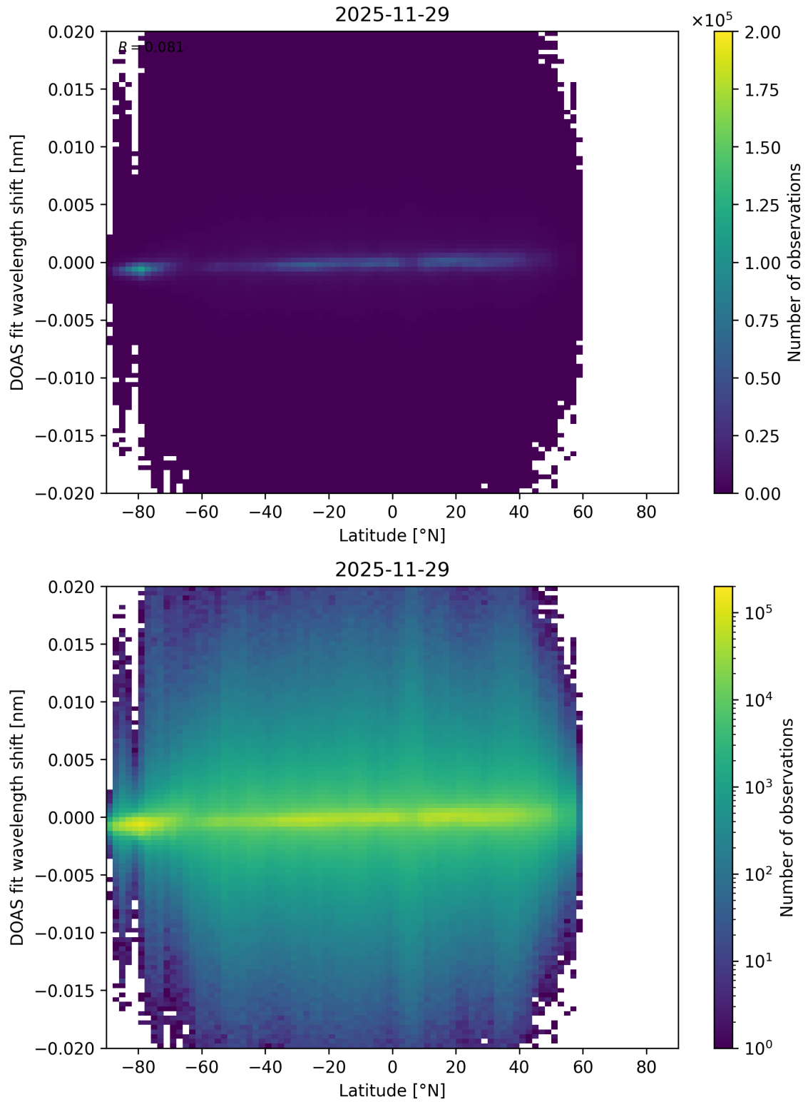
Figure 172: Scatter density plot of “Latitude” against “DOAS fit wavelength shift” for 2025-11-28 to 2025-11-30.
