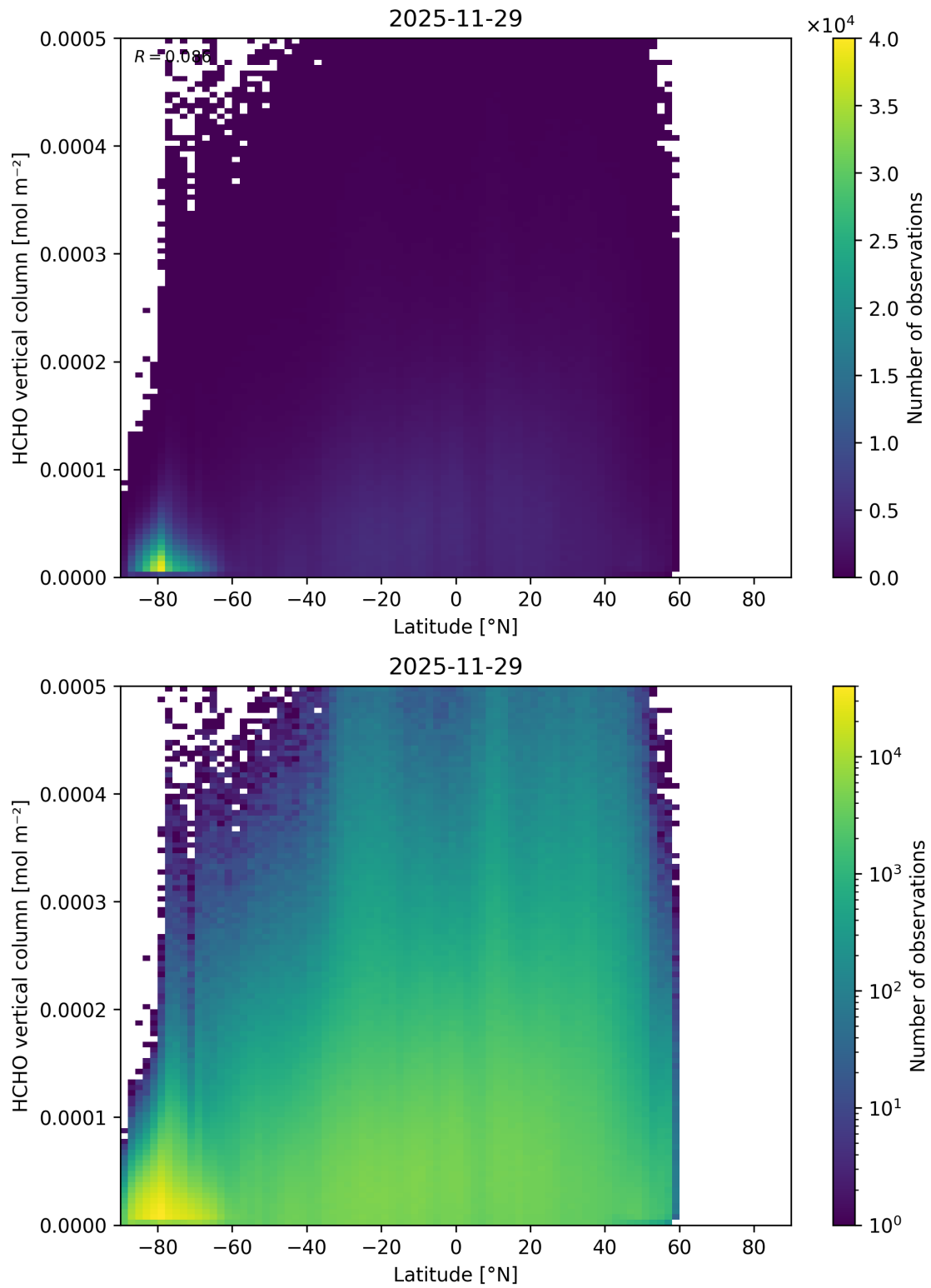
Figure 181: Scatter density plot of “Latitude” against “HCHO vertical column” for 2025-11-28 to 2025-11-30.
