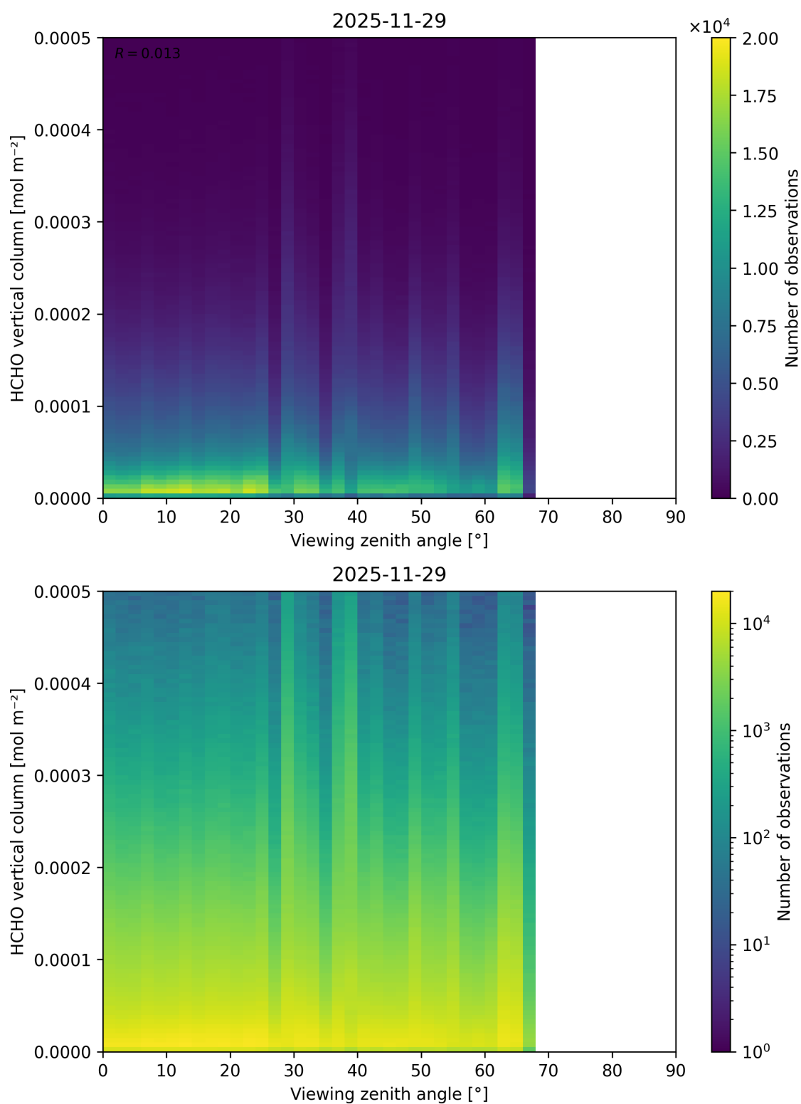
Figure 212: Scatter density plot of “Viewing zenith angle” against “HCHO vertical column” for 2025-11-28 to 2025-11-30.
