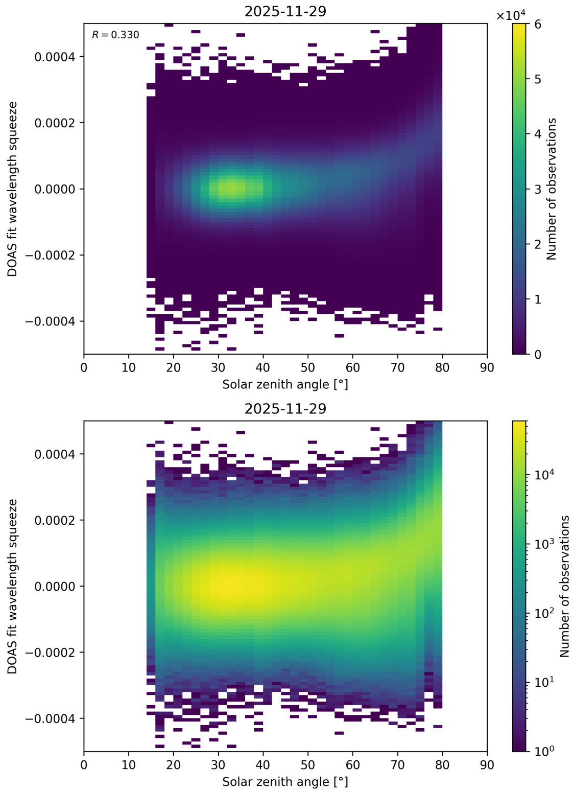
Figure 188: Scatter density plot of “Solar zenith angle” against “DOAS fit wavelength squeeze” for 2025-11-28 to 2025-11-30.
