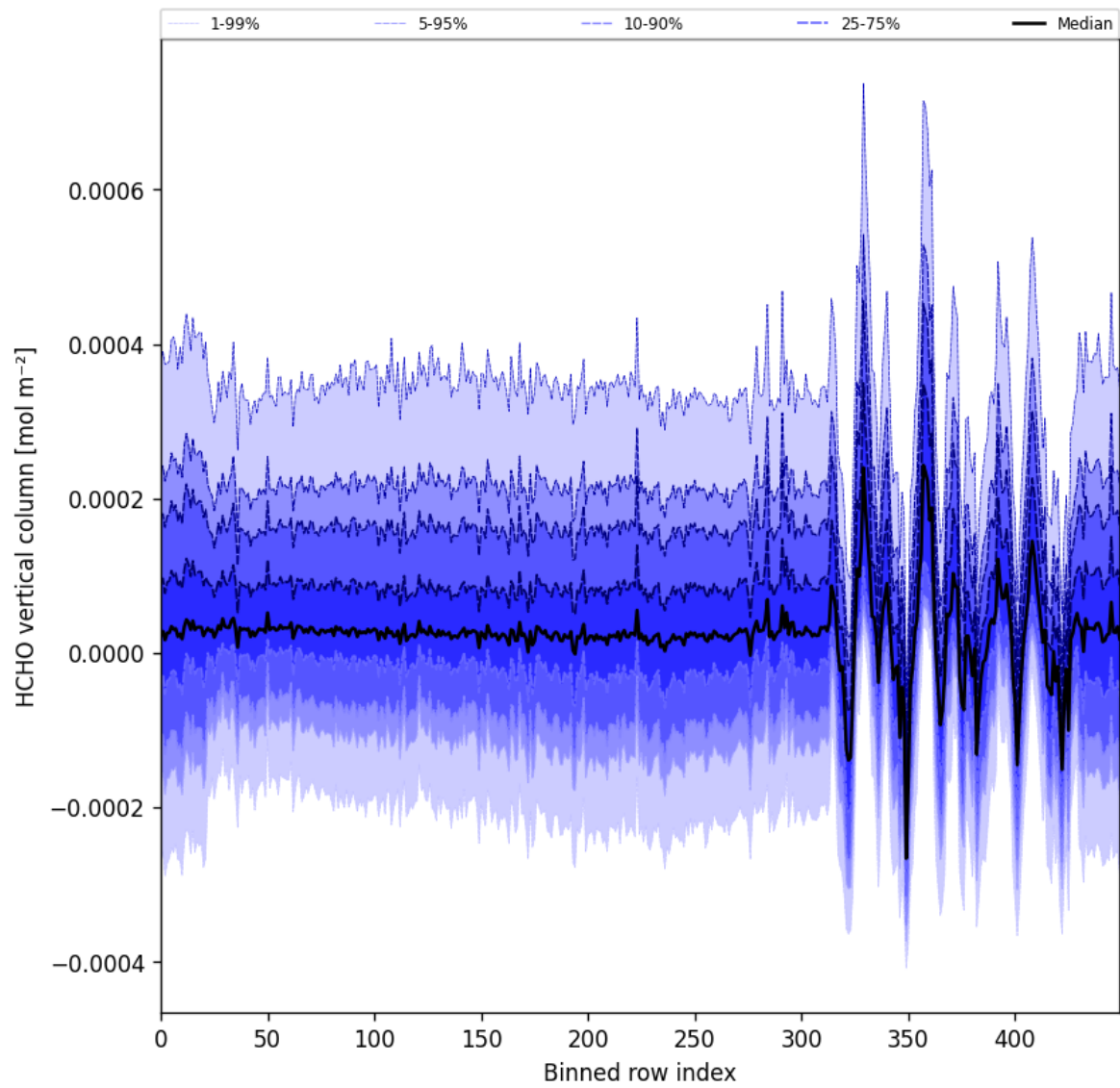
Figure 52: Along track statistics of “HCHO vertical column” for 2025-11-28 to 2025-11-30
