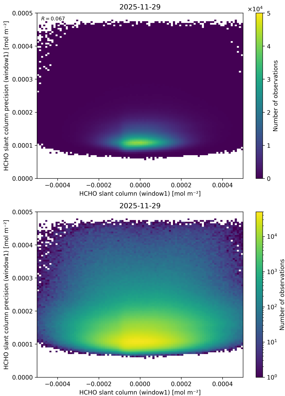
Figure 94: Scatter density plot of “HCHO slant column (window1)” against “HCHO slant column precision (window1)” for 2025-11-28 to 2025-11-30.
