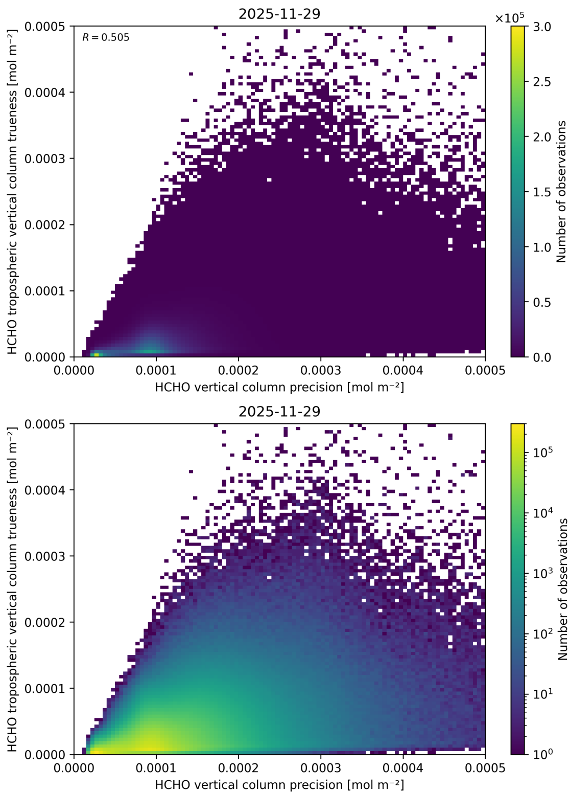
Figure 163: Scatter density plot of “HCHO vertical column precision” against “HCHO tropospheric vertical column truthness” for 2025-11-28 to 2025-11-30.
