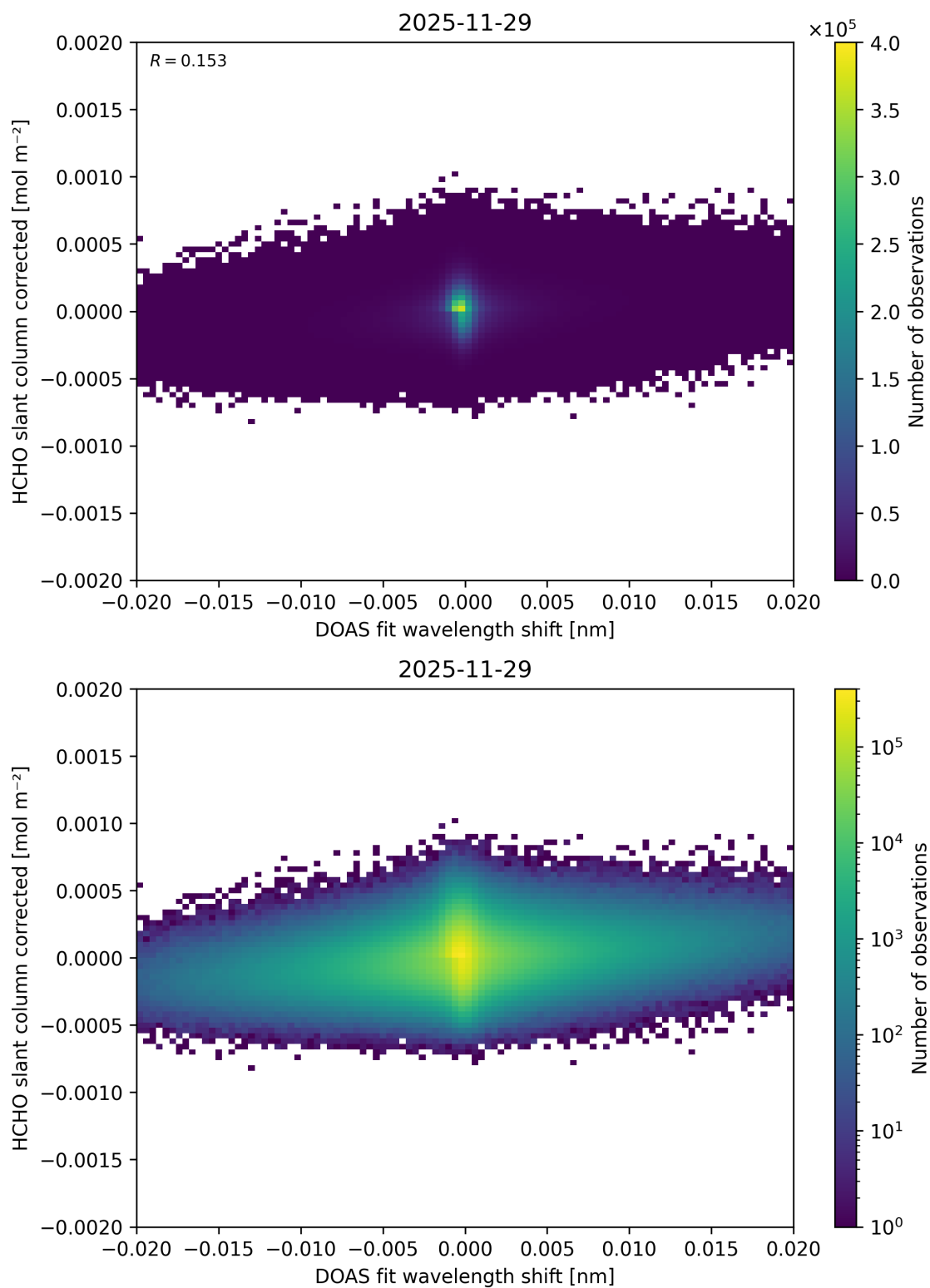
Figure 71: Scatter density plot of “DOAS fit wavelength shift” against “HCHO slant column corrected” for 2025-11-28 to 2025-11-30.
