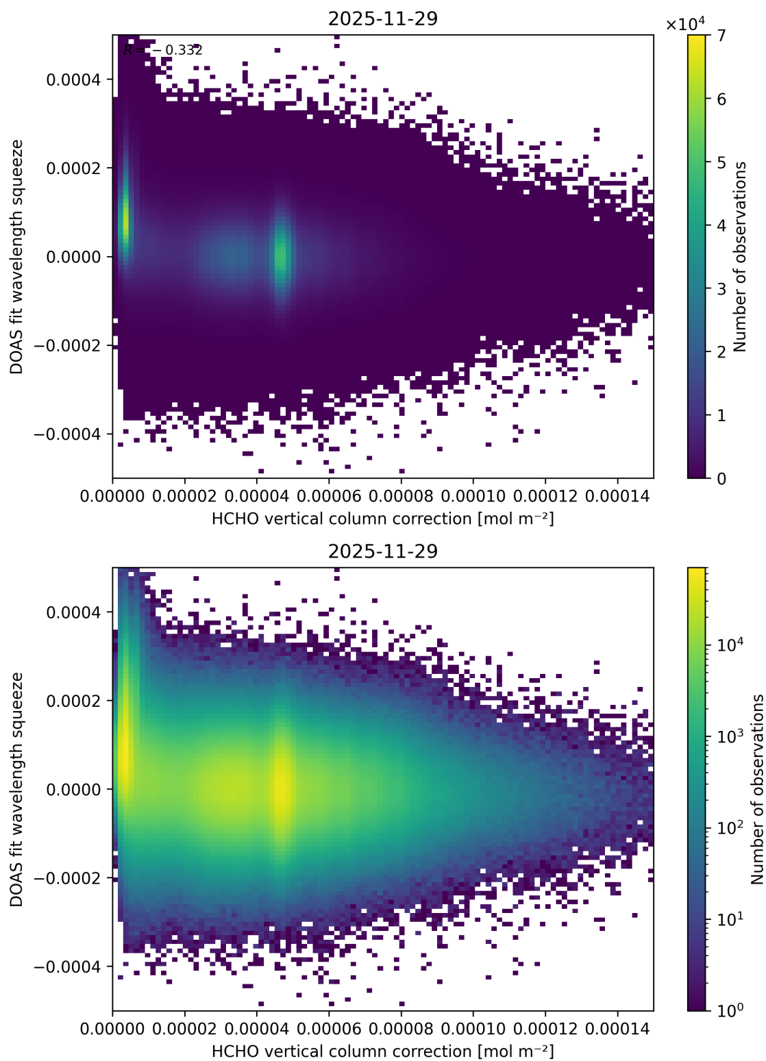
Figure 128: Scatter density plot of “HCHO vertical column correction” against “DOAS fit wavelength squeeze” for 2025-11-28 to 2025-11-30.
