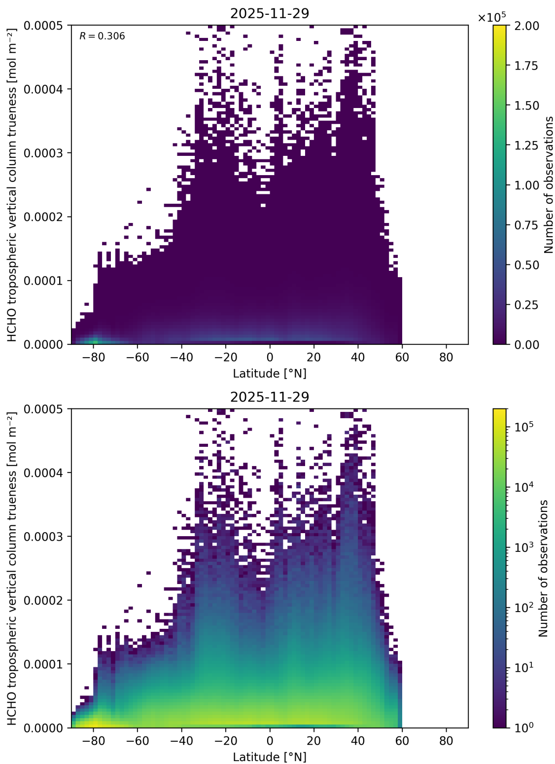
Figure 184: Scatter density plot of “Latitude” against “HCHO tropospheric vertical column trueeness” for 2025-11-28 to 2025-11-30.
