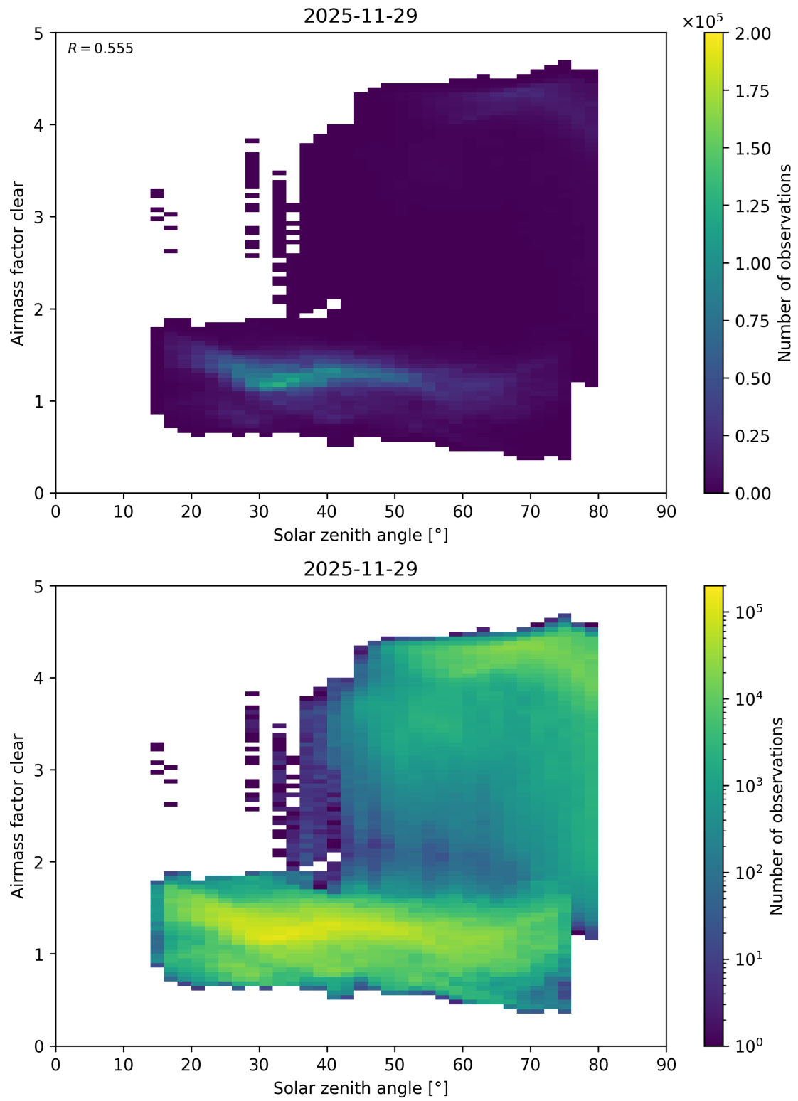
Figure 189: Scatter density plot of “Solar zenith angle” against “Airmass factor clear” for 2025-11-28 to 2025-11-30.
