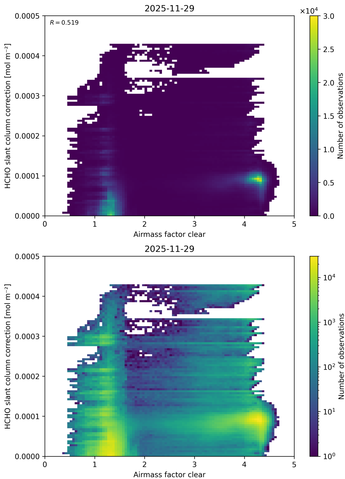
Figure 82: Scatter density plot of “Airmass factor clear” against “HCHO slant column correction” for 2025-11-28 to 2025-11-30.
