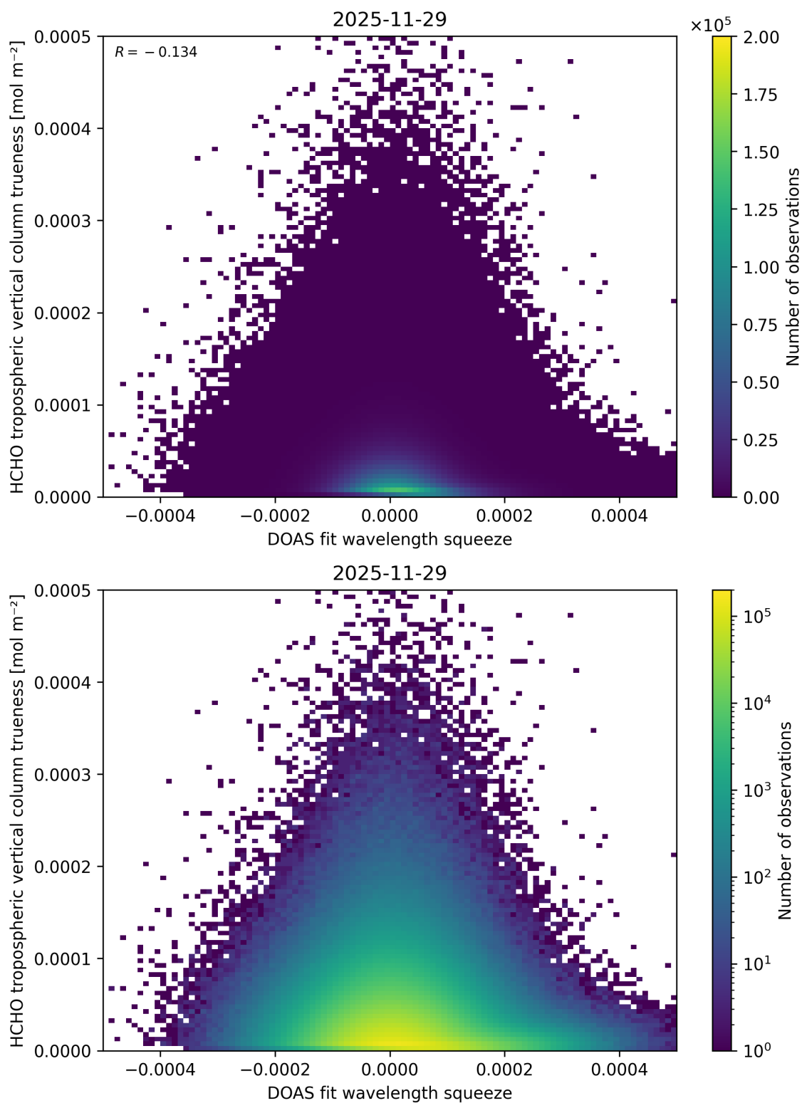
Figure 77: Scatter density plot of “DOAS fit wavelength squeeze” against “HCHO tropospheric vertical column trueness” for 2025-11-28 to 2025-11-30.
