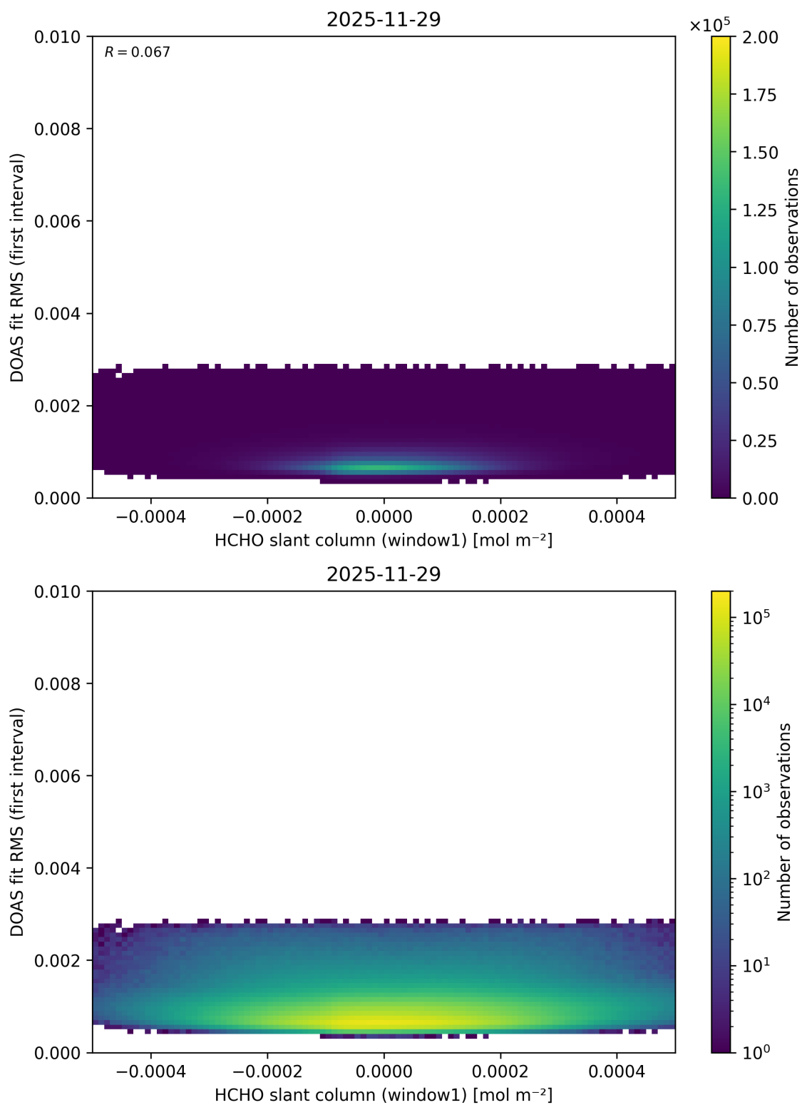
Figure 88: Scatter density plot of “HCHO slant column (window1)” against “DOAS fit RMS (first interval)” for 2025-11-28 to 2025-11-30.
