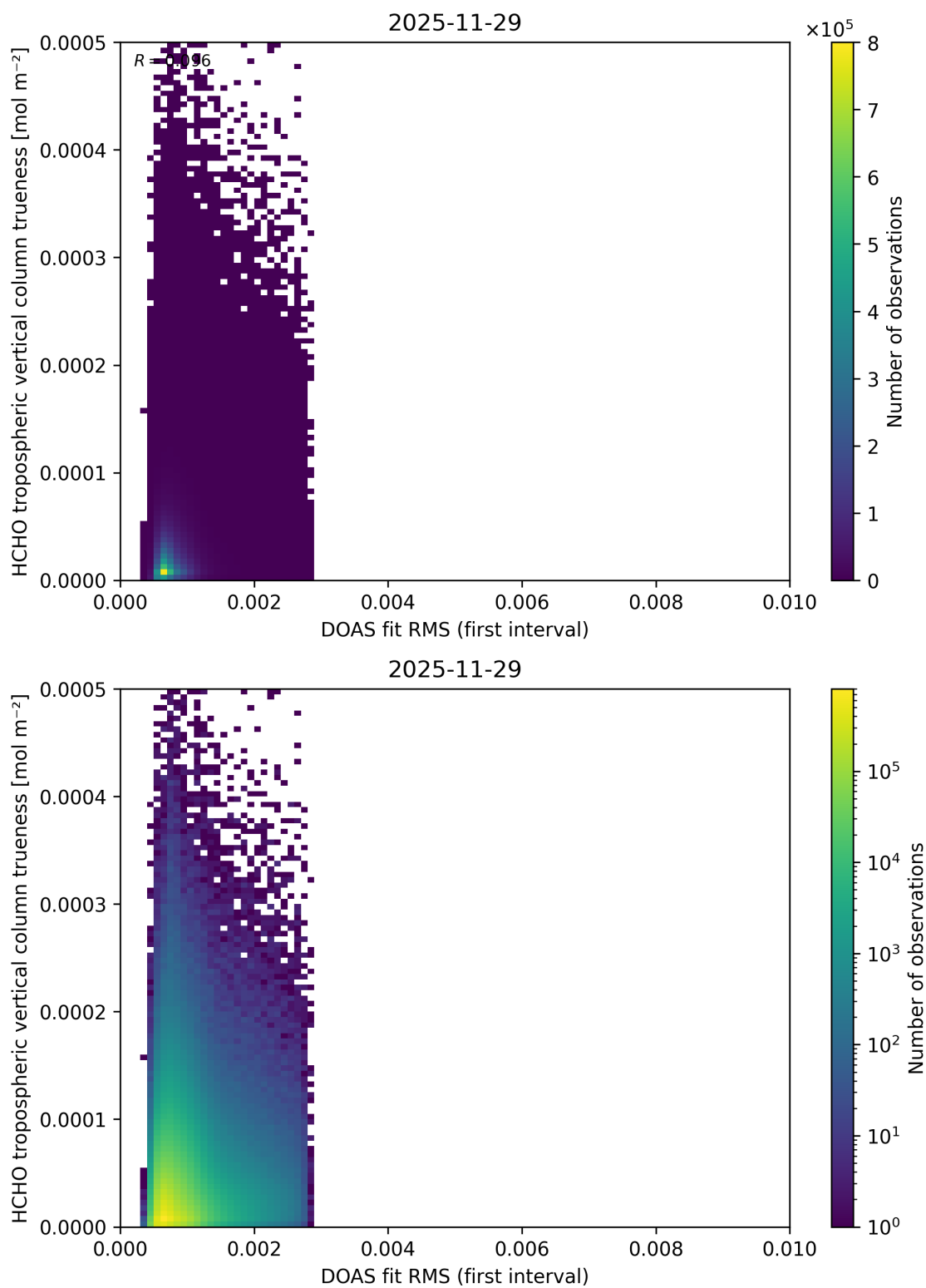
Figure 68: Scatter density plot of “DOAS fit RMS (first interval)” against “HCHO tropospheric vertical column trueness” for 2025-11-28 to 2025-11-30.
