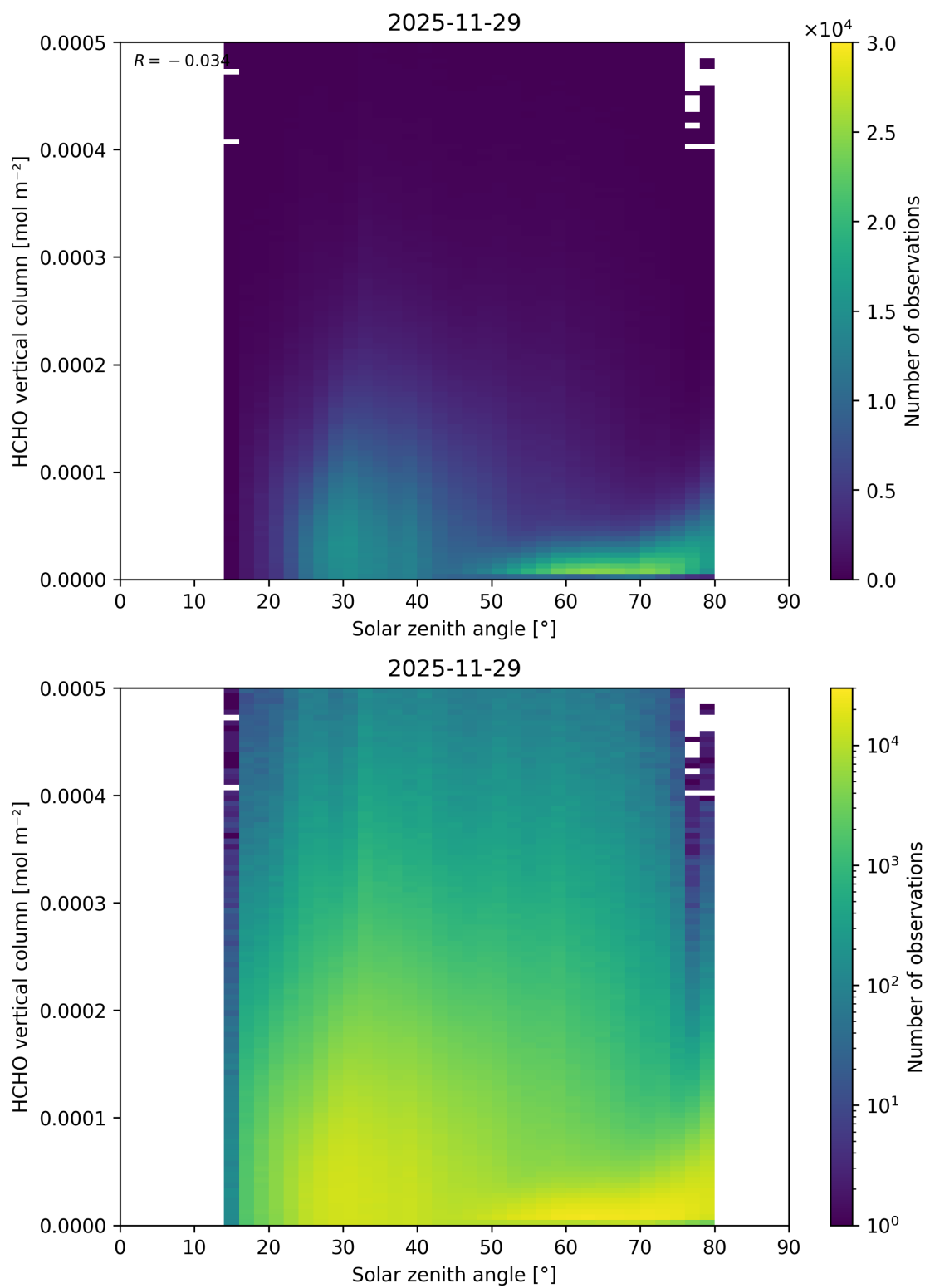
Figure 196: Scatter density plot of “Solar zenith angle” against “HCHO vertical column” for 2025-11-28 to 2025-11-30.
