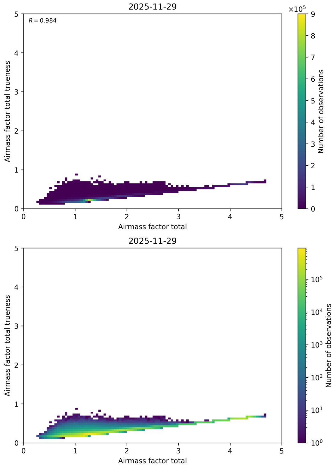
Figure 115: Scatter density plot of “Airmass factor total” against “Airmass factor total trueness” for 2025-11-28 to 2025-11-30.
