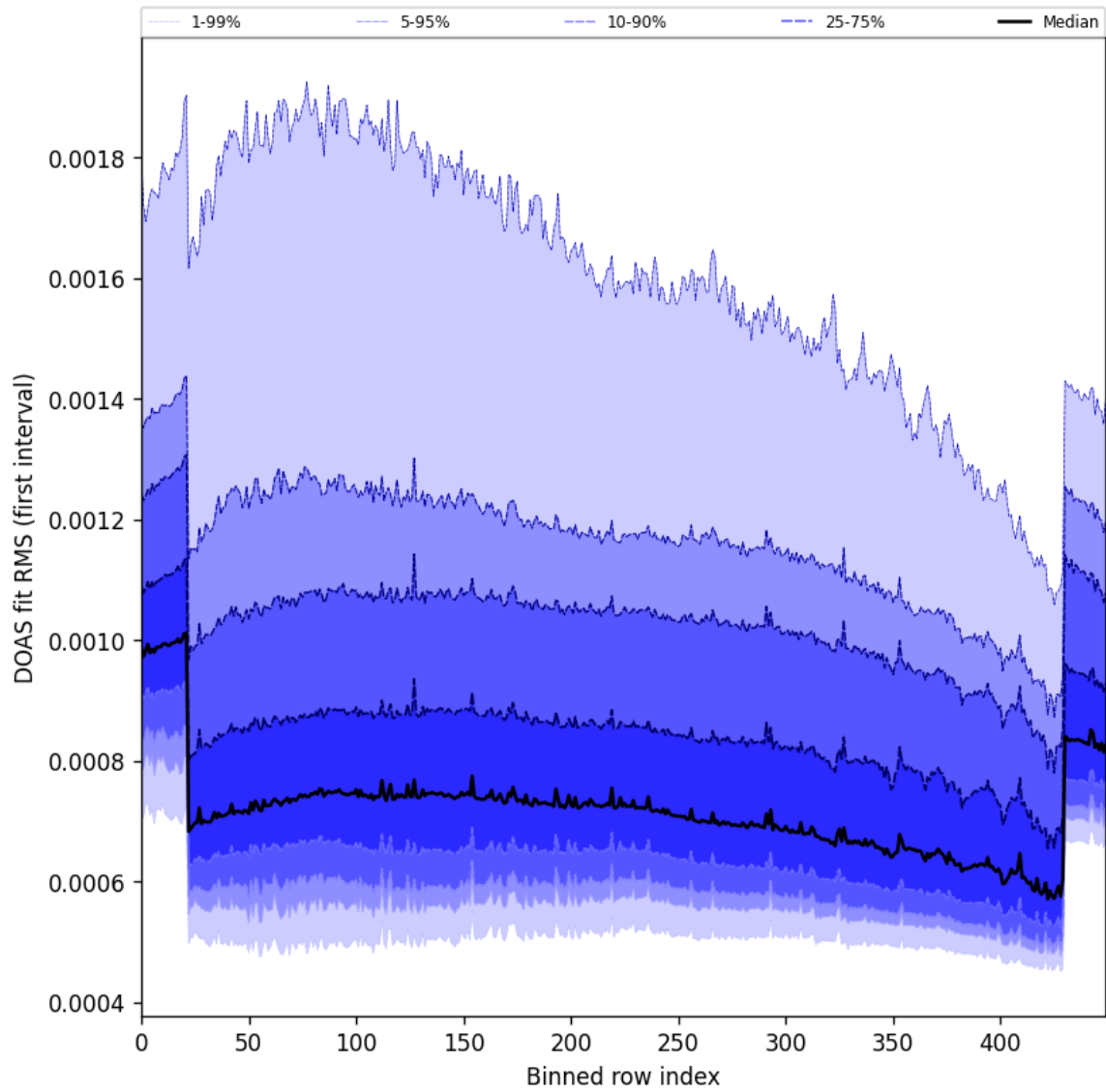
Figure 63: Along track statistics of “DOAS fit RMS (first interval)” for 2025-11-28 to 2025-11-30
