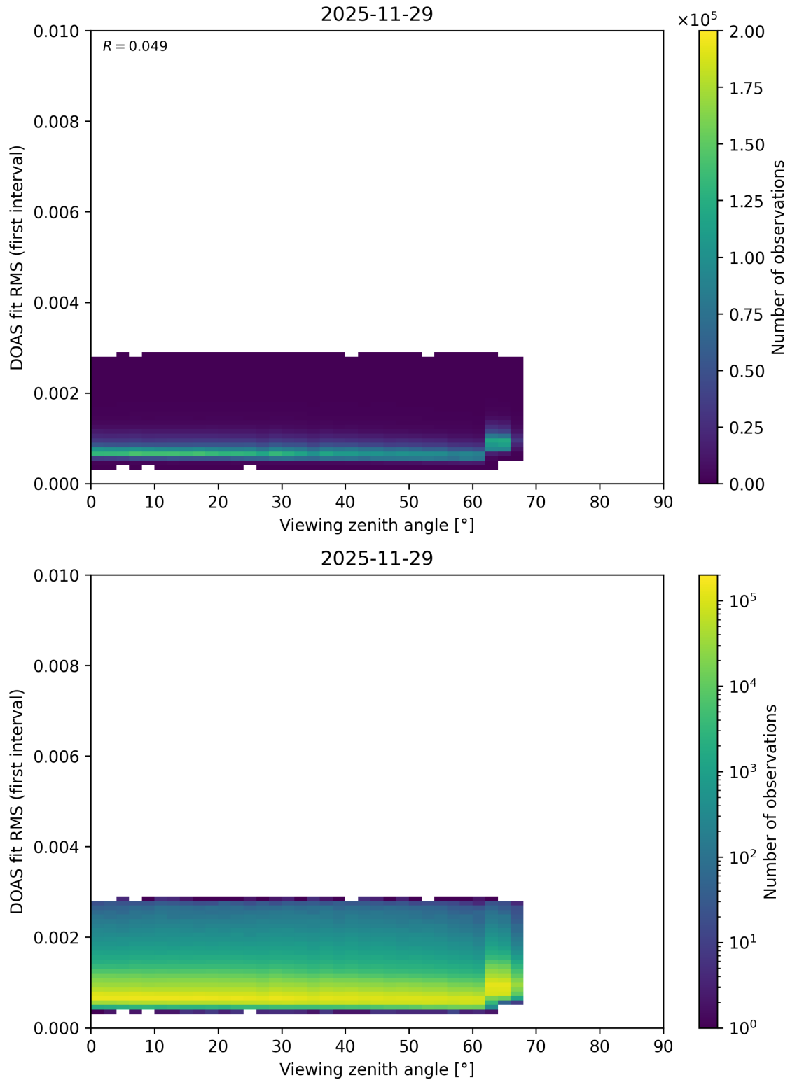
Figure 202: Scatter density plot of “Viewing zenith angle” against “DOAS fit RMS (first interval)” for 2025-11-28 to 2025-11-30.
