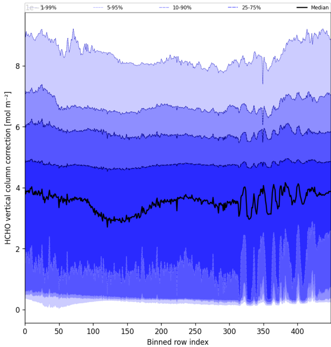
Figure 54: Along track statistics of “HCHO vertical column correction” for 2025-11-28 to 2025-11-30
