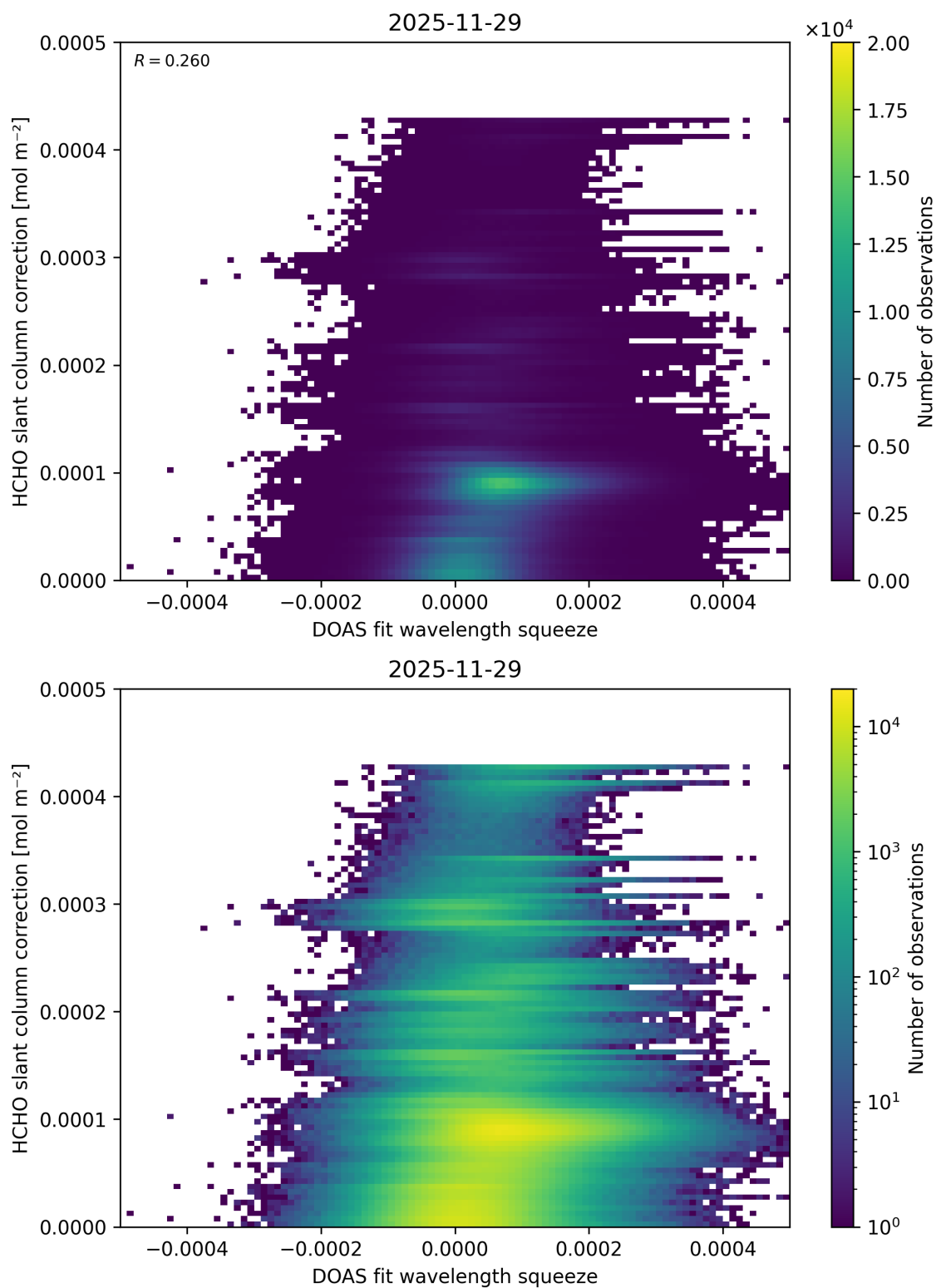
Figure 76: Scatter density plot of “DOAS fit wavelength squeeze” against “HCHO slant column correction” for 2025-11-28 to 2025-11-30.
