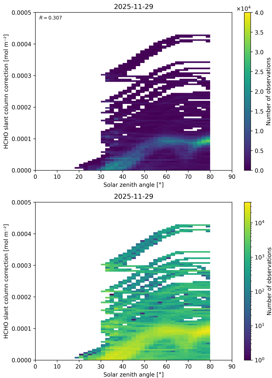
Figure 191: Scatter density plot of “Solar zenith angle” against “HCHO slant column correction” for 2025-11-28 to 2025-11-30.
