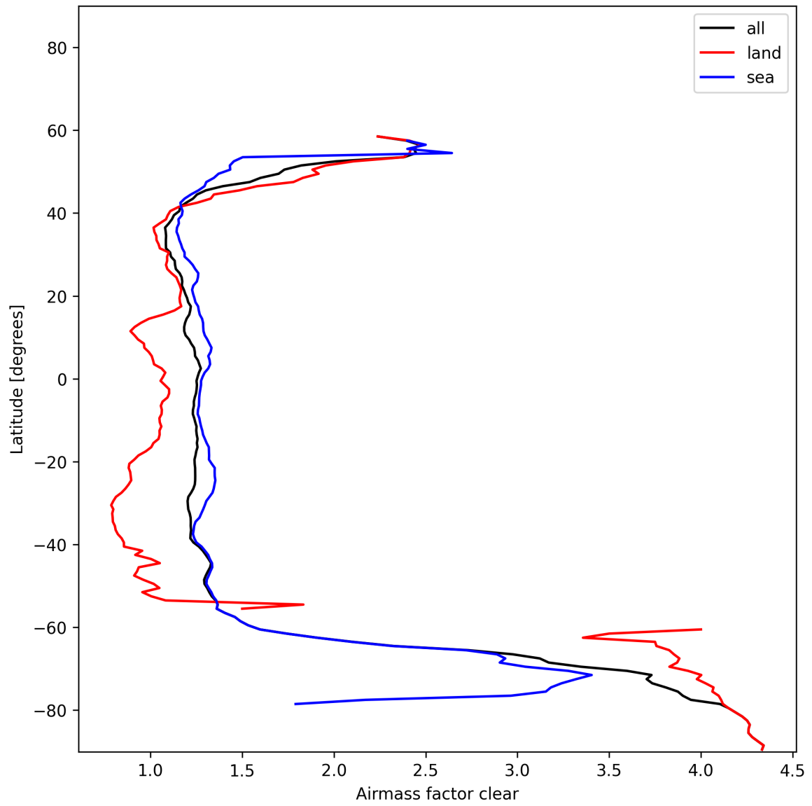
Figure 29: Zonal average of “Airmass factor clear” for 2025-11-28 to 2025-11-30.
