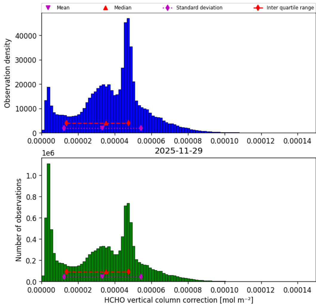
Figure 39: Histogram of “HCHO vertical column correction” for 2025-11-28 to 2025-11-30
