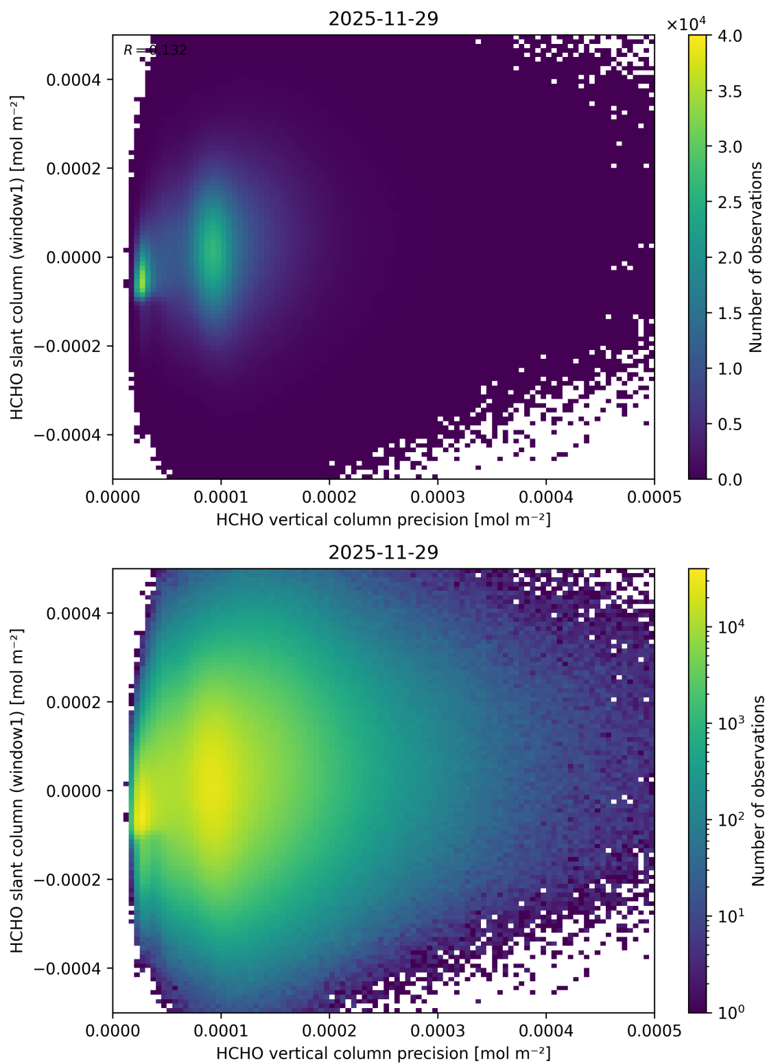
Figure 158: Scatter density plot of “HCHO vertical column precision” against “HCHO slant column (window1)” for 2025-11-28 to 2025-11-30.
