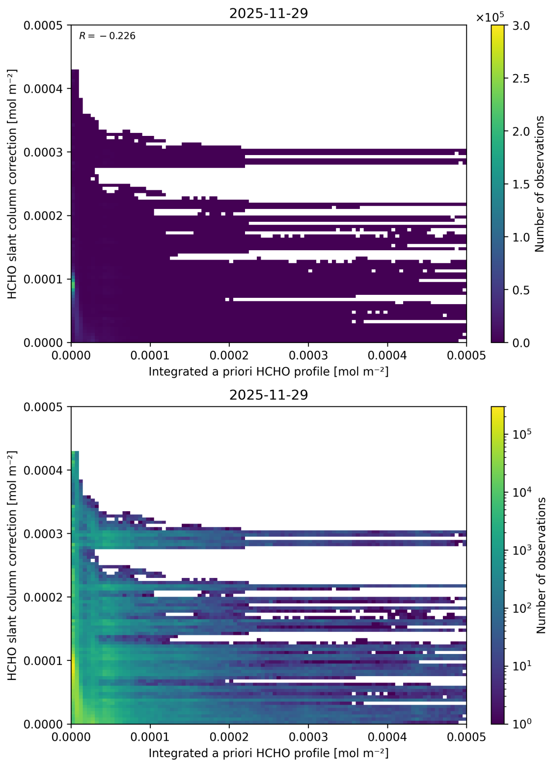
Figure 169: Scatter density plot of “Integrated a priori HCHO profile” against “HCHO slant column correction” for 2025-11-28 to 2025-11-30.
