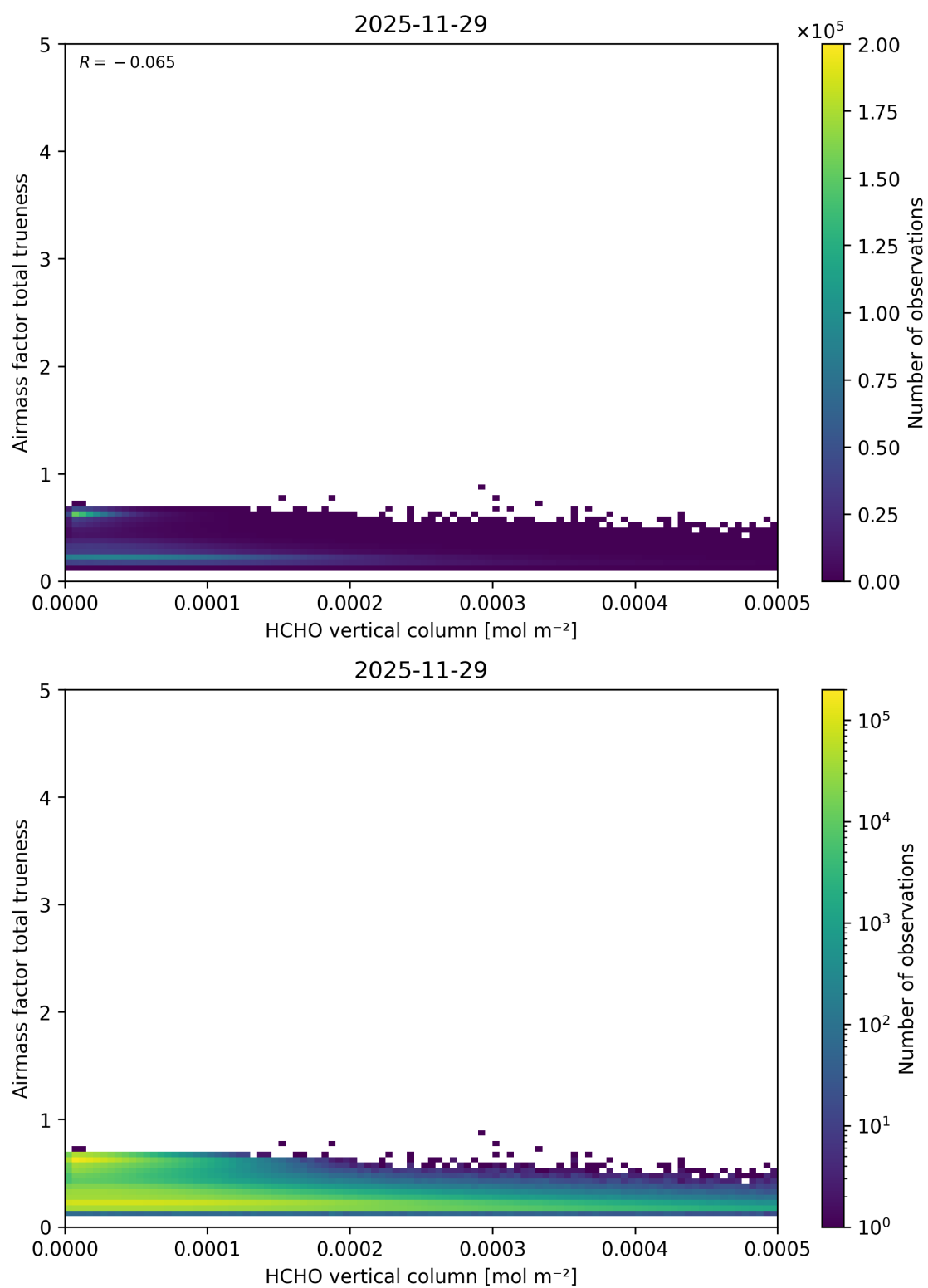
Figure 147: Scatter density plot of “HCHO vertical column” against “Airmass factor total trueneess” for 2025-11-28 to 2025-11-30.
