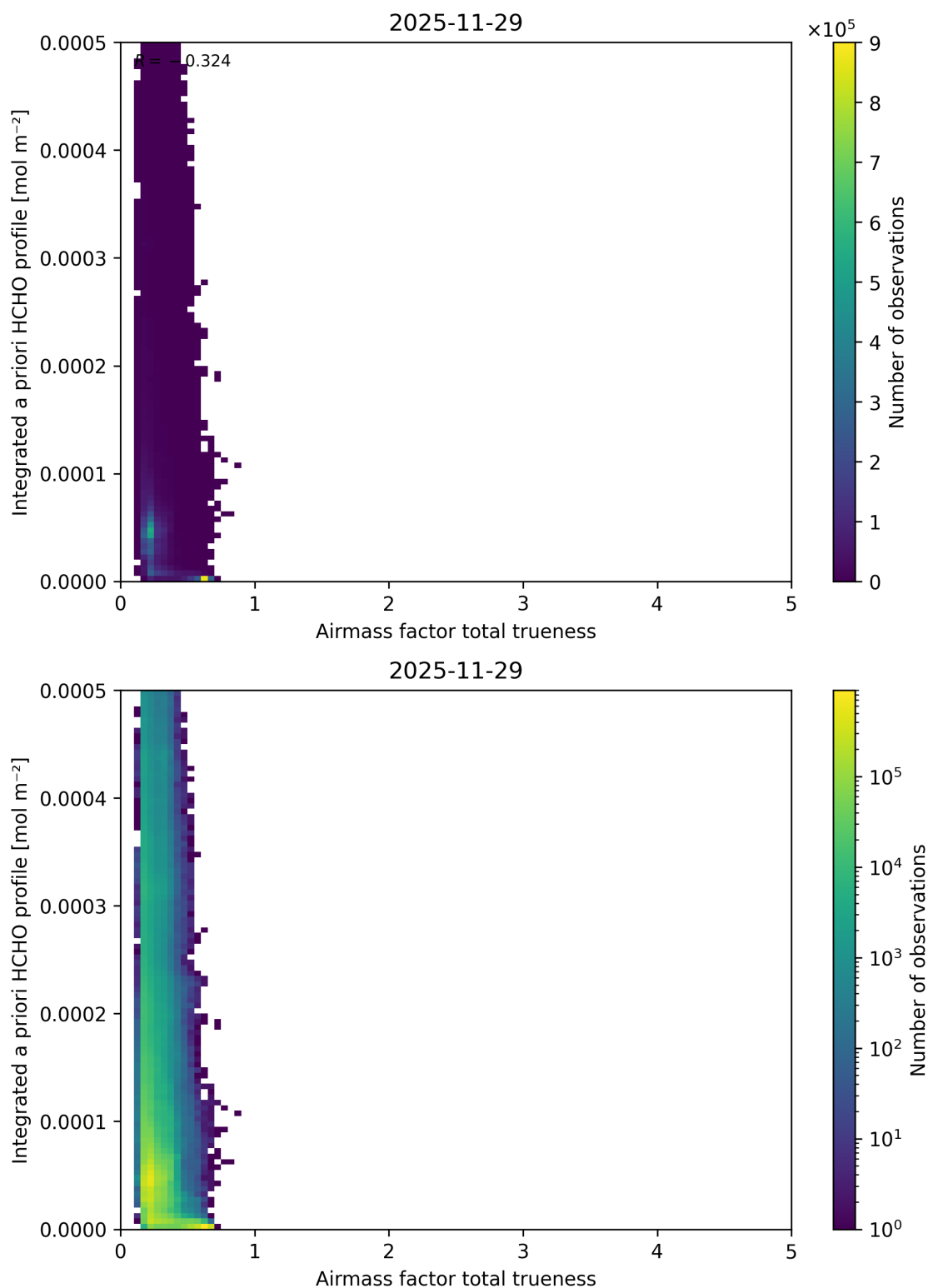
Figure 125: Scatter density plot of “Airmass factor total trueness” against “Integrated a priori HCHO profile” for 2025-11-28 to 2025-11-30.
