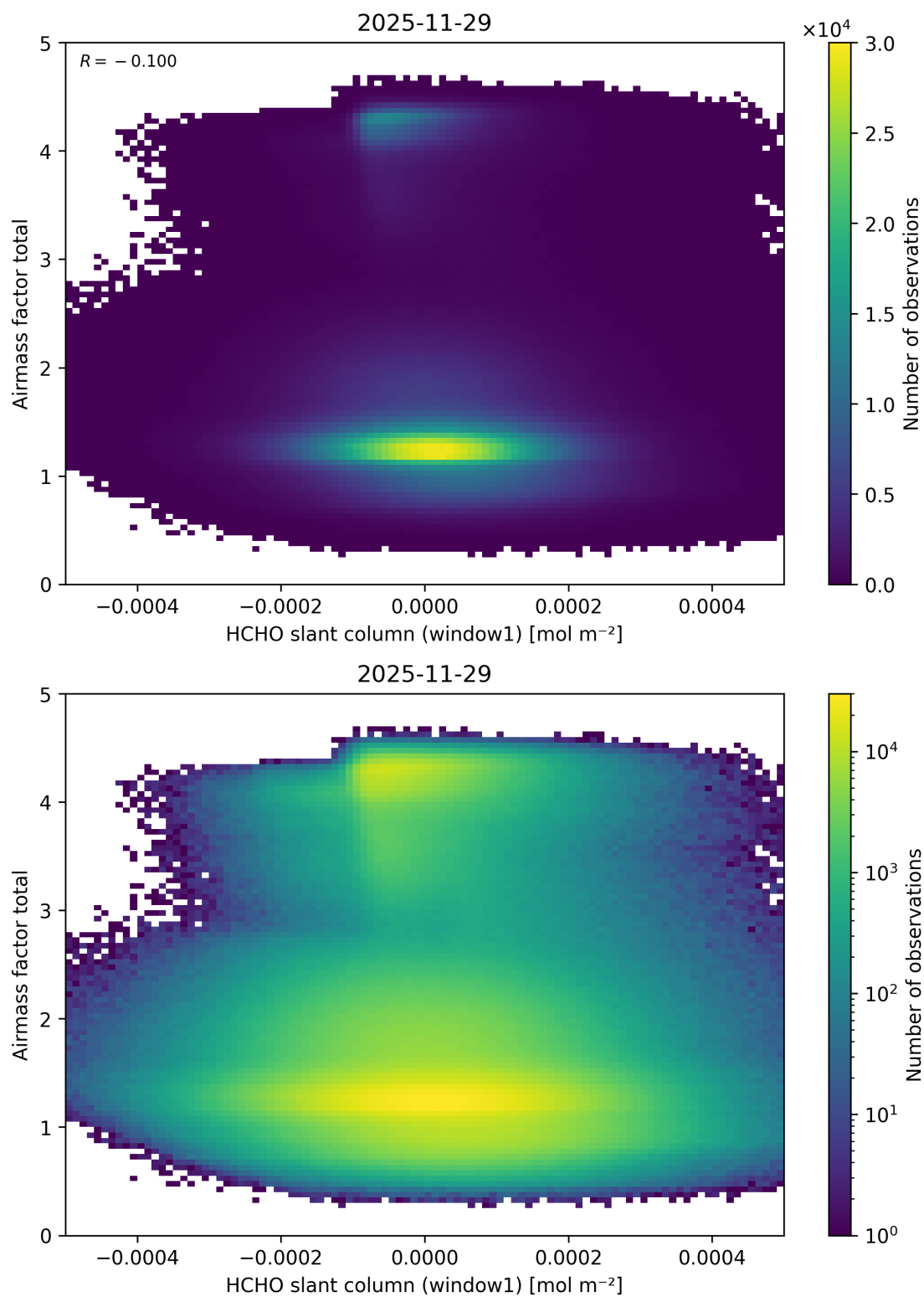
Figure 95: Scatter density plot of “HCHO slant column (window1)” against “Airmass factor total” for 2025-11-28 to 2025-11-30.
