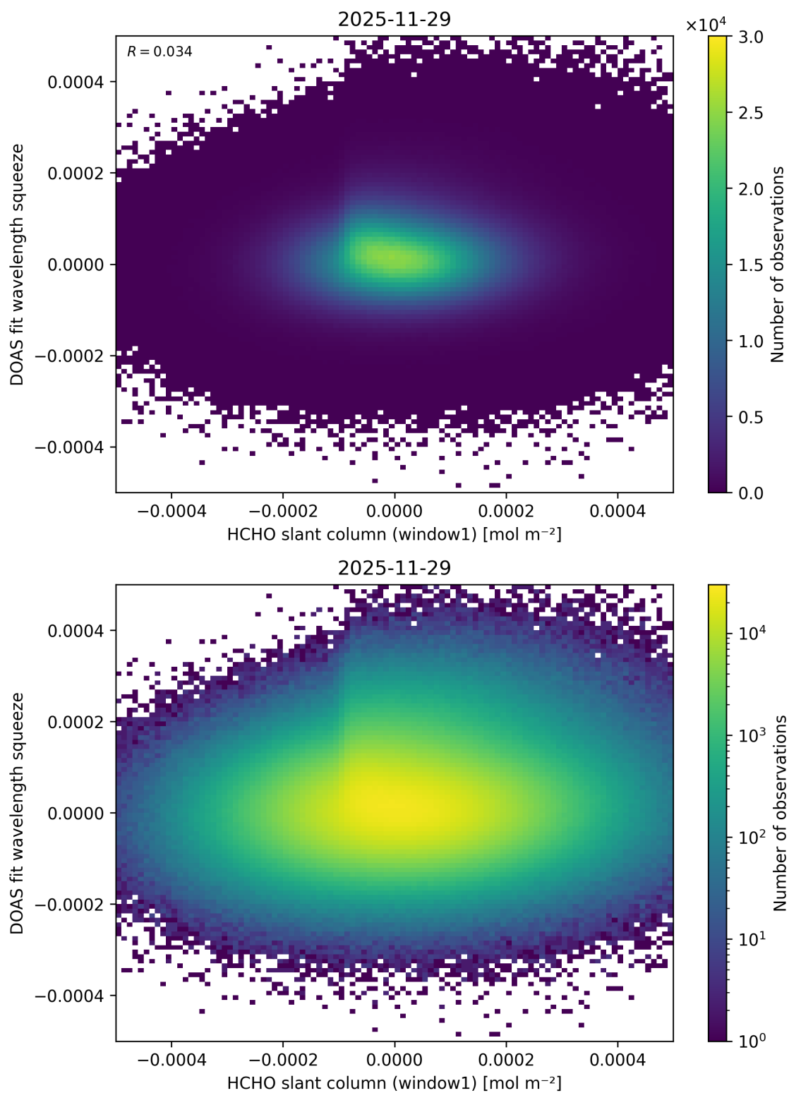
Figure 90: Scatter density plot of “HCHO slant column (window1)” against “DOAS fit wavelength squeeze” for 2025-11-28 to 2025-11-30.
