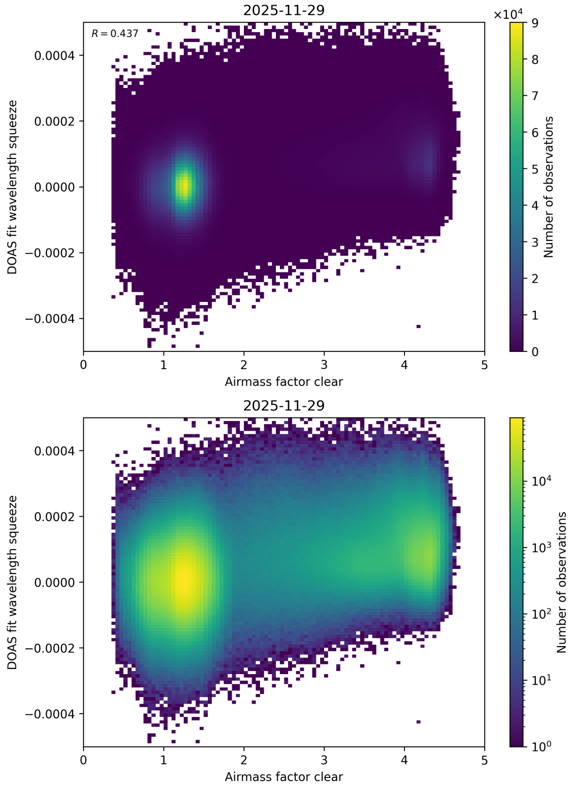
Figure 80: Scatter density plot of “Airmass factor clear” against “DOAS fit wavelength squeeze” for 2025-11-28 to 2025-11-30.
