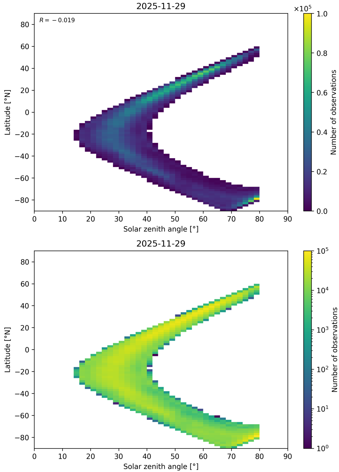
Figure 201: Scatter density plot of “Solar zenith angle” against “Latitude” for 2025-11-28 to 2025-11-30.
