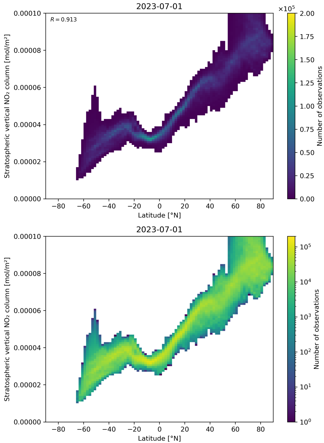
Figure 87: Scatter density plot of “Latitude” against “Stratospheric vertical \text{NO}_2 column” for 2023-06-30 to 2023-07-02.
