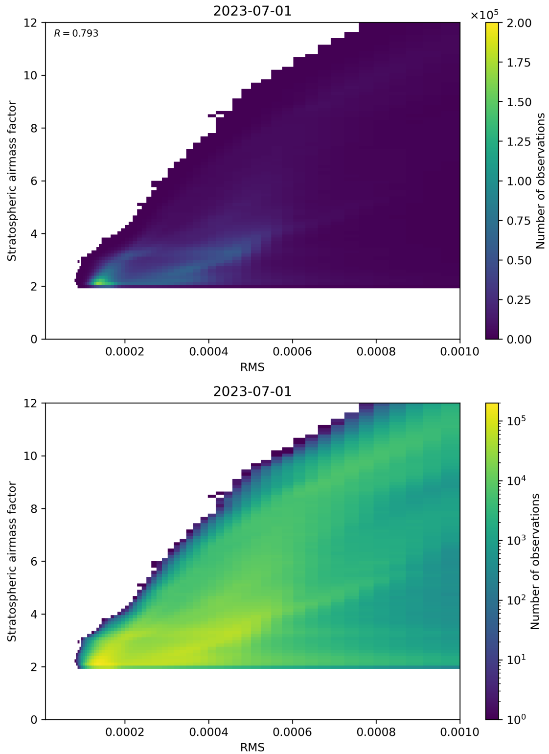
Figure 144: Scatter density plot of “RMS” against “Stratospheric airmass factor” for 2023-06-30 to 2023-07-02.
