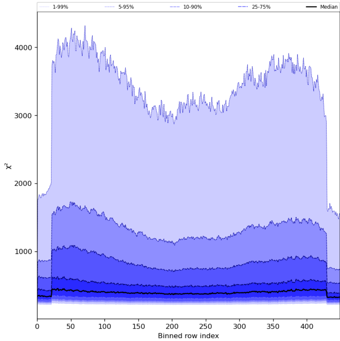
Figure 59: Along track statistics of “ \chi^2 ” for 2023-06-30 to 2023-07-02
