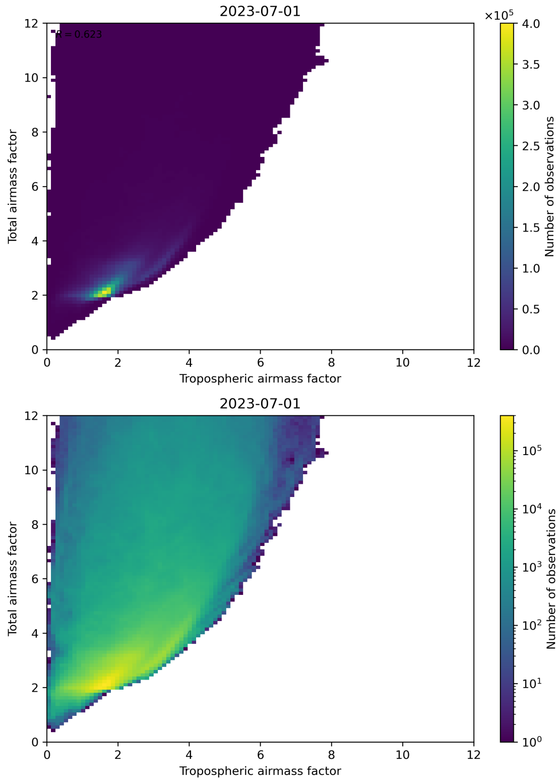
Figure 72: Scatter density plot of “Tropospheric airmass factor” against “Total airmass factor” for 2023-06-30 to 2023-07-02.
