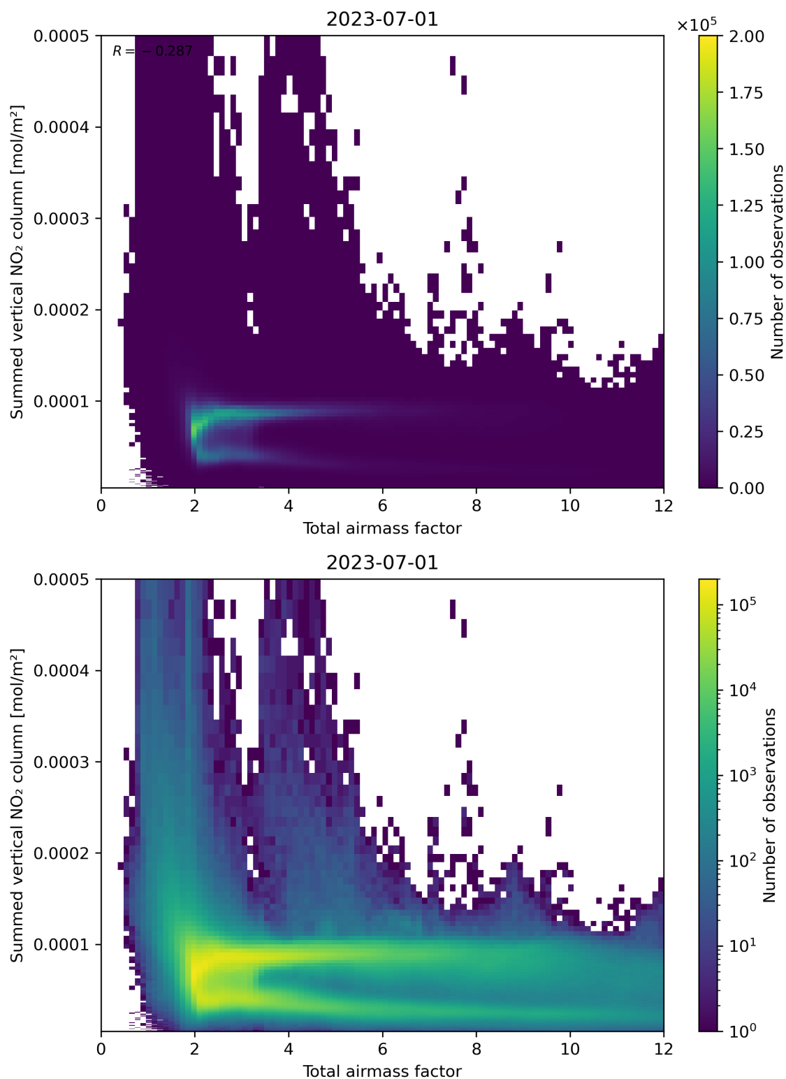
Figure 65: Scatter density plot of “Total airmass factor” against “Summed vertical NO 2 column” for 2023-06-30 to 2023-07-02.
