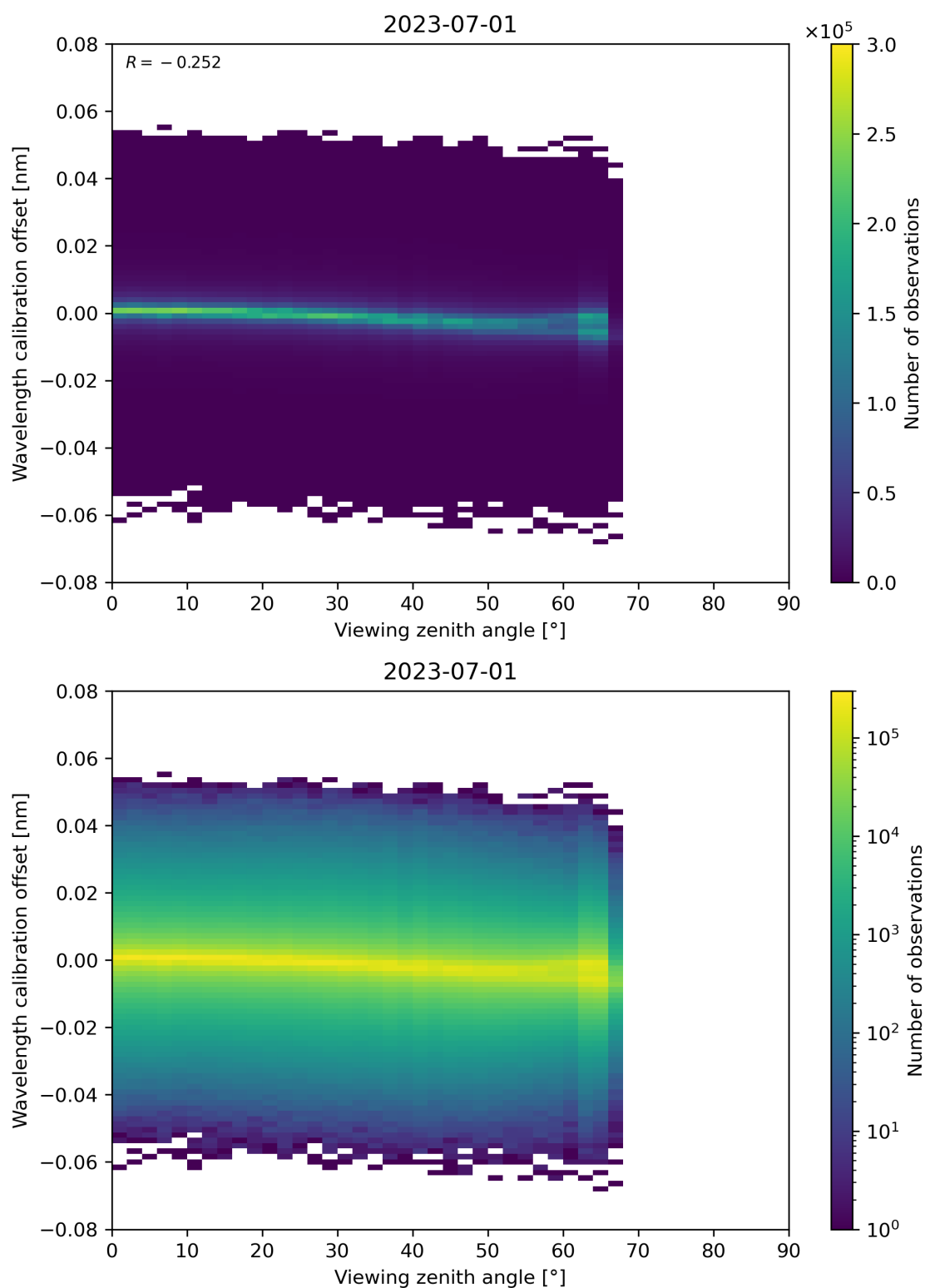
Figure 173: Scatter density plot of “Viewing zenith angle” against “Wavelength calibration offset” for 2023-06-30 to 2023-07-02.
