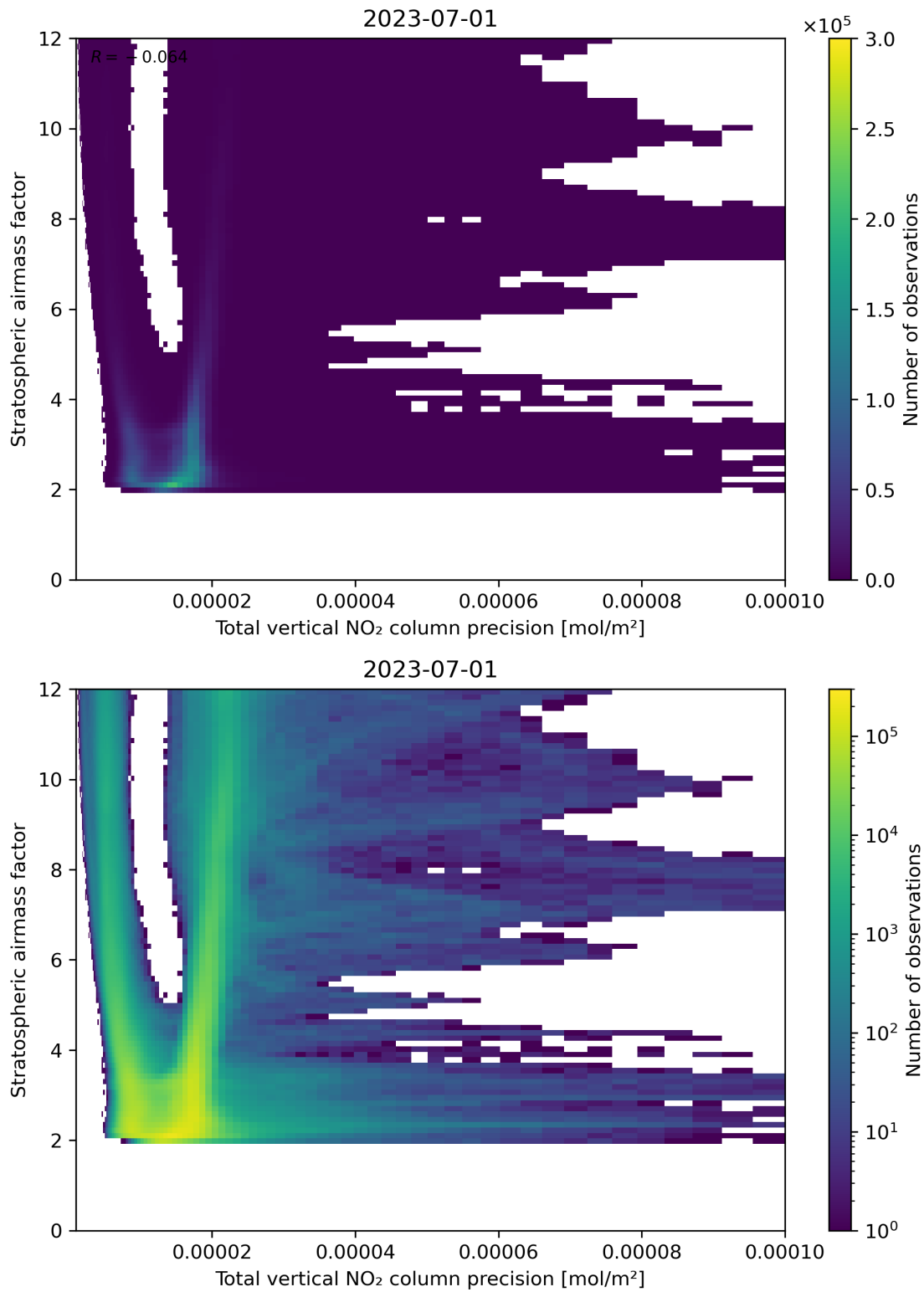
Figure 115: Scatter density plot of “Total vertical NO 2 column precision” against “Stratospheric air mass factor” for 2023-06-30 to 2023-07-02.
