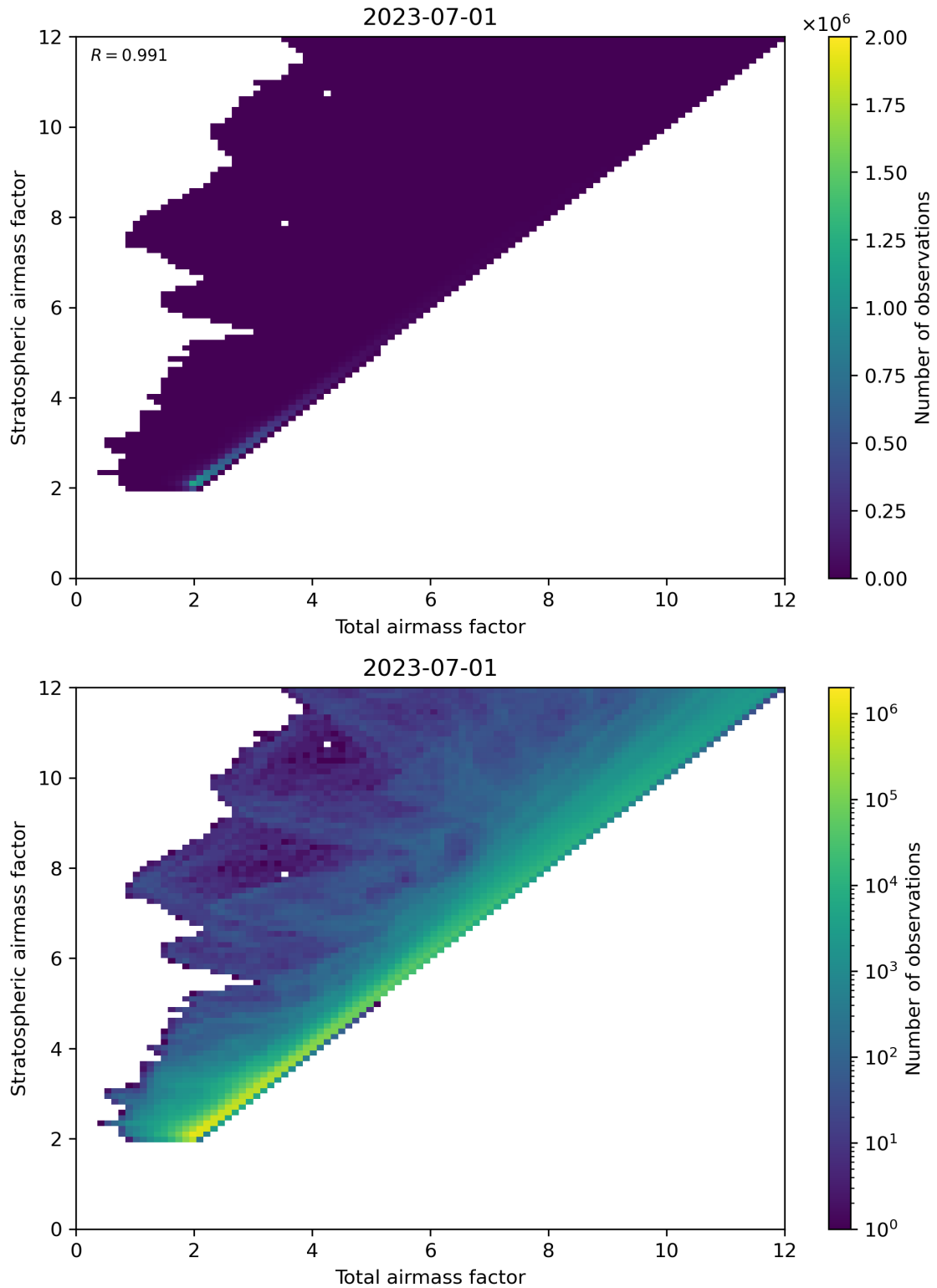
Figure 62: Scatter density plot of “Total airmass factor” against “Stratospheric airmass factor” for 2023-06-30 to 2023-07-02.
