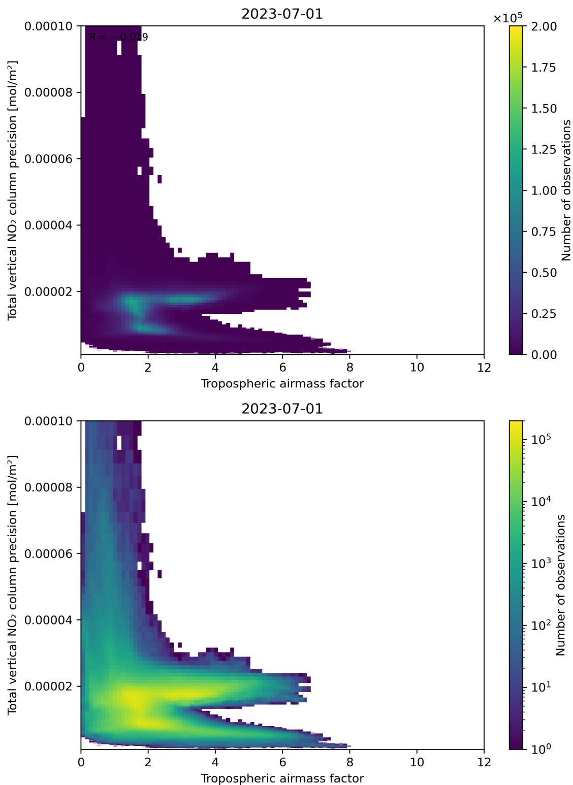
Figure 78: Scatter density plot of “Tropospheric air mass factor” against “Total vertical NO 2 column precision” for 2023-06-30 to 2023-07-02.
