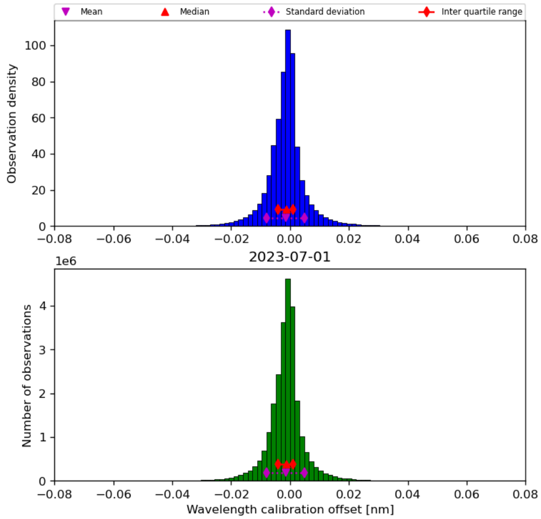
Figure 35: Histogram of “Wavelength calibration offset” for 2023-06-30 to 2023-07-02
