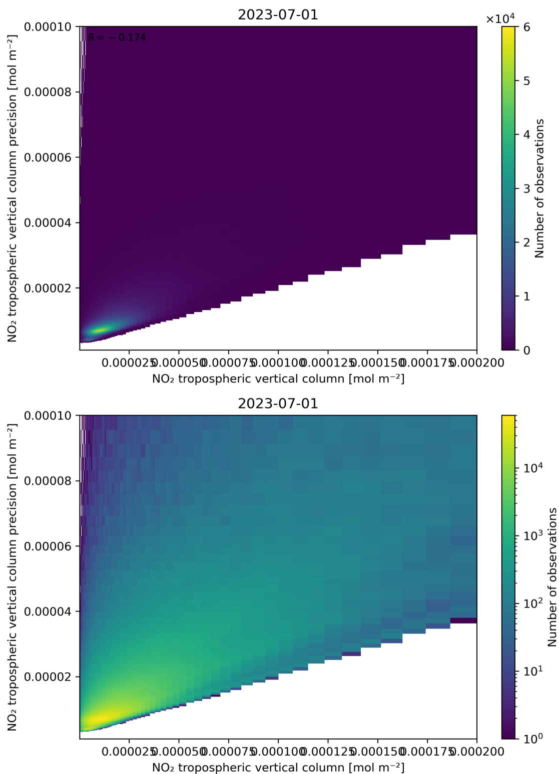
Figure 130: Scatter density plot of “NO 2 tropospheric vertical column” against “NO 2 tropospheric vertical column precision” for 2023-06-30 to 2023-07-02.
