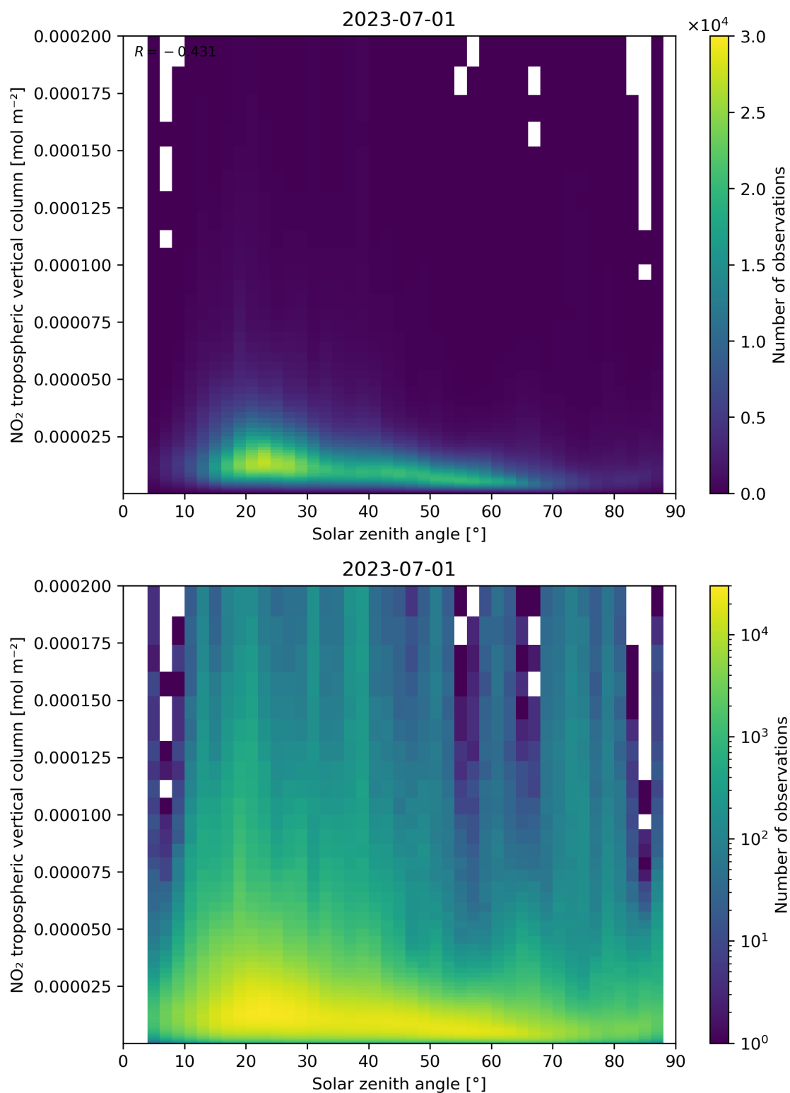
Figure 155: Scatter density plot of “Solar zenith angle” against “NO 2 tropospheric vertical column” for 2023-06-30 to 2023-07-02.
