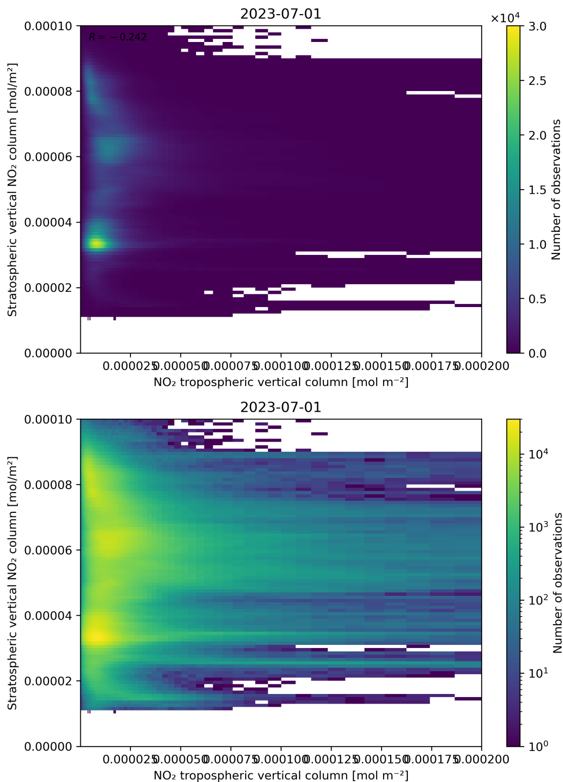
Figure 125: Scatter density plot of “NO 2 tropospheric vertical column” against “Stratospheric vertical NO 2 column” for 2023-06-30 to 2023-07-02.
