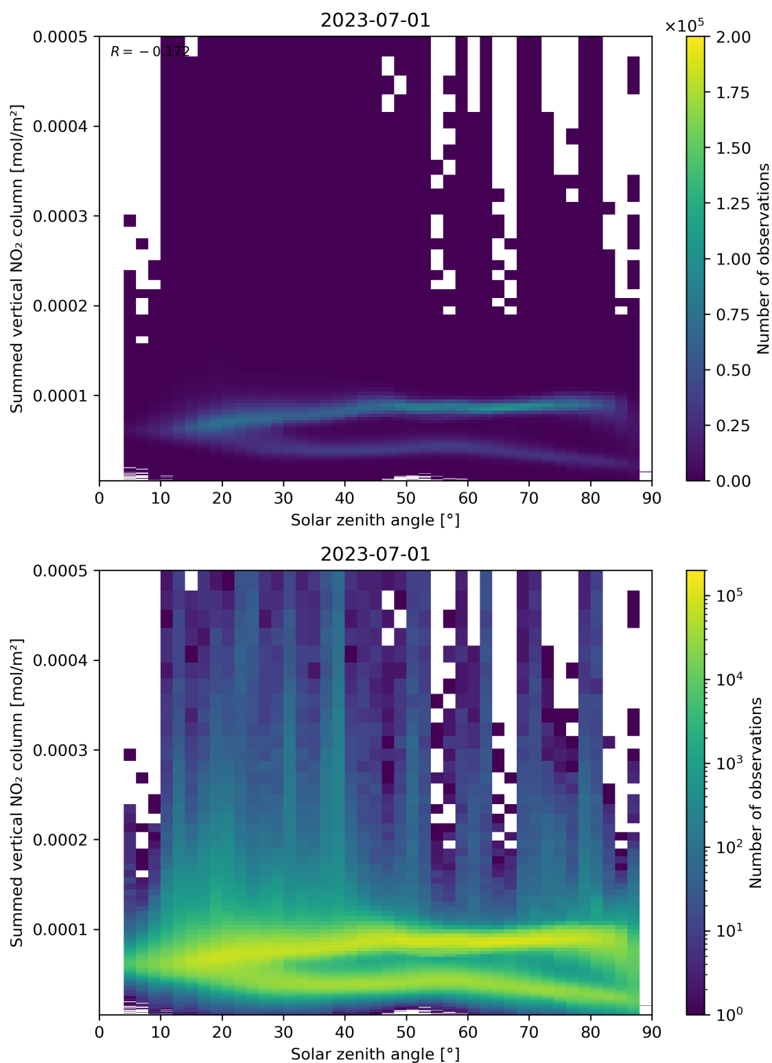
Figure 151: Scatter density plot of “Solar zenith angle” against “Summed vertical NO 2 column” for 2023-06-30 to 2023-07-02.
