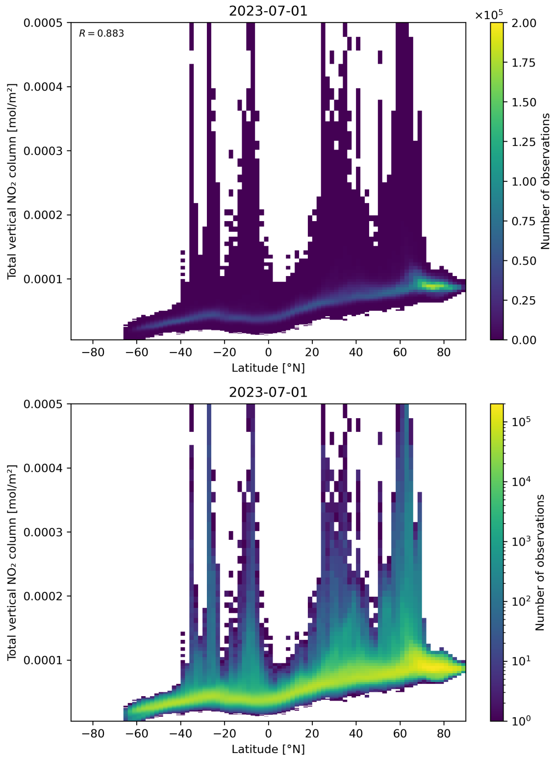
Figure 90: Scatter density plot of “Latitude” against “Total vertical NO 2 column” for 2023-06-30 to 2023-07-02.
