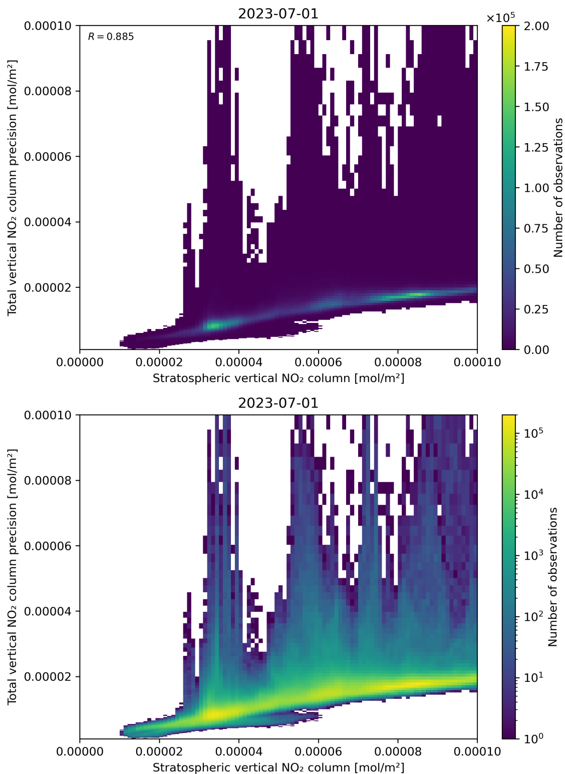
Figure 101: Scatter density plot of “Stratospheric vertical NO 2 column” against “Total vertical NO 2 column precision” for 2023-06-30 to 2023-07-02.
