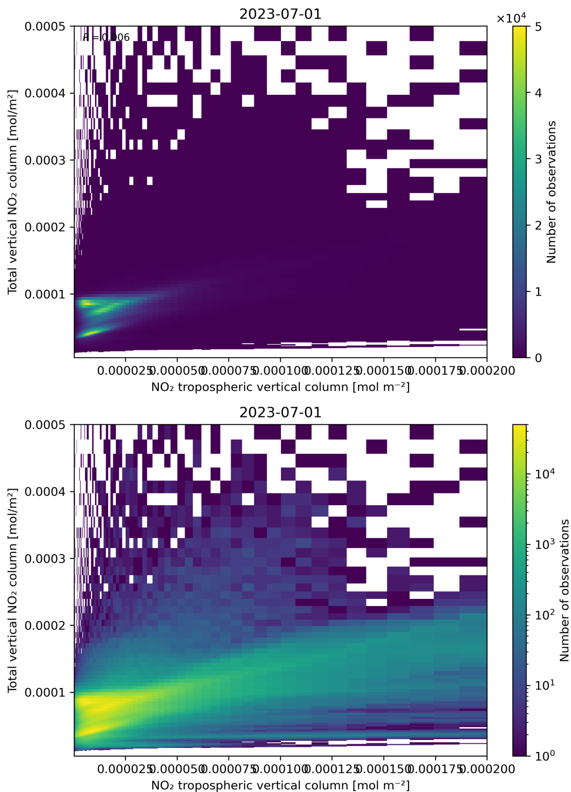
Figure 128: Scatter density plot of “NO 2 tropospheric vertical column” against “Total vertical NO 2 column” for 2023-06-30 to 2023-07-02.
