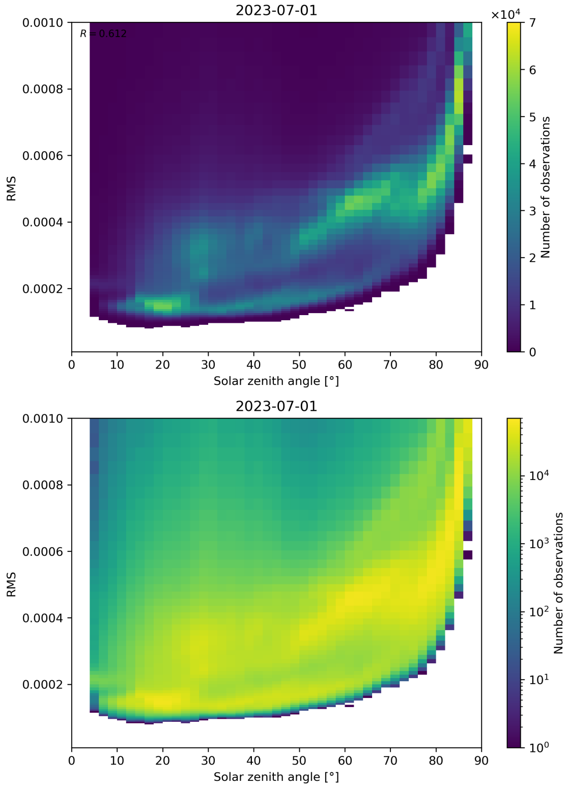
Figure 157: Scatter density plot of “Solar zenith angle” against “RMS” for 2023-06-30 to 2023-07-02.
