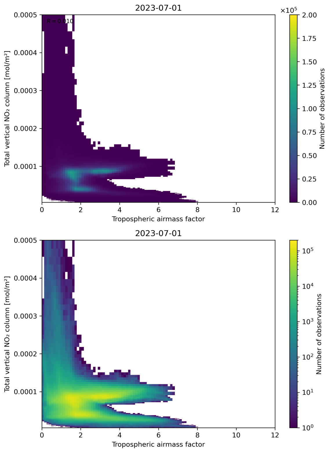
Figure 77: Scatter density plot of “Tropospheric airmass factor” against “Total vertical NO 2 column” for 2023-06-30 to 2023-07-02.
