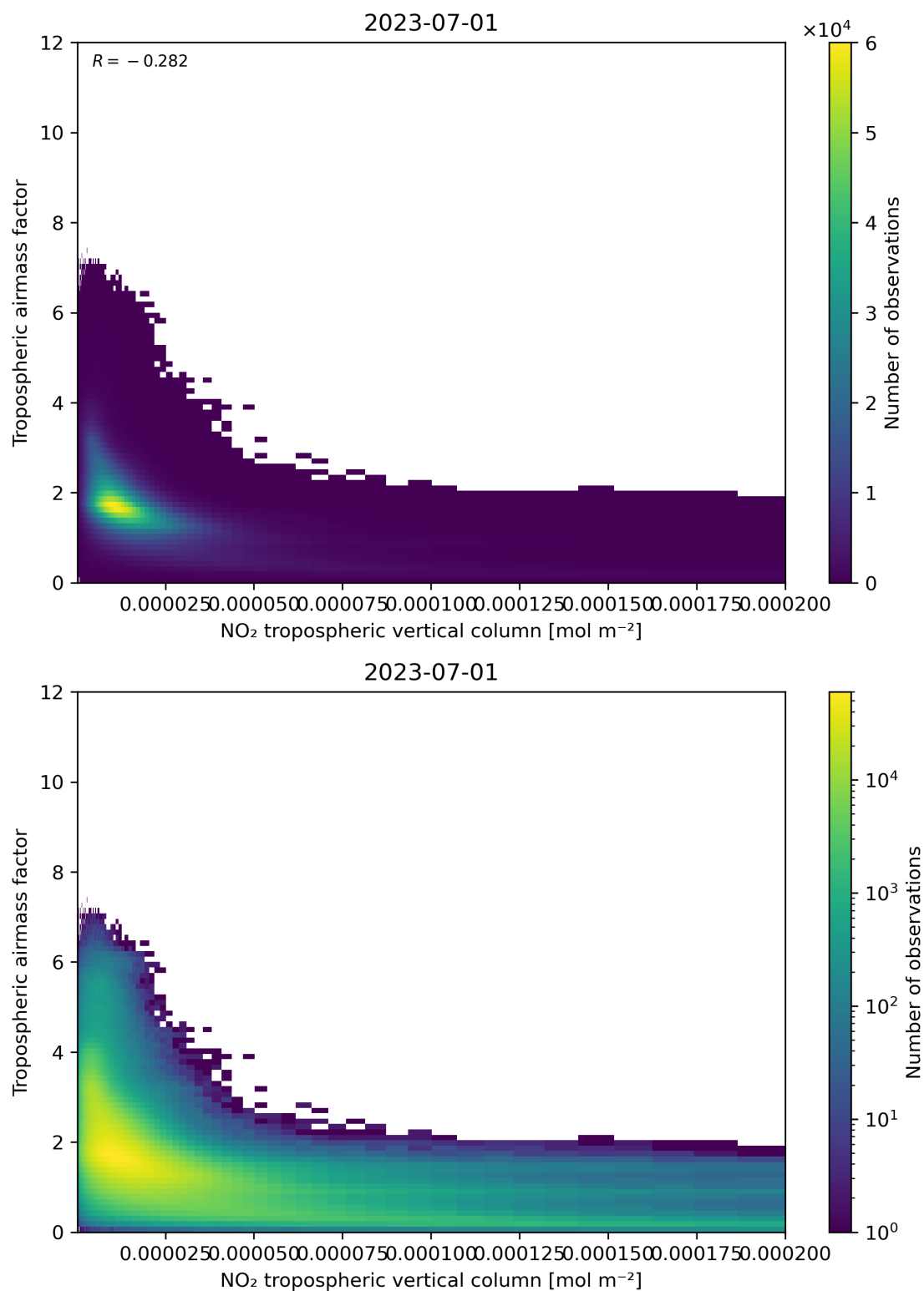
Figure 123: Scatter density plot of “NO 2 tropospheric vertical column” against “Tropospheric air mass factor” for 2023-06-30 to 2023-07-02.
