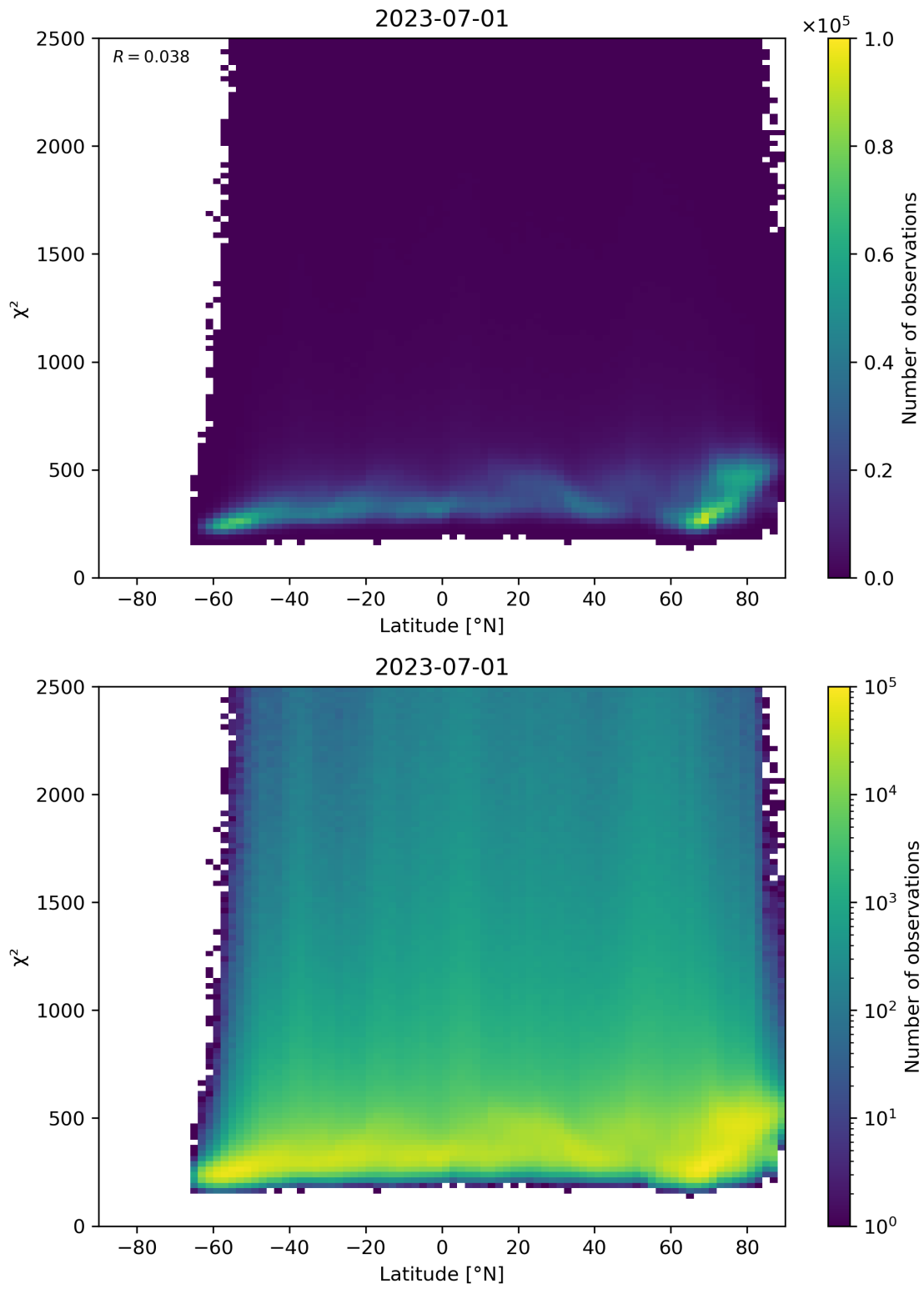
Figure 86: Scatter density plot of “Latitude” against “ \chi^2 ” for 2023-06-30 to 2023-07-02.
