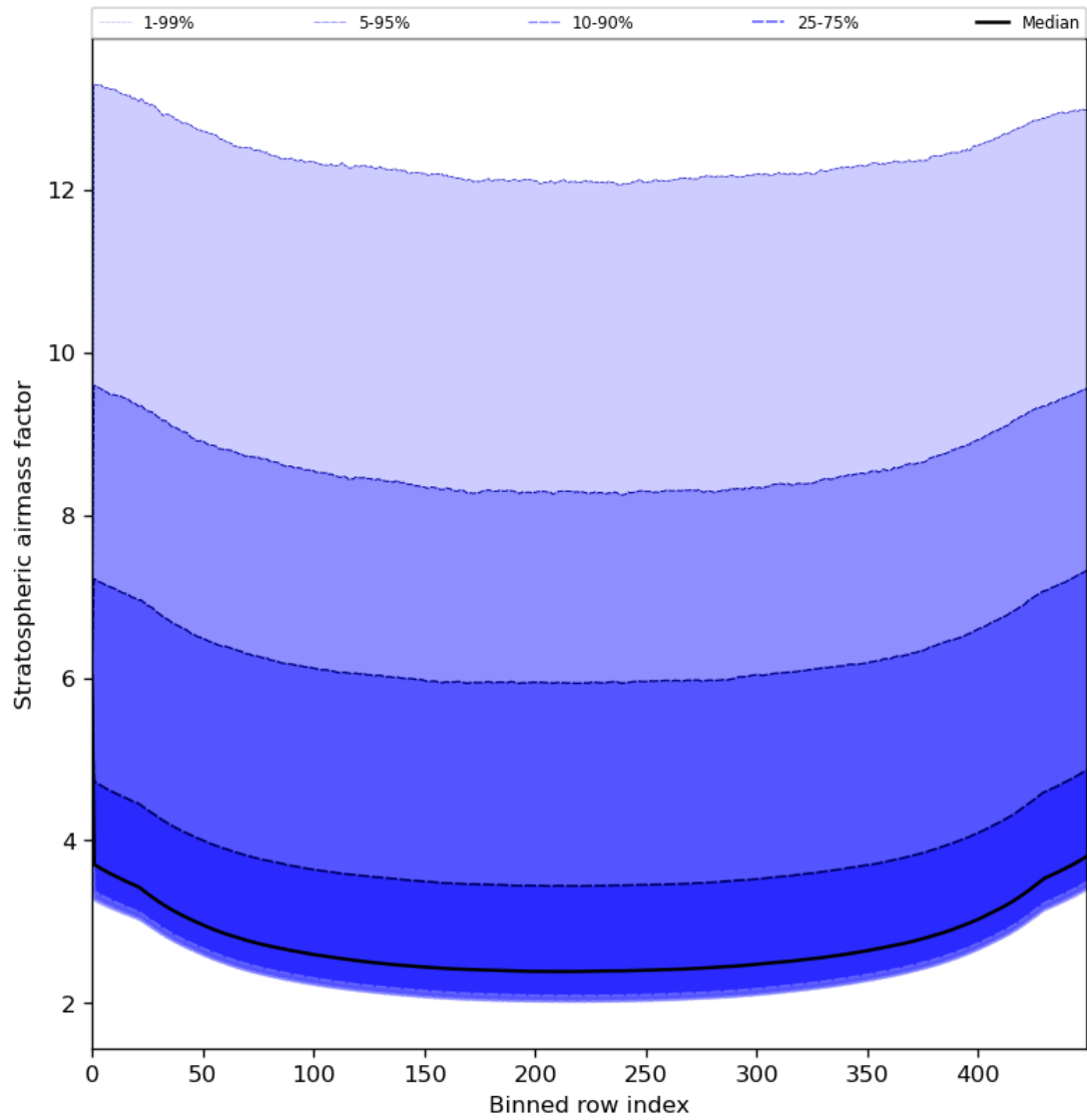
Figure 61: Along track statistics of “Stratospheric airmass factor” for 2023-06-30 to 2023-07-02
