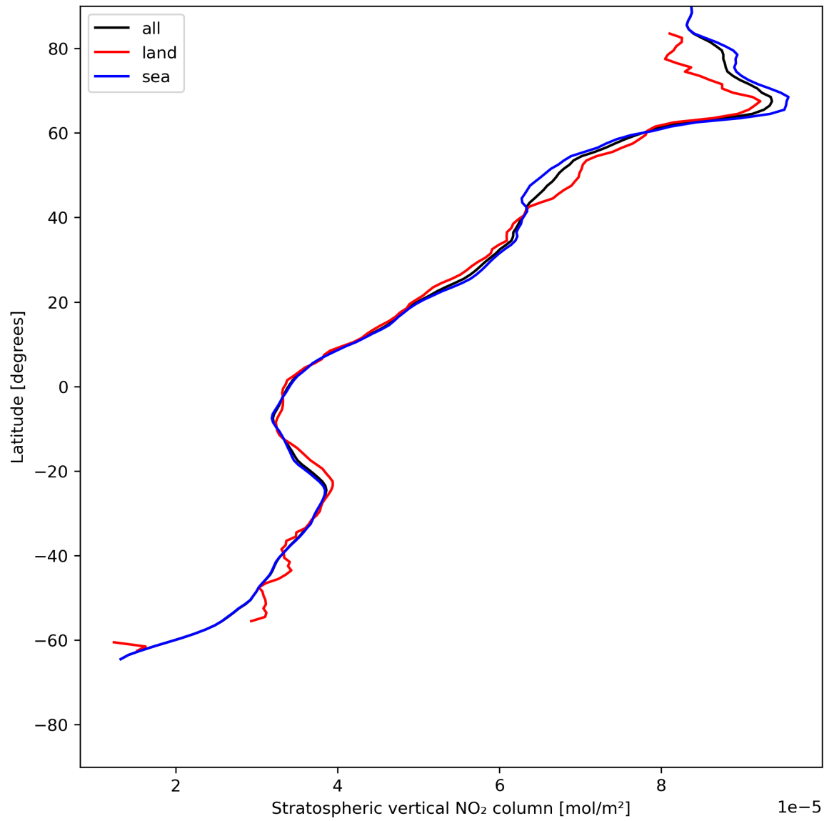
Figure 19: Zonal average of “Stratospheric vertical NO 2 column” for 2023-06-30 to 2023-07-02.
