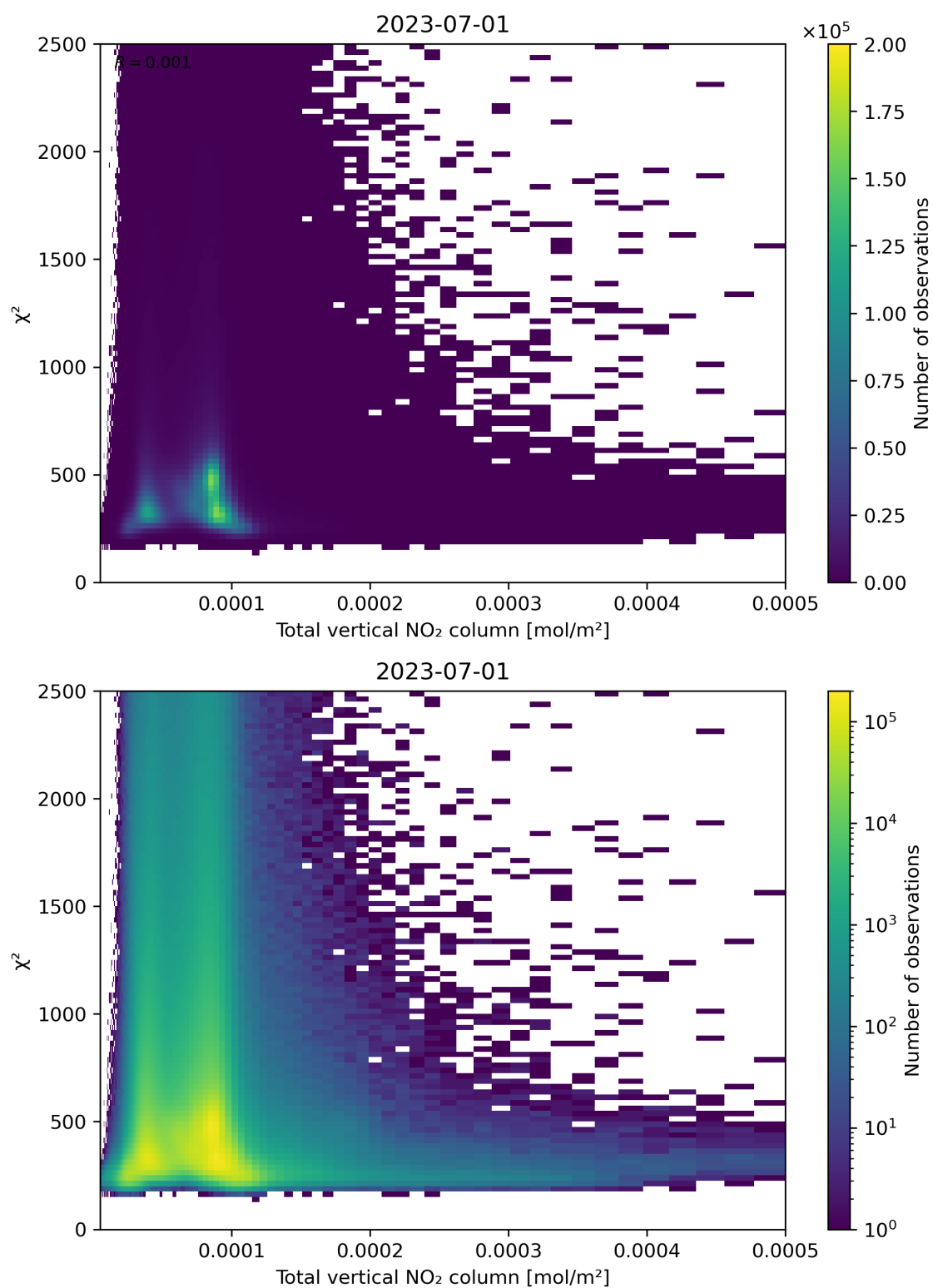
Figure 111: Scatter density plot of “Total vertical NO 2 column” against “ \chi^2 ” for 2023-06-30 to 2023-07-02.
