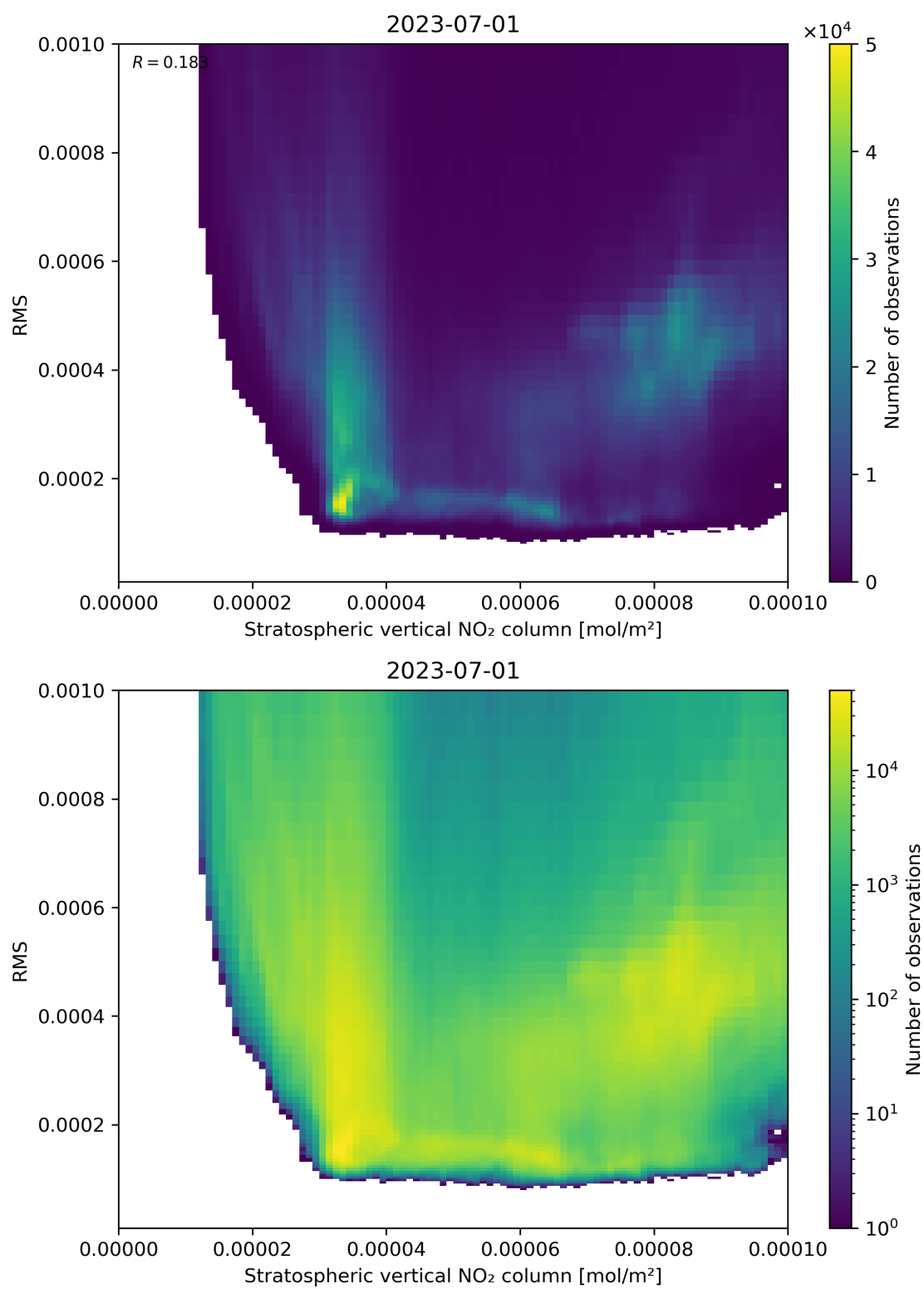
Figure 102: Scatter density plot of “Stratospheric vertical NO 2 column” against “RMS” for 2023-06-30 to 2023-07-02.
