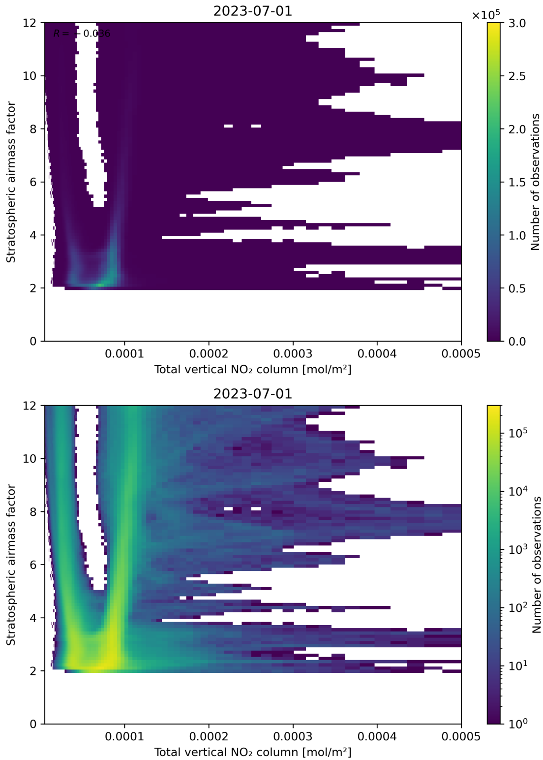
Figure 110: Scatter density plot of “Total vertical NO 2 column” against “Stratospheric air mass factor” for 2023-06-30 to 2023-07-02.
