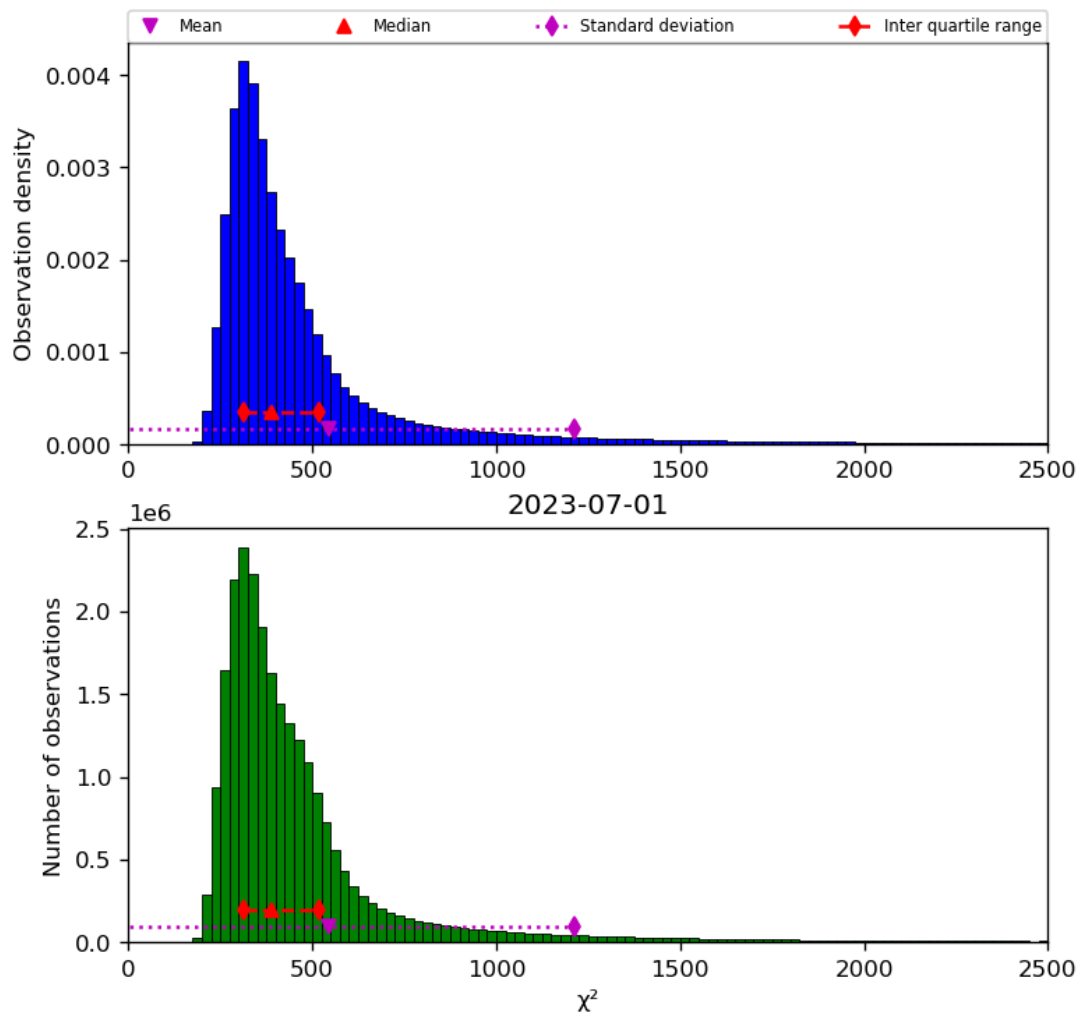
Figure 42: Histogram of “ \chi^2 ” for 2023-06-30 to 2023-07-02
