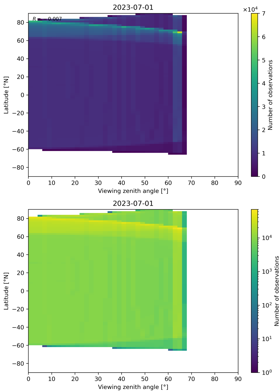
Figure 163: Scatter density plot of “Viewing zenith angle” against “Latitude” for 2023-06-30 to 2023-07-02.
