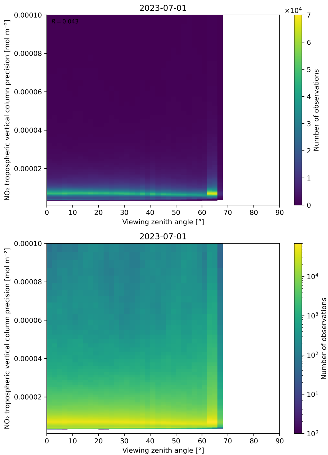
Figure 170: Scatter density plot of “Viewing zenith angle” against “NO 2 tropospheric vertical column precision” for 2023-06-30 to 2023-07-02.
