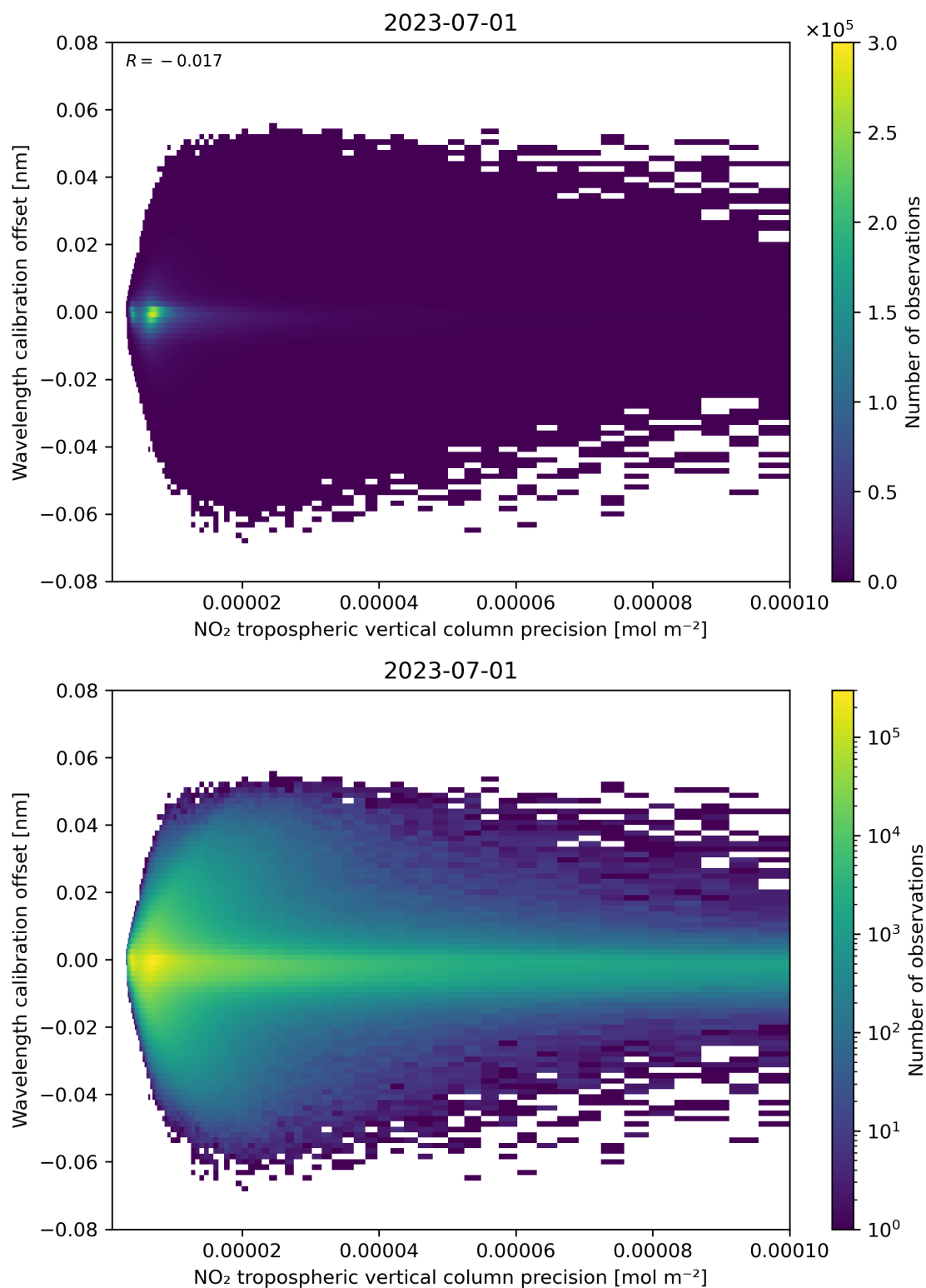
Figure 141: Scatter density plot of “NO 2 tropospheric vertical column precision” against “Wavelength calibration offset” for 2023-06-30 to 2023-07-02.
