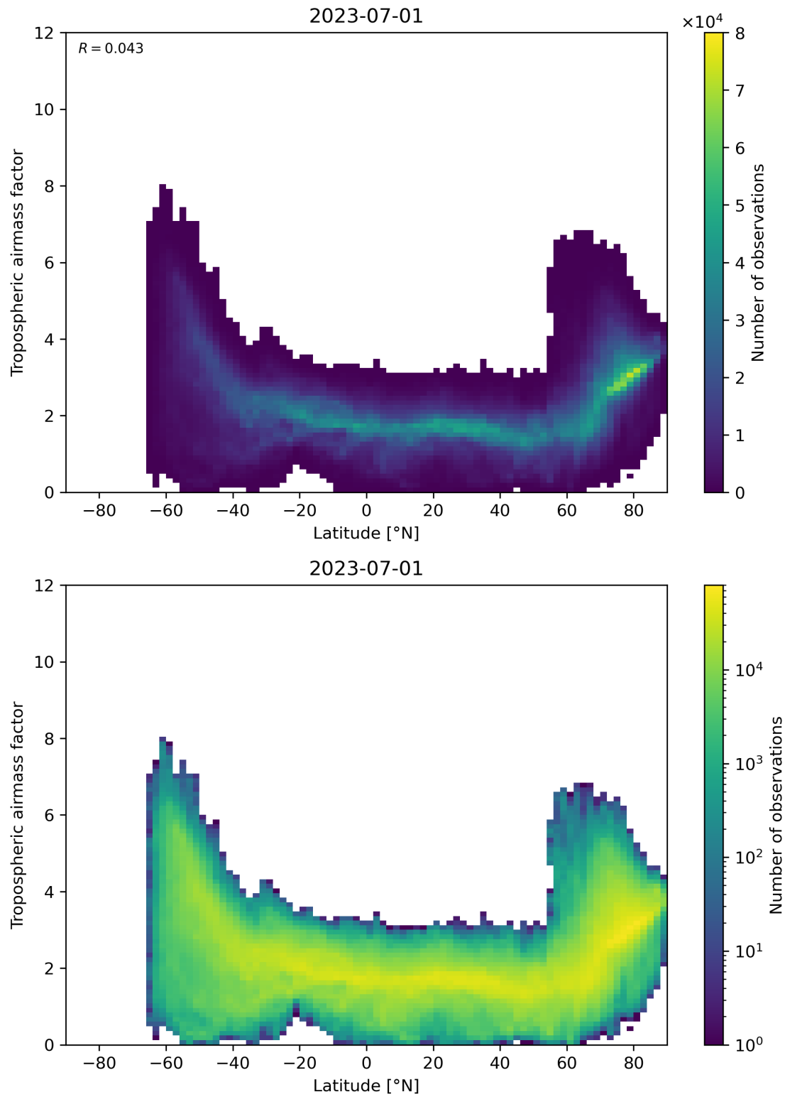
Figure 85: Scatter density plot of “Latitude” against “Tropospheric air mass factor” for 2023-06-30 to 2023-07-02.
