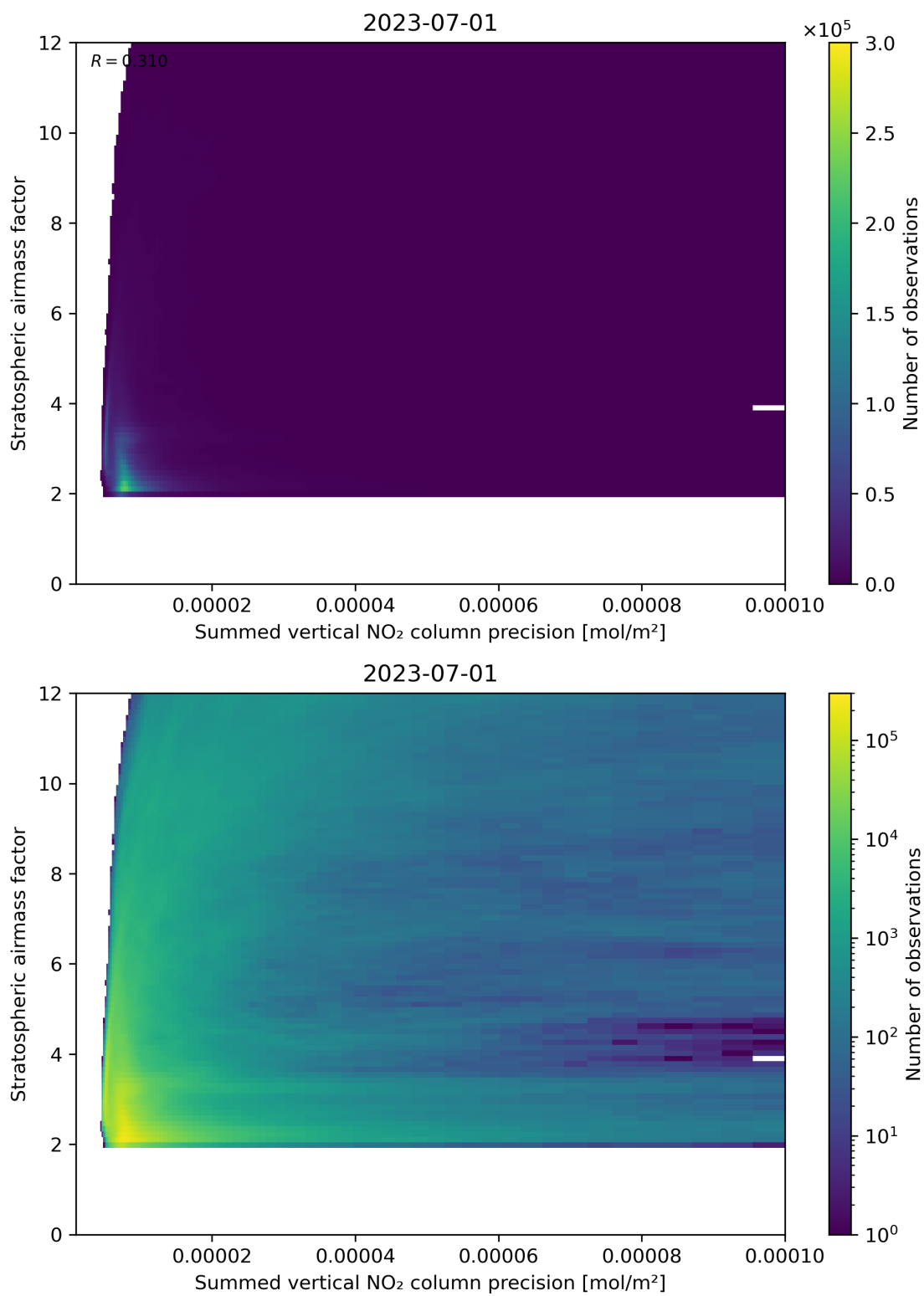
Figure 106: Scatter density plot of “Summed vertical NO 2 column precision” against “Stratospheric airmass factor” for 2023-06-30 to 2023-07-02.
