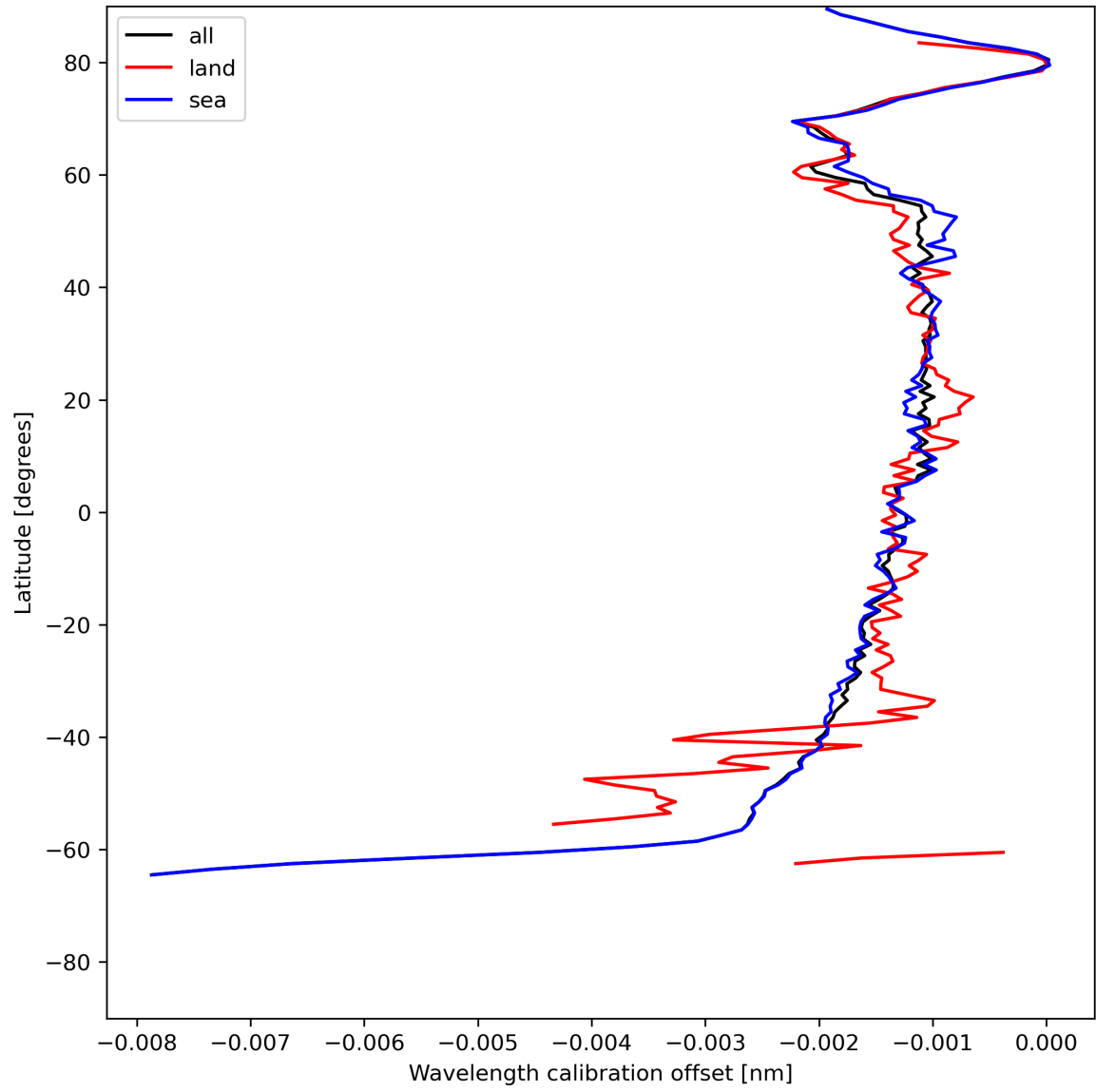
Figure 18: Zonal average of “Wavelength calibration offset” for 2023-06-30 to 2023-07-02.
