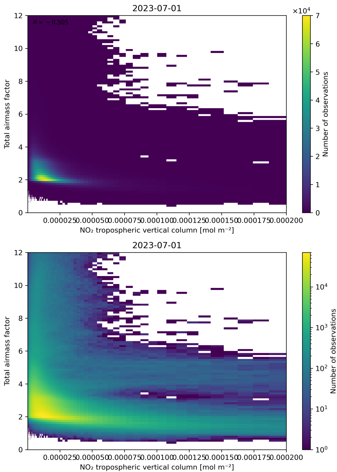
Figure 122: Scatter density plot of “NO 2 tropospheric vertical column” against “Total air mass factor” for 2023-06-30 to 2023-07-02.
