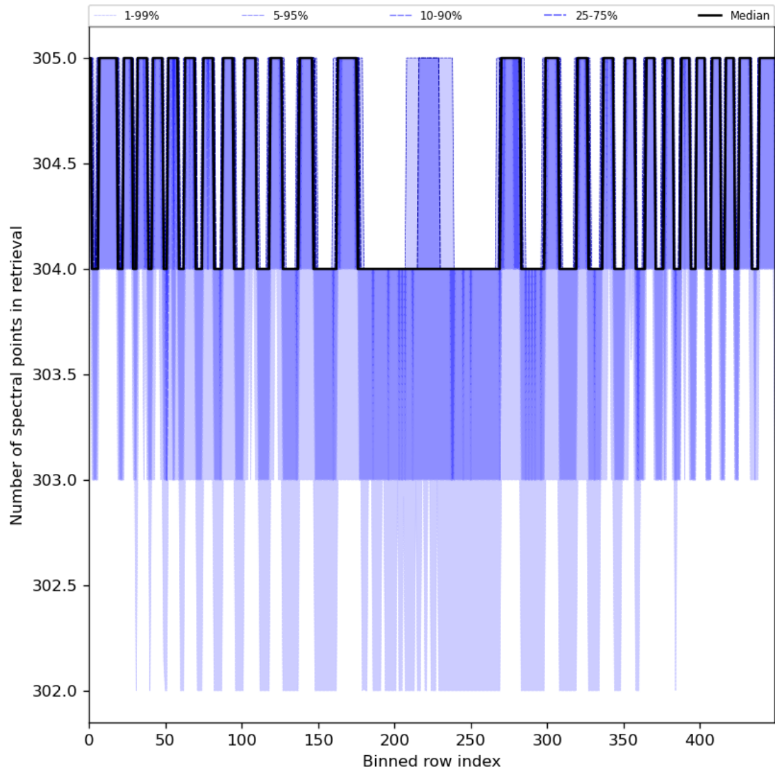
Figure 50: Along track statistics of “Number of spectral points in retrieval” for 2023-06-30 to 2023-07-02
