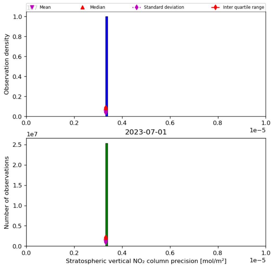
Figure 37: Histogram of “Stratospheric vertical NO 2 column precision” for 2023-06-30 to 2023-07-02
