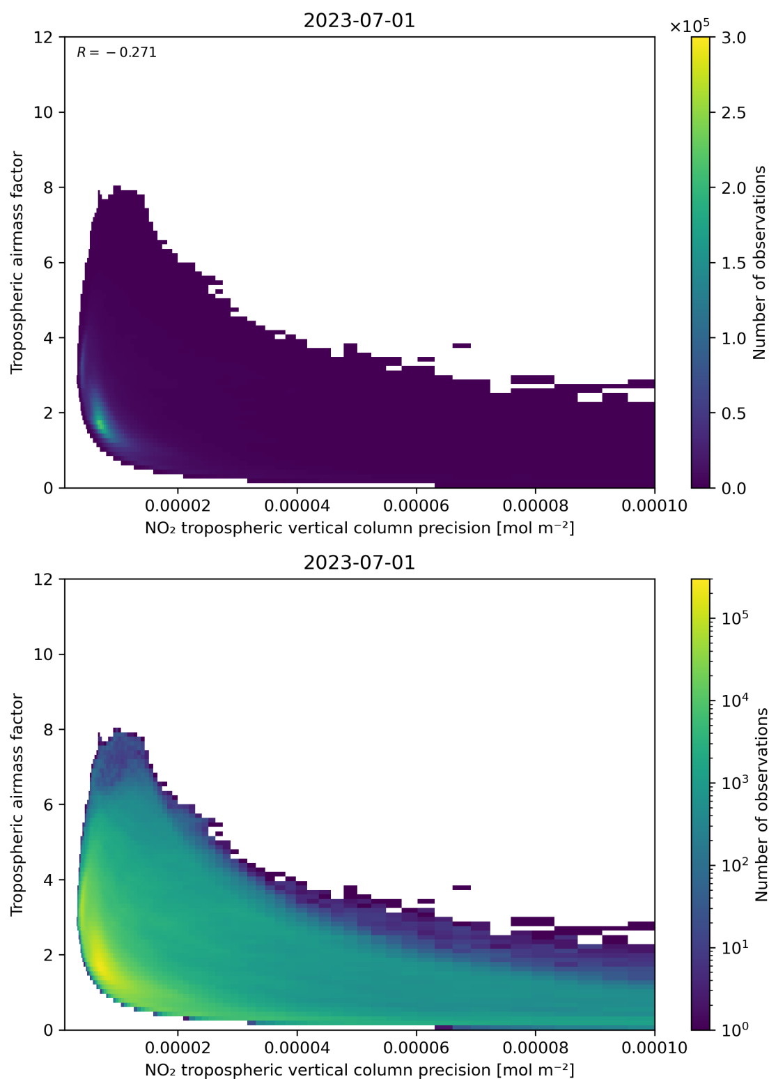
Figure 133: Scatter density plot of “NO 2 tropospheric vertical column precision” against “Tropospheric airmass factor” for 2023-06-30 to 2023-07-02.
