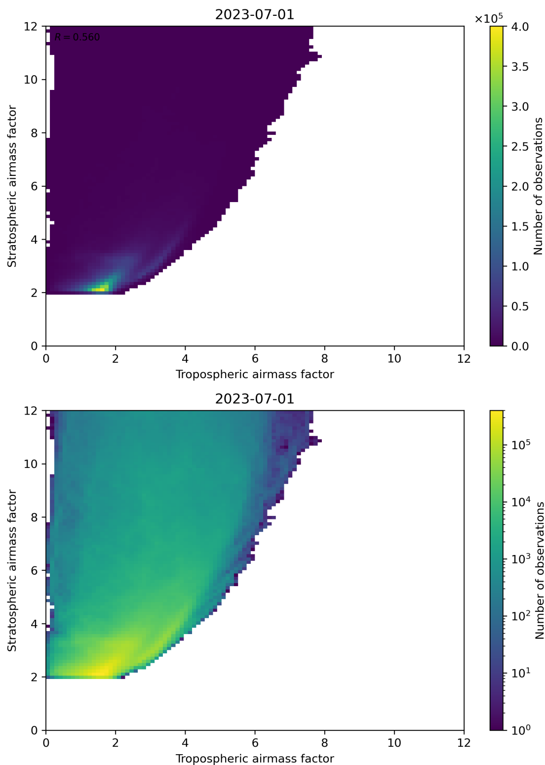
Figure 71: Scatter density plot of “Tropospheric airmass factor” against “Stratospheric airmass factor” for 2023-06-30 to 2023-07-02.
