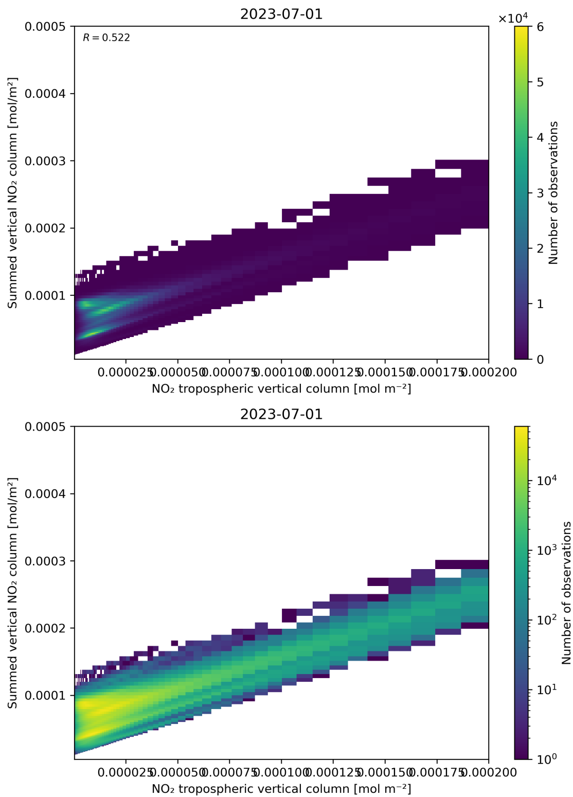
Figure 126: Scatter density plot of “NO 2 tropospheric vertical column” against “Summed vertical NO 2 column” for 2023-06-30 to 2023-07-02.
