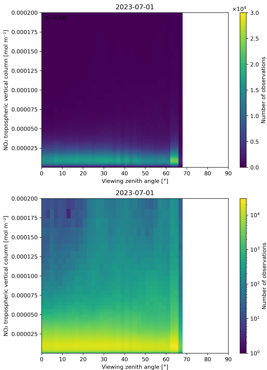
Figure 169: Scatter density plot of “Viewing zenith angle” against “NO 2 tropospheric vertical column” for 2023-06-30 to 2023-07-02.
