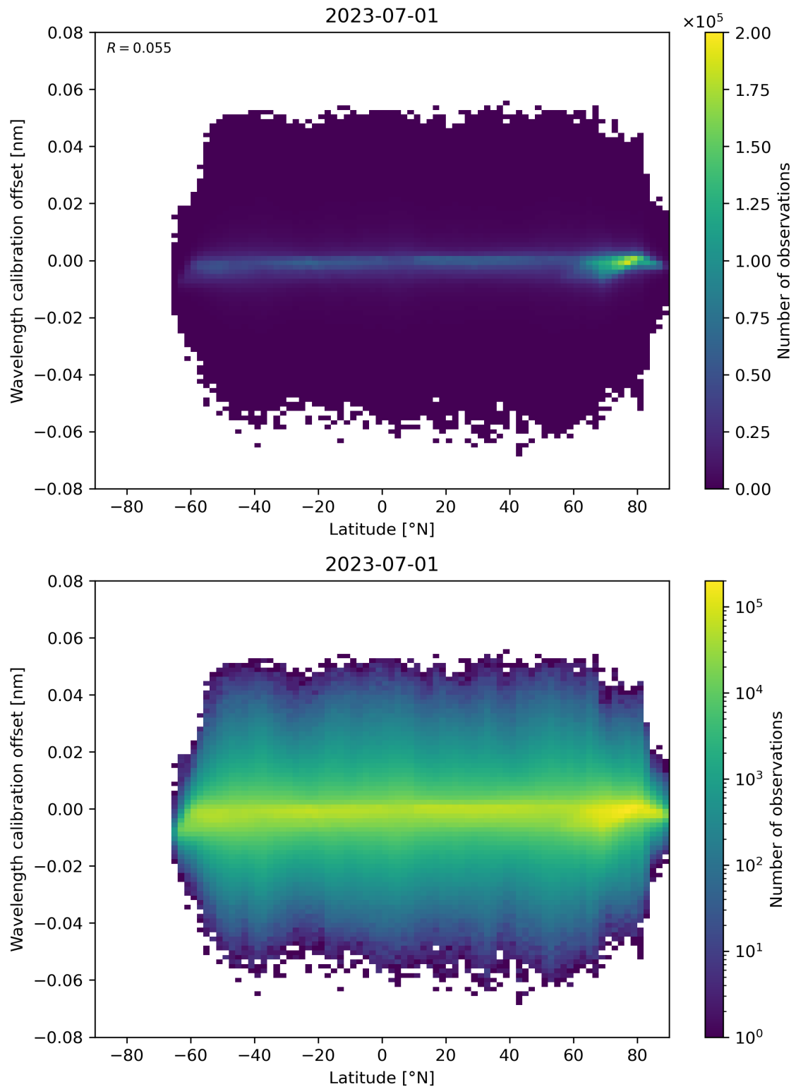
Figure 95: Scatter density plot of “Latitude” against “Wavelength calibration offset” for 2023-06-30 to 2023-07-02.
