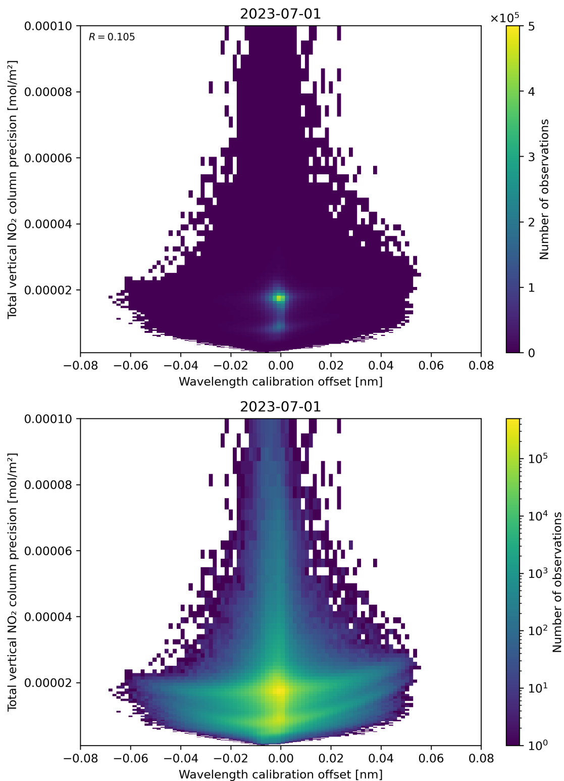
Figure 180: Scatter density plot of “Wavelength calibration offset” against “Total vertical NO 2 column precision” for 2023-06-30 to 2023-07-02.
