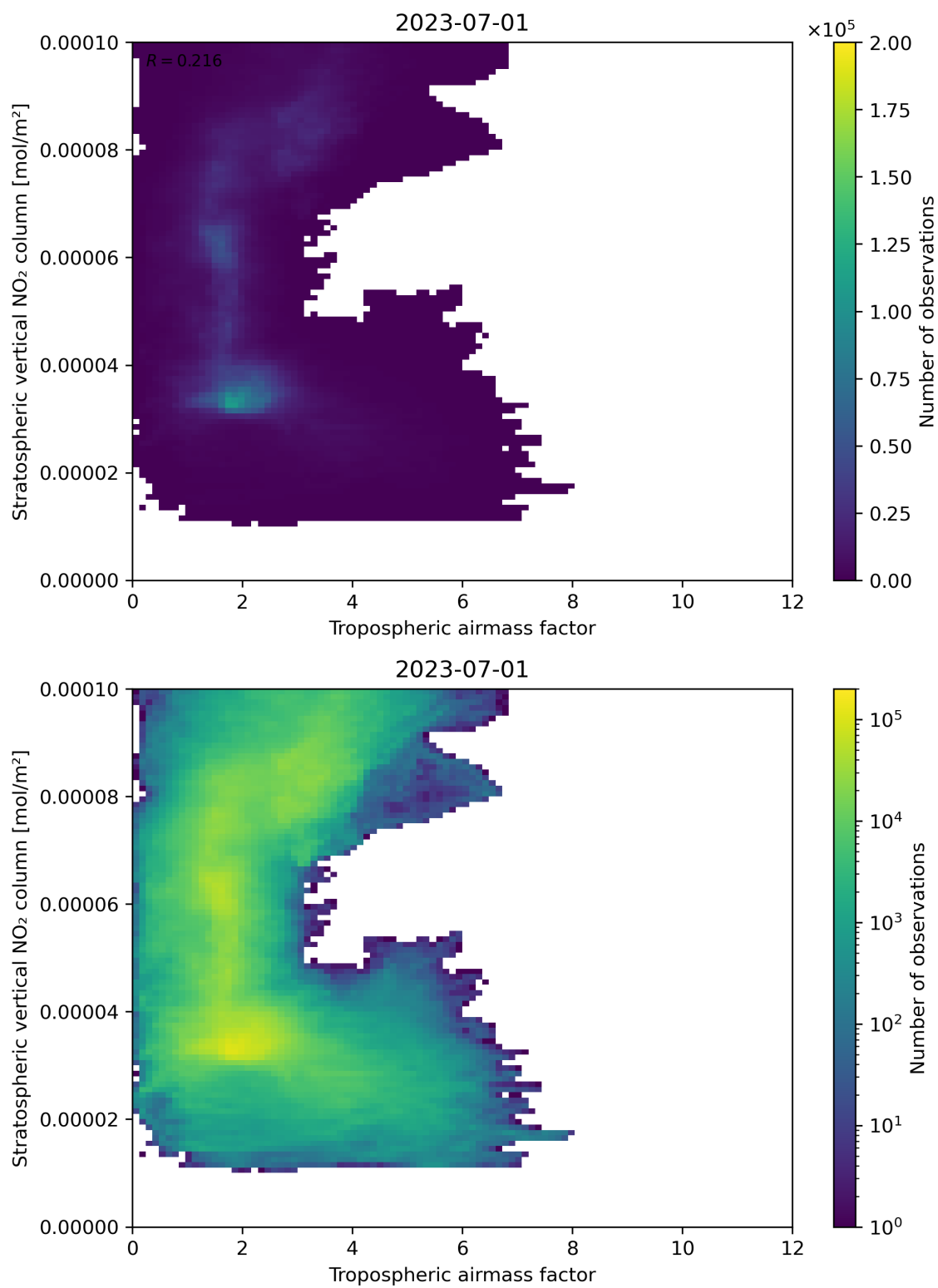
Figure 74: Scatter density plot of “Tropospheric air mass factor” against “Stratospheric vertical \text{NO}_2 column” for 2023-06-30 to 2023-07-02.
