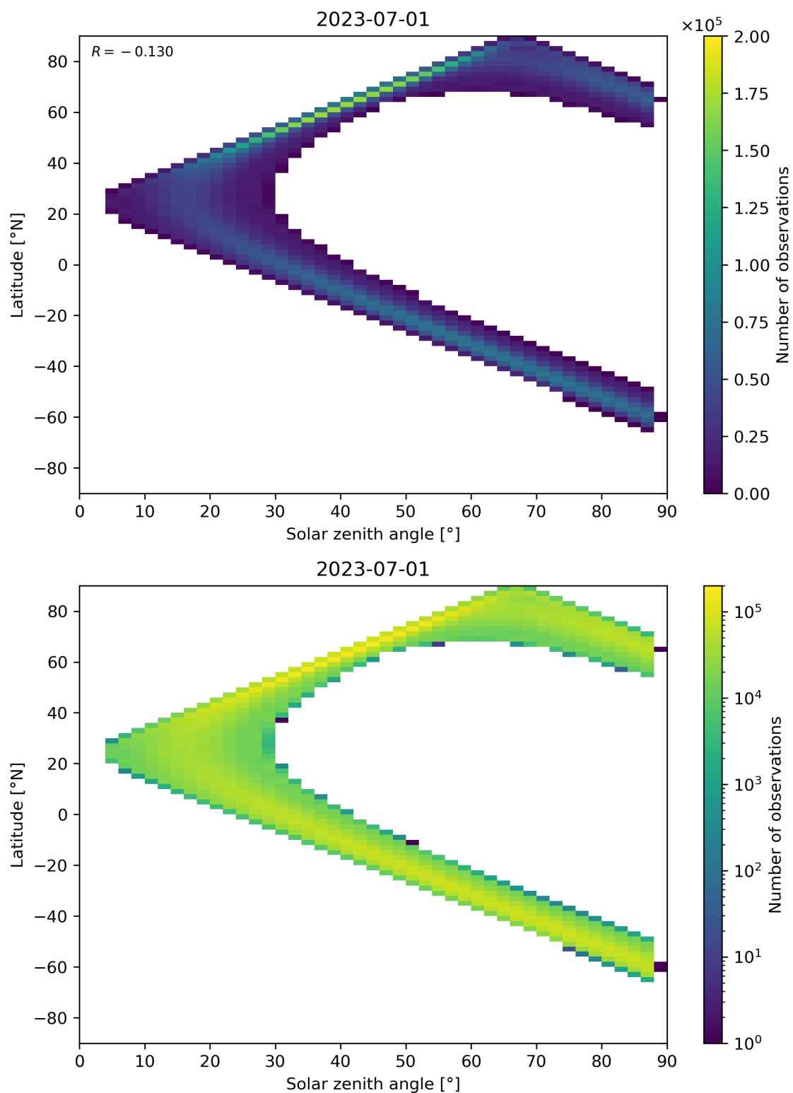
Figure 149: Scatter density plot of “Solar zenith angle” against “Latitude” for 2023-06-30 to 2023-07-02.
