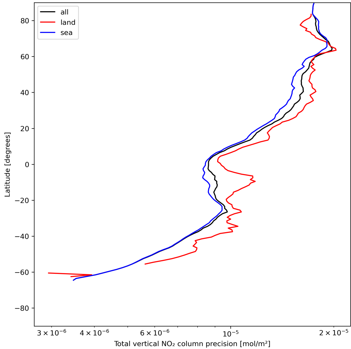
Figure 22: Zonal average of “Total vertical NO 2 column precision” for 2023-06-30 to 2023-07-02.
