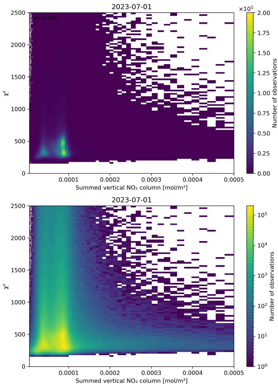
Figure 104: Scatter density plot of “Summed vertical NO 2 column” against “ \chi^2 ” for 2023-06-30 to 2023-07-02.
