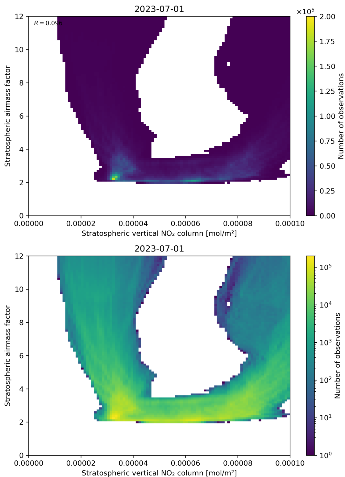
Figure 96: Scatter density plot of “Stratospheric vertical NO 2 column” against “Stratospheric airmass factor” for 2023-06-30 to 2023-07-02.
