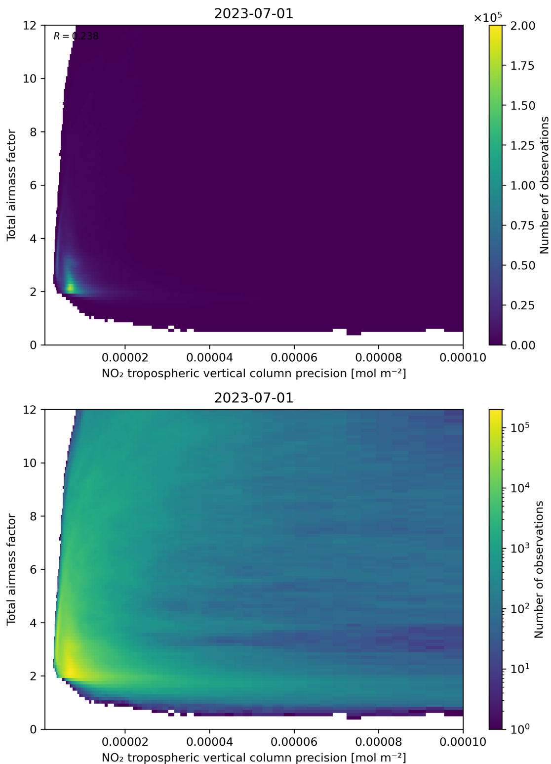
Figure 132: Scatter density plot of “NO 2 tropospheric vertical column precision” against “Total air mass factor” for 2023-06-30 to 2023-07-02.
