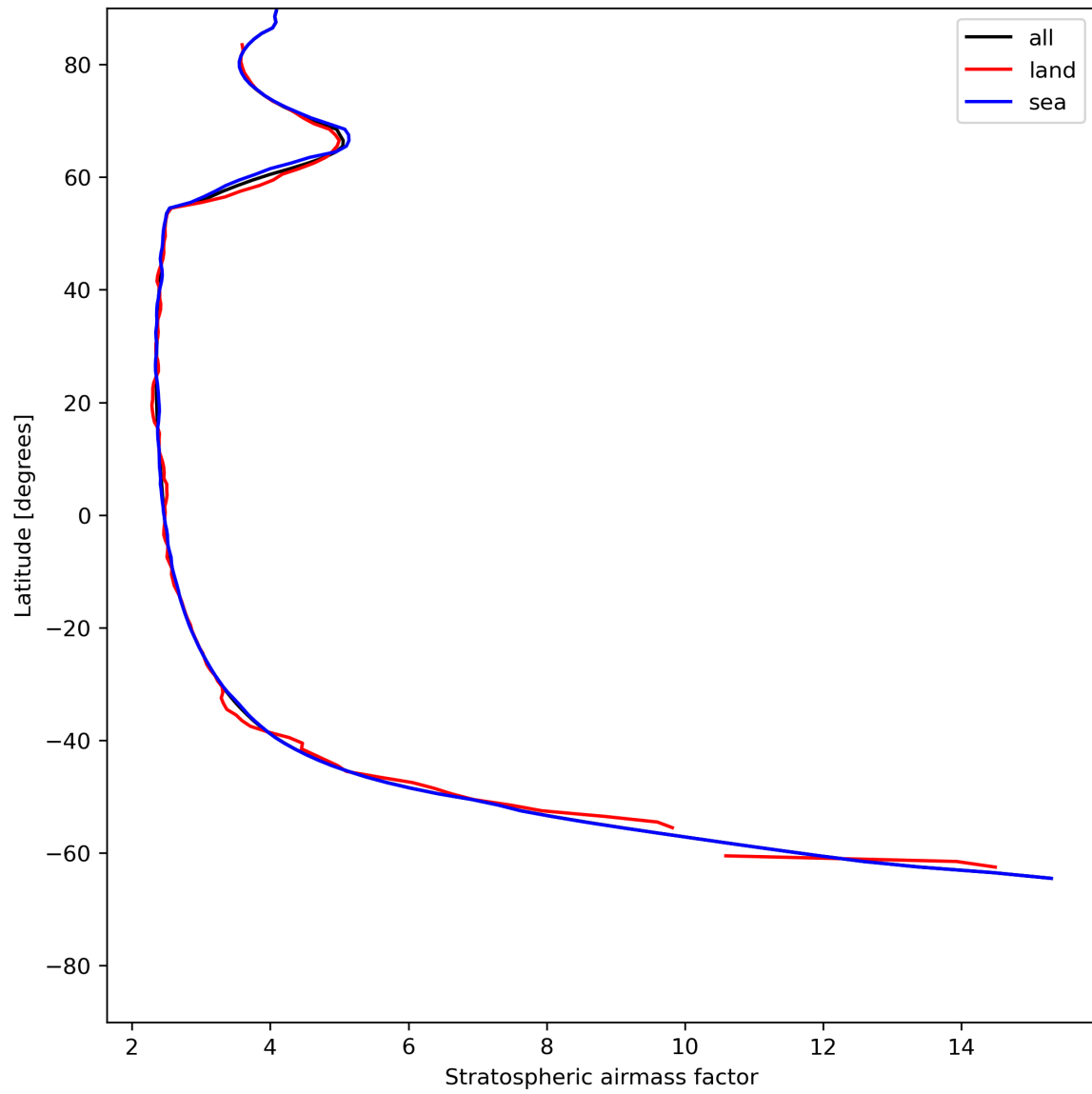
Figure 27: Zonal average of “Stratospheric airmass factor” for 2023-06-30 to 2023-07-02.
