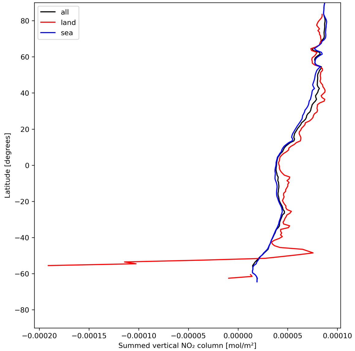
Figure 23: Zonal average of “Summed vertical NO 2 column” for 2023-06-30 to 2023-07-02.
