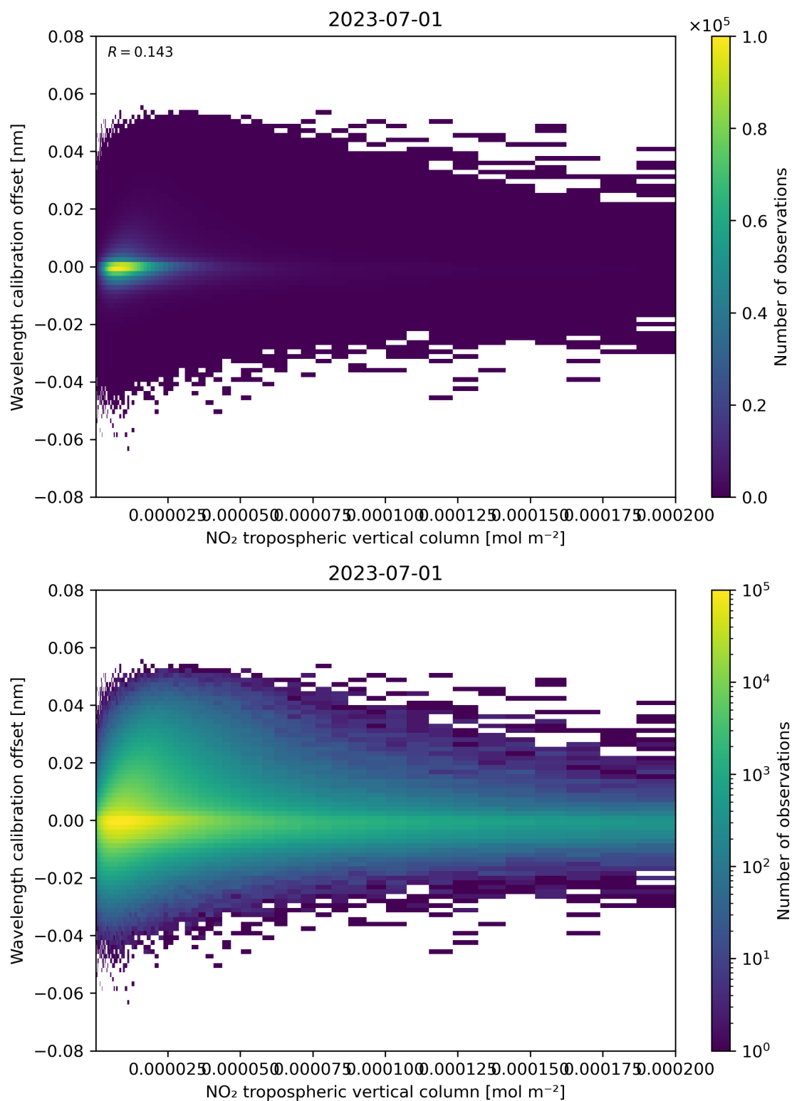
Figure 143: Scatter density plot of “NO 2 tropospheric vertical column” against “Wavelength calibration offset” for 2023-06-30 to 2023-07-02.
