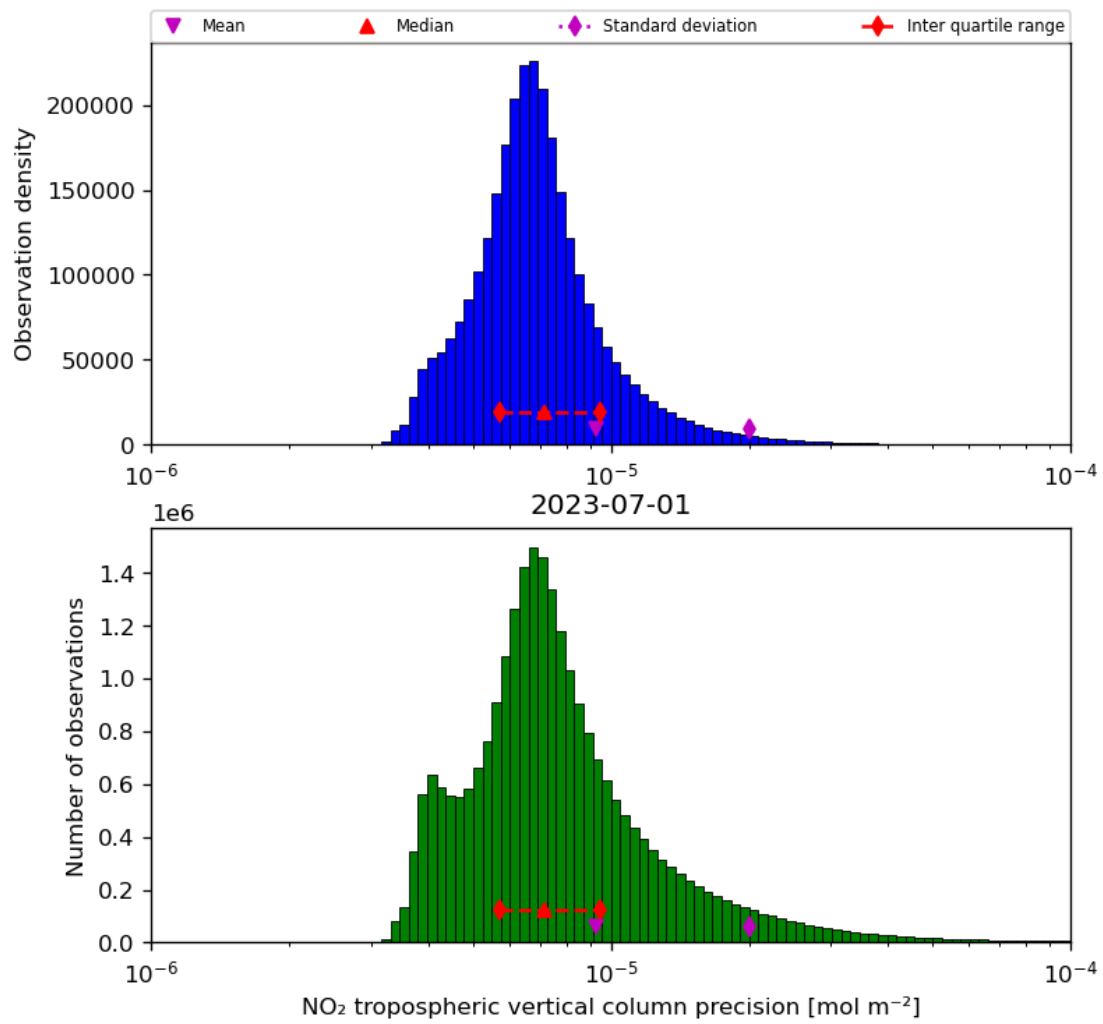
Figure 30: Histogram of “NO 2 tropospheric vertical column precision” for 2023-06-30 to 2023-07-02
