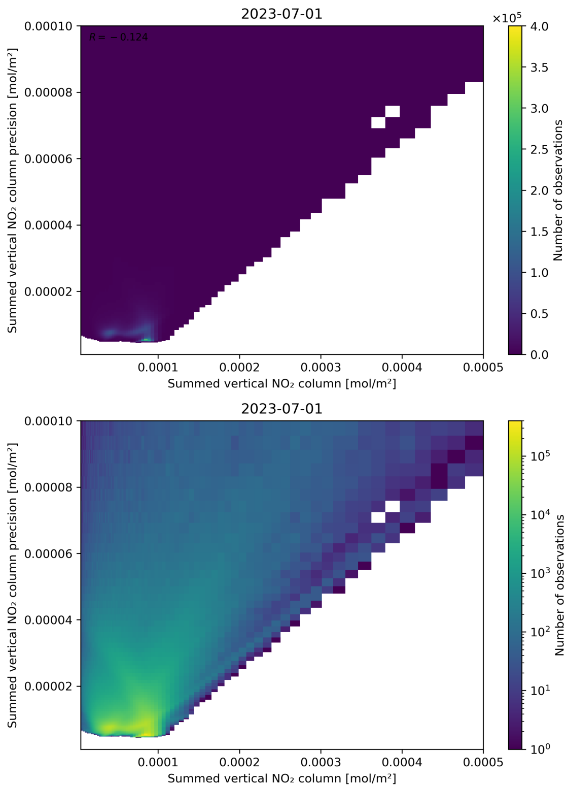
Figure 105: Scatter density plot of “Summed vertical NO 2 column” against “Summed vertical NO 2 column precision” for 2023-06-30 to 2023-07-02.
