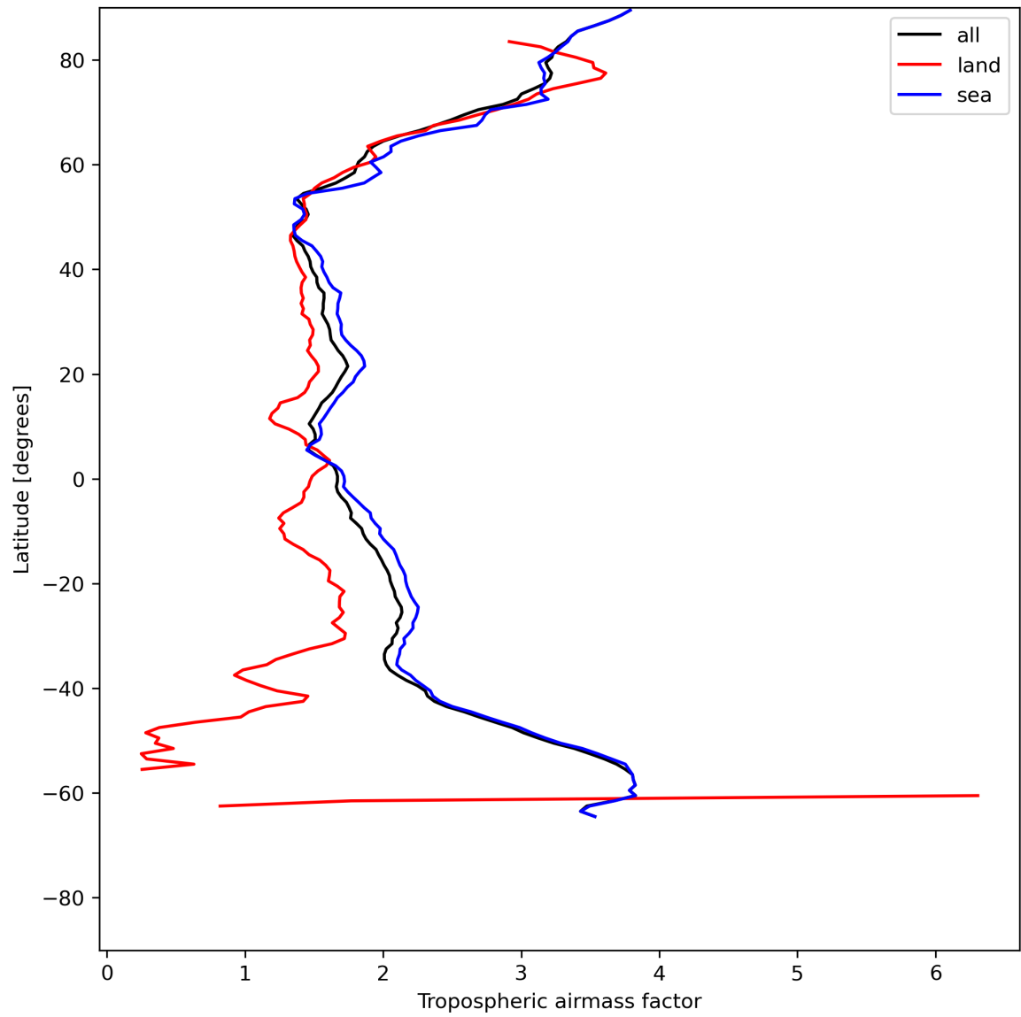
Figure 14: Zonal average of “Tropospheric airmass factor” for 2023-06-30 to 2023-07-02.
