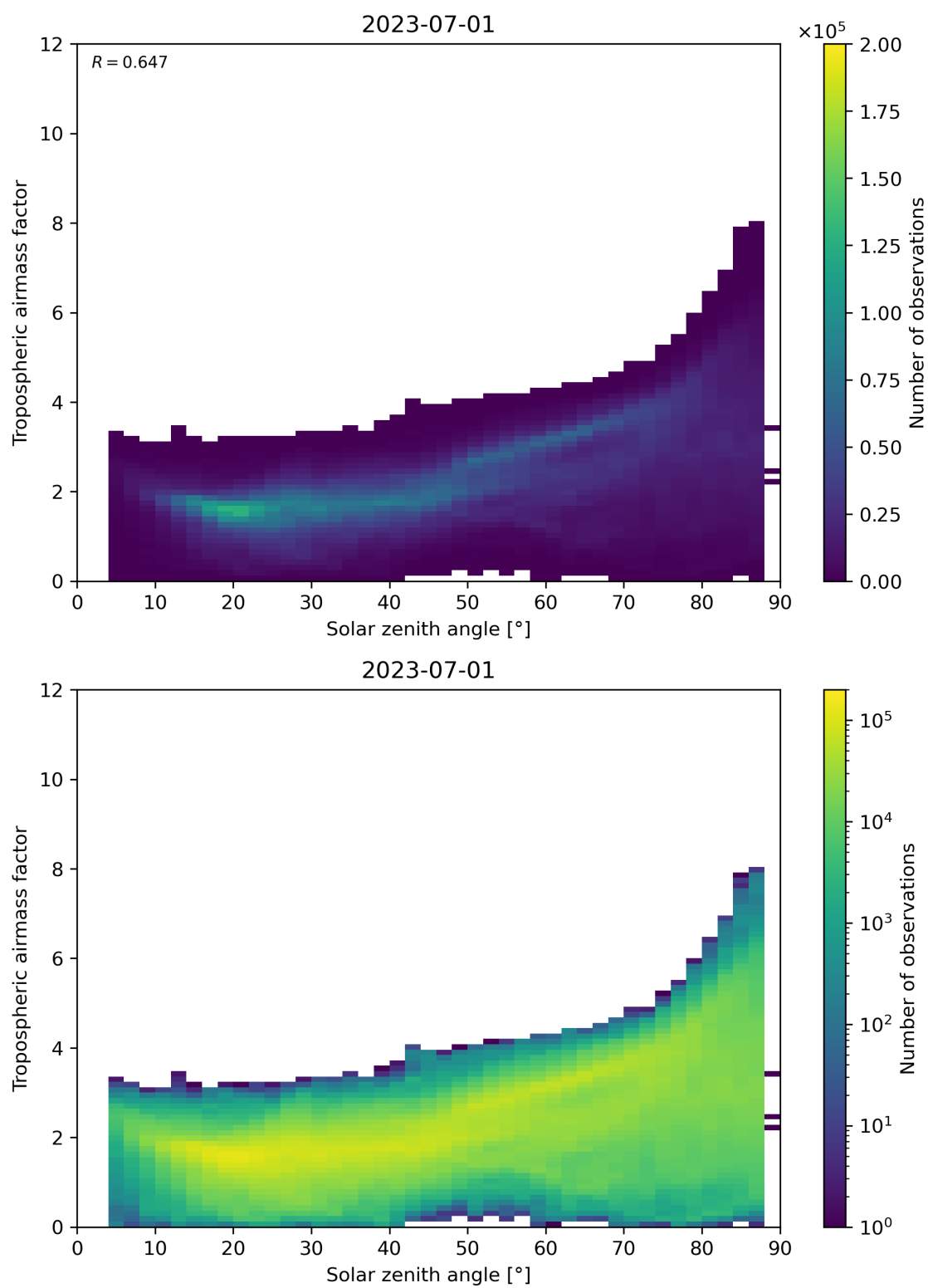
Figure 147: Scatter density plot of “Solar zenith angle” against “Tropospheric airmass factor” for 2023-06-30 to 2023-07-02.
