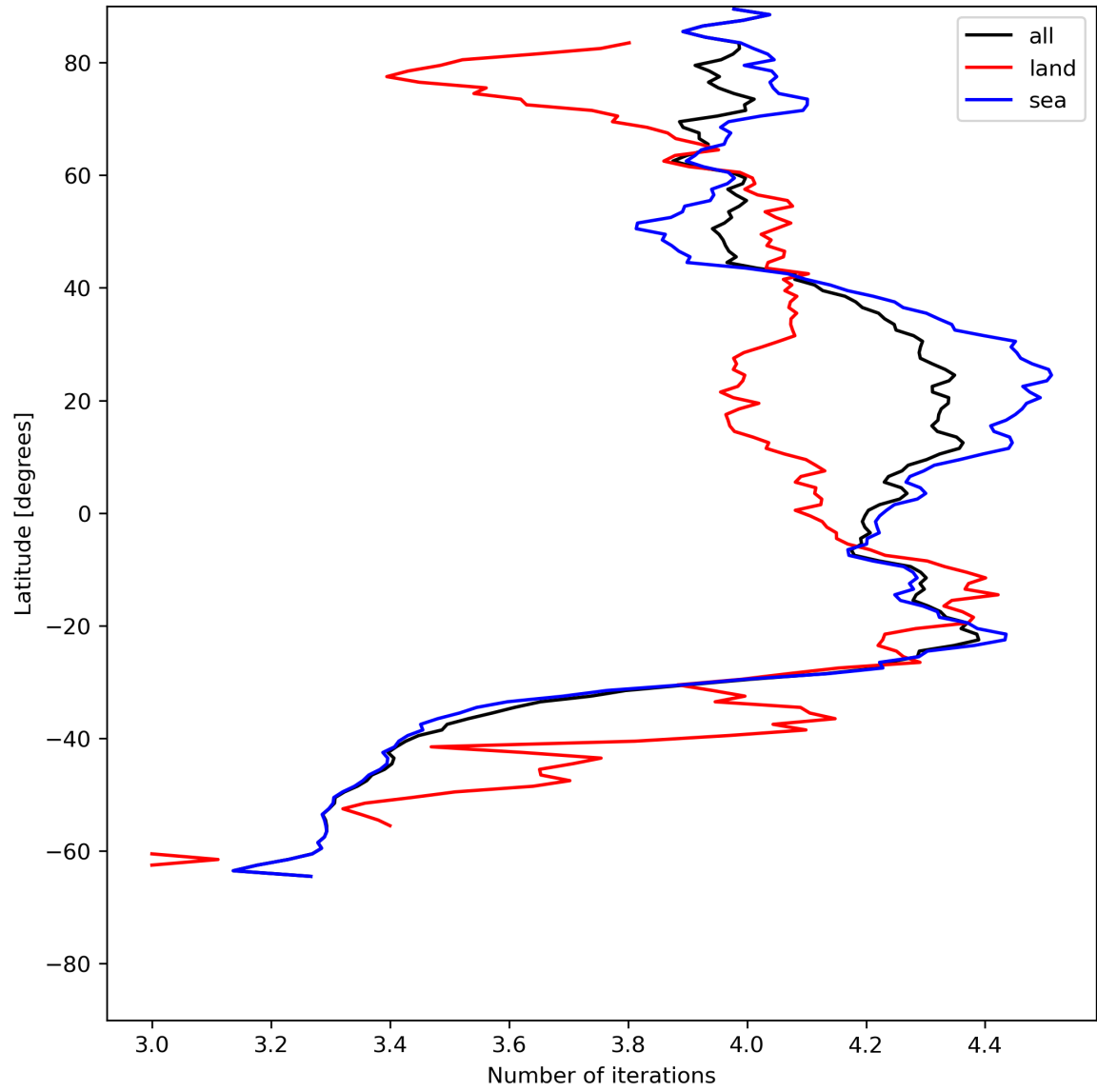
Figure 17: Zonal average of “Number of iterations” for 2023-06-30 to 2023-07-02.
