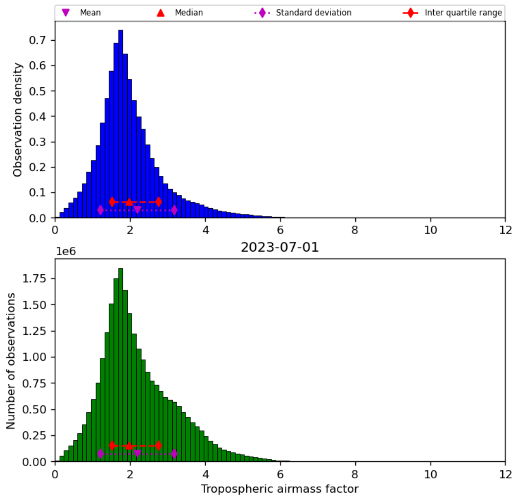
Figure 31: Histogram of “Tropospheric airmass factor” for 2023-06-30 to 2023-07-02
