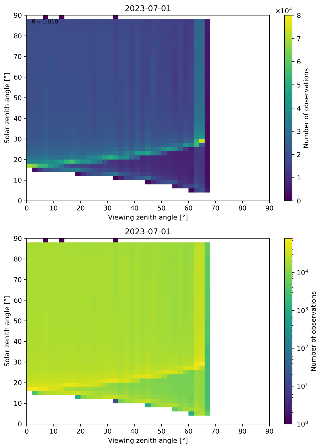
Figure 172: Scatter density plot of “Viewing zenith angle” against “Solar zenith angle” for 2023-06-30 to 2023-07-02.
