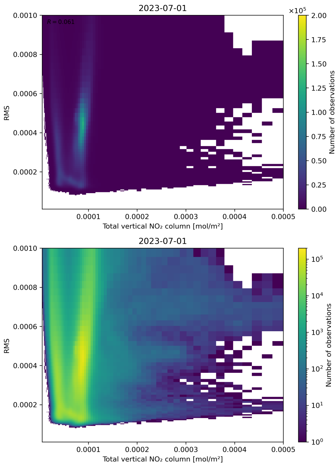
Figure 120: Scatter density plot of “Total vertical NO 2 column” against “RMS” for 2023-06-30 to 2023-07-02.
