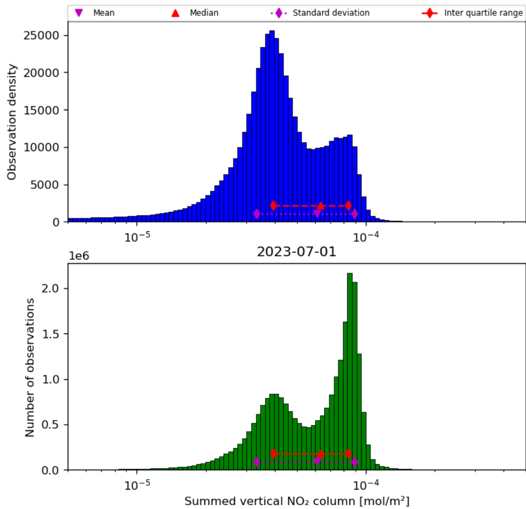
Figure 40: Histogram of “Summed vertical NO 2 column” for 2023-06-30 to 2023-07-02
