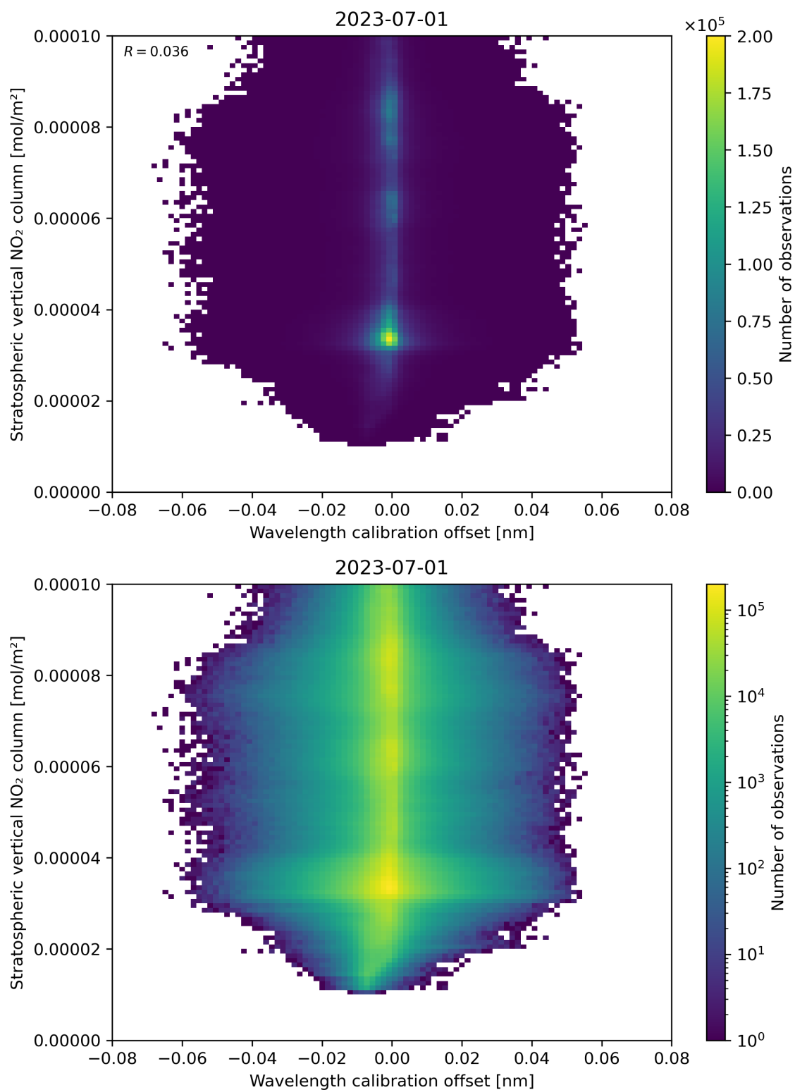
Figure 176: Scatter density plot of “Wavelength calibration offset” against “Stratospheric vertical NO 2 column” for 2023-06-30 to 2023-07-02.
