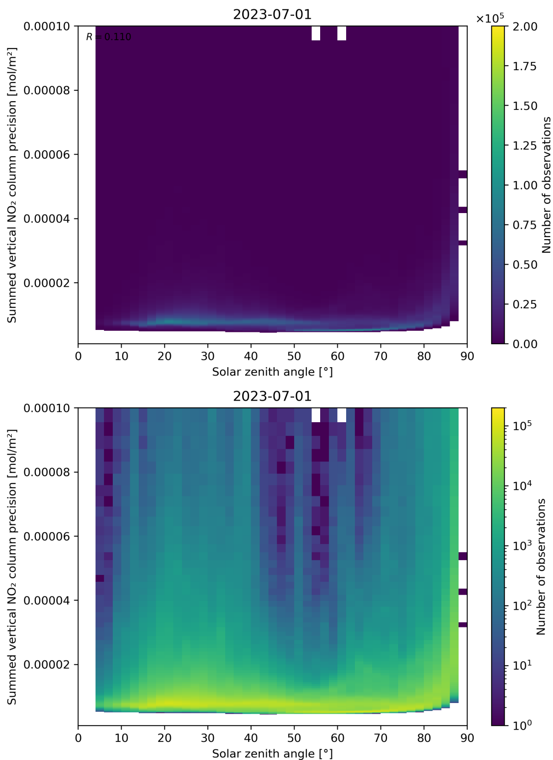
Figure 152: Scatter density plot of “Solar zenith angle” against “Summed vertical NO 2 column precision” for 2023-06-30 to 2023-07-02.
