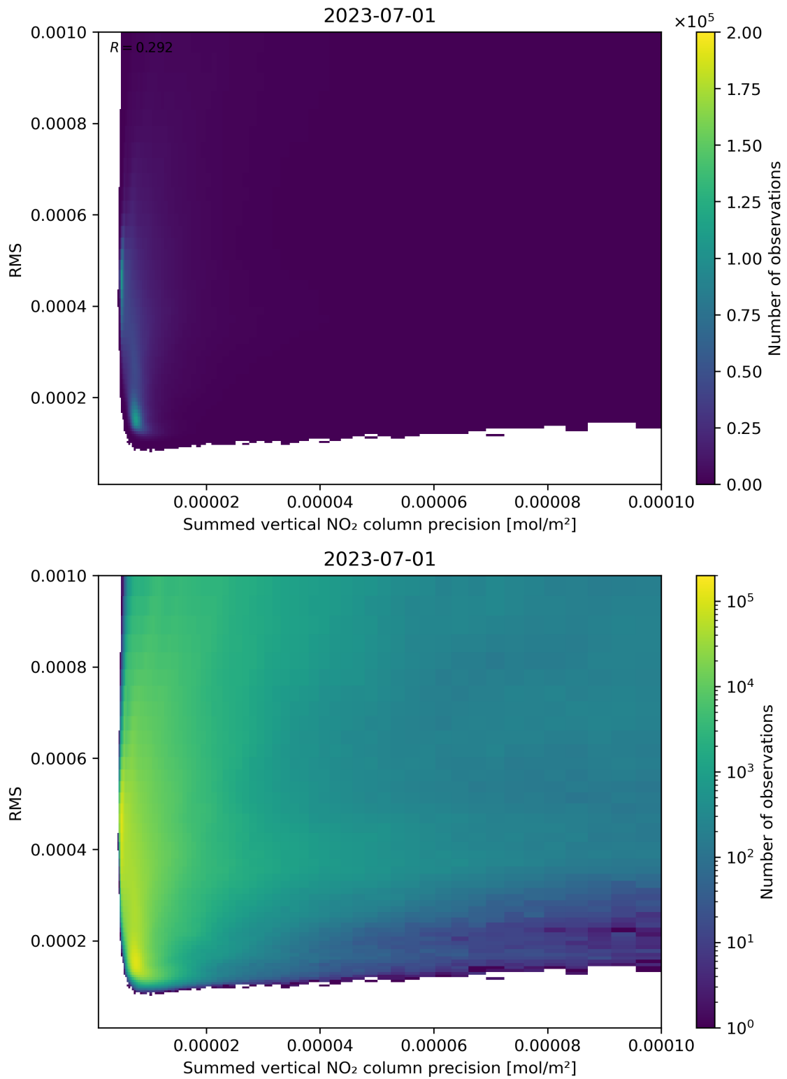
Figure 108: Scatter density plot of “Summed vertical NO 2 column precision” against “RMS” for 2023-06-30 to 2023-07-02.
