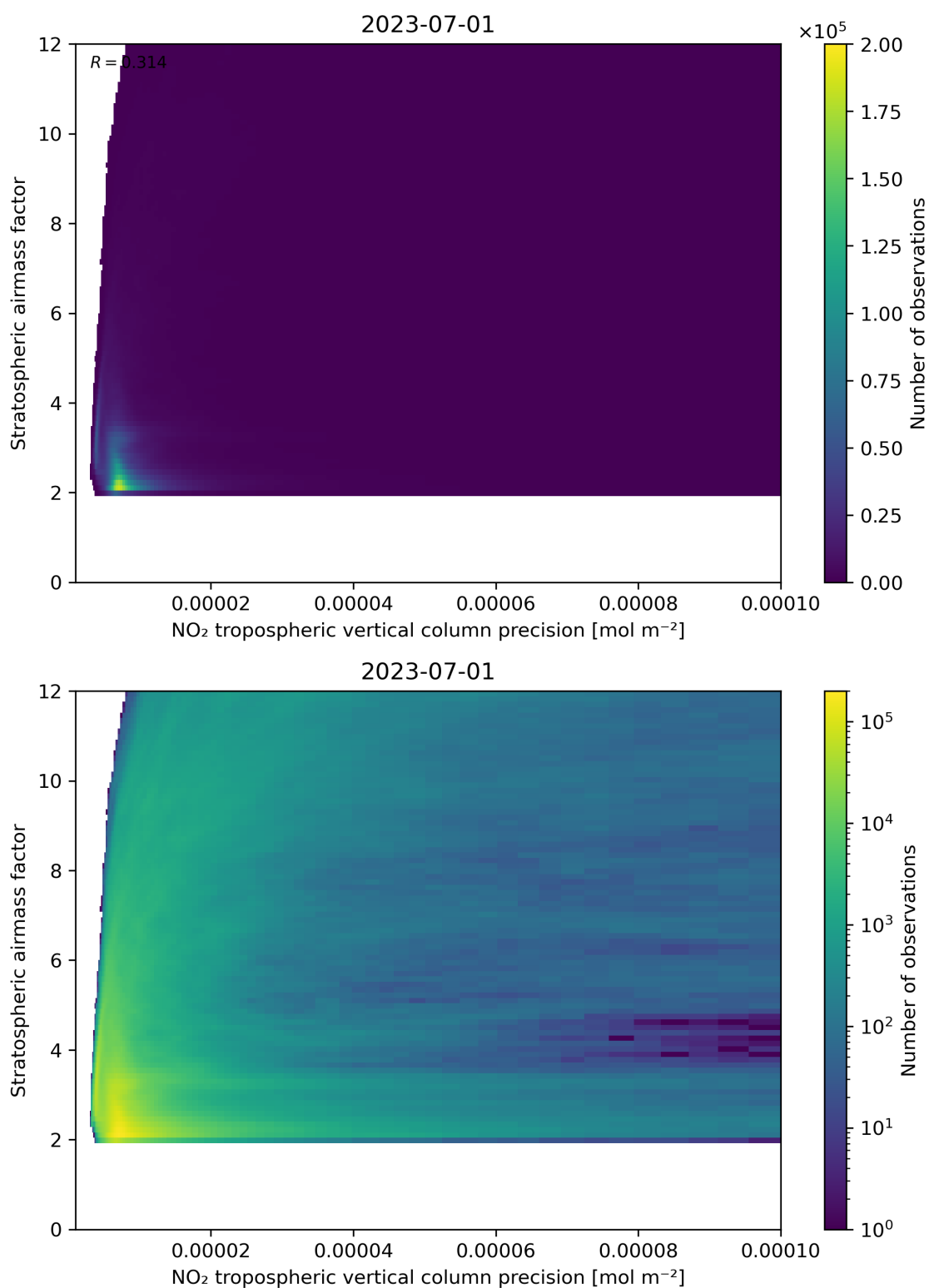
Figure 131: Scatter density plot of “NO 2 tropospheric vertical column precision” against “Stratospheric airmass factor” for 2023-06-30 to 2023-07-02.
