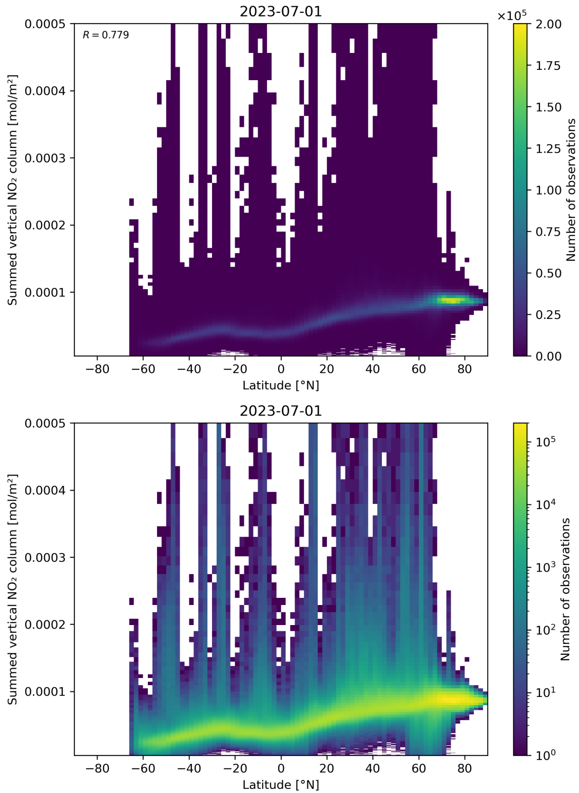
Figure 88: Scatter density plot of “Latitude” against “Summed vertical NO 2 column” for 2023-06-30 to 2023-07-02.
