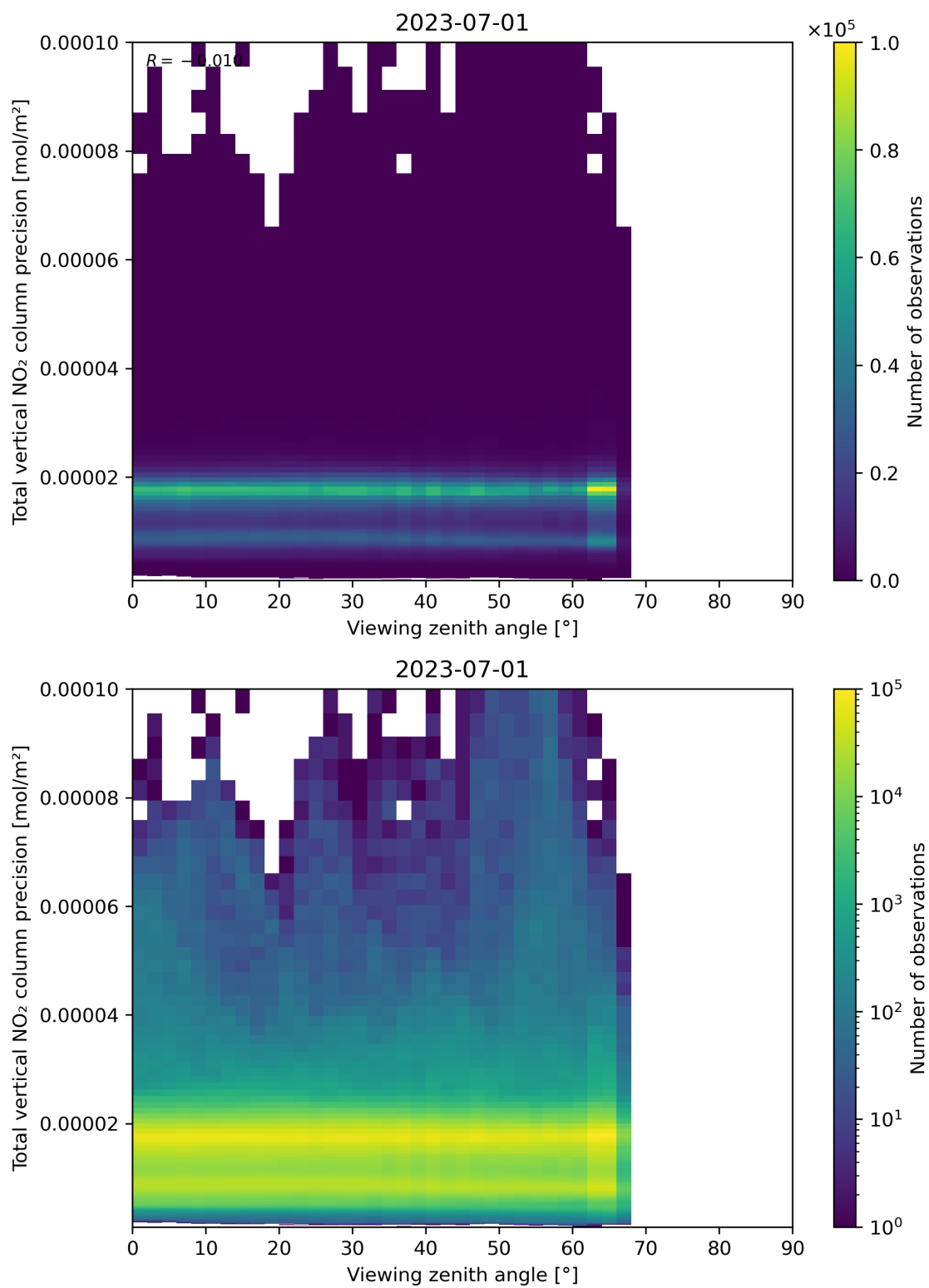
Figure 168: Scatter density plot of “Viewing zenith angle” against “Total vertical NO 2 column precision” for 2023-06-30 to 2023-07-02.
