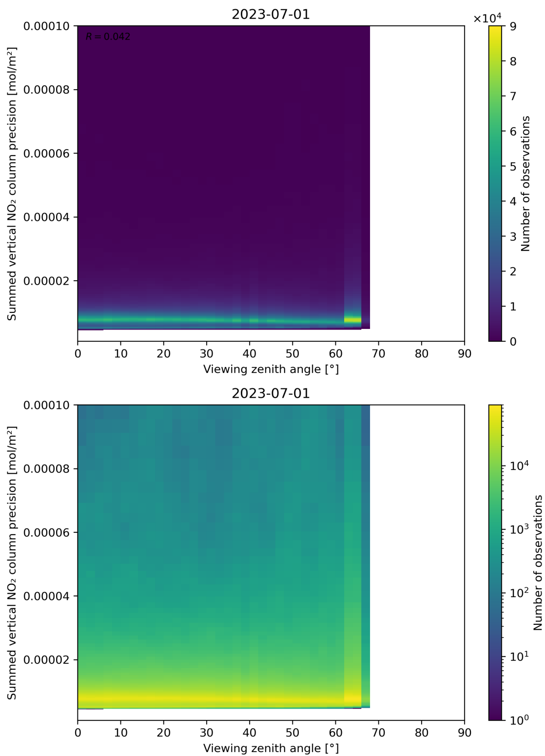
Figure 166: Scatter density plot of “Viewing zenith angle” against “Summed vertical NO 2 column precision” for 2023-06-30 to 2023-07-02.
