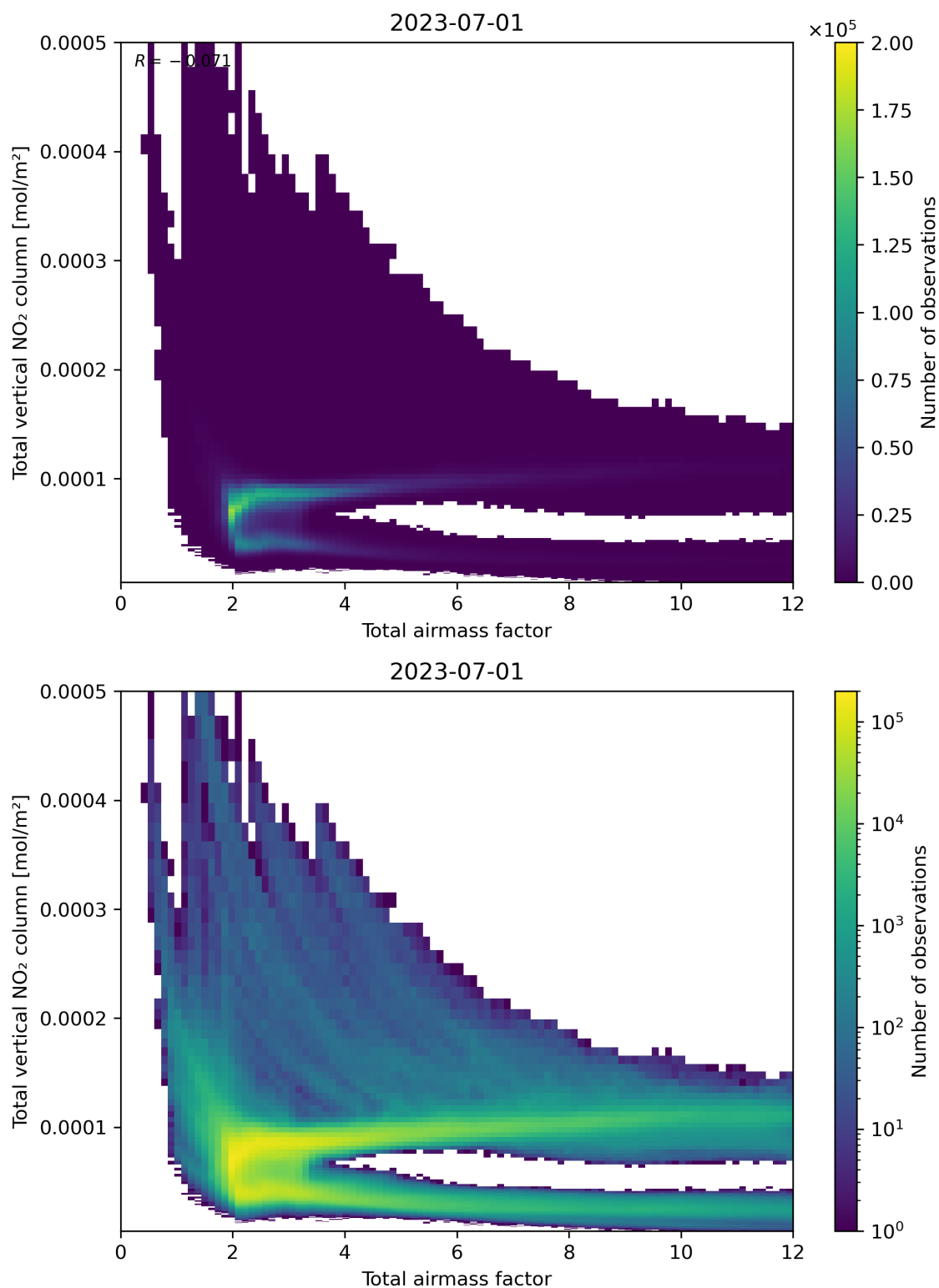
Figure 67: Scatter density plot of “Total airmass factor” against “Total vertical NO 2 column” for 2023-06-30 to 2023-07-02.
