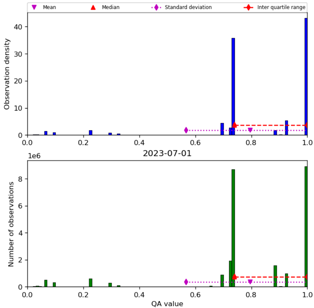
Figure 28: Histogram of “QA value” for 2023-06-30 to 2023-07-02
