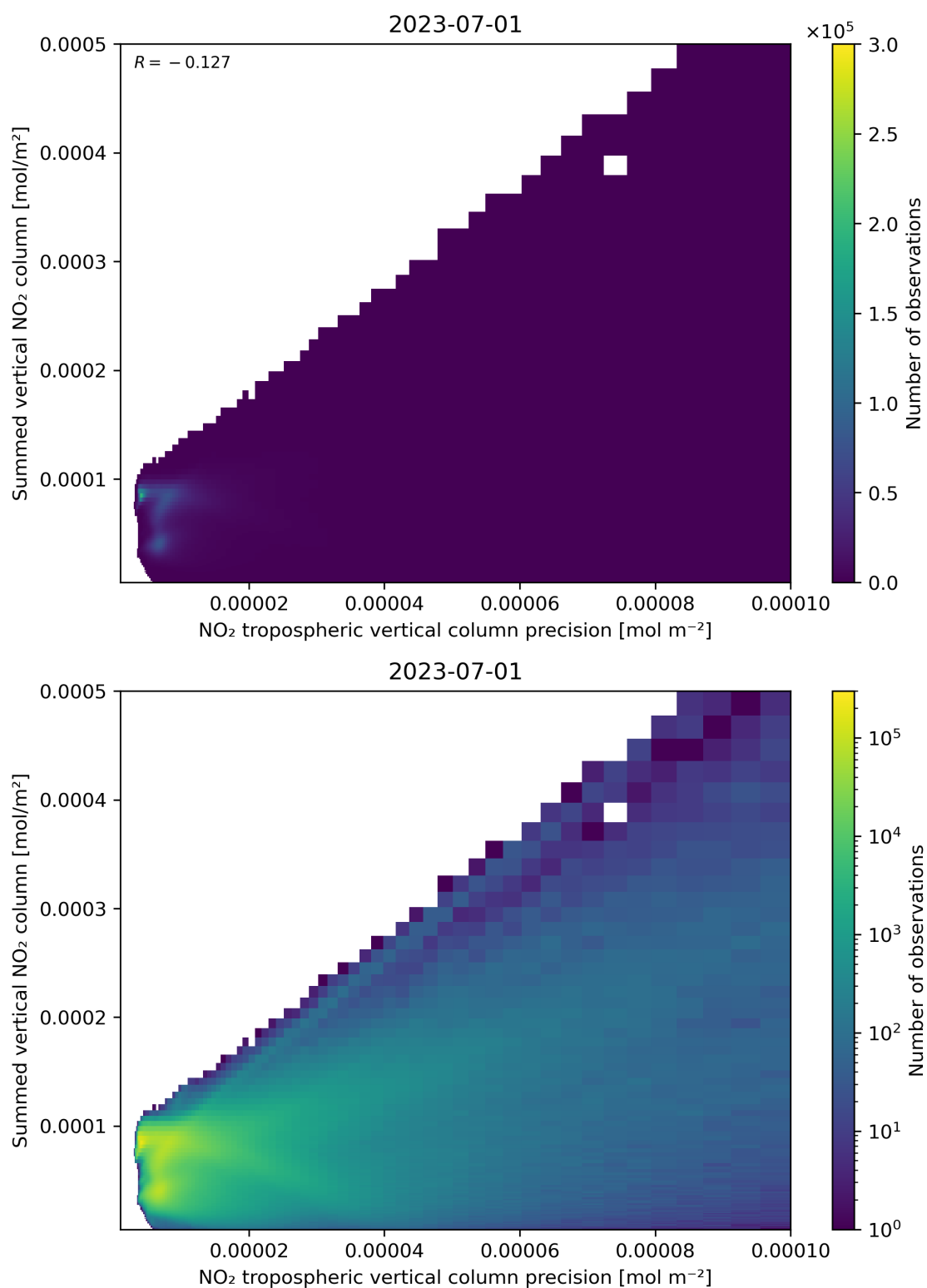
Figure 136: Scatter density plot of “NO 2 tropospheric vertical column precision” against “Summed vertical NO 2 column” for 2023-06-30 to 2023-07-02.
