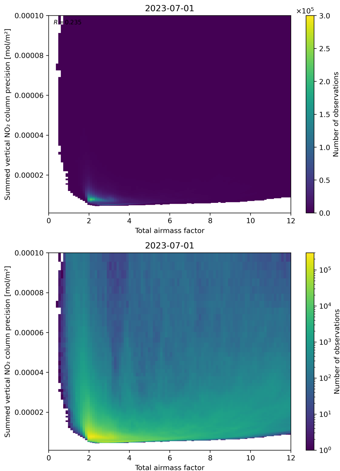
Figure 66: Scatter density plot of “Total airmass factor” against “Summed vertical NO 2 column precision” for 2023-06-30 to 2023-07-02.
