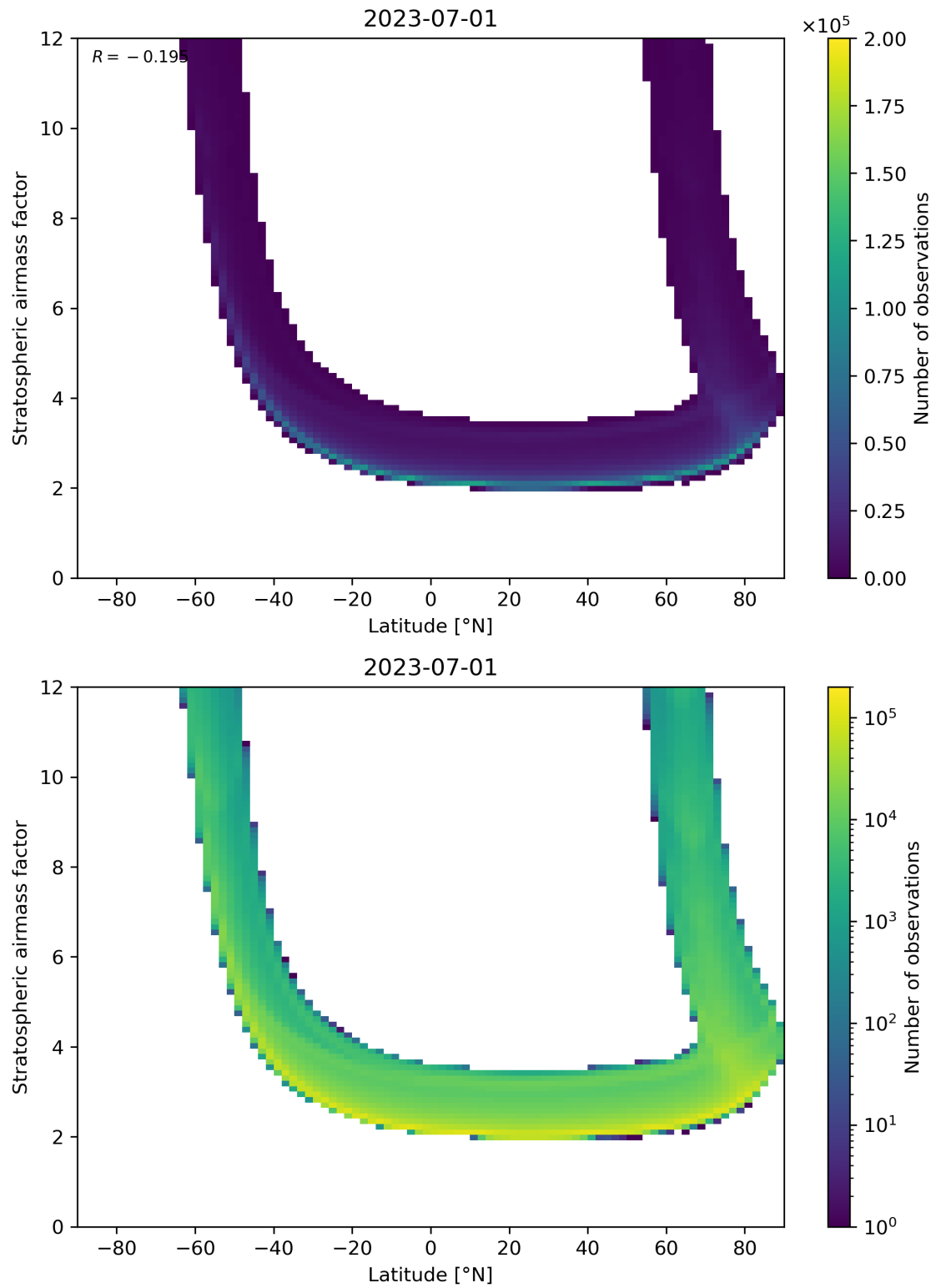
Figure 83: Scatter density plot of “Latitude” against “Stratospheric air mass factor” for 2023-06-30 to 2023-07-02.
