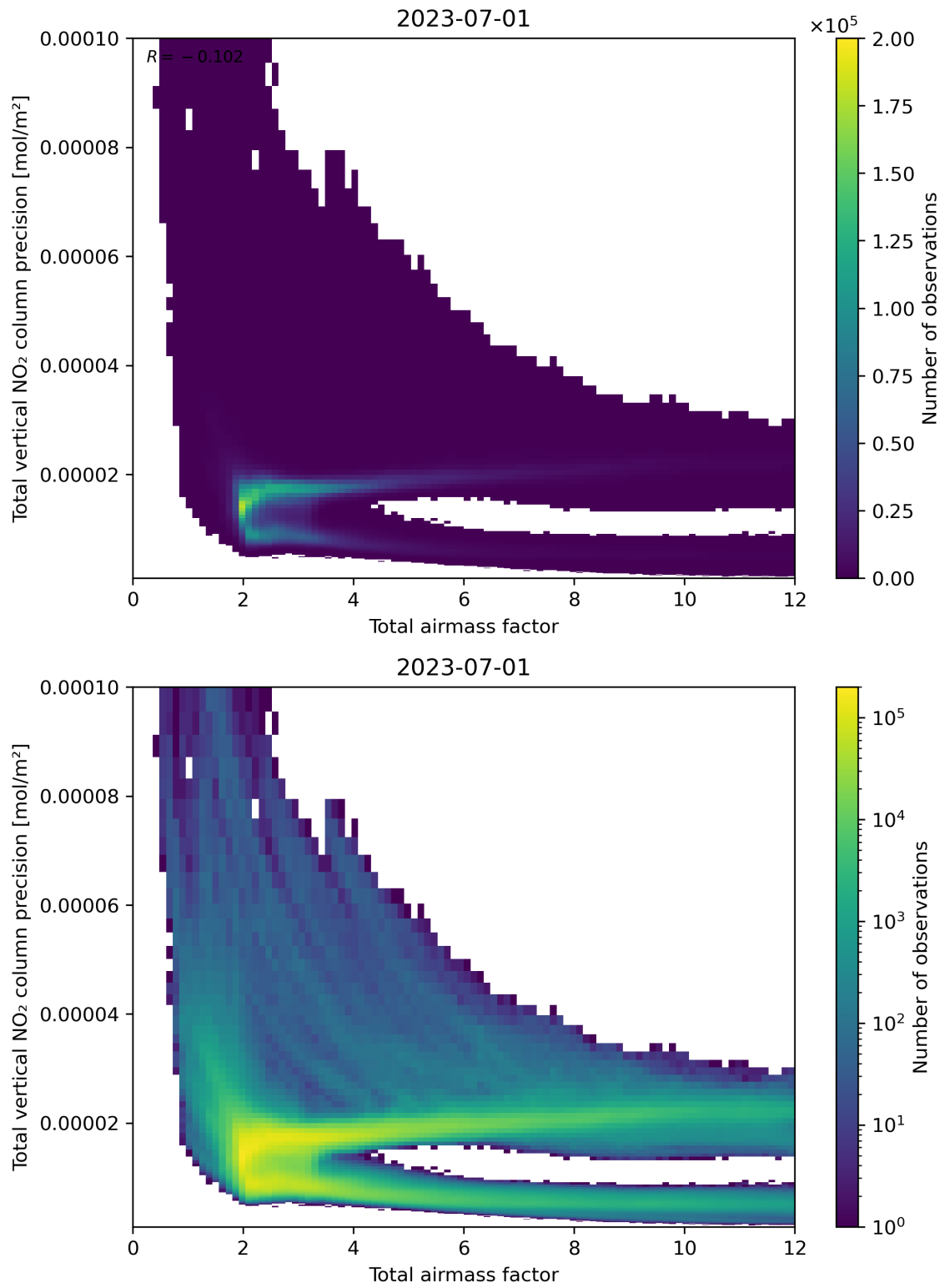
Figure 68: Scatter density plot of “Total airmass factor” against “Total vertical NO 2 column precision” for 2023-06-30 to 2023-07-02.
