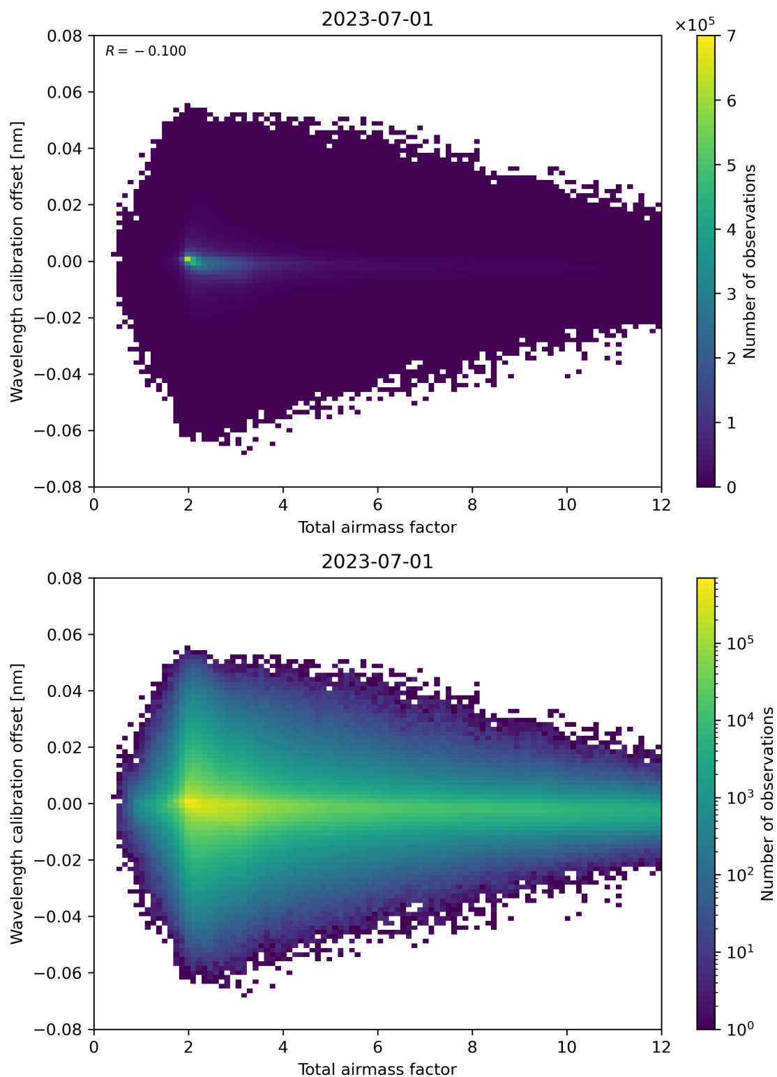
Figure 70: Scatter density plot of “Total airmass factor” against “Wavelength calibration offset” for 2023-06-30 to 2023-07-02.
