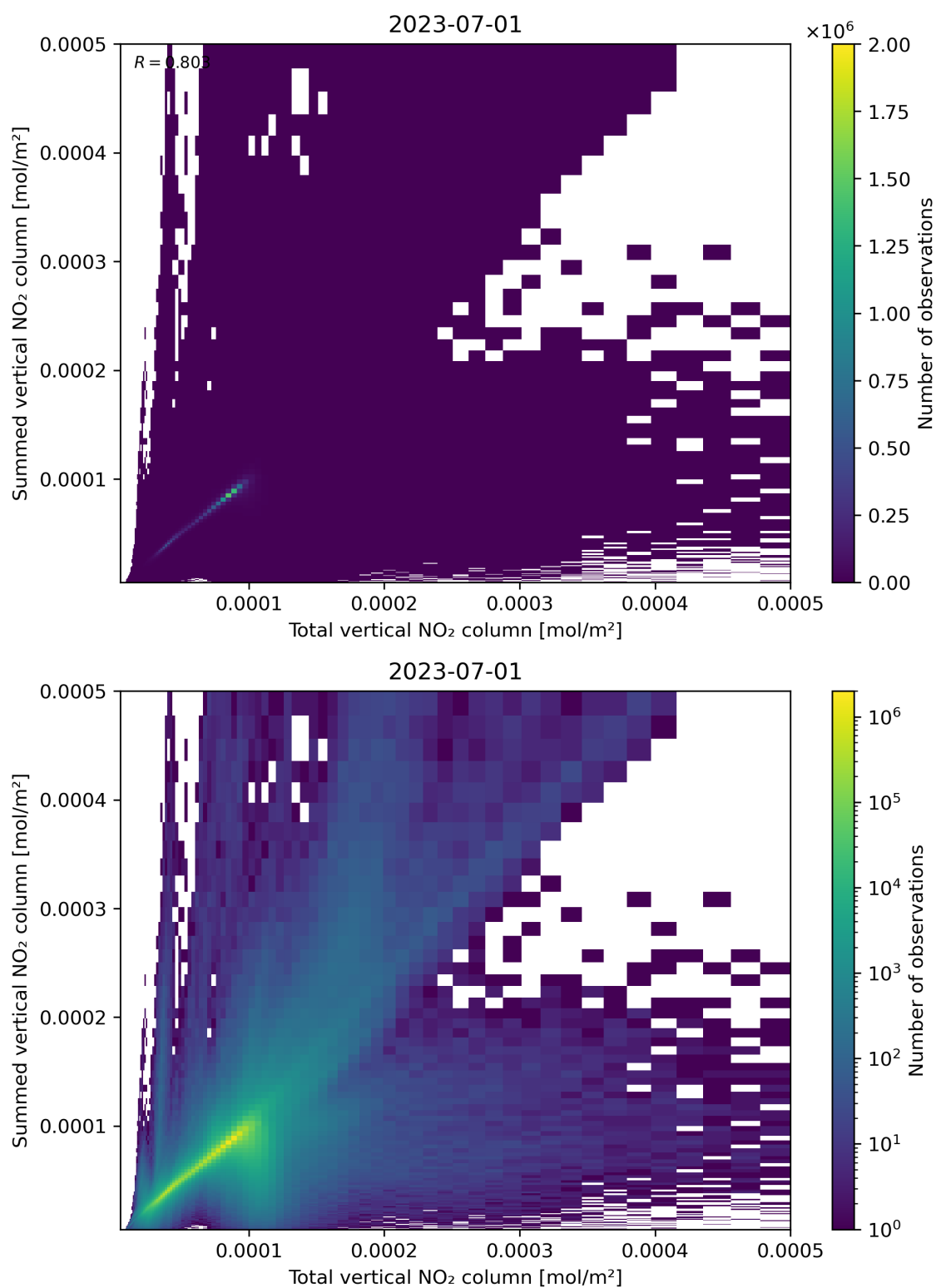
Figure 112: Scatter density plot of “Total vertical NO 2 column” against “Summed vertical NO 2 column” for 2023-06-30 to 2023-07-02.
