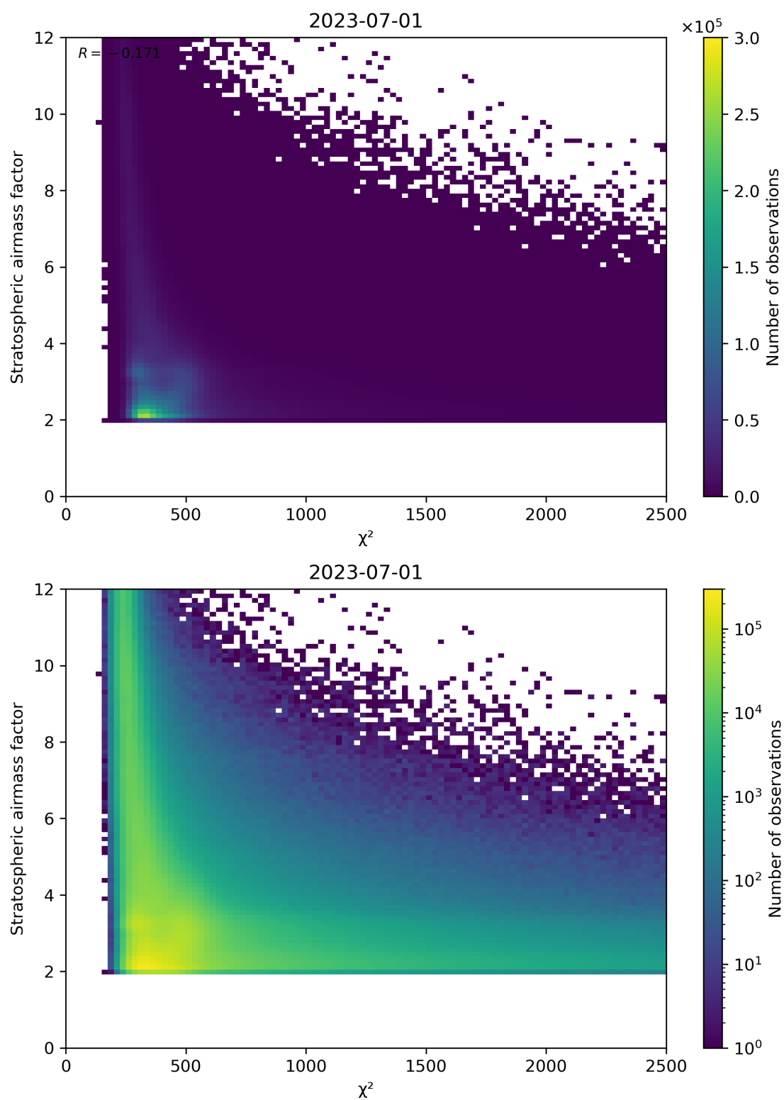
Figure 81: Scatter density plot of “ \chi^2 ” against “Stratospheric airmass factor” for 2023-06-30 to 2023-07-02.
