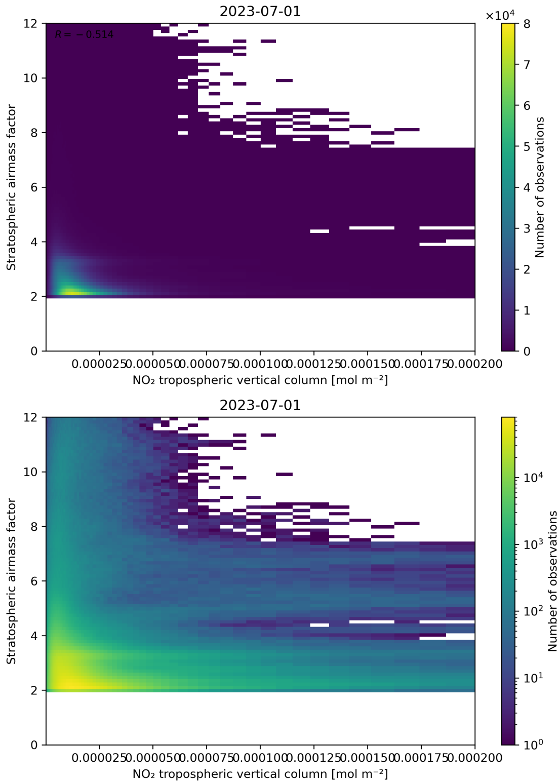
Figure 121: Scatter density plot of “NO 2 tropospheric vertical column” against “Stratospheric air mass factor” for 2023-06-30 to 2023-07-02.
