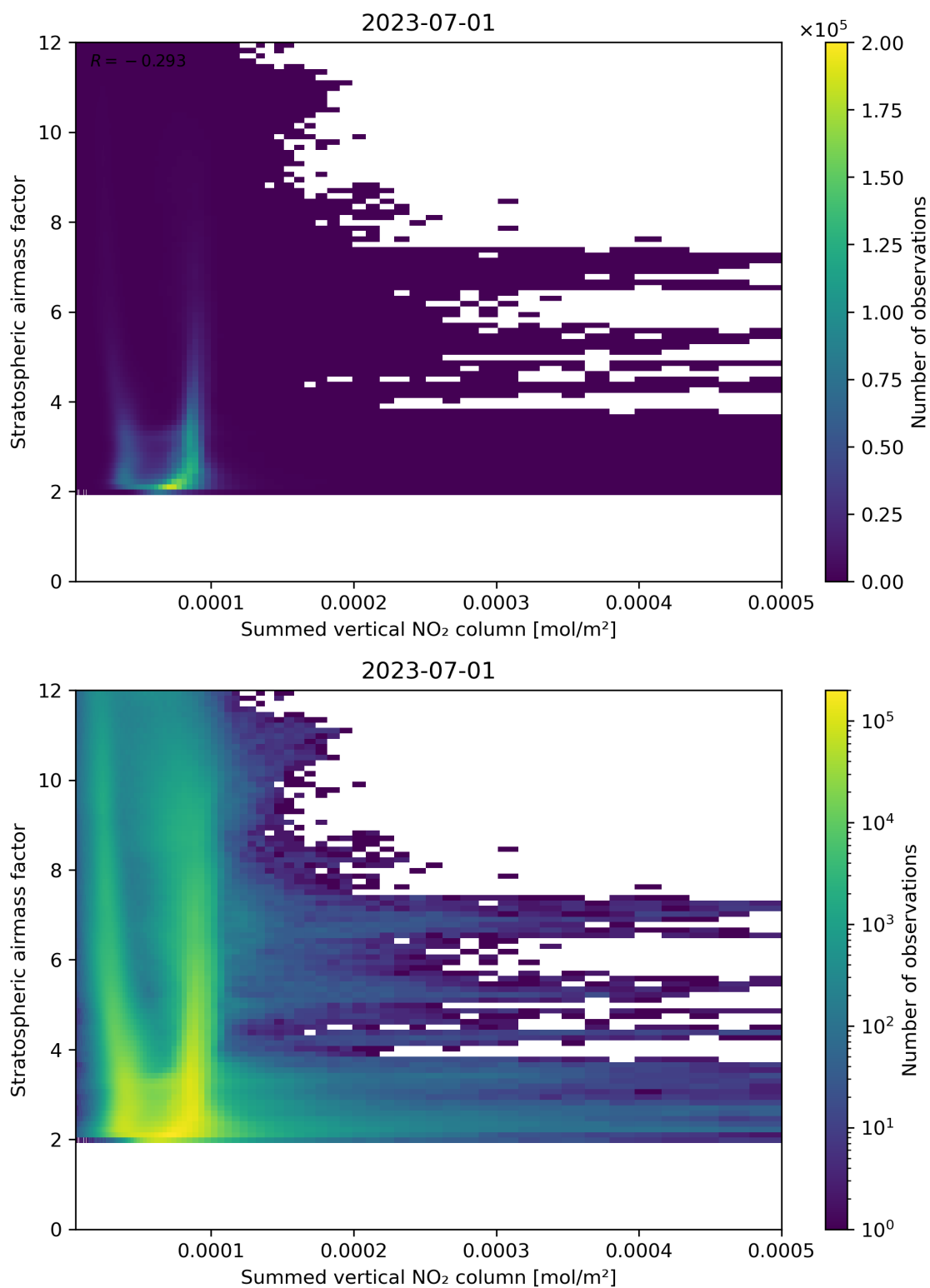
Figure 103: Scatter density plot of “Summed vertical NO 2 column” against “Stratospheric air mass factor” for 2023-06-30 to 2023-07-02.
