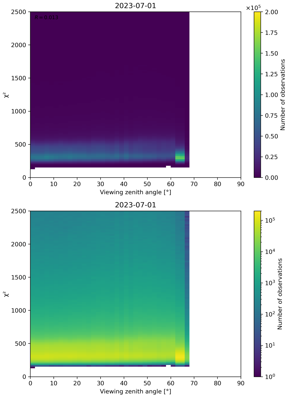
Figure 162: Scatter density plot of “Viewing zenith angle” against “ \chi^2 ” for 2023-06-30 to 2023-07-02.
