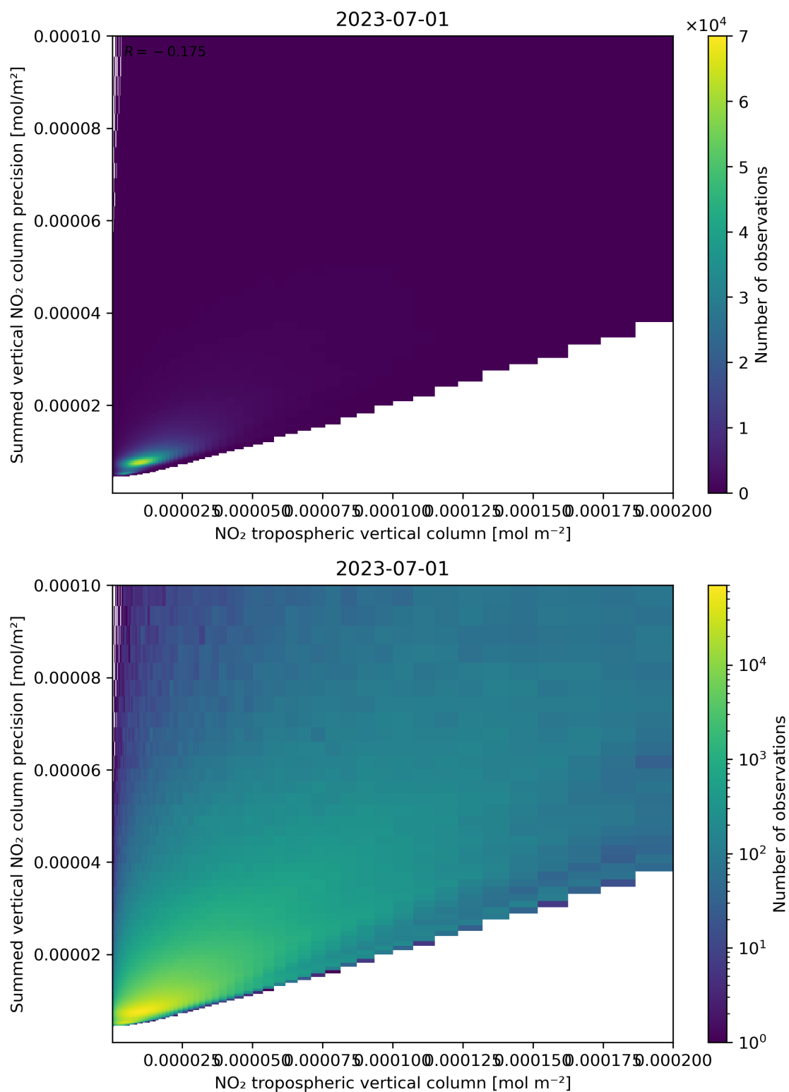
Figure 127: Scatter density plot of “NO 2 tropospheric vertical column” against “Summed vertical NO 2 column precision” for 2023-06-30 to 2023-07-02.
