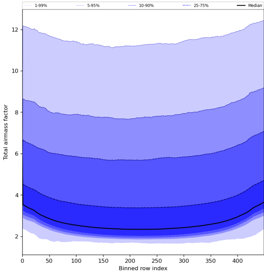
Figure 49: Along track statistics of “Total airmass factor” for 2023-06-30 to 2023-07-02
