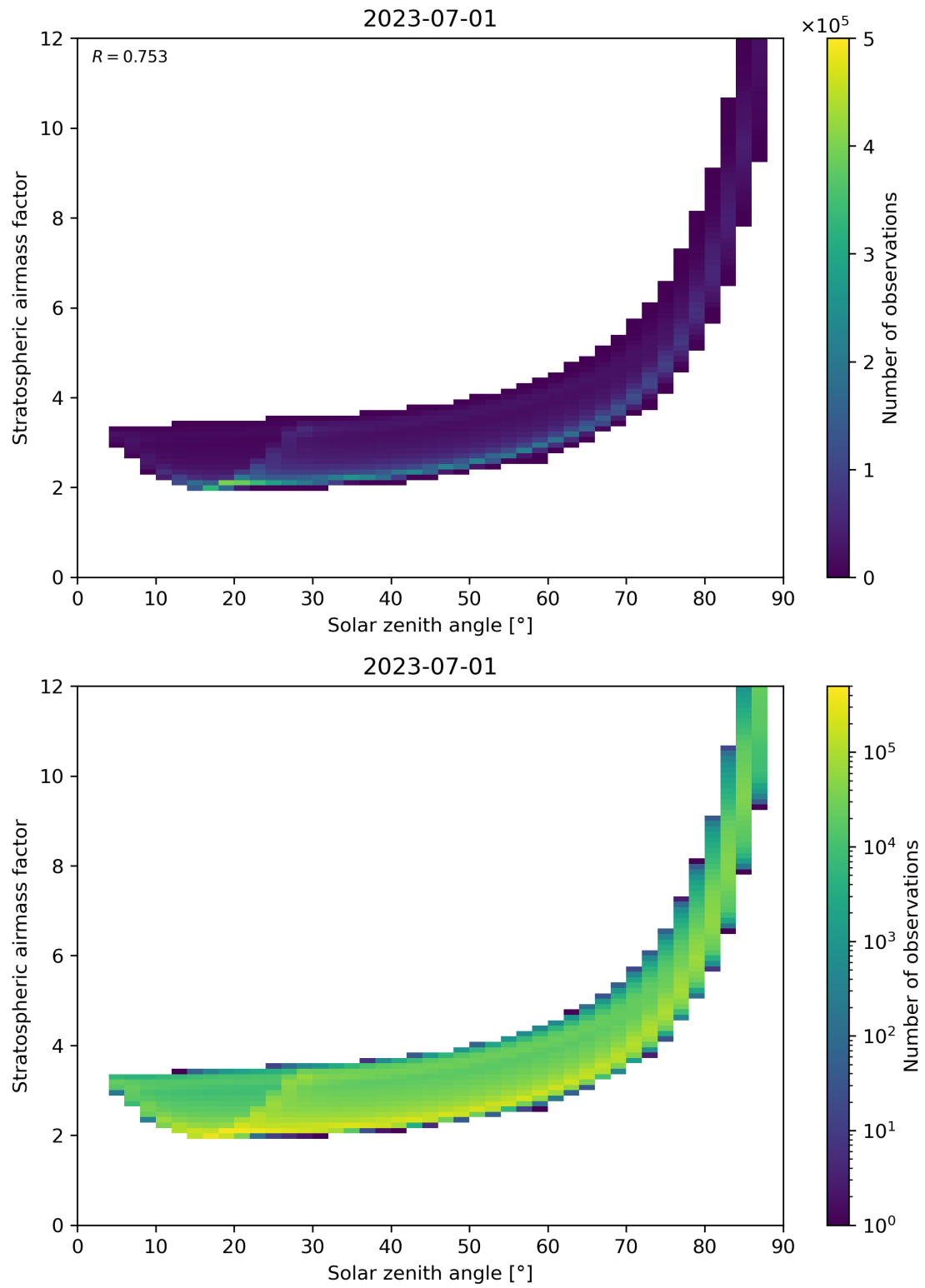
Figure 145: Scatter density plot of “Solar zenith angle” against “Stratospheric airmass factor” for 2023-06-30 to 2023-07-02.
