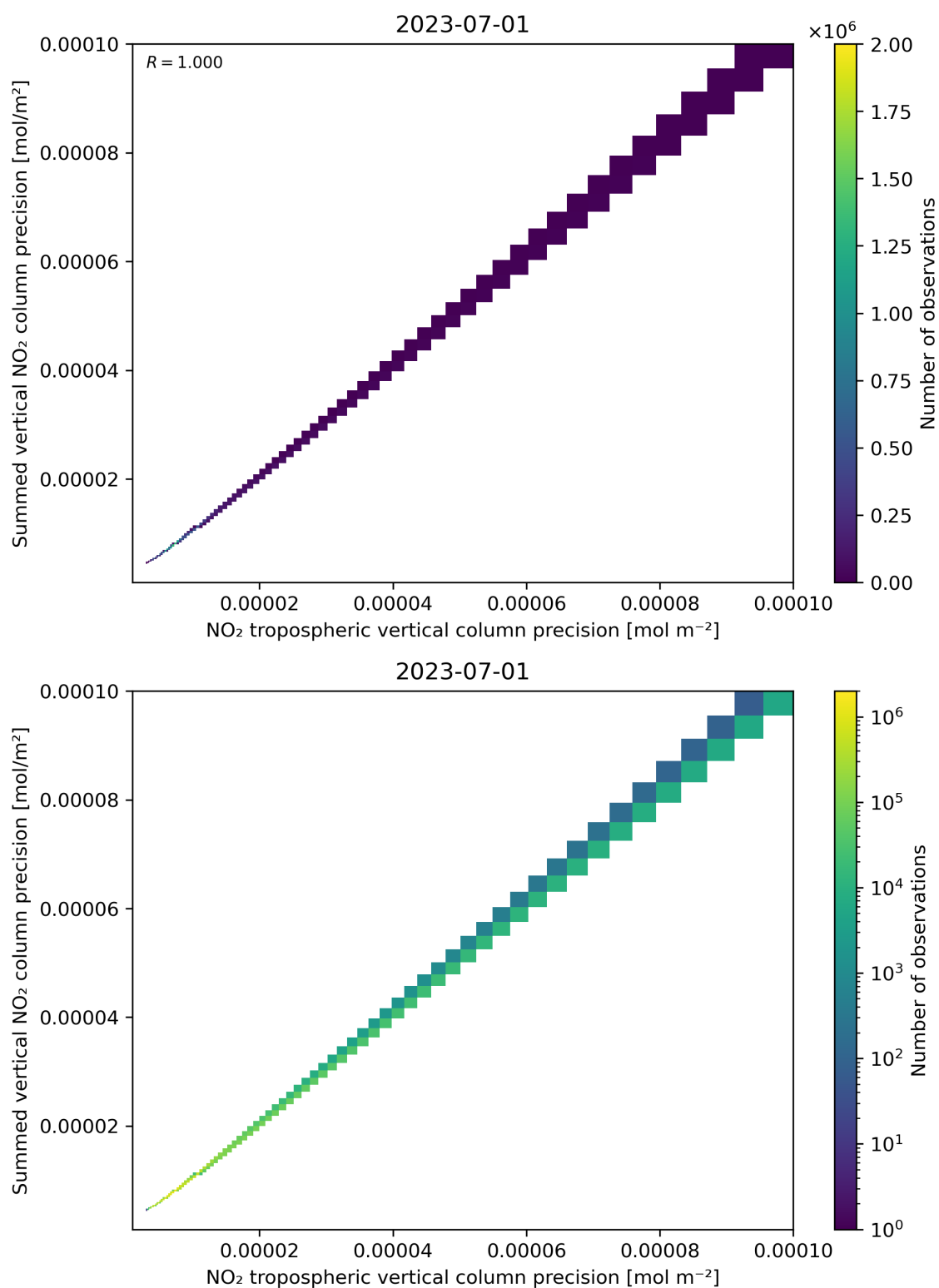
Figure 137: Scatter density plot of “NO 2 tropospheric vertical column precision” against “Summed vertical NO 2 column precision” for 2023-06-30 to 2023-07-02.
