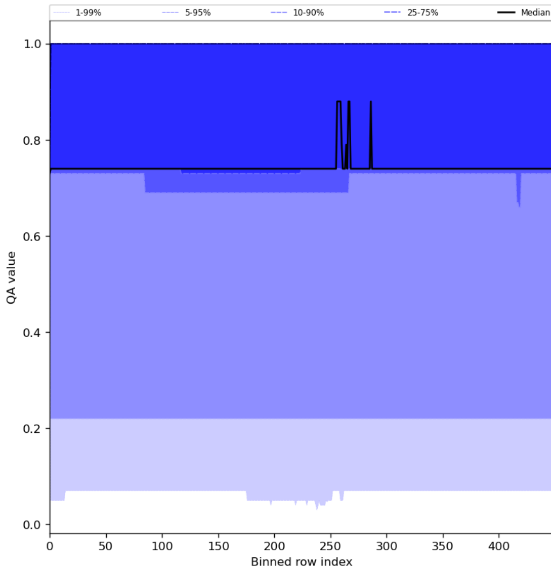
Figure 45: Along track statistics of “QA value” for 2023-06-30 to 2023-07-02
