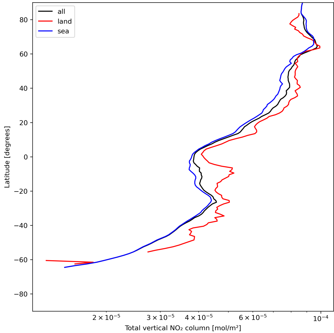
Figure 21: Zonal average of “Total vertical NO 2 column” for 2023-06-30 to 2023-07-02.
