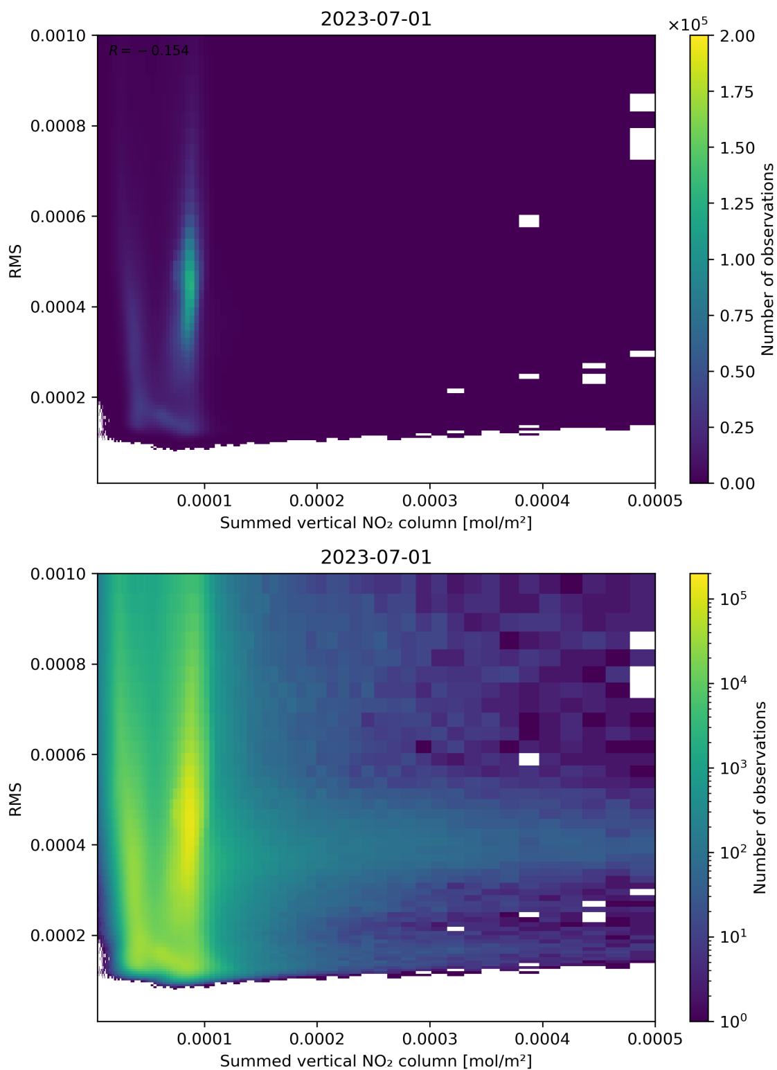
Figure 109: Scatter density plot of “Summed vertical NO 2 column” against “RMS” for 2023-06-30 to 2023-07-02.
