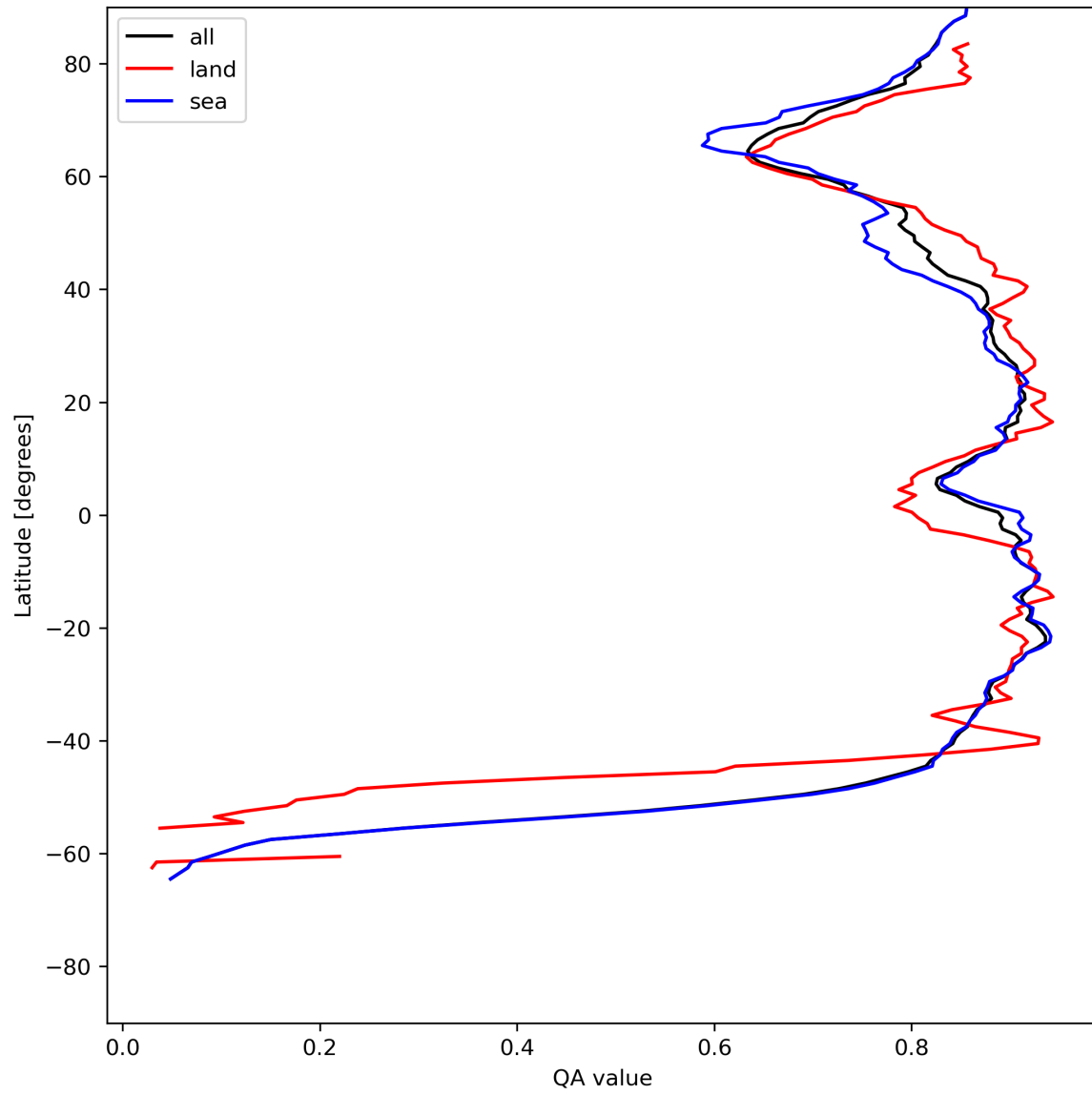
Figure 11: Zonal average of “QA value” for 2023-06-30 to 2023-07-02.
