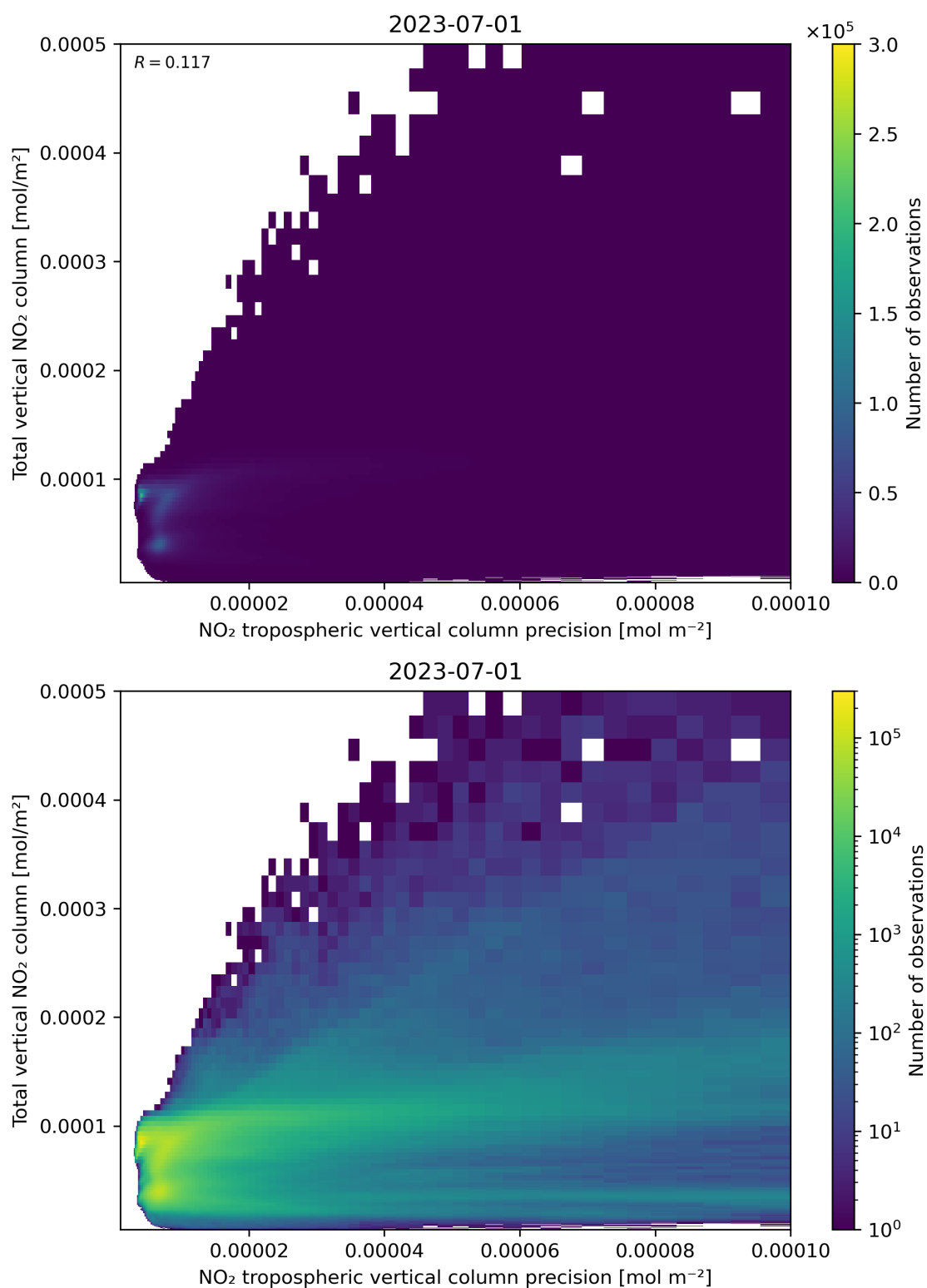
Figure 138: Scatter density plot of “NO 2 tropospheric vertical column precision” against “Total vertical NO 2 column” for 2023-06-30 to 2023-07-02.
