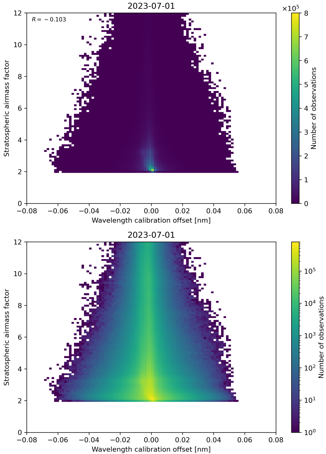
Figure 174: Scatter density plot of “Wavelength calibration offset” against “Stratospheric airmass factor” for 2023-06-30 to 2023-07-02.
