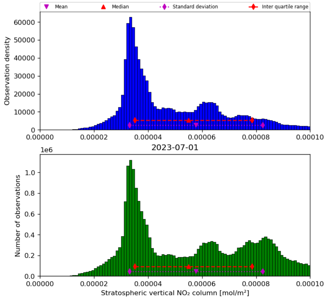
Figure 36: Histogram of “Stratospheric vertical NO 2 column” for 2023-06-30 to 2023-07-02
