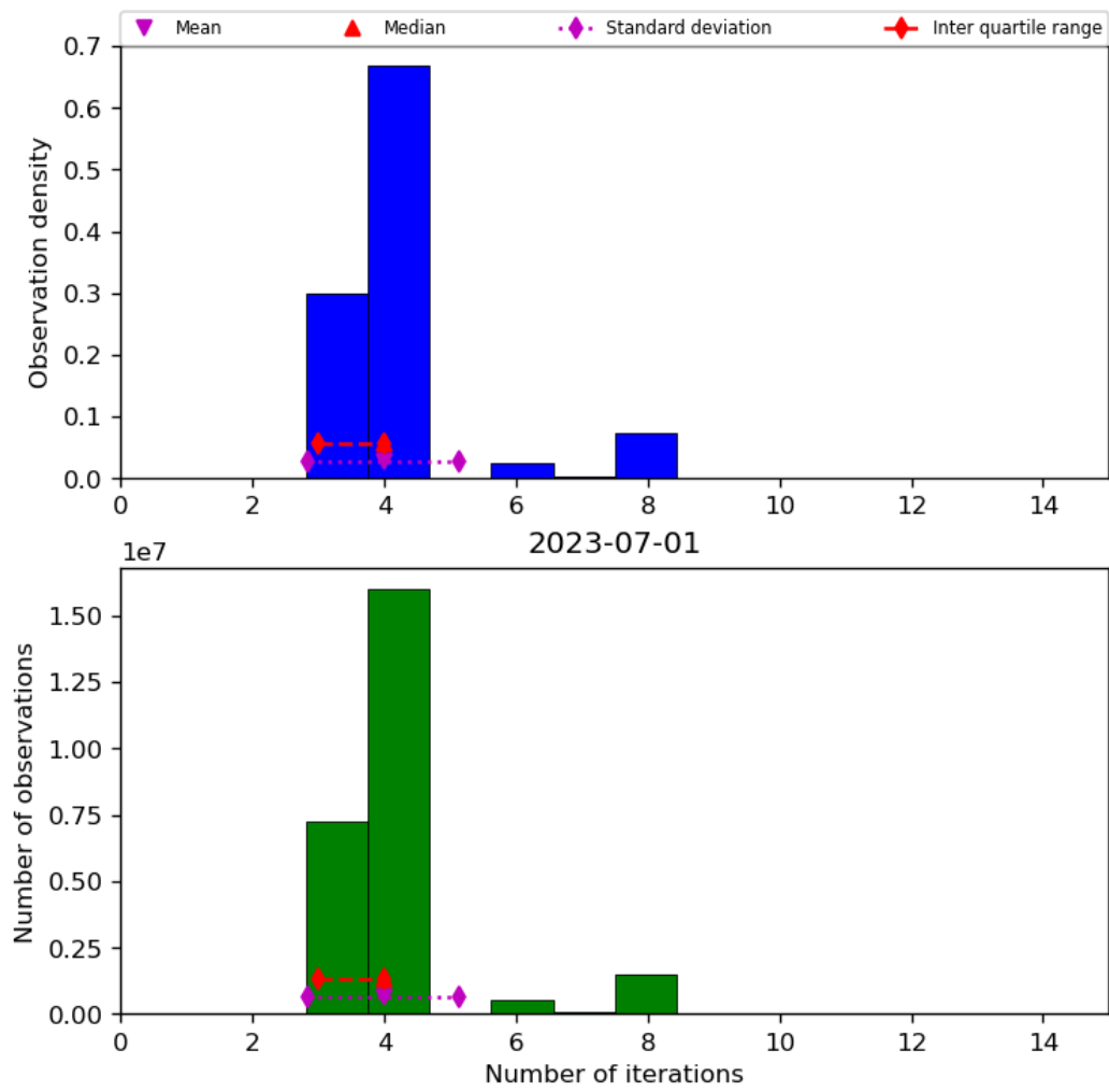
Figure 34: Histogram of “Number of iterations” for 2023-06-30 to 2023-07-02
