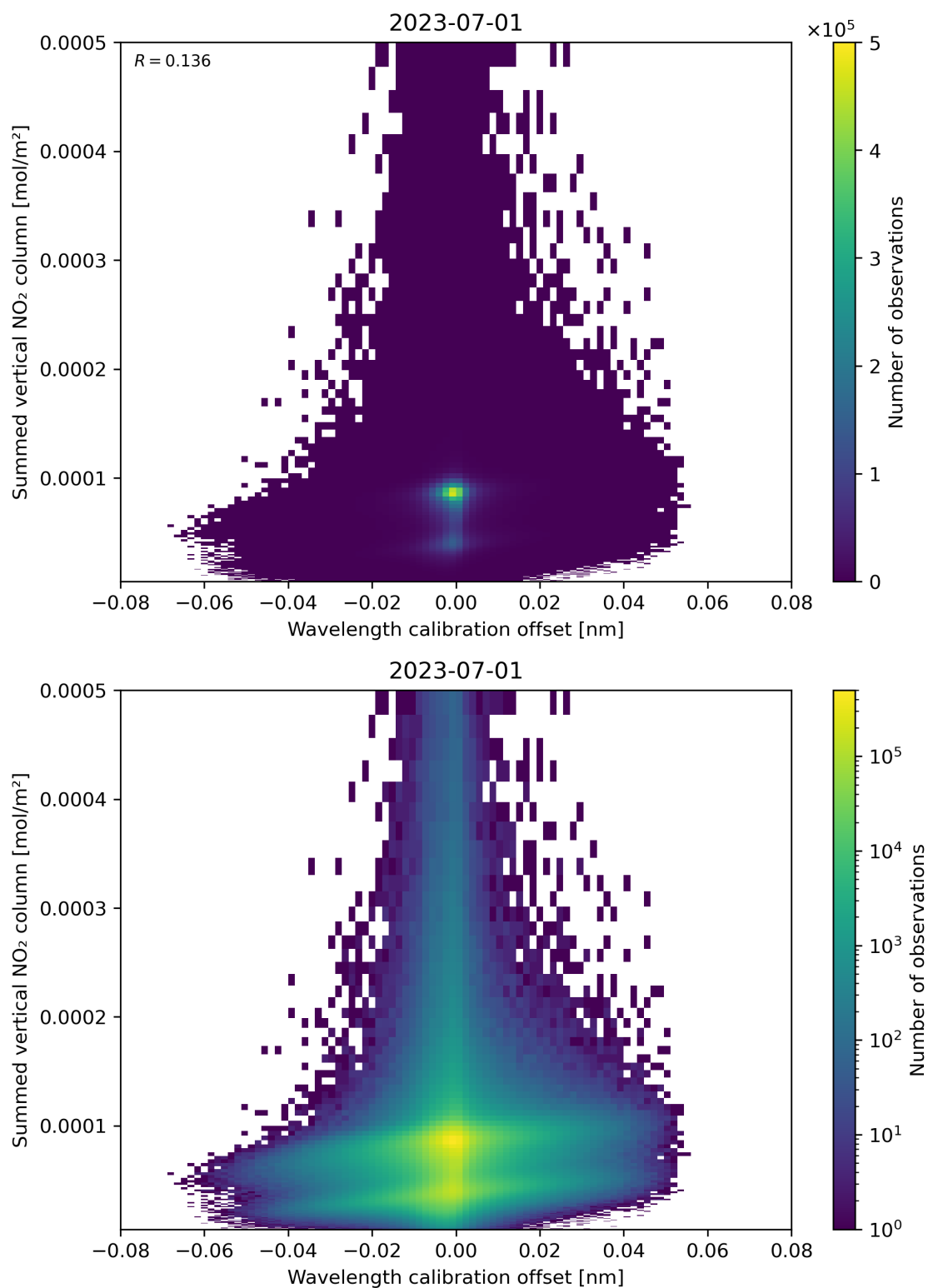
Figure 177: Scatter density plot of “Wavelength calibration offset” against “Summed vertical NO 2 column” for 2023-06-30 to 2023-07-02.
