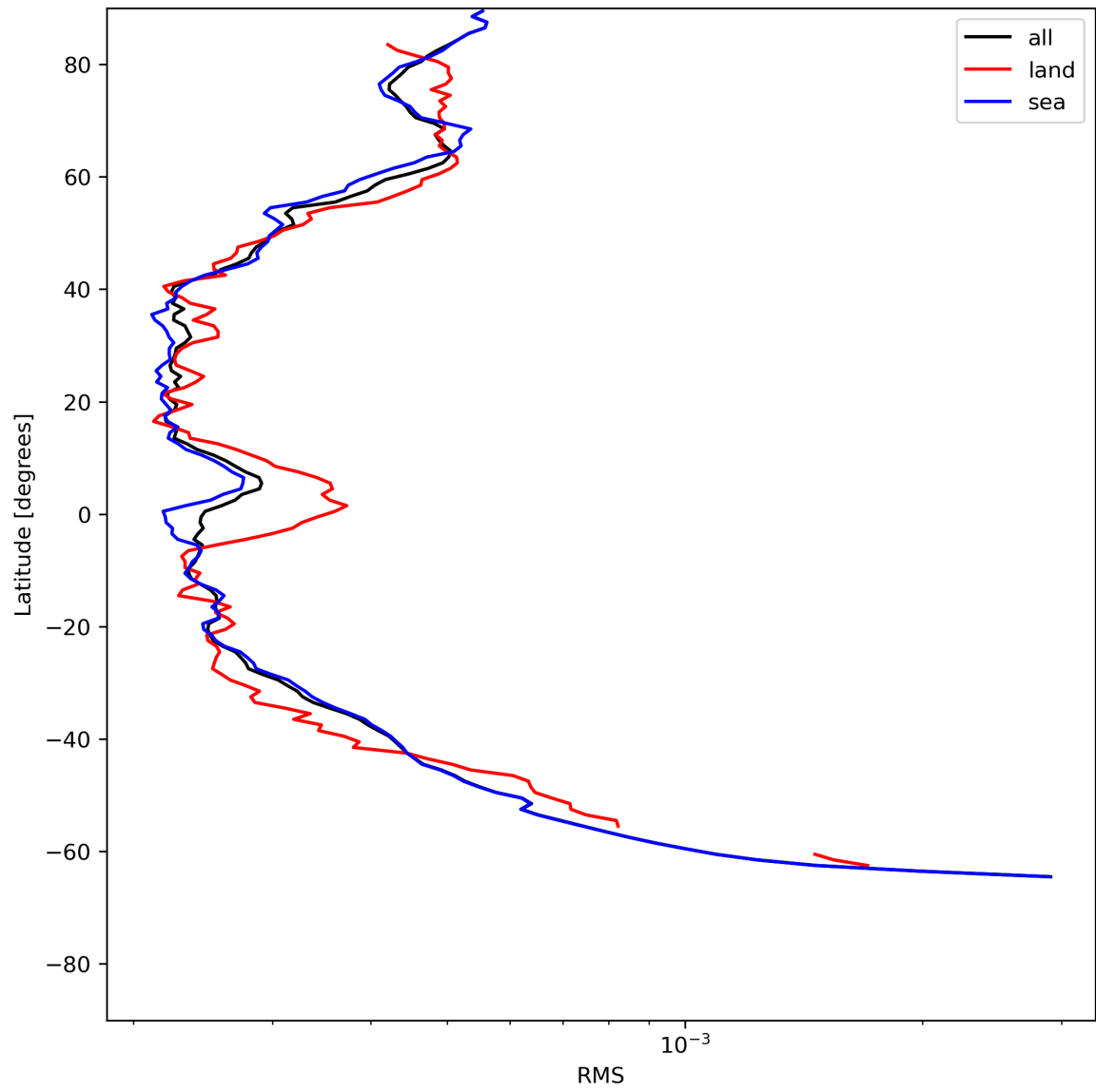
Figure 26: Zonal average of “RMS” for 2023-06-30 to 2023-07-02.
