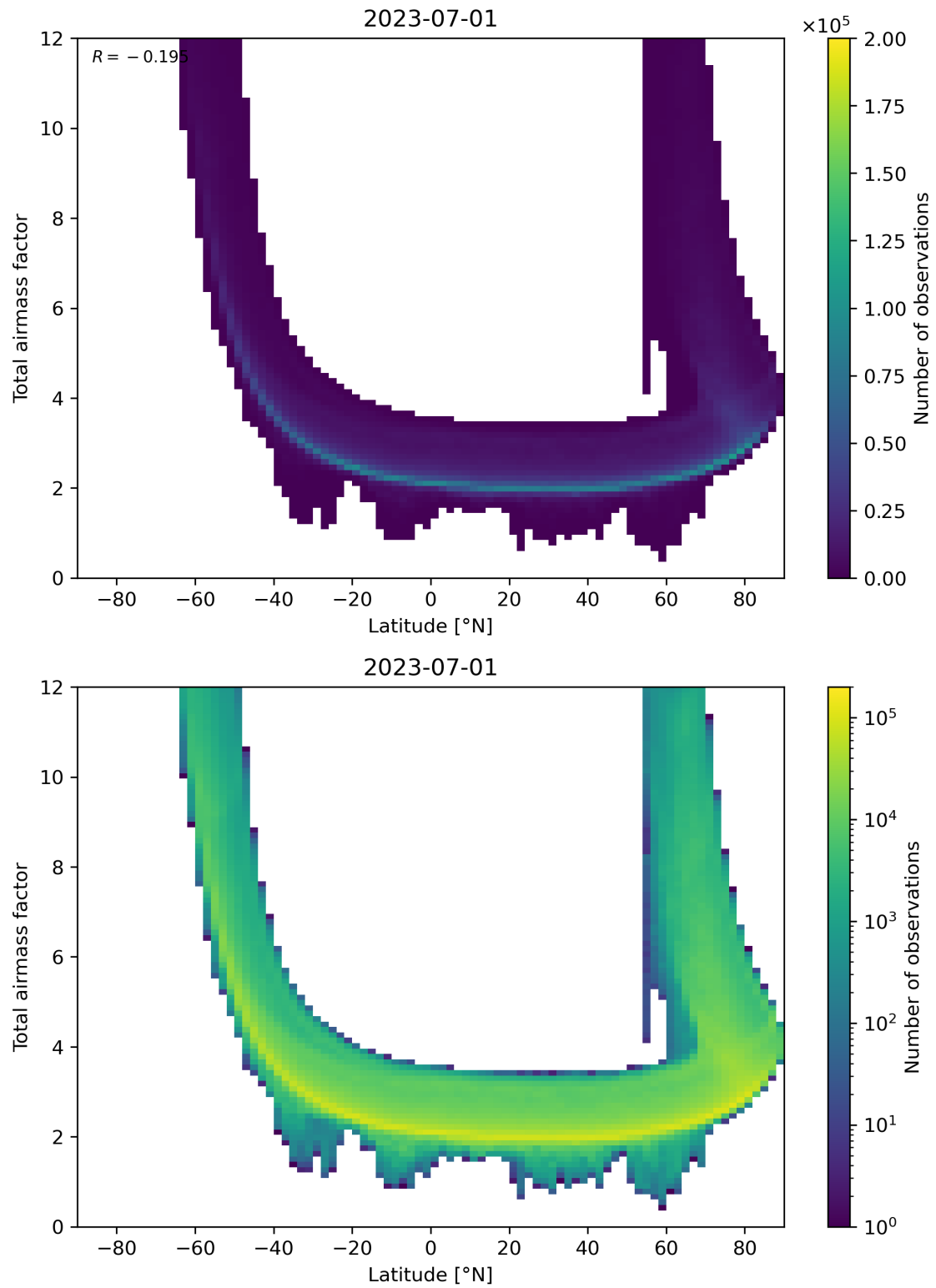
Figure 84: Scatter density plot of “Latitude” against “Total airmass factor” for 2023-06-30 to 2023-07-02.
