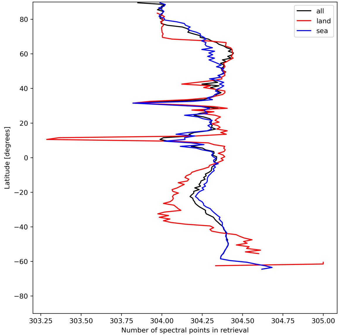
Figure 16: Zonal average of “Number of spectral points in retrieval” for 2023-06-30 to 2023-07-02.
