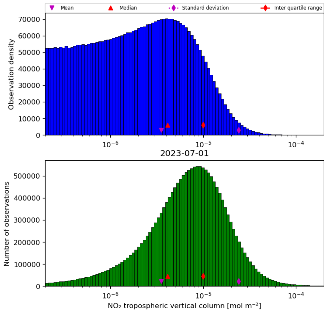
Figure 29: Histogram of “NO 2 tropospheric vertical column” for 2023-06-30 to 2023-07-02
