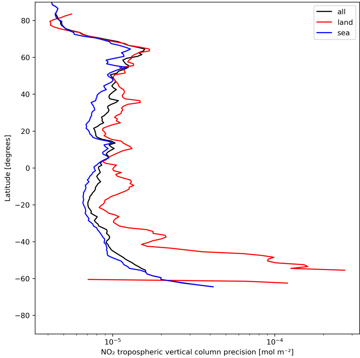
Figure 13: Zonal average of “NO 2 tropospheric vertical column precision” for 2023-06-30 to 2023-07-02.
