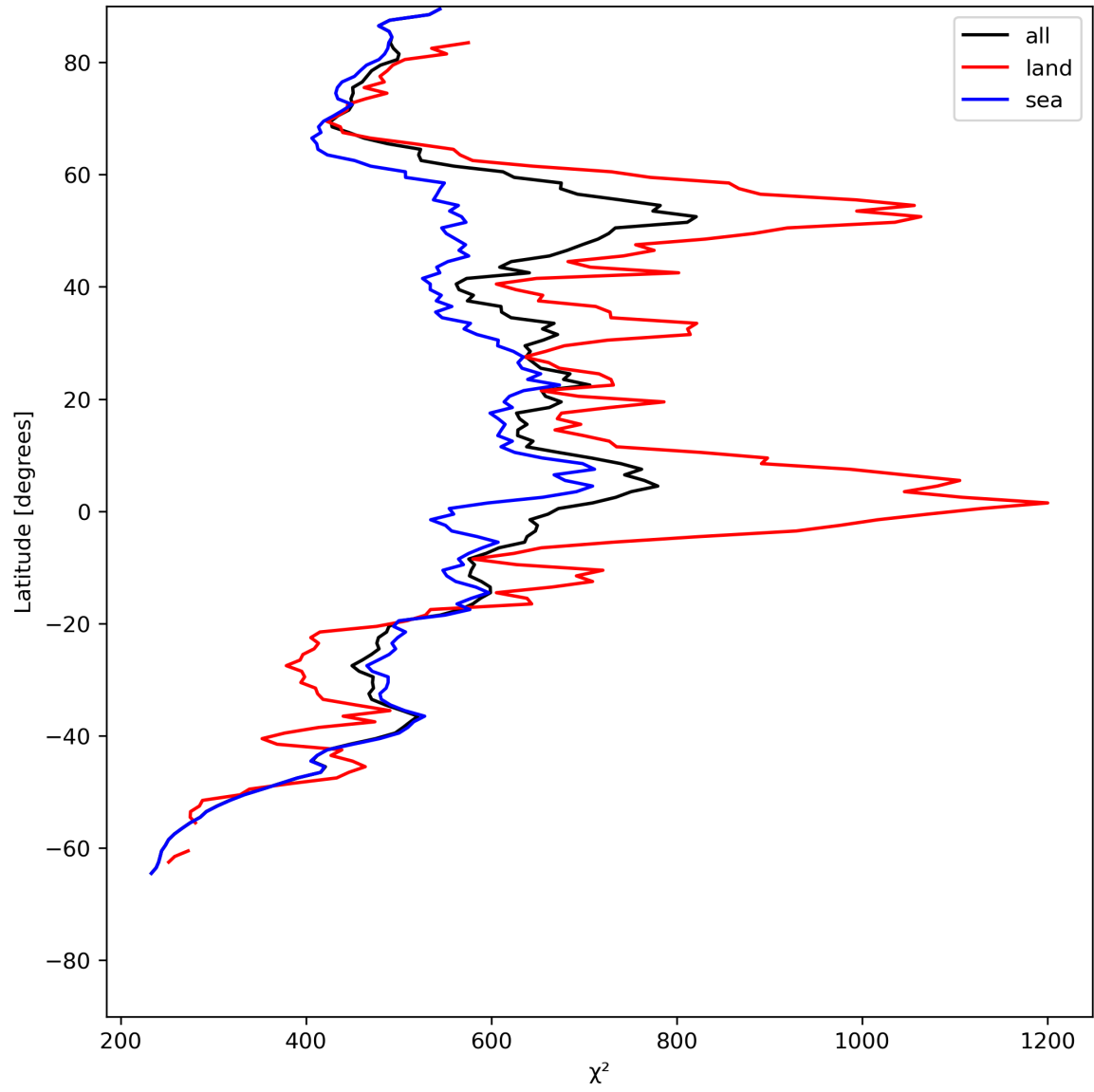
Figure 25: Zonal average of “ \chi^2 ” for 2023-06-30 to 2023-07-02.
