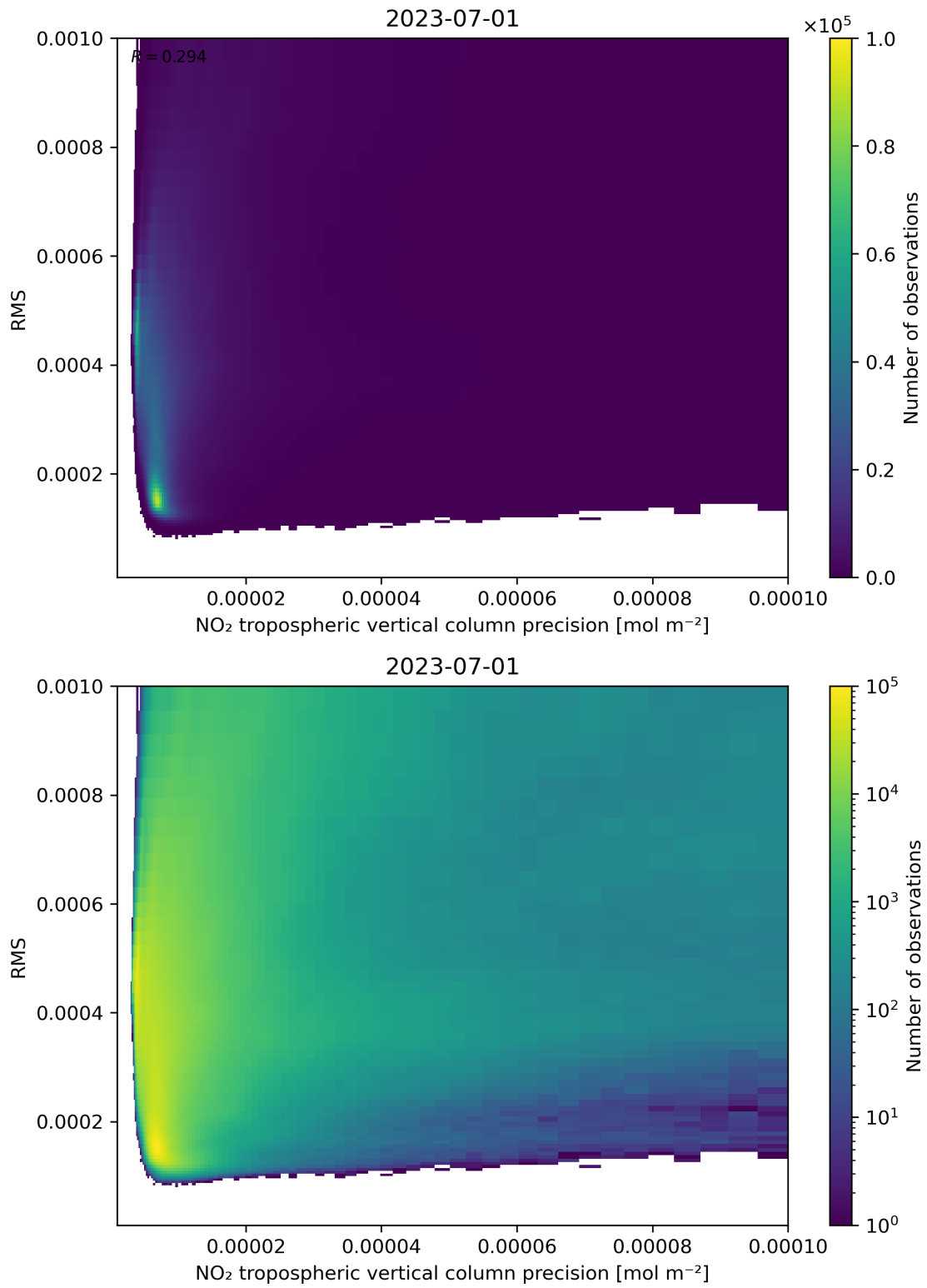
Figure 140: Scatter density plot of “NO 2 tropospheric vertical column precision” against “RMS” for 2023-06-30 to 2023-07-02.
