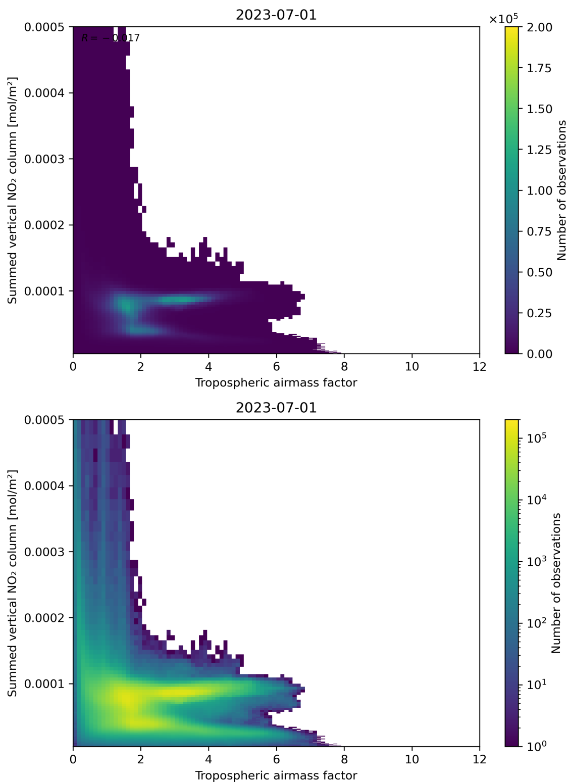
Figure 75: Scatter density plot of “Tropospheric airmass factor” against “Summed vertical NO 2 column” for 2023-06-30 to 2023-07-02.
