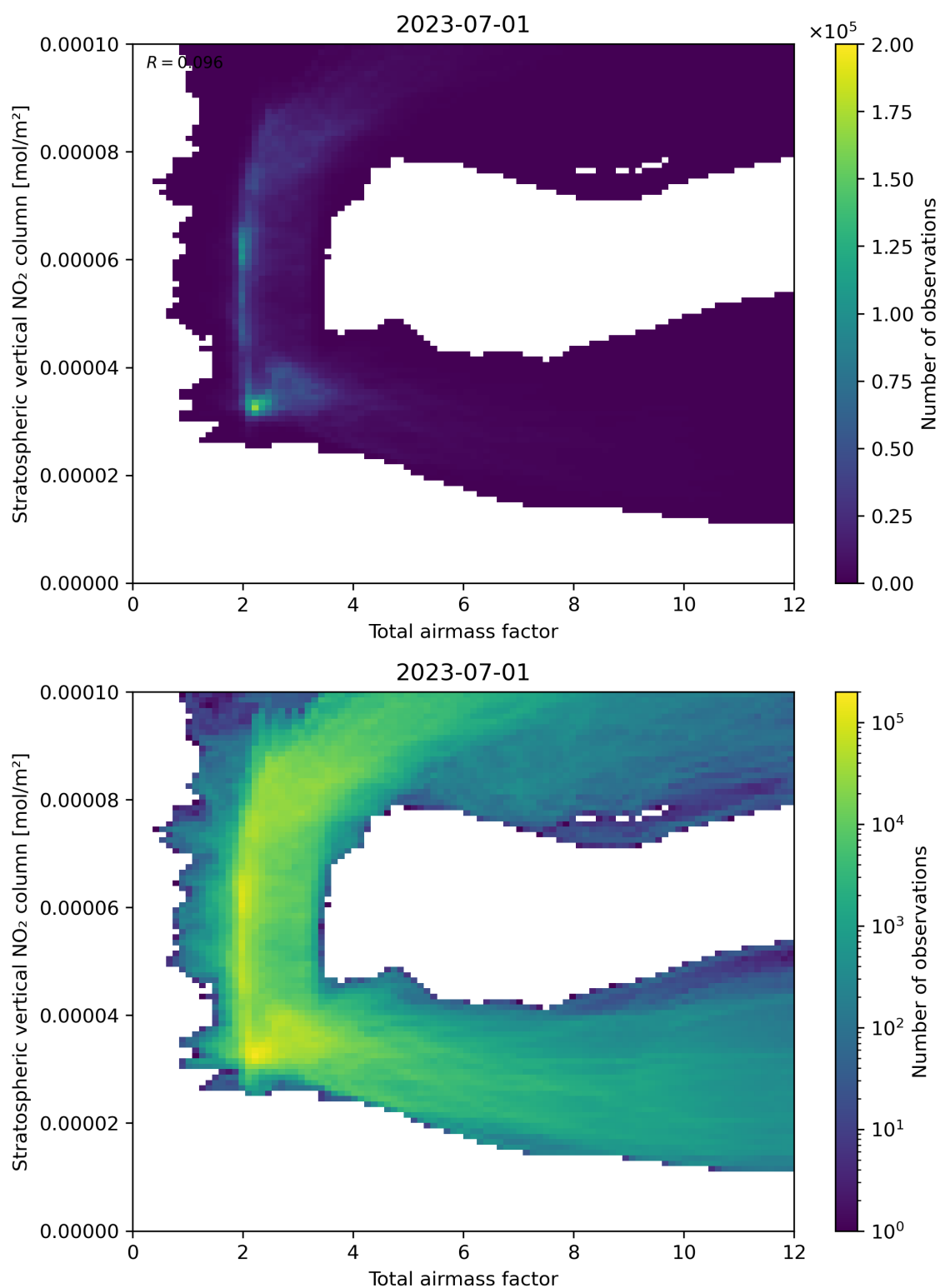
Figure 64: Scatter density plot of “Total airmass factor” against “Stratospheric vertical NO 2 column” for 2023-06-30 to 2023-07-02.
