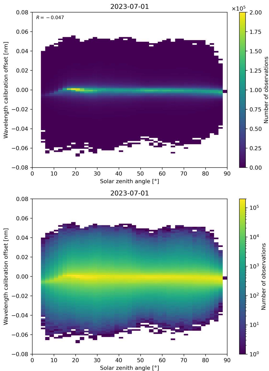
Figure 158: Scatter density plot of “Solar zenith angle” against “Wavelength calibration offset” for 2023-06-30 to 2023-07-02.
