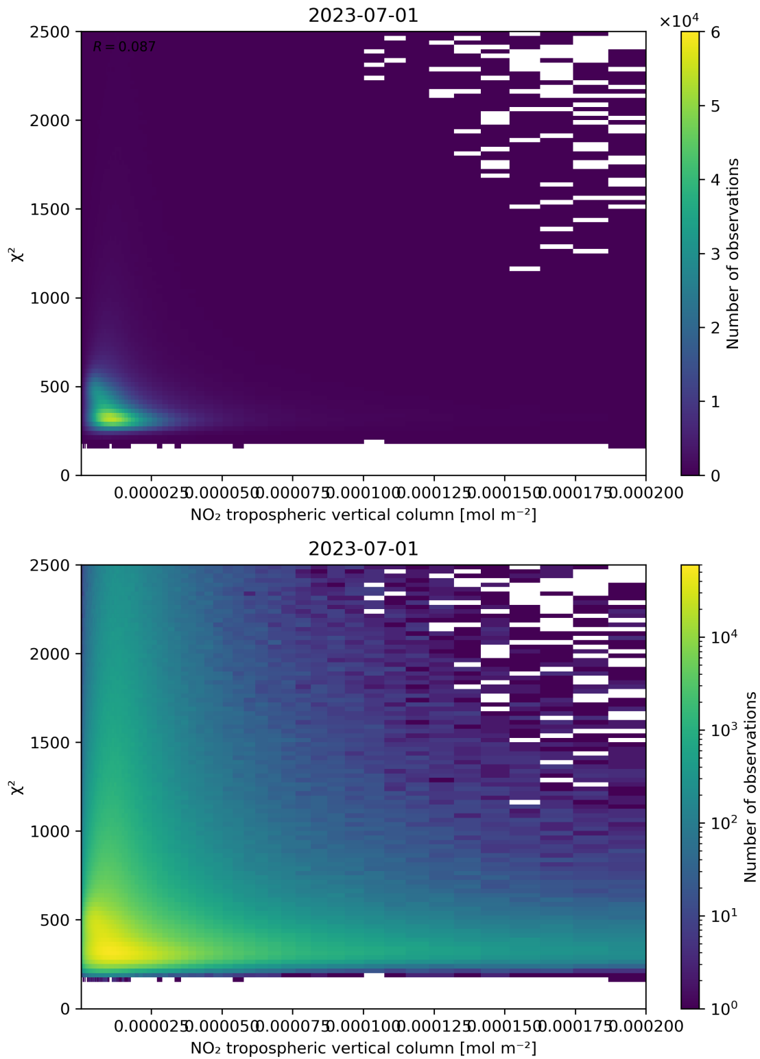
Figure 124: Scatter density plot of “NO 2 tropospheric vertical column” against “ \chi^2 ” for 2023-06-30 to 2023-07-02.
