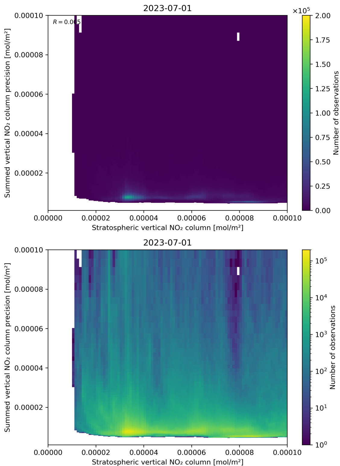
Figure 99: Scatter density plot of “Stratospheric vertical NO 2 column” against “Summed vertical NO 2 column precision” for 2023-06-30 to 2023-07-02.
