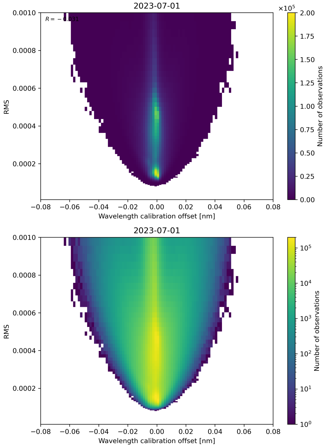
Figure 181: Scatter density plot of “Wavelength calibration offset” against “RMS” for 2023-06-30 to 2023-07-02.
