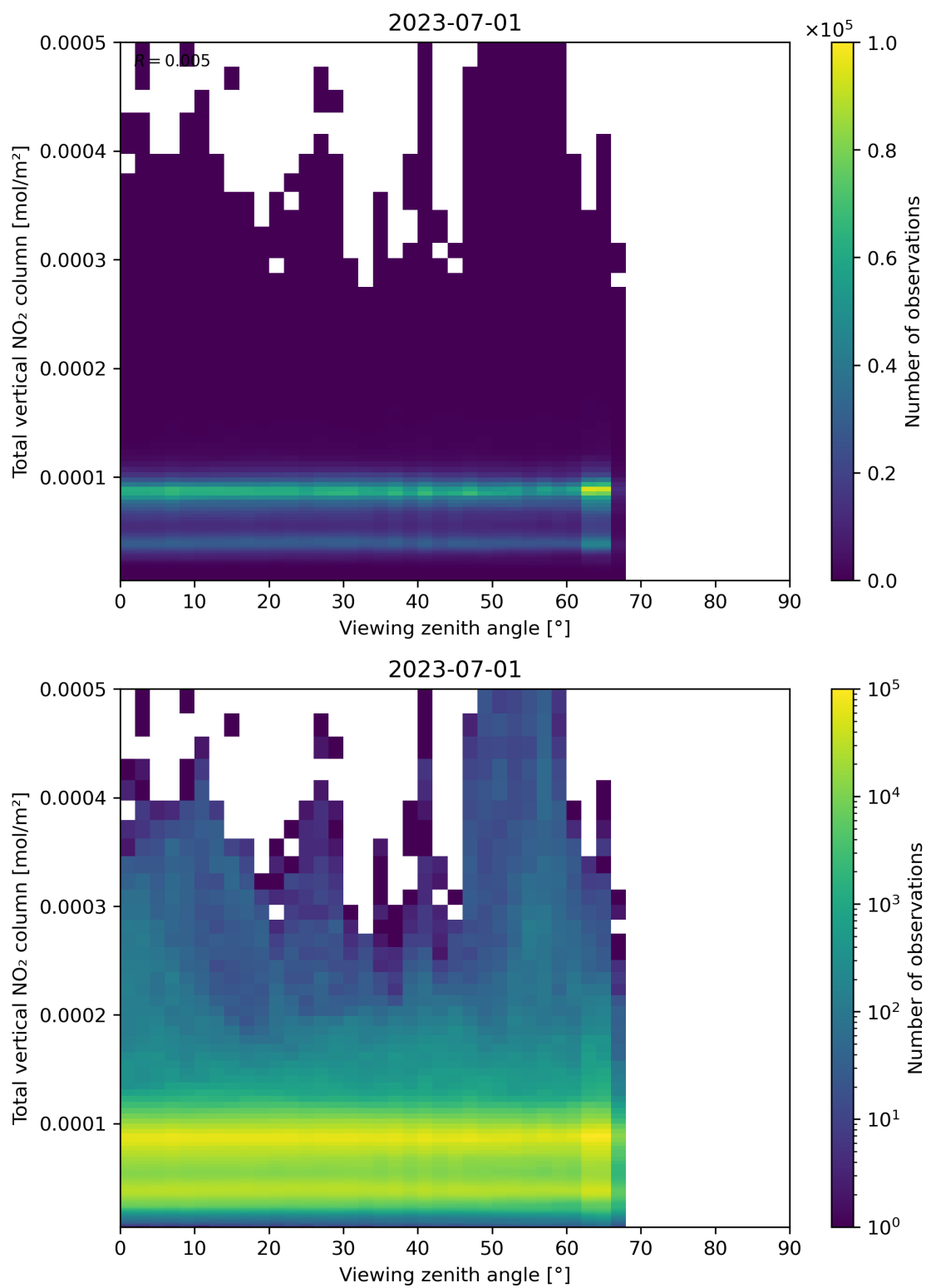
Figure 167: Scatter density plot of “Viewing zenith angle” against “Total vertical NO 2 column” for 2023-06-30 to 2023-07-02.
