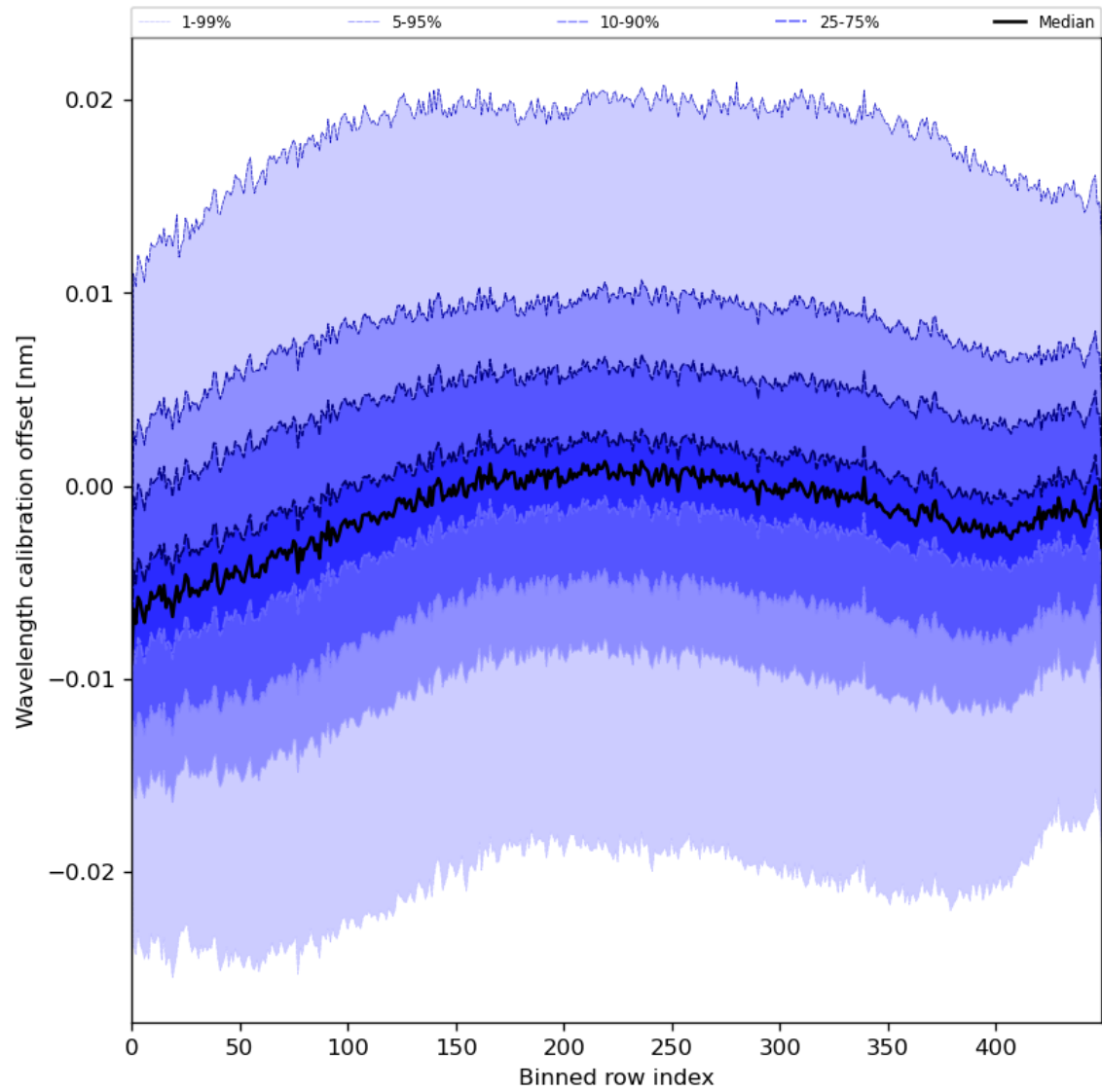
Figure 52: Along track statistics of “Wavelength calibration offset” for 2023-06-30 to 2023-07-02
