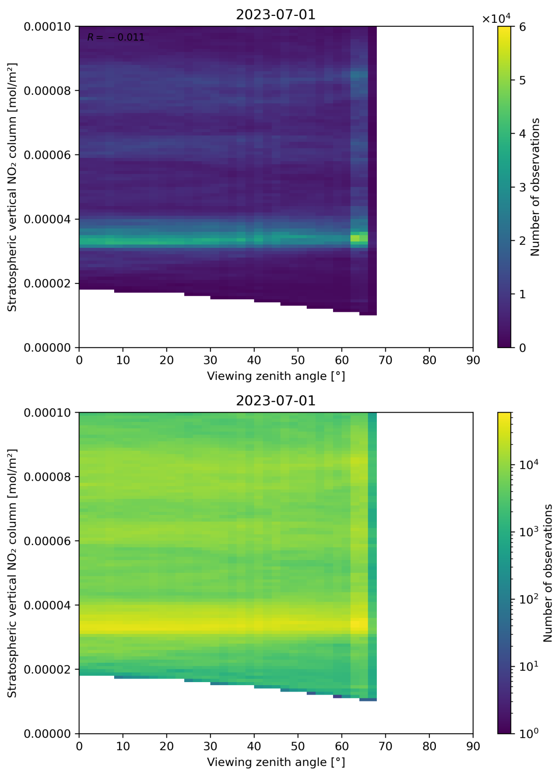
Figure 164: Scatter density plot of “Viewing zenith angle” against “Stratospheric vertical NO 2 column” for 2023-06-30 to 2023-07-02.
