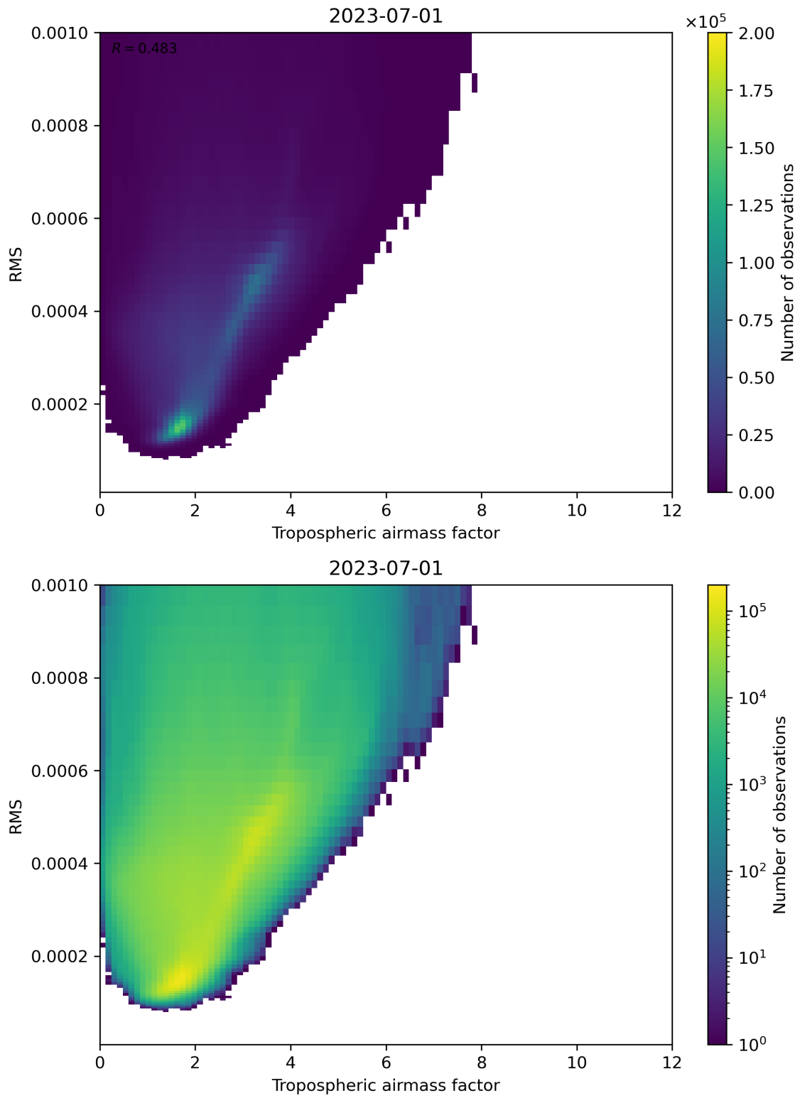
Figure 79: Scatter density plot of “Tropospheric airmass factor” against “RMS” for 2023-06-30 to 2023-07-02.
