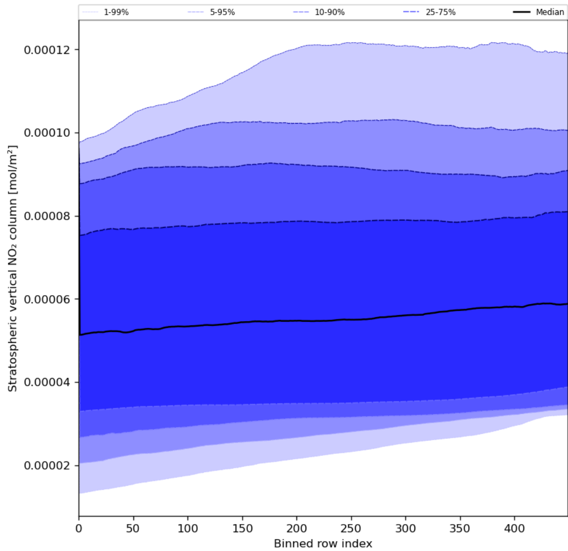
Figure 53: Along track statistics of “Stratospheric vertical NO 2 column” for 2023-06-30 to 2023-07-02
