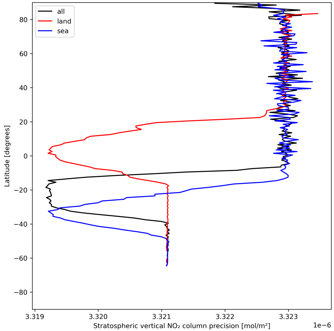
Figure 20: Zonal average of “Stratospheric vertical NO 2 column precision” for 2023-06-30 to 2023-07-02.
