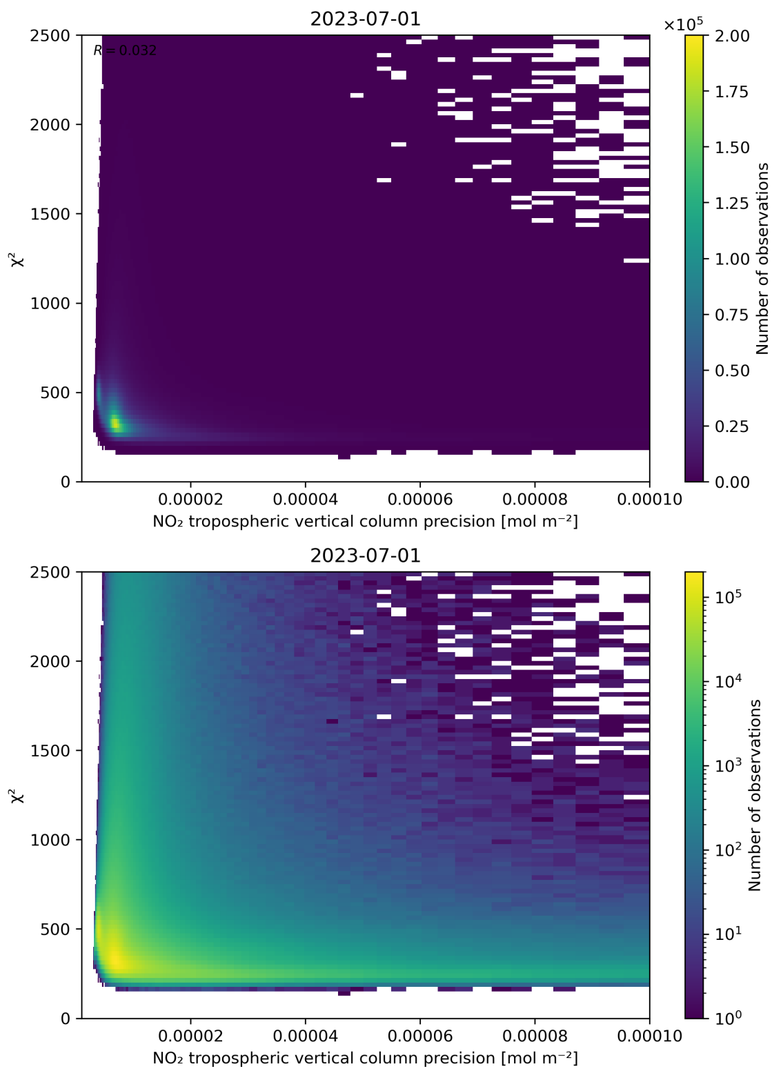
Figure 134: Scatter density plot of “NO 2 tropospheric vertical column precision” against “ \chi^2 ” for 2023-06-30 to 2023-07-02.
