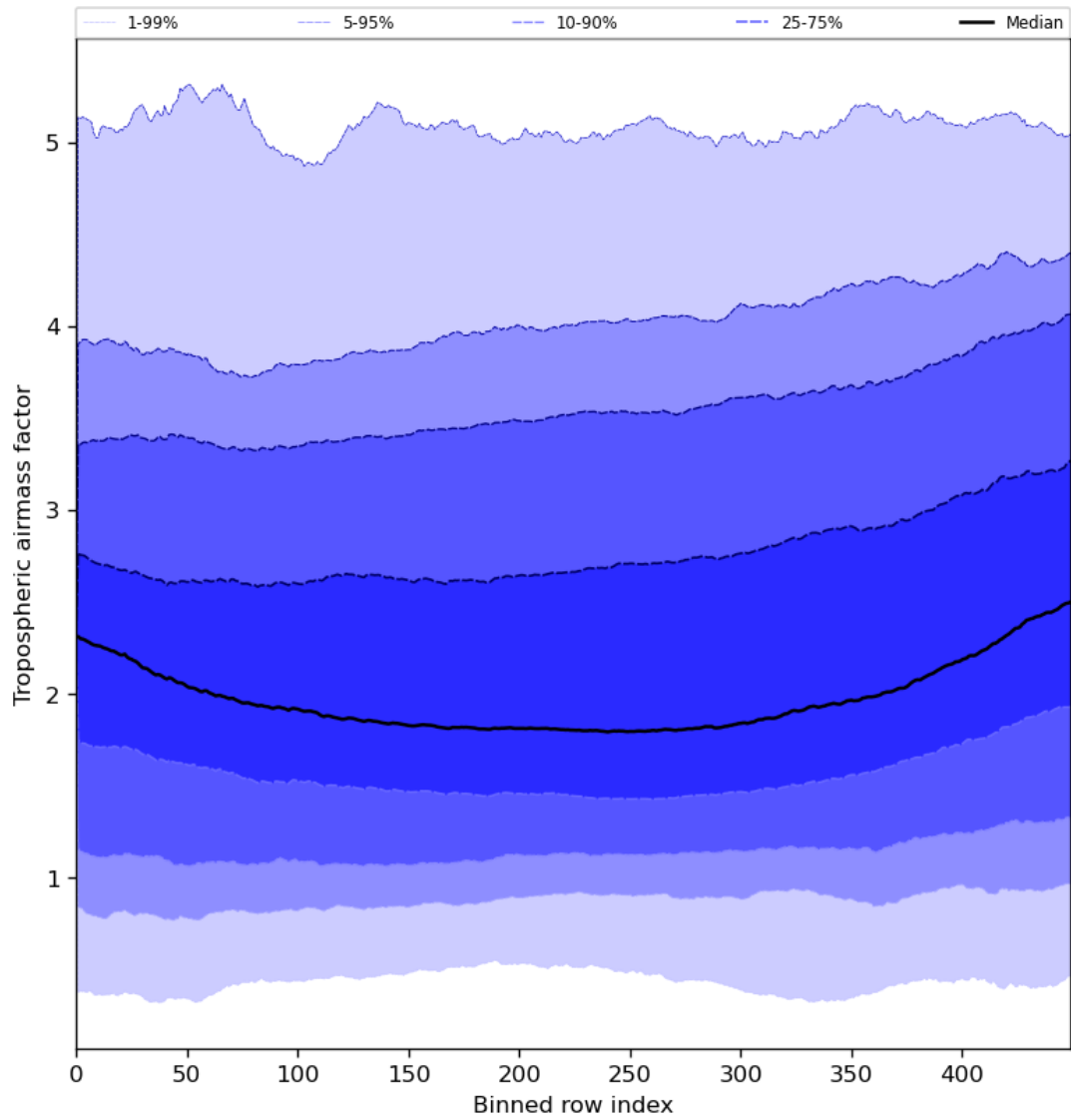
Figure 48: Along track statistics of “Tropospheric airmass factor” for 2023-06-30 to 2023-07-02
