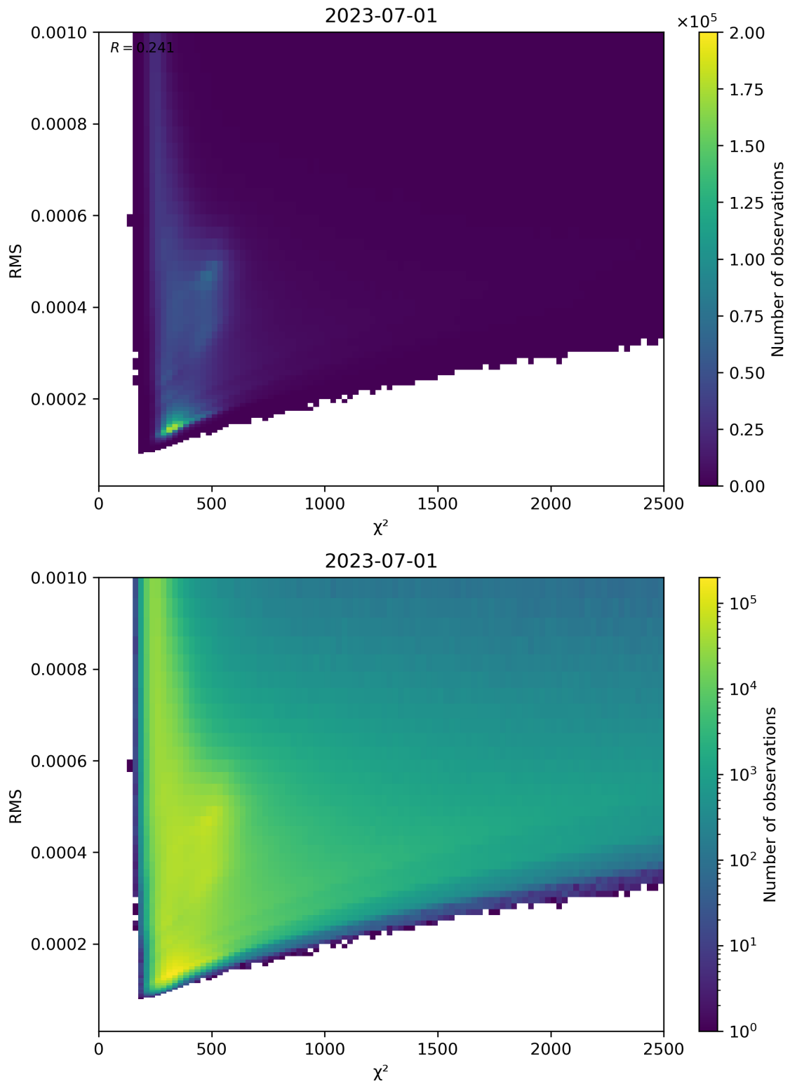
Figure 82: Scatter density plot of “ \chi^2 ” against “RMS” for 2023-06-30 to 2023-07-02.
