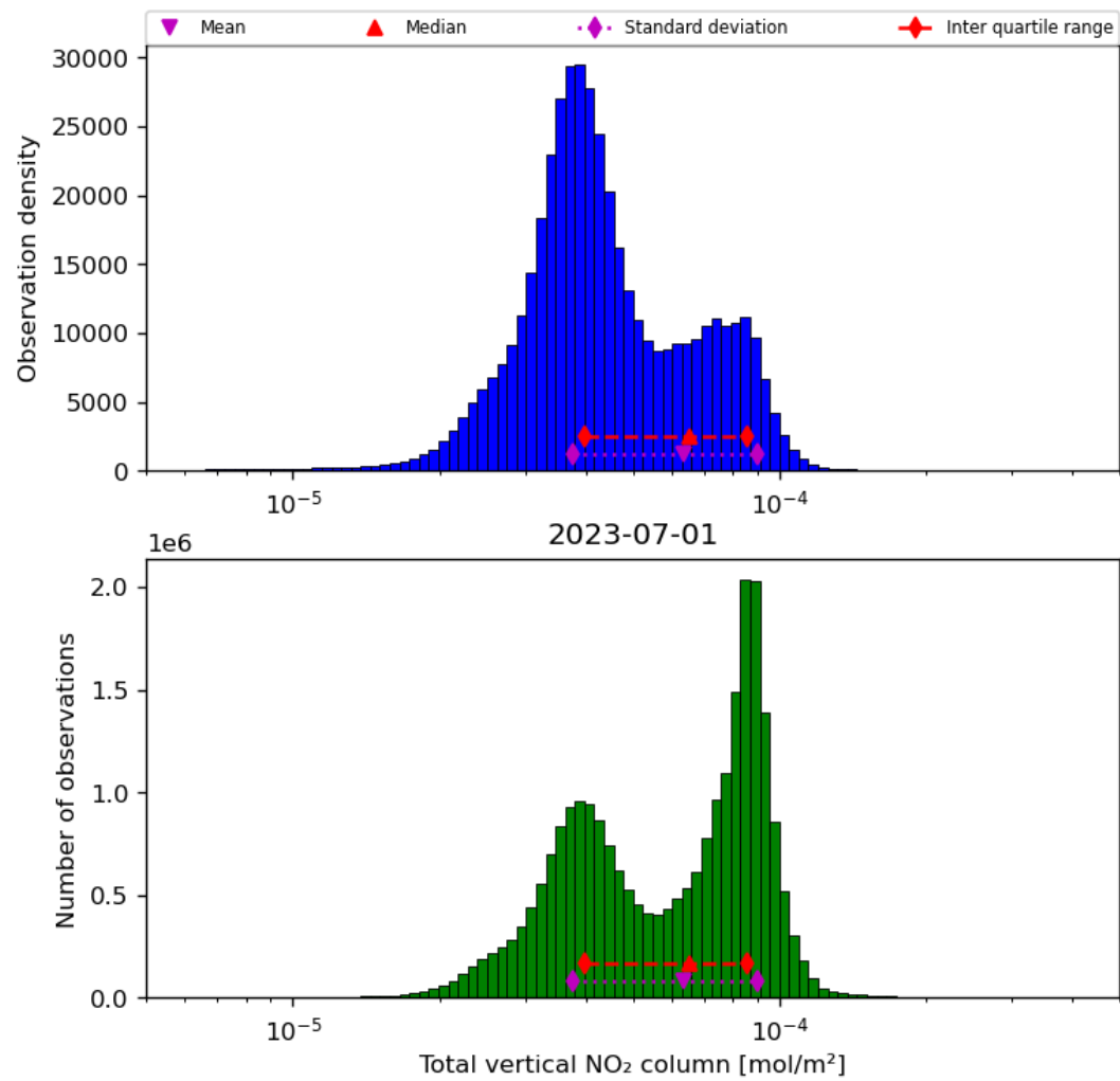
Figure 38: Histogram of “Total vertical NO 2 column” for 2023-06-30 to 2023-07-02
