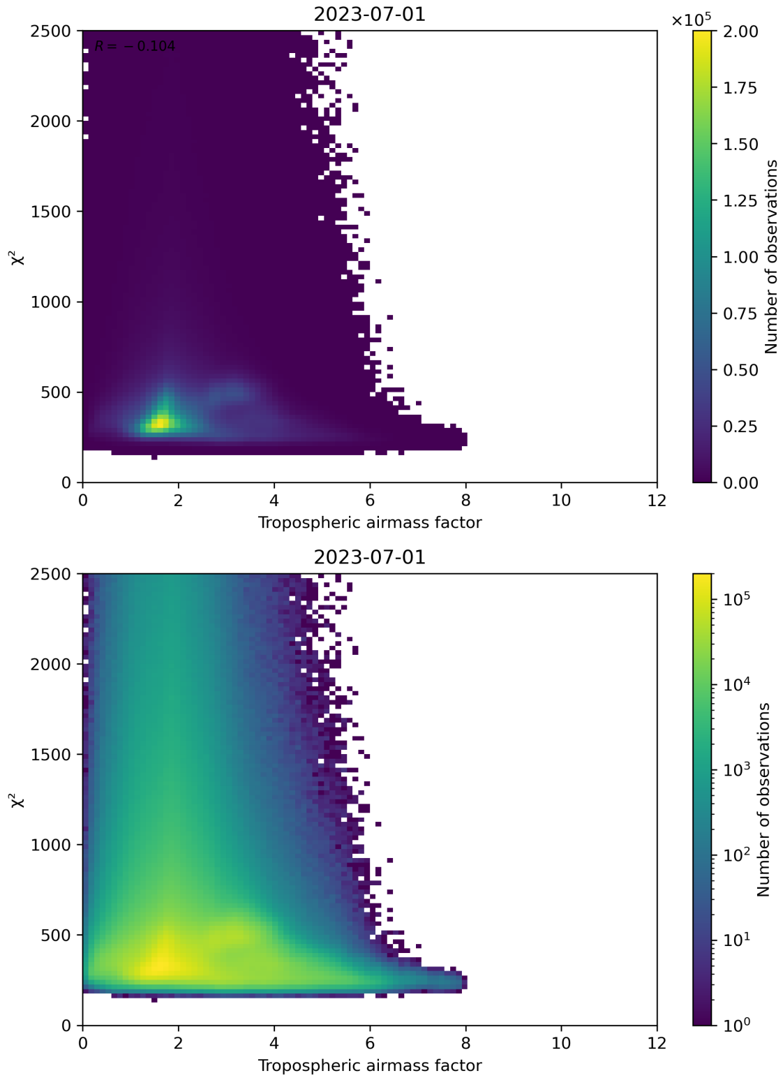
Figure 73: Scatter density plot of “Tropospheric airmass factor” against “ \chi^2 ” for 2023-06-30 to 2023-07-02.
