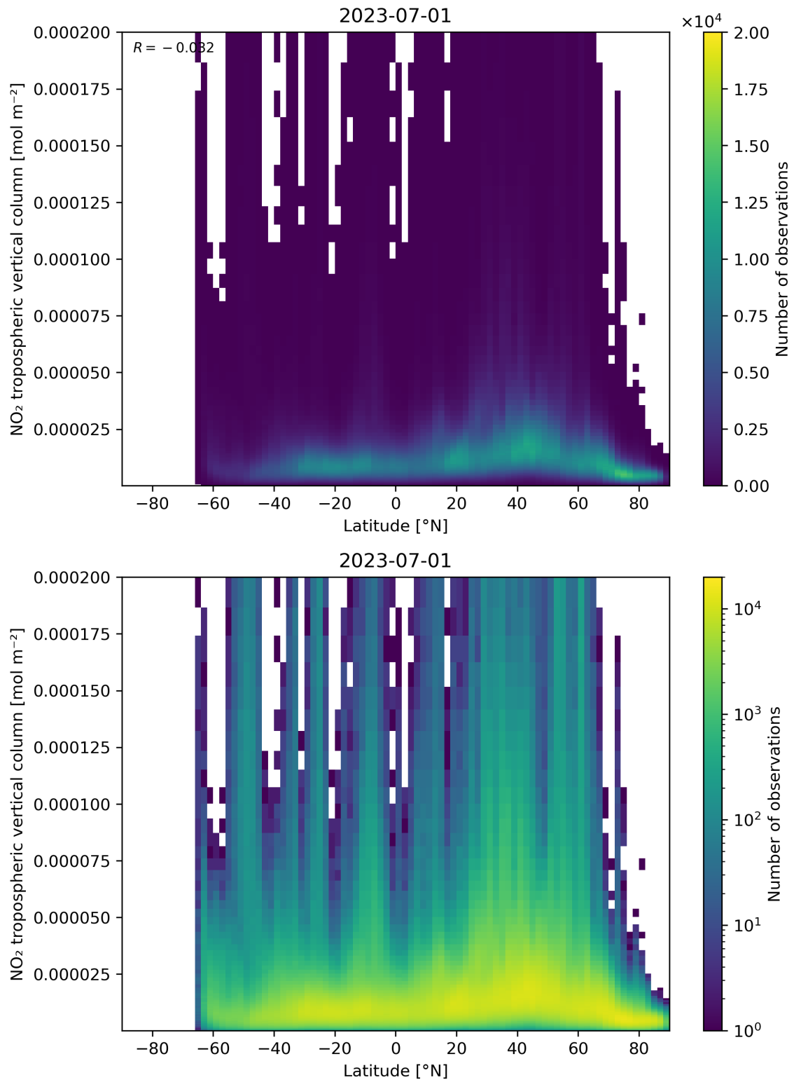
Figure 92: Scatter density plot of “Latitude” against “NO 2 tropospheric vertical column” for 2023-06-30 to 2023-07-02.
