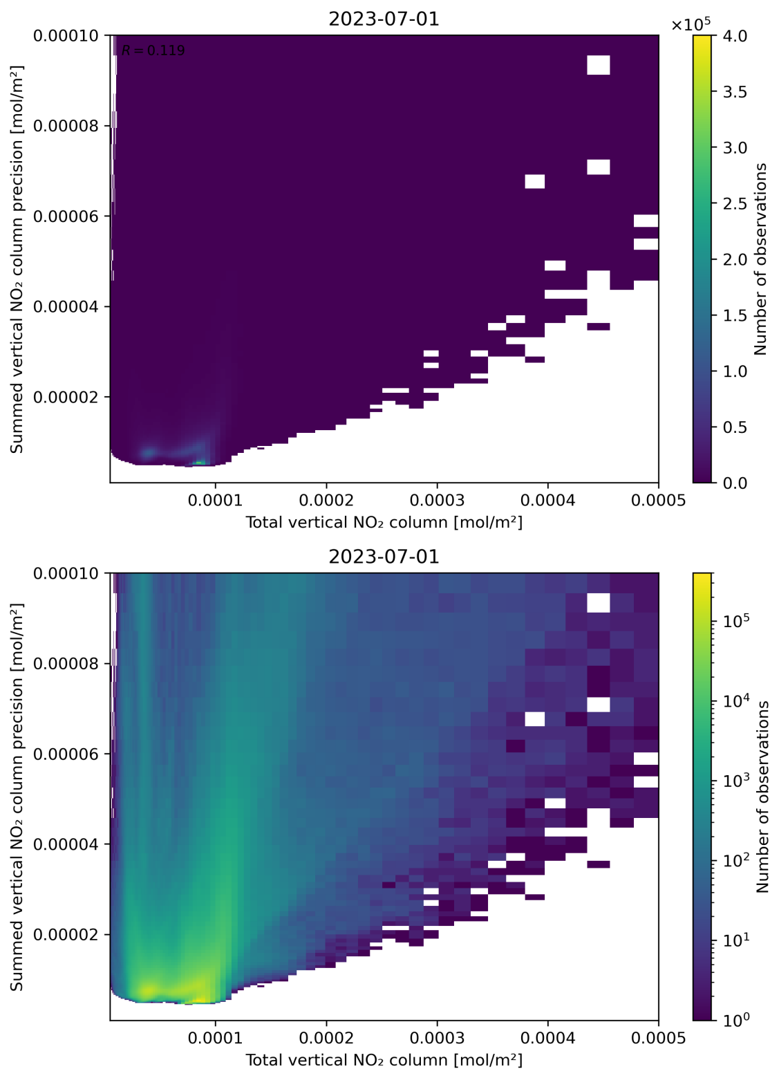
Figure 113: Scatter density plot of “Total vertical NO 2 column” against “Summed vertical NO 2 column precision” for 2023-06-30 to 2023-07-02.
