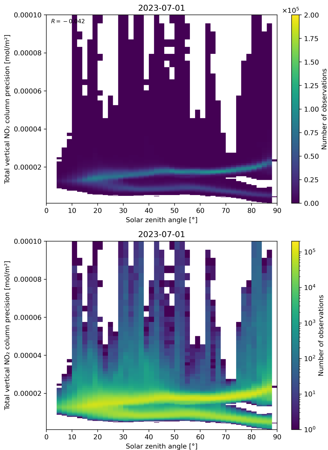
Figure 154: Scatter density plot of “Solar zenith angle” against “Total vertical NO 2 column precision” for 2023-06-30 to 2023-07-02.
