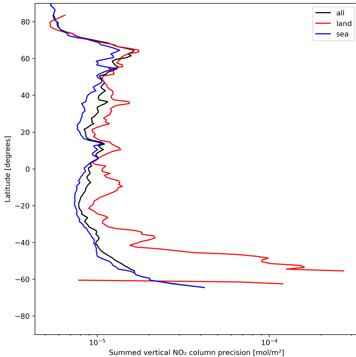
Figure 24: Zonal average of “Summed vertical NO 2 column precision” for 2023-06-30 to 2023-07-02.
