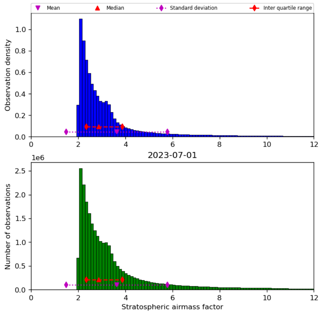
Figure 44: Histogram of “Stratospheric airmass factor” for 2023-06-30 to 2023-07-02
