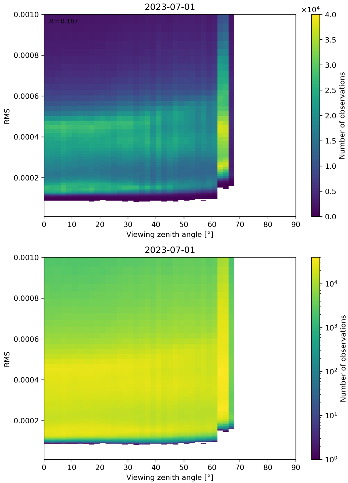
Figure 171: Scatter density plot of “Viewing zenith angle” against “RMS” for 2023-06-30 to 2023-07-02.
