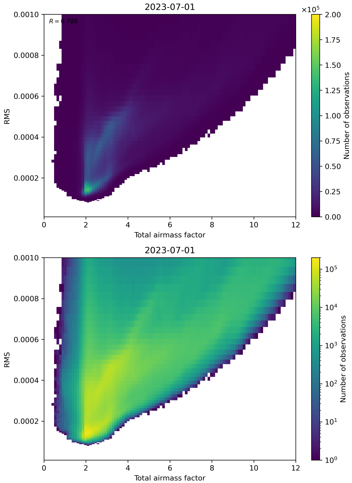
Figure 69: Scatter density plot of “Total airmass factor” against “RMS” for 2023-06-30 to 2023-07-02.
