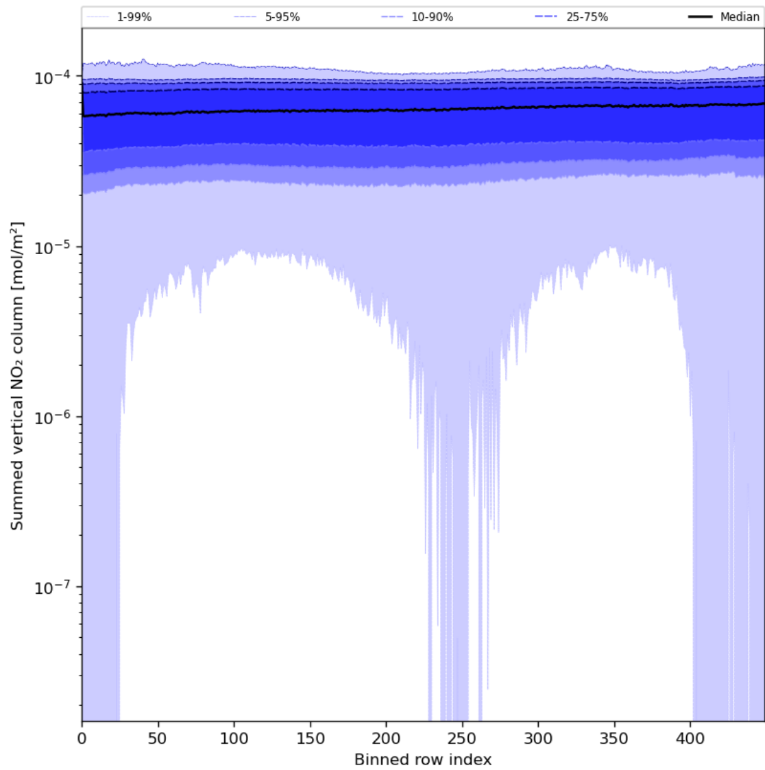
Figure 57: Along track statistics of “Summed vertical NO 2 column” for 2023-06-30 to 2023-07-02
