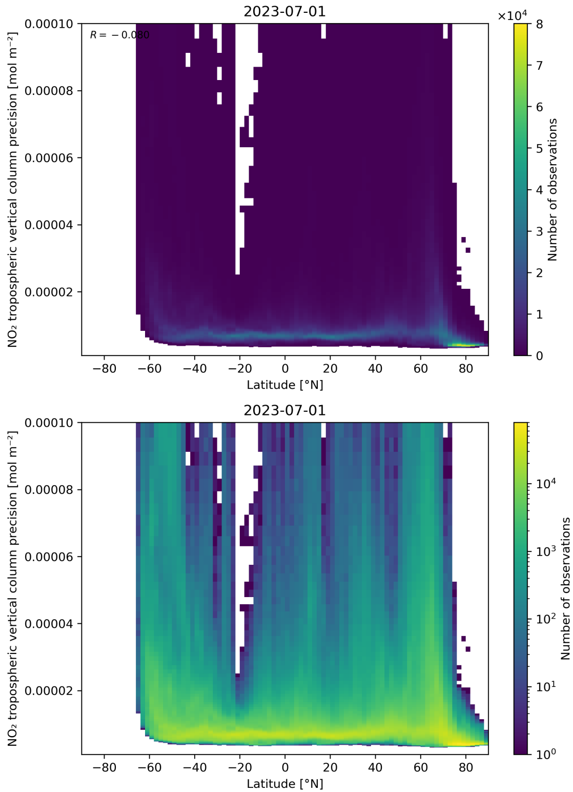
Figure 93: Scatter density plot of “Latitude” against “NO 2 tropospheric vertical column precision” for 2023-06-30 to 2023-07-02.
