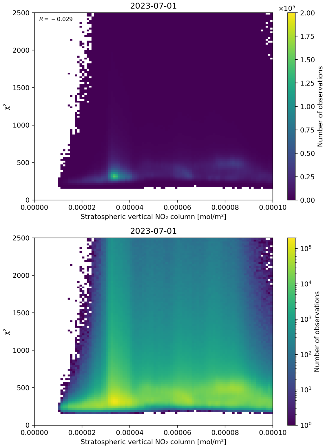
Figure 97: Scatter density plot of “Stratospheric vertical NO 2 column” against “ \chi^2 ” for 2023-06-30 to 2023-07-02.
