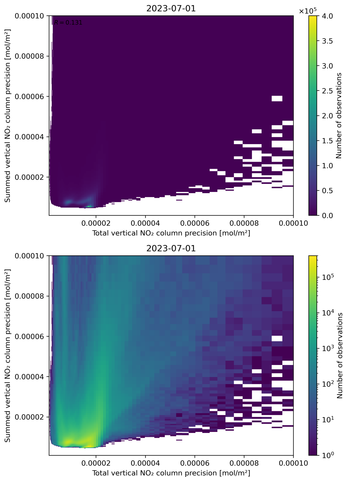
Figure 118: Scatter density plot of “Total vertical NO 2 column precision” against “Summed vertical NO 2 column precision” for 2023-06-30 to 2023-07-02.
