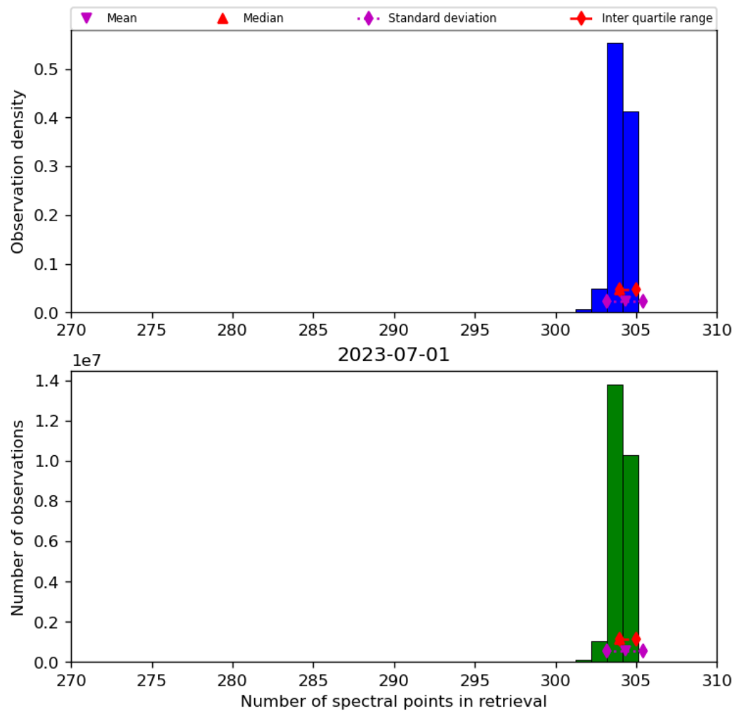
Figure 33: Histogram of “Number of spectral points in retrieval” for 2023-06-30 to 2023-07-02
