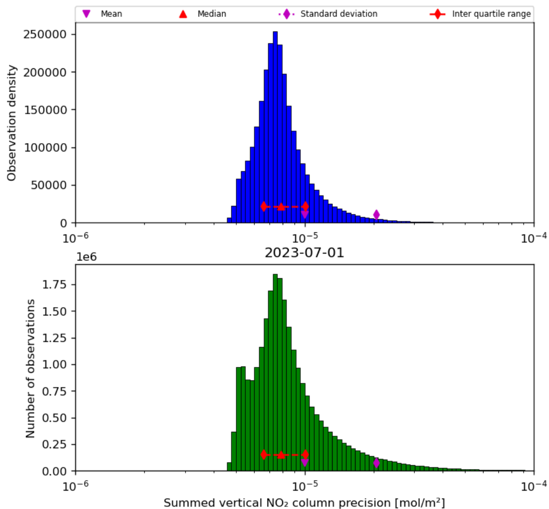
Figure 41: Histogram of “Summed vertical NO 2 column precision” for 2023-06-30 to 2023-07-02
