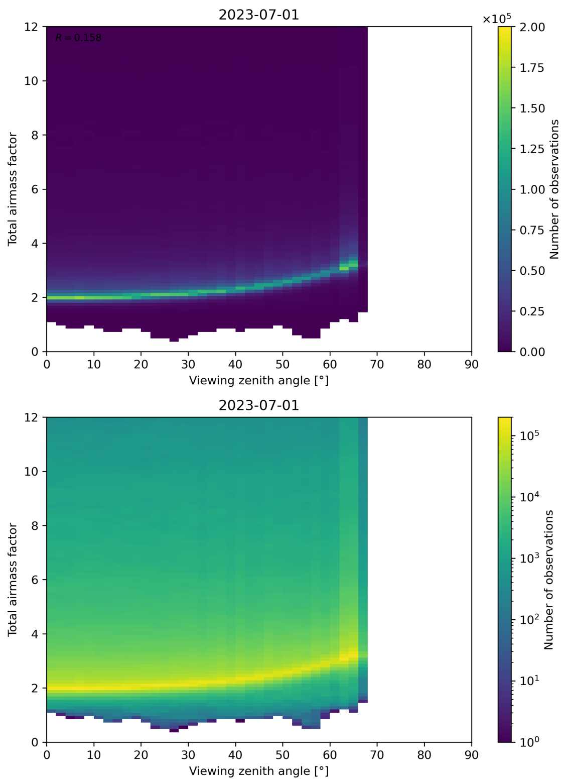
Figure 160: Scatter density plot of “Viewing zenith angle” against “Total airmass factor” for 2023-06-30 to 2023-07-02.
