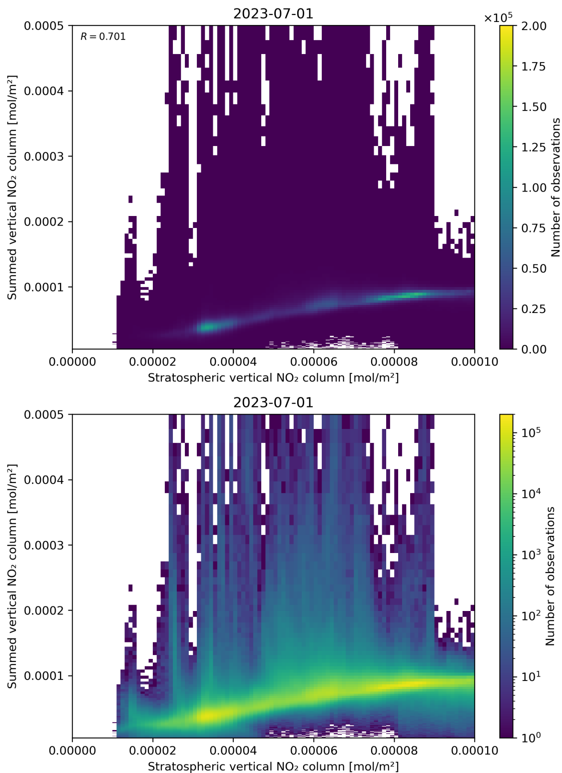
Figure 98: Scatter density plot of “Stratospheric vertical NO 2 column” against “Summed vertical NO 2 column” for 2023-06-30 to 2023-07-02.
