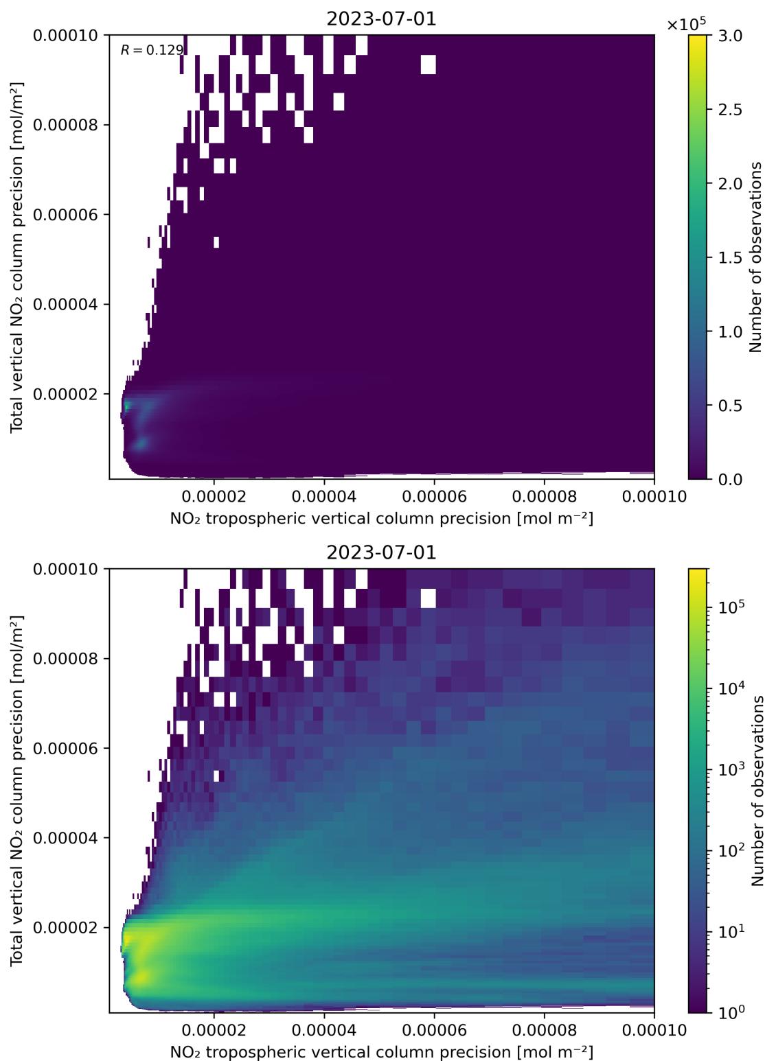
Figure 139: Scatter density plot of “NO 2 tropospheric vertical column precision” against “Total vertical NO 2 column precision” for 2023-06-30 to 2023-07-02.
