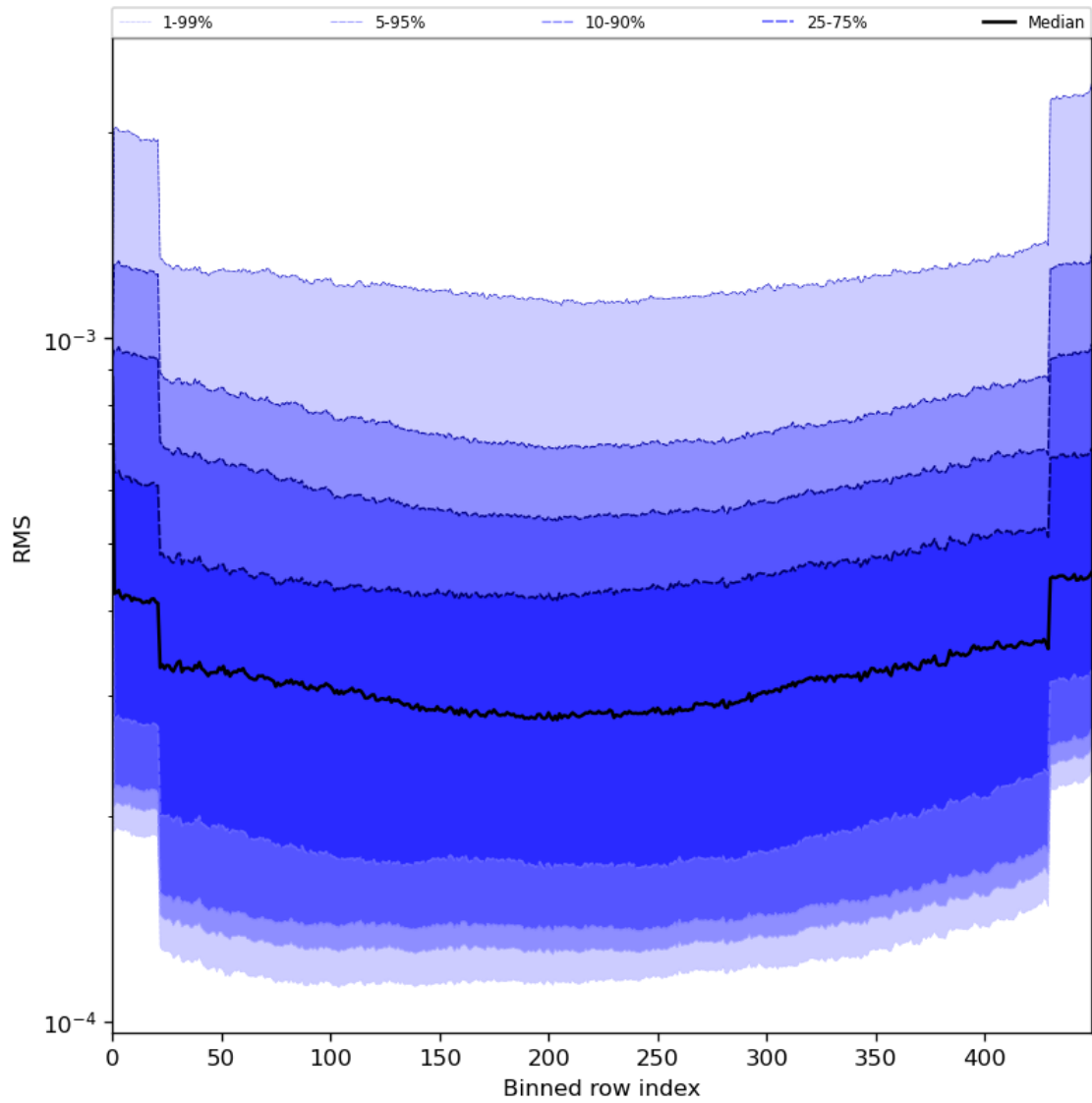
Figure 60: Along track statistics of “RMS” for 2023-06-30 to 2023-07-02
