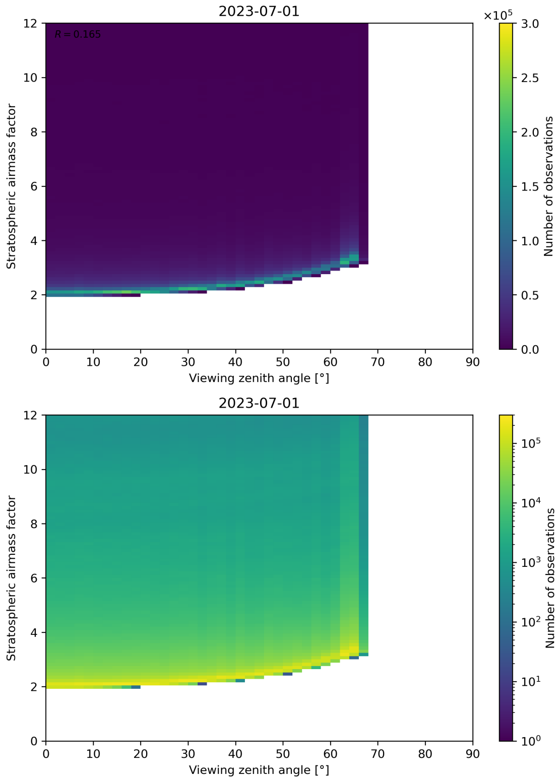
Figure 159: Scatter density plot of “Viewing zenith angle” against “Stratospheric airmass factor” for 2023-06-30 to 2023-07-02.
