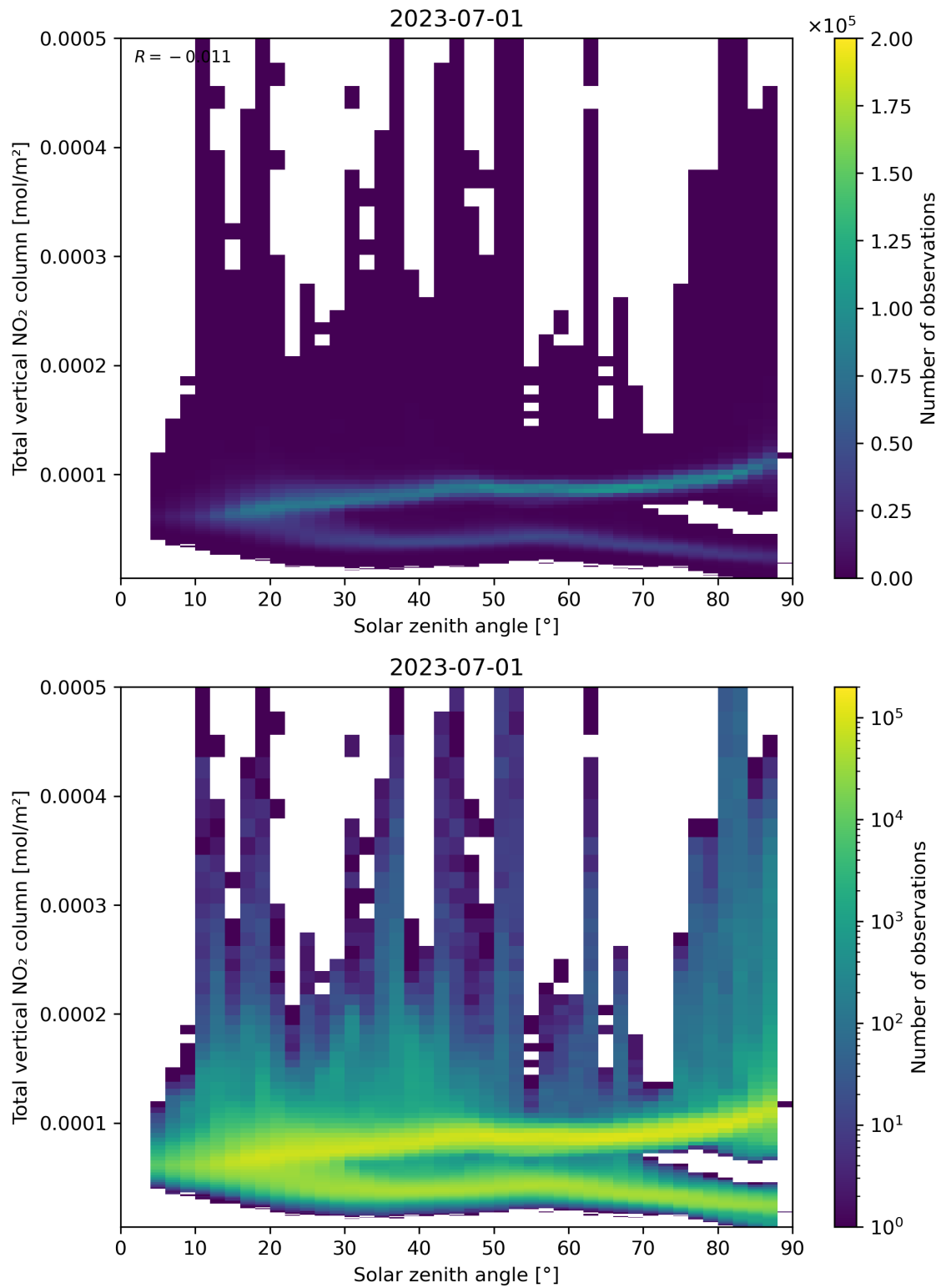
Figure 153: Scatter density plot of “Solar zenith angle” against “Total vertical NO 2 column” for 2023-06-30 to 2023-07-02.
