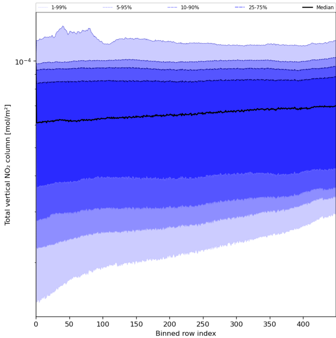
Figure 55: Along track statistics of “Total vertical NO 2 column” for 2023-06-30 to 2023-07-02
