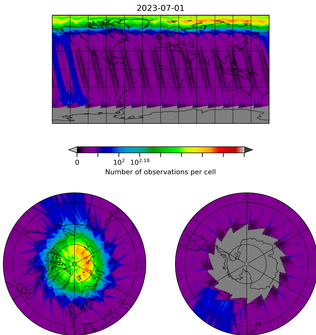
Figure 10: Map of the number of observations for 2023-06-30 to 2023-07-02
