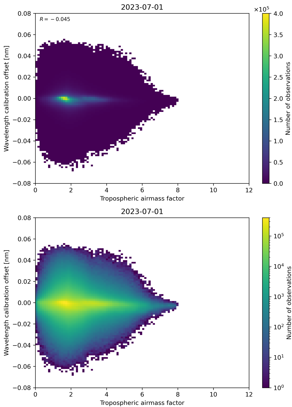
Figure 80: Scatter density plot of “Tropospheric airmass factor” against “Wavelength calibration offset” for 2023-06-30 to 2023-07-02.
