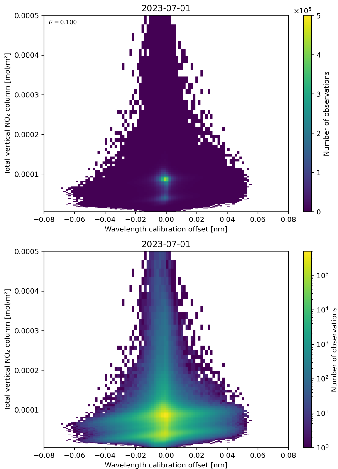
Figure 179: Scatter density plot of “Wavelength calibration offset” against “Total vertical NO 2 column” for 2023-06-30 to 2023-07-02.
