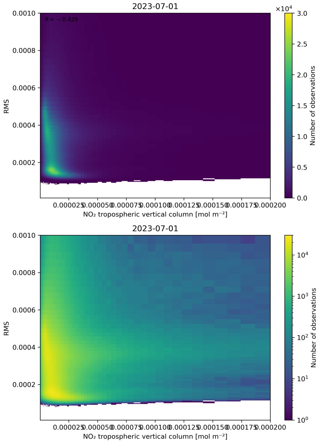
Figure 142: Scatter density plot of “NO 2 tropospheric vertical column” against “RMS” for 2023-06-30 to 2023-07-02.
