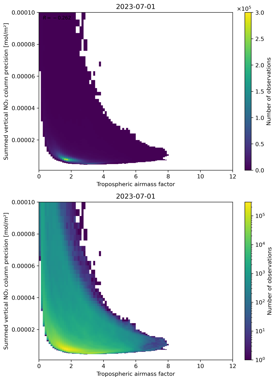
Figure 76: Scatter density plot of “Tropospheric air mass factor” against “Summed vertical NO 2 column precision” for 2023-06-30 to 2023-07-02.
