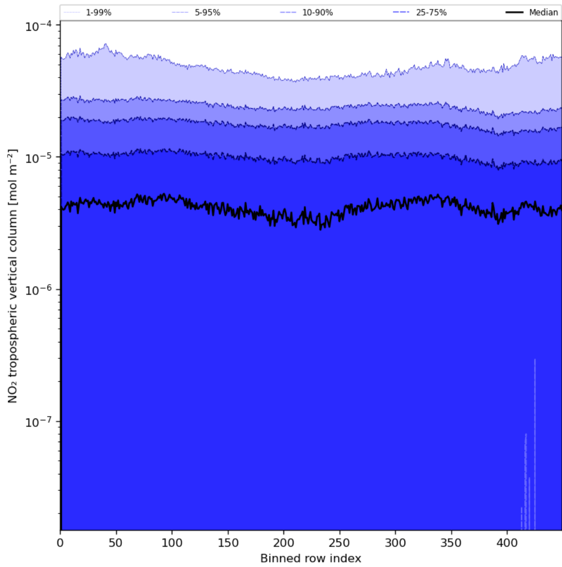
Figure 46: Along track statistics of “NO 2 tropospheric vertical column” for 2023-06-30 to 2023-07-02
