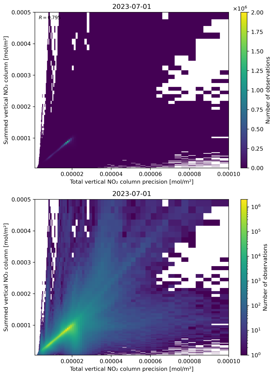
Figure 117: Scatter density plot of “Total vertical NO 2 column precision” against “Summed vertical NO 2 column” for 2023-06-30 to 2023-07-02.
