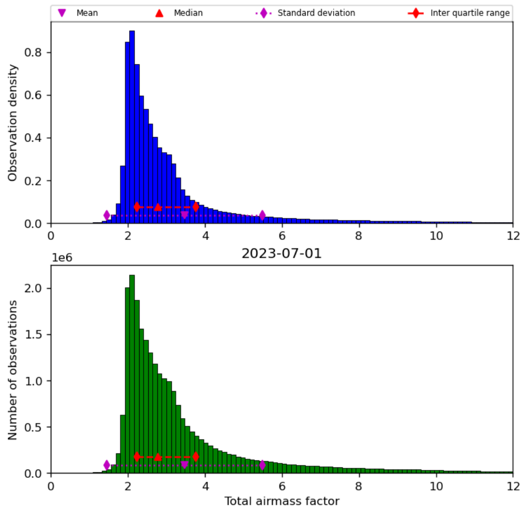
Figure 32: Histogram of “Total airmass factor” for 2023-06-30 to 2023-07-02
