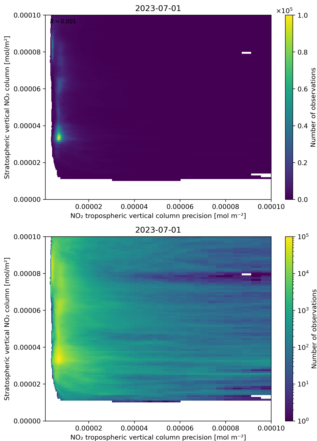
Figure 135: Scatter density plot of “NO 2 tropospheric vertical column precision” against “Stratospheric vertical NO 2 column” for 2023-06-30 to 2023-07-02.
