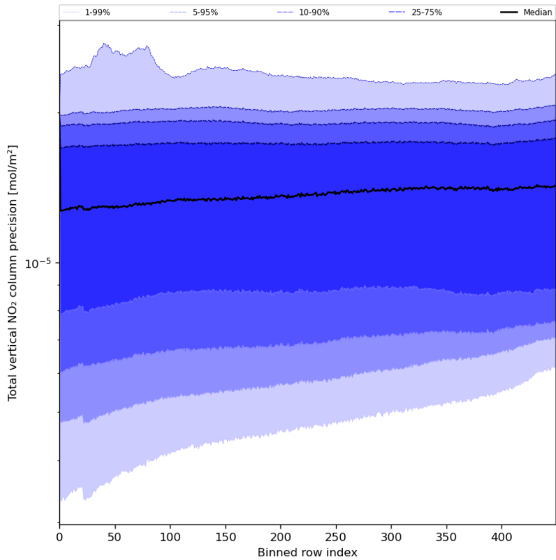
Figure 56: Along track statistics of “Total vertical NO 2 column precision” for 2023-06-30 to 2023-07-02
