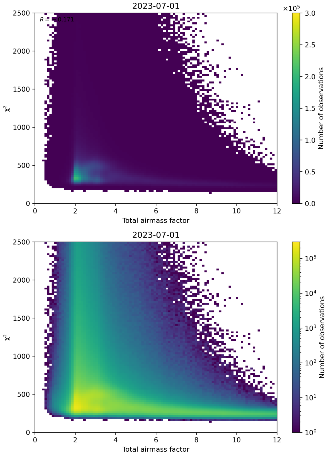
Figure 63: Scatter density plot of “Total airmass factor” against “ \chi^2 ” for 2023-06-30 to 2023-07-02.
