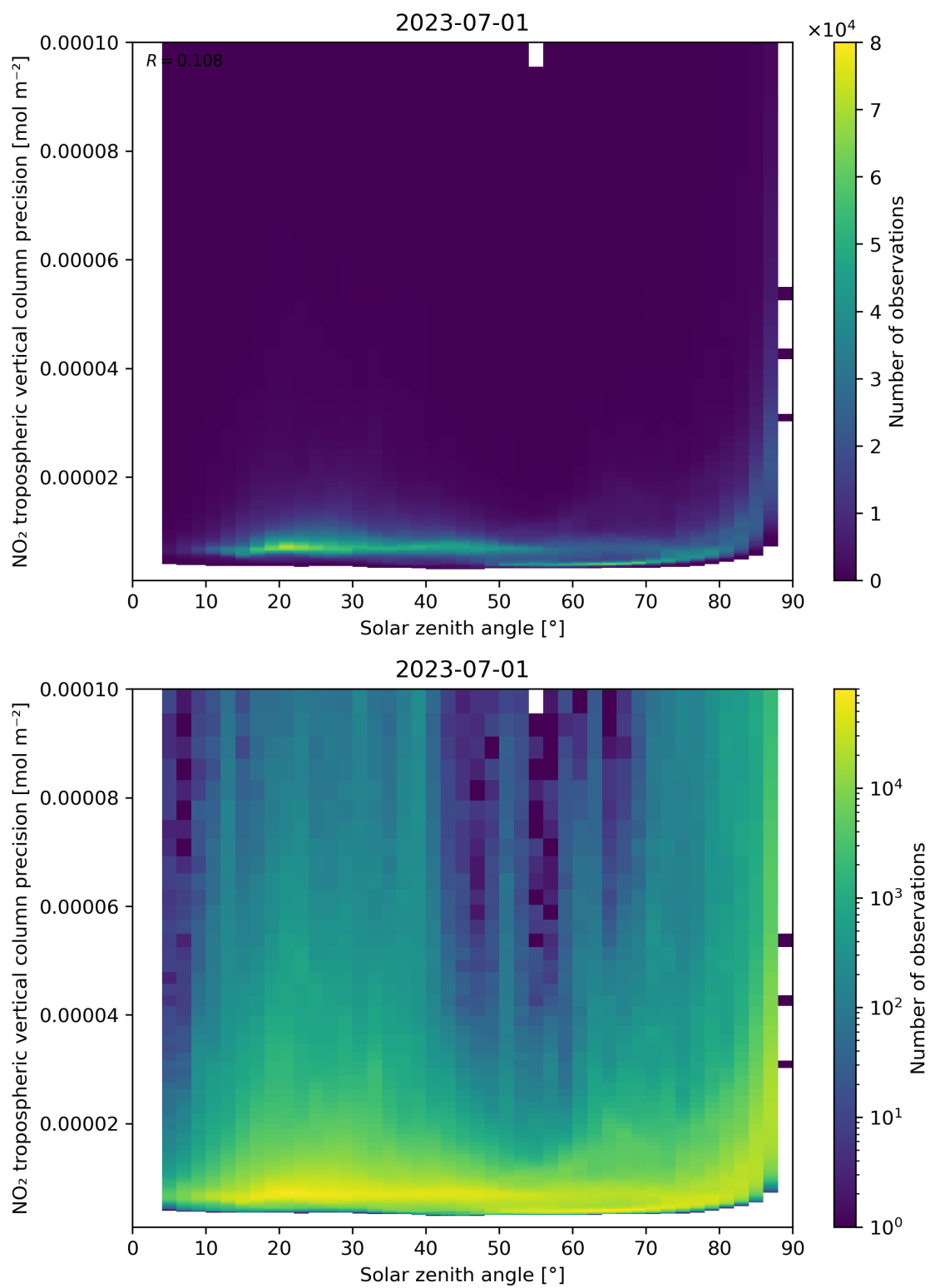
Figure 156: Scatter density plot of “Solar zenith angle” against “NO 2 tropospheric vertical column precision” for 2023-06-30 to 2023-07-02.
