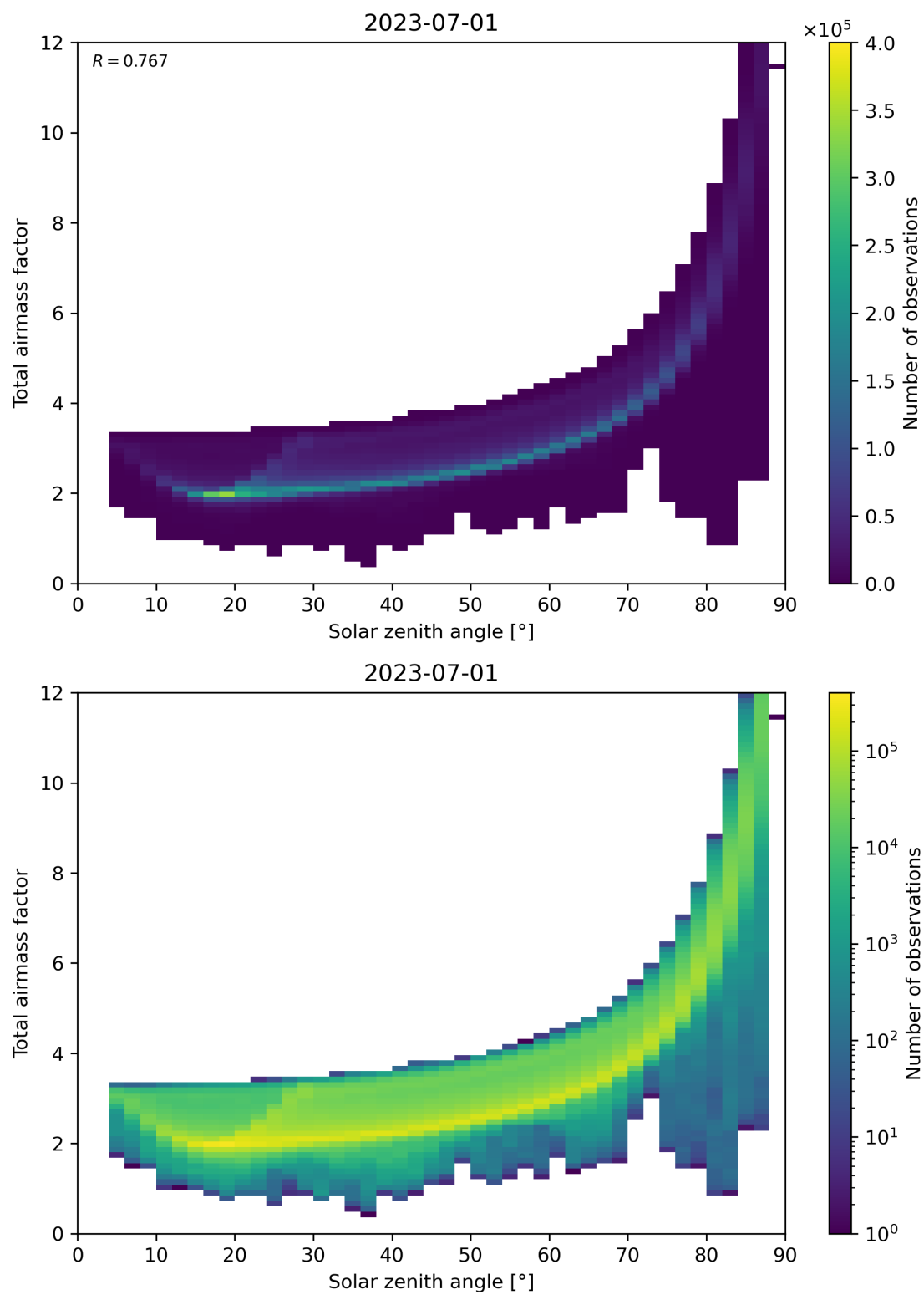
Figure 146: Scatter density plot of “Solar zenith angle” against “Total air mass factor” for 2023-06-30 to 2023-07-02.
