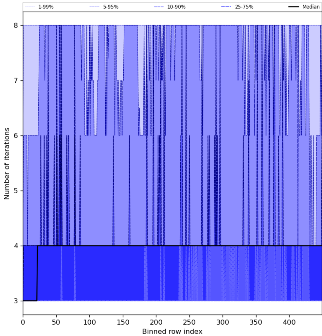
Figure 51: Along track statistics of “Number of iterations” for 2023-06-30 to 2023-07-02
