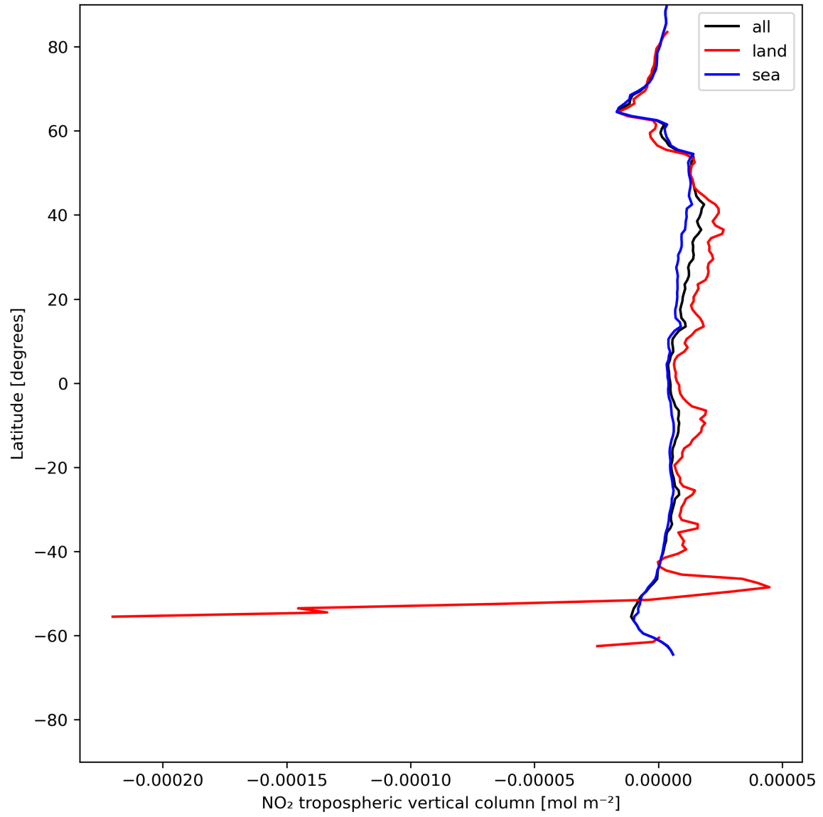
Figure 12: Zonal average of “NO 2 tropospheric vertical column” for 2023-06-30 to 2023-07-02.
