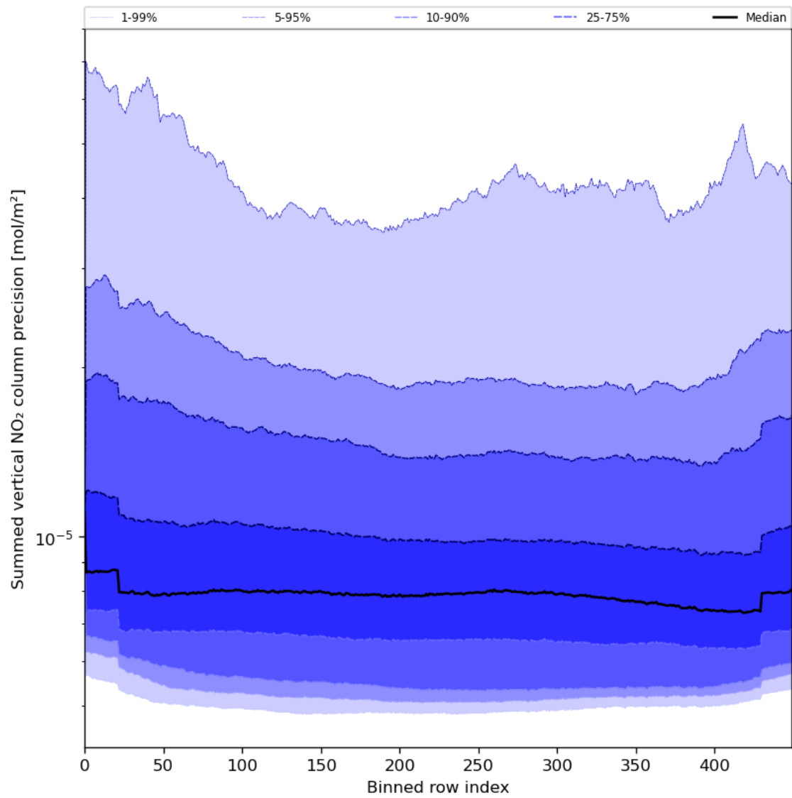
Figure 58: Along track statistics of “Summed vertical NO 2 column precision” for 2023-06-30 to 2023-07-02
