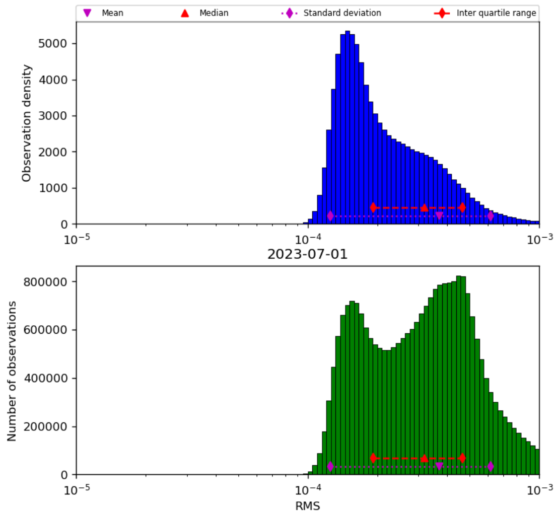
Figure 43: Histogram of “RMS” for 2023-06-30 to 2023-07-02
