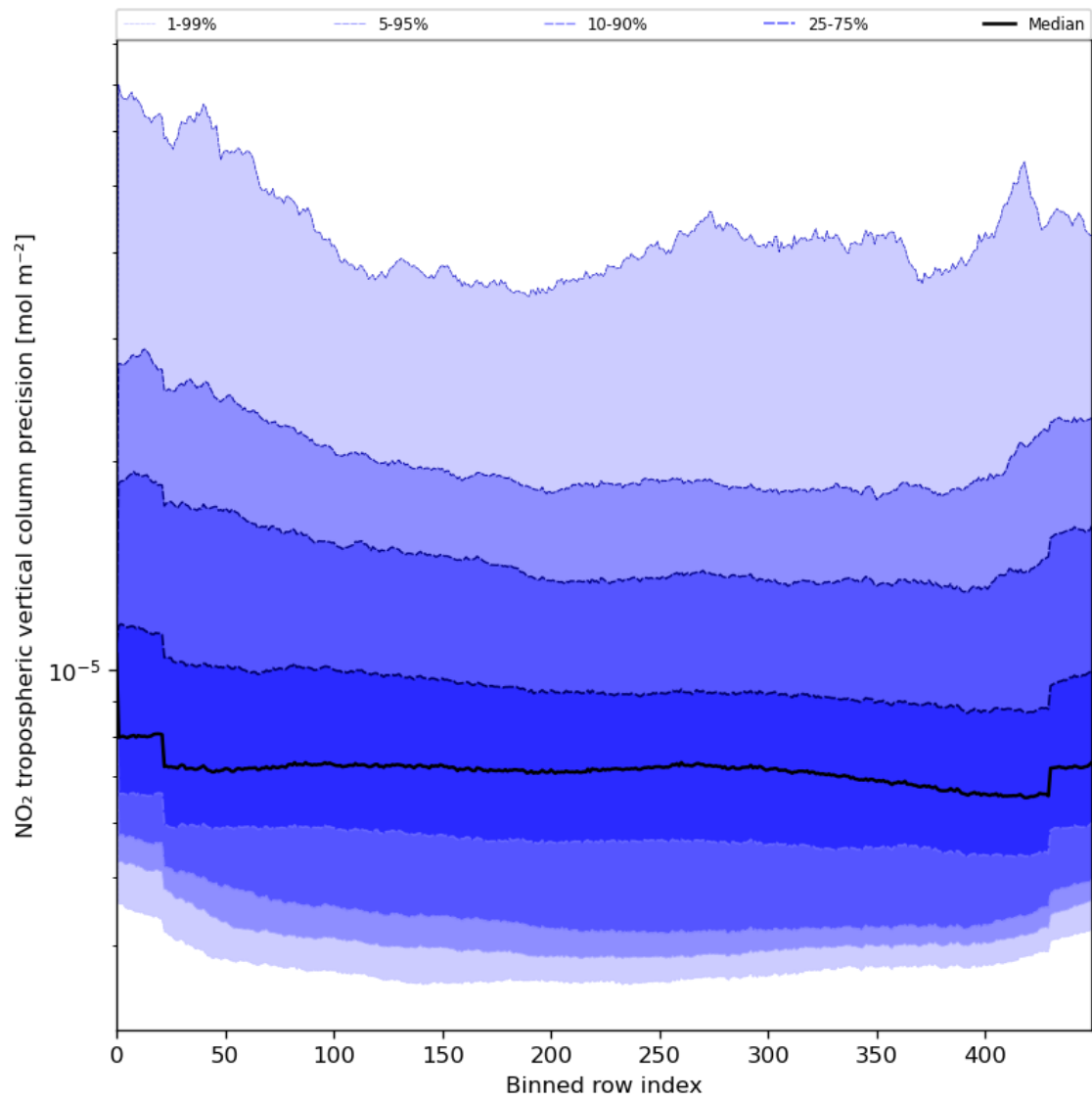
Figure 47: Along track statistics of “NO 2 tropospheric vertical column precision” for 2023-06-30 to 2023-07-02
