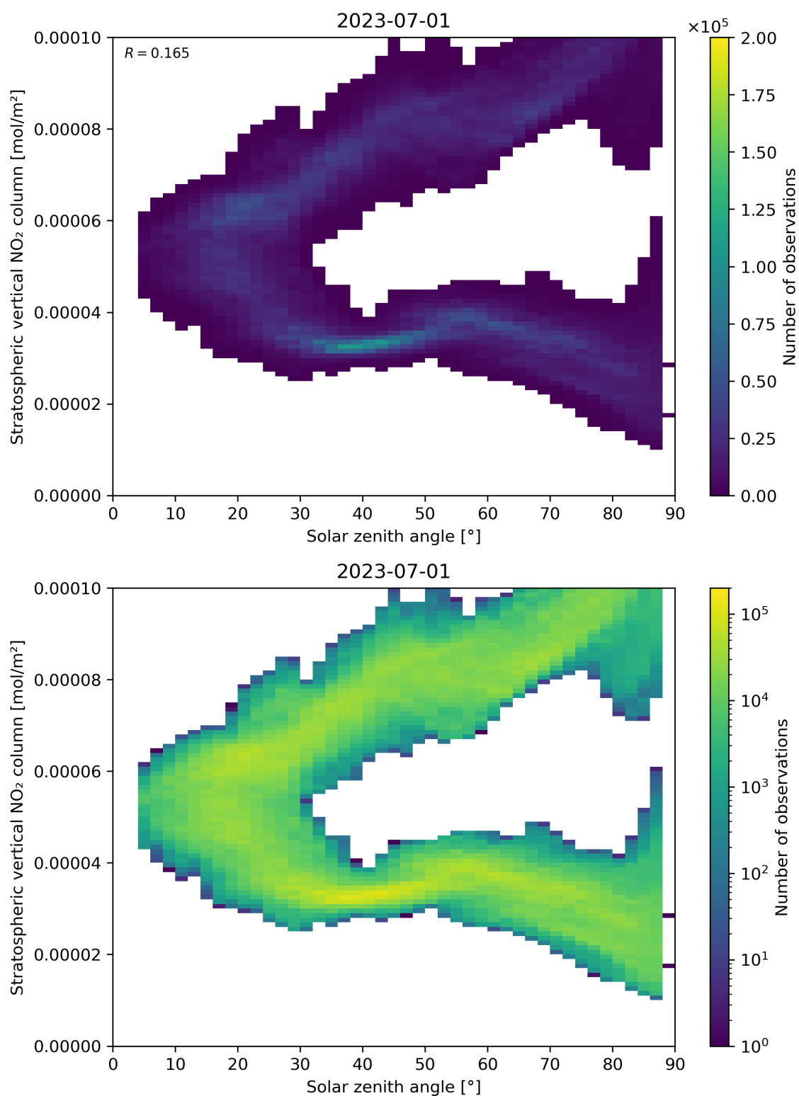
Figure 150: Scatter density plot of “Solar zenith angle” against “Stratospheric vertical NO 2 column” for 2023-06-30 to 2023-07-02.
