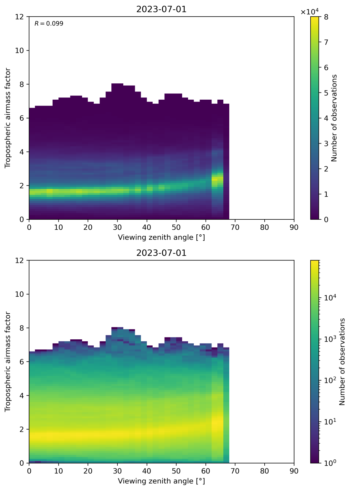
Figure 161: Scatter density plot of “Viewing zenith angle” against “Tropospheric airmass factor” for 2023-06-30 to 2023-07-02.
