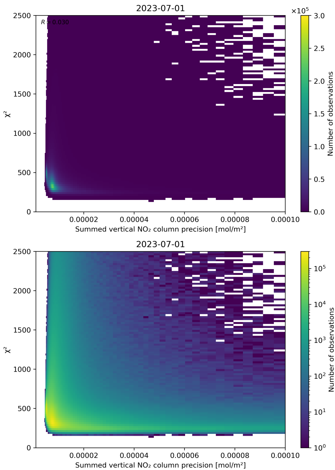
Figure 107: Scatter density plot of “Summed vertical NO 2 column precision” against “ \chi^2 ” for 2023-06-30 to 2023-07-02.
