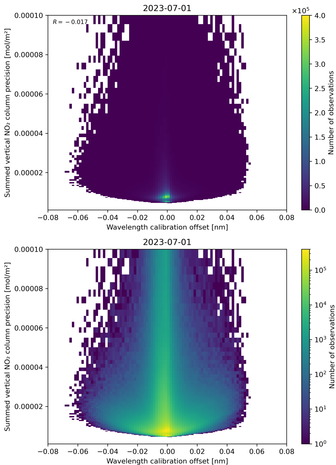
Figure 178: Scatter density plot of “Wavelength calibration offset” against “Summed vertical NO 2 column precision” for 2023-06-30 to 2023-07-02.
