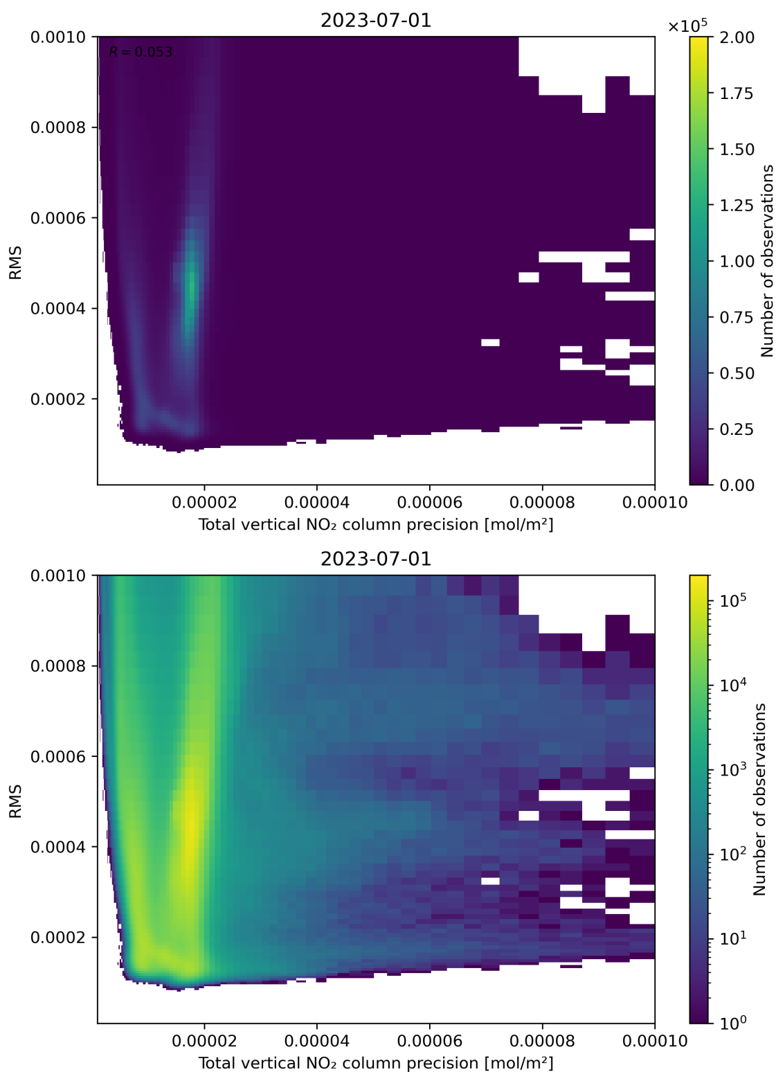
Figure 119: Scatter density plot of “Total vertical NO 2 column precision” against “RMS” for 2023-06-30 to 2023-07-02.
