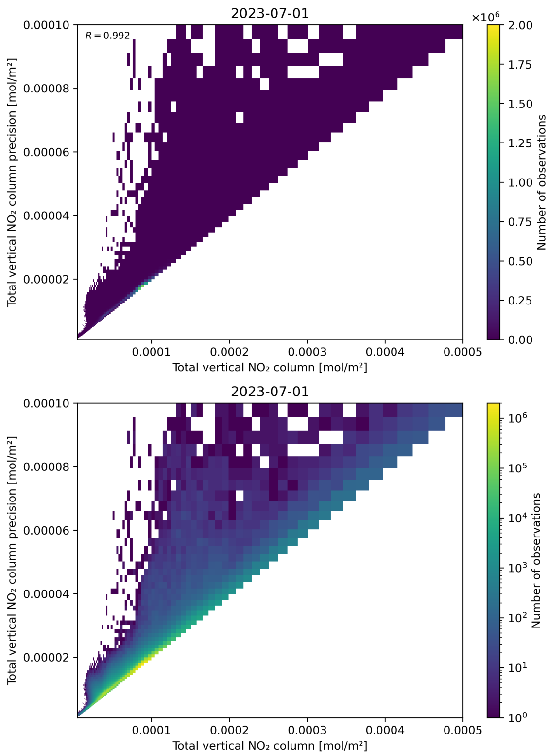
Figure 114: Scatter density plot of “Total vertical NO 2 column” against “Total vertical NO 2 column precision” for 2023-06-30 to 2023-07-02.
