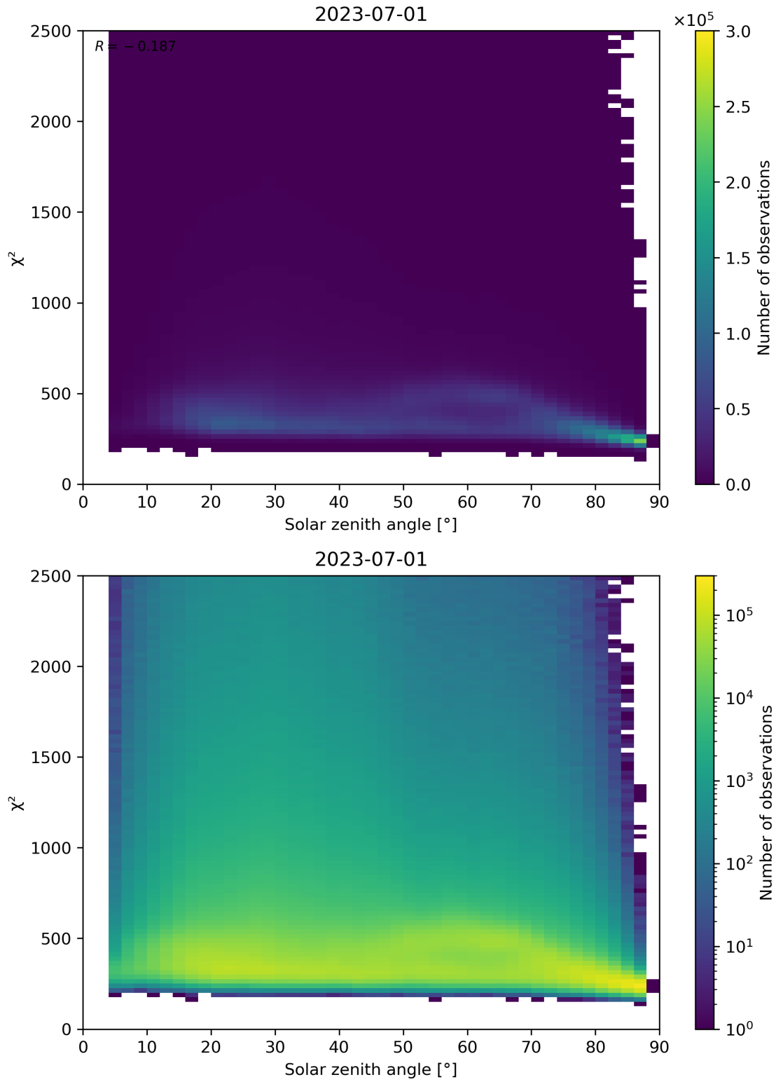
Figure 148: Scatter density plot of “Solar zenith angle” against “ \chi^2 ” for 2023-06-30 to 2023-07-02.
