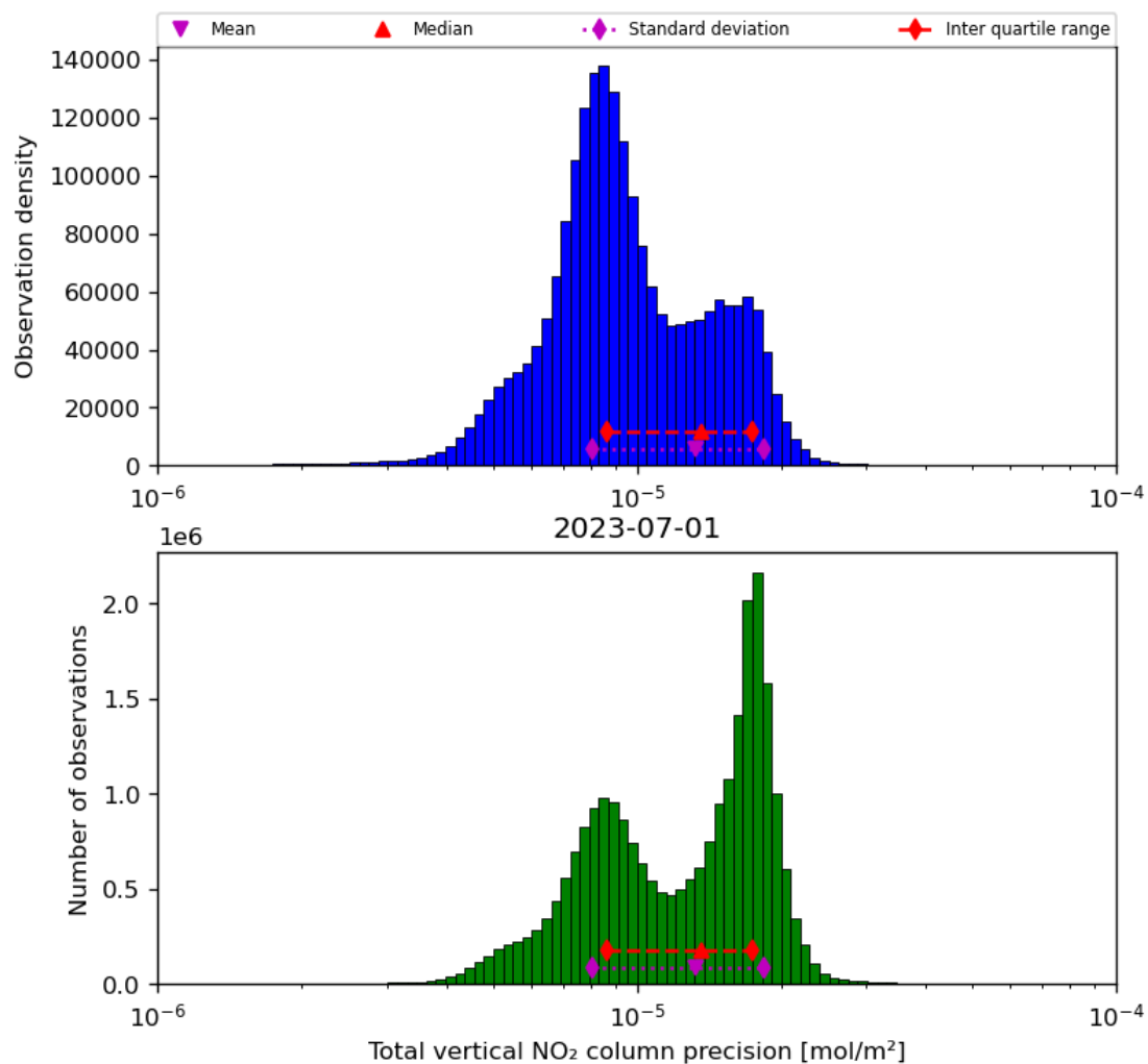
Figure 39: Histogram of “Total vertical NO 2 column precision” for 2023-06-30 to 2023-07-02
