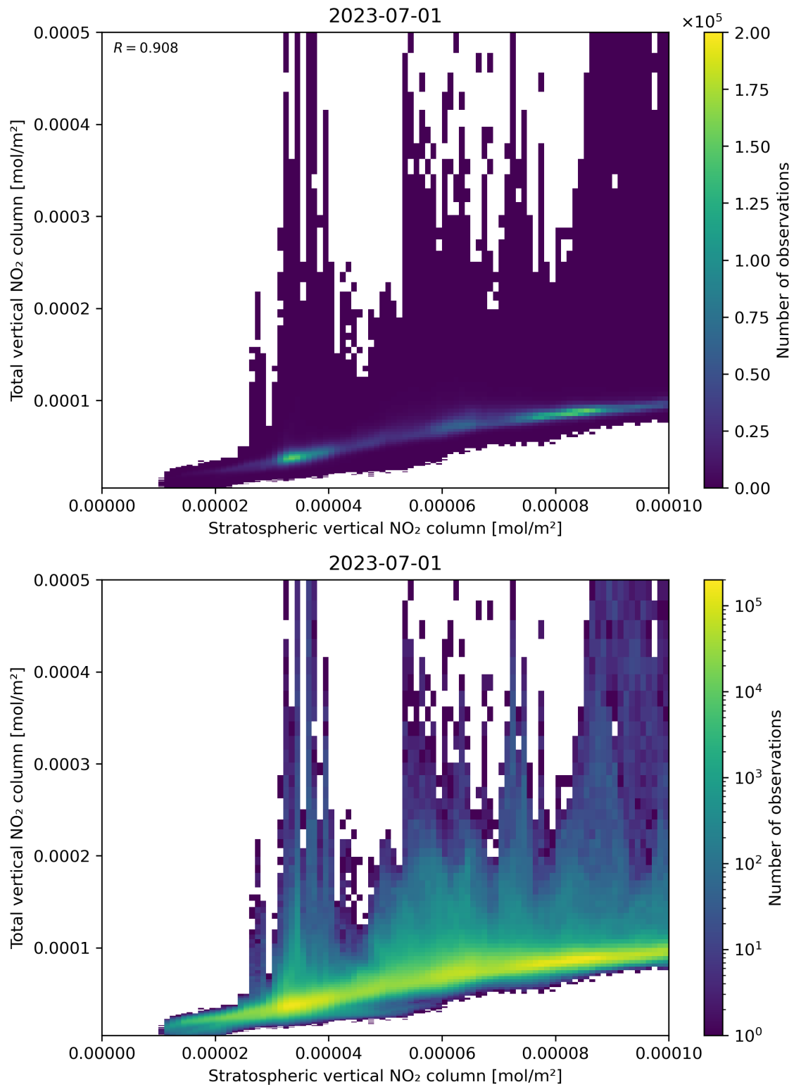
Figure 100: Scatter density plot of “Stratospheric vertical NO 2 column” against “Total vertical NO 2 column” for 2023-06-30 to 2023-07-02.
