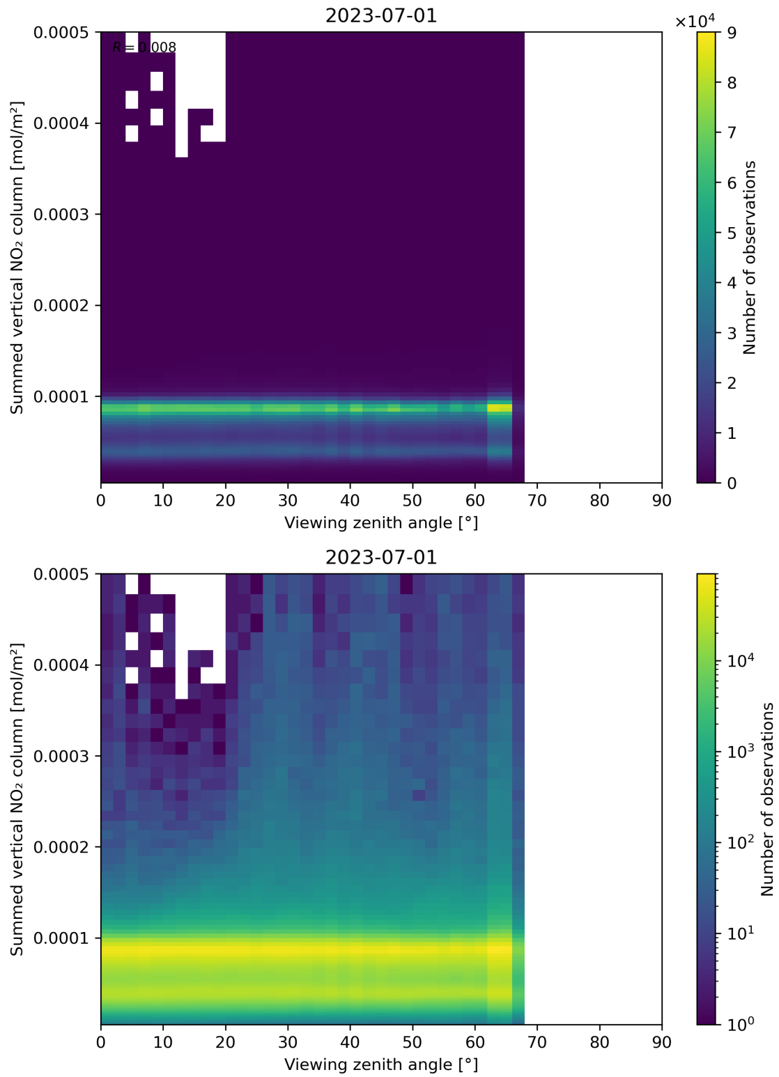
Figure 165: Scatter density plot of “Viewing zenith angle” against “Summed vertical NO 2 column” for 2023-06-30 to 2023-07-02.
