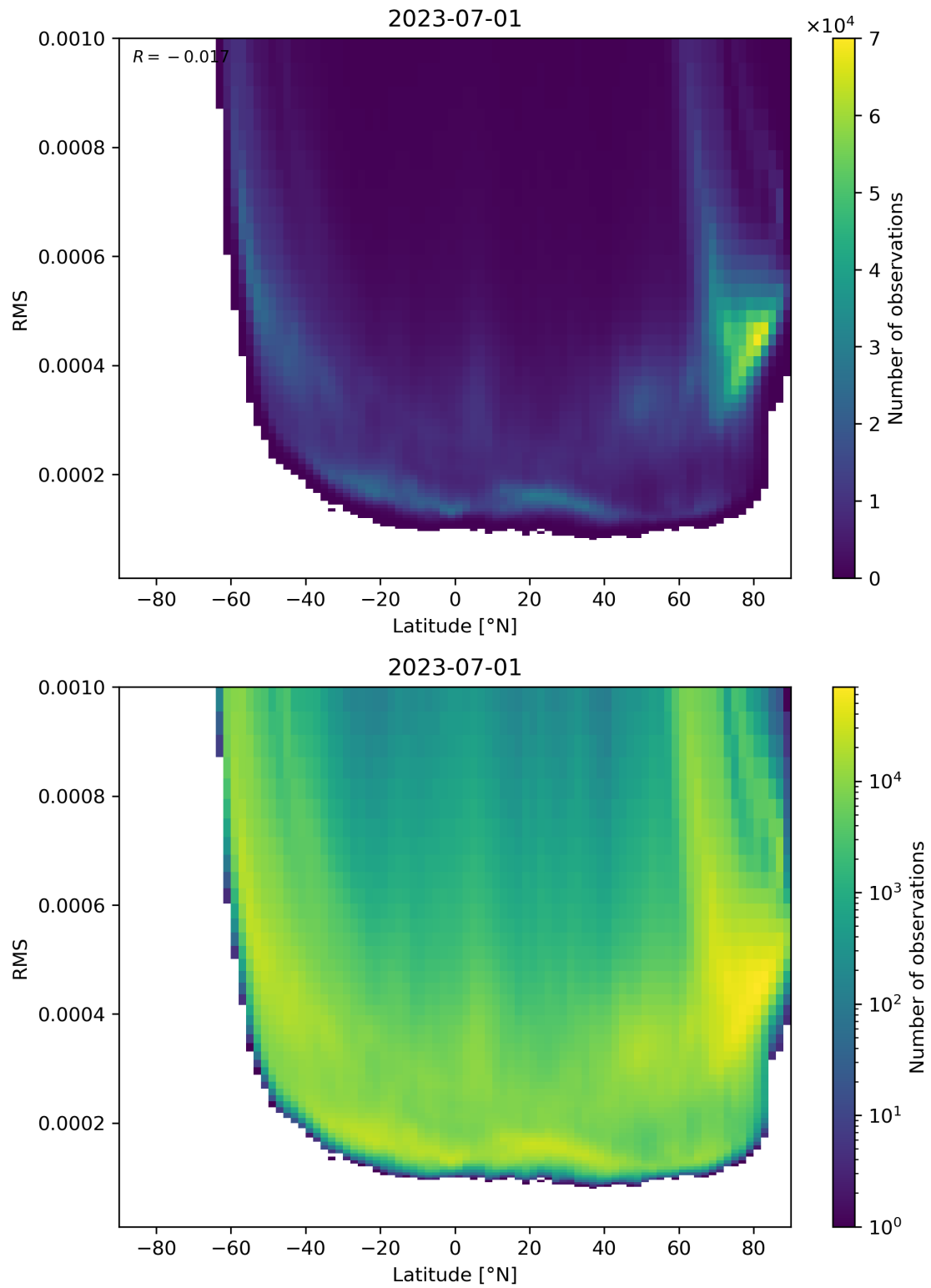
Figure 94: Scatter density plot of “Latitude” against “RMS” for 2023-06-30 to 2023-07-02.
