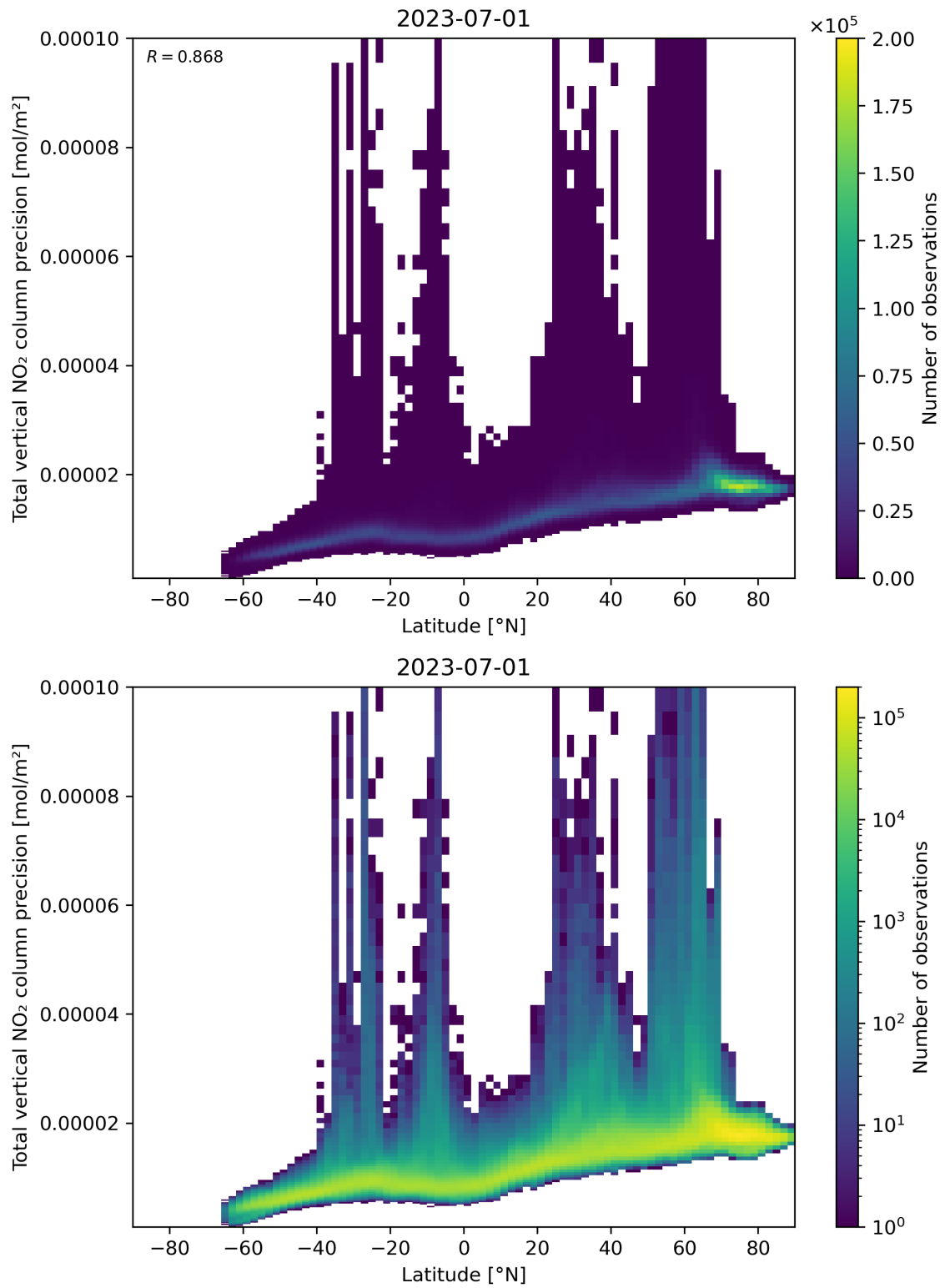
Figure 91: Scatter density plot of “Latitude” against “Total vertical NO 2 column precision” for 2023-06-30 to 2023-07-02.
