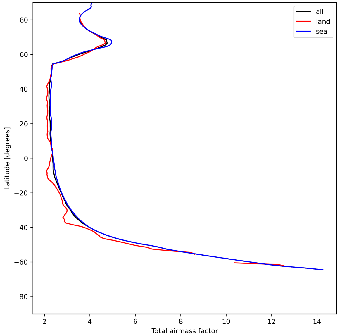
Figure 15: Zonal average of “Total airmass factor” for 2023-06-30 to 2023-07-02.
