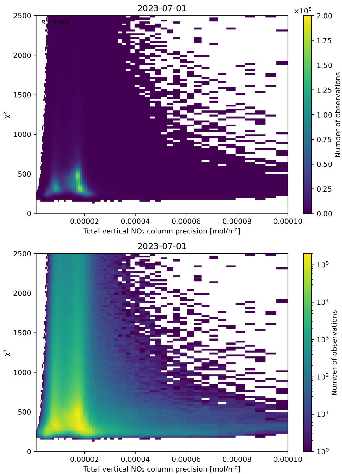
Figure 116: Scatter density plot of “Total vertical NO 2 column precision” against “ \chi^2 ” for 2023-06-30 to 2023-07-02.
