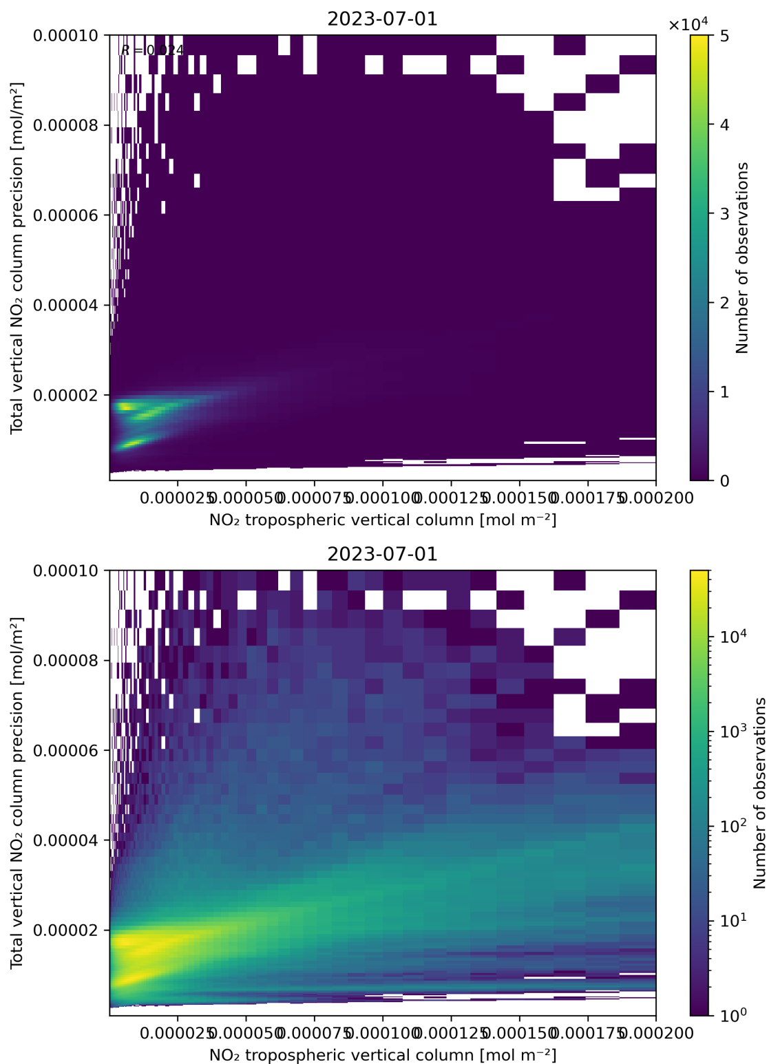
Figure 129: Scatter density plot of “NO 2 tropospheric vertical column” against “Total vertical NO 2 column precision” for 2023-06-30 to 2023-07-02.
