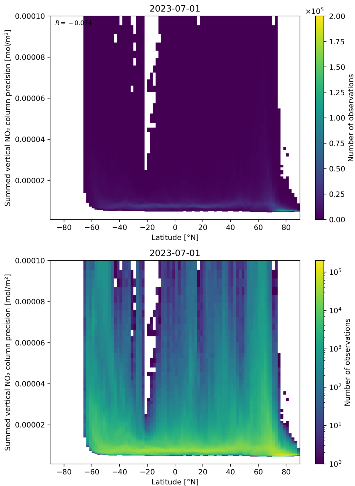
Figure 89: Scatter density plot of “Latitude” against “Summed vertical NO 2 column precision” for 2023-06-30 to 2023-07-02.
