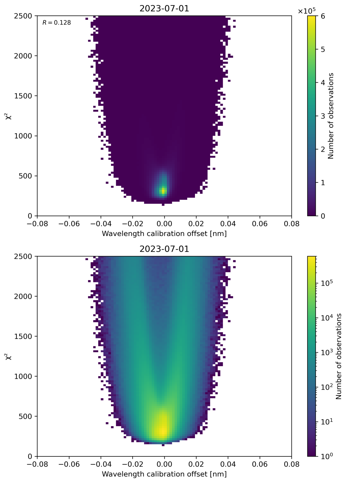
Figure 175: Scatter density plot of “Wavelength calibration offset” against “ \chi^2 ” for 2023-06-30 to 2023-07-02.
