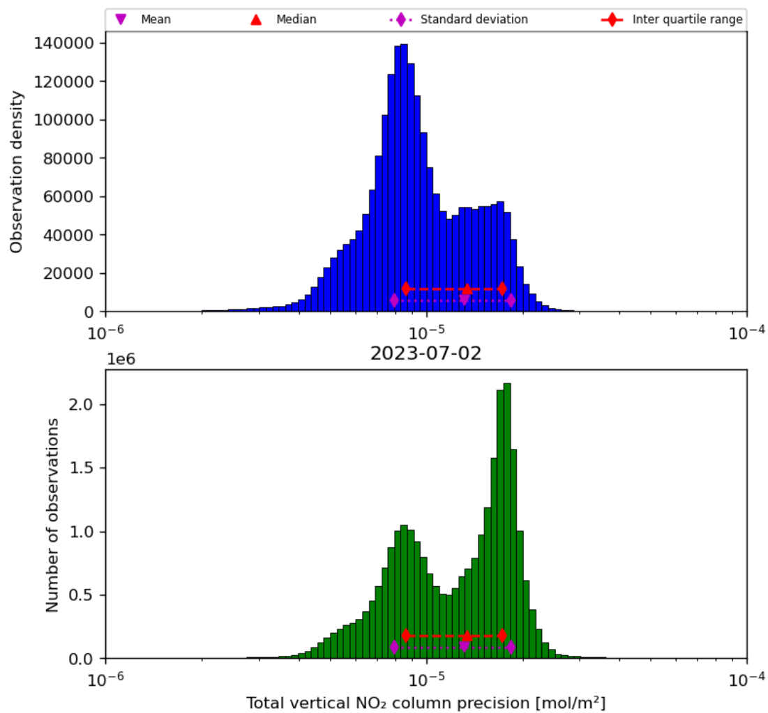
Figure 39: Histogram of “Total vertical NO 2 column precision” for 2023-07-01 to 2023-07-03
