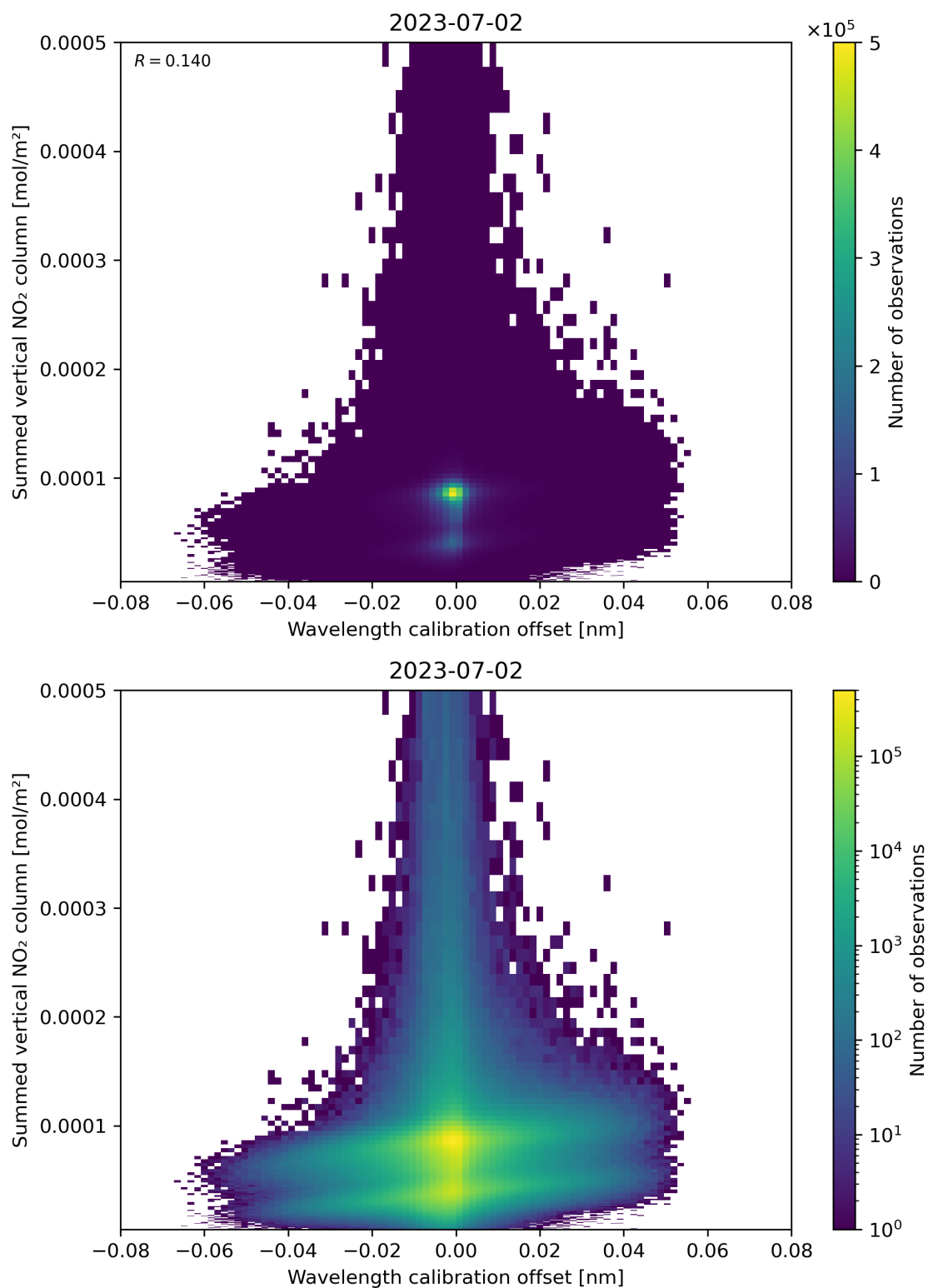
Figure 177: Scatter density plot of “Wavelength calibration offset” against “Summed vertical NO 2 column” for 2023-07-01 to 2023-07-03.
