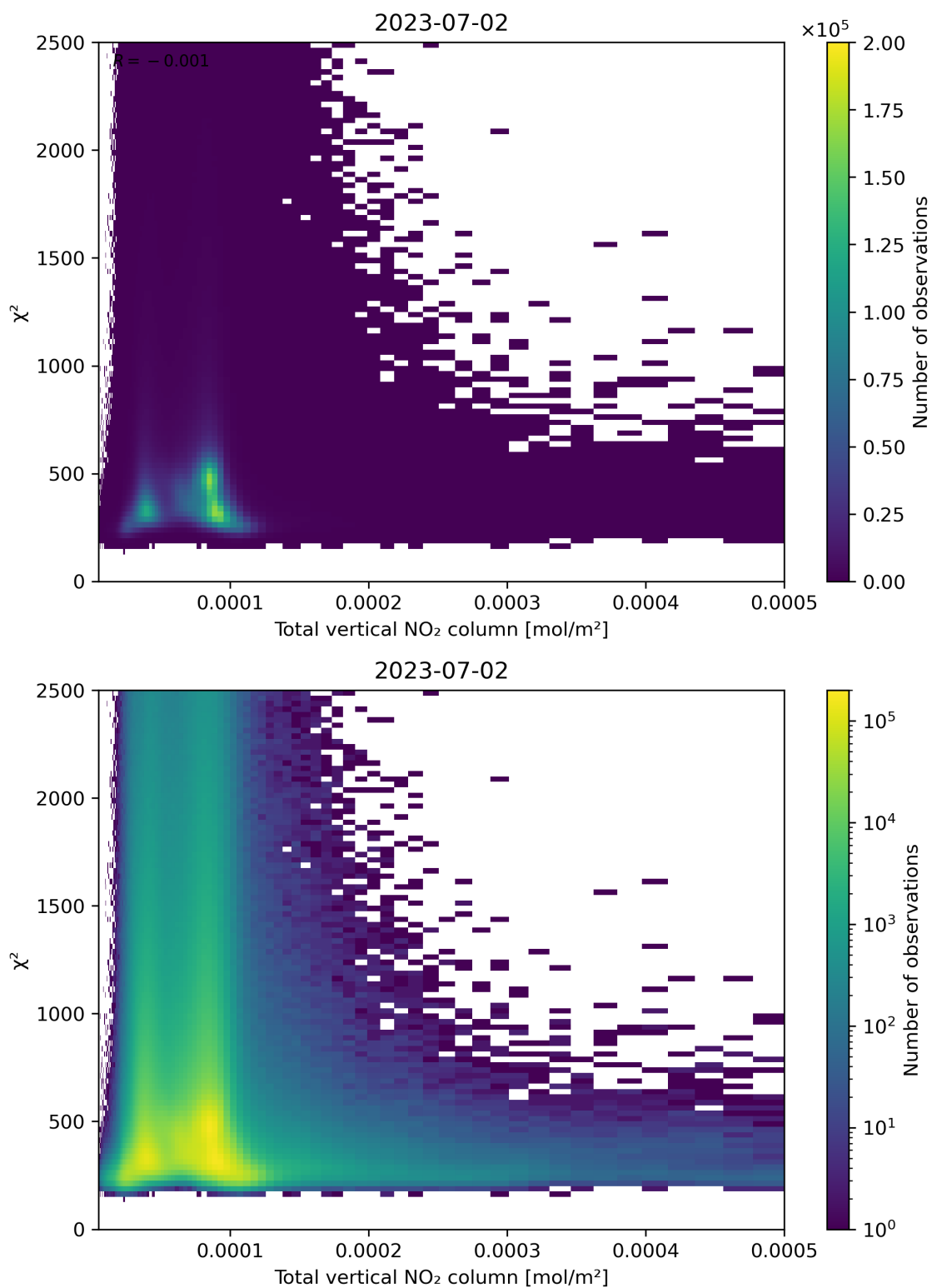
Figure 111: Scatter density plot of “Total vertical NO 2 column” against “ \chi^2 ” for 2023-07-01 to 2023-07-03.
