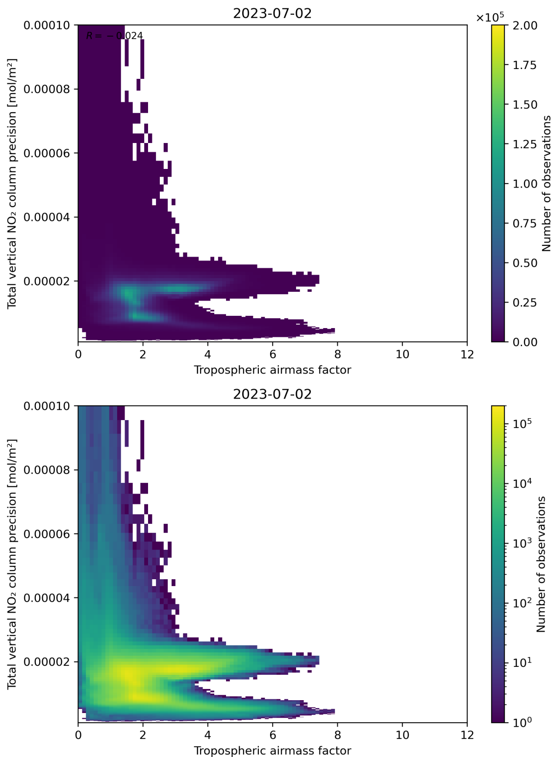
Figure 78: Scatter density plot of “Tropospheric air mass factor” against “Total vertical NO 2 column precision” for 2023-07-01 to 2023-07-03.
