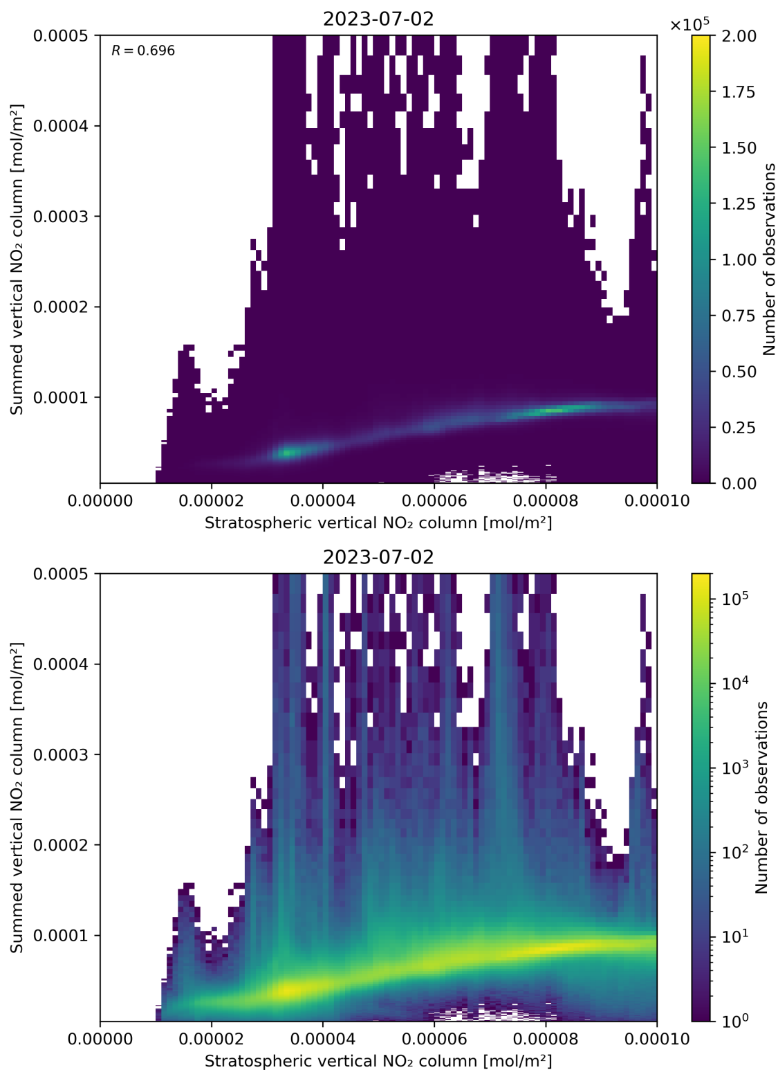
Figure 98: Scatter density plot of “Stratospheric vertical NO 2 column” against “Summed vertical NO 2 column” for 2023-07-01 to 2023-07-03.
