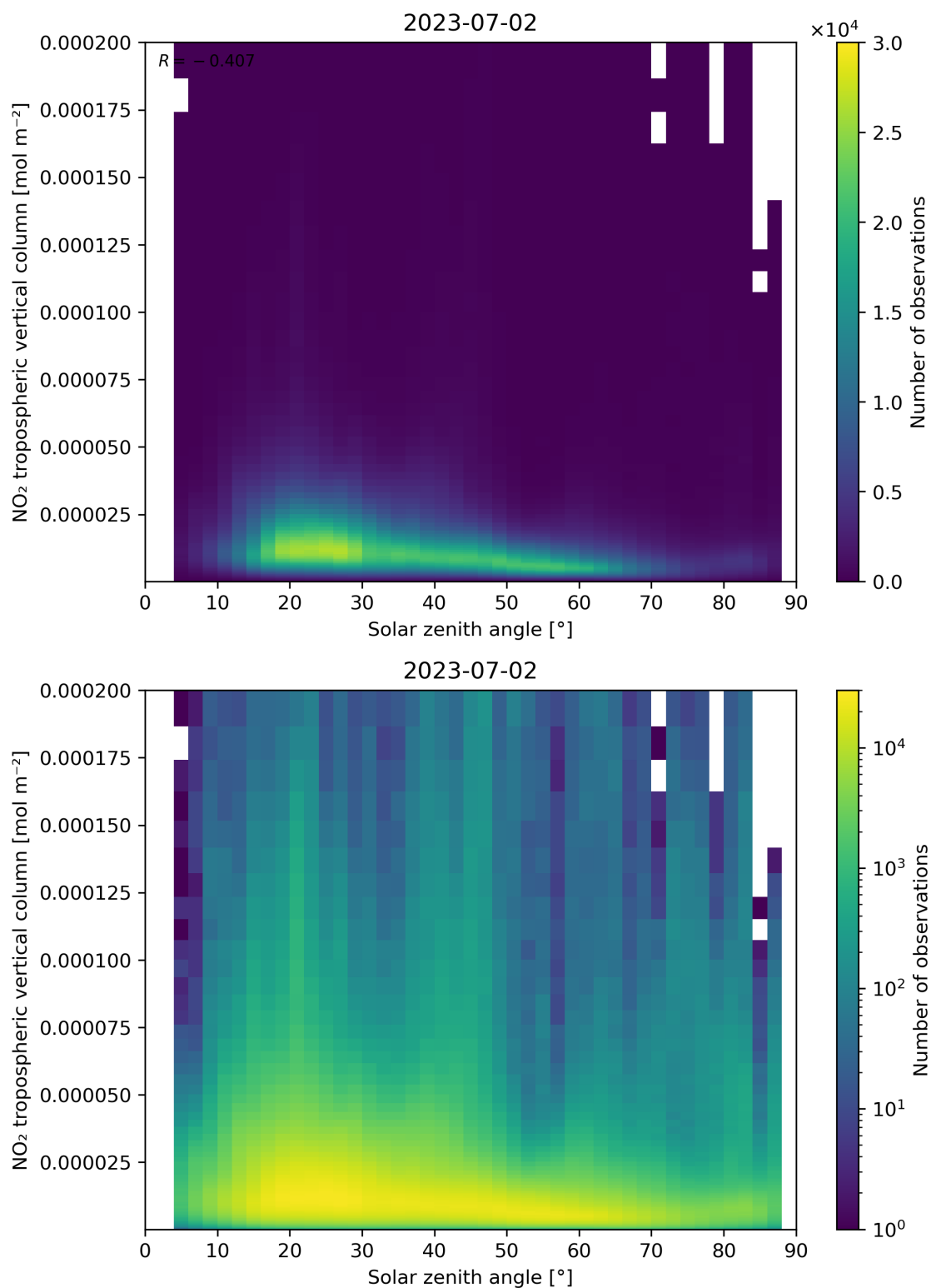
Figure 155: Scatter density plot of “Solar zenith angle” against “NO 2 tropospheric vertical column” for 2023-07-01 to 2023-07-03.
