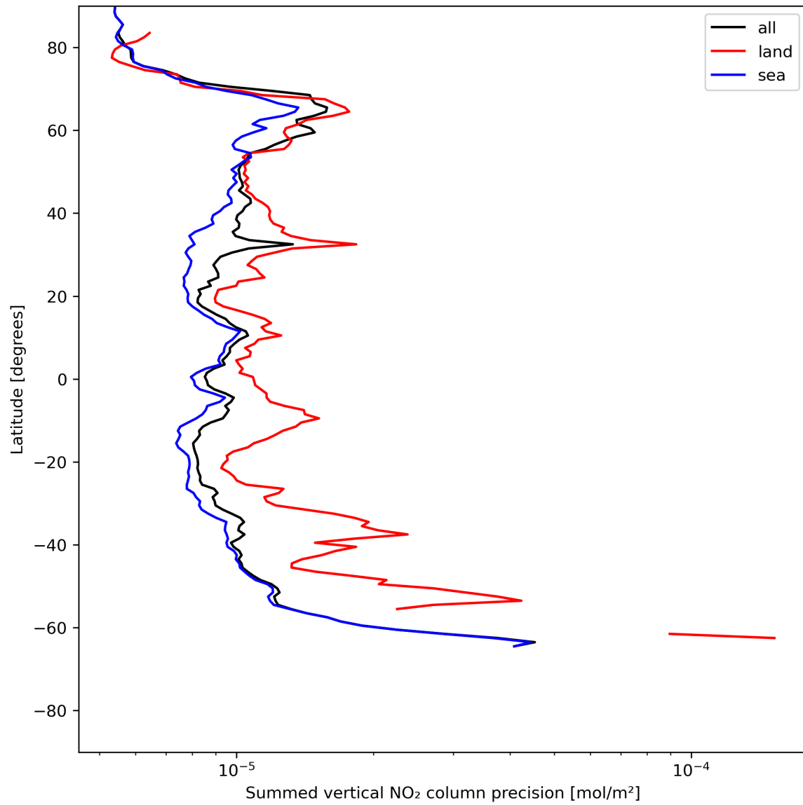
Figure 24: Zonal average of “Summed vertical NO 2 column precision” for 2023-07-01 to 2023-07-03.
