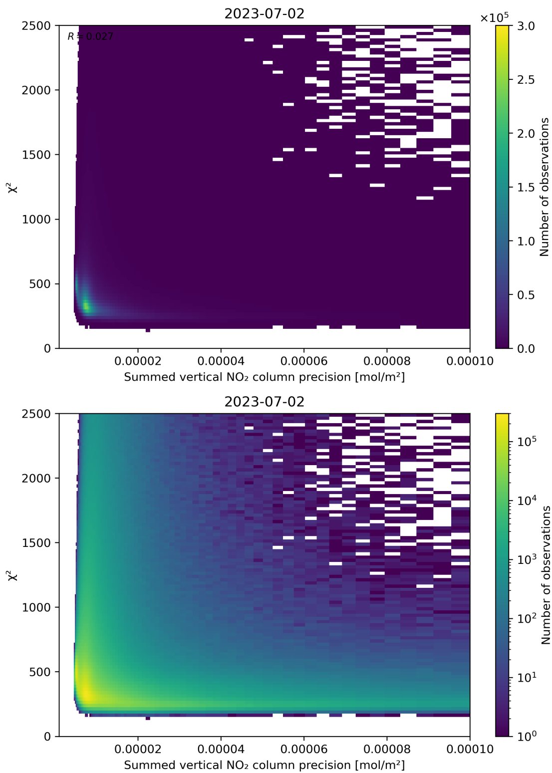
Figure 107: Scatter density plot of “Summed vertical NO 2 column precision” against “ \chi^2 ” for 2023-07-01 to 2023-07-03.
