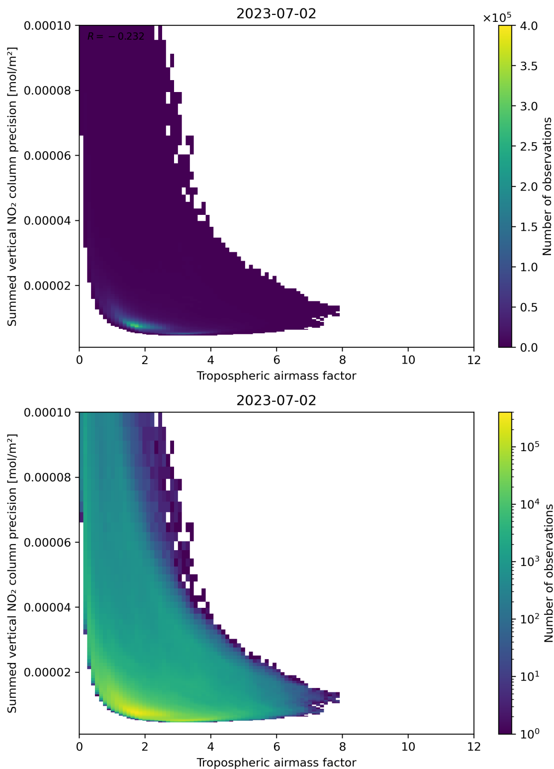
Figure 76: Scatter density plot of “Tropospheric air mass factor” against “Summed vertical NO 2 column precision” for 2023-07-01 to 2023-07-03.
