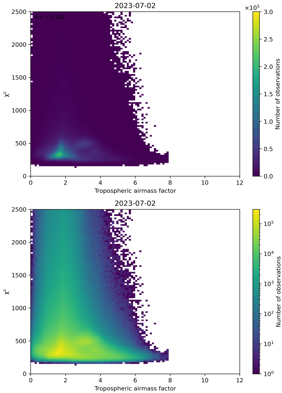
Figure 73: Scatter density plot of “Tropospheric airmass factor” against “ \chi^2 ” for 2023-07-01 to 2023-07-03.
