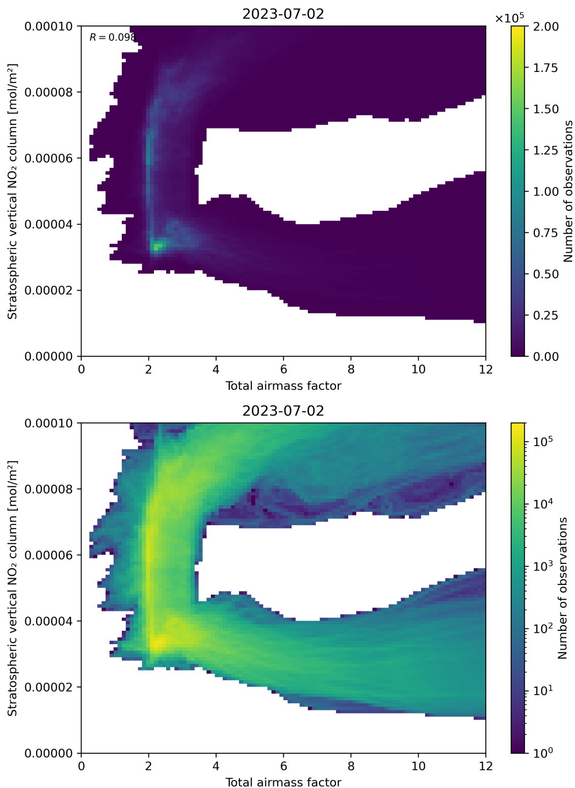
Figure 64: Scatter density plot of “Total airmass factor” against “Stratospheric vertical NO 2 column” for 2023-07-01 to 2023-07-03.
