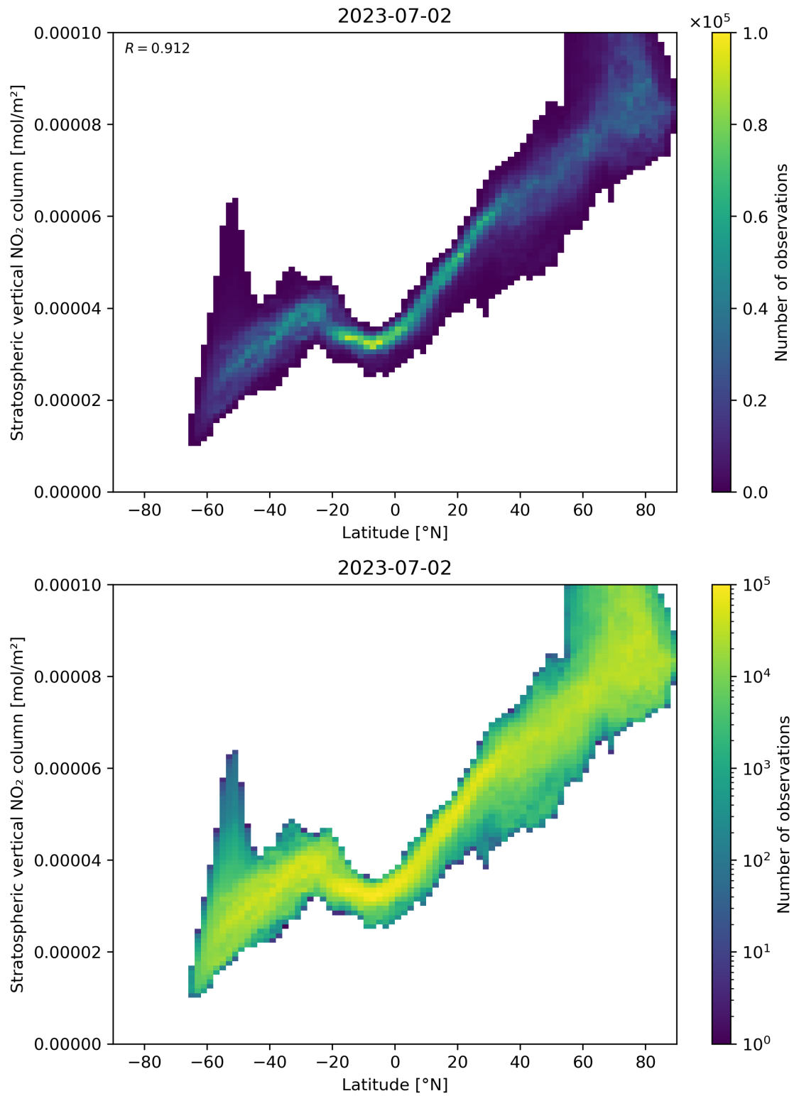
Figure 87: Scatter density plot of “Latitude” against “Stratospheric vertical NO 2 column” for 2023-07-01 to 2023-07-03.
