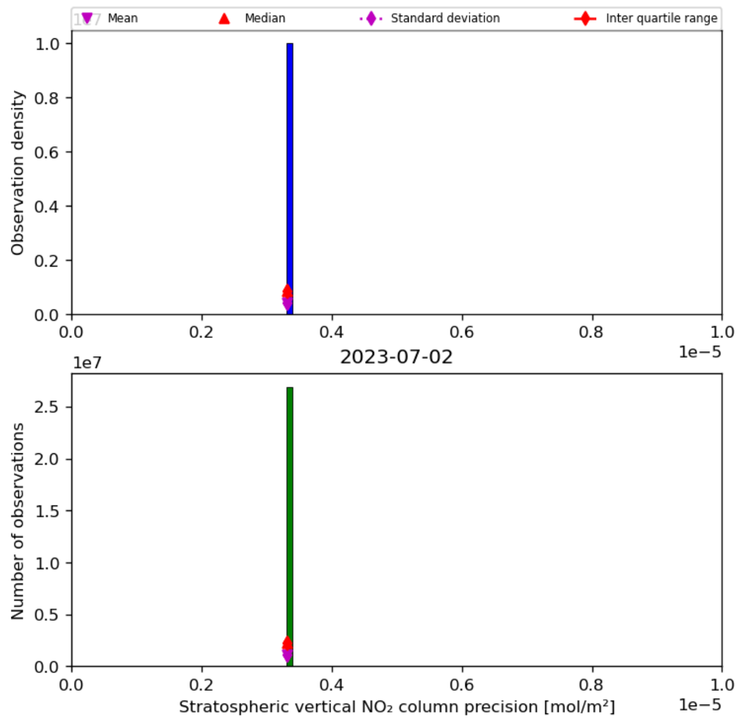
Figure 37: Histogram of “Stratospheric vertical NO 2 column precision” for 2023-07-01 to 2023-07-03
