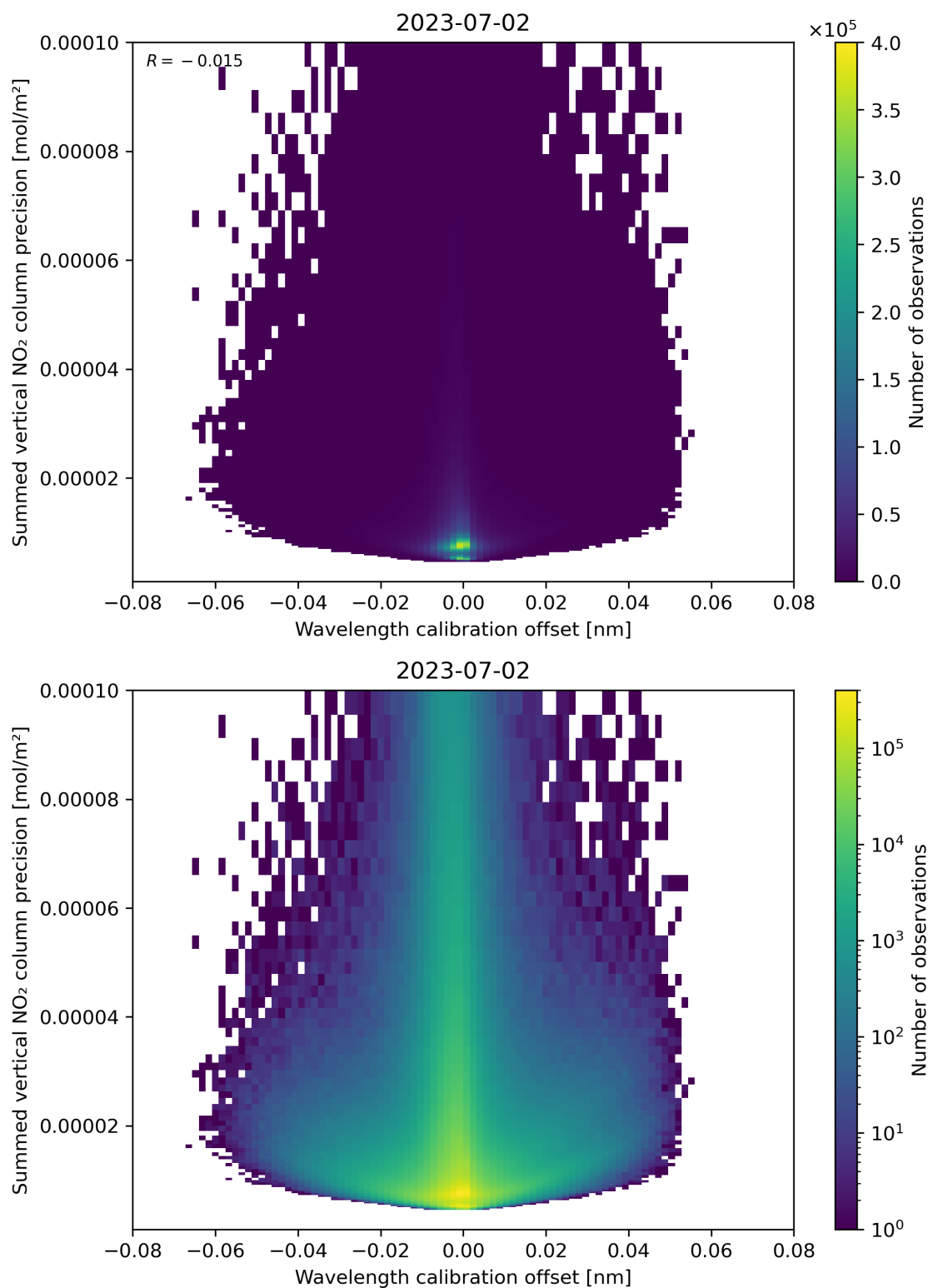
Figure 178: Scatter density plot of “Wavelength calibration offset” against “Summed vertical NO 2 column precision” for 2023-07-01 to 2023-07-03.
