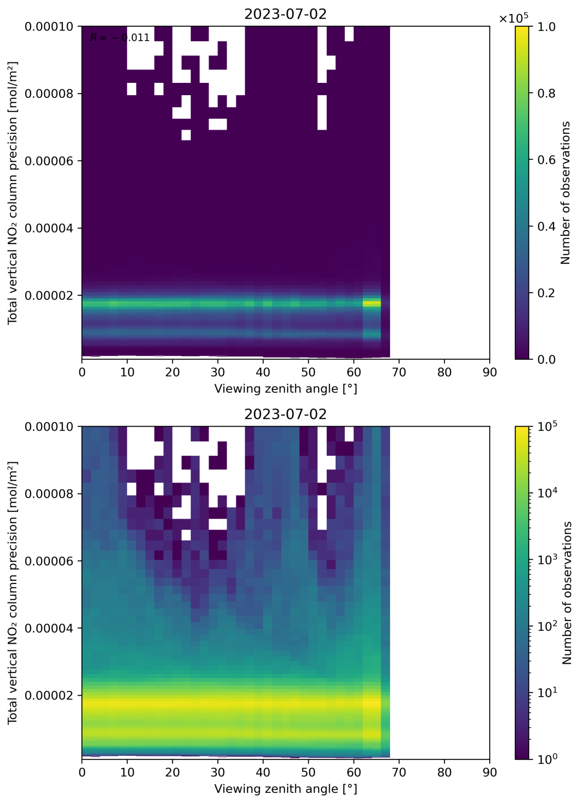
Figure 168: Scatter density plot of “Viewing zenith angle” against “Total vertical NO 2 column precision” for 2023-07-01 to 2023-07-03.
