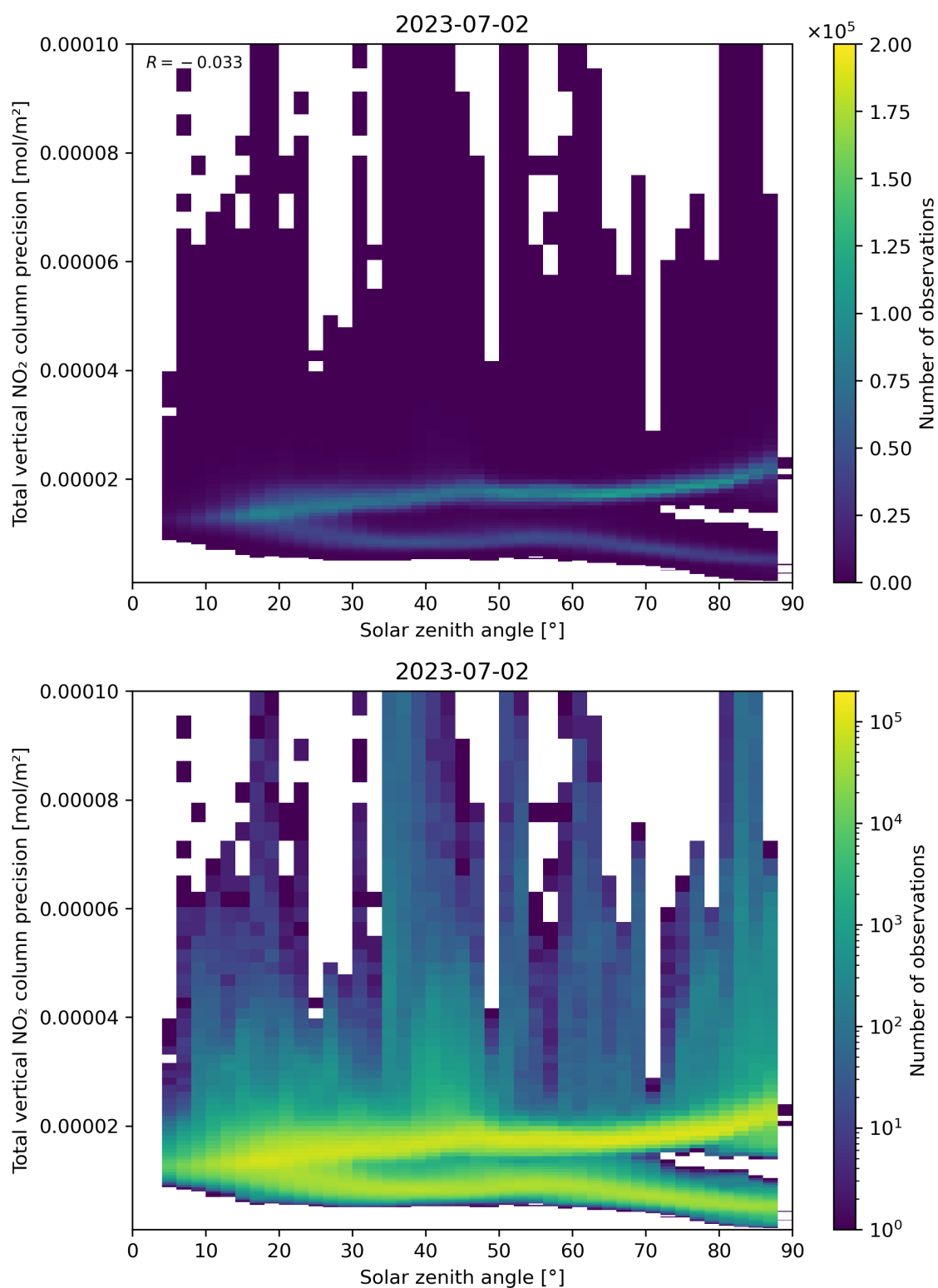
Figure 154: Scatter density plot of “Solar zenith angle” against “Total vertical NO 2 column precision” for 2023-07-01 to 2023-07-03.
