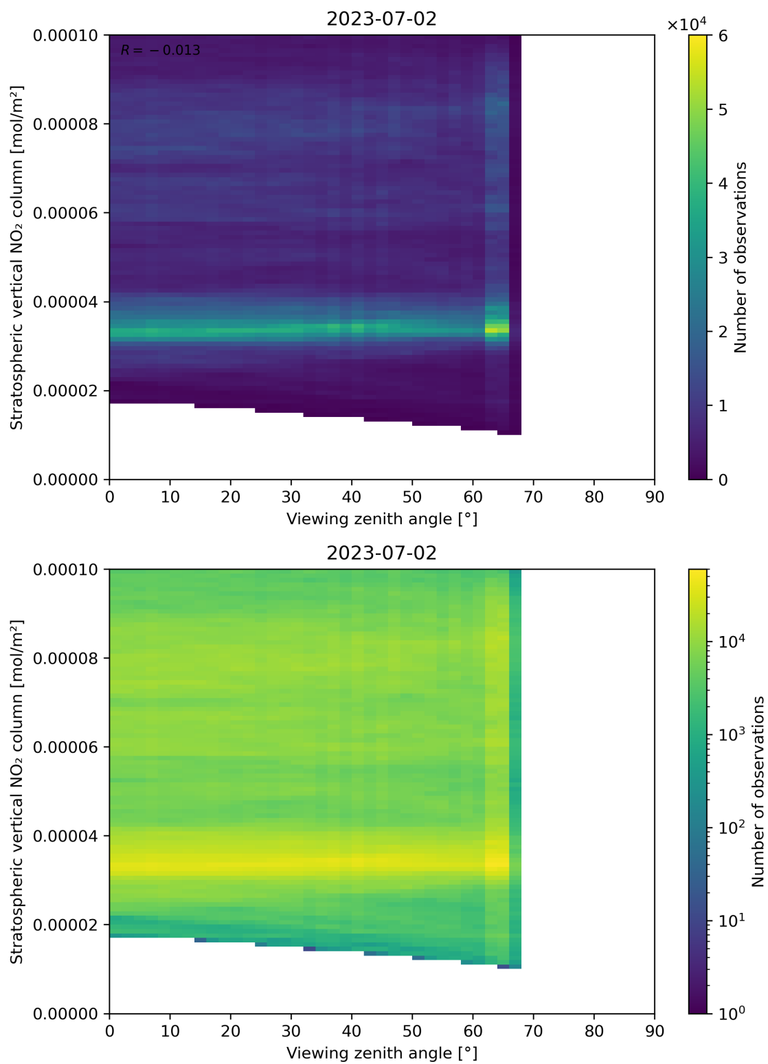
Figure 164: Scatter density plot of “Viewing zenith angle” against “Stratospheric vertical NO 2 column” for 2023-07-01 to 2023-07-03.
