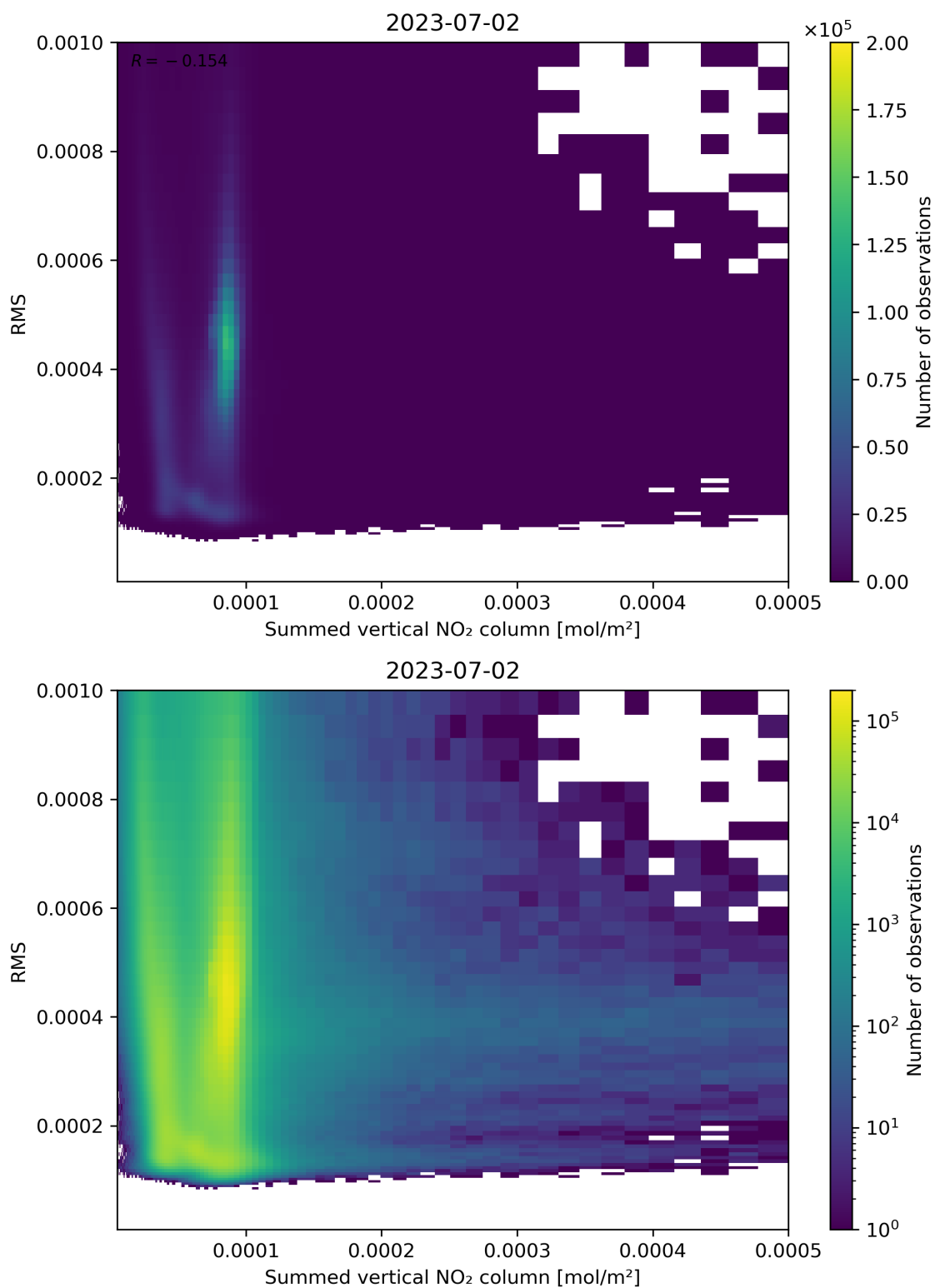
Figure 109: Scatter density plot of “Summed vertical NO 2 column” against “RMS” for 2023-07-01 to 2023-07-03.
