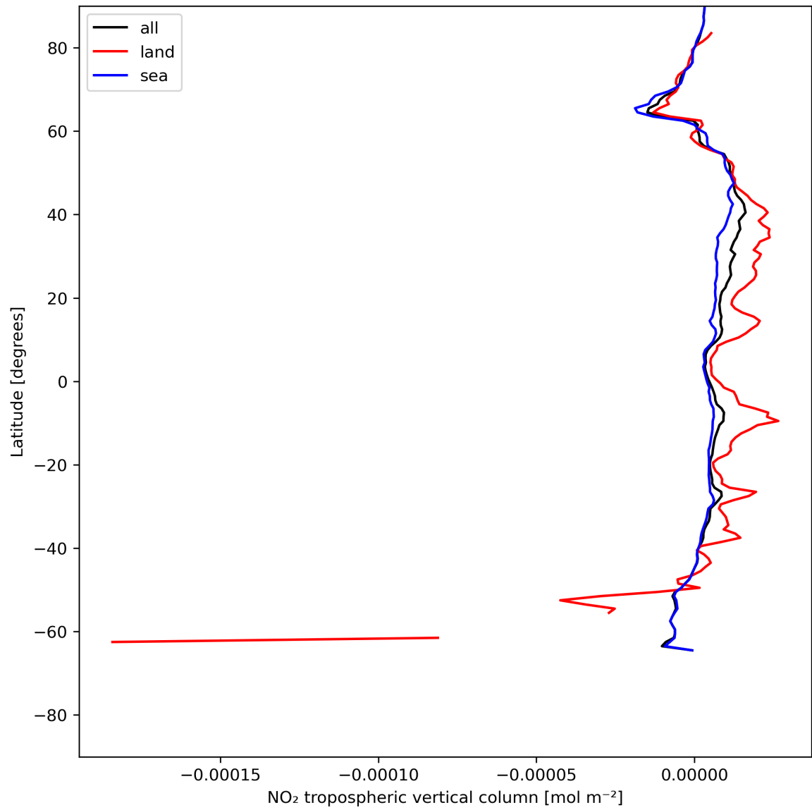
Figure 12: Zonal average of “NO 2 tropospheric vertical column” for 2023-07-01 to 2023-07-03.
