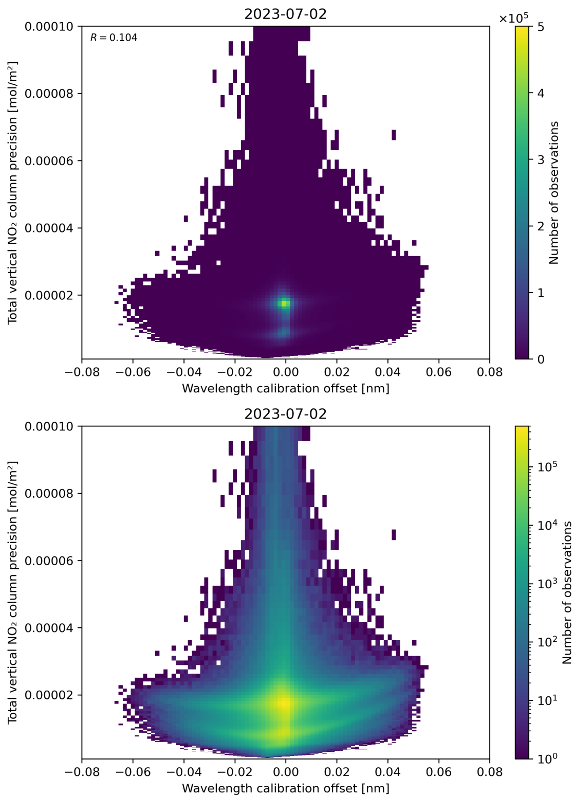
Figure 180: Scatter density plot of “Wavelength calibration offset” against “Total vertical NO 2 column precision” for 2023-07-01 to 2023-07-03.
