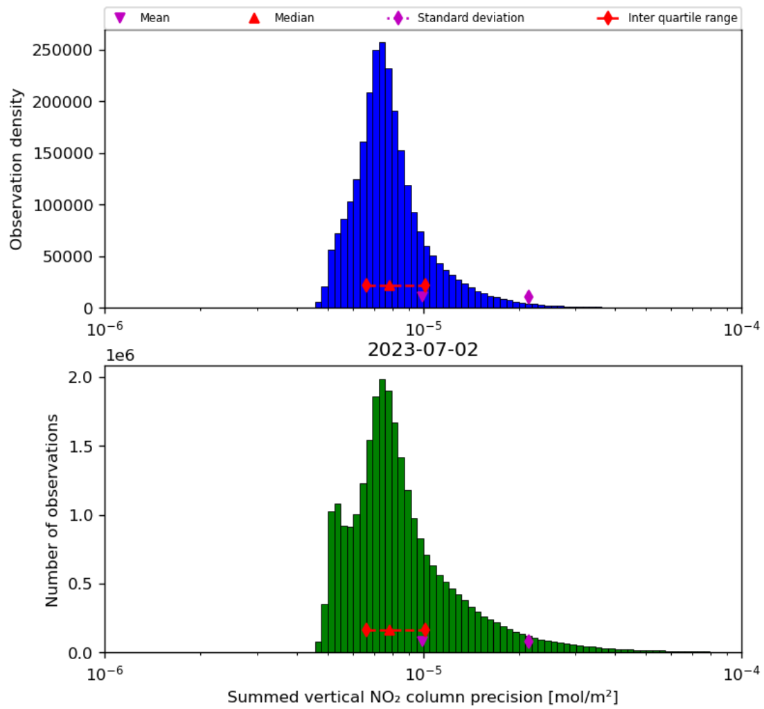
Figure 41: Histogram of “Summed vertical NO 2 column precision” for 2023-07-01 to 2023-07-03
