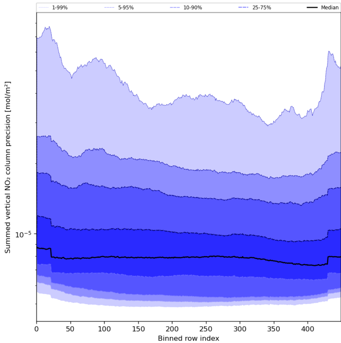
Figure 58: Along track statistics of “Summed vertical NO 2 column precision” for 2023-07-01 to 2023-07-03
