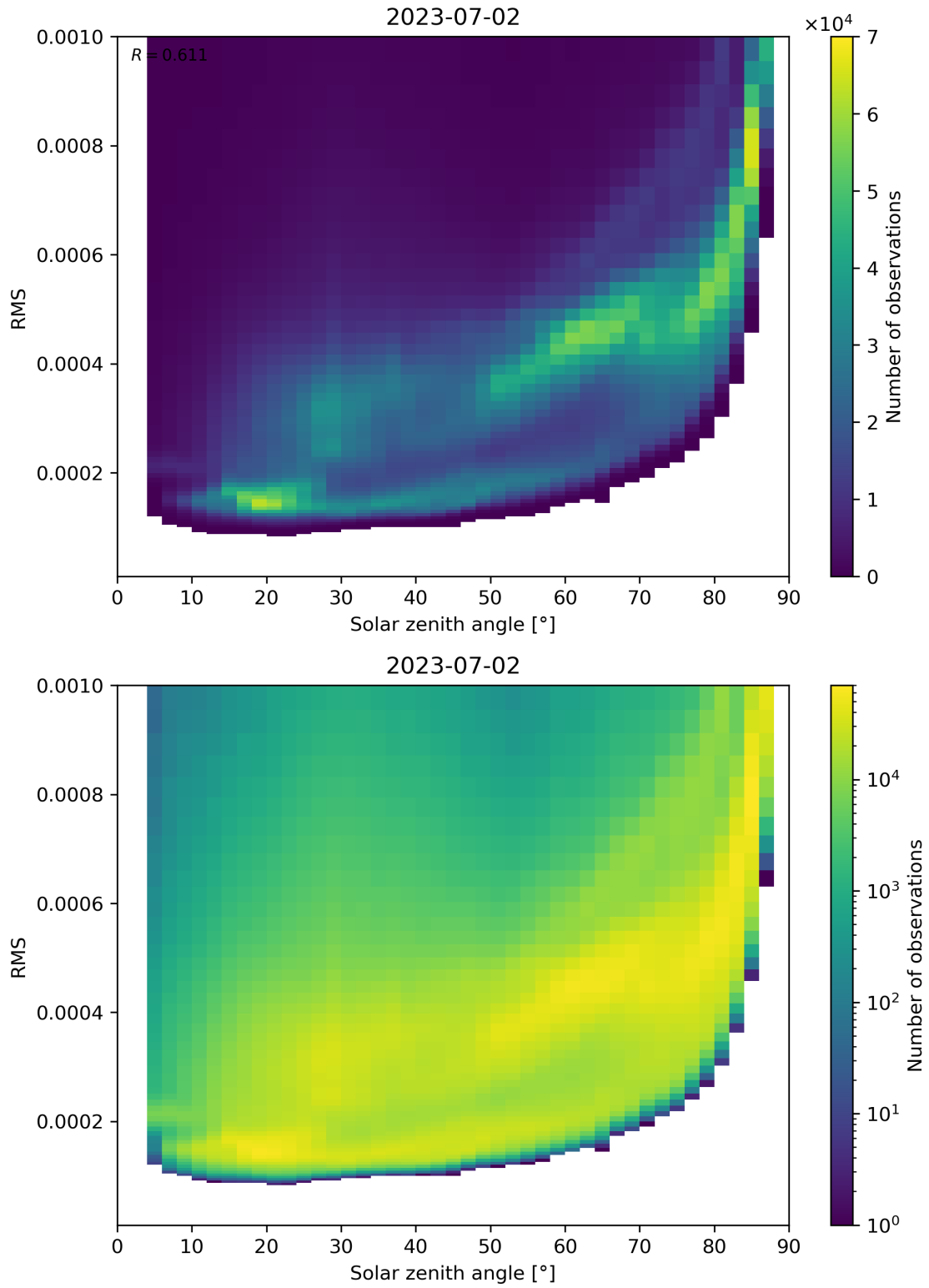
Figure 157: Scatter density plot of “Solar zenith angle” against “RMS” for 2023-07-01 to 2023-07-03.
