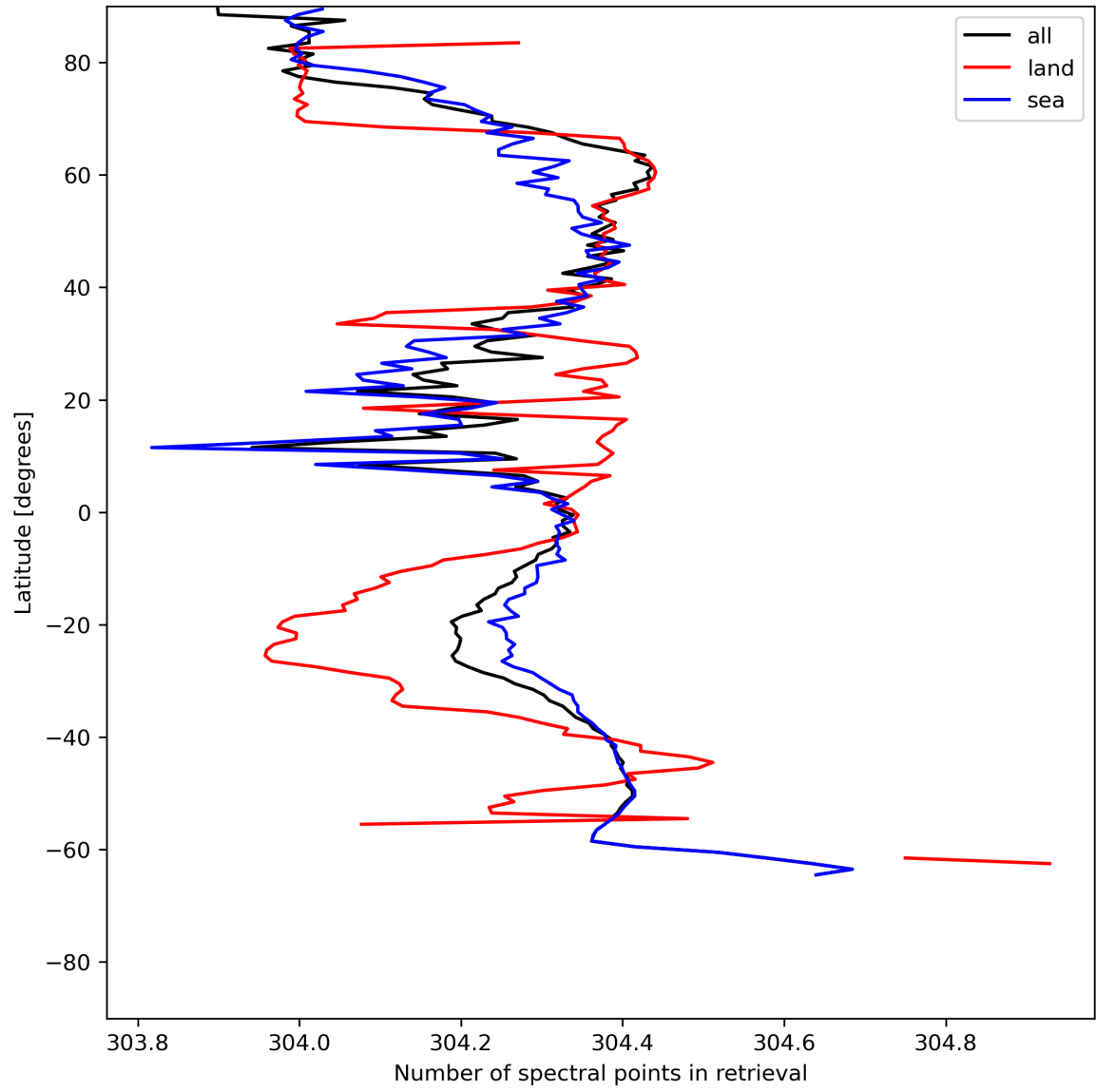
Figure 16: Zonal average of “Number of spectral points in retrieval” for 2023-07-01 to 2023-07-03.
