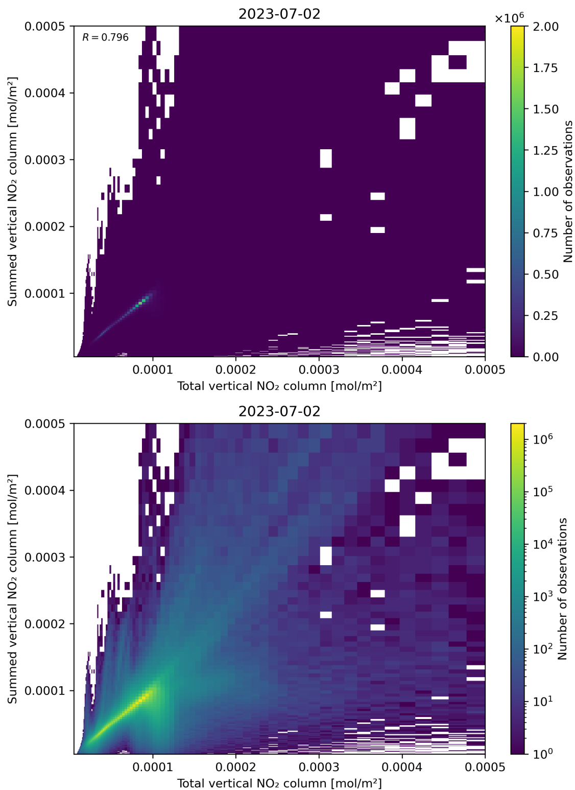
Figure 112: Scatter density plot of “Total vertical NO 2 column” against “Summed vertical NO 2 column” for 2023-07-01 to 2023-07-03.
