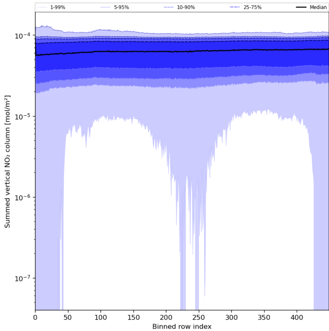
Figure 57: Along track statistics of “Summed vertical NO 2 column” for 2023-07-01 to 2023-07-03
