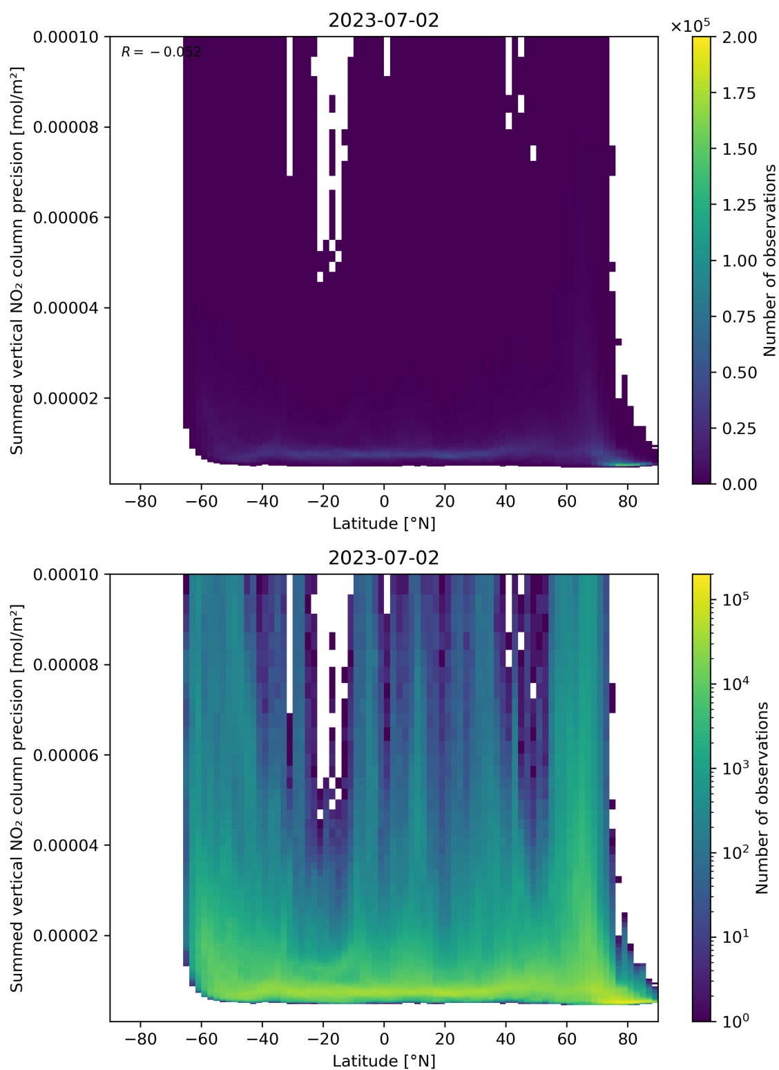
Figure 89: Scatter density plot of “Latitude” against “Summed vertical NO 2 column precision” for 2023-07-01 to 2023-07-03.
