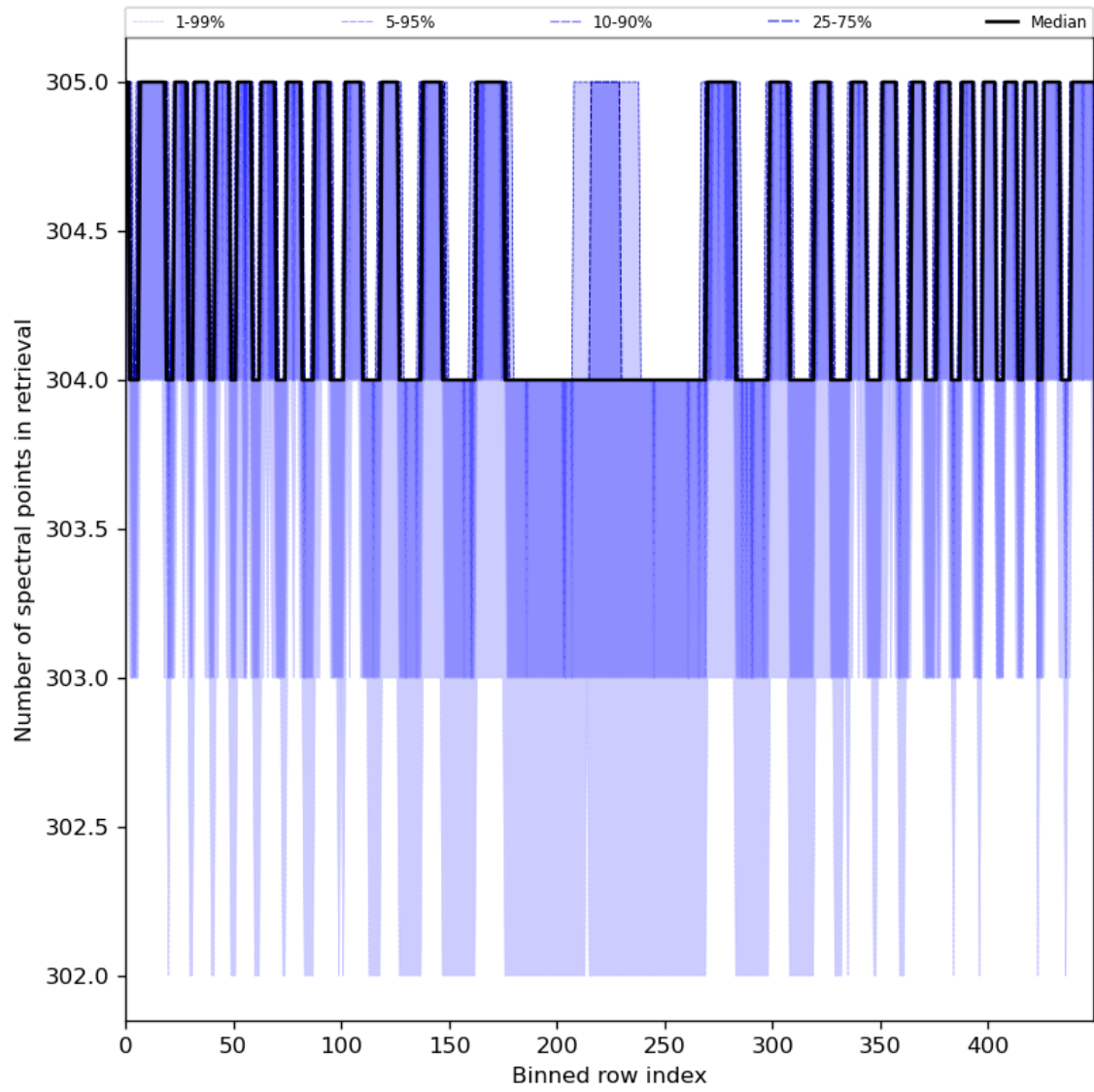
Figure 50: Along track statistics of “Number of spectral points in retrieval” for 2023-07-01 to 2023-07-03
