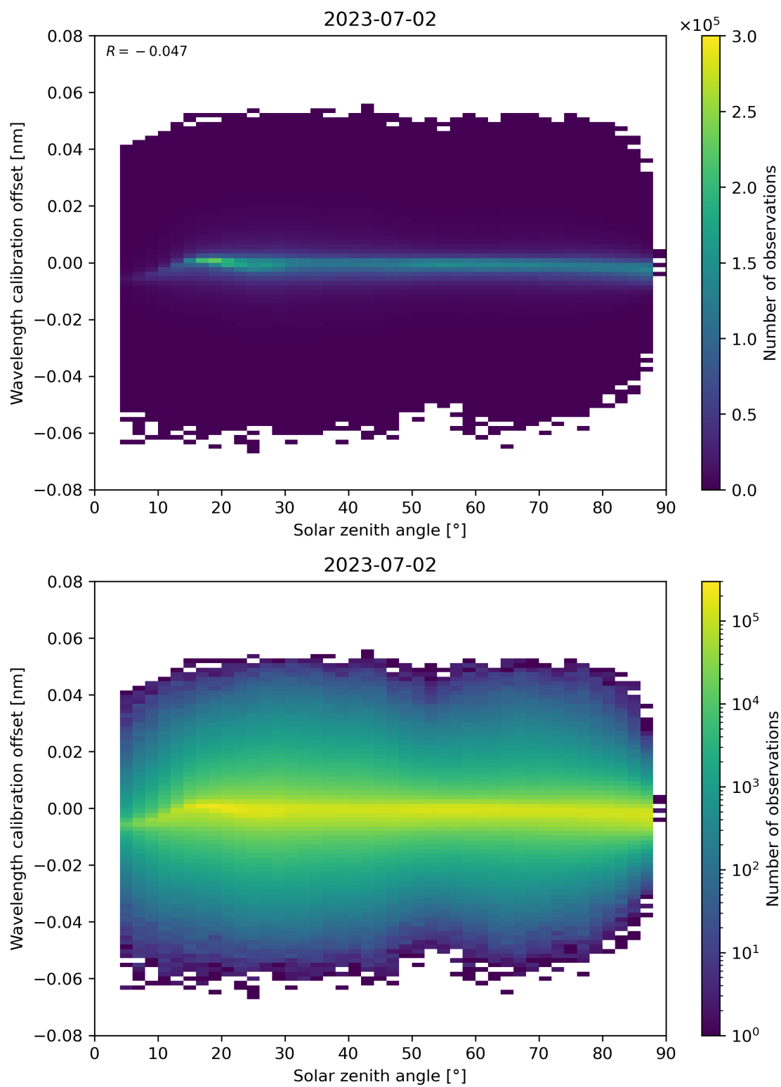
Figure 158: Scatter density plot of “Solar zenith angle” against “Wavelength calibration offset” for 2023-07-01 to 2023-07-03.
