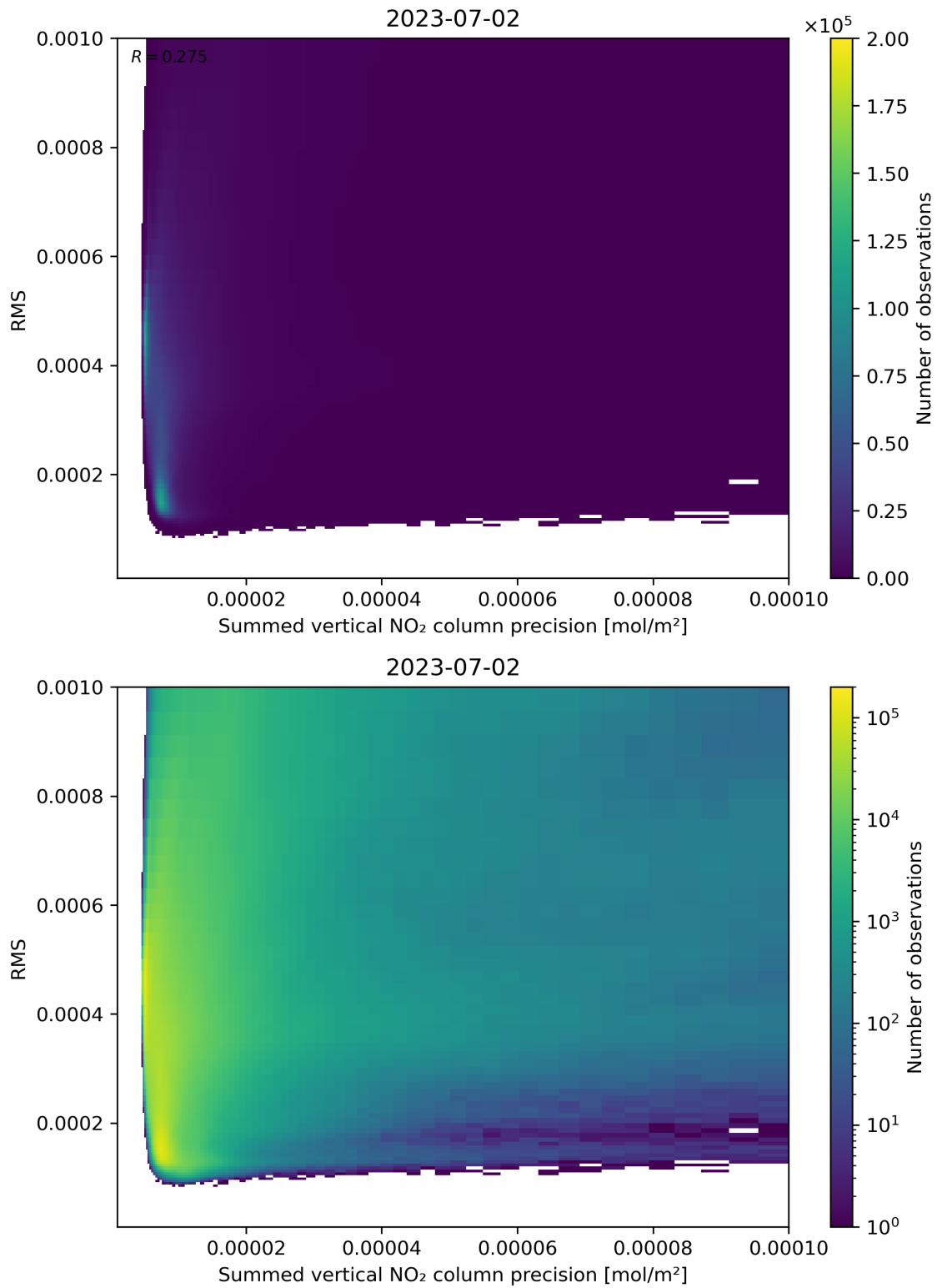
Figure 108: Scatter density plot of “Summed vertical NO 2 column precision” against “RMS” for 2023-07-01 to 2023-07-03.
