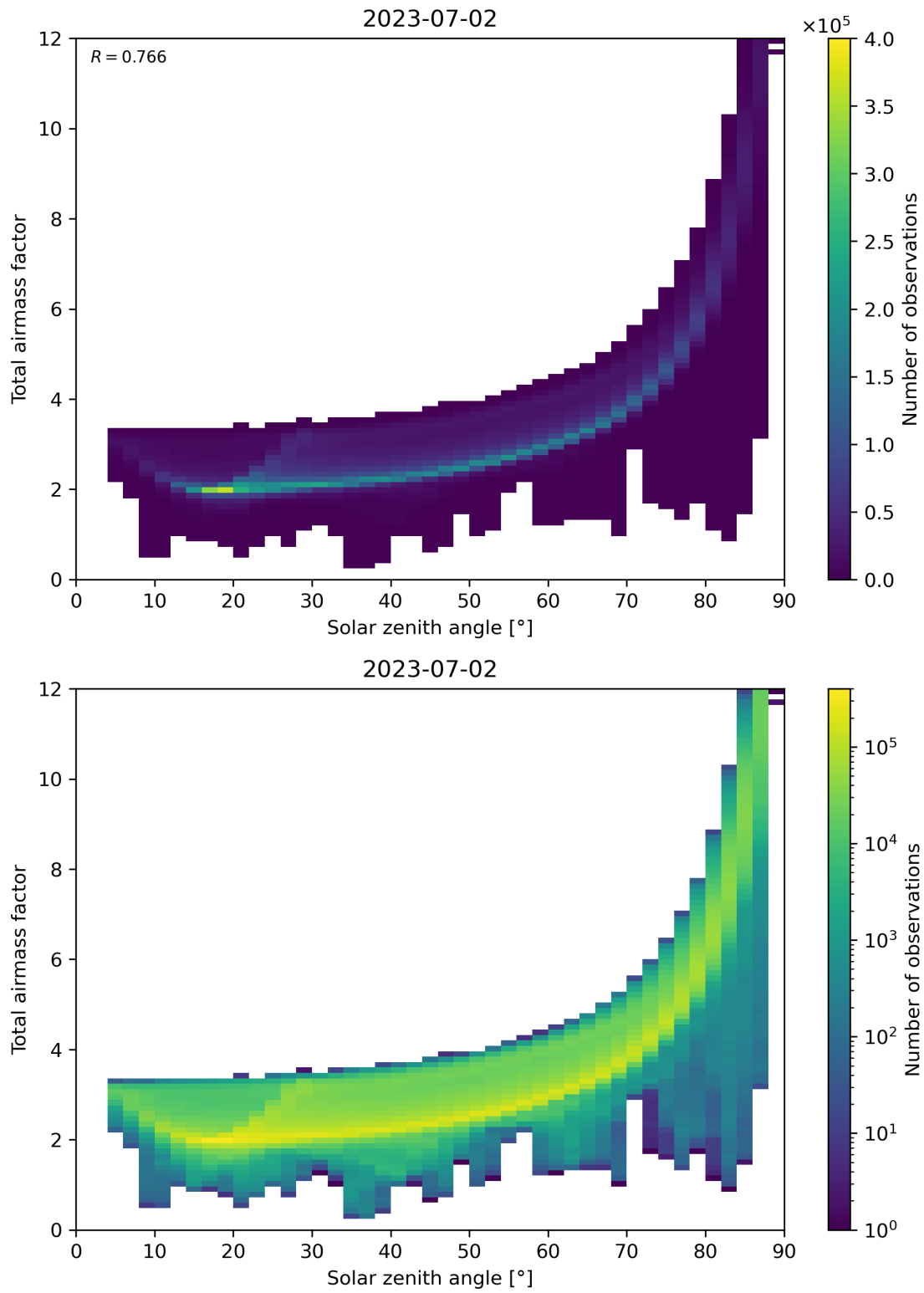
Figure 146: Scatter density plot of “Solar zenith angle” against “Total air mass factor” for 2023-07-01 to 2023-07-03.
