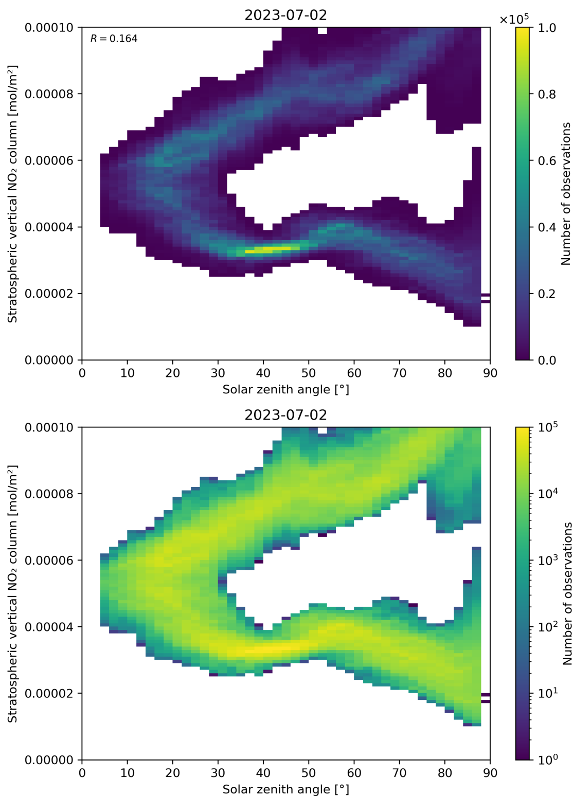
Figure 150: Scatter density plot of “Solar zenith angle” against “Stratospheric vertical NO 2 column” for 2023-07-01 to 2023-07-03.
