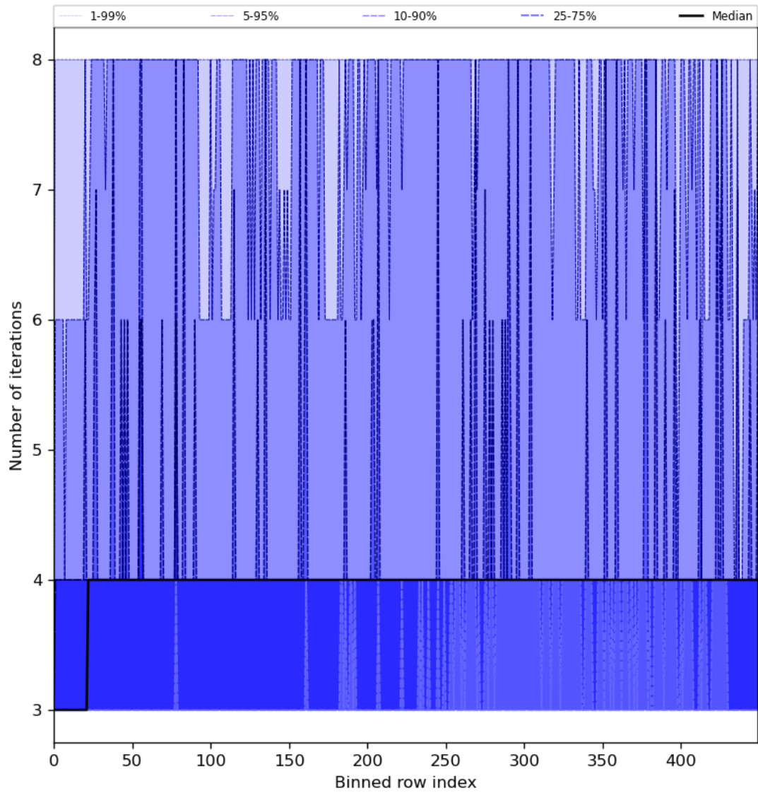
Figure 51: Along track statistics of “Number of iterations” for 2023-07-01 to 2023-07-03
