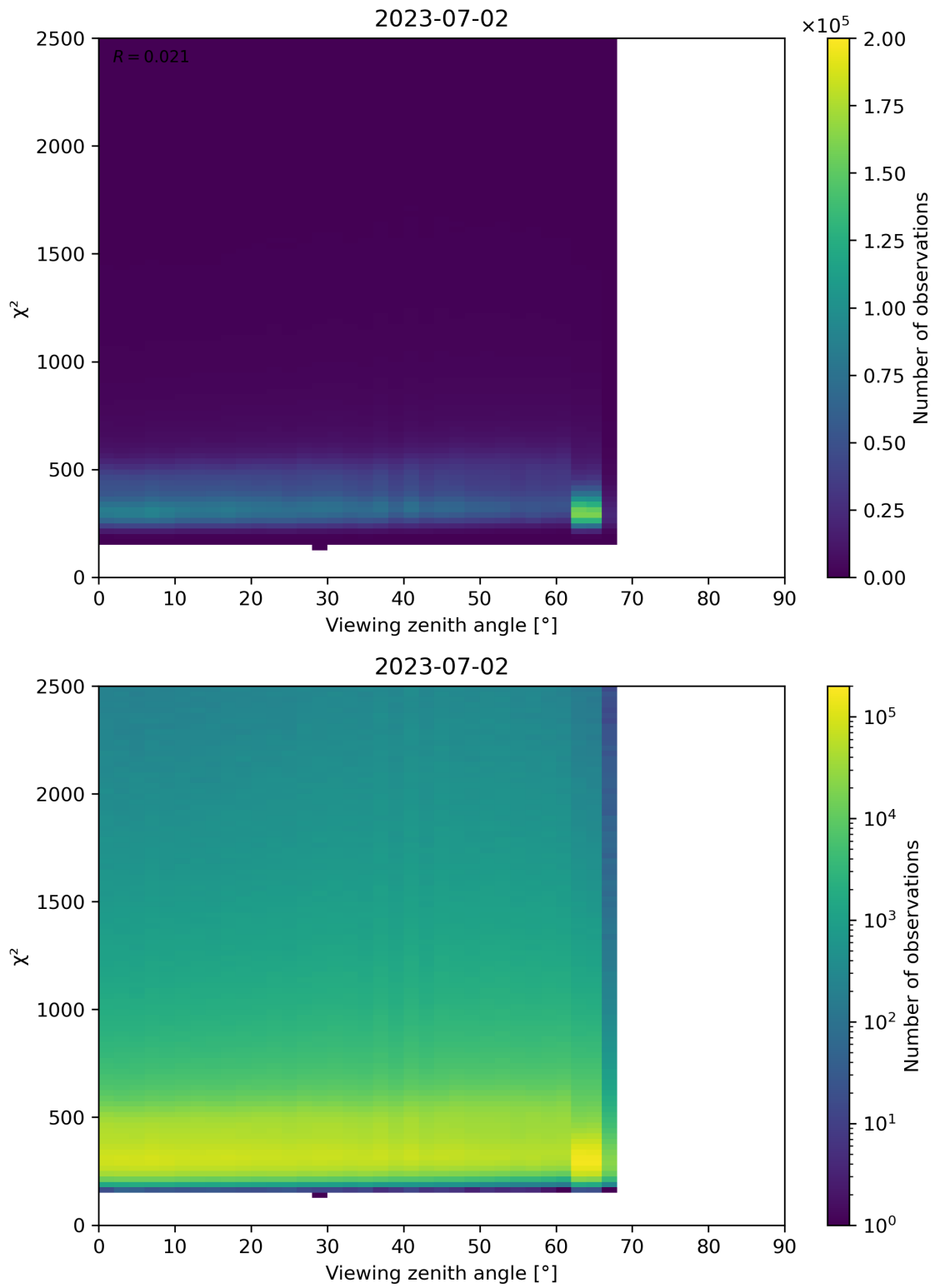
Figure 162: Scatter density plot of “Viewing zenith angle” against “ \chi^2 ” for 2023-07-01 to 2023-07-03.
