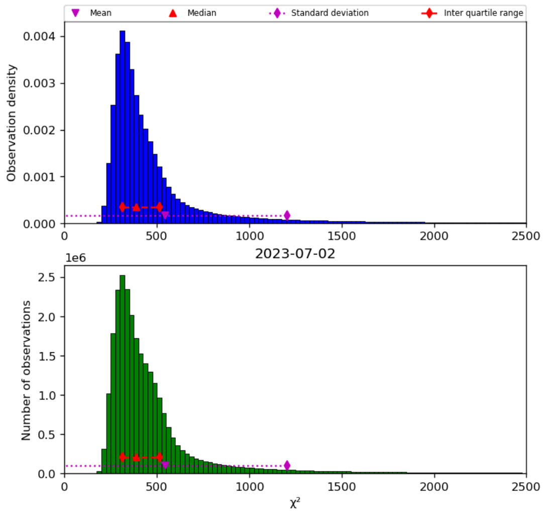
Figure 42: Histogram of “ \chi^2 ” for 2023-07-01 to 2023-07-03
