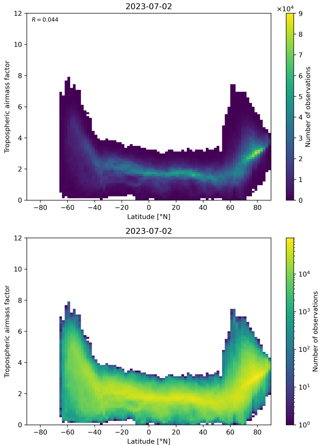
Figure 85: Scatter density plot of “Latitude” against “Tropospheric air mass factor” for 2023-07-01 to 2023-07-03.
