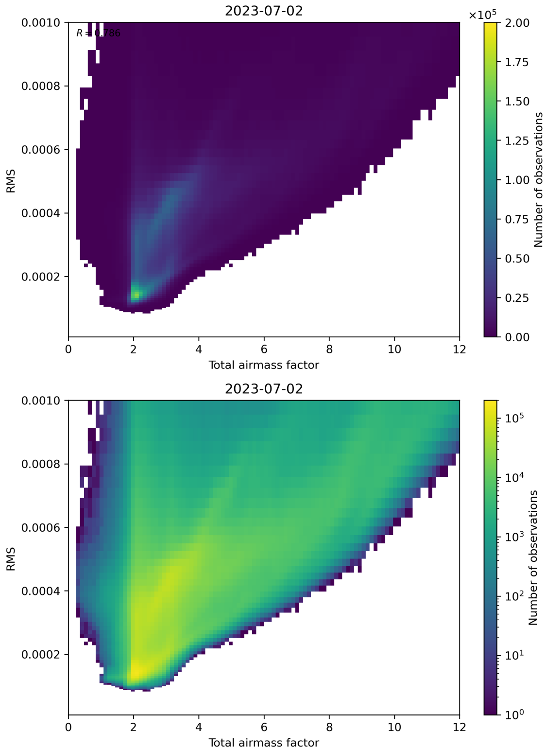
Figure 69: Scatter density plot of “Total airmass factor” against “RMS” for 2023-07-01 to 2023-07-03.
