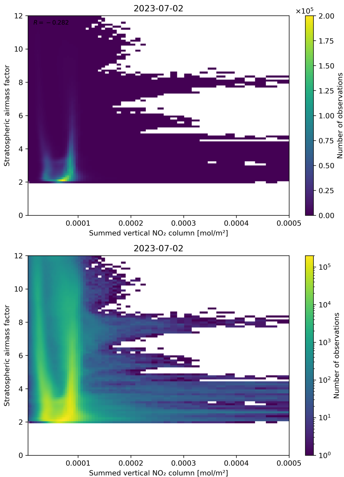
Figure 103: Scatter density plot of “Summed vertical NO 2 column” against “Stratospheric air mass factor” for 2023-07-01 to 2023-07-03.
