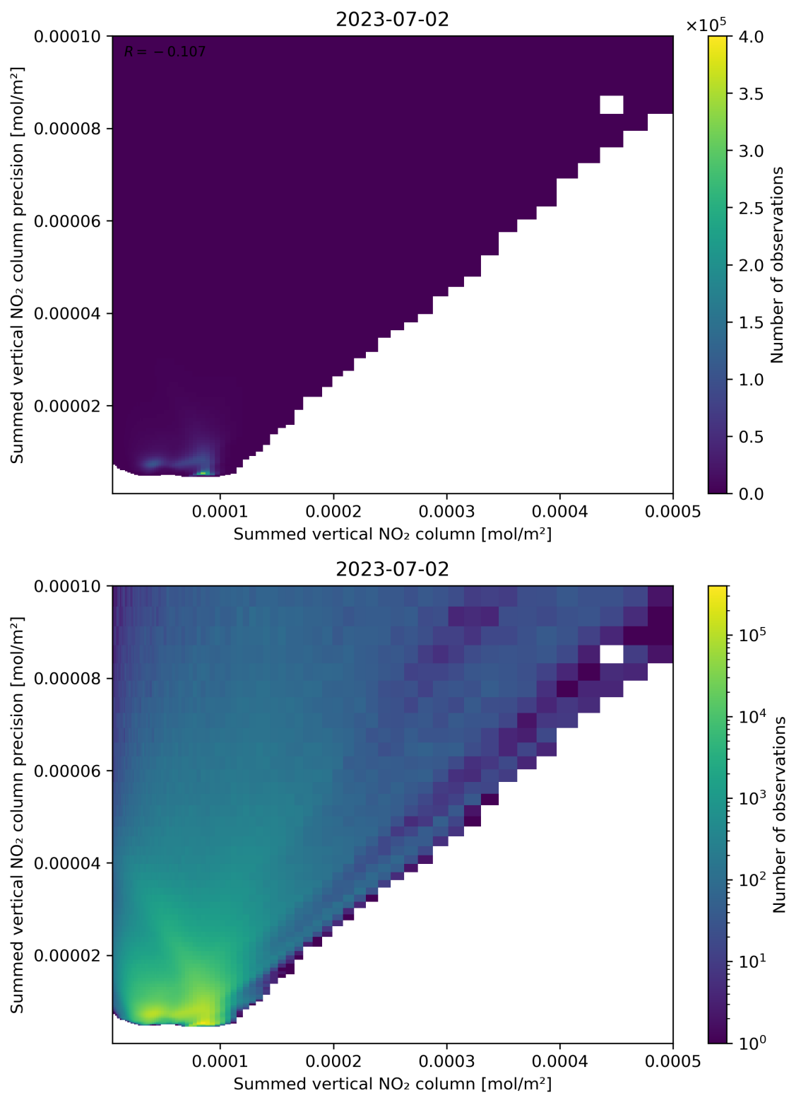
Figure 105: Scatter density plot of “Summed vertical NO 2 column” against “Summed vertical NO 2 column precision” for 2023-07-01 to 2023-07-03.
