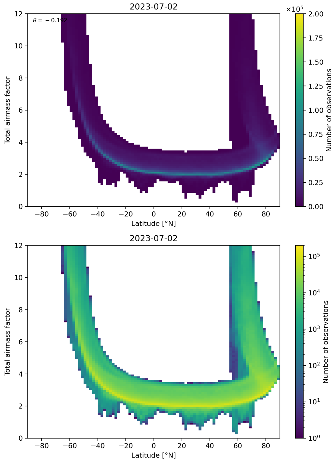
Figure 84: Scatter density plot of “Latitude” against “Total air mass factor” for 2023-07-01 to 2023-07-03.
