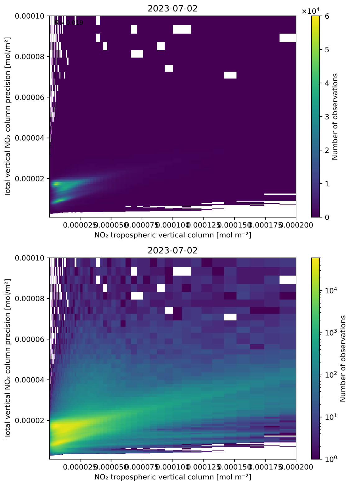
Figure 129: Scatter density plot of “NO 2 tropospheric vertical column” against “Total vertical NO 2 column precision” for 2023-07-01 to 2023-07-03.
