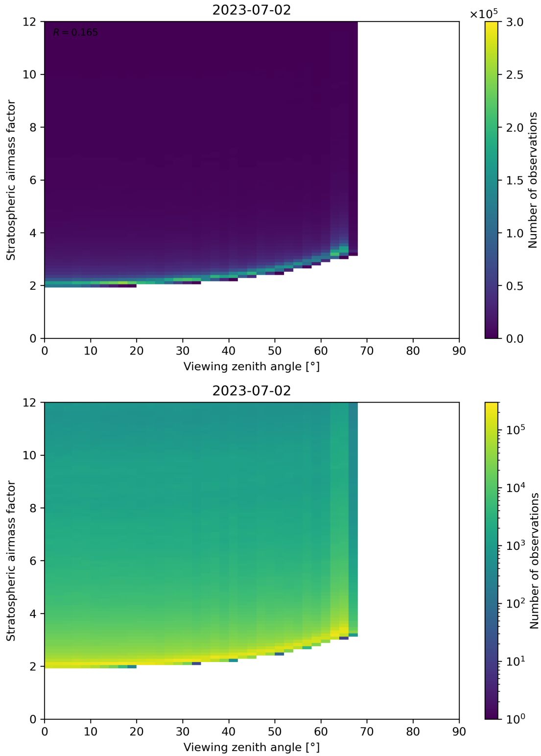
Figure 159: Scatter density plot of “Viewing zenith angle” against “Stratospheric airmass factor” for 2023-07-01 to 2023-07-03.
