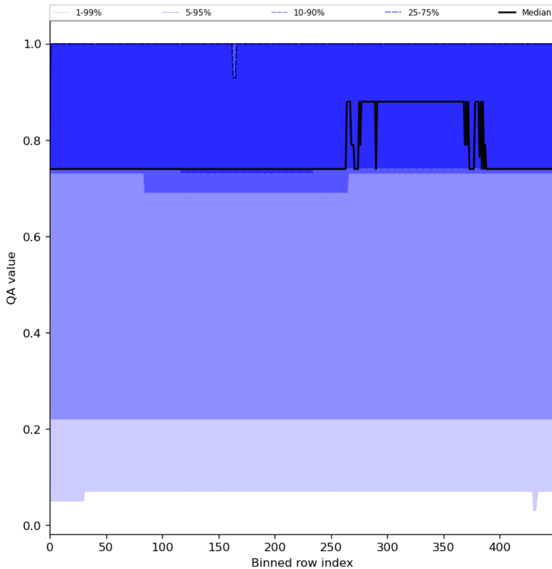
Figure 45: Along track statistics of “QA value” for 2023-07-01 to 2023-07-03
