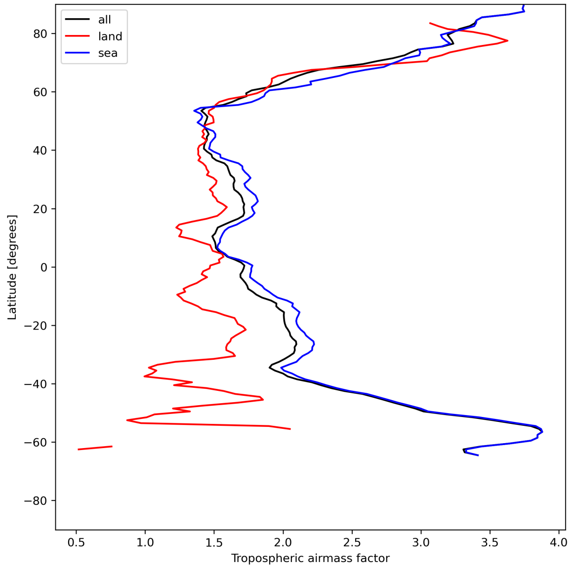
Figure 14: Zonal average of “Tropospheric air mass factor” for 2023-07-01 to 2023-07-03.
