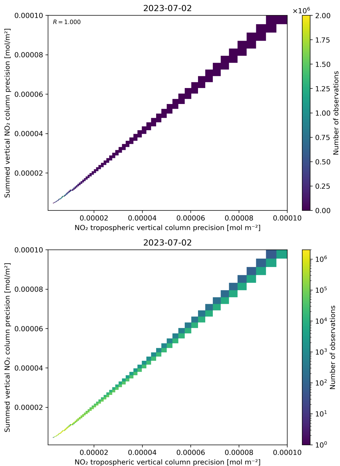
Figure 137: Scatter density plot of “NO 2 tropospheric vertical column precision” against “Summed vertical NO 2 column precision” for 2023-07-01 to 2023-07-03.
