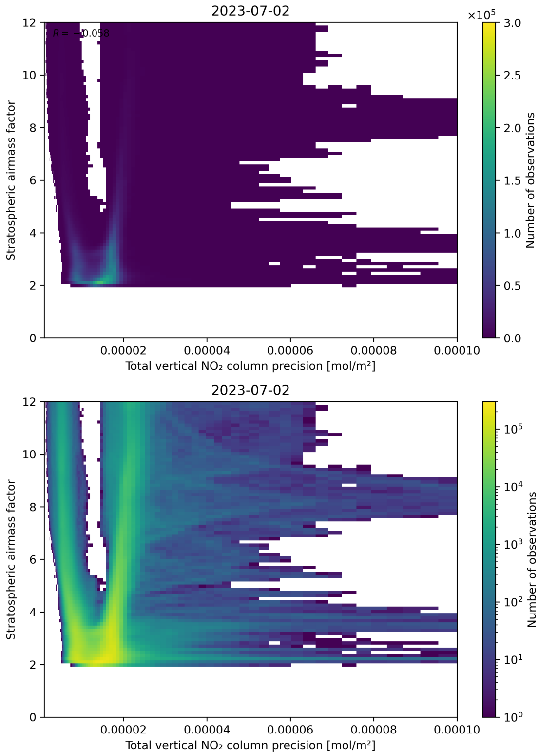
Figure 115: Scatter density plot of “Total vertical NO 2 column precision” against “Stratospheric air mass factor” for 2023-07-01 to 2023-07-03.
