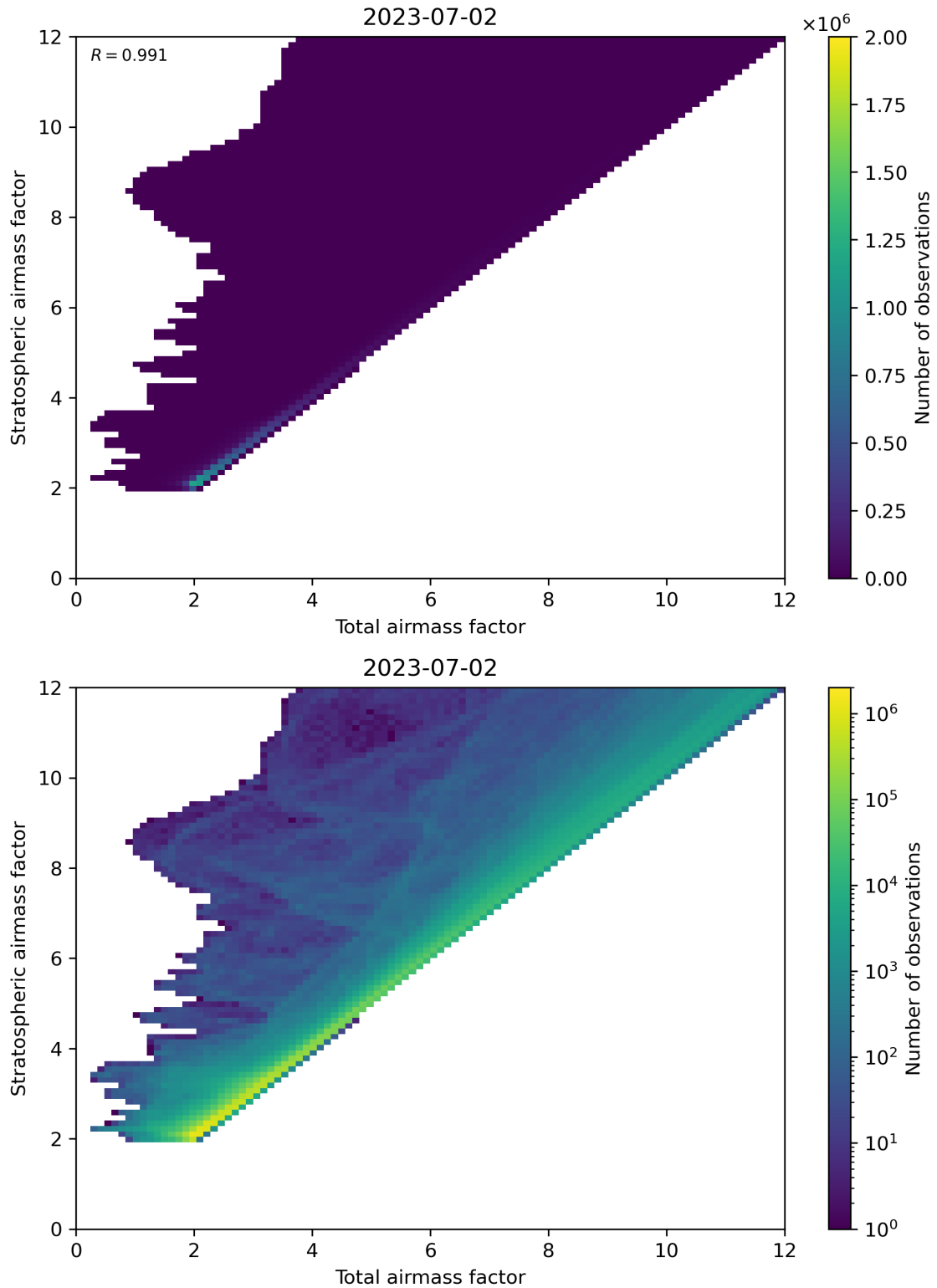
Figure 62: Scatter density plot of “Total airmass factor” against “Stratospheric airmass factor” for 2023-07-01 to 2023-07-03.
