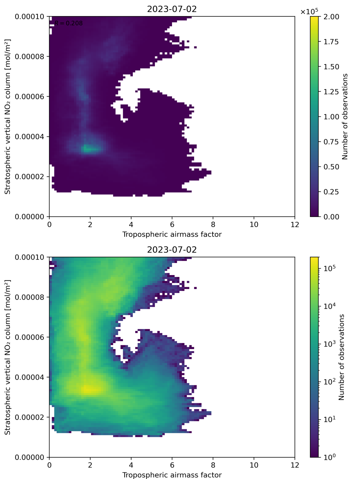
Figure 74: Scatter density plot of “Tropospheric air mass factor” against “Stratospheric vertical NO 2 column” for 2023-07-01 to 2023-07-03.
