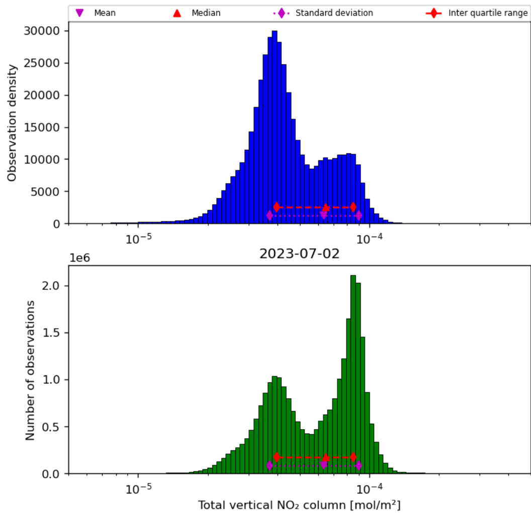
Figure 38: Histogram of “Total vertical NO 2 column” for 2023-07-01 to 2023-07-03
