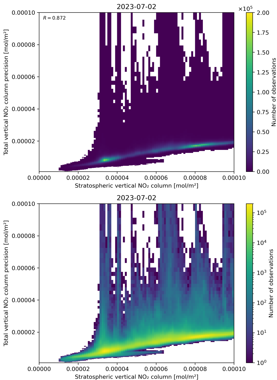
Figure 101: Scatter density plot of “Stratospheric vertical NO 2 column” against “Total vertical NO 2 column precision” for 2023-07-01 to 2023-07-03.
