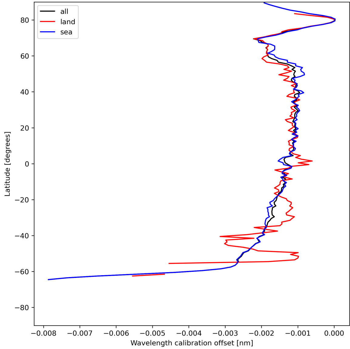
Figure 18: Zonal average of “Wavelength calibration offset” for 2023-07-01 to 2023-07-03.
