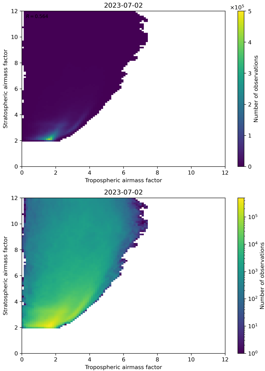
Figure 71: Scatter density plot of “Tropospheric airmass factor” against “Stratospheric airmass factor” for 2023-07-01 to 2023-07-03.
