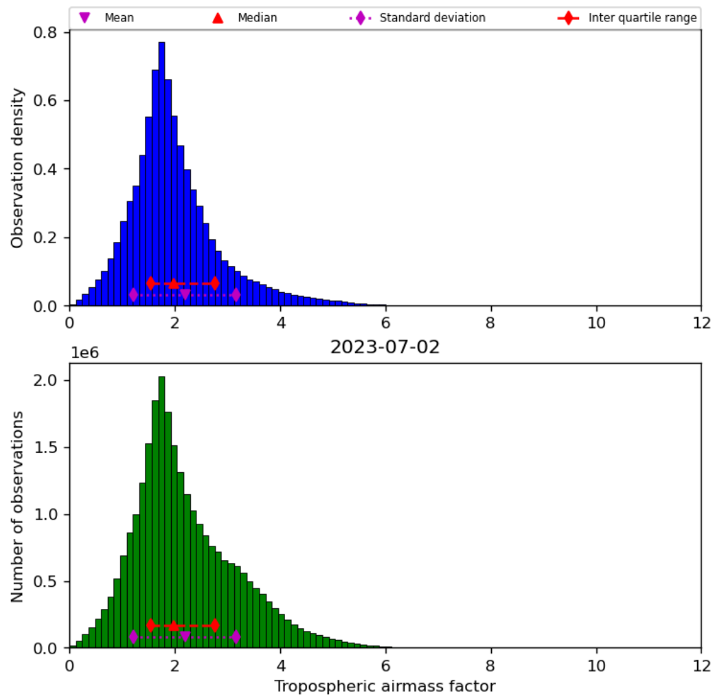
Figure 31: Histogram of “Tropospheric airmass factor” for 2023-07-01 to 2023-07-03
