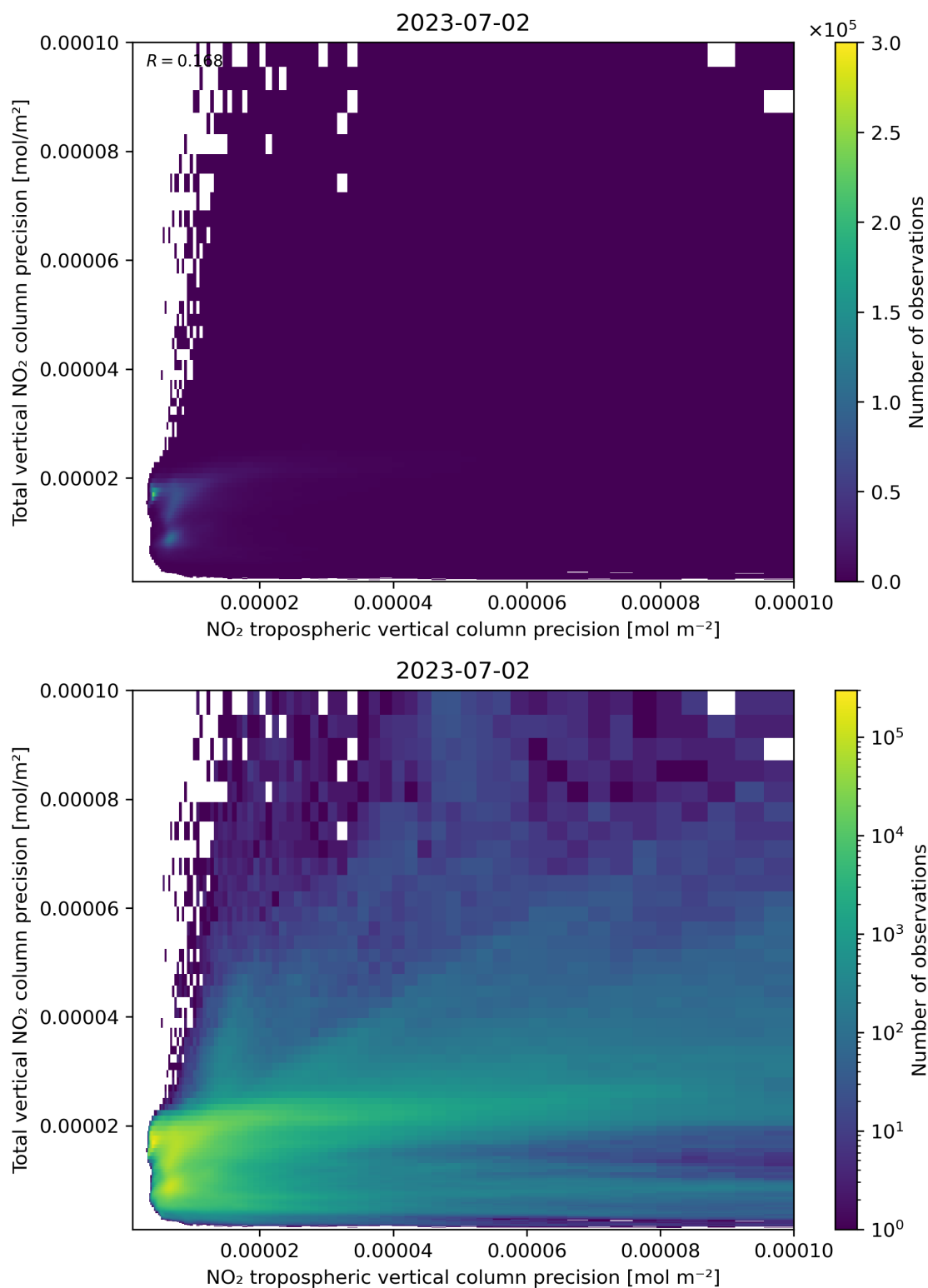
Figure 139: Scatter density plot of “NO 2 tropospheric vertical column precision” against “Total vertical NO 2 column precision” for 2023-07-01 to 2023-07-03.
