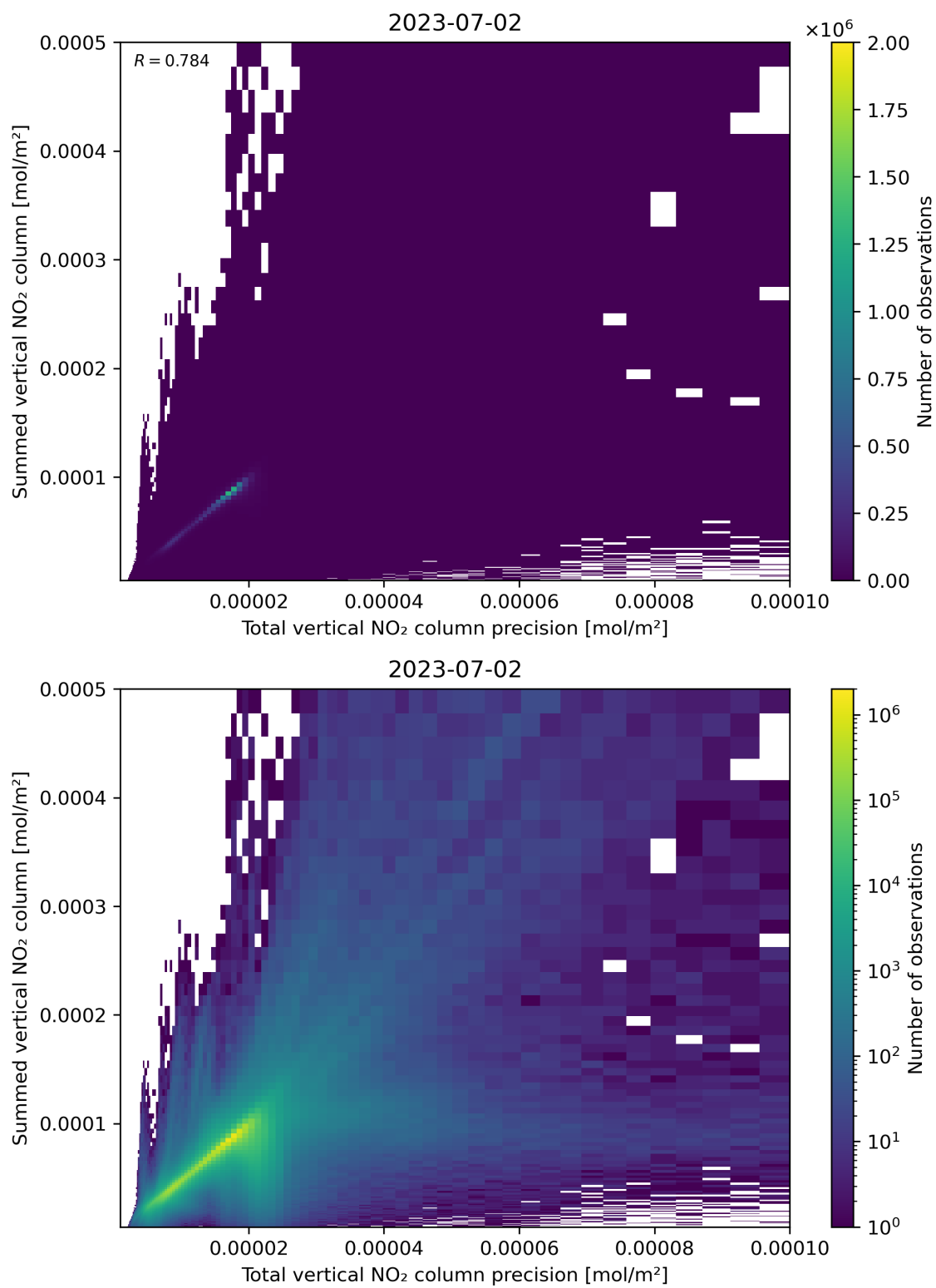
Figure 117: Scatter density plot of “Total vertical NO 2 column precision” against “Summed vertical NO 2 column” for 2023-07-01 to 2023-07-03.
