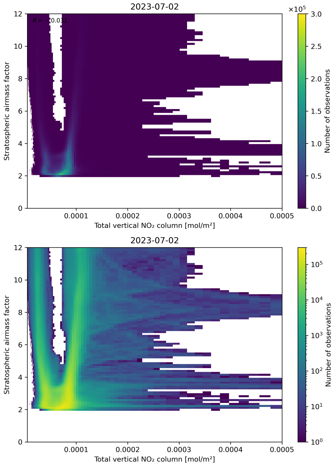
Figure 110: Scatter density plot of “Total vertical NO 2 column” against “Stratospheric air mass factor” for 2023-07-01 to 2023-07-03.
