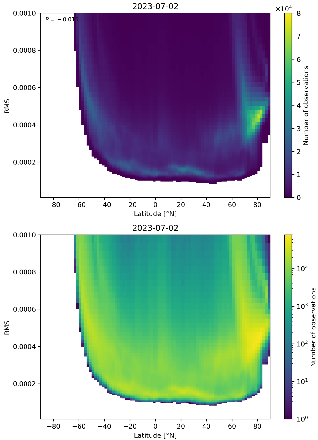
Figure 94: Scatter density plot of “Latitude” against “RMS” for 2023-07-01 to 2023-07-03.
