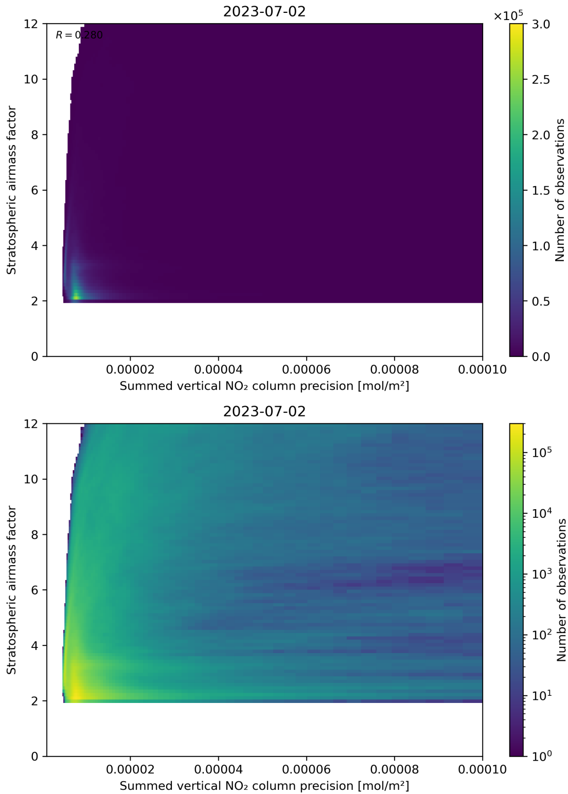
Figure 106: Scatter density plot of “Summed vertical NO 2 column precision” against “Stratospheric airmass factor” for 2023-07-01 to 2023-07-03.
