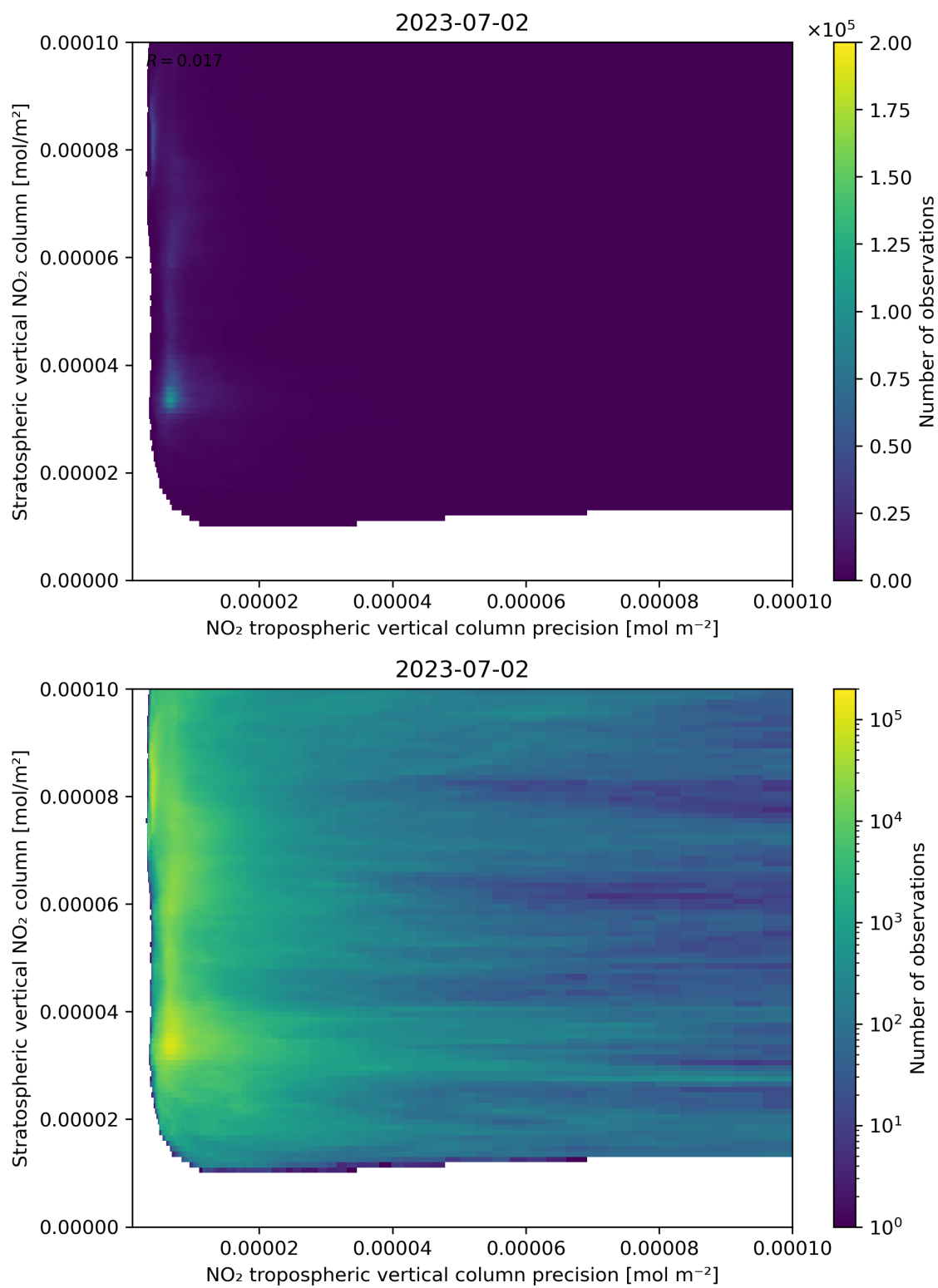
Figure 135: Scatter density plot of “NO 2 tropospheric vertical column precision” against “Stratospheric vertical NO 2 column” for 2023-07-01 to 2023-07-03.
