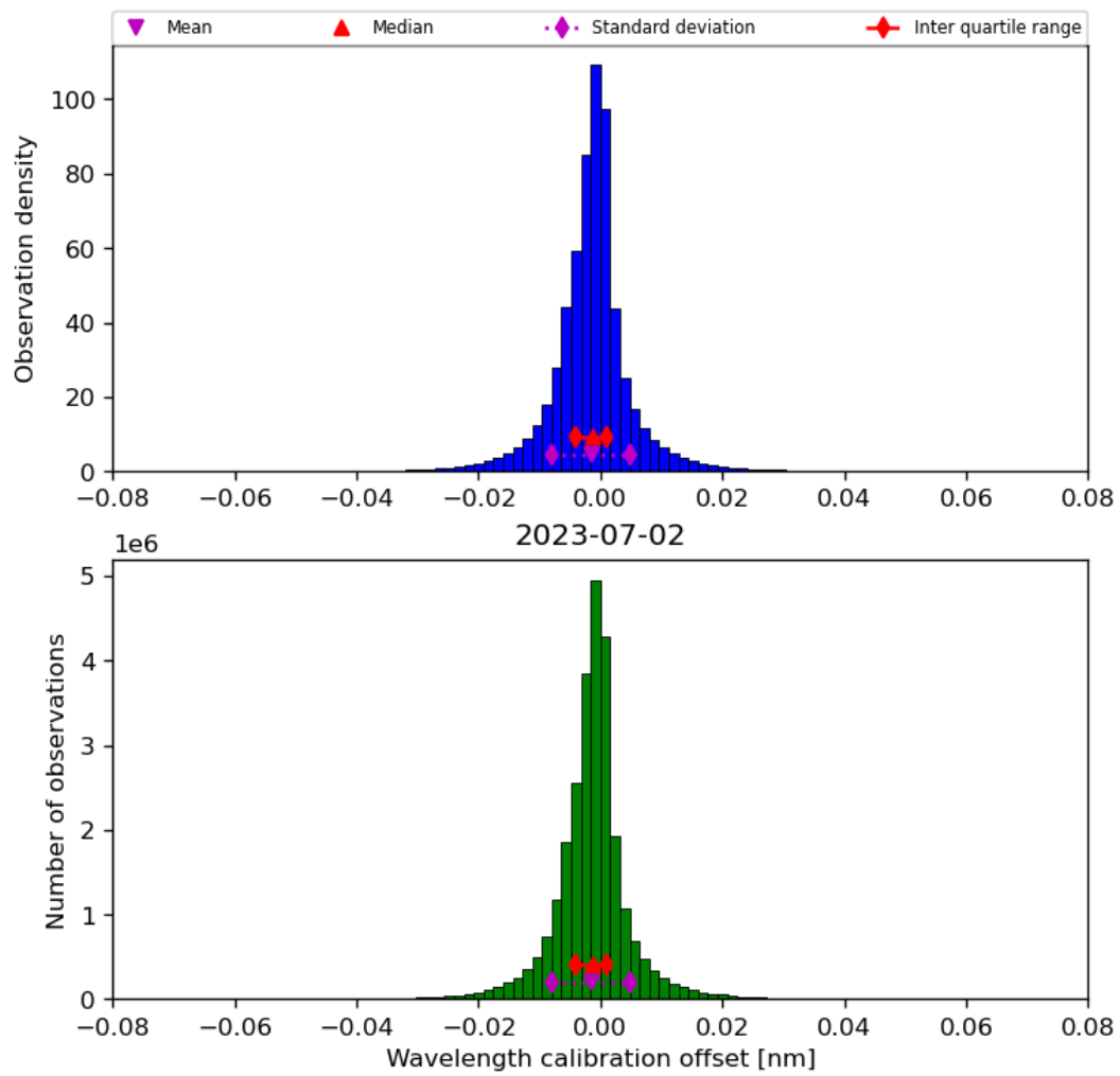
Figure 35: Histogram of “Wavelength calibration offset” for 2023-07-01 to 2023-07-03
