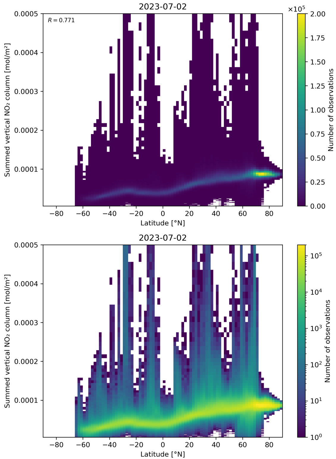
Figure 88: Scatter density plot of “Latitude” against “Summed vertical NO 2 column” for 2023-07-01 to 2023-07-03.
