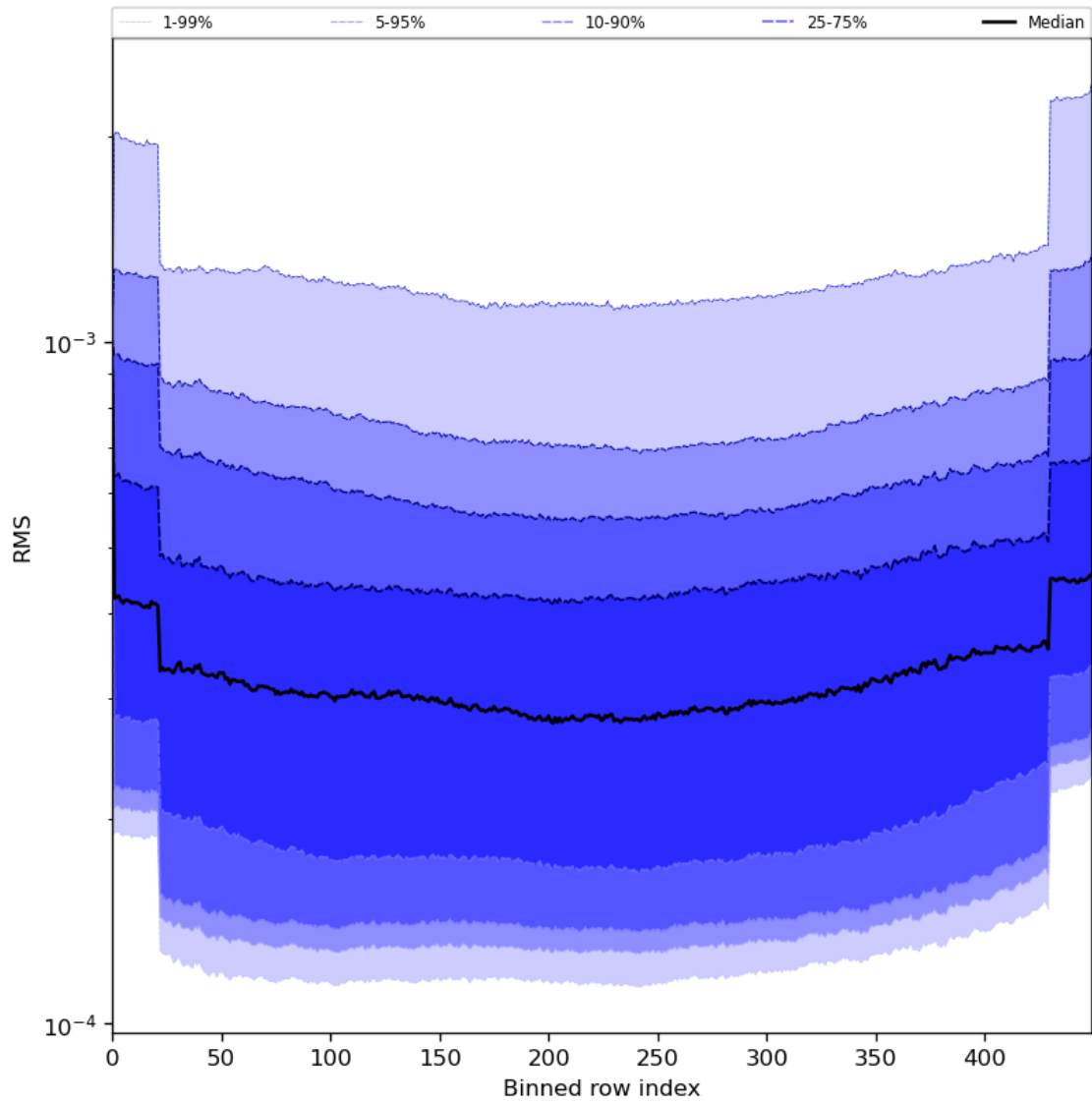
Figure 60: Along track statistics of “RMS” for 2023-07-01 to 2023-07-03
