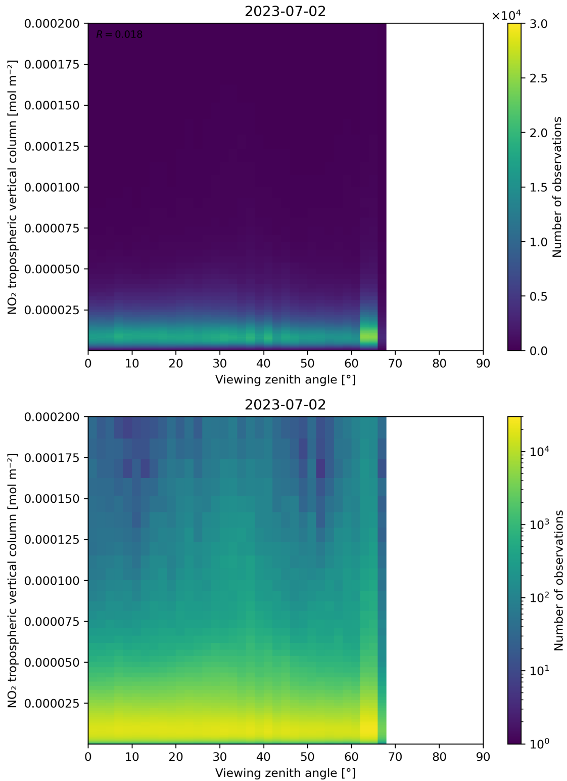
Figure 169: Scatter density plot of “Viewing zenith angle” against “NO 2 tropospheric vertical column” for 2023-07-01 to 2023-07-03.
