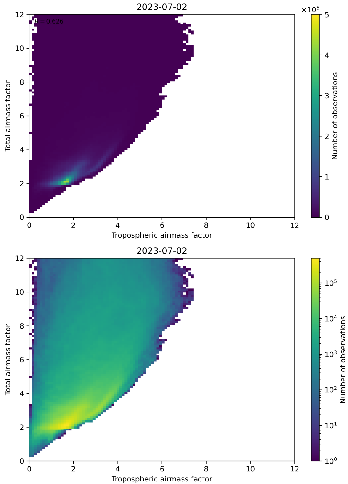
Figure 72: Scatter density plot of “Tropospheric airmass factor” against “Total airmass factor” for 2023-07-01 to 2023-07-03.
