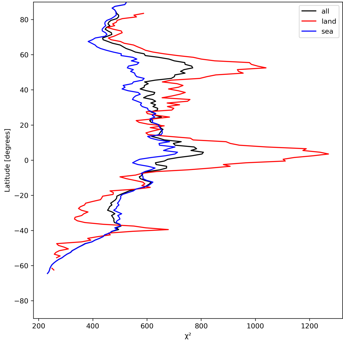
Figure 25: Zonal average of “ \chi^2 ” for 2023-07-01 to 2023-07-03.
