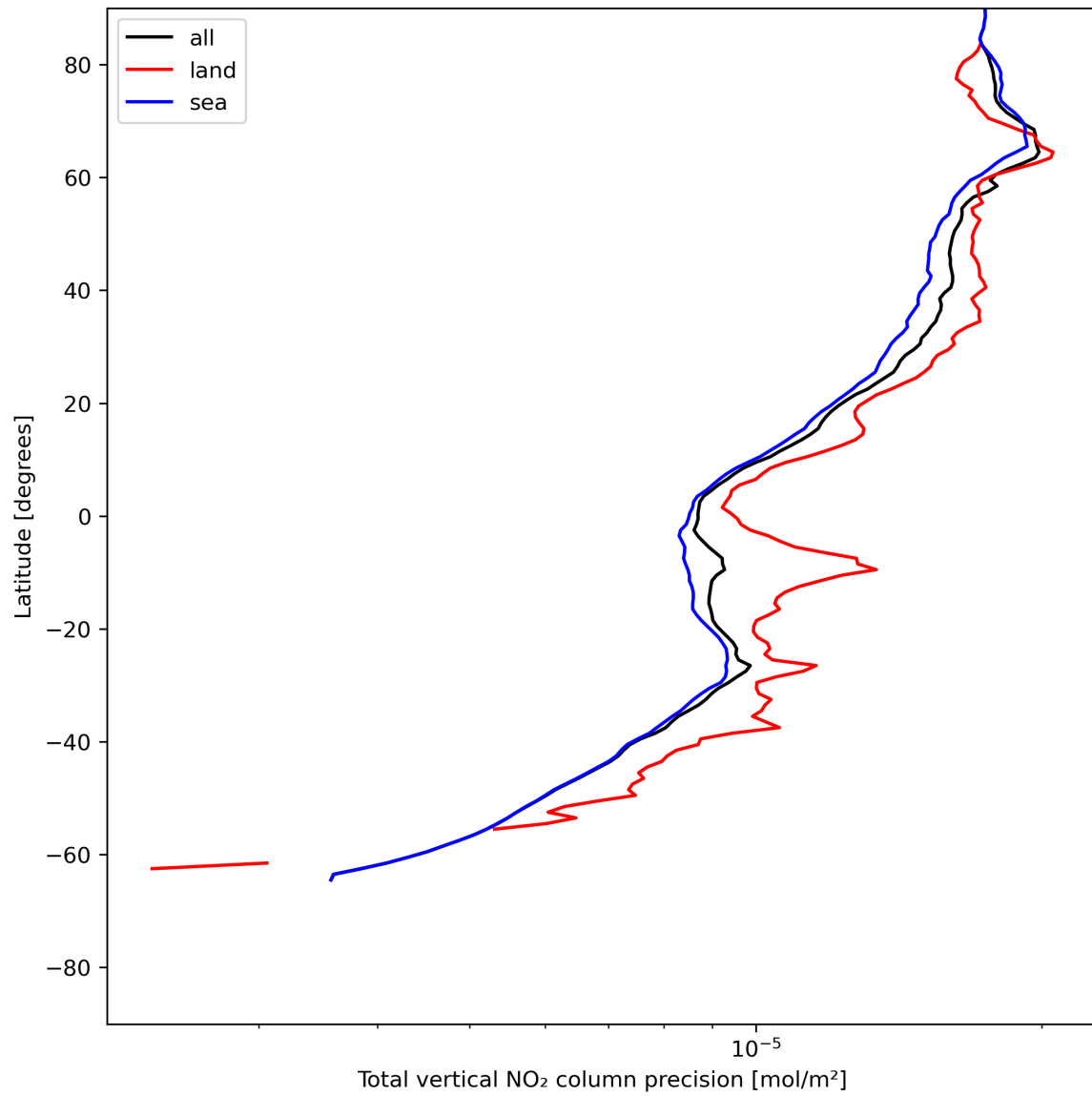
Figure 22: Zonal average of “Total vertical NO 2 column precision” for 2023-07-01 to 2023-07-03.
