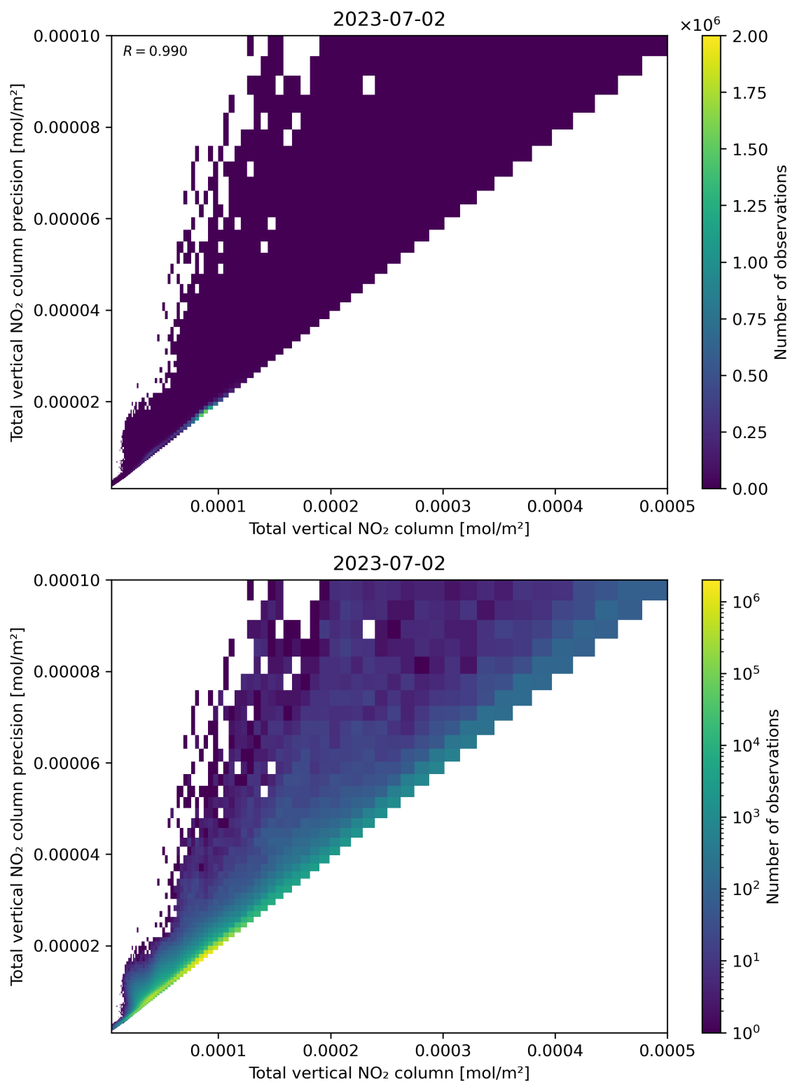
Figure 114: Scatter density plot of “Total vertical NO 2 column” against “Total vertical NO 2 column precision” for 2023-07-01 to 2023-07-03.
