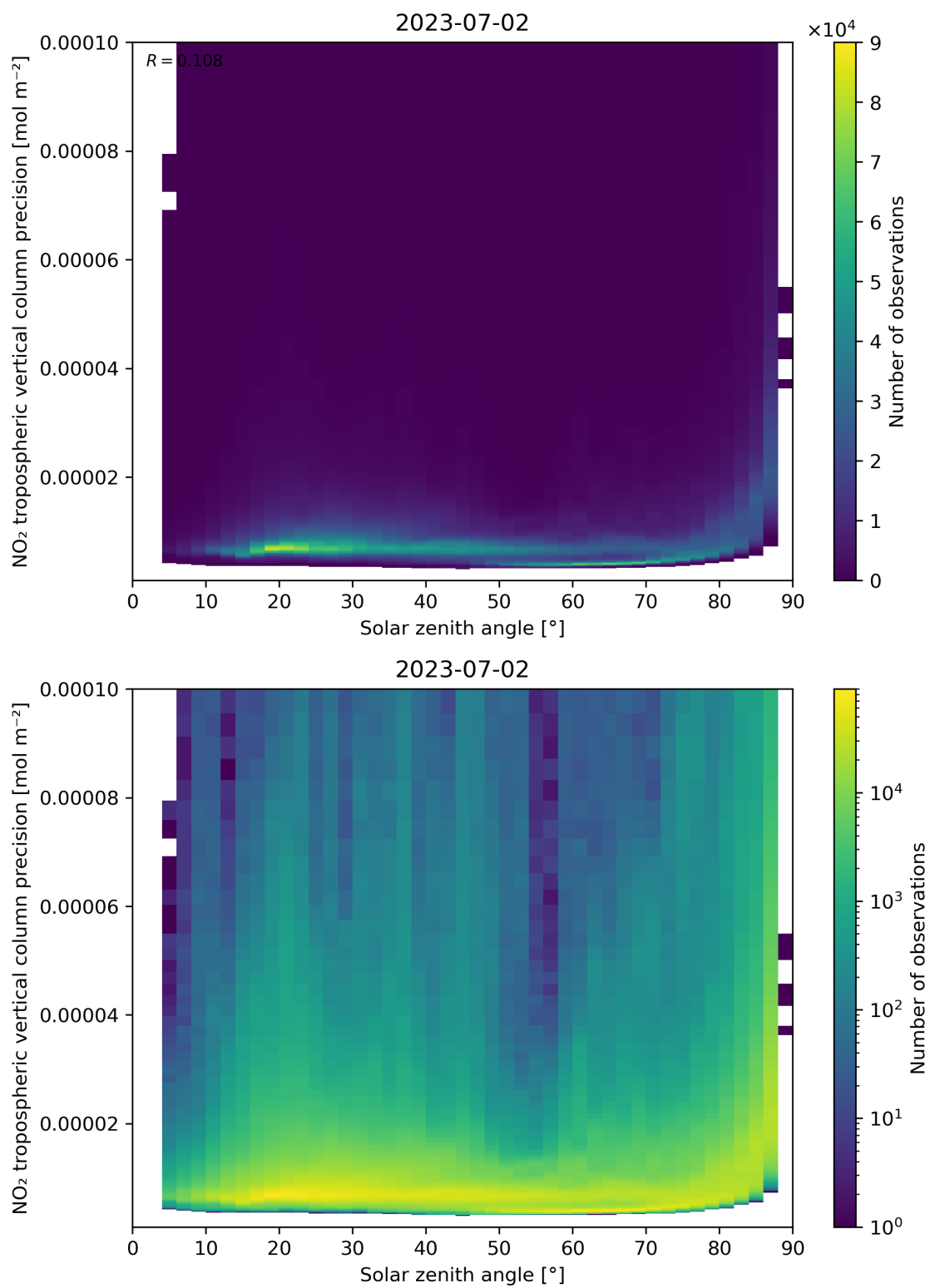
Figure 156: Scatter density plot of “Solar zenith angle” against “NO 2 tropospheric vertical column precision” for 2023-07-01 to 2023-07-03.
