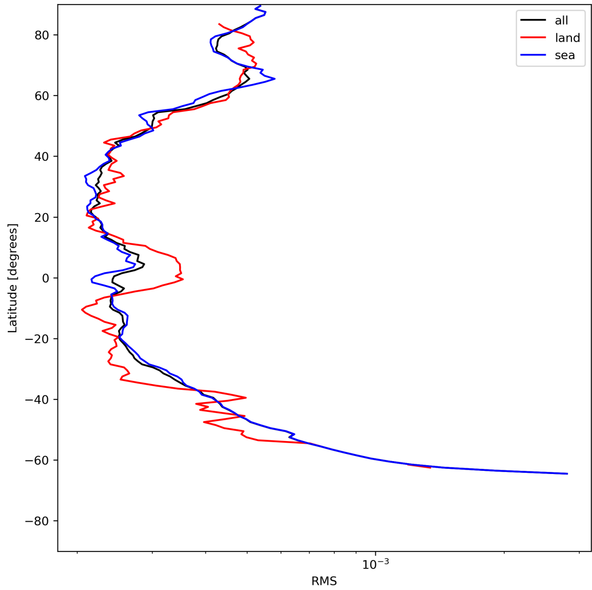
Figure 26: Zonal average of “RMS” for 2023-07-01 to 2023-07-03.
