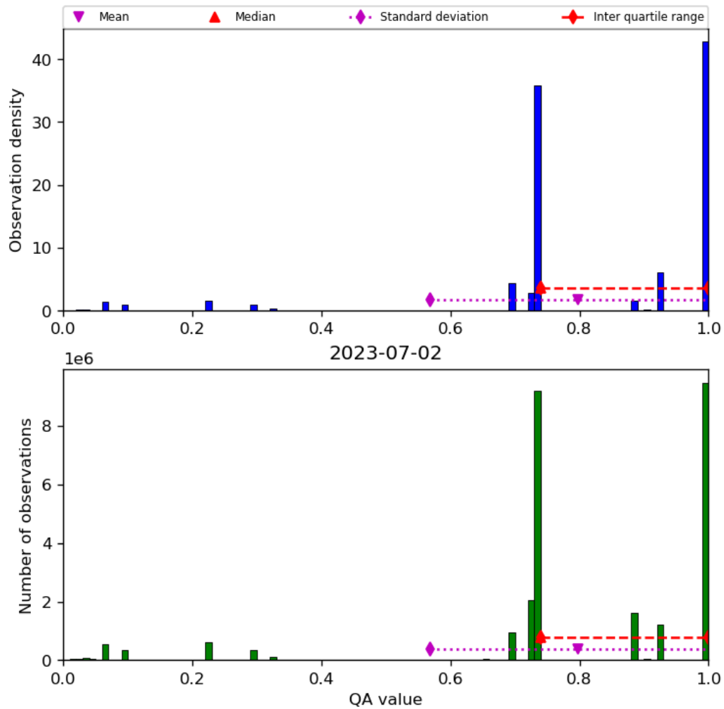
Figure 28: Histogram of “QA value” for 2023-07-01 to 2023-07-03
