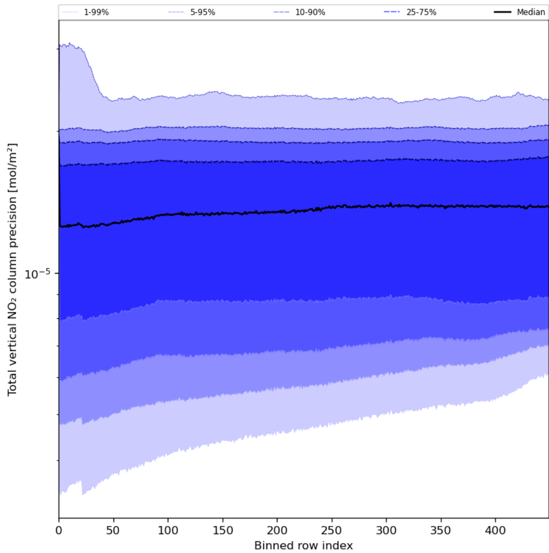
Figure 56: Along track statistics of “Total vertical NO 2 column precision” for 2023-07-01 to 2023-07-03
