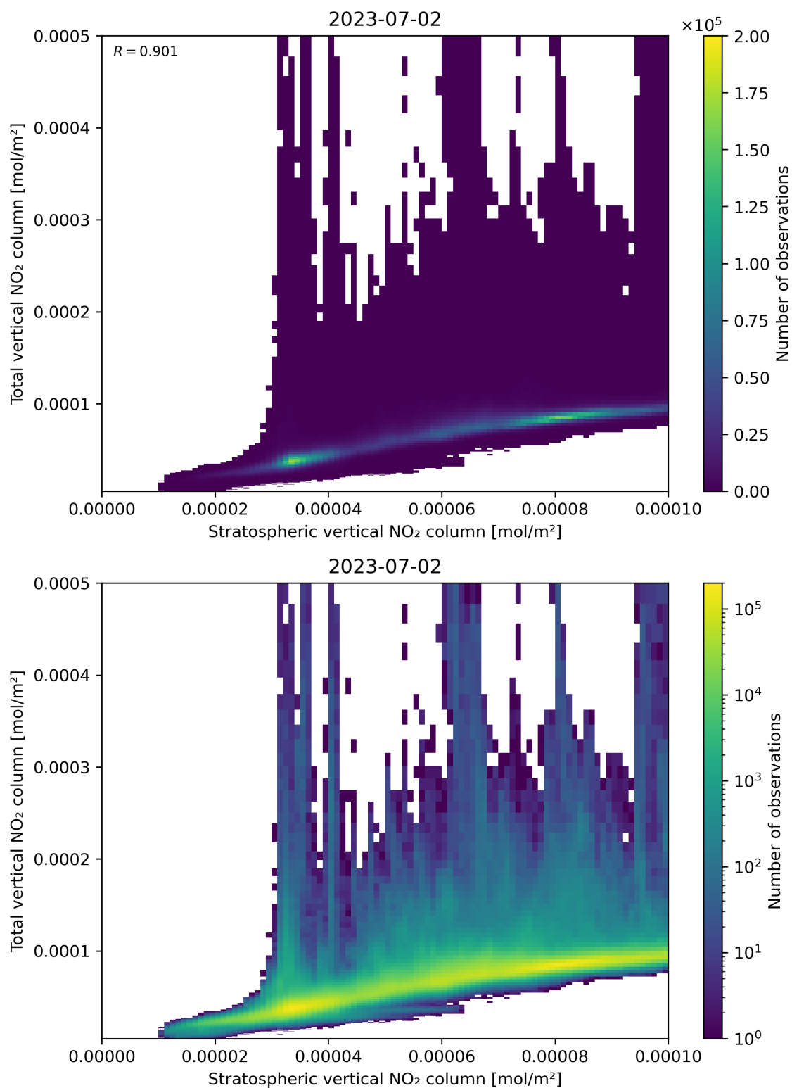
Figure 100: Scatter density plot of “Stratospheric vertical NO 2 column” against “Total vertical NO 2 column” for 2023-07-01 to 2023-07-03.
