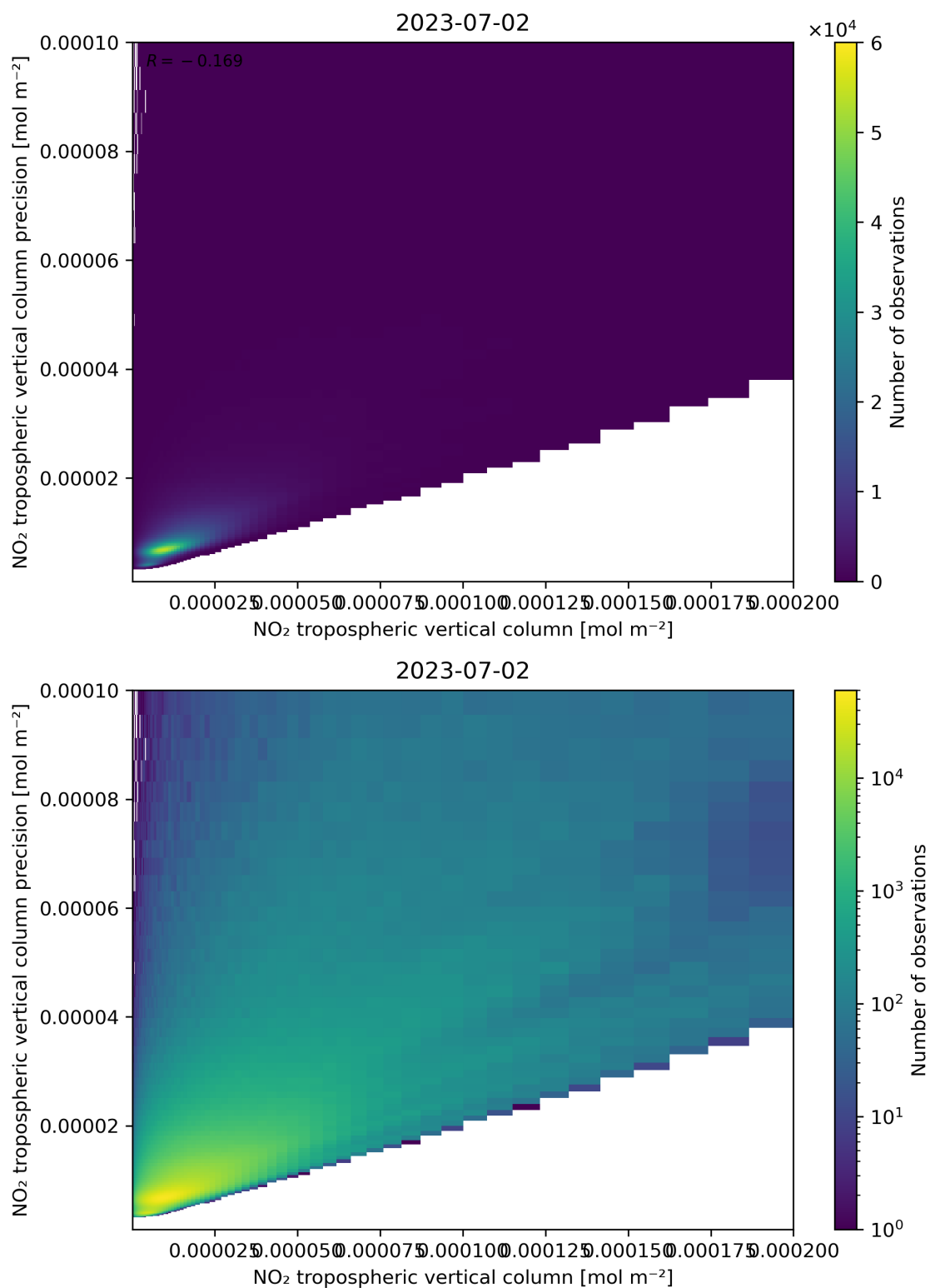
Figure 130: Scatter density plot of “NO 2 tropospheric vertical column” against “NO 2 tropospheric vertical column precision” for 2023-07-01 to 2023-07-03.
