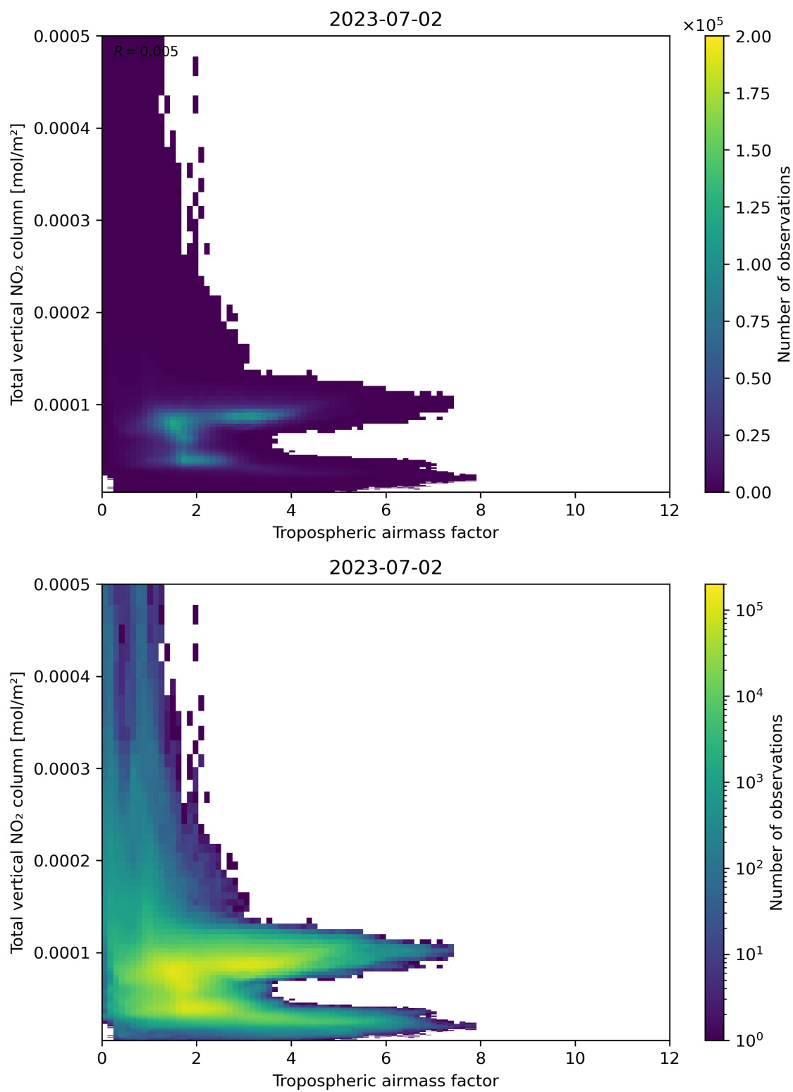
Figure 77: Scatter density plot of “Tropospheric airmass factor” against “Total vertical NO 2 column” for 2023-07-01 to 2023-07-03.
