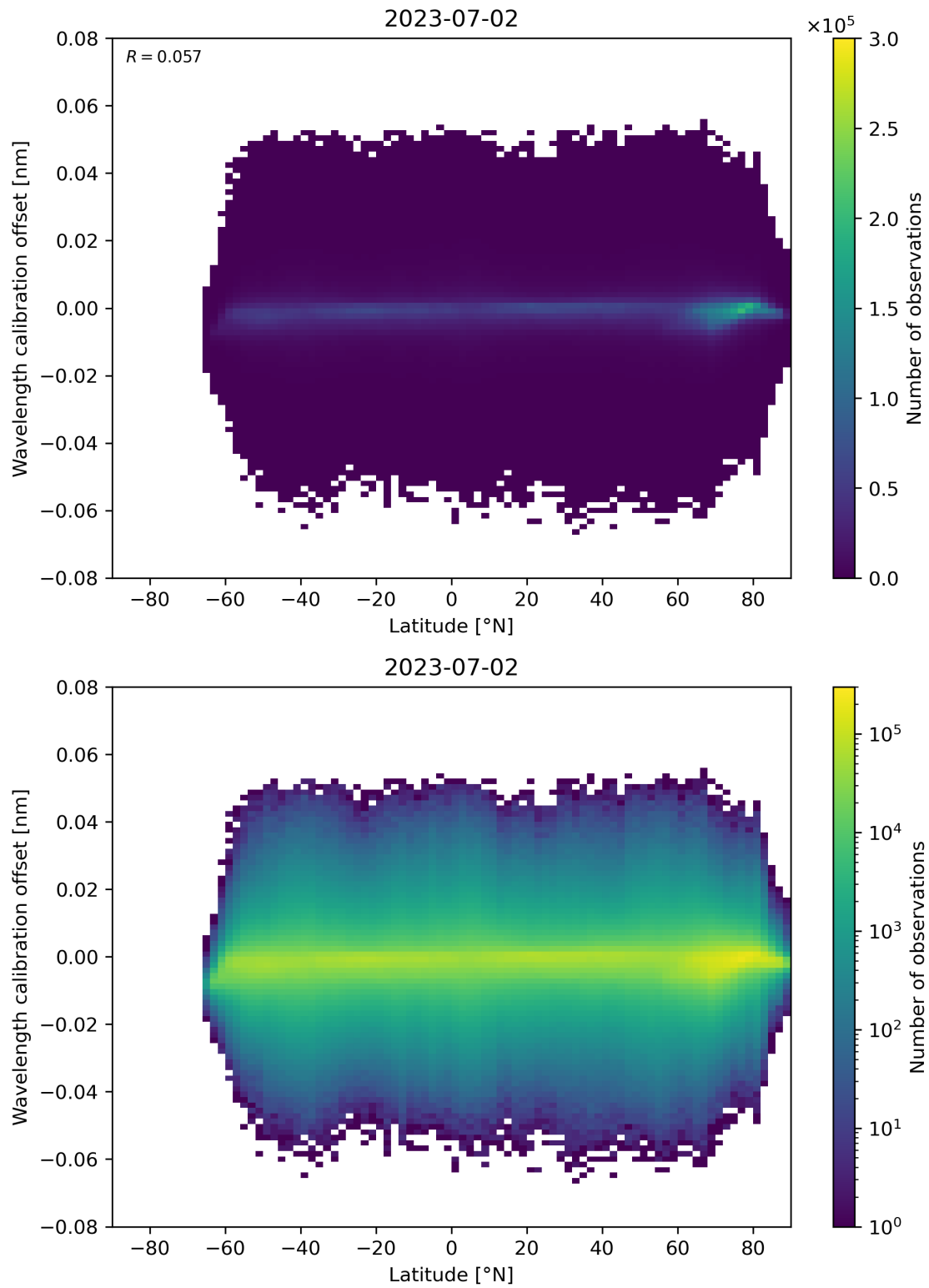
Figure 95: Scatter density plot of “Latitude” against “Wavelength calibration offset” for 2023-07-01 to 2023-07-03.
