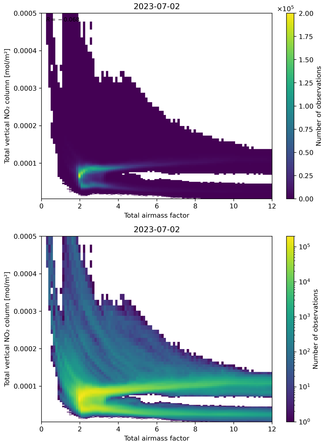
Figure 67: Scatter density plot of “Total airmass factor” against “Total vertical NO 2 column” for 2023-07-01 to 2023-07-03.
