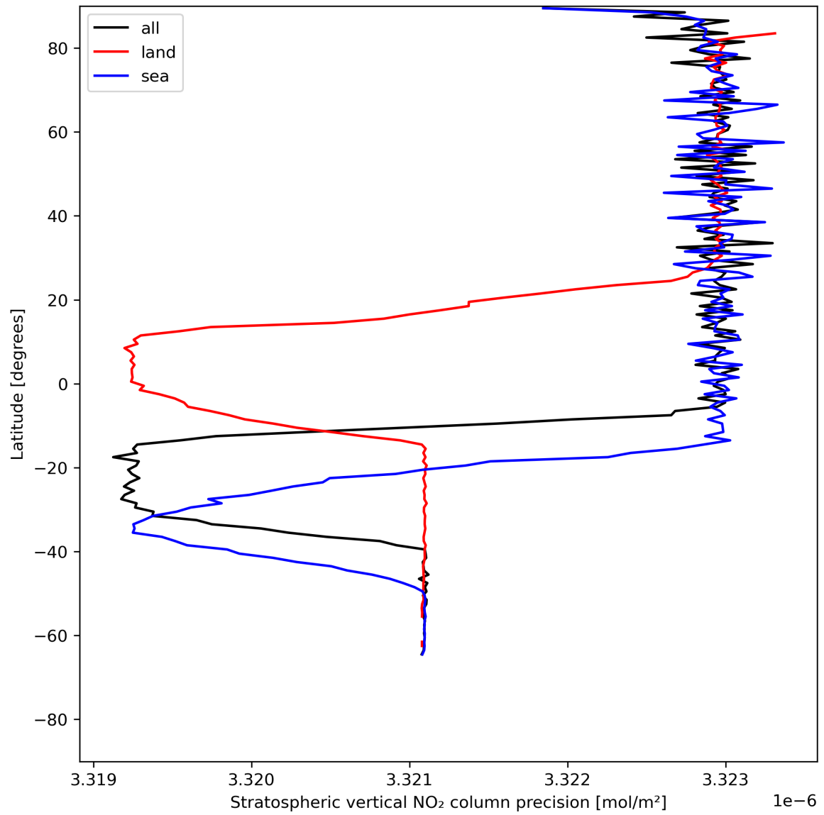
Figure 20: Zonal average of “Stratospheric vertical NO 2 column precision” for 2023-07-01 to 2023-07-03.
