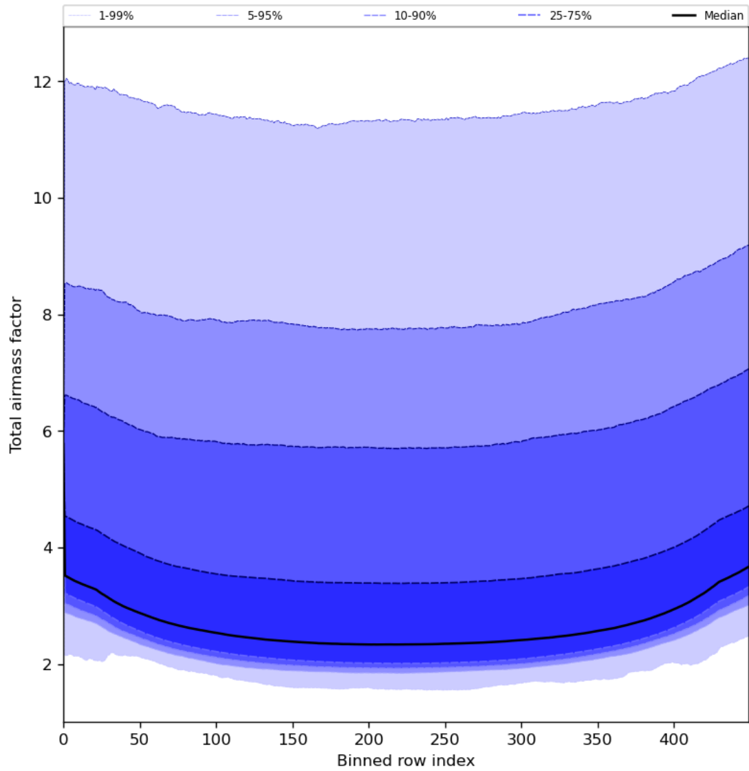
Figure 49: Along track statistics of “Total airmass factor” for 2023-07-01 to 2023-07-03
