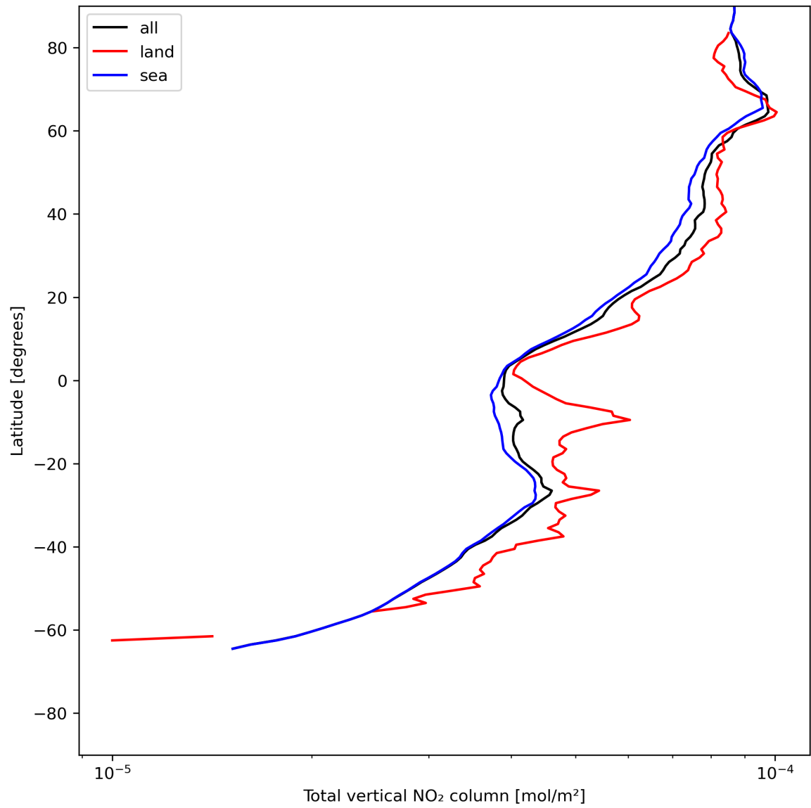
Figure 21: Zonal average of “Total vertical NO 2 column” for 2023-07-01 to 2023-07-03.
