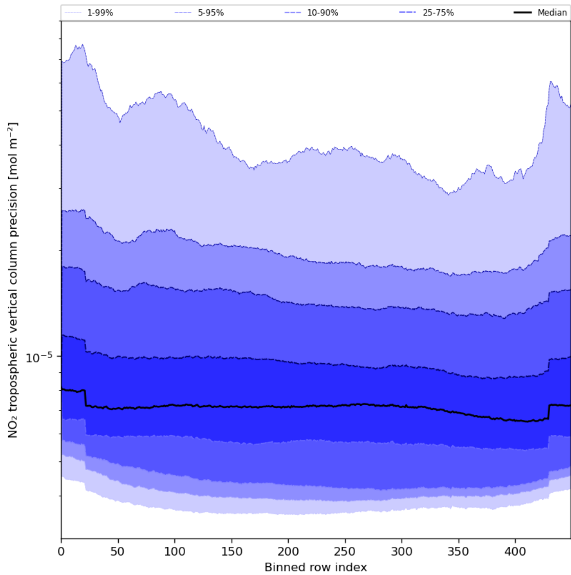
Figure 47: Along track statistics of “NO 2 tropospheric vertical column precision” for 2023-07-01 to 2023-07-03
