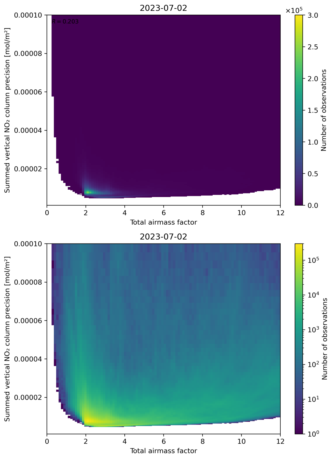
Figure 66: Scatter density plot of “Total airmass factor” against “Summed vertical NO 2 column precision” for 2023-07-01 to 2023-07-03.
