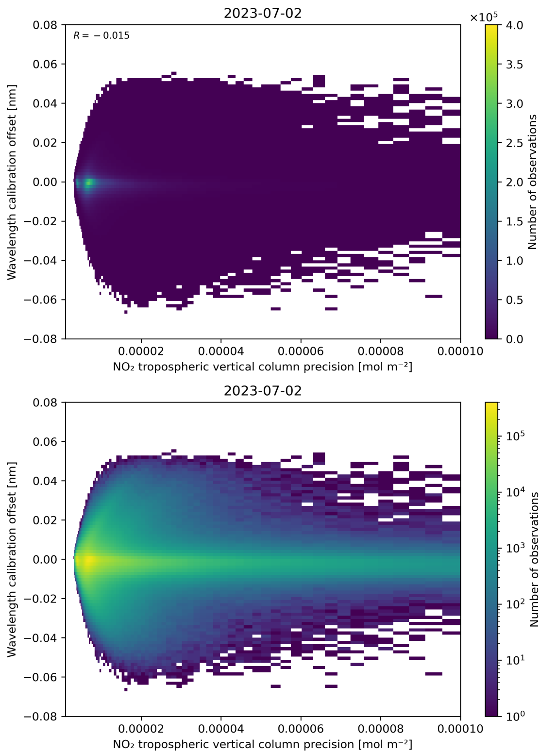
Figure 141: Scatter density plot of “NO 2 tropospheric vertical column precision” against “Wavelength calibration offset” for 2023-07-01 to 2023-07-03.
