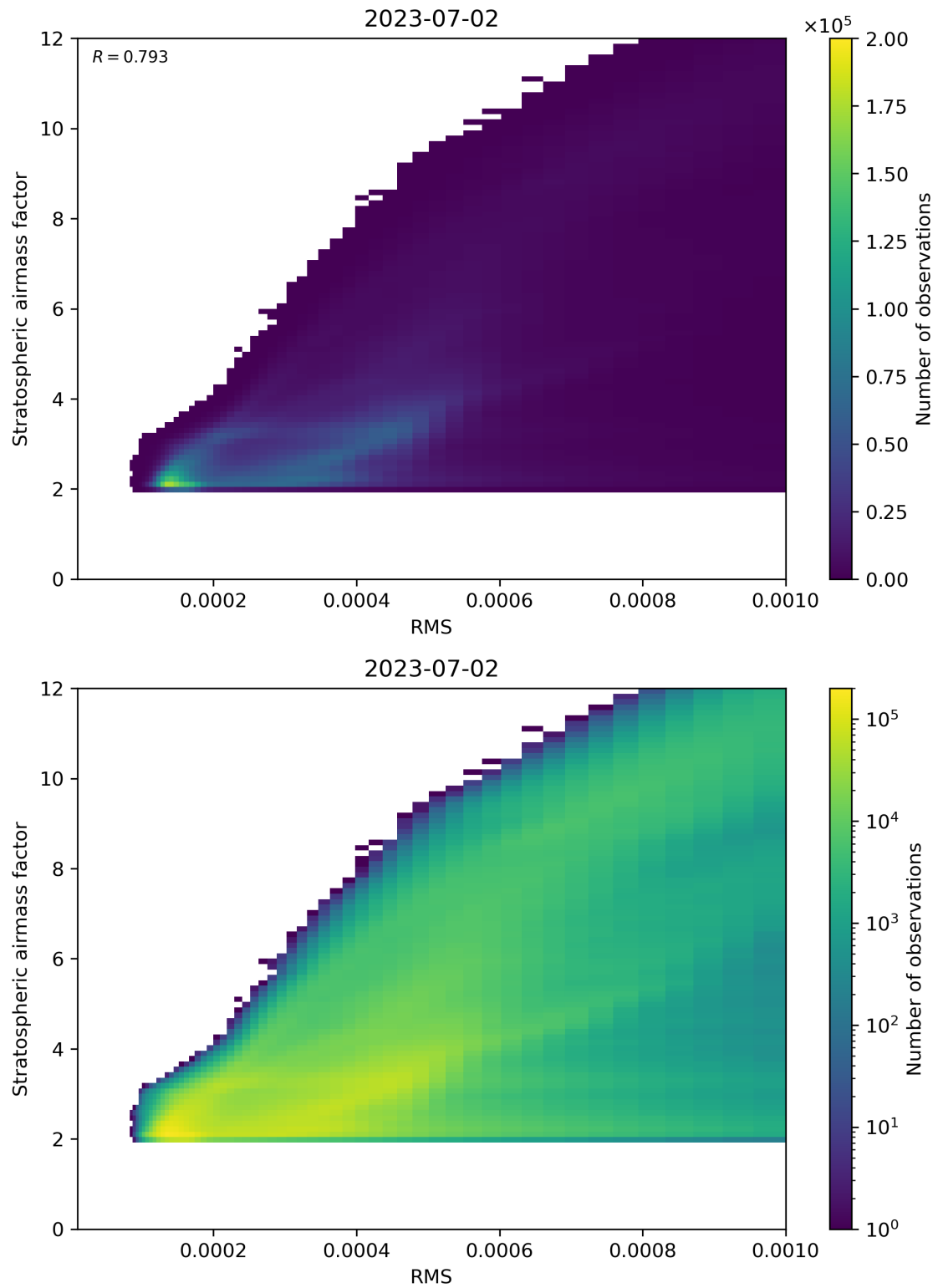
Figure 144: Scatter density plot of “RMS” against “Stratospheric airmass factor” for 2023-07-01 to 2023-07-03.
