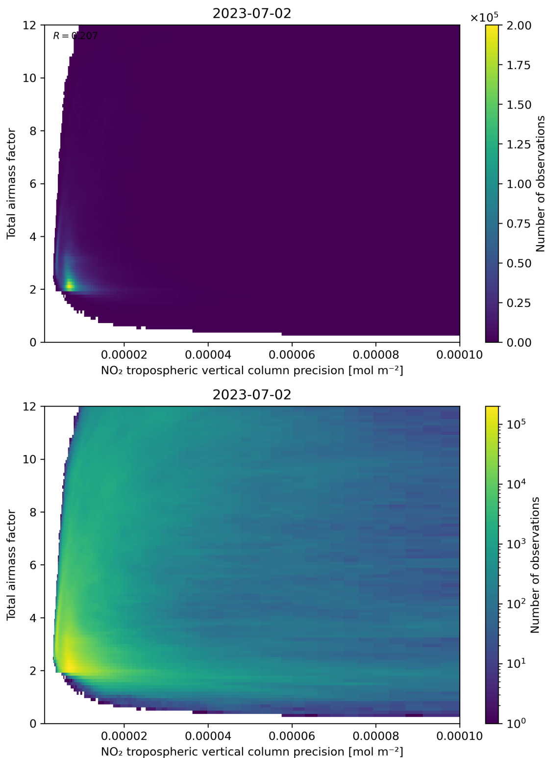
Figure 132: Scatter density plot of “NO 2 tropospheric vertical column precision” against “Total air mass factor” for 2023-07-01 to 2023-07-03.
