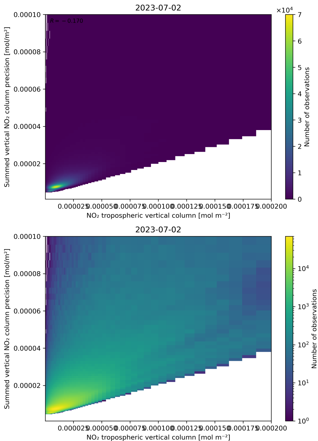
Figure 127: Scatter density plot of “NO 2 tropospheric vertical column” against “Summed vertical NO 2 column precision” for 2023-07-01 to 2023-07-03.
