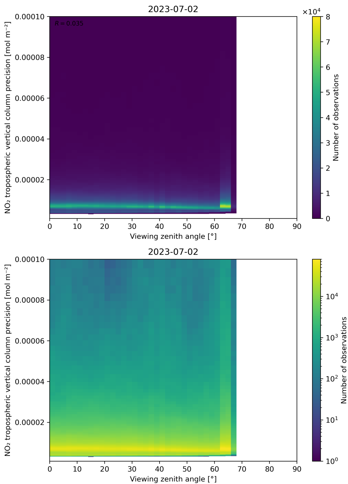
Figure 170: Scatter density plot of “Viewing zenith angle” against “NO 2 tropospheric vertical column precision” for 2023-07-01 to 2023-07-03.
