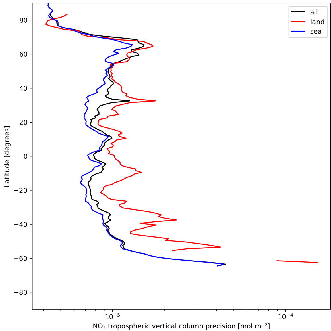
Figure 13: Zonal average of “NO 2 tropospheric vertical column precision” for 2023-07-01 to 2023-07-03.
