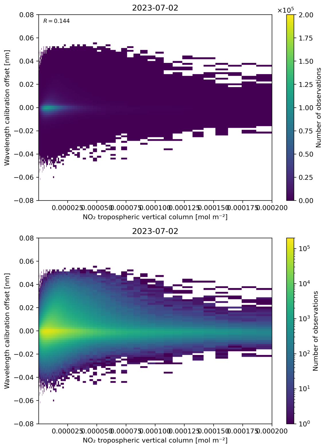
Figure 143: Scatter density plot of “NO 2 tropospheric vertical column” against “Wavelength calibration offset” for 2023-07-01 to 2023-07-03.
