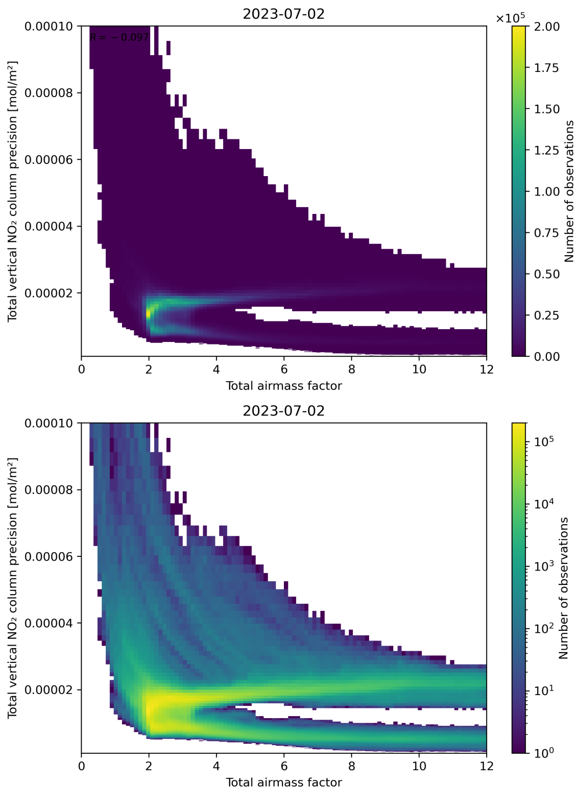
Figure 68: Scatter density plot of “Total airmass factor” against “Total vertical NO 2 column precision” for 2023-07-01 to 2023-07-03.
