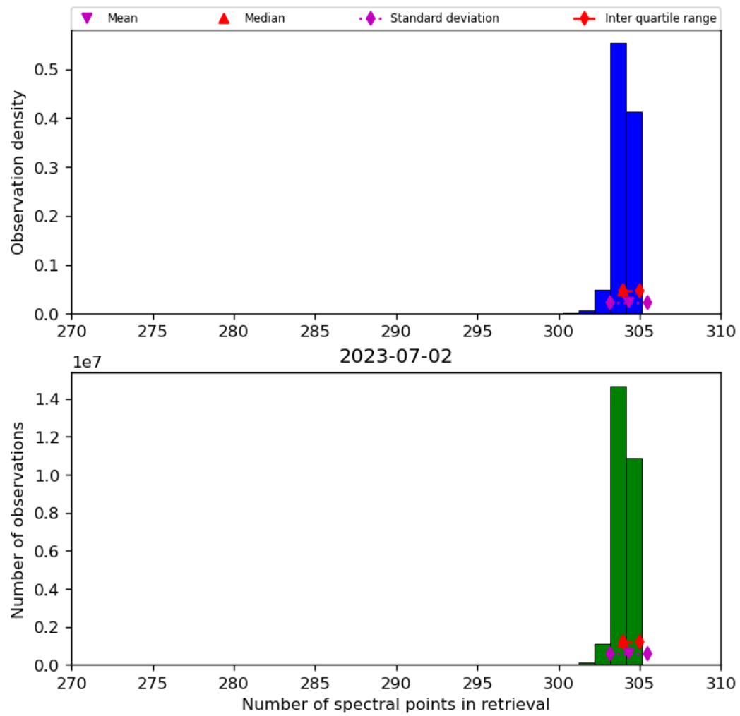
Figure 33: Histogram of “Number of spectral points in retrieval” for 2023-07-01 to 2023-07-03
