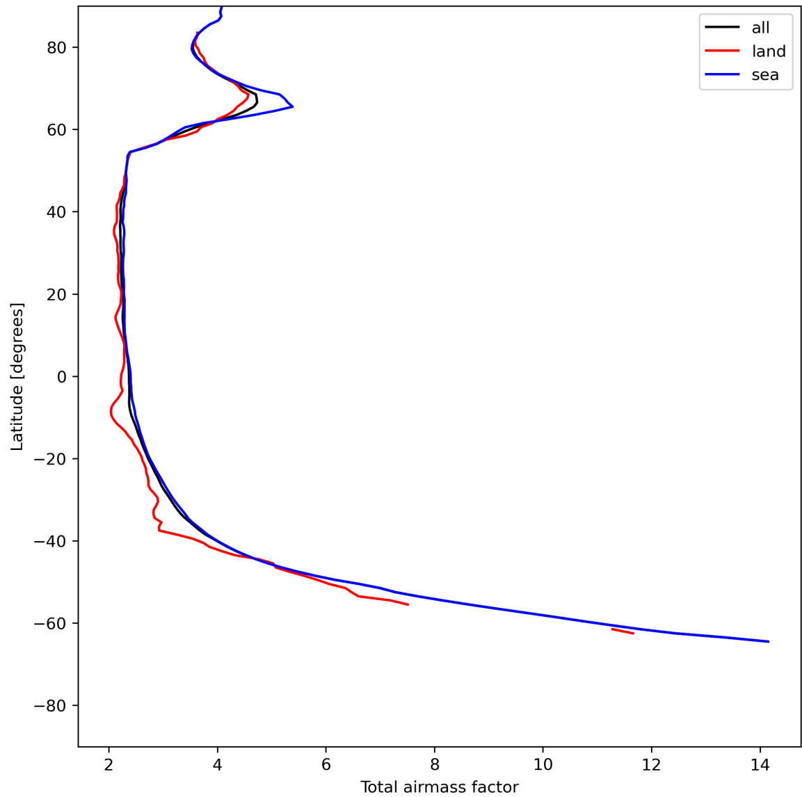
Figure 15: Zonal average of “Total airmass factor” for 2023-07-01 to 2023-07-03.
