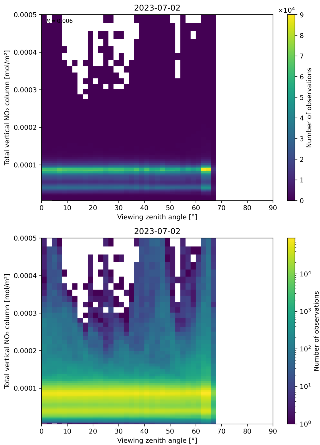
Figure 167: Scatter density plot of “Viewing zenith angle” against “Total vertical NO 2 column” for 2023-07-01 to 2023-07-03.
