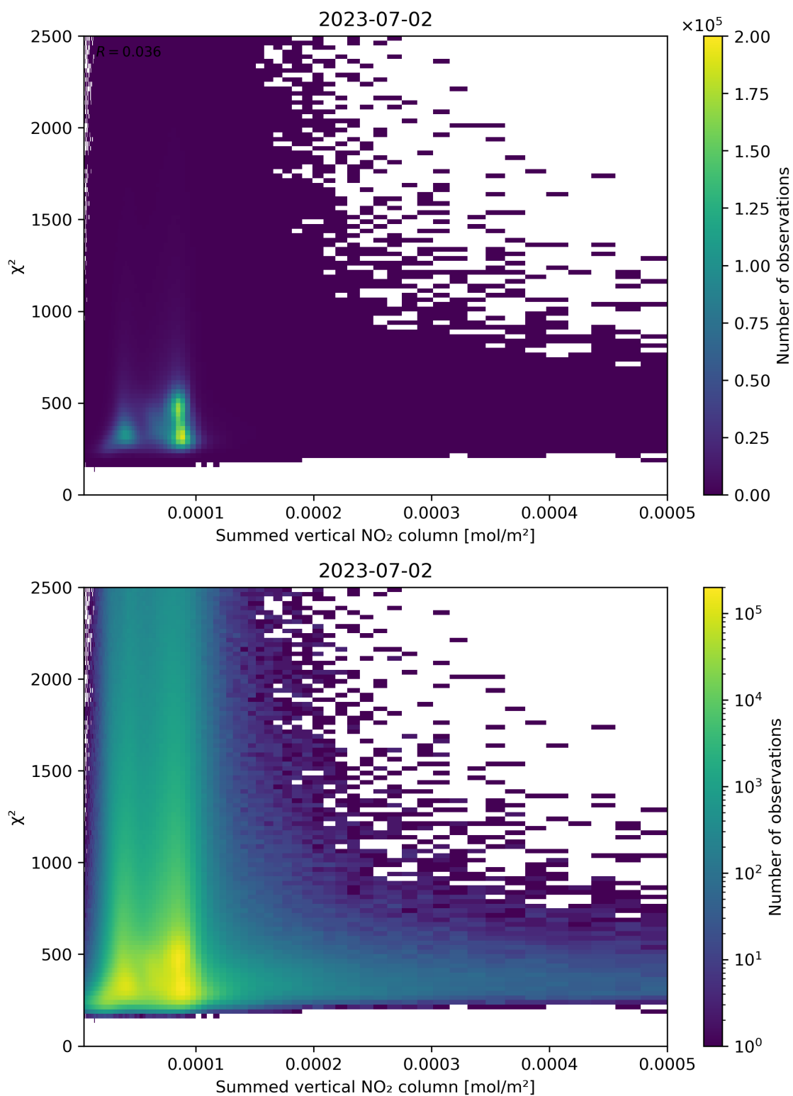
Figure 104: Scatter density plot of “Summed vertical NO 2 column” against “ \chi^2 ” for 2023-07-01 to 2023-07-03.
