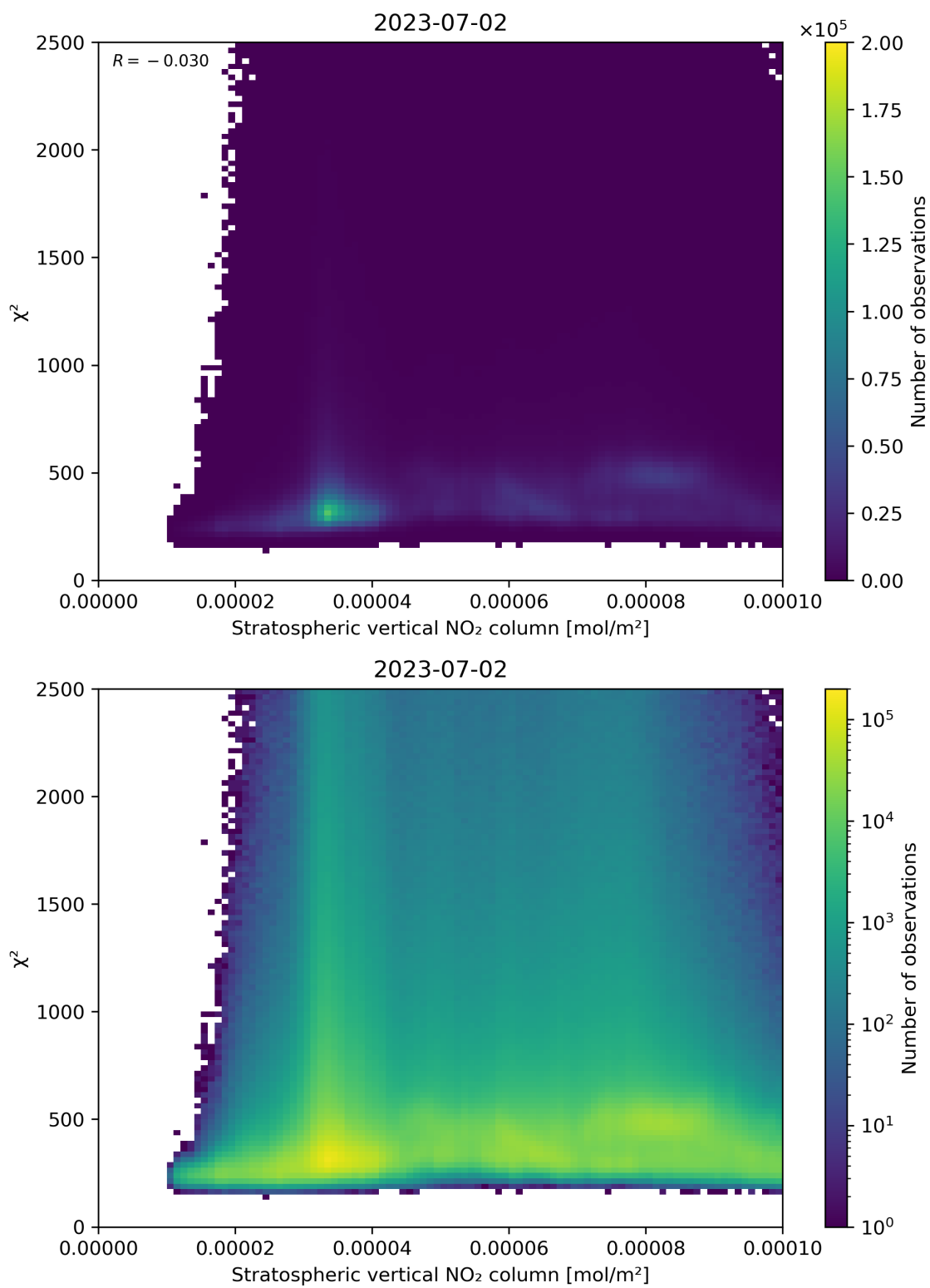
Figure 97: Scatter density plot of “Stratospheric vertical NO 2 column” against “ \chi^2 ” for 2023-07-01 to 2023-07-03.
