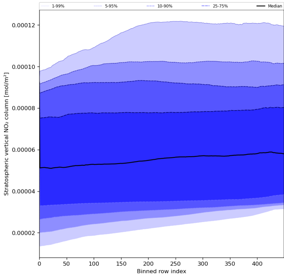
Figure 53: Along track statistics of “Stratospheric vertical NO 2 column” for 2023-07-01 to 2023-07-03
