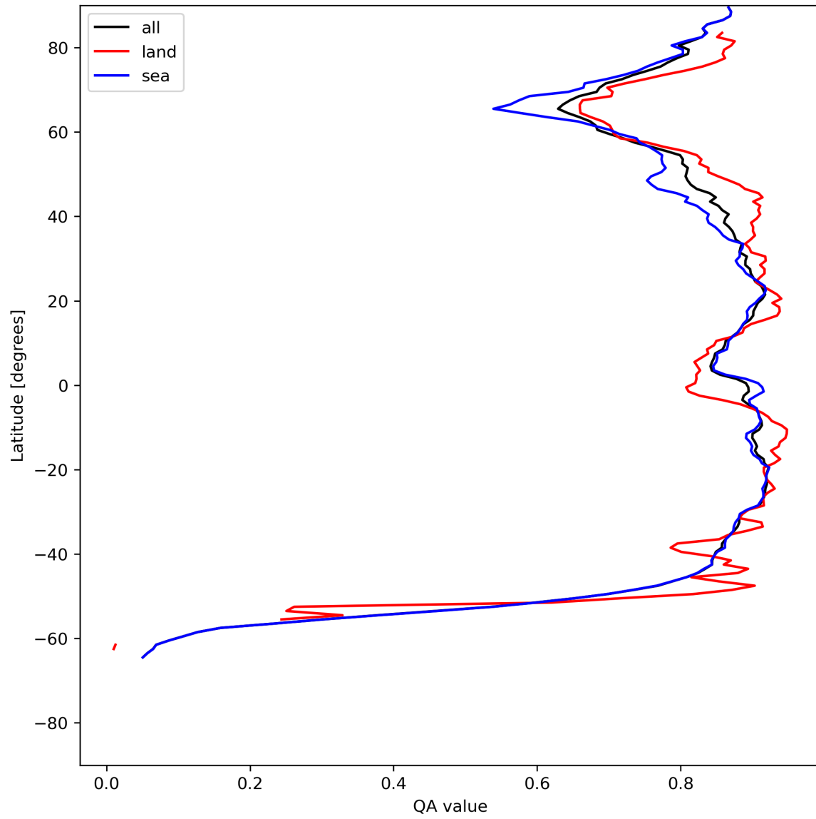
Figure 11: Zonal average of “QA value” for 2023-07-01 to 2023-07-03.
