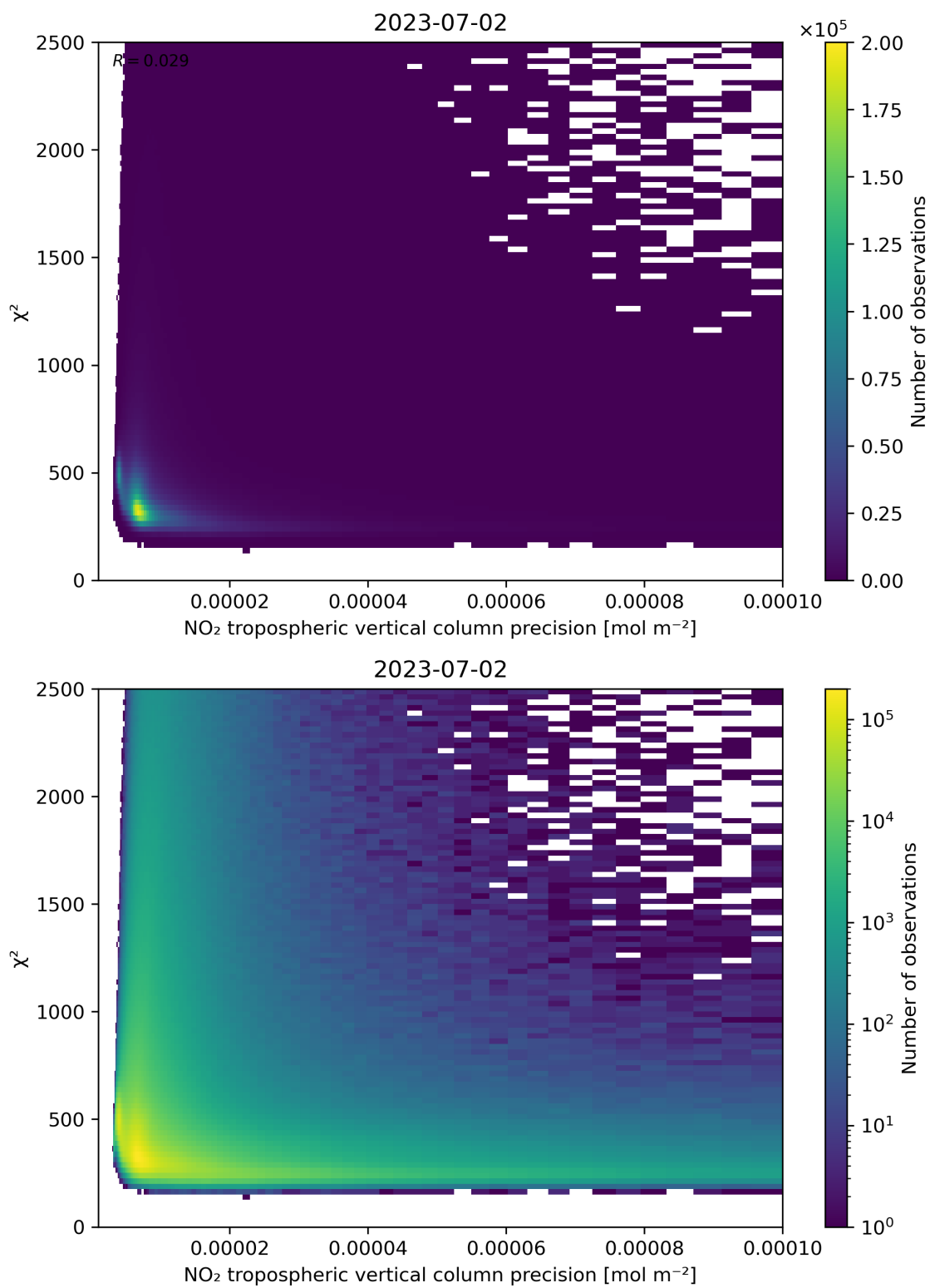
Figure 134: Scatter density plot of “NO 2 tropospheric vertical column precision” against “ \chi^2 ” for 2023-07-01 to 2023-07-03.
