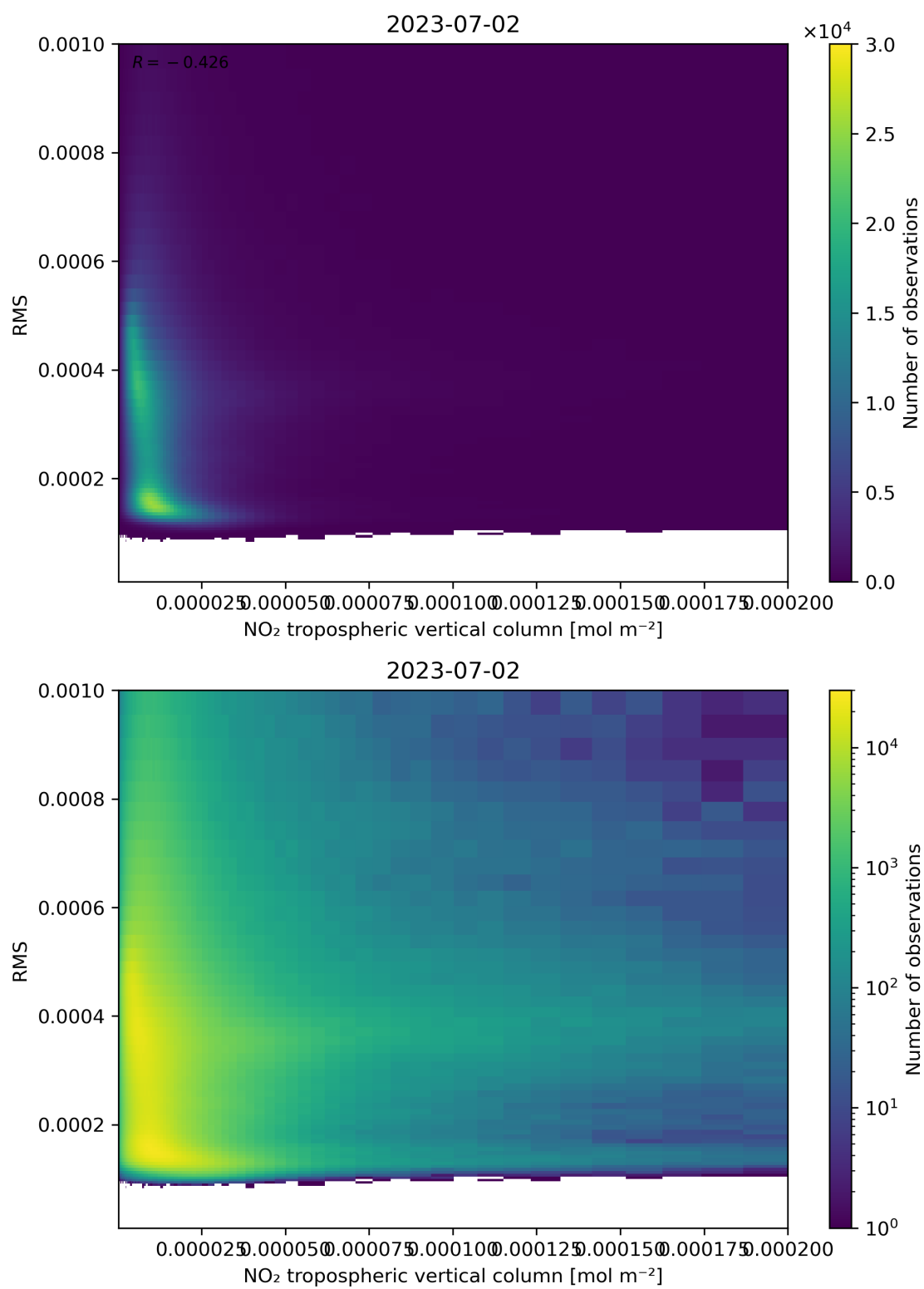
Figure 142: Scatter density plot of “NO 2 tropospheric vertical column” against “RMS” for 2023-07-01 to 2023-07-03.
