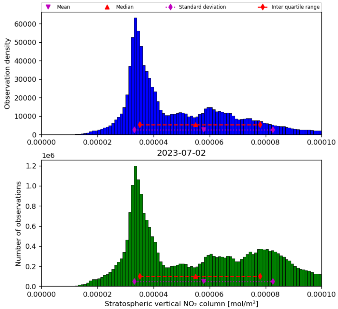
Figure 36: Histogram of “Stratospheric vertical NO 2 column” for 2023-07-01 to 2023-07-03
