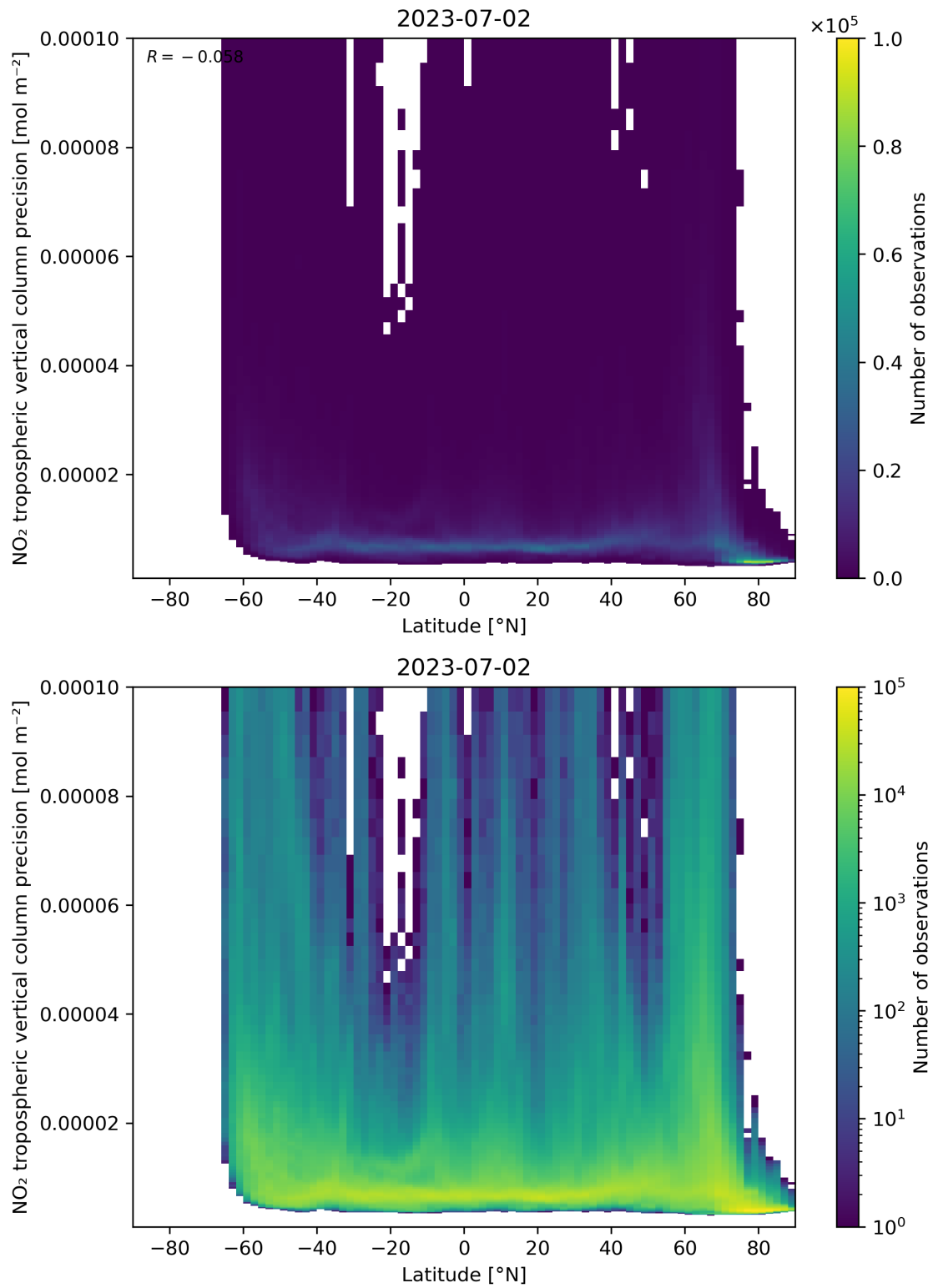
Figure 93: Scatter density plot of “Latitude” against “NO 2 tropospheric vertical column precision” for 2023-07-01 to 2023-07-03.
