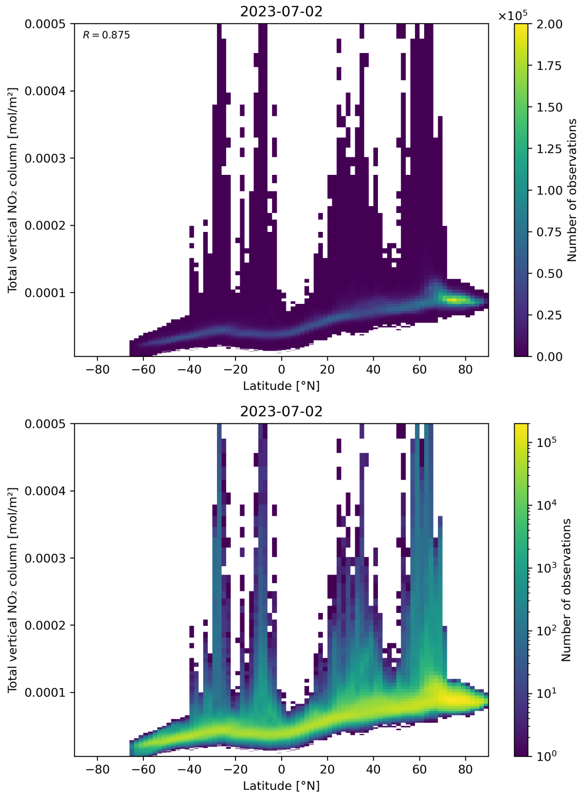
Figure 90: Scatter density plot of “Latitude” against “Total vertical NO 2 column” for 2023-07-01 to 2023-07-03.
