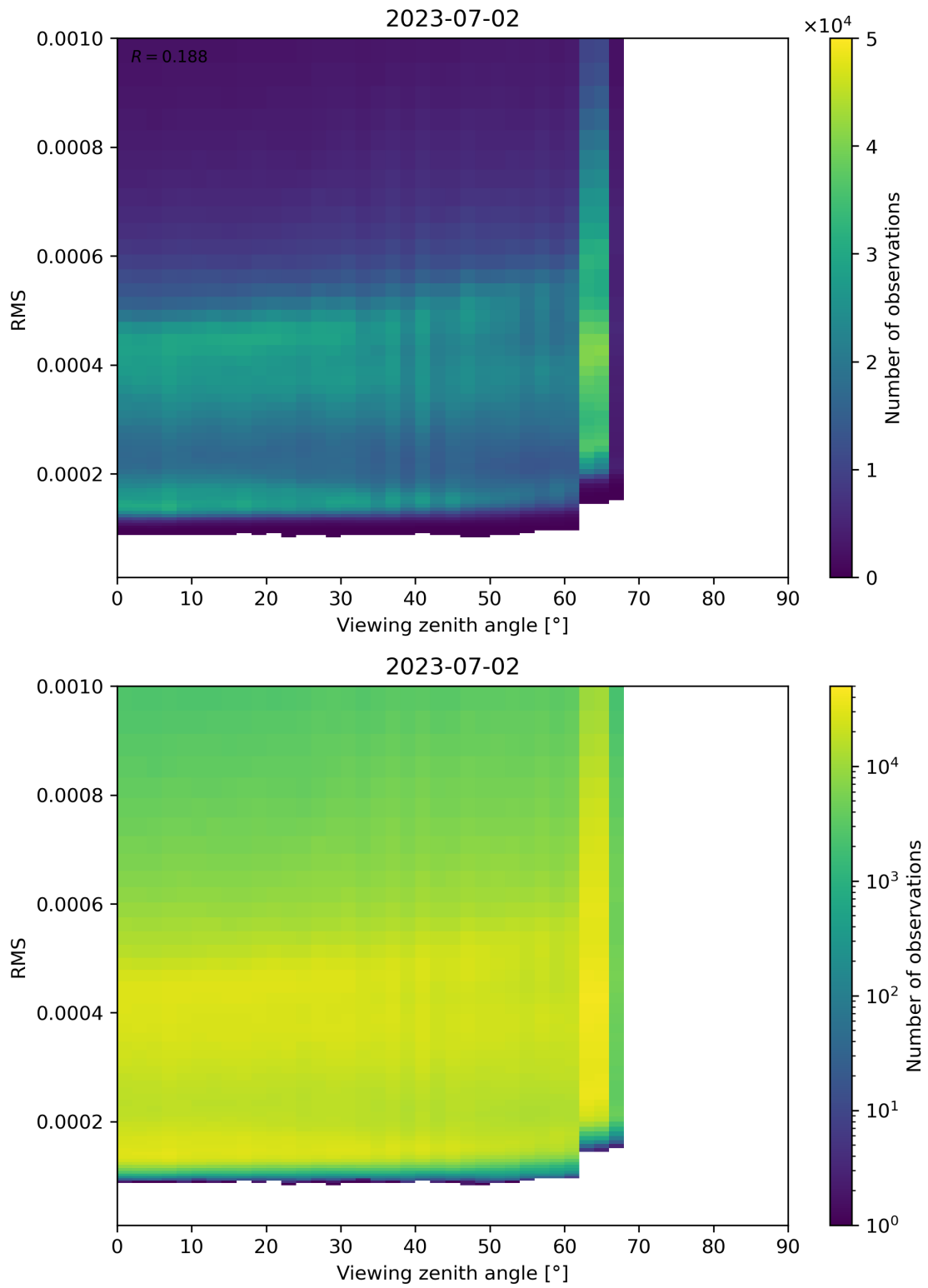
Figure 171: Scatter density plot of “Viewing zenith angle” against “RMS” for 2023-07-01 to 2023-07-03.
