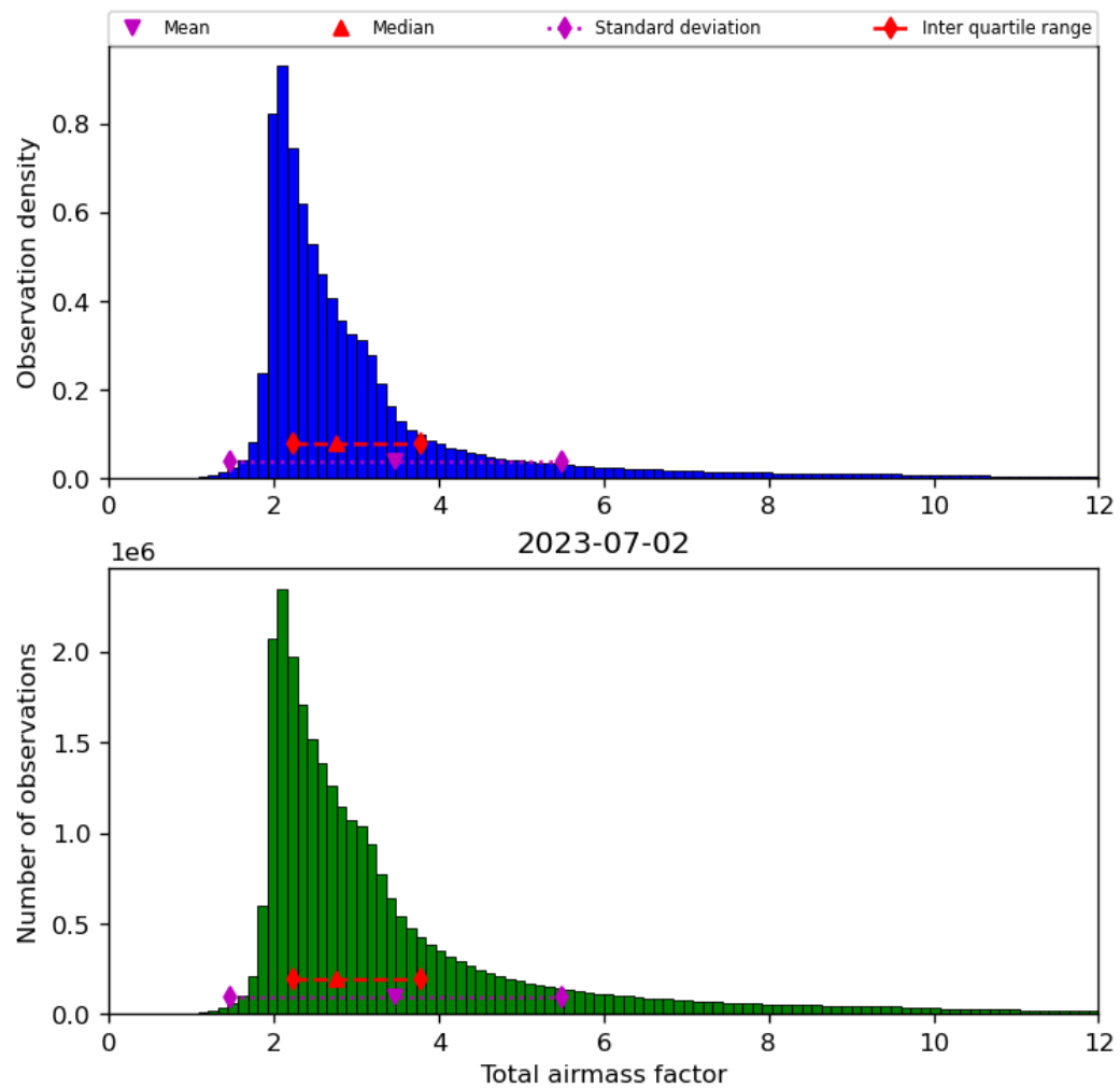
Figure 32: Histogram of “Total airmass factor” for 2023-07-01 to 2023-07-03
