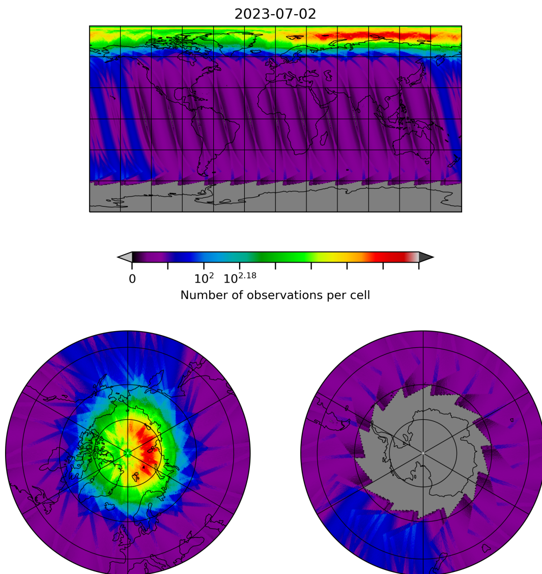
Figure 10: Map of the number of observations for 2023-07-01 to 2023-07-03
