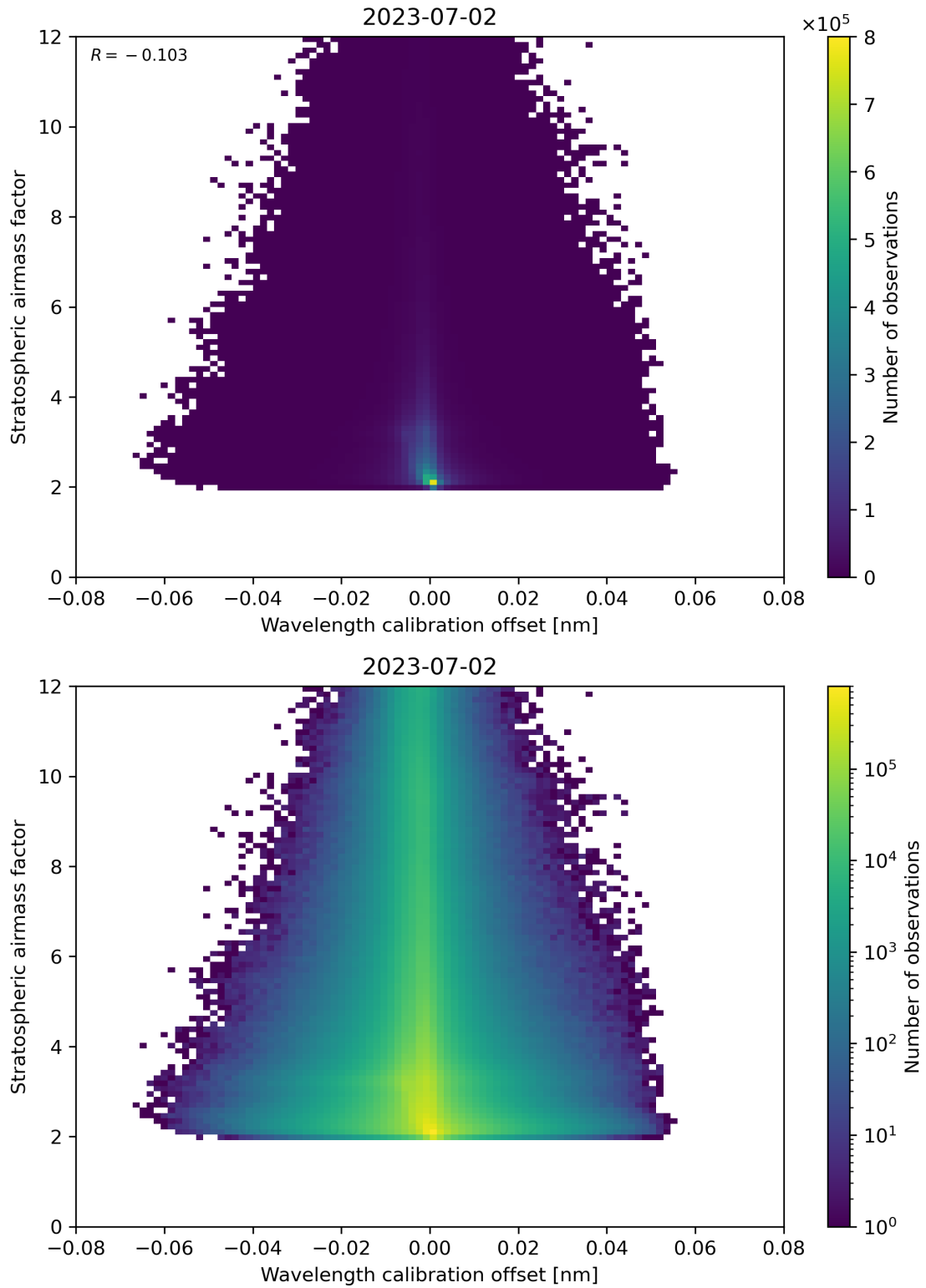
Figure 174: Scatter density plot of “Wavelength calibration offset” against “Stratospheric air mass factor” for 2023-07-01 to 2023-07-03.
