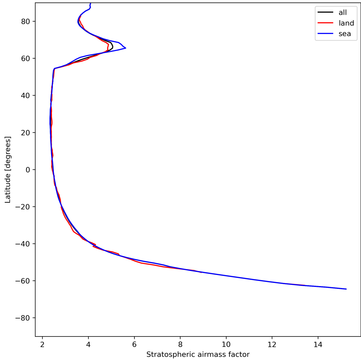
Figure 27: Zonal average of “Stratospheric air mass factor” for 2023-07-01 to 2023-07-03.
