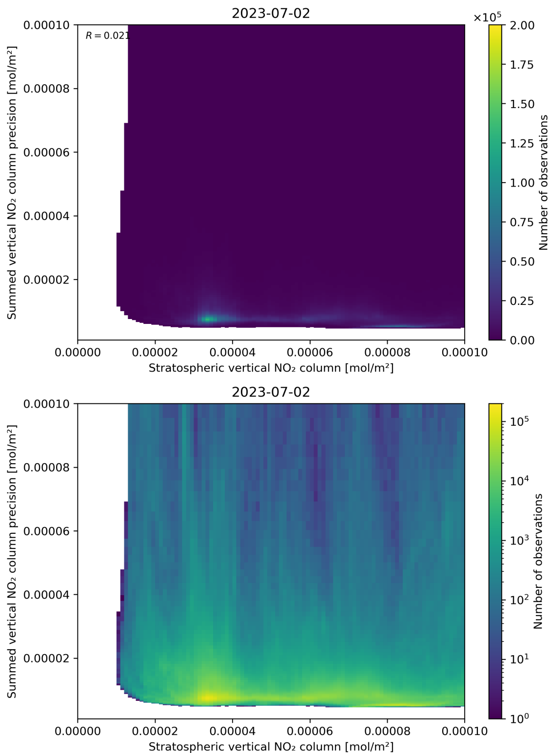
Figure 99: Scatter density plot of “Stratospheric vertical NO 2 column” against “Summed vertical NO 2 column precision” for 2023-07-01 to 2023-07-03.
