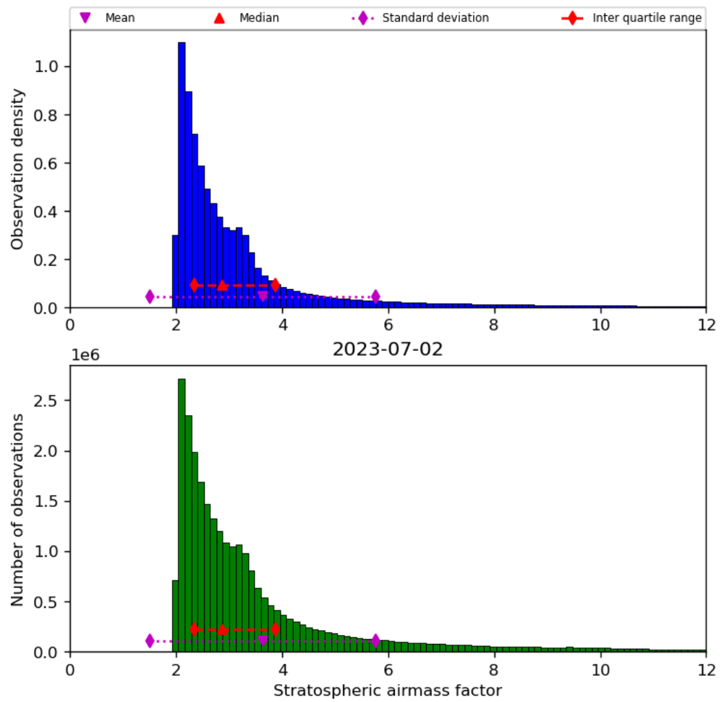
Figure 44: Histogram of “Stratospheric airmass factor” for 2023-07-01 to 2023-07-03
