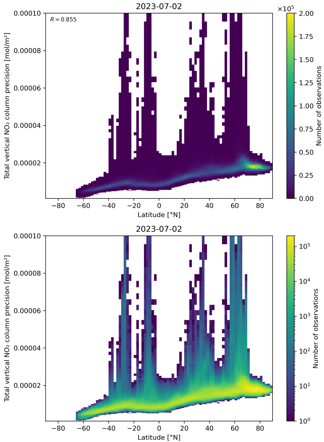
Figure 91: Scatter density plot of “Latitude” against “Total vertical NO 2 column precision” for 2023-07-01 to 2023-07-03.
