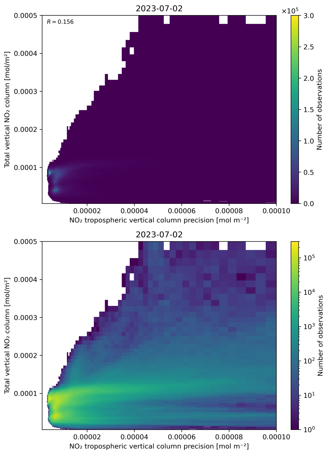
Figure 138: Scatter density plot of “NO 2 tropospheric vertical column precision” against “Total vertical NO 2 column” for 2023-07-01 to 2023-07-03.
