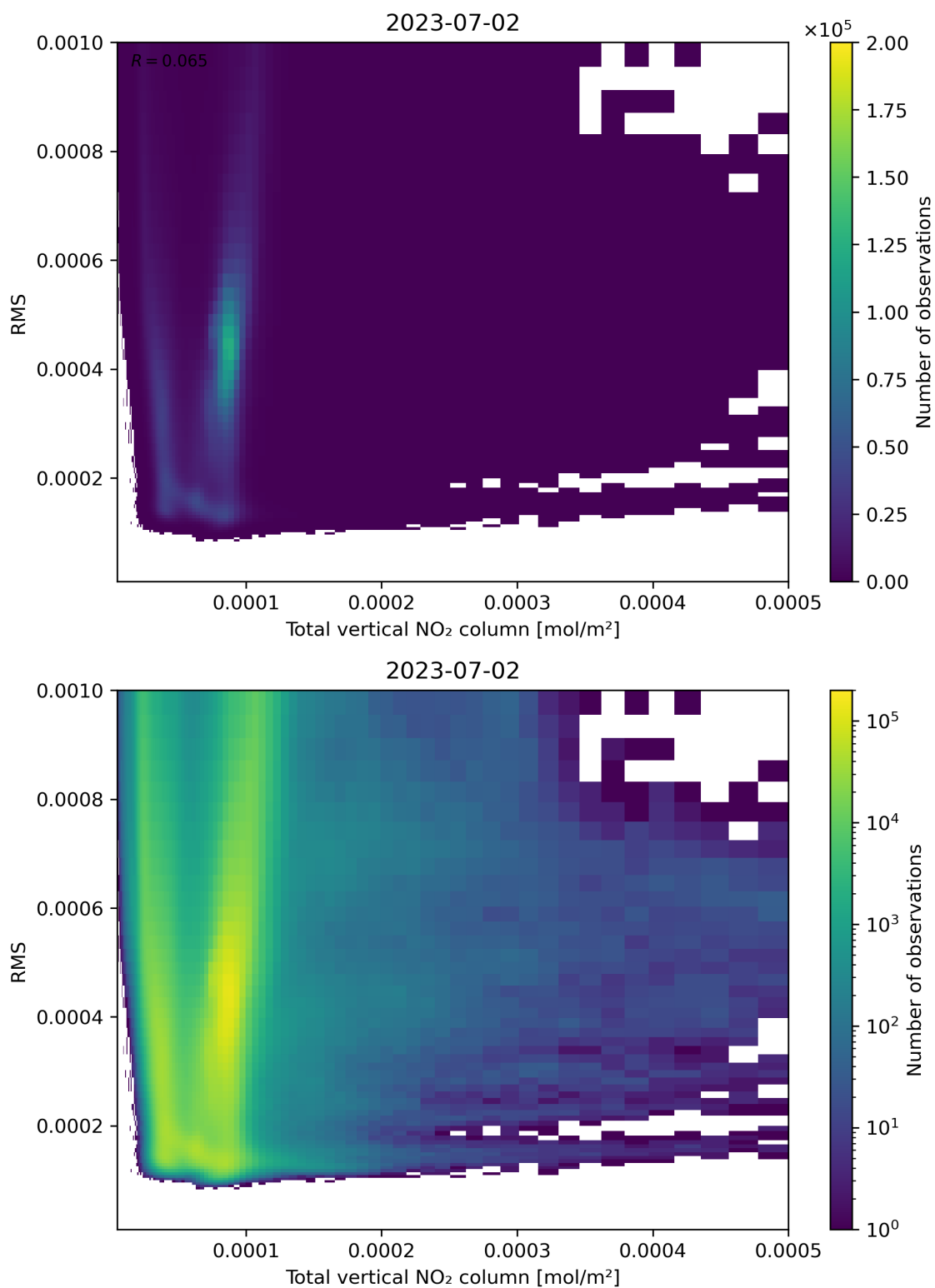
Figure 120: Scatter density plot of “Total vertical NO 2 column” against “RMS” for 2023-07-01 to 2023-07-03.
