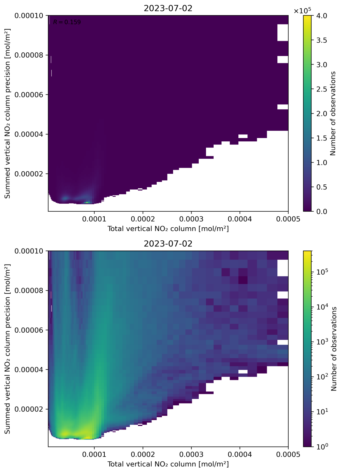
Figure 113: Scatter density plot of “Total vertical NO 2 column” against “Summed vertical NO 2 column precision” for 2023-07-01 to 2023-07-03.
