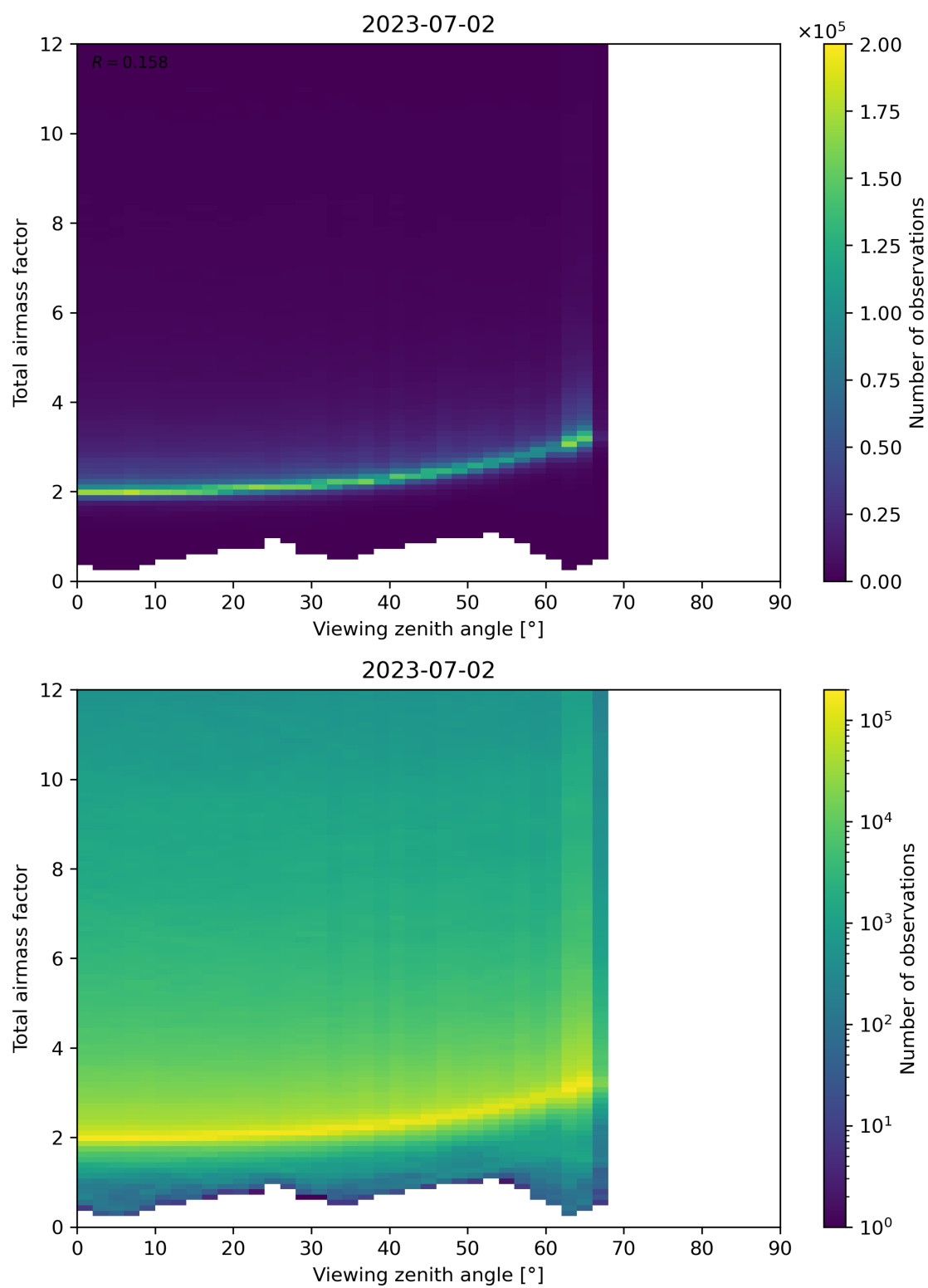
Figure 160: Scatter density plot of “Viewing zenith angle” against “Total airmass factor” for 2023-07-01 to 2023-07-03.
