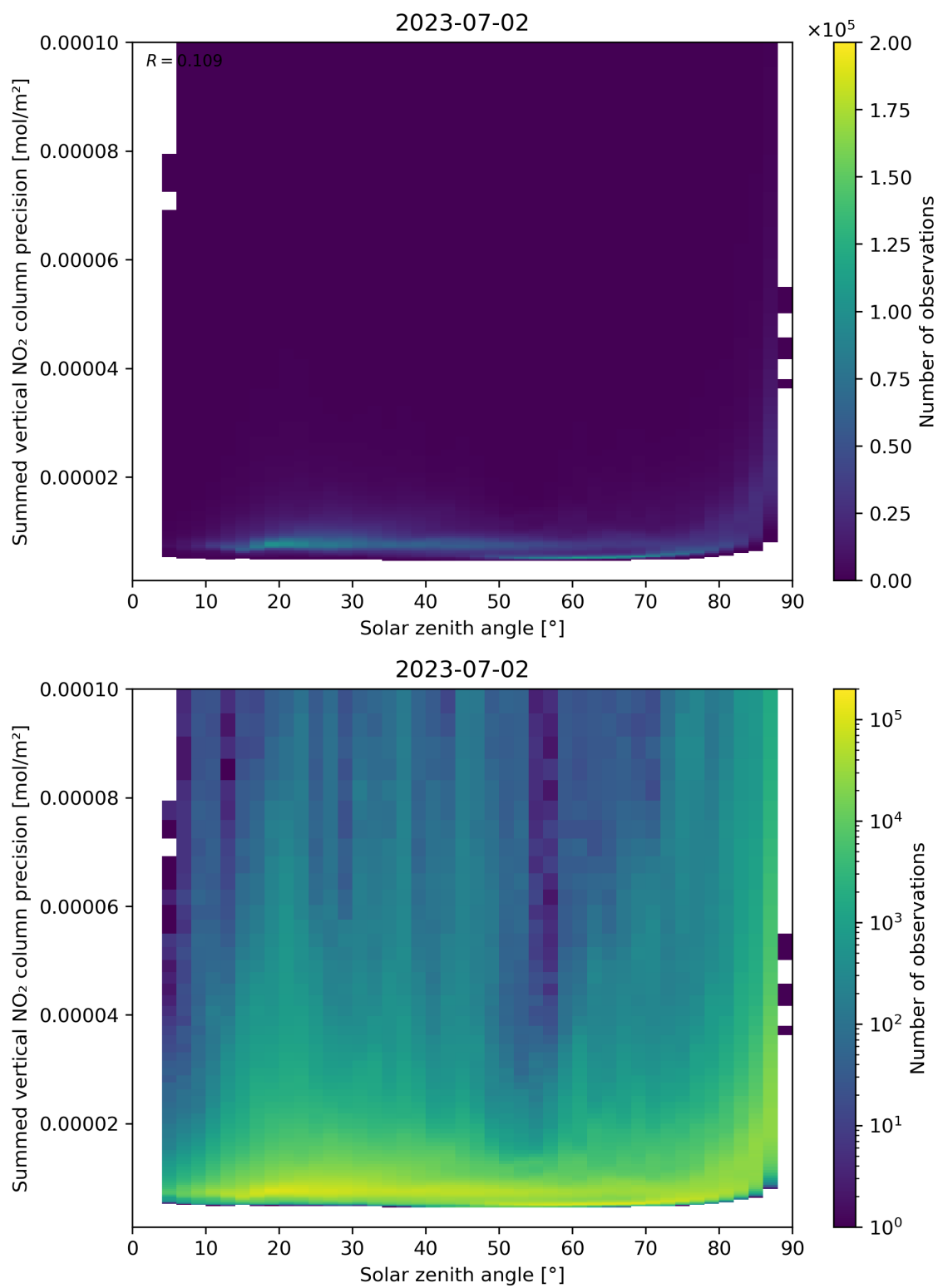
Figure 152: Scatter density plot of “Solar zenith angle” against “Summed vertical NO 2 column precision” for 2023-07-01 to 2023-07-03.
