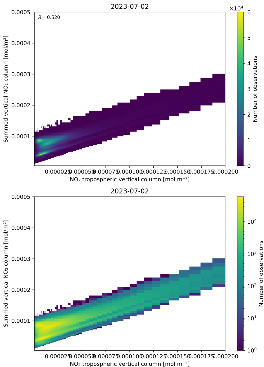
Figure 126: Scatter density plot of “NO 2 tropospheric vertical column” against “Summed vertical NO 2 column” for 2023-07-01 to 2023-07-03.
