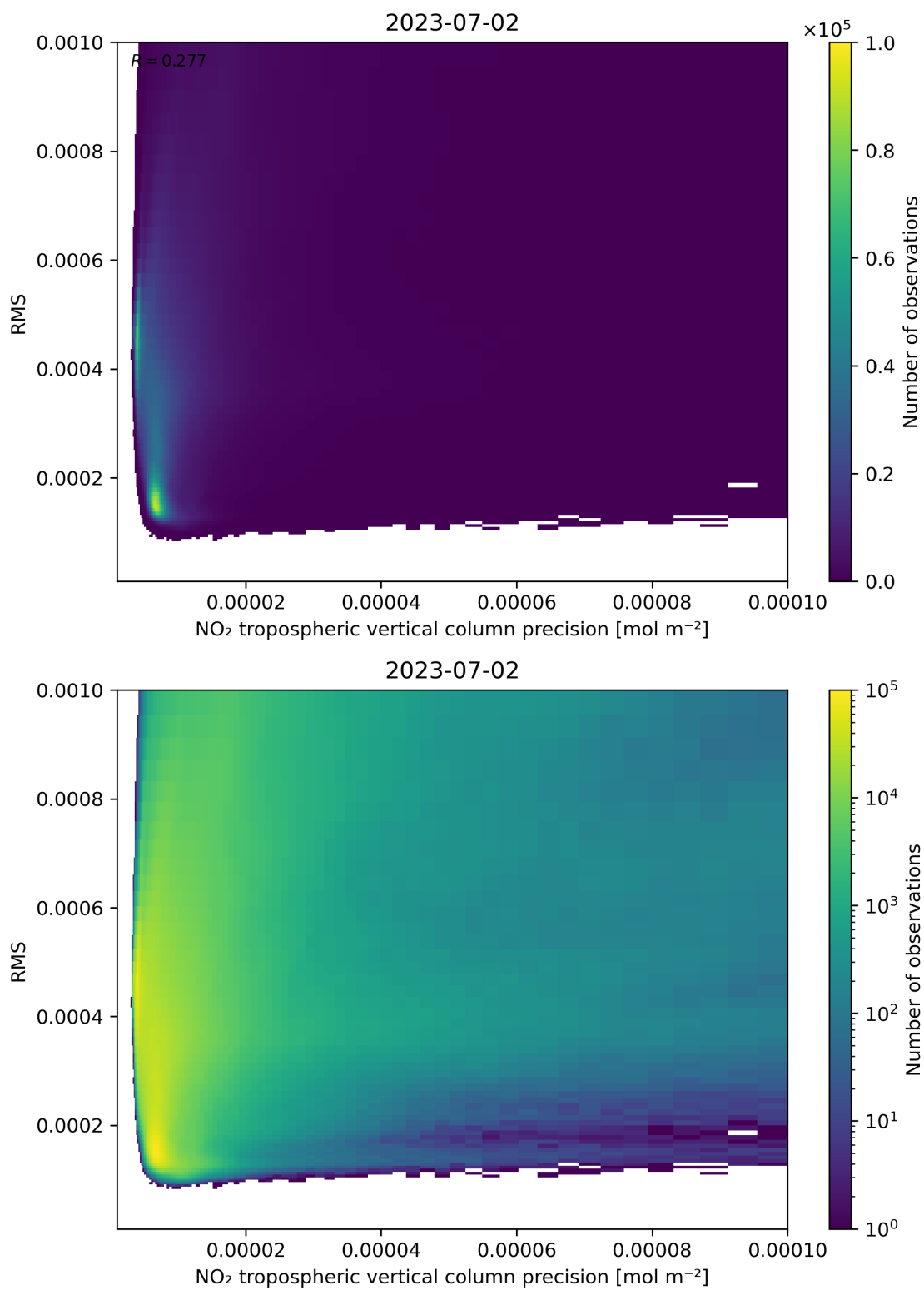
Figure 140: Scatter density plot of “NO 2 tropospheric vertical column precision” against “RMS” for 2023-07-01 to 2023-07-03.
