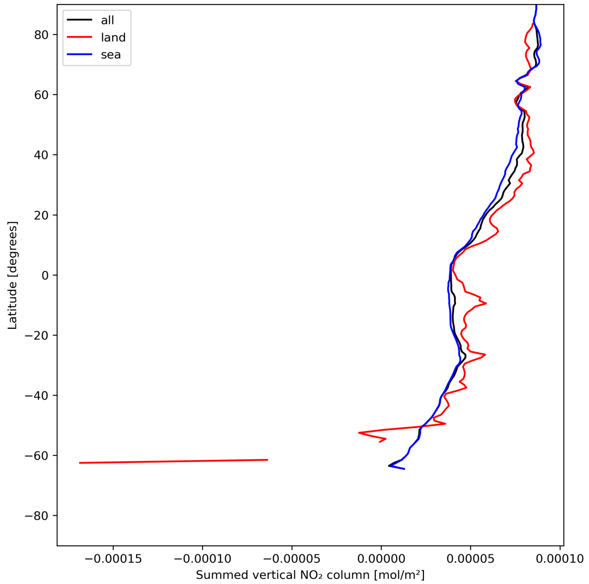
Figure 23: Zonal average of “Summed vertical NO 2 column” for 2023-07-01 to 2023-07-03.
