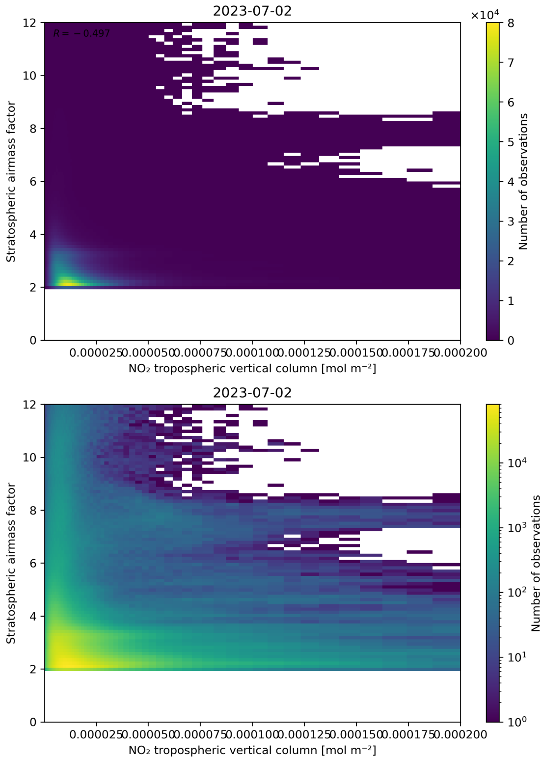
Figure 121: Scatter density plot of “NO 2 tropospheric vertical column” against “Stratospheric air mass factor” for 2023-07-01 to 2023-07-03.
