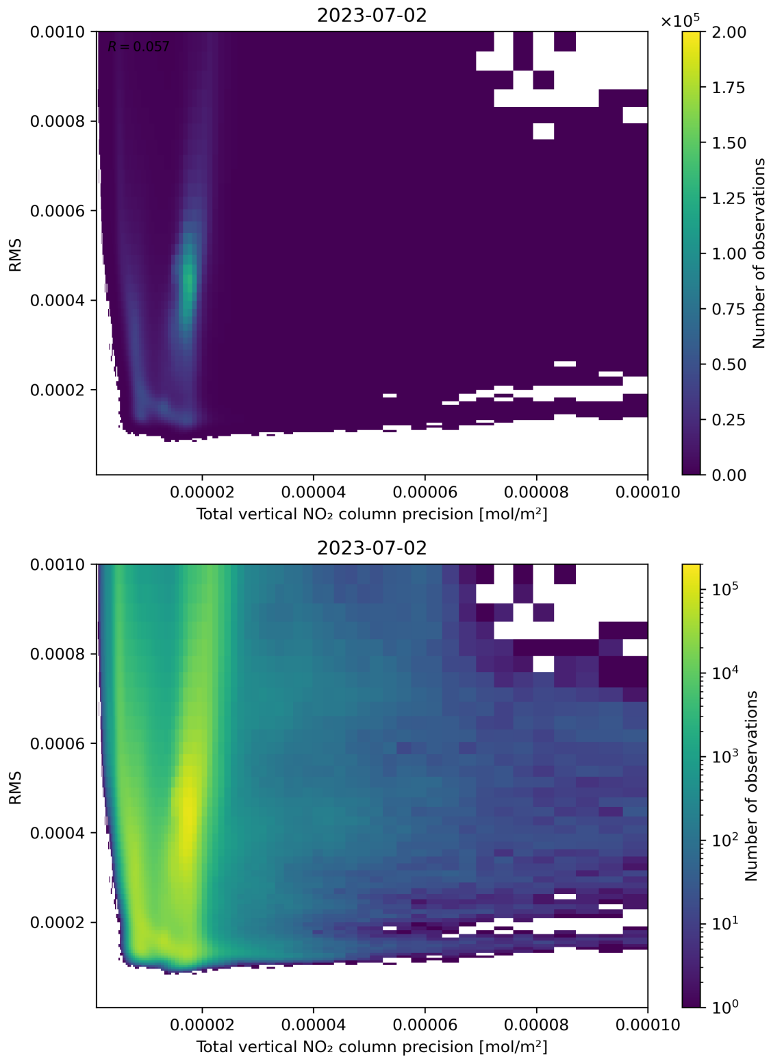
Figure 119: Scatter density plot of “Total vertical NO 2 column precision” against “RMS” for 2023-07-01 to 2023-07-03.
