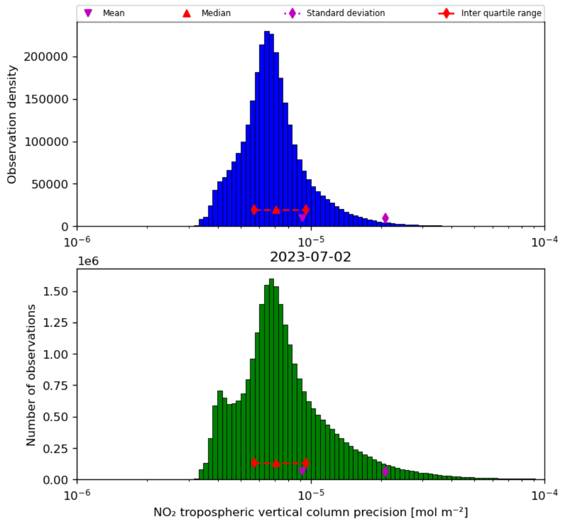
Figure 30: Histogram of “NO 2 tropospheric vertical column precision” for 2023-07-01 to 2023-07-03
