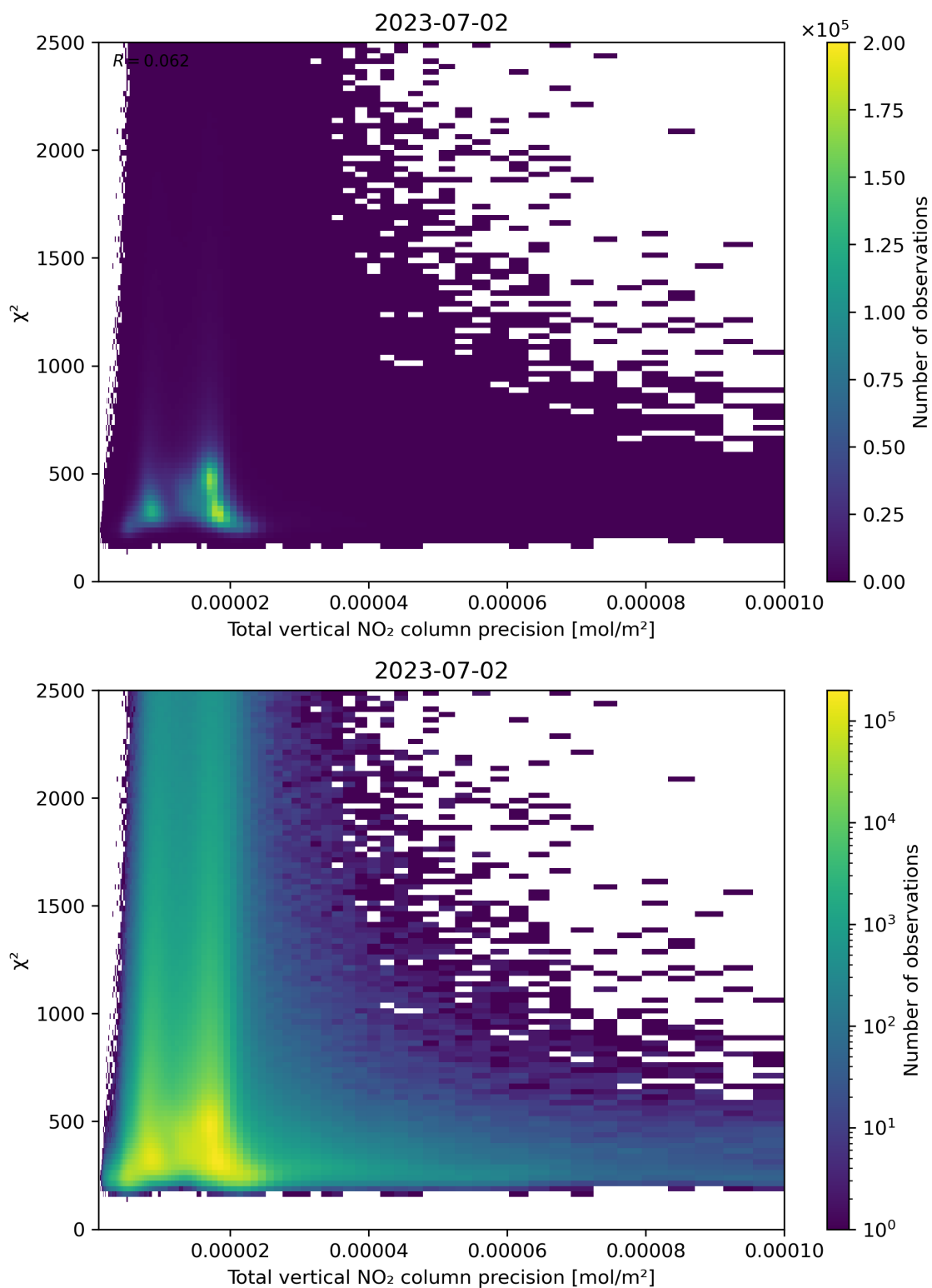
Figure 116: Scatter density plot of “Total vertical NO 2 column precision” against “ \chi^2 ” for 2023-07-01 to 2023-07-03.
