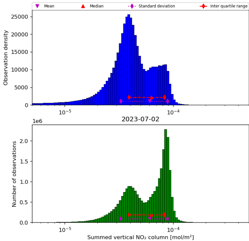
Figure 40: Histogram of “Summed vertical NO 2 column” for 2023-07-01 to 2023-07-03
