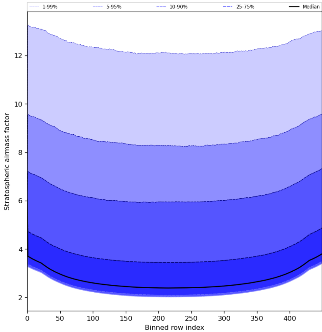
Figure 61: Along track statistics of “Stratospheric airmass factor” for 2023-07-01 to 2023-07-03
