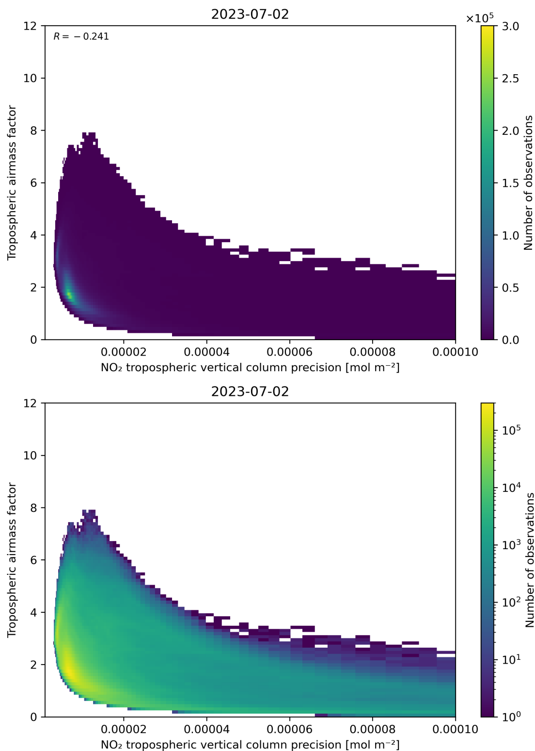
Figure 133: Scatter density plot of “NO 2 tropospheric vertical column precision” against “Tropospheric airmass factor” for 2023-07-01 to 2023-07-03.
