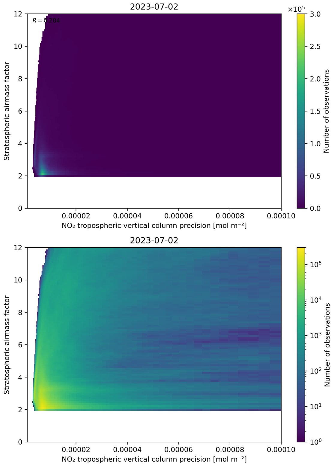
Figure 131: Scatter density plot of “NO 2 tropospheric vertical column precision” against “Stratospheric airmass factor” for 2023-07-01 to 2023-07-03.
