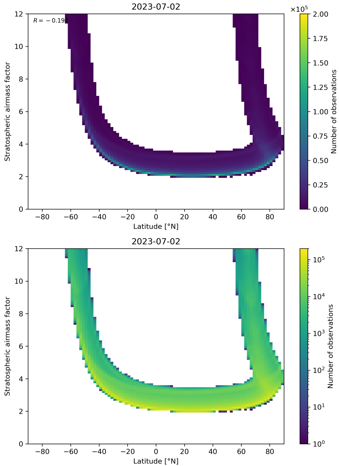
Figure 83: Scatter density plot of “Latitude” against “Stratospheric air mass factor” for 2023-07-01 to 2023-07-03.
