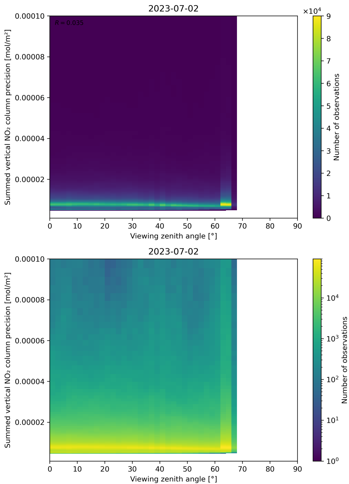
Figure 166: Scatter density plot of “Viewing zenith angle” against “Summed vertical NO 2 column precision” for 2023-07-01 to 2023-07-03.
