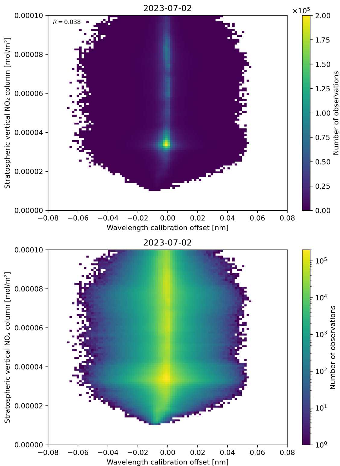
Figure 176: Scatter density plot of “Wavelength calibration offset” against “Stratospheric vertical NO 2 column” for 2023-07-01 to 2023-07-03.
