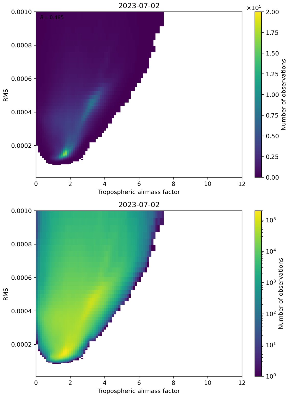
Figure 79: Scatter density plot of “Tropospheric airmass factor” against “RMS” for 2023-07-01 to 2023-07-03.
