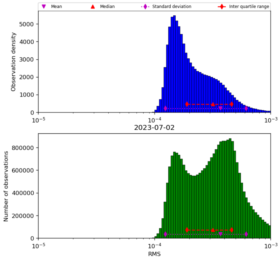
Figure 43: Histogram of “RMS” for 2023-07-01 to 2023-07-03
