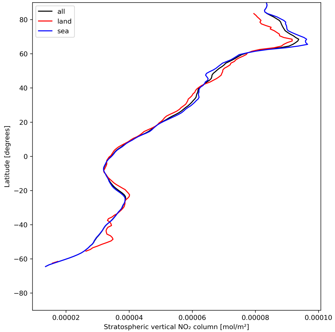
Figure 19: Zonal average of “Stratospheric vertical NO 2 column” for 2023-07-01 to 2023-07-03.
