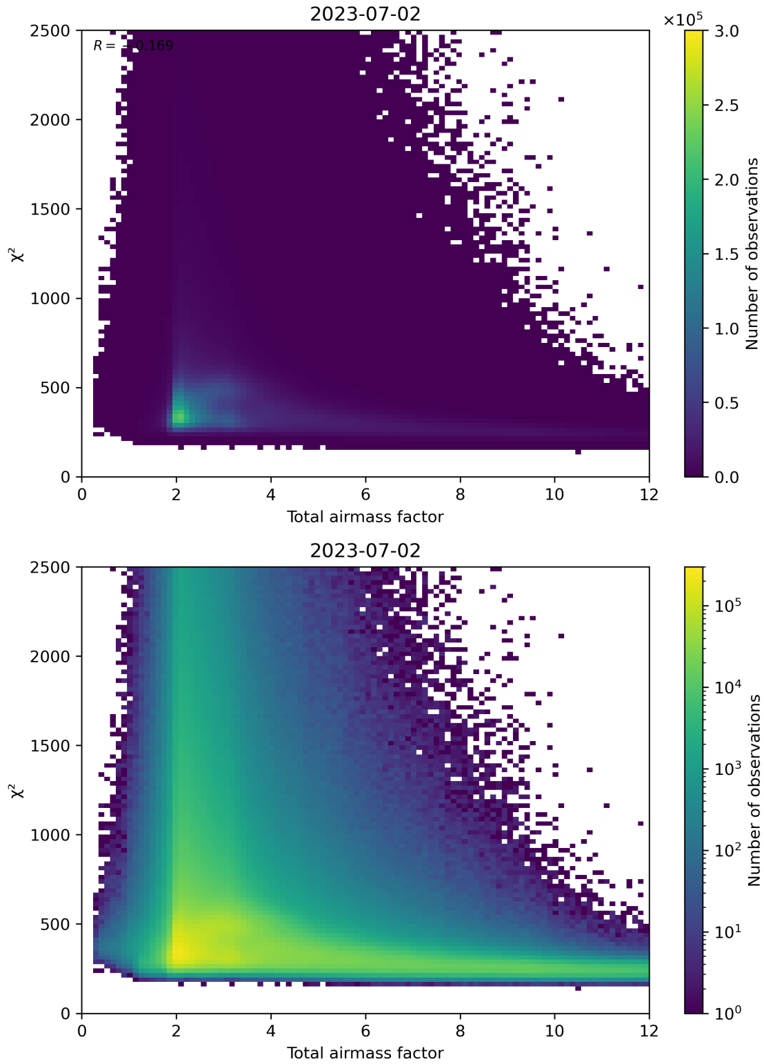
Figure 63: Scatter density plot of “Total airmass factor” against “ \chi^2 ” for 2023-07-01 to 2023-07-03.
