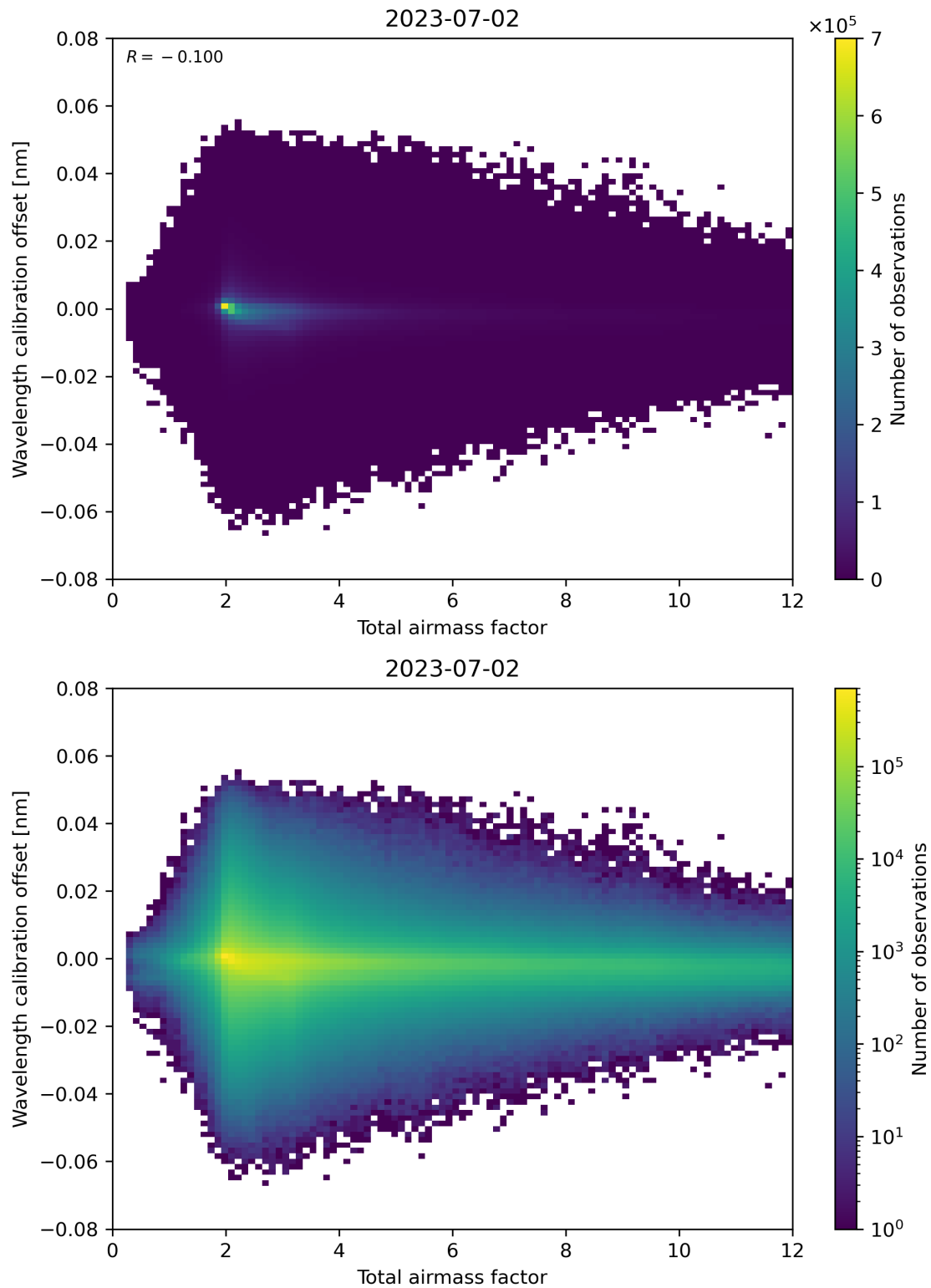
Figure 70: Scatter density plot of “Total airmass factor” against “Wavelength calibration offset” for 2023-07-01 to 2023-07-03.
