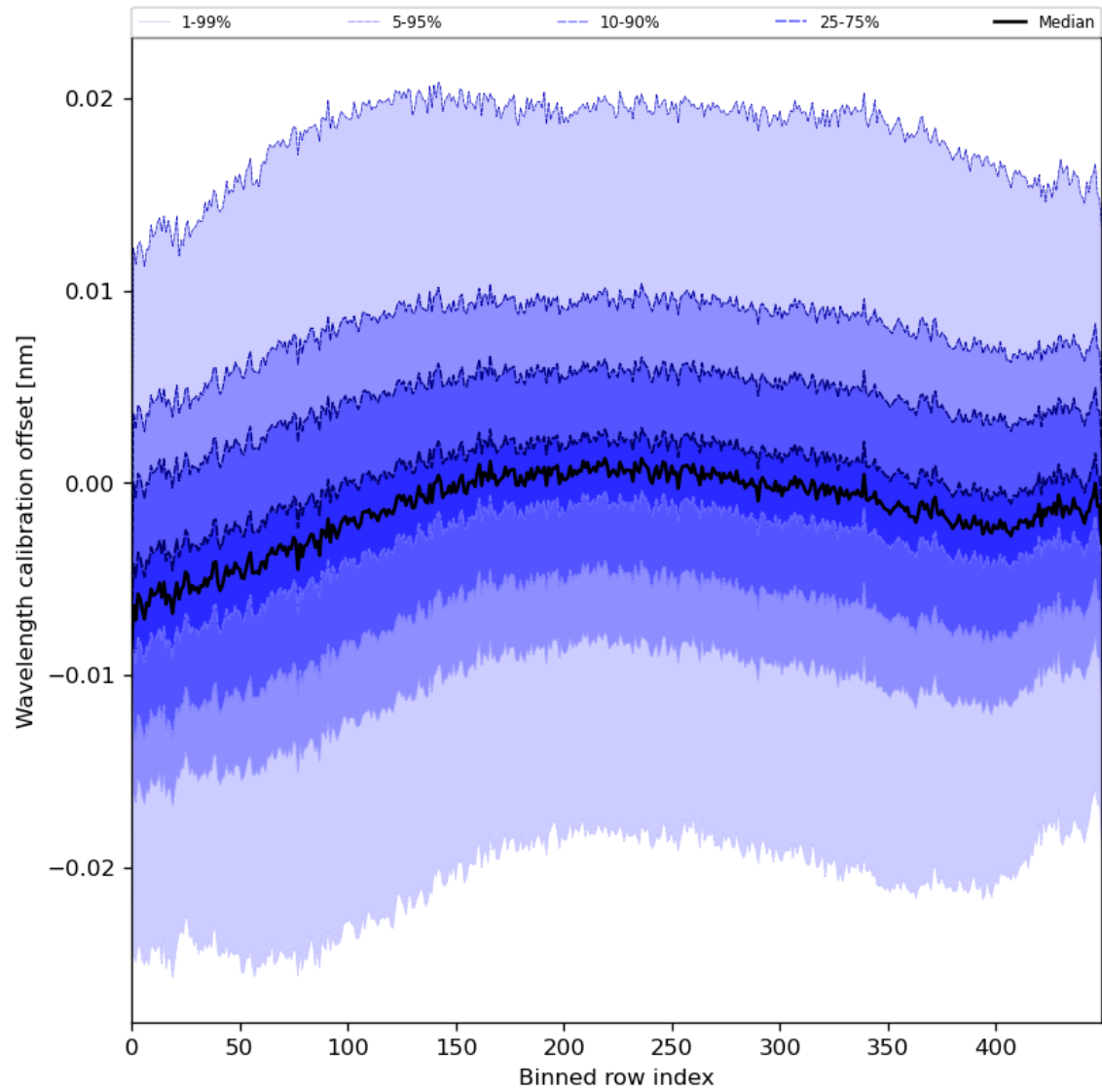
Figure 52: Along track statistics of “Wavelength calibration offset” for 2023-07-01 to 2023-07-03
