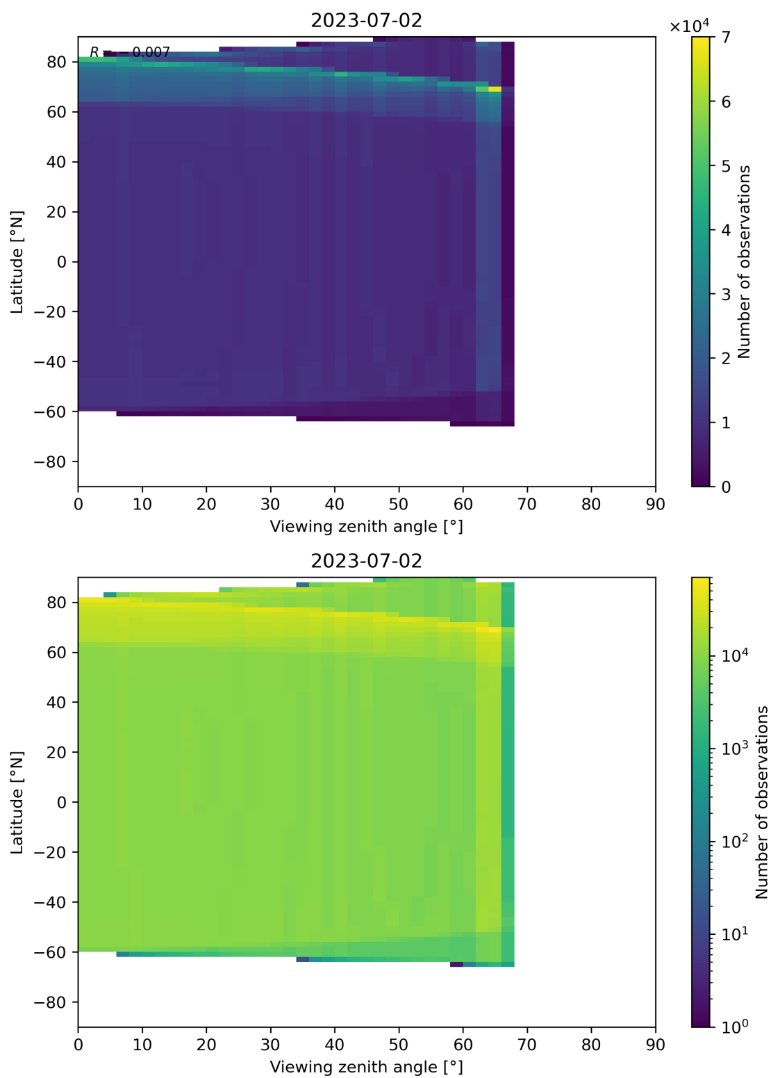
Figure 163: Scatter density plot of “Viewing zenith angle” against “Latitude” for 2023-07-01 to 2023-07-03.
