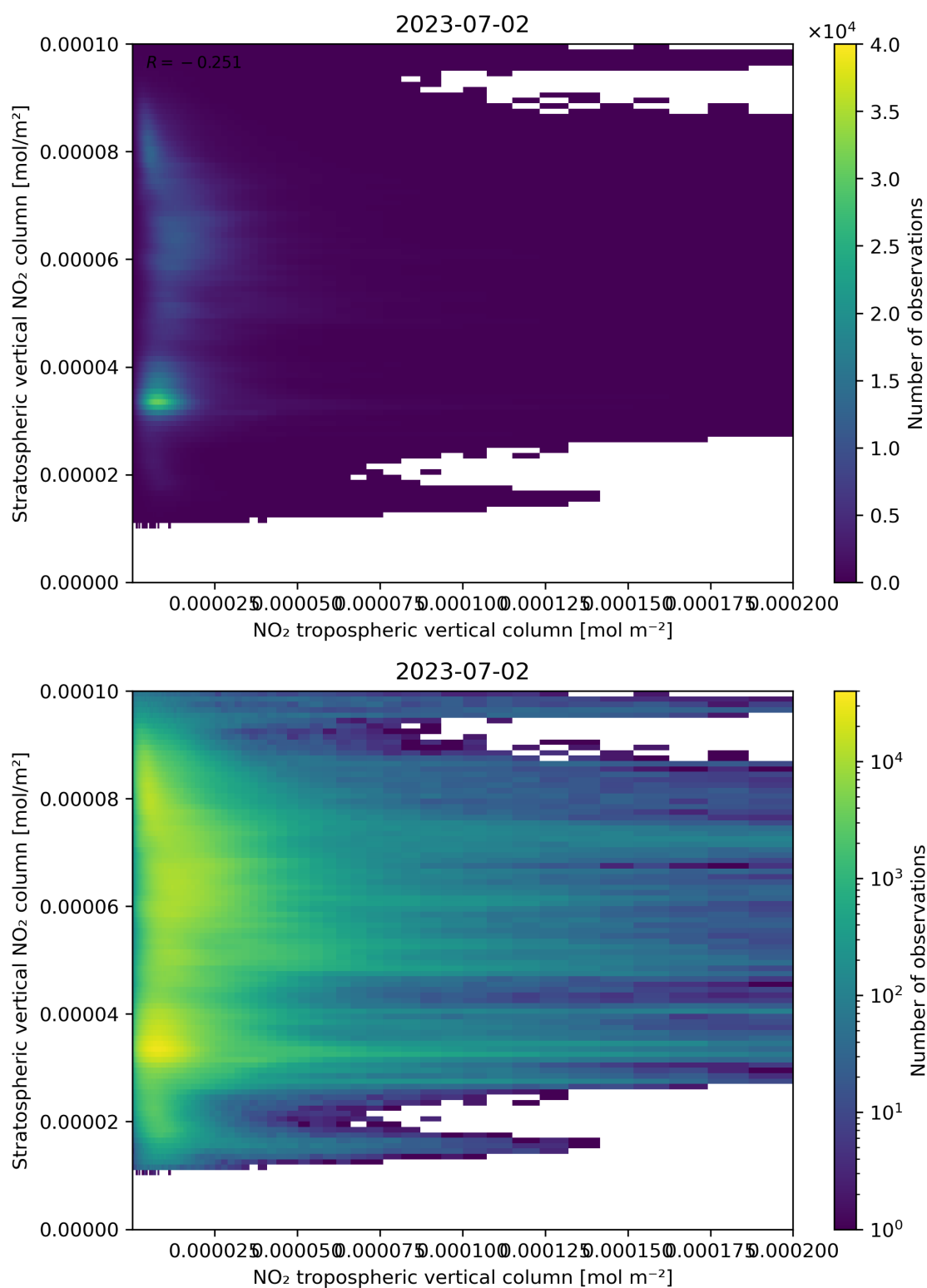
Figure 125: Scatter density plot of “NO 2 tropospheric vertical column” against “Stratospheric vertical NO 2 column” for 2023-07-01 to 2023-07-03.
