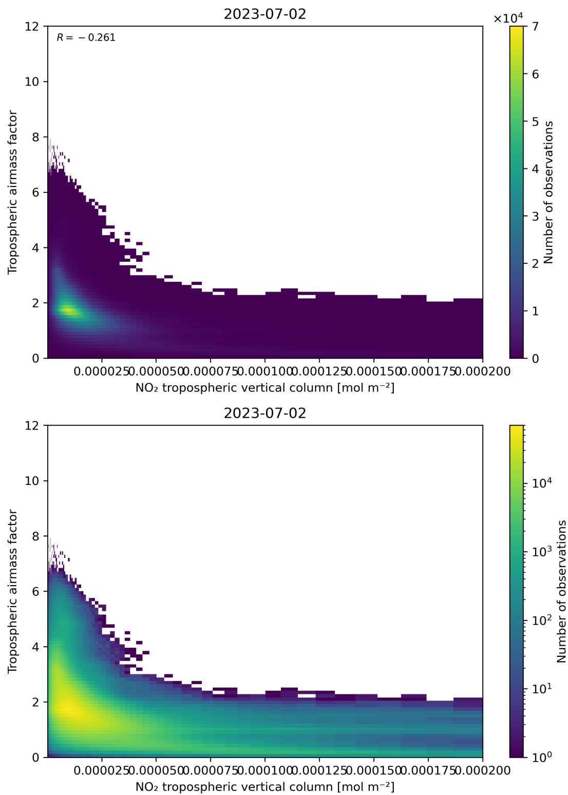
Figure 123: Scatter density plot of “NO 2 tropospheric vertical column” against “Tropospheric air mass factor” for 2023-07-01 to 2023-07-03.
