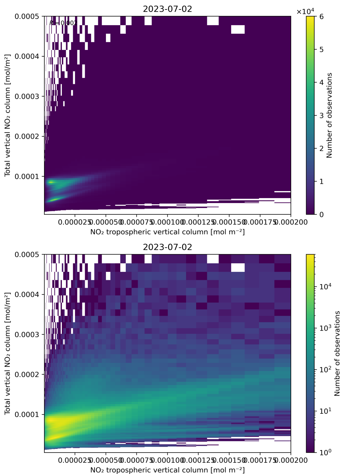
Figure 128: Scatter density plot of “NO 2 tropospheric vertical column” against “Total vertical NO 2 column” for 2023-07-01 to 2023-07-03.
