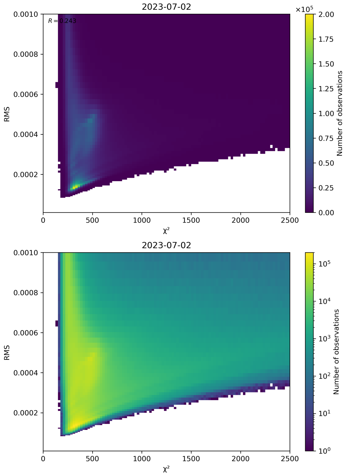
Figure 82: Scatter density plot of “ \chi^2 ” against “RMS” for 2023-07-01 to 2023-07-03.
