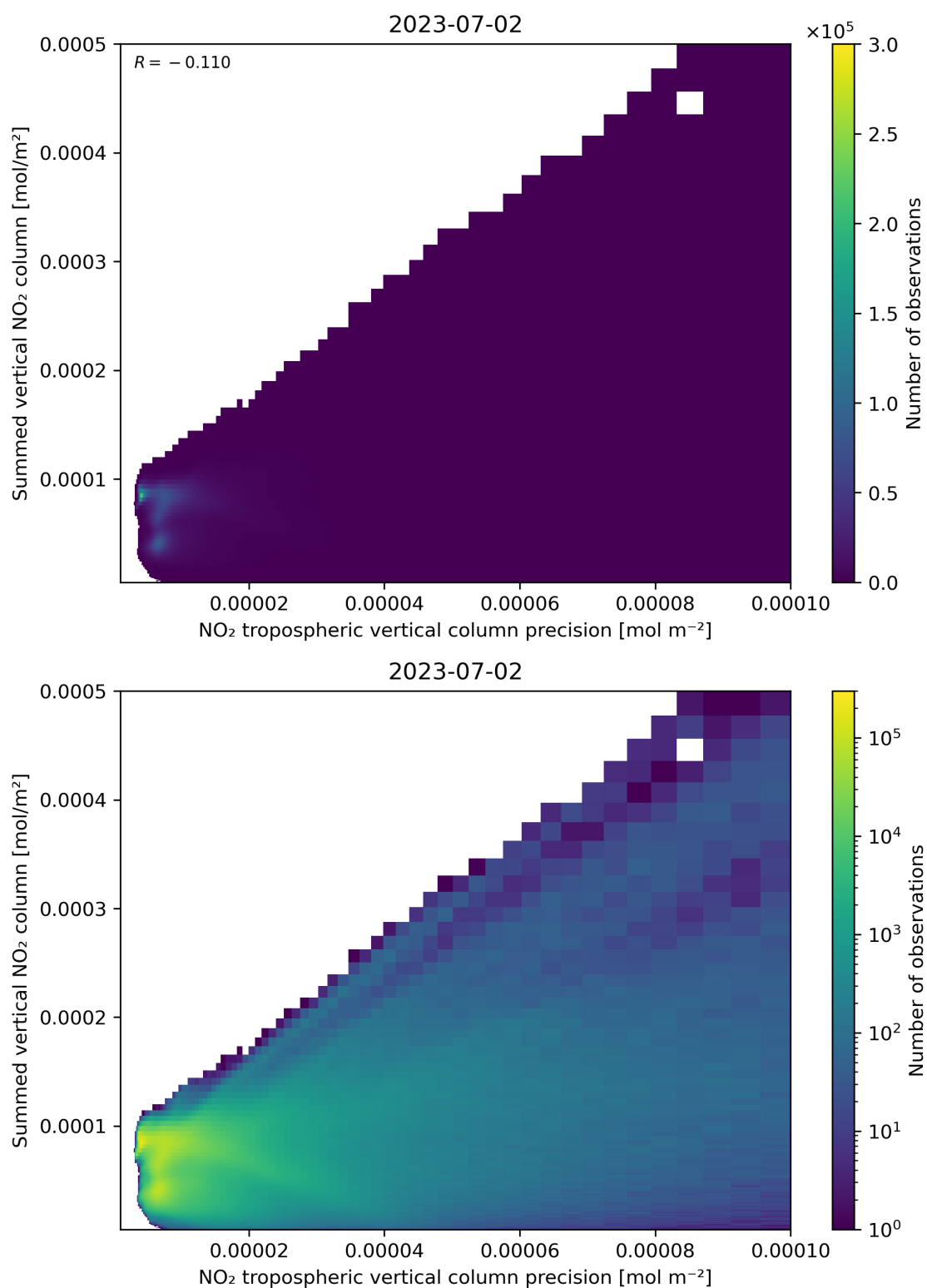
Figure 136: Scatter density plot of “NO 2 tropospheric vertical column precision” against “Summed vertical NO 2 column” for 2023-07-01 to 2023-07-03.
