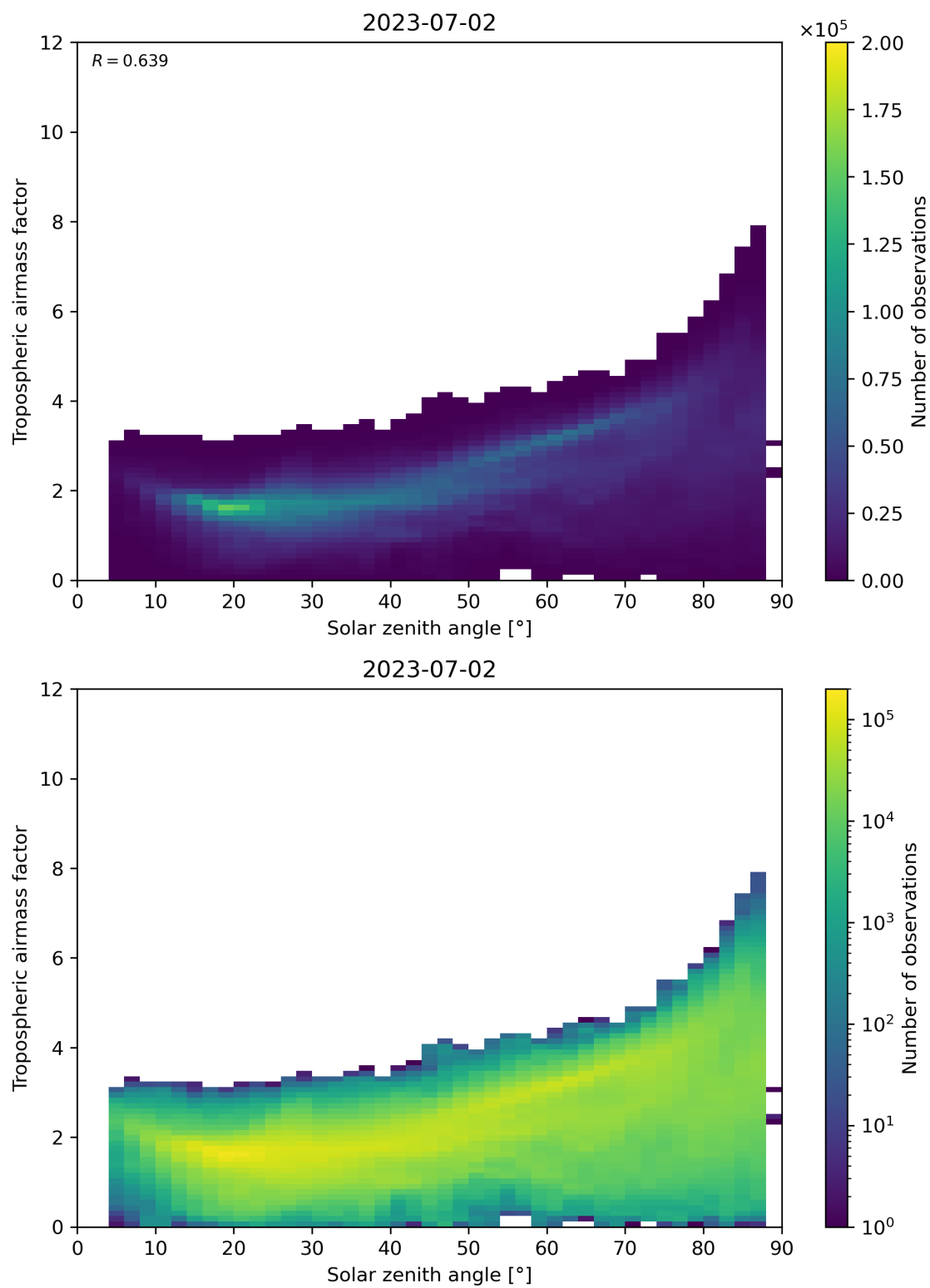
Figure 147: Scatter density plot of “Solar zenith angle” against “Tropospheric airmass factor” for 2023-07-01 to 2023-07-03.
