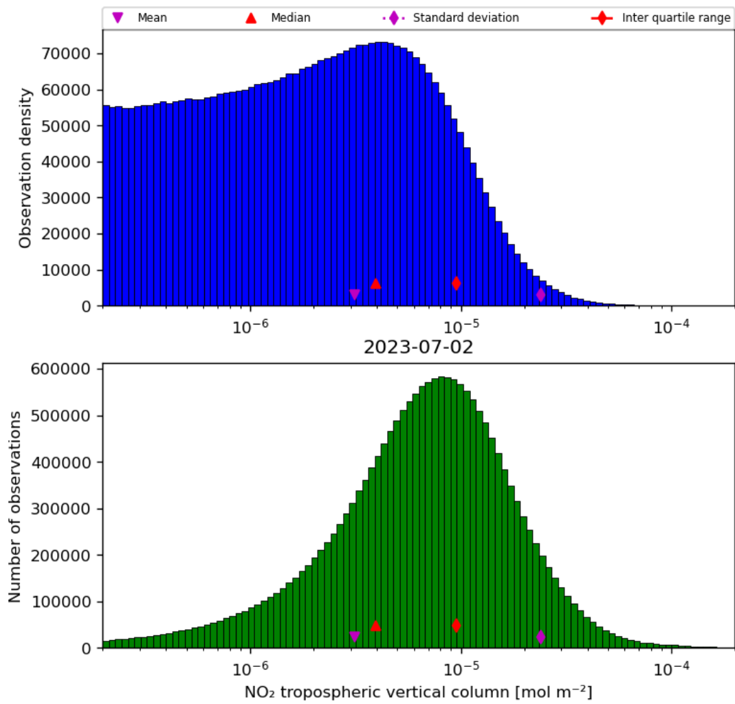
Figure 29: Histogram of “NO 2 tropospheric vertical column” for 2023-07-01 to 2023-07-03
