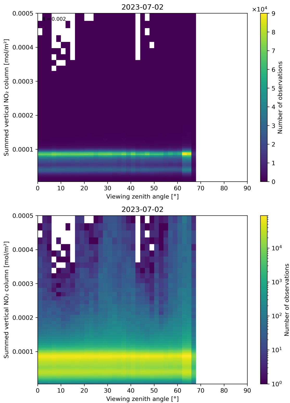
Figure 165: Scatter density plot of “Viewing zenith angle” against “Summed vertical NO 2 column” for 2023-07-01 to 2023-07-03.
