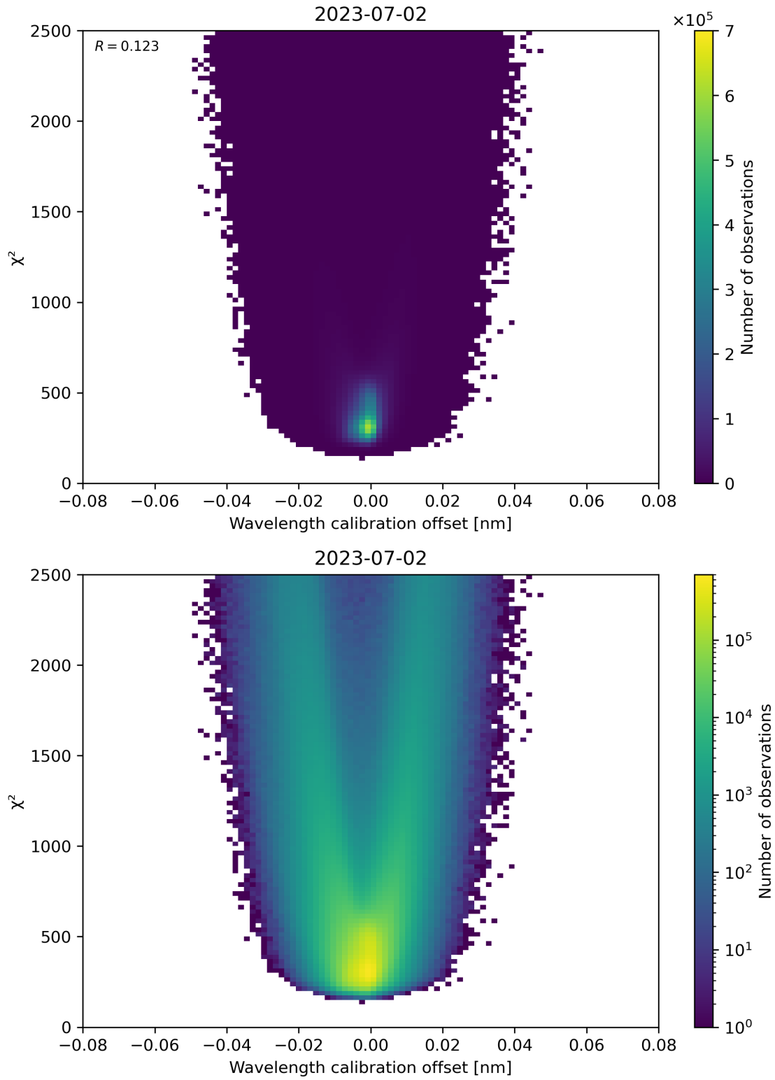
Figure 175: Scatter density plot of “Wavelength calibration offset” against “ \chi^2 ” for 2023-07-01 to 2023-07-03.
