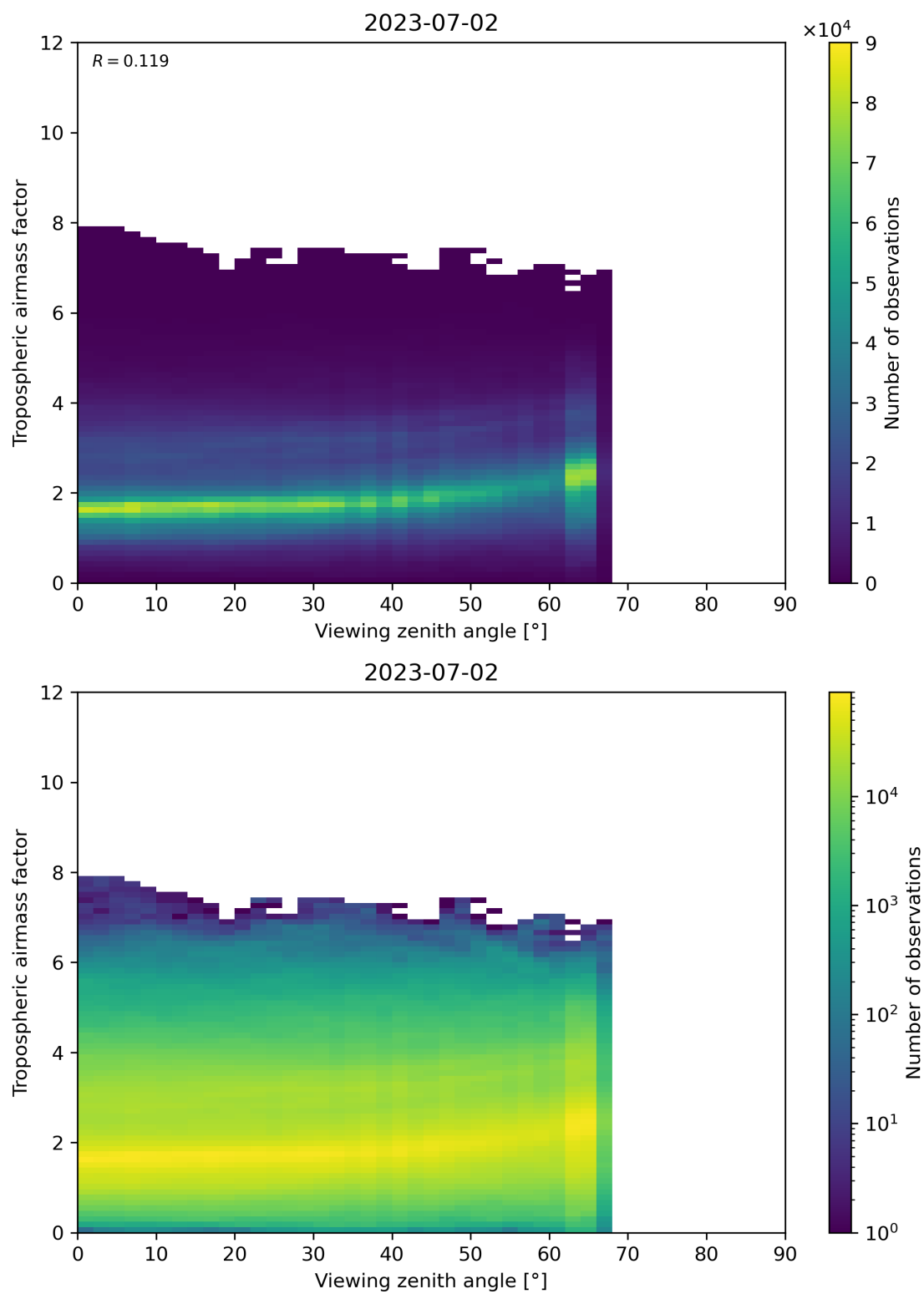
Figure 161: Scatter density plot of “Viewing zenith angle” against “Tropospheric airmass factor” for 2023-07-01 to 2023-07-03.
