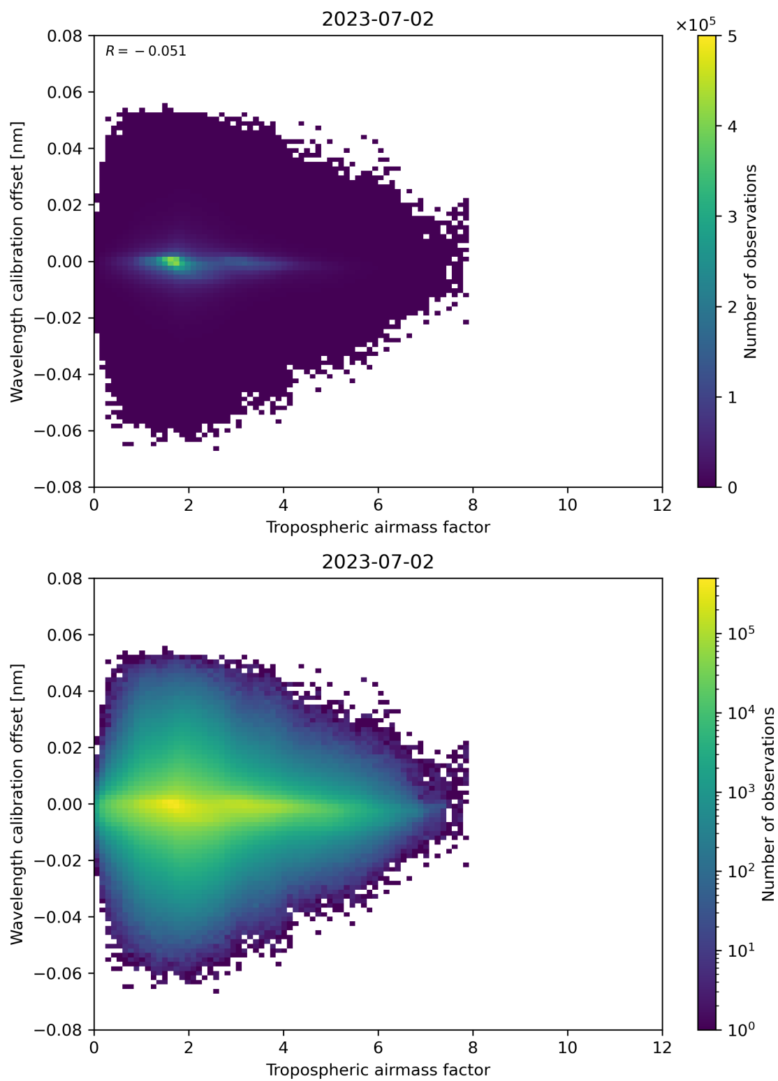
Figure 80: Scatter density plot of “Tropospheric airmass factor” against “Wavelength calibration offset” for 2023-07-01 to 2023-07-03.
