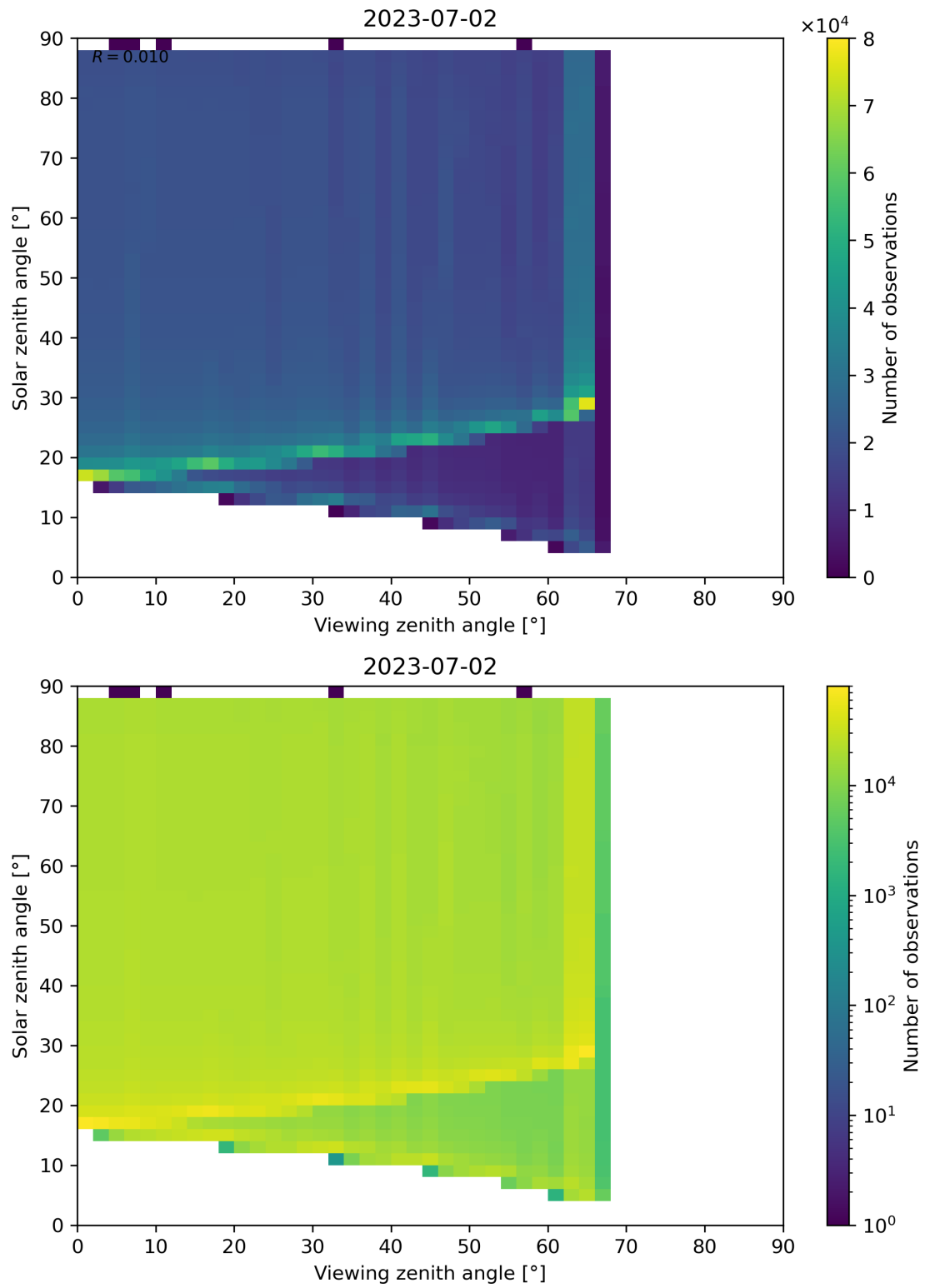
Figure 172: Scatter density plot of “Viewing zenith angle” against “Solar zenith angle” for 2023-07-01 to 2023-07-03.
