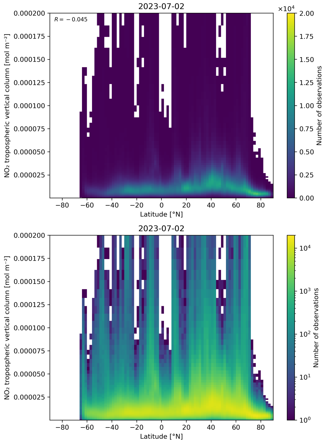
Figure 92: Scatter density plot of “Latitude” against “NO 2 tropospheric vertical column” for 2023-07-01 to 2023-07-03.
