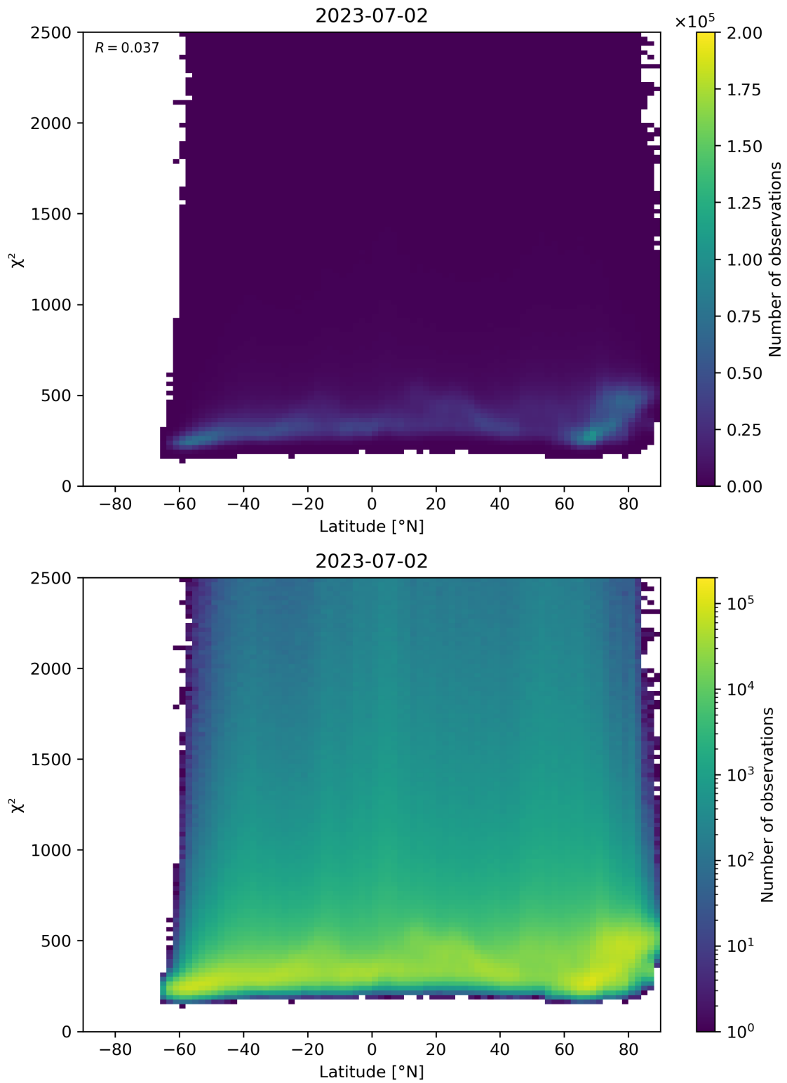
Figure 86: Scatter density plot of “Latitude” against “ \chi^2 ” for 2023-07-01 to 2023-07-03.
