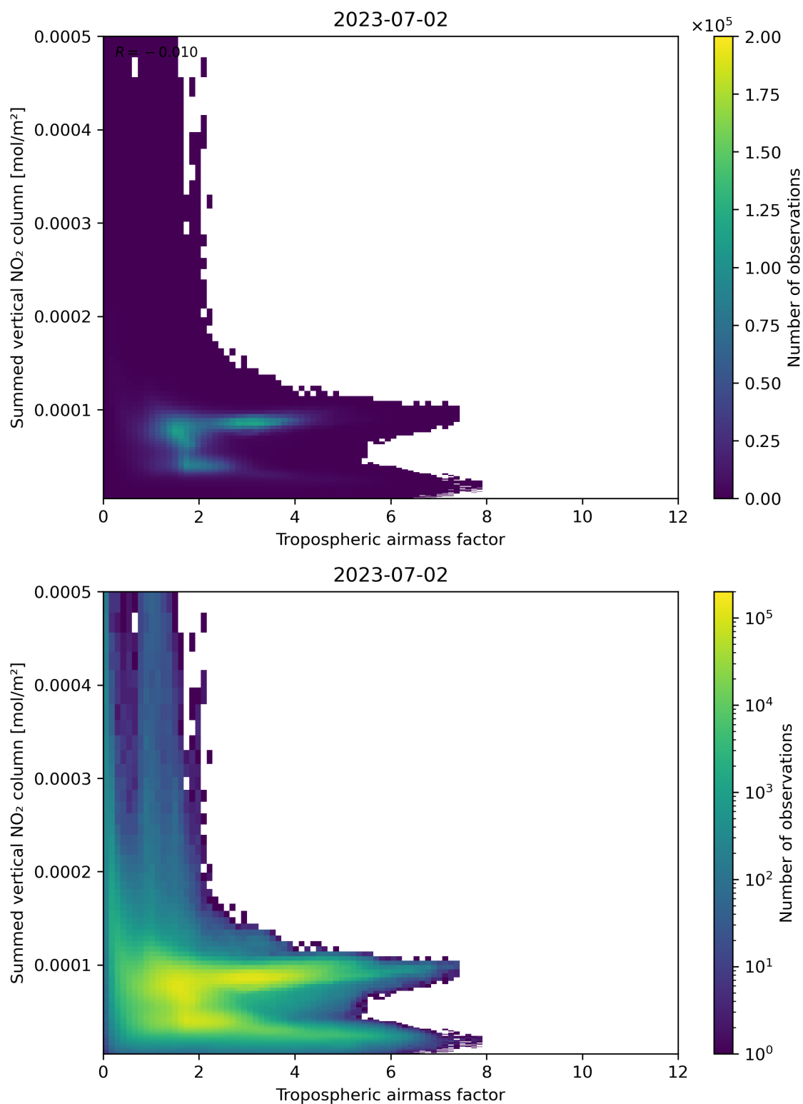
Figure 75: Scatter density plot of “Tropospheric airmass factor” against “Summed vertical NO 2 column” for 2023-07-01 to 2023-07-03.
