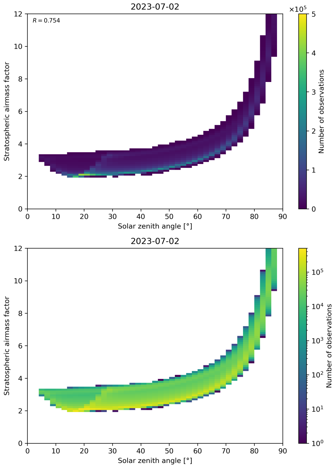
Figure 145: Scatter density plot of “Solar zenith angle” against “Stratospheric airmass factor” for 2023-07-01 to 2023-07-03.
