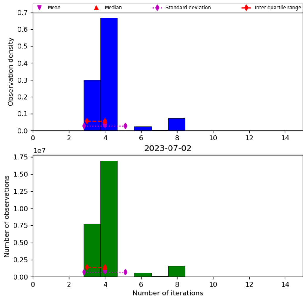
Figure 34: Histogram of “Number of iterations” for 2023-07-01 to 2023-07-03
