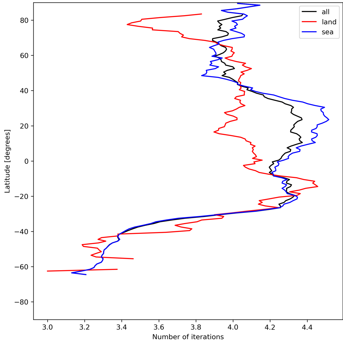
Figure 17: Zonal average of “Number of iterations” for 2023-07-01 to 2023-07-03.
