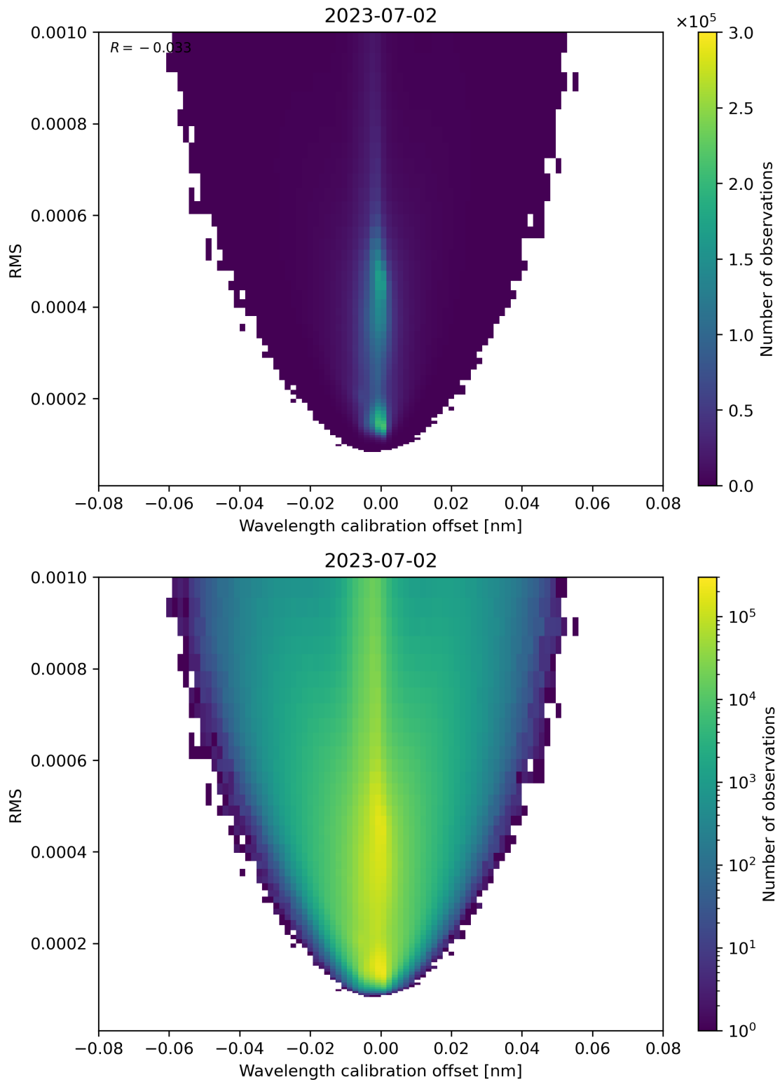
Figure 181: Scatter density plot of “Wavelength calibration offset” against “RMS” for 2023-07-01 to 2023-07-03.
