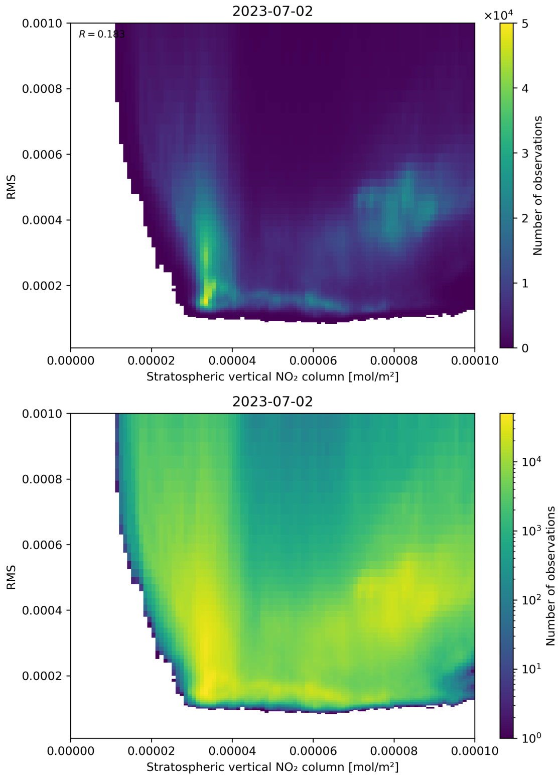
Figure 102: Scatter density plot of “Stratospheric vertical NO 2 column” against “RMS” for 2023-07-01 to 2023-07-03.
