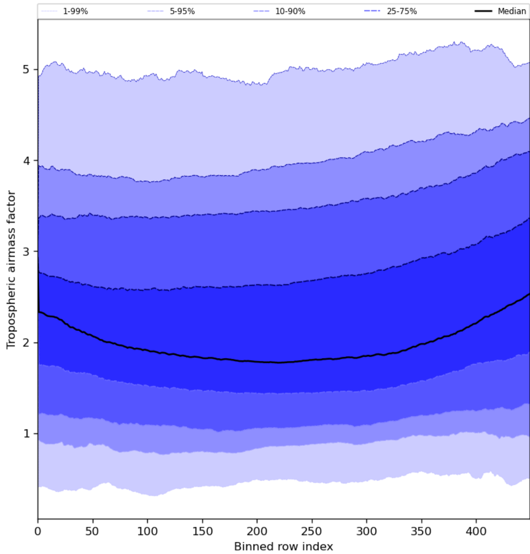
Figure 48: Along track statistics of “Tropospheric air mass factor” for 2023-07-01 to 2023-07-03
