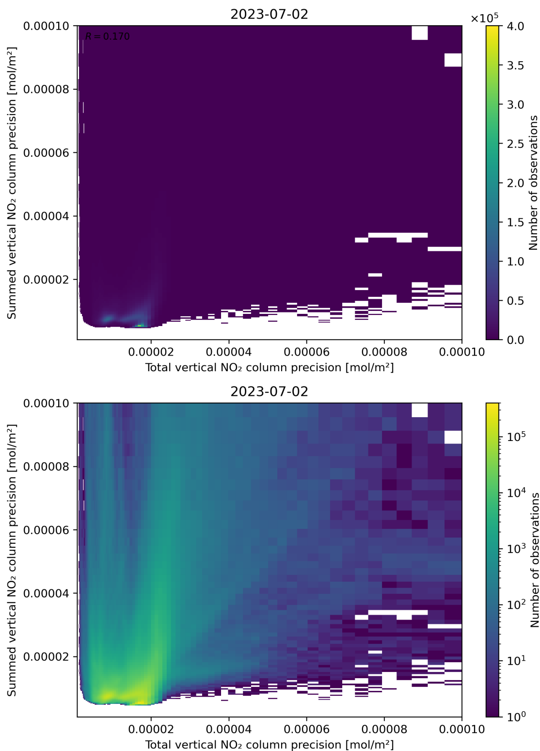
Figure 118: Scatter density plot of “Total vertical NO 2 column precision” against “Summed vertical NO 2 column precision” for 2023-07-01 to 2023-07-03.
