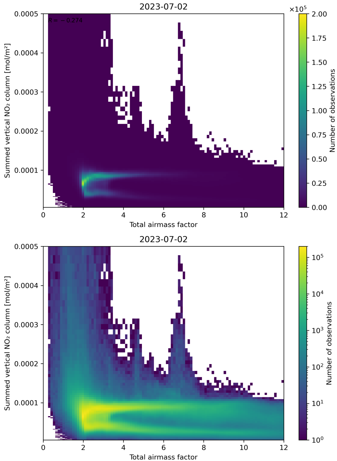
Figure 65: Scatter density plot of “Total airmass factor” against “Summed vertical NO 2 column” for 2023-07-01 to 2023-07-03.
