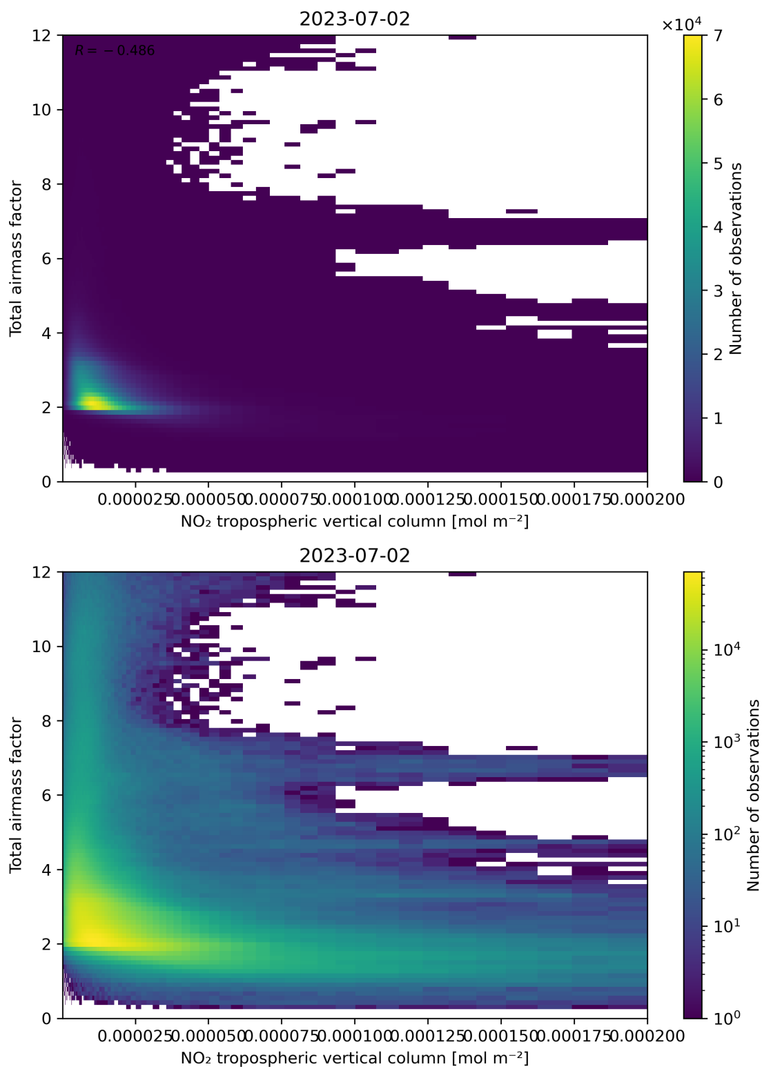
Figure 122: Scatter density plot of “NO 2 tropospheric vertical column” against “Total airmass factor” for 2023-07-01 to 2023-07-03.
