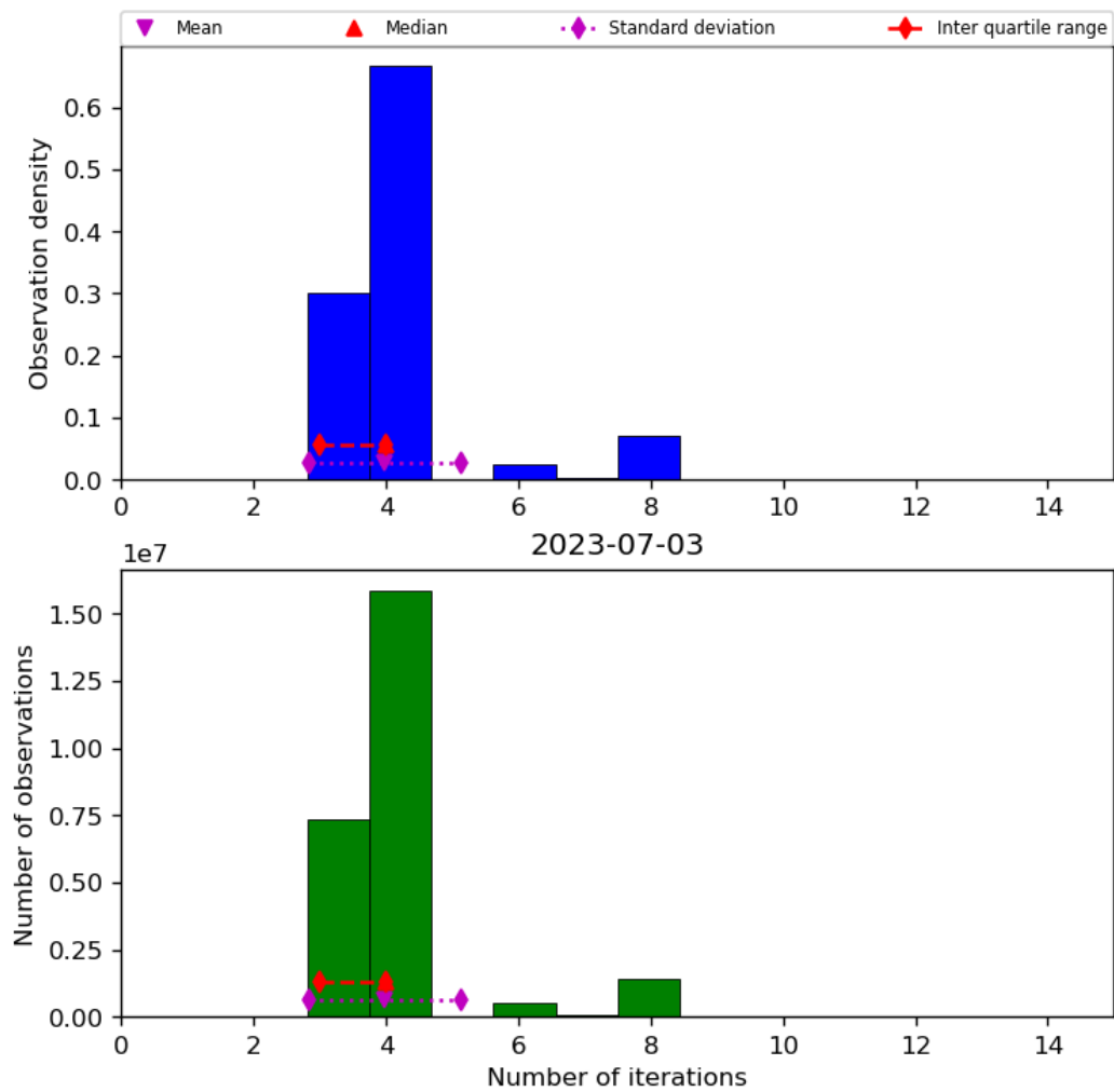
Figure 34: Histogram of “Number of iterations” for 2023-07-03 to 2023-07-04
