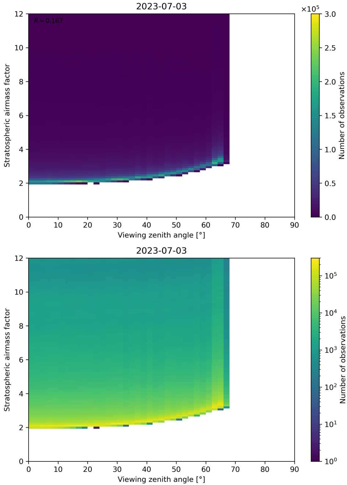
Figure 159: Scatter density plot of “Viewing zenith angle” against “Stratospheric airmass factor” for 2023-07-03 to 2023-07-04.
