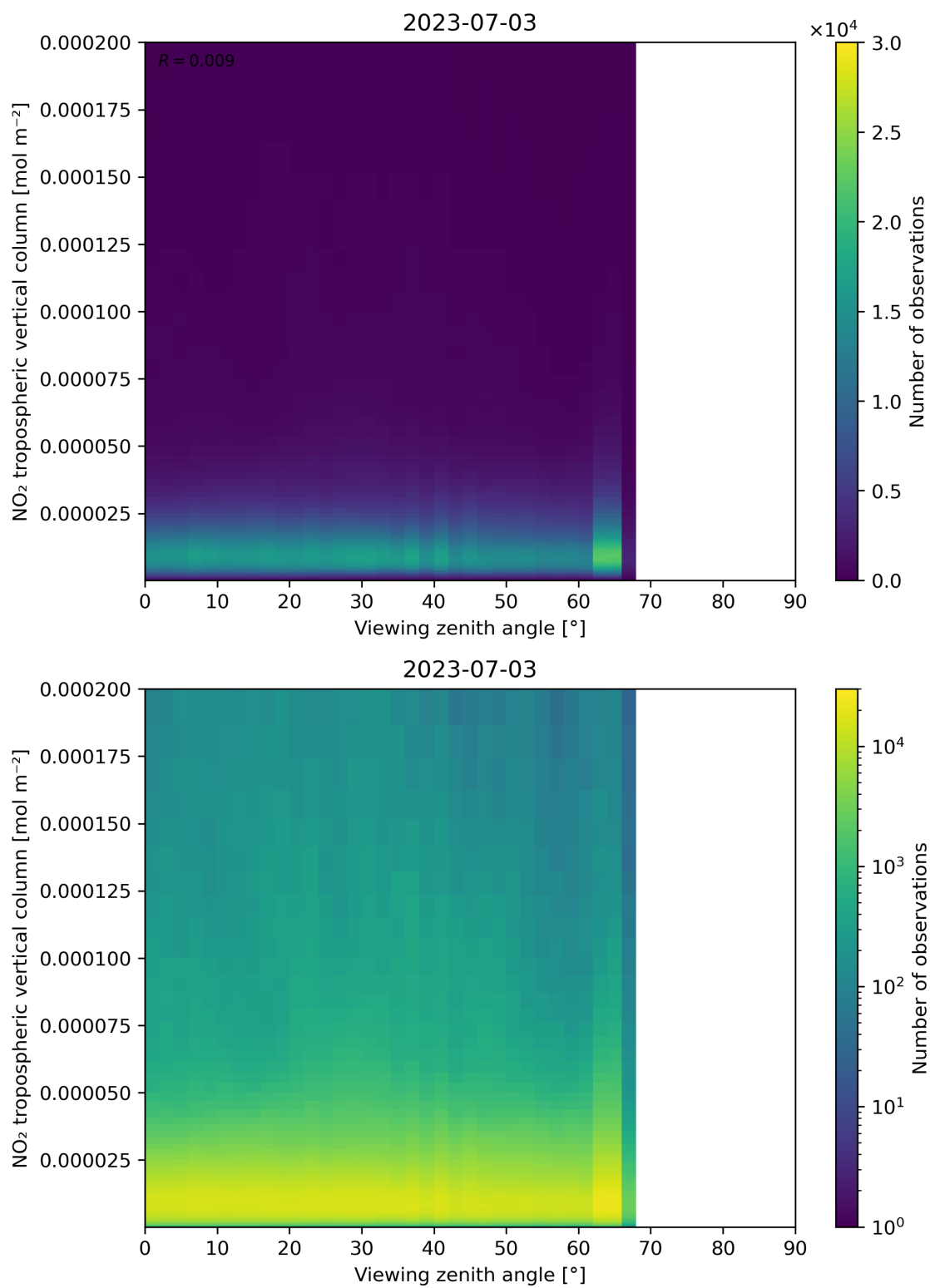
Figure 169: Scatter density plot of “Viewing zenith angle” against “NO 2 tropospheric vertical column” for 2023-07-03 to 2023-07-04.
