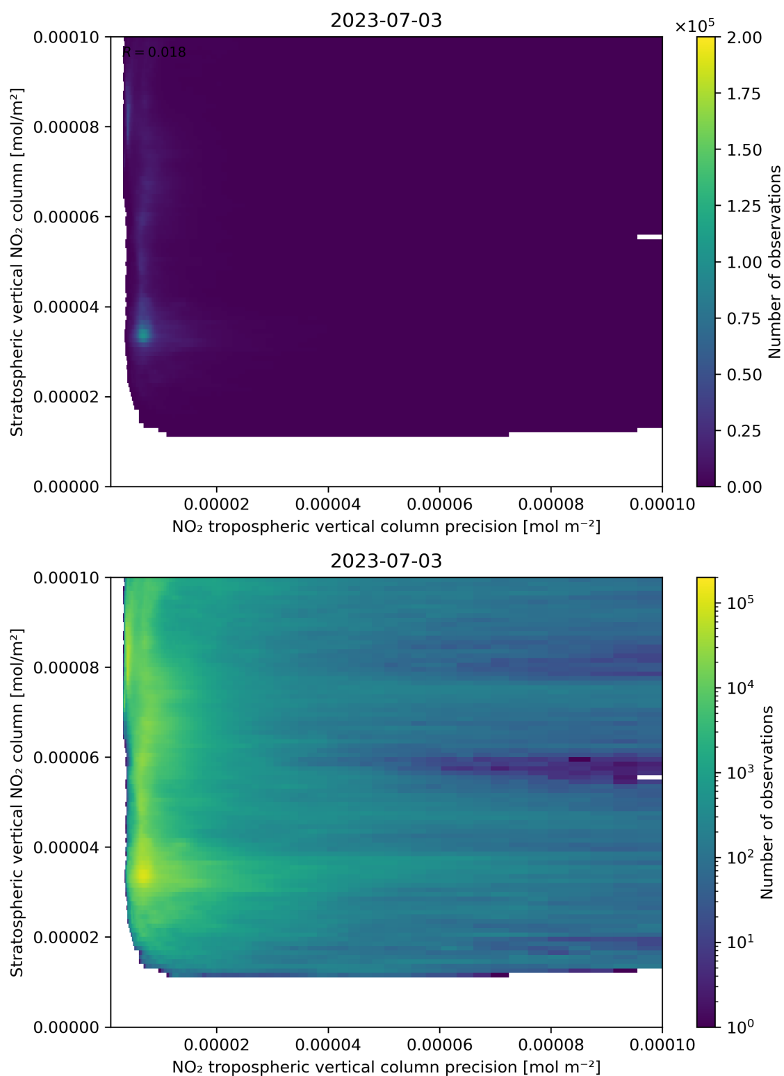
Figure 135: Scatter density plot of “NO 2 tropospheric vertical column precision” against “Stratospheric vertical NO 2 column” for 2023-07-03 to 2023-07-04.
