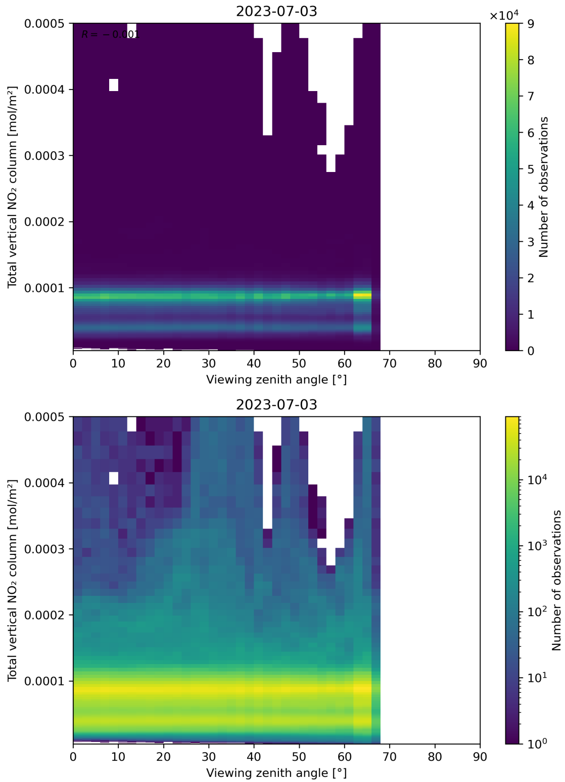
Figure 167: Scatter density plot of “Viewing zenith angle” against “Total vertical NO 2 column” for 2023-07-03 to 2023-07-04.
