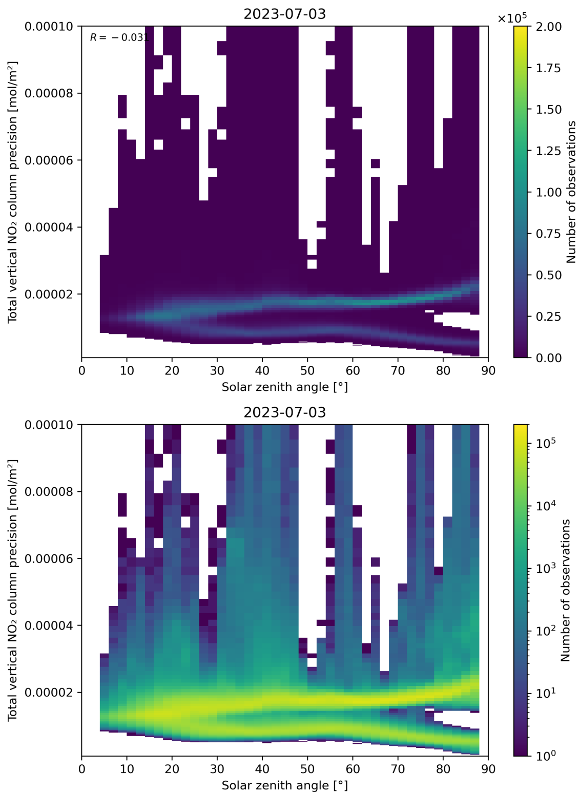
Figure 154: Scatter density plot of “Solar zenith angle” against “Total vertical NO 2 column precision” for 2023-07-03 to 2023-07-04.
