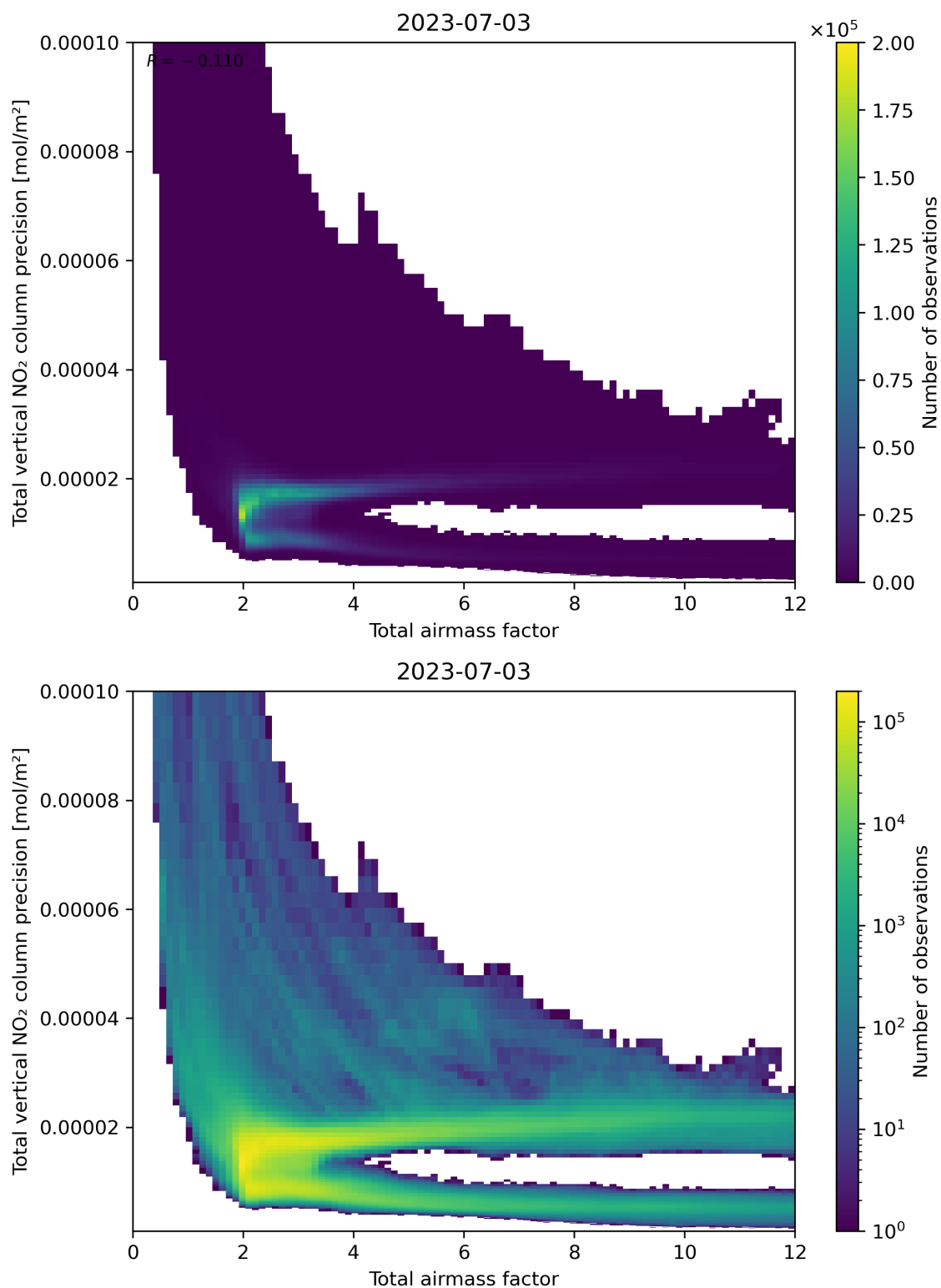
Figure 68: Scatter density plot of “Total airmass factor” against “Total vertical NO 2 column precision” for 2023-07-03 to 2023-07-04.
