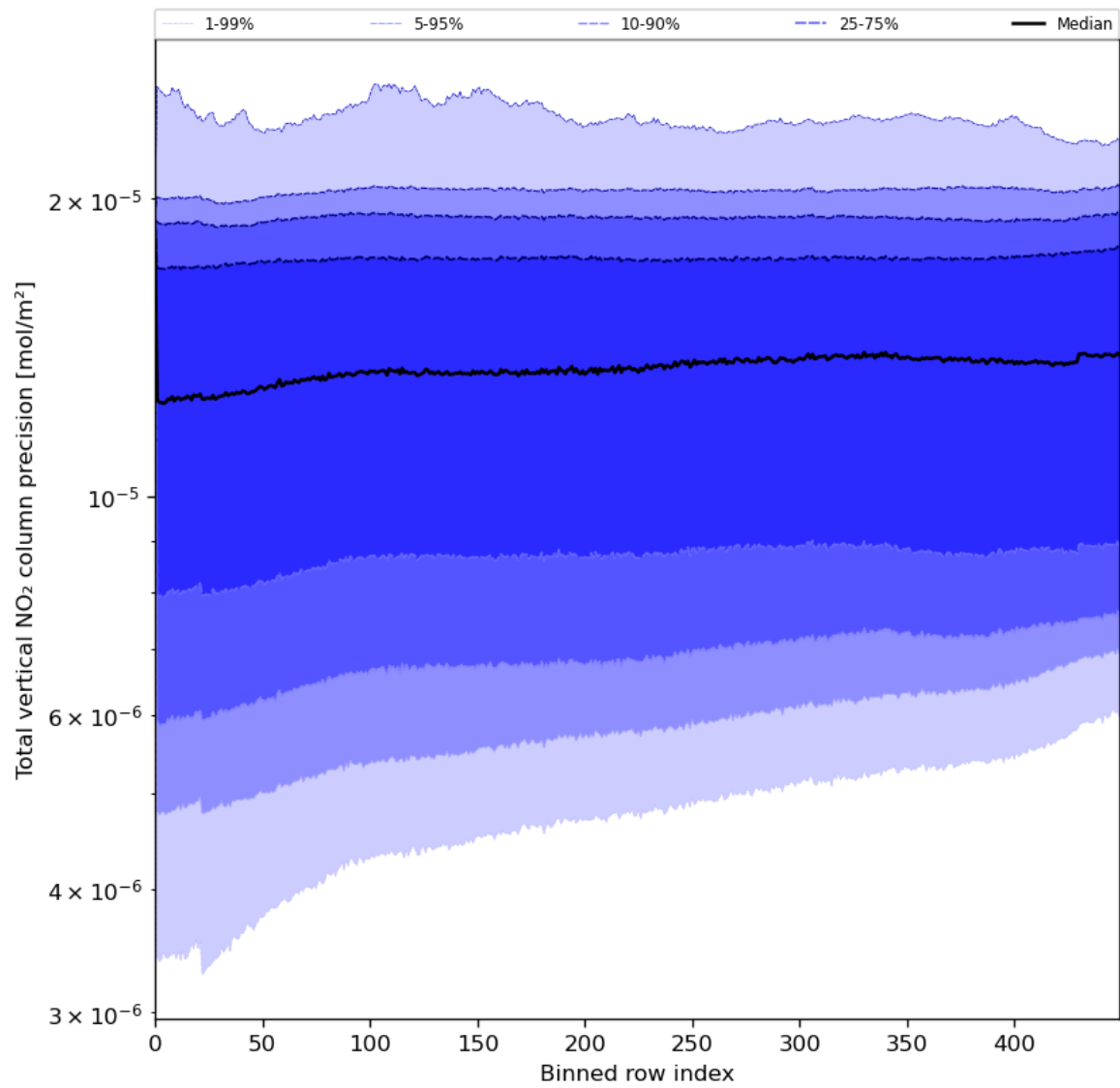
Figure 56: Along track statistics of “Total vertical NO 2 column precision” for 2023-07-03 to 2023-07-04
