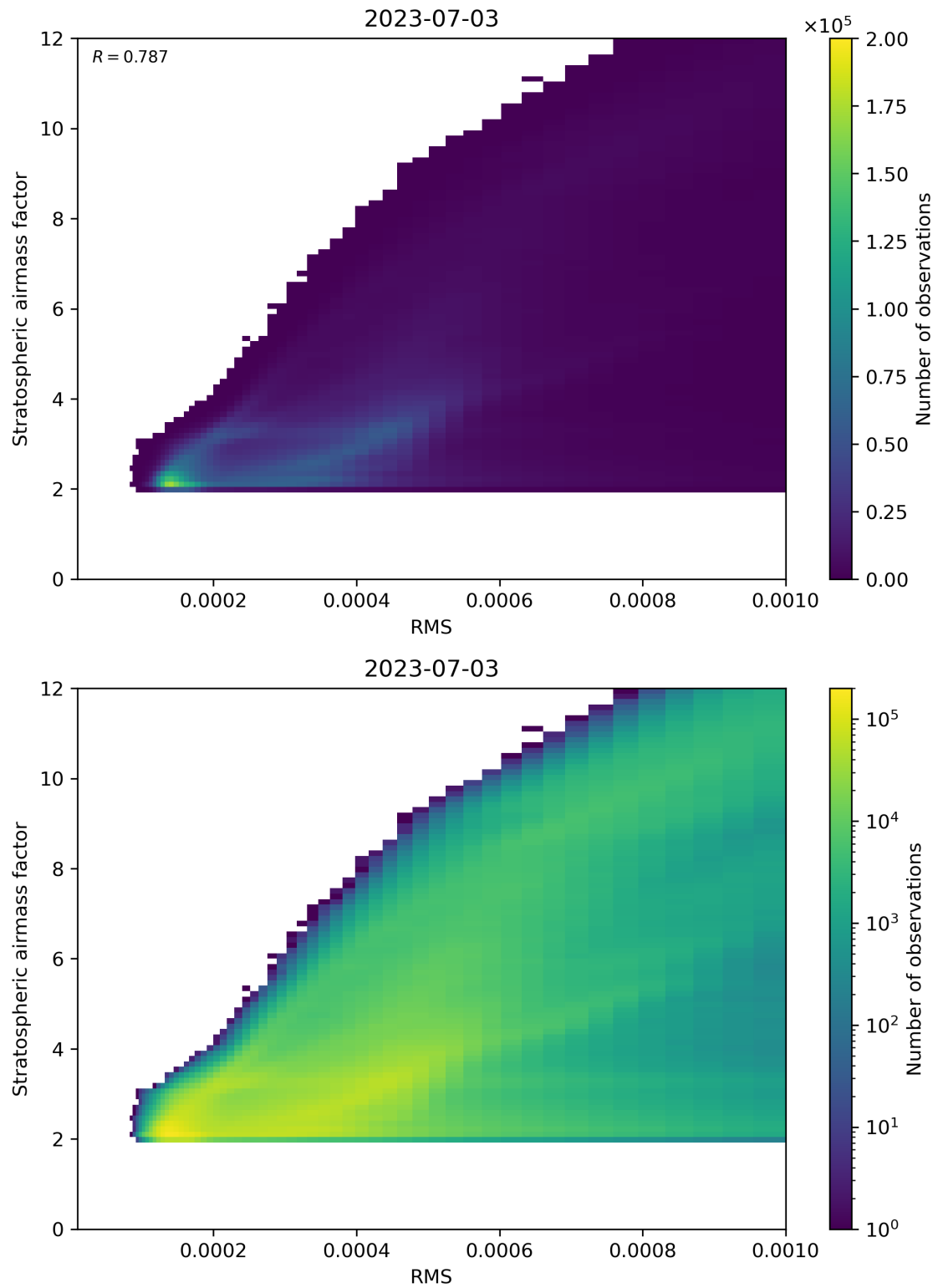
Figure 144: Scatter density plot of “RMS” against “Stratospheric airmass factor” for 2023-07-03 to 2023-07-04.
