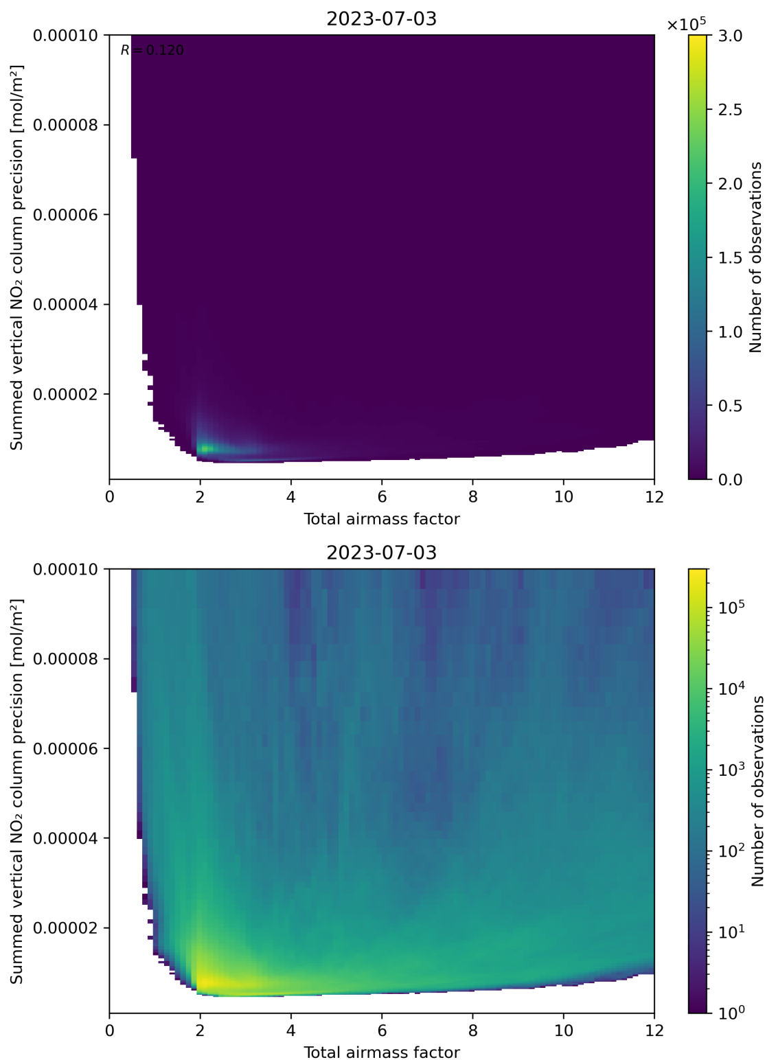
Figure 66: Scatter density plot of “Total airmass factor” against “Summed vertical NO 2 column precision” for 2023-07-03 to 2023-07-04.
