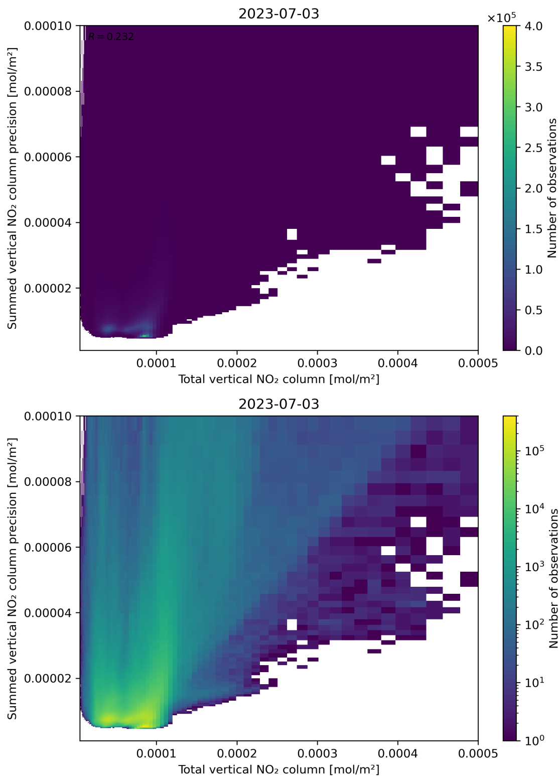
Figure 113: Scatter density plot of “Total vertical NO 2 column” against “Summed vertical NO 2 column precision” for 2023-07-03 to 2023-07-04.
