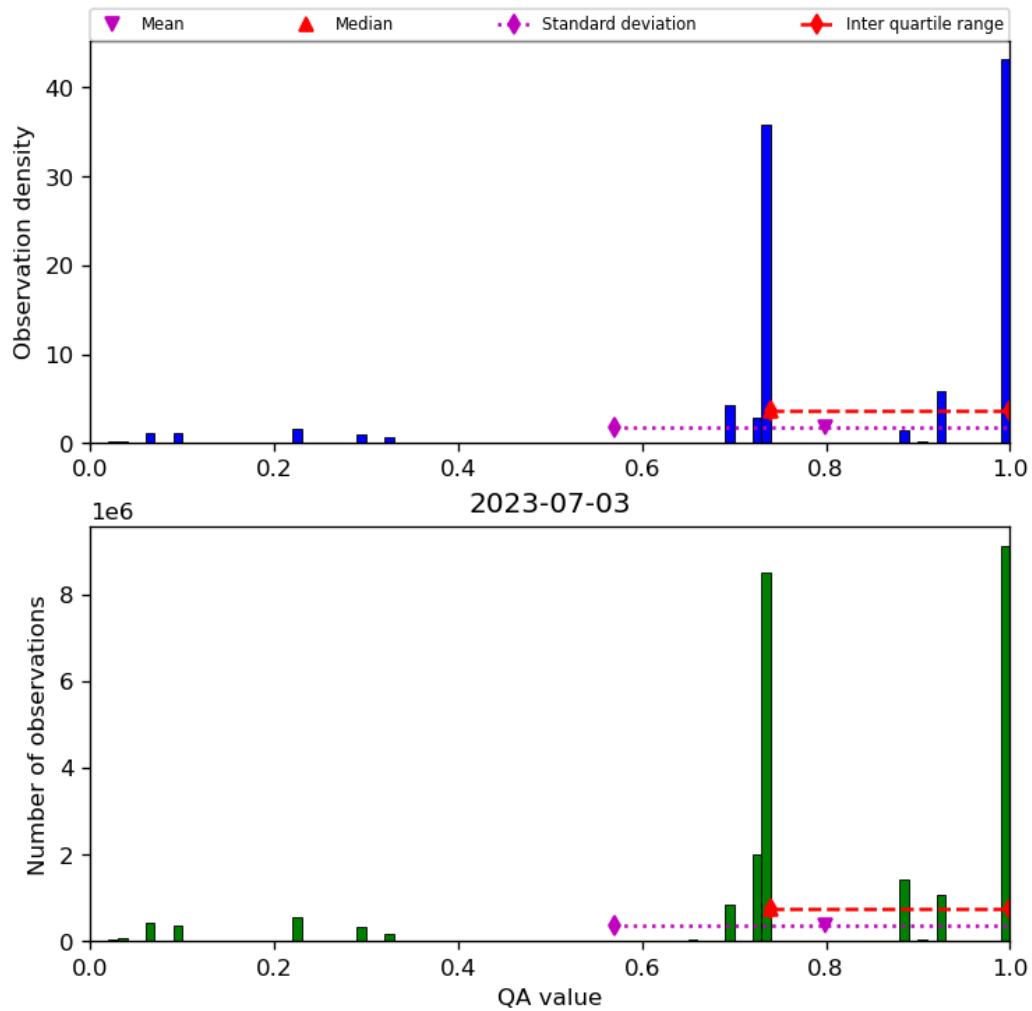
Figure 28: Histogram of “QA value” for 2023-07-03 to 2023-07-04
