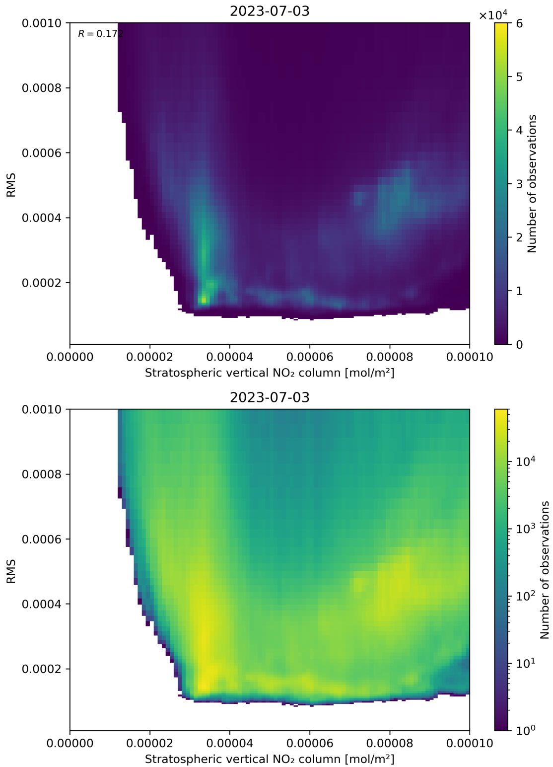
Figure 102: Scatter density plot of “Stratospheric vertical NO 2 column” against “RMS” for 2023-07-03 to 2023-07-04.
