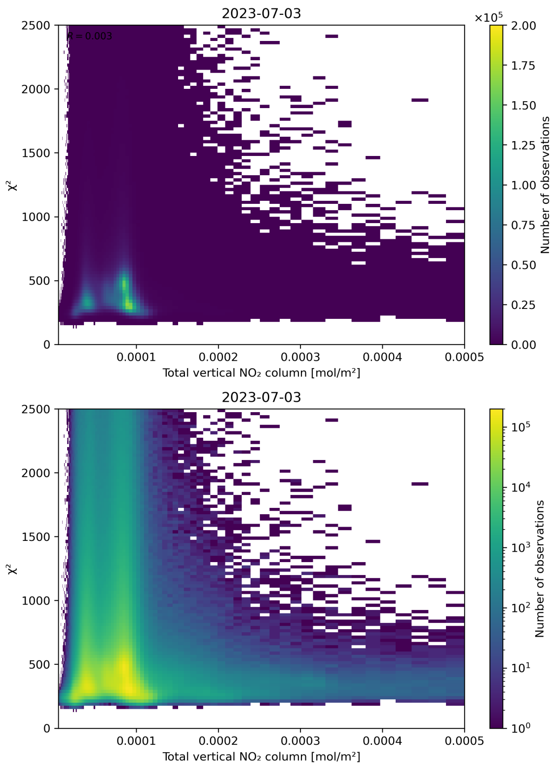
Figure 111: Scatter density plot of “Total vertical NO 2 column” against “ \chi^2 ” for 2023-07-03 to 2023-07-04.
