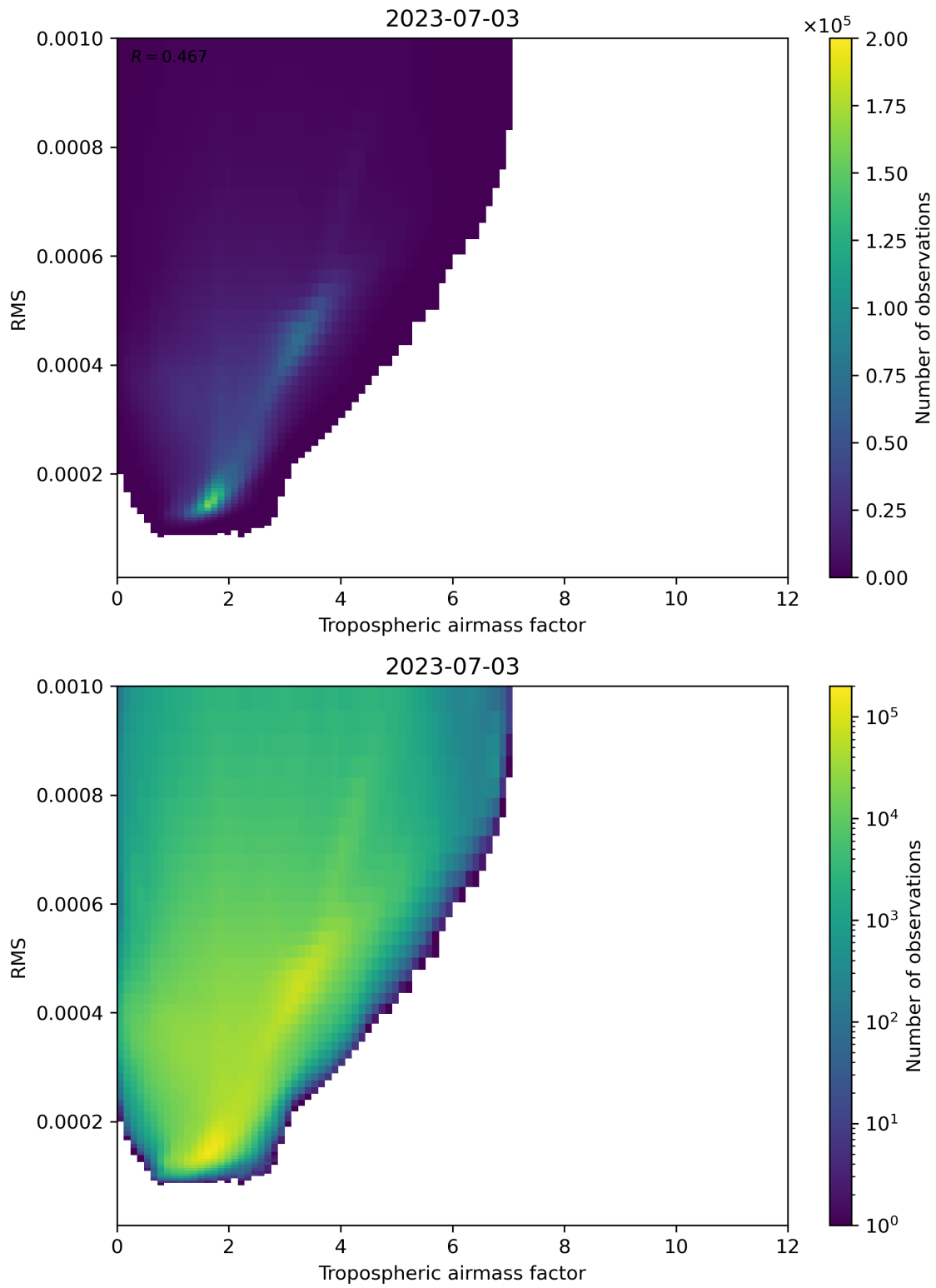
Figure 79: Scatter density plot of “Tropospheric airmass factor” against “RMS” for 2023-07-03 to 2023-07-04.
