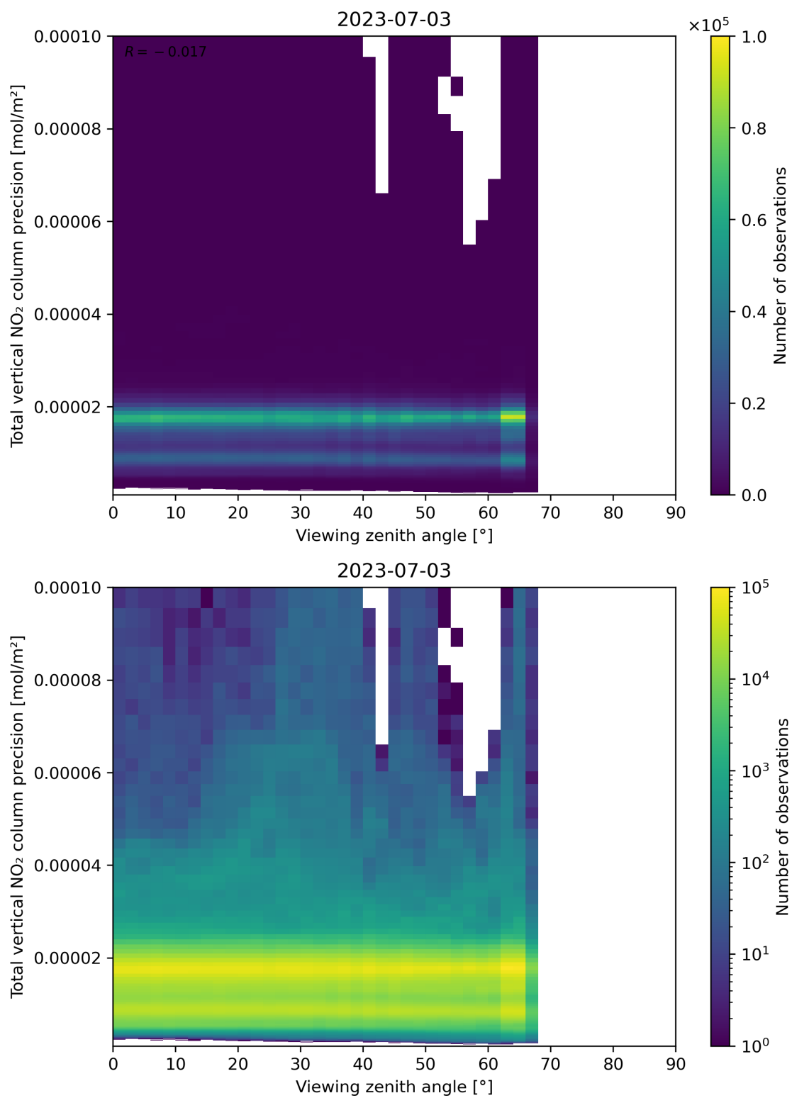
Figure 168: Scatter density plot of “Viewing zenith angle” against “Total vertical NO 2 column precision” for 2023-07-03 to 2023-07-04.
