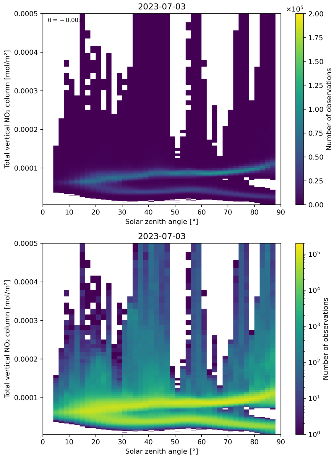
Figure 153: Scatter density plot of “Solar zenith angle” against “Total vertical NO 2 column” for 2023-07-03 to 2023-07-04.
