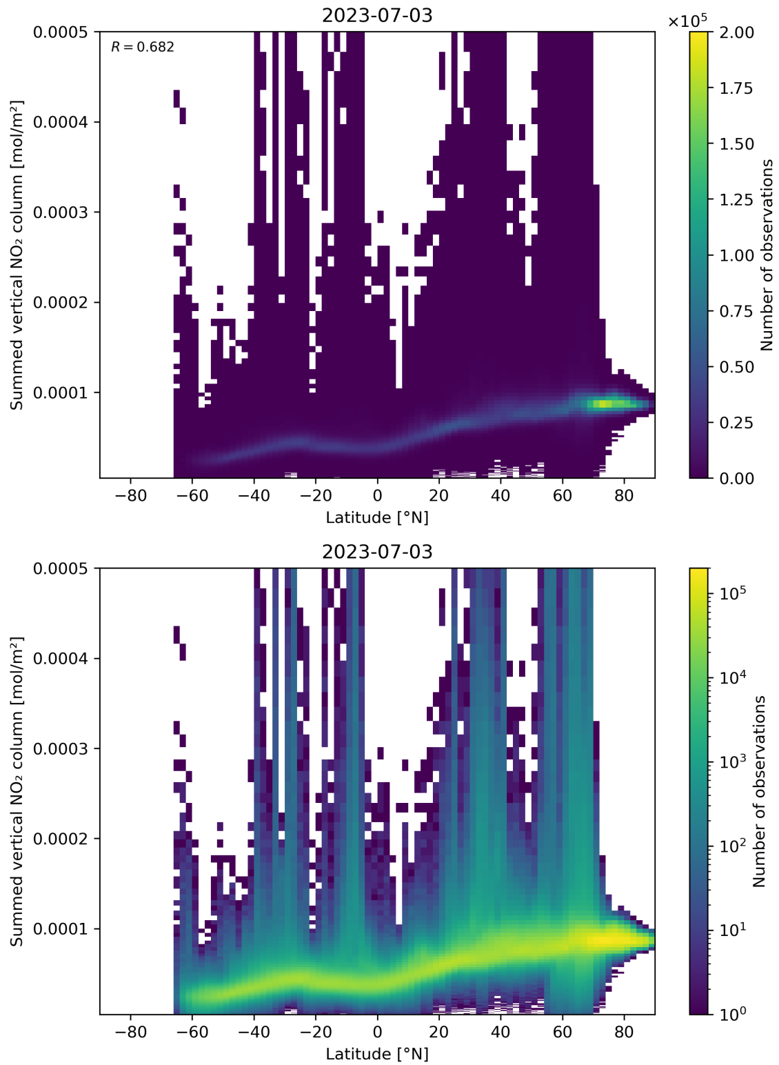
Figure 88: Scatter density plot of “Latitude” against “Summed vertical NO 2 column” for 2023-07-03 to 2023-07-04.
