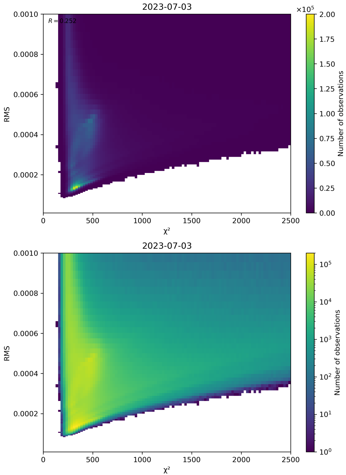
Figure 82: Scatter density plot of “ \chi^2 ” against “RMS” for 2023-07-03 to 2023-07-04.
