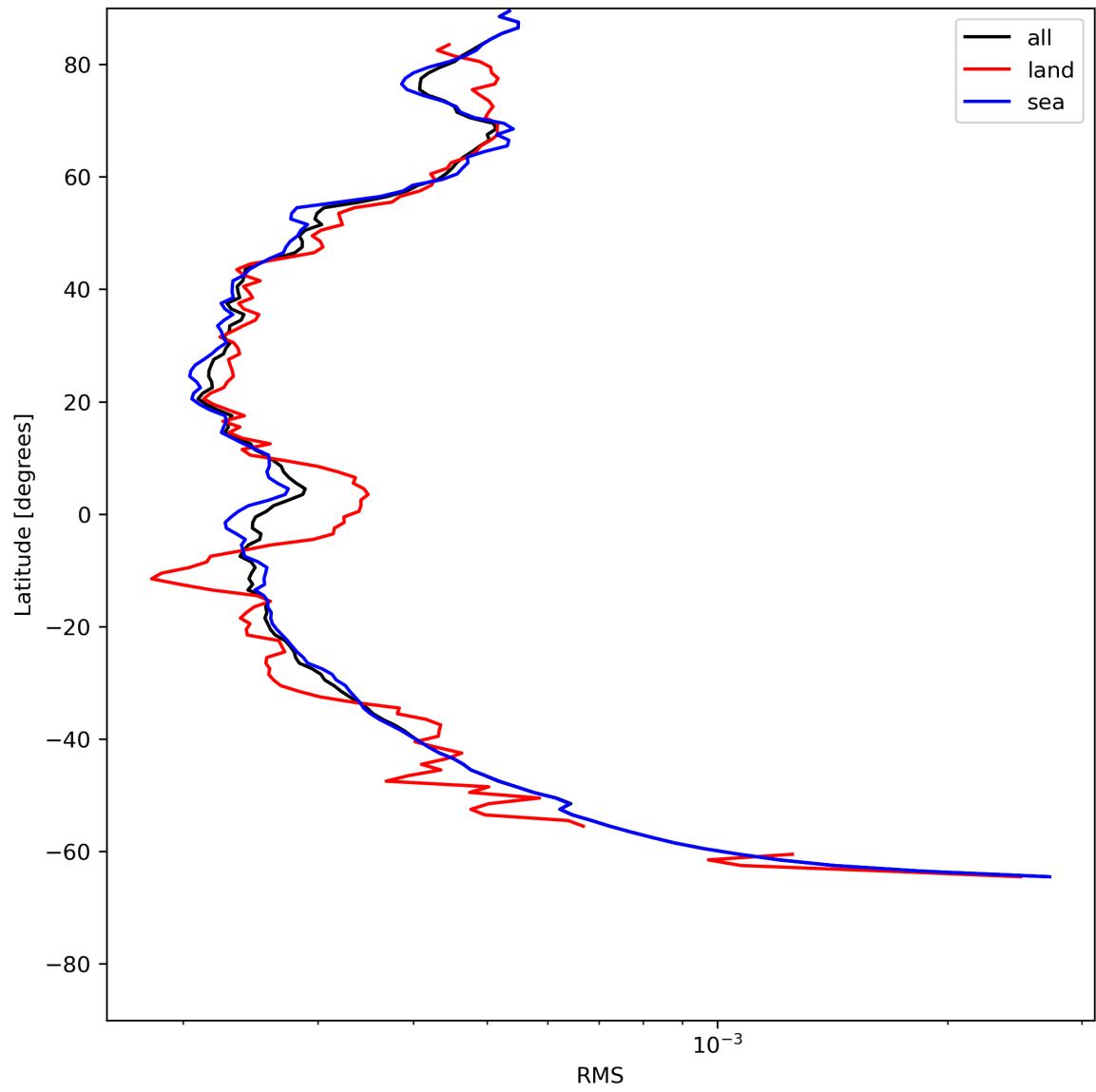
Figure 26: Zonal average of “RMS” for 2023-07-03 to 2023-07-04.
