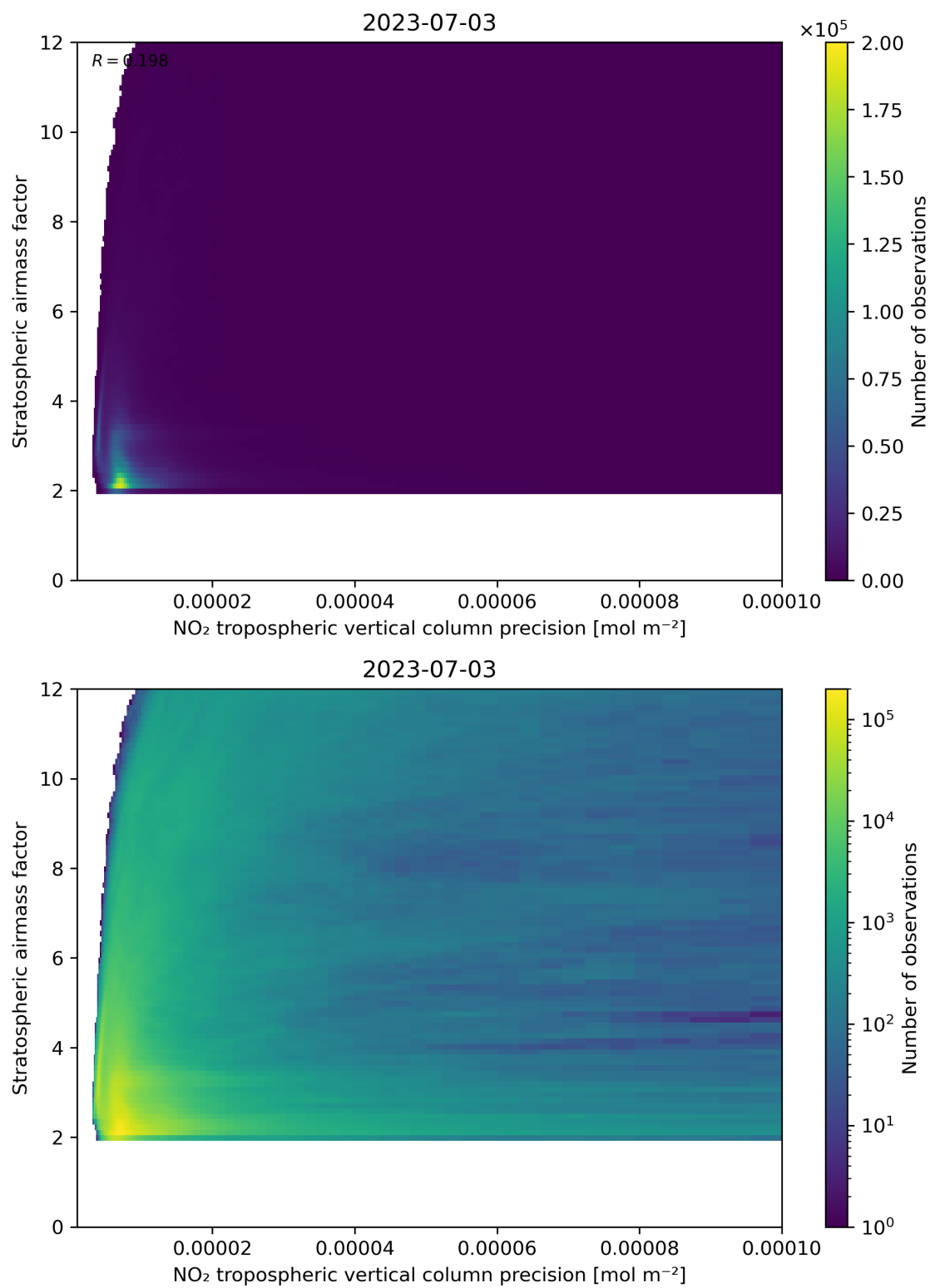
Figure 131: Scatter density plot of “NO 2 tropospheric vertical column precision” against “Stratospheric airmass factor” for 2023-07-03 to 2023-07-04.
