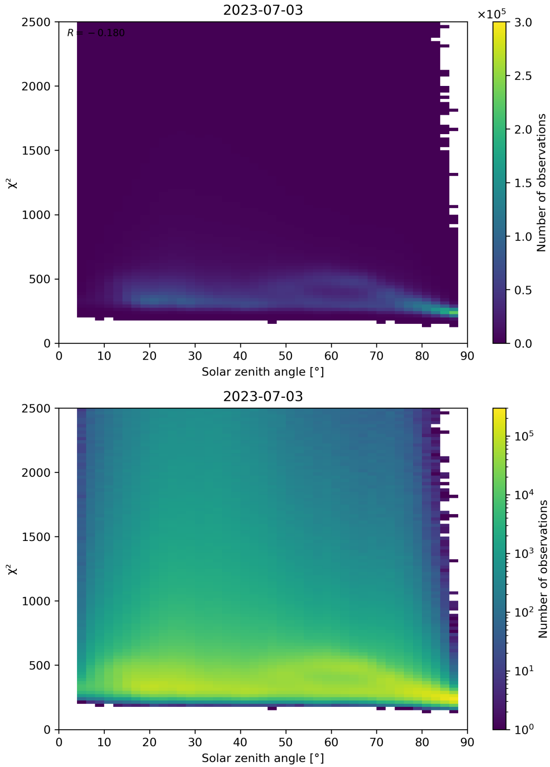
Figure 148: Scatter density plot of “Solar zenith angle” against “ \chi^2 ” for 2023-07-03 to 2023-07-04.
