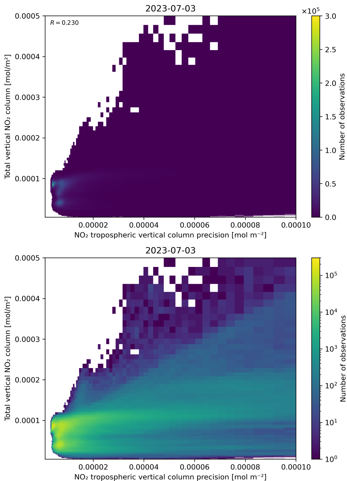
Figure 138: Scatter density plot of “NO 2 tropospheric vertical column precision” against “Total vertical NO 2 column” for 2023-07-03 to 2023-07-04.
