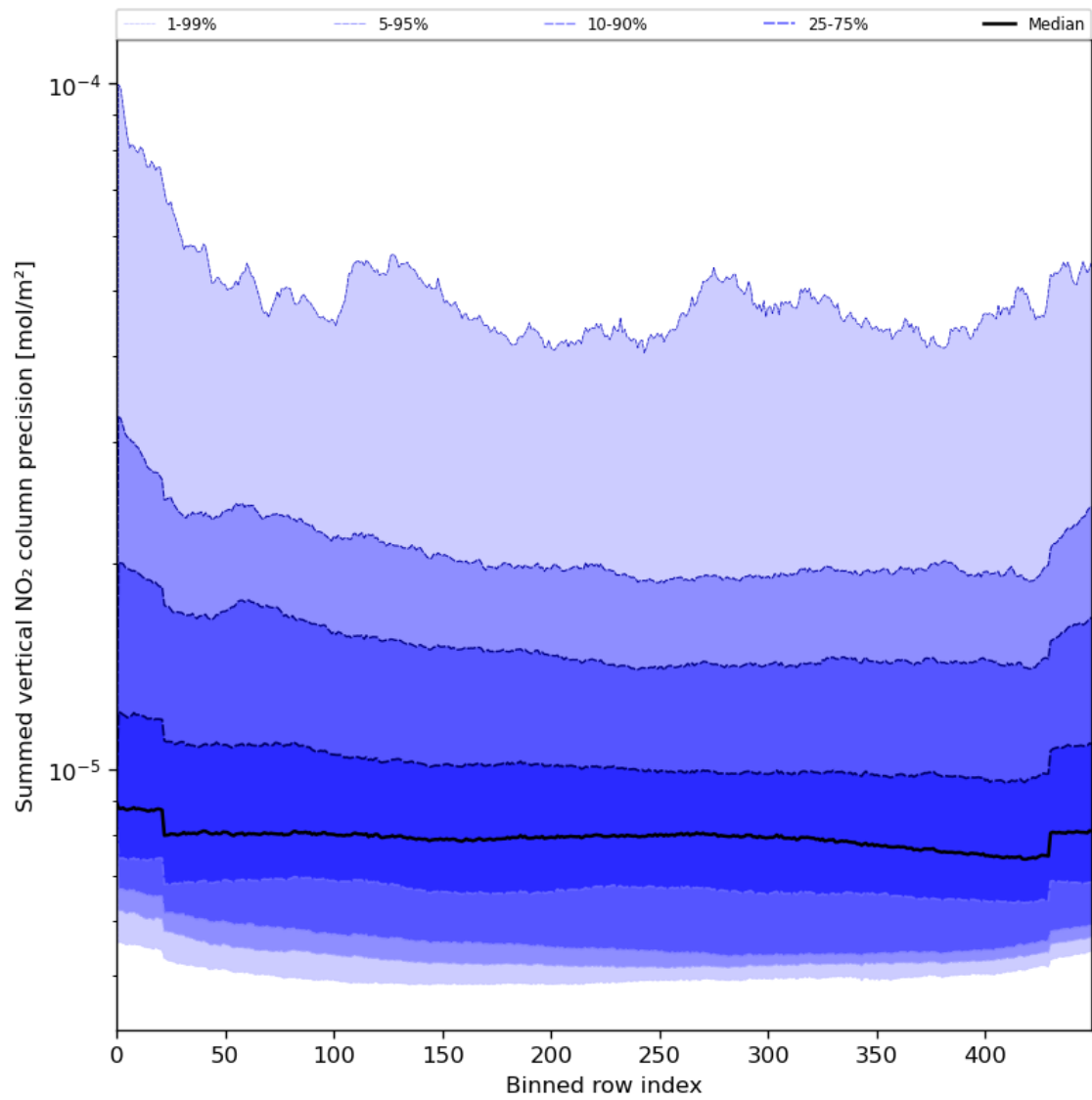
Figure 58: Along track statistics of “Summed vertical NO 2 column precision” for 2023-07-03 to 2023-07-04
