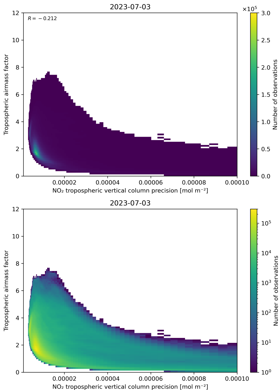
Figure 133: Scatter density plot of “NO 2 tropospheric vertical column precision” against “Tropospheric airmass factor” for 2023-07-03 to 2023-07-04.
