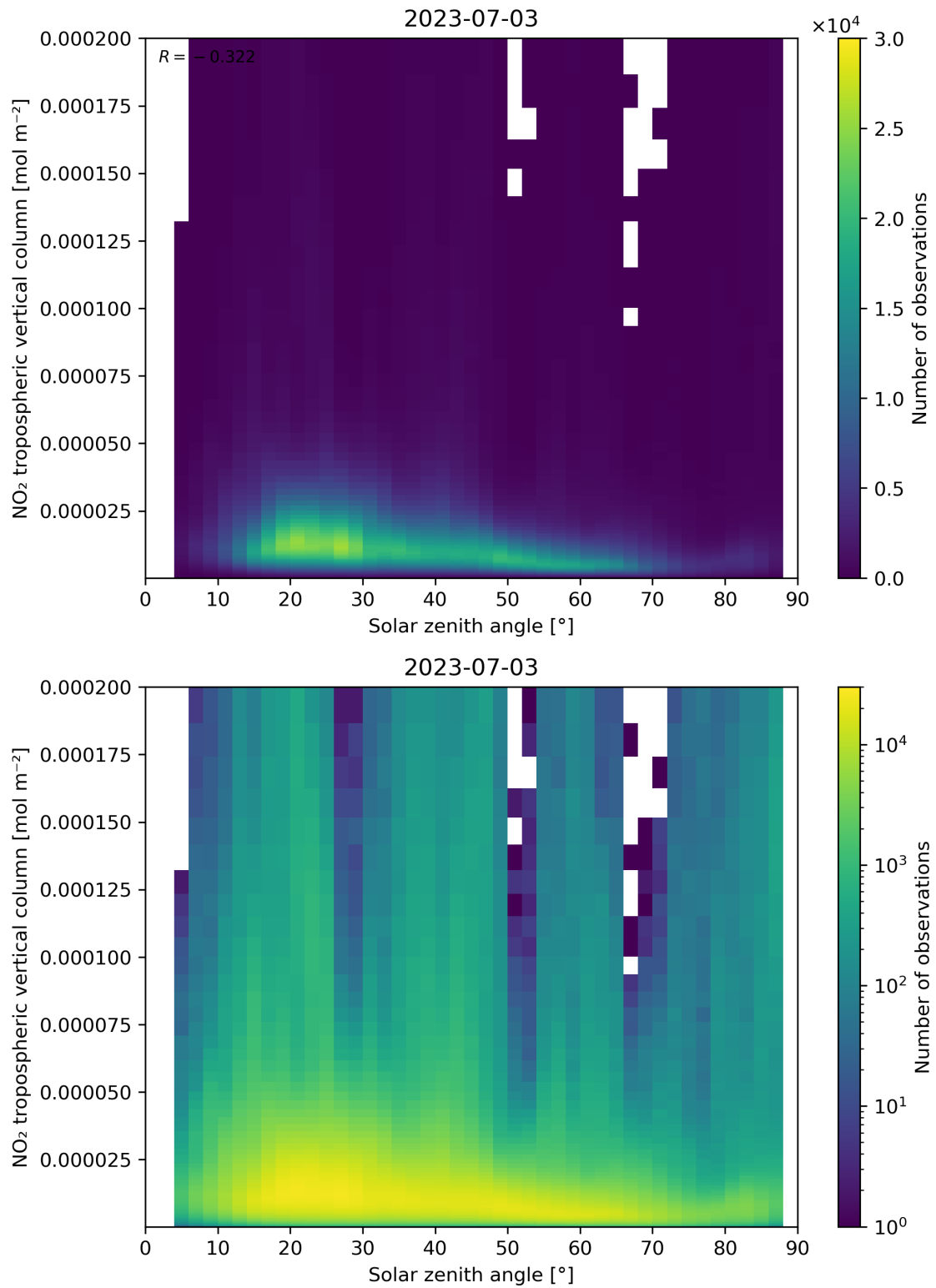
Figure 155: Scatter density plot of “Solar zenith angle” against “NO 2 tropospheric vertical column” for 2023-07-03 to 2023-07-04.
