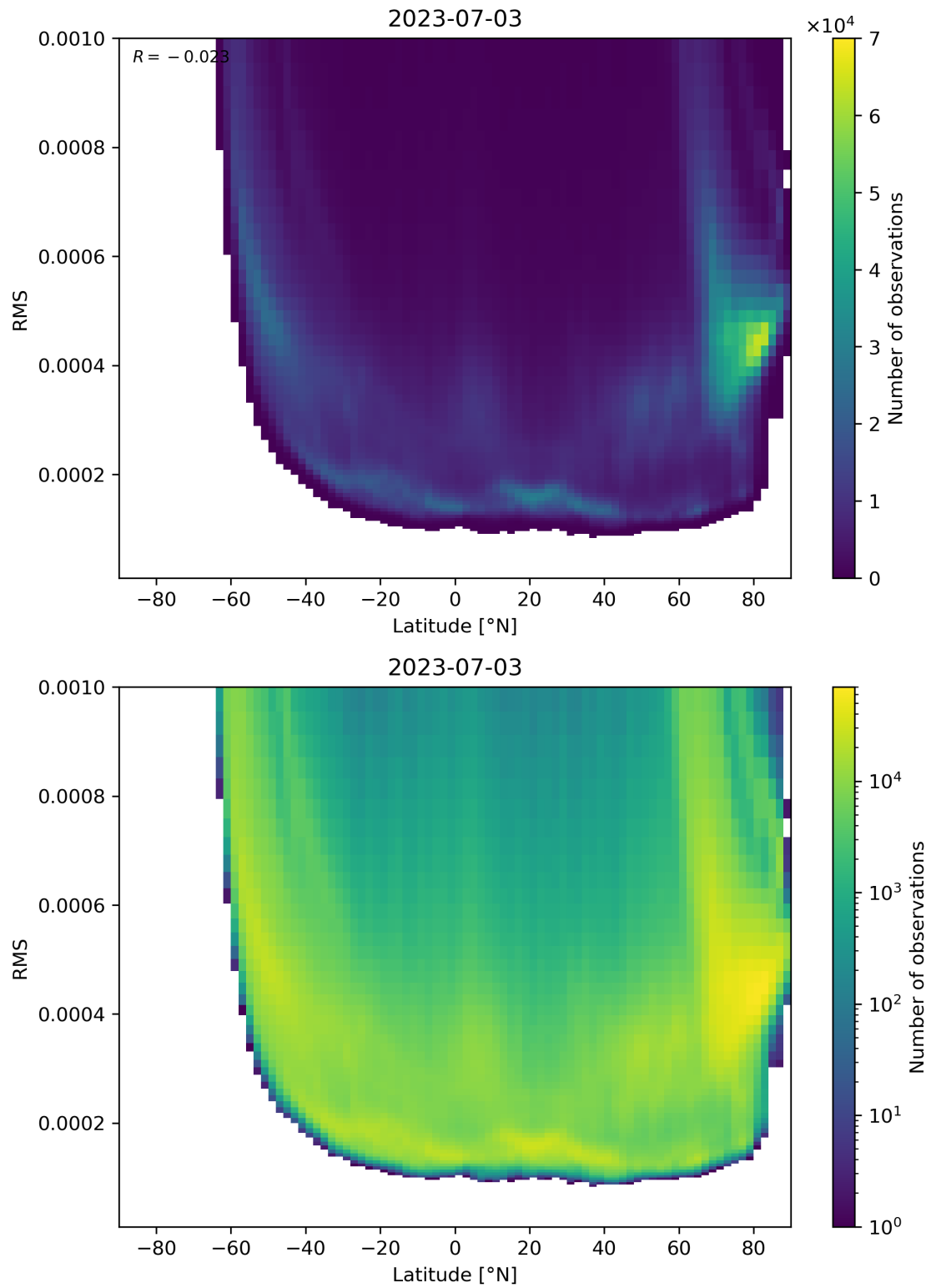
Figure 94: Scatter density plot of “Latitude” against “RMS” for 2023-07-03 to 2023-07-04.
