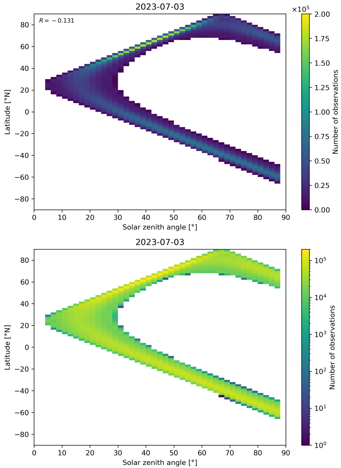
Figure 149: Scatter density plot of “Solar zenith angle” against “Latitude” for 2023-07-03 to 2023-07-04.
