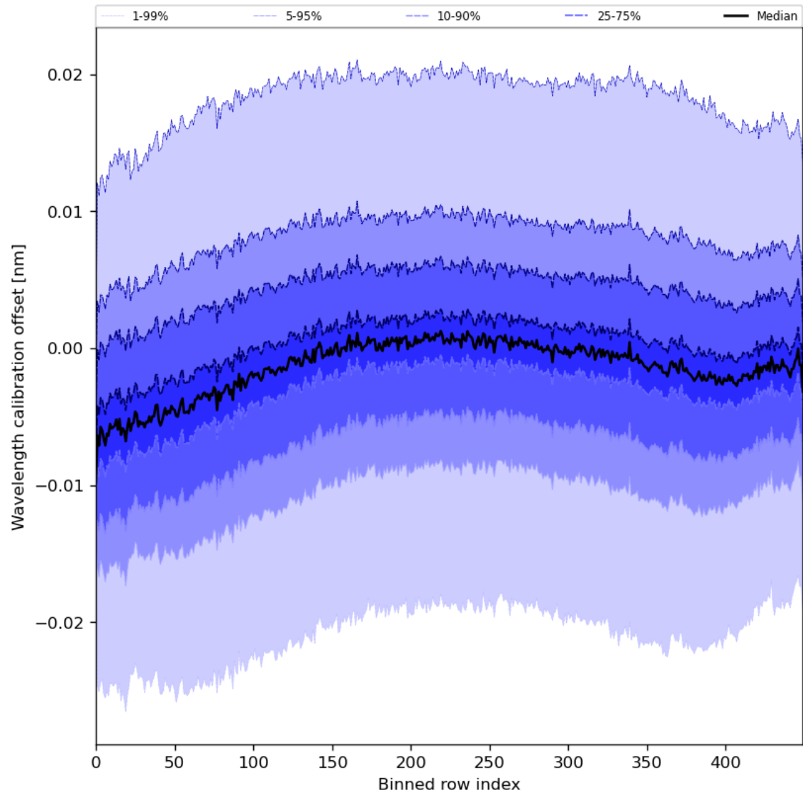
Figure 52: Along track statistics of “Wavelength calibration offset” for 2023-07-03 to 2023-07-04
