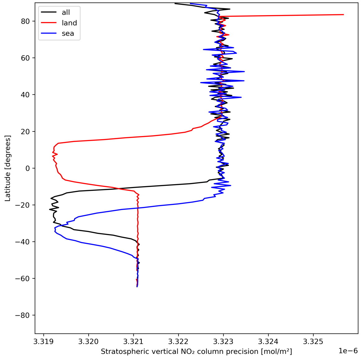
Figure 20: Zonal average of “Stratospheric vertical NO 2 column precision” for 2023-07-03 to 2023-07-04.
