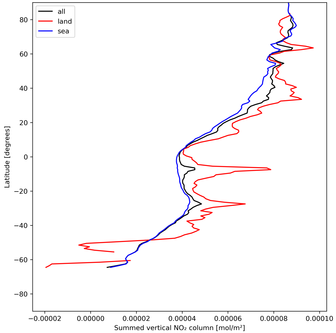
Figure 23: Zonal average of “Summed vertical NO 2 column” for 2023-07-03 to 2023-07-04.
