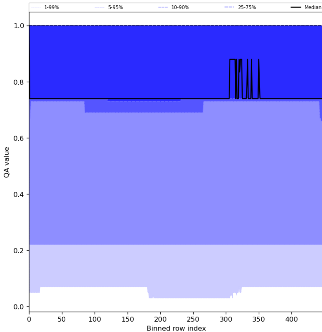
Figure 45: Along track statistics of “QA value” for 2023-07-03 to 2023-07-04
