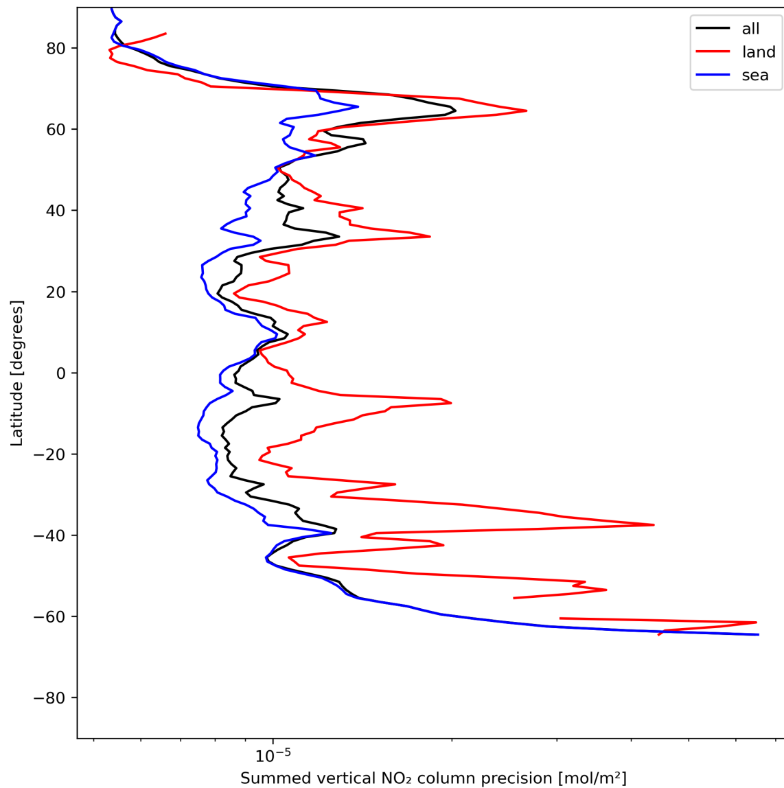
Figure 24: Zonal average of “Summed vertical NO 2 column precision” for 2023-07-03 to 2023-07-04.
