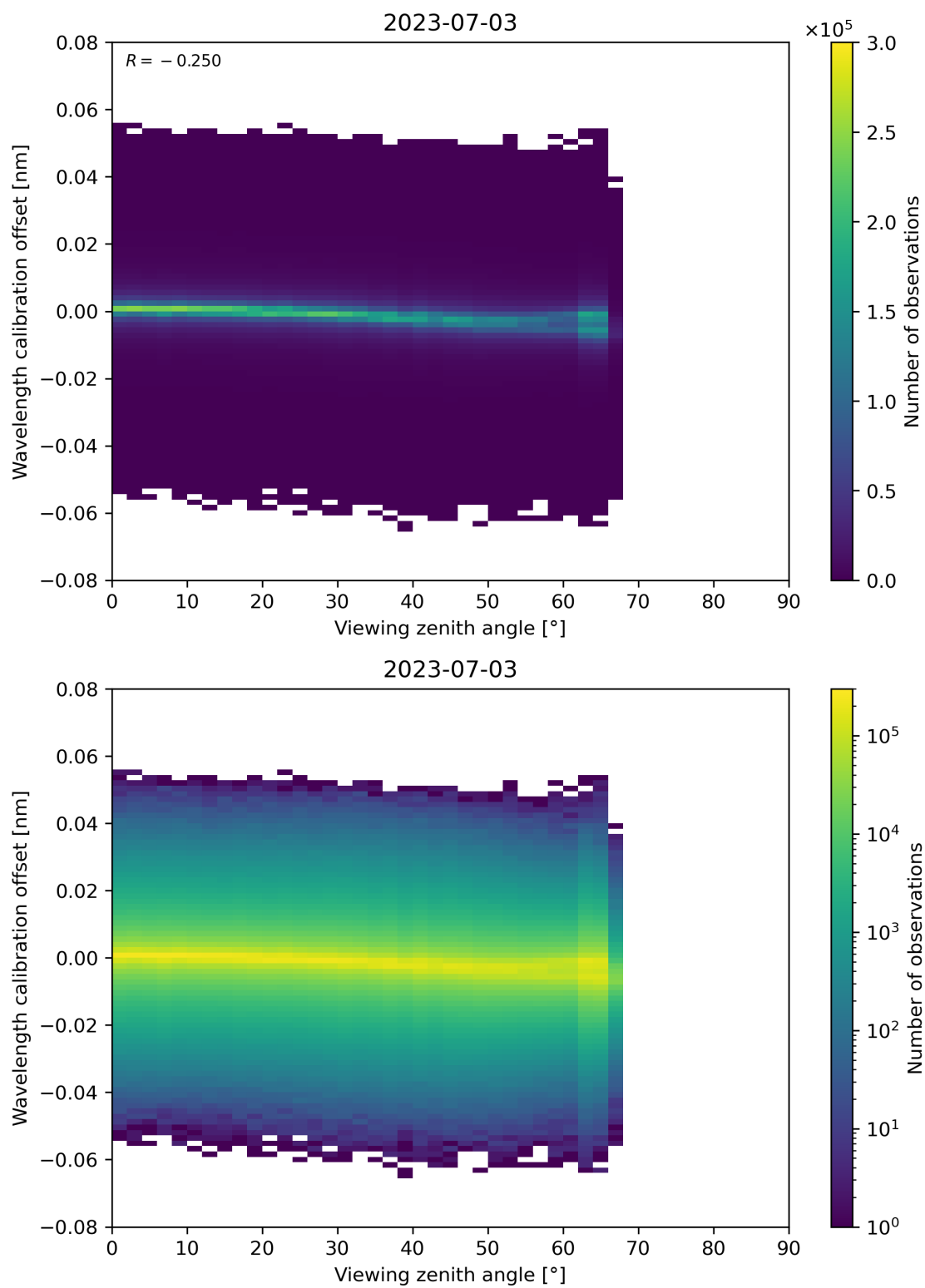
Figure 173: Scatter density plot of “Viewing zenith angle” against “Wavelength calibration offset” for 2023-07-03 to 2023-07-04.
