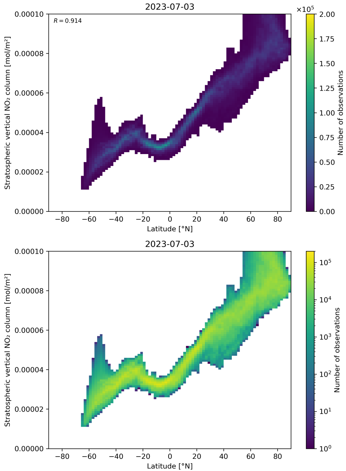
Figure 87: Scatter density plot of “Latitude” against “Stratospheric vertical NO 2 column” for 2023-07-03 to 2023-07-04.
