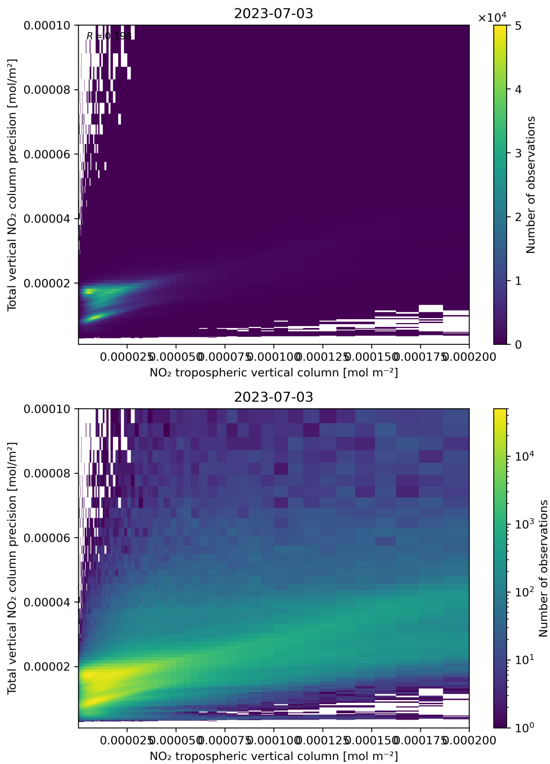
Figure 129: Scatter density plot of “NO 2 tropospheric vertical column” against “Total vertical NO 2 column precision” for 2023-07-03 to 2023-07-04.
