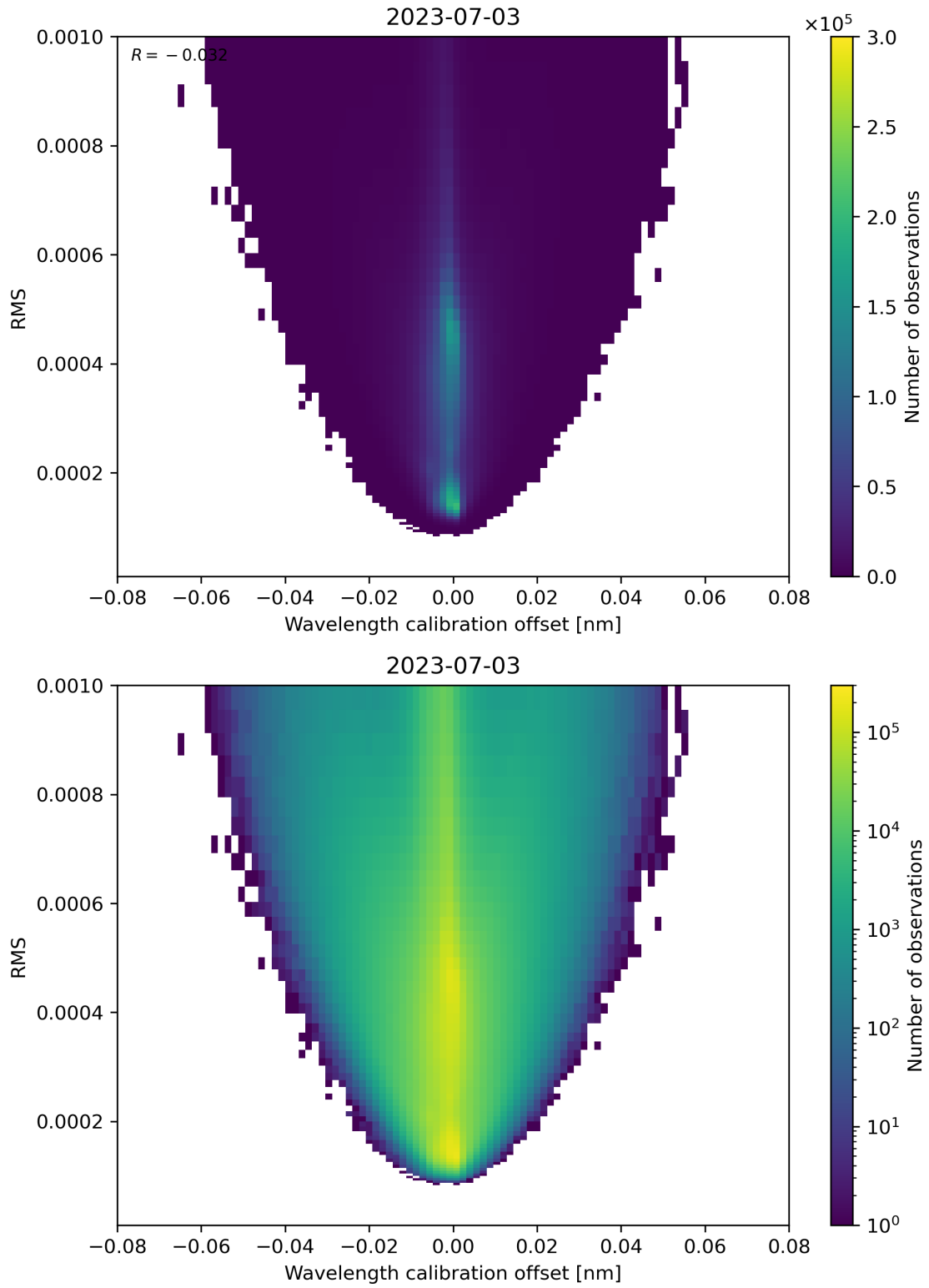
Figure 181: Scatter density plot of “Wavelength calibration offset” against “RMS” for 2023-07-03 to 2023-07-04.
