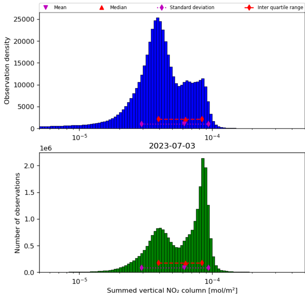
Figure 40: Histogram of “Summed vertical NO 2 column” for 2023-07-03 to 2023-07-04
