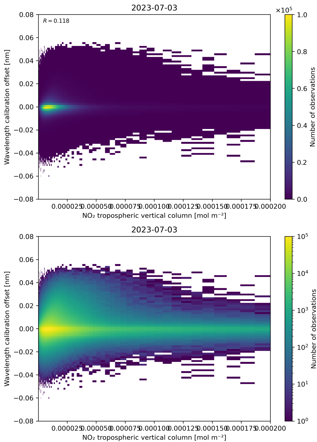
Figure 143: Scatter density plot of “NO 2 tropospheric vertical column” against “Wavelength calibration offset” for 2023-07-03 to 2023-07-04.
