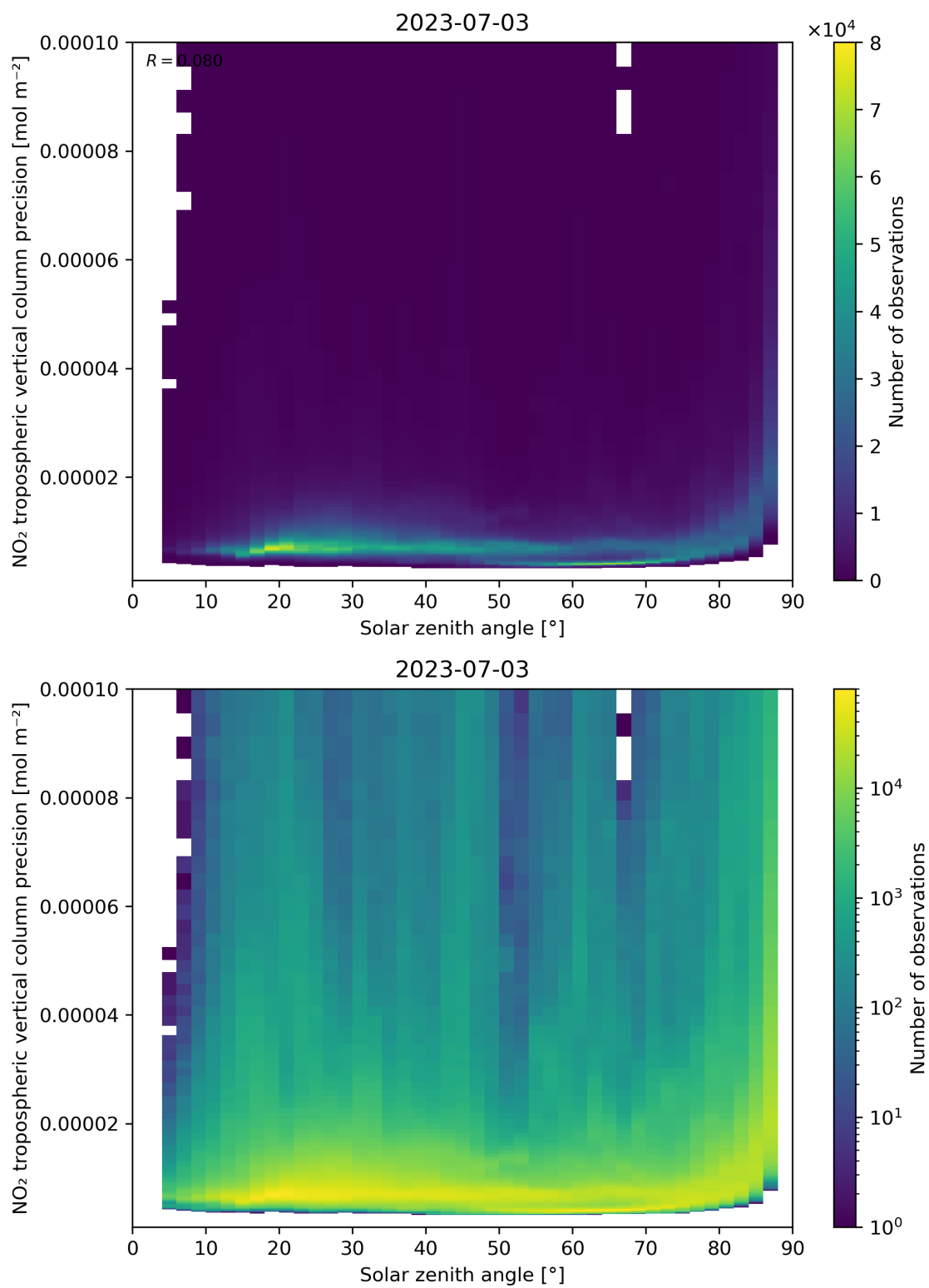
Figure 156: Scatter density plot of “Solar zenith angle” against “NO 2 tropospheric vertical column precision” for 2023-07-03 to 2023-07-04.
