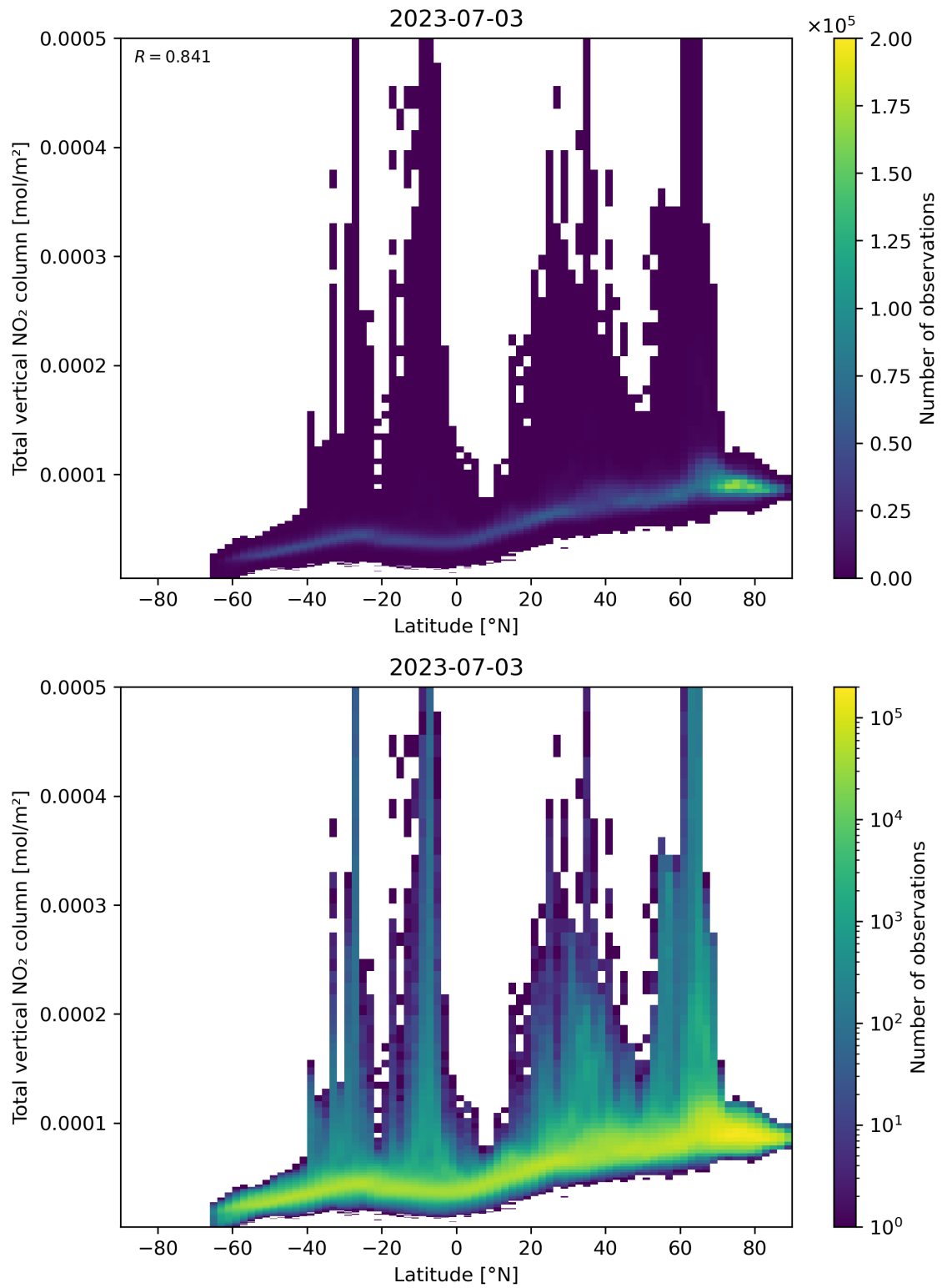
Figure 90: Scatter density plot of “Latitude” against “Total vertical NO 2 column” for 2023-07-03 to 2023-07-04.
