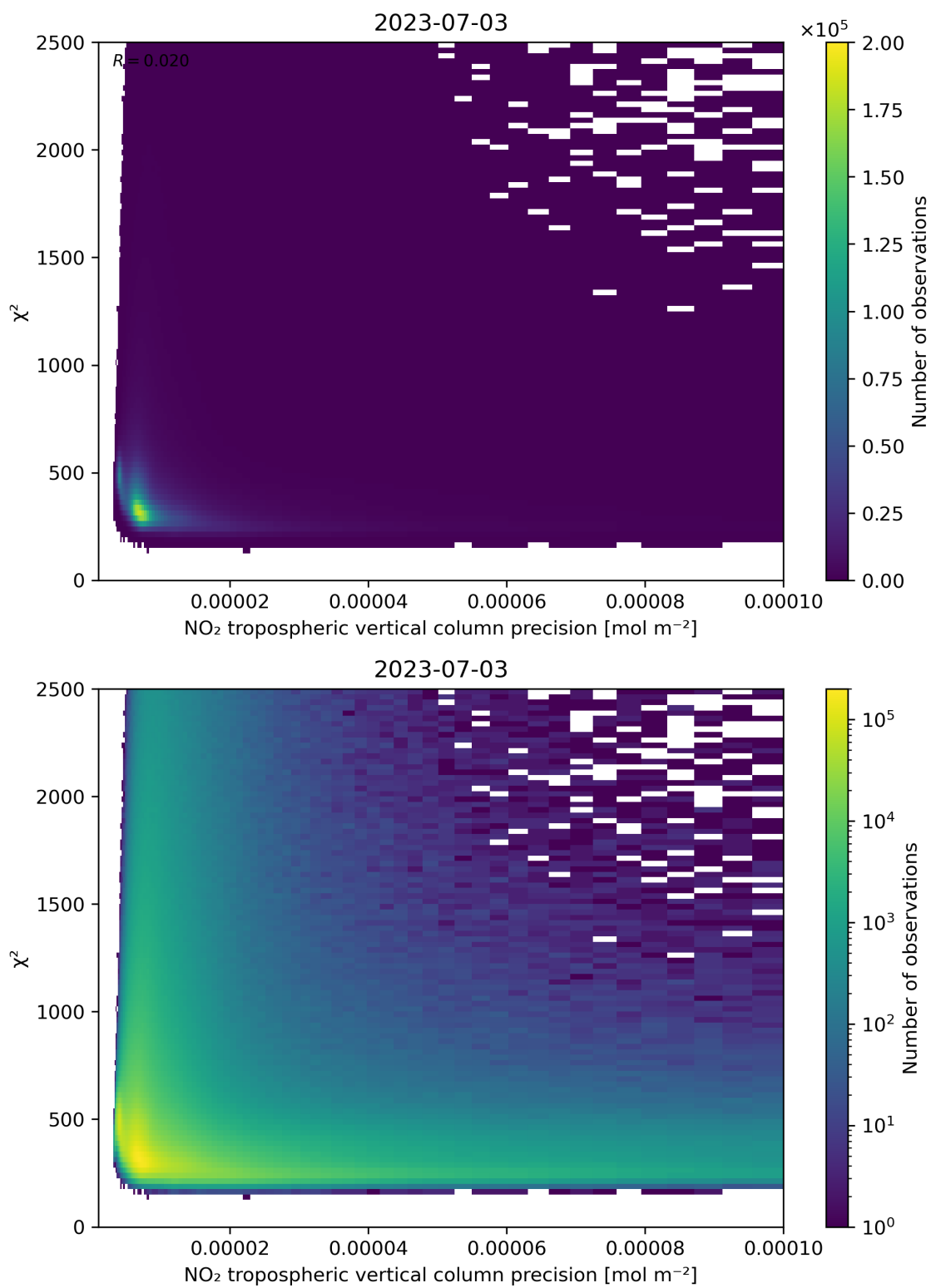
Figure 134: Scatter density plot of “NO 2 tropospheric vertical column precision” against “ \chi^2 ” for 2023-07-03 to 2023-07-04.
