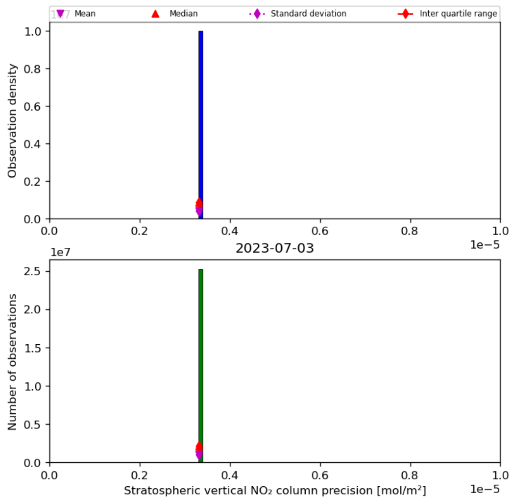
Figure 37: Histogram of “Stratospheric vertical NO 2 column precision” for 2023-07-03 to 2023-07-04
