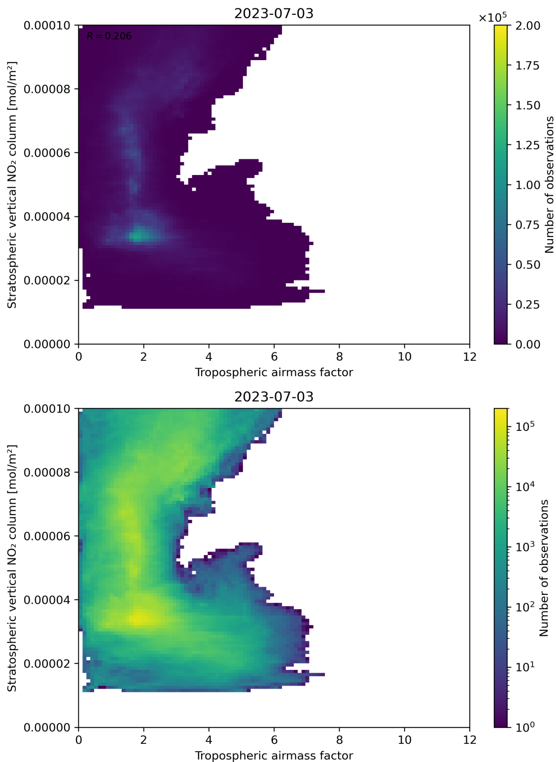
Figure 74: Scatter density plot of “Tropospheric air mass factor” against “Stratospheric vertical NO 2 column” for 2023-07-03 to 2023-07-04.
