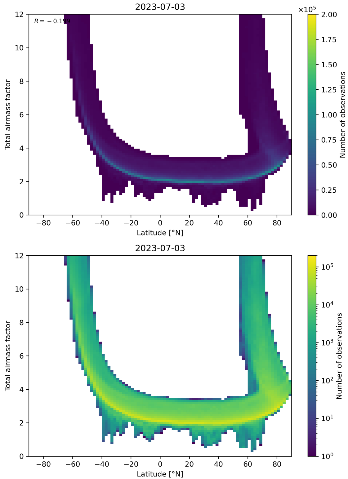
Figure 84: Scatter density plot of “Latitude” against “Total airmass factor” for 2023-07-03 to 2023-07-04.
