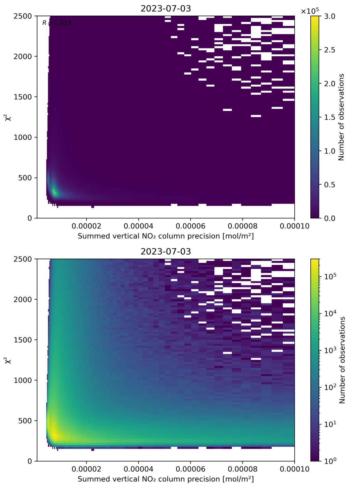
Figure 107: Scatter density plot of “Summed vertical NO 2 column precision” against “ \chi^2 ” for 2023-07-03 to 2023-07-04.
