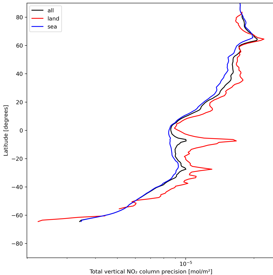
Figure 22: Zonal average of “Total vertical NO 2 column precision” for 2023-07-03 to 2023-07-04.
