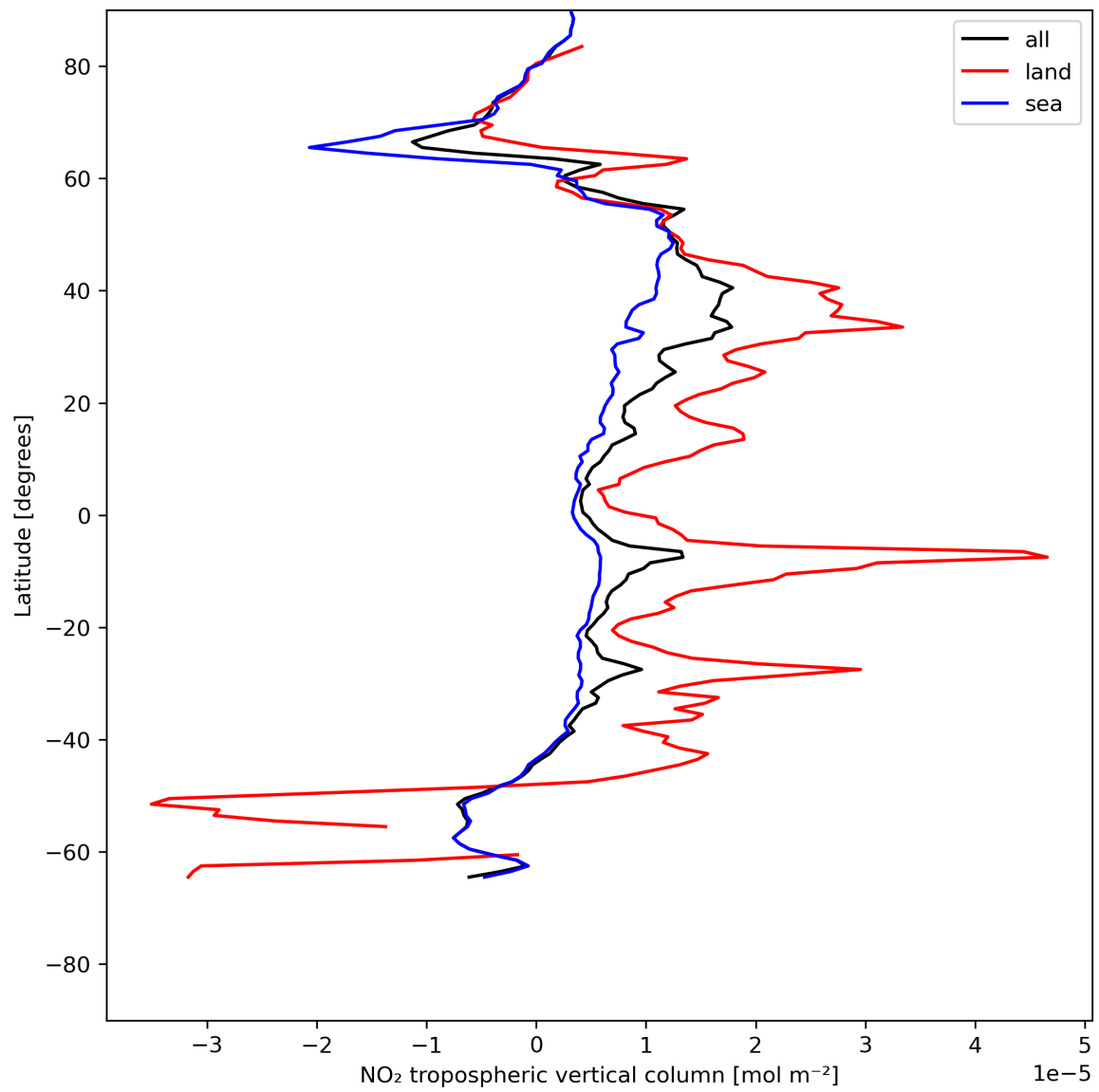
Figure 12: Zonal average of “NO 2 tropospheric vertical column” for 2023-07-03 to 2023-07-04.
