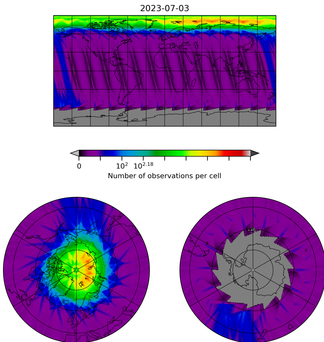
Figure 10: Map of the number of observations for 2023-07-03 to 2023-07-04
