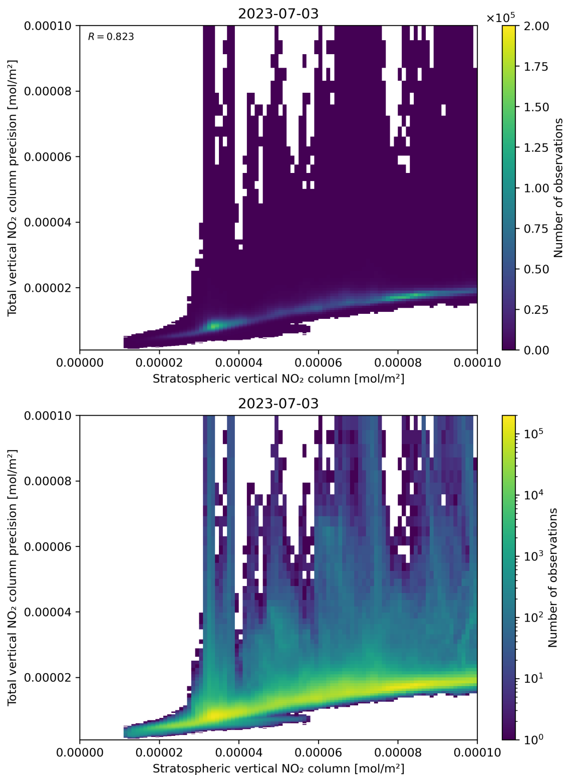
Figure 101: Scatter density plot of “Stratospheric vertical NO 2 column” against “Total vertical NO 2 column precision” for 2023-07-03 to 2023-07-04.
