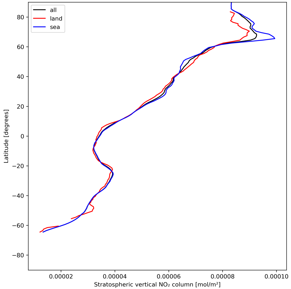
Figure 19: Zonal average of “Stratospheric vertical NO 2 column” for 2023-07-03 to 2023-07-04.
