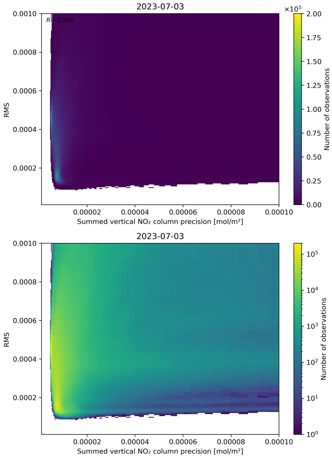
Figure 108: Scatter density plot of “Summed vertical NO 2 column precision” against “RMS” for 2023-07-03 to 2023-07-04.
