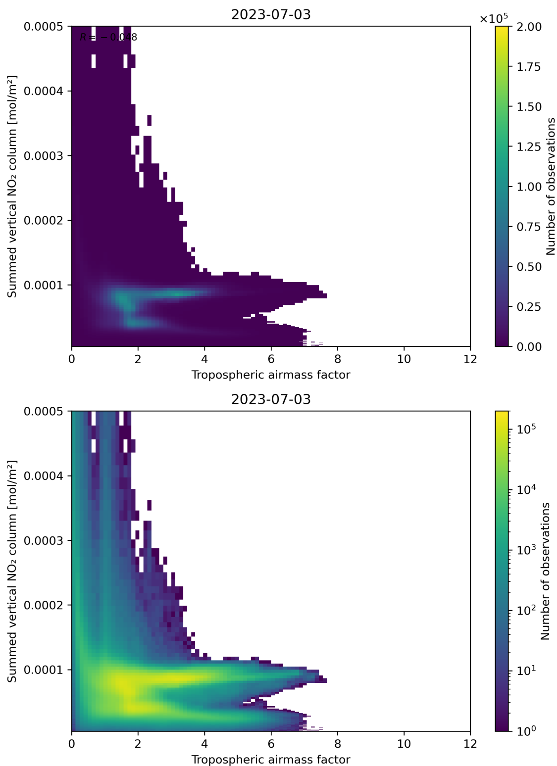
Figure 75: Scatter density plot of “Tropospheric airmass factor” against “Summed vertical NO 2 column” for 2023-07-03 to 2023-07-04.
