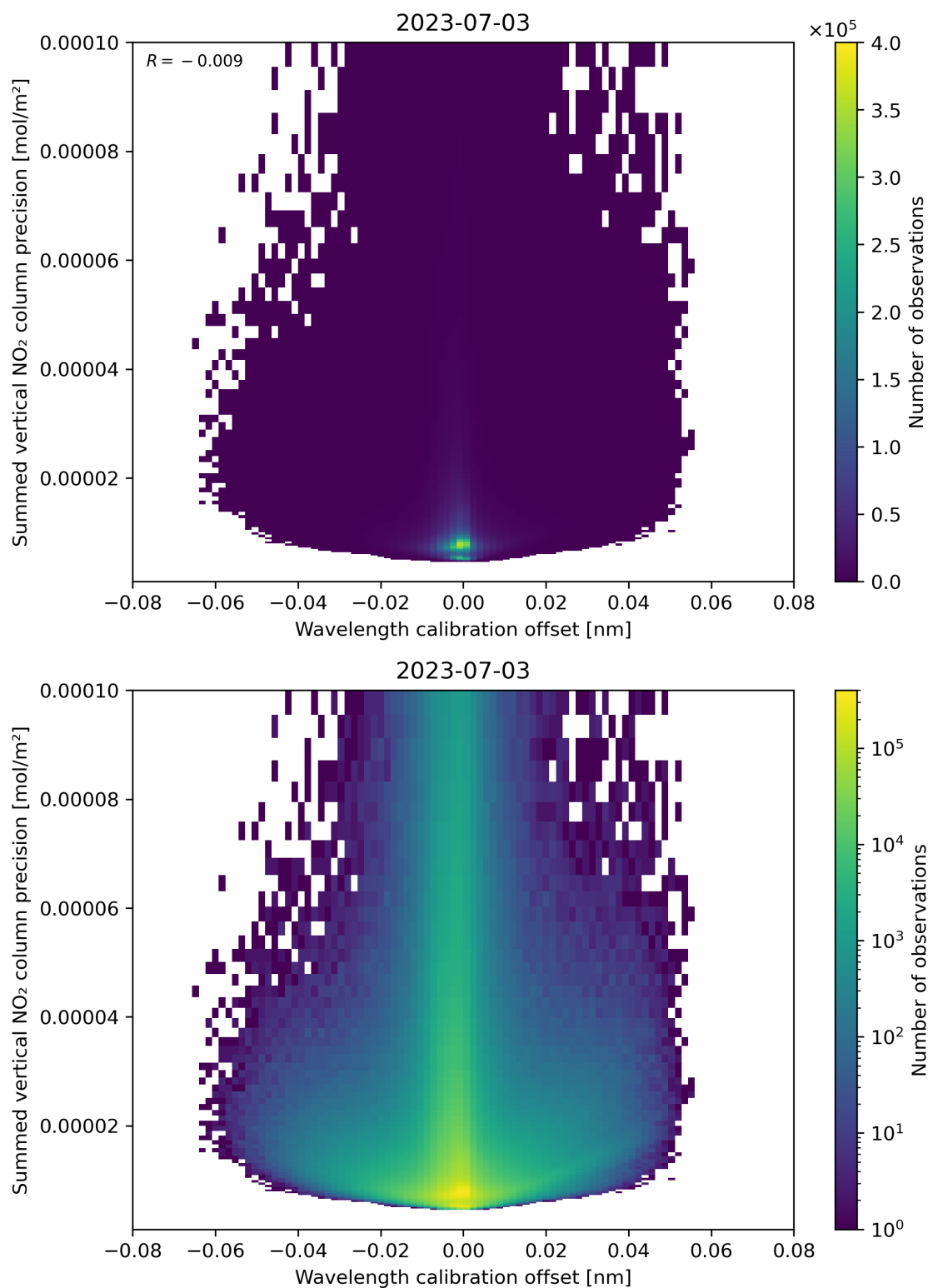
Figure 178: Scatter density plot of “Wavelength calibration offset” against “Summed vertical NO 2 column precision” for 2023-07-03 to 2023-07-04.
