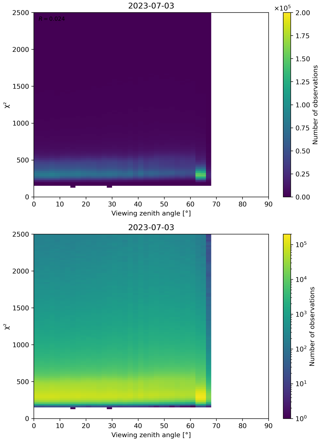
Figure 162: Scatter density plot of “Viewing zenith angle” against “ \chi^2 ” for 2023-07-03 to 2023-07-04.
