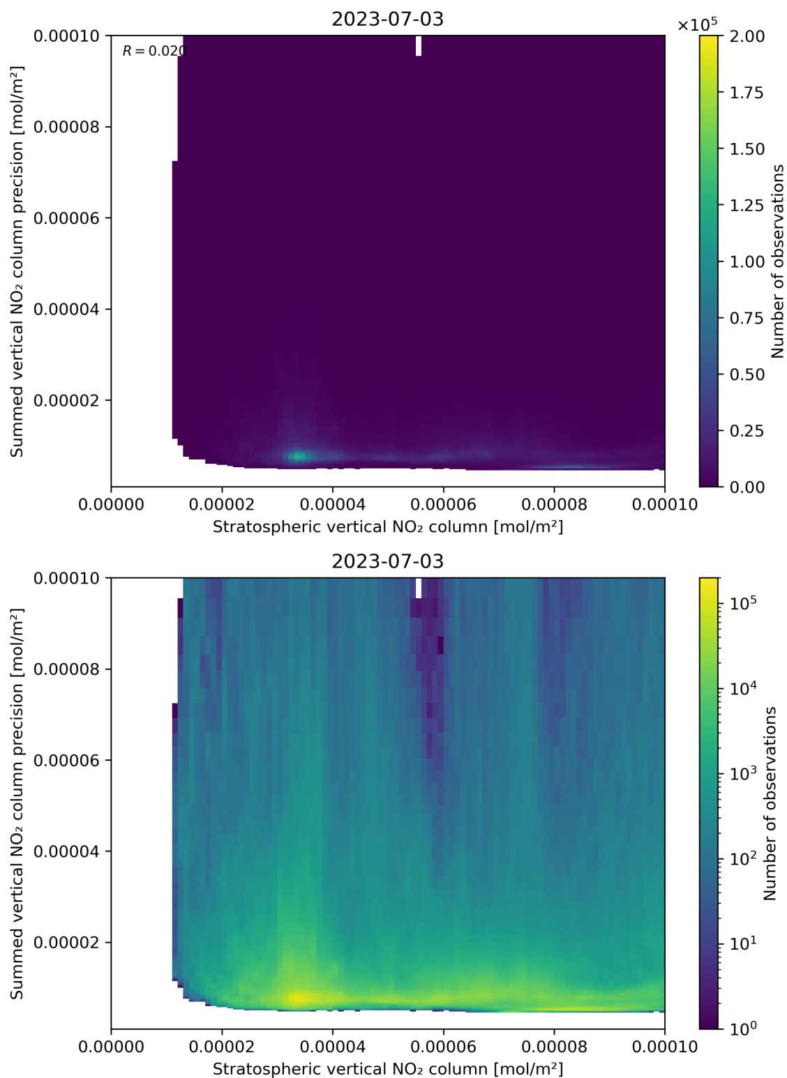
Figure 99: Scatter density plot of “Stratospheric vertical NO 2 column” against “Summed vertical NO 2 column precision” for 2023-07-03 to 2023-07-04.
