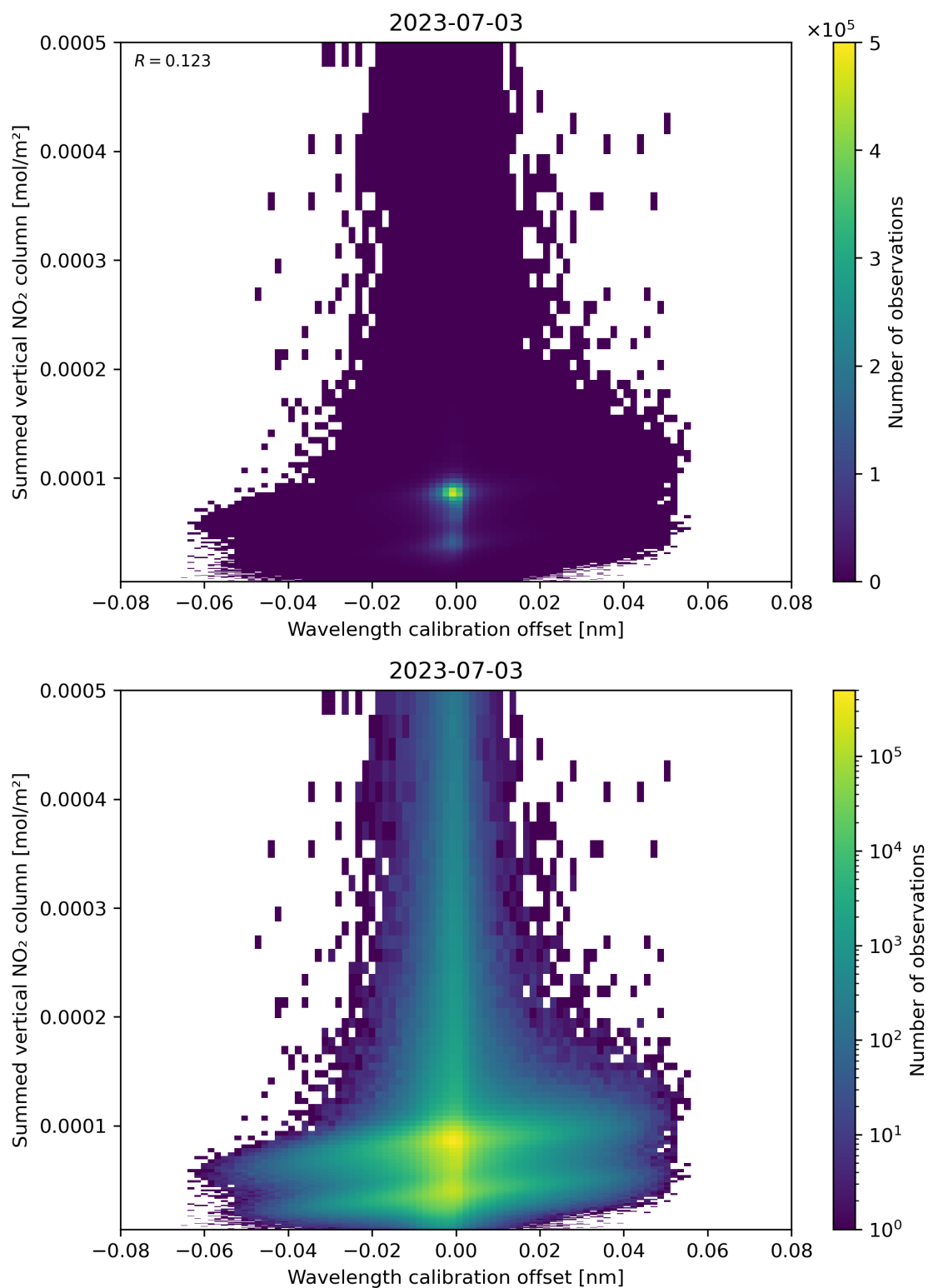
Figure 177: Scatter density plot of “Wavelength calibration offset” against “Summed vertical NO 2 column” for 2023-07-03 to 2023-07-04.
