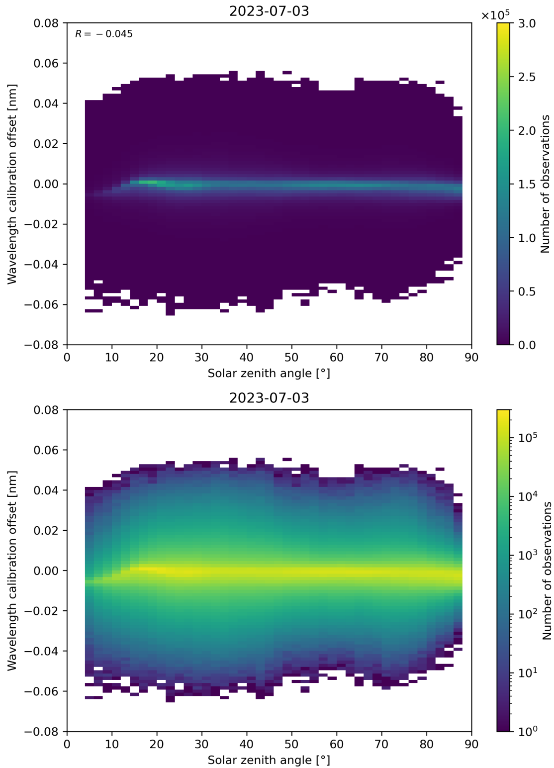
Figure 158: Scatter density plot of “Solar zenith angle” against “Wavelength calibration offset” for 2023-07-03 to 2023-07-04.
