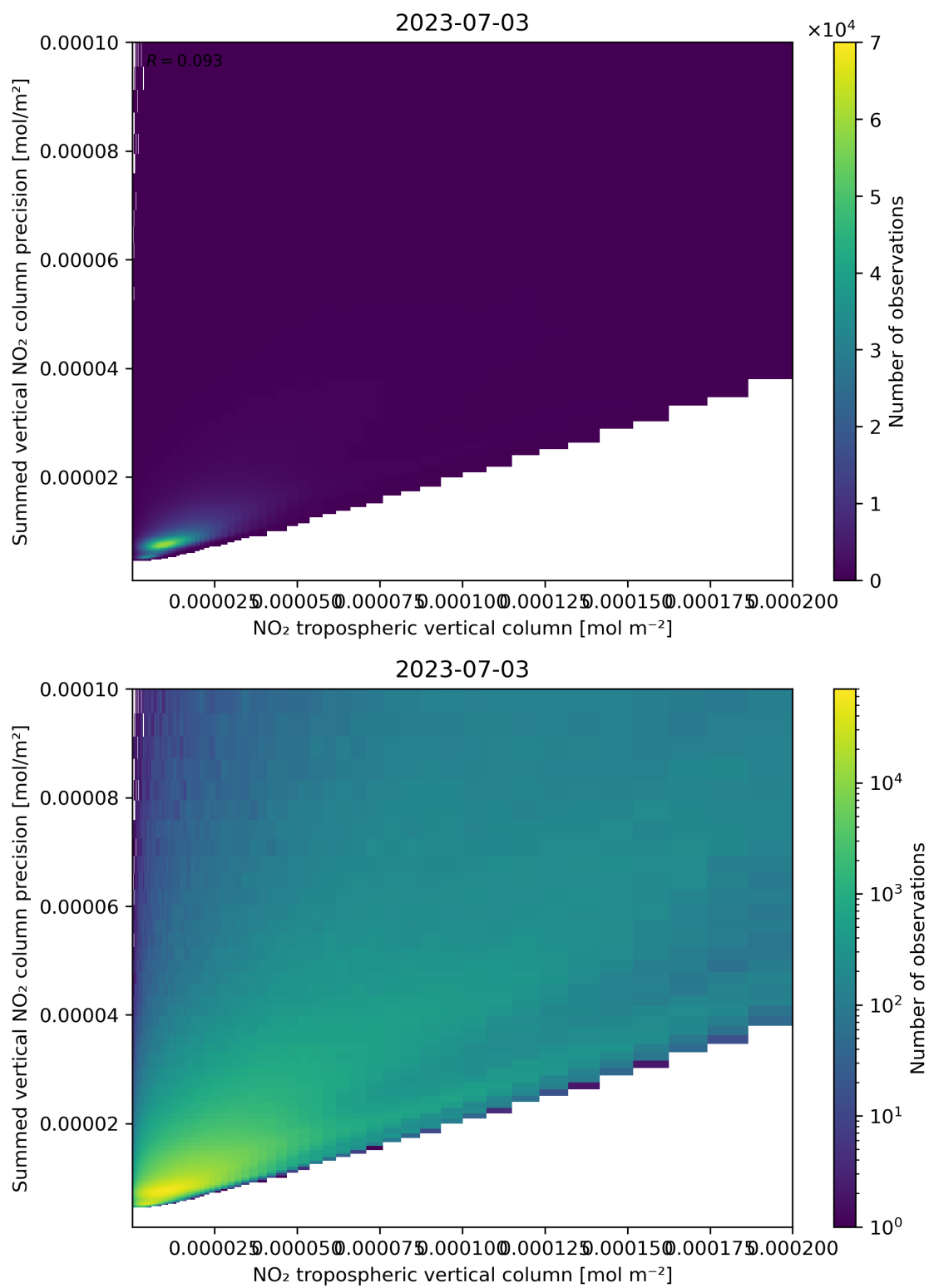
Figure 127: Scatter density plot of “NO 2 tropospheric vertical column” against “Summed vertical NO 2 column precision” for 2023-07-03 to 2023-07-04.
