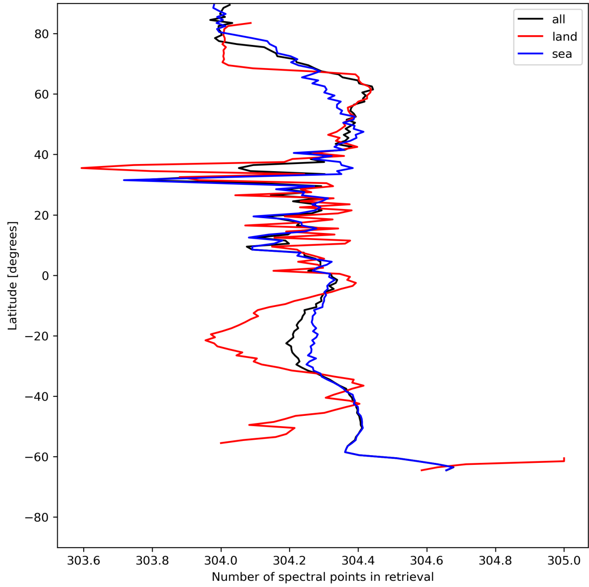
Figure 16: Zonal average of “Number of spectral points in retrieval” for 2023-07-03 to 2023-07-04.
