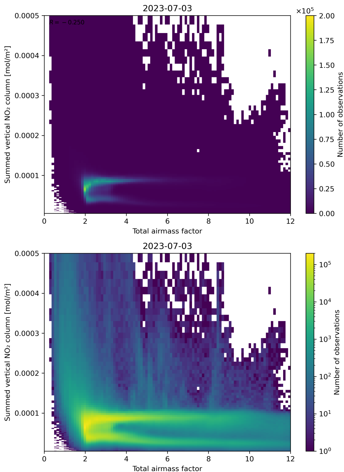
Figure 65: Scatter density plot of “Total airmass factor” against “Summed vertical NO 2 column” for 2023-07-03 to 2023-07-04.
