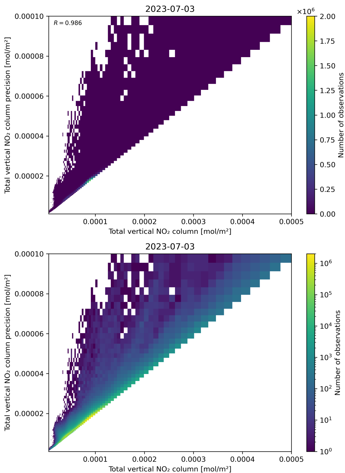
Figure 114: Scatter density plot of “Total vertical NO 2 column” against “Total vertical NO 2 column precision” for 2023-07-03 to 2023-07-04.
