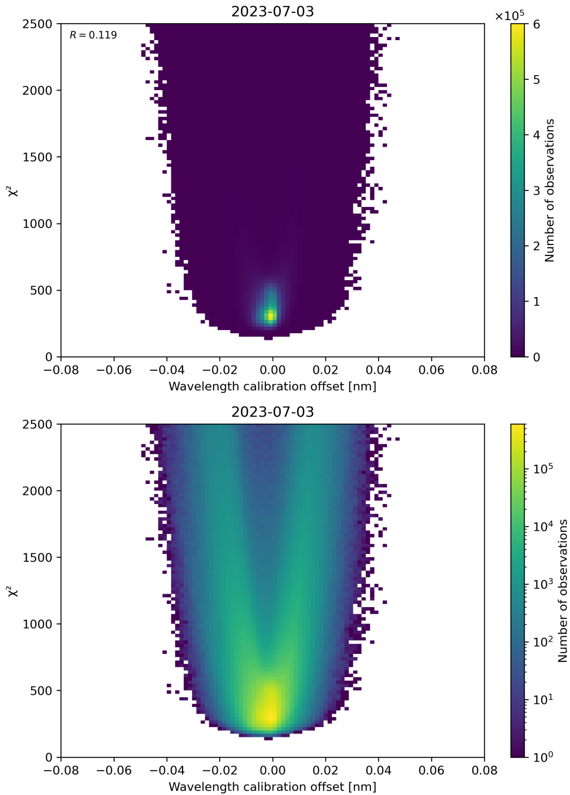
Figure 175: Scatter density plot of “Wavelength calibration offset” against “ \chi^2 ” for 2023-07-03 to 2023-07-04.
