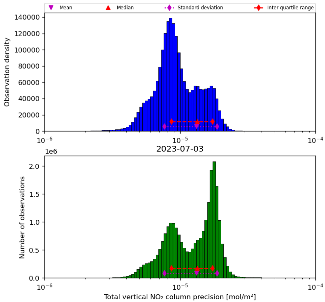
Figure 39: Histogram of “Total vertical NO 2 column precision” for 2023-07-03 to 2023-07-04
