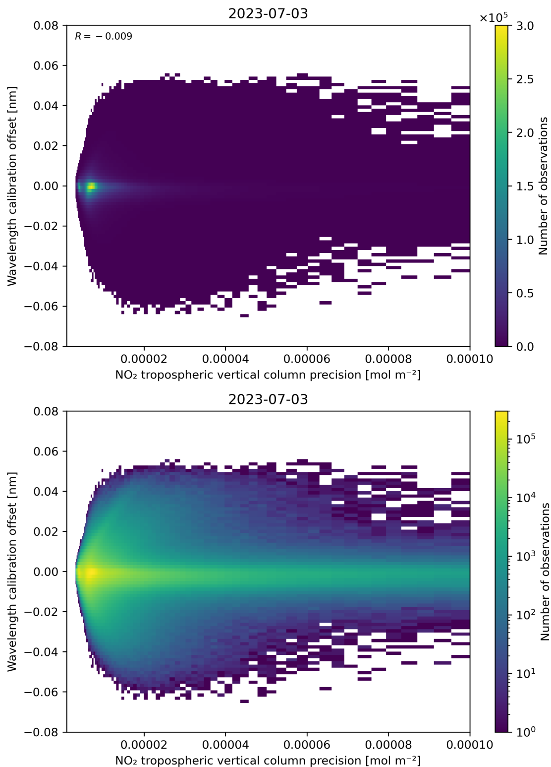
Figure 141: Scatter density plot of “NO 2 tropospheric vertical column precision” against “Wavelength calibration offset” for 2023-07-03 to 2023-07-04.
