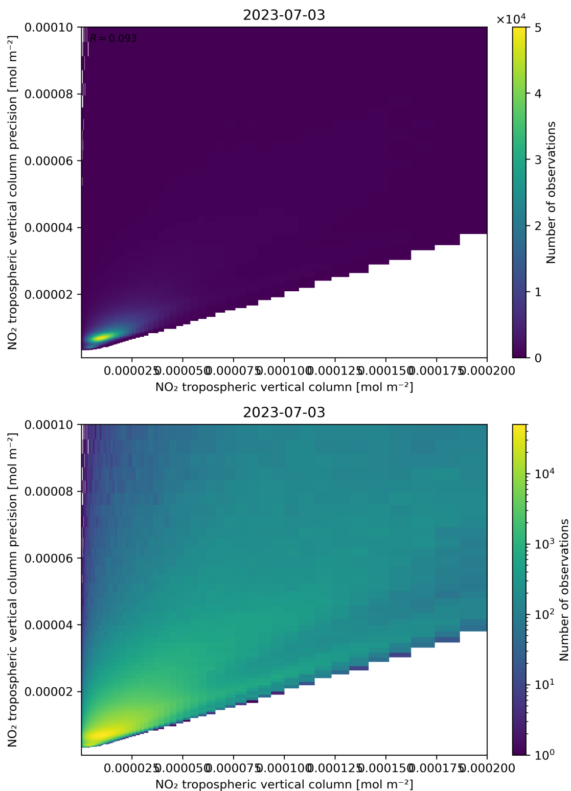
Figure 130: Scatter density plot of “NO 2 tropospheric vertical column” against “NO 2 tropospheric vertical column precision” for 2023-07-03 to 2023-07-04.
