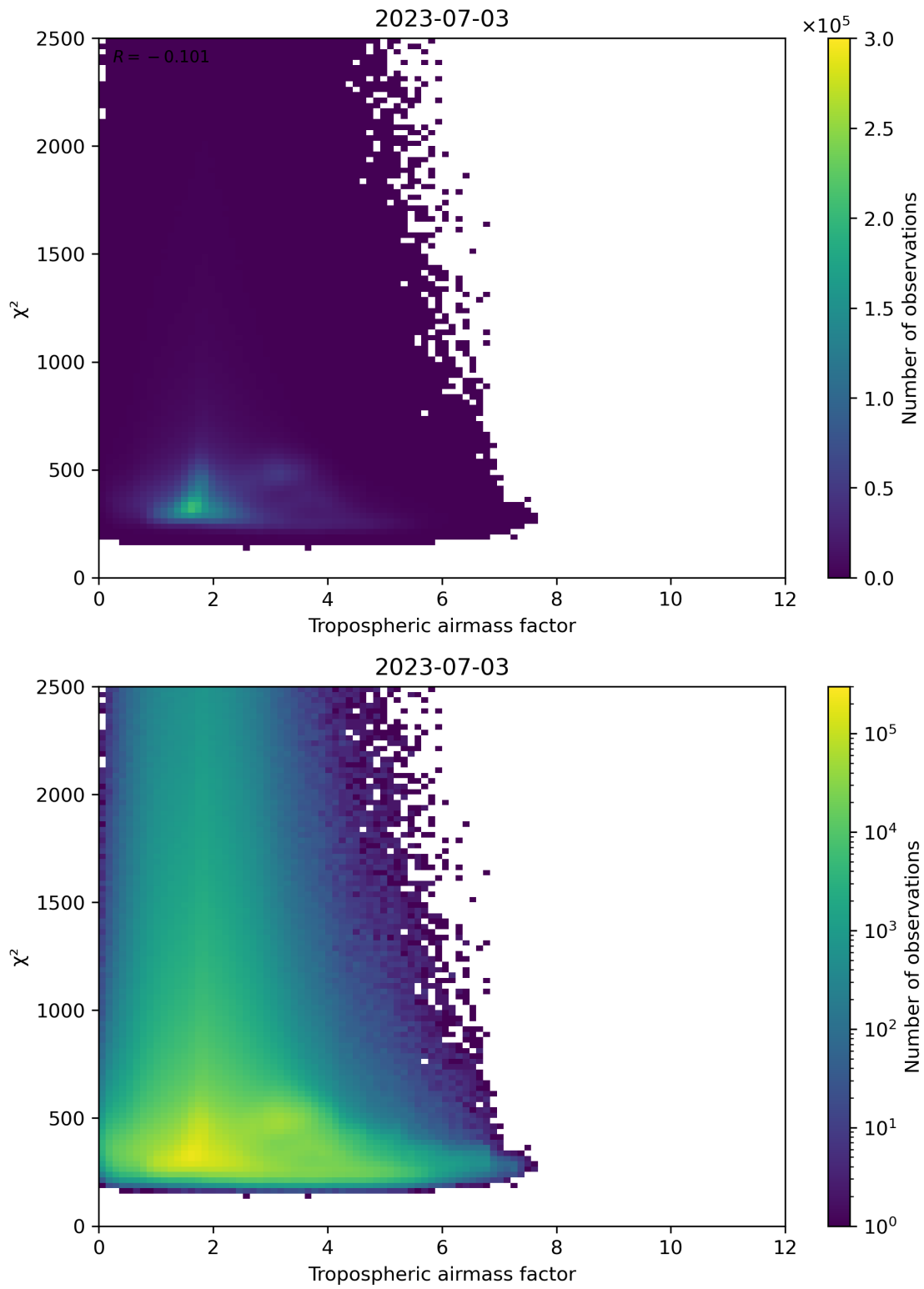
Figure 73: Scatter density plot of “Tropospheric airmass factor” against “ \chi^2 ” for 2023-07-03 to 2023-07-04.
