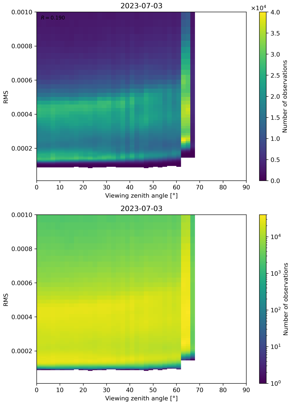
Figure 171: Scatter density plot of “Viewing zenith angle” against “RMS” for 2023-07-03 to 2023-07-04.
