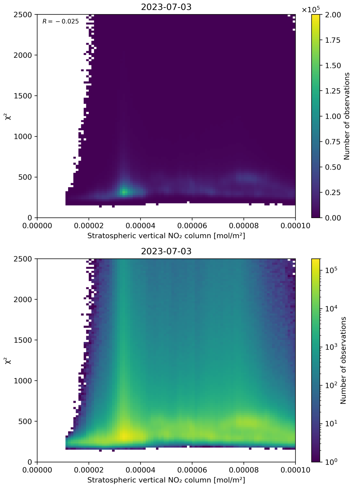
Figure 97: Scatter density plot of “Stratospheric vertical NO 2 column” against “ \chi^2 ” for 2023-07-03 to 2023-07-04.
