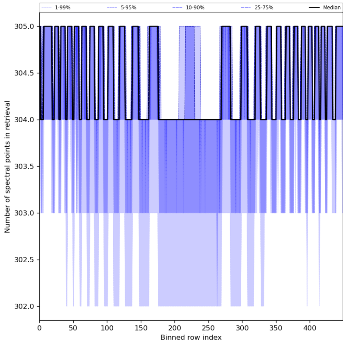
Figure 50: Along track statistics of “Number of spectral points in retrieval” for 2023-07-03 to 2023-07-04
