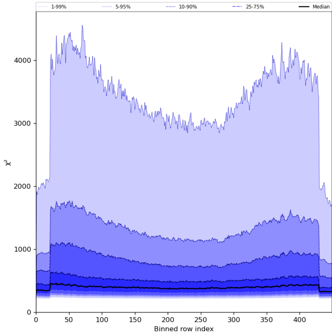
Figure 59: Along track statistics of “ \chi^2 ” for 2023-07-03 to 2023-07-04
