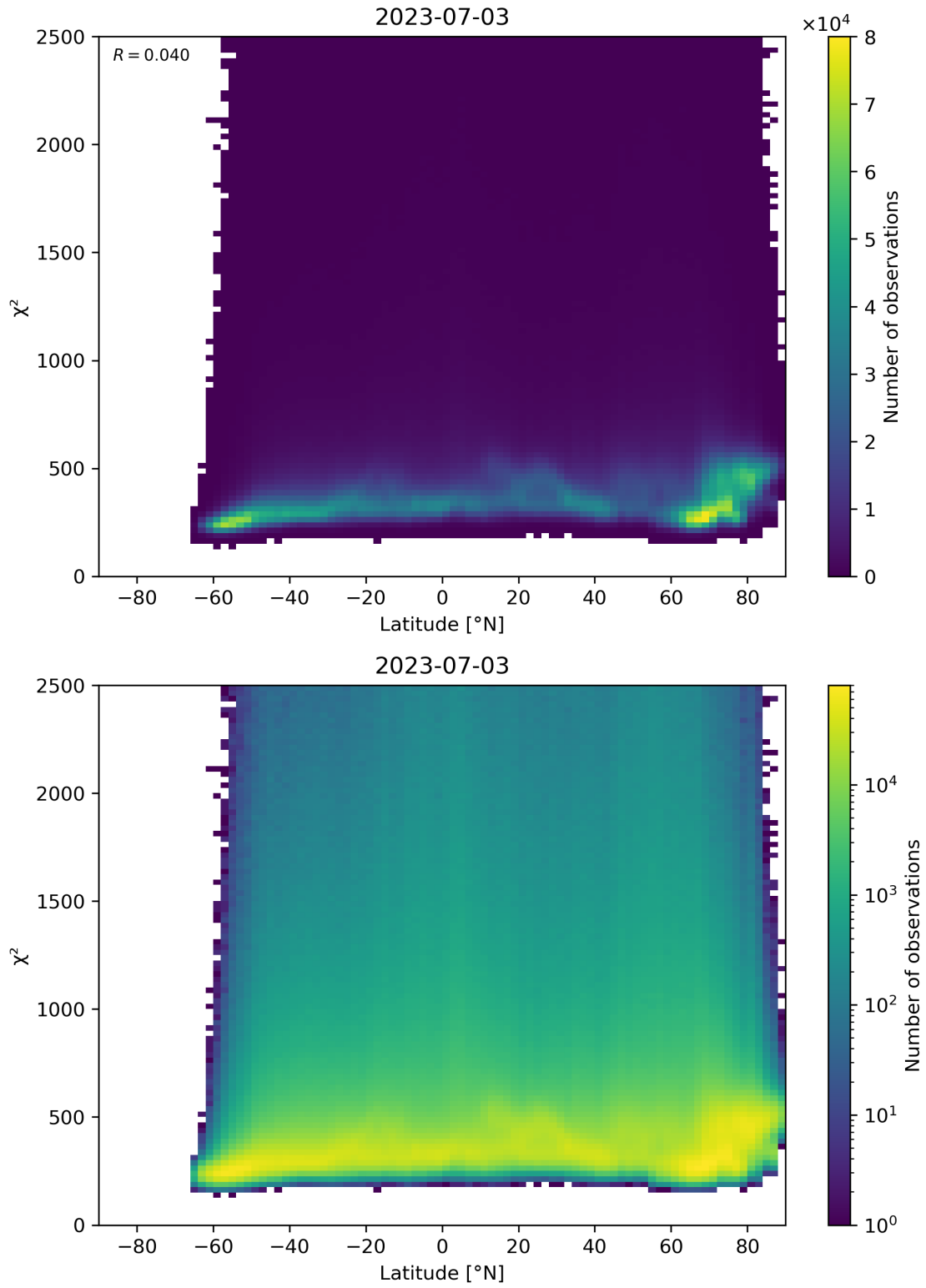
Figure 86: Scatter density plot of “Latitude” against “ \chi^2 ” for 2023-07-03 to 2023-07-04.
