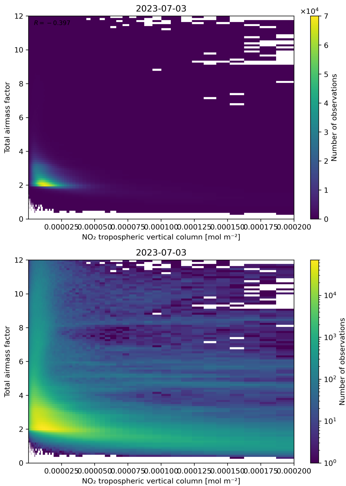
Figure 122: Scatter density plot of “NO 2 tropospheric vertical column” against “Total air mass factor” for 2023-07-03 to 2023-07-04.
