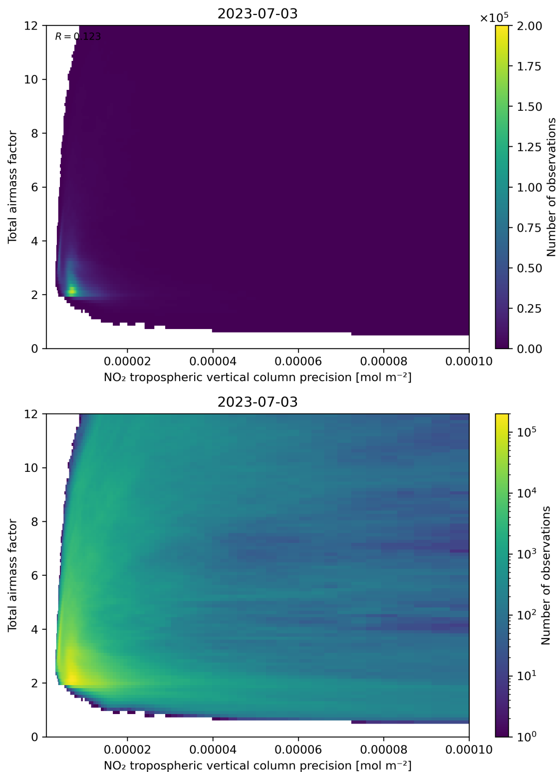
Figure 132: Scatter density plot of “NO 2 tropospheric vertical column precision” against “Total air mass factor” for 2023-07-03 to 2023-07-04.
