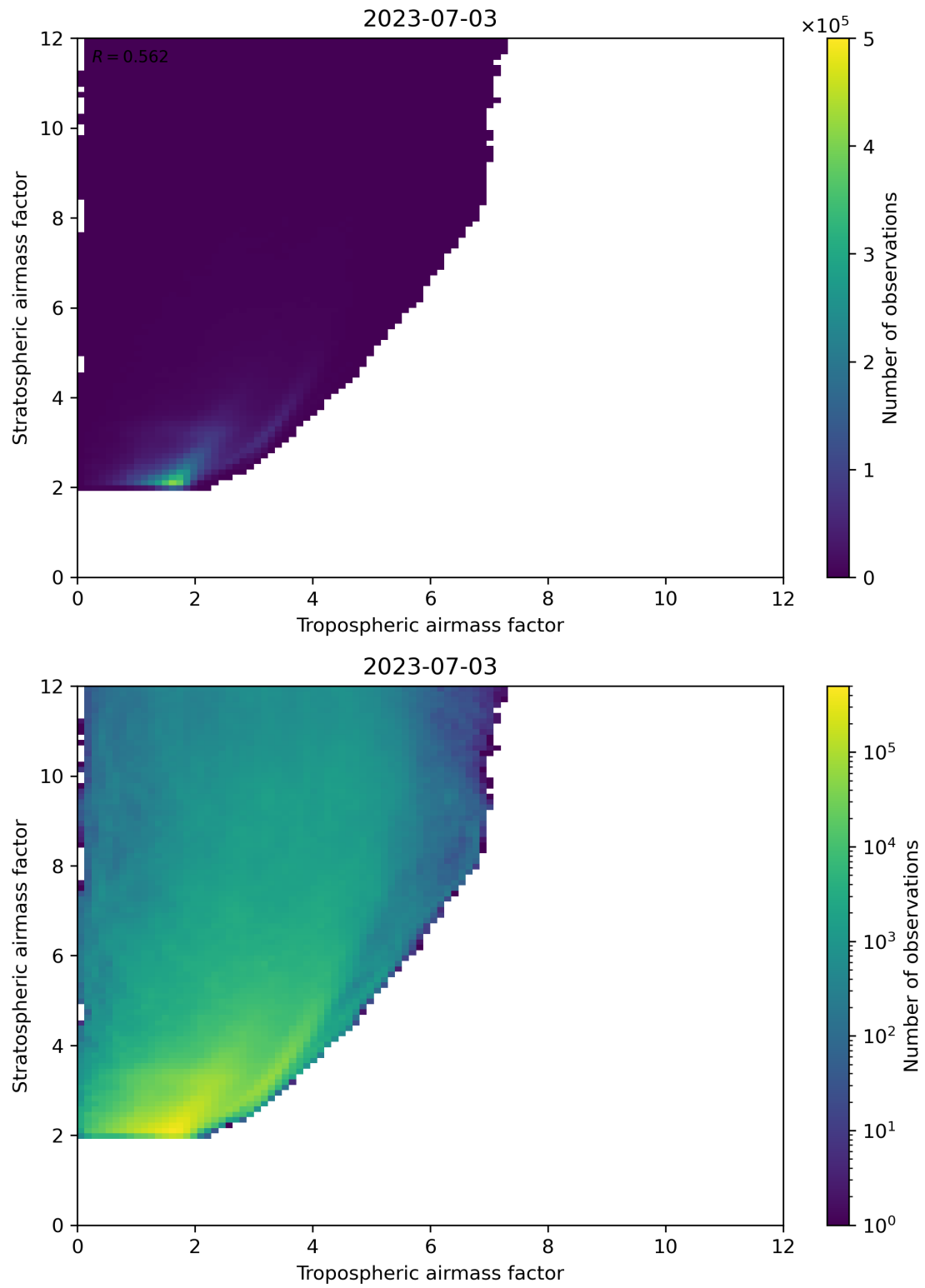
Figure 71: Scatter density plot of “Tropospheric airmass factor” against “Stratospheric airmass factor” for 2023-07-03 to 2023-07-04.
