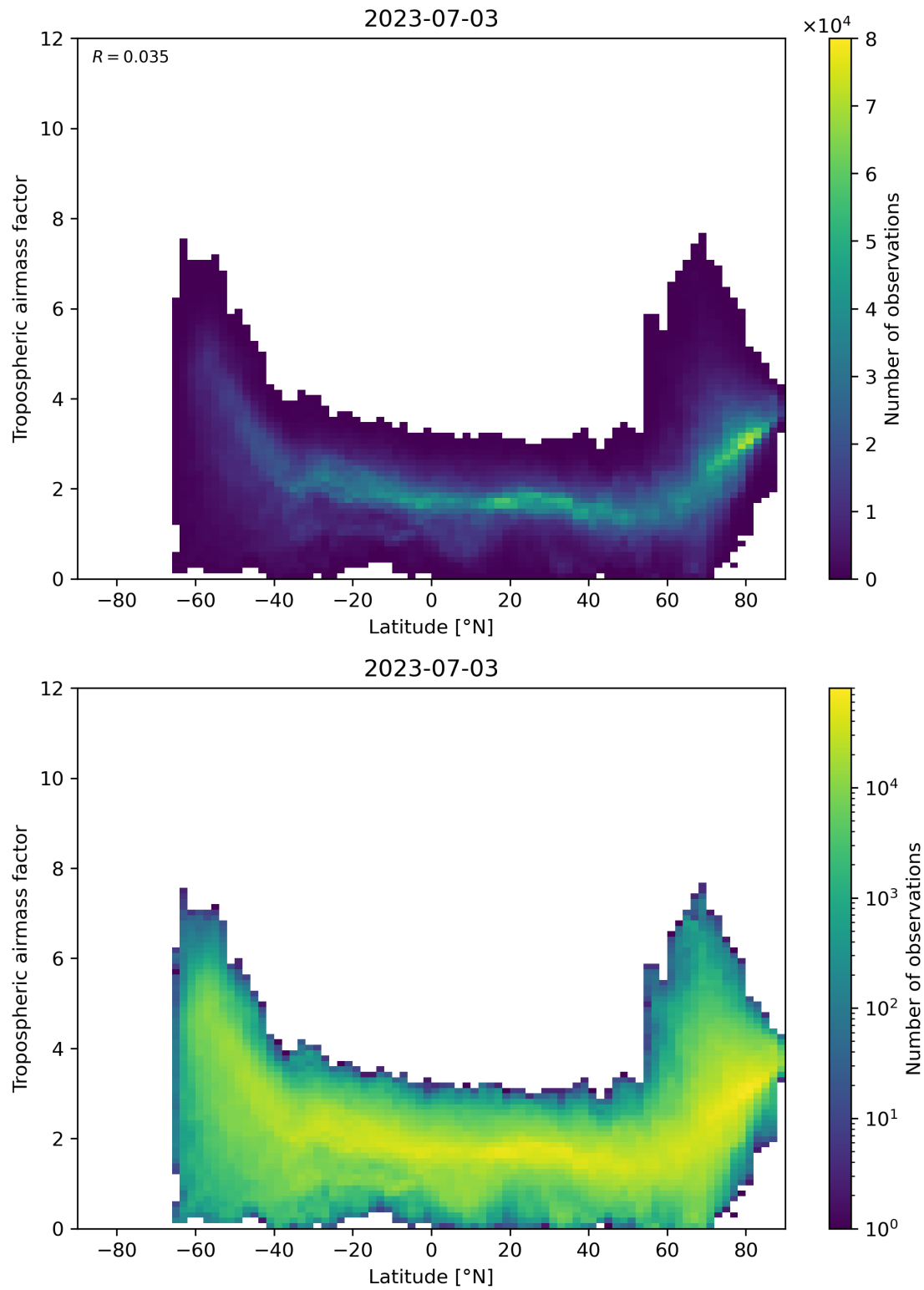
Figure 85: Scatter density plot of “Latitude” against “Tropospheric air mass factor” for 2023-07-03 to 2023-07-04.
