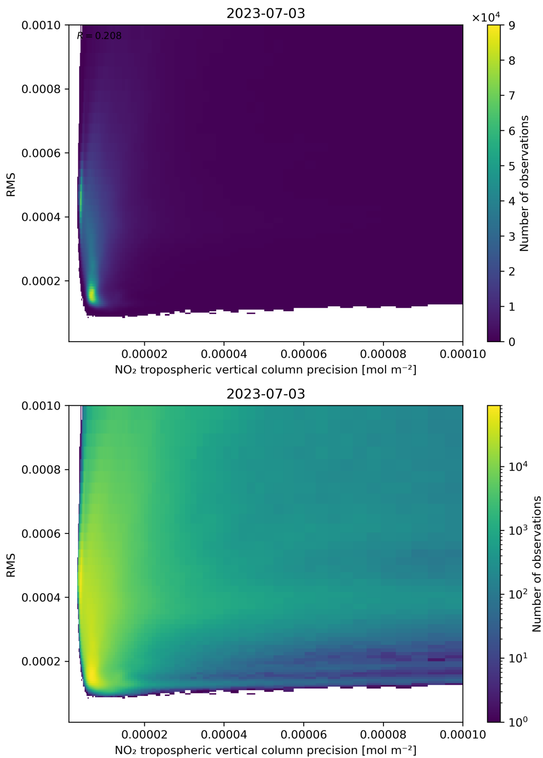
Figure 140: Scatter density plot of “NO 2 tropospheric vertical column precision” against “RMS” for 2023-07-03 to 2023-07-04.
