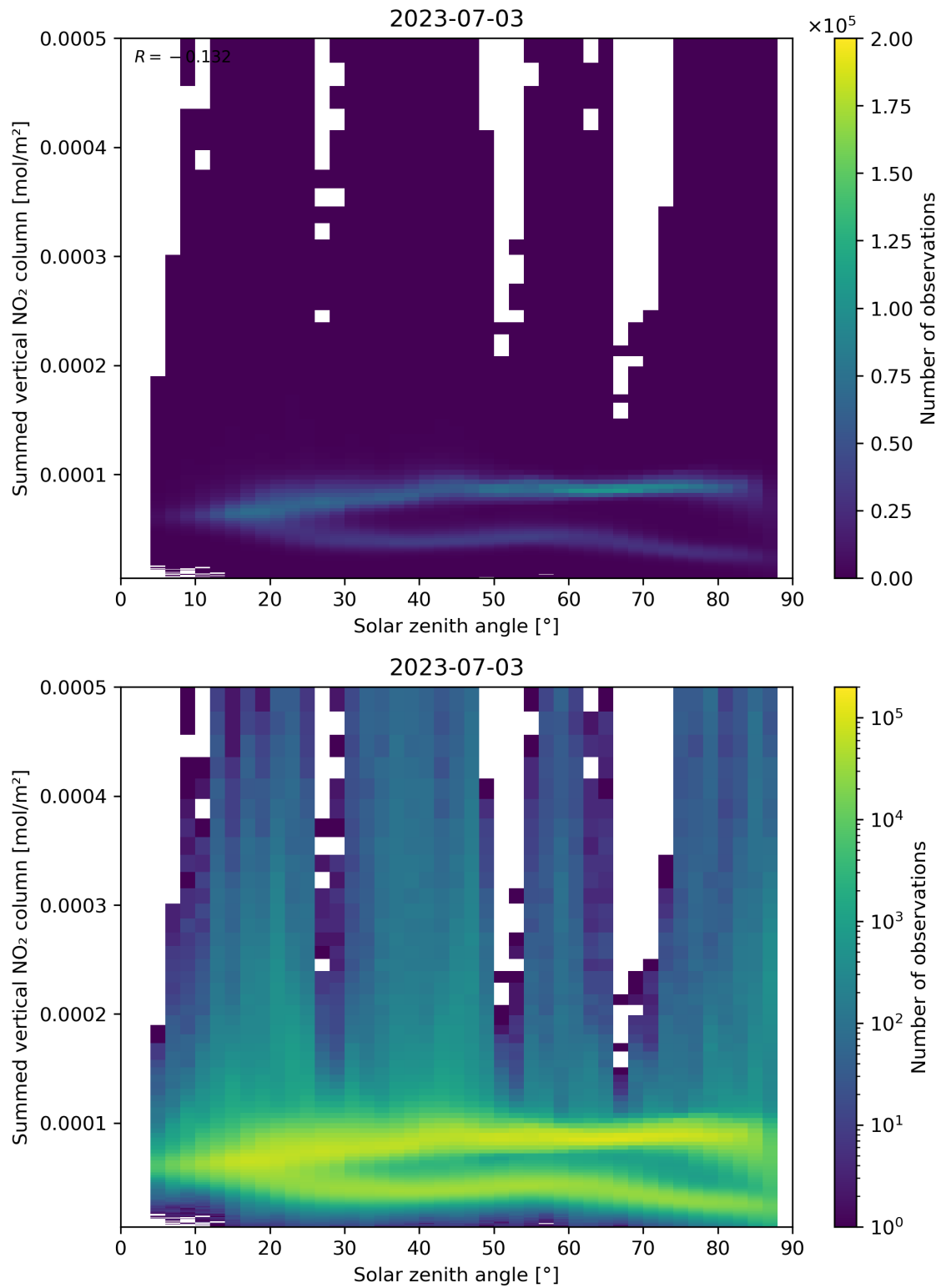
Figure 151: Scatter density plot of “Solar zenith angle” against “Summed vertical NO 2 column” for 2023-07-03 to 2023-07-04.
