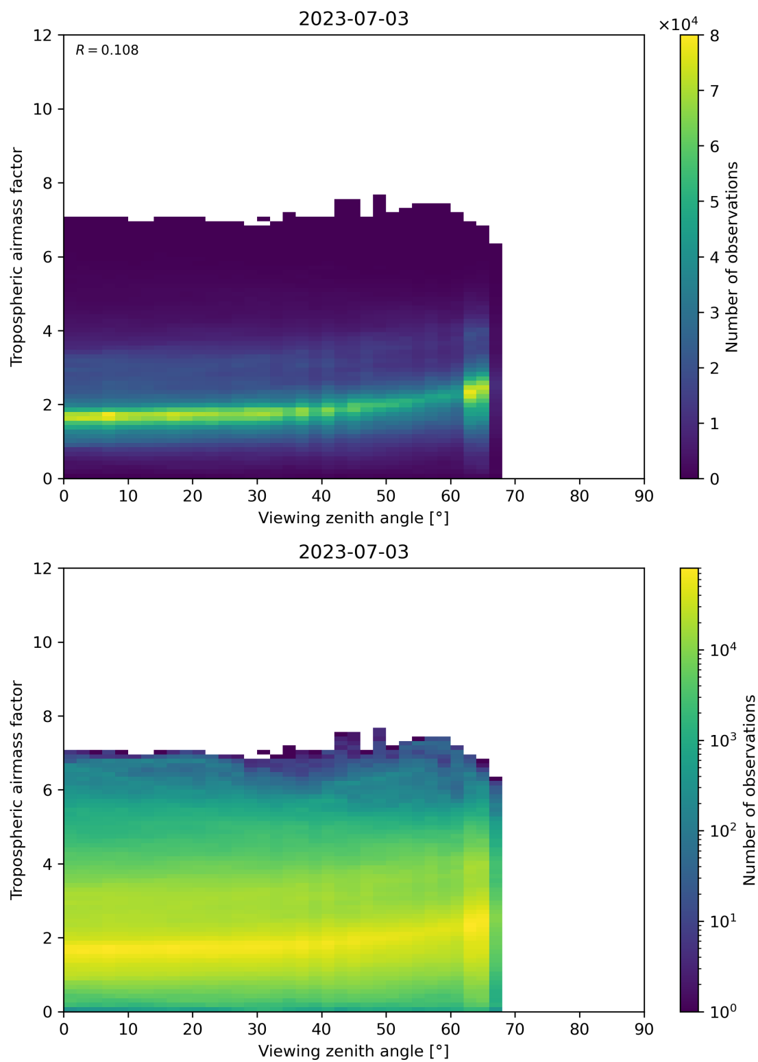
Figure 161: Scatter density plot of “Viewing zenith angle” against “Tropospheric airmass factor” for 2023-07-03 to 2023-07-04.
