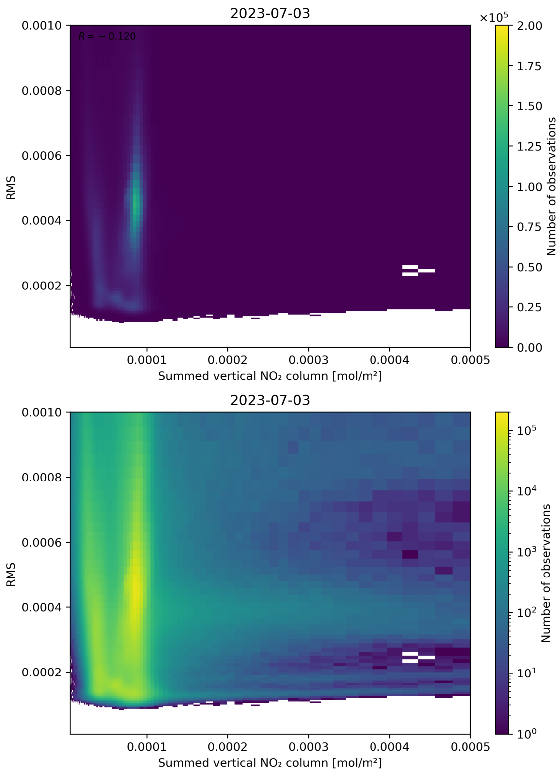
Figure 109: Scatter density plot of “Summed vertical NO 2 column” against “RMS” for 2023-07-03 to 2023-07-04.
