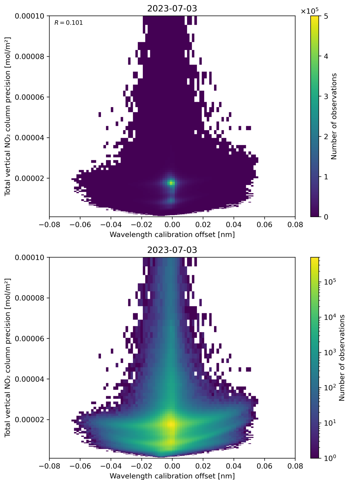
Figure 180: Scatter density plot of “Wavelength calibration offset” against “Total vertical NO 2 column precision” for 2023-07-03 to 2023-07-04.
