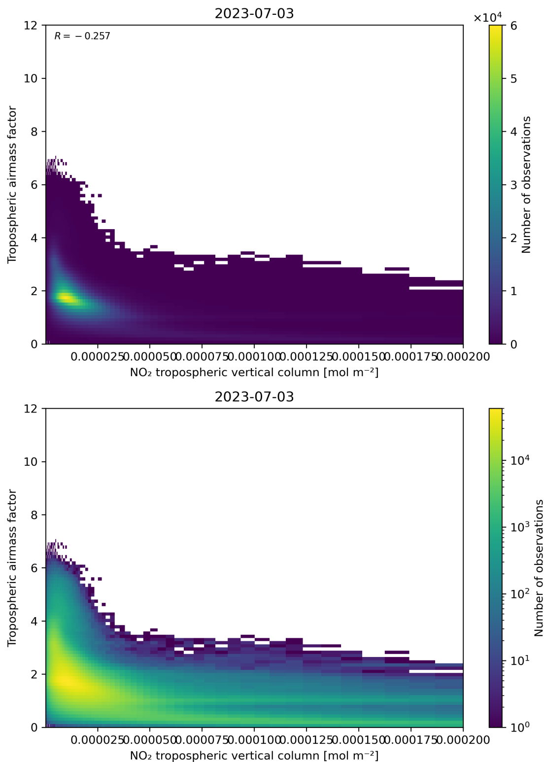
Figure 123: Scatter density plot of “NO 2 tropospheric vertical column” against “Tropospheric airmass factor” for 2023-07-03 to 2023-07-04.
