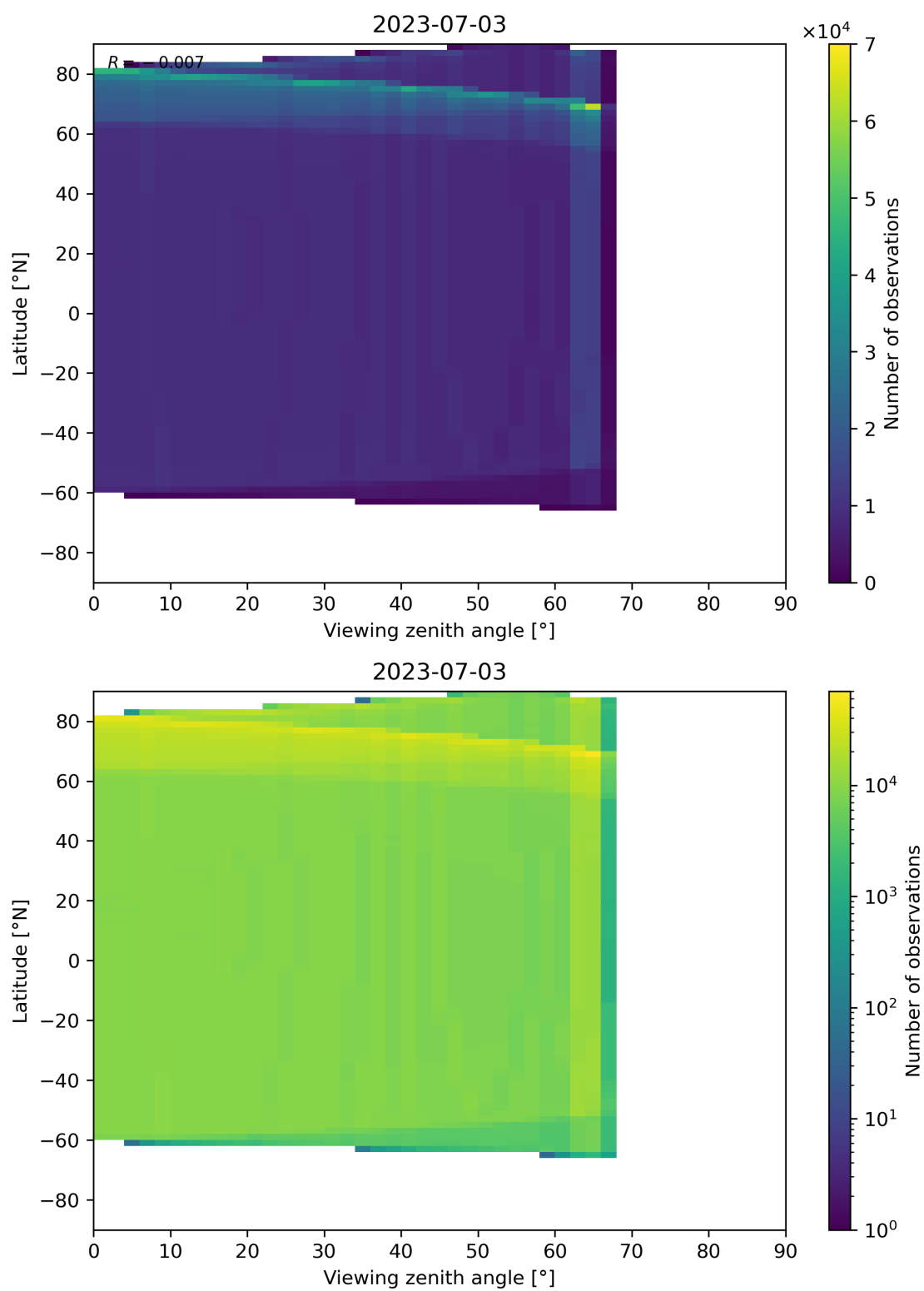
Figure 163: Scatter density plot of “Viewing zenith angle” against “Latitude” for 2023-07-03 to 2023-07-04.
