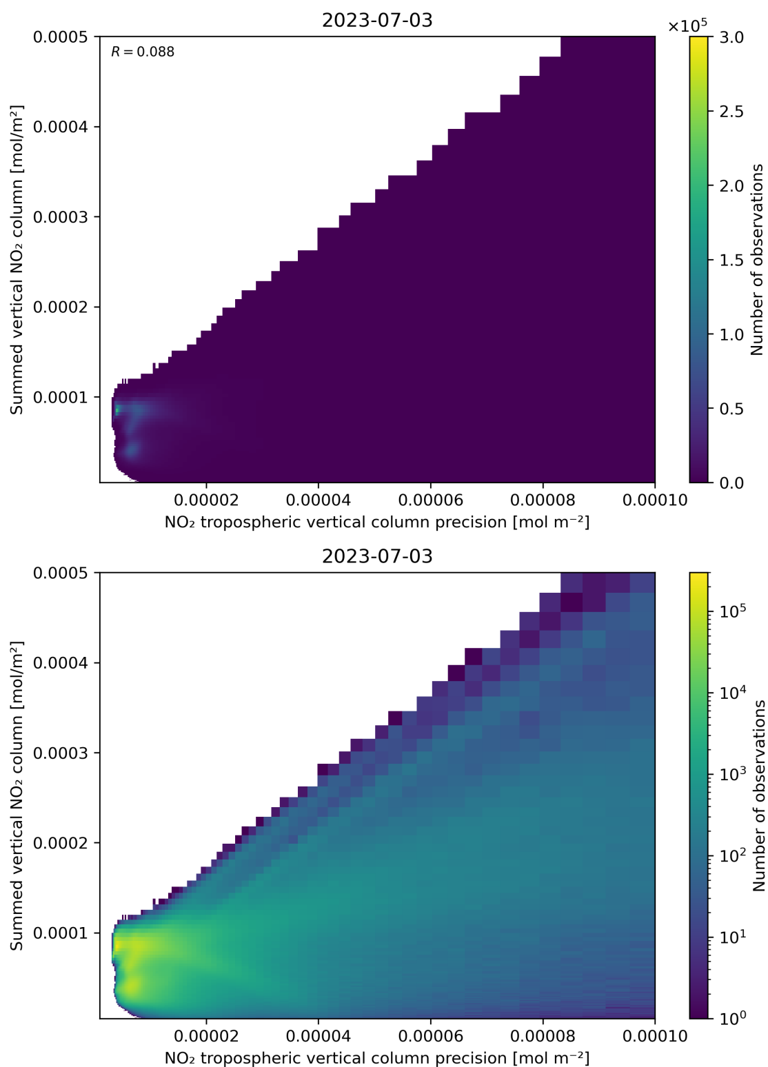
Figure 136: Scatter density plot of “NO 2 tropospheric vertical column precision” against “Summed vertical NO 2 column” for 2023-07-03 to 2023-07-04.
