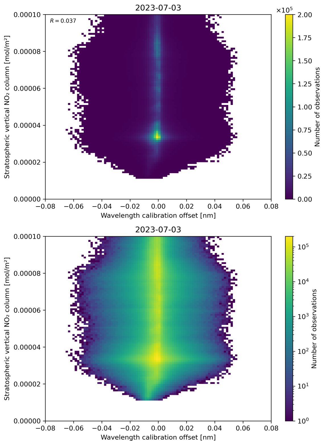
Figure 176: Scatter density plot of “Wavelength calibration offset” against “Stratospheric vertical NO 2 column” for 2023-07-03 to 2023-07-04.
