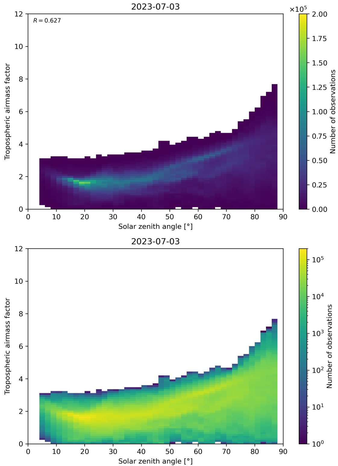
Figure 147: Scatter density plot of “Solar zenith angle” against “Tropospheric airmass factor” for 2023-07-03 to 2023-07-04.
