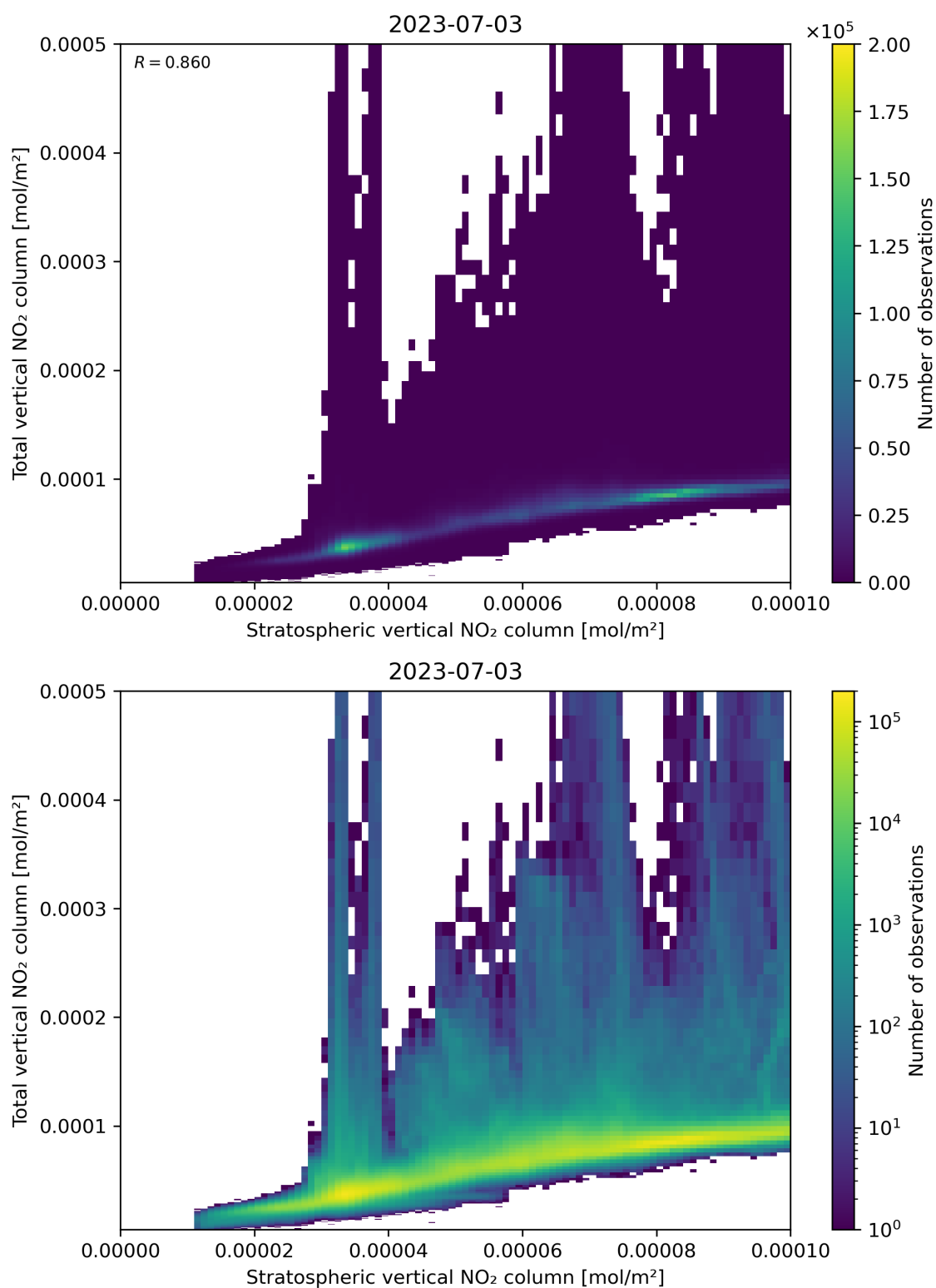
Figure 100: Scatter density plot of “Stratospheric vertical NO 2 column” against “Total vertical NO 2 column” for 2023-07-03 to 2023-07-04.
