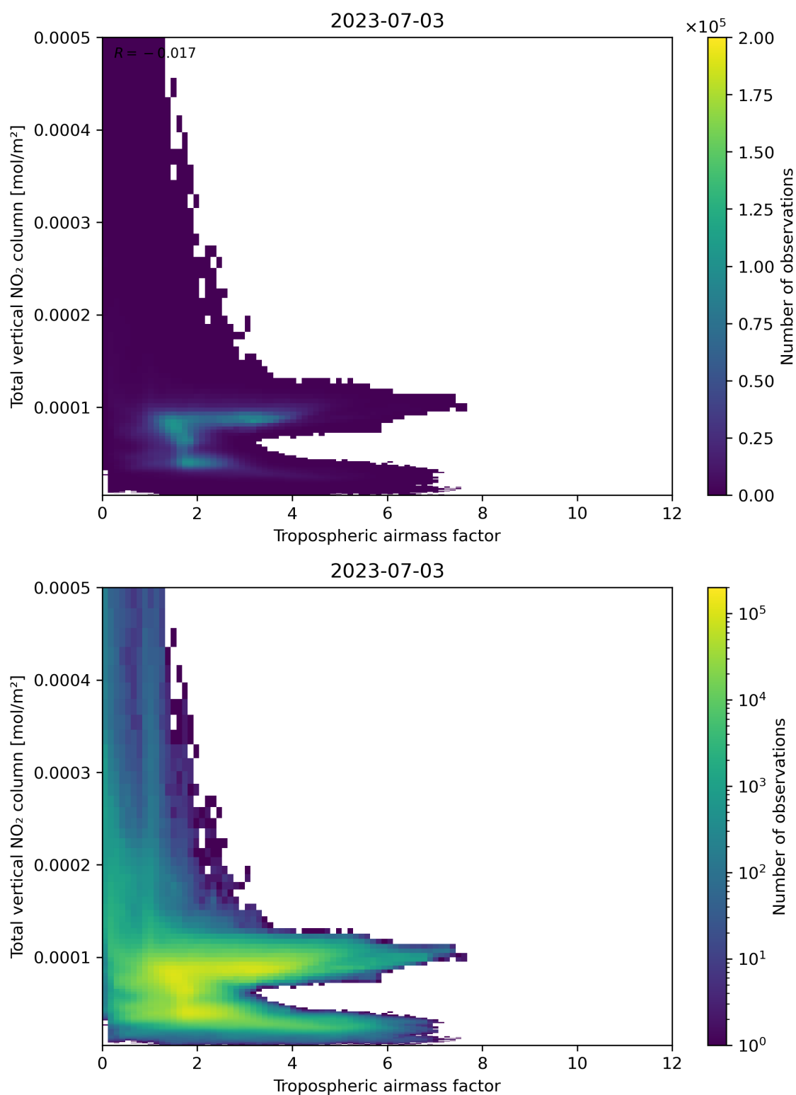
Figure 77: Scatter density plot of “Tropospheric airmass factor” against “Total vertical NO 2 column” for 2023-07-03 to 2023-07-04.
