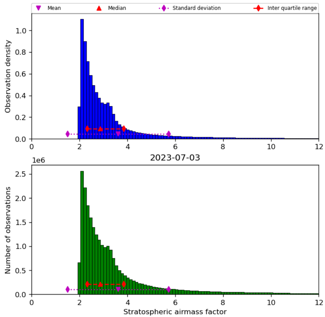
Figure 44: Histogram of “Stratospheric airmass factor” for 2023-07-03 to 2023-07-04
