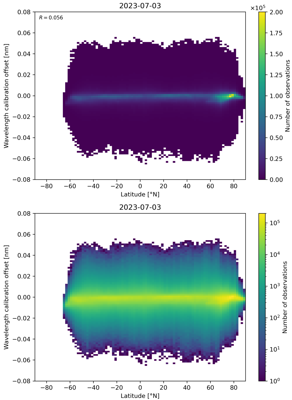
Figure 95: Scatter density plot of “Latitude” against “Wavelength calibration offset” for 2023-07-03 to 2023-07-04.
