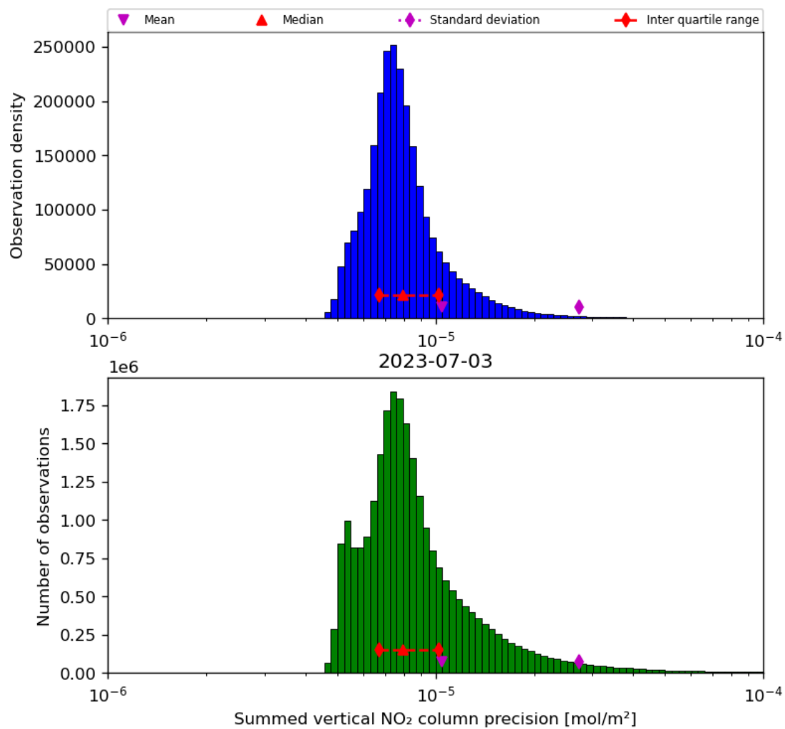
Figure 41: Histogram of “Summed vertical NO 2 column precision” for 2023-07-03 to 2023-07-04
