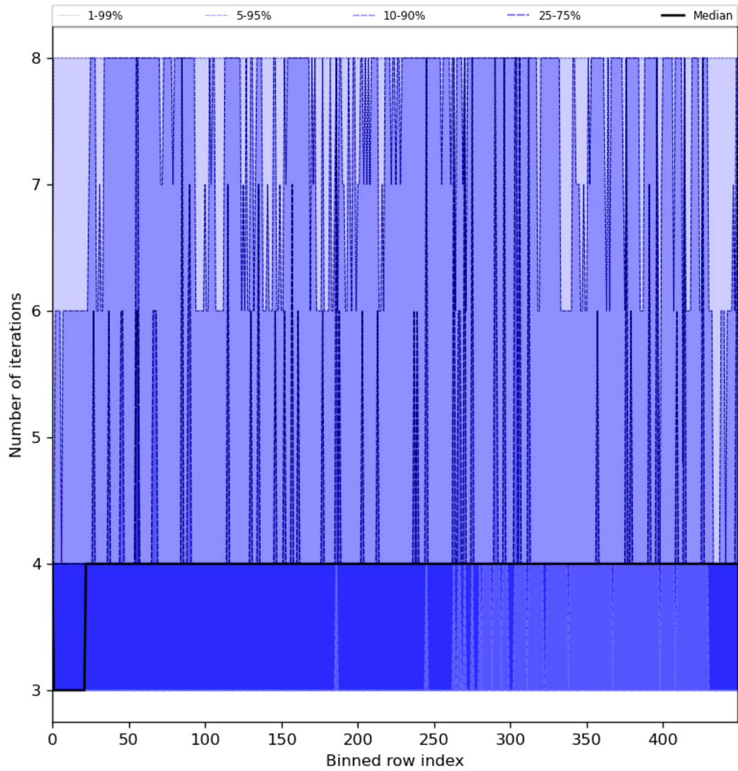
Figure 51: Along track statistics of “Number of iterations” for 2023-07-03 to 2023-07-04
