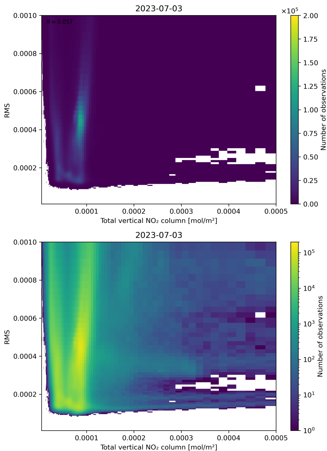
Figure 120: Scatter density plot of “Total vertical NO 2 column” against “RMS” for 2023-07-03 to 2023-07-04.
