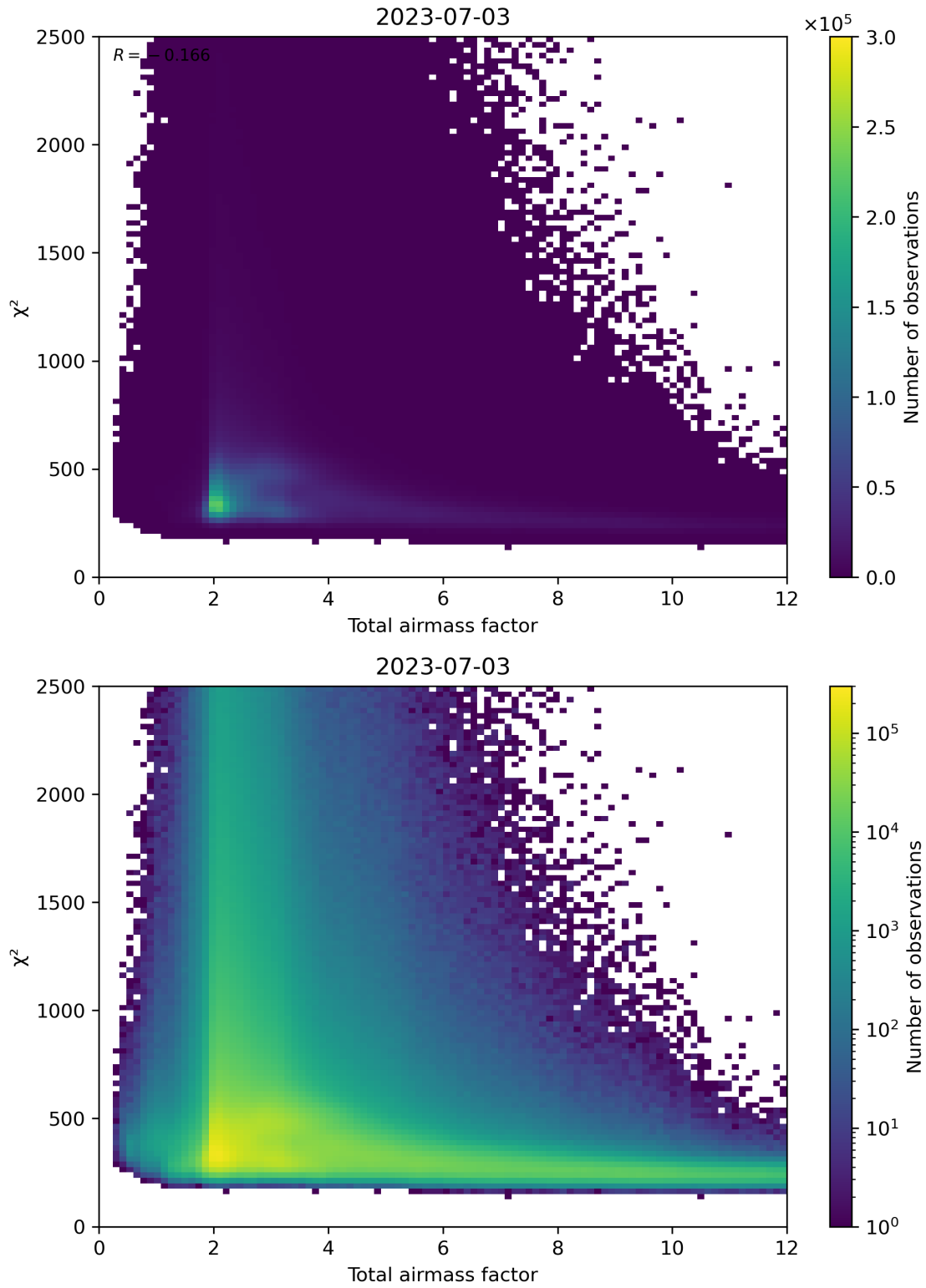
Figure 63: Scatter density plot of “Total airmass factor” against “ \chi^2 ” for 2023-07-03 to 2023-07-04.
