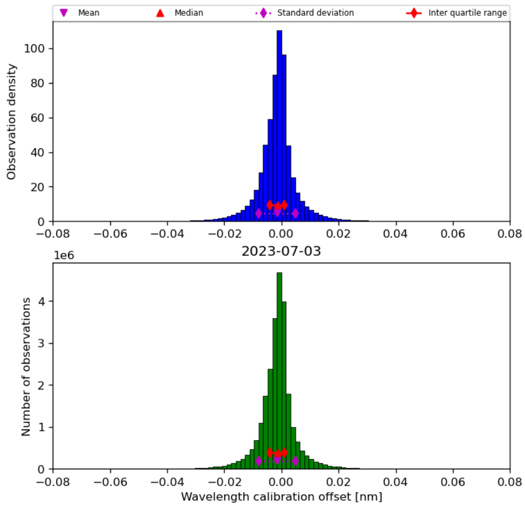
Figure 35: Histogram of “Wavelength calibration offset” for 2023-07-03 to 2023-07-04
