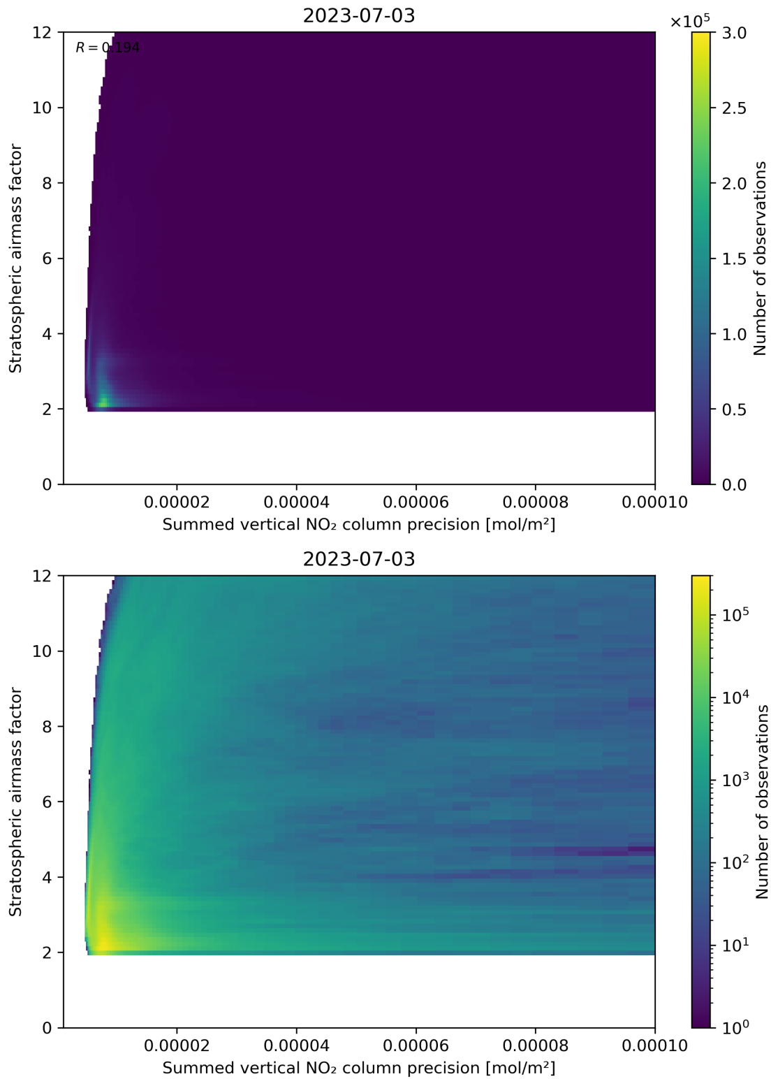
Figure 106: Scatter density plot of “Summed vertical NO 2 column precision” against “Stratospheric airmass factor” for 2023-07-03 to 2023-07-04.
