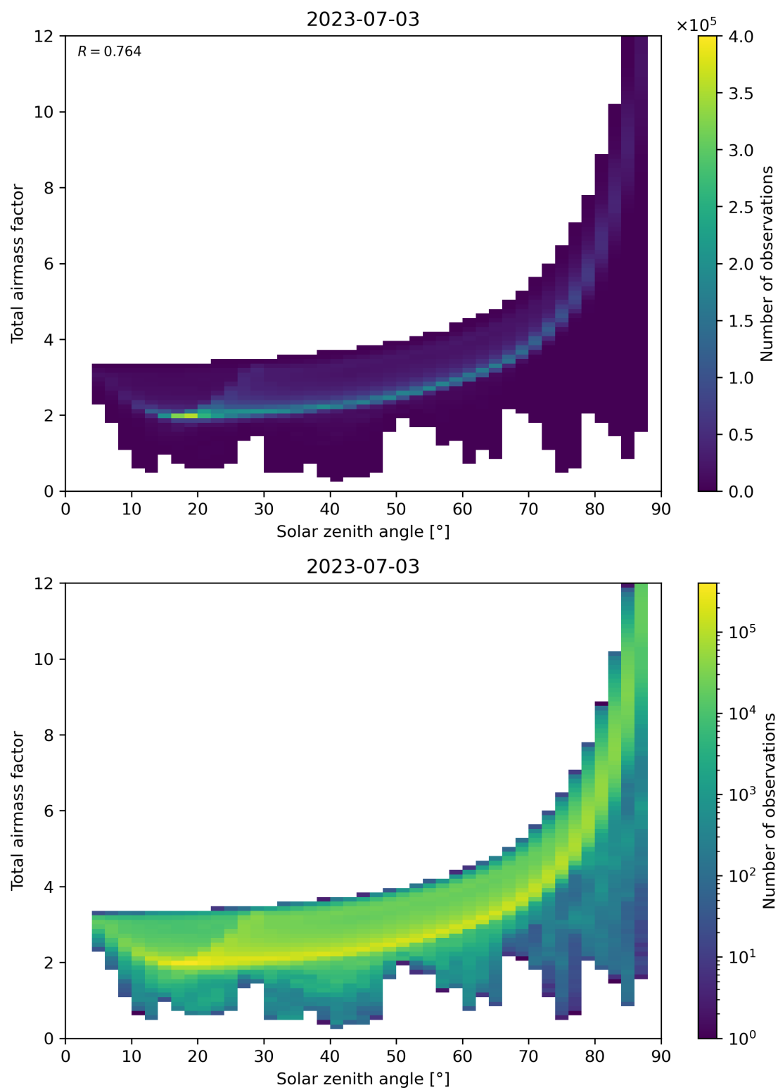
Figure 146: Scatter density plot of “Solar zenith angle” against “Total air mass factor” for 2023-07-03 to 2023-07-04.
