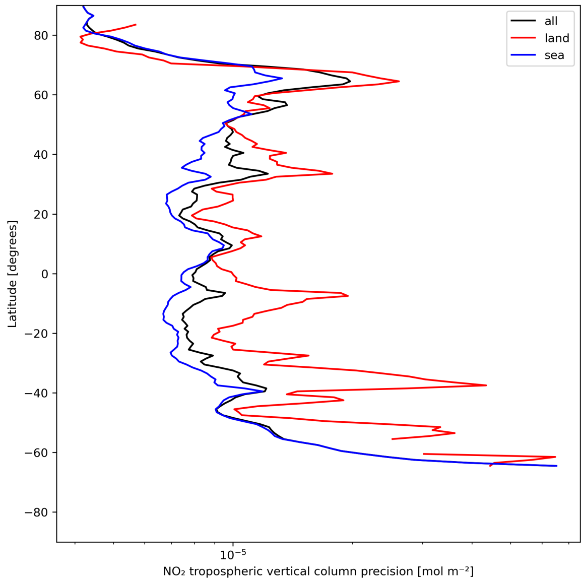
Figure 13: Zonal average of “NO 2 tropospheric vertical column precision” for 2023-07-03 to 2023-07-04.
