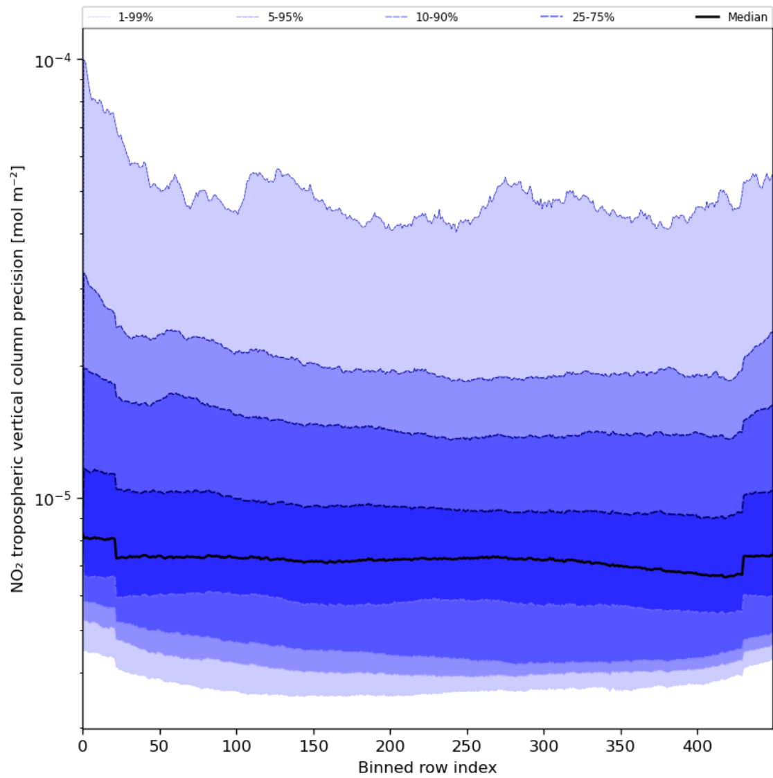
Figure 47: Along track statistics of “NO 2 tropospheric vertical column precision” for 2023-07-03 to 2023-07-04
