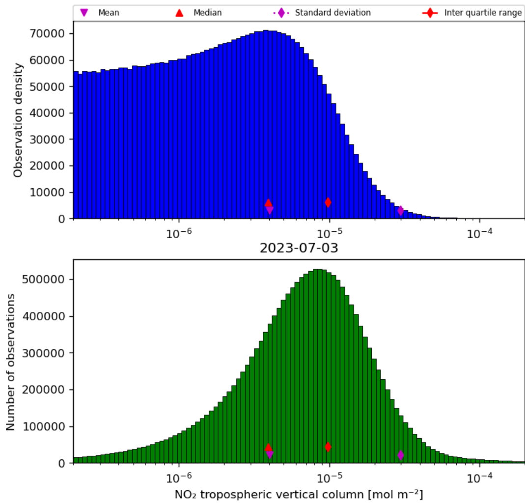
Figure 29: Histogram of “NO 2 tropospheric vertical column” for 2023-07-03 to 2023-07-04
