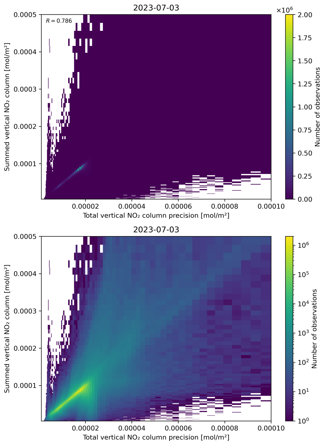
Figure 117: Scatter density plot of “Total vertical NO 2 column precision” against “Summed vertical NO 2 column” for 2023-07-03 to 2023-07-04.
