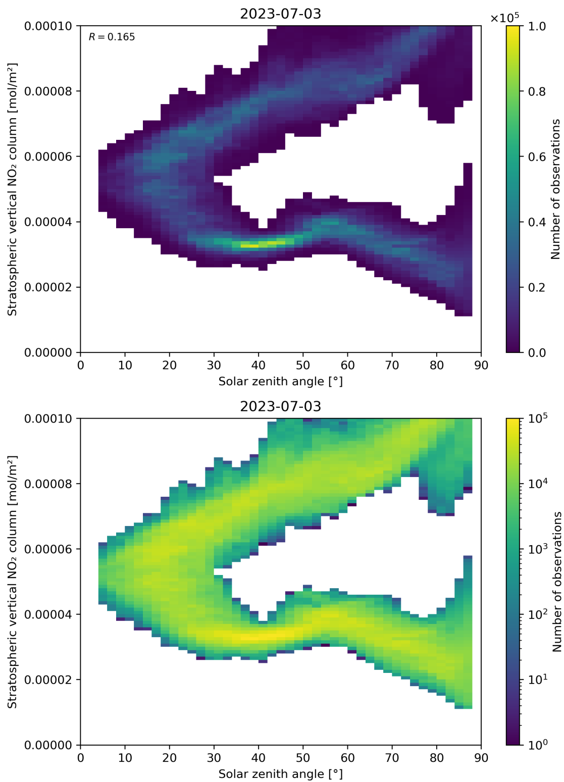
Figure 150: Scatter density plot of “Solar zenith angle” against “Stratospheric vertical NO 2 column” for 2023-07-03 to 2023-07-04.
