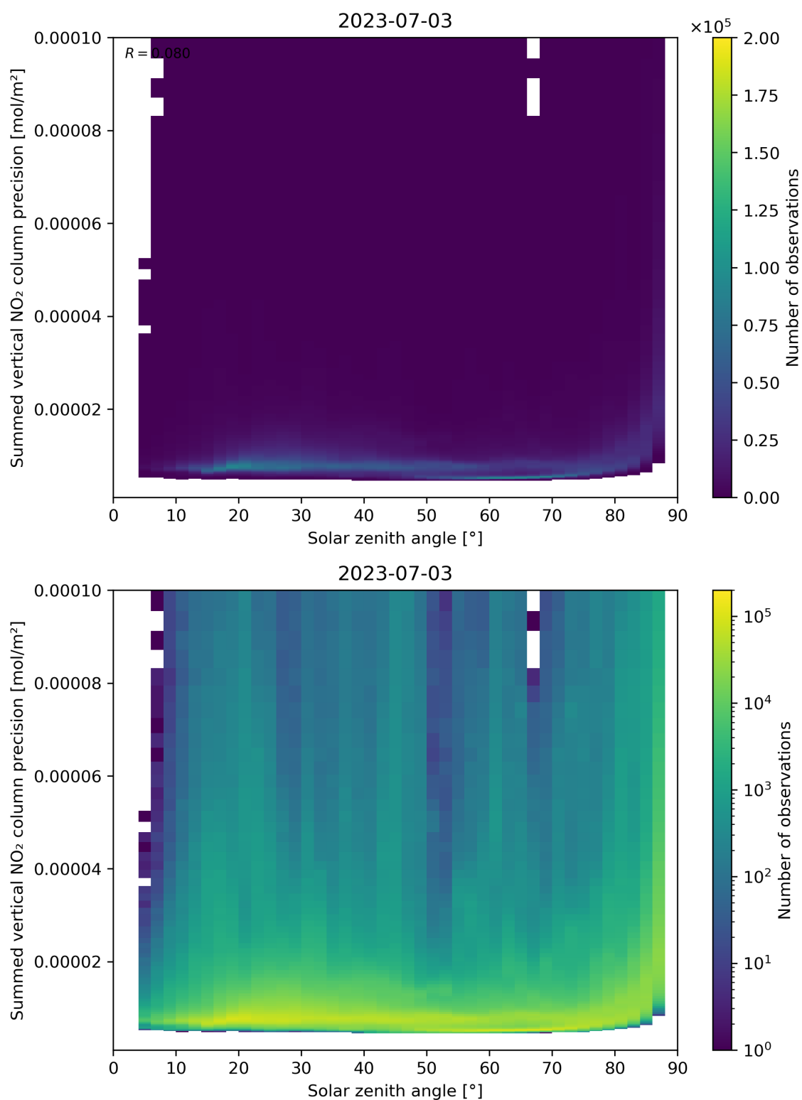
Figure 152: Scatter density plot of “Solar zenith angle” against “Summed vertical NO 2 column precision” for 2023-07-03 to 2023-07-04.
