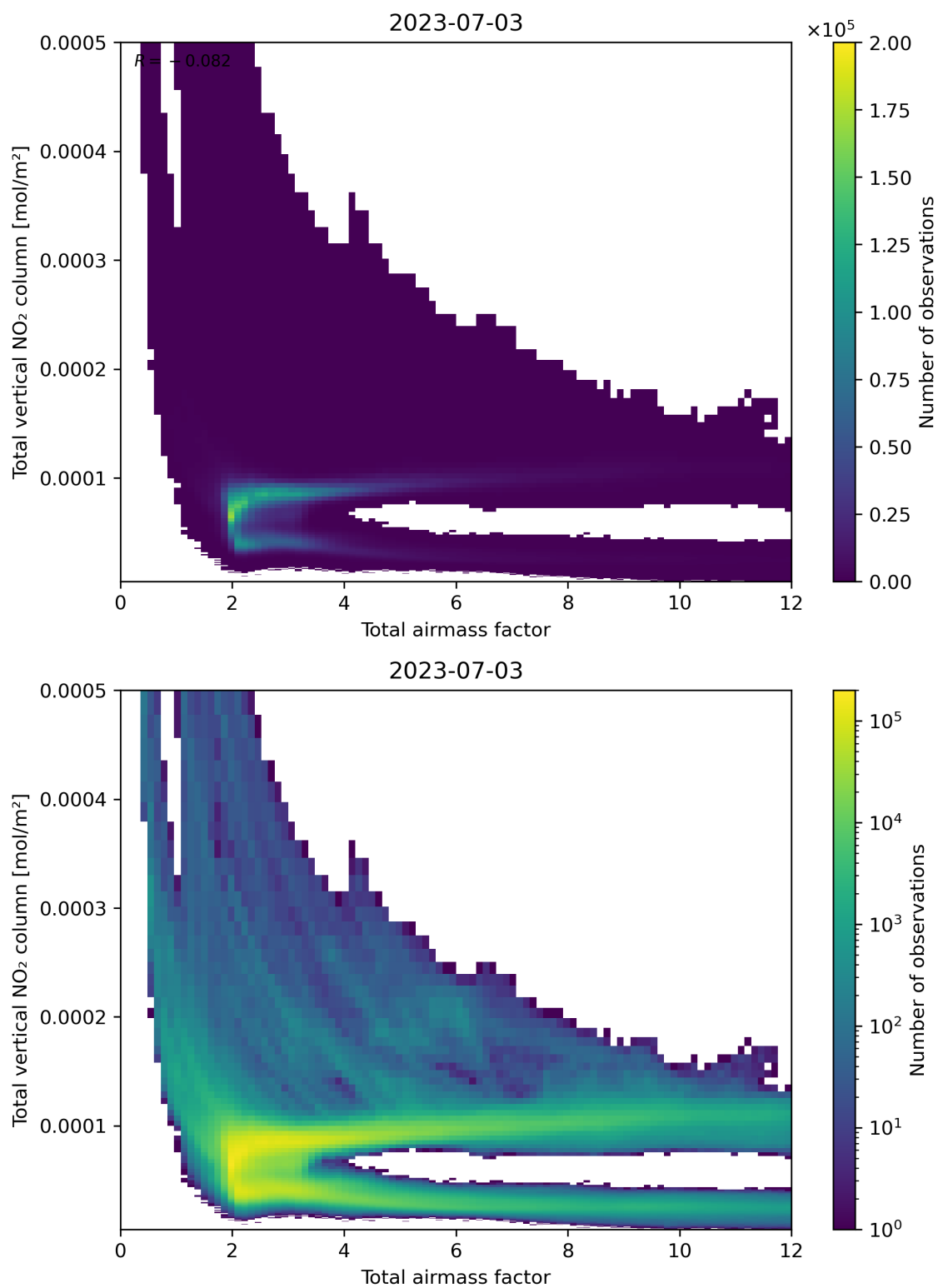
Figure 67: Scatter density plot of “Total airmass factor” against “Total vertical NO 2 column” for 2023-07-03 to 2023-07-04.
