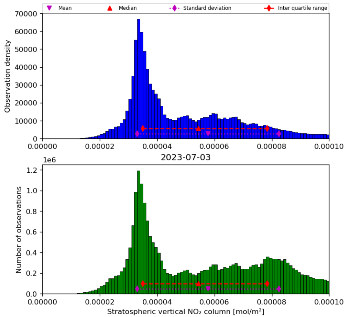
Figure 36: Histogram of “Stratospheric vertical NO 2 column” for 2023-07-03 to 2023-07-04
