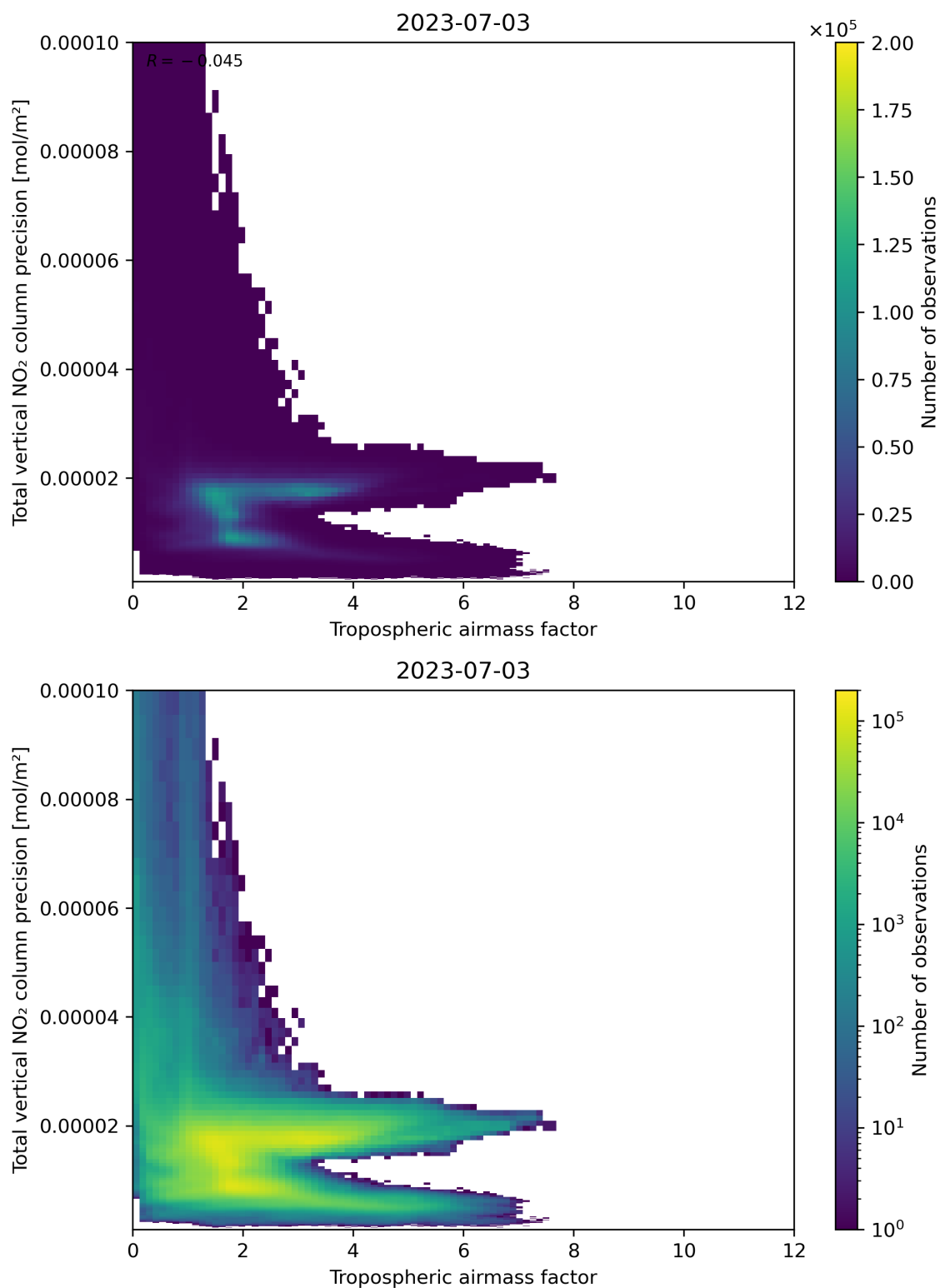
Figure 78: Scatter density plot of “Tropospheric air mass factor” against “Total vertical NO 2 column precision” for 2023-07-03 to 2023-07-04.
