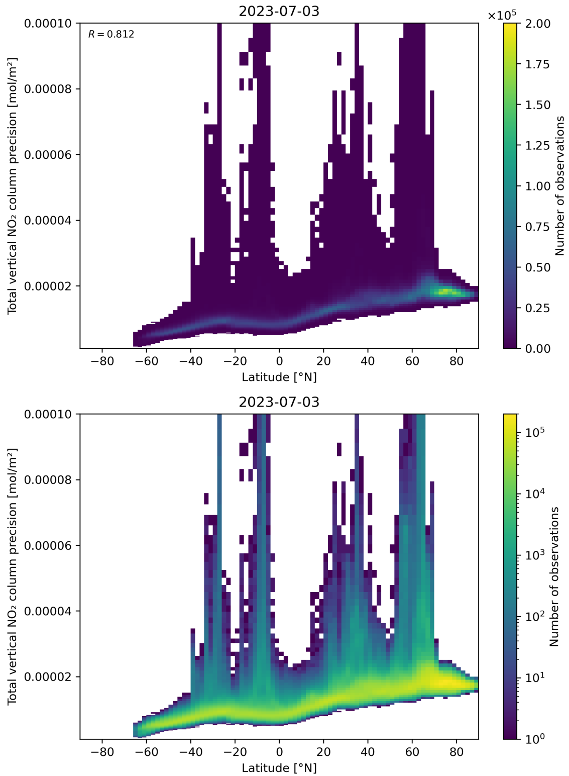
Figure 91: Scatter density plot of “Latitude” against “Total vertical NO 2 column precision” for 2023-07-03 to 2023-07-04.
