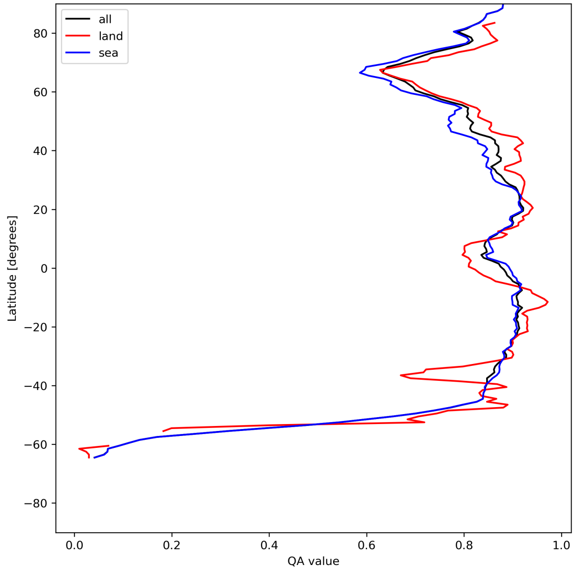
Figure 11: Zonal average of “QA value” for 2023-07-03 to 2023-07-04.
