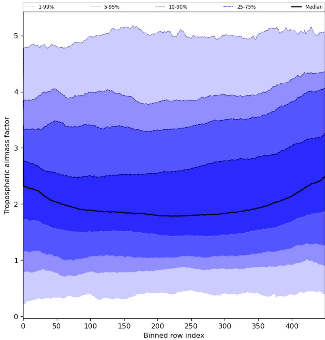
Figure 48: Along track statistics of “Tropospheric air mass factor” for 2023-07-03 to 2023-07-04
