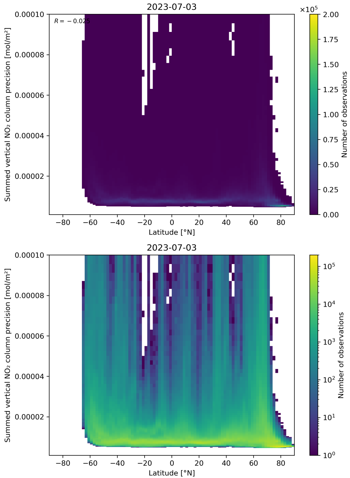
Figure 89: Scatter density plot of “Latitude” against “Summed vertical NO 2 column precision” for 2023-07-03 to 2023-07-04.
