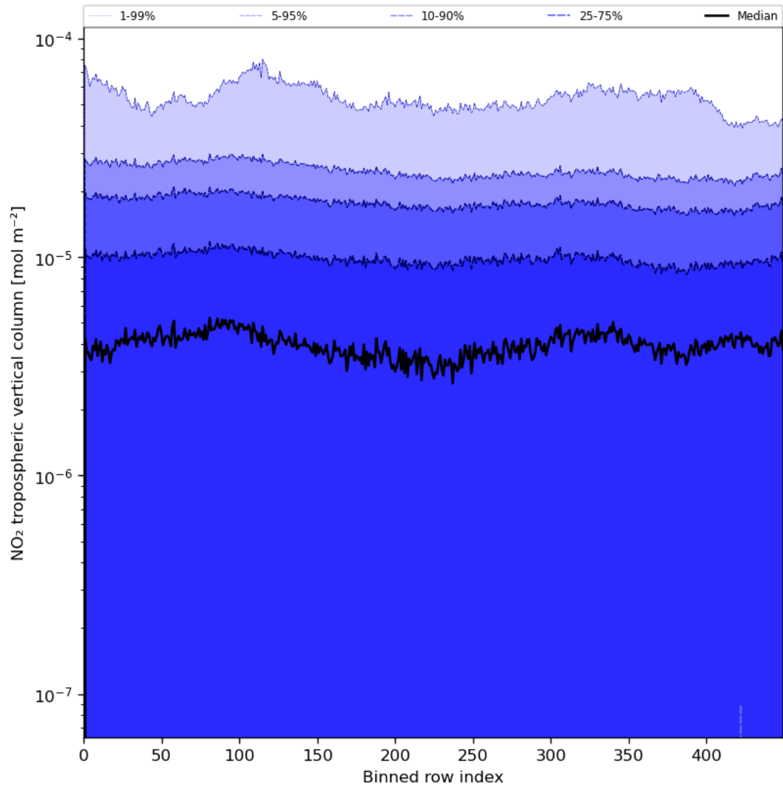
Figure 46: Along track statistics of "NO 2 tropospheric vertical column" for 2023-07-03 to 2023-07-04
