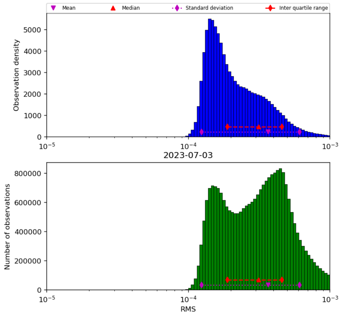
Figure 43: Histogram of “RMS” for 2023-07-03 to 2023-07-04
