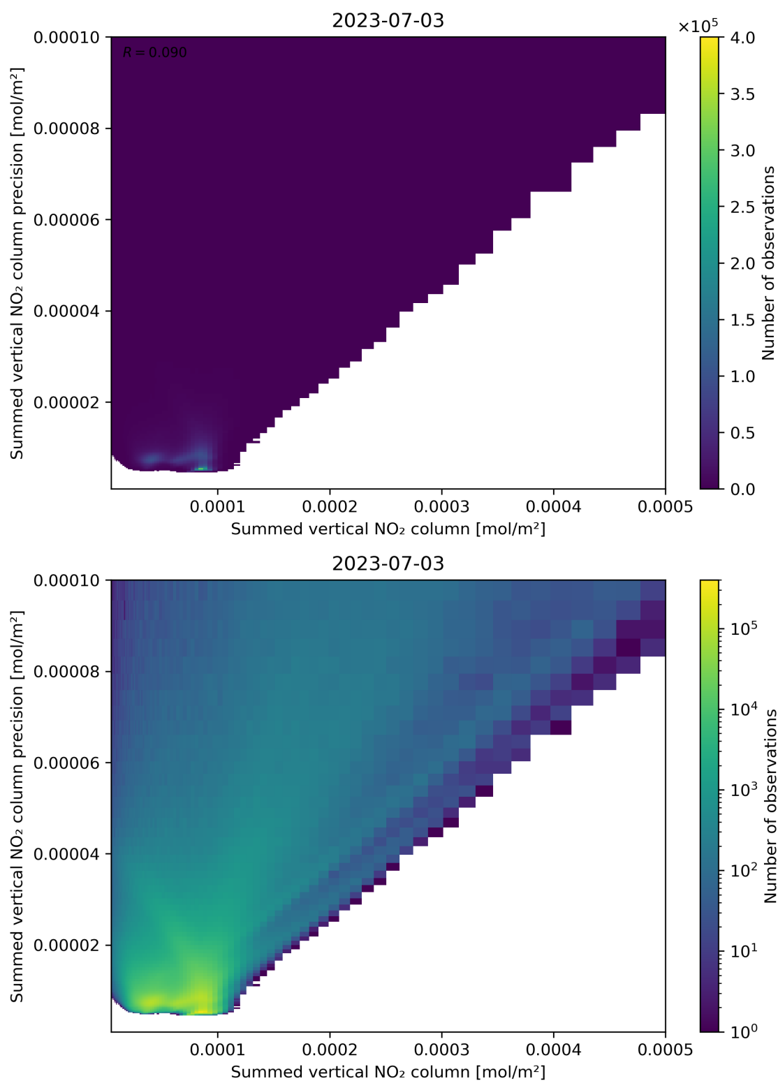
Figure 105: Scatter density plot of “Summed vertical NO 2 column” against “Summed vertical NO 2 column precision” for 2023-07-03 to 2023-07-04.
