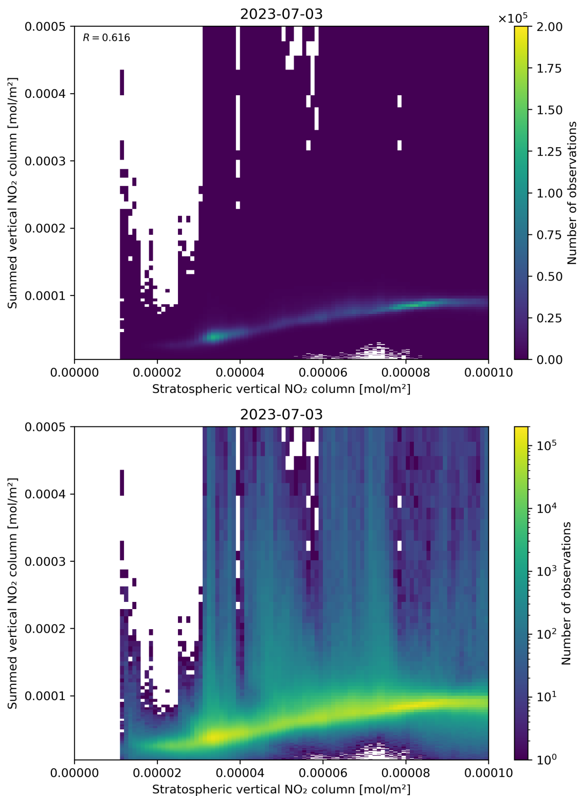
Figure 98: Scatter density plot of “Stratospheric vertical NO 2 column” against “Summed vertical NO 2 column” for 2023-07-03 to 2023-07-04.
