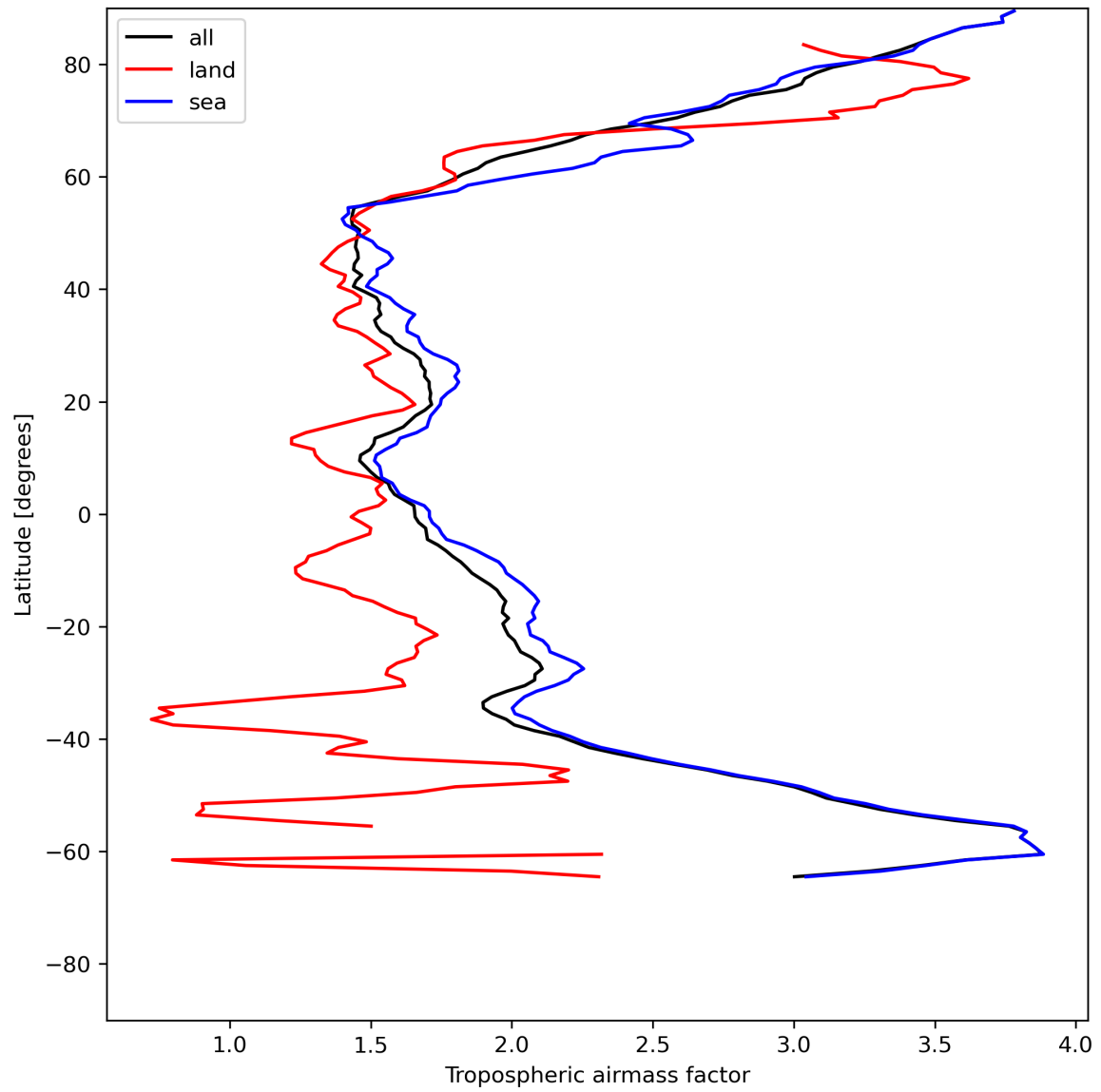
Figure 14: Zonal average of “Tropospheric airmass factor” for 2023-07-03 to 2023-07-04.
