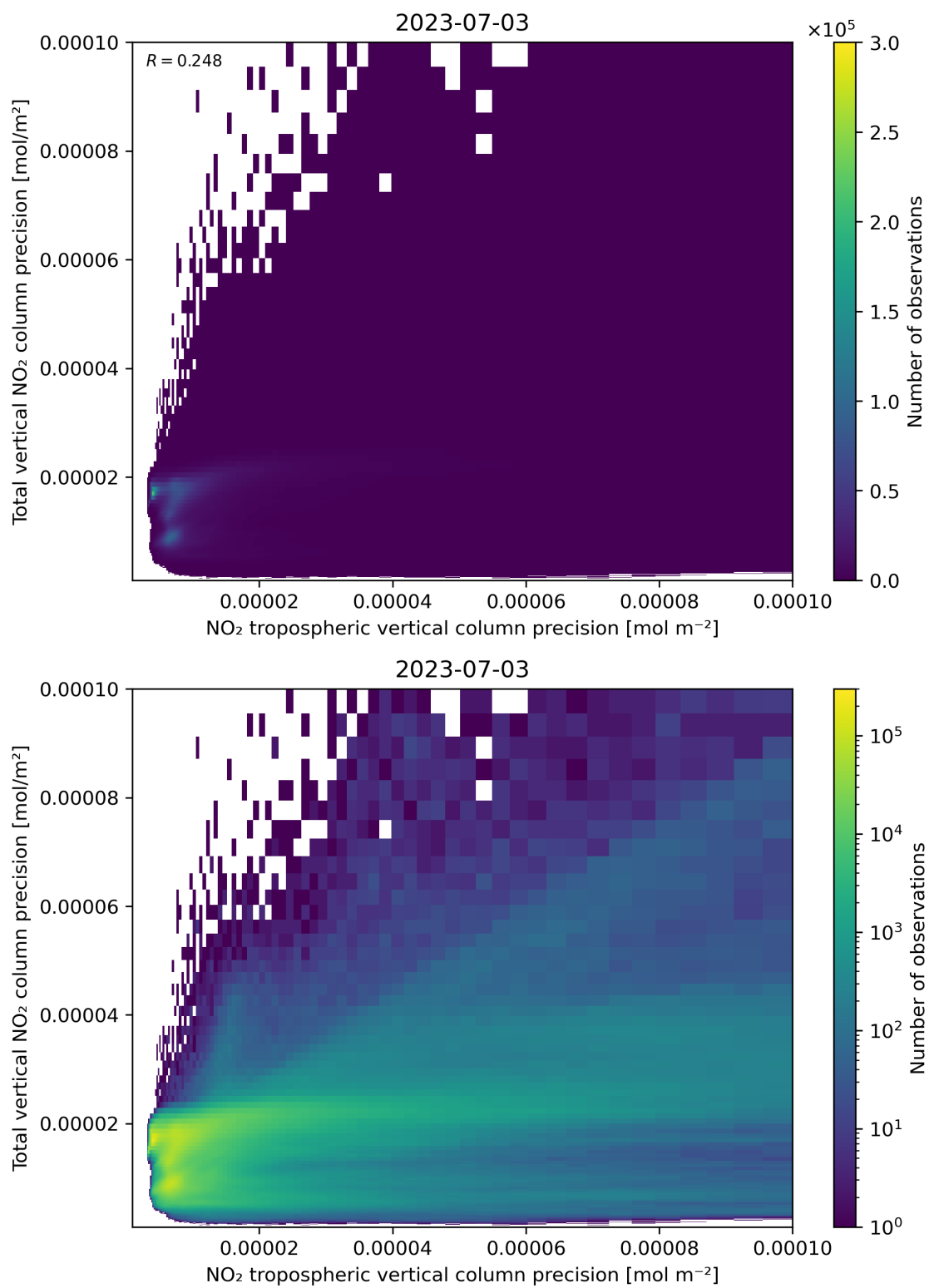
Figure 139: Scatter density plot of “NO 2 tropospheric vertical column precision” against “Total vertical NO 2 column precision” for 2023-07-03 to 2023-07-04.
