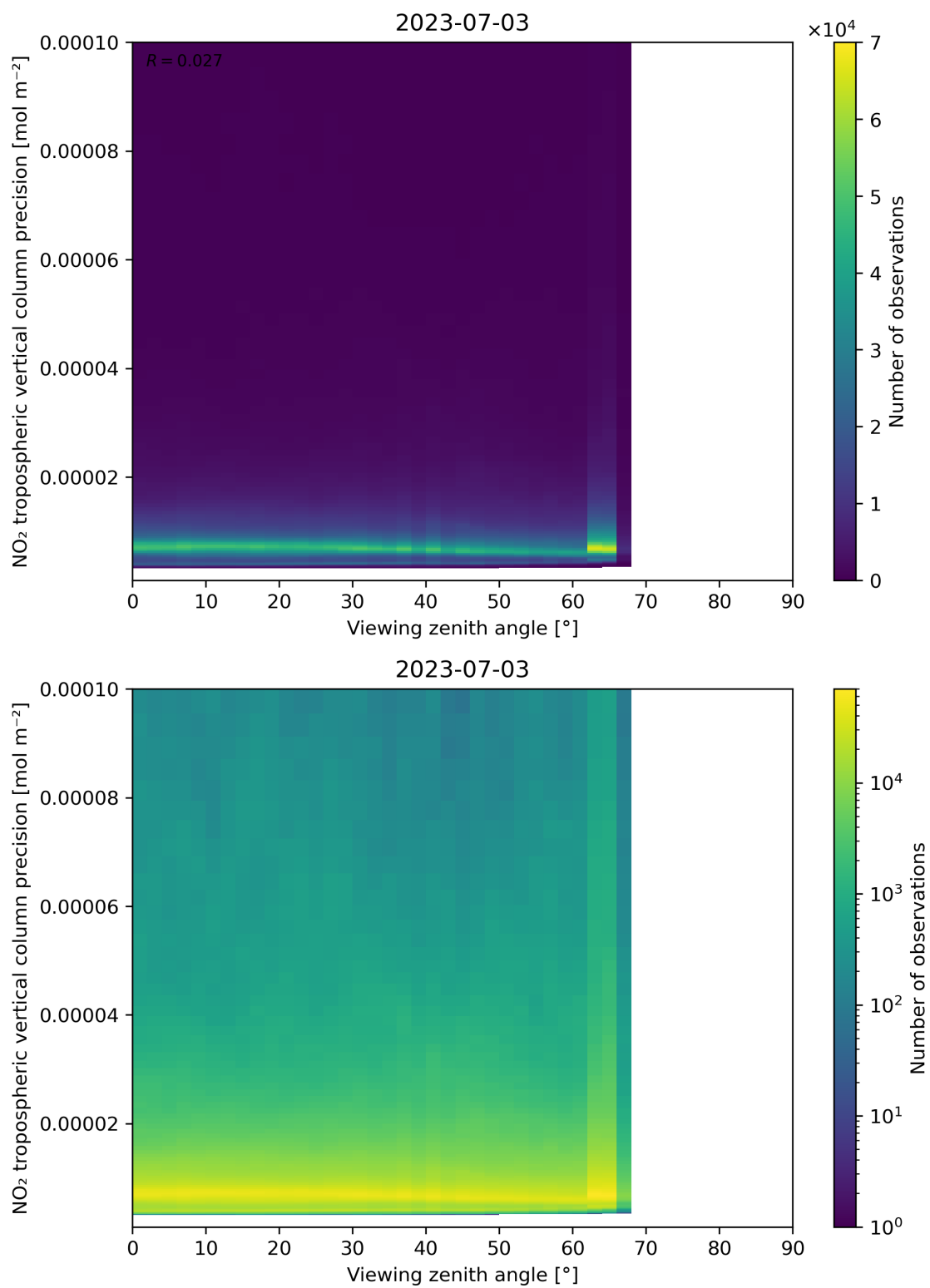
Figure 170: Scatter density plot of “Viewing zenith angle” against “NO 2 tropospheric vertical column precision” for 2023-07-03 to 2023-07-04.
