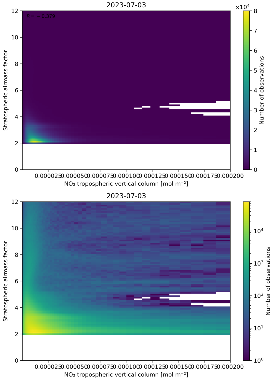
Figure 121: Scatter density plot of “NO 2 tropospheric vertical column” against “Stratospheric air mass factor” for 2023-07-03 to 2023-07-04.
