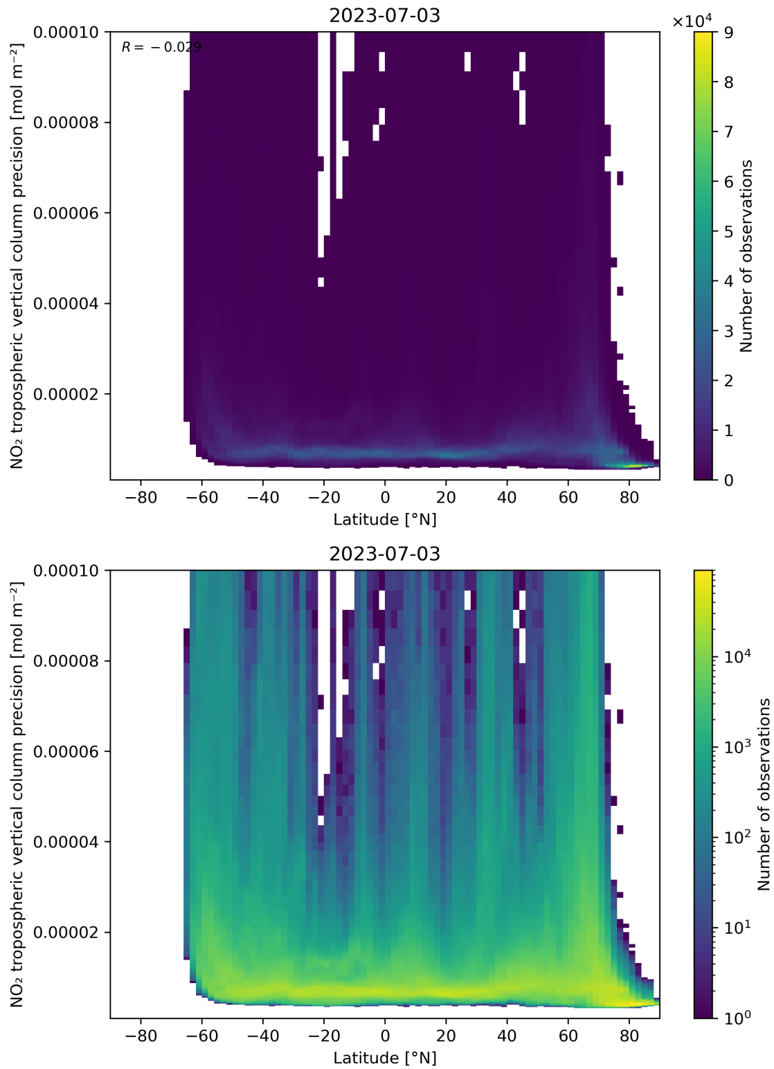
Figure 93: Scatter density plot of “Latitude” against “NO 2 tropospheric vertical column precision” for 2023-07-03 to 2023-07-04.
