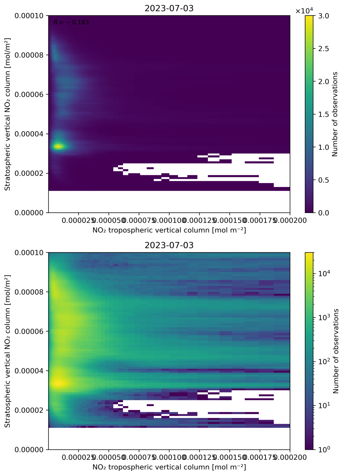
Figure 125: Scatter density plot of “NO 2 tropospheric vertical column” against “Stratospheric vertical NO 2 column” for 2023-07-03 to 2023-07-04.
