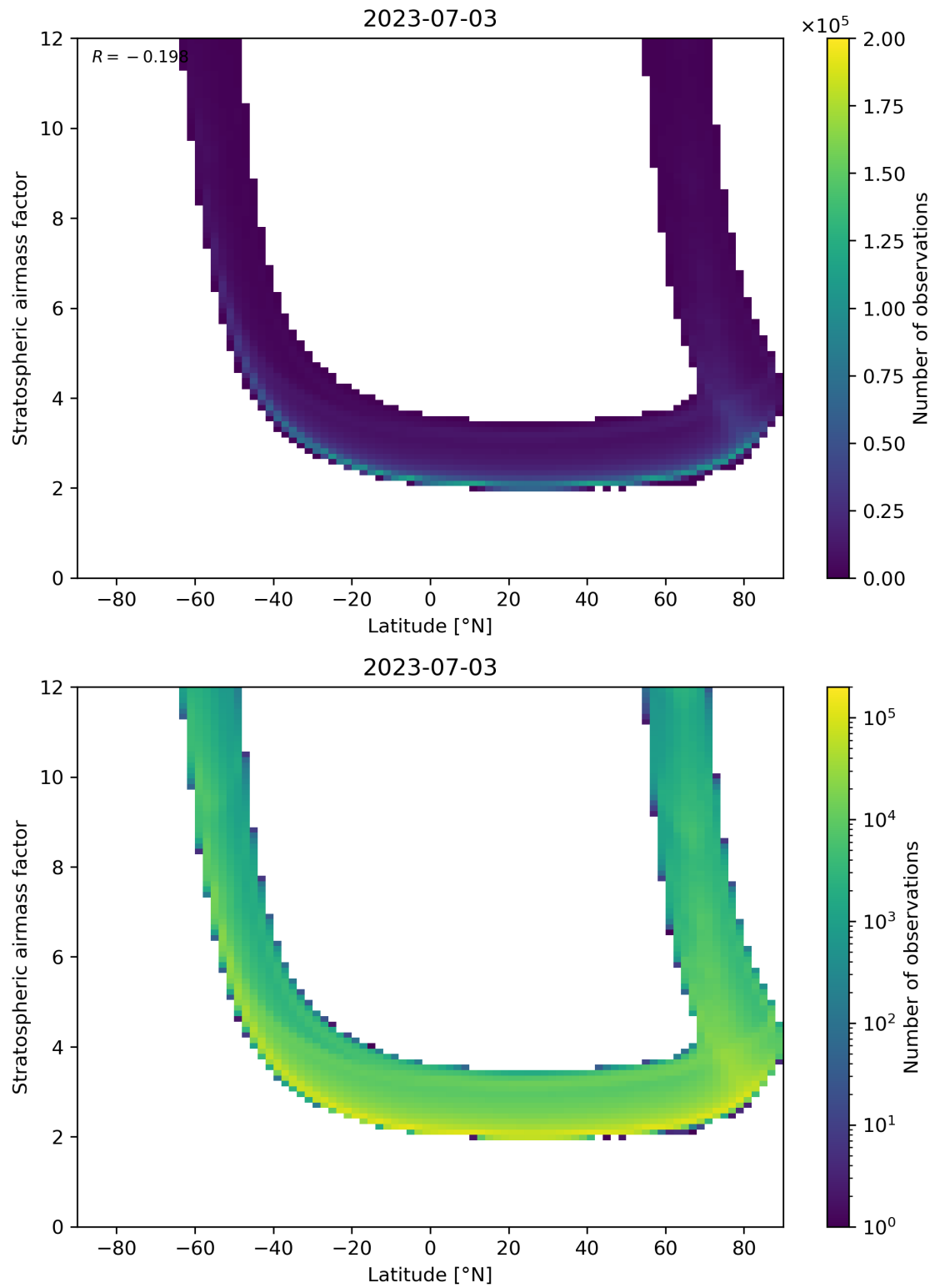
Figure 83: Scatter density plot of “Latitude” against “Stratospheric air mass factor” for 2023-07-03 to 2023-07-04.
