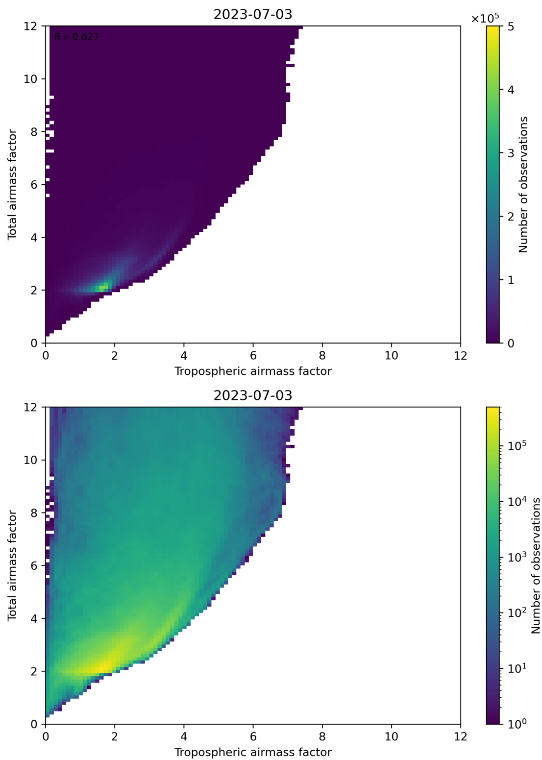
Figure 72: Scatter density plot of “Tropospheric airmass factor” against “Total airmass factor” for 2023-07-03 to 2023-07-04.
