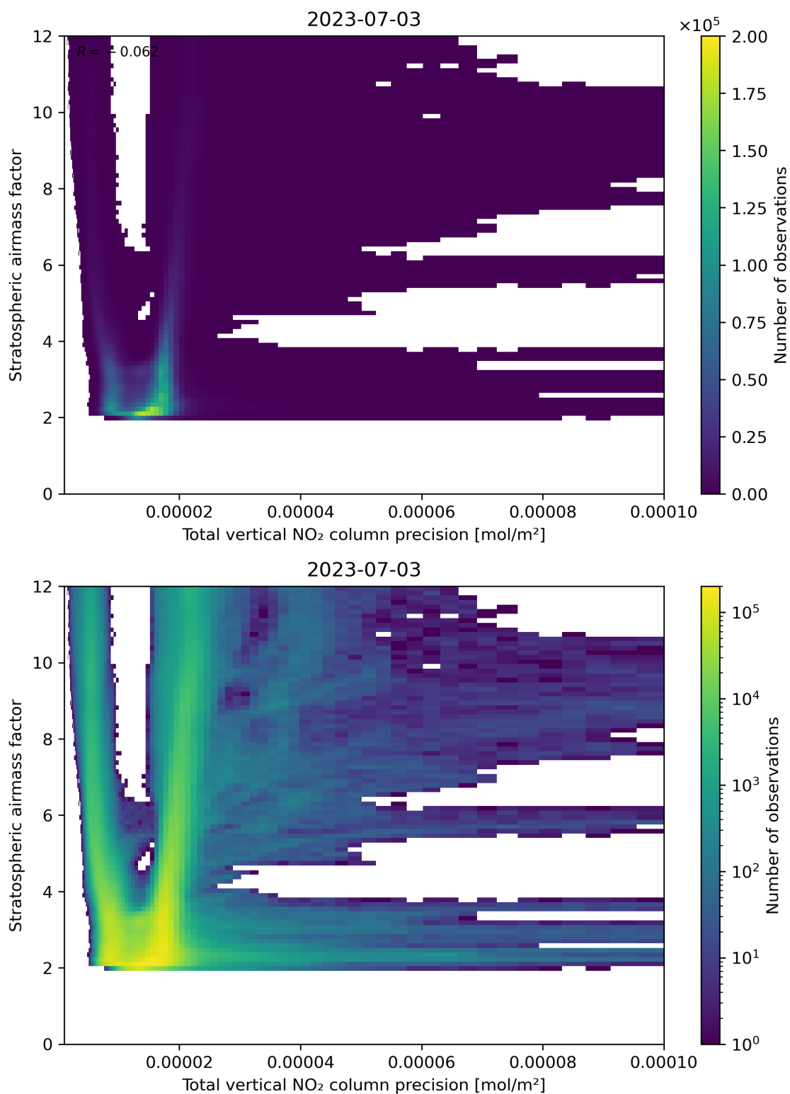
Figure 115: Scatter density plot of “Total vertical NO 2 column precision” against “Stratospheric air mass factor” for 2023-07-03 to 2023-07-04.
