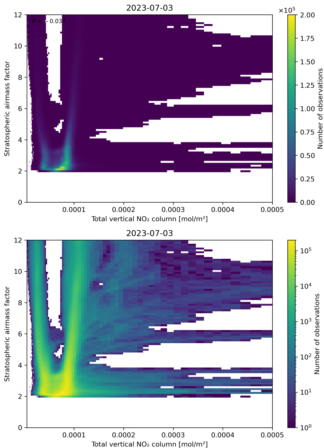
Figure 110: Scatter density plot of “Total vertical NO 2 column” against “Stratospheric airmass factor” for 2023-07-03 to 2023-07-04.
