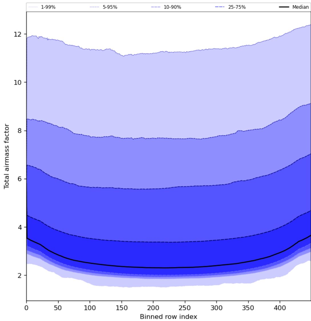
Figure 49: Along track statistics of “Total airmass factor” for 2023-07-03 to 2023-07-04
