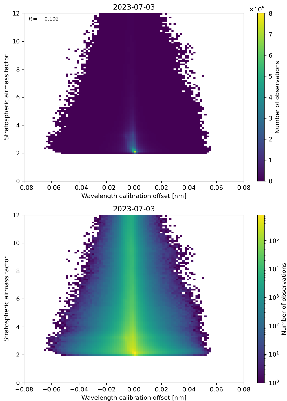
Figure 174: Scatter density plot of “Wavelength calibration offset” against “Stratospheric air mass factor” for 2023-07-03 to 2023-07-04.
