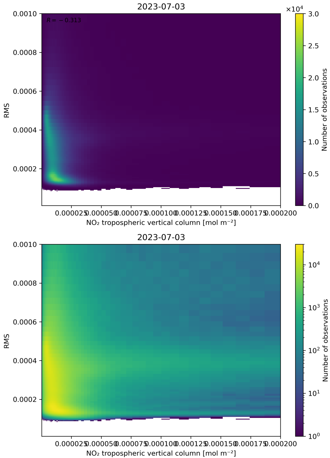
Figure 142: Scatter density plot of “NO 2 tropospheric vertical column” against “RMS” for 2023-07-03 to 2023-07-04.
