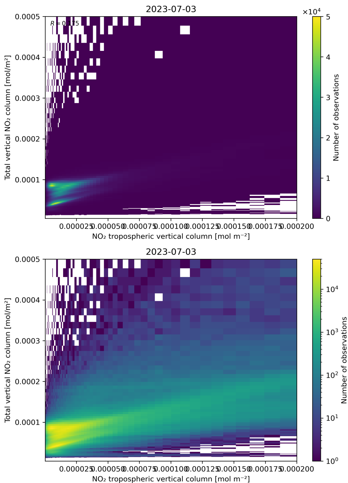
Figure 128: Scatter density plot of “NO 2 tropospheric vertical column” against “Total vertical NO 2 column” for 2023-07-03 to 2023-07-04.
