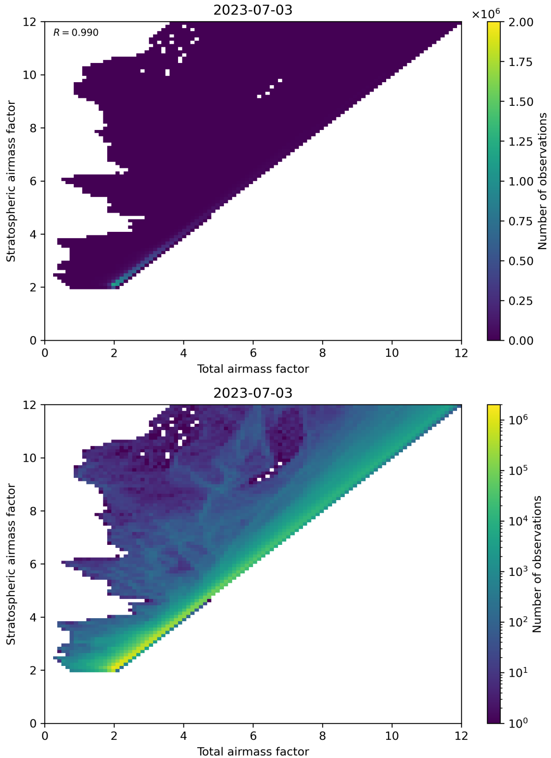
Figure 62: Scatter density plot of “Total airmass factor” against “Stratospheric airmass factor” for 2023-07-03 to 2023-07-04.
