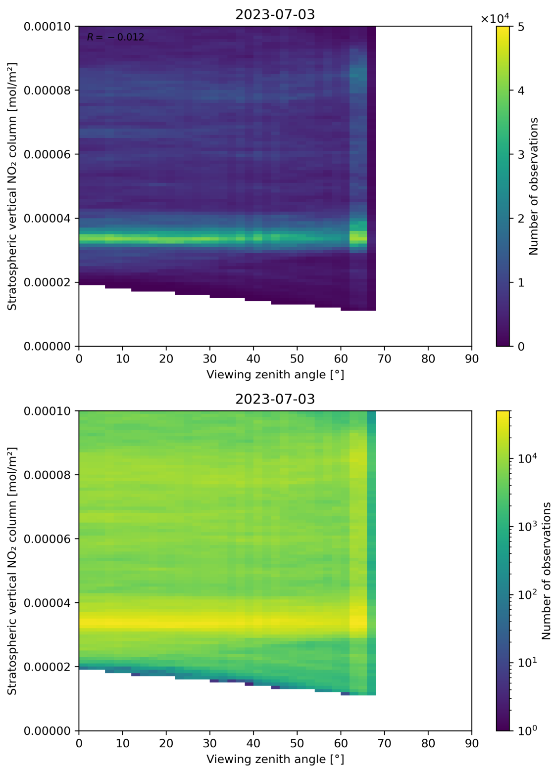
Figure 164: Scatter density plot of “Viewing zenith angle” against “Stratospheric vertical NO 2 column” for 2023-07-03 to 2023-07-04.
