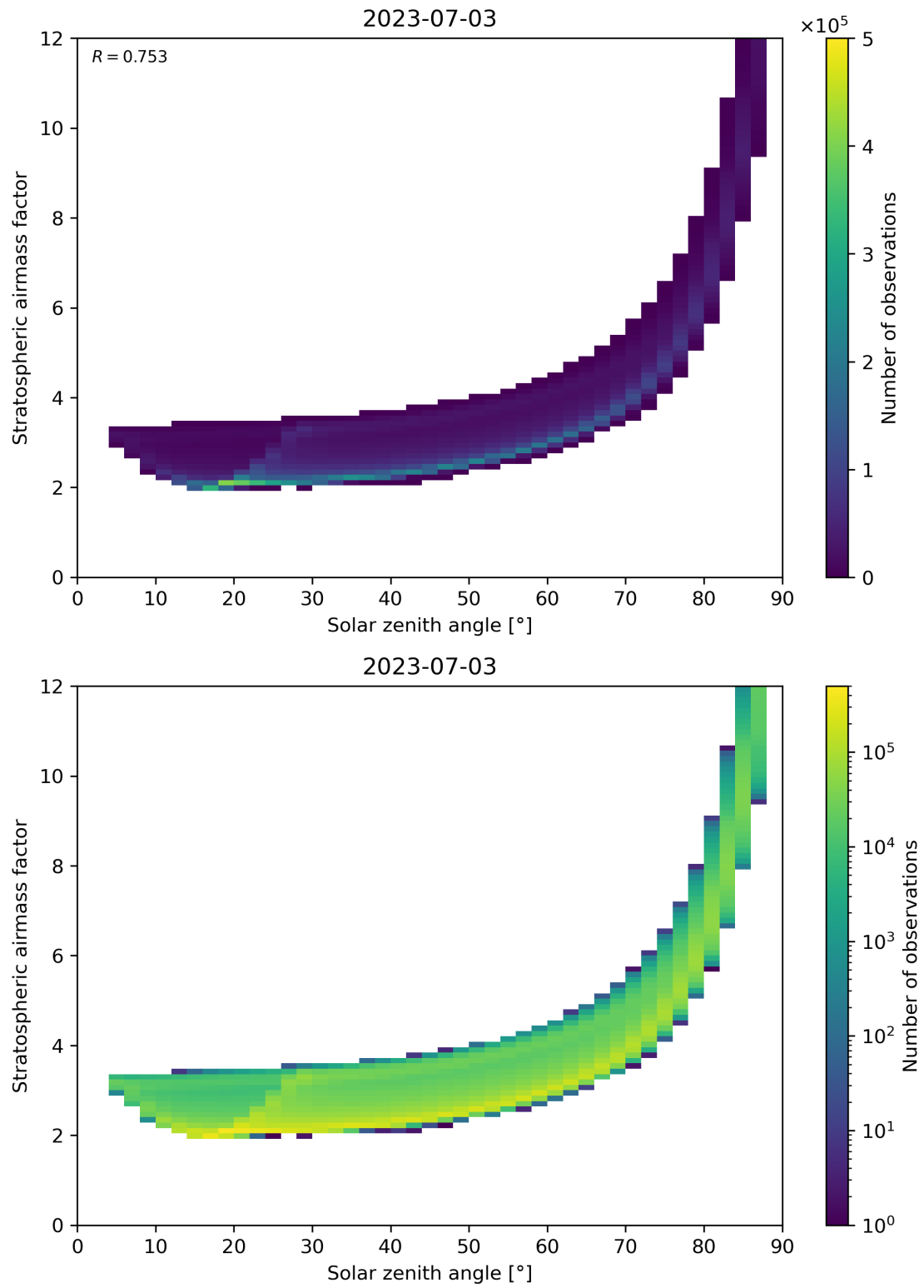
Figure 145: Scatter density plot of “Solar zenith angle” against “Stratospheric airmass factor” for 2023-07-03 to 2023-07-04.
