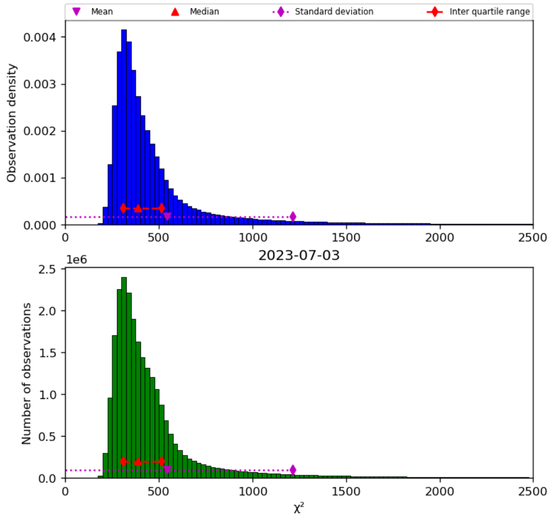
Figure 42: Histogram of “ \chi^2 ” for 2023-07-03 to 2023-07-04
