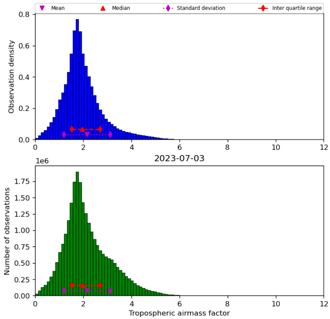
Figure 31: Histogram of “Tropospheric airmass factor” for 2023-07-03 to 2023-07-04
