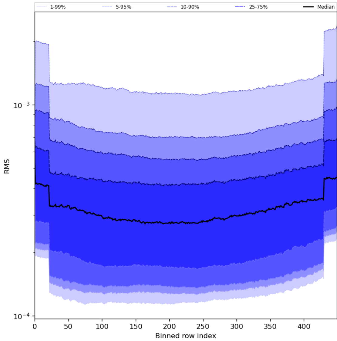
Figure 60: Along track statistics of “RMS” for 2023-07-03 to 2023-07-04
