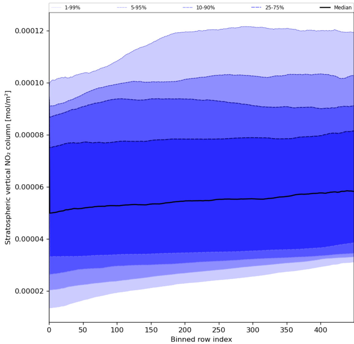
Figure 53: Along track statistics of “Stratospheric vertical NO 2 column” for 2023-07-03 to 2023-07-04
