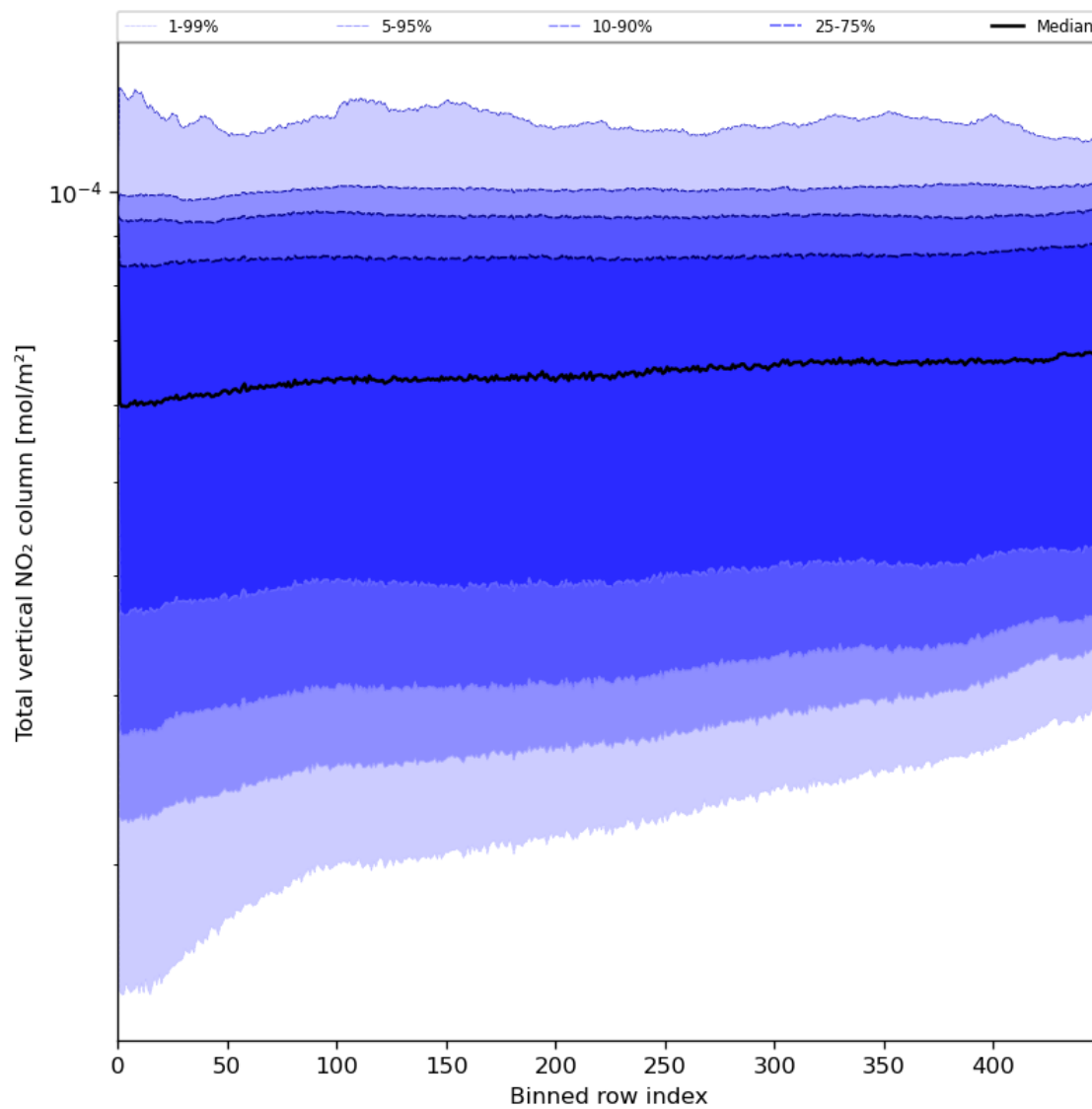
Figure 55: Along track statistics of “Total vertical NO 2 column” for 2023-07-03 to 2023-07-04
