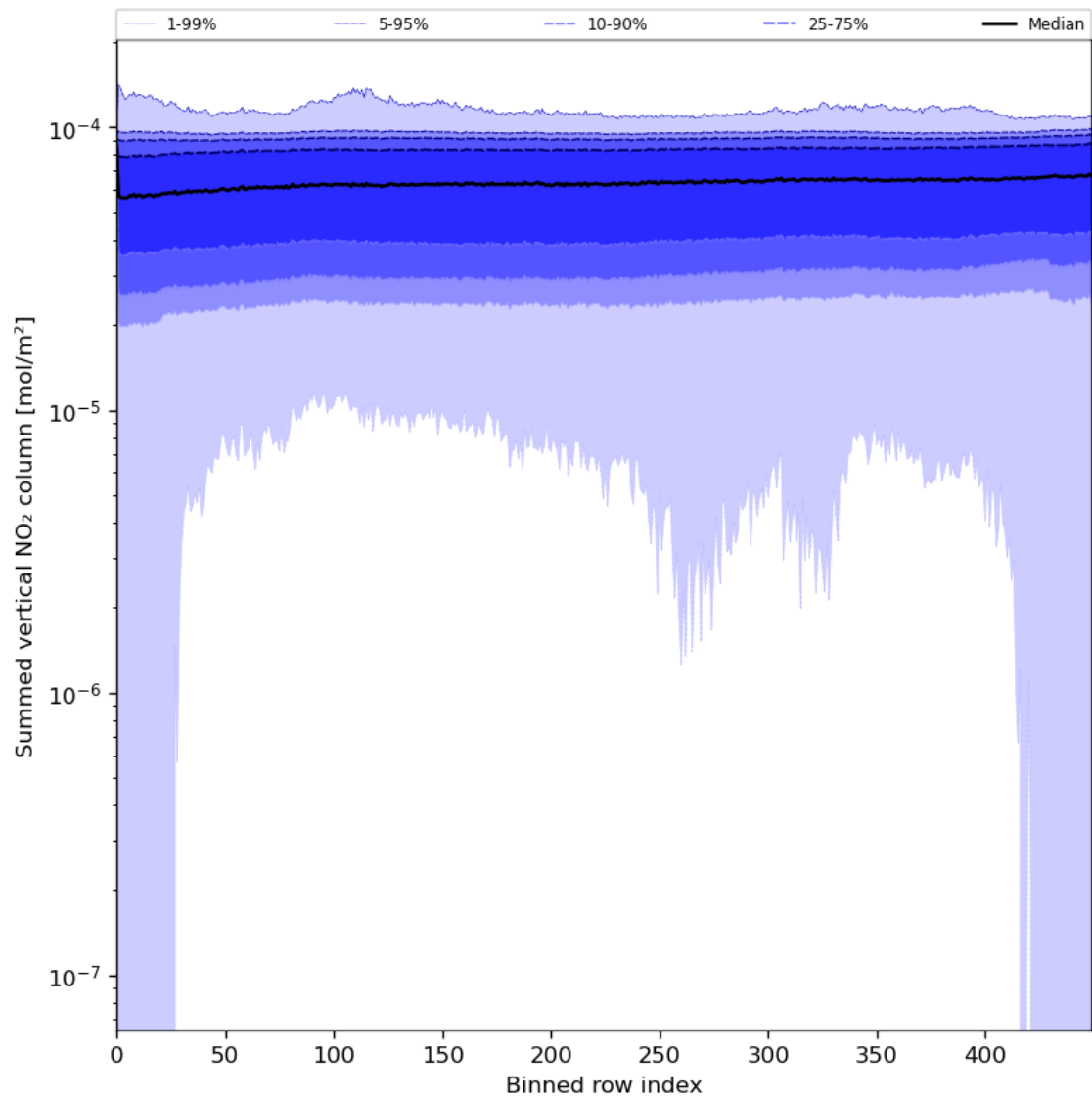
Figure 57: Along track statistics of “Summed vertical NO 2 column” for 2023-07-03 to 2023-07-04
