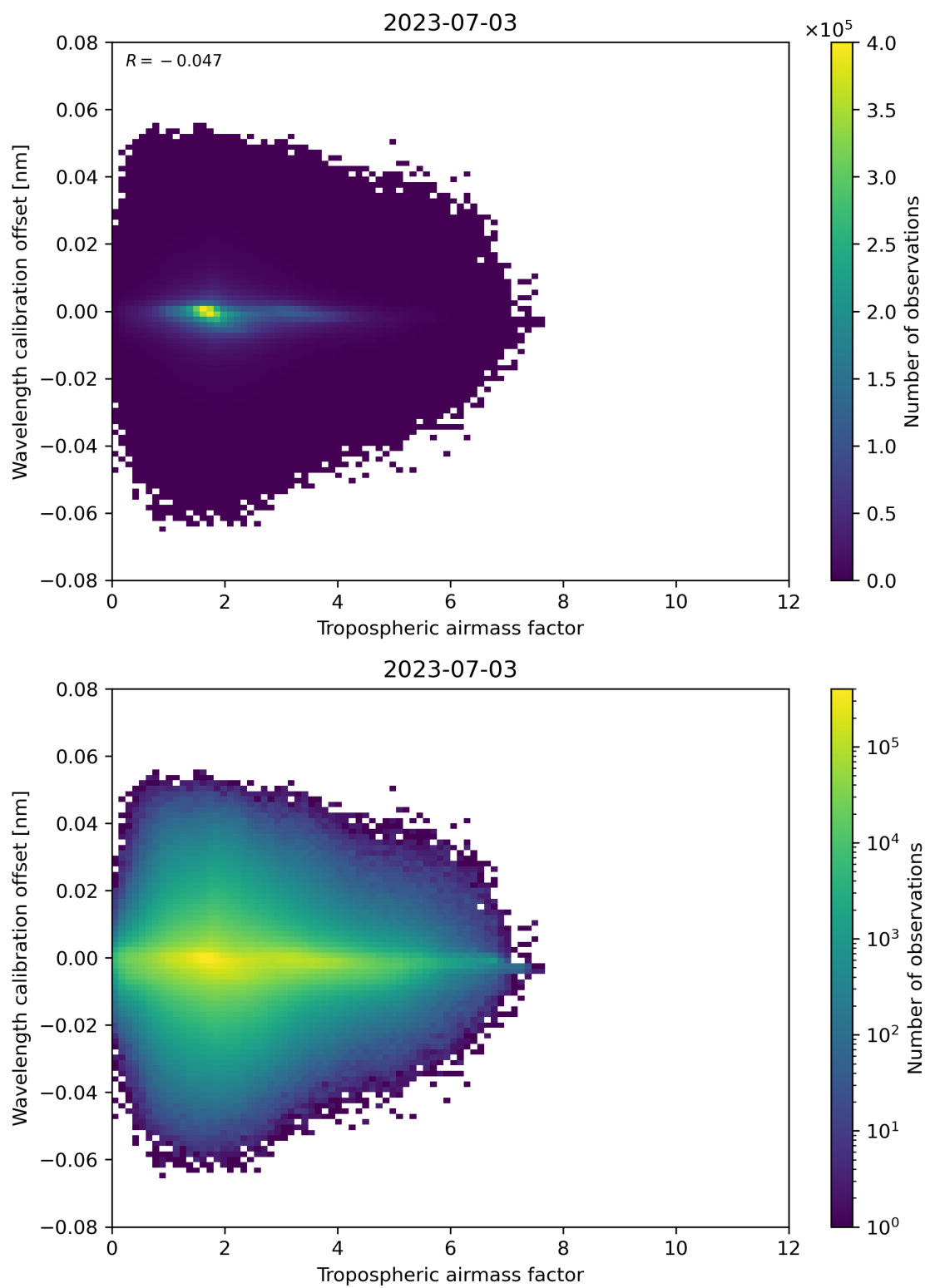
Figure 80: Scatter density plot of “Tropospheric airmass factor” against “Wavelength calibration offset” for 2023-07-03 to 2023-07-04.
