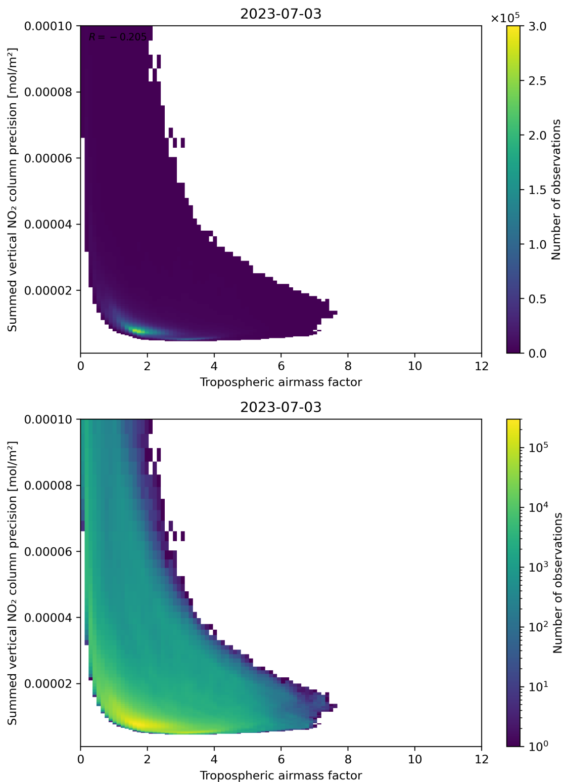
Figure 76: Scatter density plot of “Tropospheric air mass factor” against “Summed vertical NO 2 column precision” for 2023-07-03 to 2023-07-04.
