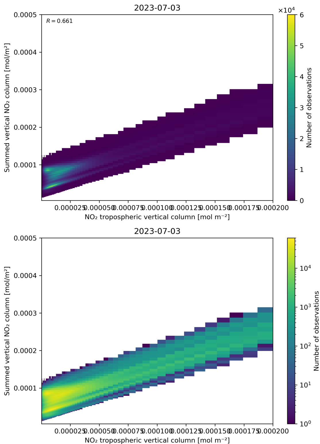
Figure 126: Scatter density plot of “NO 2 tropospheric vertical column” against “Summed vertical NO 2 column” for 2023-07-03 to 2023-07-04.
