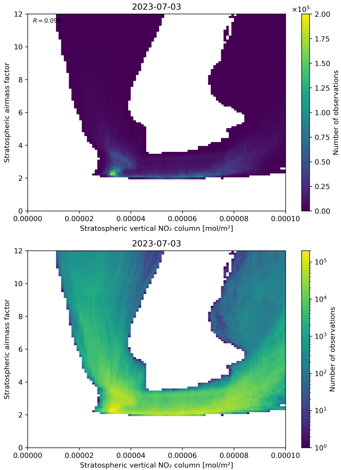
Figure 96: Scatter density plot of “Stratospheric vertical NO 2 column” against “Stratospheric airmass factor” for 2023-07-03 to 2023-07-04.
