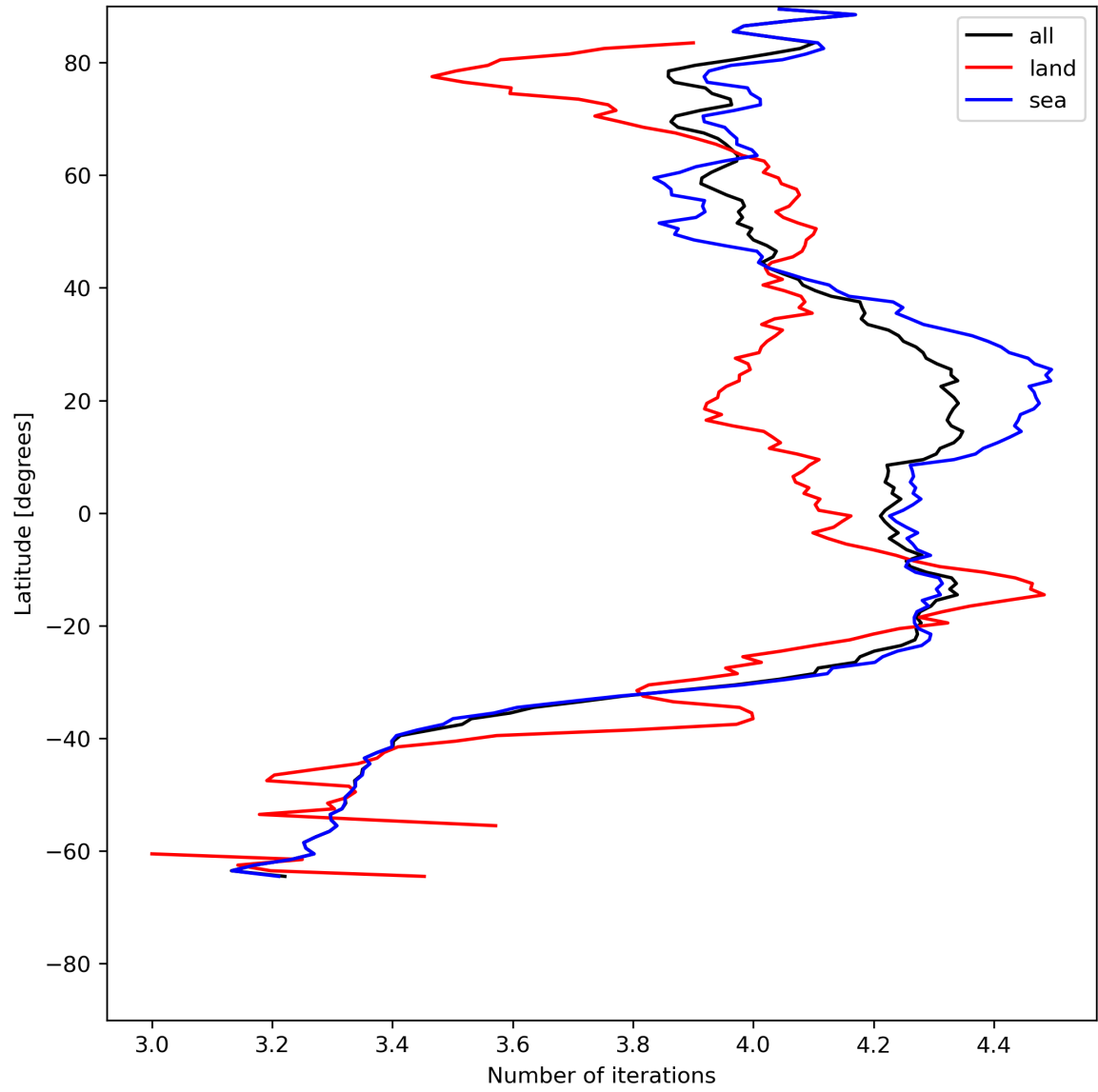
Figure 17: Zonal average of “Number of iterations” for 2023-07-03 to 2023-07-04.
