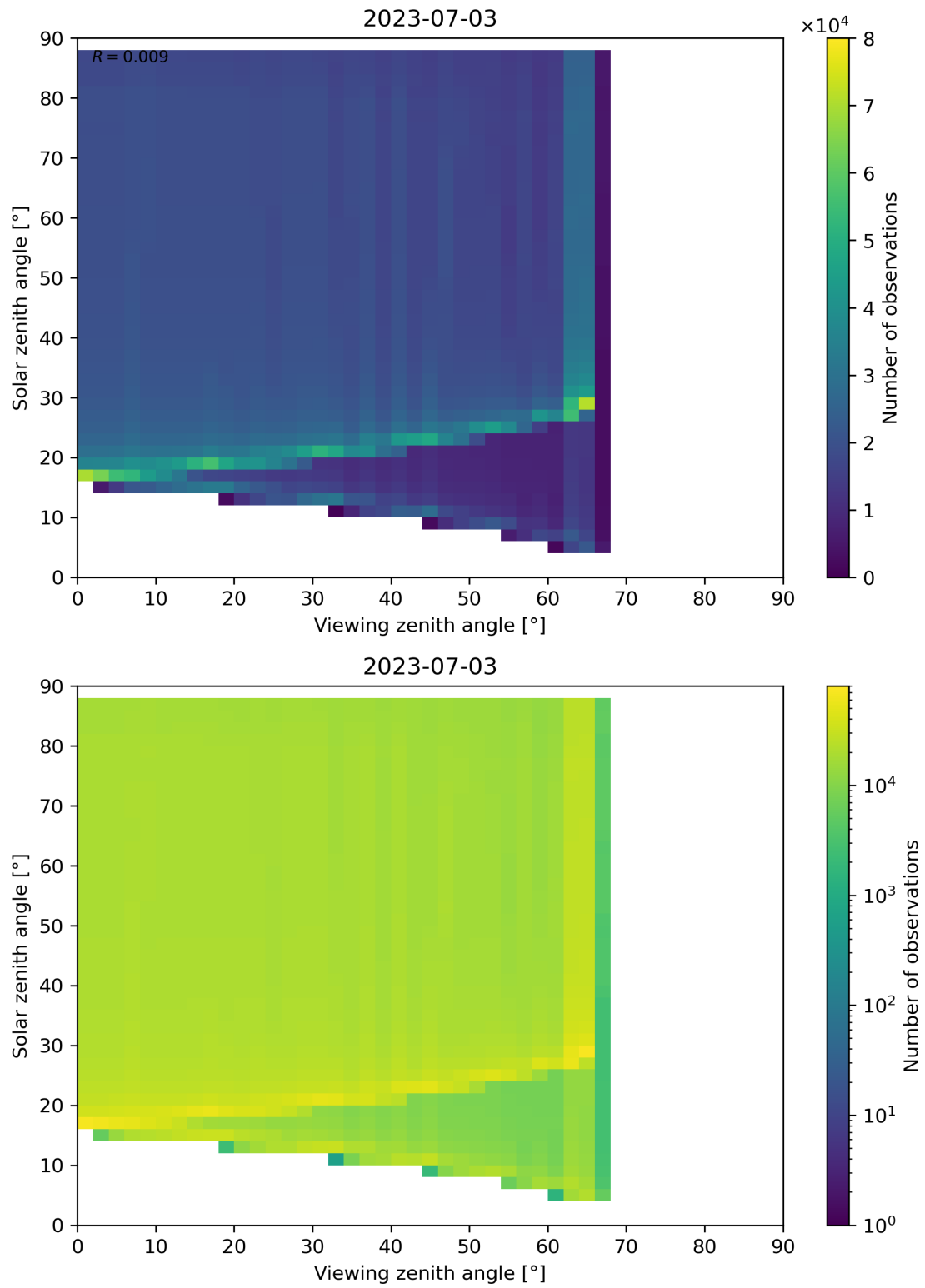
Figure 172: Scatter density plot of “Viewing zenith angle” against “Solar zenith angle” for 2023-07-03 to 2023-07-04.
