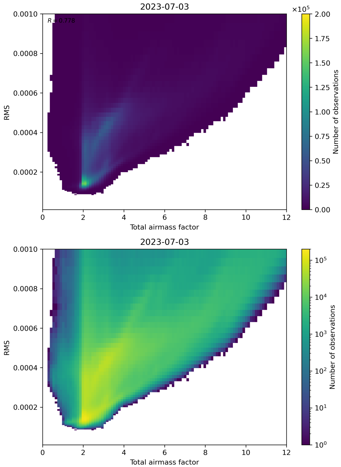
Figure 69: Scatter density plot of “Total airmass factor” against “RMS” for 2023-07-03 to 2023-07-04.
