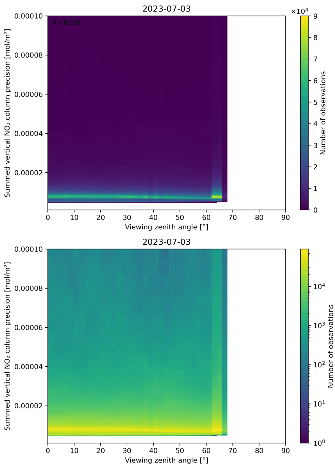
Figure 166: Scatter density plot of “Viewing zenith angle” against “Summed vertical NO 2 column precision” for 2023-07-03 to 2023-07-04.
