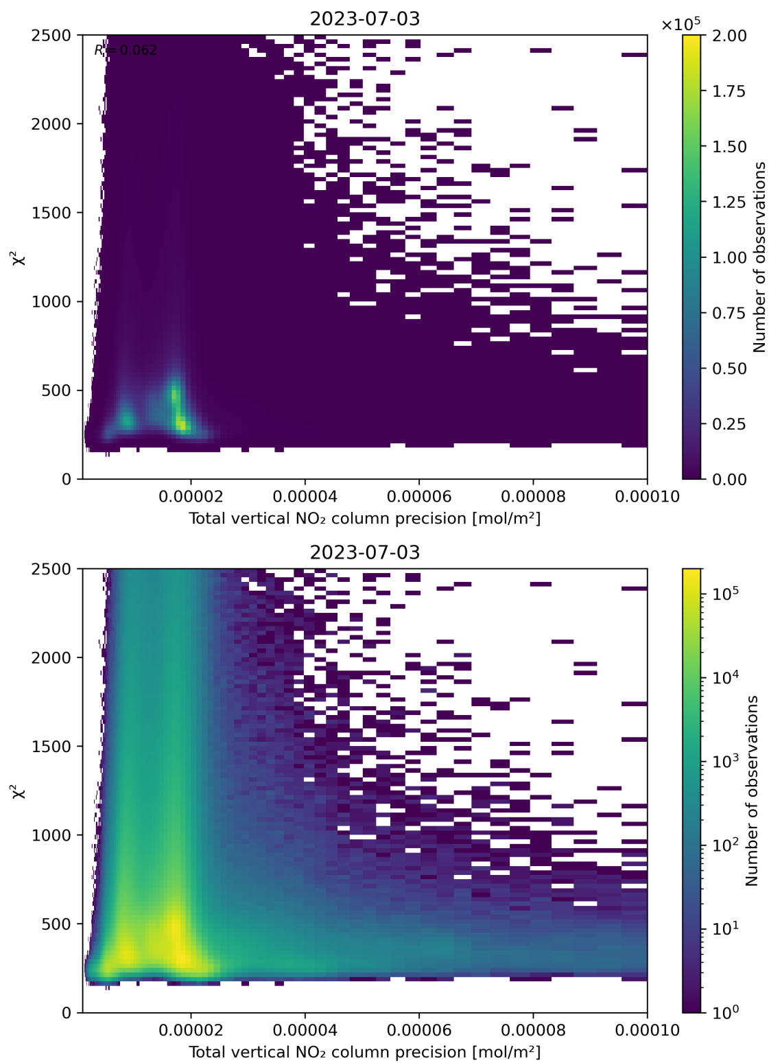
Figure 116: Scatter density plot of “Total vertical NO 2 column precision” against “ \chi^2 ” for 2023-07-03 to 2023-07-04.
