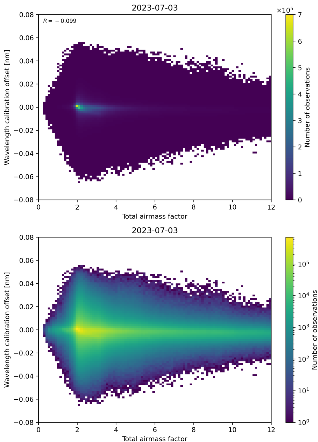
Figure 70: Scatter density plot of “Total airmass factor” against “Wavelength calibration offset” for 2023-07-03 to 2023-07-04.
