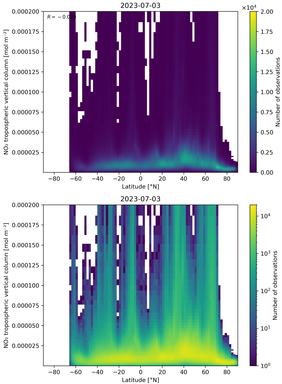
Figure 92: Scatter density plot of “Latitude” against “NO 2 tropospheric vertical column” for 2023-07-03 to 2023-07-04.
