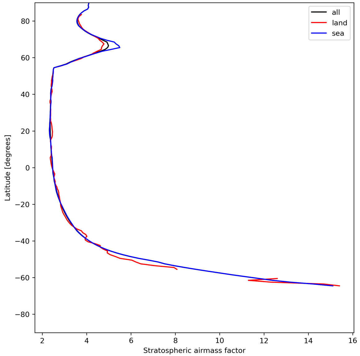
Figure 27: Zonal average of “Stratospheric airmass factor” for 2023-07-03 to 2023-07-04.
