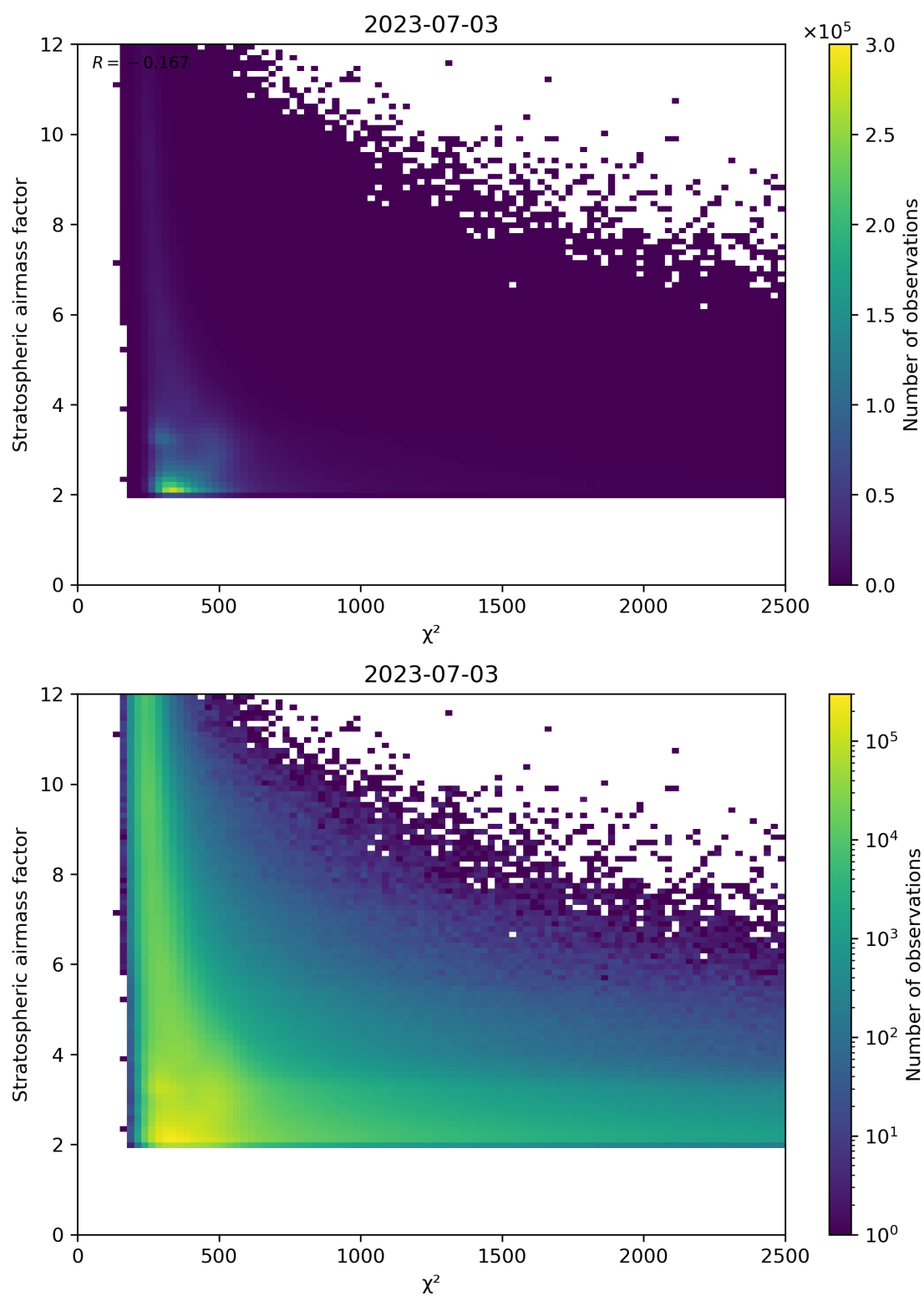
Figure 81: Scatter density plot of “ \chi^2 ” against “Stratospheric airmass factor” for 2023-07-03 to 2023-07-04.
