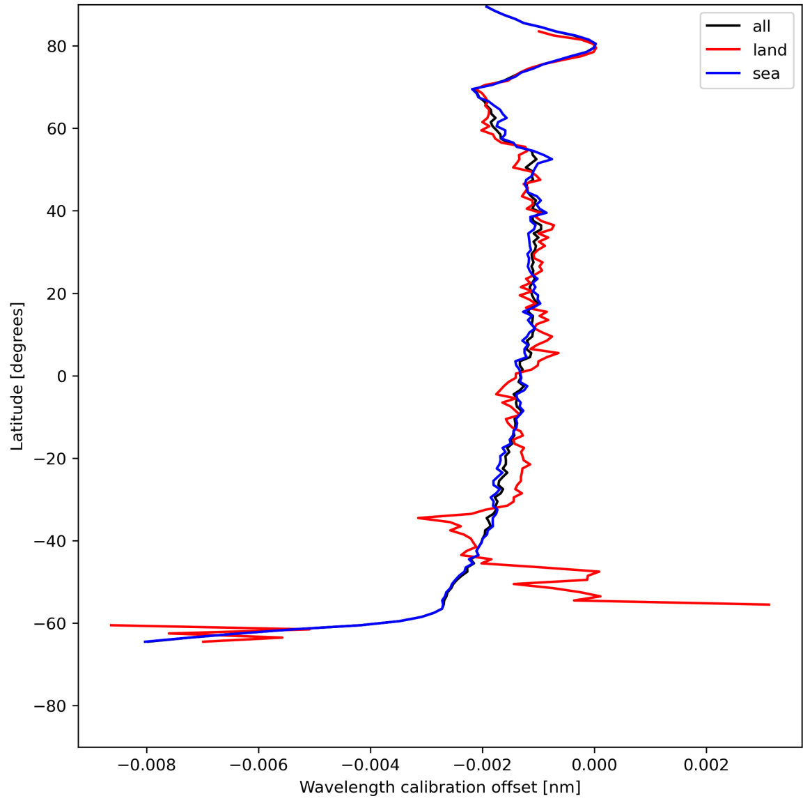
Figure 18: Zonal average of “Wavelength calibration offset” for 2023-07-03 to 2023-07-04.
