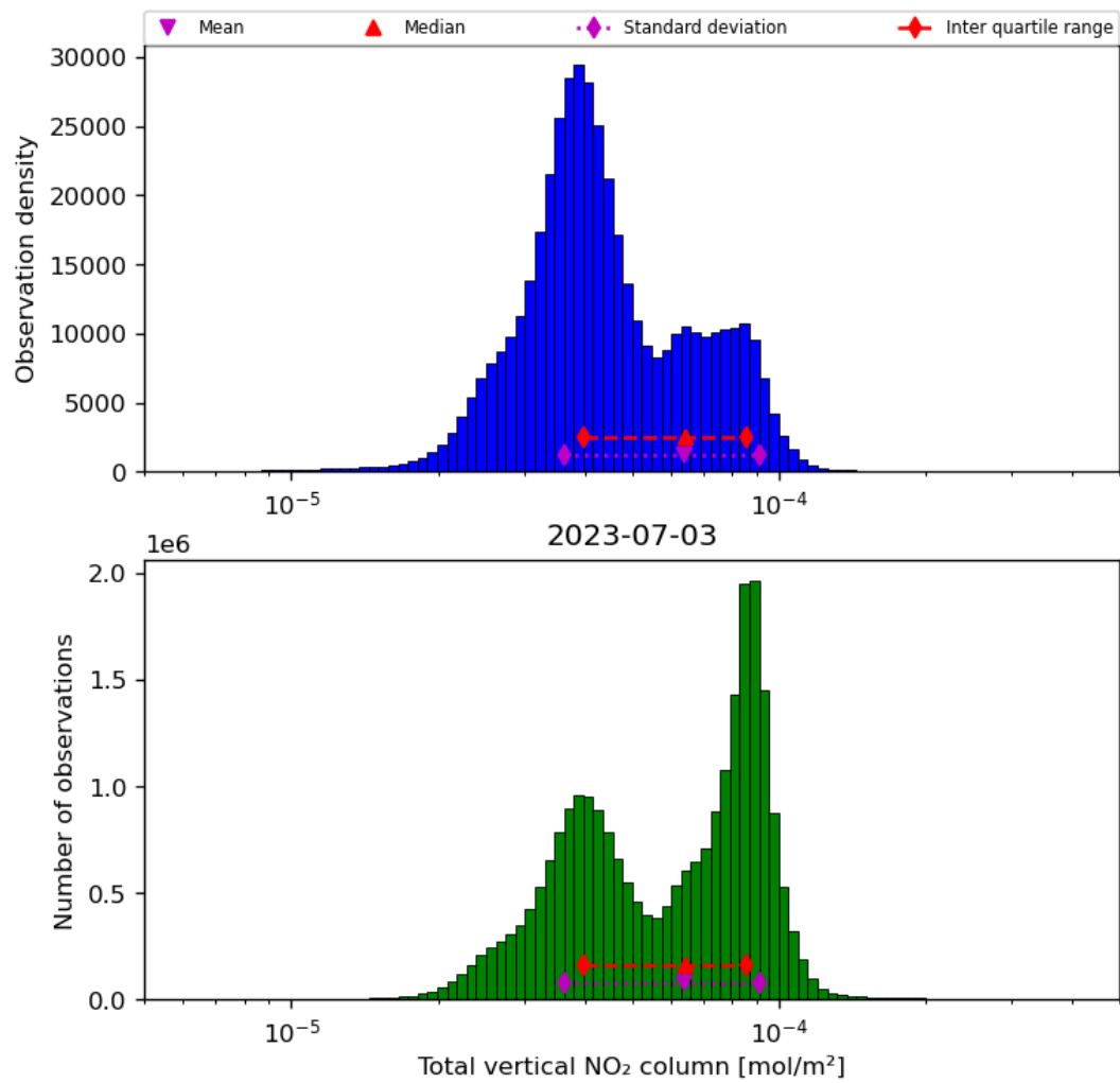
Figure 38: Histogram of “Total vertical NO 2 column” for 2023-07-03 to 2023-07-04
