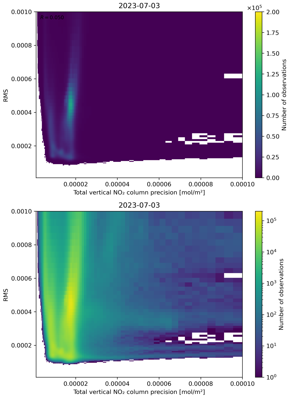
Figure 119: Scatter density plot of “Total vertical NO 2 column precision” against “RMS” for 2023-07-03 to 2023-07-04.
