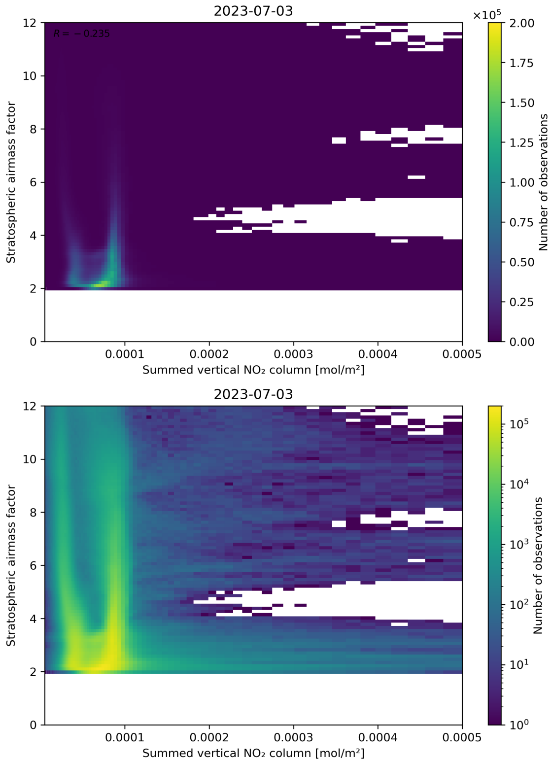
Figure 103: Scatter density plot of “Summed vertical NO 2 column” against “Stratospheric air mass factor” for 2023-07-03 to 2023-07-04.
