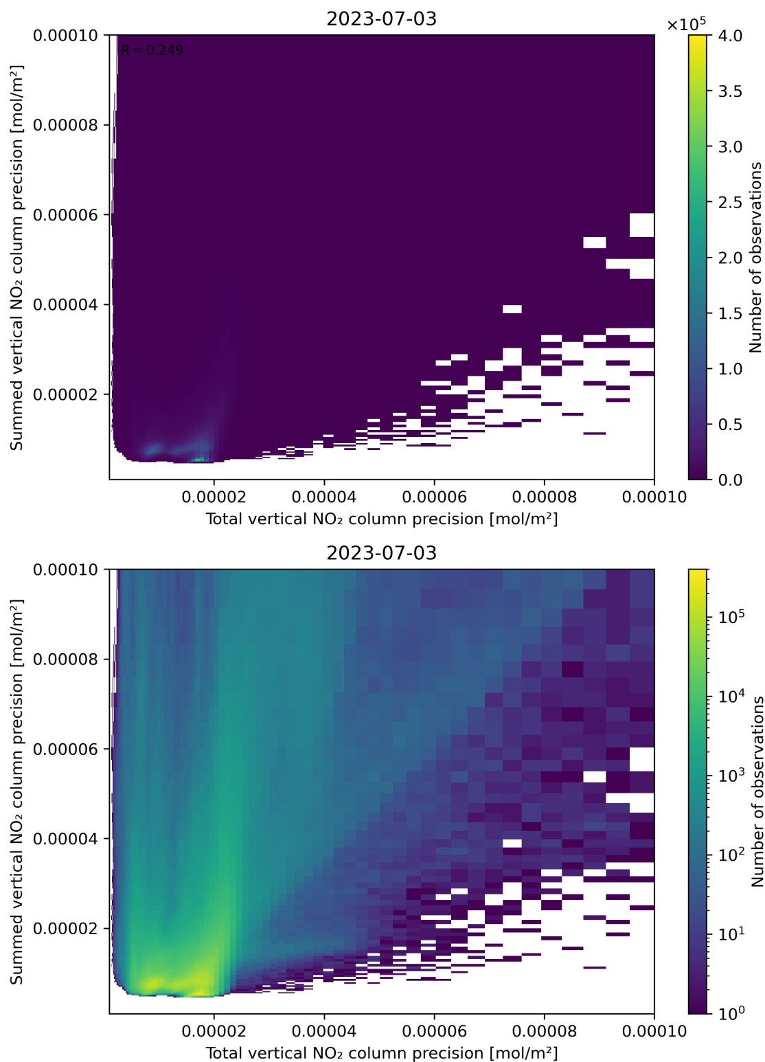
Figure 118: Scatter density plot of “Total vertical NO 2 column precision” against “Summed vertical NO 2 column precision” for 2023-07-03 to 2023-07-04.
