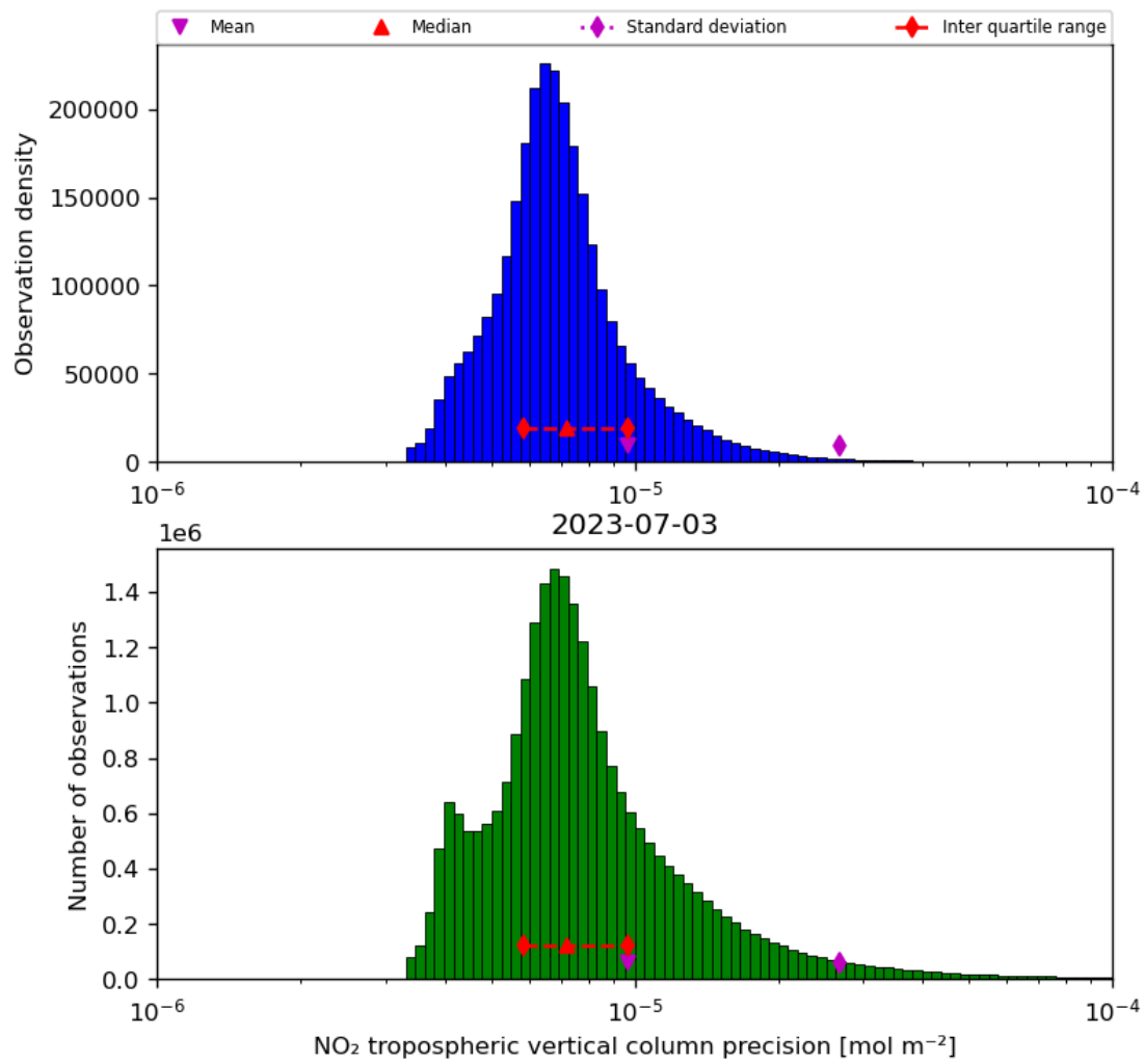
Figure 30: Histogram of “NO 2 tropospheric vertical column precision” for 2023-07-03 to 2023-07-04
