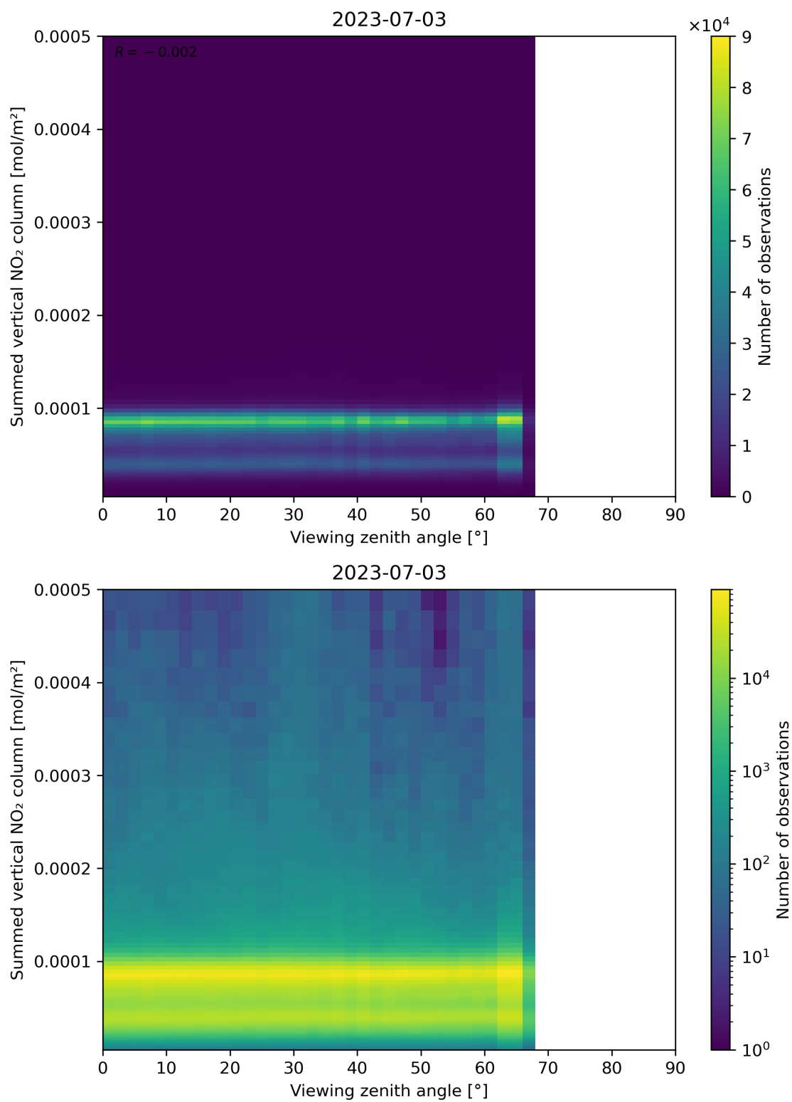
Figure 165: Scatter density plot of “Viewing zenith angle” against “Summed vertical NO 2 column” for 2023-07-03 to 2023-07-04.
