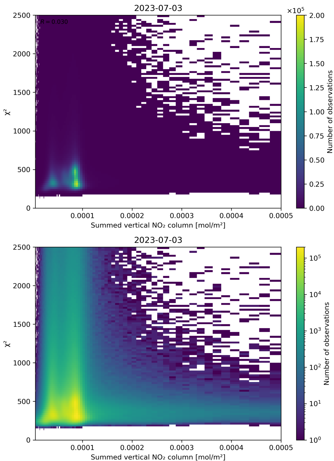
Figure 104: Scatter density plot of “Summed vertical NO 2 column” against “ \chi^2 ” for 2023-07-03 to 2023-07-04.
