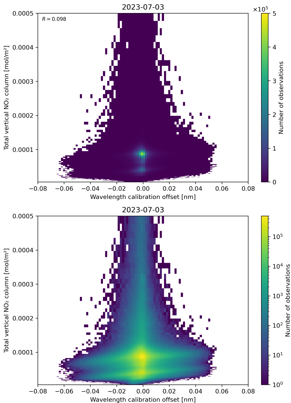
Figure 179: Scatter density plot of “Wavelength calibration offset” against “Total vertical NO 2 column” for 2023-07-03 to 2023-07-04.
