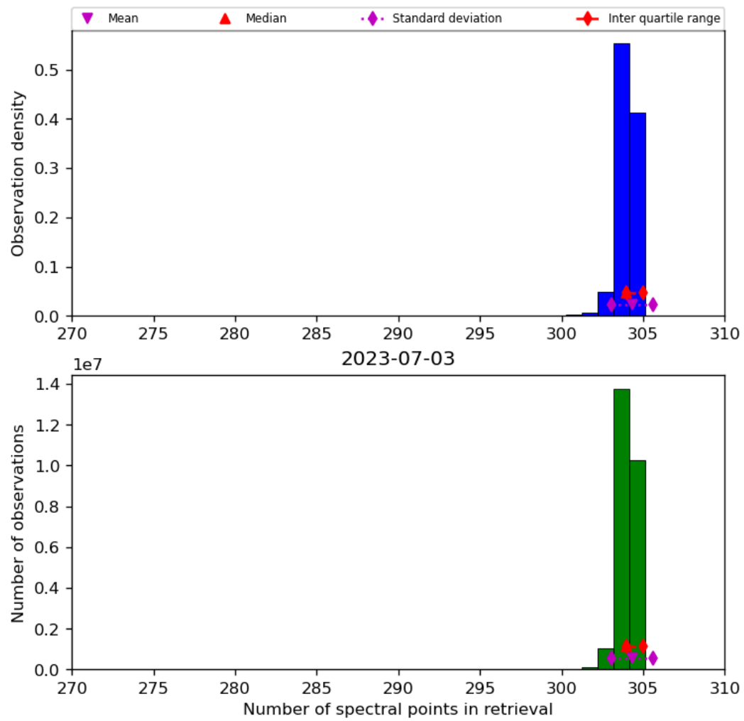
Figure 33: Histogram of “Number of spectral points in retrieval” for 2023-07-03 to 2023-07-04
