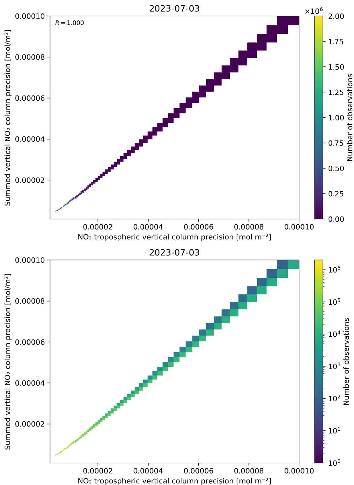
Figure 137: Scatter density plot of “NO 2 tropospheric vertical column precision” against “Summed vertical NO 2 column precision” for 2023-07-03 to 2023-07-04.
