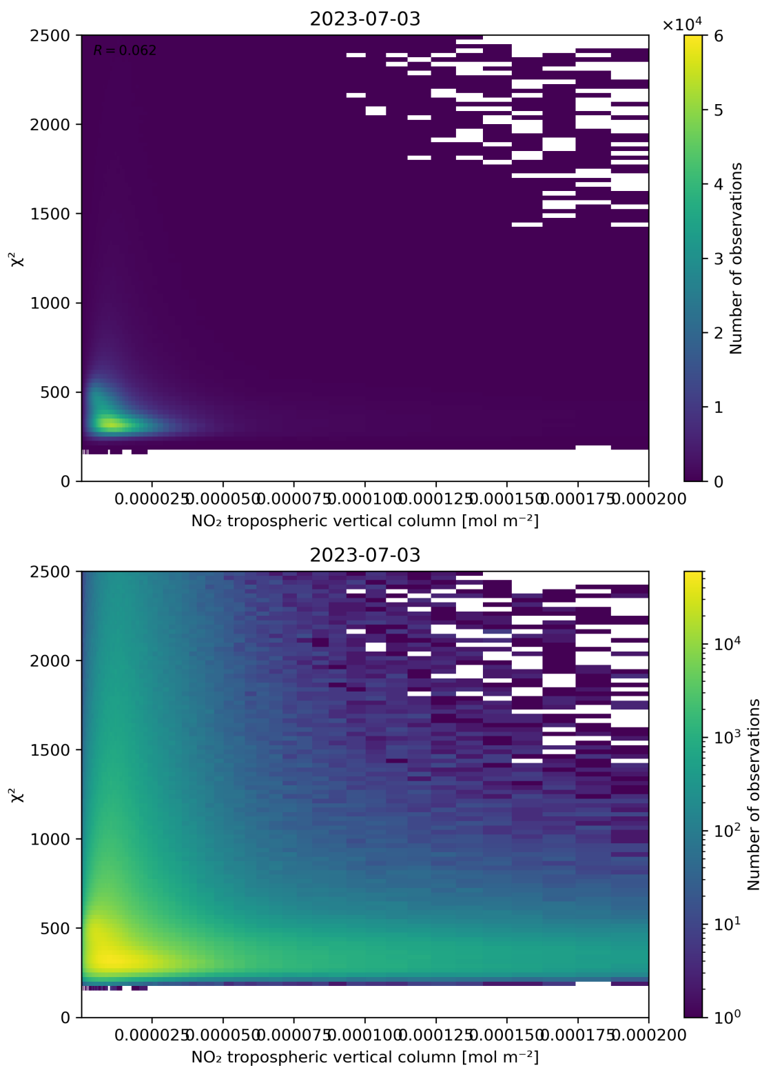
Figure 124: Scatter density plot of “NO 2 tropospheric vertical column” against “ \chi^2 ” for 2023-07-03 to 2023-07-04.
