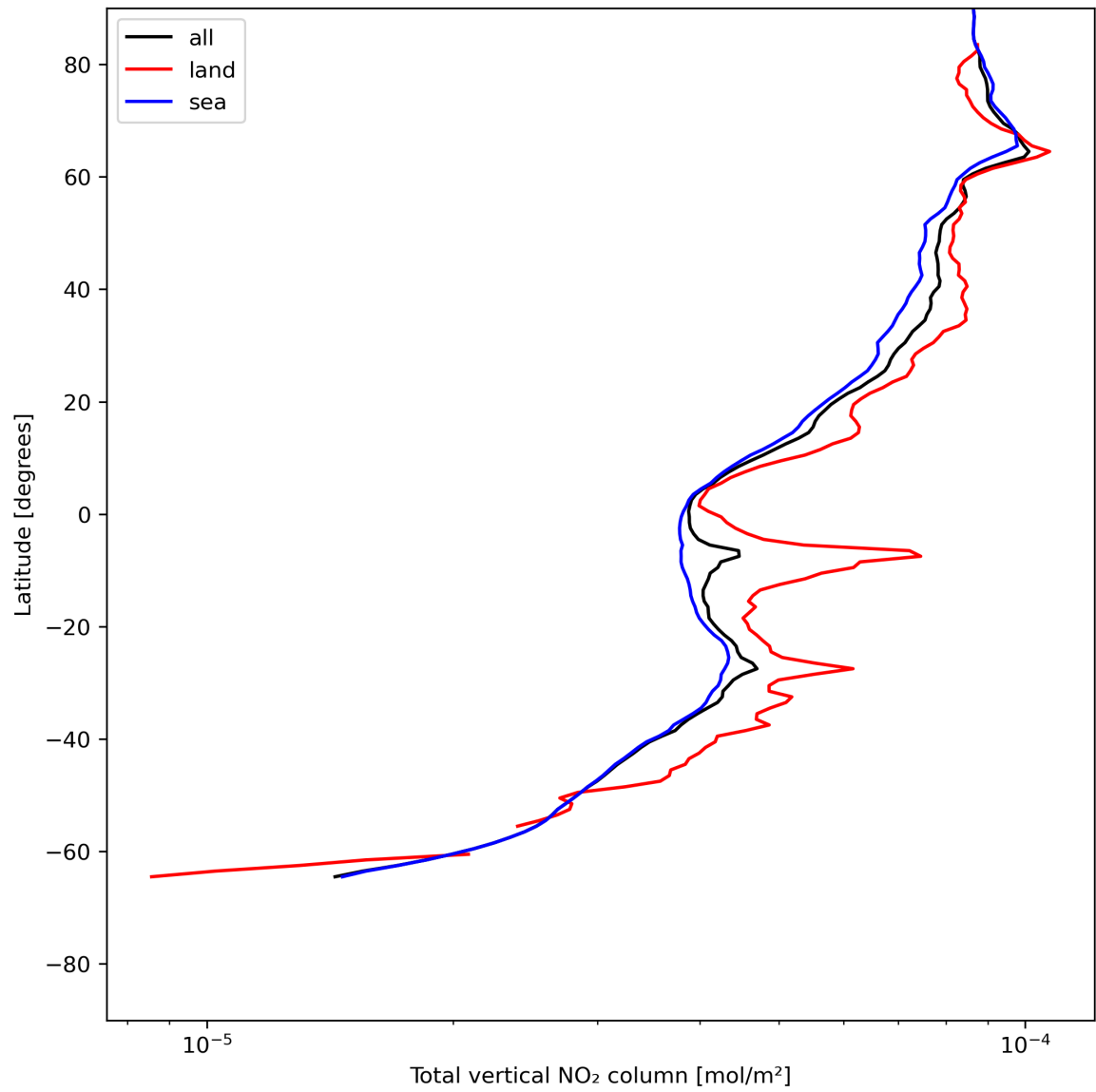
Figure 21: Zonal average of “Total vertical NO 2 column” for 2023-07-03 to 2023-07-04.
