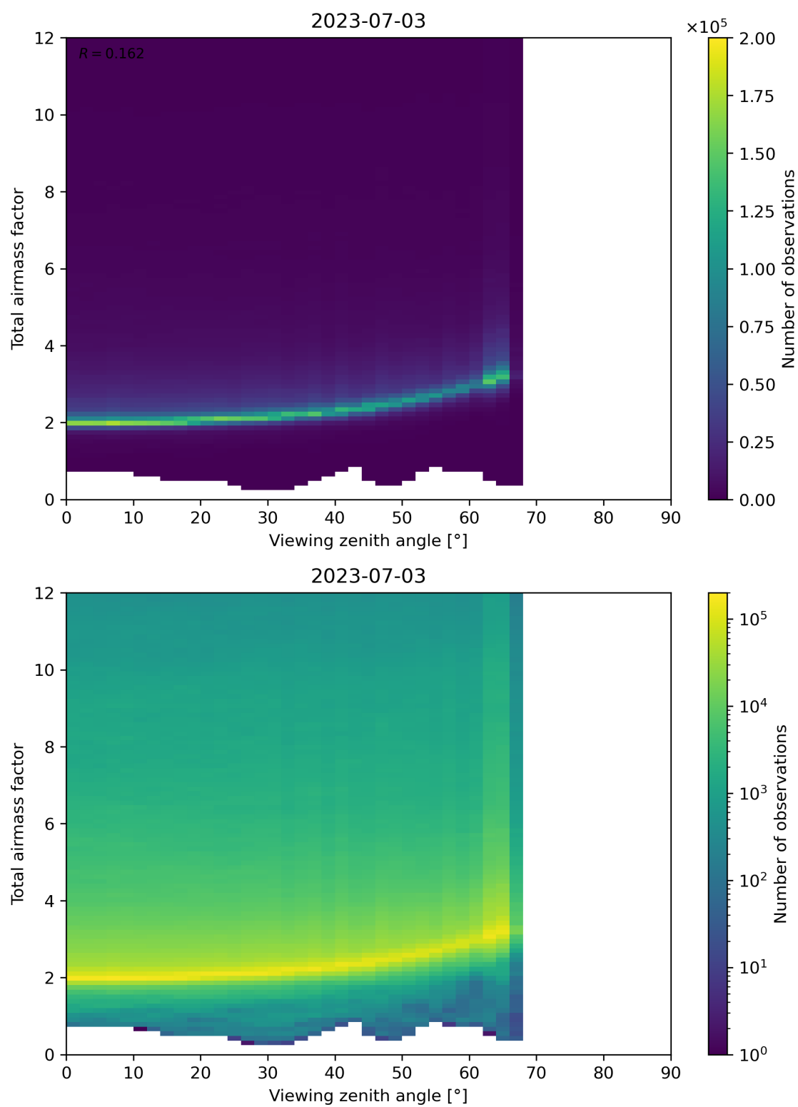
Figure 160: Scatter density plot of “Viewing zenith angle” against “Total airmass factor” for 2023-07-03 to 2023-07-04.
