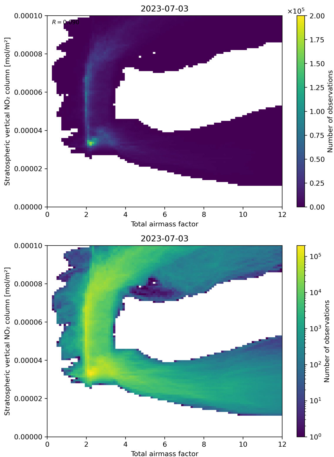
Figure 64: Scatter density plot of “Total airmass factor” against “Stratospheric vertical NO 2 column” for 2023-07-03 to 2023-07-04.
