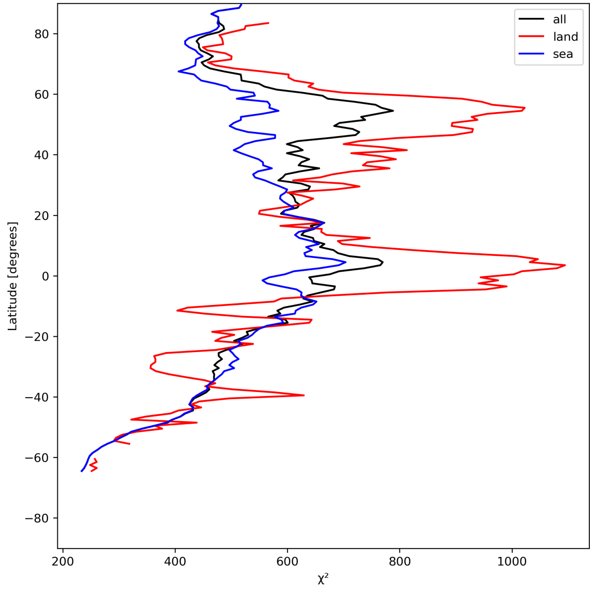
Figure 25: Zonal average of “ \chi^2 ” for 2023-07-03 to 2023-07-04.
