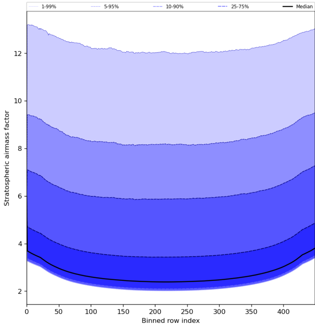
Figure 61: Along track statistics of “Stratospheric airmass factor” for 2023-07-03 to 2023-07-04
