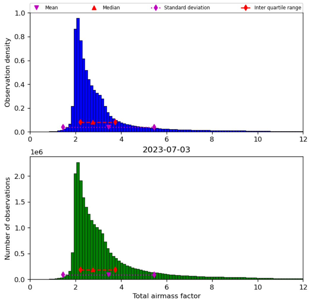
Figure 32: Histogram of “Total airmass factor” for 2023-07-03 to 2023-07-04
