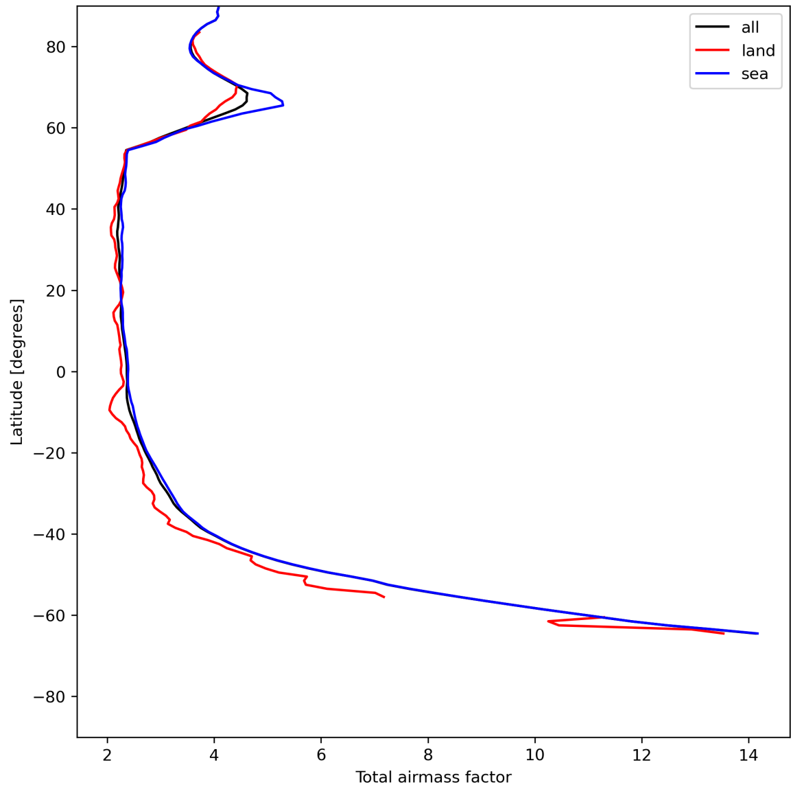
Figure 15: Zonal average of “Total airmass factor” for 2023-07-03 to 2023-07-04.
