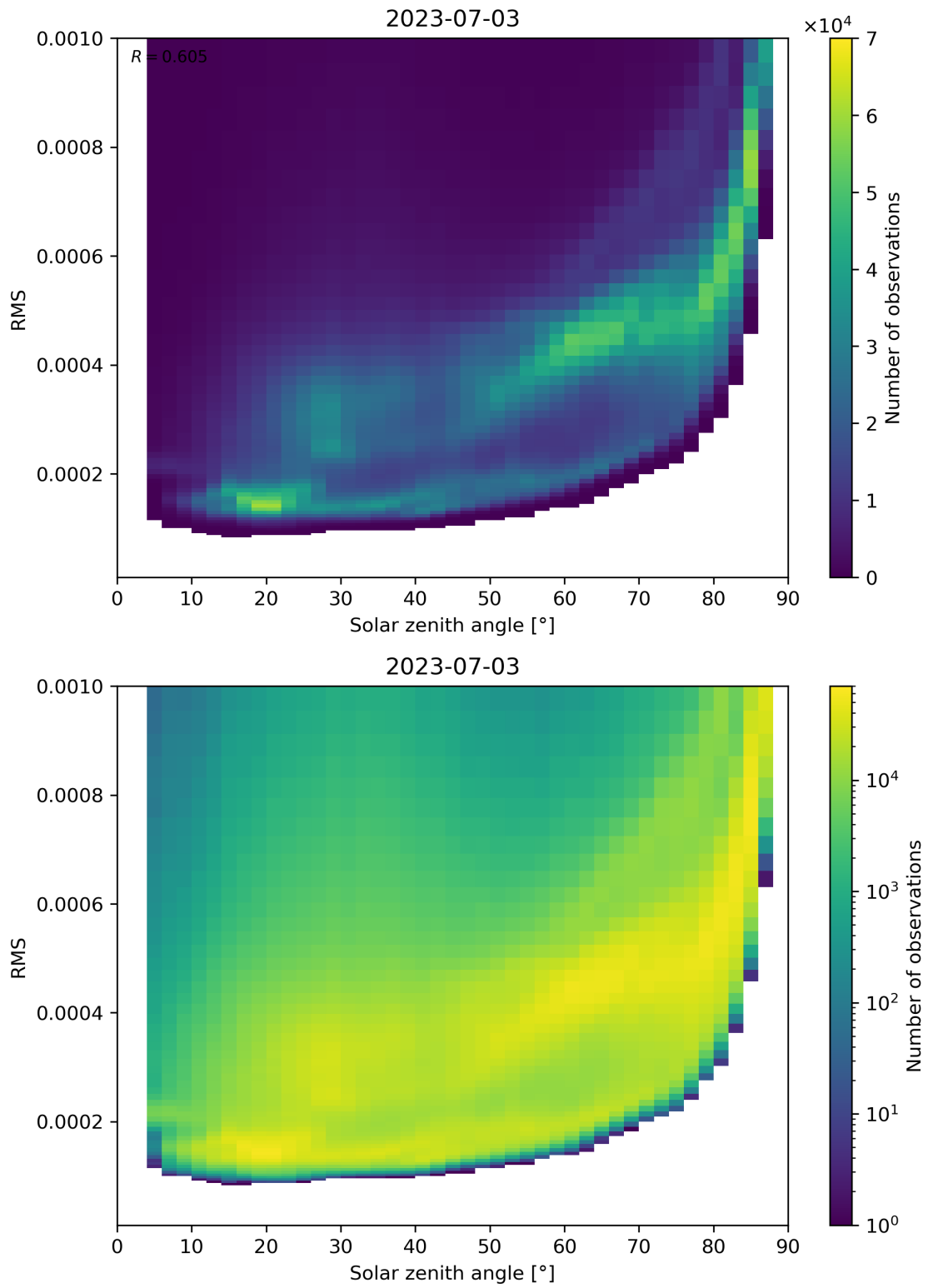
Figure 157: Scatter density plot of “Solar zenith angle” against “RMS” for 2023-07-03 to 2023-07-04.
