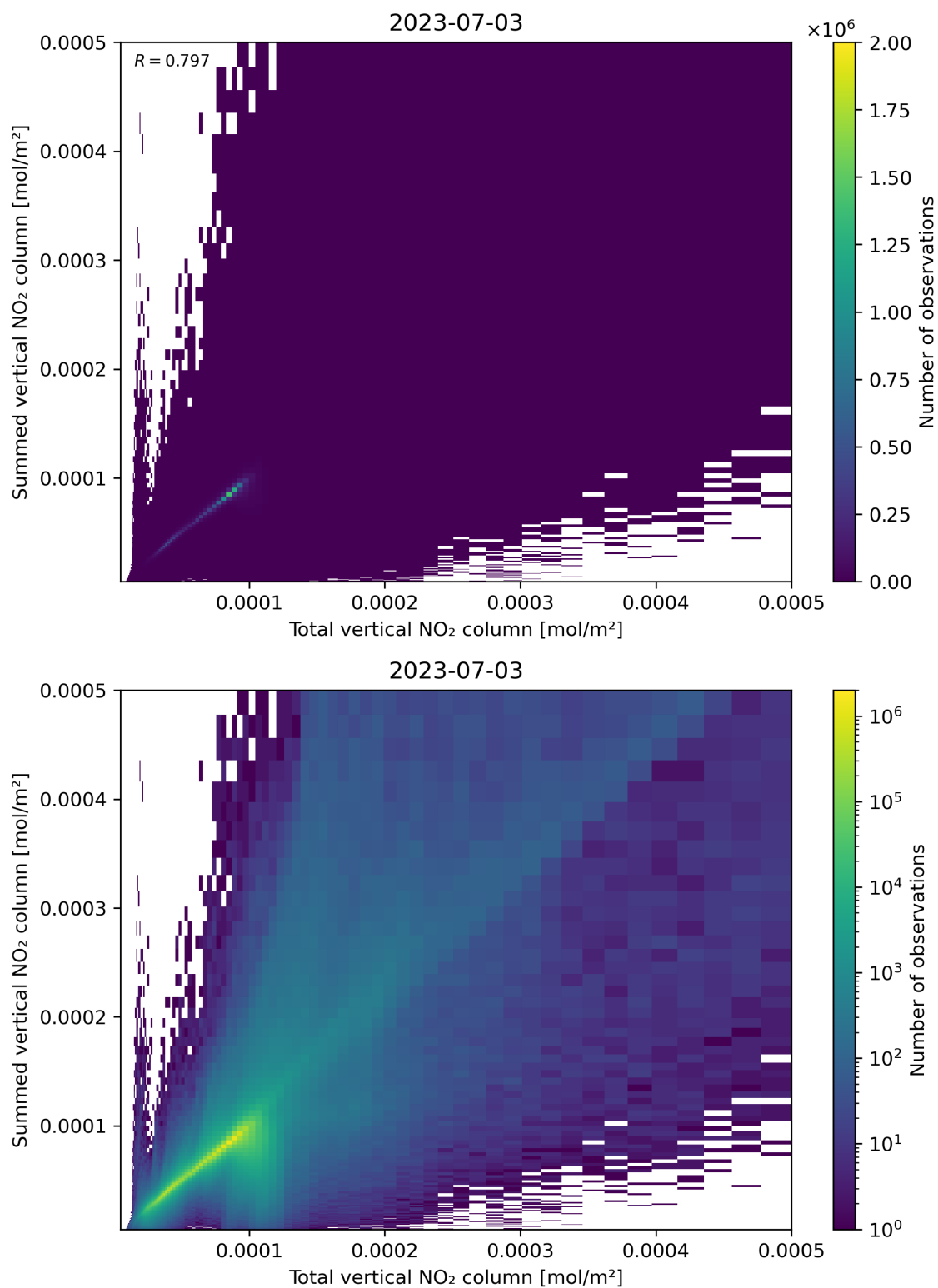
Figure 112: Scatter density plot of “Total vertical NO 2 column” against “Summed vertical NO 2 column” for 2023-07-03 to 2023-07-04.
