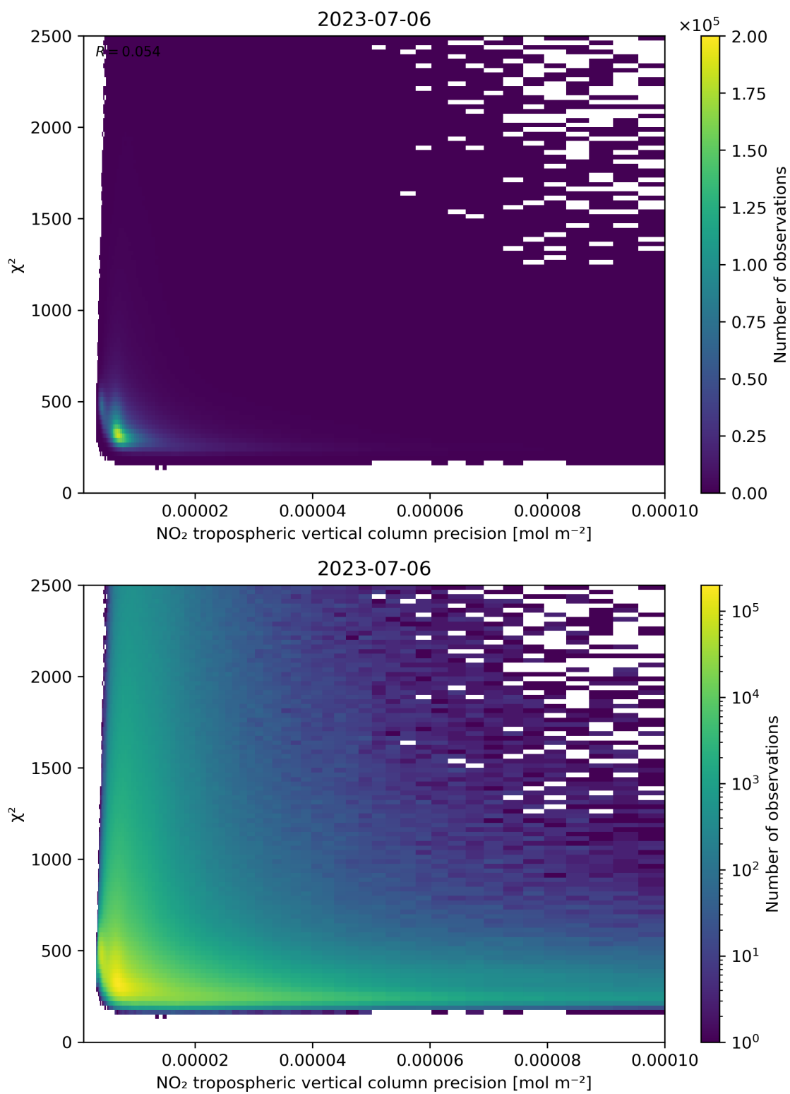
Figure 134: Scatter density plot of “NO 2 tropospheric vertical column precision” against “ \chi^2 ” for 2023-07-05 to 2023-07-07.
