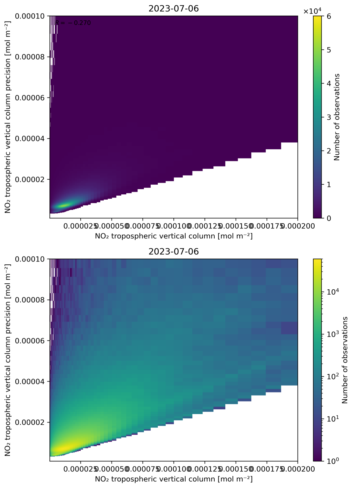
Figure 130: Scatter density plot of “NO 2 tropospheric vertical column” against “NO 2 tropospheric vertical column precision” for 2023-07-05 to 2023-07-07.
