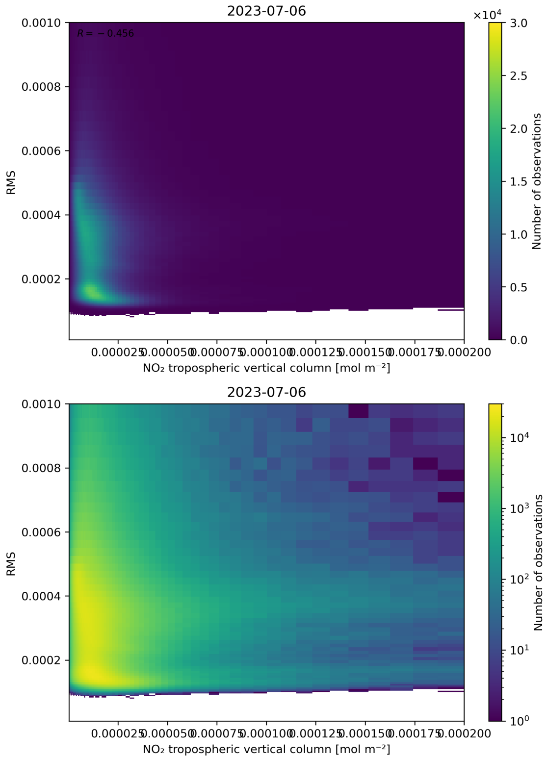
Figure 142: Scatter density plot of “NO 2 tropospheric vertical column” against “RMS” for 2023-07-05 to 2023-07-07.
