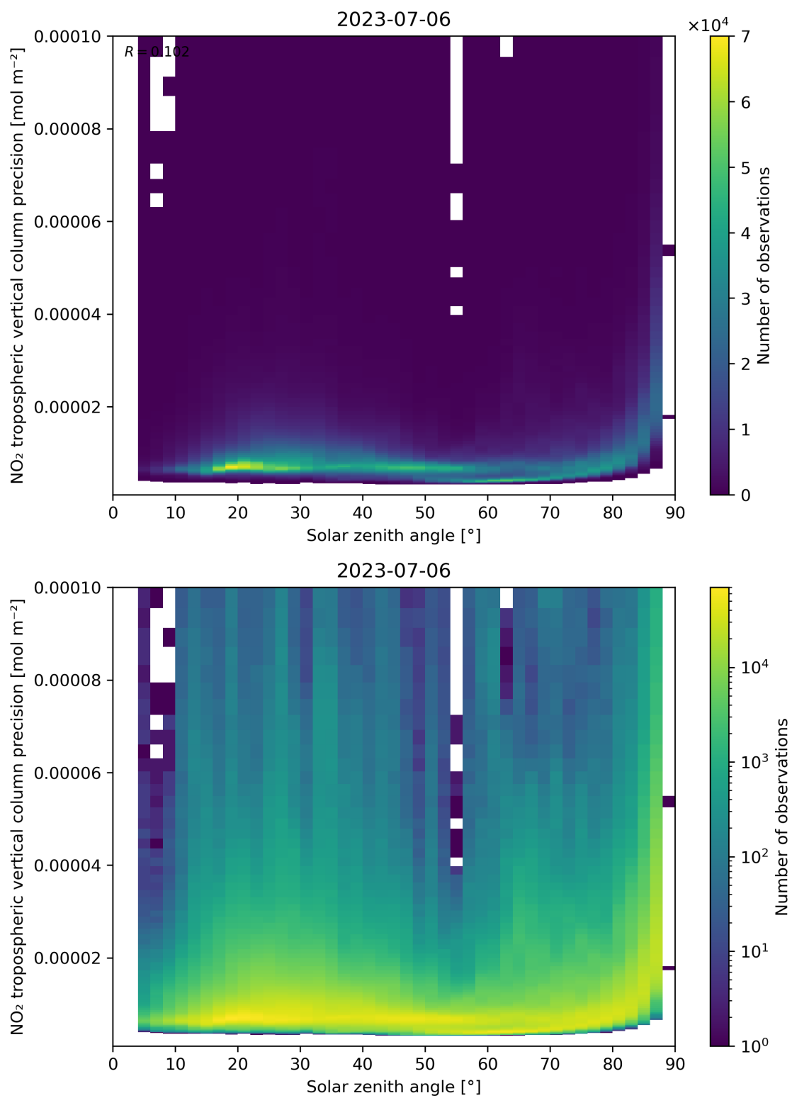
Figure 156: Scatter density plot of “Solar zenith angle” against “NO 2 tropospheric vertical column precision” for 2023-07-05 to 2023-07-07.
