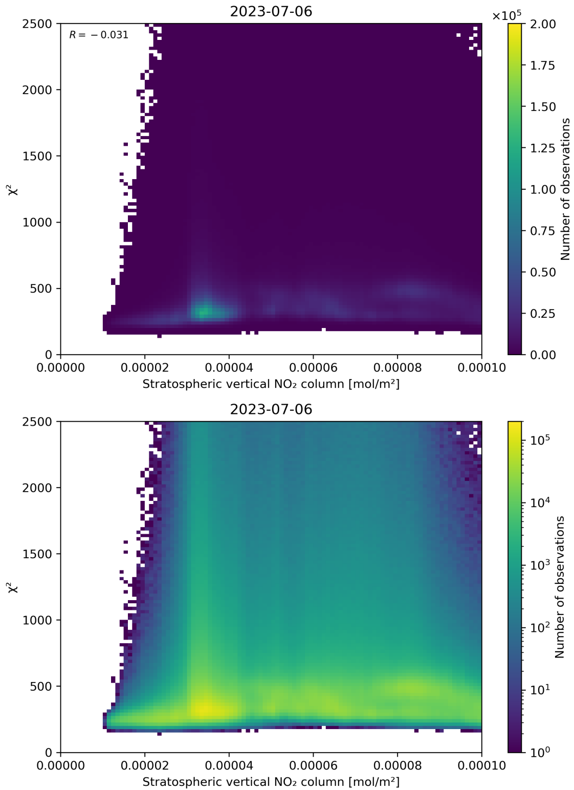
Figure 97: Scatter density plot of “Stratospheric vertical NO 2 column” against “ \chi^2 ” for 2023-07-05 to 2023-07-07.
