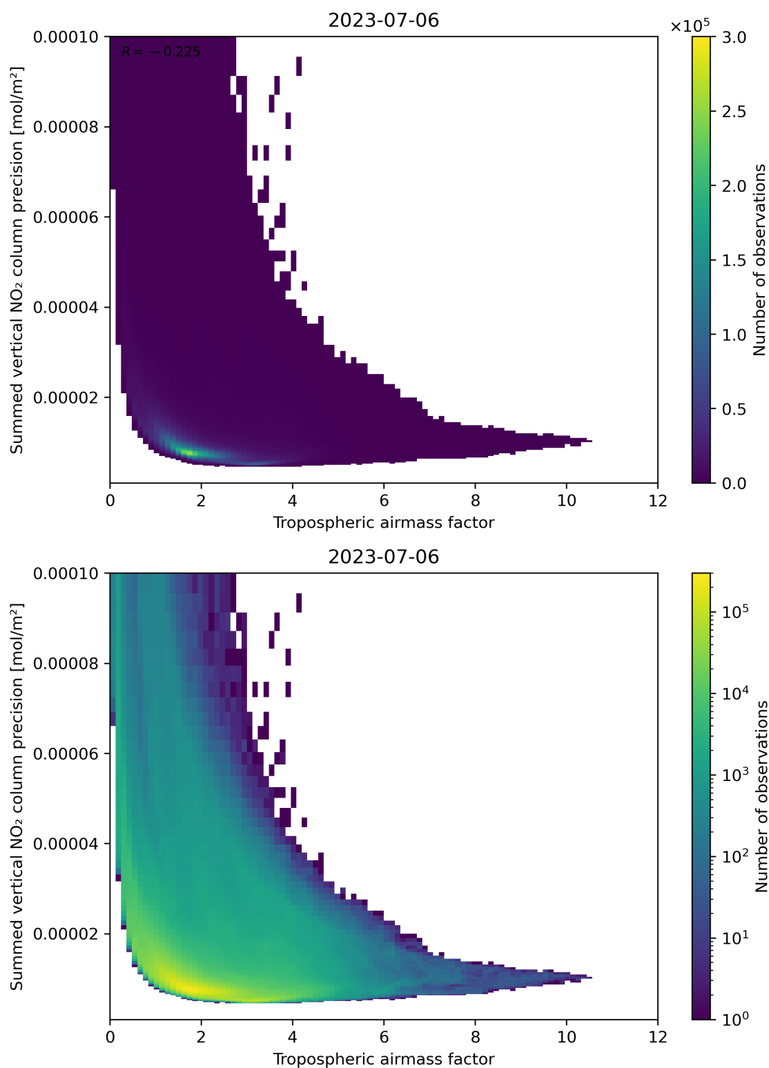
Figure 76: Scatter density plot of “Tropospheric air mass factor” against “Summed vertical NO 2 column precision” for 2023-07-05 to 2023-07-07.
