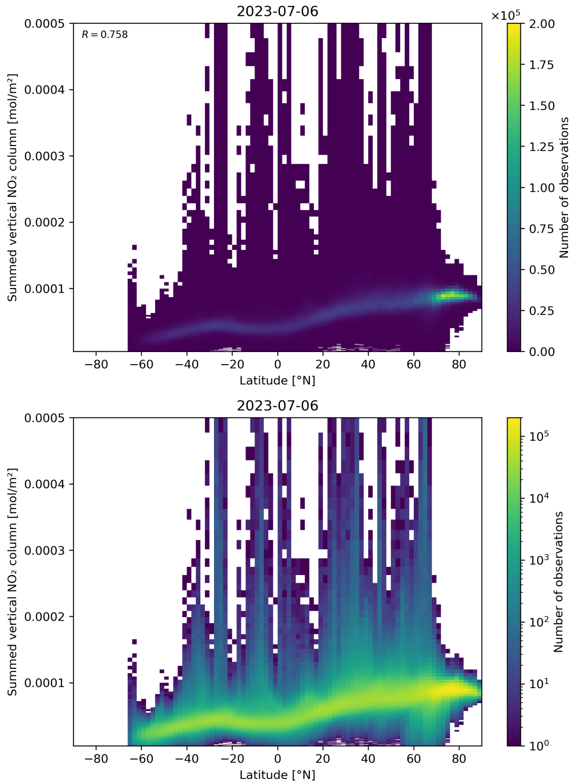
Figure 88: Scatter density plot of “Latitude” against “Summed vertical NO 2 column” for 2023-07-05 to 2023-07-07.
