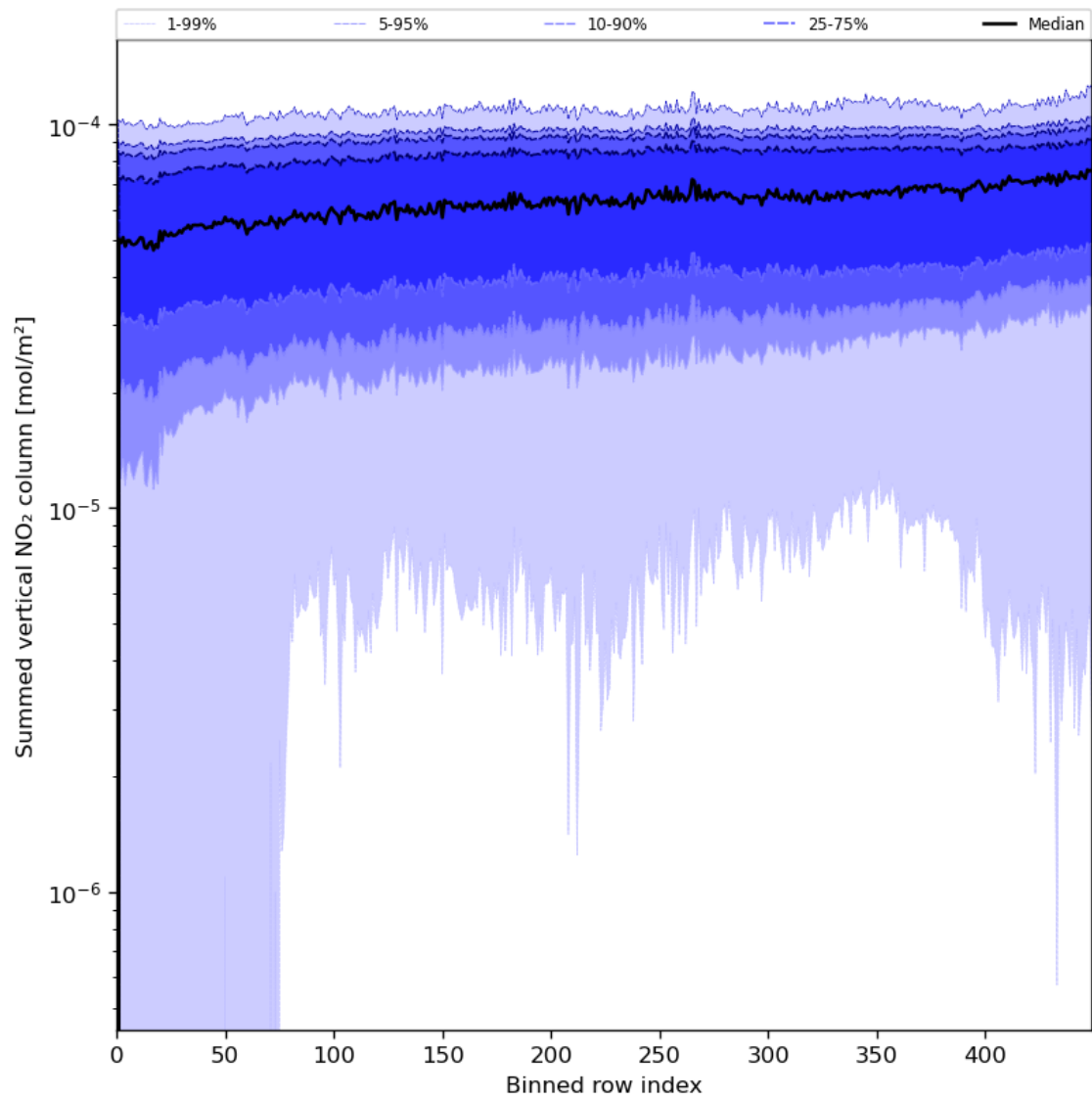
Figure 57: Along track statistics of “Summed vertical NO 2 column” for 2023-07-05 to 2023-07-07
