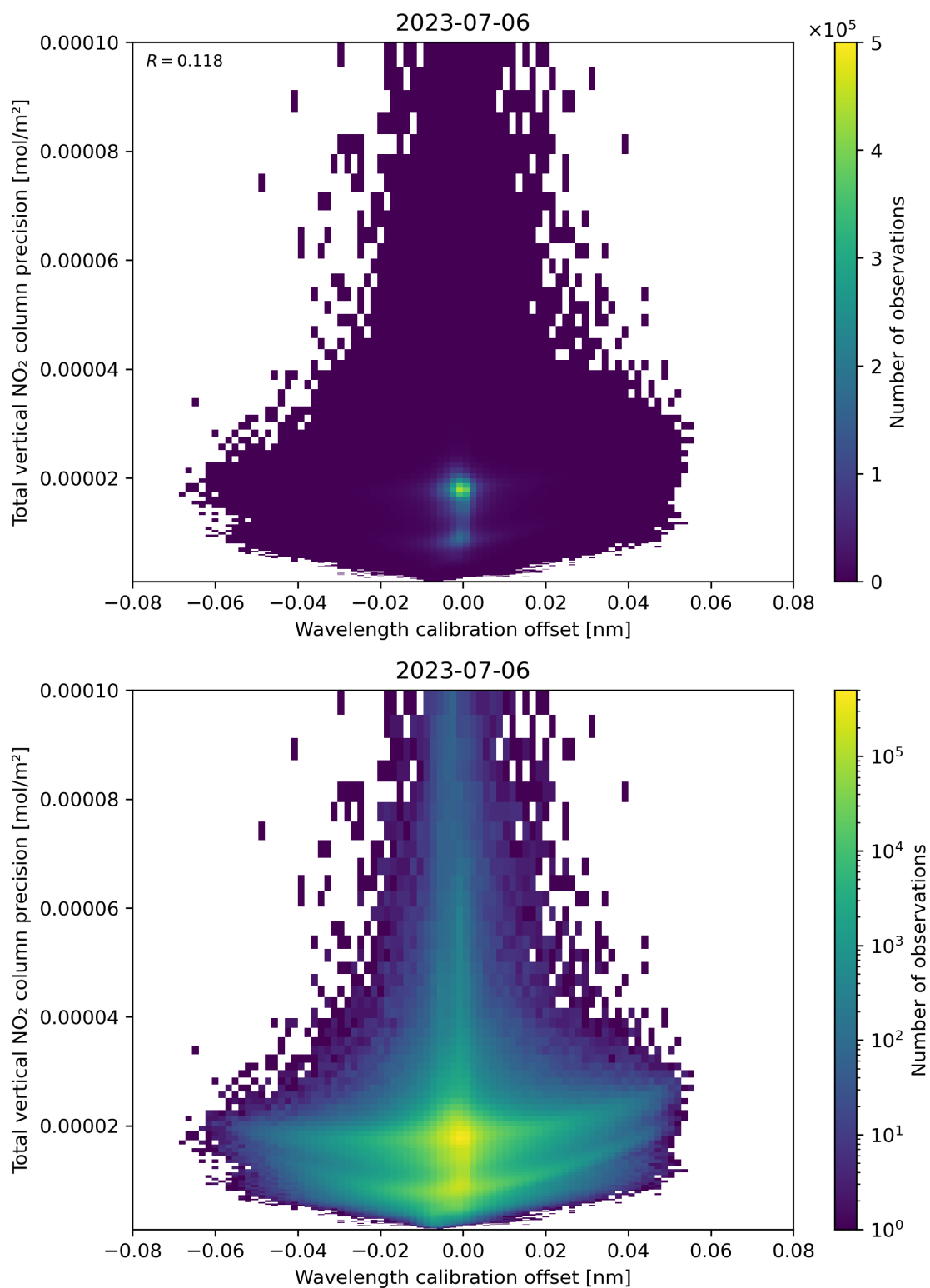
Figure 180: Scatter density plot of “Wavelength calibration offset” against “Total vertical NO 2 column precision” for 2023-07-05 to 2023-07-07.
