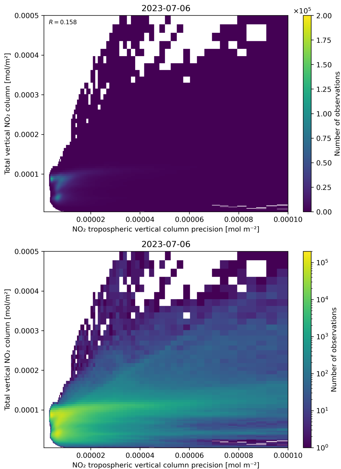
Figure 138: Scatter density plot of “NO 2 tropospheric vertical column precision” against “Total vertical NO 2 column” for 2023-07-05 to 2023-07-07.
