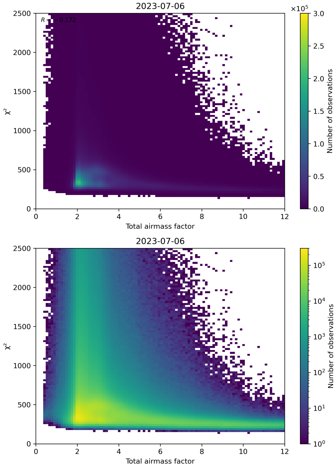
Figure 63: Scatter density plot of “Total airmass factor” against “ \chi^2 ” for 2023-07-05 to 2023-07-07.
