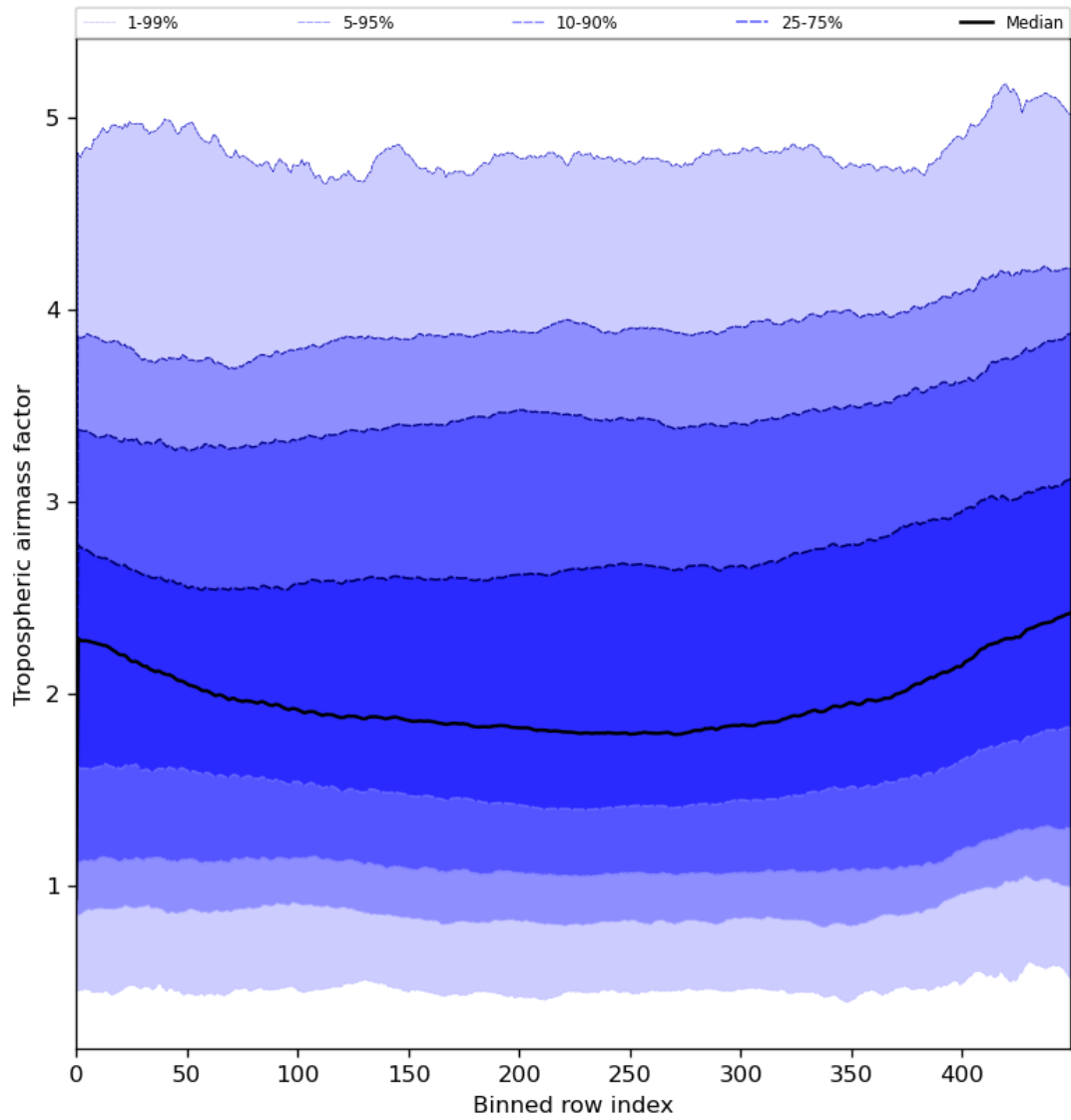
Figure 48: Along track statistics of “Tropospheric airmass factor” for 2023-07-05 to 2023-07-07
