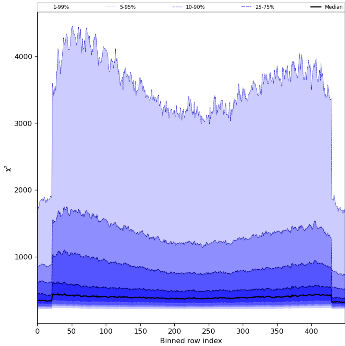
Figure 59: Along track statistics of “ \chi^2 ” for 2023-07-05 to 2023-07-07
