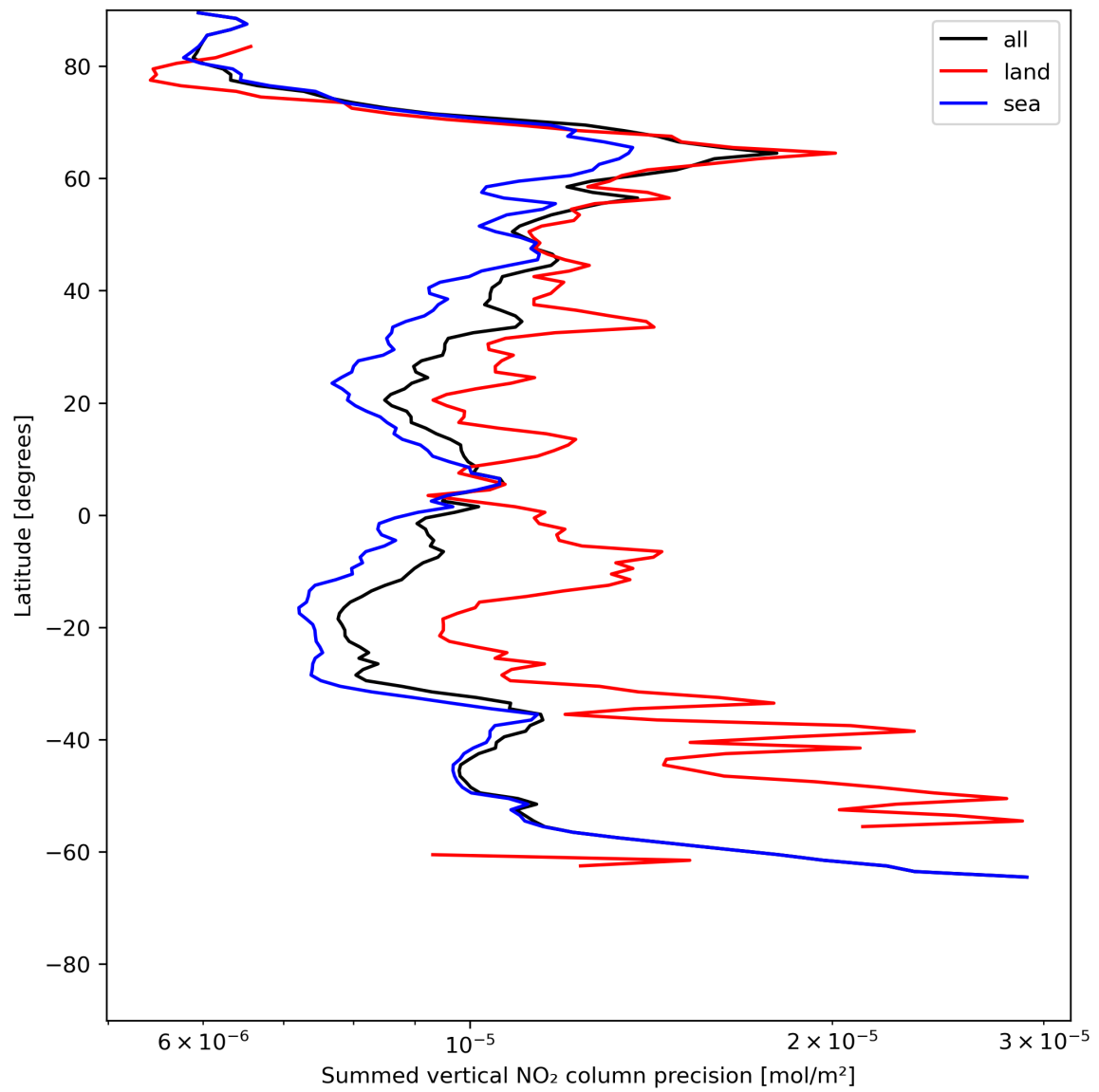
Figure 24: Zonal average of “Summed vertical NO 2 column precision” for 2023-07-05 to 2023-07-07.
