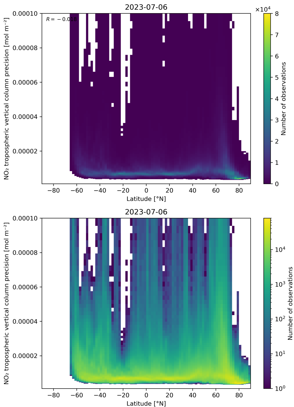
Figure 93: Scatter density plot of “Latitude” against “NO 2 tropospheric vertical column precision” for 2023-07-05 to 2023-07-07.
