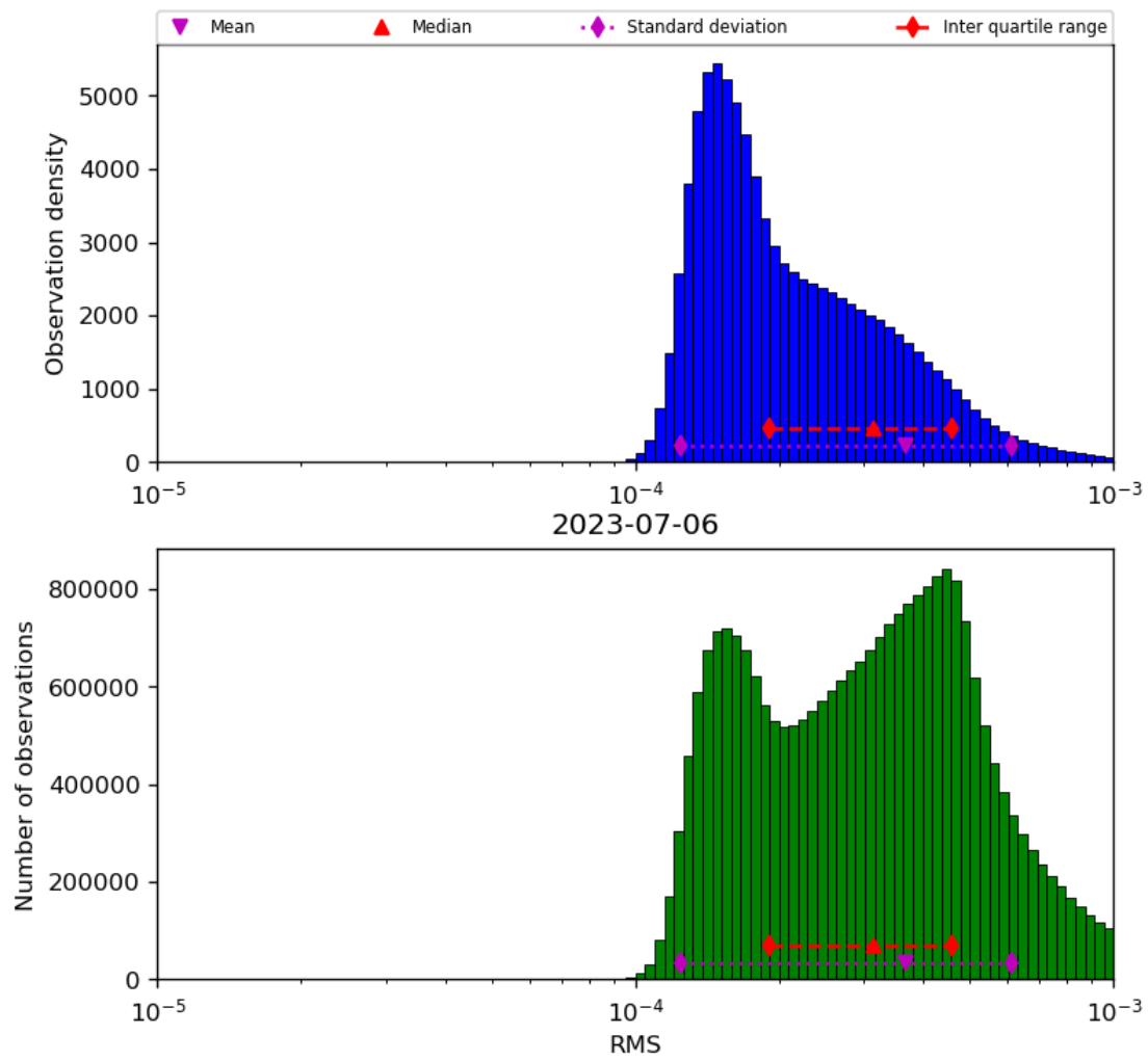
Figure 43: Histogram of “RMS” for 2023-07-05 to 2023-07-07
