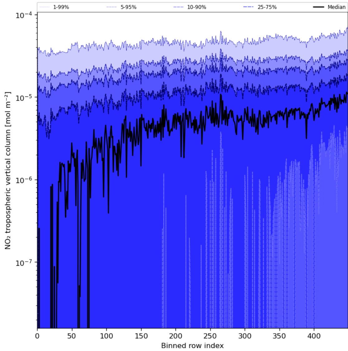
Figure 46: Along track statistics of “NO 2 tropospheric vertical column” for 2023-07-05 to 2023-07-07
