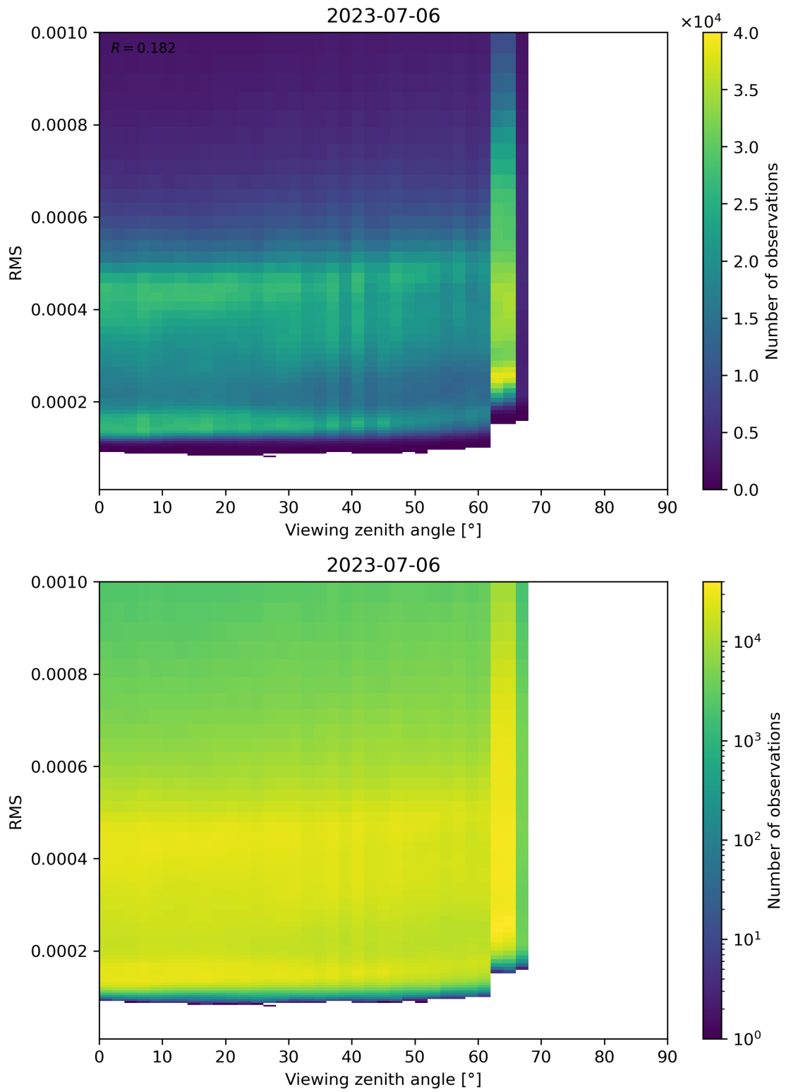
Figure 171: Scatter density plot of “Viewing zenith angle” against “RMS” for 2023-07-05 to 2023-07-07.
