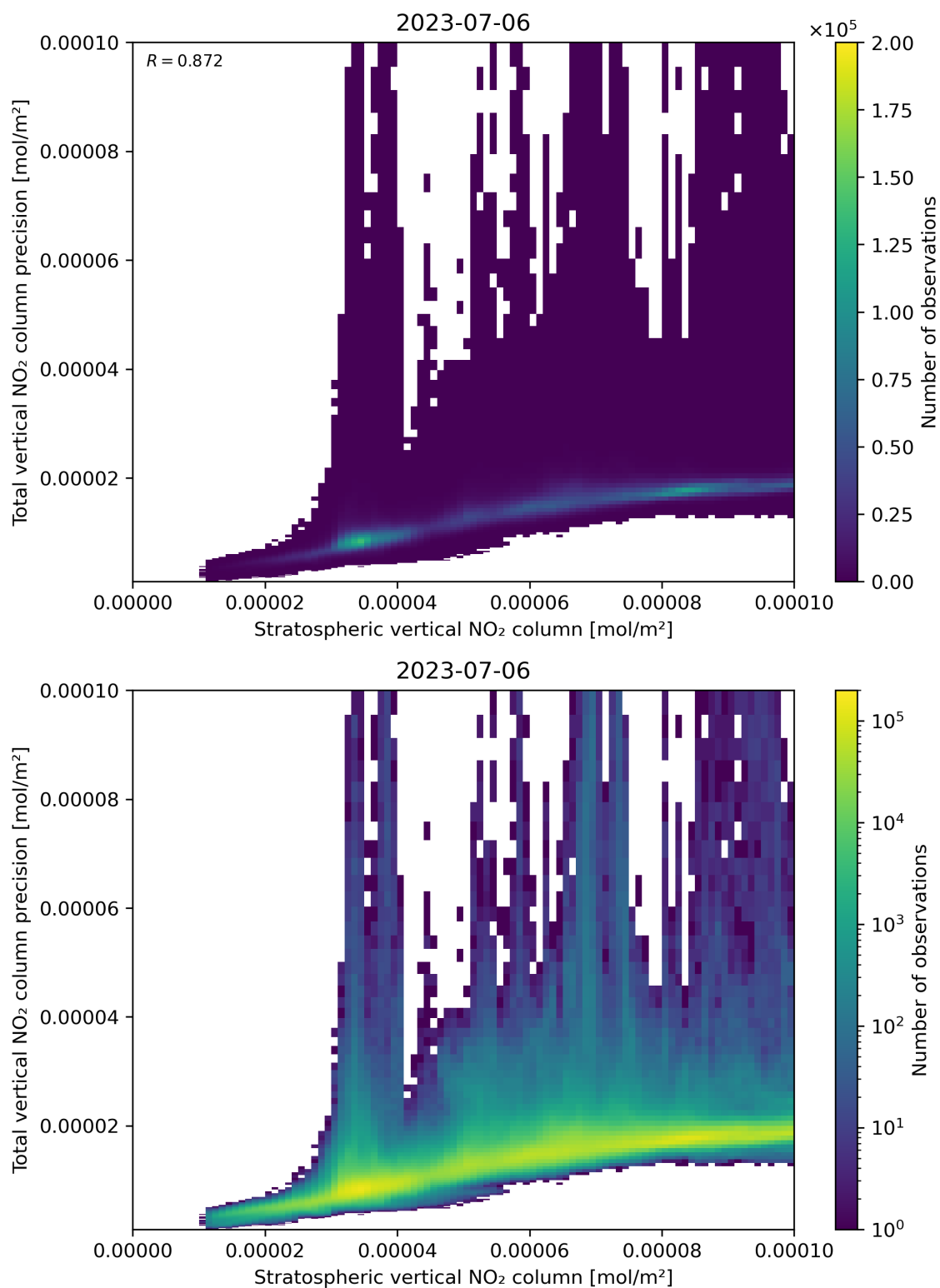
Figure 101: Scatter density plot of “Stratospheric vertical NO 2 column” against “Total vertical NO 2 column precision” for 2023-07-05 to 2023-07-07.
