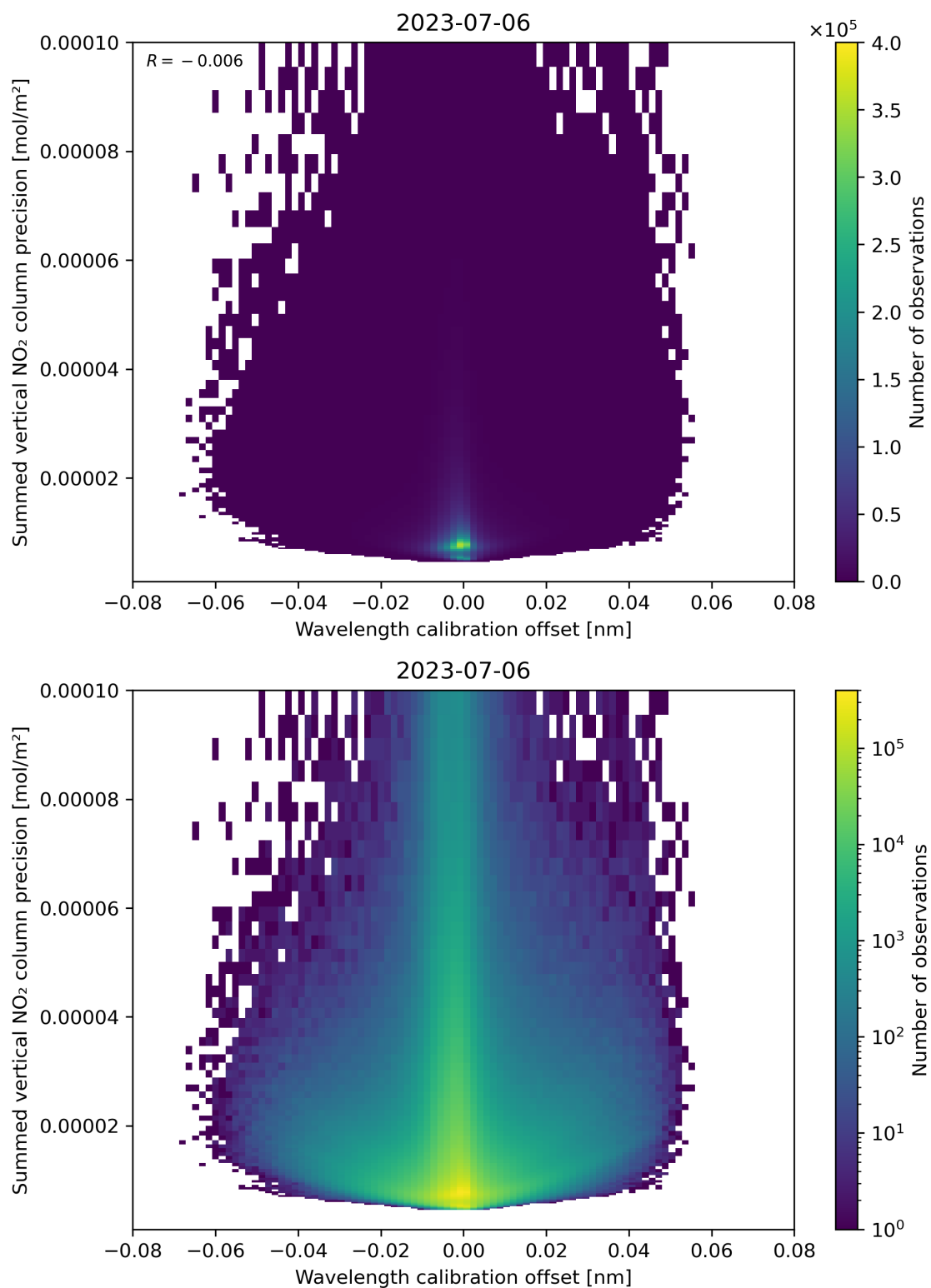
Figure 178: Scatter density plot of “Wavelength calibration offset” against “Summed vertical NO 2 column precision” for 2023-07-05 to 2023-07-07.
