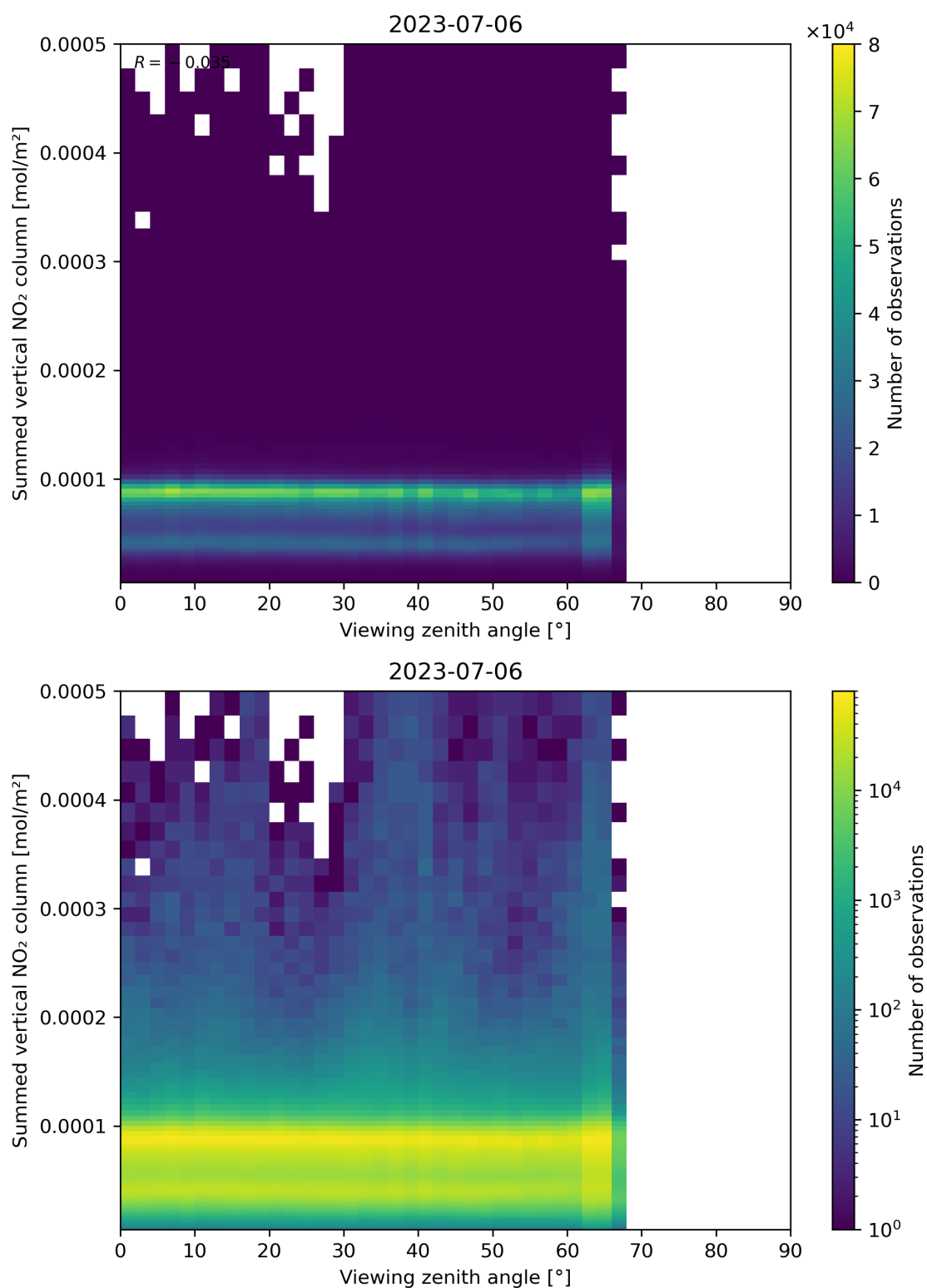
Figure 165: Scatter density plot of “Viewing zenith angle” against “Summed vertical NO 2 column” for 2023-07-05 to 2023-07-07.
