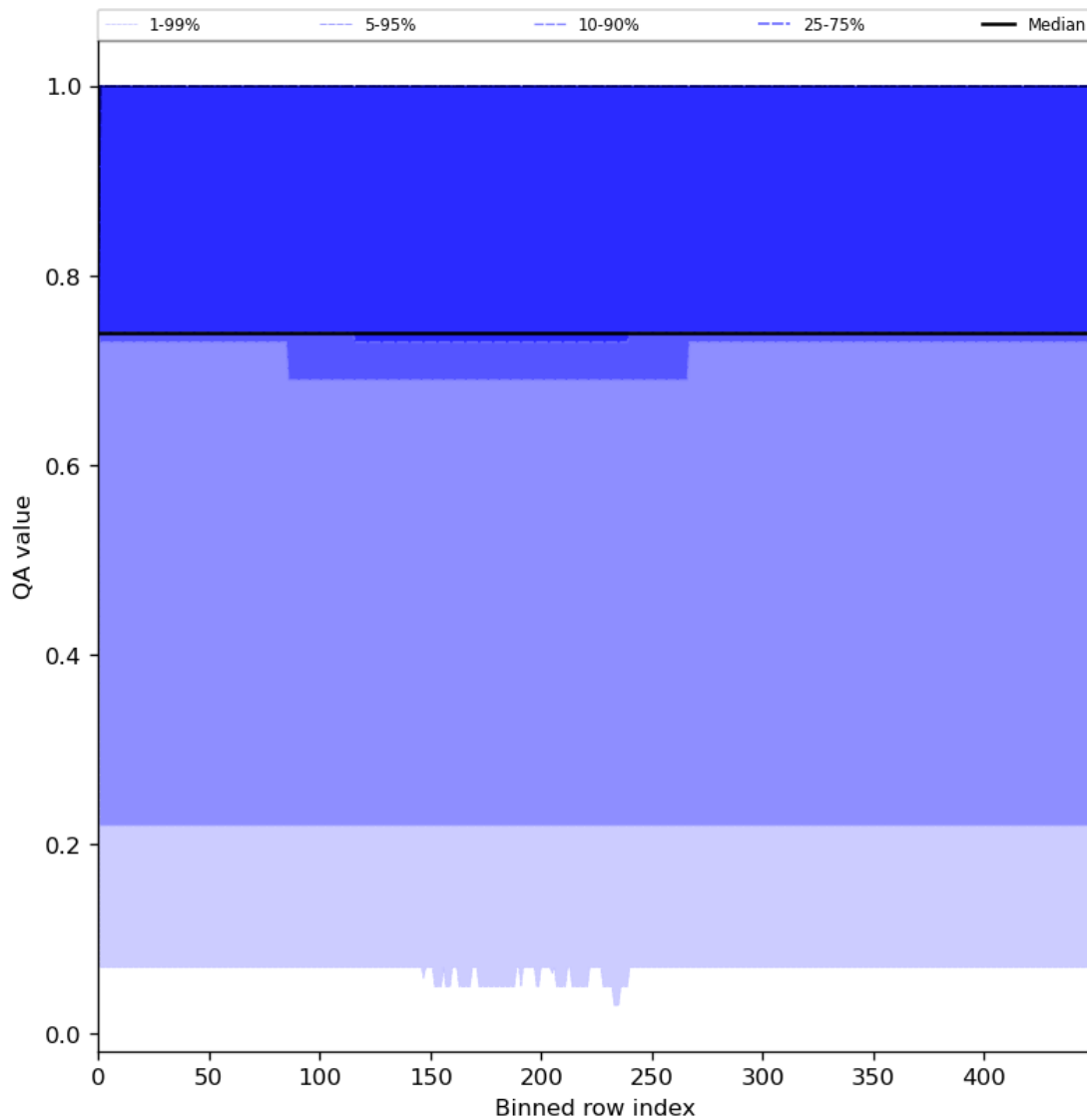
Figure 45: Along track statistics of “QA value” for 2023-07-05 to 2023-07-07
