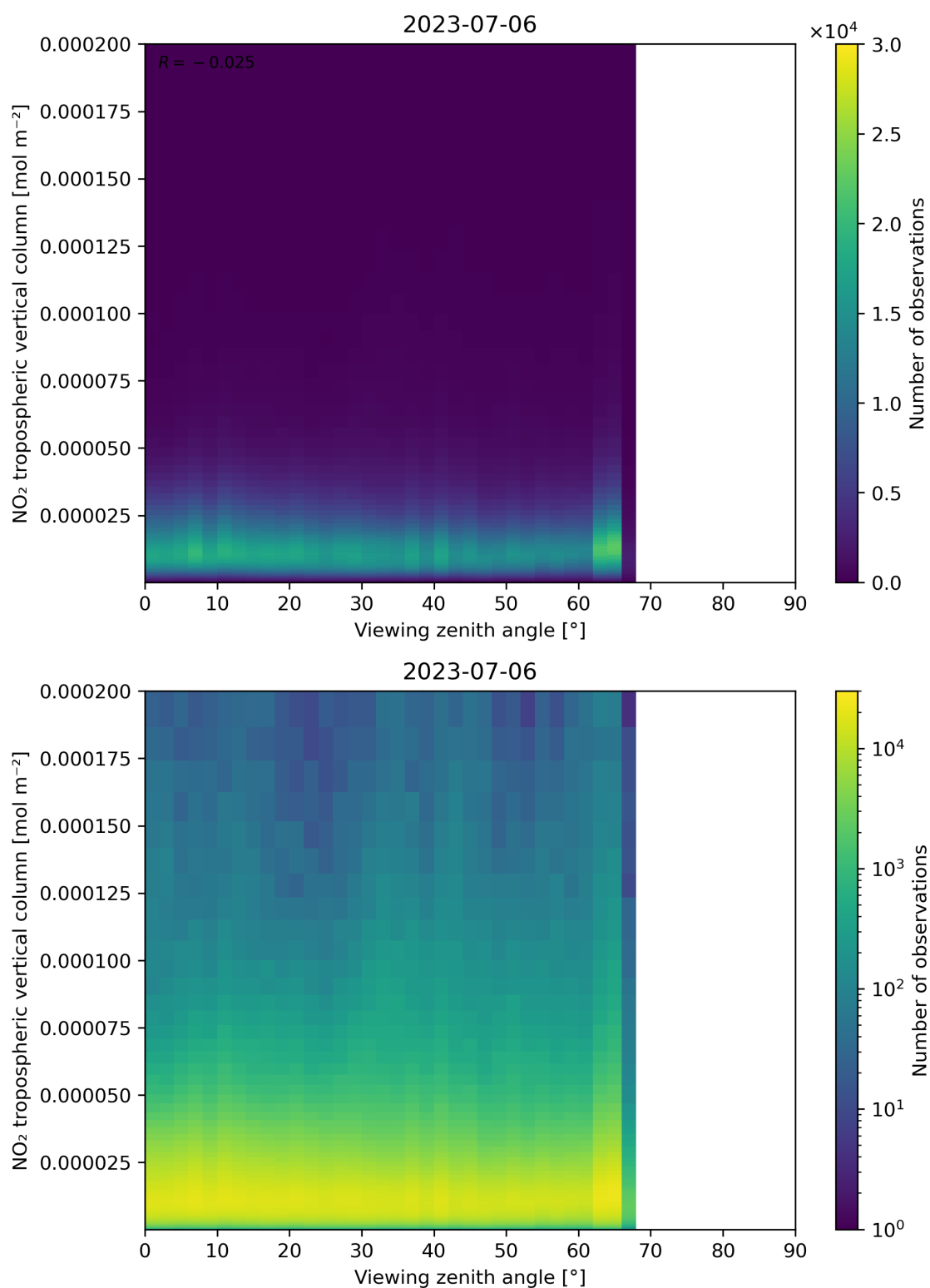
Figure 169: Scatter density plot of “Viewing zenith angle” against “NO 2 tropospheric vertical column” for 2023-07-05 to 2023-07-07.
