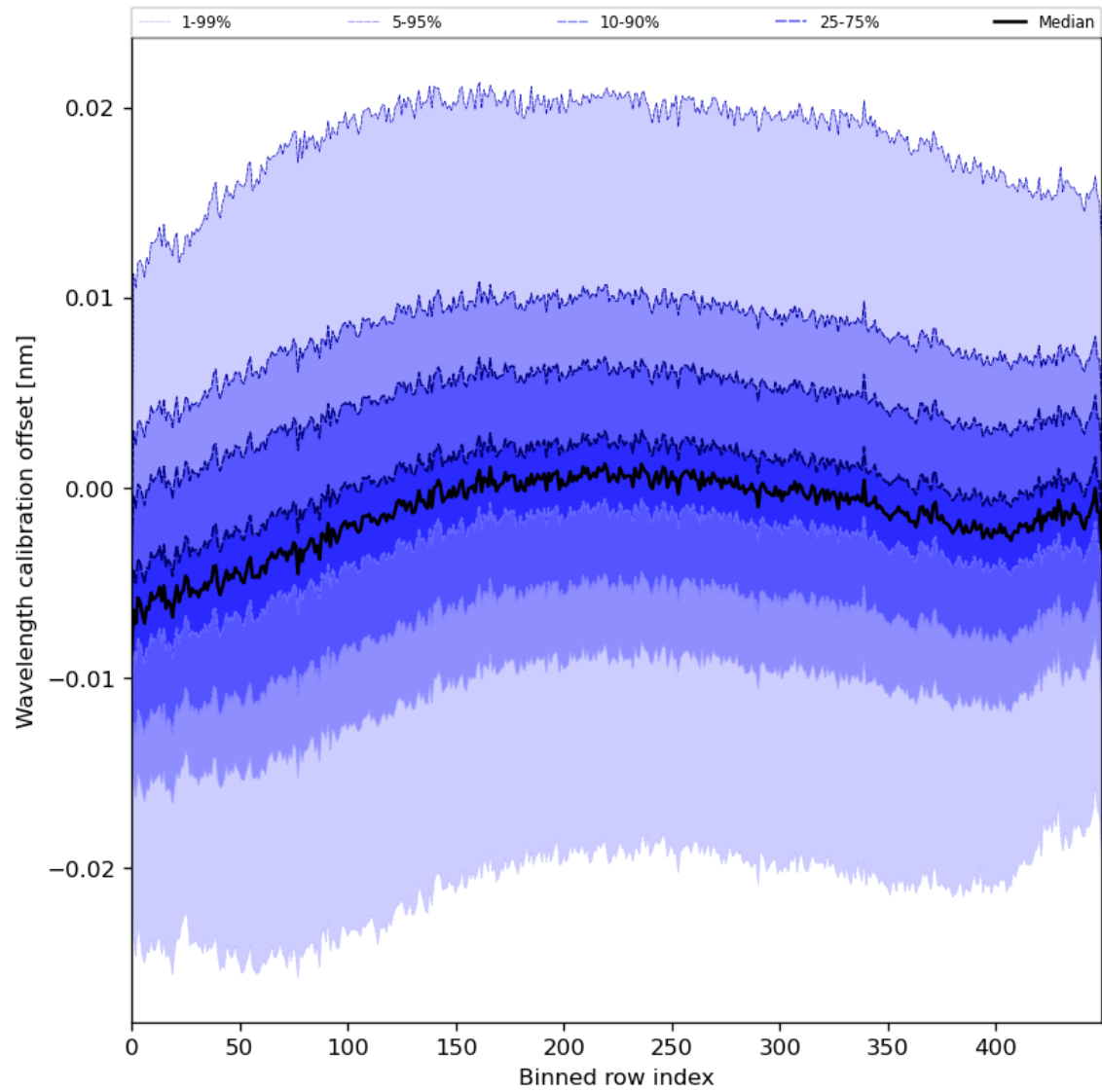
Figure 52: Along track statistics of “Wavelength calibration offset” for 2023-07-05 to 2023-07-07
