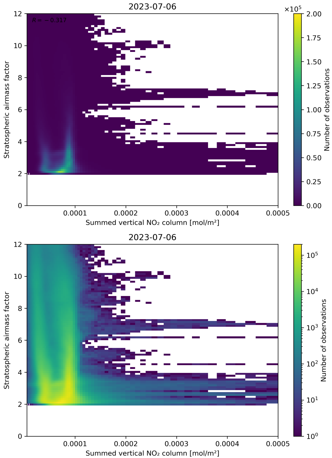
Figure 103: Scatter density plot of “Summed vertical NO 2 column” against “Stratospheric air mass factor” for 2023-07-05 to 2023-07-07.
