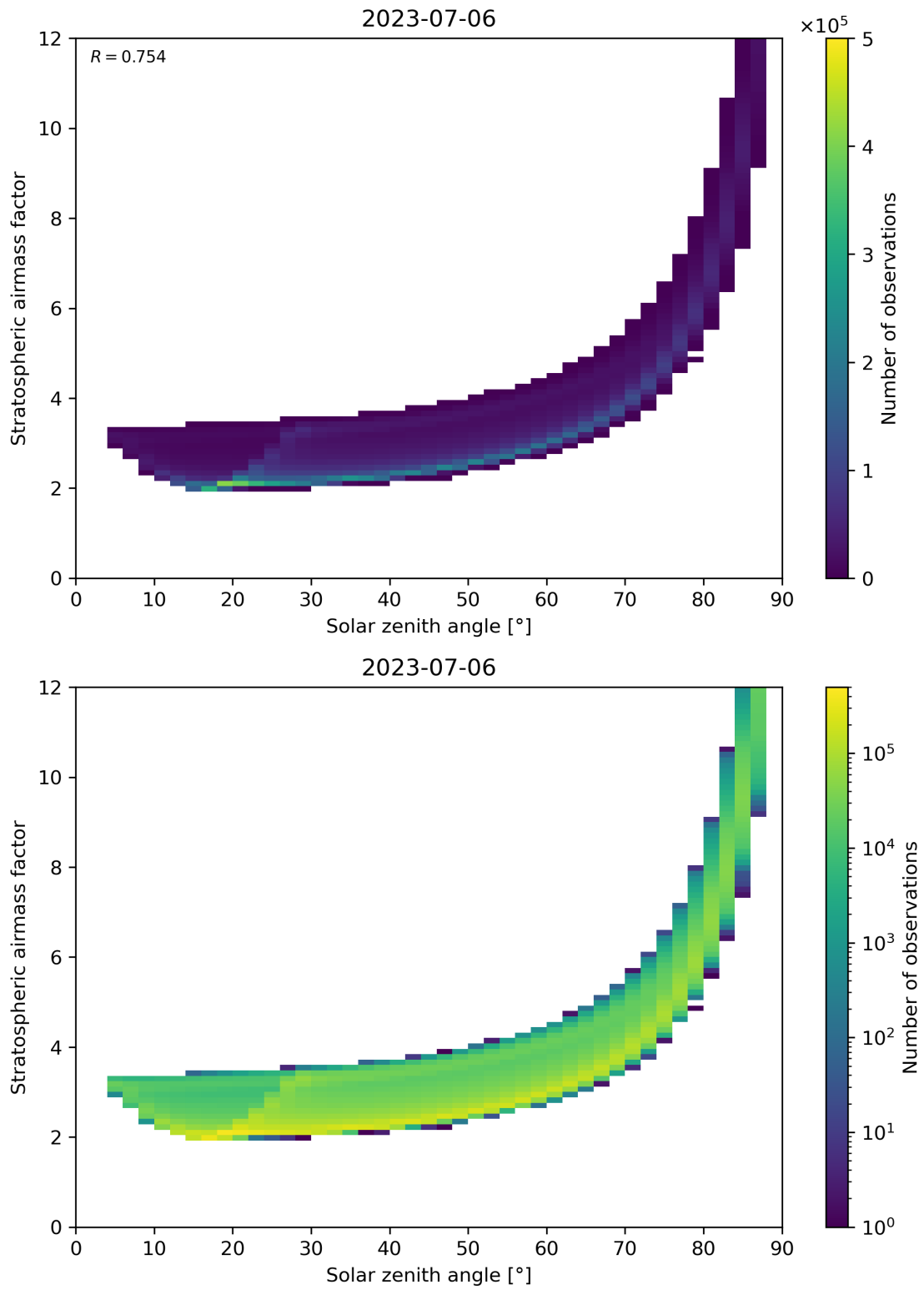
Figure 145: Scatter density plot of “Solar zenith angle” against “Stratospheric airmass factor” for 2023-07-05 to 2023-07-07.
