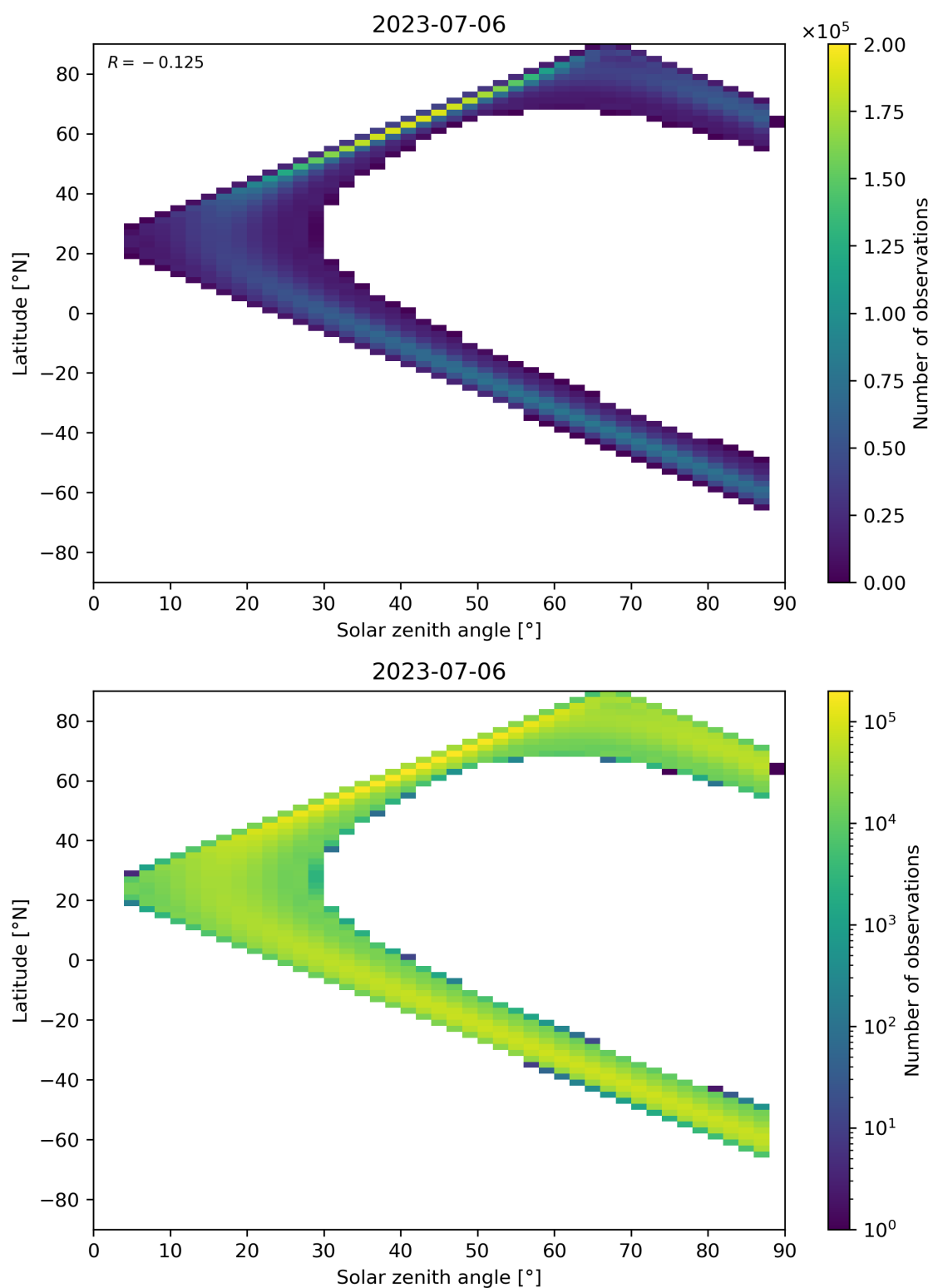
Figure 149: Scatter density plot of “Solar zenith angle” against “Latitude” for 2023-07-05 to 2023-07-07.
