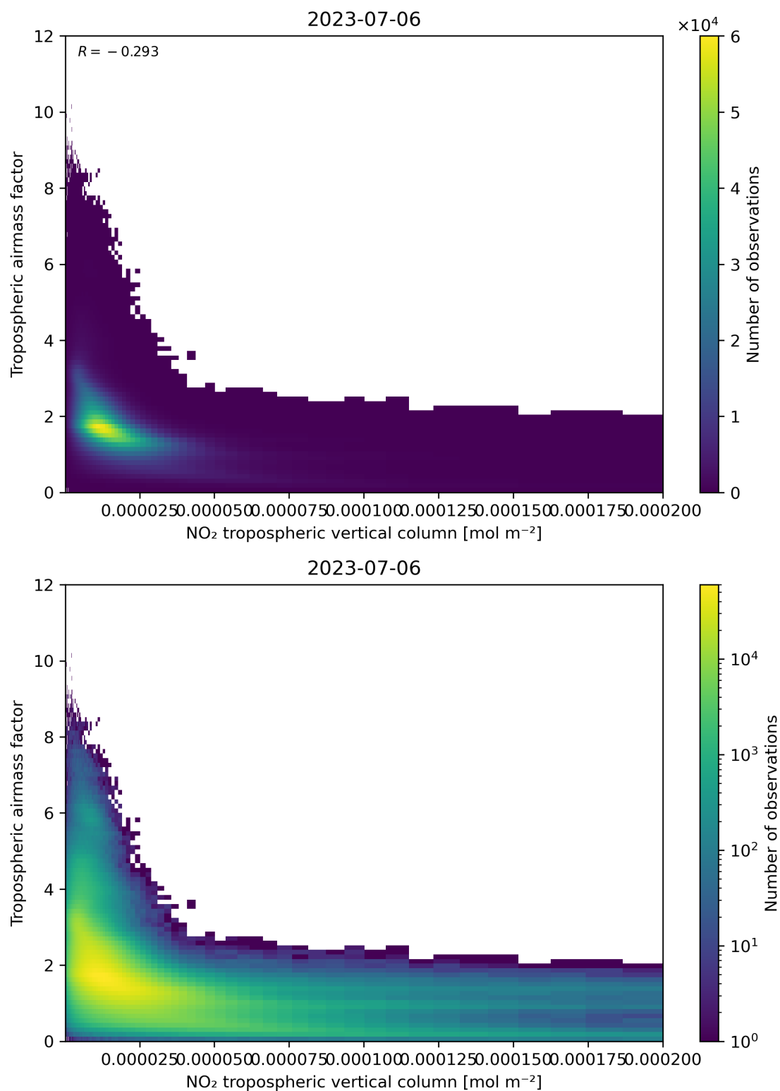
Figure 123: Scatter density plot of “NO 2 tropospheric vertical column” against “Tropospheric airmass factor” for 2023-07-05 to 2023-07-07.
