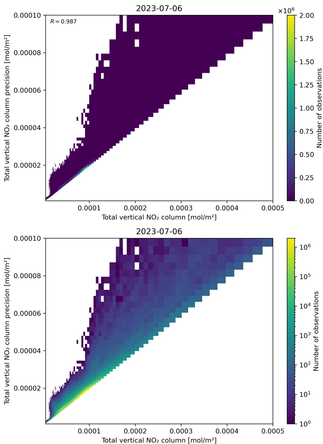
Figure 114: Scatter density plot of “Total vertical NO 2 column” against “Total vertical NO 2 column precision” for 2023-07-05 to 2023-07-07.
