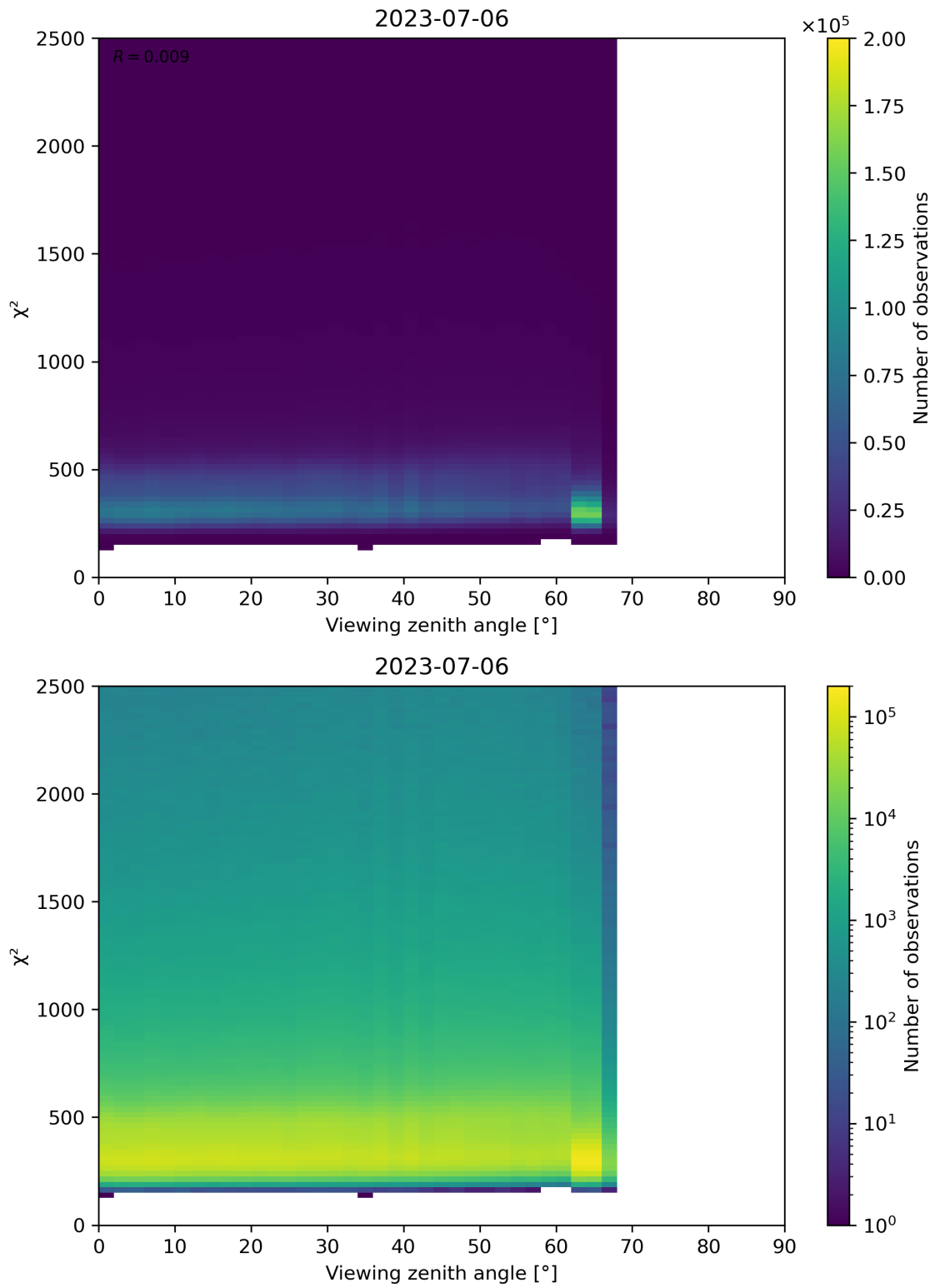
Figure 162: Scatter density plot of “Viewing zenith angle” against “ \chi^2 ” for 2023-07-05 to 2023-07-07.
