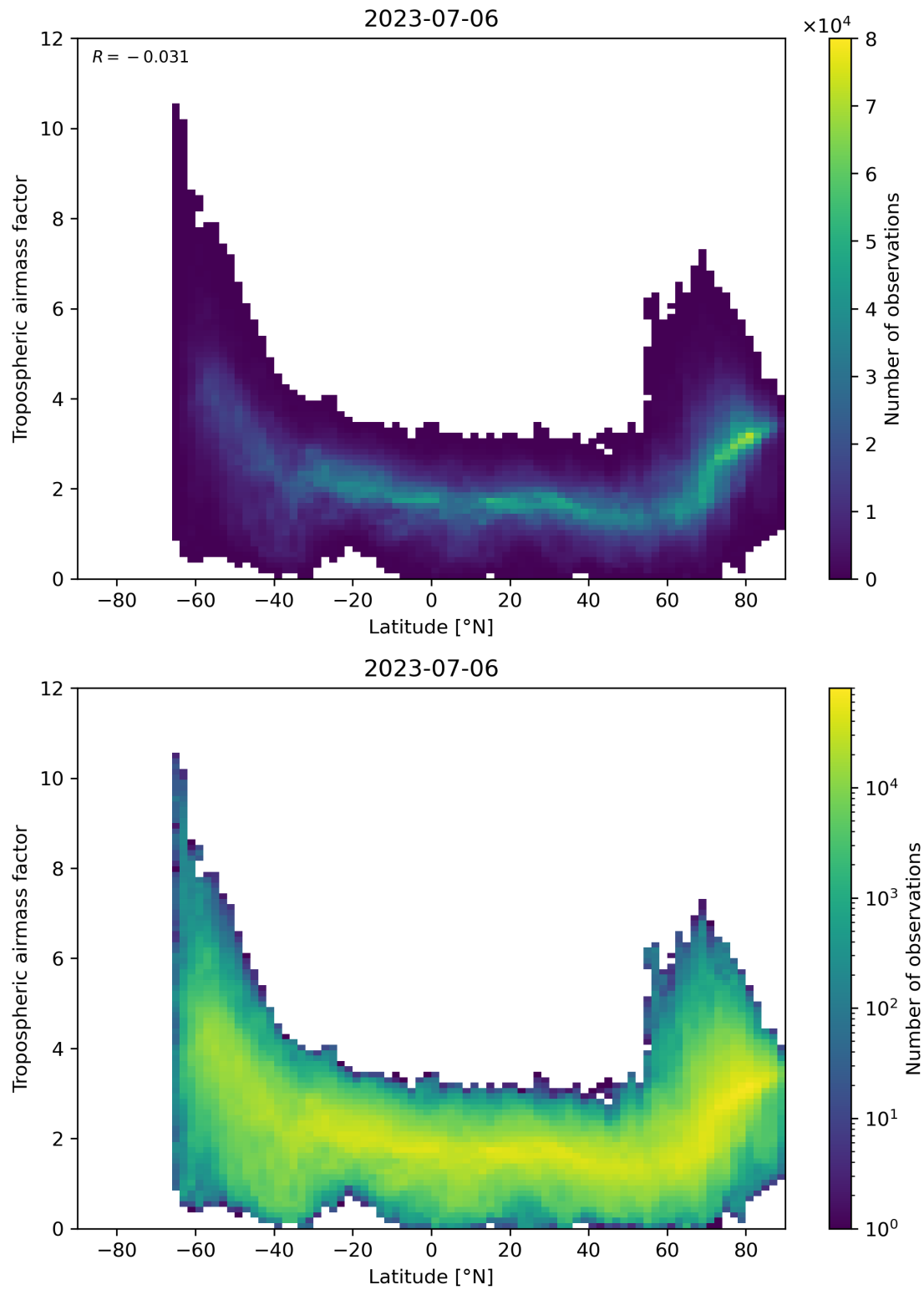
Figure 85: Scatter density plot of “Latitude” against “Tropospheric air mass factor” for 2023-07-05 to 2023-07-07.
