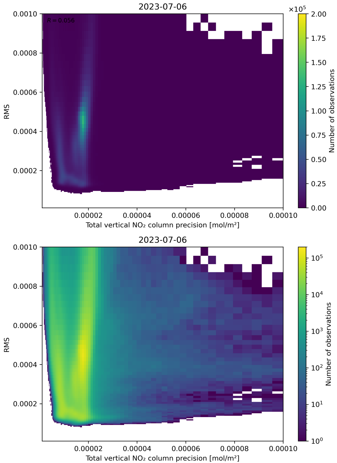
Figure 119: Scatter density plot of “Total vertical NO 2 column precision” against “RMS” for 2023-07-05 to 2023-07-07.
