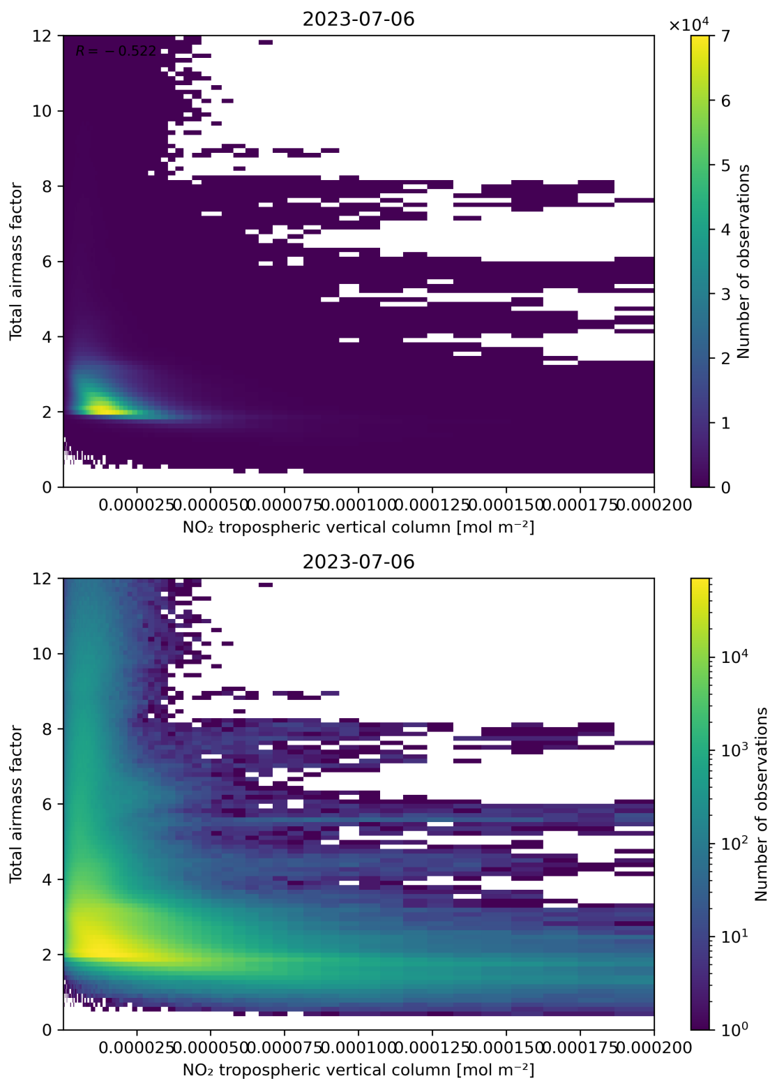
Figure 122: Scatter density plot of “NO 2 tropospheric vertical column” against “Total air mass factor” for 2023-07-05 to 2023-07-07.
