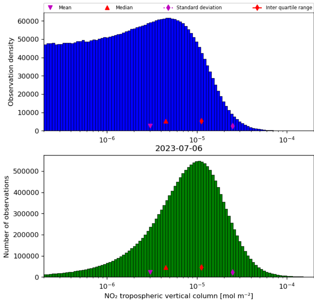
Figure 29: Histogram of “NO 2 tropospheric vertical column” for 2023-07-05 to 2023-07-07
