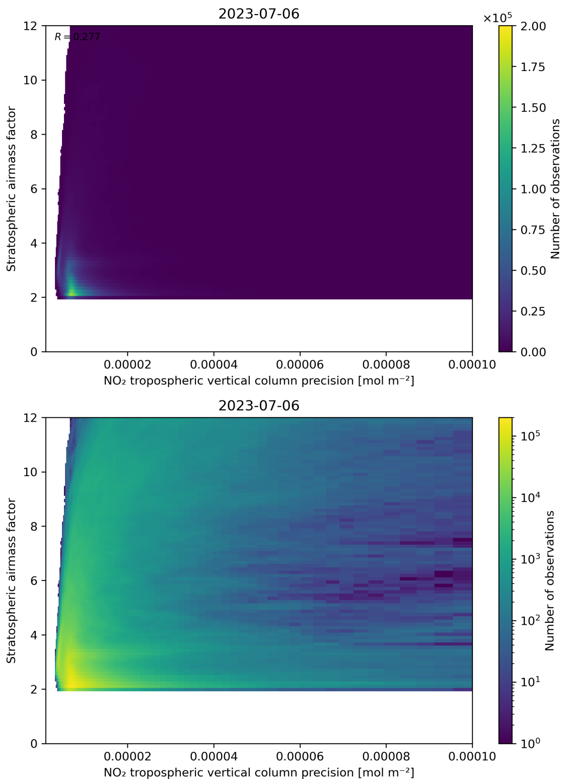
Figure 131: Scatter density plot of “NO 2 tropospheric vertical column precision” against “Stratospheric airmass factor” for 2023-07-05 to 2023-07-07.
