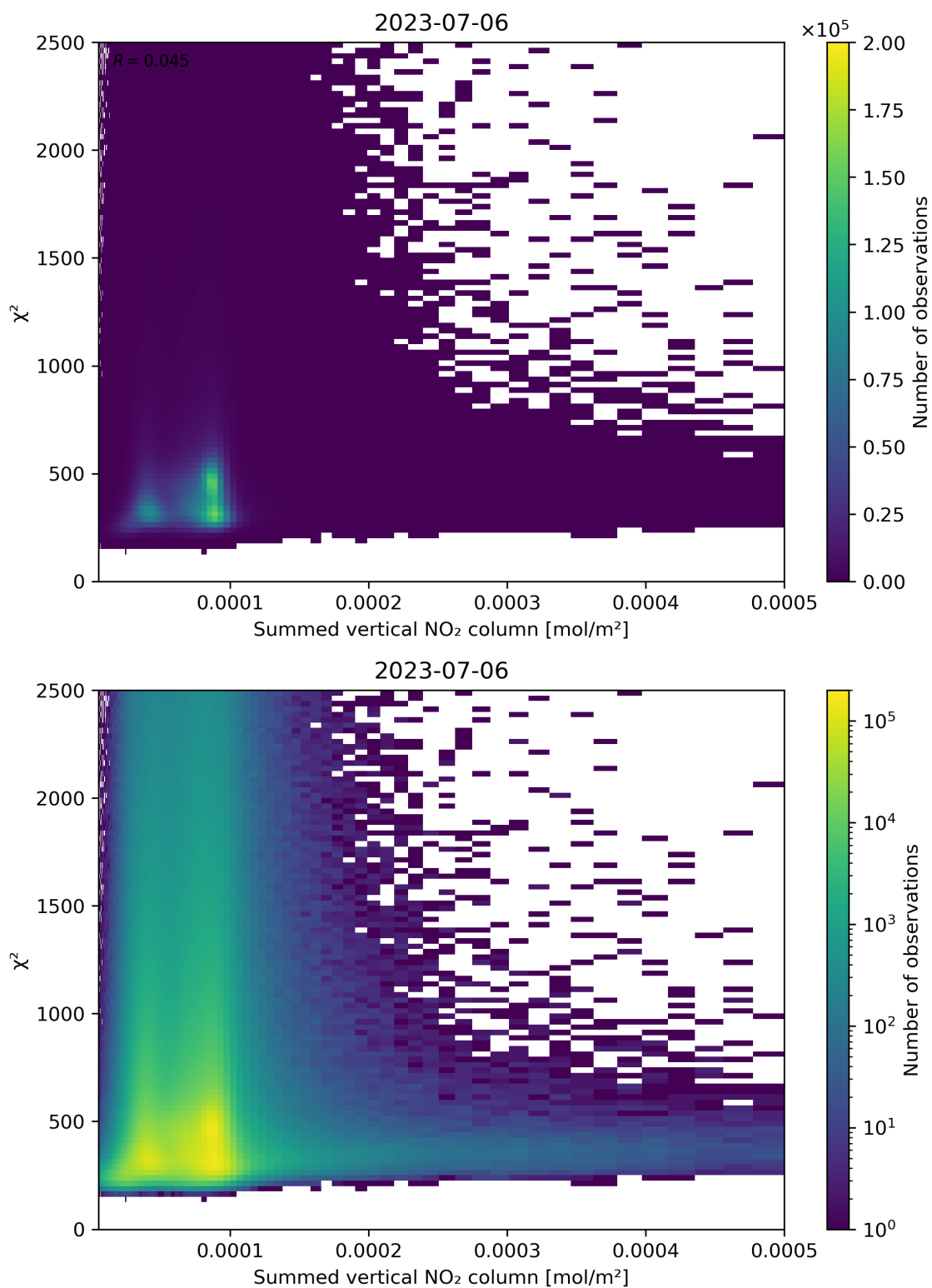
Figure 104: Scatter density plot of “Summed vertical NO 2 column” against “ \chi^2 ” for 2023-07-05 to 2023-07-07.
