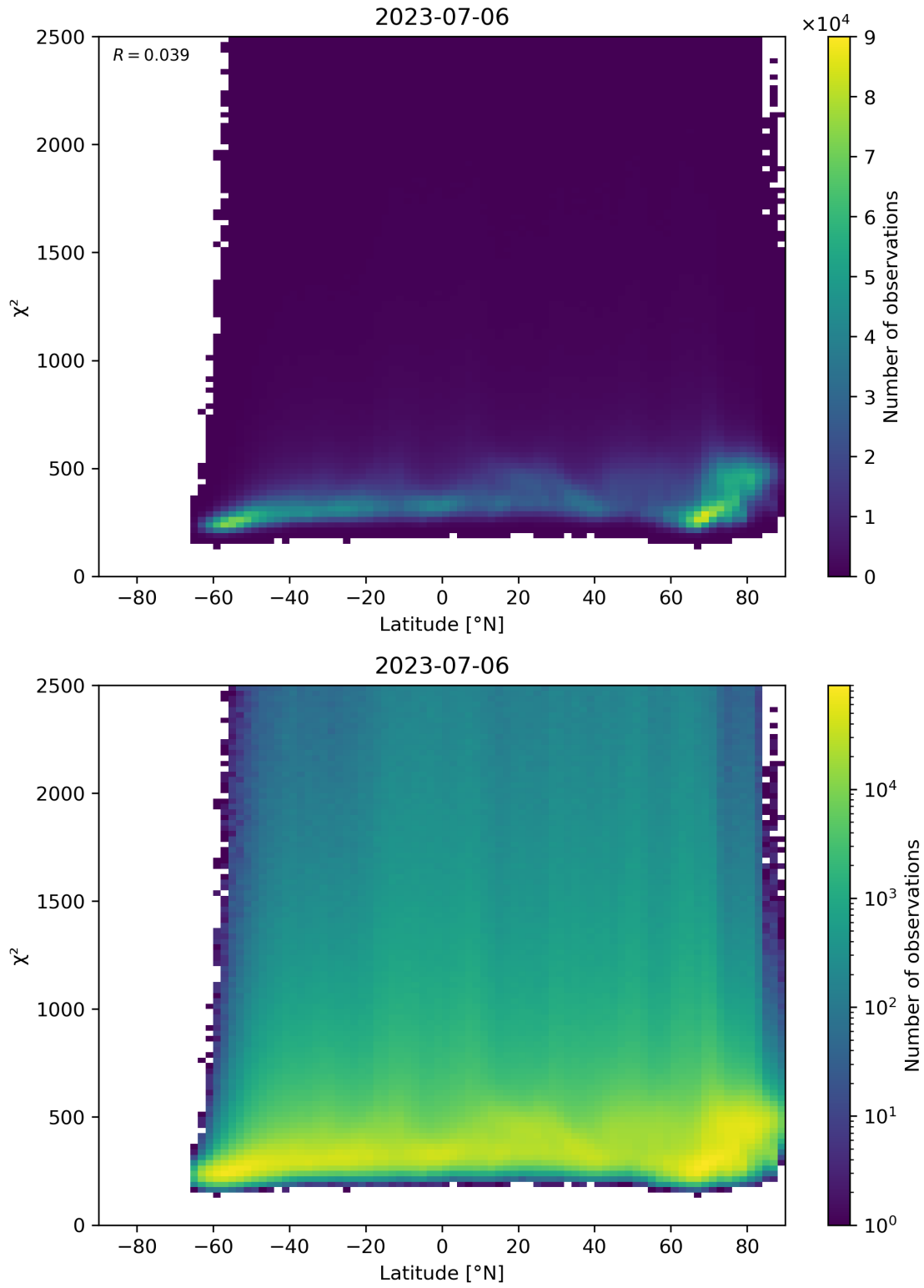
Figure 86: Scatter density plot of “Latitude” against “ \chi^2 ” for 2023-07-05 to 2023-07-07.
