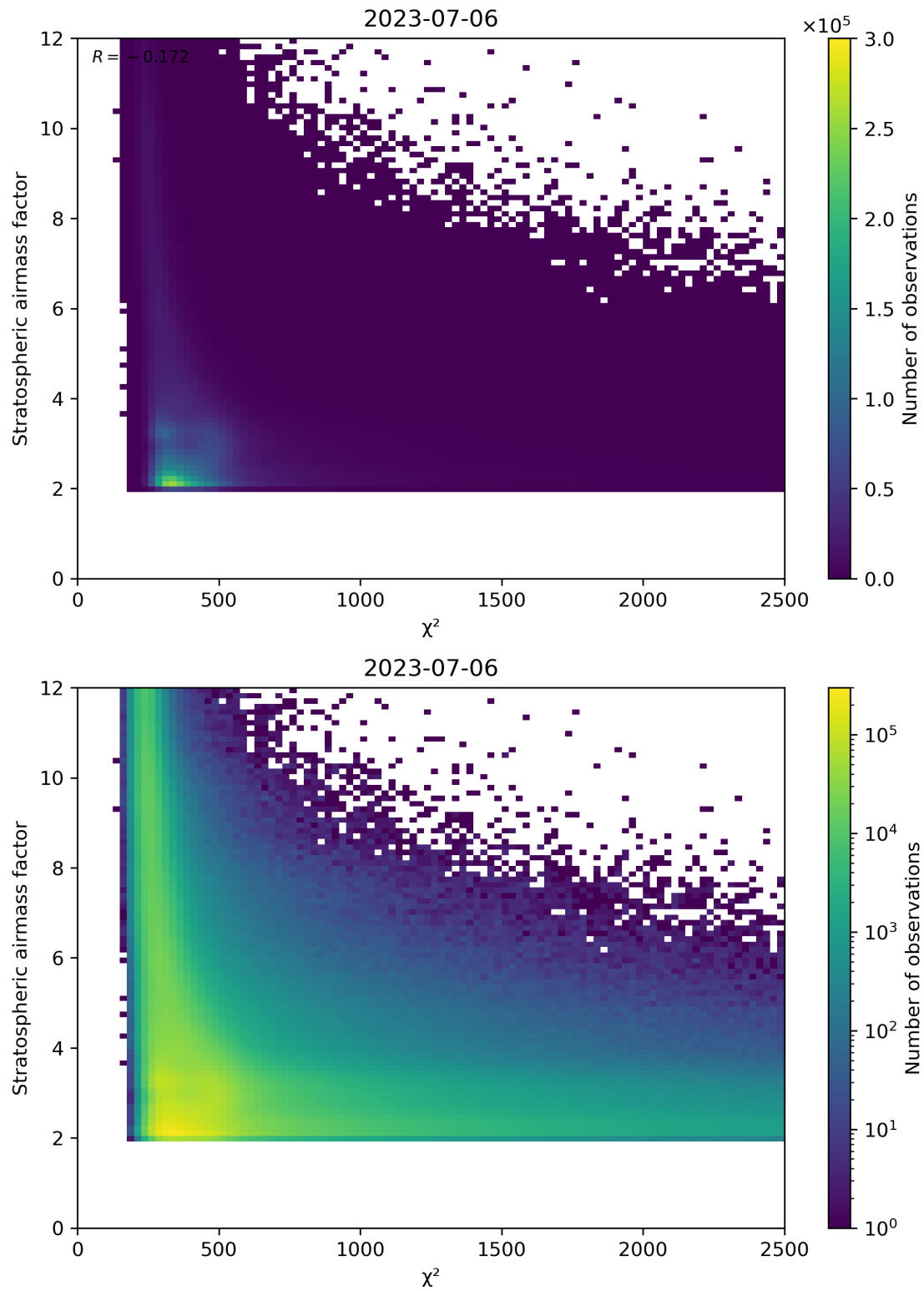
Figure 81: Scatter density plot of “ \chi^2 ” against “Stratospheric airmass factor” for 2023-07-05 to 2023-07-07.
