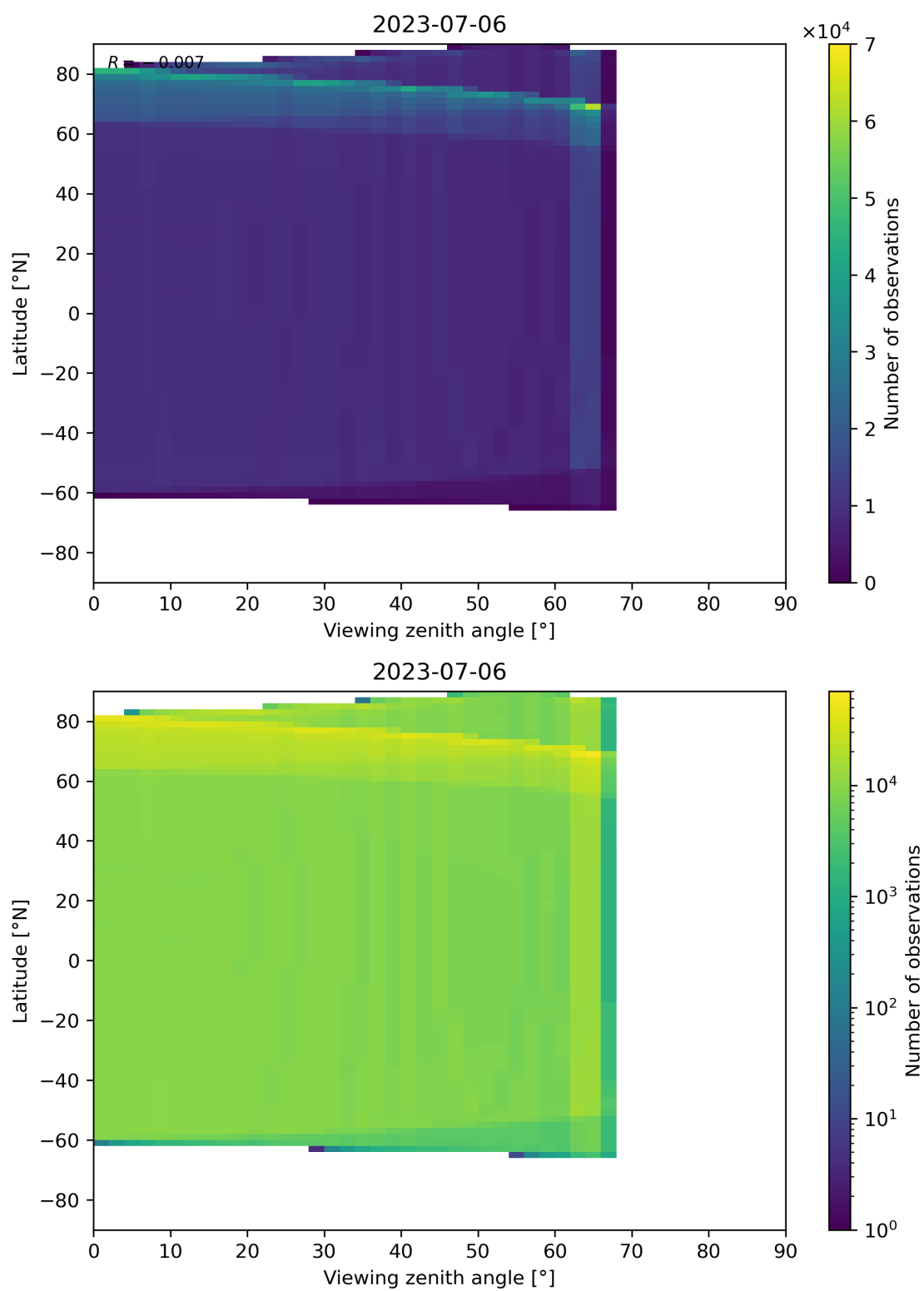
Figure 163: Scatter density plot of “Viewing zenith angle” against “Latitude” for 2023-07-05 to 2023-07-07.
