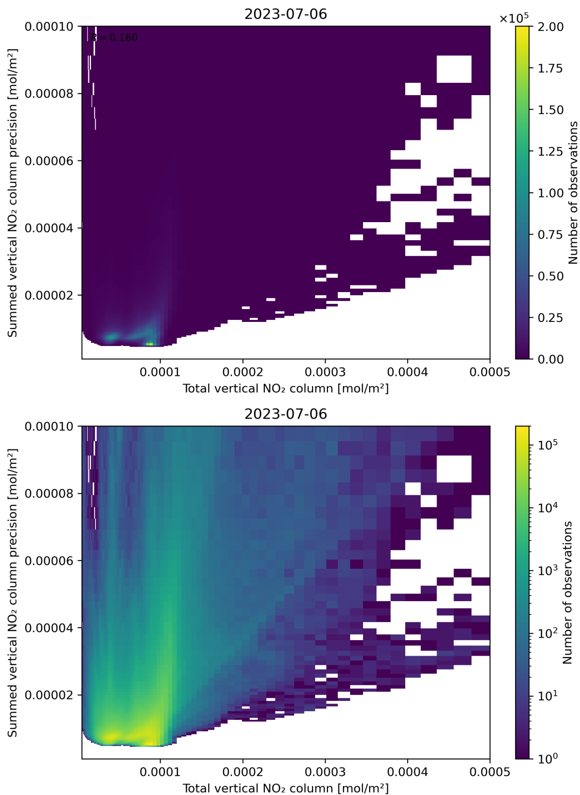
Figure 113: Scatter density plot of “Total vertical NO 2 column” against “Summed vertical NO 2 column precision” for 2023-07-05 to 2023-07-07.
