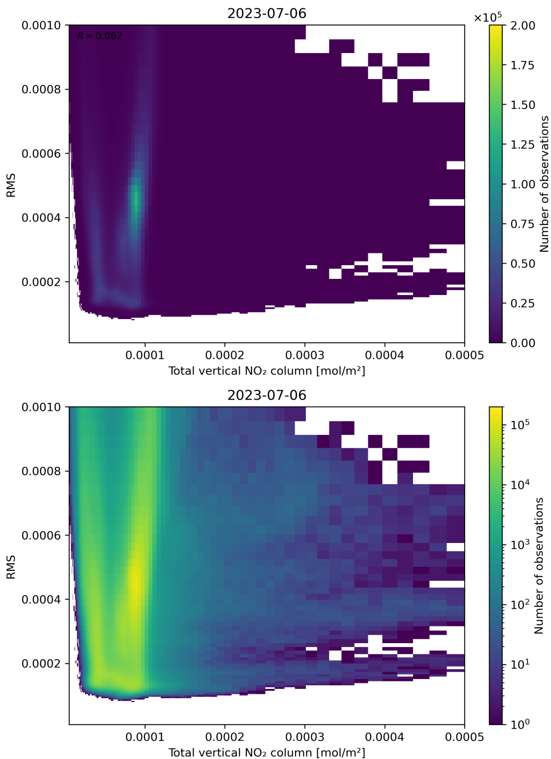
Figure 120: Scatter density plot of “Total vertical NO 2 column” against “RMS” for 2023-07-05 to 2023-07-07.
