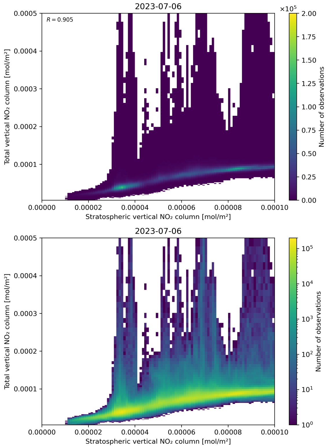
Figure 100: Scatter density plot of “Stratospheric vertical NO 2 column” against “Total vertical NO 2 column” for 2023-07-05 to 2023-07-07.
