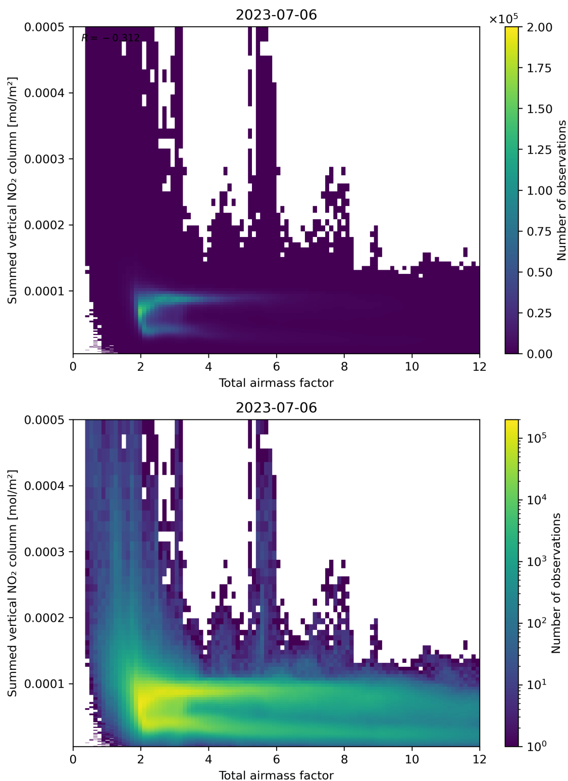
Figure 65: Scatter density plot of “Total airmass factor” against “Summed vertical NO 2 column” for 2023-07-05 to 2023-07-07.
