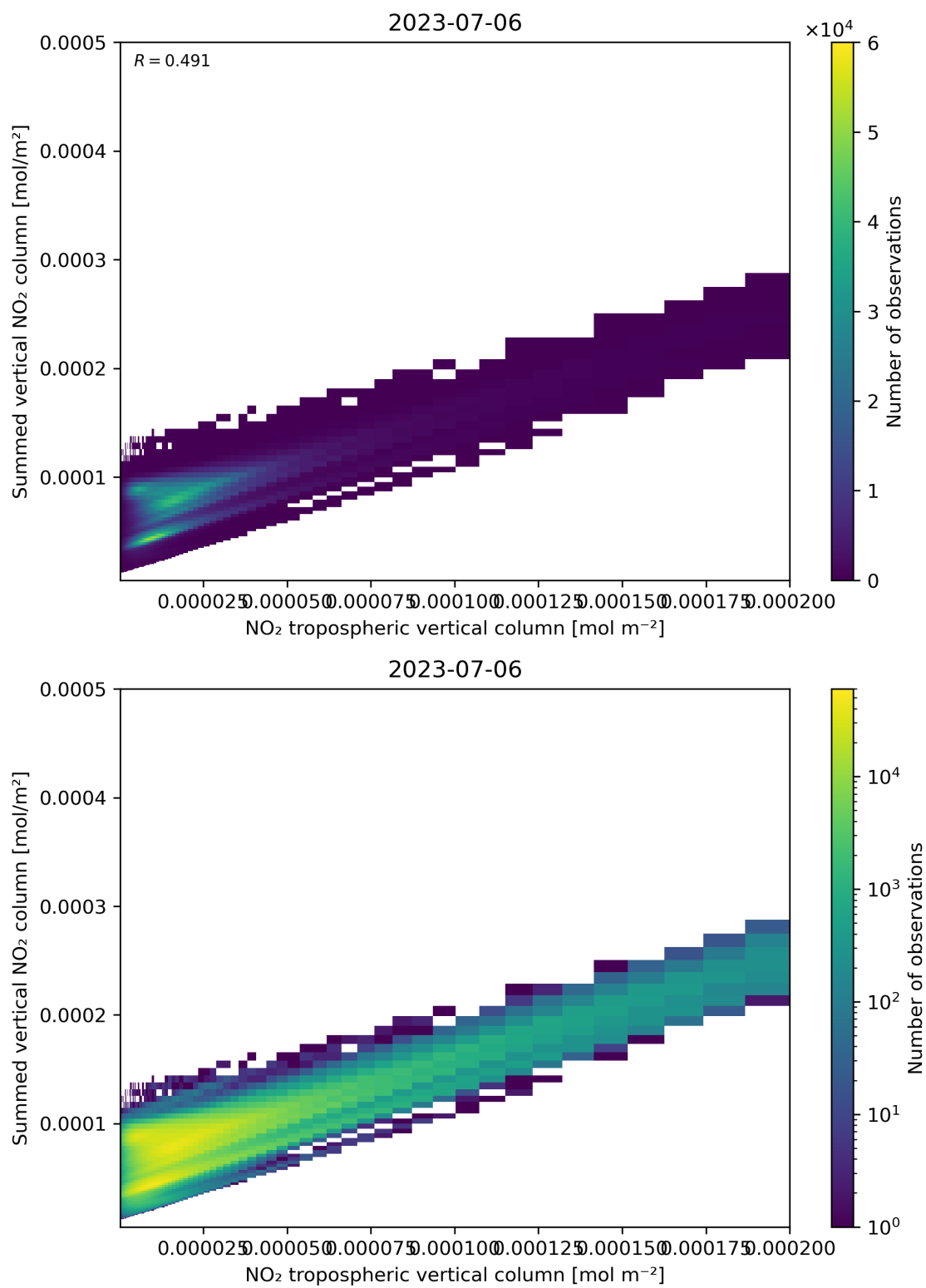
Figure 126: Scatter density plot of “NO 2 tropospheric vertical column” against “Summed vertical NO 2 column” for 2023-07-05 to 2023-07-07.
