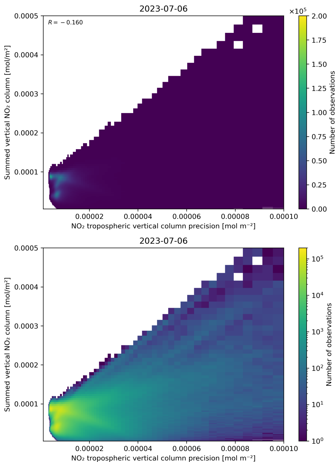
Figure 136: Scatter density plot of “NO 2 tropospheric vertical column precision” against “Summed vertical NO 2 column” for 2023-07-05 to 2023-07-07.
