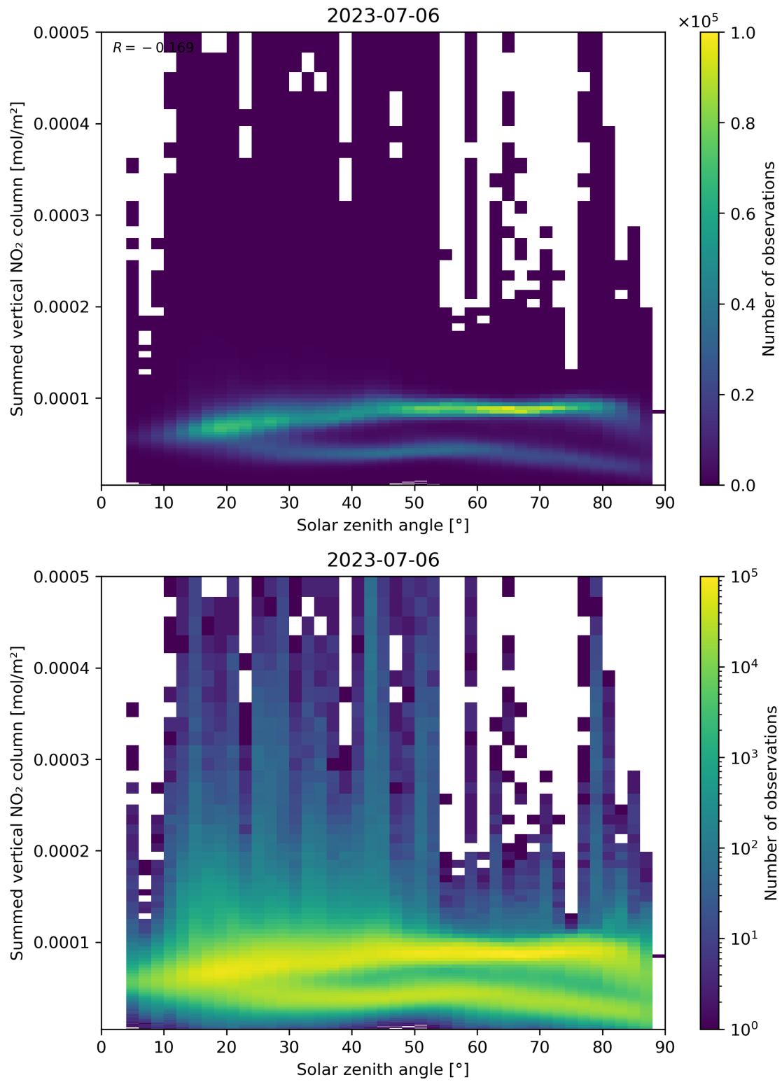
Figure 151: Scatter density plot of “Solar zenith angle” against “Summed vertical NO 2 column” for 2023-07-05 to 2023-07-07.
