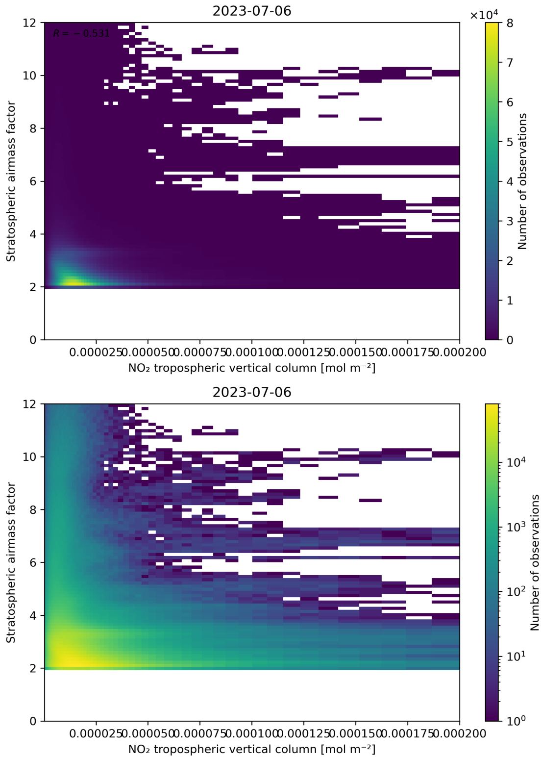
Figure 121: Scatter density plot of “NO 2 tropospheric vertical column” against “Stratospheric air mass factor” for 2023-07-05 to 2023-07-07.
