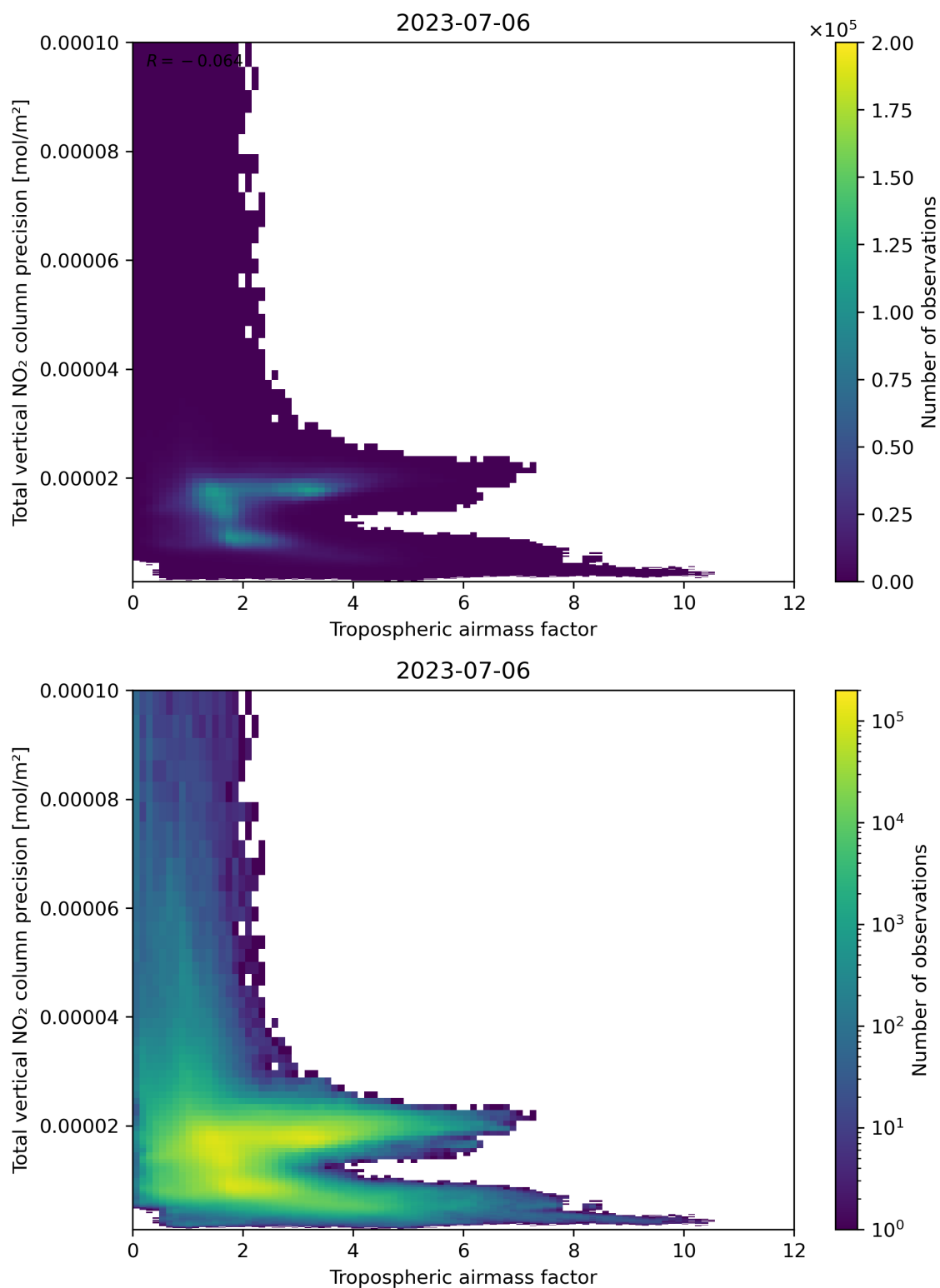
Figure 78: Scatter density plot of “Tropospheric air mass factor” against “Total vertical NO 2 column precision” for 2023-07-05 to 2023-07-07.
