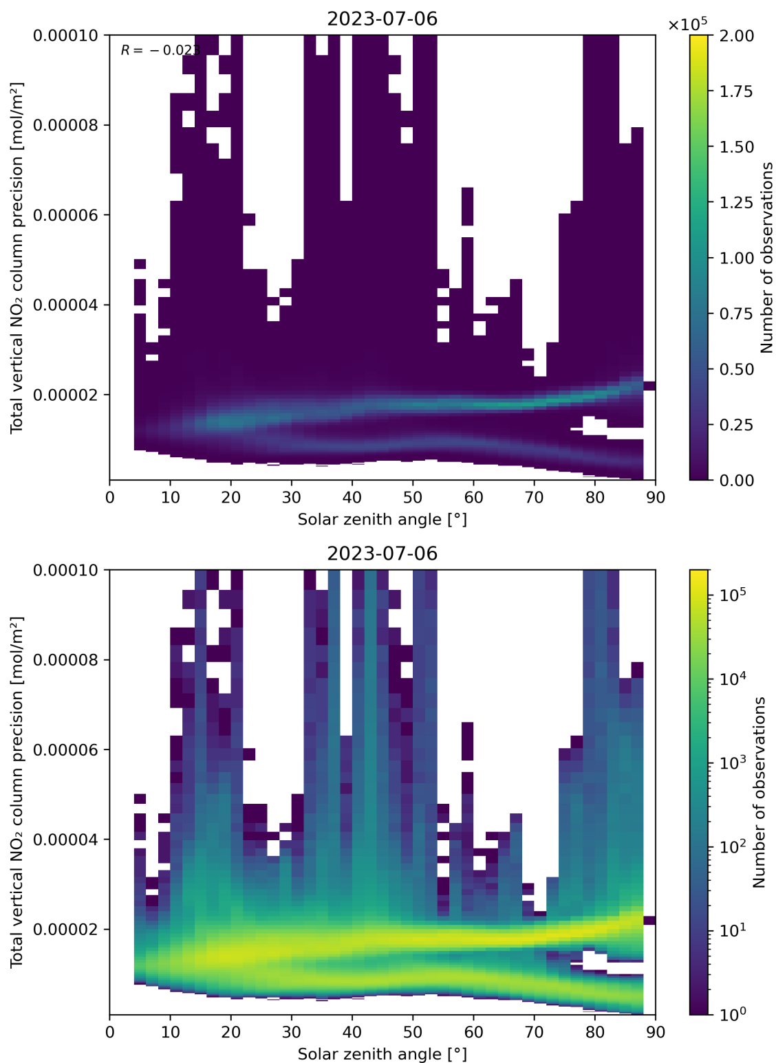
Figure 154: Scatter density plot of “Solar zenith angle” against “Total vertical NO 2 column precision” for 2023-07-05 to 2023-07-07.
