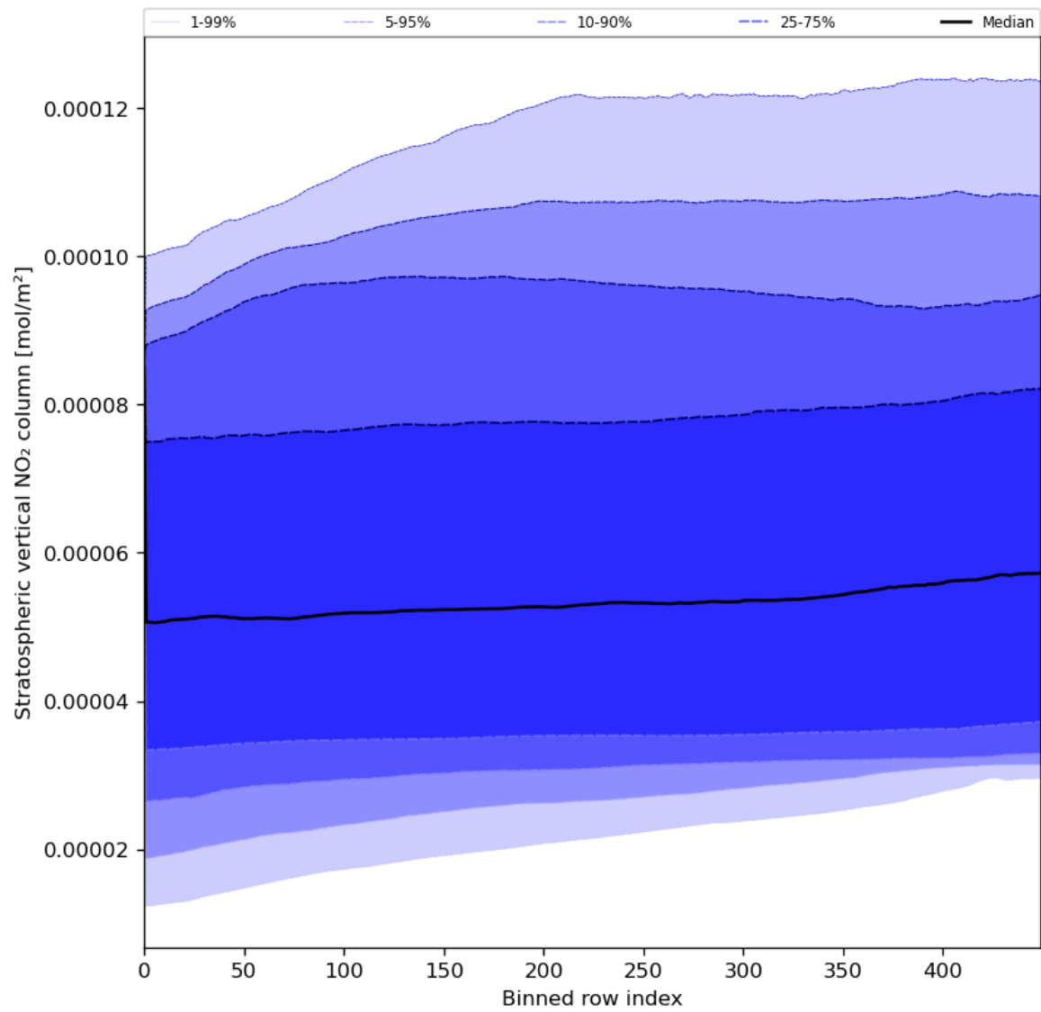
Figure 53: Along track statistics of “Stratospheric vertical NO 2 column” for 2023-07-05 to 2023-07-07
