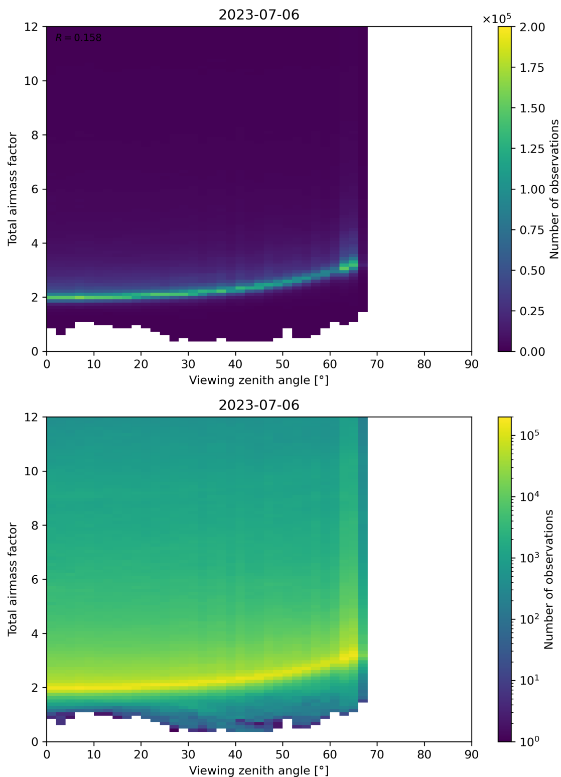
Figure 160: Scatter density plot of “Viewing zenith angle” against “Total airmass factor” for 2023-07-05 to 2023-07-07.
