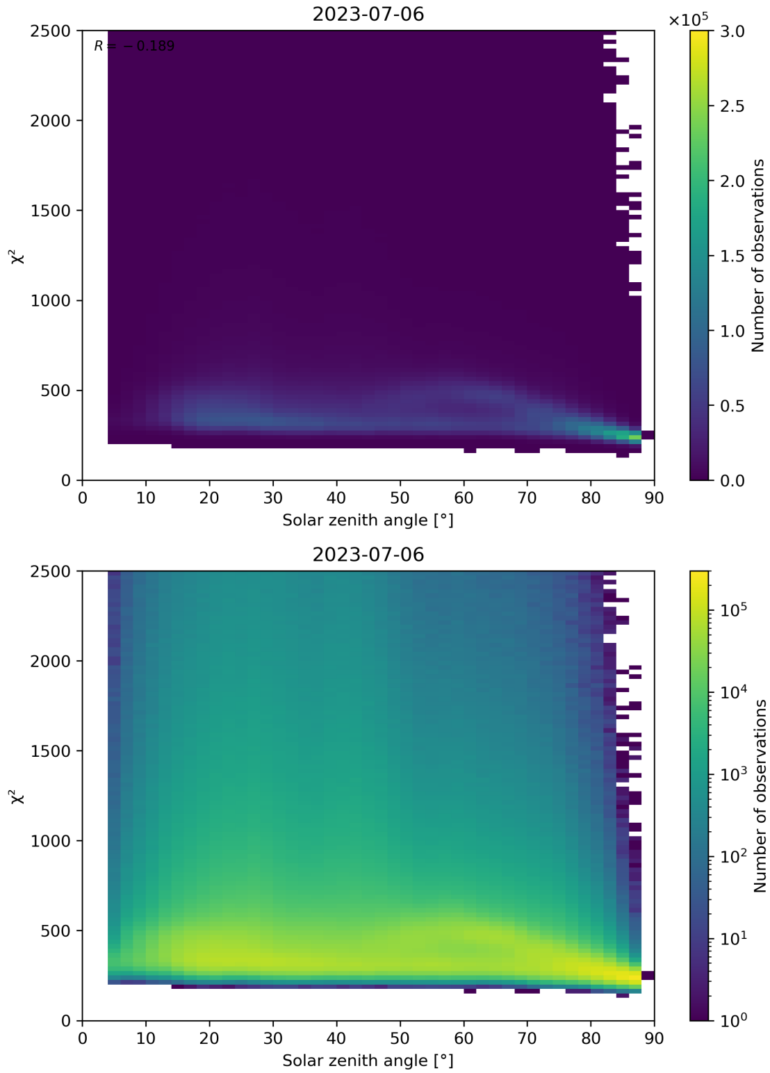
Figure 148: Scatter density plot of “Solar zenith angle” against “ \chi^2 ” for 2023-07-05 to 2023-07-07.
