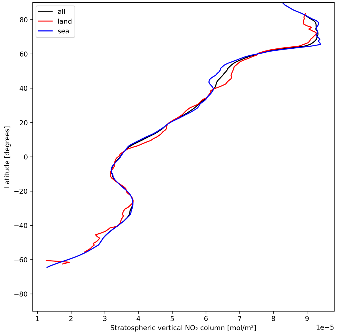
Figure 19: Zonal average of “Stratospheric vertical NO 2 column” for 2023-07-05 to 2023-07-07.
