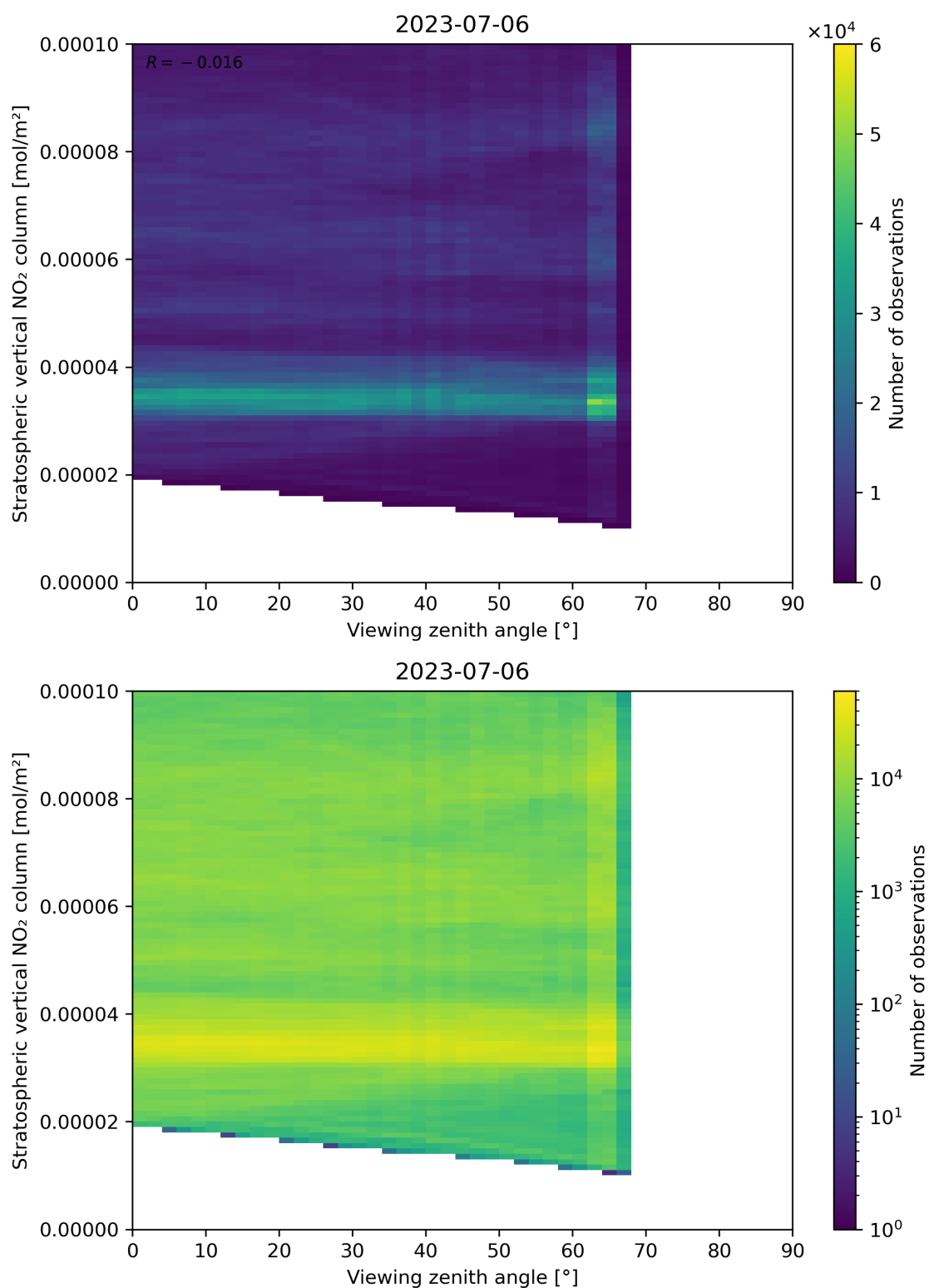
Figure 164: Scatter density plot of “Viewing zenith angle” against “Stratospheric vertical NO 2 column” for 2023-07-05 to 2023-07-07.
