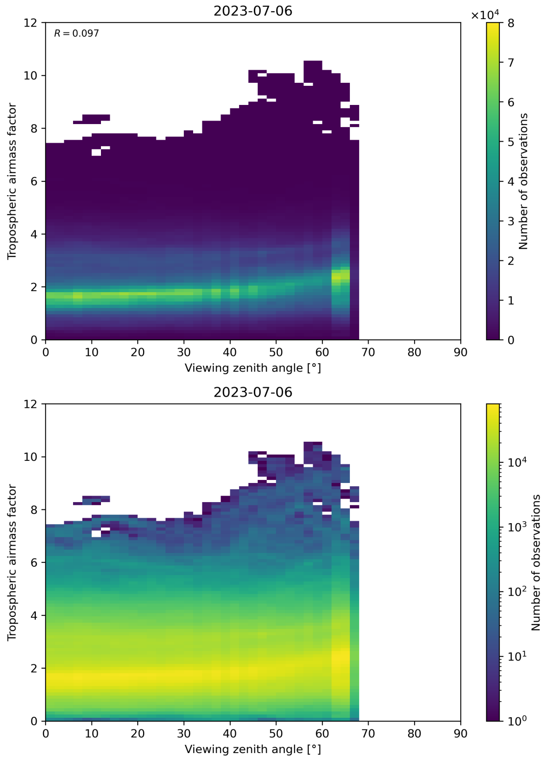
Figure 161: Scatter density plot of “Viewing zenith angle” against “Tropospheric airmass factor” for 2023-07-05 to 2023-07-07.
