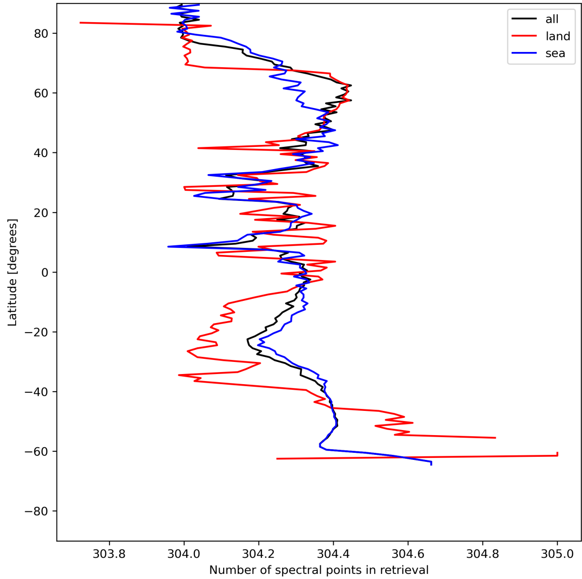
Figure 16: Zonal average of “Number of spectral points in retrieval” for 2023-07-05 to 2023-07-07.
