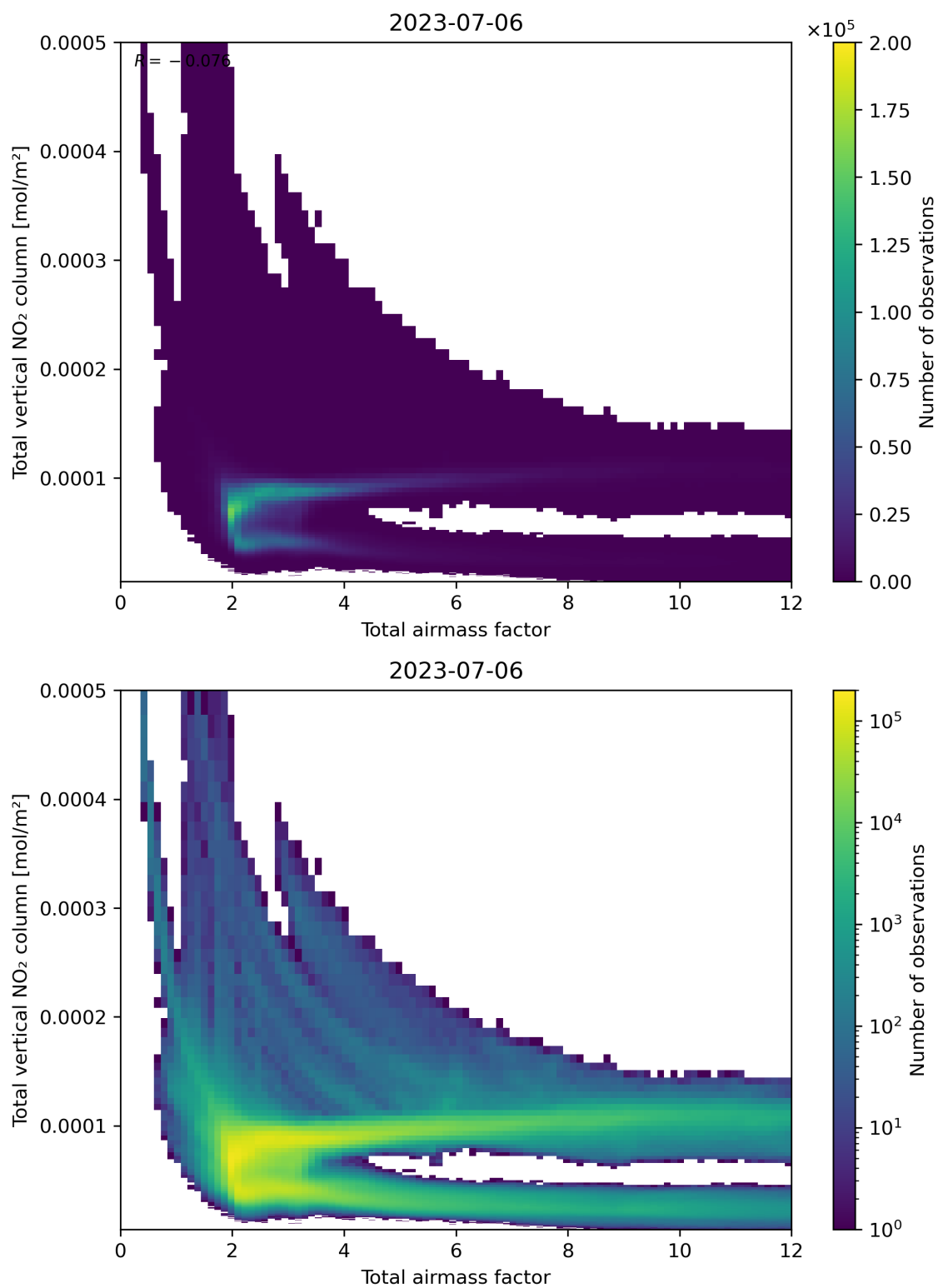
Figure 67: Scatter density plot of “Total airmass factor” against “Total vertical NO 2 column” for 2023-07-05 to 2023-07-07.
