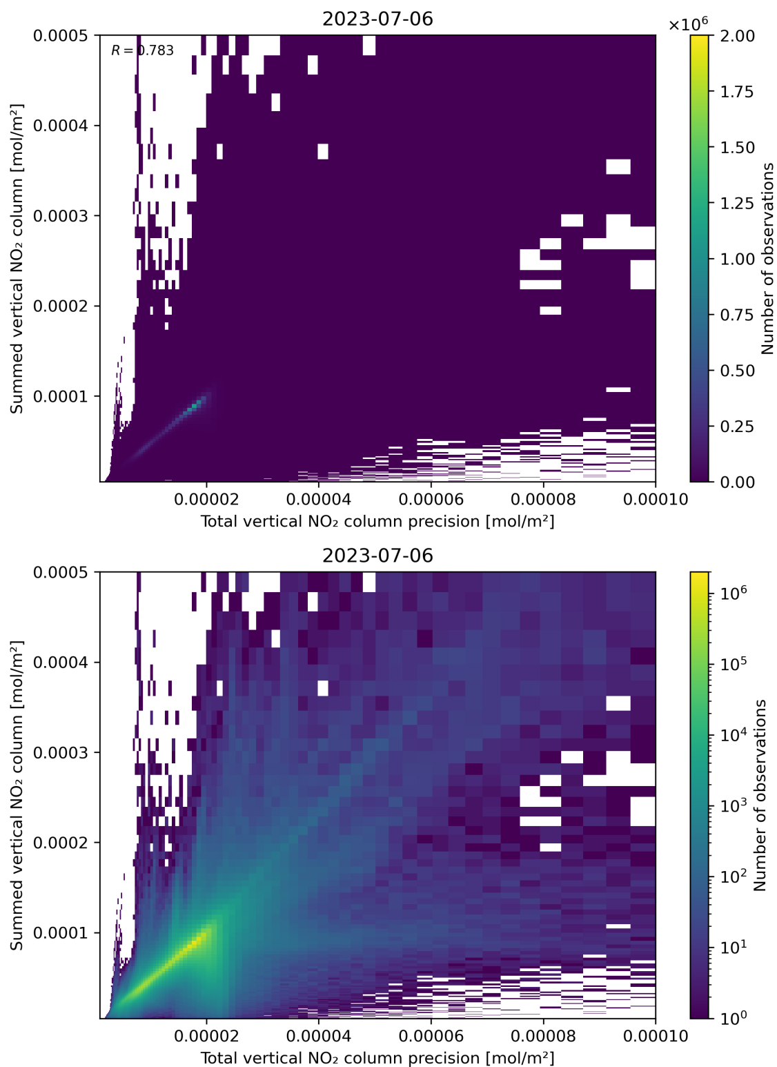
Figure 117: Scatter density plot of “Total vertical NO 2 column precision” against “Summed vertical NO 2 column” for 2023-07-05 to 2023-07-07.
