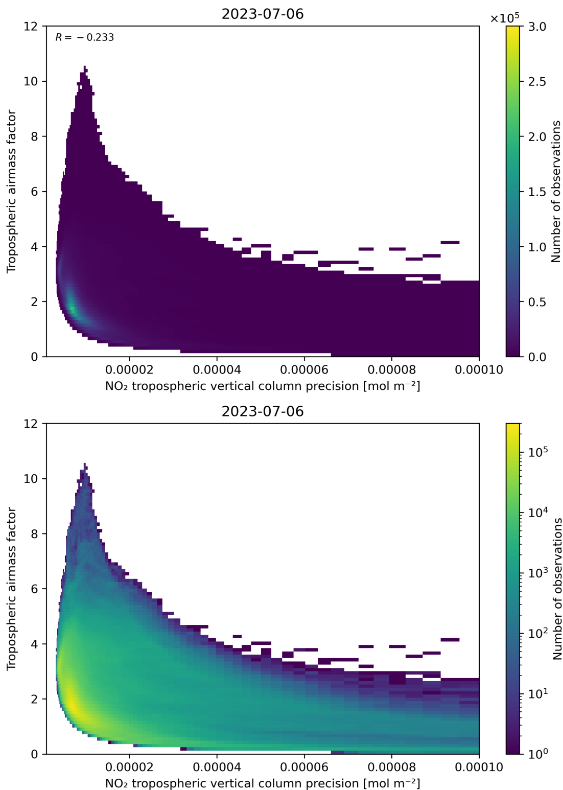
Figure 133: Scatter density plot of “NO 2 tropospheric vertical column precision” against “Tropospheric air mass factor” for 2023-07-05 to 2023-07-07.
