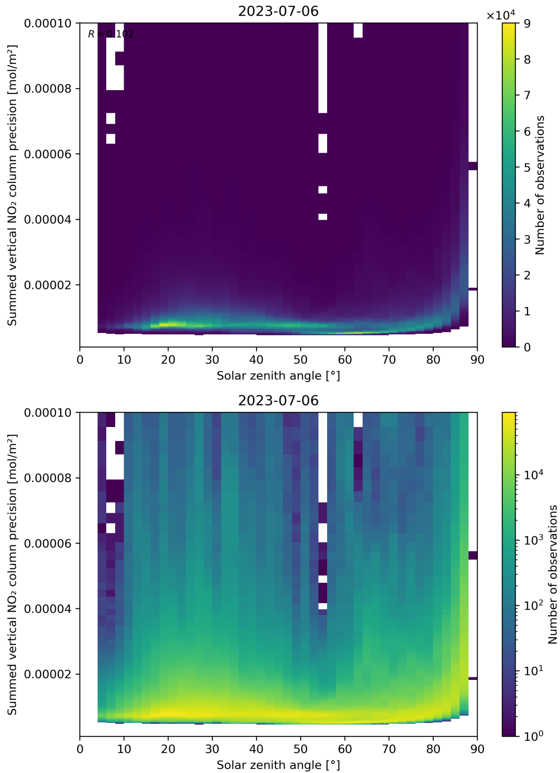
Figure 152: Scatter density plot of “Solar zenith angle” against “Summed vertical NO 2 column precision” for 2023-07-05 to 2023-07-07.
