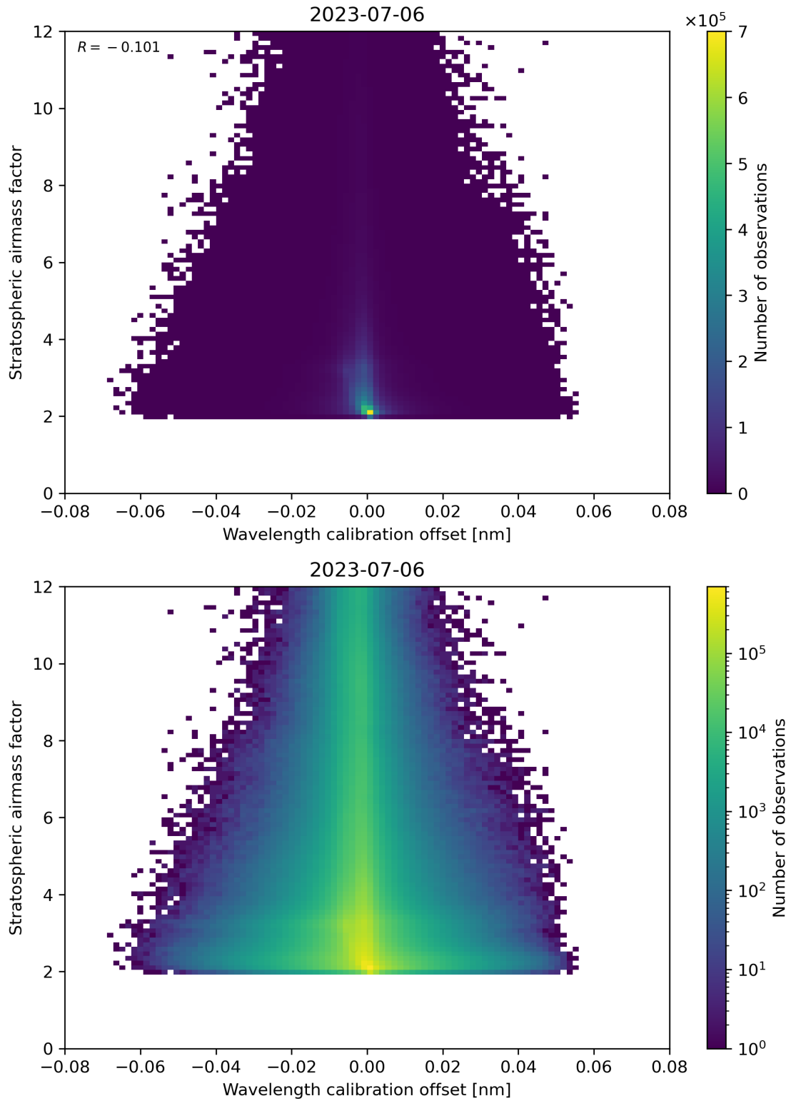
Figure 174: Scatter density plot of “Wavelength calibration offset” against “Stratospheric airmass factor” for 2023-07-05 to 2023-07-07.
