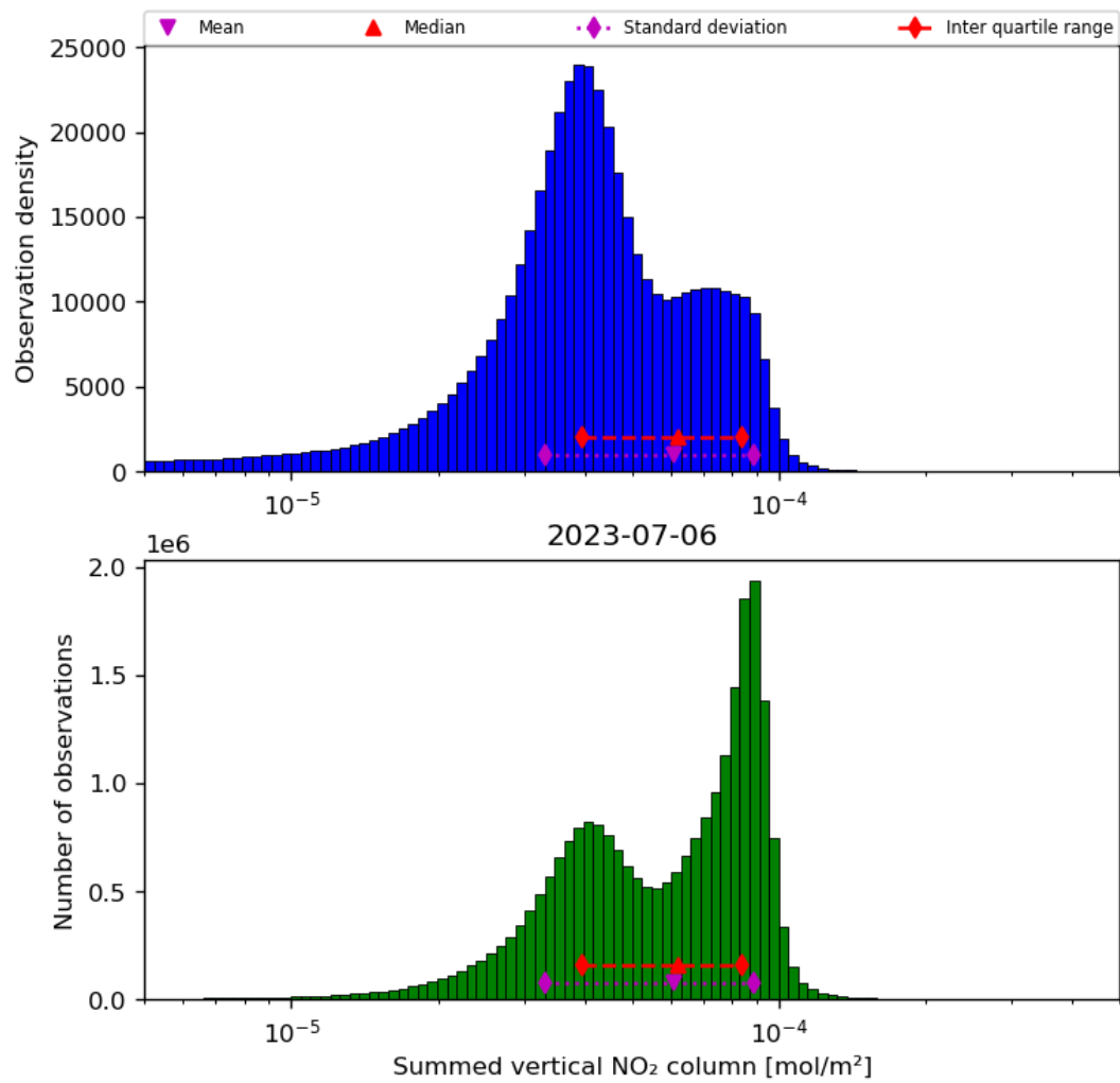
Figure 40: Histogram of “Summed vertical NO 2 column” for 2023-07-05 to 2023-07-07
