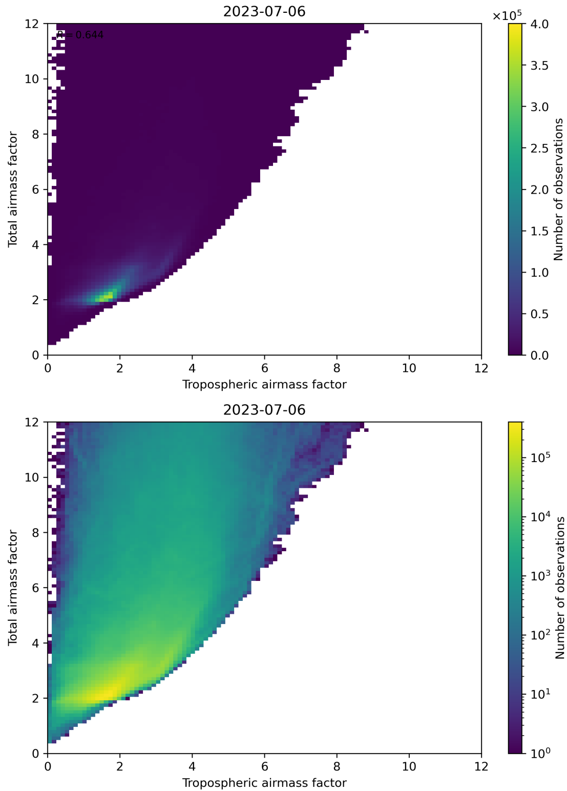
Figure 72: Scatter density plot of “Tropospheric airmass factor” against “Total airmass factor” for 2023-07-05 to 2023-07-07.
