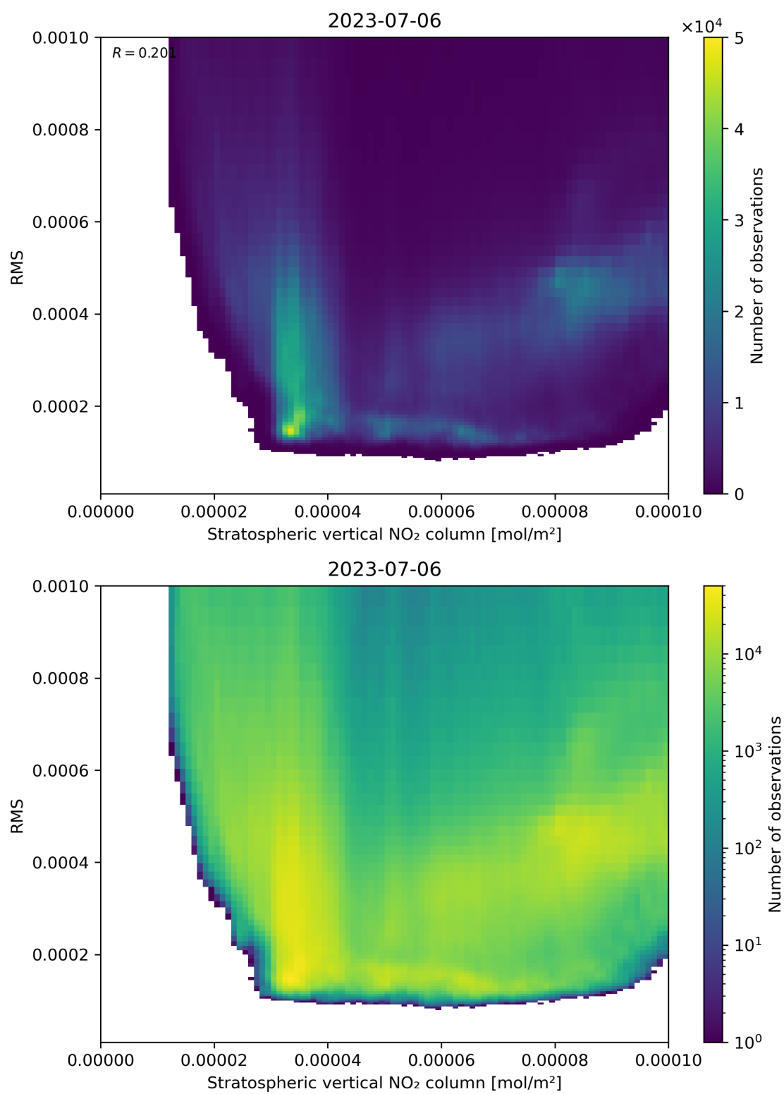
Figure 102: Scatter density plot of “Stratospheric vertical NO 2 column” against “RMS” for 2023-07-05 to 2023-07-07.
