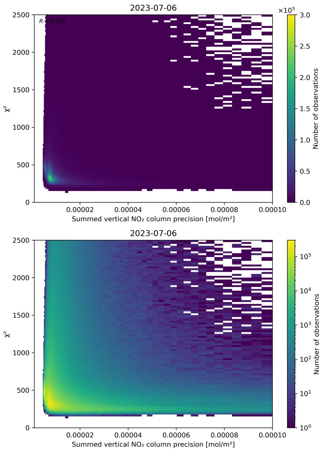
Figure 107: Scatter density plot of “Summed vertical NO 2 column precision” against “ \chi^2 ” for 2023-07-05 to 2023-07-07.
