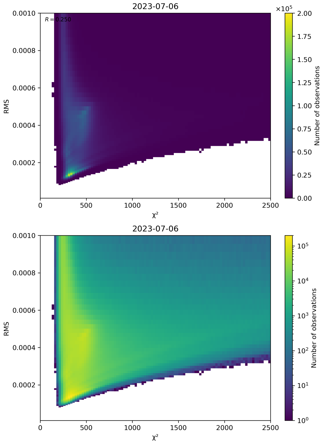
Figure 82: Scatter density plot of “ \chi^2 ” against “RMS” for 2023-07-05 to 2023-07-07.
