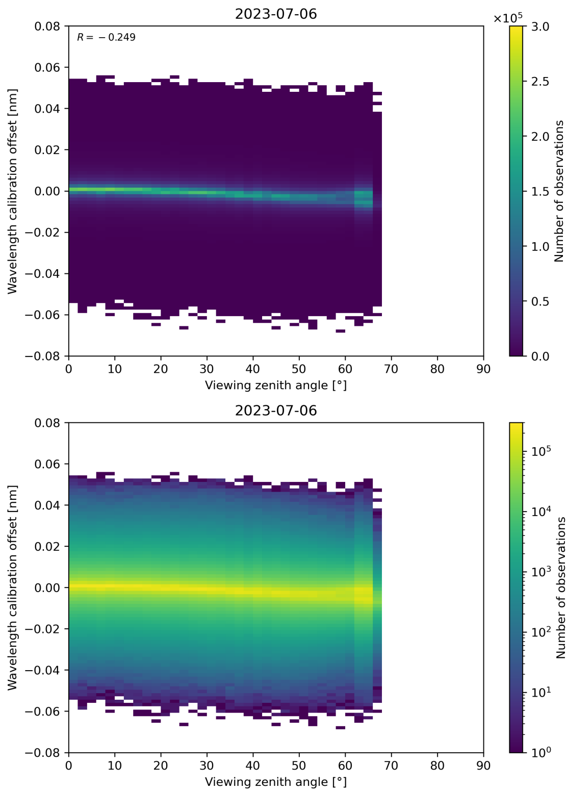
Figure 173: Scatter density plot of “Viewing zenith angle” against “Wavelength calibration offset” for 2023-07-05 to 2023-07-07.
