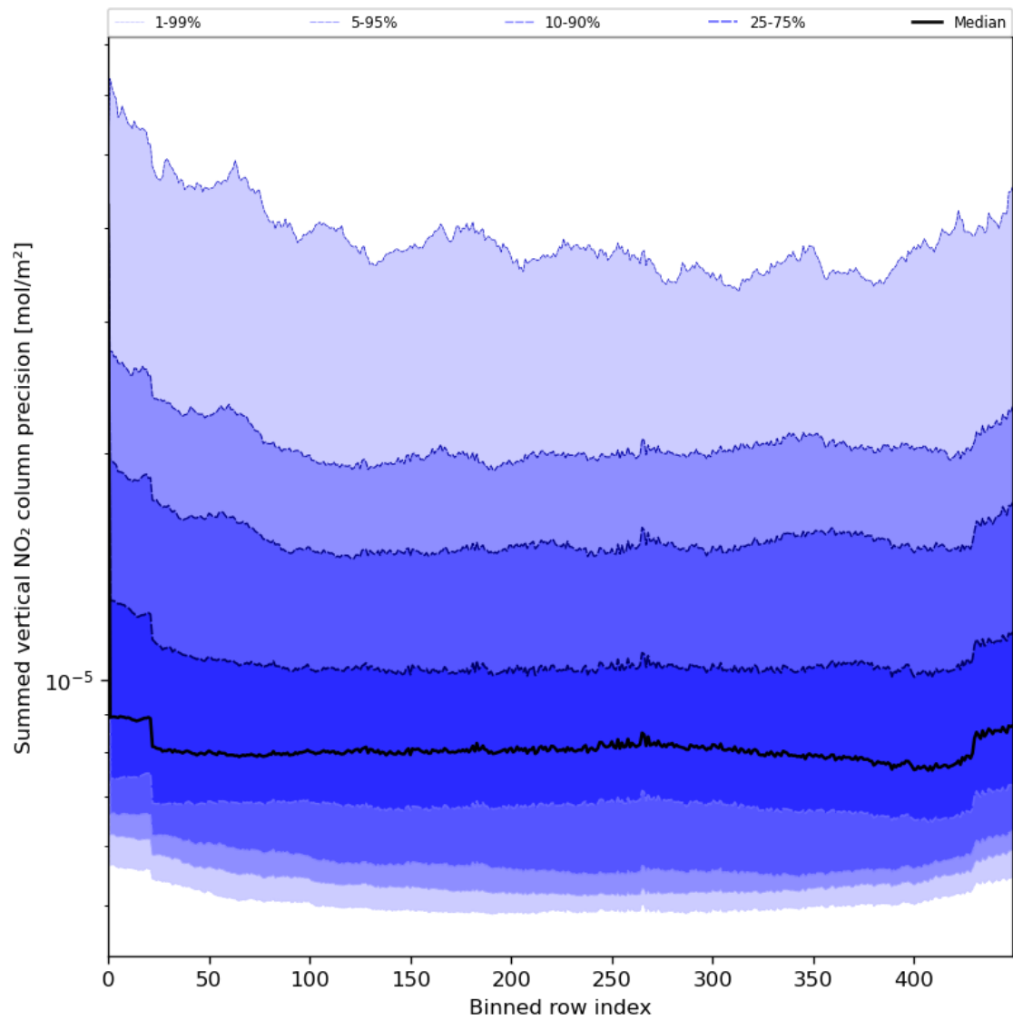
Figure 58: Along track statistics of “Summed vertical NO 2 column precision” for 2023-07-05 to 2023-07-07
