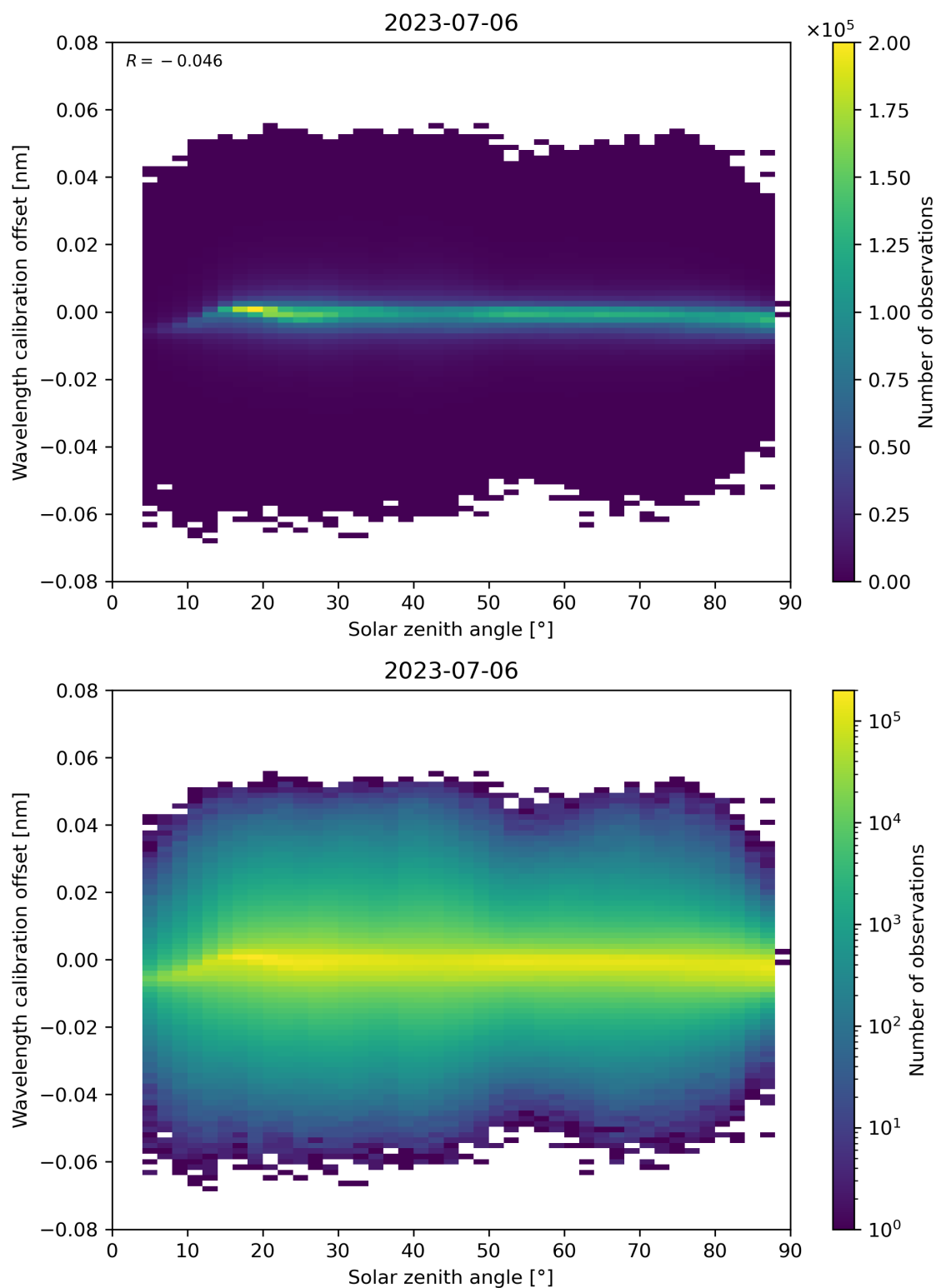
Figure 158: Scatter density plot of “Solar zenith angle” against “Wavelength calibration offset” for 2023-07-05 to 2023-07-07.
