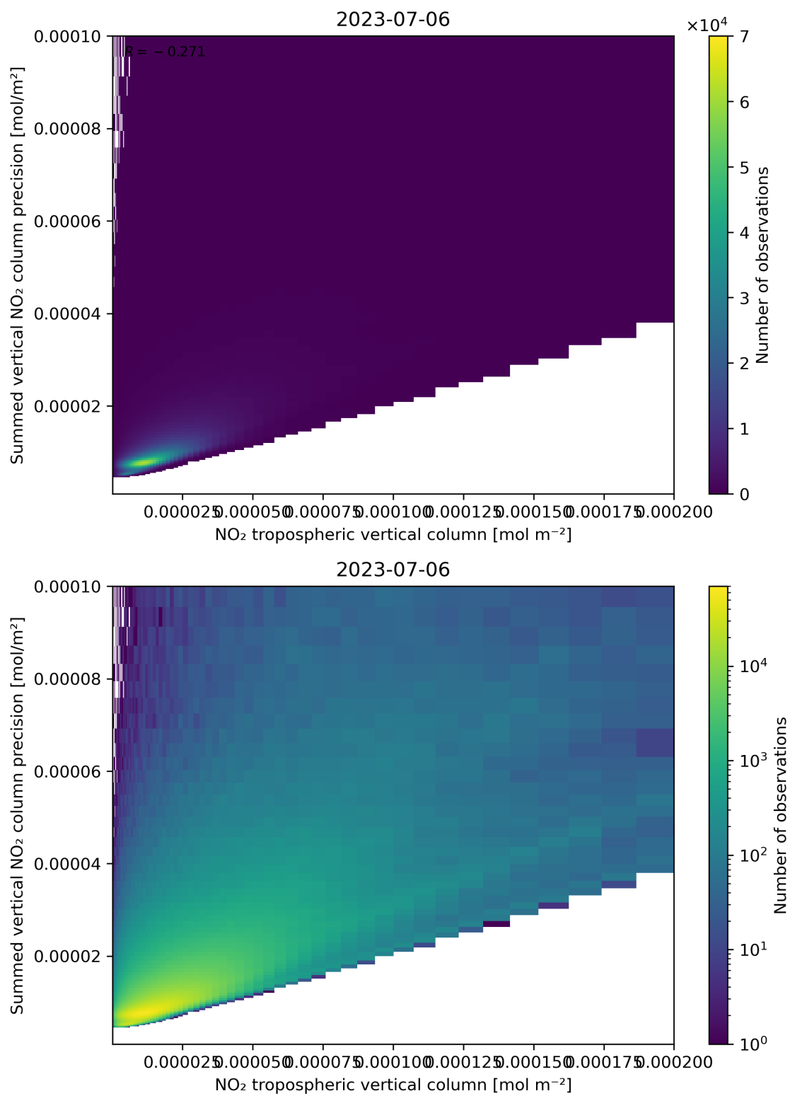
Figure 127: Scatter density plot of “NO 2 tropospheric vertical column” against “Summed vertical NO 2 column precision” for 2023-07-05 to 2023-07-07.
