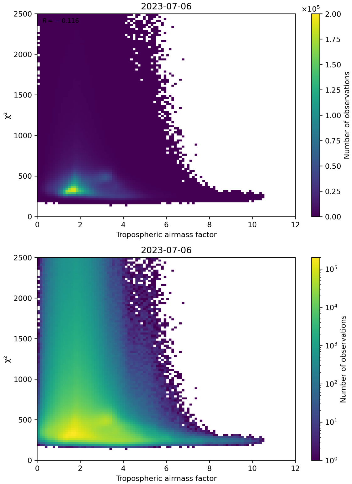
Figure 73: Scatter density plot of “Tropospheric airmass factor” against “ \chi^2 ” for 2023-07-05 to 2023-07-07.
