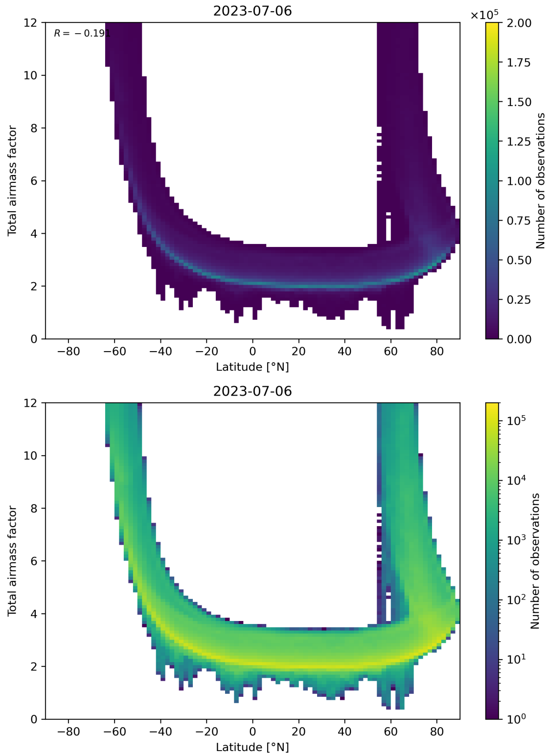
Figure 84: Scatter density plot of “Latitude” against “Total airmass factor” for 2023-07-05 to 2023-07-07.
