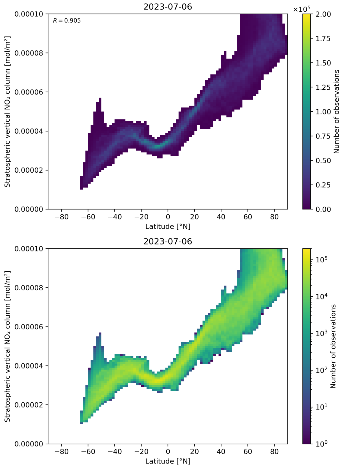
Figure 87: Scatter density plot of “Latitude” against “Stratospheric vertical NO 2 column” for 2023-07-05 to 2023-07-07.
