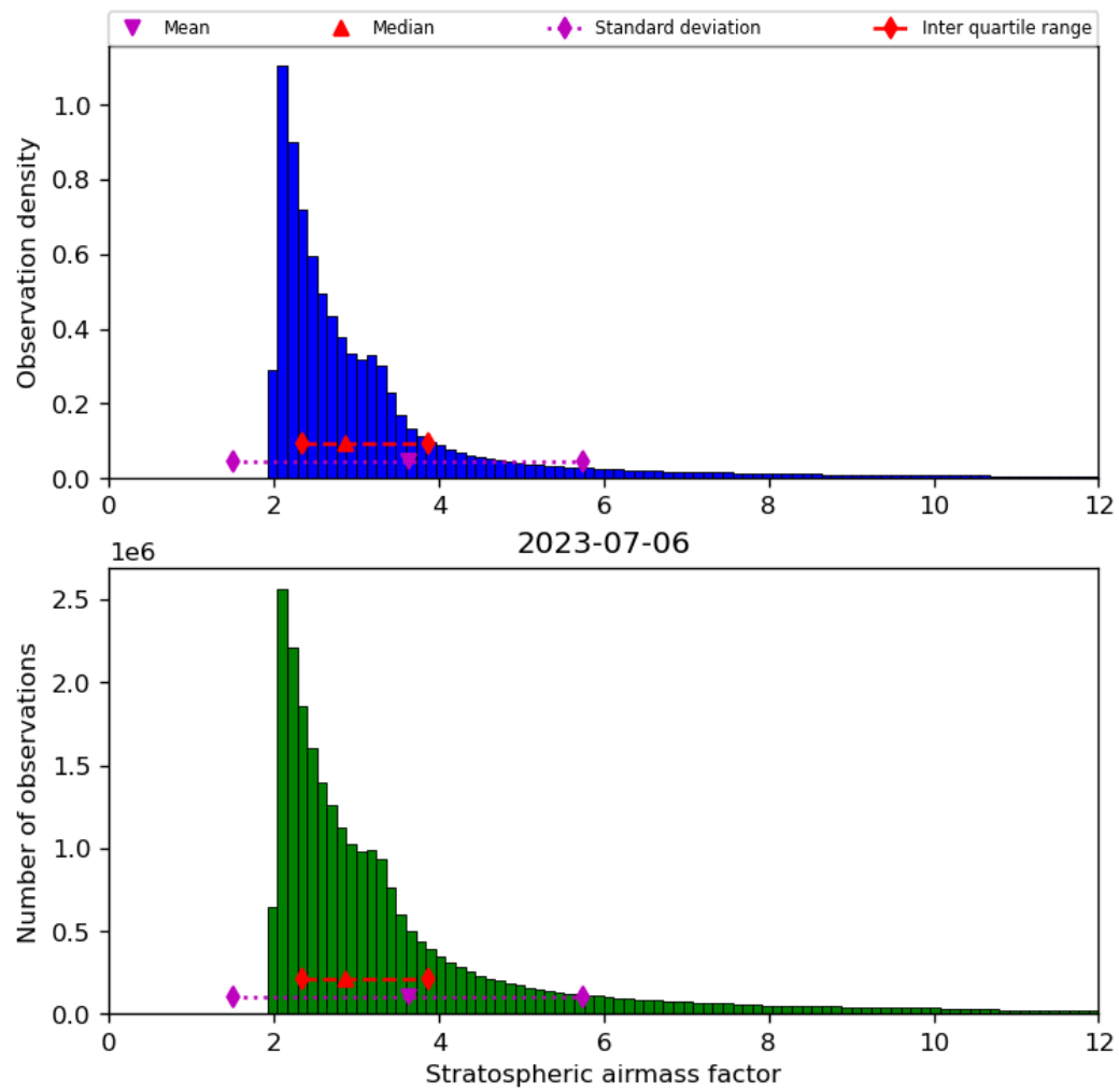
Figure 44: Histogram of “Stratospheric airmass factor” for 2023-07-05 to 2023-07-07
