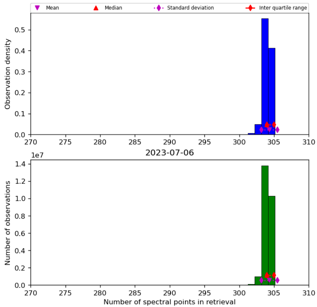
Figure 33: Histogram of “Number of spectral points in retrieval” for 2023-07-05 to 2023-07-07
