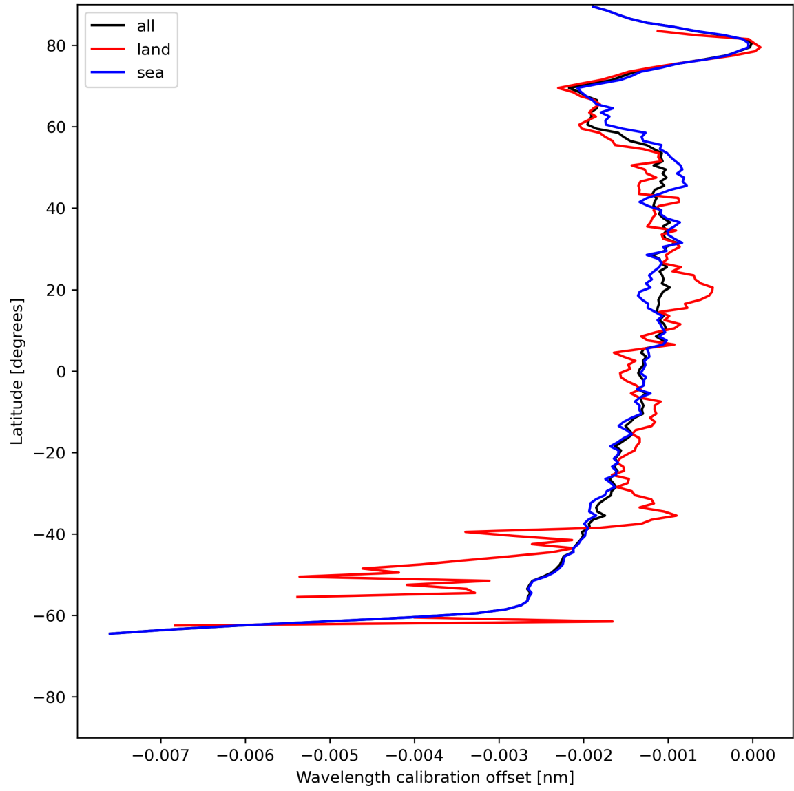
Figure 18: Zonal average of “Wavelength calibration offset” for 2023-07-05 to 2023-07-07.
