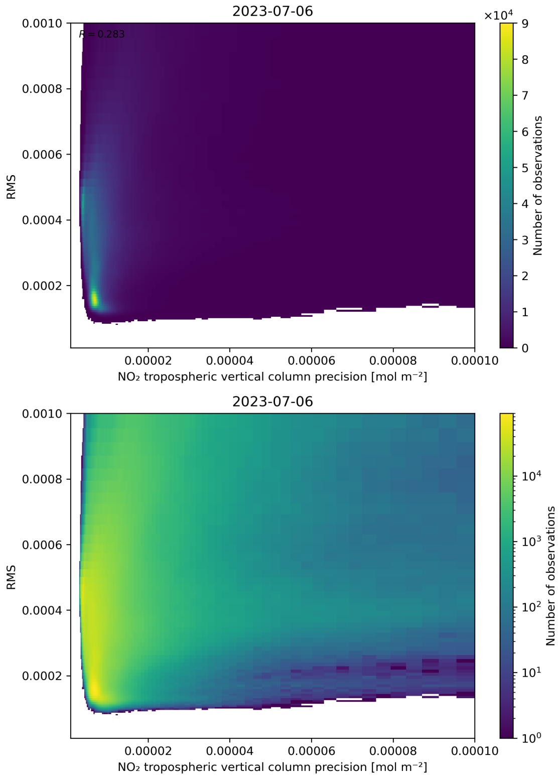
Figure 140: Scatter density plot of “NO 2 tropospheric vertical column precision” against “RMS” for 2023-07-05 to 2023-07-07.
