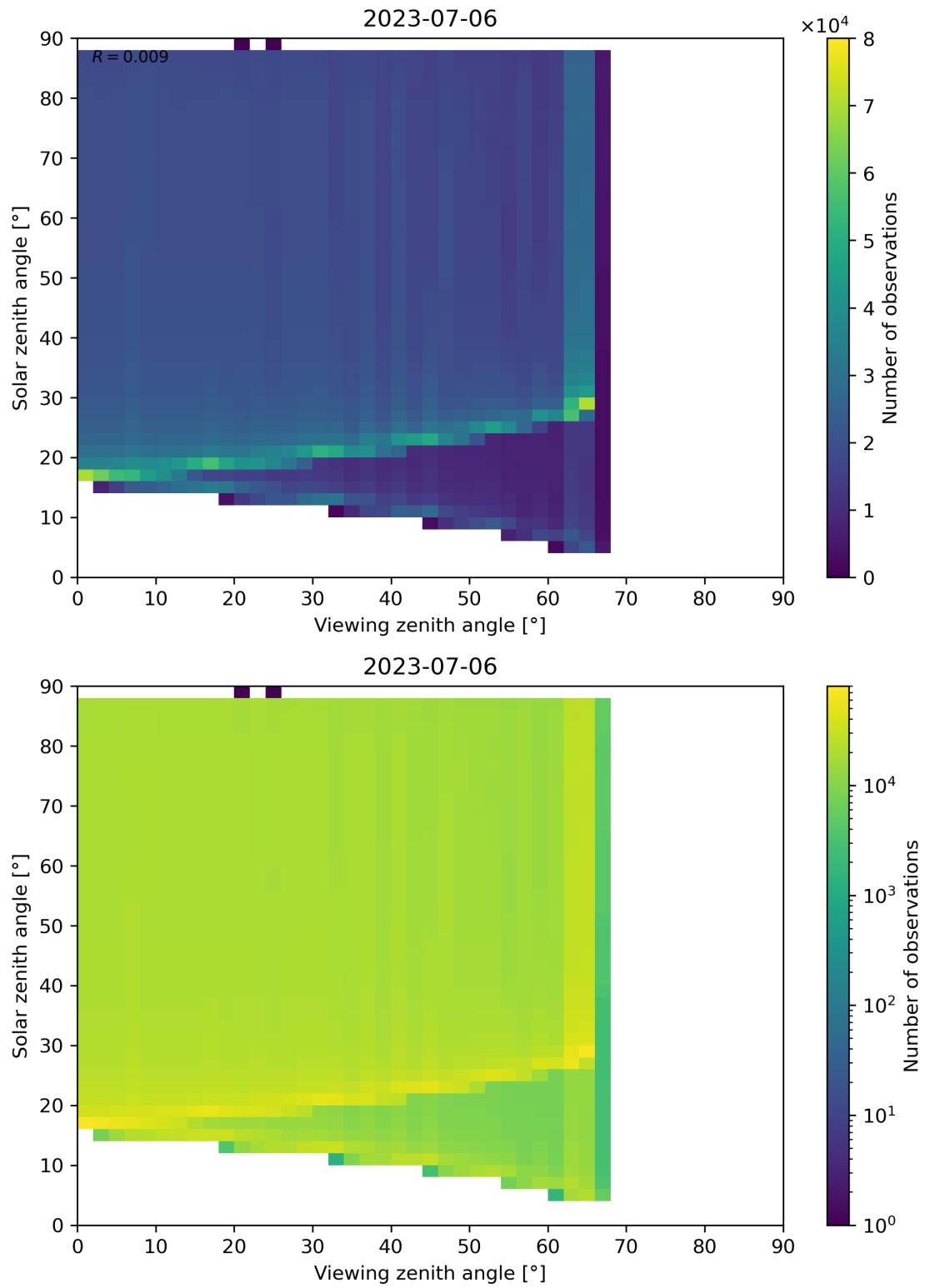
Figure 172: Scatter density plot of “Viewing zenith angle” against “Solar zenith angle” for 2023-07-05 to 2023-07-07.
