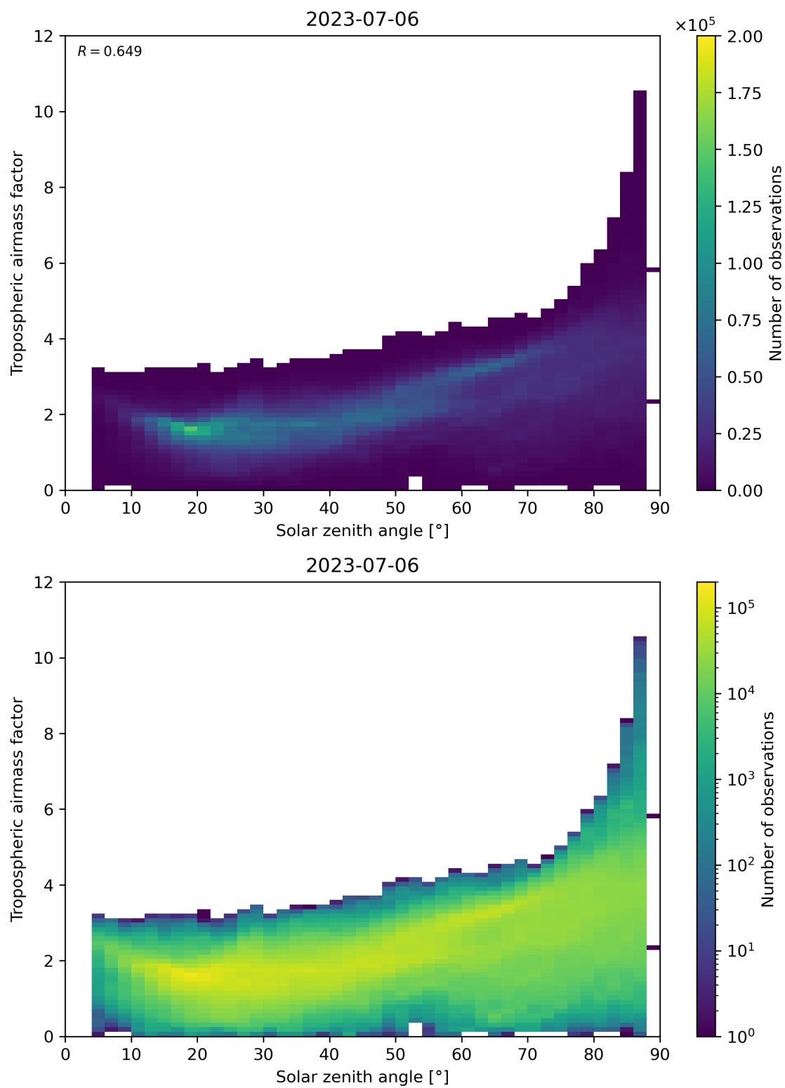
Figure 147: Scatter density plot of “Solar zenith angle” against “Tropospheric airmass factor” for 2023-07-05 to 2023-07-07.
