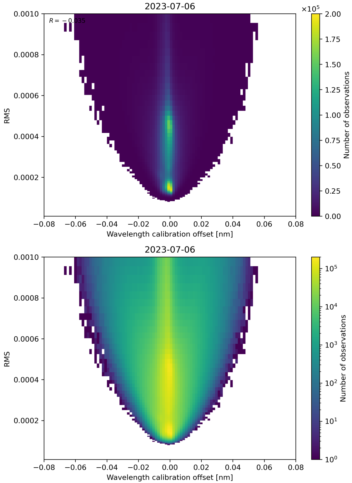
Figure 181: Scatter density plot of “Wavelength calibration offset” against “RMS” for 2023-07-05 to 2023-07-07.
