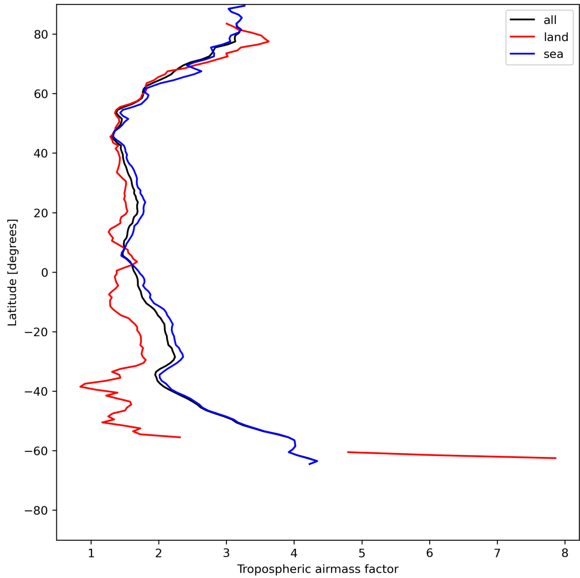
Figure 14: Zonal average of “Tropospheric airmass factor” for 2023-07-05 to 2023-07-07.
