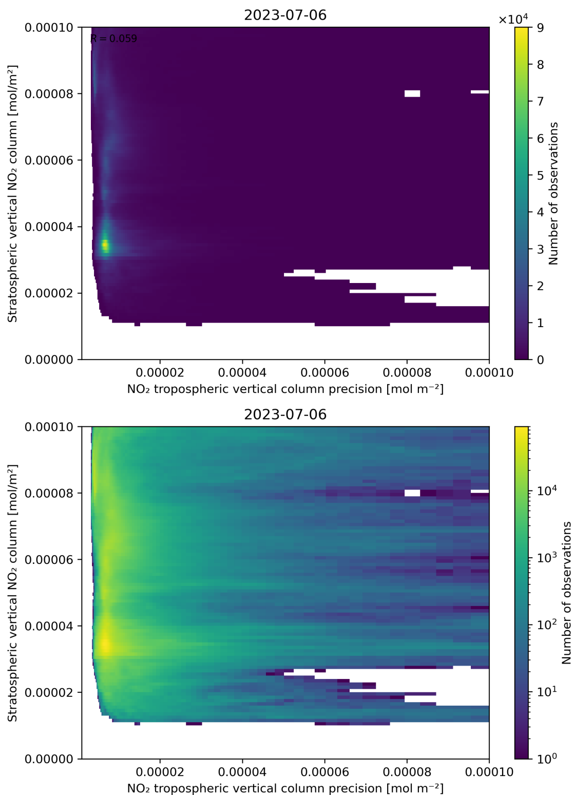
Figure 135: Scatter density plot of “NO 2 tropospheric vertical column precision” against “Stratospheric vertical NO 2 column” for 2023-07-05 to 2023-07-07.
