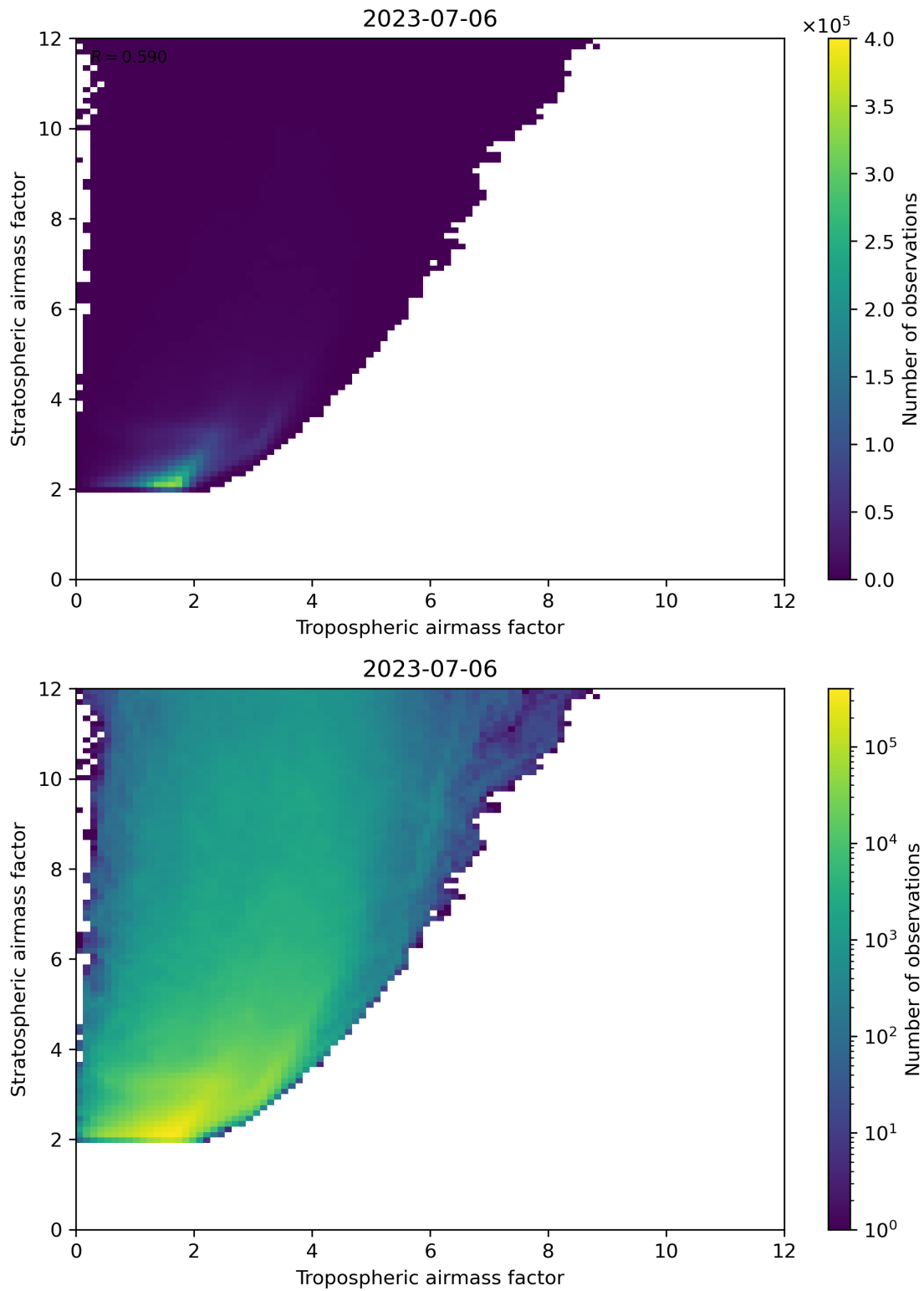
Figure 71: Scatter density plot of “Tropospheric airmass factor” against “Stratospheric airmass factor” for 2023-07-05 to 2023-07-07.
