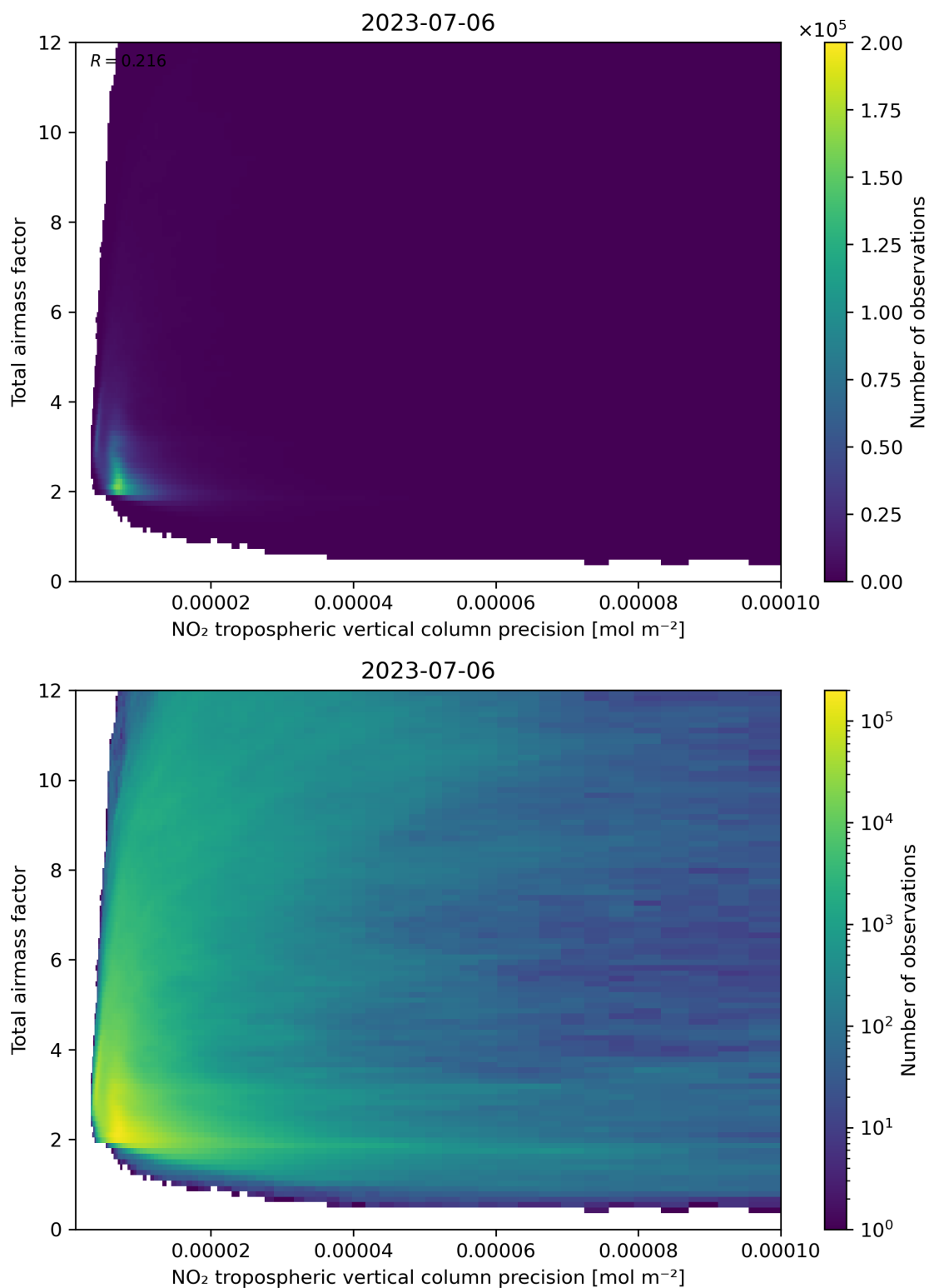
Figure 132: Scatter density plot of “NO 2 tropospheric vertical column precision” against “Total air mass factor” for 2023-07-05 to 2023-07-07.
