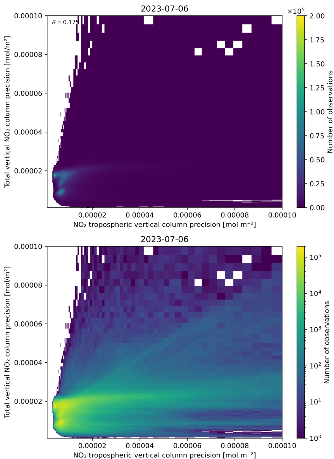
Figure 139: Scatter density plot of “NO 2 tropospheric vertical column precision” against “Total vertical NO 2 column precision” for 2023-07-05 to 2023-07-07.
