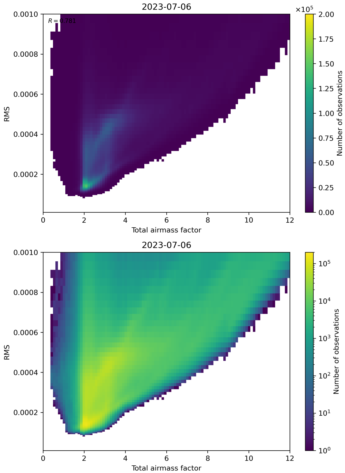
Figure 69: Scatter density plot of “Total airmass factor” against “RMS” for 2023-07-05 to 2023-07-07.
