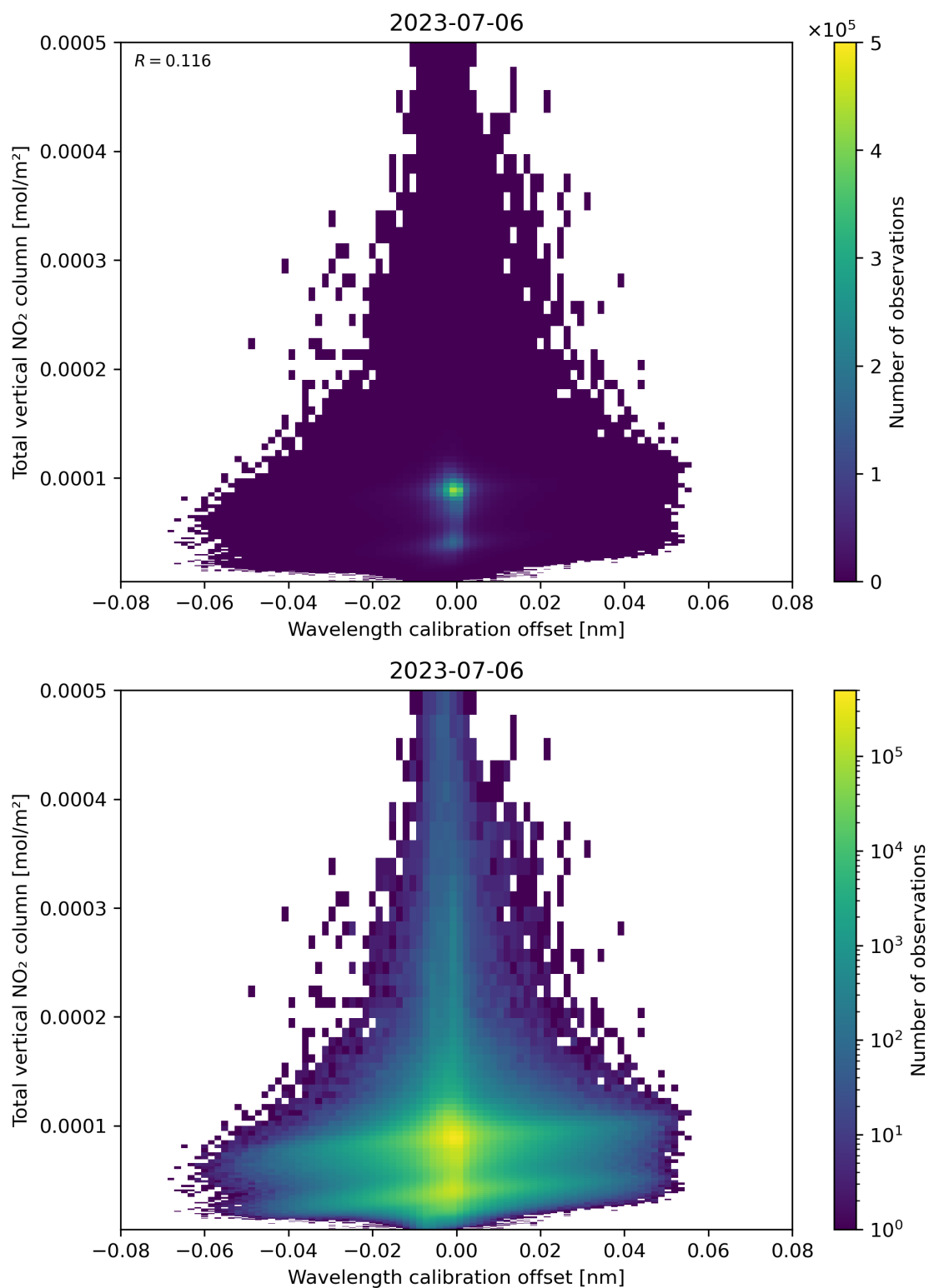
Figure 179: Scatter density plot of “Wavelength calibration offset” against “Total vertical NO 2 column” for 2023-07-05 to 2023-07-07.
