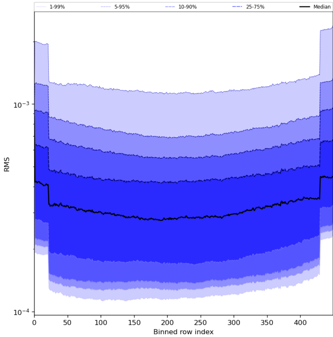
Figure 60: Along track statistics of “RMS” for 2023-07-05 to 2023-07-07
