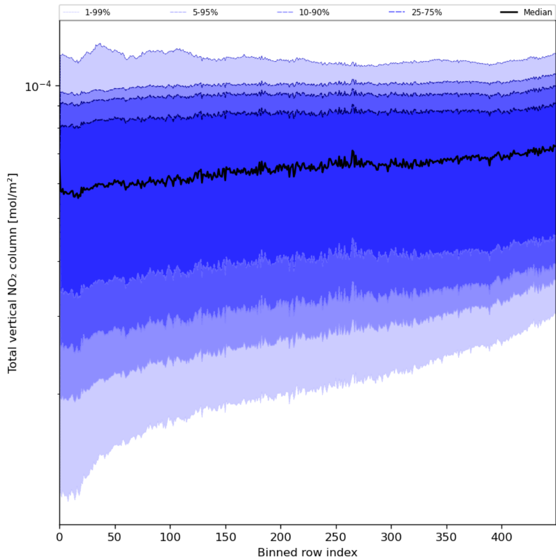
Figure 55: Along track statistics of “Total vertical NO 2 column” for 2023-07-05 to 2023-07-07
