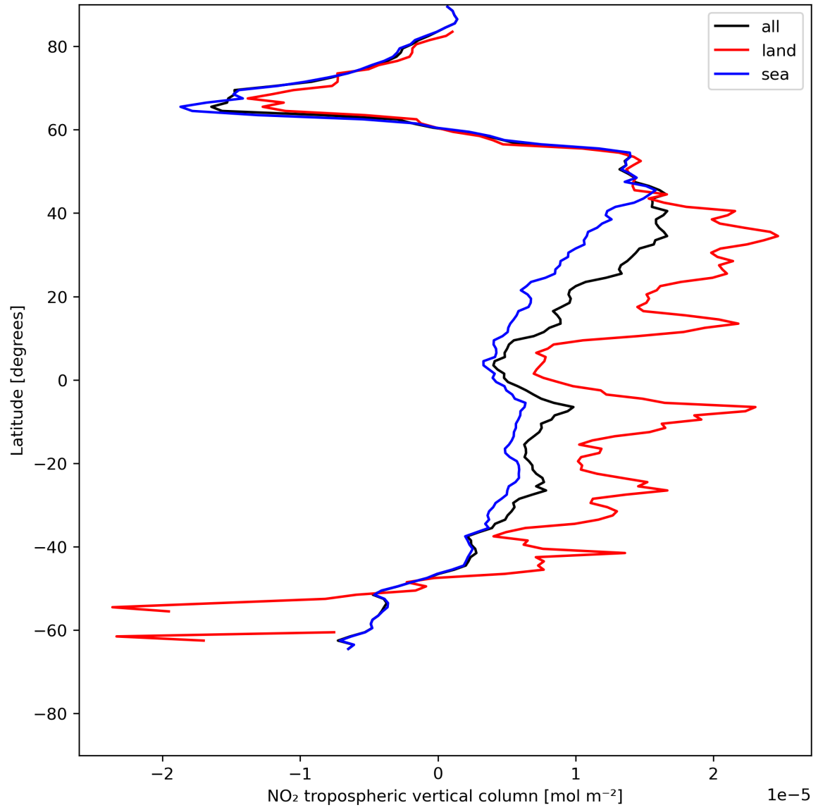
Figure 12: Zonal average of “NO 2 tropospheric vertical column” for 2023-07-05 to 2023-07-07.
