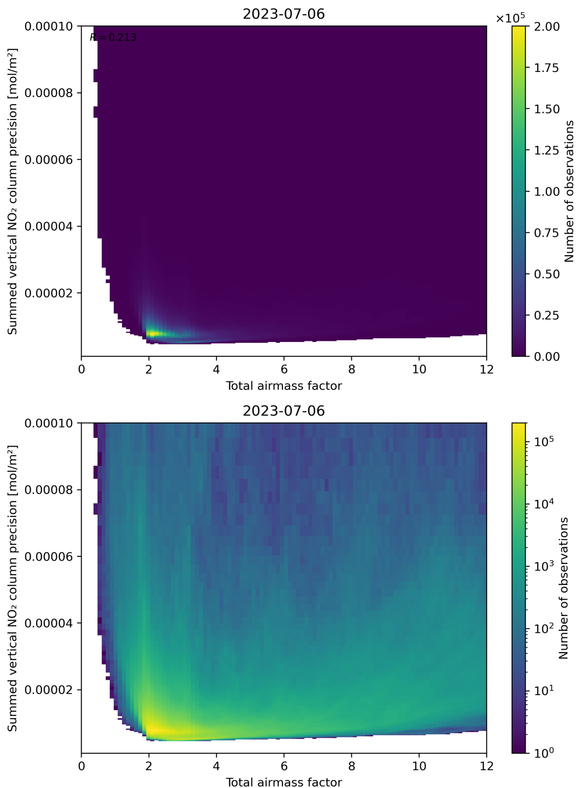
Figure 66: Scatter density plot of “Total airmass factor” against “Summed vertical NO 2 column precision” for 2023-07-05 to 2023-07-07.
