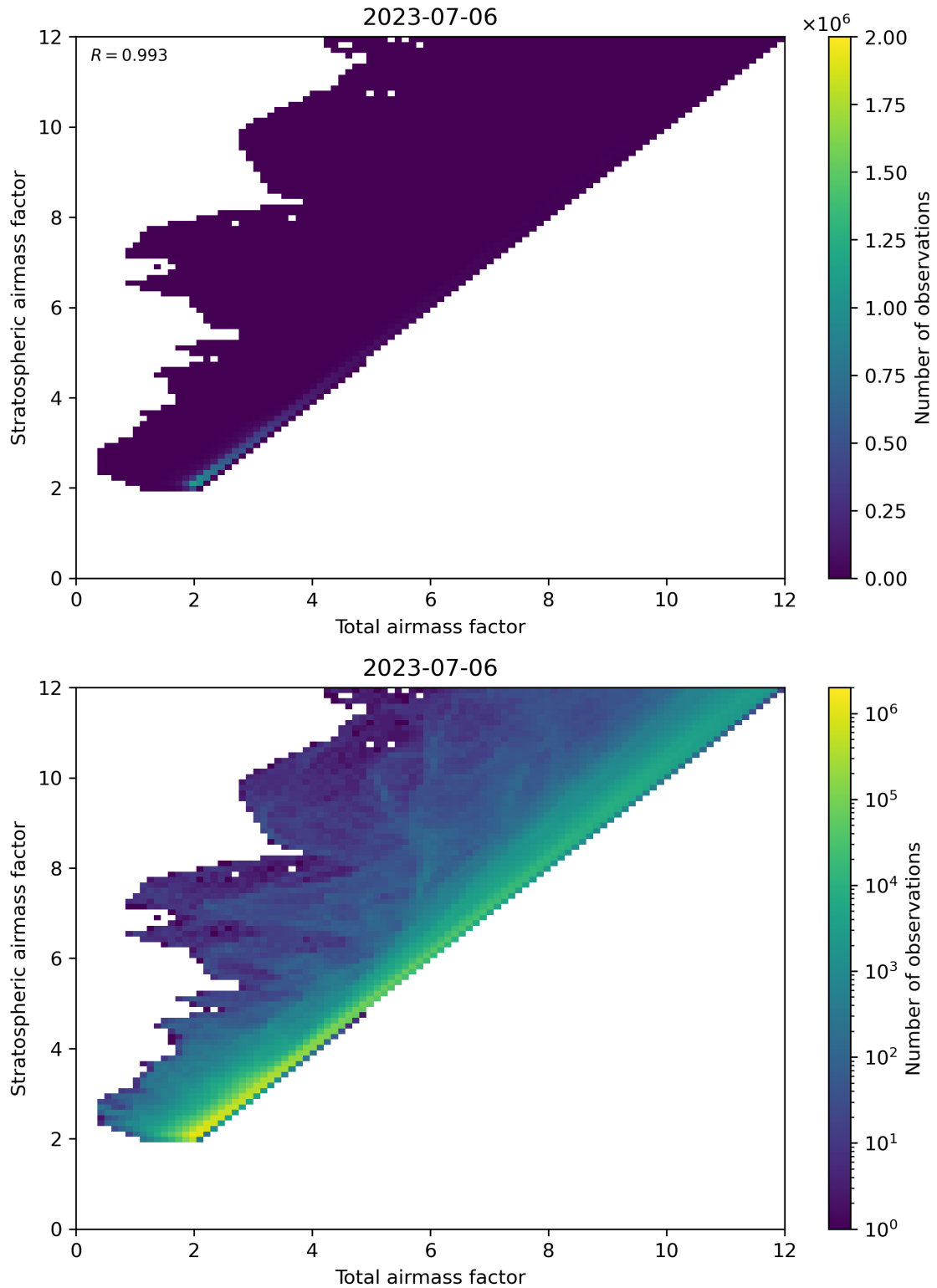
Figure 62: Scatter density plot of “Total airmass factor” against “Stratospheric airmass factor” for 2023-07-05 to 2023-07-07.
