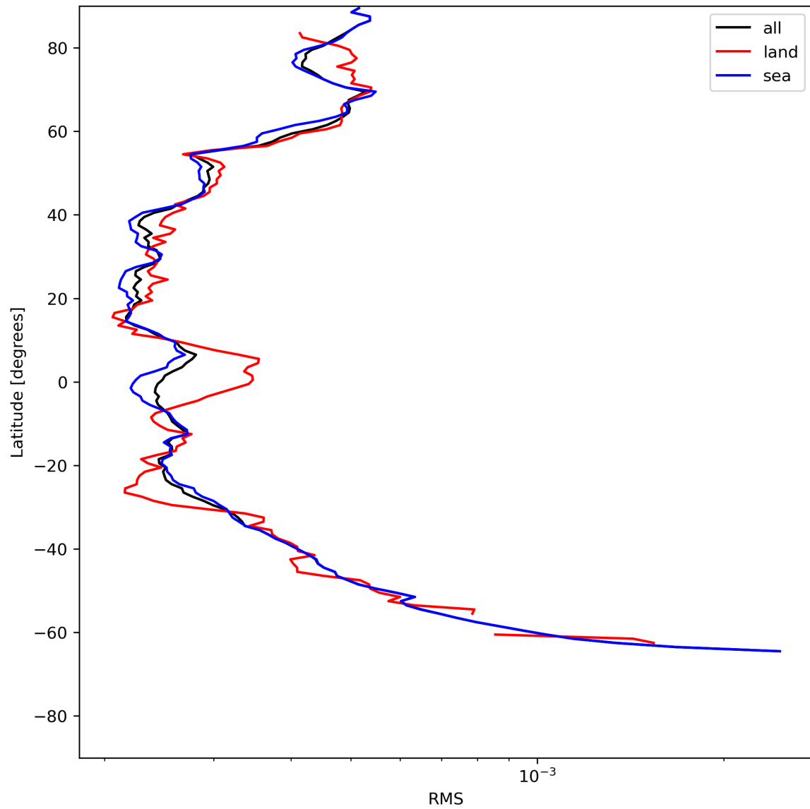
Figure 26: Zonal average of “RMS” for 2023-07-05 to 2023-07-07.
