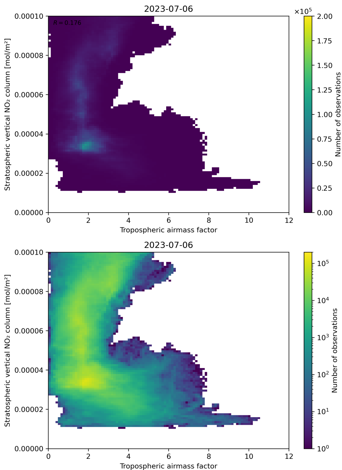
Figure 74: Scatter density plot of “Tropospheric air mass factor” against “Stratospheric vertical NO 2 column” for 2023-07-05 to 2023-07-07.
