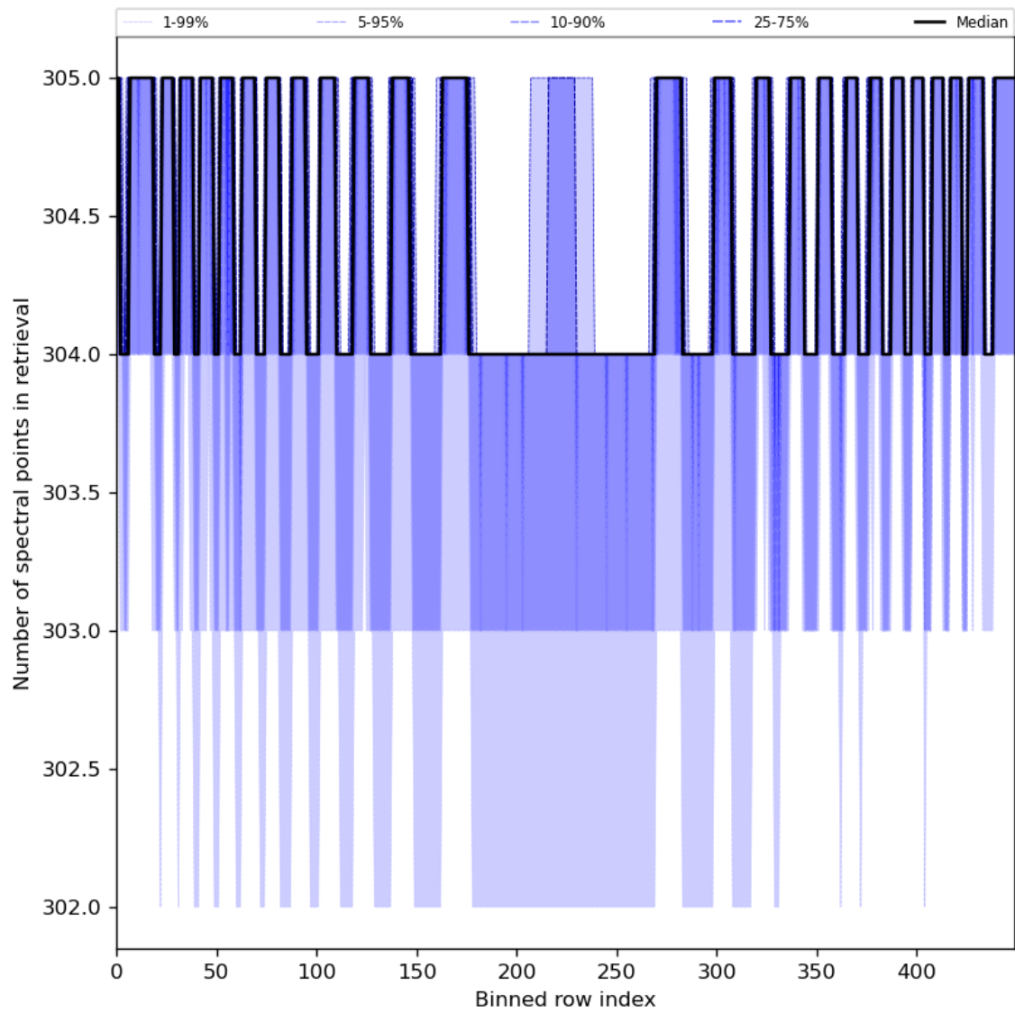
Figure 50: Along track statistics of “Number of spectral points in retrieval” for 2023-07-05 to 2023-07-07
