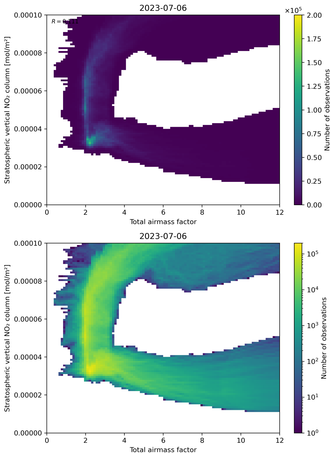
Figure 64: Scatter density plot of “Total airmass factor” against “Stratospheric vertical NO 2 column” for 2023-07-05 to 2023-07-07.
