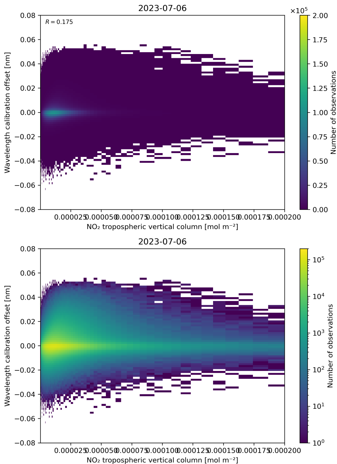
Figure 143: Scatter density plot of “NO 2 tropospheric vertical column” against “Wavelength calibration offset” for 2023-07-05 to 2023-07-07.
