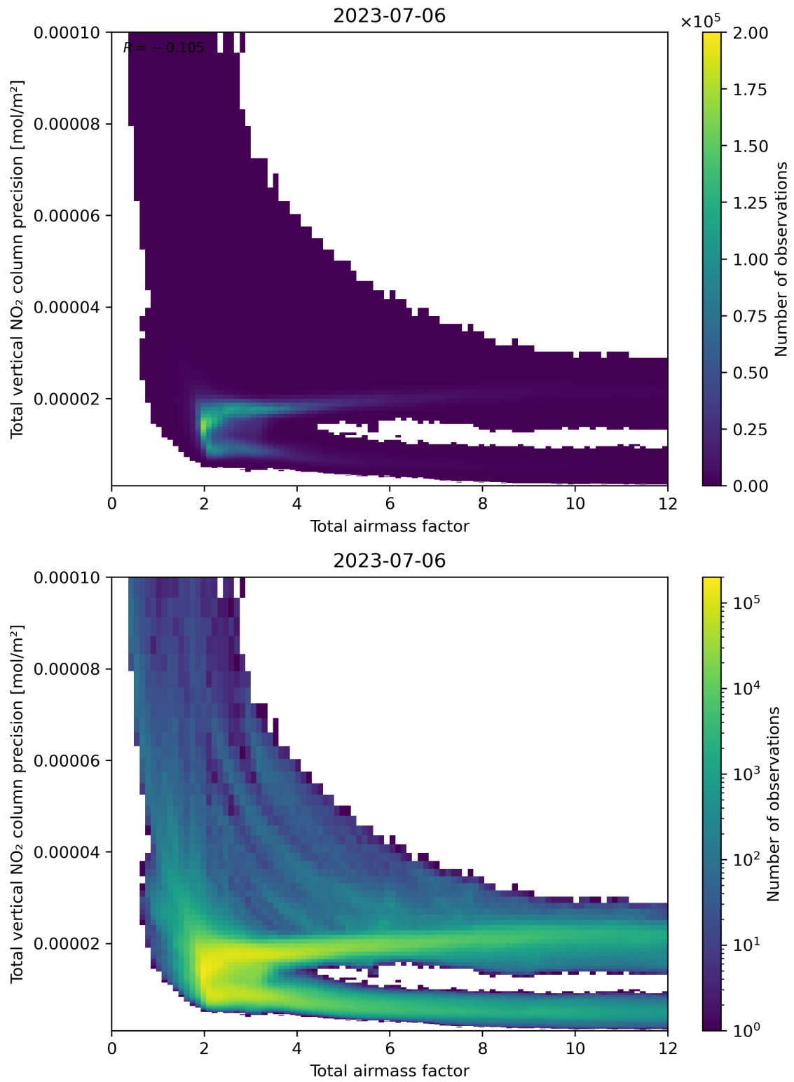
Figure 68: Scatter density plot of “Total airmass factor” against “Total vertical NO 2 column precision” for 2023-07-05 to 2023-07-07.
