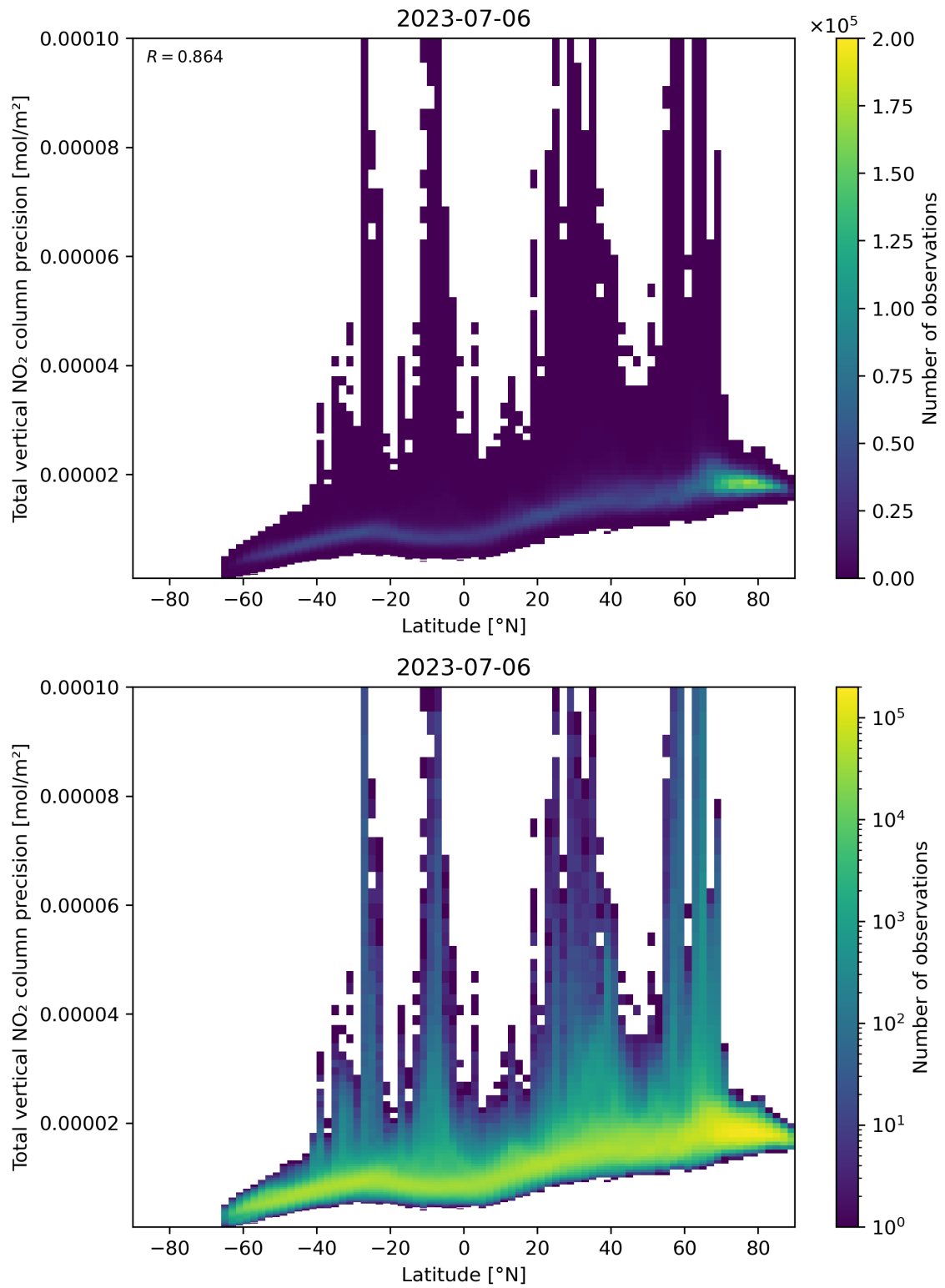
Figure 91: Scatter density plot of “Latitude” against “Total vertical NO 2 column precision” for 2023-07-05 to 2023-07-07.
