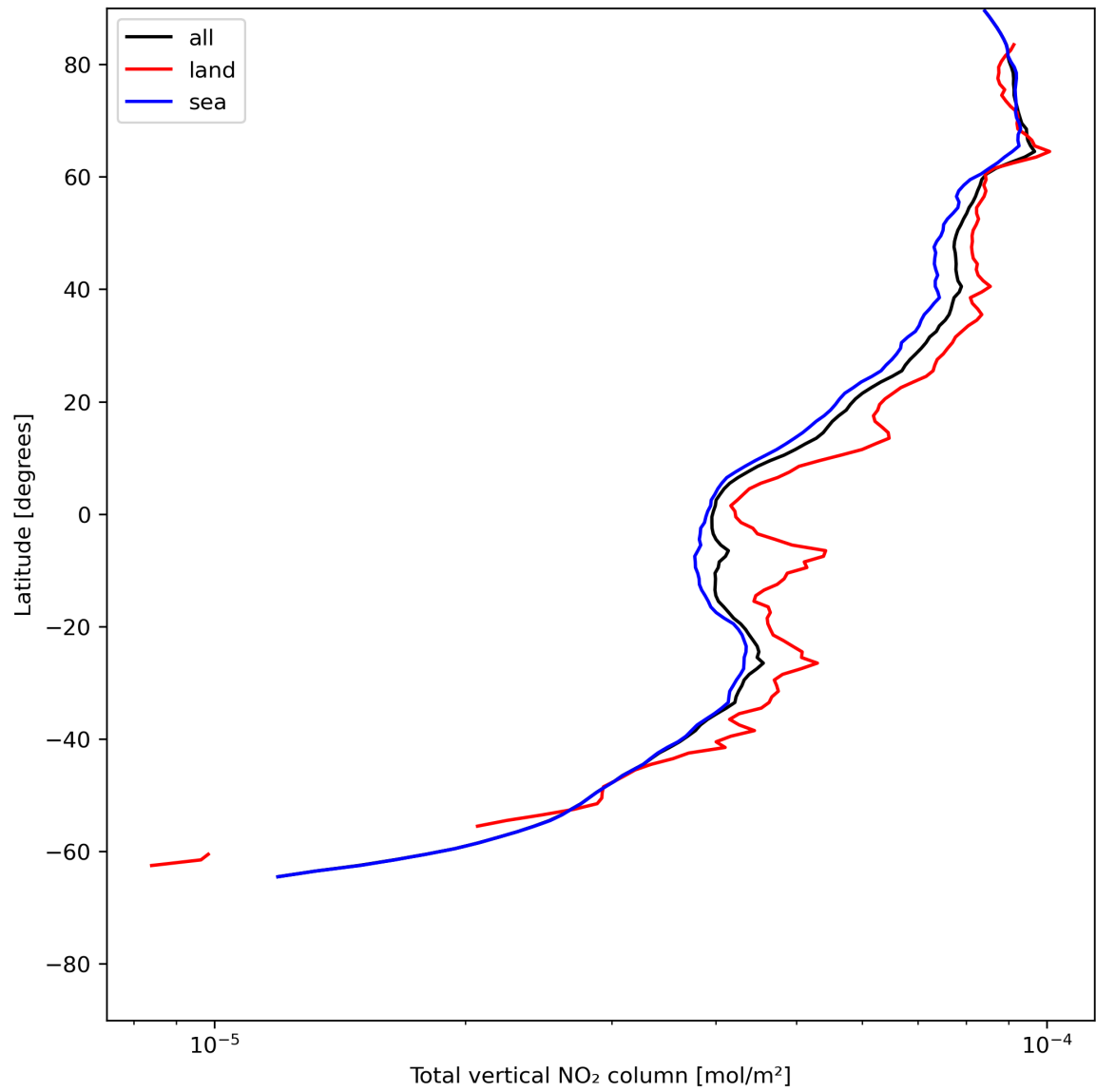
Figure 21: Zonal average of “Total vertical NO 2 column” for 2023-07-05 to 2023-07-07.
