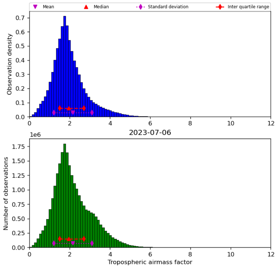
Figure 31: Histogram of “Tropospheric airmass factor” for 2023-07-05 to 2023-07-07
