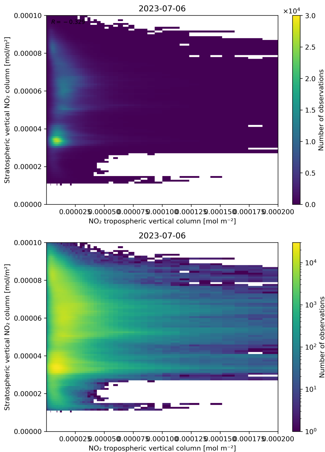
Figure 125: Scatter density plot of “NO 2 tropospheric vertical column” against “Stratospheric vertical NO 2 column” for 2023-07-05 to 2023-07-07.
