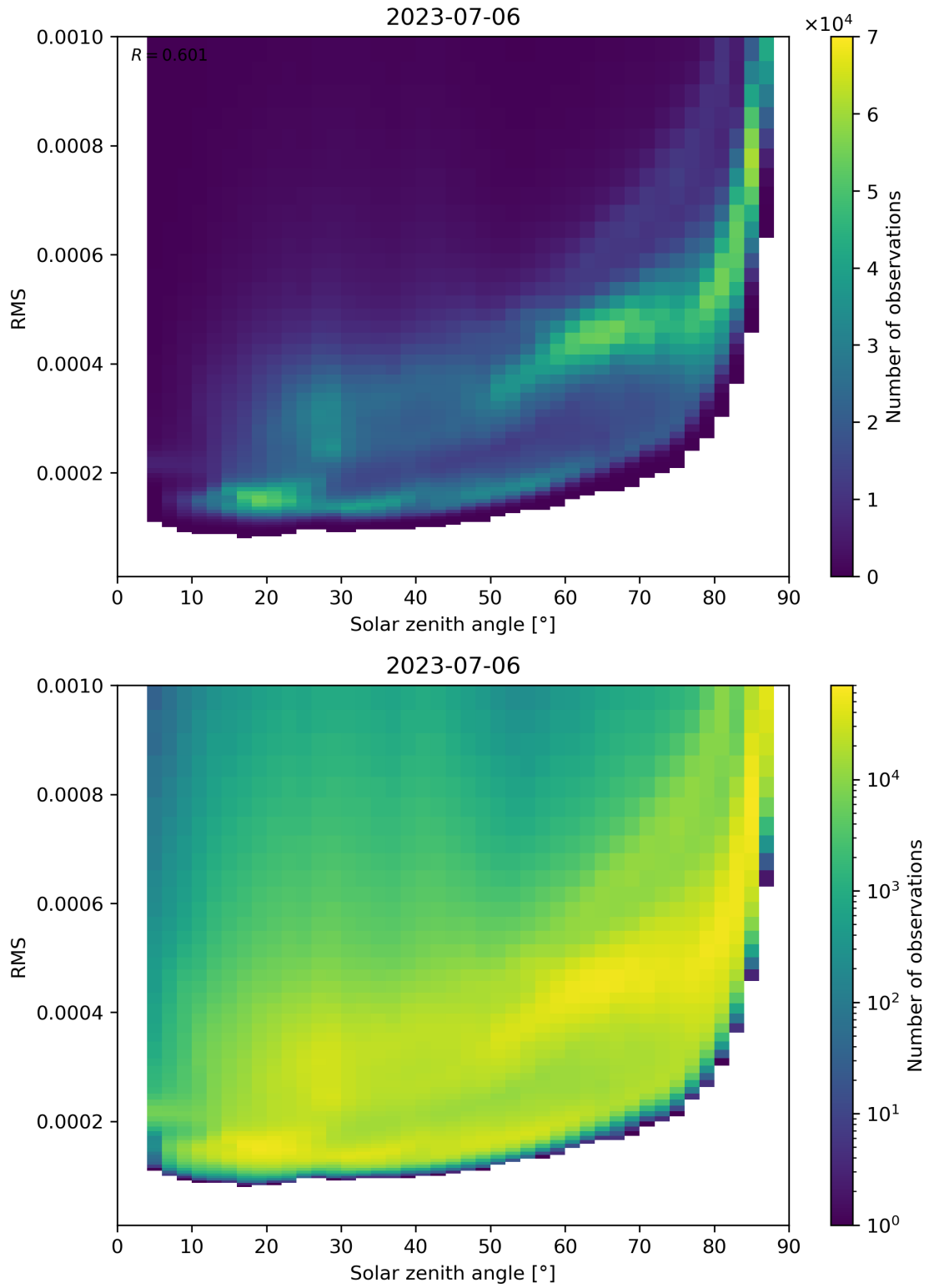
Figure 157: Scatter density plot of “Solar zenith angle” against “RMS” for 2023-07-05 to 2023-07-07.
