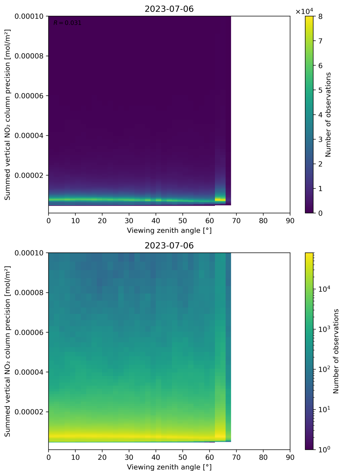
Figure 166: Scatter density plot of “Viewing zenith angle” against “Summed vertical NO 2 column precision” for 2023-07-05 to 2023-07-07.
