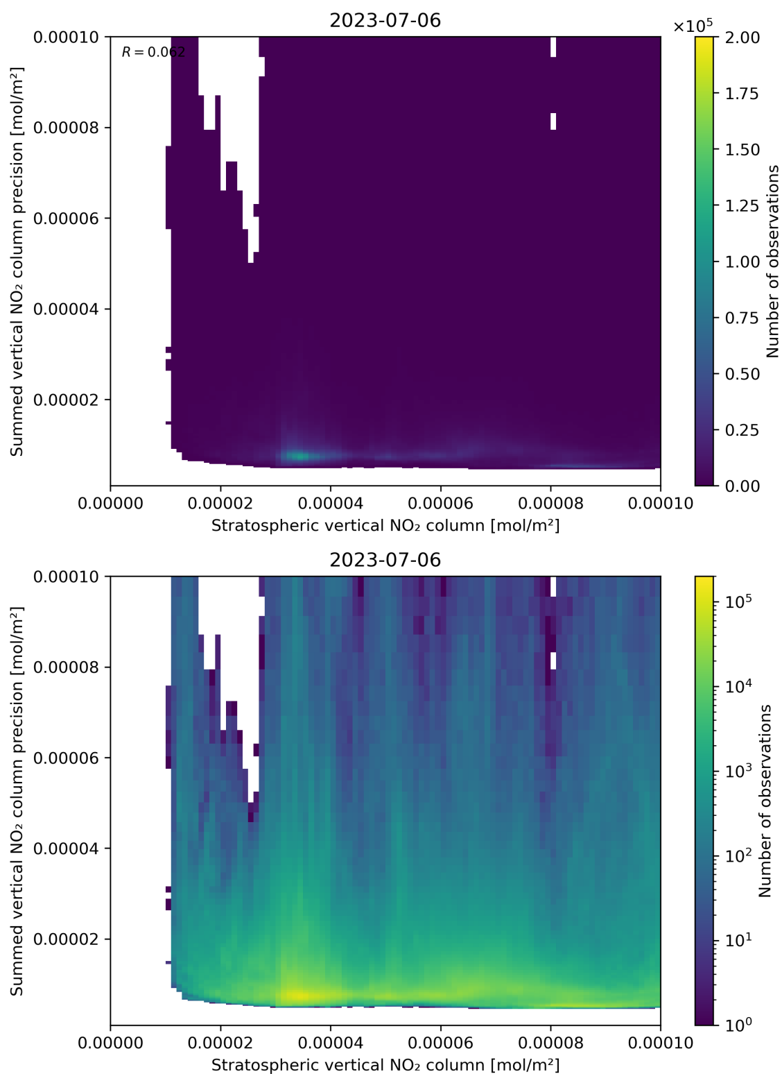
Figure 99: Scatter density plot of “Stratospheric vertical NO 2 column” against “Summed vertical NO 2 column precision” for 2023-07-05 to 2023-07-07.
