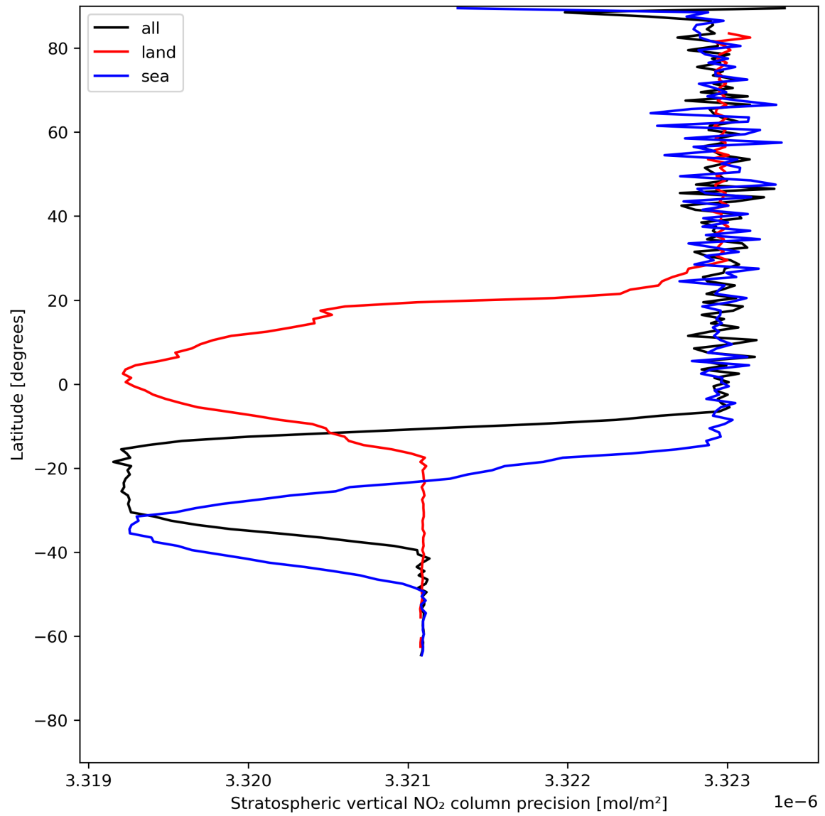
Figure 20: Zonal average of “Stratospheric vertical NO 2 column precision” for 2023-07-05 to 2023-07-07.
