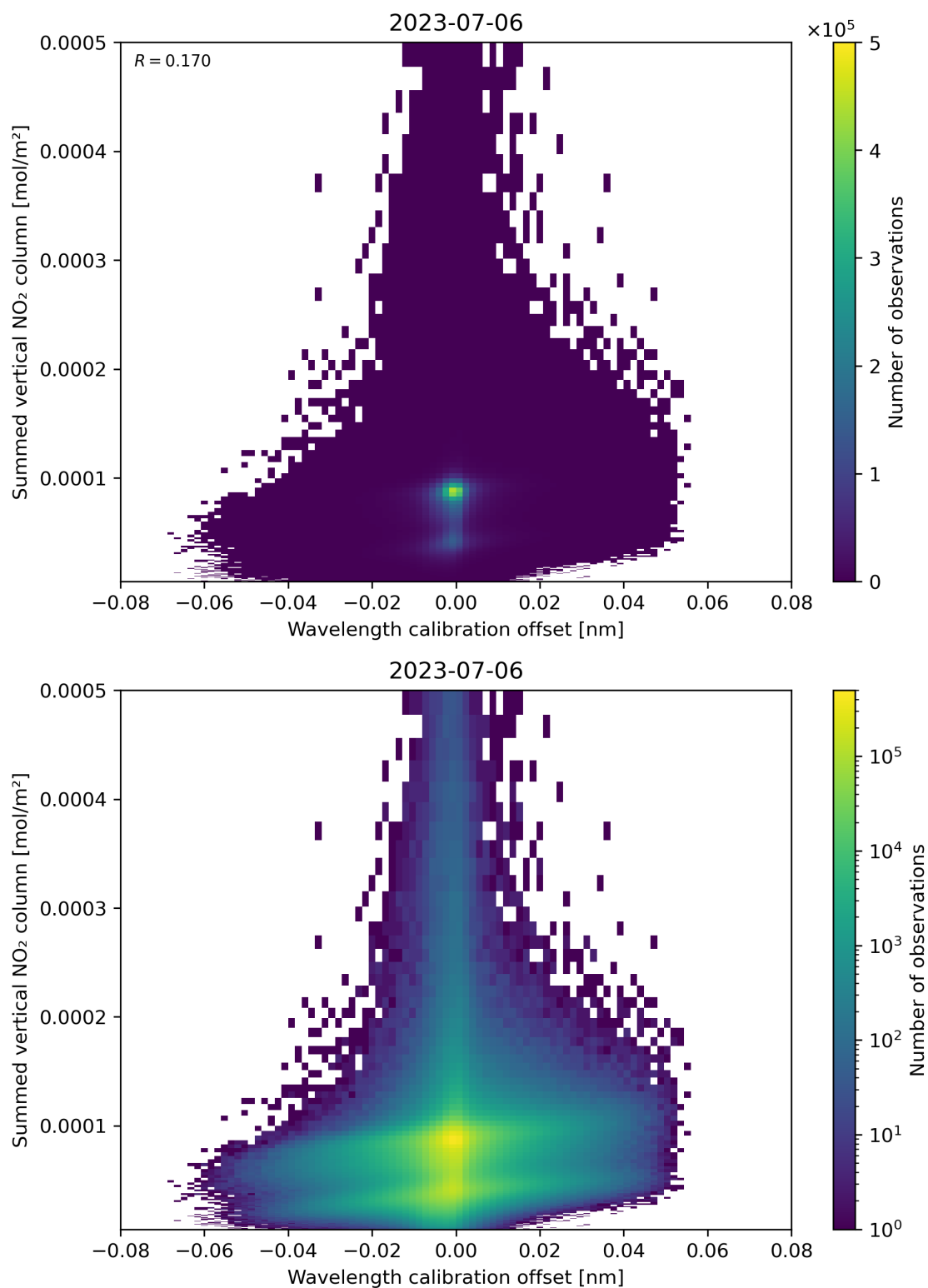
Figure 177: Scatter density plot of “Wavelength calibration offset” against “Summed vertical NO 2 column” for 2023-07-05 to 2023-07-07.
