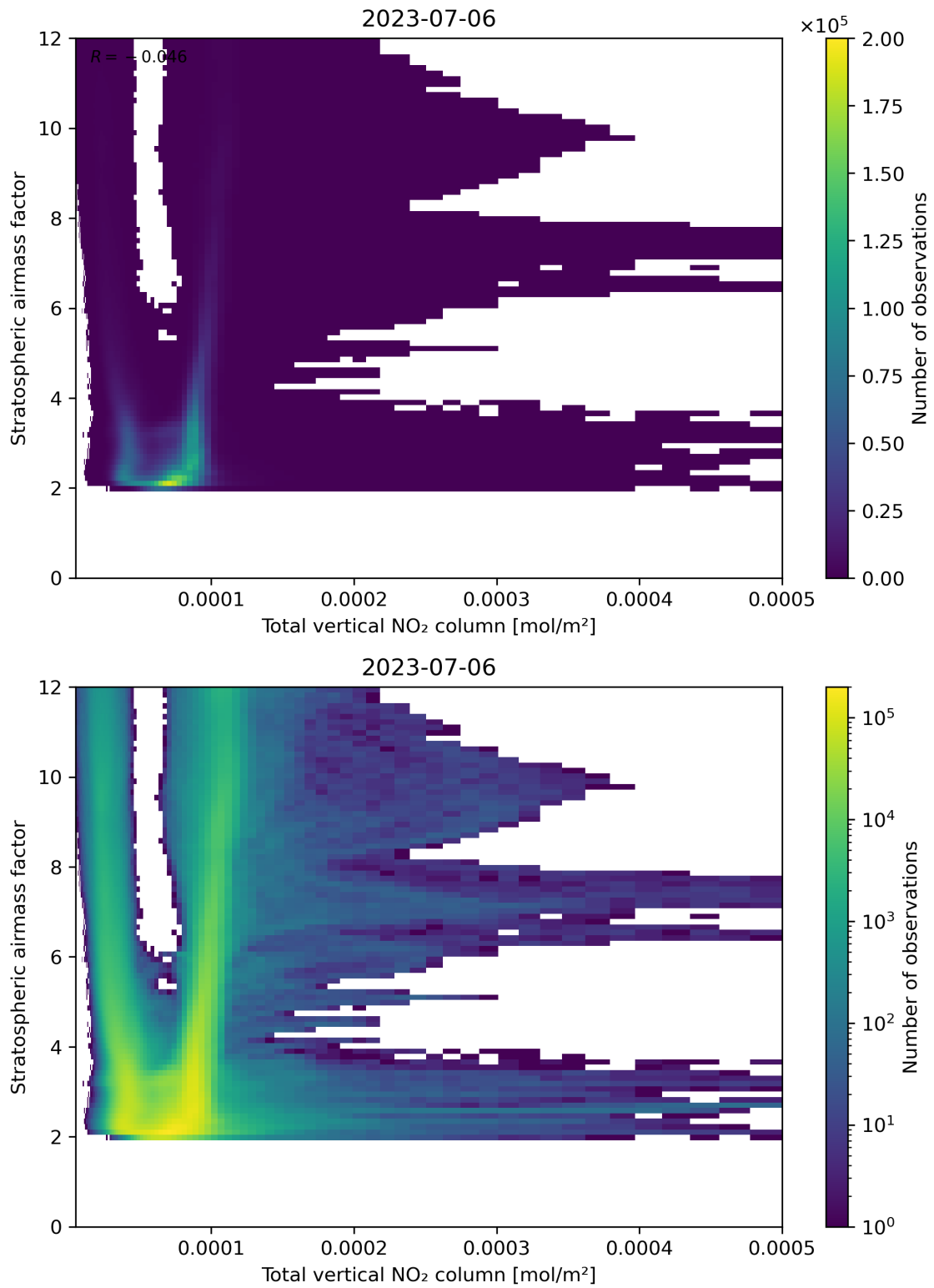
Figure 110: Scatter density plot of “Total vertical NO 2 column” against “Stratospheric airmass factor” for 2023-07-05 to 2023-07-07.
