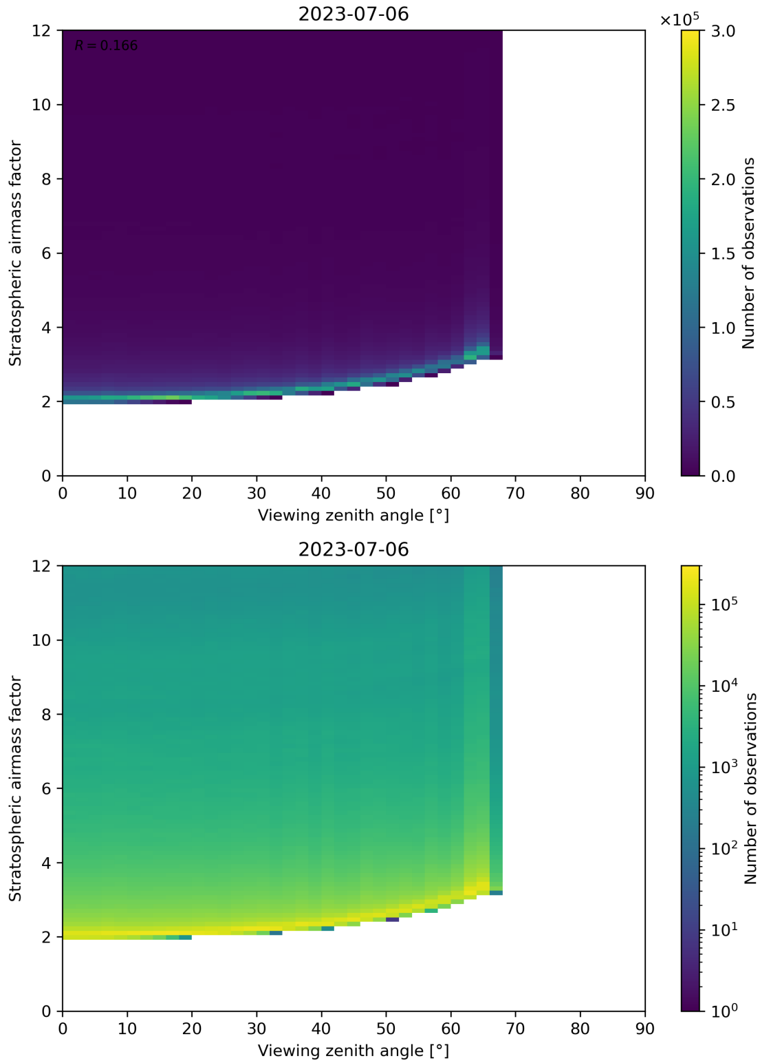
Figure 159: Scatter density plot of “Viewing zenith angle” against “Stratospheric airmass factor” for 2023-07-05 to 2023-07-07.
