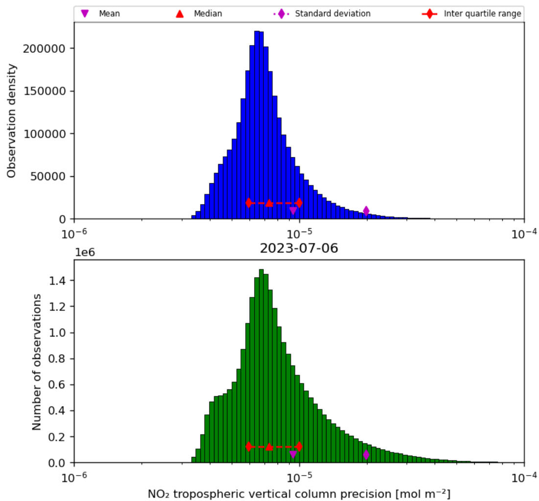
Figure 30: Histogram of “NO 2 tropospheric vertical column precision” for 2023-07-05 to 2023-07-07
