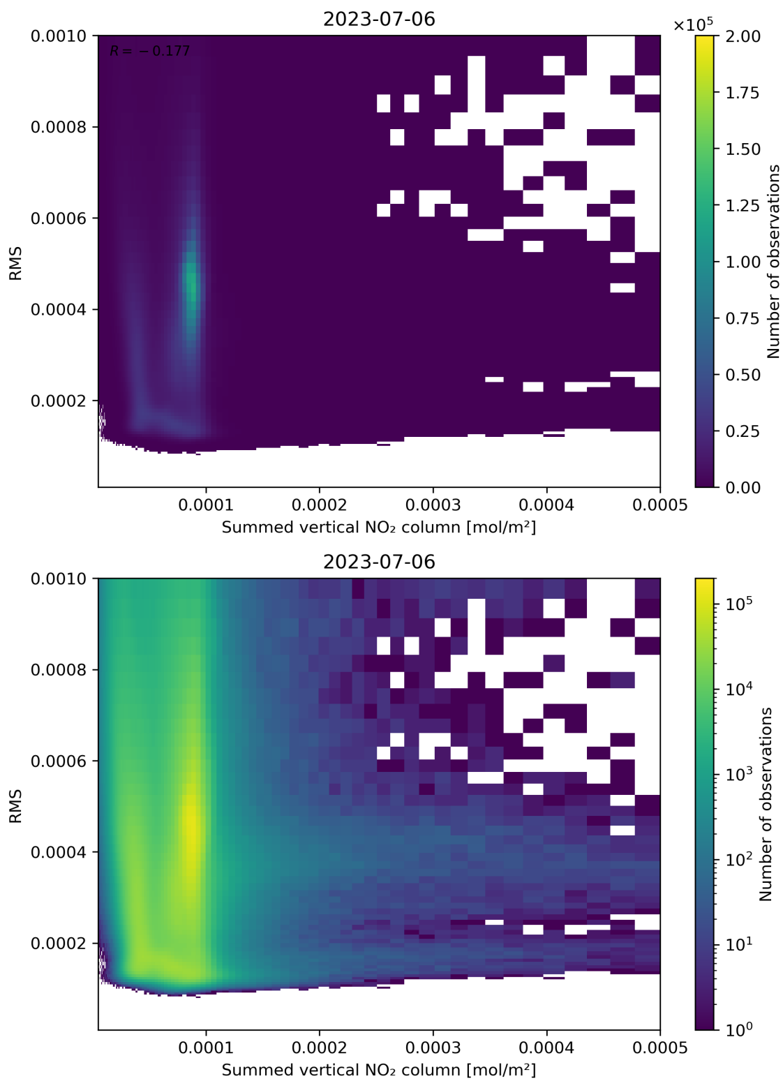
Figure 109: Scatter density plot of “Summed vertical NO 2 column” against “RMS” for 2023-07-05 to 2023-07-07.
