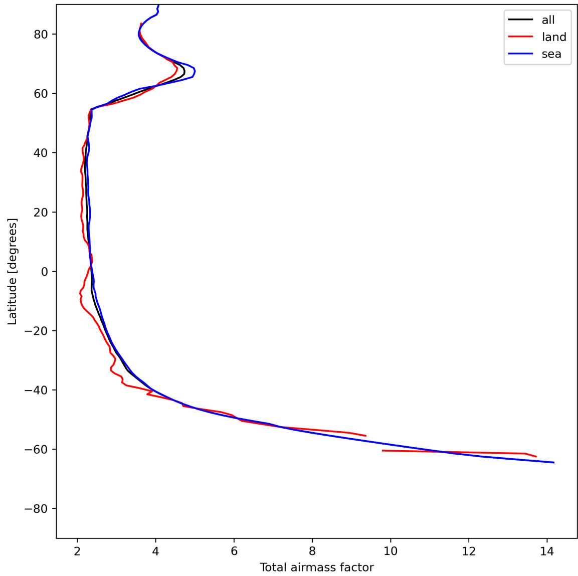
Figure 15: Zonal average of “Total airmass factor” for 2023-07-05 to 2023-07-07.
