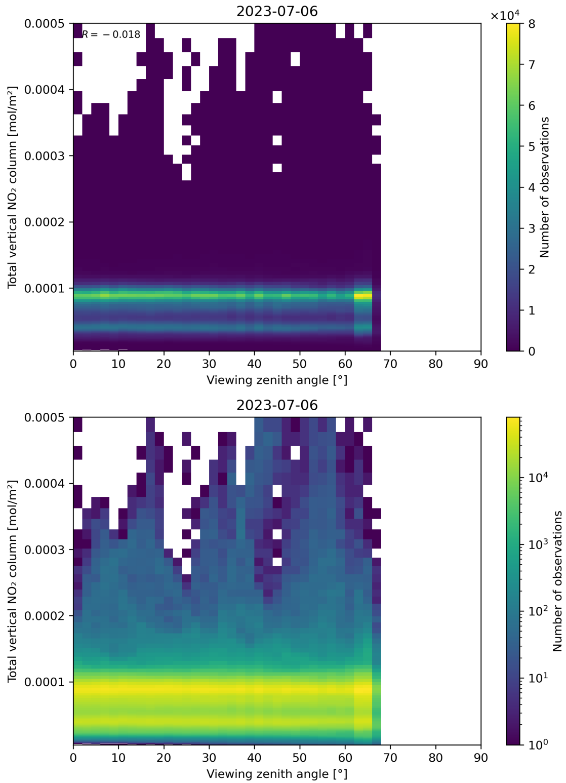
Figure 167: Scatter density plot of “Viewing zenith angle” against “Total vertical NO 2 column” for 2023-07-05 to 2023-07-07.
