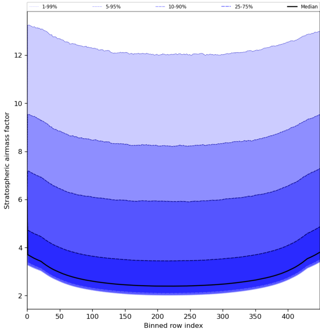
Figure 61: Along track statistics of “Stratospheric airmass factor” for 2023-07-05 to 2023-07-07
