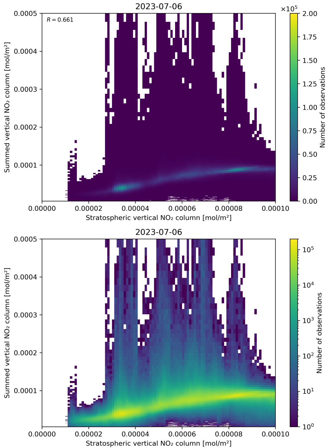
Figure 98: Scatter density plot of “Stratospheric vertical NO 2 column” against “Summed vertical NO 2 column” for 2023-07-05 to 2023-07-07.
