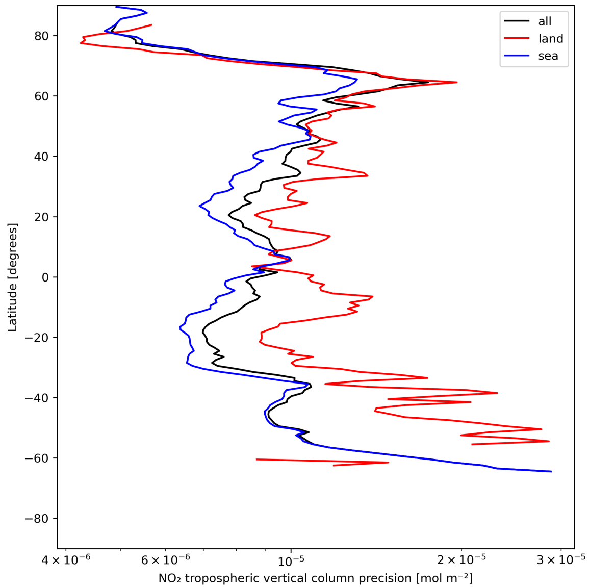
Figure 13: Zonal average of “NO 2 tropospheric vertical column precision” for 2023-07-05 to 2023-07-07.
