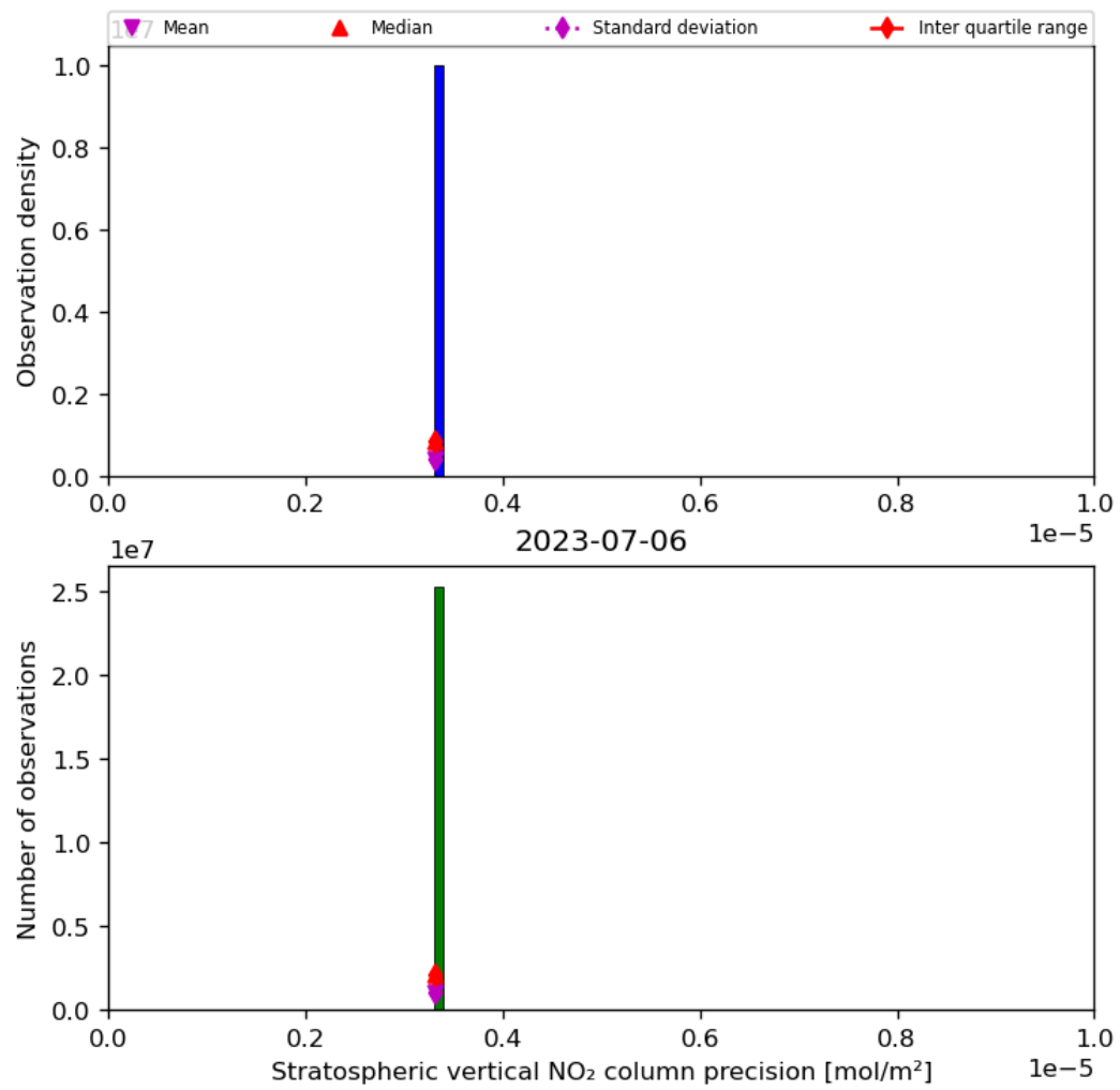
Figure 37: Histogram of “Stratospheric vertical NO 2 column precision” for 2023-07-05 to 2023-07-07
