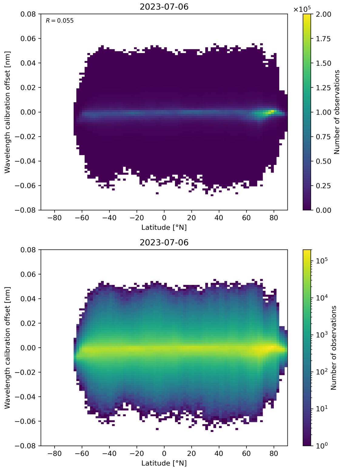
Figure 95: Scatter density plot of “Latitude” against “Wavelength calibration offset” for 2023-07-05 to 2023-07-07.
