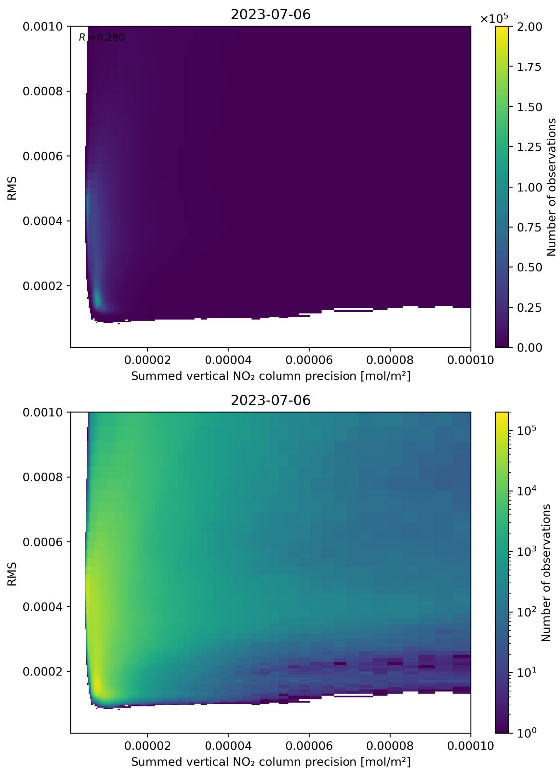
Figure 108: Scatter density plot of “Summed vertical NO 2 column precision” against “RMS” for 2023-07-05 to 2023-07-07.
