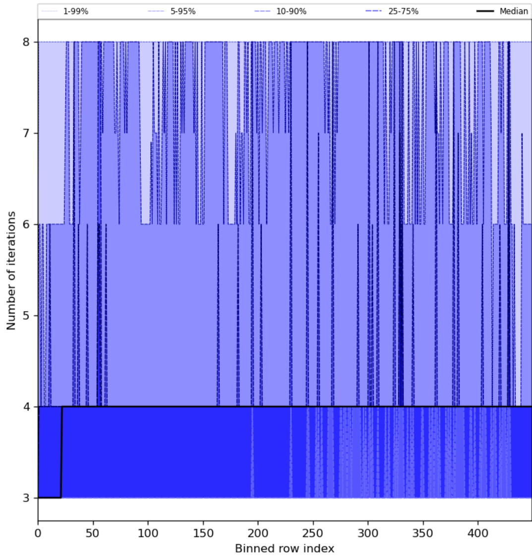
Figure 51: Along track statistics of “Number of iterations” for 2023-07-05 to 2023-07-07
