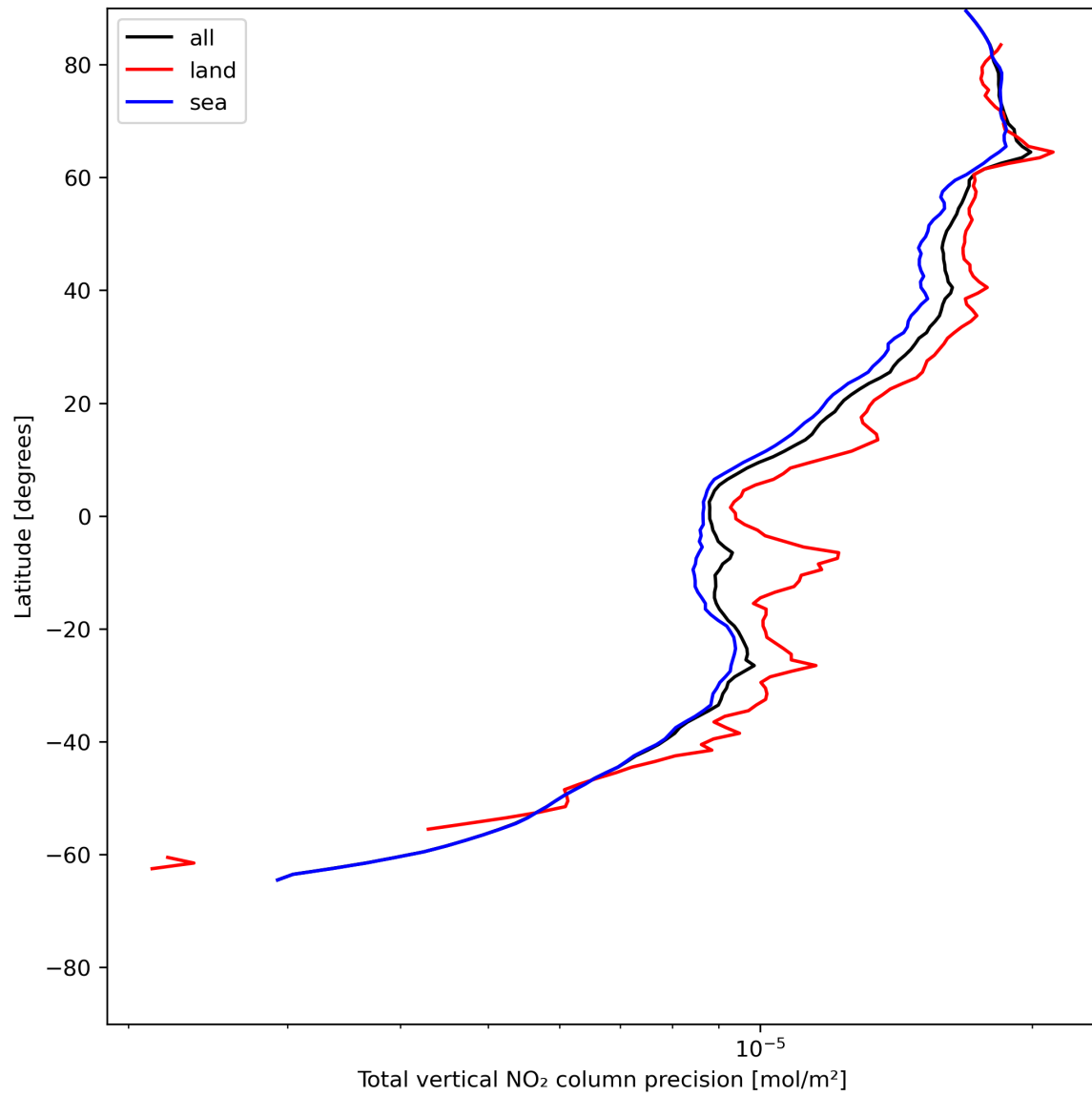
Figure 22: Zonal average of “Total vertical NO 2 column precision” for 2023-07-05 to 2023-07-07.
