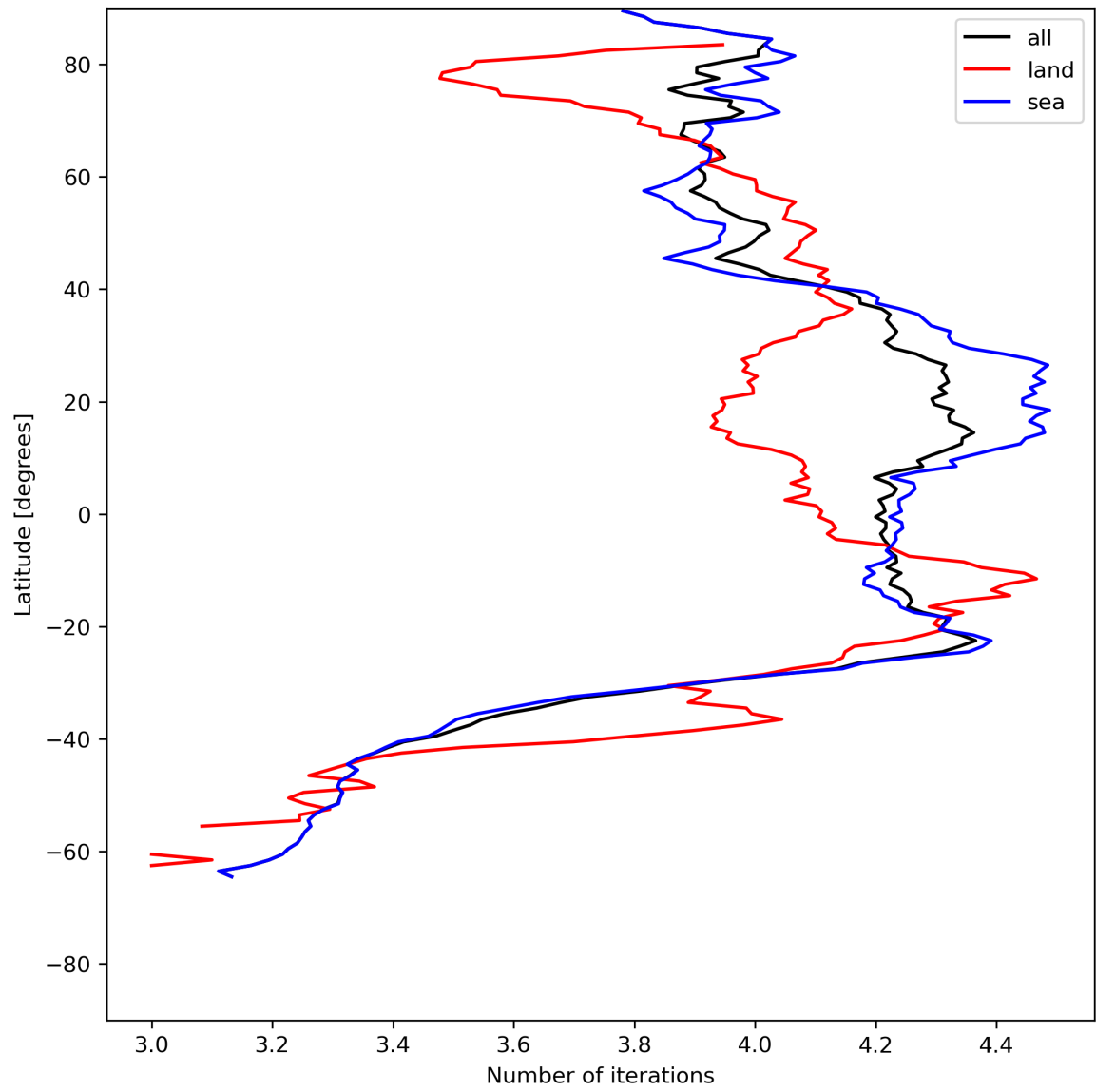
Figure 17: Zonal average of “Number of iterations” for 2023-07-05 to 2023-07-07.
