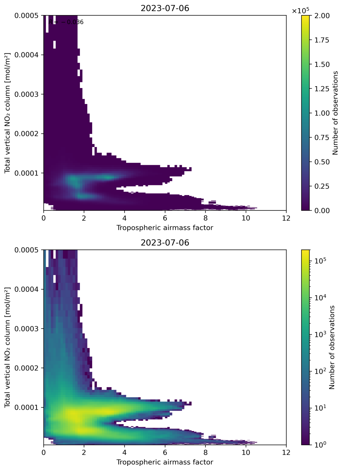
Figure 77: Scatter density plot of “Tropospheric airmass factor” against “Total vertical NO 2 column” for 2023-07-05 to 2023-07-07.
