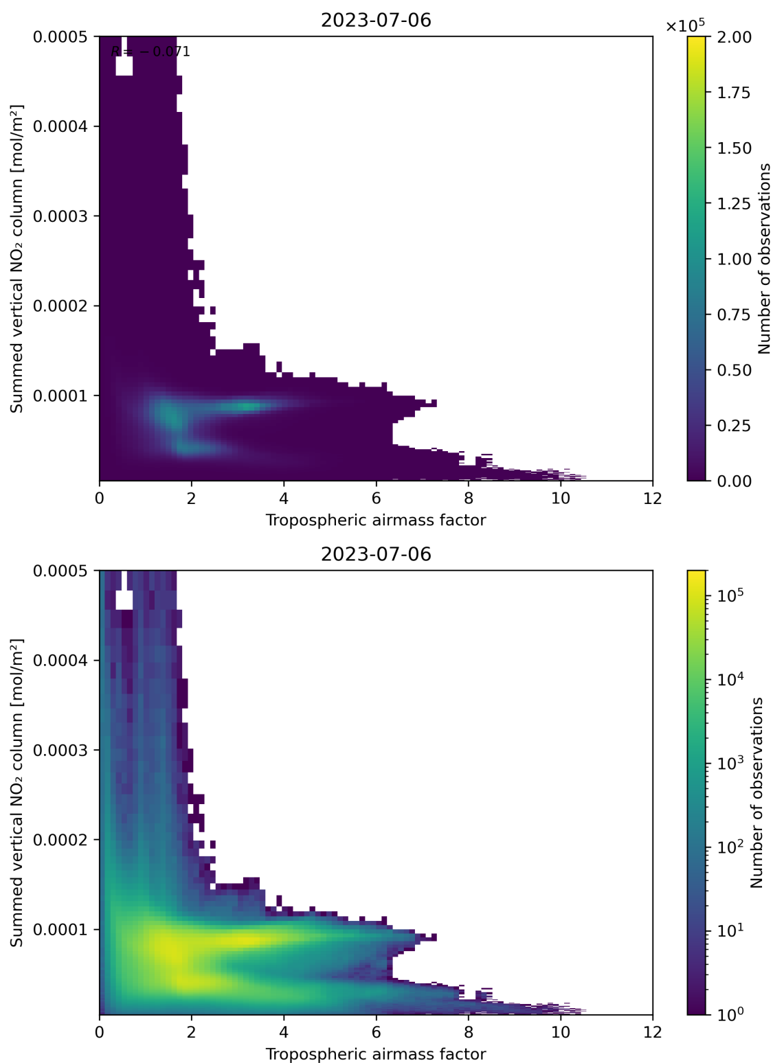
Figure 75: Scatter density plot of “Tropospheric airmass factor” against “Summed vertical NO 2 column” for 2023-07-05 to 2023-07-07.
