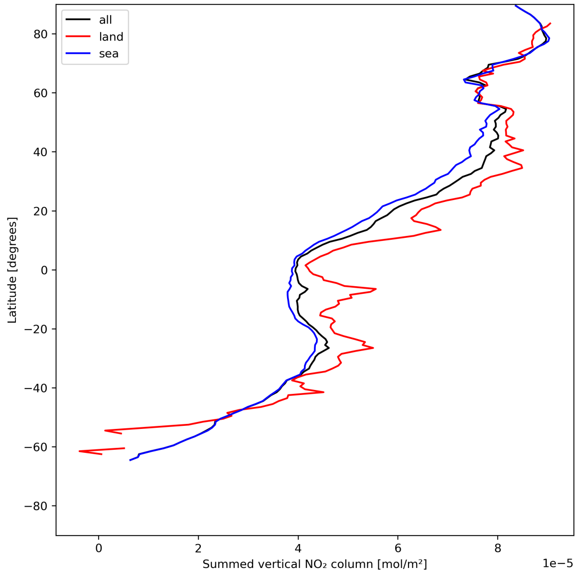
Figure 23: Zonal average of “Summed vertical NO 2 column” for 2023-07-05 to 2023-07-07.
