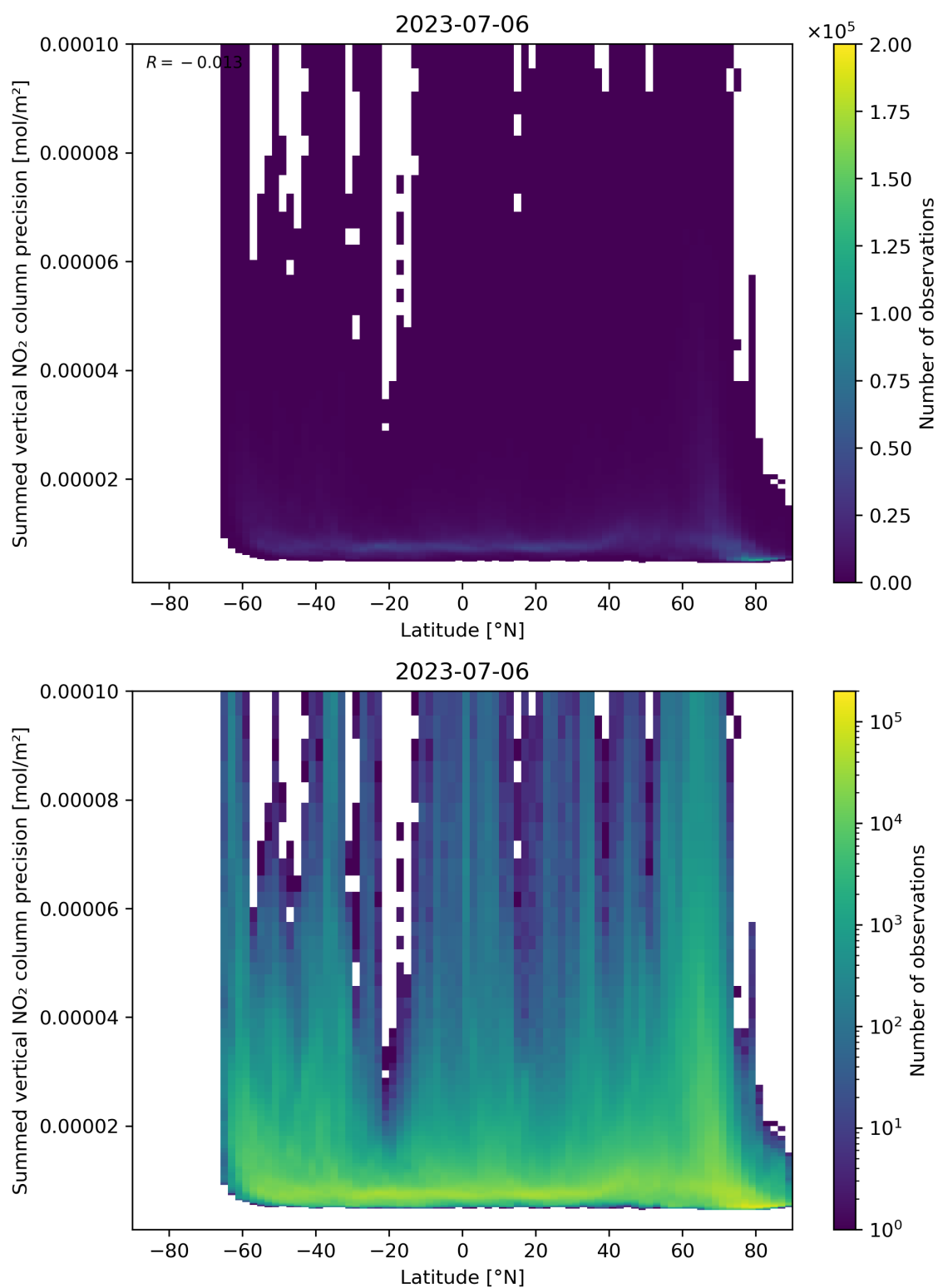
Figure 89: Scatter density plot of “Latitude” against “Summed vertical NO 2 column precision” for 2023-07-05 to 2023-07-07.
