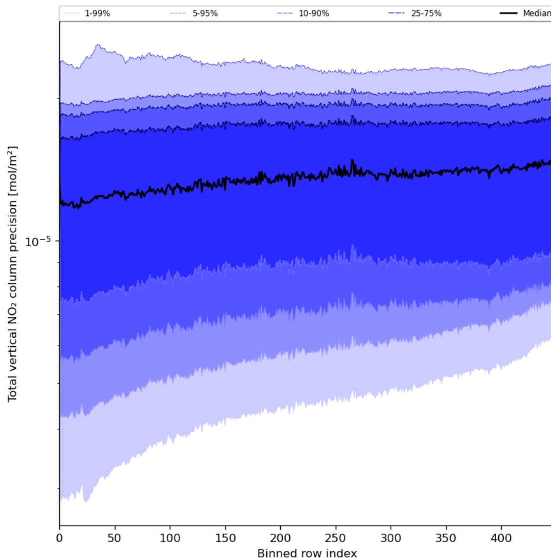
Figure 56: Along track statistics of “Total vertical NO 2 column precision” for 2023-07-05 to 2023-07-07
