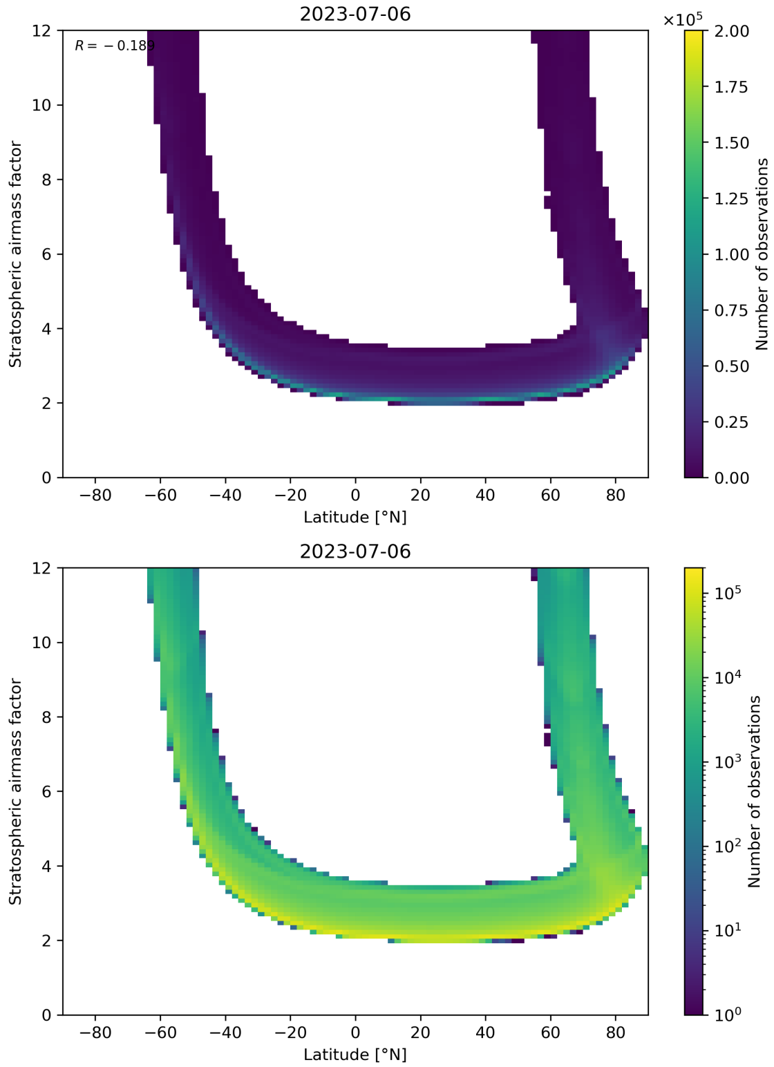
Figure 83: Scatter density plot of “Latitude” against “Stratospheric air mass factor” for 2023-07-05 to 2023-07-07.
