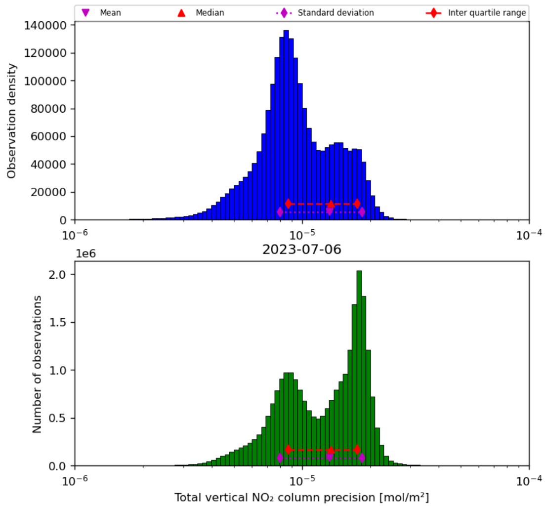
Figure 39: Histogram of “Total vertical NO 2 column precision” for 2023-07-05 to 2023-07-07
