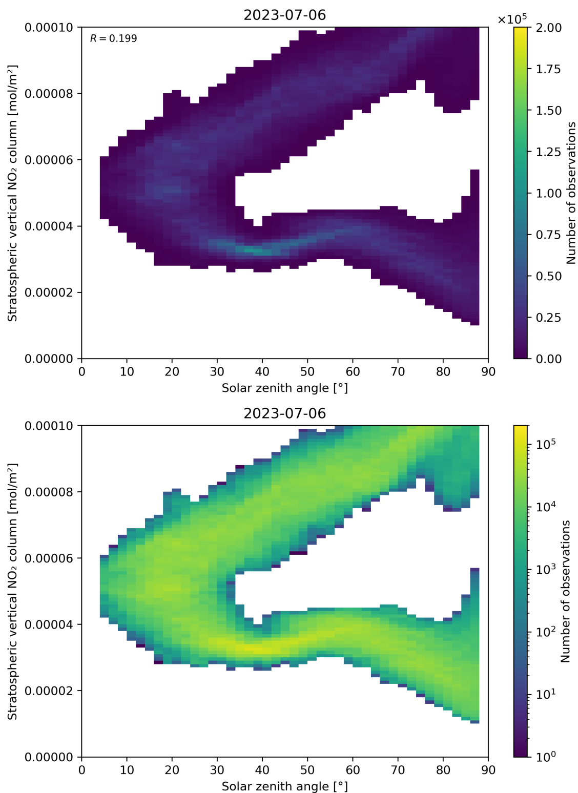
Figure 150: Scatter density plot of “Solar zenith angle” against “Stratospheric vertical NO 2 column” for 2023-07-05 to 2023-07-07.
