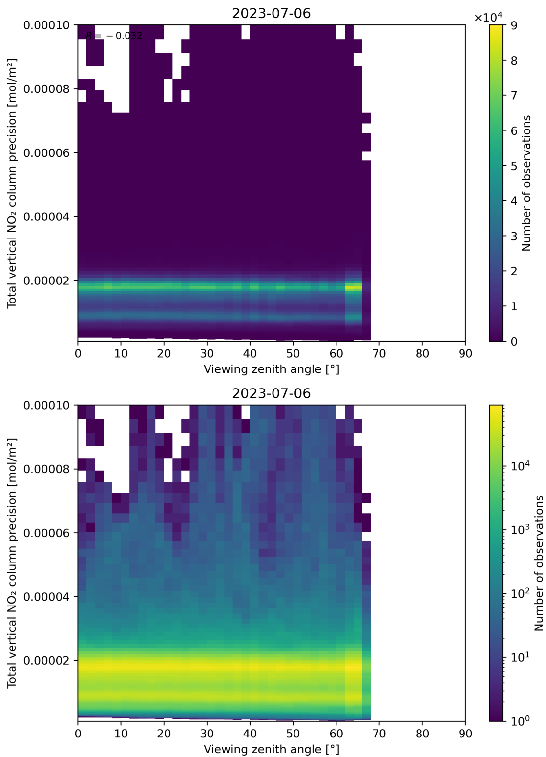
Figure 168: Scatter density plot of “Viewing zenith angle” against “Total vertical NO 2 column precision” for 2023-07-05 to 2023-07-07.
