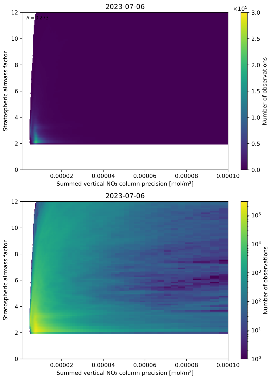
Figure 106: Scatter density plot of “Summed vertical NO 2 column precision” against “Stratospheric airmass factor” for 2023-07-05 to 2023-07-07.
