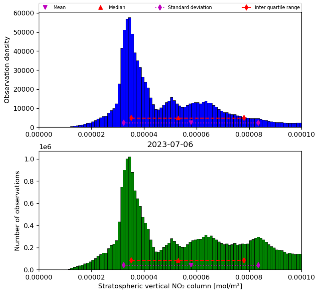
Figure 36: Histogram of “Stratospheric vertical NO 2 column” for 2023-07-05 to 2023-07-07
