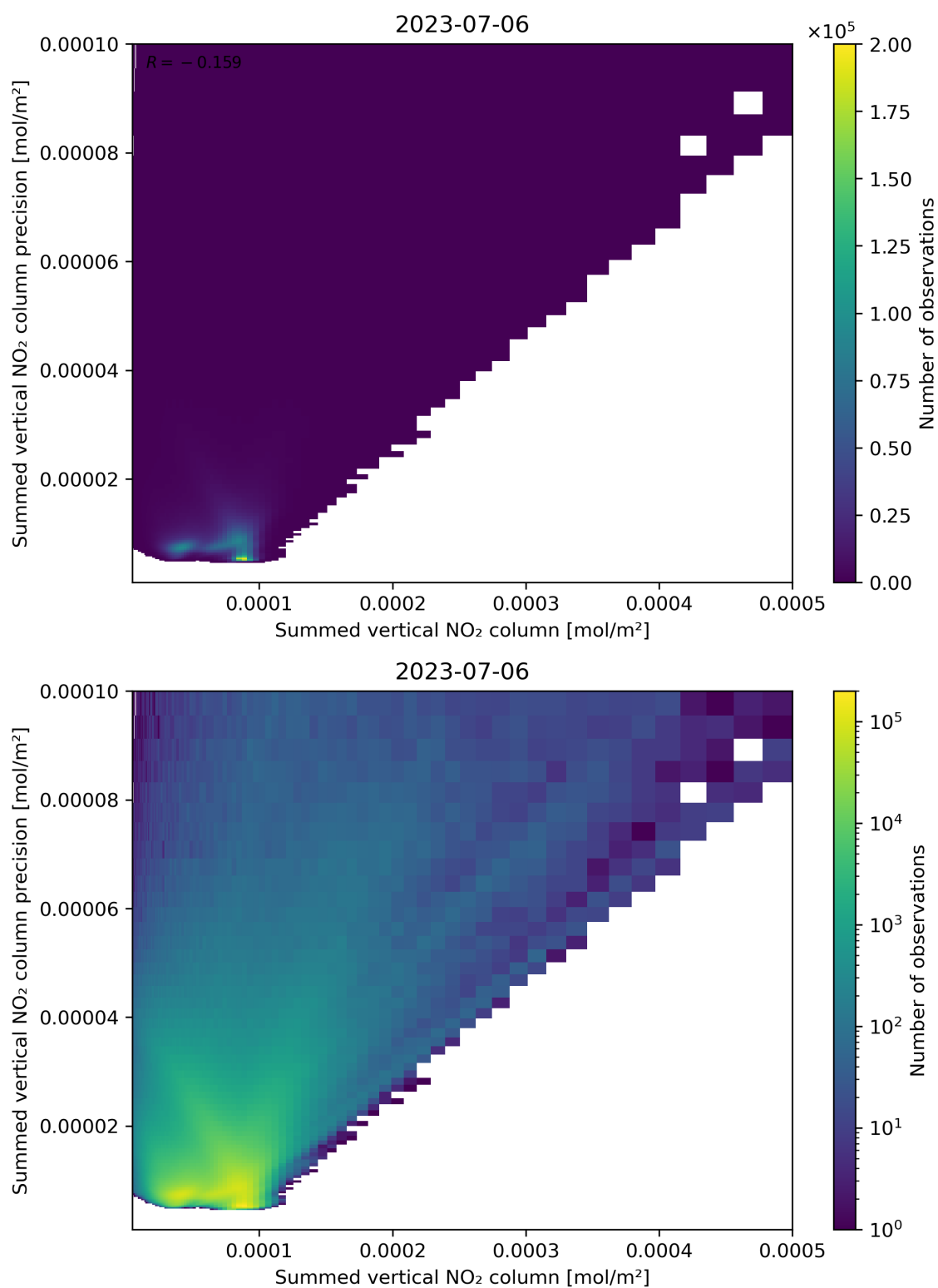
Figure 105: Scatter density plot of “Summed vertical NO 2 column” against “Summed vertical NO 2 column precision” for 2023-07-05 to 2023-07-07.
