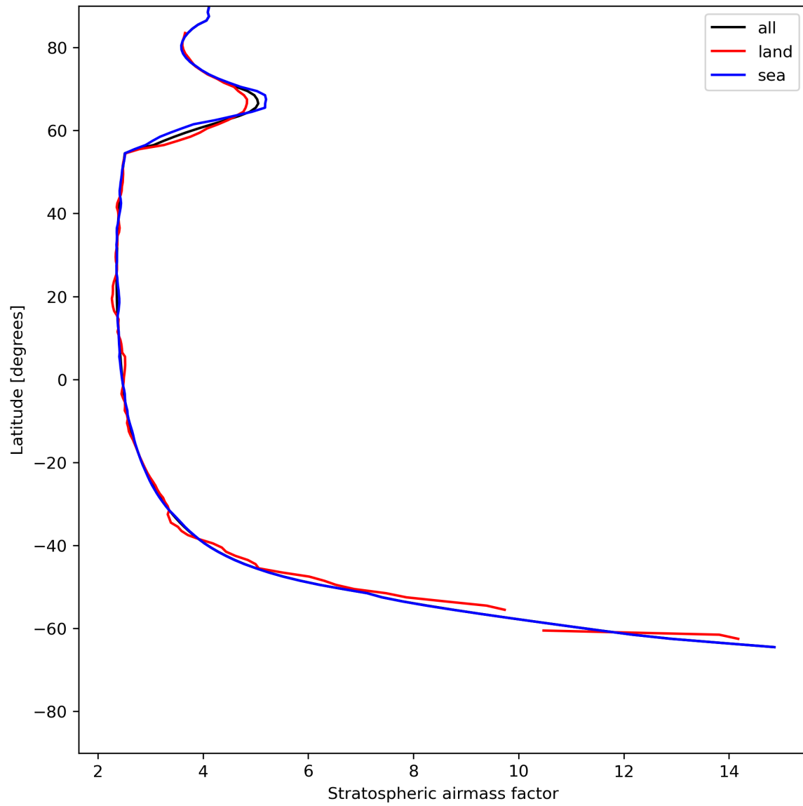
Figure 27: Zonal average of “Stratospheric air mass factor” for 2023-07-05 to 2023-07-07.
