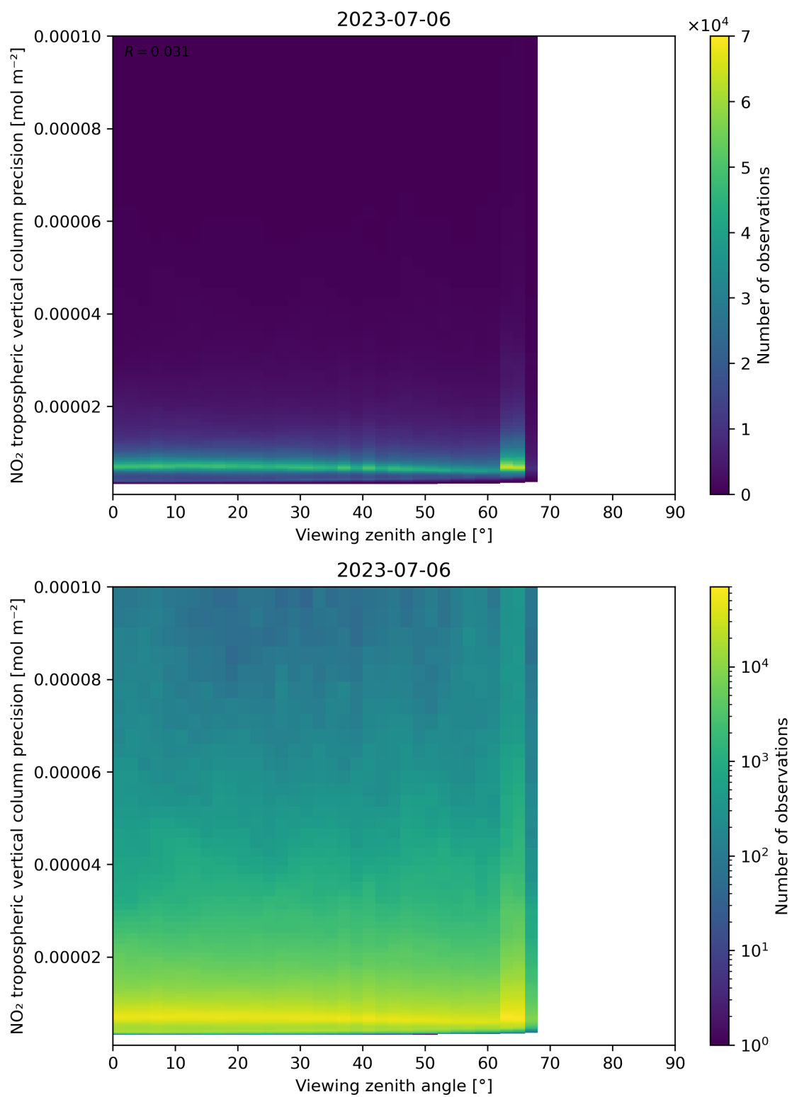
Figure 170: Scatter density plot of “Viewing zenith angle” against “NO 2 tropospheric vertical column precision” for 2023-07-05 to 2023-07-07.
