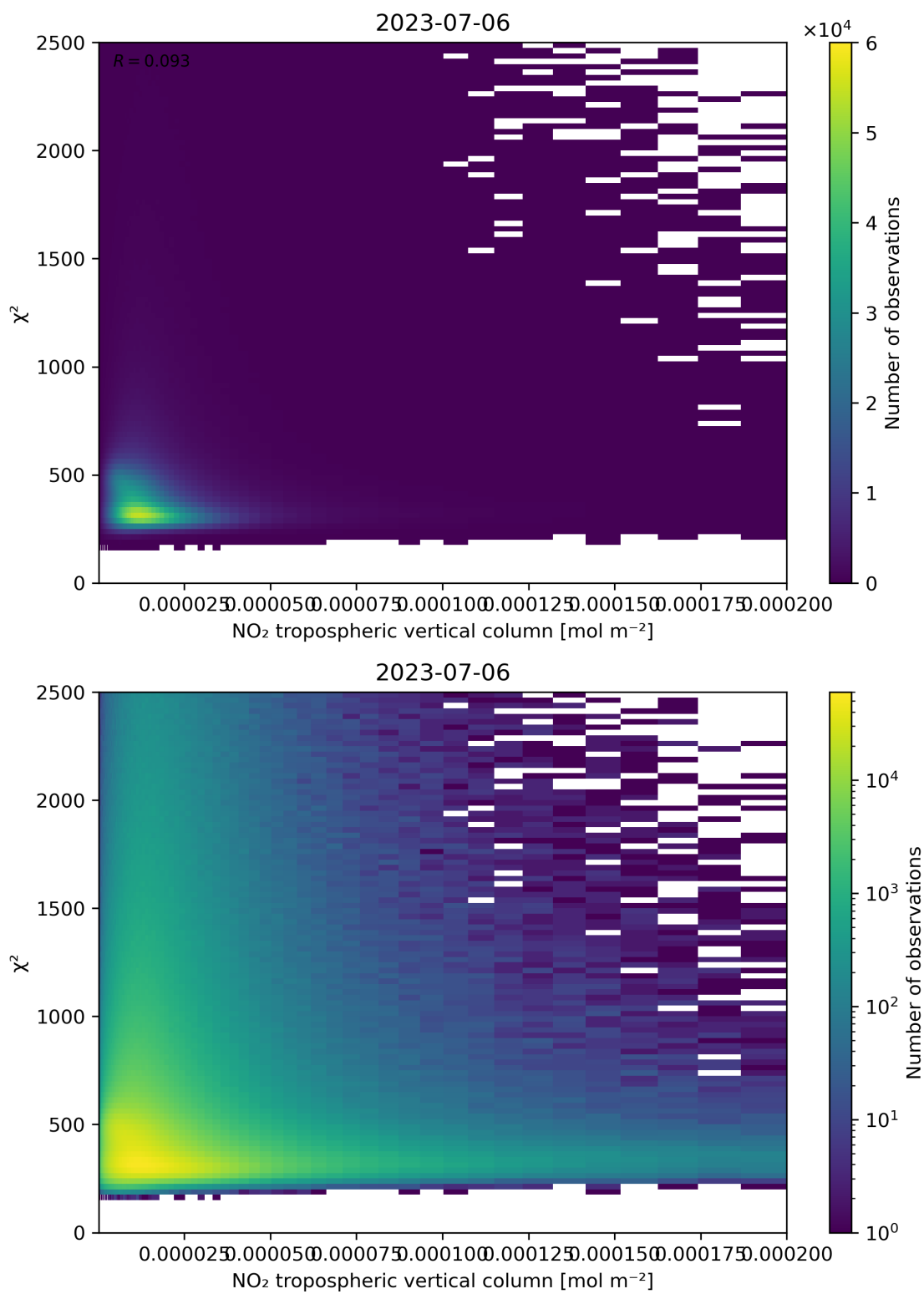
Figure 124: Scatter density plot of “NO 2 tropospheric vertical column” against “ \chi^2 ” for 2023-07-05 to 2023-07-07.
