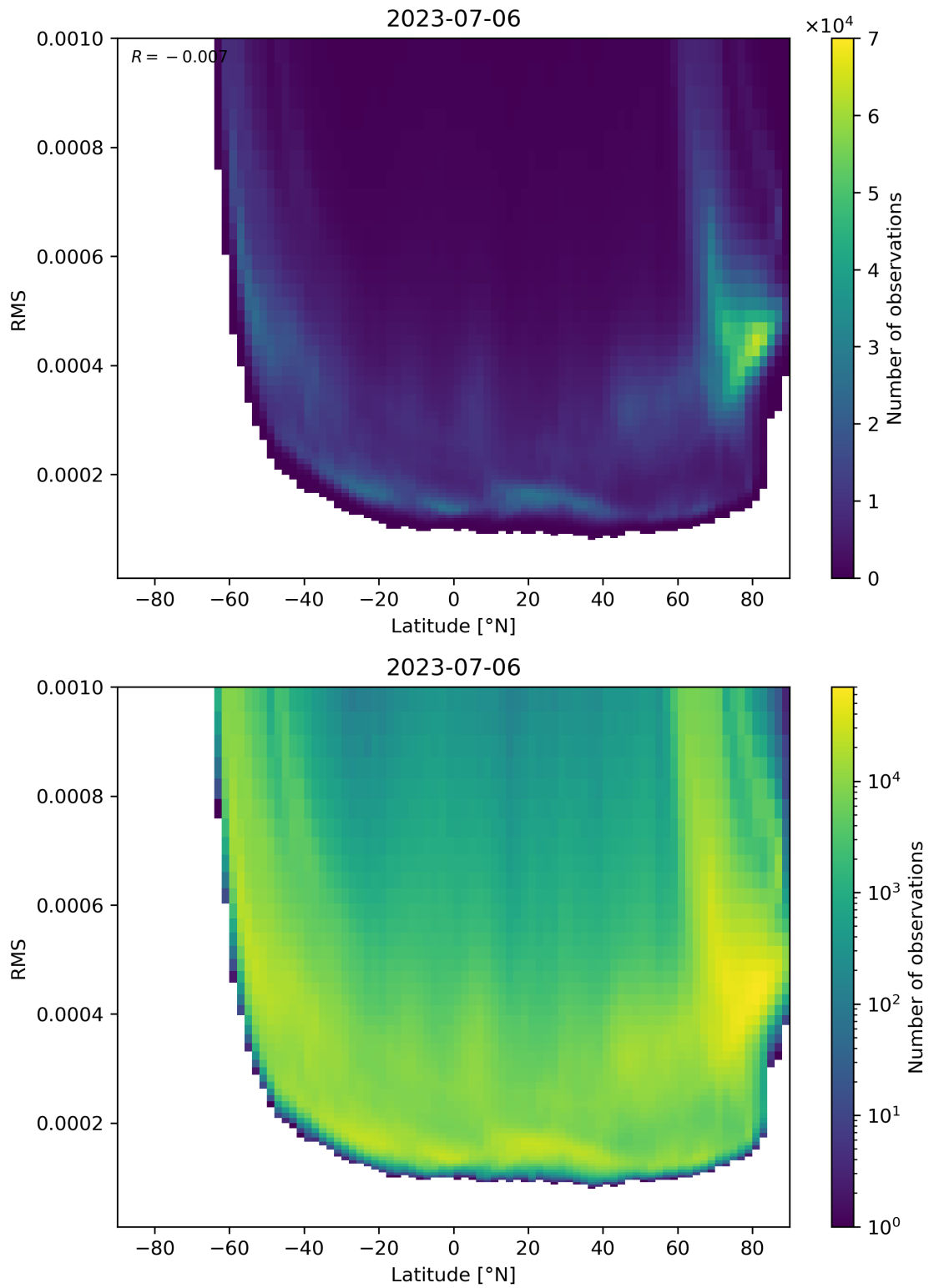
Figure 94: Scatter density plot of “Latitude” against “RMS” for 2023-07-05 to 2023-07-07.
