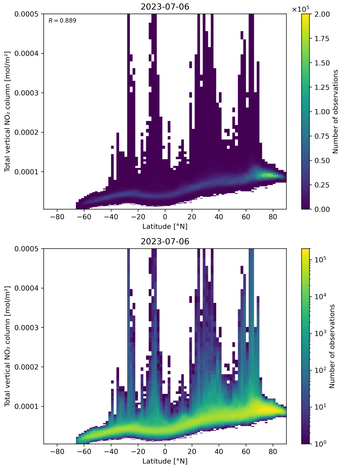
Figure 90: Scatter density plot of “Latitude” against “Total vertical NO 2 column” for 2023-07-05 to 2023-07-07.
