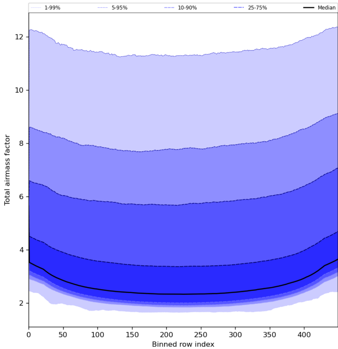
Figure 49: Along track statistics of “Total airmass factor” for 2023-07-05 to 2023-07-07
