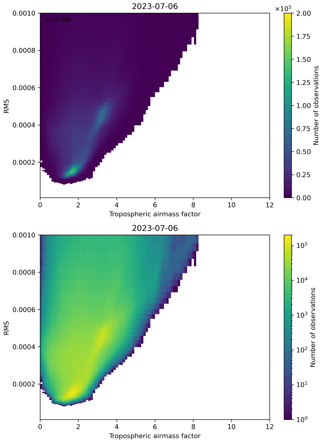
Figure 79: Scatter density plot of “Tropospheric airmass factor” against “RMS” for 2023-07-05 to 2023-07-07.
