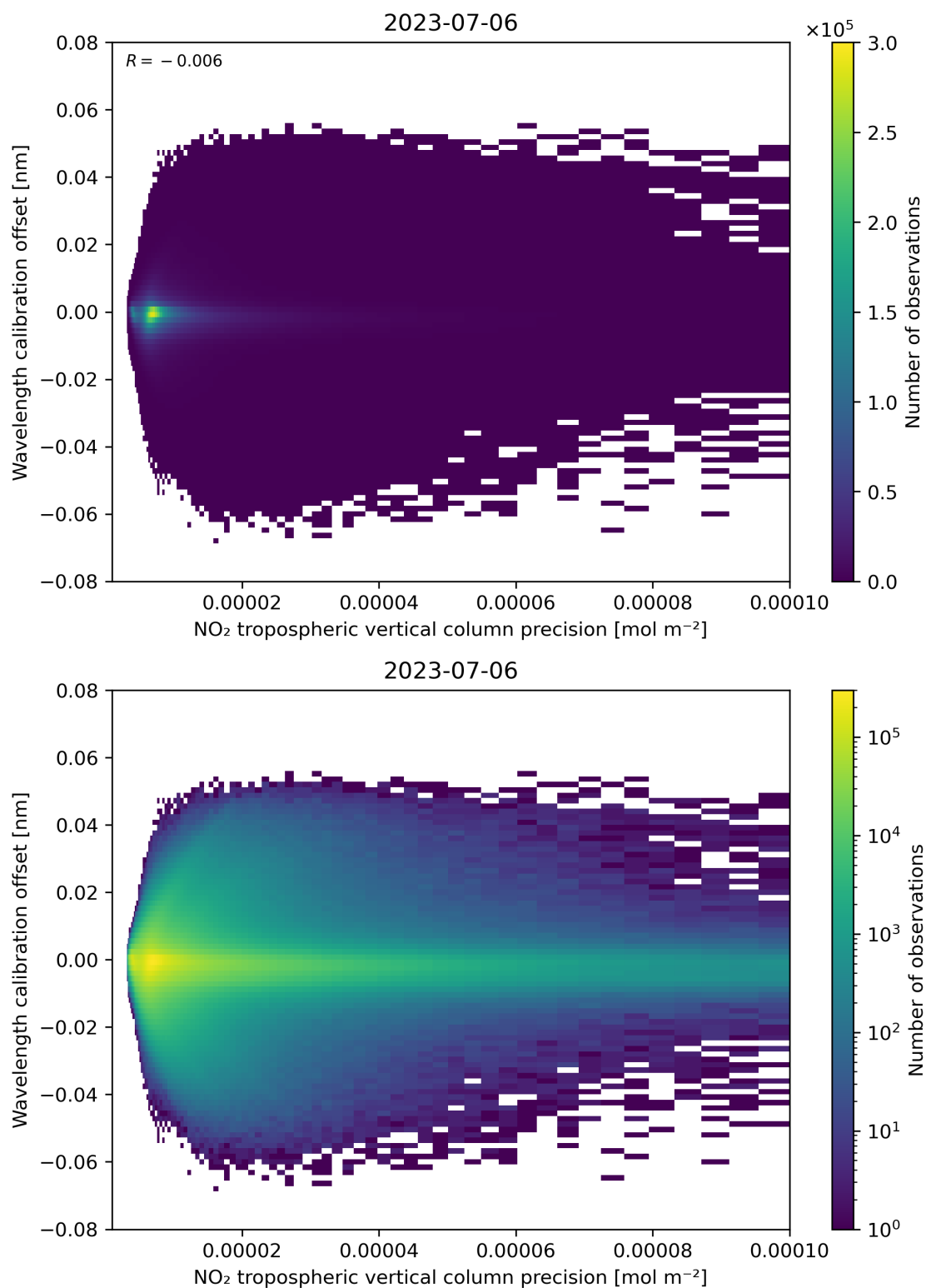
Figure 141: Scatter density plot of “NO 2 tropospheric vertical column precision” against “Wavelength calibration offset” for 2023-07-05 to 2023-07-07.
