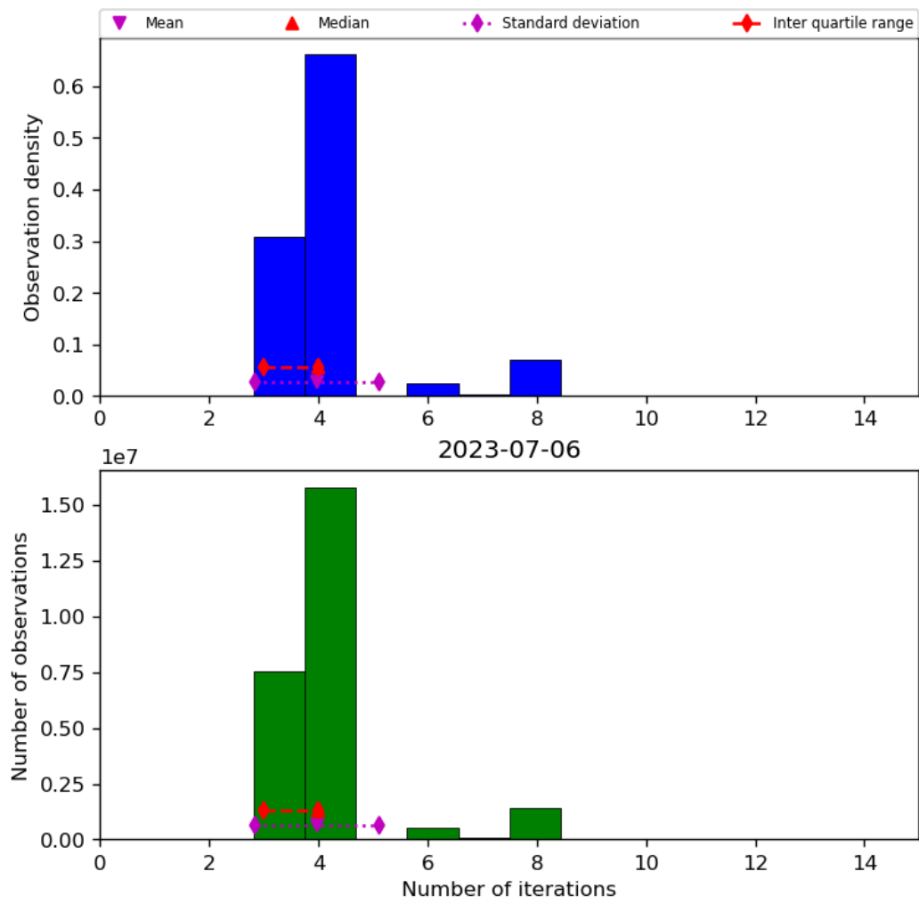
Figure 34: Histogram of “Number of iterations” for 2023-07-05 to 2023-07-07
