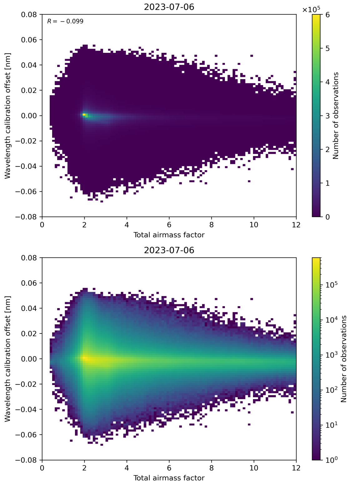
Figure 70: Scatter density plot of “Total airmass factor” against “Wavelength calibration offset” for 2023-07-05 to 2023-07-07.
