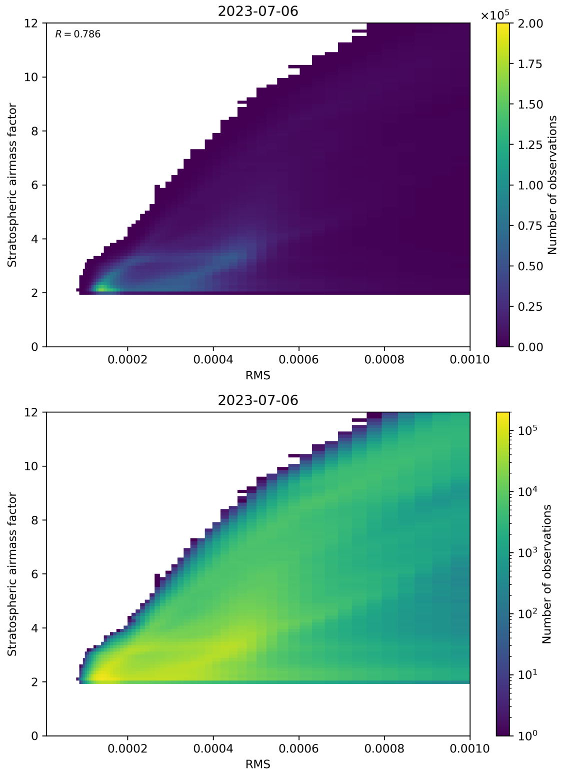
Figure 144: Scatter density plot of “RMS” against “Stratospheric airmass factor” for 2023-07-05 to 2023-07-07.
