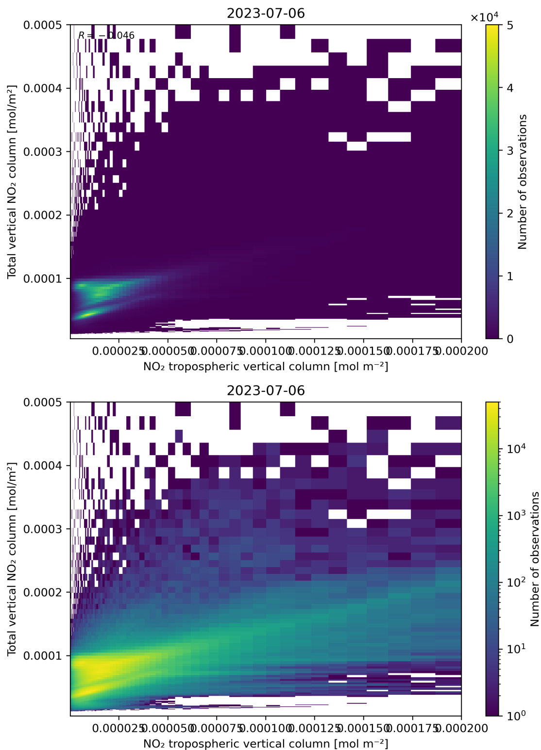
Figure 128: Scatter density plot of “NO 2 tropospheric vertical column” against “Total vertical NO 2 column” for 2023-07-05 to 2023-07-07.
