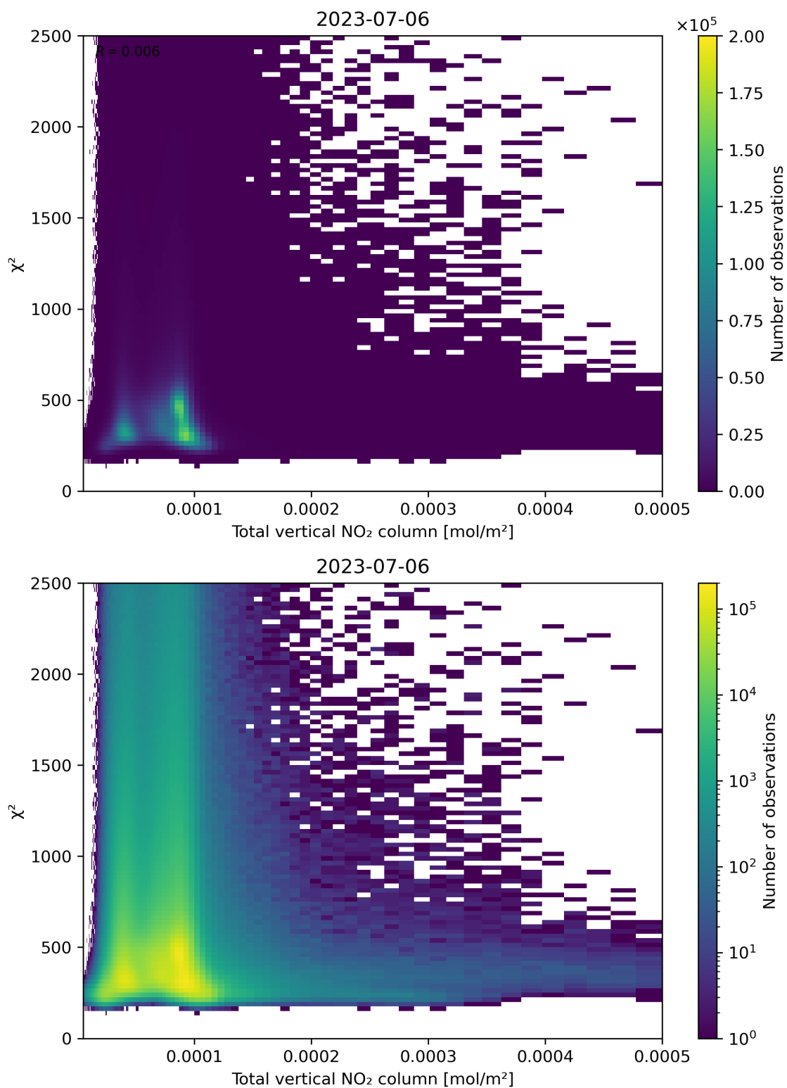
Figure 111: Scatter density plot of “Total vertical NO 2 column” against “ \chi^2 ” for 2023-07-05 to 2023-07-07.
