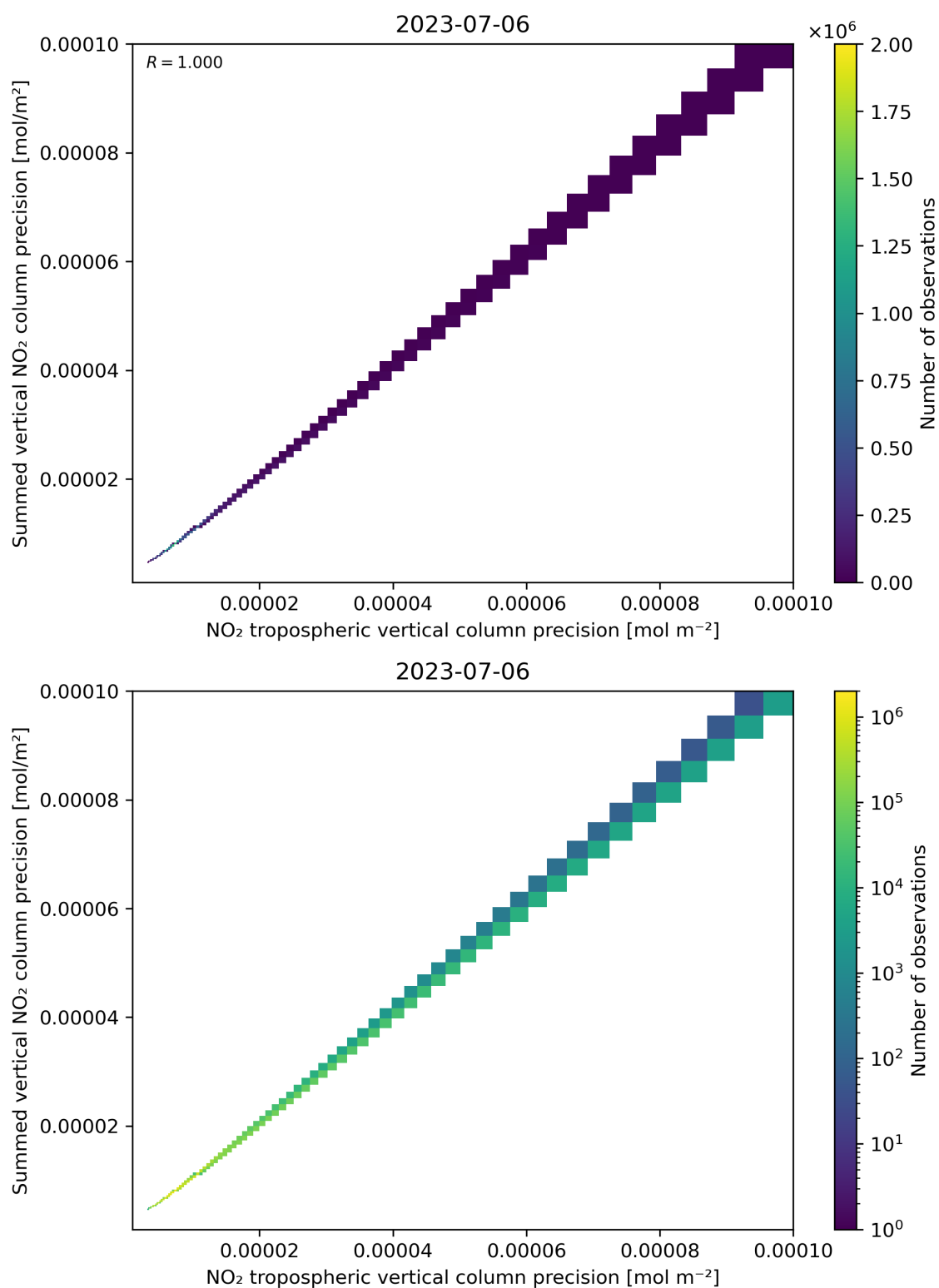
Figure 137: Scatter density plot of “NO 2 tropospheric vertical column precision” against “Summed vertical NO 2 column precision” for 2023-07-05 to 2023-07-07.
