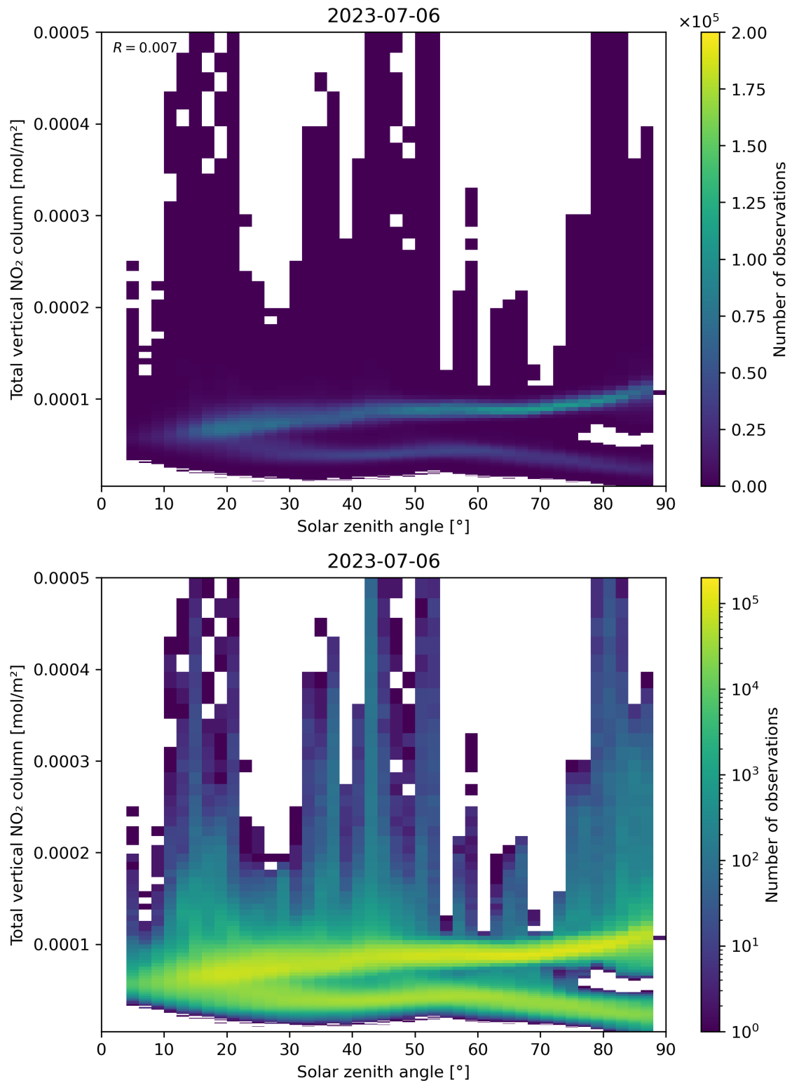
Figure 153: Scatter density plot of “Solar zenith angle” against “Total vertical NO 2 column” for 2023-07-05 to 2023-07-07.
