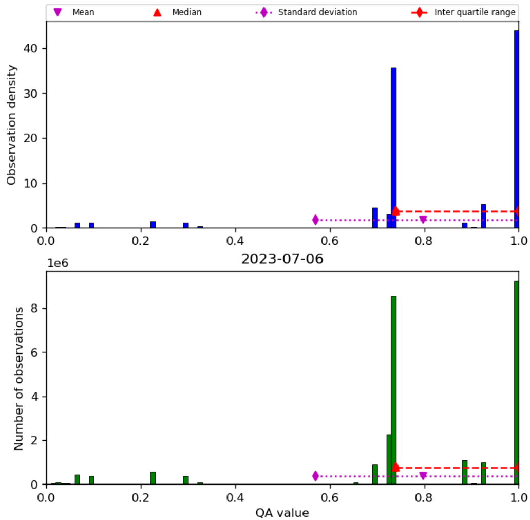
Figure 28: Histogram of “QA value” for 2023-07-05 to 2023-07-07
