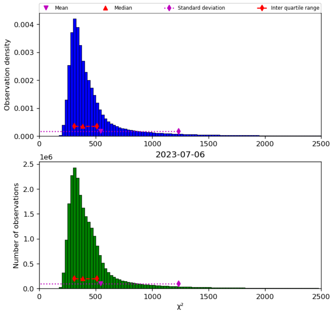
Figure 42: Histogram of “ \chi^2 ” for 2023-07-05 to 2023-07-07
