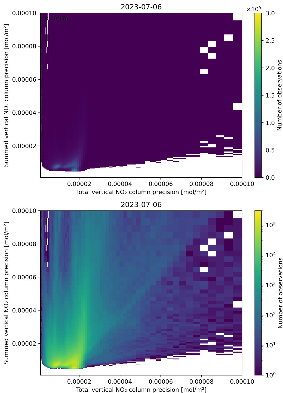
Figure 118: Scatter density plot of “Total vertical NO 2 column precision” against “Summed vertical NO 2 column precision” for 2023-07-05 to 2023-07-07.
