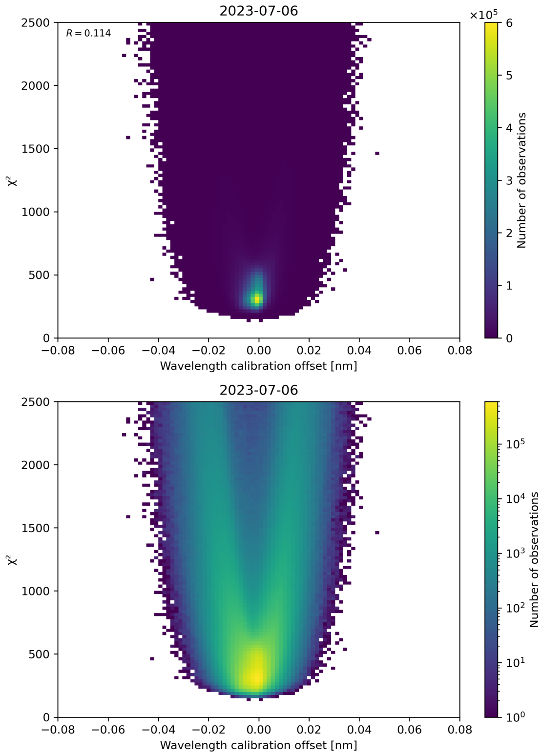
Figure 175: Scatter density plot of “Wavelength calibration offset” against “ \chi^2 ” for 2023-07-05 to 2023-07-07.
