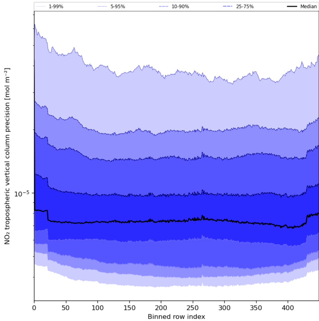
Figure 47: Along track statistics of “NO 2 tropospheric vertical column precision” for 2023-07-05 to 2023-07-07
