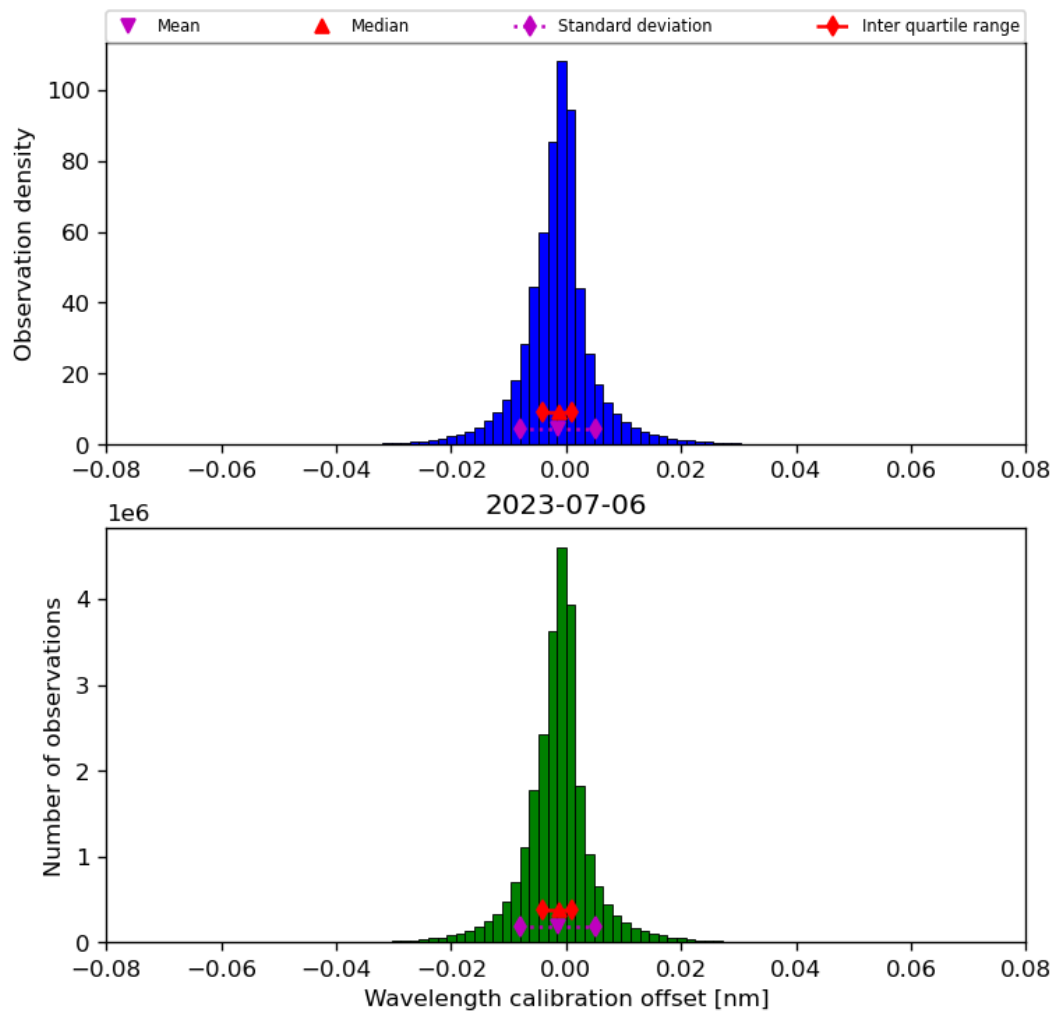
Figure 35: Histogram of “Wavelength calibration offset” for 2023-07-05 to 2023-07-07
