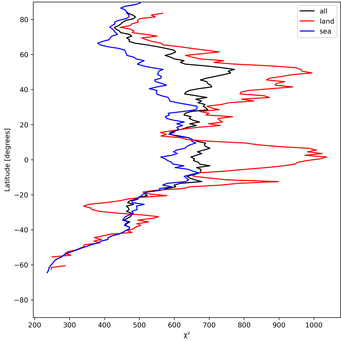
Figure 25: Zonal average of “ \chi^2 ” for 2023-07-05 to 2023-07-07.
