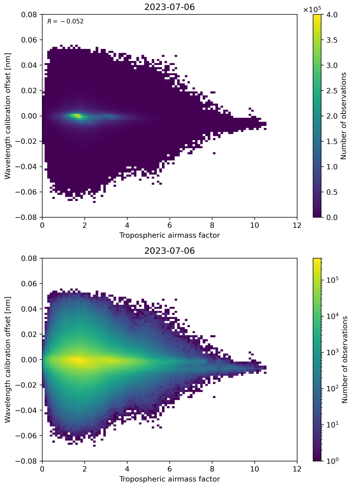
Figure 80: Scatter density plot of “Tropospheric airmass factor” against “Wavelength calibration offset” for 2023-07-05 to 2023-07-07.
