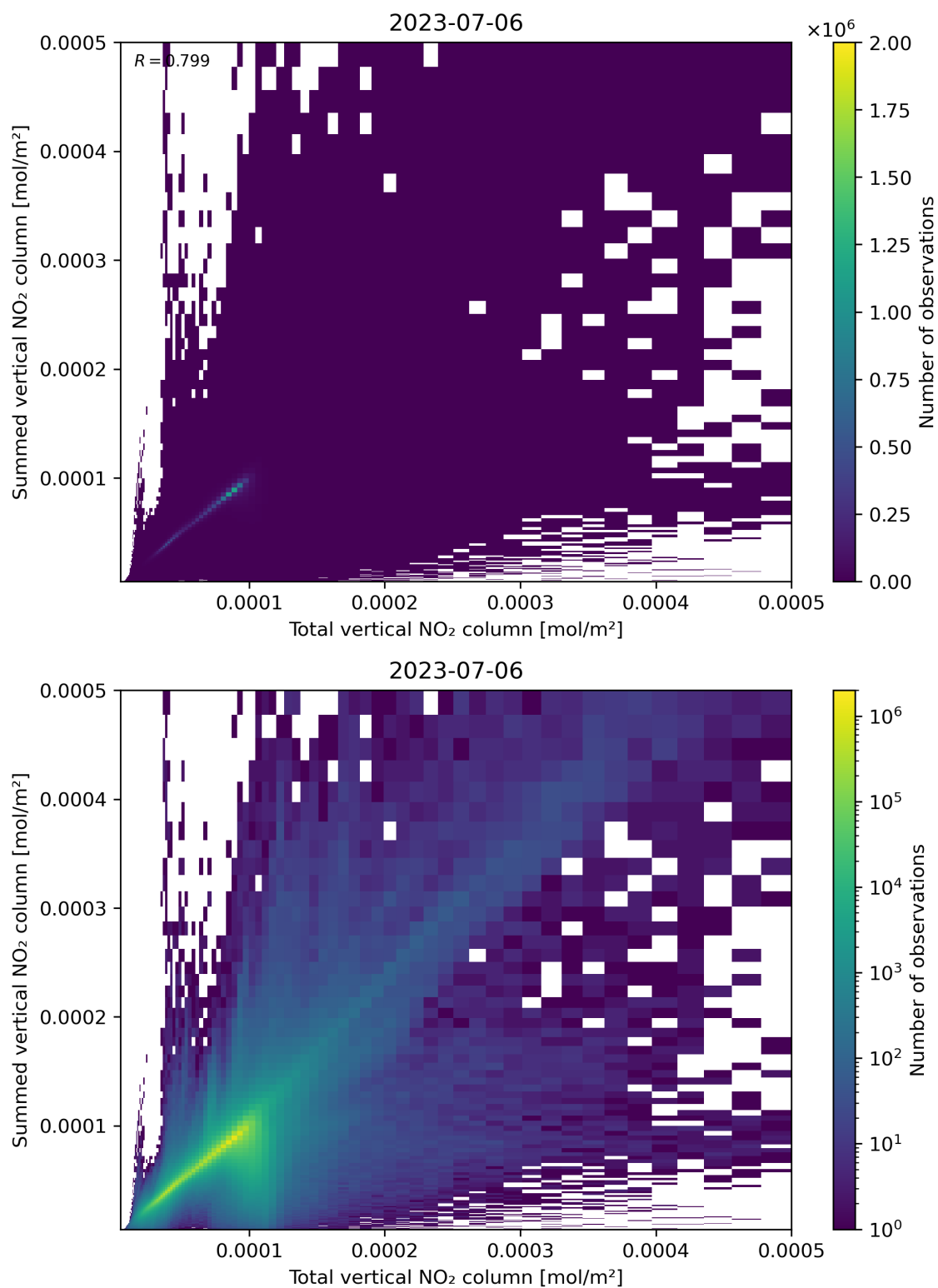
Figure 112: Scatter density plot of “Total vertical NO 2 column” against “Summed vertical NO 2 column” for 2023-07-05 to 2023-07-07.
