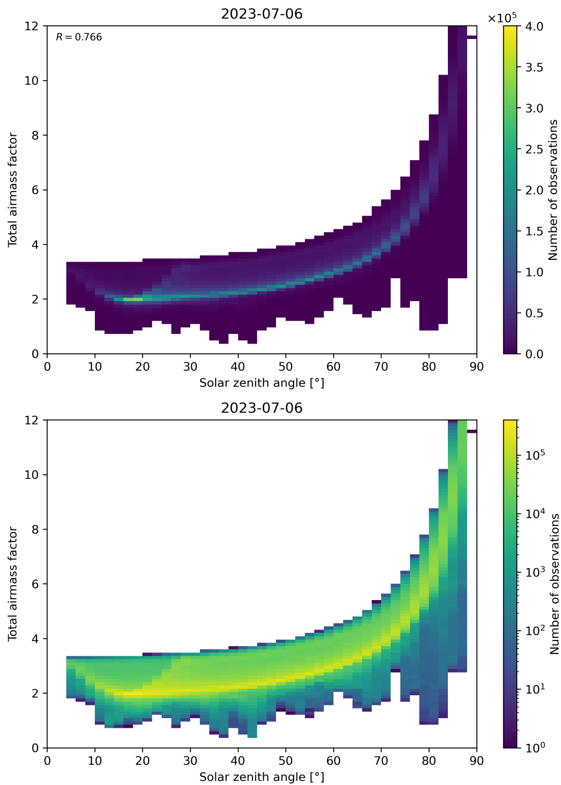
Figure 146: Scatter density plot of “Solar zenith angle” against “Total air mass factor” for 2023-07-05 to 2023-07-07.
