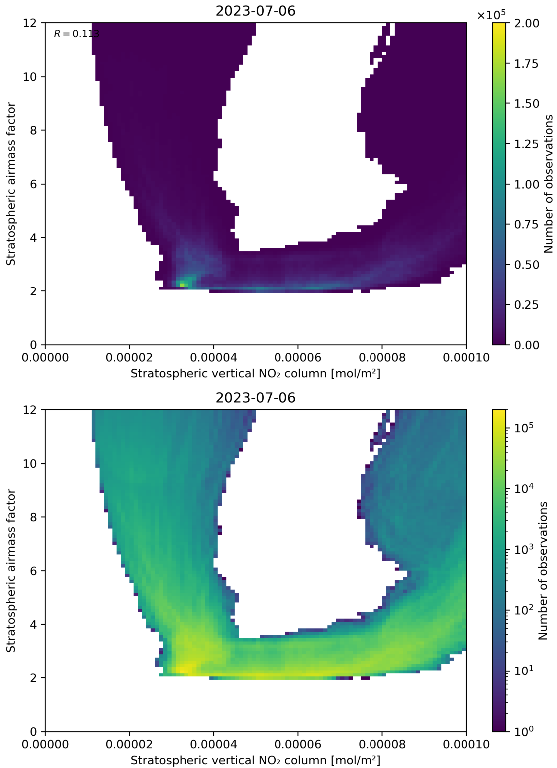
Figure 96: Scatter density plot of “Stratospheric vertical NO 2 column” against “Stratospheric airmass factor” for 2023-07-05 to 2023-07-07.
