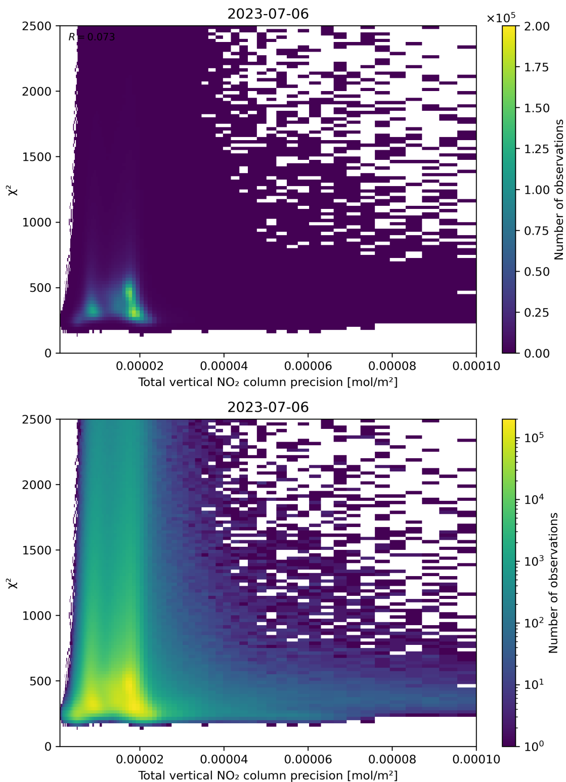
Figure 116: Scatter density plot of “Total vertical NO 2 column precision” against “ \chi^2 ” for 2023-07-05 to 2023-07-07.
