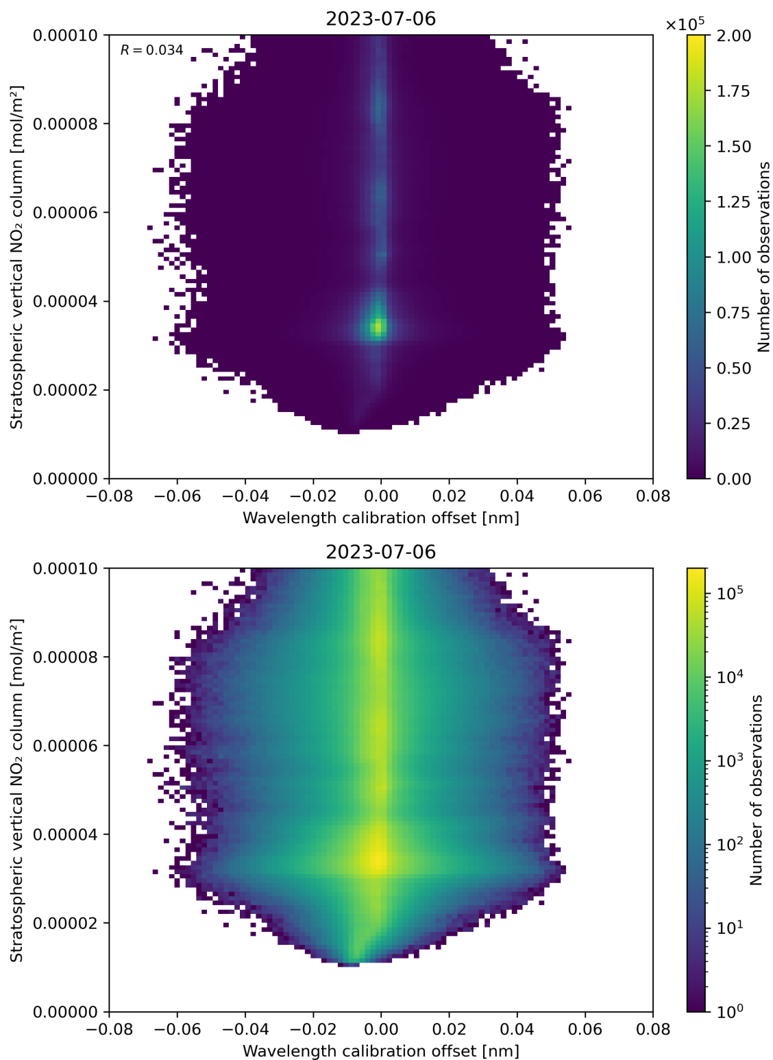
Figure 176: Scatter density plot of “Wavelength calibration offset” against “Stratospheric vertical NO 2 column” for 2023-07-05 to 2023-07-07.
