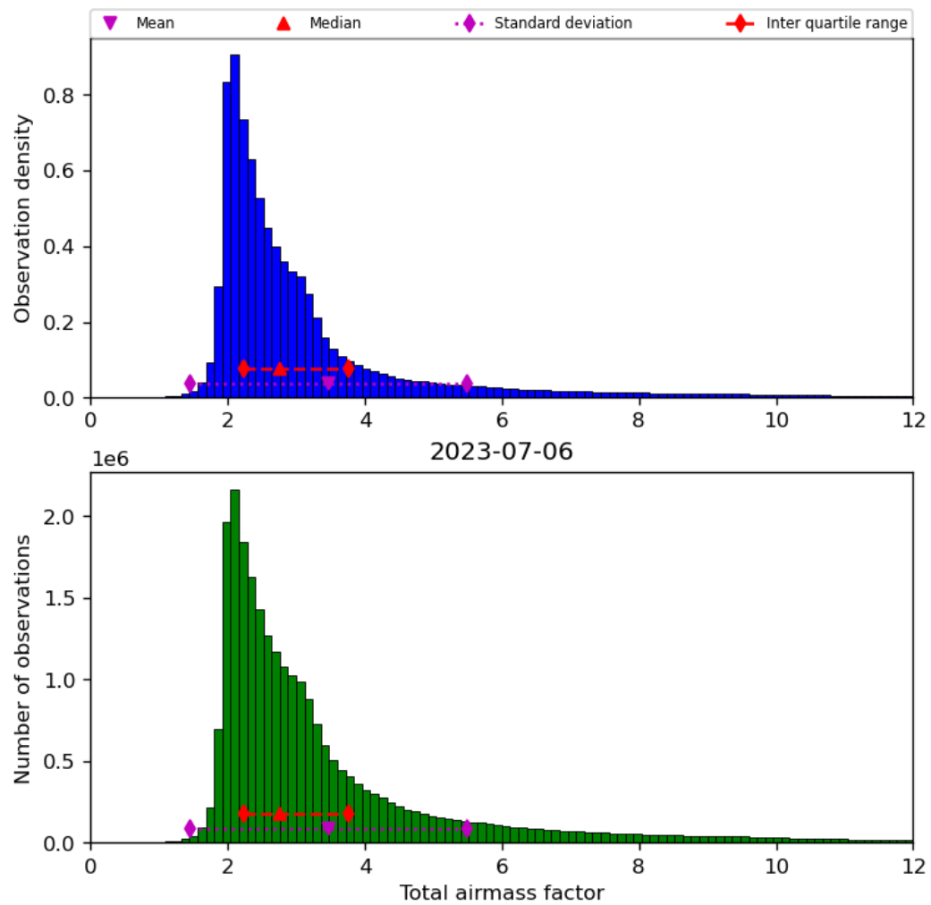
Figure 32: Histogram of “Total airmass factor” for 2023-07-05 to 2023-07-07
