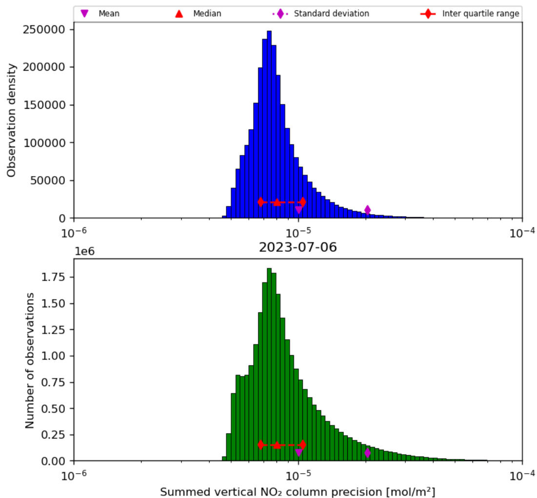
Figure 41: Histogram of “Summed vertical NO 2 column precision” for 2023-07-05 to 2023-07-07
