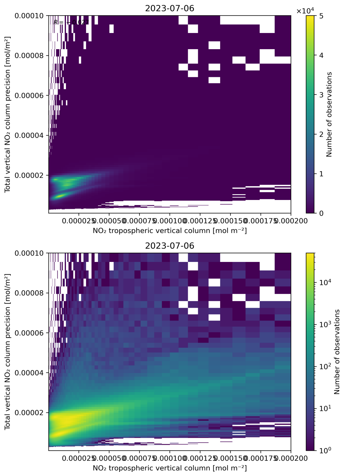
Figure 129: Scatter density plot of “NO 2 tropospheric vertical column” against “Total vertical NO 2 column precision” for 2023-07-05 to 2023-07-07.
