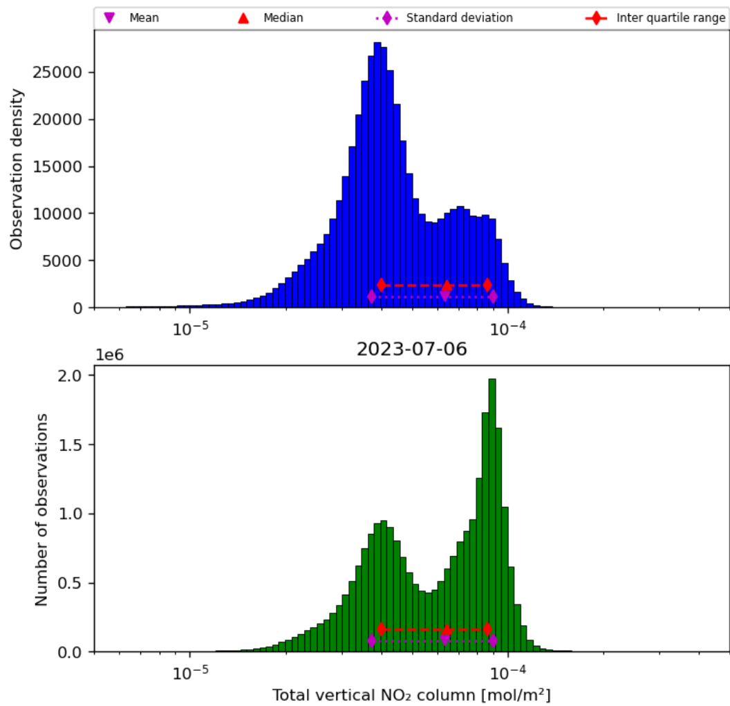
Figure 38: Histogram of “Total vertical NO 2 column” for 2023-07-05 to 2023-07-07
