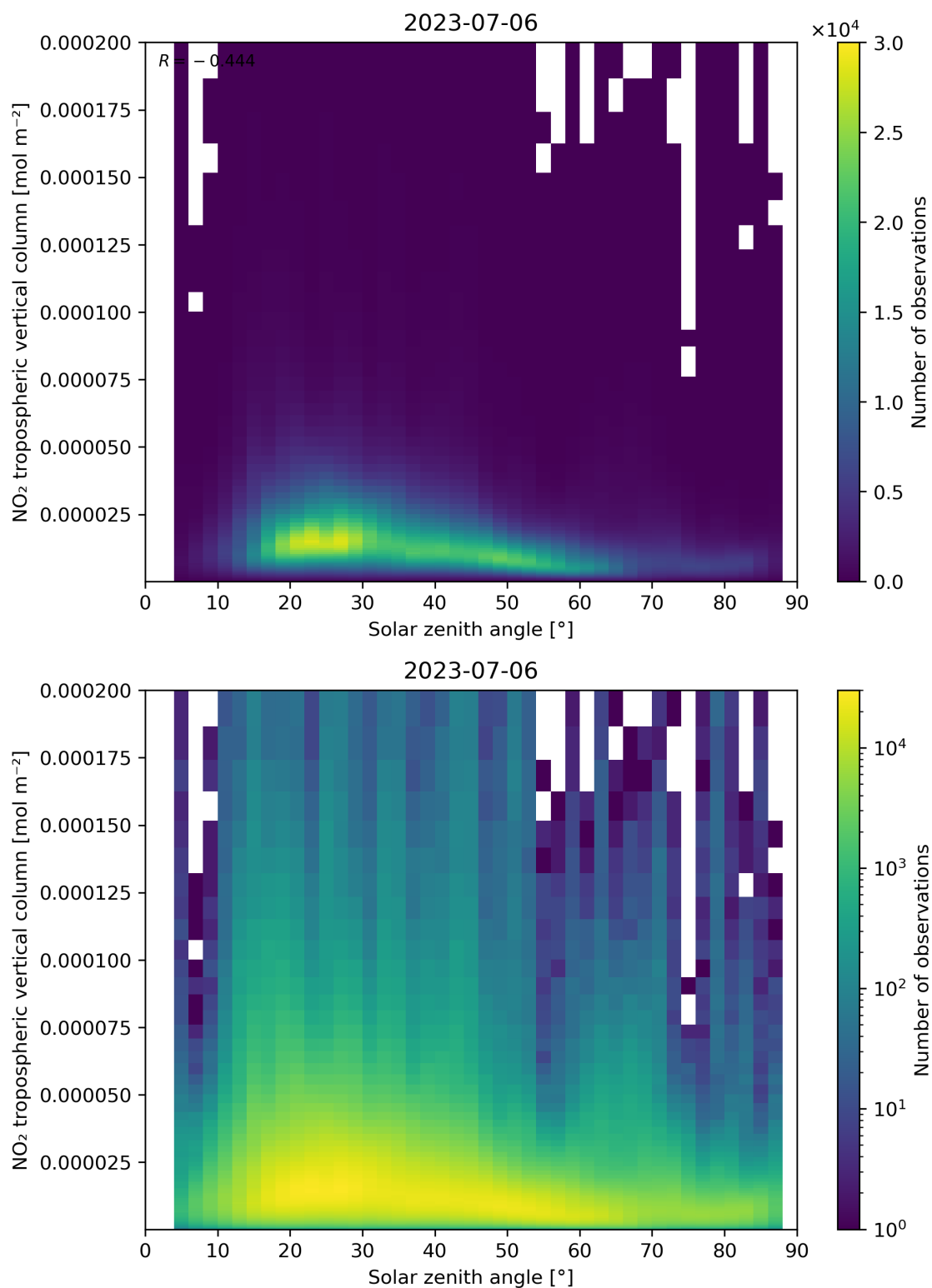
Figure 155: Scatter density plot of “Solar zenith angle” against “NO 2 tropospheric vertical column” for 2023-07-05 to 2023-07-07.
