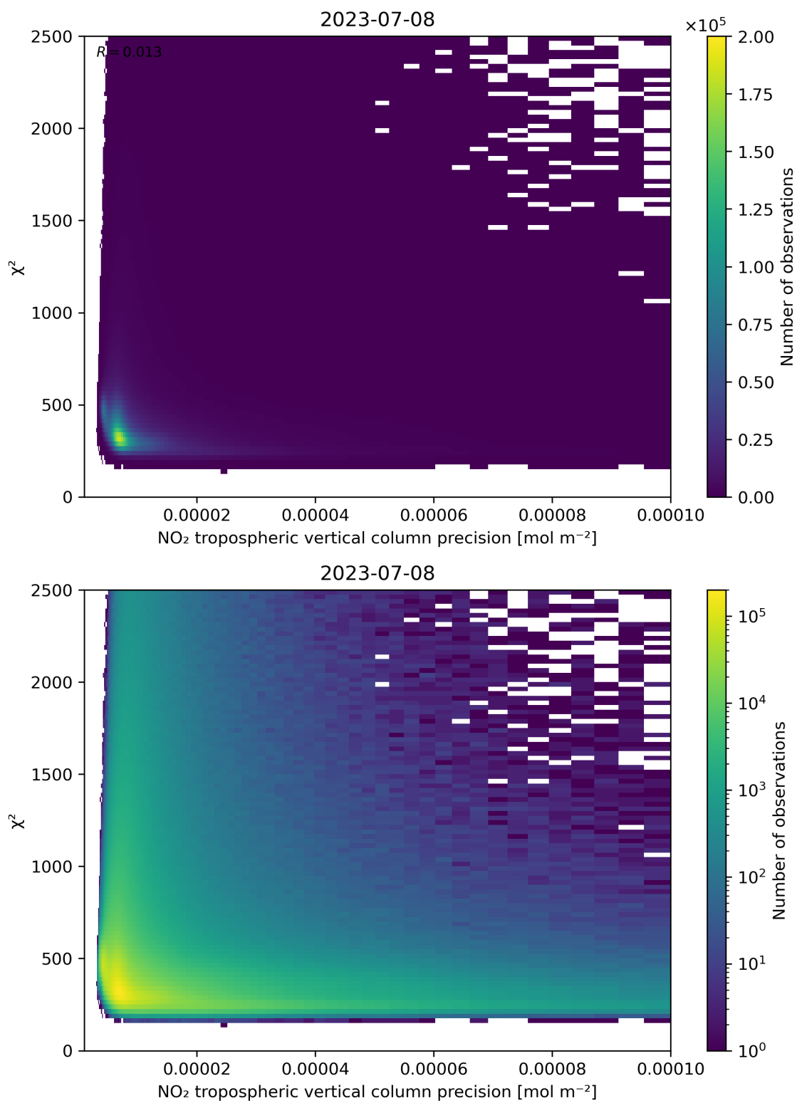
Figure 134: Scatter density plot of “NO 2 tropospheric vertical column precision” against “ \chi^2 ” for 2023-07-08 to 2023-07-09.
