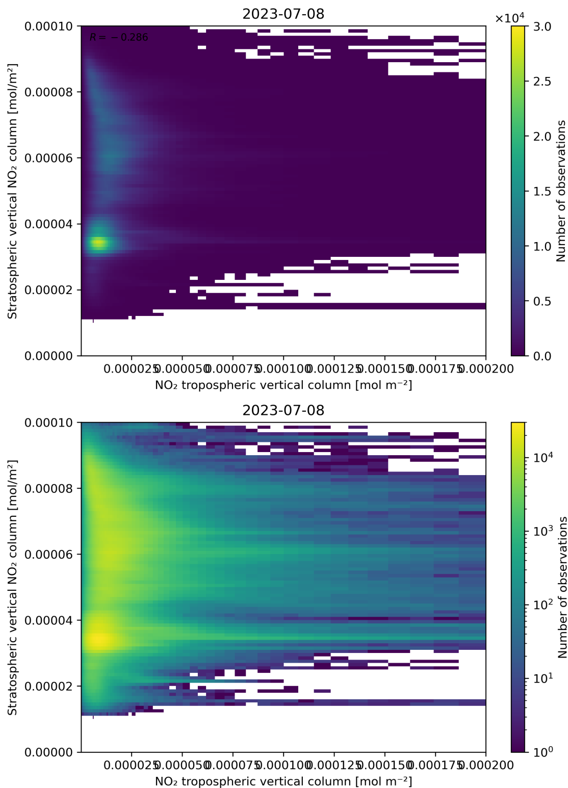
Figure 125: Scatter density plot of “NO 2 tropospheric vertical column” against “Stratospheric vertical NO 2 column” for 2023-07-08 to 2023-07-09.
