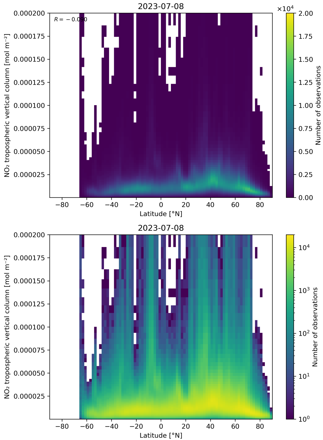
Figure 92: Scatter density plot of “Latitude” against “NO 2 tropospheric vertical column” for 2023-07-08 to 2023-07-09.
