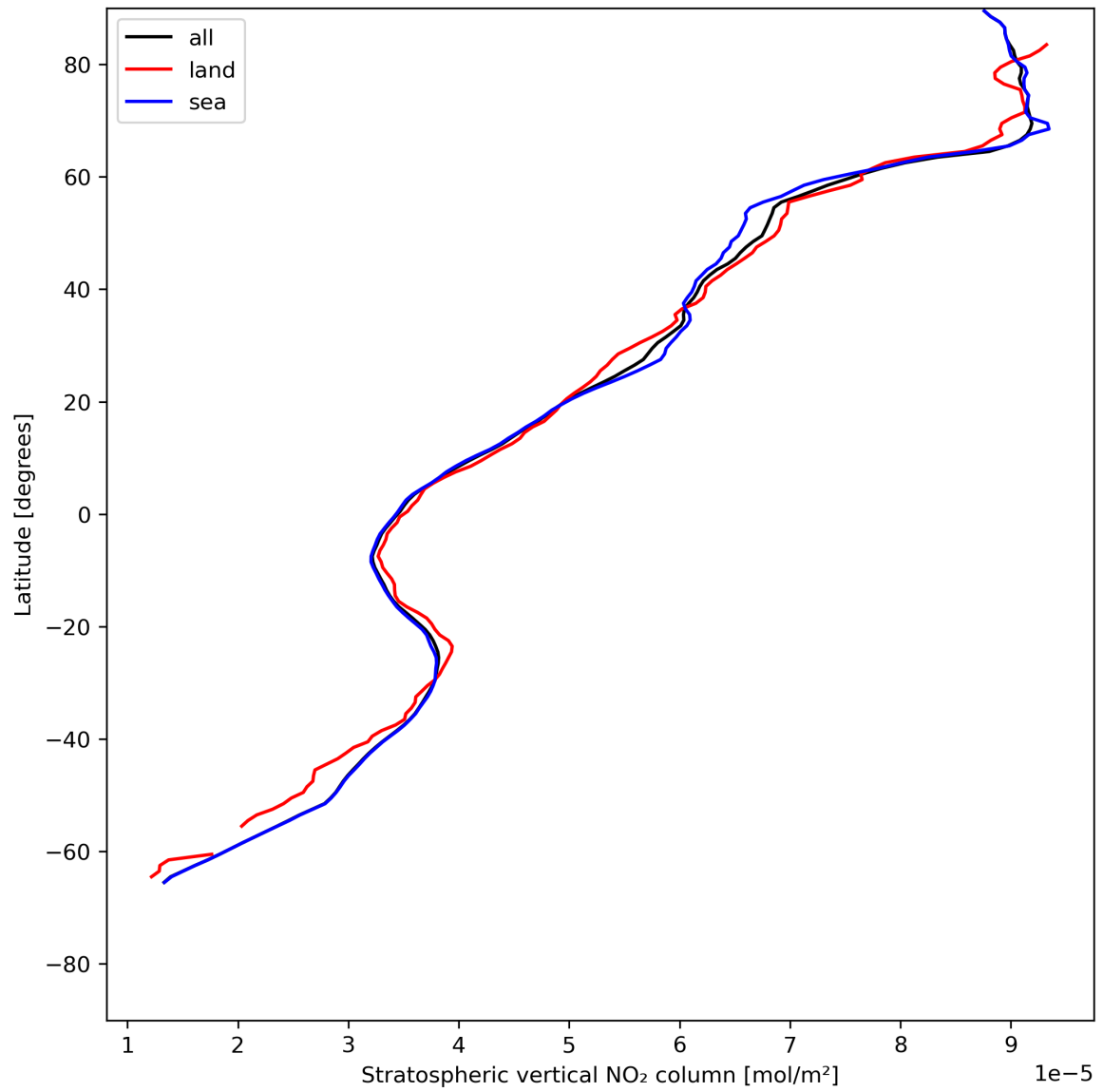
Figure 19: Zonal average of “Stratospheric vertical NO 2 column” for 2023-07-08 to 2023-07-09.
