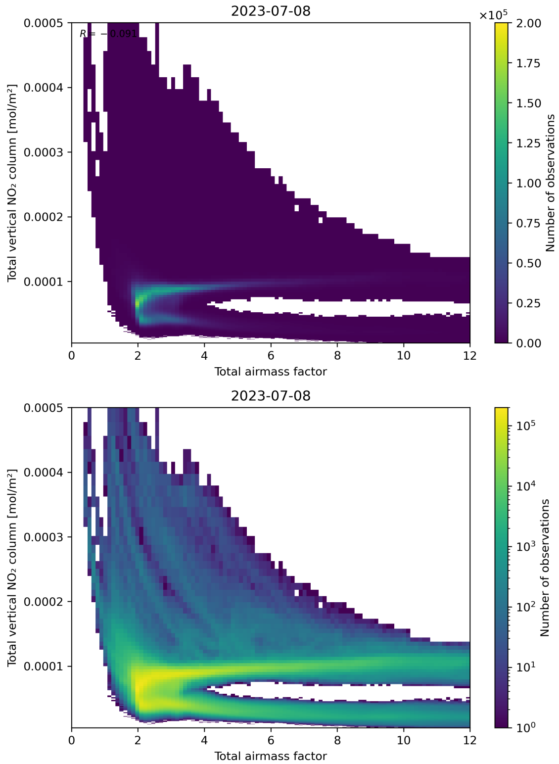
Figure 67: Scatter density plot of “Total airmass factor” against “Total vertical NO 2 column” for 2023-07-08 to 2023-07-09.
