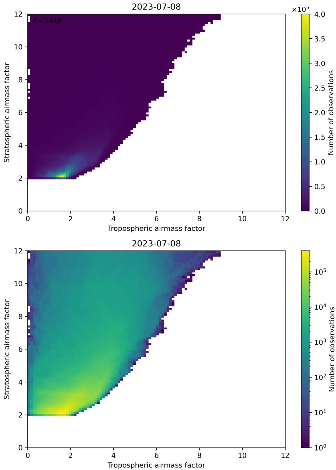
Figure 71: Scatter density plot of “Tropospheric airmass factor” against “Stratospheric airmass factor” for 2023-07-08 to 2023-07-09.
