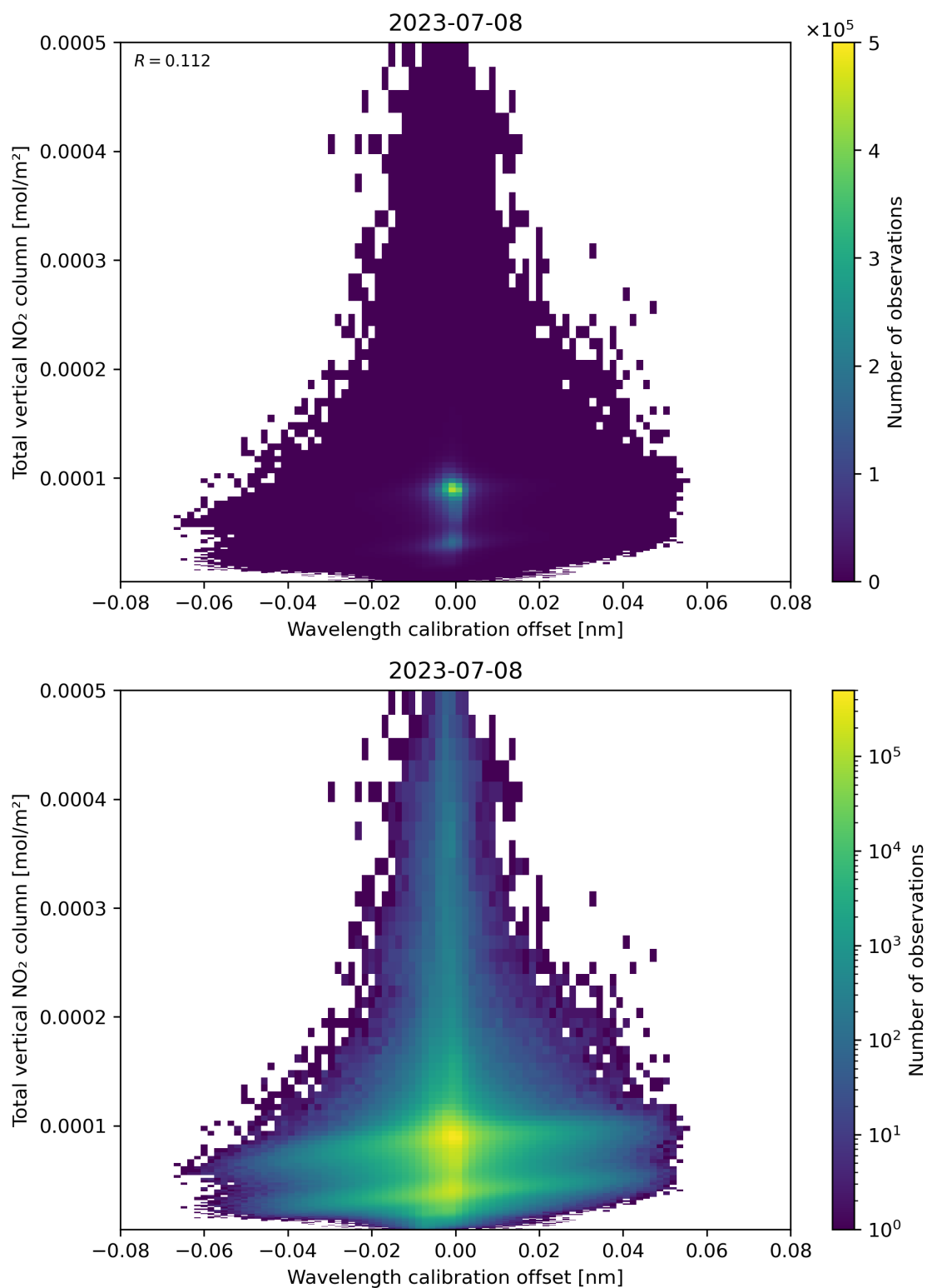
Figure 179: Scatter density plot of “Wavelength calibration offset” against “Total vertical NO 2 column” for 2023-07-08 to 2023-07-09.
