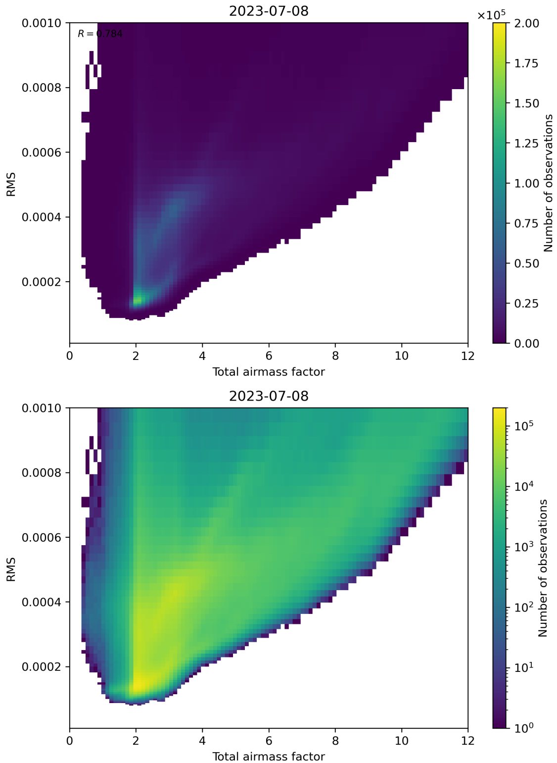
Figure 69: Scatter density plot of “Total airmass factor” against “RMS” for 2023-07-08 to 2023-07-09.
