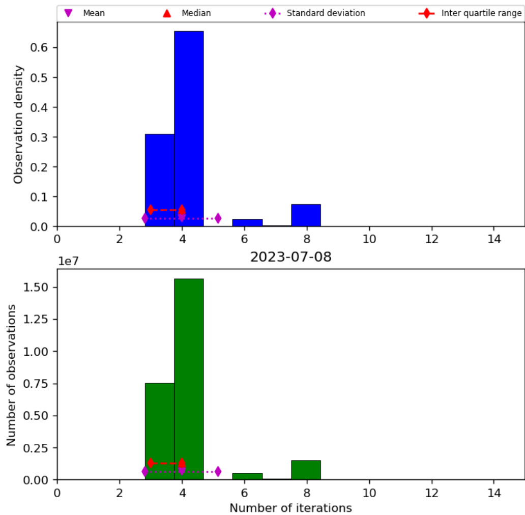
Figure 34: Histogram of “Number of iterations” for 2023-07-08 to 2023-07-09
