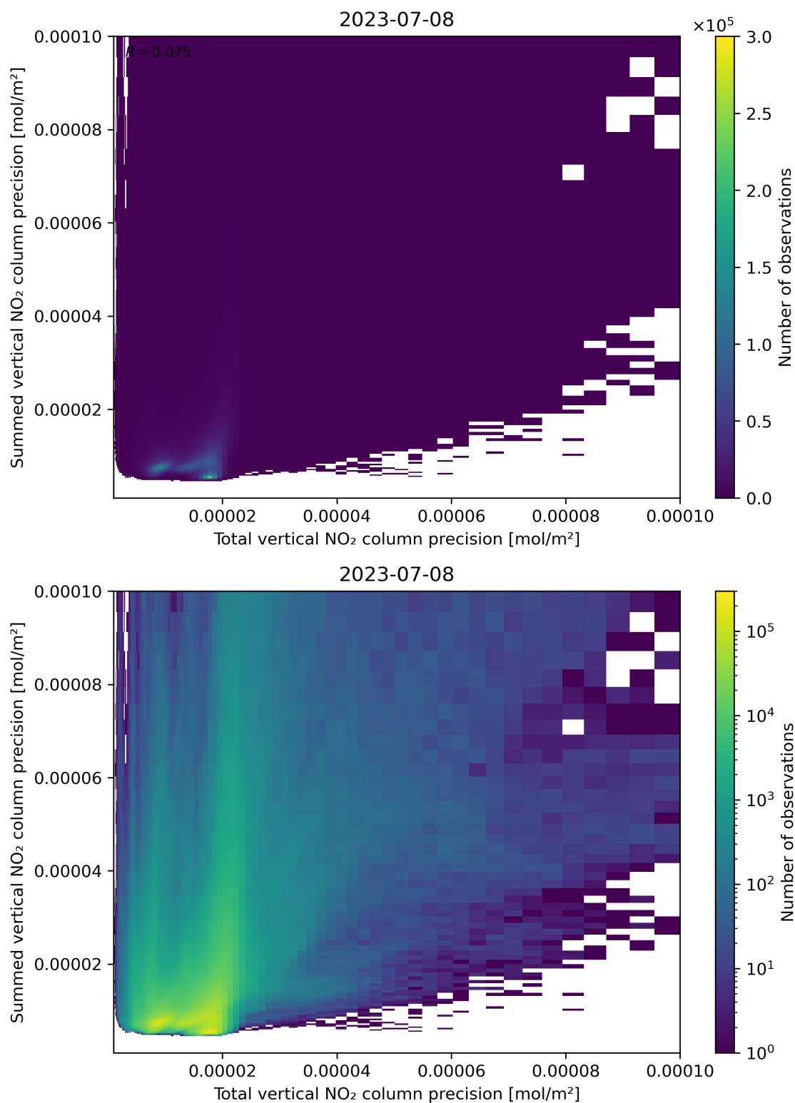
Figure 118: Scatter density plot of “Total vertical NO 2 column precision” against “Summed vertical NO 2 column precision” for 2023-07-08 to 2023-07-09.
