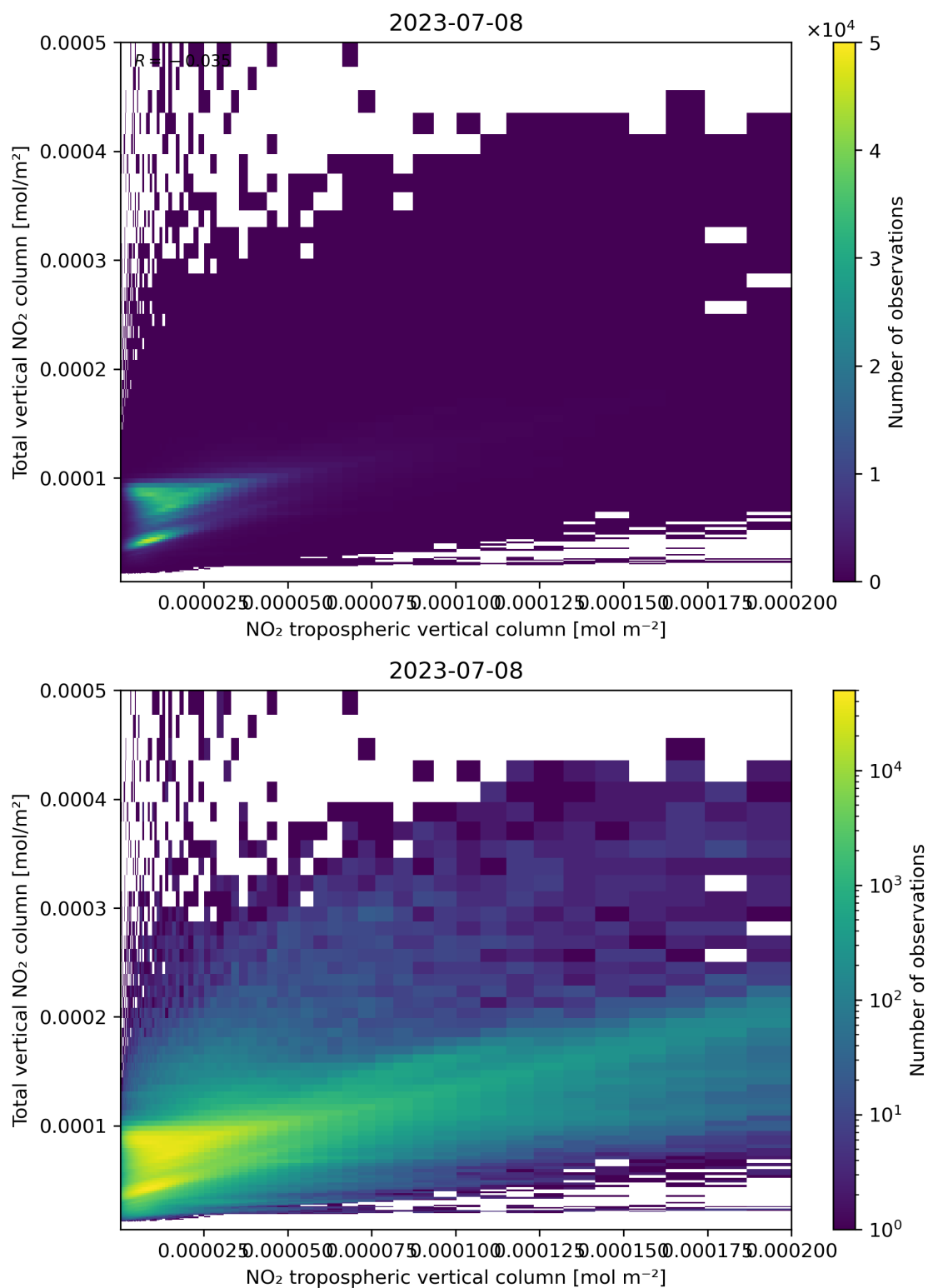
Figure 128: Scatter density plot of “NO 2 tropospheric vertical column” against “Total vertical NO 2 column” for 2023-07-08 to 2023-07-09.
