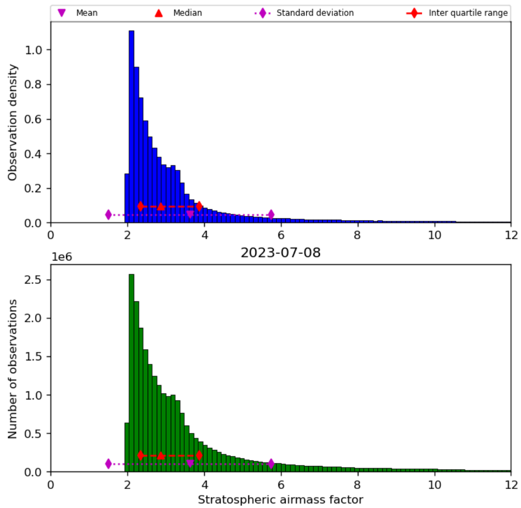
Figure 44: Histogram of “Stratospheric airmass factor” for 2023-07-08 to 2023-07-09
