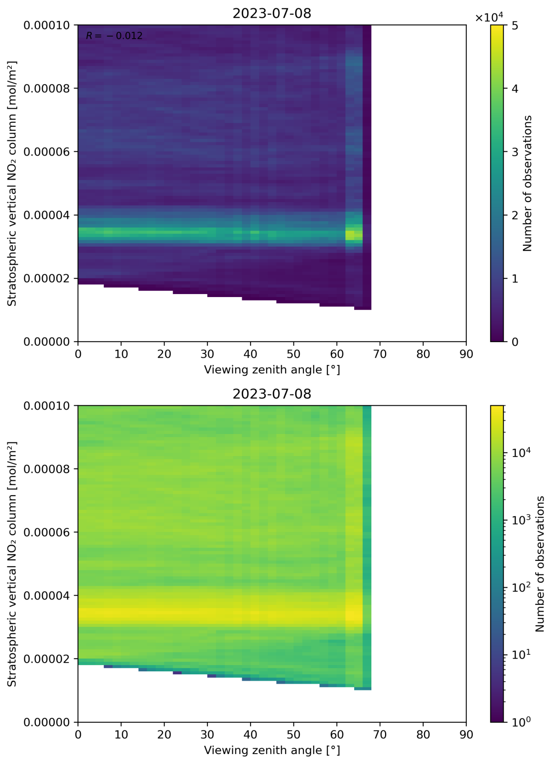
Figure 164: Scatter density plot of “Viewing zenith angle” against “Stratospheric vertical NO 2 column” for 2023-07-08 to 2023-07-09.
