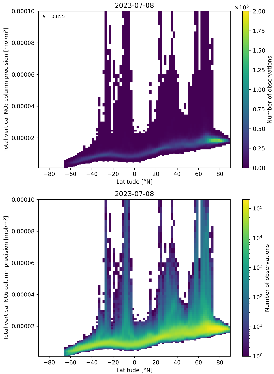
Figure 91: Scatter density plot of “Latitude” against “Total vertical NO 2 column precision” for 2023-07-08 to 2023-07-09.
