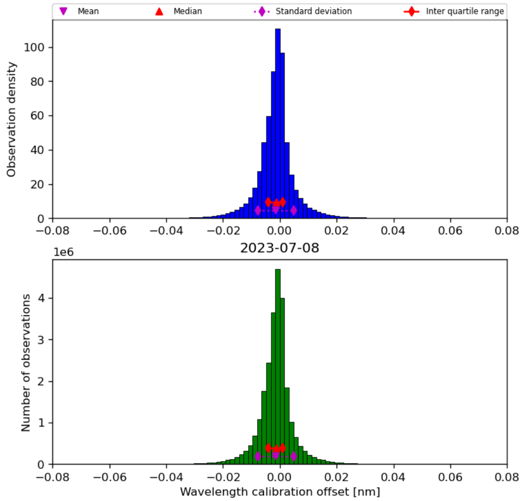
Figure 35: Histogram of “Wavelength calibration offset” for 2023-07-08 to 2023-07-09
