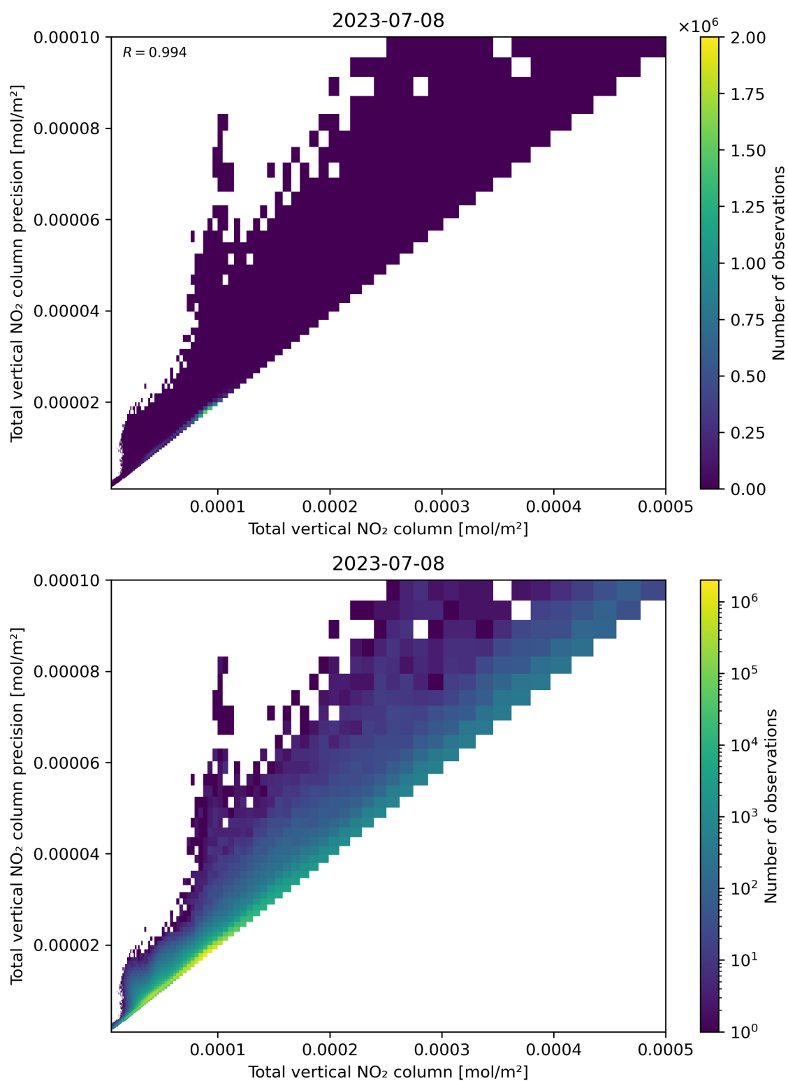
Figure 114: Scatter density plot of “Total vertical NO 2 column” against “Total vertical NO 2 column precision” for 2023-07-08 to 2023-07-09.
