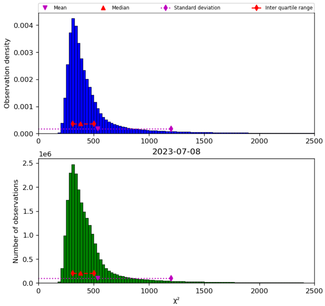
Figure 42: Histogram of “ \chi^2 ” for 2023-07-08 to 2023-07-09
