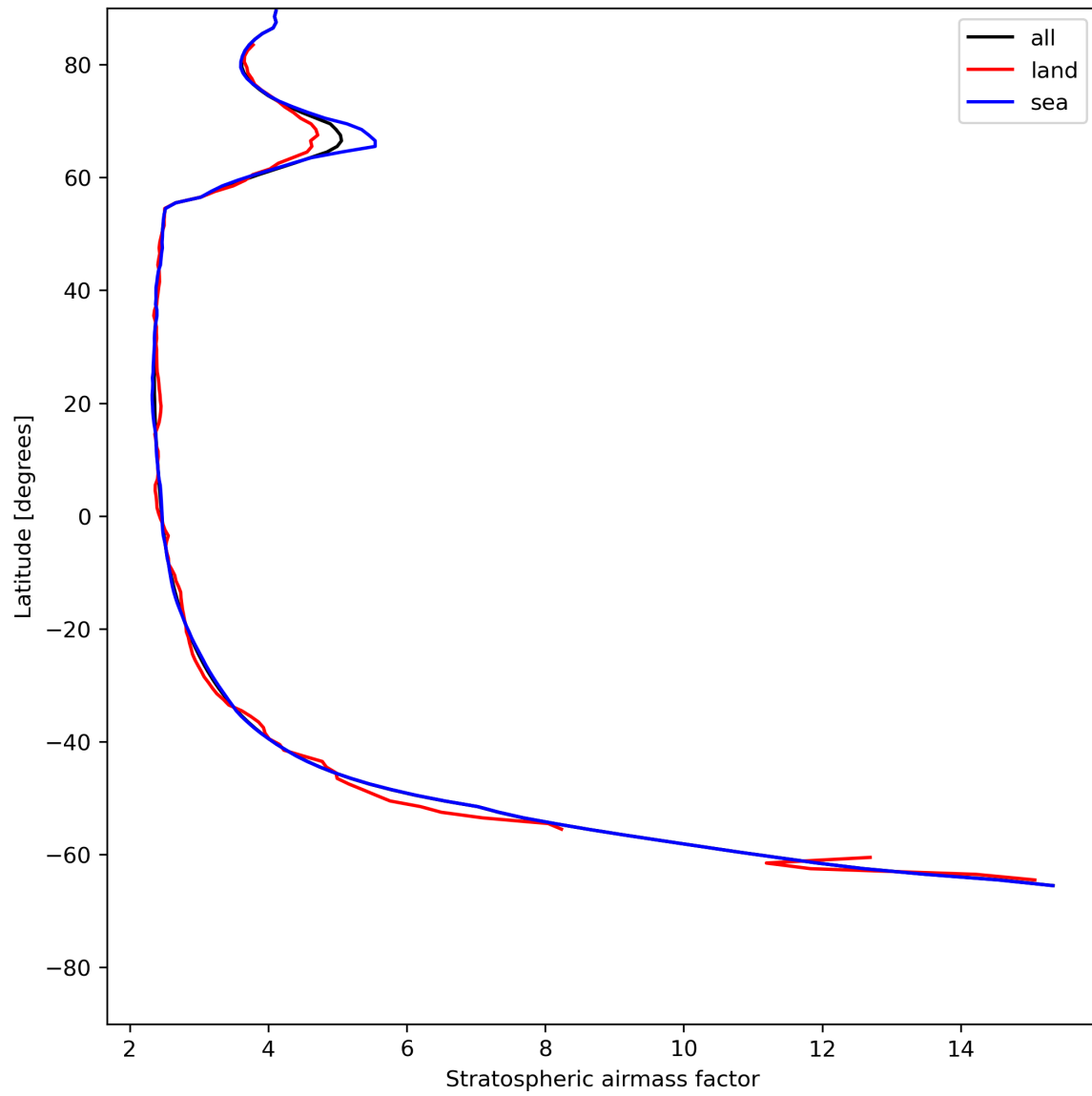
Figure 27: Zonal average of “Stratospheric airmass factor” for 2023-07-08 to 2023-07-09.
