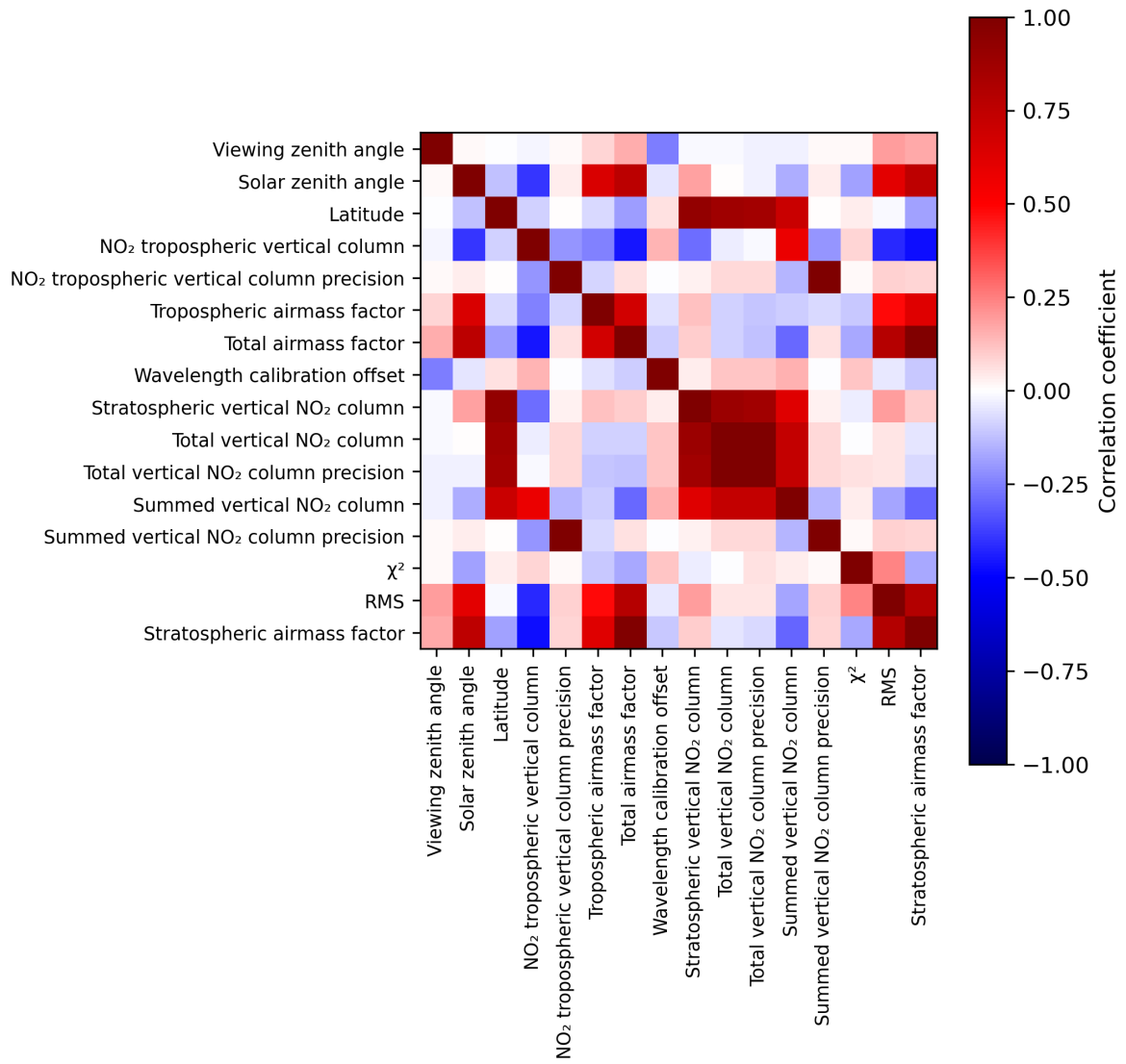
Figure 2: Map of correlation matrix for 2023-07-08 to 2023-07-09.
