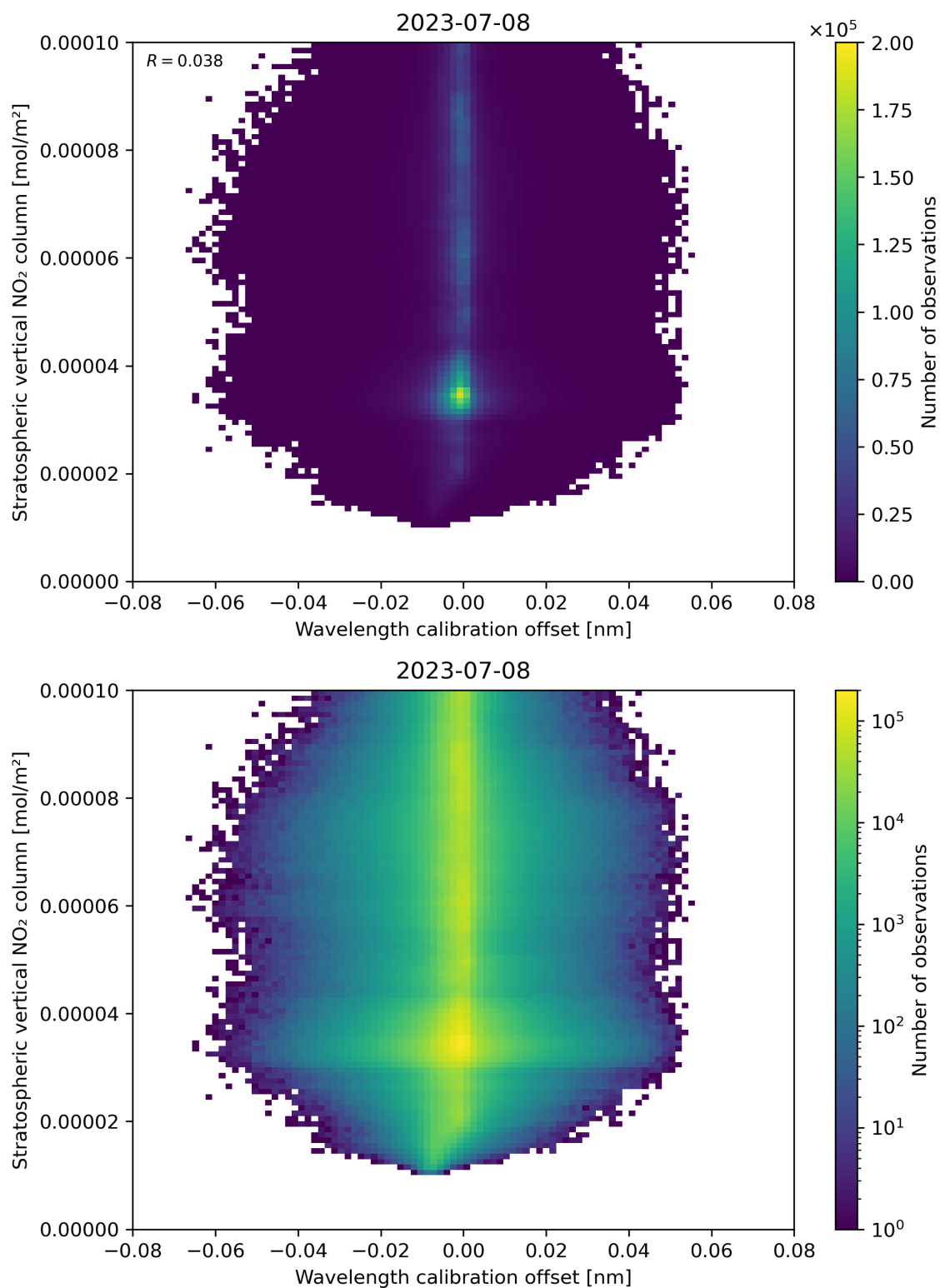
Figure 176: Scatter density plot of “Wavelength calibration offset” against “Stratospheric vertical NO 2 column” for 2023-07-08 to 2023-07-09.
