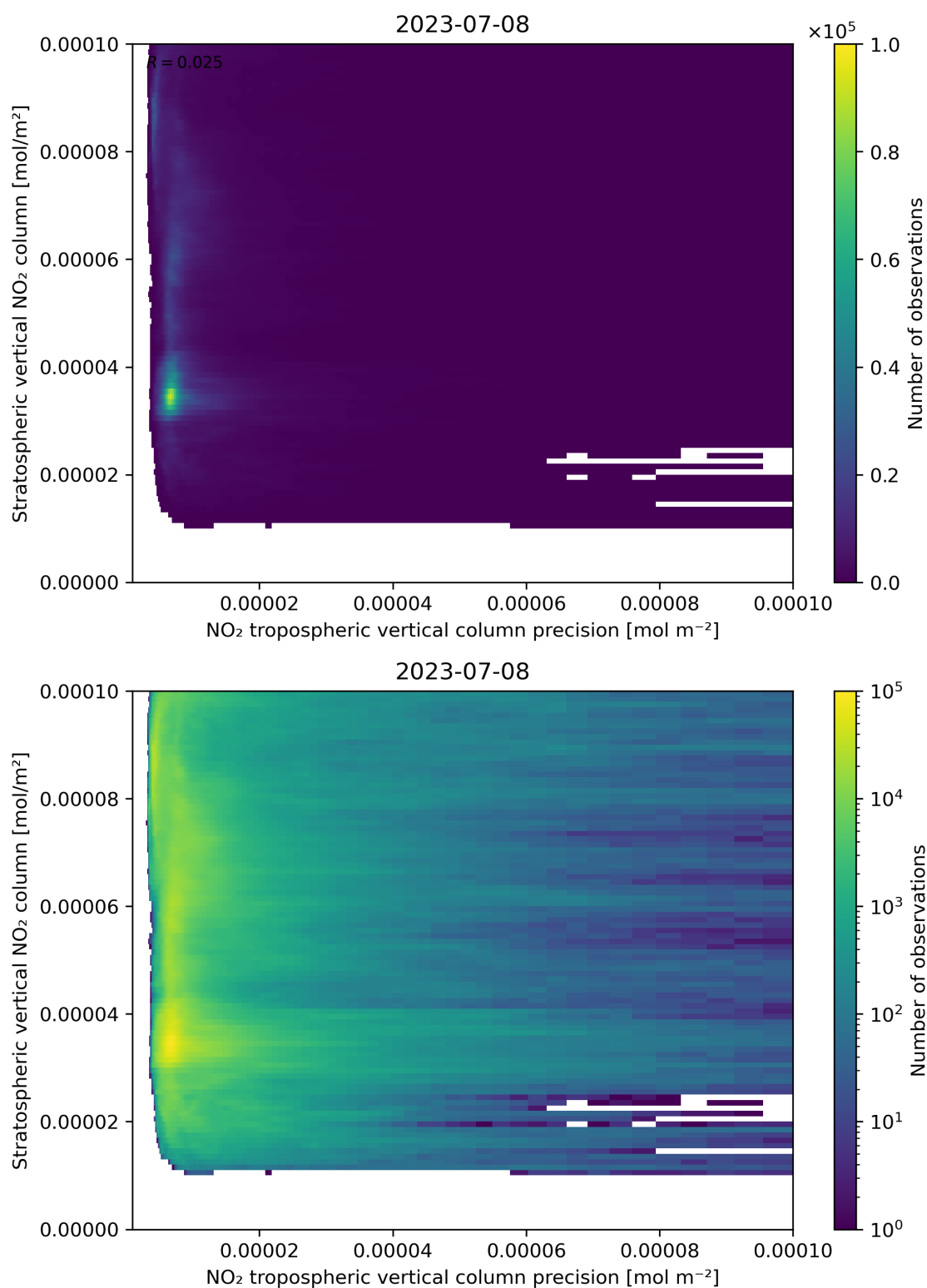
Figure 135: Scatter density plot of “NO 2 tropospheric vertical column precision” against “Stratospheric vertical NO 2 column” for 2023-07-08 to 2023-07-09.
