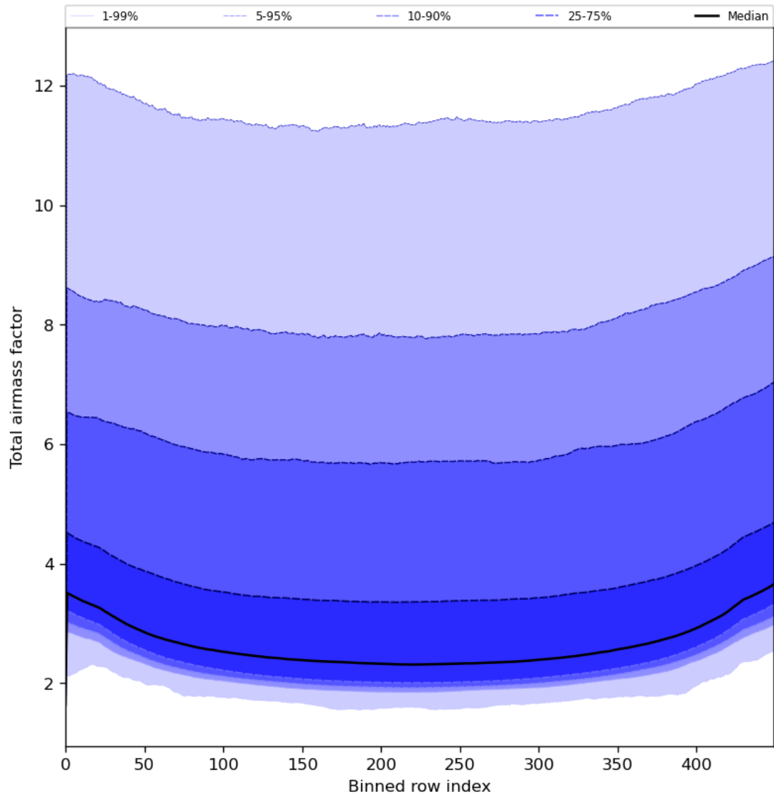
Figure 49: Along track statistics of “Total airmass factor” for 2023-07-08 to 2023-07-09
