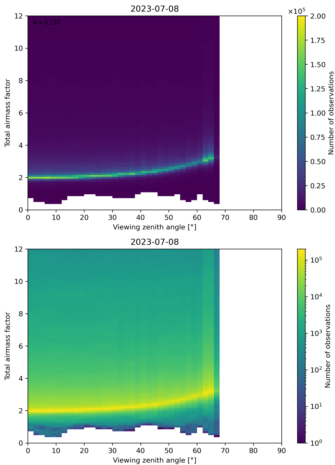
Figure 160: Scatter density plot of “Viewing zenith angle” against “Total airmass factor” for 2023-07-08 to 2023-07-09.
