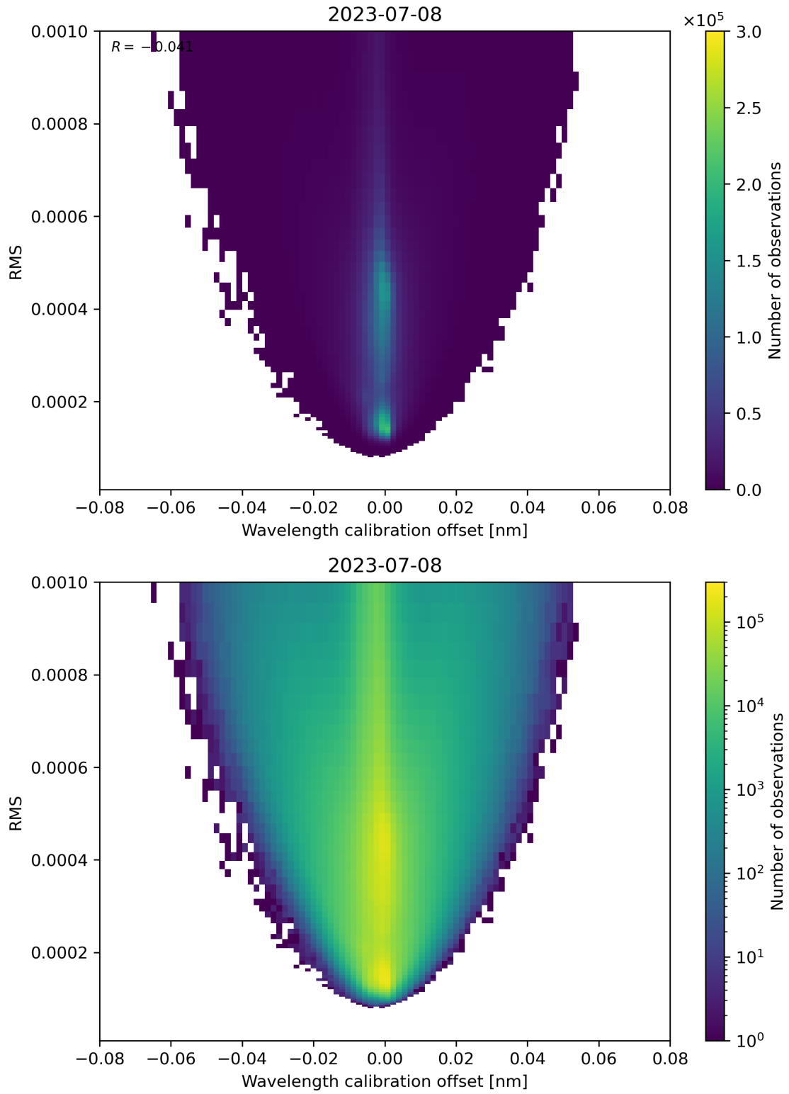
Figure 181: Scatter density plot of “Wavelength calibration offset” against “RMS” for 2023-07-08 to 2023-07-09.
