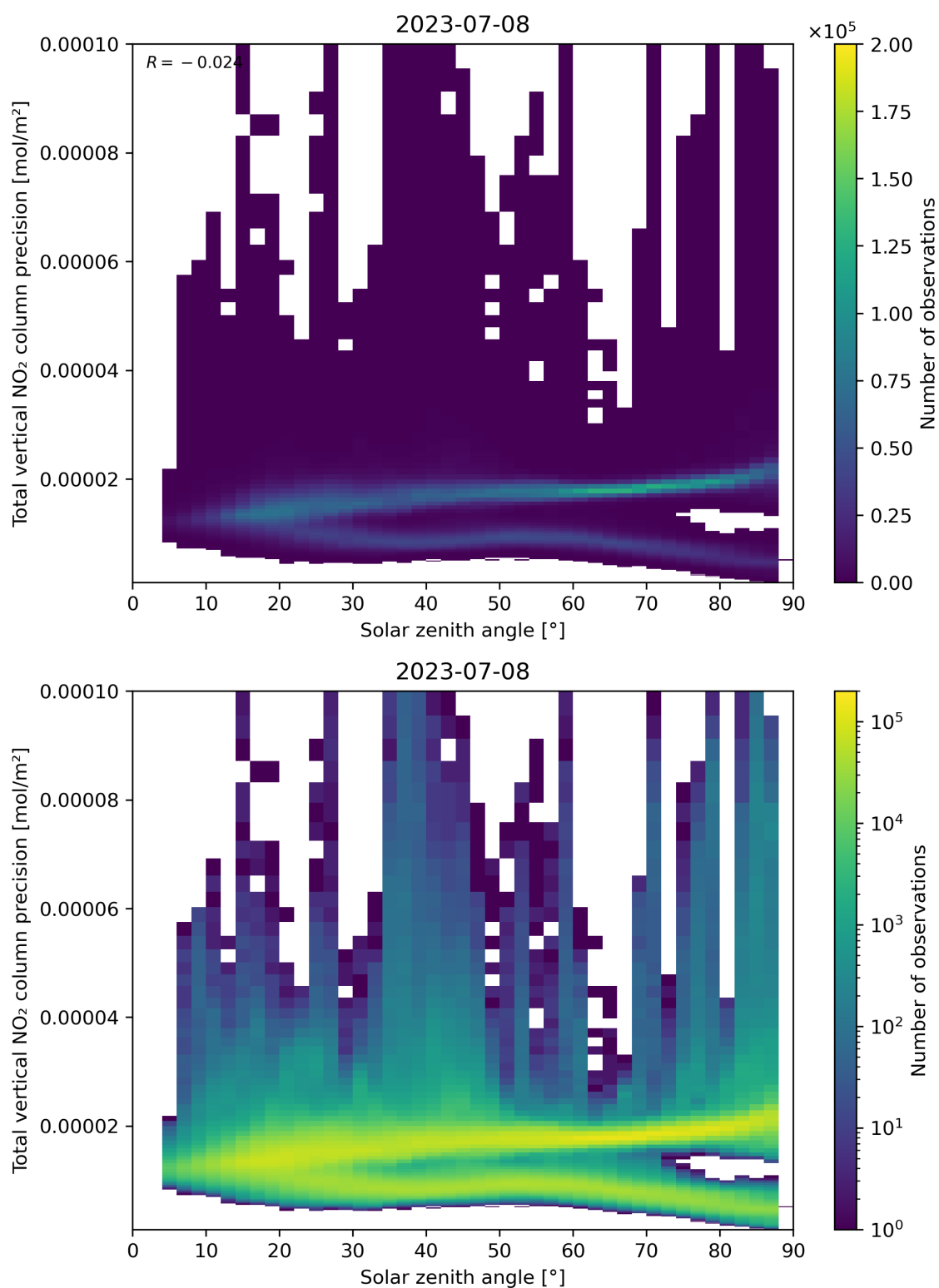
Figure 154: Scatter density plot of “Solar zenith angle” against “Total vertical NO 2 column precision” for 2023-07-08 to 2023-07-09.
