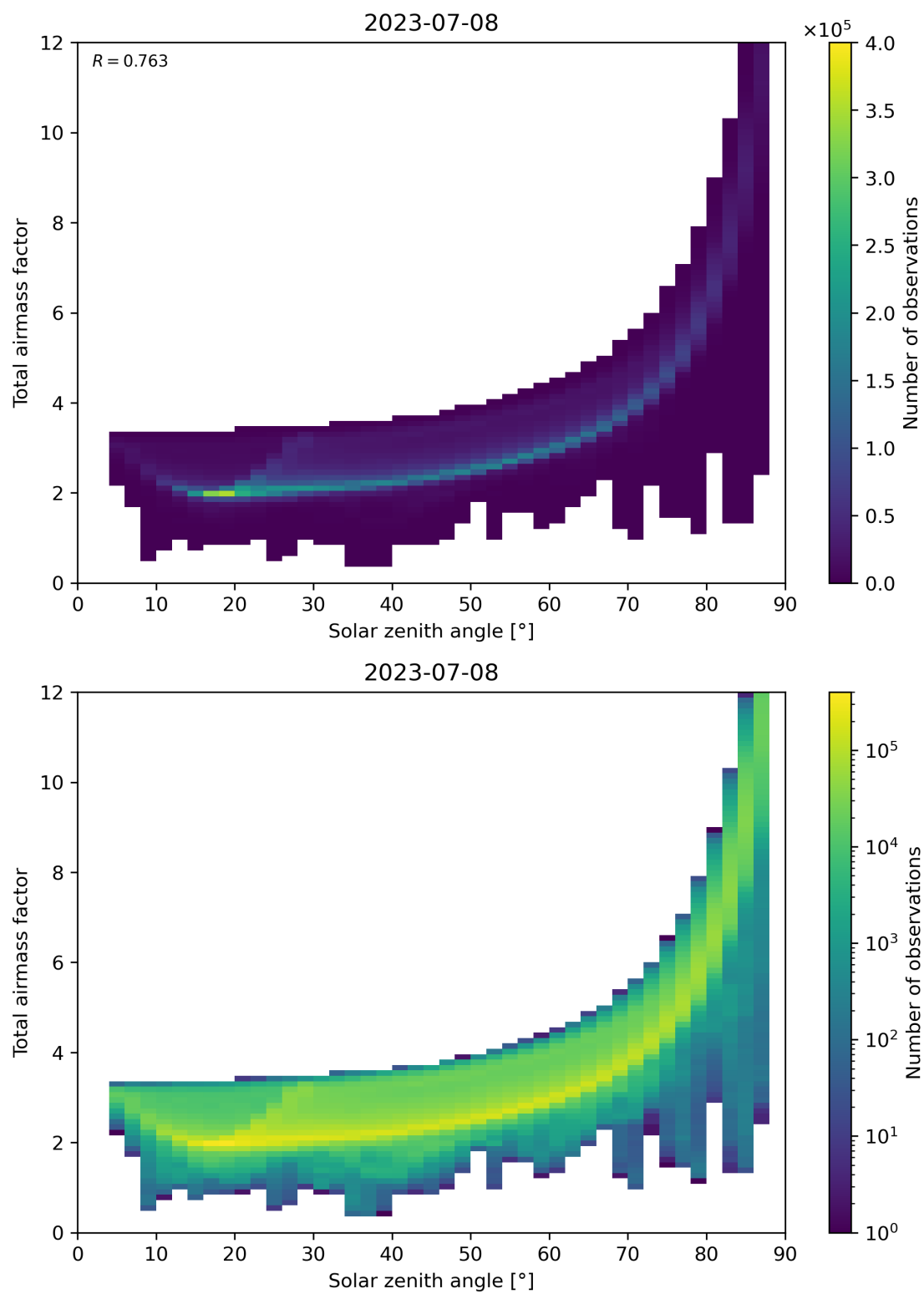
Figure 146: Scatter density plot of “Solar zenith angle” against “Total air mass factor” for 2023-07-08 to 2023-07-09.
