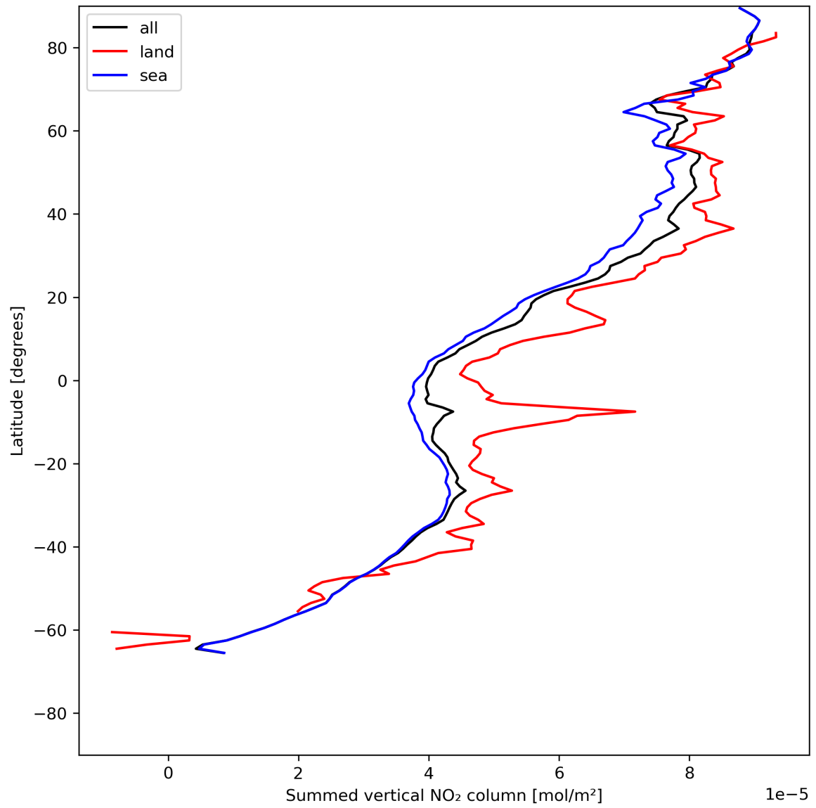
Figure 23: Zonal average of “Summed vertical NO 2 column” for 2023-07-08 to 2023-07-09.
