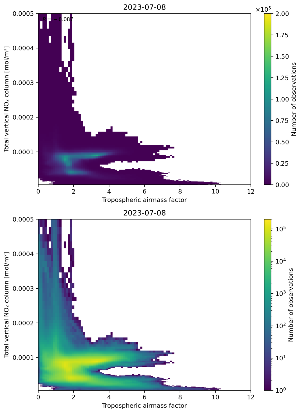
Figure 77: Scatter density plot of “Tropospheric airmass factor” against “Total vertical NO 2 column” for 2023-07-08 to 2023-07-09.
