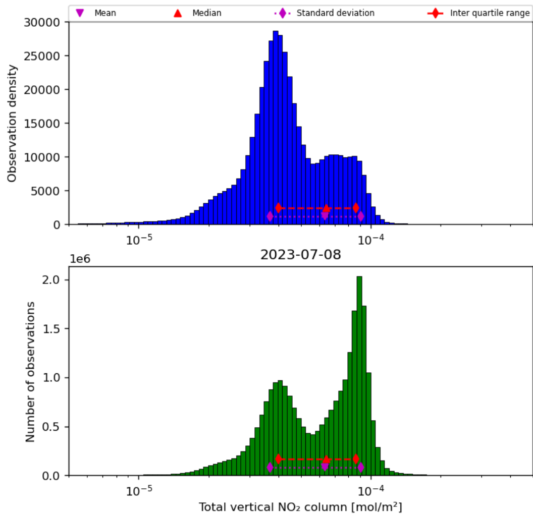
Figure 38: Histogram of “Total vertical NO 2 column” for 2023-07-08 to 2023-07-09
