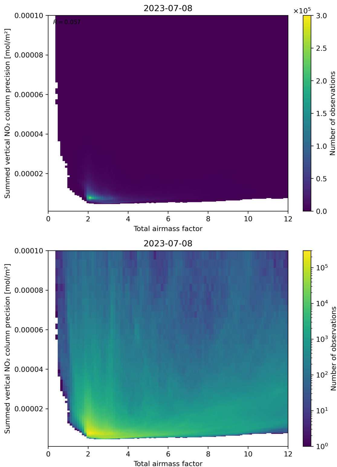
Figure 66: Scatter density plot of “Total airmass factor” against “Summed vertical NO 2 column precision” for 2023-07-08 to 2023-07-09.
