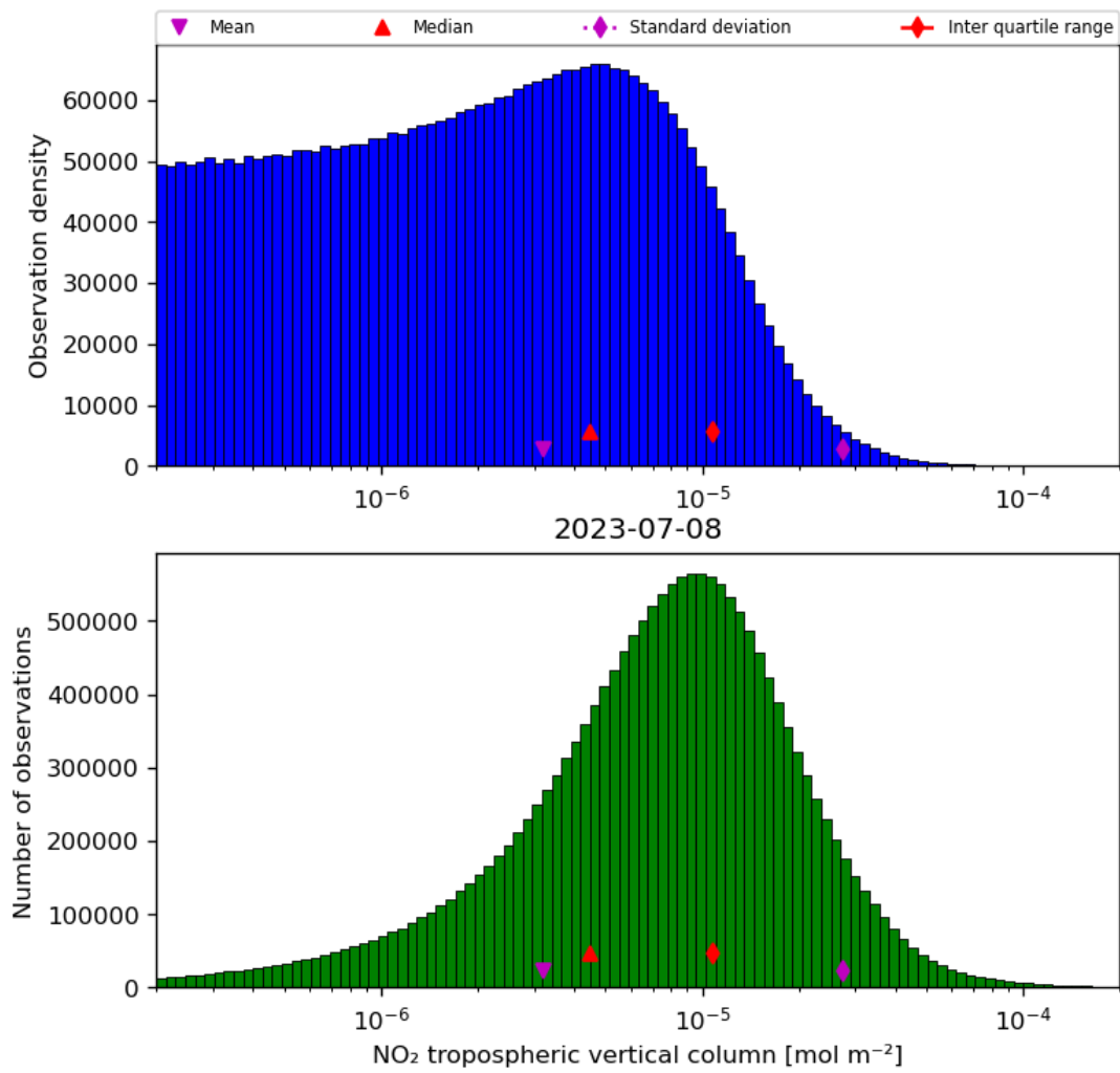
Figure 29: Histogram of “NO 2 tropospheric vertical column” for 2023-07-08 to 2023-07-09
