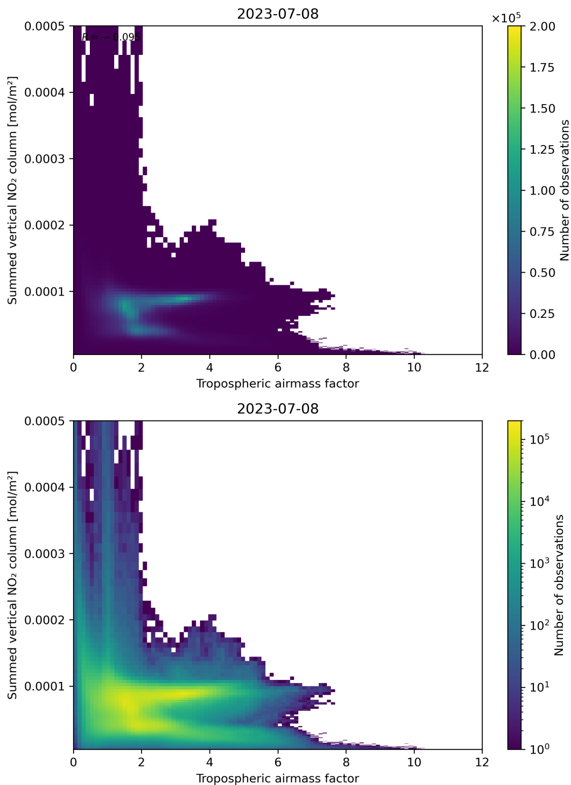
Figure 75: Scatter density plot of “Tropospheric airmass factor” against “Summed vertical NO 2 column” for 2023-07-08 to 2023-07-09.
