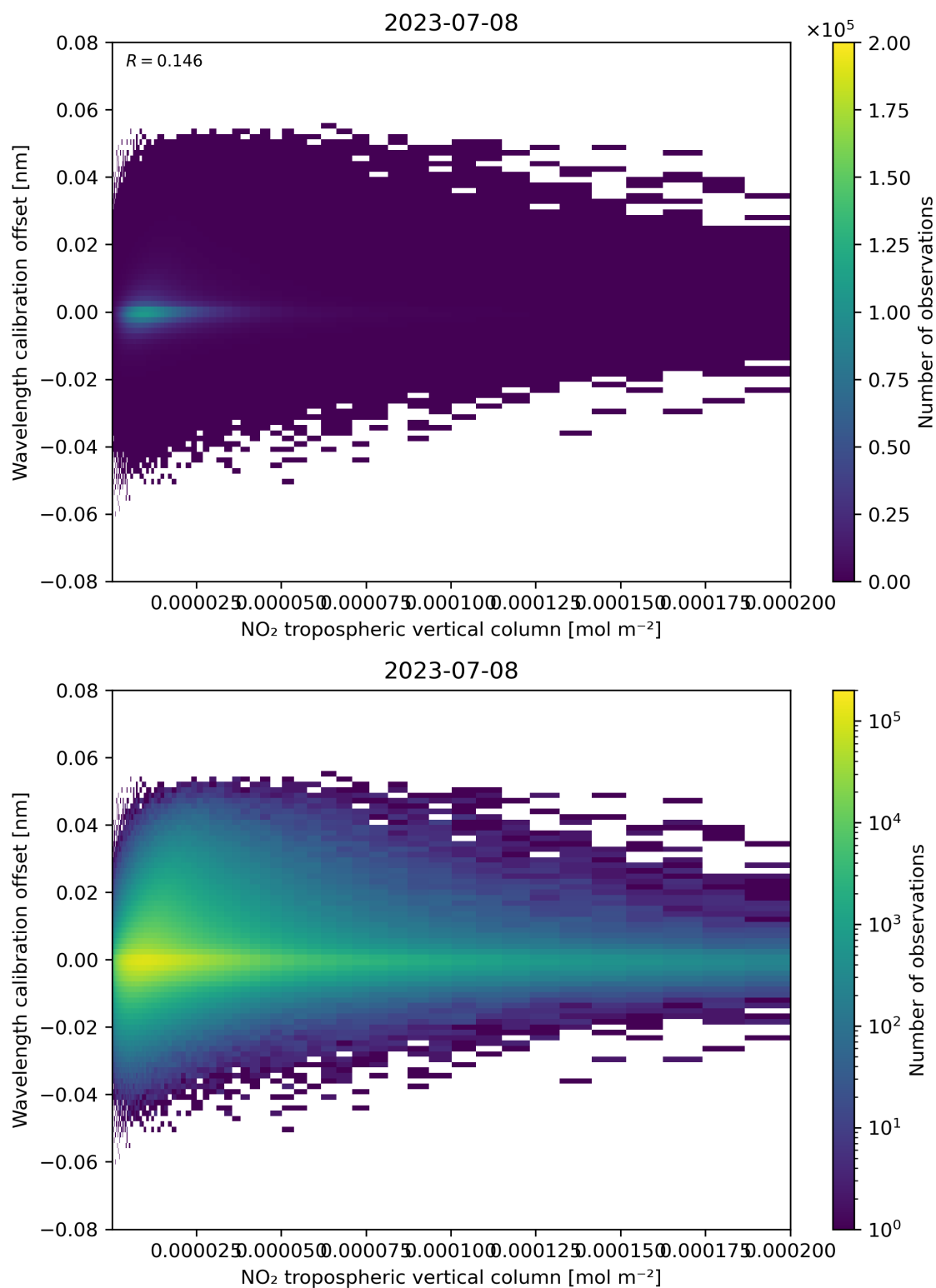
Figure 143: Scatter density plot of “NO 2 tropospheric vertical column” against “Wavelength calibration offset” for 2023-07-08 to 2023-07-09.
