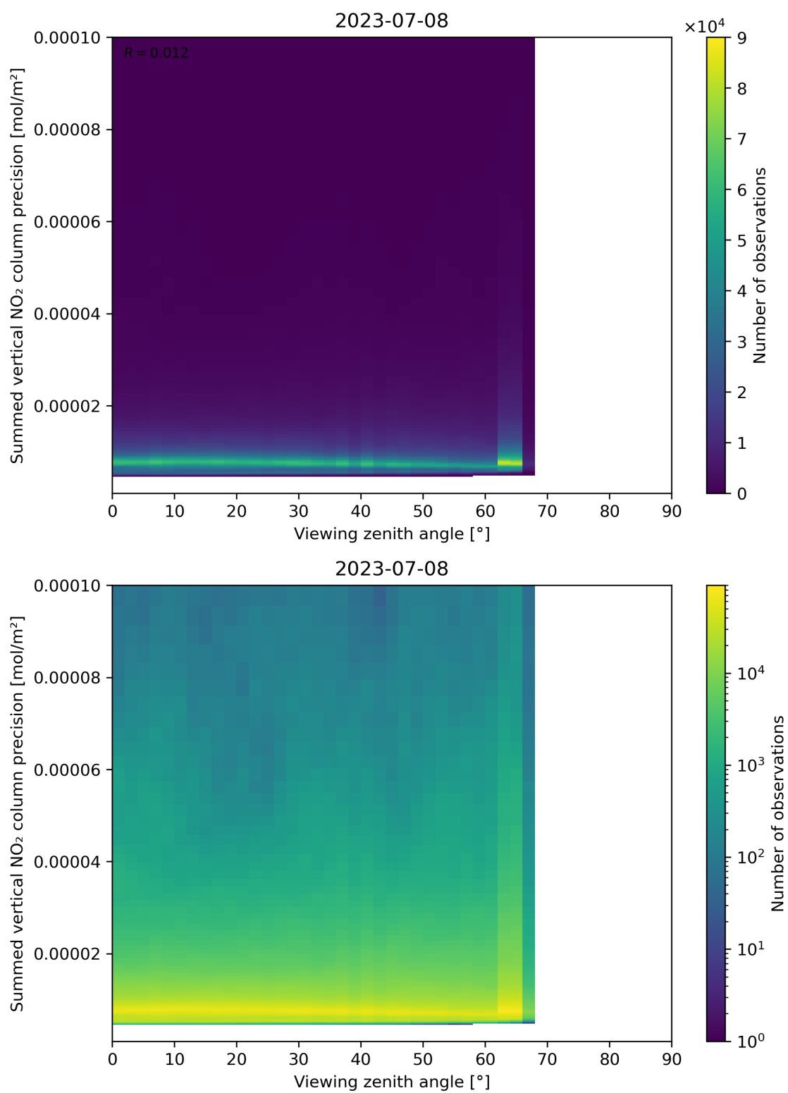
Figure 166: Scatter density plot of “Viewing zenith angle” against “Summed vertical NO 2 column precision” for 2023-07-08 to 2023-07-09.
