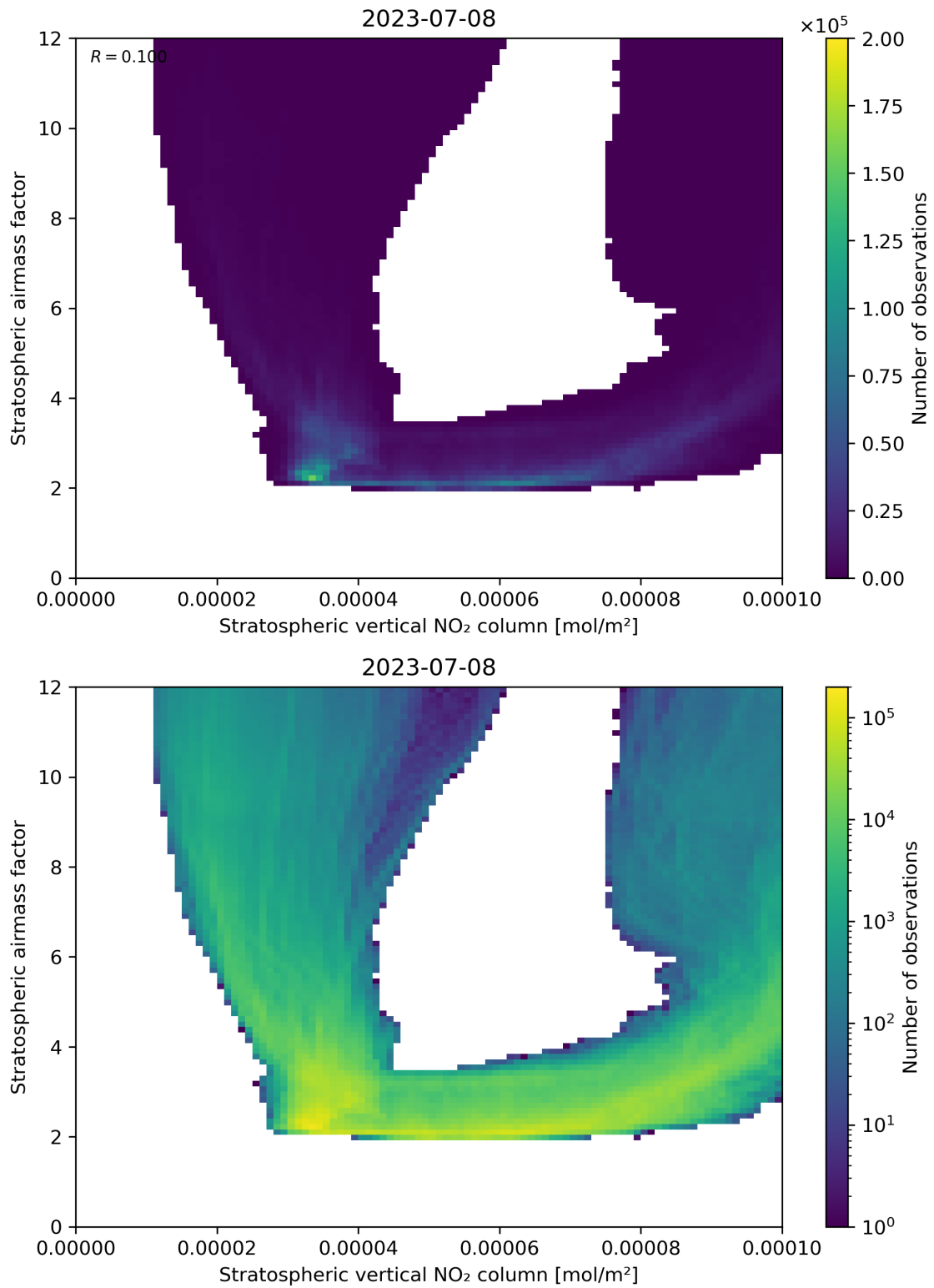
Figure 96: Scatter density plot of “Stratospheric vertical NO 2 column” against “Stratospheric airmass factor” for 2023-07-08 to 2023-07-09.
