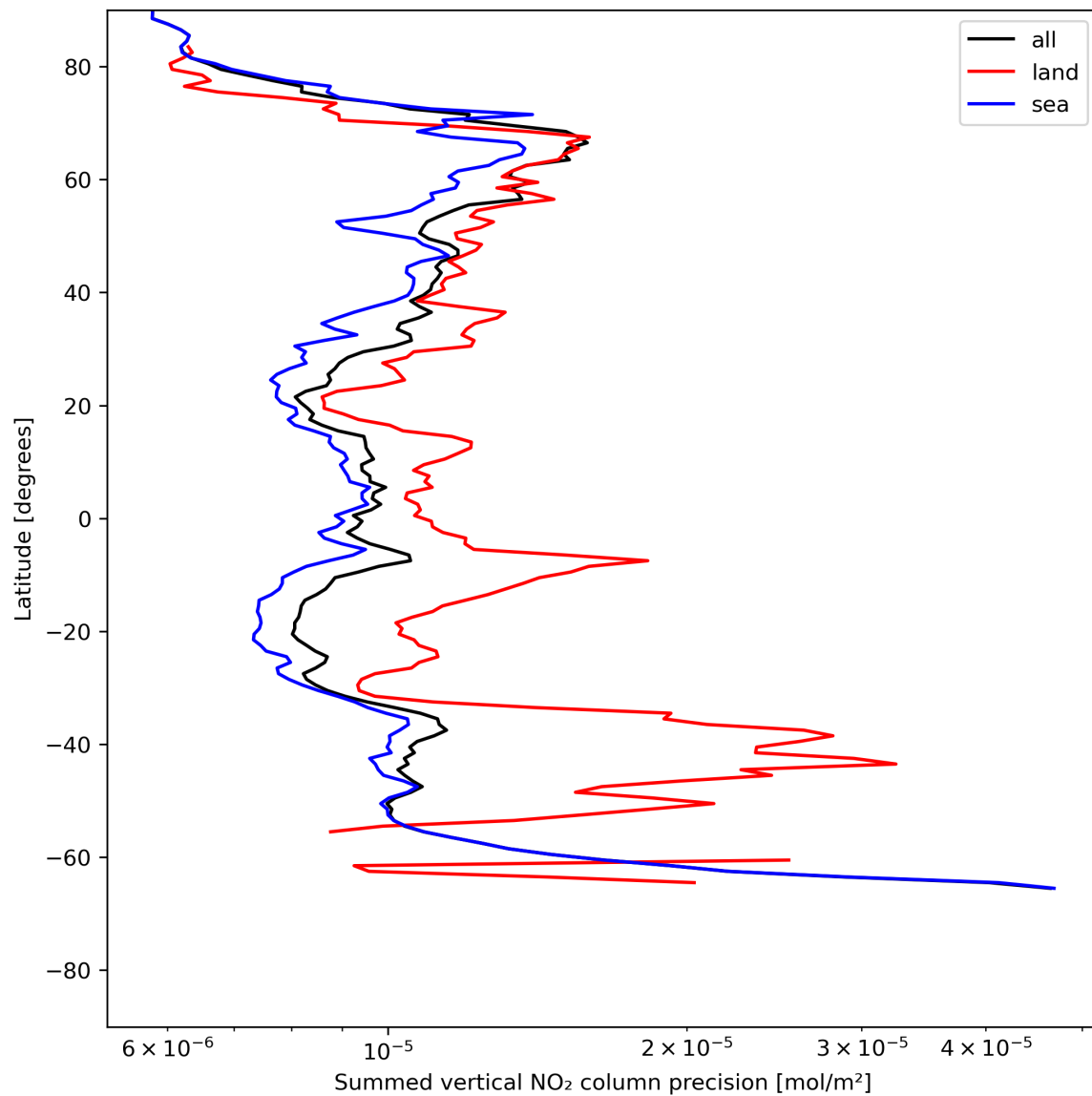
Figure 24: Zonal average of “Summed vertical NO 2 column precision” for 2023-07-08 to 2023-07-09.
