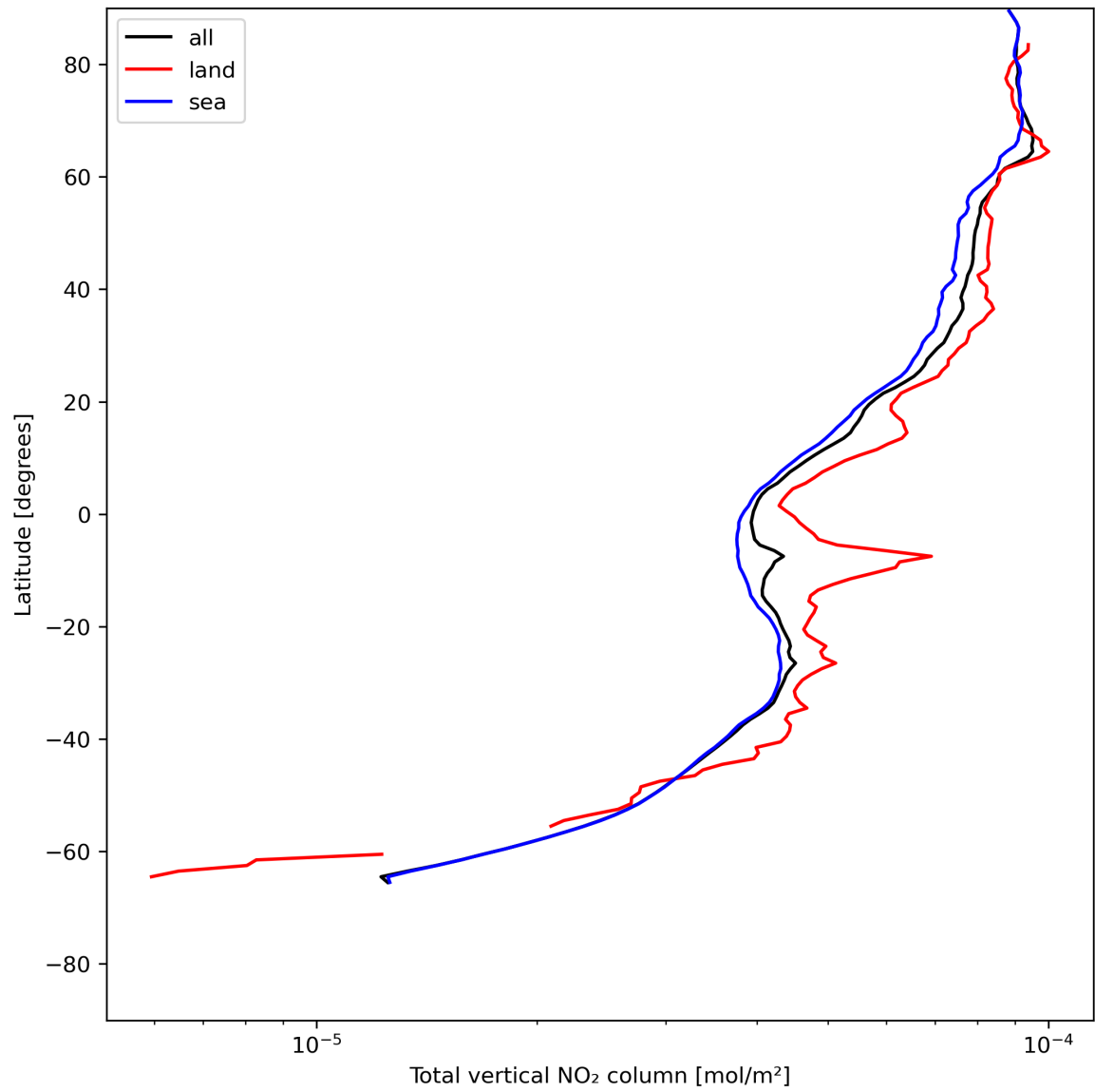
Figure 21: Zonal average of “Total vertical NO 2 column” for 2023-07-08 to 2023-07-09.
