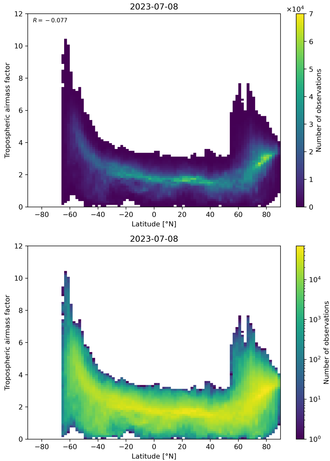
Figure 85: Scatter density plot of “Latitude” against “Tropospheric airmass factor” for 2023-07-08 to 2023-07-09.
