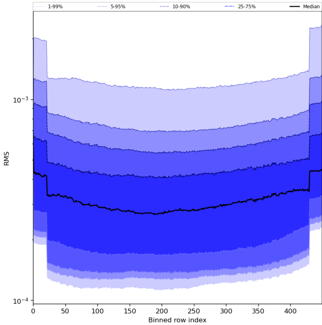
Figure 60: Along track statistics of “RMS” for 2023-07-08 to 2023-07-09
