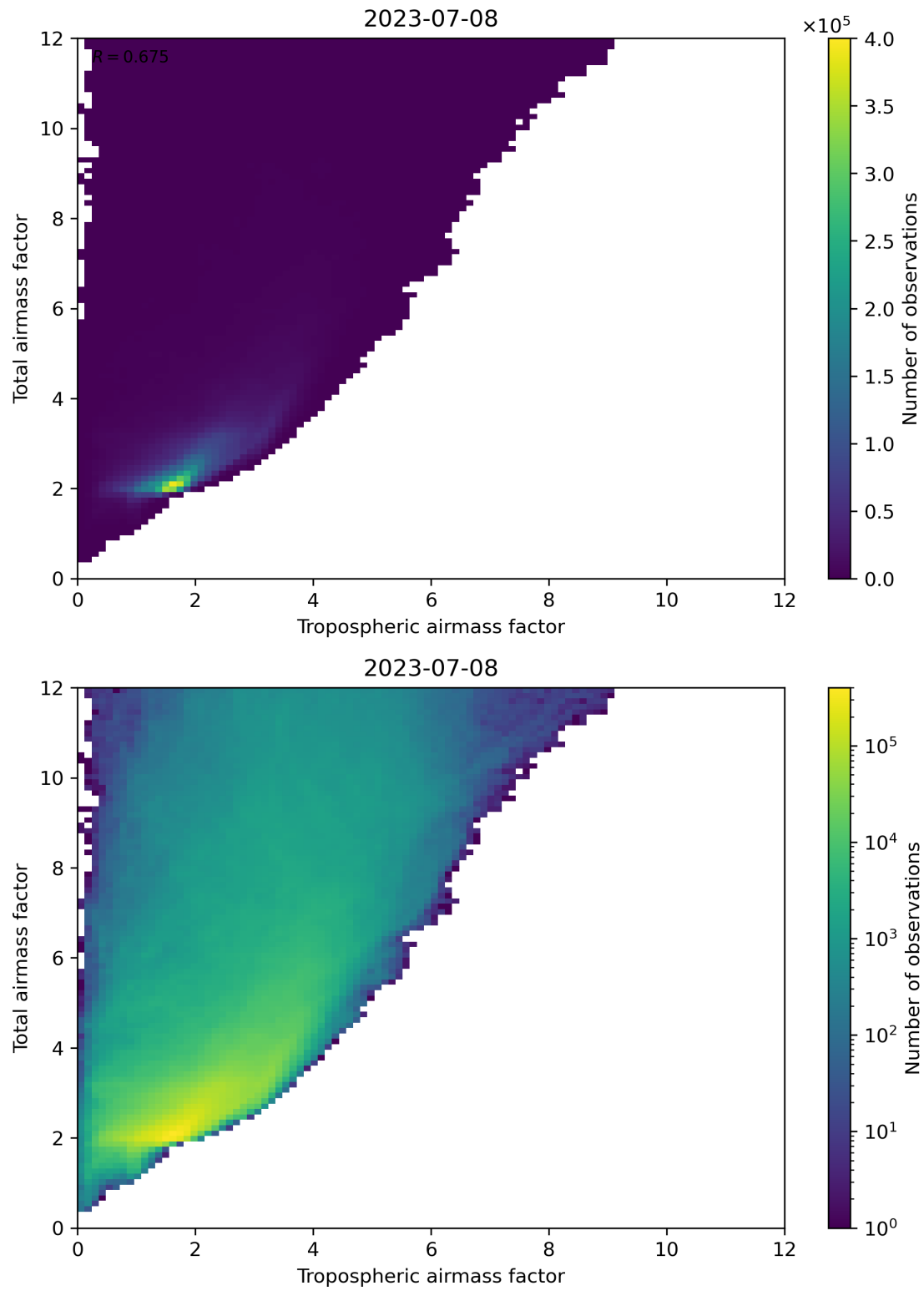
Figure 72: Scatter density plot of “Tropospheric airmass factor” against “Total airmass factor” for 2023-07-08 to 2023-07-09.
