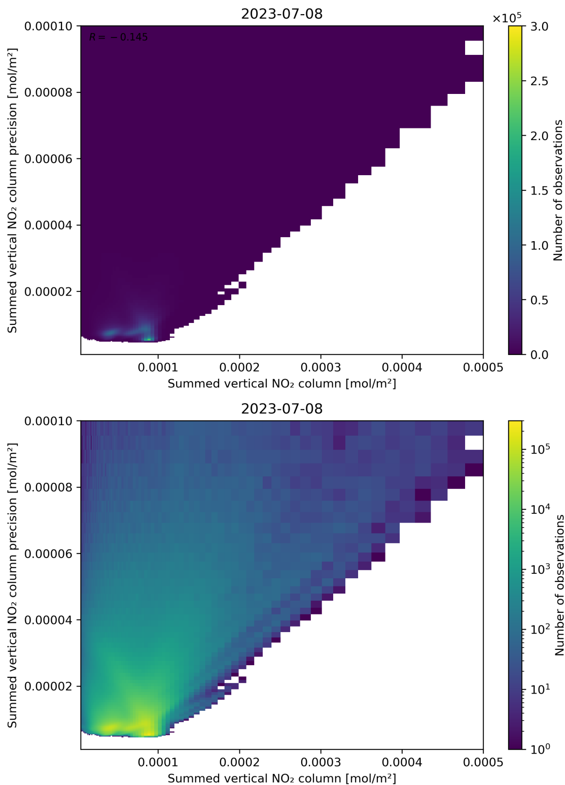
Figure 105: Scatter density plot of “Summed vertical NO 2 column” against “Summed vertical NO 2 column precision” for 2023-07-08 to 2023-07-09.
