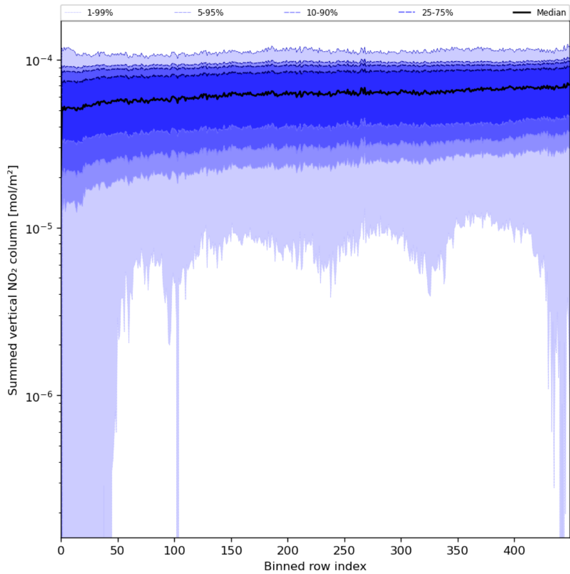
Figure 57: Along track statistics of “Summed vertical NO 2 column” for 2023-07-08 to 2023-07-09
