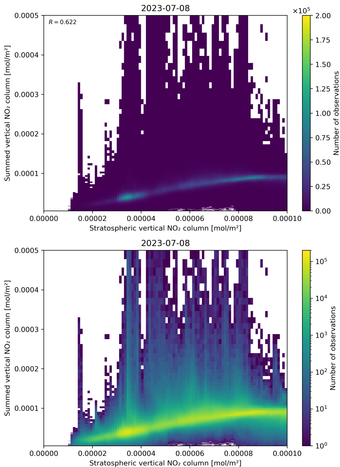
Figure 98: Scatter density plot of “Stratospheric vertical NO 2 column” against “Summed vertical NO 2 column” for 2023-07-08 to 2023-07-09.
