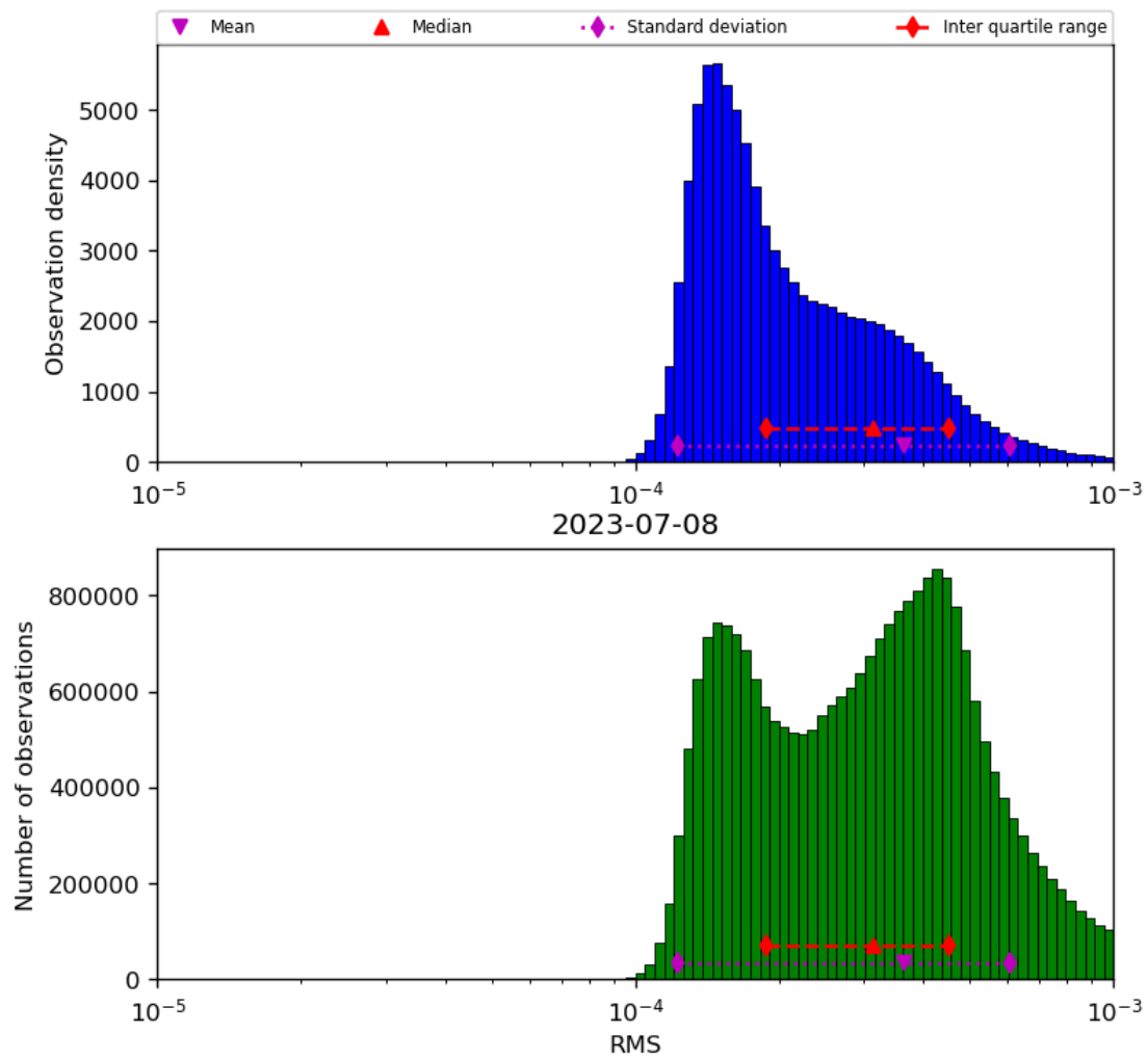
Figure 43: Histogram of “RMS” for 2023-07-08 to 2023-07-09
