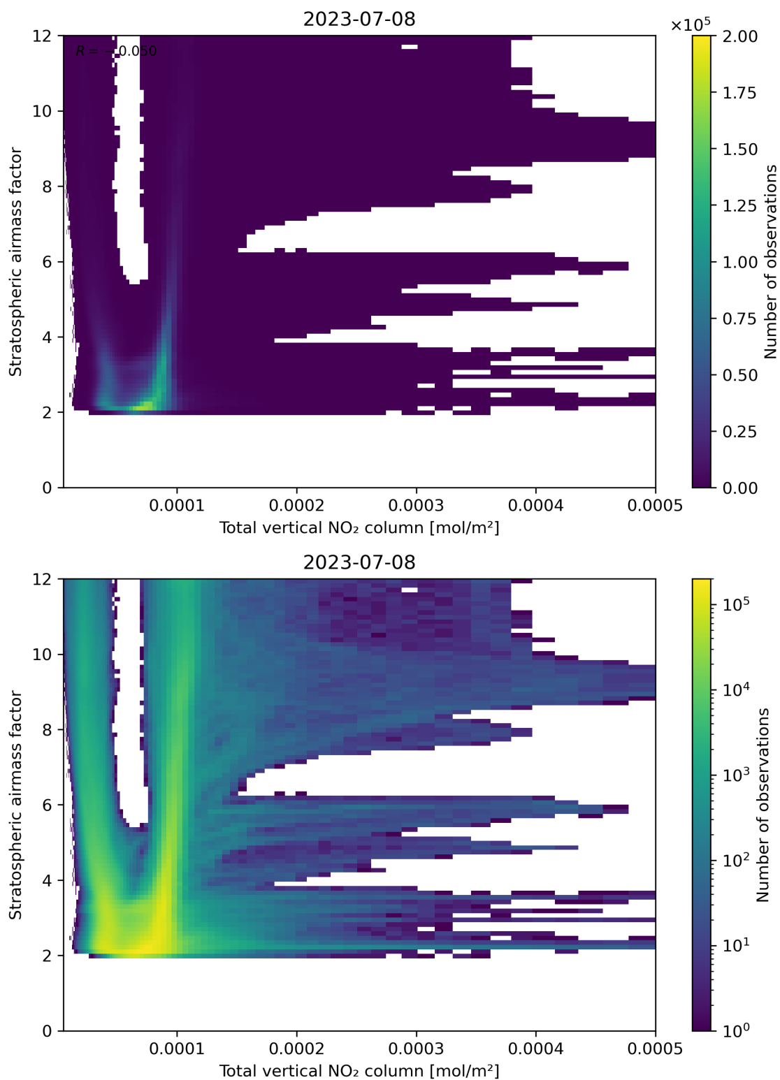
Figure 110: Scatter density plot of “Total vertical NO 2 column” against “Stratospheric airmass factor” for 2023-07-08 to 2023-07-09.
