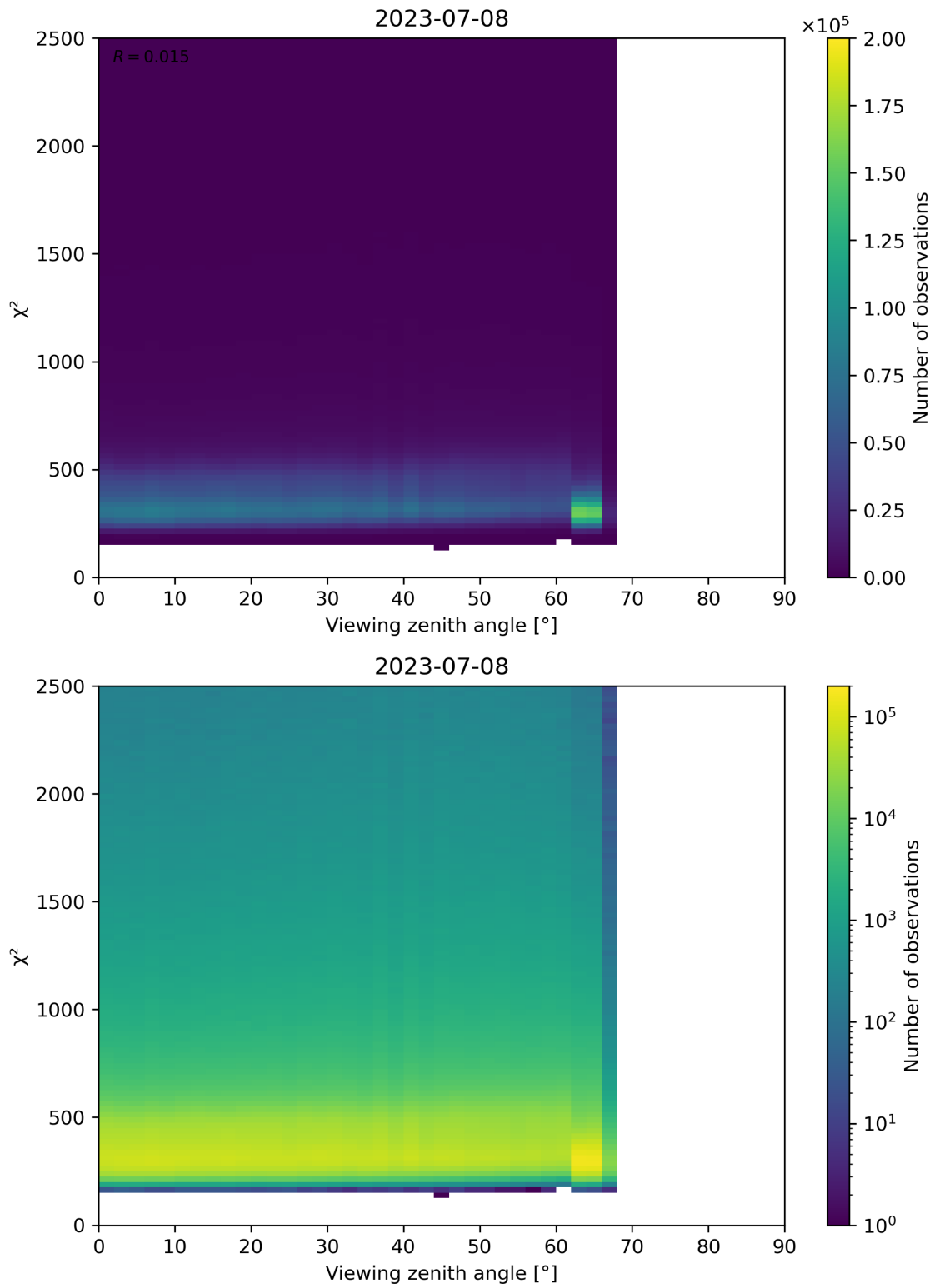
Figure 162: Scatter density plot of “Viewing zenith angle” against “ \chi^2 ” for 2023-07-08 to 2023-07-09.
