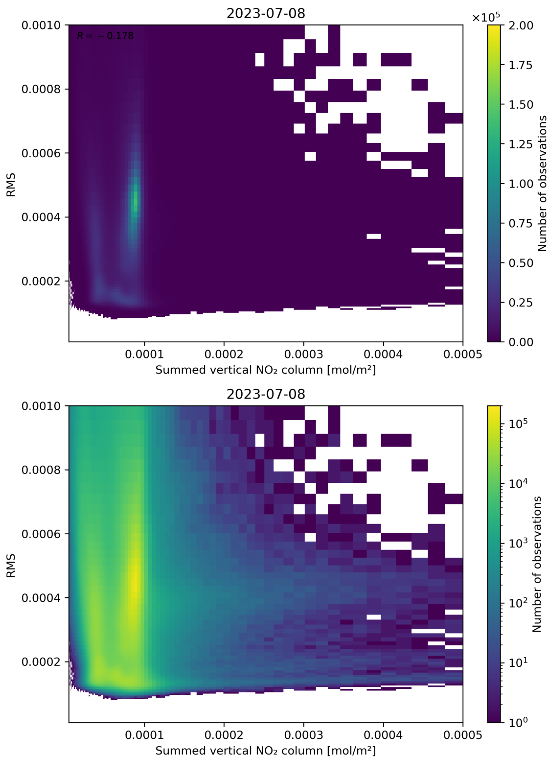
Figure 109: Scatter density plot of “Summed vertical NO 2 column” against “RMS” for 2023-07-08 to 2023-07-09.
