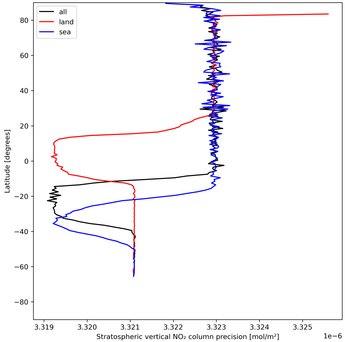
Figure 20: Zonal average of “Stratospheric vertical NO 2 column precision” for 2023-07-08 to 2023-07-09.
