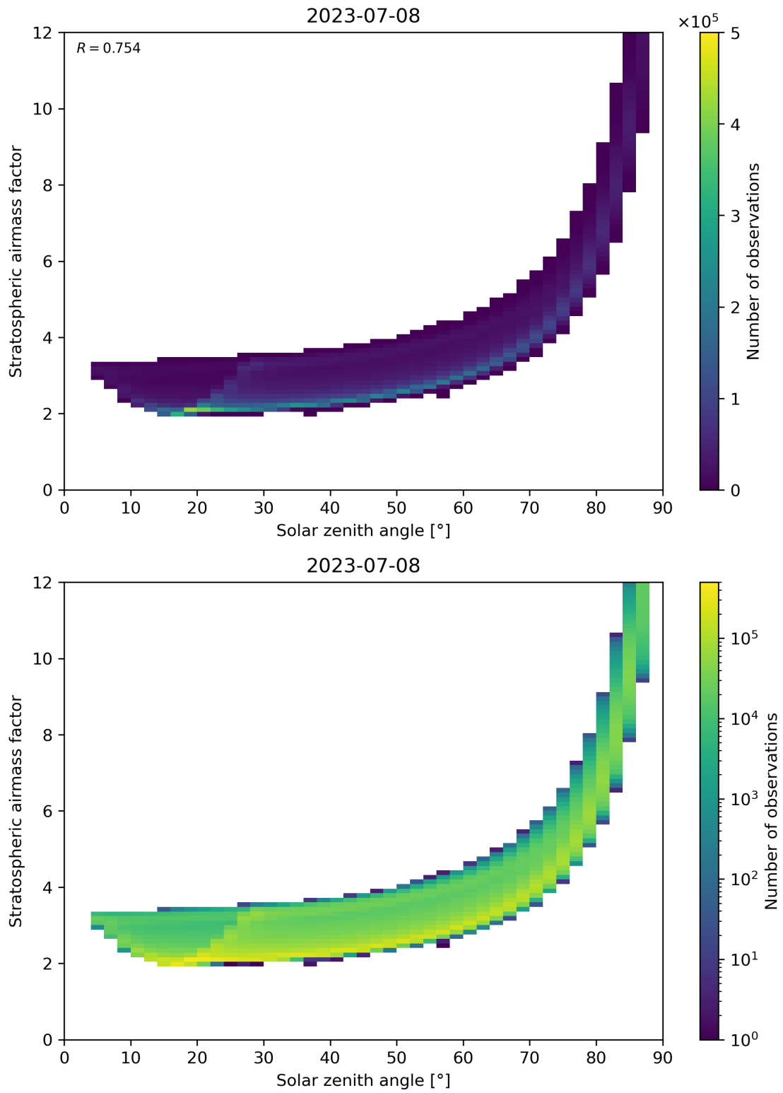
Figure 145: Scatter density plot of “Solar zenith angle” against “Stratospheric airmass factor” for 2023-07-08 to 2023-07-09.
