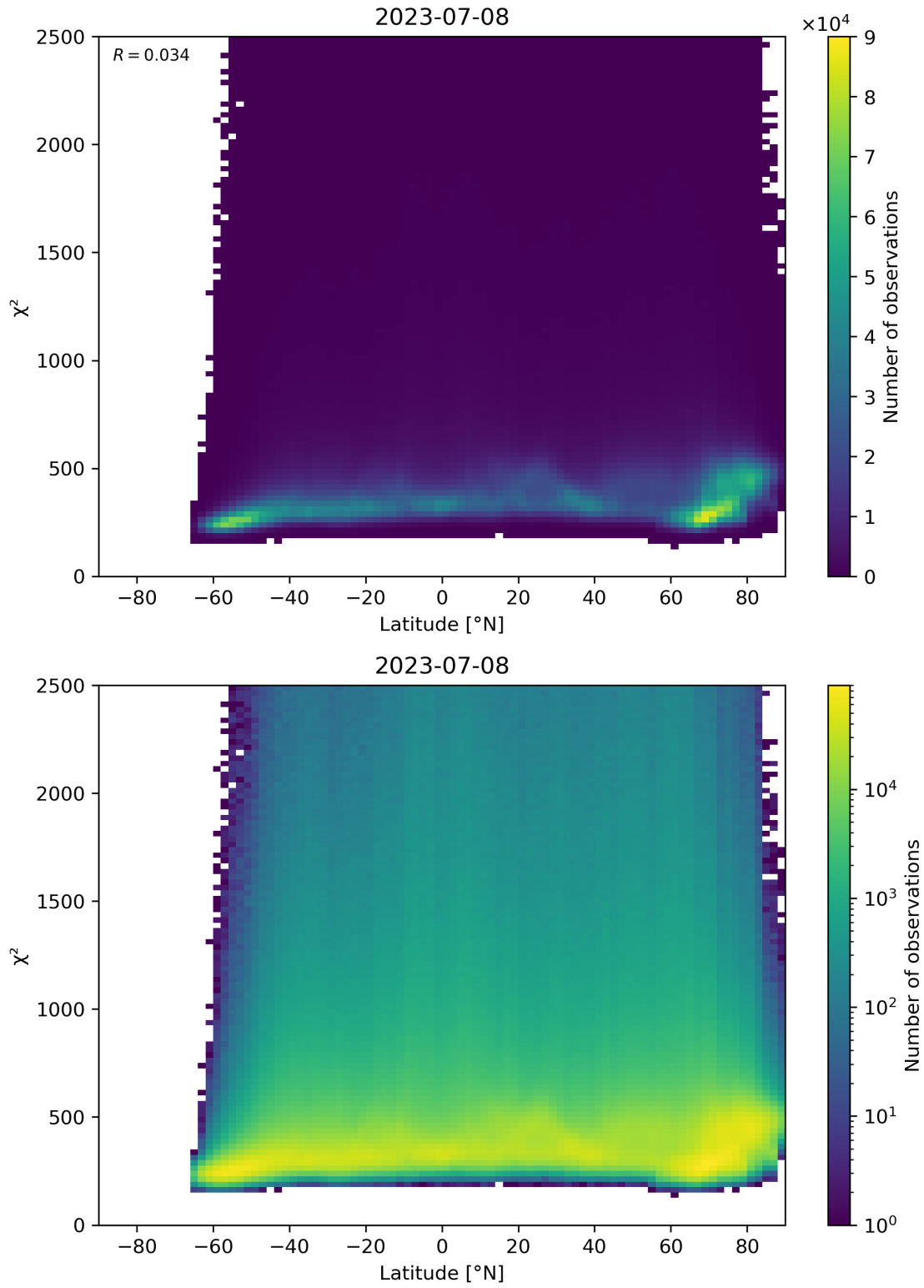
Figure 86: Scatter density plot of “Latitude” against “ \chi^2 ” for 2023-07-08 to 2023-07-09.
