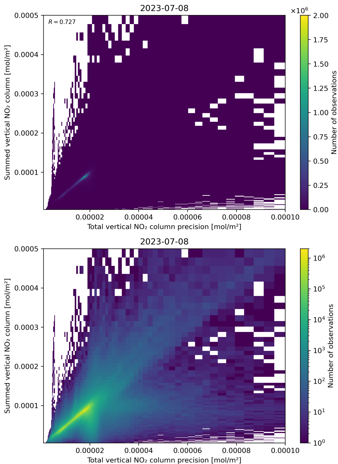
Figure 117: Scatter density plot of “Total vertical NO 2 column precision” against “Summed vertical NO 2 column” for 2023-07-08 to 2023-07-09.
