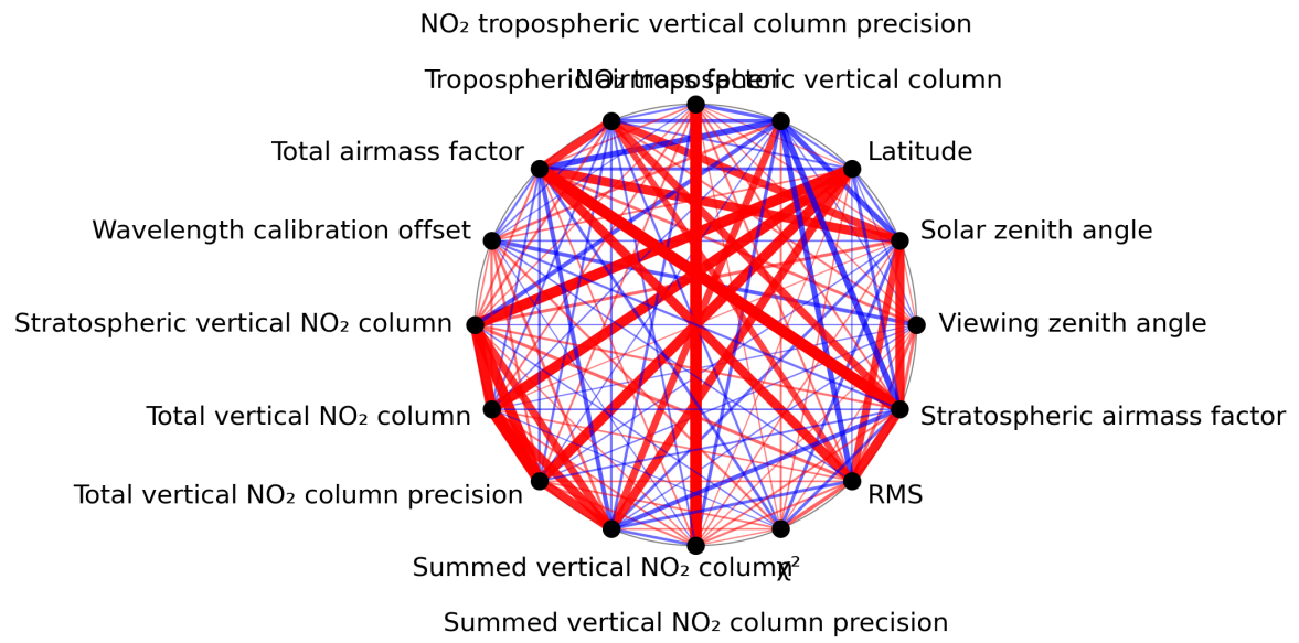
Figure 1: Map of correlation graph for 2023-07-08 to 2023-07-09.
