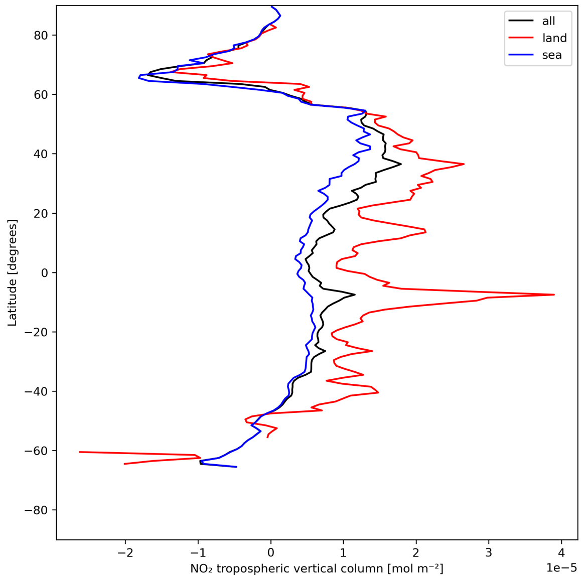
Figure 12: Zonal average of “NO 2 tropospheric vertical column” for 2023-07-08 to 2023-07-09.
