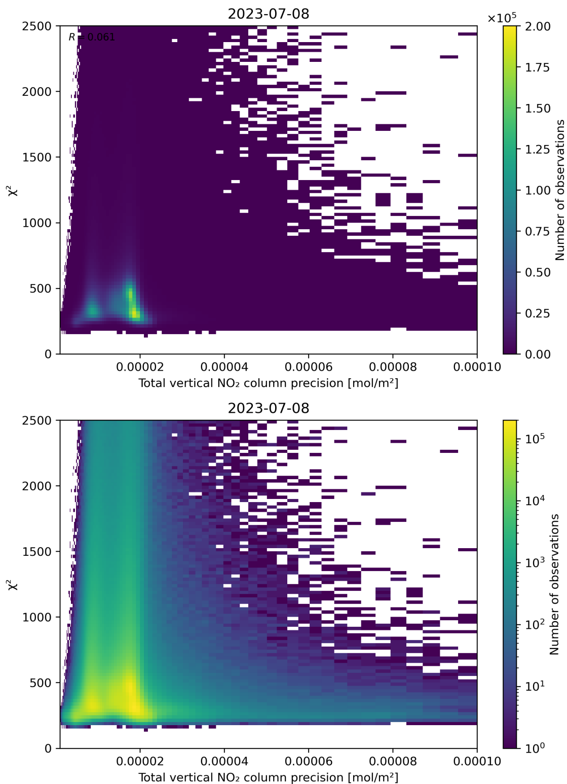
Figure 116: Scatter density plot of “Total vertical NO 2 column precision” against “ \chi^2 ” for 2023-07-08 to 2023-07-09.
