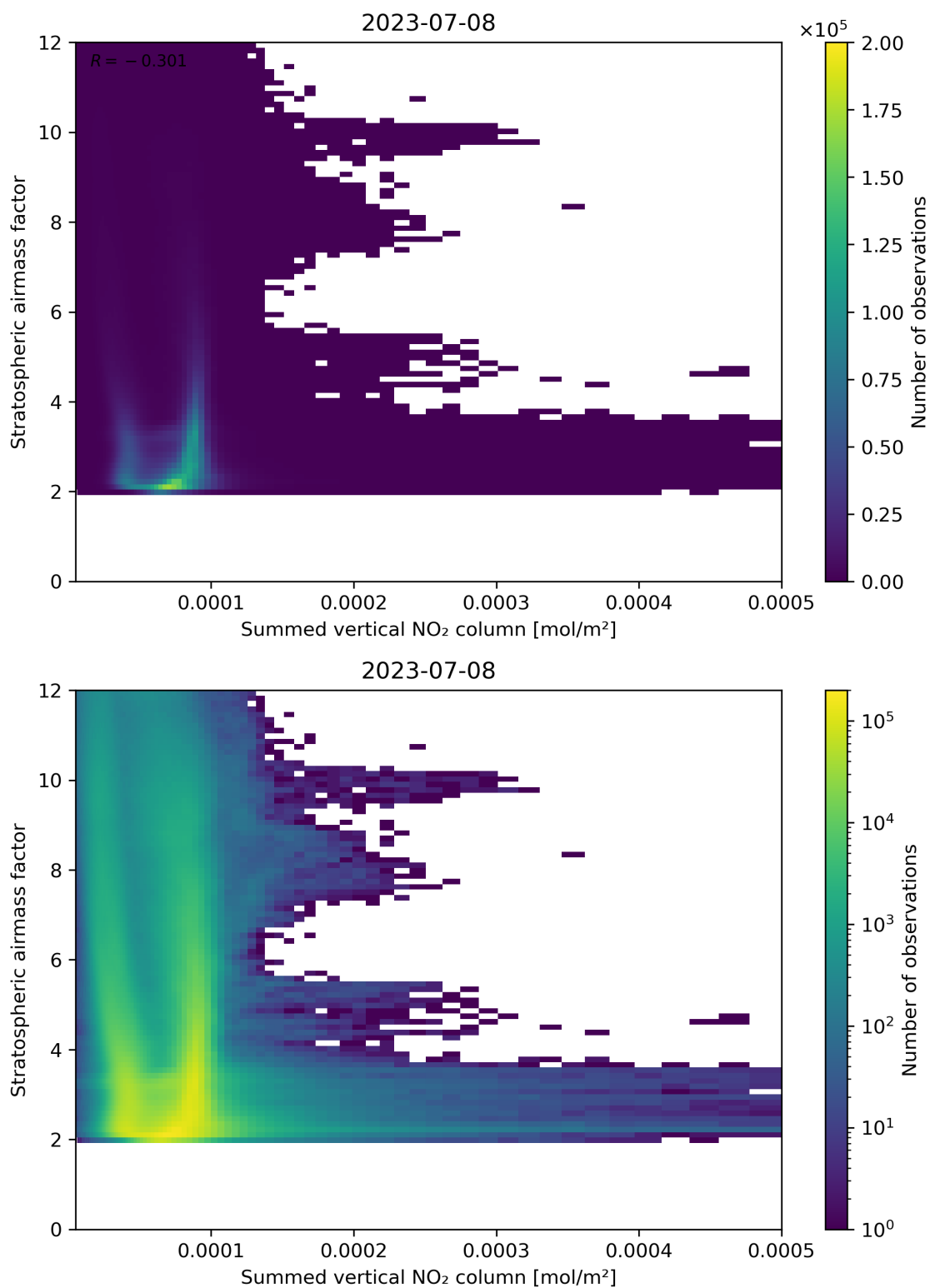
Figure 103: Scatter density plot of “Summed vertical NO 2 column” against “Stratospheric air mass factor” for 2023-07-08 to 2023-07-09.
