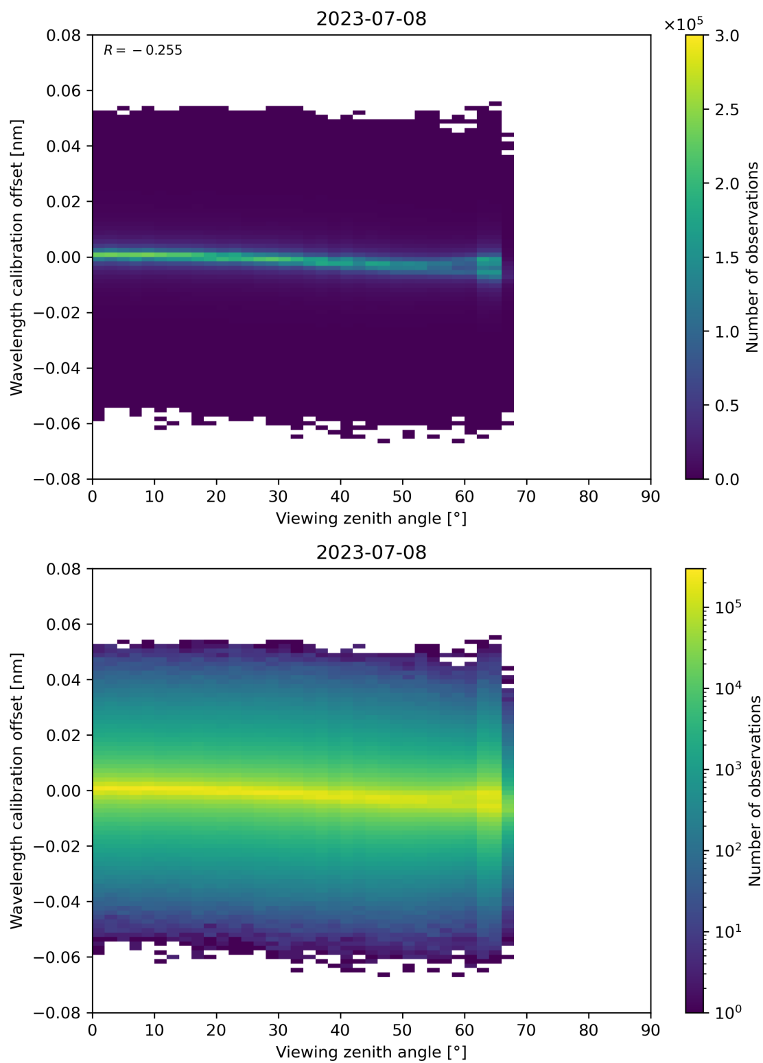
Figure 173: Scatter density plot of “Viewing zenith angle” against “Wavelength calibration offset” for 2023-07-08 to 2023-07-09.
