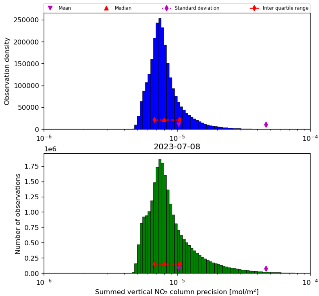
Figure 41: Histogram of “Summed vertical NO 2 column precision” for 2023-07-08 to 2023-07-09
