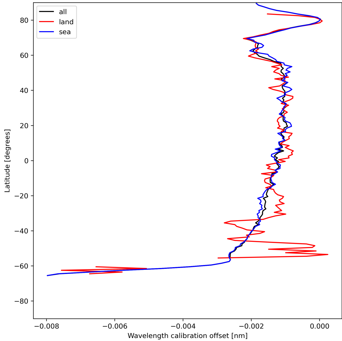
Figure 18: Zonal average of “Wavelength calibration offset” for 2023-07-08 to 2023-07-09.
