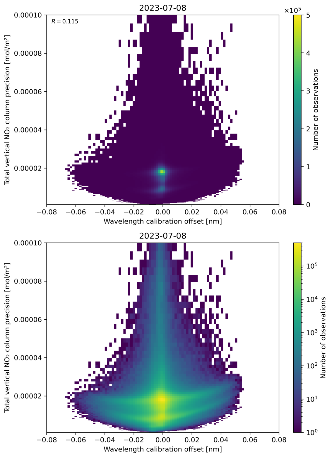
Figure 180: Scatter density plot of “Wavelength calibration offset” against “Total vertical NO 2 column precision” for 2023-07-08 to 2023-07-09.
