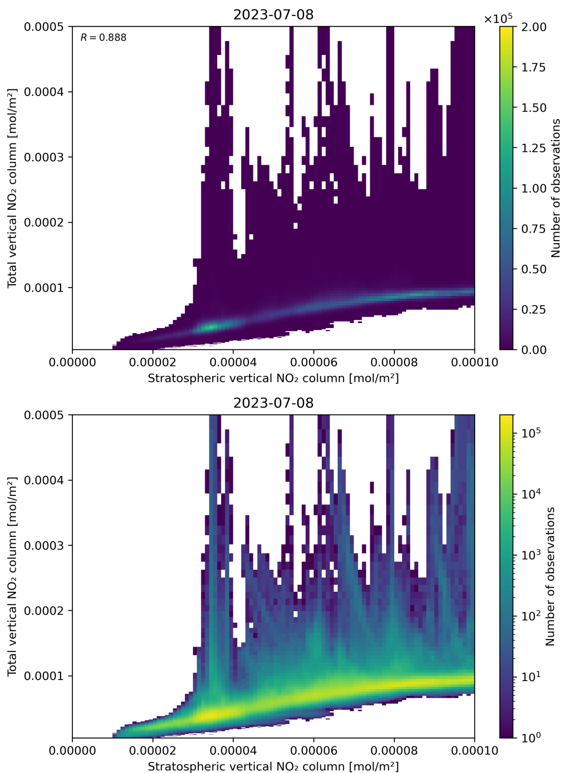
Figure 100: Scatter density plot of “Stratospheric vertical NO 2 column” against “Total vertical NO 2 column” for 2023-07-08 to 2023-07-09.
