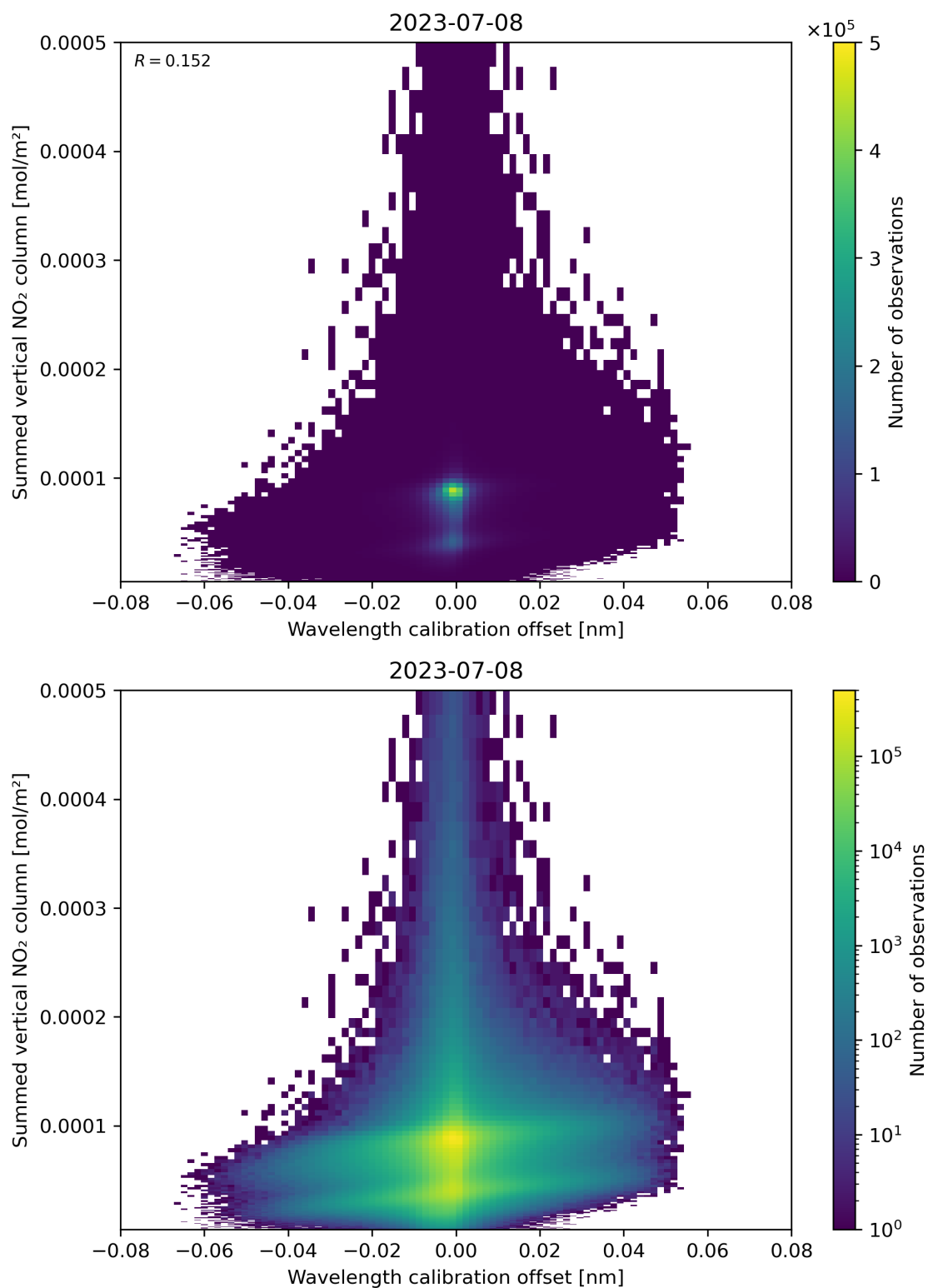
Figure 177: Scatter density plot of “Wavelength calibration offset” against “Summed vertical NO 2 column” for 2023-07-08 to 2023-07-09.
