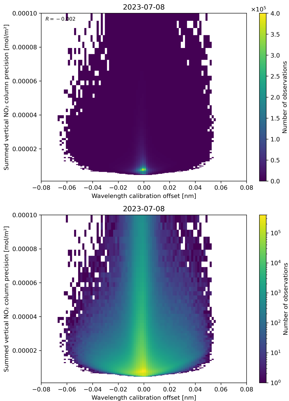
Figure 178: Scatter density plot of “Wavelength calibration offset” against “Summed vertical NO 2 column precision” for 2023-07-08 to 2023-07-09.
