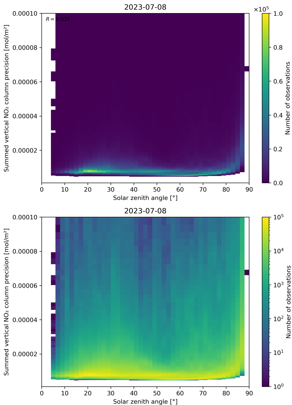
Figure 152: Scatter density plot of “Solar zenith angle” against “Summed vertical NO 2 column precision” for 2023-07-08 to 2023-07-09.
