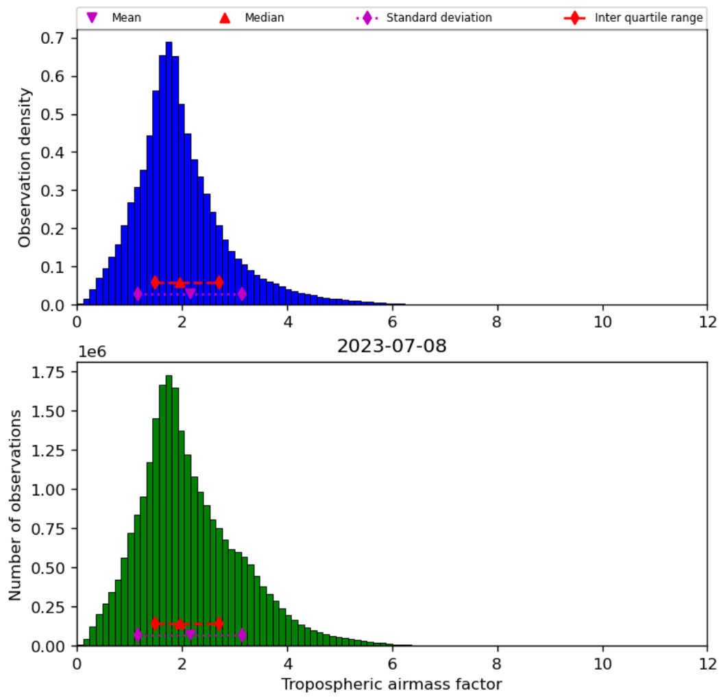
Figure 31: Histogram of “Tropospheric airmass factor” for 2023-07-08 to 2023-07-09
