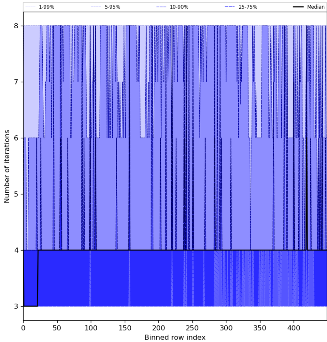
Figure 51: Along track statistics of “Number of iterations” for 2023-07-08 to 2023-07-09
