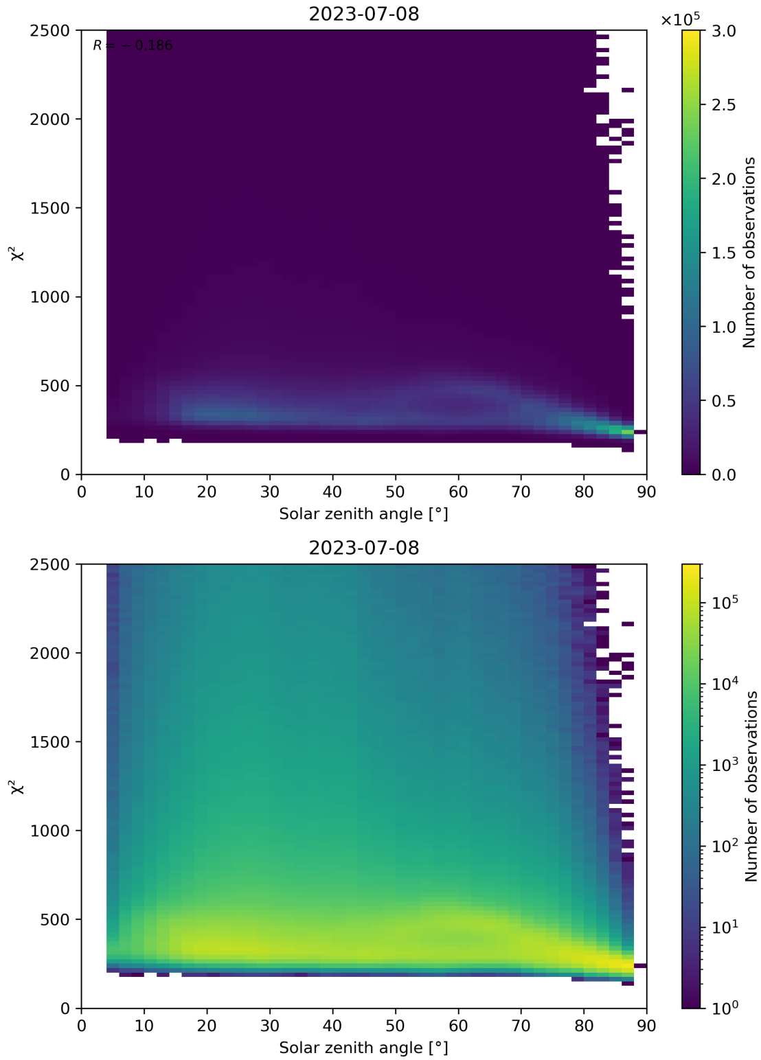
Figure 148: Scatter density plot of “Solar zenith angle” against “ \chi^2 ” for 2023-07-08 to 2023-07-09.
