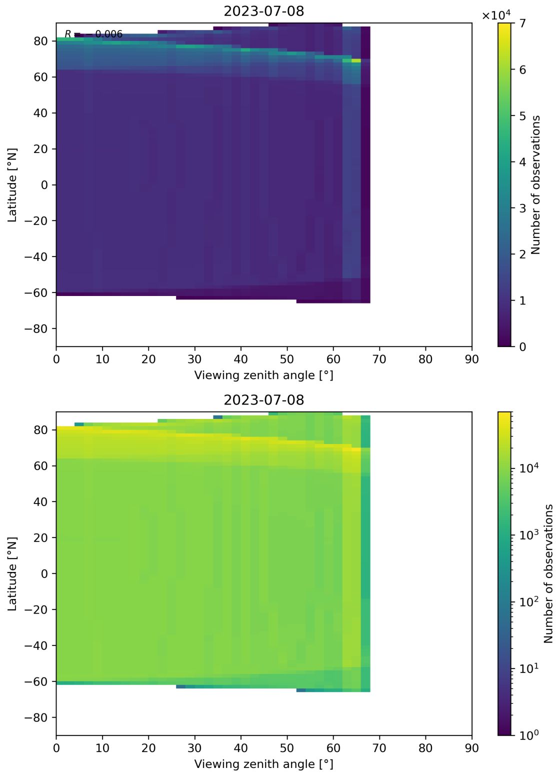
Figure 163: Scatter density plot of “Viewing zenith angle” against “Latitude” for 2023-07-08 to 2023-07-09.
