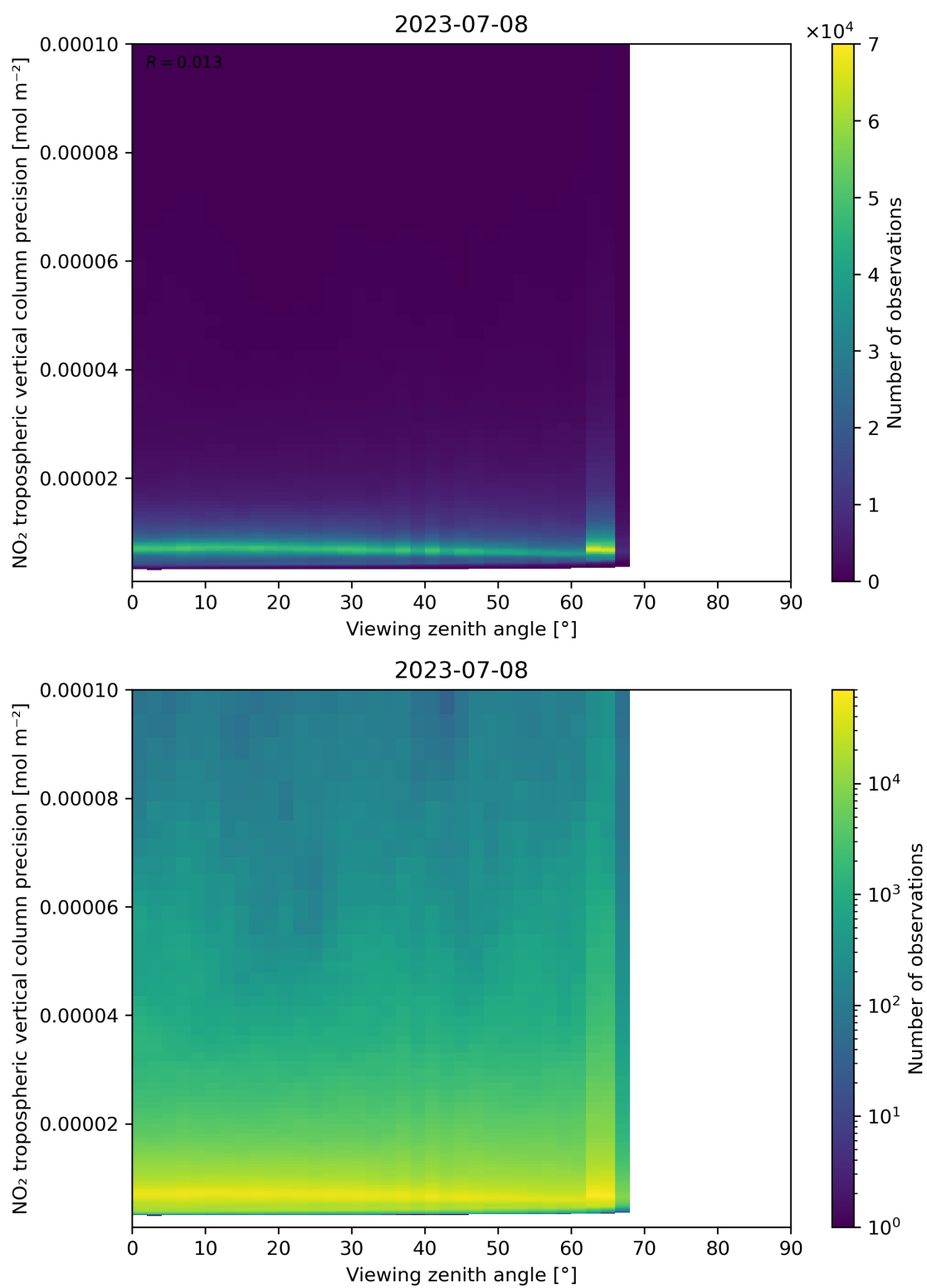
Figure 170: Scatter density plot of “Viewing zenith angle” against “NO 2 tropospheric vertical column precision” for 2023-07-08 to 2023-07-09.
