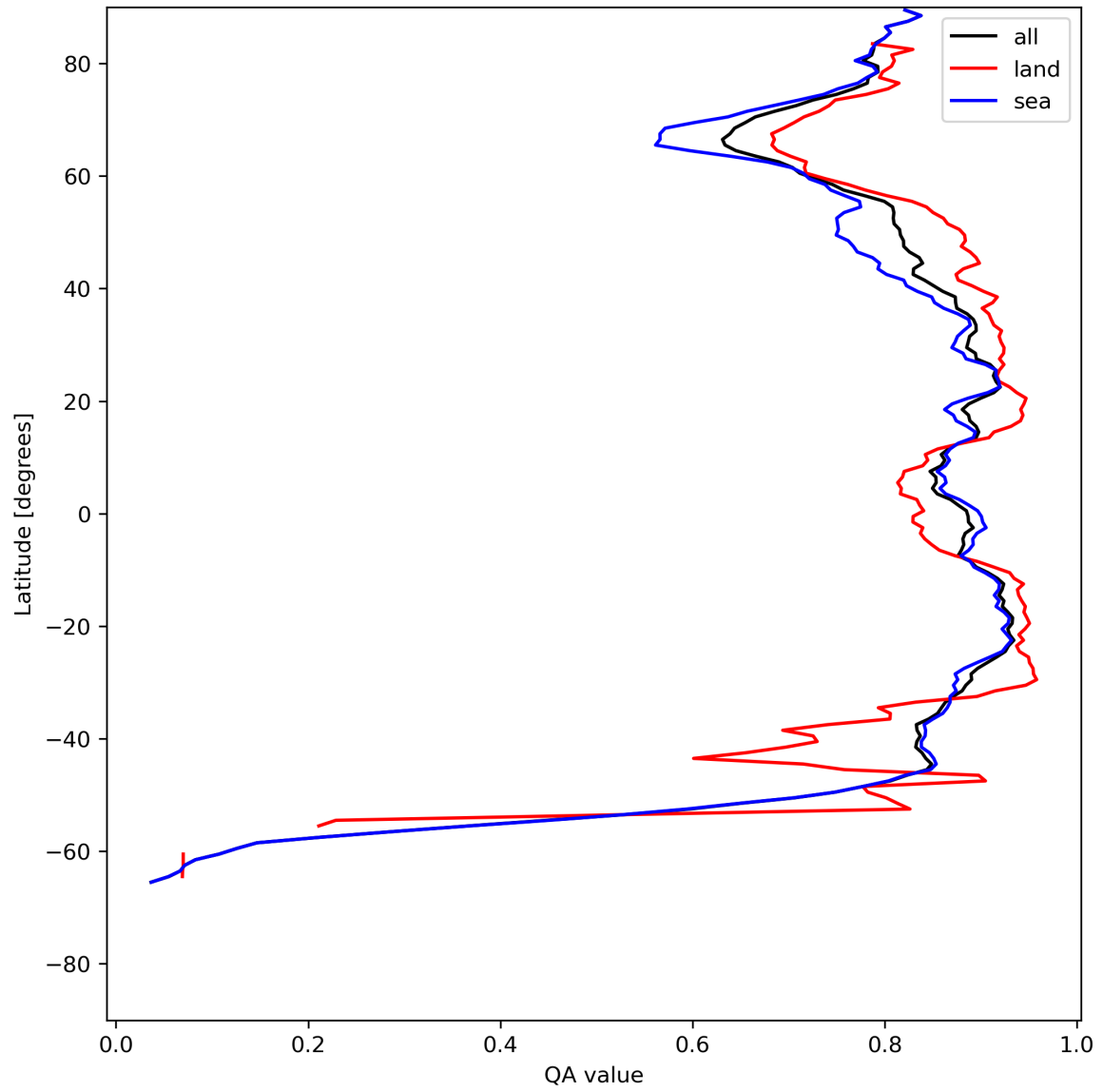
Figure 11: Zonal average of “QA value” for 2023-07-08 to 2023-07-09.
