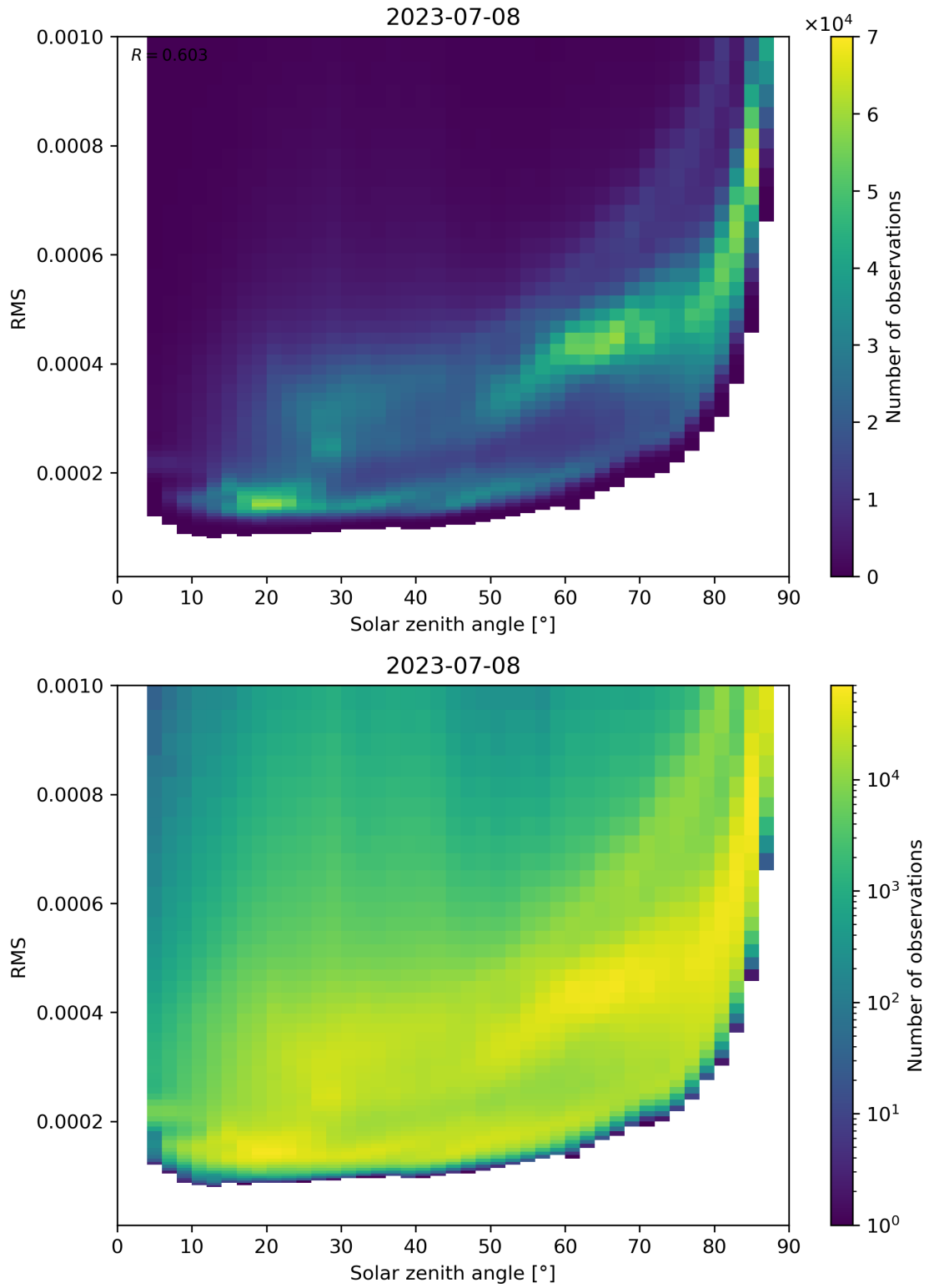
Figure 157: Scatter density plot of “Solar zenith angle” against “RMS” for 2023-07-08 to 2023-07-09.
