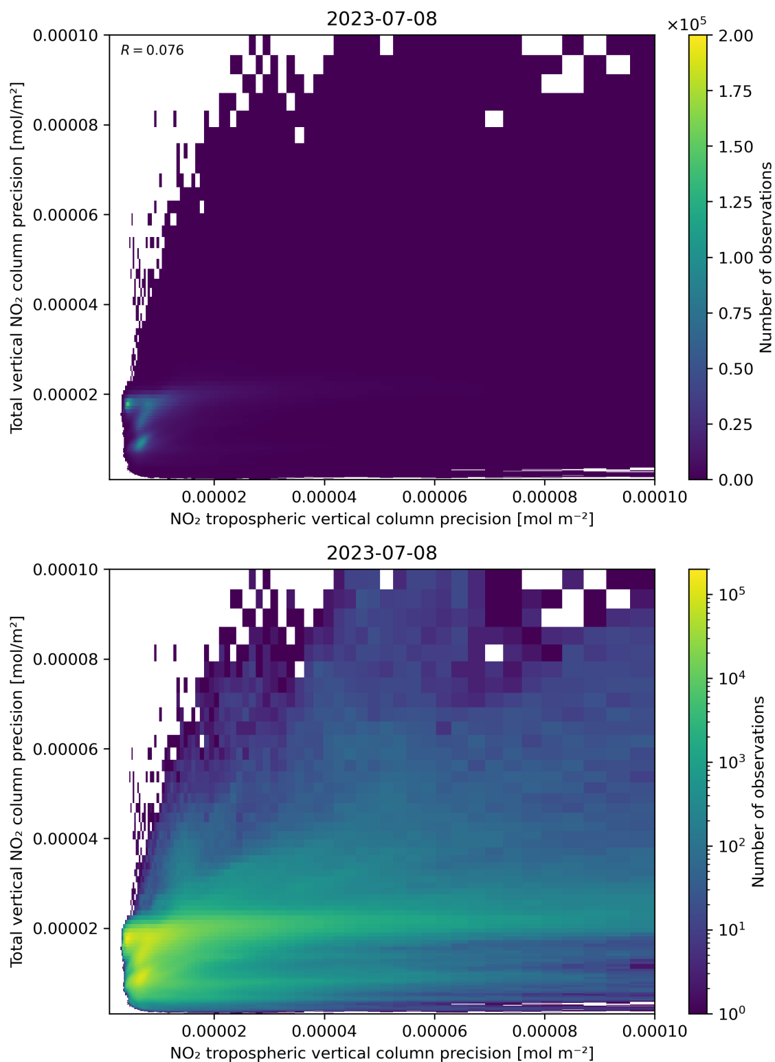
Figure 139: Scatter density plot of “NO 2 tropospheric vertical column precision” against “Total vertical NO 2 column precision” for 2023-07-08 to 2023-07-09.
