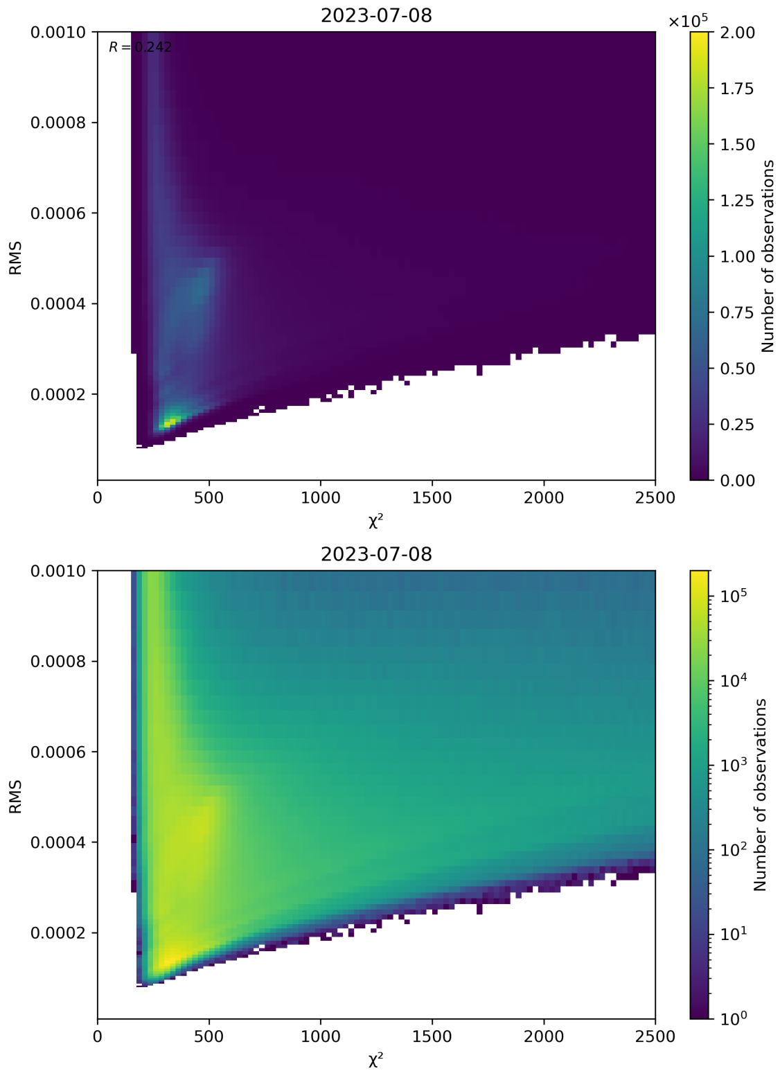
Figure 82: Scatter density plot of “ \chi^2 ” against “RMS” for 2023-07-08 to 2023-07-09.
