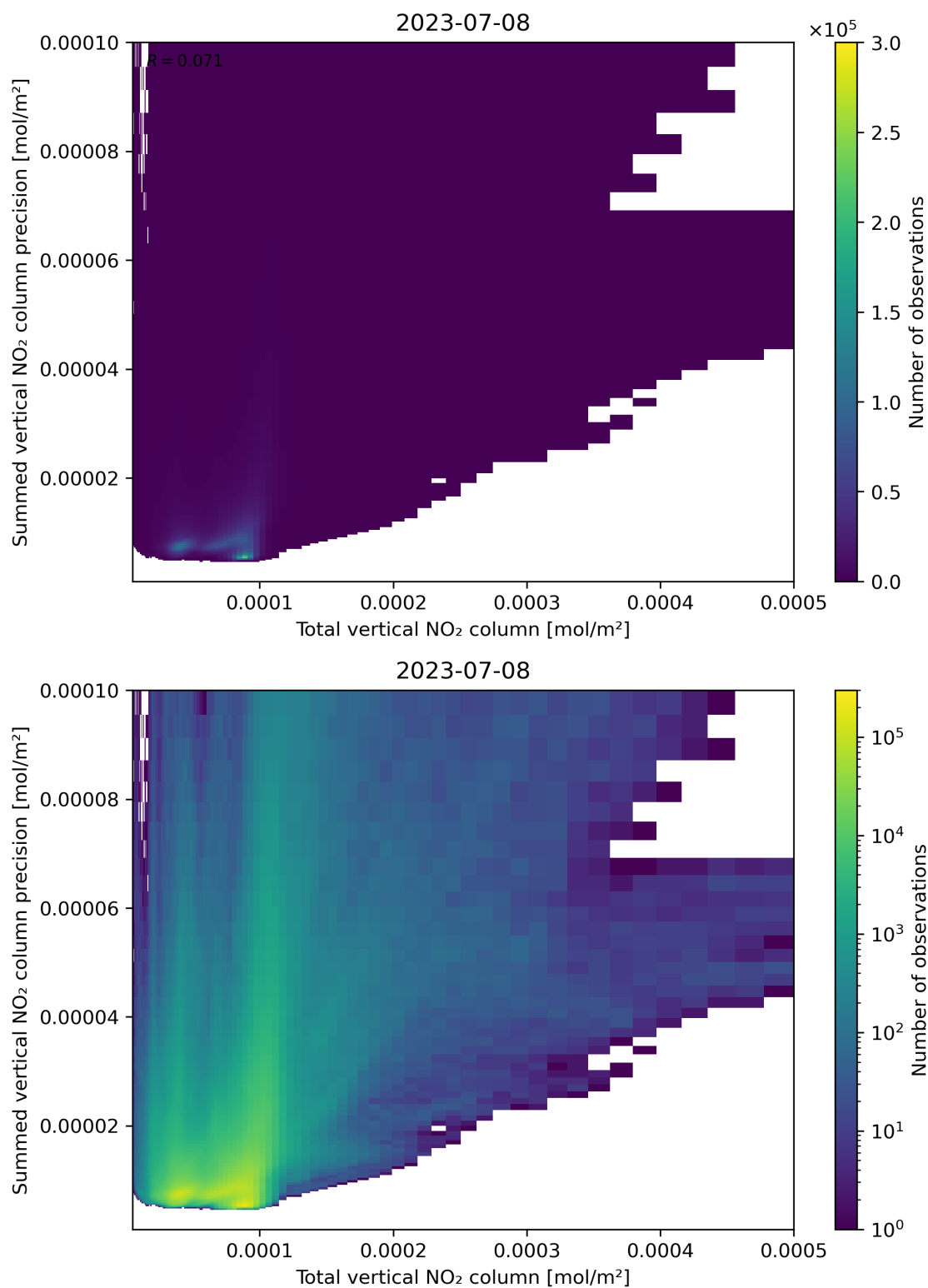
Figure 113: Scatter density plot of “Total vertical NO 2 column” against “Summed vertical NO 2 column precision” for 2023-07-08 to 2023-07-09.
