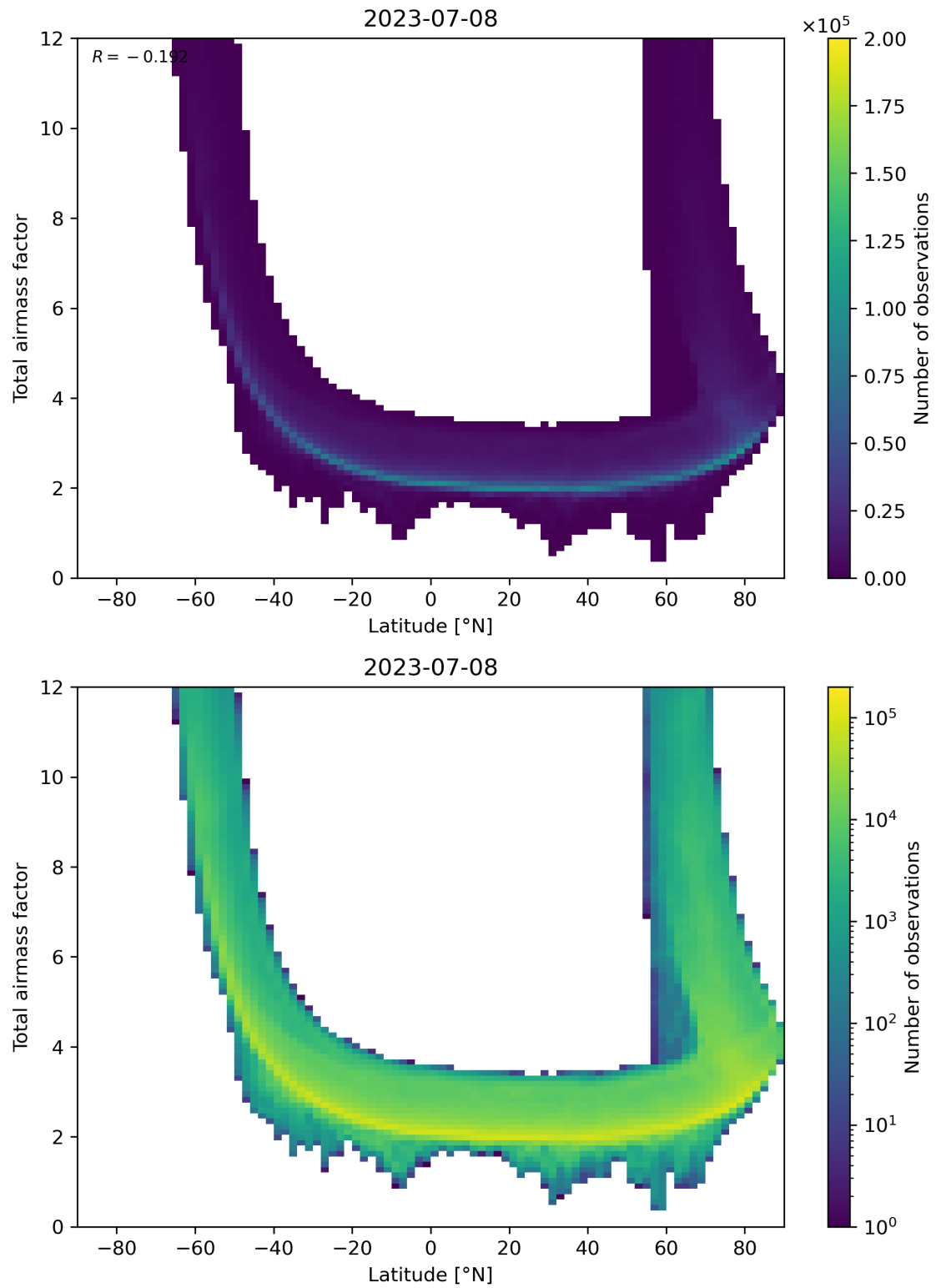
Figure 84: Scatter density plot of “Latitude” against “Total airmass factor” for 2023-07-08 to 2023-07-09.
