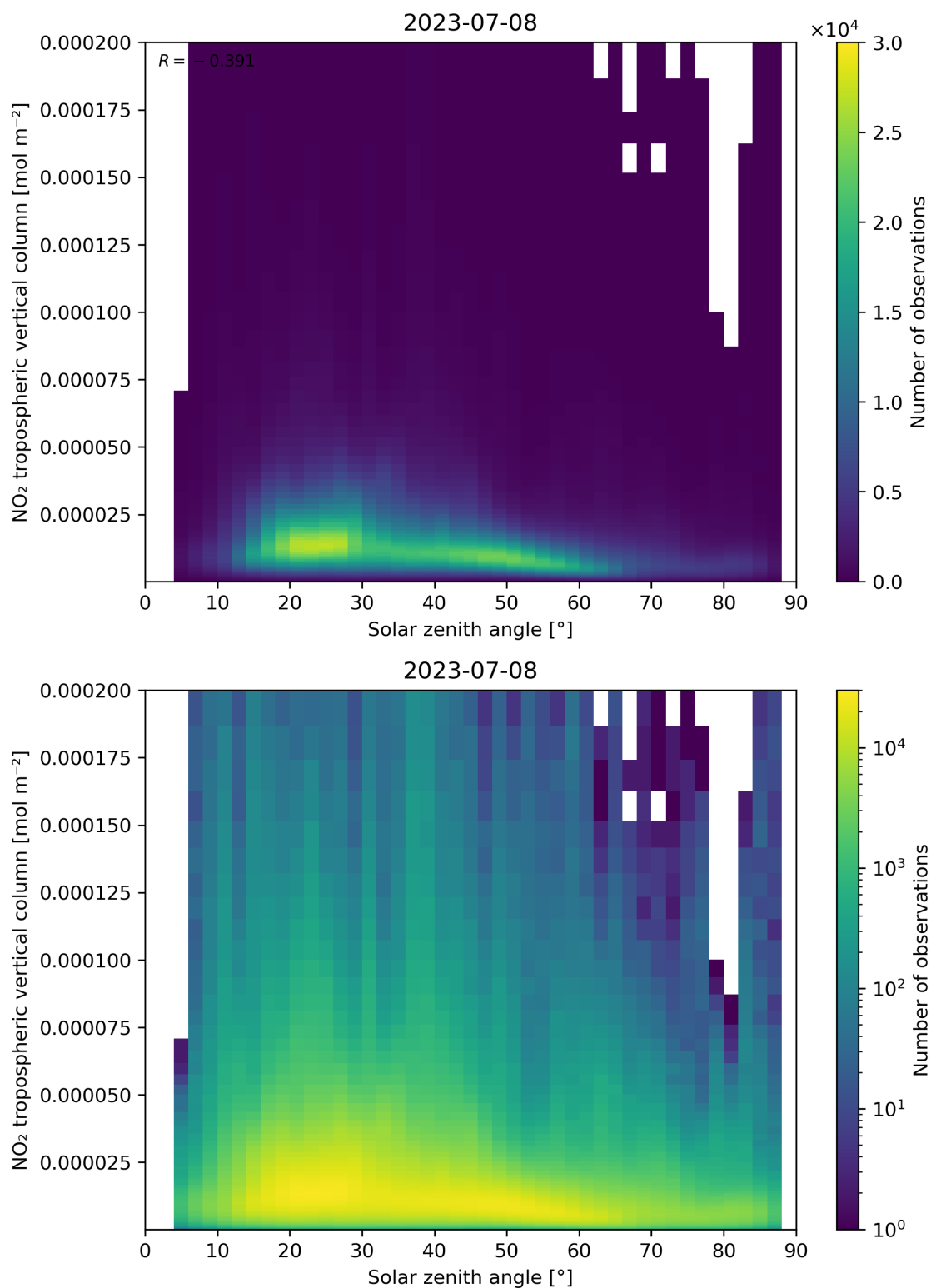
Figure 155: Scatter density plot of “Solar zenith angle” against “NO 2 tropospheric vertical column” for 2023-07-08 to 2023-07-09.
