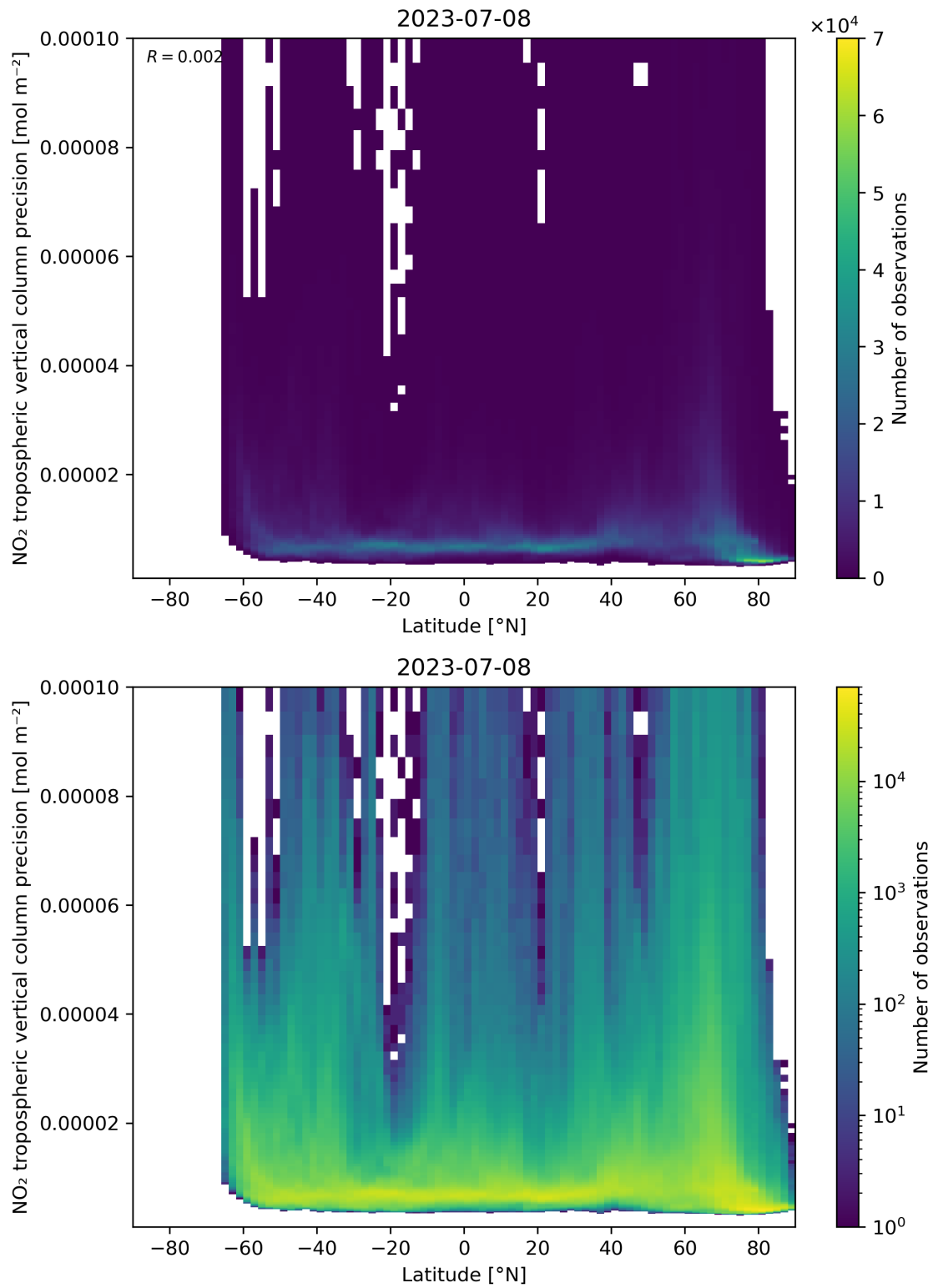
Figure 93: Scatter density plot of “Latitude” against “NO 2 tropospheric vertical column precision” for 2023-07-08 to 2023-07-09.
