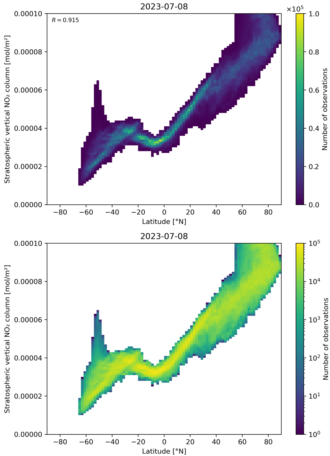
Figure 87: Scatter density plot of “Latitude” against “Stratospheric vertical NO 2 column” for 2023-07-08 to 2023-07-09.
