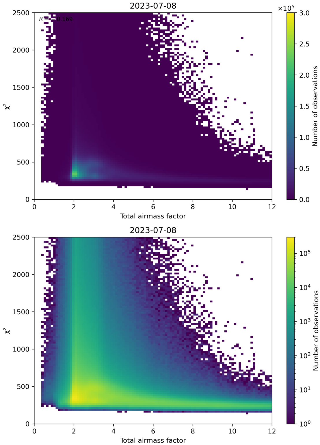
Figure 63: Scatter density plot of “Total airmass factor” against “ \chi^2 ” for 2023-07-08 to 2023-07-09.
