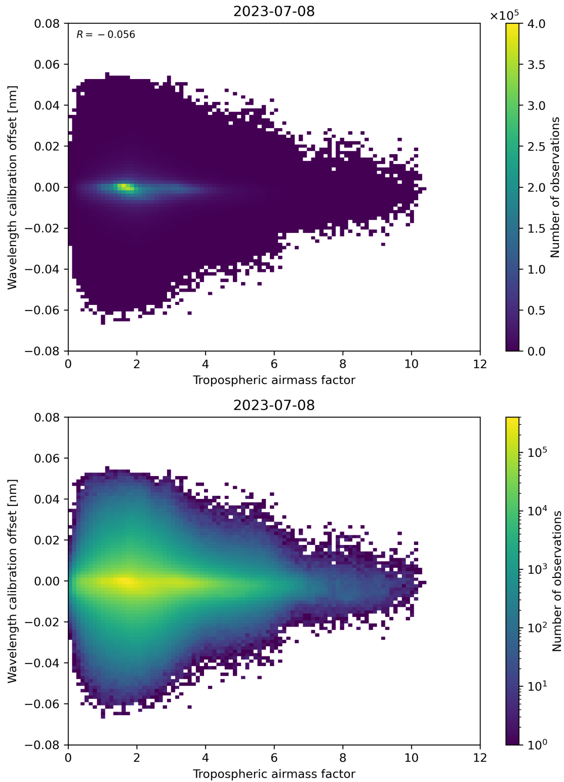
Figure 80: Scatter density plot of “Tropospheric air mass factor” against “Wavelength calibration offset” for 2023-07-08 to 2023-07-09.
