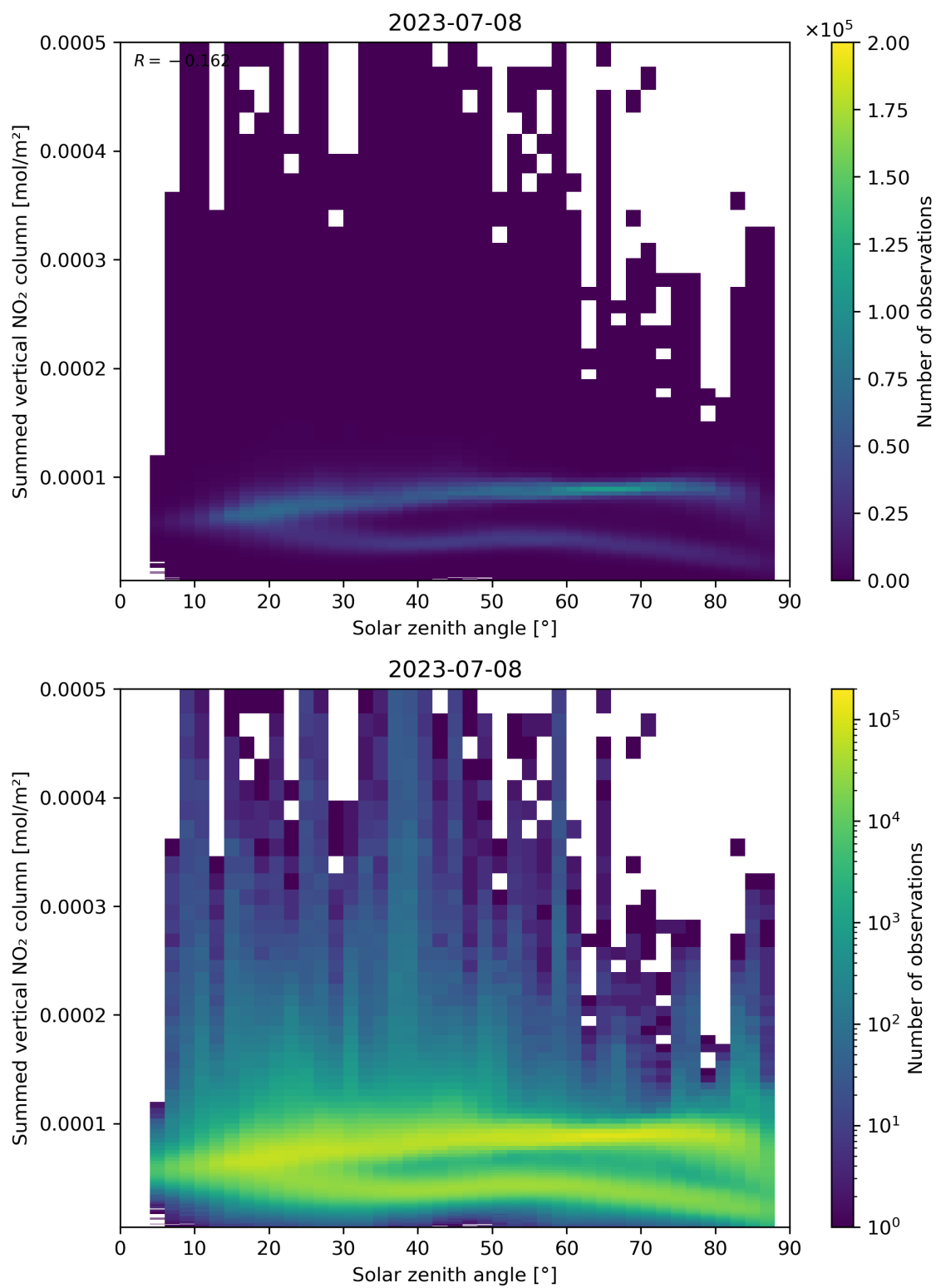
Figure 151: Scatter density plot of “Solar zenith angle” against “Summed vertical NO 2 column” for 2023-07-08 to 2023-07-09.
