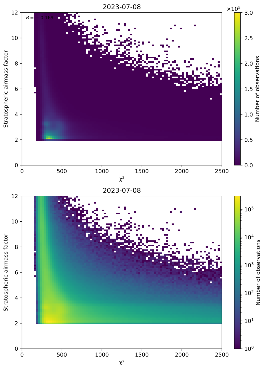
Figure 81: Scatter density plot of “ \chi^2 ” against “Stratospheric air mass factor” for 2023-07-08 to 2023-07-09.
