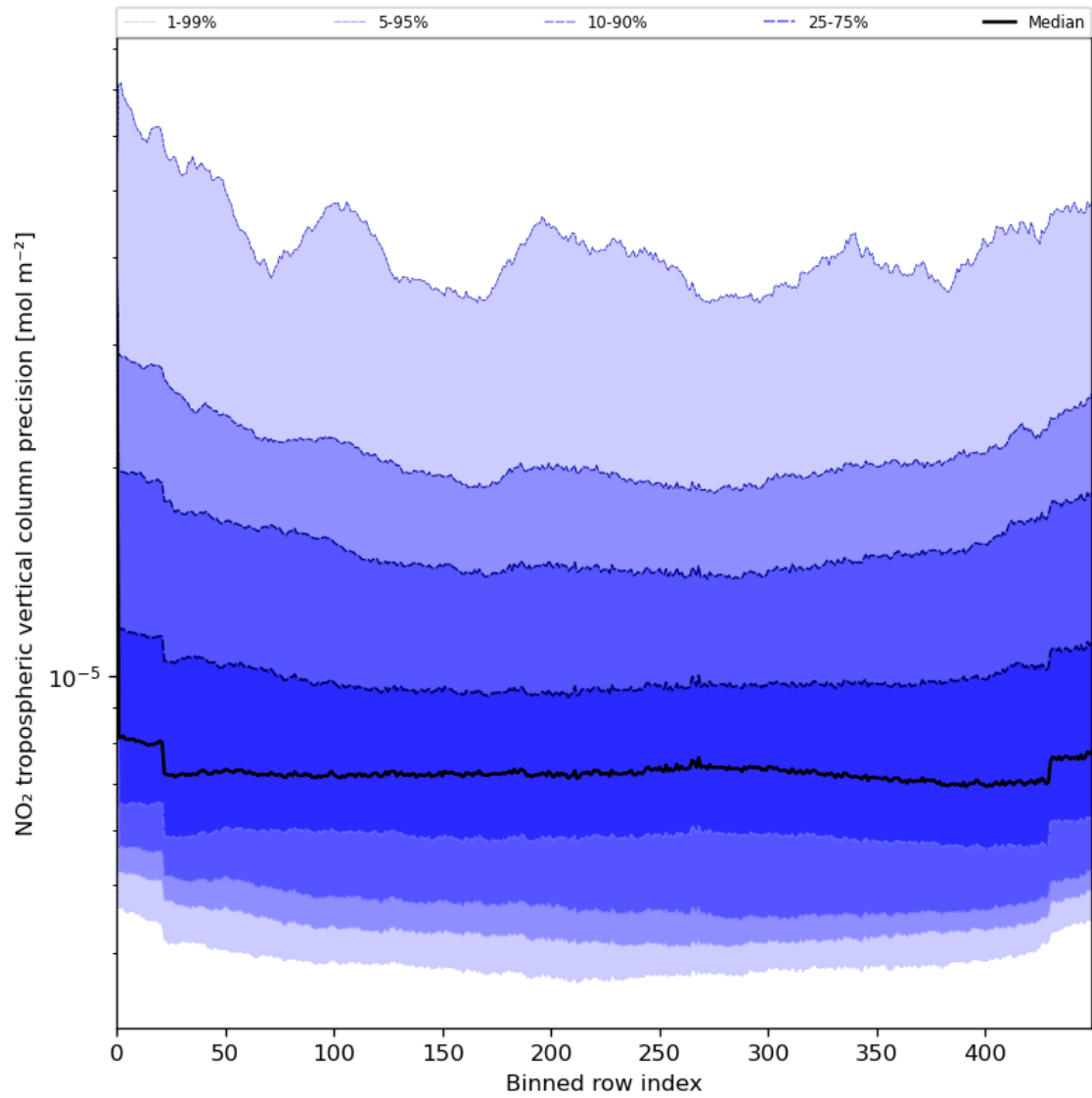
Figure 47: Along track statistics of “NO 2 tropospheric vertical column precision” for 2023-07-08 to 2023-07-09
