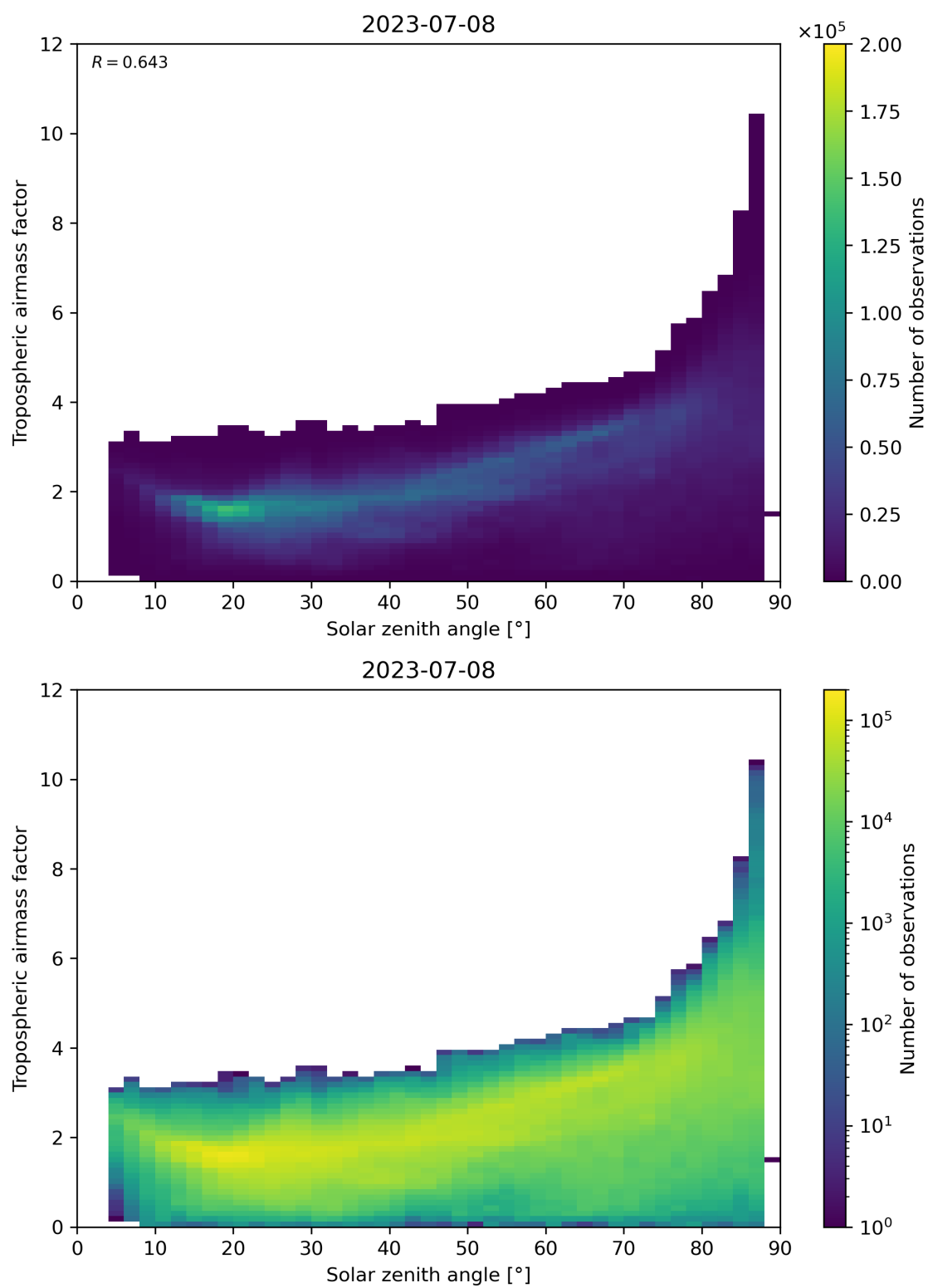
Figure 147: Scatter density plot of “Solar zenith angle” against “Tropospheric airmass factor” for 2023-07-08 to 2023-07-09.
