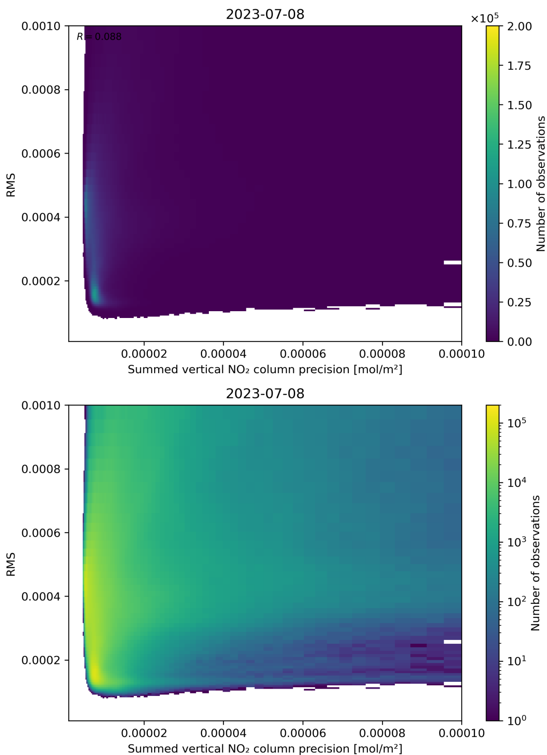
Figure 108: Scatter density plot of “Summed vertical NO 2 column precision” against “RMS” for 2023-07-08 to 2023-07-09.
