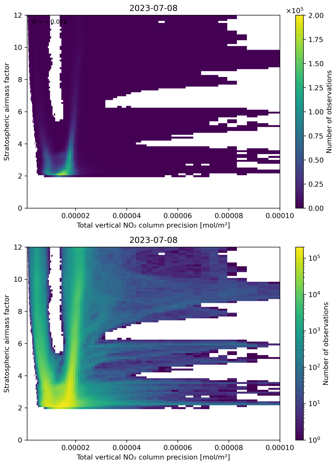
Figure 115: Scatter density plot of “Total vertical NO 2 column precision” against “Stratospheric air mass factor” for 2023-07-08 to 2023-07-09.
