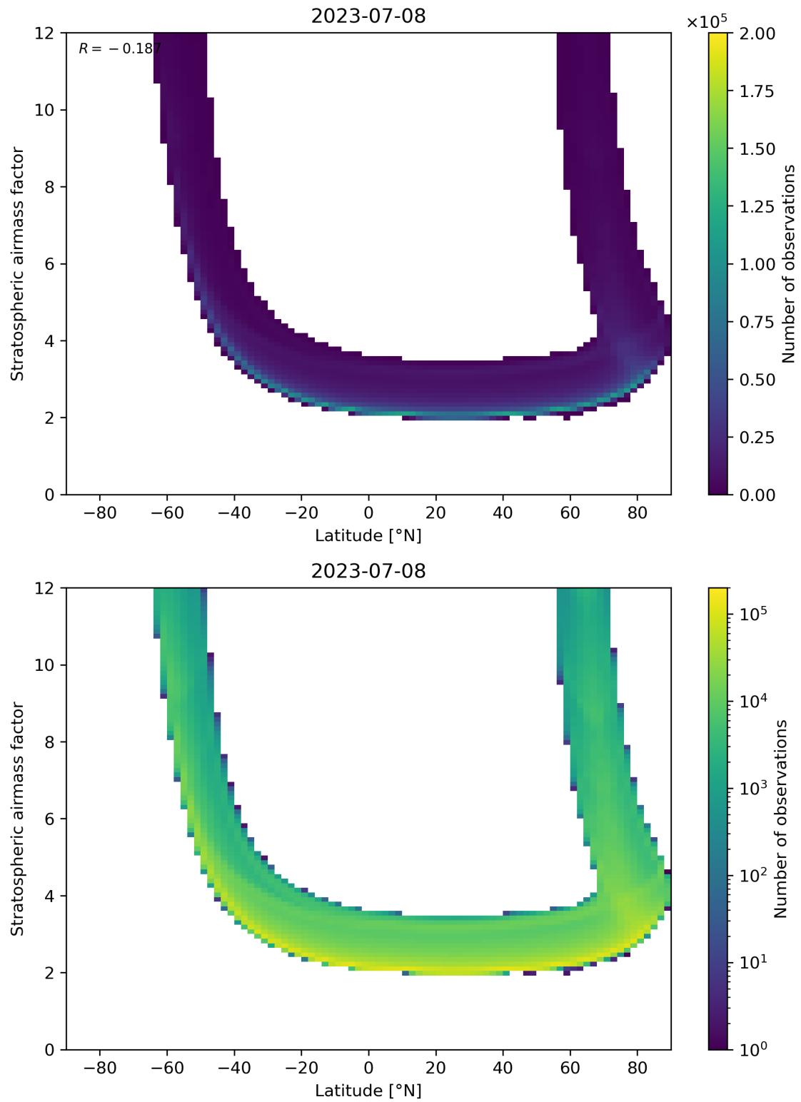
Figure 83: Scatter density plot of “Latitude” against “Stratospheric air mass factor” for 2023-07-08 to 2023-07-09.
