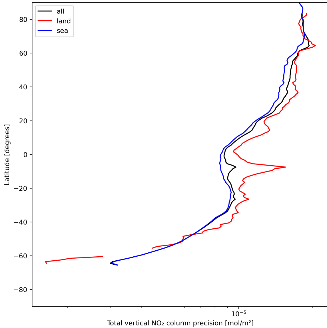
Figure 22: Zonal average of “Total vertical NO 2 column precision” for 2023-07-08 to 2023-07-09.
