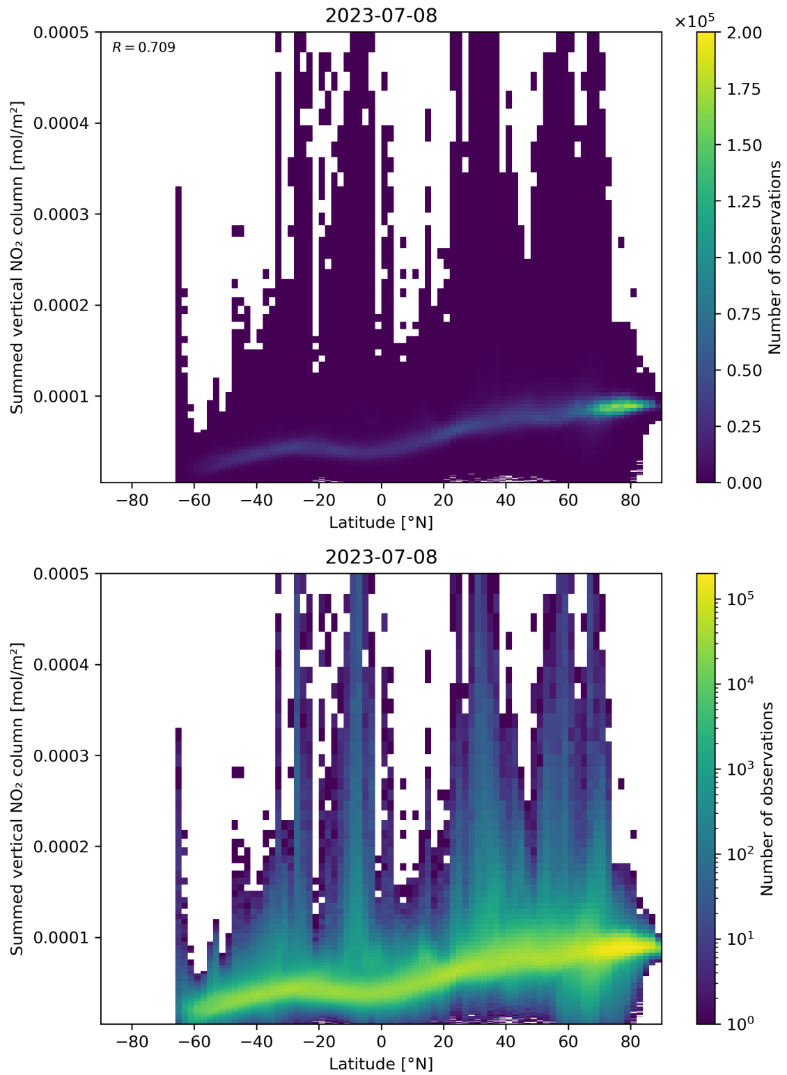
Figure 88: Scatter density plot of “Latitude” against “Summed vertical NO 2 column” for 2023-07-08 to 2023-07-09.
