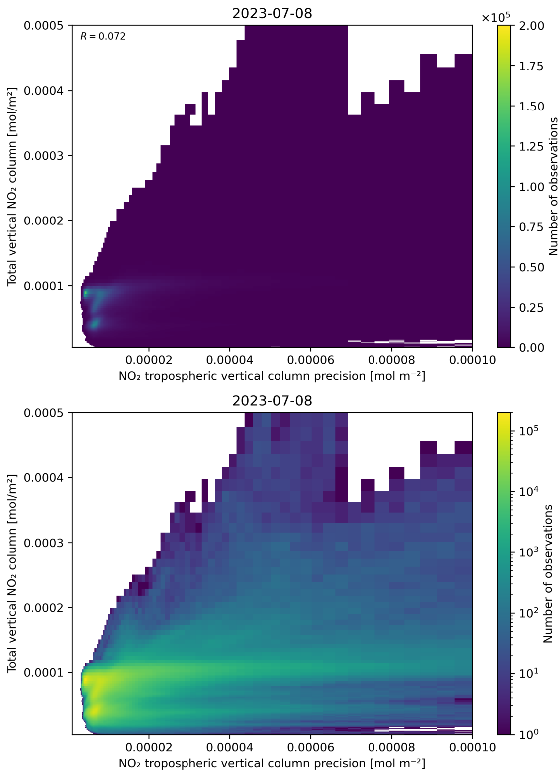
Figure 138: Scatter density plot of “NO 2 tropospheric vertical column precision” against “Total vertical NO 2 column” for 2023-07-08 to 2023-07-09.
