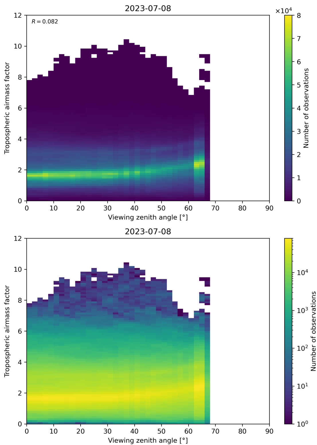
Figure 161: Scatter density plot of “Viewing zenith angle” against “Tropospheric airmass factor” for 2023-07-08 to 2023-07-09.
