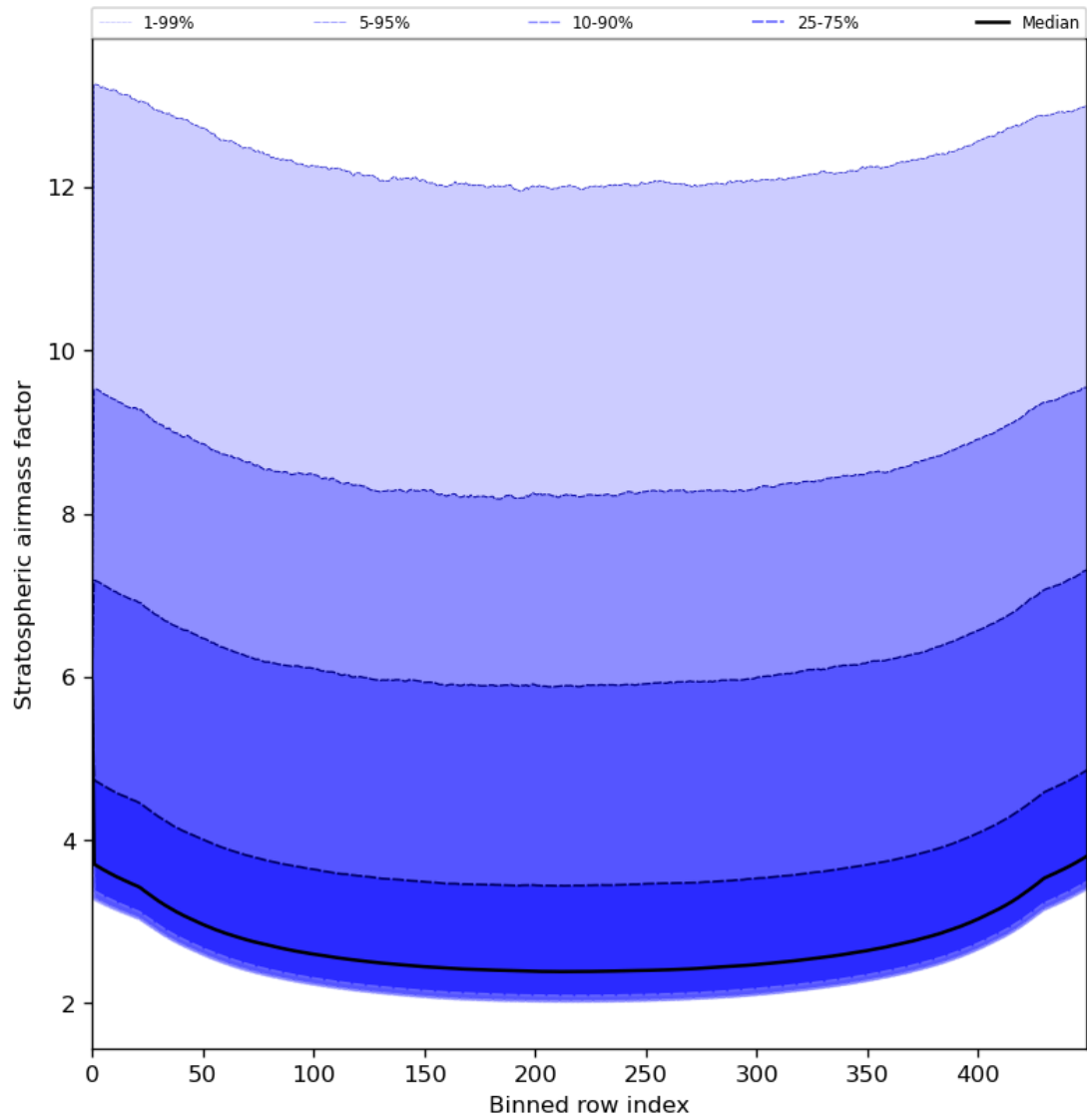
Figure 61: Along track statistics of “Stratospheric airmass factor” for 2023-07-08 to 2023-07-09
