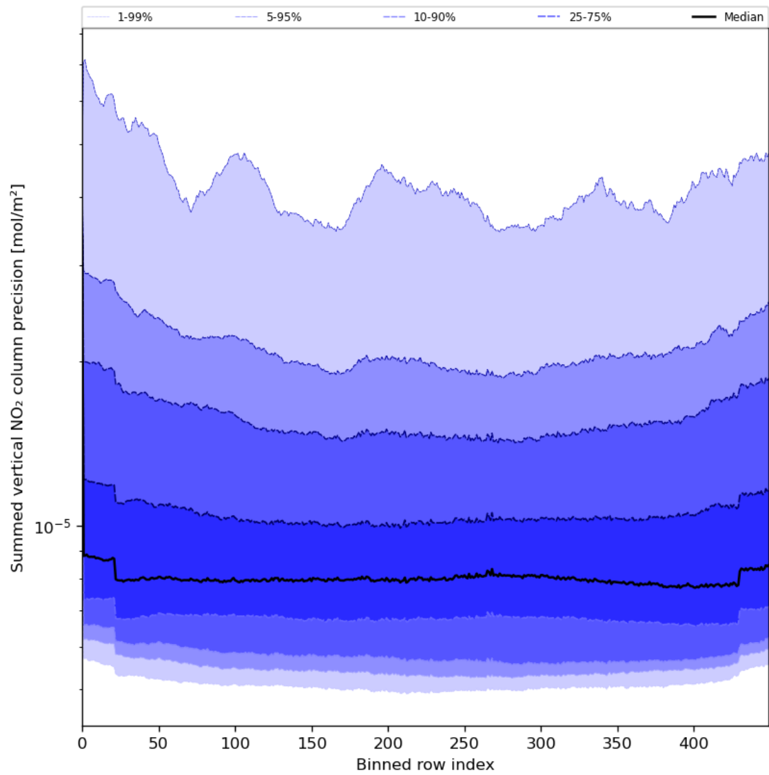
Figure 58: Along track statistics of “Summed vertical NO 2 column precision” for 2023-07-08 to 2023-07-09
