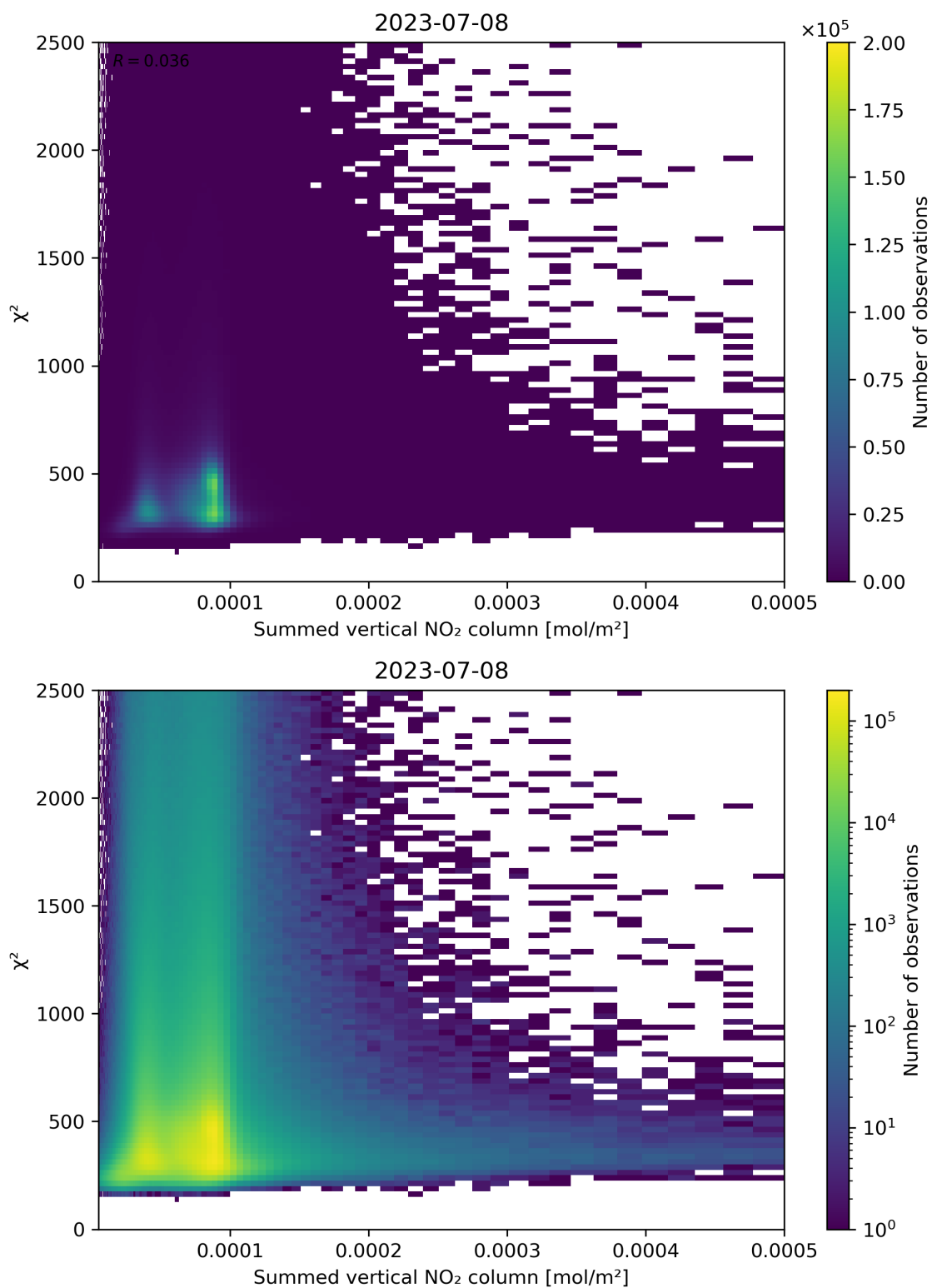
Figure 104: Scatter density plot of “Summed vertical NO 2 column” against “ \chi^2 ” for 2023-07-08 to 2023-07-09.
