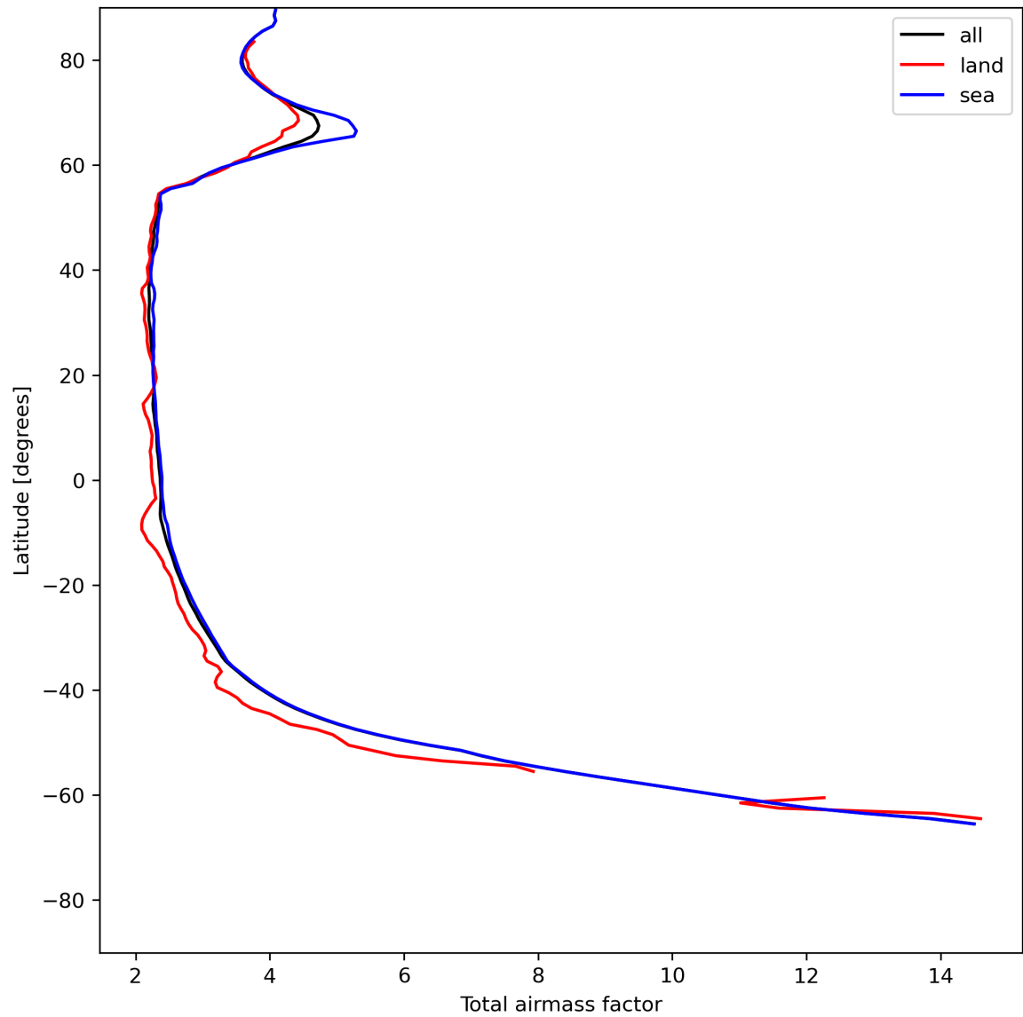
Figure 15: Zonal average of “Total airmass factor” for 2023-07-08 to 2023-07-09.
