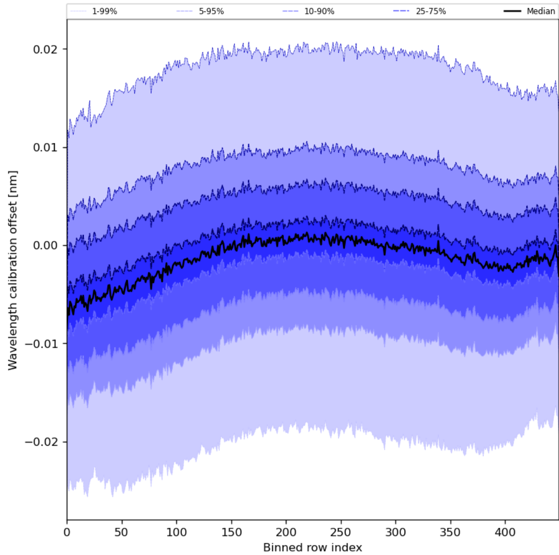
Figure 52: Along track statistics of “Wavelength calibration offset” for 2023-07-08 to 2023-07-09
