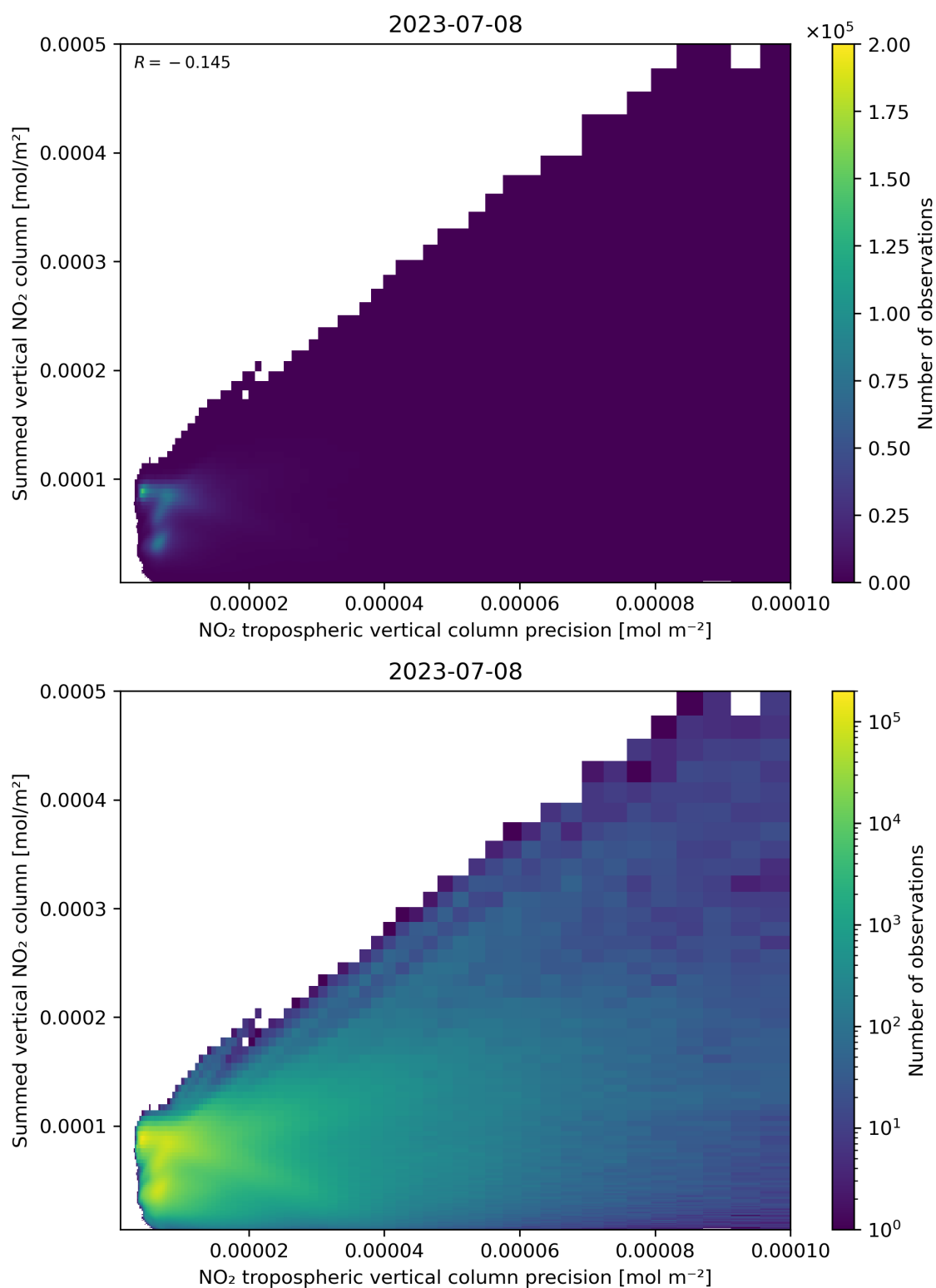
Figure 136: Scatter density plot of “NO 2 tropospheric vertical column precision” against “Summed vertical NO 2 column” for 2023-07-08 to 2023-07-09.
