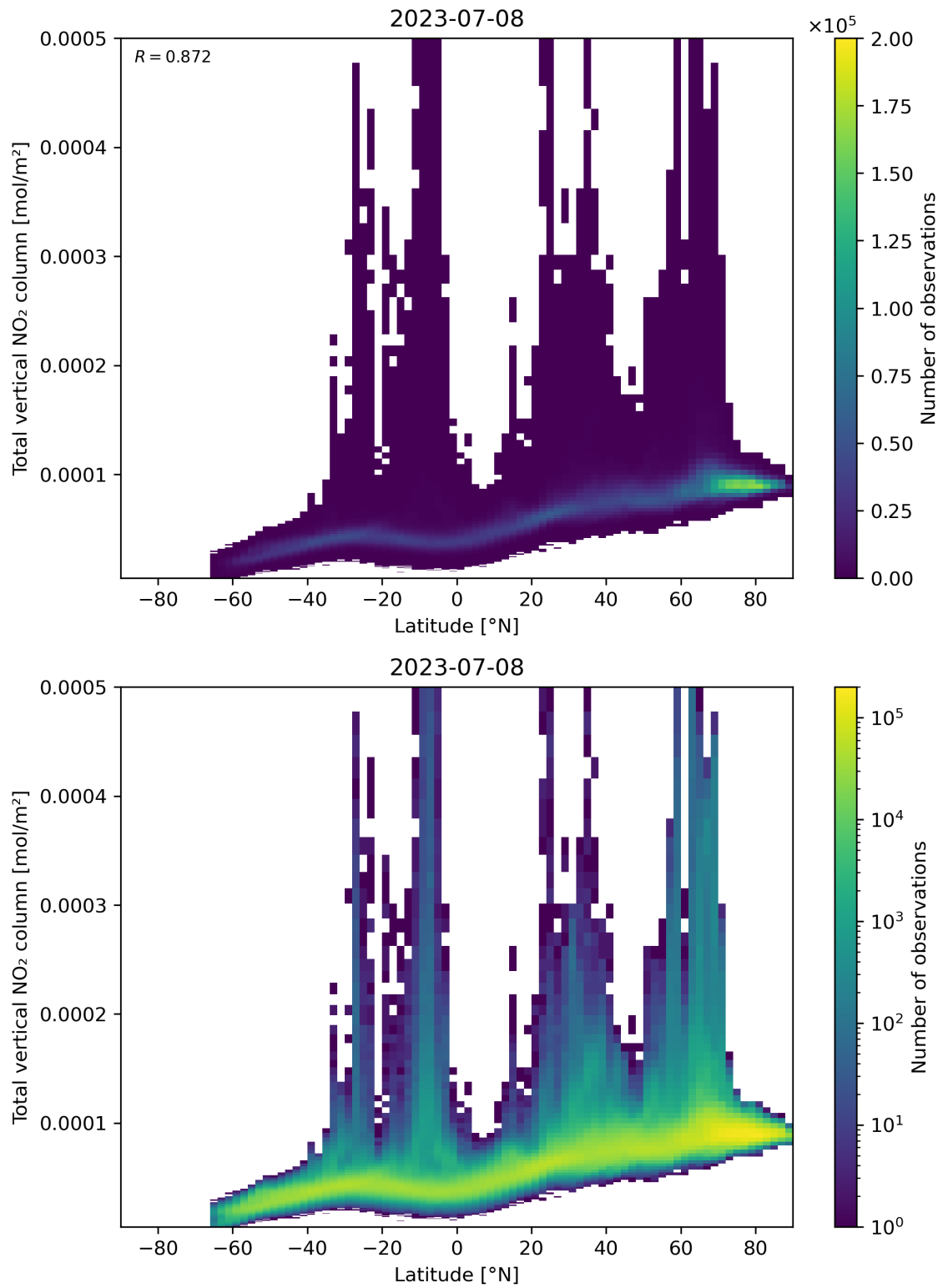
Figure 90: Scatter density plot of “Latitude” against “Total vertical NO 2 column” for 2023-07-08 to 2023-07-09.
