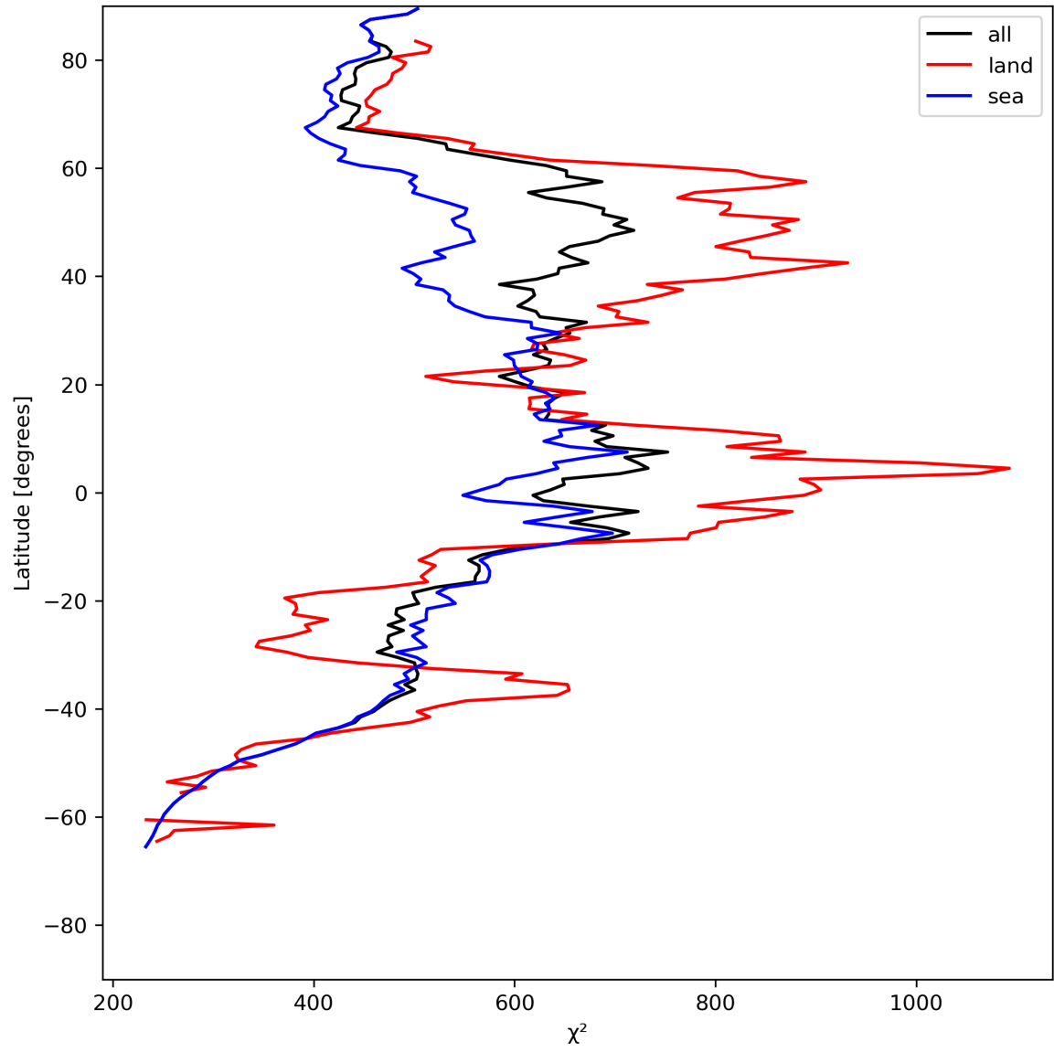
Figure 25: Zonal average of “ \chi^2 ” for 2023-07-08 to 2023-07-09.
