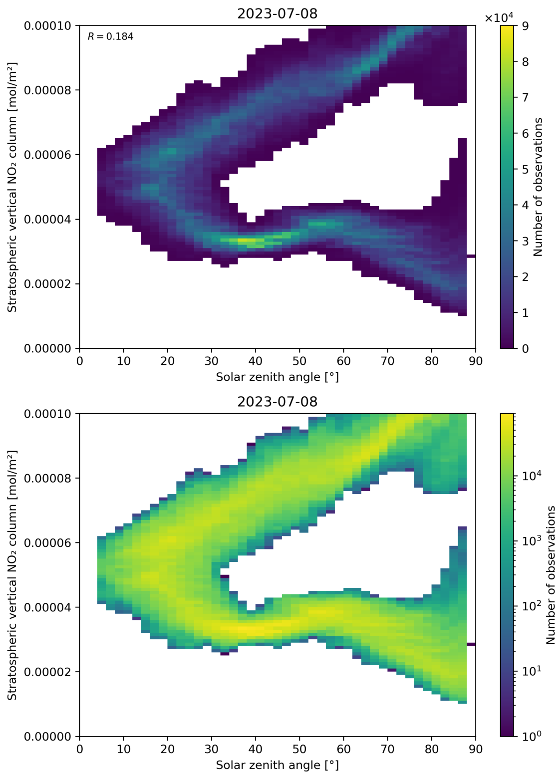
Figure 150: Scatter density plot of “Solar zenith angle” against “Stratospheric vertical NO 2 column” for 2023-07-08 to 2023-07-09.
