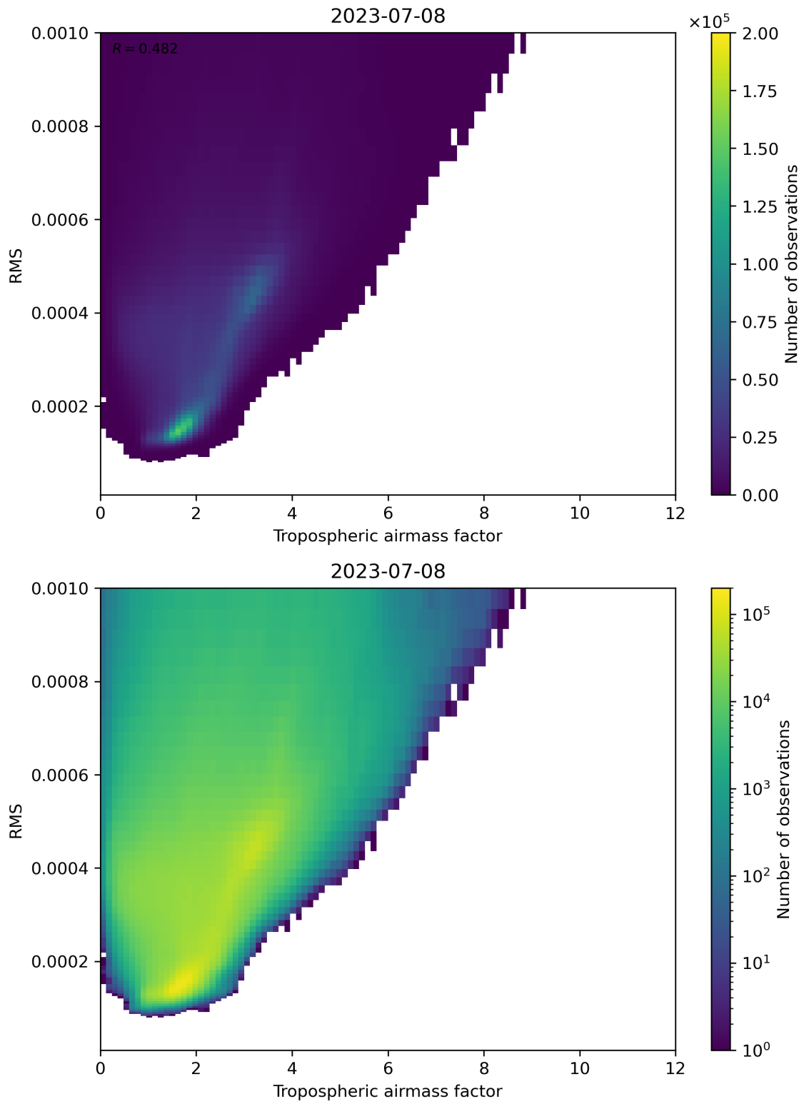
Figure 79: Scatter density plot of “Tropospheric airmass factor” against “RMS” for 2023-07-08 to 2023-07-09.
