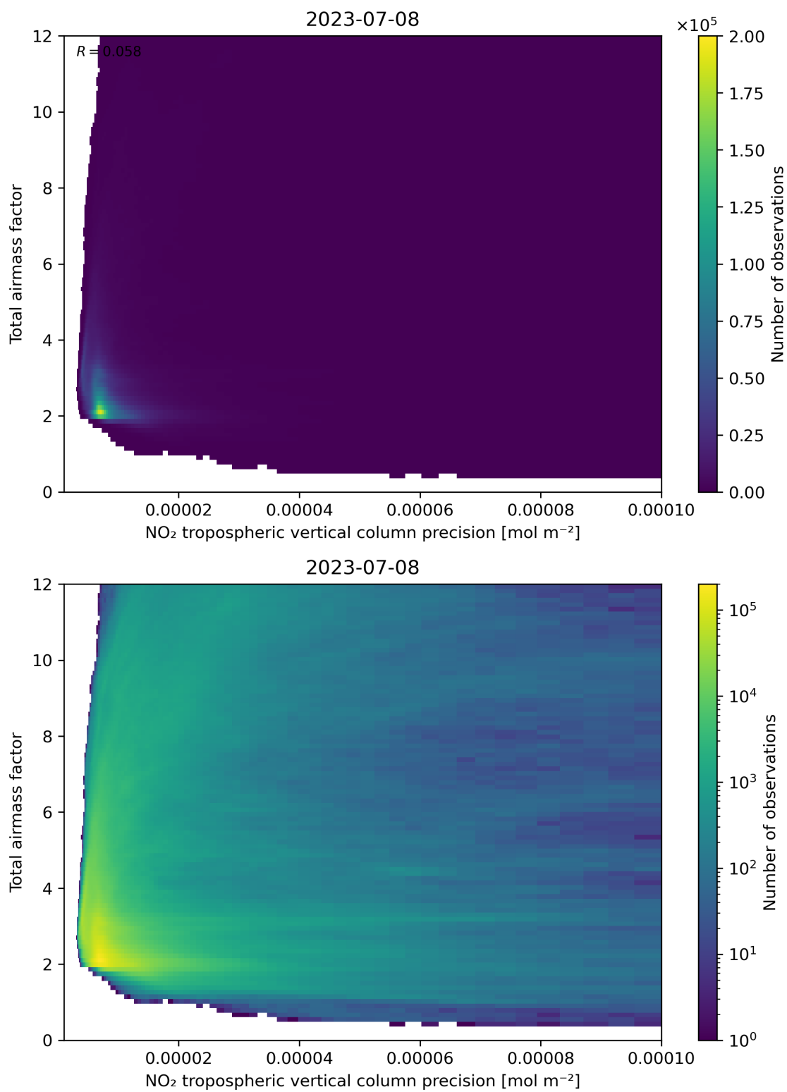
Figure 132: Scatter density plot of “NO 2 tropospheric vertical column precision” against “Total air mass factor” for 2023-07-08 to 2023-07-09.
