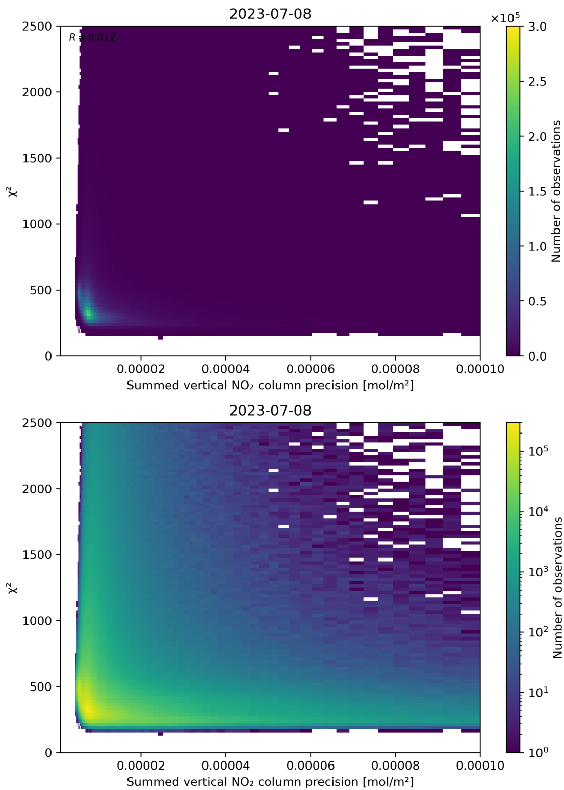
Figure 107: Scatter density plot of “Summed vertical NO 2 column precision” against “ \chi^2 ” for 2023-07-08 to 2023-07-09.
