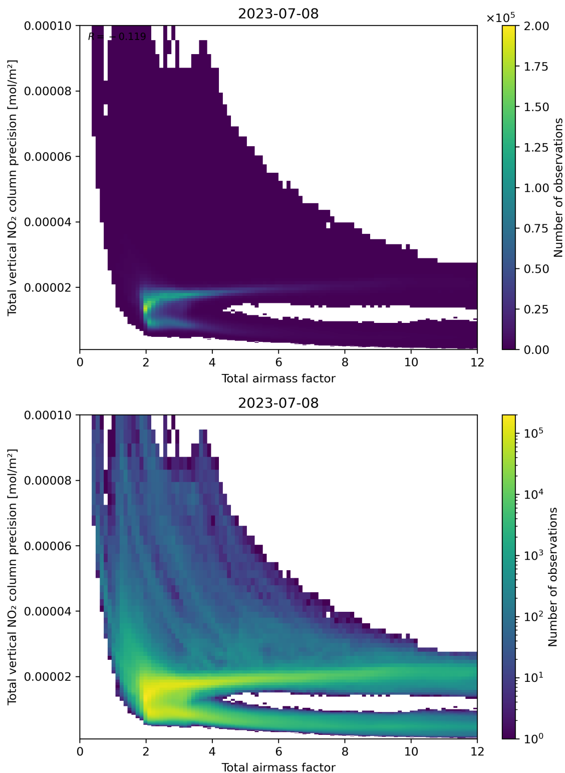
Figure 68: Scatter density plot of “Total airmass factor” against “Total vertical NO 2 column precision” for 2023-07-08 to 2023-07-09.
