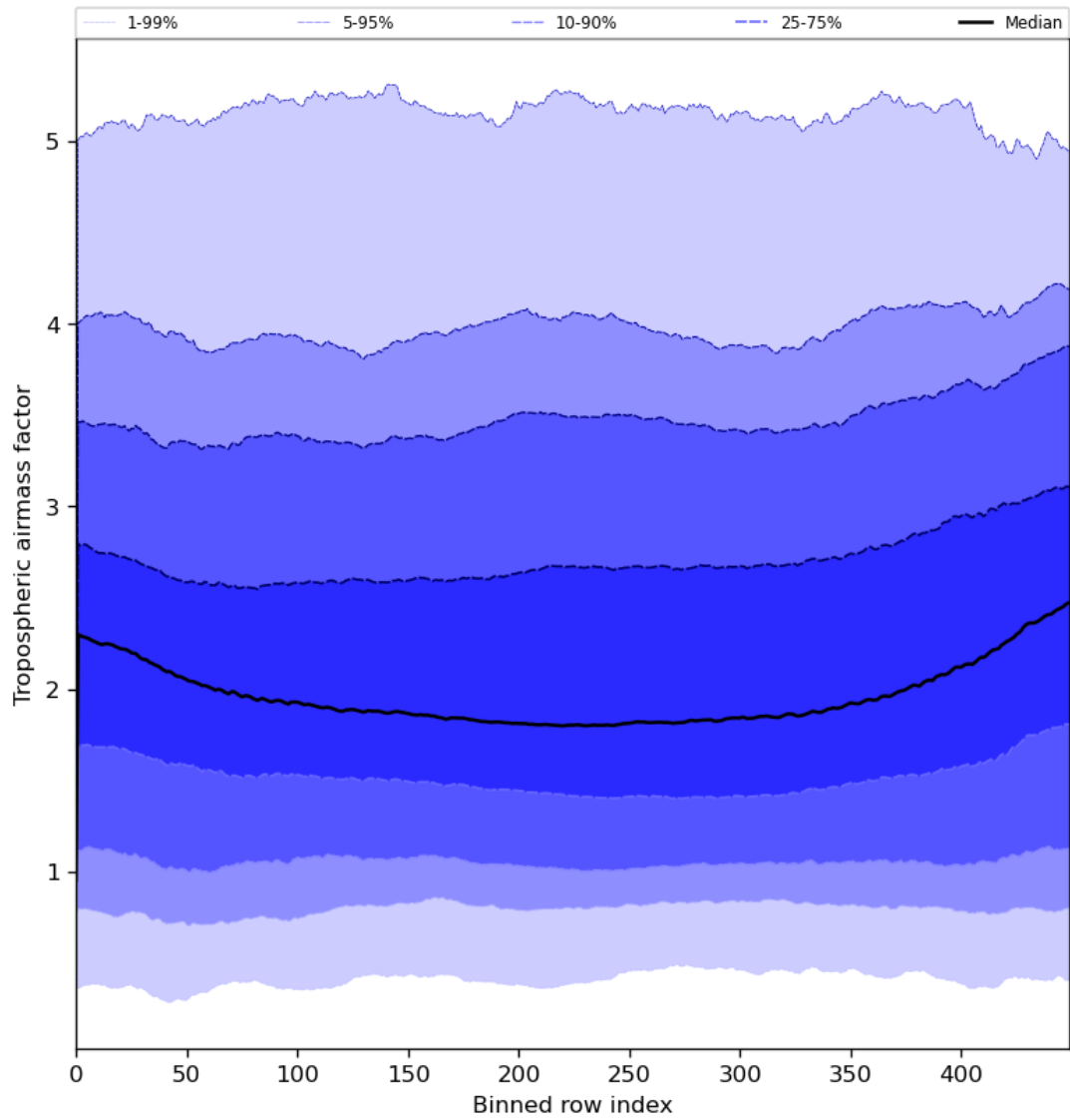
Figure 48: Along track statistics of “Tropospheric airmass factor” for 2023-07-08 to 2023-07-09
