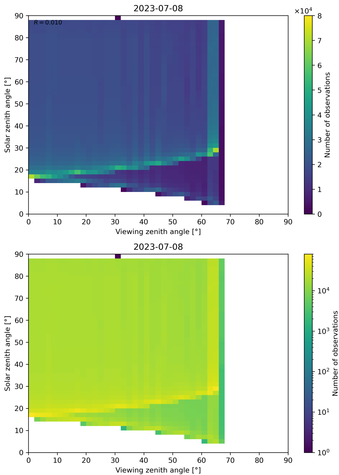
Figure 172: Scatter density plot of “Viewing zenith angle” against “Solar zenith angle” for 2023-07-08 to 2023-07-09.
