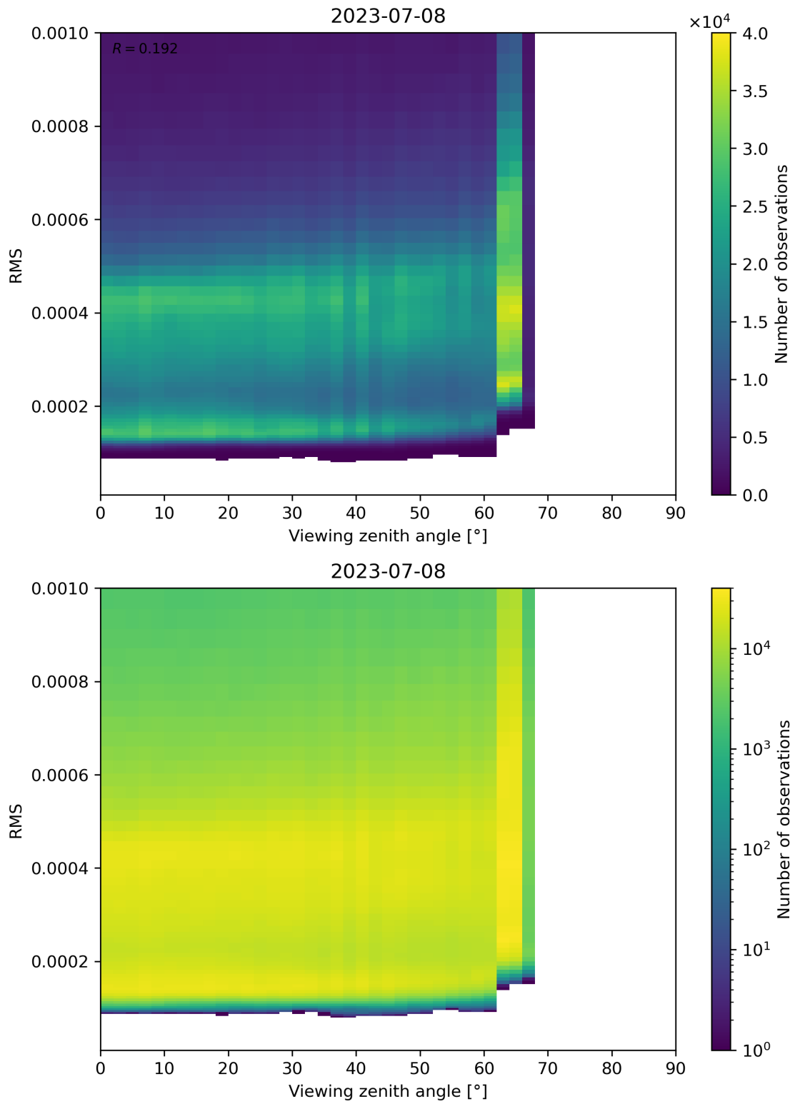
Figure 171: Scatter density plot of “Viewing zenith angle” against “RMS” for 2023-07-08 to 2023-07-09.
