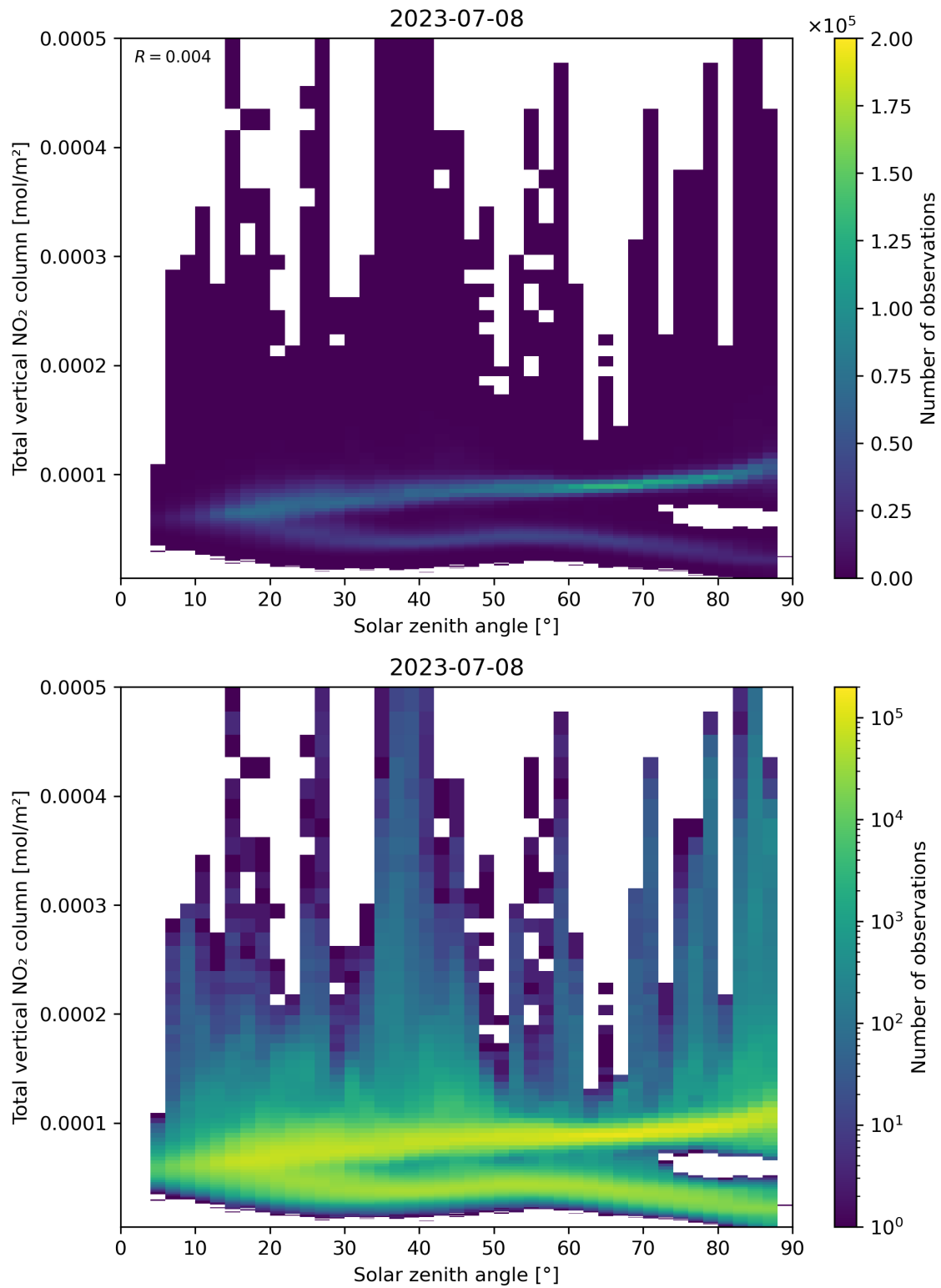
Figure 153: Scatter density plot of “Solar zenith angle” against “Total vertical NO 2 column” for 2023-07-08 to 2023-07-09.
