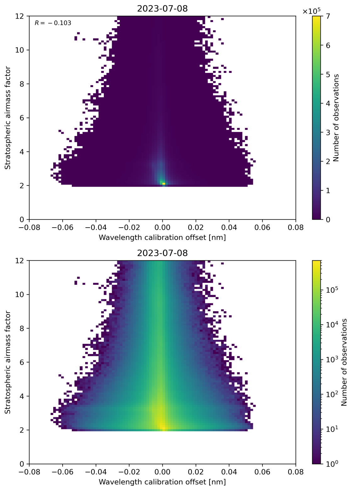
Figure 174: Scatter density plot of “Wavelength calibration offset” against “Stratospheric airmass factor” for 2023-07-08 to 2023-07-09.
