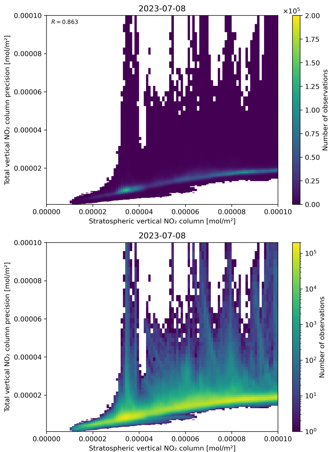
Figure 101: Scatter density plot of “Stratospheric vertical NO 2 column” against “Total vertical NO 2 column precision” for 2023-07-08 to 2023-07-09.
