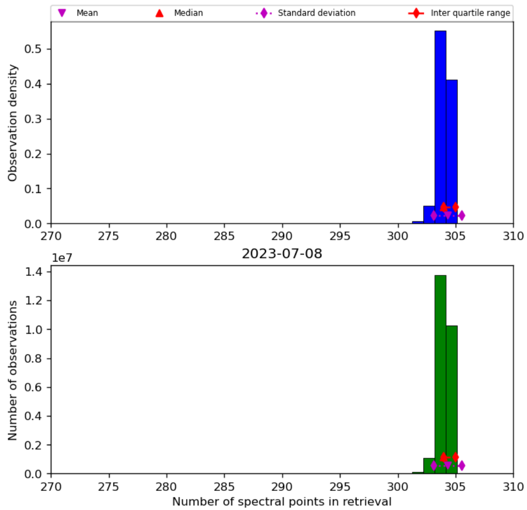
Figure 33: Histogram of “Number of spectral points in retrieval” for 2023-07-08 to 2023-07-09
