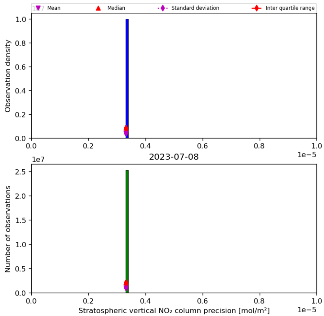
Figure 37: Histogram of “Stratospheric vertical NO 2 column precision” for 2023-07-08 to 2023-07-09
