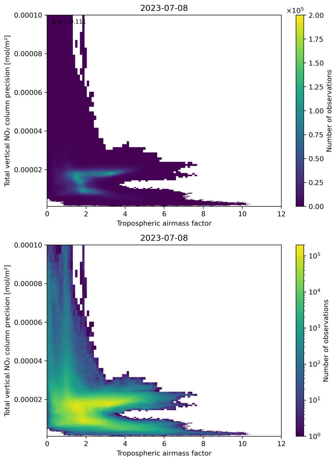
Figure 78: Scatter density plot of “Tropospheric air mass factor” against “Total vertical NO 2 column precision” for 2023-07-08 to 2023-07-09.
