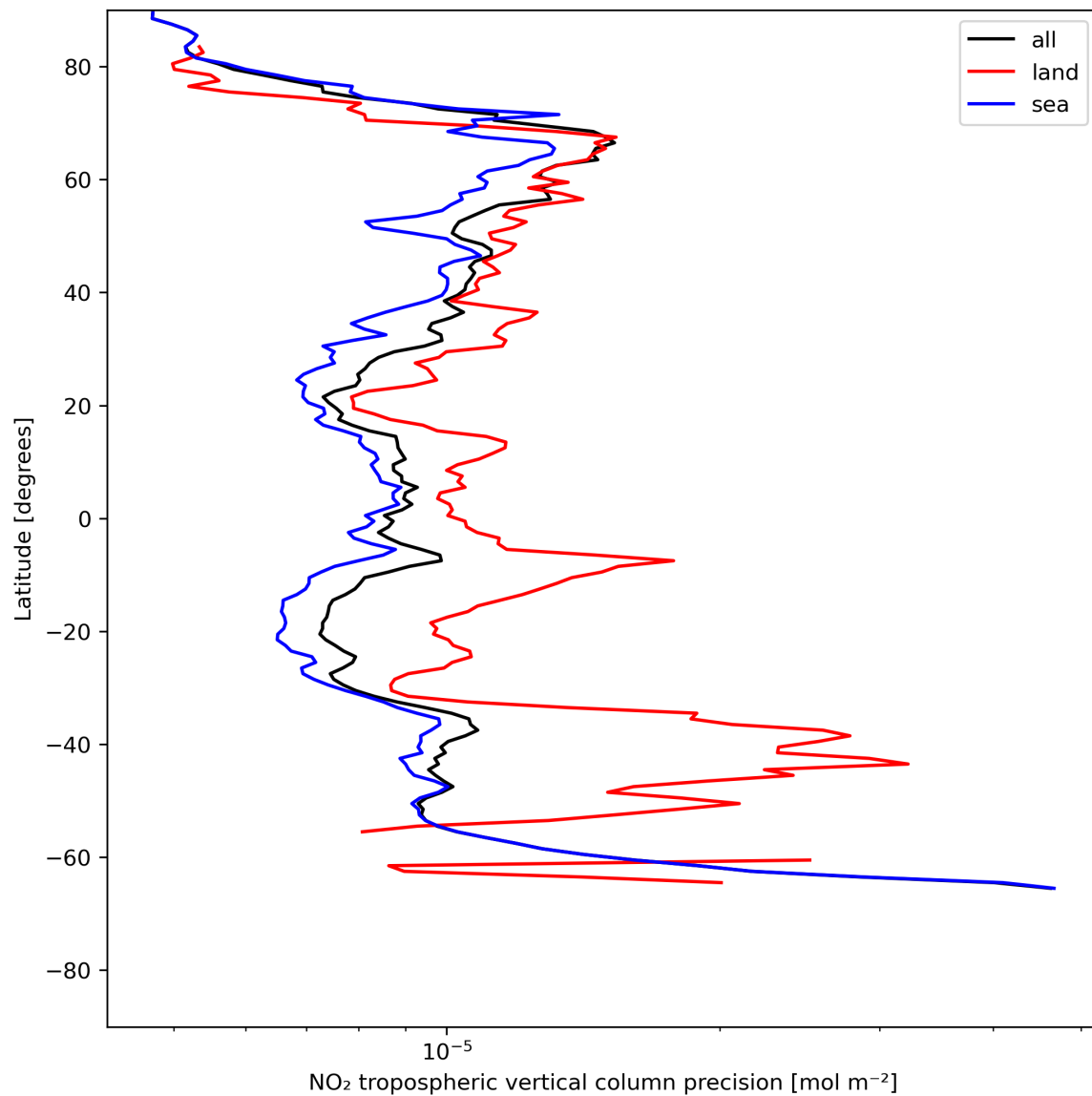
Figure 13: Zonal average of “NO 2 tropospheric vertical column precision” for 2023-07-08 to 2023-07-09.
