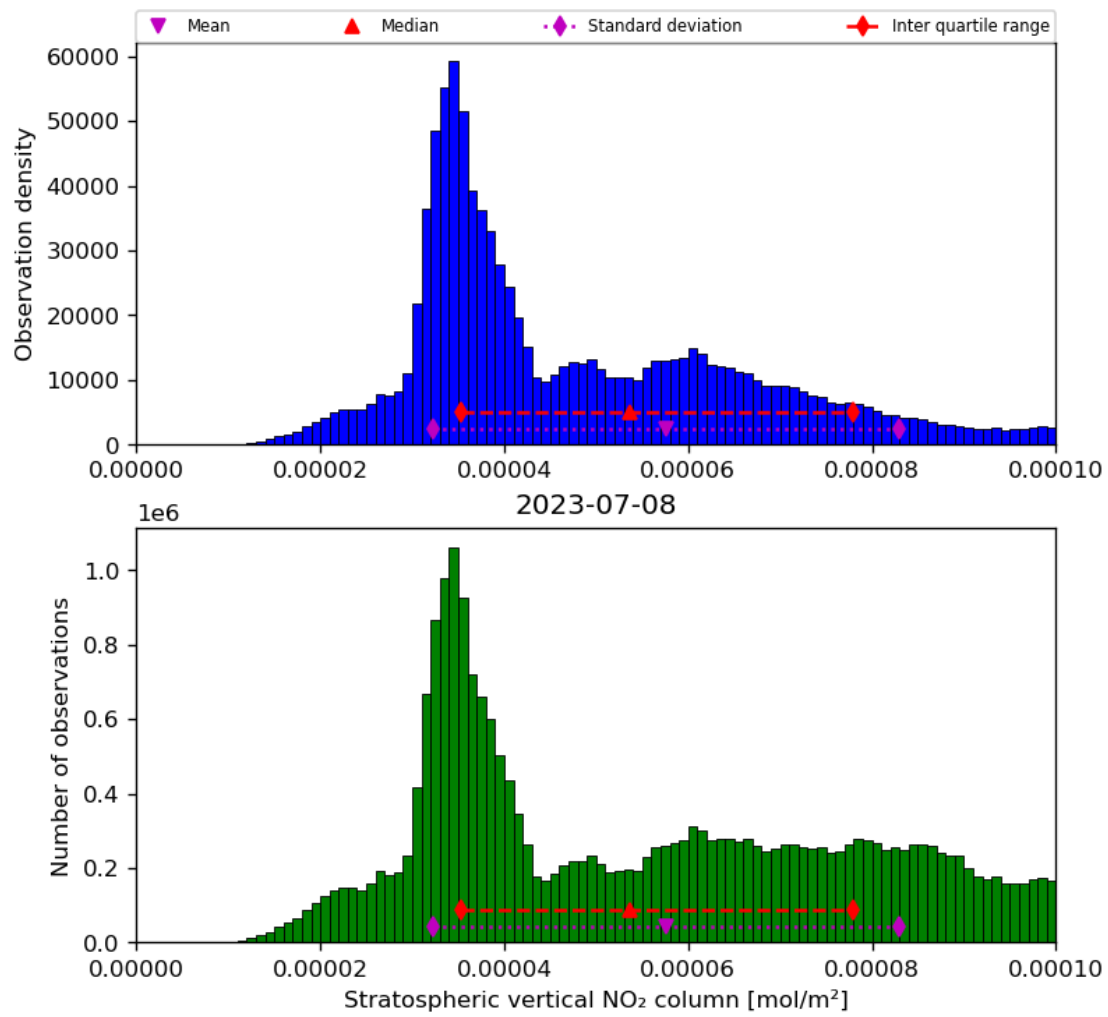
Figure 36: Histogram of “Stratospheric vertical NO 2 column” for 2023-07-08 to 2023-07-09
