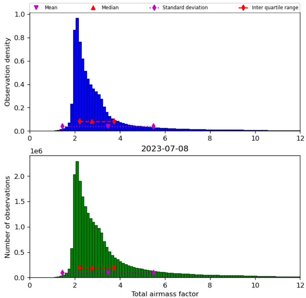
Figure 32: Histogram of “Total airmass factor” for 2023-07-08 to 2023-07-09
