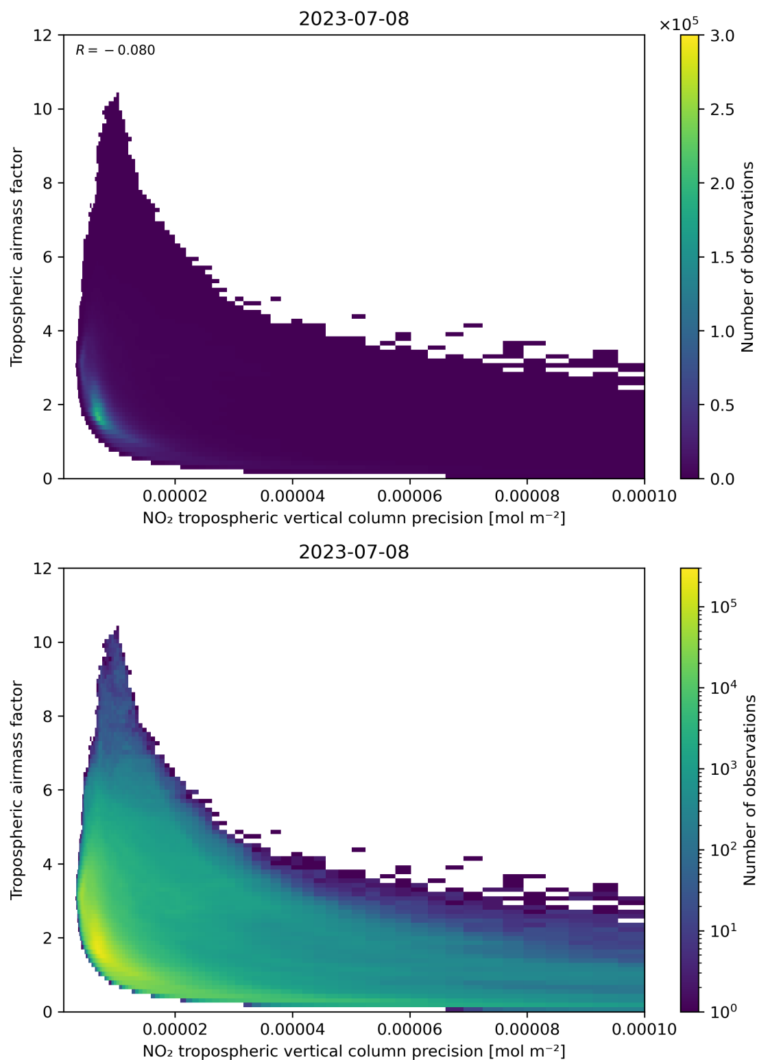
Figure 133: Scatter density plot of “NO 2 tropospheric vertical column precision” against “Tropospheric airmass factor” for 2023-07-08 to 2023-07-09.
