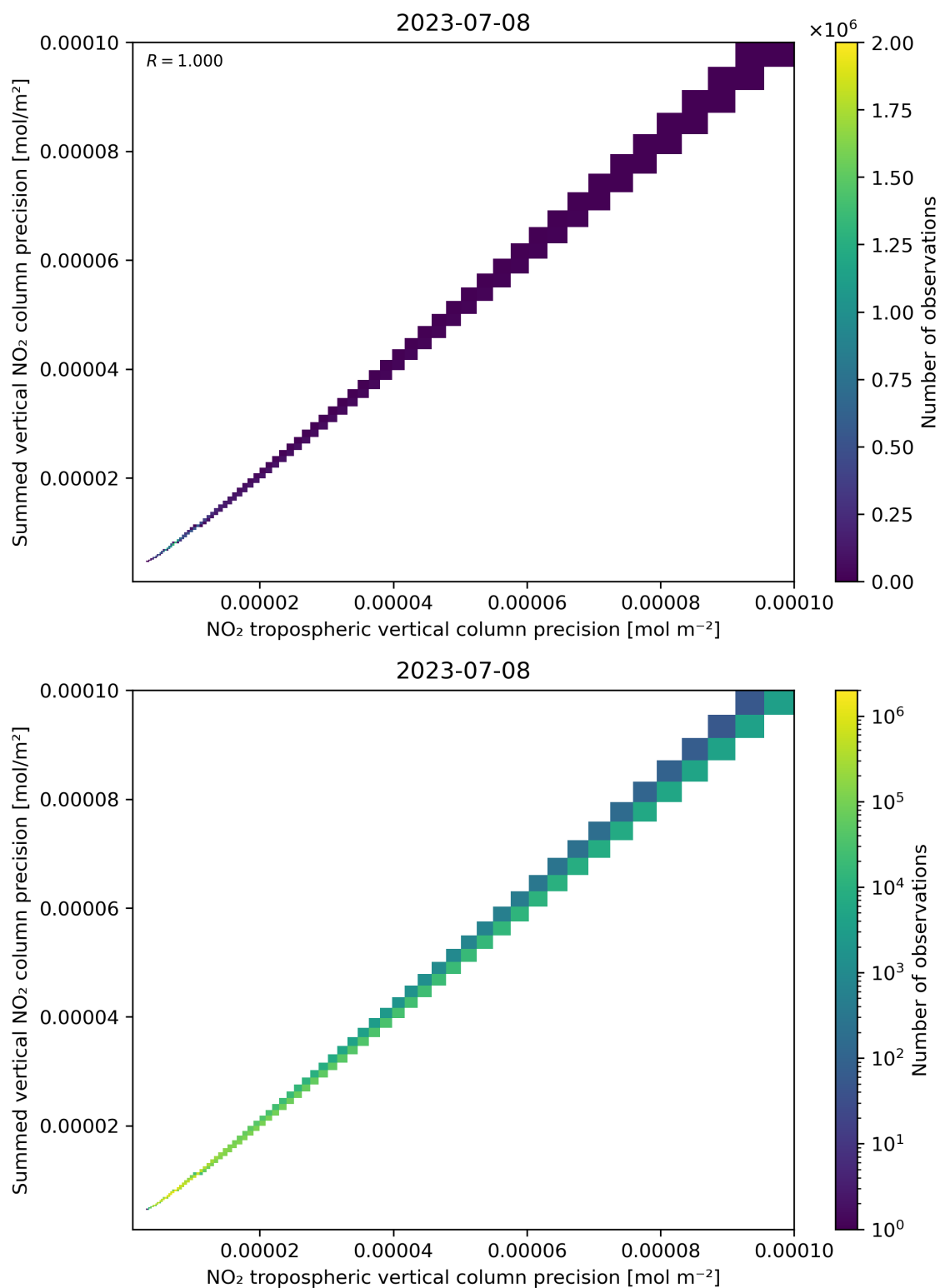
Figure 137: Scatter density plot of “NO 2 tropospheric vertical column precision” against “Summed vertical NO 2 column precision” for 2023-07-08 to 2023-07-09.
