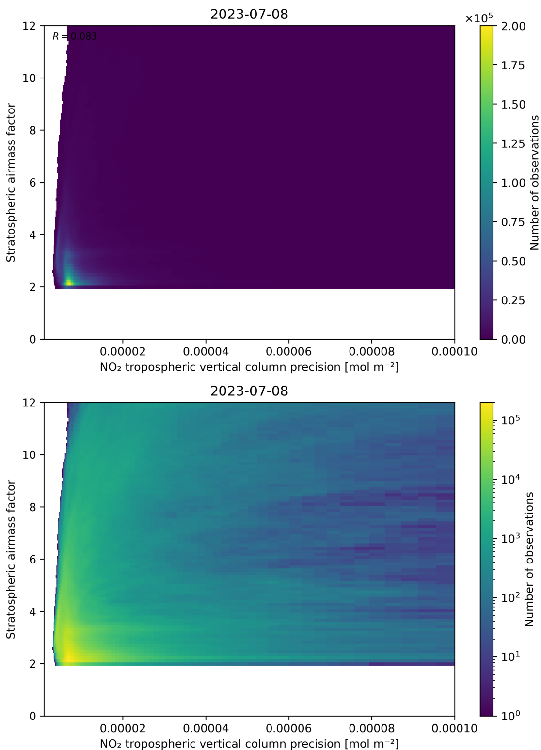
Figure 131: Scatter density plot of “NO 2 tropospheric vertical column precision” against “Stratospheric airmass factor” for 2023-07-08 to 2023-07-09.
