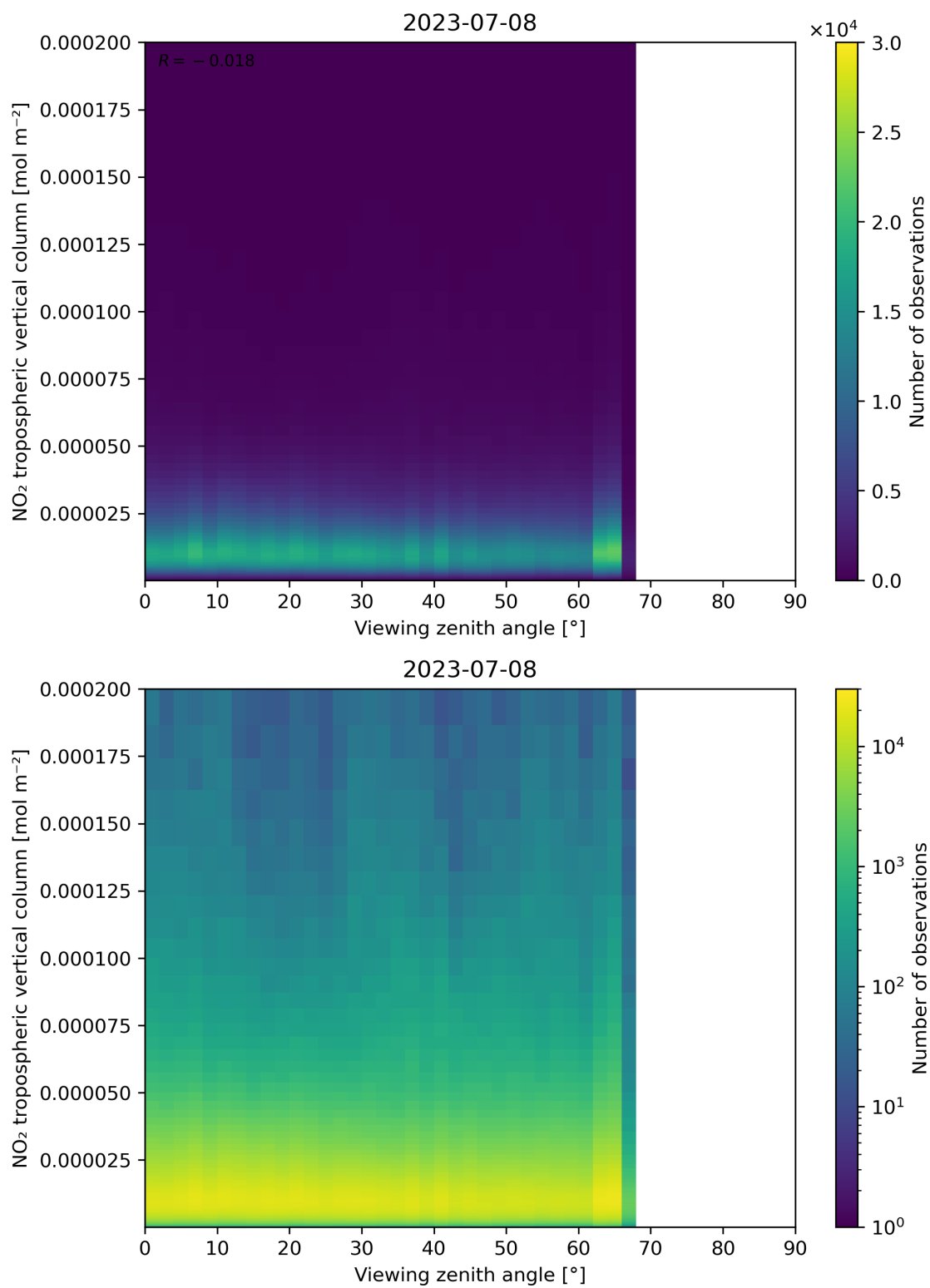
Figure 169: Scatter density plot of “Viewing zenith angle” against “NO 2 tropospheric vertical column” for 2023-07-08 to 2023-07-09.
