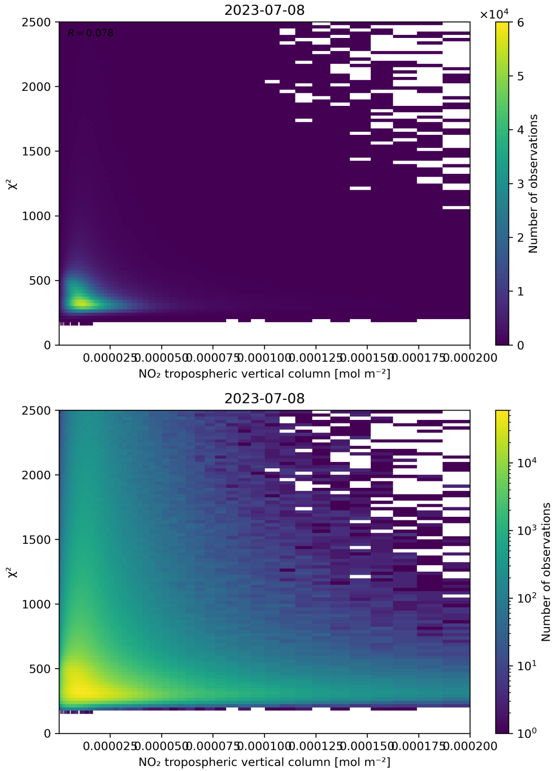
Figure 124: Scatter density plot of “NO 2 tropospheric vertical column” against “ \chi^2 ” for 2023-07-08 to 2023-07-09.
