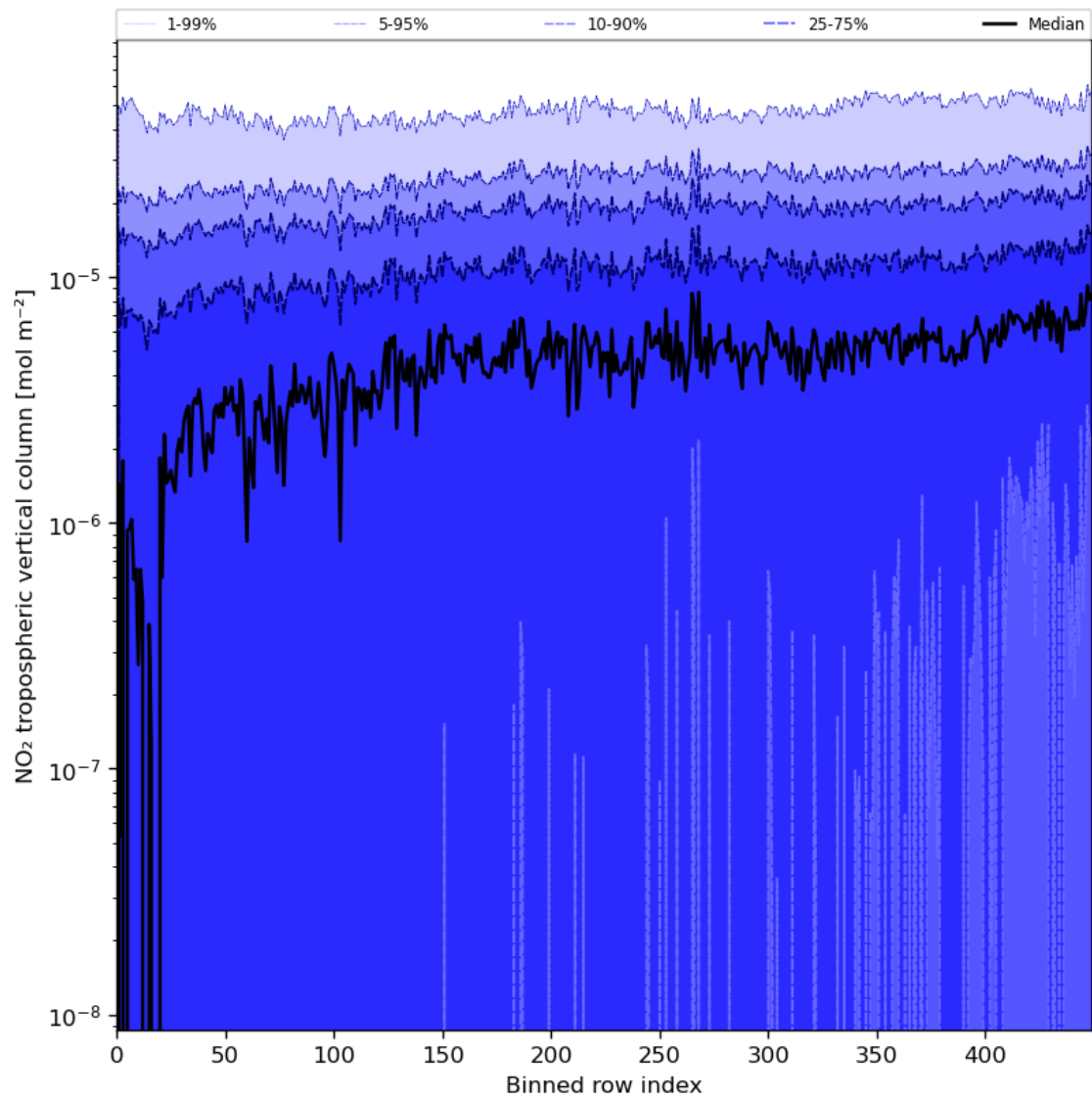
Figure 46: Along track statistics of “NO 2 tropospheric vertical column” for 2023-07-08 to 2023-07-09
