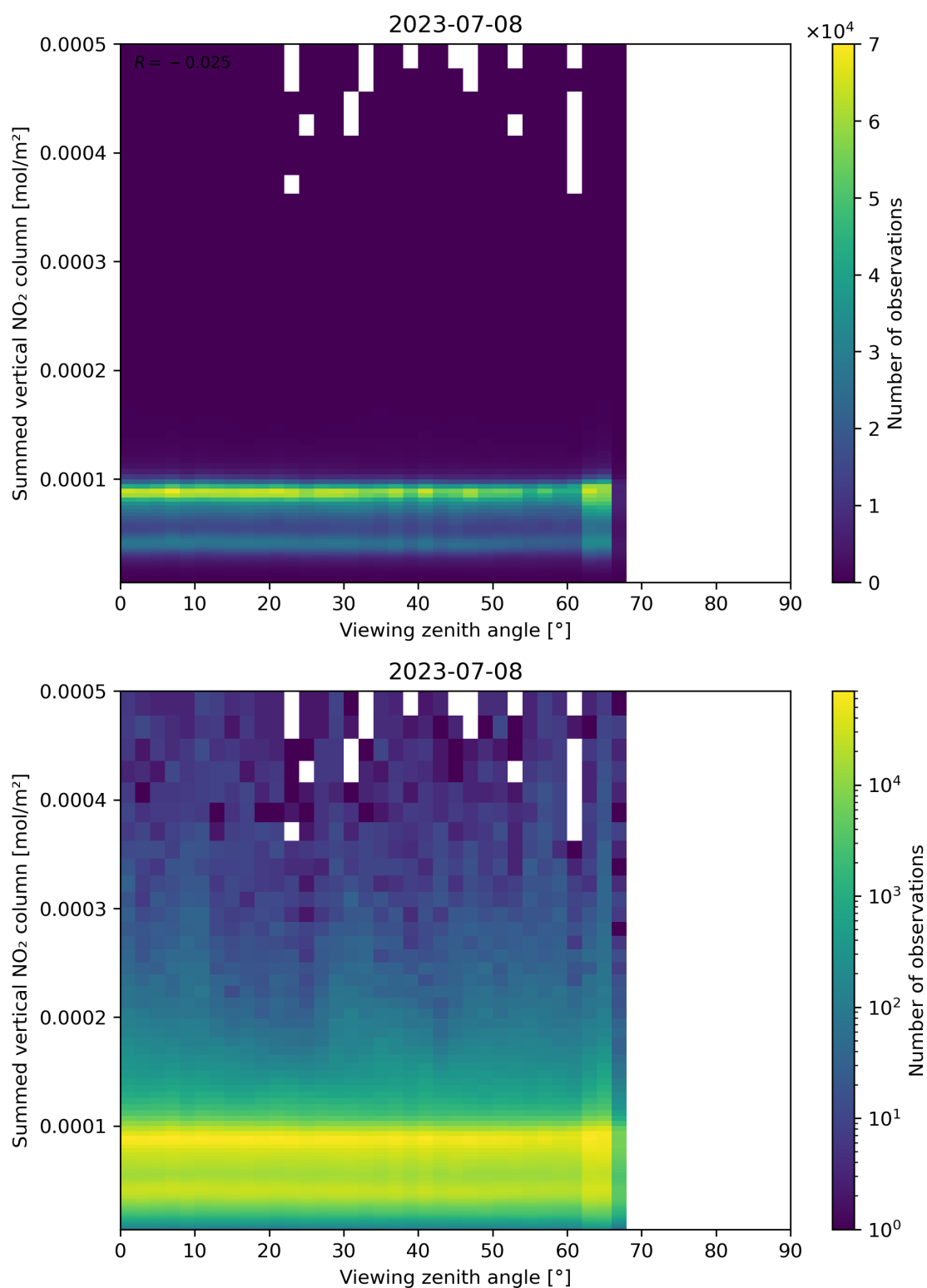
Figure 165: Scatter density plot of “Viewing zenith angle” against “Summed vertical NO 2 column” for 2023-07-08 to 2023-07-09.
