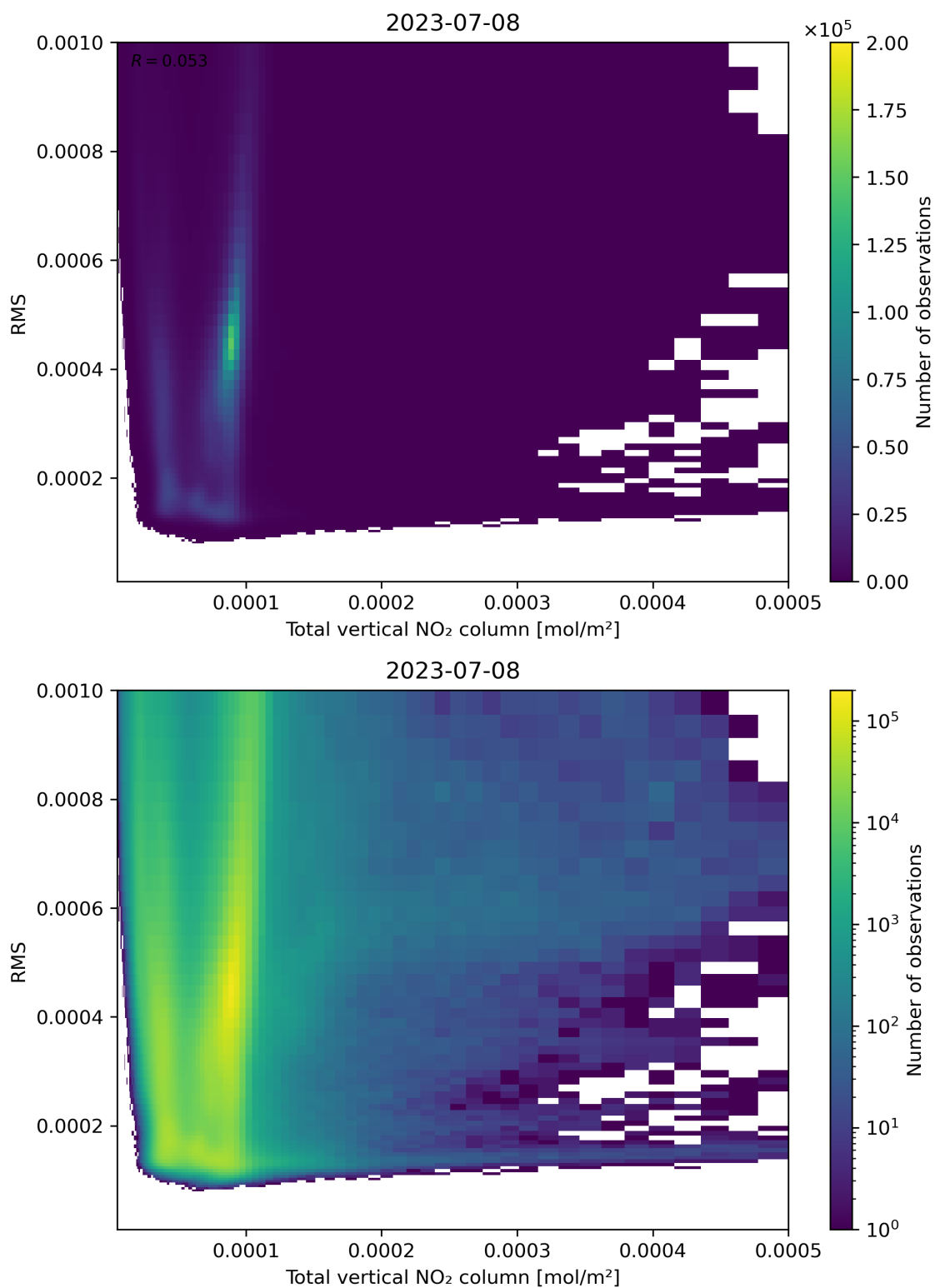
Figure 120: Scatter density plot of “Total vertical NO 2 column” against “RMS” for 2023-07-08 to 2023-07-09.
