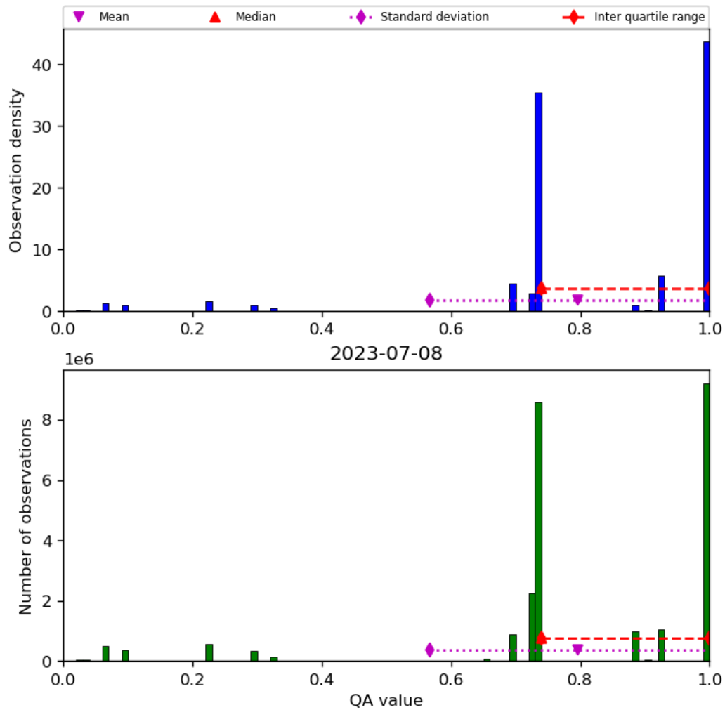
Figure 28: Histogram of “QA value” for 2023-07-08 to 2023-07-09
