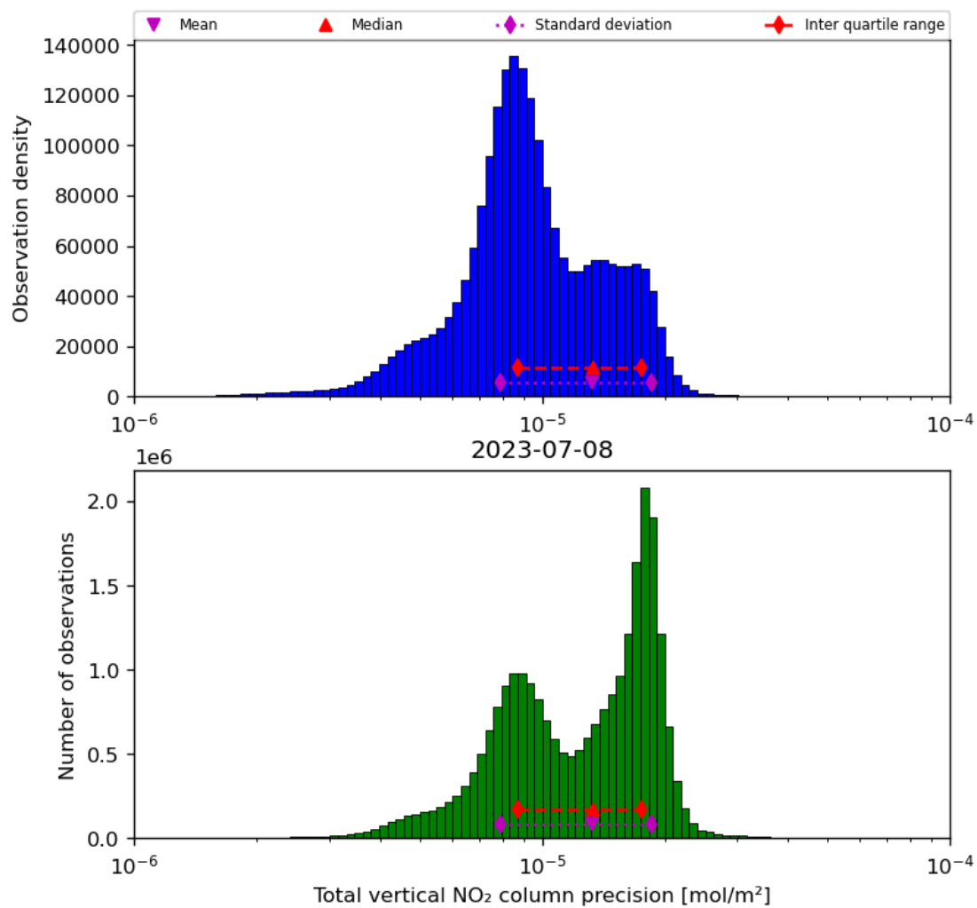
Figure 39: Histogram of “Total vertical NO 2 column precision” for 2023-07-08 to 2023-07-09
