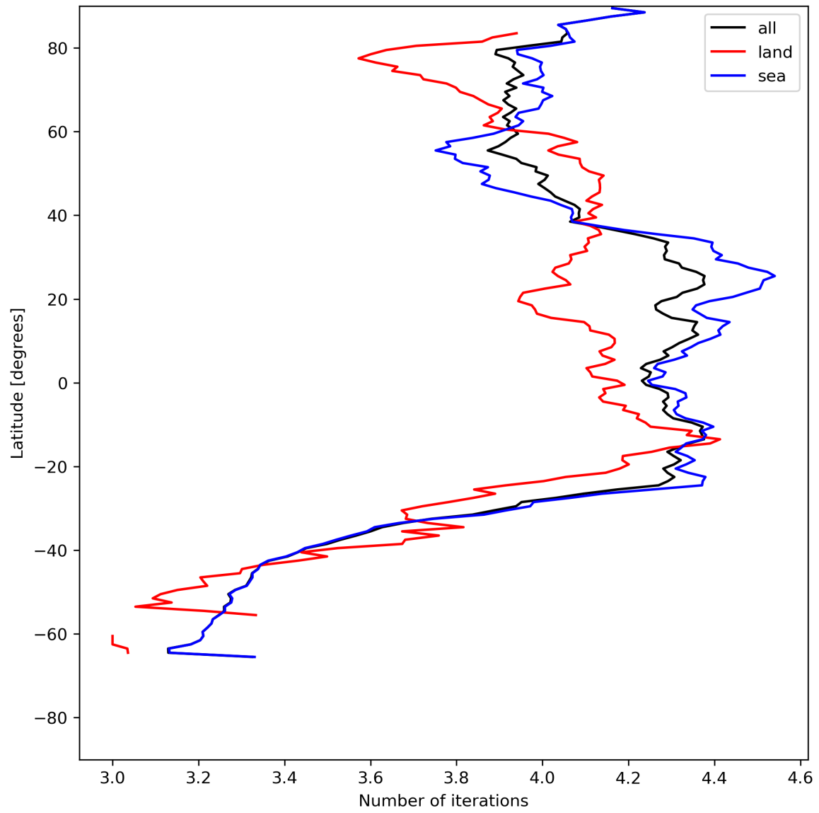
Figure 17: Zonal average of “Number of iterations” for 2023-07-08 to 2023-07-09.
