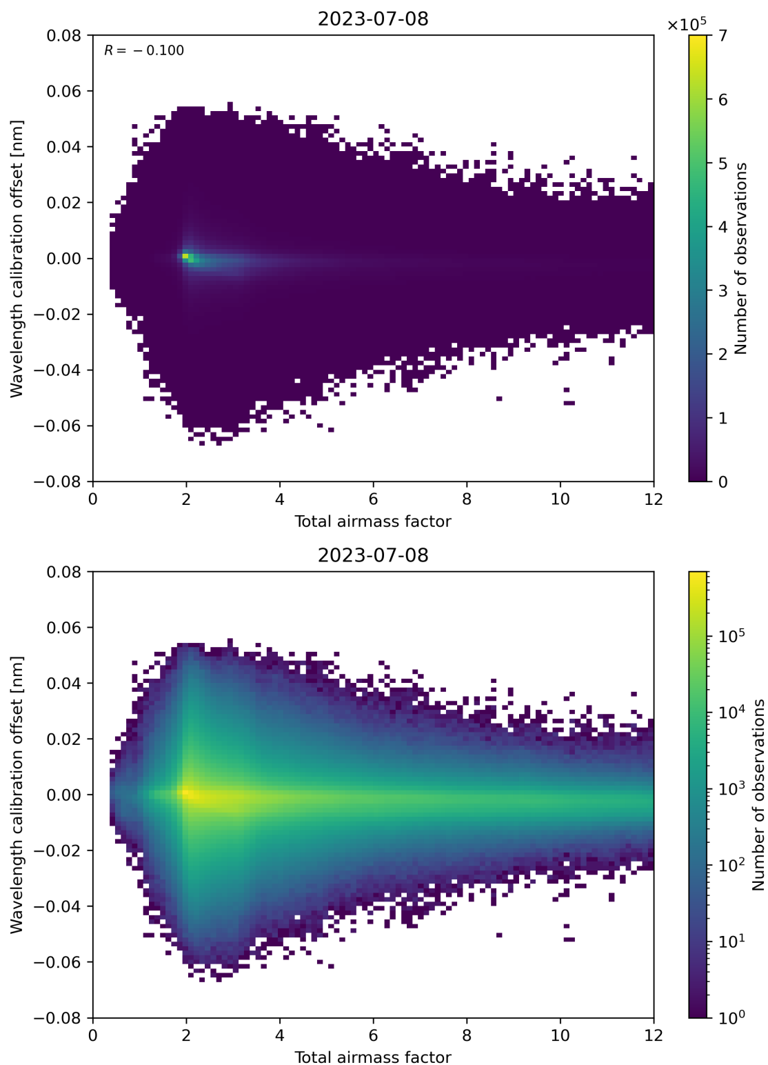
Figure 70: Scatter density plot of “Total airmass factor” against “Wavelength calibration offset” for 2023-07-08 to 2023-07-09.
