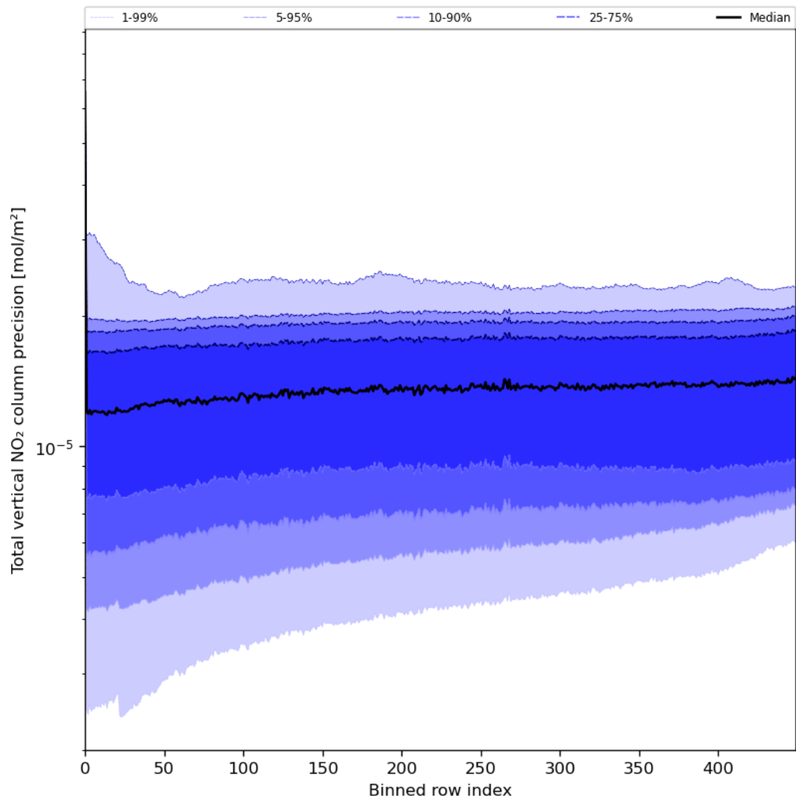
Figure 56: Along track statistics of “Total vertical NO 2 column precision” for 2023-07-08 to 2023-07-09
