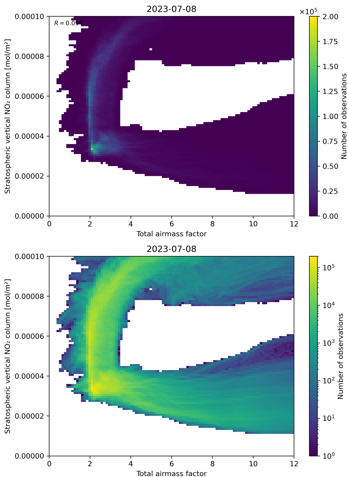
Figure 64: Scatter density plot of “Total airmass factor” against “Stratospheric vertical NO 2 column” for 2023-07-08 to 2023-07-09.
