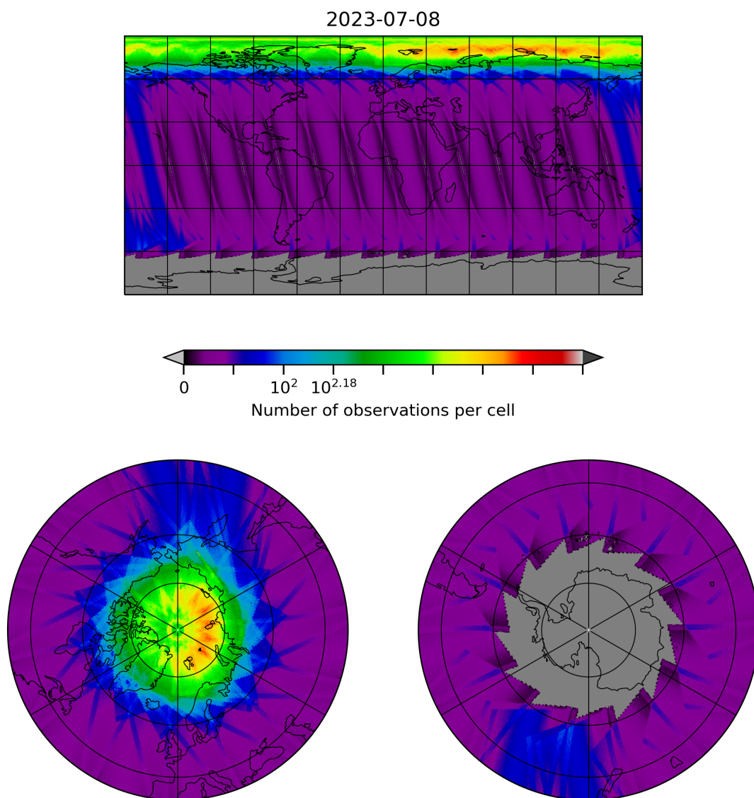
Figure 10: Map of the number of observations for 2023-07-08 to 2023-07-09
