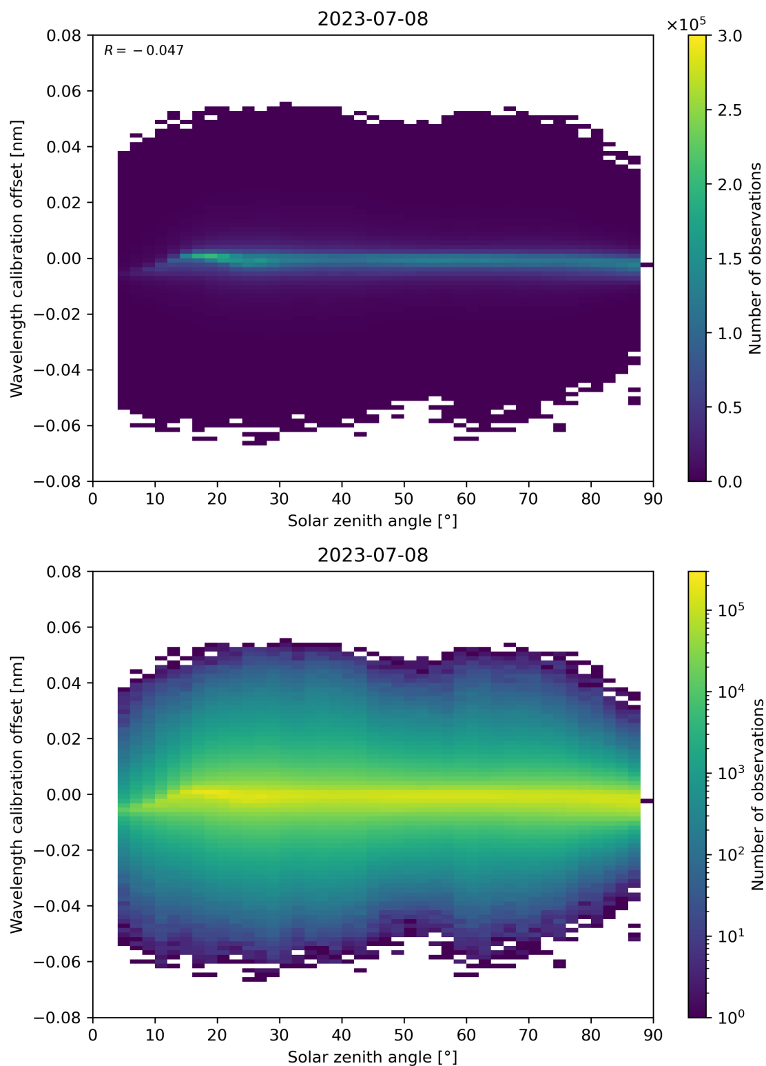
Figure 158: Scatter density plot of “Solar zenith angle” against “Wavelength calibration offset” for 2023-07-08 to 2023-07-09.
