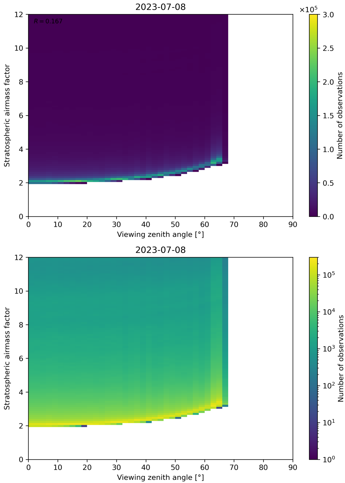
Figure 159: Scatter density plot of “Viewing zenith angle” against “Stratospheric airmass factor” for 2023-07-08 to 2023-07-09.
