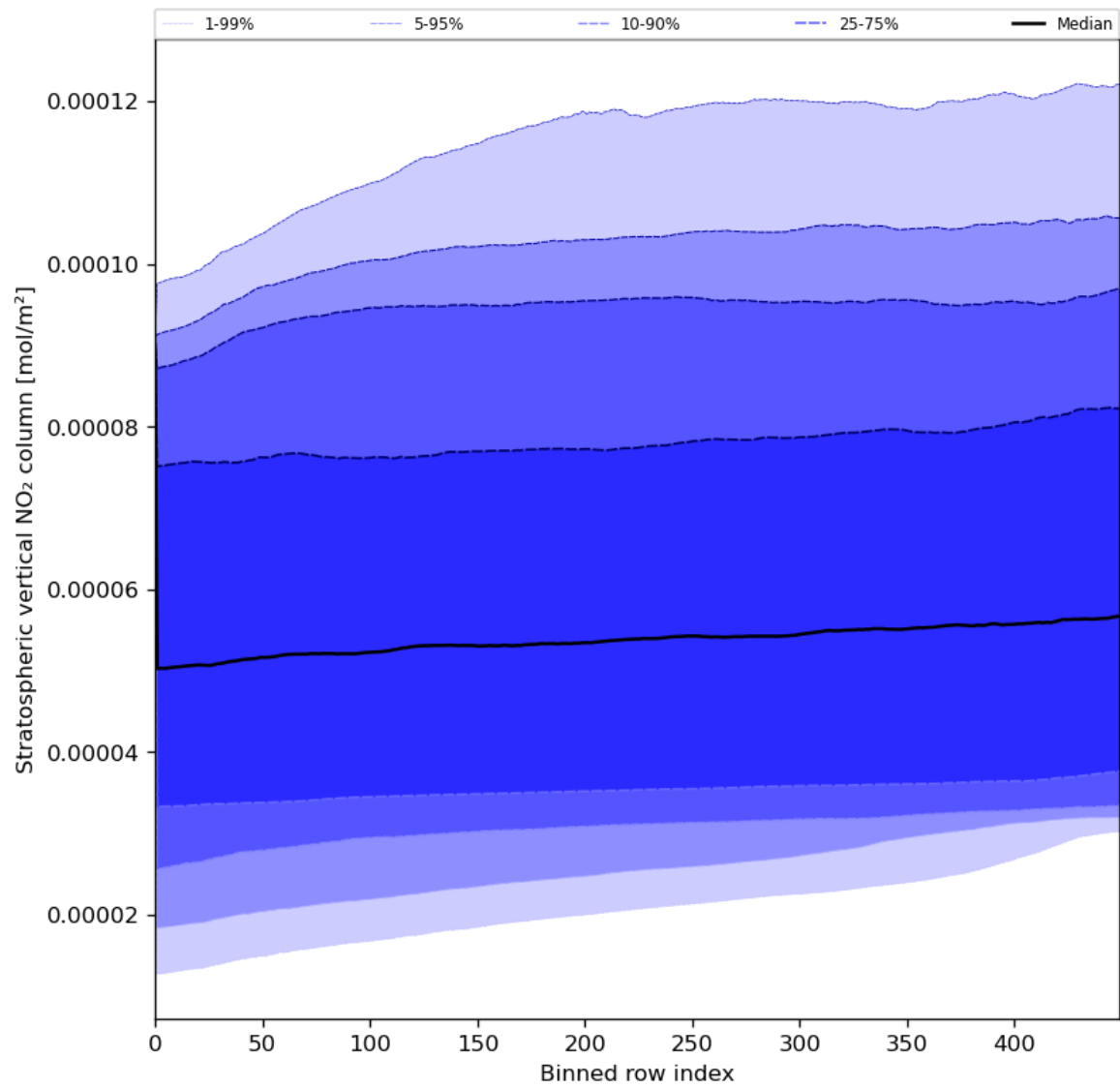
Figure 53: Along track statistics of “Stratospheric vertical NO 2 column” for 2023-07-08 to 2023-07-09
