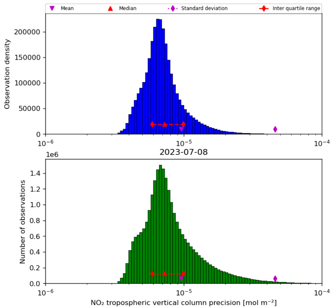
Figure 30: Histogram of “NO 2 tropospheric vertical column precision” for 2023-07-08 to 2023-07-09
