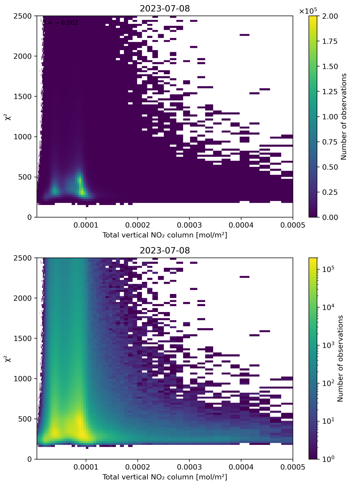
Figure 111: Scatter density plot of “Total vertical NO 2 column” against “ \chi^2 ” for 2023-07-08 to 2023-07-09.
