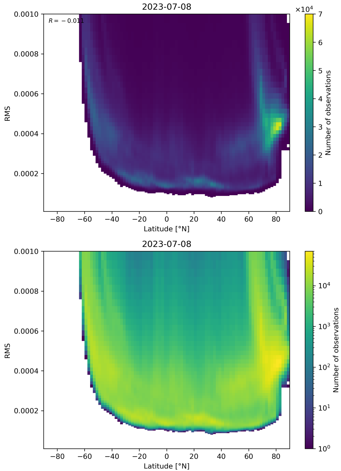
Figure 94: Scatter density plot of “Latitude” against “RMS” for 2023-07-08 to 2023-07-09.
