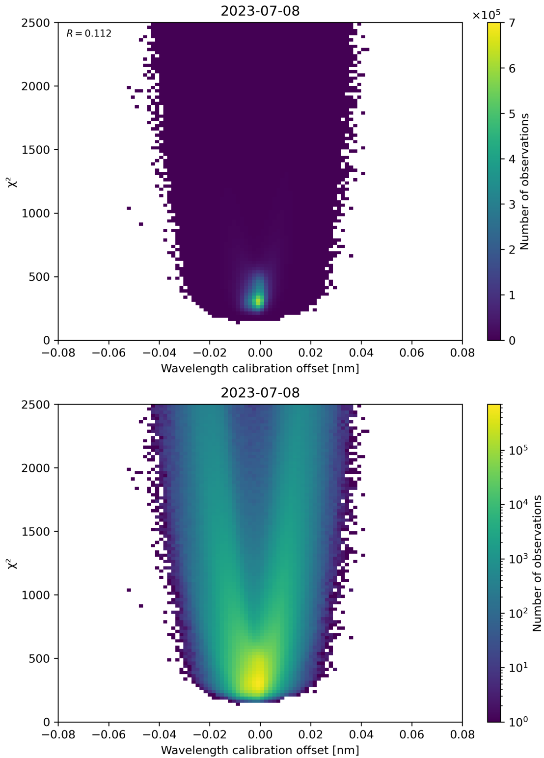
Figure 175: Scatter density plot of “Wavelength calibration offset” against “ \chi^2 ” for 2023-07-08 to 2023-07-09.
