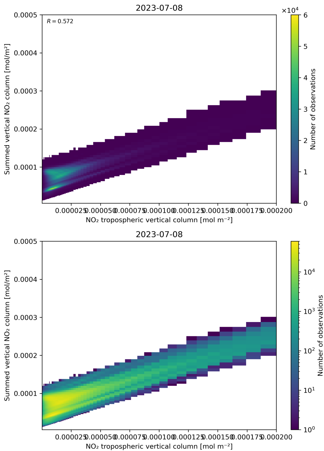
Figure 126: Scatter density plot of “NO 2 tropospheric vertical column” against “Summed vertical NO 2 column” for 2023-07-08 to 2023-07-09.
