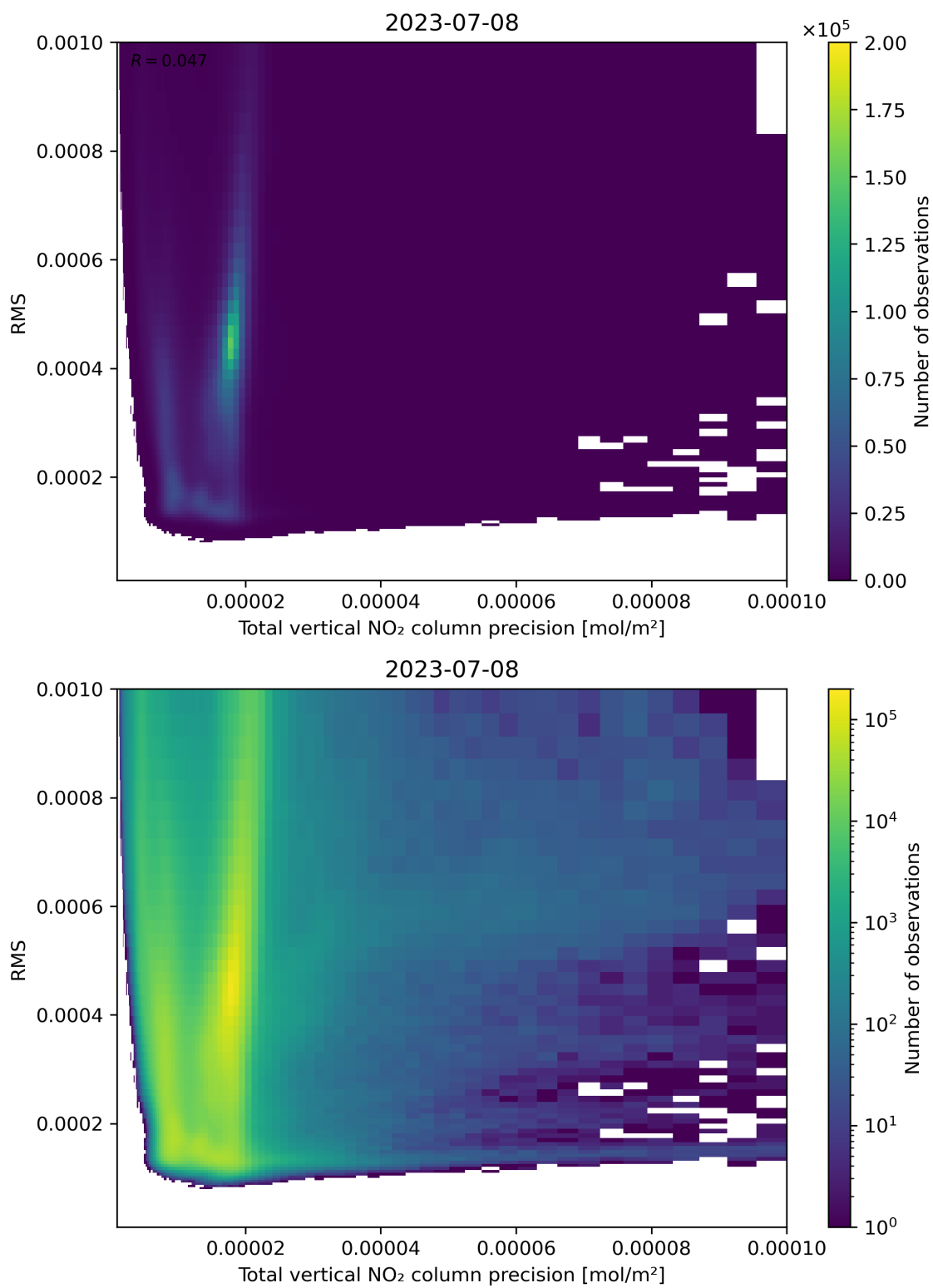
Figure 119: Scatter density plot of “Total vertical NO 2 column precision” against “RMS” for 2023-07-08 to 2023-07-09.
