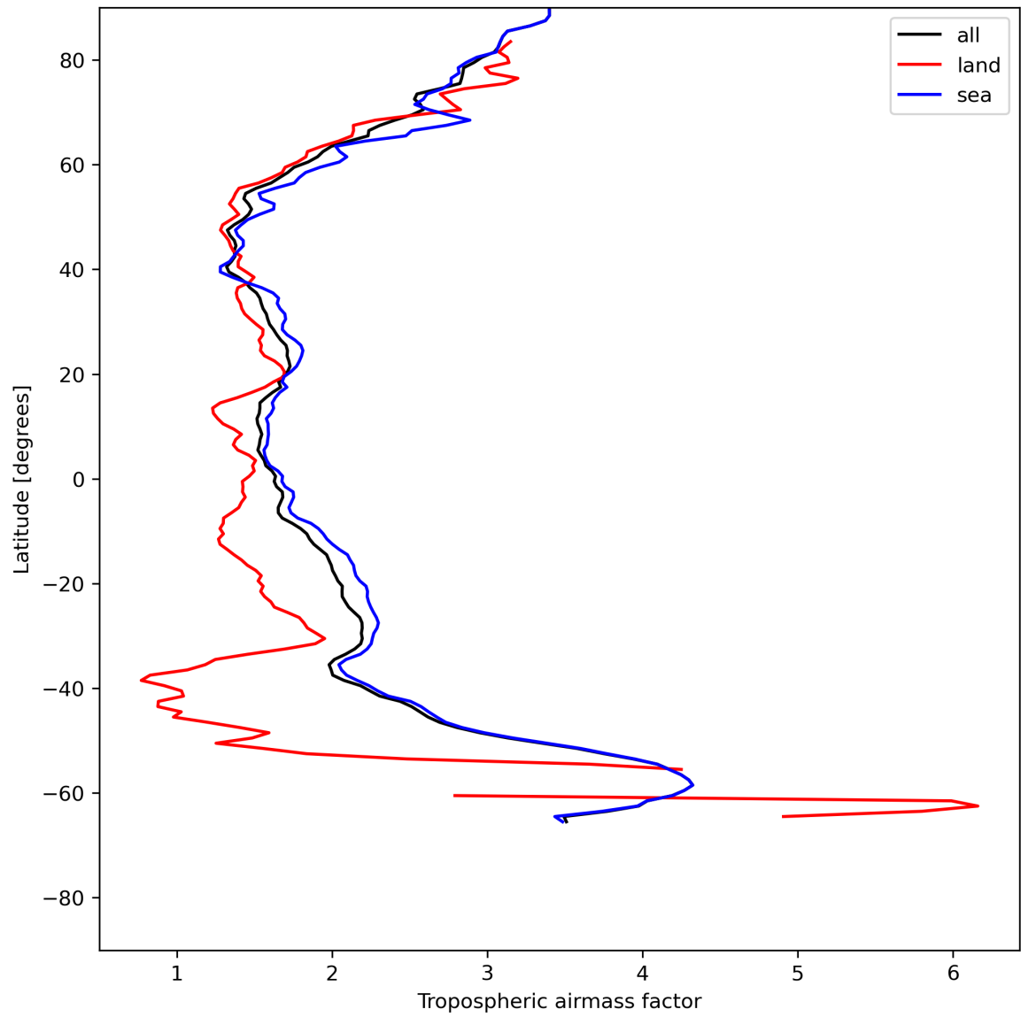
Figure 14: Zonal average of “Tropospheric airmass factor” for 2023-07-08 to 2023-07-09.
