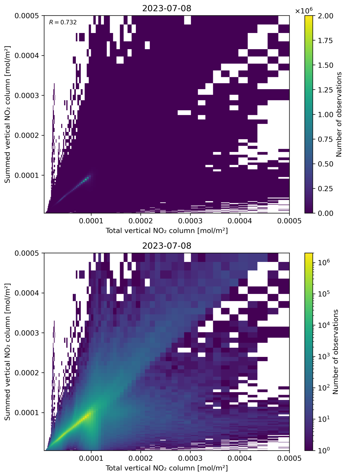
Figure 112: Scatter density plot of “Total vertical NO 2 column” against “Summed vertical NO 2 column” for 2023-07-08 to 2023-07-09.
