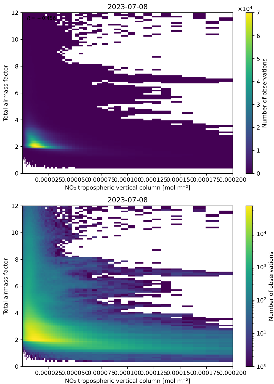
Figure 122: Scatter density plot of “NO 2 tropospheric vertical column” against “Total air mass factor” for 2023-07-08 to 2023-07-09.
