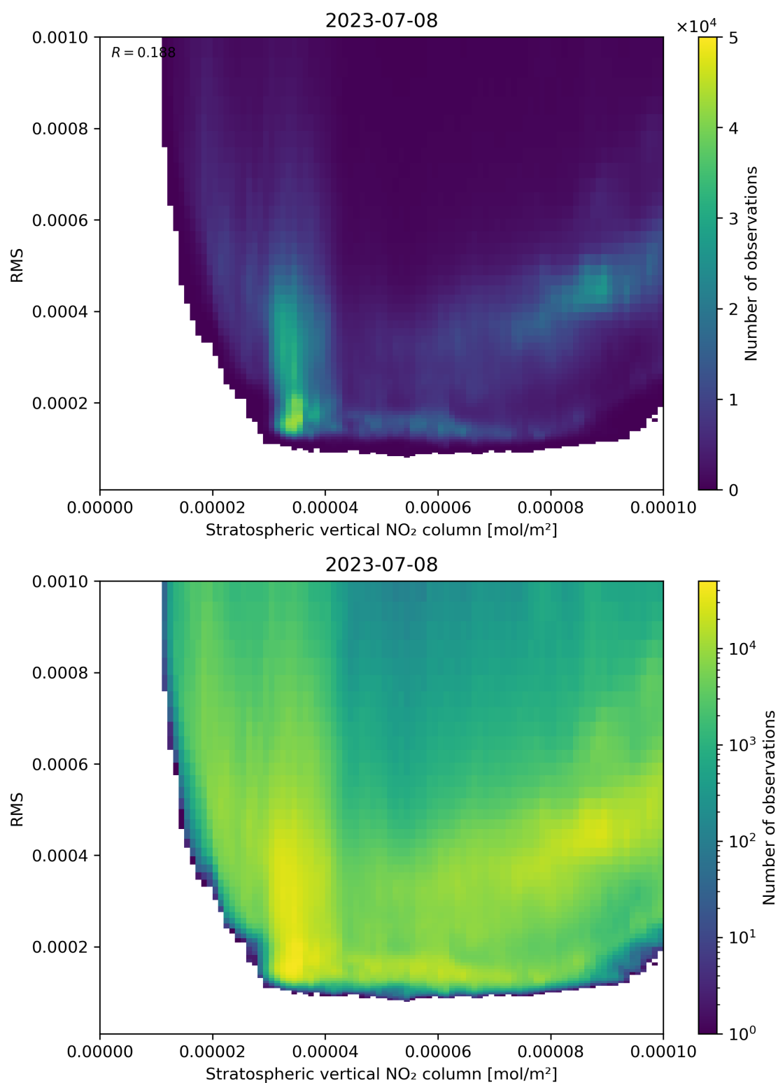
Figure 102: Scatter density plot of “Stratospheric vertical NO 2 column” against “RMS” for 2023-07-08 to 2023-07-09.
