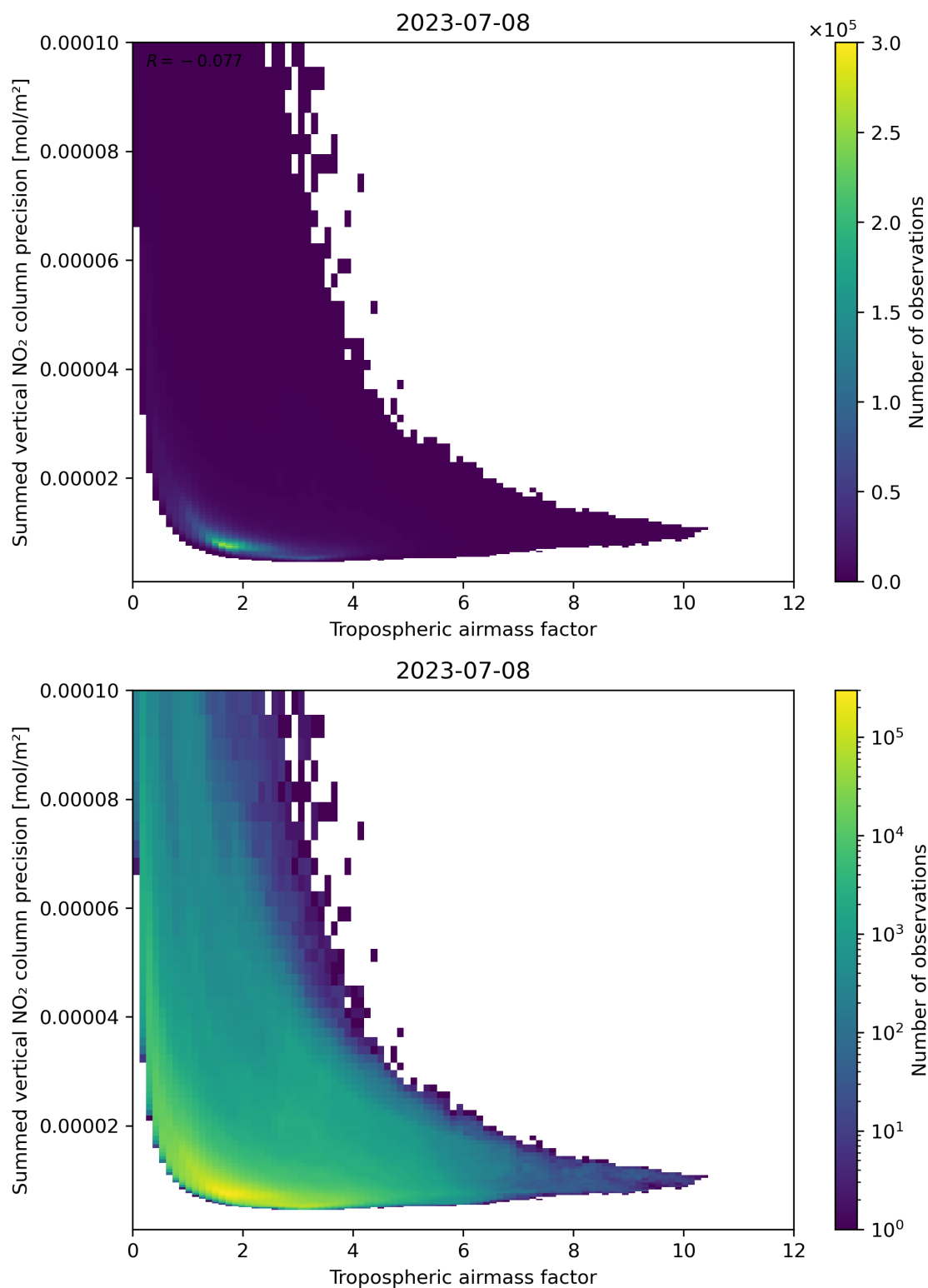
Figure 76: Scatter density plot of “Tropospheric air mass factor” against “Summed vertical NO 2 column precision” for 2023-07-08 to 2023-07-09.
