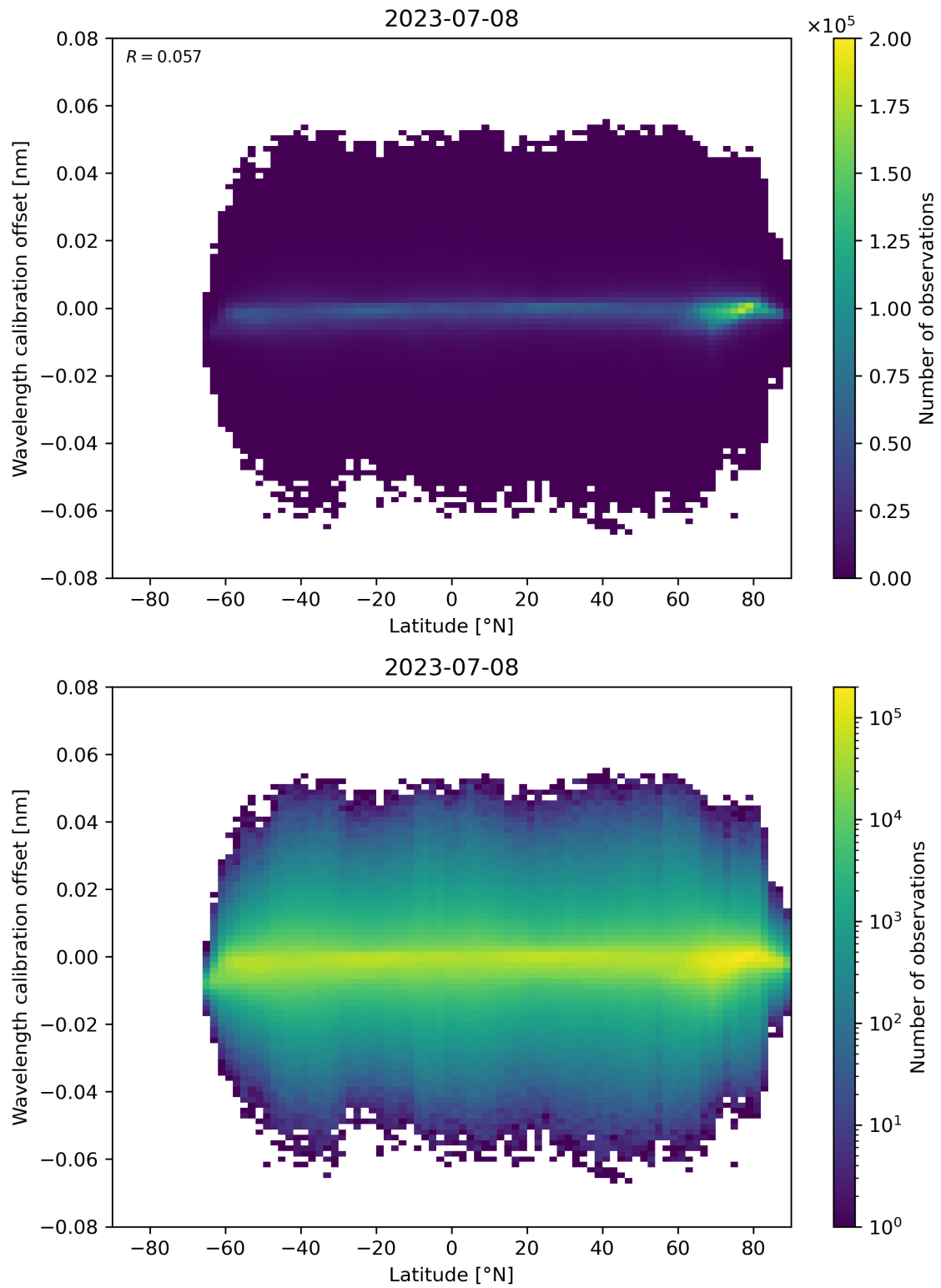
Figure 95: Scatter density plot of “Latitude” against “Wavelength calibration offset” for 2023-07-08 to 2023-07-09.
