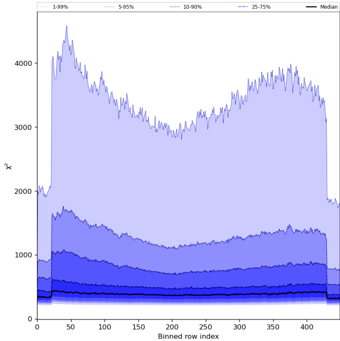
Figure 59: Along track statistics of “ \chi^2 ” for 2023-07-08 to 2023-07-09
