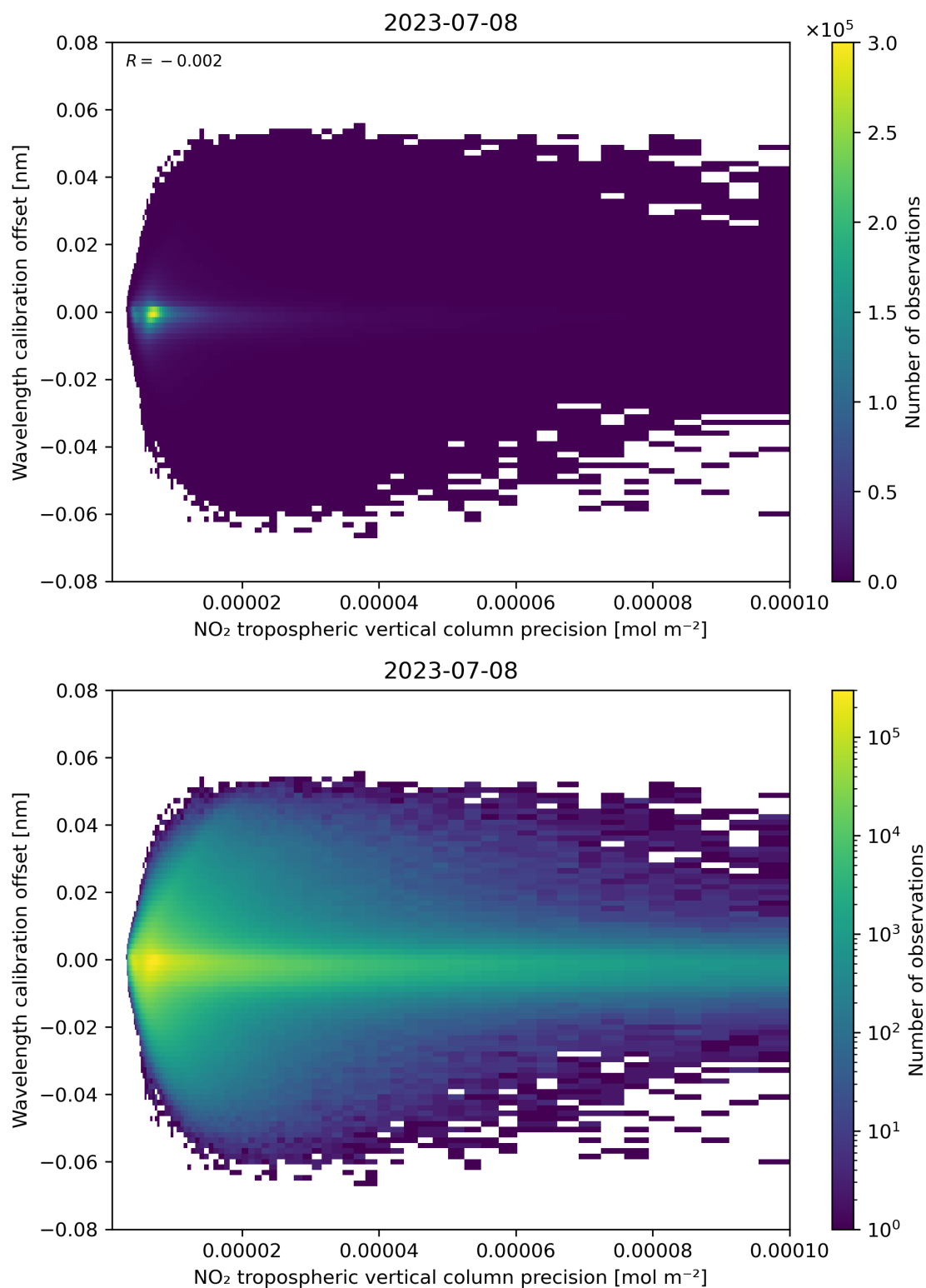
Figure 141: Scatter density plot of “NO 2 tropospheric vertical column precision” against “Wavelength calibration offset” for 2023-07-08 to 2023-07-09.
