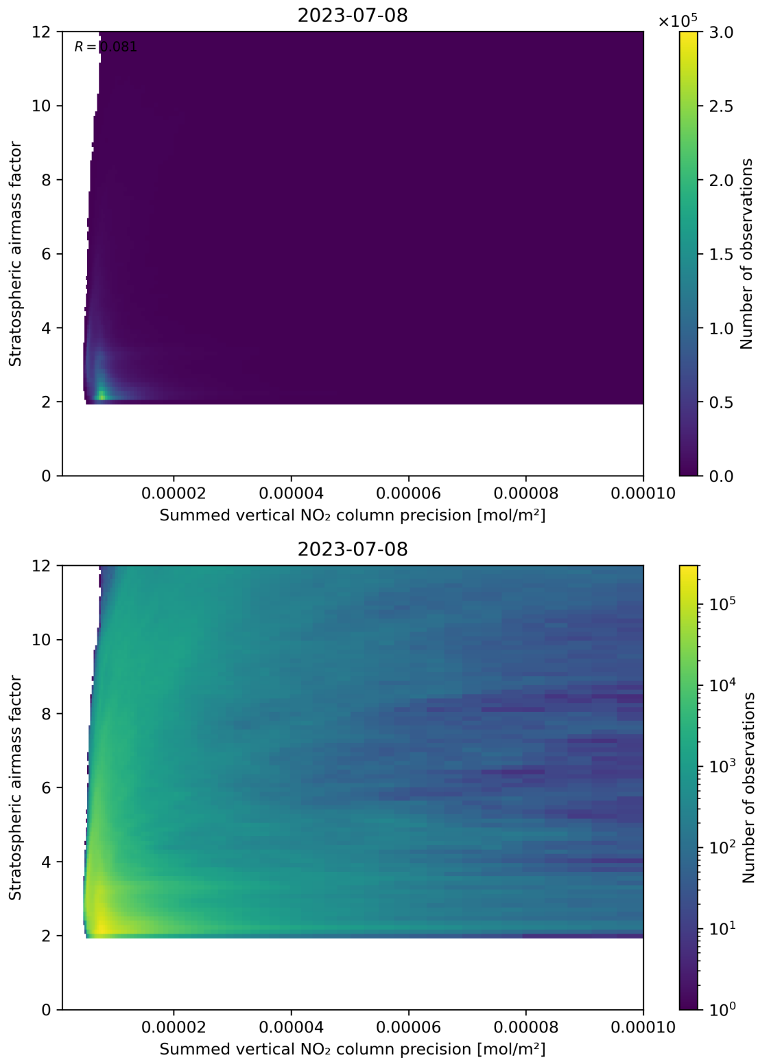
Figure 106: Scatter density plot of “Summed vertical NO 2 column precision” against “Stratospheric airmass factor” for 2023-07-08 to 2023-07-09.
