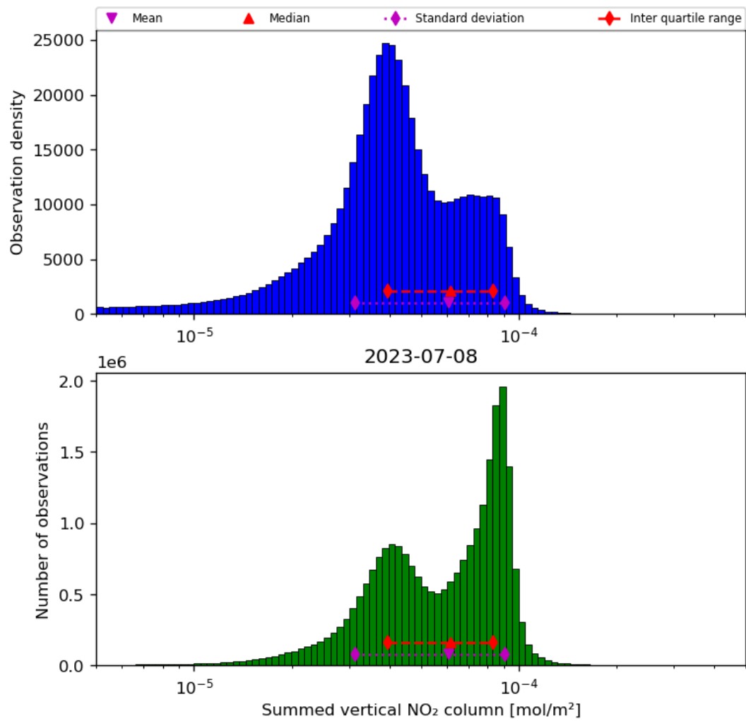
Figure 40: Histogram of “Summed vertical NO 2 column” for 2023-07-08 to 2023-07-09
