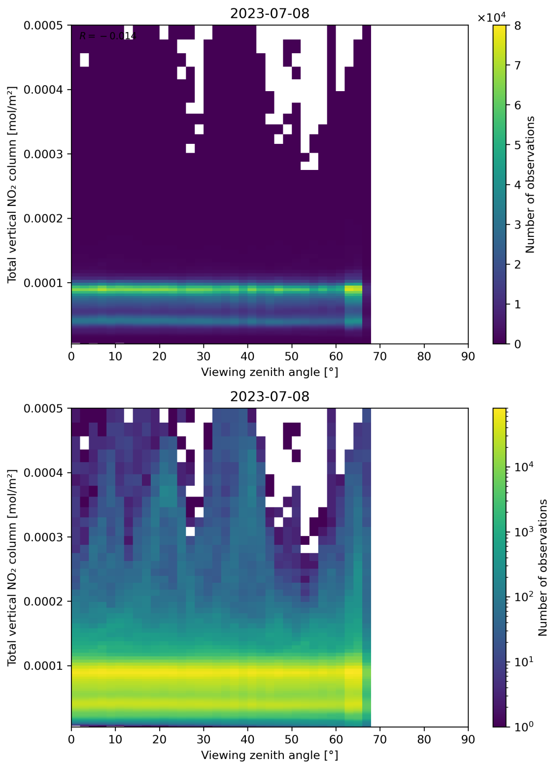
Figure 167: Scatter density plot of “Viewing zenith angle” against “Total vertical NO 2 column” for 2023-07-08 to 2023-07-09.
