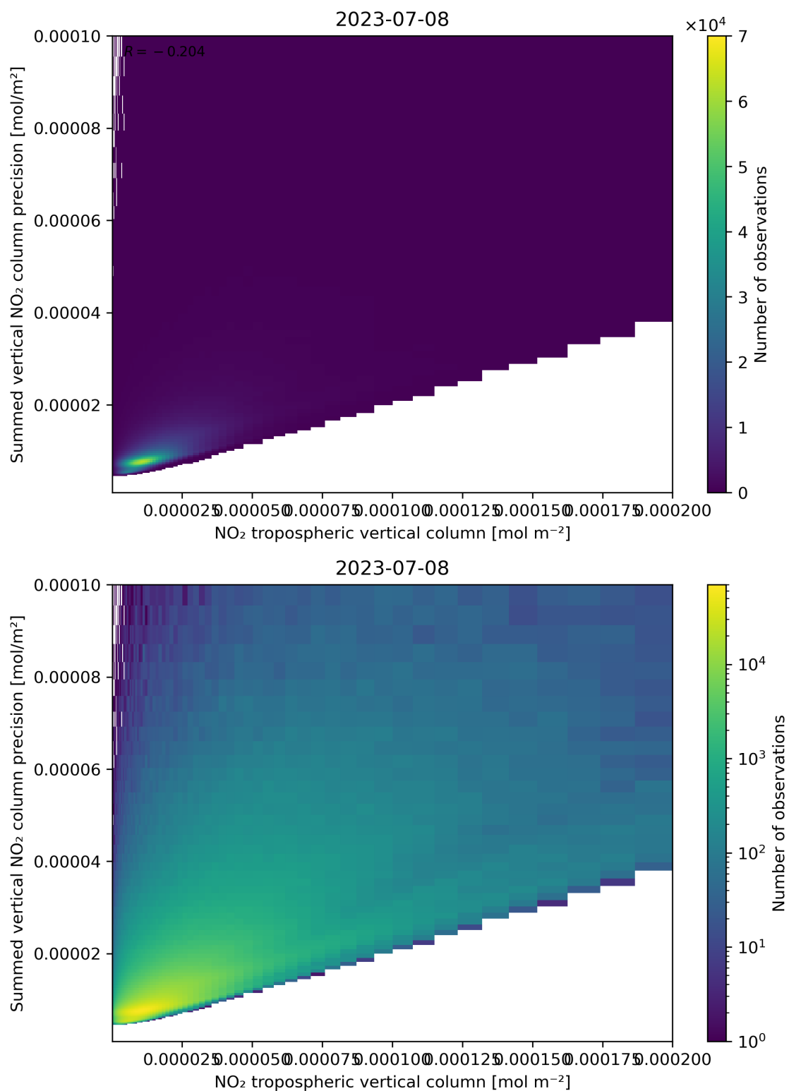
Figure 127: Scatter density plot of “NO 2 tropospheric vertical column” against “Summed vertical NO 2 column precision” for 2023-07-08 to 2023-07-09.
