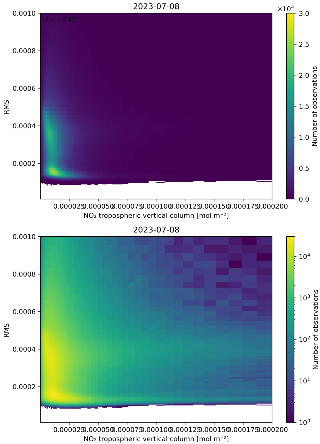
Figure 142: Scatter density plot of “NO 2 tropospheric vertical column” against “RMS” for 2023-07-08 to 2023-07-09.
