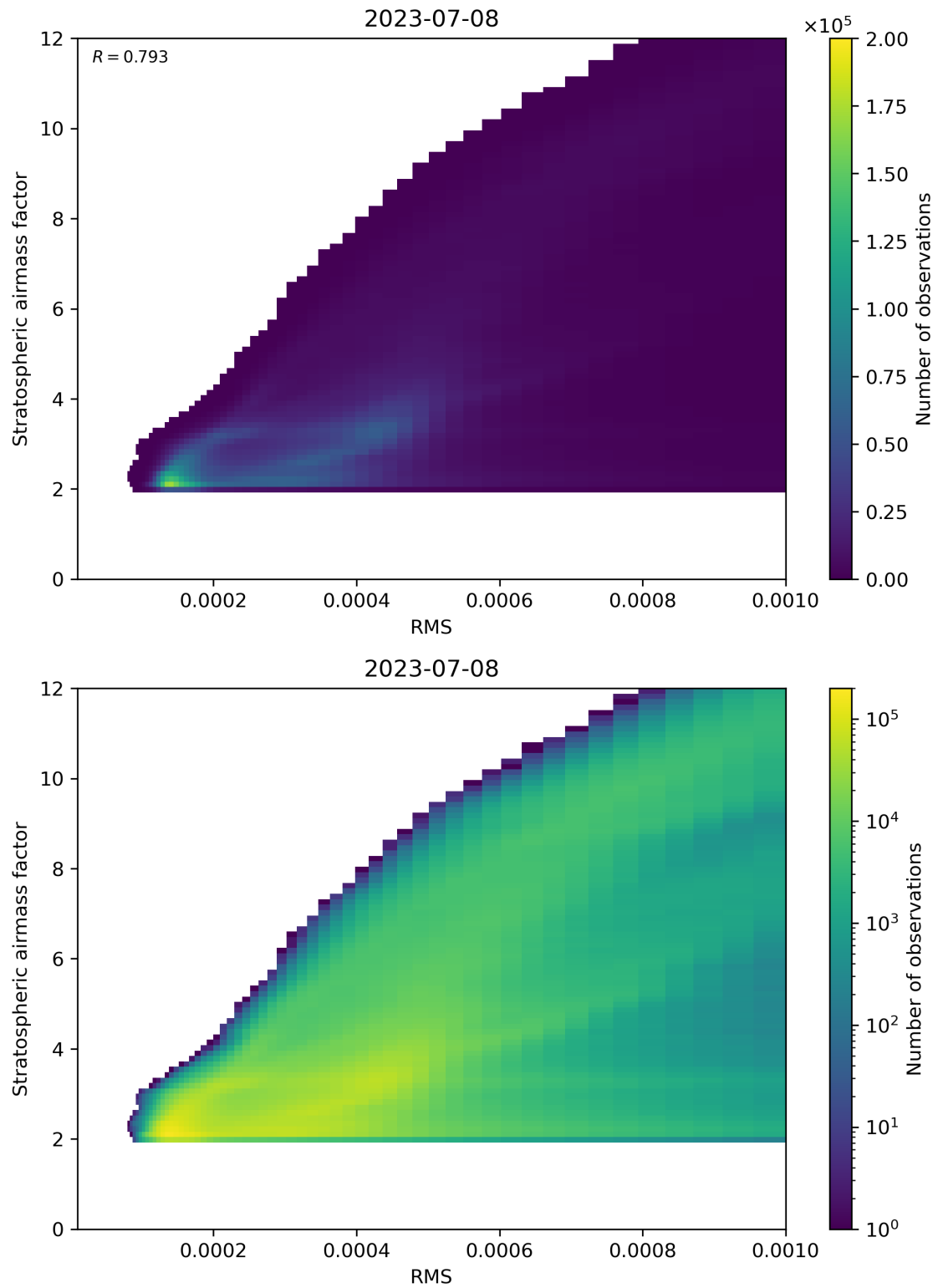
Figure 144: Scatter density plot of “RMS” against “Stratospheric airmass factor” for 2023-07-08 to 2023-07-09.
