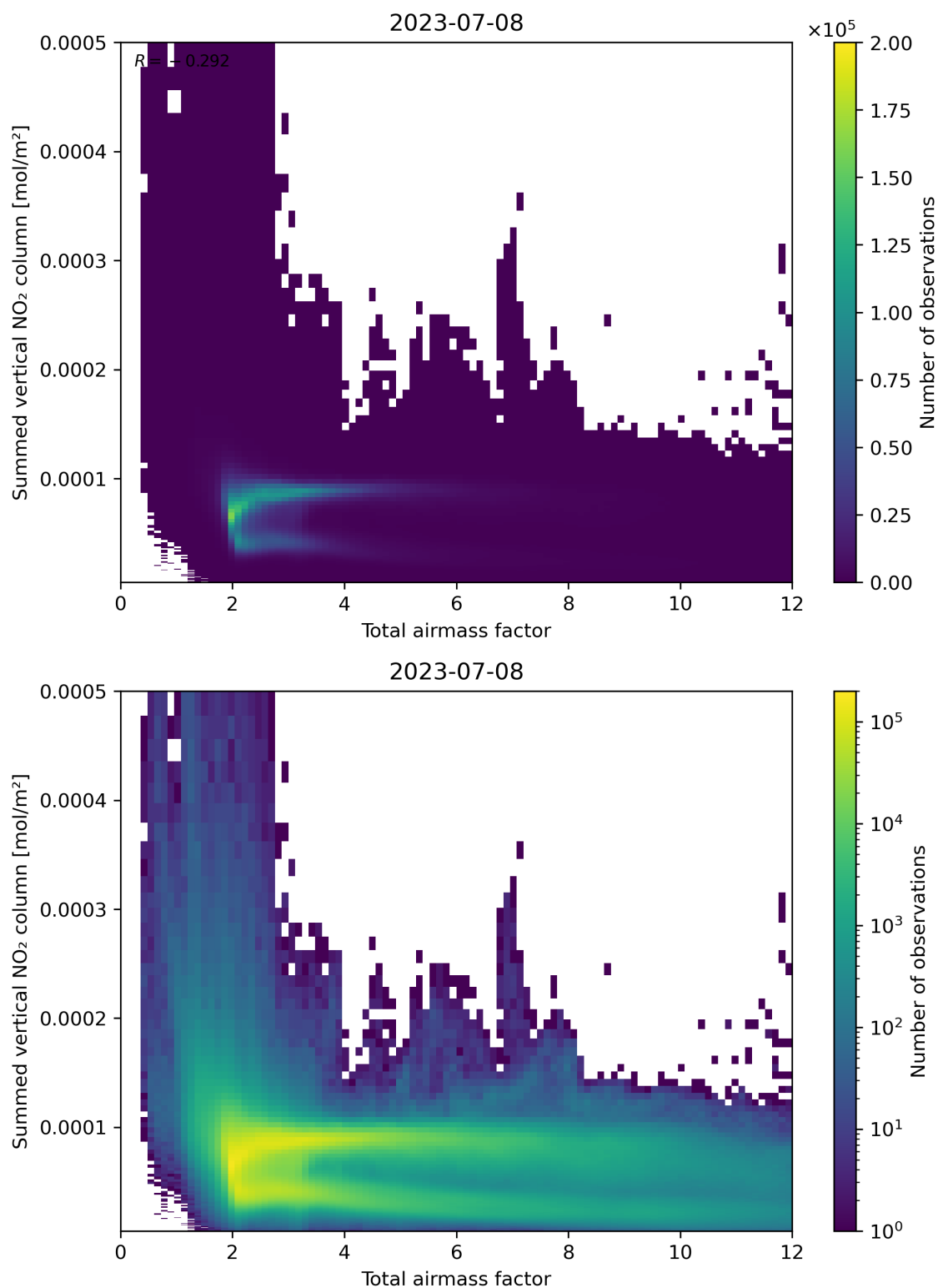
Figure 65: Scatter density plot of “Total airmass factor” against “Summed vertical NO 2 column” for 2023-07-08 to 2023-07-09.
