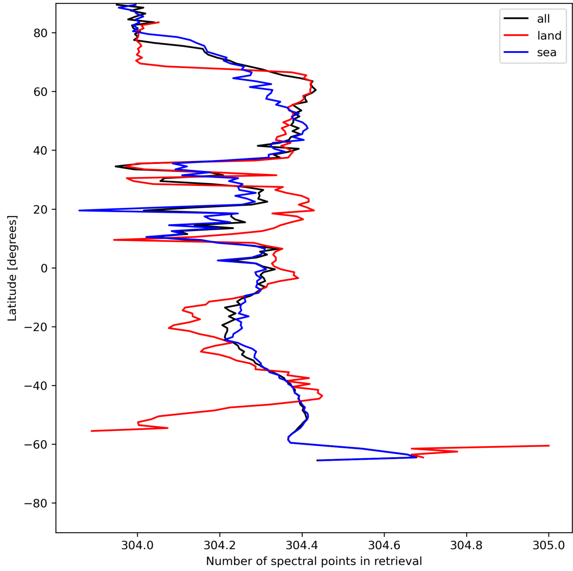
Figure 16: Zonal average of “Number of spectral points in retrieval” for 2023-07-08 to 2023-07-09.
