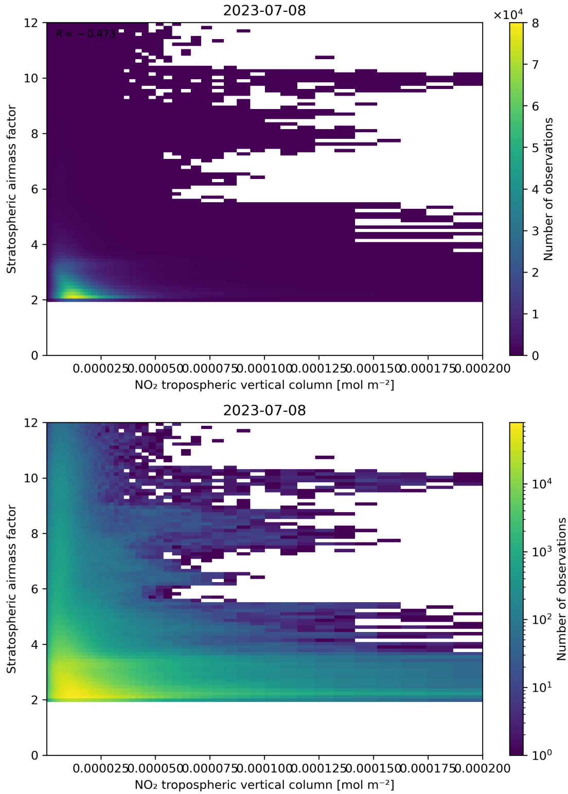
Figure 121: Scatter density plot of “NO 2 tropospheric vertical column” against “Stratospheric air mass factor” for 2023-07-08 to 2023-07-09.
