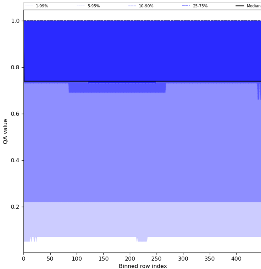
Figure 45: Along track statistics of “QA value” for 2023-07-08 to 2023-07-09
