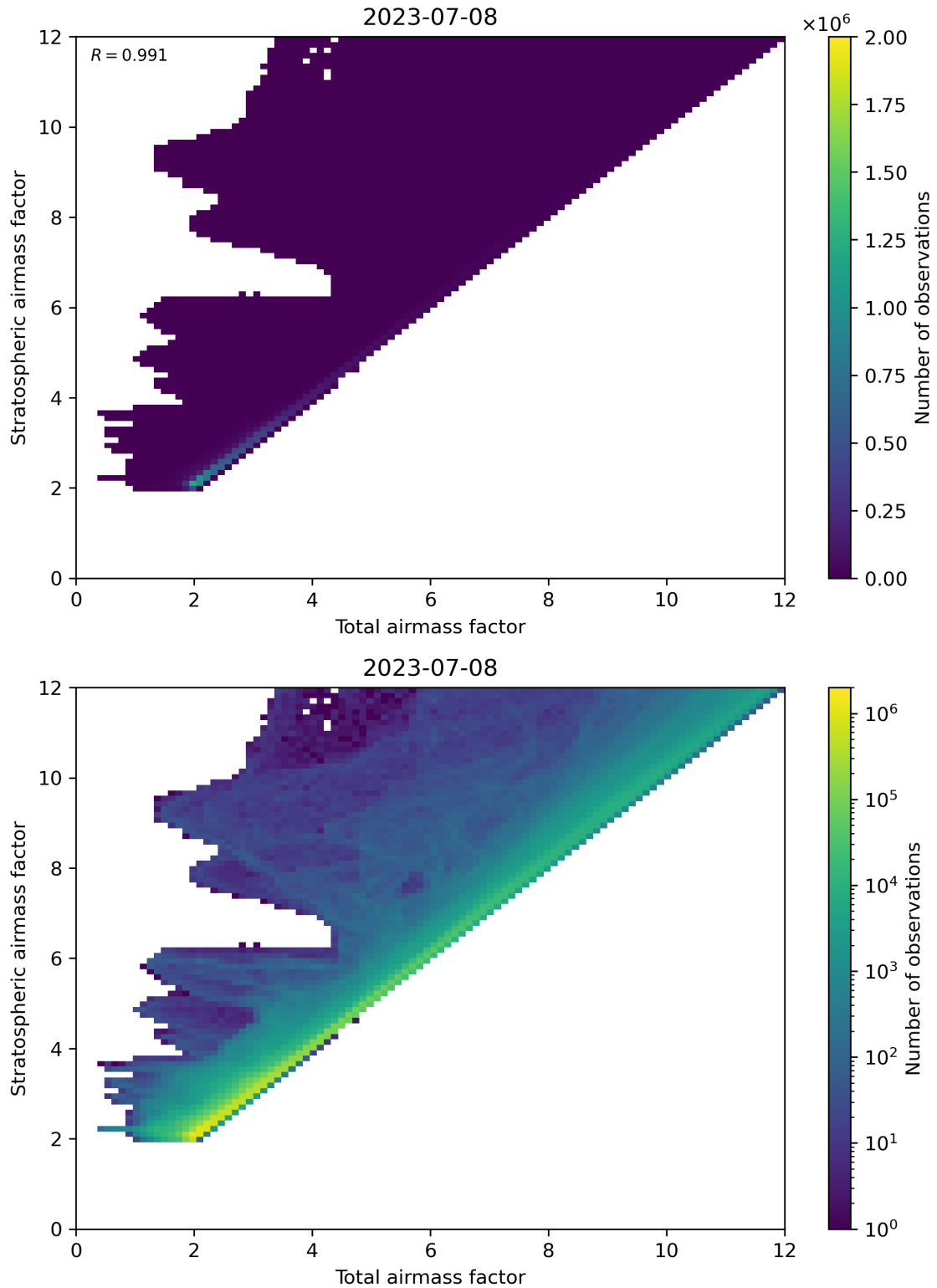
Figure 62: Scatter density plot of “Total airmass factor” against “Stratospheric airmass factor” for 2023-07-08 to 2023-07-09.
