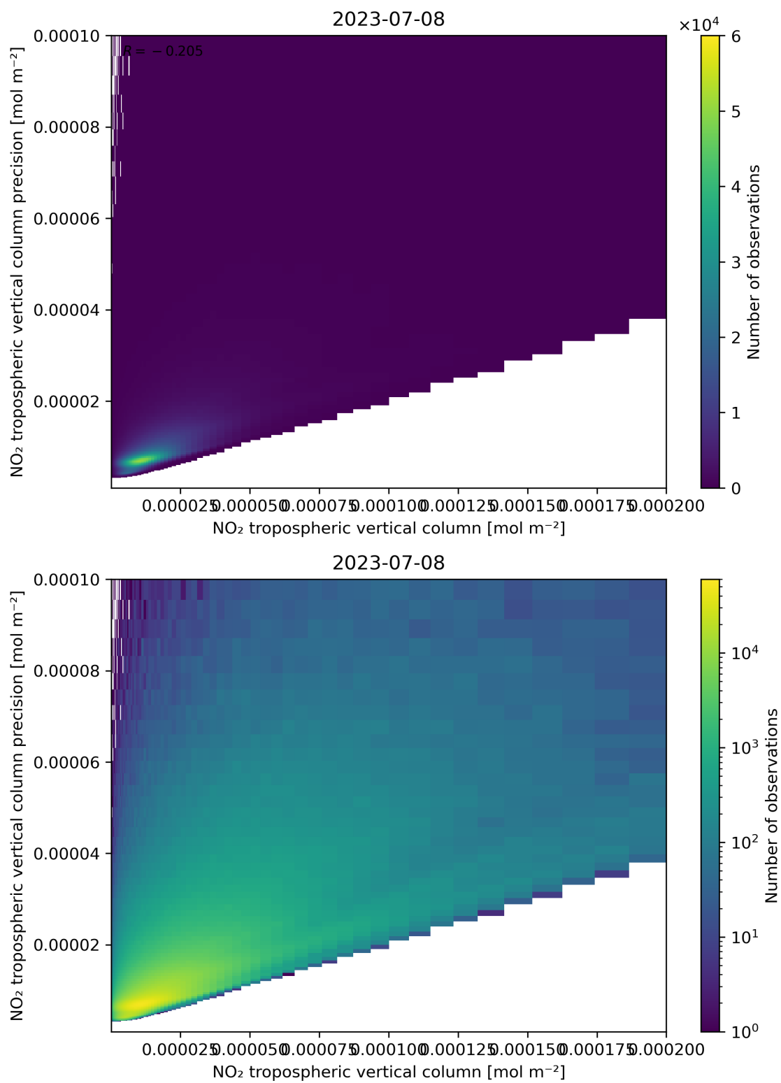
Figure 130: Scatter density plot of “NO 2 tropospheric vertical column” against “NO 2 tropospheric vertical column precision” for 2023-07-08 to 2023-07-09.
