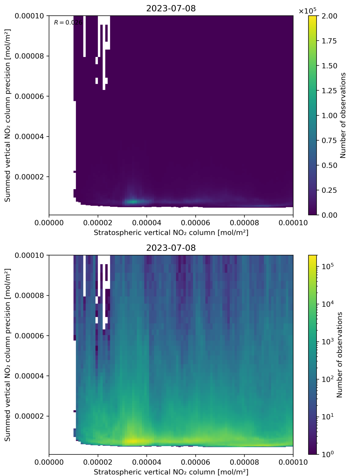
Figure 99: Scatter density plot of “Stratospheric vertical NO 2 column” against “Summed vertical NO 2 column precision” for 2023-07-08 to 2023-07-09.
