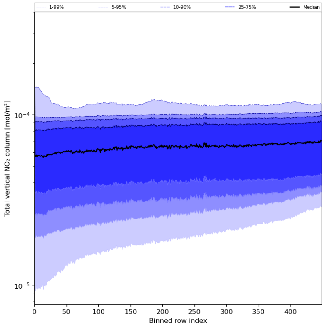
Figure 55: Along track statistics of “Total vertical NO 2 column” for 2023-07-08 to 2023-07-09
