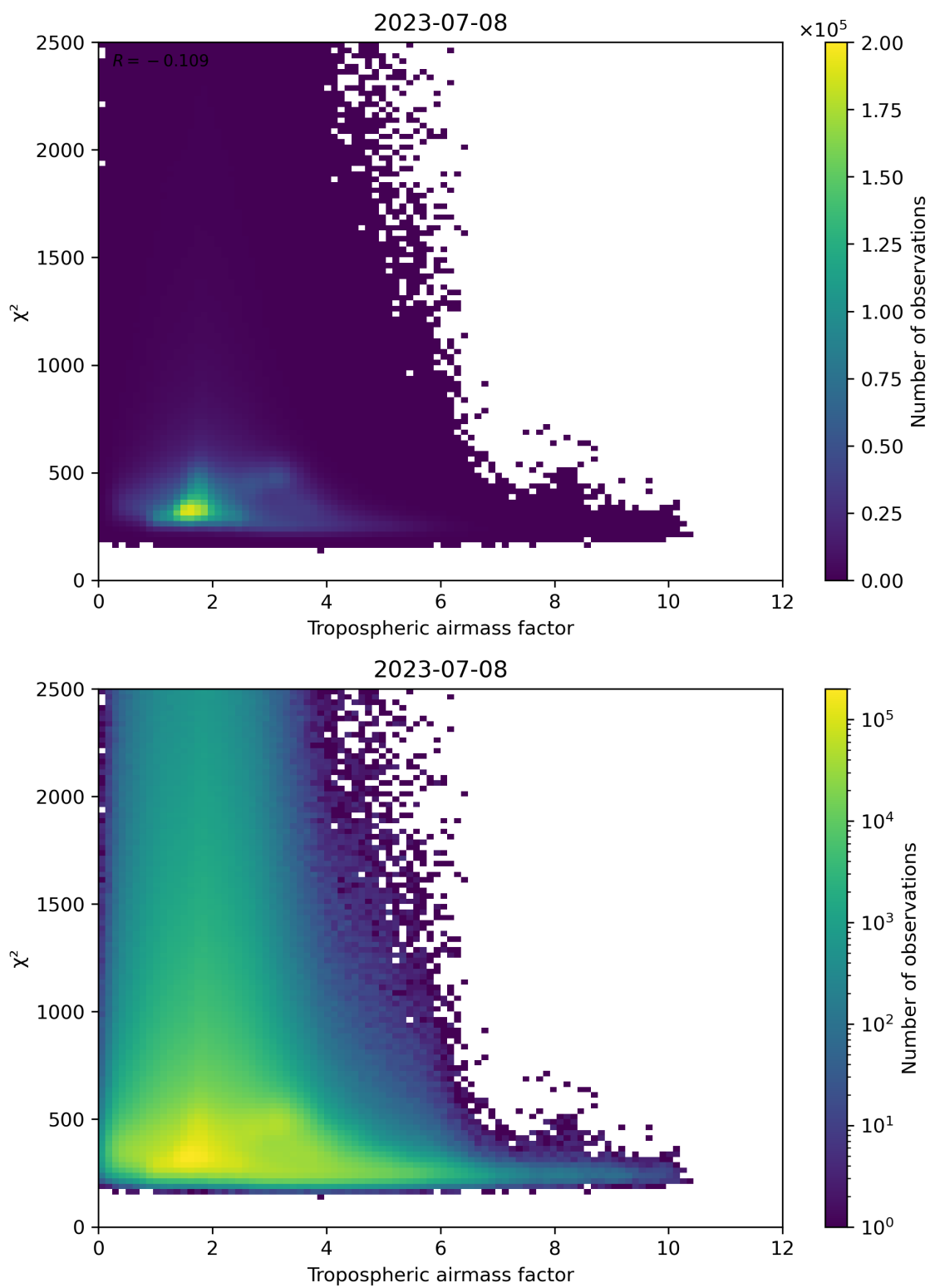
Figure 73: Scatter density plot of “Tropospheric airmass factor” against “ \chi^2 ” for 2023-07-08 to 2023-07-09.
