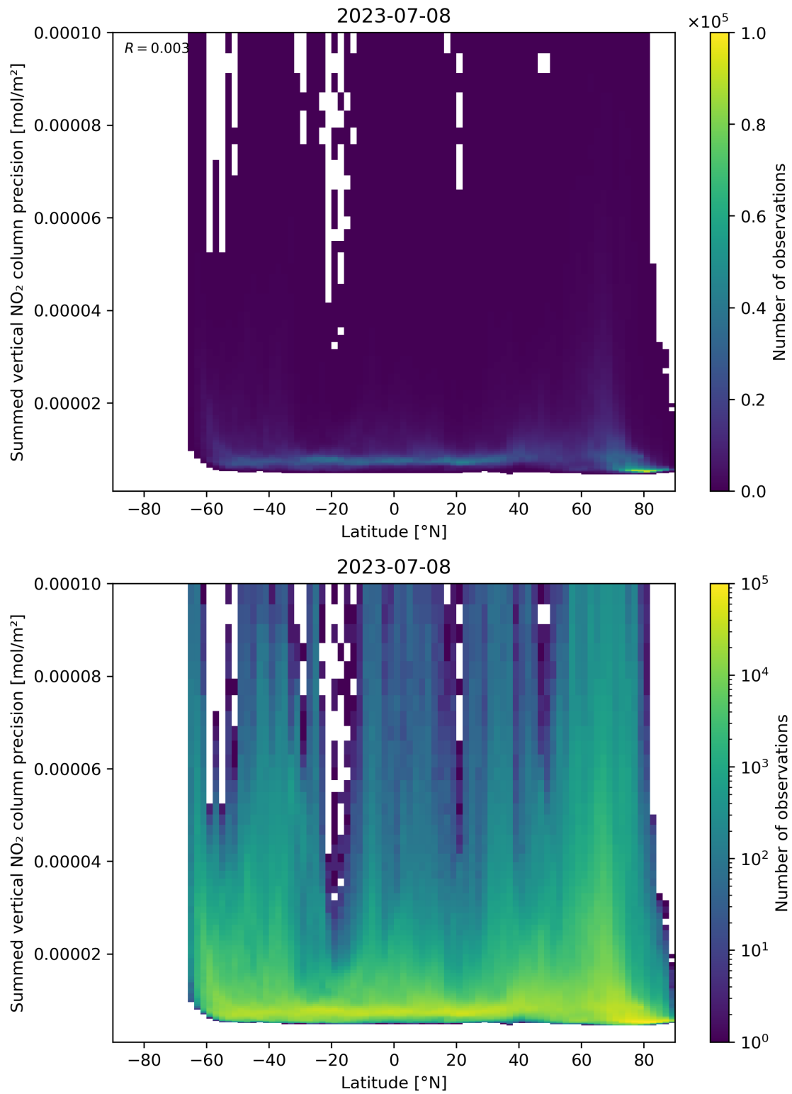
Figure 89: Scatter density plot of “Latitude” against “Summed vertical NO 2 column precision” for 2023-07-08 to 2023-07-09.
