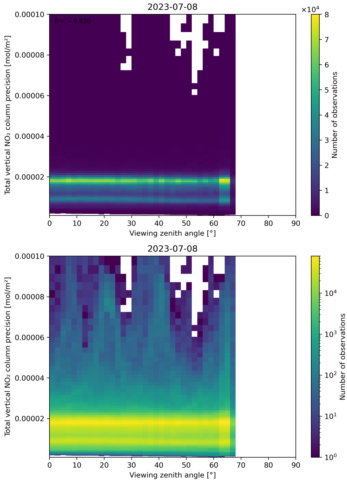
Figure 168: Scatter density plot of “Viewing zenith angle” against “Total vertical NO 2 column precision” for 2023-07-08 to 2023-07-09.
