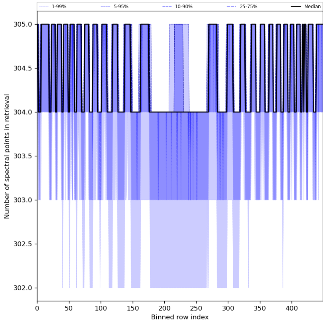
Figure 50: Along track statistics of “Number of spectral points in retrieval” for 2023-07-08 to 2023-07-09
