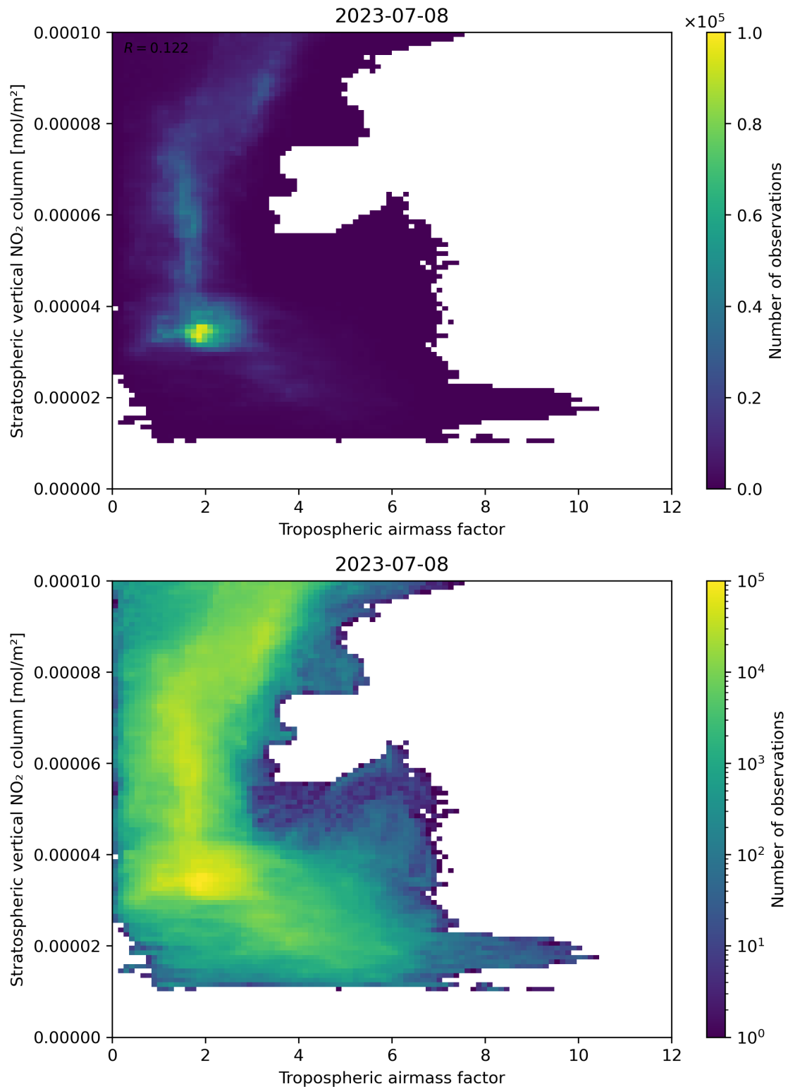
Figure 74: Scatter density plot of “Tropospheric air mass factor” against “Stratospheric vertical NO 2 column” for 2023-07-08 to 2023-07-09.
