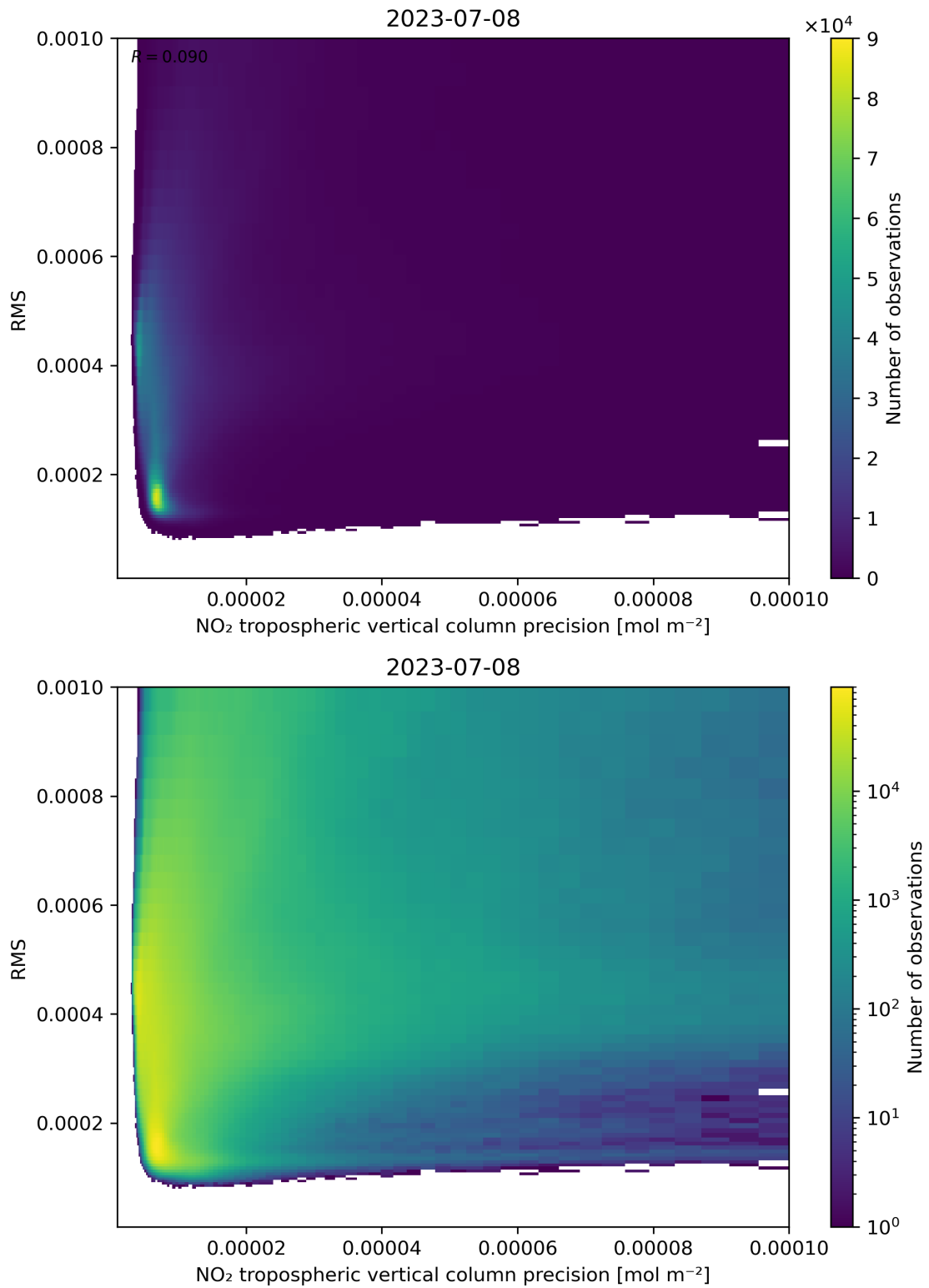
Figure 140: Scatter density plot of “NO 2 tropospheric vertical column precision” against “RMS” for 2023-07-08 to 2023-07-09.
