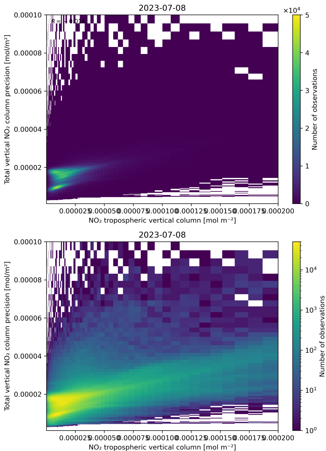
Figure 129: Scatter density plot of “NO 2 tropospheric vertical column” against “Total vertical NO 2 column precision” for 2023-07-08 to 2023-07-09.
