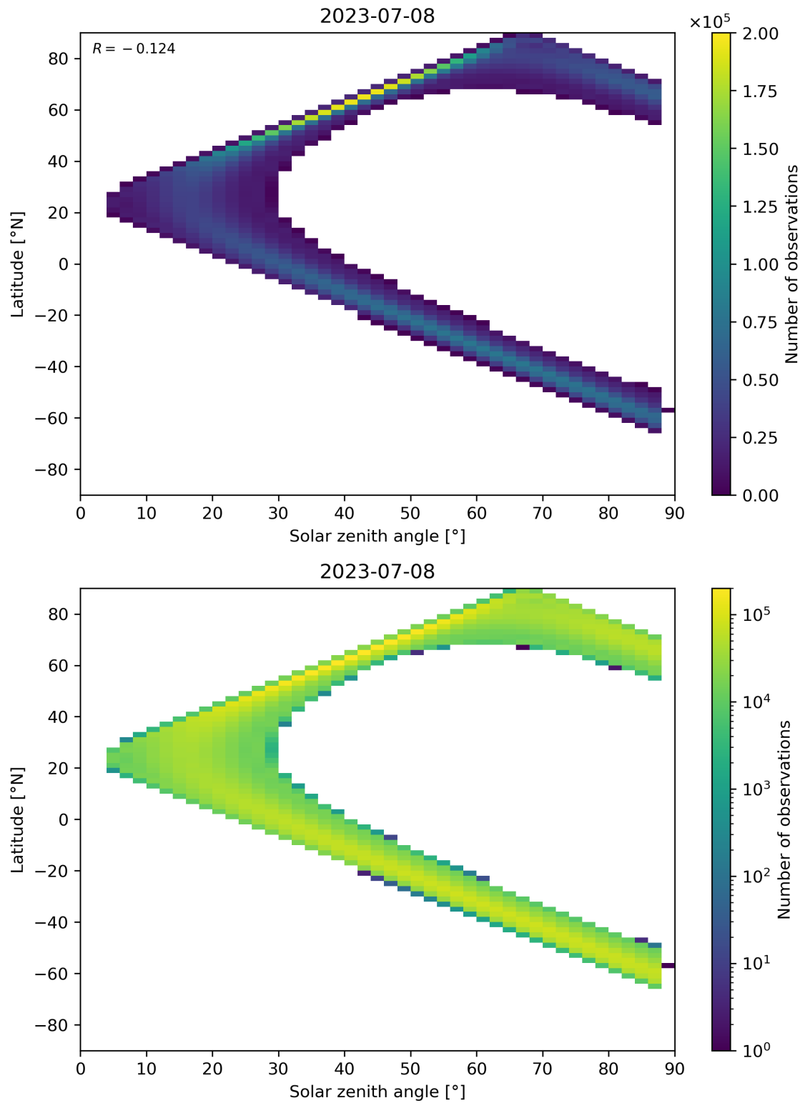
Figure 149: Scatter density plot of “Solar zenith angle” against “Latitude” for 2023-07-08 to 2023-07-09.
