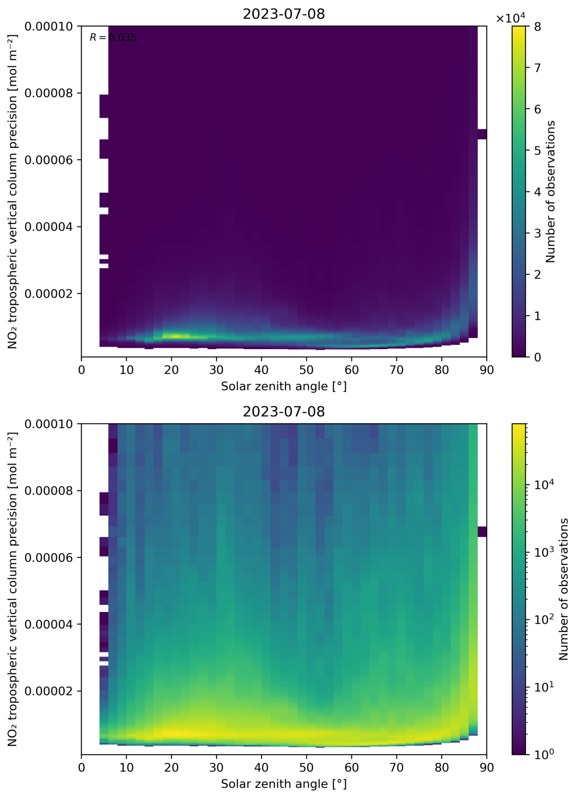
Figure 156: Scatter density plot of “Solar zenith angle” against “NO 2 tropospheric vertical column precision” for 2023-07-08 to 2023-07-09.
