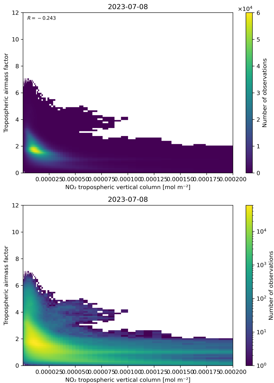
Figure 123: Scatter density plot of “NO 2 tropospheric vertical column” against “Tropospheric air mass factor” for 2023-07-08 to 2023-07-09.
