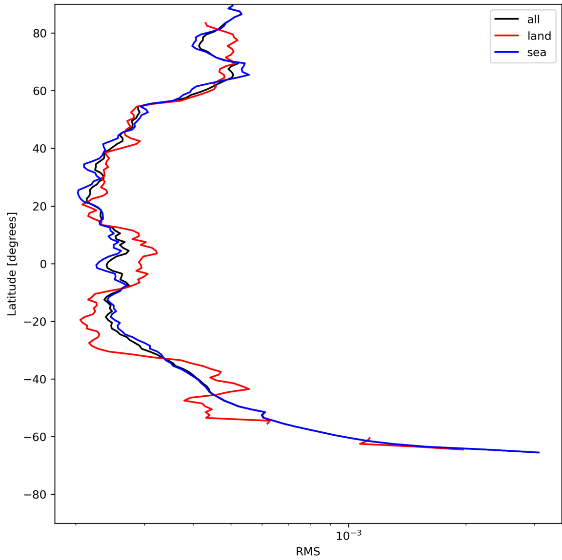
Figure 26: Zonal average of “RMS” for 2023-07-08 to 2023-07-09.
