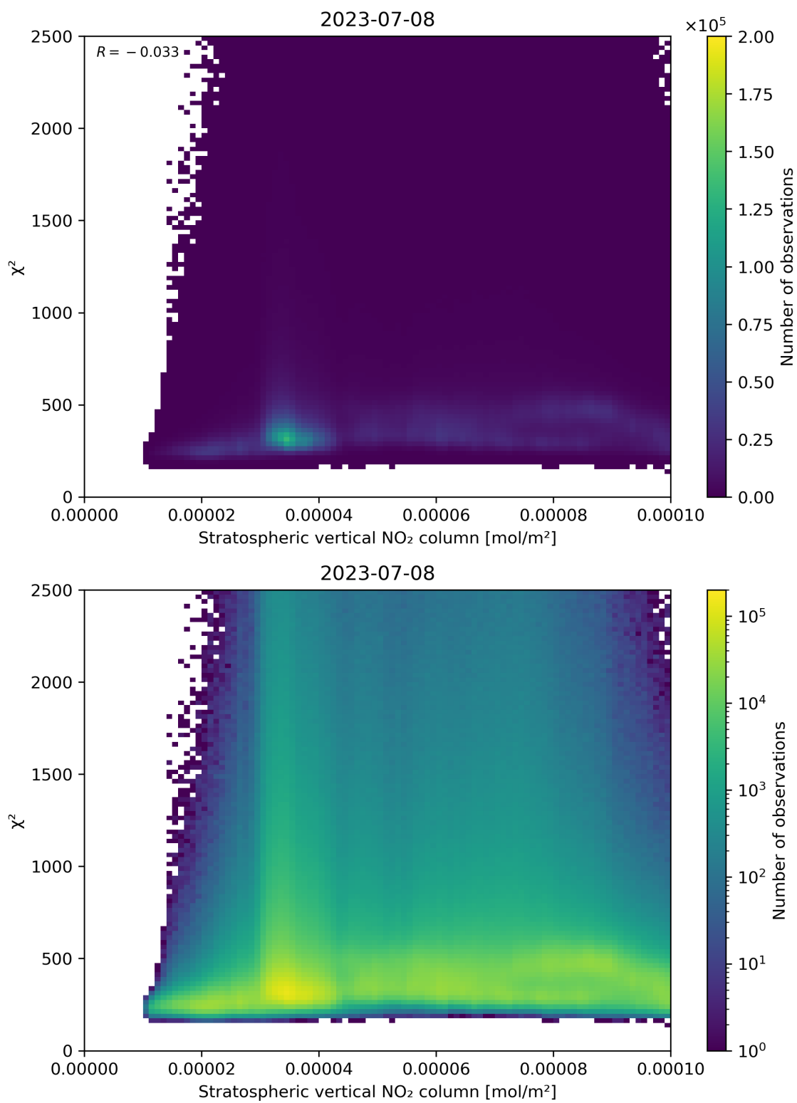
Figure 97: Scatter density plot of “Stratospheric vertical NO 2 column” against “ \chi^2 ” for 2023-07-08 to 2023-07-09.
