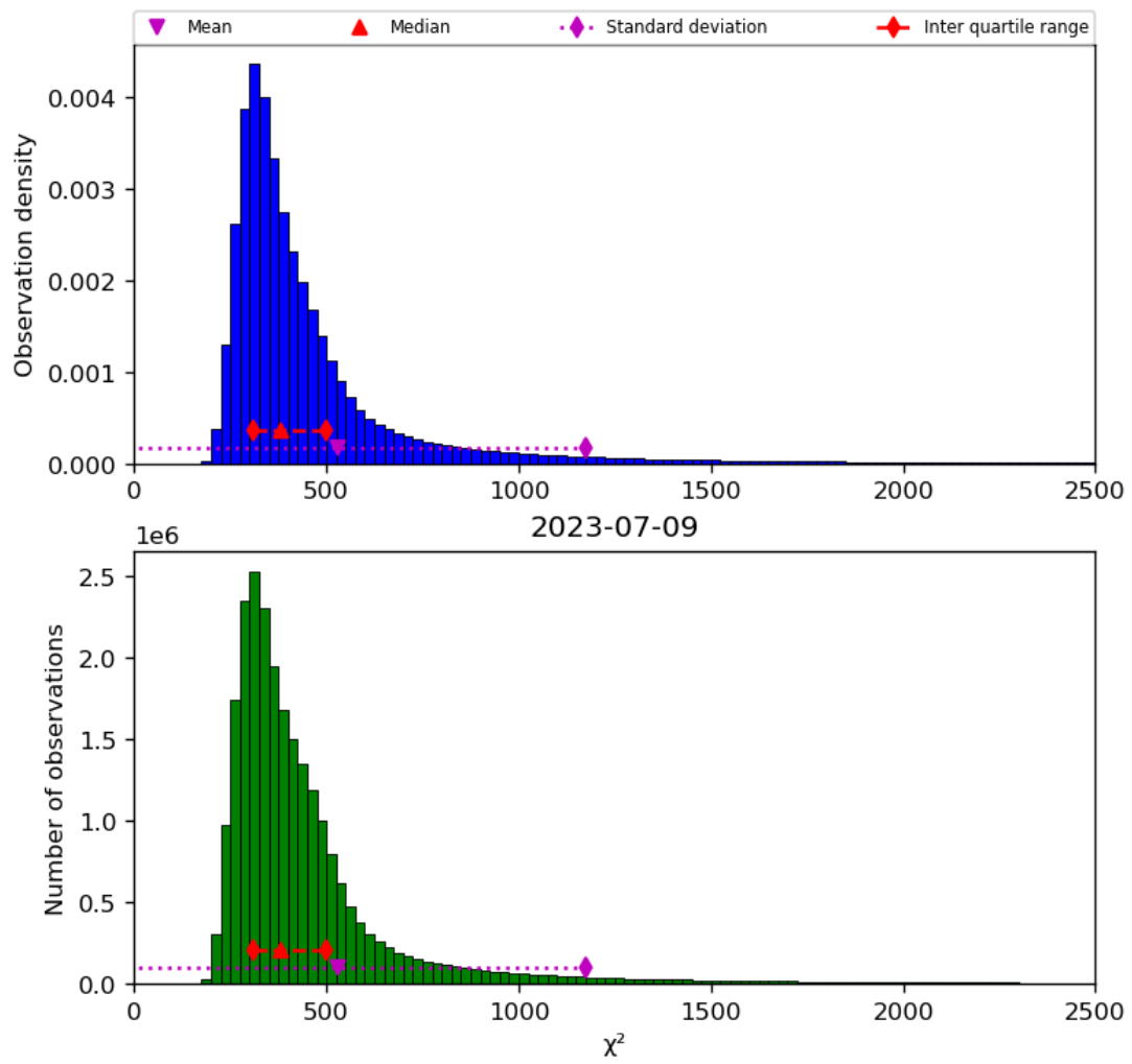
Figure 42: Histogram of “ \chi^2 ” for 2023-07-08 to 2023-07-10
