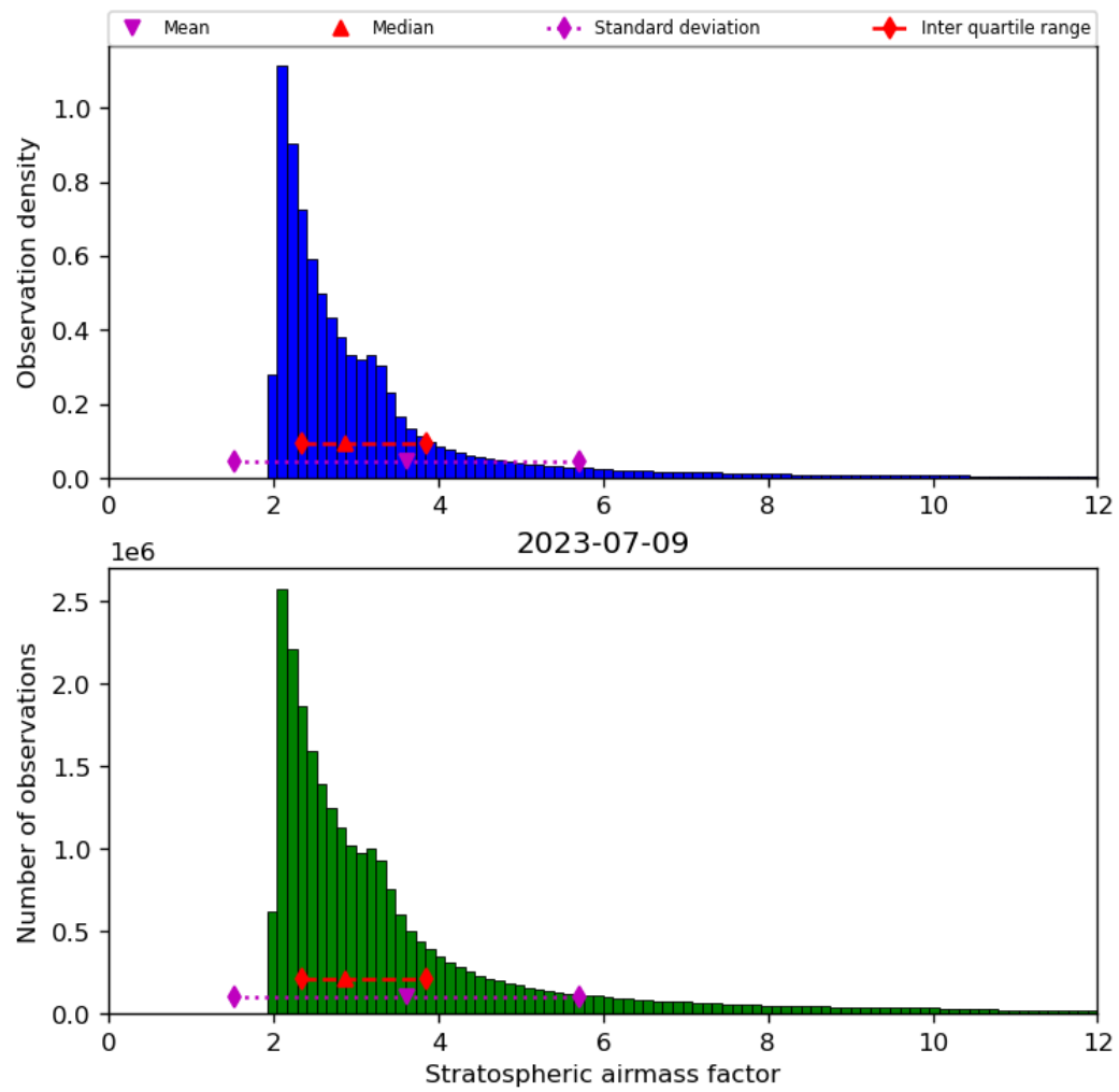
Figure 44: Histogram of “Stratospheric airmass factor” for 2023-07-08 to 2023-07-10
