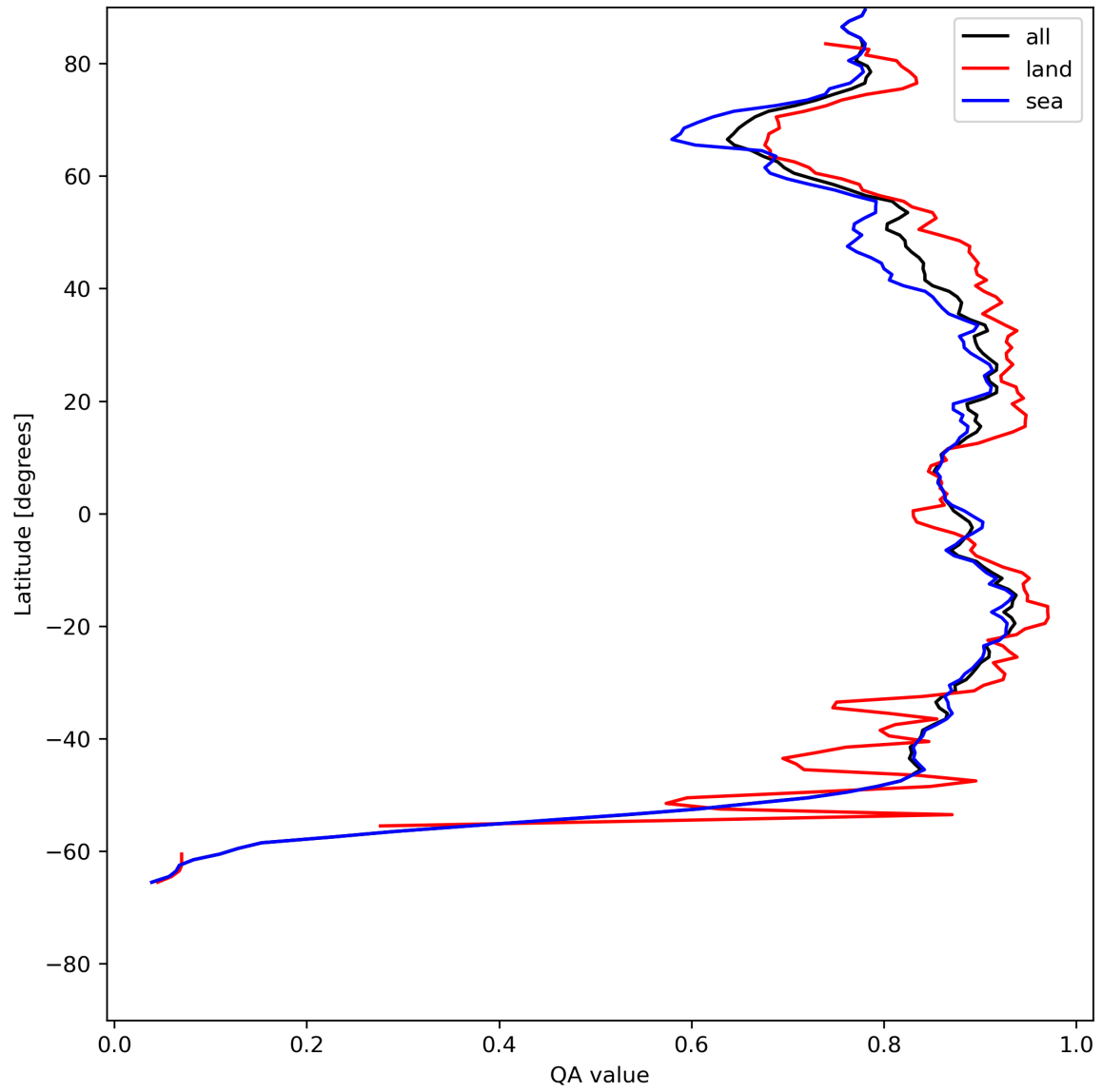
Figure 11: Zonal average of “QA value” for 2023-07-08 to 2023-07-10.
