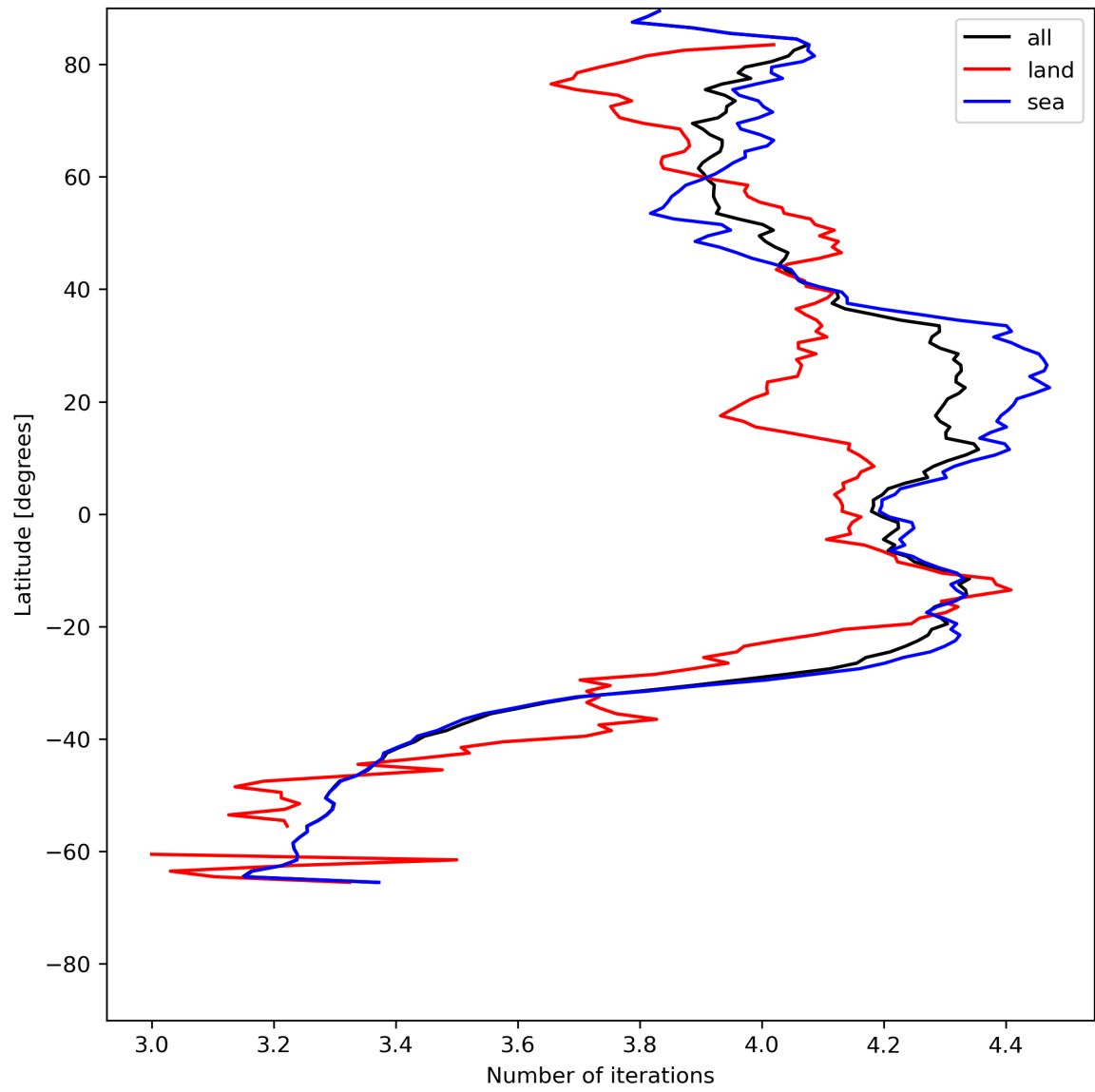
Figure 17: Zonal average of “Number of iterations” for 2023-07-08 to 2023-07-10.
