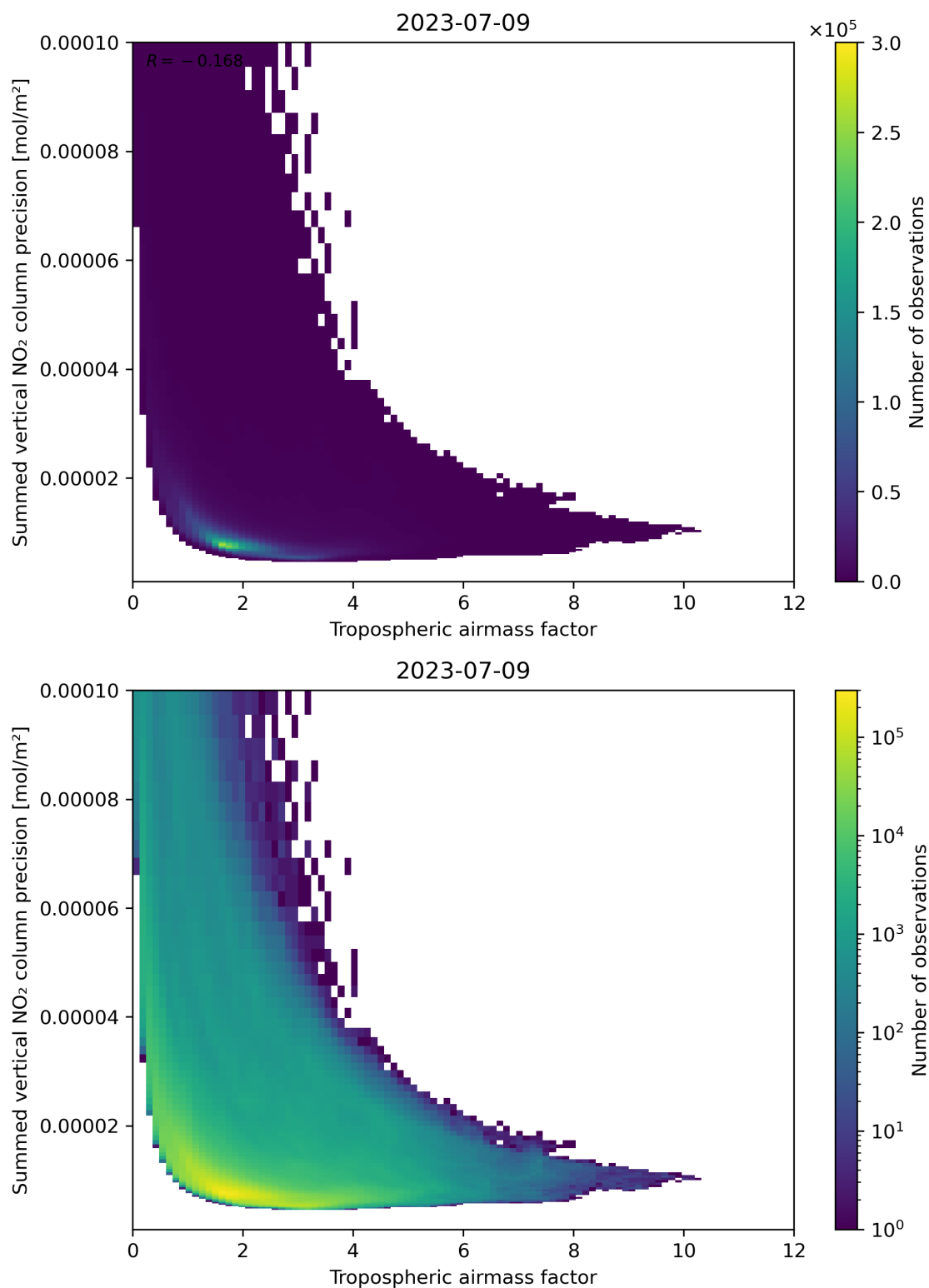
Figure 76: Scatter density plot of “Tropospheric air mass factor” against “Summed vertical NO 2 column precision” for 2023-07-08 to 2023-07-10.
