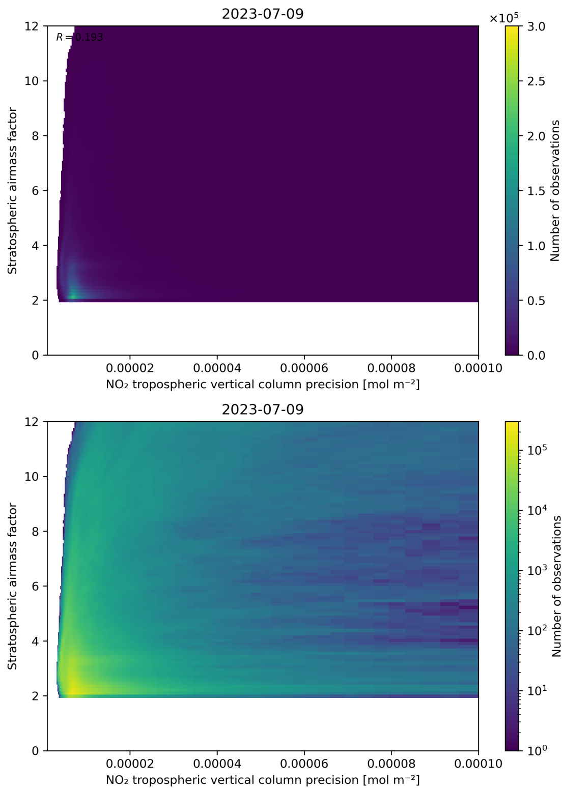
Figure 131: Scatter density plot of “NO 2 tropospheric vertical column precision” against “Stratospheric airmass factor” for 2023-07-08 to 2023-07-10.
