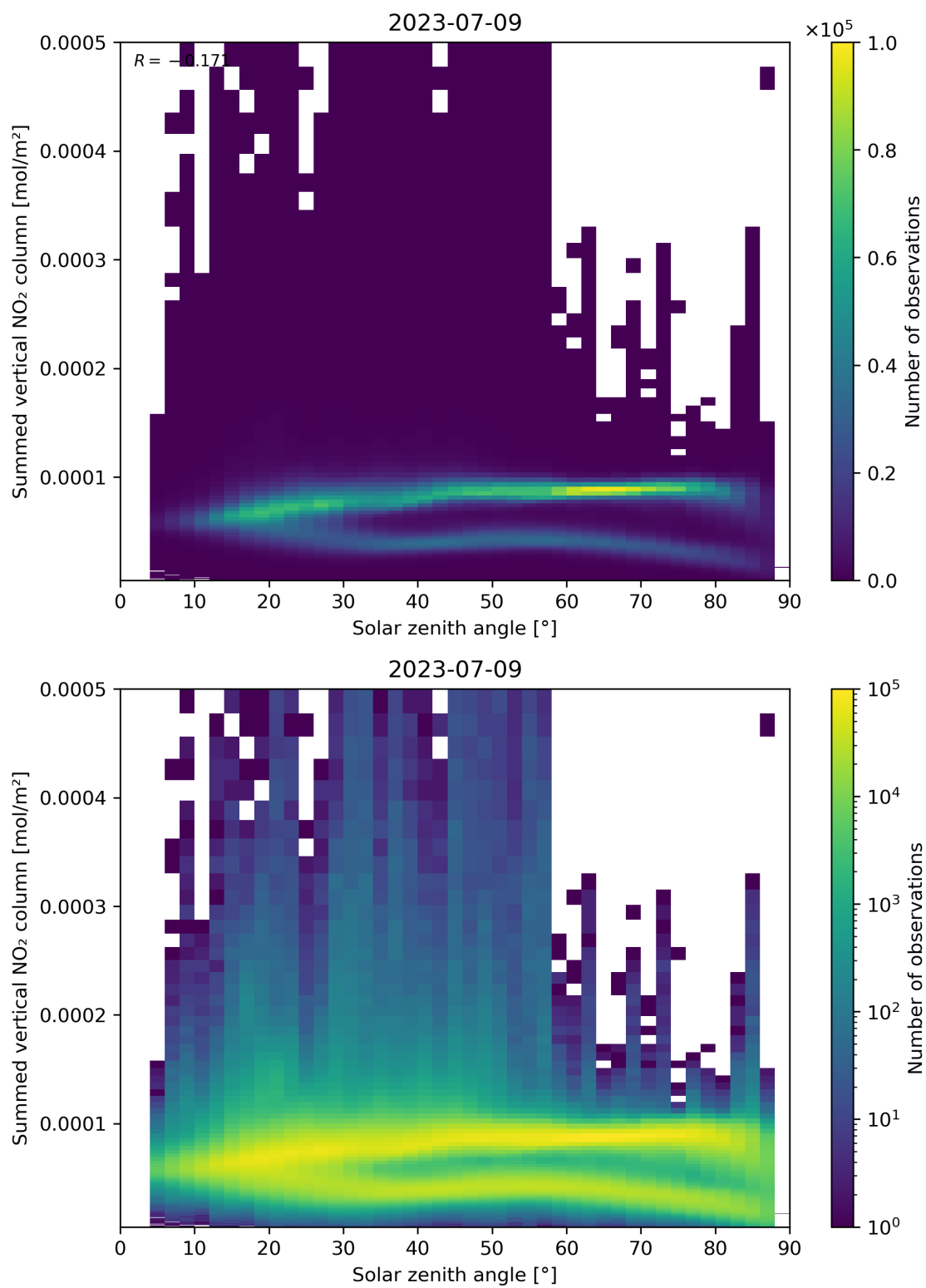
Figure 151: Scatter density plot of “Solar zenith angle” against “Summed vertical NO 2 column” for 2023-07-08 to 2023-07-10.
