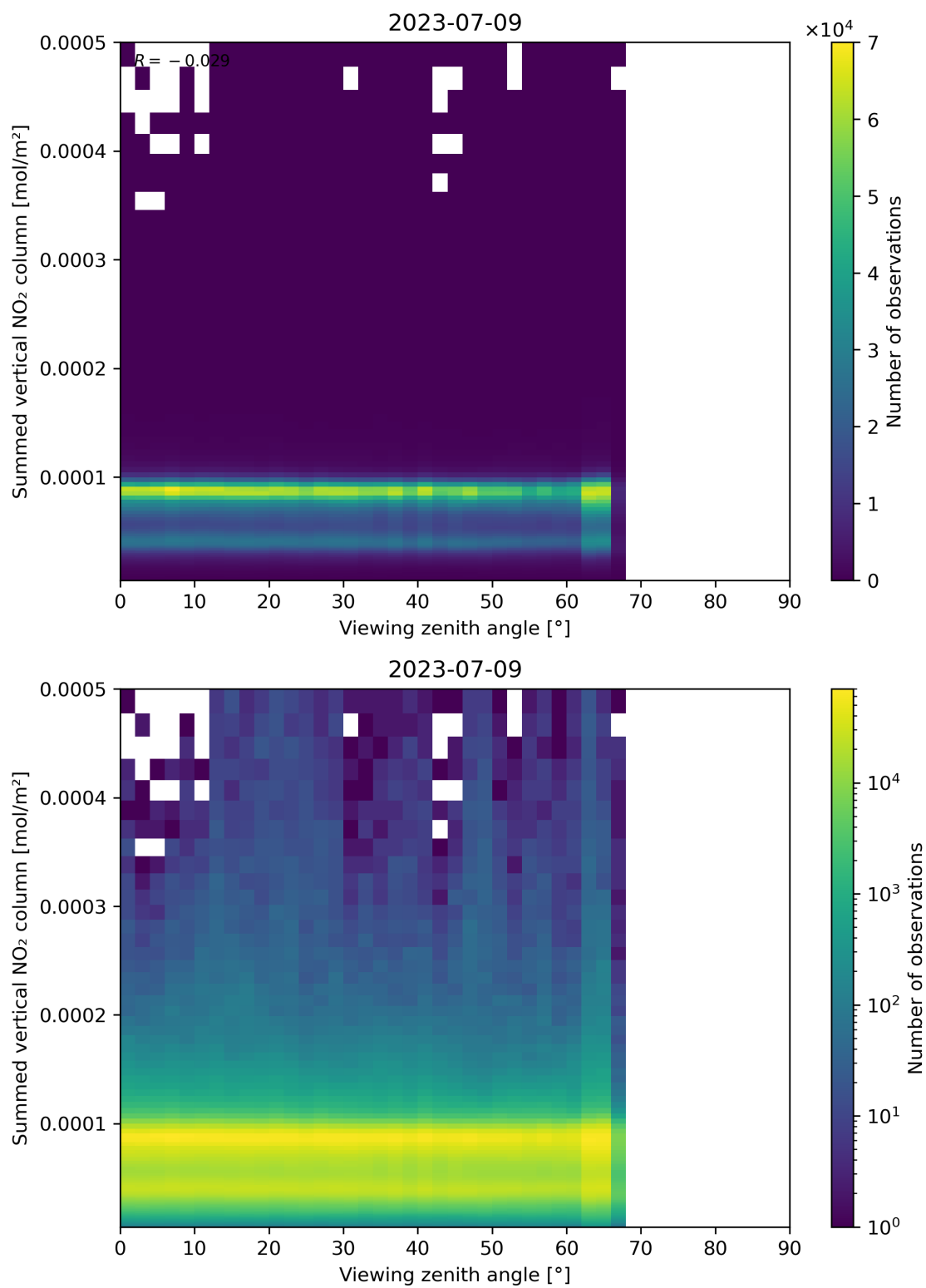
Figure 165: Scatter density plot of “Viewing zenith angle” against “Summed vertical NO 2 column” for 2023-07-08 to 2023-07-10.
