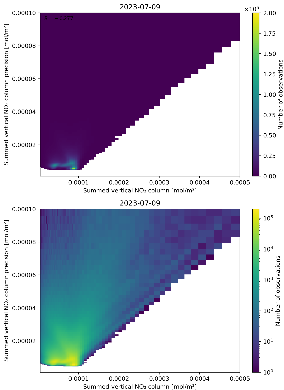
Figure 105: Scatter density plot of “Summed vertical NO 2 column” against “Summed vertical NO 2 column precision” for 2023-07-08 to 2023-07-10.
