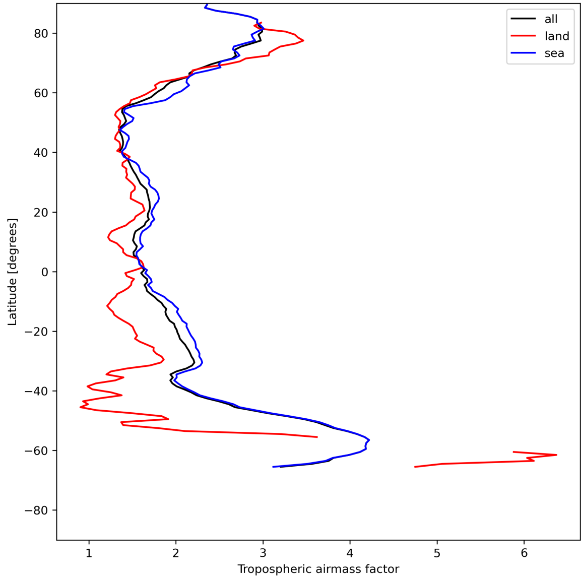
Figure 14: Zonal average of “Tropospheric airmass factor” for 2023-07-08 to 2023-07-10.
