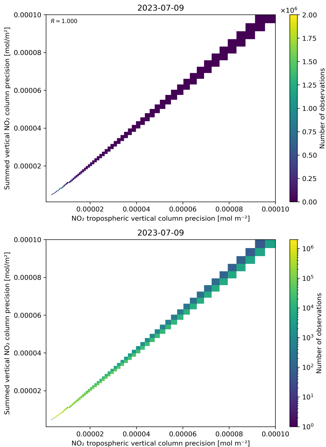
Figure 137: Scatter density plot of “NO 2 tropospheric vertical column precision” against “Summed vertical NO 2 column precision” for 2023-07-08 to 2023-07-10.
