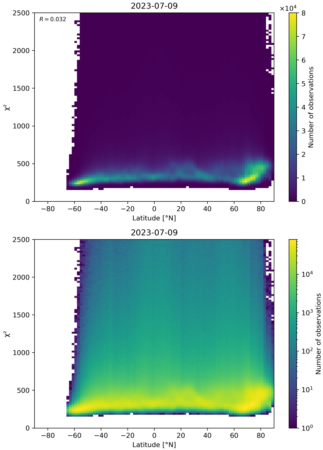
Figure 86: Scatter density plot of “Latitude” against “ \chi^2 ” for 2023-07-08 to 2023-07-10.
