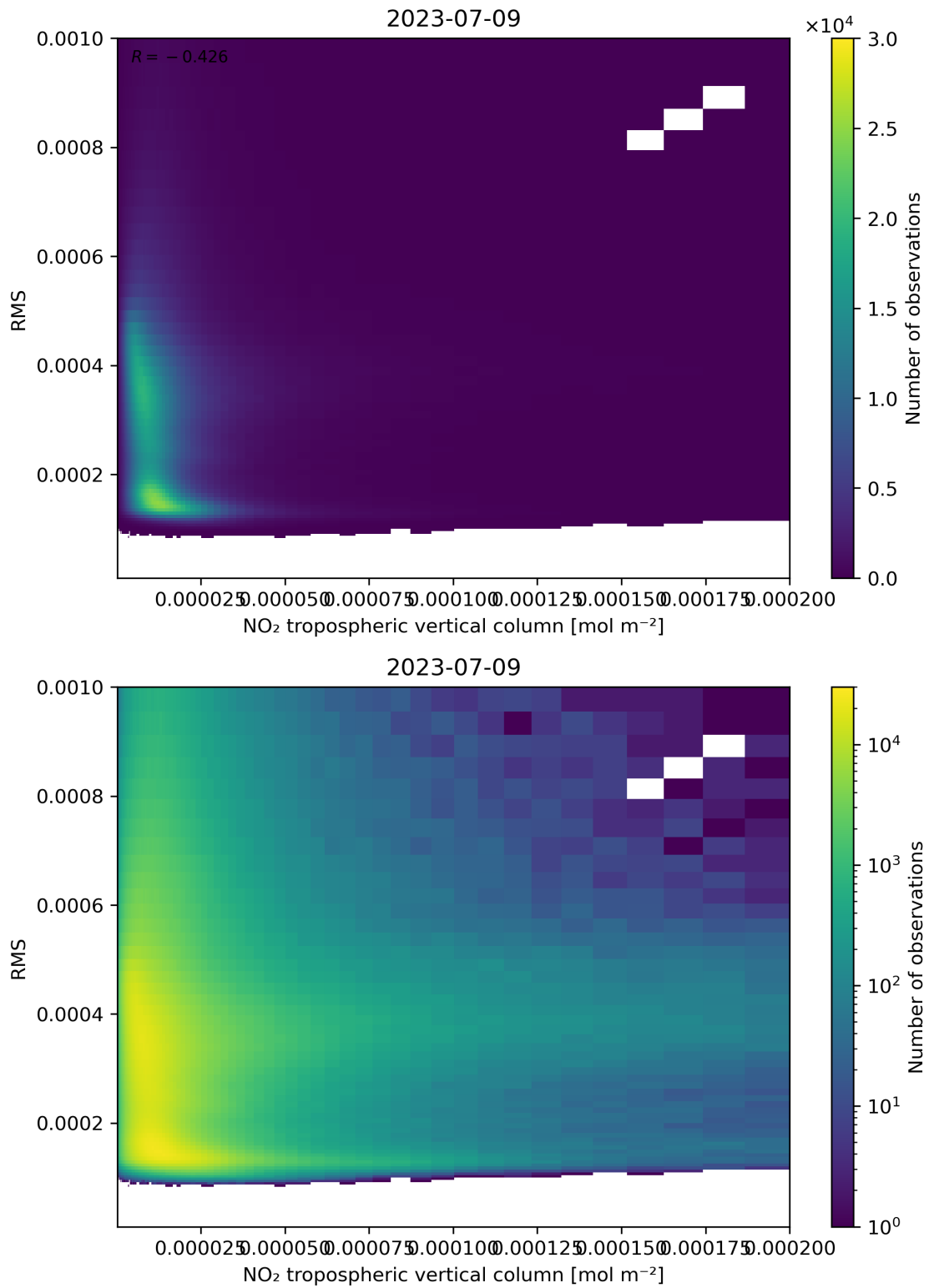
Figure 142: Scatter density plot of “NO 2 tropospheric vertical column” against “RMS” for 2023-07-08 to 2023-07-10.
