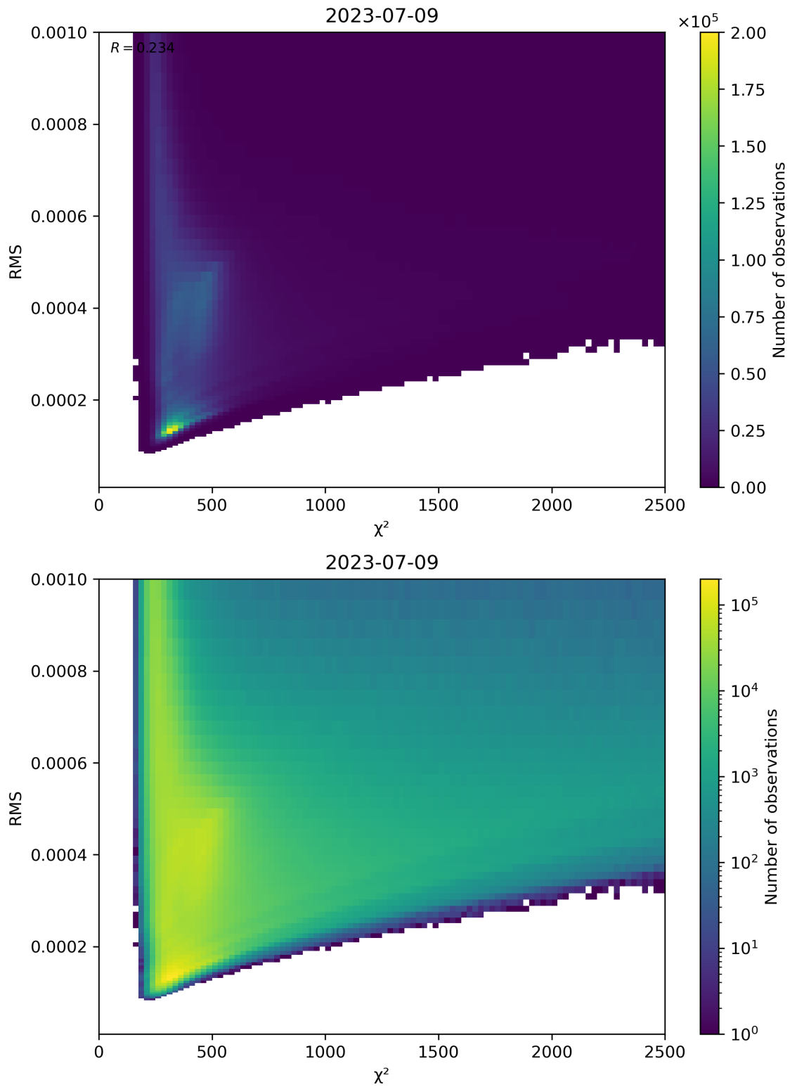
Figure 82: Scatter density plot of “ \chi^2 ” against “RMS” for 2023-07-08 to 2023-07-10.
