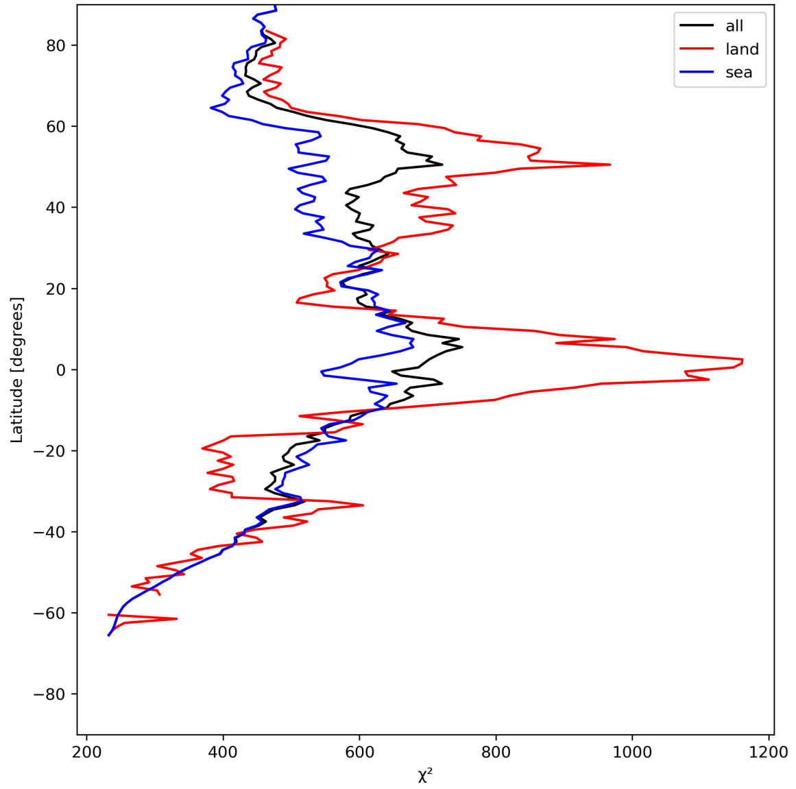
Figure 25: Zonal average of “ \chi^2 ” for 2023-07-08 to 2023-07-10.
