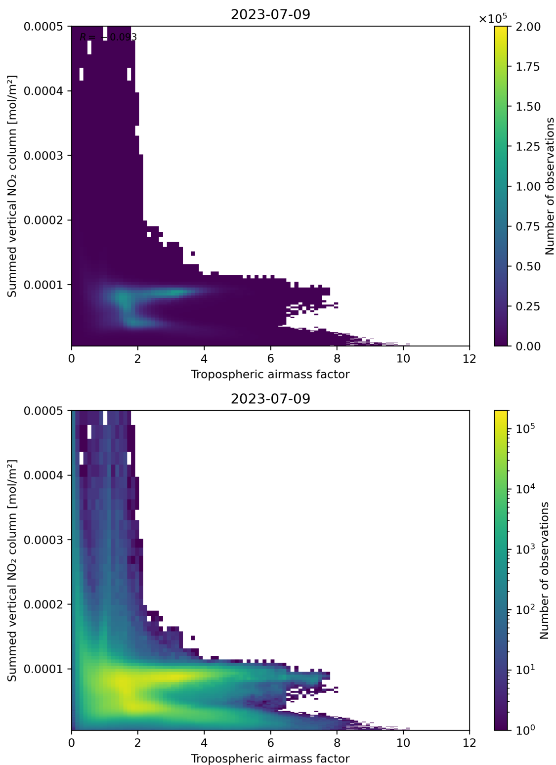
Figure 75: Scatter density plot of “Tropospheric airmass factor” against “Summed vertical NO 2 column” for 2023-07-08 to 2023-07-10.
