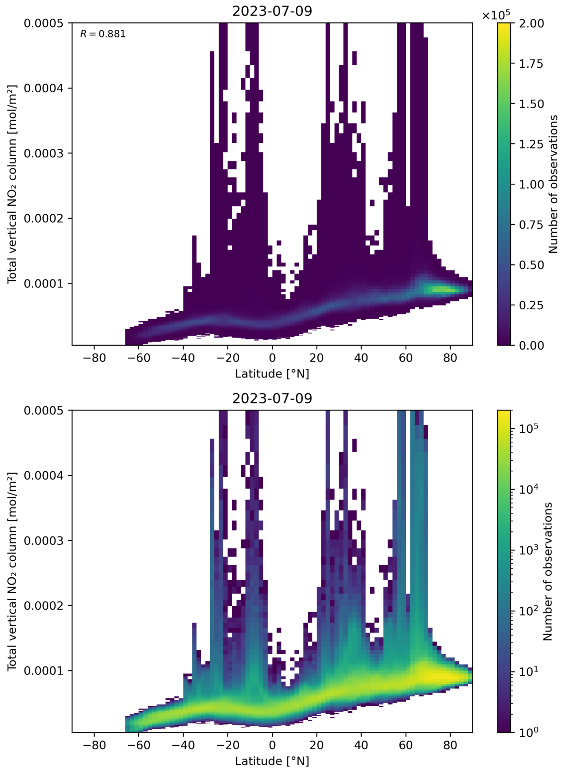
Figure 90: Scatter density plot of “Latitude” against “Total vertical NO 2 column” for 2023-07-08 to 2023-07-10.
