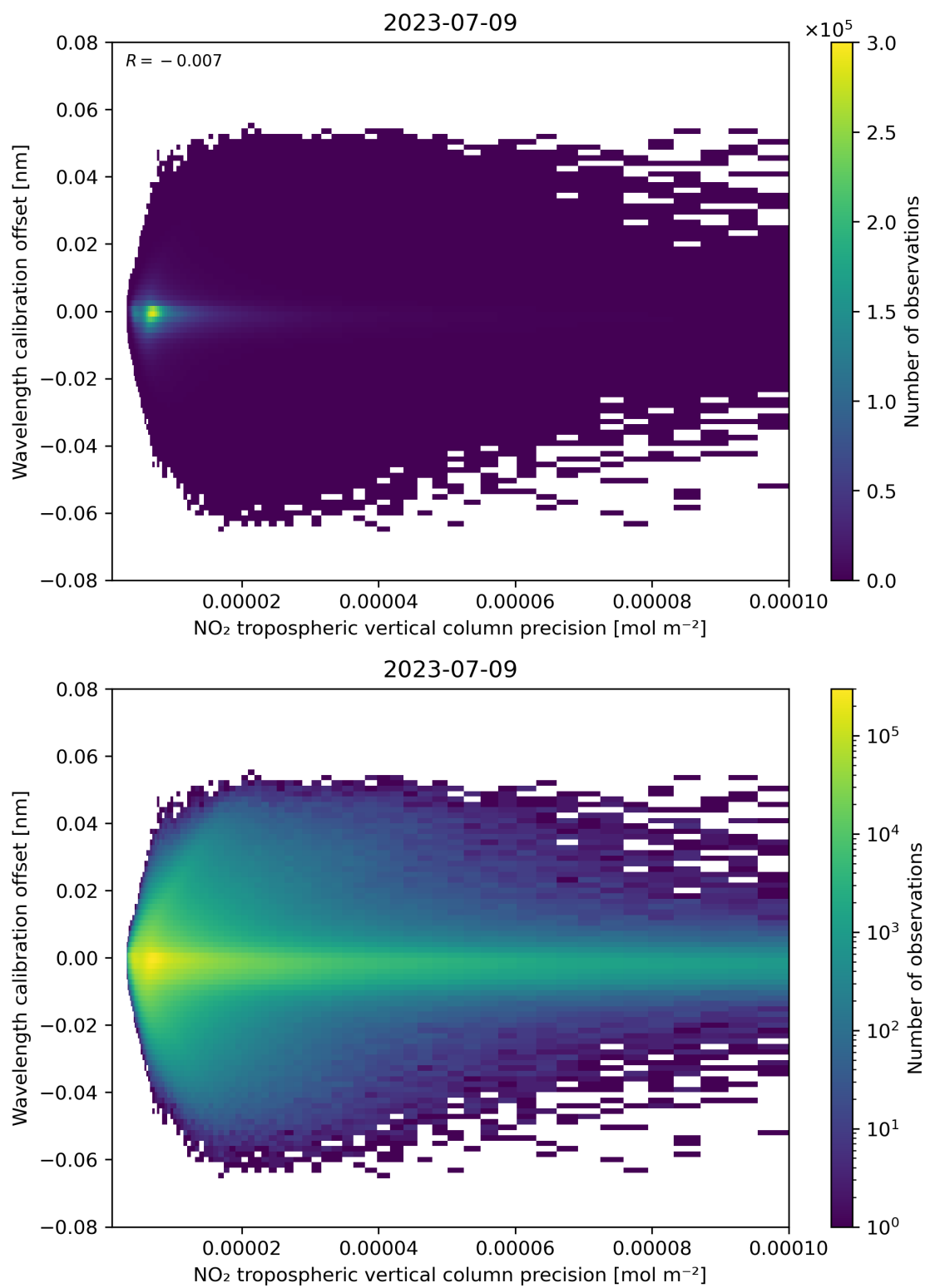
Figure 141: Scatter density plot of “NO 2 tropospheric vertical column precision” against “Wavelength calibration offset” for 2023-07-08 to 2023-07-10.
