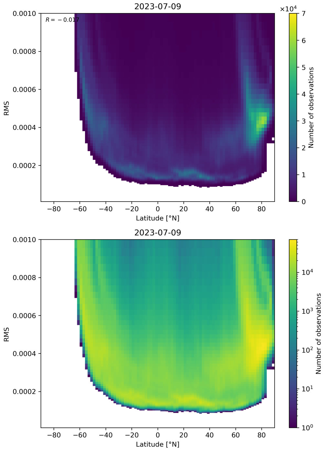
Figure 94: Scatter density plot of “Latitude” against “RMS” for 2023-07-08 to 2023-07-10.
