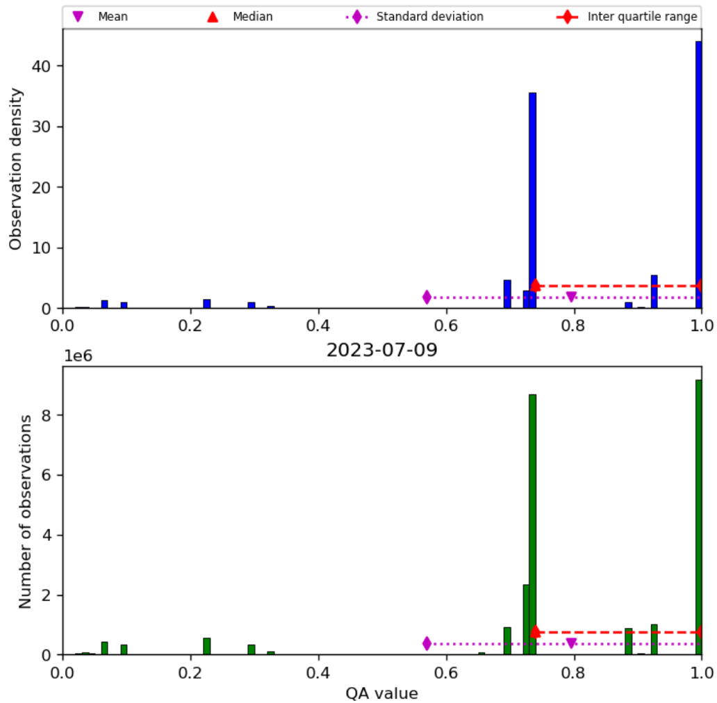
Figure 28: Histogram of “QA value” for 2023-07-08 to 2023-07-10
