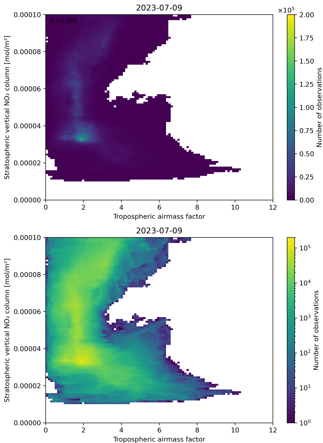
Figure 74: Scatter density plot of “Tropospheric air mass factor” against “Stratospheric vertical \text{NO}_2 column” for 2023-07-08 to 2023-07-10.
