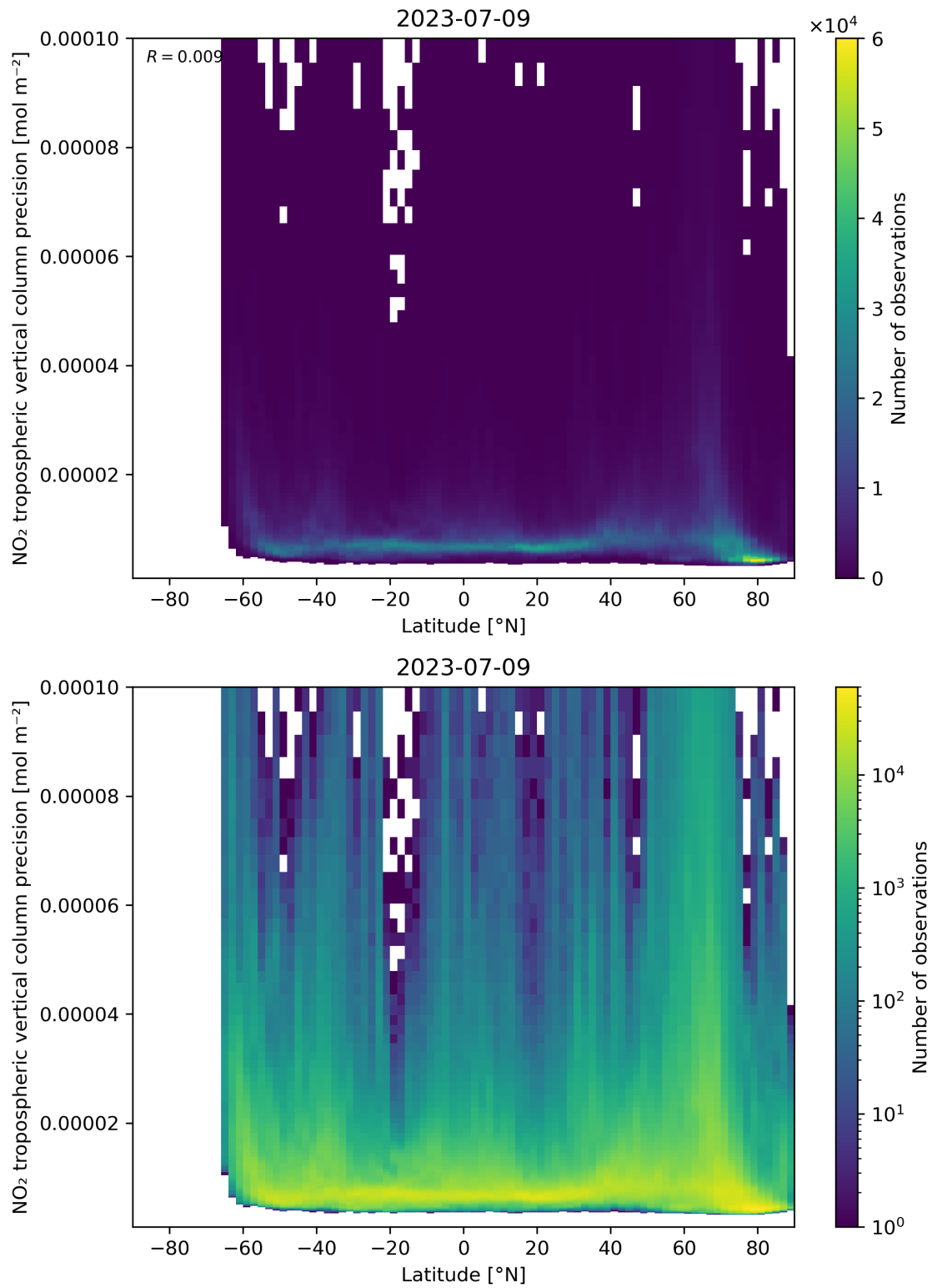
Figure 93: Scatter density plot of “Latitude” against “NO 2 tropospheric vertical column precision” for 2023-07-08 to 2023-07-10.
