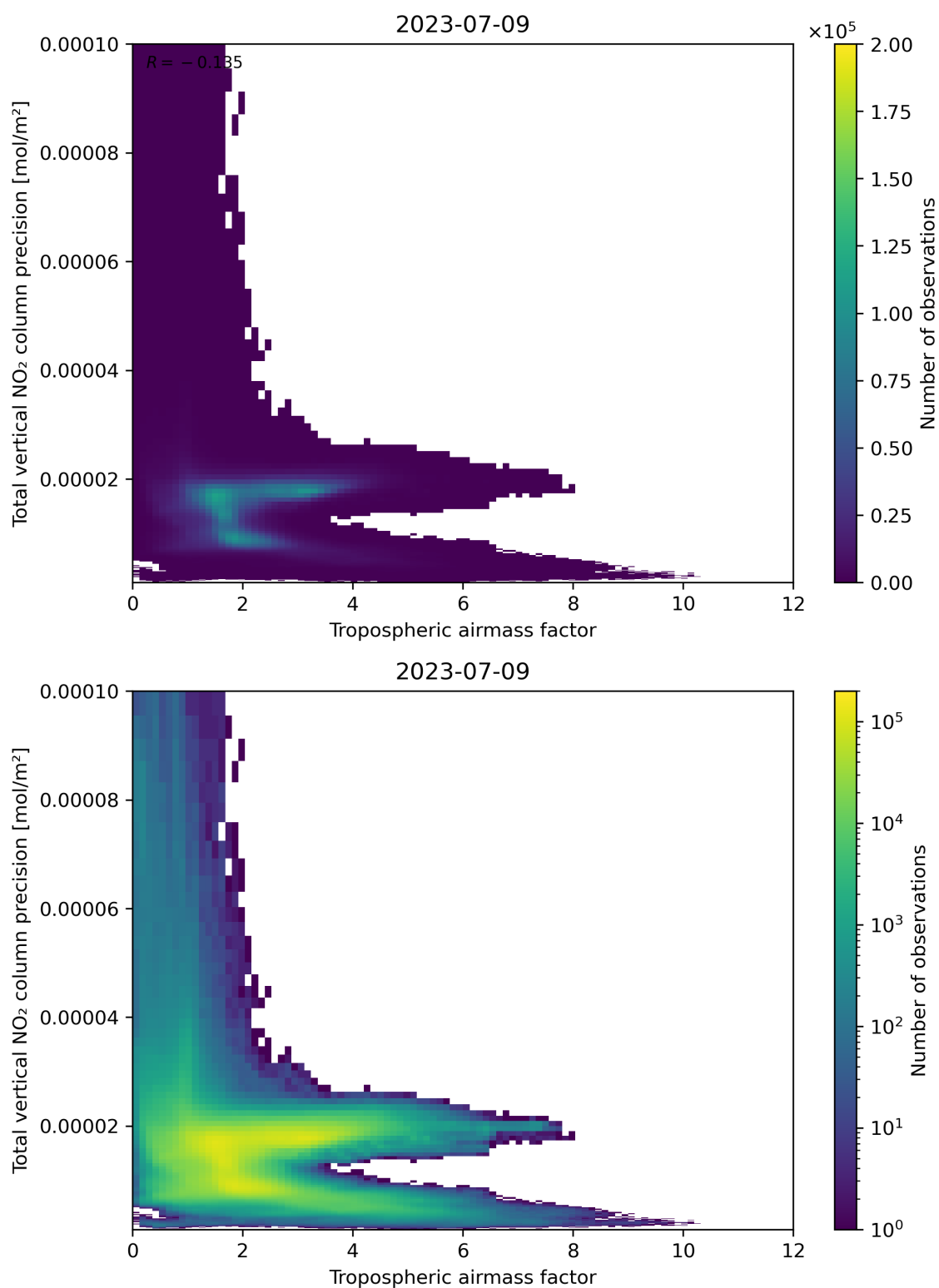
Figure 78: Scatter density plot of “Tropospheric airmass factor” against “Total vertical NO 2 column precision” for 2023-07-08 to 2023-07-10.
