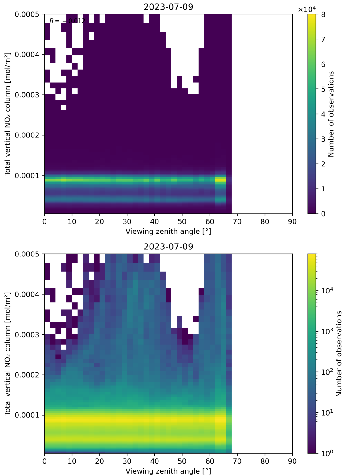
Figure 167: Scatter density plot of “Viewing zenith angle” against “Total vertical NO 2 column” for 2023-07-08 to 2023-07-10.
