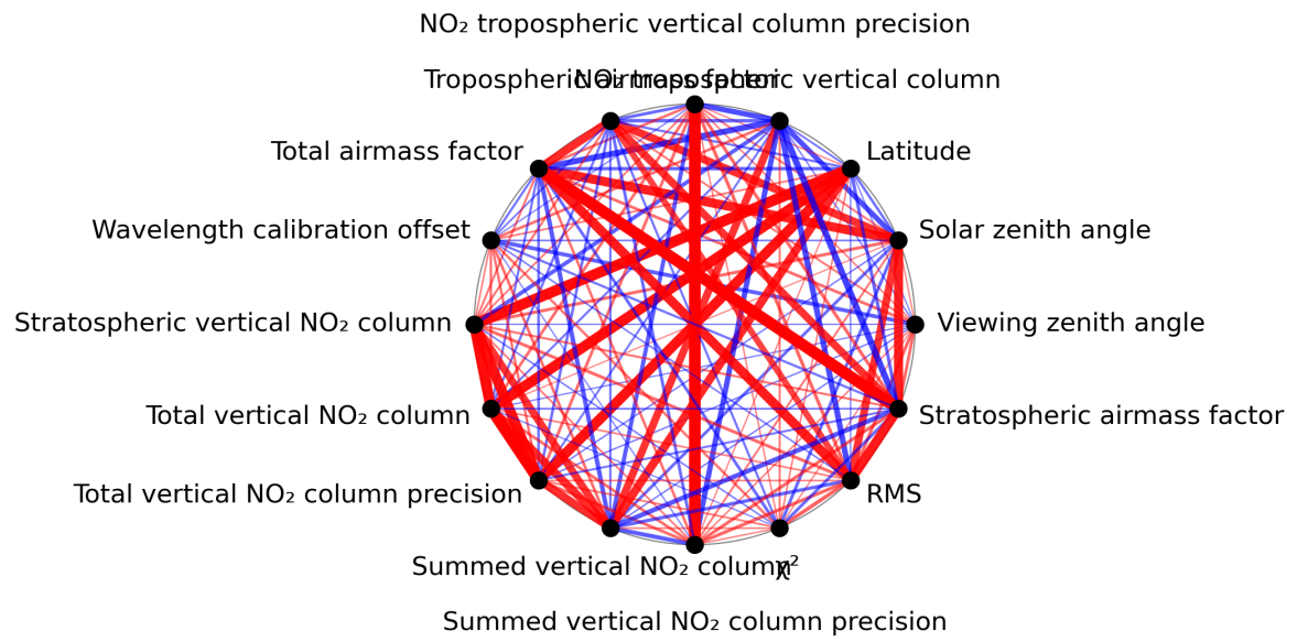
Figure 1: Map of correlation graph for 2023-07-08 to 2023-07-10.
