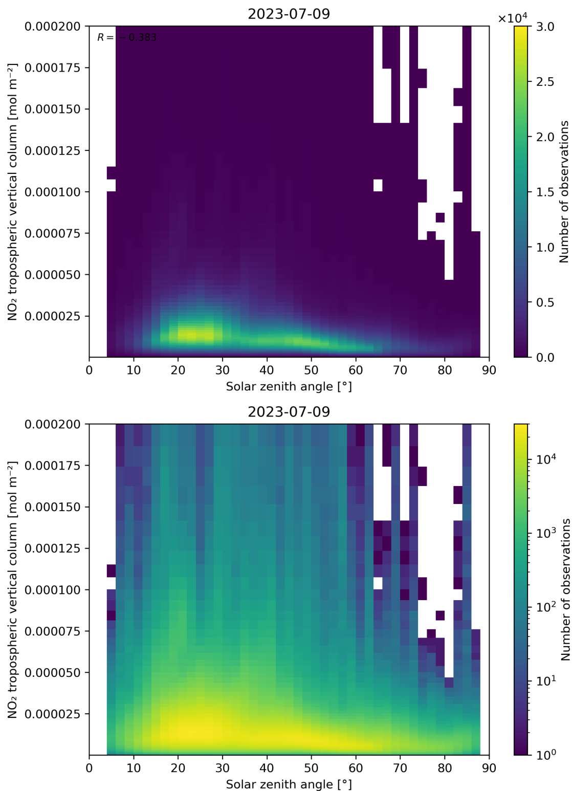
Figure 155: Scatter density plot of “Solar zenith angle” against “NO 2 tropospheric vertical column” for 2023-07-08 to 2023-07-10.
