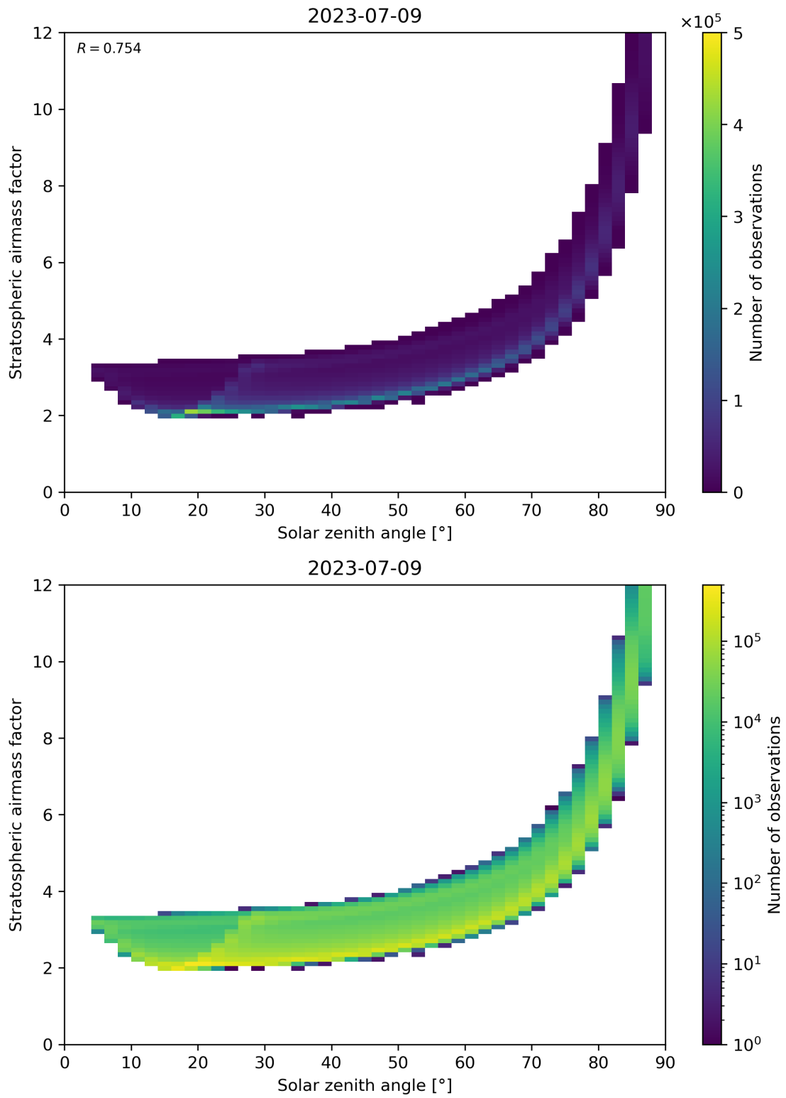
Figure 145: Scatter density plot of “Solar zenith angle” against “Stratospheric airmass factor” for 2023-07-08 to 2023-07-10.
