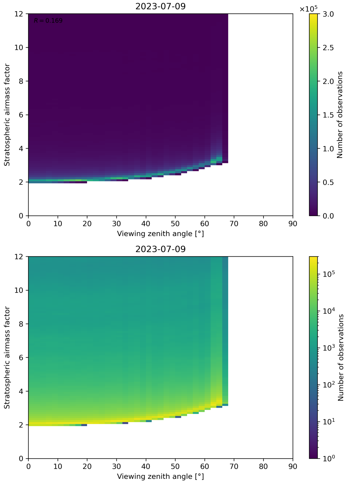
Figure 159: Scatter density plot of “Viewing zenith angle” against “Stratospheric airmass factor” for 2023-07-08 to 2023-07-10.
