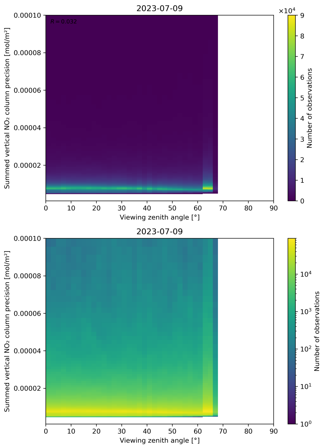
Figure 166: Scatter density plot of “Viewing zenith angle” against “Summed vertical NO 2 column precision” for 2023-07-08 to 2023-07-10.
