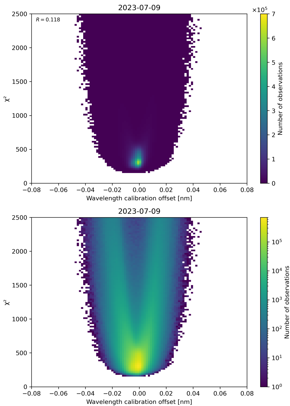
Figure 175: Scatter density plot of “Wavelength calibration offset” against “ \chi^2 ” for 2023-07-08 to 2023-07-10.
