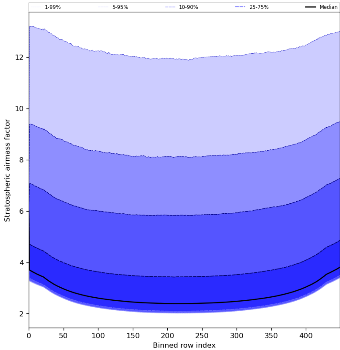
Figure 61: Along track statistics of “Stratospheric airmass factor” for 2023-07-08 to 2023-07-10
