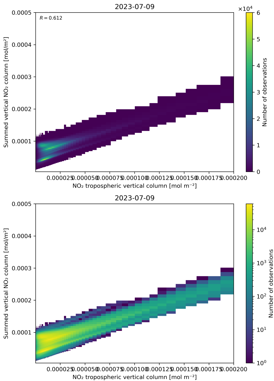
Figure 126: Scatter density plot of “NO 2 tropospheric vertical column” against “Summed vertical NO 2 column” for 2023-07-08 to 2023-07-10.
