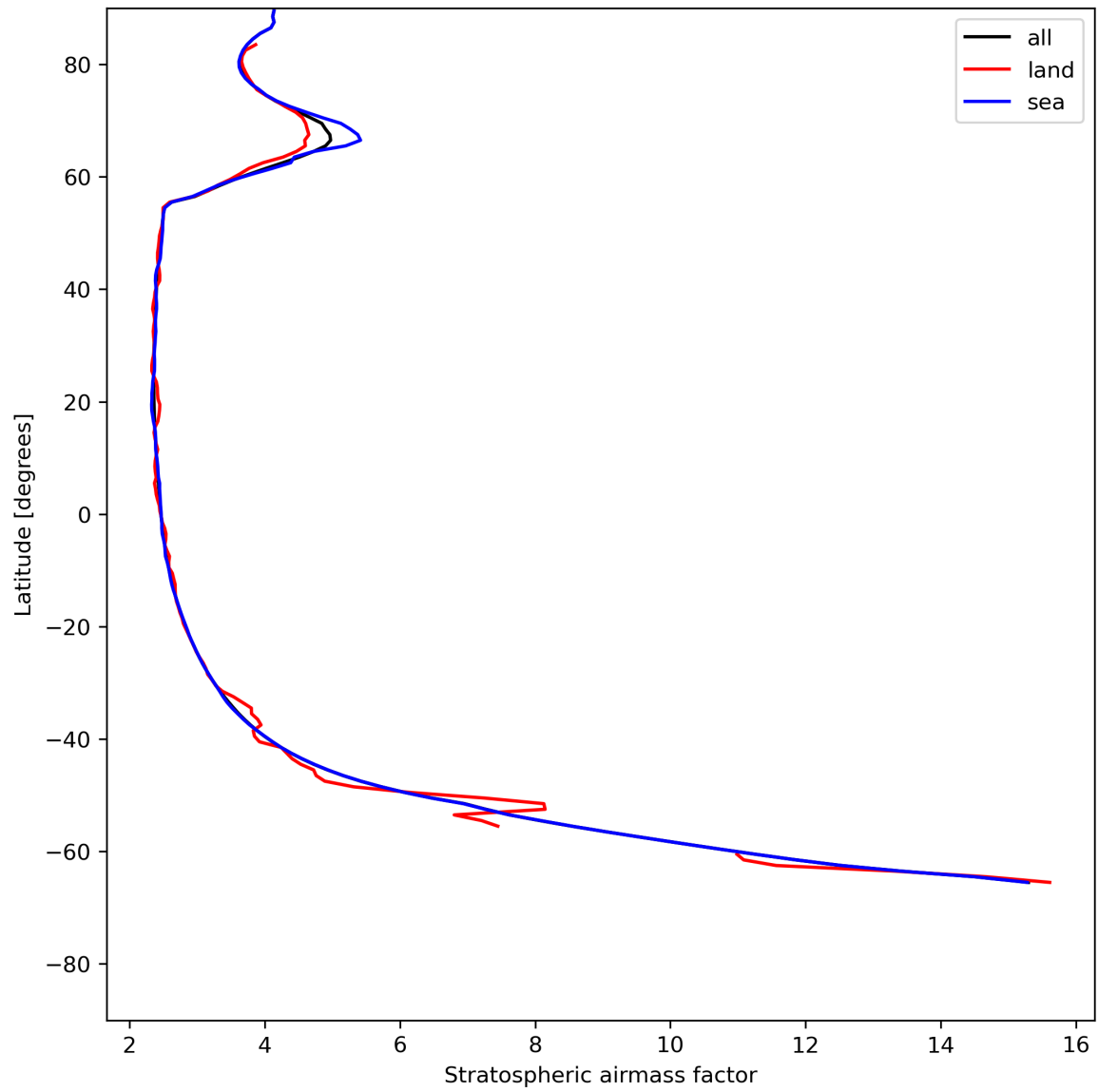
Figure 27: Zonal average of “Stratospheric air mass factor” for 2023-07-08 to 2023-07-10.
