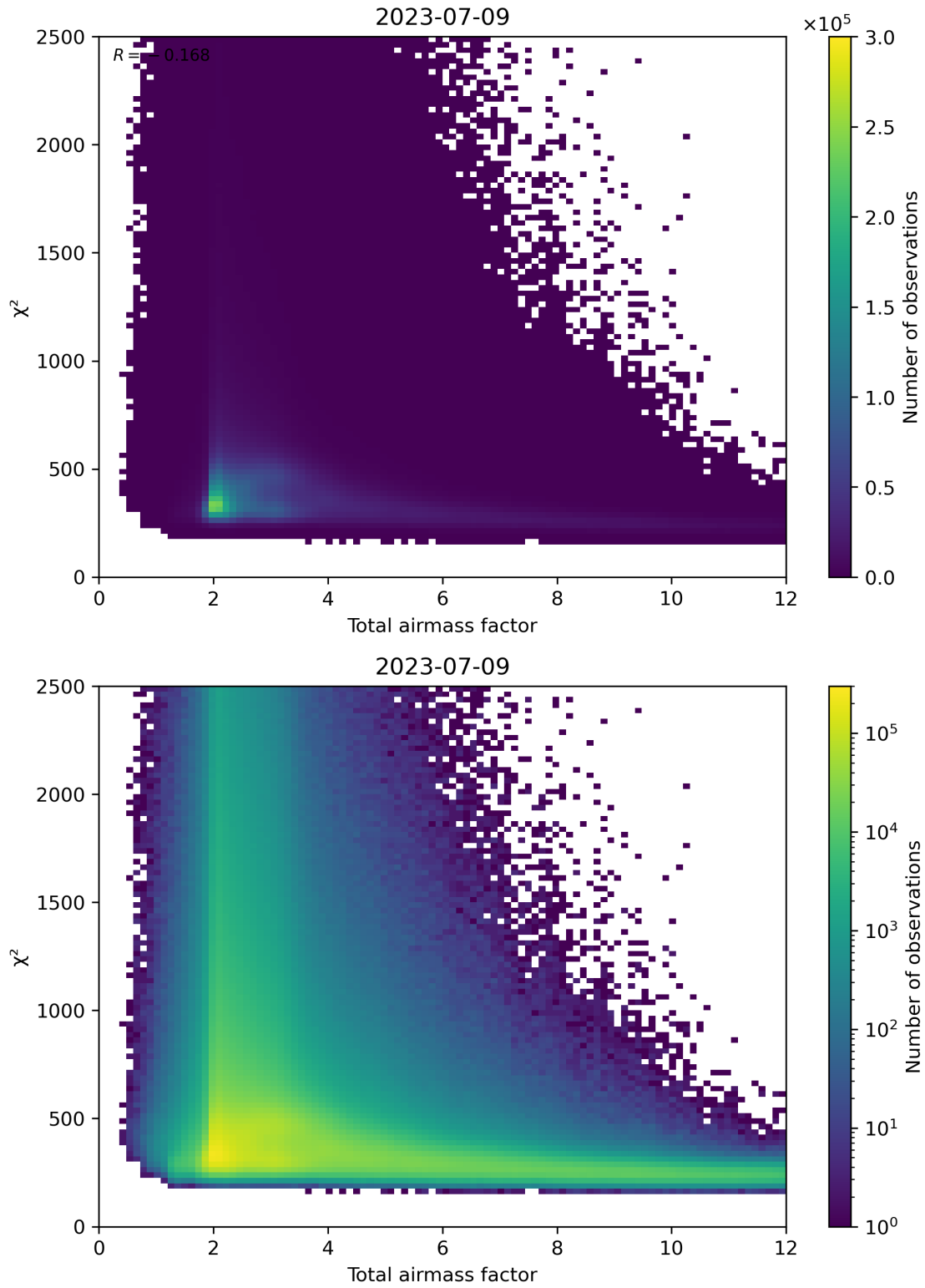
Figure 63: Scatter density plot of “Total airmass factor” against “ \chi^2 ” for 2023-07-08 to 2023-07-10.
