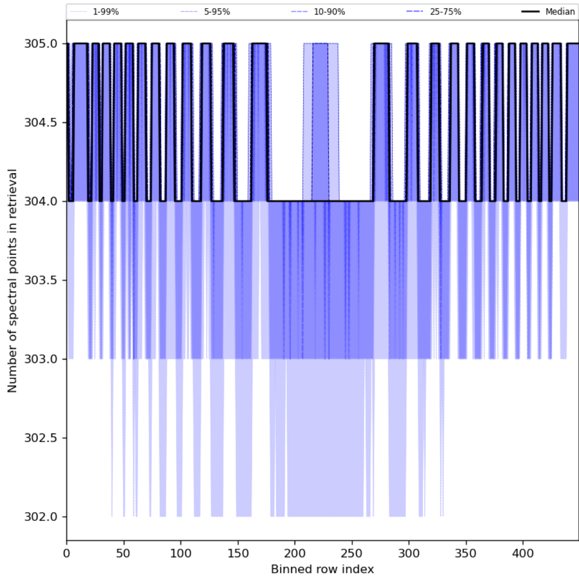
Figure 50: Along track statistics of “Number of spectral points in retrieval” for 2023-07-08 to 2023-07-10
