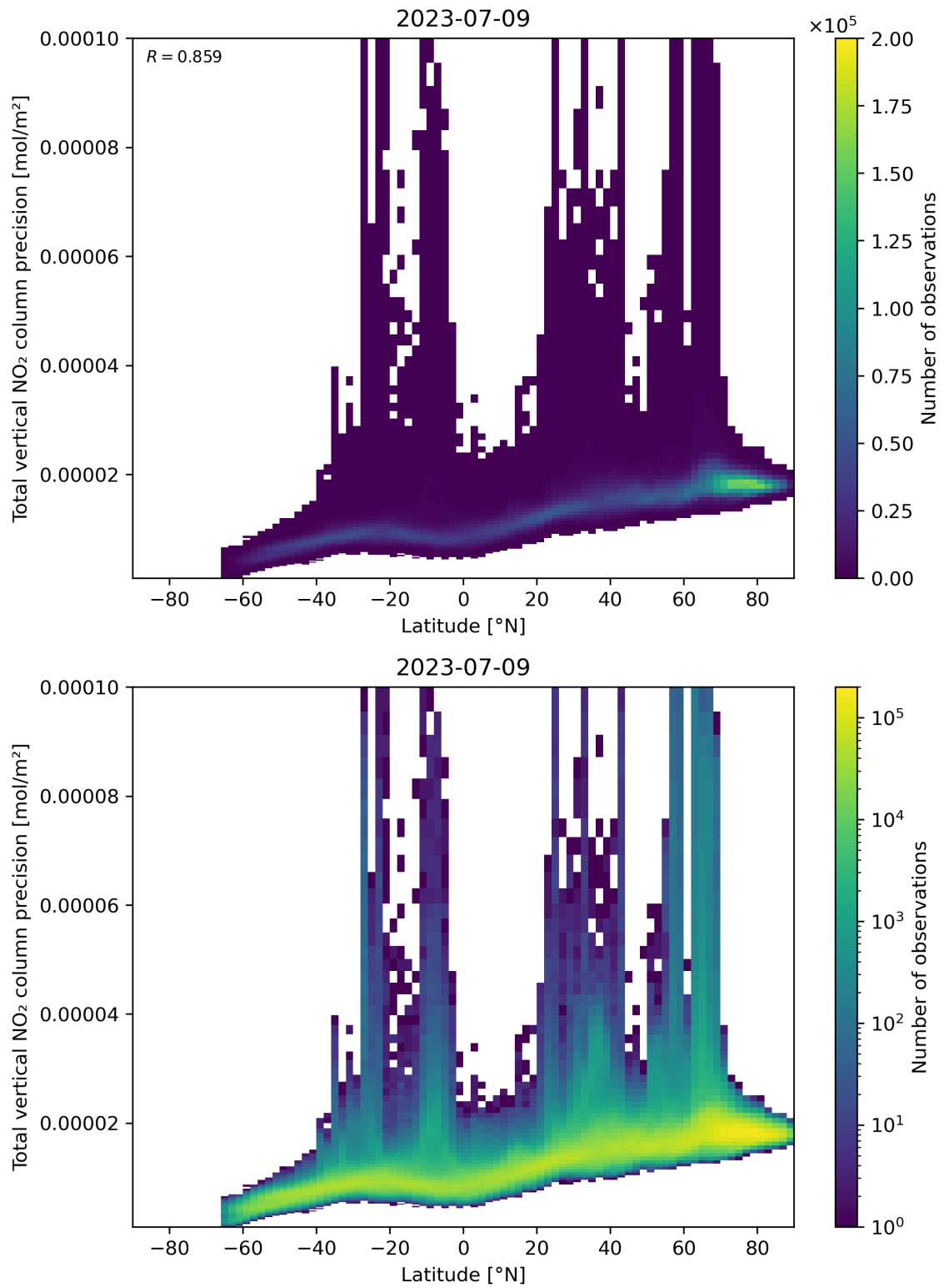
Figure 91: Scatter density plot of “Latitude” against “Total vertical NO 2 column precision” for 2023-07-08 to 2023-07-10.
