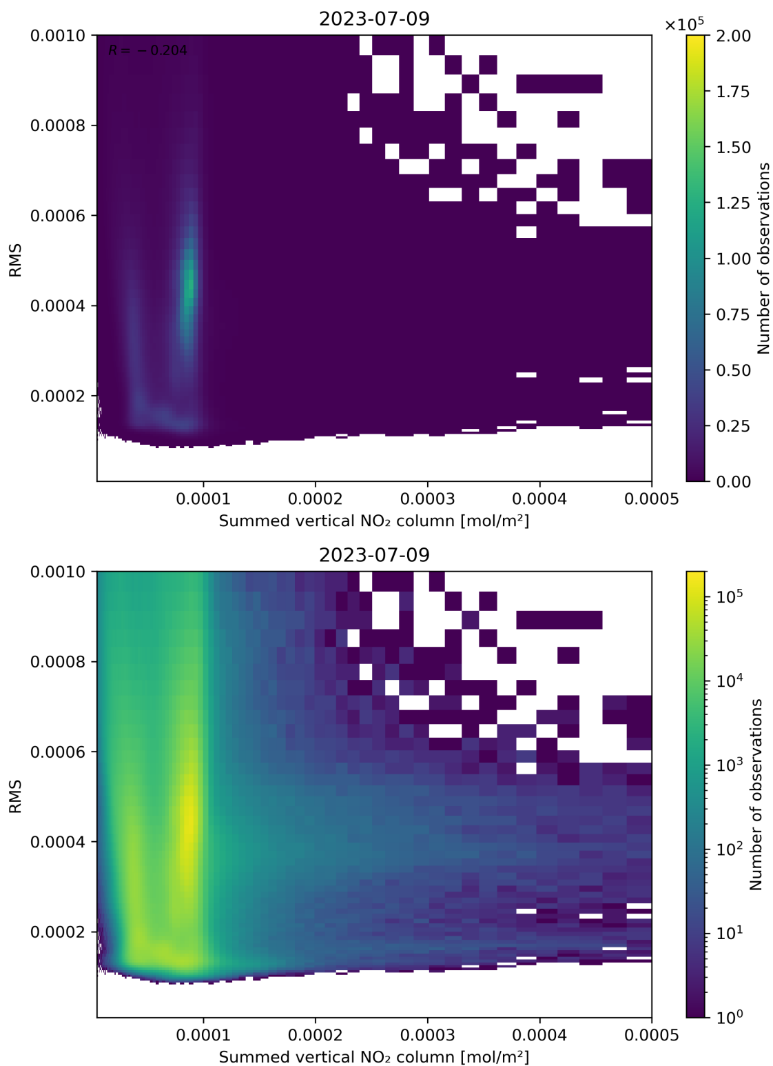
Figure 109: Scatter density plot of “Summed vertical NO 2 column” against “RMS” for 2023-07-08 to 2023-07-10.
