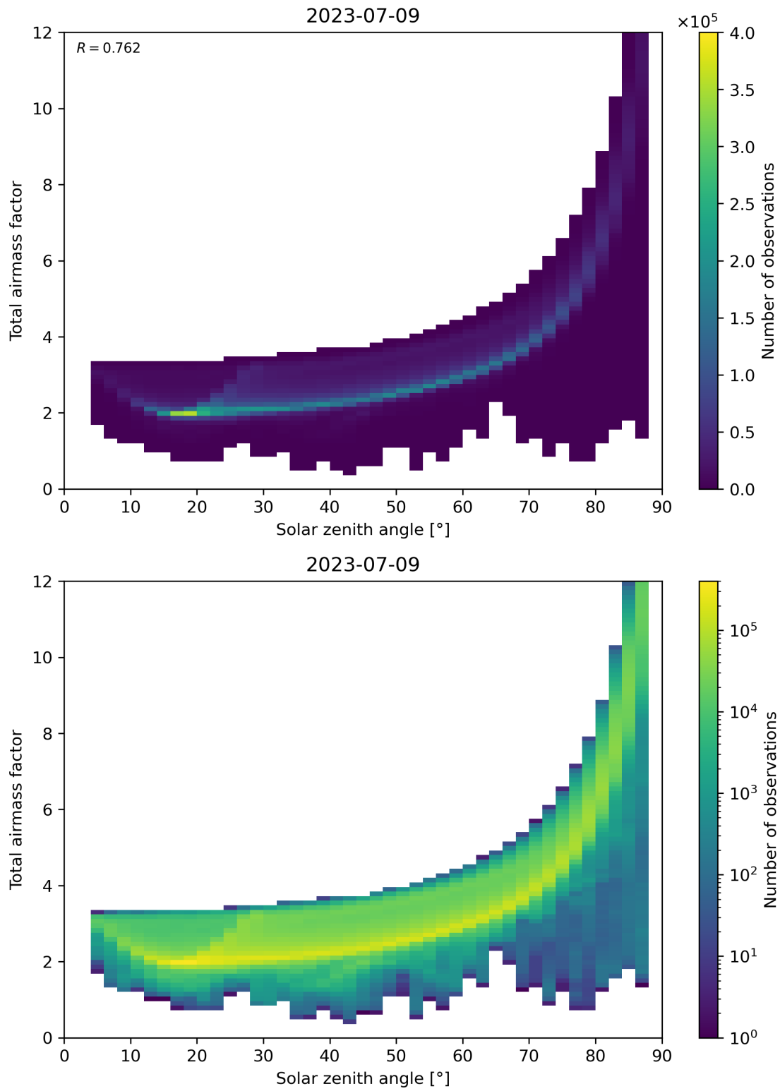
Figure 146: Scatter density plot of “Solar zenith angle” against “Total airmass factor” for 2023-07-08 to 2023-07-10.
