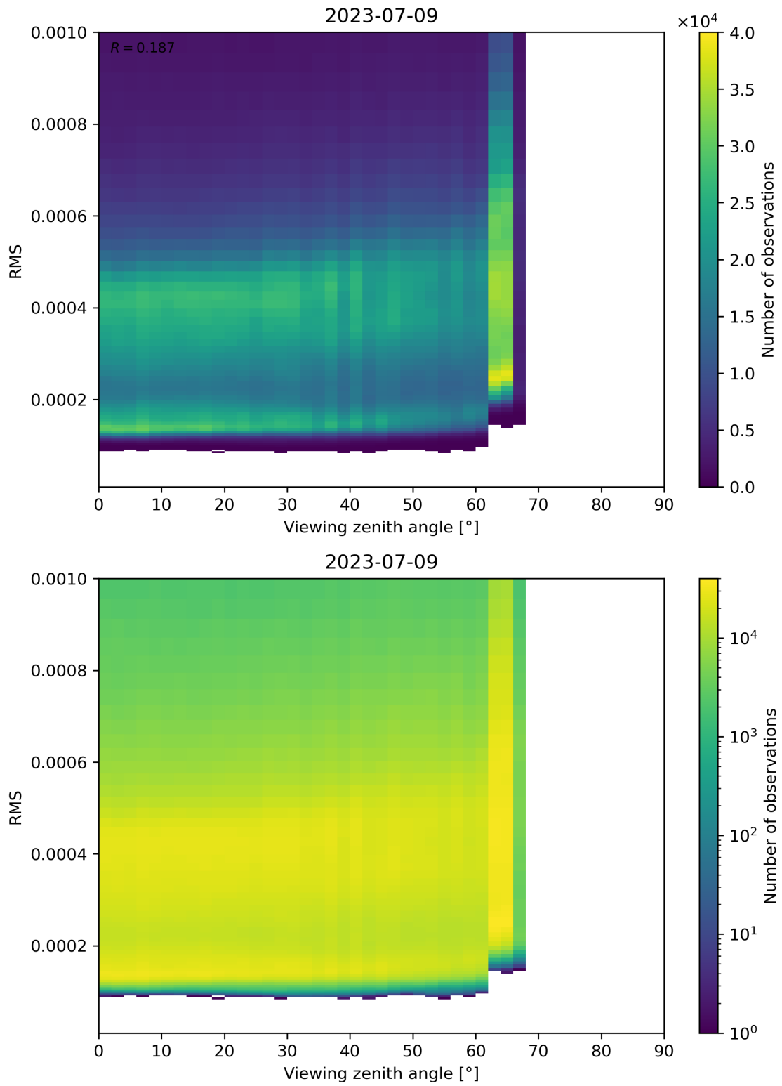
Figure 171: Scatter density plot of “Viewing zenith angle” against “RMS” for 2023-07-08 to 2023-07-10.
