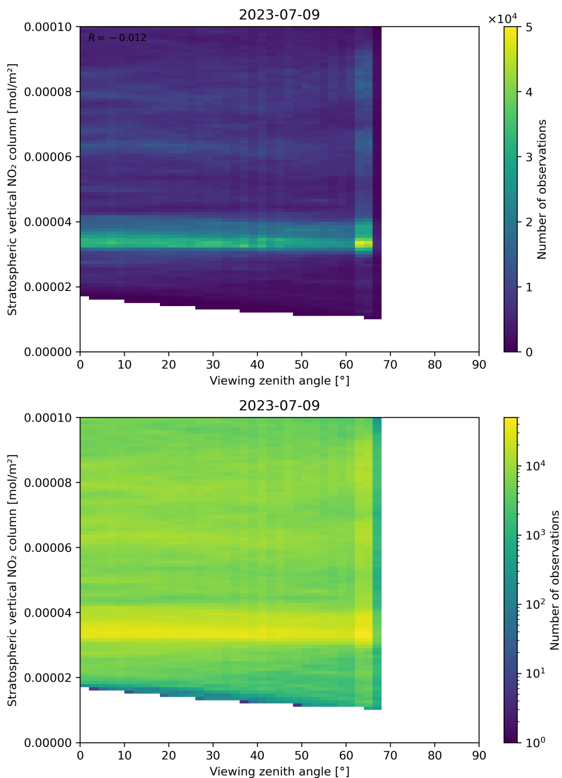
Figure 164: Scatter density plot of “Viewing zenith angle” against “Stratospheric vertical NO 2 column” for 2023-07-08 to 2023-07-10.
