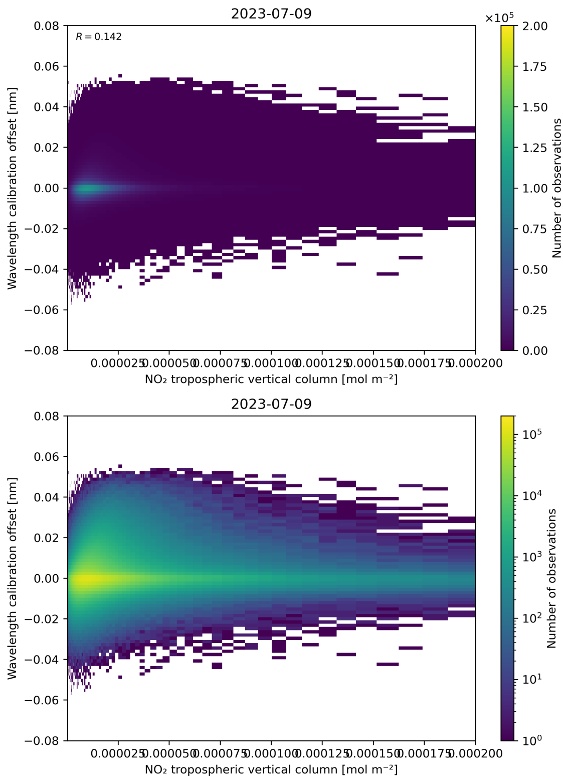
Figure 143: Scatter density plot of “NO 2 tropospheric vertical column” against “Wavelength calibration offset” for 2023-07-08 to 2023-07-10.
