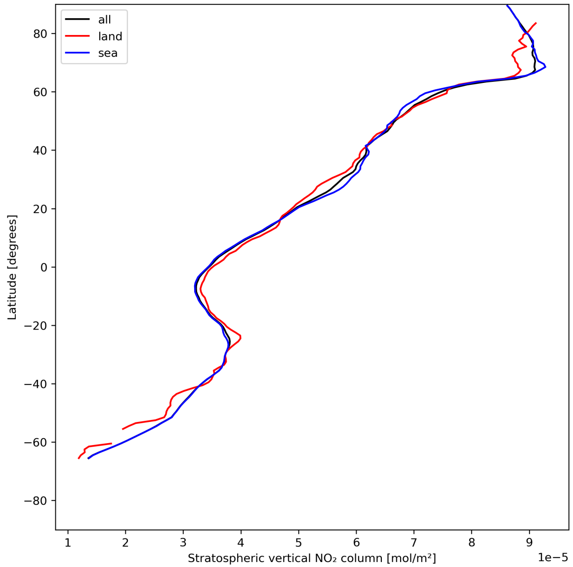
Figure 19: Zonal average of “Stratospheric vertical NO 2 column” for 2023-07-08 to 2023-07-10.
