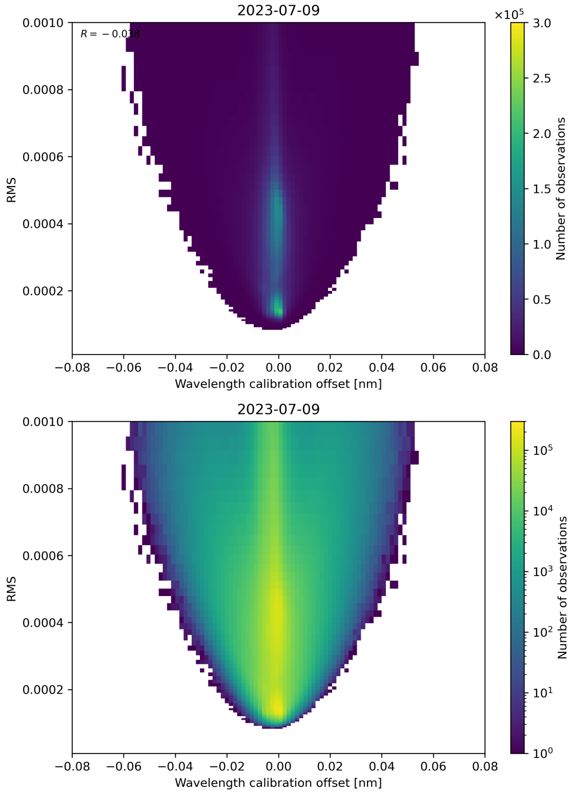
Figure 181: Scatter density plot of “Wavelength calibration offset” against “RMS” for 2023-07-08 to 2023-07-10.
