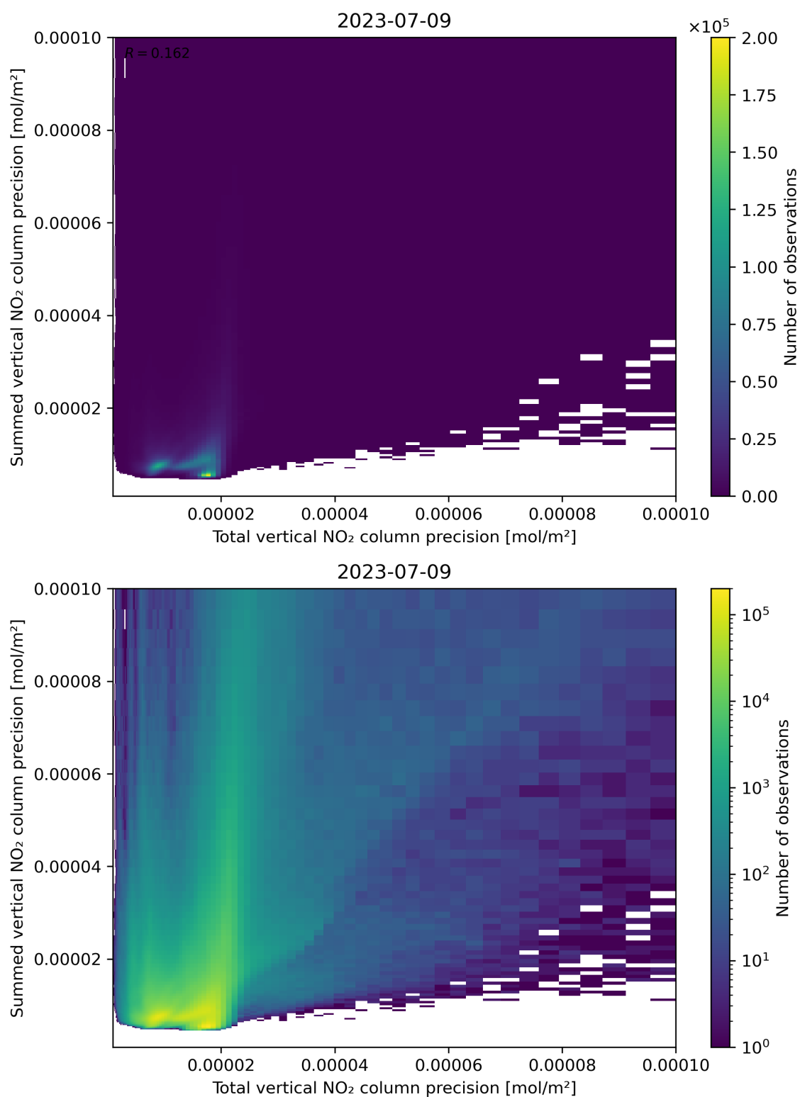
Figure 118: Scatter density plot of “Total vertical NO 2 column precision” against “Summed vertical NO 2 column precision” for 2023-07-08 to 2023-07-10.
