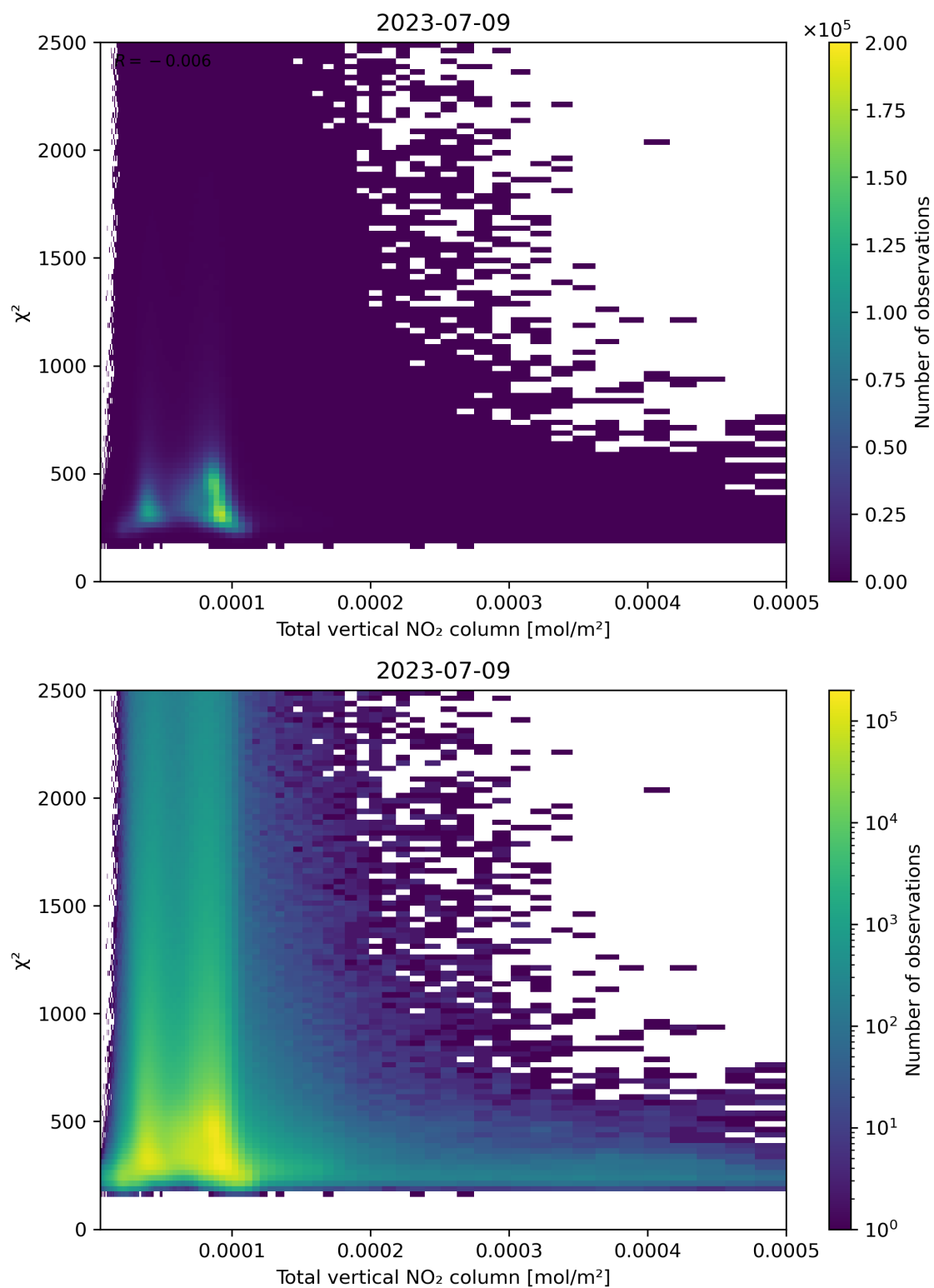
Figure 111: Scatter density plot of “Total vertical NO 2 column” against “ \chi^2 ” for 2023-07-08 to 2023-07-10.
