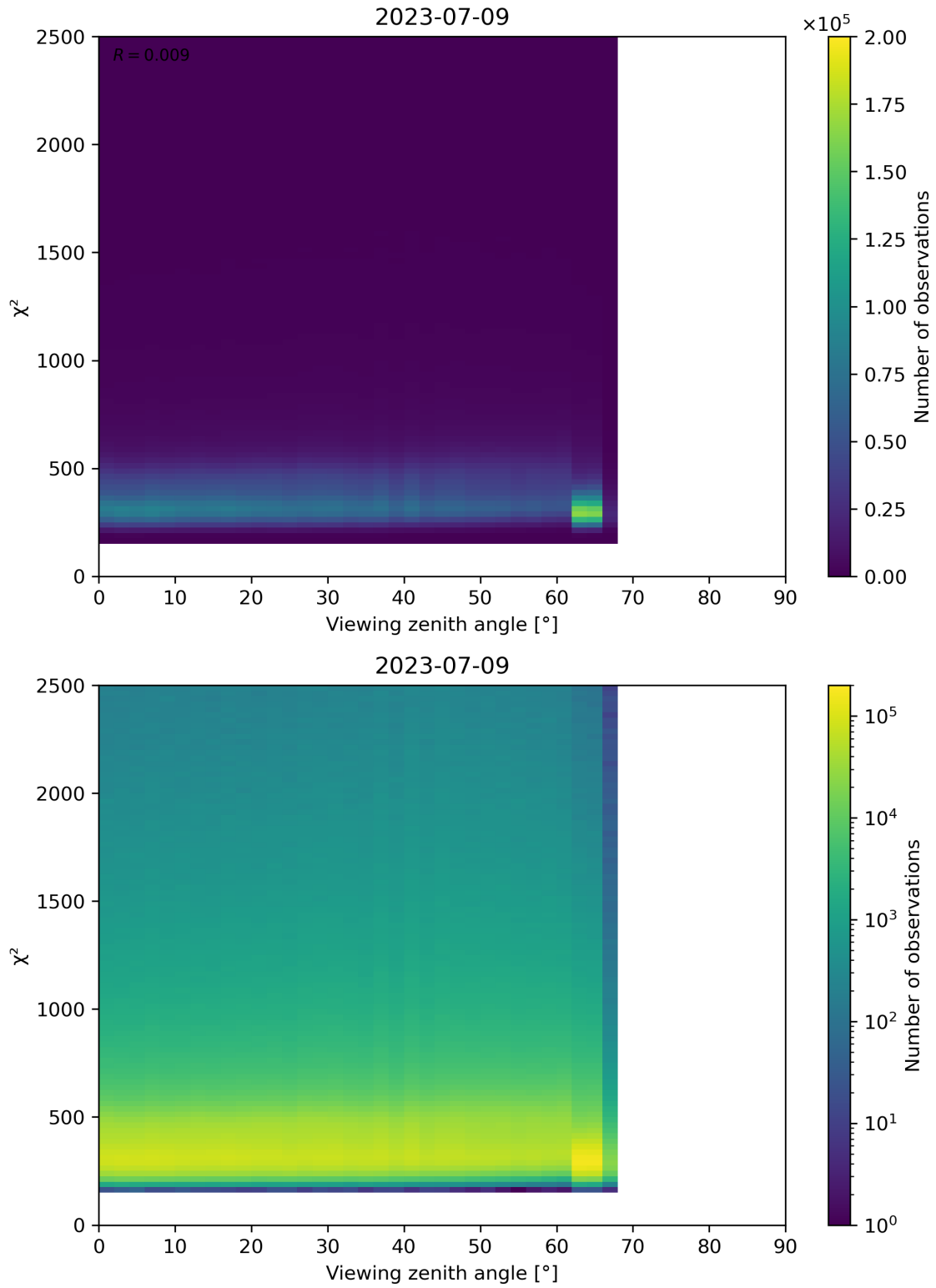
Figure 162: Scatter density plot of “Viewing zenith angle” against “ \chi^2 ” for 2023-07-08 to 2023-07-10.
