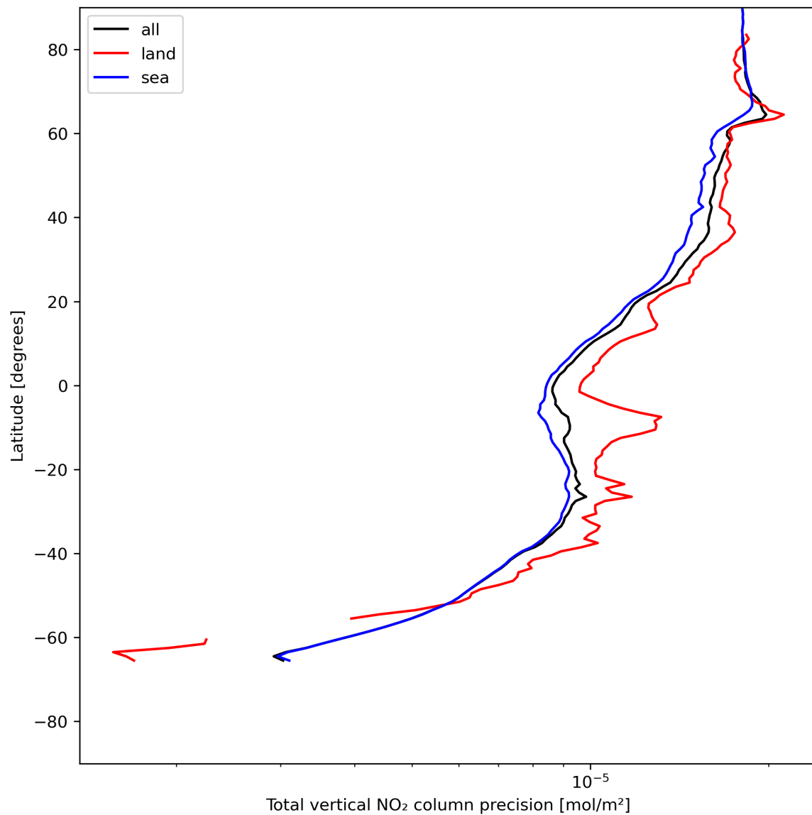
Figure 22: Zonal average of “Total vertical NO 2 column precision” for 2023-07-08 to 2023-07-10.
