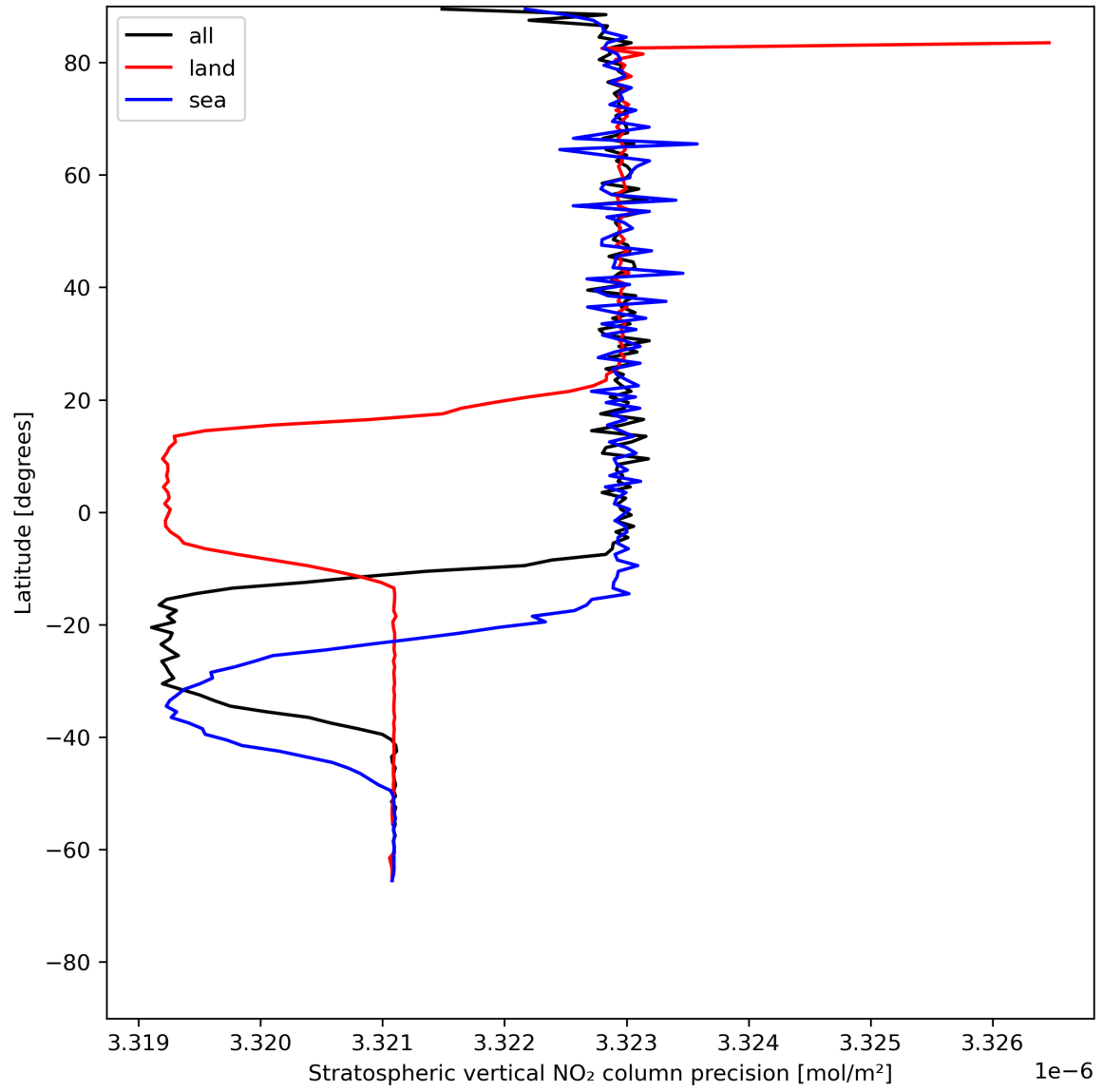
Figure 20: Zonal average of “Stratospheric vertical NO 2 column precision” for 2023-07-08 to 2023-07-10.
