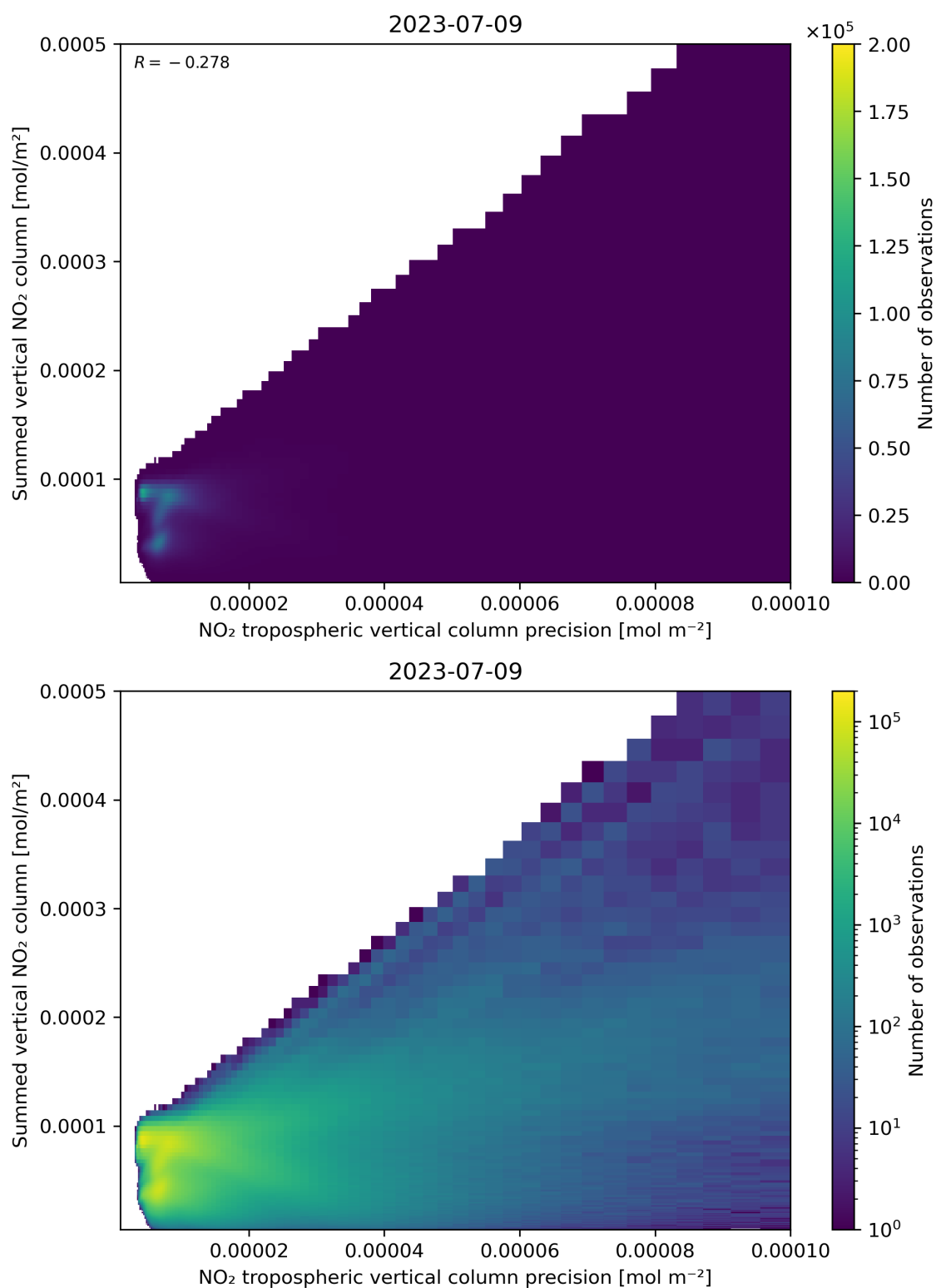
Figure 136: Scatter density plot of “NO 2 tropospheric vertical column precision” against “Summed vertical NO 2 column” for 2023-07-08 to 2023-07-10.
