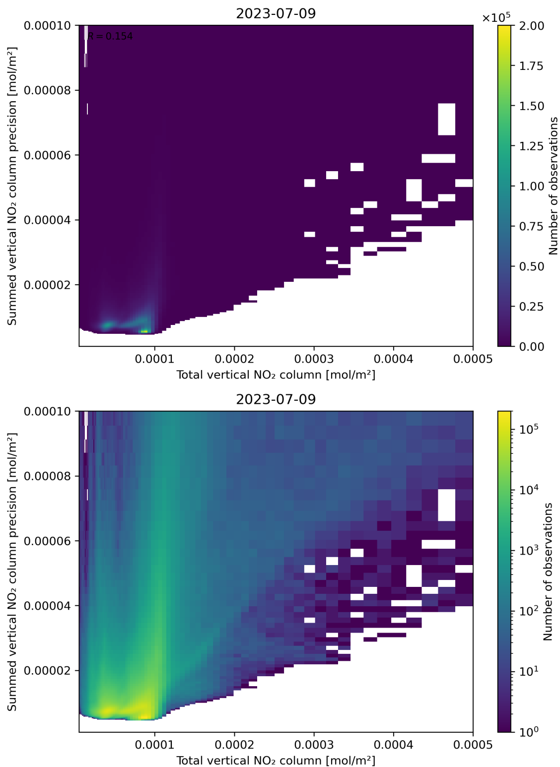
Figure 113: Scatter density plot of “Total vertical NO 2 column” against “Summed vertical NO 2 column precision” for 2023-07-08 to 2023-07-10.
