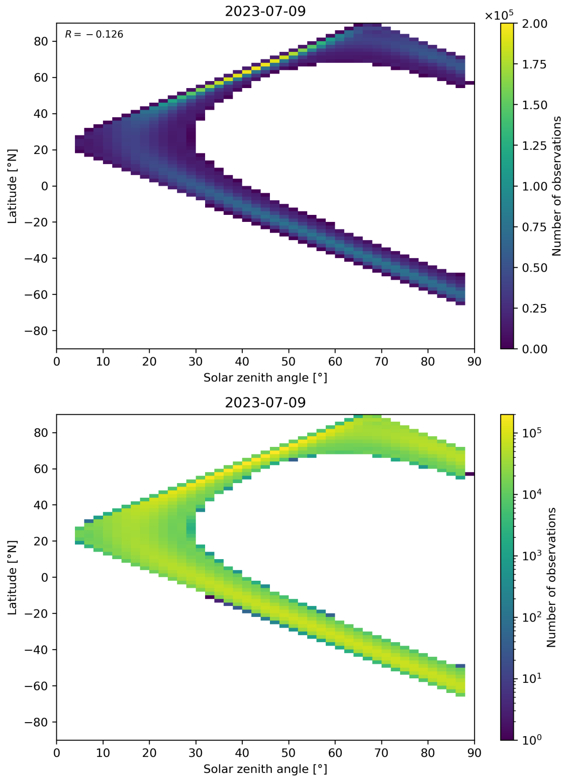
Figure 149: Scatter density plot of “Solar zenith angle” against “Latitude” for 2023-07-08 to 2023-07-10.
