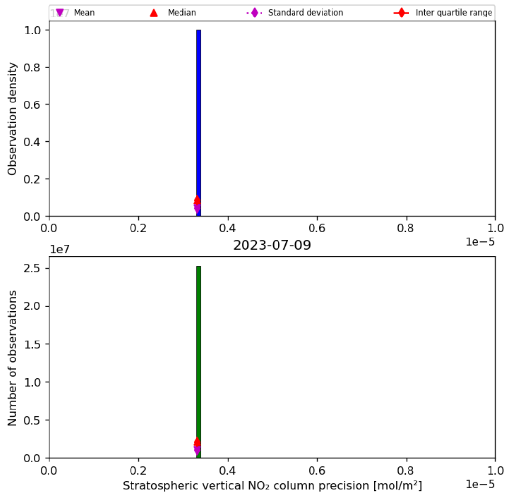
Figure 37: Histogram of “Stratospheric vertical NO 2 column precision” for 2023-07-08 to 2023-07-10
