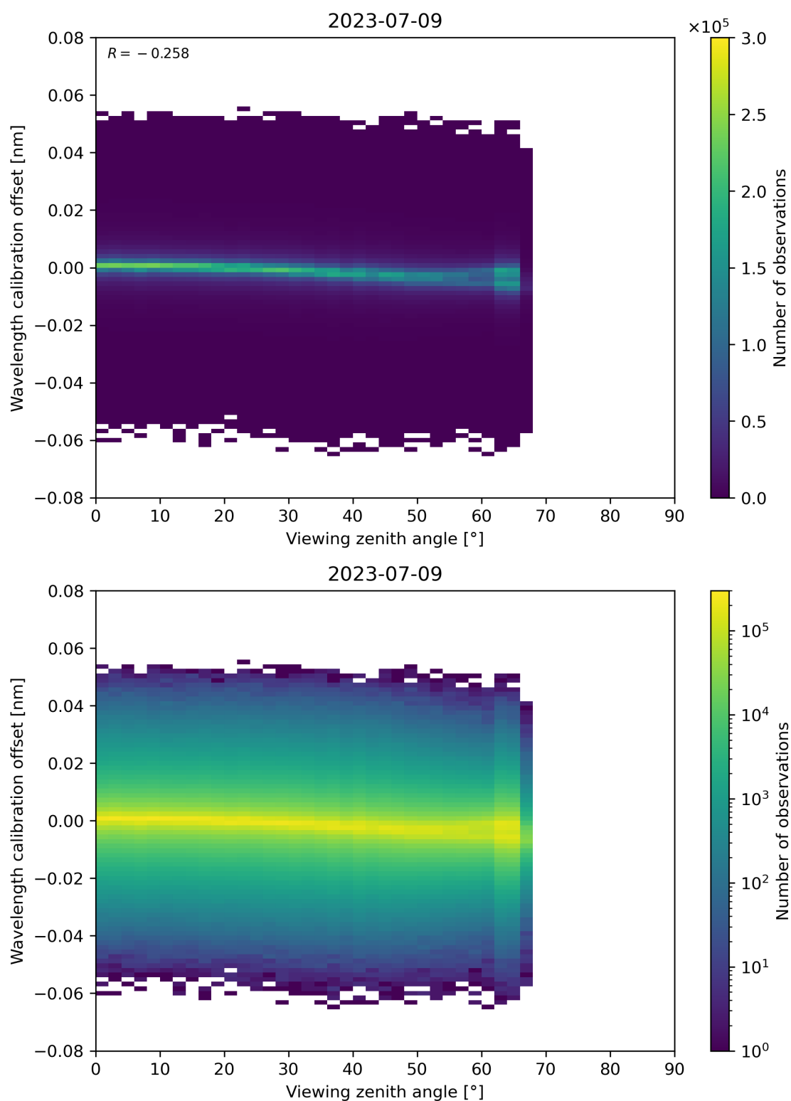
Figure 173: Scatter density plot of “Viewing zenith angle” against “Wavelength calibration offset” for 2023-07-08 to 2023-07-10.
