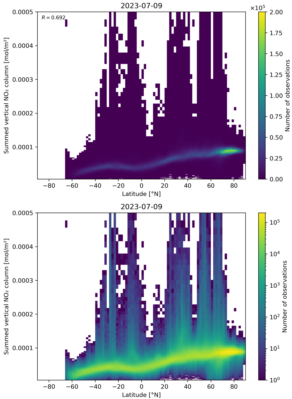
Figure 88: Scatter density plot of “Latitude” against “Summed vertical NO 2 column” for 2023-07-08 to 2023-07-10.
