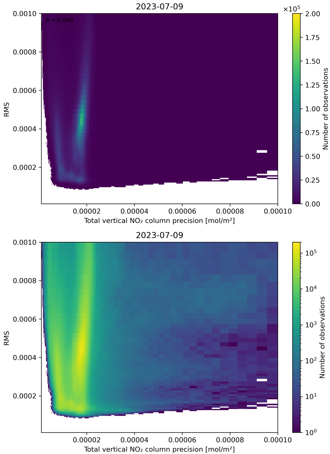
Figure 119: Scatter density plot of “Total vertical NO 2 column precision” against “RMS” for 2023-07-08 to 2023-07-10.
