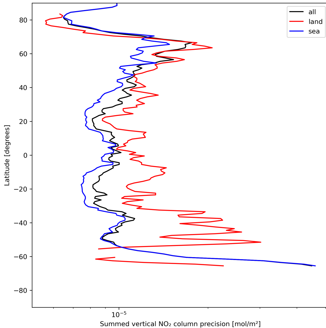
Figure 24: Zonal average of “Summed vertical NO 2 column precision” for 2023-07-08 to 2023-07-10.
