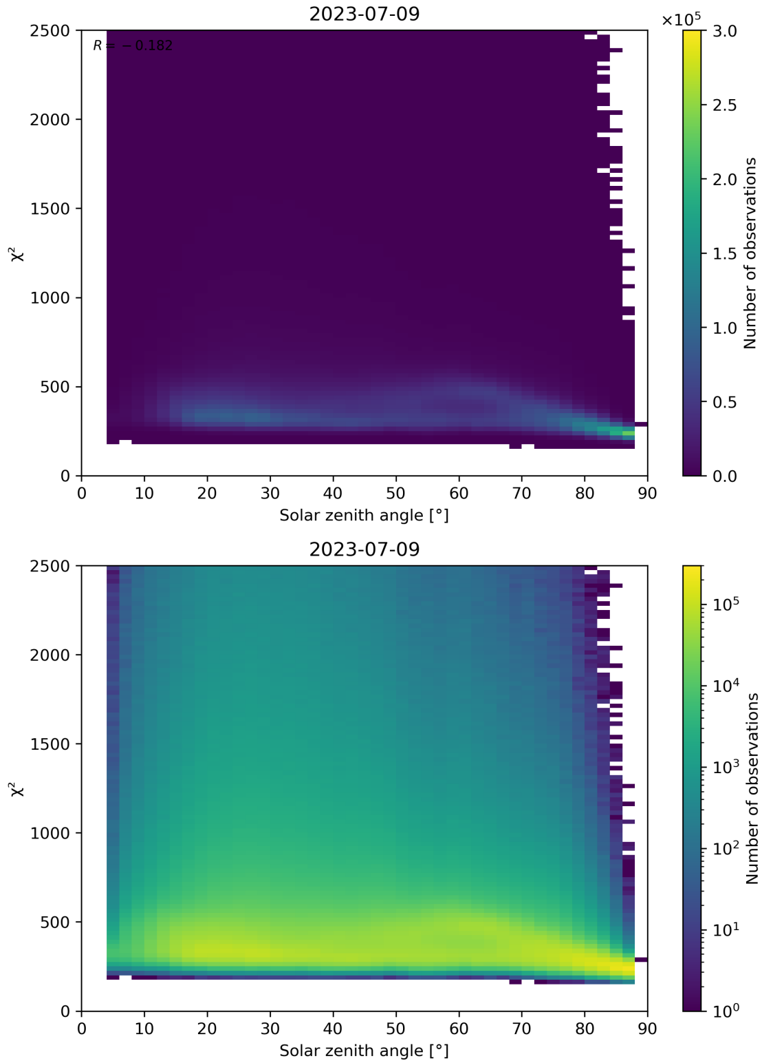
Figure 148: Scatter density plot of “Solar zenith angle” against “ \chi^2 ” for 2023-07-08 to 2023-07-10.
