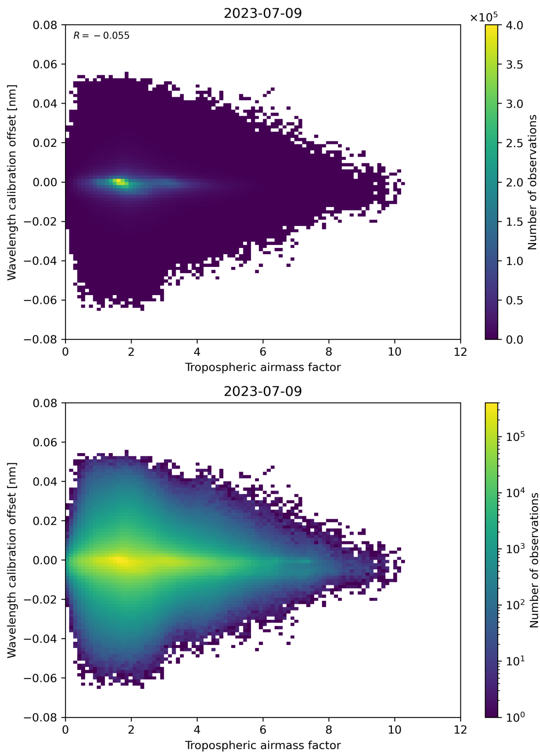
Figure 80: Scatter density plot of “Tropospheric airmass factor” against “Wavelength calibration offset” for 2023-07-08 to 2023-07-10.
