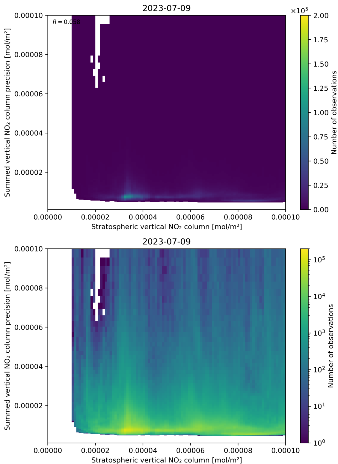
Figure 99: Scatter density plot of “Stratospheric vertical NO 2 column” against “Summed vertical NO 2 column precision” for 2023-07-08 to 2023-07-10.
