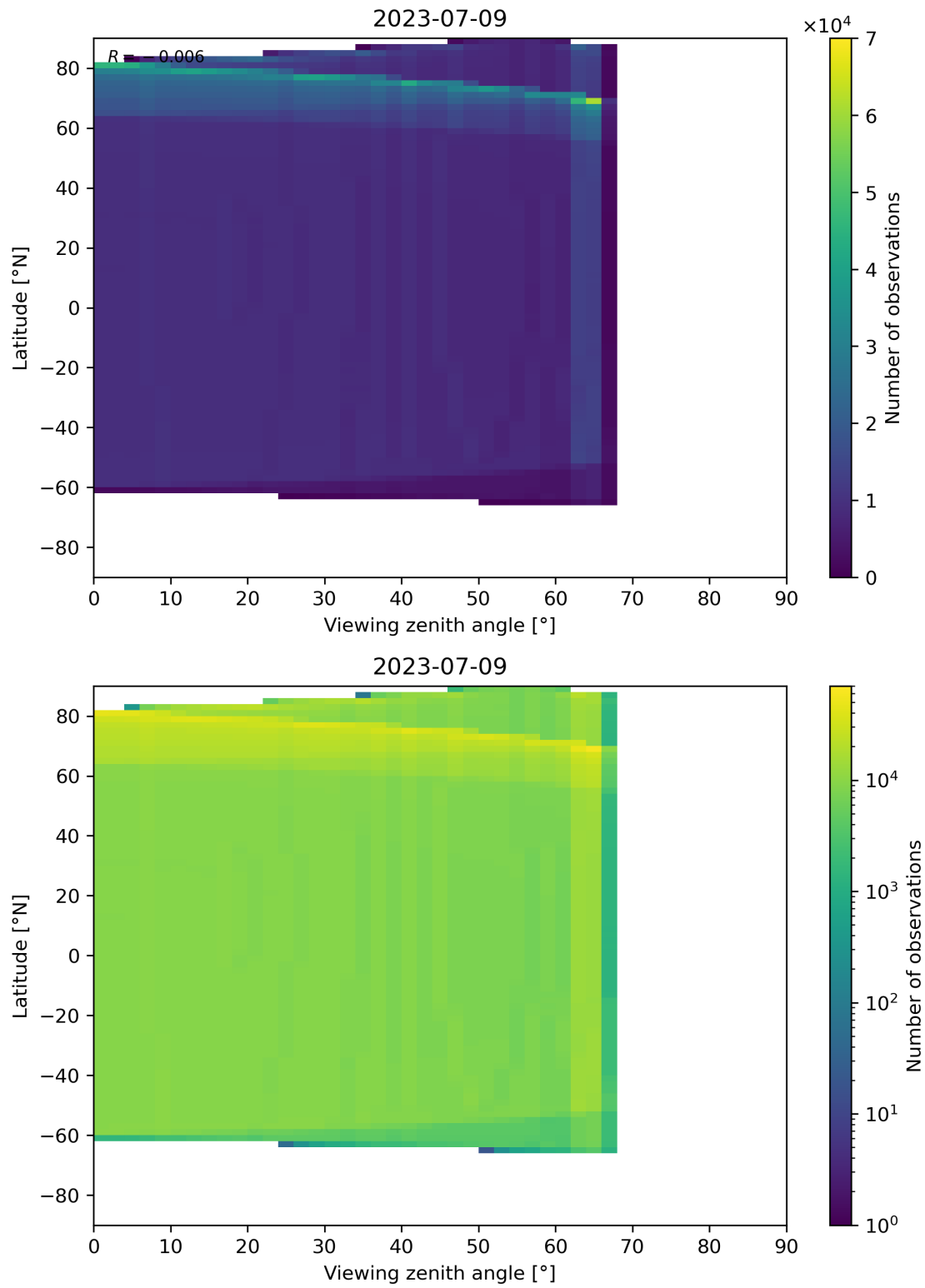
Figure 163: Scatter density plot of “Viewing zenith angle” against “Latitude” for 2023-07-08 to 2023-07-10.
