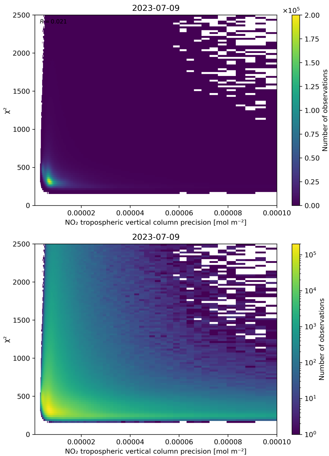
Figure 134: Scatter density plot of “NO 2 tropospheric vertical column precision” against “ \chi^2 ” for 2023-07-08 to 2023-07-10.
