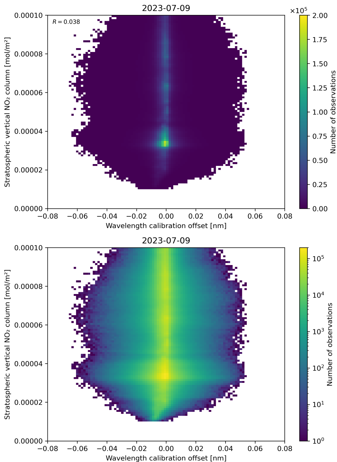
Figure 176: Scatter density plot of “Wavelength calibration offset” against “Stratospheric vertical NO 2 column” for 2023-07-08 to 2023-07-10.
