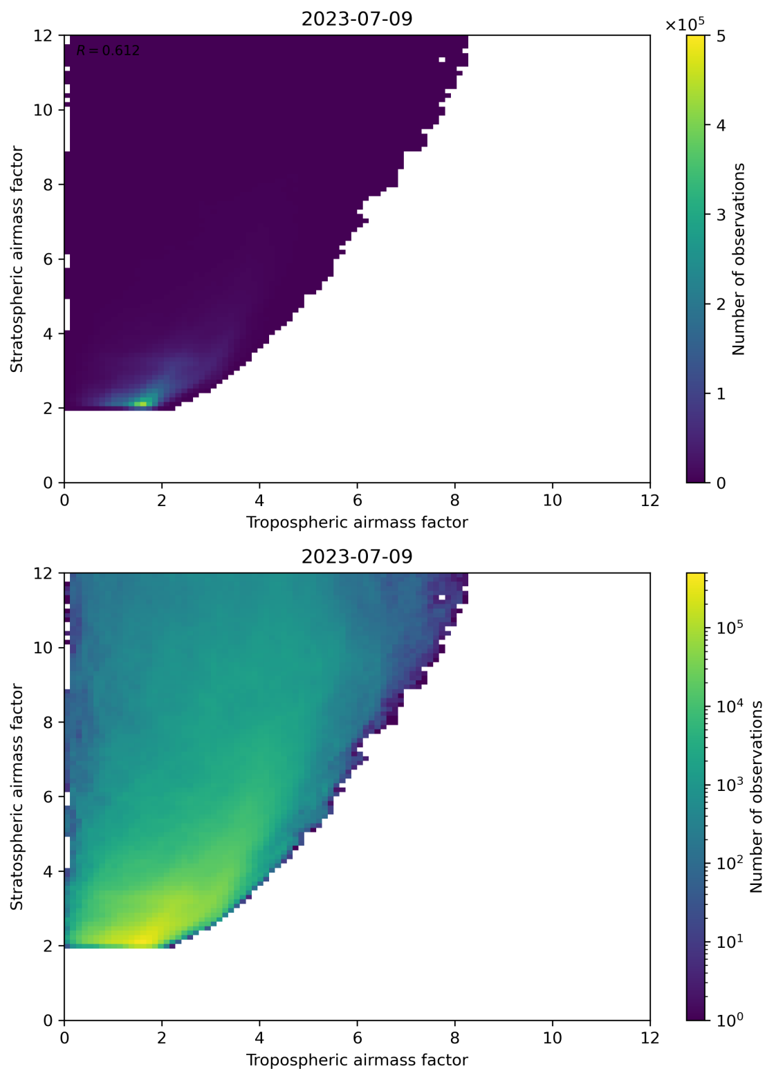
Figure 71: Scatter density plot of “Tropospheric airmass factor” against “Stratospheric airmass factor” for 2023-07-08 to 2023-07-10.
