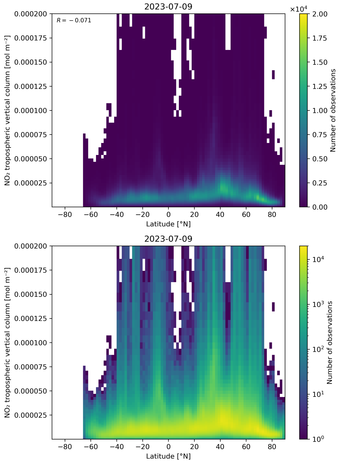
Figure 92: Scatter density plot of “Latitude” against “NO 2 tropospheric vertical column” for 2023-07-08 to 2023-07-10.
