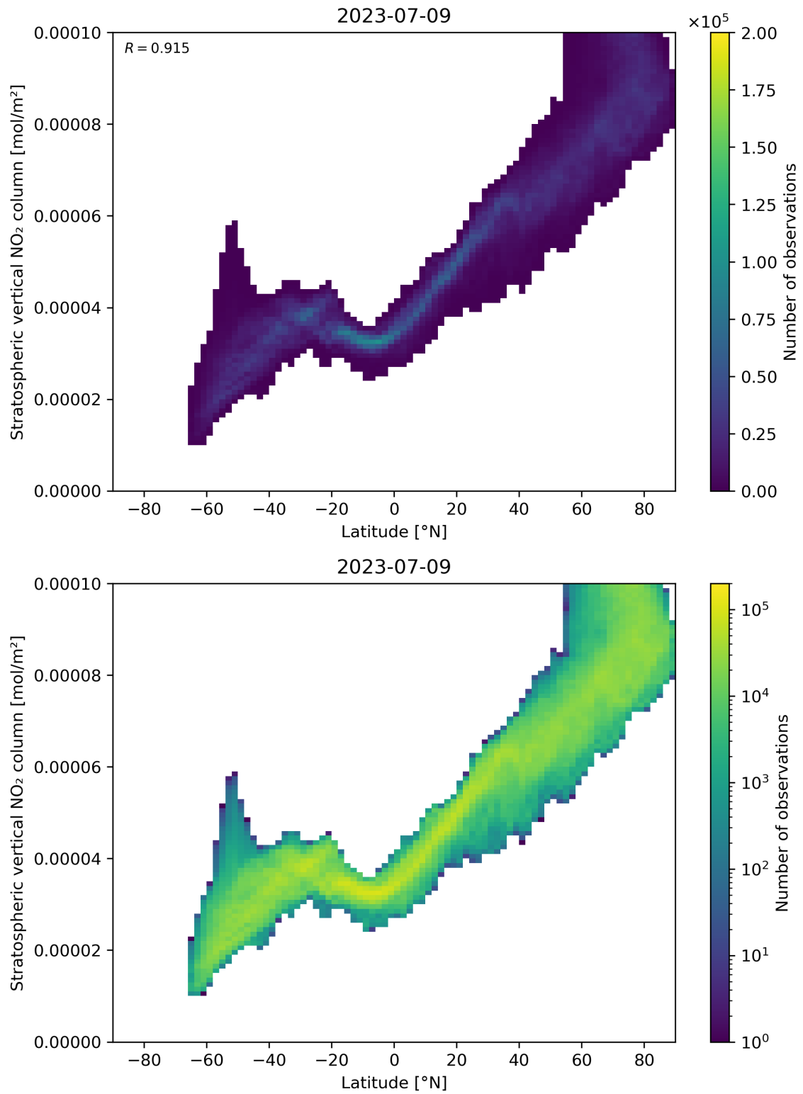
Figure 87: Scatter density plot of “Latitude” against “Stratospheric vertical NO 2 column” for 2023-07-08 to 2023-07-10.
