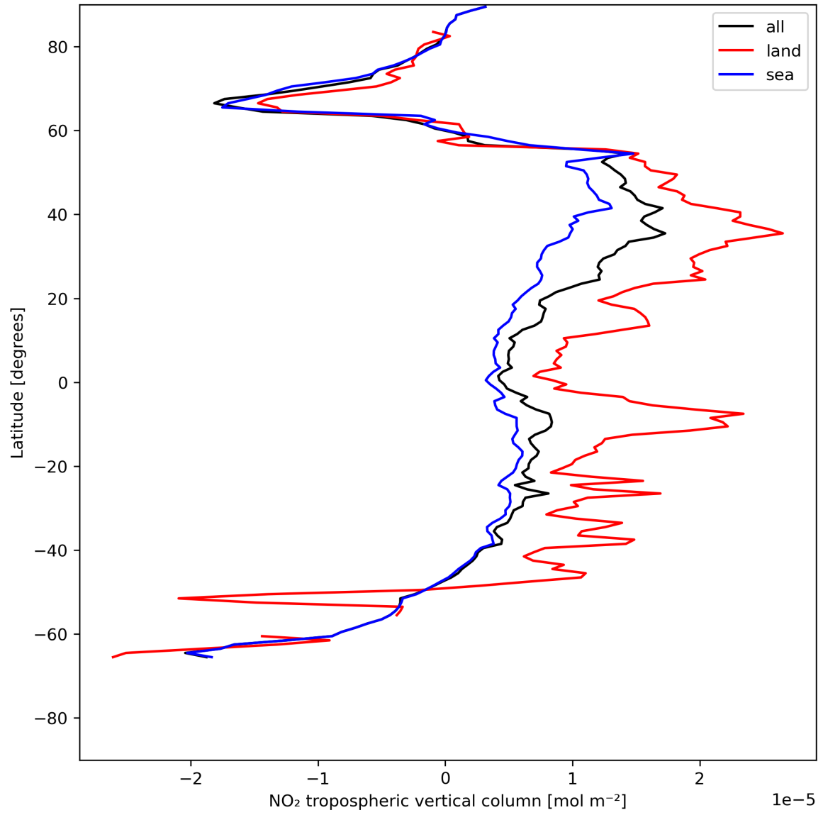
Figure 12: Zonal average of “NO 2 tropospheric vertical column” for 2023-07-08 to 2023-07-10.
