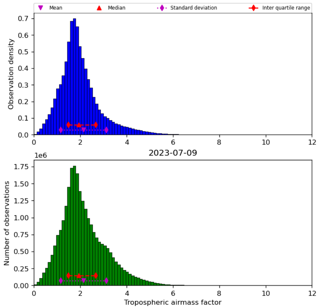
Figure 31: Histogram of “Tropospheric airmass factor” for 2023-07-08 to 2023-07-10
