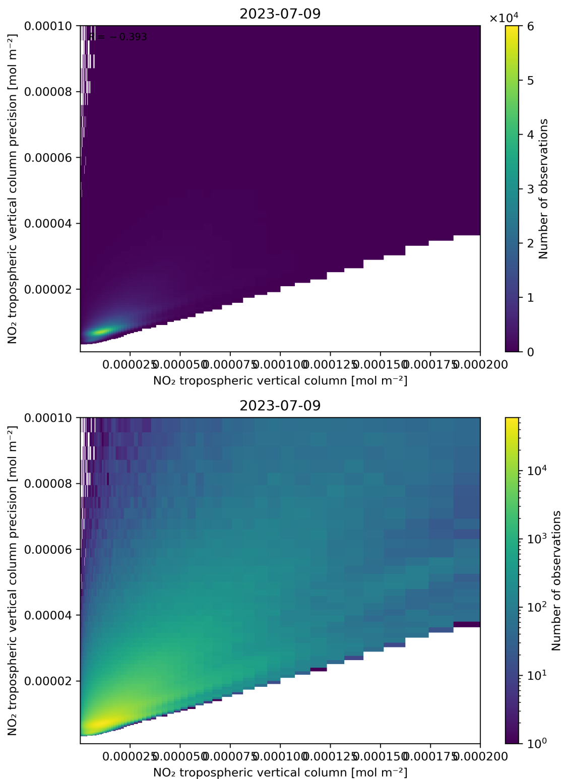
Figure 130: Scatter density plot of “NO 2 tropospheric vertical column” against “NO 2 tropospheric vertical column precision” for 2023-07-08 to 2023-07-10.
