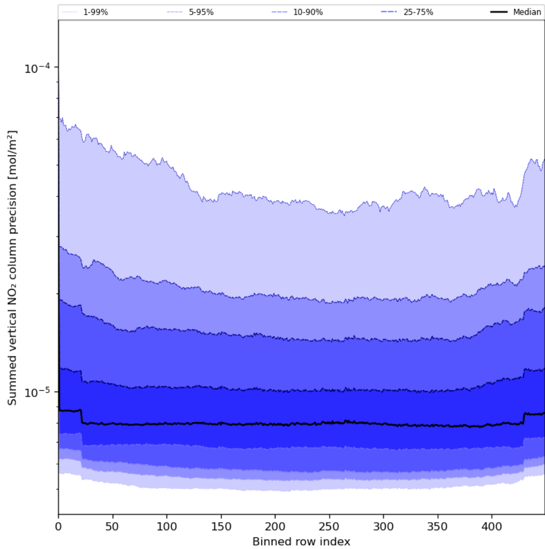
Figure 58: Along track statistics of “Summed vertical NO 2 column precision” for 2023-07-08 to 2023-07-10
