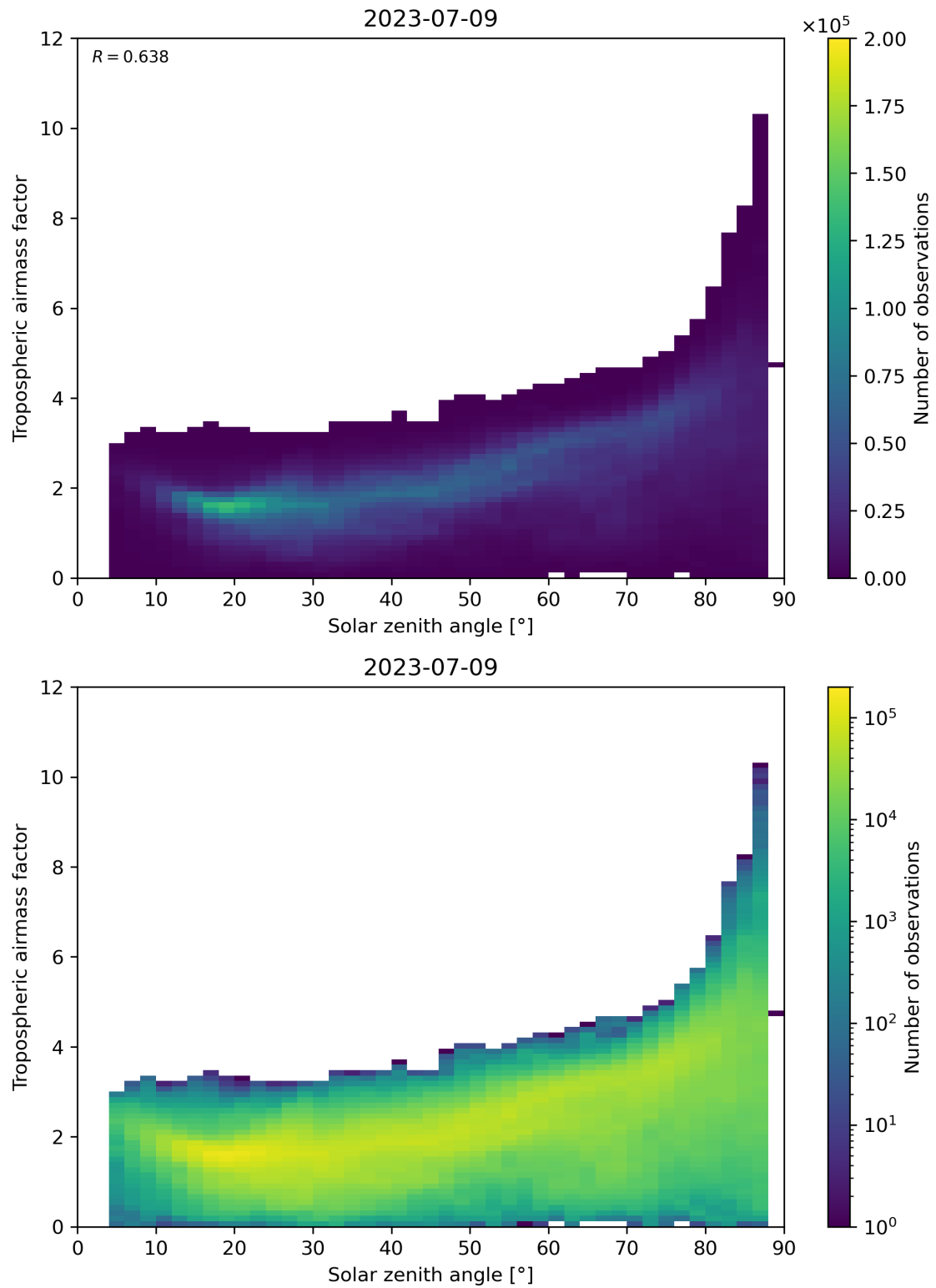
Figure 147: Scatter density plot of “Solar zenith angle” against “Tropospheric airmass factor” for 2023-07-08 to 2023-07-10.
