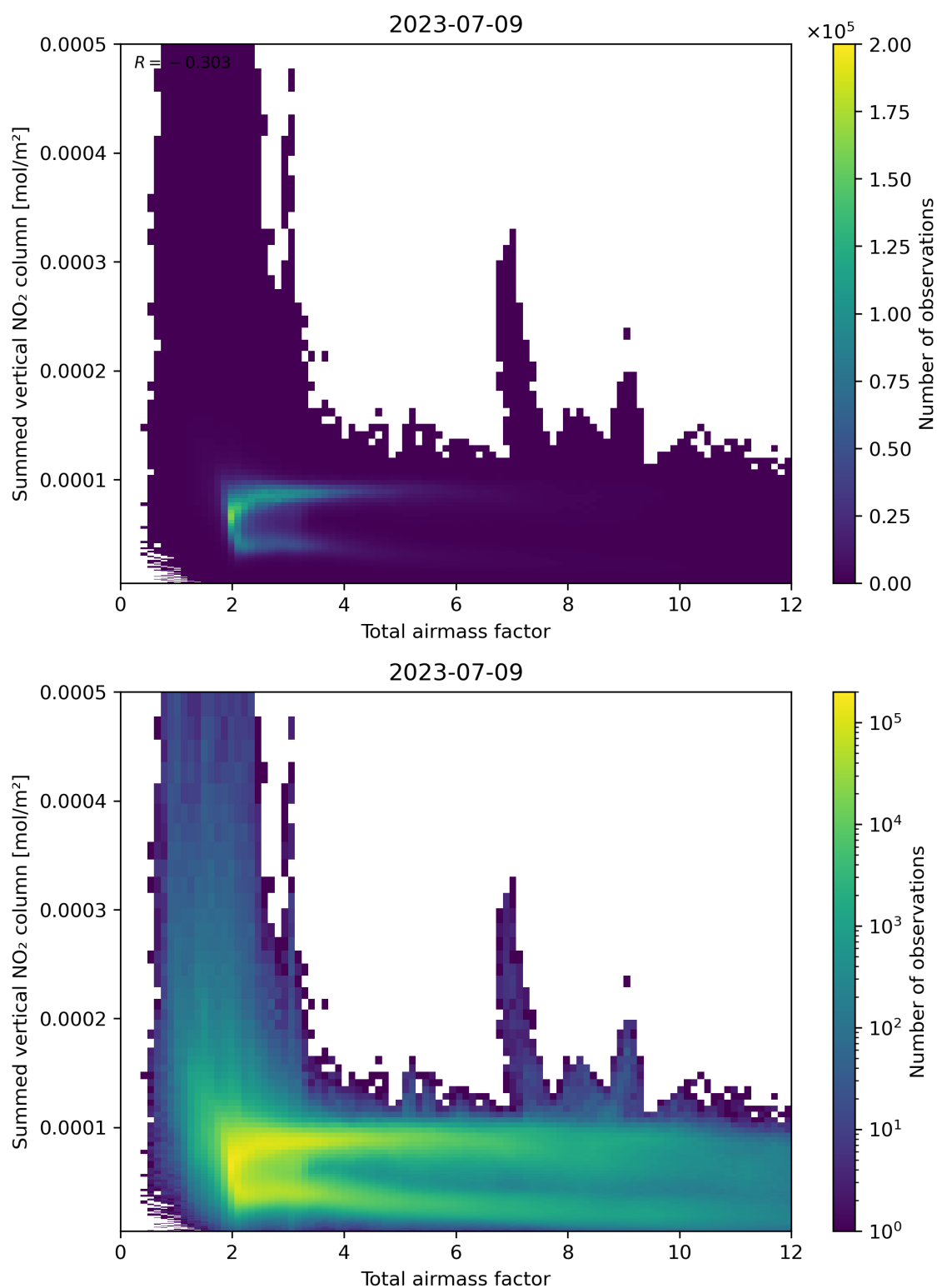
Figure 65: Scatter density plot of “Total airmass factor” against “Summed vertical NO 2 column” for 2023-07-08 to 2023-07-10.
