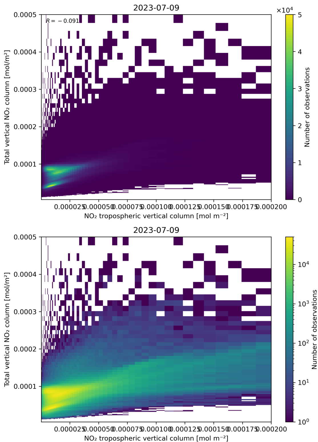
Figure 128: Scatter density plot of “NO 2 tropospheric vertical column” against “Total vertical NO 2 column” for 2023-07-08 to 2023-07-10.
