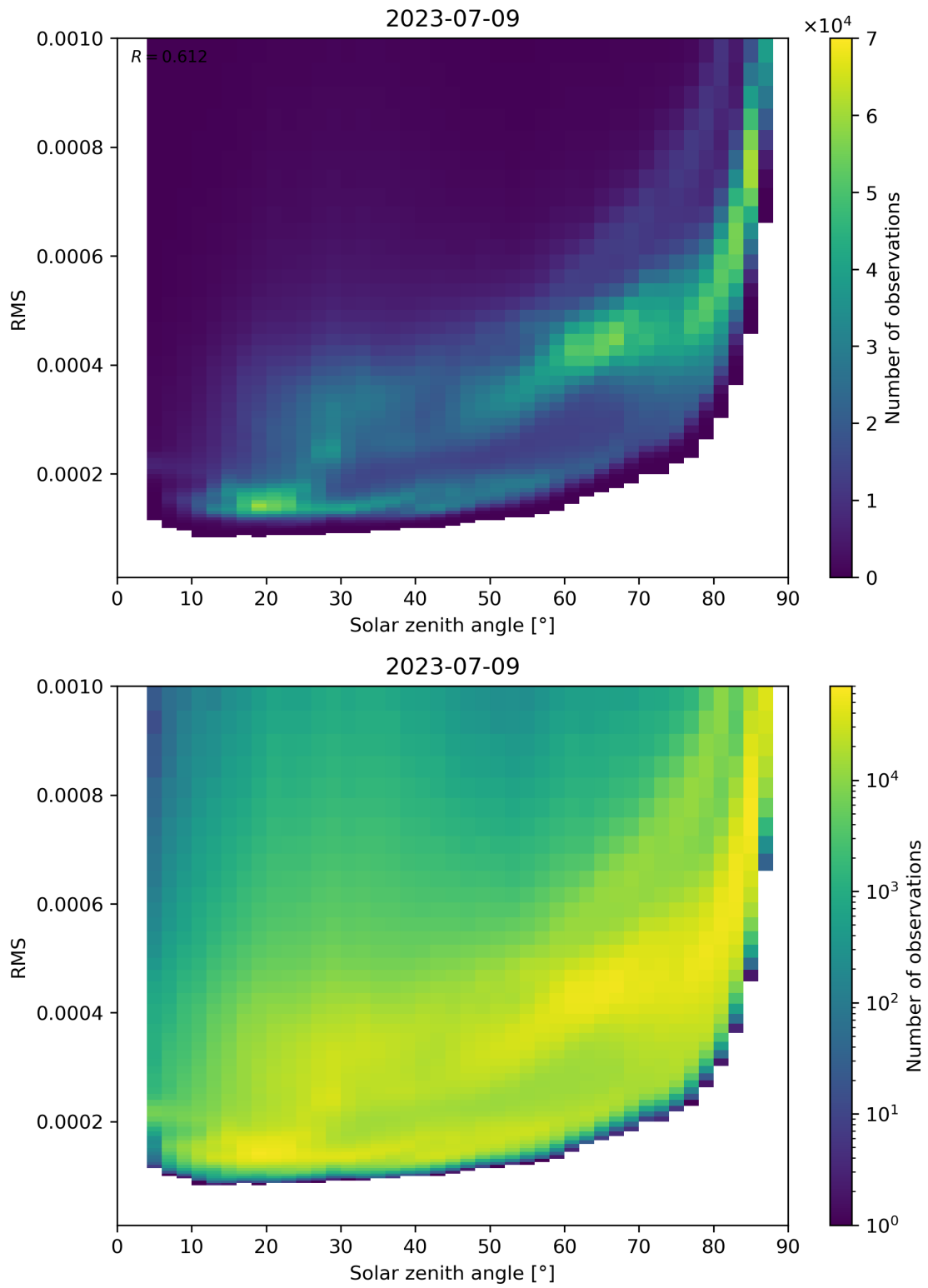
Figure 157: Scatter density plot of “Solar zenith angle” against “RMS” for 2023-07-08 to 2023-07-10.
