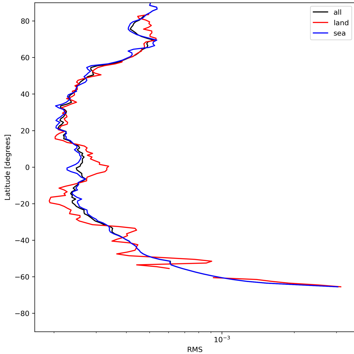
Figure 26: Zonal average of “RMS” for 2023-07-08 to 2023-07-10.
