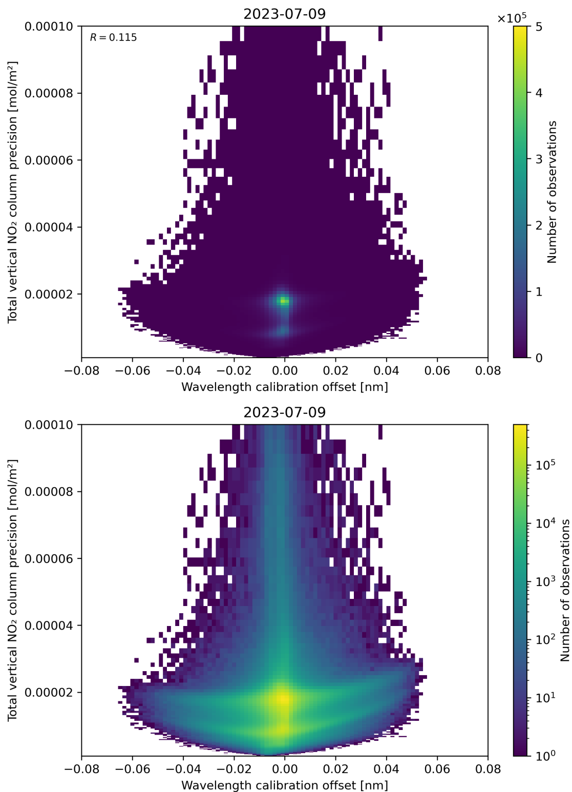
Figure 180: Scatter density plot of “Wavelength calibration offset” against “Total vertical NO 2 column precision” for 2023-07-08 to 2023-07-10.
