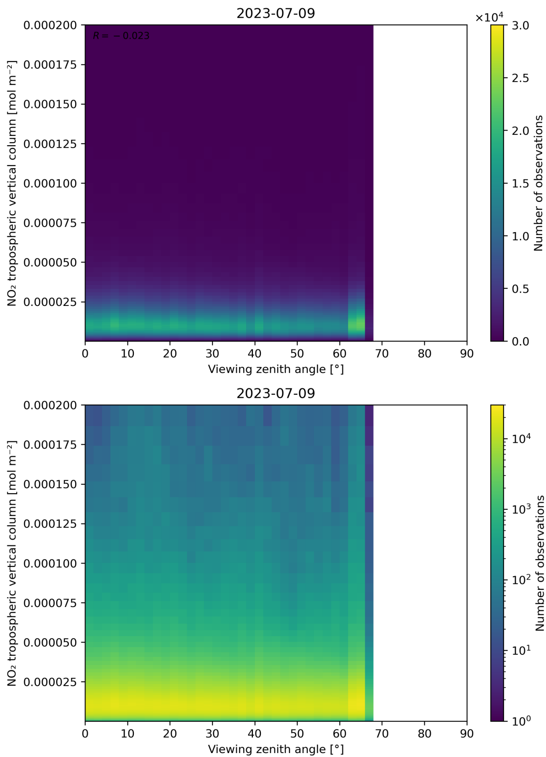
Figure 169: Scatter density plot of “Viewing zenith angle” against “NO 2 tropospheric vertical column” for 2023-07-08 to 2023-07-10.
