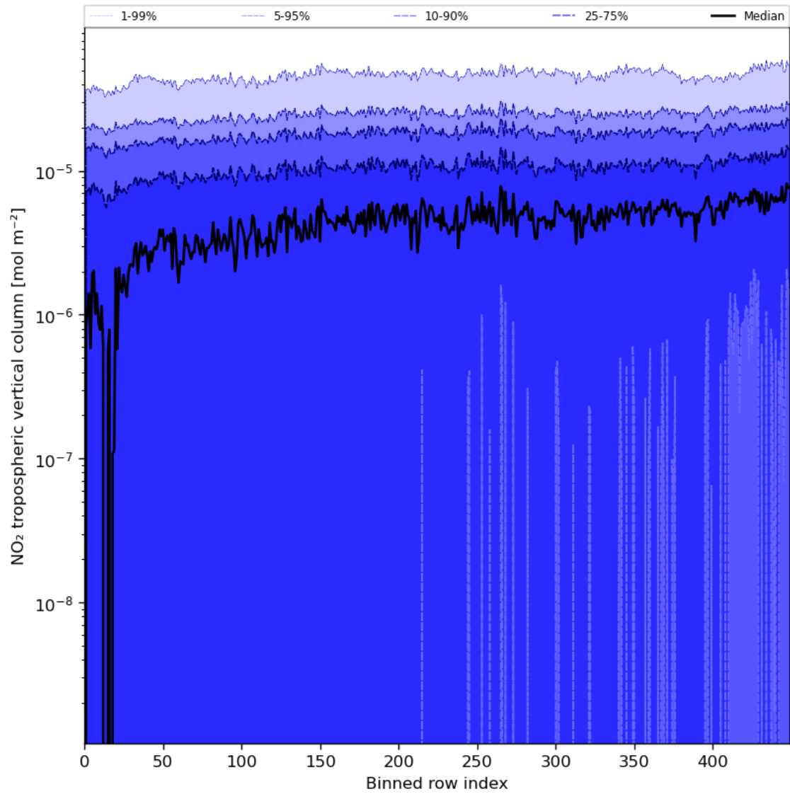
Figure 46: Along track statistics of “NO 2 tropospheric vertical column” for 2023-07-08 to 2023-07-10
