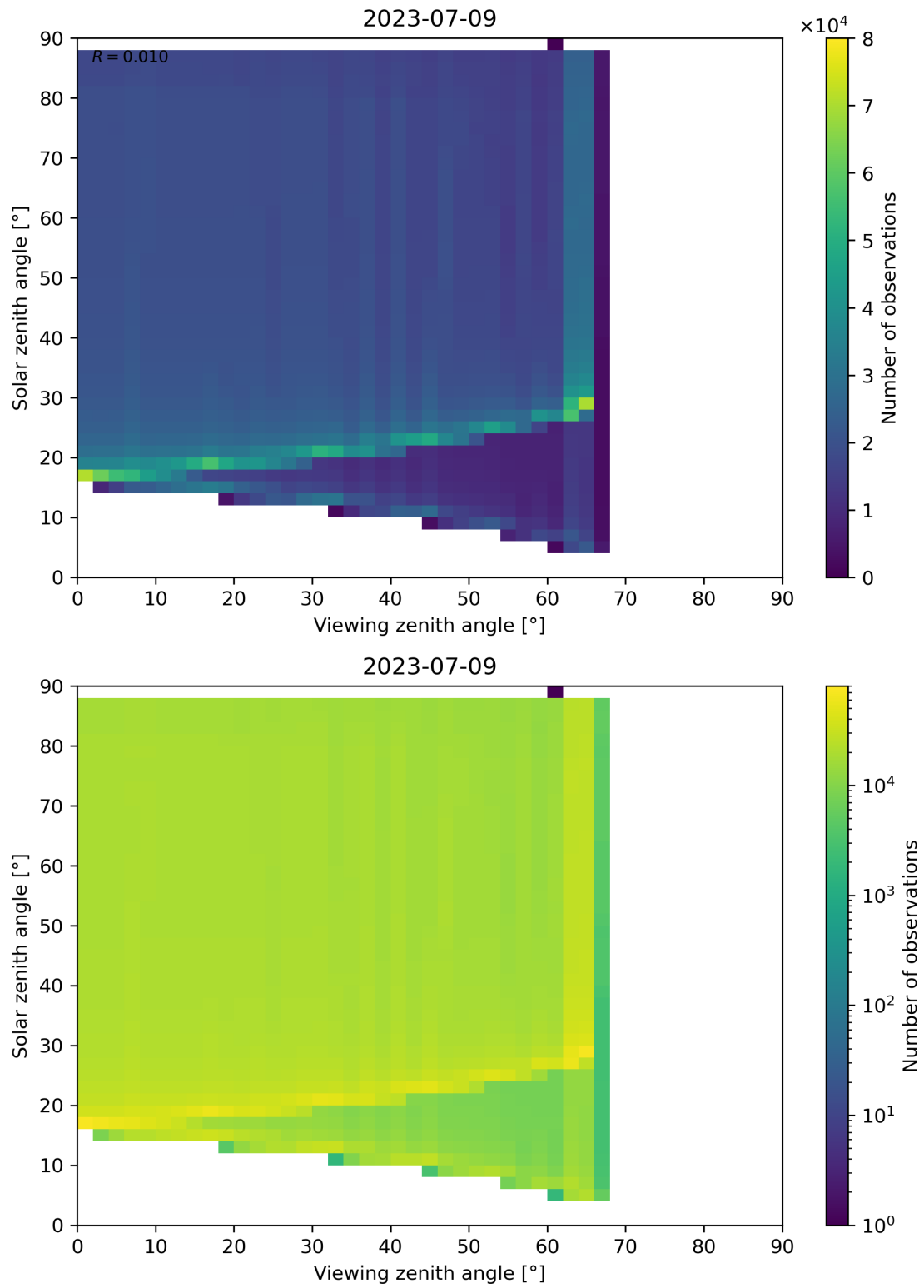
Figure 172: Scatter density plot of “Viewing zenith angle” against “Solar zenith angle” for 2023-07-08 to 2023-07-10.
