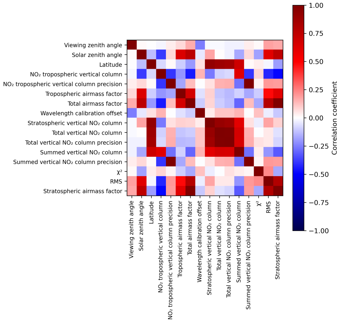
Figure 2: Map of correlation matrix for 2023-07-08 to 2023-07-10.
