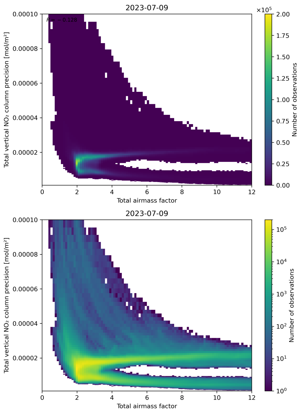
Figure 68: Scatter density plot of “Total airmass factor” against “Total vertical NO 2 column precision” for 2023-07-08 to 2023-07-10.
