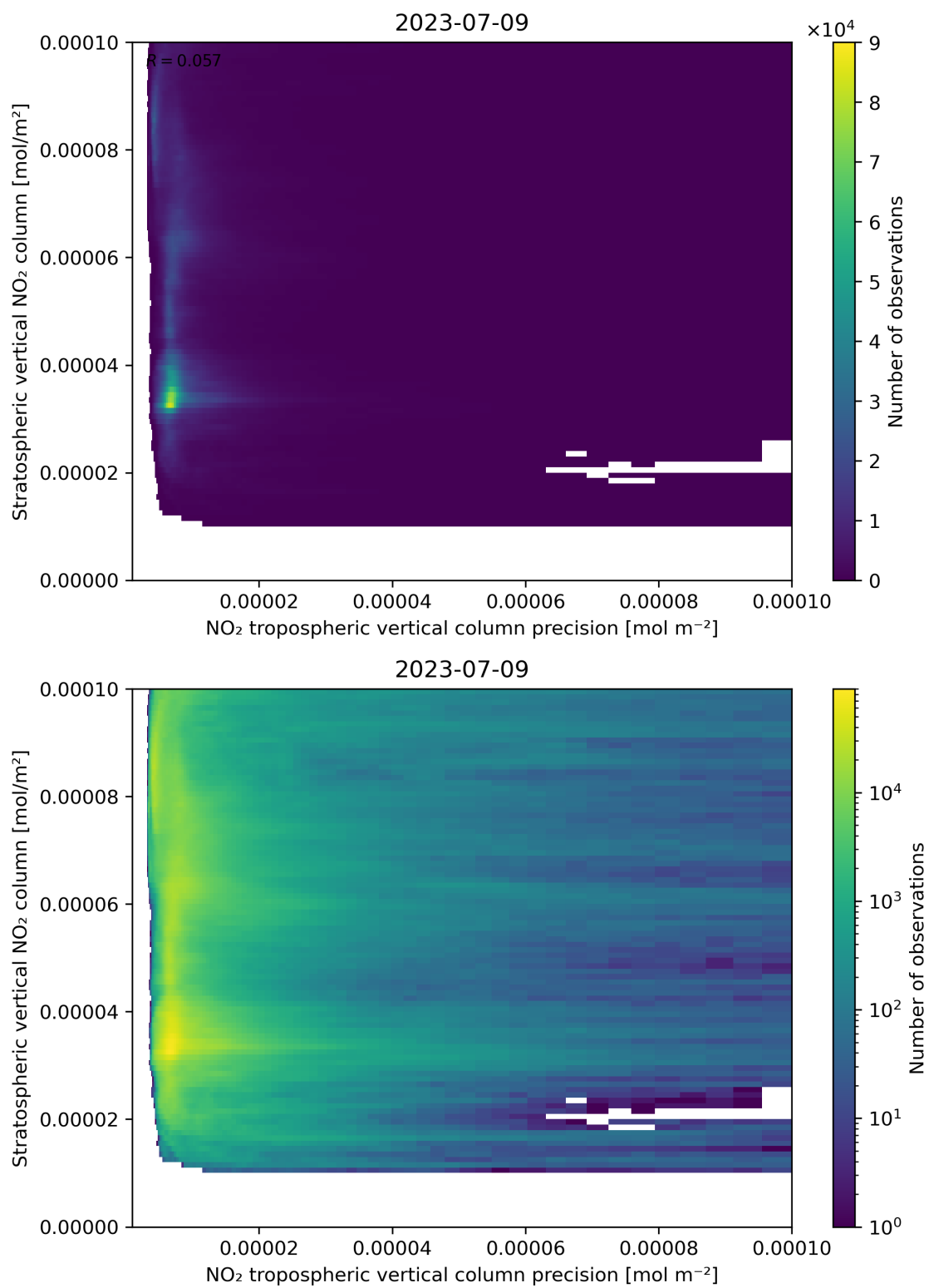
Figure 135: Scatter density plot of “NO 2 tropospheric vertical column precision” against “Stratospheric vertical NO 2 column” for 2023-07-08 to 2023-07-10.
