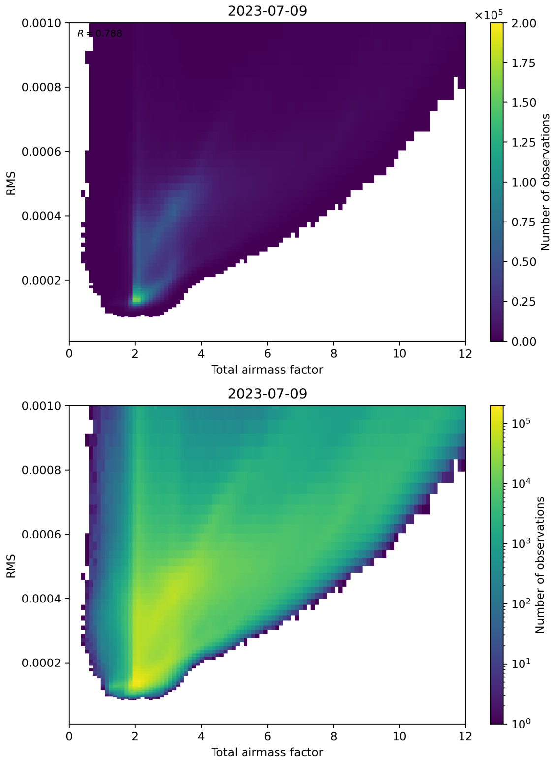
Figure 69: Scatter density plot of “Total airmass factor” against “RMS” for 2023-07-08 to 2023-07-10.
