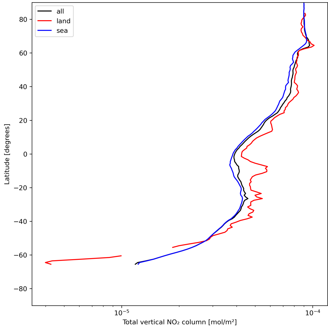
Figure 21: Zonal average of “Total vertical NO 2 column” for 2023-07-08 to 2023-07-10.
