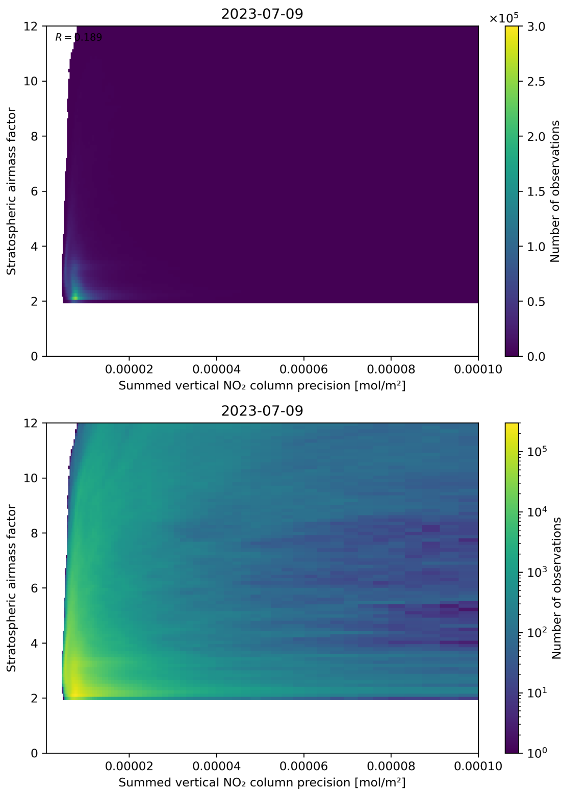
Figure 106: Scatter density plot of “Summed vertical NO 2 column precision” against “Stratospheric airmass factor” for 2023-07-08 to 2023-07-10.
