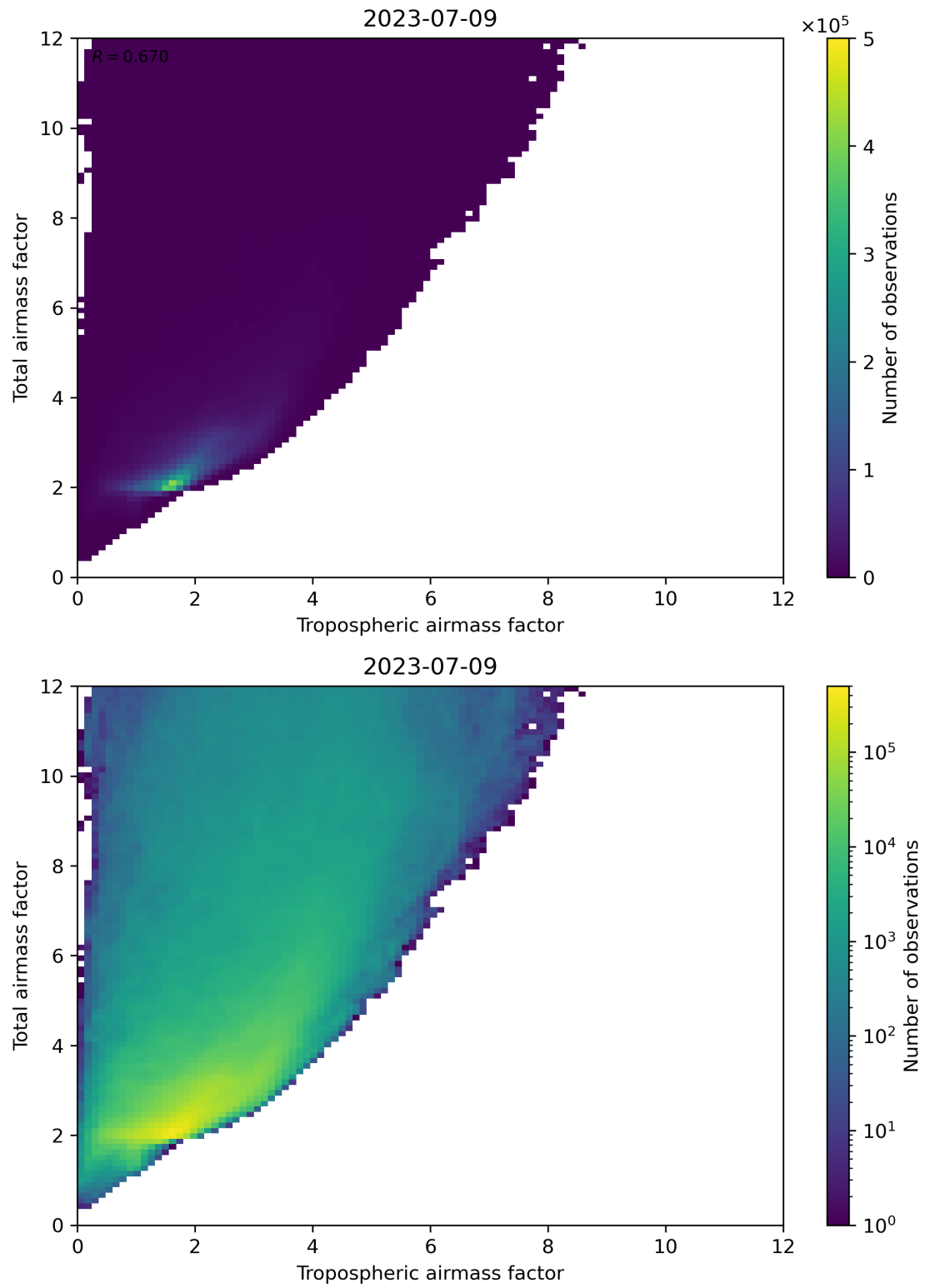
Figure 72: Scatter density plot of “Tropospheric airmass factor” against “Total airmass factor” for 2023-07-08 to 2023-07-10.
