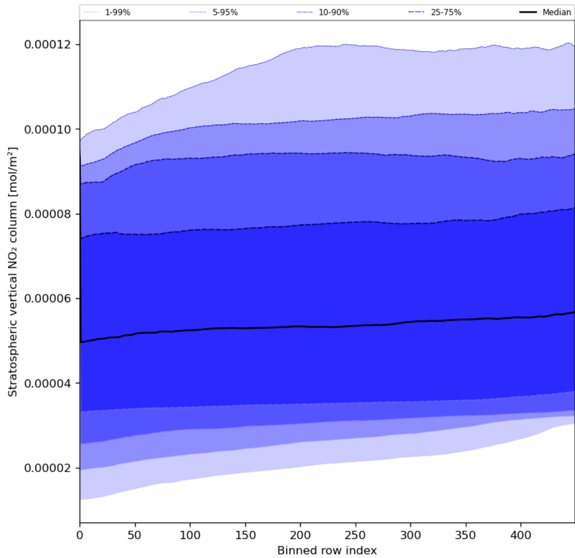
Figure 53: Along track statistics of “Stratospheric vertical NO 2 column” for 2023-07-08 to 2023-07-10
