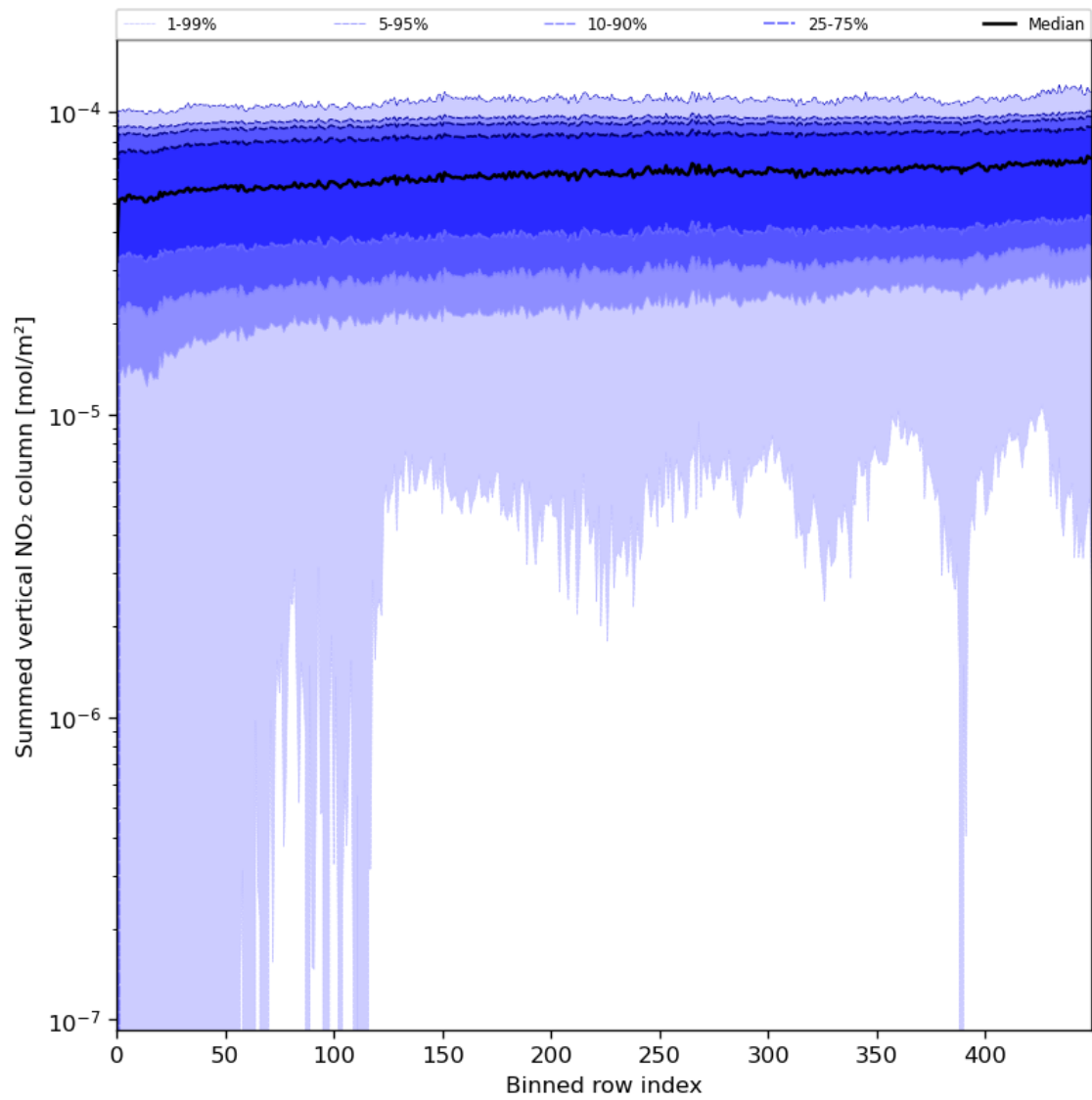
Figure 57: Along track statistics of “Summed vertical NO 2 column” for 2023-07-08 to 2023-07-10
