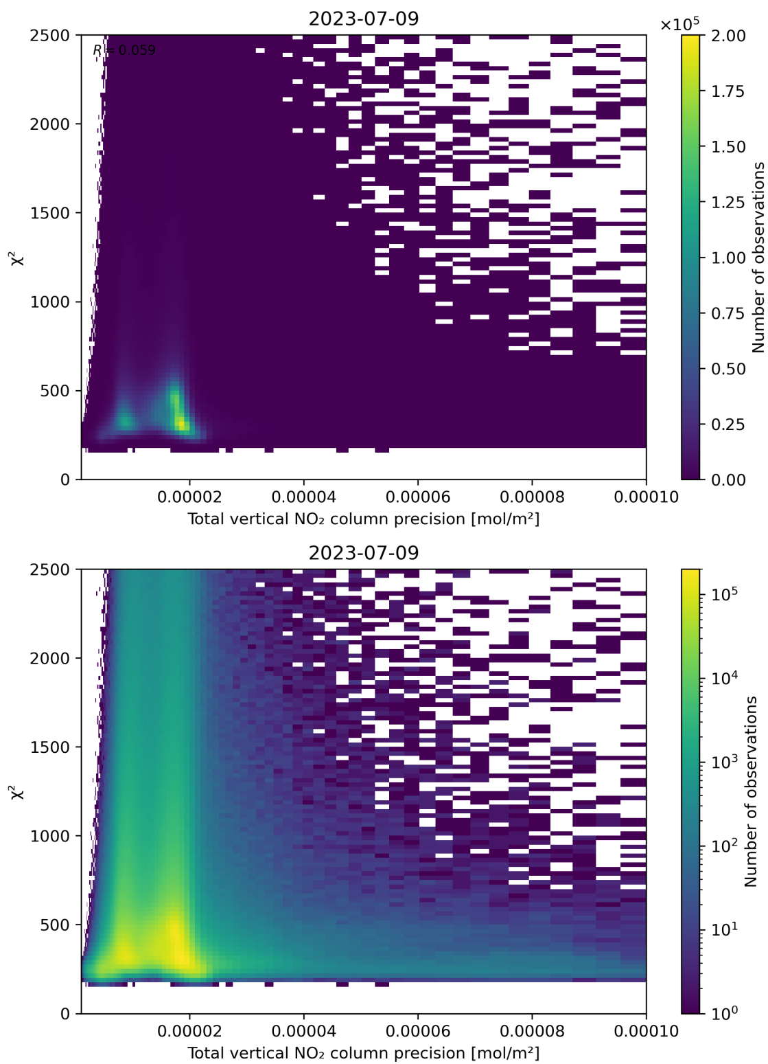
Figure 116: Scatter density plot of “Total vertical NO 2 column precision” against “ \chi^2 ” for 2023-07-08 to 2023-07-10.
