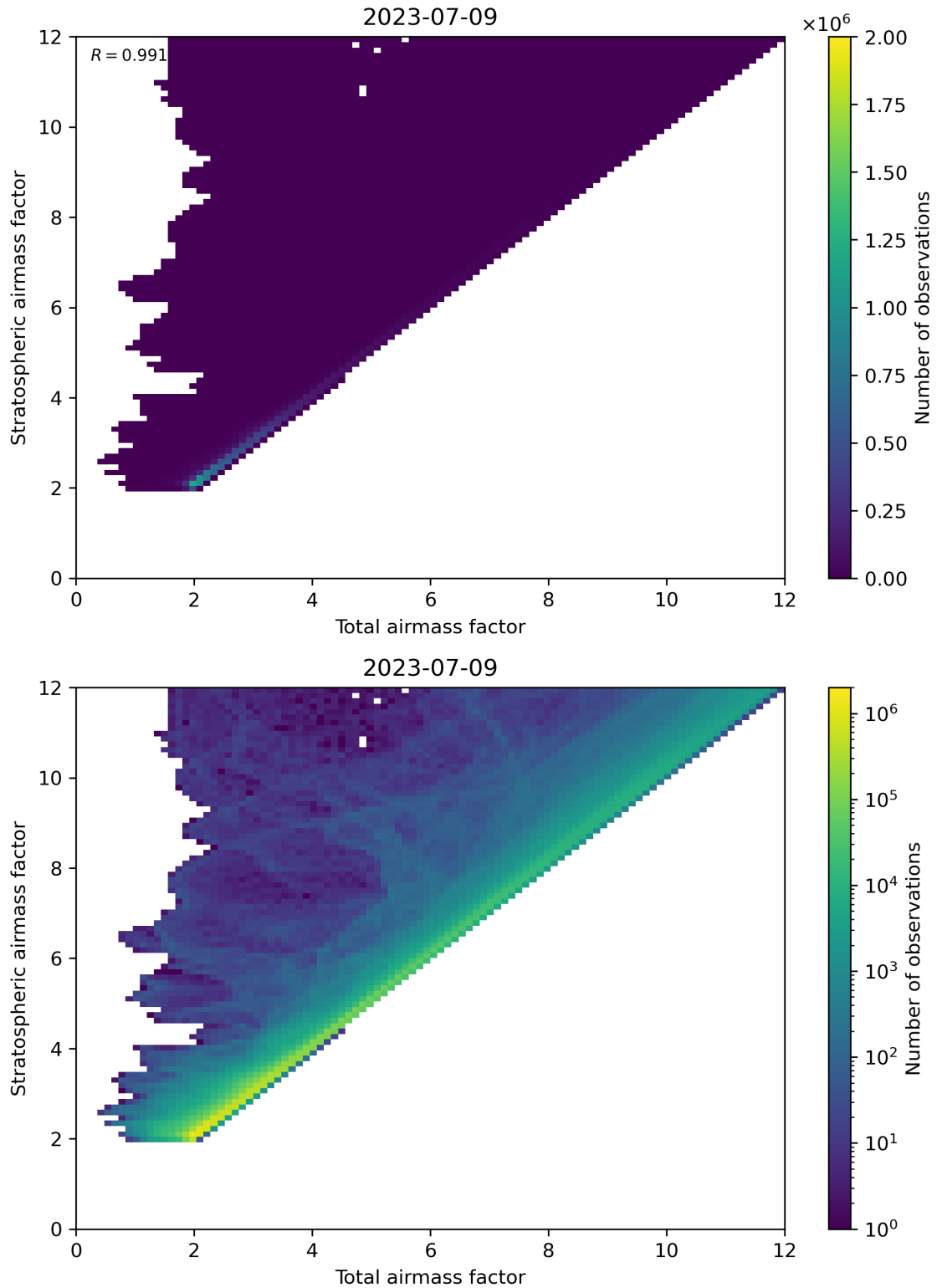
Figure 62: Scatter density plot of “Total airmass factor” against “Stratospheric airmass factor” for 2023-07-08 to 2023-07-10.
