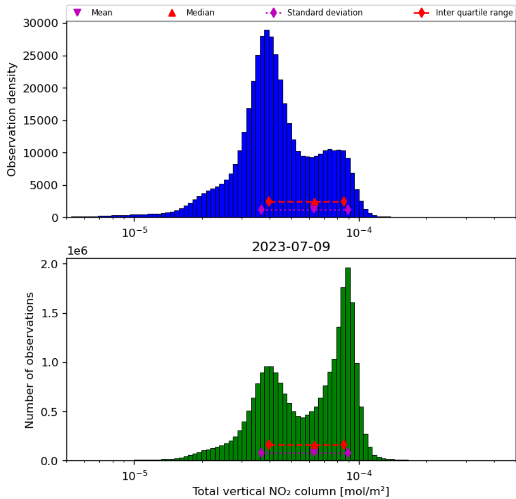
Figure 38: Histogram of “Total vertical NO 2 column” for 2023-07-08 to 2023-07-10
