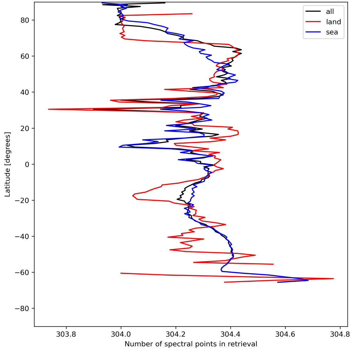
Figure 16: Zonal average of “Number of spectral points in retrieval” for 2023-07-08 to 2023-07-10.
