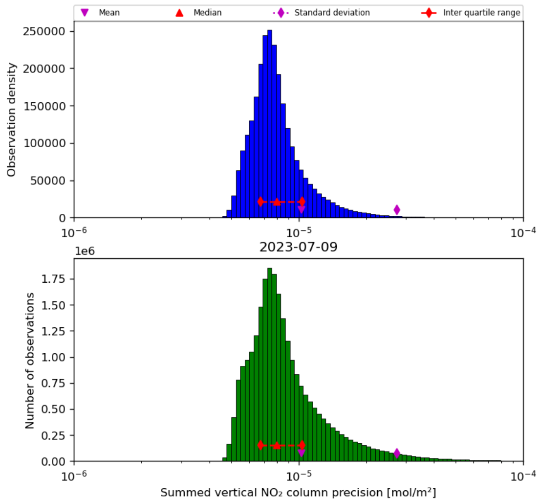
Figure 41: Histogram of “Summed vertical NO 2 column precision” for 2023-07-08 to 2023-07-10
