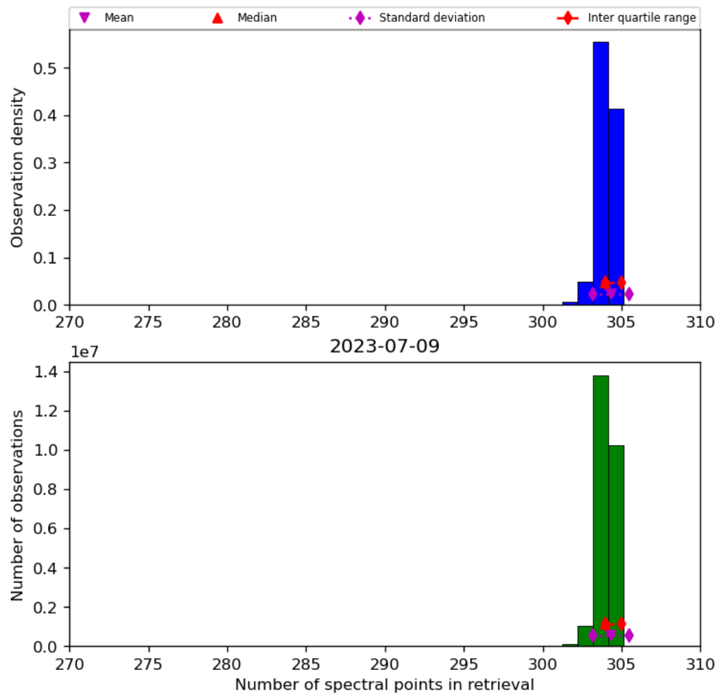
Figure 33: Histogram of “Number of spectral points in retrieval” for 2023-07-08 to 2023-07-10
