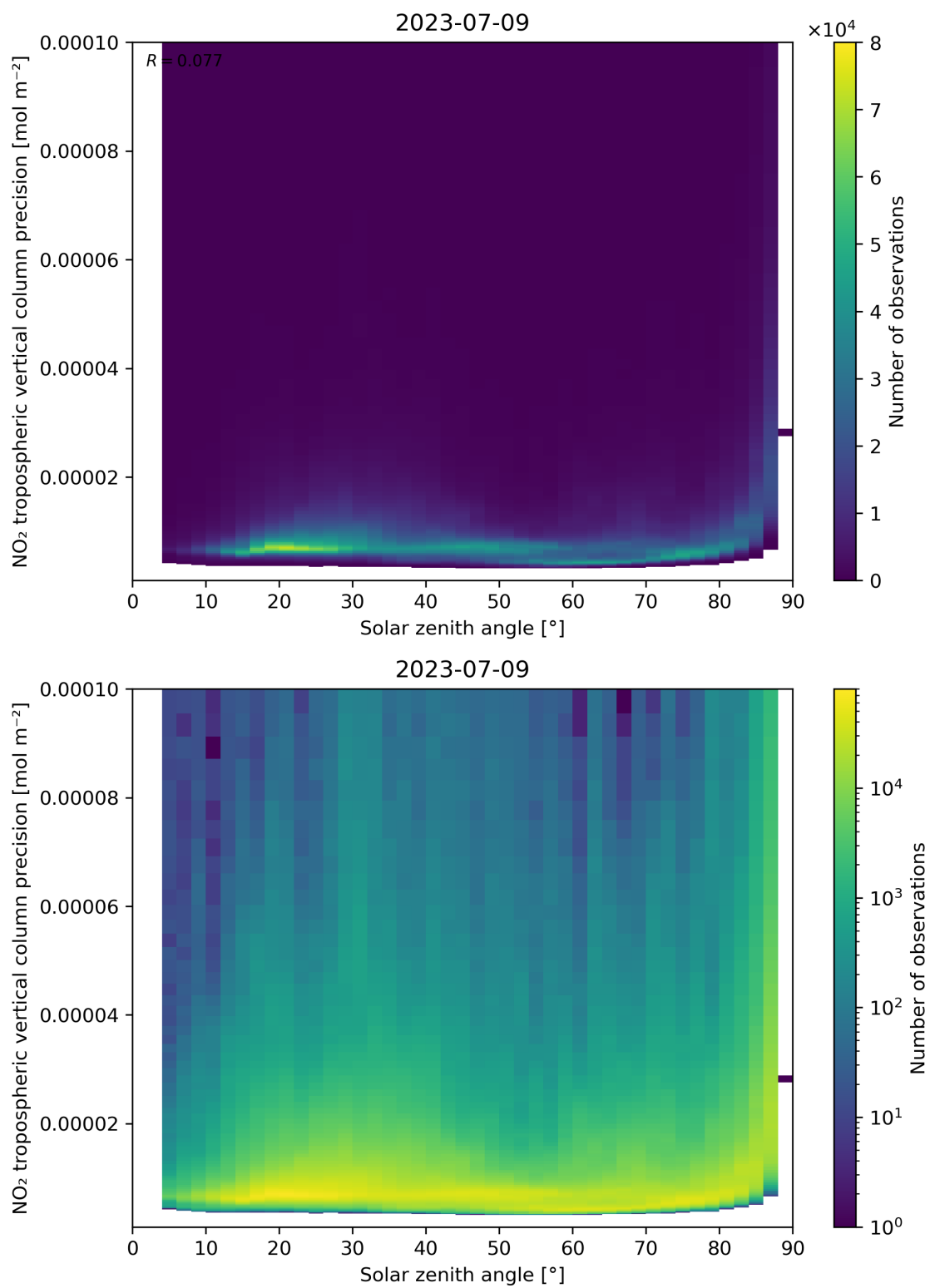
Figure 156: Scatter density plot of “Solar zenith angle” against “NO 2 tropospheric vertical column precision” for 2023-07-08 to 2023-07-10.
