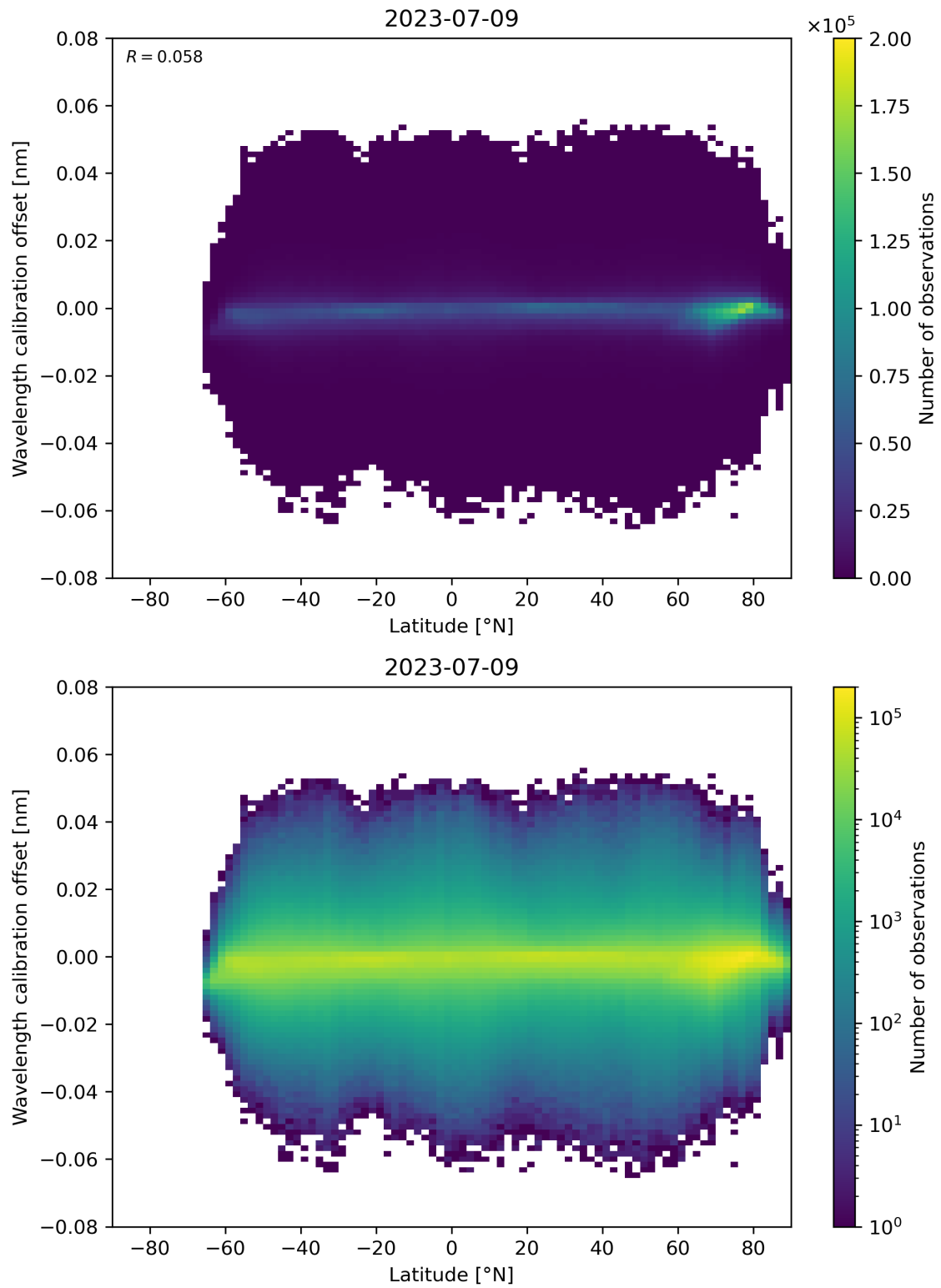
Figure 95: Scatter density plot of “Latitude” against “Wavelength calibration offset” for 2023-07-08 to 2023-07-10.
