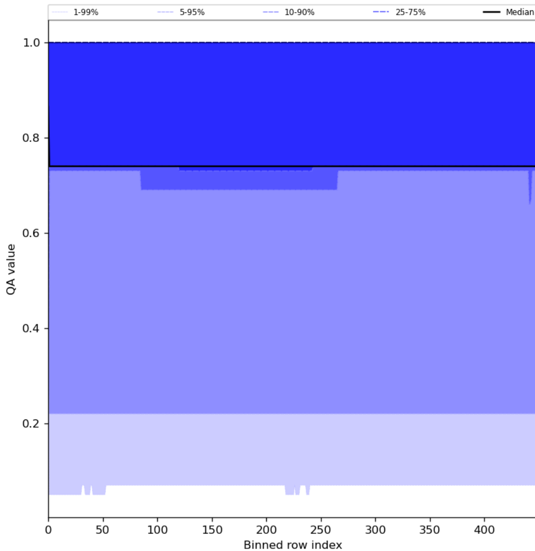
Figure 45: Along track statistics of “QA value” for 2023-07-08 to 2023-07-10
