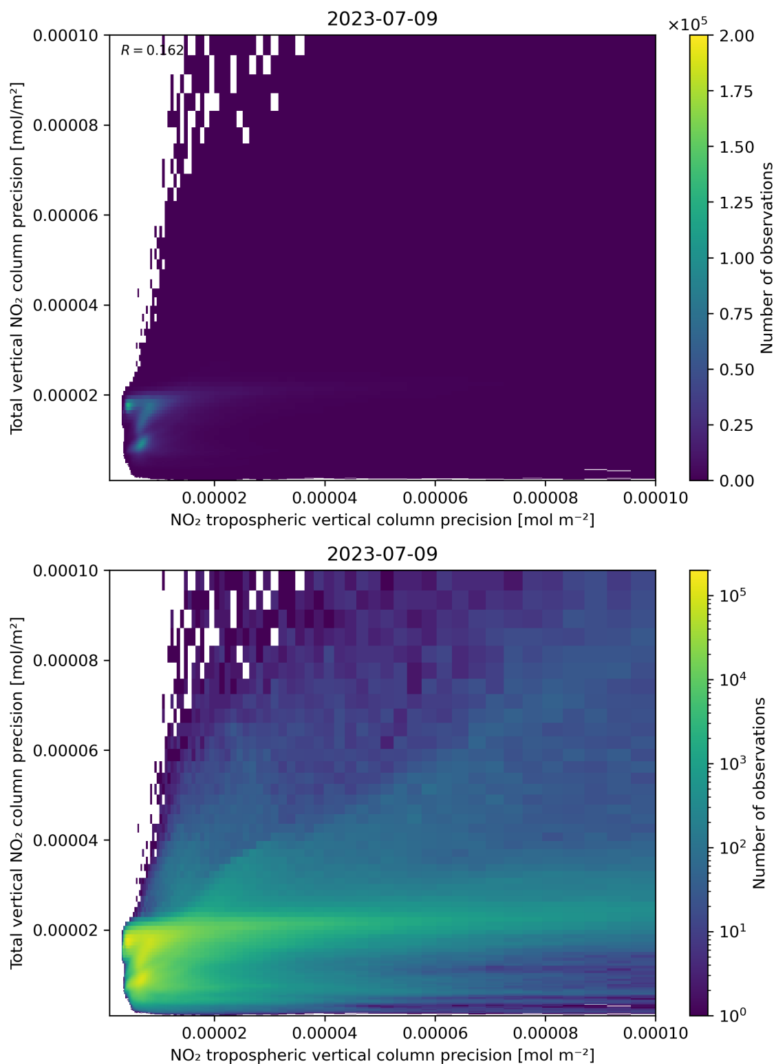
Figure 139: Scatter density plot of “NO 2 tropospheric vertical column precision” against “Total vertical NO 2 column precision” for 2023-07-08 to 2023-07-10.
