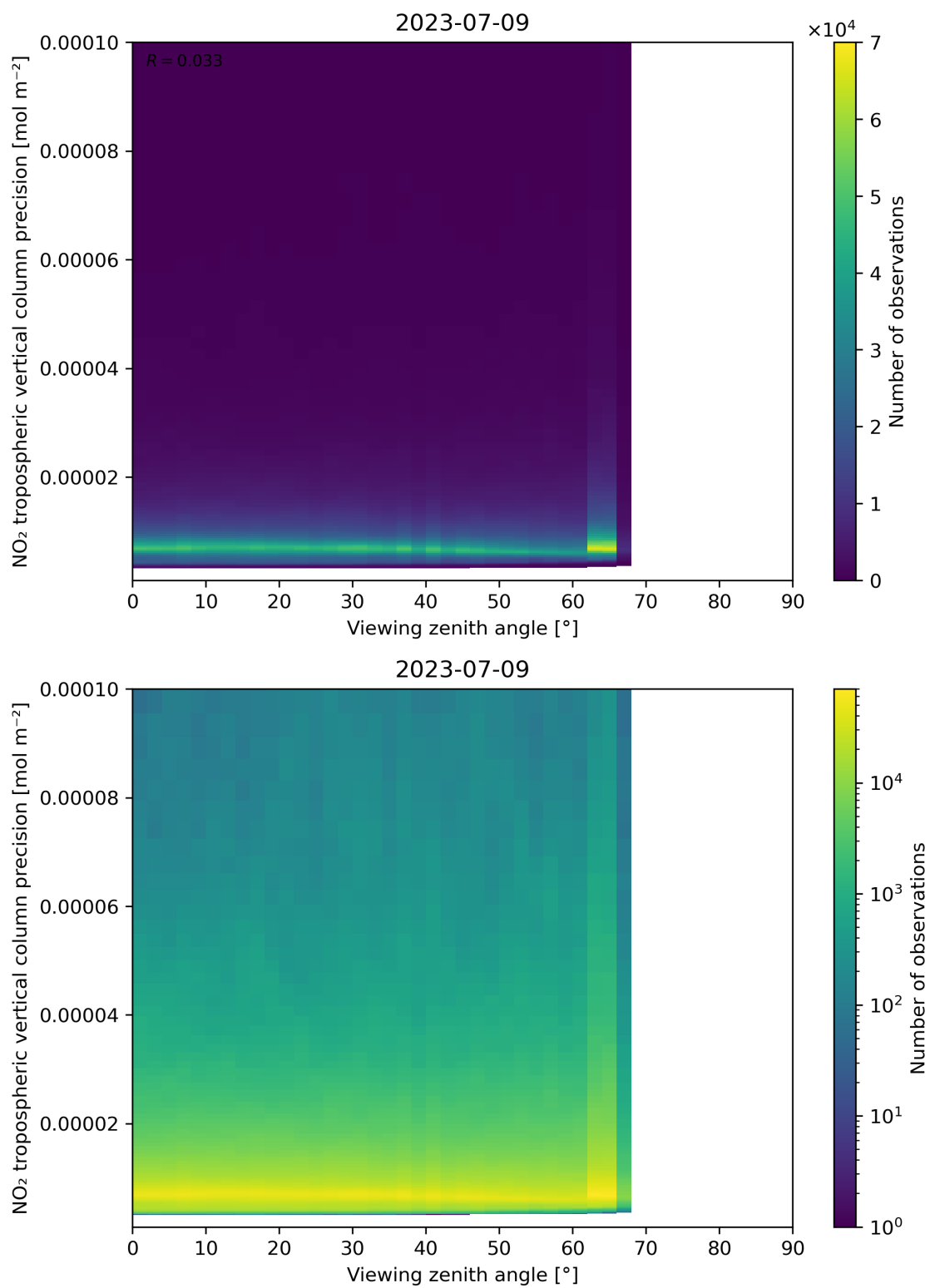
Figure 170: Scatter density plot of “Viewing zenith angle” against “NO 2 tropospheric vertical column precision” for 2023-07-08 to 2023-07-10.
