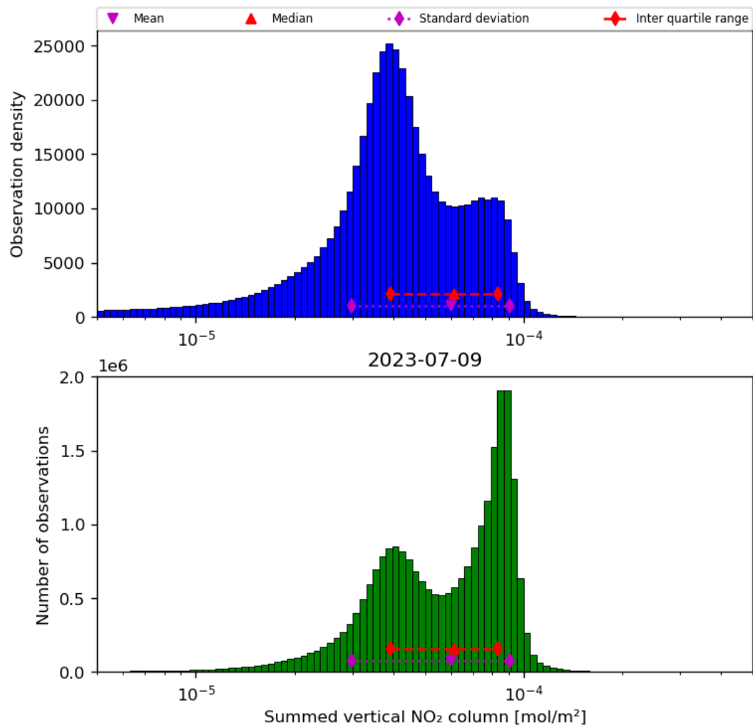
Figure 40: Histogram of “Summed vertical NO 2 column” for 2023-07-08 to 2023-07-10
