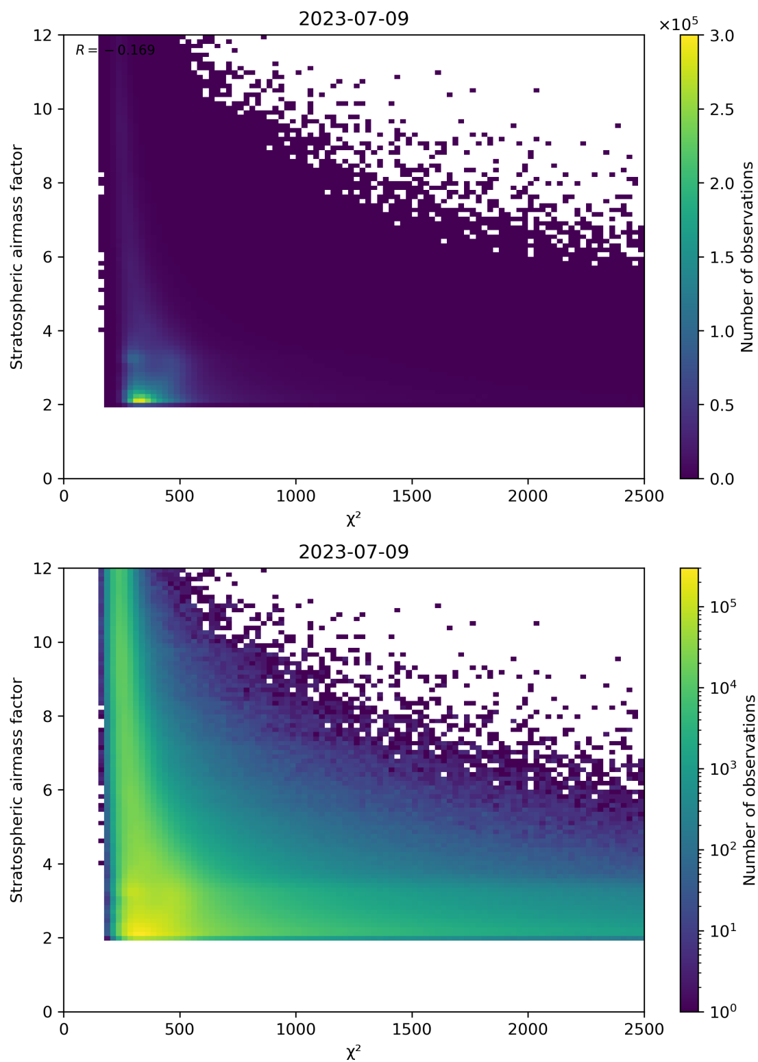
Figure 81: Scatter density plot of “ \chi^2 ” against “Stratospheric airmass factor” for 2023-07-08 to 2023-07-10.
