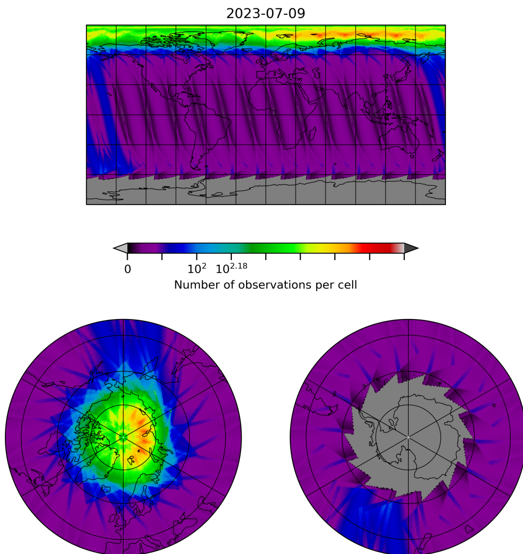
Figure 10: Map of the number of observations for 2023-07-08 to 2023-07-10
