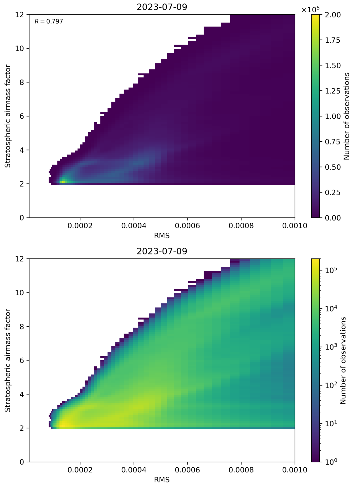
Figure 144: Scatter density plot of “RMS” against “Stratospheric airmass factor” for 2023-07-08 to 2023-07-10.
