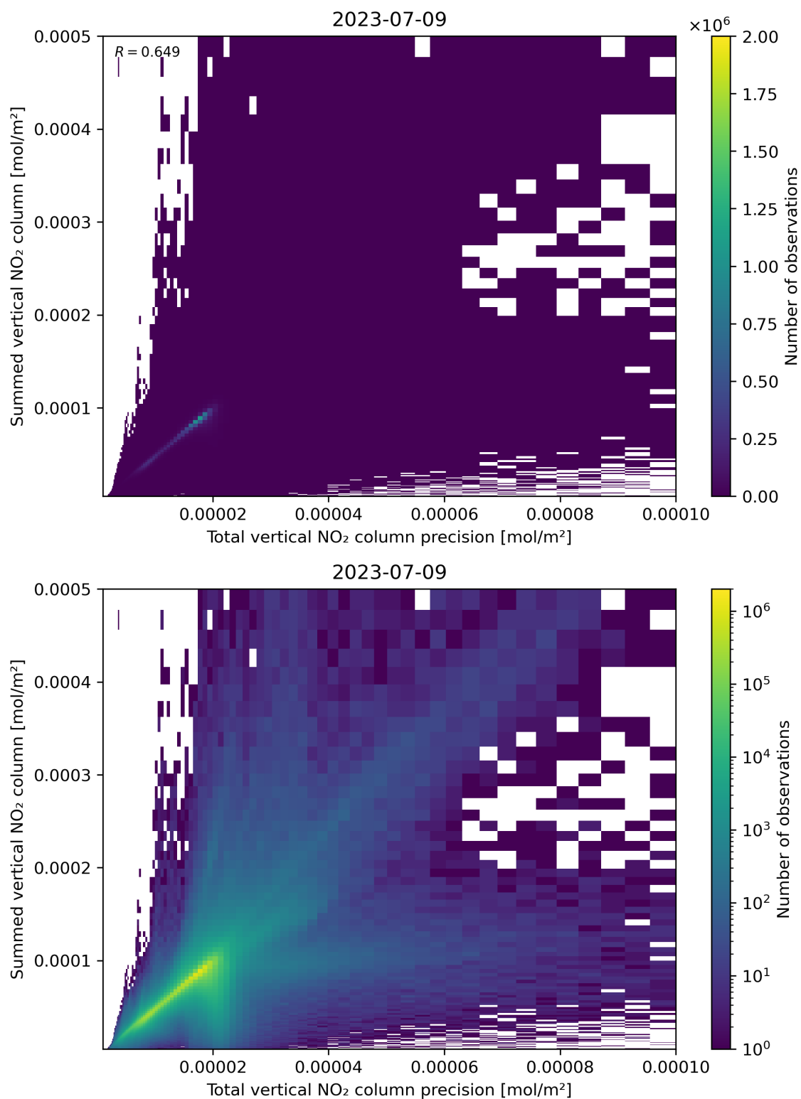
Figure 117: Scatter density plot of “Total vertical NO 2 column precision” against “Summed vertical NO 2 column” for 2023-07-08 to 2023-07-10.
