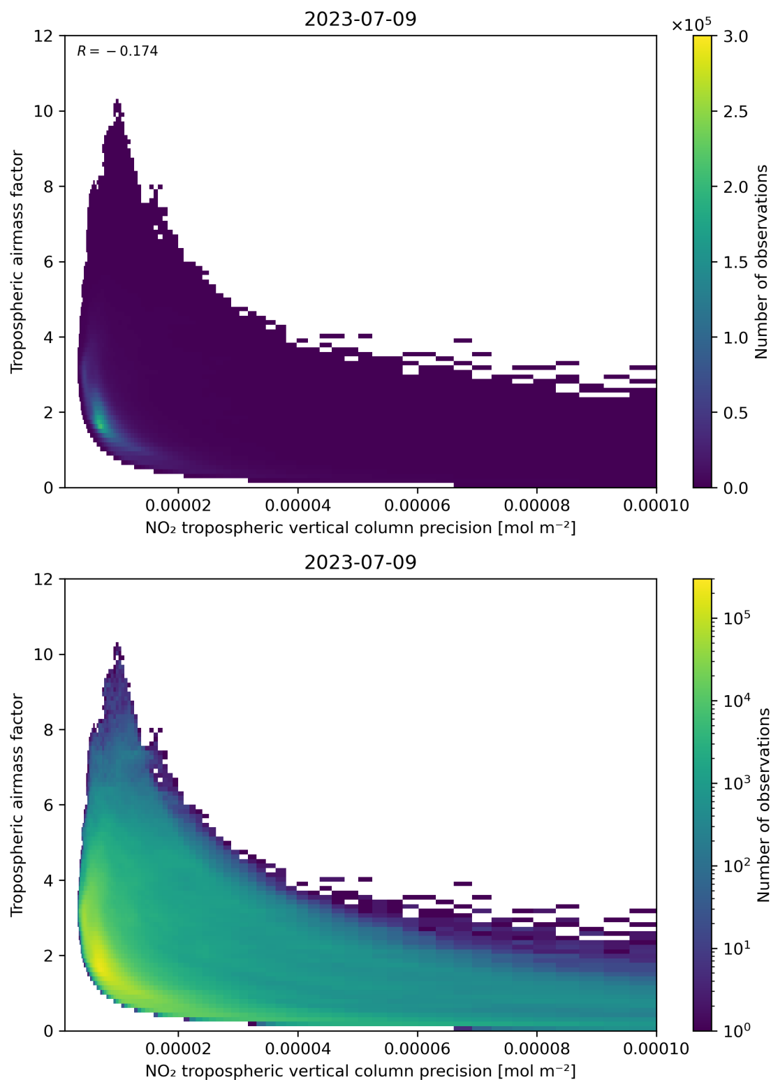
Figure 133: Scatter density plot of “NO 2 tropospheric vertical column precision” against “Tropospheric airmass factor” for 2023-07-08 to 2023-07-10.
