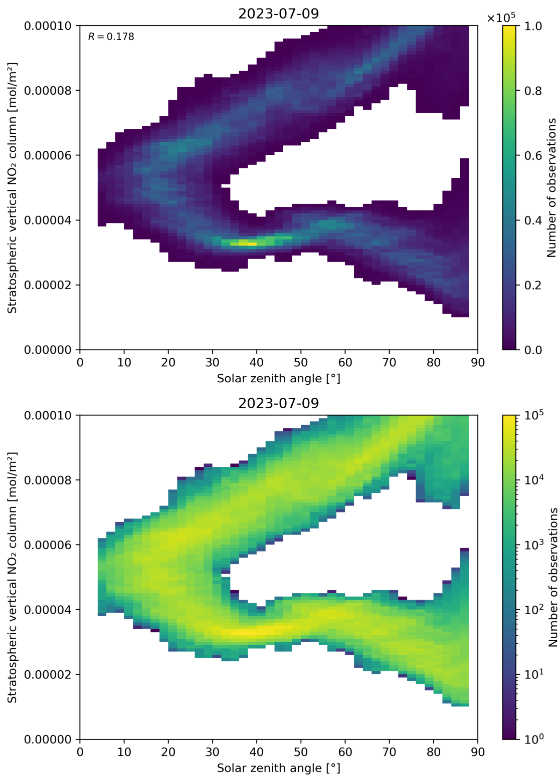
Figure 150: Scatter density plot of “Solar zenith angle” against “Stratospheric vertical NO 2 column” for 2023-07-08 to 2023-07-10.
