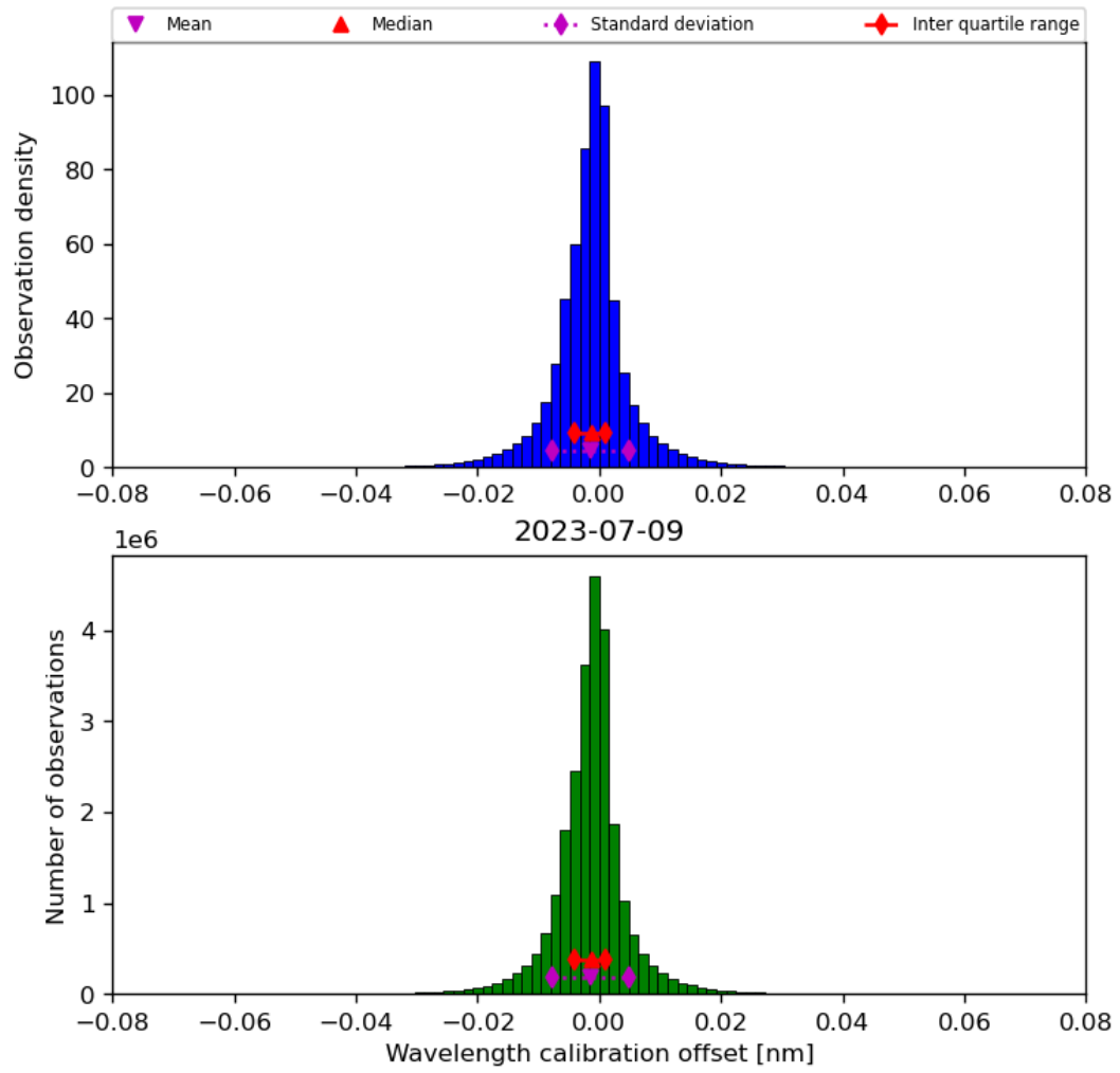
Figure 35: Histogram of “Wavelength calibration offset” for 2023-07-08 to 2023-07-10
