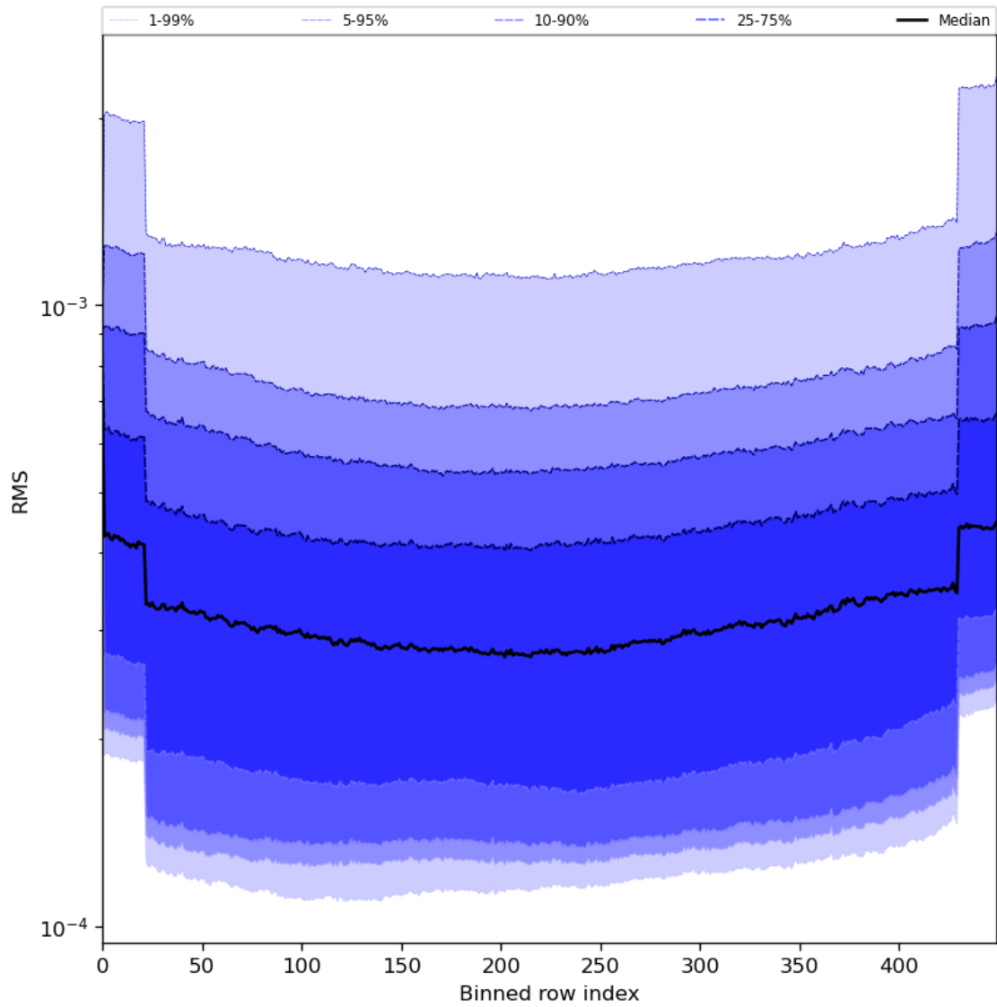
Figure 60: Along track statistics of “RMS” for 2023-07-08 to 2023-07-10
