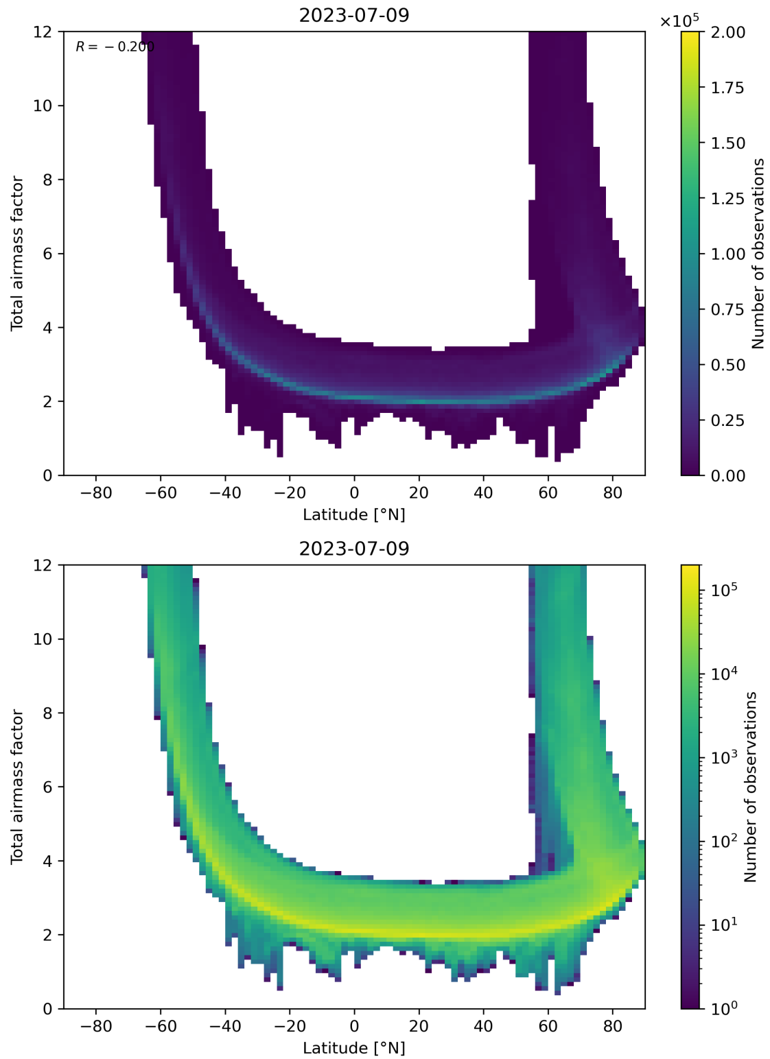
Figure 84: Scatter density plot of “Latitude” against “Total airmass factor” for 2023-07-08 to 2023-07-10.
