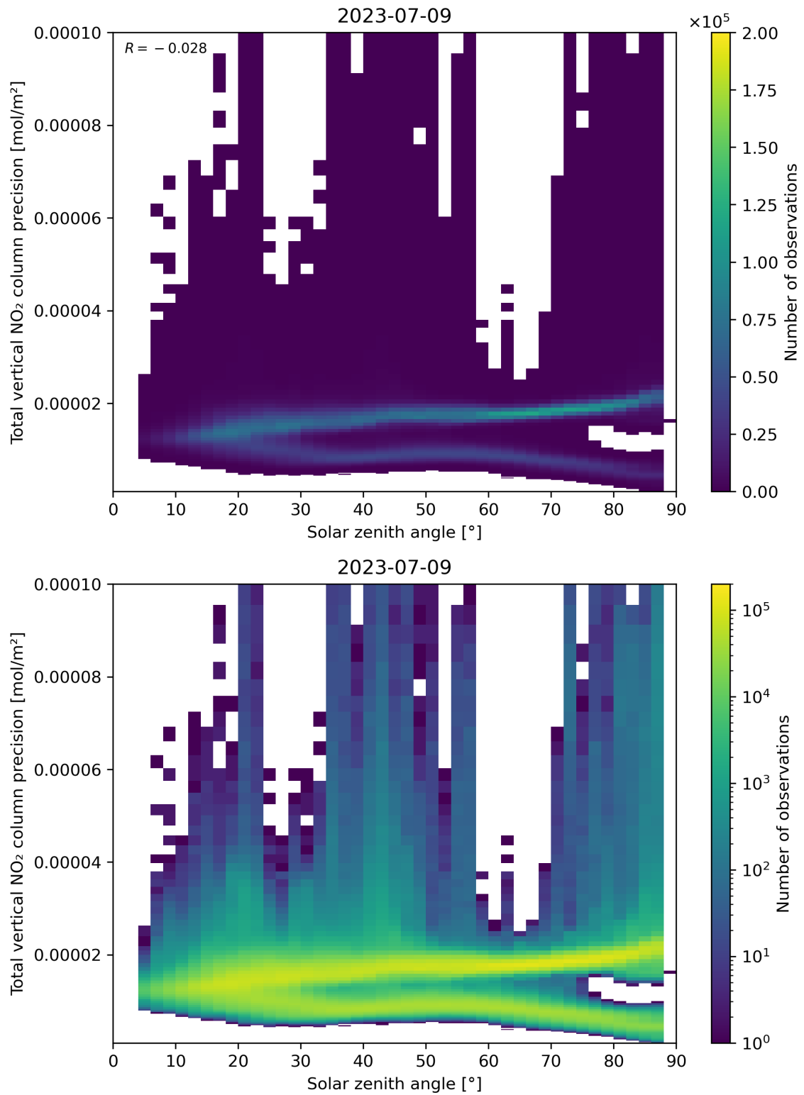
Figure 154: Scatter density plot of “Solar zenith angle” against “Total vertical NO 2 column precision” for 2023-07-08 to 2023-07-10.
