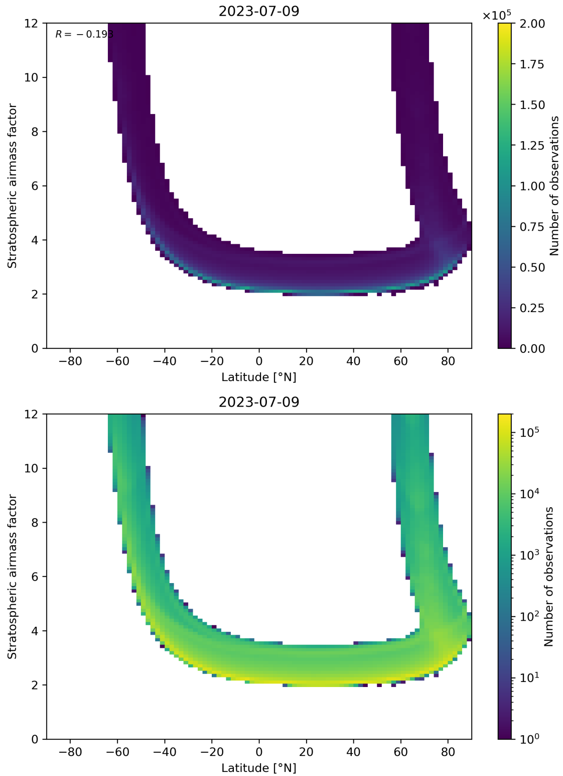
Figure 83: Scatter density plot of “Latitude” against “Stratospheric airmass factor” for 2023-07-08 to 2023-07-10.
