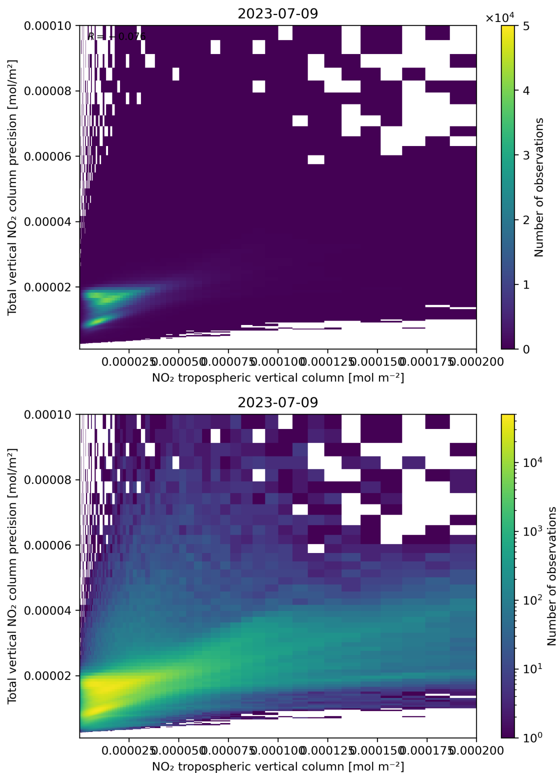
Figure 129: Scatter density plot of “NO 2 tropospheric vertical column” against “Total vertical NO 2 column precision” for 2023-07-08 to 2023-07-10.
