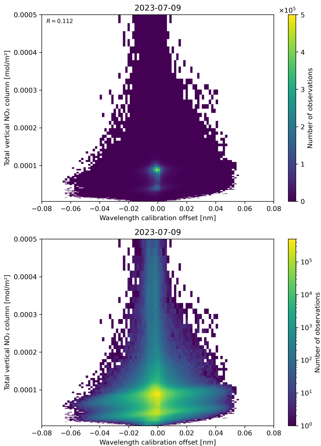
Figure 179: Scatter density plot of “Wavelength calibration offset” against “Total vertical NO 2 column” for 2023-07-08 to 2023-07-10.
