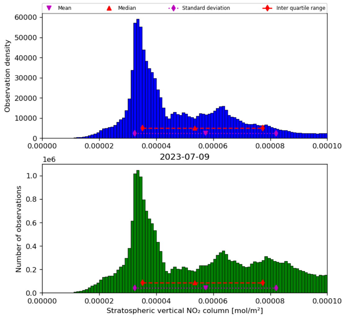
Figure 36: Histogram of “Stratospheric vertical NO 2 column” for 2023-07-08 to 2023-07-10
