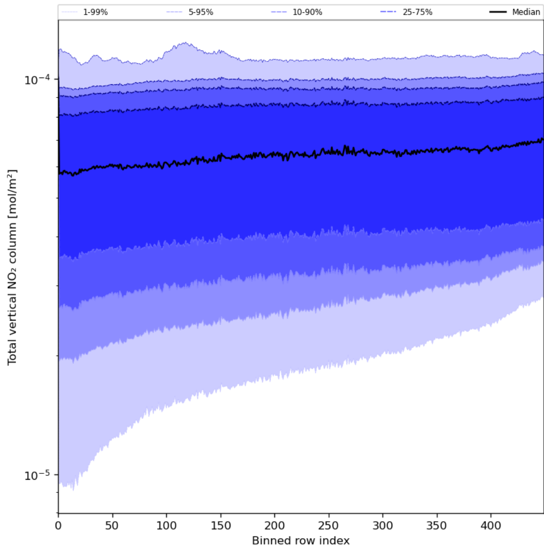
Figure 55: Along track statistics of “Total vertical NO 2 column” for 2023-07-08 to 2023-07-10
