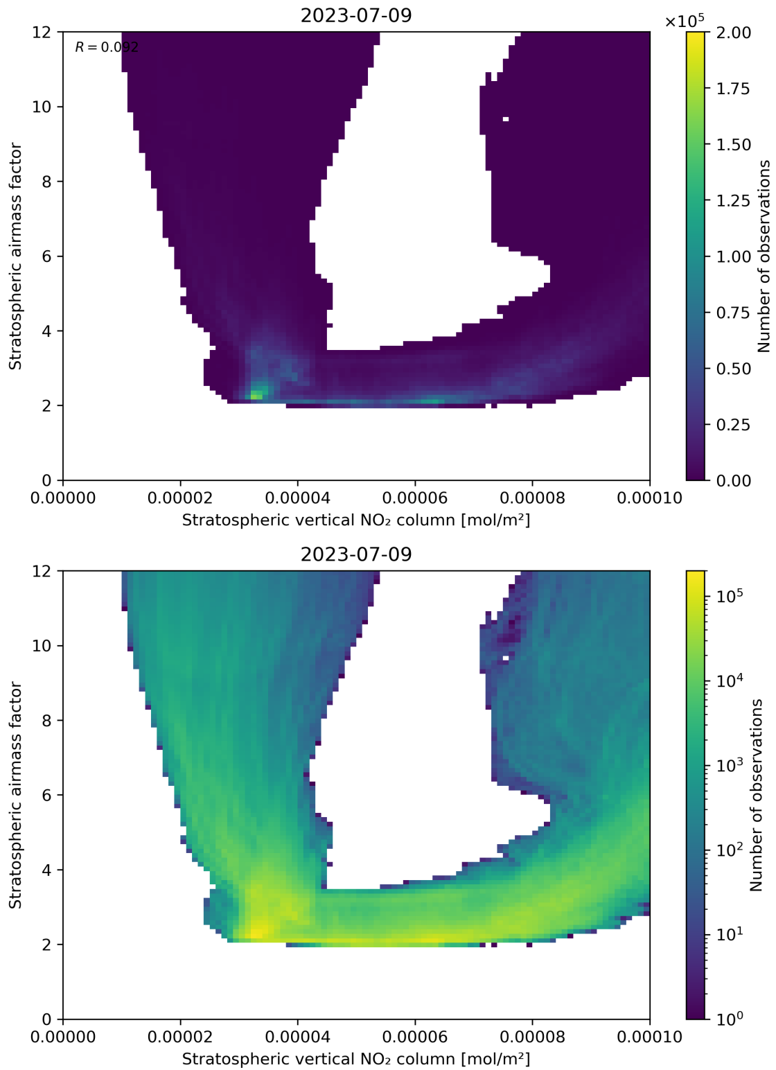
Figure 96: Scatter density plot of “Stratospheric vertical NO 2 column” against “Stratospheric airmass factor” for 2023-07-08 to 2023-07-10.
