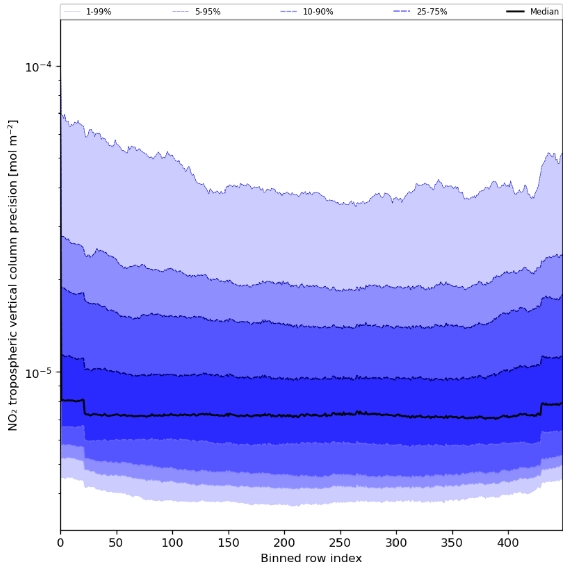
Figure 47: Along track statistics of “NO 2 tropospheric vertical column precision” for 2023-07-08 to 2023-07-10
