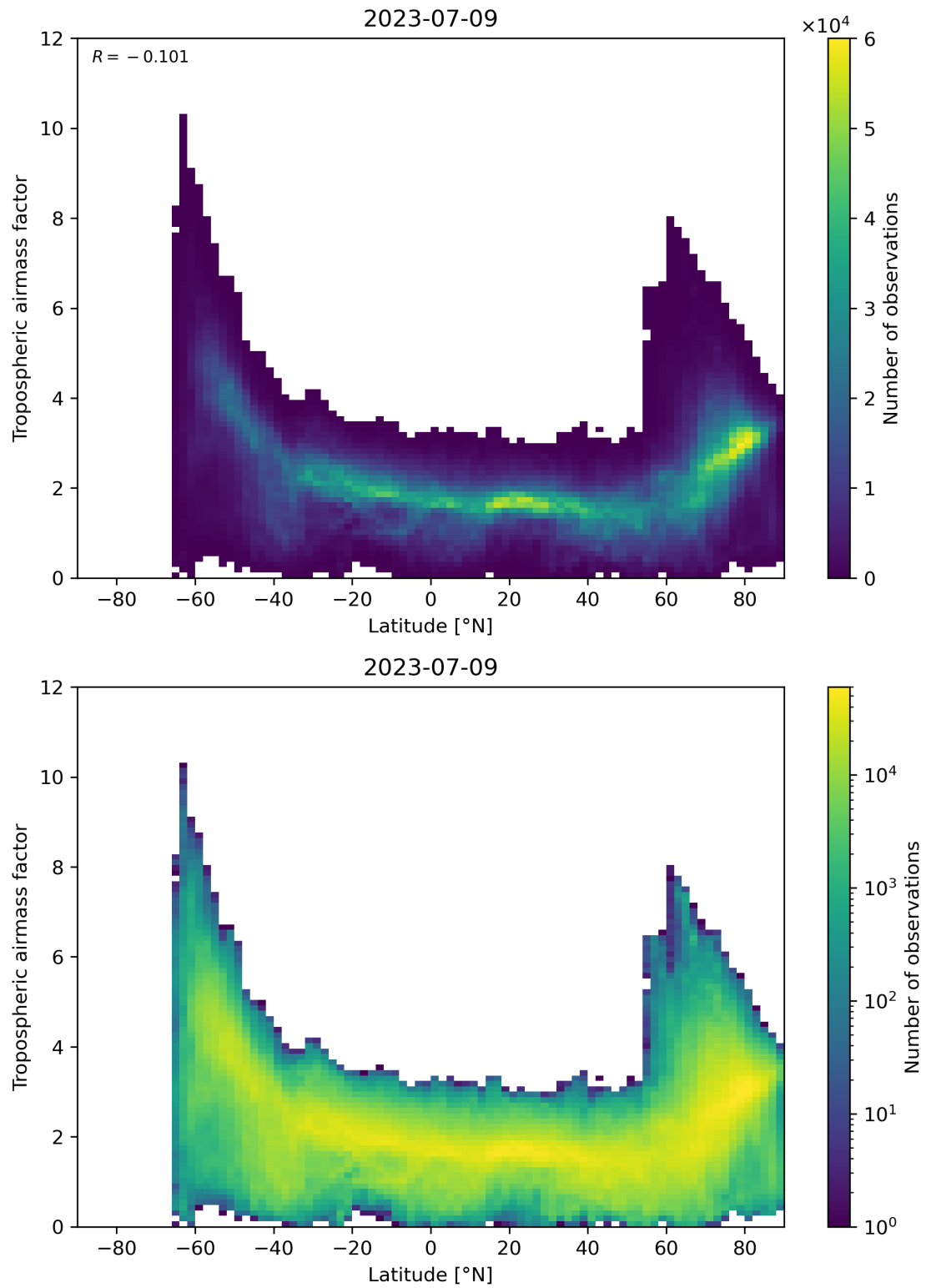
Figure 85: Scatter density plot of “Latitude” against “Tropospheric airmass factor” for 2023-07-08 to 2023-07-10.
