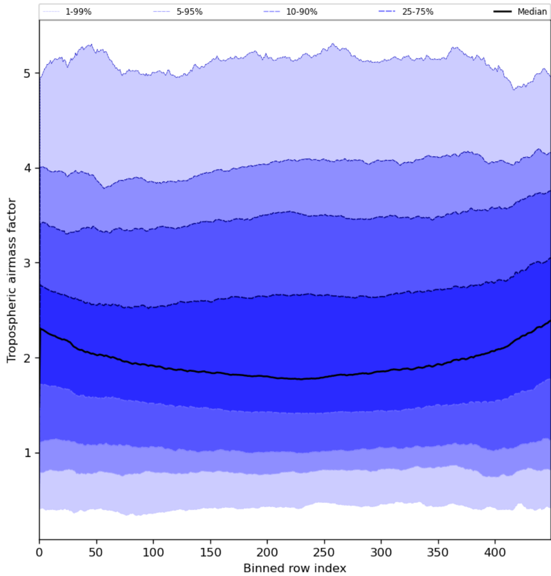
Figure 48: Along track statistics of “Tropospheric airmass factor” for 2023-07-08 to 2023-07-10
