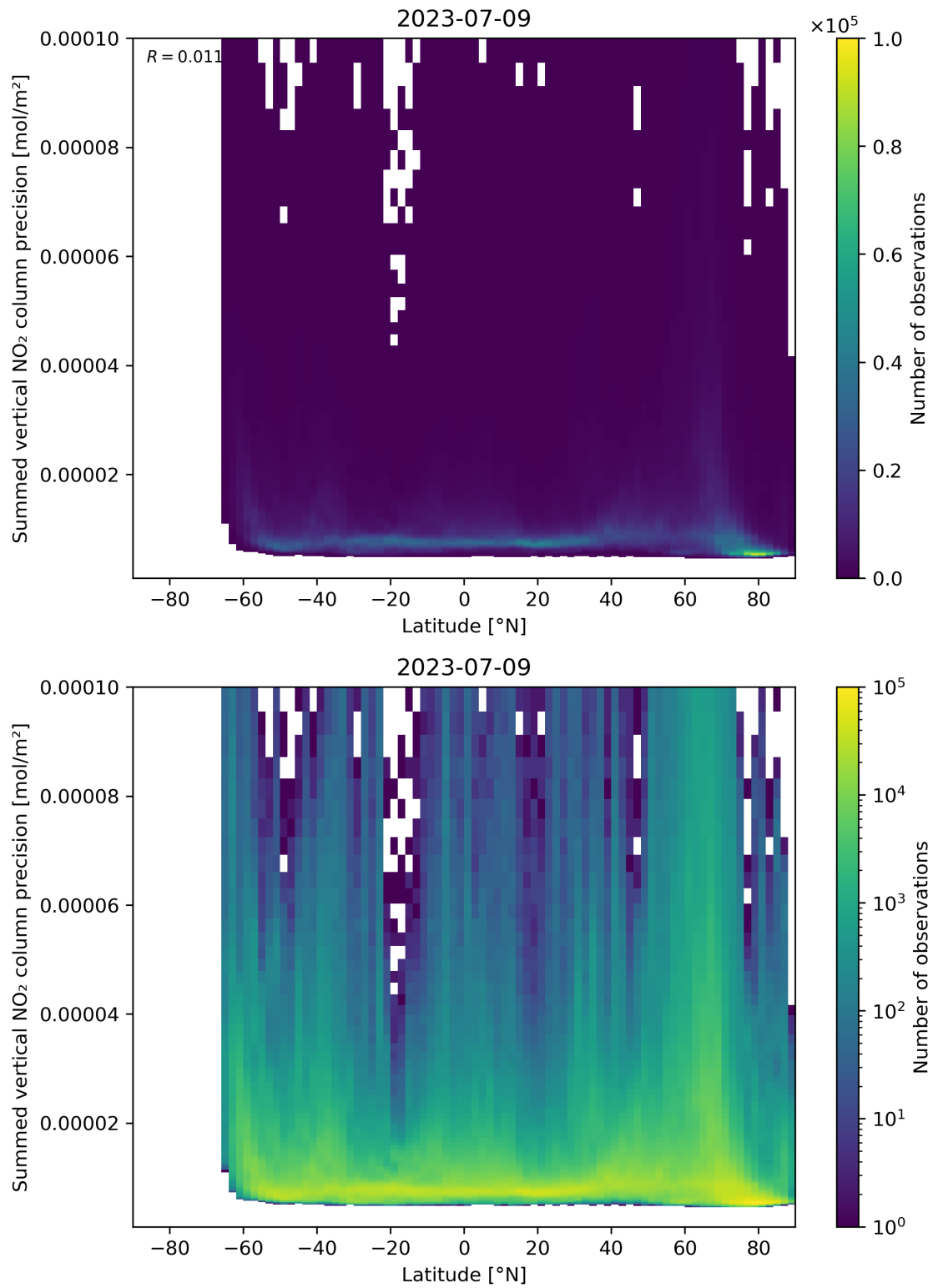
Figure 89: Scatter density plot of “Latitude” against “Summed vertical NO 2 column precision” for 2023-07-08 to 2023-07-10.
