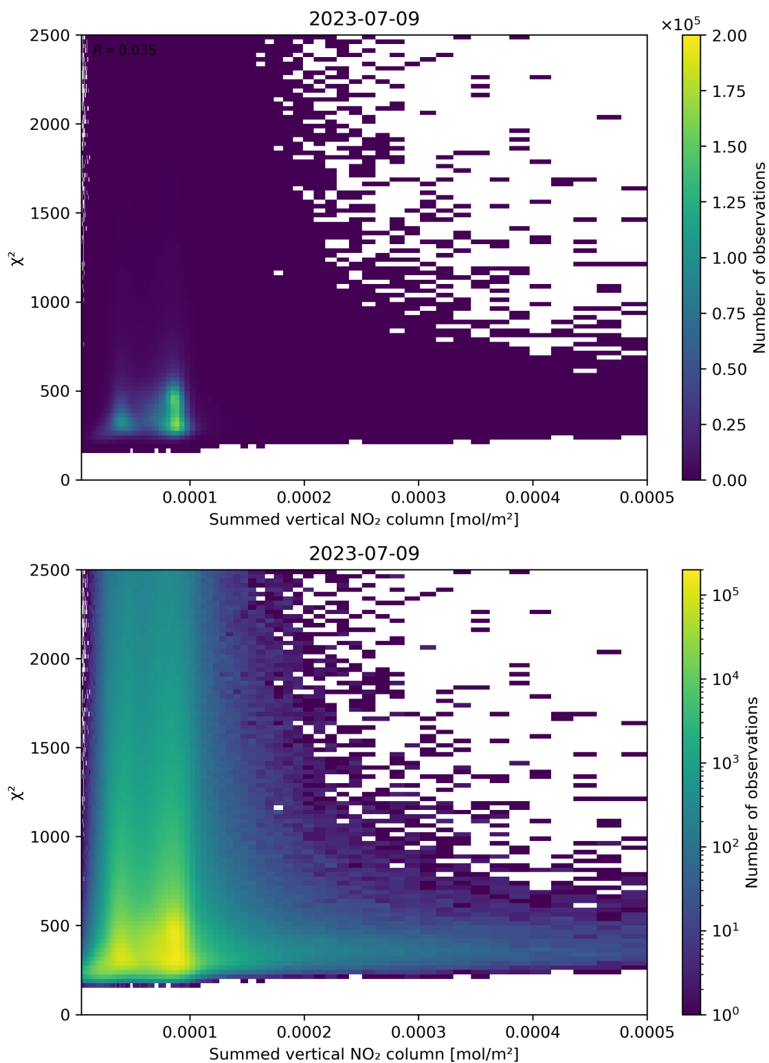
Figure 104: Scatter density plot of “Summed vertical NO 2 column” against “ \chi^2 ” for 2023-07-08 to 2023-07-10.
