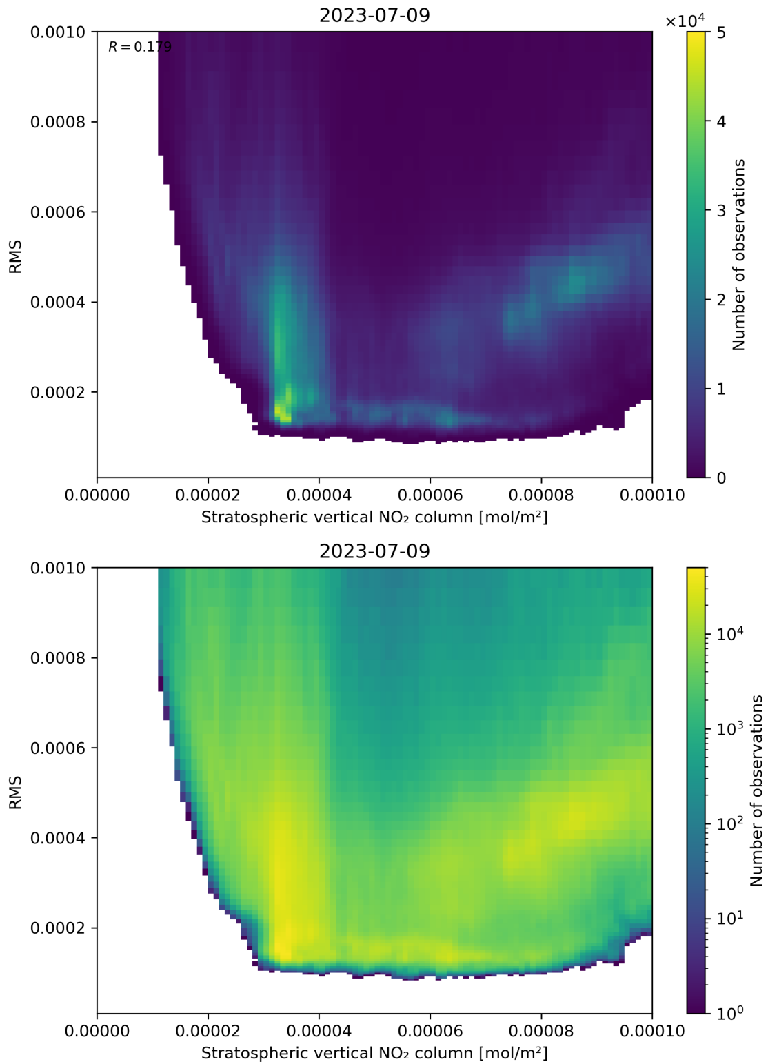
Figure 102: Scatter density plot of “Stratospheric vertical NO 2 column” against “RMS” for 2023-07-08 to 2023-07-10.
