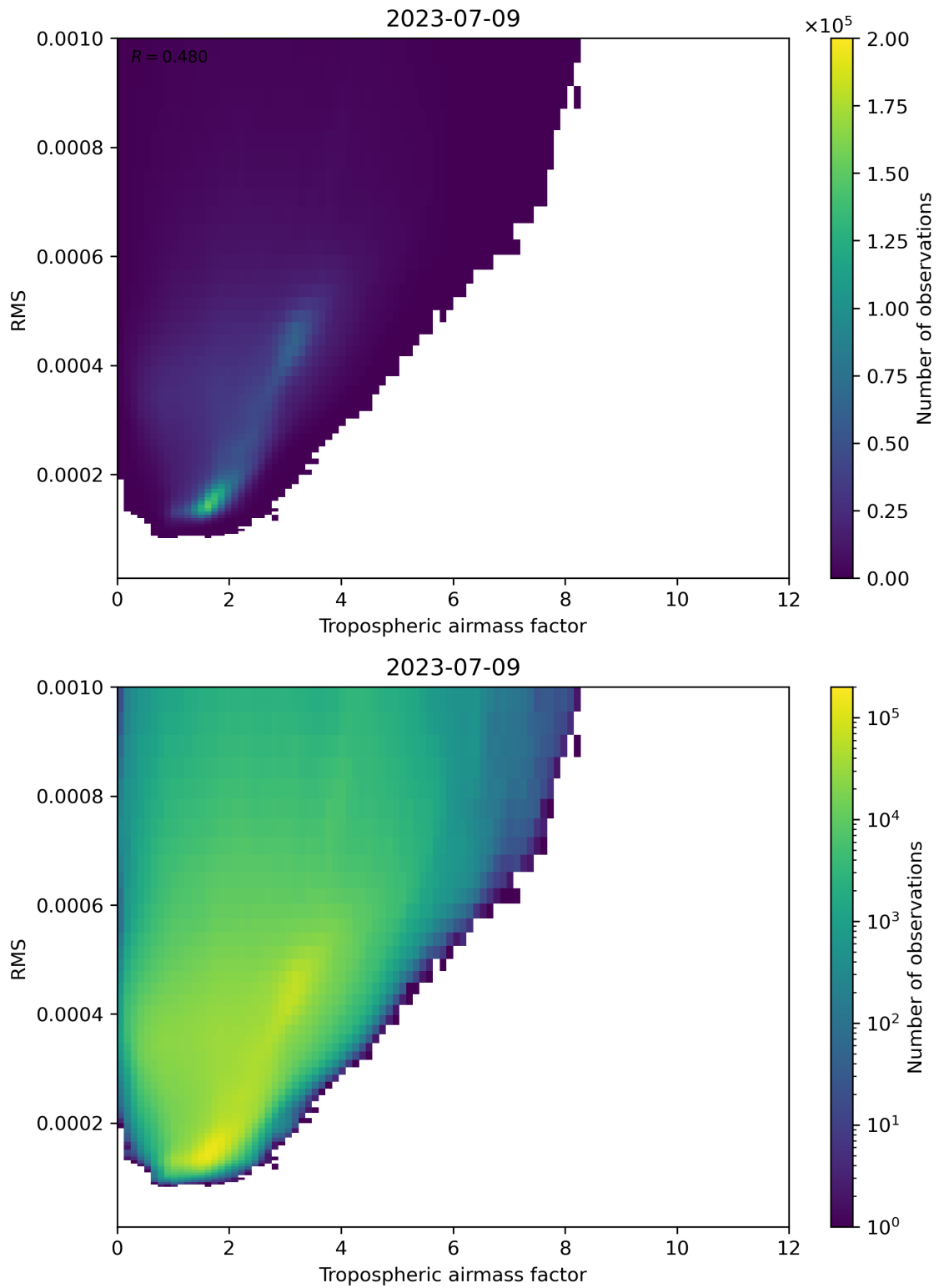
Figure 79: Scatter density plot of “Tropospheric airmass factor” against “RMS” for 2023-07-08 to 2023-07-10.
