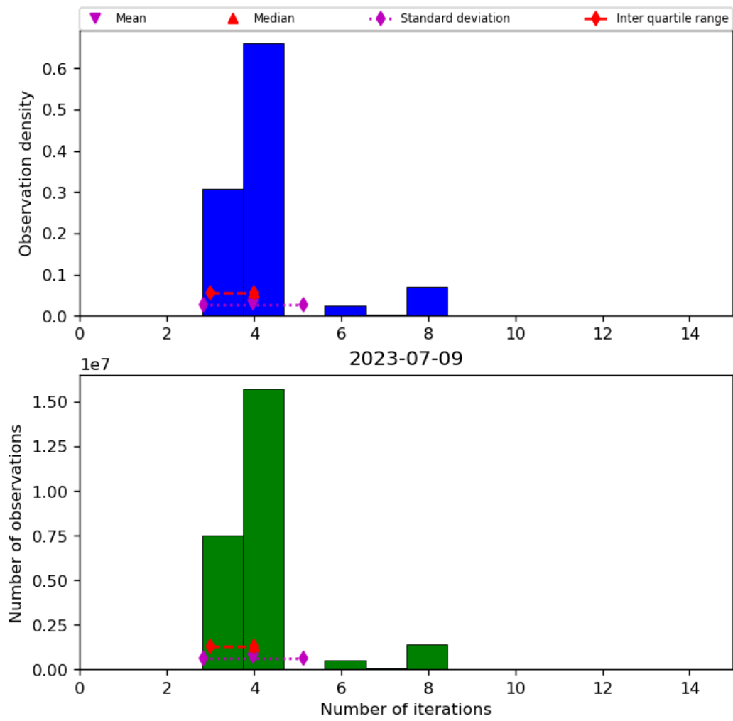
Figure 34: Histogram of “Number of iterations” for 2023-07-08 to 2023-07-10
