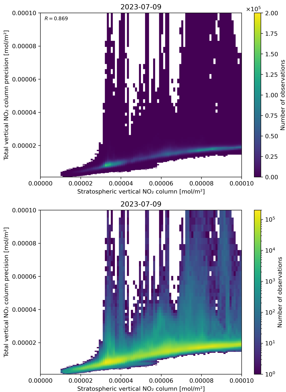
Figure 101: Scatter density plot of “Stratospheric vertical NO 2 column” against “Total vertical NO 2 column precision” for 2023-07-08 to 2023-07-10.
