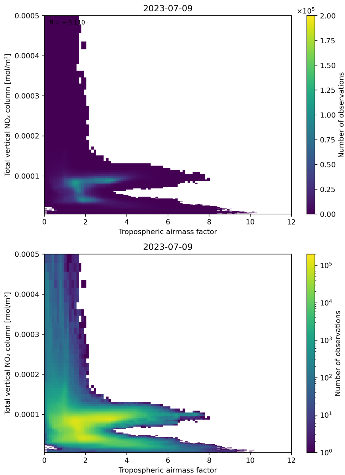
Figure 77: Scatter density plot of “Tropospheric airmass factor” against “Total vertical NO 2 column” for 2023-07-08 to 2023-07-10.
