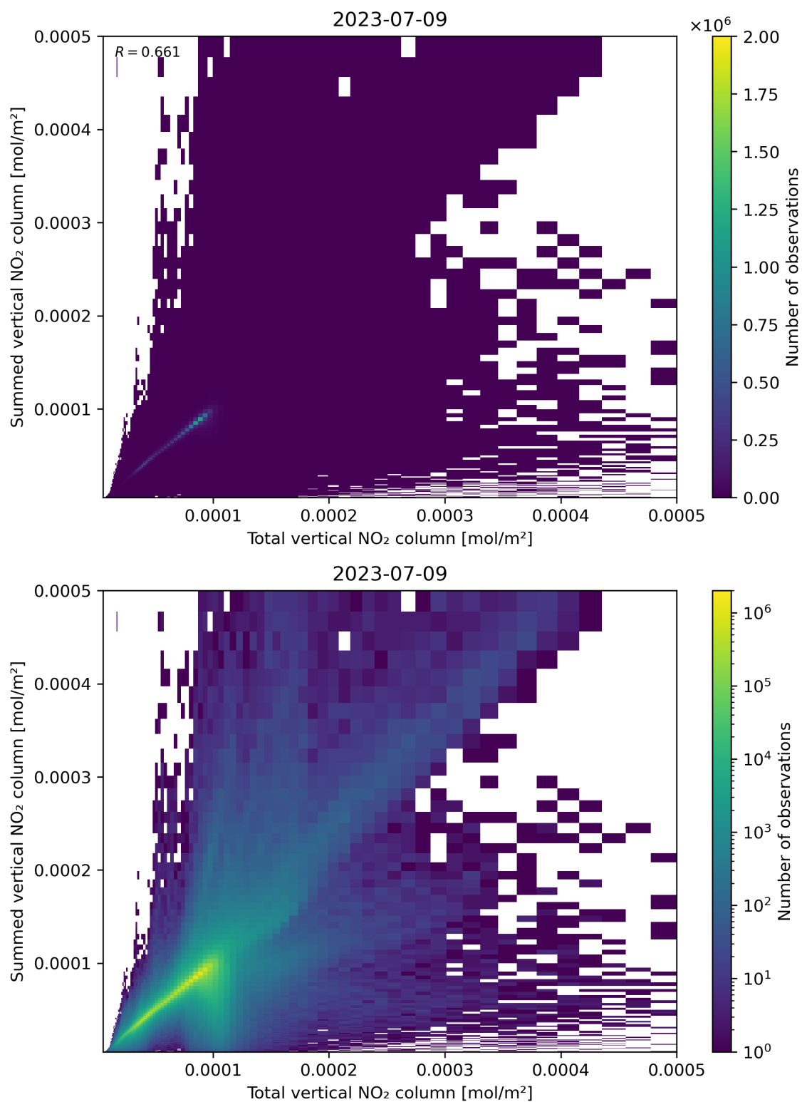
Figure 112: Scatter density plot of “Total vertical NO 2 column” against “Summed vertical NO 2 column” for 2023-07-08 to 2023-07-10.
