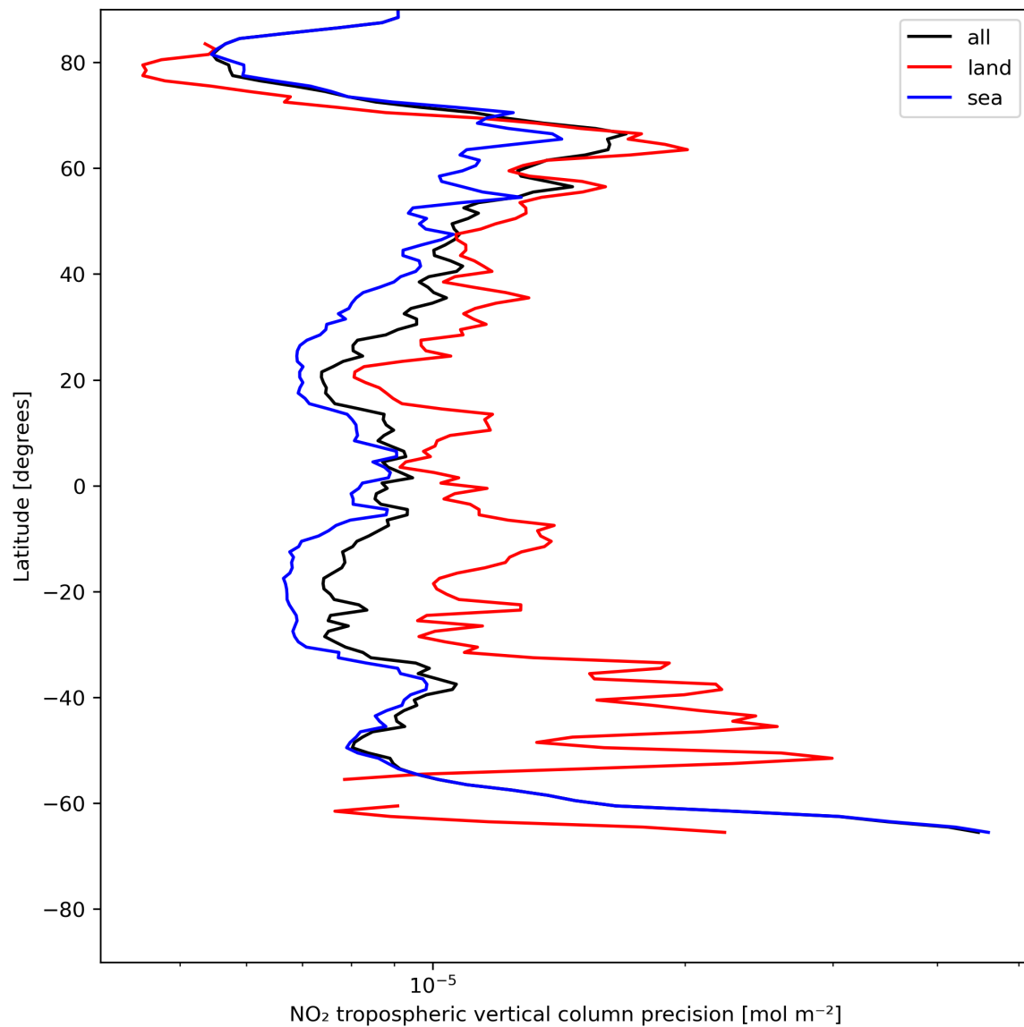
Figure 13: Zonal average of “NO 2 tropospheric vertical column precision” for 2023-07-08 to 2023-07-10.
