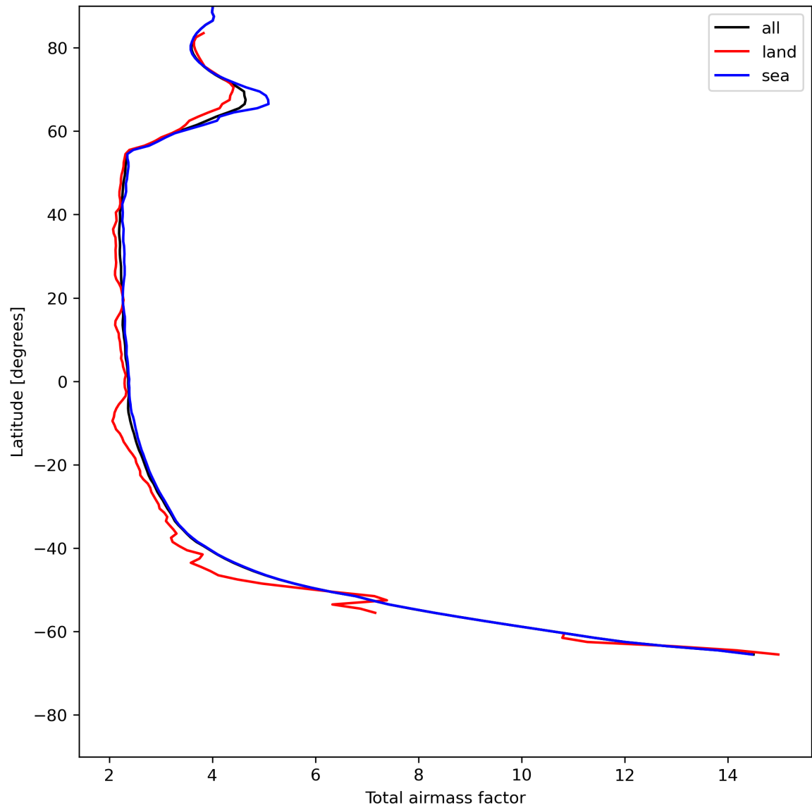
Figure 15: Zonal average of “Total airmass factor” for 2023-07-08 to 2023-07-10.
