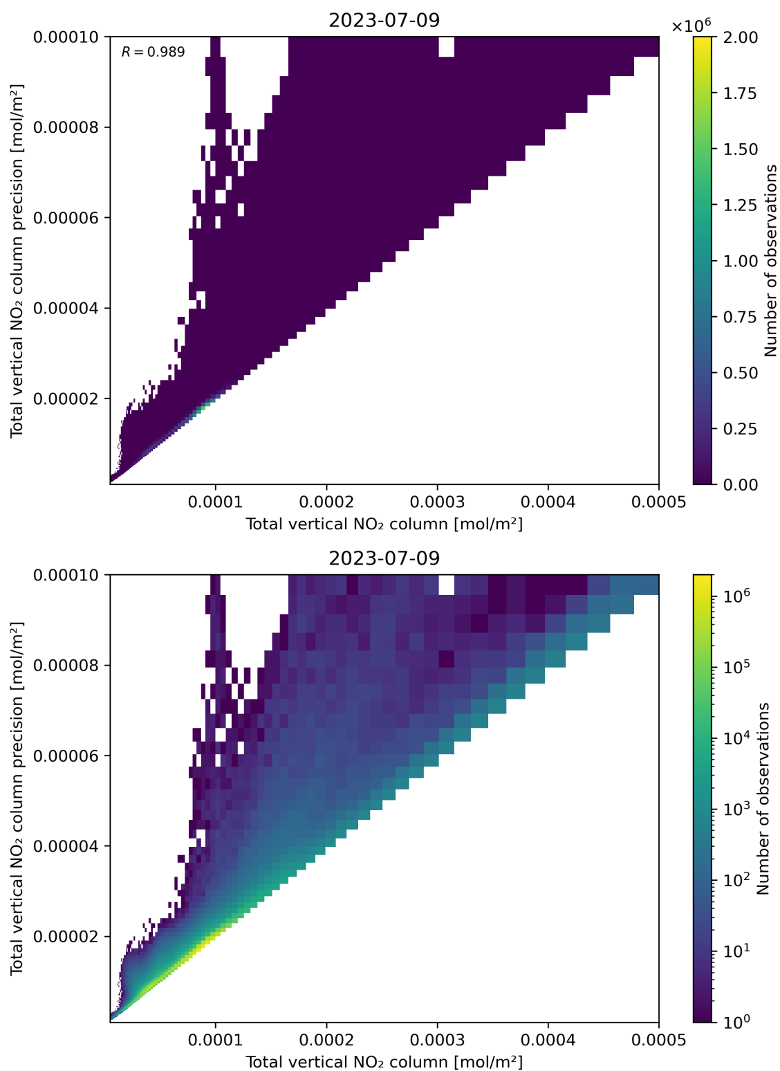
Figure 114: Scatter density plot of “Total vertical NO 2 column” against “Total vertical NO 2 column precision” for 2023-07-08 to 2023-07-10.
