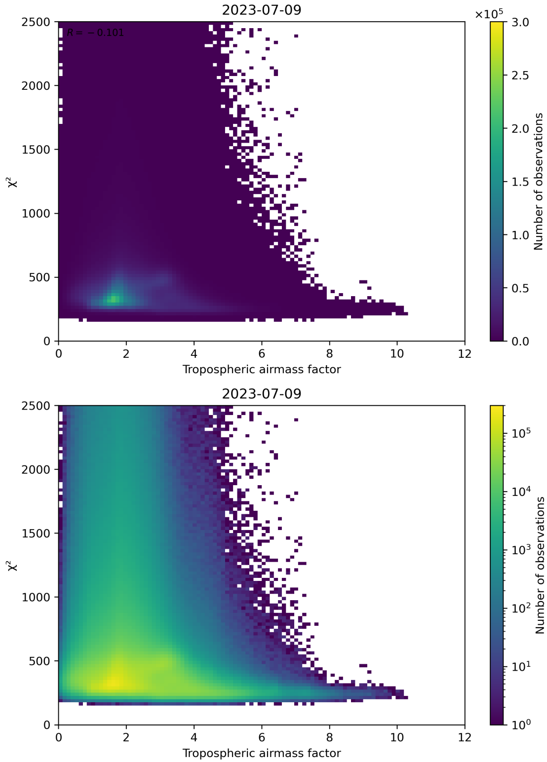
Figure 73: Scatter density plot of “Tropospheric airmass factor” against “ \chi^2 ” for 2023-07-08 to 2023-07-10.
