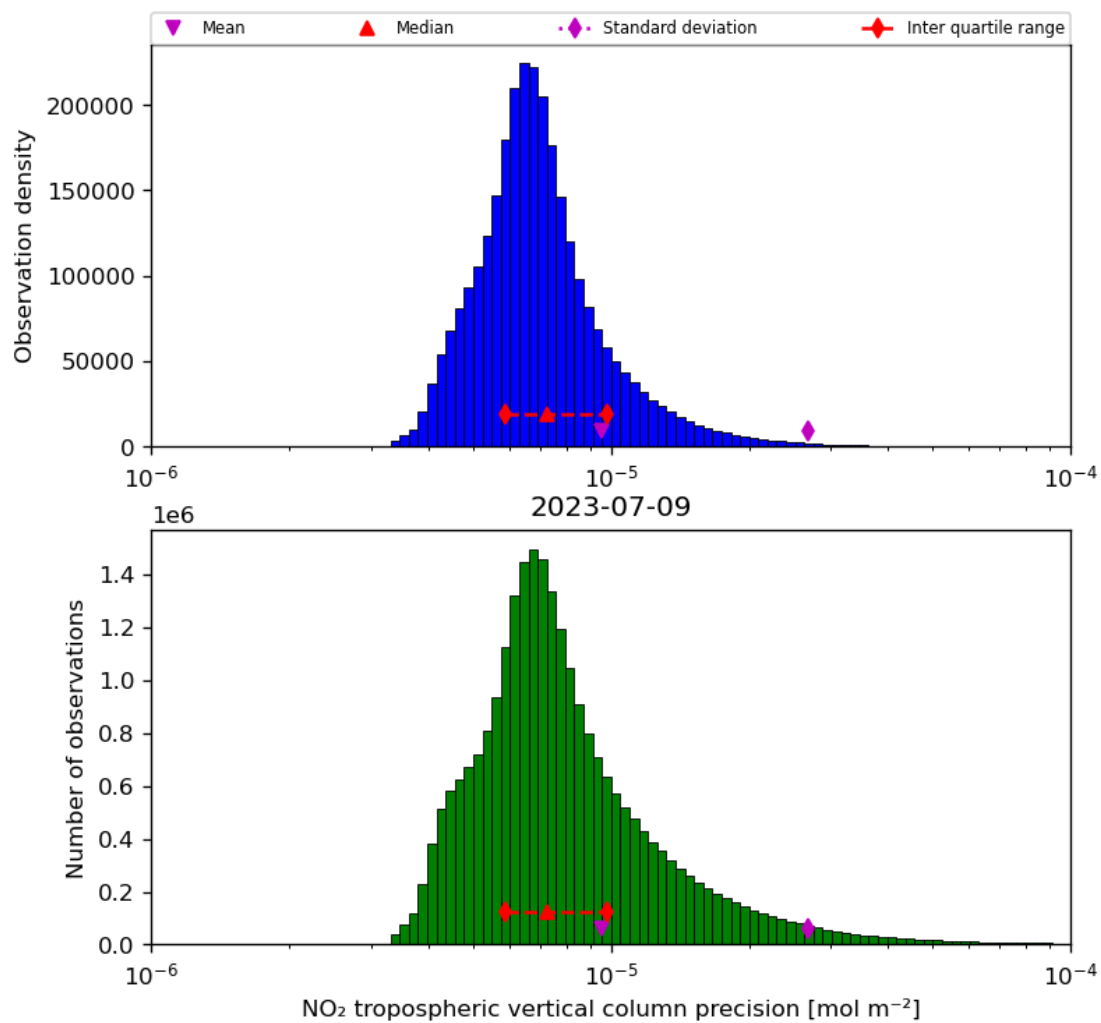
Figure 30: Histogram of “NO 2 tropospheric vertical column precision” for 2023-07-08 to 2023-07-10
