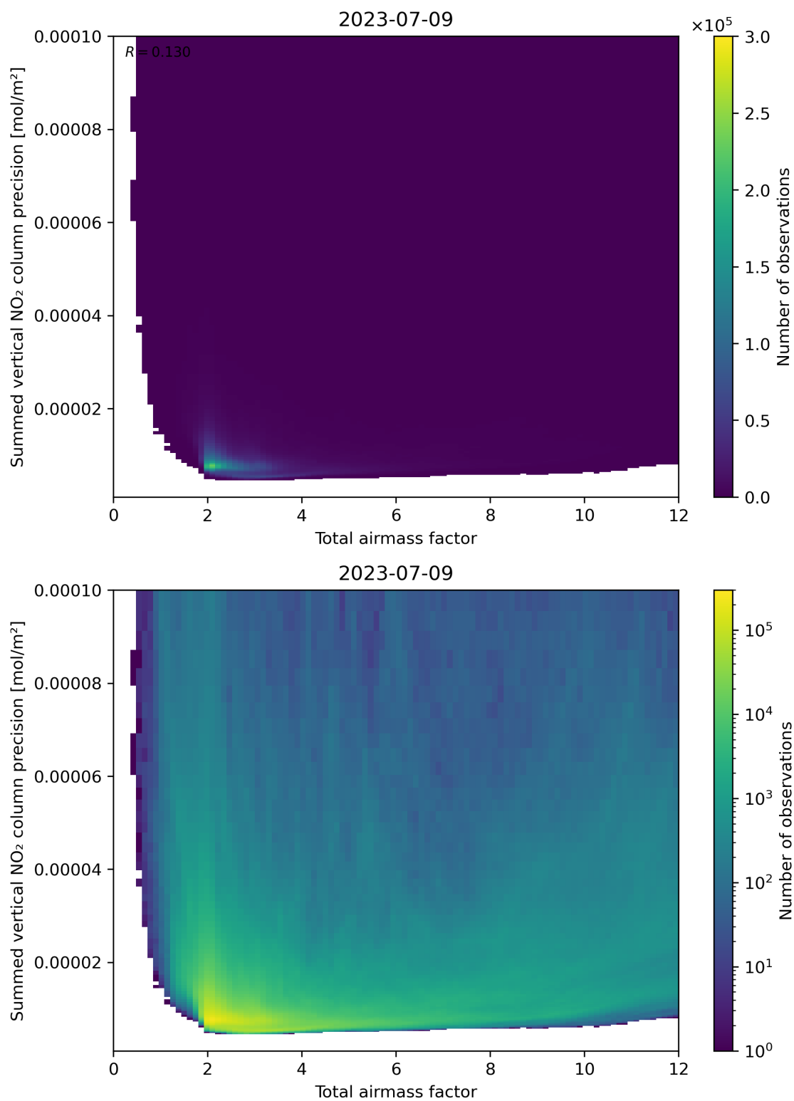
Figure 66: Scatter density plot of “Total airmass factor” against “Summed vertical NO 2 column precision” for 2023-07-08 to 2023-07-10.
