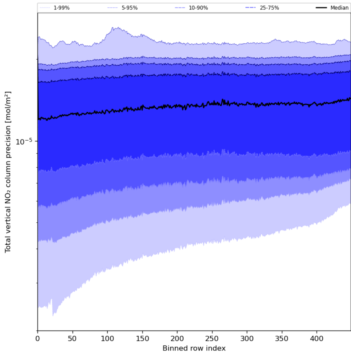
Figure 56: Along track statistics of “Total vertical NO 2 column precision” for 2023-07-08 to 2023-07-10
