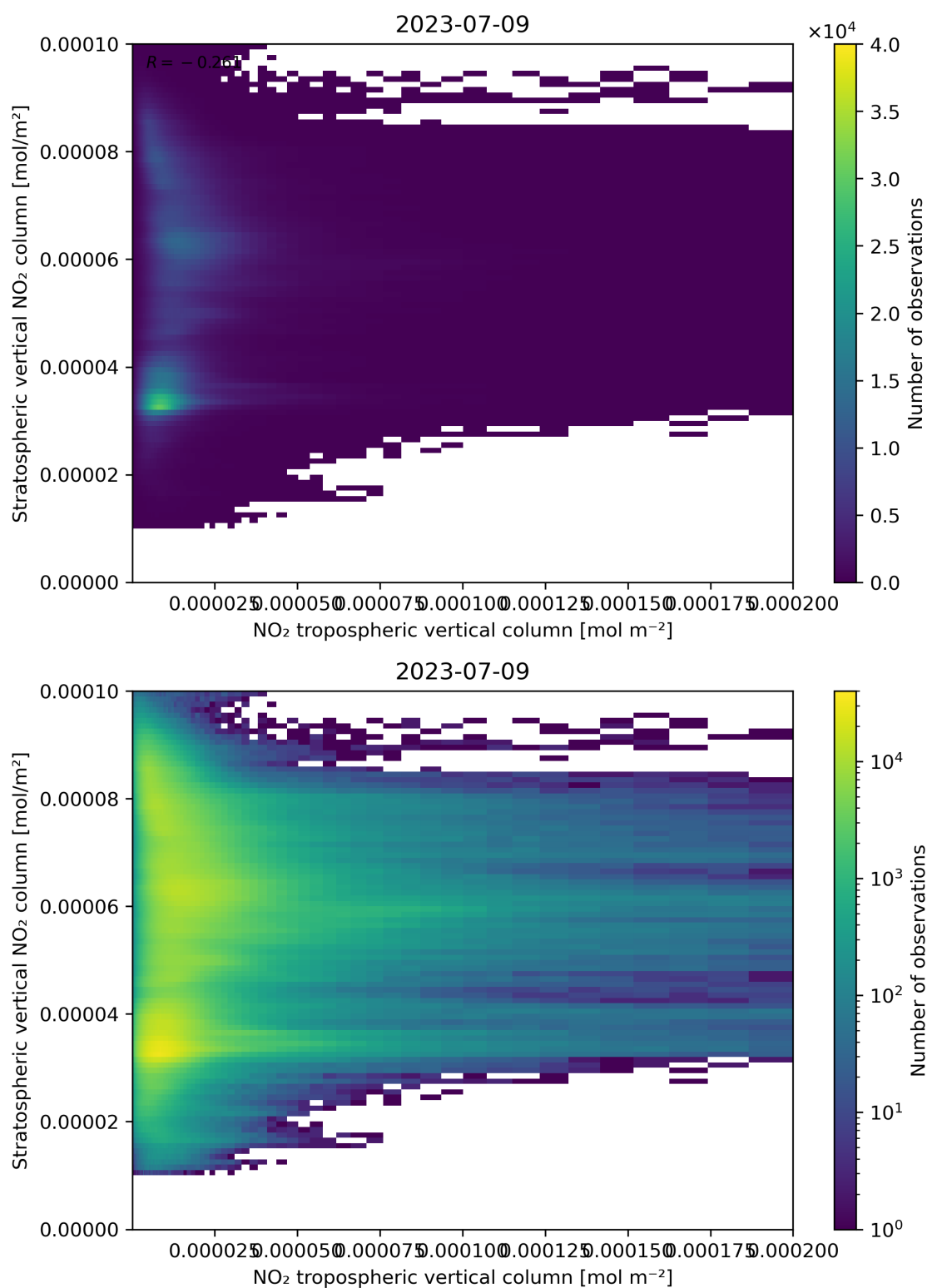
Figure 125: Scatter density plot of “NO 2 tropospheric vertical column” against “Stratospheric vertical NO 2 column” for 2023-07-08 to 2023-07-10.
