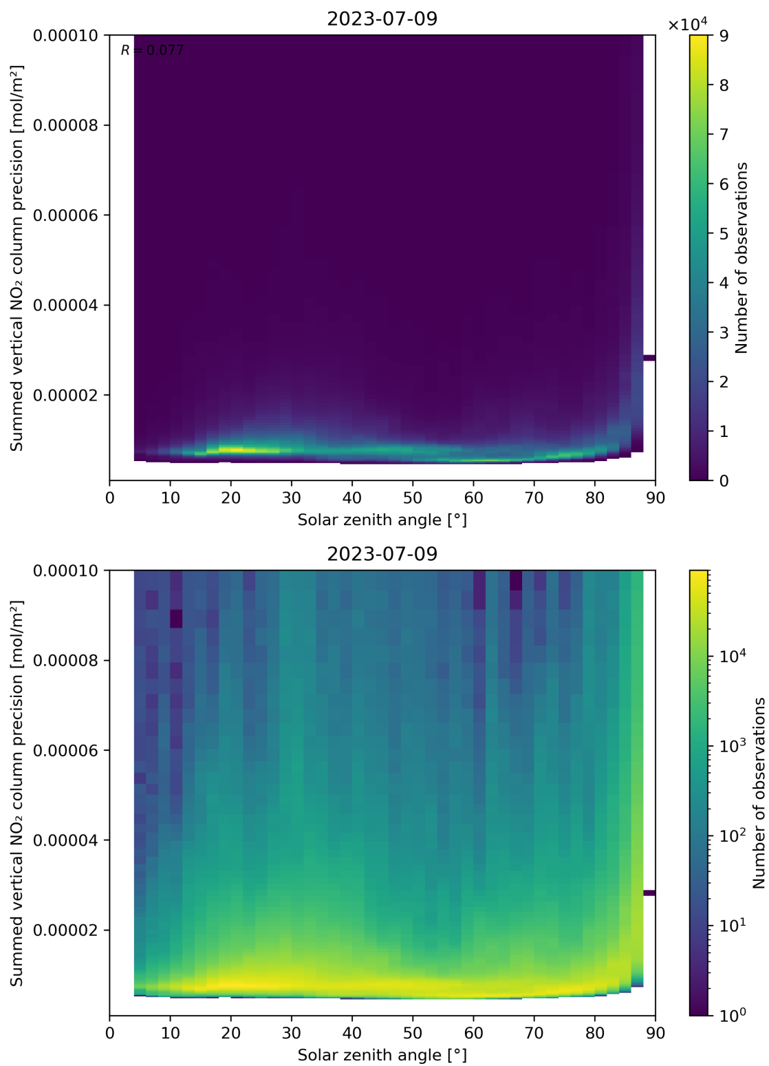
Figure 152: Scatter density plot of “Solar zenith angle” against “Summed vertical NO 2 column precision” for 2023-07-08 to 2023-07-10.
