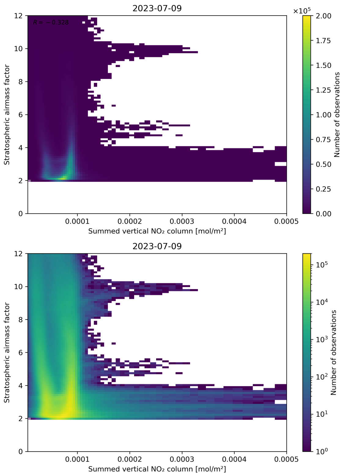
Figure 103: Scatter density plot of “Summed vertical NO 2 column” against “Stratospheric airmass factor” for 2023-07-08 to 2023-07-10.
