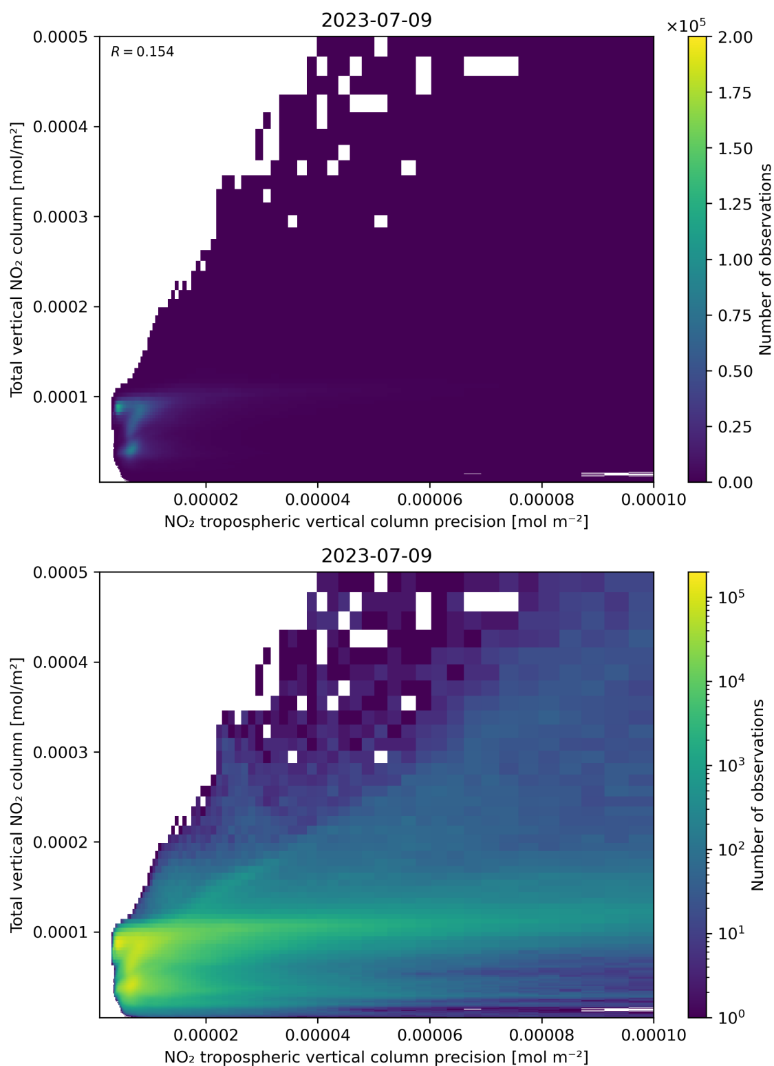
Figure 138: Scatter density plot of “NO 2 tropospheric vertical column precision” against “Total vertical NO 2 column” for 2023-07-08 to 2023-07-10.
