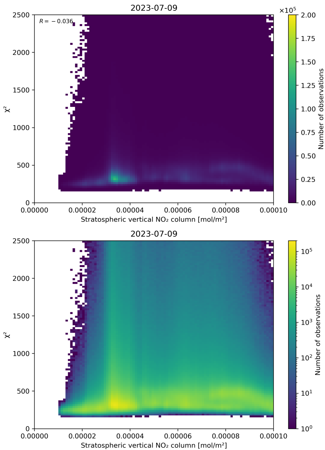
Figure 97: Scatter density plot of “Stratospheric vertical NO 2 column” against “ \chi^2 ” for 2023-07-08 to 2023-07-10.
