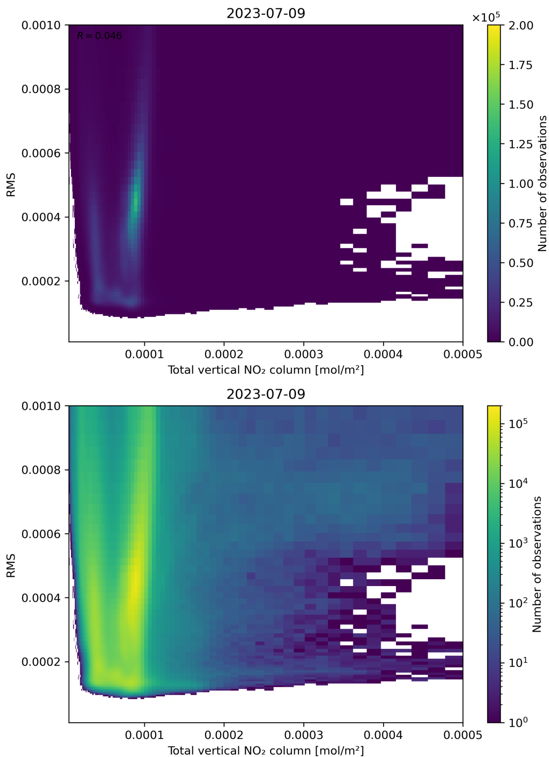
Figure 120: Scatter density plot of “Total vertical NO 2 column” against “RMS” for 2023-07-08 to 2023-07-10.
