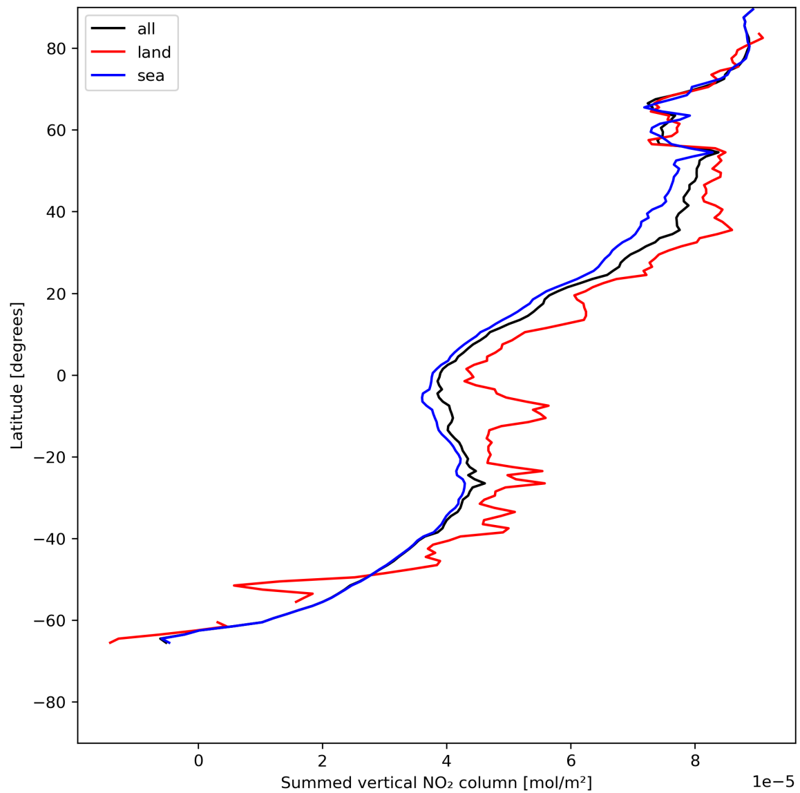
Figure 23: Zonal average of “Summed vertical NO 2 column” for 2023-07-08 to 2023-07-10.
