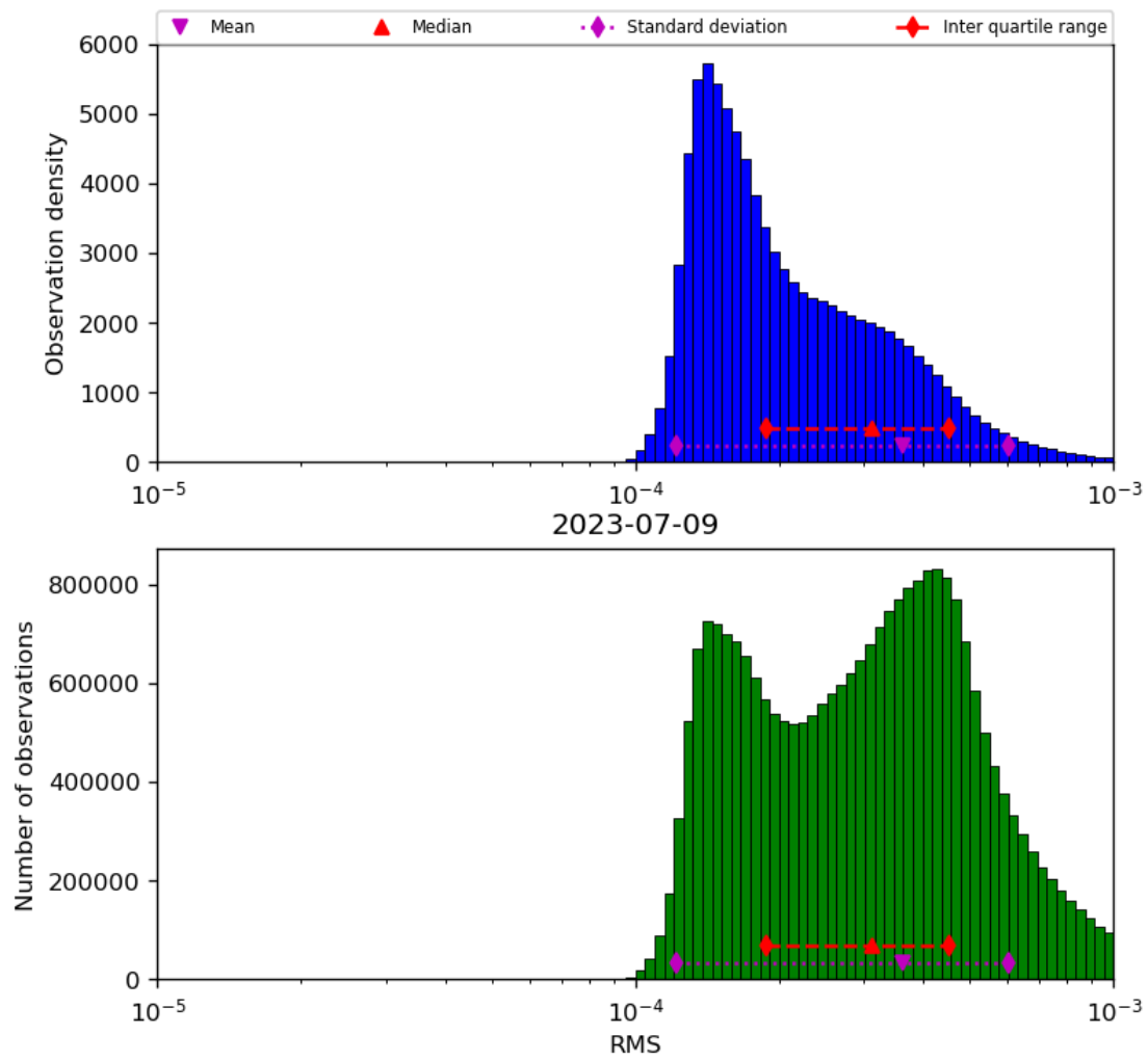
Figure 43: Histogram of “RMS” for 2023-07-08 to 2023-07-10
