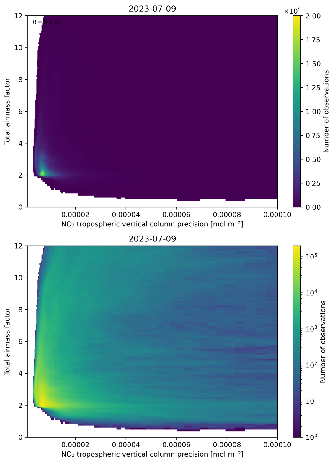
Figure 132: Scatter density plot of “NO 2 tropospheric vertical column precision” against “Total air mass factor” for 2023-07-08 to 2023-07-10.
