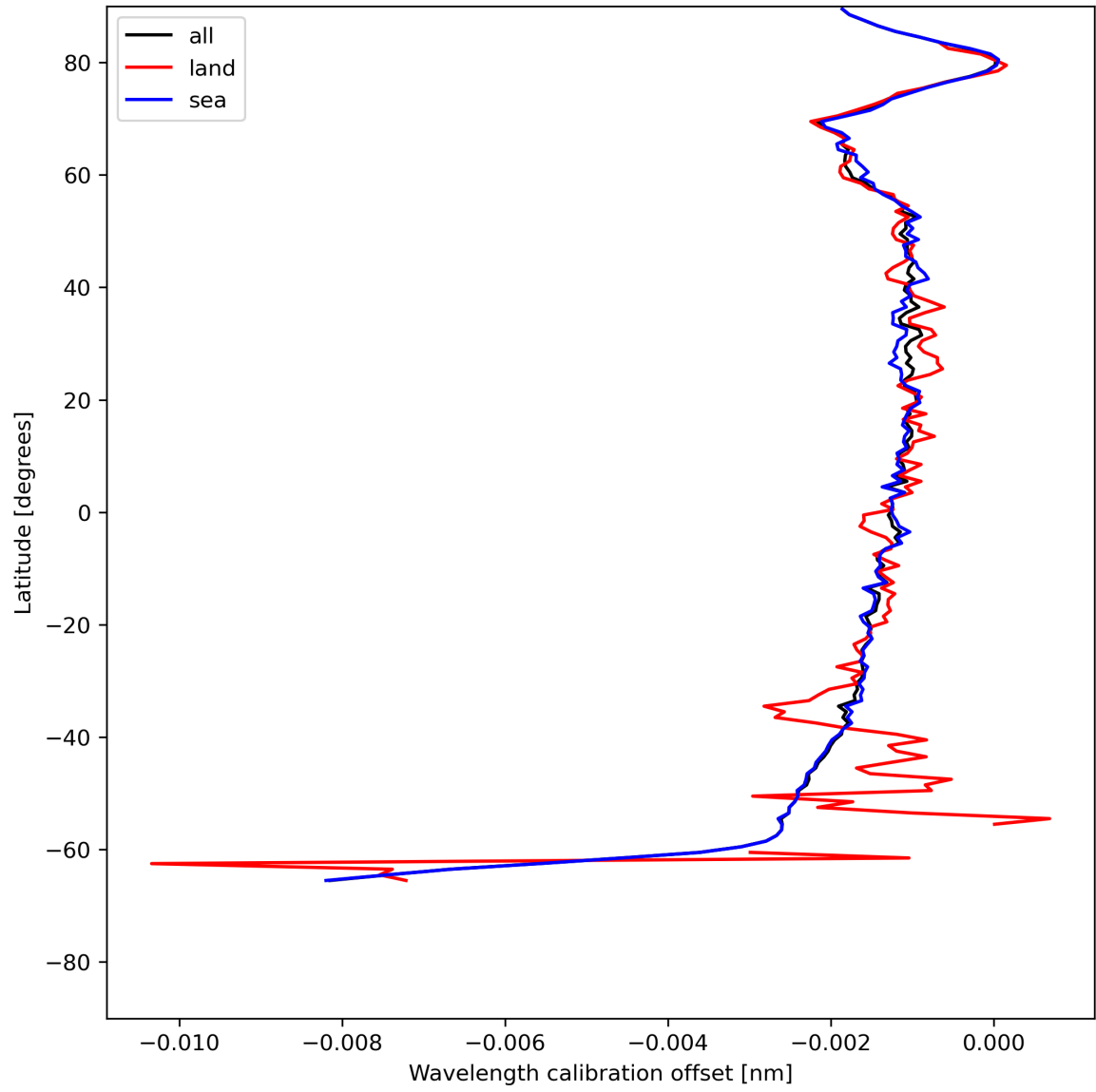
Figure 18: Zonal average of “Wavelength calibration offset” for 2023-07-08 to 2023-07-10.
