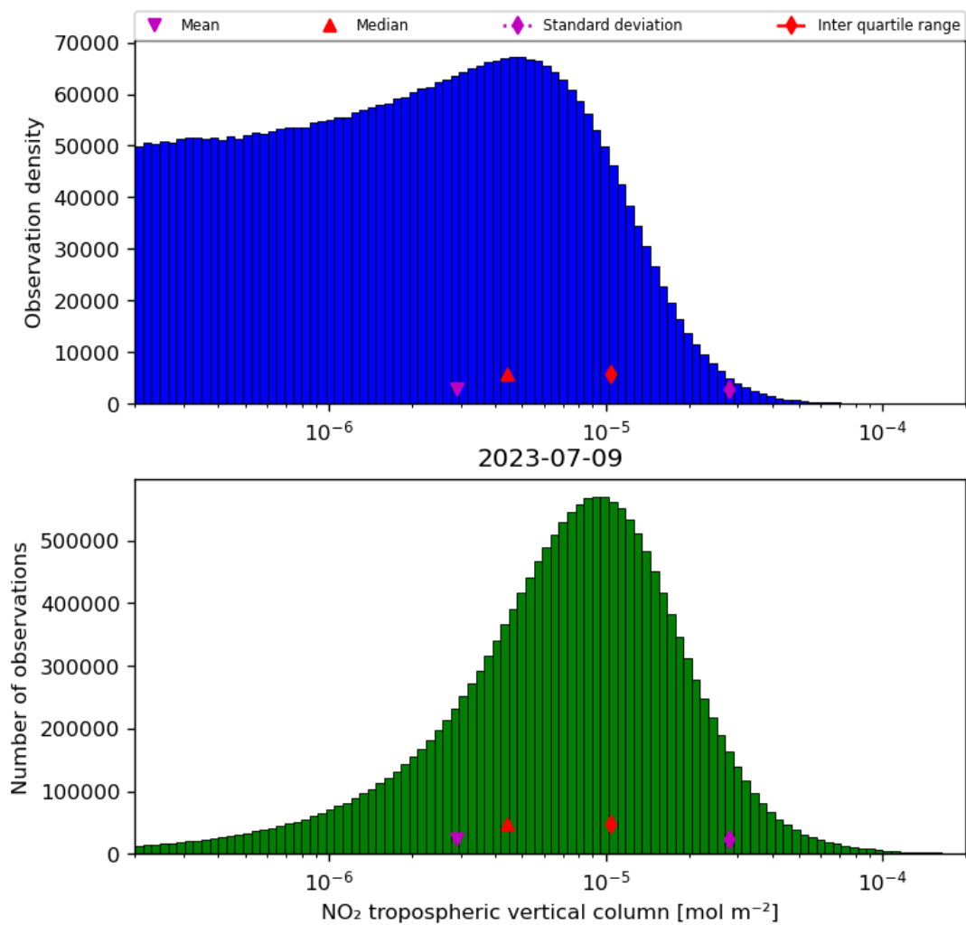
Figure 29: Histogram of “ \text{NO}_2 tropospheric vertical column” for 2023-07-08 to 2023-07-10
