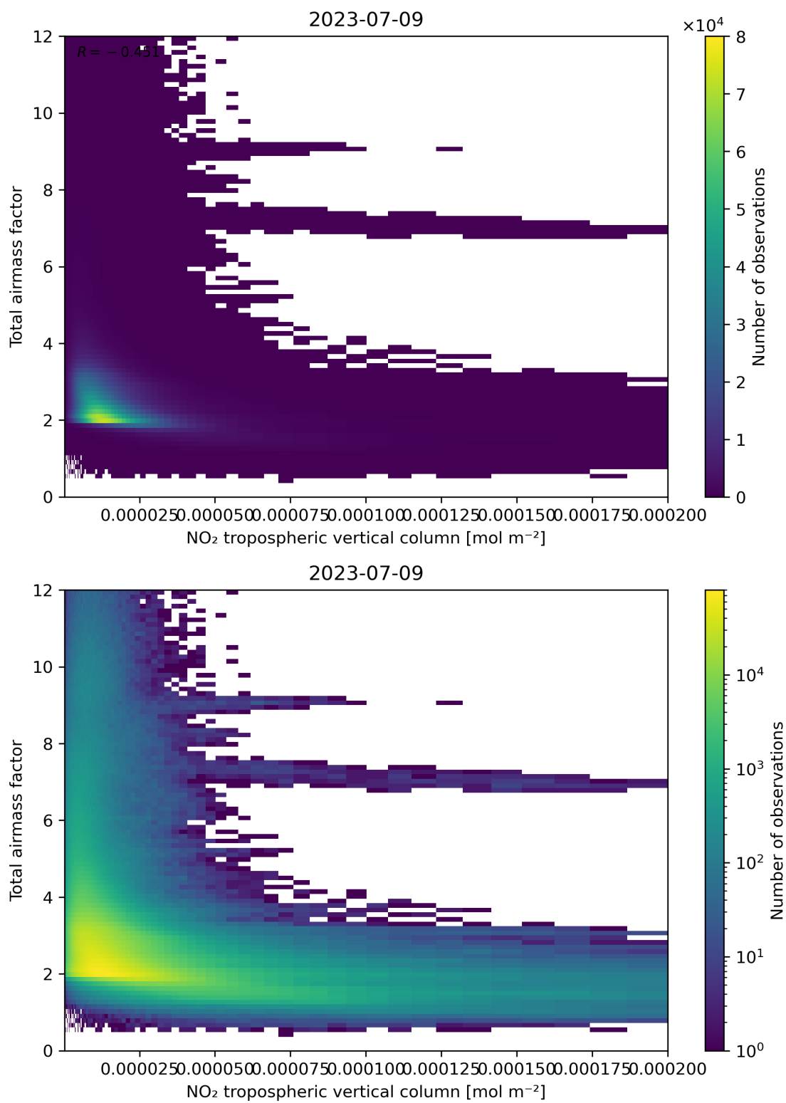
Figure 122: Scatter density plot of “NO 2 tropospheric vertical column” against “Total air mass factor” for 2023-07-08 to 2023-07-10.
