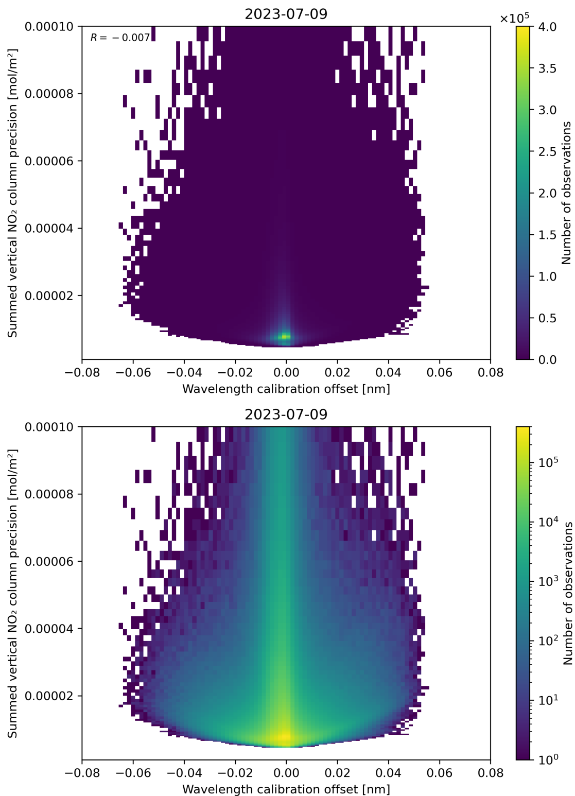
Figure 178: Scatter density plot of “Wavelength calibration offset” against “Summed vertical NO 2 column precision” for 2023-07-08 to 2023-07-10.
