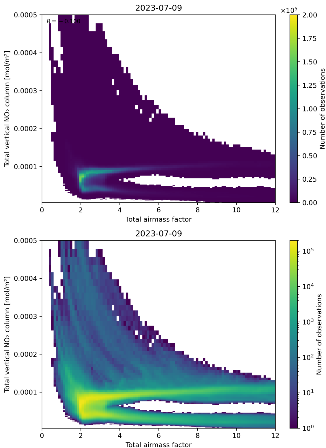
Figure 67: Scatter density plot of “Total airmass factor” against “Total vertical NO 2 column” for 2023-07-08 to 2023-07-10.
