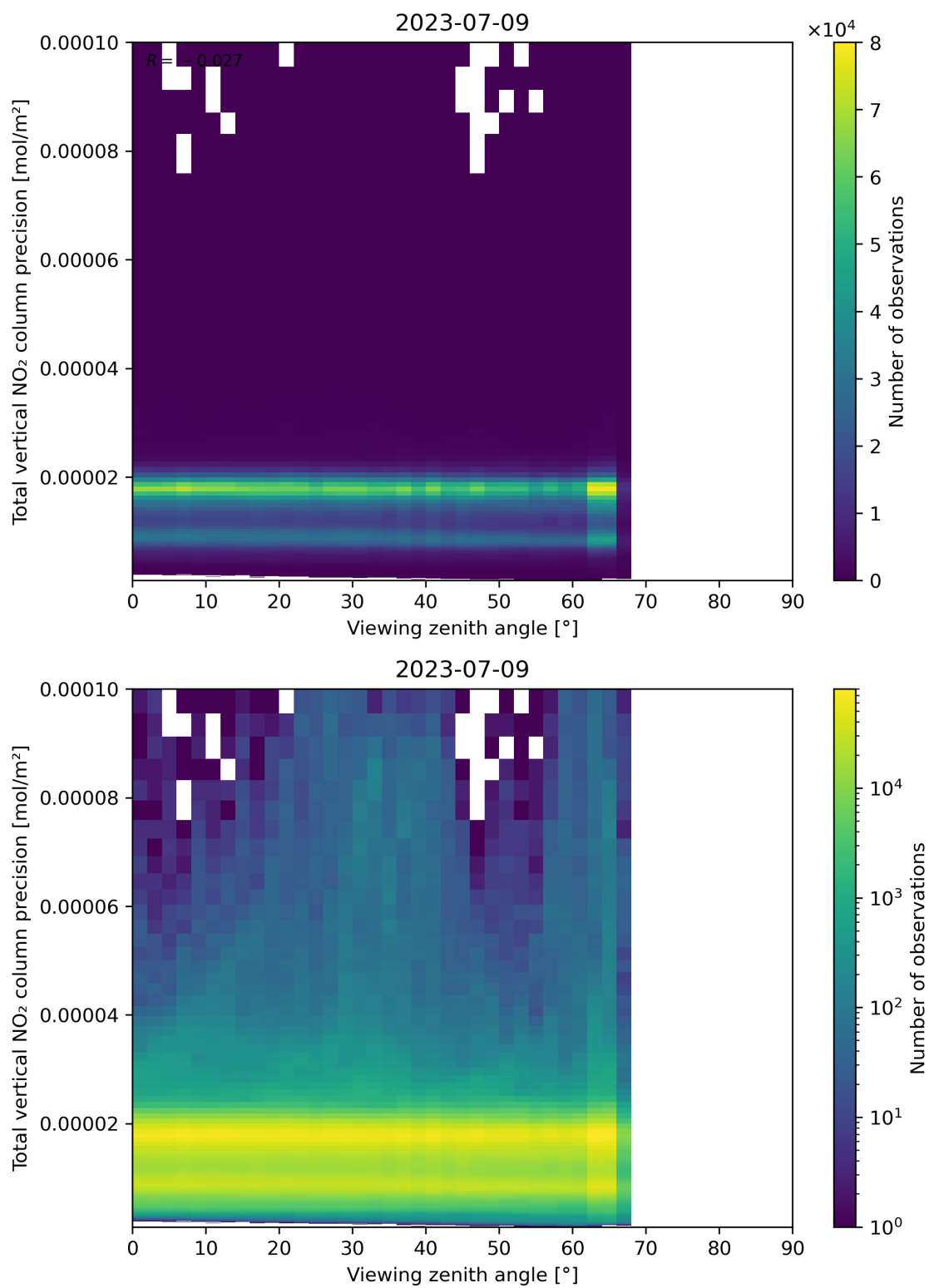
Figure 168: Scatter density plot of “Viewing zenith angle” against “Total vertical NO 2 column precision” for 2023-07-08 to 2023-07-10.
