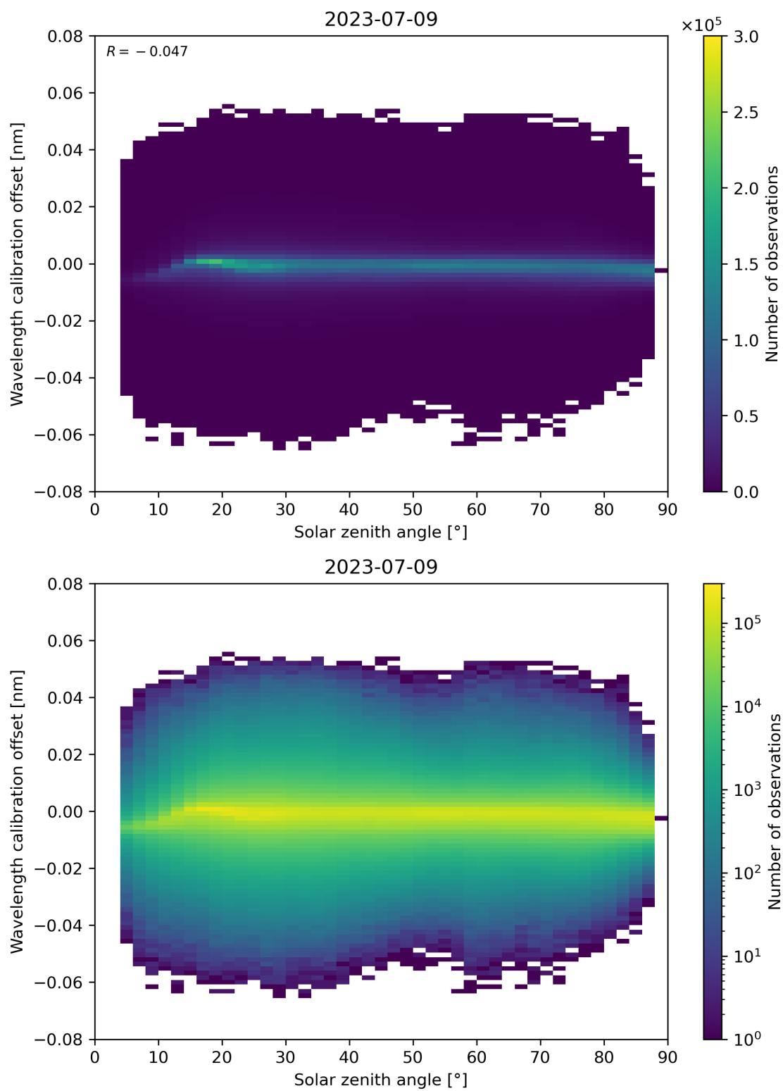
Figure 158: Scatter density plot of “Solar zenith angle” against “Wavelength calibration offset” for 2023-07-08 to 2023-07-10.
