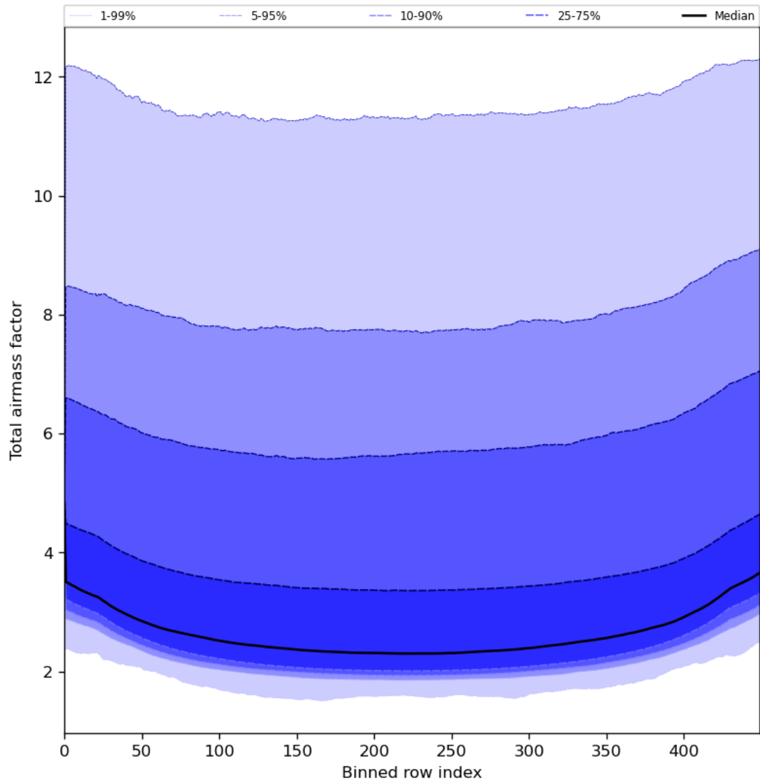
Figure 49: Along track statistics of “Total airmass factor” for 2023-07-08 to 2023-07-10
