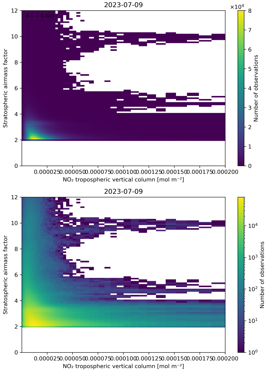
Figure 121: Scatter density plot of “NO 2 tropospheric vertical column” against “Stratospheric air mass factor” for 2023-07-08 to 2023-07-10.
