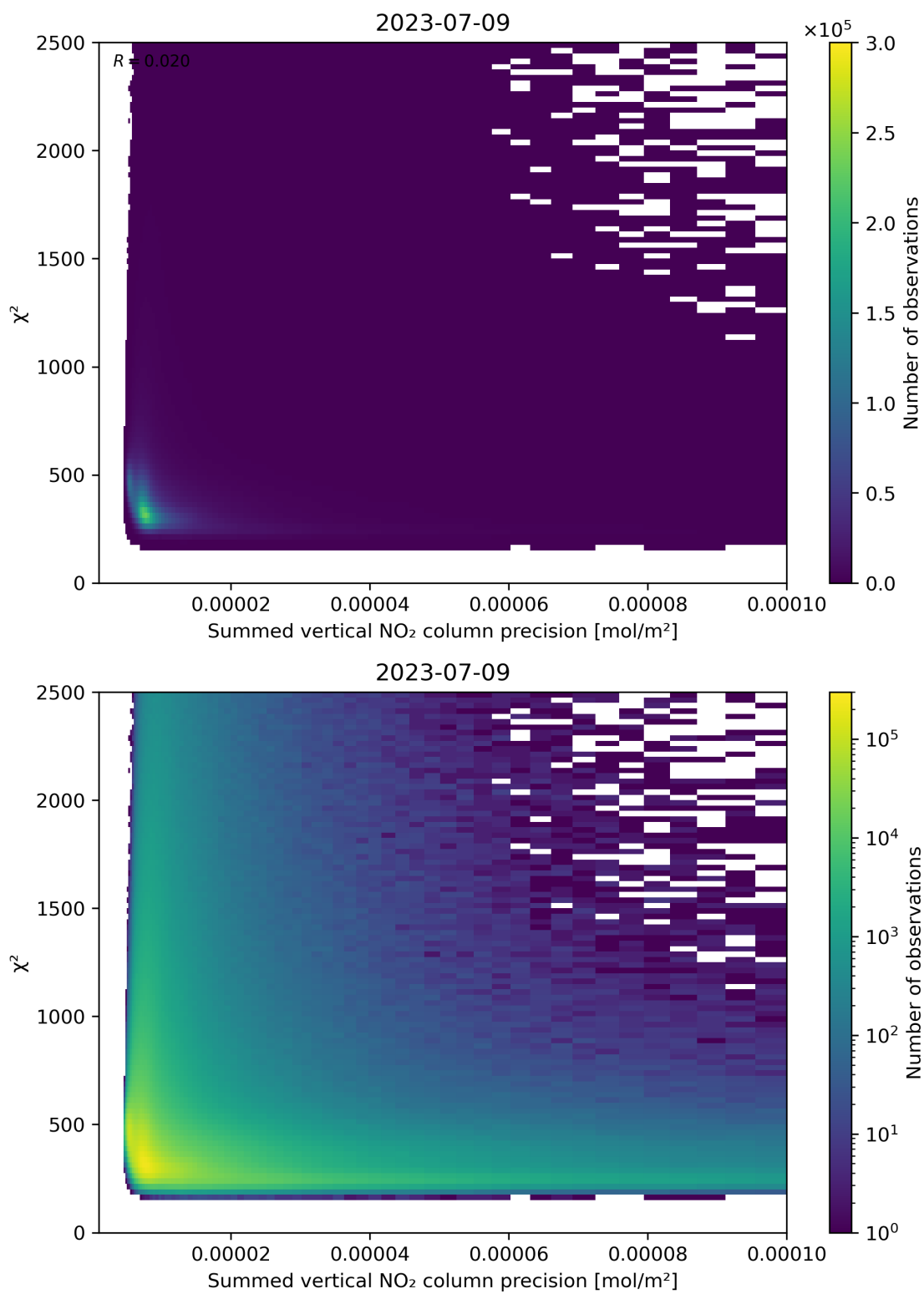
Figure 107: Scatter density plot of “Summed vertical NO 2 column precision” against “ \chi^2 ” for 2023-07-08 to 2023-07-10.
