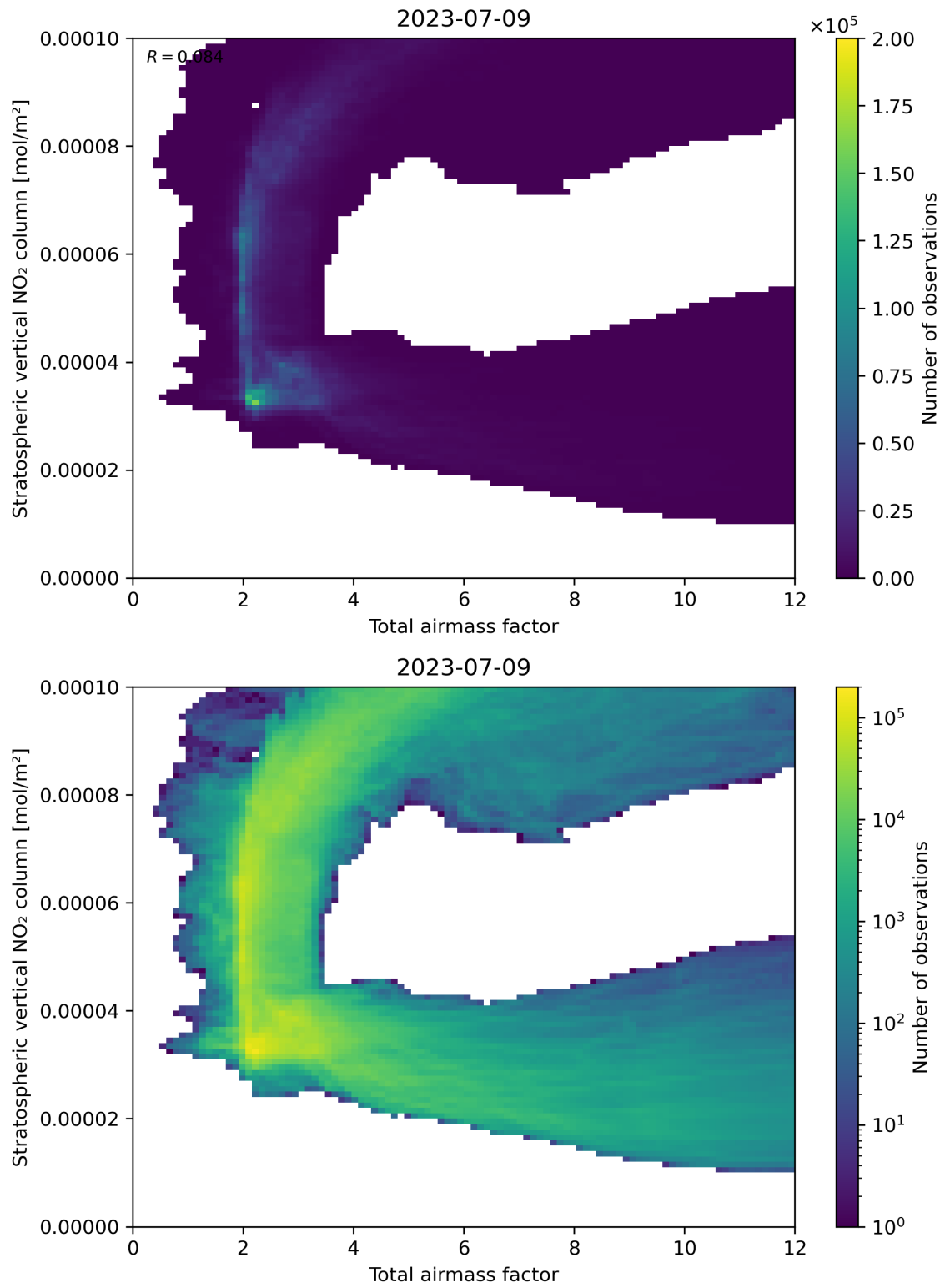
Figure 64: Scatter density plot of “Total airmass factor” against “Stratospheric vertical NO 2 column” for 2023-07-08 to 2023-07-10.
