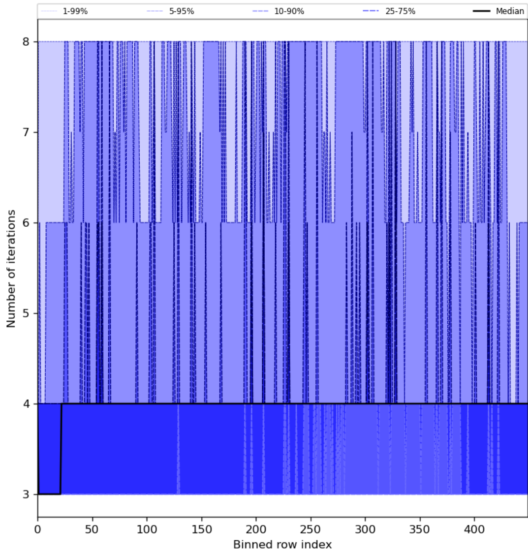
Figure 51: Along track statistics of “Number of iterations” for 2023-07-08 to 2023-07-10
