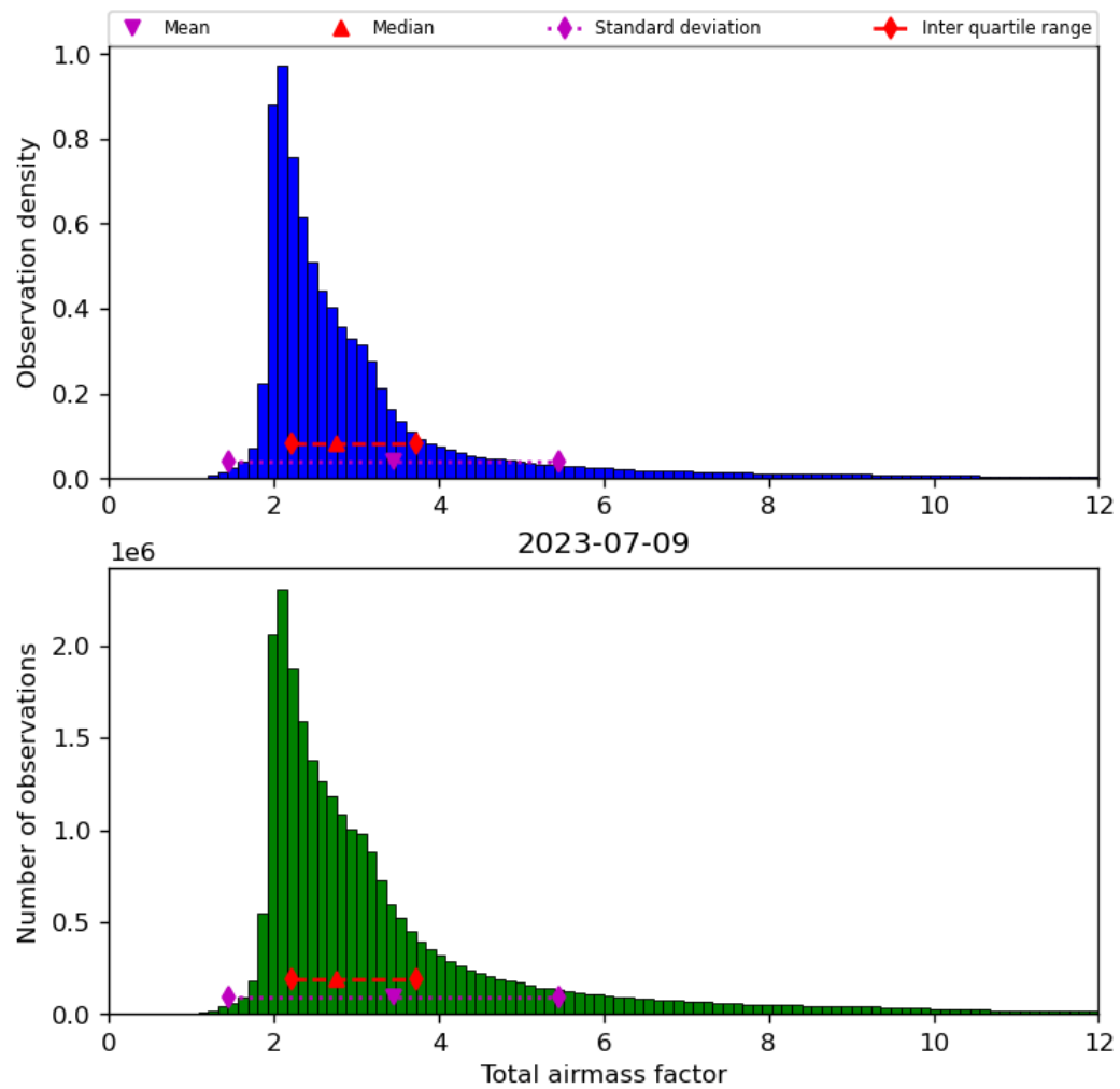
Figure 32: Histogram of “Total airmass factor” for 2023-07-08 to 2023-07-10
