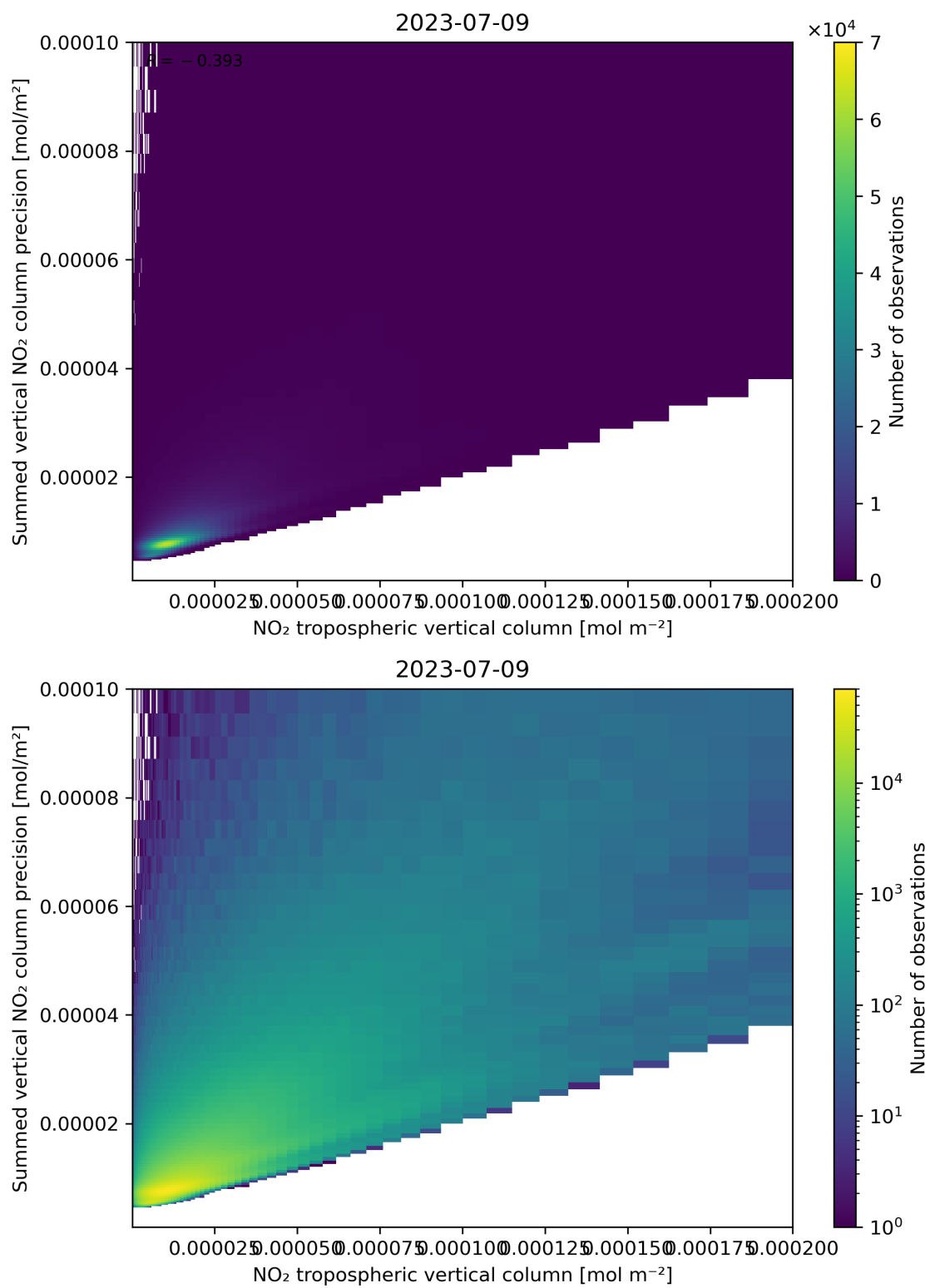
Figure 127: Scatter density plot of “NO 2 tropospheric vertical column” against “Summed vertical NO 2 column precision” for 2023-07-08 to 2023-07-10.
