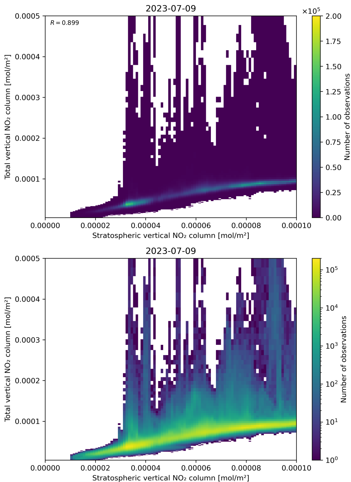
Figure 100: Scatter density plot of “Stratospheric vertical NO 2 column” against “Total vertical NO 2 column” for 2023-07-08 to 2023-07-10.
