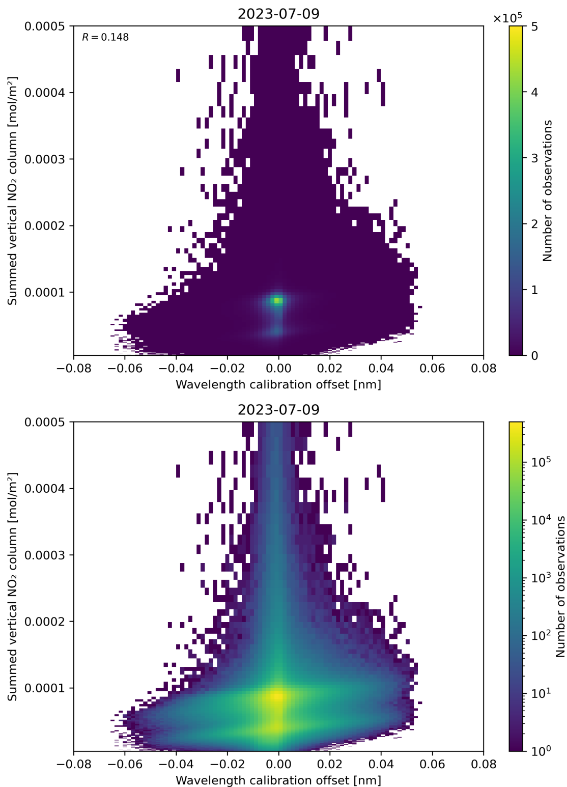
Figure 177: Scatter density plot of “Wavelength calibration offset” against “Summed vertical NO 2 column” for 2023-07-08 to 2023-07-10.
