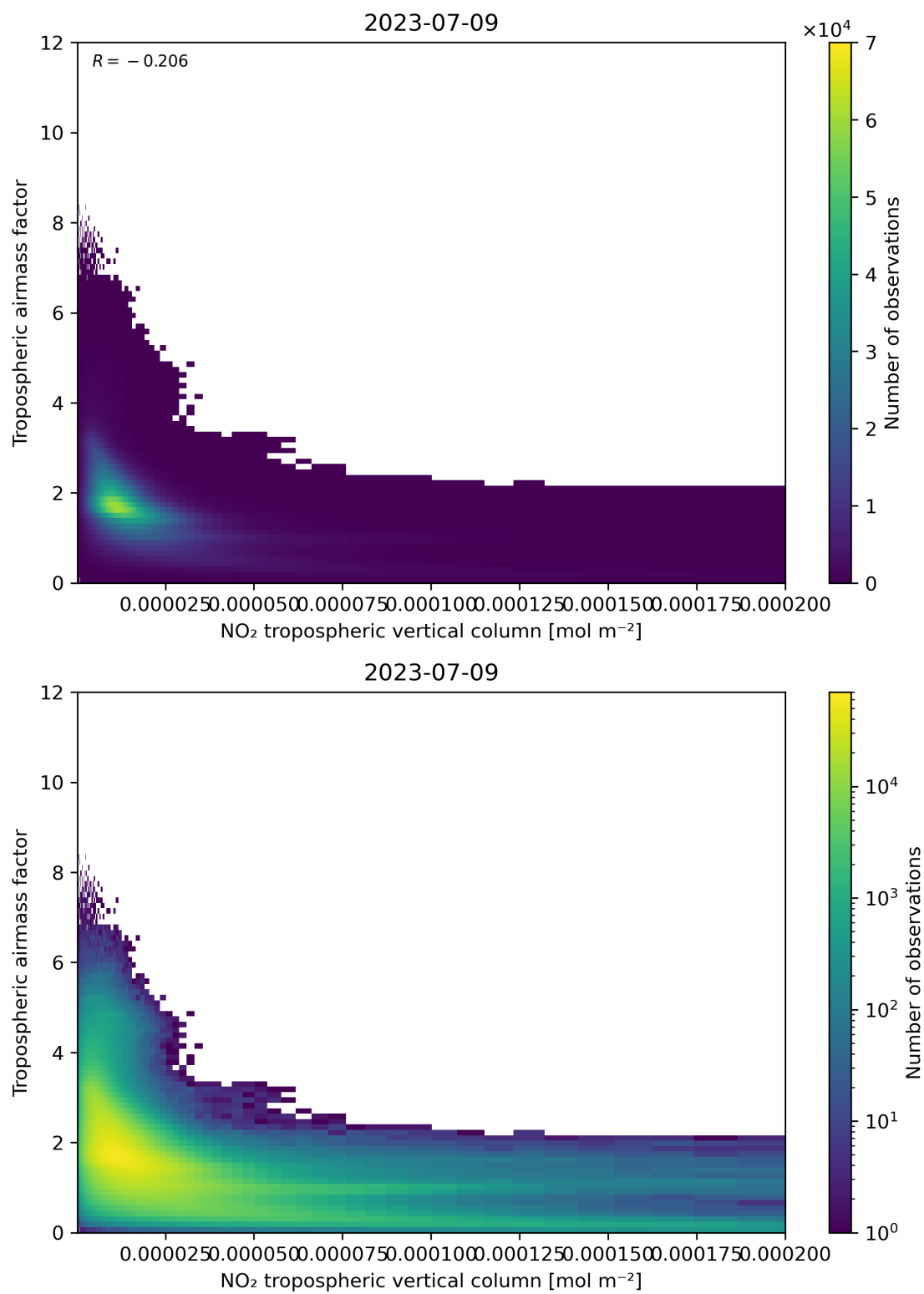
Figure 123: Scatter density plot of “NO 2 tropospheric vertical column” against “Tropospheric air mass factor” for 2023-07-08 to 2023-07-10.
