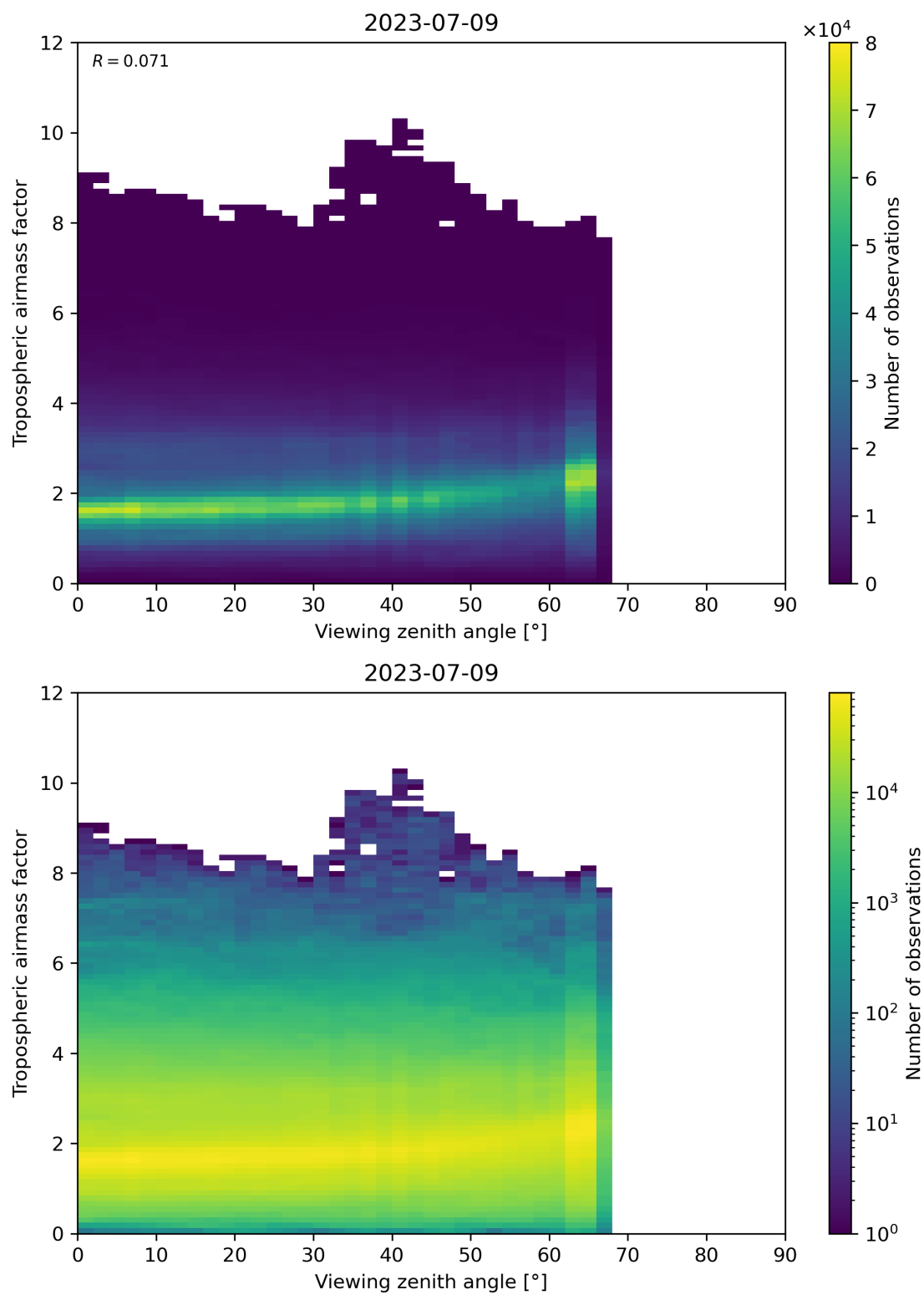
Figure 161: Scatter density plot of “Viewing zenith angle” against “Tropospheric airmass factor” for 2023-07-08 to 2023-07-10.
