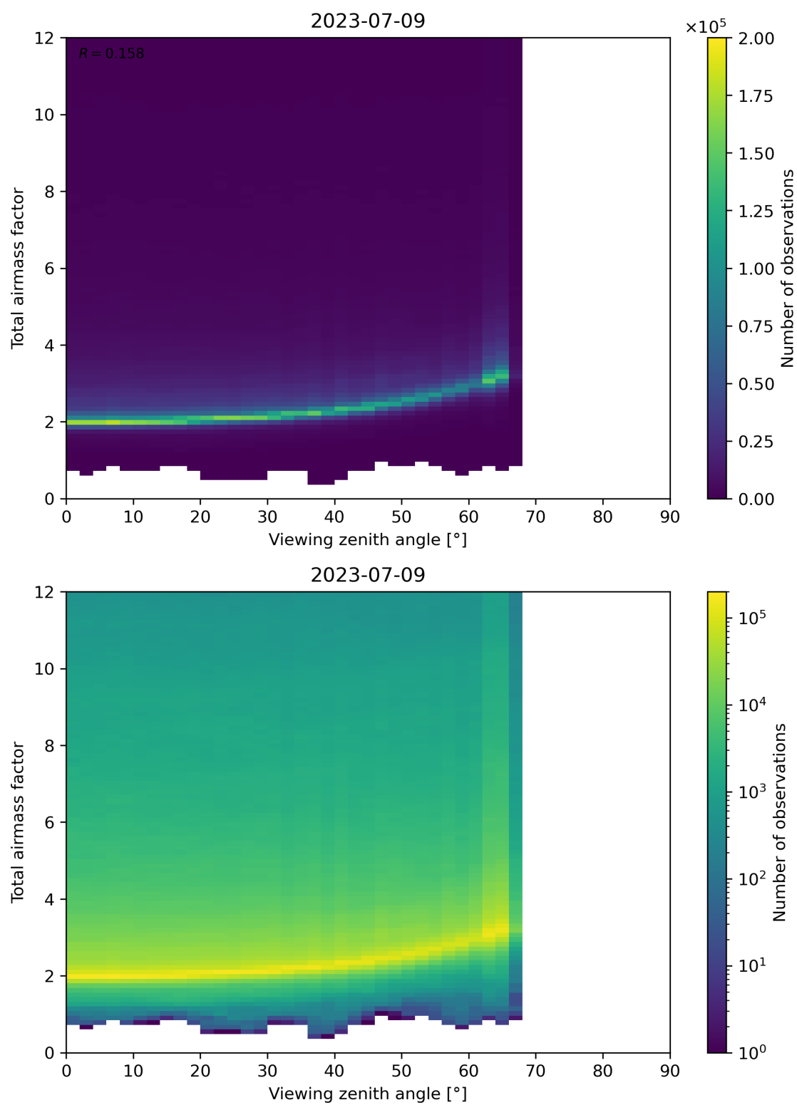
Figure 160: Scatter density plot of “Viewing zenith angle” against “Total airmass factor” for 2023-07-08 to 2023-07-10.
