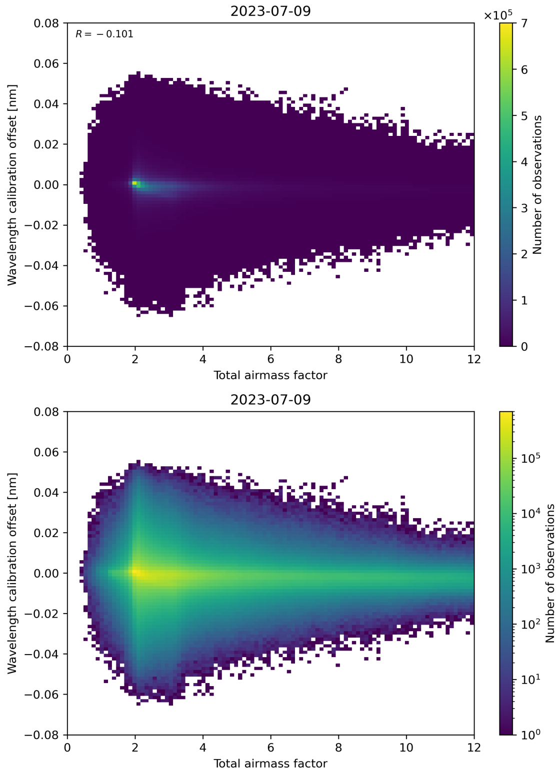
Figure 70: Scatter density plot of “Total airmass factor” against “Wavelength calibration offset” for 2023-07-08 to 2023-07-10.
