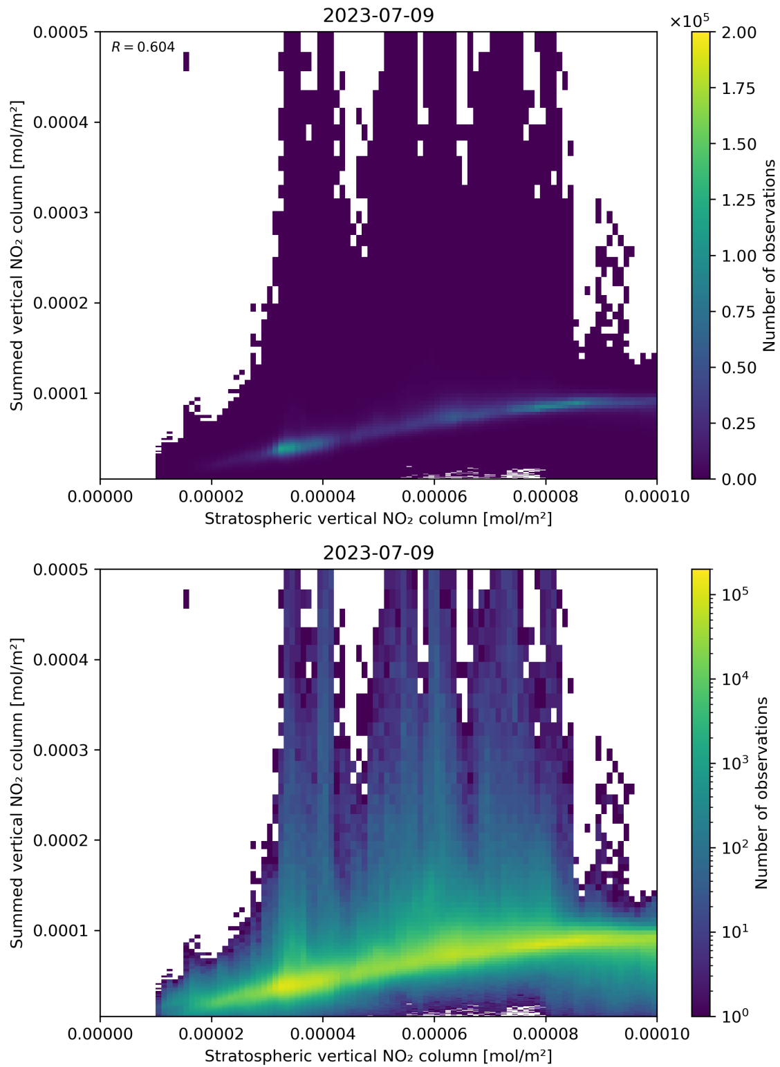
Figure 98: Scatter density plot of “Stratospheric vertical NO 2 column” against “Summed vertical NO 2 column” for 2023-07-08 to 2023-07-10.
