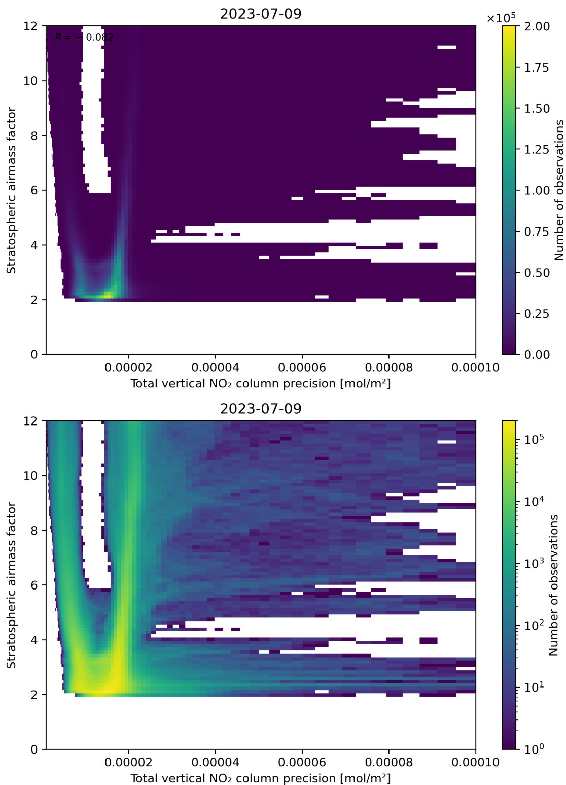
Figure 115: Scatter density plot of “Total vertical NO 2 column precision” against “Stratospheric airmass factor” for 2023-07-08 to 2023-07-10.
