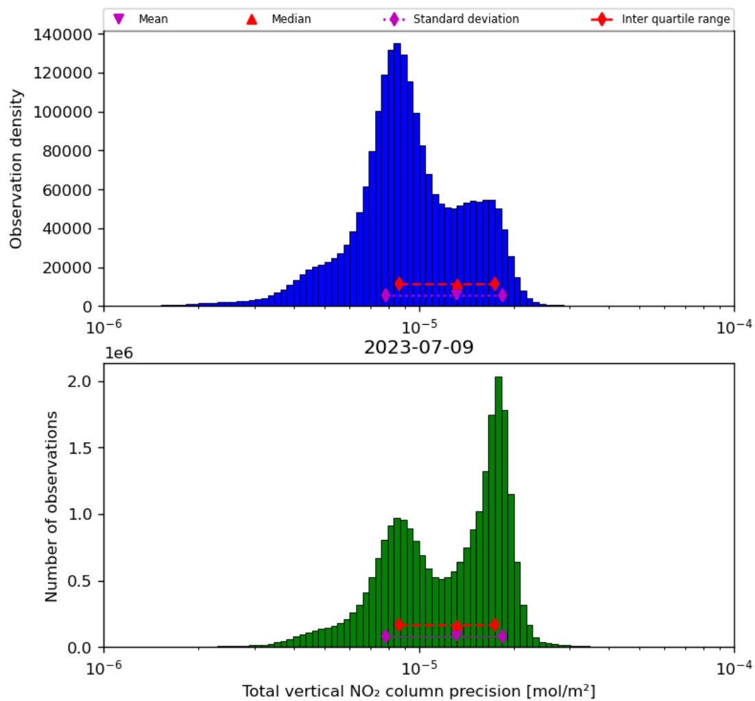
Figure 39: Histogram of “Total vertical NO 2 column precision” for 2023-07-08 to 2023-07-10
