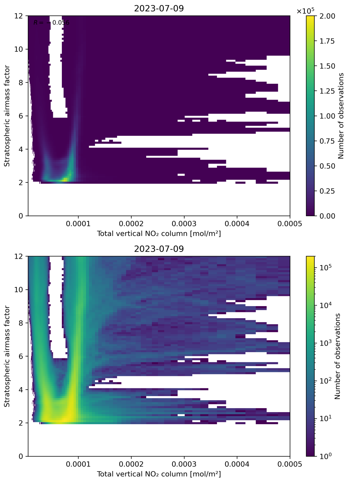
Figure 110: Scatter density plot of “Total vertical NO 2 column” against “Stratospheric air mass factor” for 2023-07-08 to 2023-07-10.
