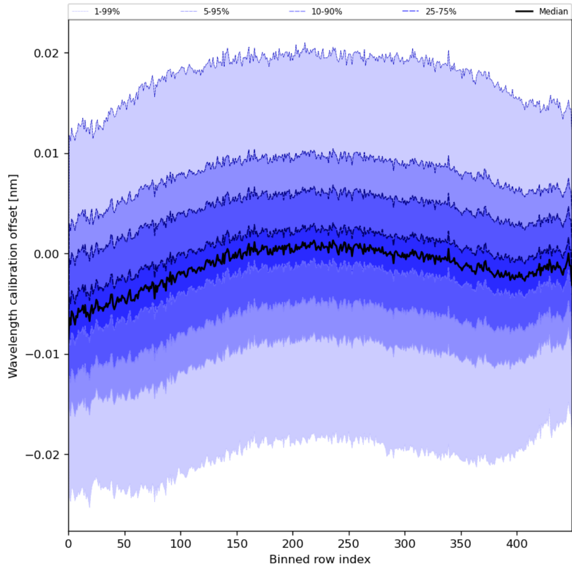
Figure 52: Along track statistics of “Wavelength calibration offset” for 2023-07-08 to 2023-07-10
