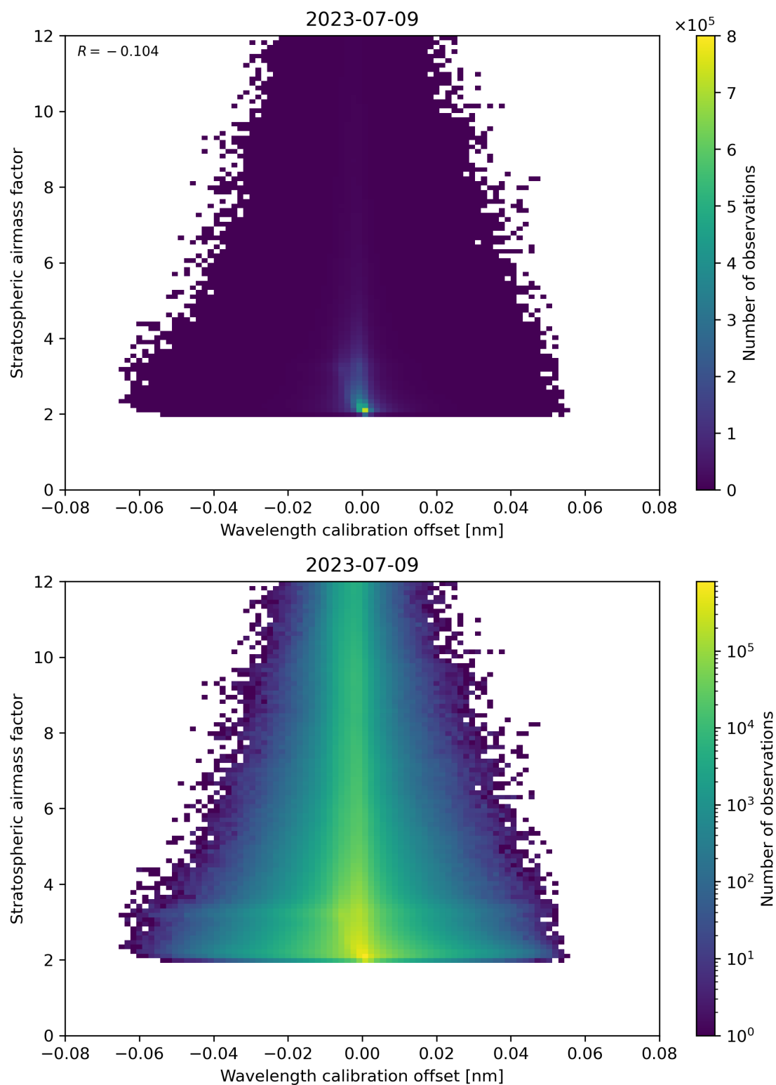
Figure 174: Scatter density plot of “Wavelength calibration offset” against “Stratospheric airmass factor” for 2023-07-08 to 2023-07-10.
