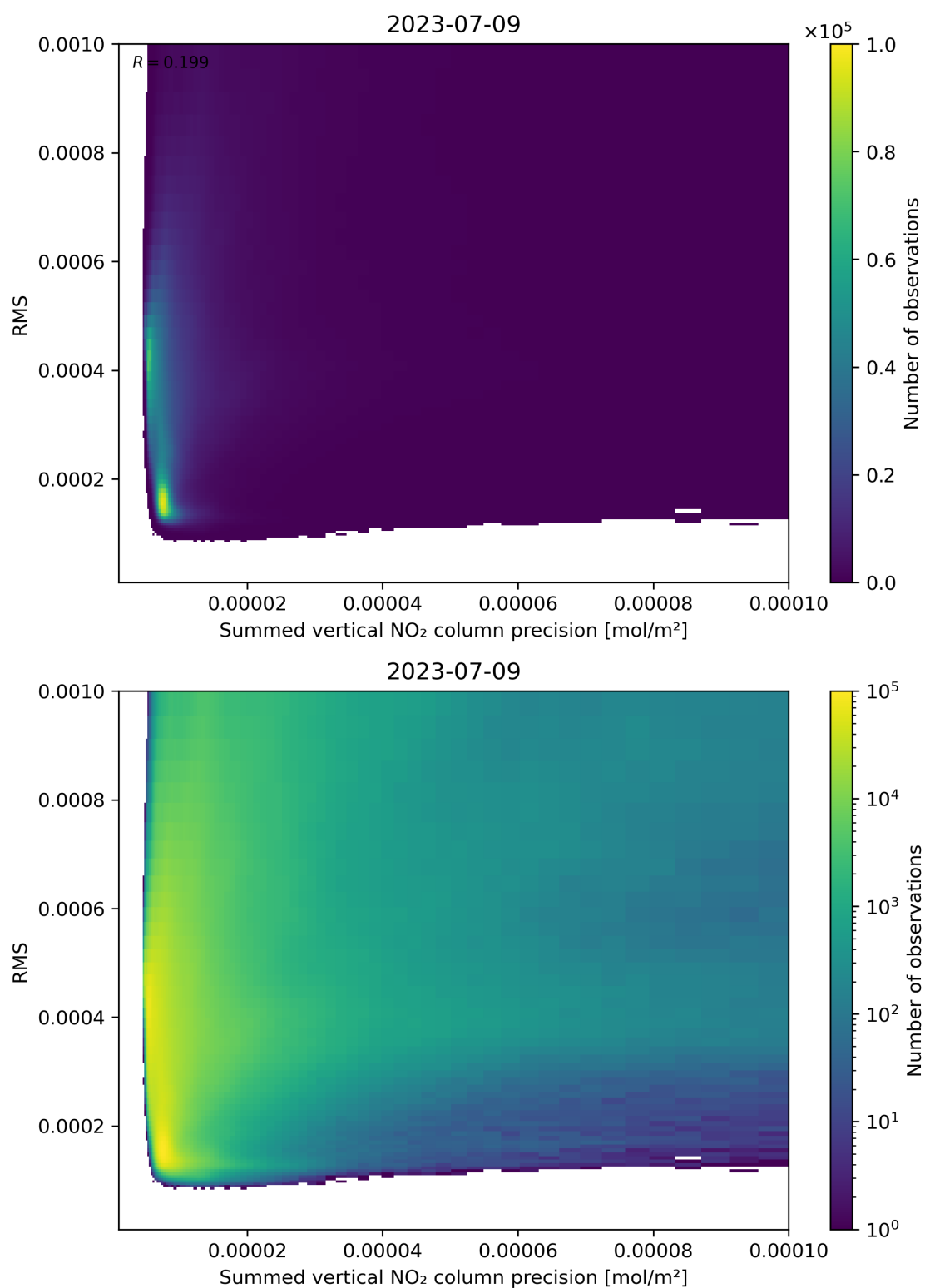
Figure 108: Scatter density plot of “Summed vertical NO 2 column precision” against “RMS” for 2023-07-08 to 2023-07-10.
