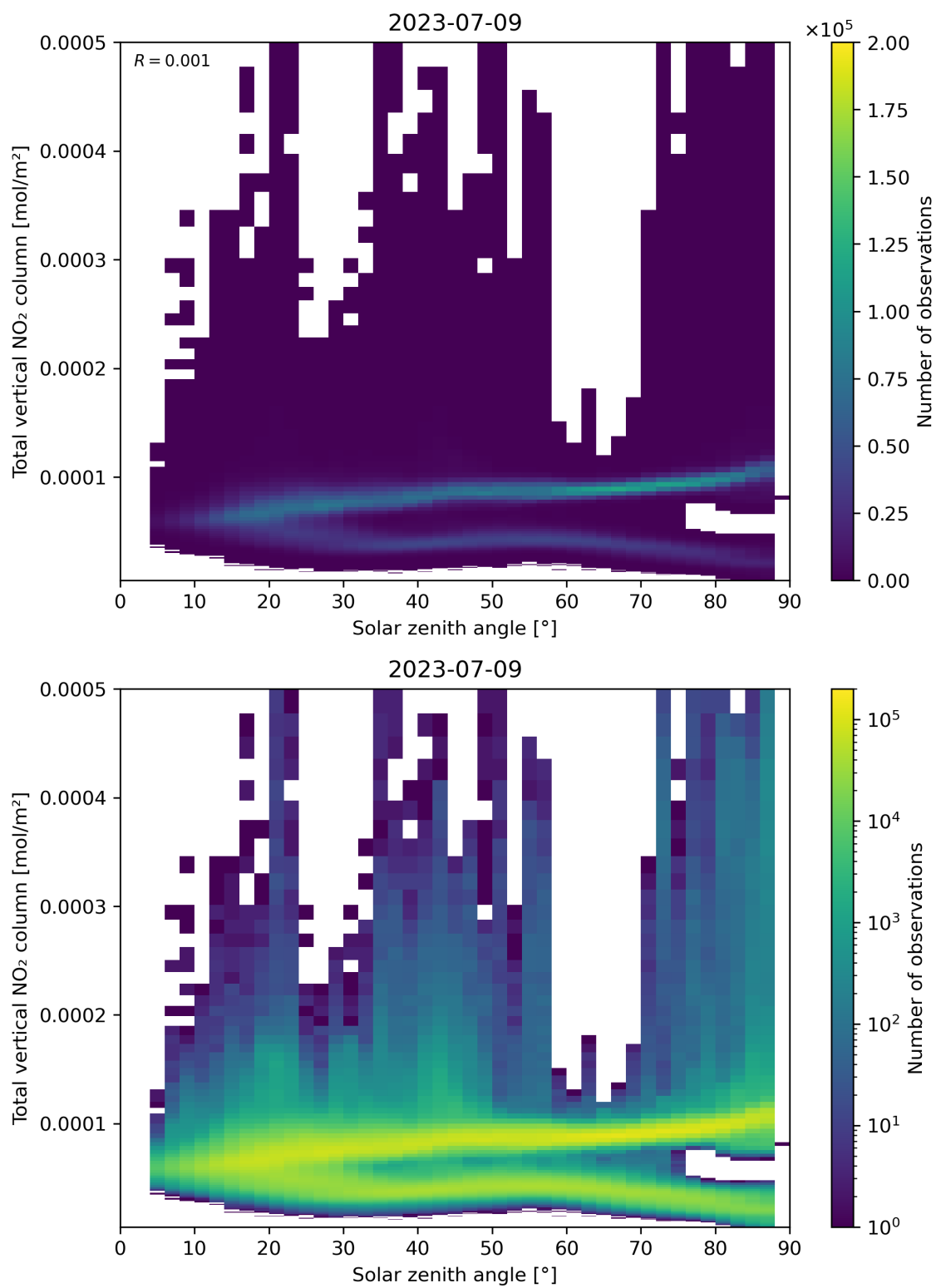
Figure 153: Scatter density plot of “Solar zenith angle” against “Total vertical NO 2 column” for 2023-07-08 to 2023-07-10.
