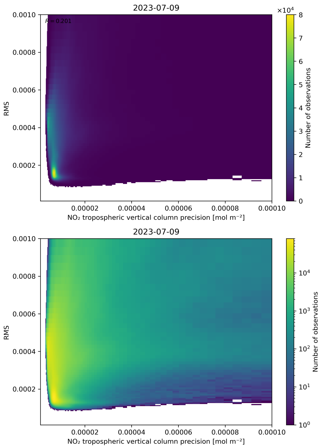
Figure 140: Scatter density plot of “NO 2 tropospheric vertical column precision” against “RMS” for 2023-07-08 to 2023-07-10.
