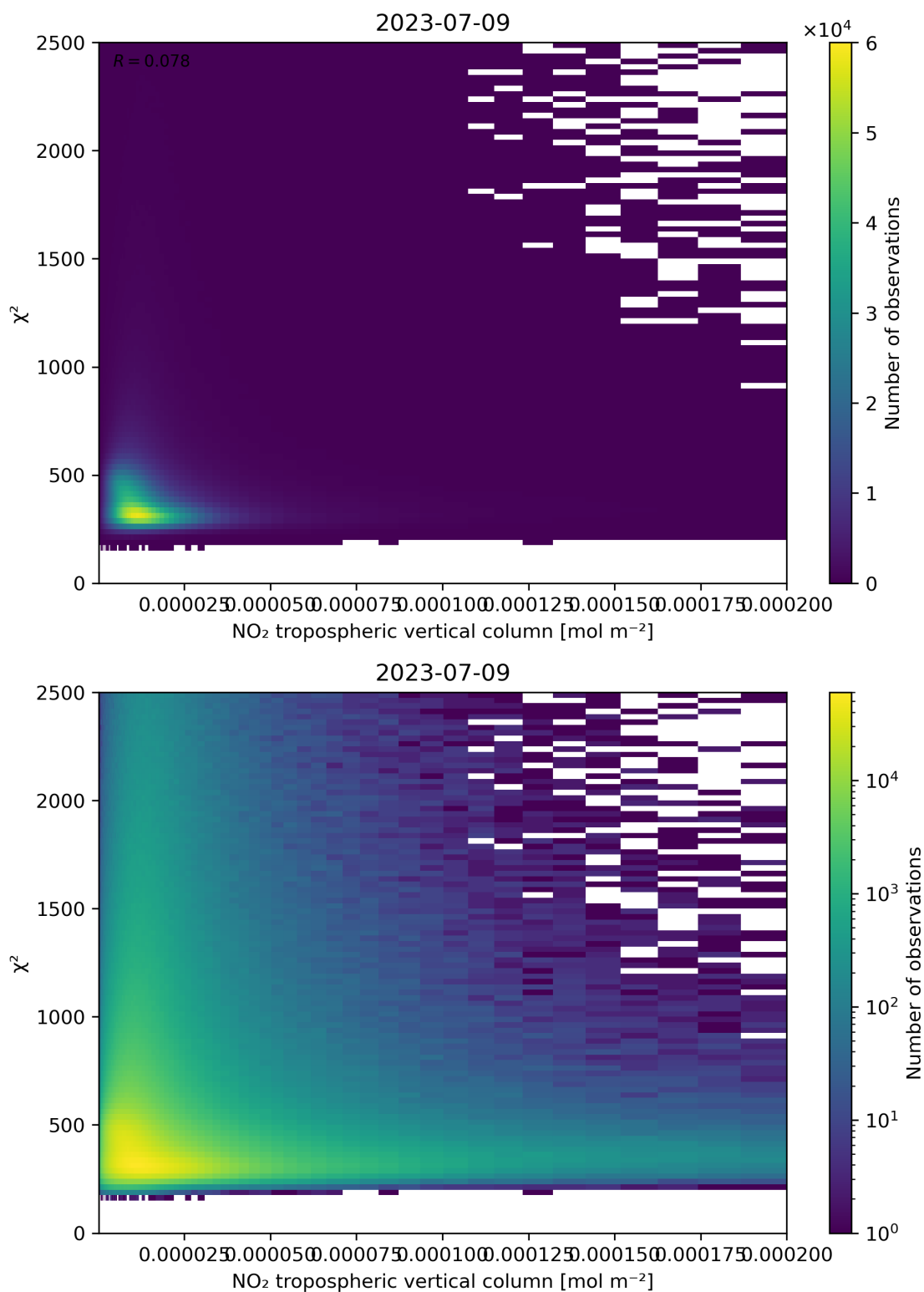
Figure 124: Scatter density plot of “NO 2 tropospheric vertical column” against “ \chi^2 ” for 2023-07-08 to 2023-07-10.
