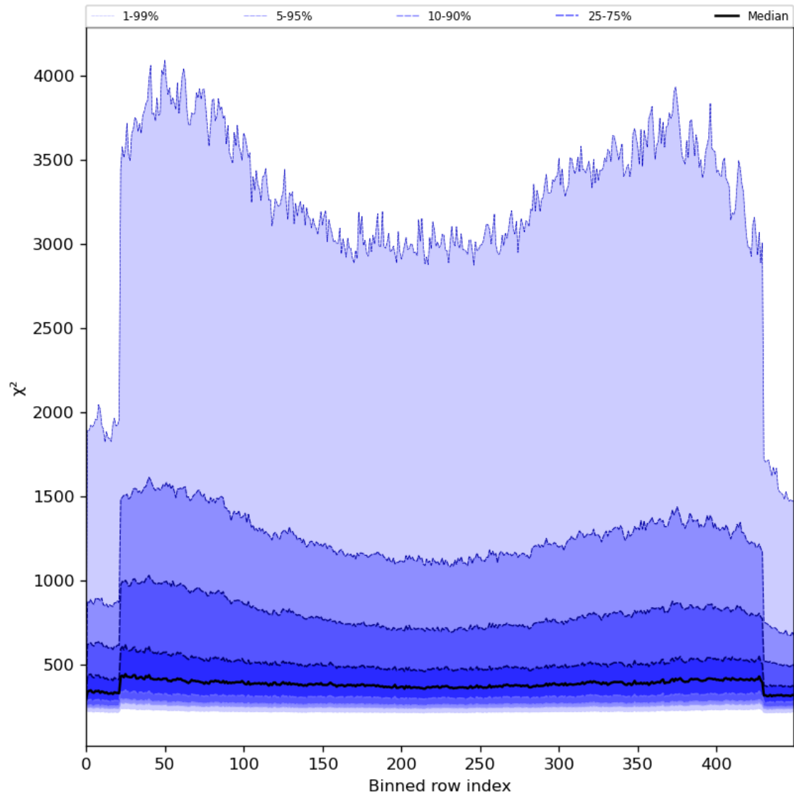
Figure 59: Along track statistics of “ \chi^2 ” for 2023-07-08 to 2023-07-10
