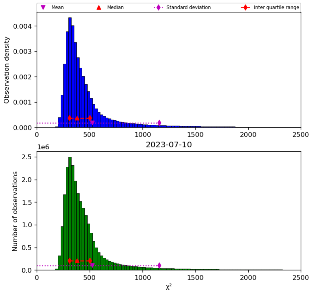
Figure 42: Histogram of “ \chi^2 ” for 2023-07-09 to 2023-07-11
