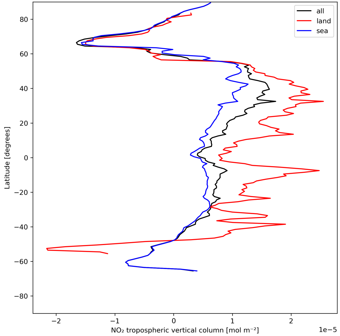
Figure 12: Zonal average of “NO 2 tropospheric vertical column” for 2023-07-09 to 2023-07-11.
