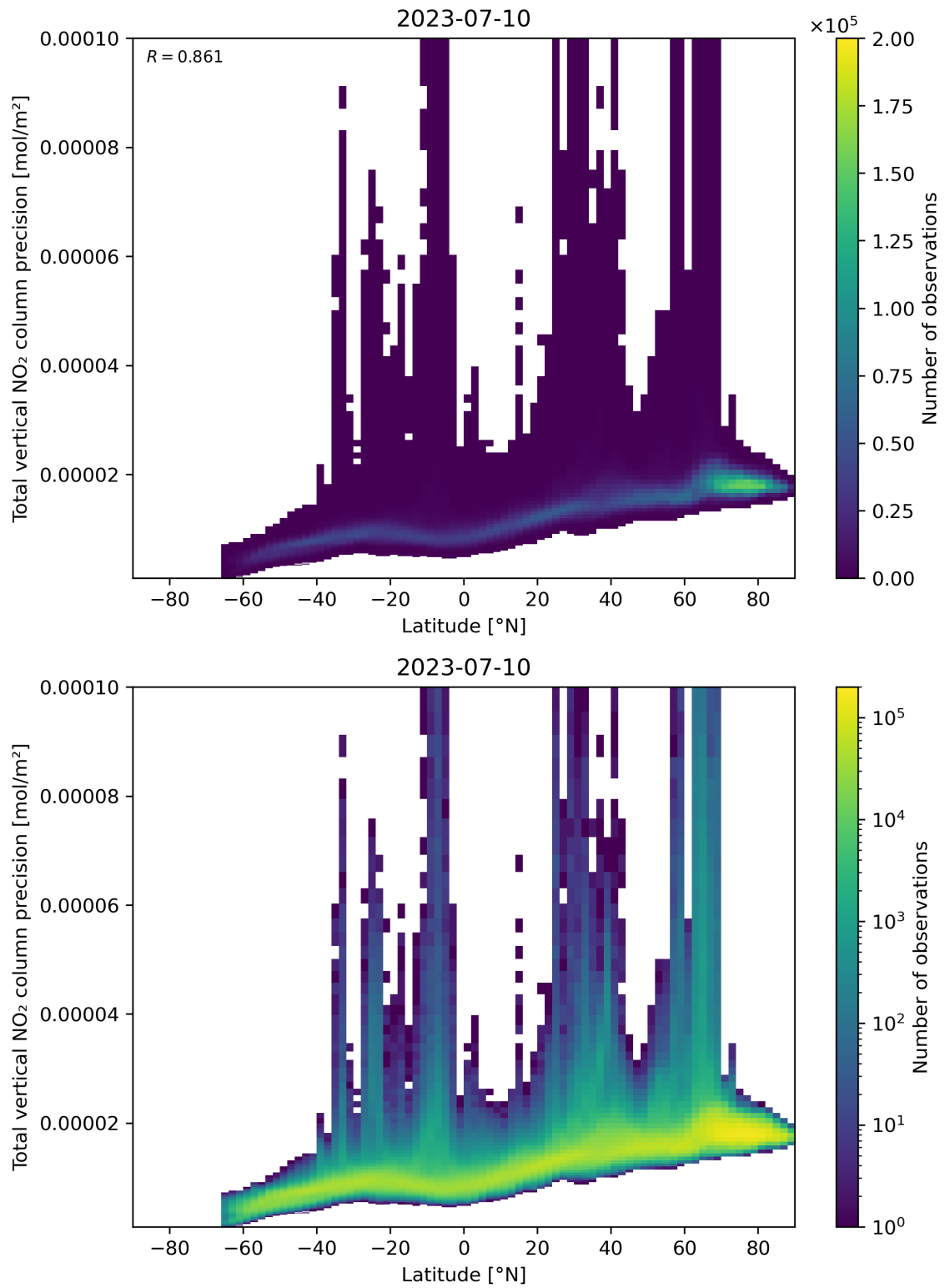
Figure 91: Scatter density plot of “Latitude” against “Total vertical NO 2 column precision” for 2023-07-09 to 2023-07-11.
