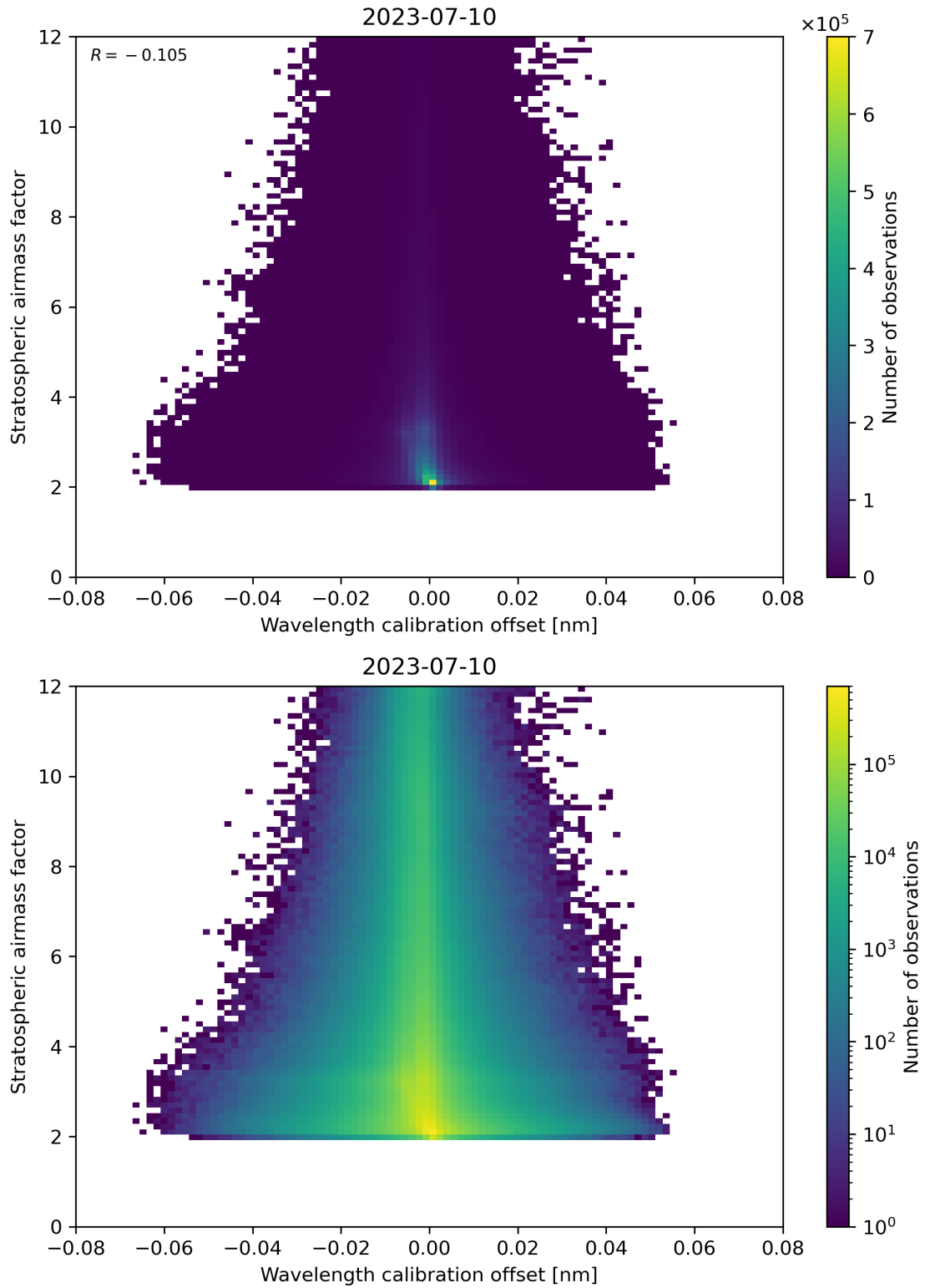
Figure 174: Scatter density plot of “Wavelength calibration offset” against “Stratospheric airmass factor” for 2023-07-09 to 2023-07-11.
