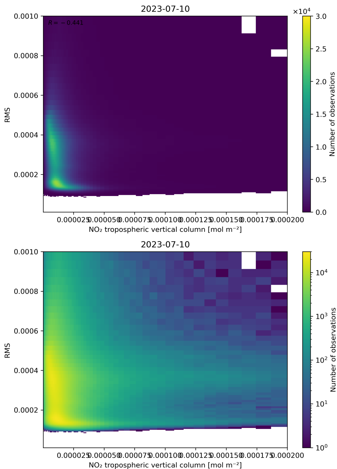
Figure 142: Scatter density plot of “NO 2 tropospheric vertical column” against “RMS” for 2023-07-09 to 2023-07-11.
