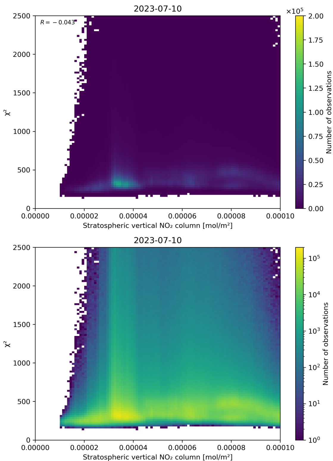
Figure 97: Scatter density plot of “Stratospheric vertical NO 2 column” against “ \chi^2 ” for 2023-07-09 to 2023-07-11.
