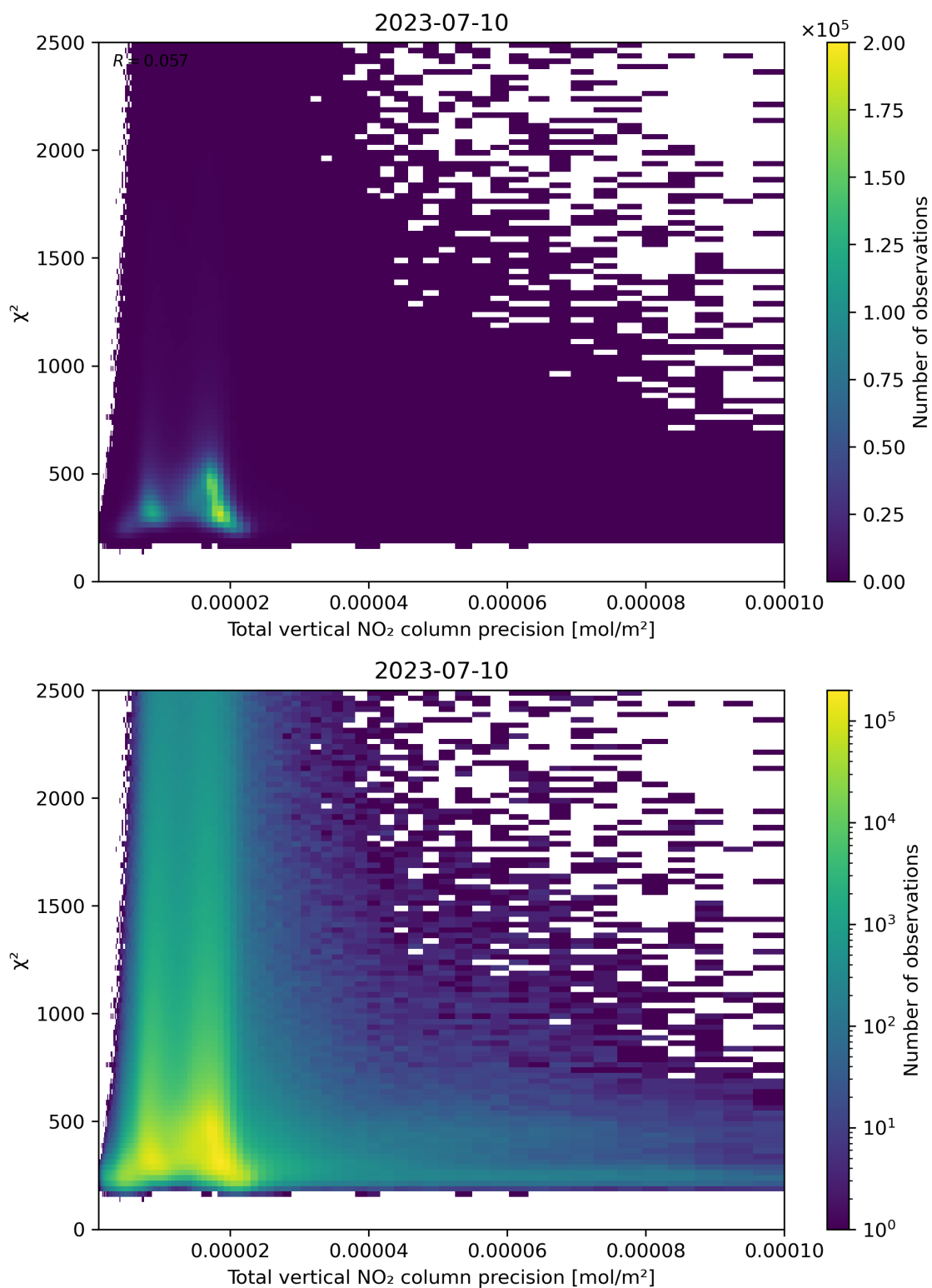
Figure 116: Scatter density plot of “Total vertical NO 2 column precision” against “ \chi^2 ” for 2023-07-09 to 2023-07-11.
