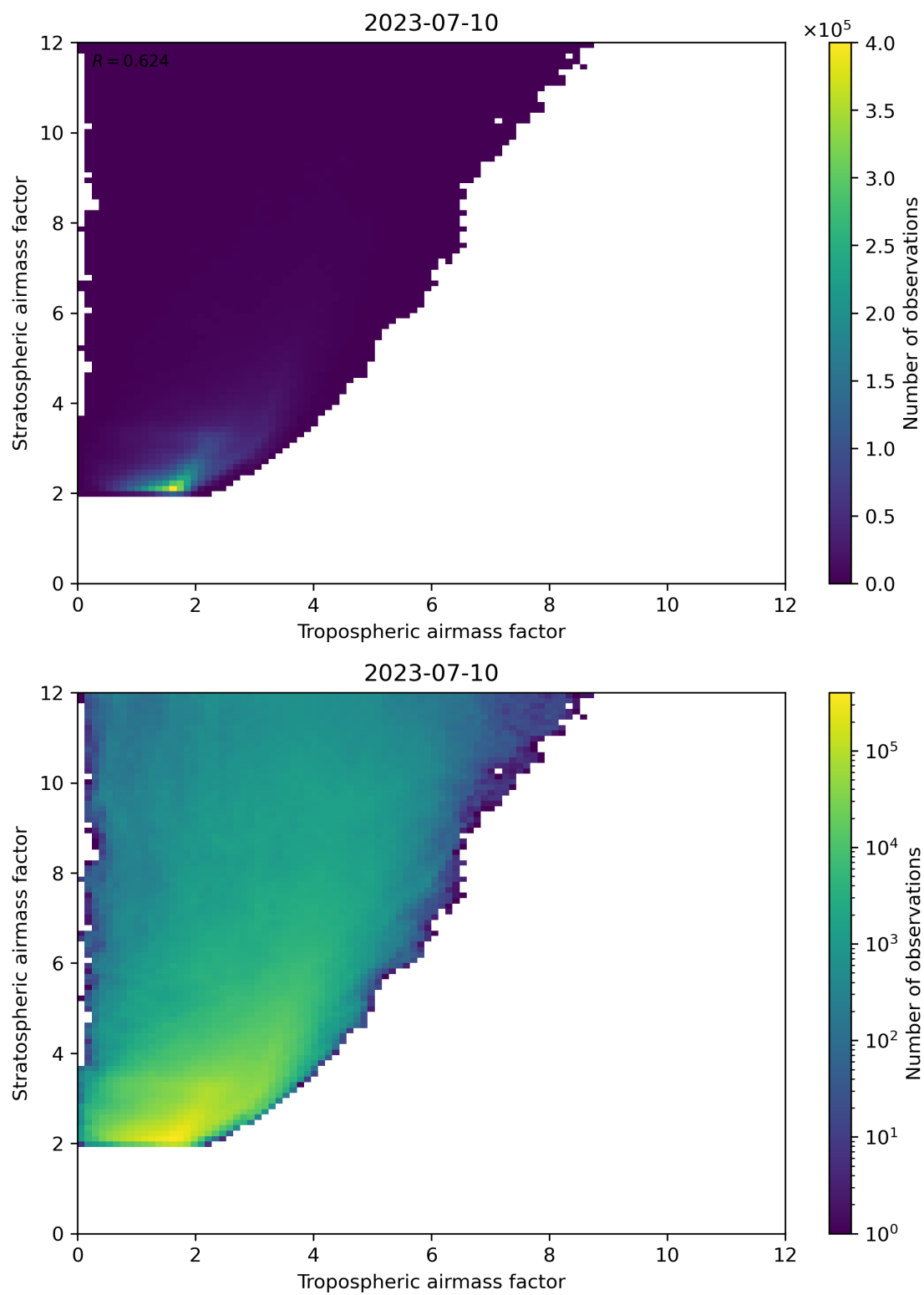
Figure 71: Scatter density plot of “Tropospheric airmass factor” against “Stratospheric airmass factor” for 2023-07-09 to 2023-07-11.
