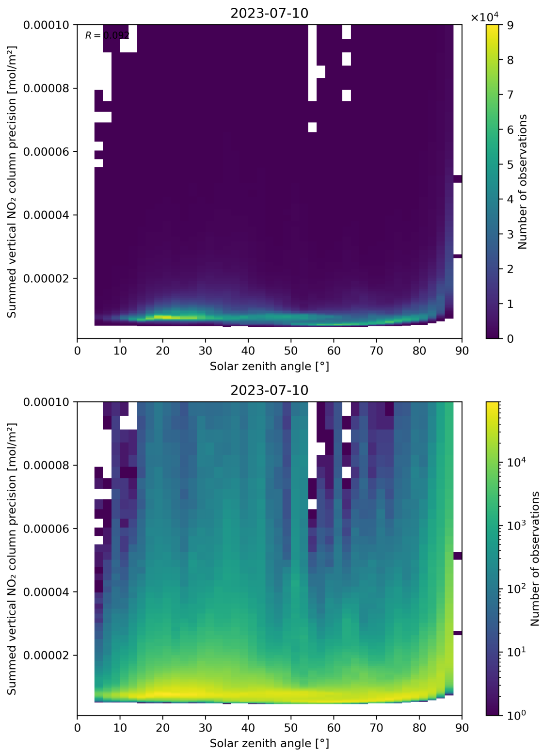
Figure 152: Scatter density plot of “Solar zenith angle” against “Summed vertical NO 2 column precision” for 2023-07-09 to 2023-07-11.
