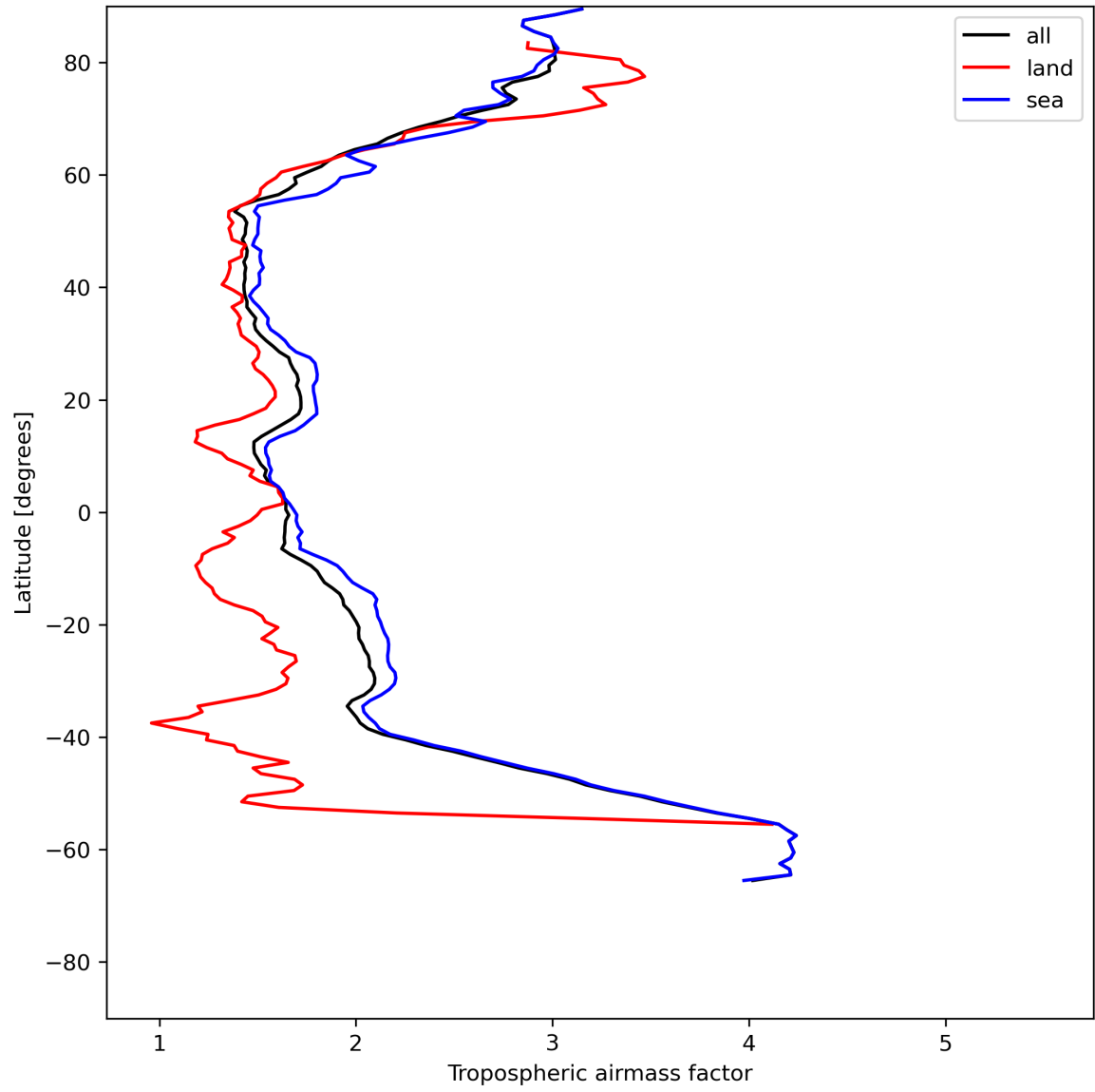
Figure 14: Zonal average of “Tropospheric airmass factor” for 2023-07-09 to 2023-07-11.
