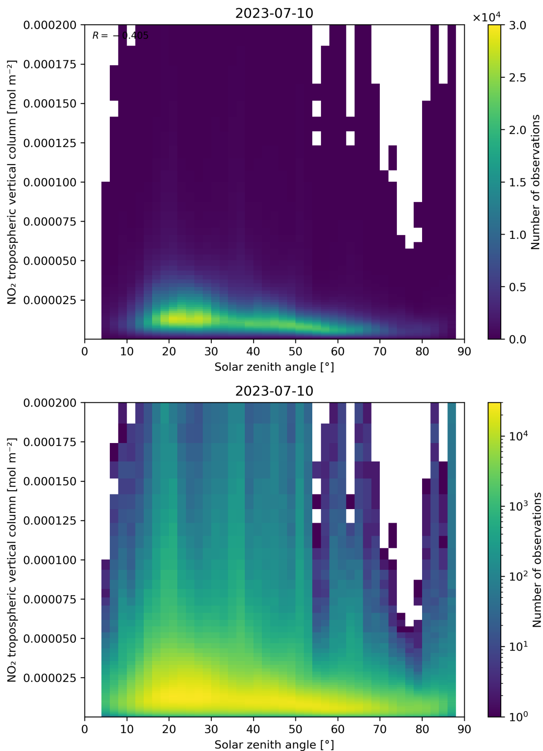
Figure 155: Scatter density plot of “Solar zenith angle” against “NO 2 tropospheric vertical column” for 2023-07-09 to 2023-07-11.
