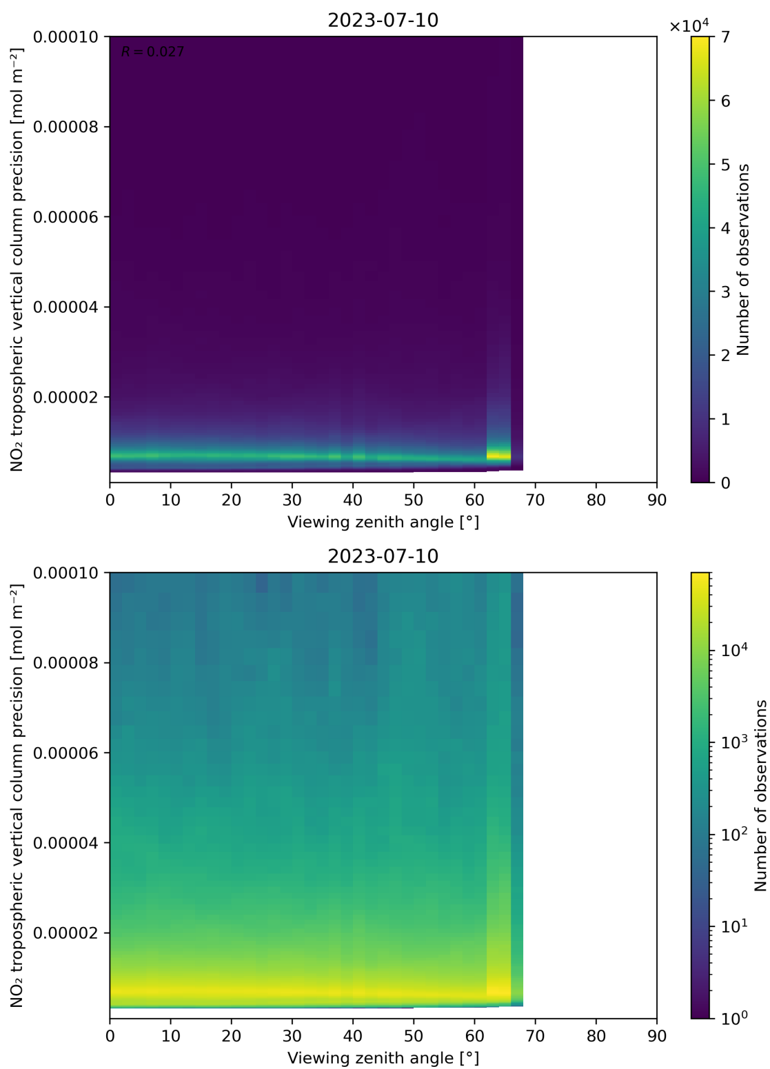
Figure 170: Scatter density plot of “Viewing zenith angle” against “NO 2 tropospheric vertical column precision” for 2023-07-09 to 2023-07-11.
