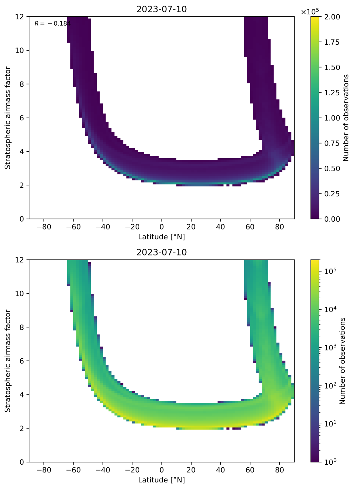
Figure 83: Scatter density plot of “Latitude” against “Stratospheric air mass factor” for 2023-07-09 to 2023-07-11.
