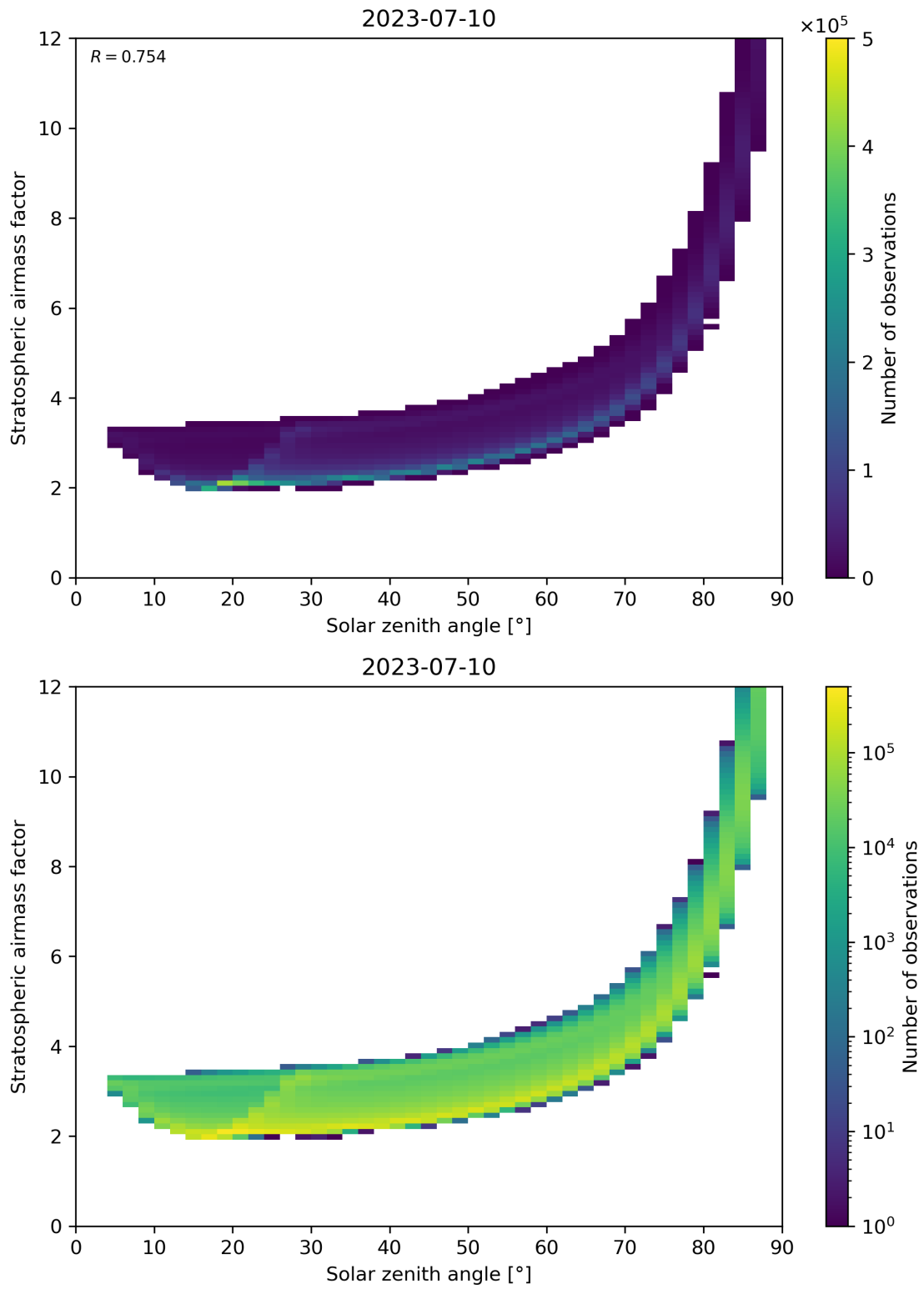
Figure 145: Scatter density plot of “Solar zenith angle” against “Stratospheric airmass factor” for 2023-07-09 to 2023-07-11.
