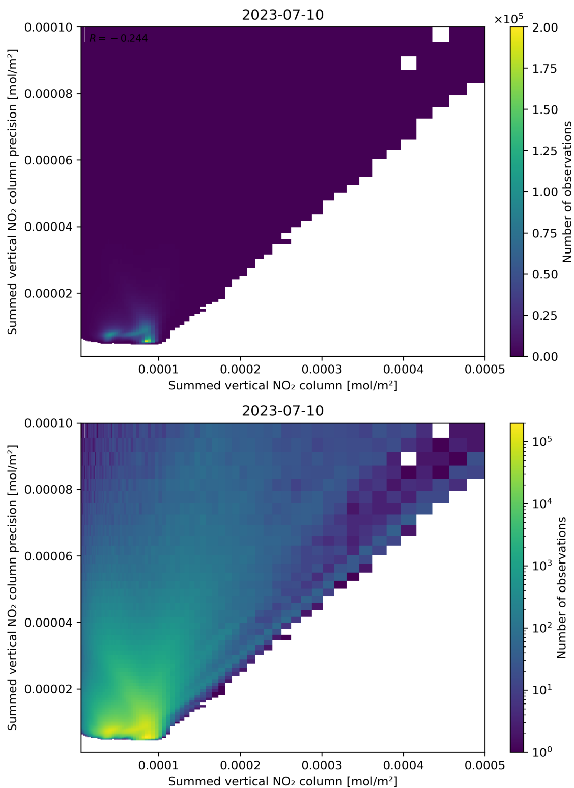
Figure 105: Scatter density plot of “Summed vertical NO 2 column” against “Summed vertical NO 2 column precision” for 2023-07-09 to 2023-07-11.
