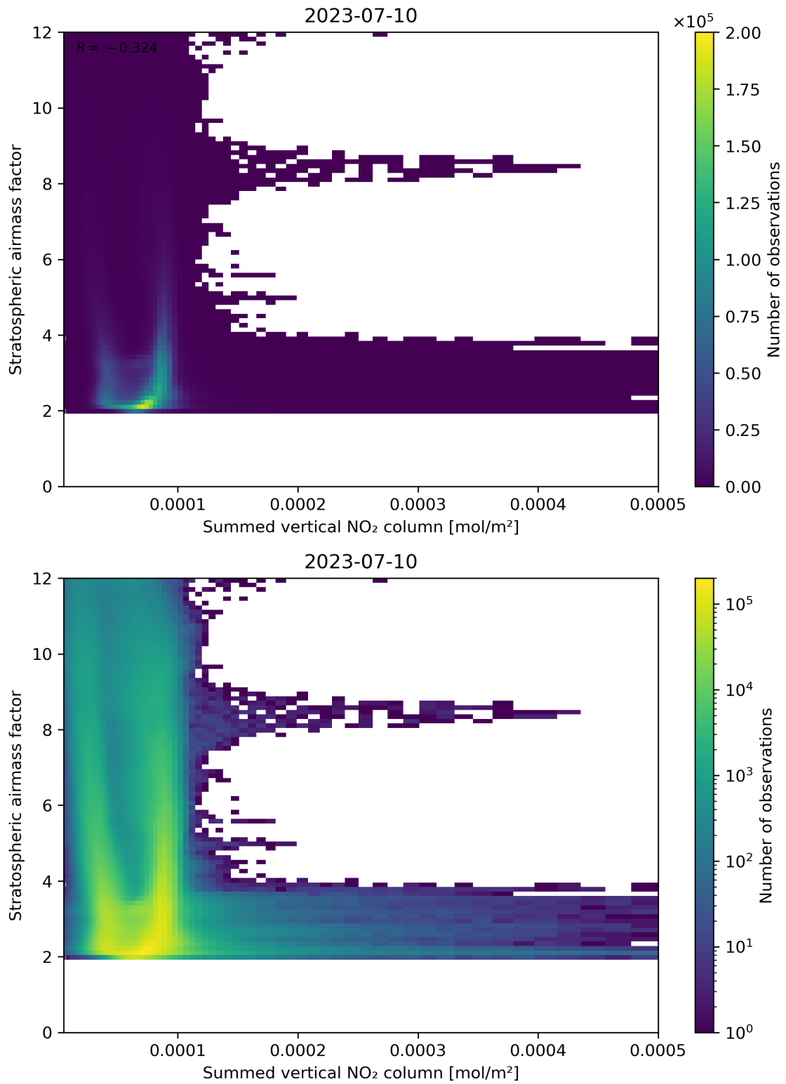
Figure 103: Scatter density plot of “Summed vertical NO 2 column” against “Stratospheric air mass factor” for 2023-07-09 to 2023-07-11.
