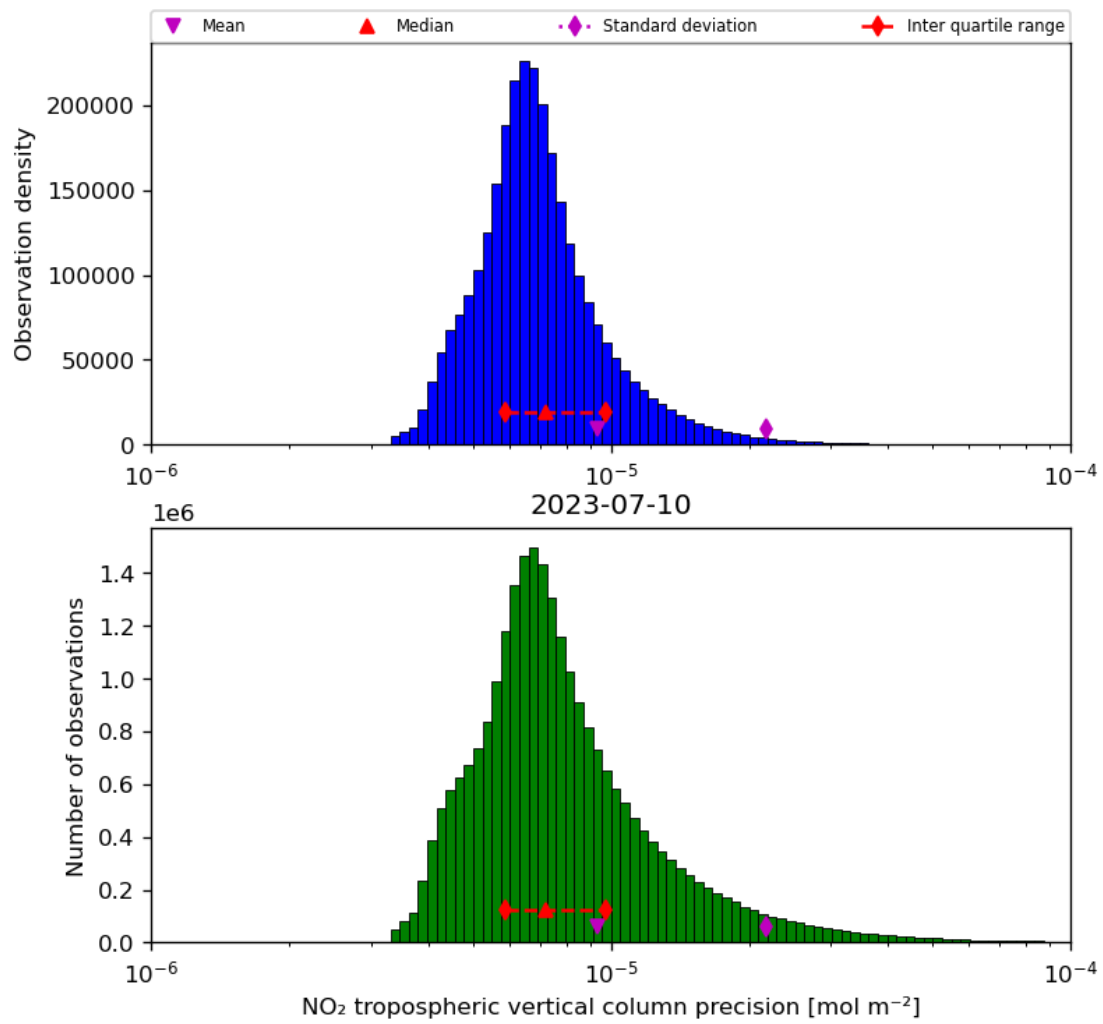
Figure 30: Histogram of “NO 2 tropospheric vertical column precision” for 2023-07-09 to 2023-07-11
