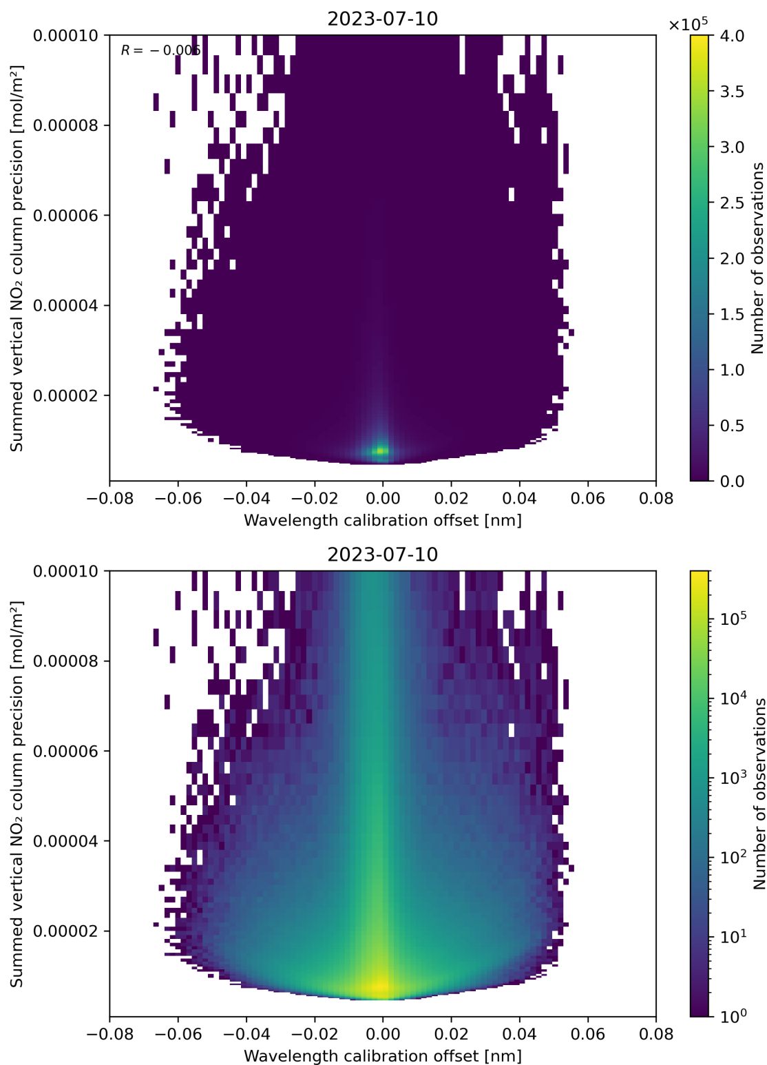
Figure 178: Scatter density plot of “Wavelength calibration offset” against “Summed vertical NO 2 column precision” for 2023-07-09 to 2023-07-11.
