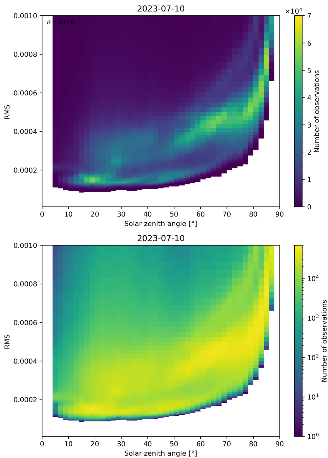
Figure 157: Scatter density plot of “Solar zenith angle” against “RMS” for 2023-07-09 to 2023-07-11.
