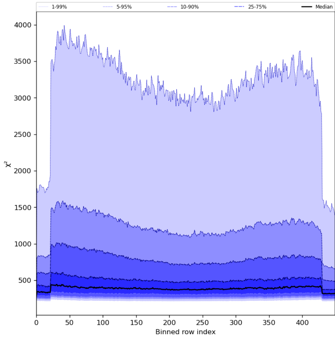
Figure 59: Along track statistics of “ \chi^2 ” for 2023-07-09 to 2023-07-11
