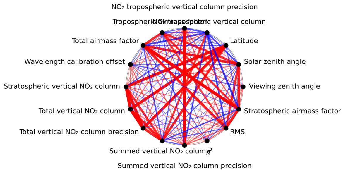
Figure 1: Map of correlation graph for 2023-07-09 to 2023-07-11.
