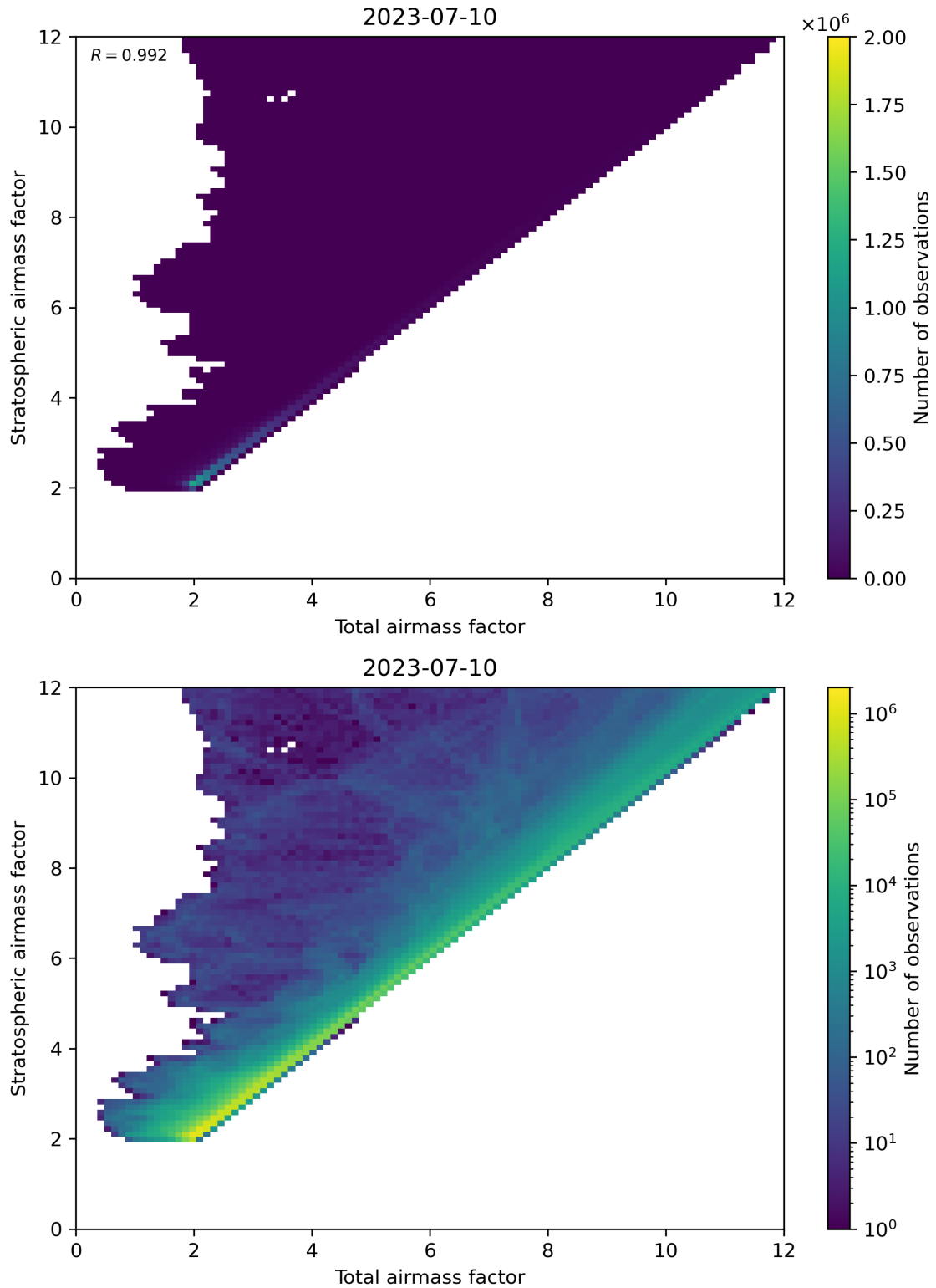
Figure 62: Scatter density plot of “Total airmass factor” against “Stratospheric airmass factor” for 2023-07-09 to 2023-07-11.
