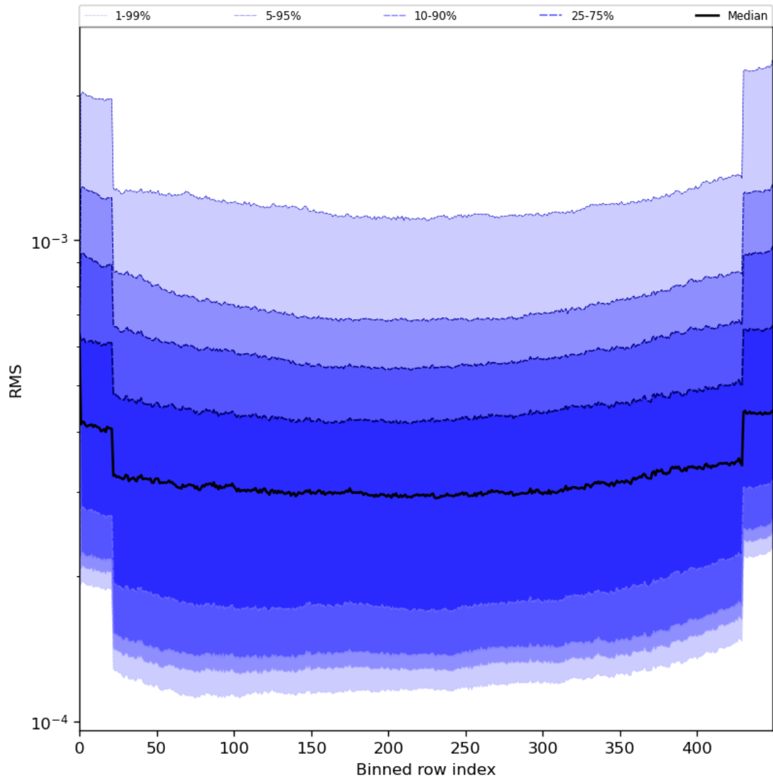
Figure 60: Along track statistics of “RMS” for 2023-07-09 to 2023-07-11
