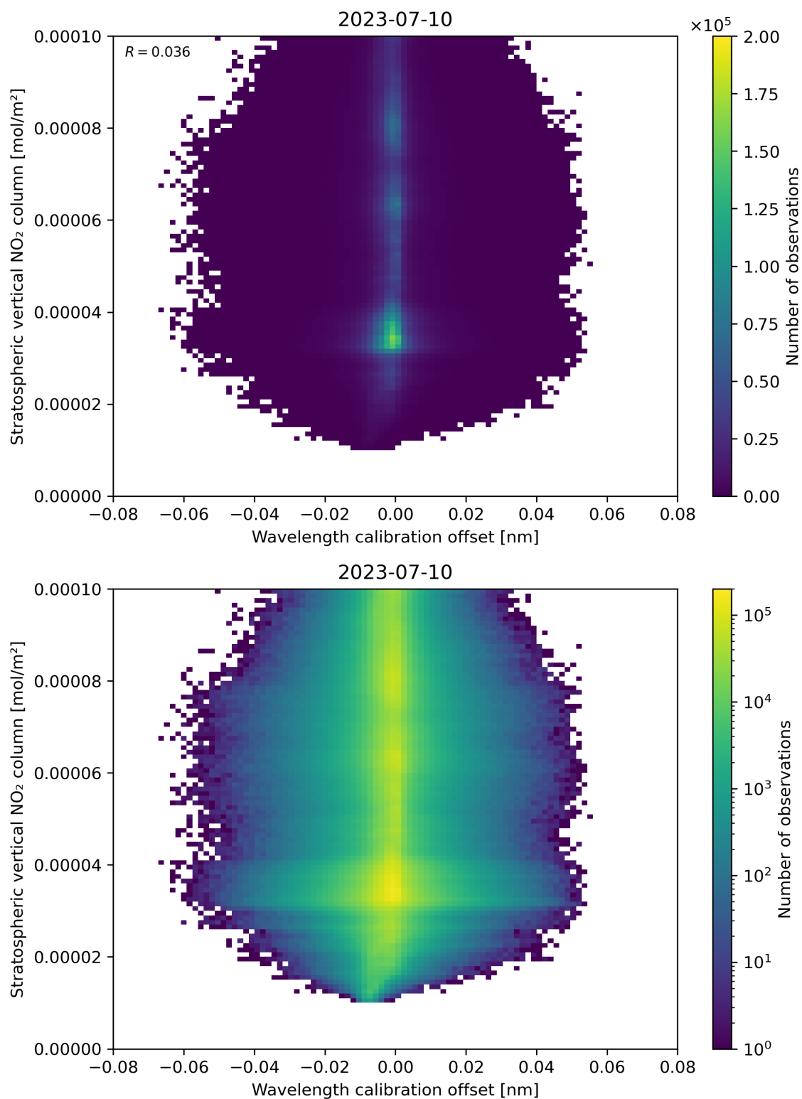
Figure 176: Scatter density plot of “Wavelength calibration offset” against “Stratospheric vertical NO 2 column” for 2023-07-09 to 2023-07-11.
