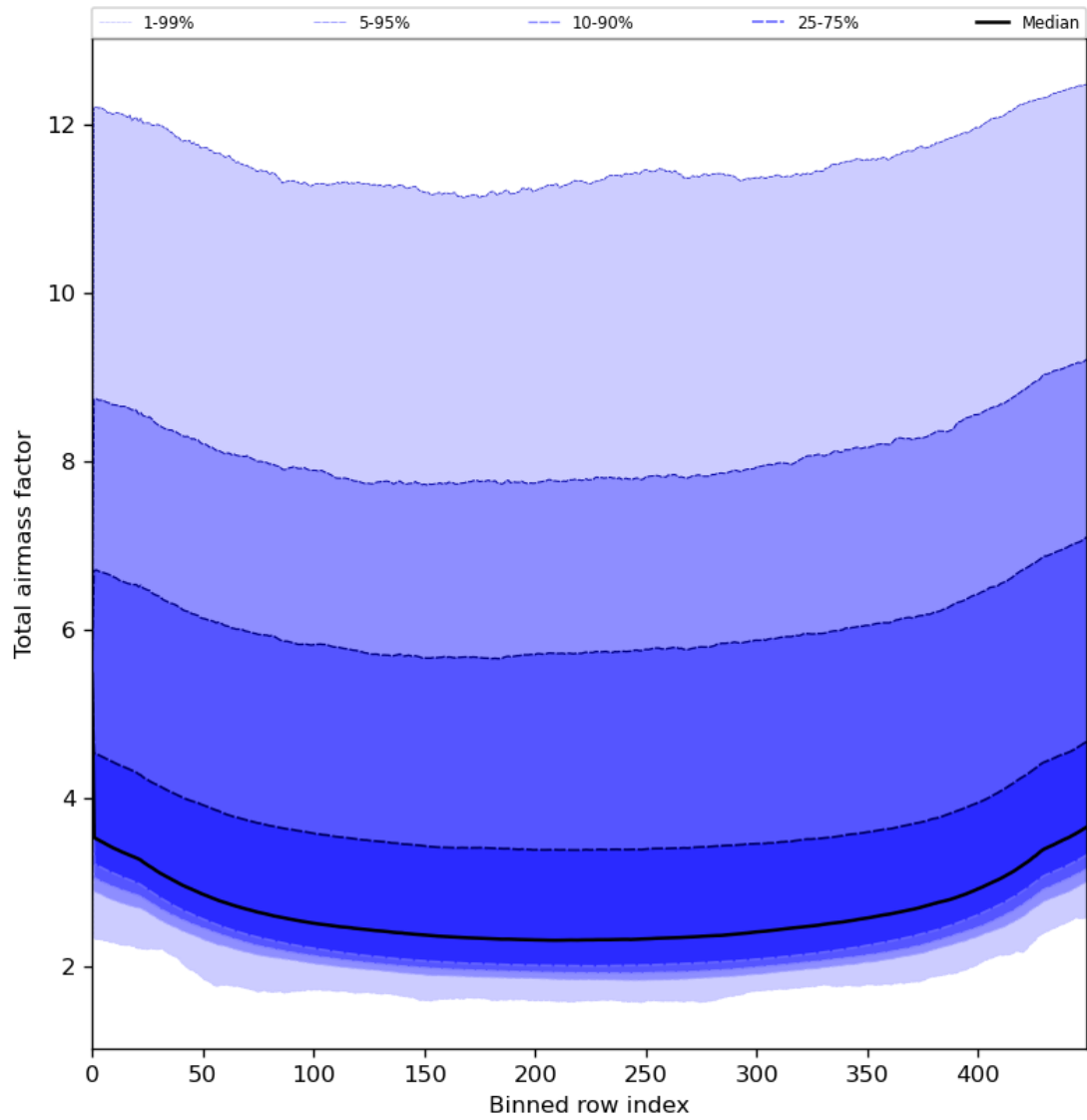
Figure 49: Along track statistics of “Total airmass factor” for 2023-07-09 to 2023-07-11
