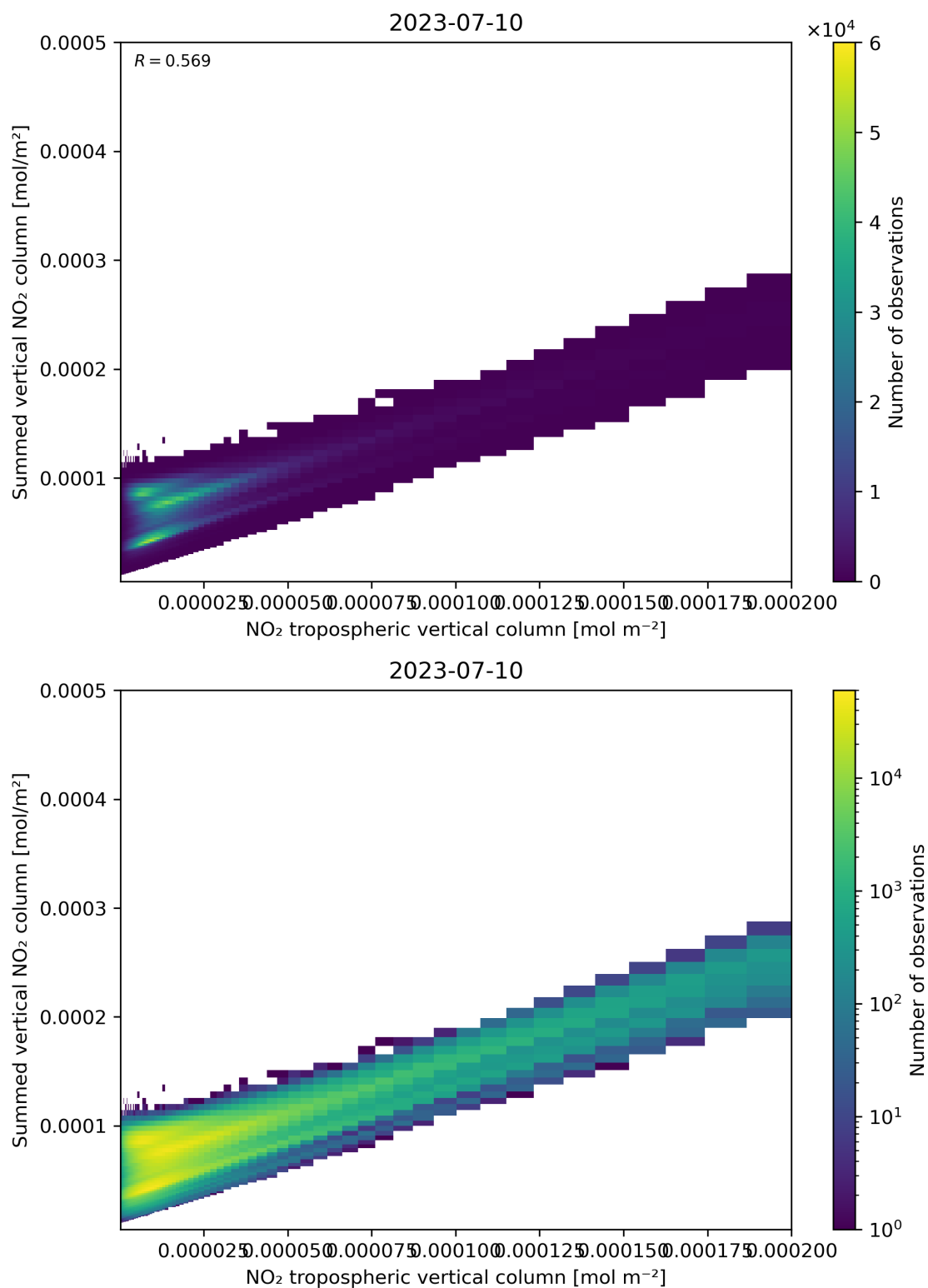
Figure 126: Scatter density plot of “NO 2 tropospheric vertical column” against “Summed vertical NO 2 column” for 2023-07-09 to 2023-07-11.
