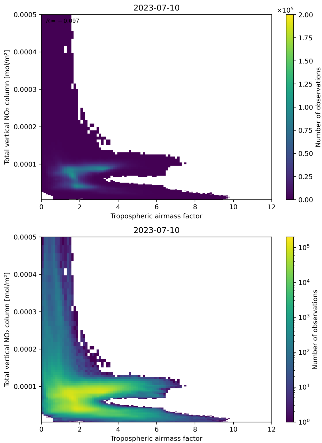
Figure 77: Scatter density plot of “Tropospheric airmass factor” against “Total vertical NO 2 column” for 2023-07-09 to 2023-07-11.
