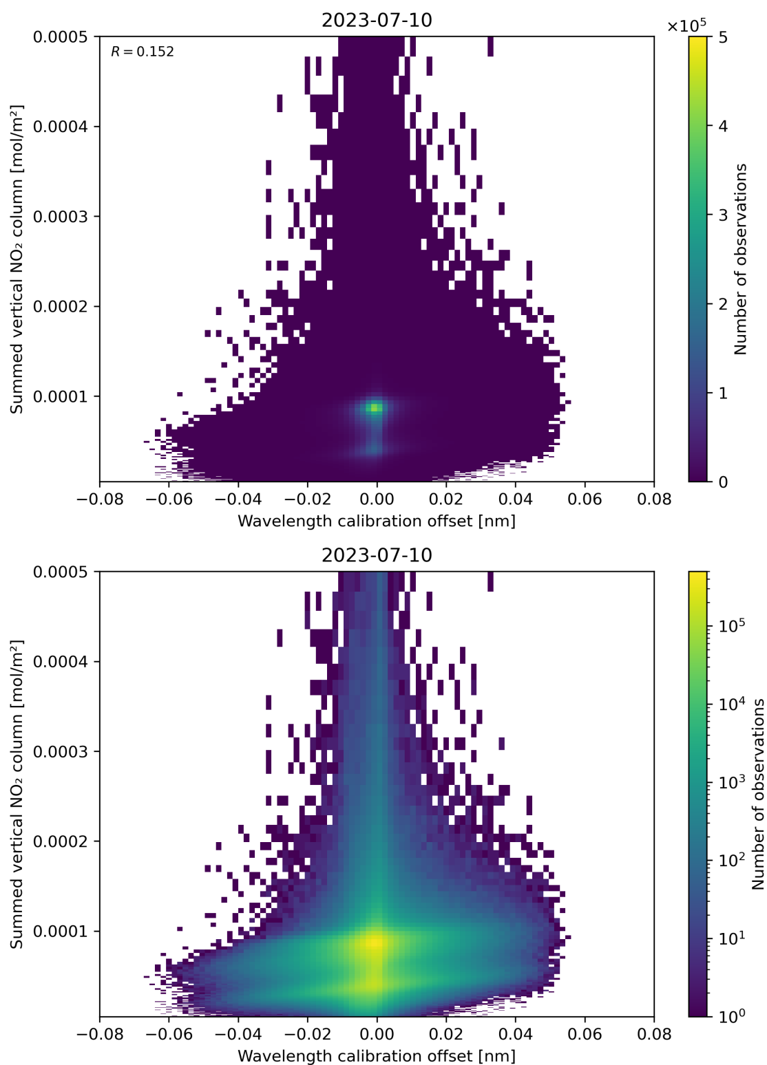
Figure 177: Scatter density plot of “Wavelength calibration offset” against “Summed vertical NO 2 column” for 2023-07-09 to 2023-07-11.
