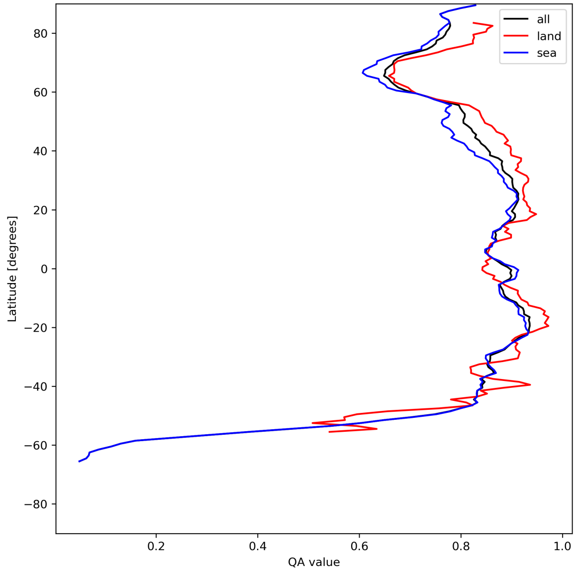
Figure 11: Zonal average of “QA value” for 2023-07-09 to 2023-07-11.
