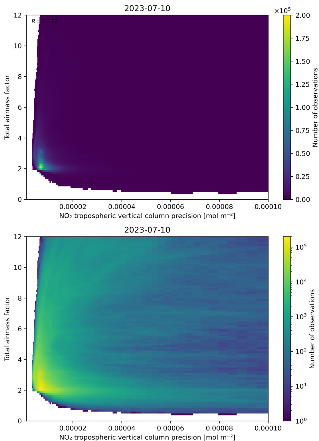
Figure 132: Scatter density plot of “NO 2 tropospheric vertical column precision” against “Total air mass factor” for 2023-07-09 to 2023-07-11.
