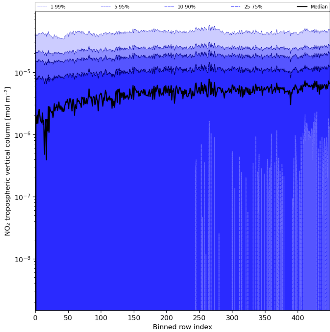
Figure 46: Along track statistics of “NO 2 tropospheric vertical column” for 2023-07-09 to 2023-07-11
