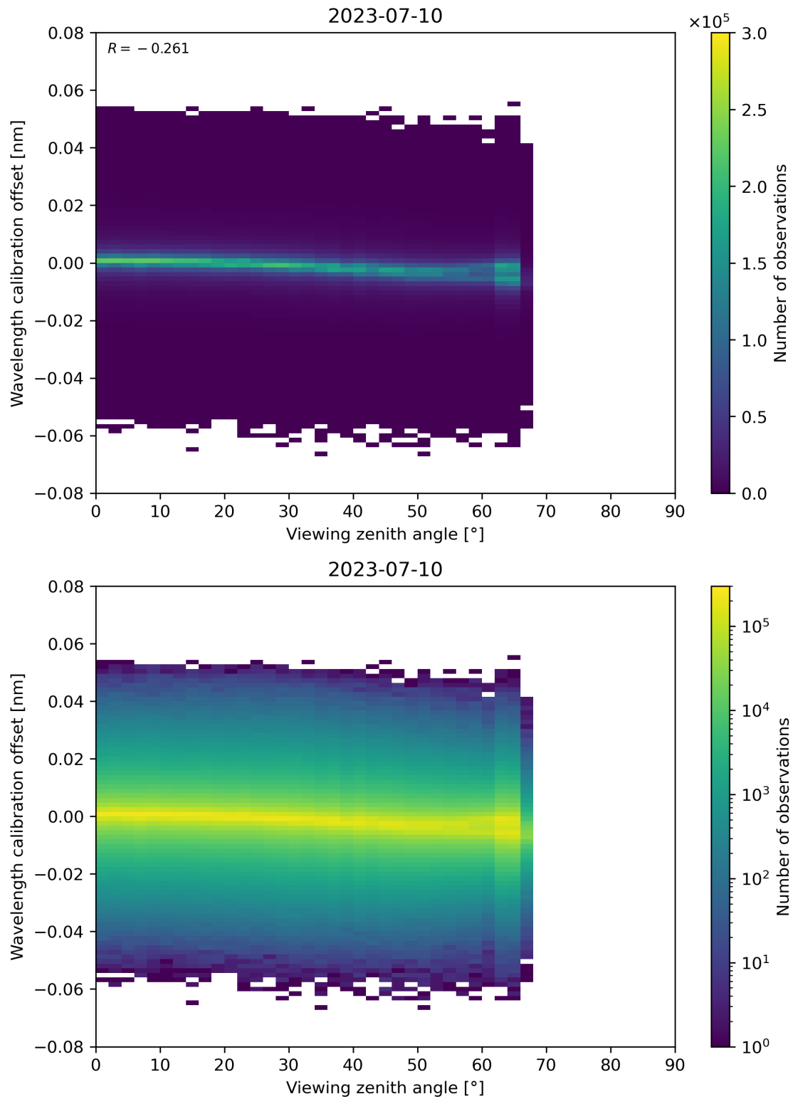
Figure 173: Scatter density plot of “Viewing zenith angle” against “Wavelength calibration offset” for 2023-07-09 to 2023-07-11.
