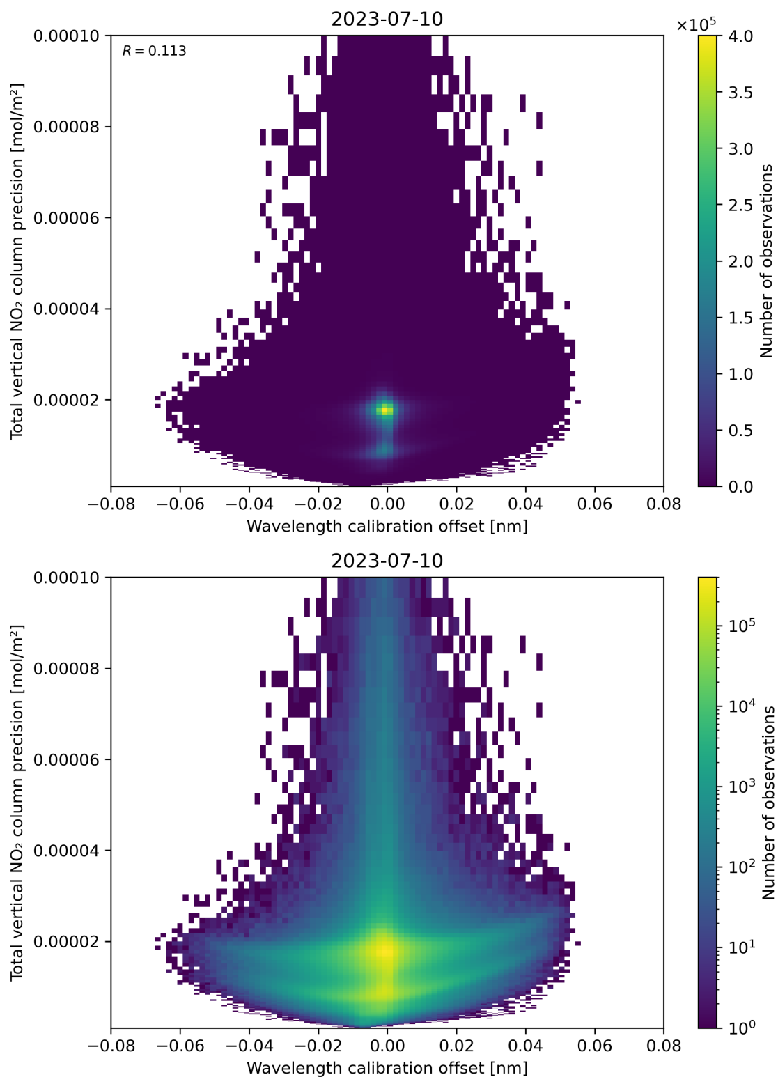
Figure 180: Scatter density plot of “Wavelength calibration offset” against “Total vertical NO 2 column precision” for 2023-07-09 to 2023-07-11.
