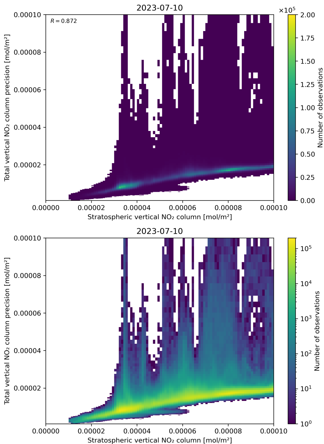
Figure 101: Scatter density plot of “Stratospheric vertical NO 2 column” against “Total vertical NO 2 column precision” for 2023-07-09 to 2023-07-11.
