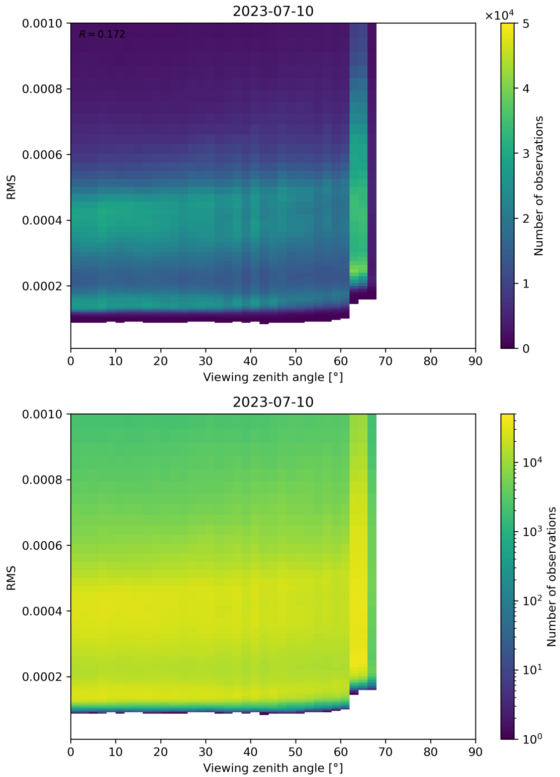
Figure 171: Scatter density plot of “Viewing zenith angle” against “RMS” for 2023-07-09 to 2023-07-11.
