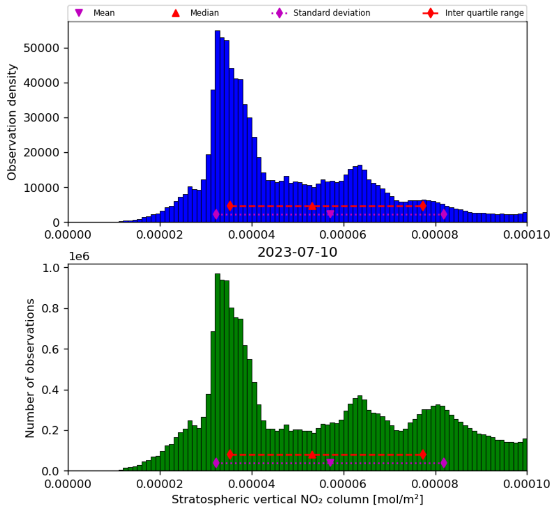
Figure 36: Histogram of “Stratospheric vertical NO 2 column” for 2023-07-09 to 2023-07-11
