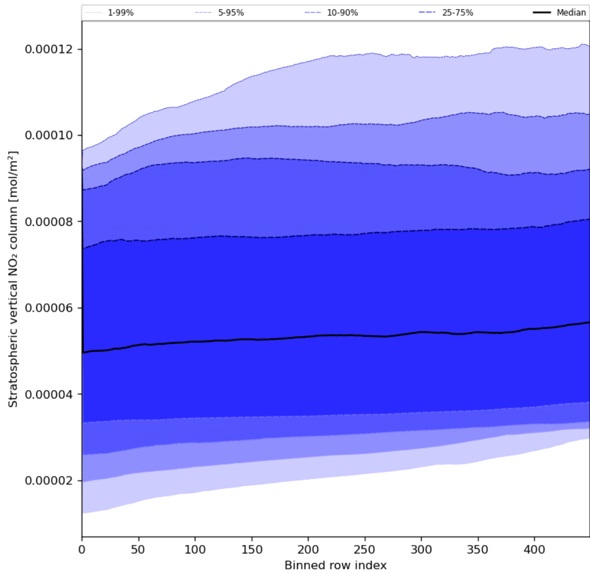
Figure 53: Along track statistics of “Stratospheric vertical NO 2 column” for 2023-07-09 to 2023-07-11
