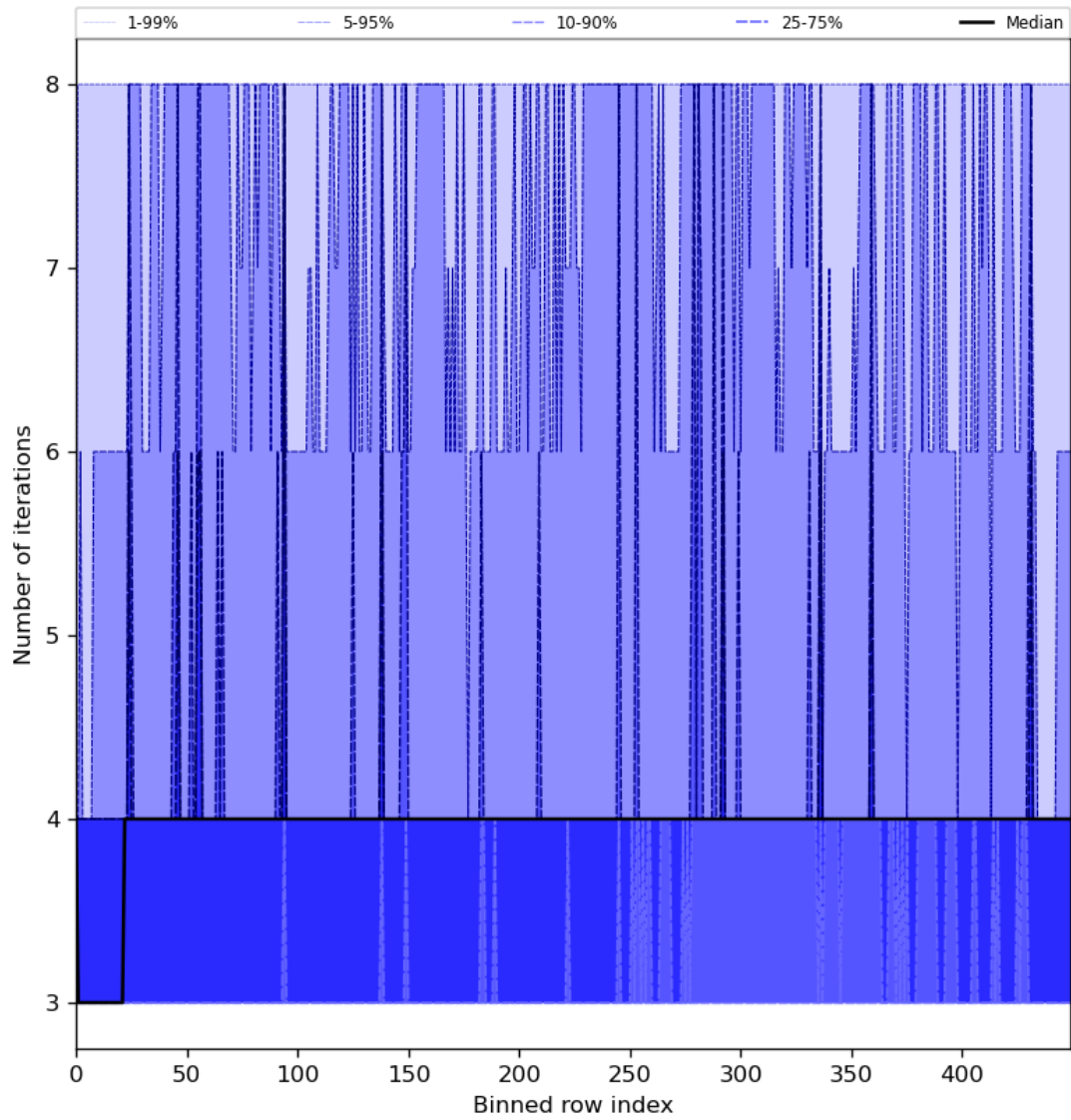
Figure 51: Along track statistics of “Number of iterations” for 2023-07-09 to 2023-07-11
