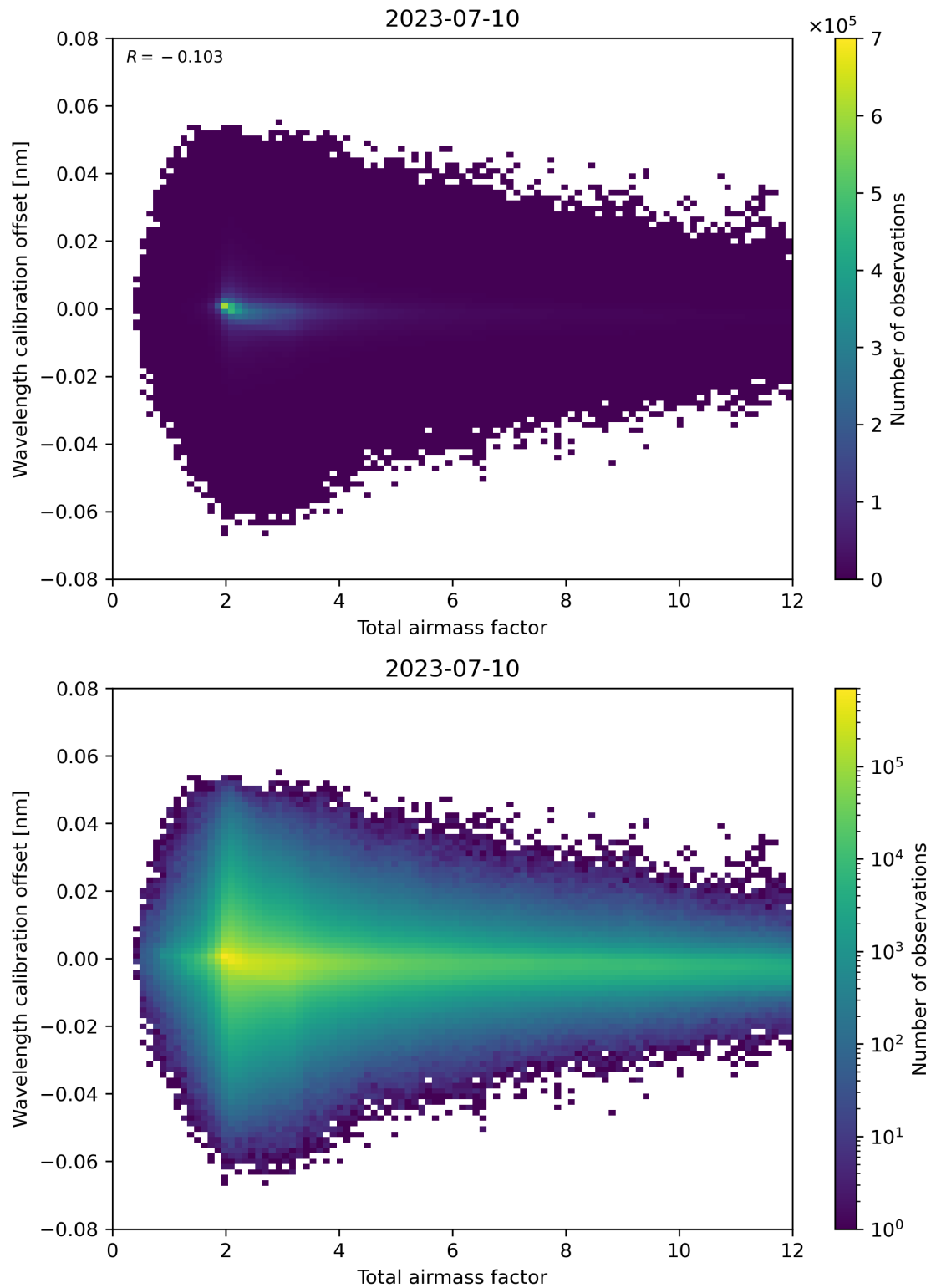
Figure 70: Scatter density plot of “Total airmass factor” against “Wavelength calibration offset” for 2023-07-09 to 2023-07-11.
