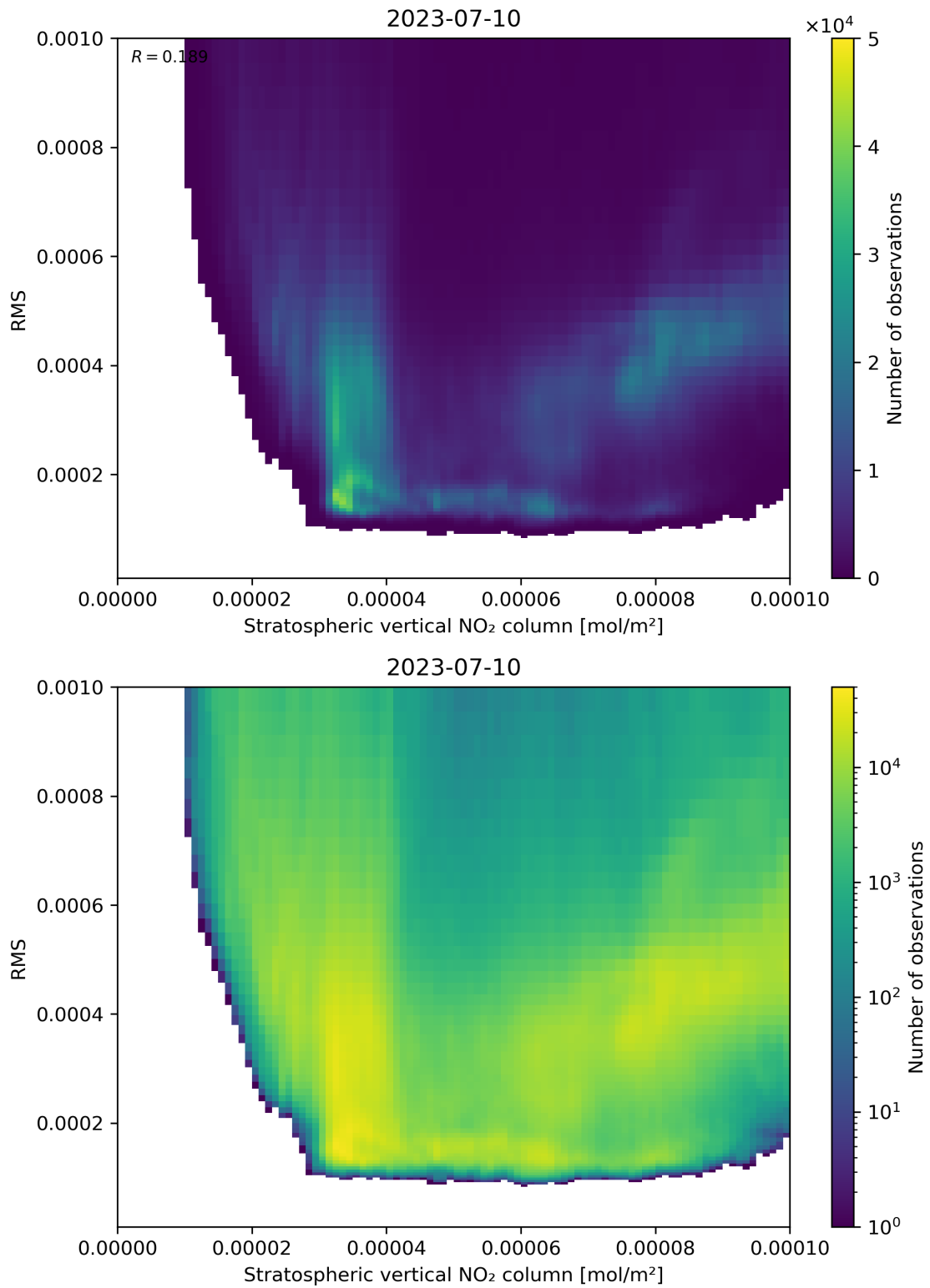
Figure 102: Scatter density plot of “Stratospheric vertical NO 2 column” against “RMS” for 2023-07-09 to 2023-07-11.
