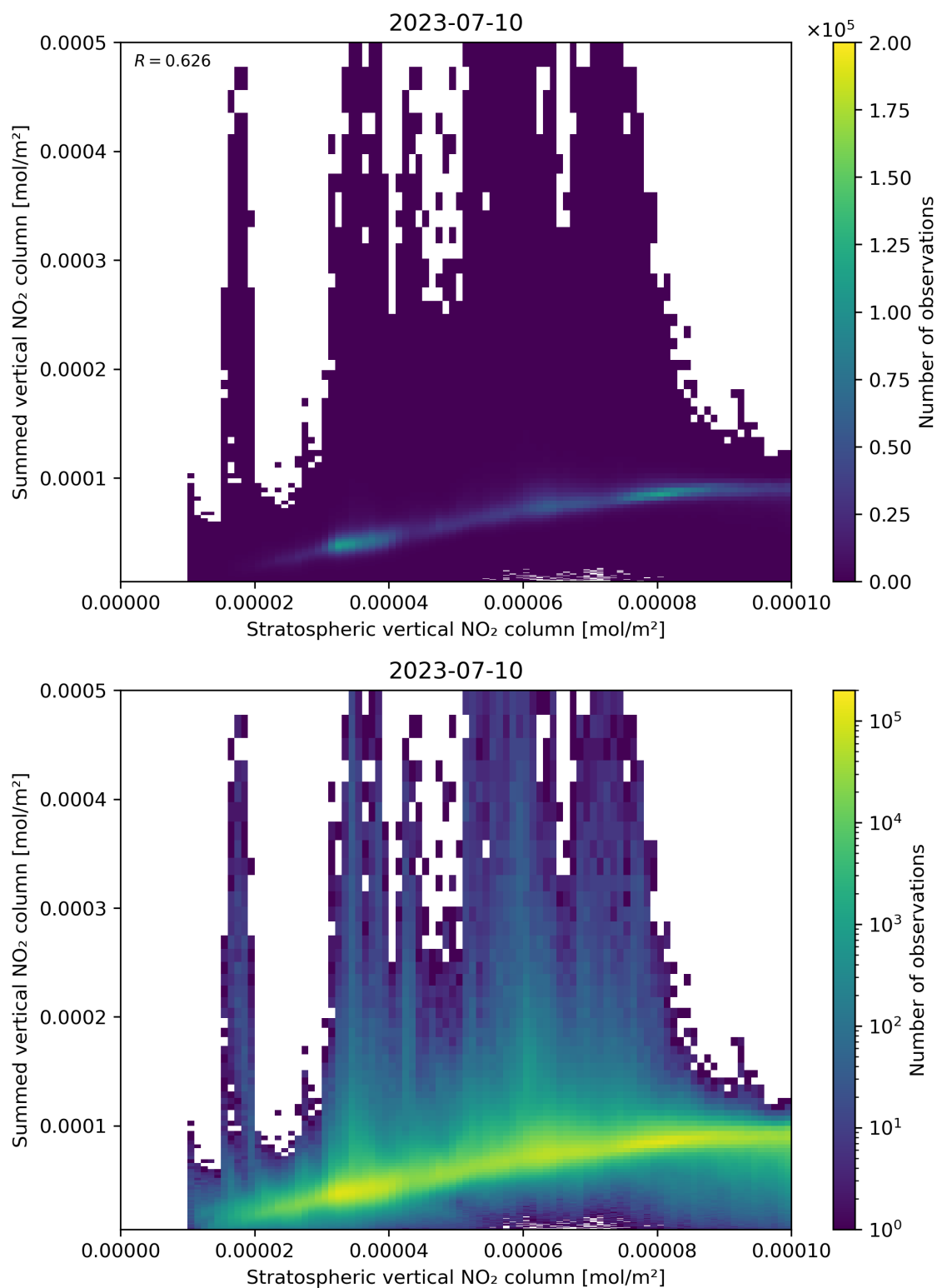
Figure 98: Scatter density plot of “Stratospheric vertical NO 2 column” against “Summed vertical NO 2 column” for 2023-07-09 to 2023-07-11.
