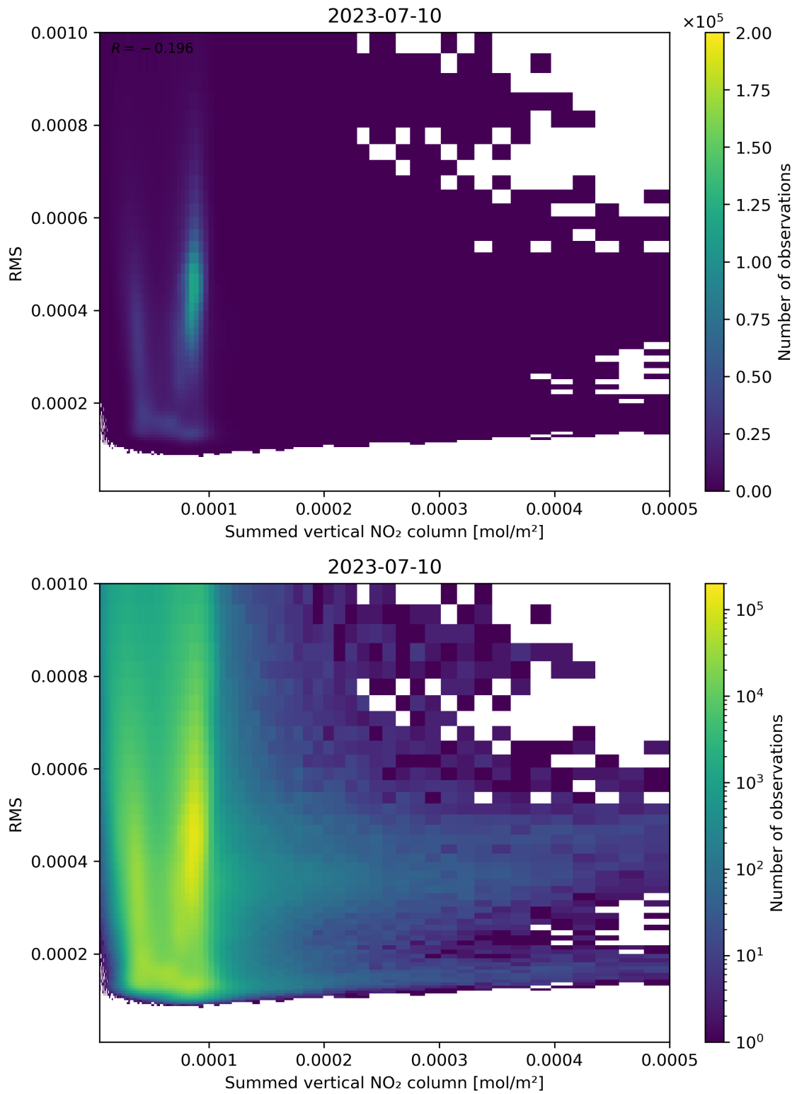
Figure 109: Scatter density plot of “Summed vertical NO 2 column” against “RMS” for 2023-07-09 to 2023-07-11.
