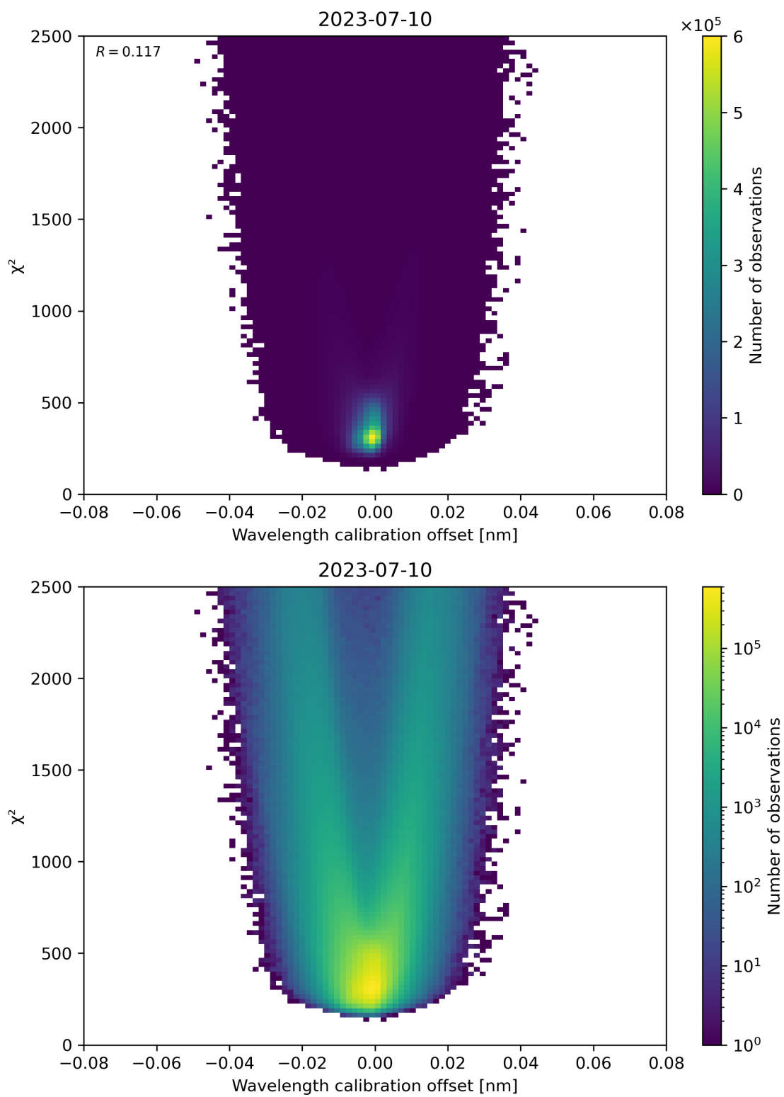
Figure 175: Scatter density plot of “Wavelength calibration offset” against “ \chi^2 ” for 2023-07-09 to 2023-07-11.
