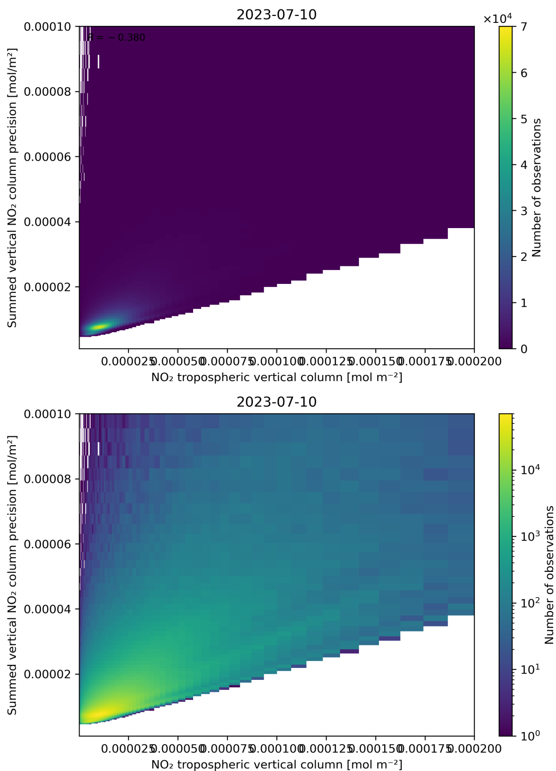
Figure 127: Scatter density plot of “NO 2 tropospheric vertical column” against “Summed vertical NO 2 column precision” for 2023-07-09 to 2023-07-11.
