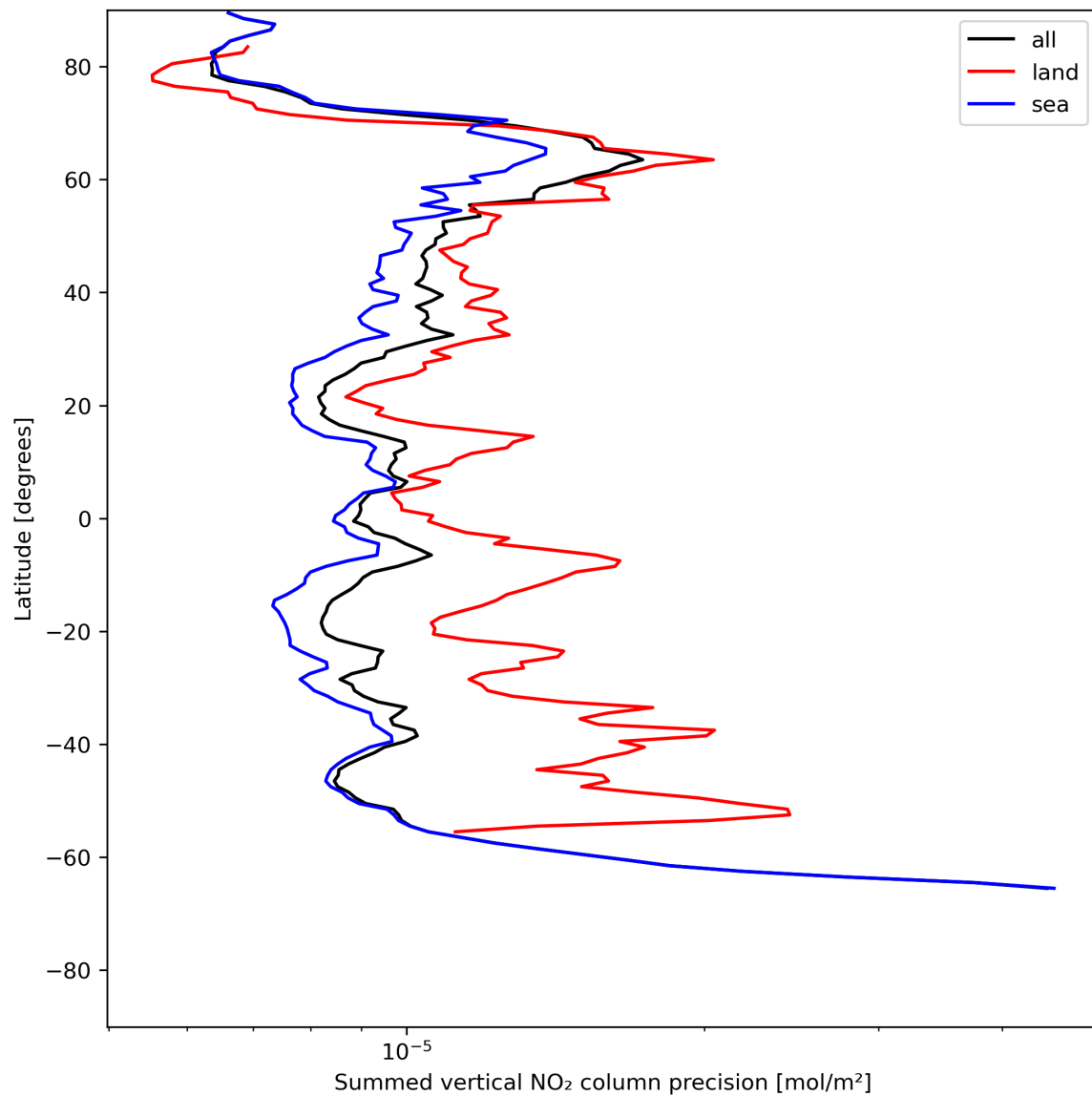
Figure 24: Zonal average of “Summed vertical NO 2 column precision” for 2023-07-09 to 2023-07-11.
