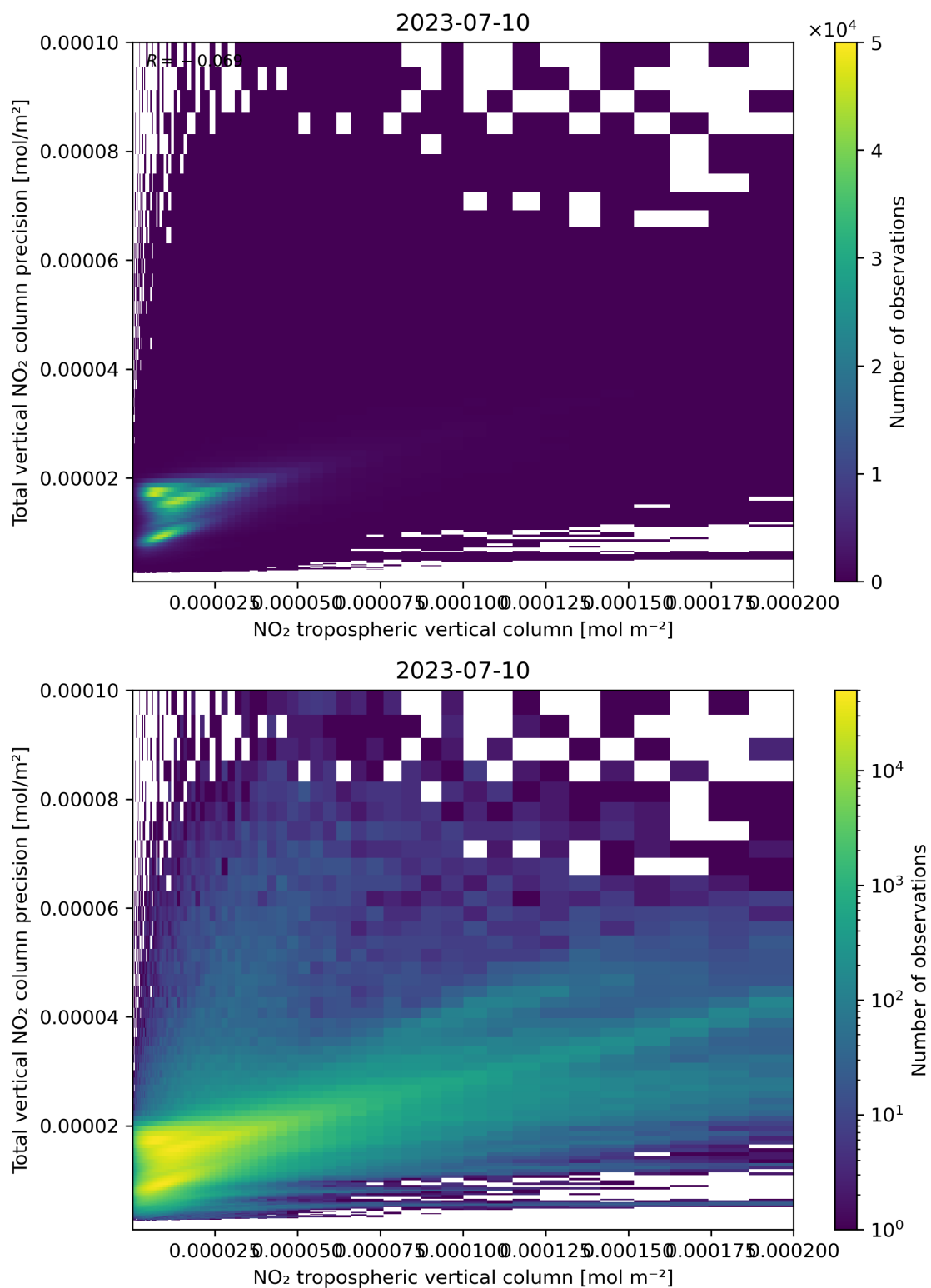
Figure 129: Scatter density plot of “NO 2 tropospheric vertical column” against “Total vertical NO 2 column precision” for 2023-07-09 to 2023-07-11.
