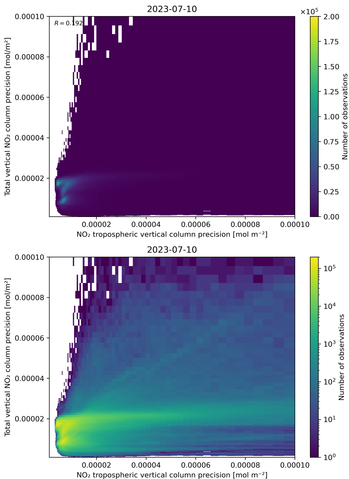
Figure 139: Scatter density plot of “NO 2 tropospheric vertical column precision” against “Total vertical NO 2 column precision” for 2023-07-09 to 2023-07-11.
