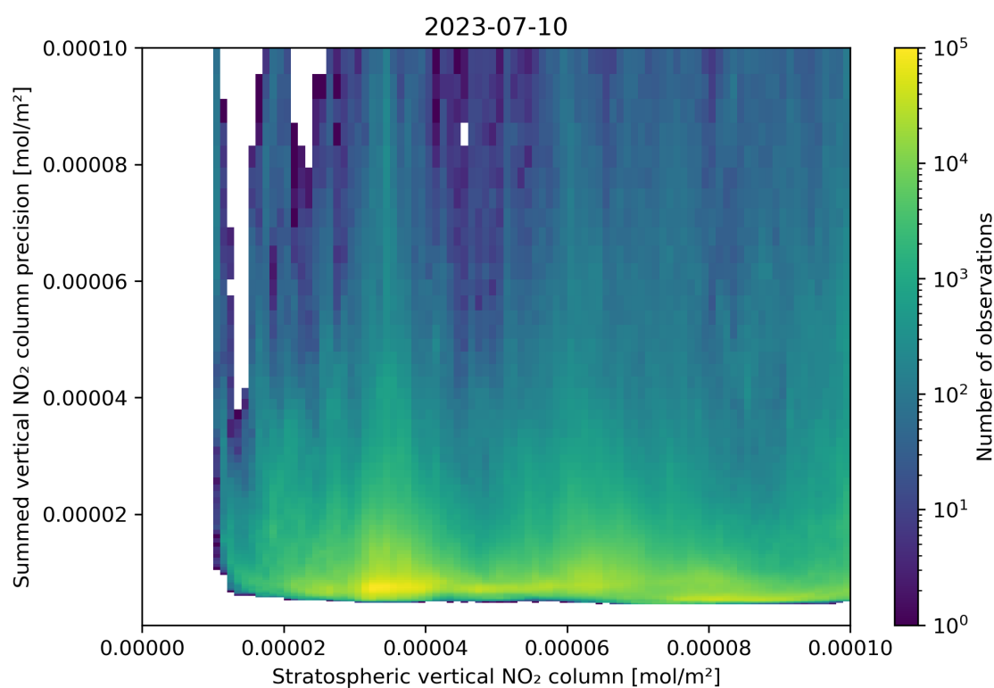
Figure 99: Scatter density plot of “Stratospheric vertical NO 2 column” against “Summed vertical NO 2 column precision” for 2023-07-09 to 2023-07-11.
