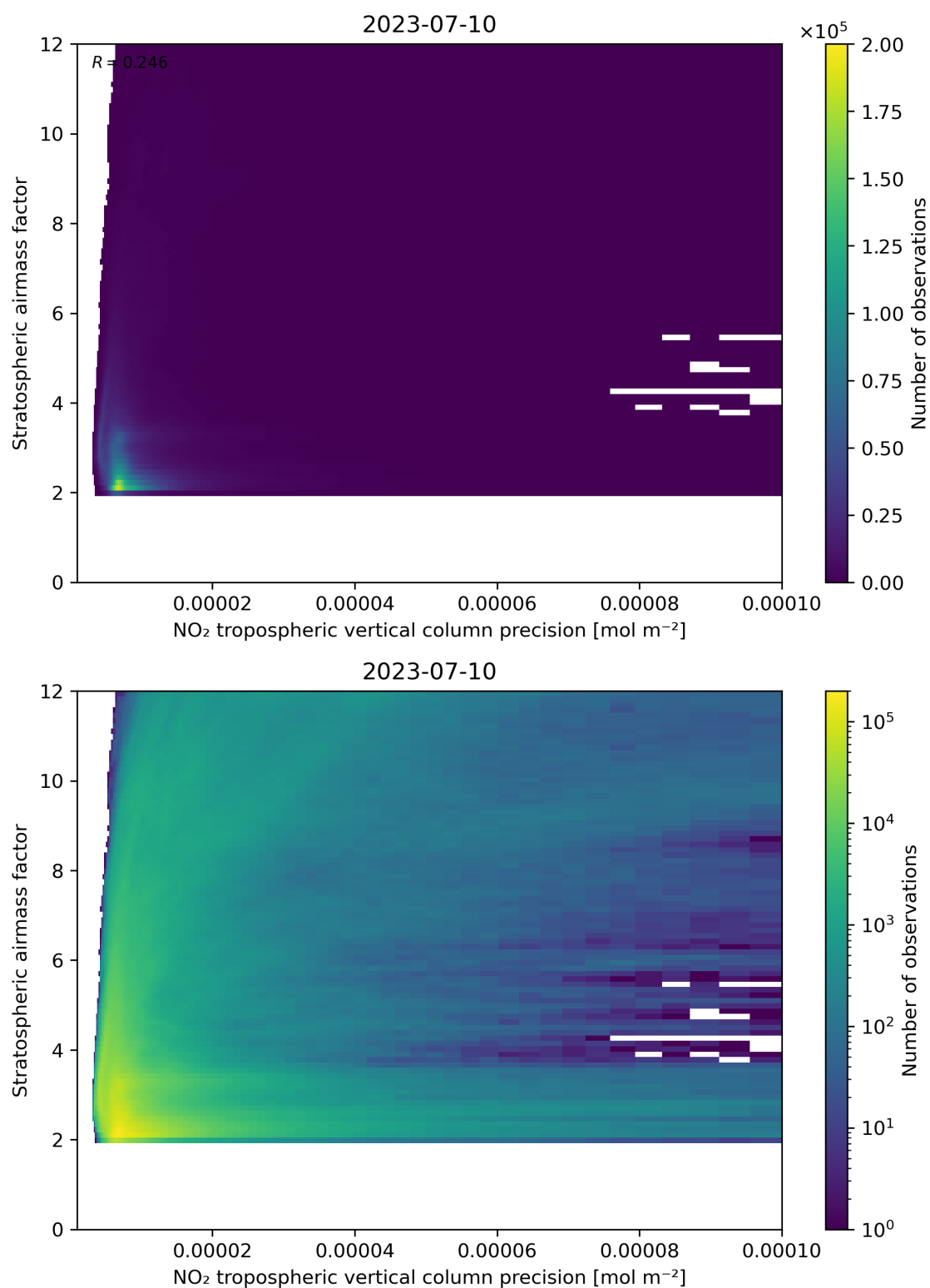
Figure 131: Scatter density plot of “NO 2 tropospheric vertical column precision” against “Stratospheric airmass factor” for 2023-07-09 to 2023-07-11.
