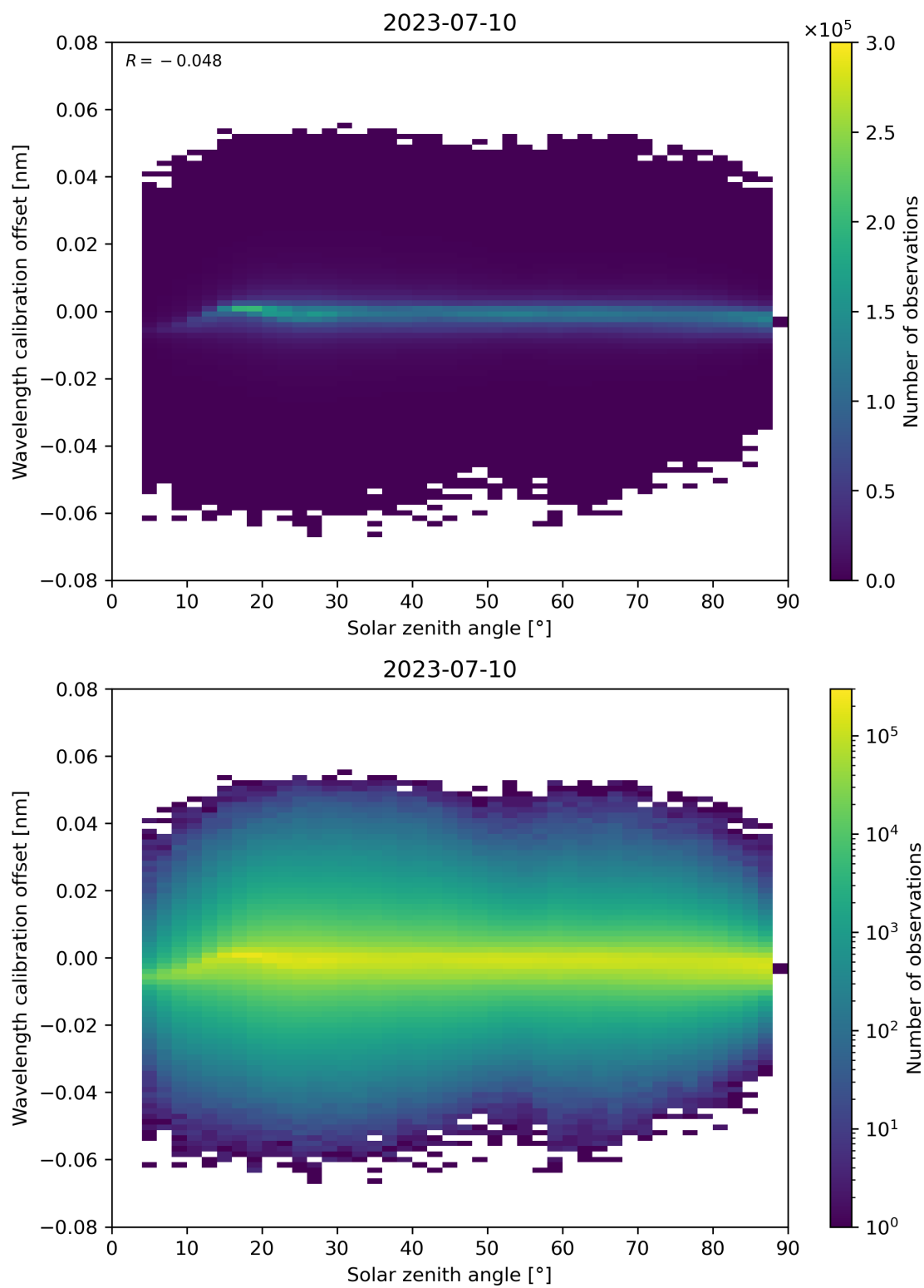
Figure 158: Scatter density plot of “Solar zenith angle” against “Wavelength calibration offset” for 2023-07-09 to 2023-07-11.
