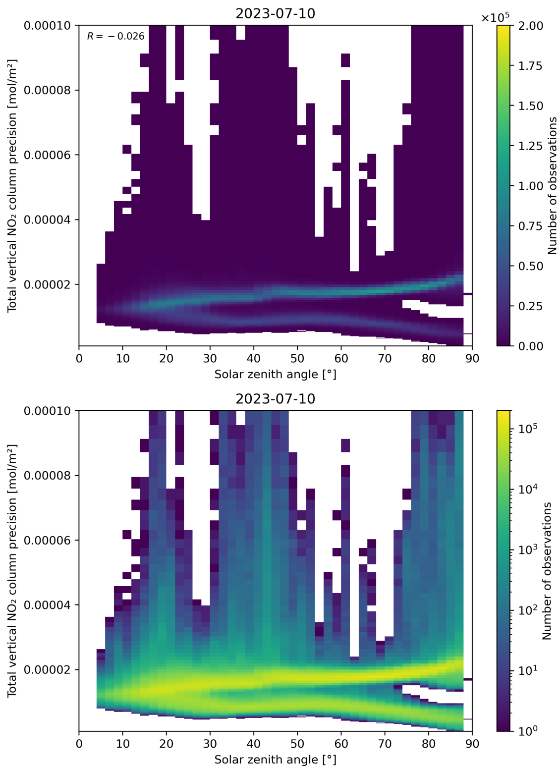
Figure 154: Scatter density plot of “Solar zenith angle” against “Total vertical NO 2 column precision” for 2023-07-09 to 2023-07-11.
