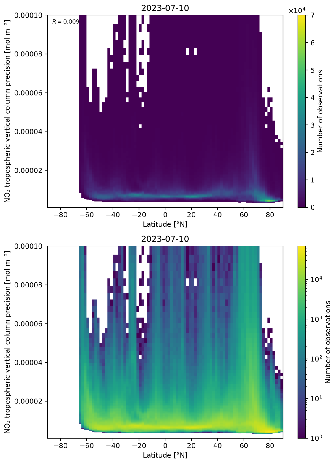
Figure 93: Scatter density plot of “Latitude” against “NO 2 tropospheric vertical column precision” for 2023-07-09 to 2023-07-11.
