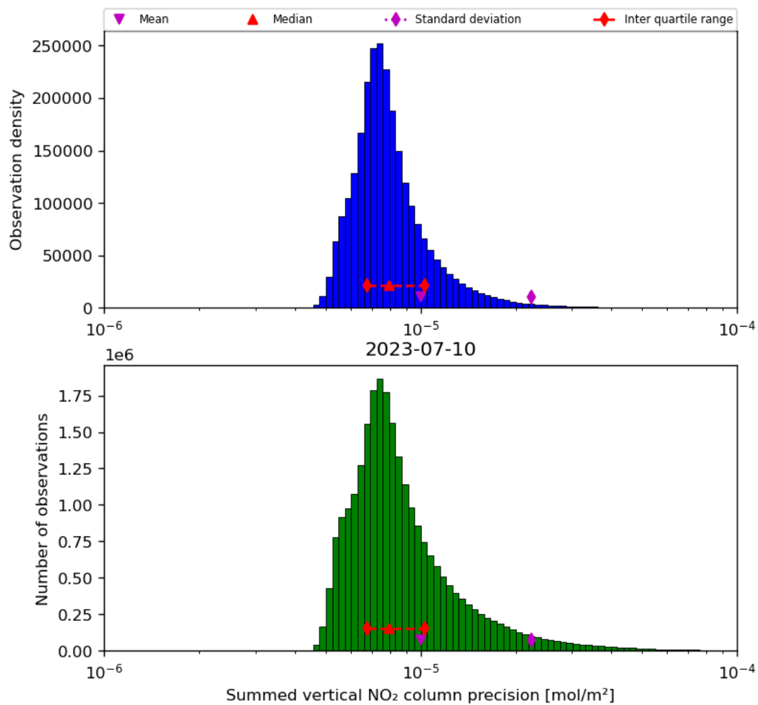
Figure 41: Histogram of “Summed vertical NO 2 column precision” for 2023-07-09 to 2023-07-11
