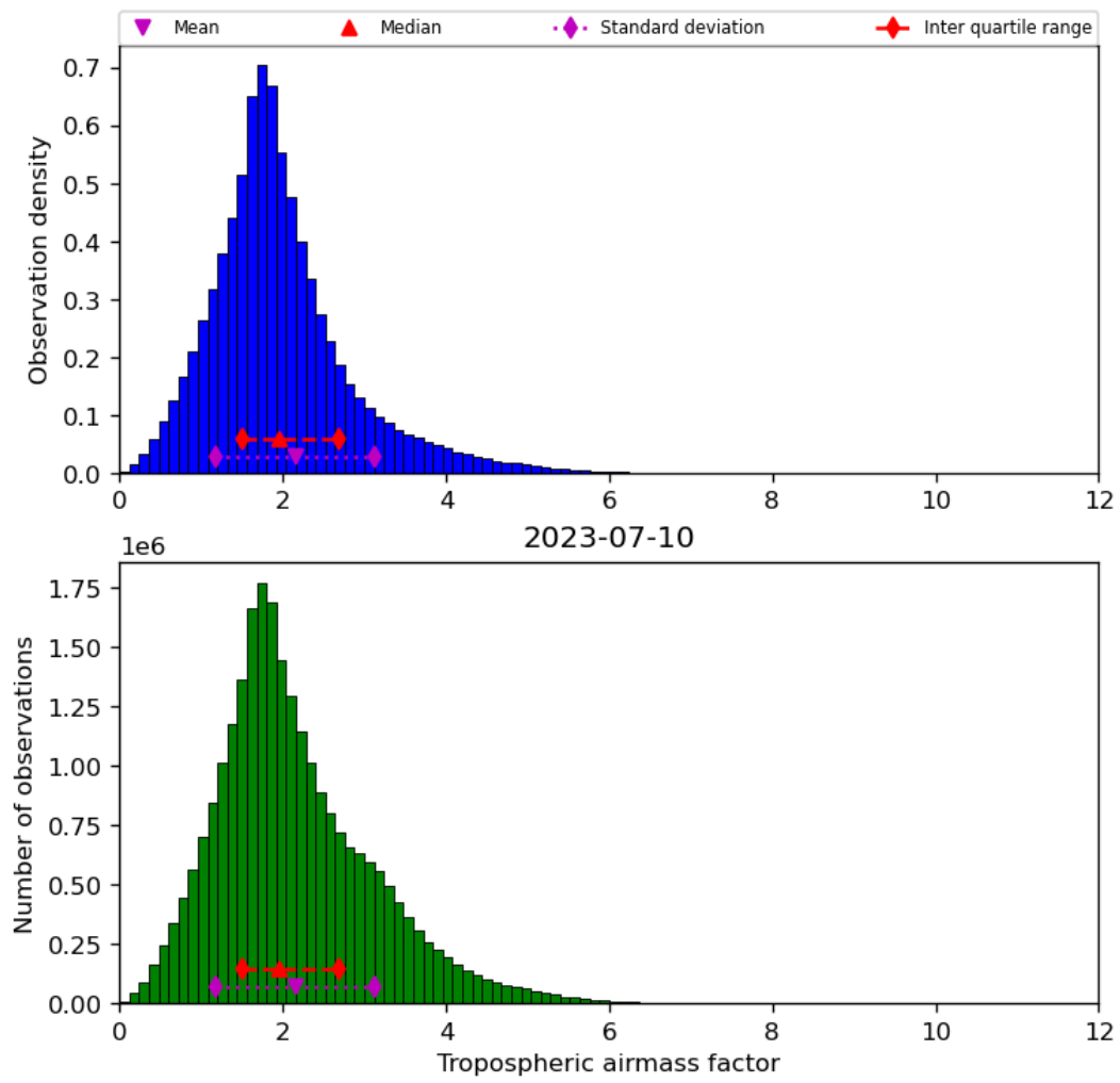
Figure 31: Histogram of “Tropospheric airmass factor” for 2023-07-09 to 2023-07-11
