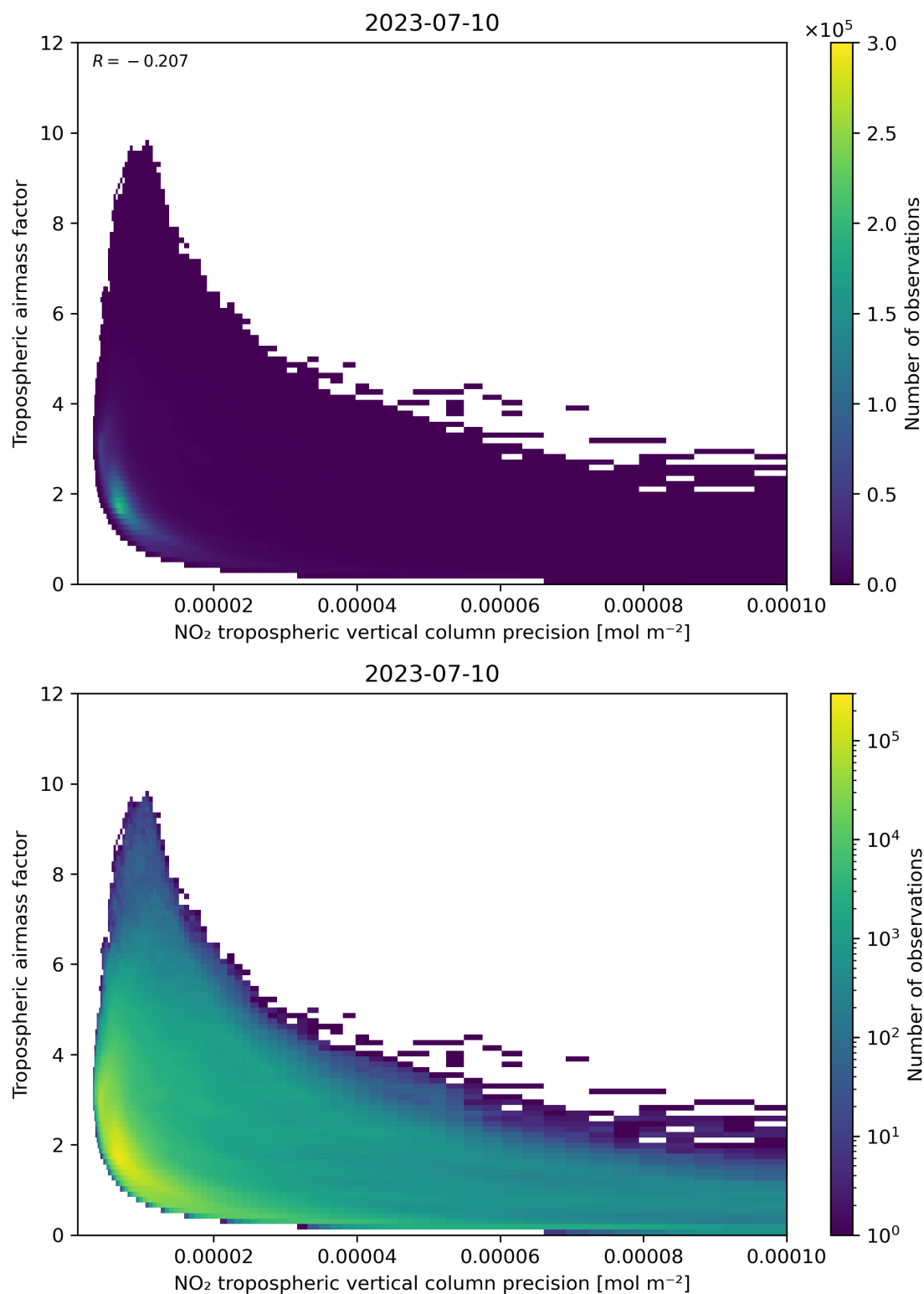
Figure 133: Scatter density plot of “NO 2 tropospheric vertical column precision” against “Tropospheric airmass factor” for 2023-07-09 to 2023-07-11.
