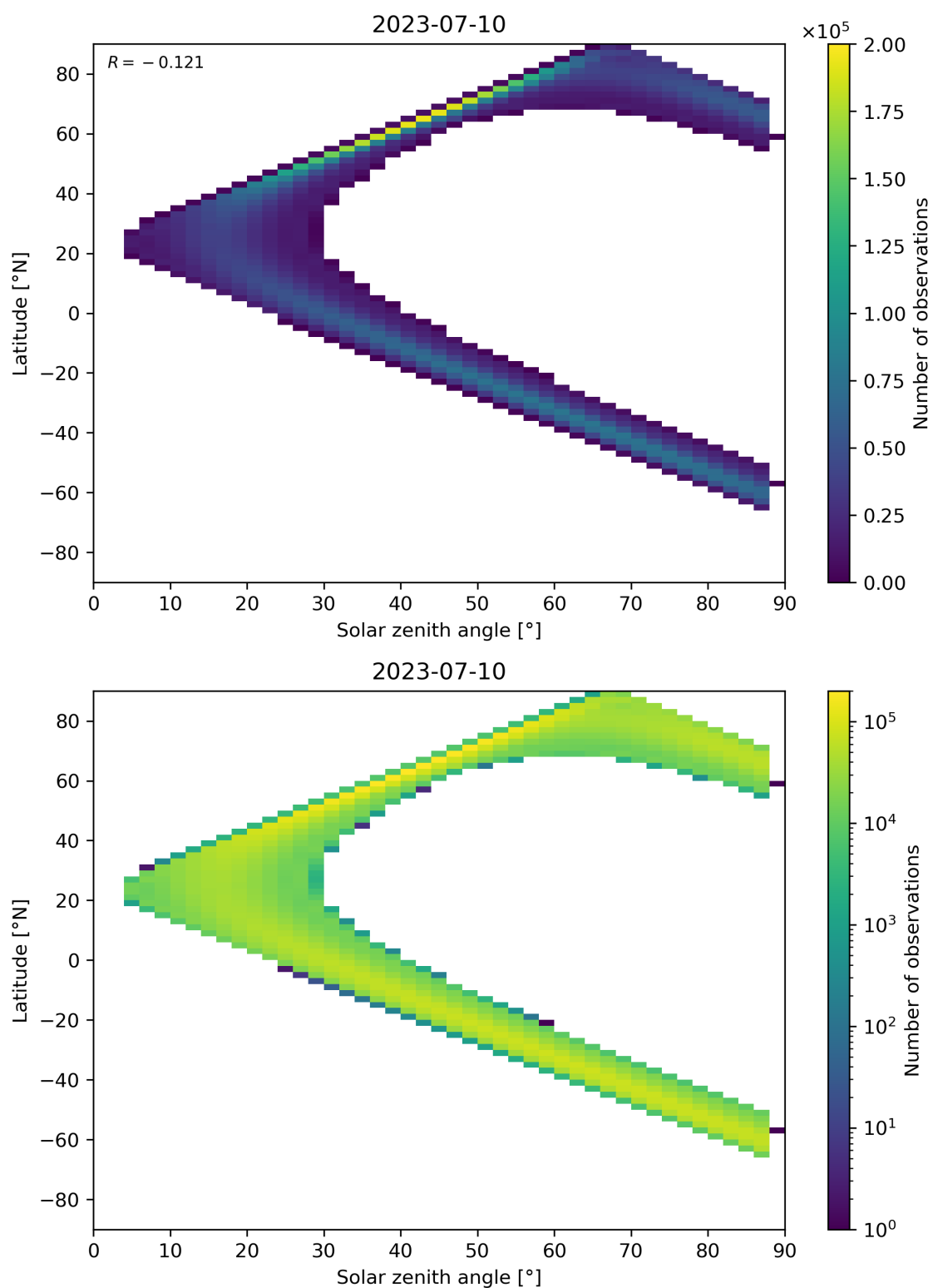
Figure 149: Scatter density plot of “Solar zenith angle” against “Latitude” for 2023-07-09 to 2023-07-11.
