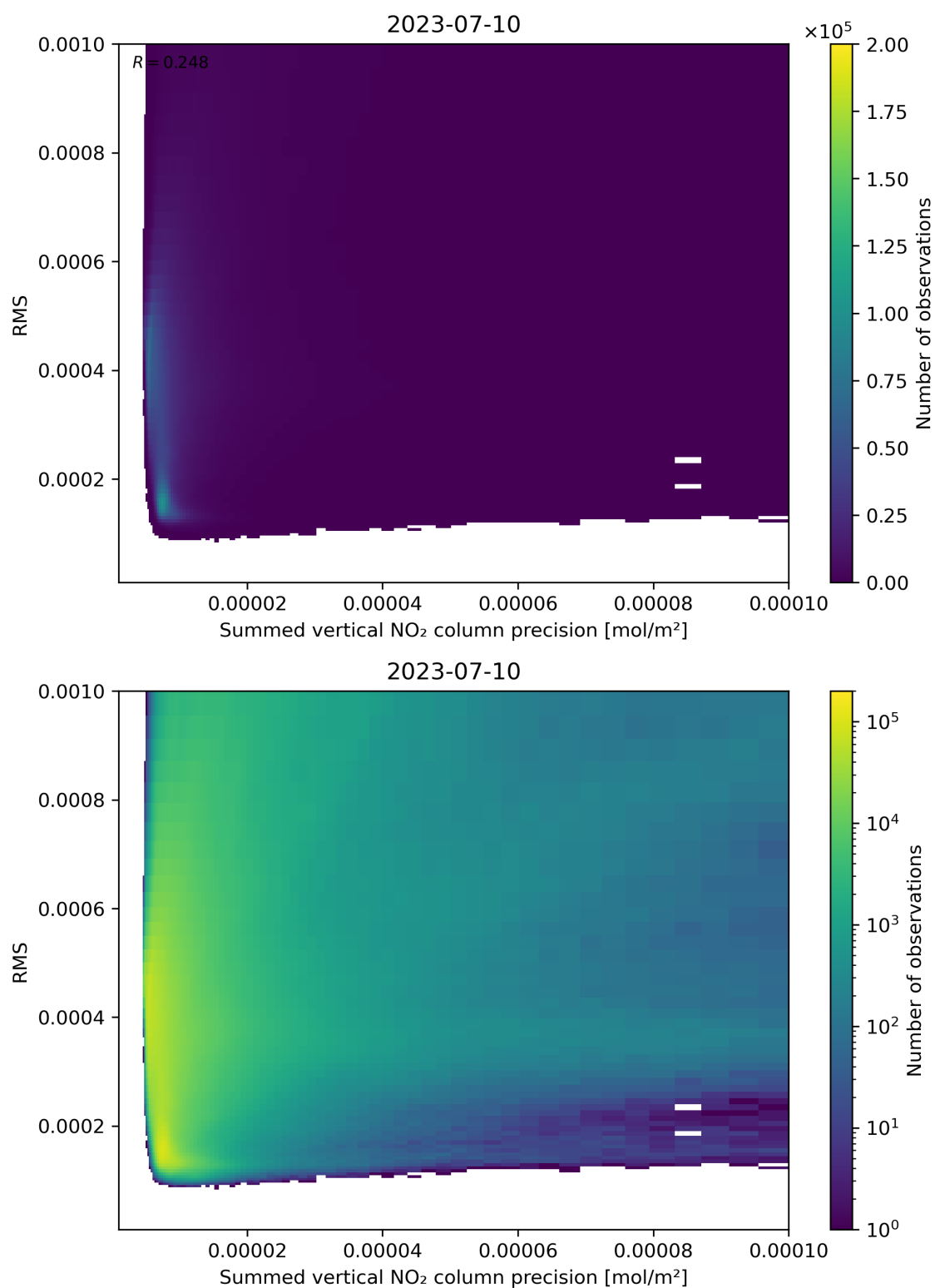
Figure 108: Scatter density plot of “Summed vertical NO 2 column precision” against “RMS” for 2023-07-09 to 2023-07-11.
