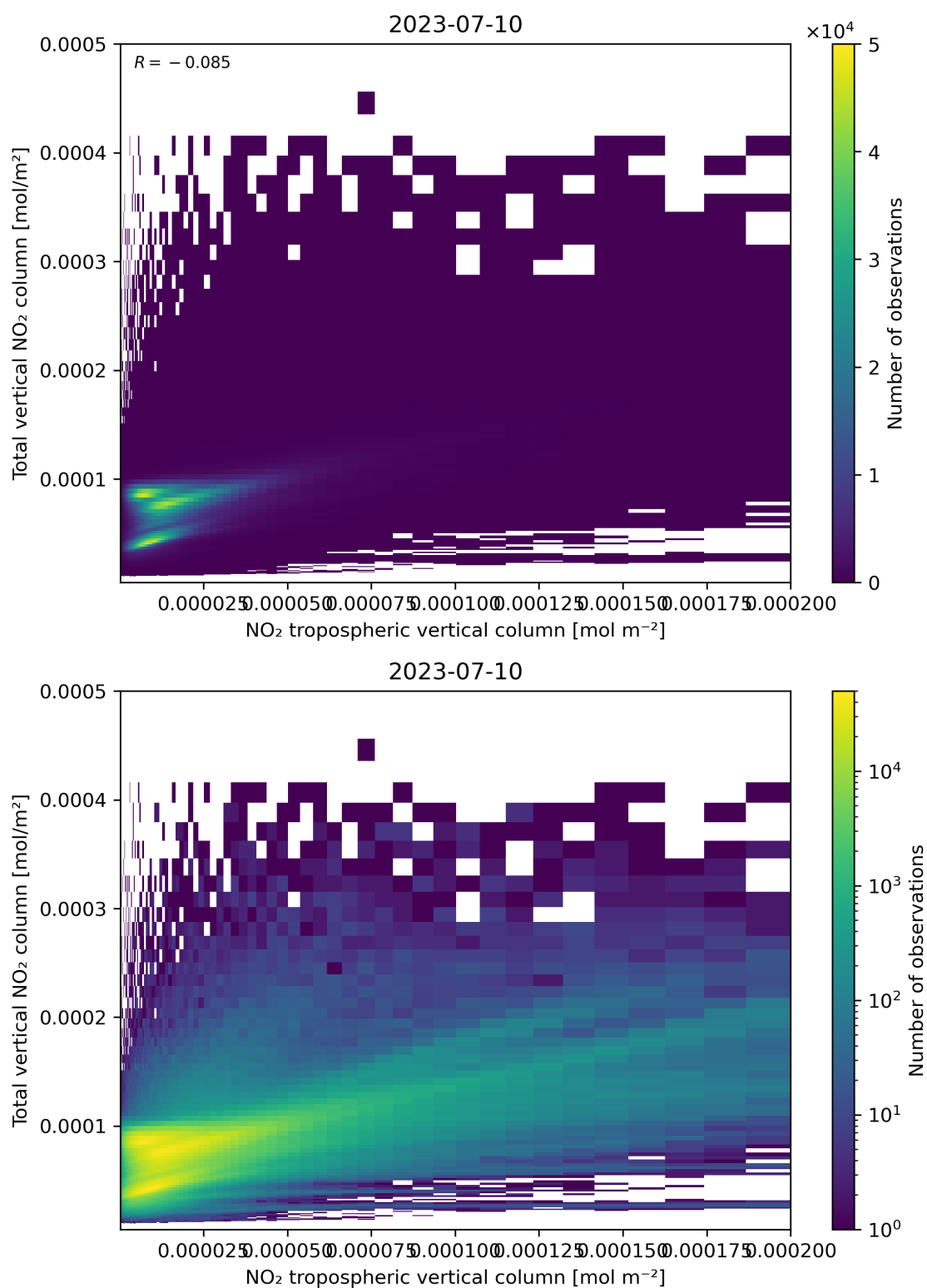
Figure 128: Scatter density plot of “NO 2 tropospheric vertical column” against “Total vertical NO 2 column” for 2023-07-09 to 2023-07-11.
