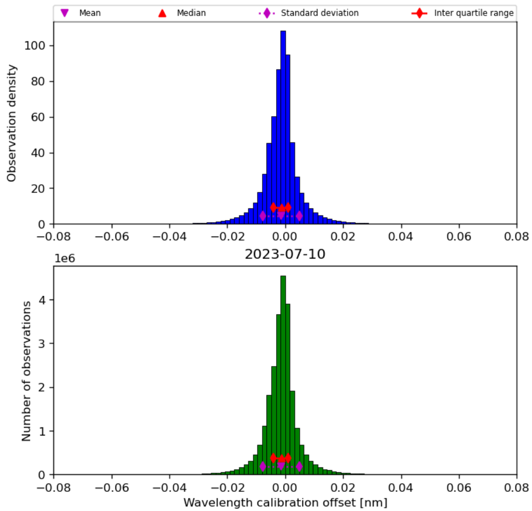
Figure 35: Histogram of “Wavelength calibration offset” for 2023-07-09 to 2023-07-11
