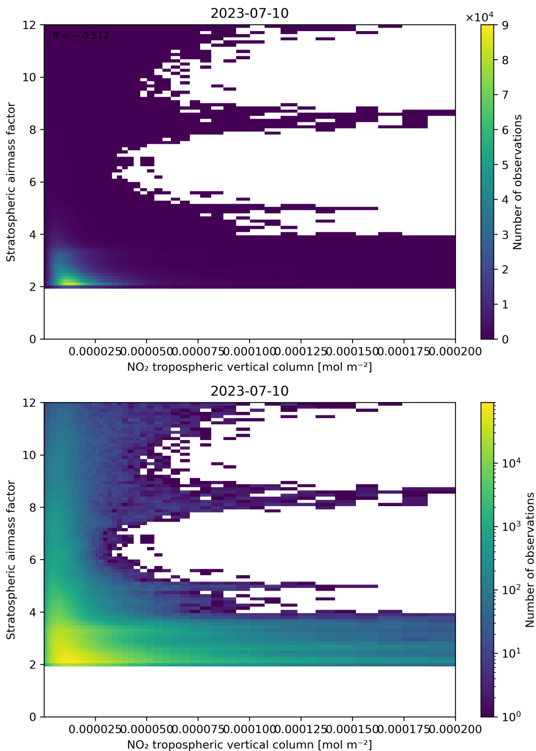
Figure 121: Scatter density plot of “NO 2 tropospheric vertical column” against “Stratospheric airmass factor” for 2023-07-09 to 2023-07-11.
