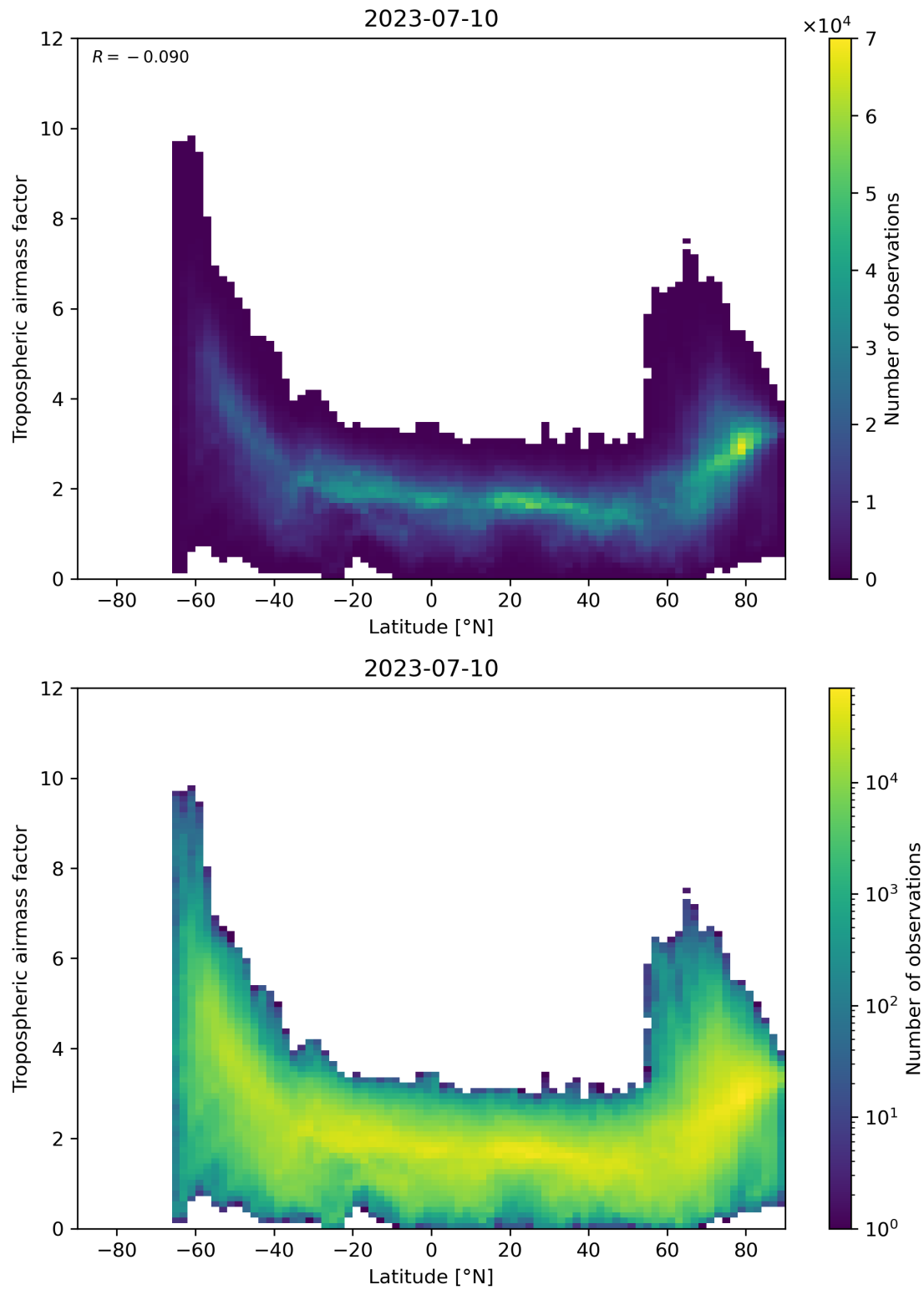
Figure 85: Scatter density plot of “Latitude” against “Tropospheric air mass factor” for 2023-07-09 to 2023-07-11.
