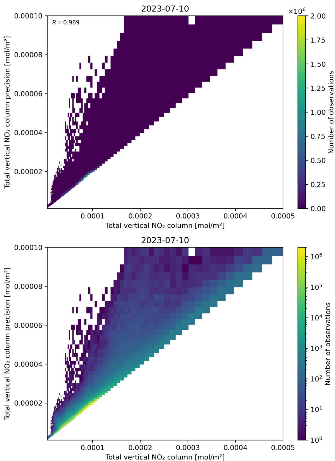
Figure 114: Scatter density plot of “Total vertical NO 2 column” against “Total vertical NO 2 column precision” for 2023-07-09 to 2023-07-11.
