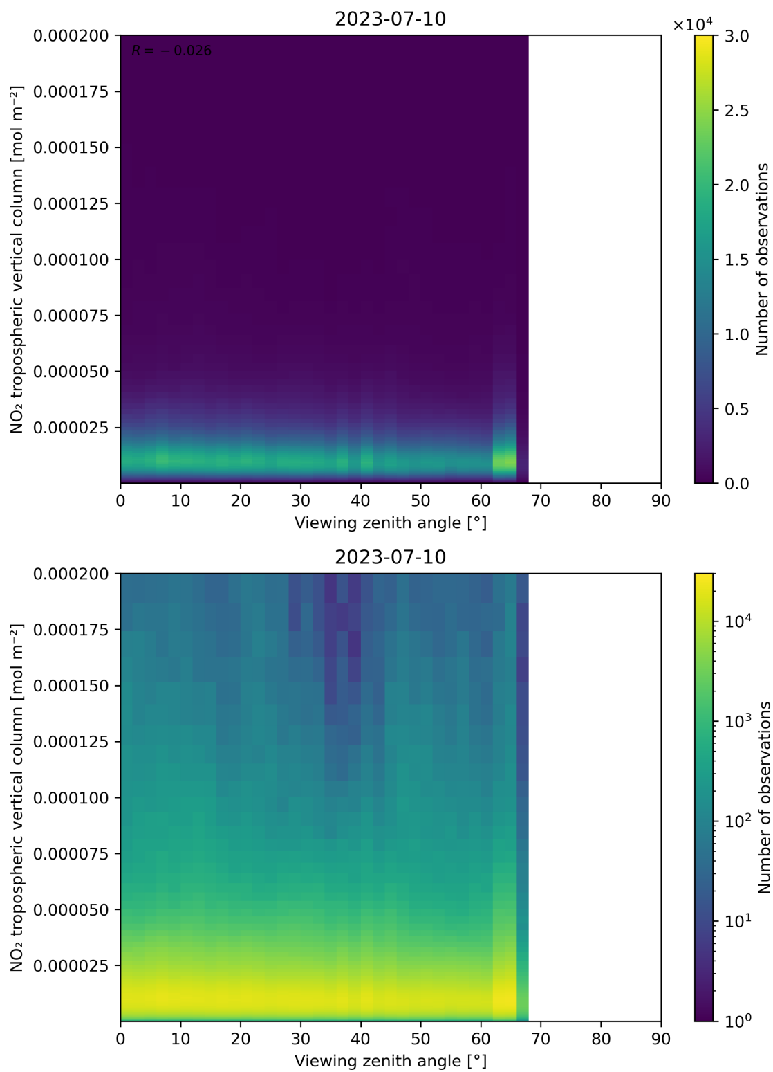
Figure 169: Scatter density plot of “Viewing zenith angle” against “NO 2 tropospheric vertical column” for 2023-07-09 to 2023-07-11.
