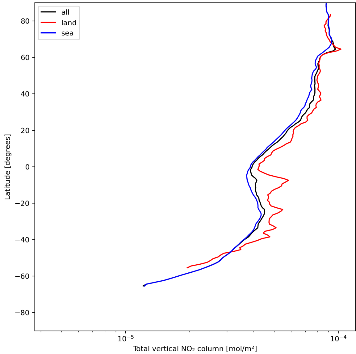
Figure 21: Zonal average of “Total vertical NO 2 column” for 2023-07-09 to 2023-07-11.
