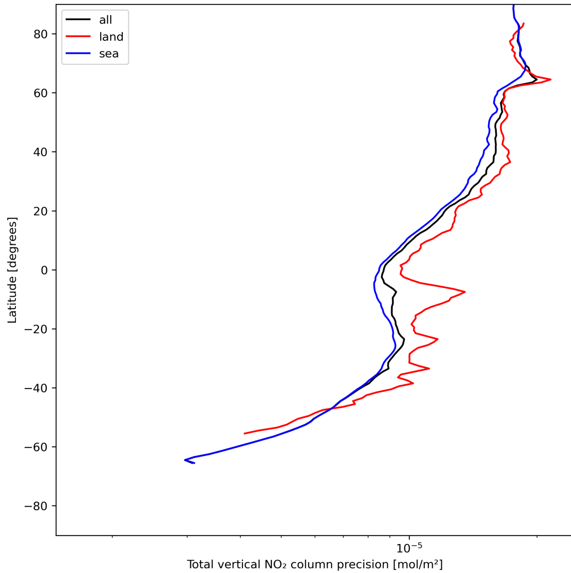
Figure 22: Zonal average of “Total vertical NO 2 column precision” for 2023-07-09 to 2023-07-11.
