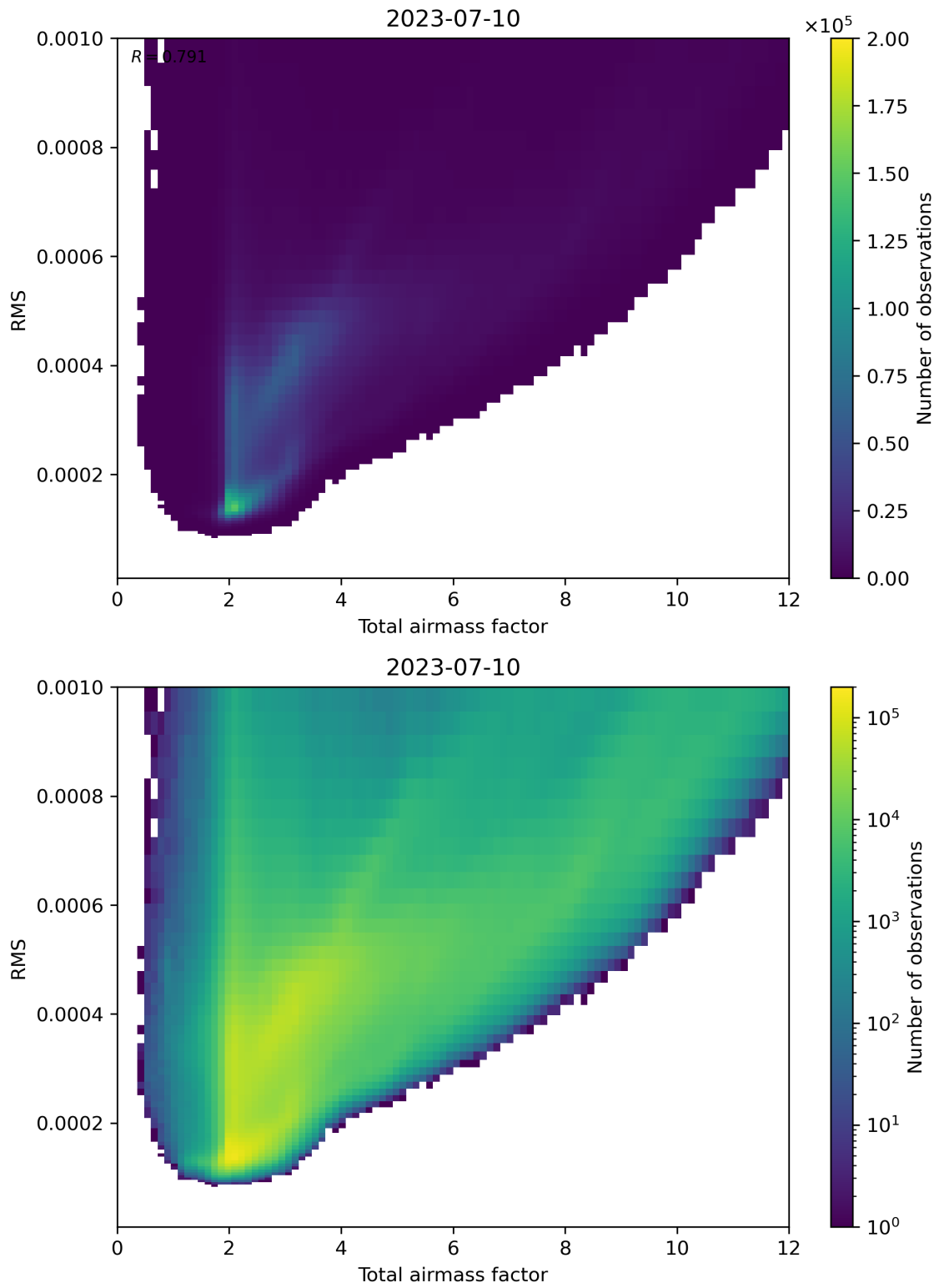
Figure 69: Scatter density plot of “Total airmass factor” against “RMS” for 2023-07-09 to 2023-07-11.
