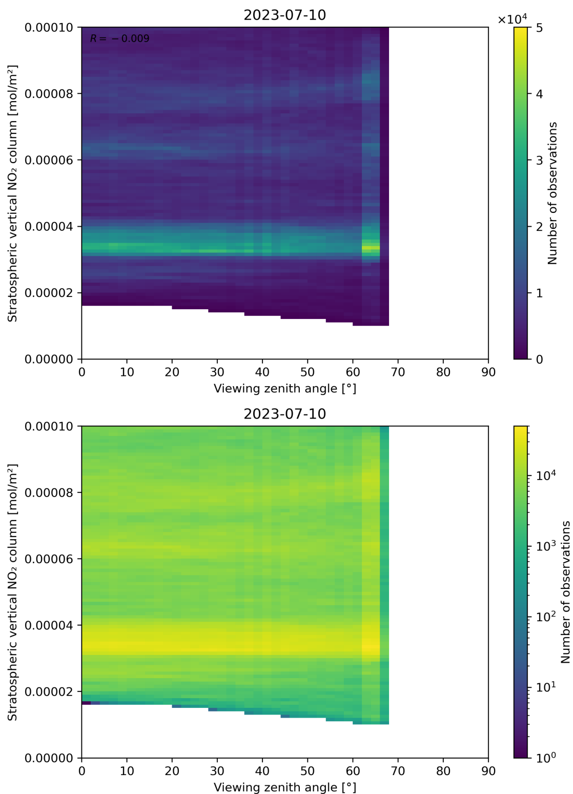
Figure 164: Scatter density plot of “Viewing zenith angle” against “Stratospheric vertical NO 2 column” for 2023-07-09 to 2023-07-11.
