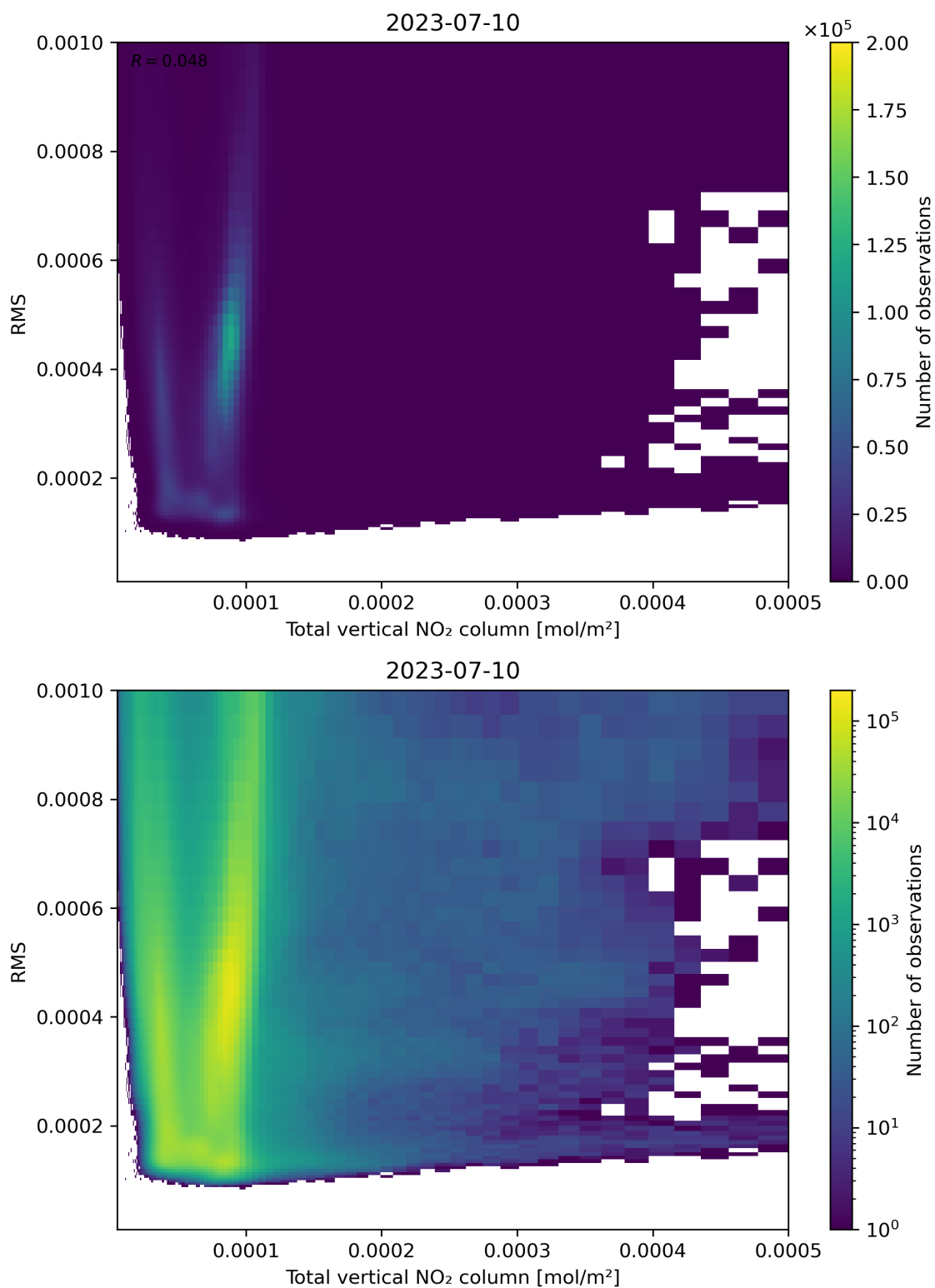
Figure 120: Scatter density plot of “Total vertical NO 2 column” against “RMS” for 2023-07-09 to 2023-07-11.
