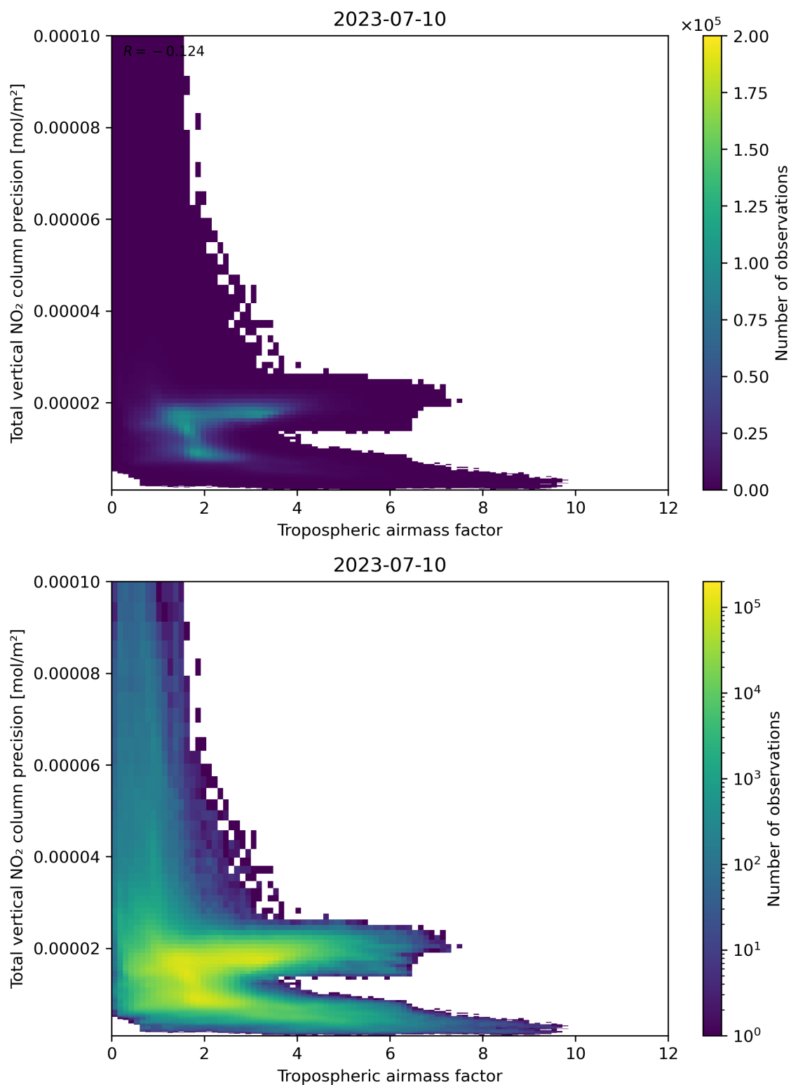
Figure 78: Scatter density plot of “Tropospheric air mass factor” against “Total vertical NO 2 column precision” for 2023-07-09 to 2023-07-11.
