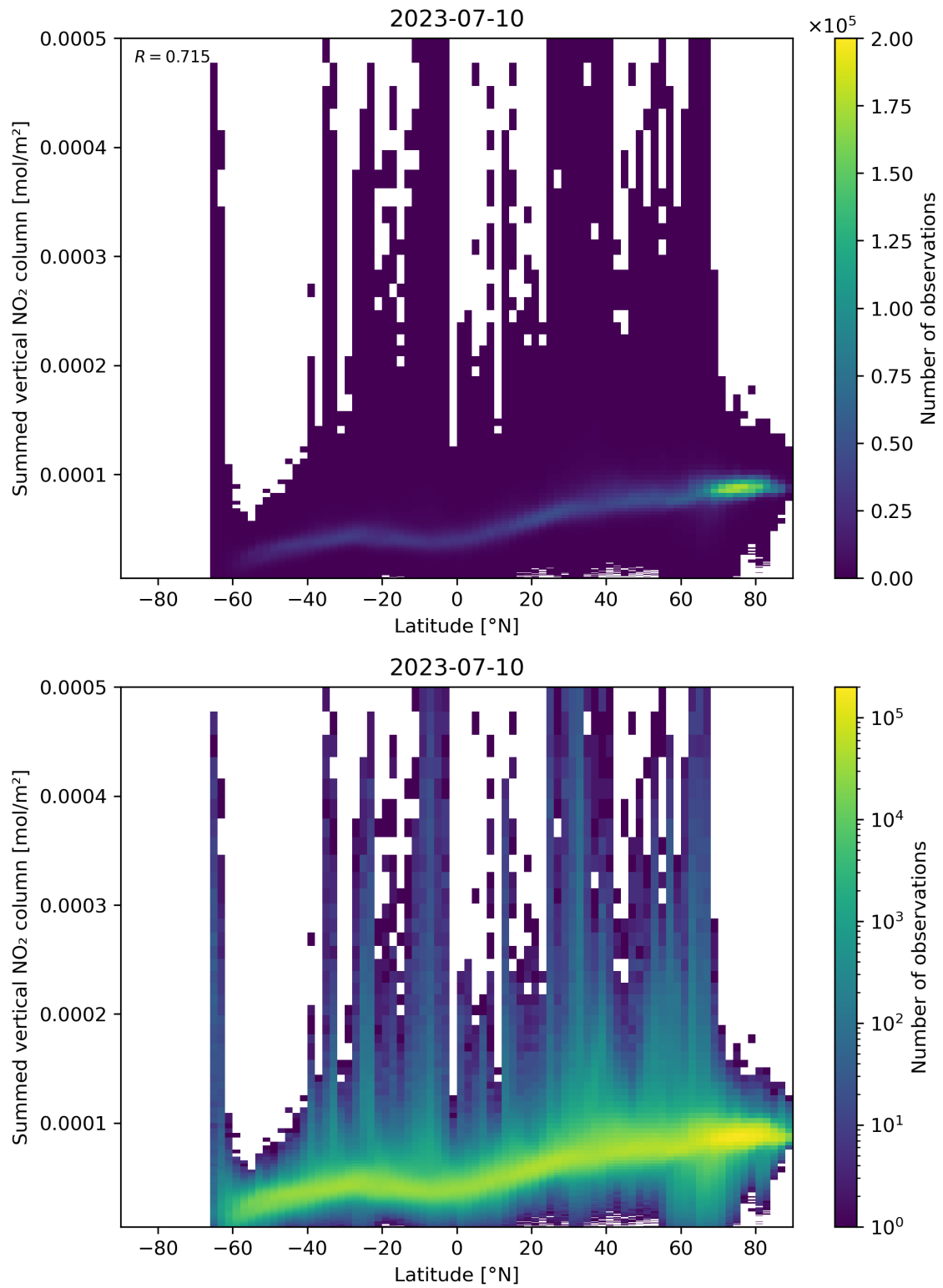
Figure 88: Scatter density plot of “Latitude” against “Summed vertical NO 2 column” for 2023-07-09 to 2023-07-11.
