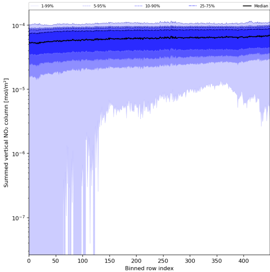
Figure 57: Along track statistics of “Summed vertical NO 2 column” for 2023-07-09 to 2023-07-11
