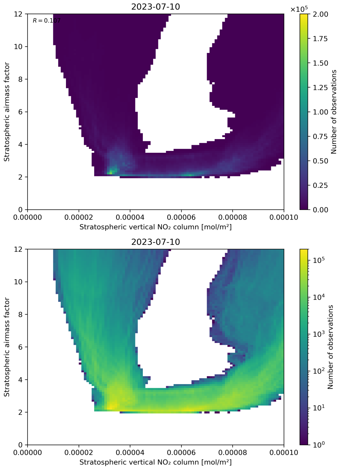
Figure 96: Scatter density plot of “Stratospheric vertical NO 2 column” against “Stratospheric airmass factor” for 2023-07-09 to 2023-07-11.
