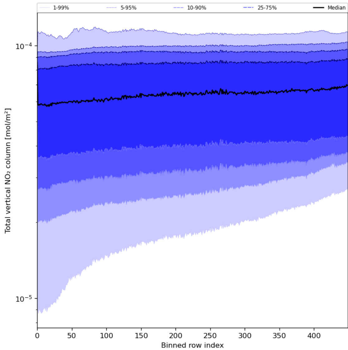
Figure 55: Along track statistics of “Total vertical NO 2 column” for 2023-07-09 to 2023-07-11
