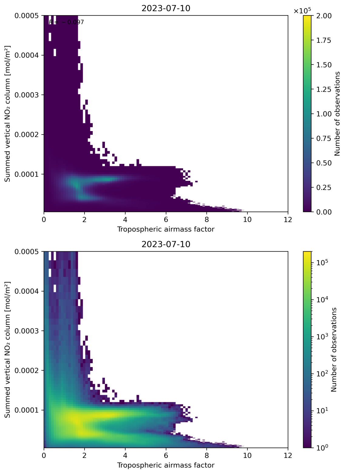
Figure 75: Scatter density plot of “Tropospheric airmass factor” against “Summed vertical NO 2 column” for 2023-07-09 to 2023-07-11.
