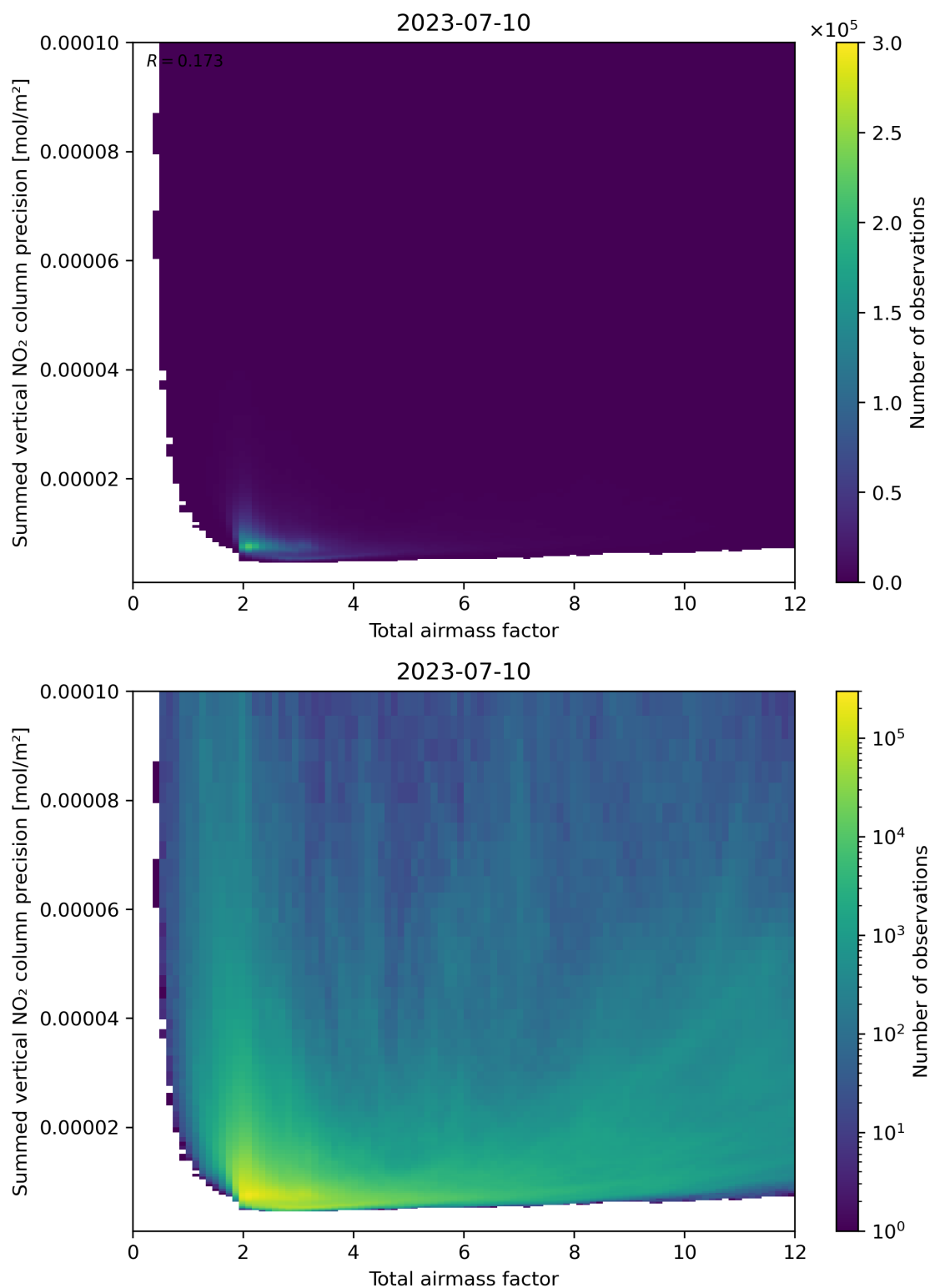
Figure 66: Scatter density plot of “Total airmass factor” against “Summed vertical NO 2 column precision” for 2023-07-09 to 2023-07-11.
