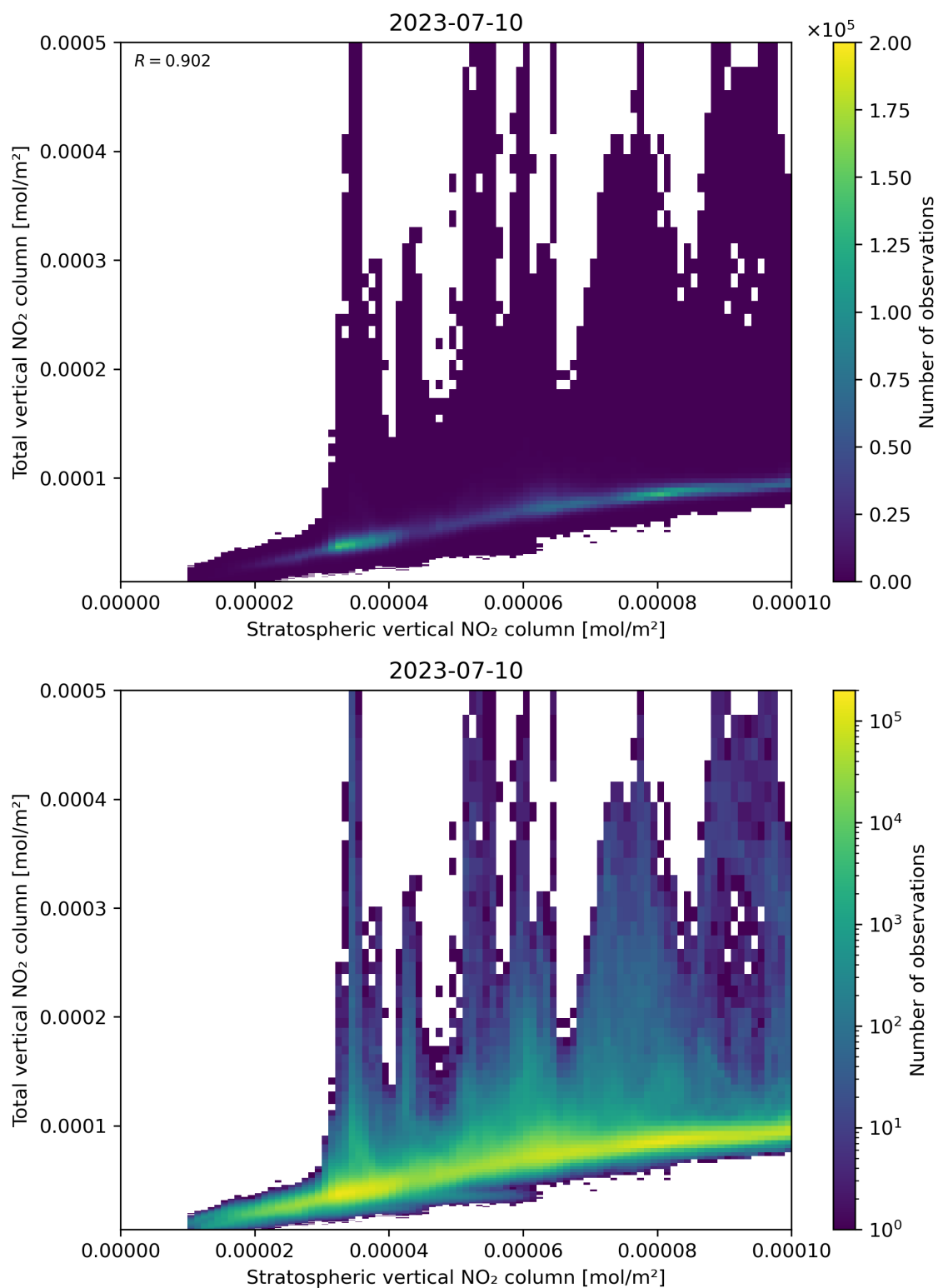
Figure 100: Scatter density plot of “Stratospheric vertical NO 2 column” against “Total vertical NO 2 column” for 2023-07-09 to 2023-07-11.
