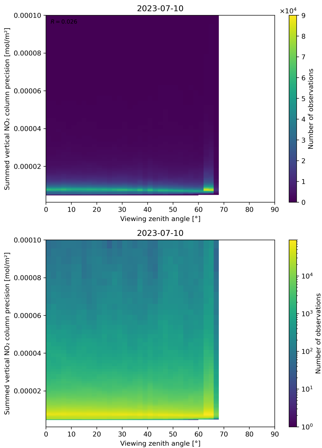
Figure 166: Scatter density plot of “Viewing zenith angle” against “Summed vertical NO 2 column precision” for 2023-07-09 to 2023-07-11.
