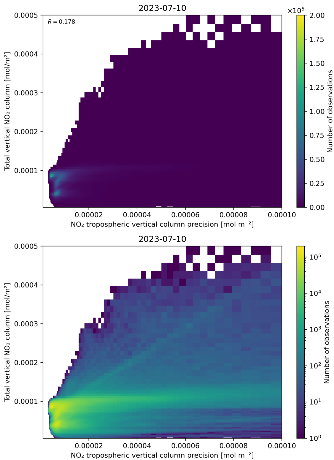
Figure 138: Scatter density plot of “NO 2 tropospheric vertical column precision” against “Total vertical NO 2 column” for 2023-07-09 to 2023-07-11.
