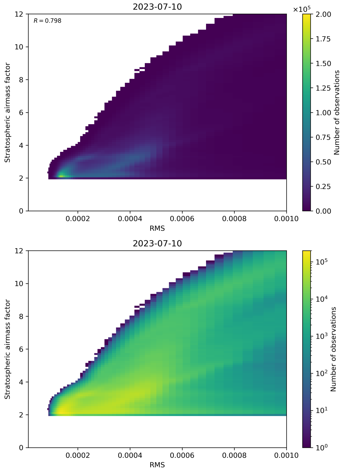
Figure 144: Scatter density plot of “RMS” against “Stratospheric airmass factor” for 2023-07-09 to 2023-07-11.
