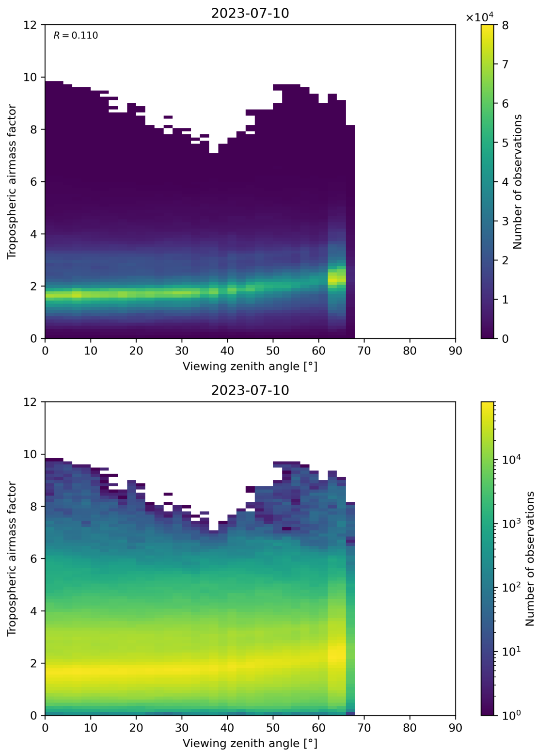
Figure 161: Scatter density plot of “Viewing zenith angle” against “Tropospheric airmass factor” for 2023-07-09 to 2023-07-11.
