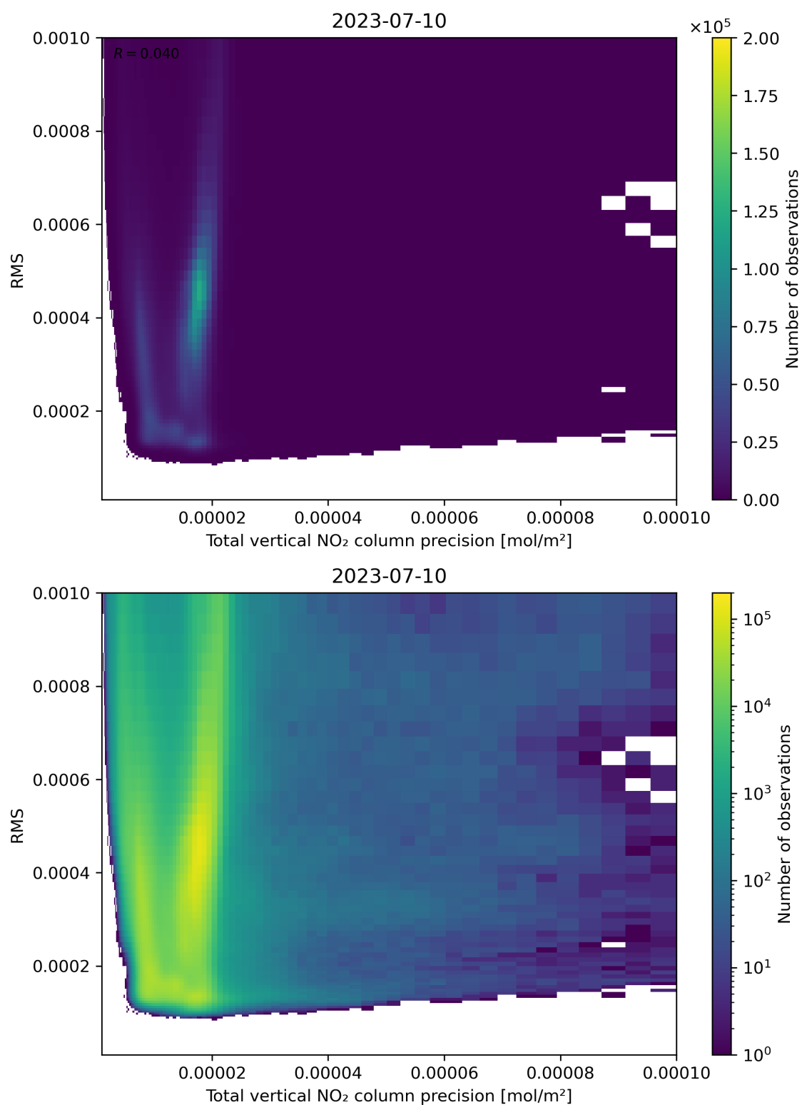
Figure 119: Scatter density plot of “Total vertical NO 2 column precision” against “RMS” for 2023-07-09 to 2023-07-11.
