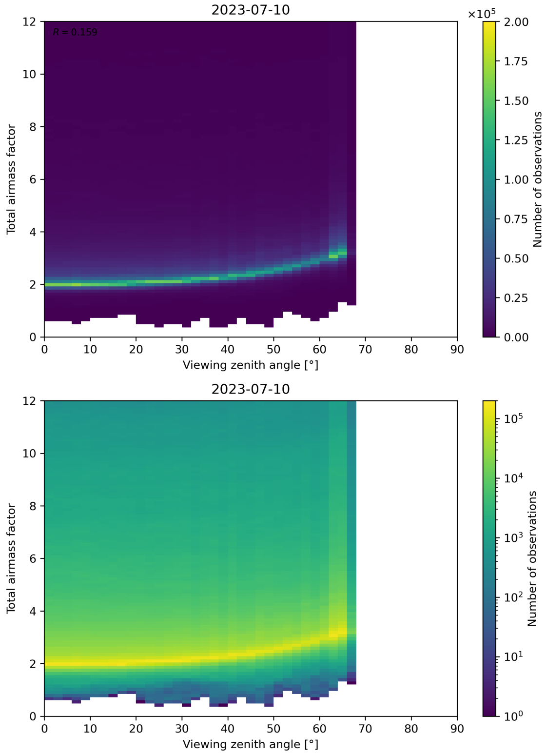
Figure 160: Scatter density plot of “Viewing zenith angle” against “Total airmass factor” for 2023-07-09 to 2023-07-11.
