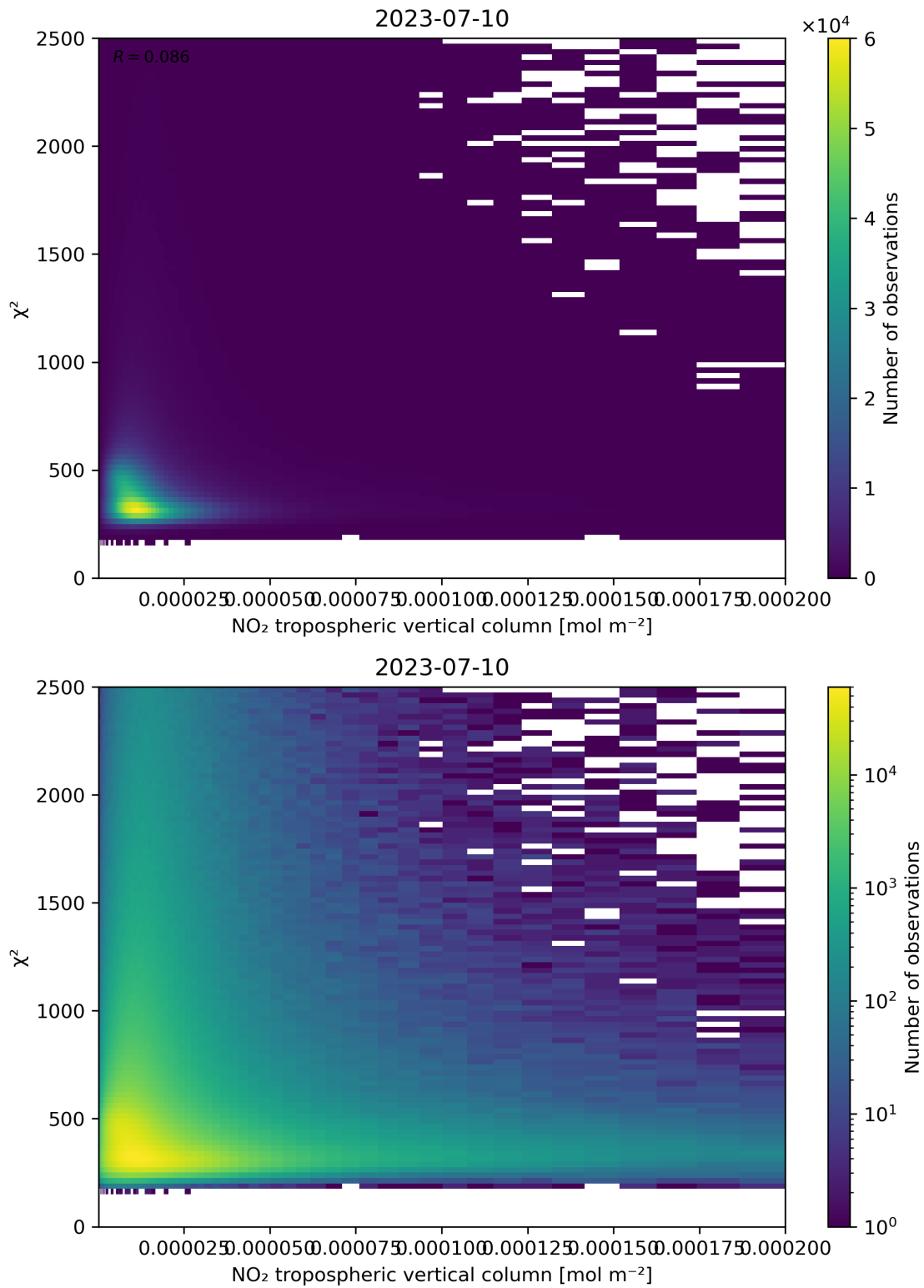
Figure 124: Scatter density plot of “NO 2 tropospheric vertical column” against “ \chi^2 ” for 2023-07-09 to 2023-07-11.
