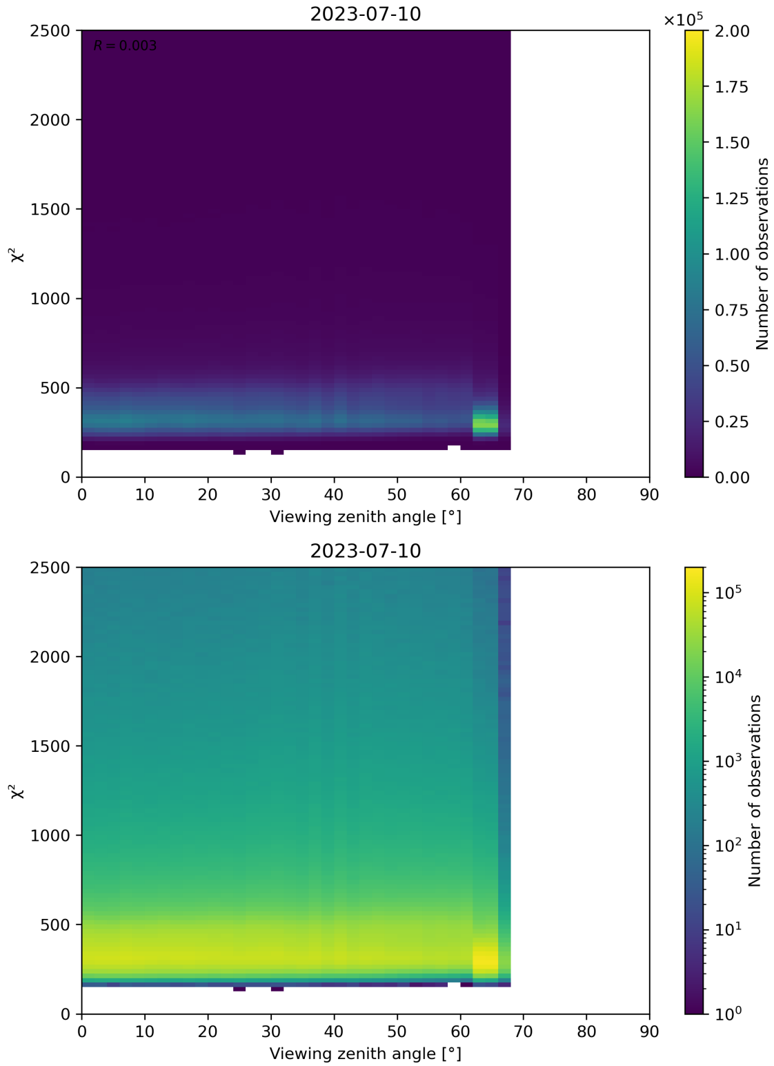
Figure 162: Scatter density plot of “Viewing zenith angle” against “ \chi^2 ” for 2023-07-09 to 2023-07-11.
