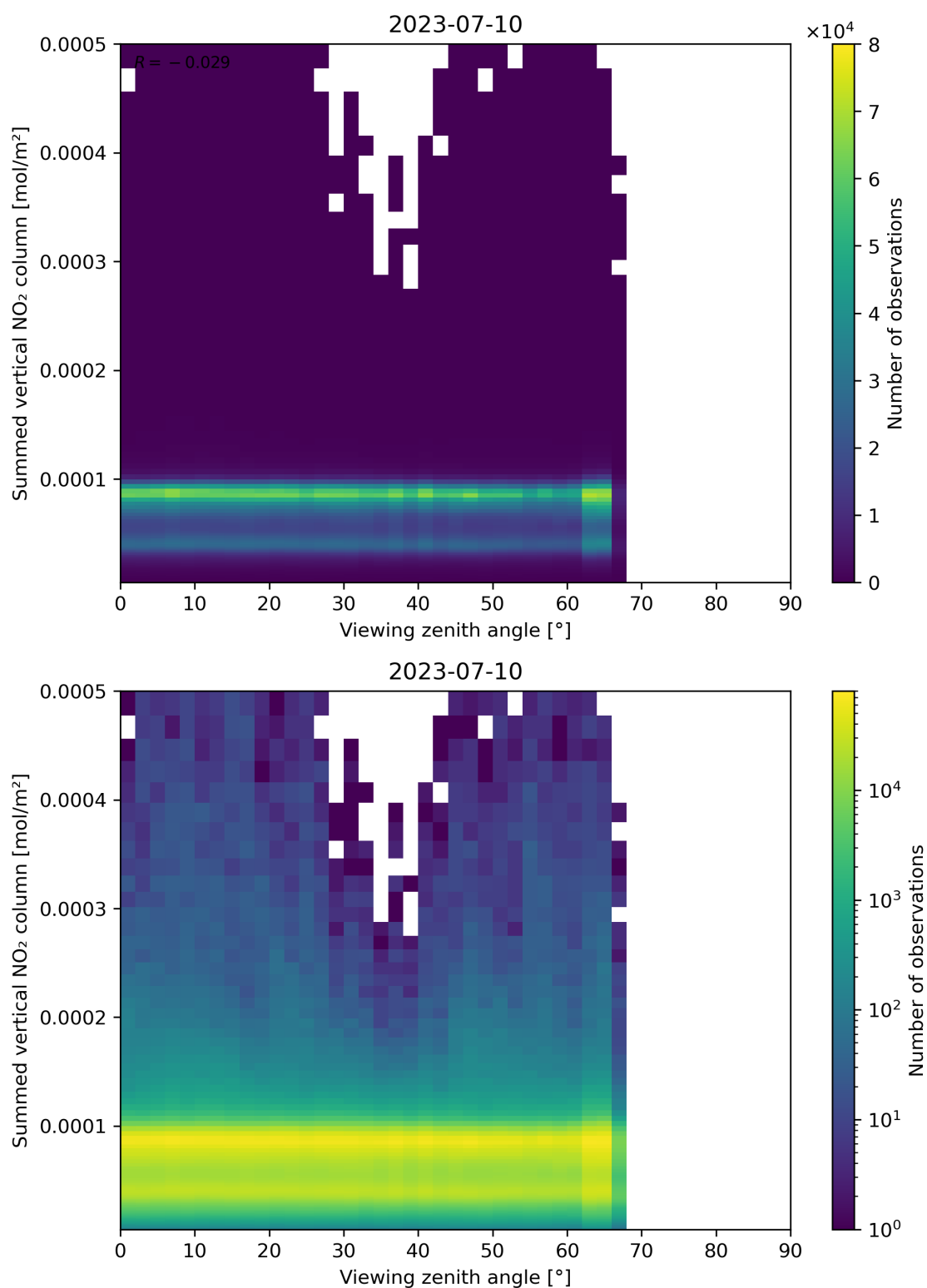
Figure 165: Scatter density plot of “Viewing zenith angle” against “Summed vertical NO 2 column” for 2023-07-09 to 2023-07-11.
