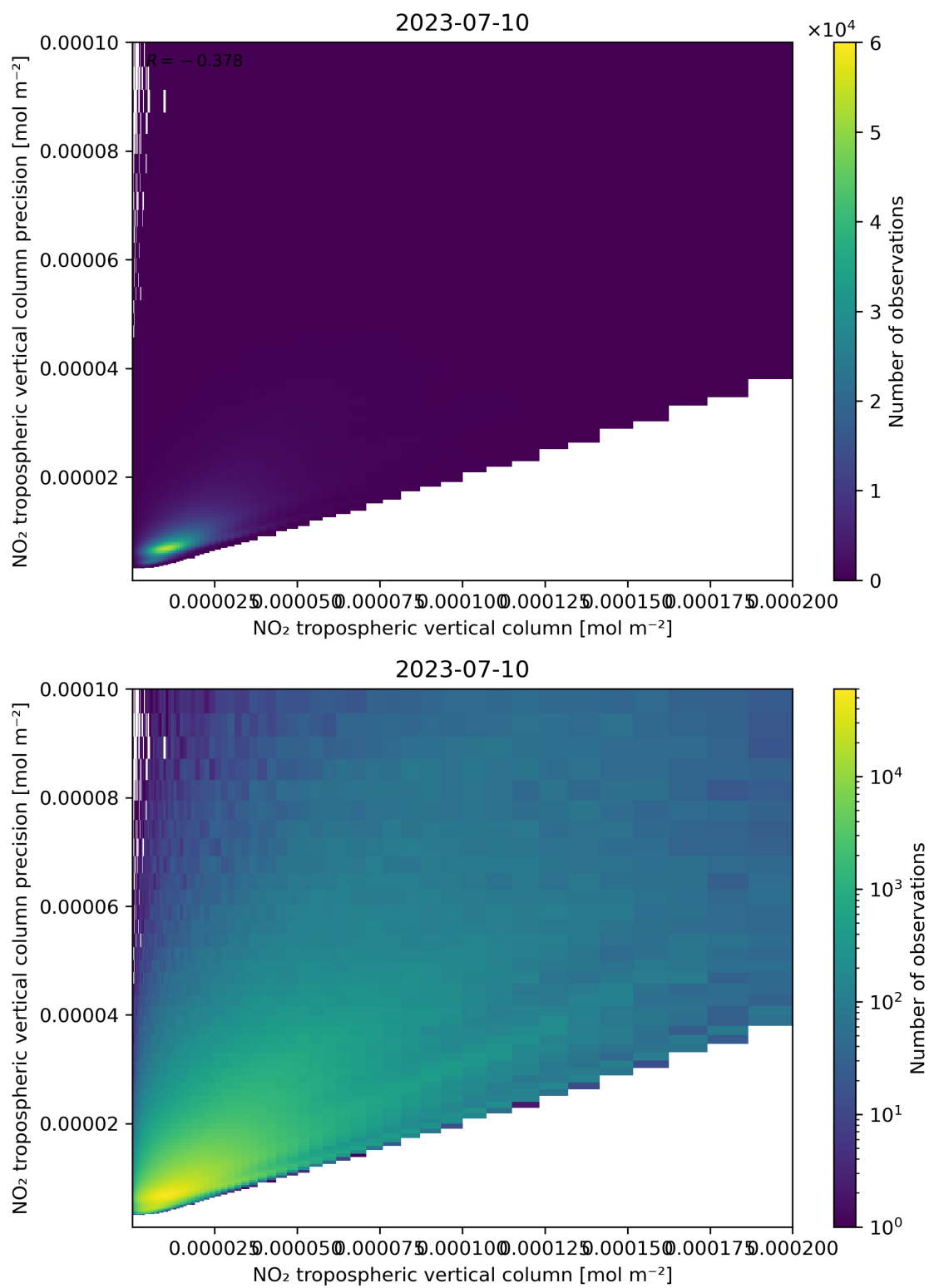
Figure 130: Scatter density plot of “NO 2 tropospheric vertical column” against “NO 2 tropospheric vertical column precision” for 2023-07-09 to 2023-07-11.
