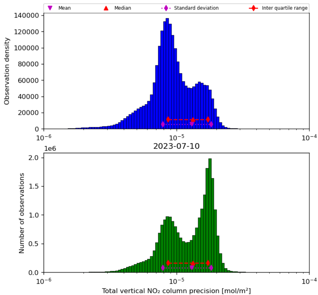
Figure 39: Histogram of “Total vertical NO 2 column precision” for 2023-07-09 to 2023-07-11
