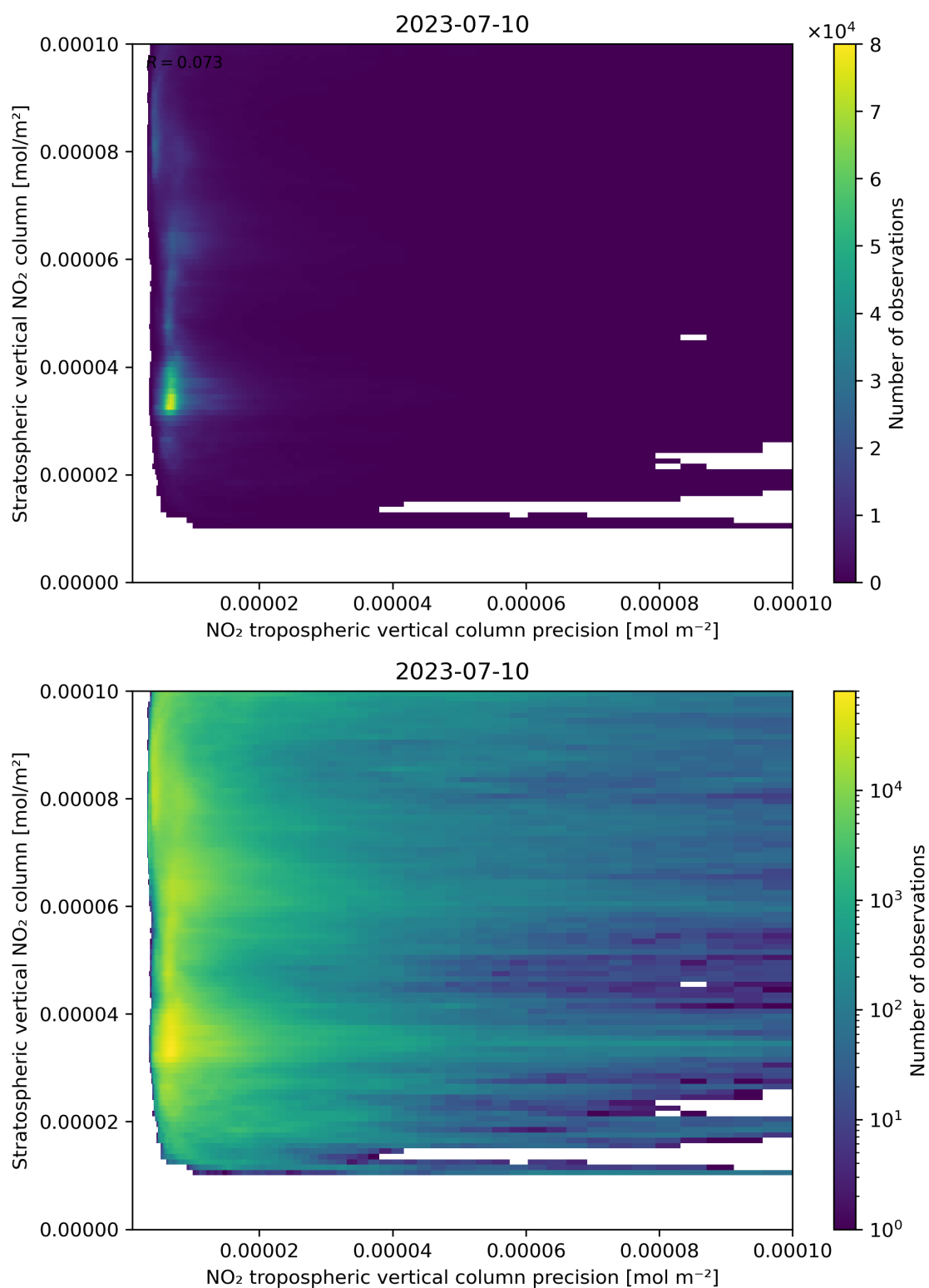
Figure 135: Scatter density plot of “NO 2 tropospheric vertical column precision” against “Stratospheric vertical NO 2 column” for 2023-07-09 to 2023-07-11.
