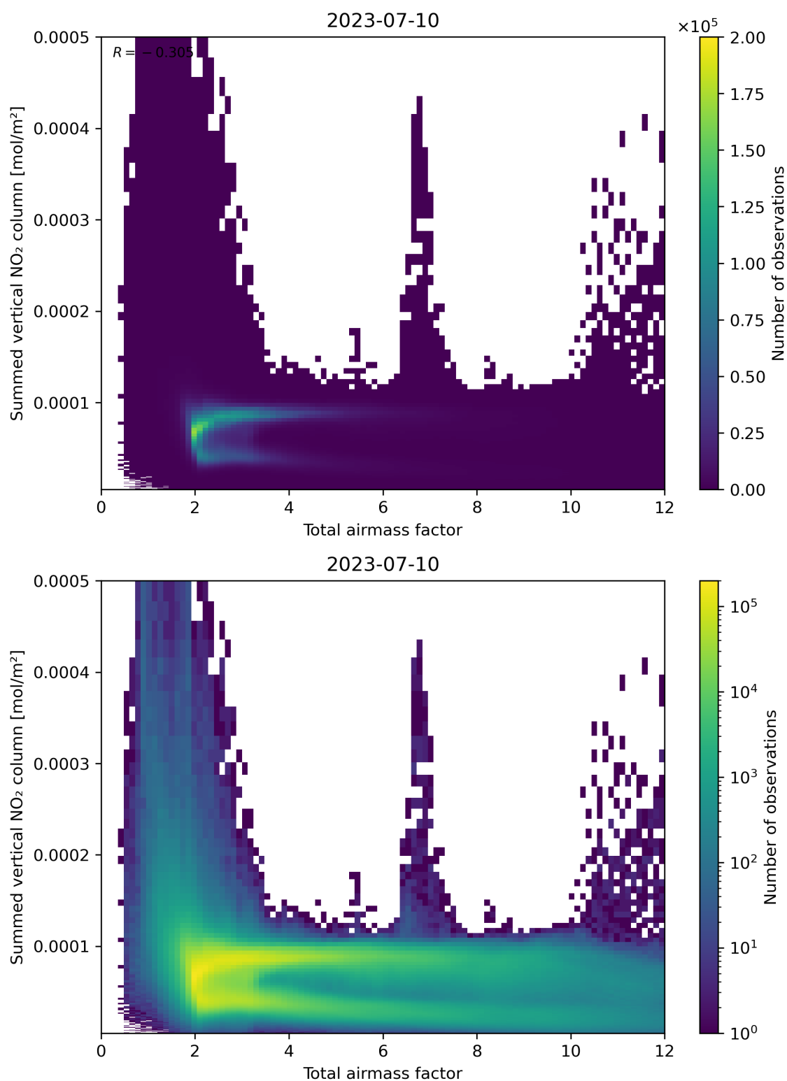
Figure 65: Scatter density plot of “Total airmass factor” against “Summed vertical NO 2 column” for 2023-07-09 to 2023-07-11.
