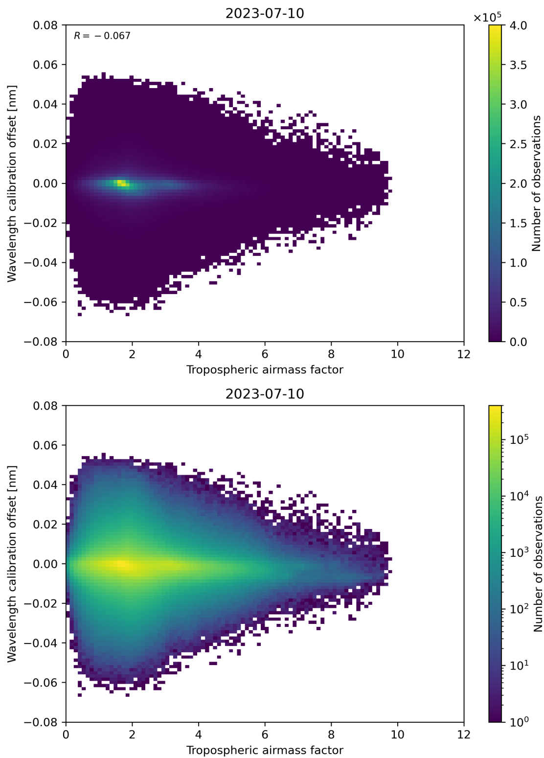
Figure 80: Scatter density plot of “Tropospheric airmass factor” against “Wavelength calibration offset” for 2023-07-09 to 2023-07-11.
