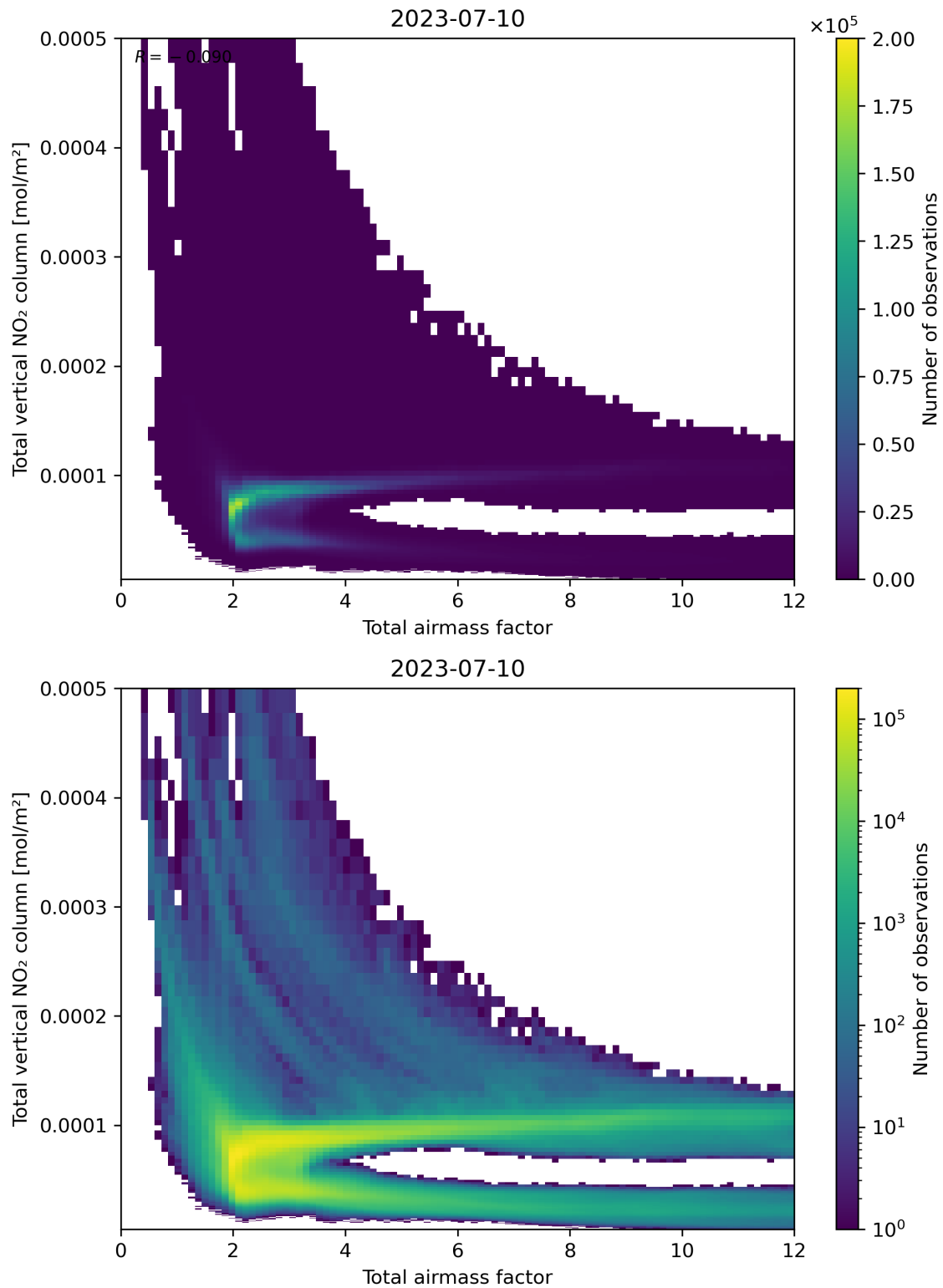
Figure 67: Scatter density plot of “Total airmass factor” against “Total vertical NO 2 column” for 2023-07-09 to 2023-07-11.
