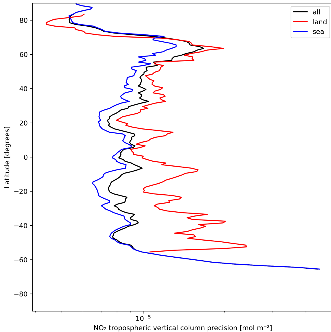
Figure 13: Zonal average of “NO 2 tropospheric vertical column precision” for 2023-07-09 to 2023-07-11.
