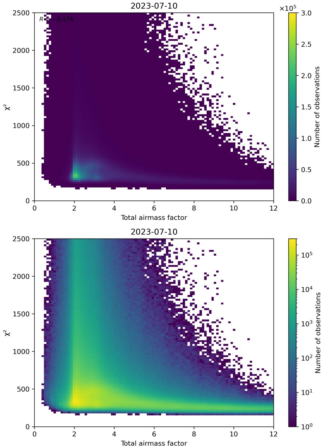
Figure 63: Scatter density plot of “Total airmass factor” against “ \chi^2 ” for 2023-07-09 to 2023-07-11.
