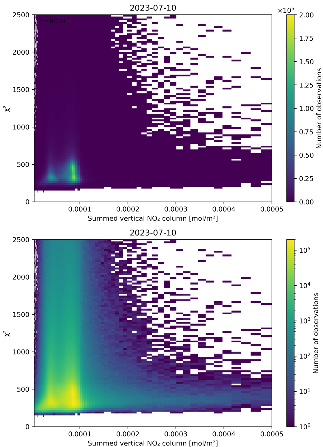
Figure 104: Scatter density plot of “Summed vertical NO 2 column” against “ \chi^2 ” for 2023-07-09 to 2023-07-11.
