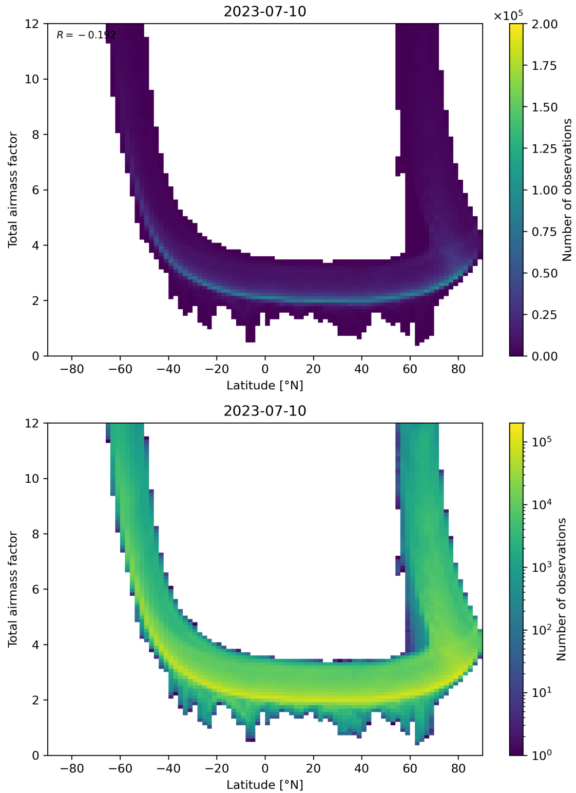
Figure 84: Scatter density plot of “Latitude” against “Total airmass factor” for 2023-07-09 to 2023-07-11.
