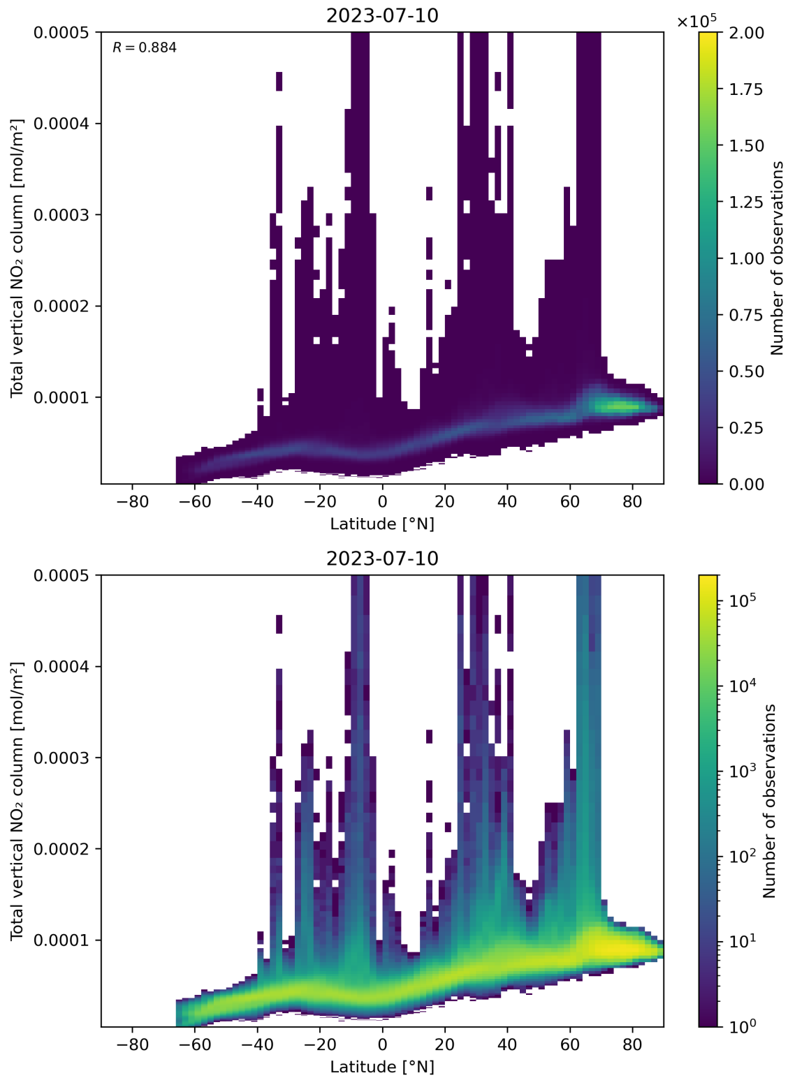
Figure 90: Scatter density plot of “Latitude” against “Total vertical NO 2 column” for 2023-07-09 to 2023-07-11.
