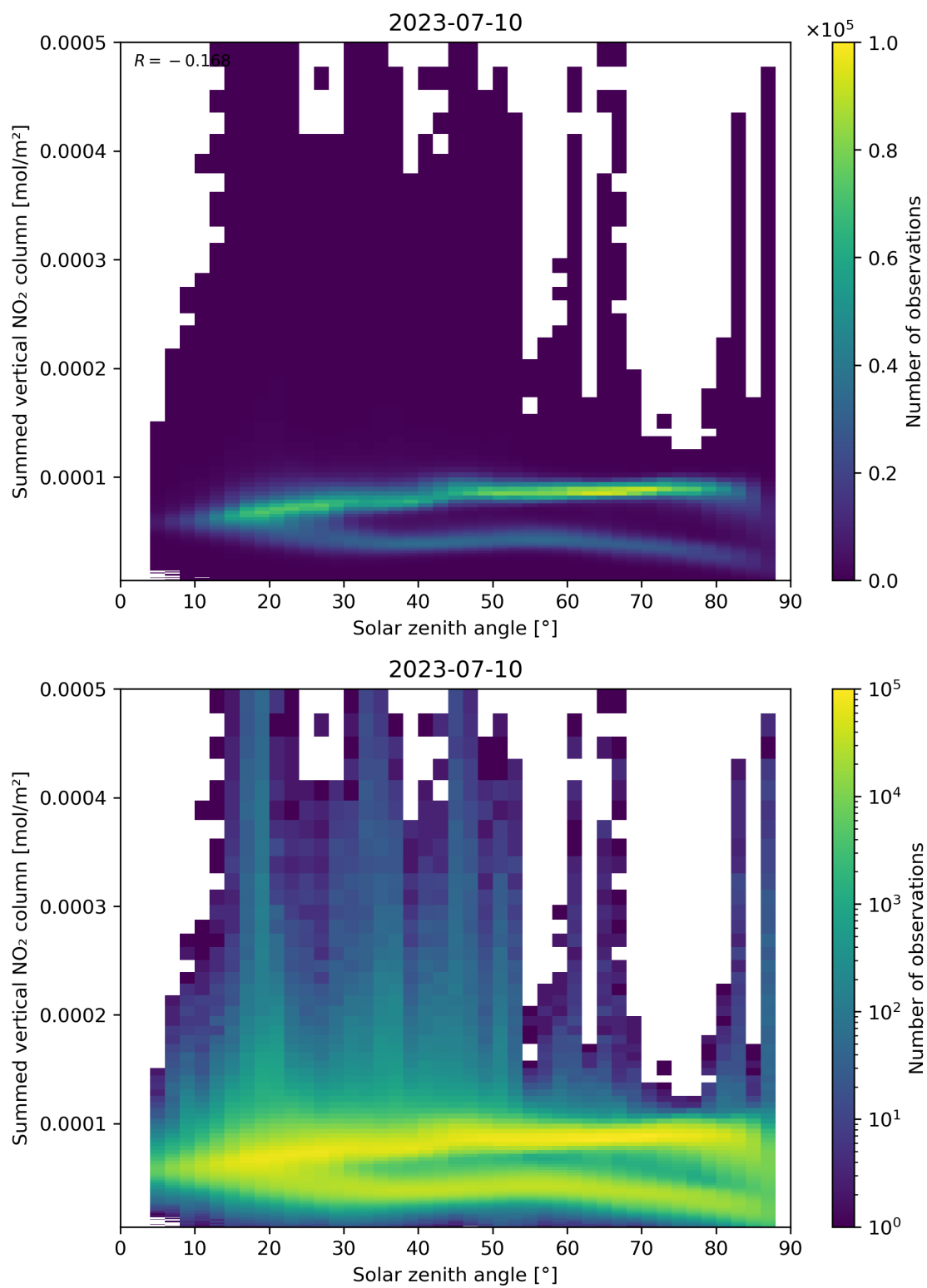
Figure 151: Scatter density plot of “Solar zenith angle” against “Summed vertical NO 2 column” for 2023-07-09 to 2023-07-11.
