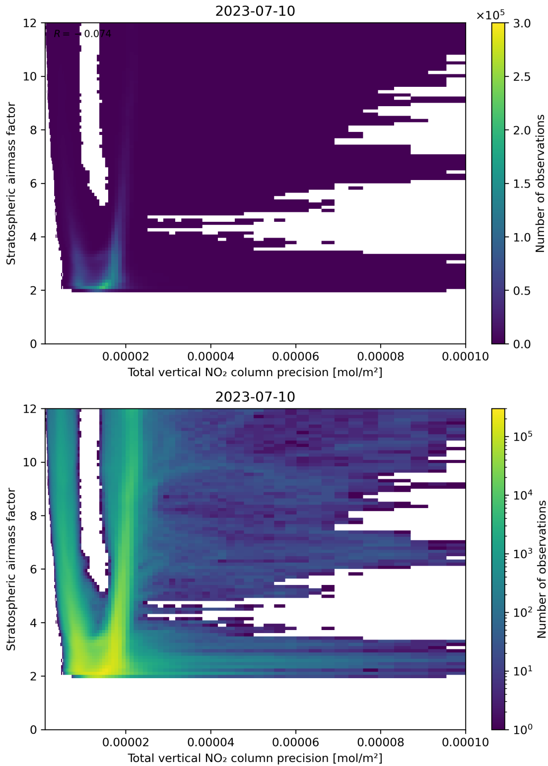
Figure 115: Scatter density plot of “Total vertical NO 2 column precision” against “Stratospheric airmass factor” for 2023-07-09 to 2023-07-11.
