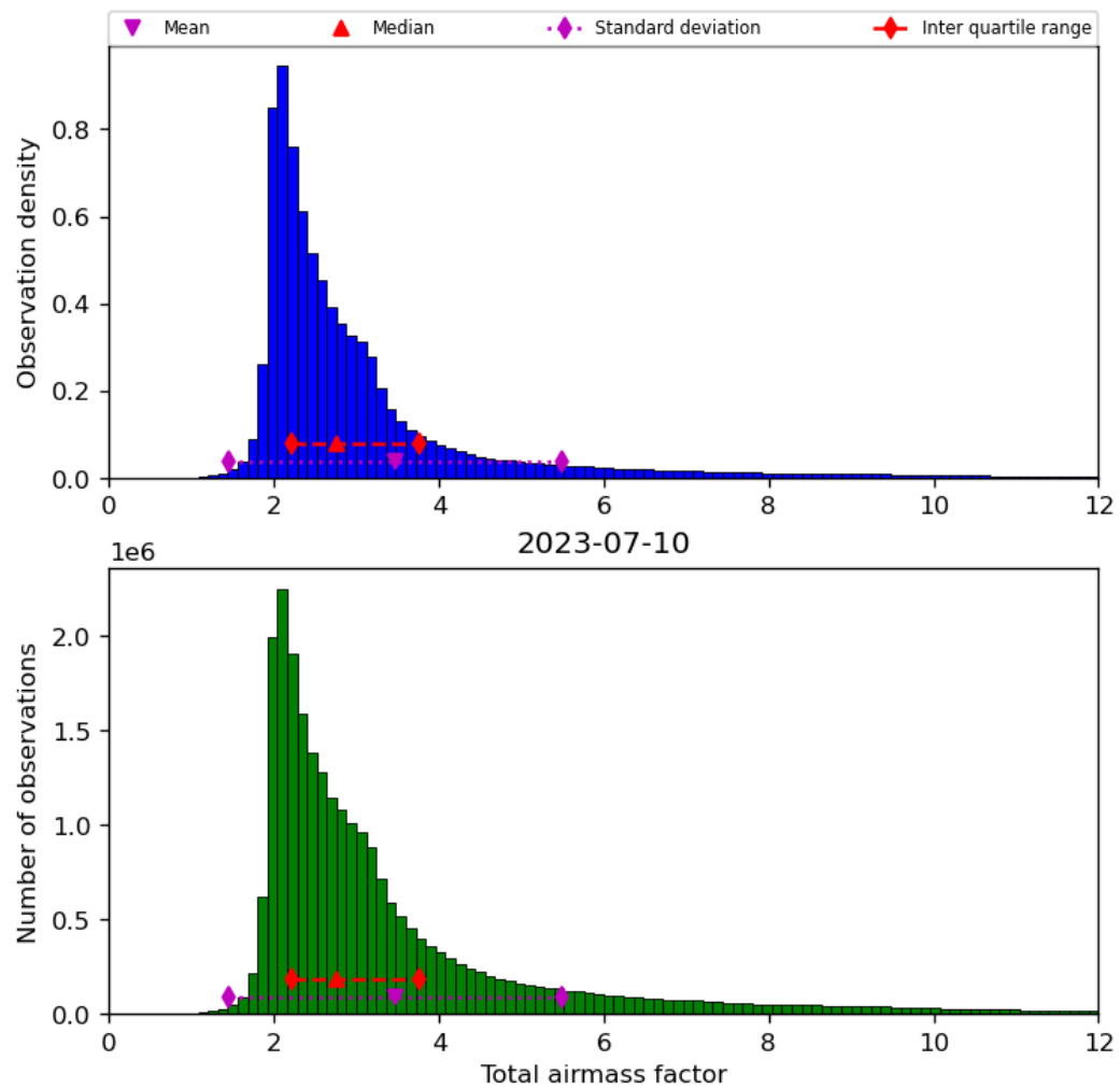
Figure 32: Histogram of “Total airmass factor” for 2023-07-09 to 2023-07-11
