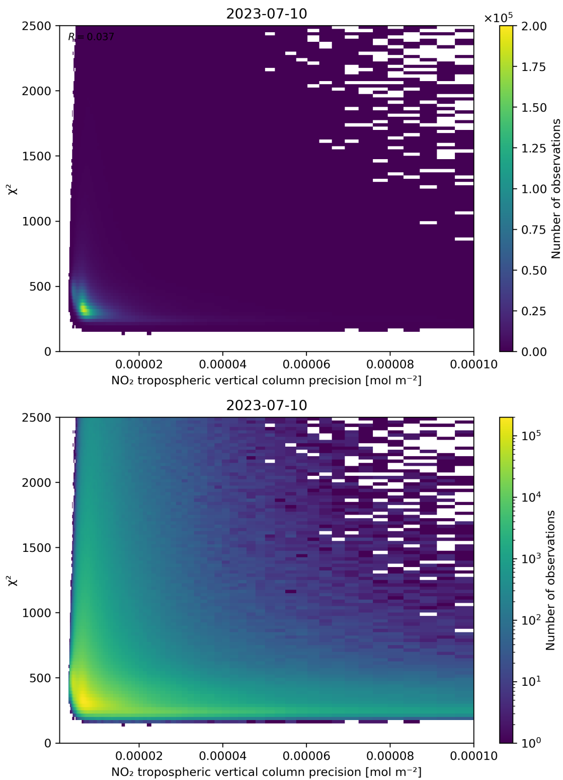
Figure 134: Scatter density plot of “NO 2 tropospheric vertical column precision” against “ \chi^2 ” for 2023-07-09 to 2023-07-11.
