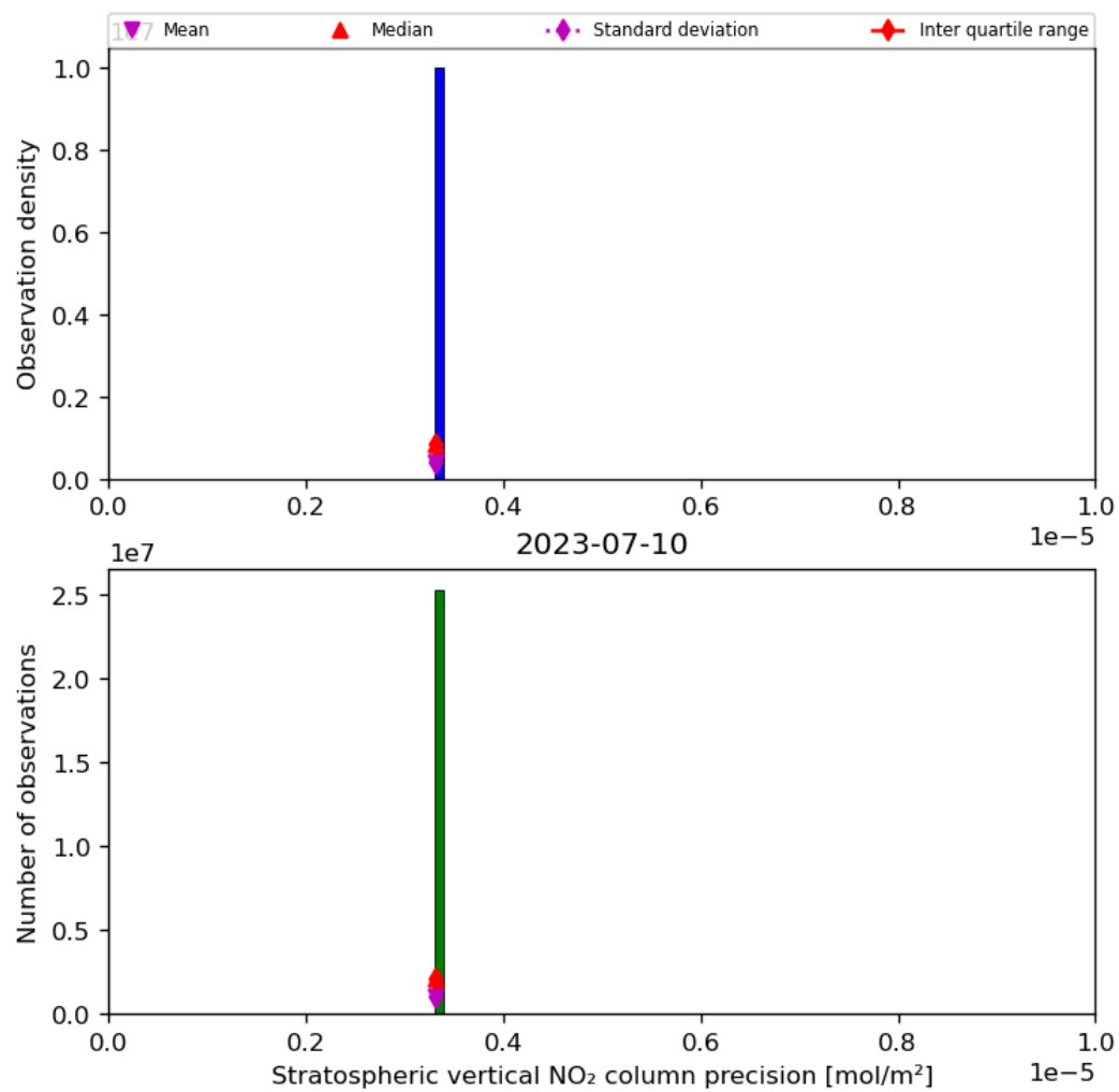
Figure 37: Histogram of “Stratospheric vertical NO 2 column precision” for 2023-07-09 to 2023-07-11
