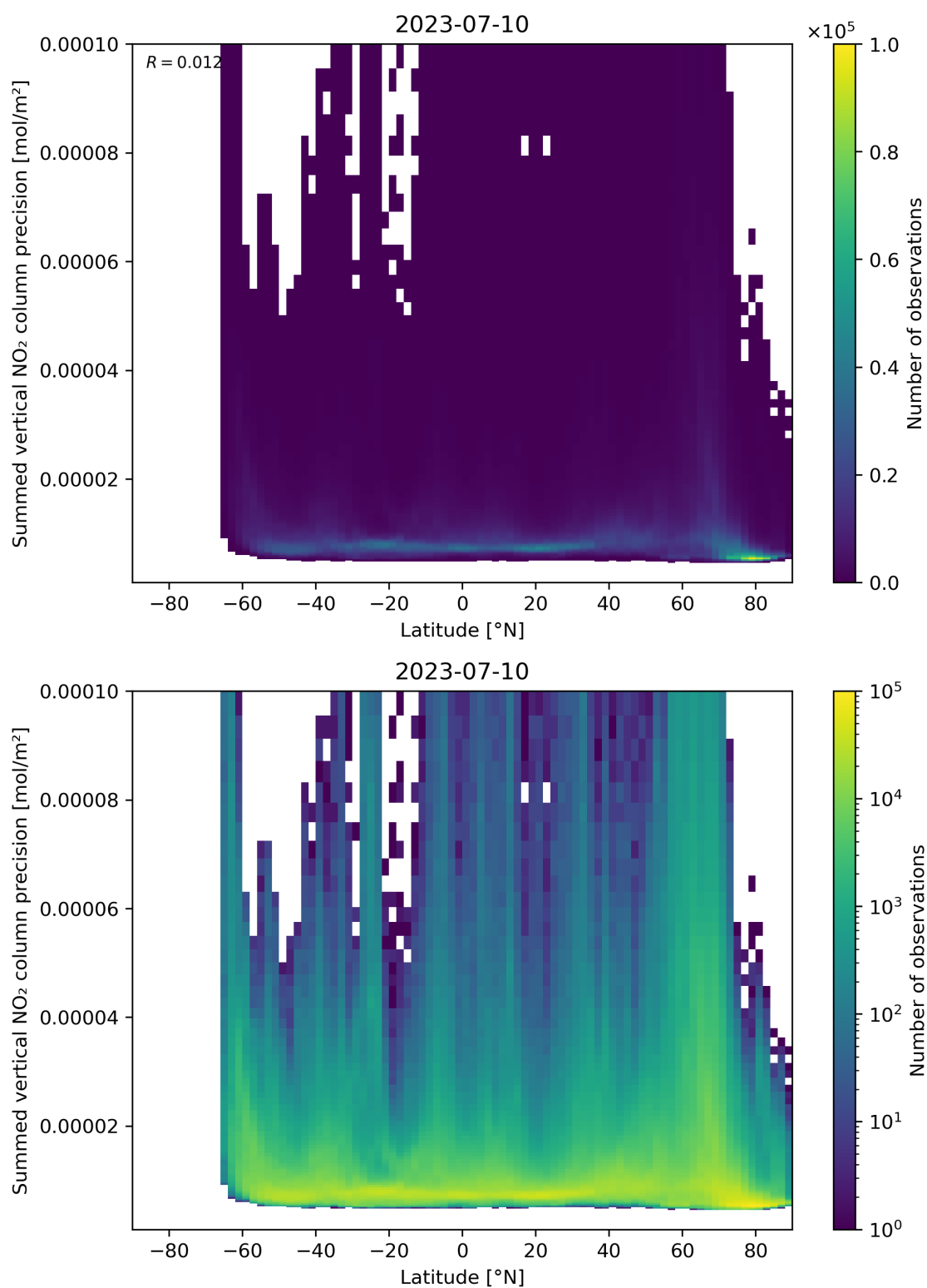
Figure 89: Scatter density plot of “Latitude” against “Summed vertical NO 2 column precision” for 2023-07-09 to 2023-07-11.
