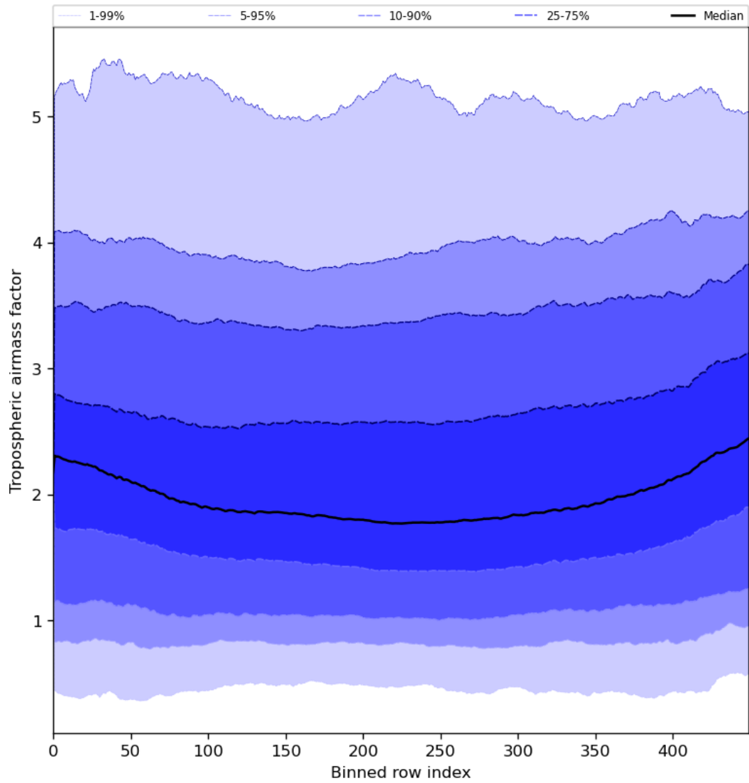
Figure 48: Along track statistics of “Tropospheric airmass factor” for 2023-07-09 to 2023-07-11
