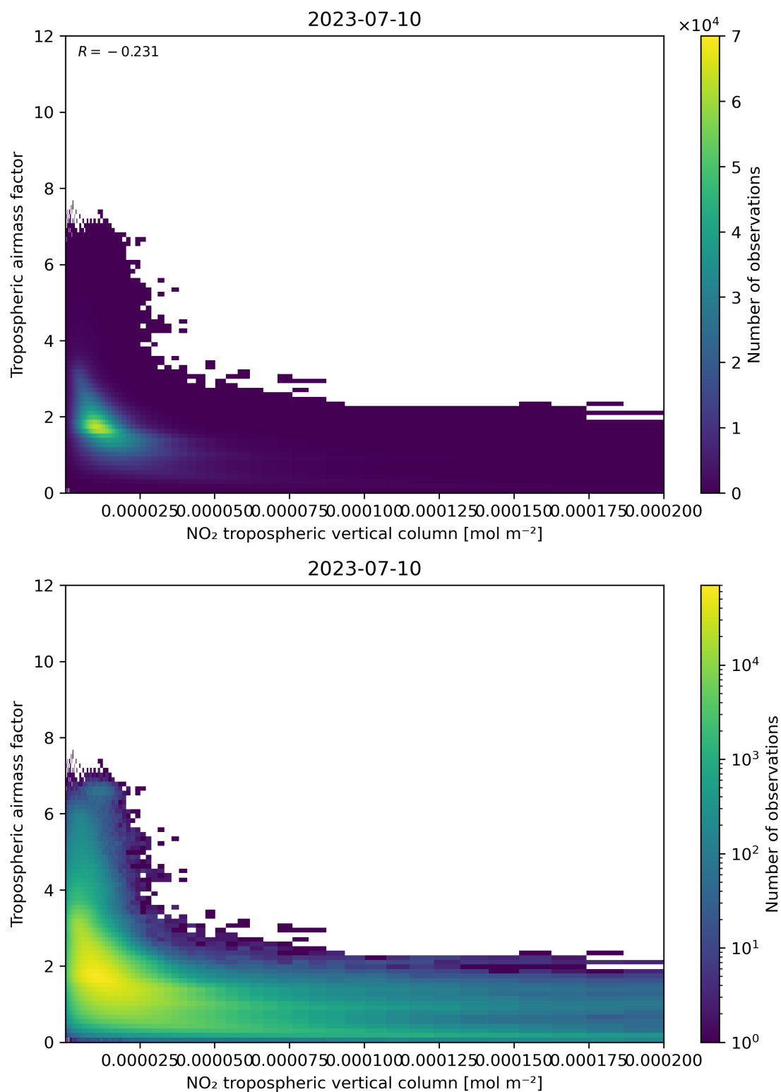
Figure 123: Scatter density plot of “NO 2 tropospheric vertical column” against “Tropospheric air mass factor” for 2023-07-09 to 2023-07-11.
