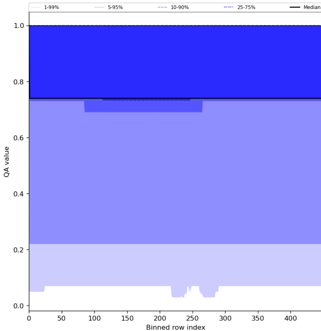
Figure 45: Along track statistics of “QA value” for 2023-07-09 to 2023-07-11
