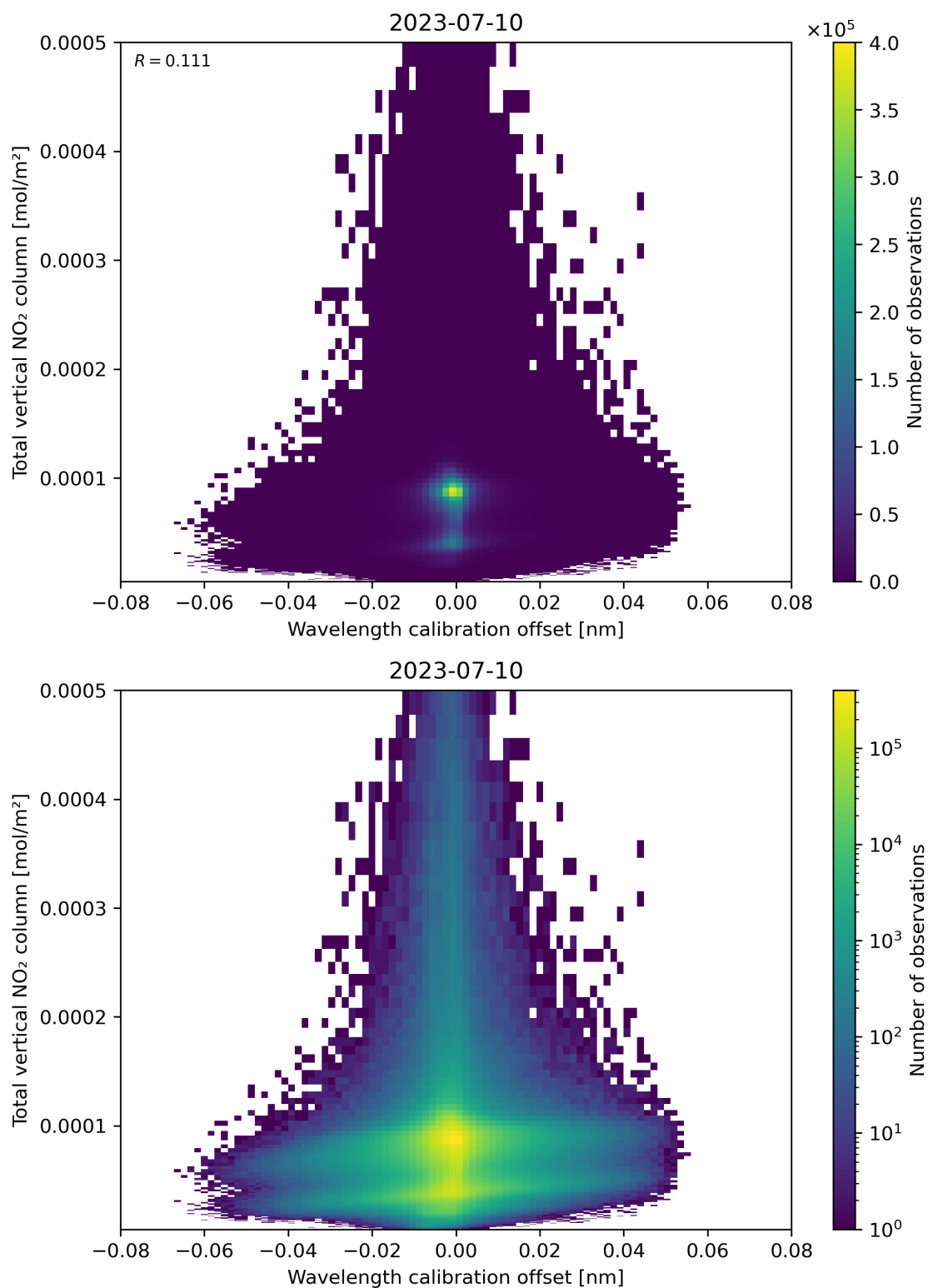
Figure 179: Scatter density plot of “Wavelength calibration offset” against “Total vertical NO 2 column” for 2023-07-09 to 2023-07-11.
