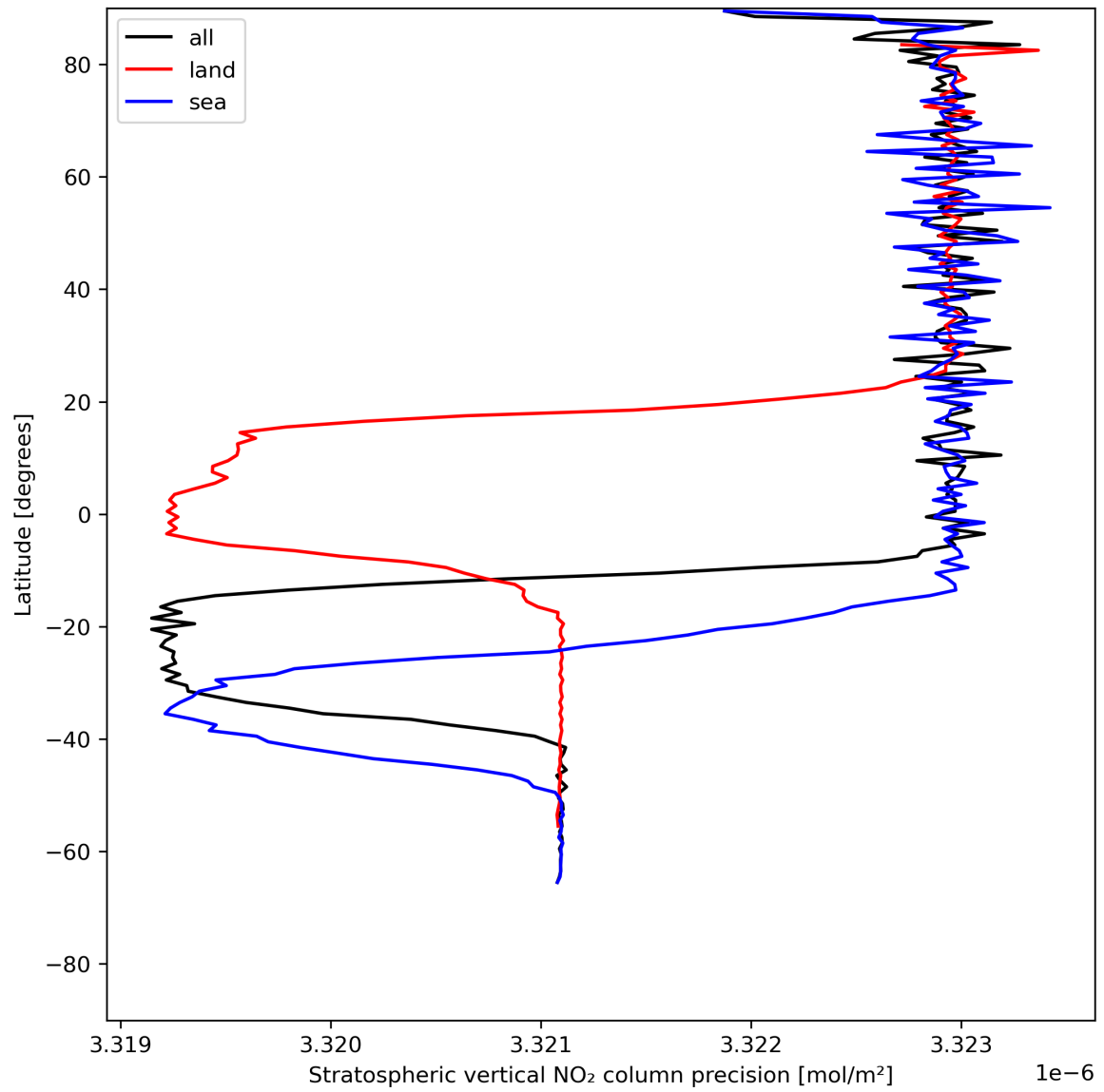
Figure 20: Zonal average of “Stratospheric vertical NO 2 column precision” for 2023-07-09 to 2023-07-11.
