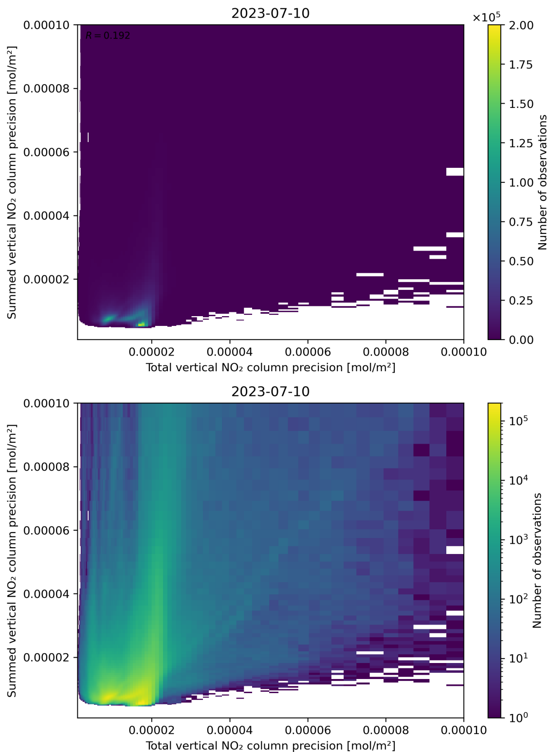
Figure 118: Scatter density plot of “Total vertical NO 2 column precision” against “Summed vertical NO 2 column precision” for 2023-07-09 to 2023-07-11.
