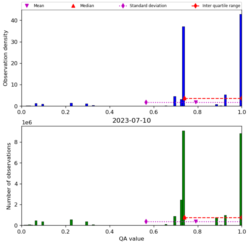
Figure 28: Histogram of “QA value” for 2023-07-09 to 2023-07-11
