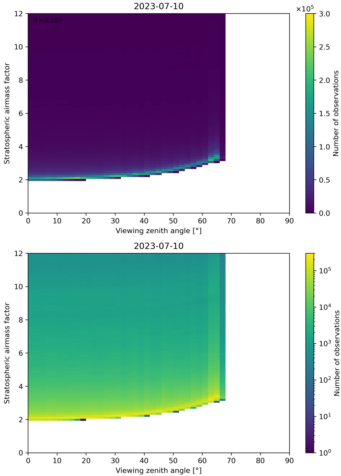
Figure 159: Scatter density plot of “Viewing zenith angle” against “Stratospheric airmass factor” for 2023-07-09 to 2023-07-11.
