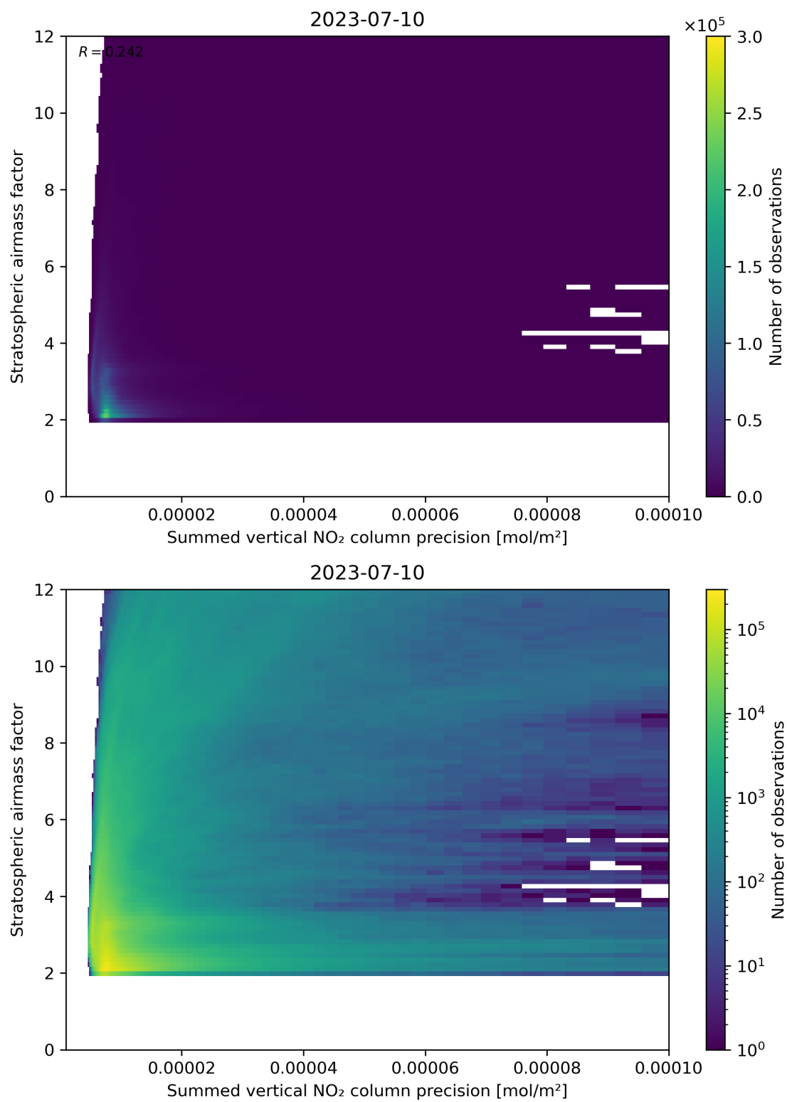
Figure 106: Scatter density plot of “Summed vertical NO 2 column precision” against “Stratospheric airmass factor” for 2023-07-09 to 2023-07-11.
