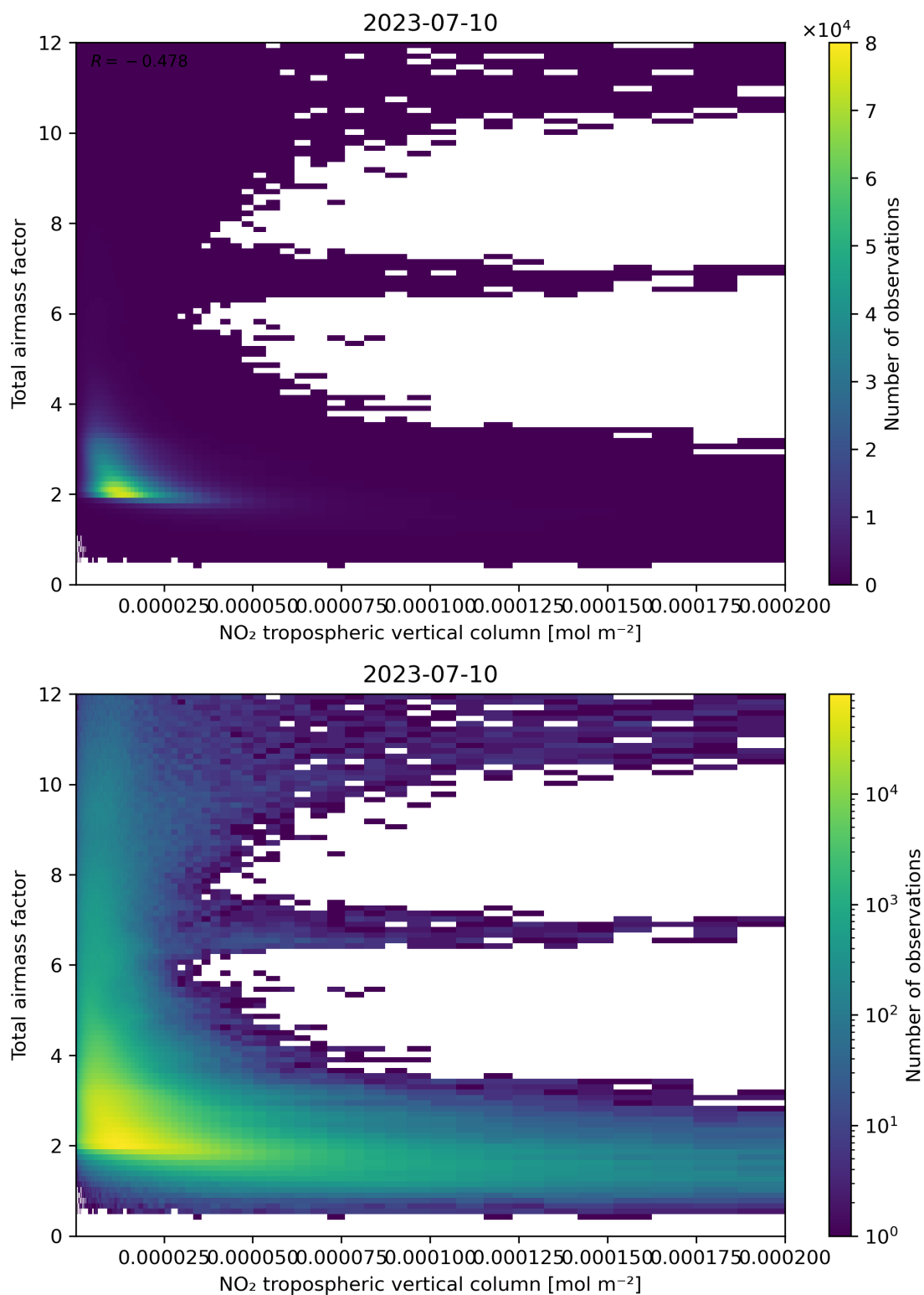
Figure 122: Scatter density plot of “NO 2 tropospheric vertical column” against “Total air mass factor” for 2023-07-09 to 2023-07-11.
