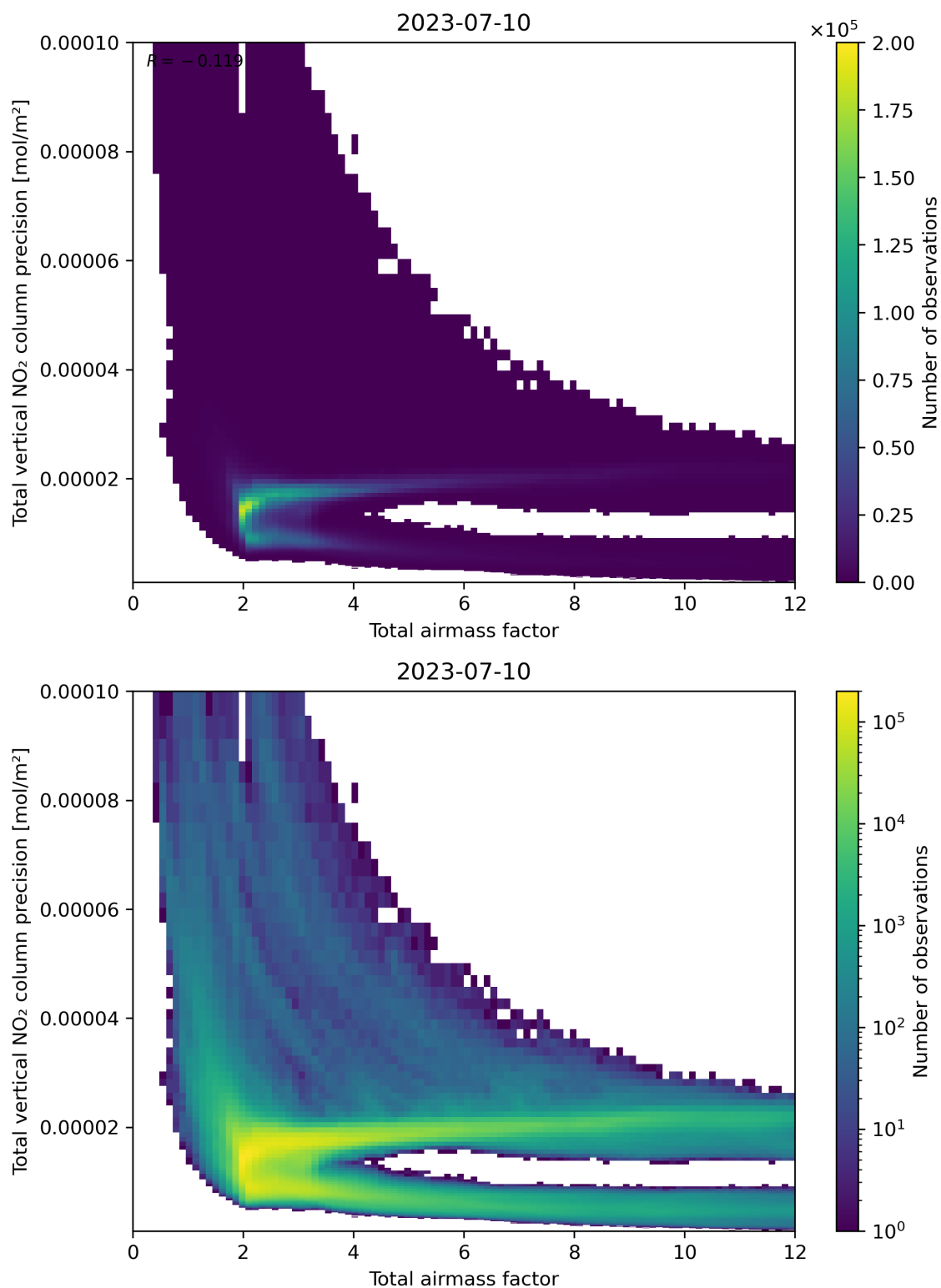
Figure 68: Scatter density plot of “Total airmass factor” against “Total vertical NO 2 column precision” for 2023-07-09 to 2023-07-11.
