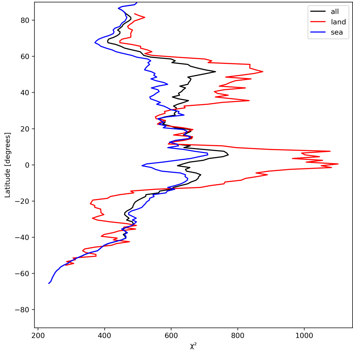
Figure 25: Zonal average of “ \chi^2 ” for 2023-07-09 to 2023-07-11.
