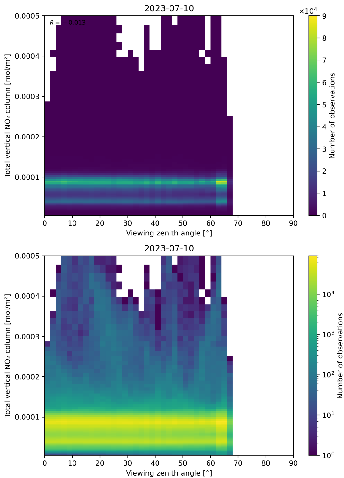
Figure 167: Scatter density plot of “Viewing zenith angle” against “Total vertical NO 2 column” for 2023-07-09 to 2023-07-11.
