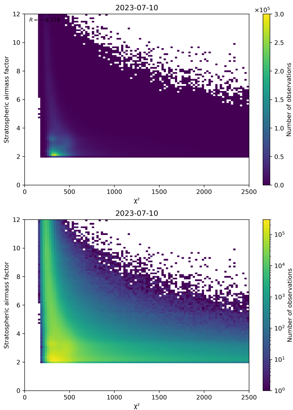
Figure 81: Scatter density plot of “ \chi^2 ” against “Stratospheric airmass factor” for 2023-07-09 to 2023-07-11.
