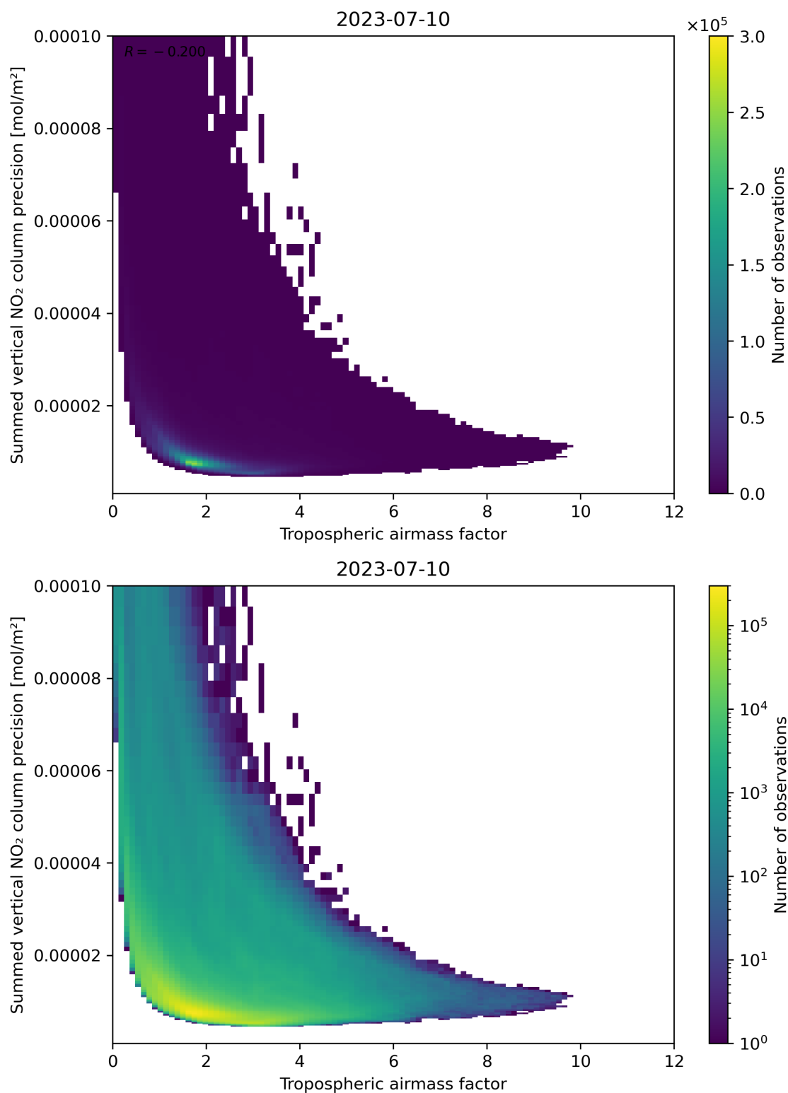
Figure 76: Scatter density plot of “Tropospheric air mass factor” against “Summed vertical NO 2 column precision” for 2023-07-09 to 2023-07-11.
