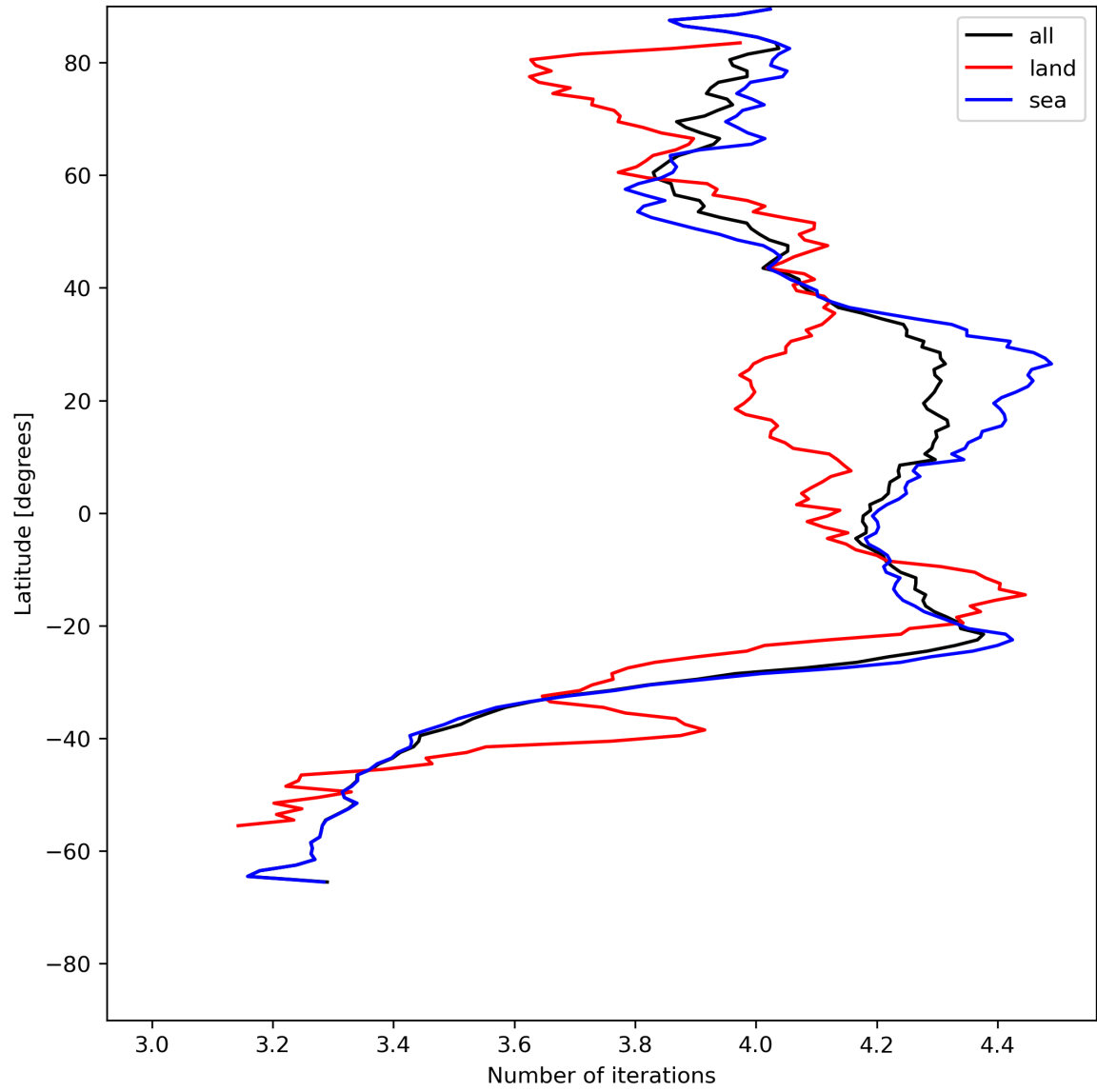
Figure 17: Zonal average of “Number of iterations” for 2023-07-09 to 2023-07-11.
