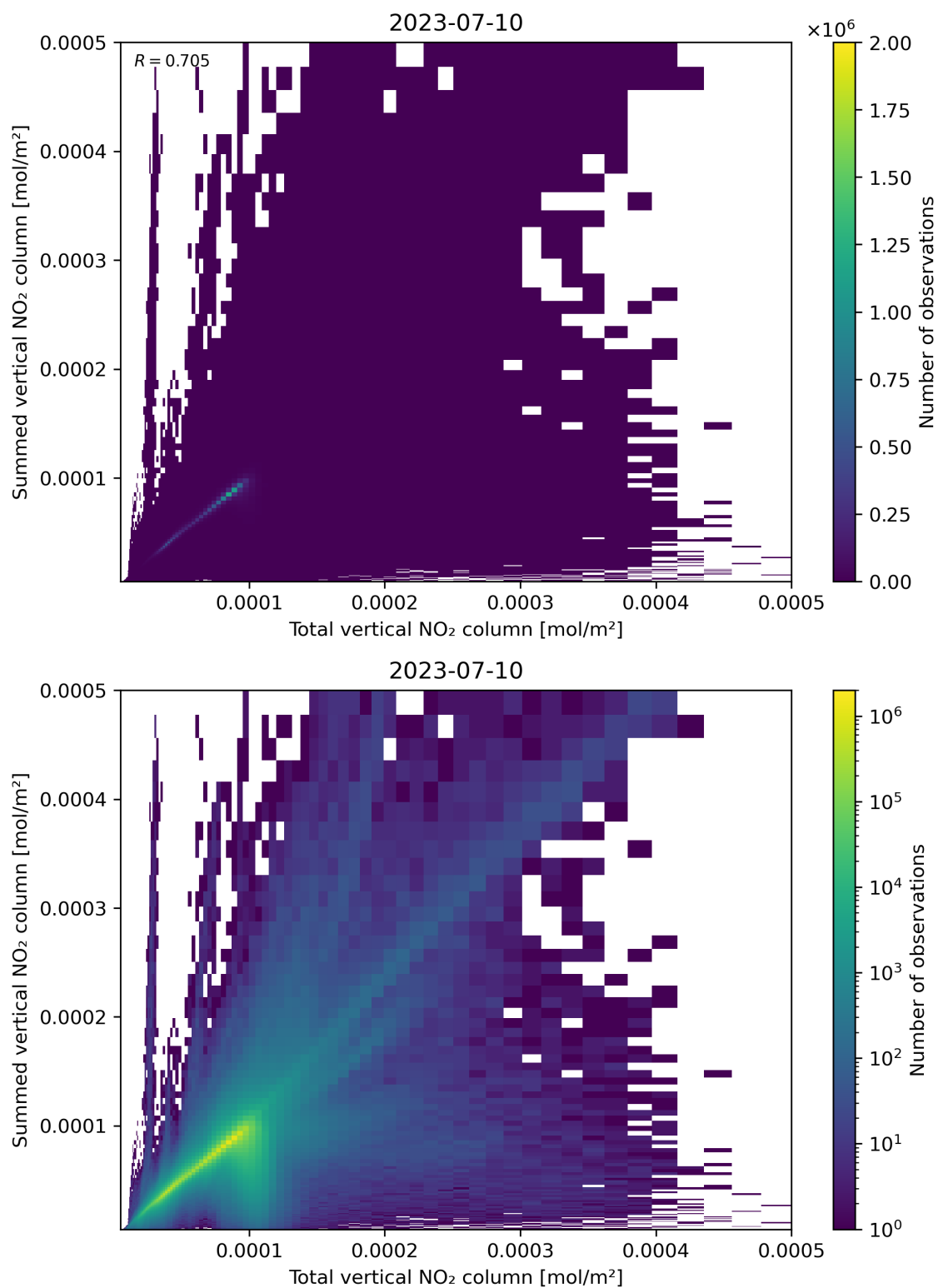
Figure 112: Scatter density plot of “Total vertical NO 2 column” against “Summed vertical NO 2 column” for 2023-07-09 to 2023-07-11.
