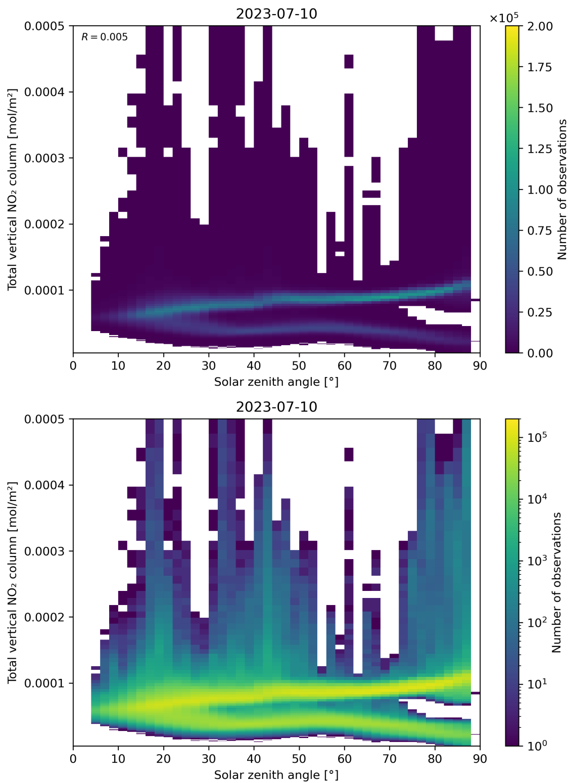
Figure 153: Scatter density plot of “Solar zenith angle” against “Total vertical NO 2 column” for 2023-07-09 to 2023-07-11.
