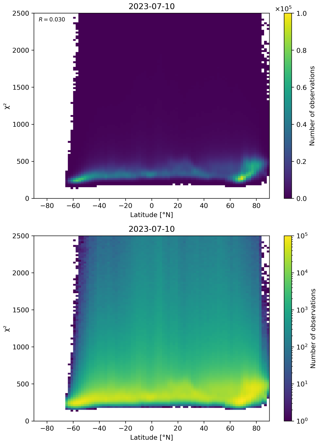
Figure 86: Scatter density plot of “Latitude” against “ \chi^2 ” for 2023-07-09 to 2023-07-11.
