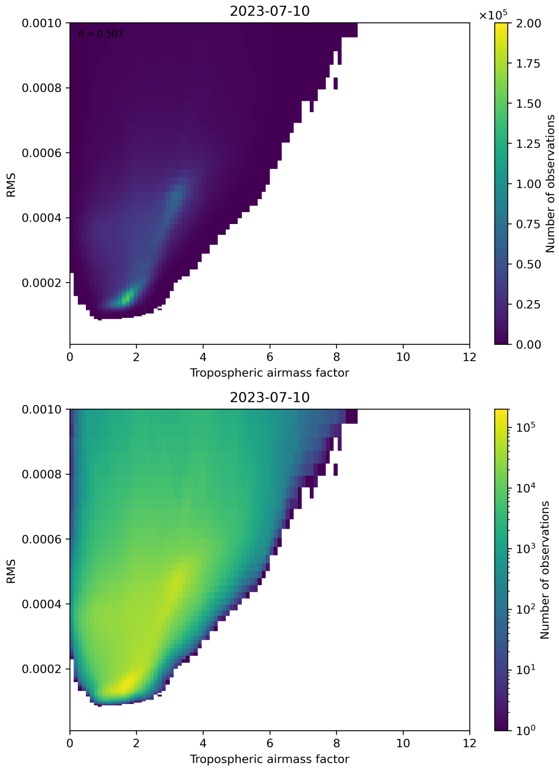
Figure 79: Scatter density plot of “Tropospheric airmass factor” against “RMS” for 2023-07-09 to 2023-07-11.
