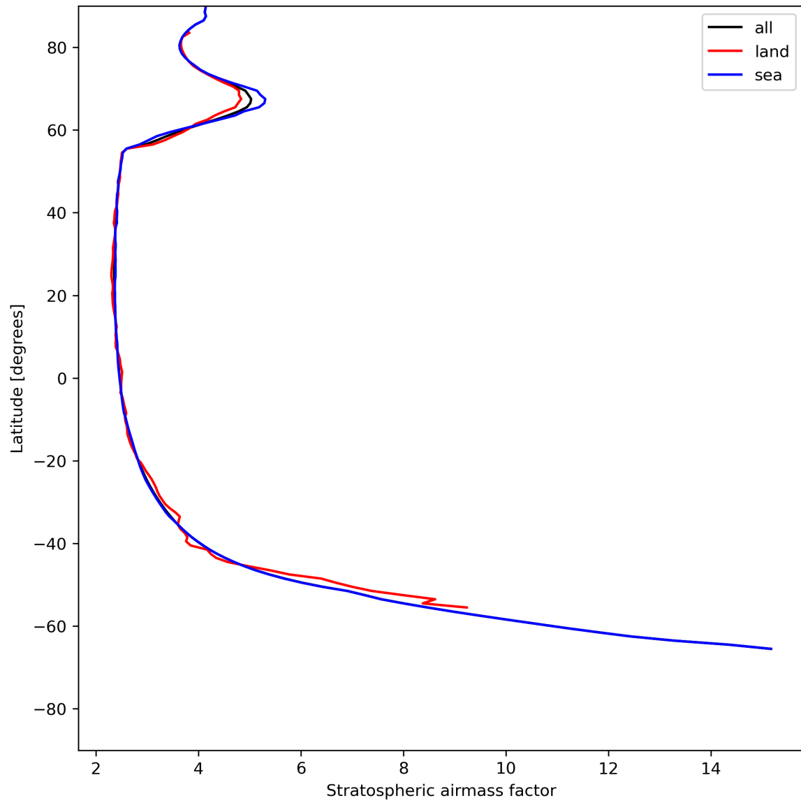
Figure 27: Zonal average of “Stratospheric airmass factor” for 2023-07-09 to 2023-07-11.
