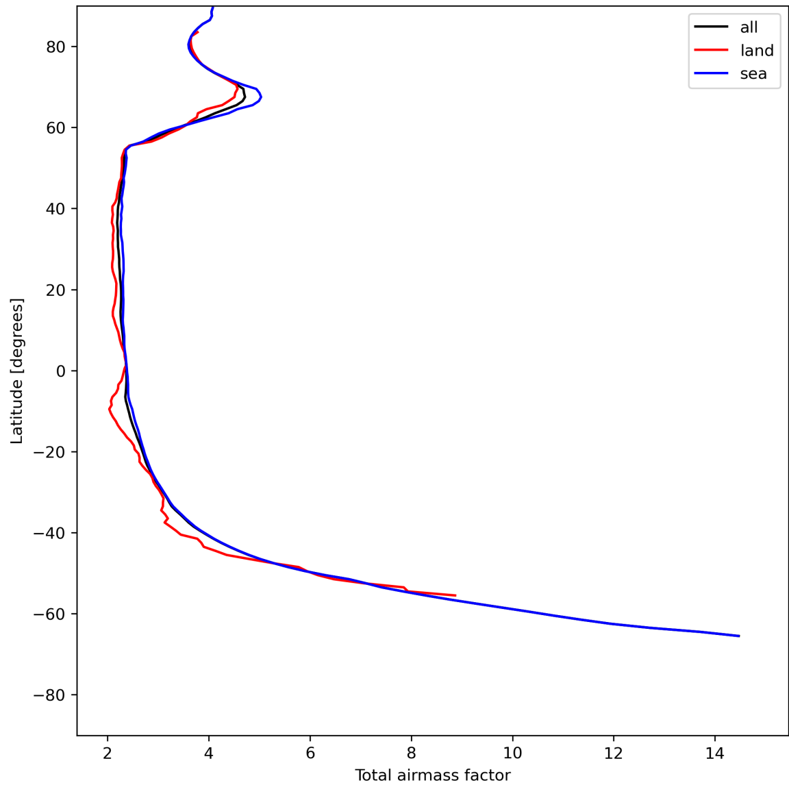
Figure 15: Zonal average of “Total airmass factor” for 2023-07-09 to 2023-07-11.
