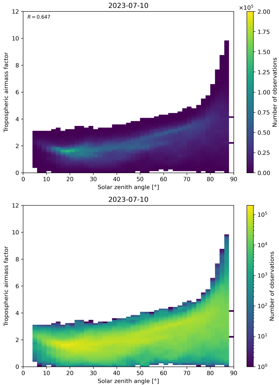
Figure 147: Scatter density plot of “Solar zenith angle” against “Tropospheric airmass factor” for 2023-07-09 to 2023-07-11.
