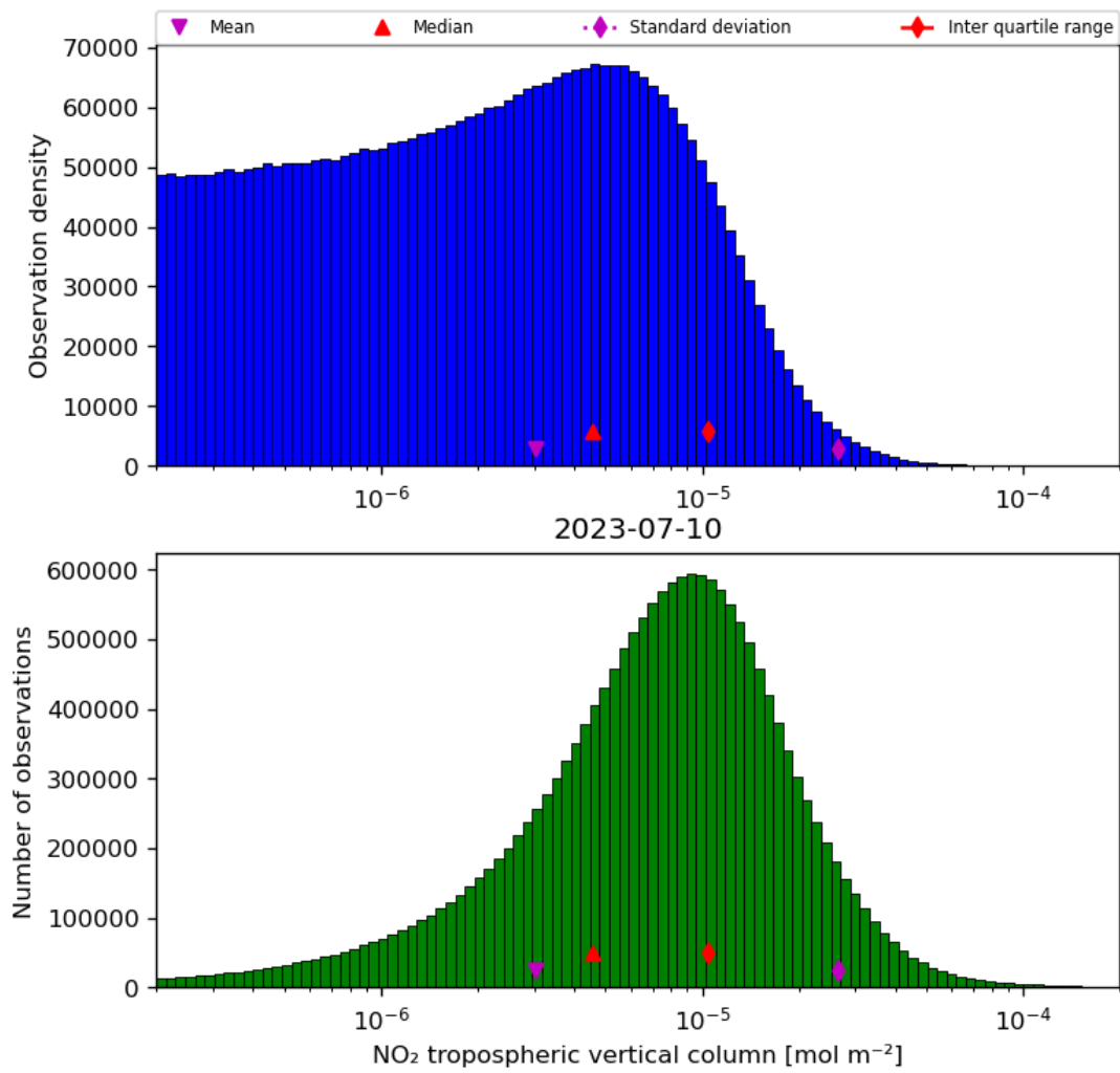
Figure 29: Histogram of “NO 2 tropospheric vertical column” for 2023-07-09 to 2023-07-11
