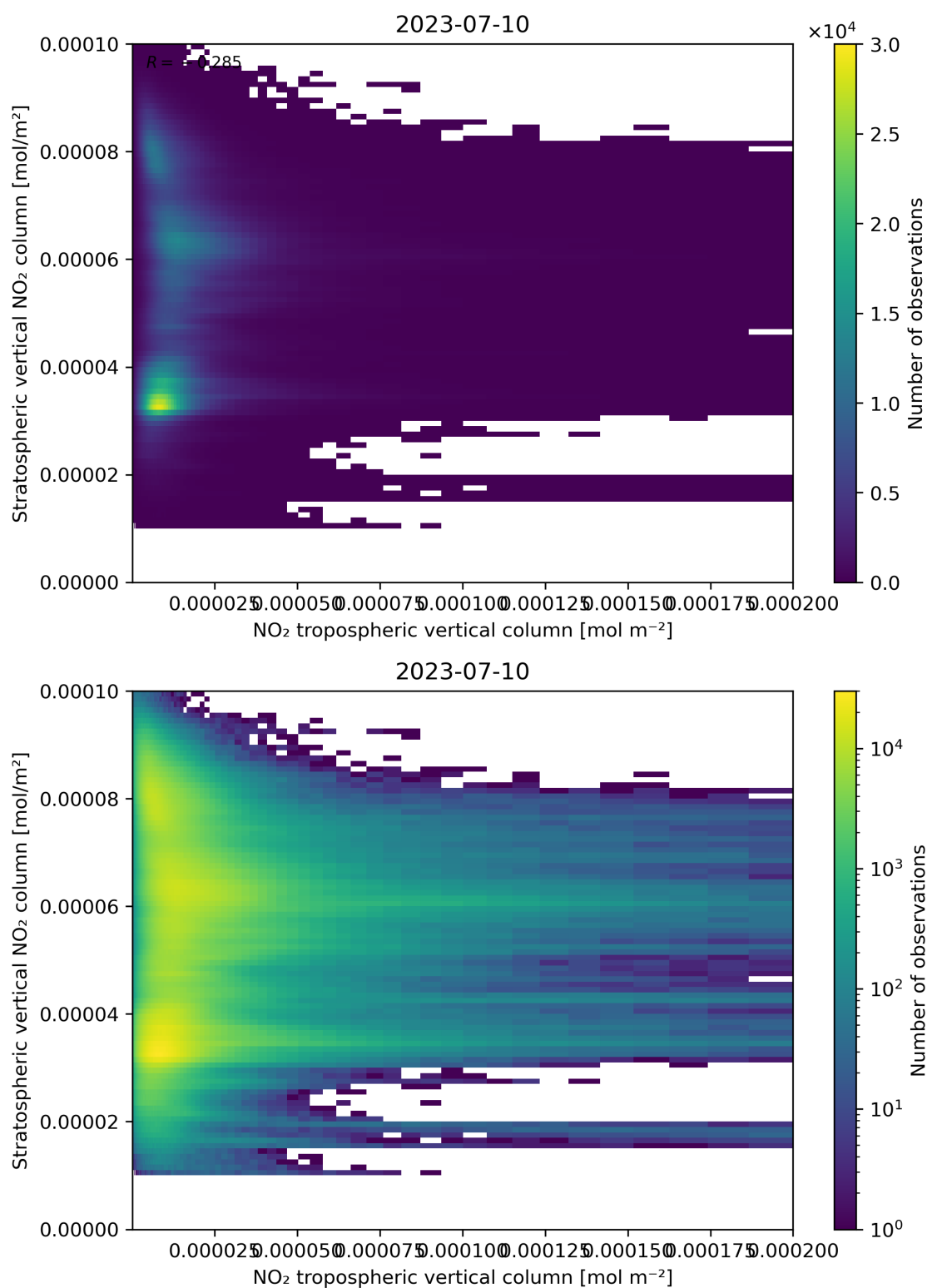
Figure 125: Scatter density plot of “NO 2 tropospheric vertical column” against “Stratospheric vertical NO 2 column” for 2023-07-09 to 2023-07-11.
