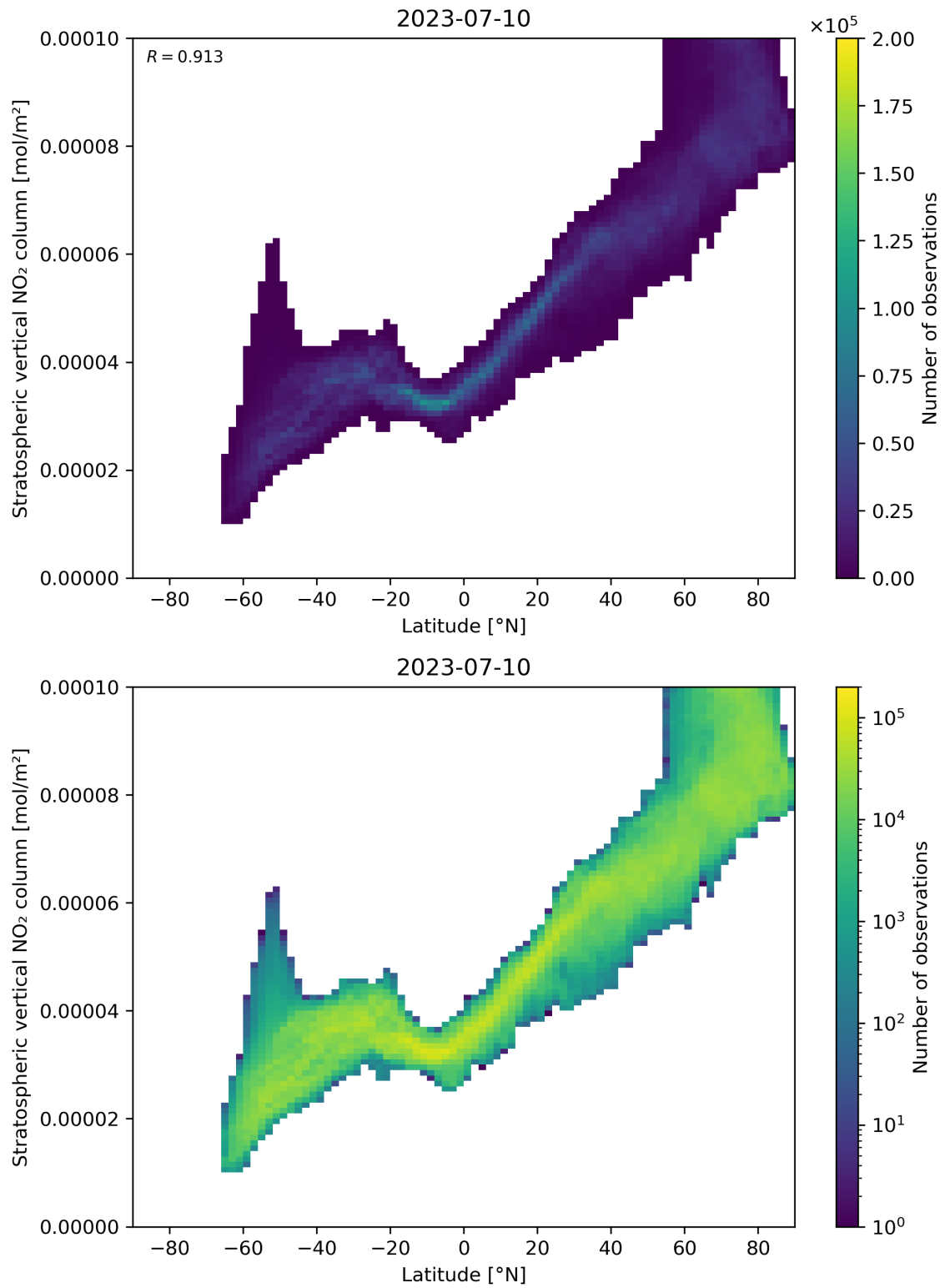
Figure 87: Scatter density plot of “Latitude” against “Stratospheric vertical \text{NO}_2 column” for 2023-07-09 to 2023-07-11.
