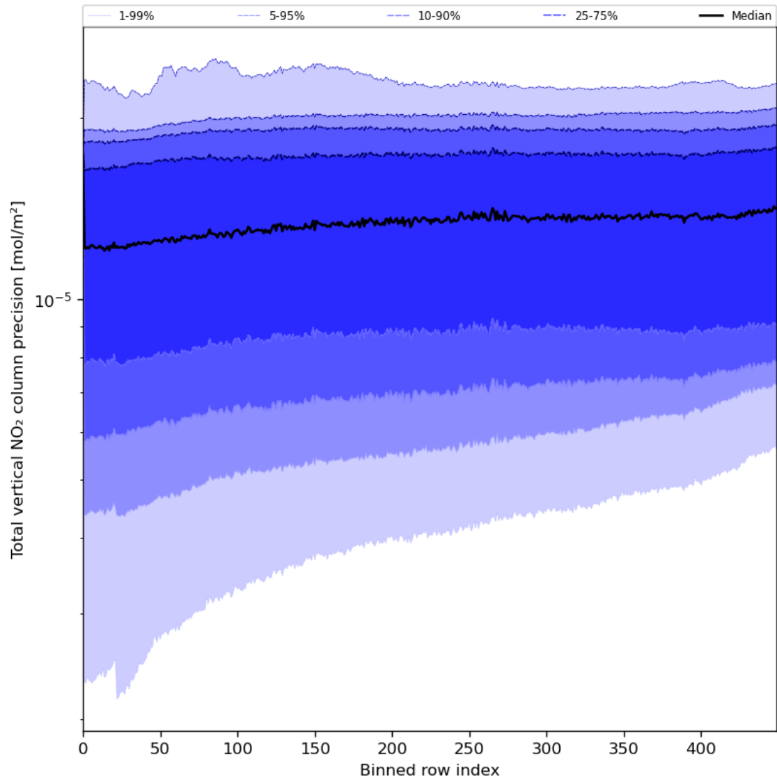
Figure 56: Along track statistics of “Total vertical NO 2 column precision” for 2023-07-09 to 2023-07-11
