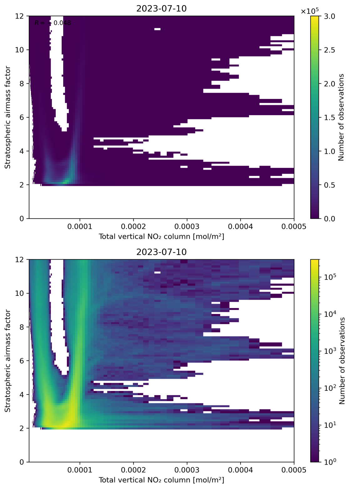
Figure 110: Scatter density plot of “Total vertical NO 2 column” against “Stratospheric air mass factor” for 2023-07-09 to 2023-07-11.
