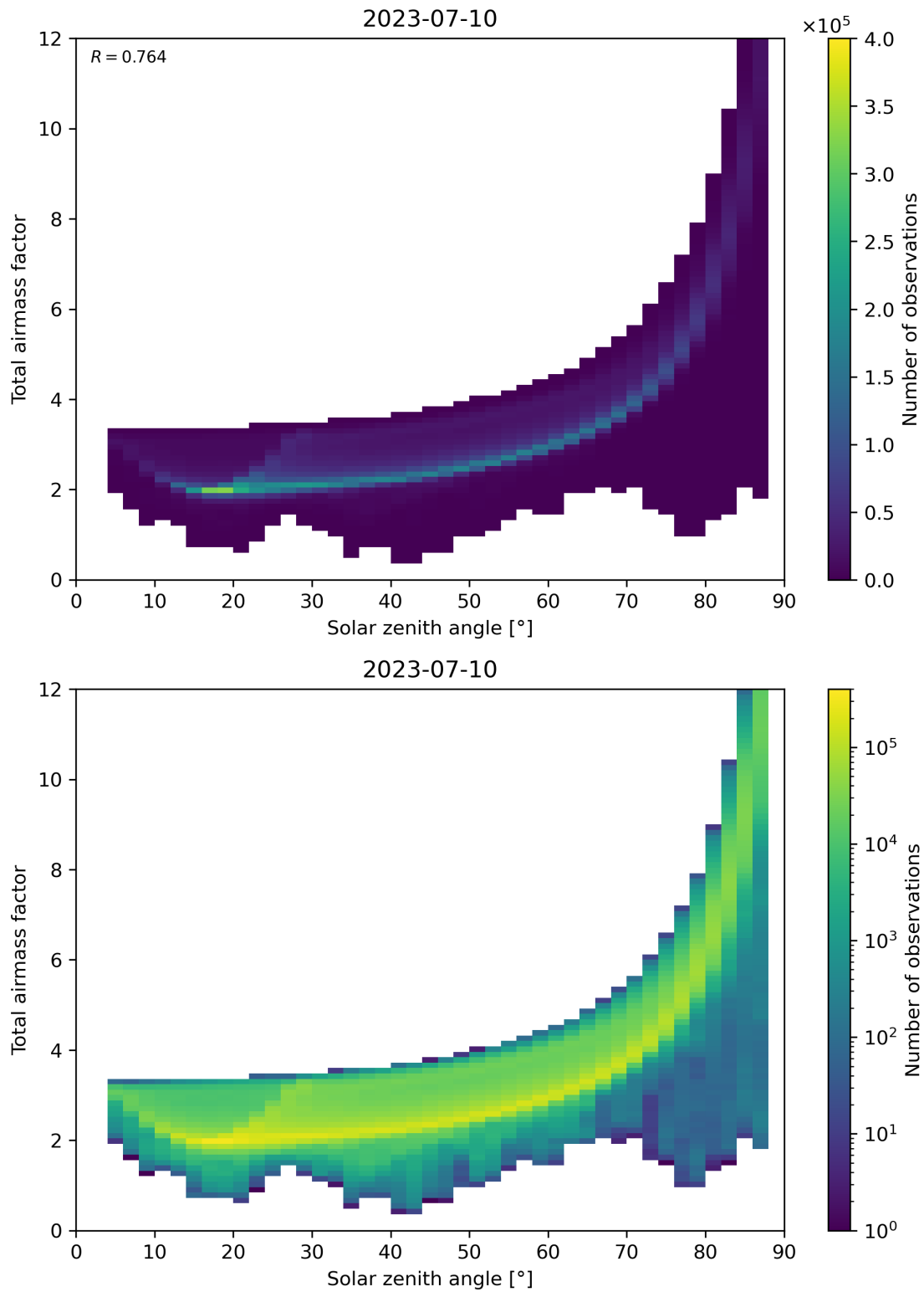
Figure 146: Scatter density plot of “Solar zenith angle” against “Total air mass factor” for 2023-07-09 to 2023-07-11.
