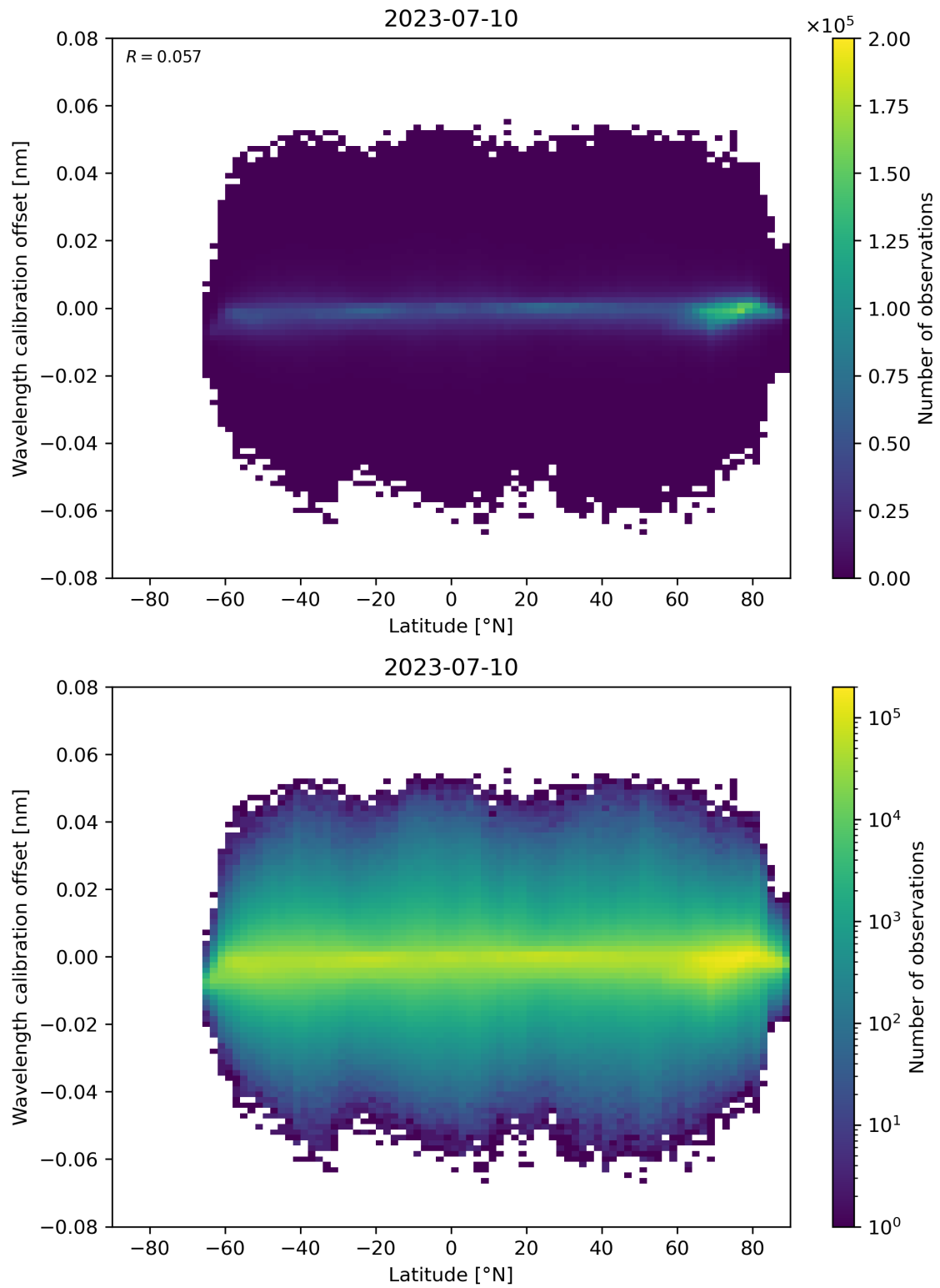
Figure 95: Scatter density plot of “Latitude” against “Wavelength calibration offset” for 2023-07-09 to 2023-07-11.
