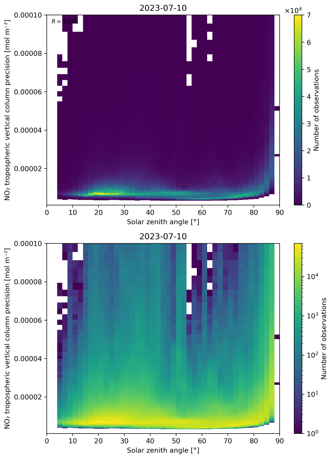
Figure 156: Scatter density plot of “Solar zenith angle” against “NO 2 tropospheric vertical column precision” for 2023-07-09 to 2023-07-11.
