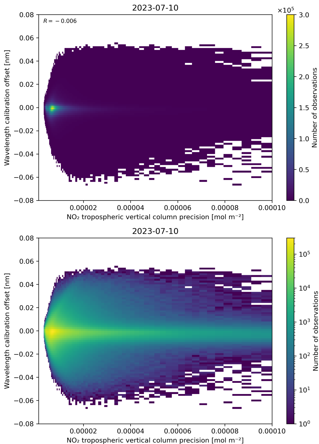
Figure 141: Scatter density plot of “NO 2 tropospheric vertical column precision” against “Wavelength calibration offset” for 2023-07-09 to 2023-07-11.
