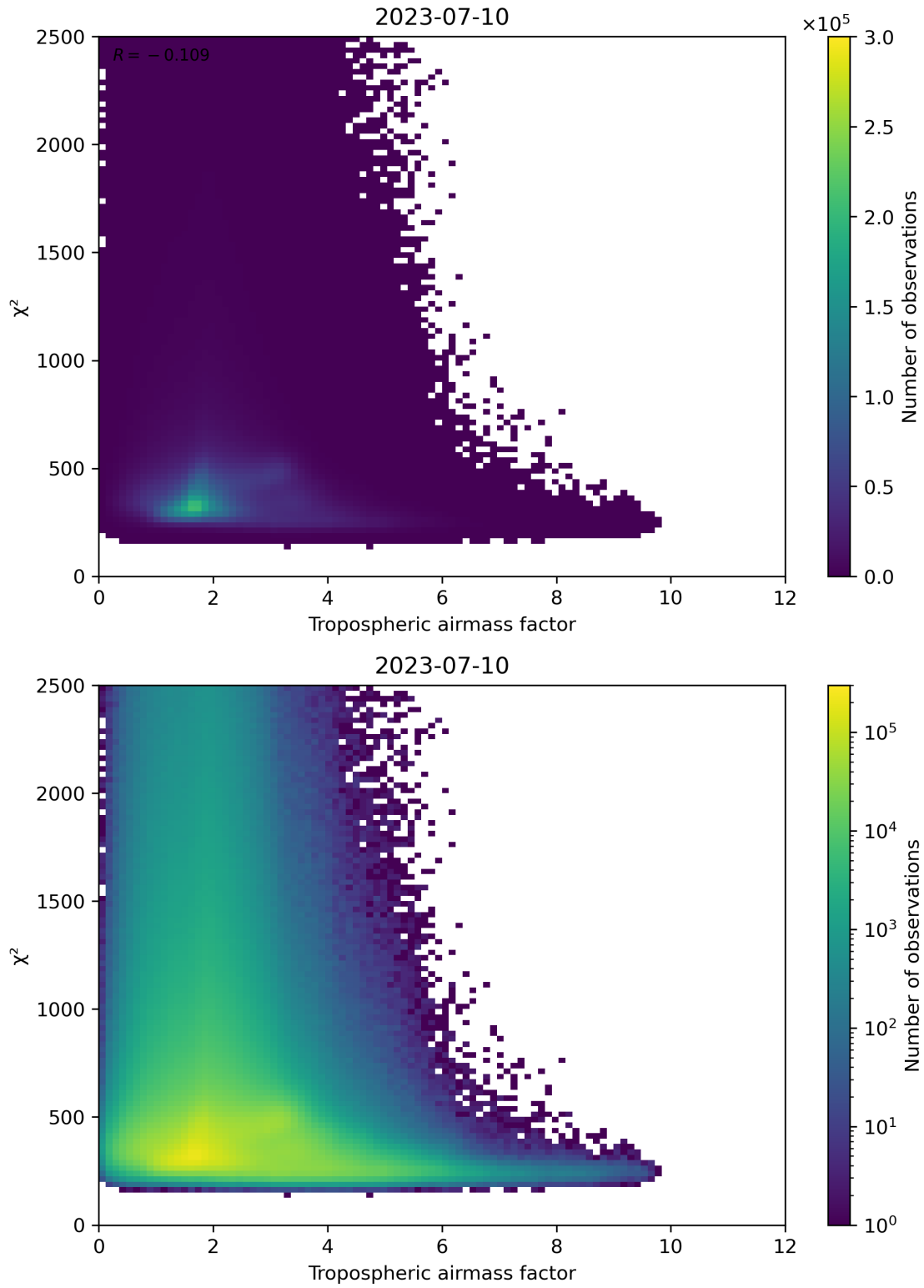
Figure 73: Scatter density plot of “Tropospheric airmass factor” against “ \chi^2 ” for 2023-07-09 to 2023-07-11.
