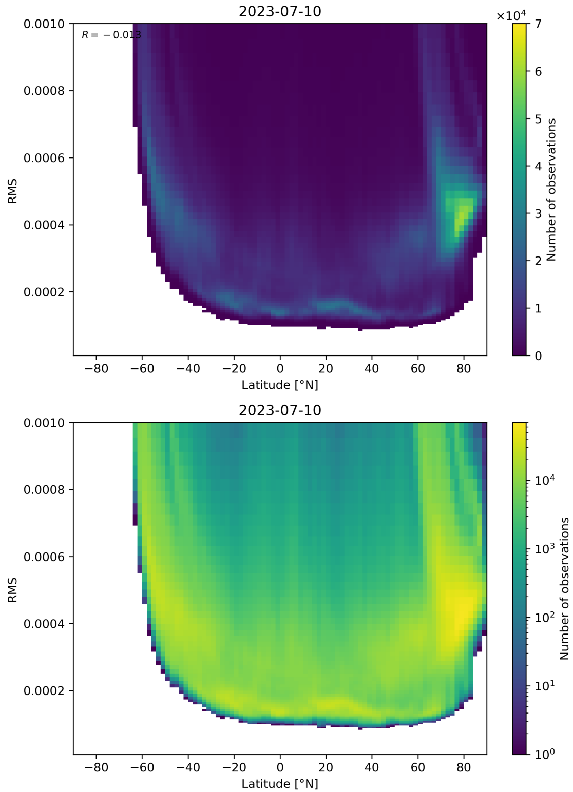
Figure 94: Scatter density plot of “Latitude” against “RMS” for 2023-07-09 to 2023-07-11.
