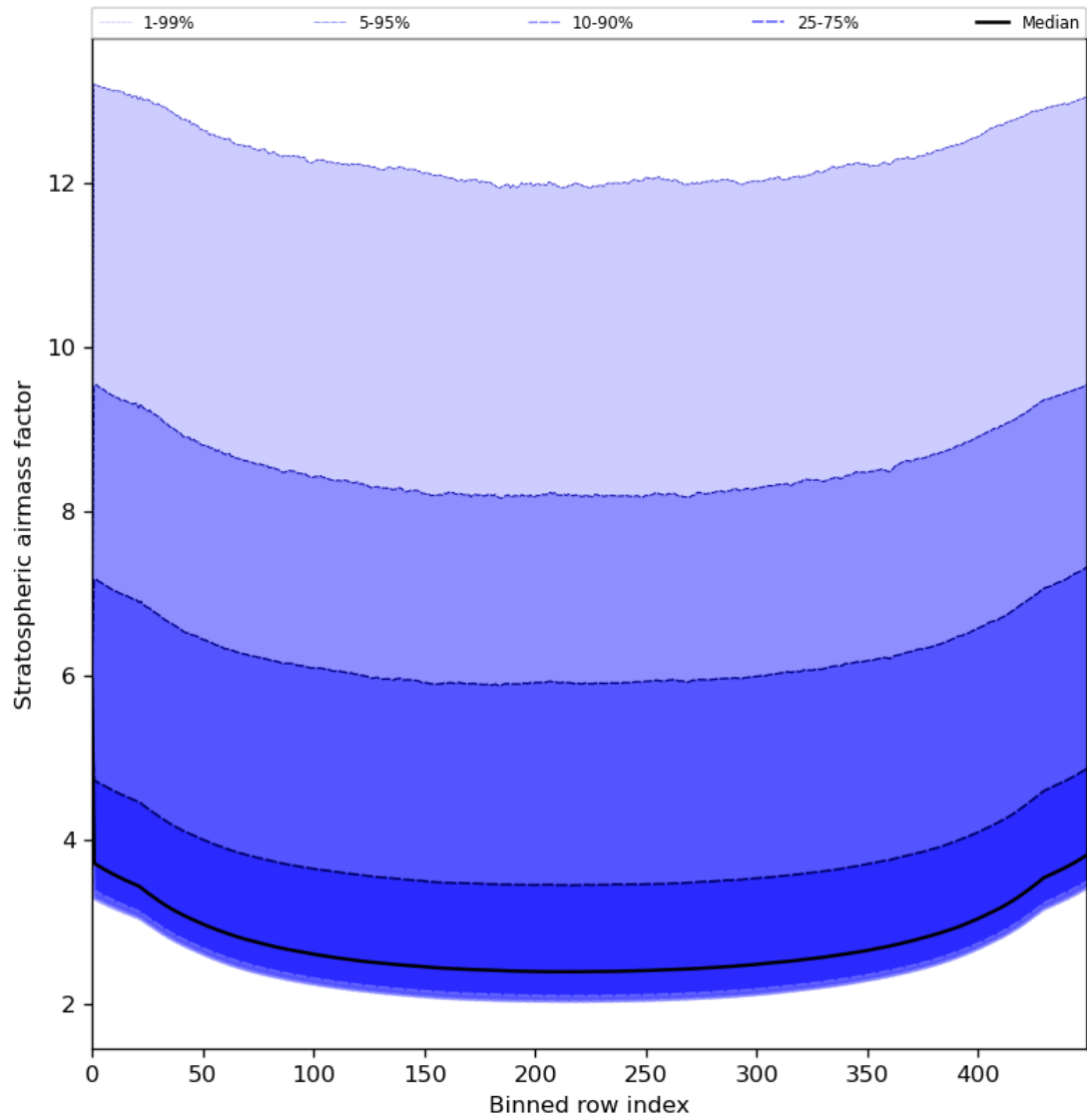
Figure 61: Along track statistics of “Stratospheric airmass factor” for 2023-07-09 to 2023-07-11
