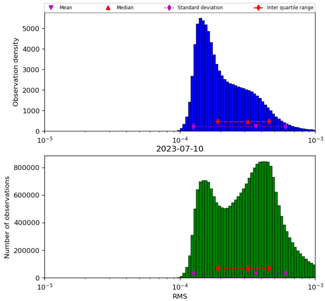
Figure 43: Histogram of “RMS” for 2023-07-09 to 2023-07-11
