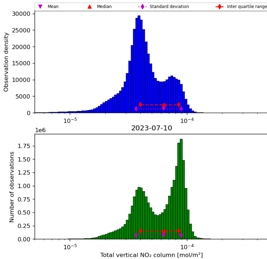
Figure 38: Histogram of “Total vertical NO 2 column” for 2023-07-09 to 2023-07-11
