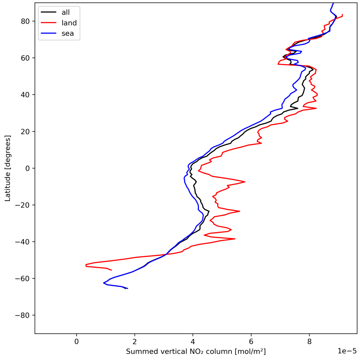
Figure 23: Zonal average of “Summed vertical NO 2 column” for 2023-07-09 to 2023-07-11.
