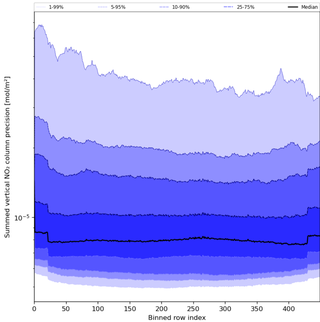
Figure 58: Along track statistics of “Summed vertical NO 2 column precision” for 2023-07-09 to 2023-07-11
