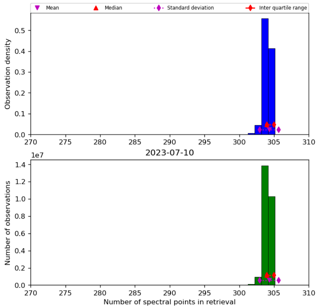
Figure 33: Histogram of “Number of spectral points in retrieval” for 2023-07-09 to 2023-07-11
