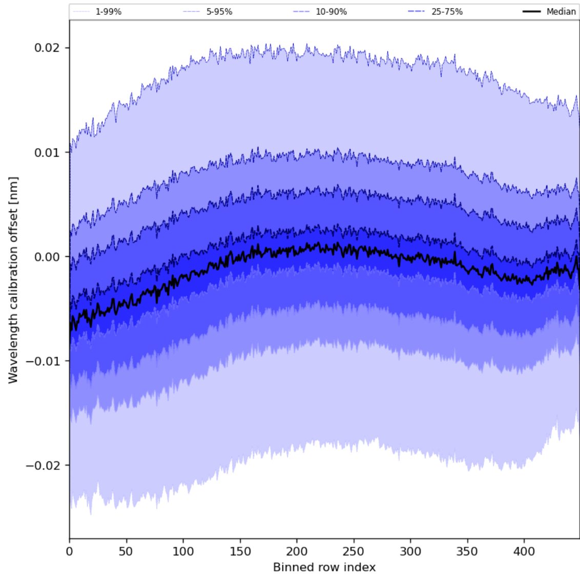
Figure 52: Along track statistics of “Wavelength calibration offset” for 2023-07-09 to 2023-07-11
