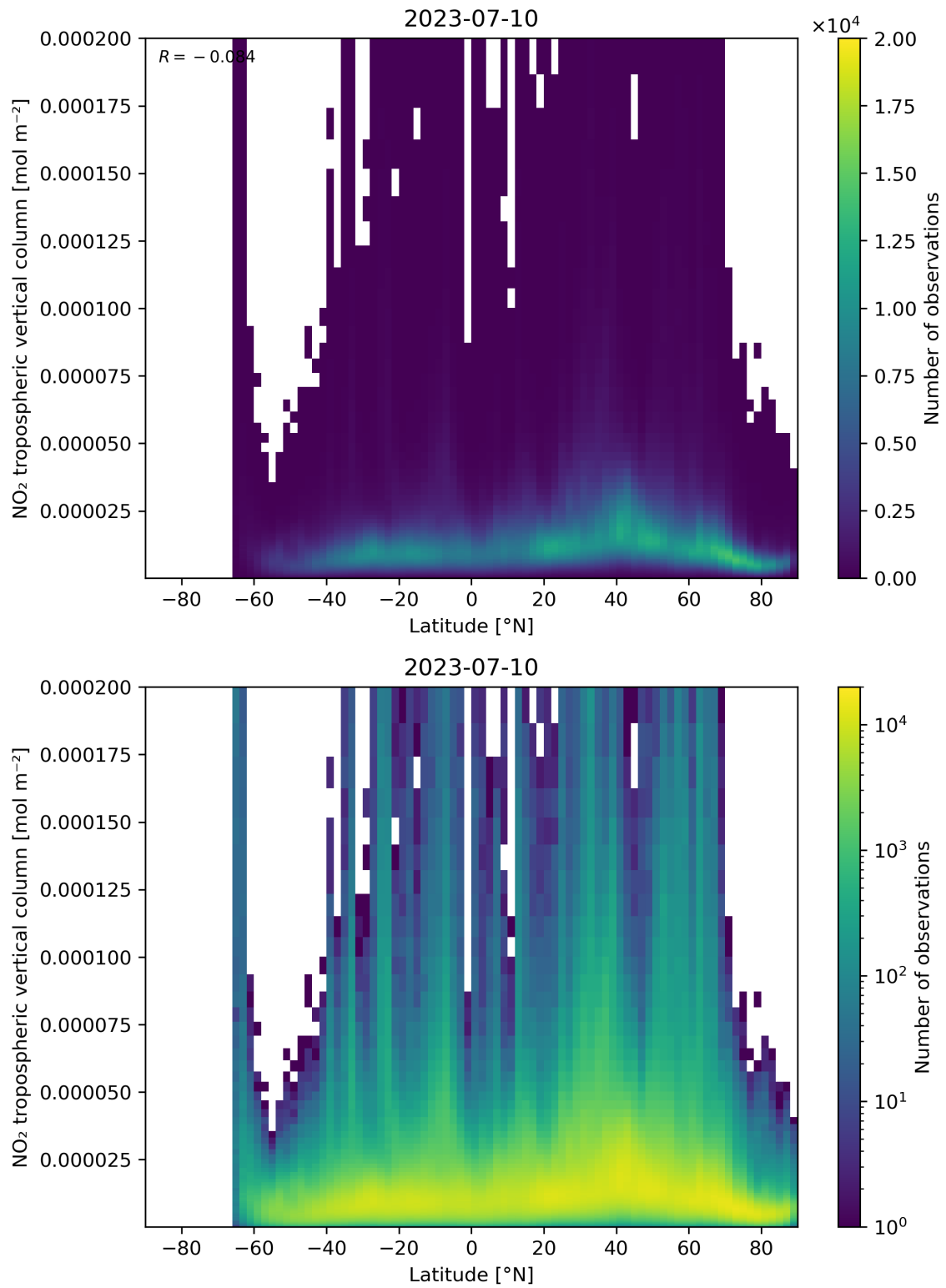
Figure 92: Scatter density plot of “Latitude” against “NO 2 tropospheric vertical column” for 2023-07-09 to 2023-07-11.
