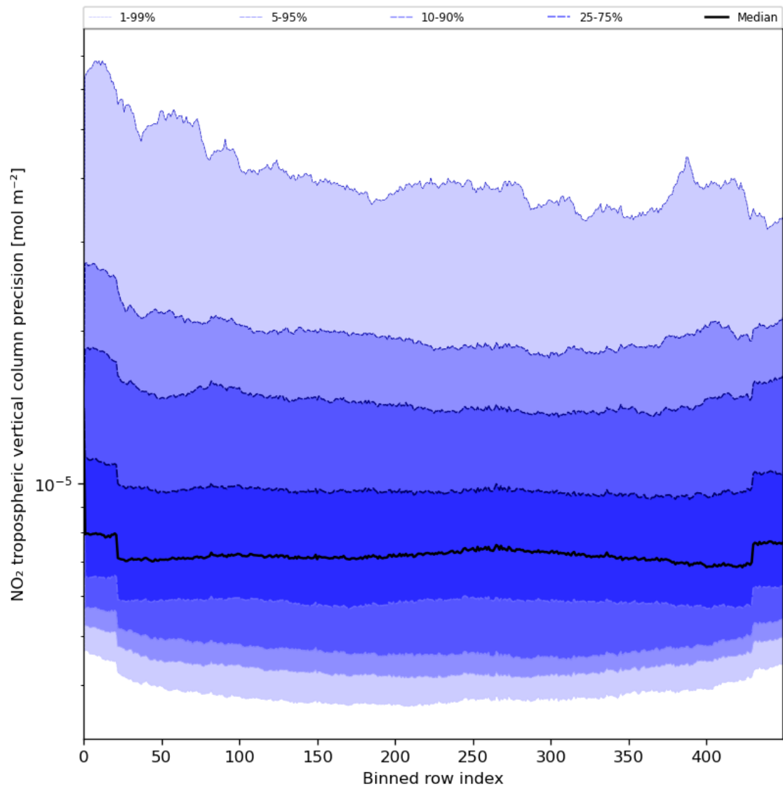
Figure 47: Along track statistics of “NO 2 tropospheric vertical column precision” for 2023-07-09 to 2023-07-11
