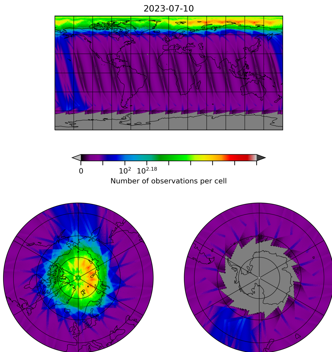
Figure 10: Map of the number of observations for 2023-07-09 to 2023-07-11
