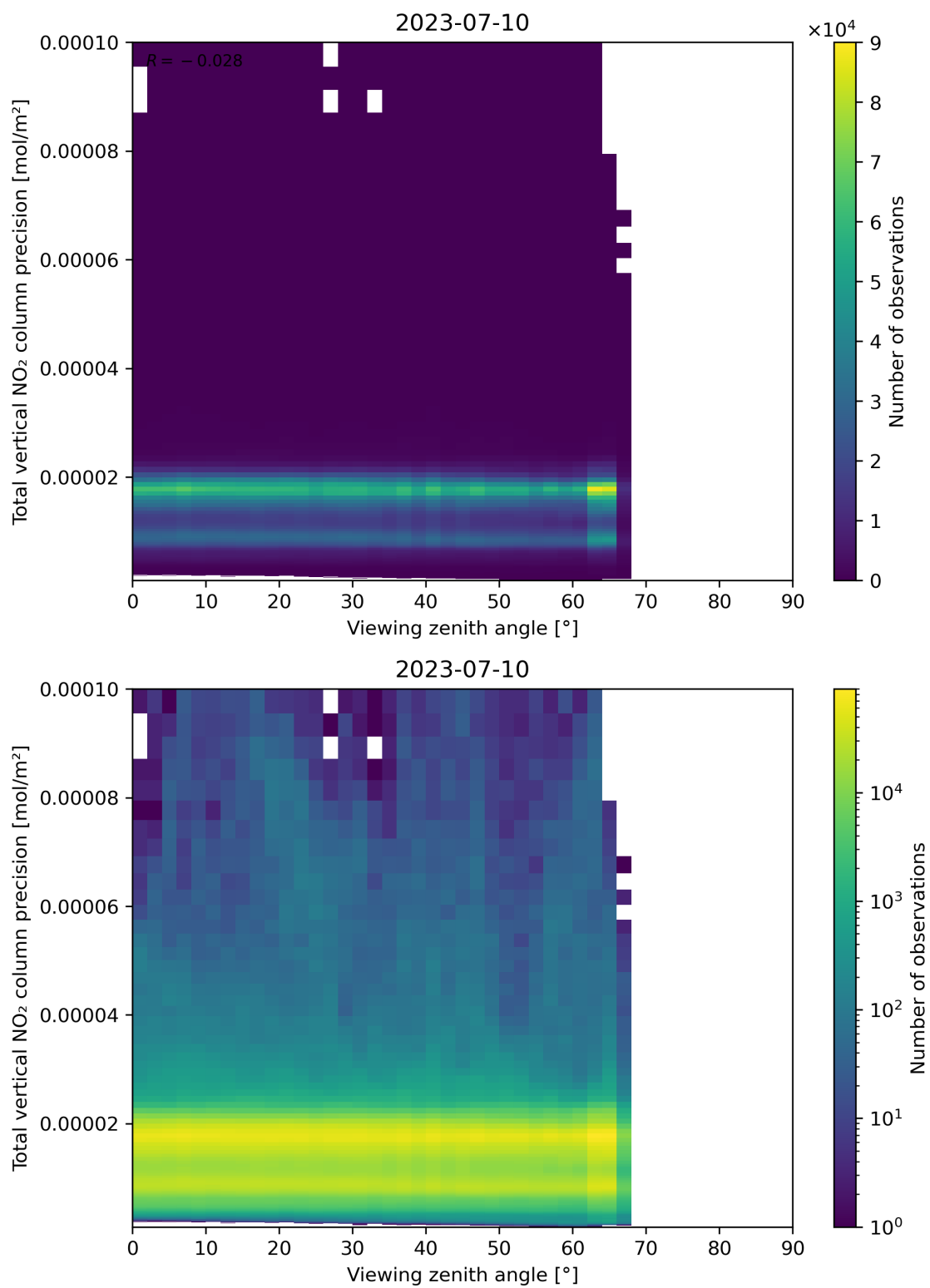
Figure 168: Scatter density plot of “Viewing zenith angle” against “Total vertical NO 2 column precision” for 2023-07-09 to 2023-07-11.
