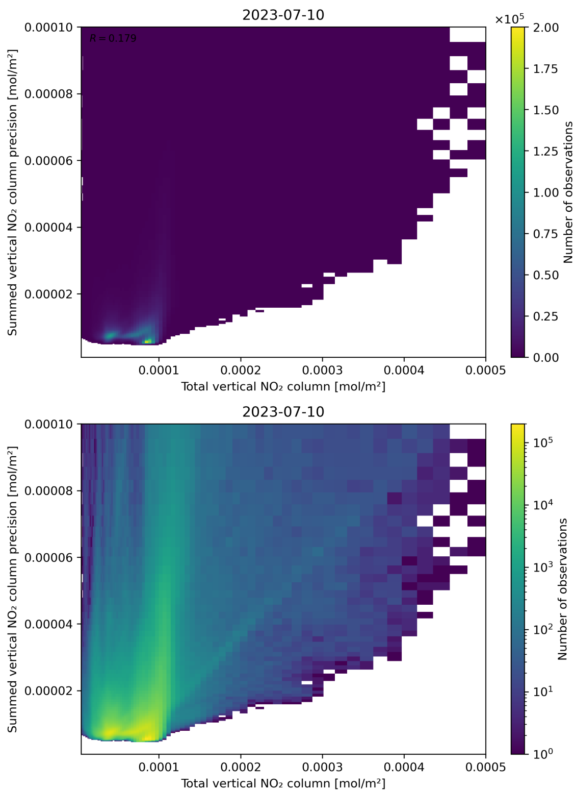
Figure 113: Scatter density plot of “Total vertical NO 2 column” against “Summed vertical NO 2 column precision” for 2023-07-09 to 2023-07-11.
