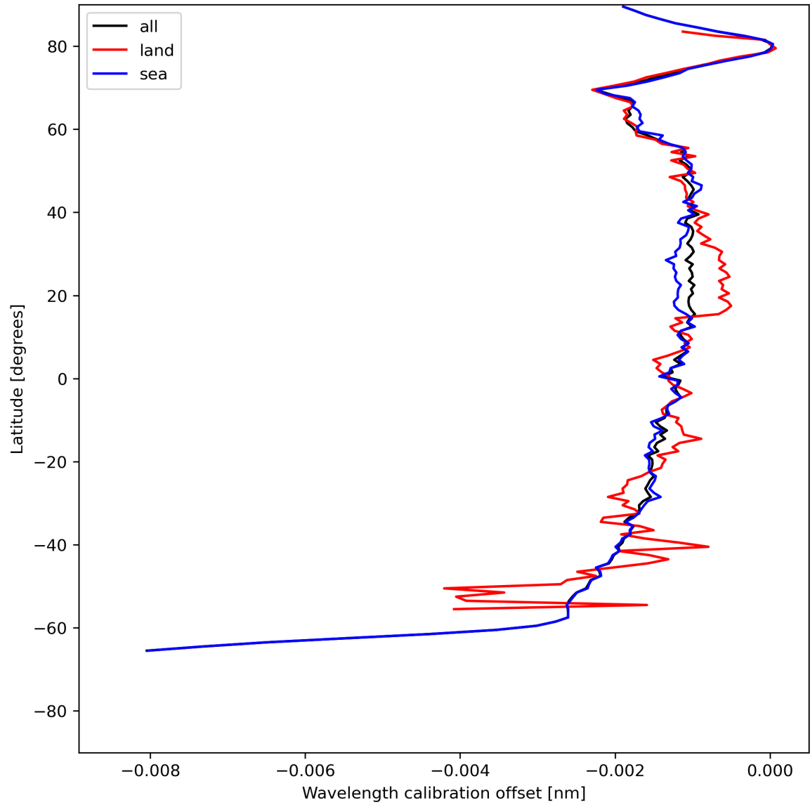
Figure 18: Zonal average of “Wavelength calibration offset” for 2023-07-09 to 2023-07-11.
