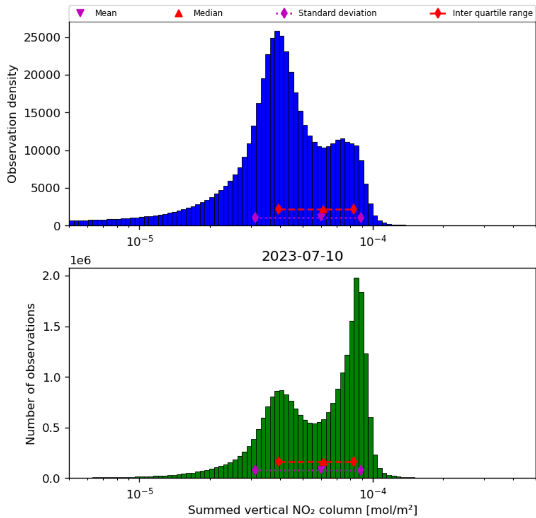
Figure 40: Histogram of “Summed vertical NO 2 column” for 2023-07-09 to 2023-07-11
