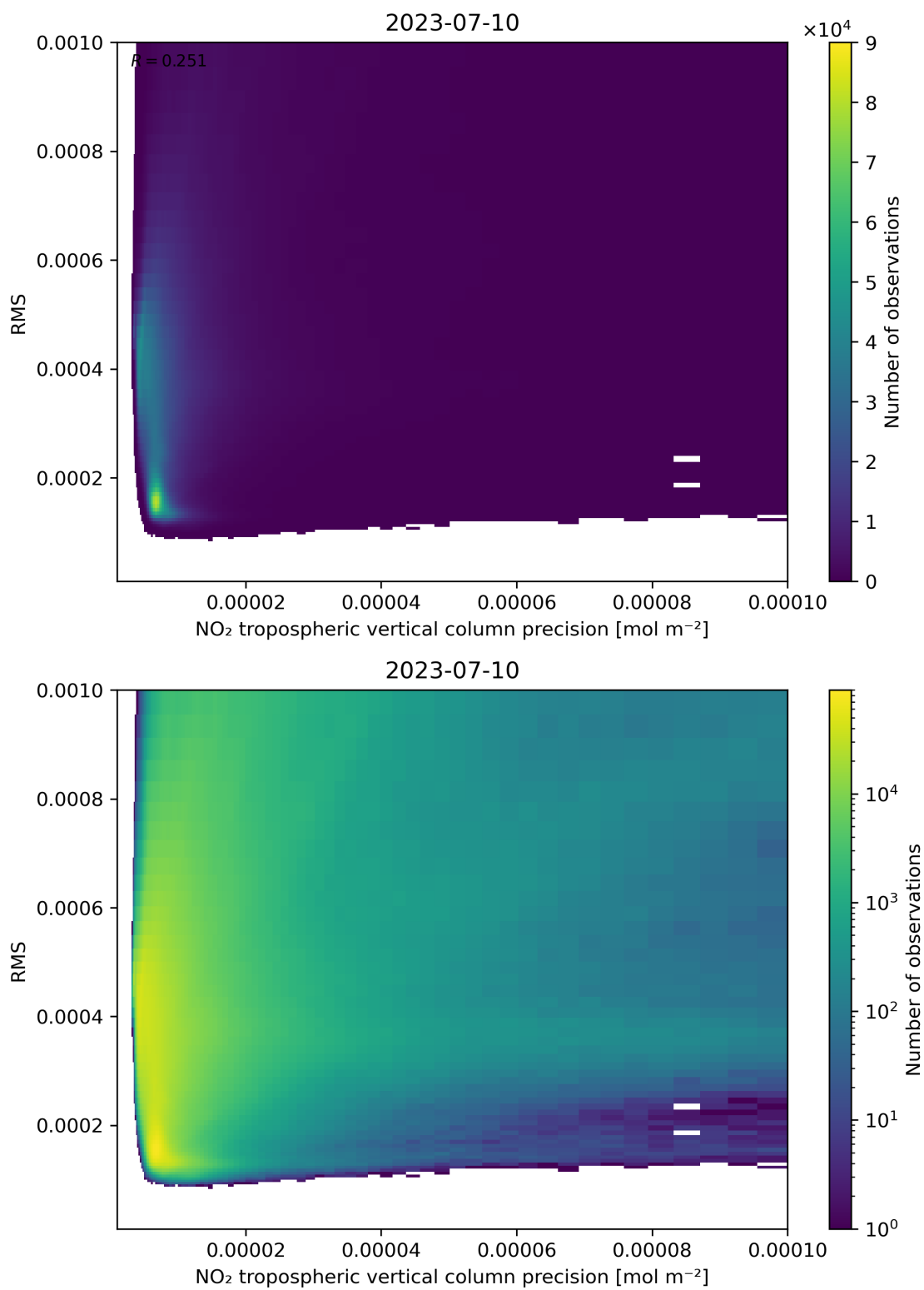
Figure 140: Scatter density plot of “NO 2 tropospheric vertical column precision” against “RMS” for 2023-07-09 to 2023-07-11.
