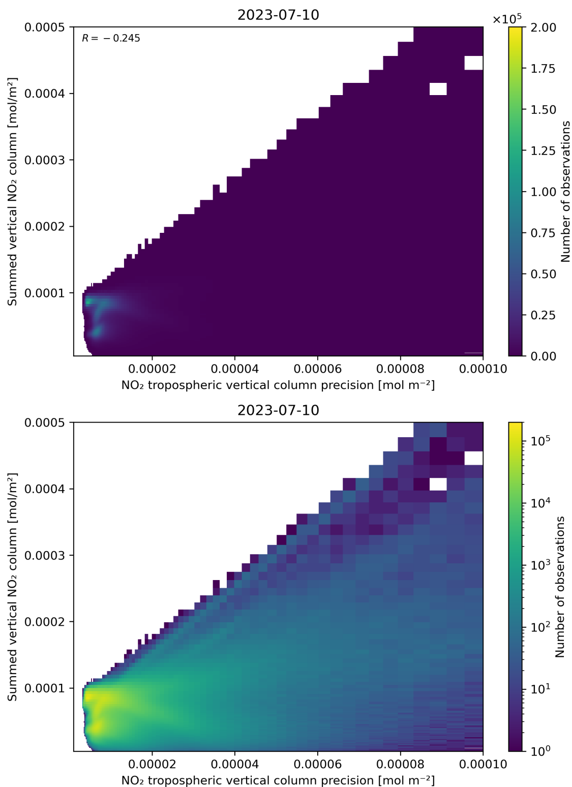
Figure 136: Scatter density plot of “NO 2 tropospheric vertical column precision” against “Summed vertical NO 2 column” for 2023-07-09 to 2023-07-11.
