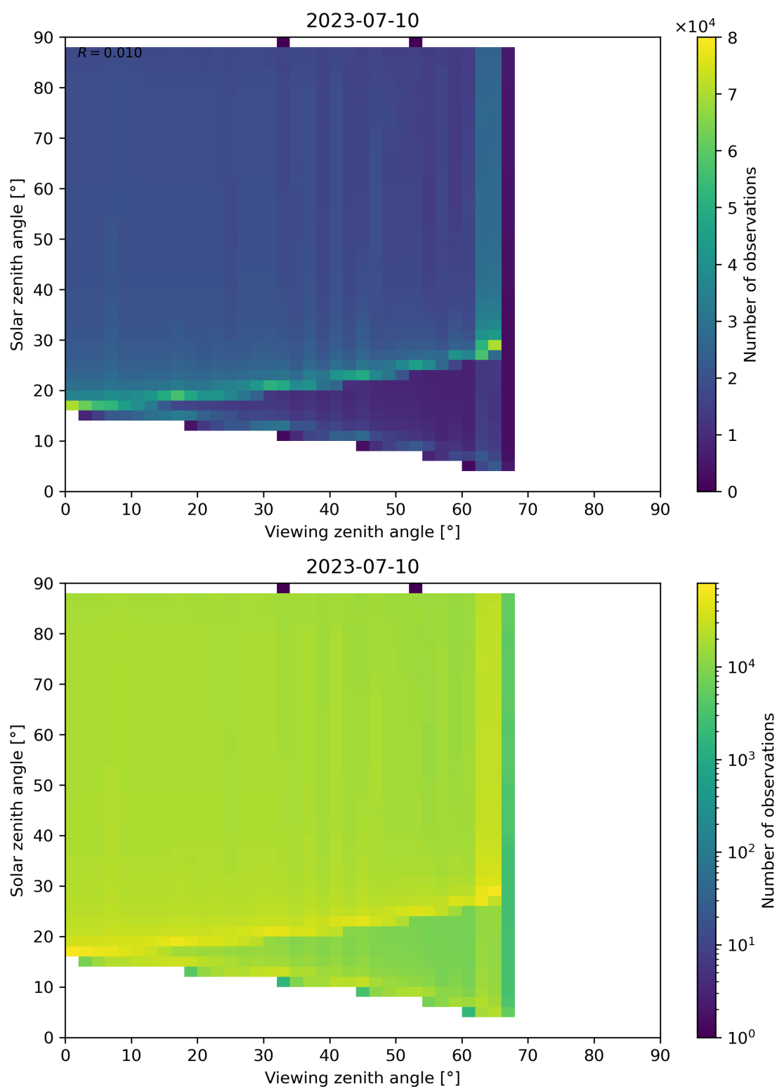
Figure 172: Scatter density plot of “Viewing zenith angle” against “Solar zenith angle” for 2023-07-09 to 2023-07-11.
