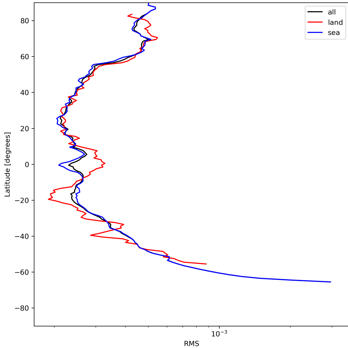
Figure 26: Zonal average of “RMS” for 2023-07-09 to 2023-07-11.
