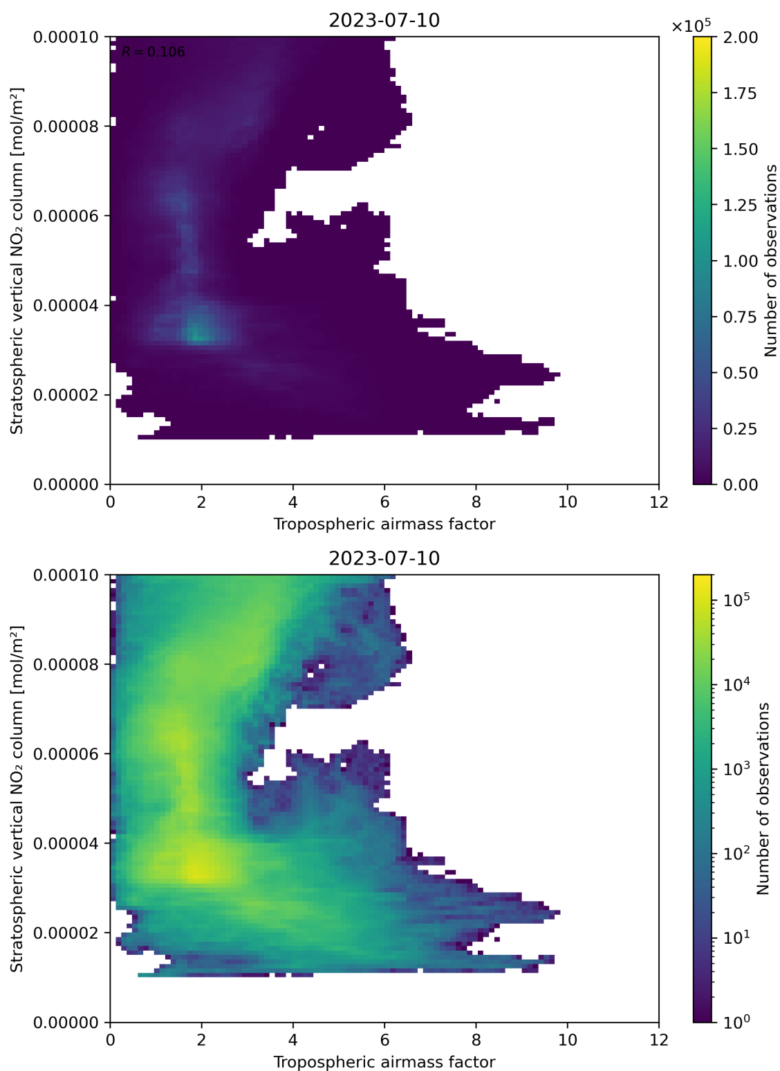
Figure 74: Scatter density plot of “Tropospheric air mass factor” against “Stratospheric vertical NO 2 column” for 2023-07-09 to 2023-07-11.
