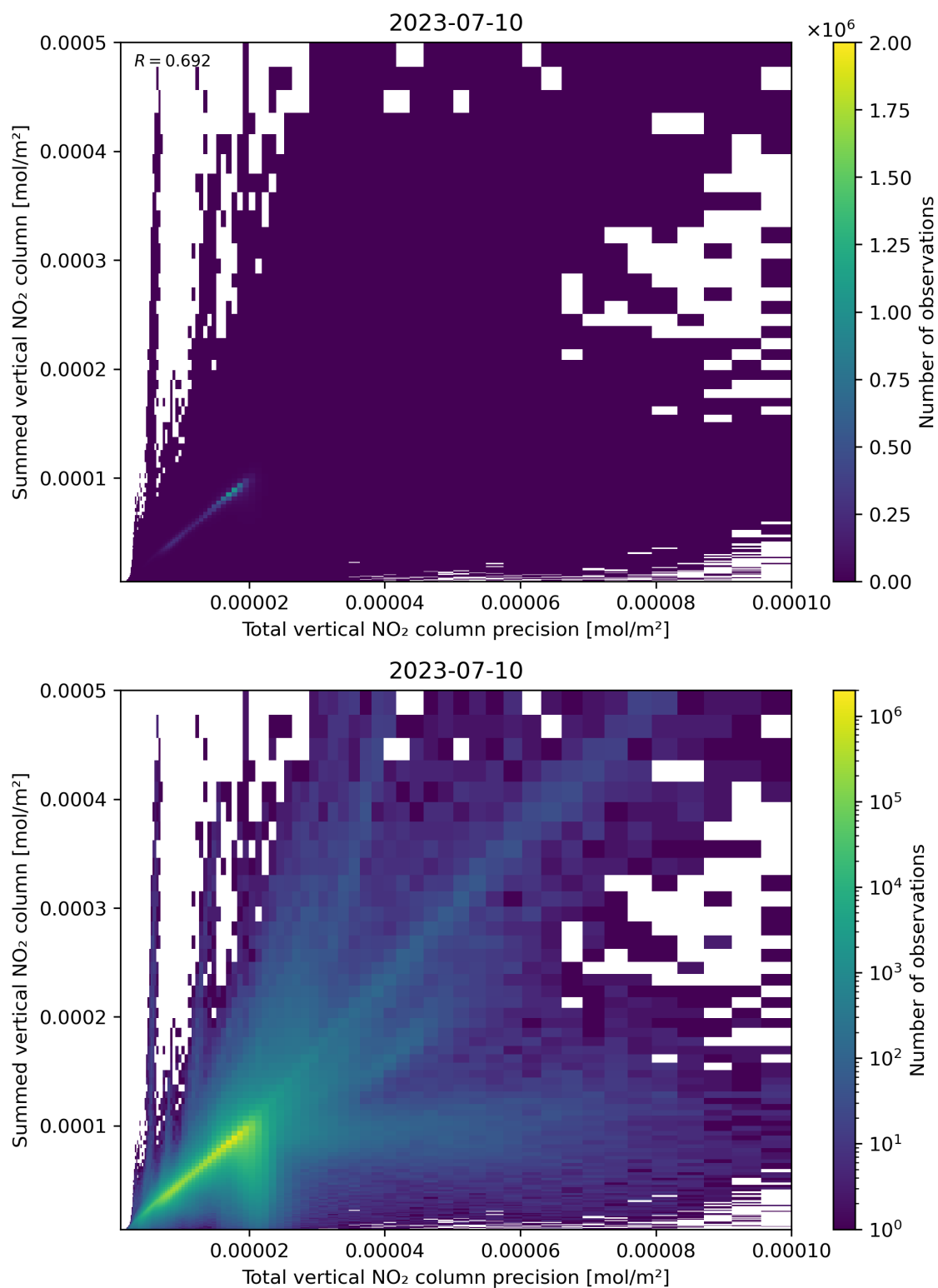
Figure 117: Scatter density plot of “Total vertical NO 2 column precision” against “Summed vertical NO 2 column” for 2023-07-09 to 2023-07-11.
