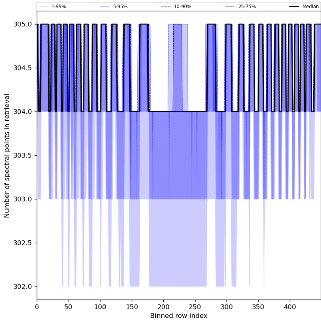
Figure 50: Along track statistics of “Number of spectral points in retrieval” for 2023-07-09 to 2023-07-11
