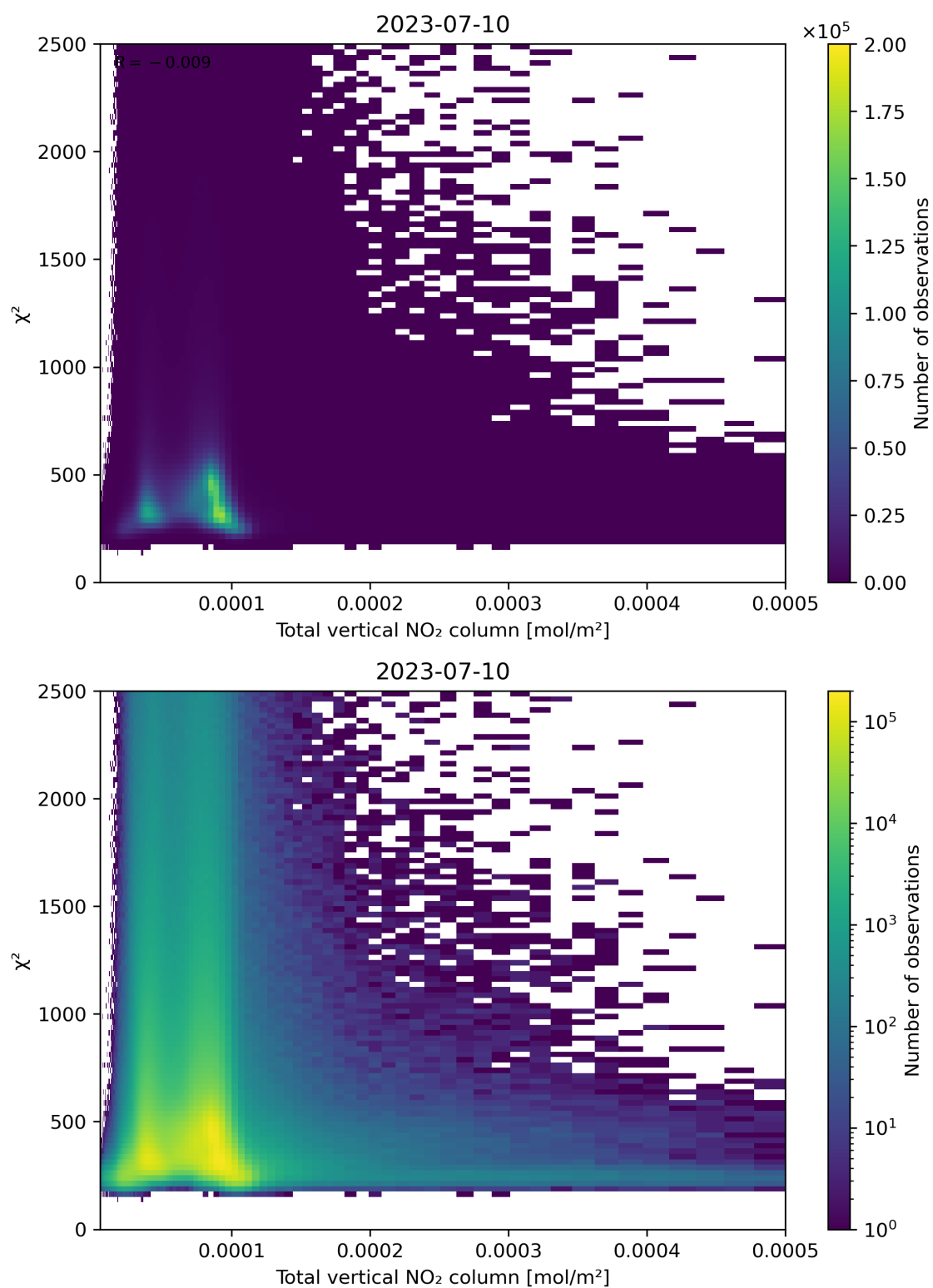
Figure 111: Scatter density plot of “Total vertical NO 2 column” against “ \chi^2 ” for 2023-07-09 to 2023-07-11.
