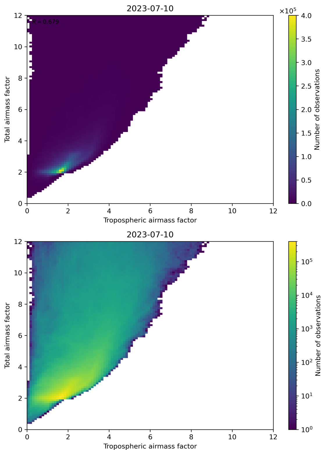
Figure 72: Scatter density plot of “Tropospheric airmass factor” against “Total airmass factor” for 2023-07-09 to 2023-07-11.
