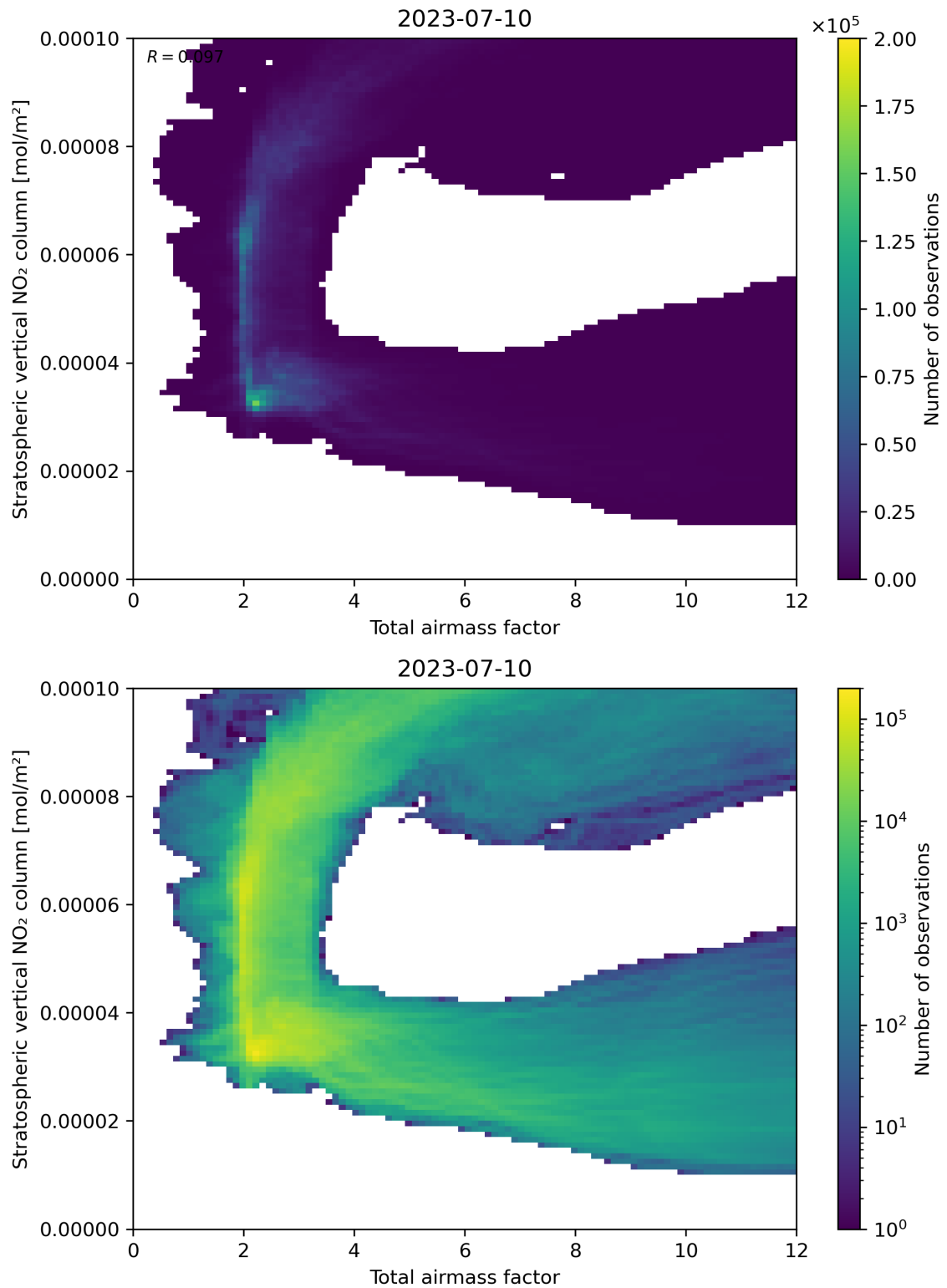
Figure 64: Scatter density plot of “Total airmass factor” against “Stratospheric vertical NO 2 column” for 2023-07-09 to 2023-07-11.
