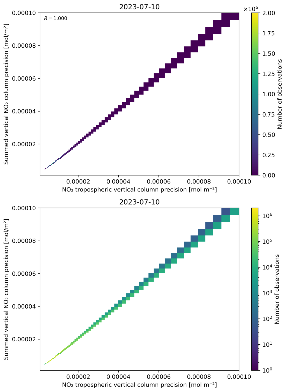
Figure 137: Scatter density plot of “NO 2 tropospheric vertical column precision” against “Summed vertical NO 2 column precision” for 2023-07-09 to 2023-07-11.
