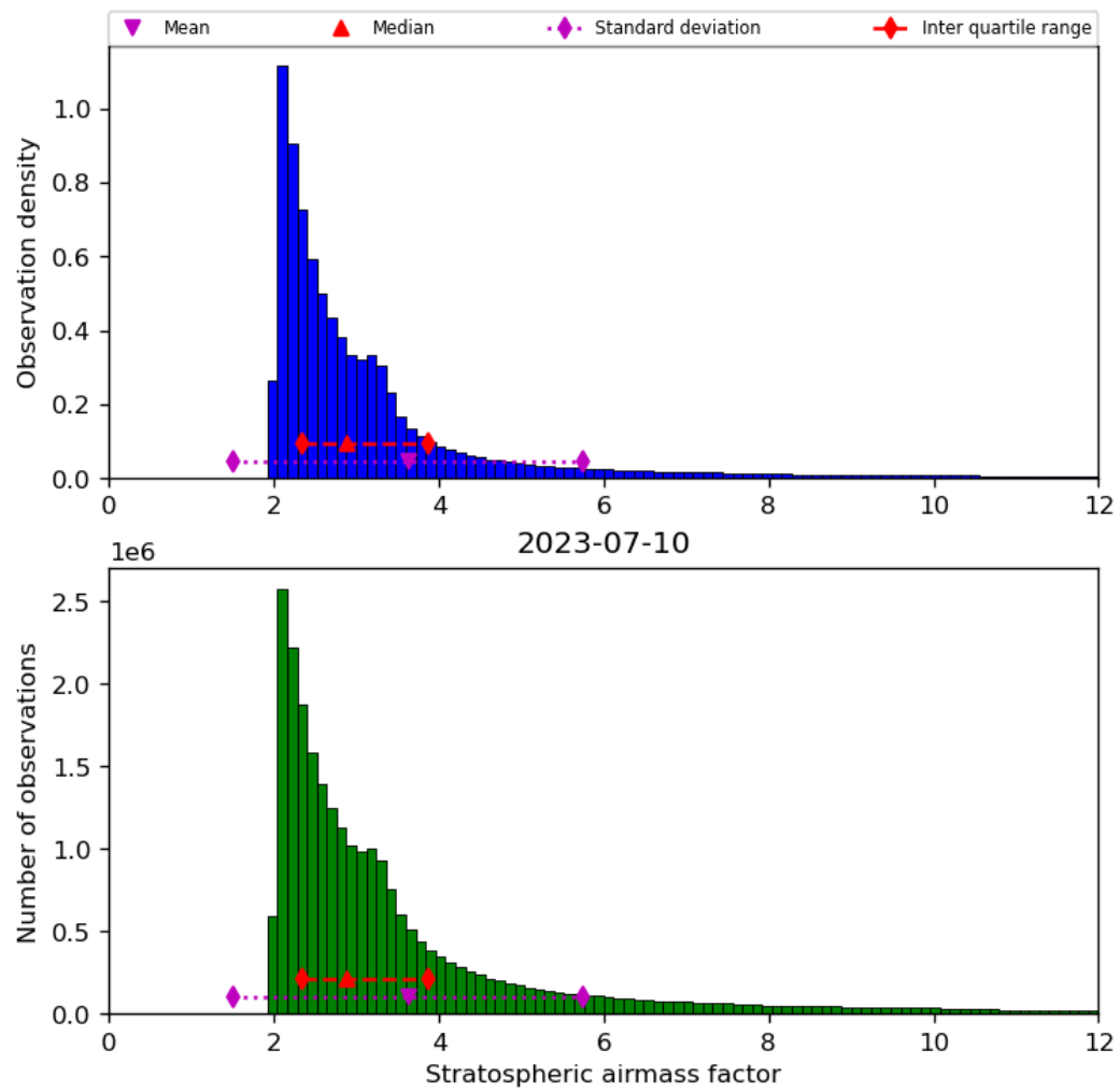
Figure 44: Histogram of “Stratospheric airmass factor” for 2023-07-09 to 2023-07-11
