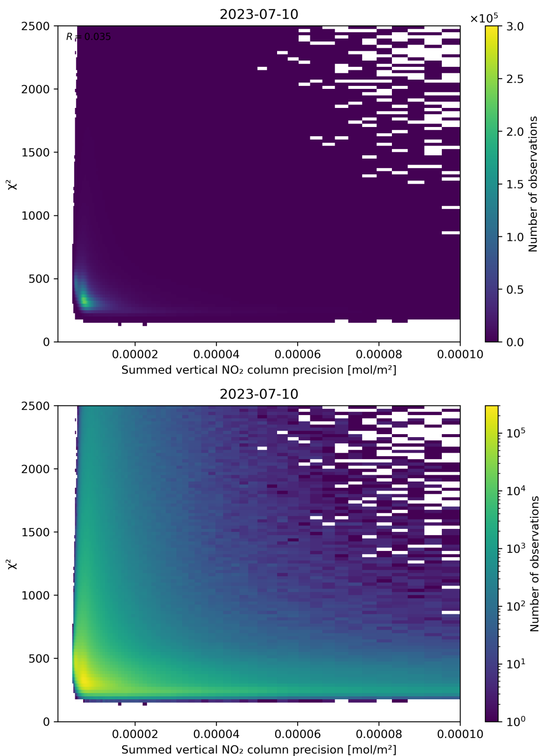
Figure 107: Scatter density plot of “Summed vertical NO 2 column precision” against “ \chi^2 ” for 2023-07-09 to 2023-07-11.
