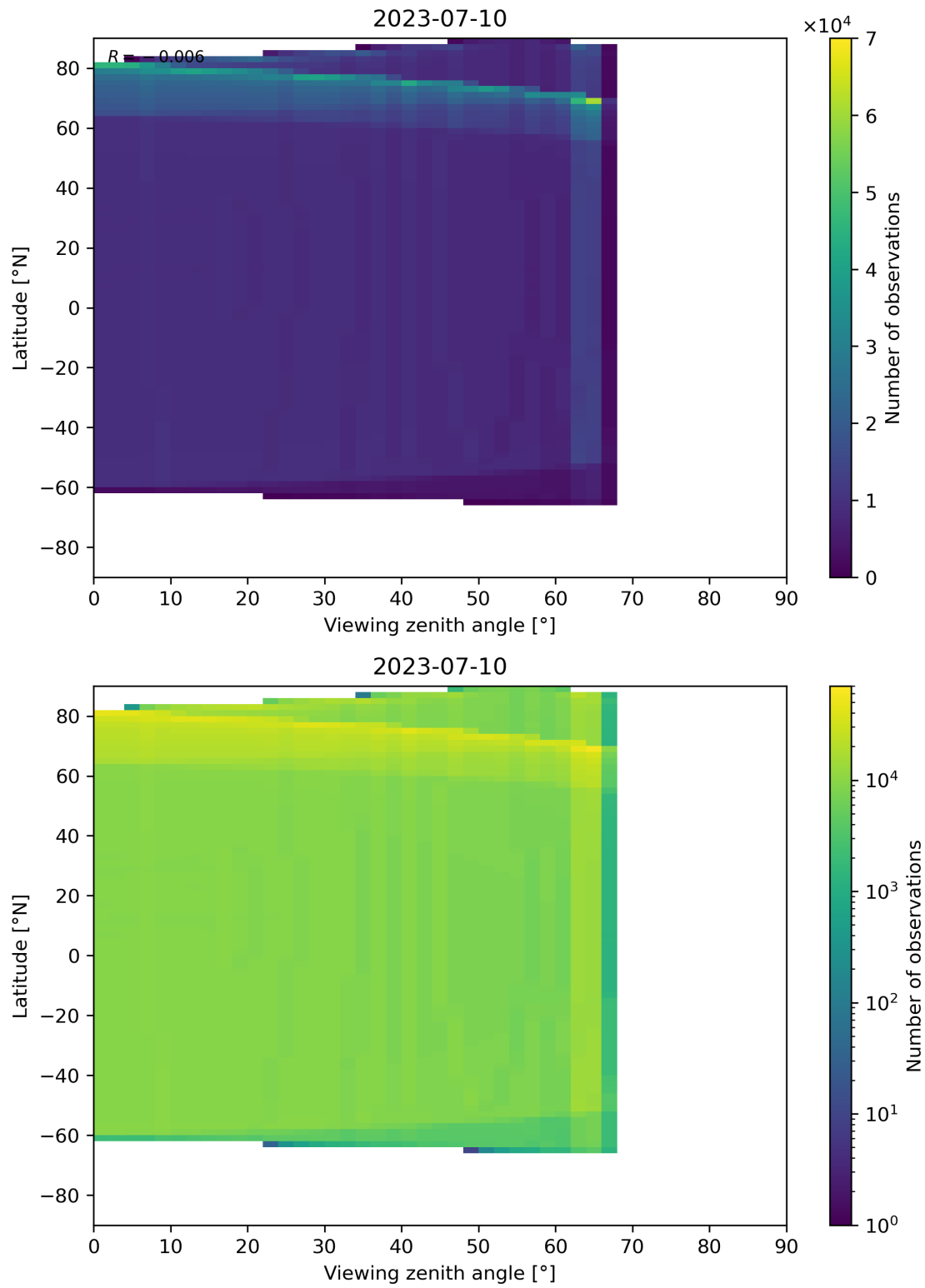
Figure 163: Scatter density plot of “Viewing zenith angle” against “Latitude” for 2023-07-09 to 2023-07-11.
