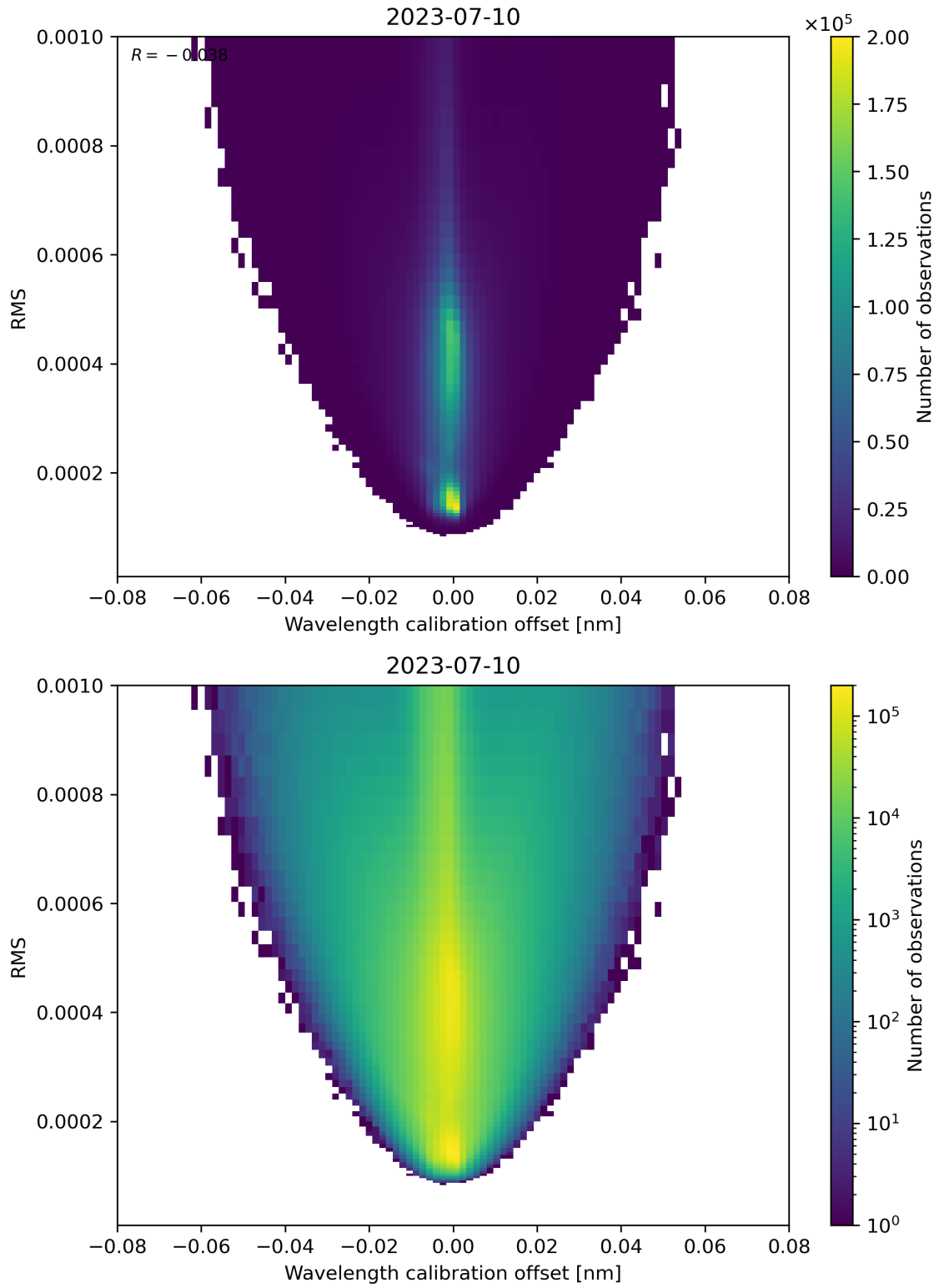
Figure 181: Scatter density plot of “Wavelength calibration offset” against “RMS” for 2023-07-09 to 2023-07-11.
