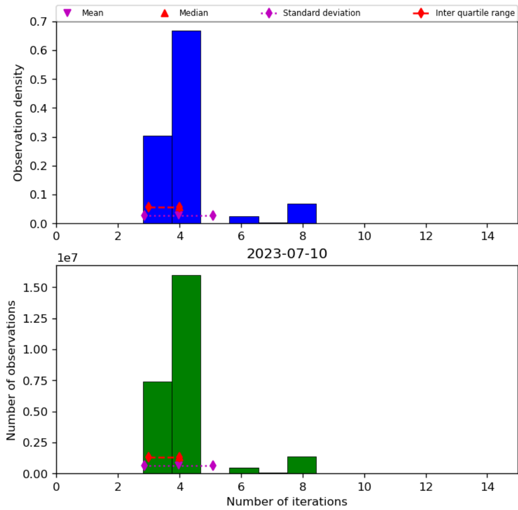
Figure 34: Histogram of “Number of iterations” for 2023-07-09 to 2023-07-11
