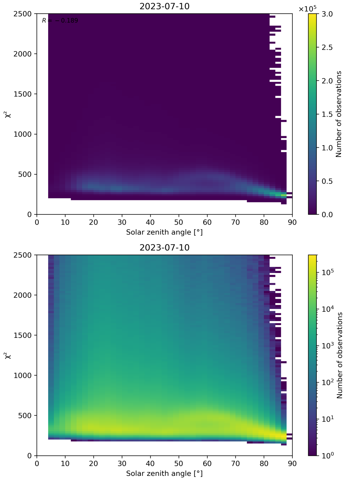
Figure 148: Scatter density plot of “Solar zenith angle” against “ \chi^2 ” for 2023-07-09 to 2023-07-11.
