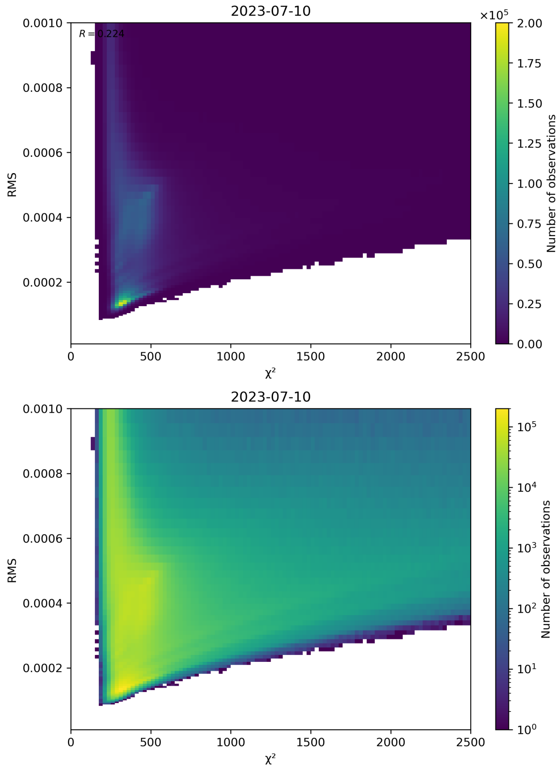
Figure 82: Scatter density plot of “ \chi^2 ” against “RMS” for 2023-07-09 to 2023-07-11.
