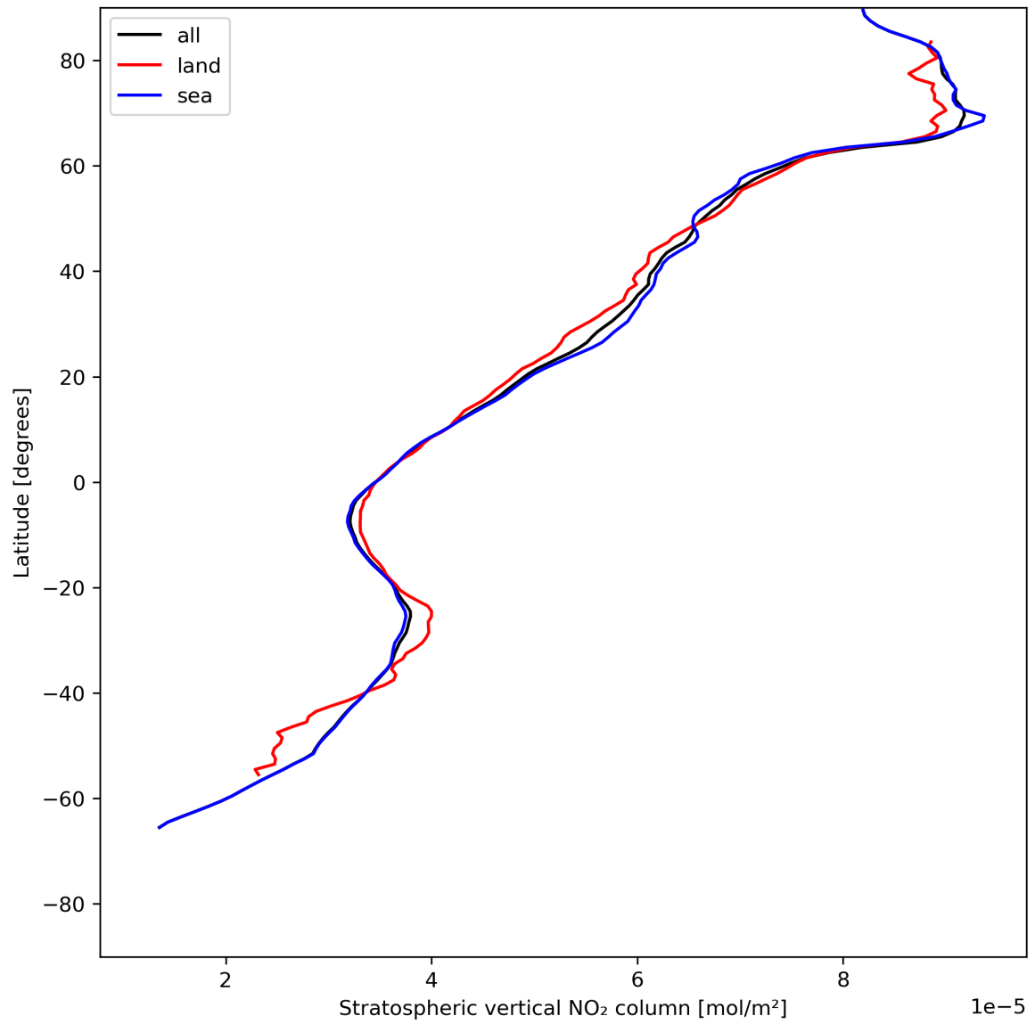
Figure 19: Zonal average of “Stratospheric vertical NO 2 column” for 2023-07-09 to 2023-07-11.
