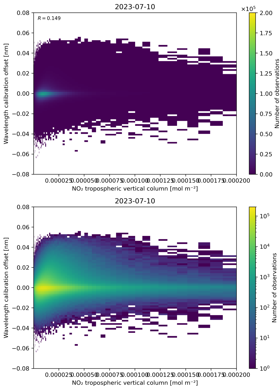
Figure 143: Scatter density plot of “NO 2 tropospheric vertical column” against “Wavelength calibration offset” for 2023-07-09 to 2023-07-11.
