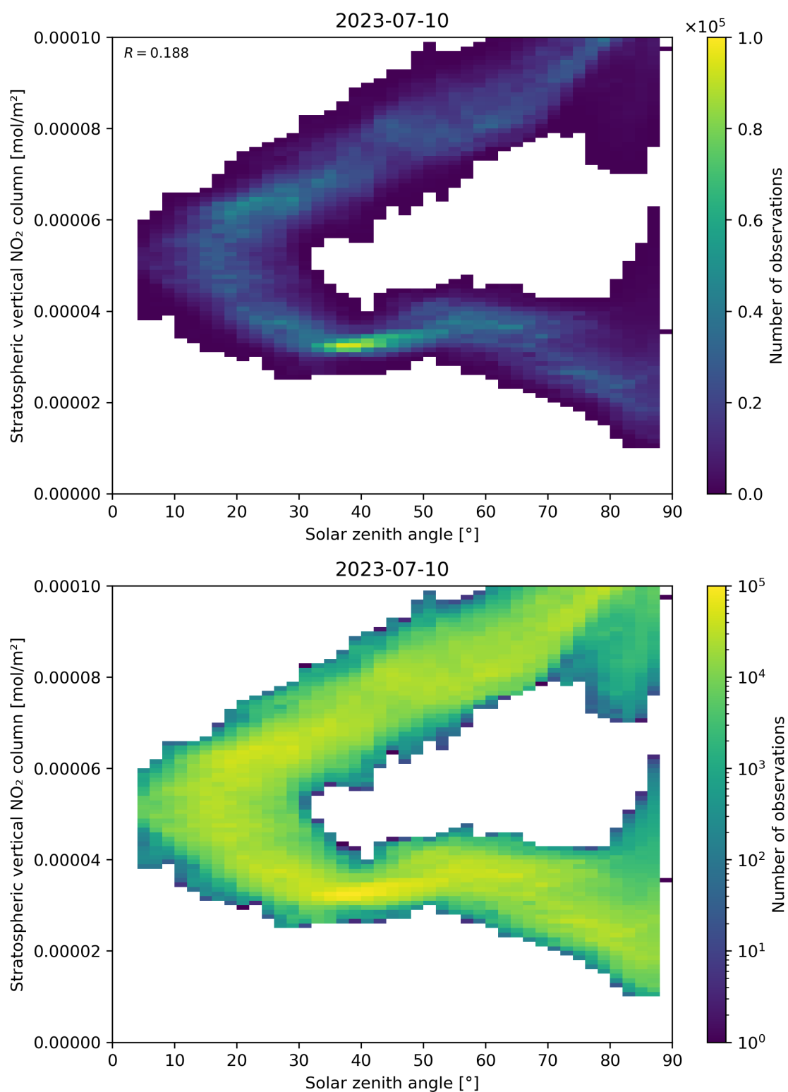
Figure 150: Scatter density plot of “Solar zenith angle” against “Stratospheric vertical NO 2 column” for 2023-07-09 to 2023-07-11.
