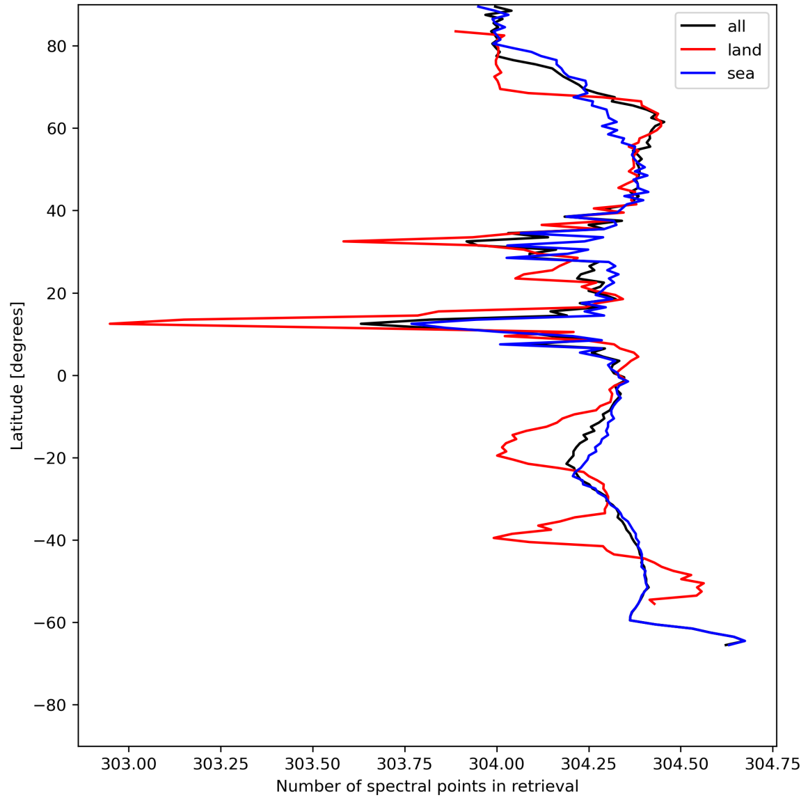
Figure 16: Zonal average of “Number of spectral points in retrieval” for 2023-07-09 to 2023-07-11.
