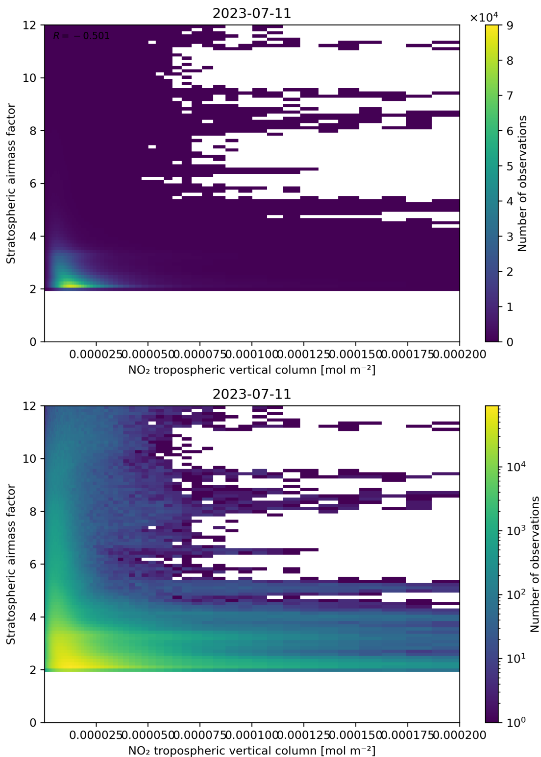
Figure 121: Scatter density plot of “NO 2 tropospheric vertical column” against “Stratospheric air mass factor” for 2023-07-10 to 2023-07-12.
