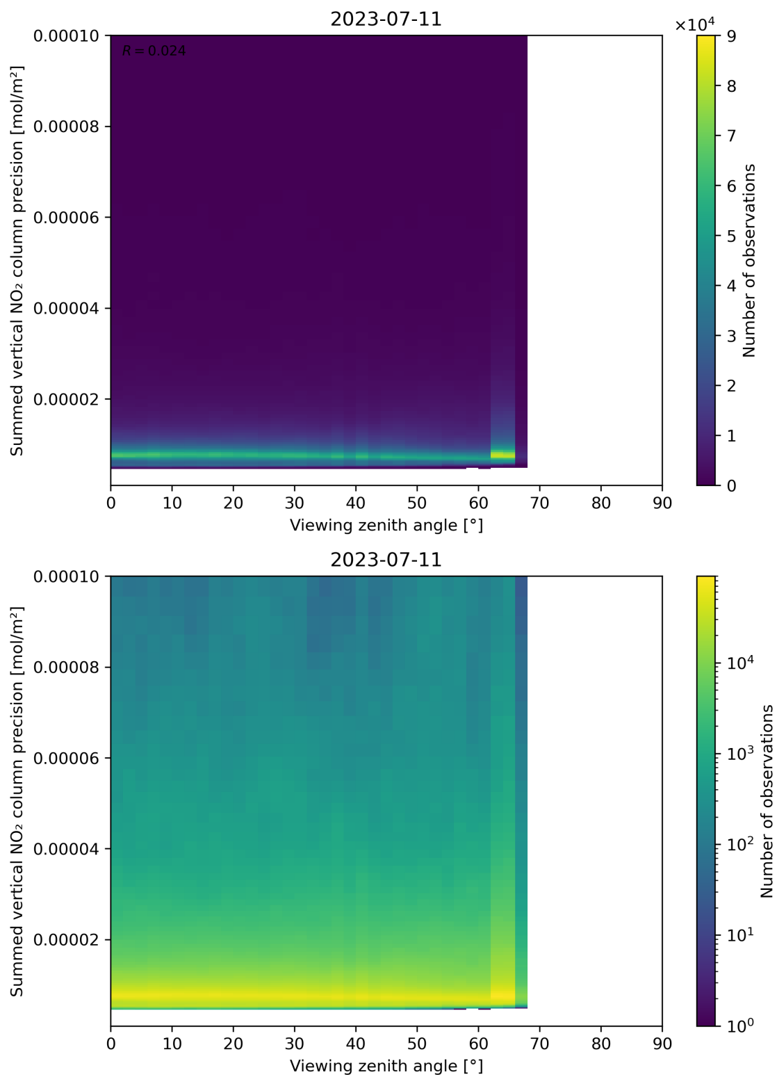
Figure 166: Scatter density plot of “Viewing zenith angle” against “Summed vertical NO 2 column precision” for 2023-07-10 to 2023-07-12.
