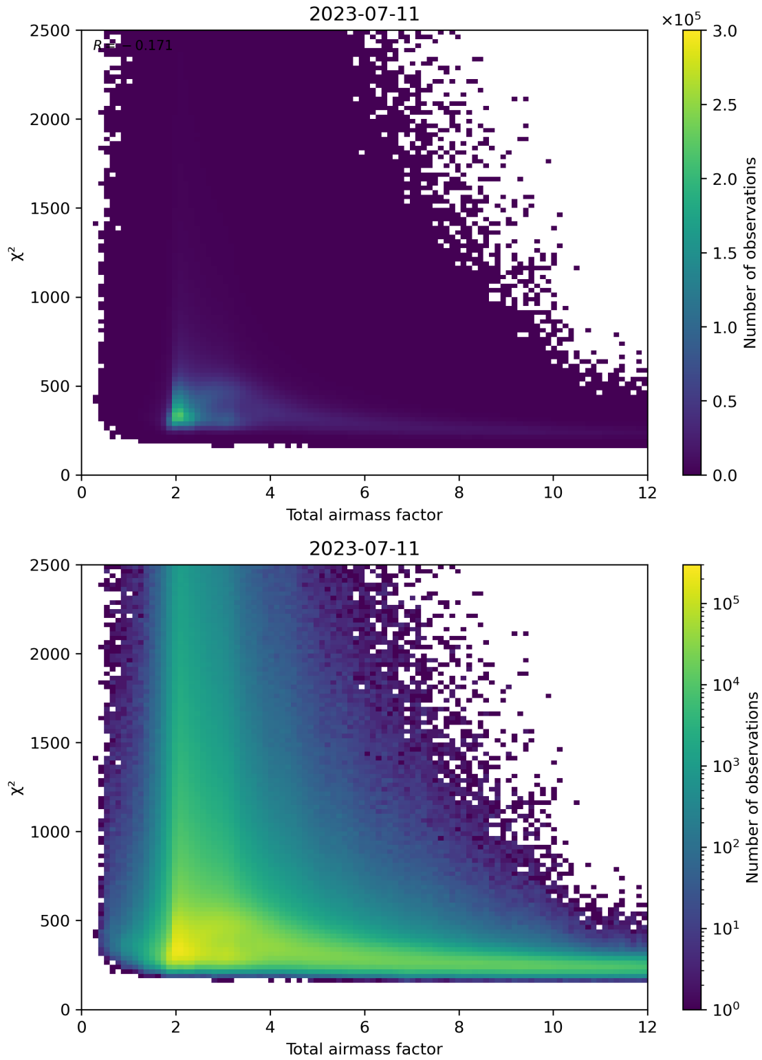
Figure 63: Scatter density plot of “Total airmass factor” against “ \chi^2 ” for 2023-07-10 to 2023-07-12.
