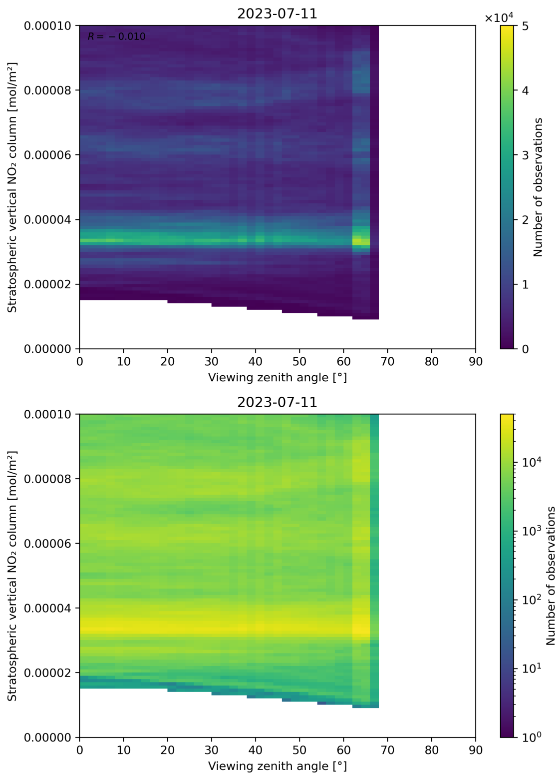
Figure 164: Scatter density plot of “Viewing zenith angle” against “Stratospheric vertical NO 2 column” for 2023-07-10 to 2023-07-12.
