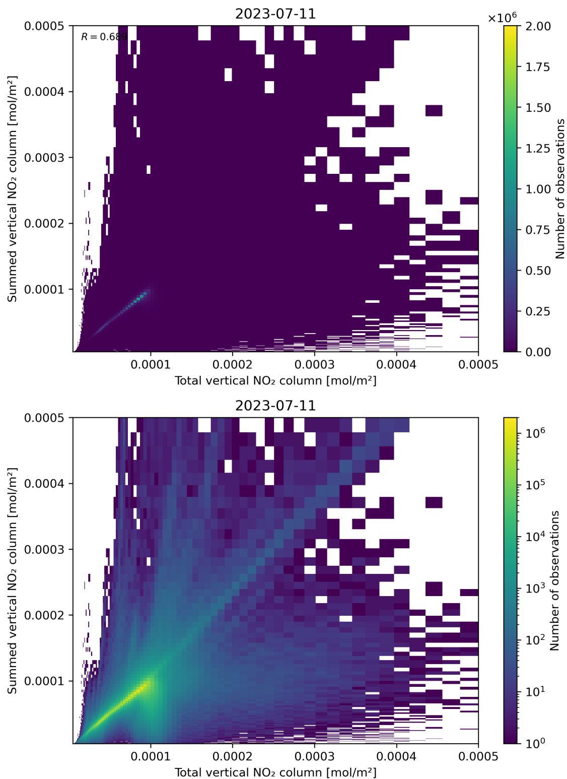
Figure 112: Scatter density plot of “Total vertical NO 2 column” against “Summed vertical NO 2 column” for 2023-07-10 to 2023-07-12.
