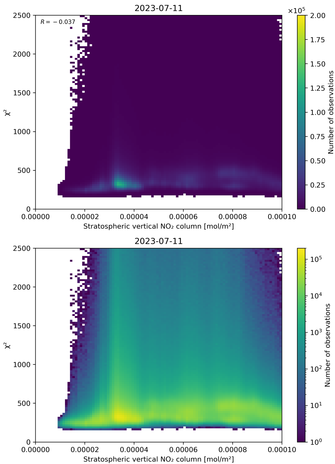
Figure 97: Scatter density plot of “Stratospheric vertical NO 2 column” against “ \chi^2 ” for 2023-07-10 to 2023-07-12.
