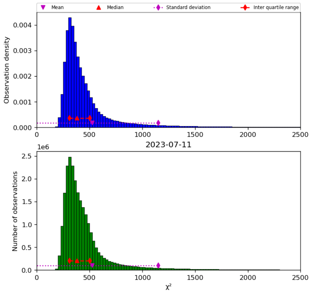
Figure 42: Histogram of “ \chi^2 ” for 2023-07-10 to 2023-07-12
