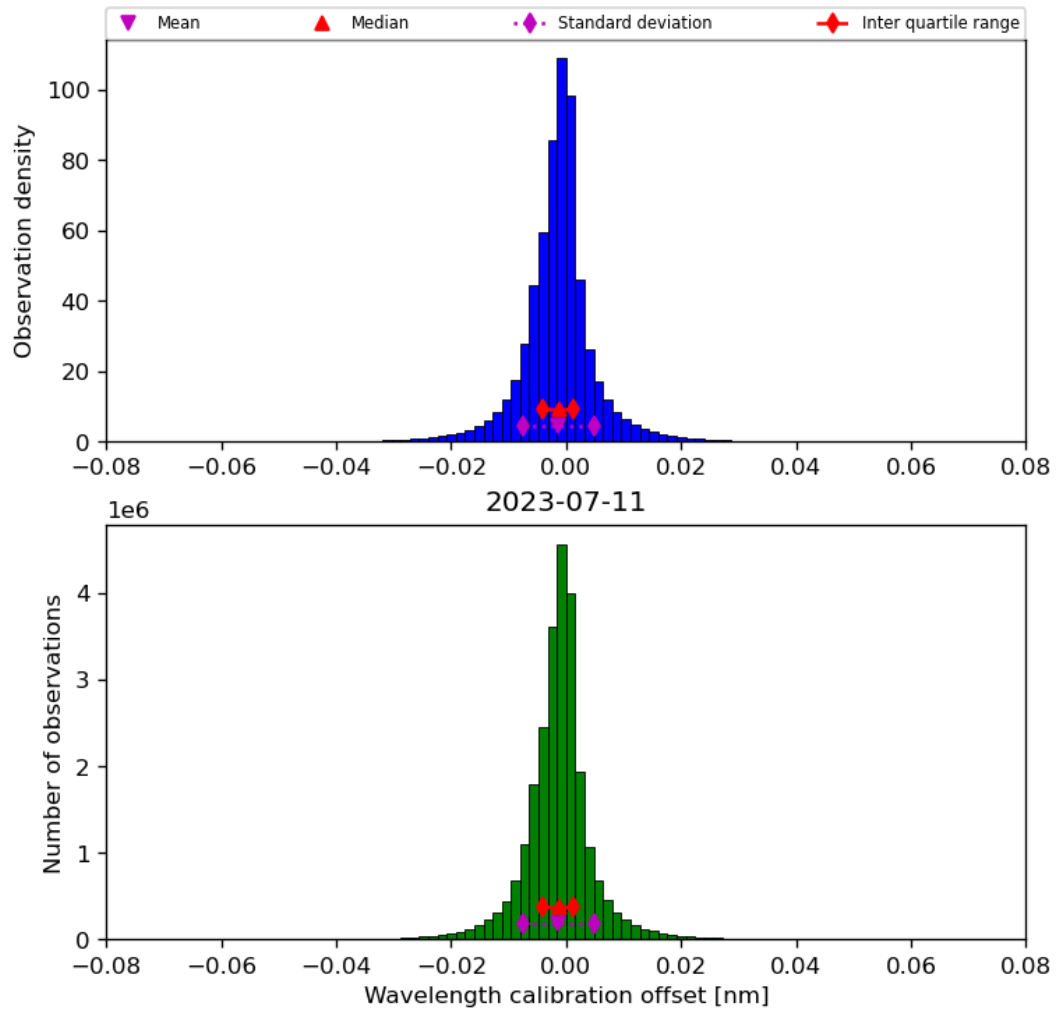
Figure 35: Histogram of “Wavelength calibration offset” for 2023-07-10 to 2023-07-12
