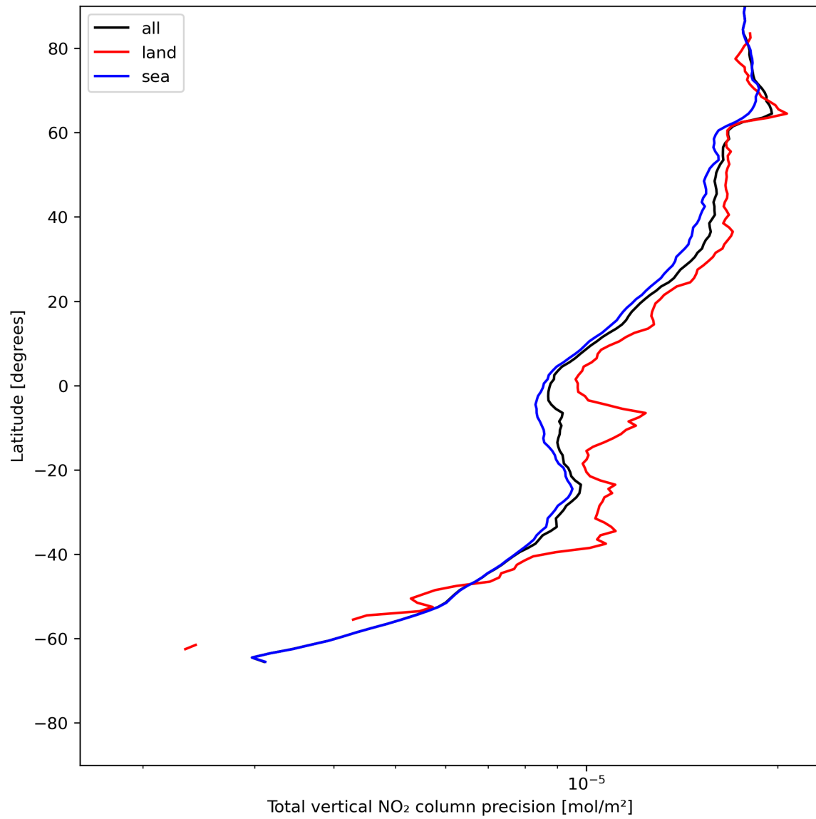
Figure 22: Zonal average of “Total vertical NO 2 column precision” for 2023-07-10 to 2023-07-12.
