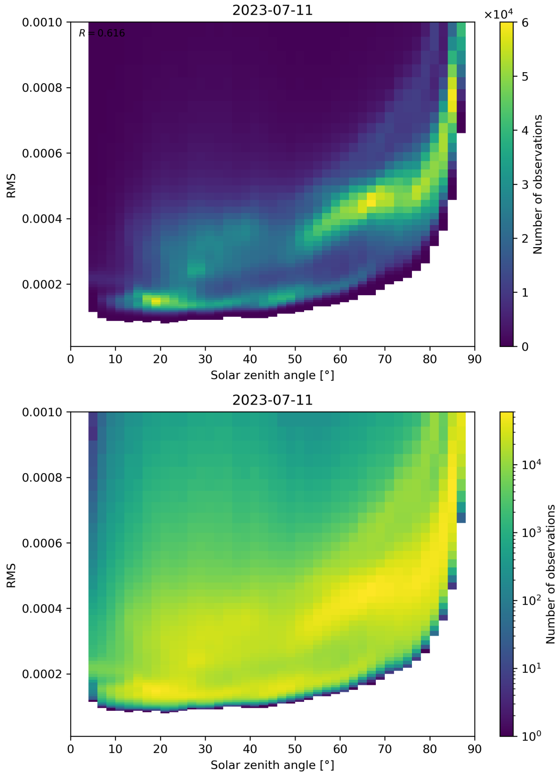
Figure 157: Scatter density plot of “Solar zenith angle” against “RMS” for 2023-07-10 to 2023-07-12.
