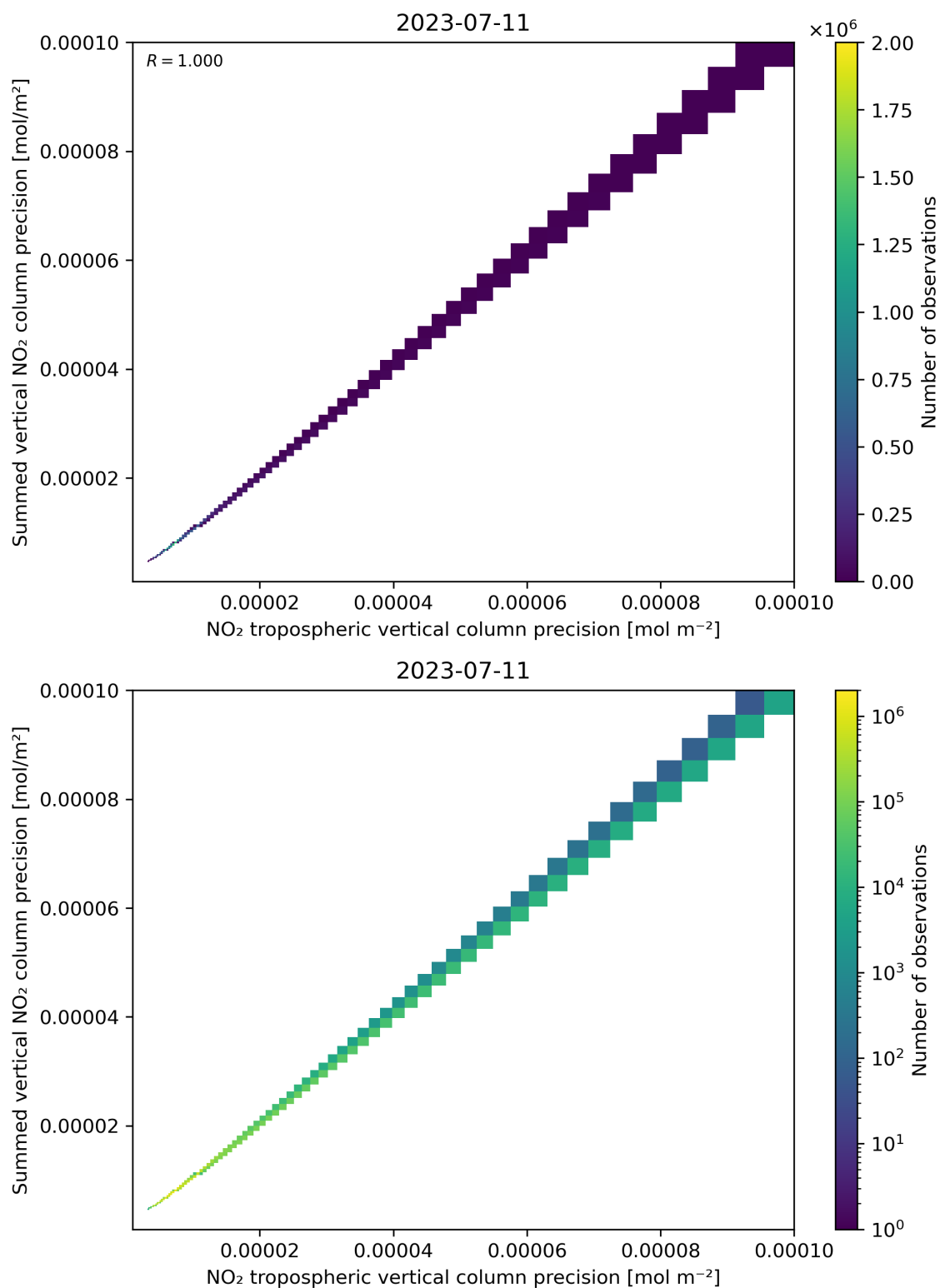
Figure 137: Scatter density plot of “NO 2 tropospheric vertical column precision” against “Summed vertical NO 2 column precision” for 2023-07-10 to 2023-07-12.
