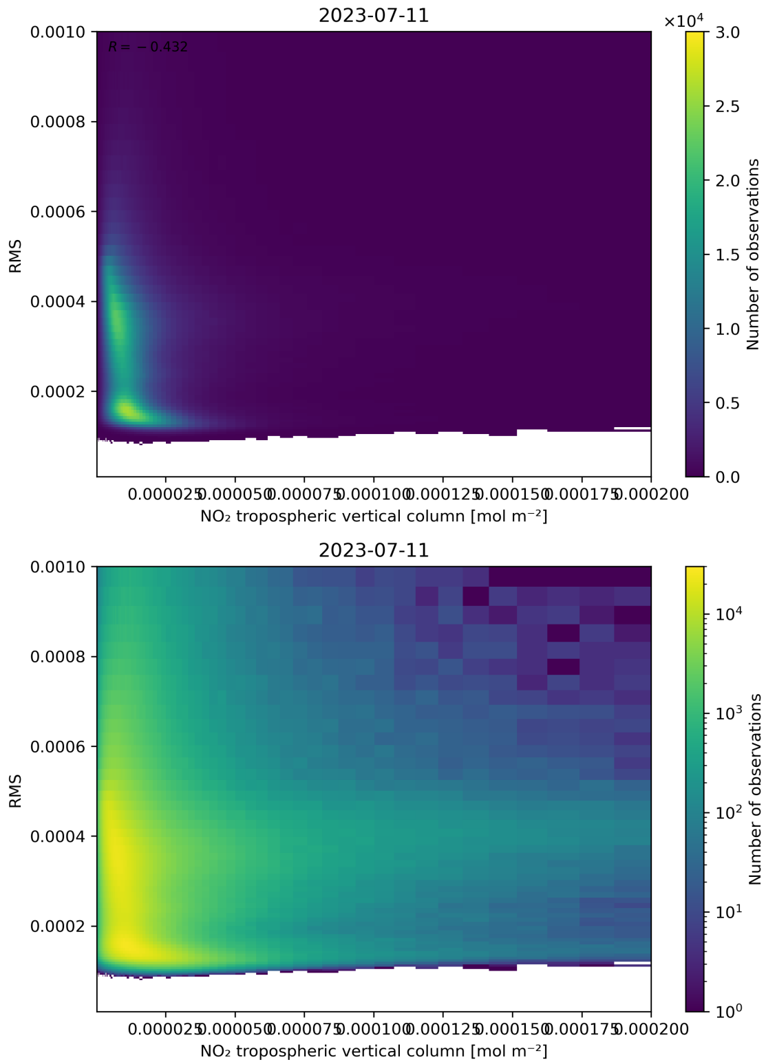
Figure 142: Scatter density plot of “NO 2 tropospheric vertical column” against “RMS” for 2023-07-10 to 2023-07-12.
