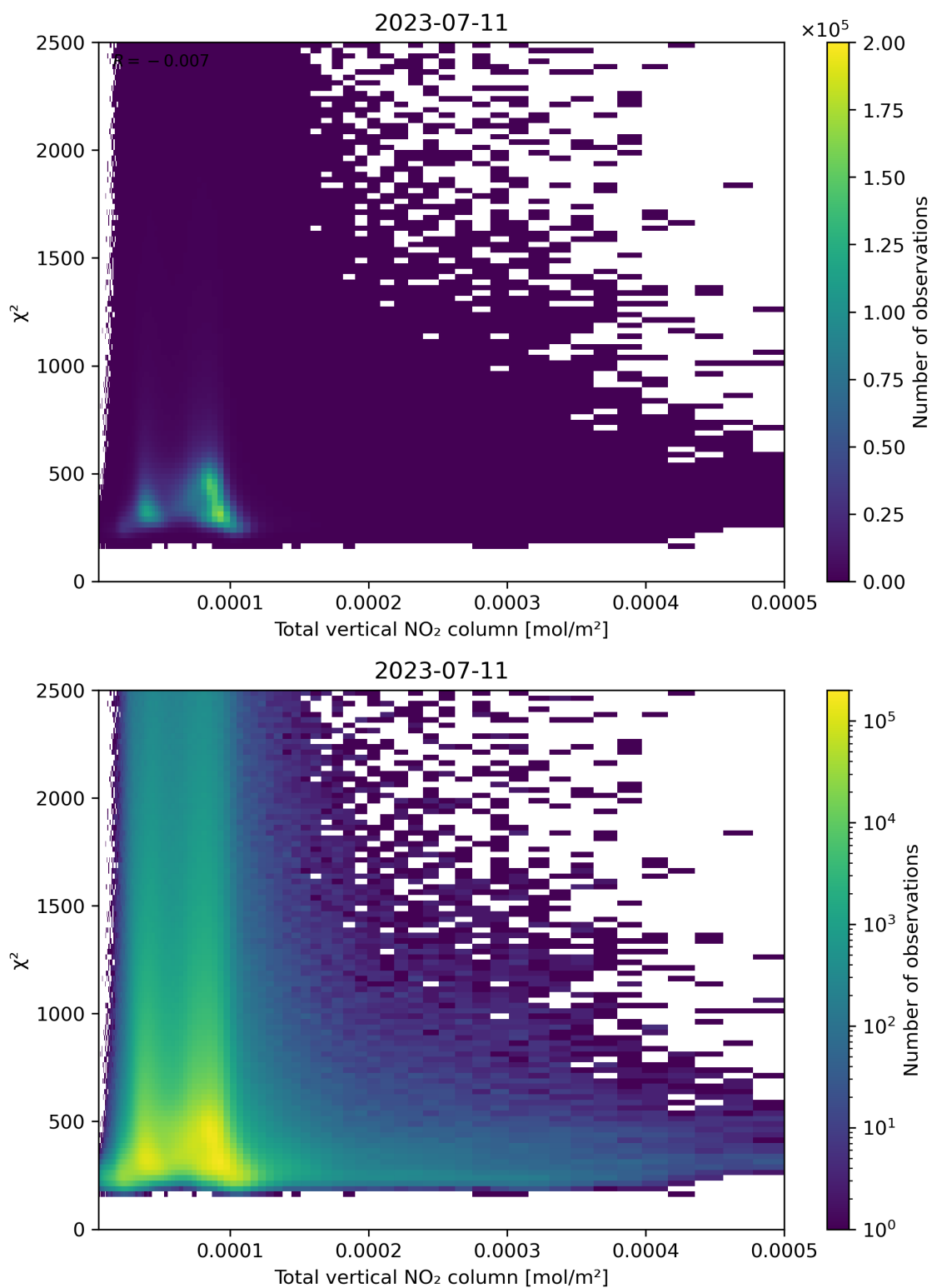
Figure 111: Scatter density plot of “Total vertical NO 2 column” against “ \chi^2 ” for 2023-07-10 to 2023-07-12.
