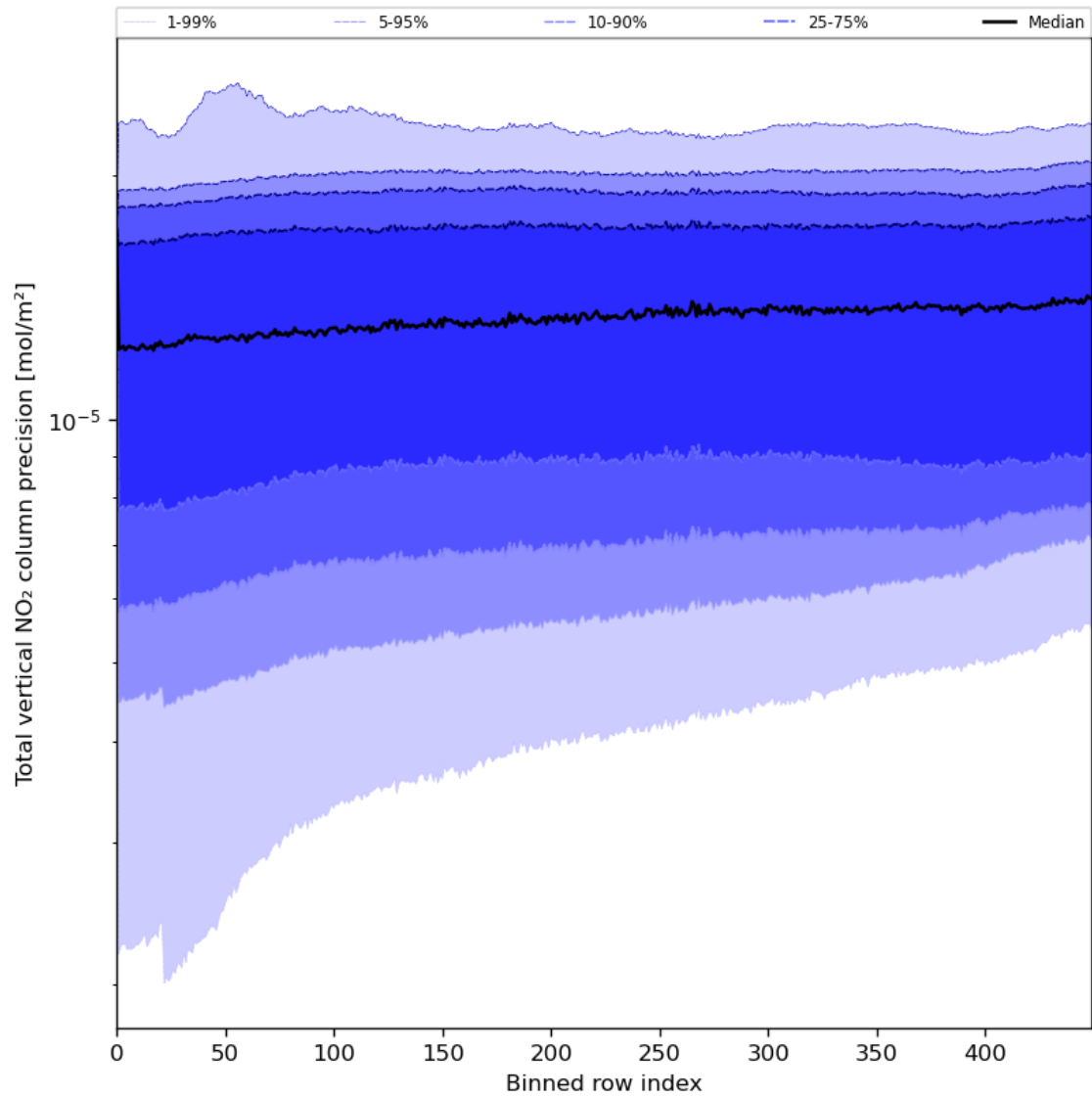
Figure 56: Along track statistics of “Total vertical NO 2 column precision” for 2023-07-10 to 2023-07-12
