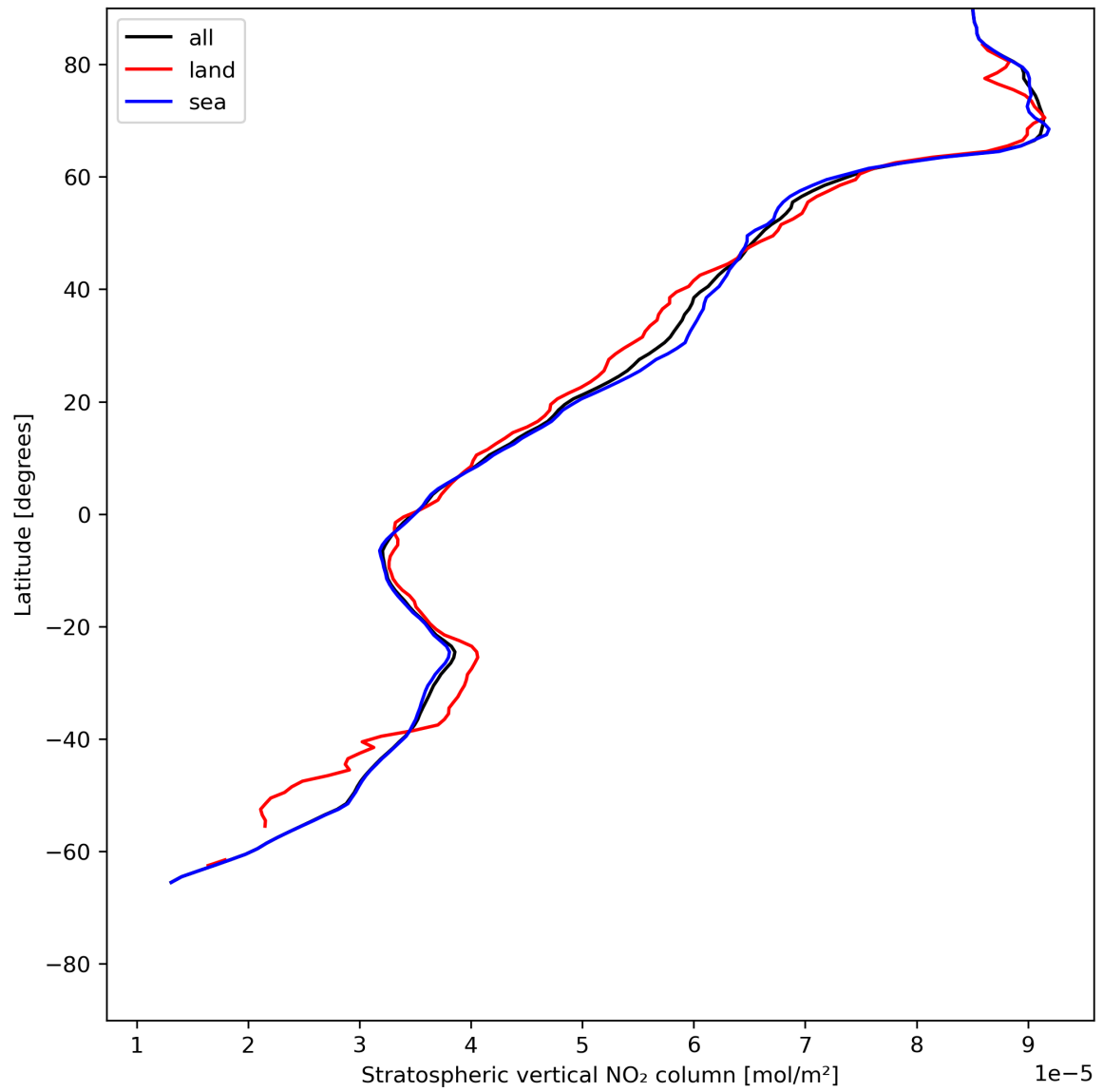
Figure 19: Zonal average of “Stratospheric vertical NO 2 column” for 2023-07-10 to 2023-07-12.
