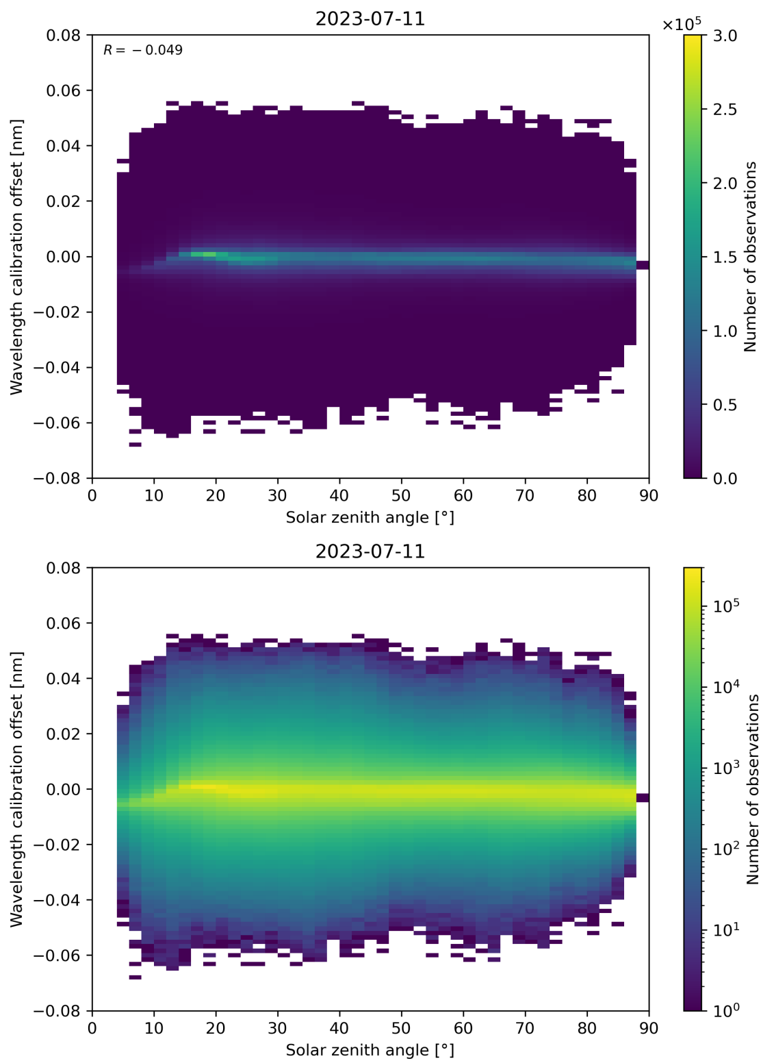
Figure 158: Scatter density plot of “Solar zenith angle” against “Wavelength calibration offset” for 2023-07-10 to 2023-07-12.
