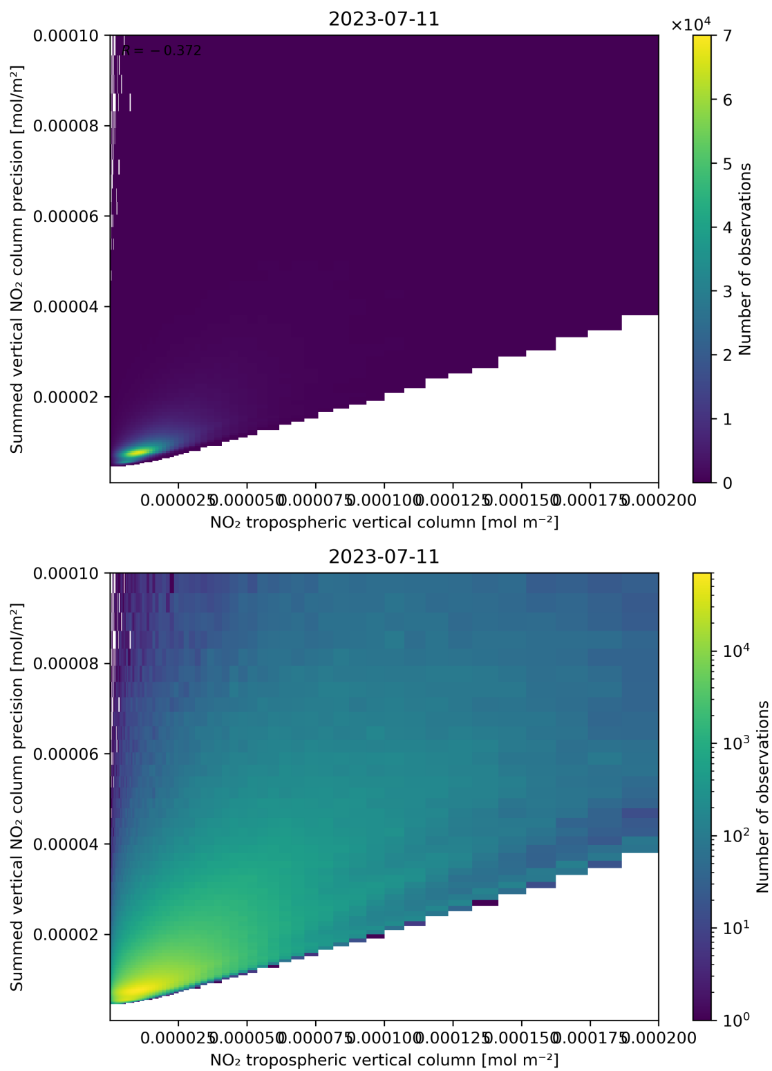
Figure 127: Scatter density plot of “NO 2 tropospheric vertical column” against “Summed vertical NO 2 column precision” for 2023-07-10 to 2023-07-12.
