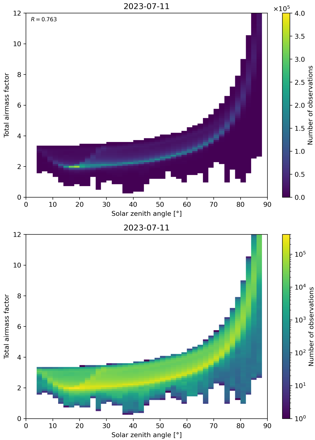
Figure 146: Scatter density plot of “Solar zenith angle” against “Total air mass factor” for 2023-07-10 to 2023-07-12.
