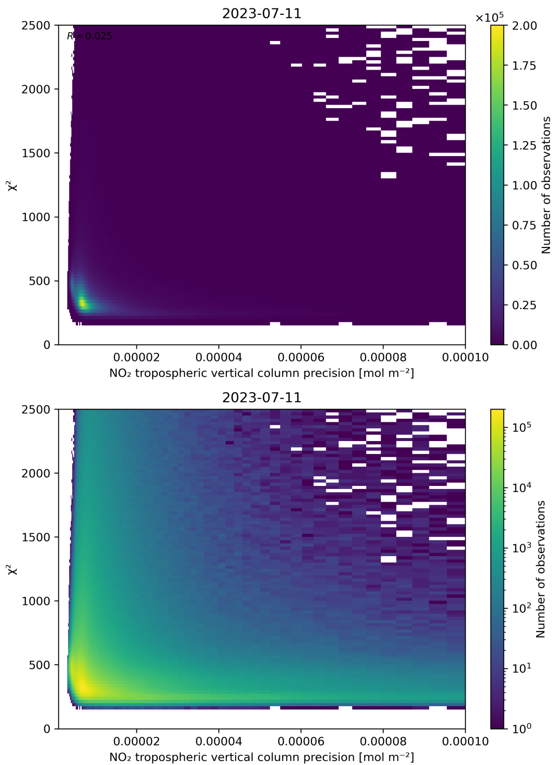
Figure 134: Scatter density plot of “NO 2 tropospheric vertical column precision” against “ \chi^2 ” for 2023-07-10 to 2023-07-12.
