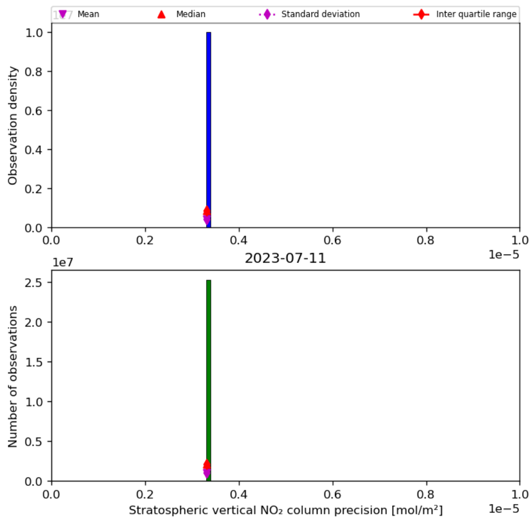
Figure 37: Histogram of “Stratospheric vertical NO 2 column precision” for 2023-07-10 to 2023-07-12
