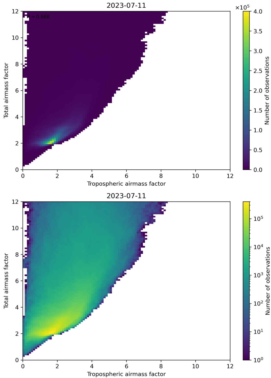
Figure 72: Scatter density plot of “Tropospheric airmass factor” against “Total airmass factor” for 2023-07-10 to 2023-07-12.
