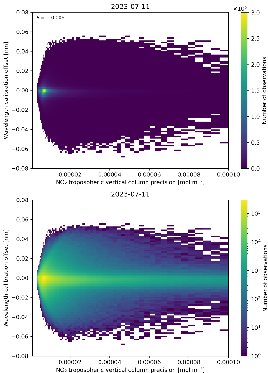
Figure 141: Scatter density plot of “NO 2 tropospheric vertical column precision” against “Wavelength calibration offset” for 2023-07-10 to 2023-07-12.
