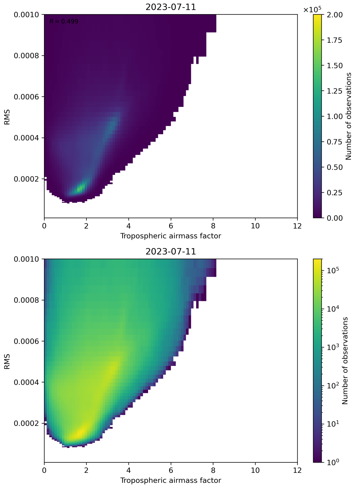
Figure 79: Scatter density plot of “Tropospheric airmass factor” against “RMS” for 2023-07-10 to 2023-07-12.
