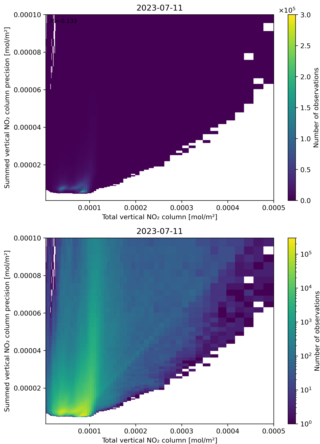
Figure 113: Scatter density plot of “Total vertical NO 2 column” against “Summed vertical NO 2 column precision” for 2023-07-10 to 2023-07-12.
