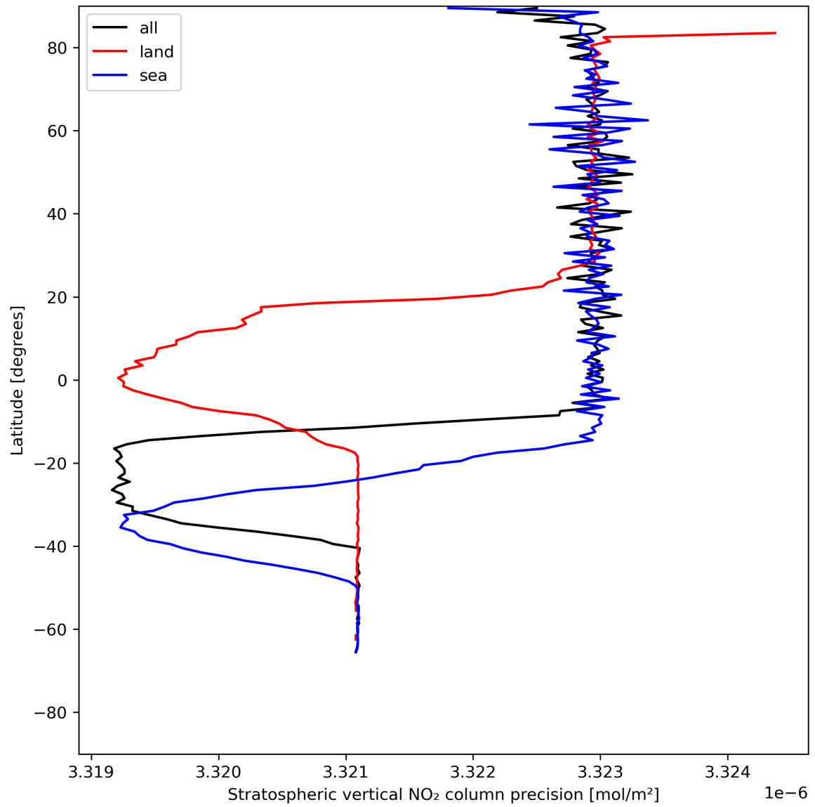
Figure 20: Zonal average of “Stratospheric vertical NO 2 column precision” for 2023-07-10 to 2023-07-12.
