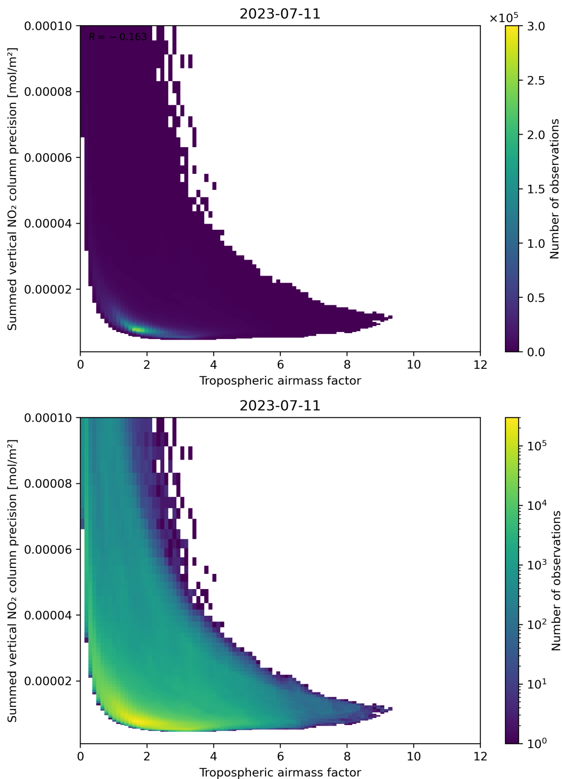
Figure 76: Scatter density plot of “Tropospheric air mass factor” against “Summed vertical NO 2 column precision” for 2023-07-10 to 2023-07-12.
