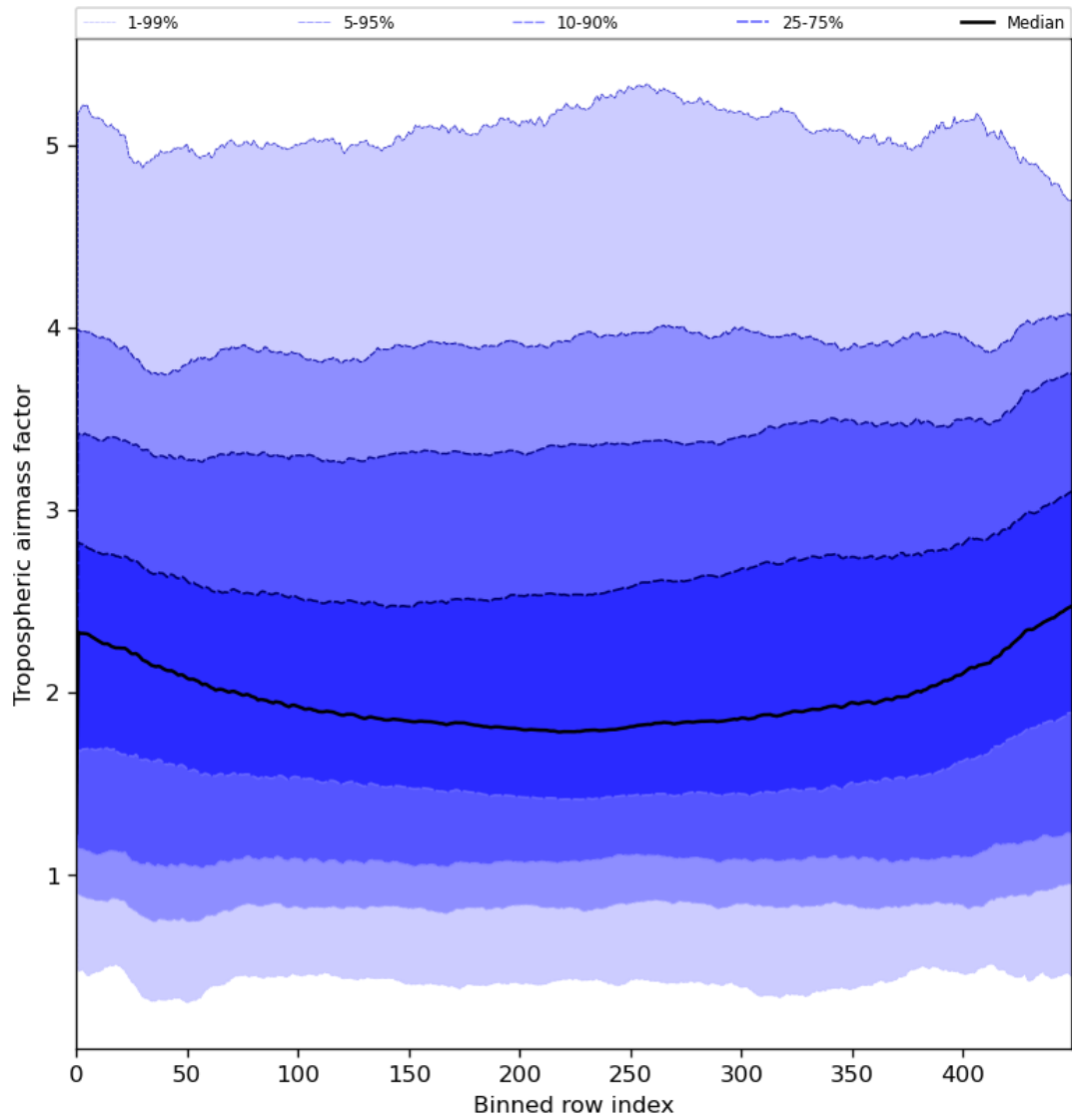
Figure 48: Along track statistics of “Tropospheric airmass factor” for 2023-07-10 to 2023-07-12
