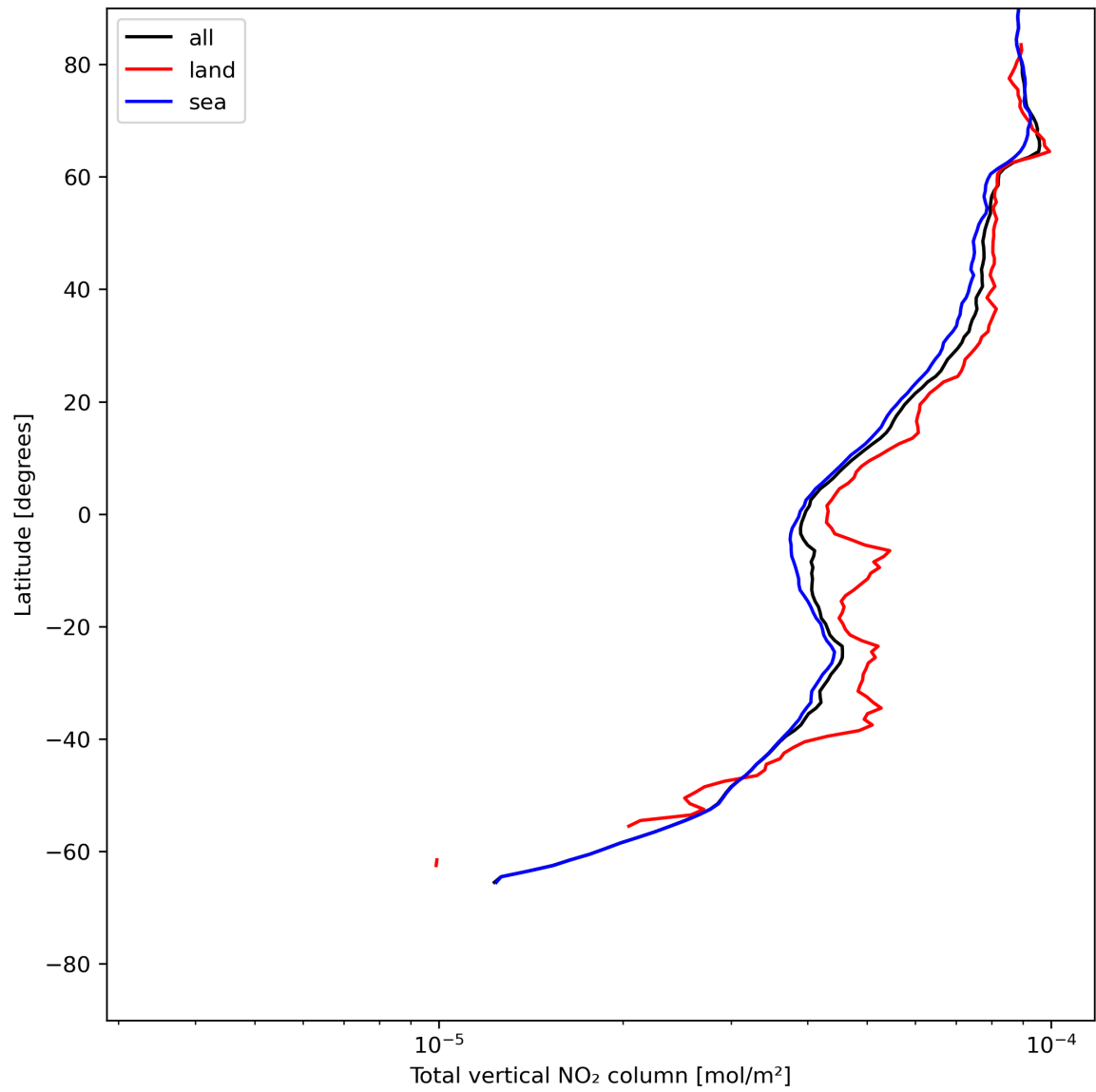
Figure 21: Zonal average of “Total vertical NO 2 column” for 2023-07-10 to 2023-07-12.
