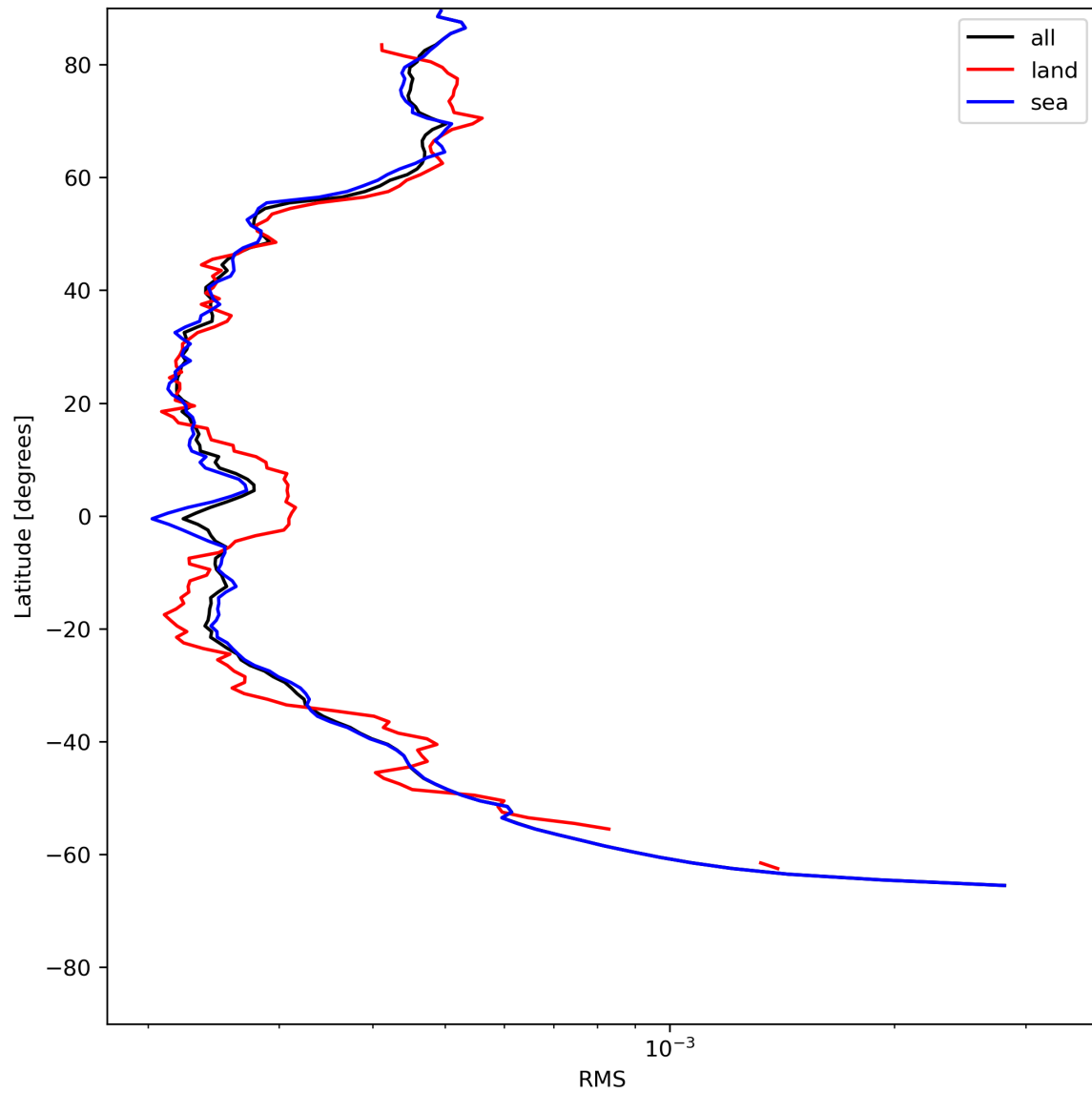
Figure 26: Zonal average of “RMS” for 2023-07-10 to 2023-07-12.
