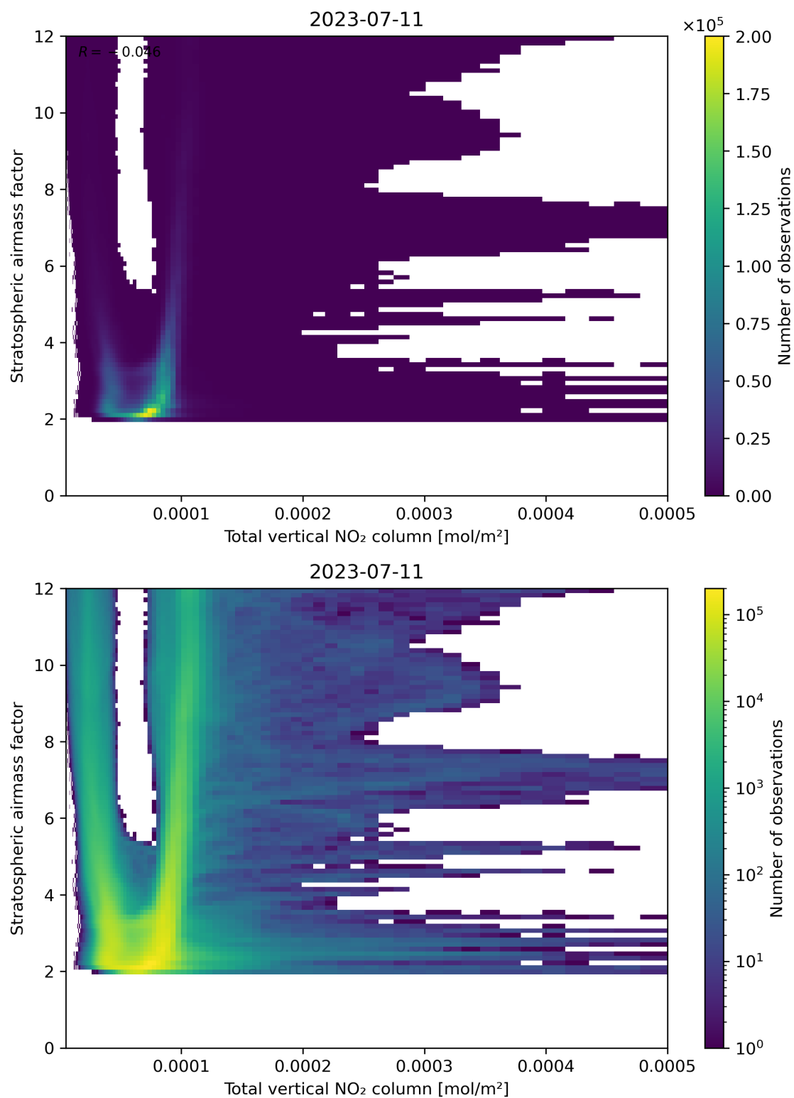
Figure 110: Scatter density plot of “Total vertical NO 2 column” against “Stratospheric airmass factor” for 2023-07-10 to 2023-07-12.
