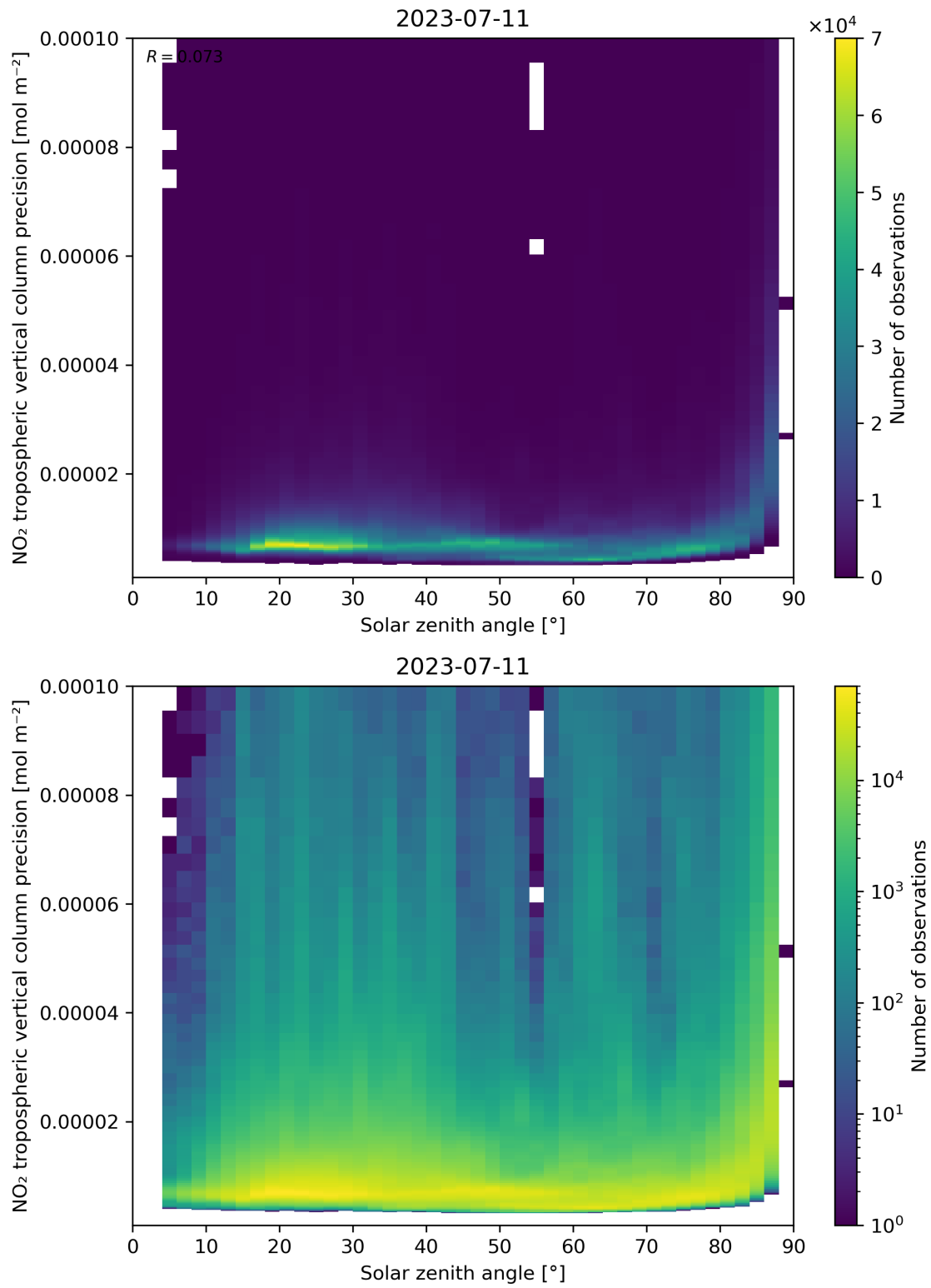
Figure 156: Scatter density plot of “Solar zenith angle” against “NO 2 tropospheric vertical column precision” for 2023-07-10 to 2023-07-12.
