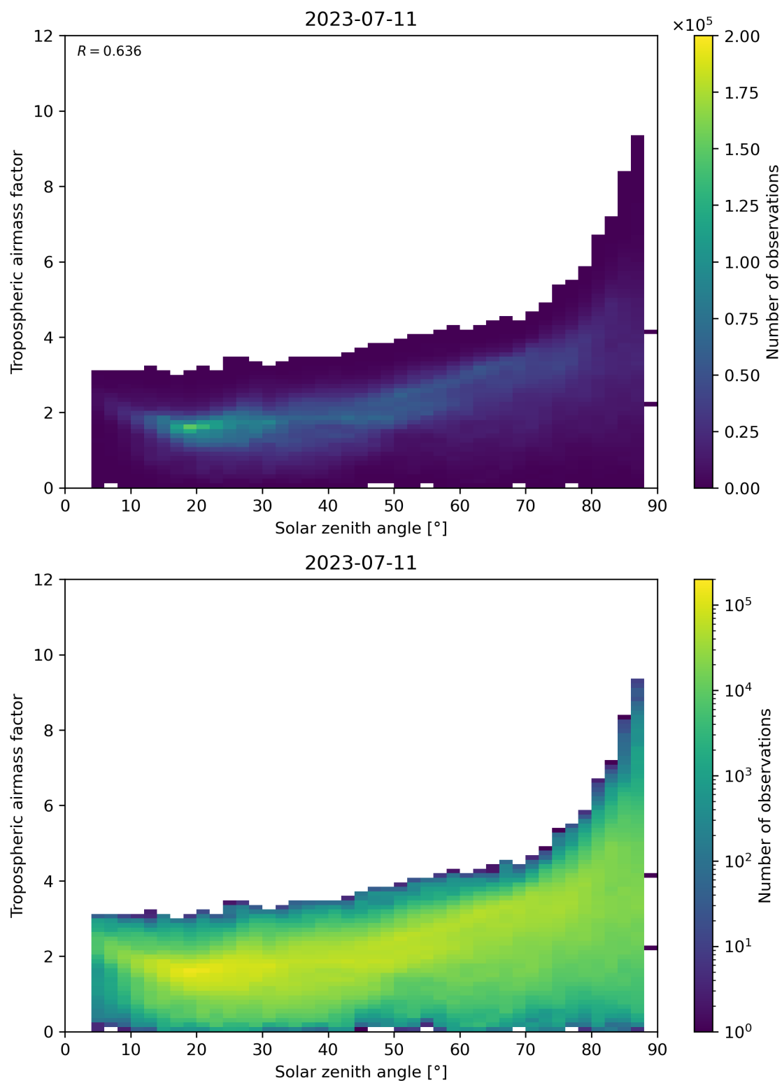
Figure 147: Scatter density plot of “Solar zenith angle” against “Tropospheric airmass factor” for 2023-07-10 to 2023-07-12.
