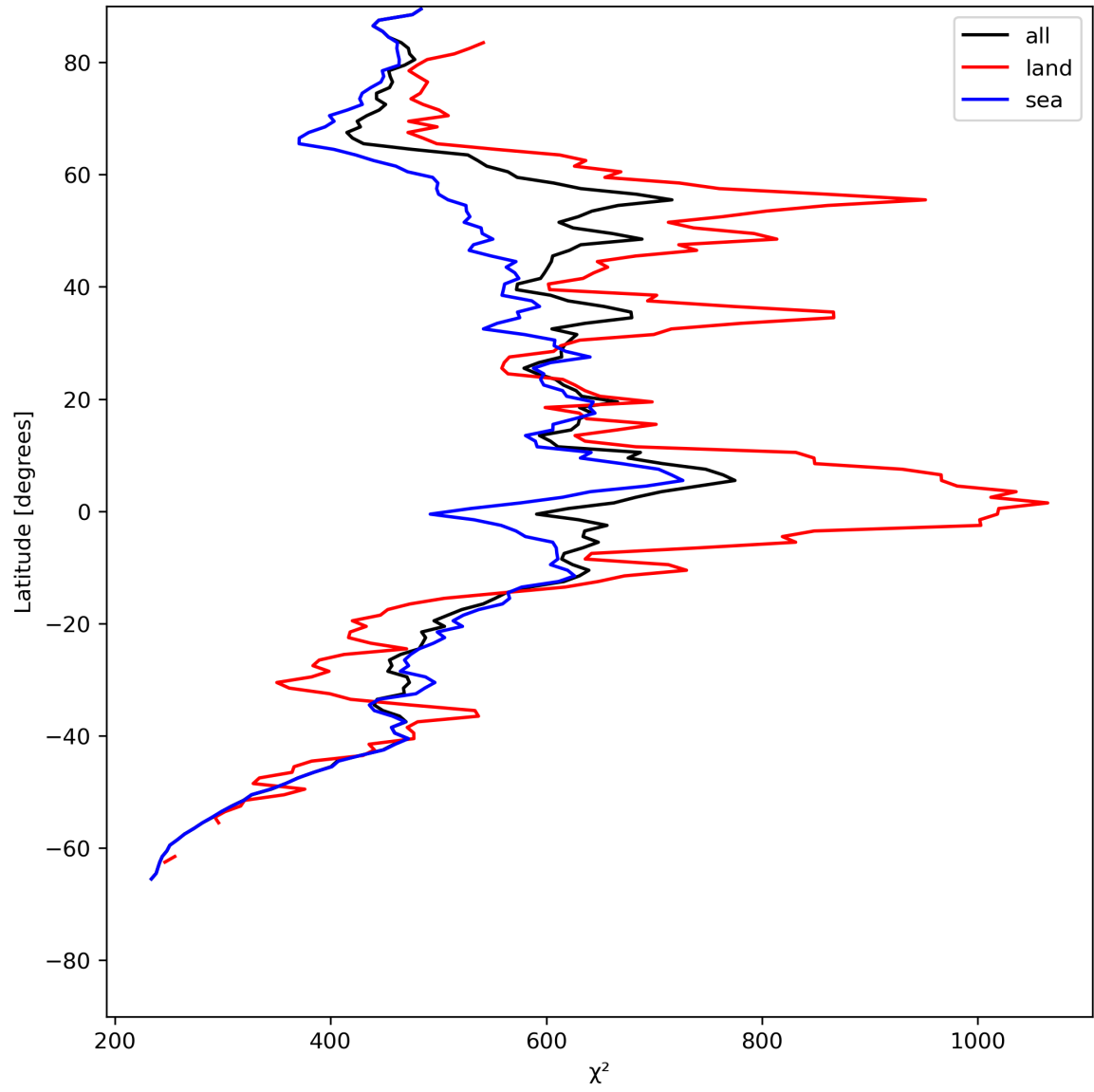
Figure 25: Zonal average of “ \chi^2 ” for 2023-07-10 to 2023-07-12.
