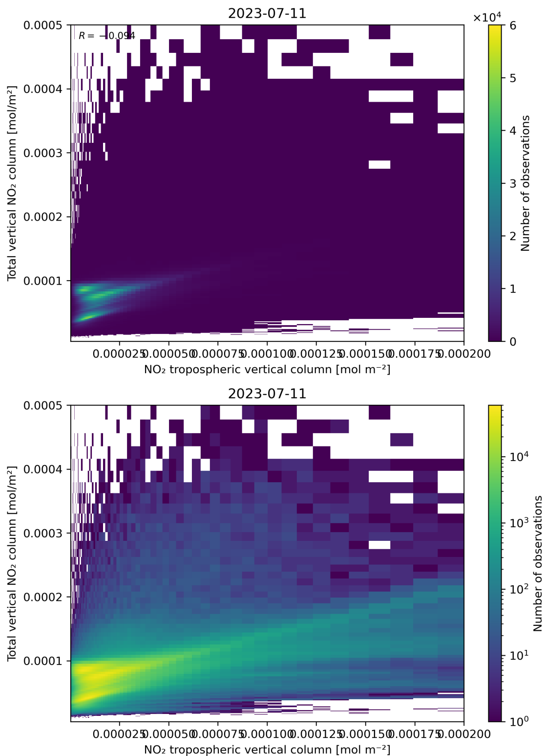
Figure 128: Scatter density plot of “NO 2 tropospheric vertical column” against “Total vertical NO 2 column” for 2023-07-10 to 2023-07-12.
