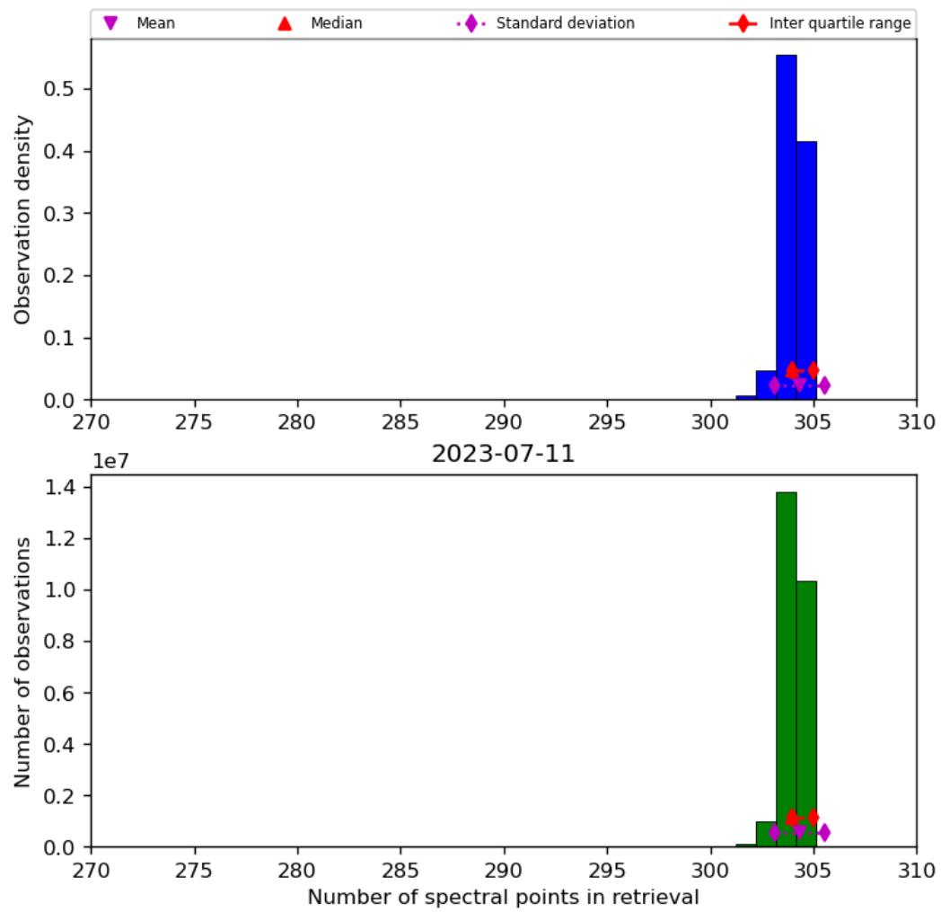
Figure 33: Histogram of “Number of spectral points in retrieval” for 2023-07-10 to 2023-07-12
