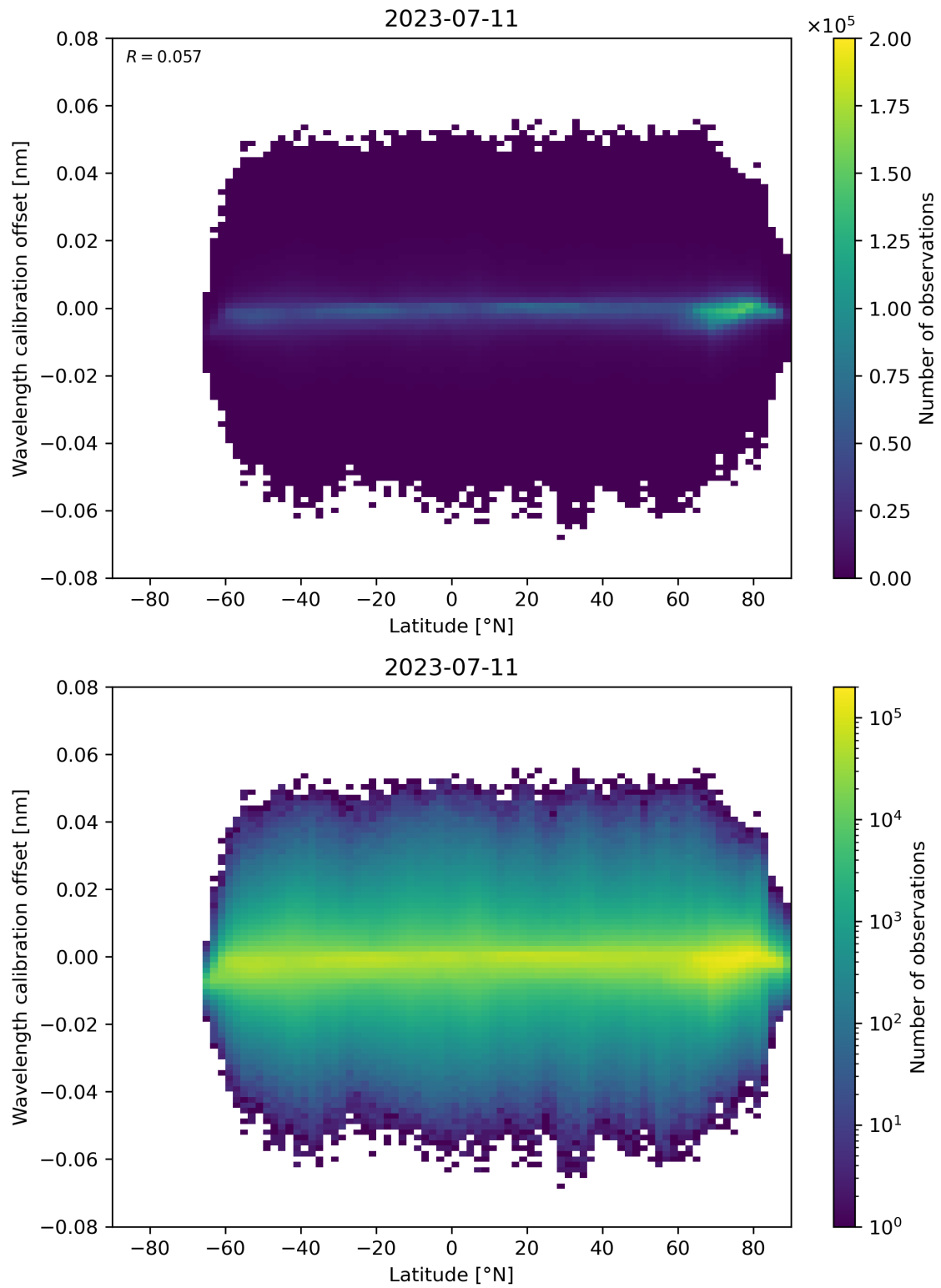
Figure 95: Scatter density plot of “Latitude” against “Wavelength calibration offset” for 2023-07-10 to 2023-07-12.
