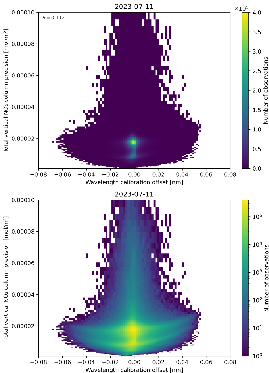
Figure 180: Scatter density plot of “Wavelength calibration offset” against “Total vertical NO 2 column precision” for 2023-07-10 to 2023-07-12.
