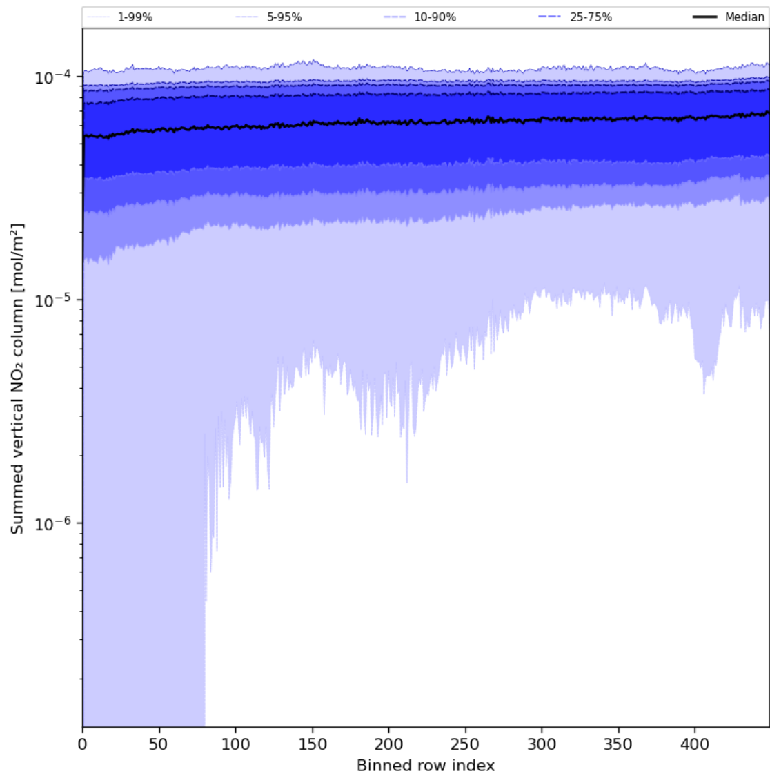
Figure 57: Along track statistics of “Summed vertical NO 2 column” for 2023-07-10 to 2023-07-12
