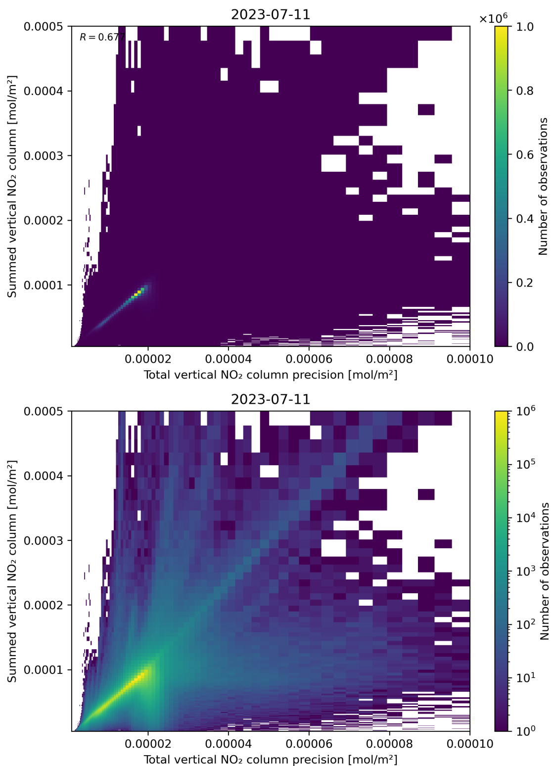
Figure 117: Scatter density plot of “Total vertical NO 2 column precision” against “Summed vertical NO 2 column” for 2023-07-10 to 2023-07-12.
