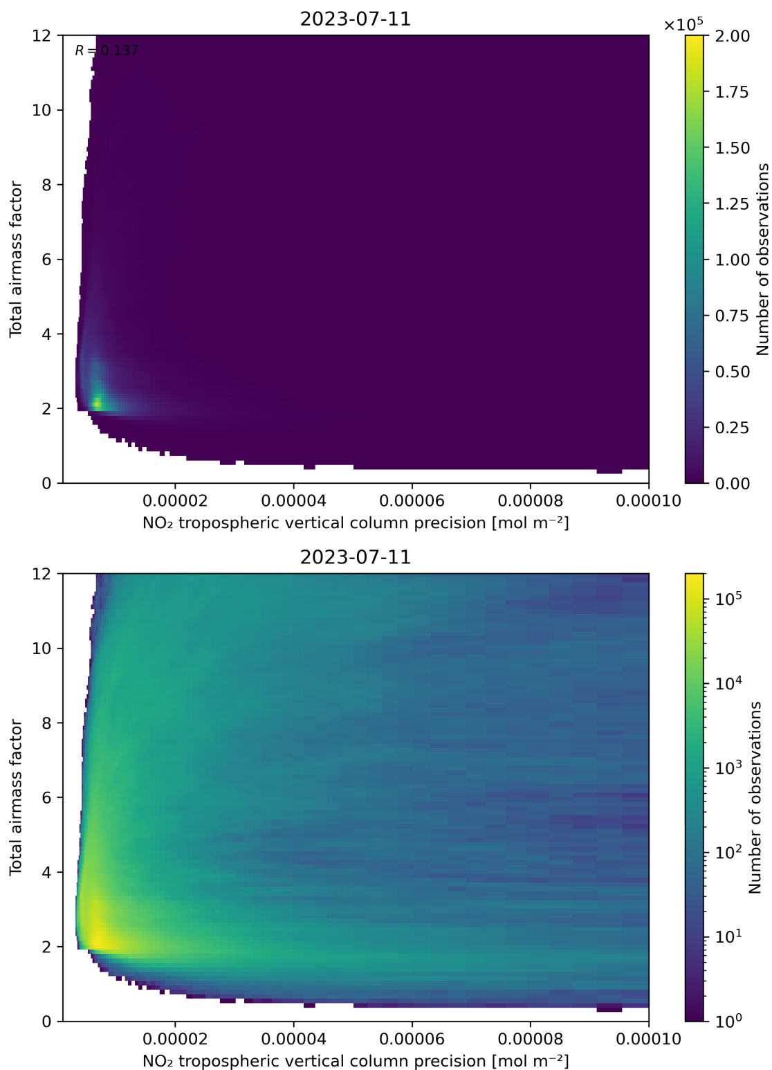
Figure 132: Scatter density plot of “NO 2 tropospheric vertical column precision” against “Total air mass factor” for 2023-07-10 to 2023-07-12.
