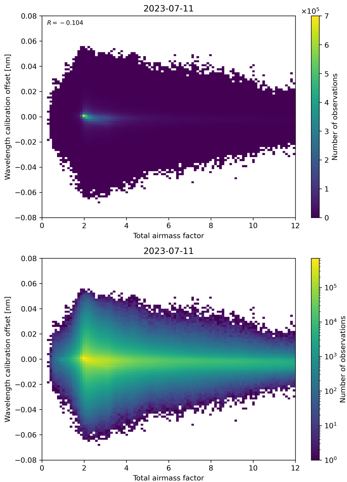
Figure 70: Scatter density plot of “Total airmass factor” against “Wavelength calibration offset” for 2023-07-10 to 2023-07-12.
