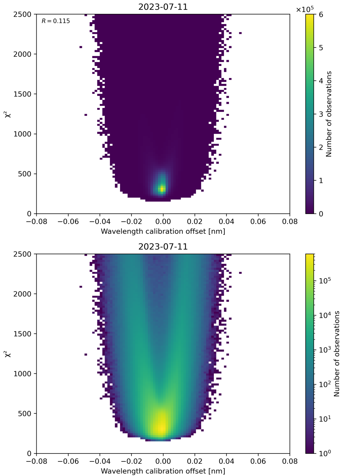
Figure 175: Scatter density plot of “Wavelength calibration offset” against “ \chi^2 ” for 2023-07-10 to 2023-07-12.
