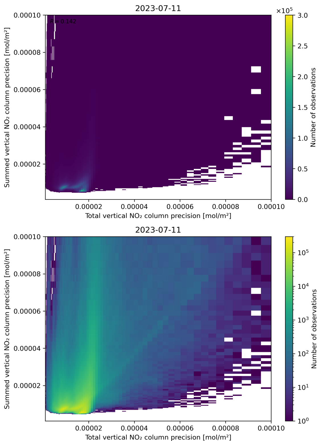
Figure 118: Scatter density plot of “Total vertical NO 2 column precision” against “Summed vertical NO 2 column precision” for 2023-07-10 to 2023-07-12.
