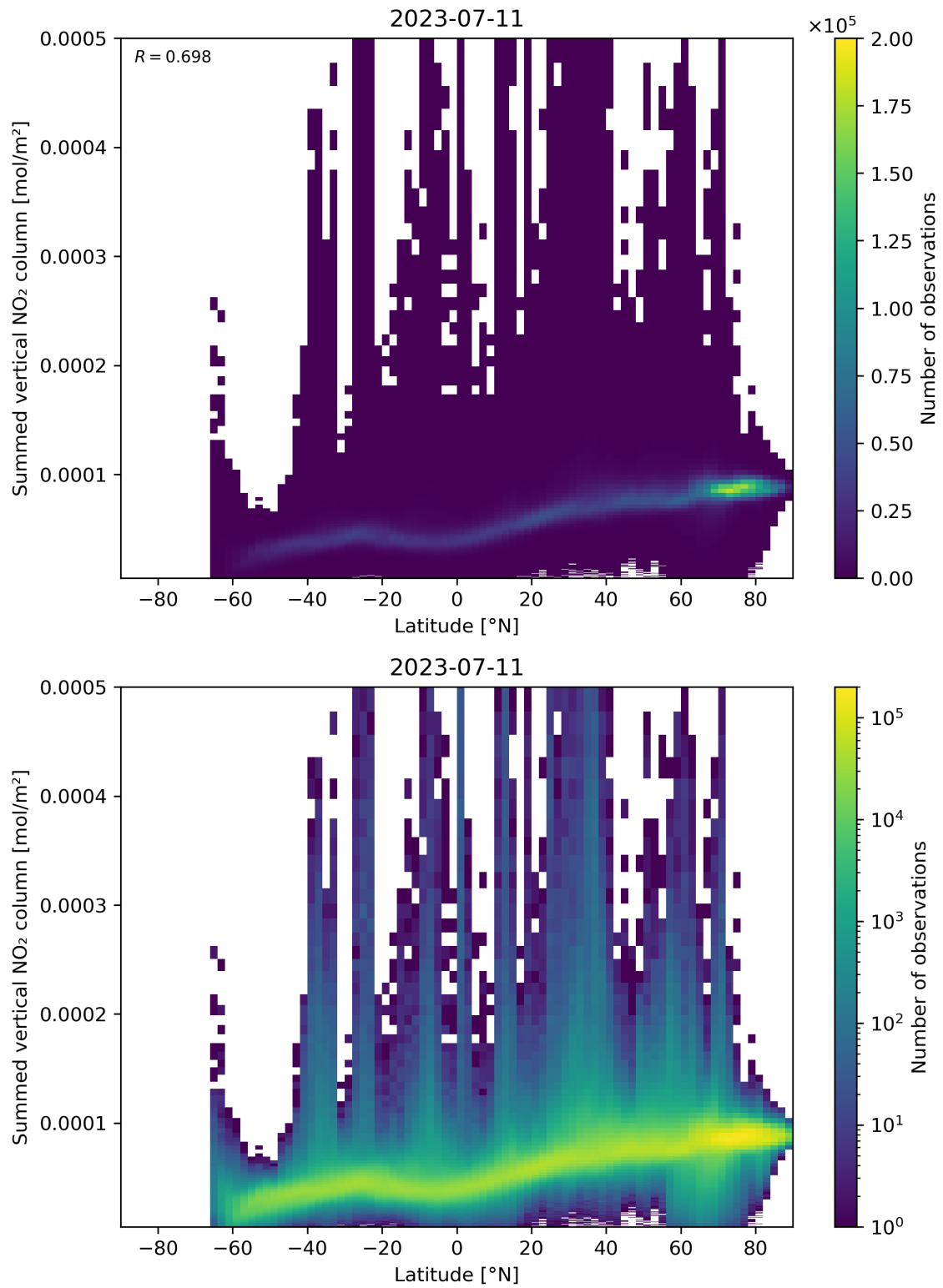
Figure 88: Scatter density plot of “Latitude” against “Summed vertical NO 2 column” for 2023-07-10 to 2023-07-12.
