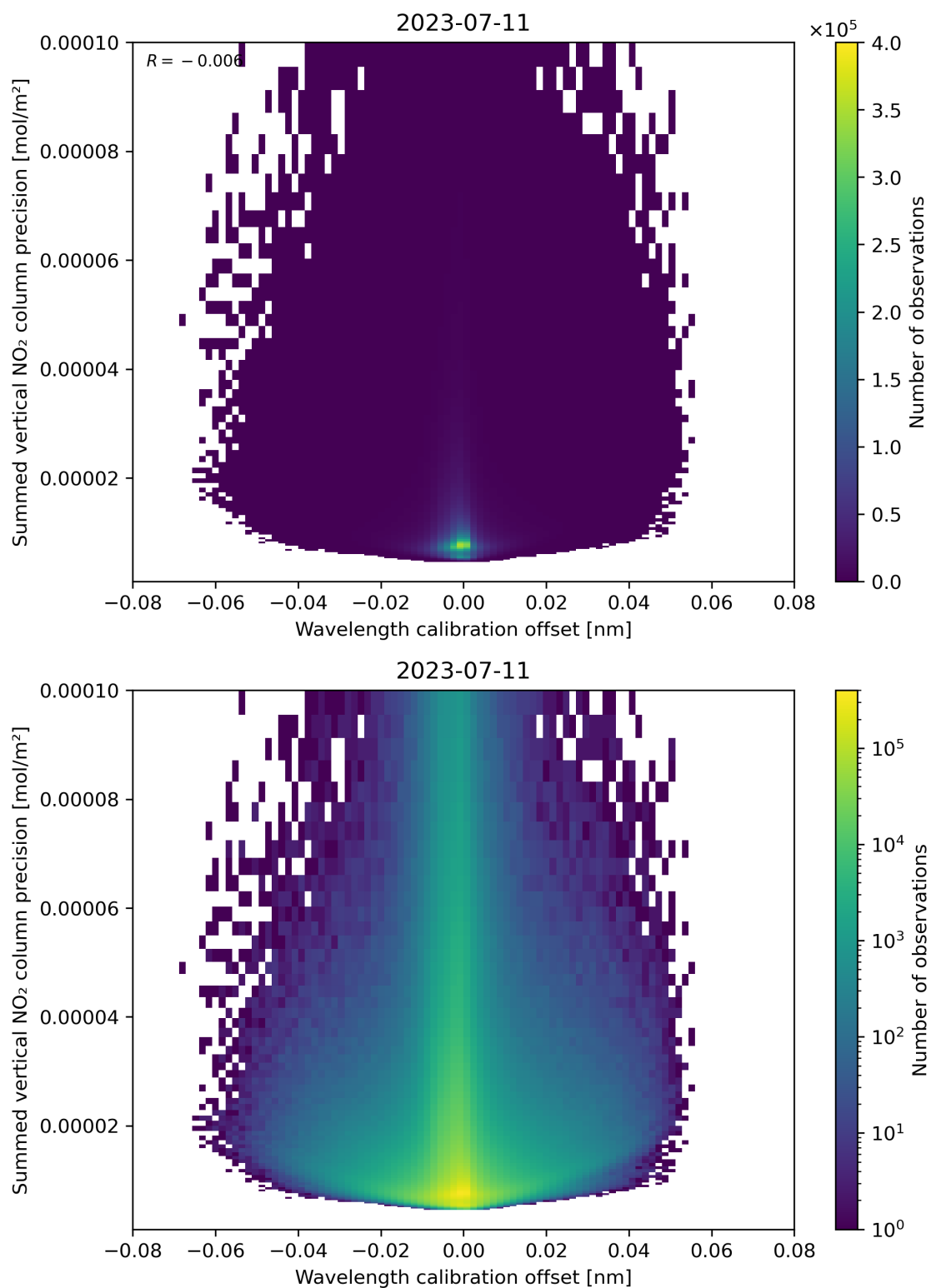
Figure 178: Scatter density plot of “Wavelength calibration offset” against “Summed vertical NO 2 column precision” for 2023-07-10 to 2023-07-12.
