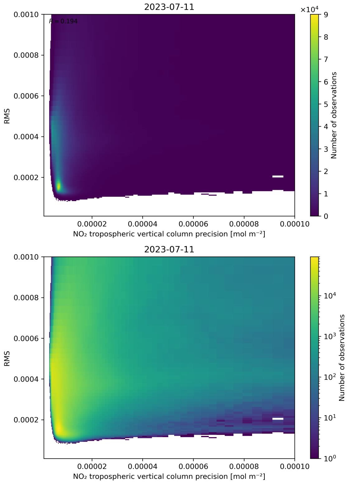
Figure 140: Scatter density plot of “NO 2 tropospheric vertical column precision” against “RMS” for 2023-07-10 to 2023-07-12.
