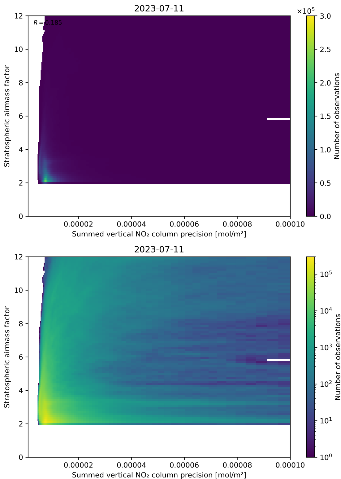
Figure 106: Scatter density plot of “Summed vertical NO 2 column precision” against “Stratospheric airmass factor” for 2023-07-10 to 2023-07-12.
