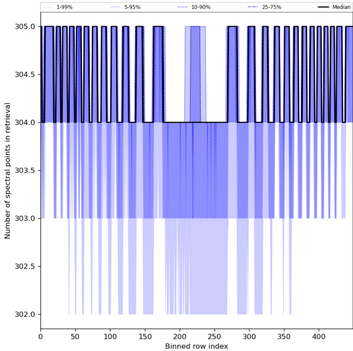
Figure 50: Along track statistics of “Number of spectral points in retrieval” for 2023-07-10 to 2023-07-12
