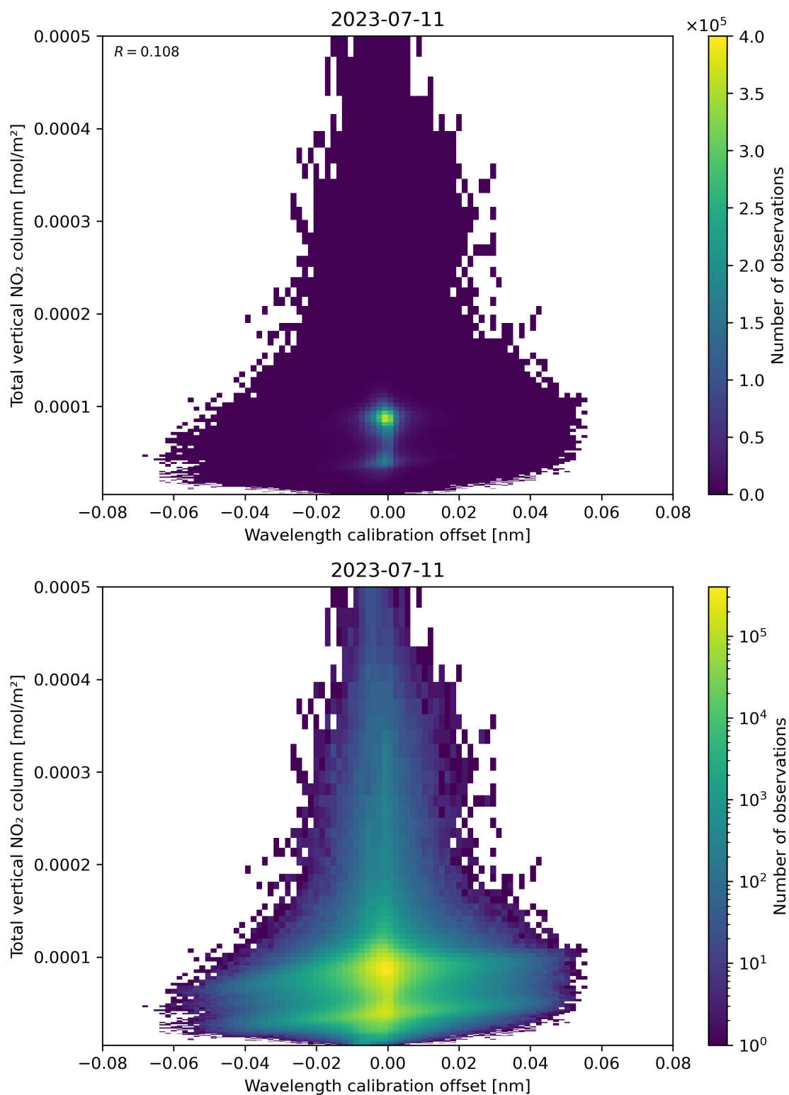
Figure 179: Scatter density plot of “Wavelength calibration offset” against “Total vertical NO 2 column” for 2023-07-10 to 2023-07-12.
