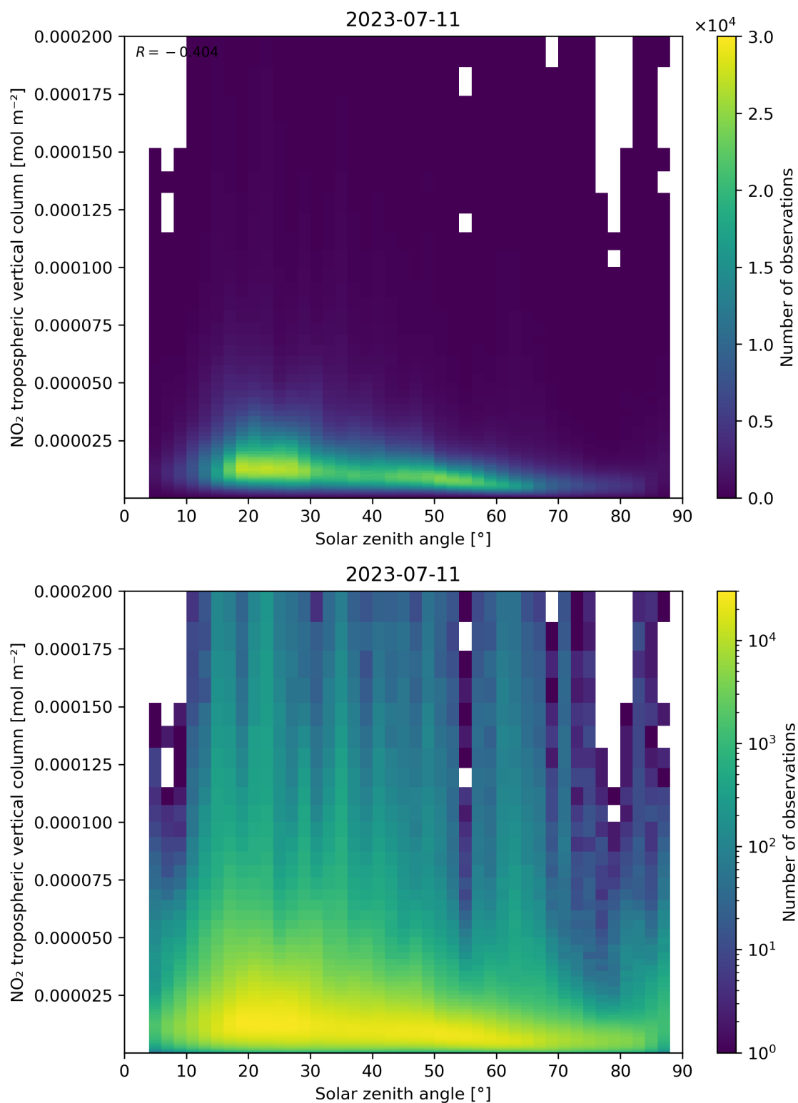
Figure 155: Scatter density plot of “Solar zenith angle” against “NO 2 tropospheric vertical column” for 2023-07-10 to 2023-07-12.
