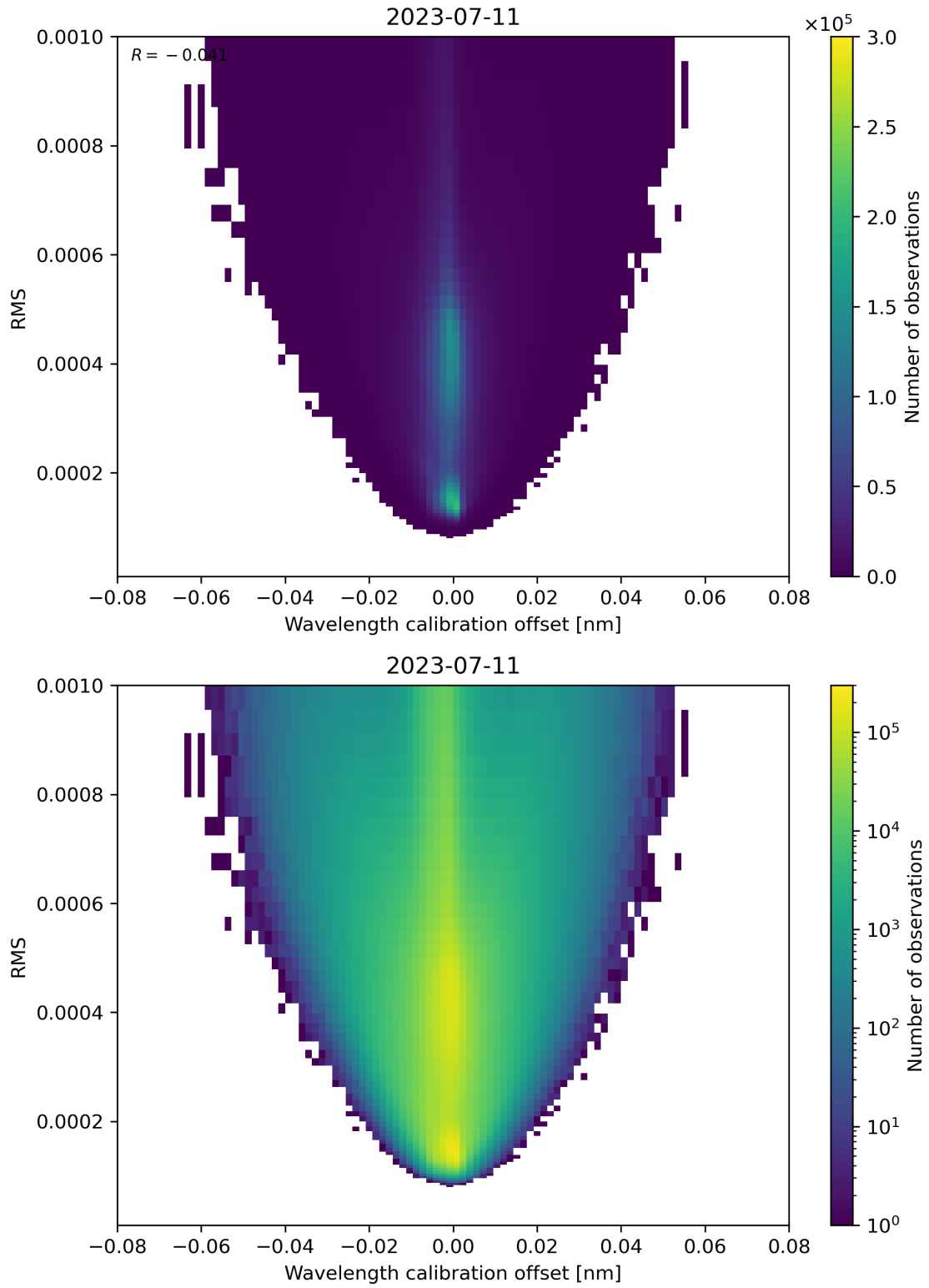
Figure 181: Scatter density plot of “Wavelength calibration offset” against “RMS” for 2023-07-10 to 2023-07-12.
