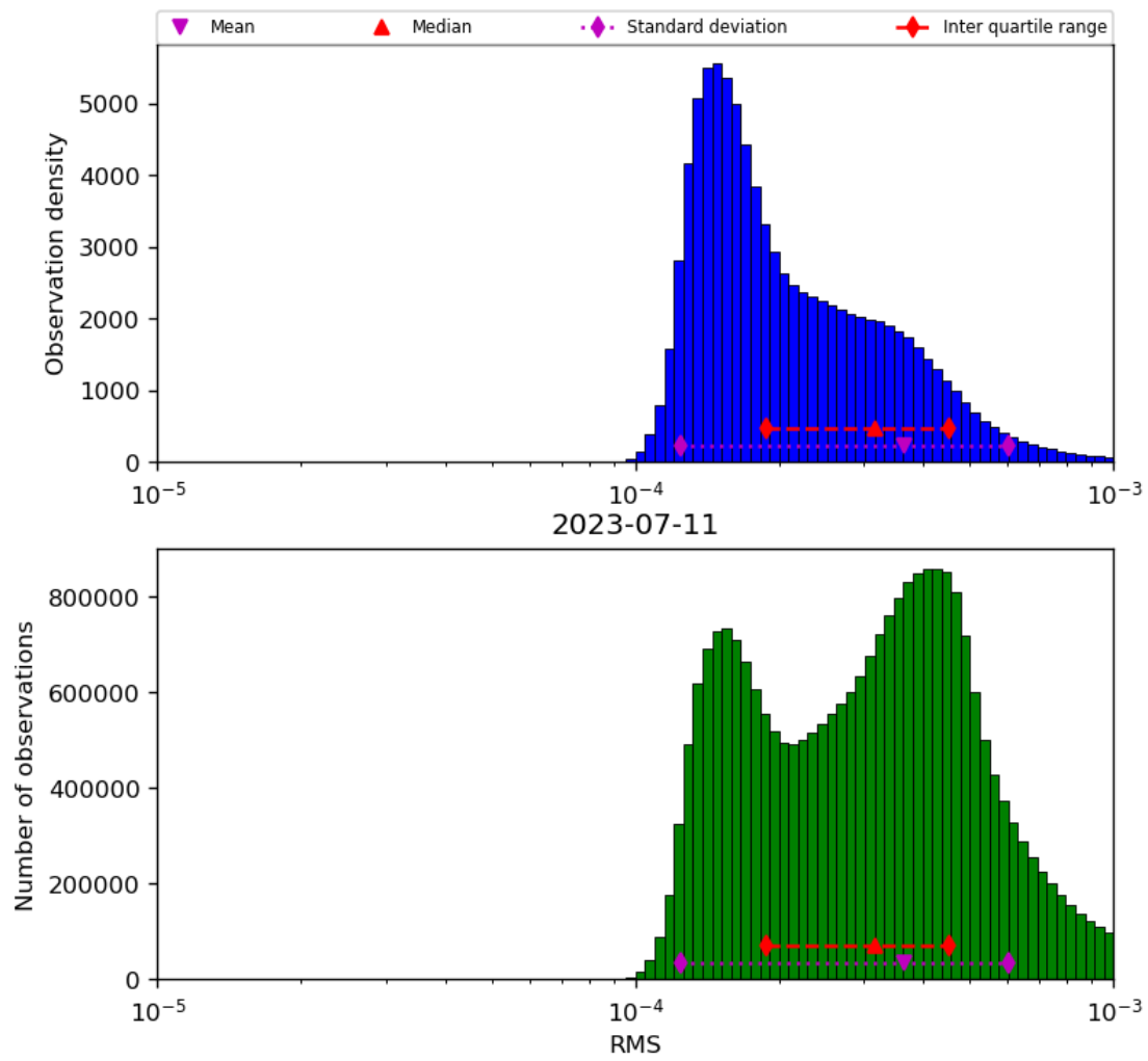
Figure 43: Histogram of “RMS” for 2023-07-10 to 2023-07-12
