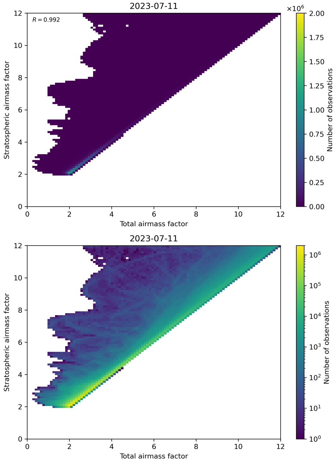
Figure 62: Scatter density plot of “Total airmass factor” against “Stratospheric airmass factor” for 2023-07-10 to 2023-07-12.
