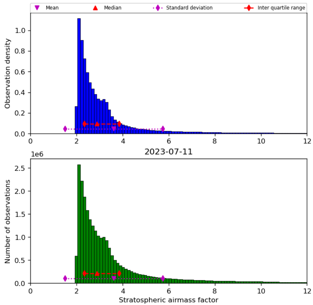
Figure 44: Histogram of “Stratospheric airmass factor” for 2023-07-10 to 2023-07-12
