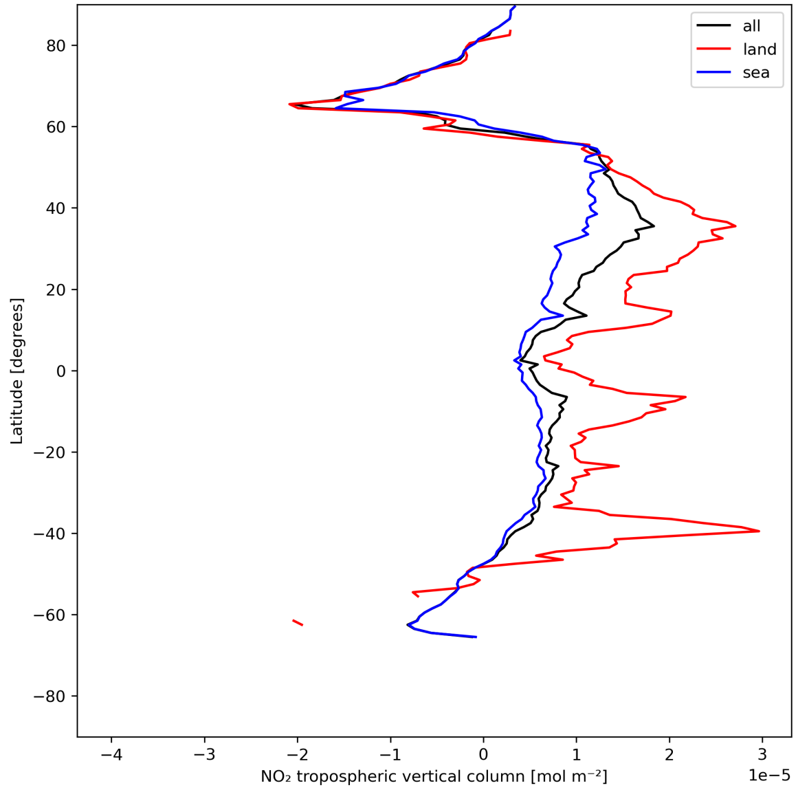
Figure 12: Zonal average of “NO 2 tropospheric vertical column” for 2023-07-10 to 2023-07-12.
