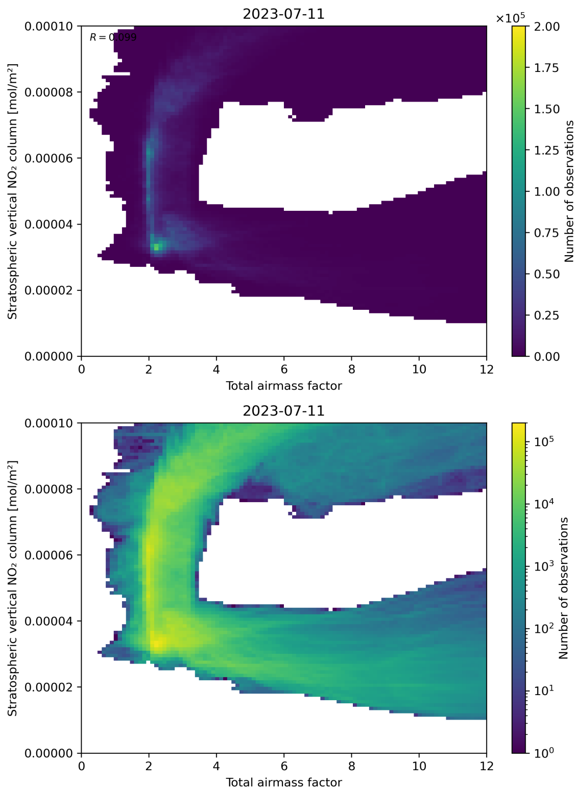
Figure 64: Scatter density plot of “Total airmass factor” against “Stratospheric vertical \text{NO}_2 column” for 2023-07-10 to 2023-07-12.
