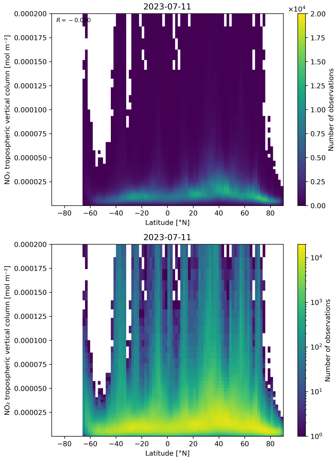
Figure 92: Scatter density plot of “Latitude” against “NO 2 tropospheric vertical column” for 2023-07-10 to 2023-07-12.
