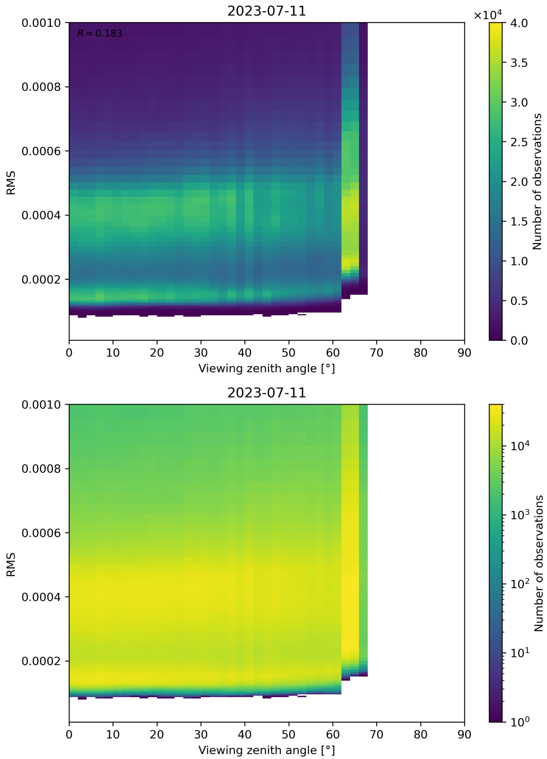
Figure 171: Scatter density plot of “Viewing zenith angle” against “RMS” for 2023-07-10 to 2023-07-12.
