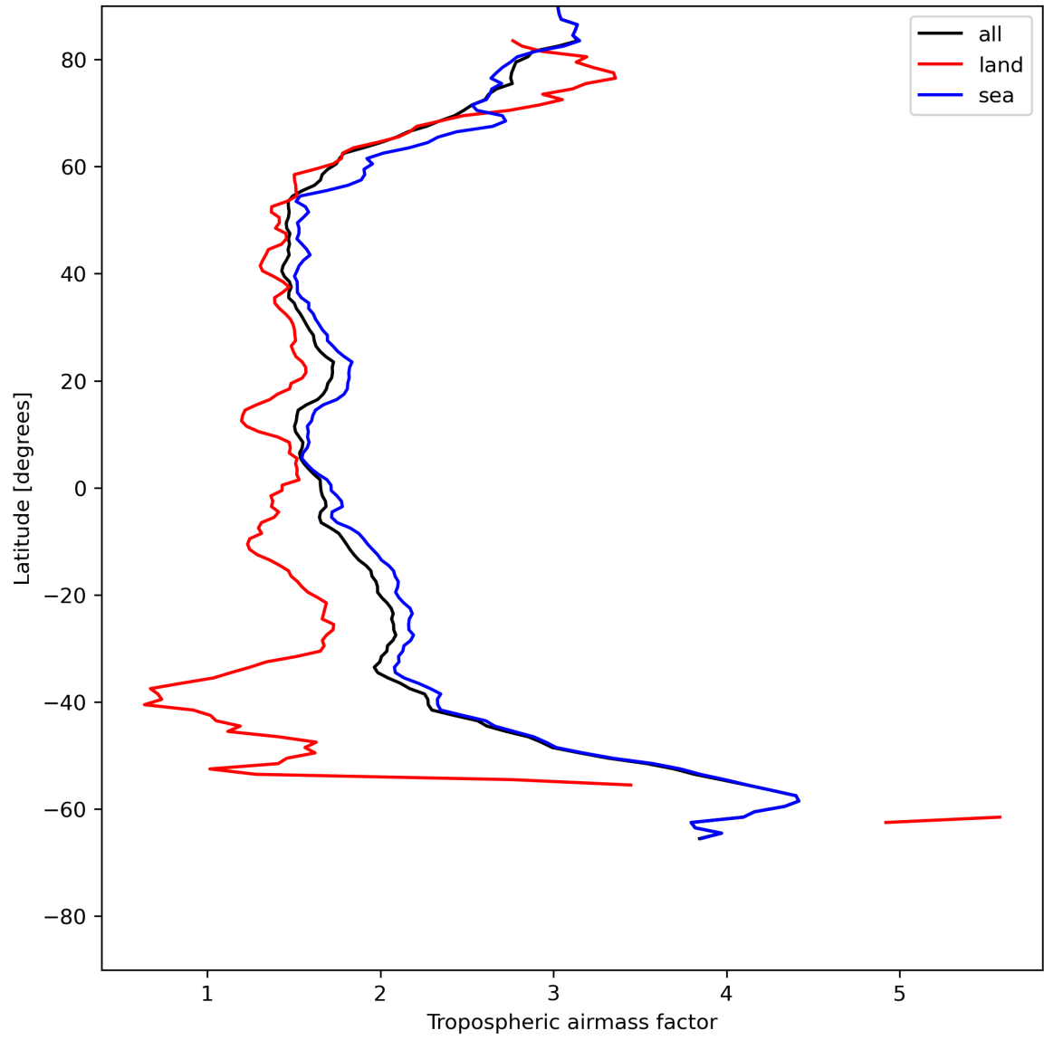
Figure 14: Zonal average of “Tropospheric airmass factor” for 2023-07-10 to 2023-07-12.
