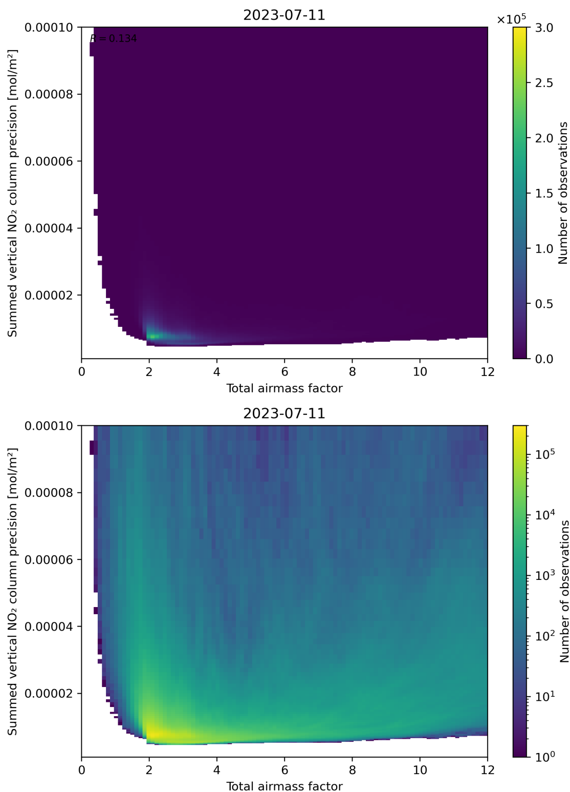
Figure 66: Scatter density plot of “Total airmass factor” against “Summed vertical NO 2 column precision” for 2023-07-10 to 2023-07-12.
