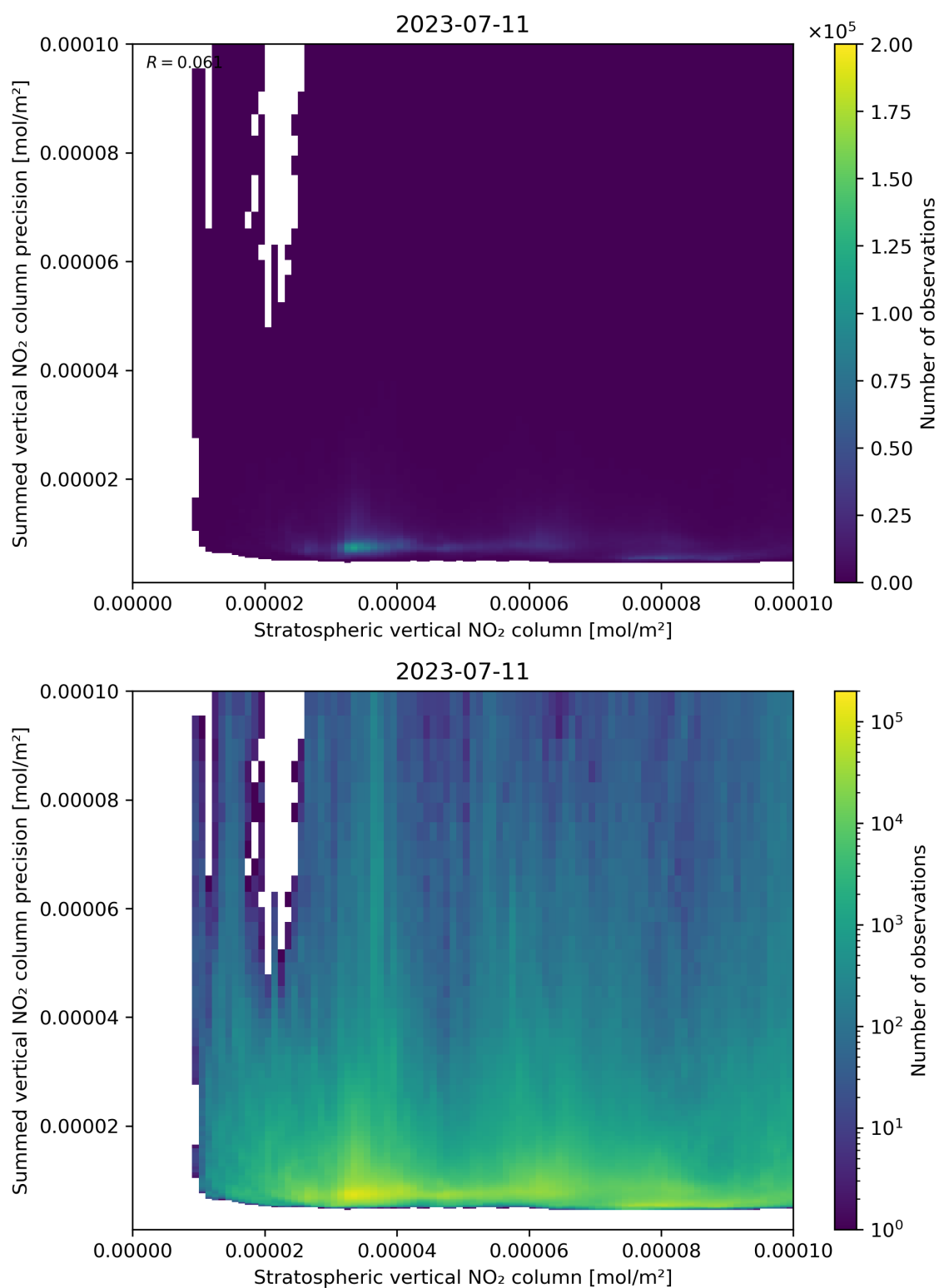
Figure 99: Scatter density plot of “Stratospheric vertical NO 2 column” against “Summed vertical NO 2 column precision” for 2023-07-10 to 2023-07-12.
