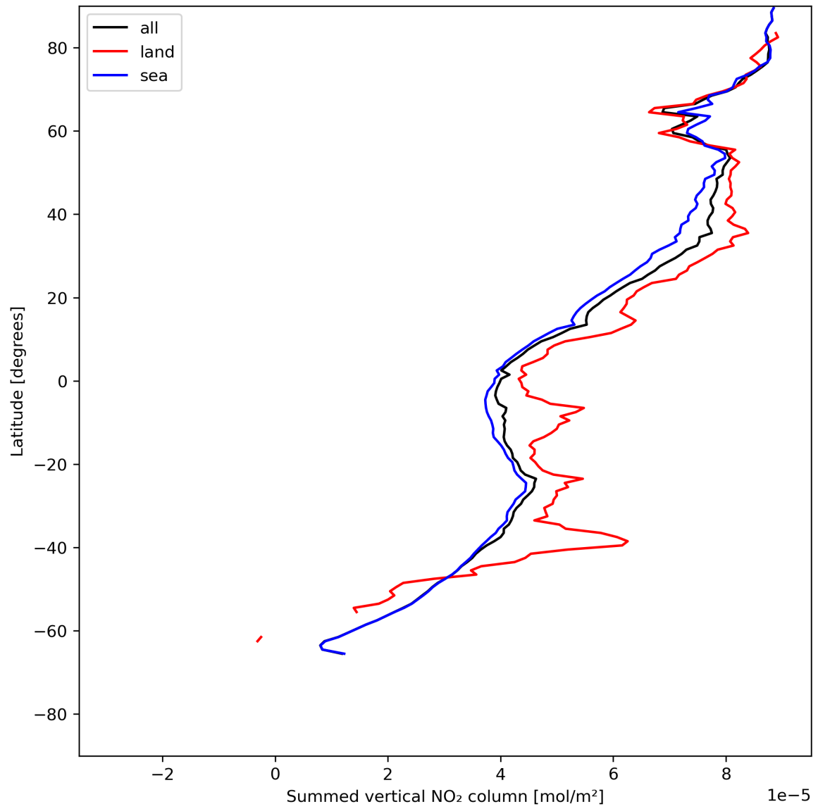
Figure 23: Zonal average of “Summed vertical NO 2 column” for 2023-07-10 to 2023-07-12.
