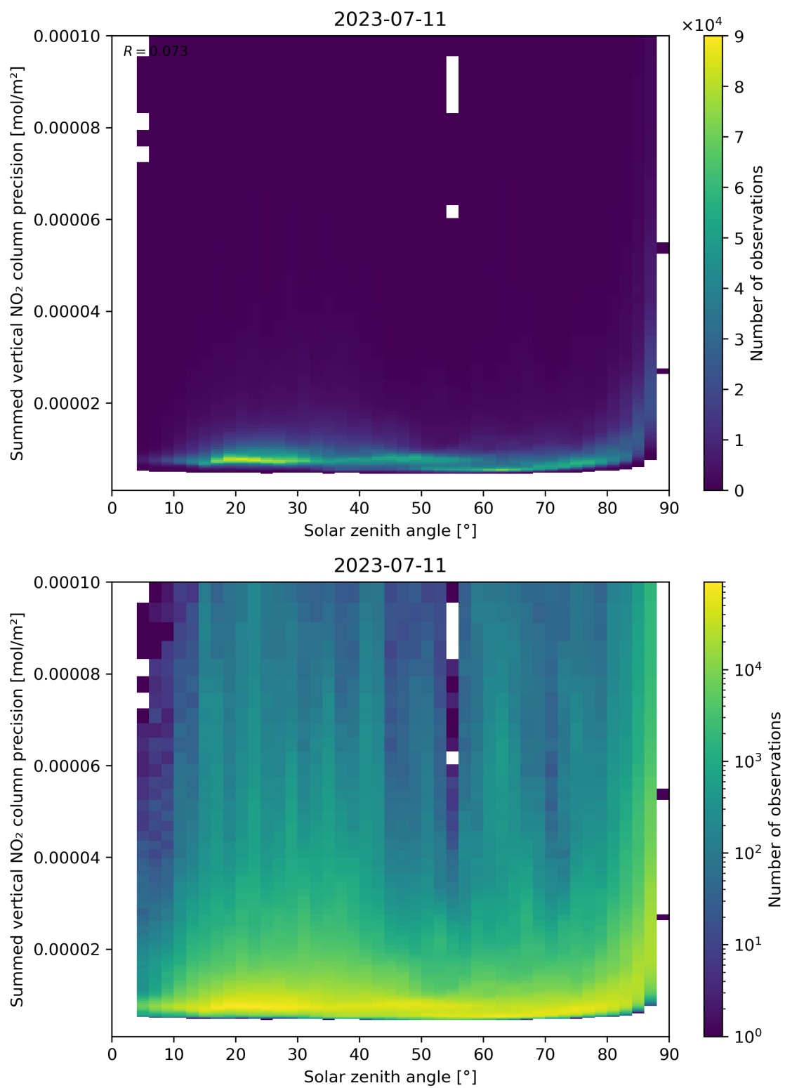
Figure 152: Scatter density plot of “Solar zenith angle” against “Summed vertical NO 2 column precision” for 2023-07-10 to 2023-07-12.
