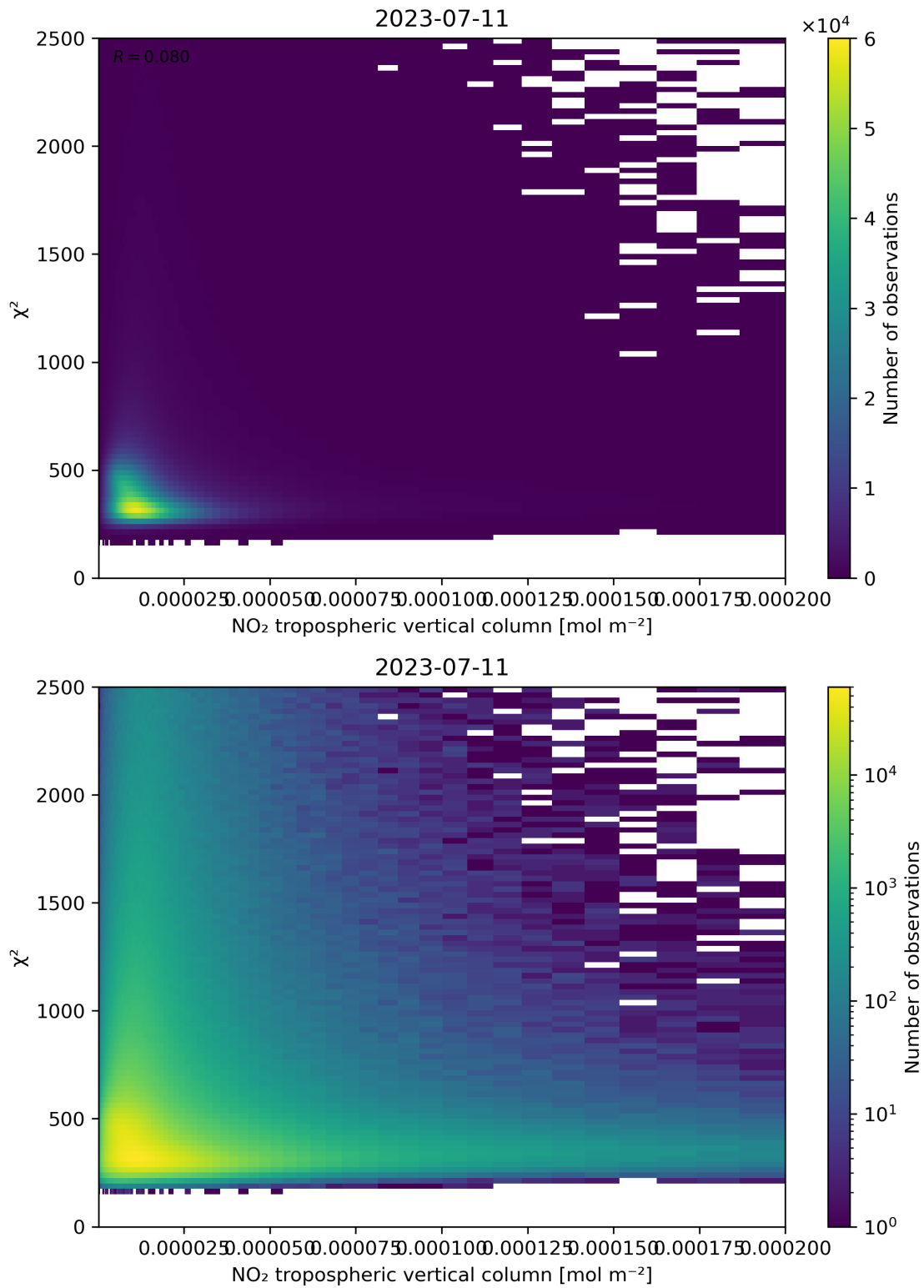
Figure 124: Scatter density plot of “NO 2 tropospheric vertical column” against “ \chi^2 ” for 2023-07-10 to 2023-07-12.
