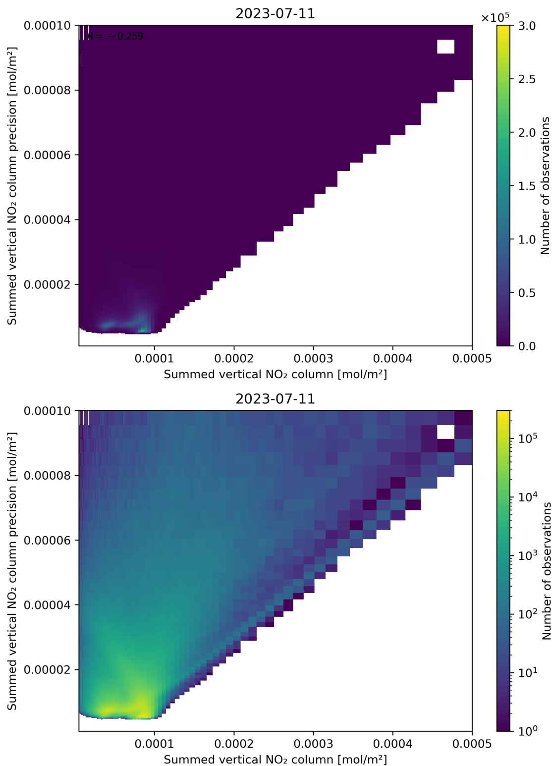
Figure 105: Scatter density plot of “Summed vertical NO 2 column” against “Summed vertical NO 2 column precision” for 2023-07-10 to 2023-07-12.
