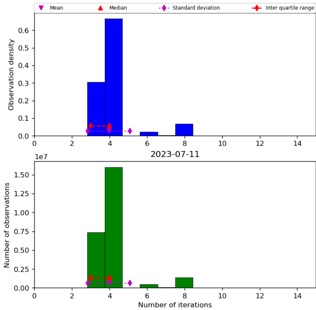
Figure 34: Histogram of “Number of iterations” for 2023-07-10 to 2023-07-12
