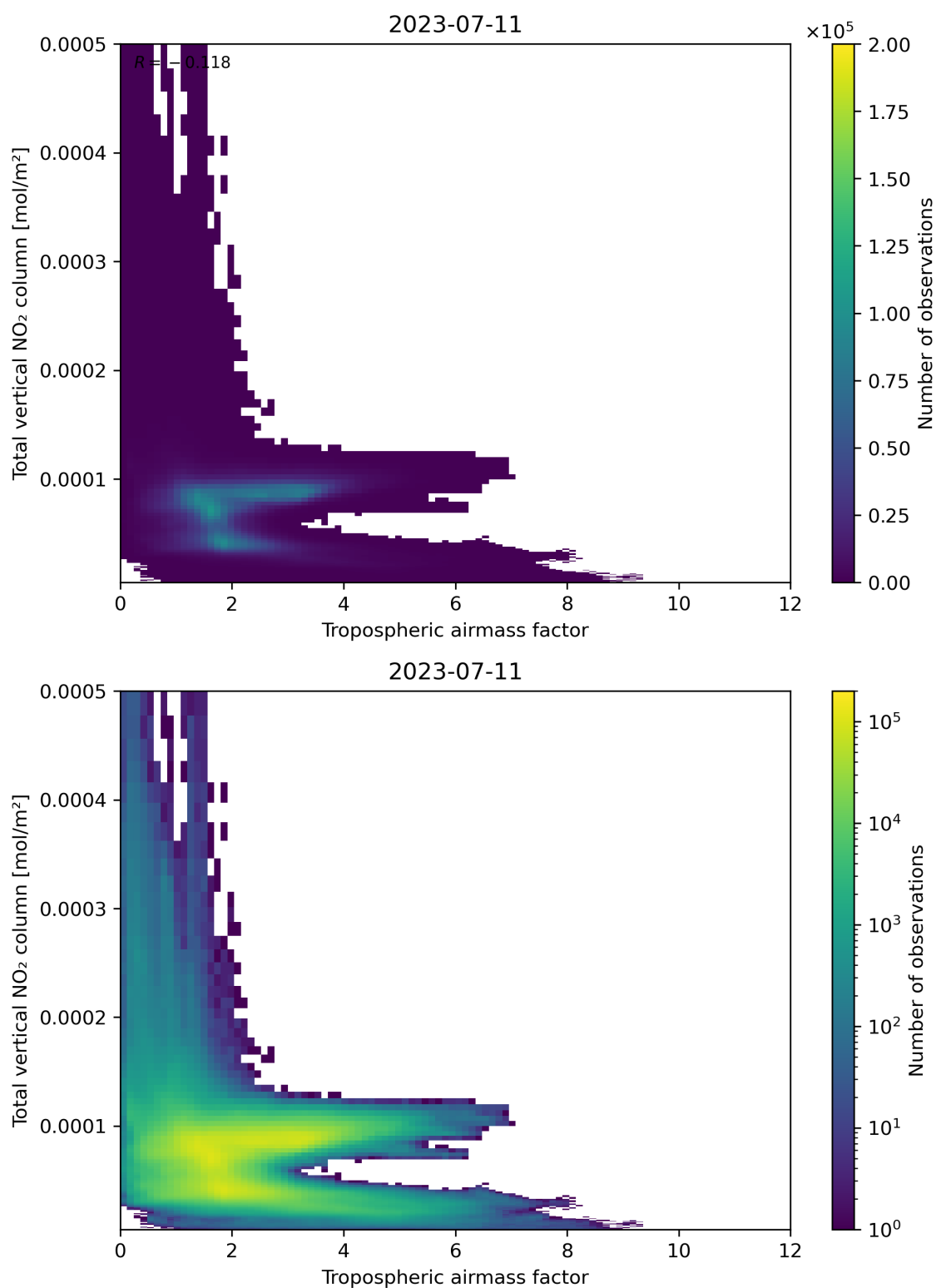
Figure 77: Scatter density plot of “Tropospheric airmass factor” against “Total vertical NO 2 column” for 2023-07-10 to 2023-07-12.
