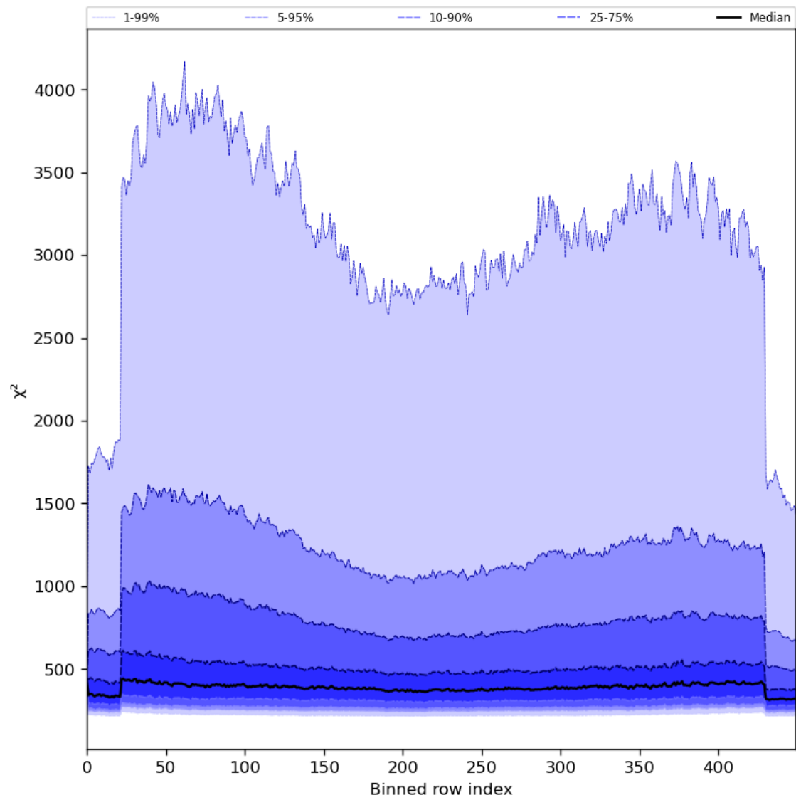
Figure 59: Along track statistics of “ \chi^2 ” for 2023-07-10 to 2023-07-12
