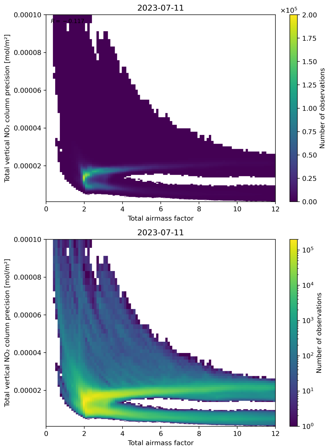
Figure 68: Scatter density plot of “Total airmass factor” against “Total vertical NO 2 column precision” for 2023-07-10 to 2023-07-12.
