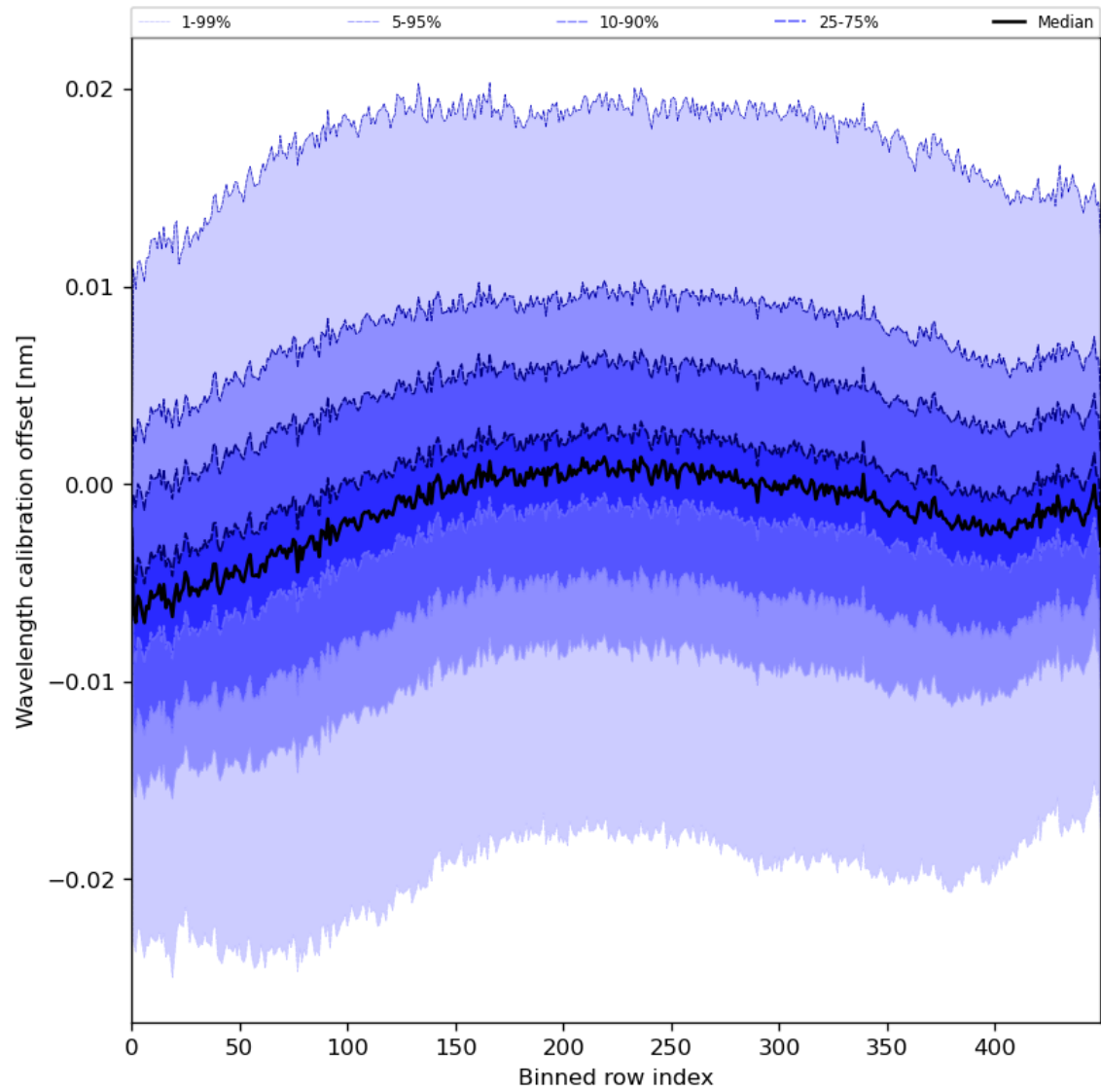
Figure 52: Along track statistics of “Wavelength calibration offset” for 2023-07-10 to 2023-07-12
