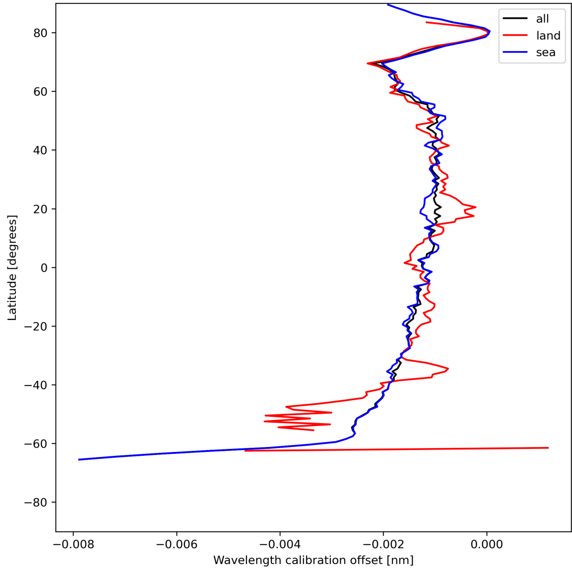
Figure 18: Zonal average of “Wavelength calibration offset” for 2023-07-10 to 2023-07-12.
