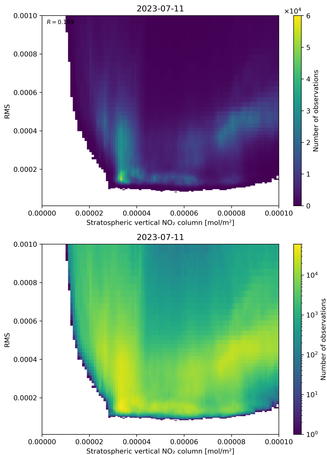
Figure 102: Scatter density plot of “Stratospheric vertical NO 2 column” against “RMS” for 2023-07-10 to 2023-07-12.
