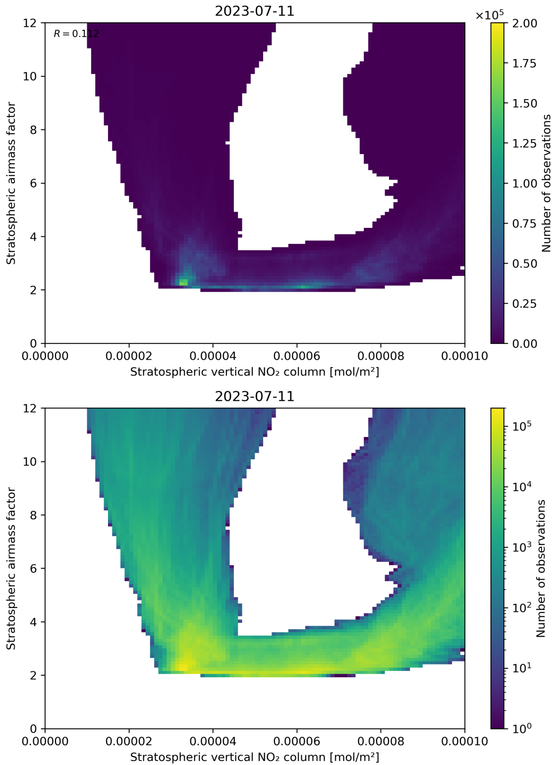
Figure 96: Scatter density plot of “Stratospheric vertical NO 2 column” against “Stratospheric airmass factor” for 2023-07-10 to 2023-07-12.
