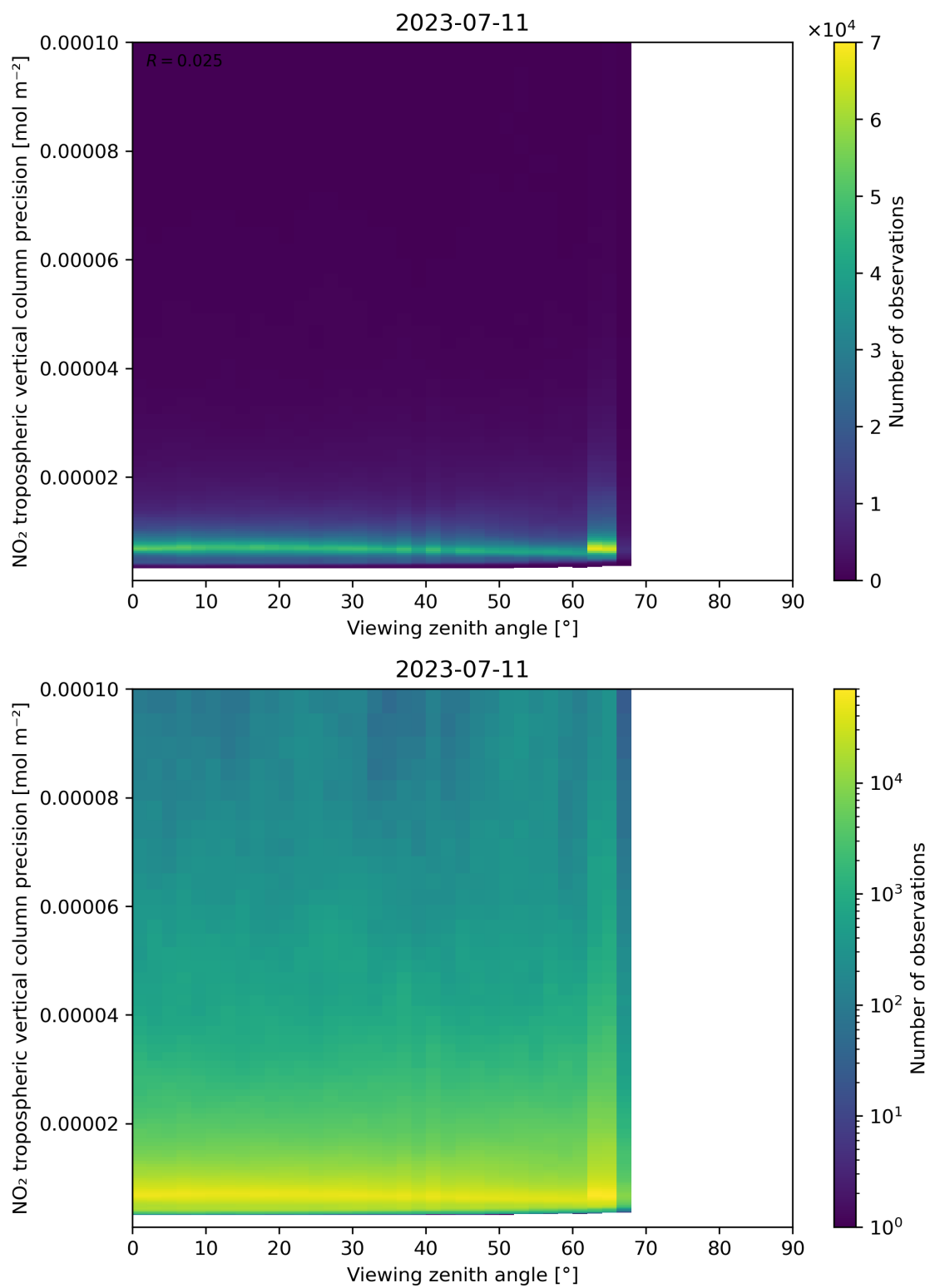
Figure 170: Scatter density plot of “Viewing zenith angle” against “NO 2 tropospheric vertical column precision” for 2023-07-10 to 2023-07-12.
