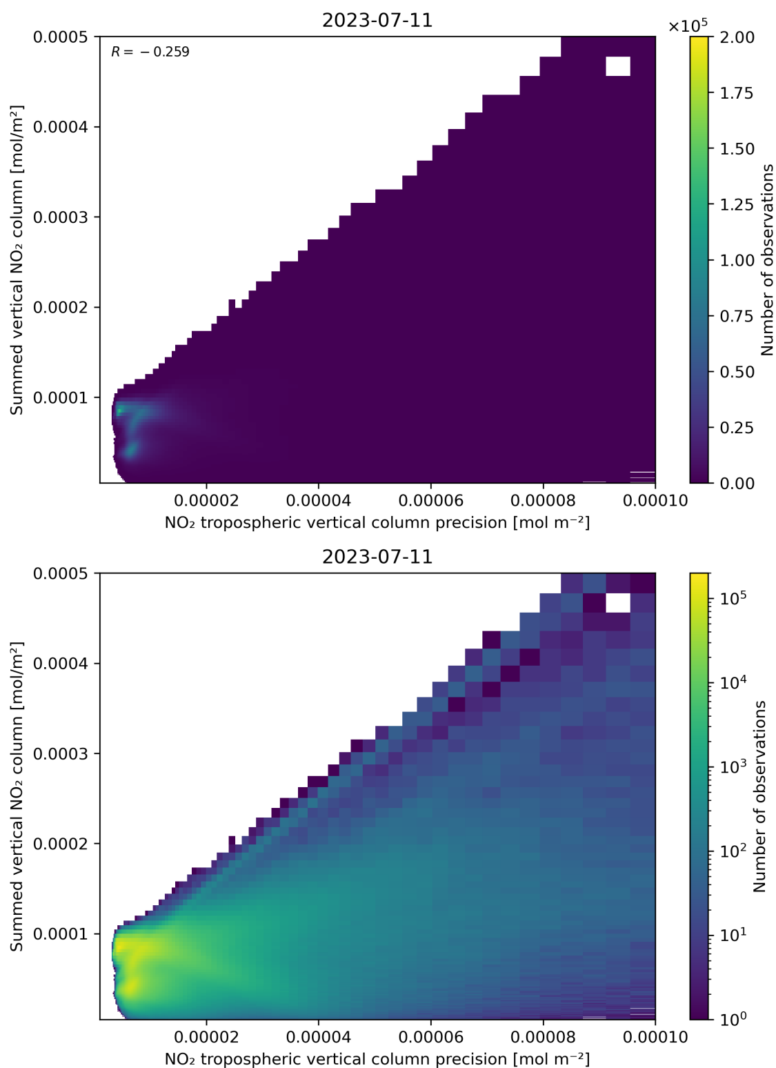
Figure 136: Scatter density plot of “NO 2 tropospheric vertical column precision” against “Summed vertical NO 2 column” for 2023-07-10 to 2023-07-12.
