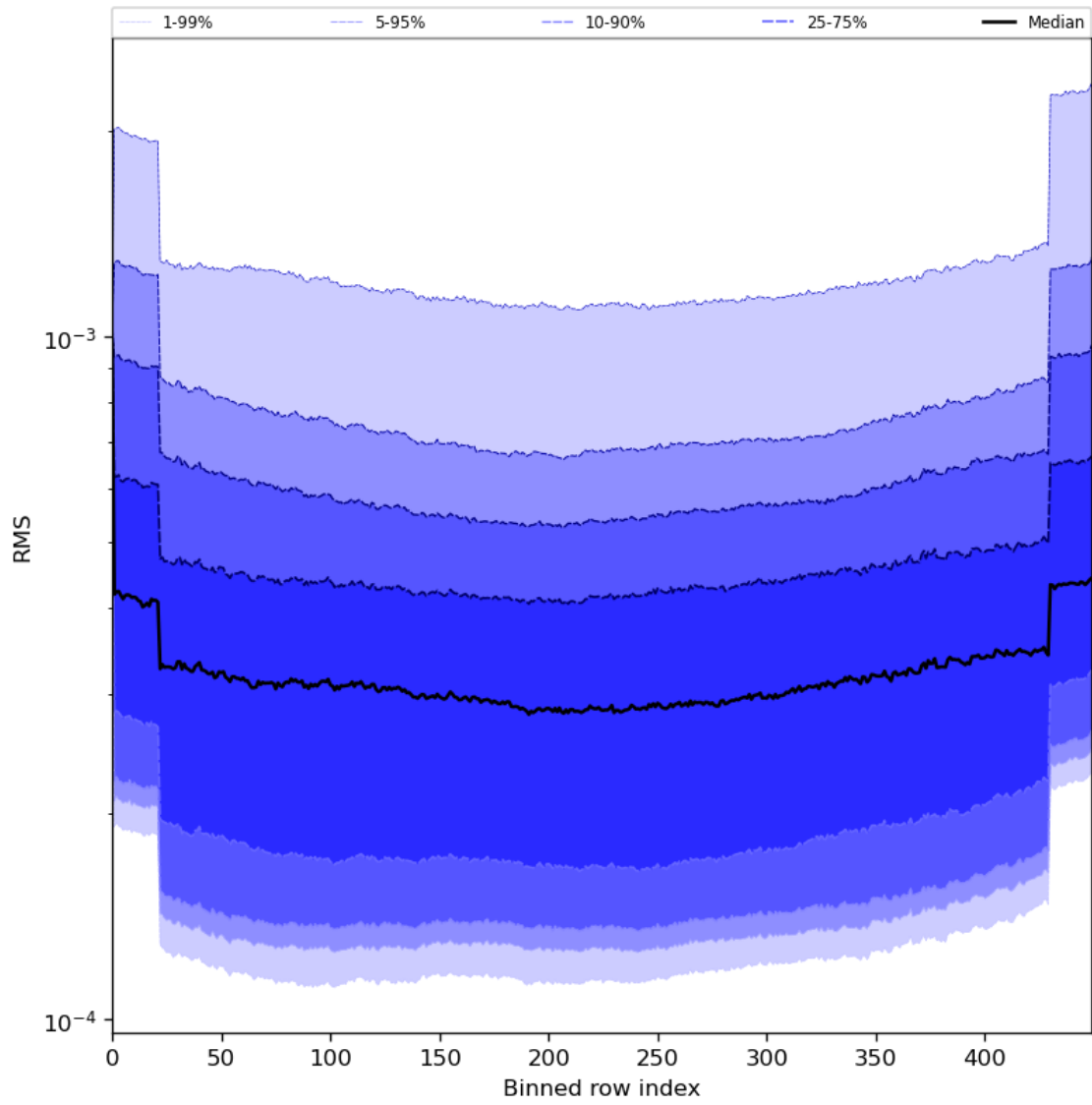
Figure 60: Along track statistics of “RMS” for 2023-07-10 to 2023-07-12
