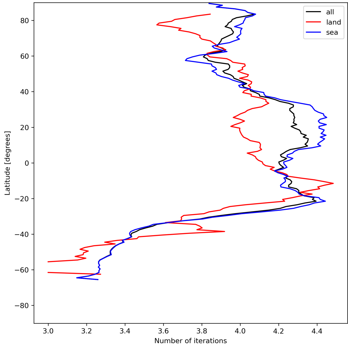
Figure 17: Zonal average of “Number of iterations” for 2023-07-10 to 2023-07-12.
