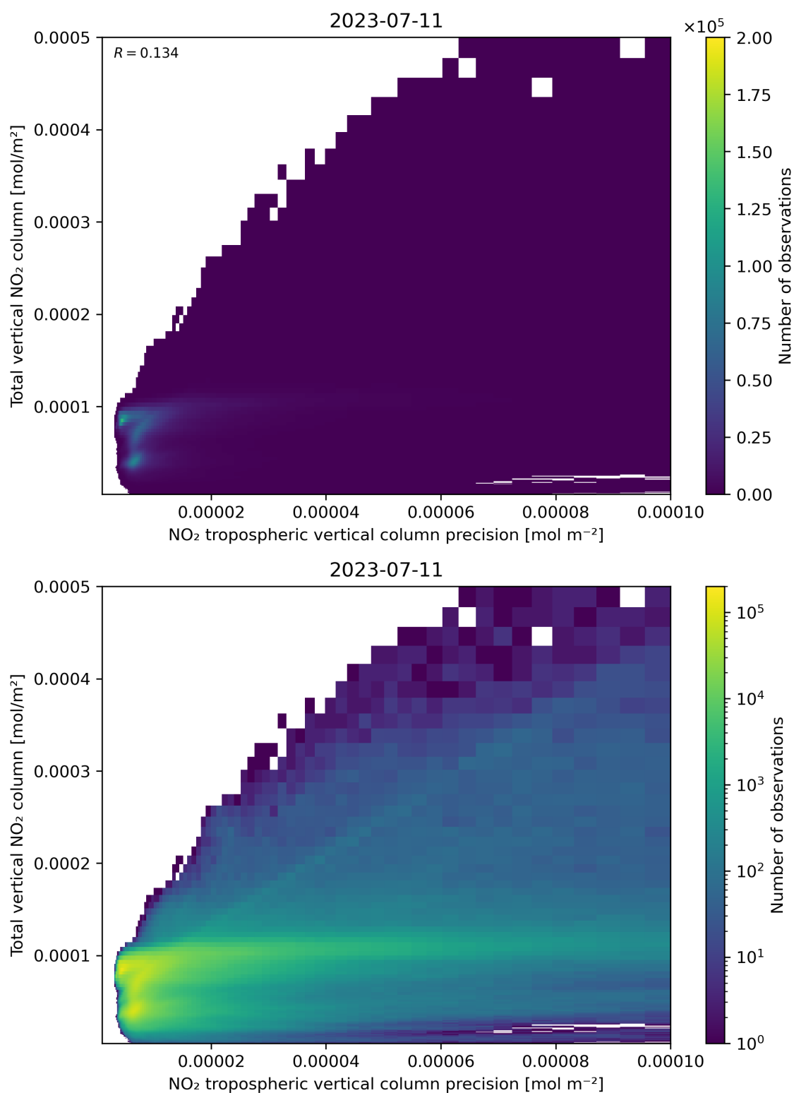
Figure 138: Scatter density plot of “NO 2 tropospheric vertical column precision” against “Total vertical NO 2 column” for 2023-07-10 to 2023-07-12.
