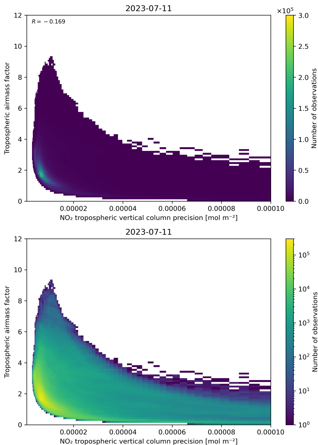
Figure 133: Scatter density plot of “NO 2 tropospheric vertical column precision” against “Tropospheric airmass factor” for 2023-07-10 to 2023-07-12.
