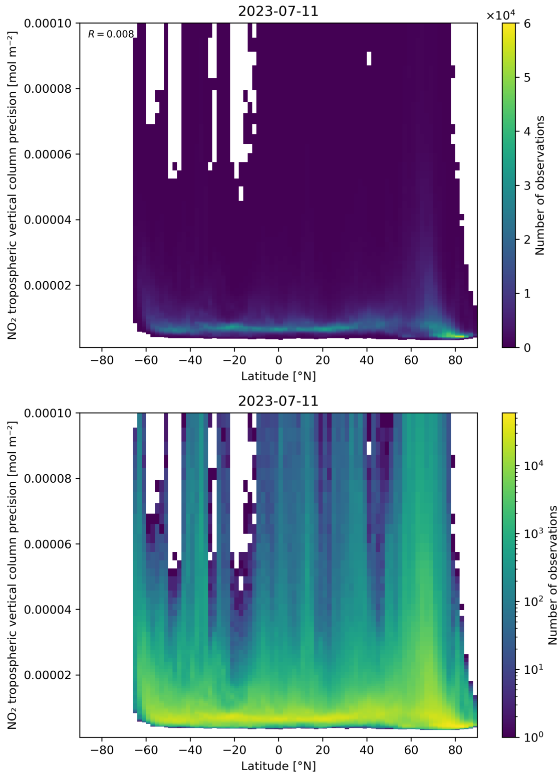
Figure 93: Scatter density plot of “Latitude” against “NO 2 tropospheric vertical column precision” for 2023-07-10 to 2023-07-12.
