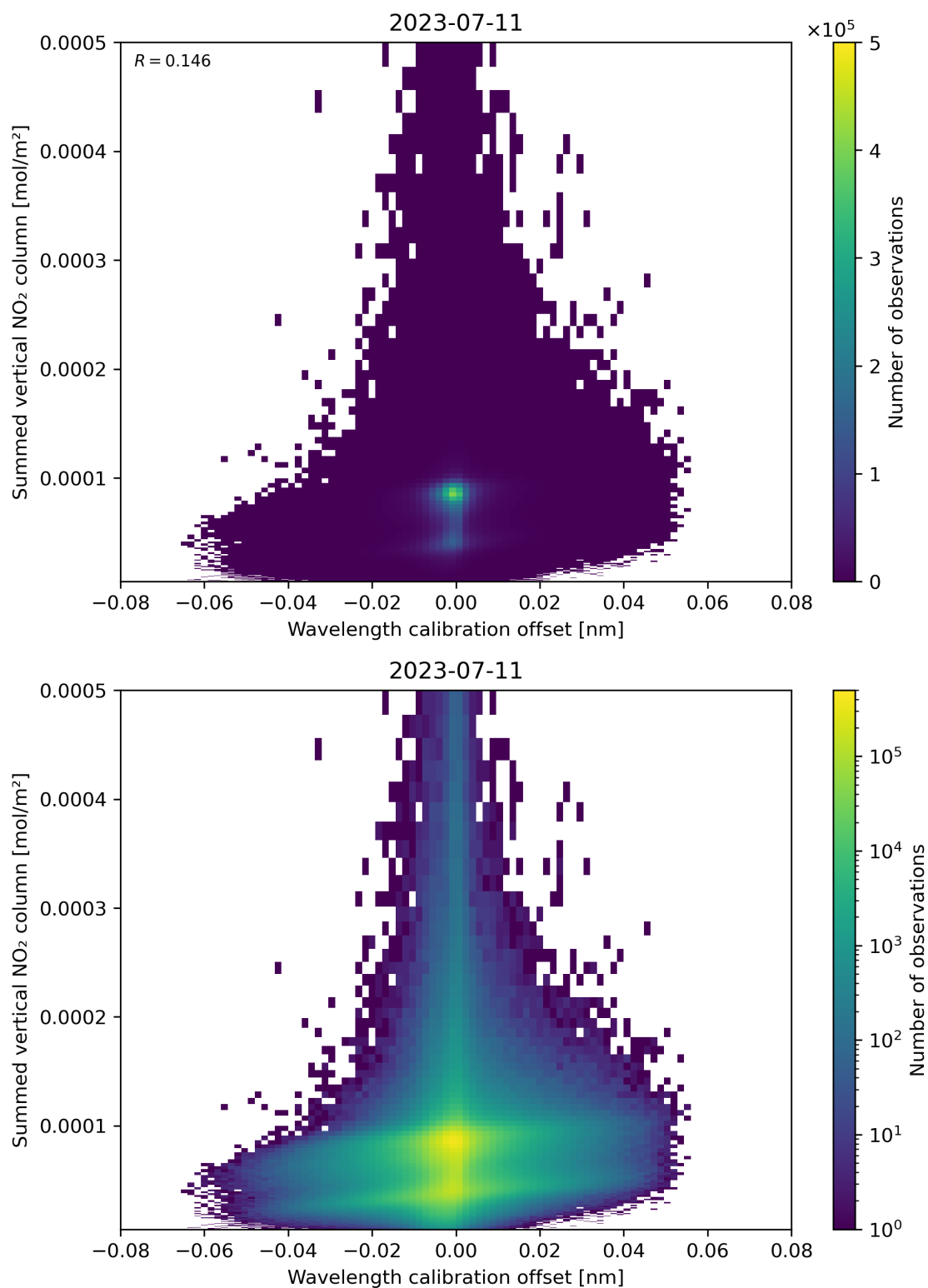
Figure 177: Scatter density plot of “Wavelength calibration offset” against “Summed vertical NO 2 column” for 2023-07-10 to 2023-07-12.
