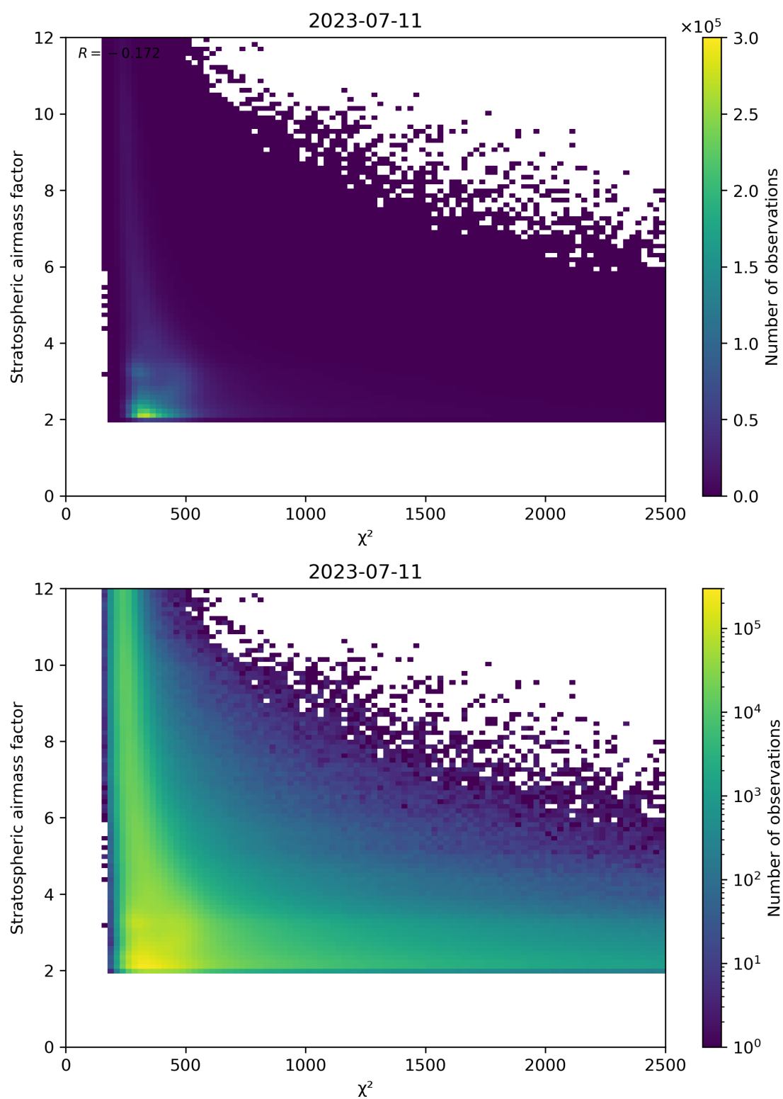
Figure 81: Scatter density plot of “ \chi^2 ” against “Stratospheric airmass factor” for 2023-07-10 to 2023-07-12.
