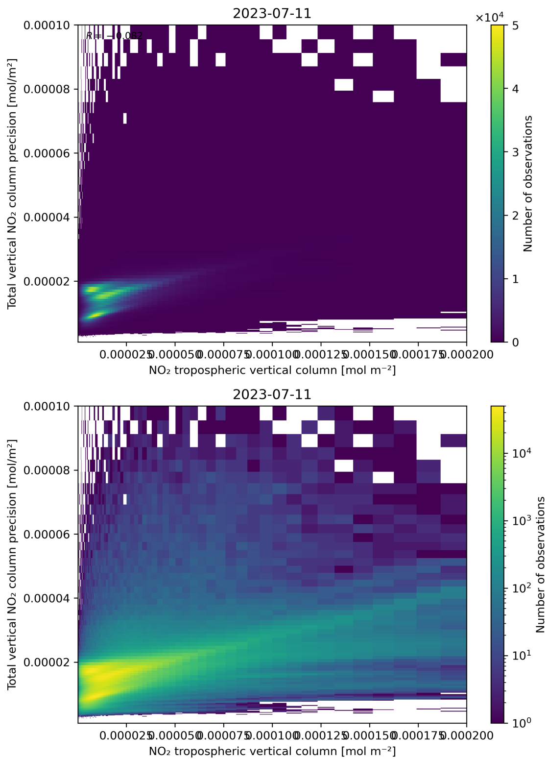
Figure 129: Scatter density plot of “NO 2 tropospheric vertical column” against “Total vertical NO 2 column precision” for 2023-07-10 to 2023-07-12.
