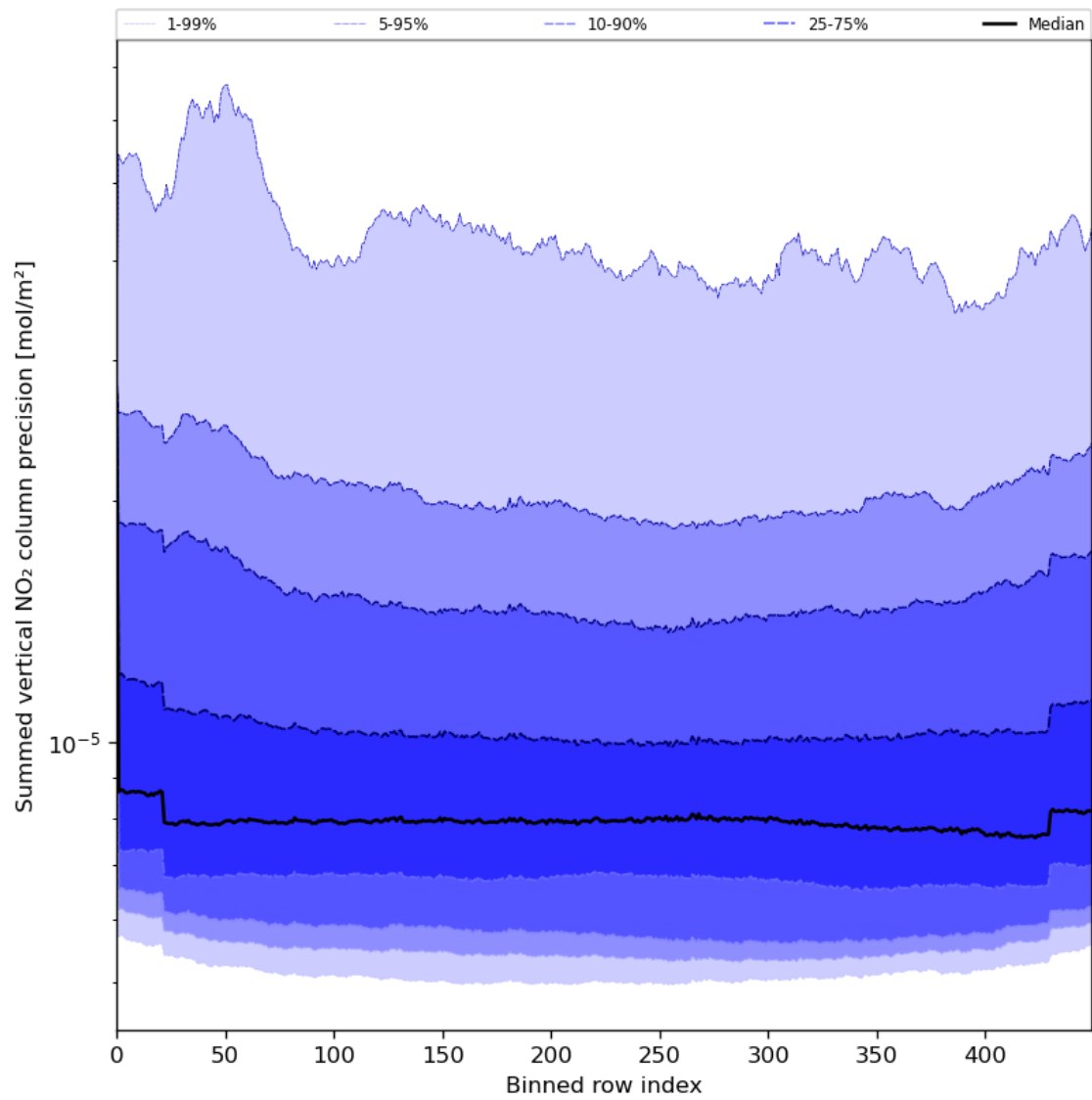
Figure 58: Along track statistics of “Summed vertical NO 2 column precision” for 2023-07-10 to 2023-07-12
