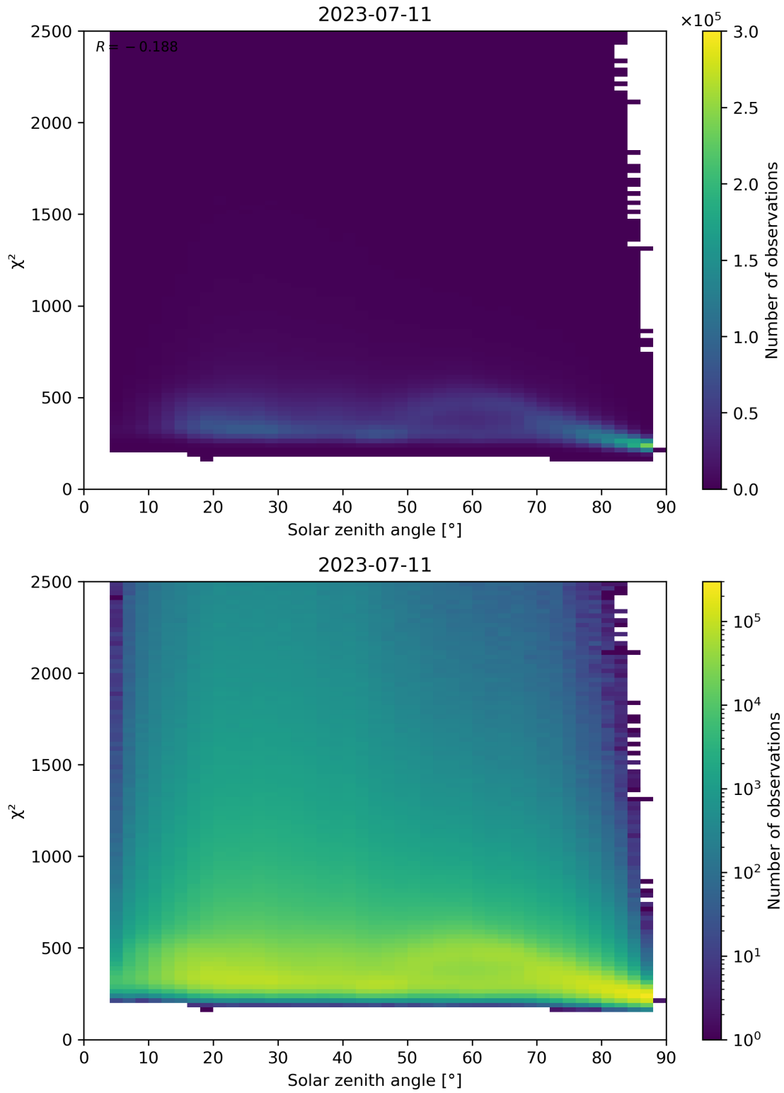
Figure 148: Scatter density plot of “Solar zenith angle” against “ \chi^2 ” for 2023-07-10 to 2023-07-12.
