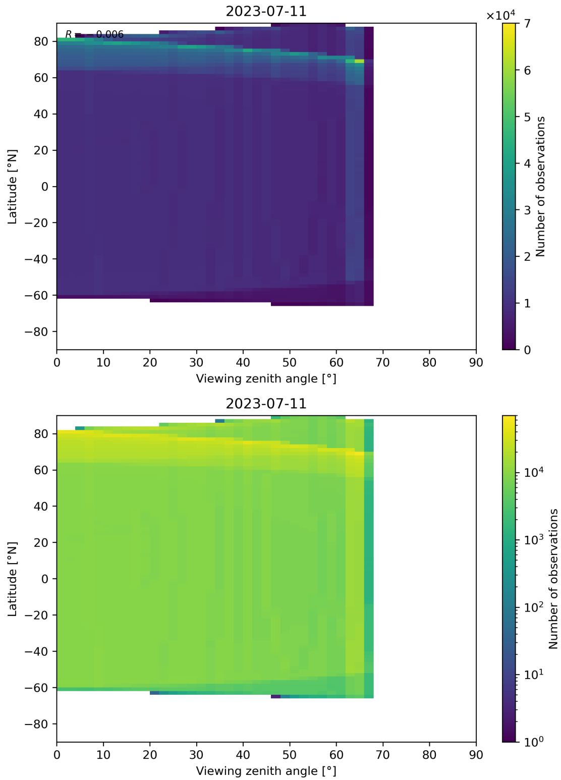
Figure 163: Scatter density plot of “Viewing zenith angle” against “Latitude” for 2023-07-10 to 2023-07-12.
