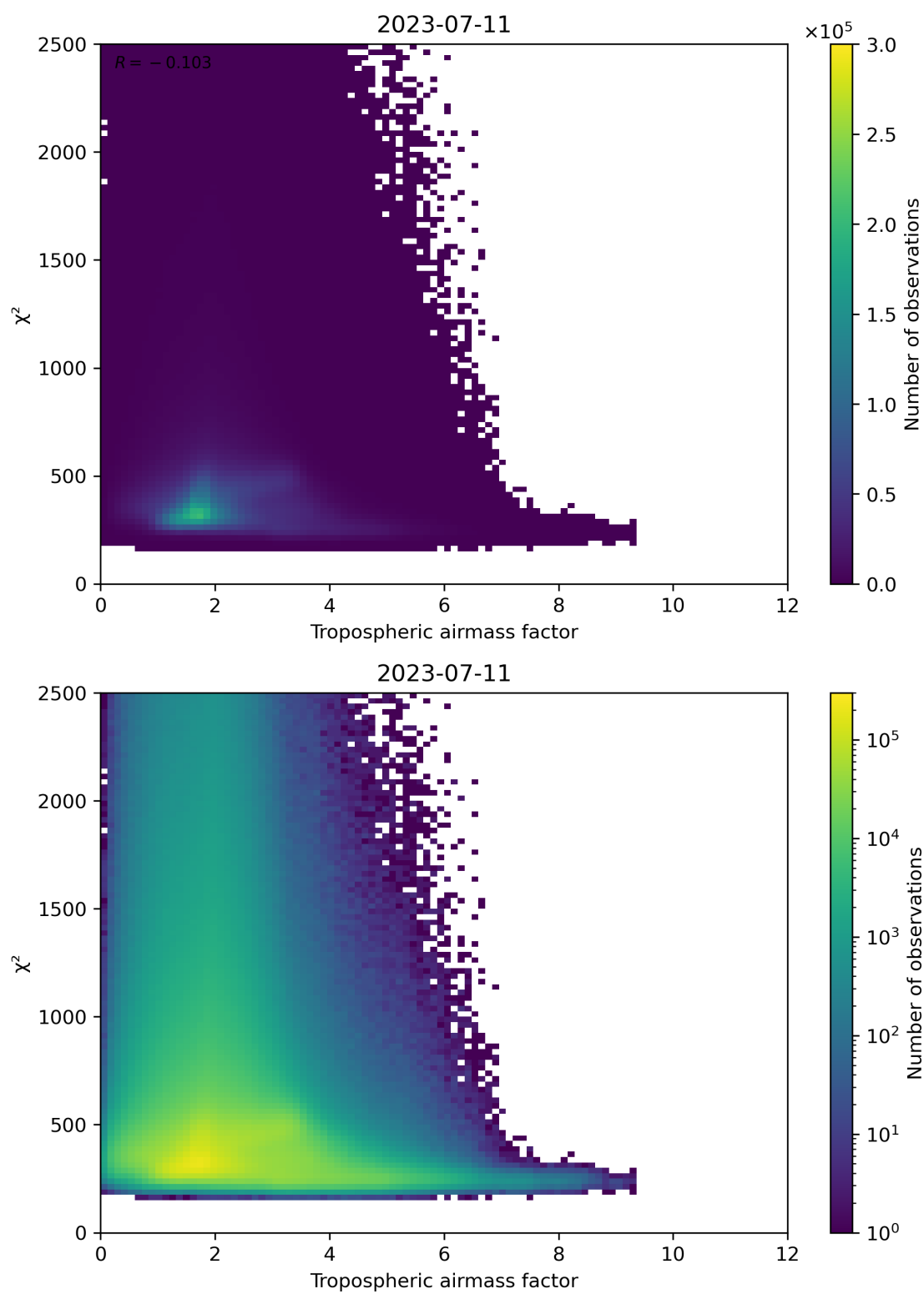
Figure 73: Scatter density plot of “Tropospheric airmass factor” against “ \chi^2 ” for 2023-07-10 to 2023-07-12.
