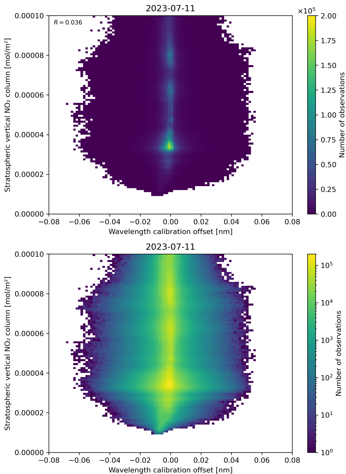
Figure 176: Scatter density plot of “Wavelength calibration offset” against “Stratospheric vertical NO 2 column” for 2023-07-10 to 2023-07-12.
