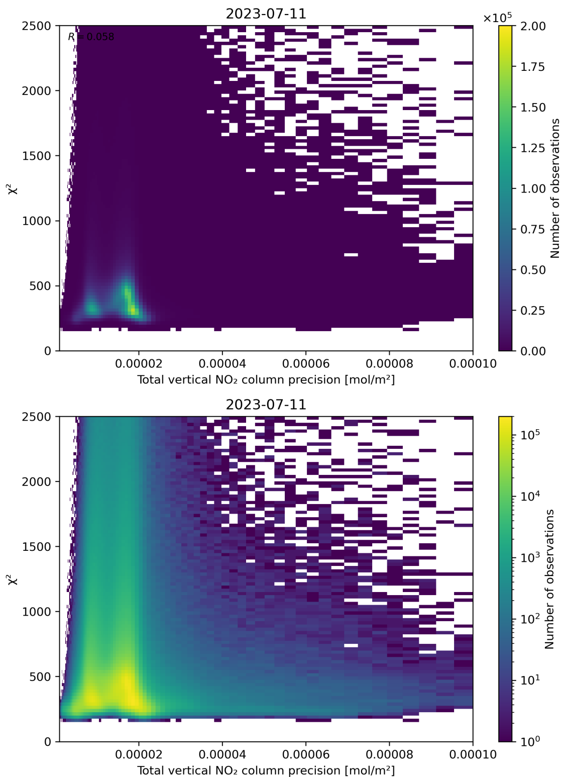
Figure 116: Scatter density plot of “Total vertical NO 2 column precision” against “ \chi^2 ” for 2023-07-10 to 2023-07-12.
