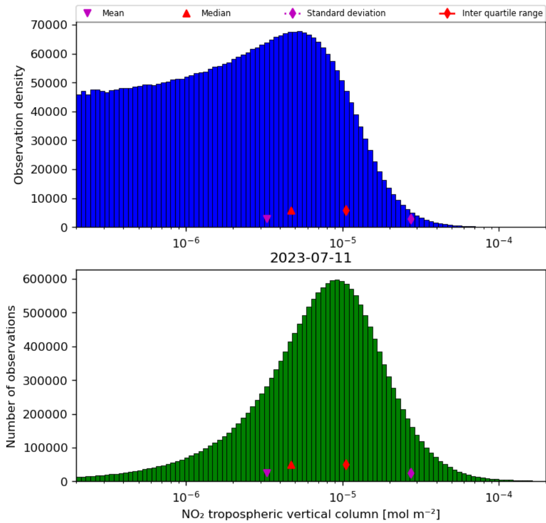
Figure 29: Histogram of “NO 2 tropospheric vertical column” for 2023-07-10 to 2023-07-12
