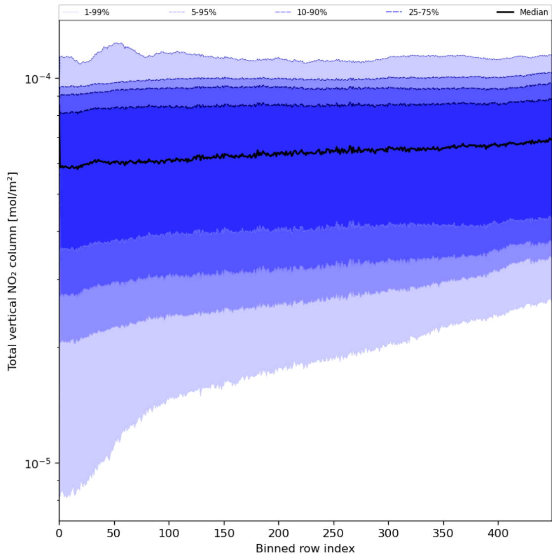
Figure 55: Along track statistics of “Total vertical NO 2 column” for 2023-07-10 to 2023-07-12
