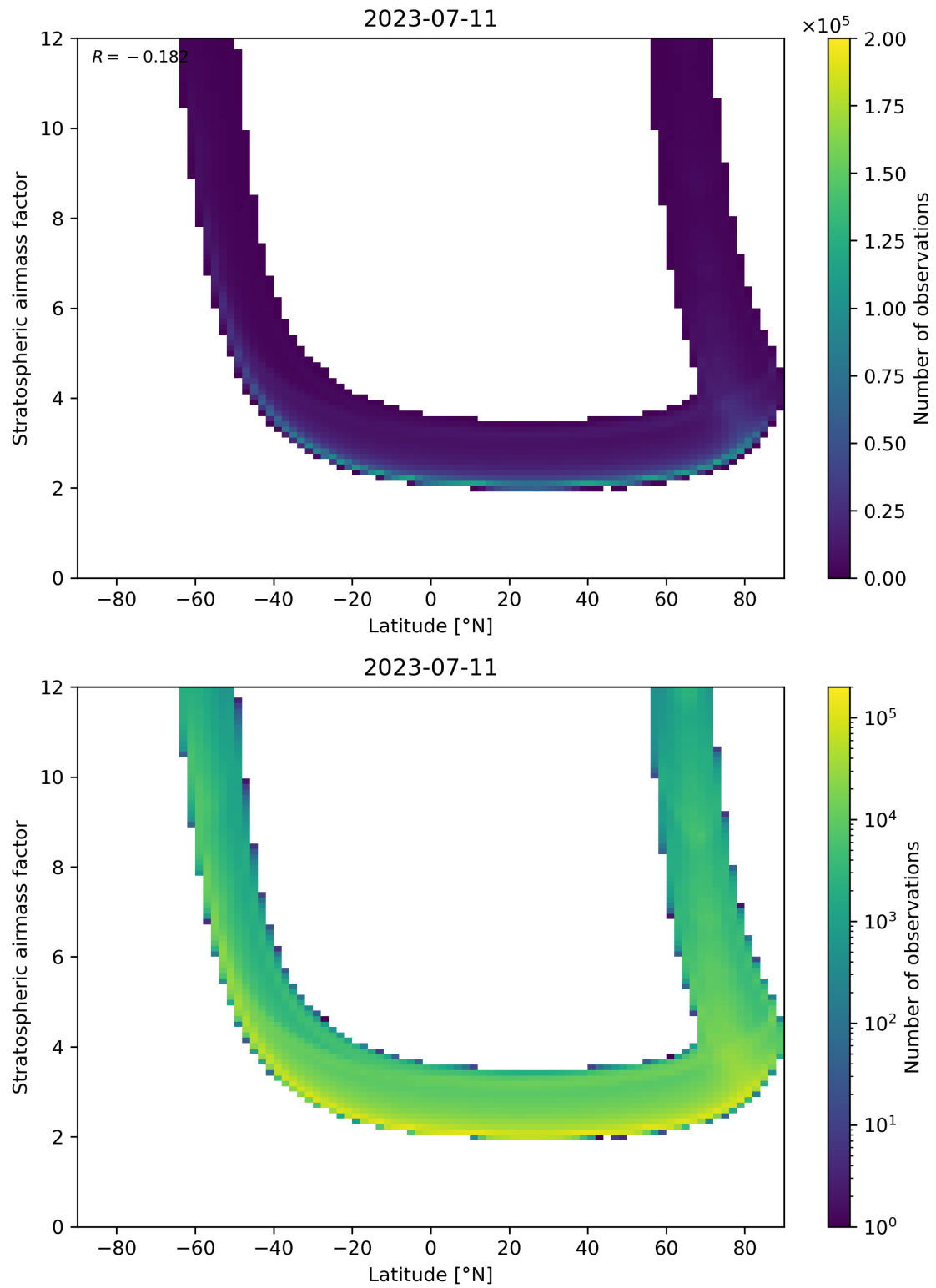
Figure 83: Scatter density plot of “Latitude” against “Stratospheric air mass factor” for 2023-07-10 to 2023-07-12.
