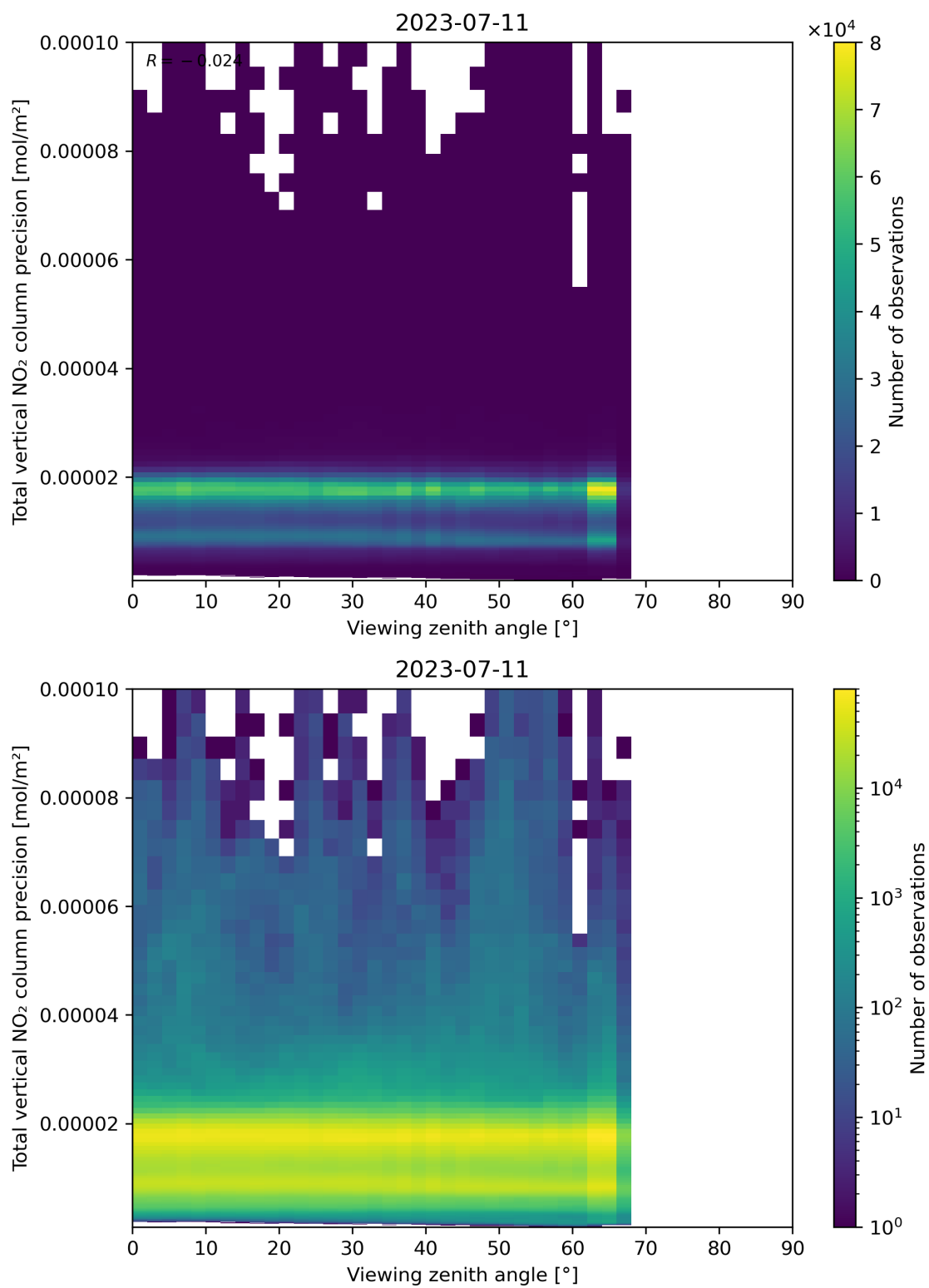
Figure 168: Scatter density plot of “Viewing zenith angle” against “Total vertical NO 2 column precision” for 2023-07-10 to 2023-07-12.
