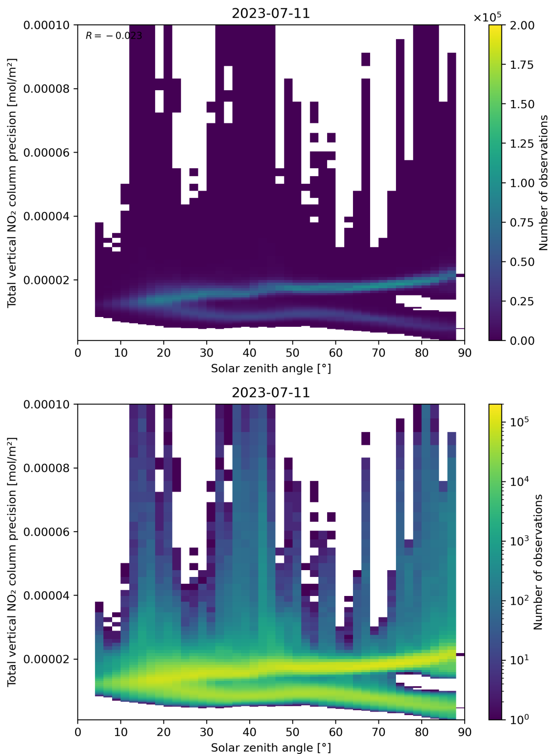
Figure 154: Scatter density plot of “Solar zenith angle” against “Total vertical NO 2 column precision” for 2023-07-10 to 2023-07-12.
