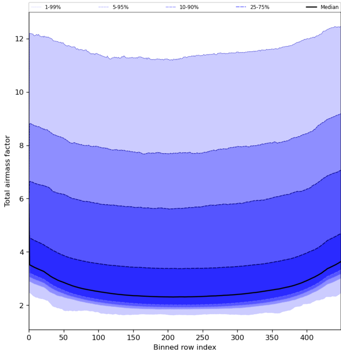
Figure 49: Along track statistics of “Total airmass factor” for 2023-07-10 to 2023-07-12
