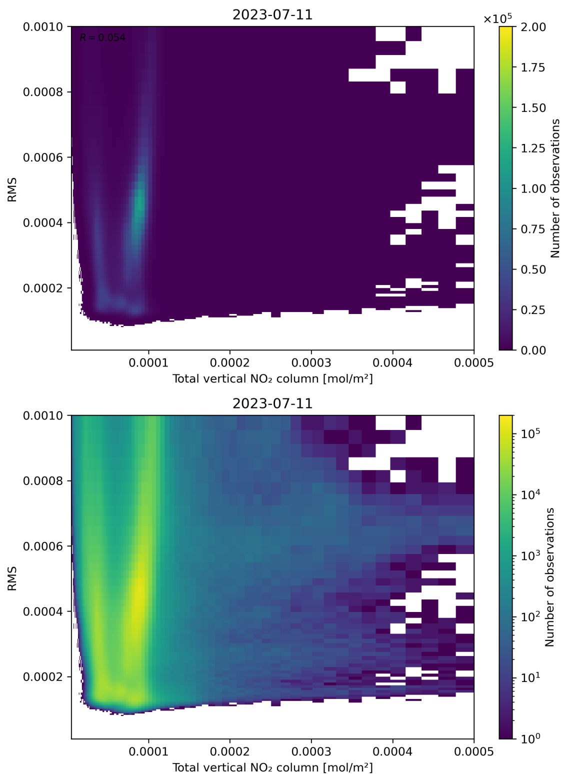
Figure 120: Scatter density plot of “Total vertical NO 2 column” against “RMS” for 2023-07-10 to 2023-07-12.
