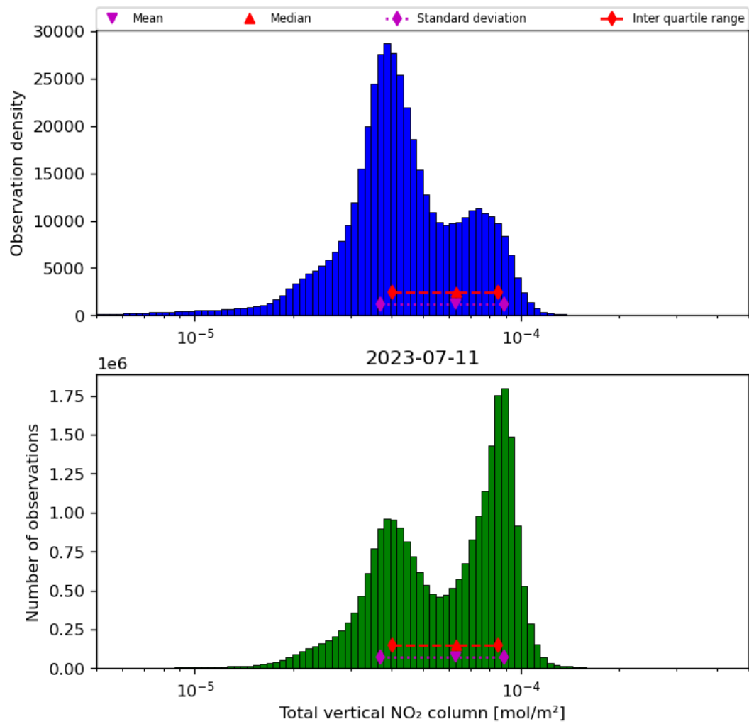
Figure 38: Histogram of “Total vertical NO 2 column” for 2023-07-10 to 2023-07-12
