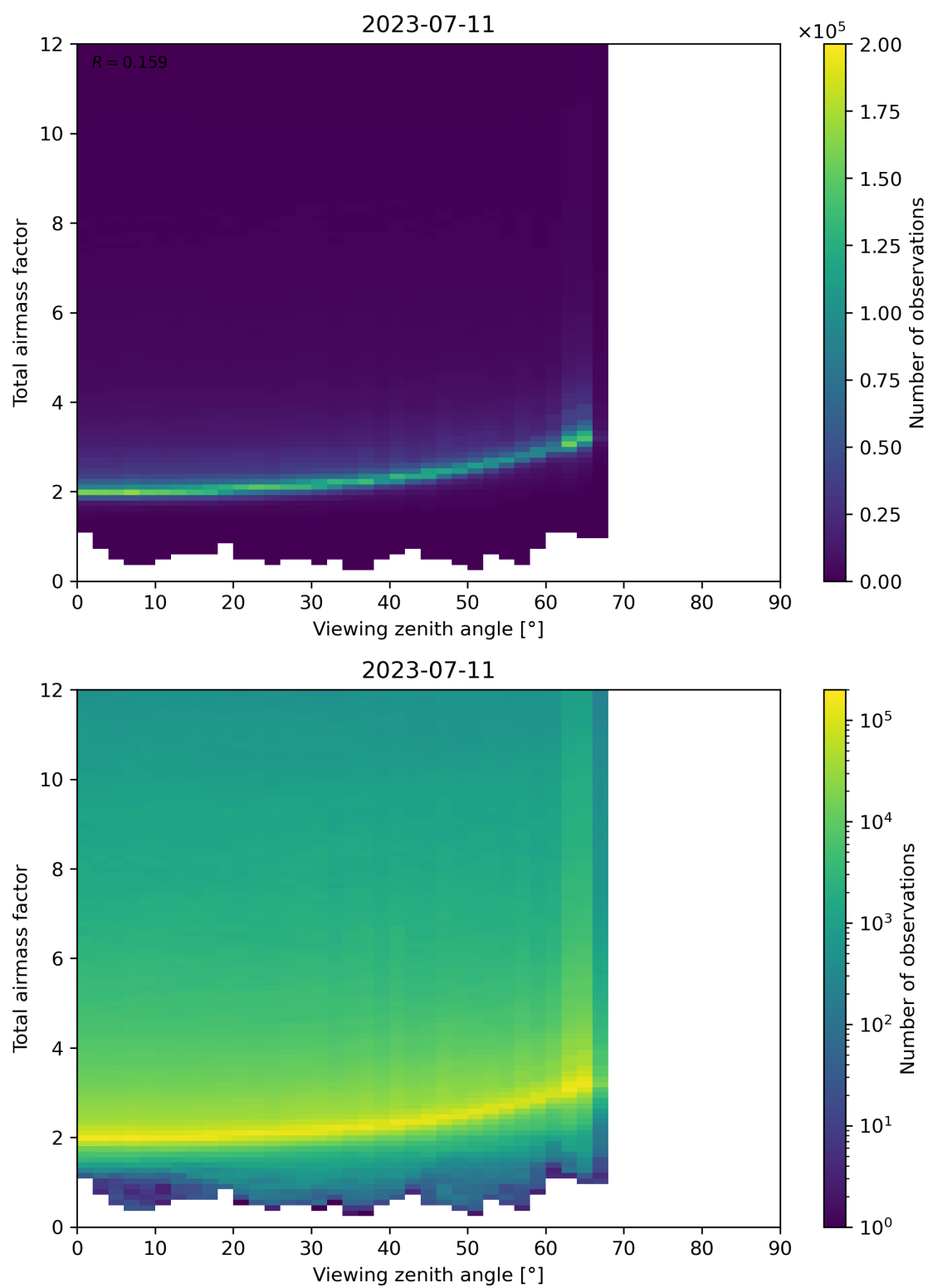
Figure 160: Scatter density plot of “Viewing zenith angle” against “Total airmass factor” for 2023-07-10 to 2023-07-12.
