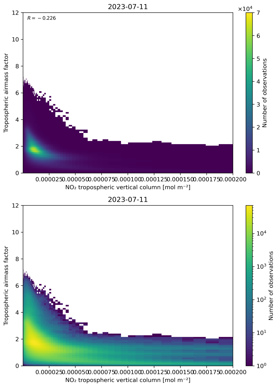
Figure 123: Scatter density plot of “NO 2 tropospheric vertical column” against “Tropospheric air mass factor” for 2023-07-10 to 2023-07-12.
