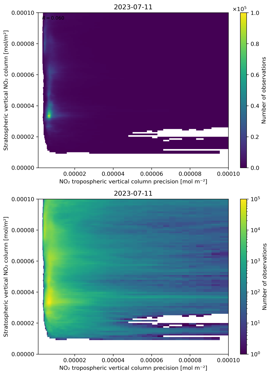
Figure 135: Scatter density plot of “NO 2 tropospheric vertical column precision” against “Stratospheric vertical NO 2 column” for 2023-07-10 to 2023-07-12.
