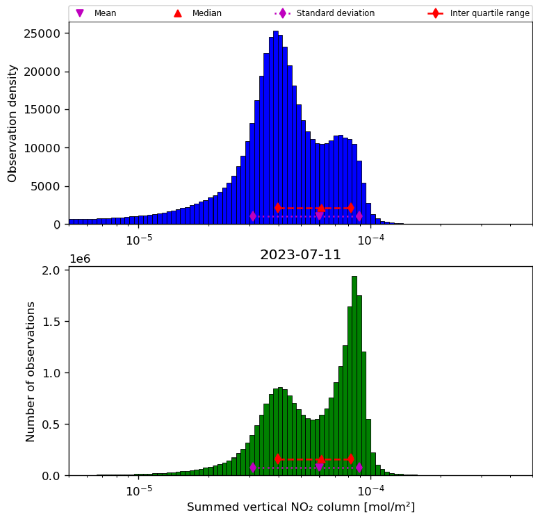
Figure 40: Histogram of “Summed vertical NO 2 column” for 2023-07-10 to 2023-07-12
