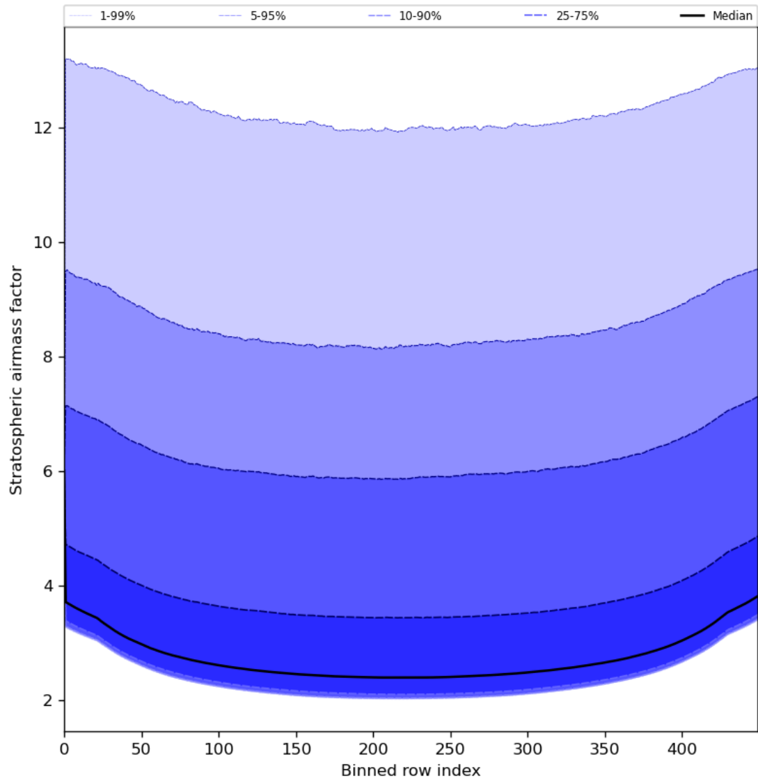
Figure 61: Along track statistics of “Stratospheric airmass factor” for 2023-07-10 to 2023-07-12
