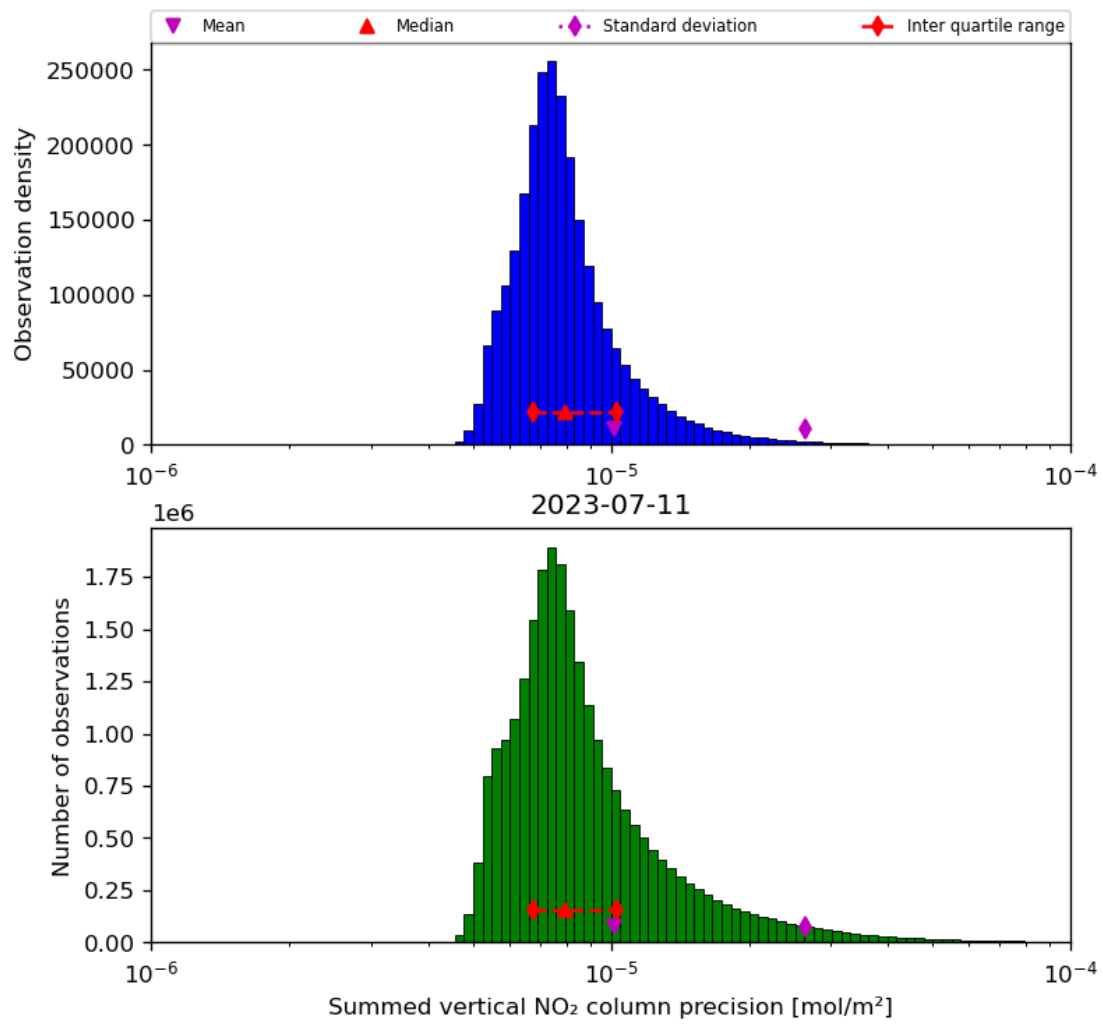
Figure 41: Histogram of "Summed vertical NO 2 column precision" for 2023-07-10 to 2023-07-12
