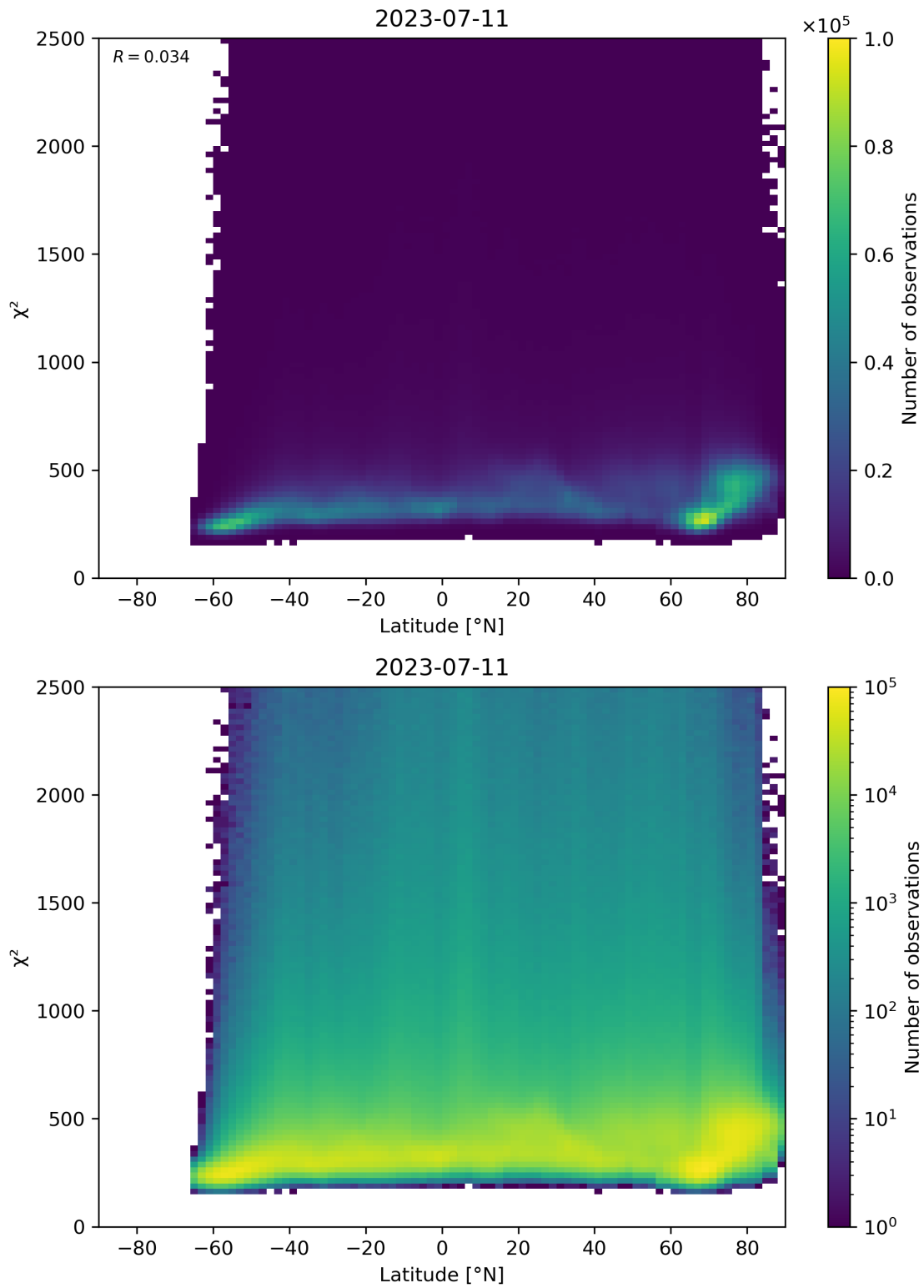
Figure 86: Scatter density plot of “Latitude” against “ \chi^2 ” for 2023-07-10 to 2023-07-12.
