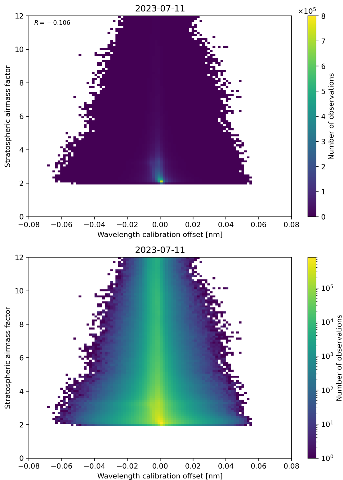
Figure 174: Scatter density plot of “Wavelength calibration offset” against “Stratospheric airmass factor” for 2023-07-10 to 2023-07-12.
