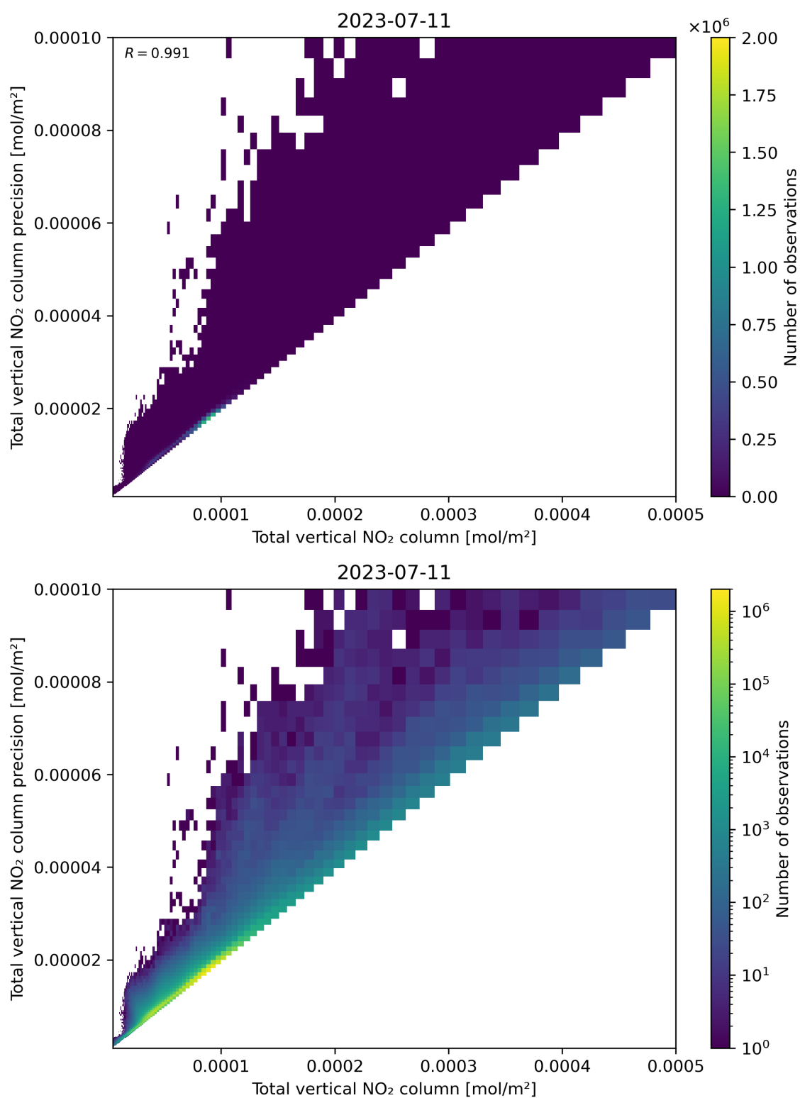
Figure 114: Scatter density plot of “Total vertical NO 2 column” against “Total vertical NO 2 column precision” for 2023-07-10 to 2023-07-12.
