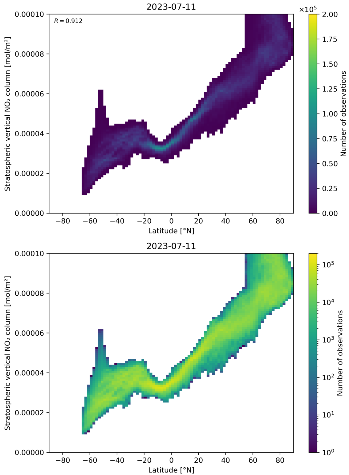
Figure 87: Scatter density plot of “Latitude” against “Stratospheric vertical NO 2 column” for 2023-07-10 to 2023-07-12.
