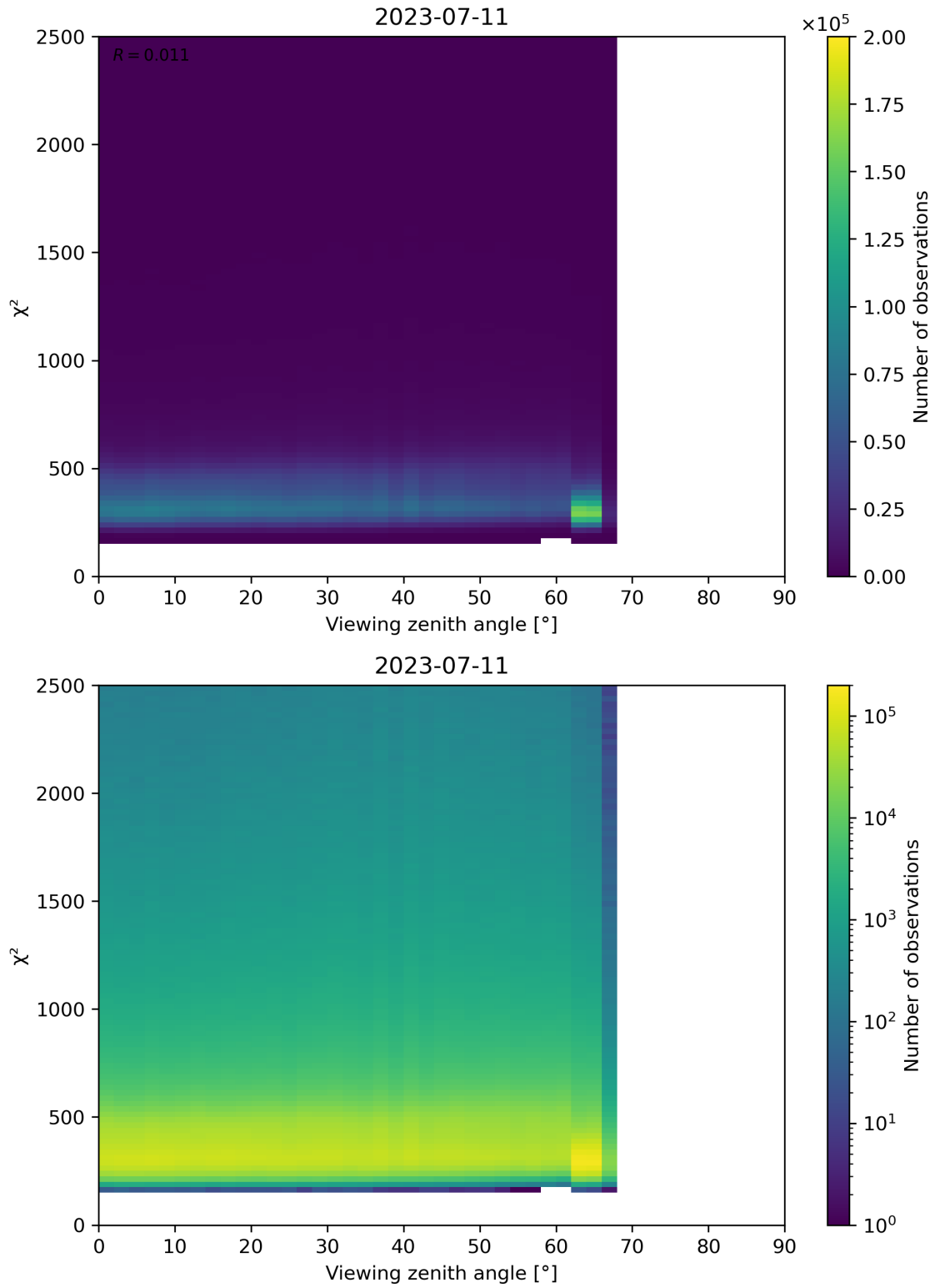
Figure 162: Scatter density plot of “Viewing zenith angle” against “ \chi^2 ” for 2023-07-10 to 2023-07-12.
