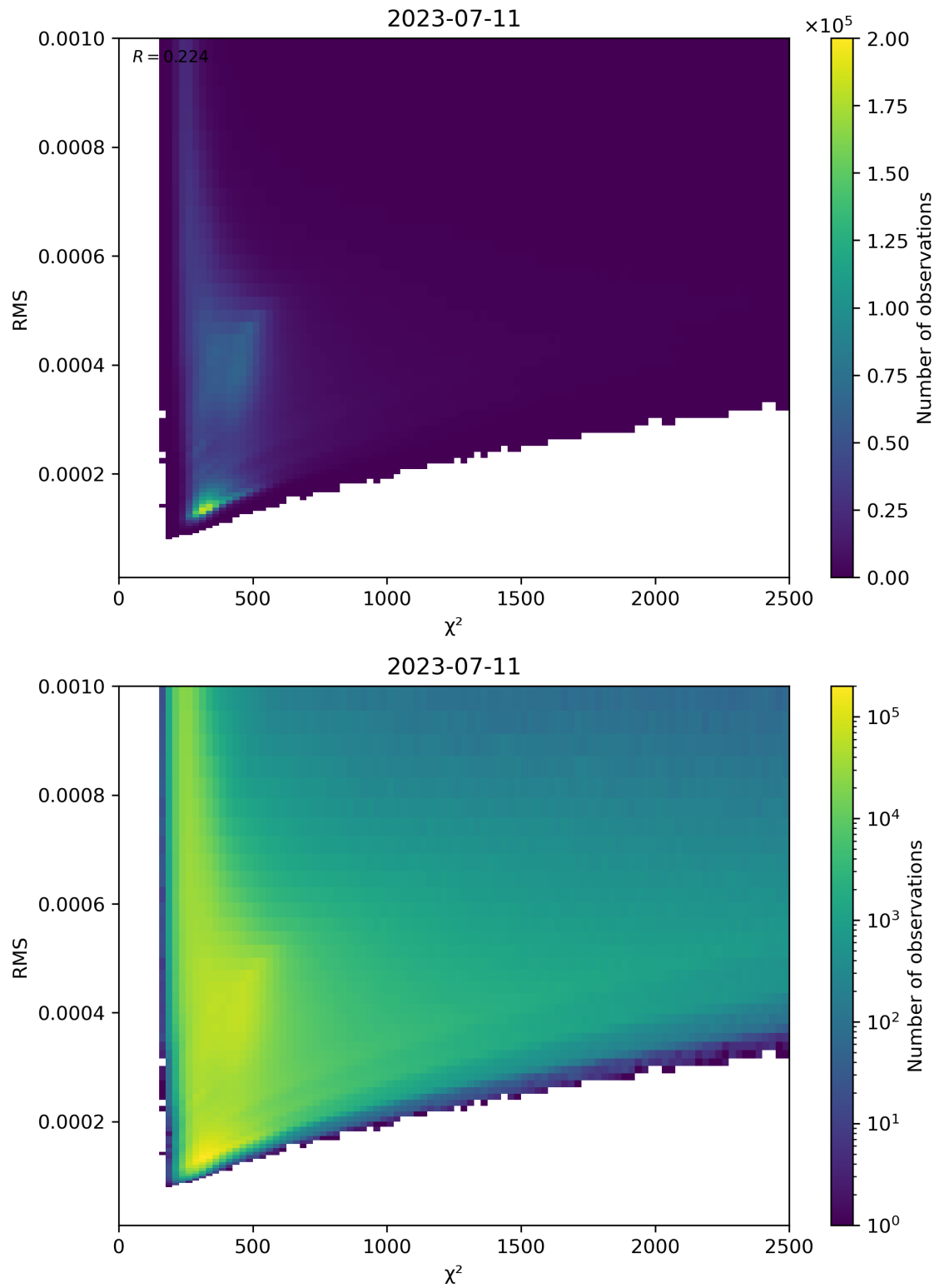
Figure 82: Scatter density plot of “ \chi^2 ” against “RMS” for 2023-07-10 to 2023-07-12.
