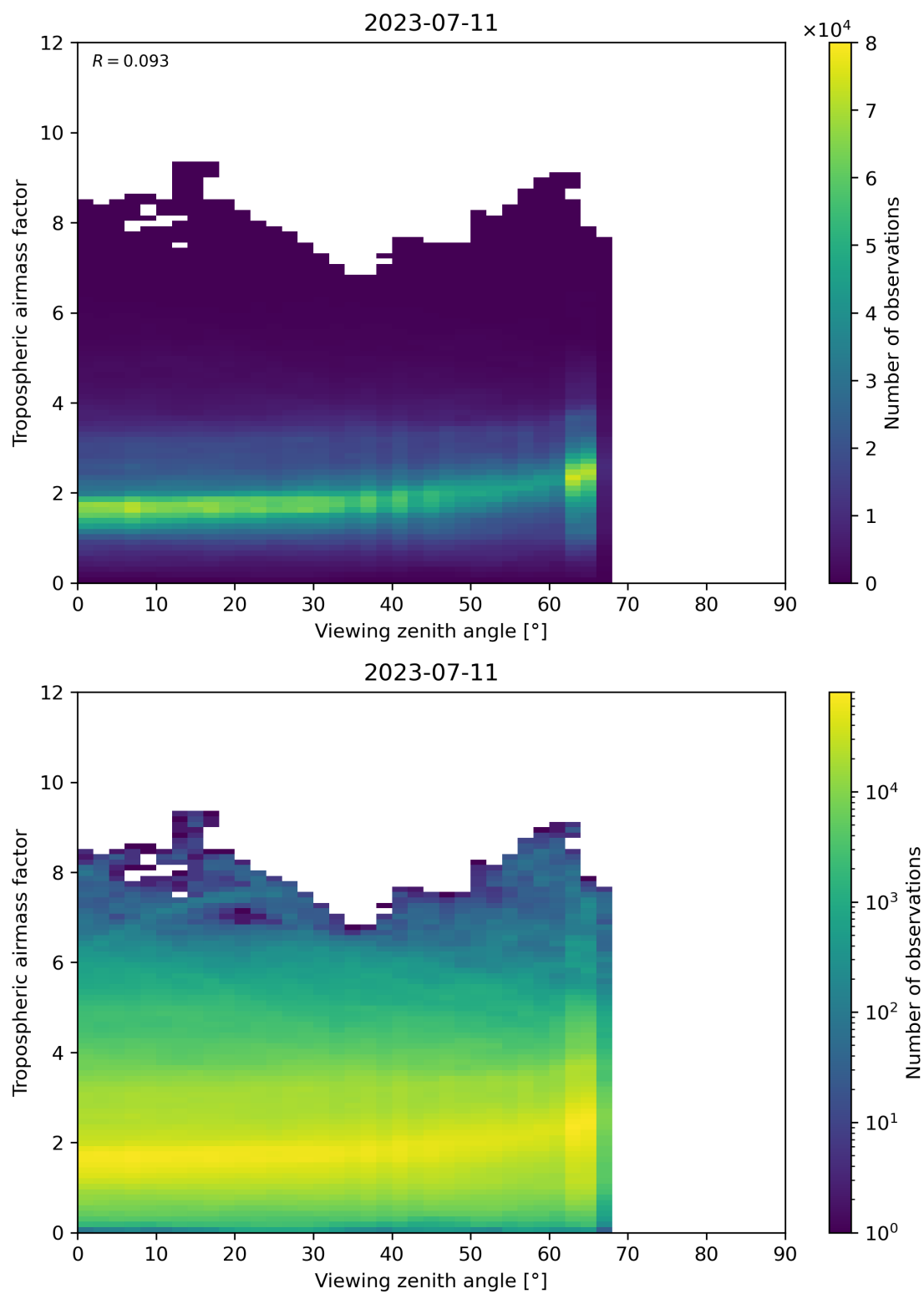
Figure 161: Scatter density plot of “Viewing zenith angle” against “Tropospheric airmass factor” for 2023-07-10 to 2023-07-12.
