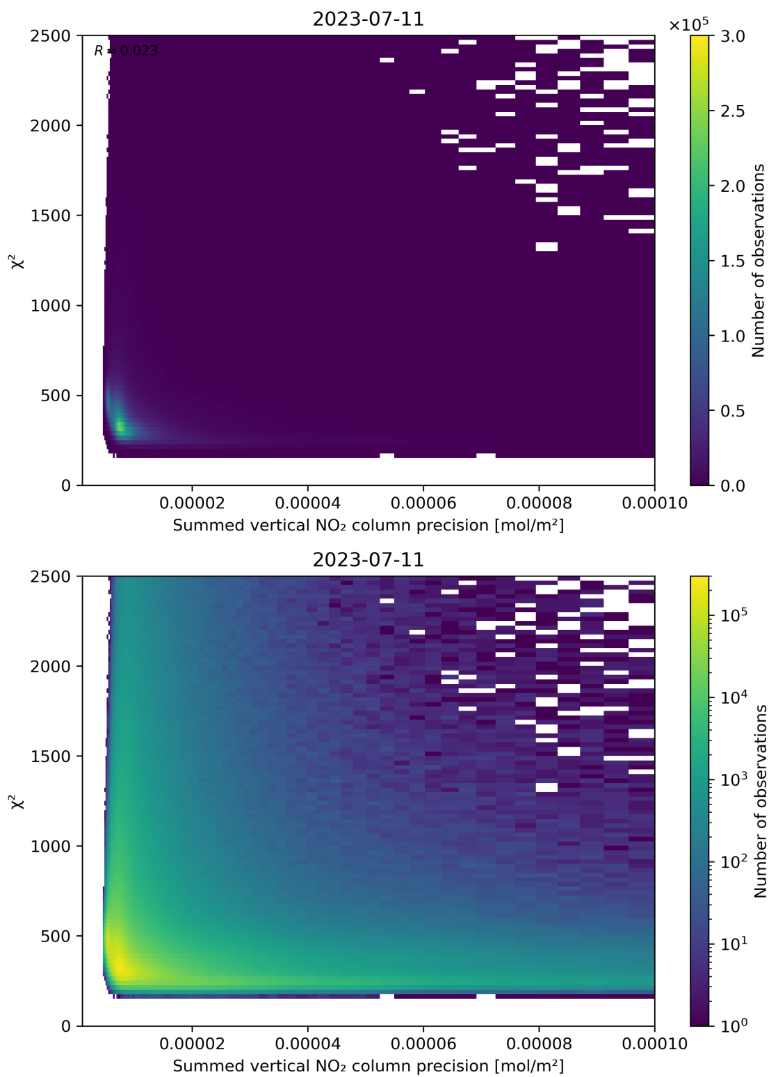
Figure 107: Scatter density plot of “Summed vertical NO 2 column precision” against “ \chi^2 ” for 2023-07-10 to 2023-07-12.
