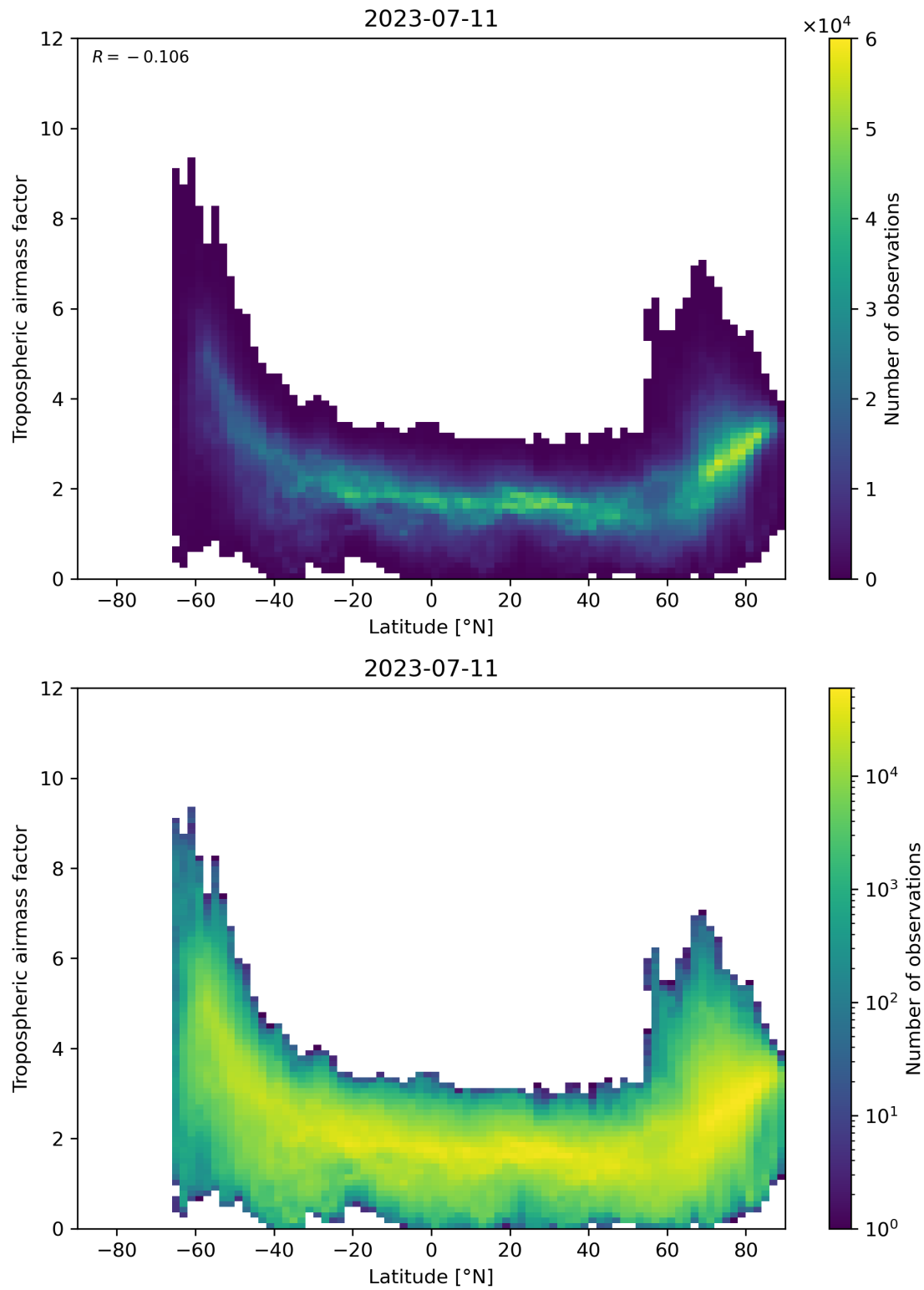
Figure 85: Scatter density plot of “Latitude” against “Tropospheric air mass factor” for 2023-07-10 to 2023-07-12.
