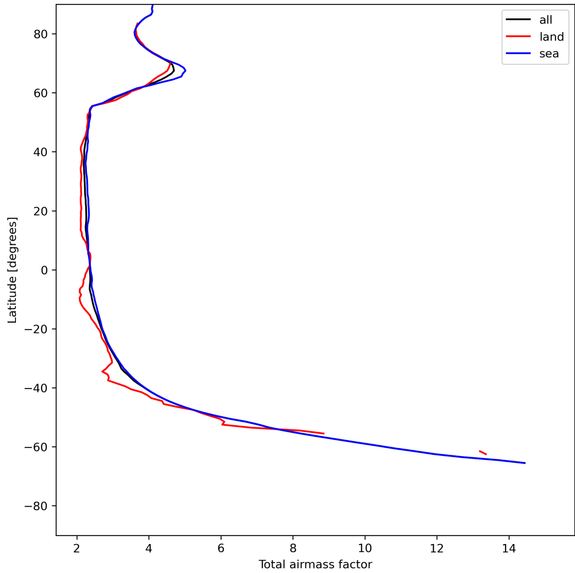
Figure 15: Zonal average of “Total airmass factor” for 2023-07-10 to 2023-07-12.
