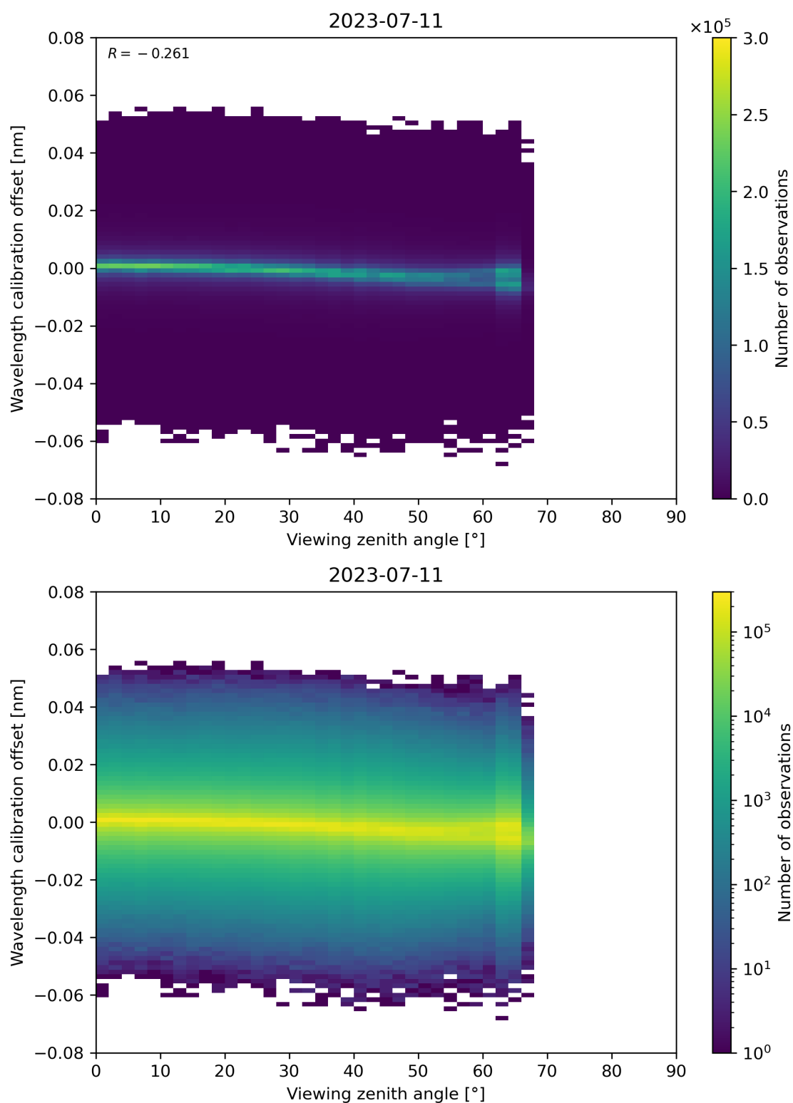
Figure 173: Scatter density plot of “Viewing zenith angle” against “Wavelength calibration offset” for 2023-07-10 to 2023-07-12.
