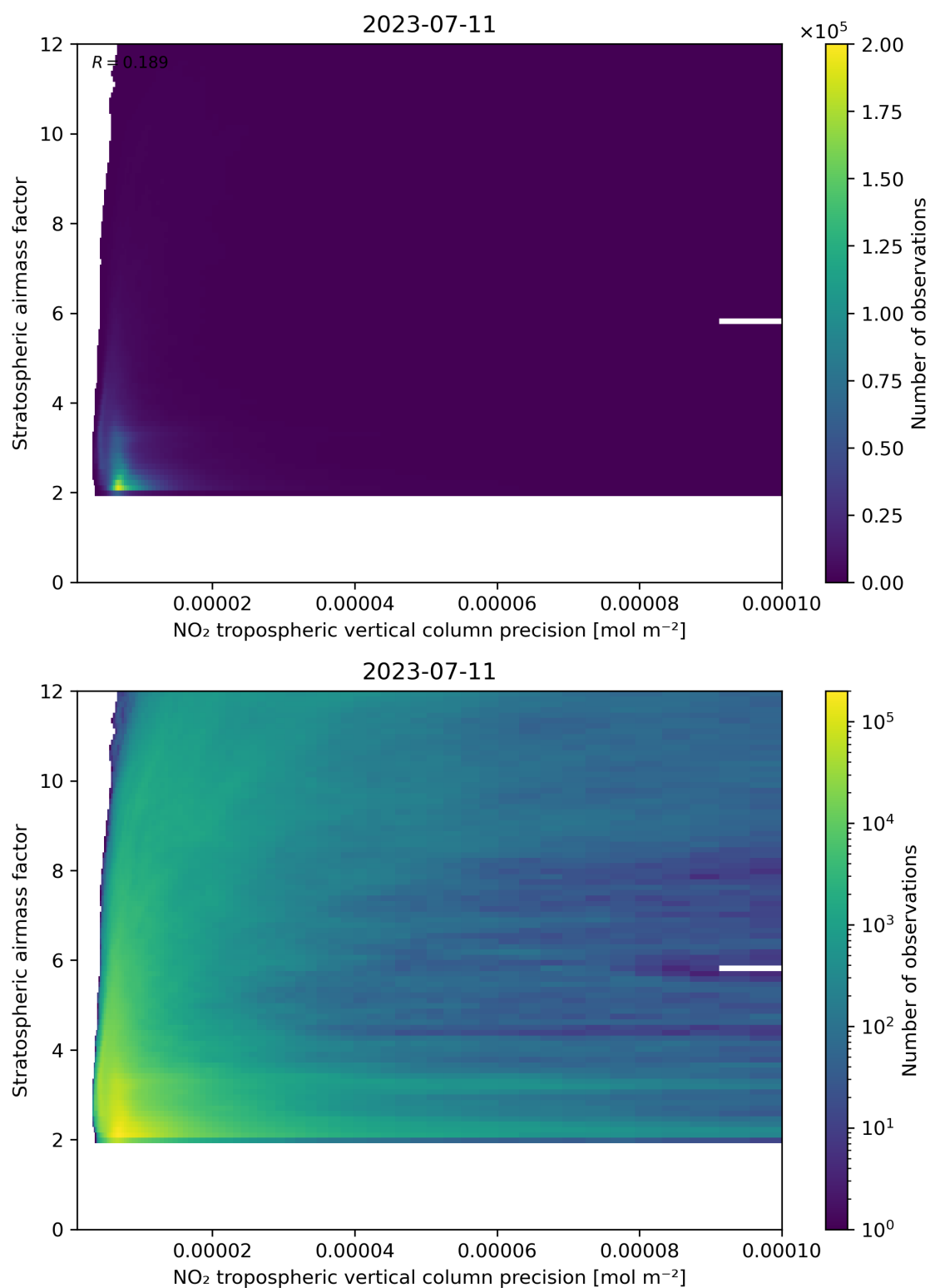
Figure 131: Scatter density plot of “NO 2 tropospheric vertical column precision” against “Stratospheric airmass factor” for 2023-07-10 to 2023-07-12.
