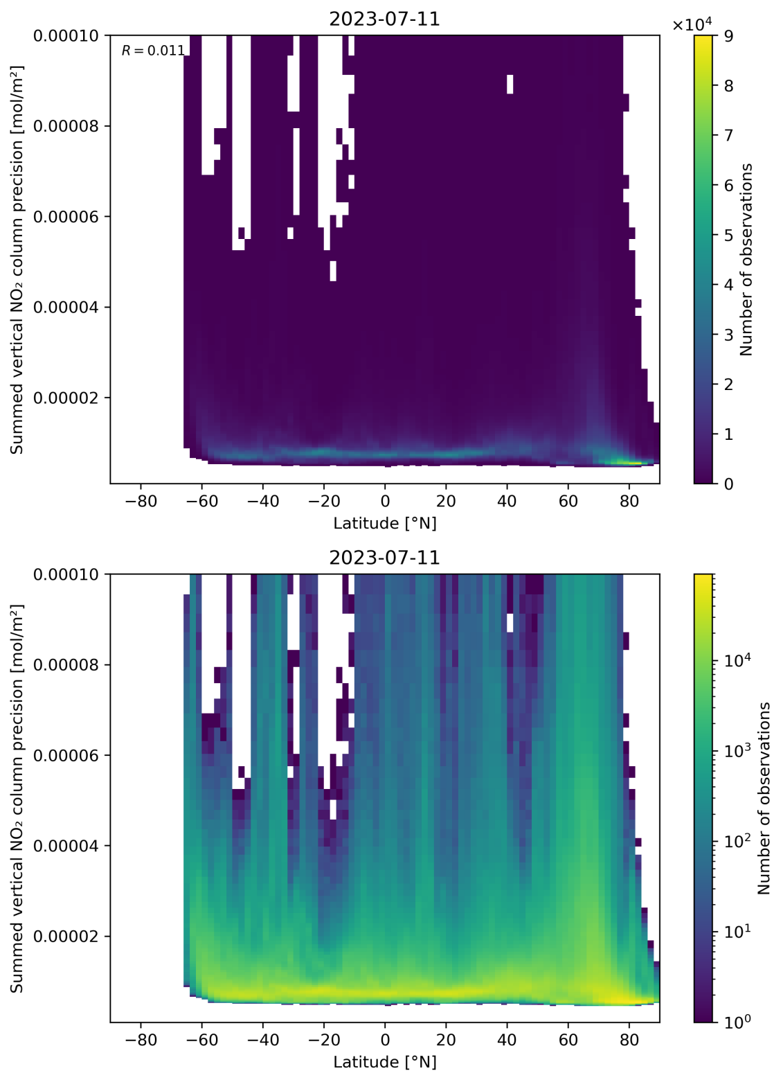
Figure 89: Scatter density plot of “Latitude” against “Summed vertical NO 2 column precision” for 2023-07-10 to 2023-07-12.
