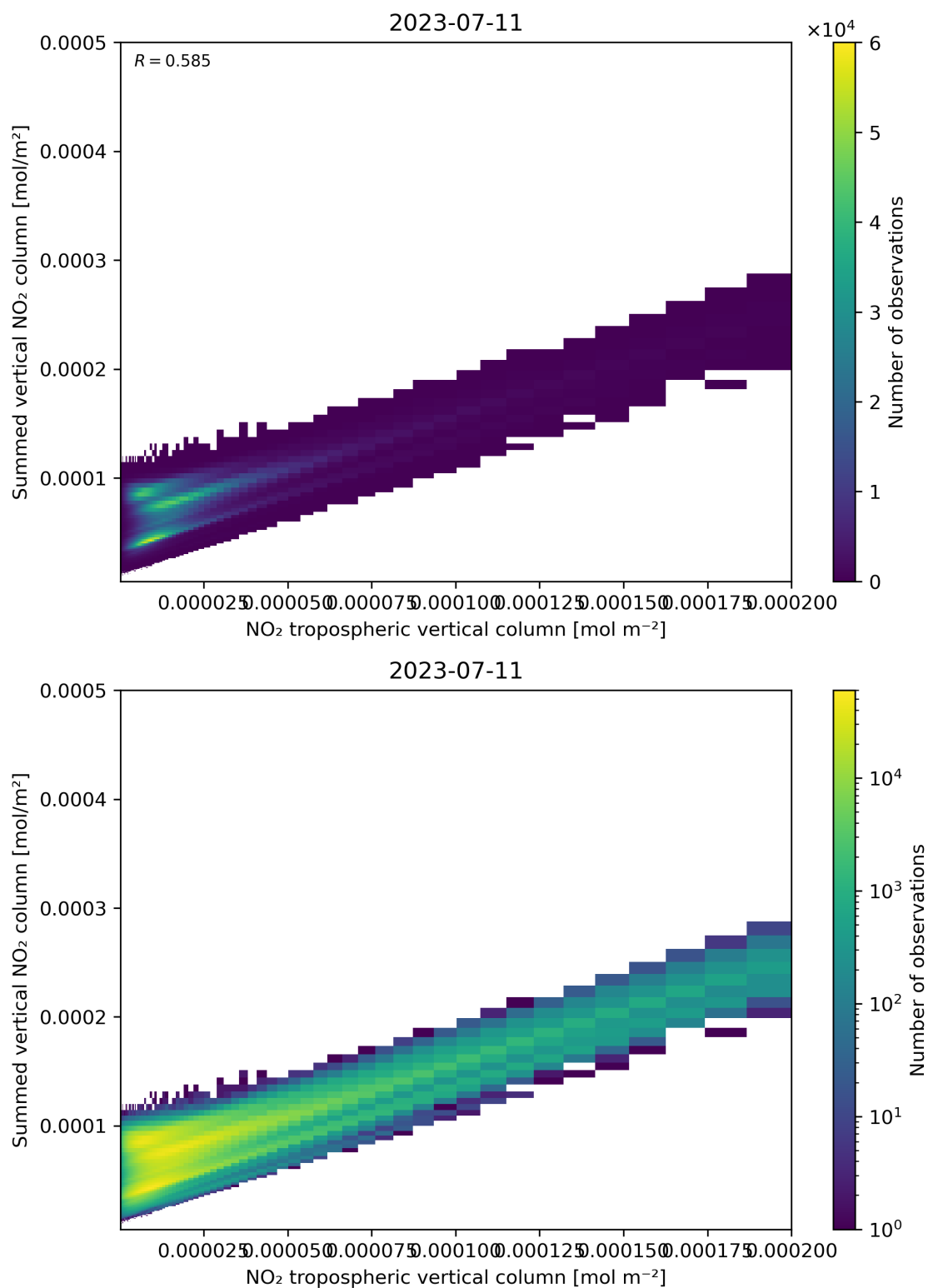
Figure 126: Scatter density plot of “NO 2 tropospheric vertical column” against “Summed vertical NO 2 column” for 2023-07-10 to 2023-07-12.
