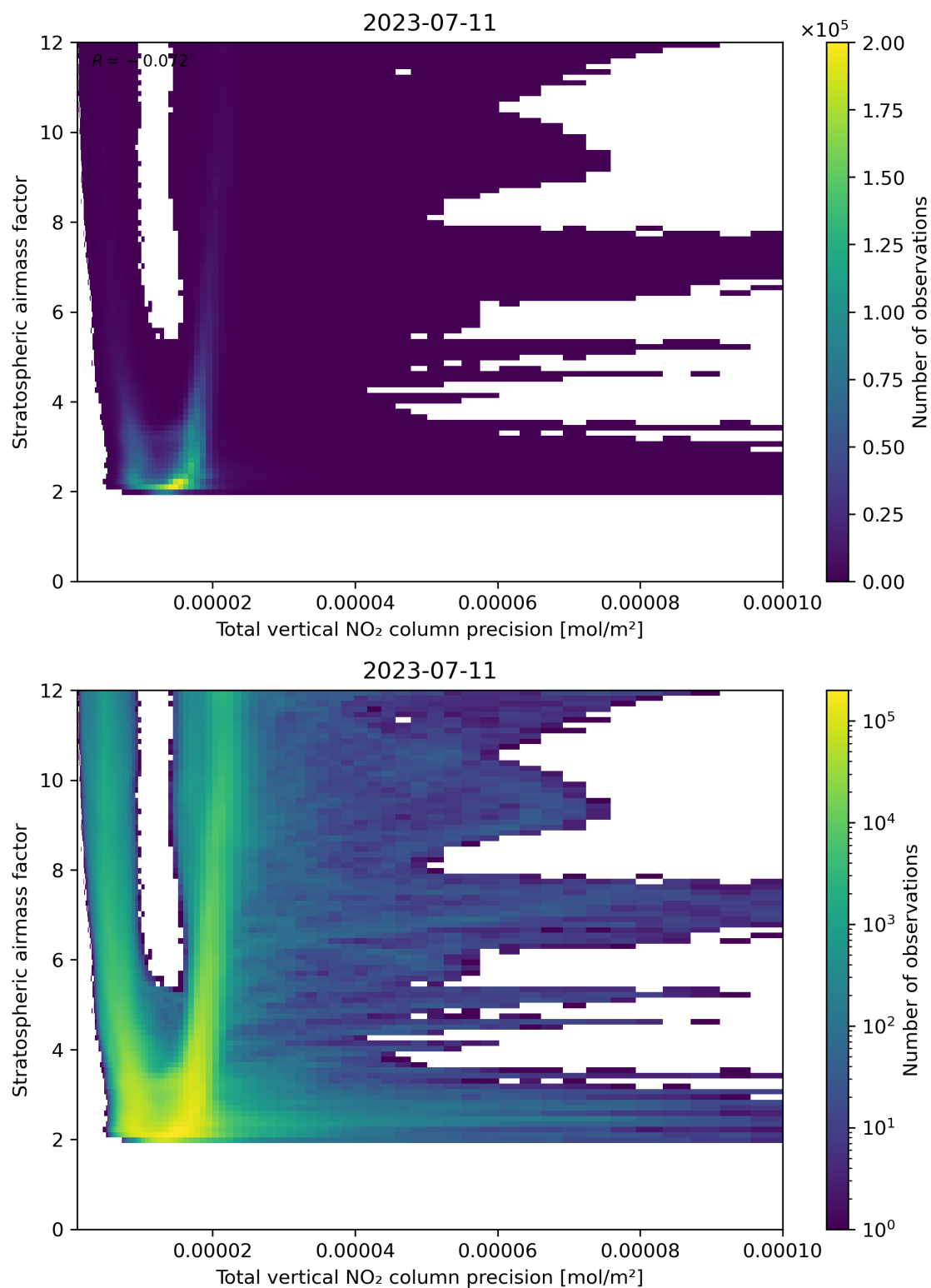
Figure 115: Scatter density plot of “Total vertical NO 2 column precision” against “Stratospheric air mass factor” for 2023-07-10 to 2023-07-12.
