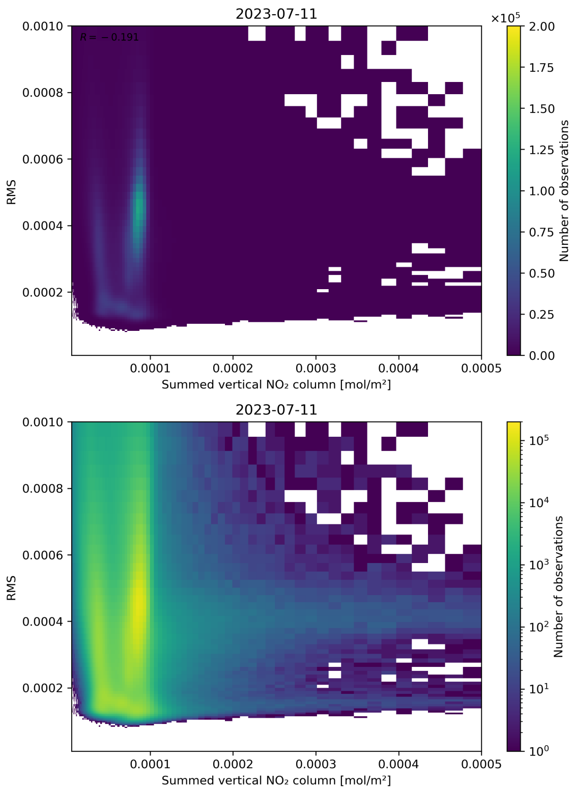
Figure 109: Scatter density plot of “Summed vertical NO 2 column” against “RMS” for 2023-07-10 to 2023-07-12.
