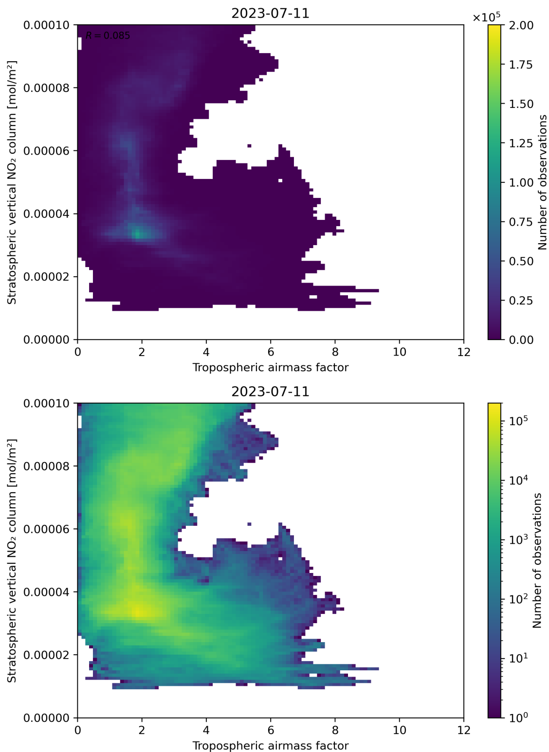
Figure 74: Scatter density plot of “Tropospheric air mass factor” against “Stratospheric vertical NO 2 column” for 2023-07-10 to 2023-07-12.
