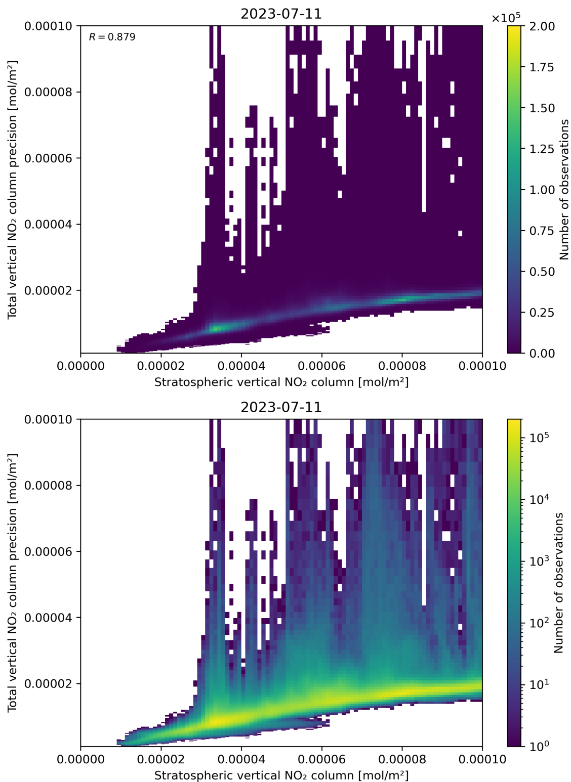
Figure 101: Scatter density plot of “Stratospheric vertical NO 2 column” against “Total vertical NO 2 column precision” for 2023-07-10 to 2023-07-12.
