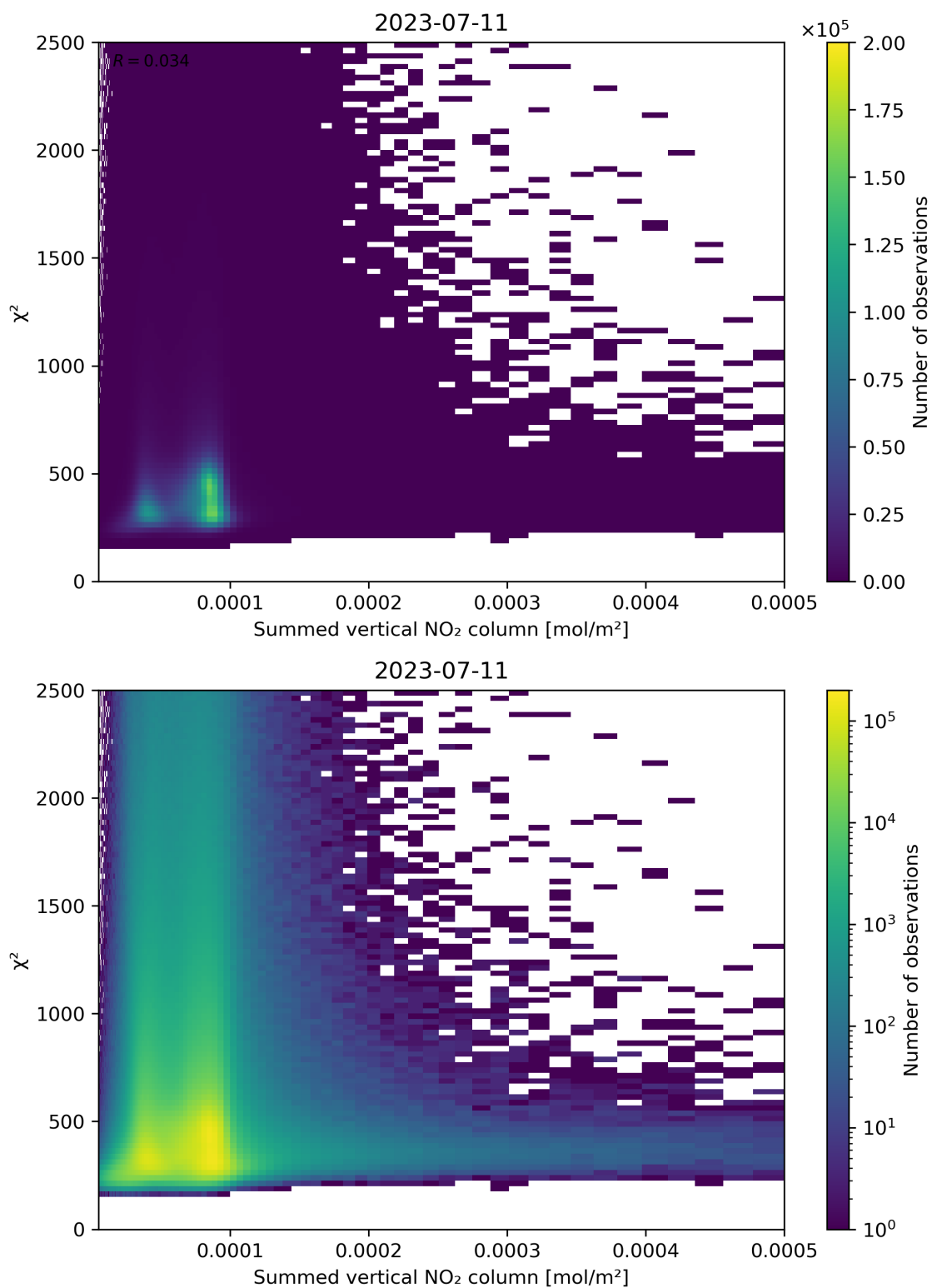
Figure 104: Scatter density plot of “Summed vertical NO 2 column” against “ \chi^2 ” for 2023-07-10 to 2023-07-12.
