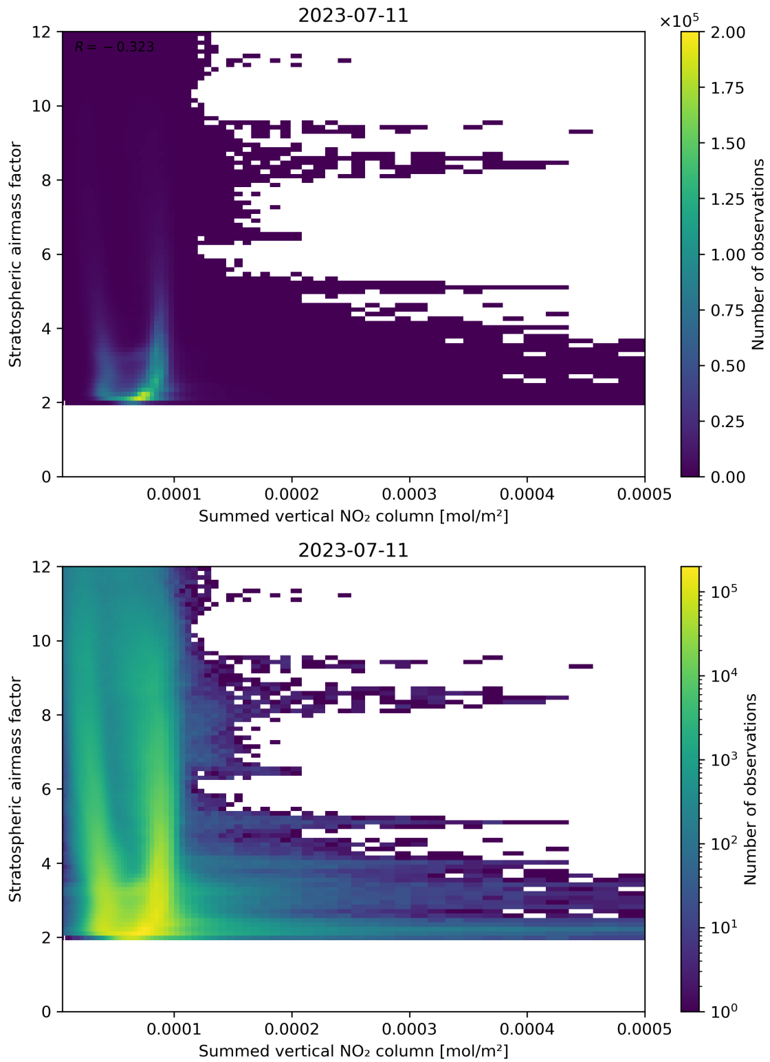
Figure 103: Scatter density plot of “Summed vertical NO 2 column” against “Stratospheric airmass factor” for 2023-07-10 to 2023-07-12.
