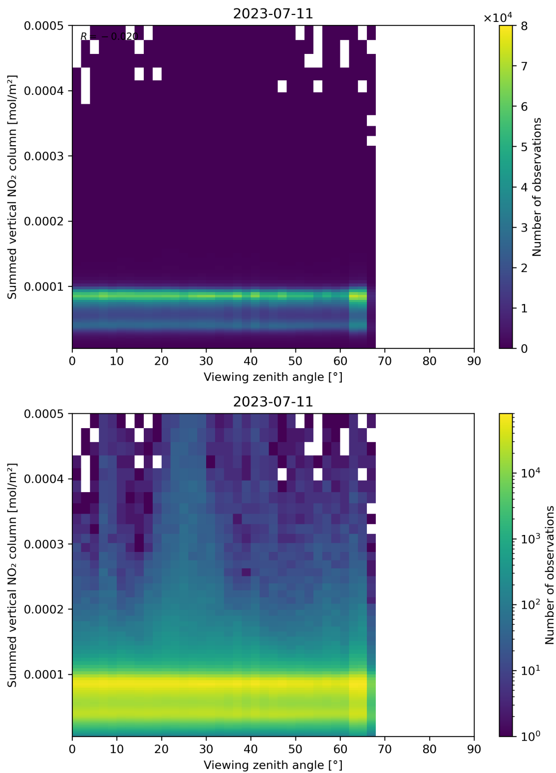
Figure 165: Scatter density plot of “Viewing zenith angle” against “Summed vertical NO 2 column” for 2023-07-10 to 2023-07-12.
