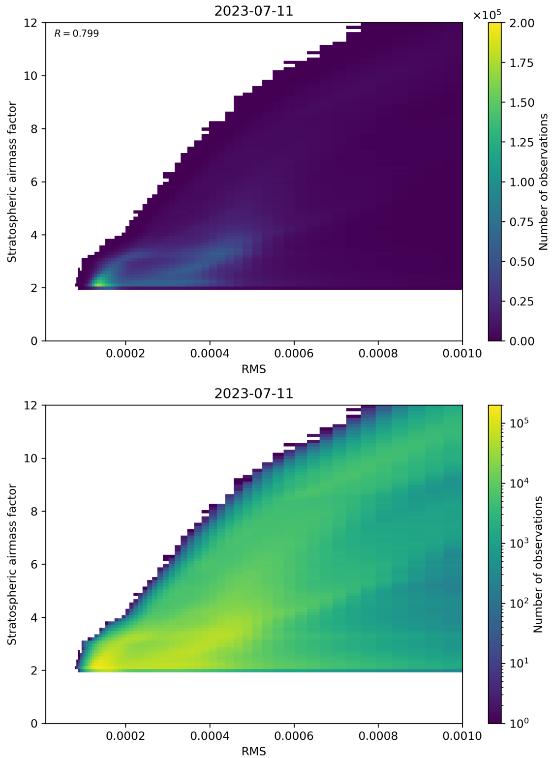
Figure 144: Scatter density plot of “RMS” against “Stratospheric airmass factor” for 2023-07-10 to 2023-07-12.
