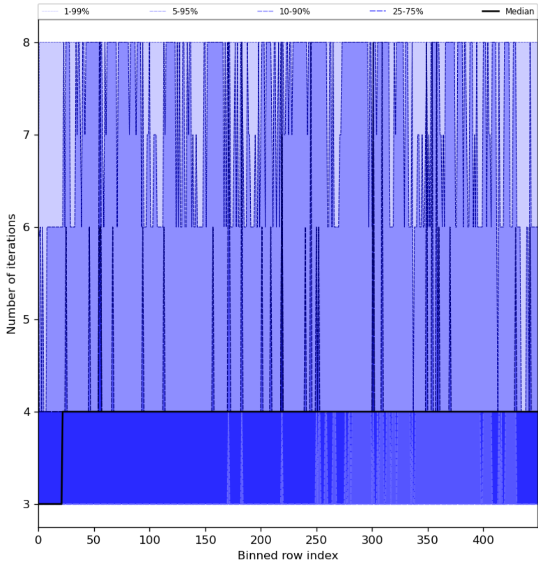
Figure 51: Along track statistics of “Number of iterations” for 2023-07-10 to 2023-07-12
