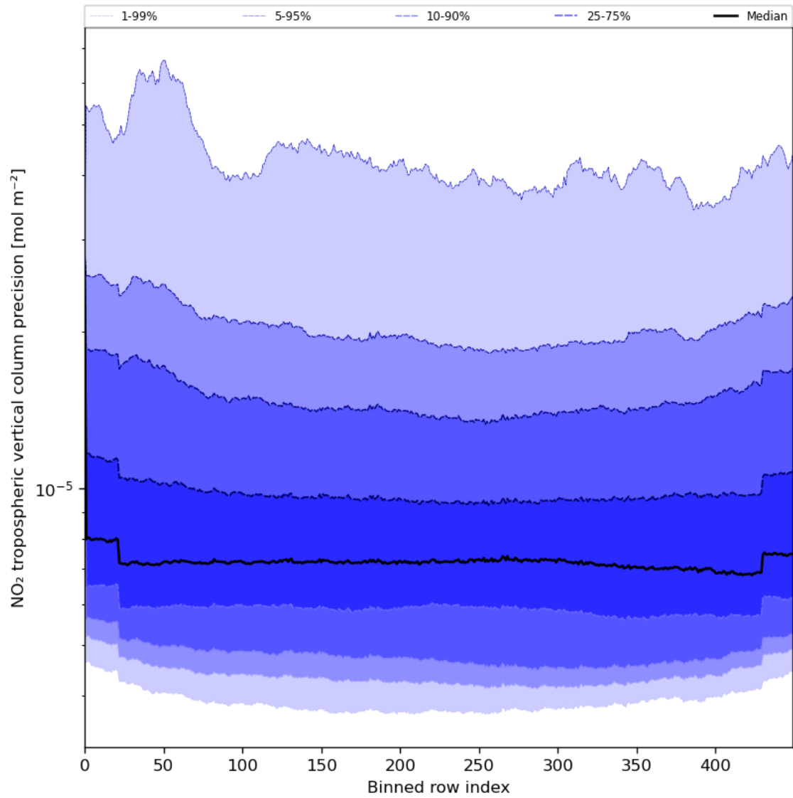
Figure 47: Along track statistics of “NO 2 tropospheric vertical column precision” for 2023-07-10 to 2023-07-12
