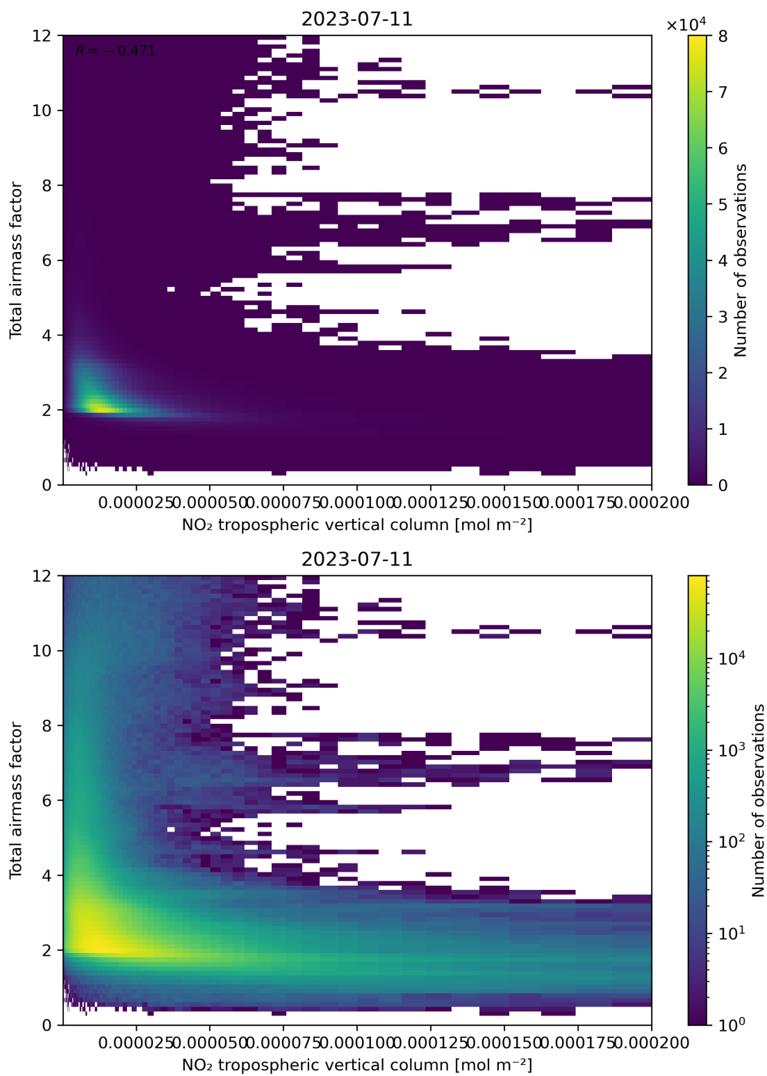
Figure 122: Scatter density plot of “NO 2 tropospheric vertical column” against “Total air mass factor” for 2023-07-10 to 2023-07-12.
