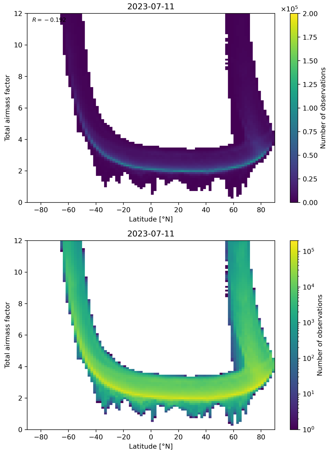
Figure 84: Scatter density plot of “Latitude” against “Total airmass factor” for 2023-07-10 to 2023-07-12.
