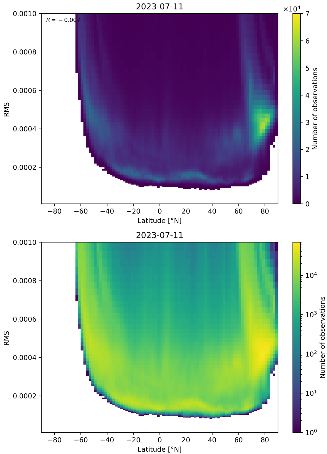
Figure 94: Scatter density plot of “Latitude” against “RMS” for 2023-07-10 to 2023-07-12.
