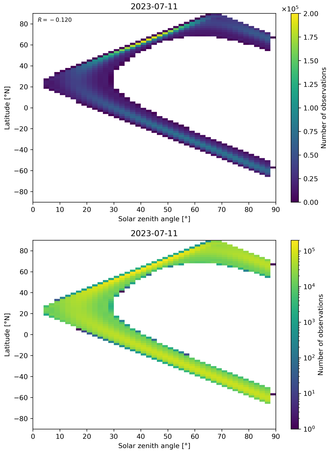
Figure 149: Scatter density plot of “Solar zenith angle” against “Latitude” for 2023-07-10 to 2023-07-12.
