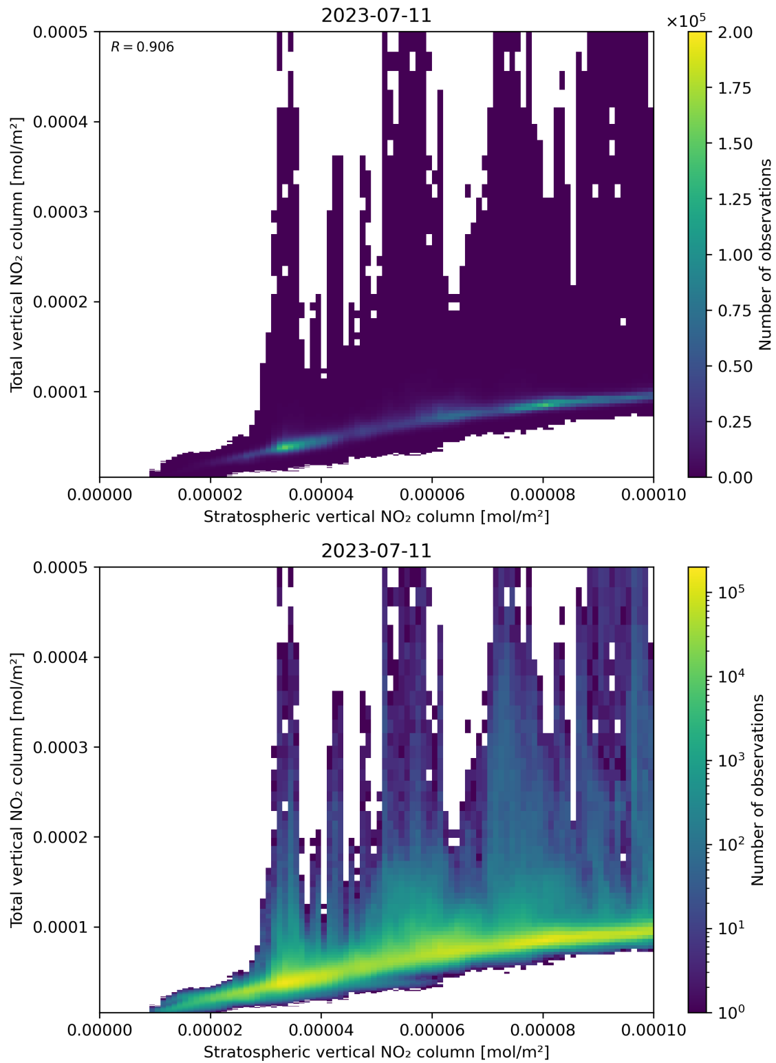
Figure 100: Scatter density plot of “Stratospheric vertical NO 2 column” against “Total vertical NO 2 column” for 2023-07-10 to 2023-07-12.
