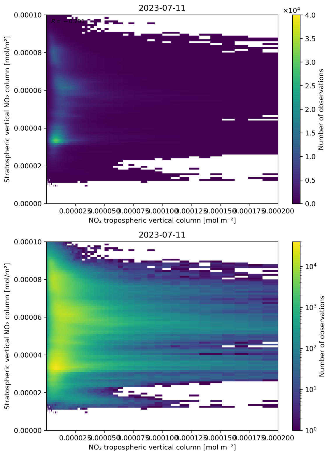
Figure 125: Scatter density plot of “NO 2 tropospheric vertical column” against “Stratospheric vertical NO 2 column” for 2023-07-10 to 2023-07-12.
