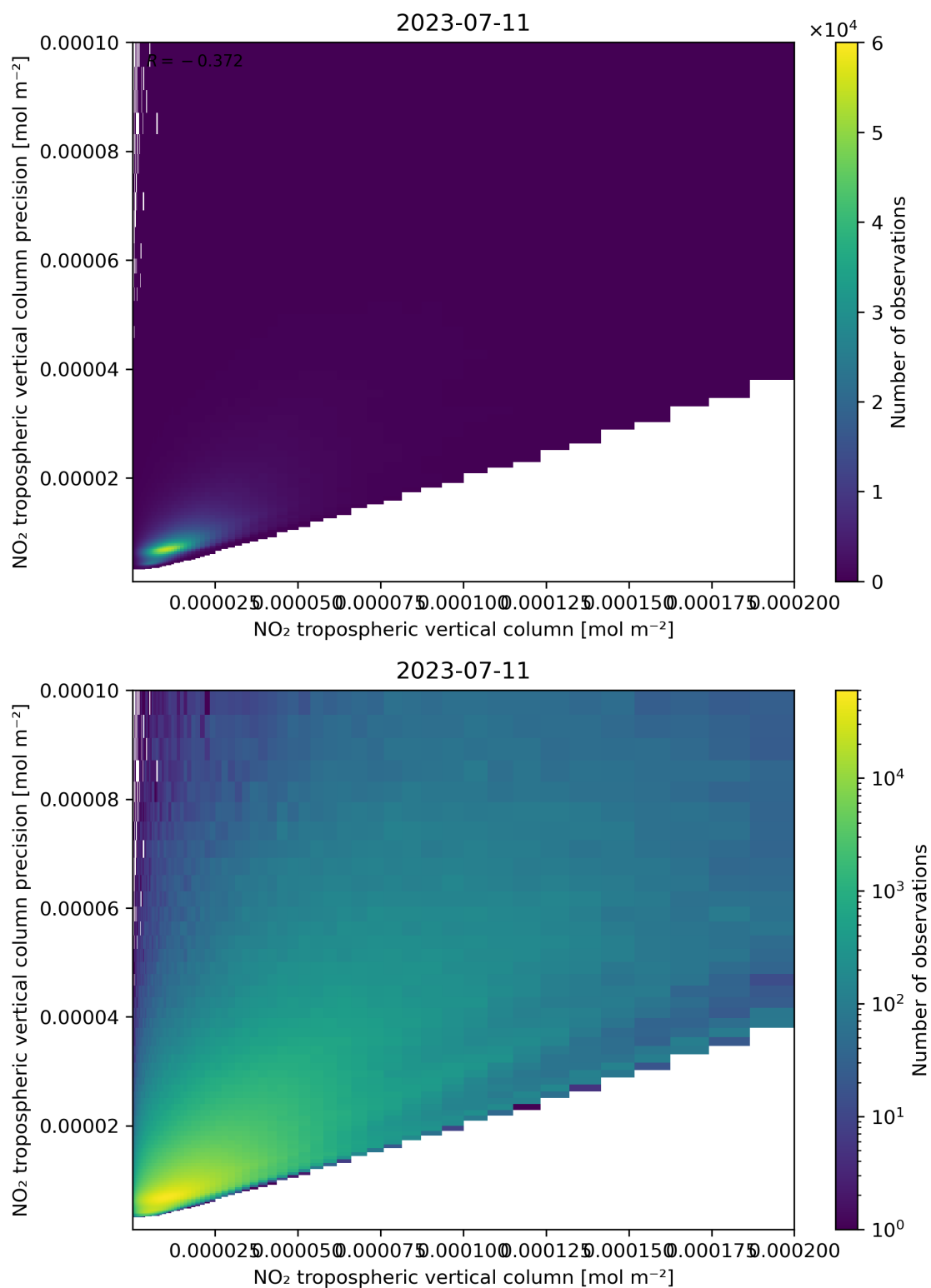
Figure 130: Scatter density plot of “NO 2 tropospheric vertical column” against “NO 2 tropospheric vertical column precision” for 2023-07-10 to 2023-07-12.
