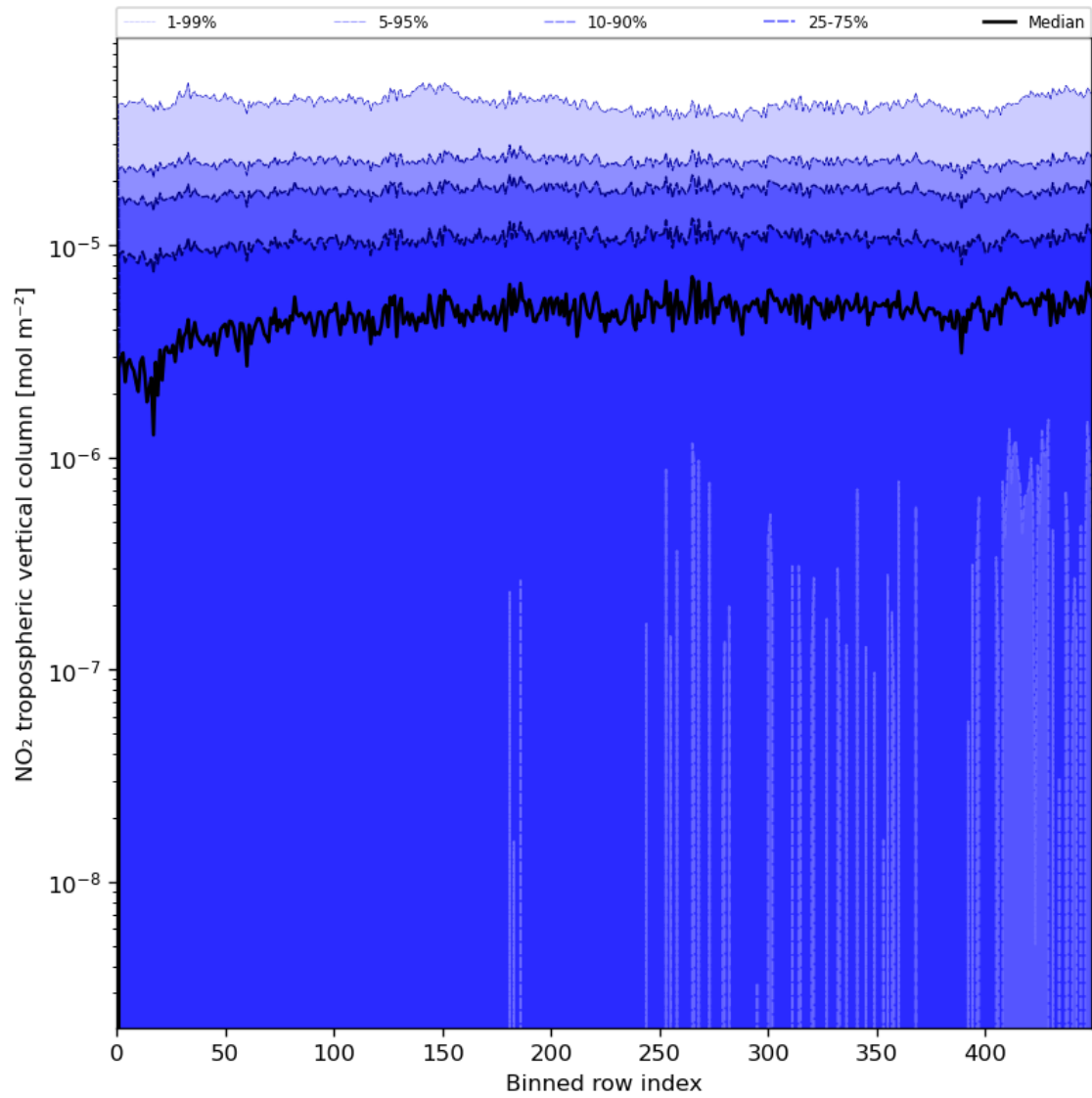
Figure 46: Along track statistics of "NO 2 tropospheric vertical column" for 2023-07-10 to 2023-07-12
