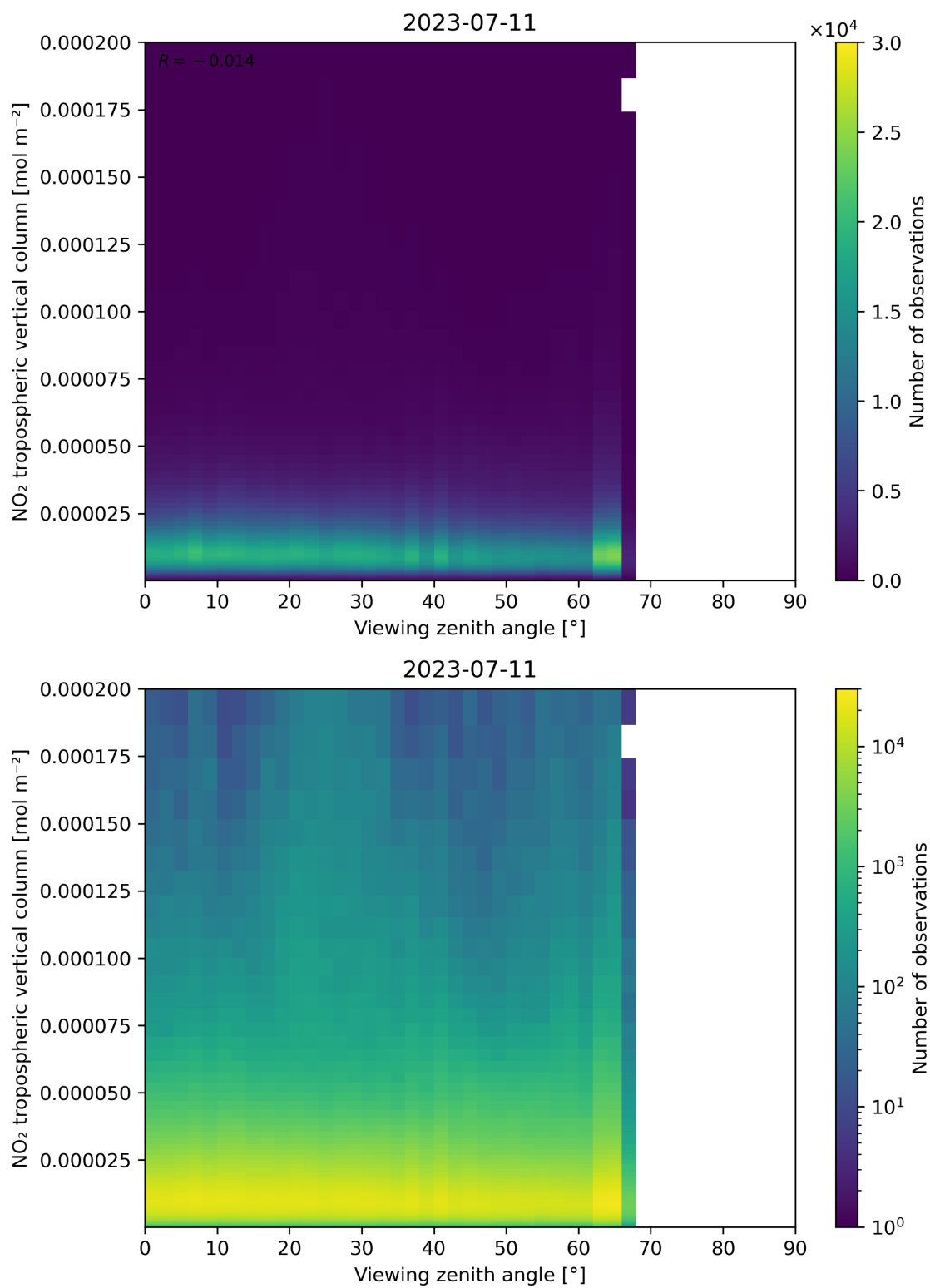
Figure 169: Scatter density plot of “Viewing zenith angle” against “NO 2 tropospheric vertical column” for 2023-07-10 to 2023-07-12.
