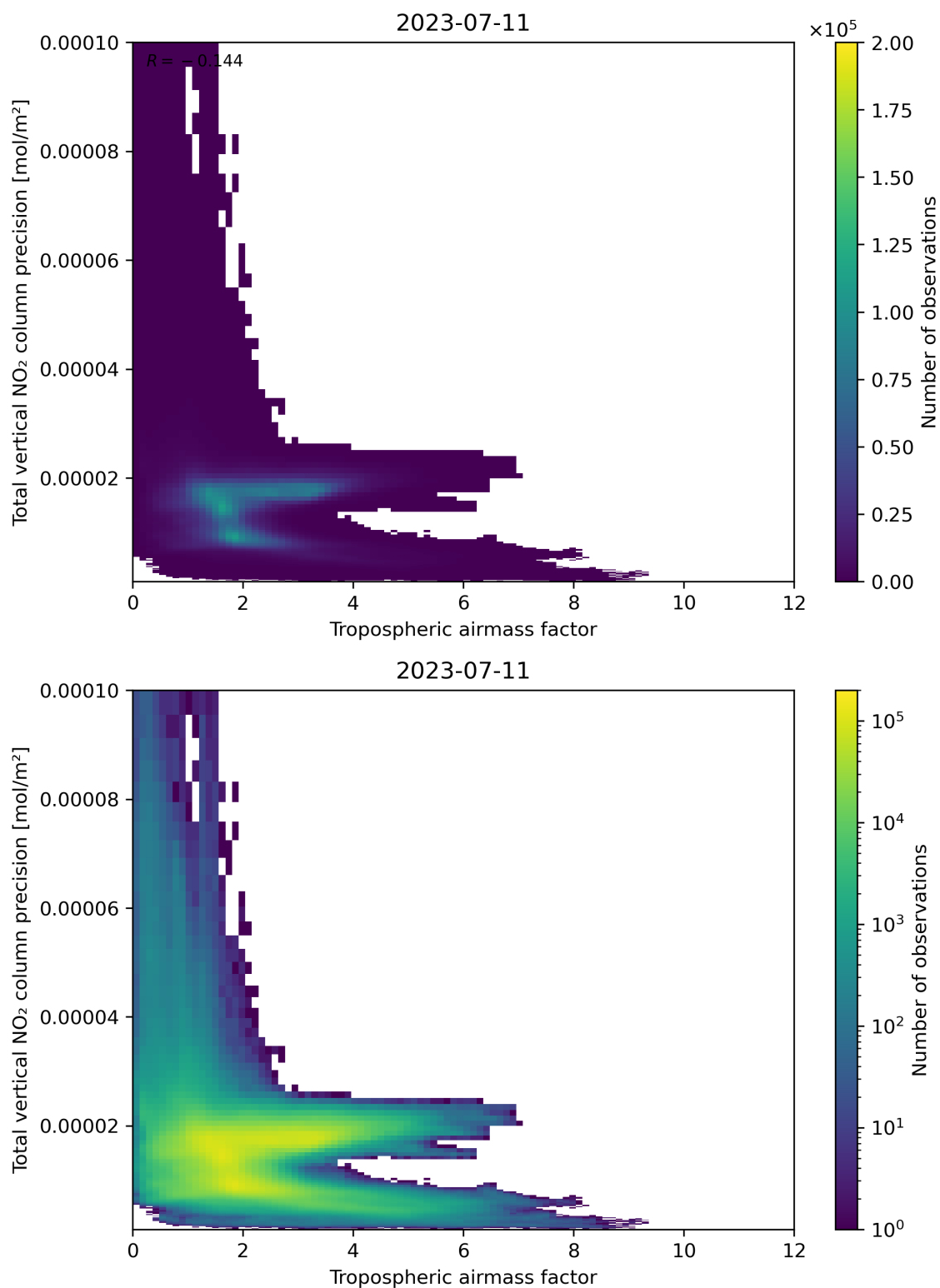
Figure 78: Scatter density plot of “Tropospheric air mass factor” against “Total vertical NO 2 column precision” for 2023-07-10 to 2023-07-12.
