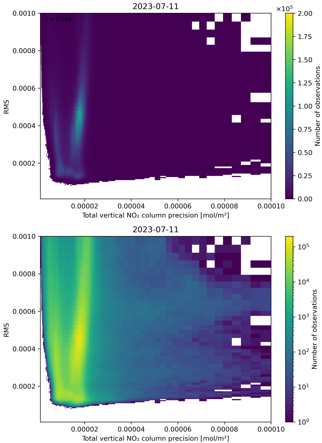
Figure 119: Scatter density plot of “Total vertical NO 2 column precision” against “RMS” for 2023-07-10 to 2023-07-12.
