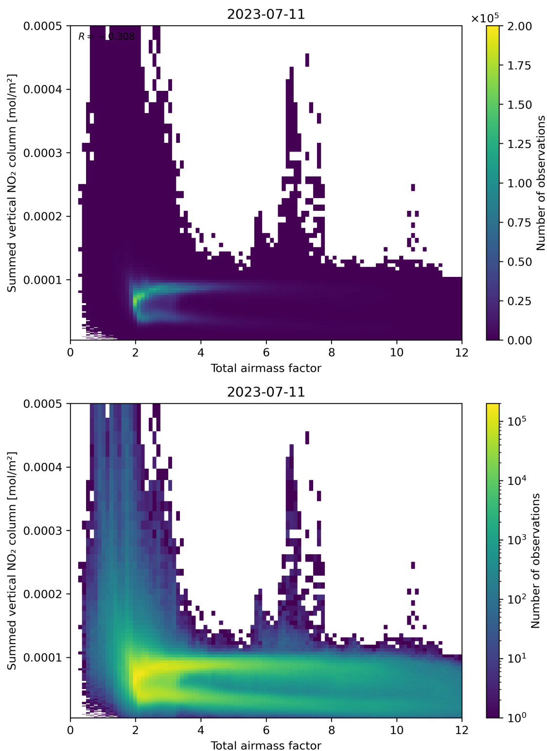
Figure 65: Scatter density plot of “Total airmass factor” against “Summed vertical NO 2 column” for 2023-07-10 to 2023-07-12.
