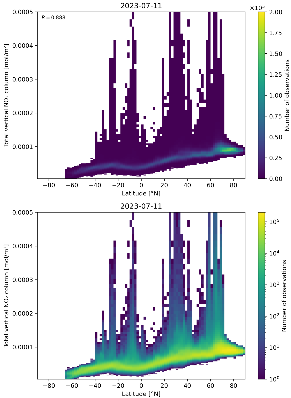
Figure 90: Scatter density plot of “Latitude” against “Total vertical NO 2 column” for 2023-07-10 to 2023-07-12.
