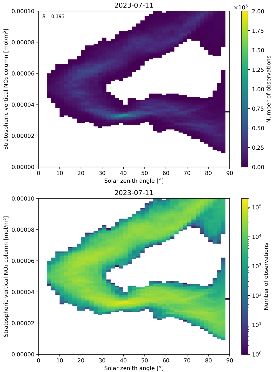
Figure 150: Scatter density plot of “Solar zenith angle” against “Stratospheric vertical NO 2 column” for 2023-07-10 to 2023-07-12.
