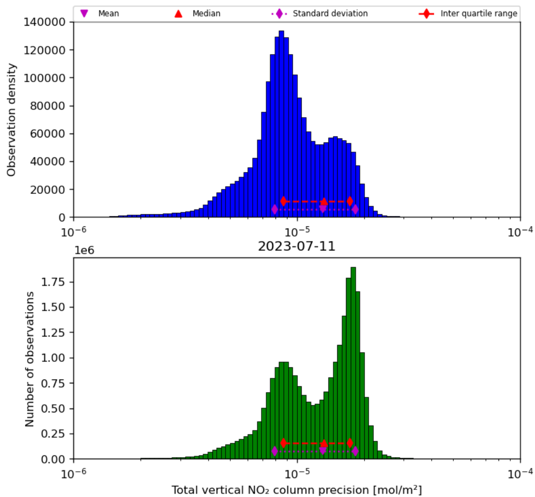
Figure 39: Histogram of “Total vertical NO 2 column precision” for 2023-07-10 to 2023-07-12
