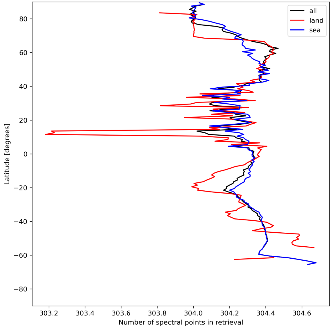
Figure 16: Zonal average of “Number of spectral points in retrieval” for 2023-07-10 to 2023-07-12.
