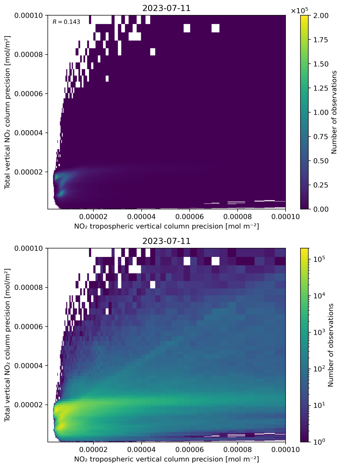
Figure 139: Scatter density plot of “NO 2 tropospheric vertical column precision” against “Total vertical NO 2 column precision” for 2023-07-10 to 2023-07-12.
