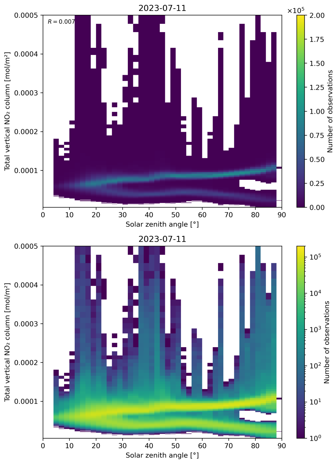
Figure 153: Scatter density plot of “Solar zenith angle” against “Total vertical NO 2 column” for 2023-07-10 to 2023-07-12.
