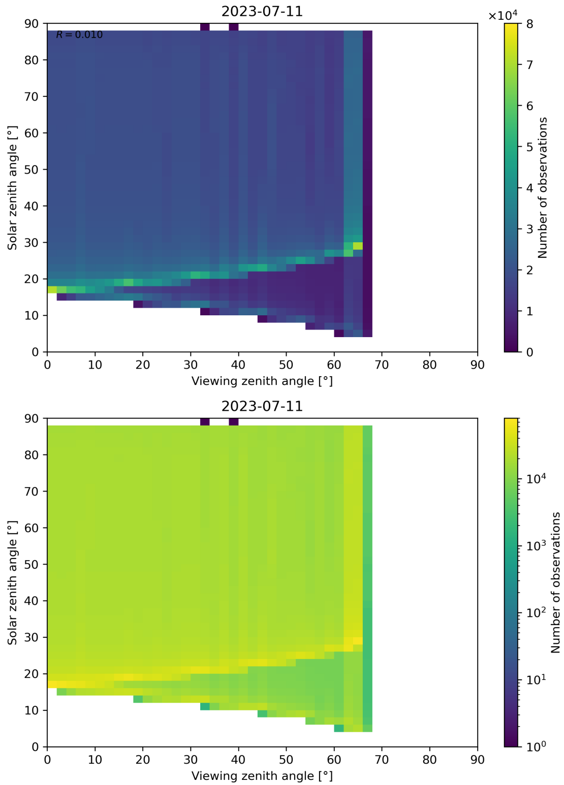
Figure 172: Scatter density plot of “Viewing zenith angle” against “Solar zenith angle” for 2023-07-10 to 2023-07-12.
