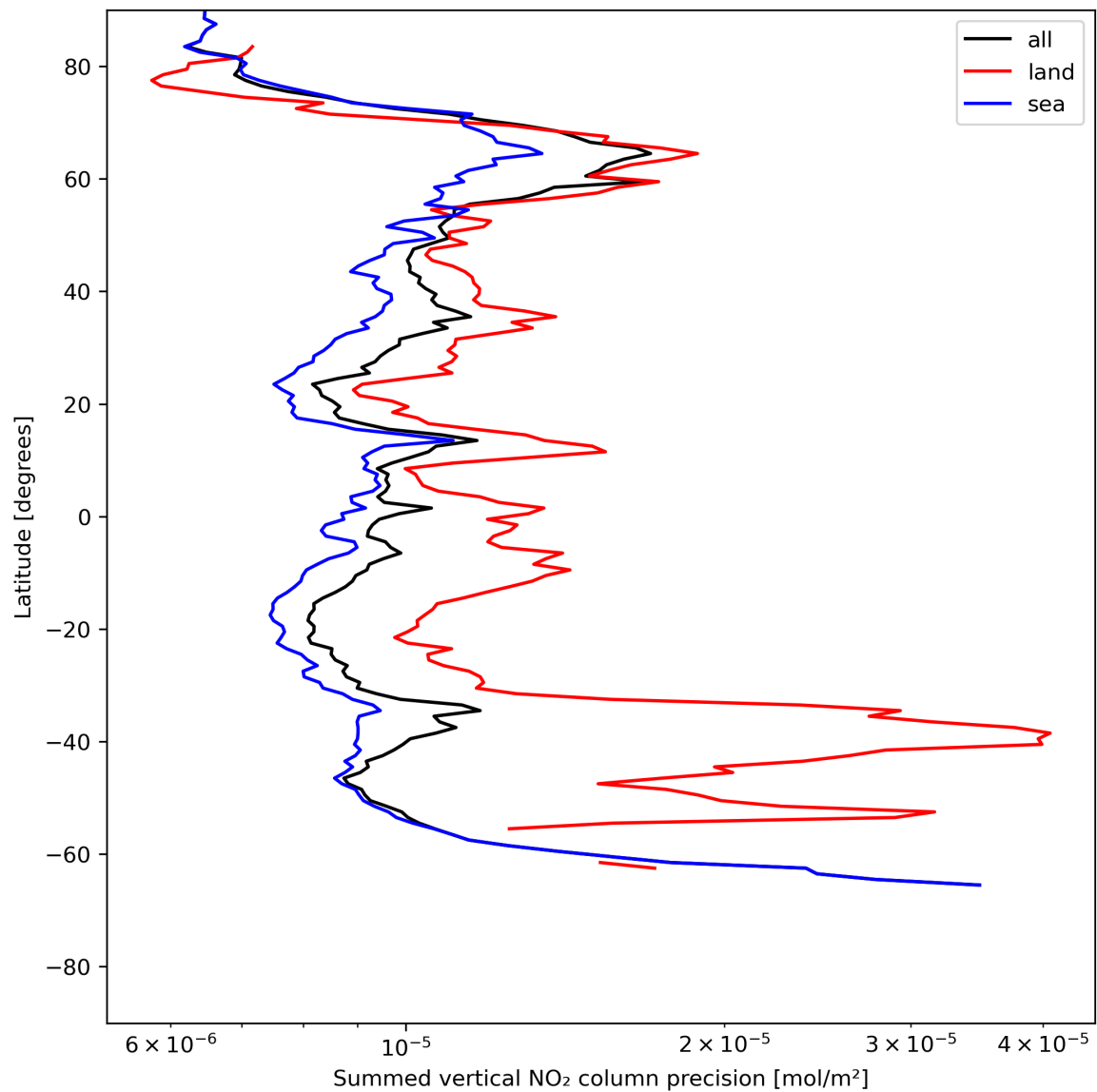
Figure 24: Zonal average of “Summed vertical NO 2 column precision” for 2023-07-10 to 2023-07-12.
