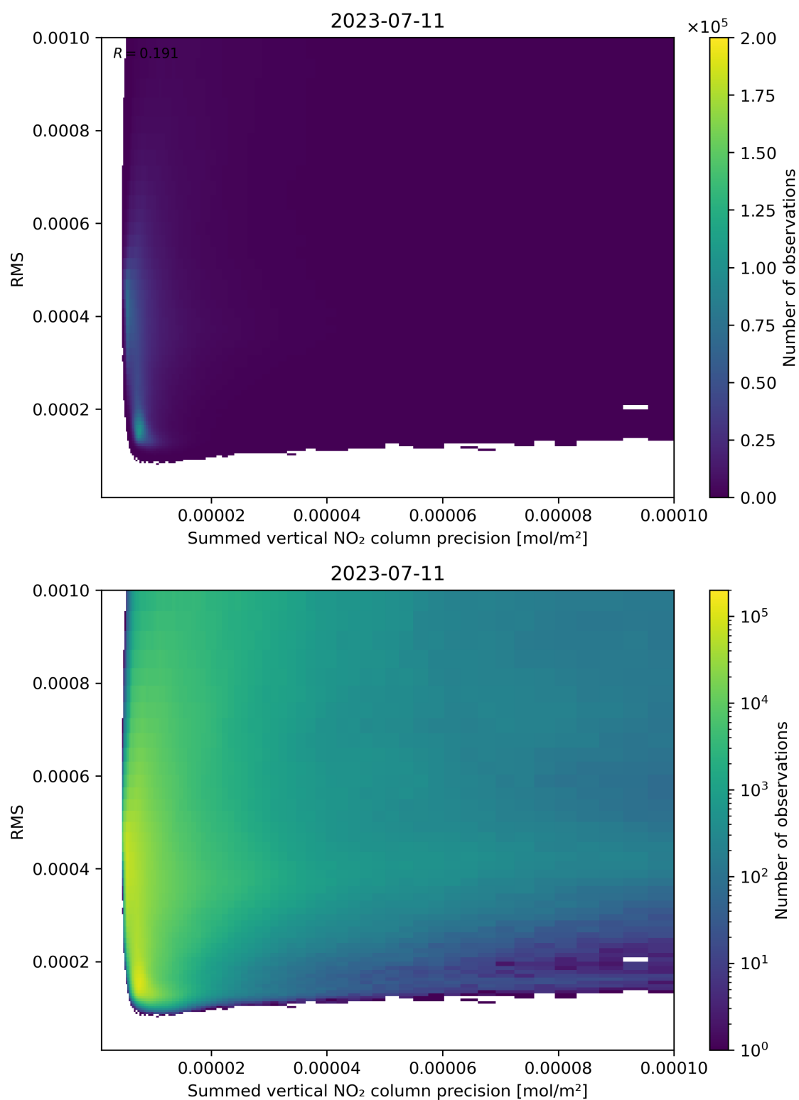
Figure 108: Scatter density plot of “Summed vertical NO 2 column precision” against “RMS” for 2023-07-10 to 2023-07-12.
