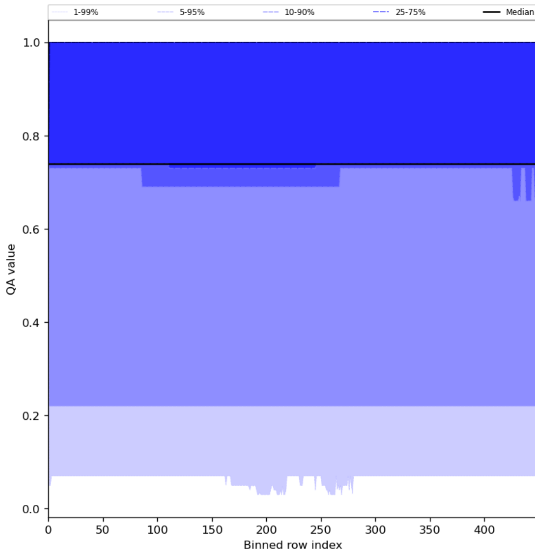
Figure 45: Along track statistics of “QA value” for 2023-07-10 to 2023-07-12
