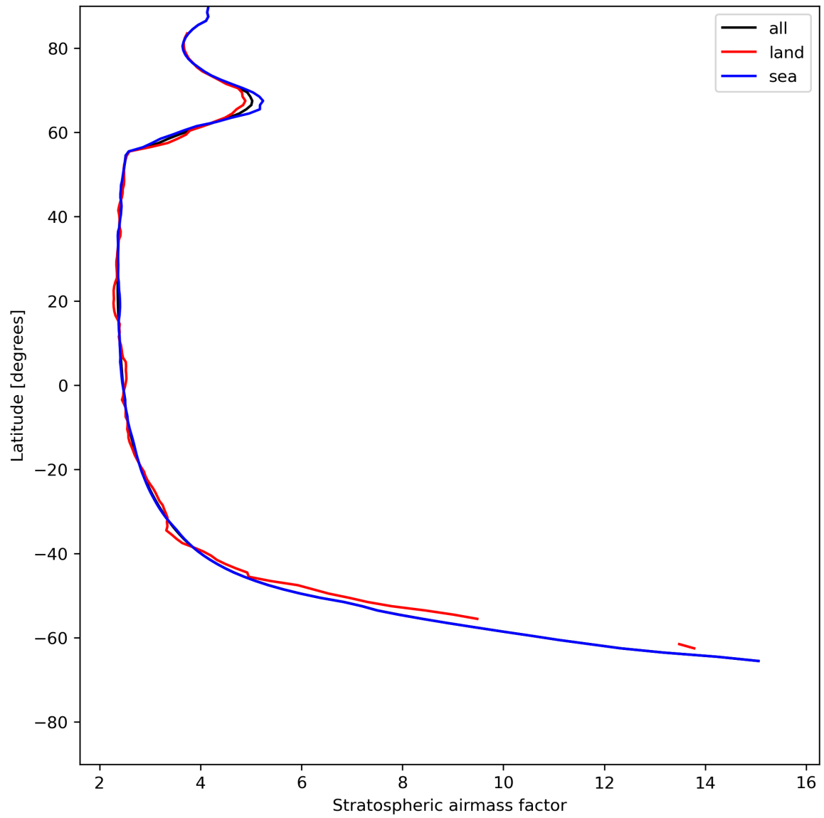
Figure 27: Zonal average of “Stratospheric airmass factor” for 2023-07-10 to 2023-07-12.
