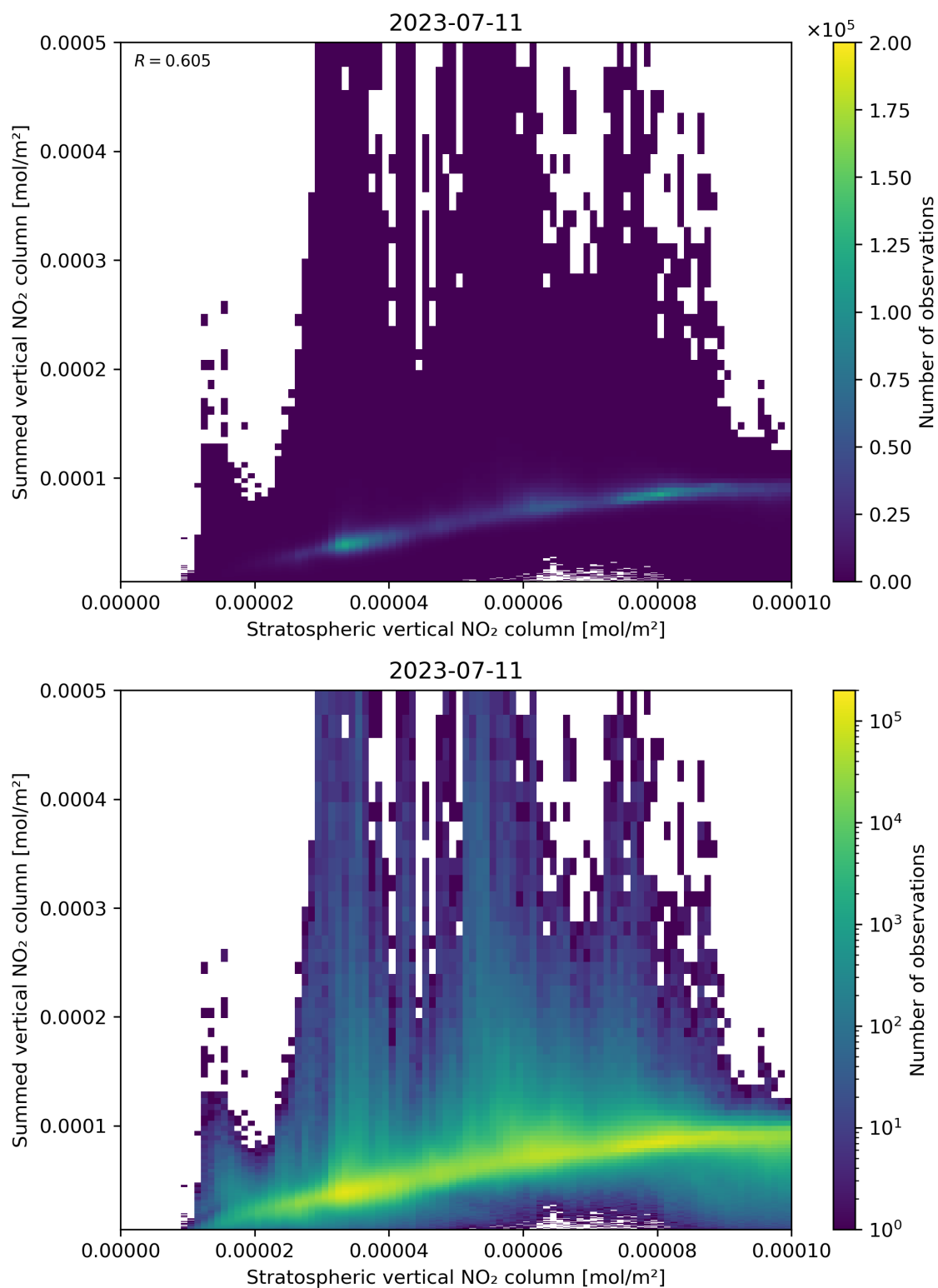
Figure 98: Scatter density plot of “Stratospheric vertical NO 2 column” against “Summed vertical NO 2 column” for 2023-07-10 to 2023-07-12.
