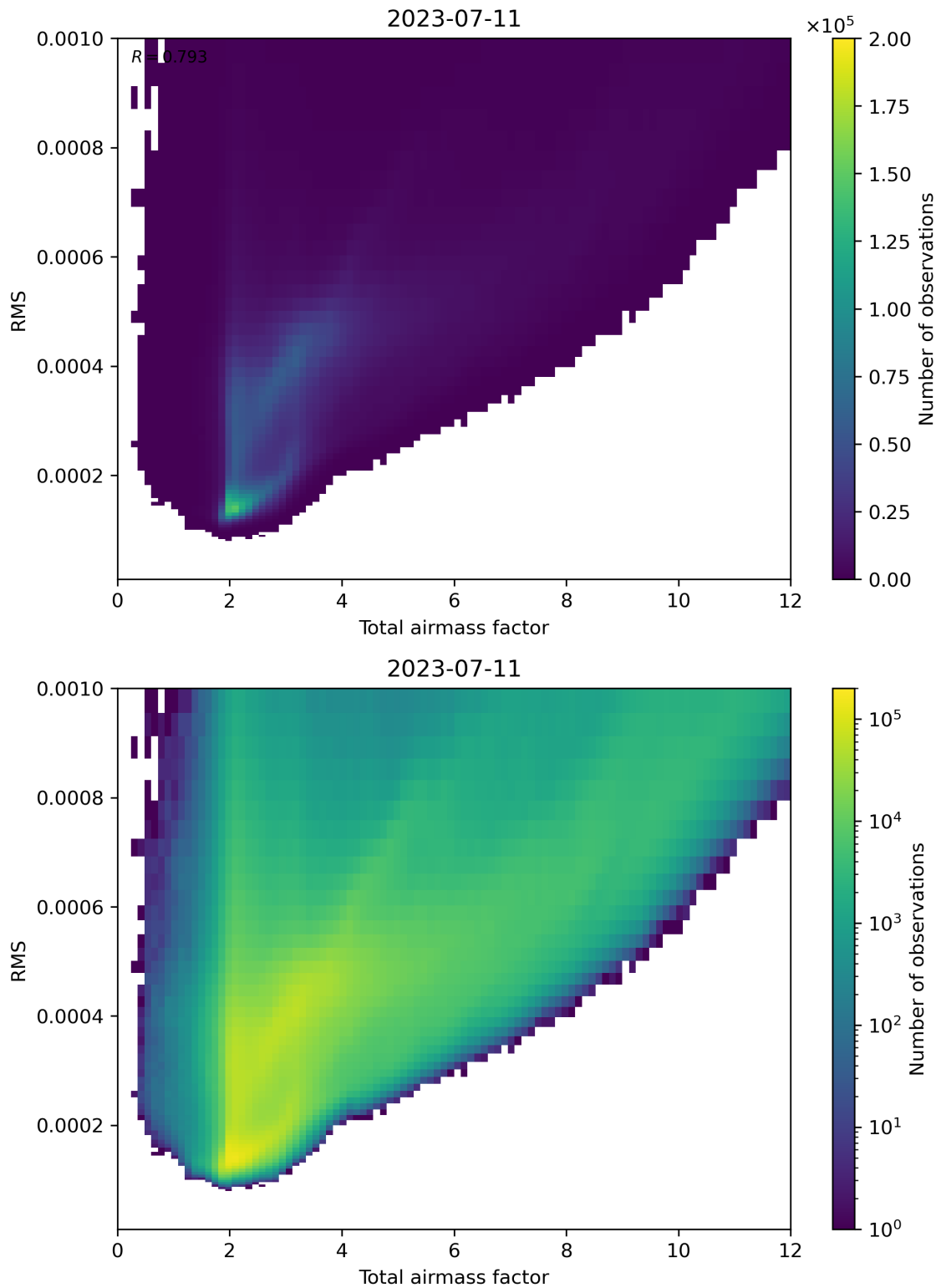
Figure 69: Scatter density plot of “Total airmass factor” against “RMS” for 2023-07-10 to 2023-07-12.
