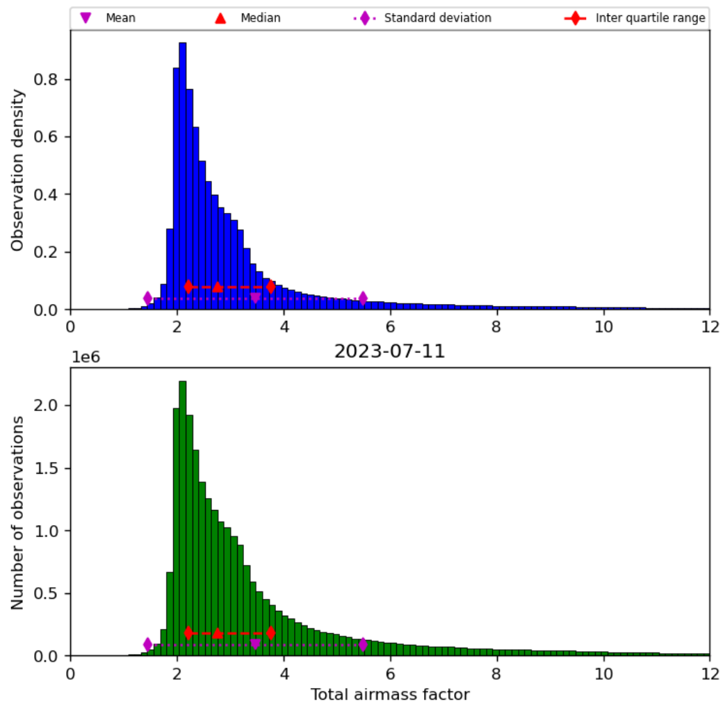
Figure 32: Histogram of “Total airmass factor” for 2023-07-10 to 2023-07-12
