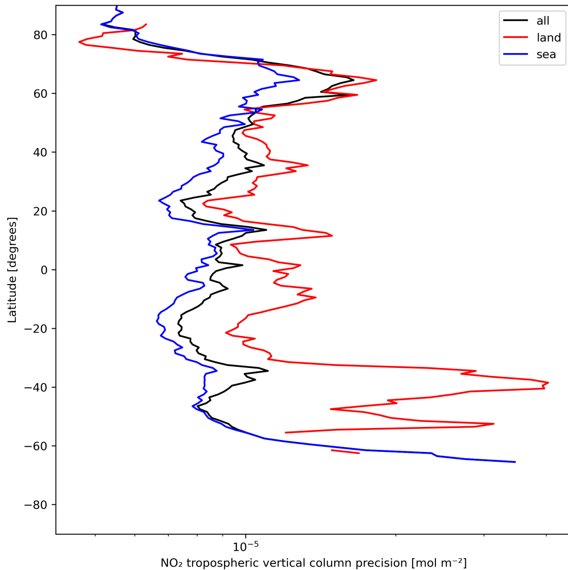
Figure 13: Zonal average of “NO 2 tropospheric vertical column precision” for 2023-07-10 to 2023-07-12.
