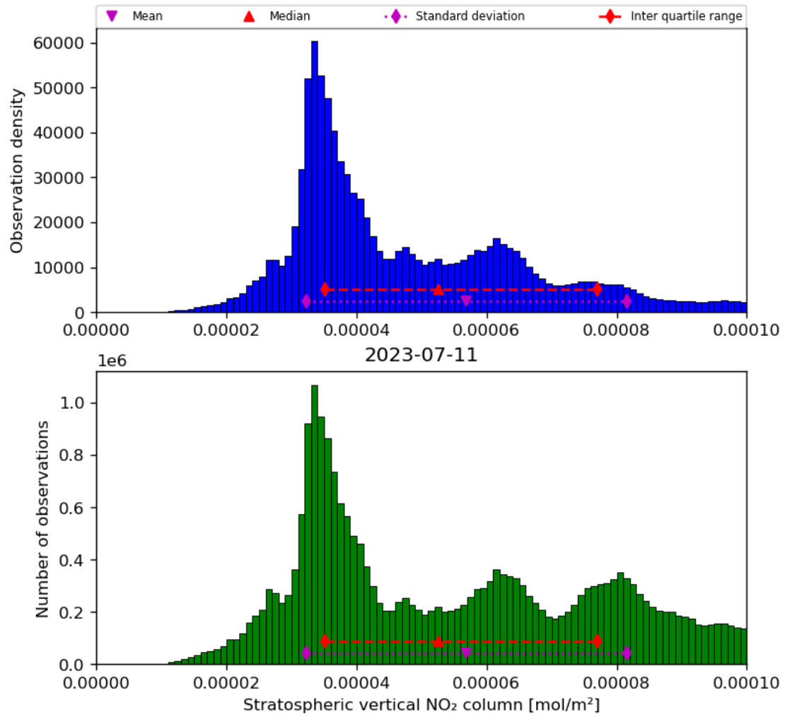
Figure 36: Histogram of “Stratospheric vertical NO 2 column” for 2023-07-10 to 2023-07-12
