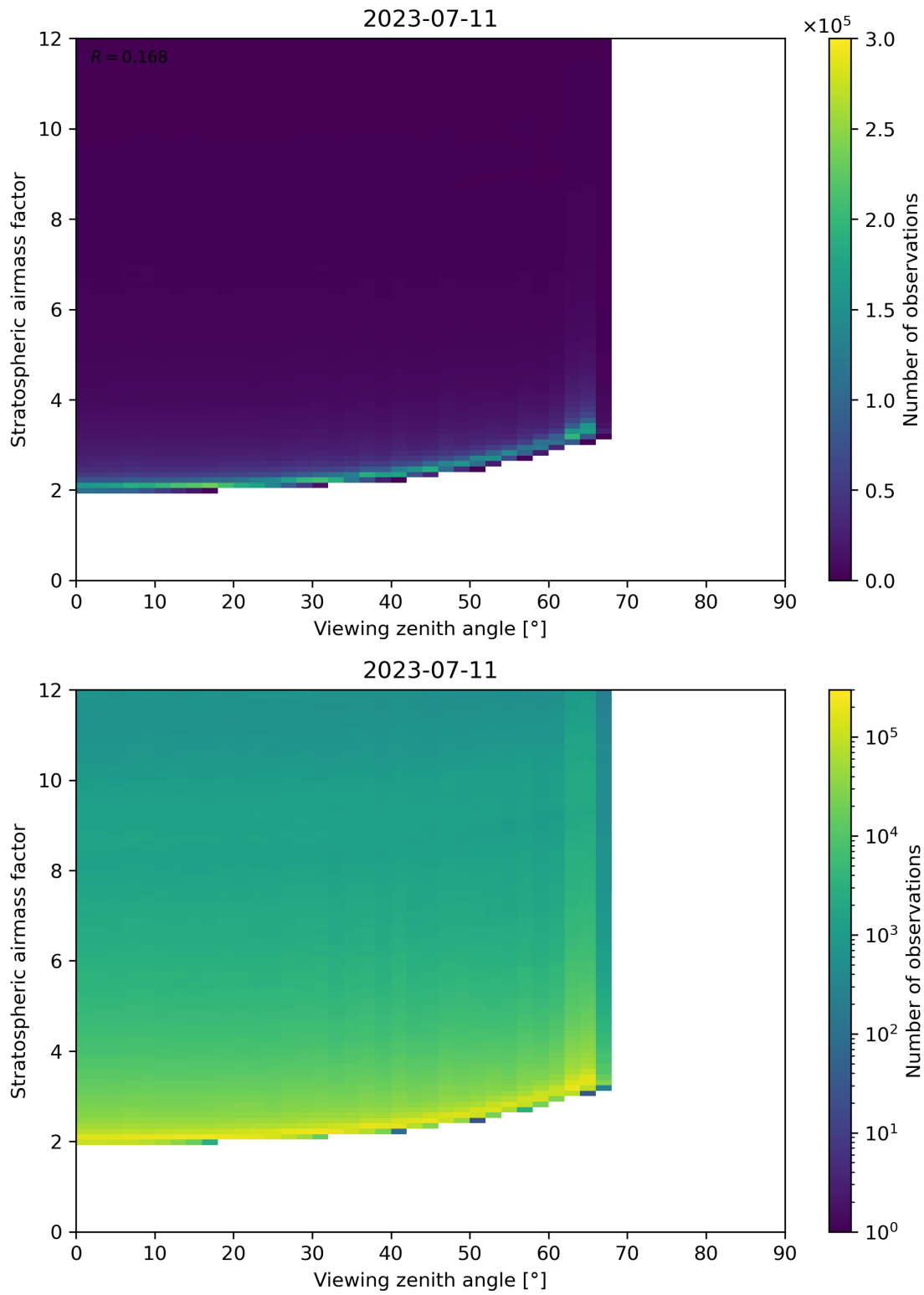
Figure 159: Scatter density plot of “Viewing zenith angle” against “Stratospheric airmass factor” for 2023-07-10 to 2023-07-12.
