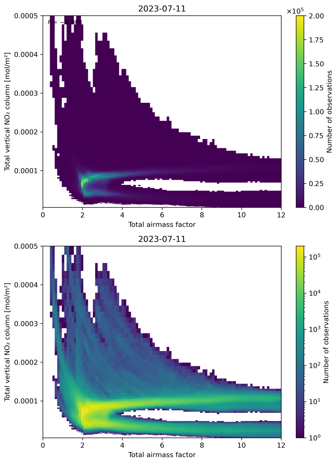
Figure 67: Scatter density plot of “Total airmass factor” against “Total vertical NO 2 column” for 2023-07-10 to 2023-07-12.
