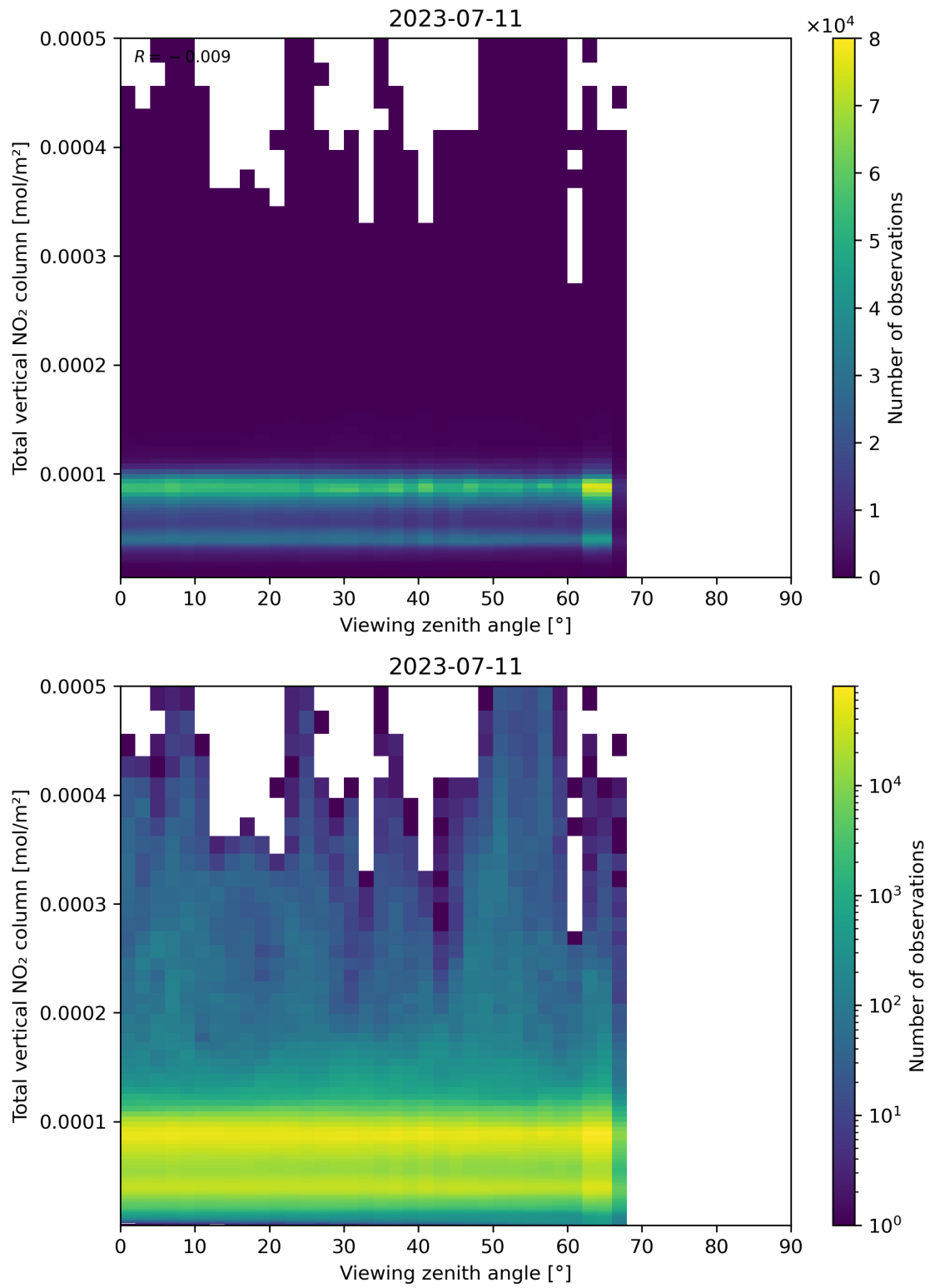
Figure 167: Scatter density plot of “Viewing zenith angle” against “Total vertical NO 2 column” for 2023-07-10 to 2023-07-12.
