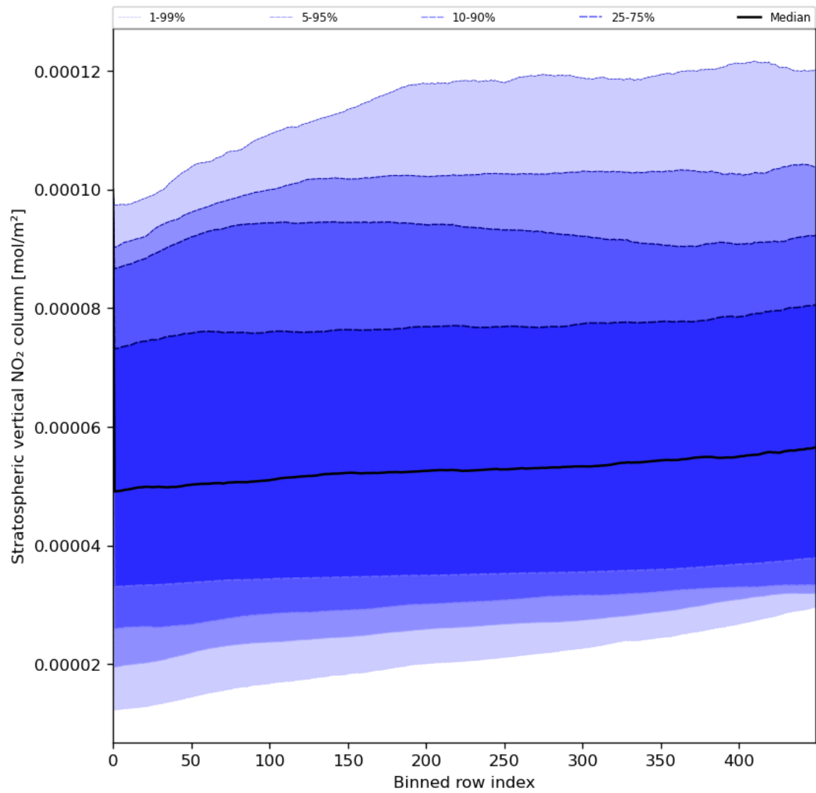
Figure 53: Along track statistics of “Stratospheric vertical NO 2 column” for 2023-07-10 to 2023-07-12
