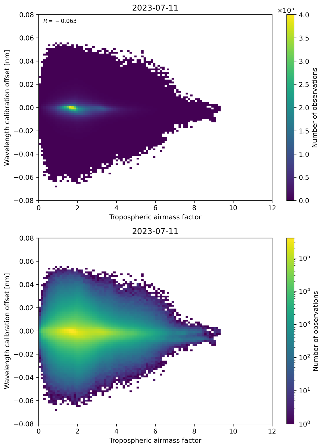
Figure 80: Scatter density plot of “Tropospheric airmass factor” against “Wavelength calibration offset” for 2023-07-10 to 2023-07-12.
