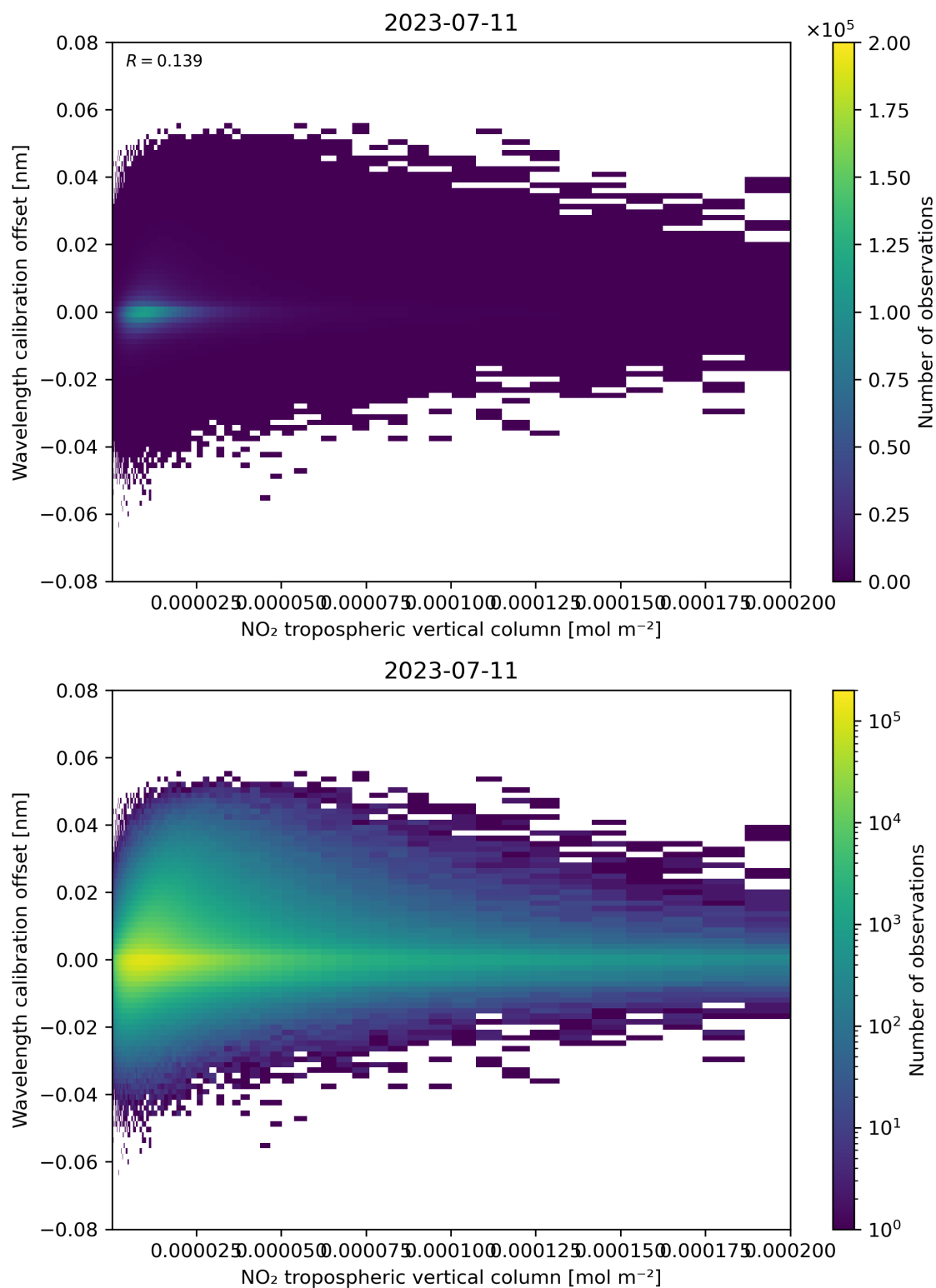
Figure 143: Scatter density plot of “NO 2 tropospheric vertical column” against “Wavelength calibration offset” for 2023-07-10 to 2023-07-12.
