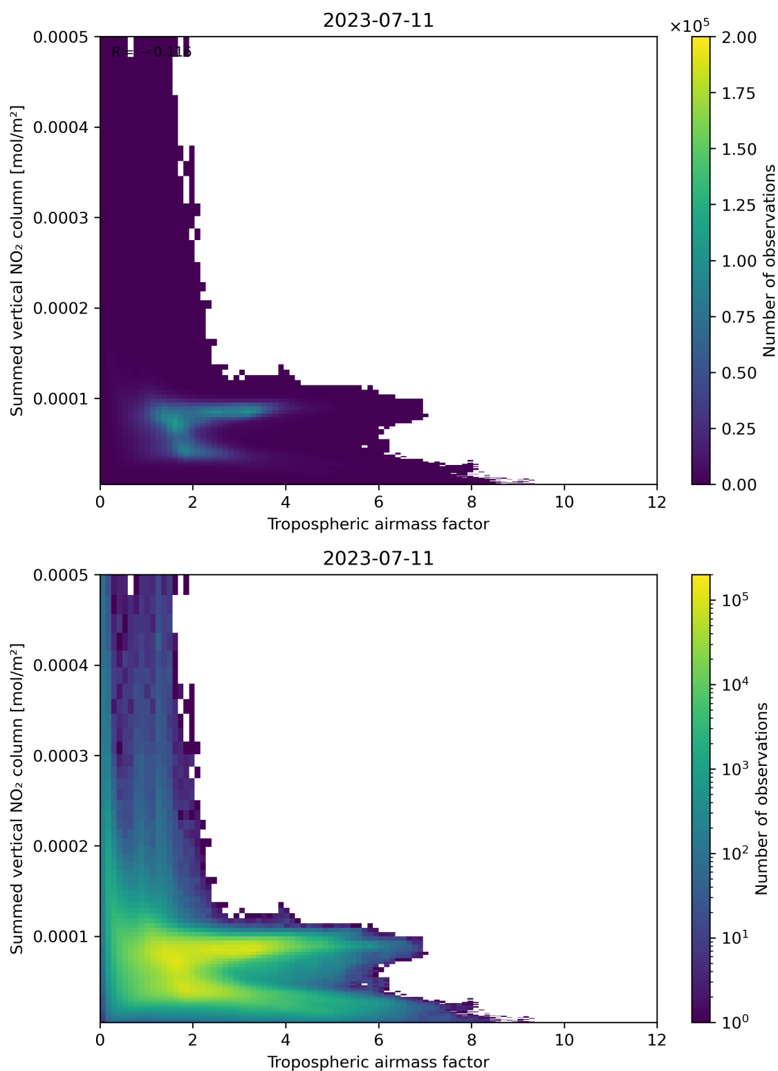
Figure 75: Scatter density plot of “Tropospheric airmass factor” against “Summed vertical NO 2 column” for 2023-07-10 to 2023-07-12.
