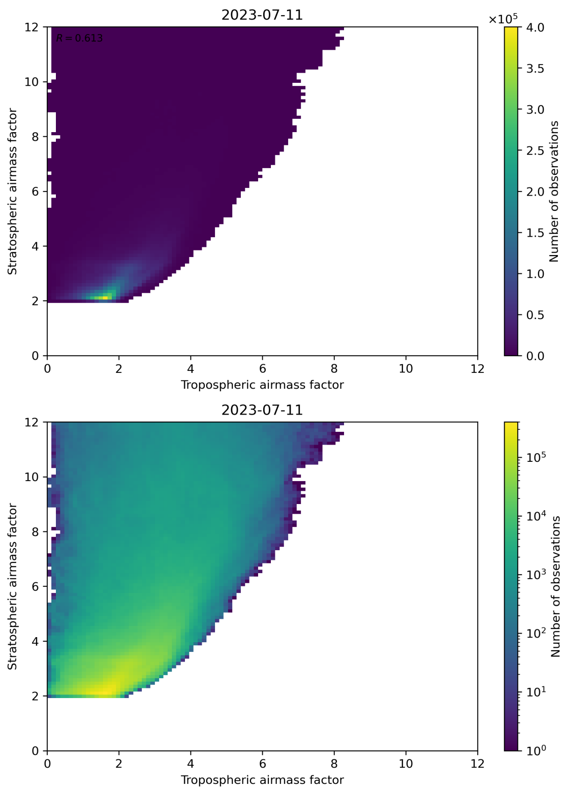
Figure 71: Scatter density plot of “Tropospheric airmass factor” against “Stratospheric airmass factor” for 2023-07-10 to 2023-07-12.
