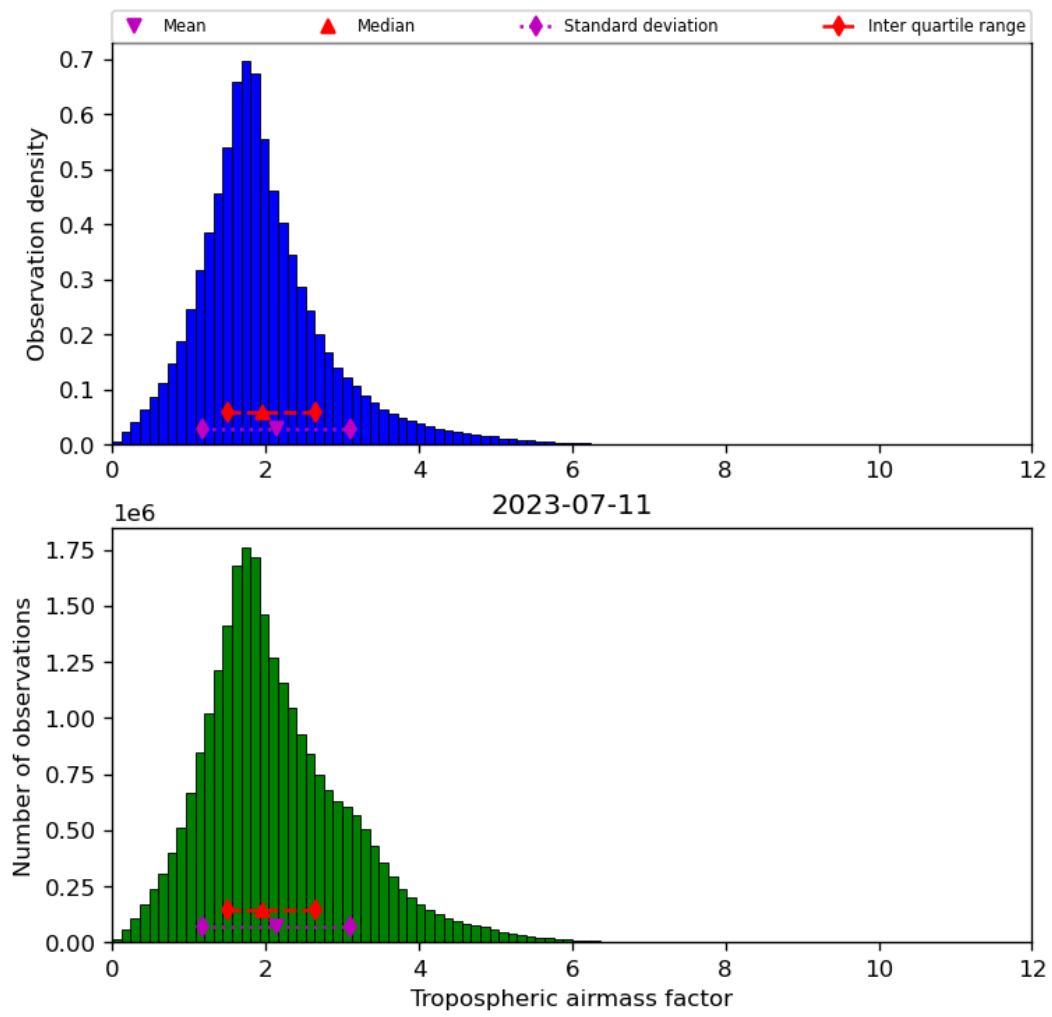
Figure 31: Histogram of “Tropospheric airmass factor” for 2023-07-10 to 2023-07-12
