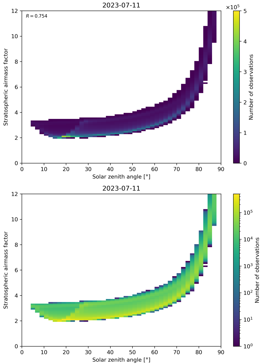
Figure 145: Scatter density plot of “Solar zenith angle” against “Stratospheric airmass factor” for 2023-07-10 to 2023-07-12.
