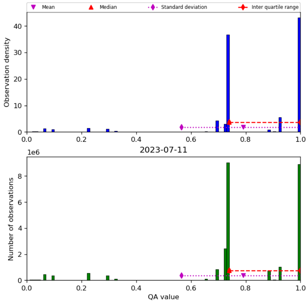
Figure 28: Histogram of “QA value” for 2023-07-10 to 2023-07-12
