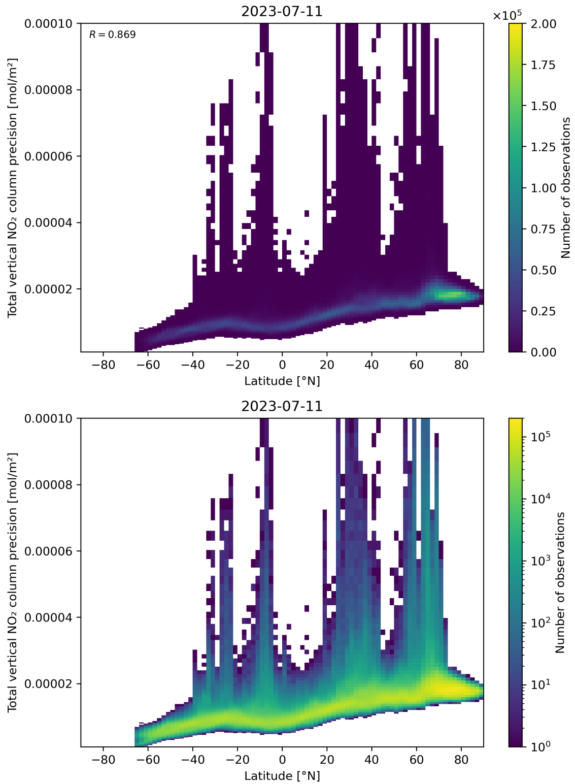
Figure 91: Scatter density plot of “Latitude” against “Total vertical NO 2 column precision” for 2023-07-10 to 2023-07-12.
