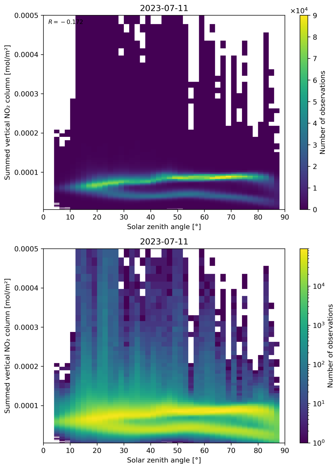
Figure 151: Scatter density plot of “Solar zenith angle” against “Summed vertical NO 2 column” for 2023-07-10 to 2023-07-12.
