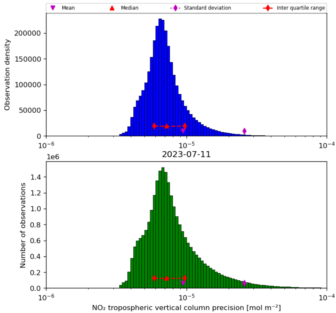
Figure 30: Histogram of “NO 2 tropospheric vertical column precision” for 2023-07-10 to 2023-07-12
