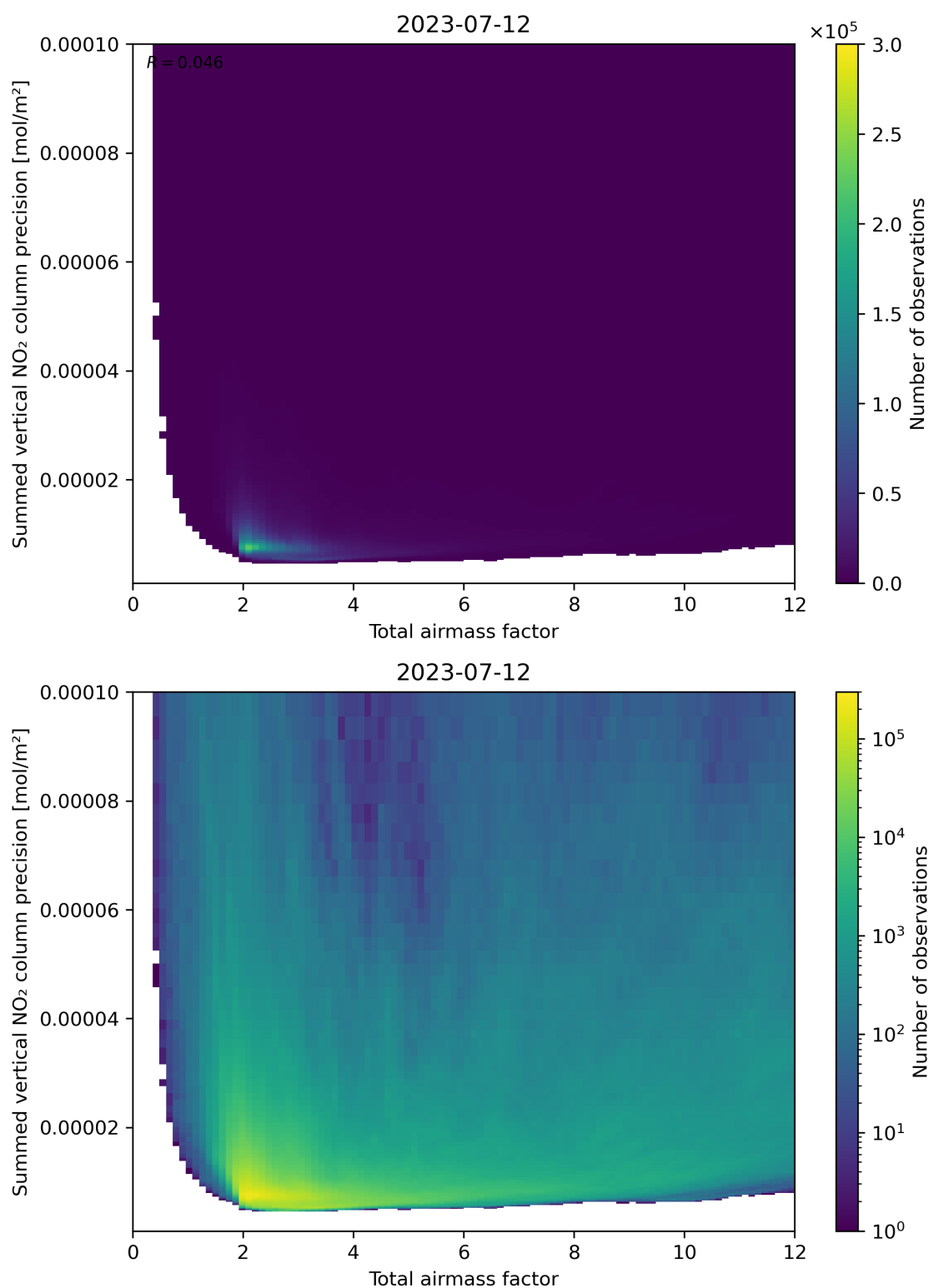
Figure 66: Scatter density plot of “Total airmass factor” against “Summed vertical NO 2 column precision” for 2023-07-11 to 2023-07-13.
