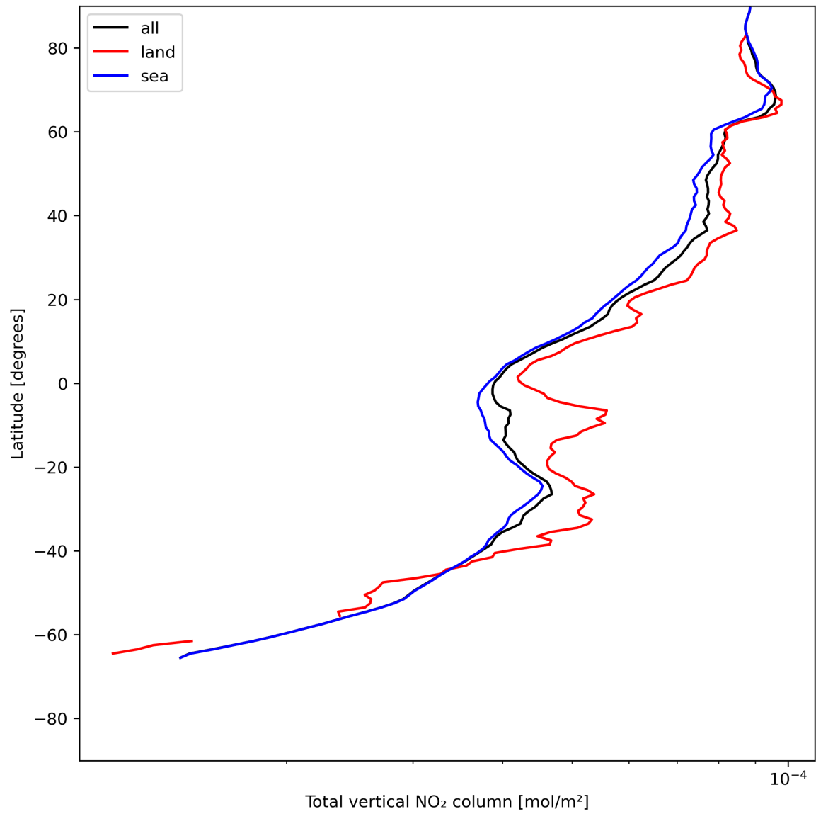
Figure 21: Zonal average of “Total vertical NO 2 column” for 2023-07-11 to 2023-07-13.
