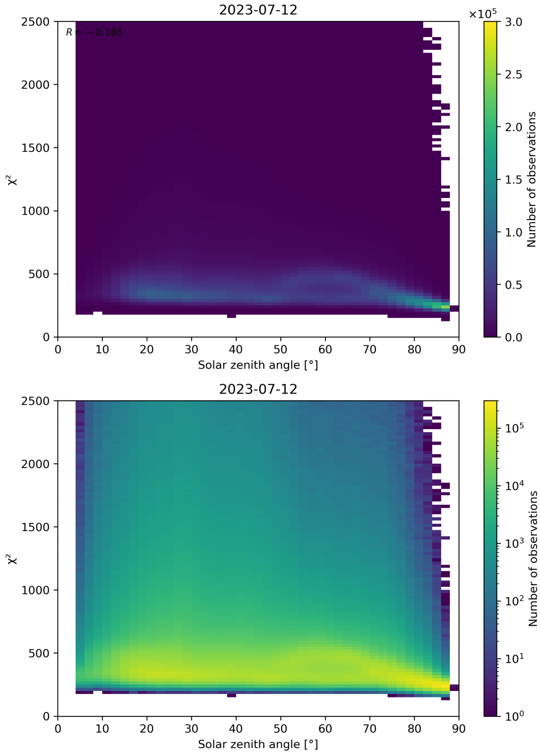
Figure 148: Scatter density plot of “Solar zenith angle” against “ \chi^2 ” for 2023-07-11 to 2023-07-13.
