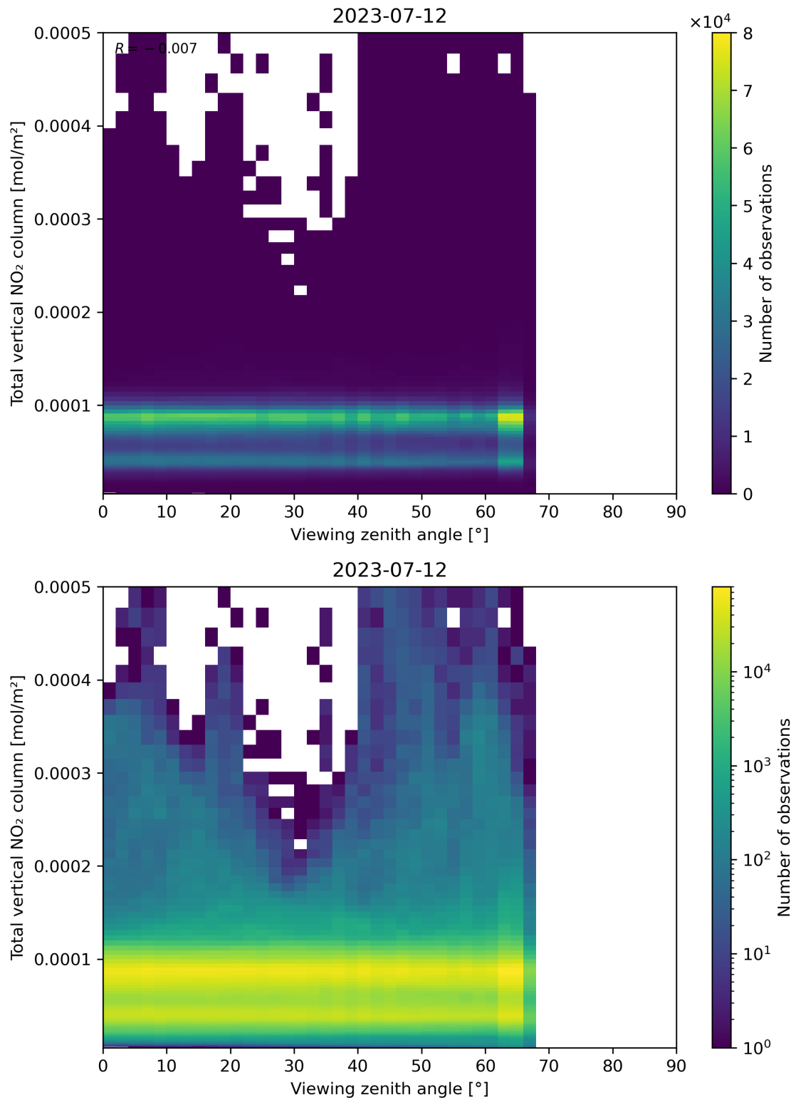
Figure 167: Scatter density plot of “Viewing zenith angle” against “Total vertical NO 2 column” for 2023-07-11 to 2023-07-13.
