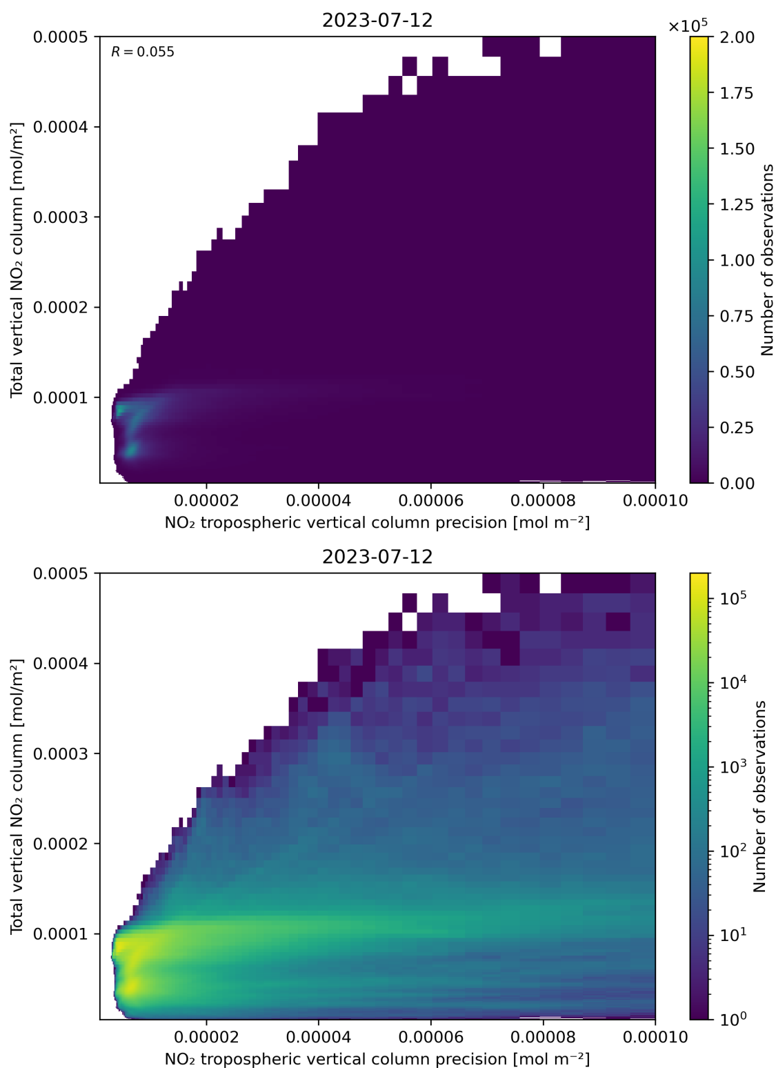
Figure 138: Scatter density plot of “NO 2 tropospheric vertical column precision” against “Total vertical NO 2 column” for 2023-07-11 to 2023-07-13.
