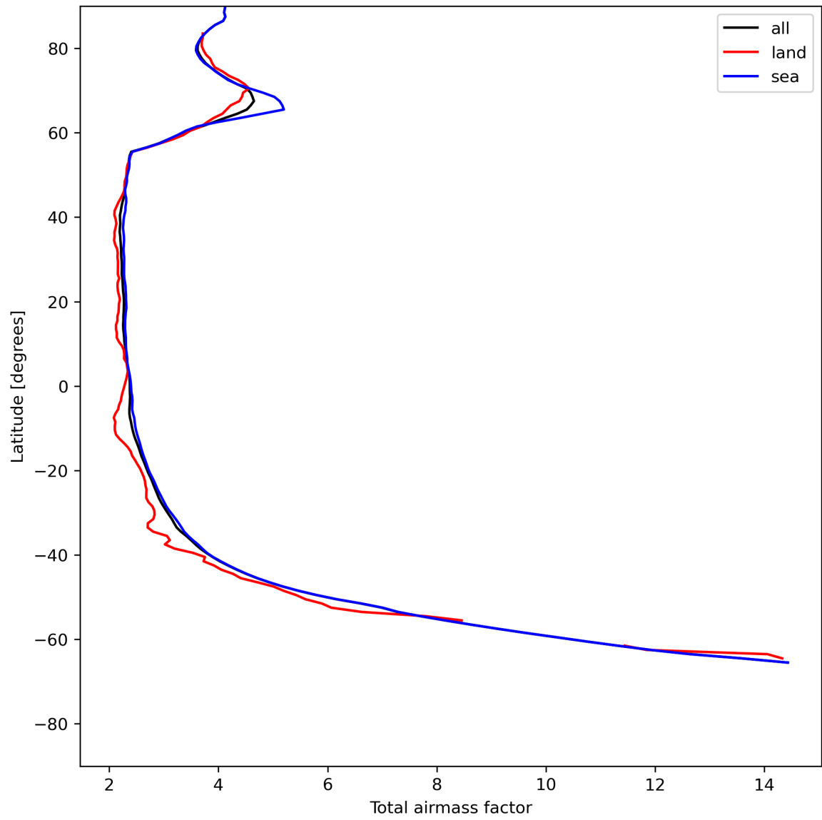
Figure 15: Zonal average of “Total airmass factor” for 2023-07-11 to 2023-07-13.
