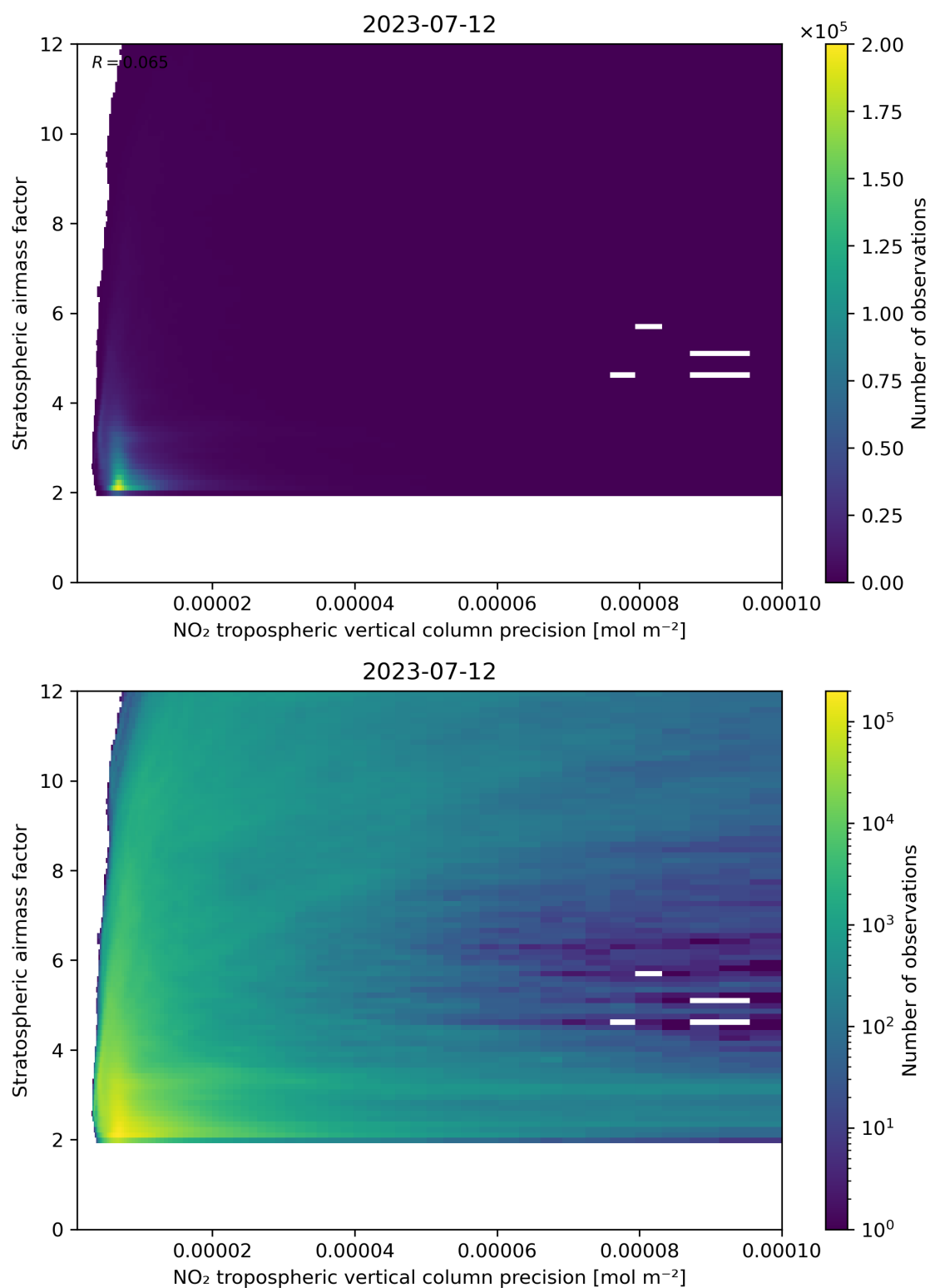
Figure 131: Scatter density plot of “NO 2 tropospheric vertical column precision” against “Stratospheric airmass factor” for 2023-07-11 to 2023-07-13.
