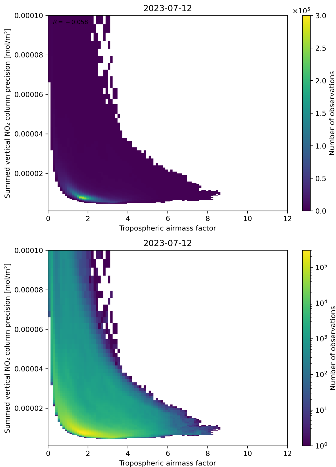
Figure 76: Scatter density plot of “Tropospheric air mass factor” against “Summed vertical NO 2 column precision” for 2023-07-11 to 2023-07-13.
