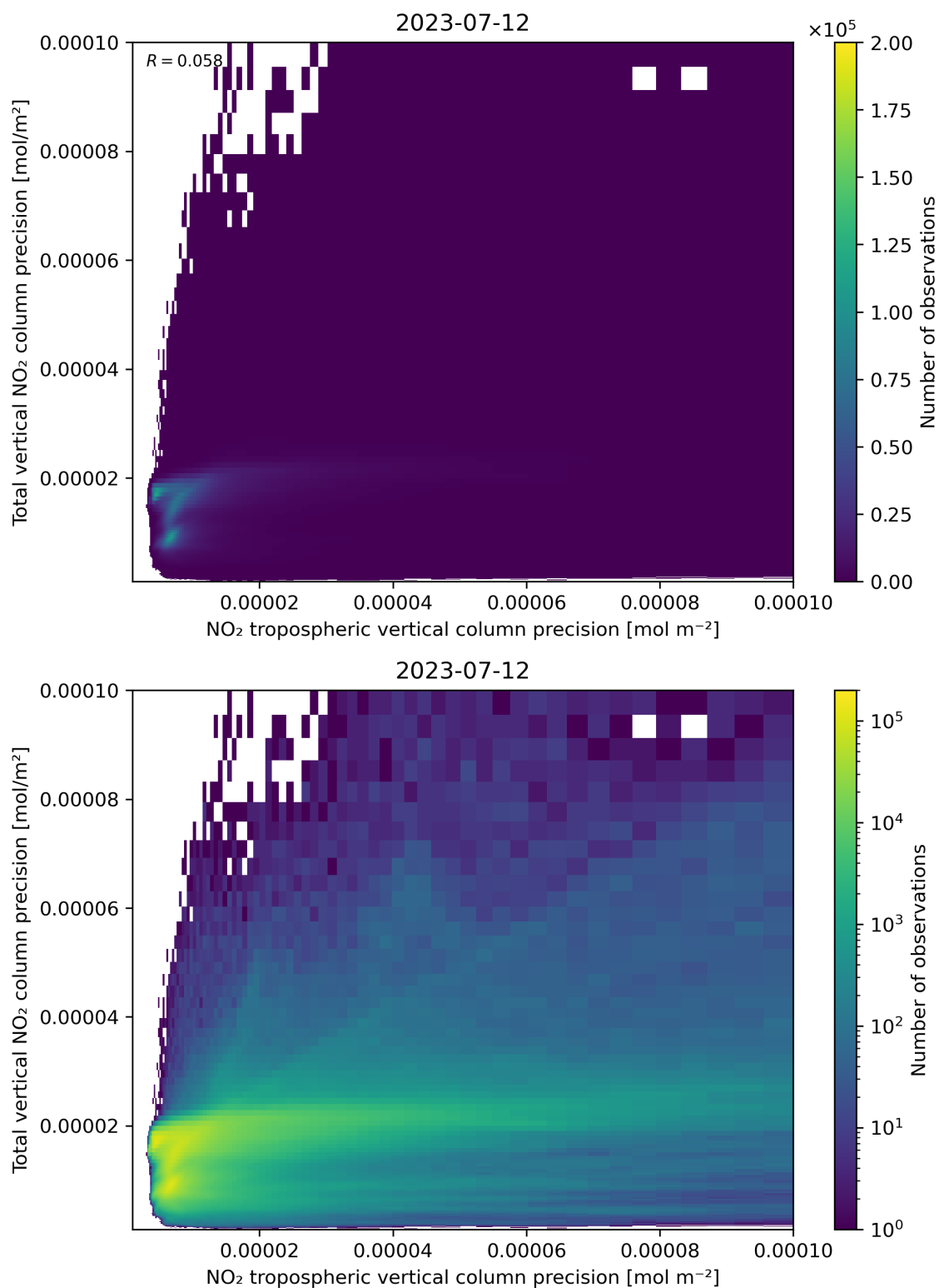
Figure 139: Scatter density plot of “NO 2 tropospheric vertical column precision” against “Total vertical NO 2 column precision” for 2023-07-11 to 2023-07-13.
