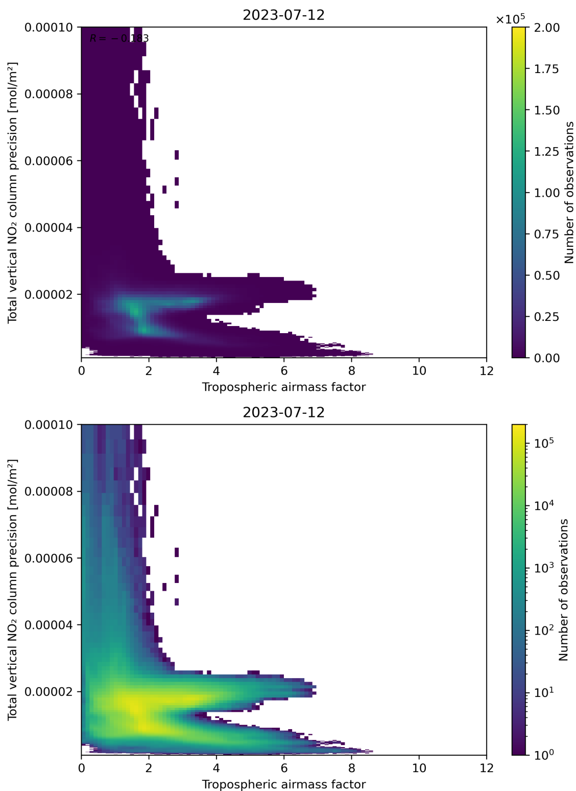
Figure 78: Scatter density plot of “Tropospheric air mass factor” against “Total vertical NO 2 column precision” for 2023-07-11 to 2023-07-13.
