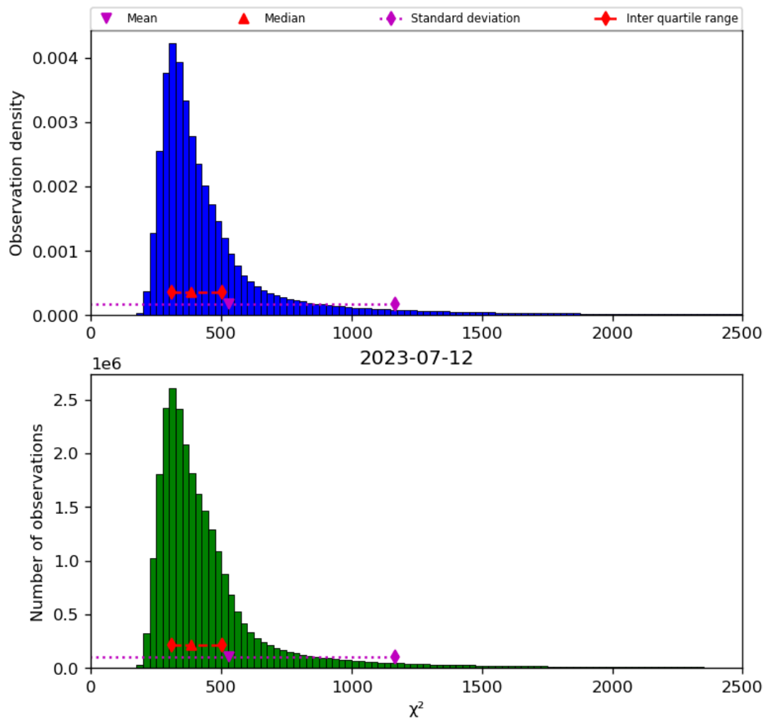
Figure 42: Histogram of “ \chi^2 ” for 2023-07-11 to 2023-07-13
