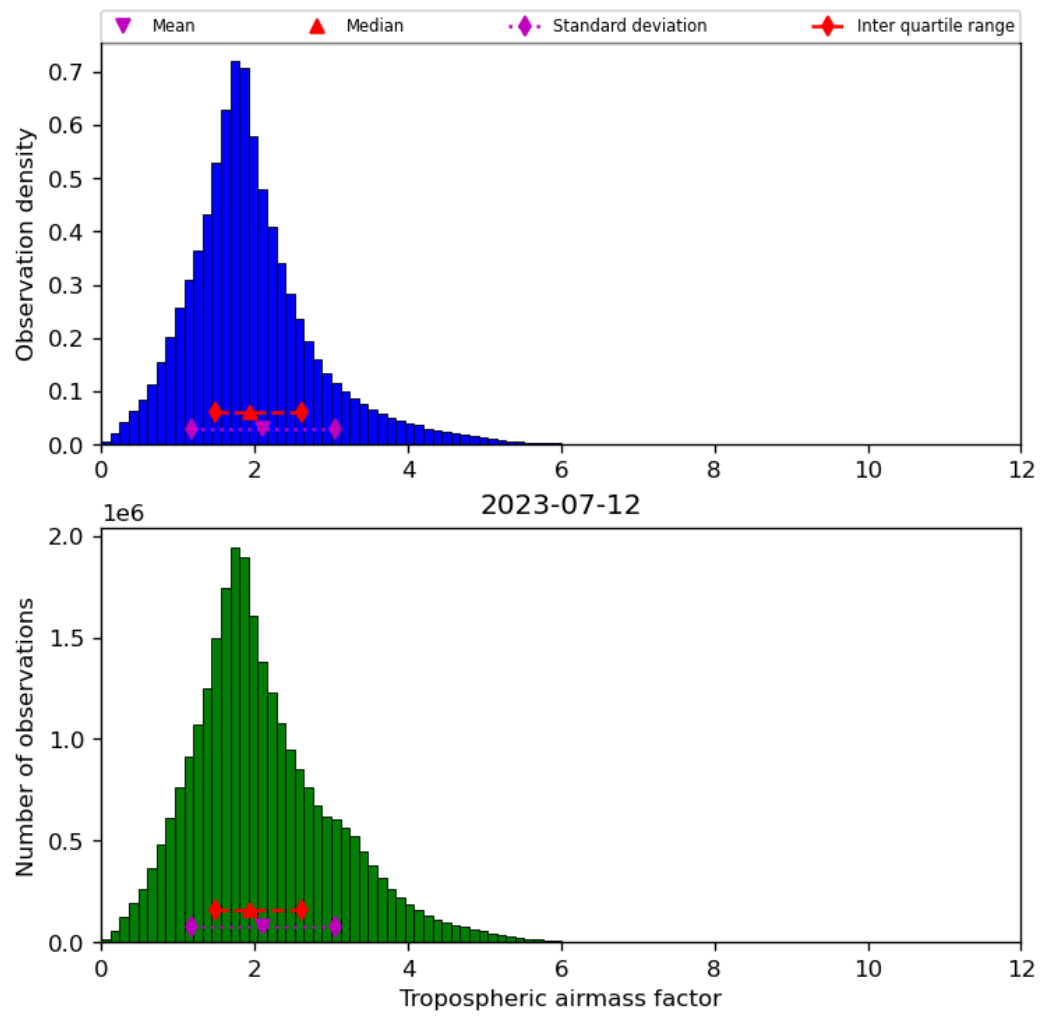
Figure 31: Histogram of “Tropospheric airmass factor” for 2023-07-11 to 2023-07-13
