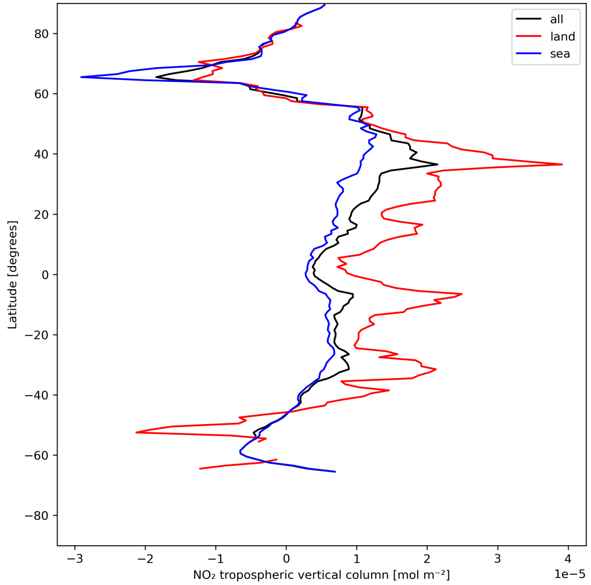
Figure 12: Zonal average of “NO 2 tropospheric vertical column” for 2023-07-11 to 2023-07-13.
