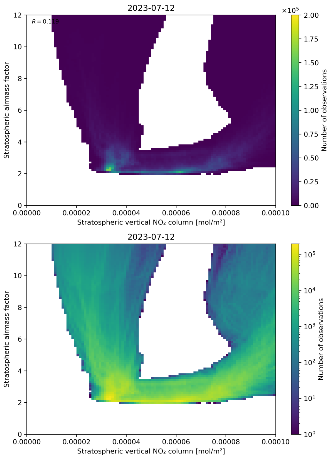
Figure 96: Scatter density plot of “Stratospheric vertical NO 2 column” against “Stratospheric airmass factor” for 2023-07-11 to 2023-07-13.
