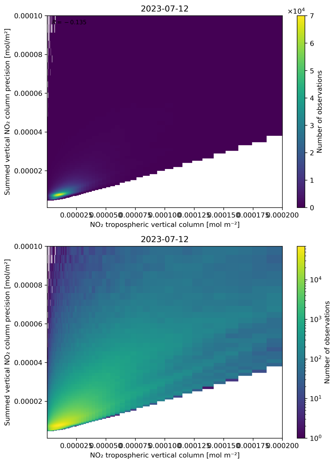
Figure 127: Scatter density plot of “NO 2 tropospheric vertical column” against “Summed vertical NO 2 column precision” for 2023-07-11 to 2023-07-13.
