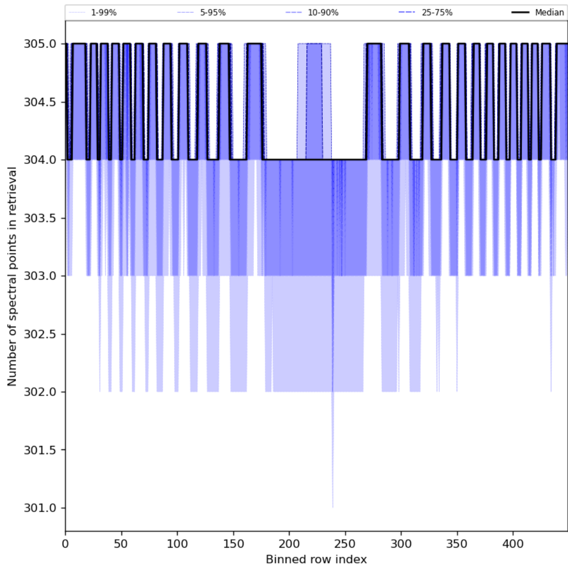
Figure 50: Along track statistics of “Number of spectral points in retrieval” for 2023-07-11 to 2023-07-13
