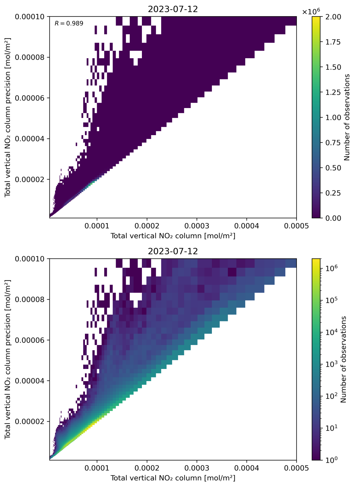
Figure 114: Scatter density plot of “Total vertical NO 2 column” against “Total vertical NO 2 column precision” for 2023-07-11 to 2023-07-13.
