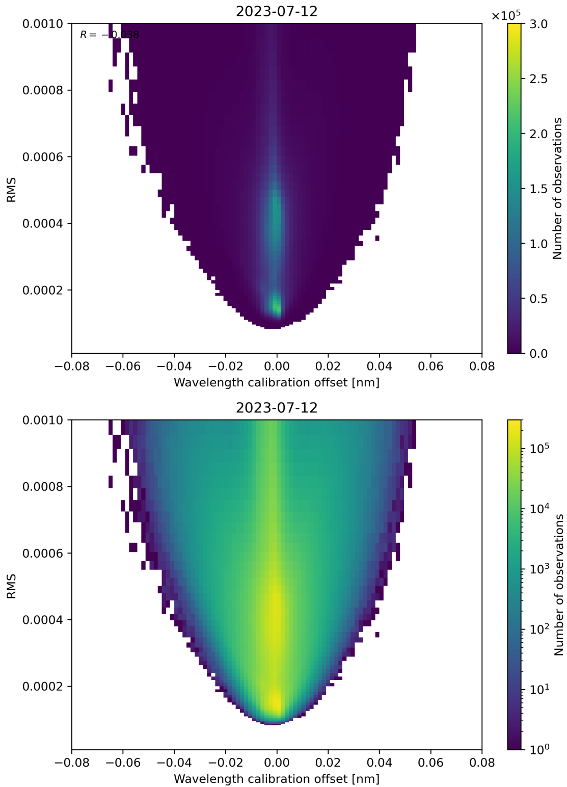
Figure 181: Scatter density plot of “Wavelength calibration offset” against “RMS” for 2023-07-11 to 2023-07-13.
