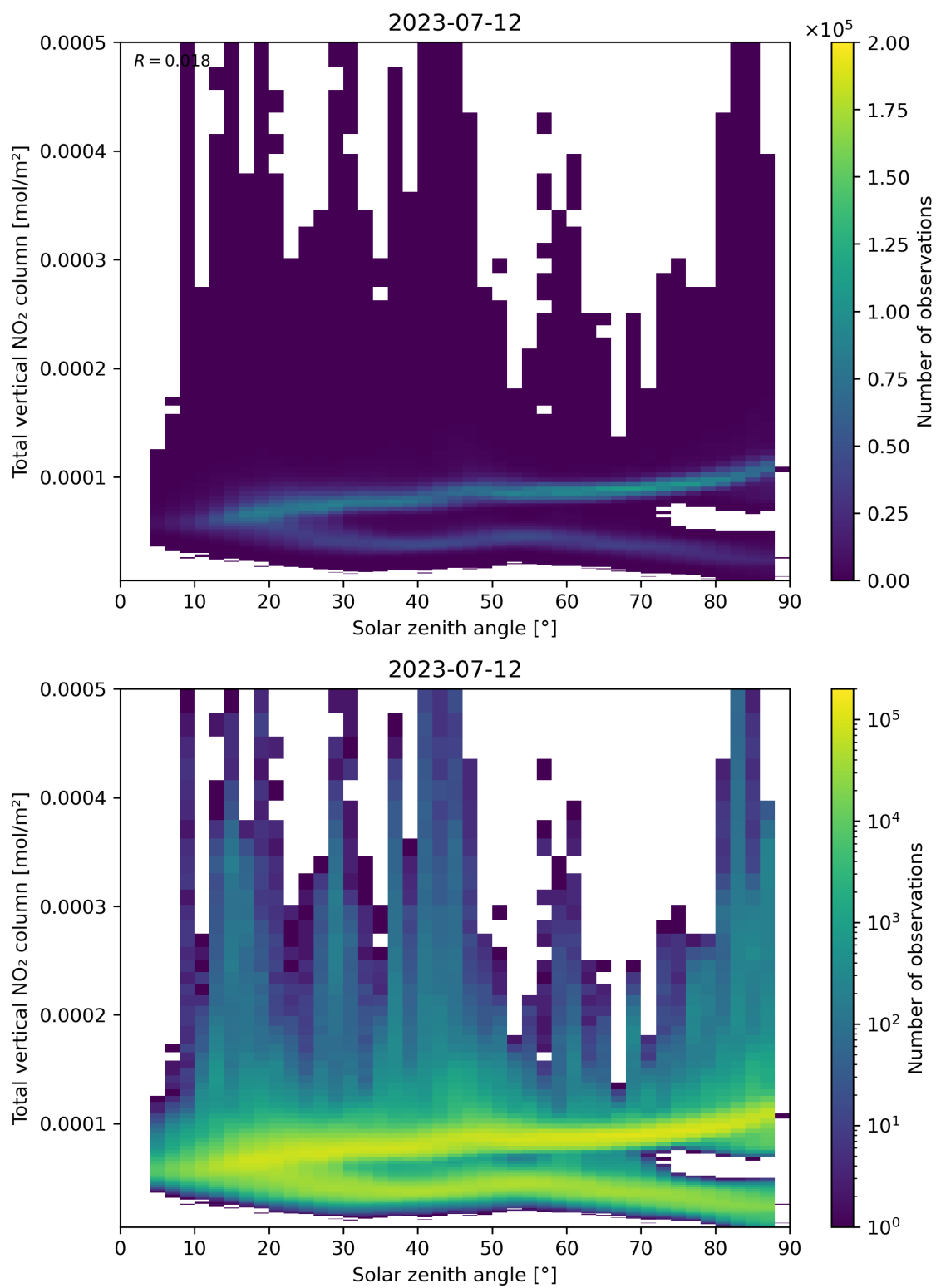
Figure 153: Scatter density plot of “Solar zenith angle” against “Total vertical NO 2 column” for 2023-07-11 to 2023-07-13.
