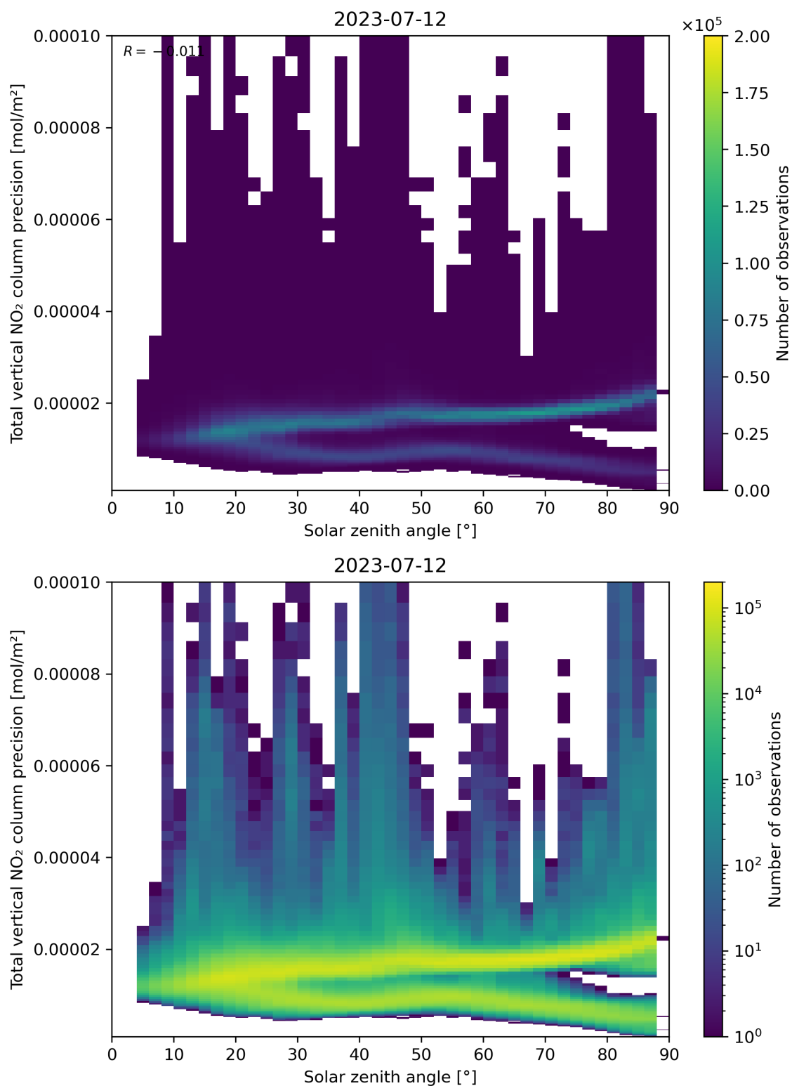
Figure 154: Scatter density plot of “Solar zenith angle” against “Total vertical NO 2 column precision” for 2023-07-11 to 2023-07-13.
