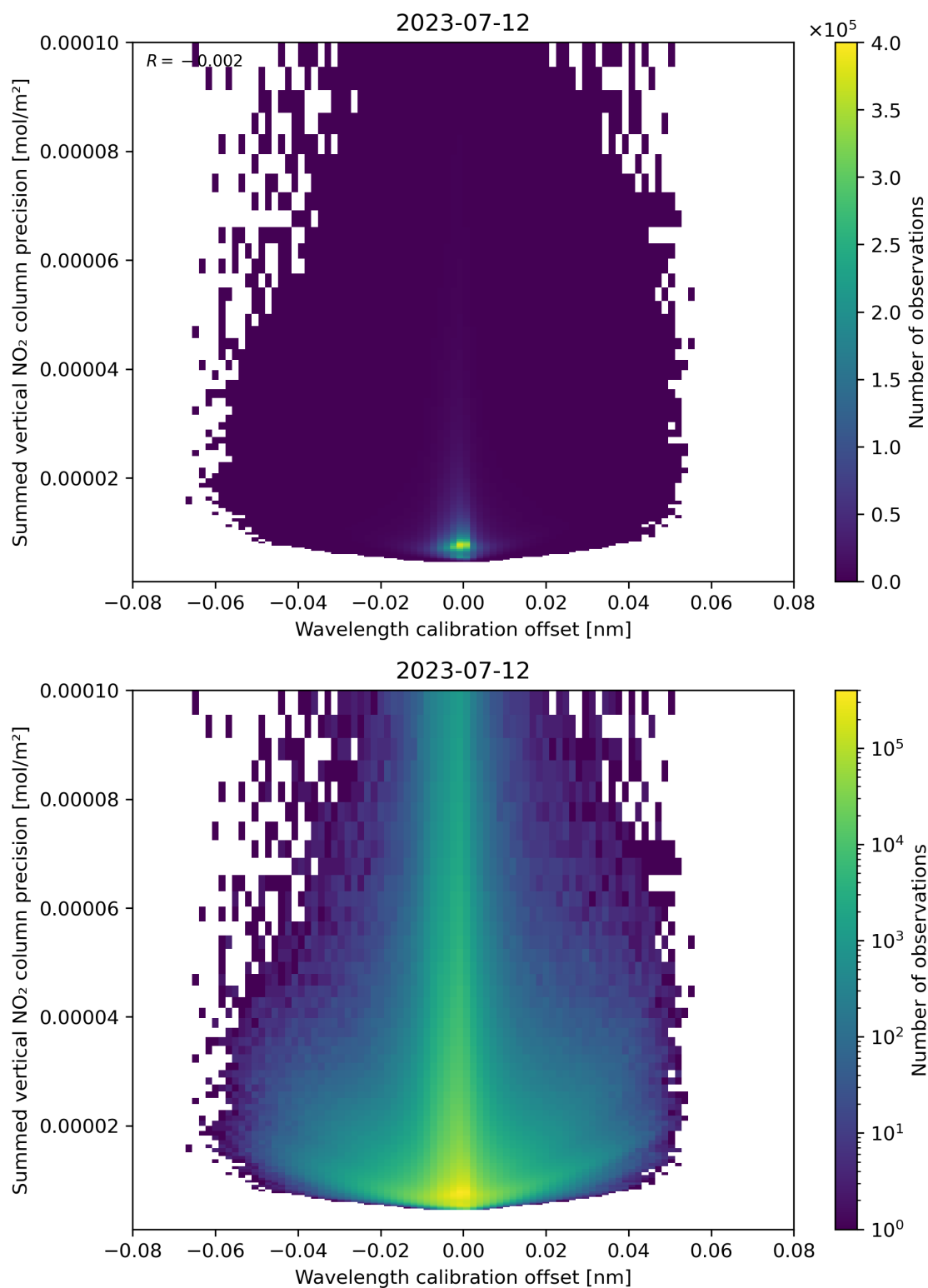
Figure 178: Scatter density plot of “Wavelength calibration offset” against “Summed vertical NO 2 column precision” for 2023-07-11 to 2023-07-13.
