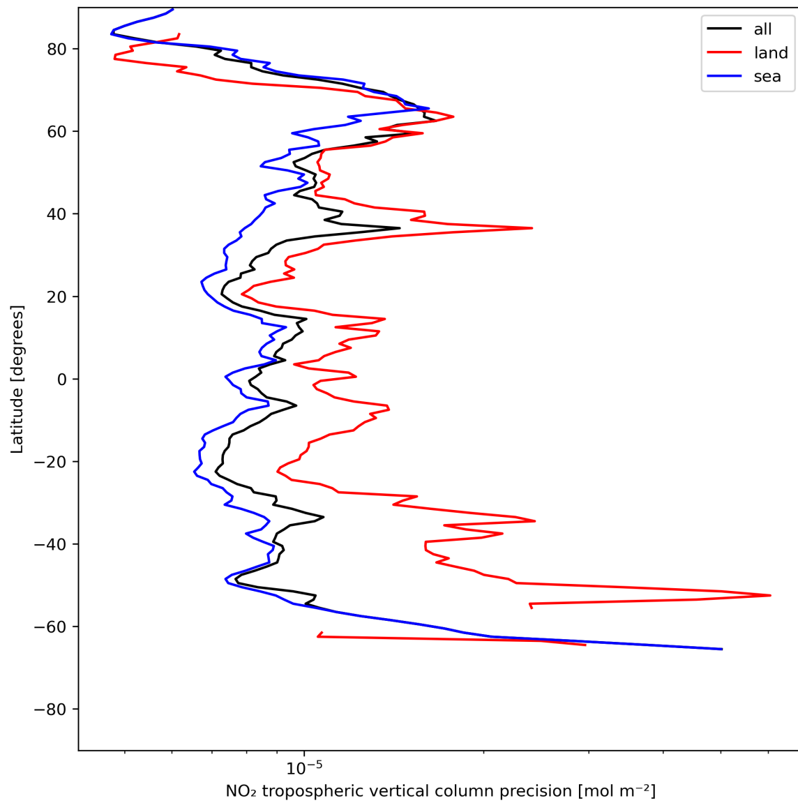
Figure 13: Zonal average of “NO 2 tropospheric vertical column precision” for 2023-07-11 to 2023-07-13.
