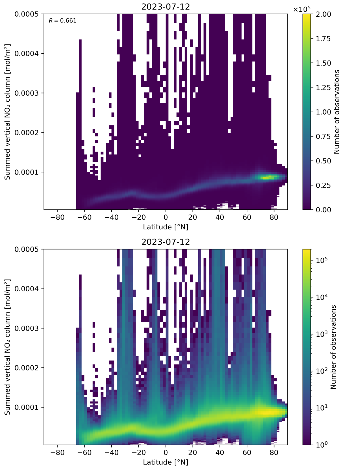
Figure 88: Scatter density plot of “Latitude” against “Summed vertical NO 2 column” for 2023-07-11 to 2023-07-13.
