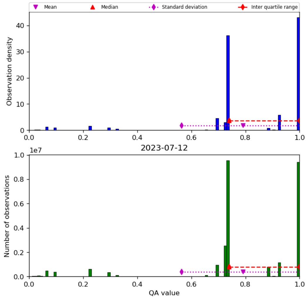
Figure 28: Histogram of “QA value” for 2023-07-11 to 2023-07-13
