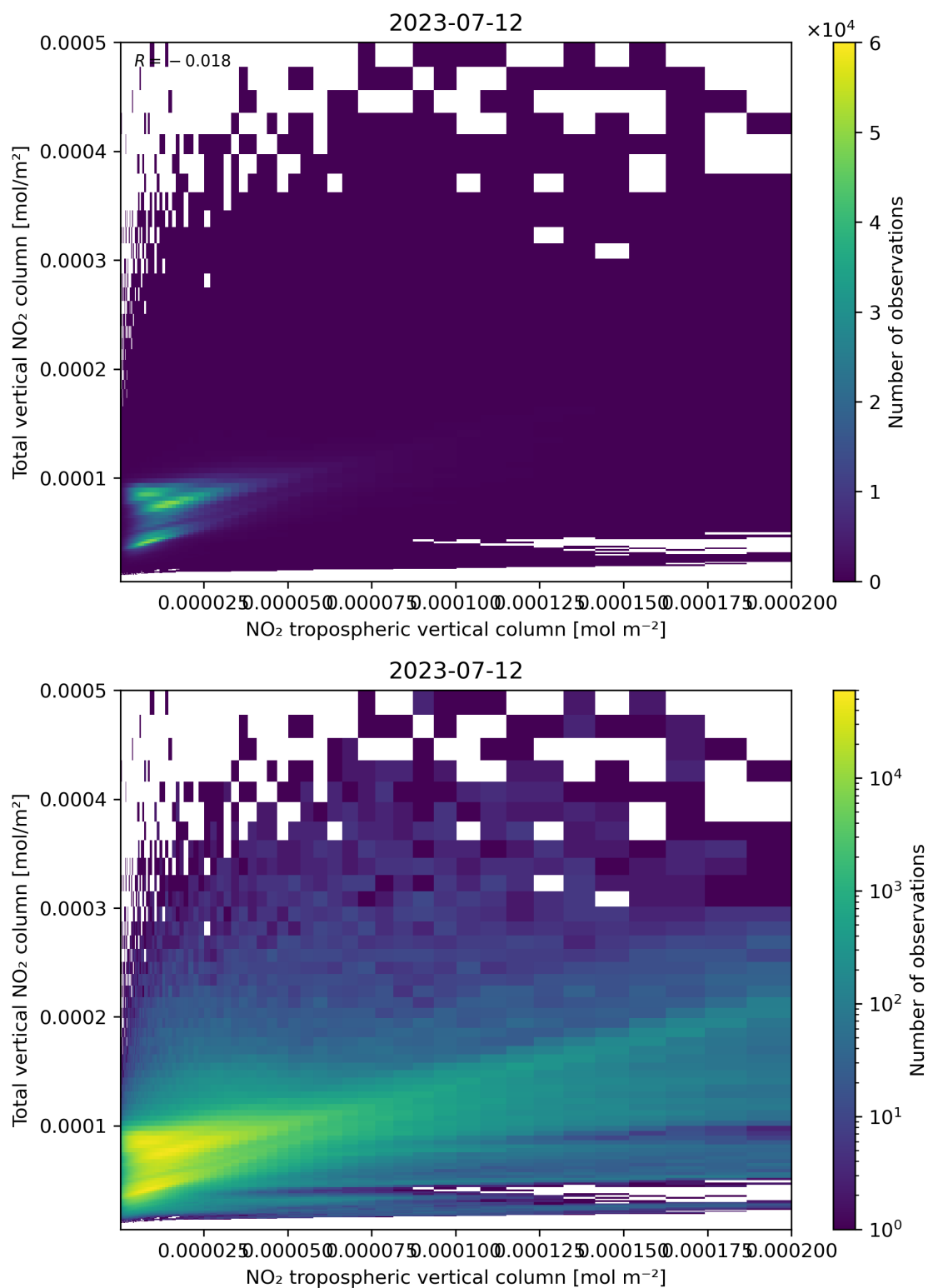
Figure 128: Scatter density plot of “NO 2 tropospheric vertical column” against “Total vertical NO 2 column” for 2023-07-11 to 2023-07-13.
