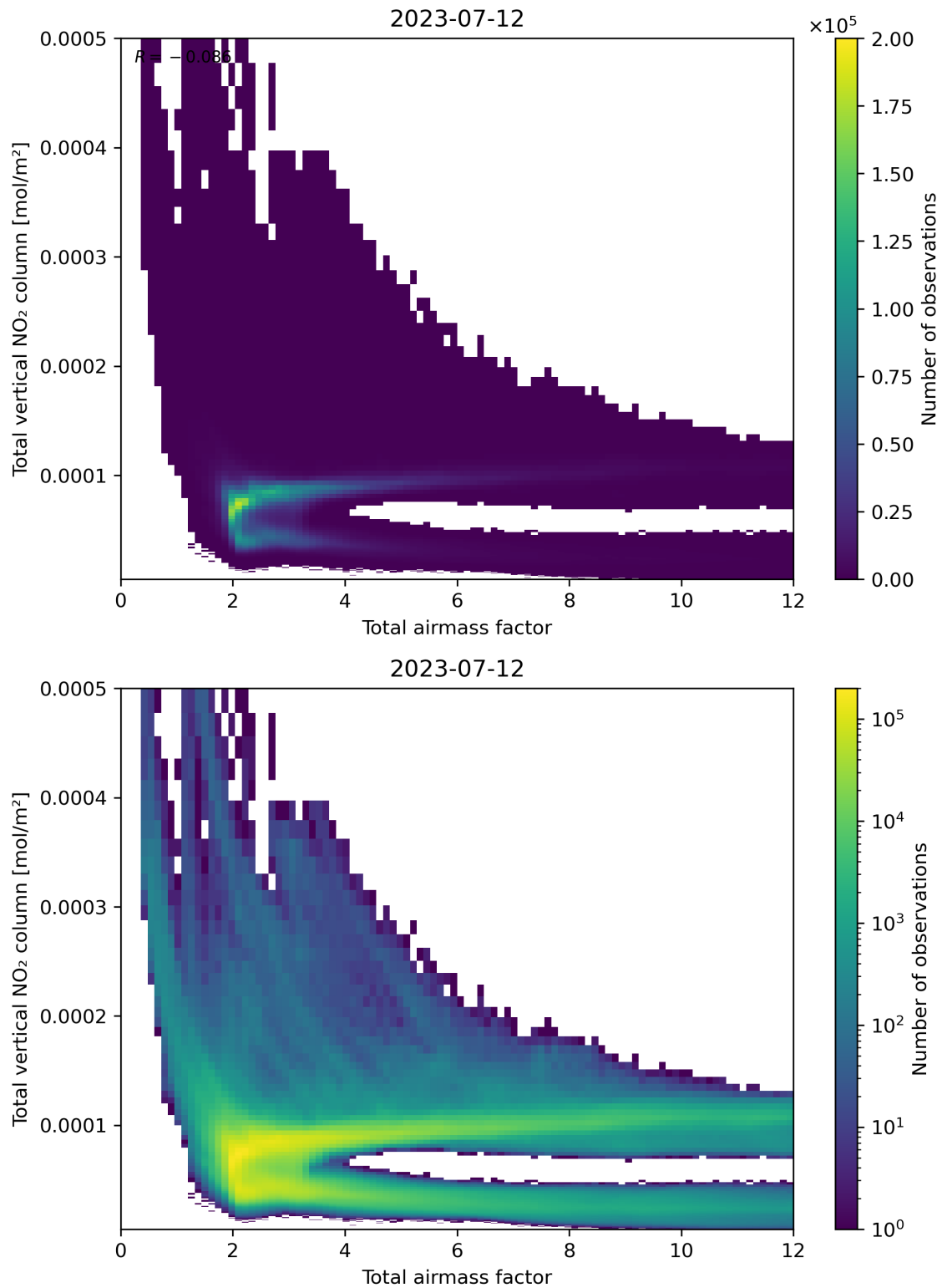
Figure 67: Scatter density plot of “Total airmass factor” against “Total vertical NO 2 column” for 2023-07-11 to 2023-07-13.
