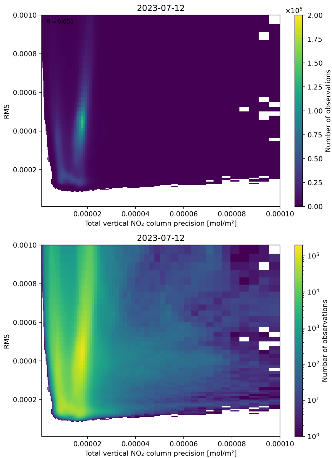
Figure 119: Scatter density plot of “Total vertical NO 2 column precision” against “RMS” for 2023-07-11 to 2023-07-13.
