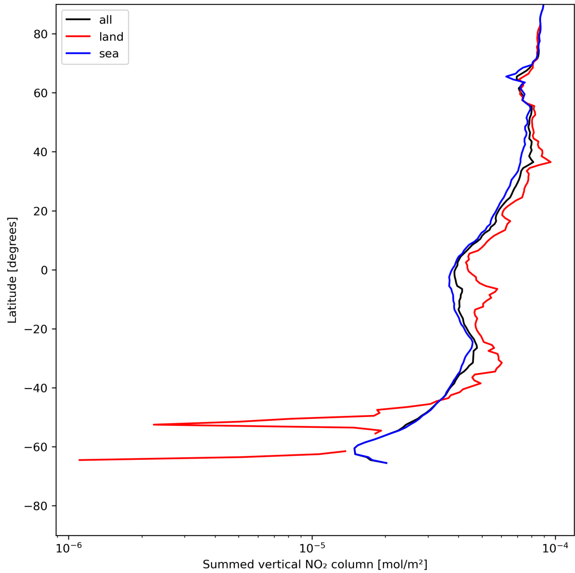
Figure 23: Zonal average of “Summed vertical NO 2 column” for 2023-07-11 to 2023-07-13.
