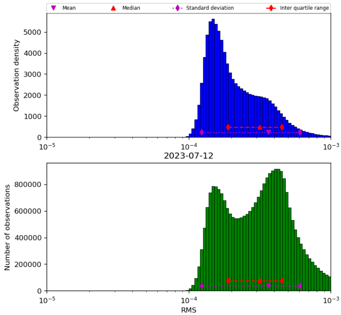
Figure 43: Histogram of “RMS” for 2023-07-11 to 2023-07-13
