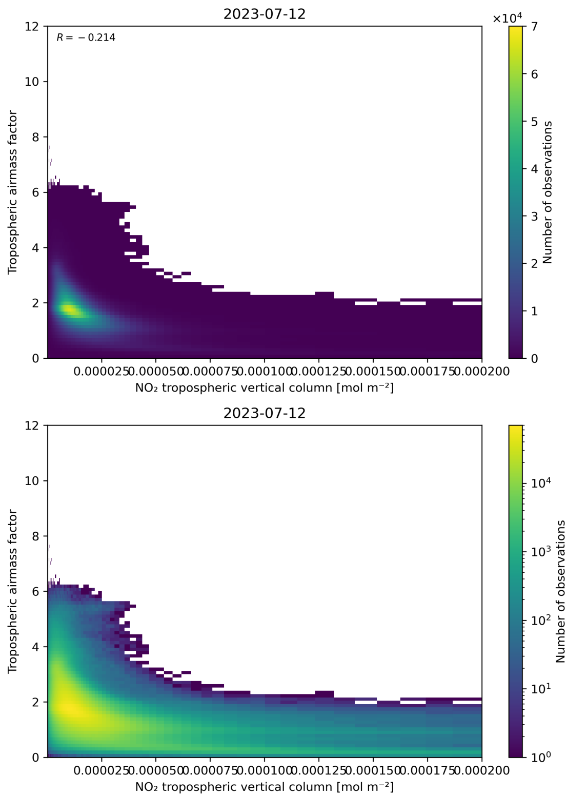
Figure 123: Scatter density plot of “NO 2 tropospheric vertical column” against “Tropospheric air mass factor” for 2023-07-11 to 2023-07-13.
