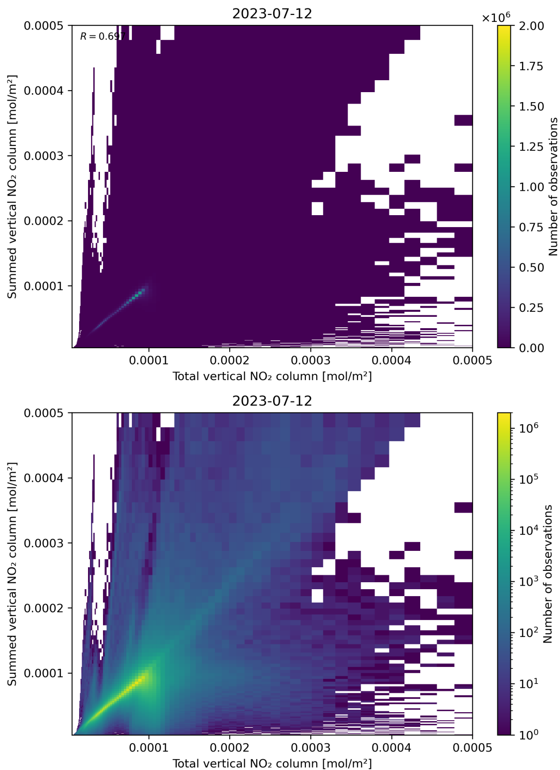
Figure 112: Scatter density plot of “Total vertical NO 2 column” against “Summed vertical NO 2 column” for 2023-07-11 to 2023-07-13.
