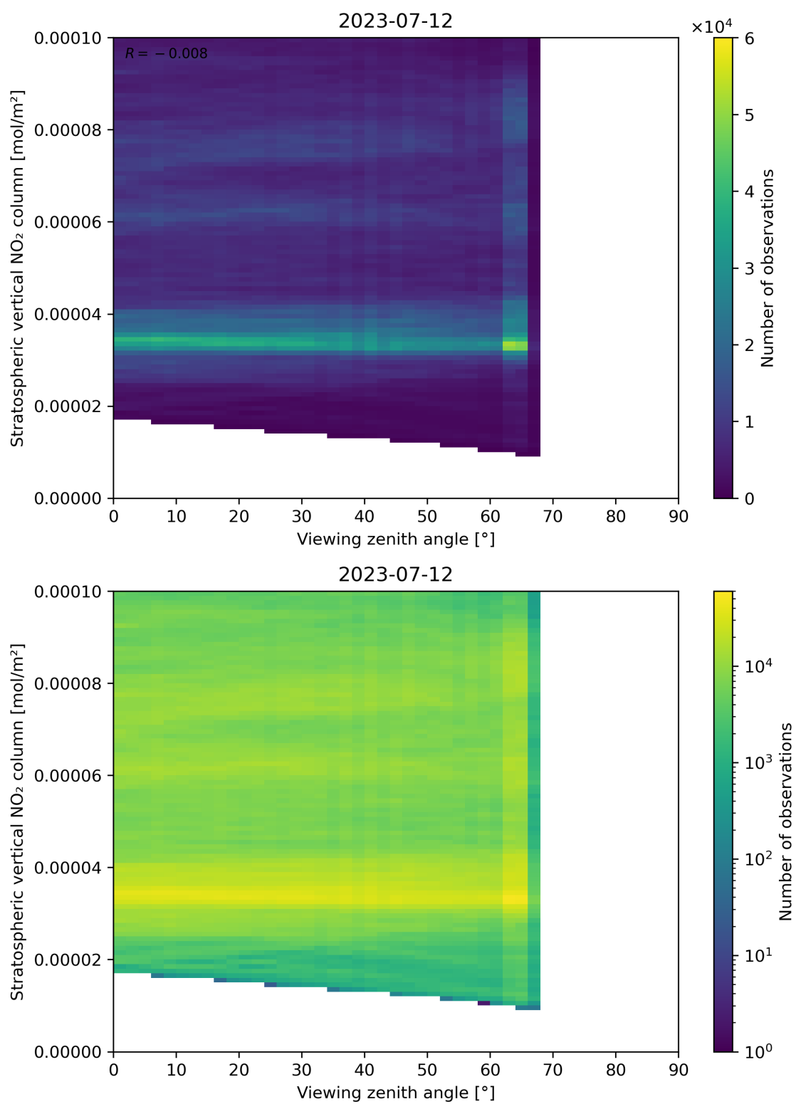
Figure 164: Scatter density plot of “Viewing zenith angle” against “Stratospheric vertical NO 2 column” for 2023-07-11 to 2023-07-13.
