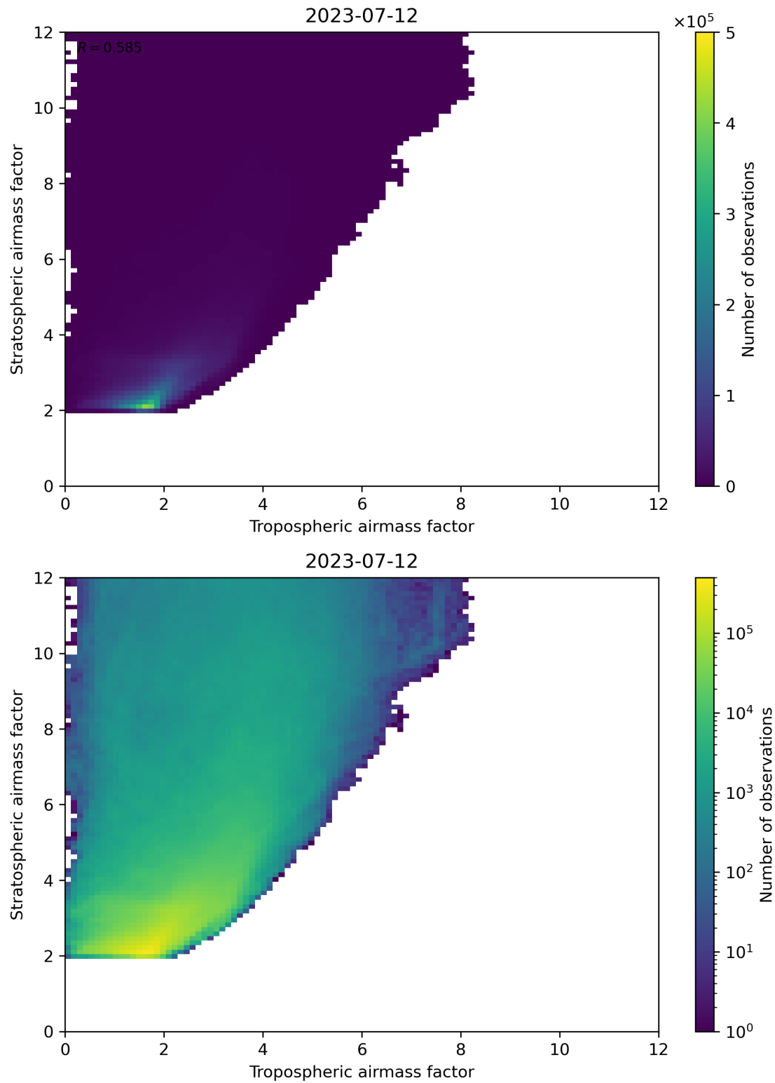
Figure 71: Scatter density plot of “Tropospheric air mass factor” against “Stratospheric air mass factor” for 2023-07-11 to 2023-07-13.
