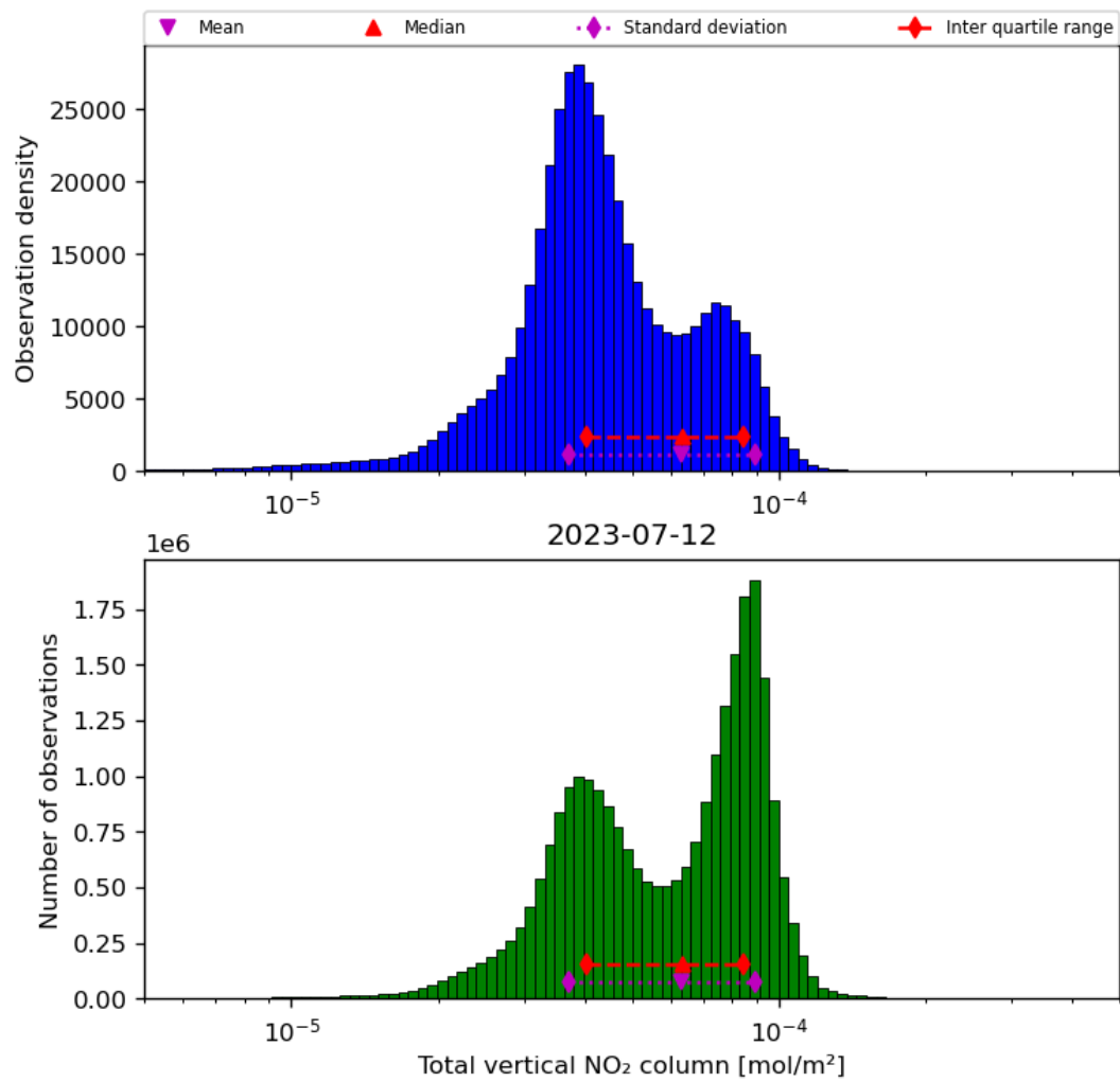
Figure 38: Histogram of “Total vertical NO 2 column” for 2023-07-11 to 2023-07-13
