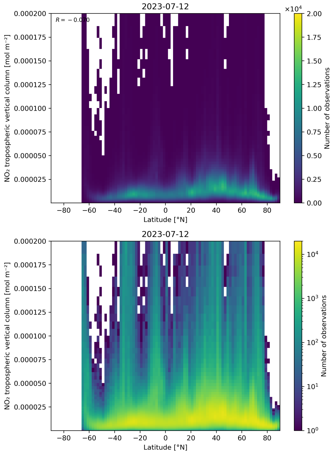
Figure 92: Scatter density plot of “Latitude” against “NO 2 tropospheric vertical column” for 2023-07-11 to 2023-07-13.
