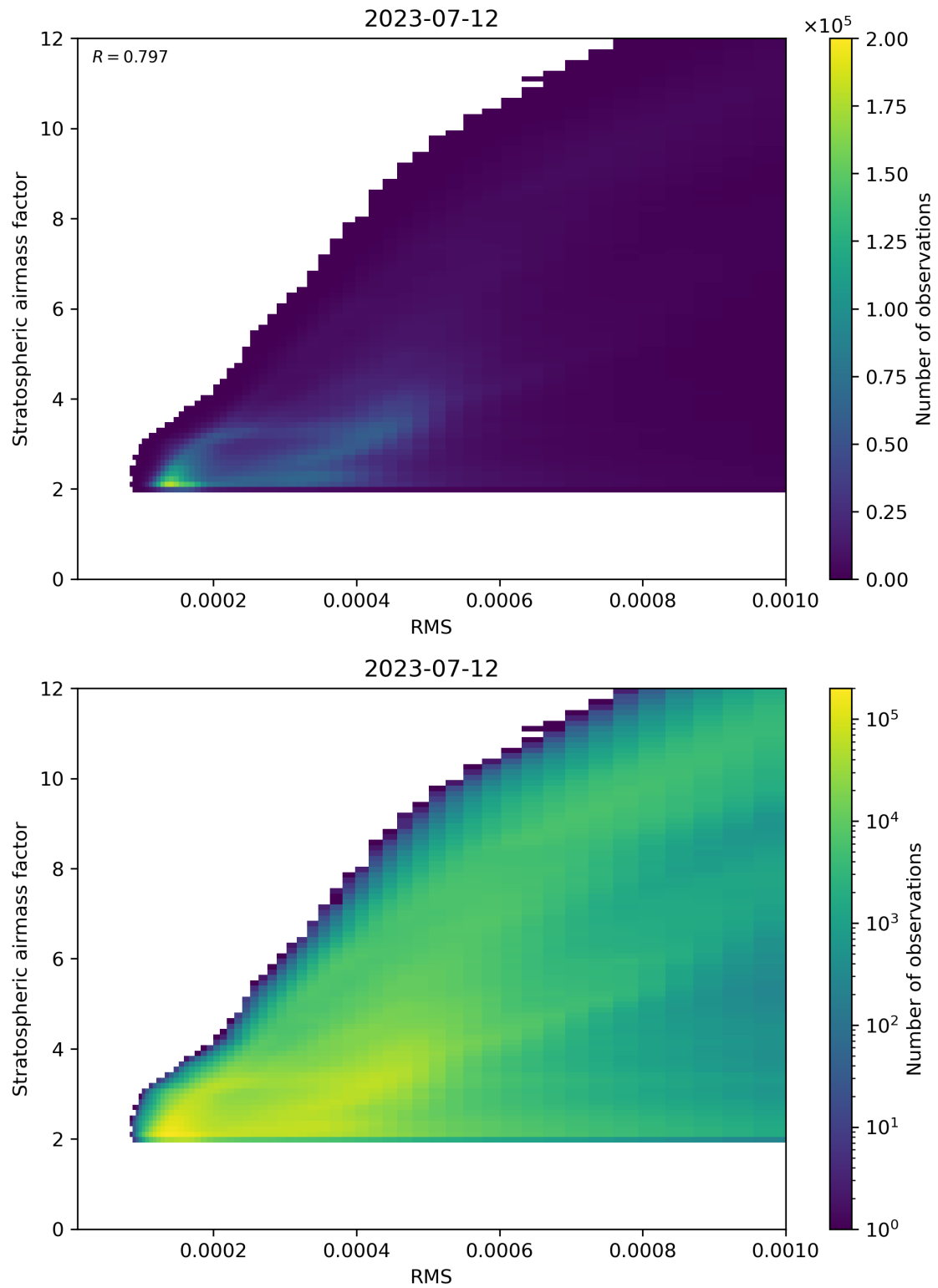
Figure 144: Scatter density plot of “RMS” against “Stratospheric airmass factor” for 2023-07-11 to 2023-07-13.
