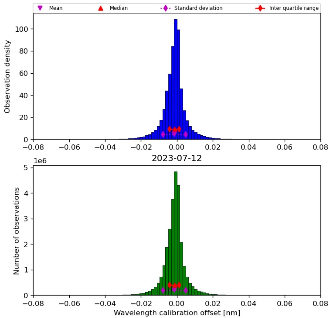
Figure 35: Histogram of “Wavelength calibration offset” for 2023-07-11 to 2023-07-13
