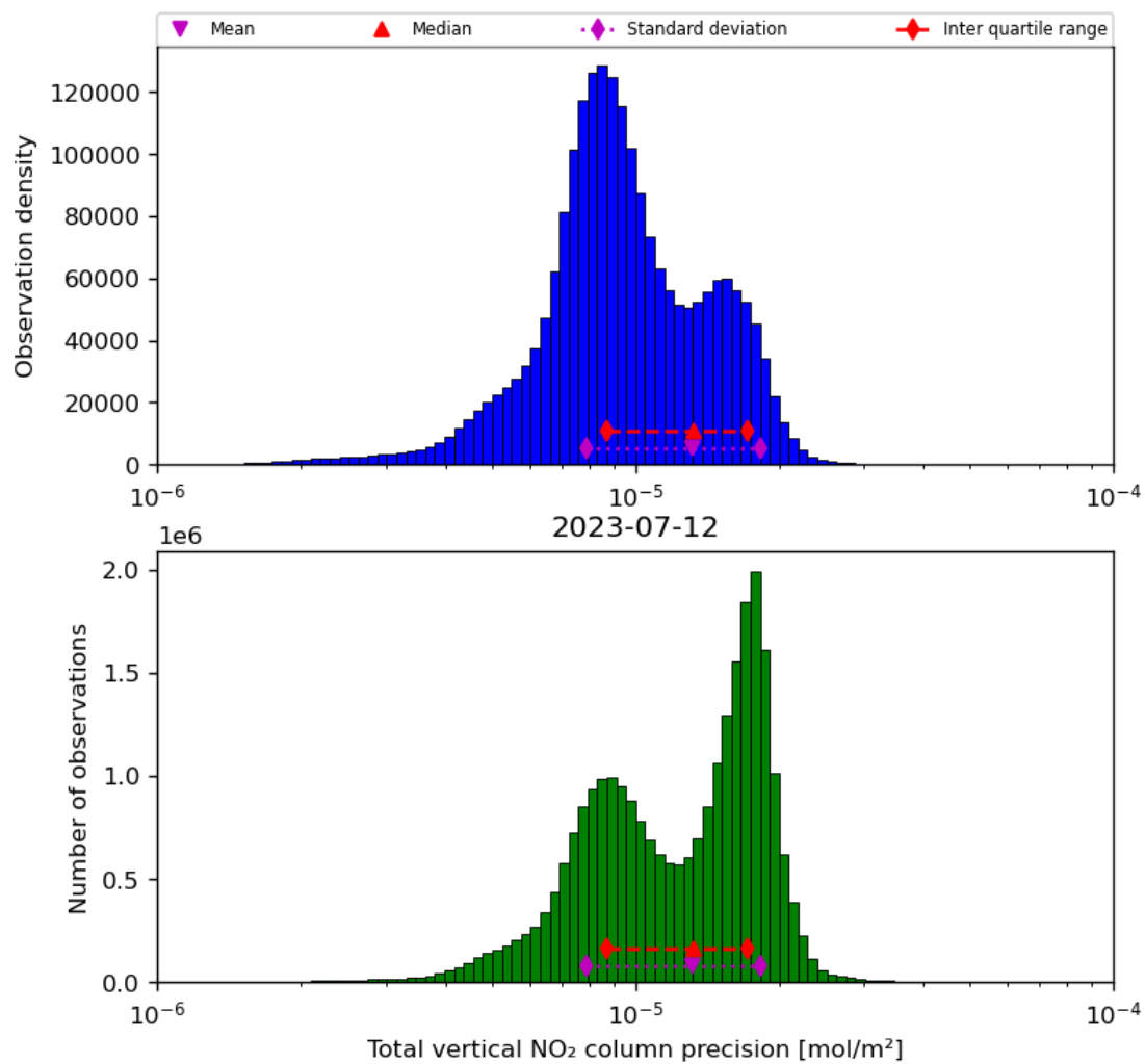
Figure 39: Histogram of “Total vertical NO 2 column precision” for 2023-07-11 to 2023-07-13
