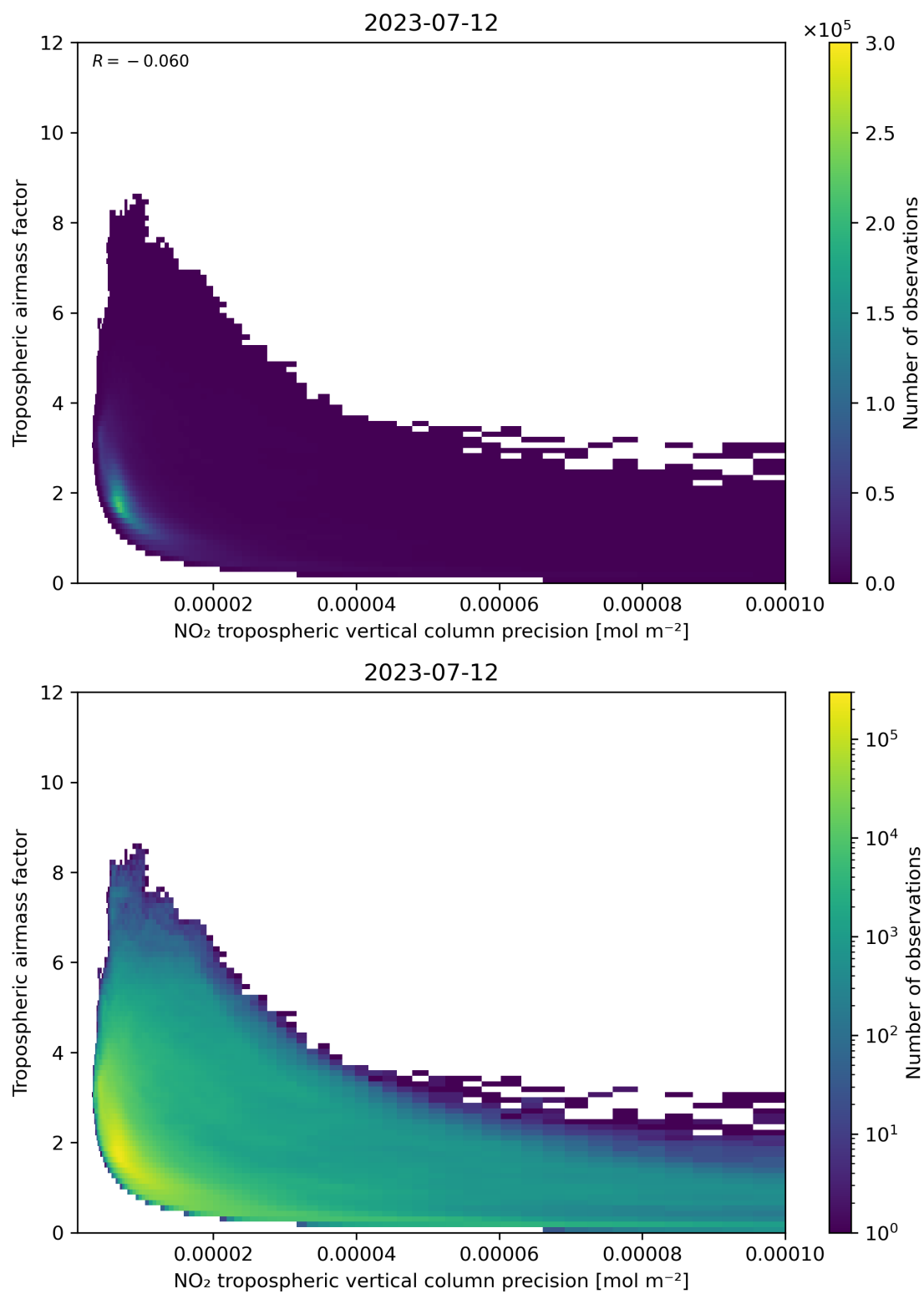
Figure 133: Scatter density plot of “NO 2 tropospheric vertical column precision” against “Tropospheric airmass factor” for 2023-07-11 to 2023-07-13.
