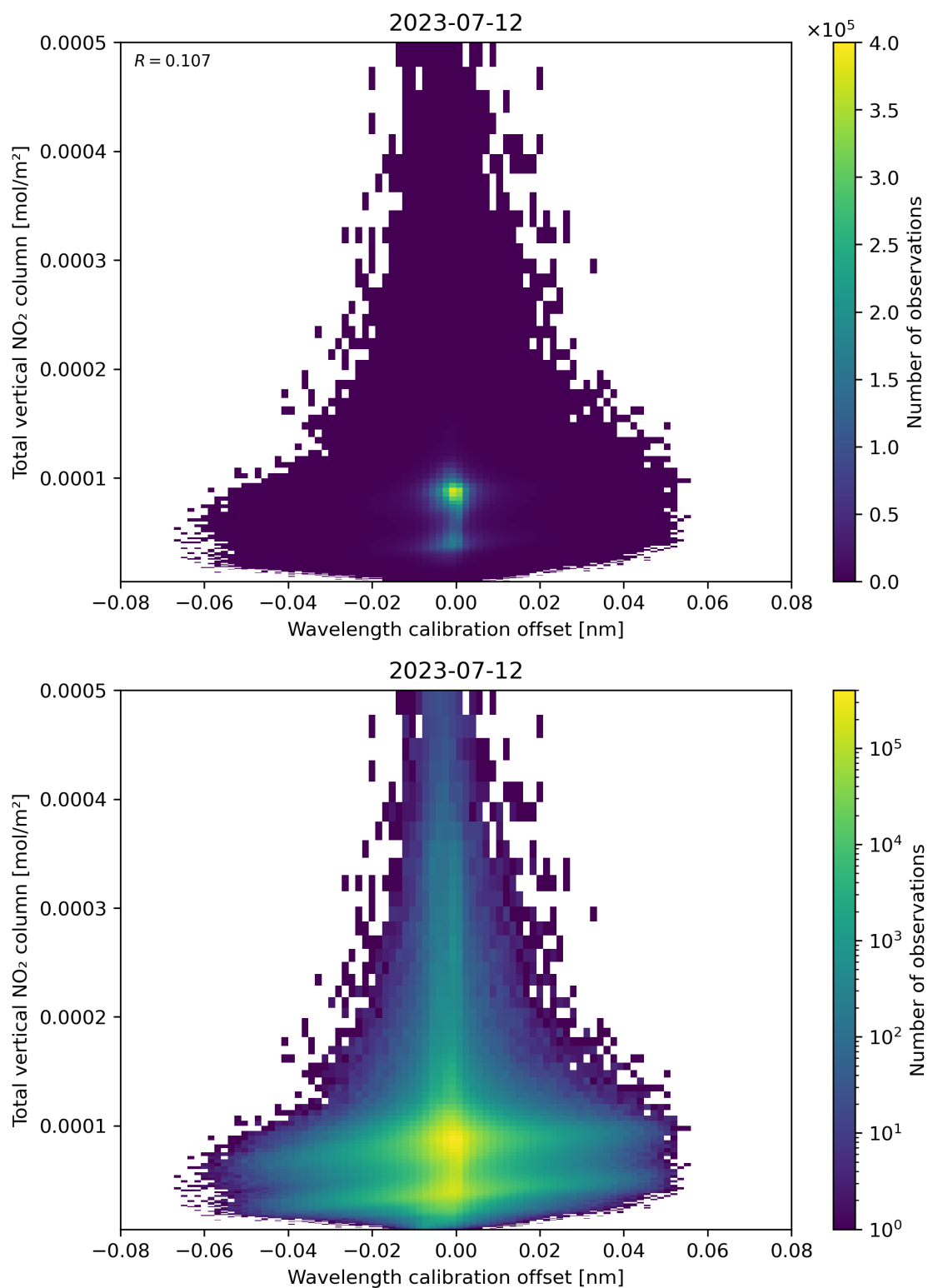
Figure 179: Scatter density plot of “Wavelength calibration offset” against “Total vertical NO 2 column” for 2023-07-11 to 2023-07-13.
