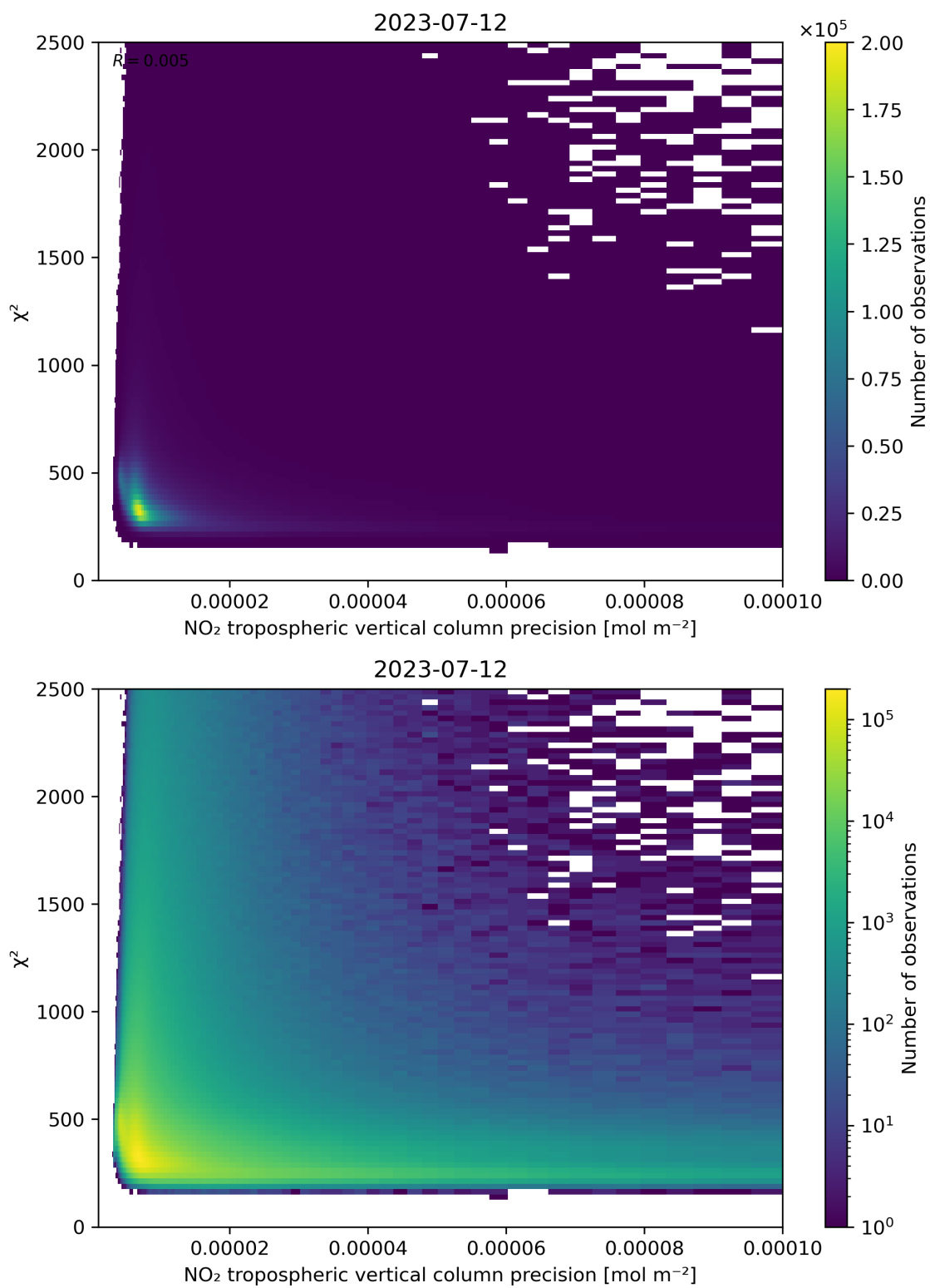
Figure 134: Scatter density plot of “NO 2 tropospheric vertical column precision” against “ \chi^2 ” for 2023-07-11 to 2023-07-13.
