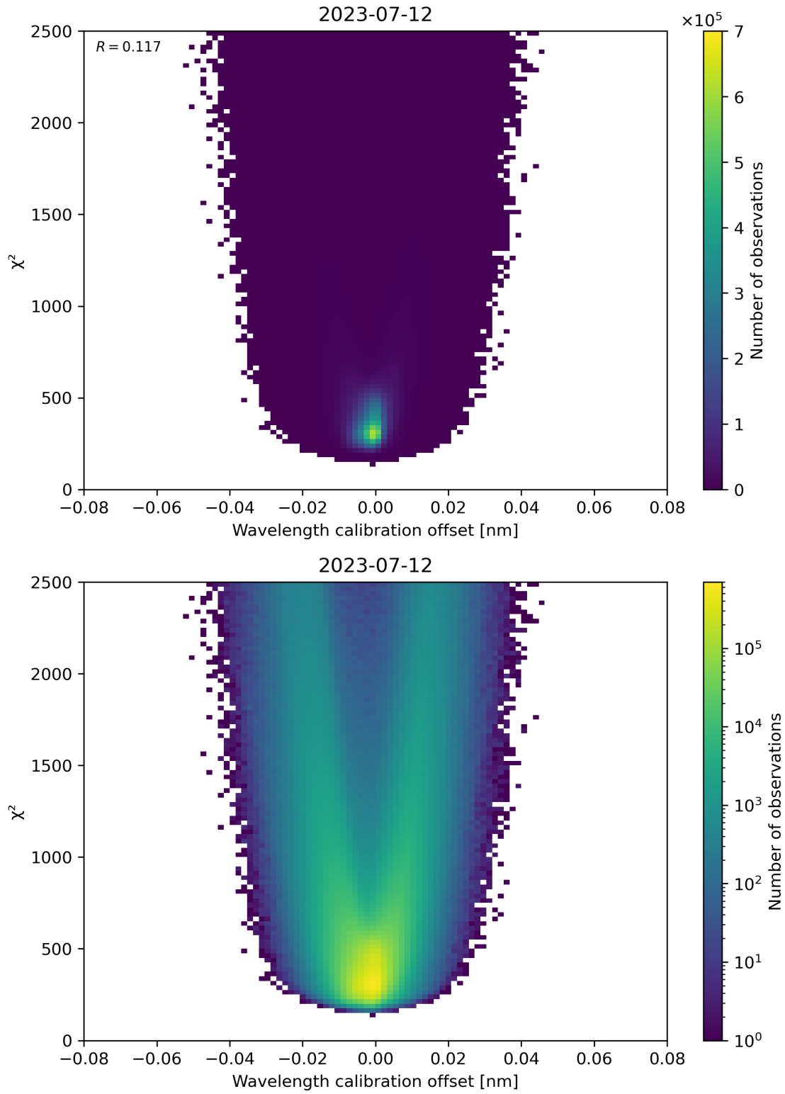
Figure 175: Scatter density plot of “Wavelength calibration offset” against “ \chi^2 ” for 2023-07-11 to 2023-07-13.
