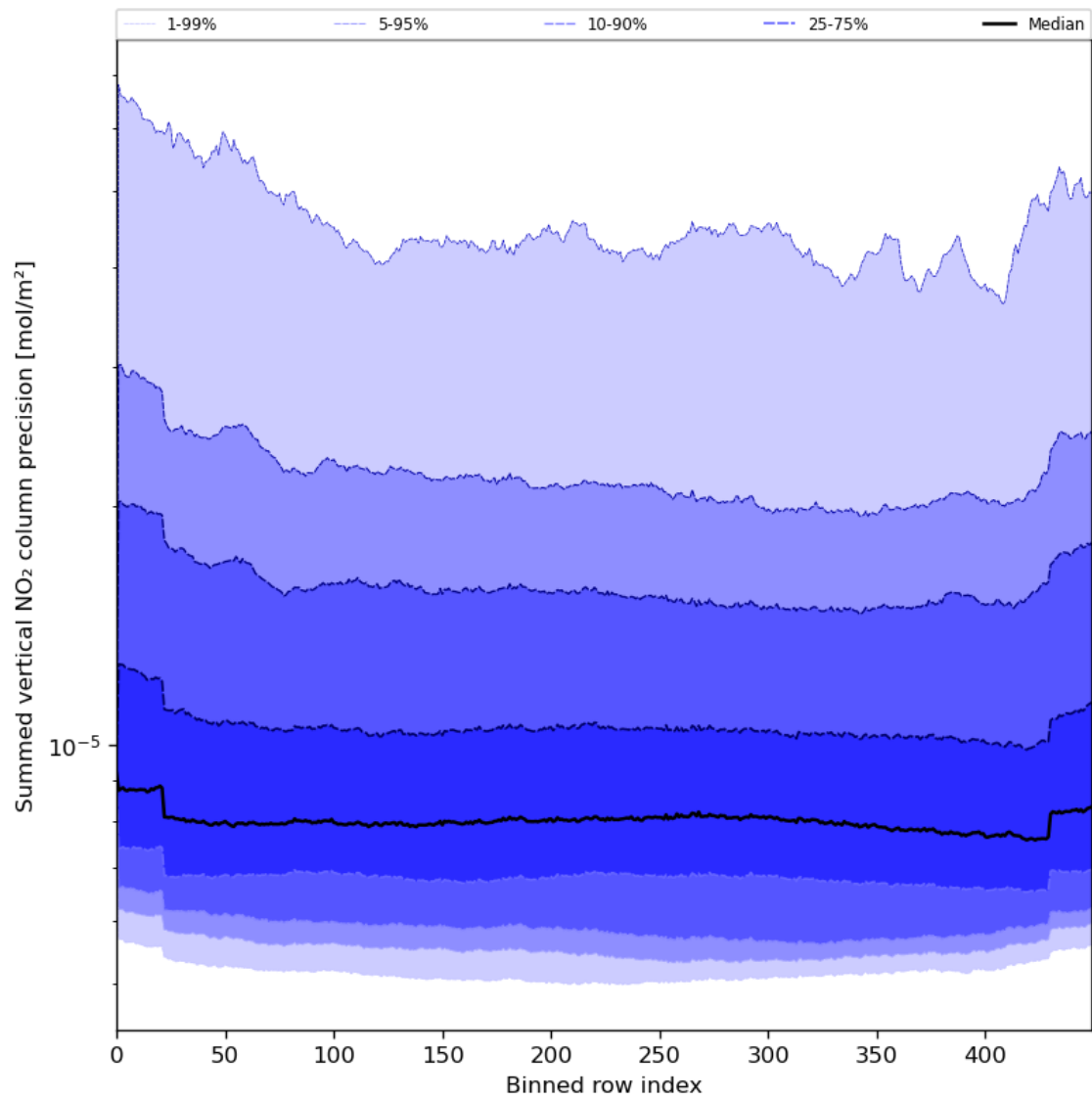
Figure 58: Along track statistics of “Summed vertical NO 2 column precision” for 2023-07-11 to 2023-07-13
