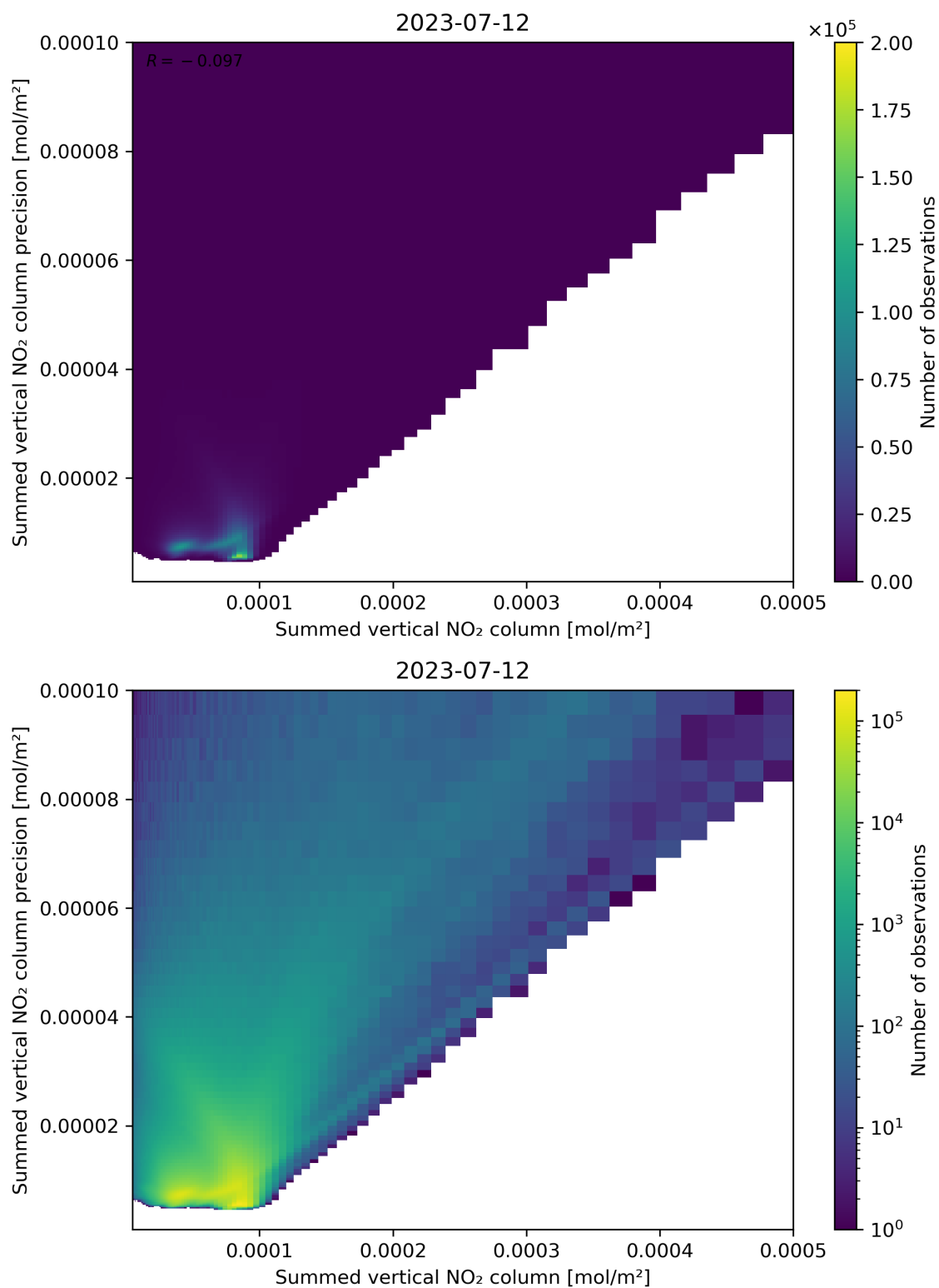
Figure 105: Scatter density plot of “Summed vertical NO 2 column” against “Summed vertical NO 2 column precision” for 2023-07-11 to 2023-07-13.
