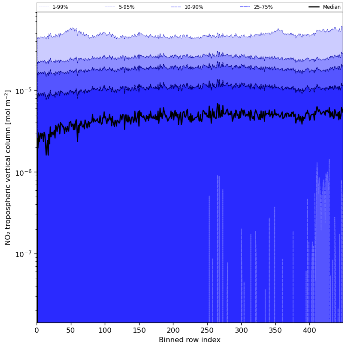
Figure 46: Along track statistics of “NO 2 tropospheric vertical column” for 2023-07-11 to 2023-07-13
