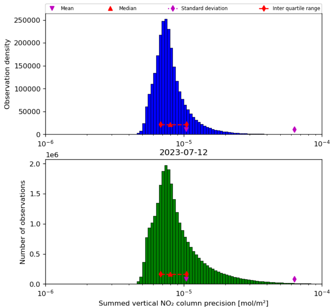
Figure 41: Histogram of "Summed vertical NO 2 column precision" for 2023-07-11 to 2023-07-13
