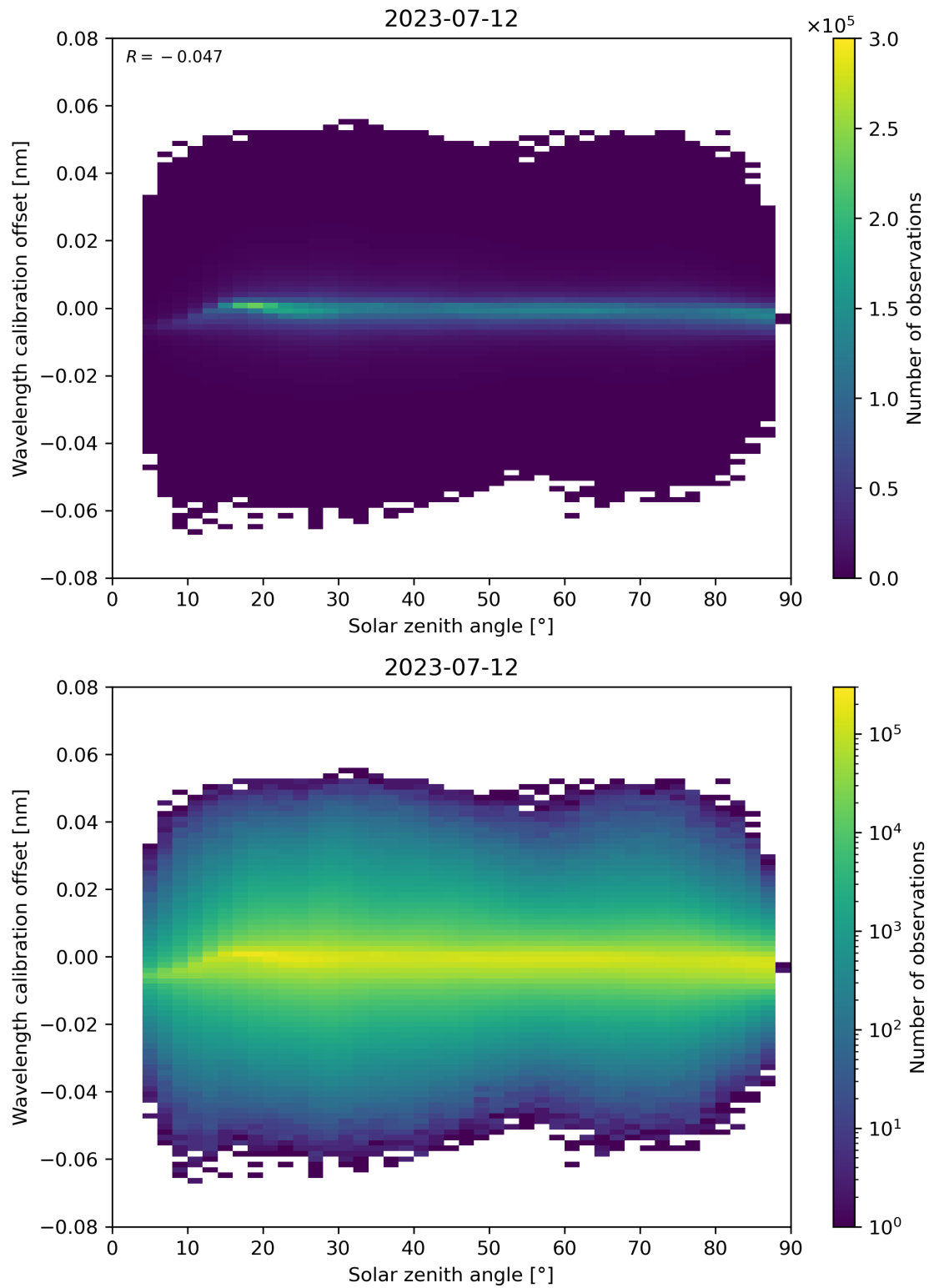
Figure 158: Scatter density plot of “Solar zenith angle” against “Wavelength calibration offset” for 2023-07-11 to 2023-07-13.
