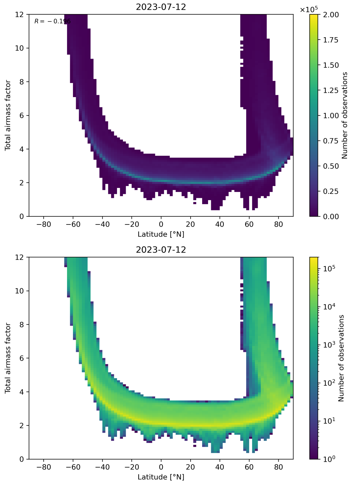
Figure 84: Scatter density plot of “Latitude” against “Total airmass factor” for 2023-07-11 to 2023-07-13.
