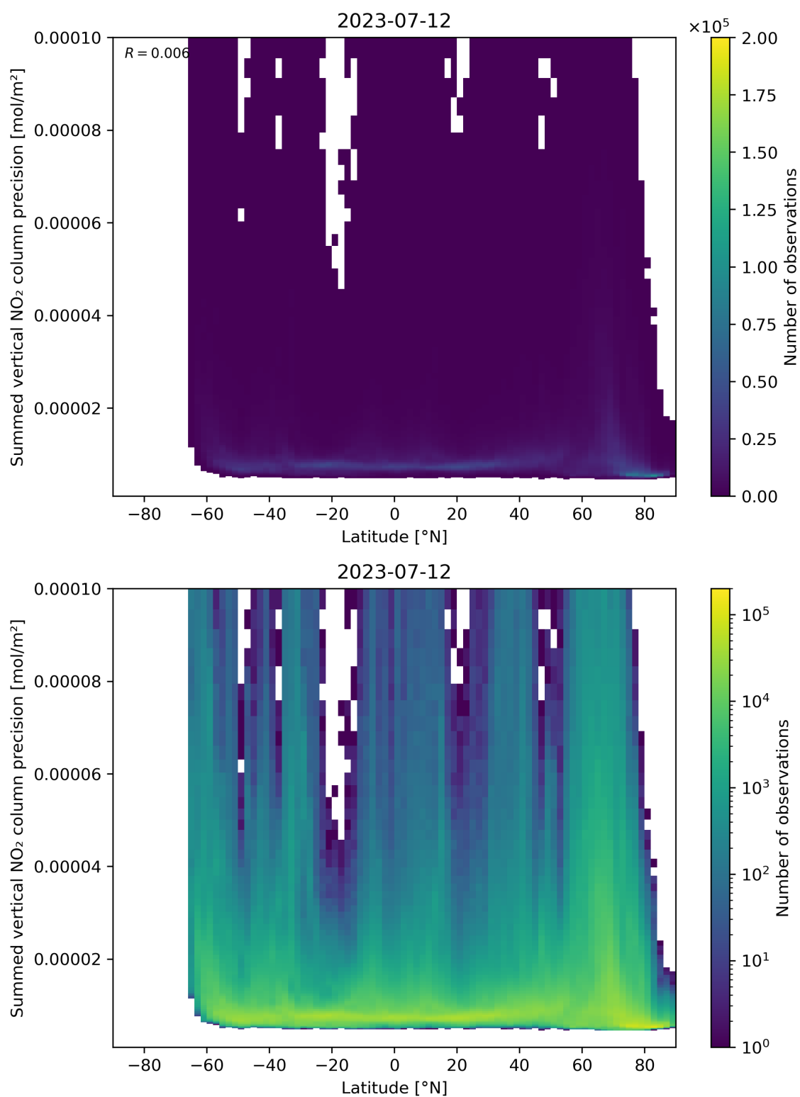
Figure 89: Scatter density plot of “Latitude” against “Summed vertical NO 2 column precision” for 2023-07-11 to 2023-07-13.
