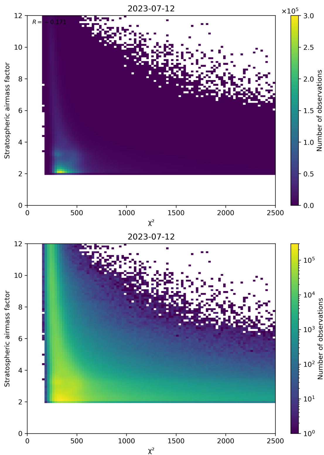
Figure 81: Scatter density plot of “ \chi^2 ” against “Stratospheric airmass factor” for 2023-07-11 to 2023-07-13.
