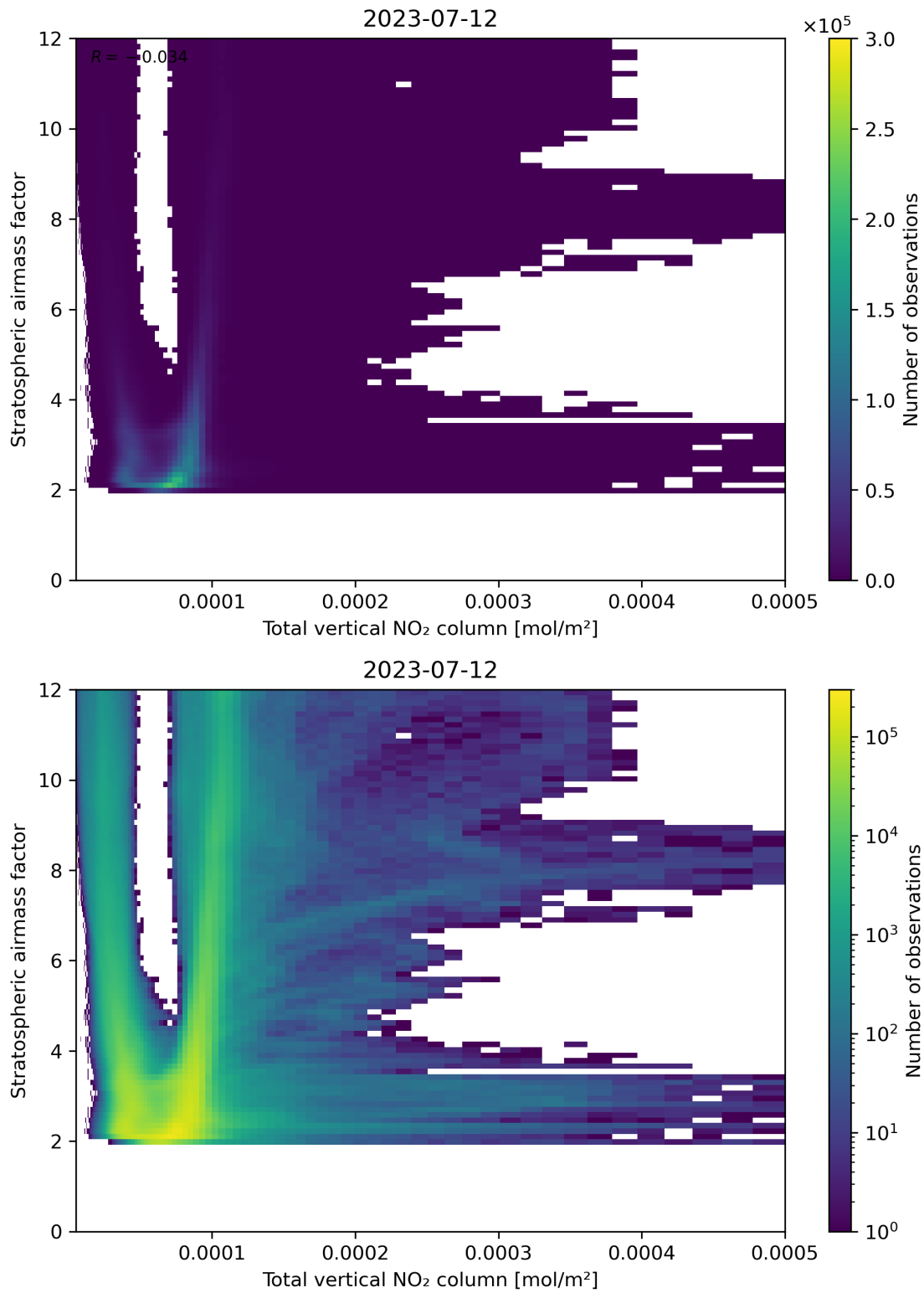
Figure 110: Scatter density plot of “Total vertical NO 2 column” against “Stratospheric airmass factor” for 2023-07-11 to 2023-07-13.
