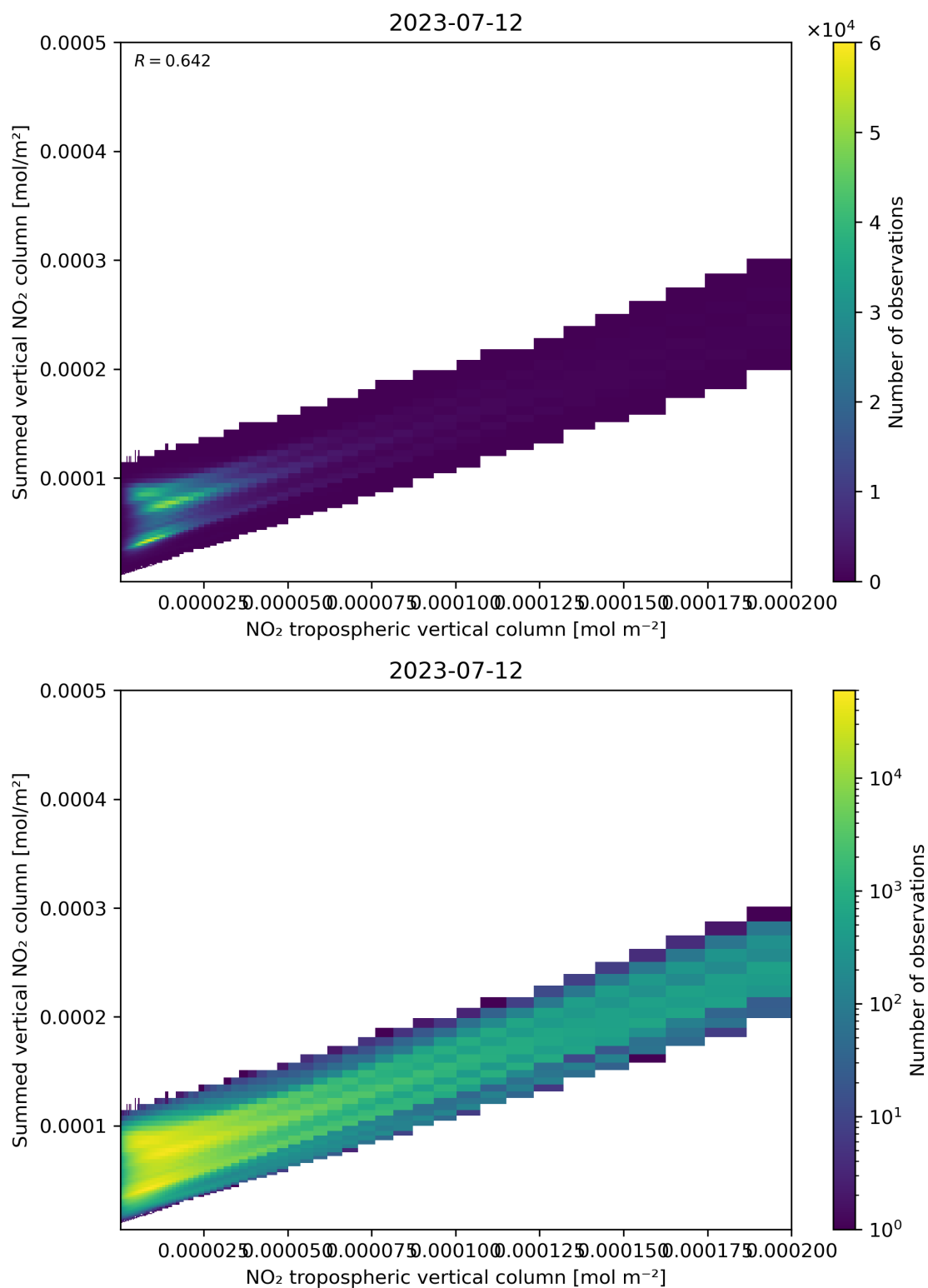
Figure 126: Scatter density plot of “NO 2 tropospheric vertical column” against “Summed vertical NO 2 column” for 2023-07-11 to 2023-07-13.
