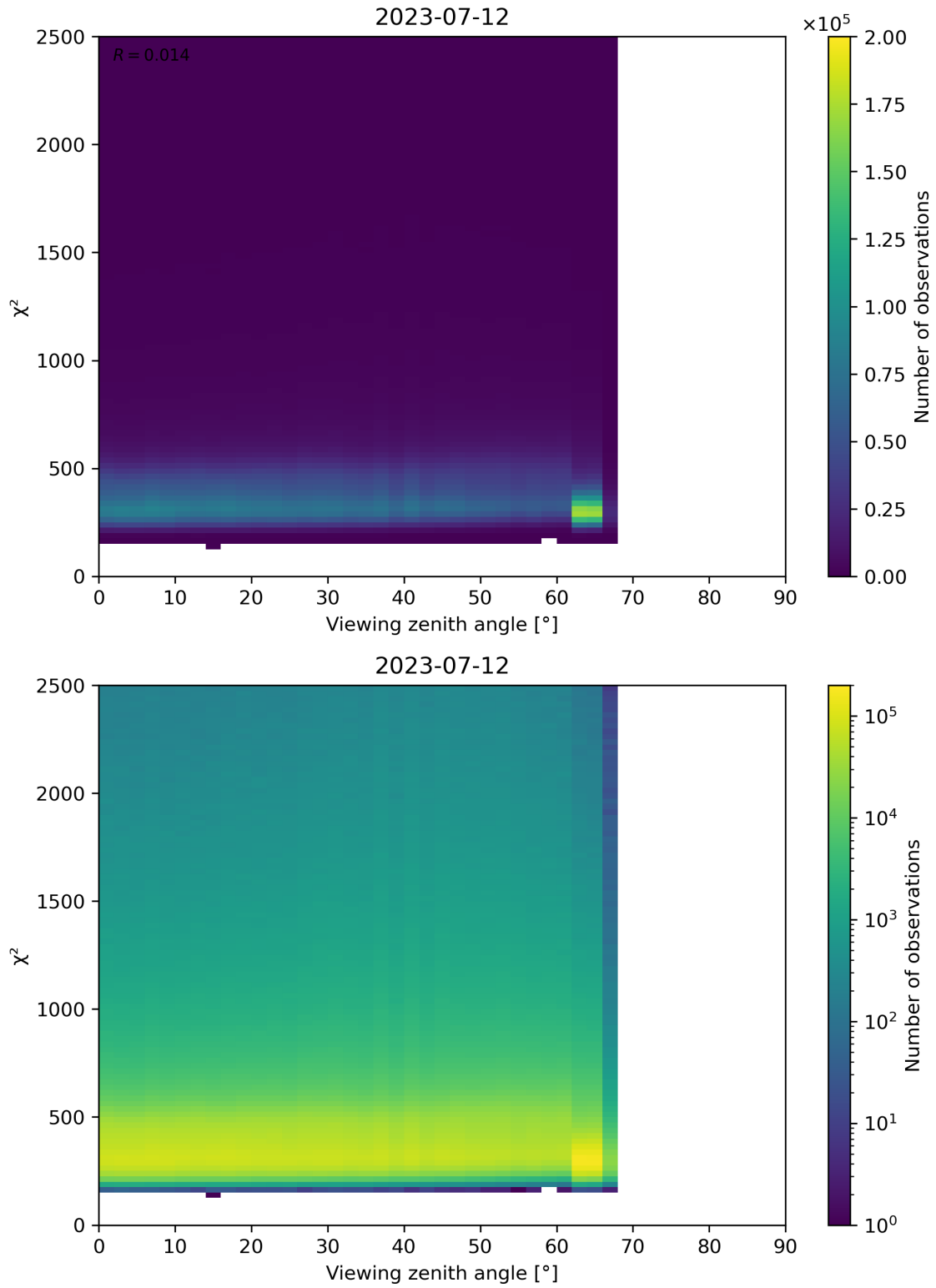
Figure 162: Scatter density plot of “Viewing zenith angle” against “ \chi^2 ” for 2023-07-11 to 2023-07-13.
