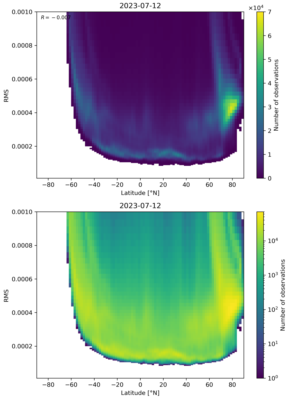
Figure 94: Scatter density plot of “Latitude” against “RMS” for 2023-07-11 to 2023-07-13.
