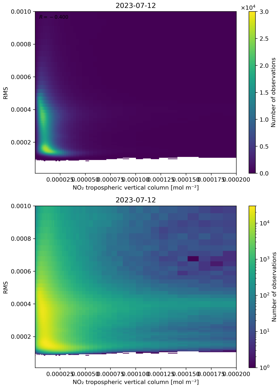
Figure 142: Scatter density plot of “NO 2 tropospheric vertical column” against “RMS” for 2023-07-11 to 2023-07-13.
