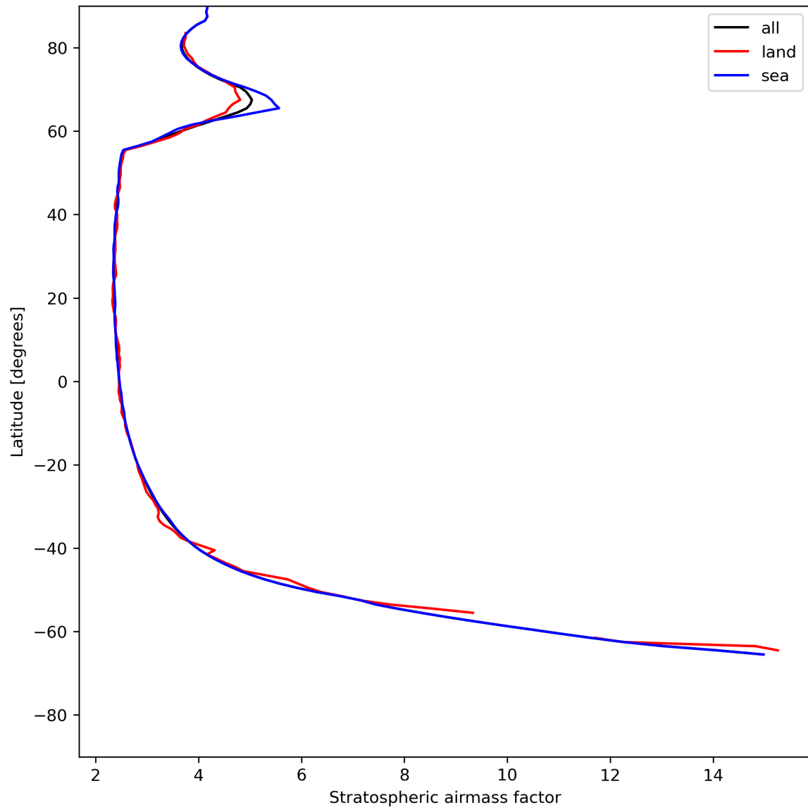
Figure 27: Zonal average of “Stratospheric airmass factor” for 2023-07-11 to 2023-07-13.
