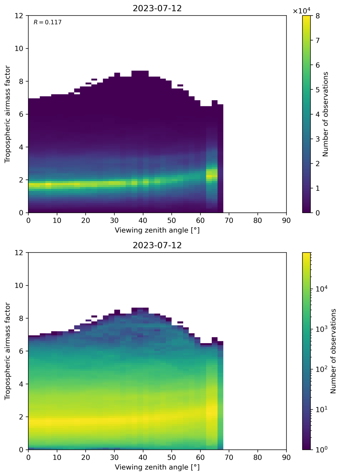
Figure 161: Scatter density plot of “Viewing zenith angle” against “Tropospheric airmass factor” for 2023-07-11 to 2023-07-13.
