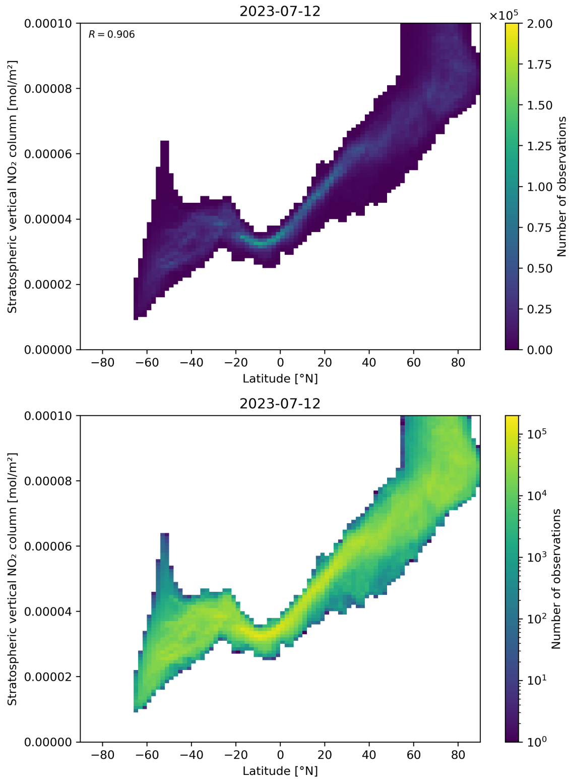
Figure 87: Scatter density plot of “Latitude” against “Stratospheric vertical \text{NO}_2 column” for 2023-07-11 to 2023-07-13.
