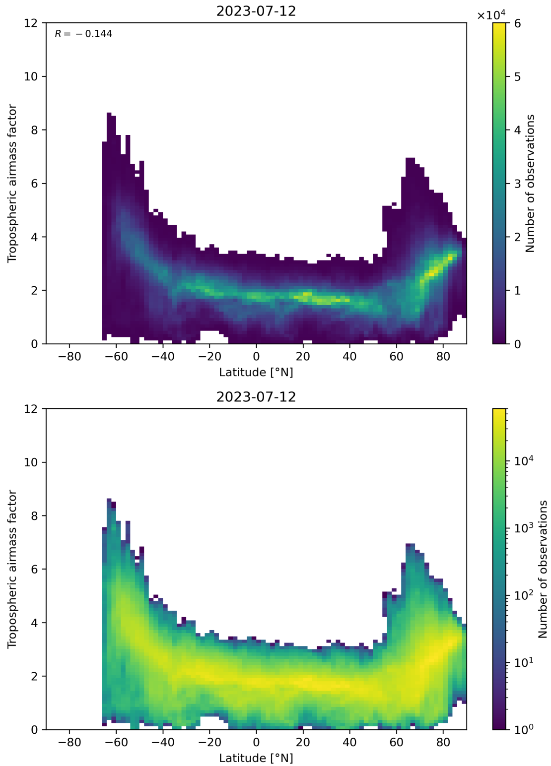
Figure 85: Scatter density plot of “Latitude” against “Tropospheric air mass factor” for 2023-07-11 to 2023-07-13.
