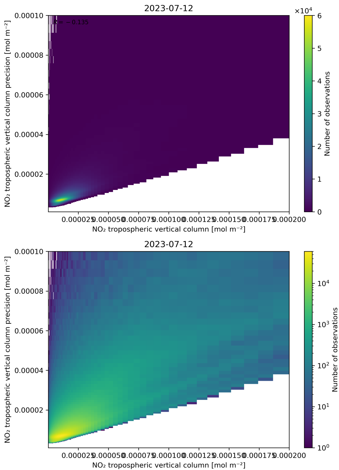
Figure 130: Scatter density plot of “NO 2 tropospheric vertical column” against “NO 2 tropospheric vertical column precision” for 2023-07-11 to 2023-07-13.
