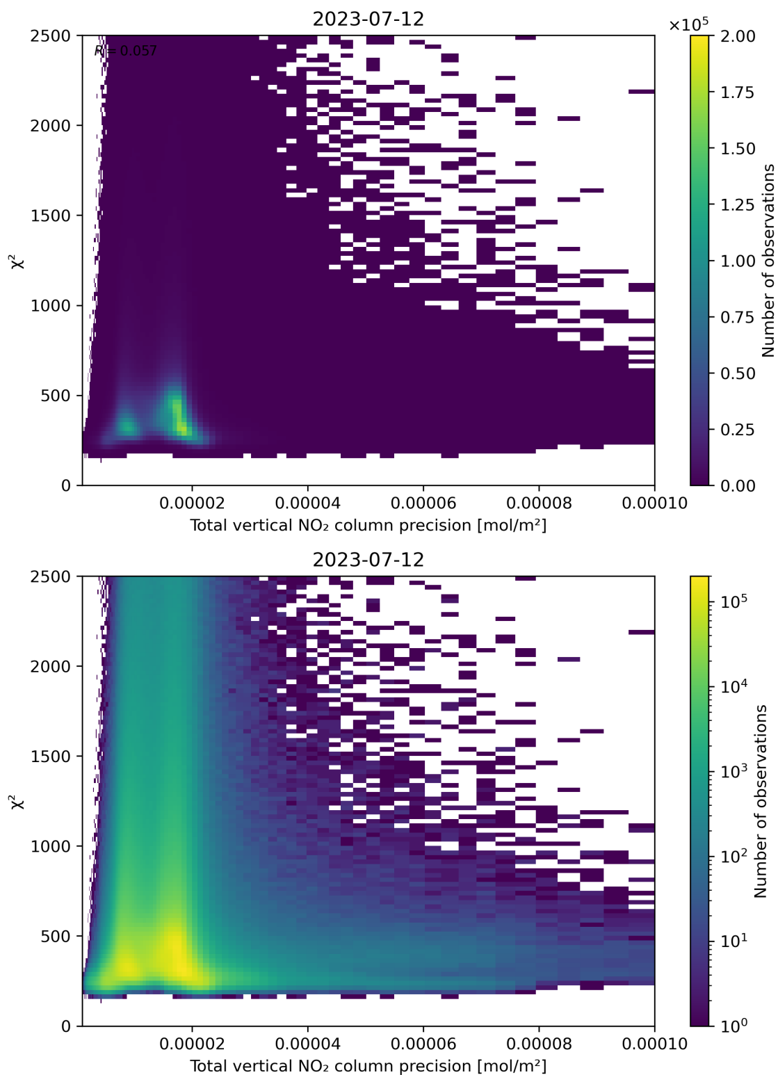
Figure 116: Scatter density plot of “Total vertical NO 2 column precision” against “ \chi^2 ” for 2023-07-11 to 2023-07-13.
