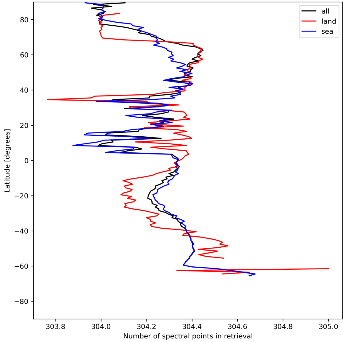
Figure 16: Zonal average of “Number of spectral points in retrieval” for 2023-07-11 to 2023-07-13.
