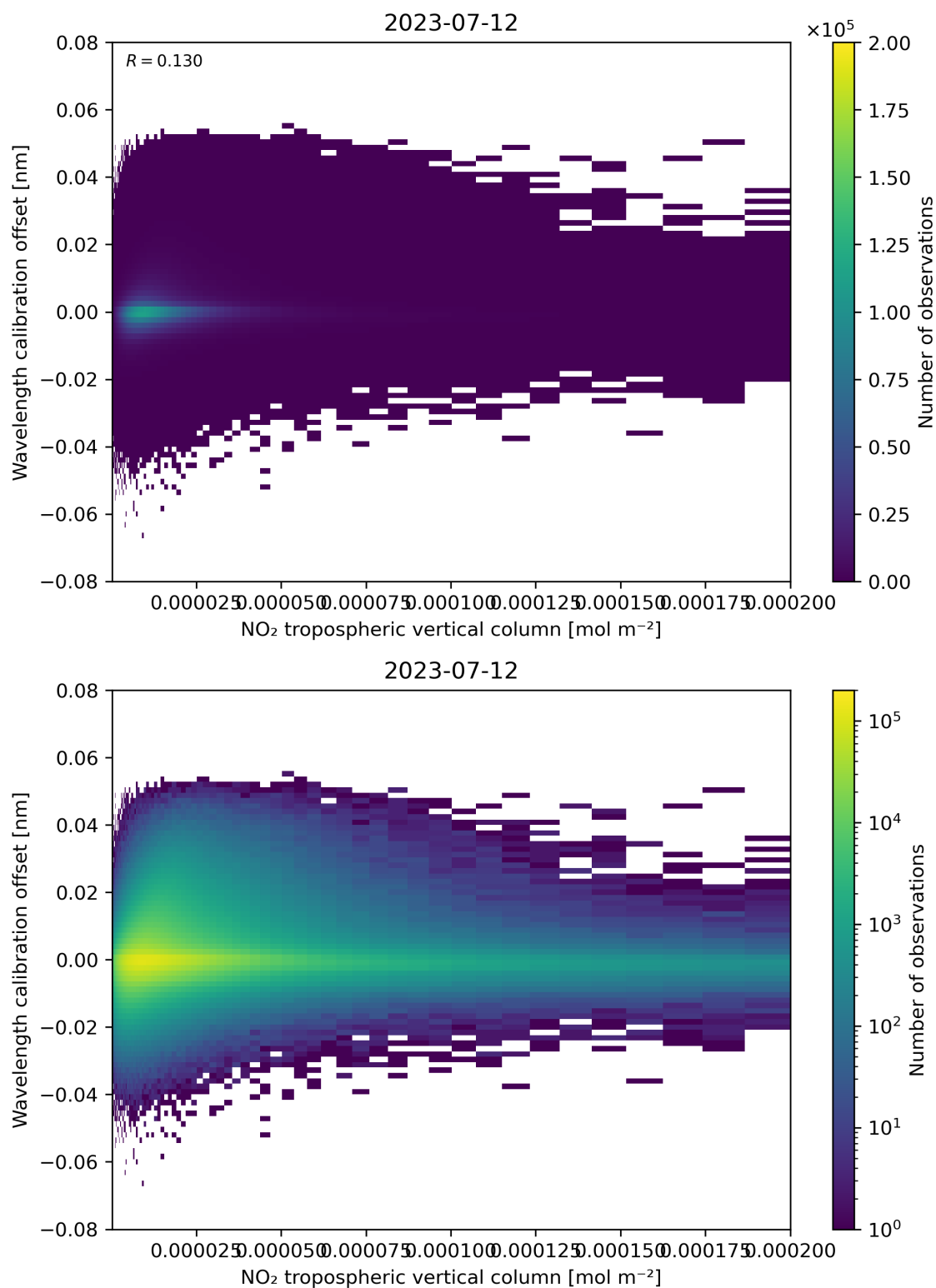
Figure 143: Scatter density plot of “NO 2 tropospheric vertical column” against “Wavelength calibration offset” for 2023-07-11 to 2023-07-13.
