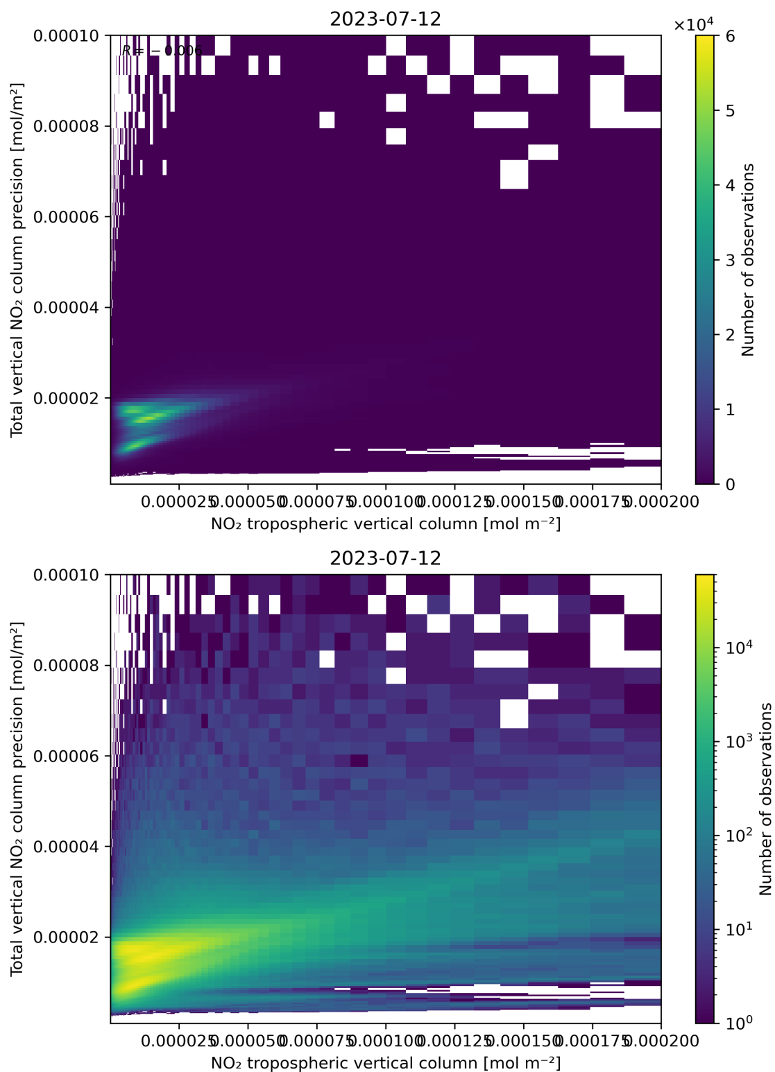
Figure 129: Scatter density plot of “NO 2 tropospheric vertical column” against “Total vertical NO 2 column precision” for 2023-07-11 to 2023-07-13.
