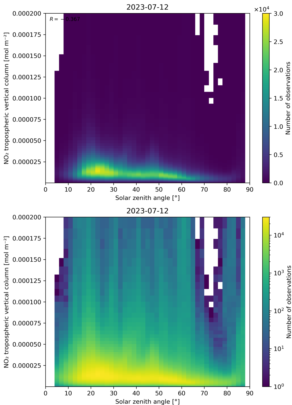
Figure 155: Scatter density plot of “Solar zenith angle” against “NO 2 tropospheric vertical column” for 2023-07-11 to 2023-07-13.
