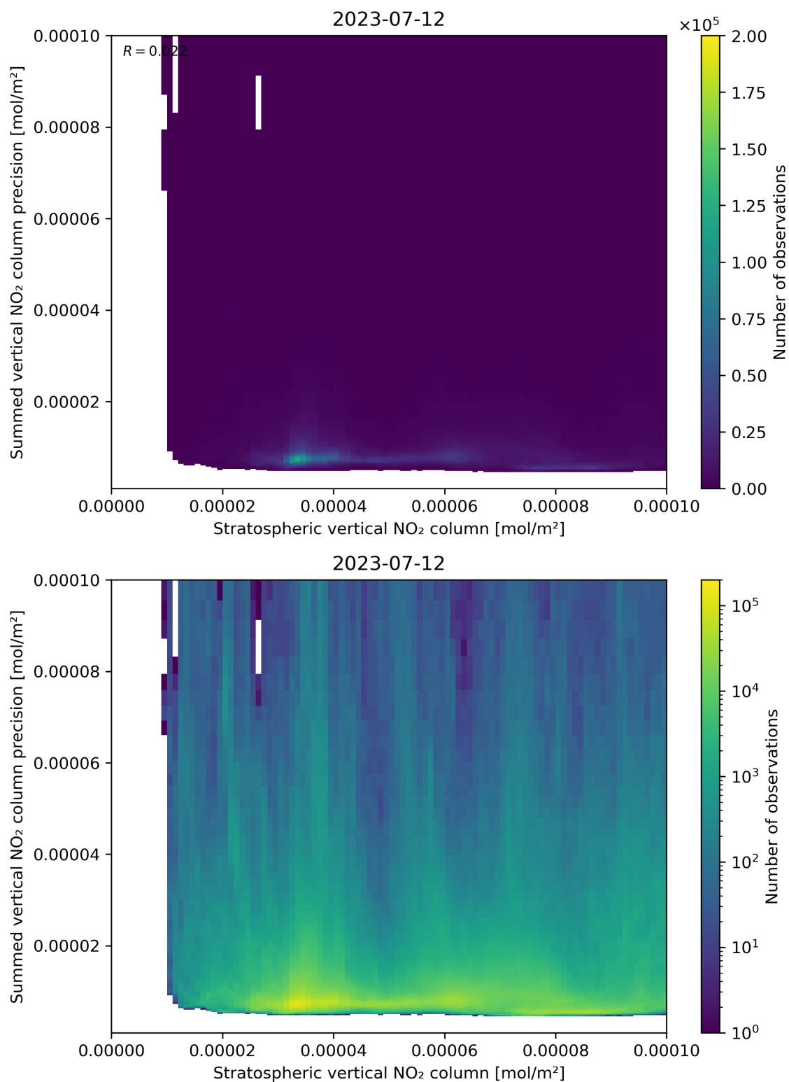
Figure 99: Scatter density plot of “Stratospheric vertical NO 2 column” against “Summed vertical NO 2 column precision” for 2023-07-11 to 2023-07-13.
