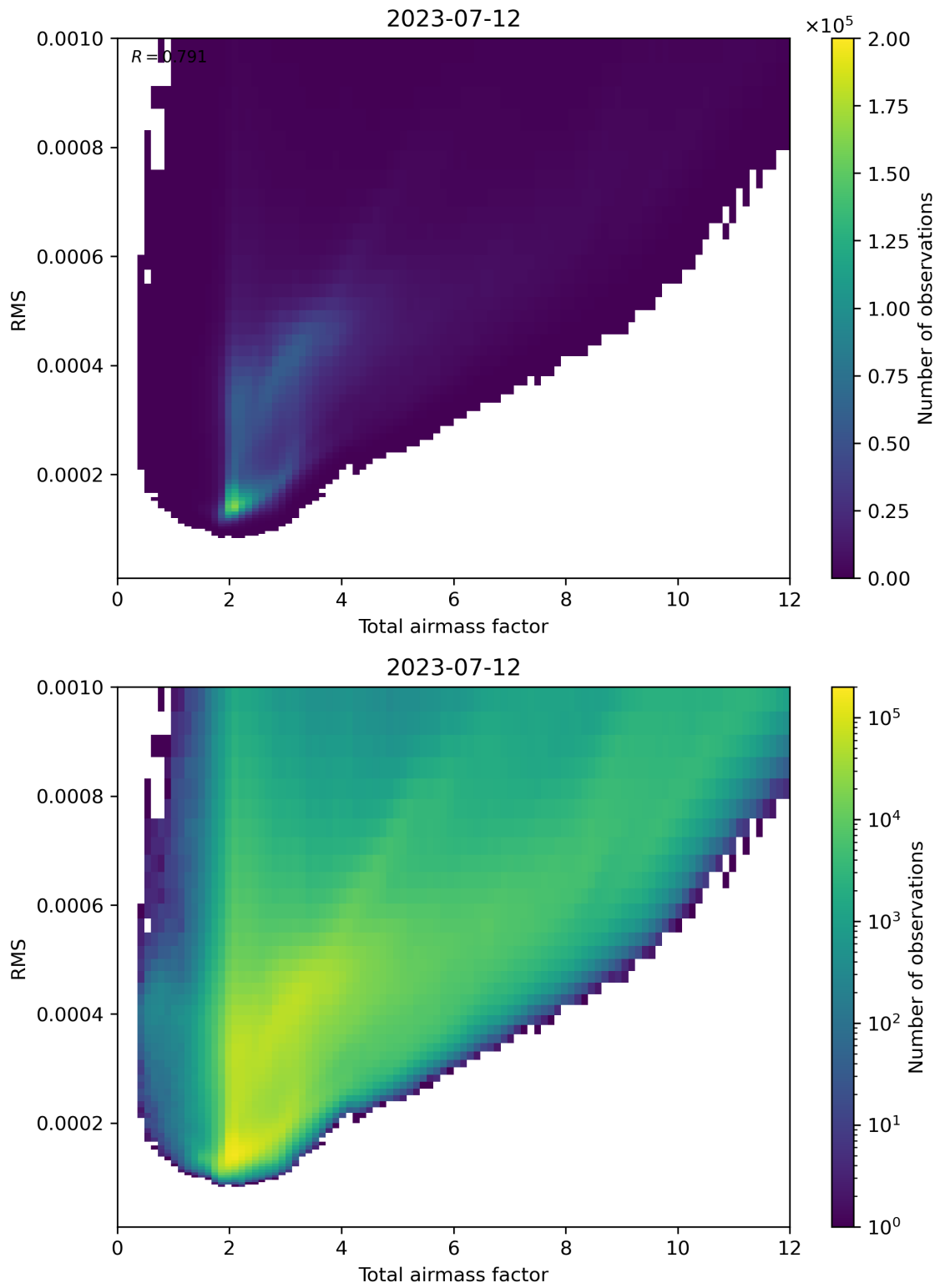
Figure 69: Scatter density plot of “Total airmass factor” against “RMS” for 2023-07-11 to 2023-07-13.
