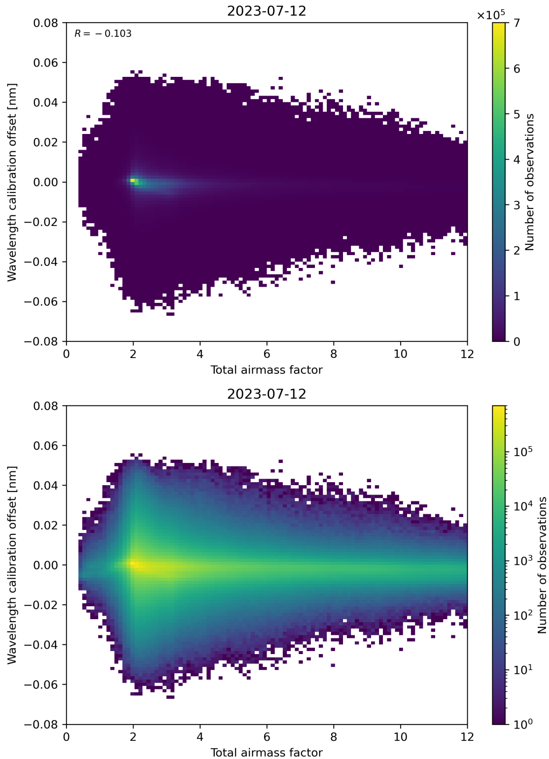
Figure 70: Scatter density plot of “Total airmass factor” against “Wavelength calibration offset” for 2023-07-11 to 2023-07-13.
