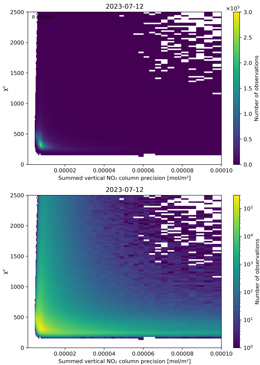
Figure 107: Scatter density plot of “Summed vertical NO 2 column precision” against “ \chi^2 ” for 2023-07-11 to 2023-07-13.
