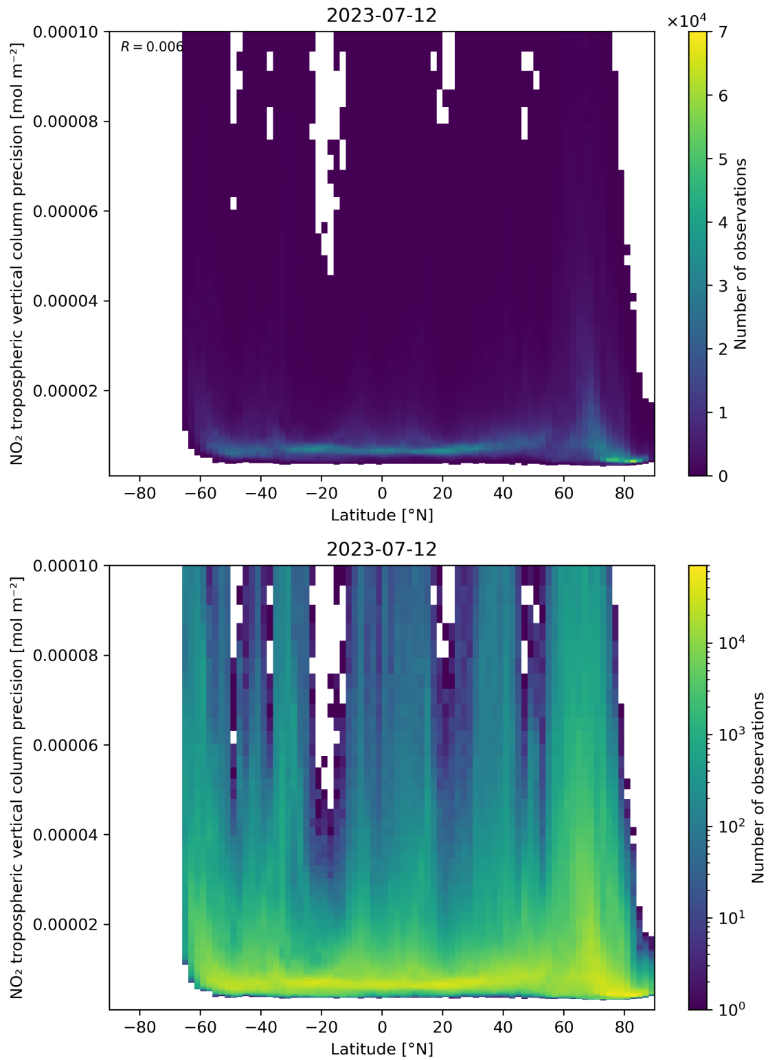
Figure 93: Scatter density plot of “Latitude” against “NO 2 tropospheric vertical column precision” for 2023-07-11 to 2023-07-13.
