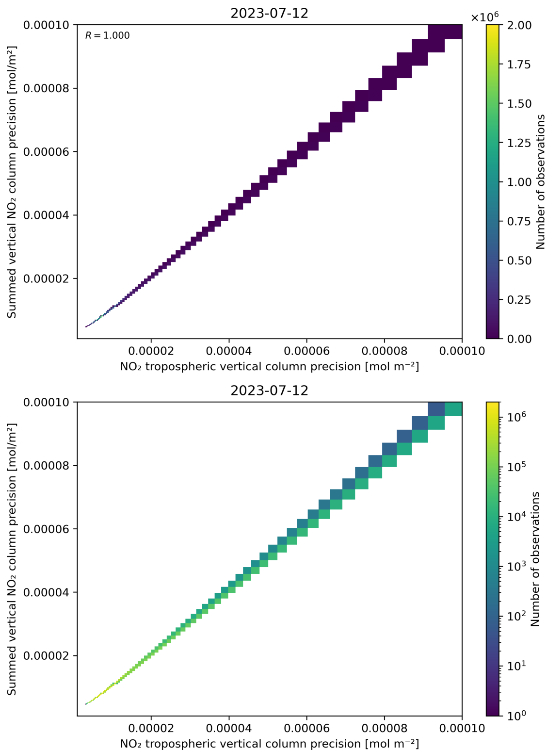
Figure 137: Scatter density plot of “NO 2 tropospheric vertical column precision” against “Summed vertical NO 2 column precision” for 2023-07-11 to 2023-07-13.
