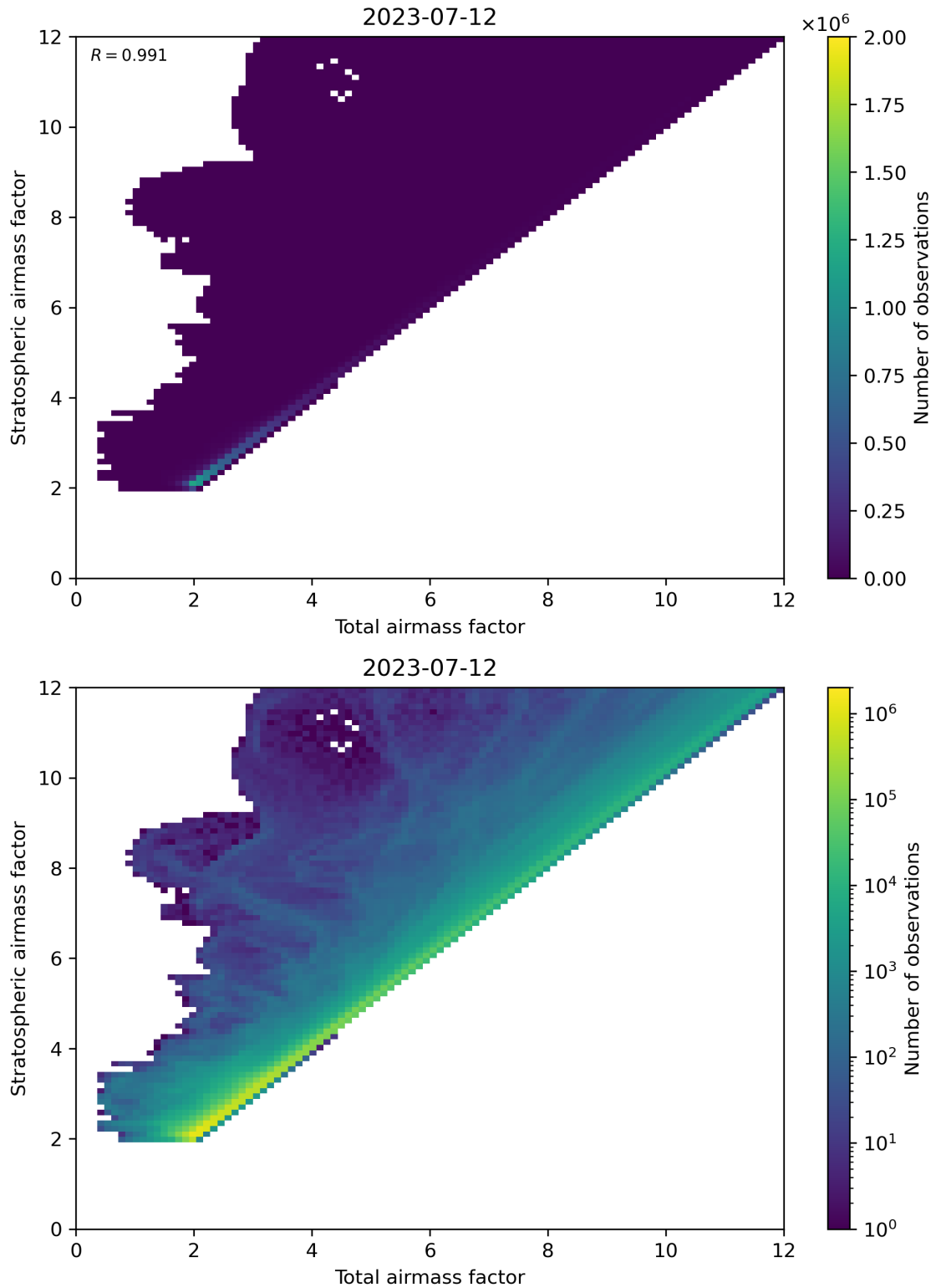
Figure 62: Scatter density plot of “Total air mass factor” against “Stratospheric air mass factor” for 2023-07-11 to 2023-07-13.
