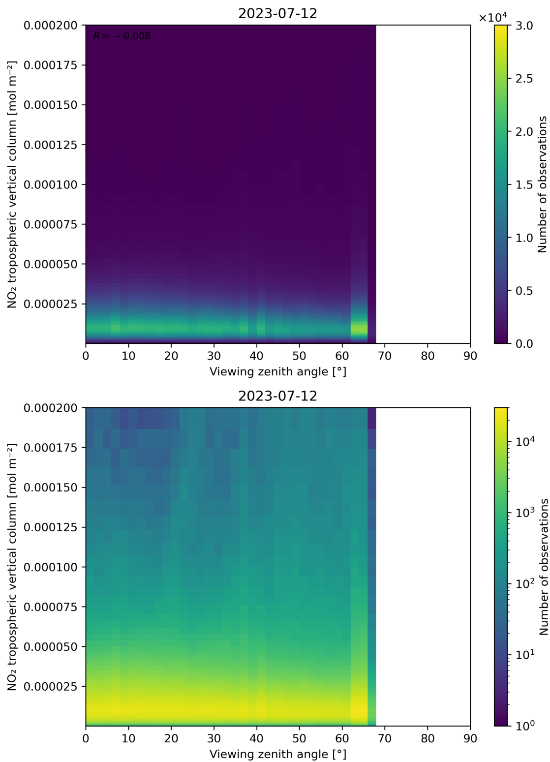
Figure 169: Scatter density plot of “Viewing zenith angle” against “NO 2 tropospheric vertical column” for 2023-07-11 to 2023-07-13.
