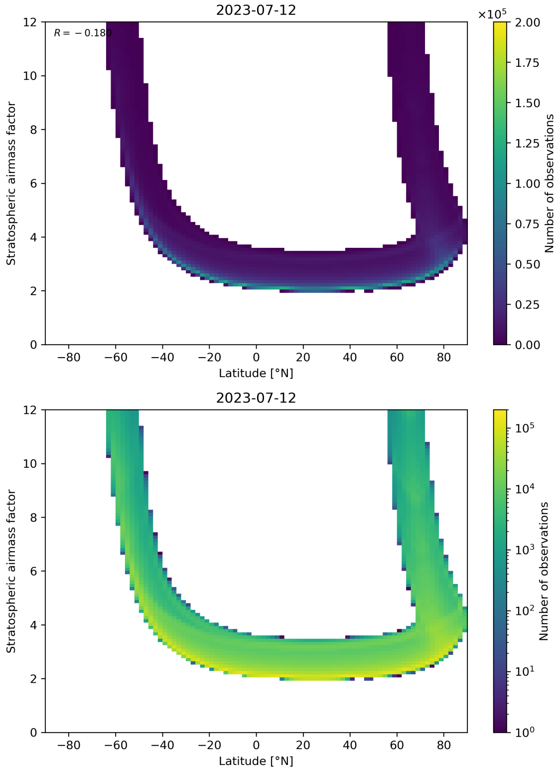
Figure 83: Scatter density plot of “Latitude” against “Stratospheric airmass factor” for 2023-07-11 to 2023-07-13.
