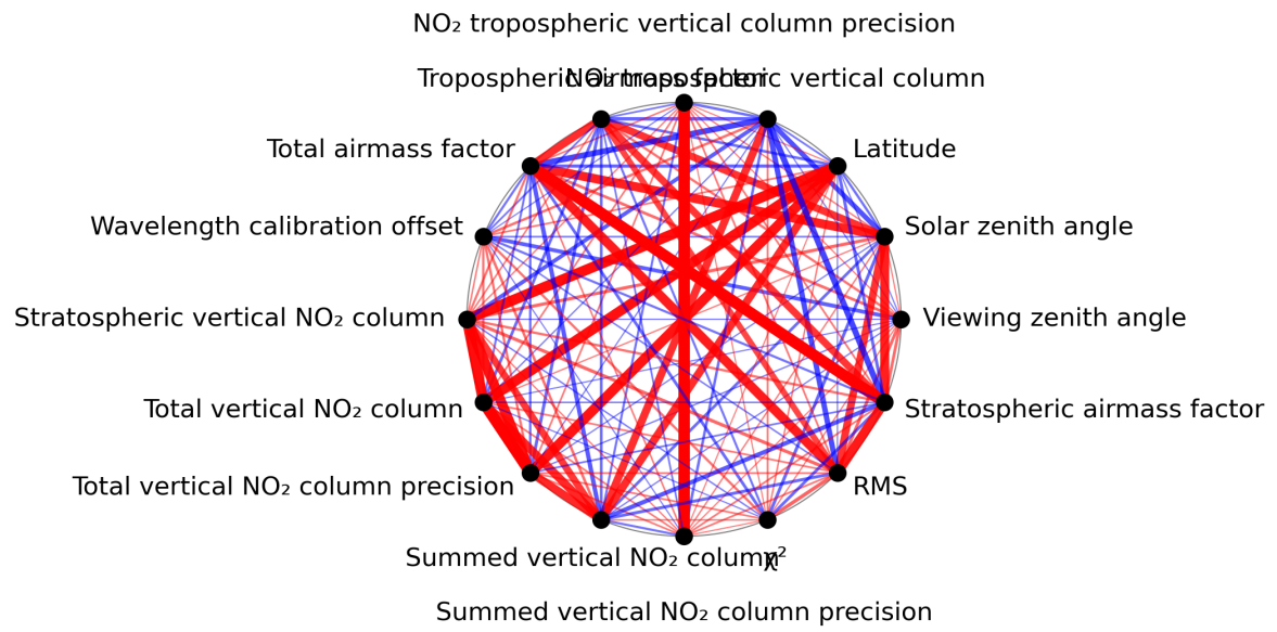
Figure 1: Map of correlation graph for 2023-07-11 to 2023-07-13.
