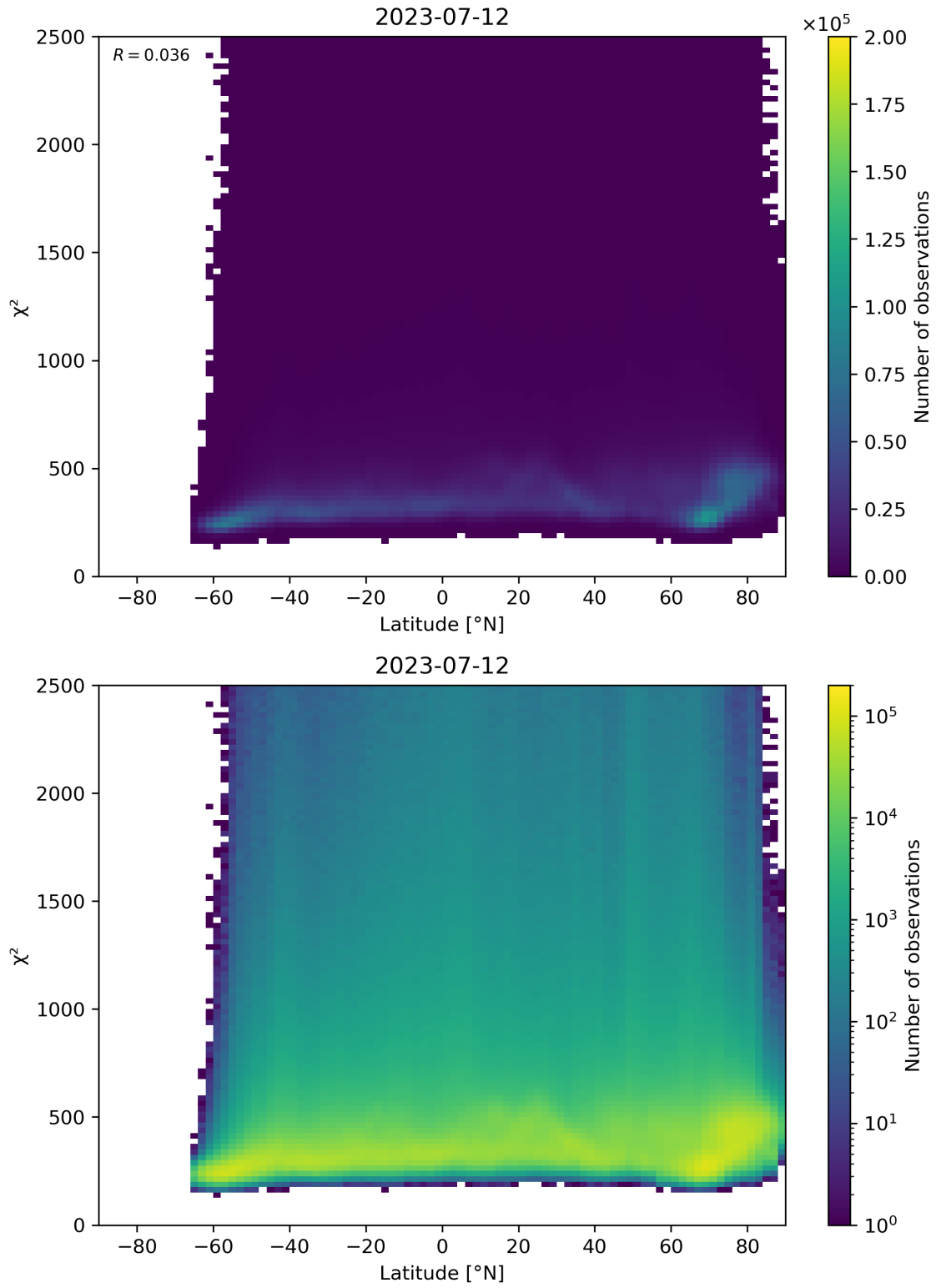
Figure 86: Scatter density plot of “Latitude” against “ \chi^2 ” for 2023-07-11 to 2023-07-13.
