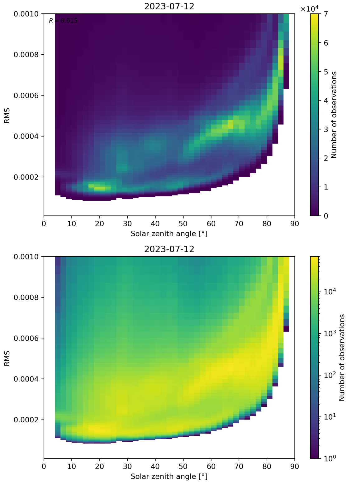
Figure 157: Scatter density plot of “Solar zenith angle” against “RMS” for 2023-07-11 to 2023-07-13.
