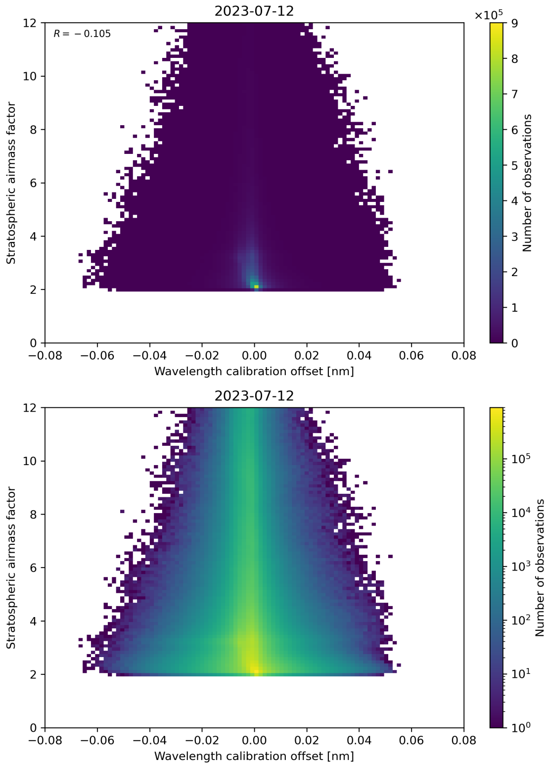
Figure 174: Scatter density plot of “Wavelength calibration offset” against “Stratospheric airmass factor” for 2023-07-11 to 2023-07-13.
