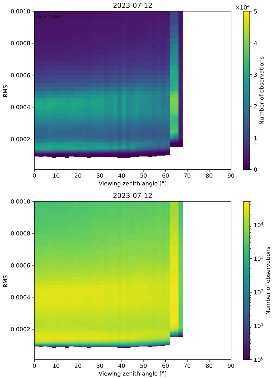
Figure 171: Scatter density plot of “Viewing zenith angle” against “RMS” for 2023-07-11 to 2023-07-13.
