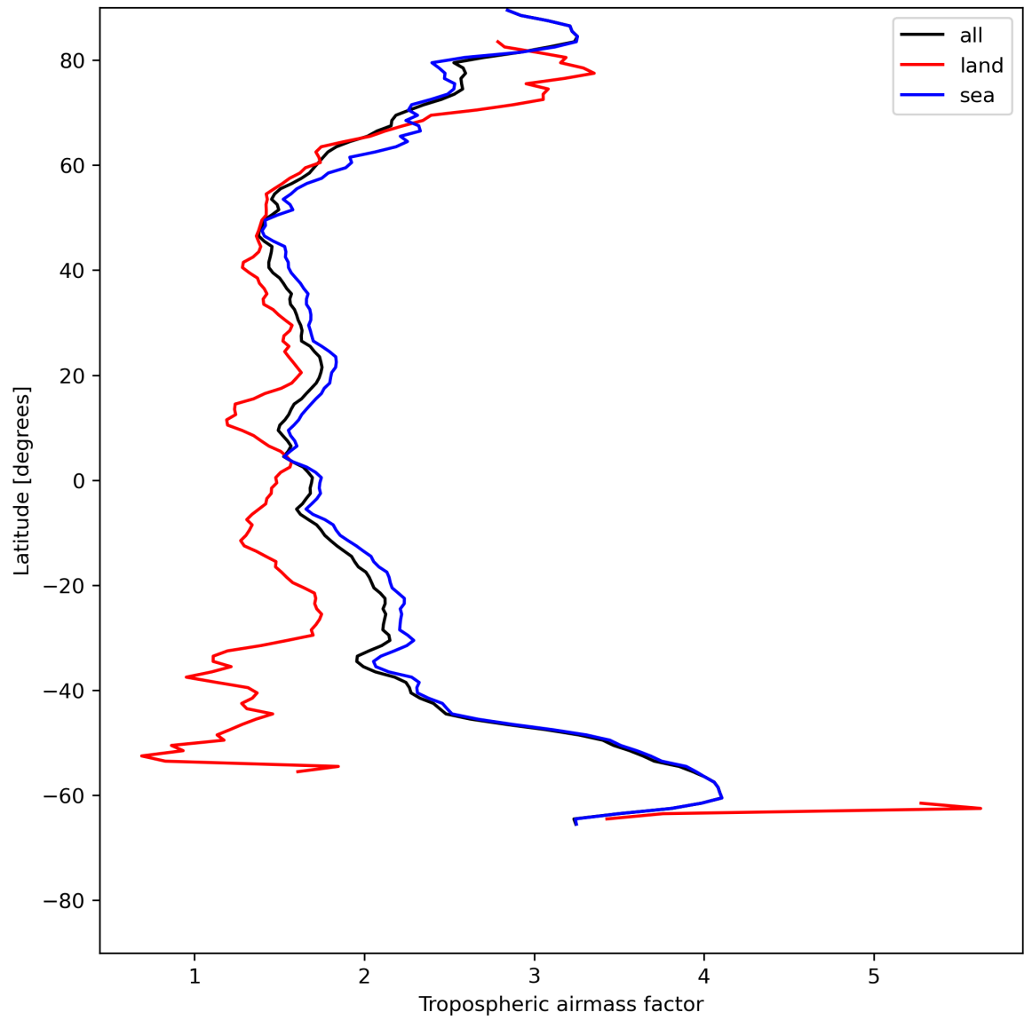
Figure 14: Zonal average of “Tropospheric airmass factor” for 2023-07-11 to 2023-07-13.
