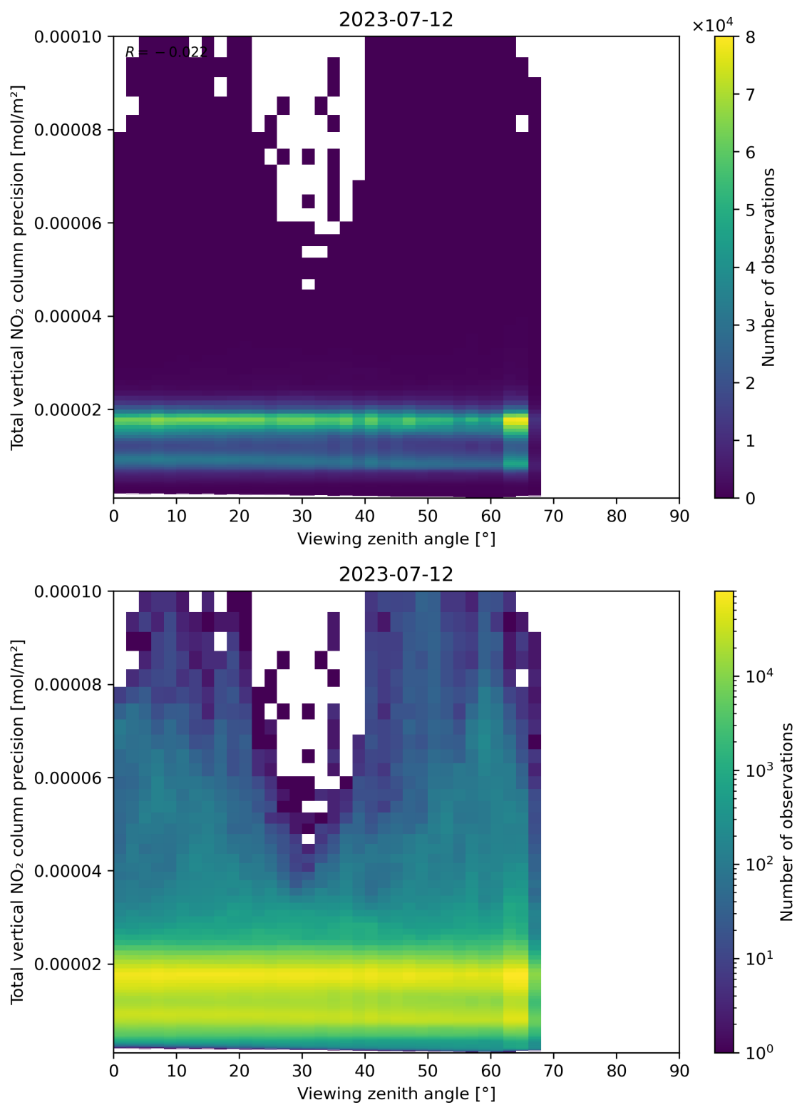
Figure 168: Scatter density plot of “Viewing zenith angle” against “Total vertical NO 2 column precision” for 2023-07-11 to 2023-07-13.
