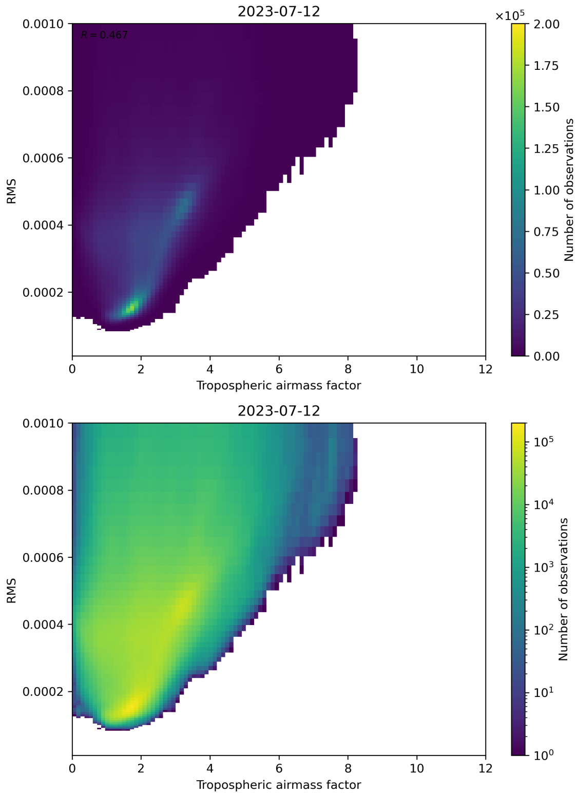
Figure 79: Scatter density plot of “Tropospheric airmass factor” against “RMS” for 2023-07-11 to 2023-07-13.
