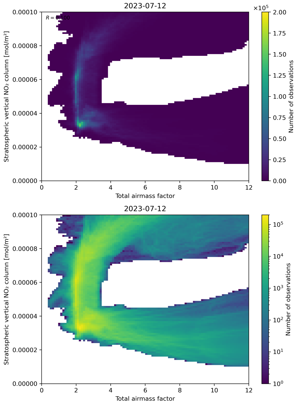
Figure 64: Scatter density plot of “Total airmass factor” against “Stratospheric vertical NO 2 column” for 2023-07-11 to 2023-07-13.
