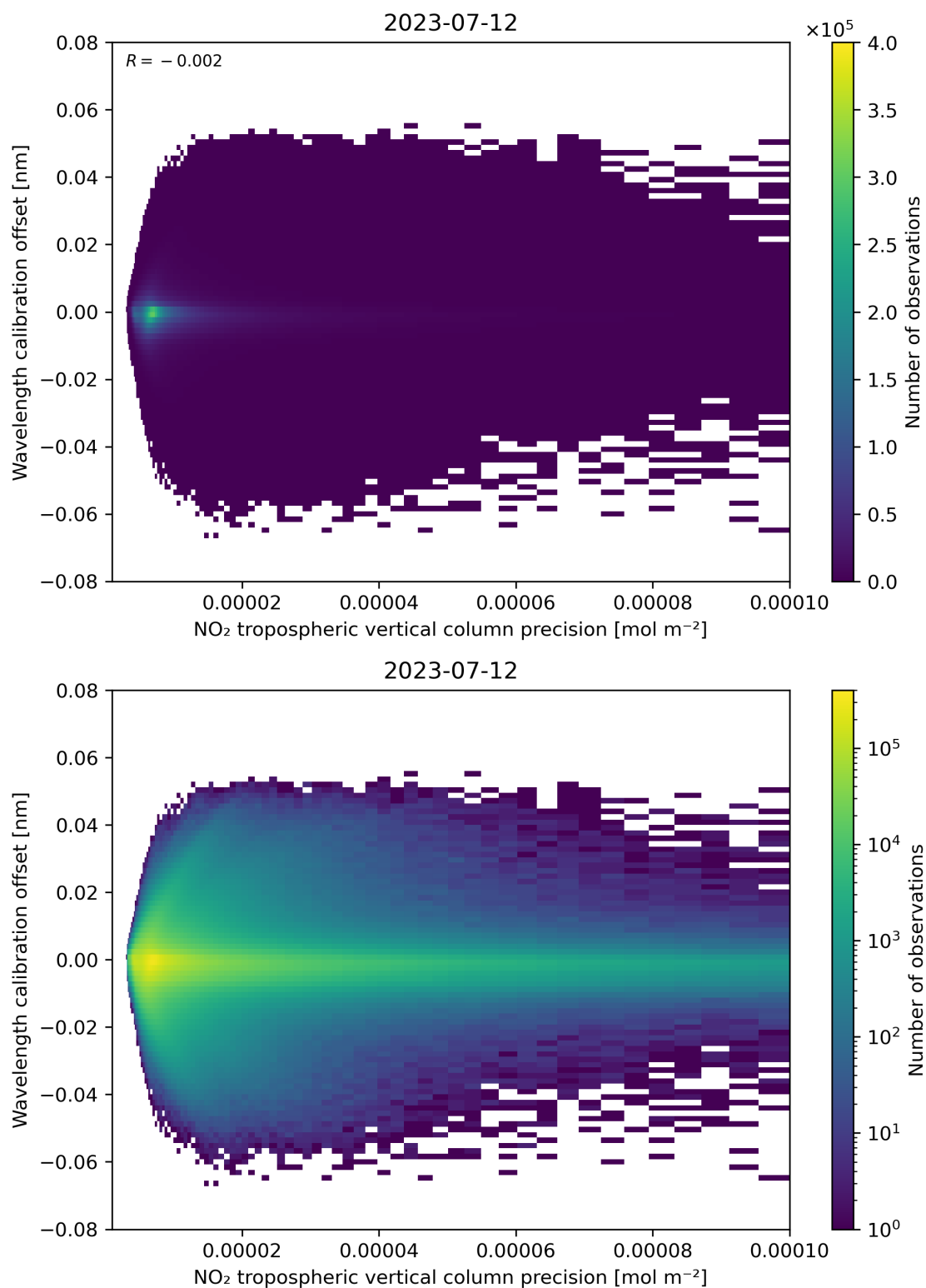
Figure 141: Scatter density plot of “NO 2 tropospheric vertical column precision” against “Wavelength calibration offset” for 2023-07-11 to 2023-07-13.
