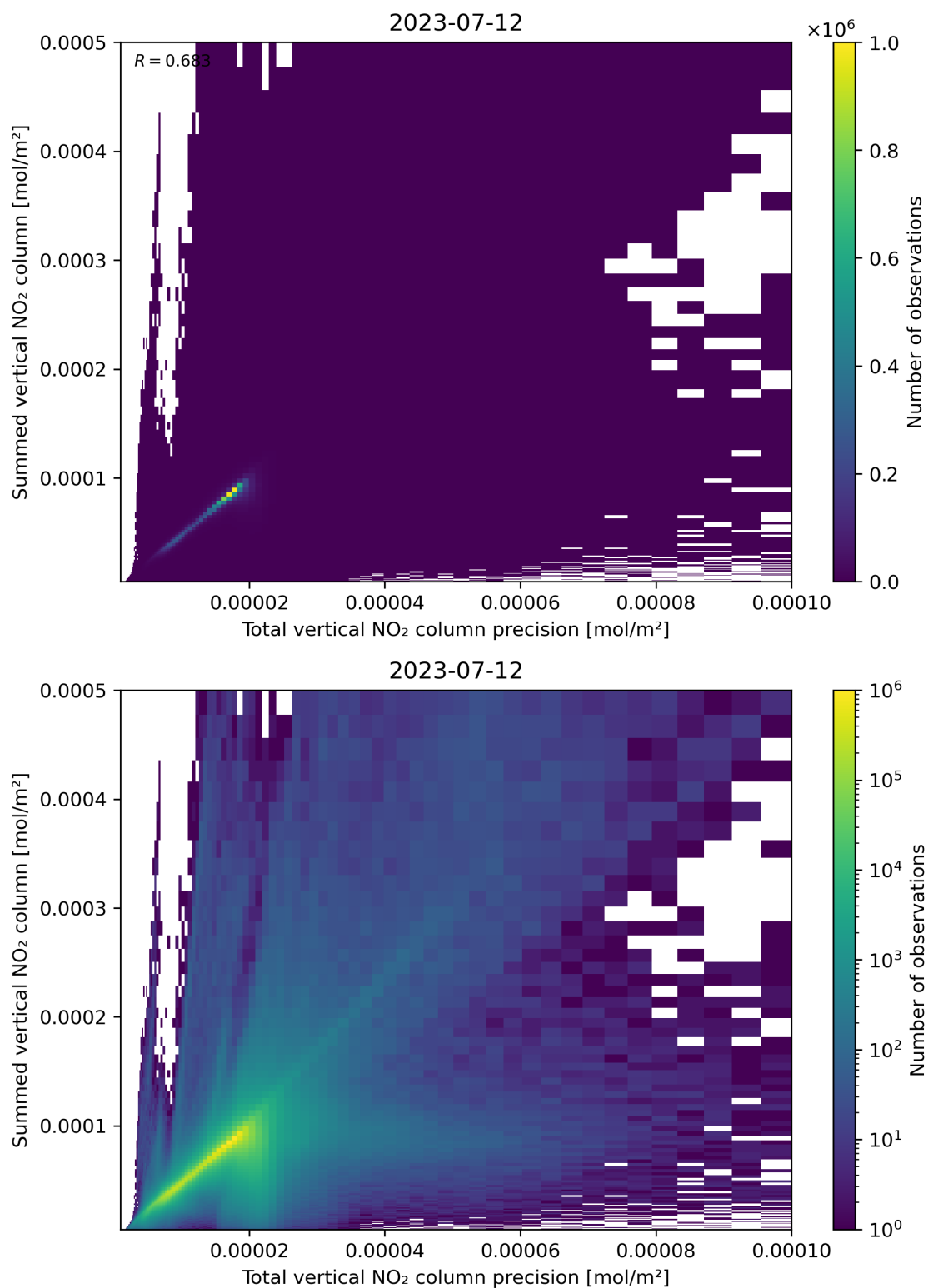
Figure 117: Scatter density plot of “Total vertical NO 2 column precision” against “Summed vertical NO 2 column” for 2023-07-11 to 2023-07-13.
