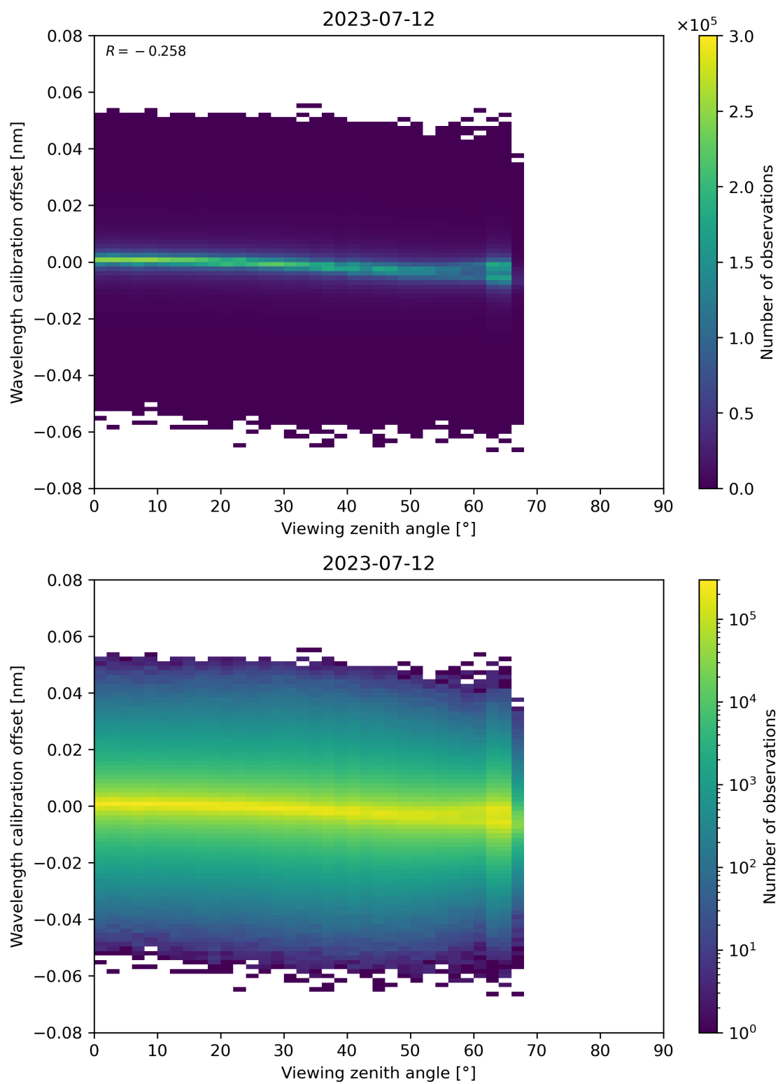
Figure 173: Scatter density plot of “Viewing zenith angle” against “Wavelength calibration offset” for 2023-07-11 to 2023-07-13.
