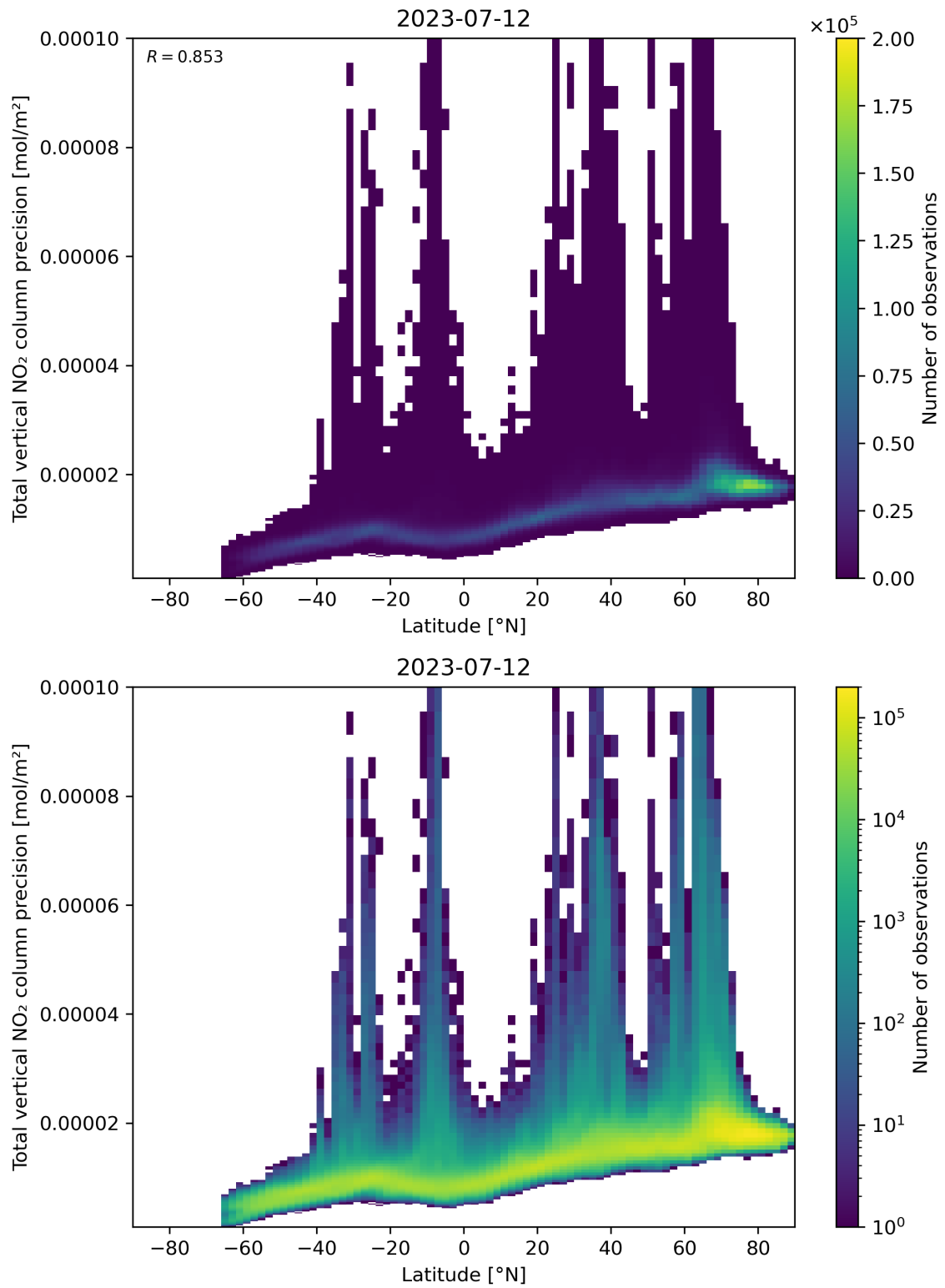
Figure 91: Scatter density plot of “Latitude” against “Total vertical NO 2 column precision” for 2023-07-11 to 2023-07-13.
