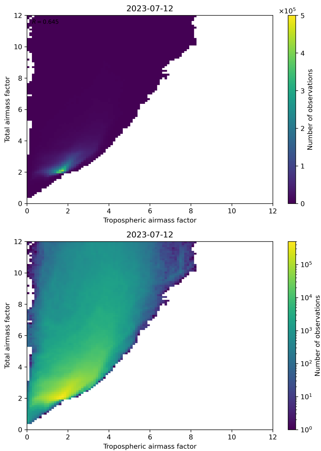
Figure 72: Scatter density plot of “Tropospheric airmass factor” against “Total airmass factor” for 2023-07-11 to 2023-07-13.
