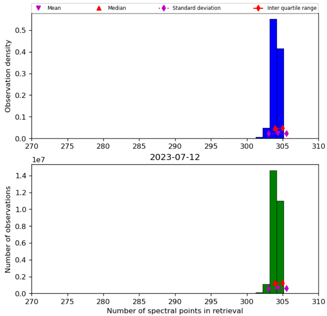
Figure 33: Histogram of “Number of spectral points in retrieval” for 2023-07-11 to 2023-07-13
