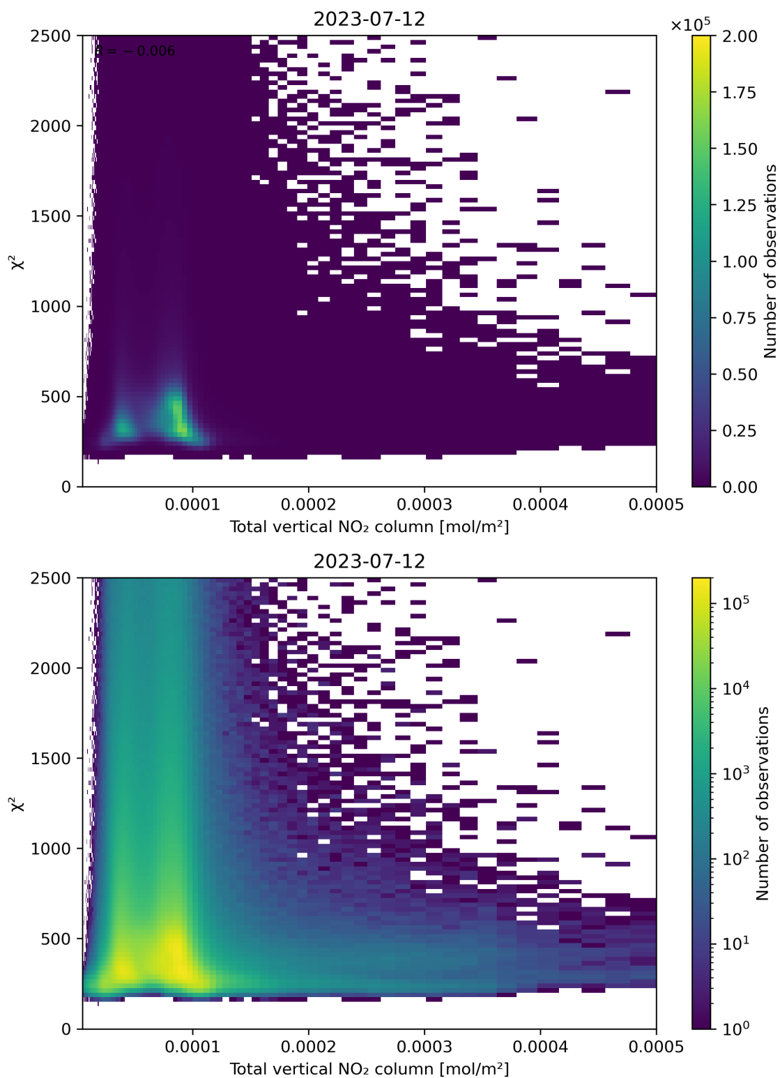
Figure 111: Scatter density plot of “Total vertical NO 2 column” against “ \chi^2 ” for 2023-07-11 to 2023-07-13.
