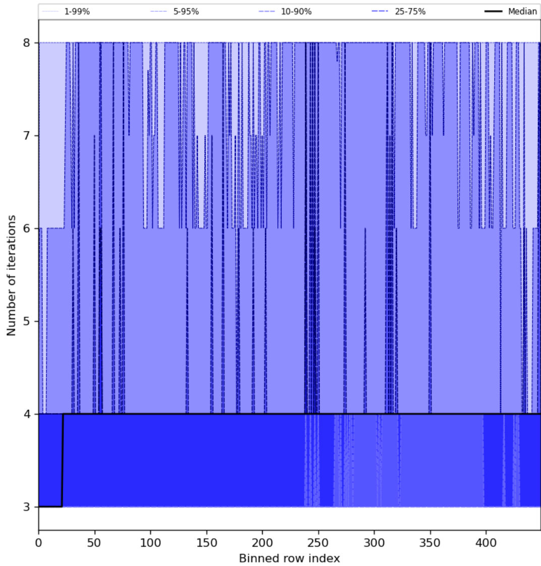
Figure 51: Along track statistics of “Number of iterations” for 2023-07-11 to 2023-07-13
