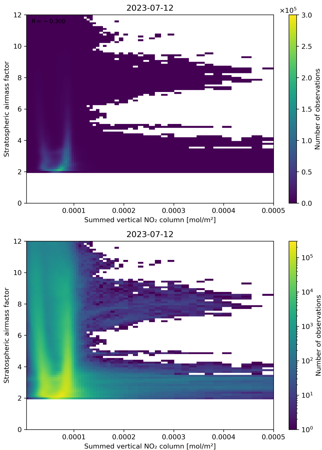
Figure 103: Scatter density plot of “Summed vertical NO 2 column” against “Stratospheric airmass factor” for 2023-07-11 to 2023-07-13.
