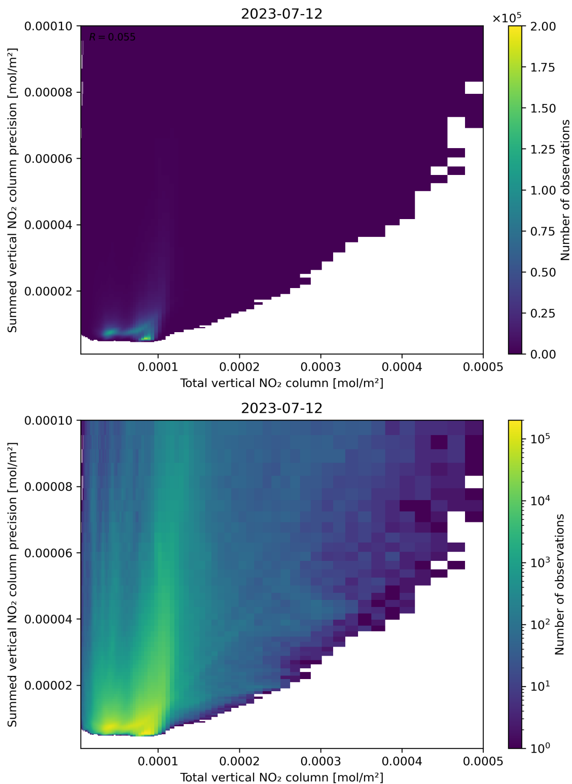
Figure 113: Scatter density plot of “Total vertical NO 2 column” against “Summed vertical NO 2 column precision” for 2023-07-11 to 2023-07-13.
