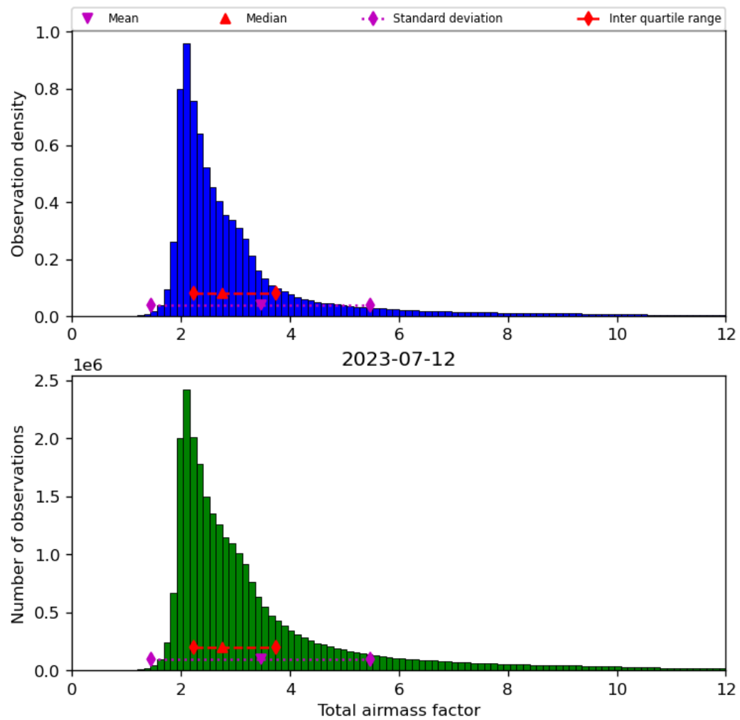
Figure 32: Histogram of “Total airmass factor” for 2023-07-11 to 2023-07-13
