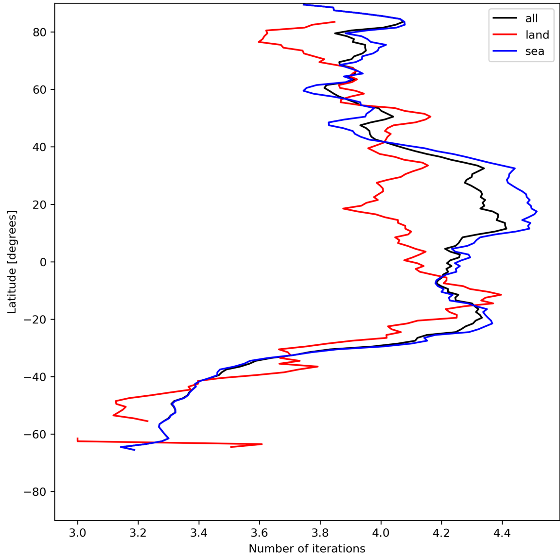
Figure 17: Zonal average of “Number of iterations” for 2023-07-11 to 2023-07-13.
