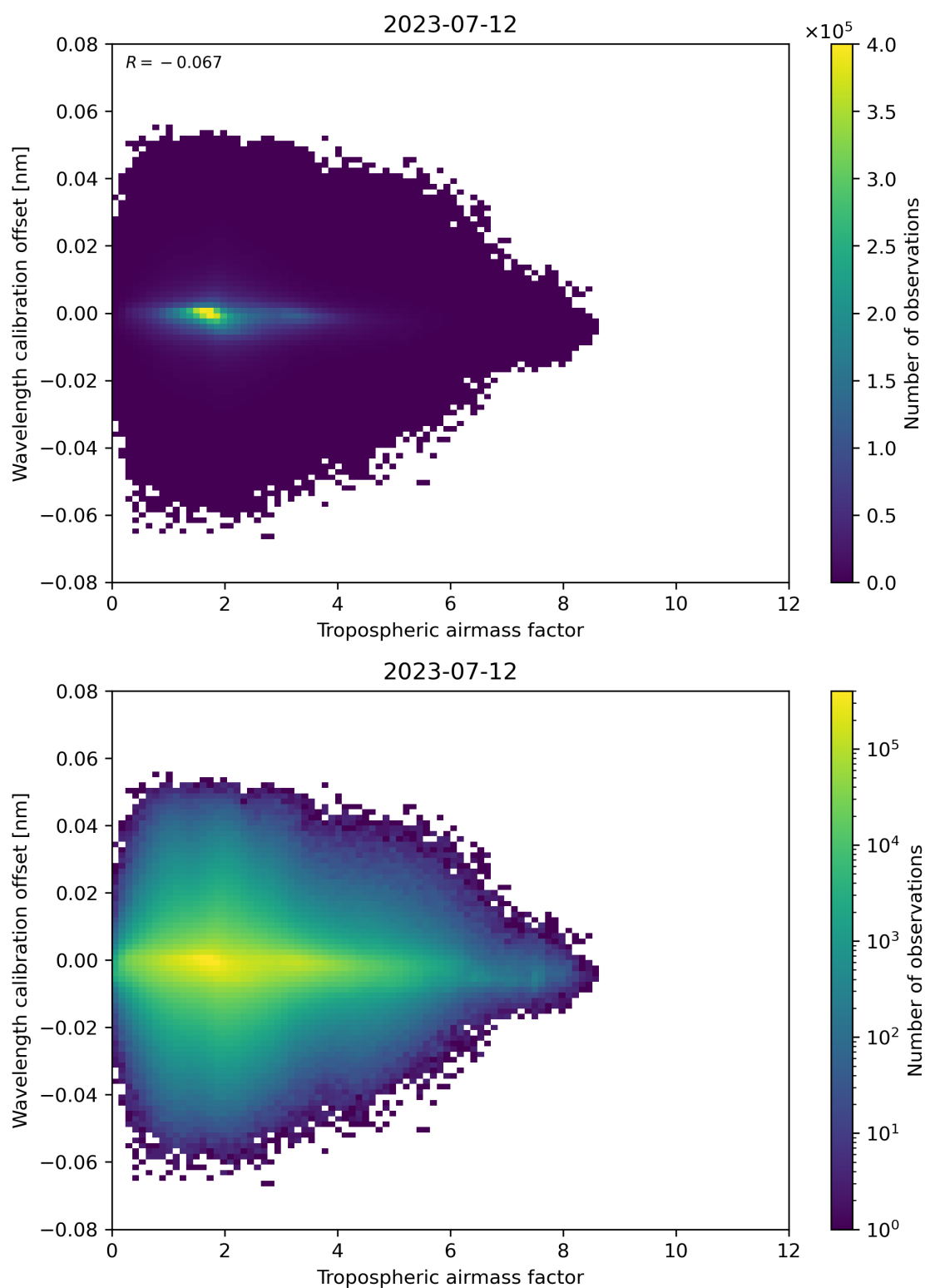
Figure 80: Scatter density plot of “Tropospheric air mass factor” against “Wavelength calibration offset” for 2023-07-11 to 2023-07-13.
