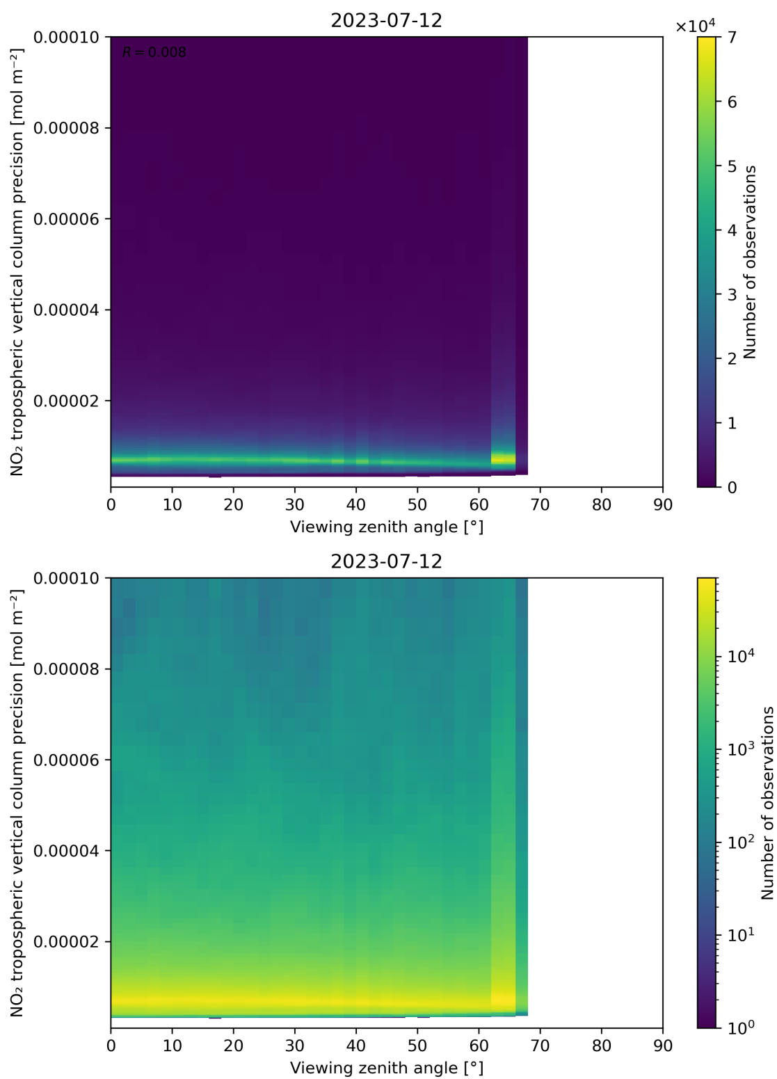
Figure 170: Scatter density plot of “Viewing zenith angle” against “NO 2 tropospheric vertical column precision” for 2023-07-11 to 2023-07-13.
