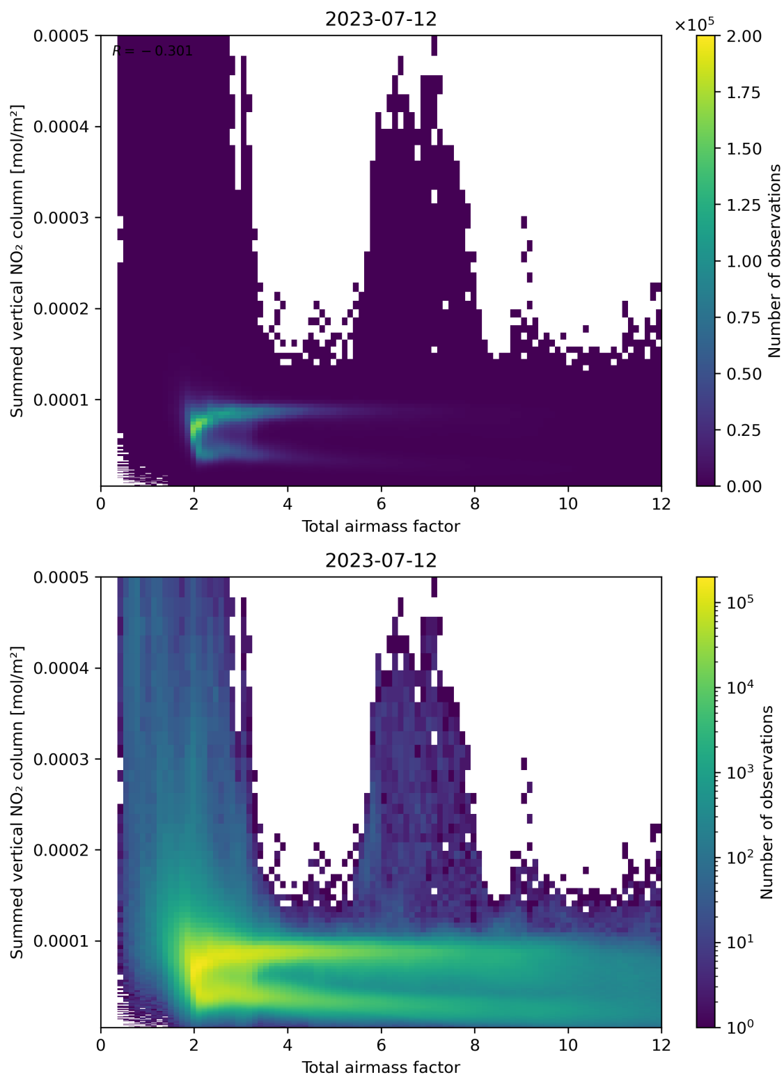
Figure 65: Scatter density plot of “Total airmass factor” against “Summed vertical NO 2 column” for 2023-07-11 to 2023-07-13.
