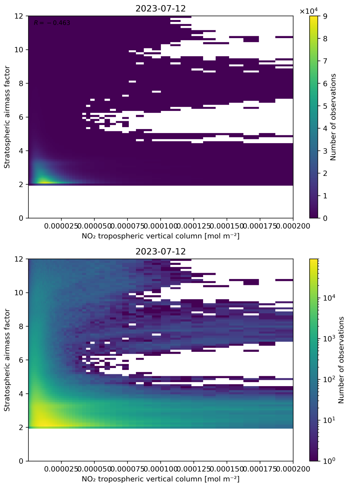
Figure 121: Scatter density plot of “NO 2 tropospheric vertical column” against “Stratospheric air mass factor” for 2023-07-11 to 2023-07-13.
