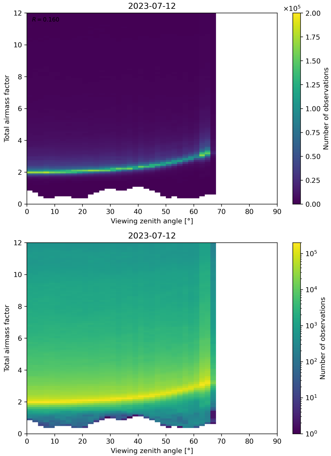
Figure 160: Scatter density plot of “Viewing zenith angle” against “Total airmass factor” for 2023-07-11 to 2023-07-13.
