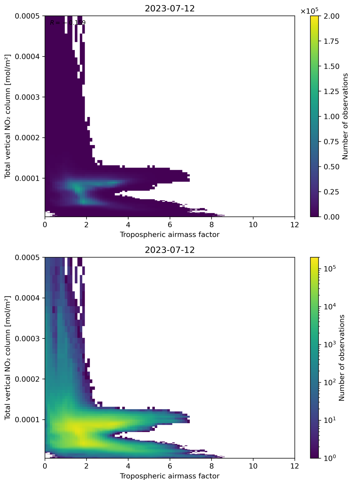
Figure 77: Scatter density plot of “Tropospheric airmass factor” against “Total vertical NO 2 column” for 2023-07-11 to 2023-07-13.
