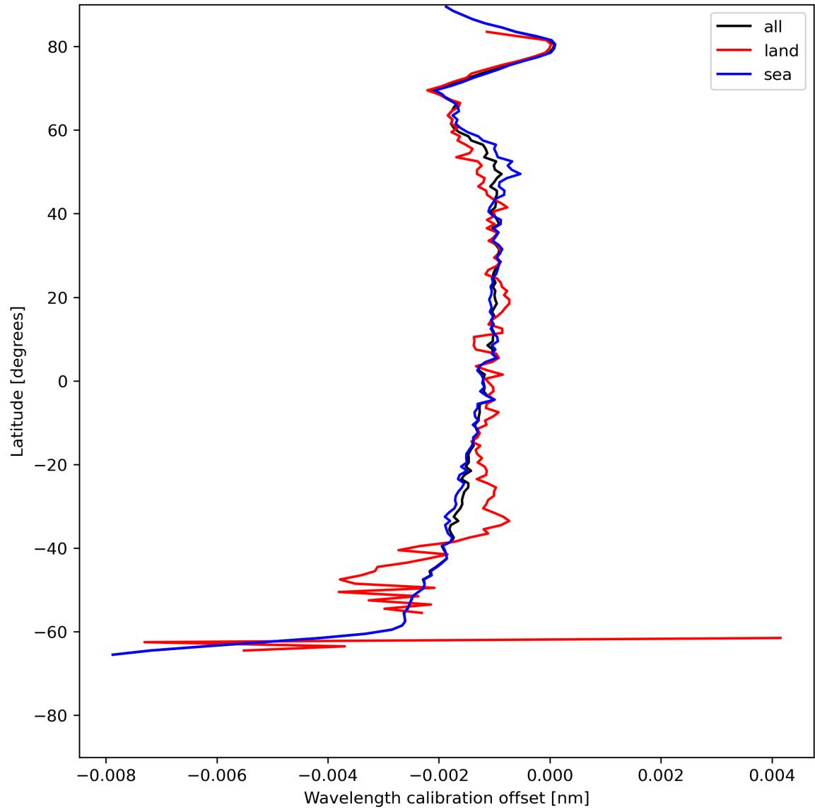
Figure 18: Zonal average of “Wavelength calibration offset” for 2023-07-11 to 2023-07-13.
