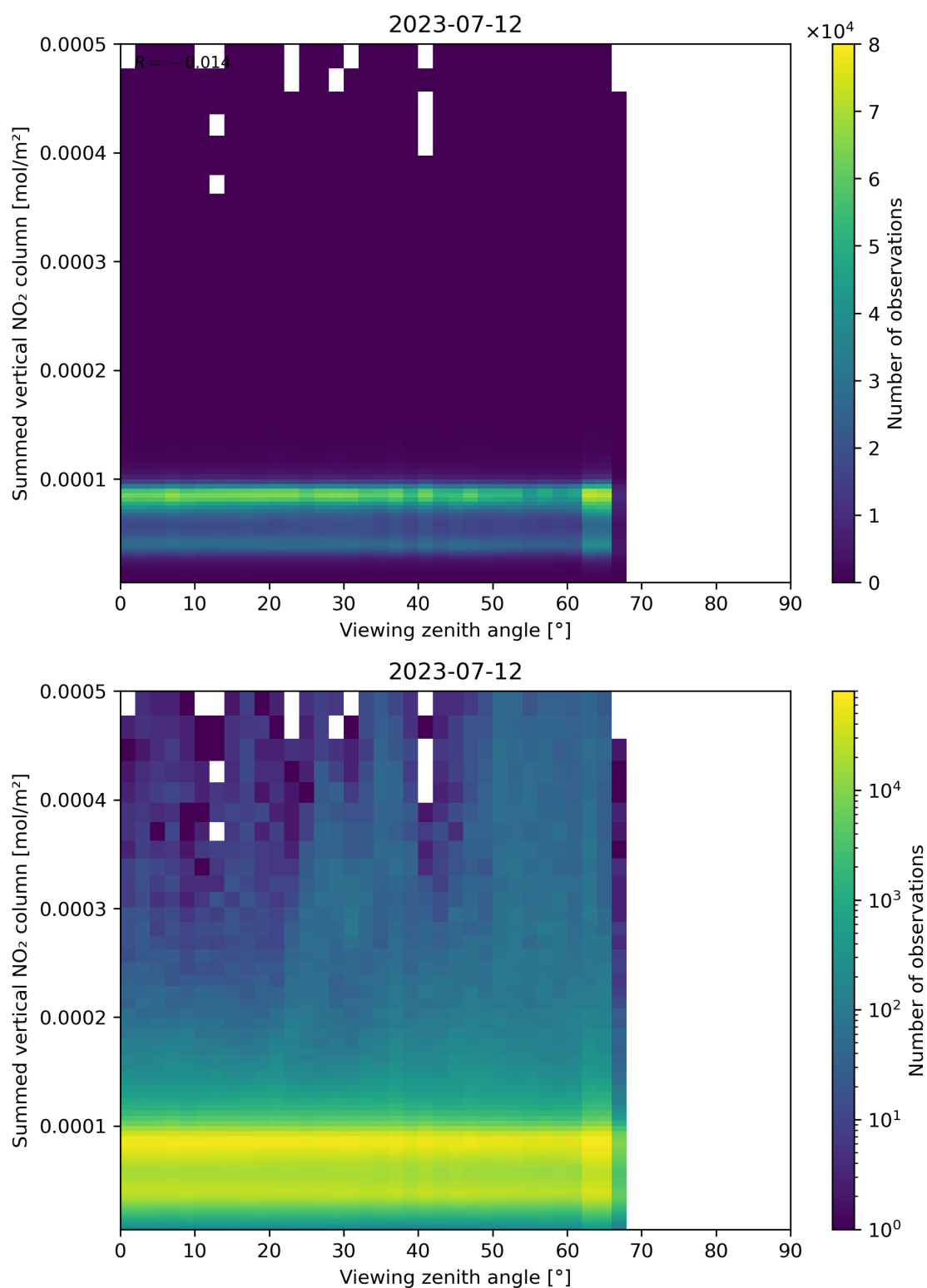
Figure 165: Scatter density plot of “Viewing zenith angle” against “Summed vertical NO 2 column” for 2023-07-11 to 2023-07-13.
