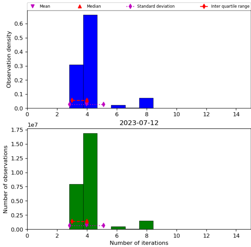
Figure 34: Histogram of “Number of iterations” for 2023-07-11 to 2023-07-13
