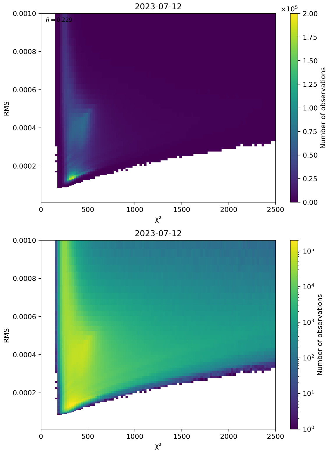
Figure 82: Scatter density plot of “ \chi^2 ” against “RMS” for 2023-07-11 to 2023-07-13.
