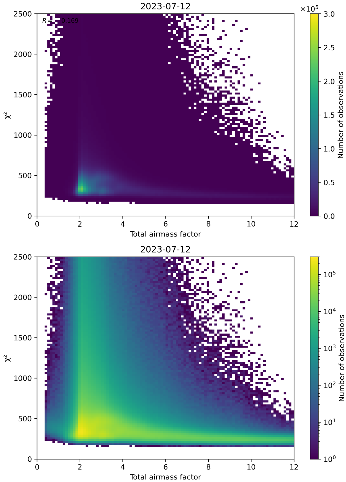
Figure 63: Scatter density plot of “Total airmass factor” against “ \chi^2 ” for 2023-07-11 to 2023-07-13.
