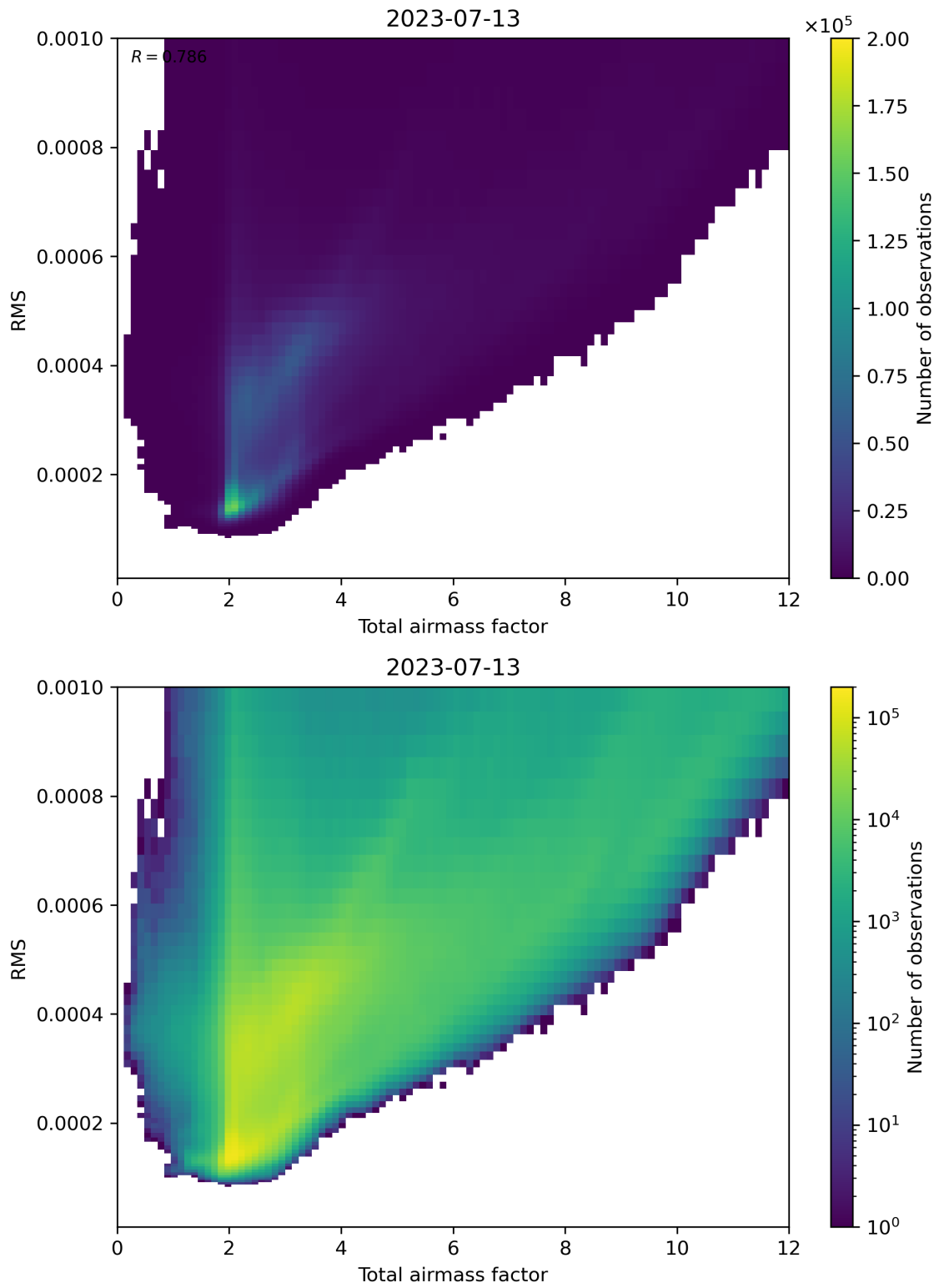
Figure 69: Scatter density plot of “Total airmass factor” against “RMS” for 2023-07-13 to 2023-07-14.
