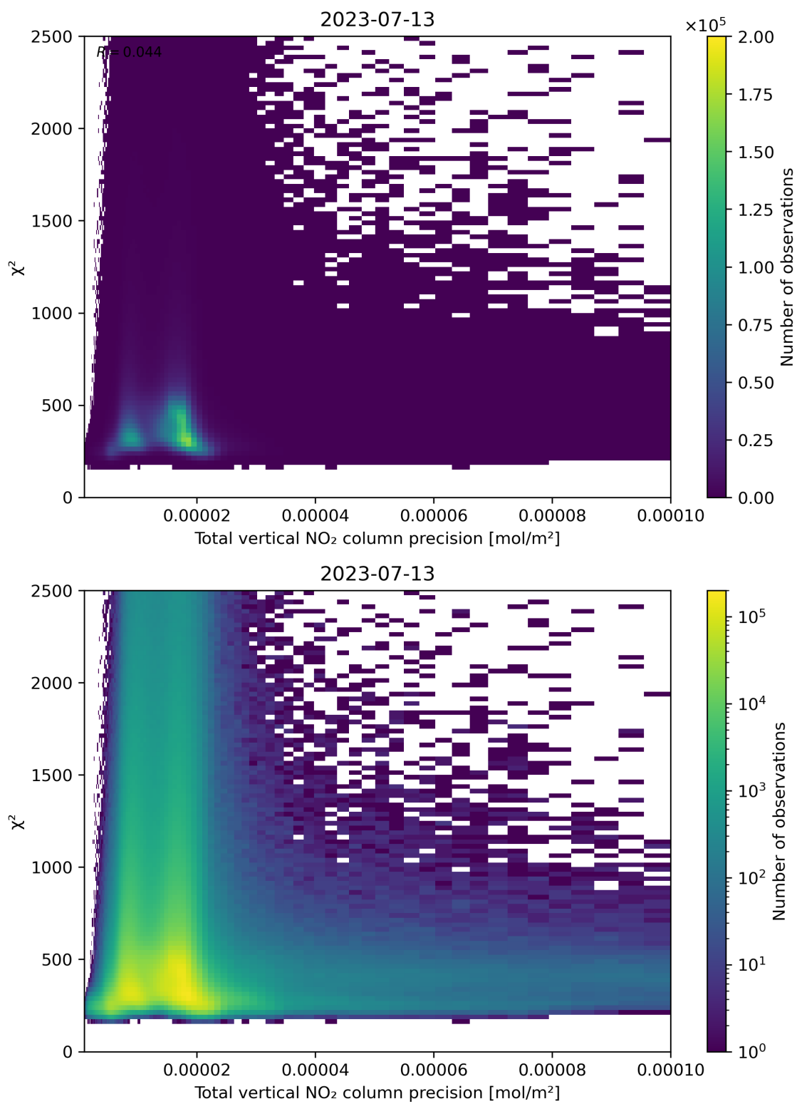
Figure 116: Scatter density plot of “Total vertical NO 2 column precision” against “ \chi^2 ” for 2023-07-13 to 2023-07-14.
