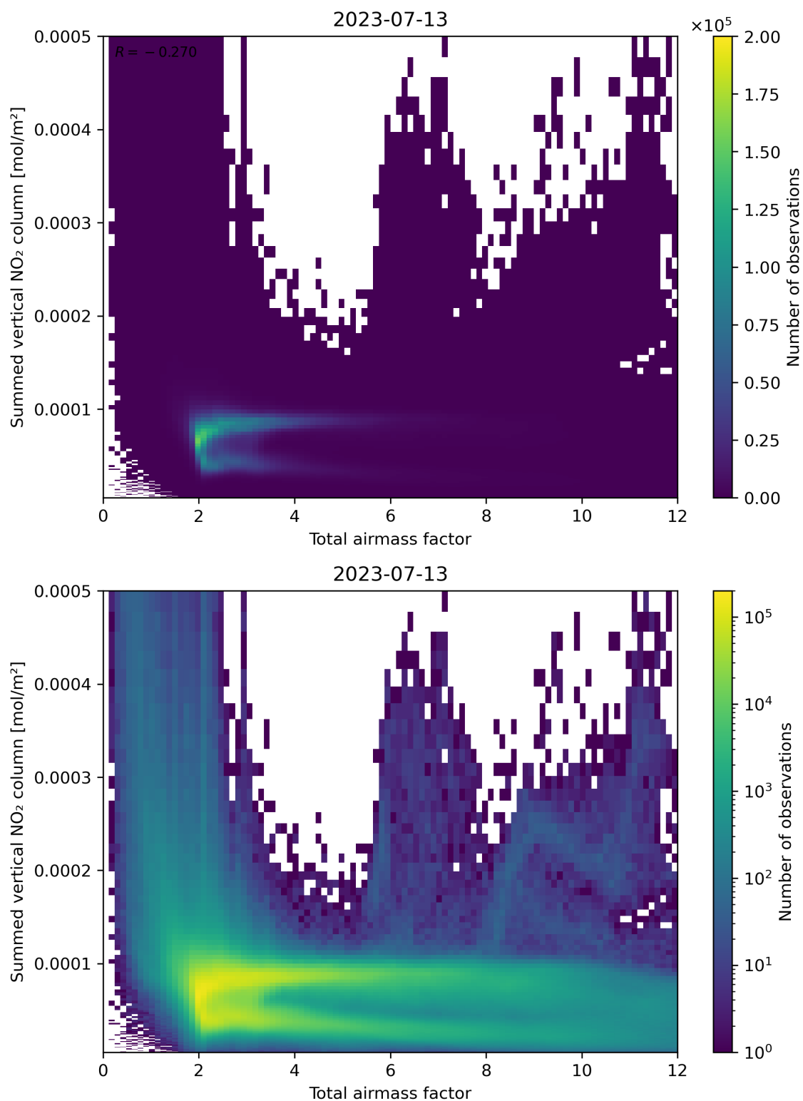
Figure 65: Scatter density plot of “Total airmass factor” against “Summed vertical NO 2 column” for 2023-07-13 to 2023-07-14.
