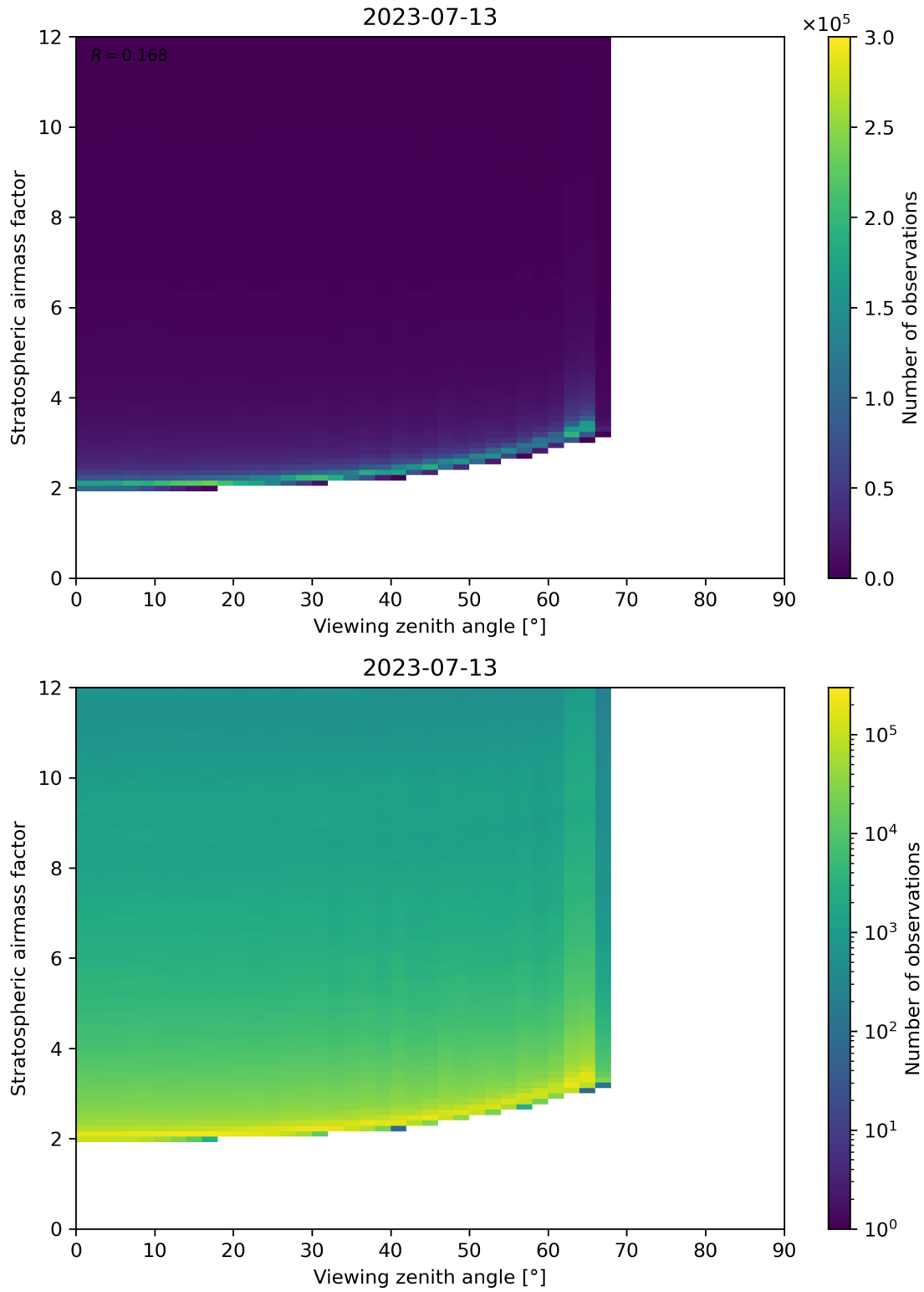
Figure 159: Scatter density plot of “Viewing zenith angle” against “Stratospheric airmass factor” for 2023-07-13 to 2023-07-14.
