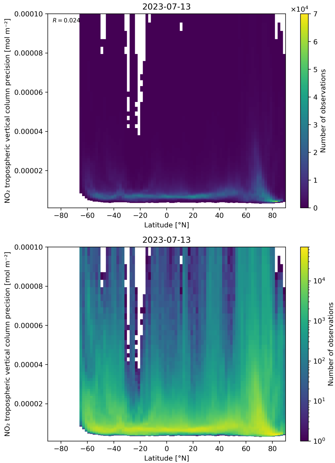
Figure 93: Scatter density plot of “Latitude” against “NO 2 tropospheric vertical column precision” for 2023-07-13 to 2023-07-14.
