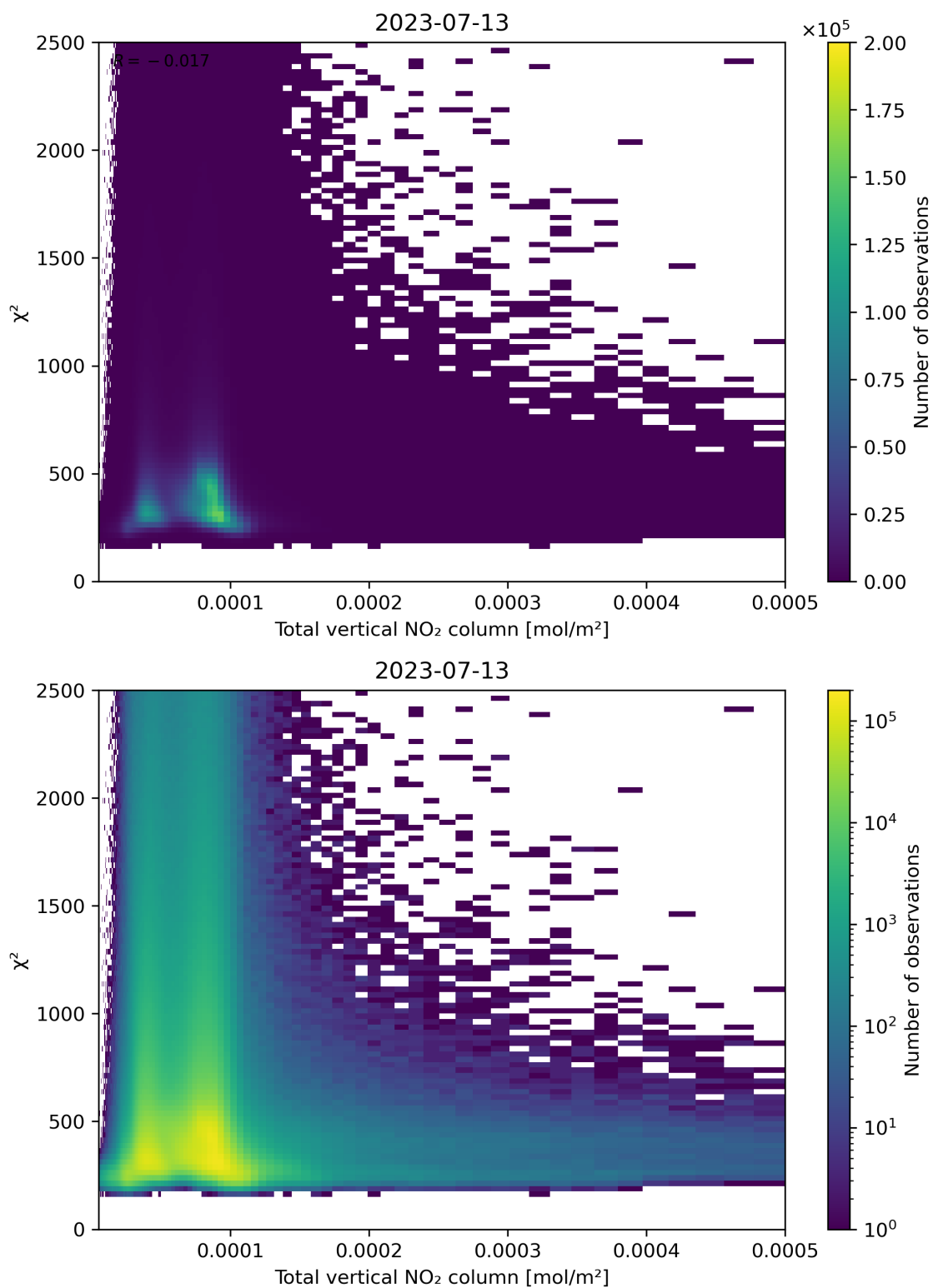
Figure 111: Scatter density plot of “Total vertical NO 2 column” against “ \chi^2 ” for 2023-07-13 to 2023-07-14.
