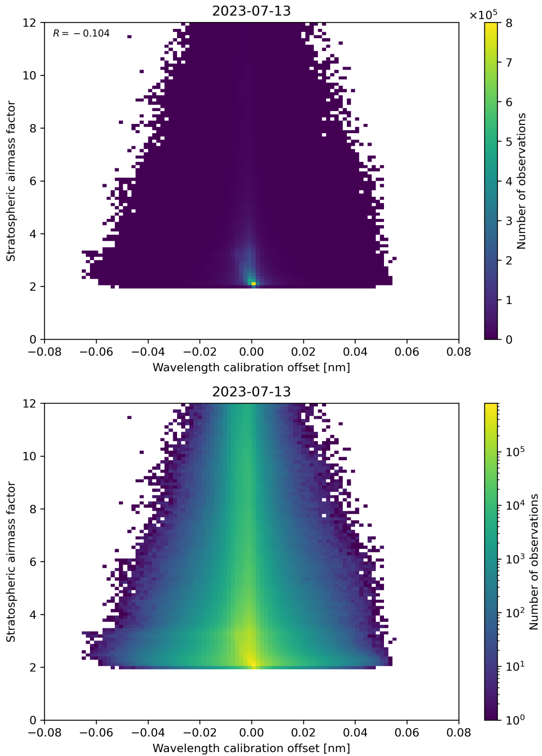
Figure 174: Scatter density plot of “Wavelength calibration offset” against “Stratospheric airmass factor” for 2023-07-13 to 2023-07-14.
