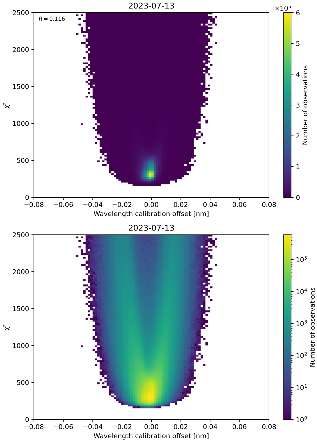
Figure 175: Scatter density plot of “Wavelength calibration offset” against “ \chi^2 ” for 2023-07-13 to 2023-07-14.
