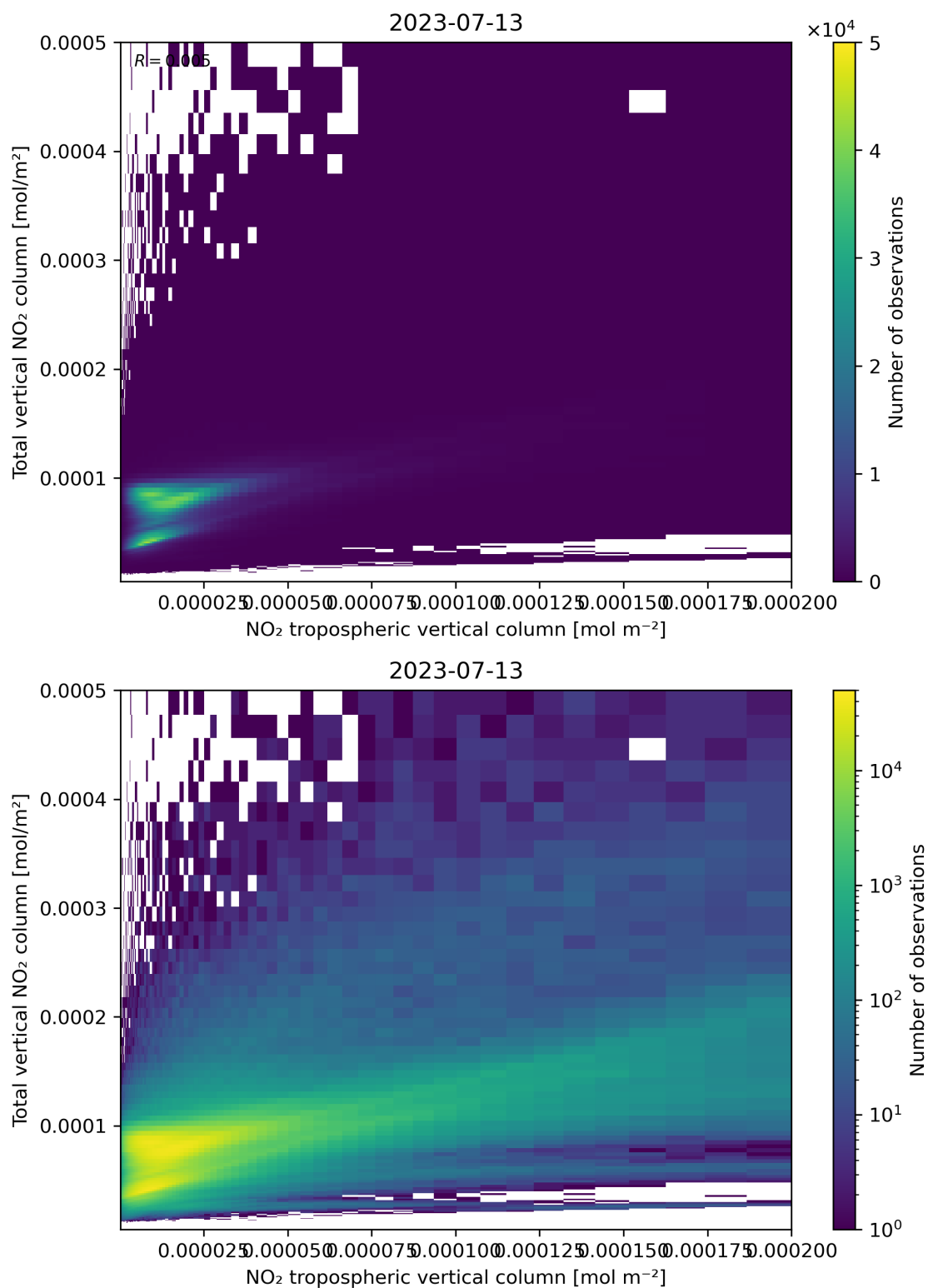
Figure 128: Scatter density plot of “NO 2 tropospheric vertical column” against “Total vertical NO 2 column” for 2023-07-13 to 2023-07-14.
