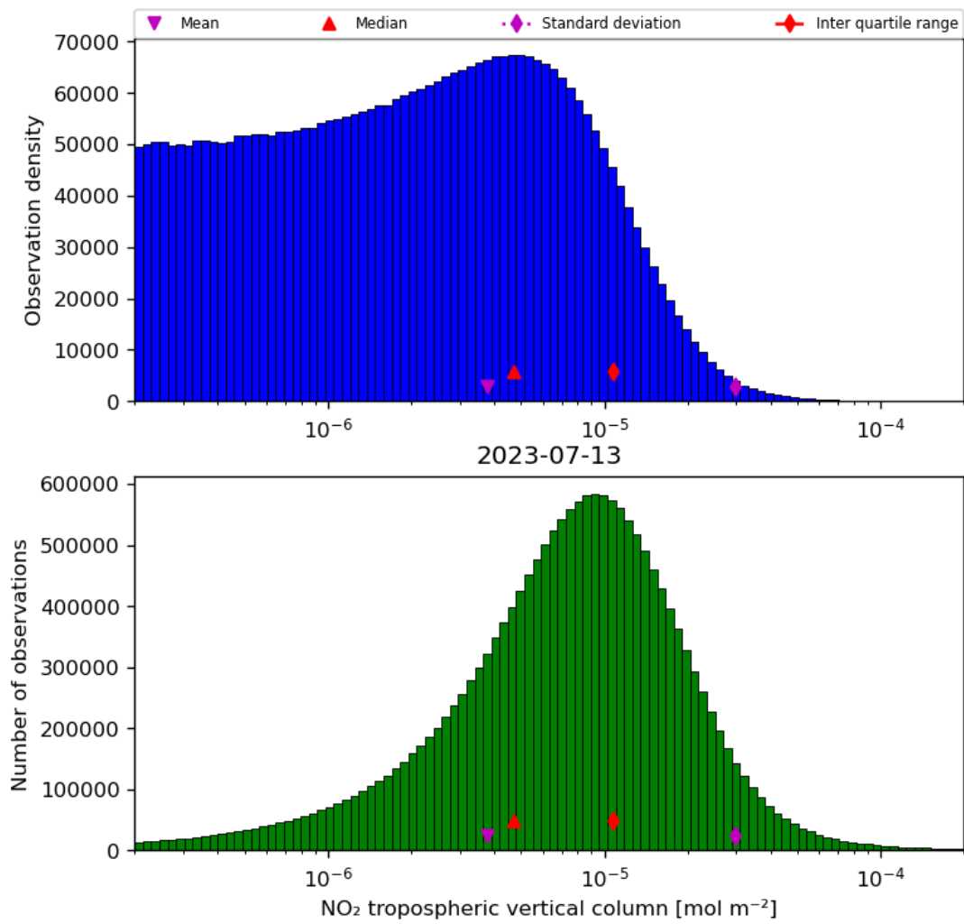
Figure 29: Histogram of “NO 2 tropospheric vertical column” for 2023-07-13 to 2023-07-14
