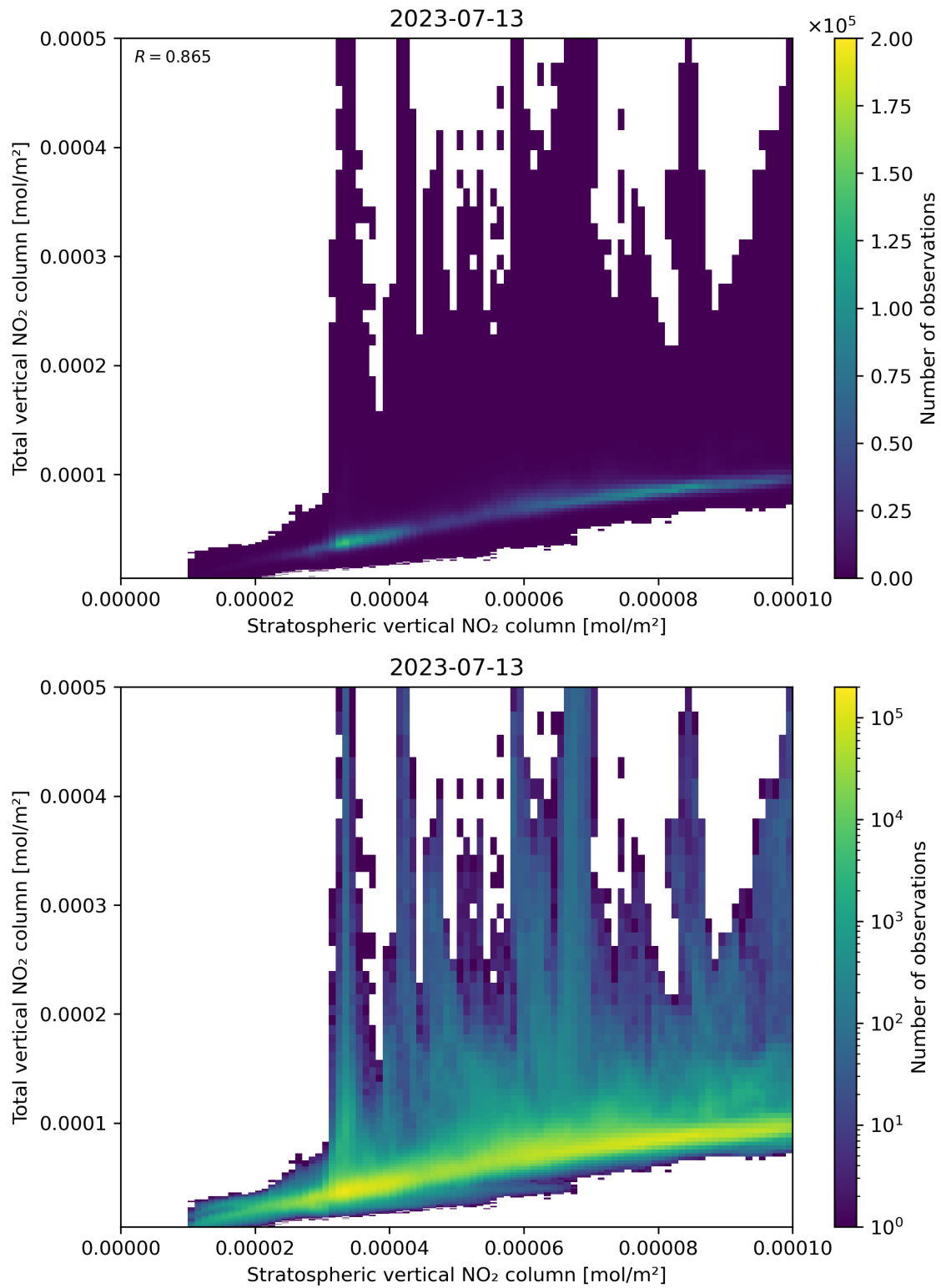
Figure 100: Scatter density plot of “Stratospheric vertical NO 2 column” against “Total vertical NO 2 column” for 2023-07-13 to 2023-07-14.
