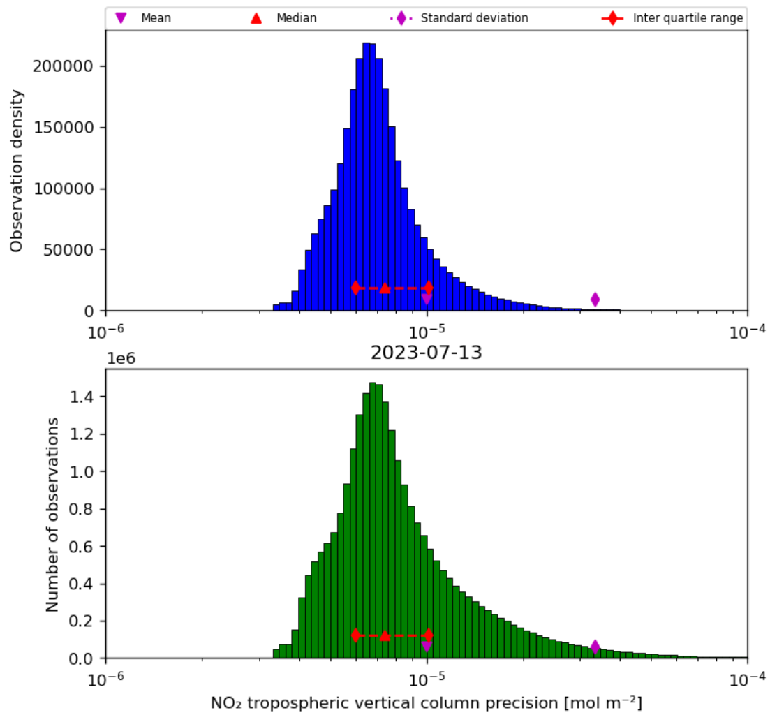
Figure 30: Histogram of “NO 2 tropospheric vertical column precision” for 2023-07-13 to 2023-07-14
