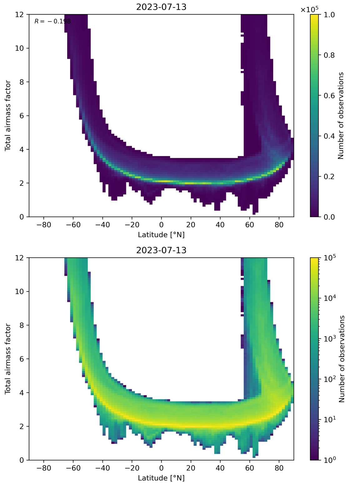
Figure 84: Scatter density plot of “Latitude” against “Total airmass factor” for 2023-07-13 to 2023-07-14.
