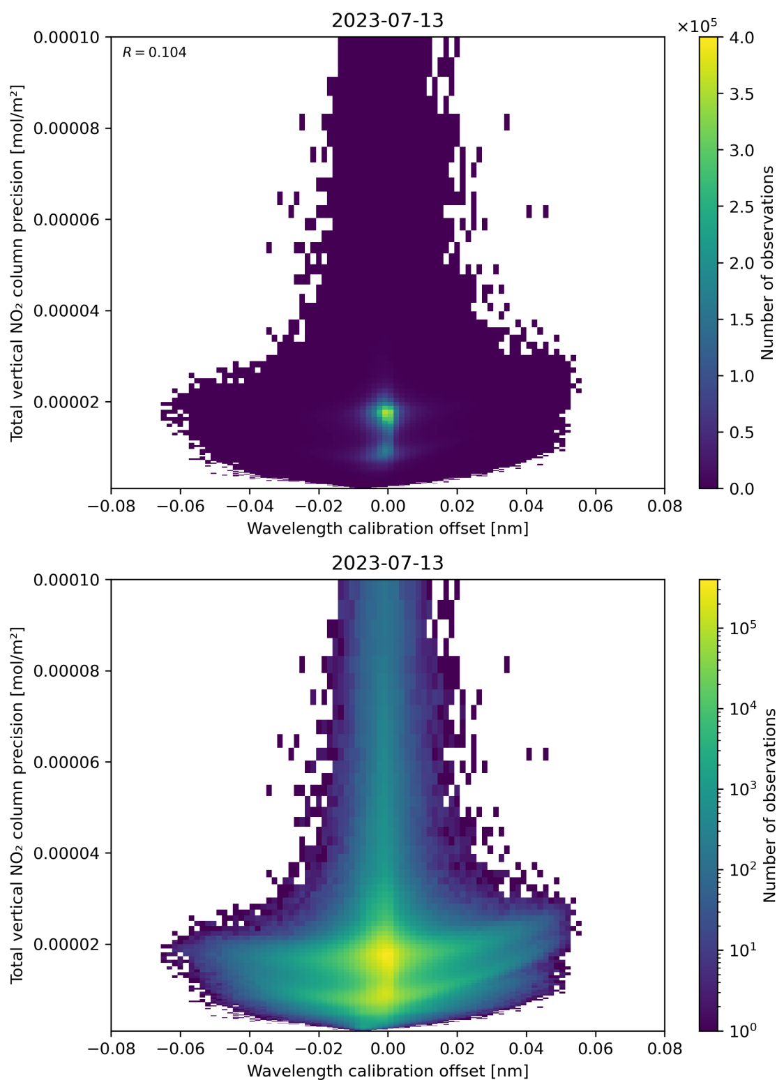
Figure 180: Scatter density plot of “Wavelength calibration offset” against “Total vertical NO 2 column precision” for 2023-07-13 to 2023-07-14.
