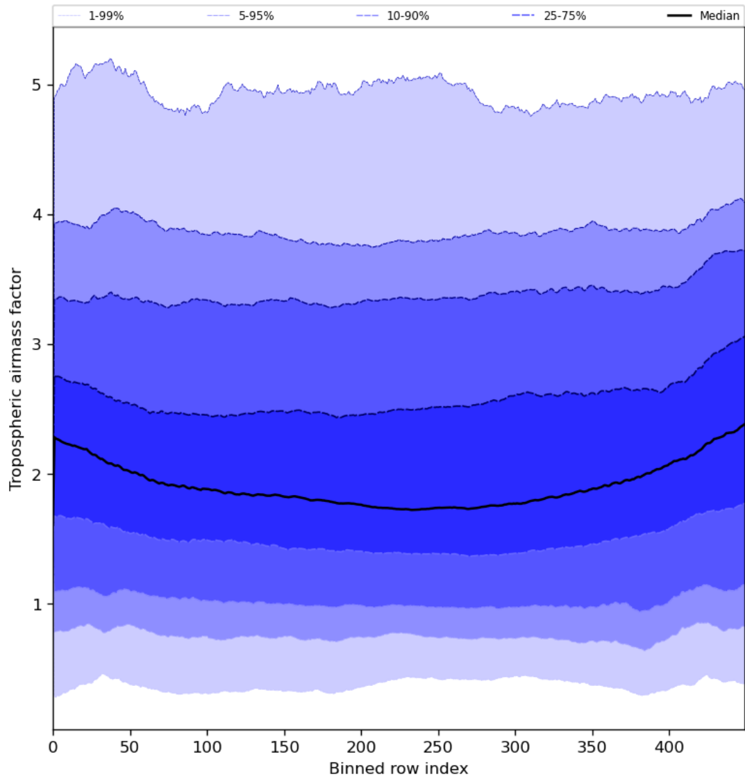
Figure 48: Along track statistics of “Tropospheric airmass factor” for 2023-07-13 to 2023-07-14
