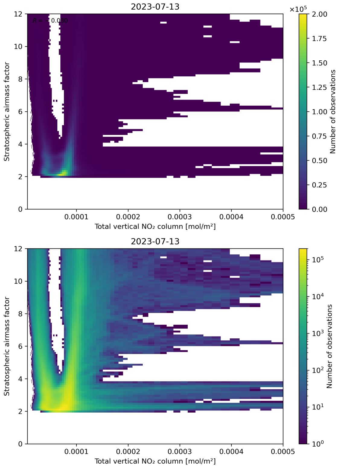
Figure 110: Scatter density plot of “Total vertical NO 2 column” against “Stratospheric airmass factor” for 2023-07-13 to 2023-07-14.
