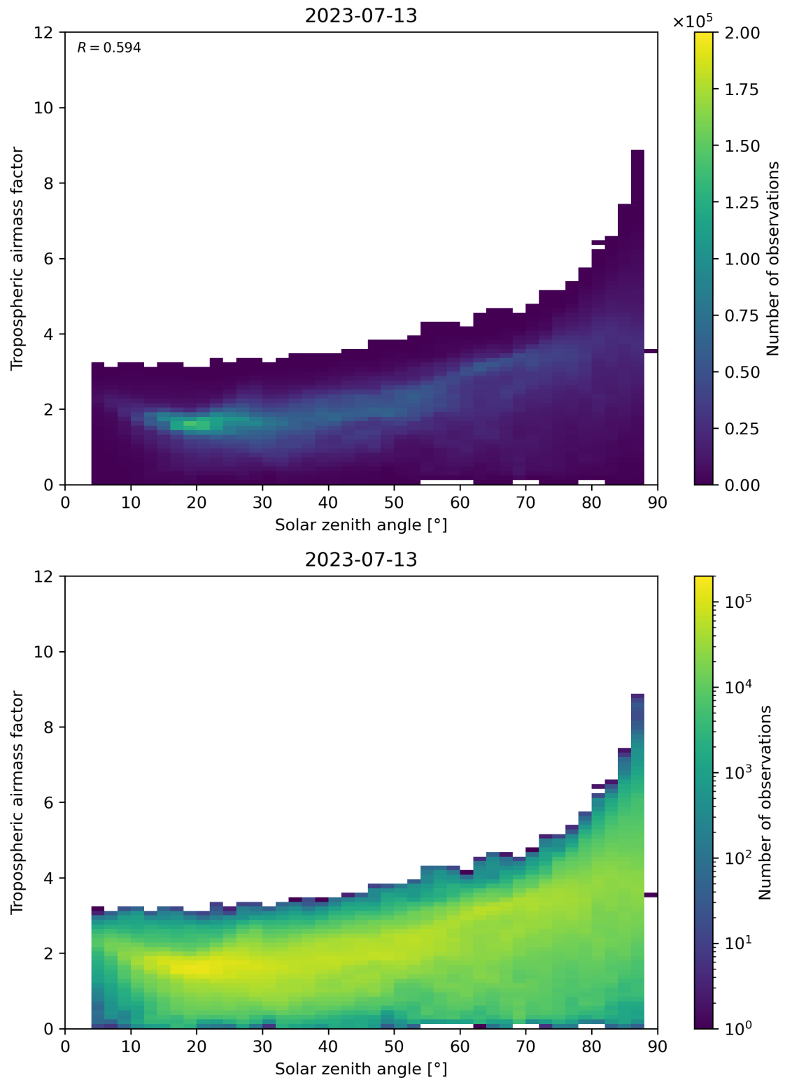
Figure 147: Scatter density plot of “Solar zenith angle” against “Tropospheric airmass factor” for 2023-07-13 to 2023-07-14.
