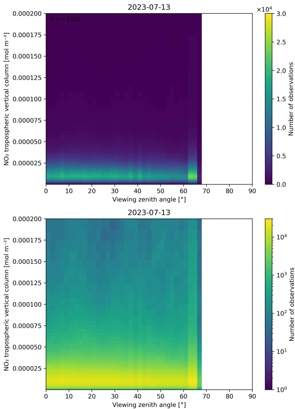
Figure 169: Scatter density plot of “Viewing zenith angle” against “NO 2 tropospheric vertical column” for 2023-07-13 to 2023-07-14.
