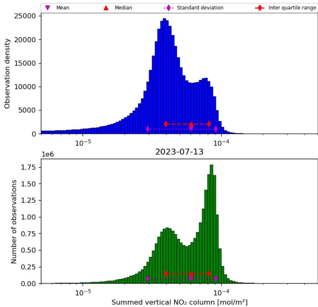
Figure 40: Histogram of "Summed vertical NO 2 column" for 2023-07-13 to 2023-07-14
