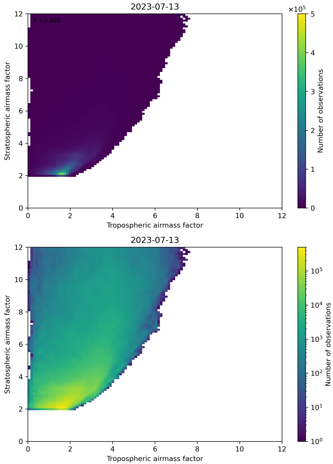
Figure 71: Scatter density plot of “Tropospheric airmass factor” against “Stratospheric airmass factor” for 2023-07-13 to 2023-07-14.
