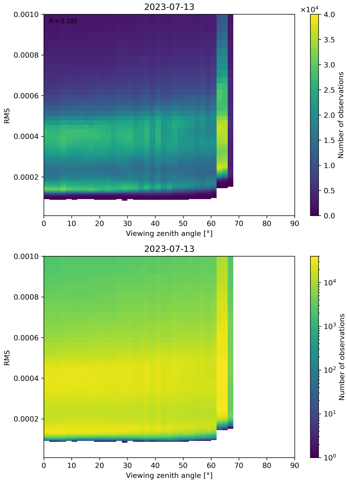
Figure 171: Scatter density plot of “Viewing zenith angle” against “RMS” for 2023-07-13 to 2023-07-14.
