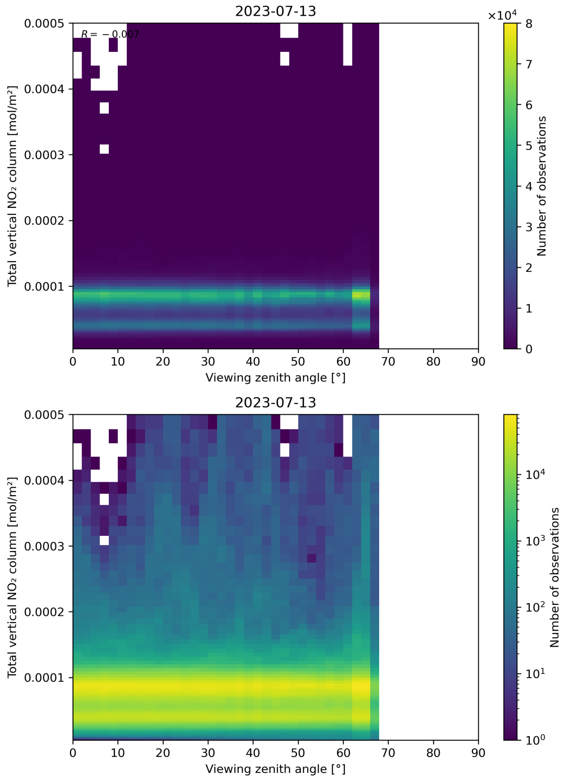
Figure 167: Scatter density plot of “Viewing zenith angle” against “Total vertical NO 2 column” for 2023-07-13 to 2023-07-14.
