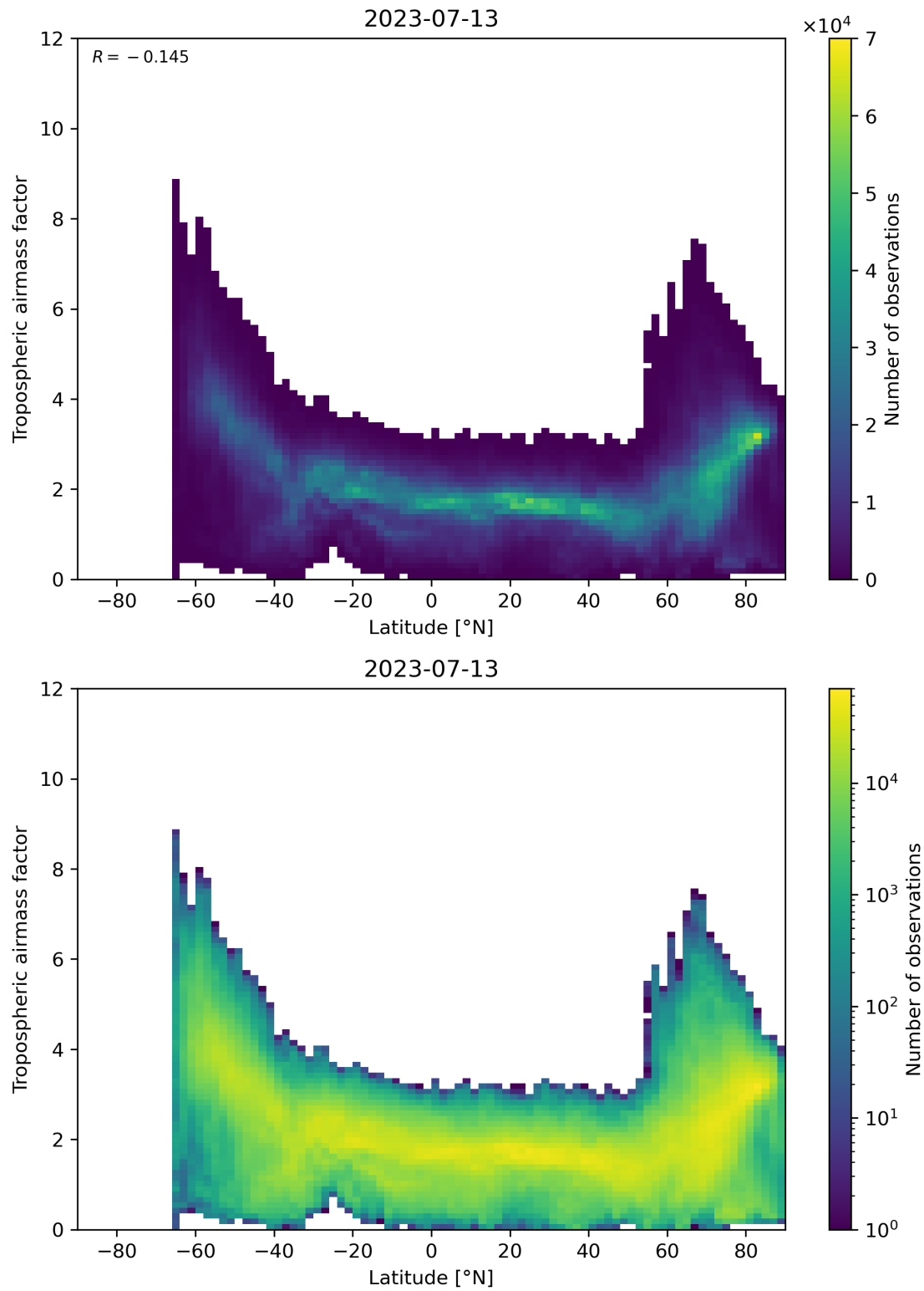
Figure 85: Scatter density plot of “Latitude” against “Tropospheric airmass factor” for 2023-07-13 to 2023-07-14.
