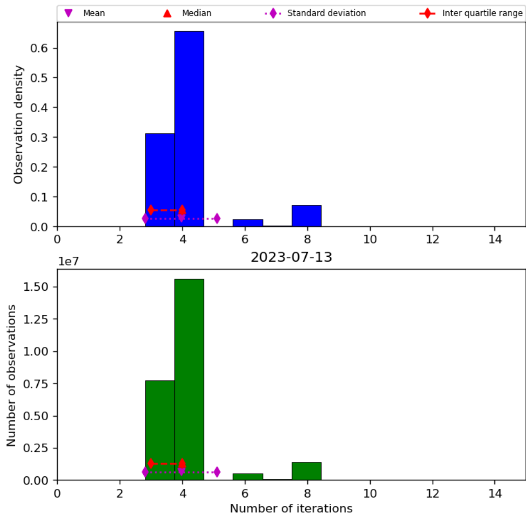
Figure 34: Histogram of “Number of iterations” for 2023-07-13 to 2023-07-14
