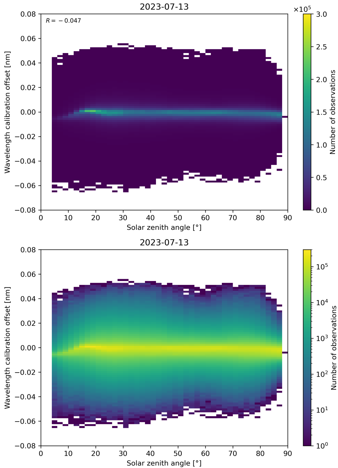
Figure 158: Scatter density plot of “Solar zenith angle” against “Wavelength calibration offset” for 2023-07-13 to 2023-07-14.
