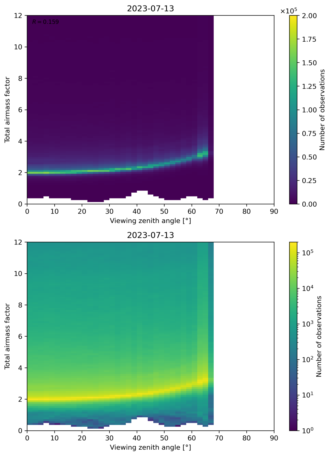
Figure 160: Scatter density plot of “Viewing zenith angle” against “Total airmass factor” for 2023-07-13 to 2023-07-14.
