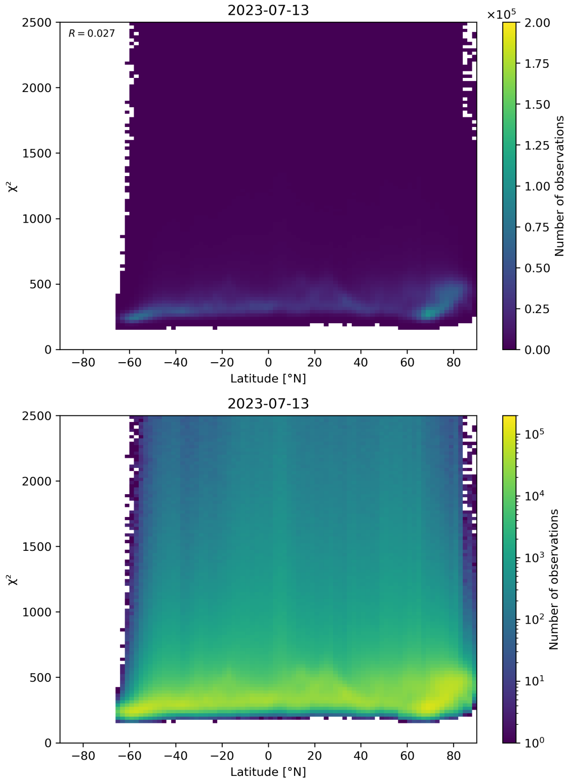
Figure 86: Scatter density plot of “Latitude” against “ \chi^2 ” for 2023-07-13 to 2023-07-14.
