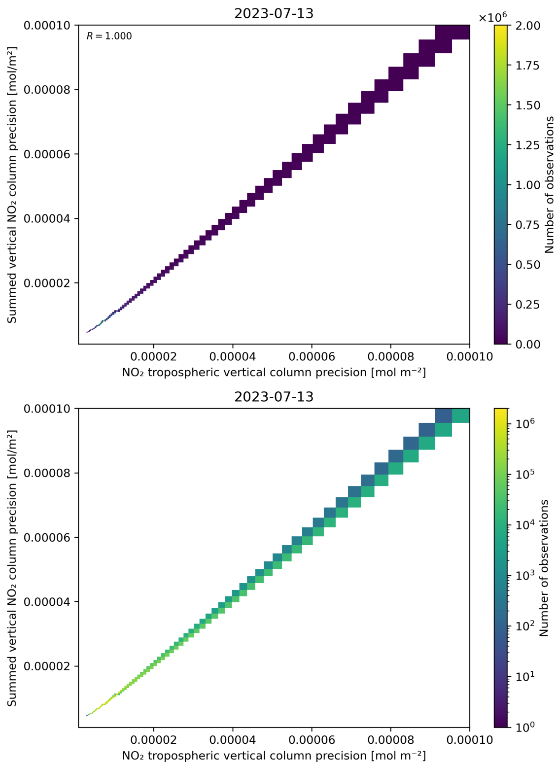
Figure 137: Scatter density plot of “NO 2 tropospheric vertical column precision” against “Summed vertical NO 2 column precision” for 2023-07-13 to 2023-07-14.
