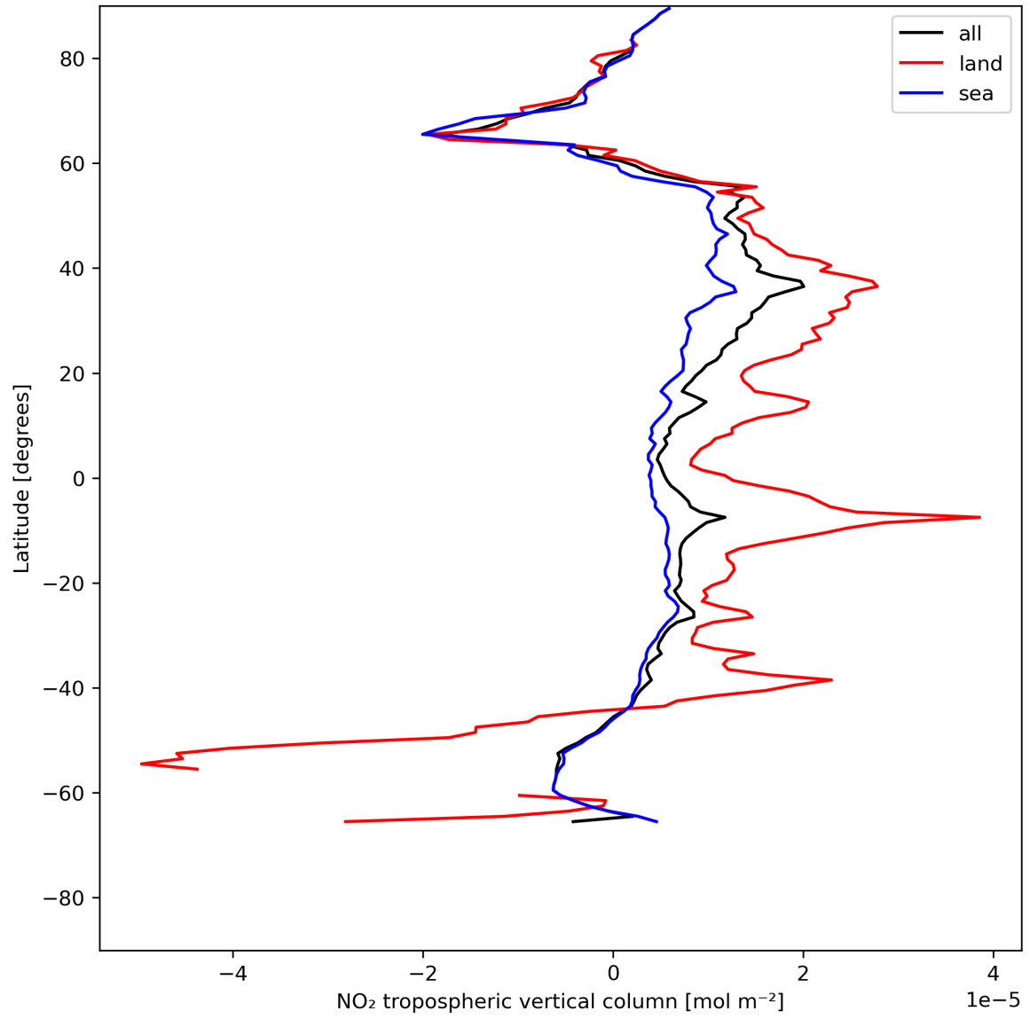
Figure 12: Zonal average of “NO 2 tropospheric vertical column” for 2023-07-13 to 2023-07-14.
