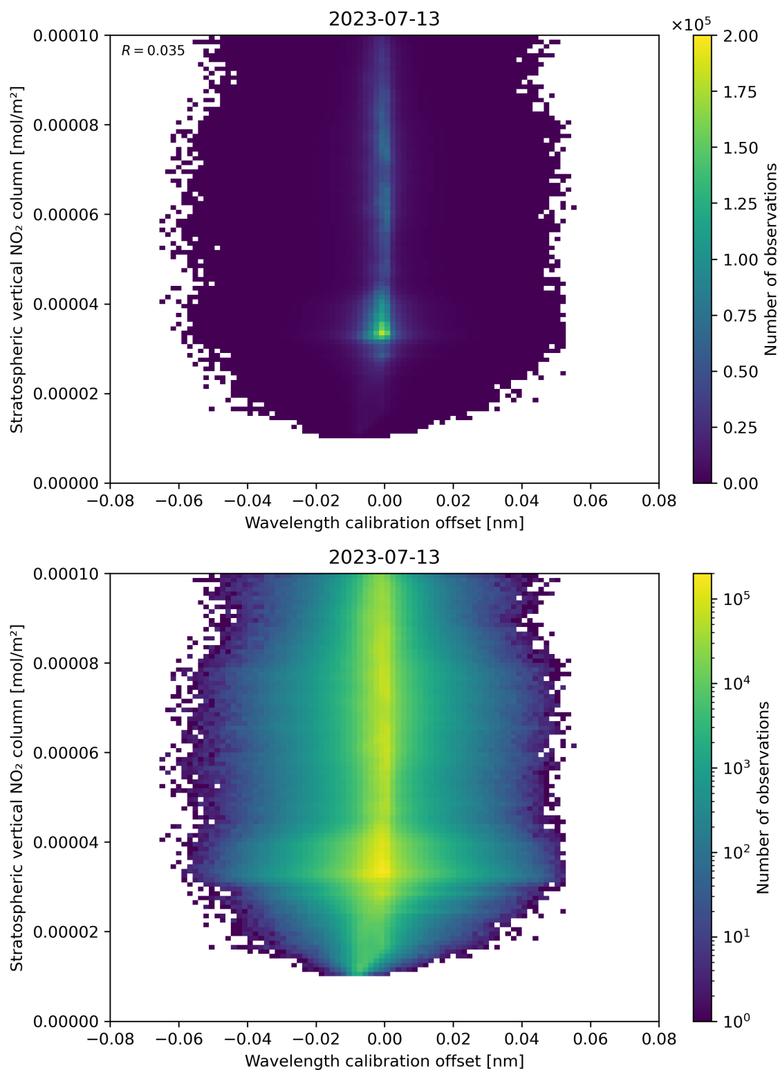
Figure 176: Scatter density plot of “Wavelength calibration offset” against “Stratospheric vertical NO 2 column” for 2023-07-13 to 2023-07-14.
