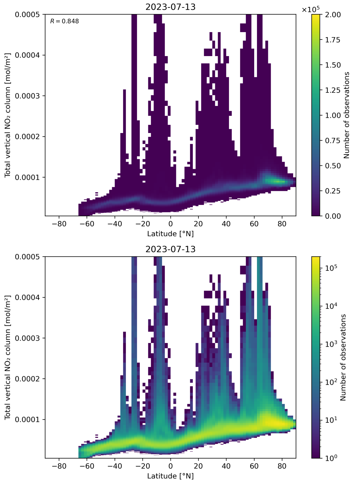
Figure 90: Scatter density plot of “Latitude” against “Total vertical NO 2 column” for 2023-07-13 to 2023-07-14.
