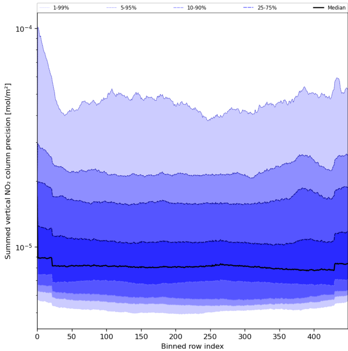
Figure 58: Along track statistics of “Summed vertical NO 2 column precision” for 2023-07-13 to 2023-07-14
