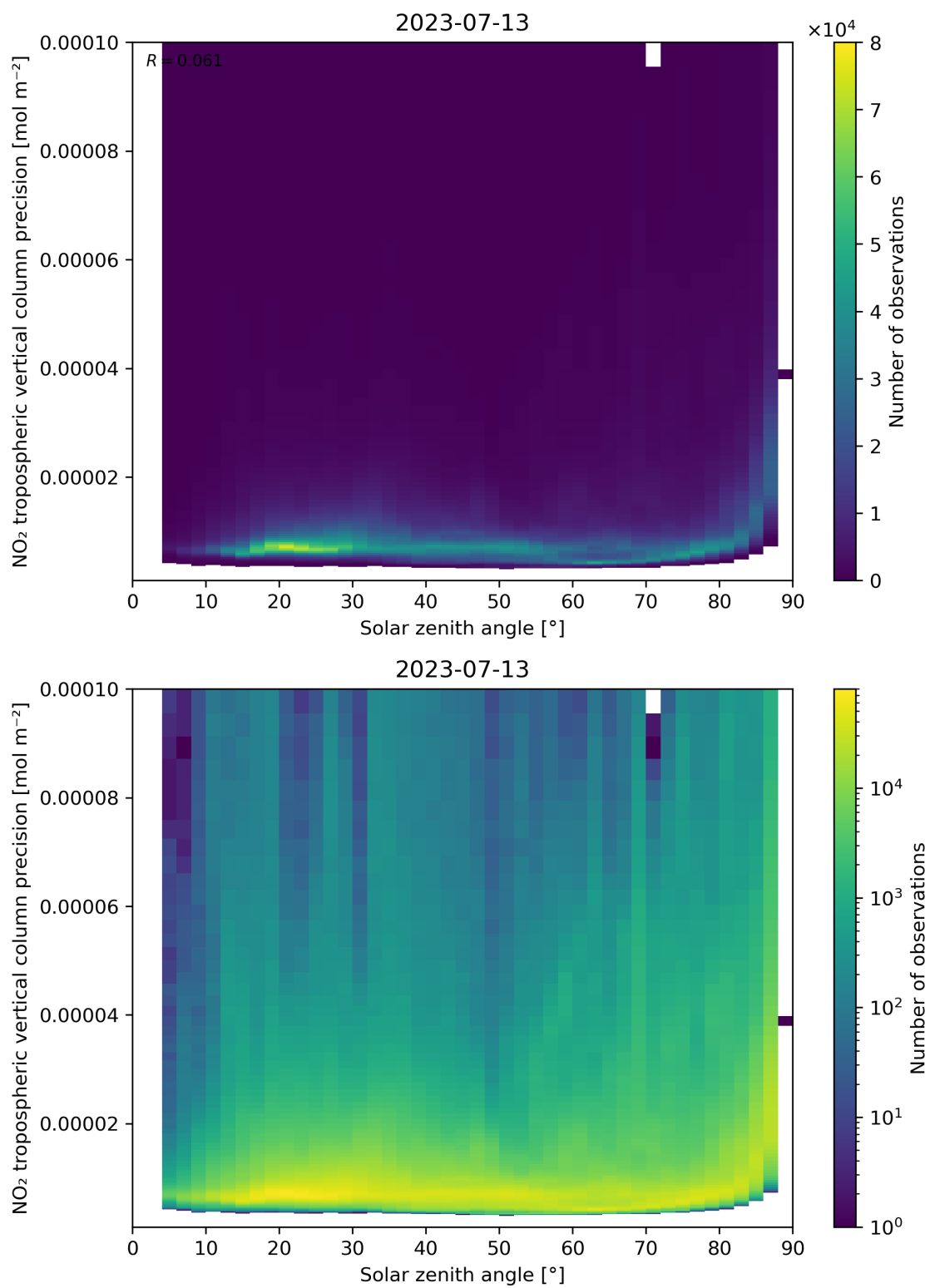
Figure 156: Scatter density plot of “Solar zenith angle” against “NO 2 tropospheric vertical column precision” for 2023-07-13 to 2023-07-14.
