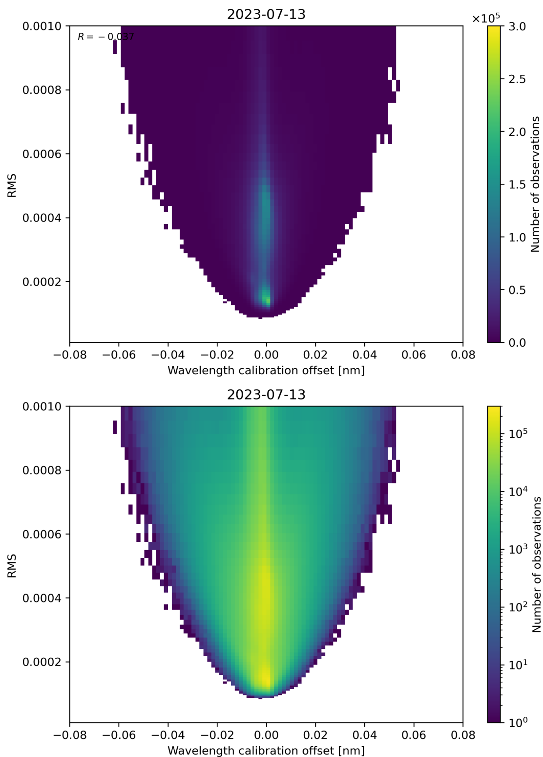
Figure 181: Scatter density plot of “Wavelength calibration offset” against “RMS” for 2023-07-13 to 2023-07-14.
