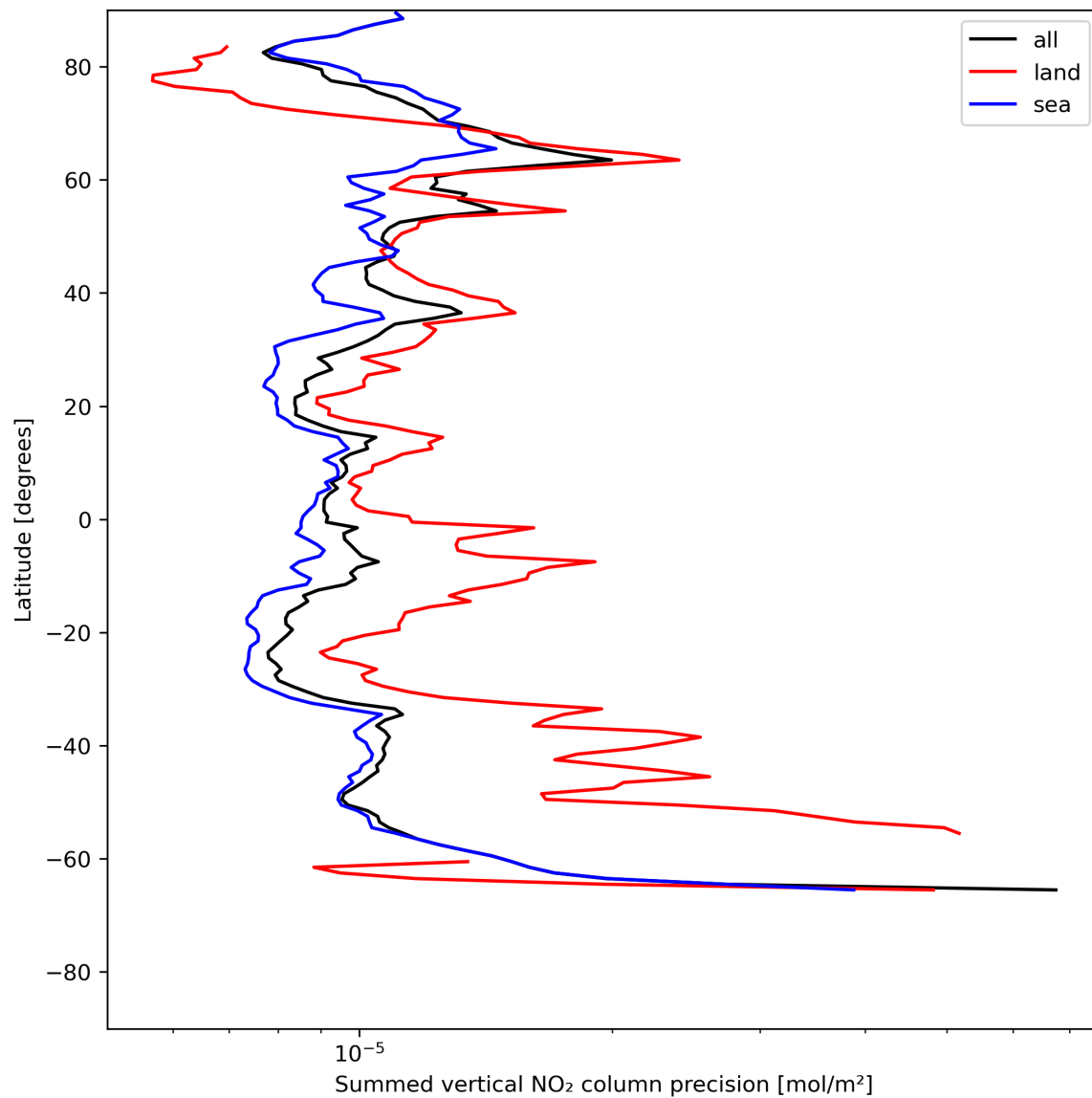
Figure 24: Zonal average of “Summed vertical NO 2 column precision” for 2023-07-13 to 2023-07-14.
