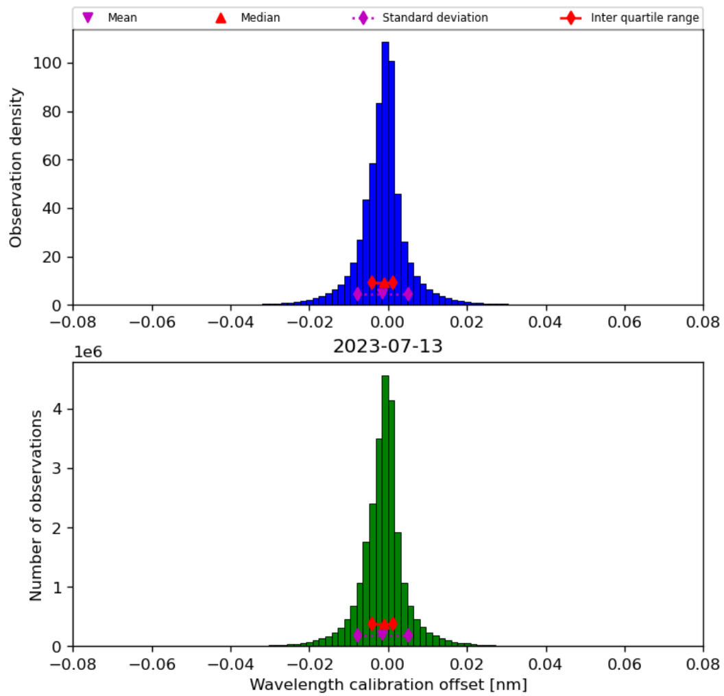
Figure 35: Histogram of “Wavelength calibration offset” for 2023-07-13 to 2023-07-14
