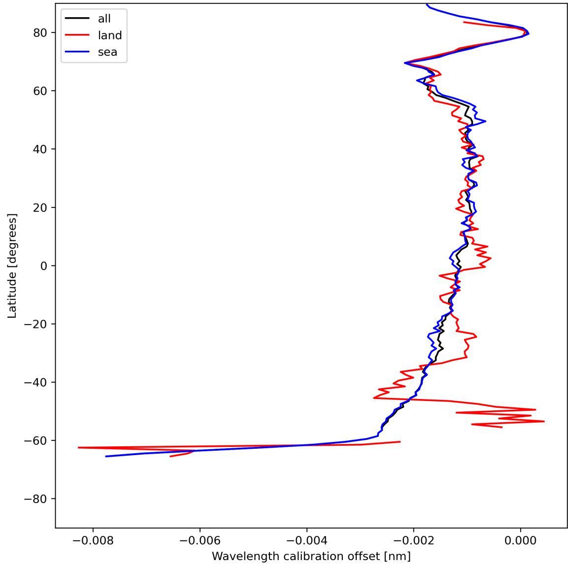
Figure 18: Zonal average of “Wavelength calibration offset” for 2023-07-13 to 2023-07-14.
