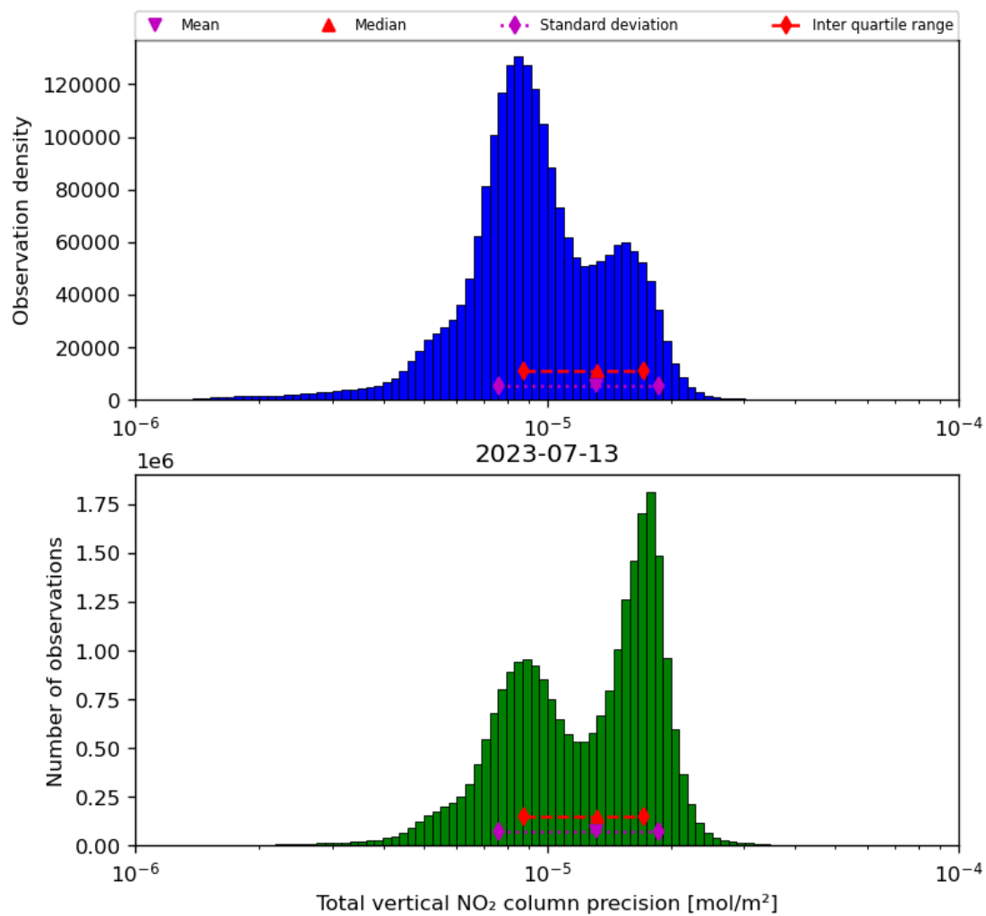
Figure 39: Histogram of “Total vertical NO 2 column precision” for 2023-07-13 to 2023-07-14
