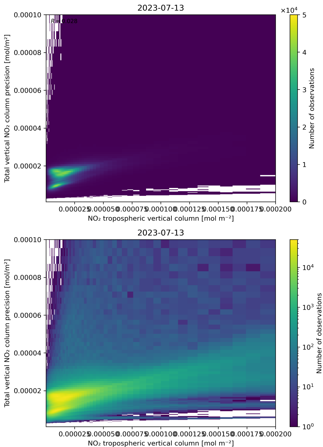
Figure 129: Scatter density plot of “NO 2 tropospheric vertical column” against “Total vertical NO 2 column precision” for 2023-07-13 to 2023-07-14.
