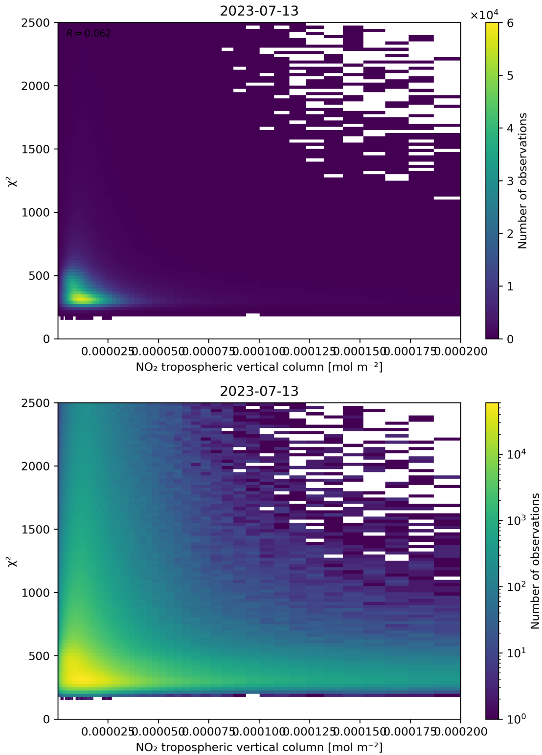
Figure 124: Scatter density plot of “NO 2 tropospheric vertical column” against “ \chi^2 ” for 2023-07-13 to 2023-07-14.
