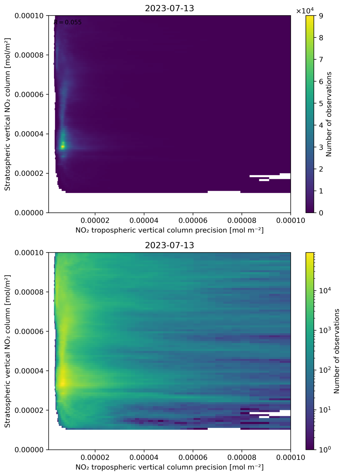
Figure 135: Scatter density plot of “NO 2 tropospheric vertical column precision” against “Stratospheric vertical NO 2 column” for 2023-07-13 to 2023-07-14.
