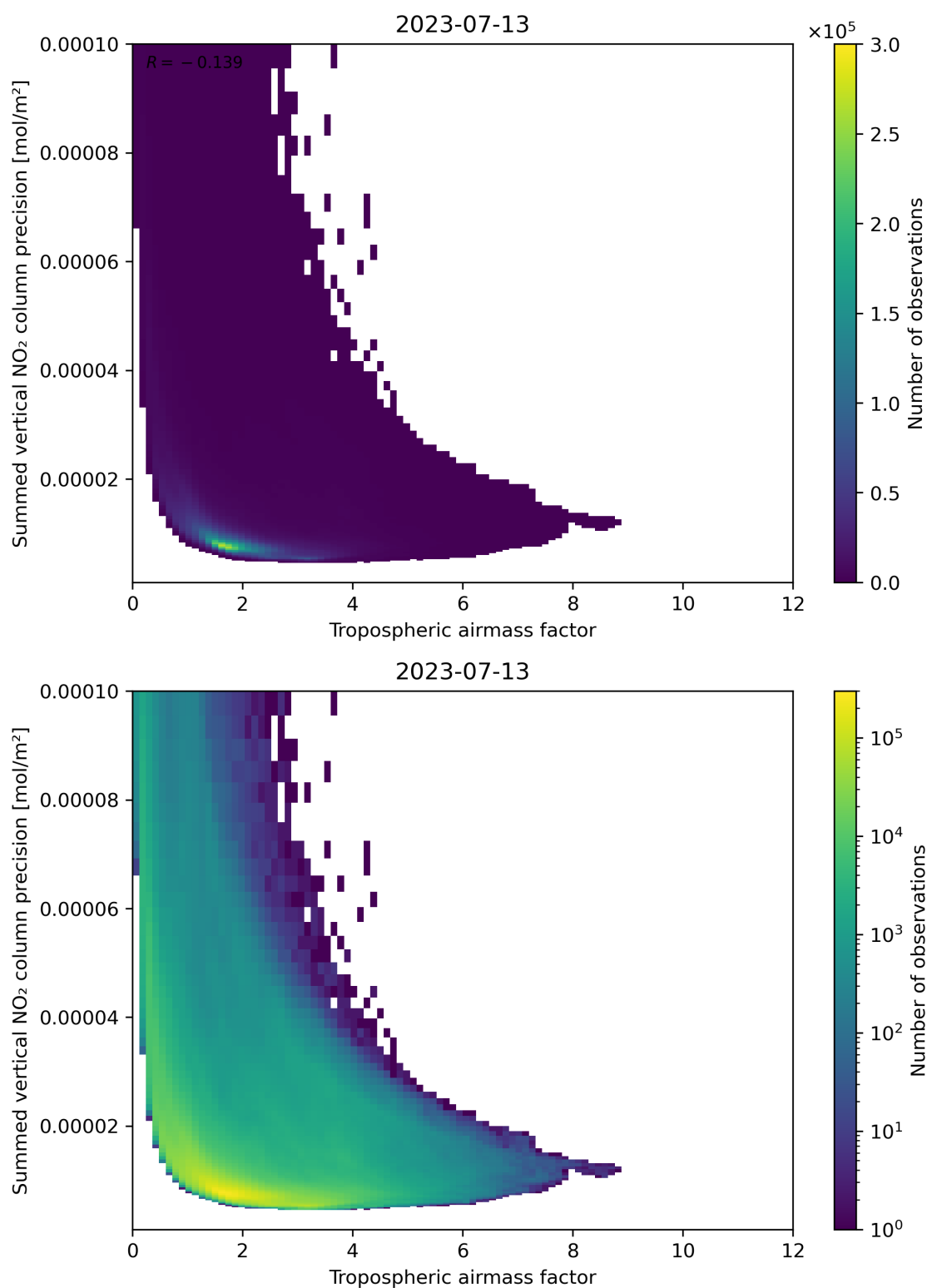
Figure 76: Scatter density plot of “Tropospheric air mass factor” against “Summed vertical NO 2 column precision” for 2023-07-13 to 2023-07-14.
