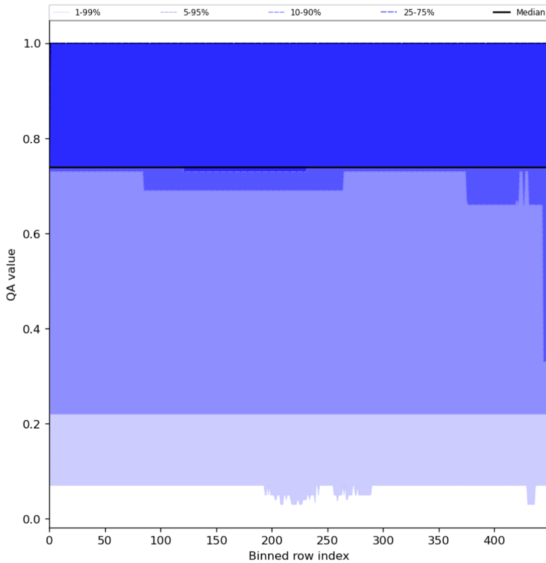
Figure 45: Along track statistics of “QA value” for 2023-07-13 to 2023-07-14
