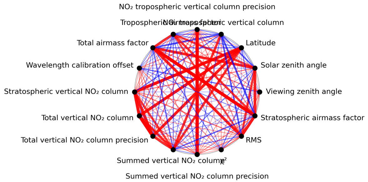
Figure 1: Map of correlation graph for 2023-07-13 to 2023-07-14.
