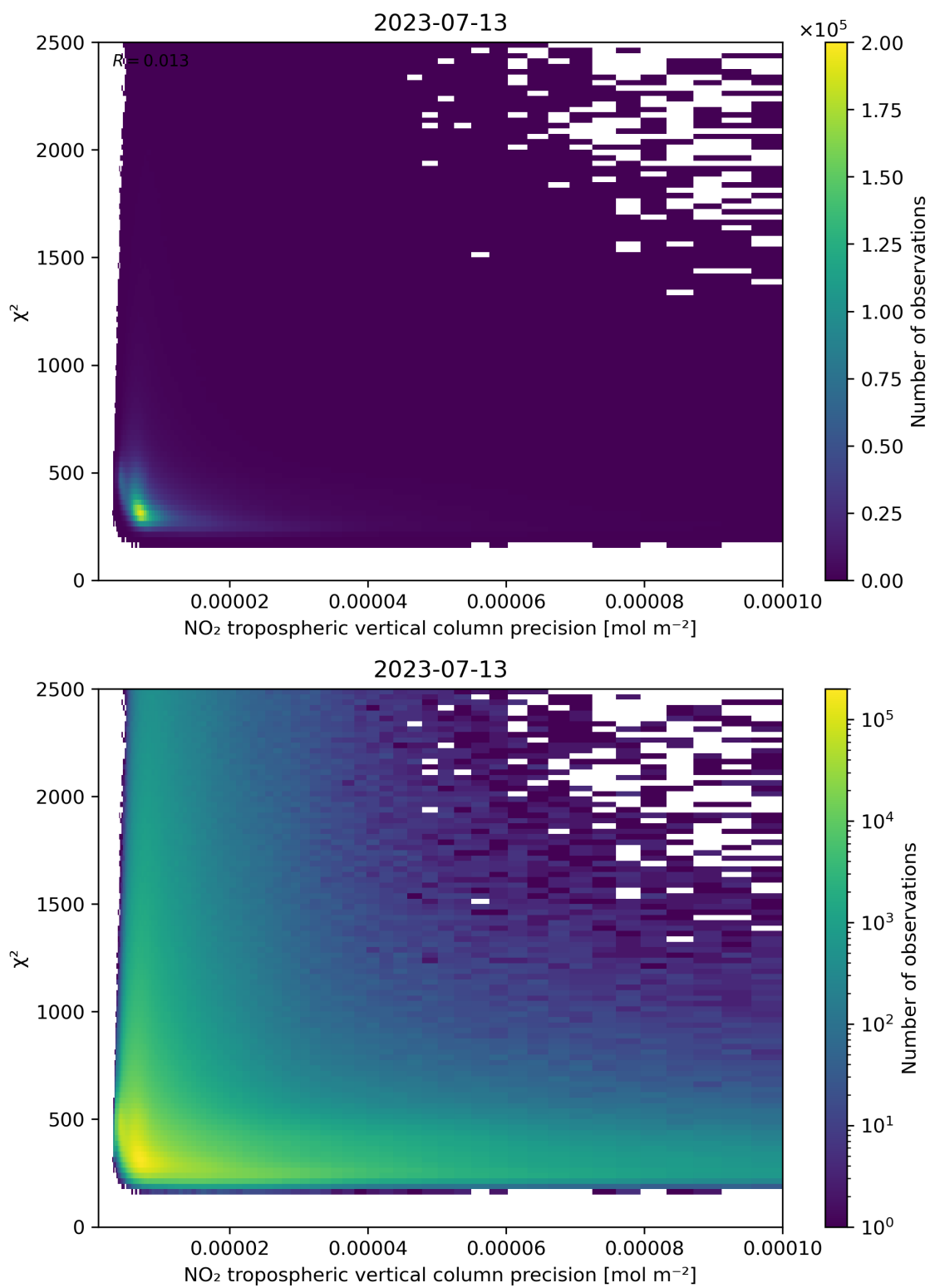
Figure 134: Scatter density plot of “NO 2 tropospheric vertical column precision” against “ \chi^2 ” for 2023-07-13 to 2023-07-14.
