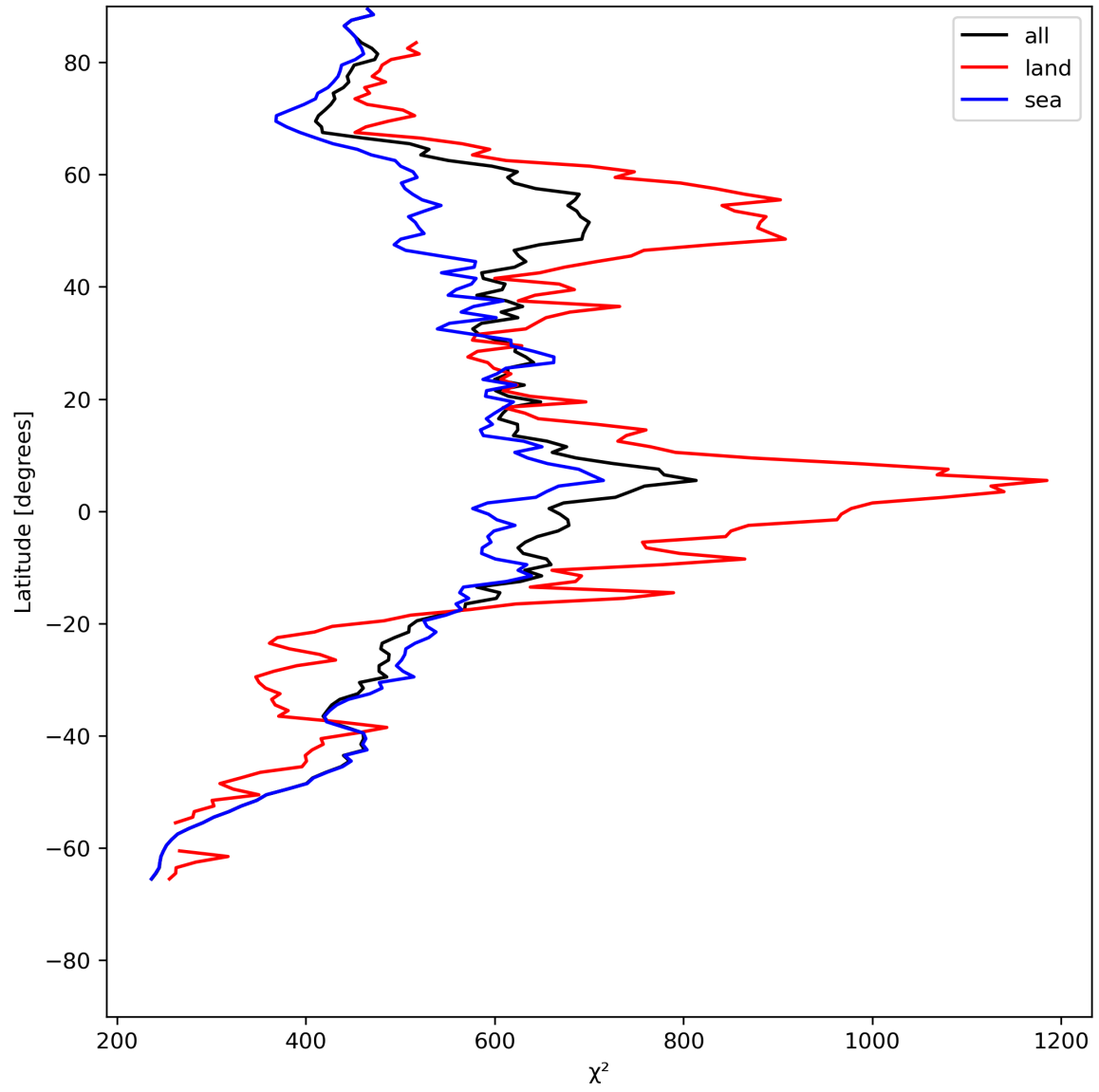
Figure 25: Zonal average of “ \chi^2 ” for 2023-07-13 to 2023-07-14.
