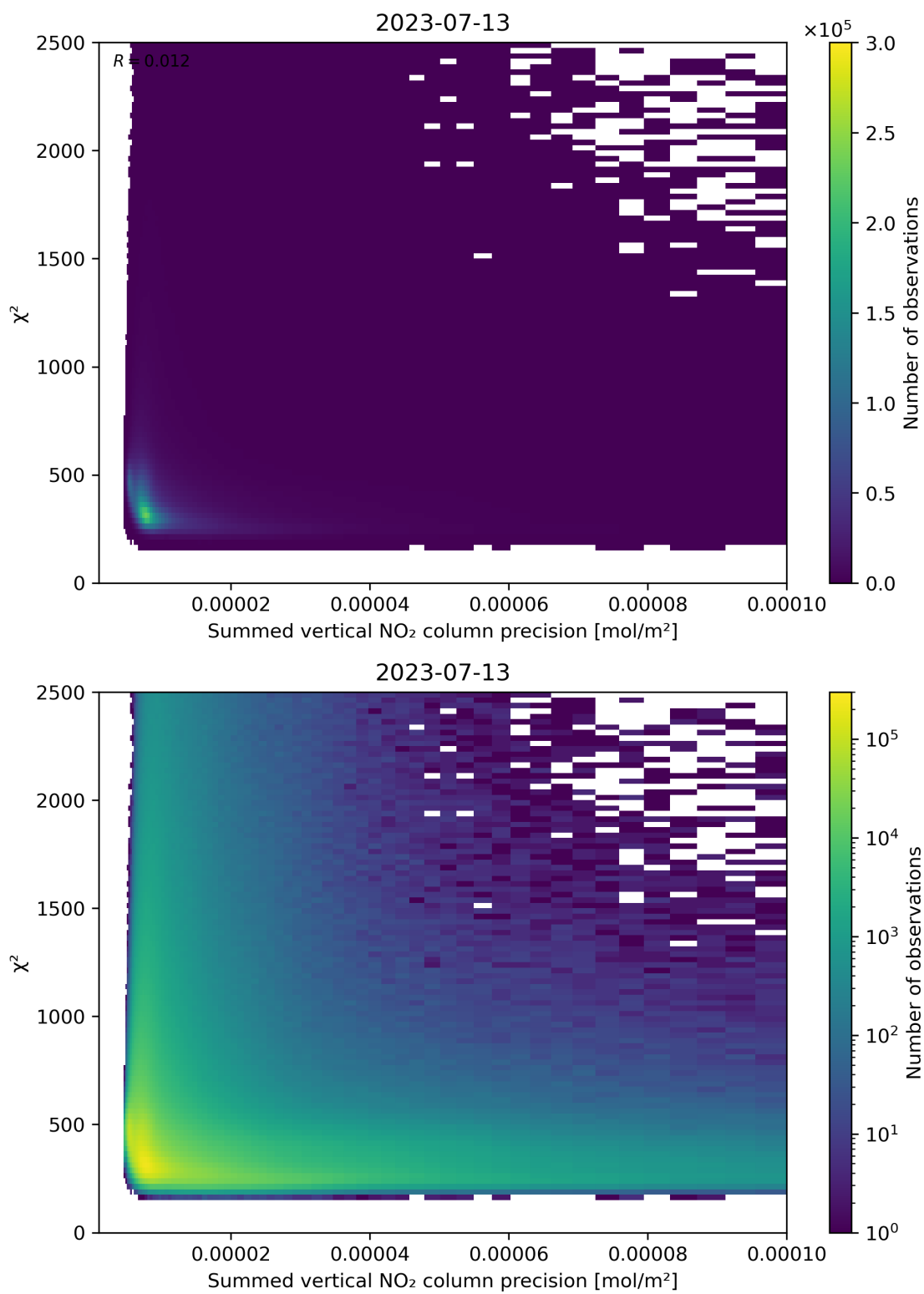
Figure 107: Scatter density plot of “Summed vertical NO 2 column precision” against “ \chi^2 ” for 2023-07-13 to 2023-07-14.
