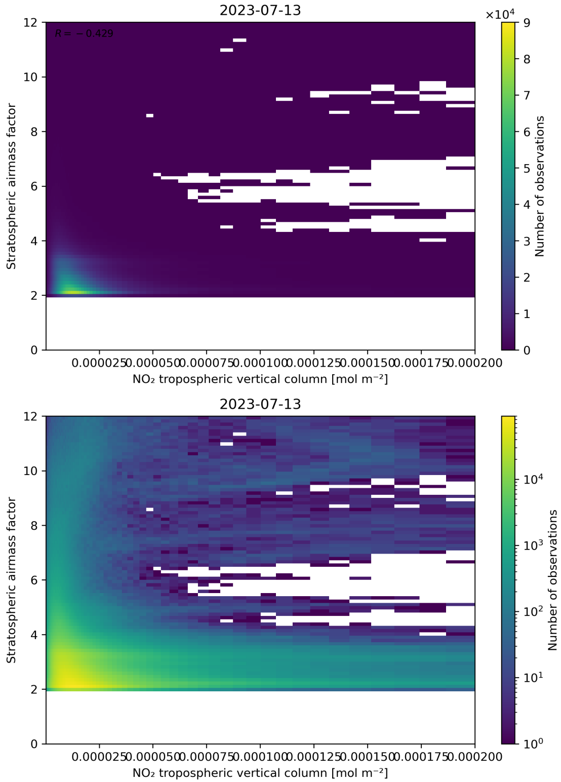
Figure 121: Scatter density plot of “NO 2 tropospheric vertical column” against “Stratospheric air mass factor” for 2023-07-13 to 2023-07-14.
