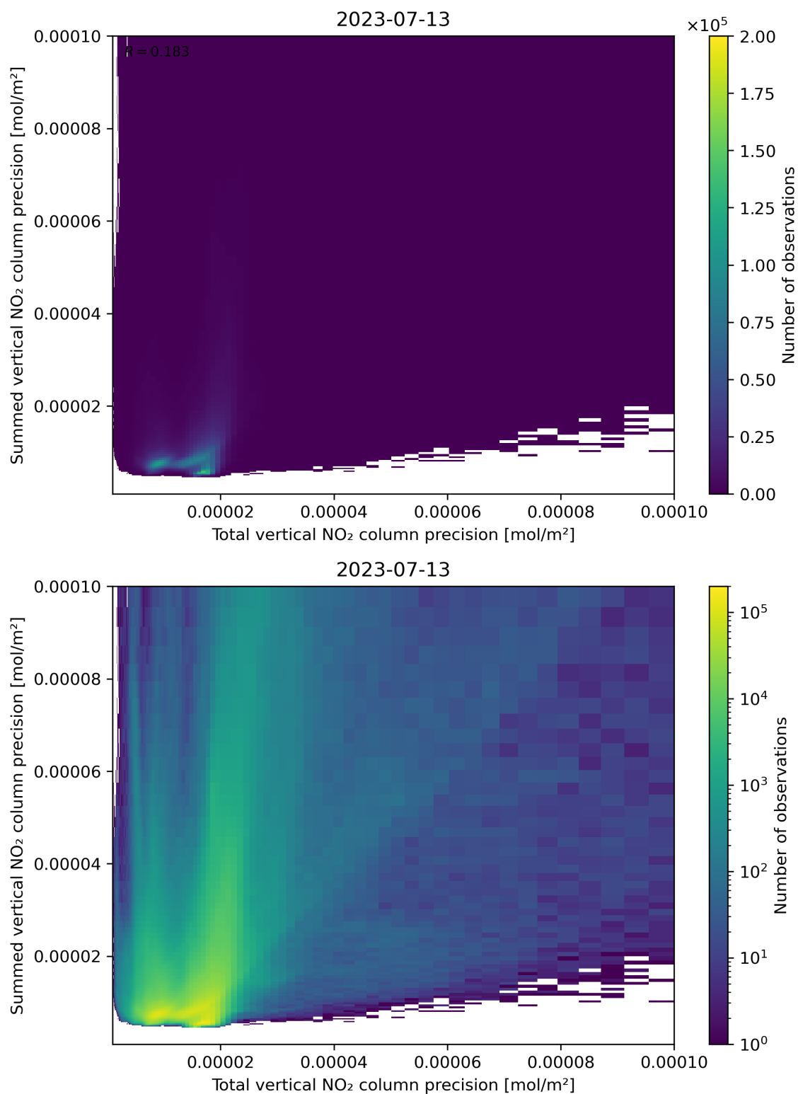
Figure 118: Scatter density plot of “Total vertical NO 2 column precision” against “Summed vertical NO 2 column precision” for 2023-07-13 to 2023-07-14.
