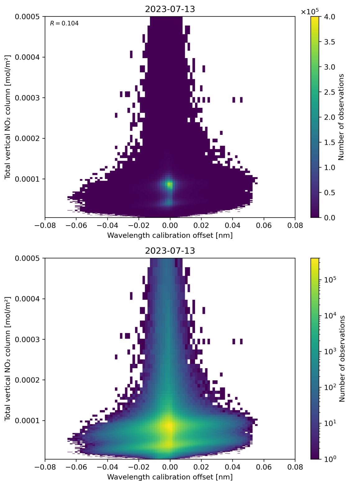
Figure 179: Scatter density plot of “Wavelength calibration offset” against “Total vertical NO 2 column” for 2023-07-13 to 2023-07-14.
