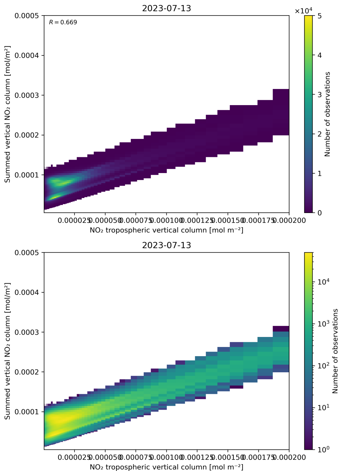
Figure 126: Scatter density plot of “NO 2 tropospheric vertical column” against “Summed vertical NO 2 column” for 2023-07-13 to 2023-07-14.
