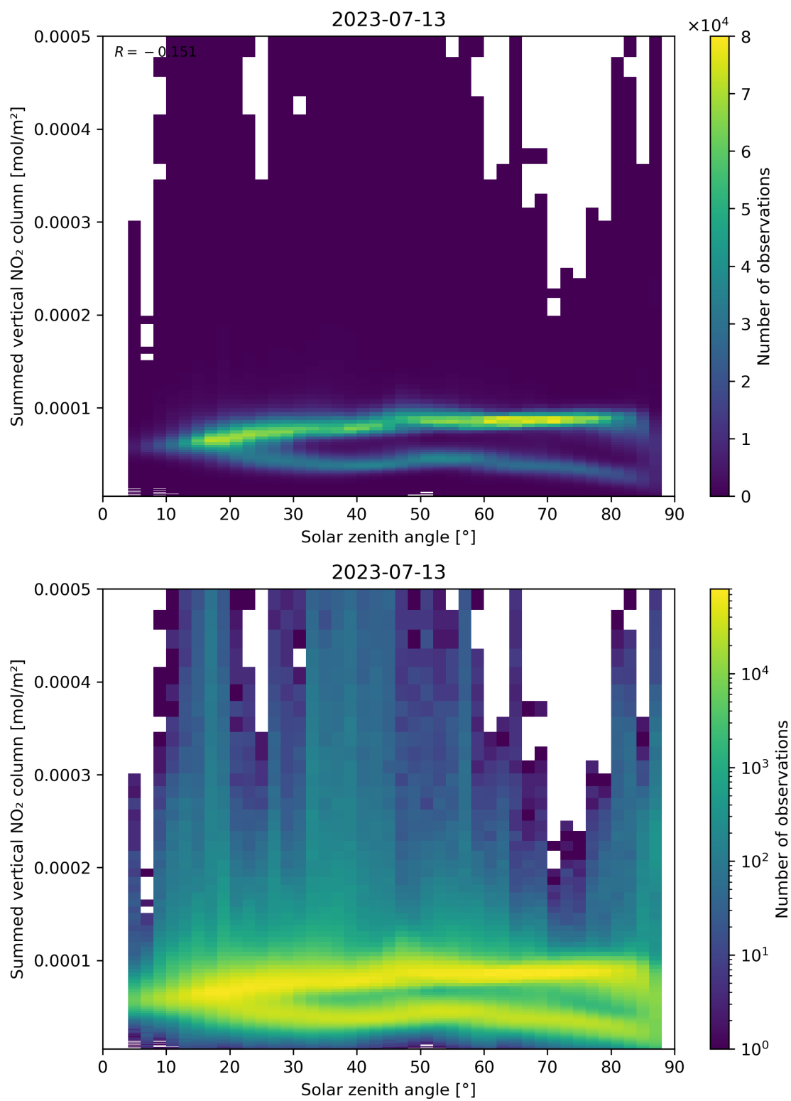
Figure 151: Scatter density plot of “Solar zenith angle” against “Summed vertical NO 2 column” for 2023-07-13 to 2023-07-14.
