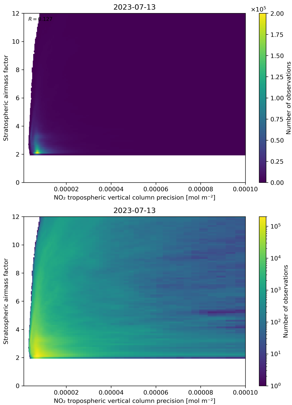
Figure 131: Scatter density plot of “NO 2 tropospheric vertical column precision” against “Stratospheric airmass factor” for 2023-07-13 to 2023-07-14.
