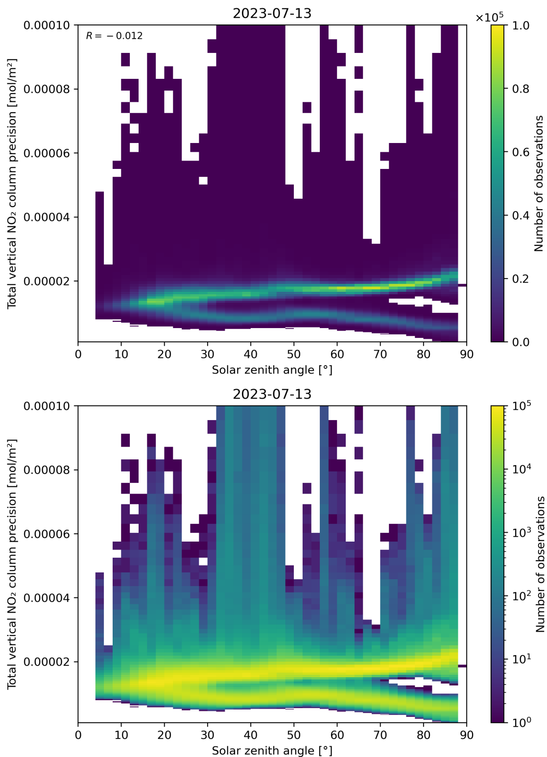
Figure 154: Scatter density plot of “Solar zenith angle” against “Total vertical NO 2 column precision” for 2023-07-13 to 2023-07-14.
