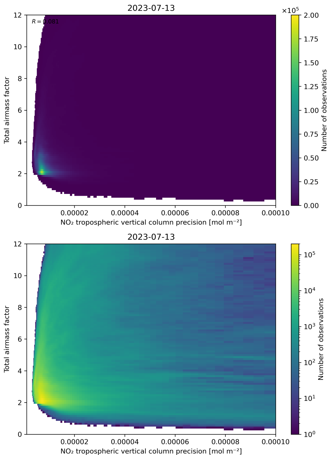
Figure 132: Scatter density plot of “NO 2 tropospheric vertical column precision” against “Total air mass factor” for 2023-07-13 to 2023-07-14.
