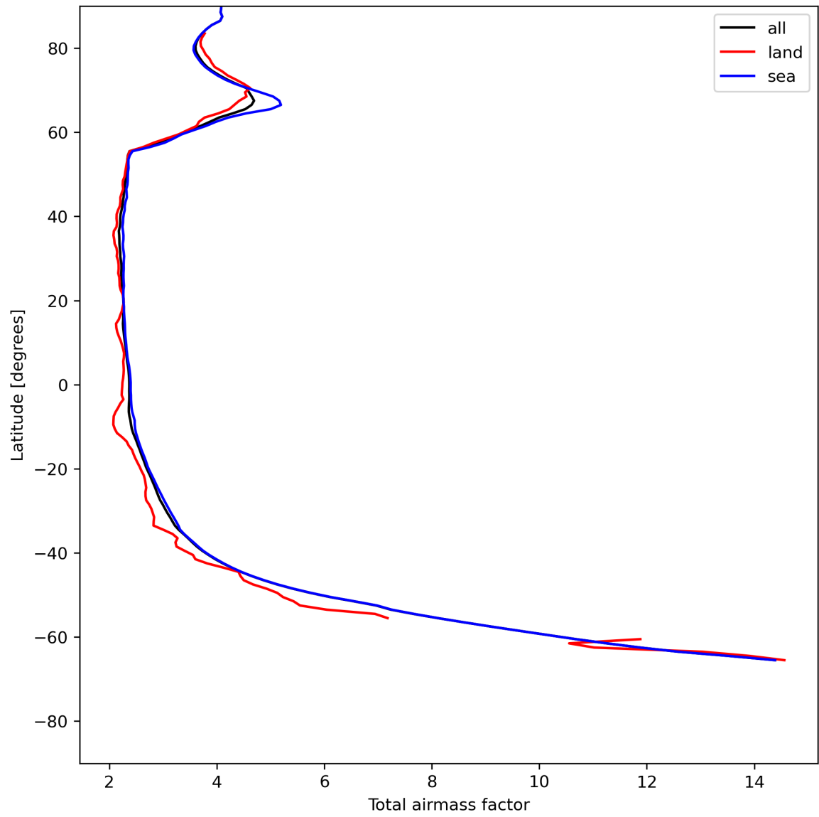
Figure 15: Zonal average of “Total airmass factor” for 2023-07-13 to 2023-07-14.
