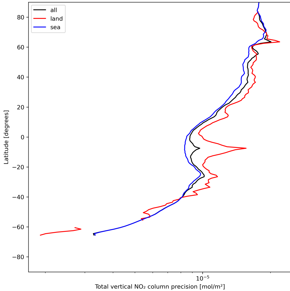
Figure 22: Zonal average of “Total vertical NO 2 column precision” for 2023-07-13 to 2023-07-14.
