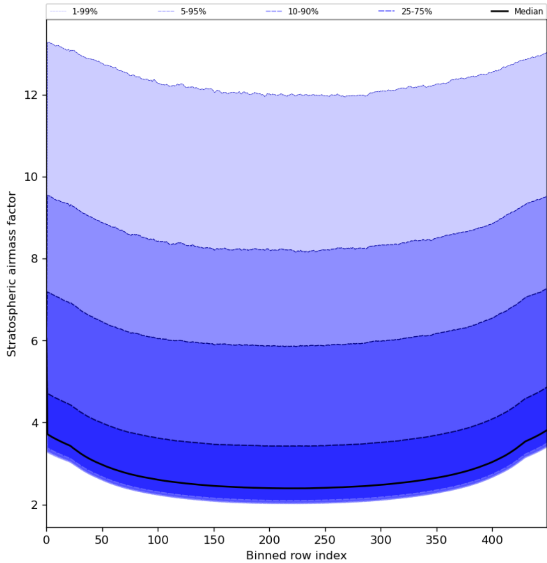
Figure 61: Along track statistics of “Stratospheric airmass factor” for 2023-07-13 to 2023-07-14
