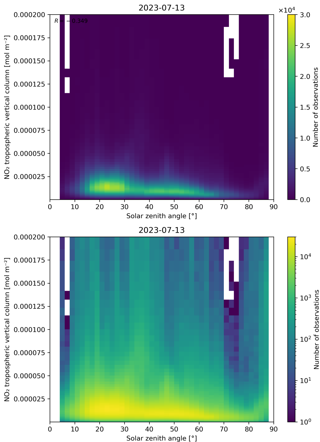
Figure 155: Scatter density plot of “Solar zenith angle” against “NO 2 tropospheric vertical column” for 2023-07-13 to 2023-07-14.
