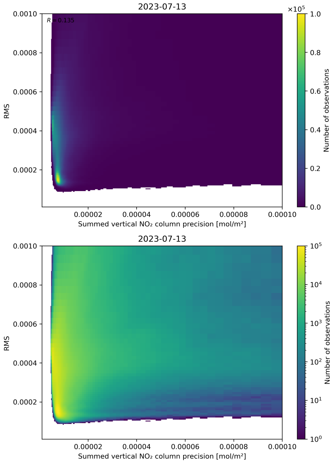
Figure 108: Scatter density plot of “Summed vertical NO 2 column precision” against “RMS” for 2023-07-13 to 2023-07-14.
