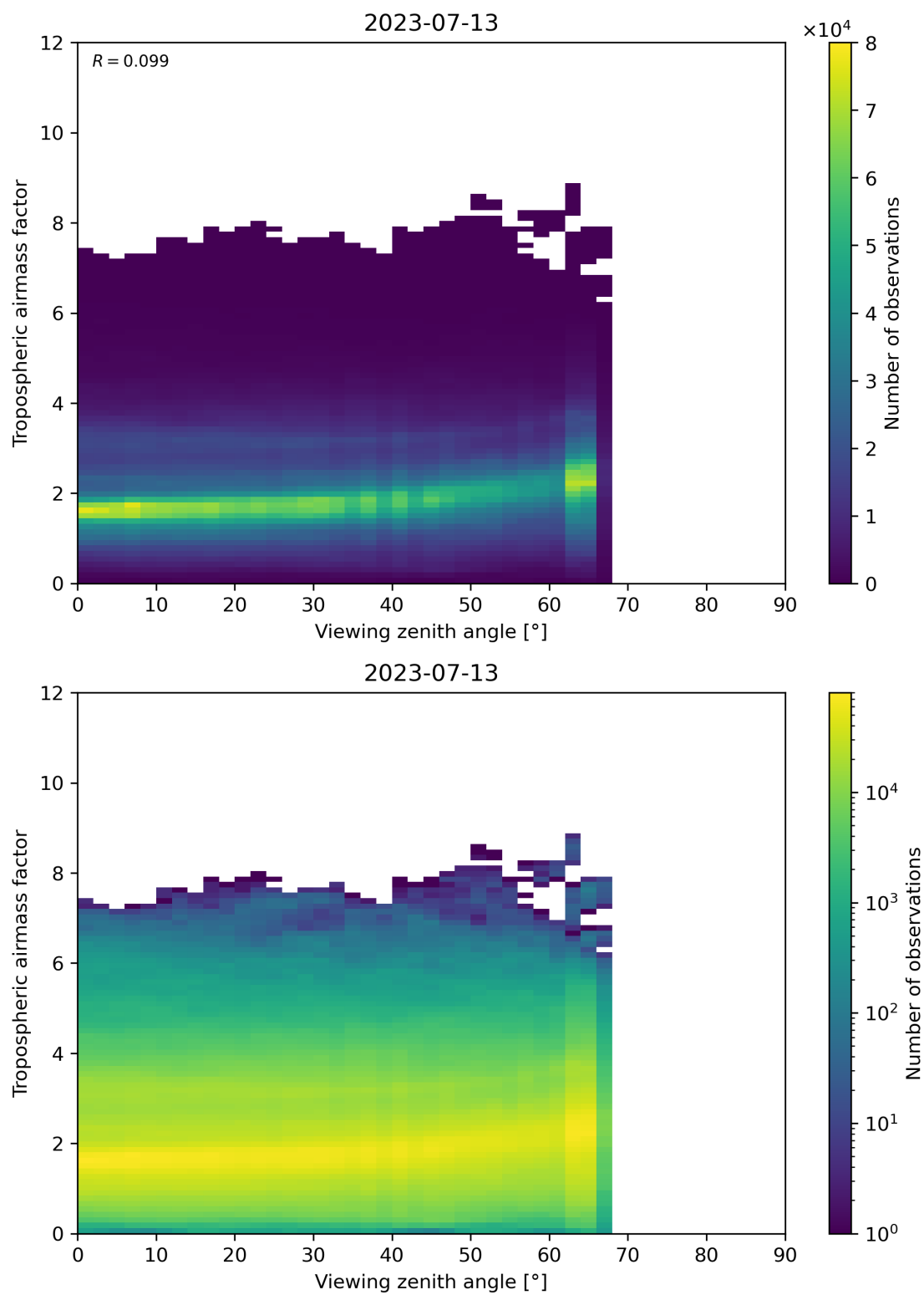
Figure 161: Scatter density plot of “Viewing zenith angle” against “Tropospheric airmass factor” for 2023-07-13 to 2023-07-14.
