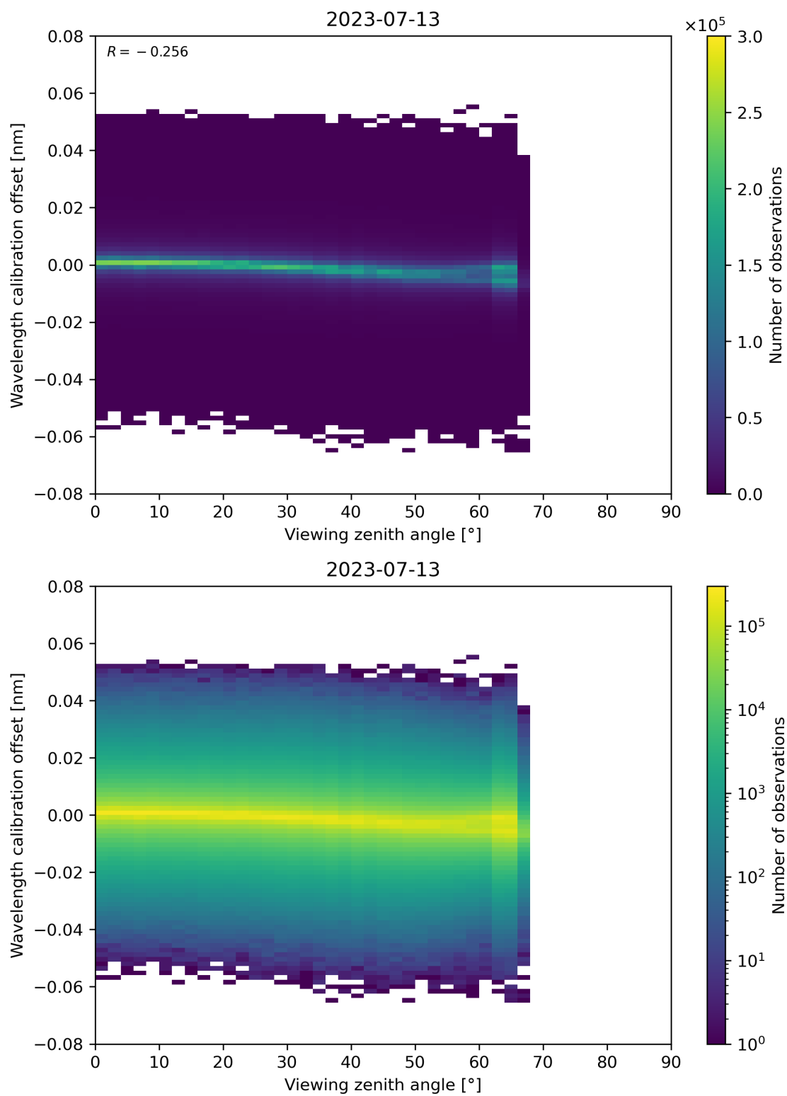
Figure 173: Scatter density plot of “Viewing zenith angle” against “Wavelength calibration offset” for 2023-07-13 to 2023-07-14.
