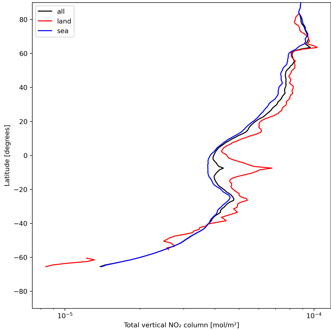
Figure 21: Zonal average of “Total vertical NO 2 column” for 2023-07-13 to 2023-07-14.
