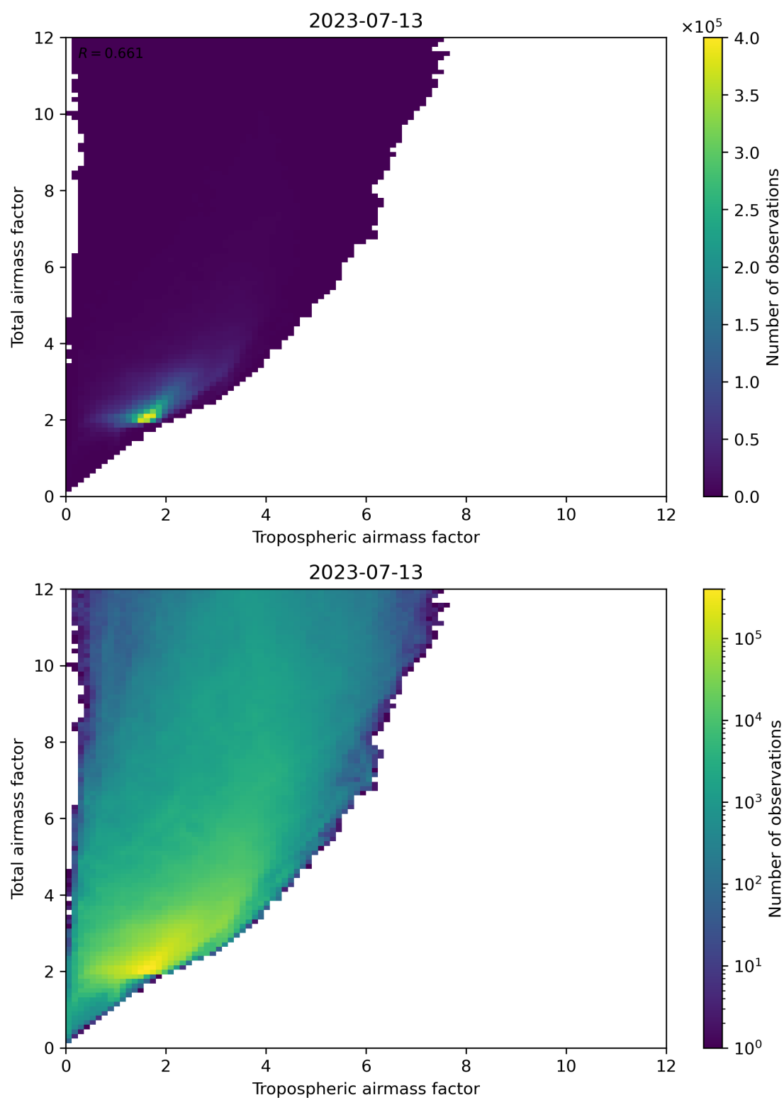
Figure 72: Scatter density plot of “Tropospheric airmass factor” against “Total airmass factor” for 2023-07-13 to 2023-07-14.
