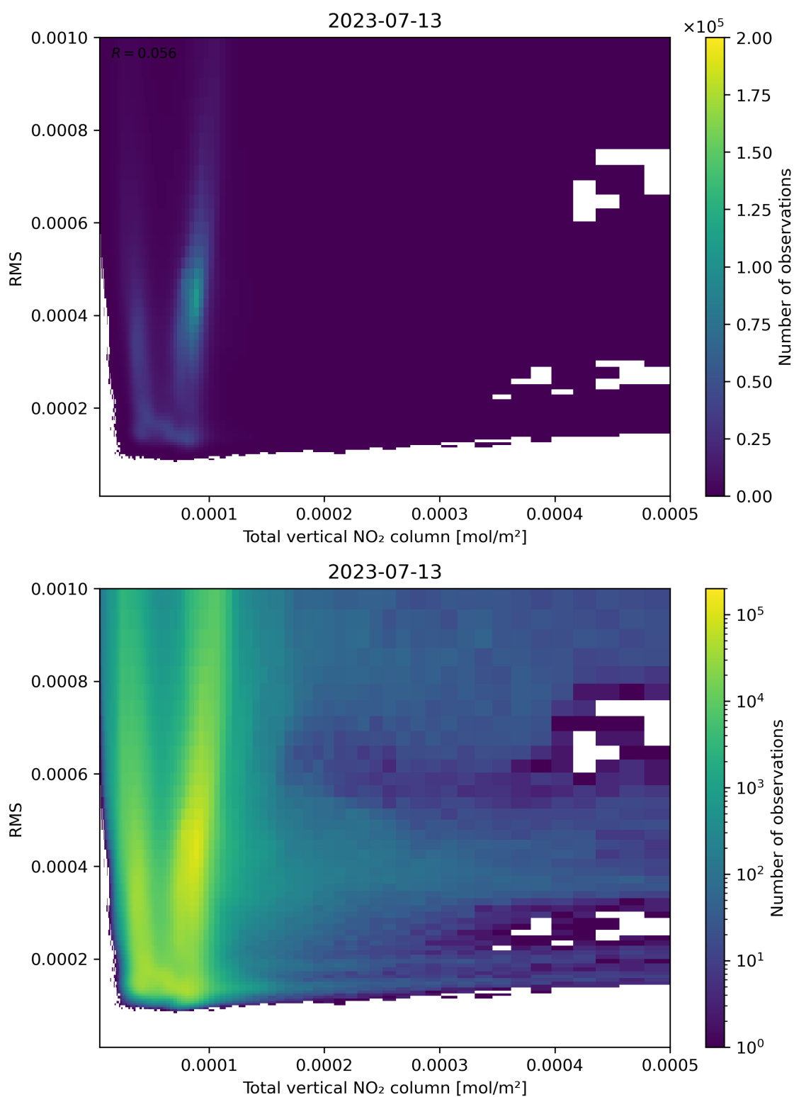
Figure 120: Scatter density plot of “Total vertical NO 2 column” against “RMS” for 2023-07-13 to 2023-07-14.
