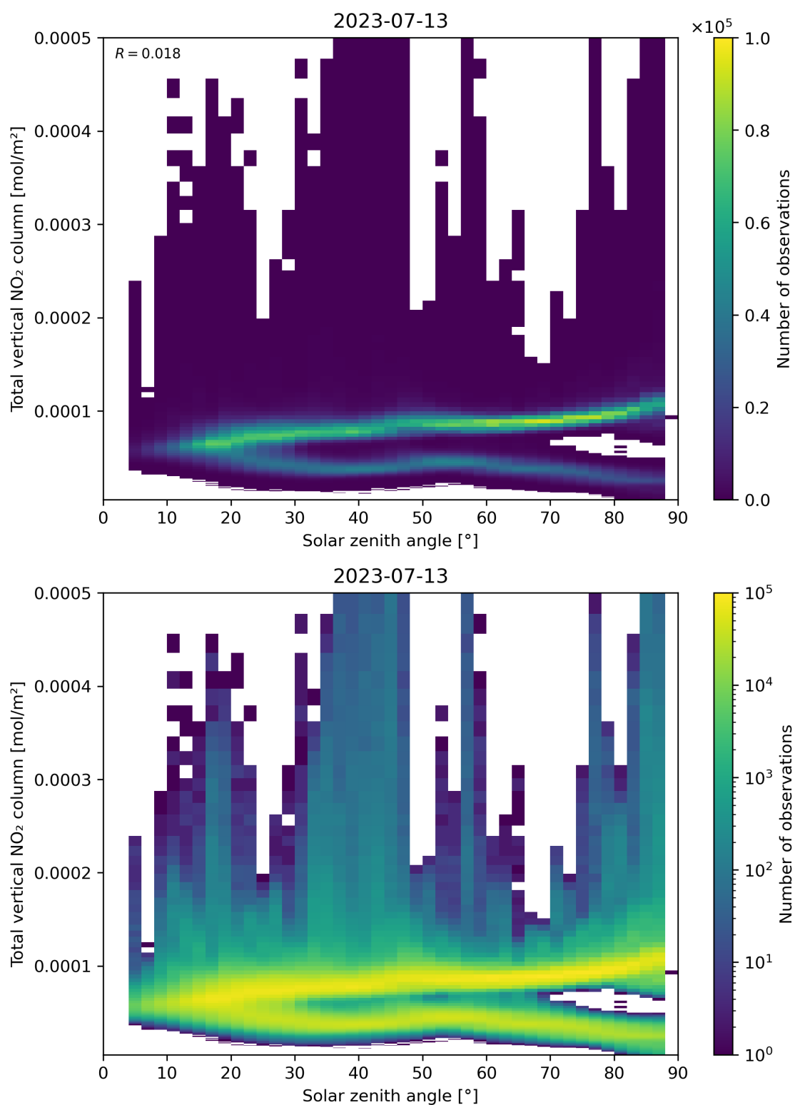
Figure 153: Scatter density plot of “Solar zenith angle” against “Total vertical NO 2 column” for 2023-07-13 to 2023-07-14.
