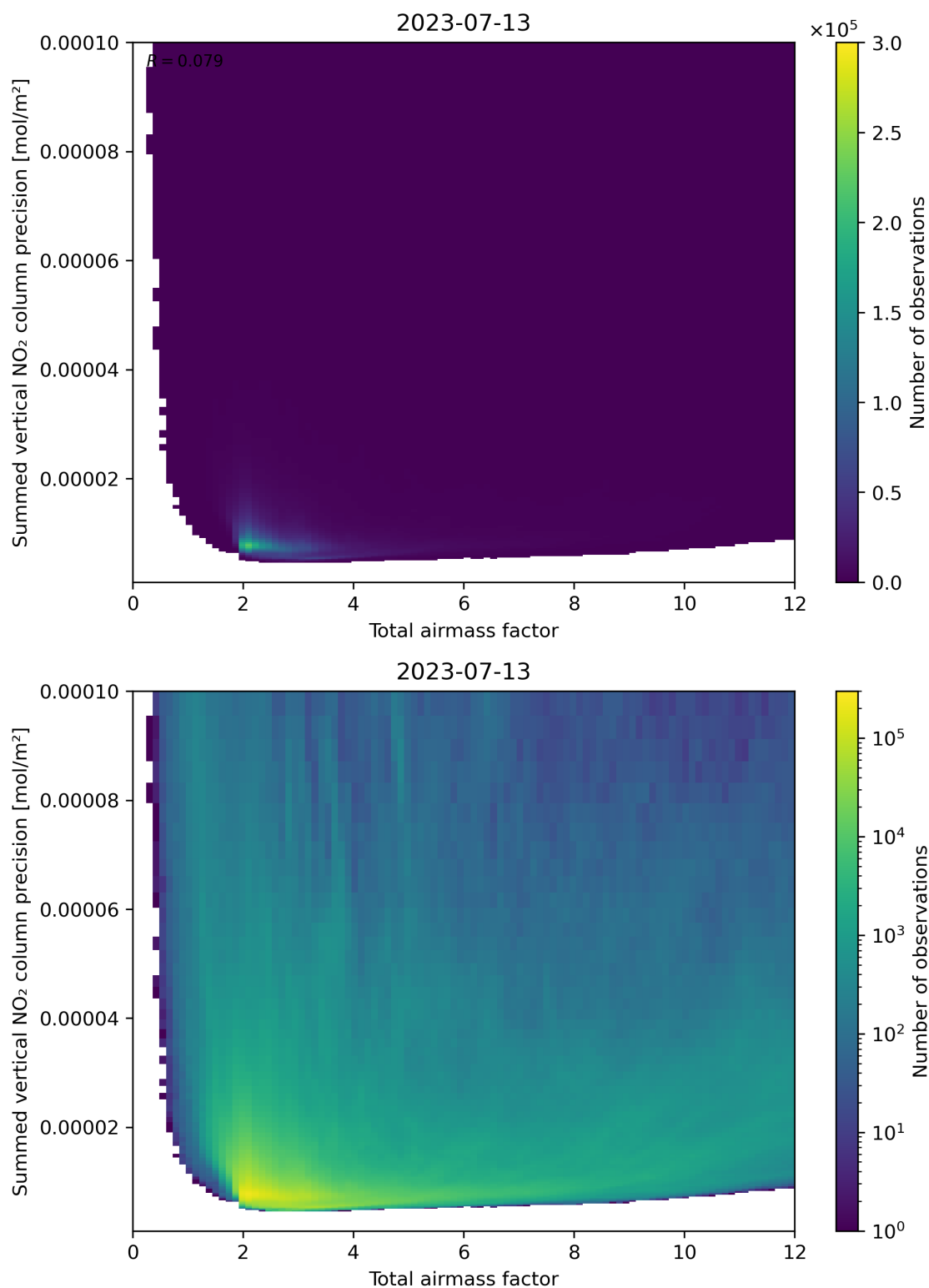
Figure 66: Scatter density plot of “Total airmass factor” against “Summed vertical NO 2 column precision” for 2023-07-13 to 2023-07-14.
