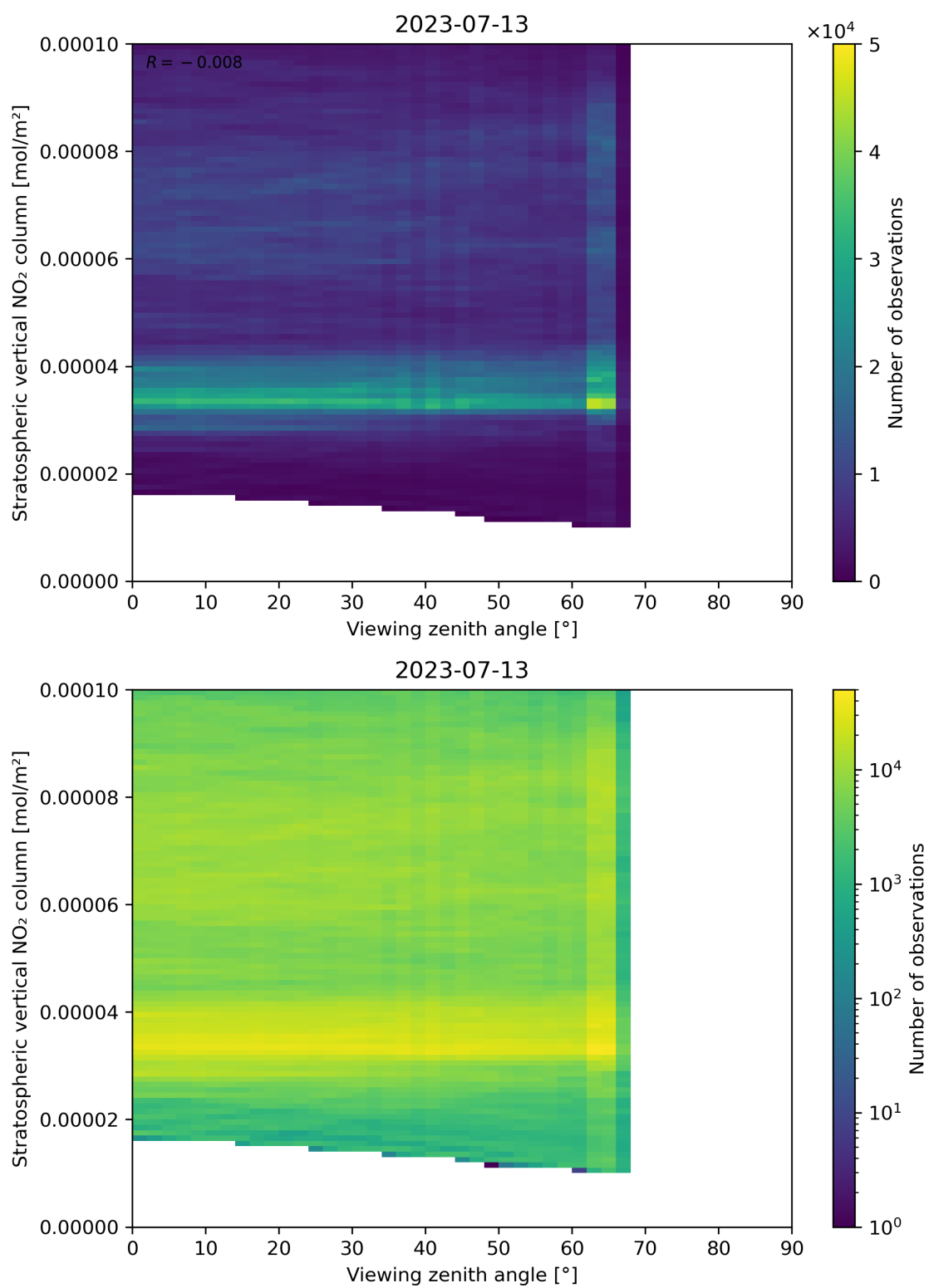
Figure 164: Scatter density plot of “Viewing zenith angle” against “Stratospheric vertical NO 2 column” for 2023-07-13 to 2023-07-14.
