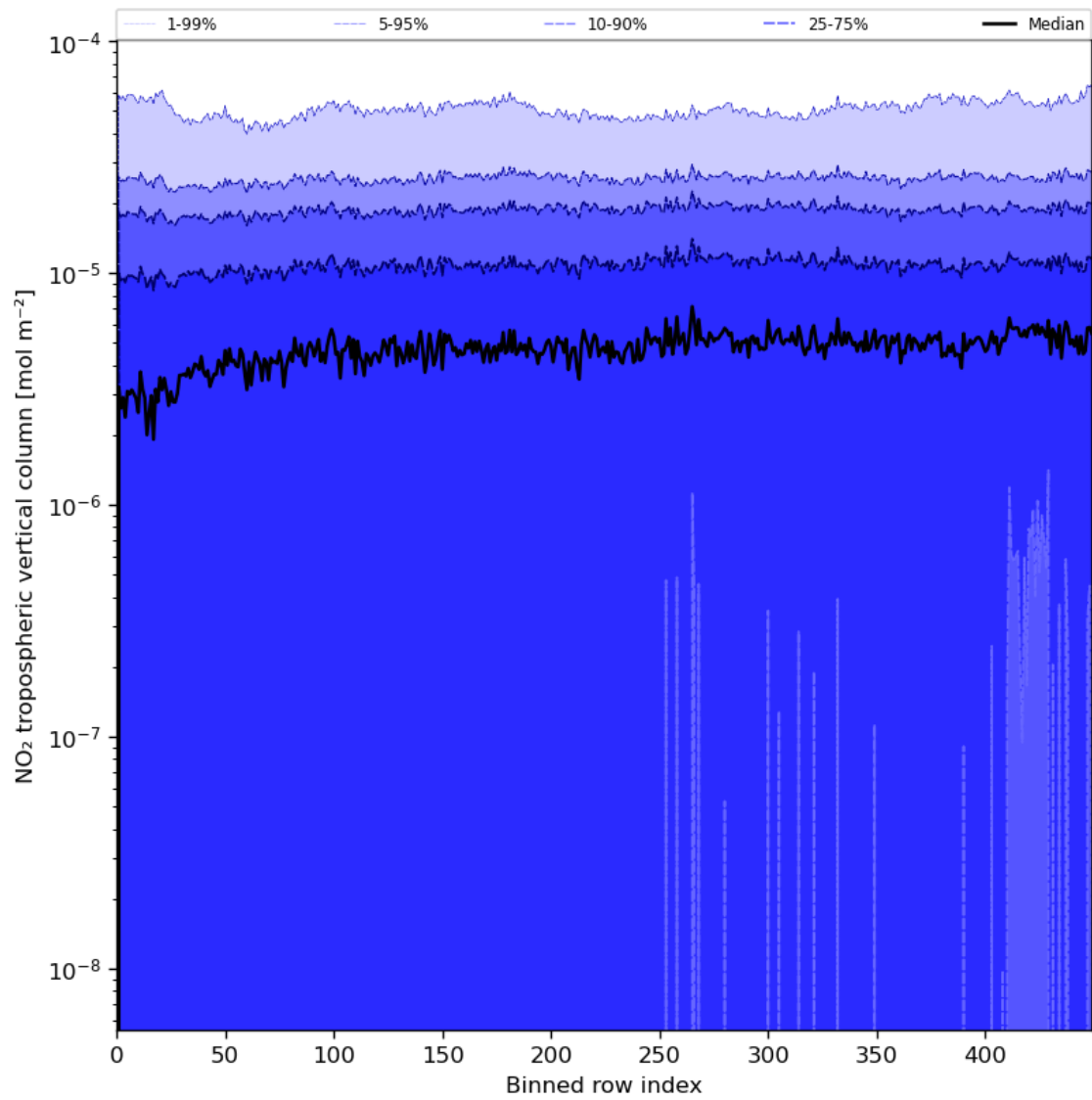
Figure 46: Along track statistics of “NO 2 tropospheric vertical column” for 2023-07-13 to 2023-07-14
