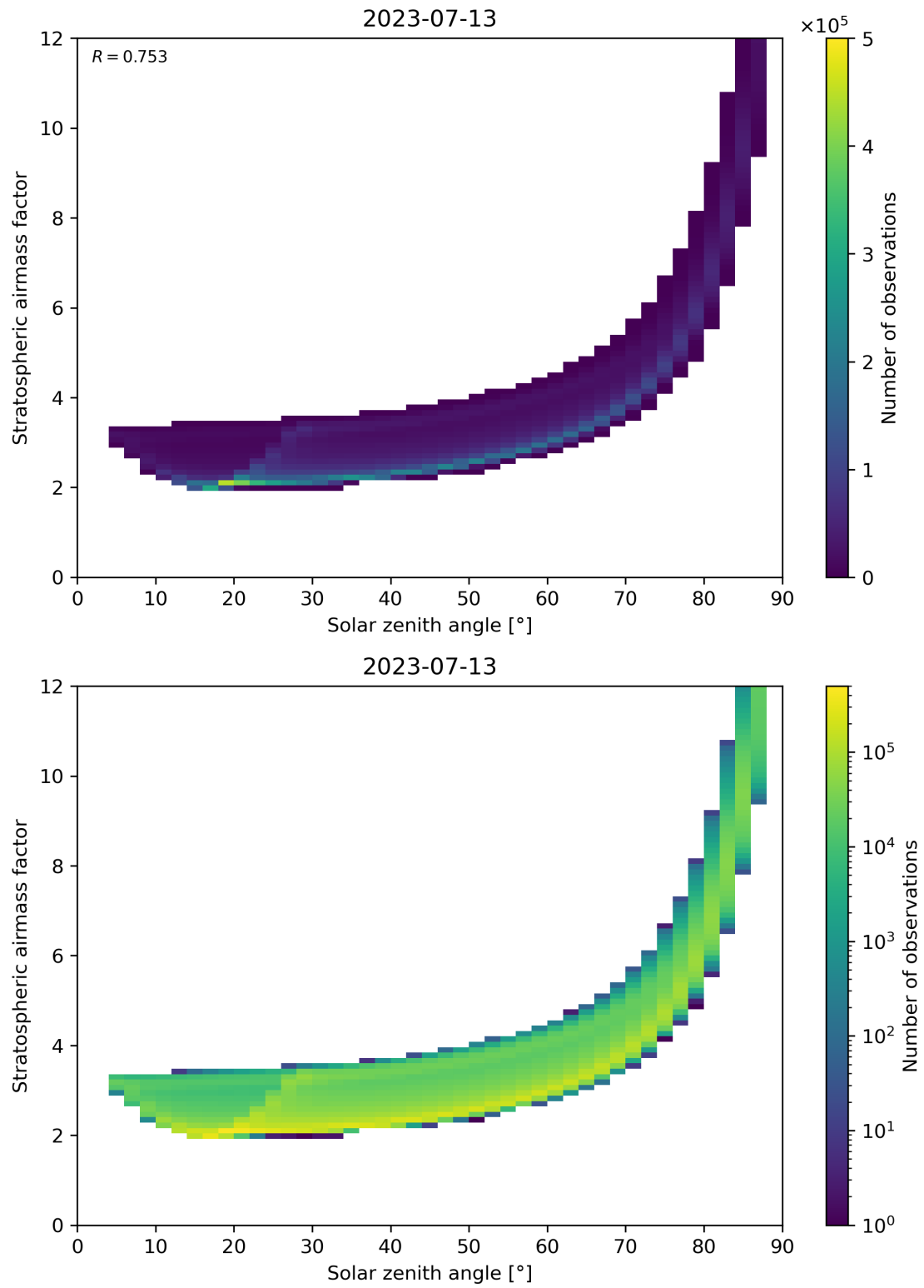
Figure 145: Scatter density plot of “Solar zenith angle” against “Stratospheric airmass factor” for 2023-07-13 to 2023-07-14.
