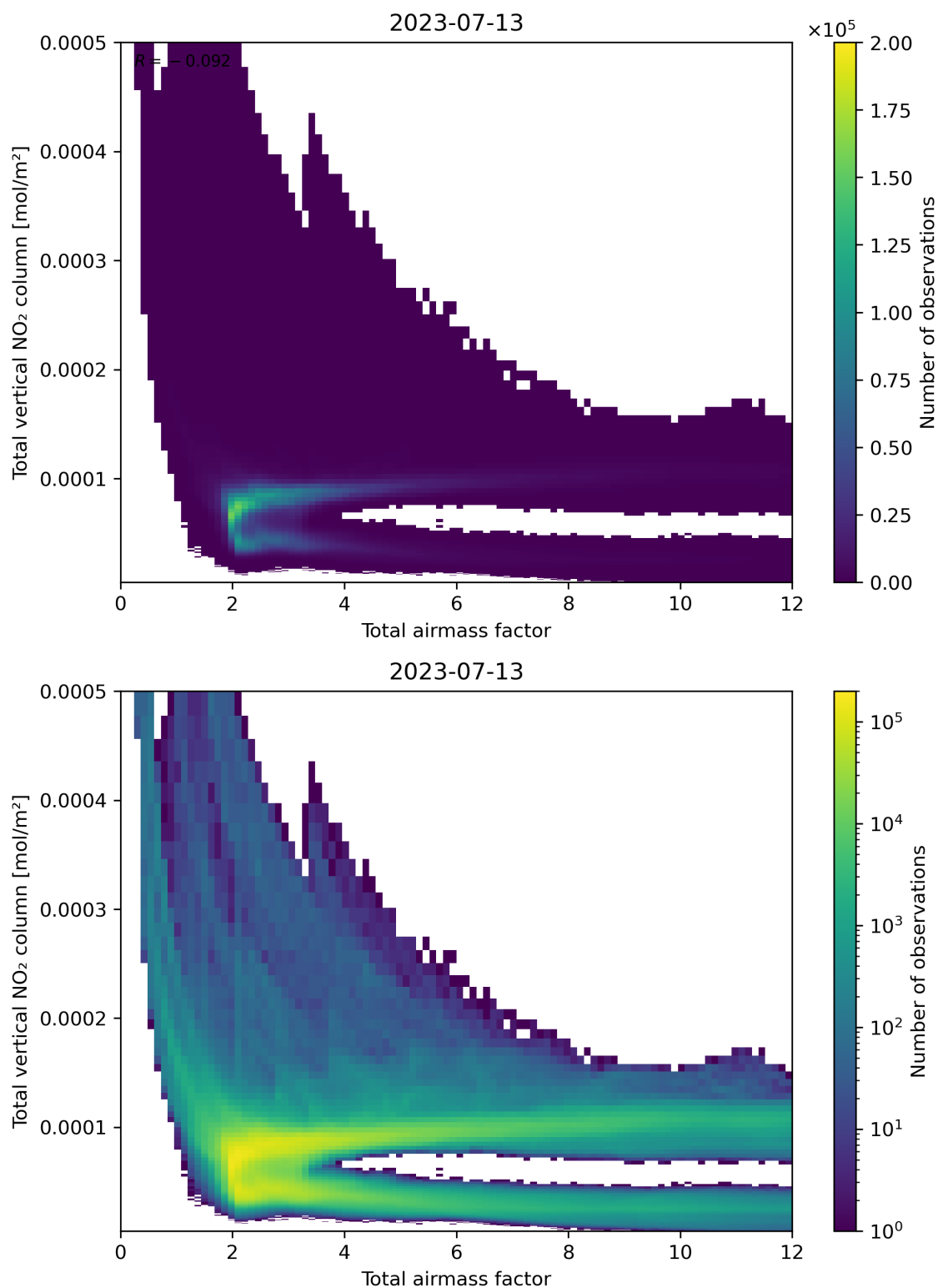
Figure 67: Scatter density plot of “Total airmass factor” against “Total vertical NO 2 column” for 2023-07-13 to 2023-07-14.
