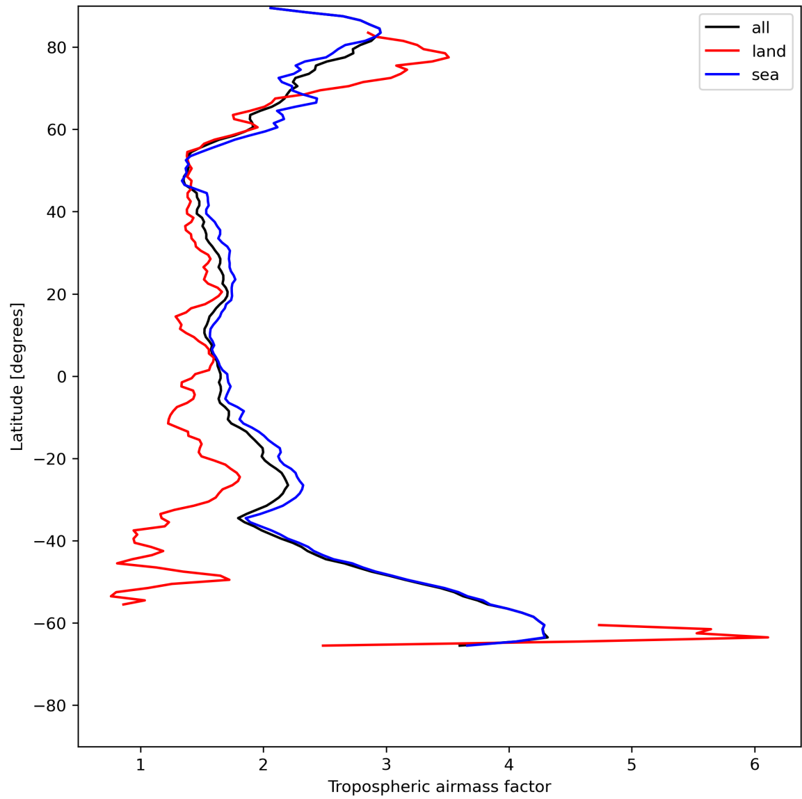
Figure 14: Zonal average of “Tropospheric air mass factor” for 2023-07-13 to 2023-07-14.
