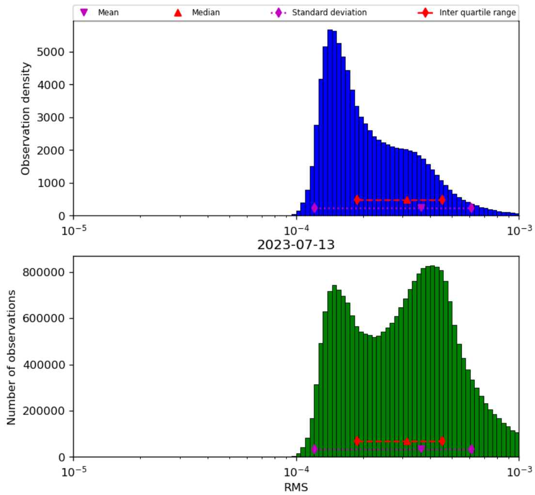
Figure 43: Histogram of “RMS” for 2023-07-13 to 2023-07-14
