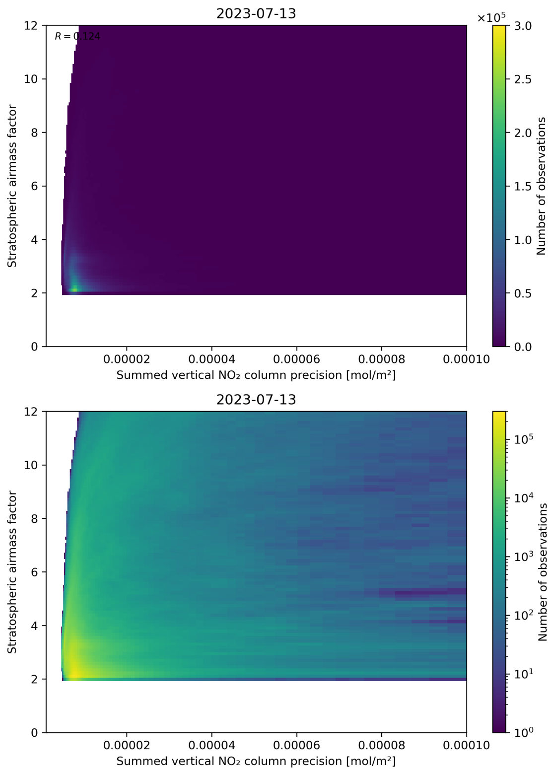
Figure 106: Scatter density plot of “Summed vertical NO 2 column precision” against “Stratospheric airmass factor” for 2023-07-13 to 2023-07-14.
