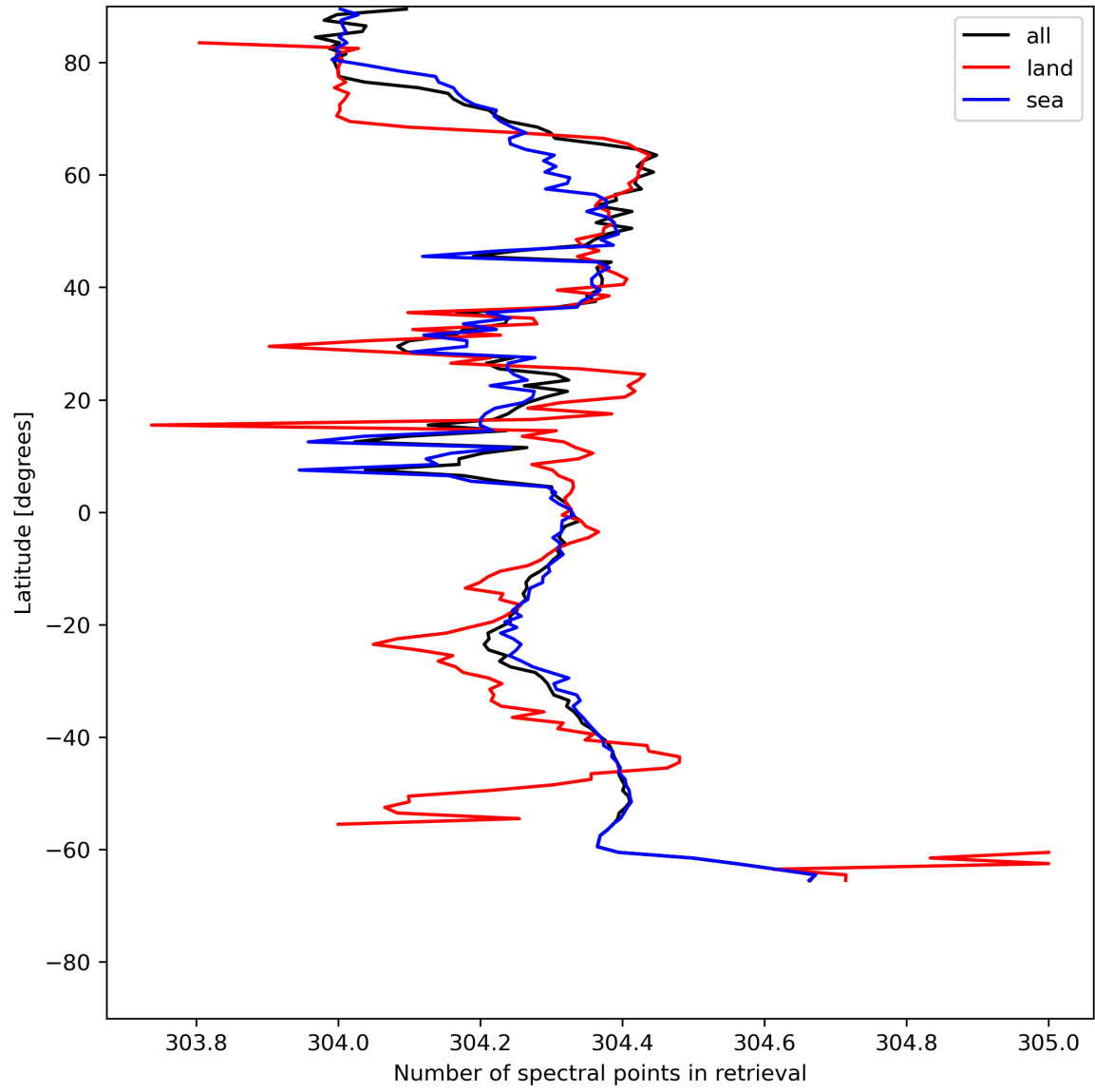
Figure 16: Zonal average of “Number of spectral points in retrieval” for 2023-07-13 to 2023-07-14.
