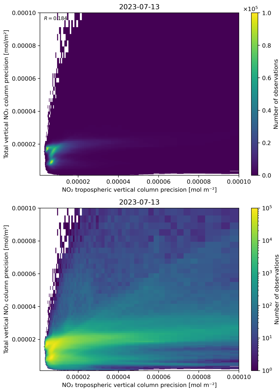
Figure 139: Scatter density plot of “NO 2 tropospheric vertical column precision” against “Total vertical NO 2 column precision” for 2023-07-13 to 2023-07-14.
