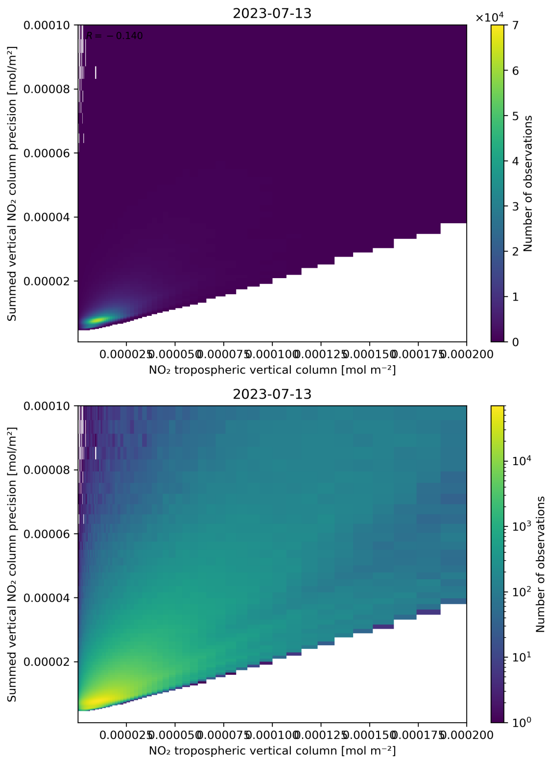
Figure 127: Scatter density plot of “NO 2 tropospheric vertical column” against “Summed vertical NO 2 column precision” for 2023-07-13 to 2023-07-14.
