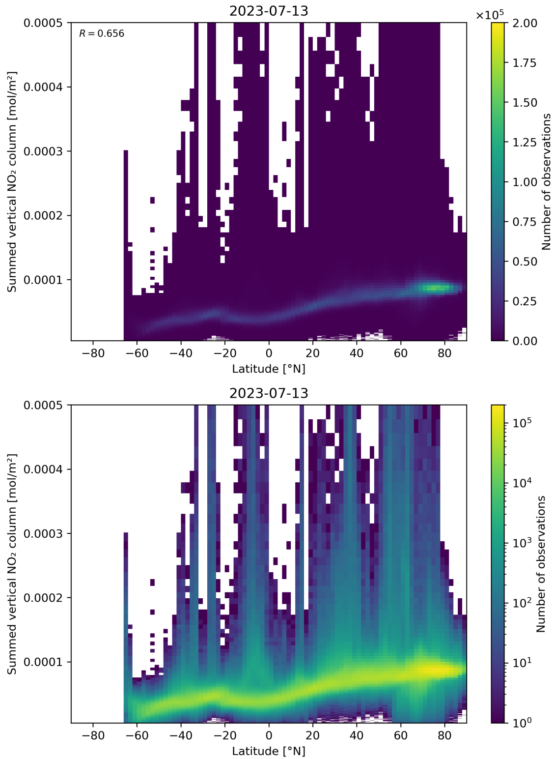
Figure 88: Scatter density plot of “Latitude” against “Summed vertical NO 2 column” for 2023-07-13 to 2023-07-14.
