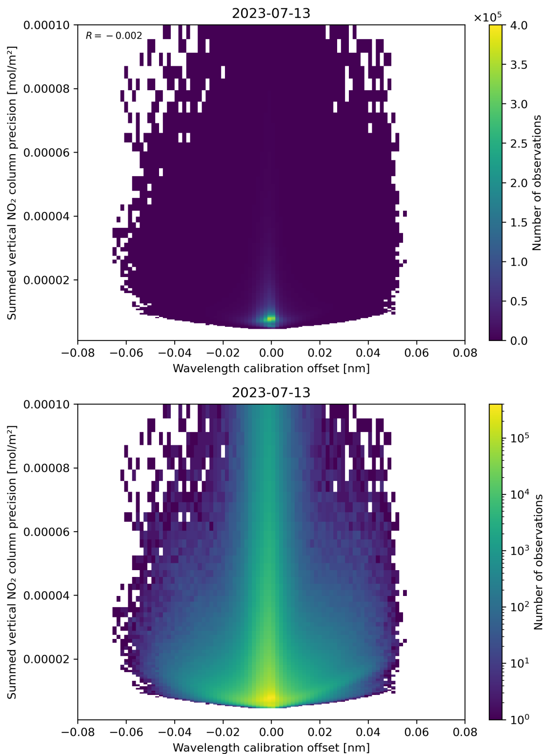
Figure 178: Scatter density plot of “Wavelength calibration offset” against “Summed vertical NO 2 column precision” for 2023-07-13 to 2023-07-14.
