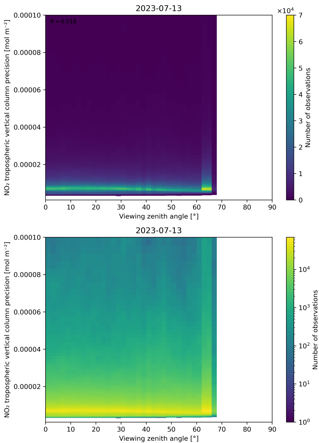
Figure 170: Scatter density plot of “Viewing zenith angle” against “NO 2 tropospheric vertical column precision” for 2023-07-13 to 2023-07-14.
