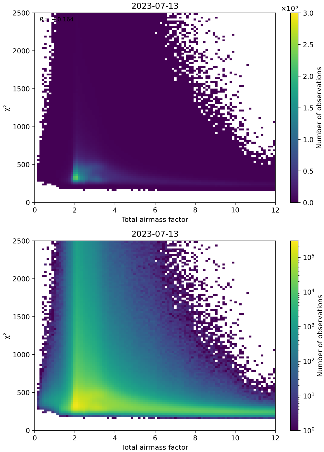
Figure 63: Scatter density plot of “Total airmass factor” against “ \chi^2 ” for 2023-07-13 to 2023-07-14.
