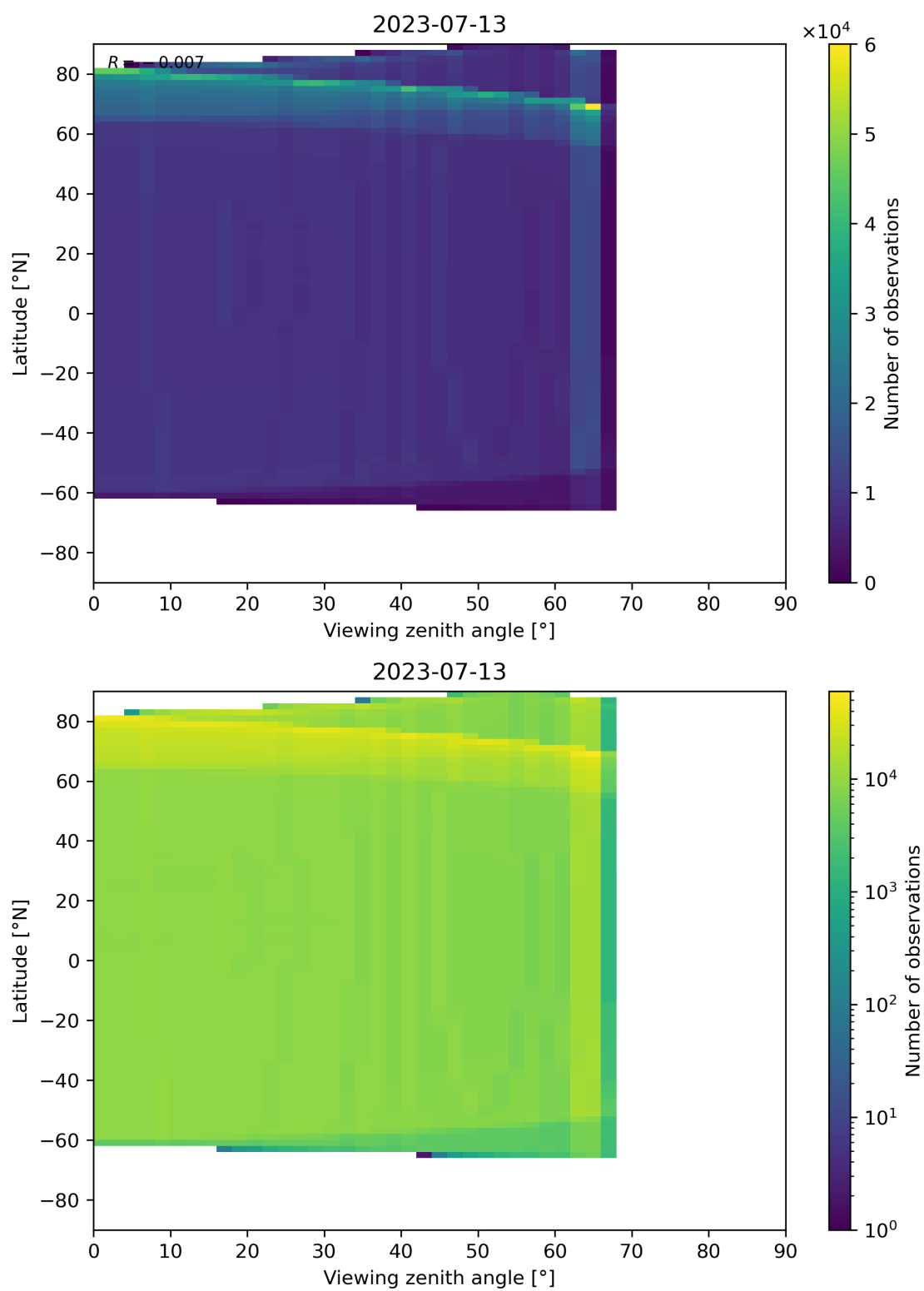
Figure 163: Scatter density plot of “Viewing zenith angle” against “Latitude” for 2023-07-13 to 2023-07-14.
