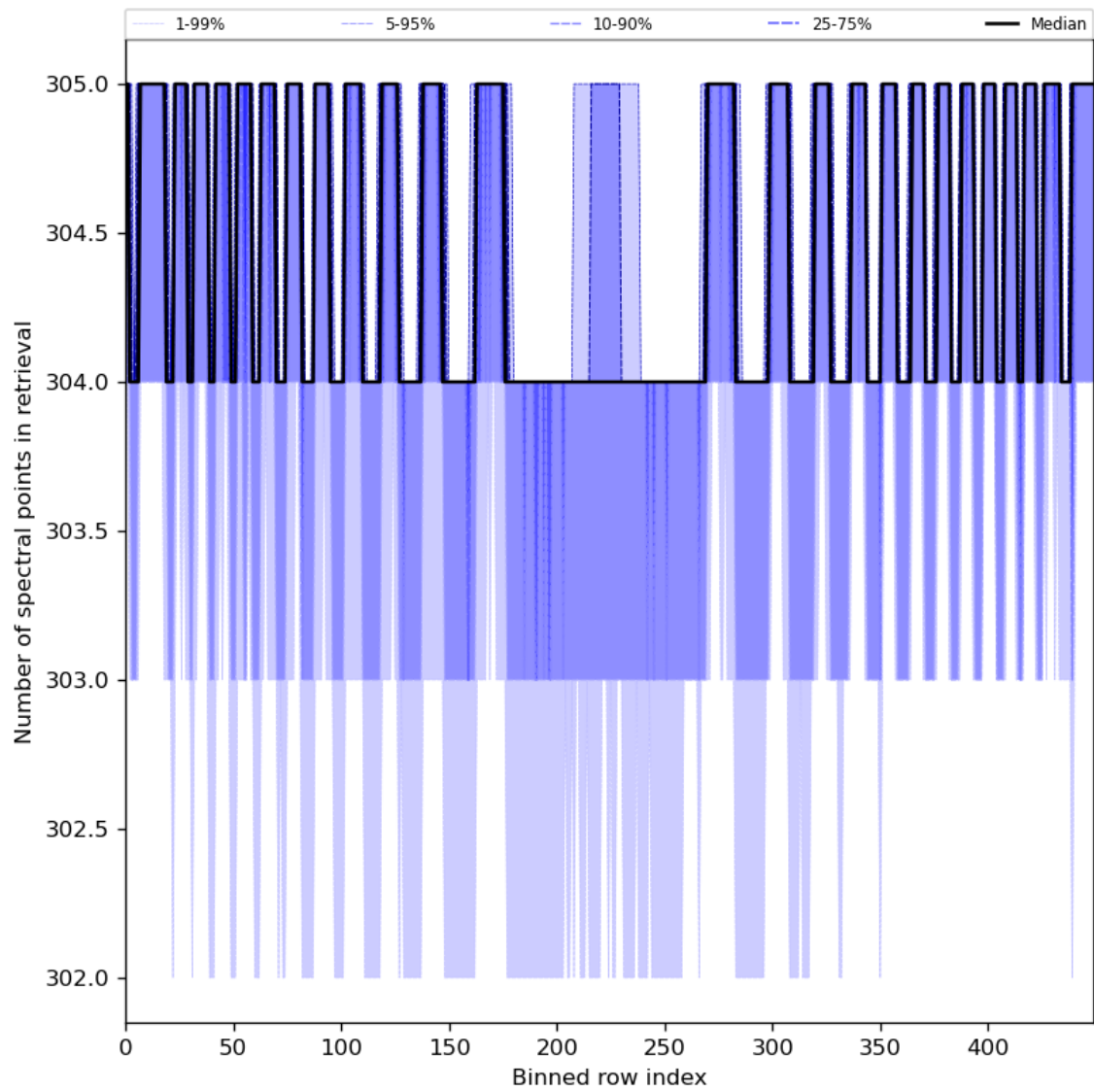
Figure 50: Along track statistics of “Number of spectral points in retrieval” for 2023-07-13 to 2023-07-14
