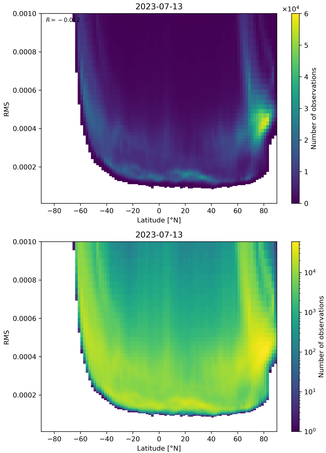
Figure 94: Scatter density plot of “Latitude” against “RMS” for 2023-07-13 to 2023-07-14.
