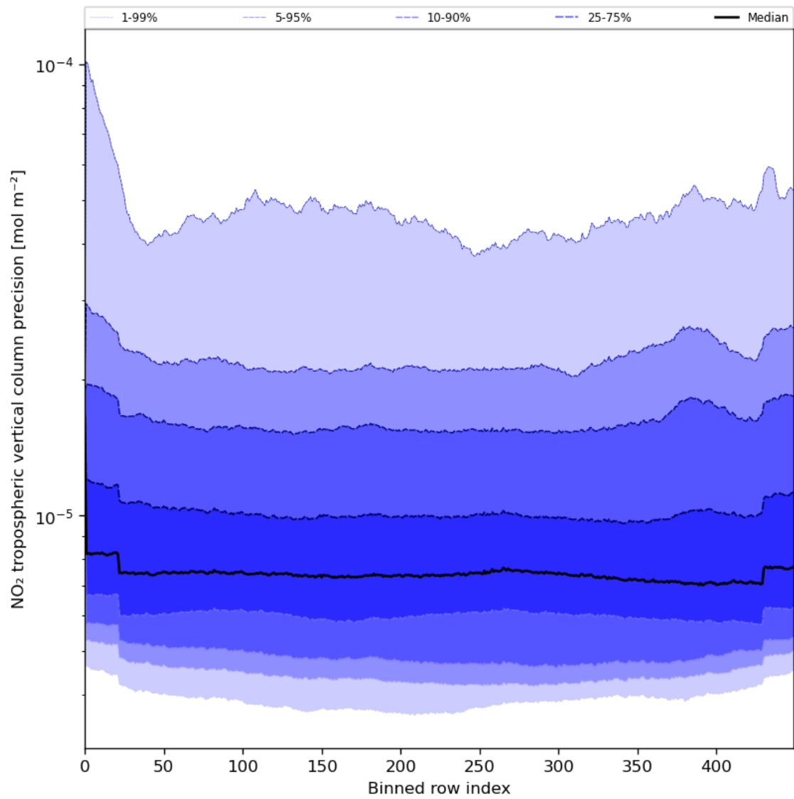
Figure 47: Along track statistics of “NO 2 tropospheric vertical column precision” for 2023-07-13 to 2023-07-14
