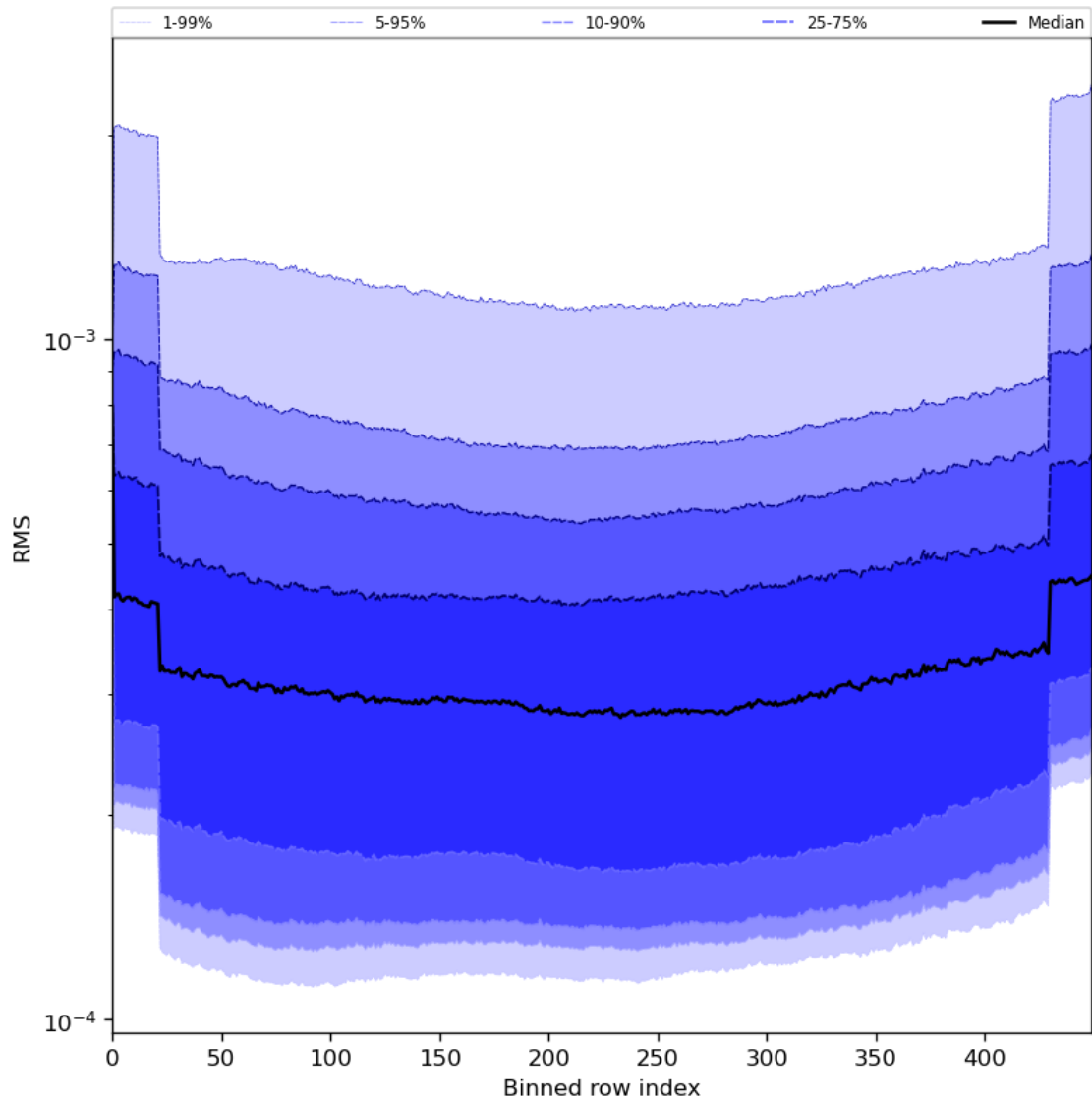
Figure 60: Along track statistics of “RMS” for 2023-07-13 to 2023-07-14
