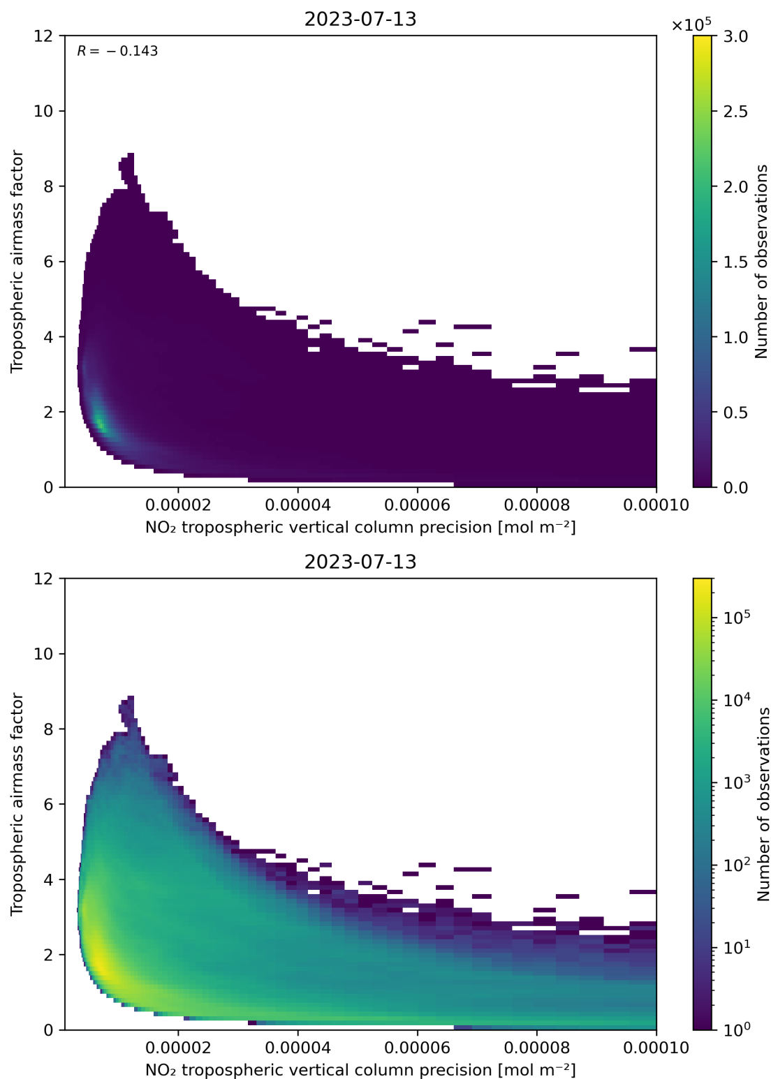
Figure 133: Scatter density plot of “NO 2 tropospheric vertical column precision” against “Tropospheric airmass factor” for 2023-07-13 to 2023-07-14.
