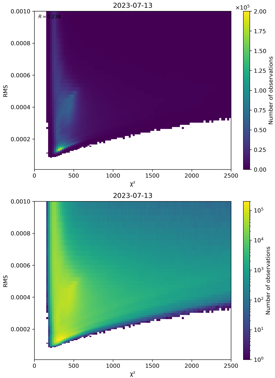
Figure 82: Scatter density plot of “ \chi^2 ” against “RMS” for 2023-07-13 to 2023-07-14.
