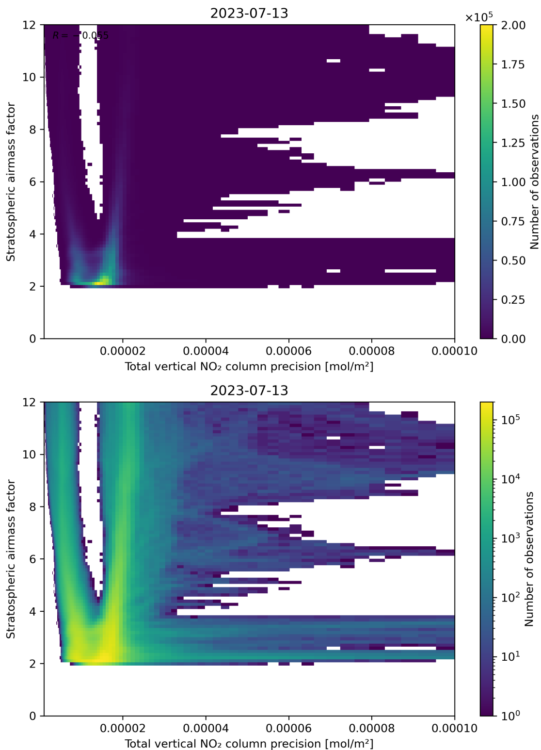
Figure 115: Scatter density plot of “Total vertical NO 2 column precision” against “Stratospheric air mass factor” for 2023-07-13 to 2023-07-14.
