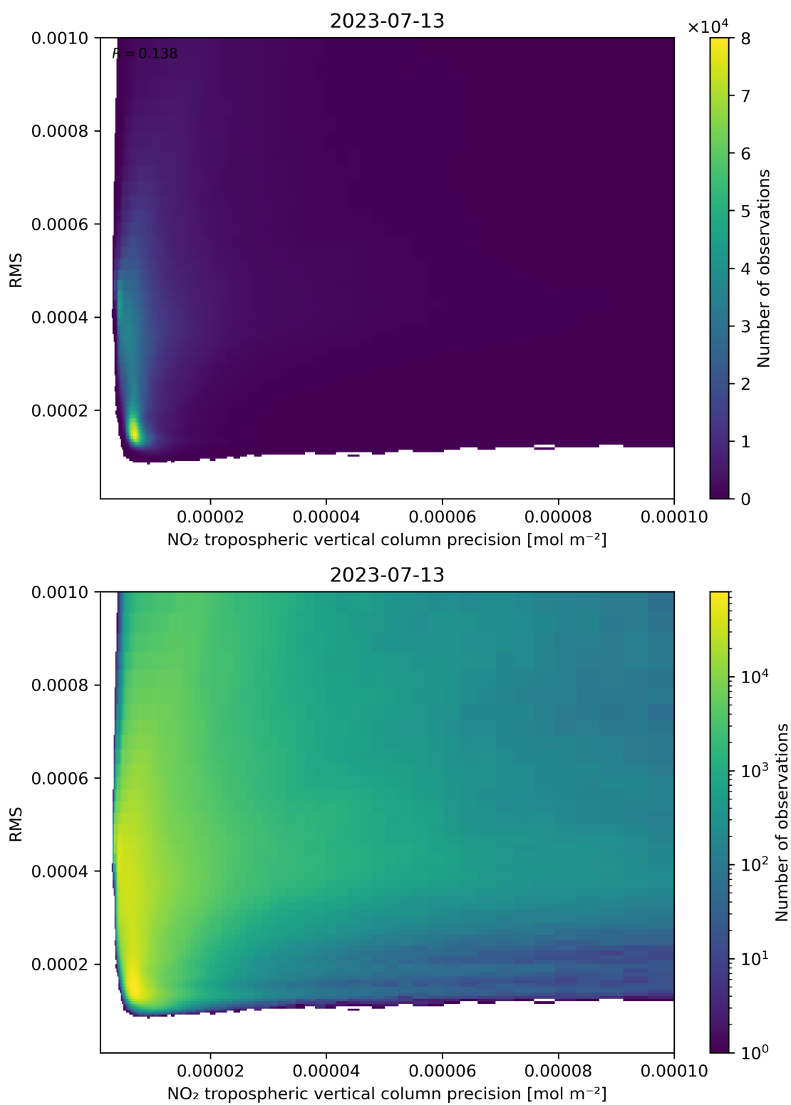
Figure 140: Scatter density plot of “NO 2 tropospheric vertical column precision” against “RMS” for 2023-07-13 to 2023-07-14.
