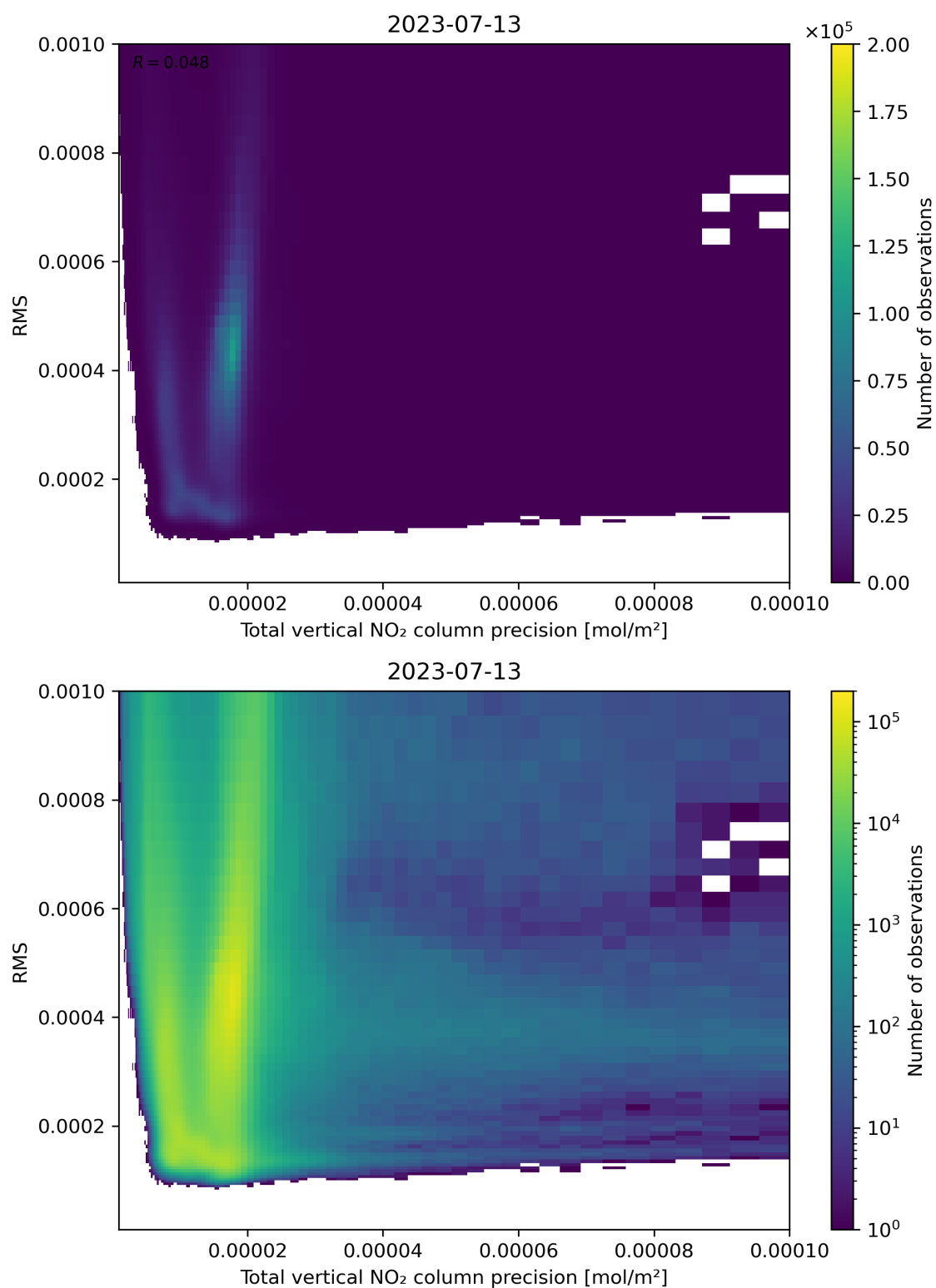
Figure 119: Scatter density plot of “Total vertical NO 2 column precision” against “RMS” for 2023-07-13 to 2023-07-14.
