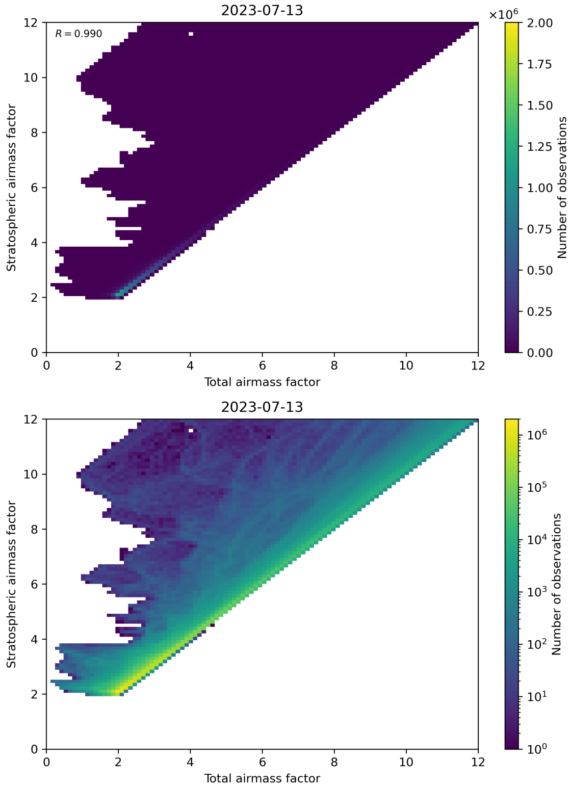
Figure 62: Scatter density plot of “Total airmass factor” against “Stratospheric airmass factor” for 2023-07-13 to 2023-07-14.
