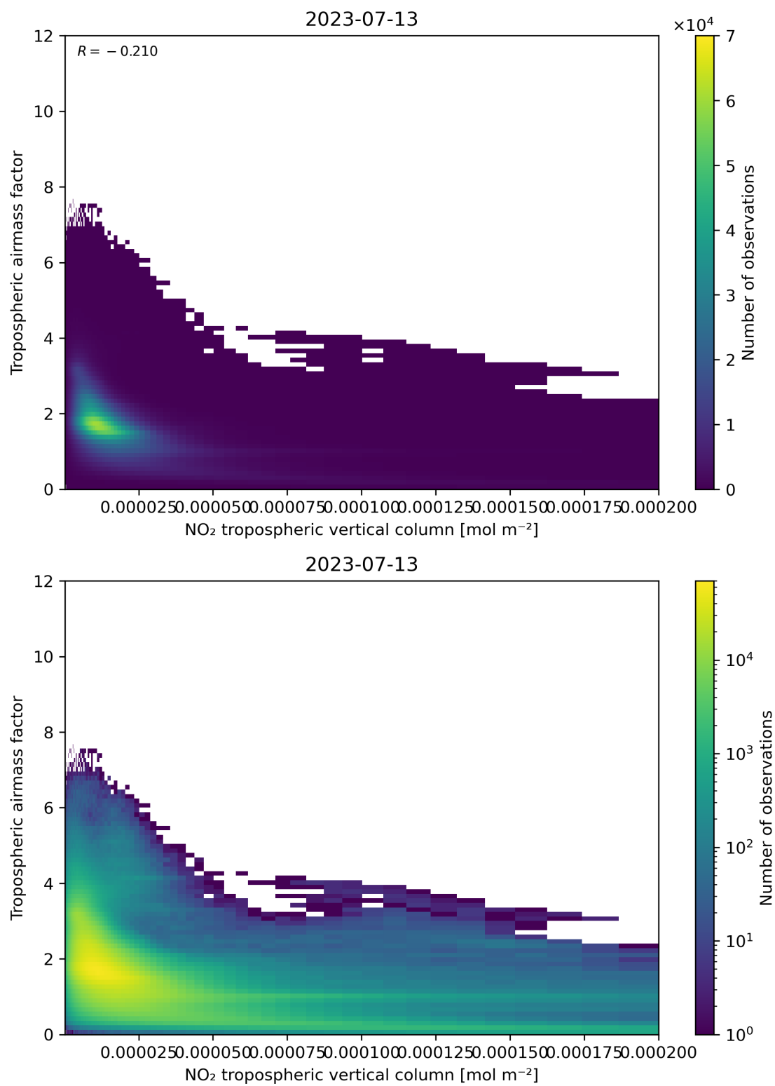
Figure 123: Scatter density plot of “NO 2 tropospheric vertical column” against “Tropospheric air mass factor” for 2023-07-13 to 2023-07-14.
