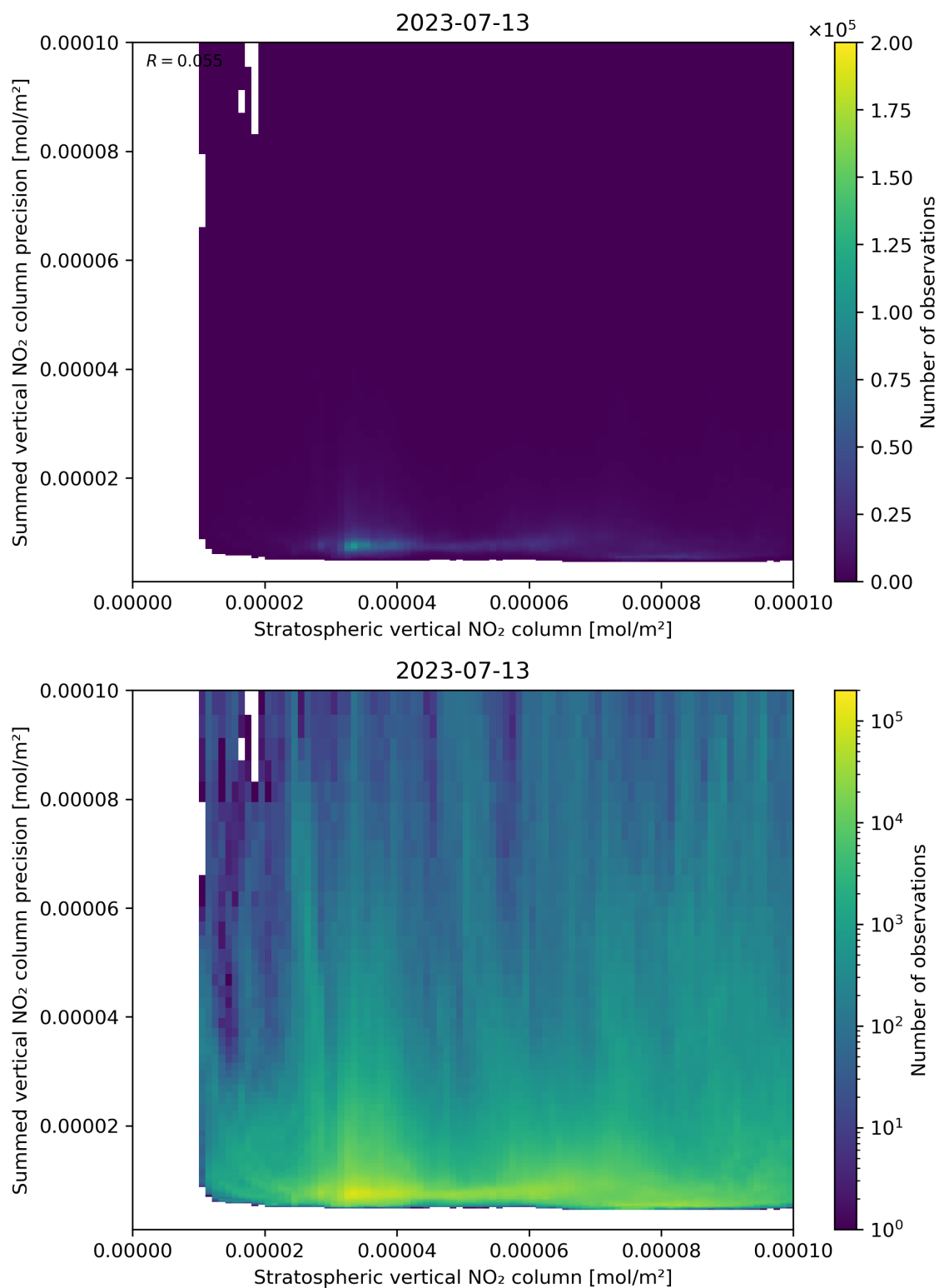
Figure 99: Scatter density plot of “Stratospheric vertical NO 2 column” against “Summed vertical NO 2 column precision” for 2023-07-13 to 2023-07-14.
