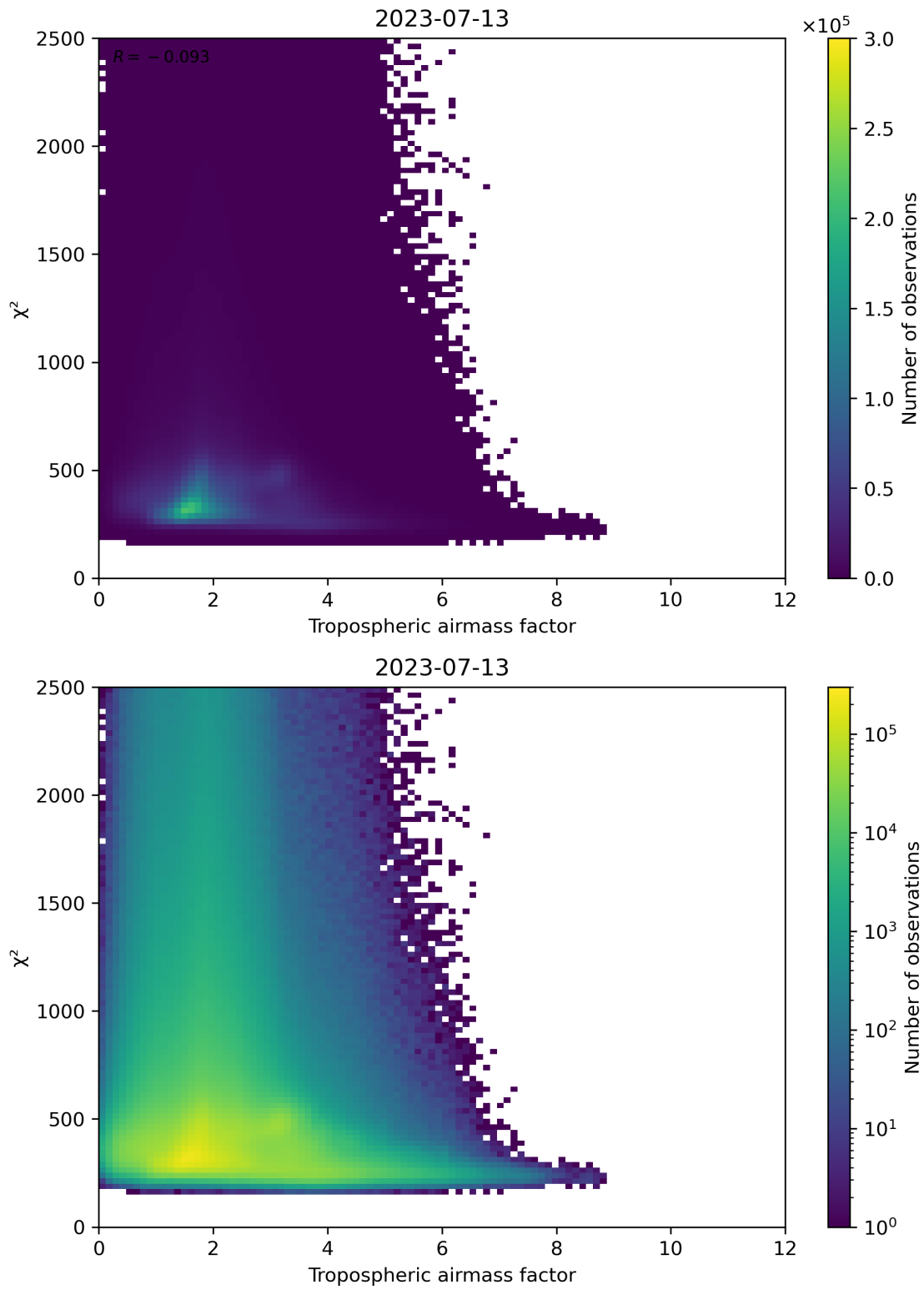
Figure 73: Scatter density plot of “Tropospheric airmass factor” against “ \chi^2 ” for 2023-07-13 to 2023-07-14.
