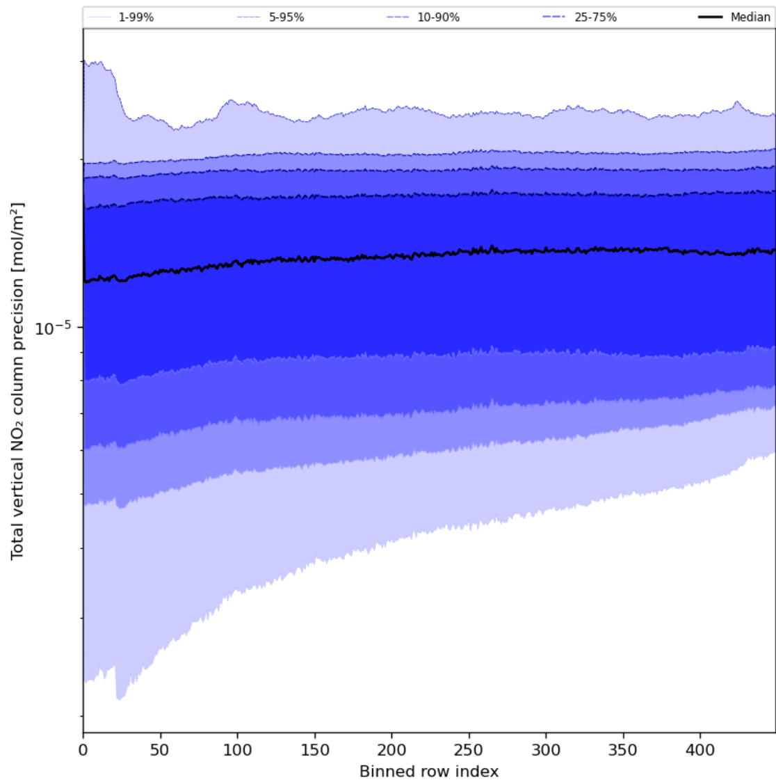
Figure 56: Along track statistics of “Total vertical NO 2 column precision” for 2023-07-13 to 2023-07-14
