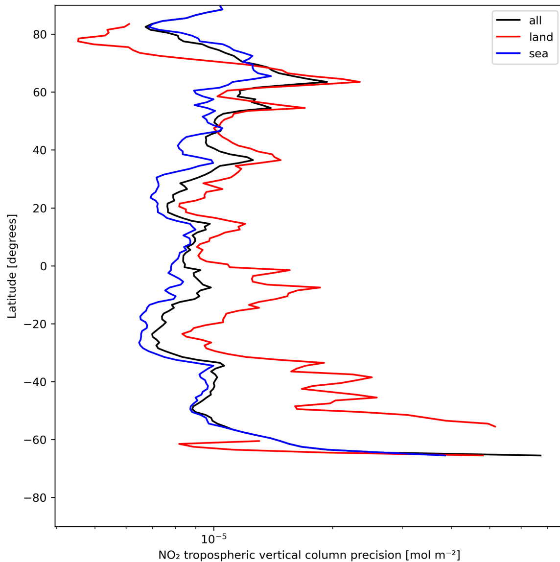
Figure 13: Zonal average of “NO 2 tropospheric vertical column precision” for 2023-07-13 to 2023-07-14.
