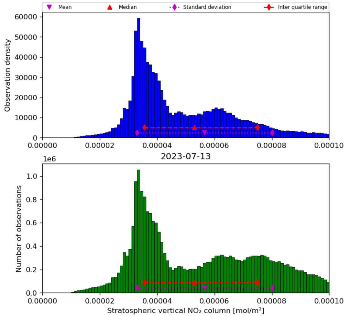
Figure 36: Histogram of “Stratospheric vertical NO 2 column” for 2023-07-13 to 2023-07-14
