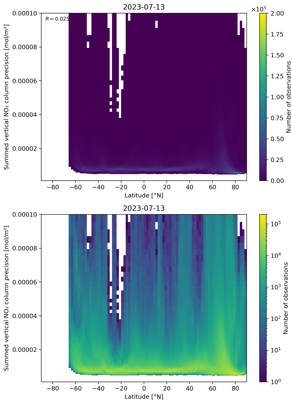
Figure 89: Scatter density plot of “Latitude” against “Summed vertical NO 2 column precision” for 2023-07-13 to 2023-07-14.
