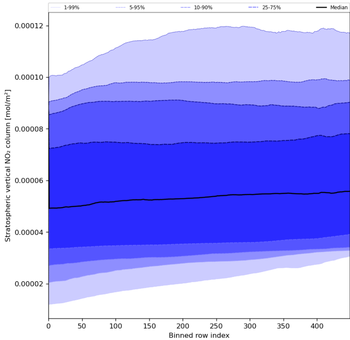
Figure 53: Along track statistics of “Stratospheric vertical NO 2 column” for 2023-07-13 to 2023-07-14
