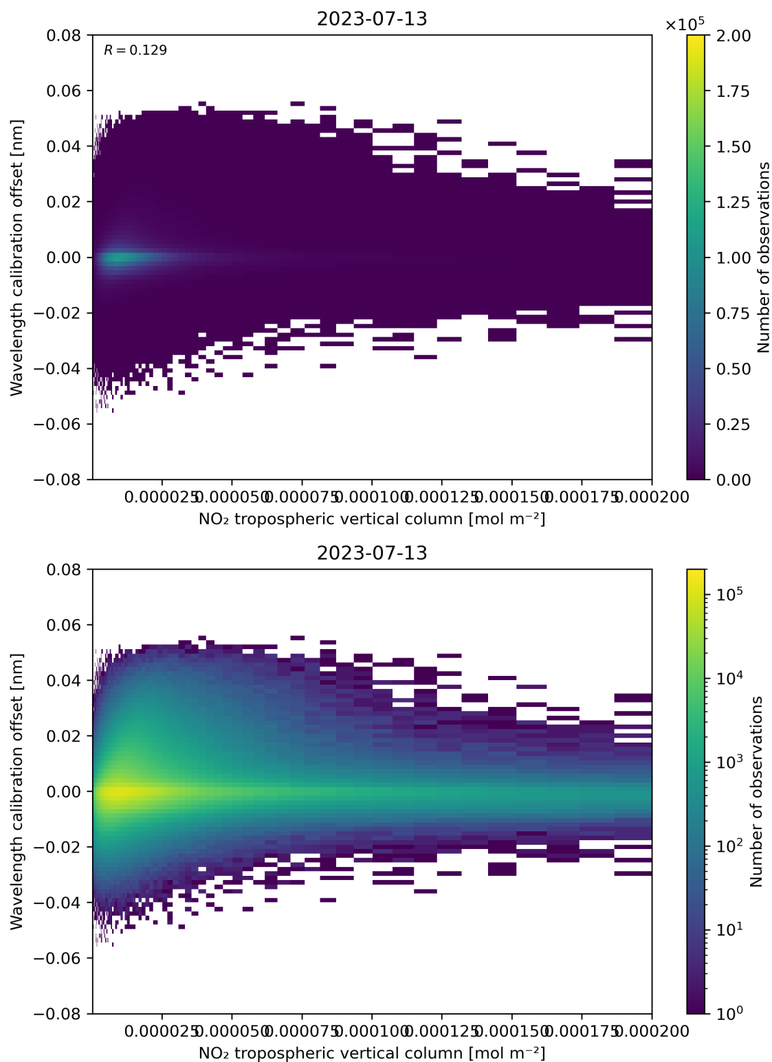
Figure 143: Scatter density plot of “NO 2 tropospheric vertical column” against “Wavelength calibration offset” for 2023-07-13 to 2023-07-14.
