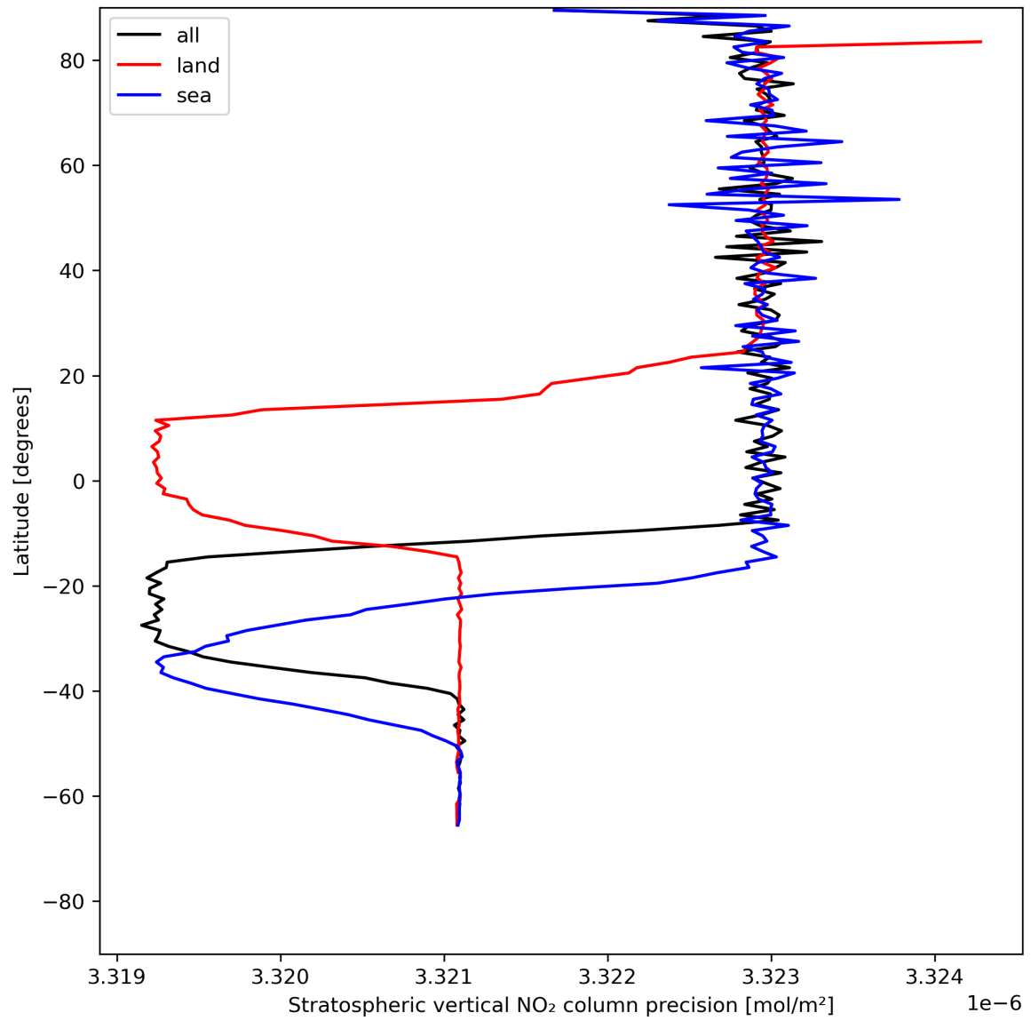
Figure 20: Zonal average of “Stratospheric vertical NO 2 column precision” for 2023-07-13 to 2023-07-14.
