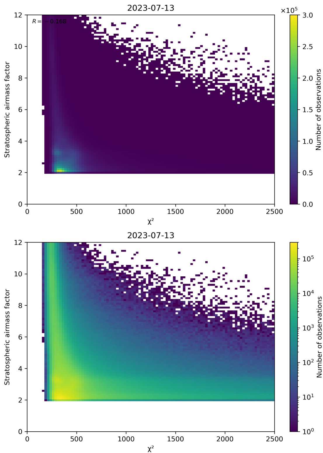
Figure 81: Scatter density plot of " \chi^2 " against "Stratospheric airmass factor" for 2023-07-13 to 2023-07-14.
