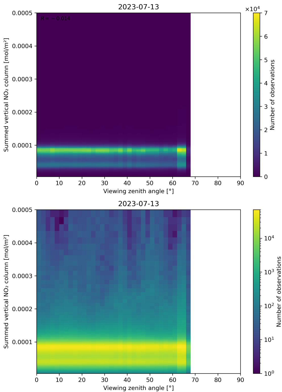
Figure 165: Scatter density plot of “Viewing zenith angle” against “Summed vertical NO 2 column” for 2023-07-13 to 2023-07-14.
