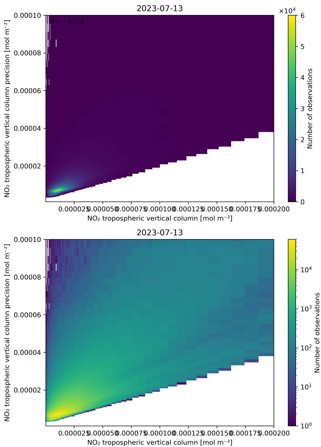
Figure 130: Scatter density plot of “NO 2 tropospheric vertical column” against “NO 2 tropospheric vertical column precision” for 2023-07-13 to 2023-07-14.
