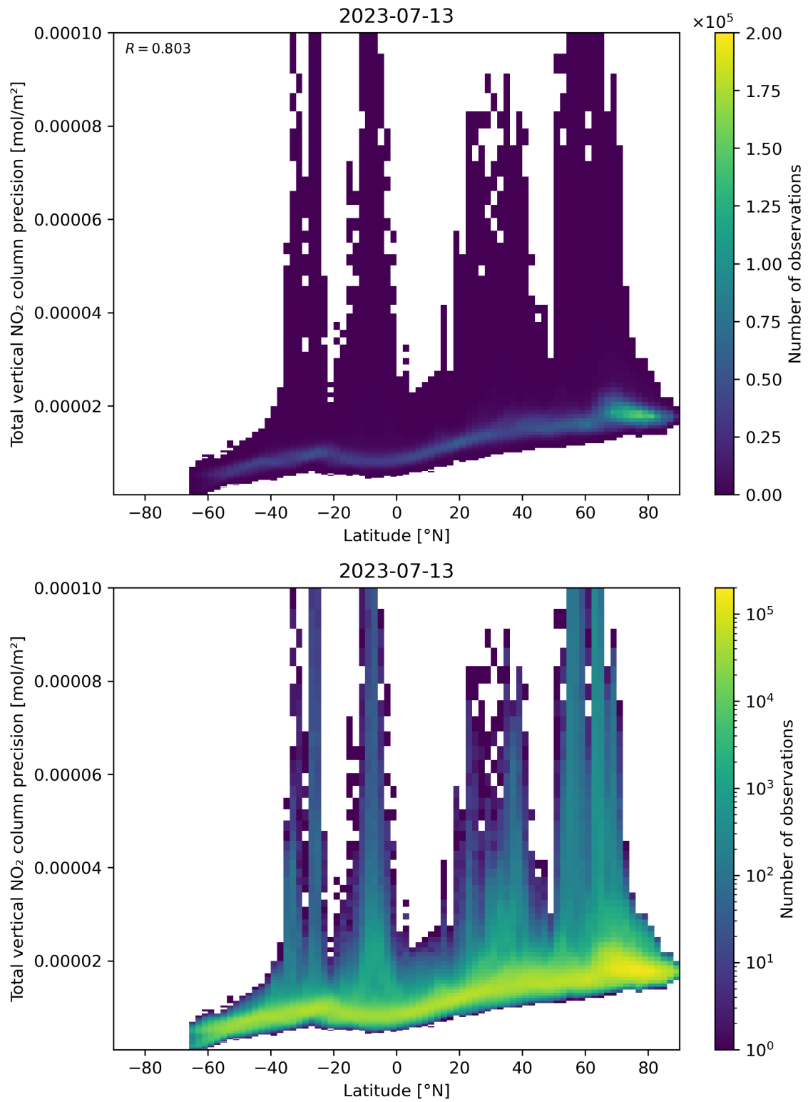
Figure 91: Scatter density plot of “Latitude” against “Total vertical NO 2 column precision” for 2023-07-13 to 2023-07-14.
