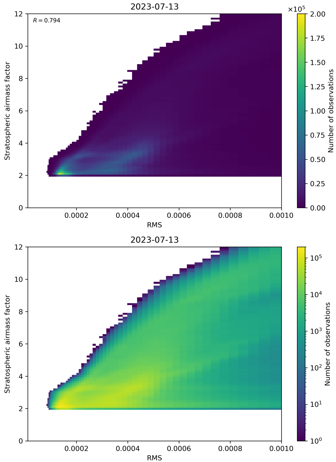
Figure 144: Scatter density plot of “RMS” against “Stratospheric airmass factor” for 2023-07-13 to 2023-07-14.
