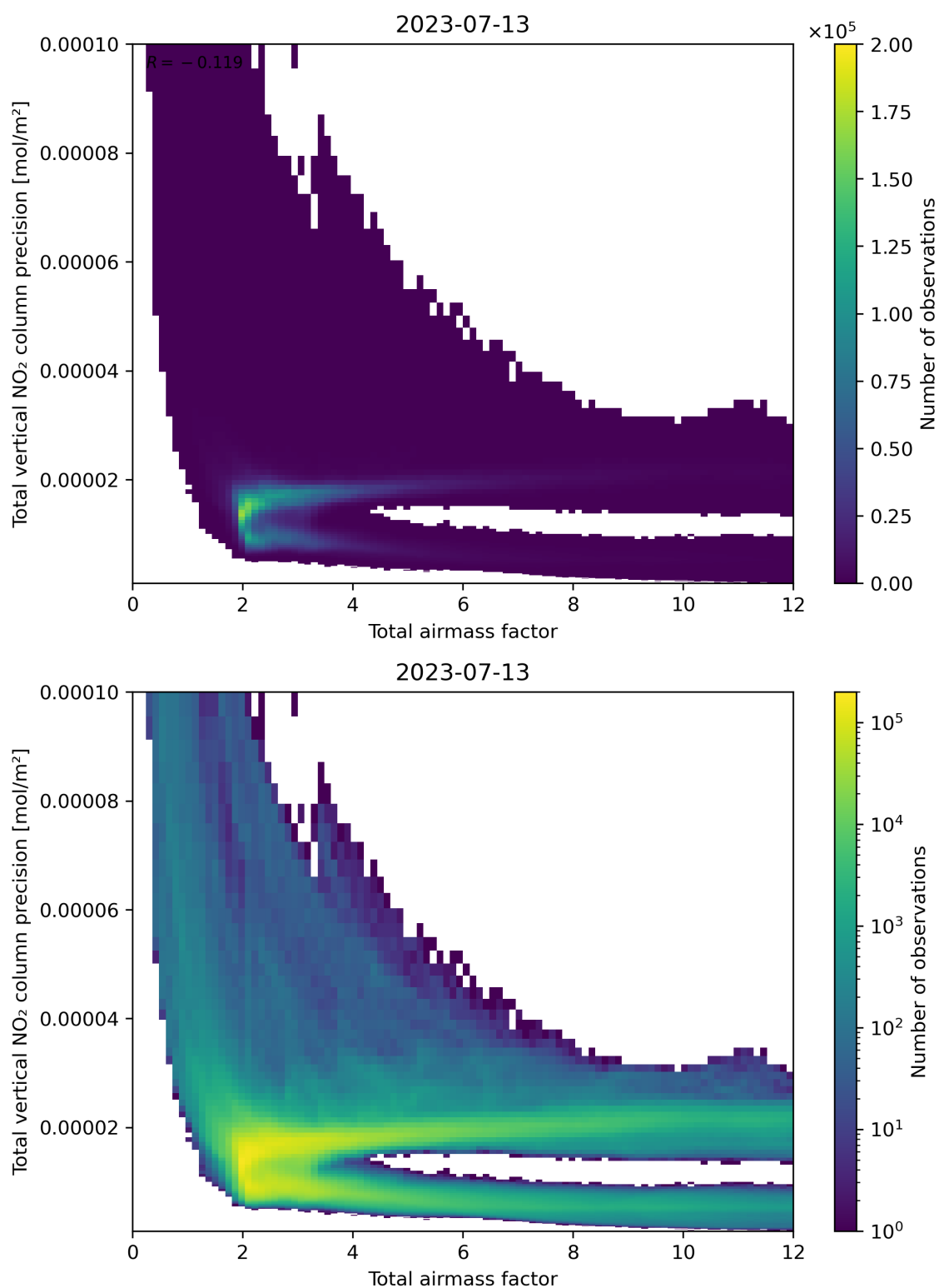
Figure 68: Scatter density plot of “Total airmass factor” against “Total vertical NO 2 column precision” for 2023-07-13 to 2023-07-14.
