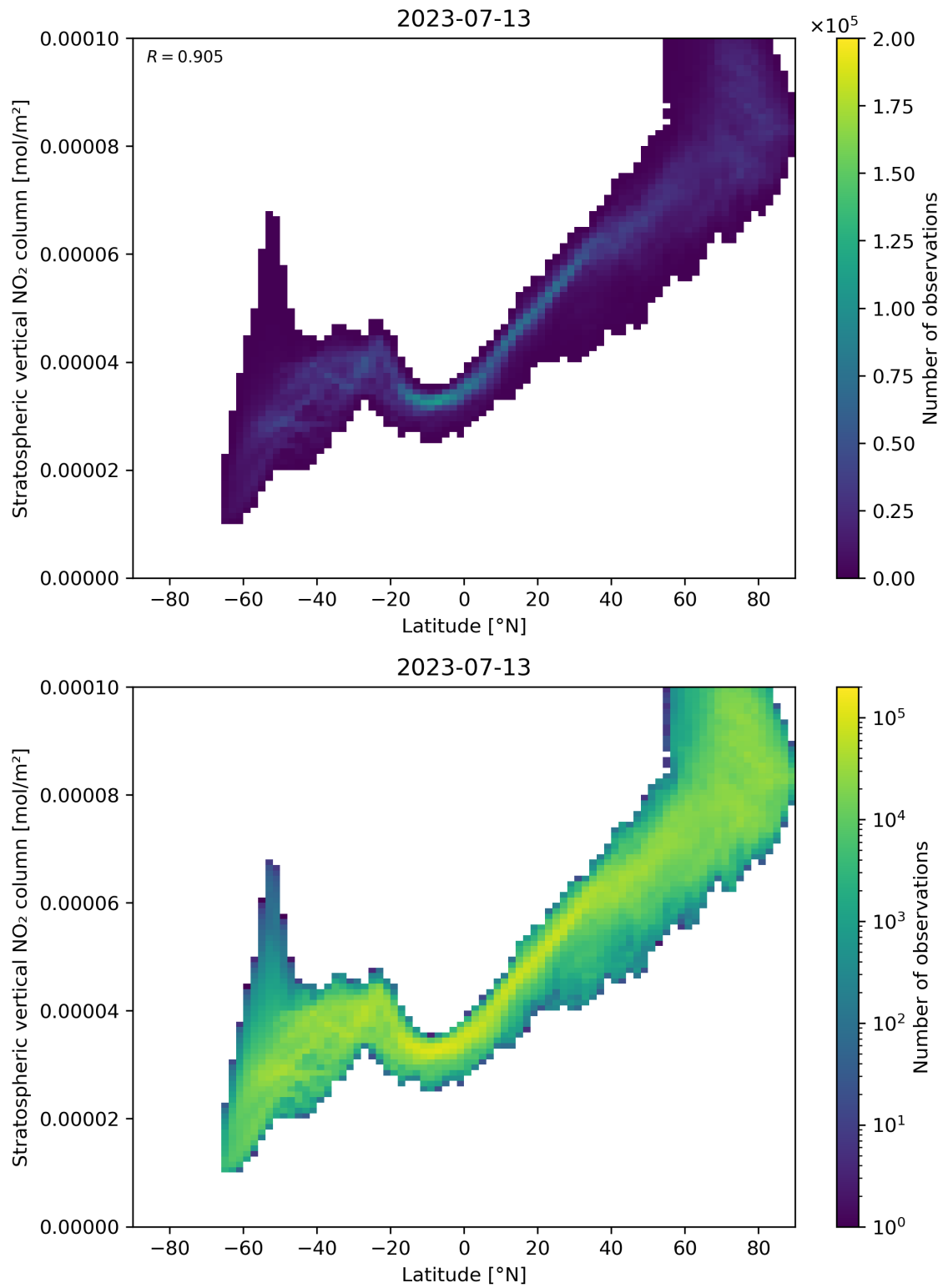
Figure 87: Scatter density plot of “Latitude” against “Stratospheric vertical NO 2 column” for 2023-07-13 to 2023-07-14.
