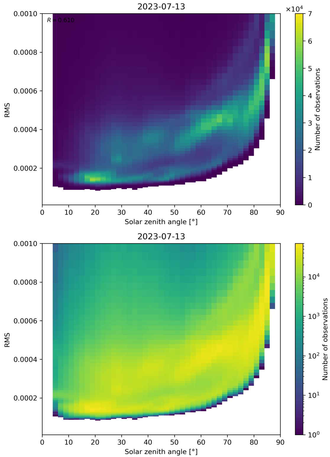
Figure 157: Scatter density plot of “Solar zenith angle” against “RMS” for 2023-07-13 to 2023-07-14.
