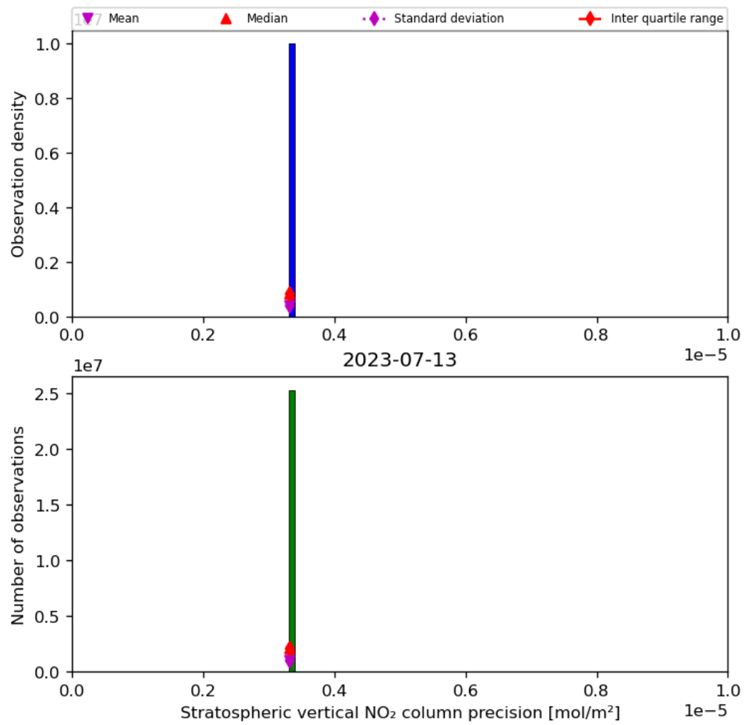
Figure 37: Histogram of “Stratospheric vertical NO 2 column precision” for 2023-07-13 to 2023-07-14
