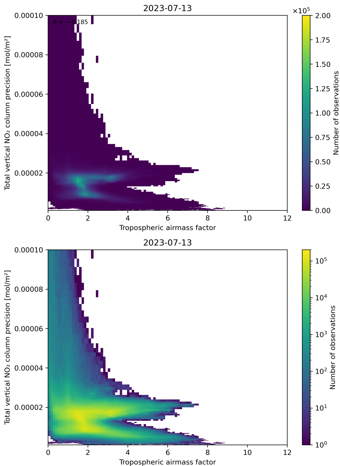
Figure 78: Scatter density plot of “Tropospheric air mass factor” against “Total vertical NO 2 column precision” for 2023-07-13 to 2023-07-14.
