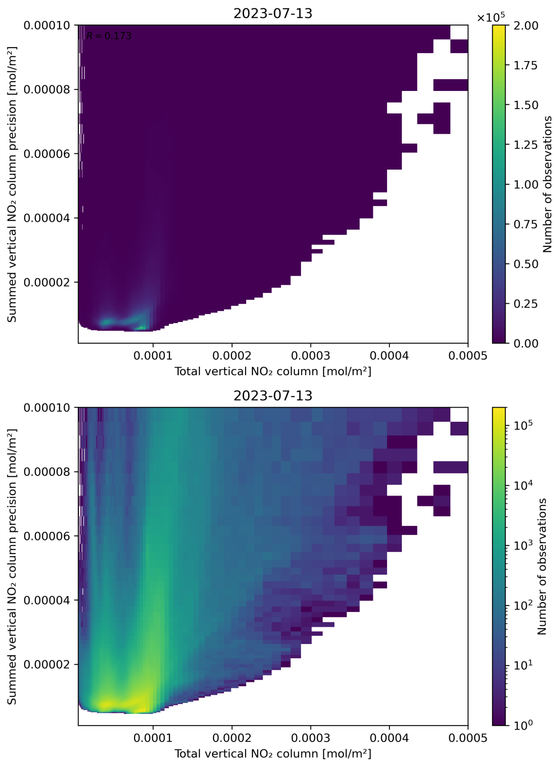
Figure 113: Scatter density plot of “Total vertical NO 2 column” against “Summed vertical NO 2 column precision” for 2023-07-13 to 2023-07-14.
