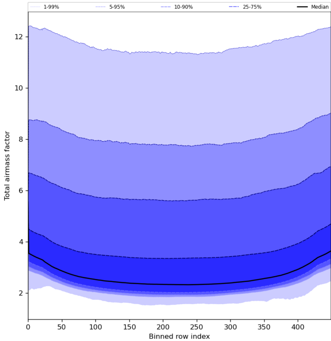
Figure 49: Along track statistics of “Total airmass factor” for 2023-07-13 to 2023-07-14
