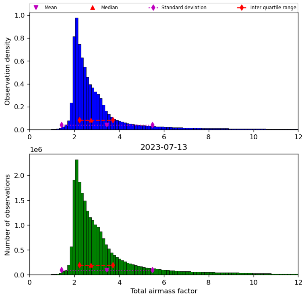
Figure 32: Histogram of “Total airmass factor” for 2023-07-13 to 2023-07-14
