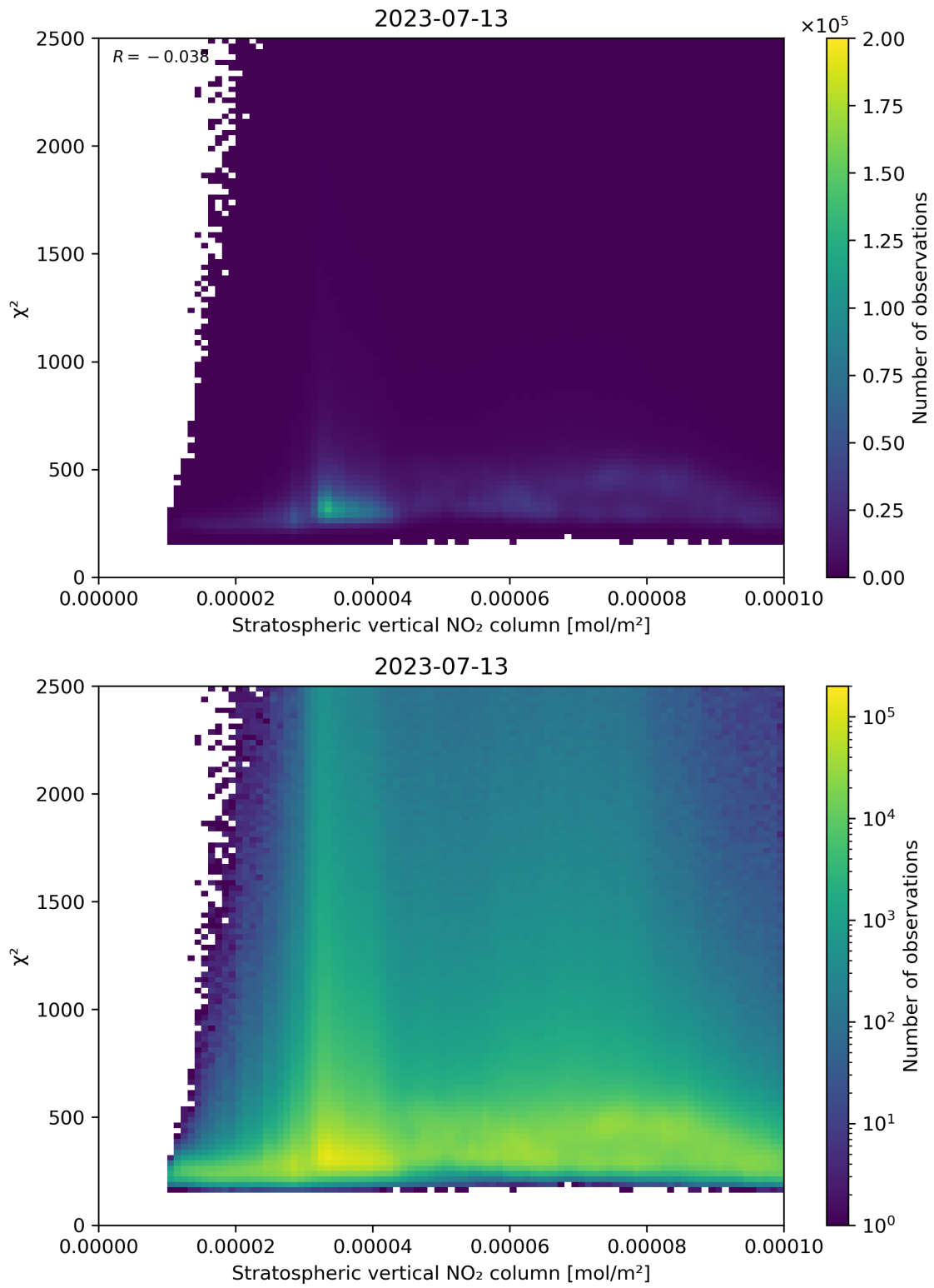
Figure 97: Scatter density plot of “Stratospheric vertical NO 2 column” against “ \chi^2 ” for 2023-07-13 to 2023-07-14.
