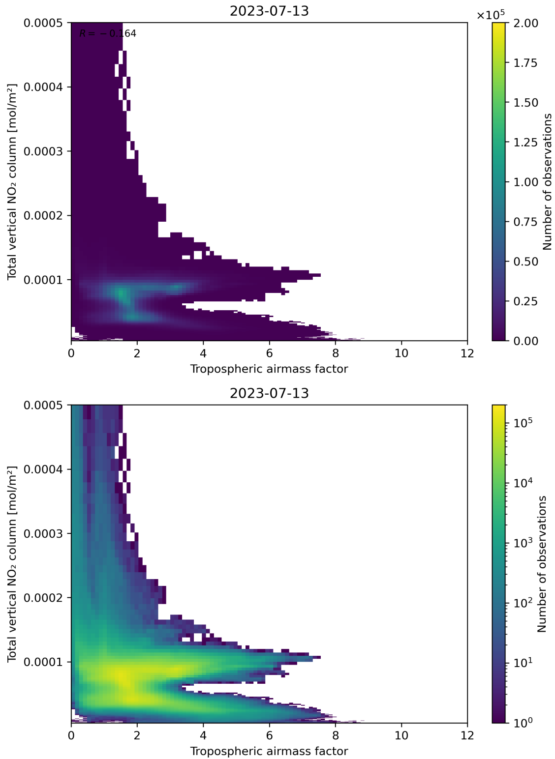
Figure 77: Scatter density plot of “Tropospheric airmass factor” against “Total vertical NO 2 column” for 2023-07-13 to 2023-07-14.
