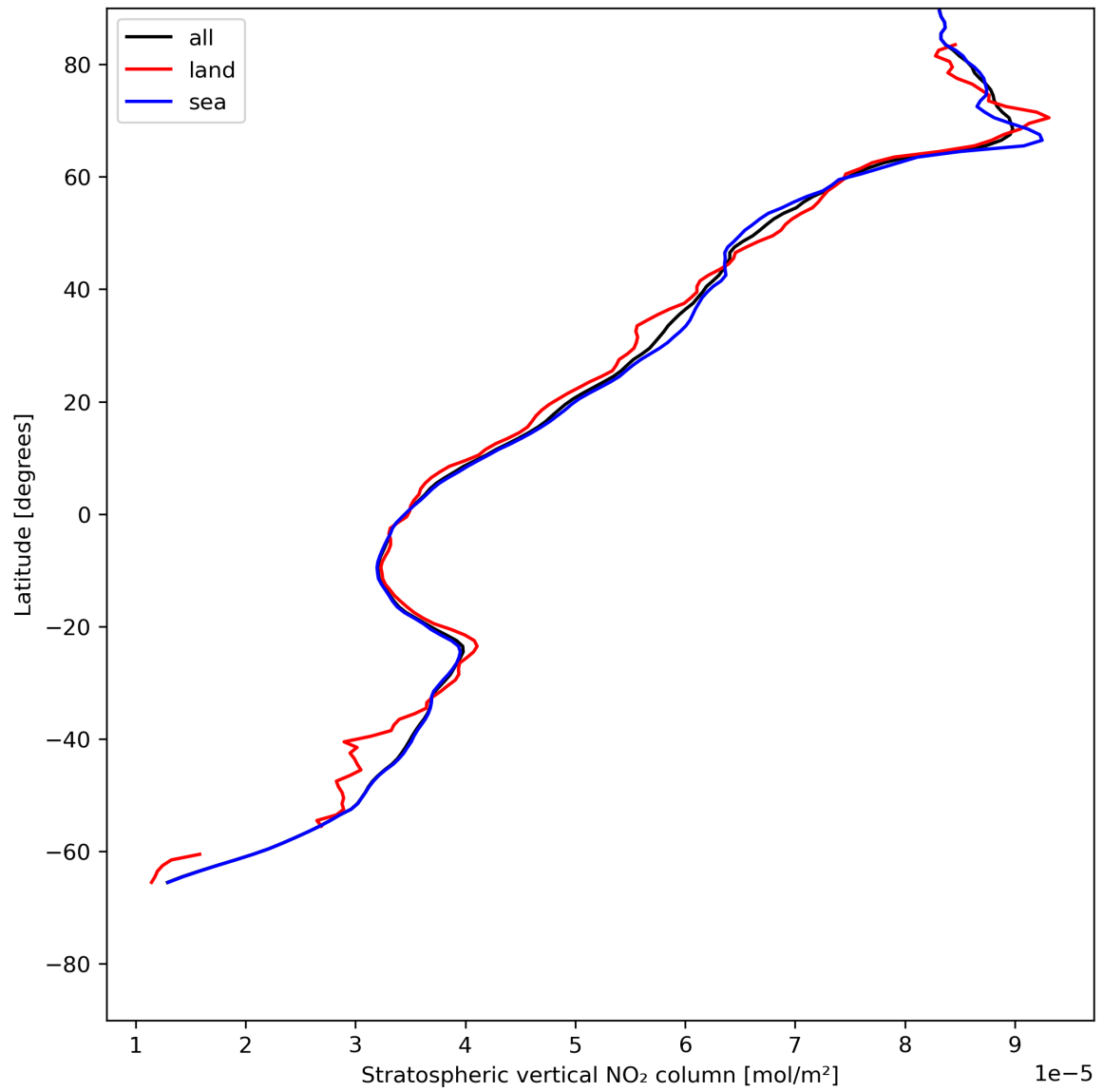
Figure 19: Zonal average of “Stratospheric vertical NO 2 column” for 2023-07-13 to 2023-07-14.
