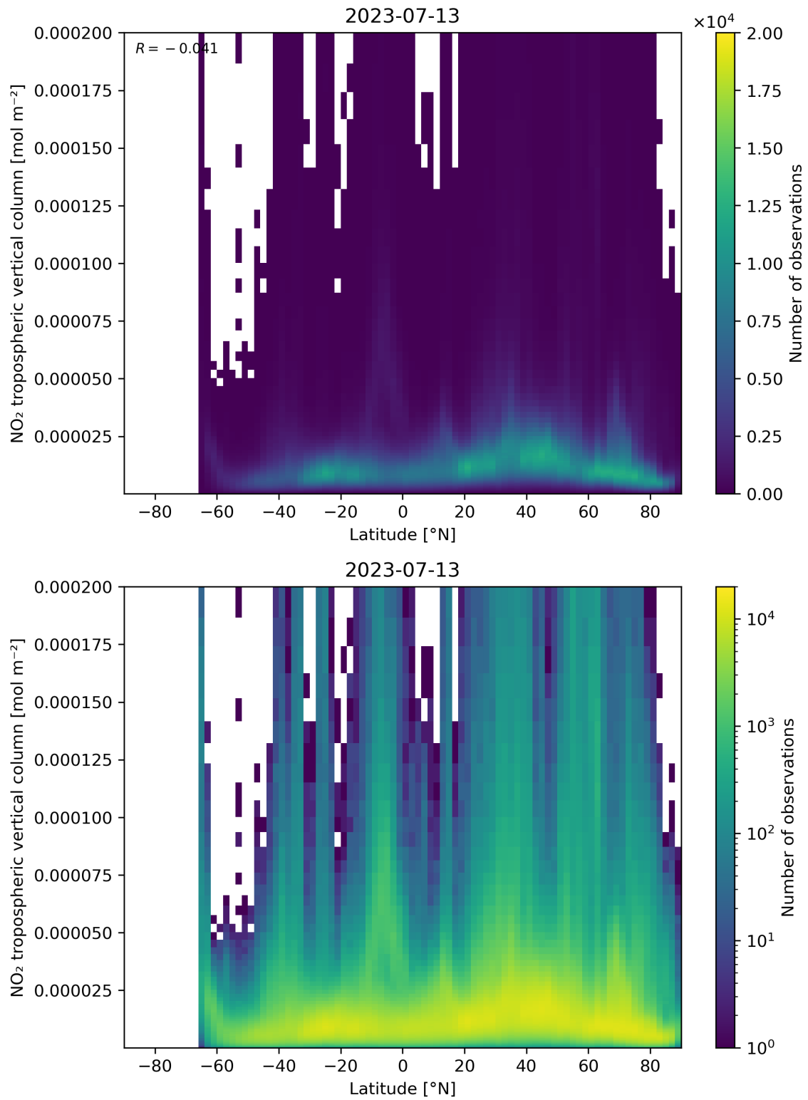
Figure 92: Scatter density plot of “Latitude” against “NO 2 tropospheric vertical column” for 2023-07-13 to 2023-07-14.
