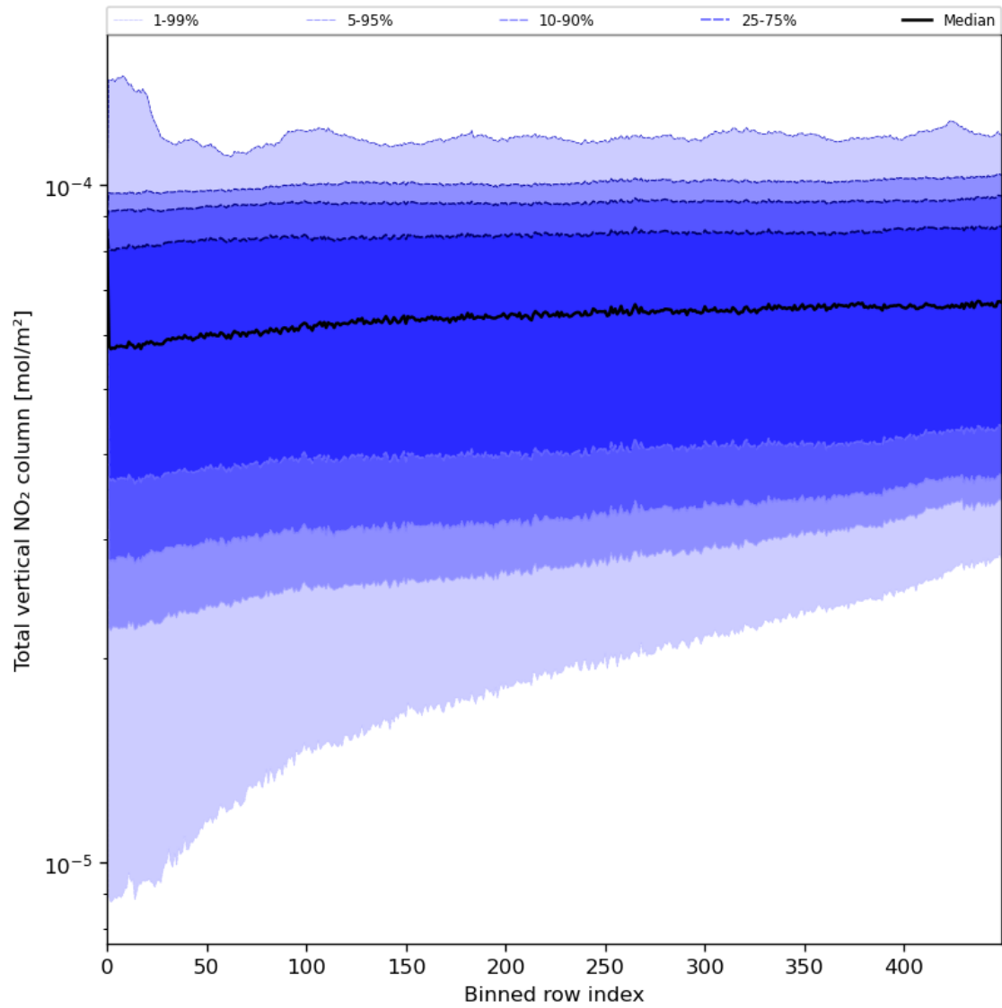
Figure 55: Along track statistics of “Total vertical NO 2 column” for 2023-07-13 to 2023-07-14
