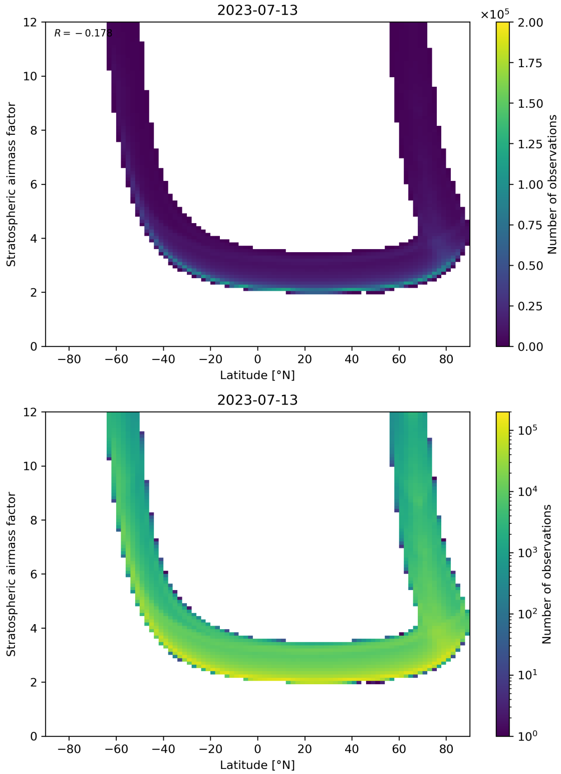
Figure 83: Scatter density plot of “Latitude” against “Stratospheric air mass factor” for 2023-07-13 to 2023-07-14.
