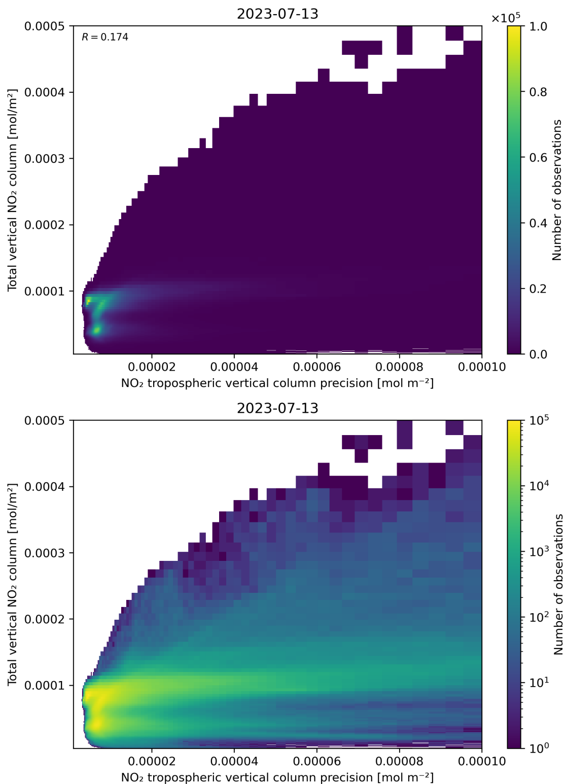
Figure 138: Scatter density plot of “NO 2 tropospheric vertical column precision” against “Total vertical NO 2 column” for 2023-07-13 to 2023-07-14.
