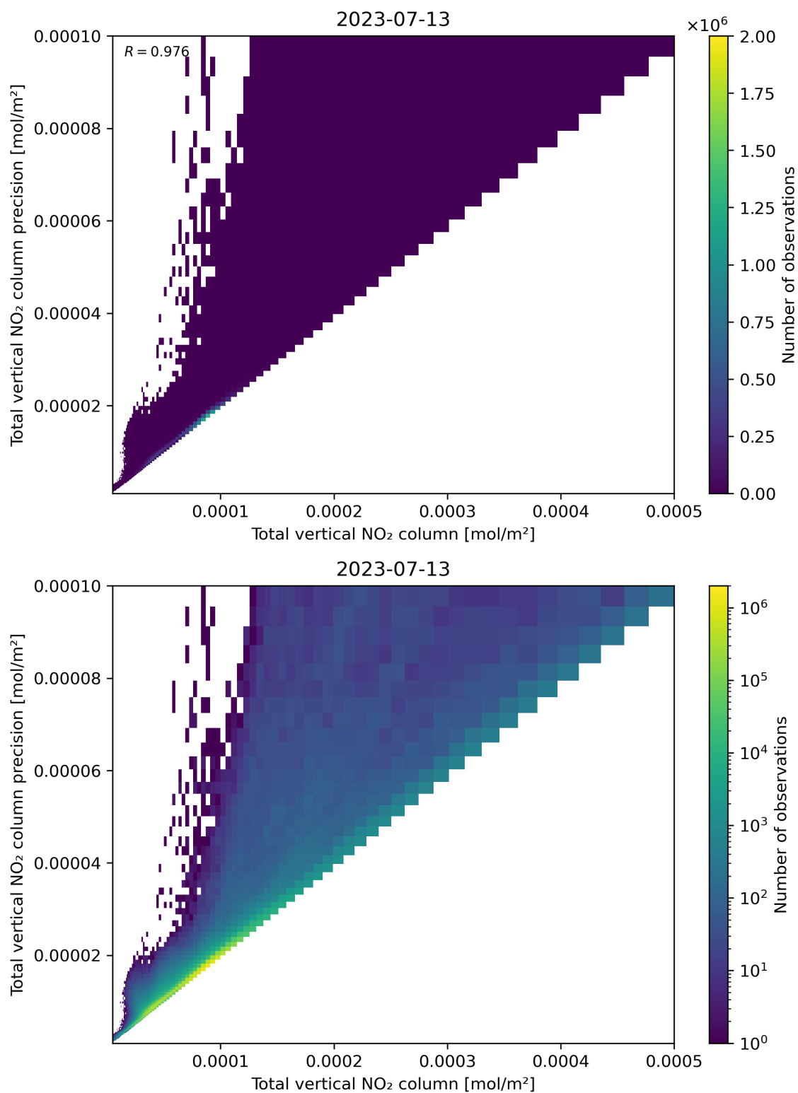
Figure 114: Scatter density plot of “Total vertical NO 2 column” against “Total vertical NO 2 column precision” for 2023-07-13 to 2023-07-14.
