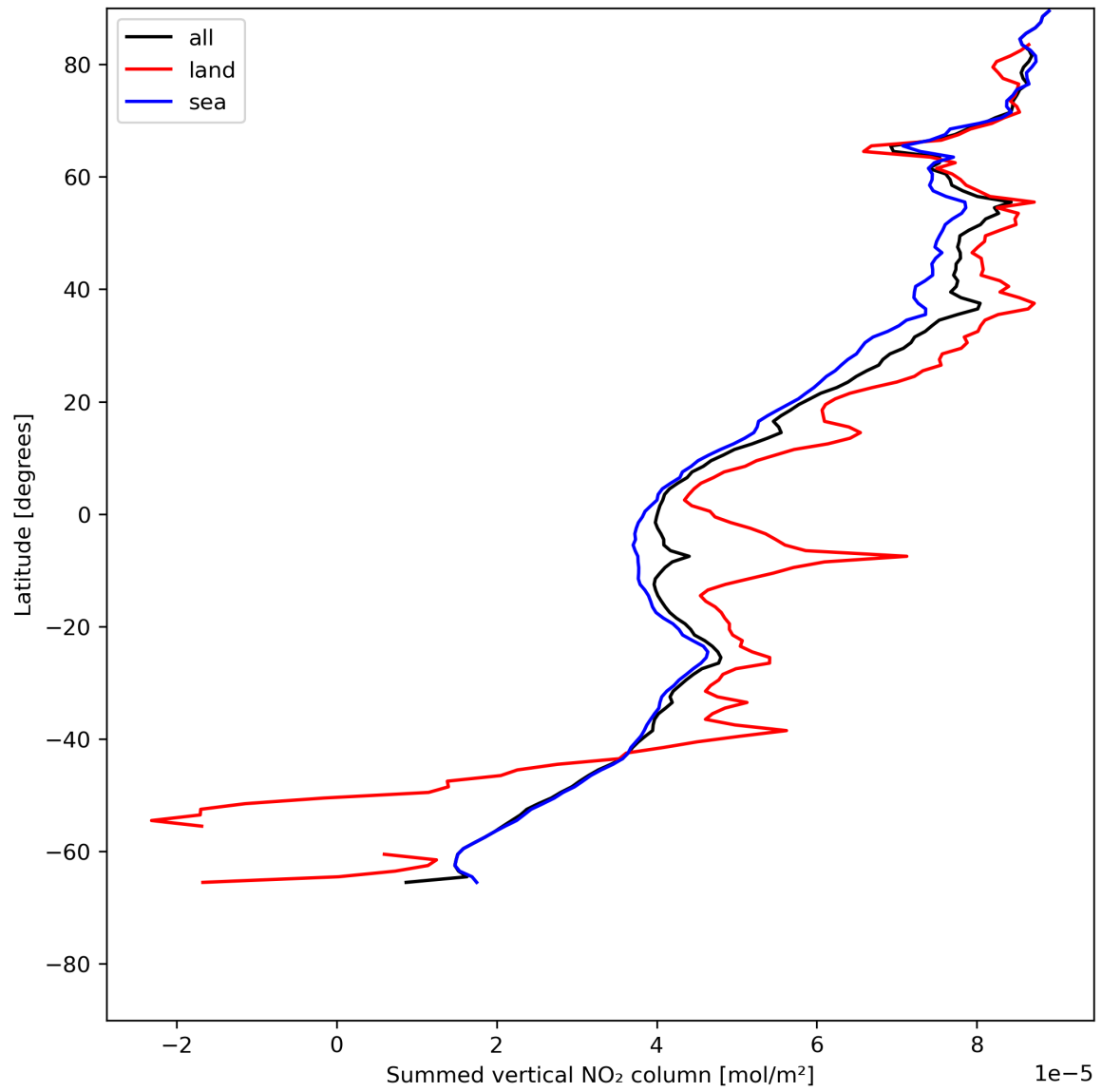
Figure 23: Zonal average of “Summed vertical NO 2 column” for 2023-07-13 to 2023-07-14.
