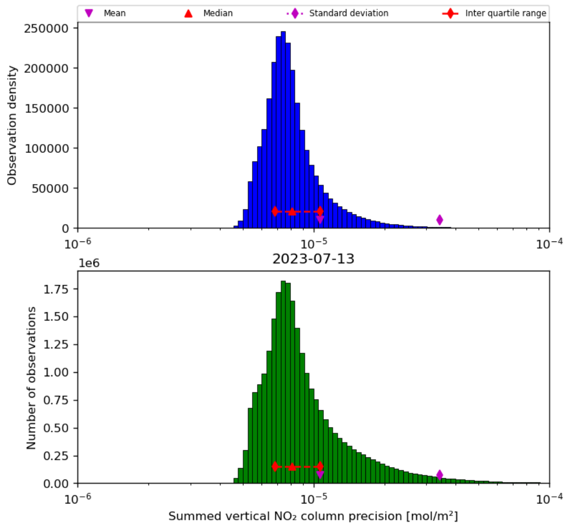
Figure 41: Histogram of “Summed vertical NO 2 column precision” for 2023-07-13 to 2023-07-14
