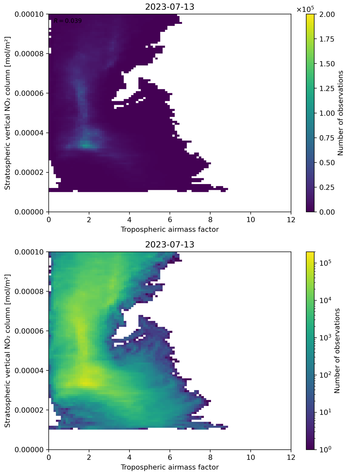
Figure 74: Scatter density plot of “Tropospheric air mass factor” against “Stratospheric vertical NO 2 column” for 2023-07-13 to 2023-07-14.
