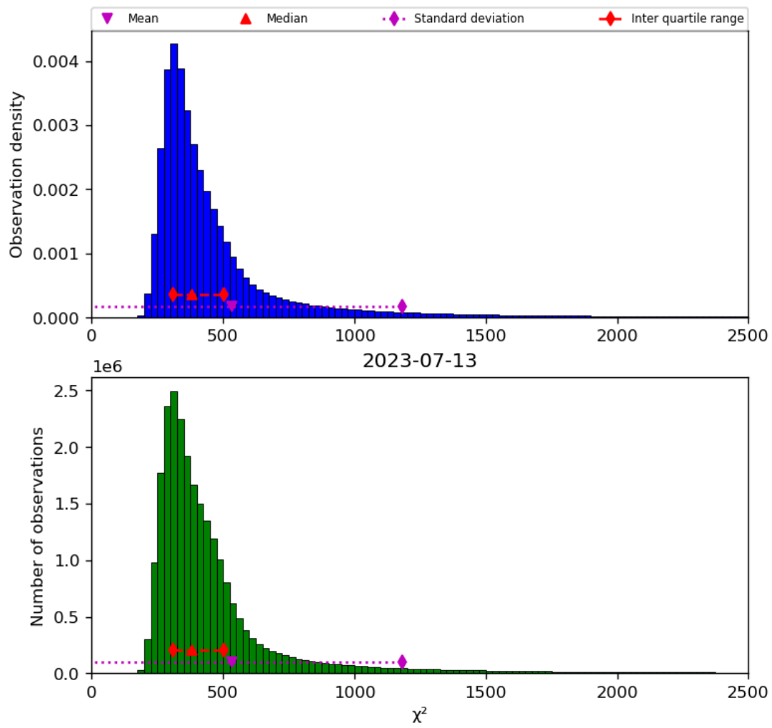
Figure 42: Histogram of " \chi^2 " for 2023-07-13 to 2023-07-14
