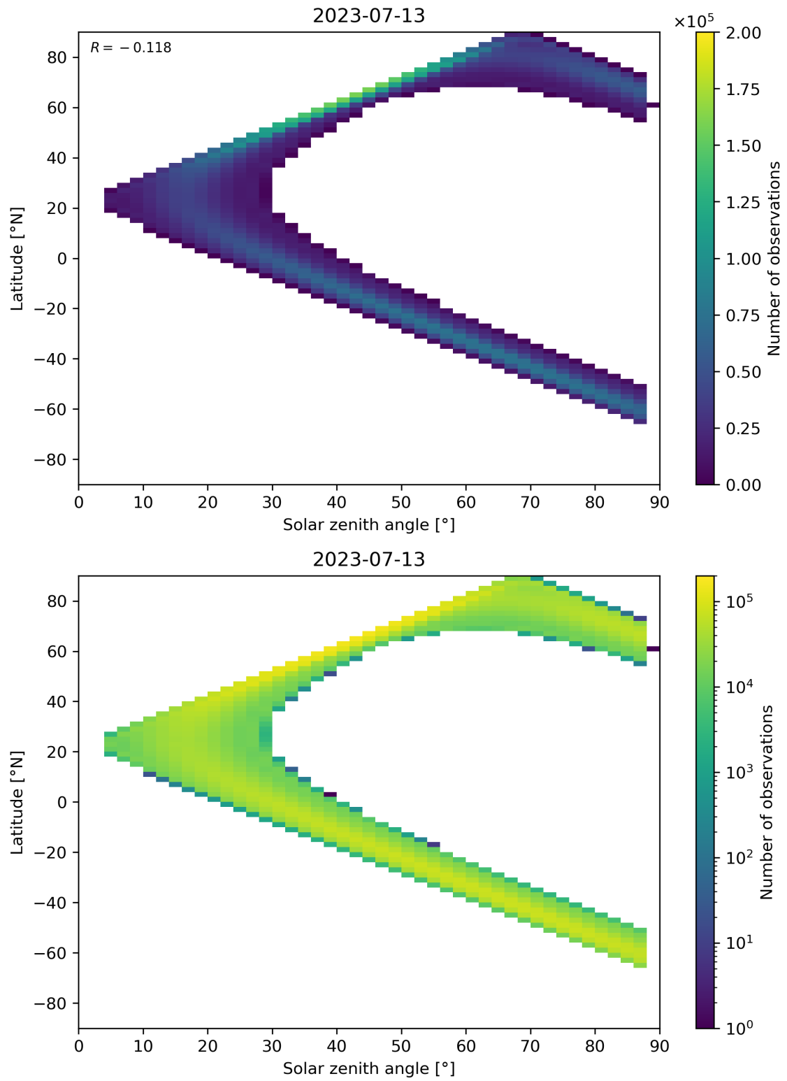
Figure 149: Scatter density plot of “Solar zenith angle” against “Latitude” for 2023-07-13 to 2023-07-14.
