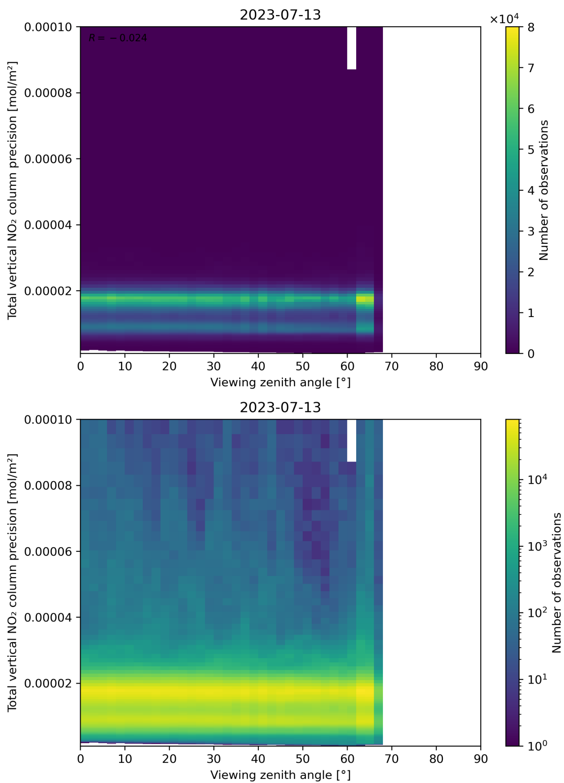
Figure 168: Scatter density plot of “Viewing zenith angle” against “Total vertical NO 2 column precision” for 2023-07-13 to 2023-07-14.
