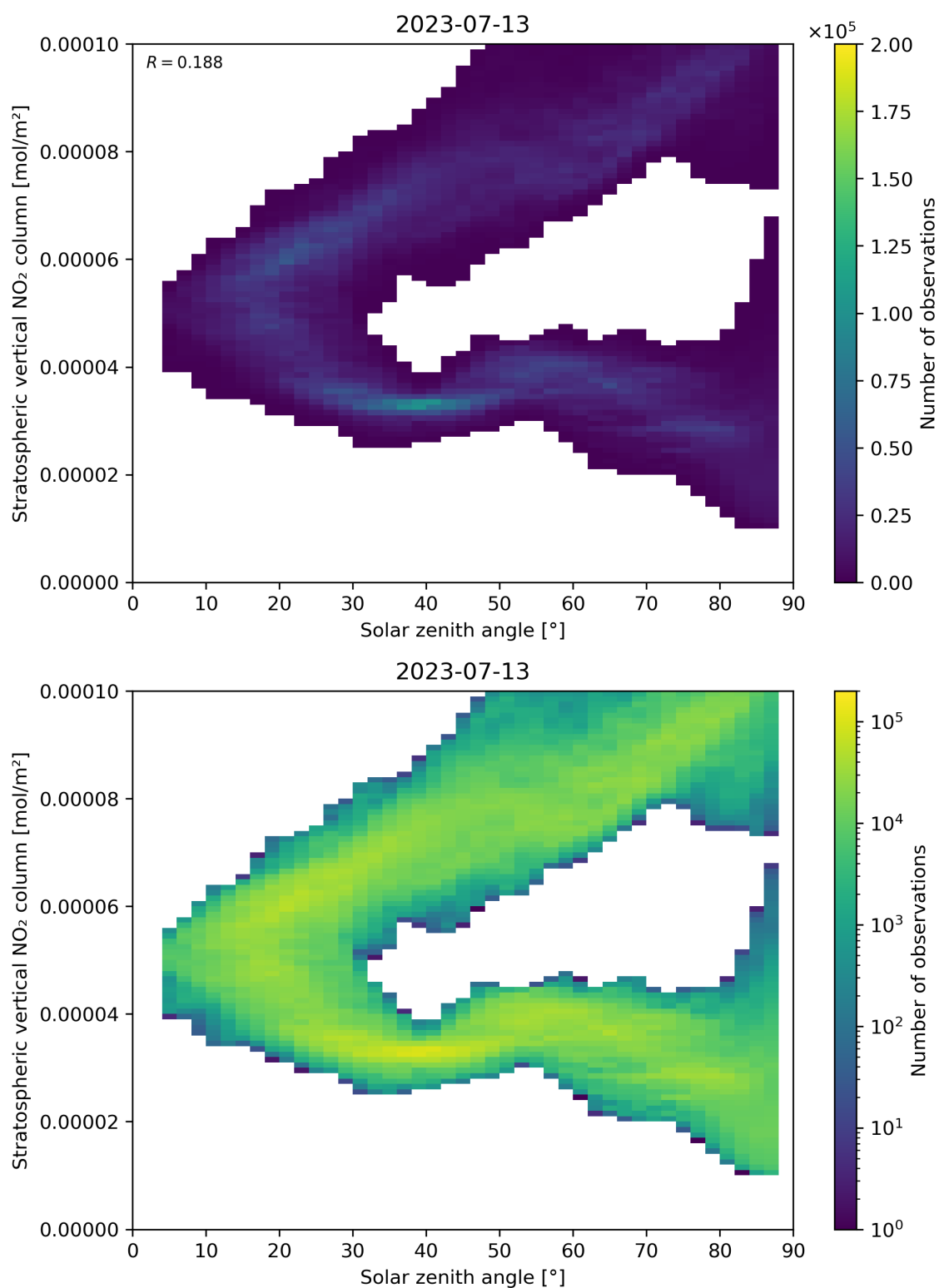
Figure 150: Scatter density plot of “Solar zenith angle” against “Stratospheric vertical NO 2 column” for 2023-07-13 to 2023-07-14.
