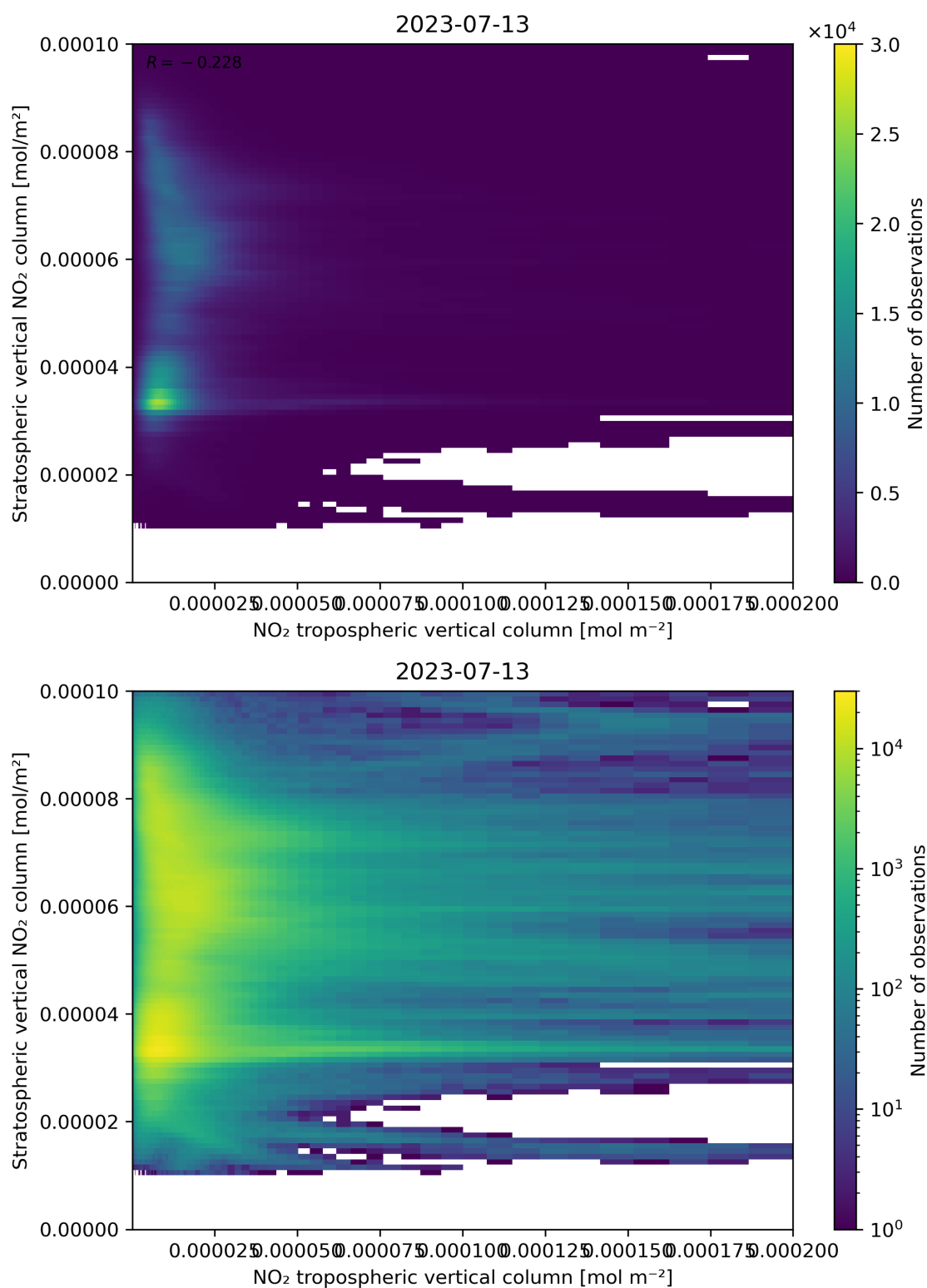
Figure 125: Scatter density plot of “NO 2 tropospheric vertical column” against “Stratospheric vertical NO 2 column” for 2023-07-13 to 2023-07-14.
