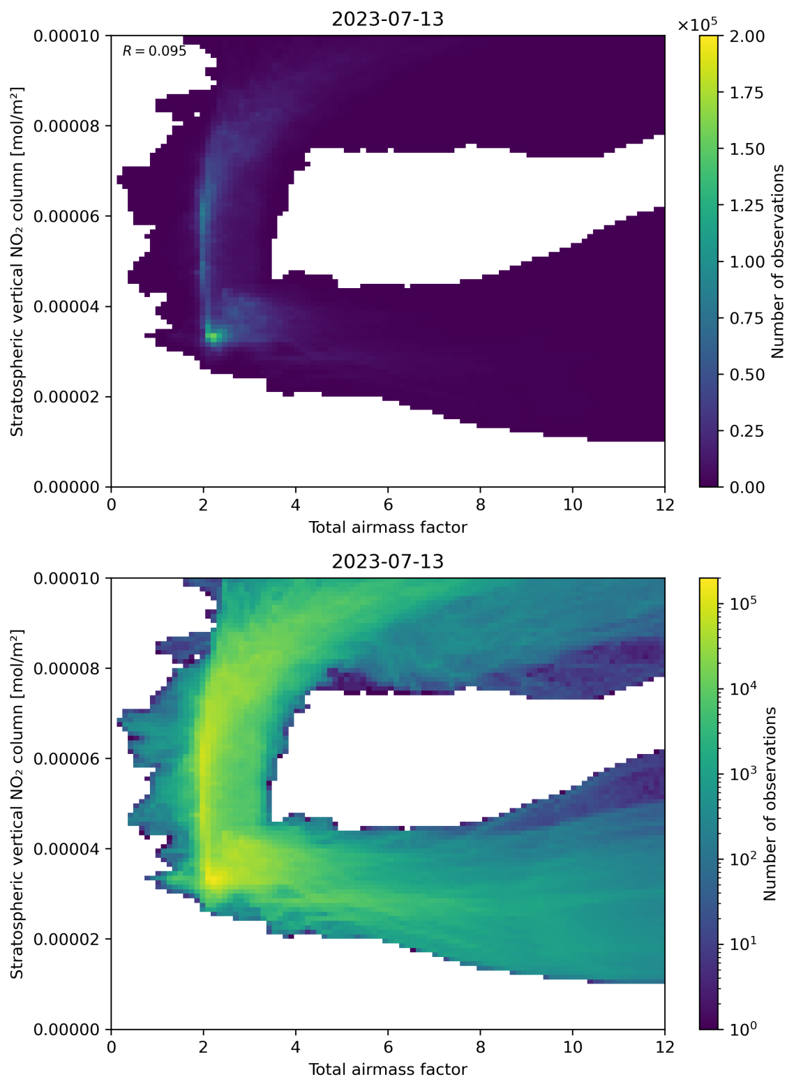
Figure 64: Scatter density plot of “Total airmass factor” against “Stratospheric vertical NO 2 column” for 2023-07-13 to 2023-07-14.
