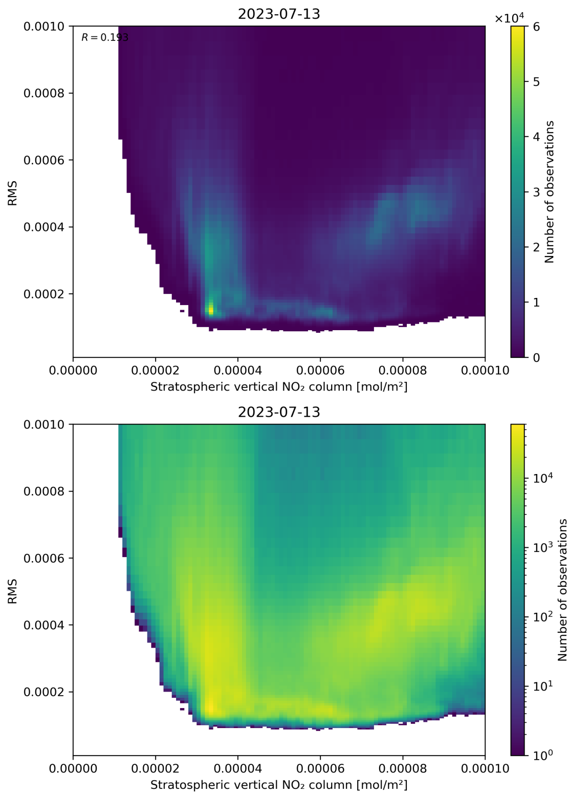
Figure 102: Scatter density plot of “Stratospheric vertical NO 2 column” against “RMS” for 2023-07-13 to 2023-07-14.
