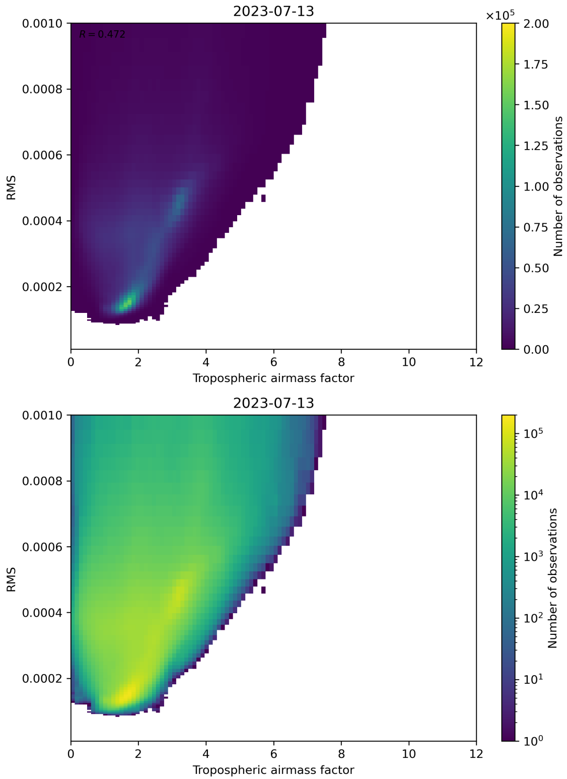
Figure 79: Scatter density plot of “Tropospheric airmass factor” against “RMS” for 2023-07-13 to 2023-07-14.
