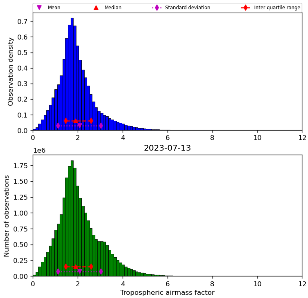
Figure 31: Histogram of “Tropospheric airmass factor” for 2023-07-13 to 2023-07-14
