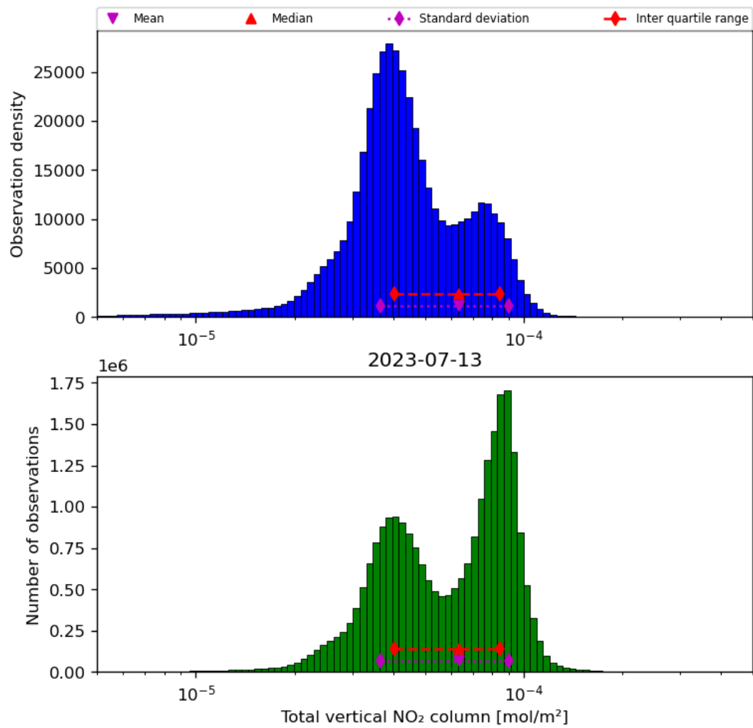
Figure 38: Histogram of “Total vertical NO 2 column” for 2023-07-13 to 2023-07-14
