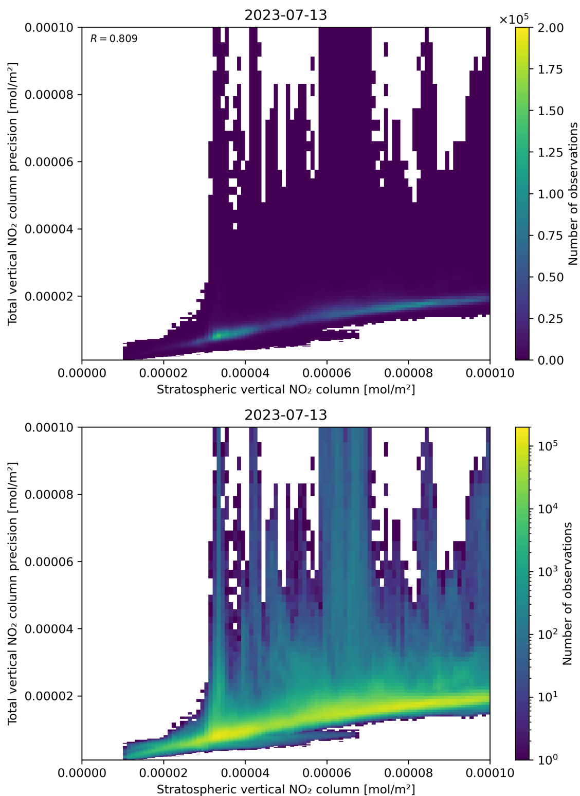
Figure 101: Scatter density plot of “Stratospheric vertical NO 2 column” against “Total vertical NO 2 column precision” for 2023-07-13 to 2023-07-14.
