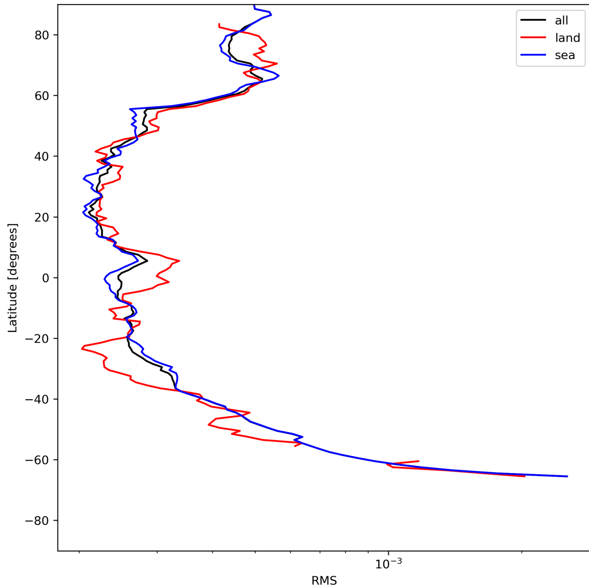
Figure 26: Zonal average of “RMS” for 2023-07-13 to 2023-07-14.
