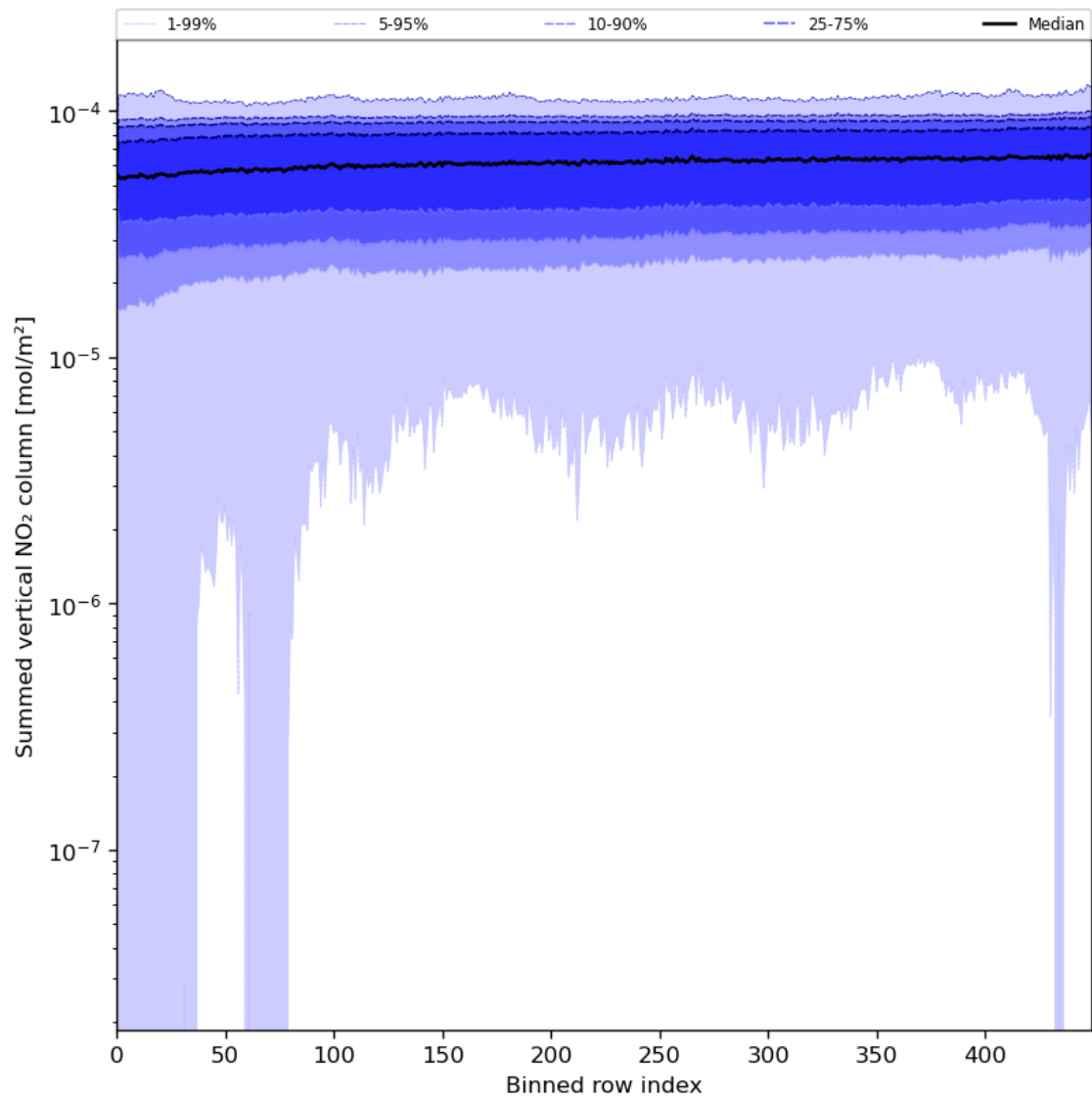
Figure 57: Along track statistics of “Summed vertical NO 2 column” for 2023-07-13 to 2023-07-14
