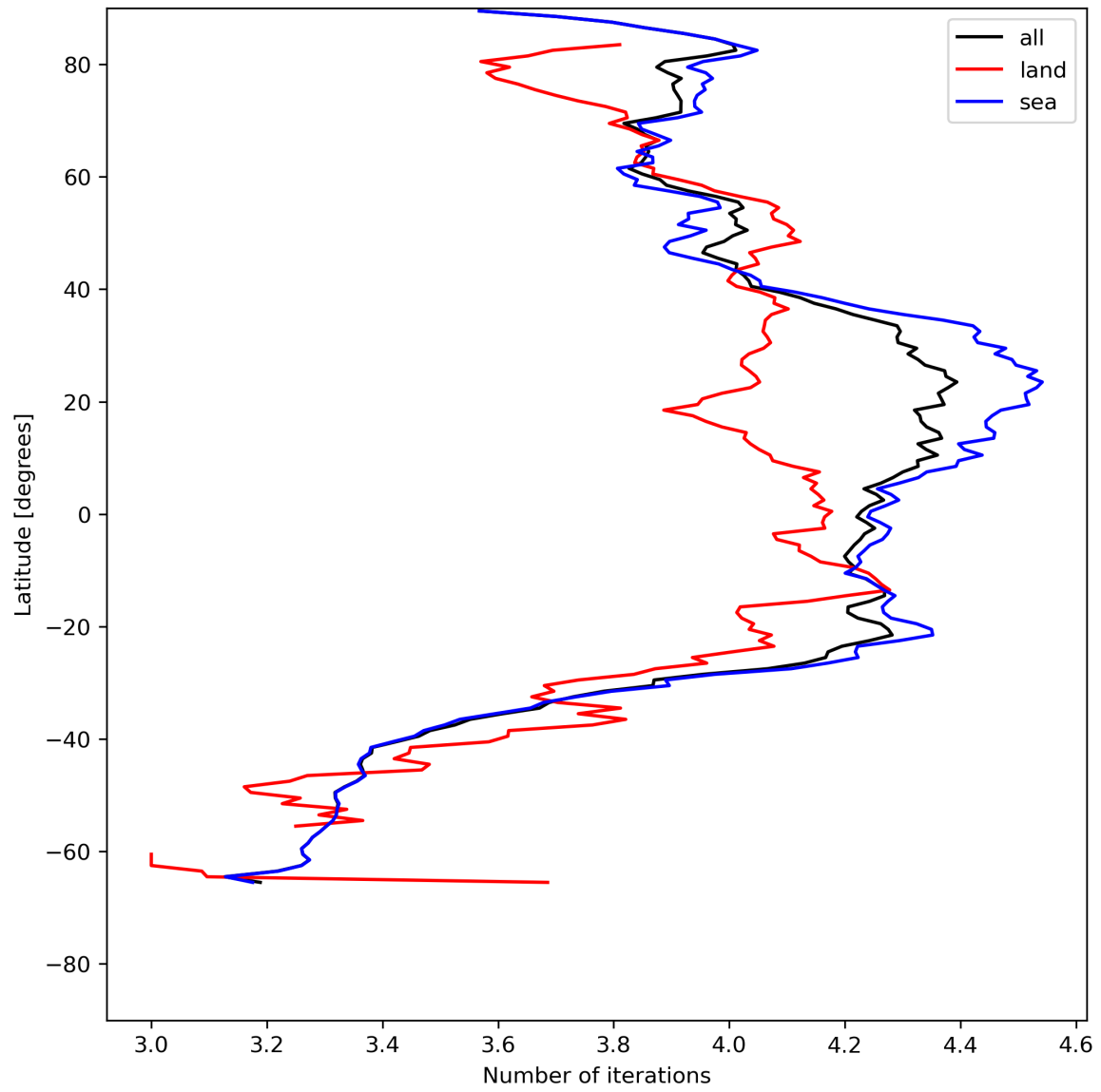
Figure 17: Zonal average of “Number of iterations” for 2023-07-13 to 2023-07-14.
