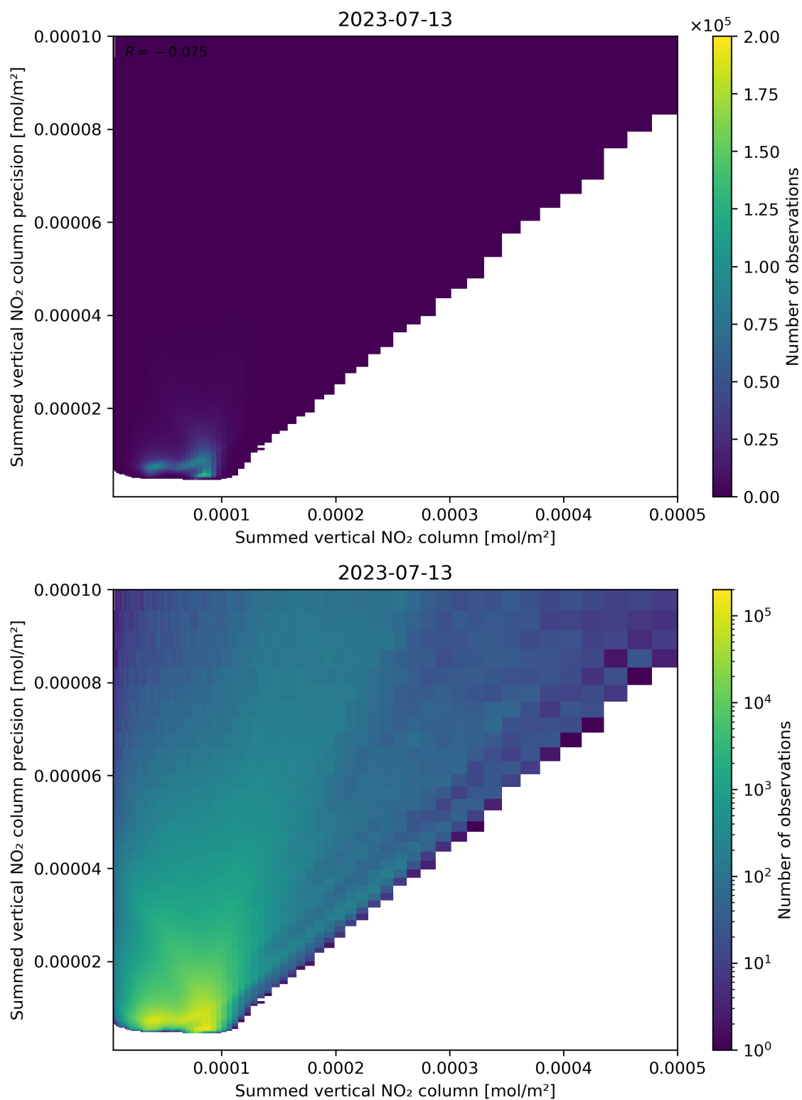
Figure 105: Scatter density plot of “Summed vertical NO 2 column” against “Summed vertical NO 2 column precision” for 2023-07-13 to 2023-07-14.
