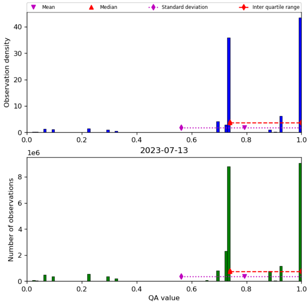
Figure 28: Histogram of “QA value” for 2023-07-13 to 2023-07-14
