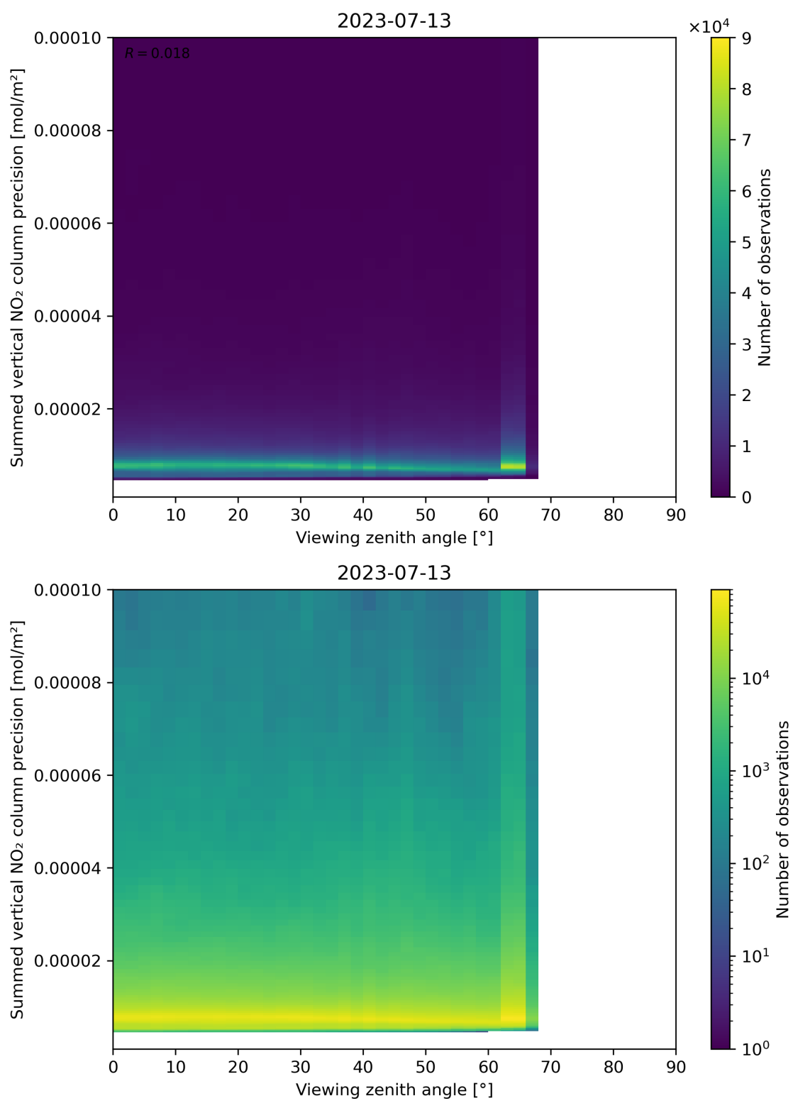
Figure 166: Scatter density plot of “Viewing zenith angle” against “Summed vertical NO 2 column precision” for 2023-07-13 to 2023-07-14.
