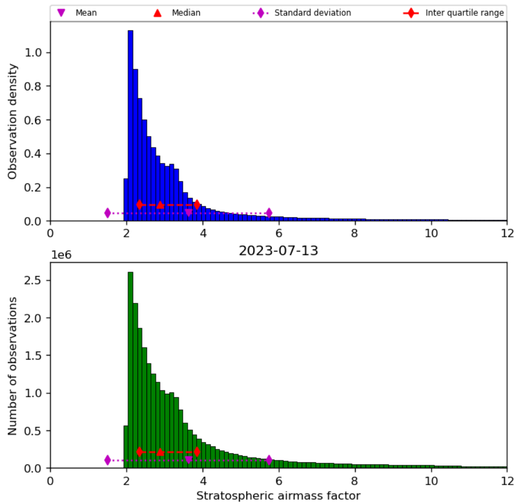
Figure 44: Histogram of “Stratospheric airmass factor” for 2023-07-13 to 2023-07-14
