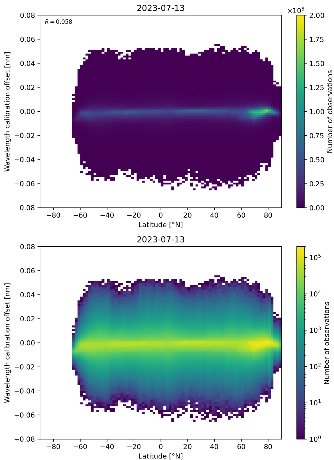
Figure 95: Scatter density plot of “Latitude” against “Wavelength calibration offset” for 2023-07-13 to 2023-07-14.
