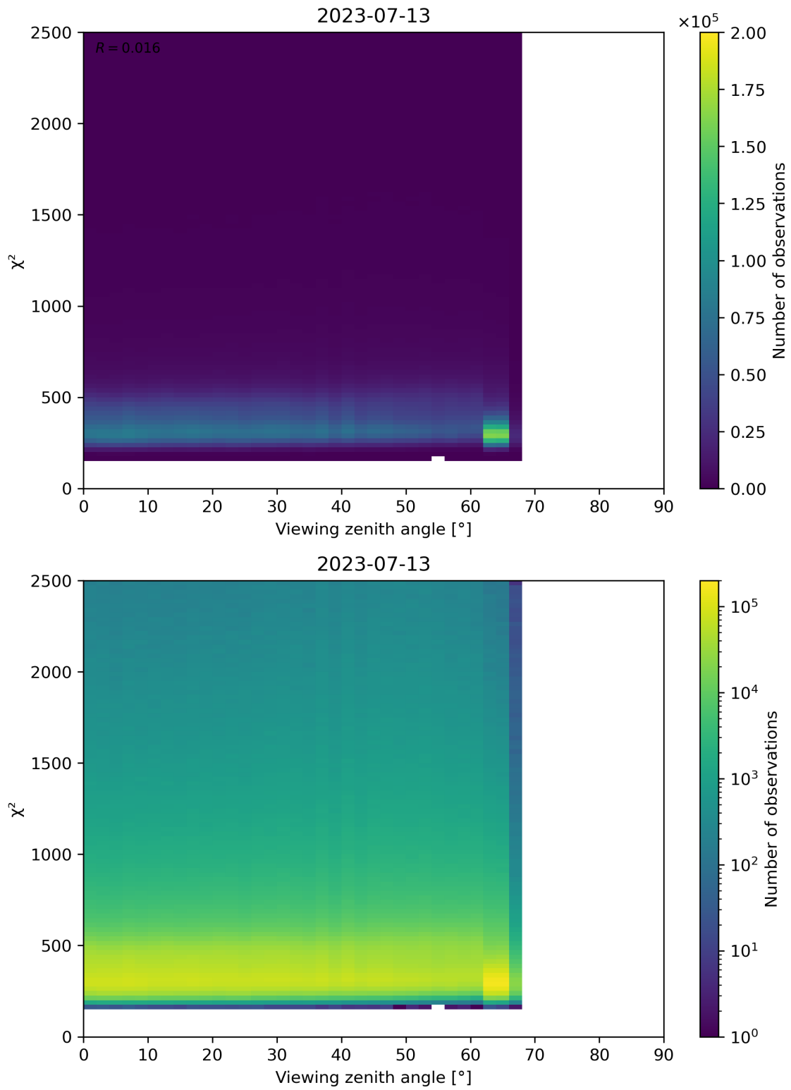
Figure 162: Scatter density plot of “Viewing zenith angle” against “ \chi^2 ” for 2023-07-13 to 2023-07-14.
