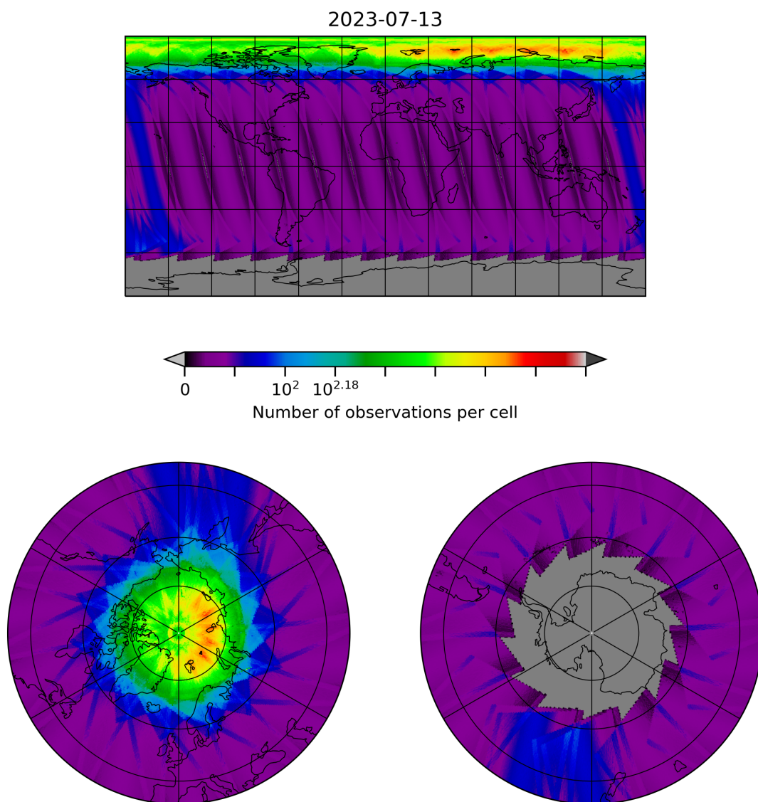
Figure 10: Map of the number of observations for 2023-07-13 to 2023-07-14
