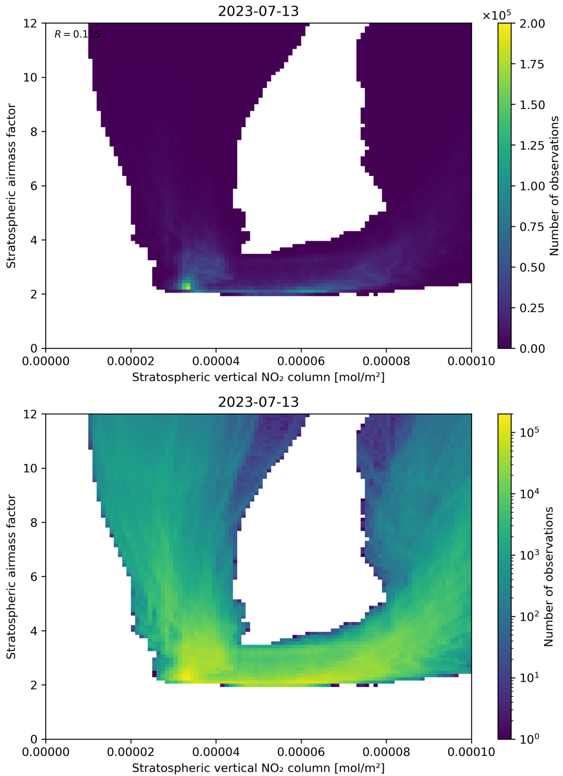
Figure 96: Scatter density plot of “Stratospheric vertical NO 2 column” against “Stratospheric airmass factor” for 2023-07-13 to 2023-07-14.
