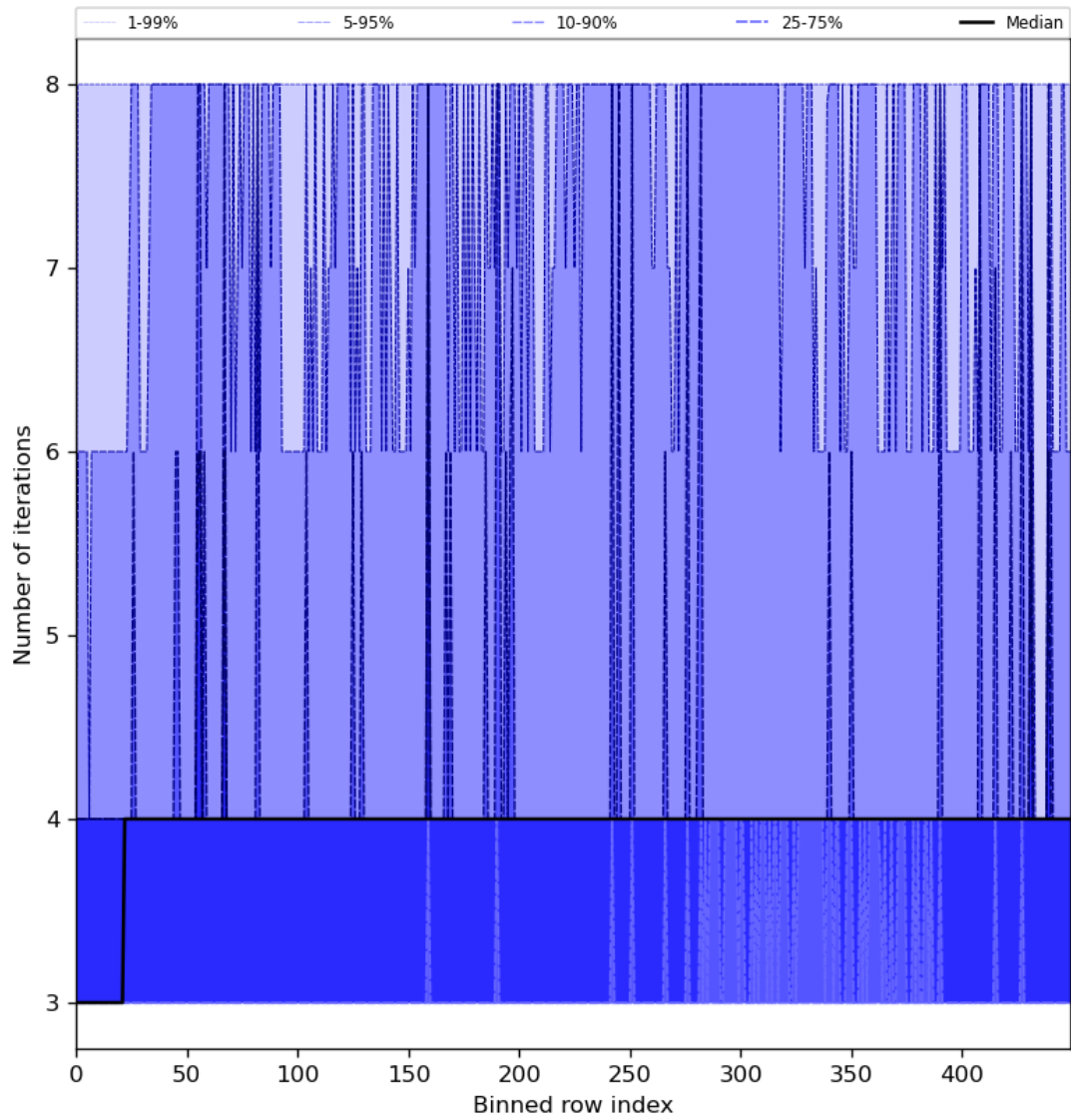
Figure 51: Along track statistics of “Number of iterations” for 2023-07-13 to 2023-07-14
