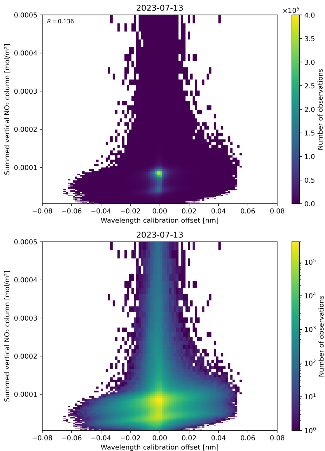
Figure 177: Scatter density plot of “Wavelength calibration offset” against “Summed vertical NO 2 column” for 2023-07-13 to 2023-07-14.
