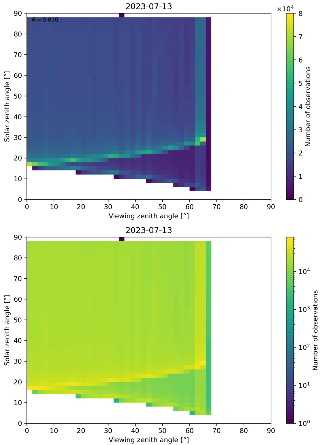
Figure 172: Scatter density plot of “Viewing zenith angle” against “Solar zenith angle” for 2023-07-13 to 2023-07-14.
