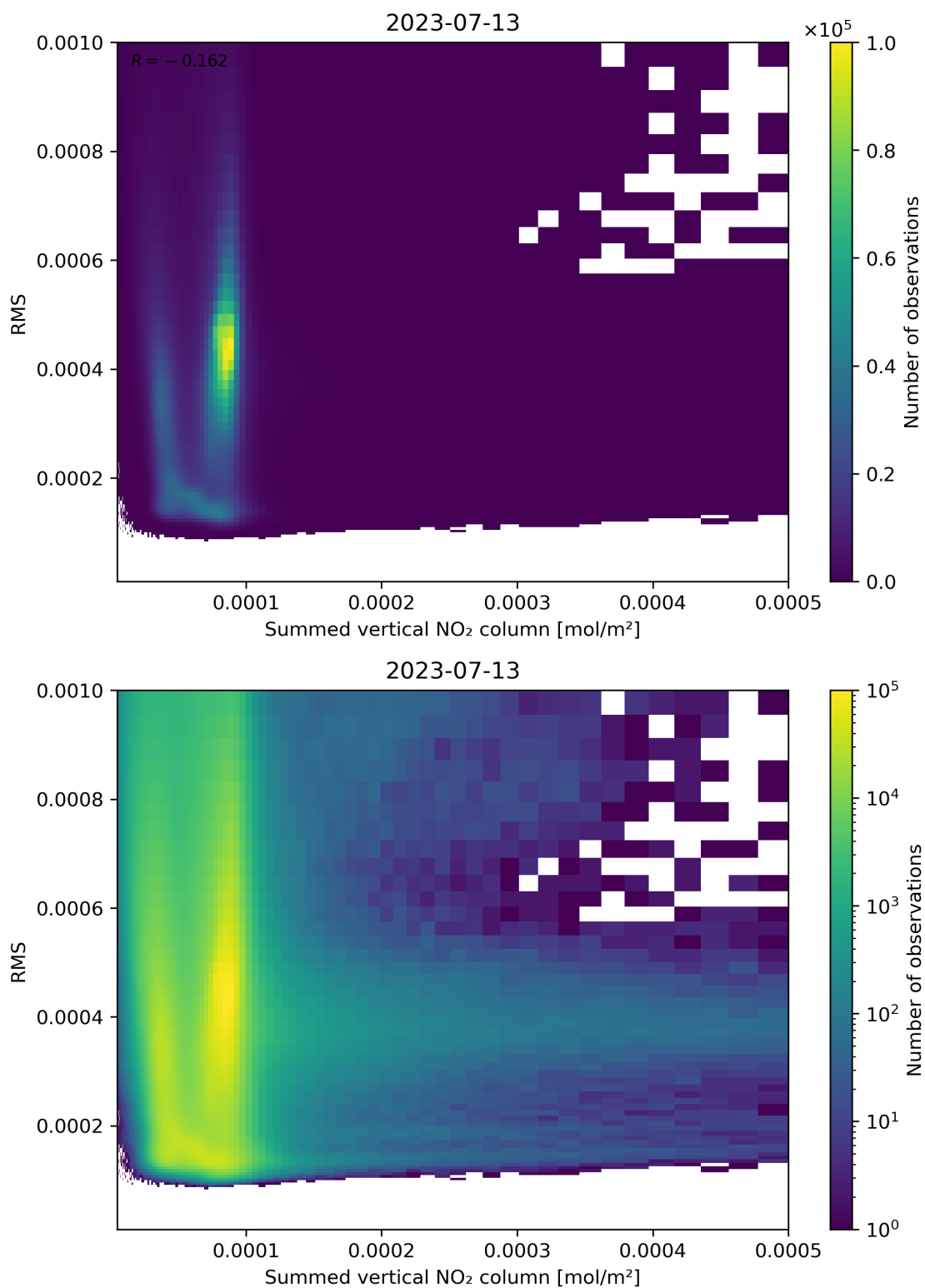
Figure 109: Scatter density plot of “Summed vertical NO 2 column” against “RMS” for 2023-07-13 to 2023-07-14.
