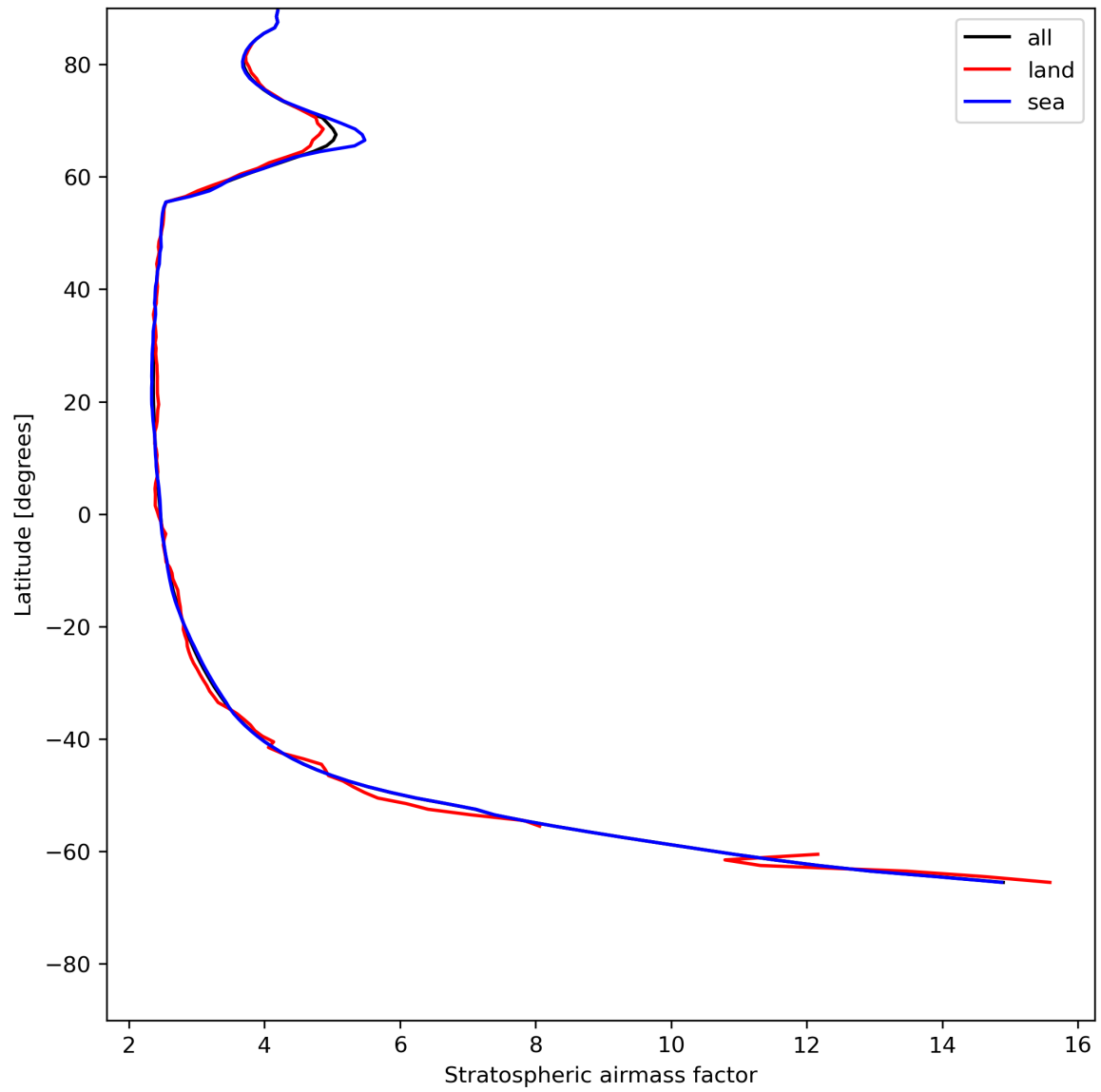
Figure 27: Zonal average of “Stratospheric airmass factor” for 2023-07-13 to 2023-07-14.
