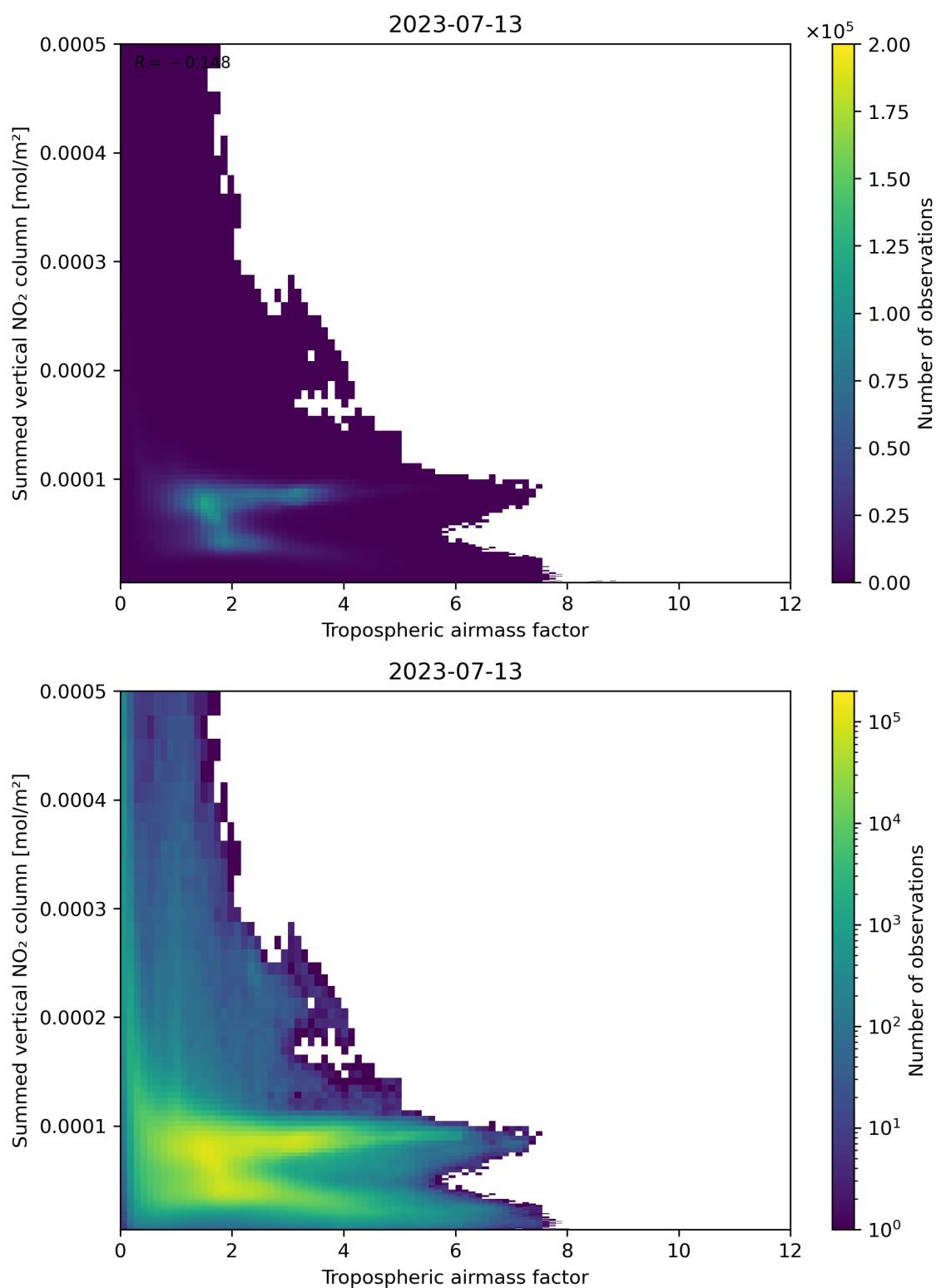
Figure 75: Scatter density plot of “Tropospheric airmass factor” against “Summed vertical NO 2 column” for 2023-07-13 to 2023-07-14.
