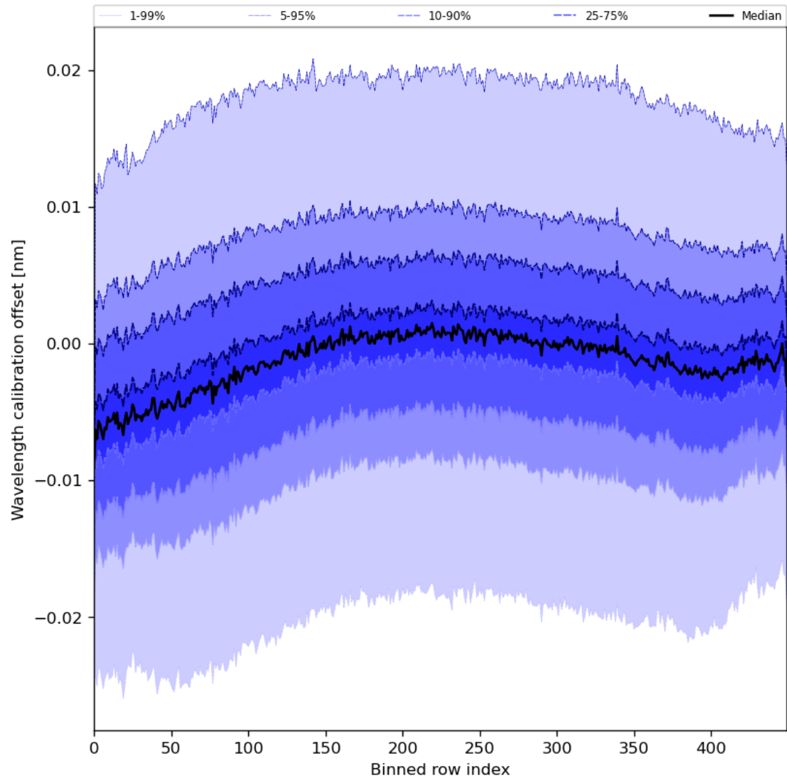
Figure 52: Along track statistics of “Wavelength calibration offset” for 2023-07-13 to 2023-07-14
