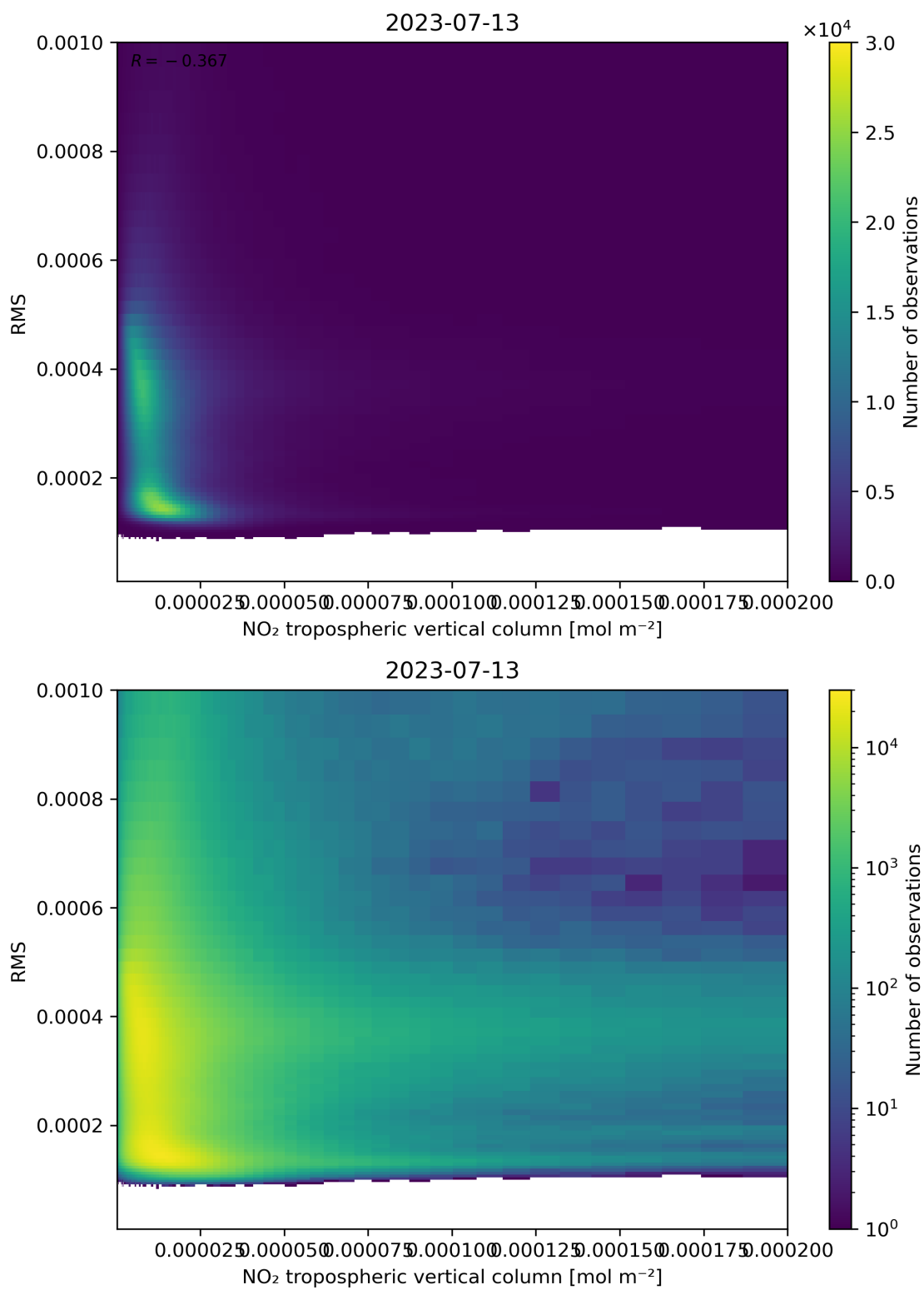
Figure 142: Scatter density plot of “NO 2 tropospheric vertical column” against “RMS” for 2023-07-13 to 2023-07-14.
