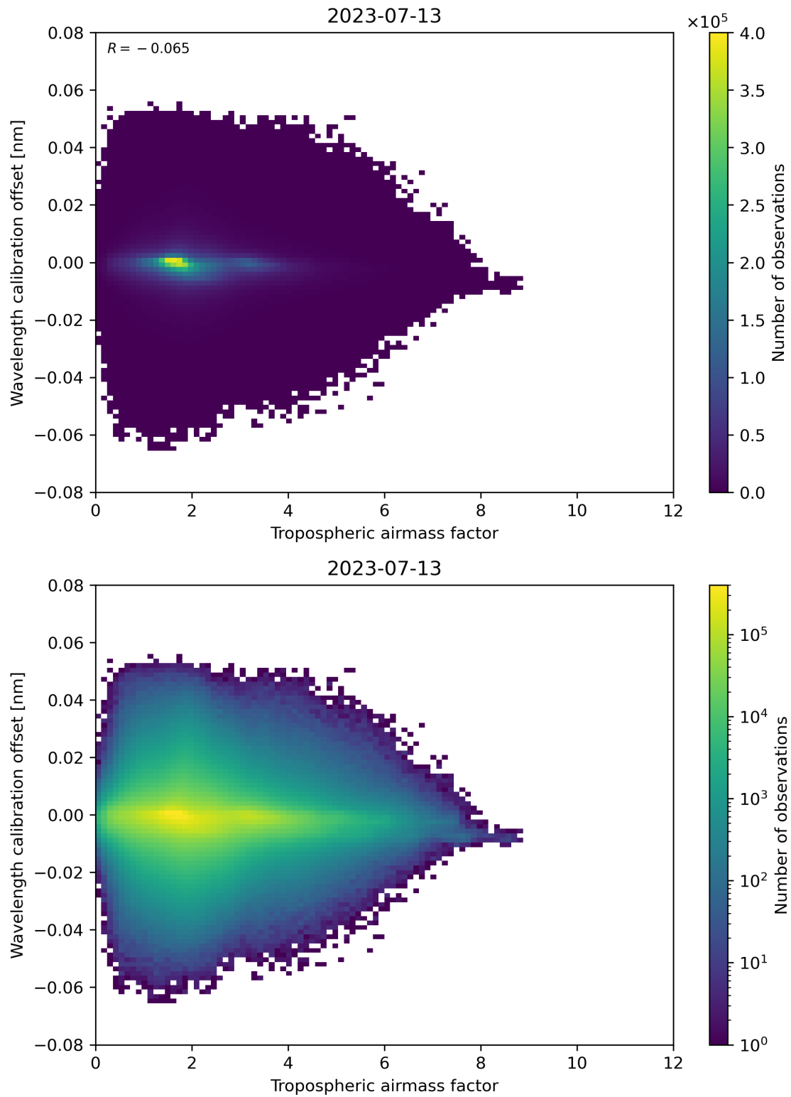
Figure 80: Scatter density plot of “Tropospheric air mass factor” against “Wavelength calibration offset” for 2023-07-13 to 2023-07-14.
