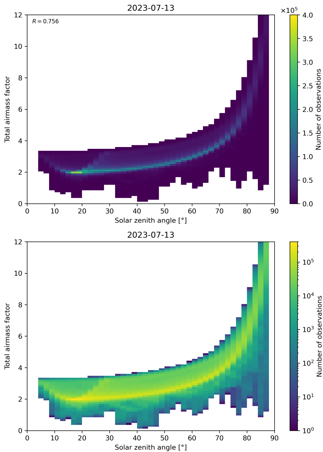
Figure 146: Scatter density plot of “Solar zenith angle” against “Total air mass factor” for 2023-07-13 to 2023-07-14.
