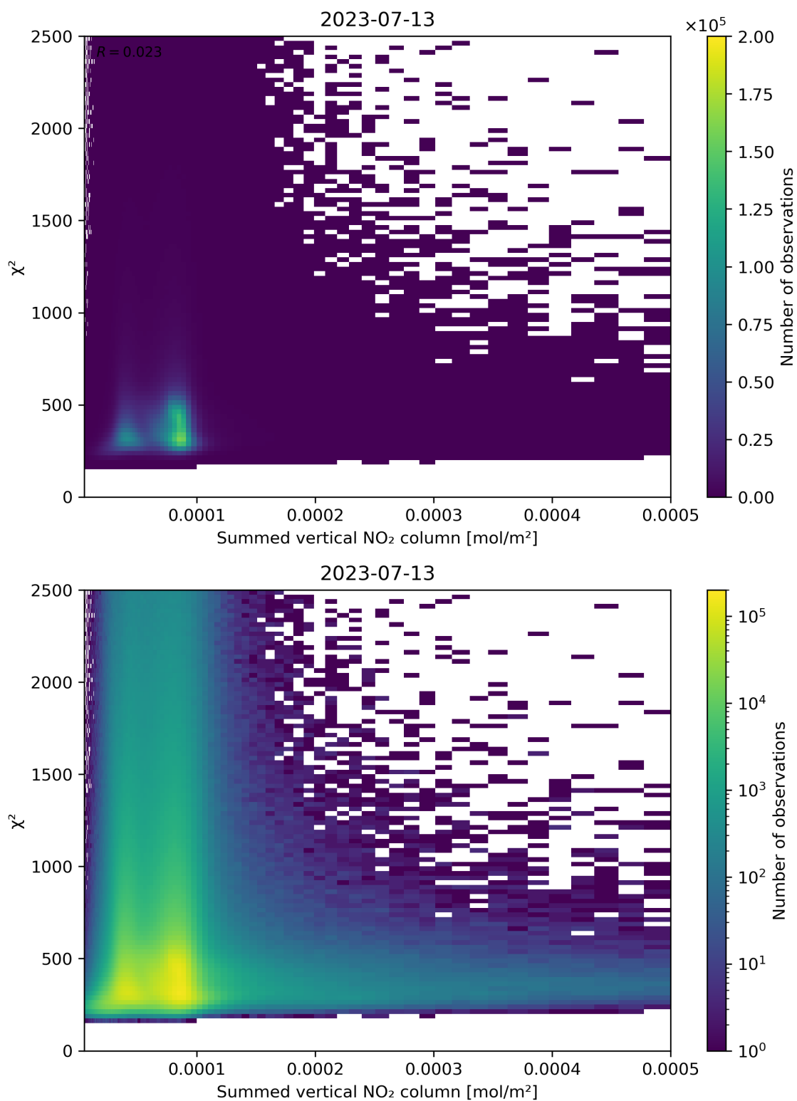
Figure 104: Scatter density plot of “Summed vertical NO 2 column” against “ \chi^2 ” for 2023-07-13 to 2023-07-14.
