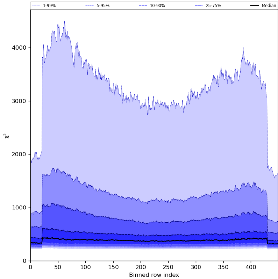
Figure 59: Along track statistics of “ \chi^2 ” for 2023-07-13 to 2023-07-14
