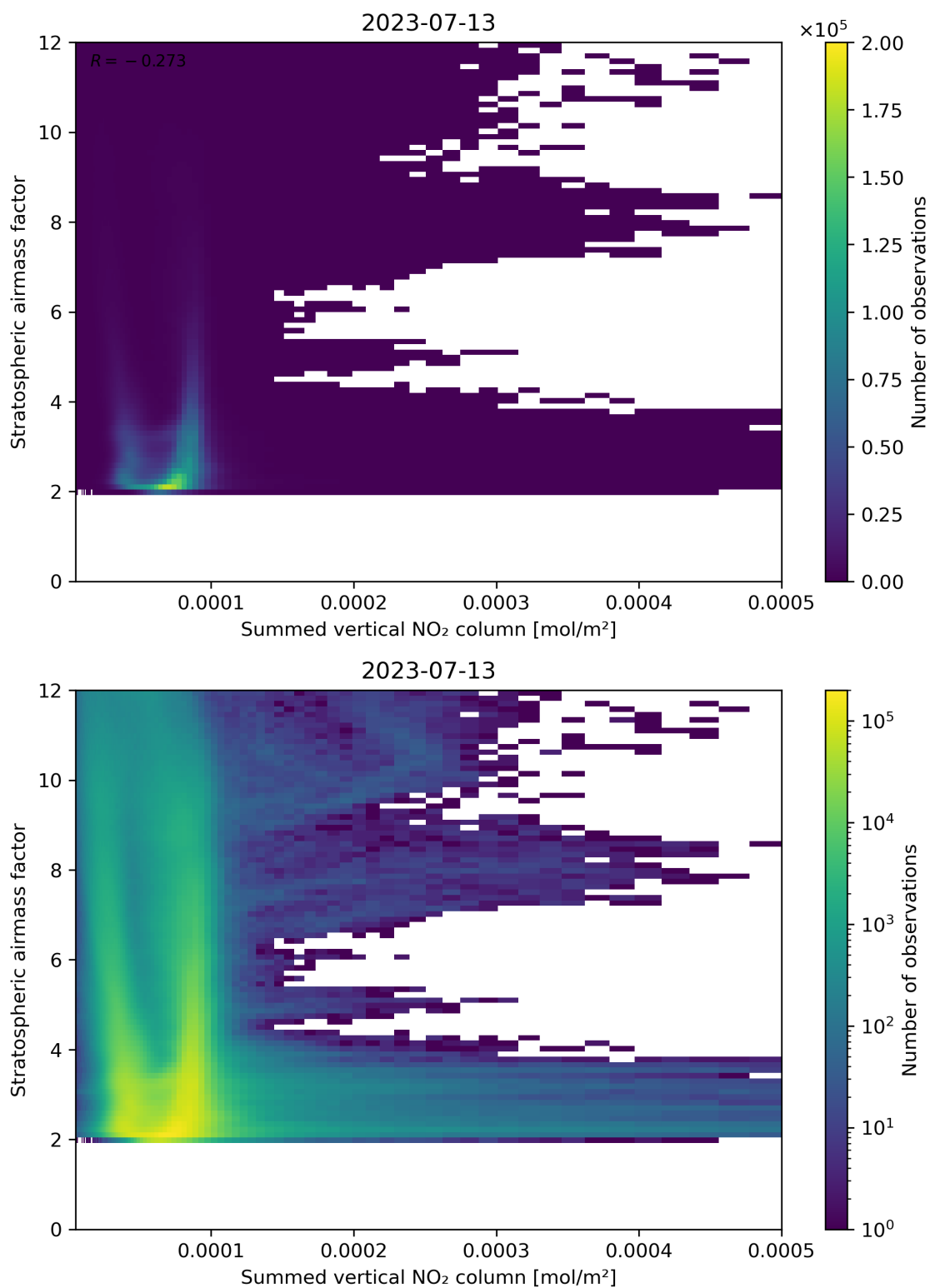
Figure 103: Scatter density plot of “Summed vertical NO 2 column” against “Stratospheric air mass factor” for 2023-07-13 to 2023-07-14.
