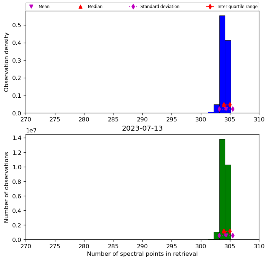
Figure 33: Histogram of “Number of spectral points in retrieval” for 2023-07-13 to 2023-07-14
