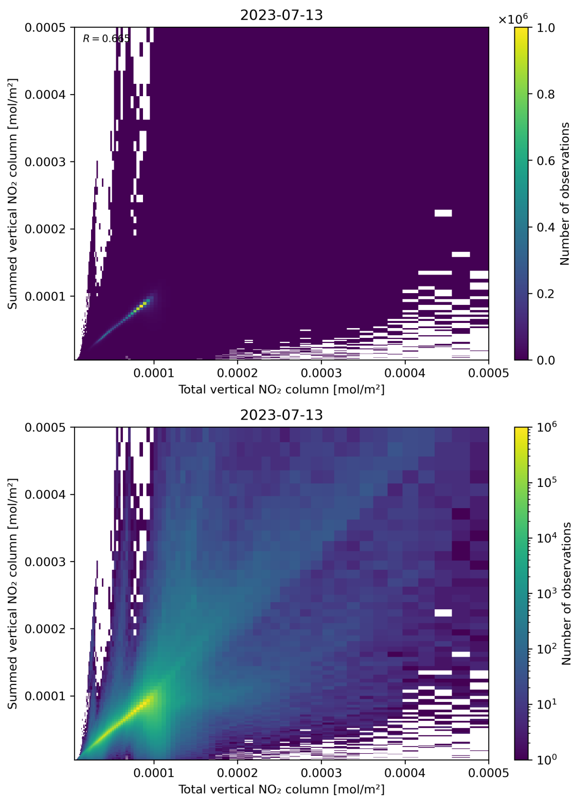
Figure 112: Scatter density plot of “Total vertical NO 2 column” against “Summed vertical NO 2 column” for 2023-07-13 to 2023-07-14.
