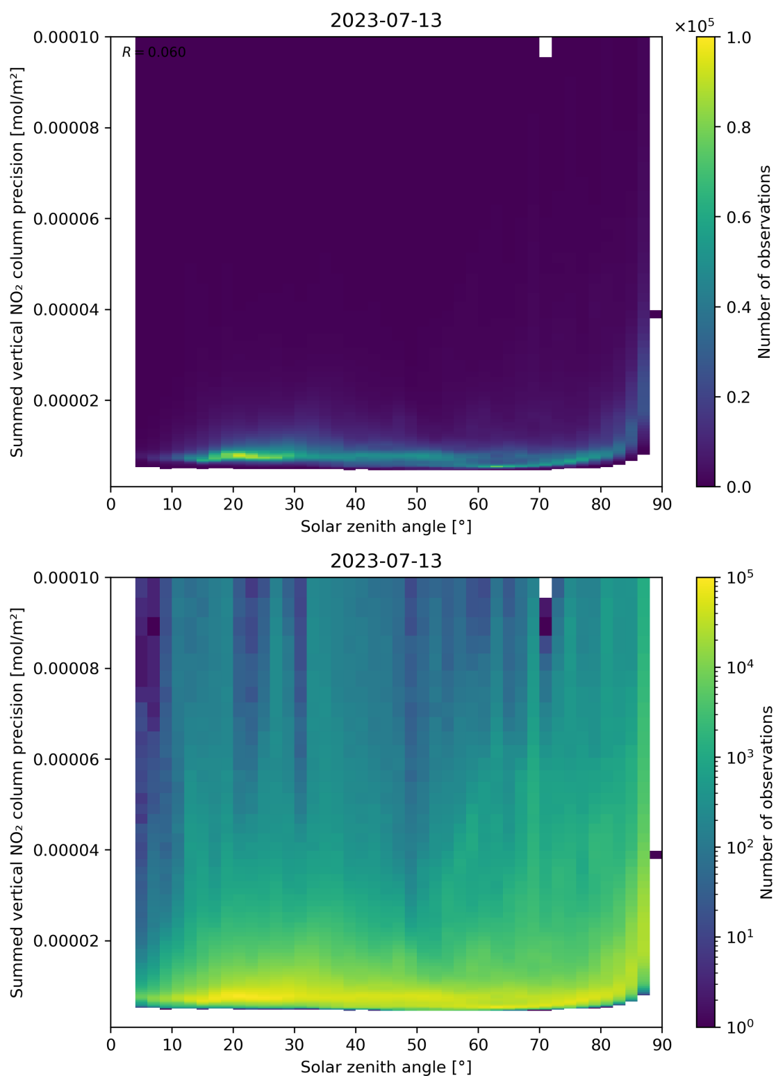
Figure 152: Scatter density plot of “Solar zenith angle” against “Summed vertical NO 2 column precision” for 2023-07-13 to 2023-07-14.
