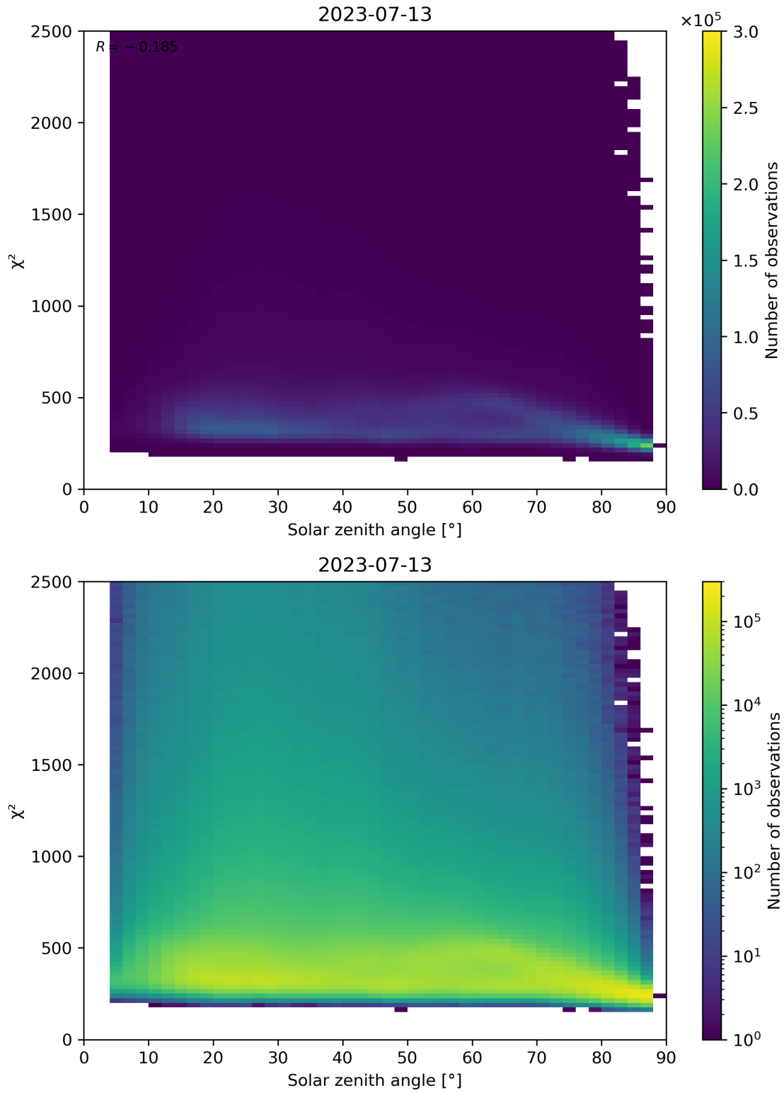
Figure 148: Scatter density plot of “Solar zenith angle” against “ \chi^2 ” for 2023-07-13 to 2023-07-14.
