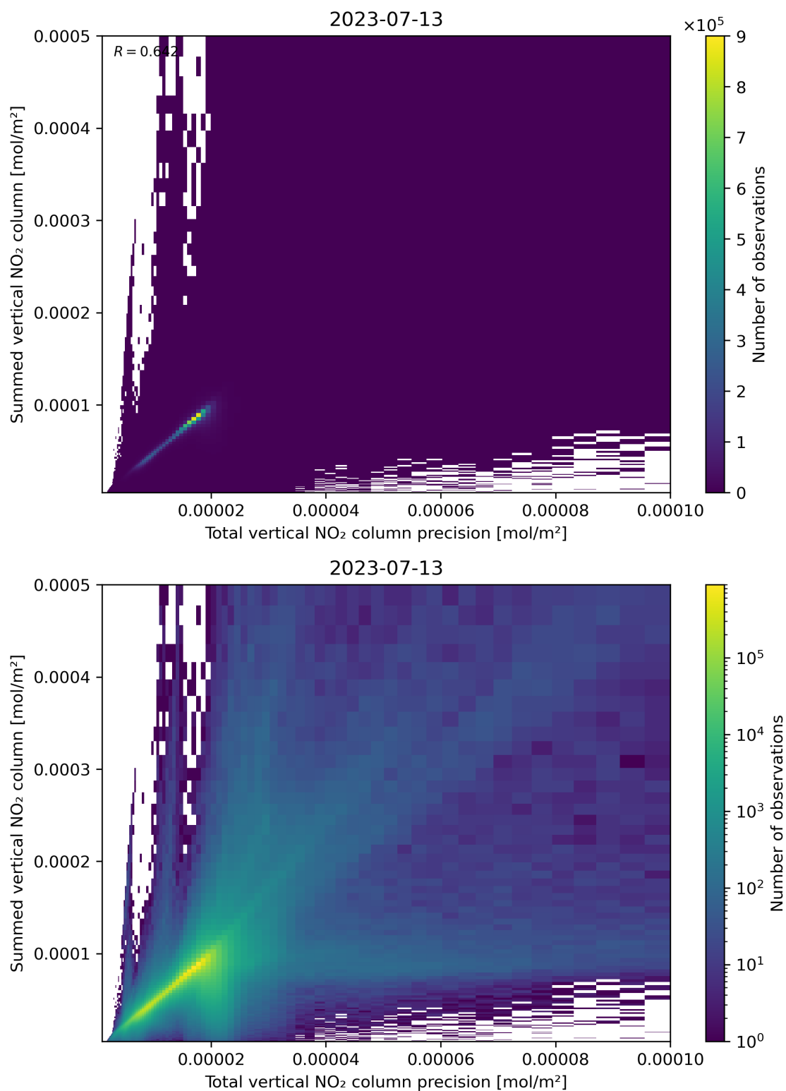
Figure 117: Scatter density plot of “Total vertical NO 2 column precision” against “Summed vertical NO 2 column” for 2023-07-13 to 2023-07-14.
