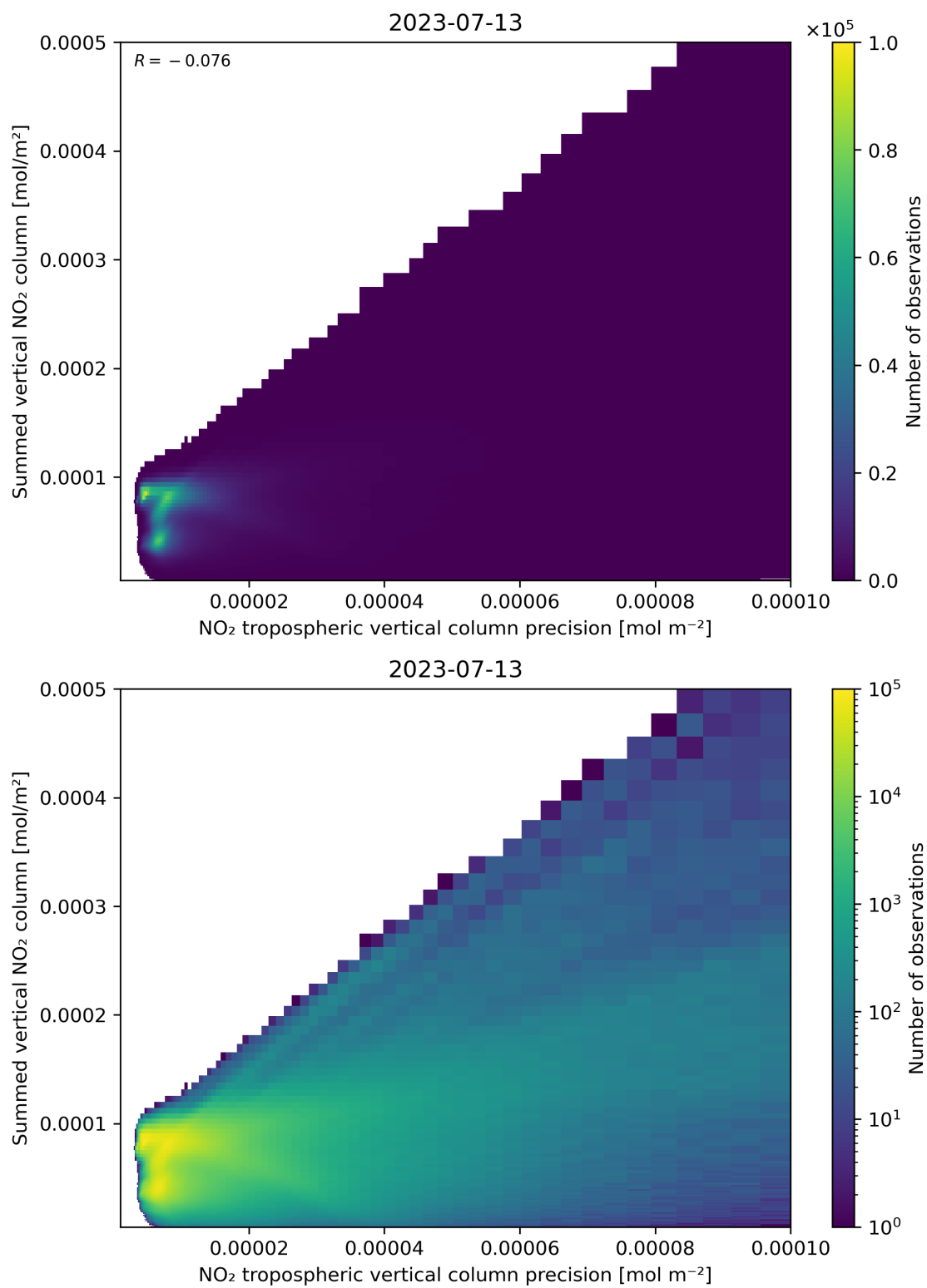
Figure 136: Scatter density plot of “NO 2 tropospheric vertical column precision” against “Summed vertical NO 2 column” for 2023-07-13 to 2023-07-14.
