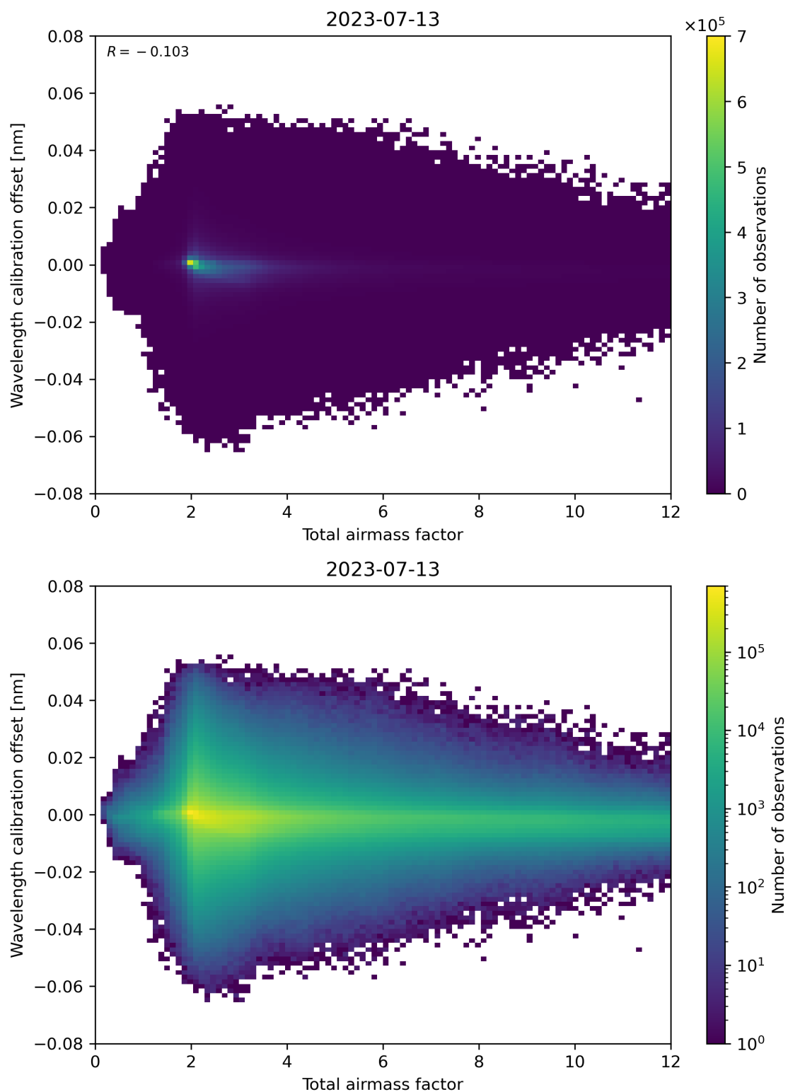
Figure 70: Scatter density plot of “Total airmass factor” against “Wavelength calibration offset” for 2023-07-13 to 2023-07-14.
