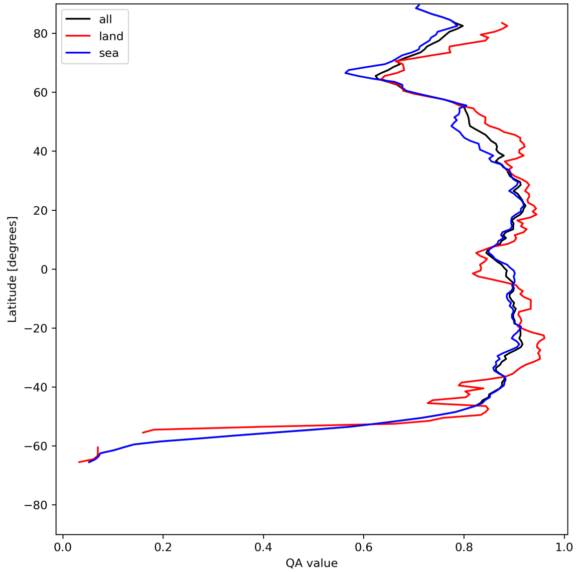
Figure 11: Zonal average of “QA value” for 2023-07-13 to 2023-07-14.
