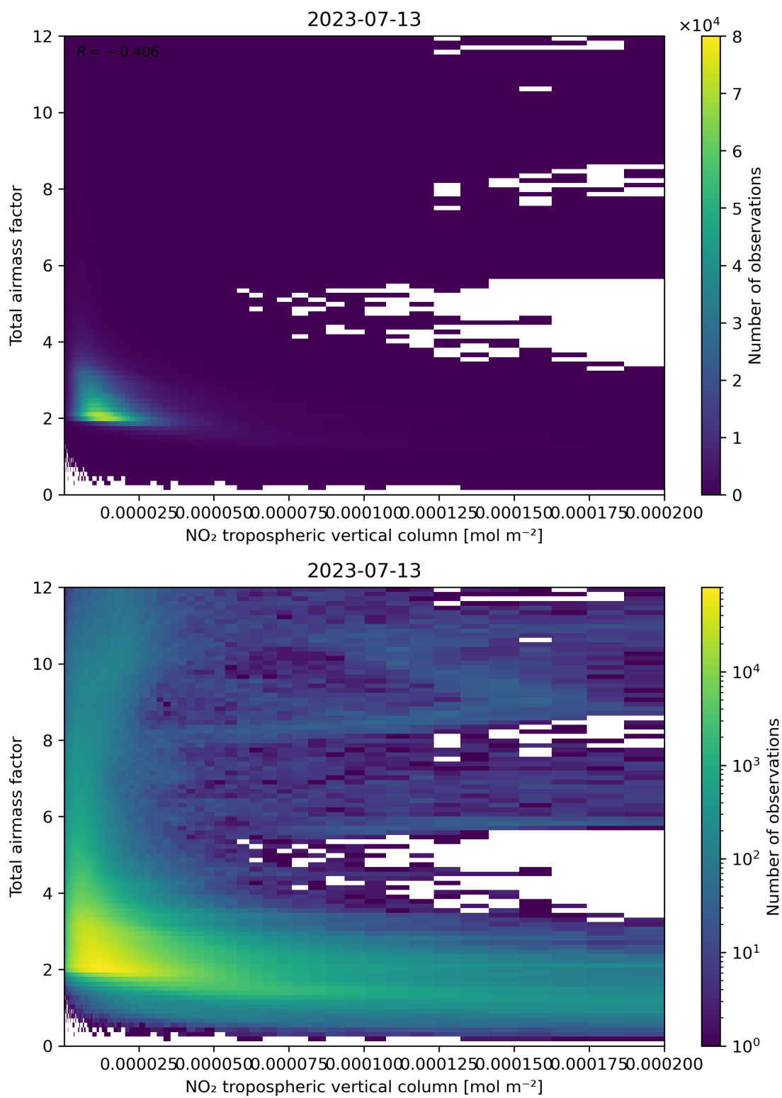
Figure 122: Scatter density plot of “NO 2 tropospheric vertical column” against “Total air mass factor” for 2023-07-13 to 2023-07-14.
