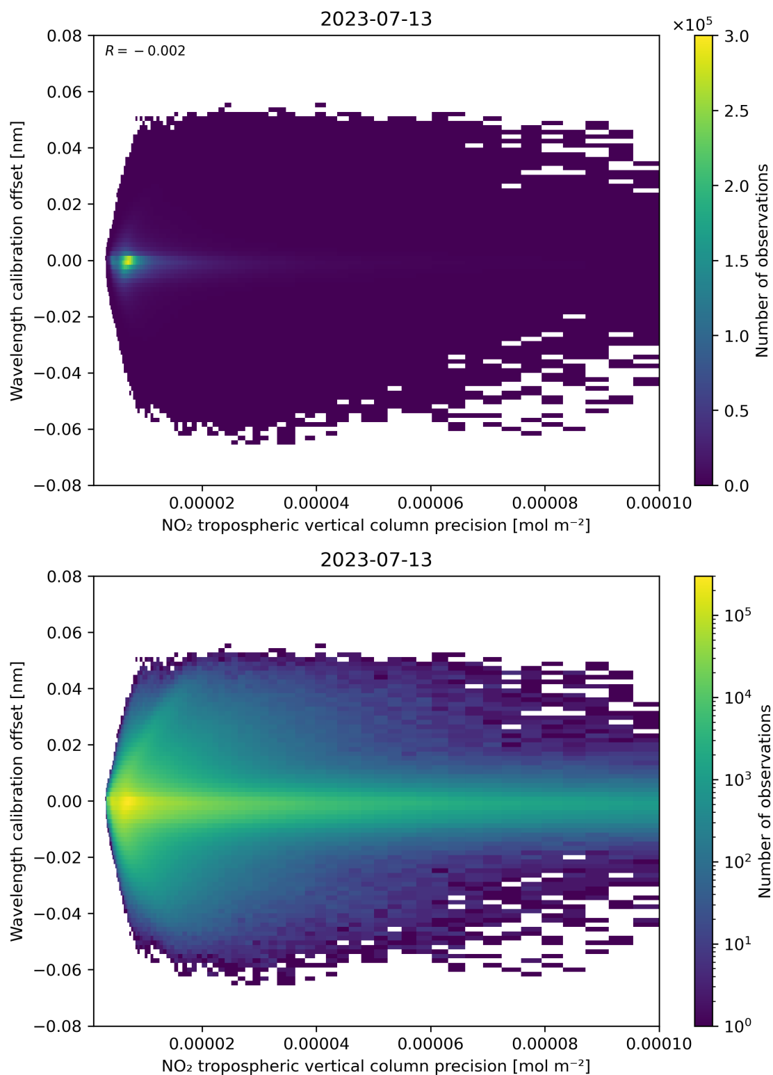
Figure 141: Scatter density plot of “NO 2 tropospheric vertical column precision” against “Wavelength calibration offset” for 2023-07-13 to 2023-07-14.
