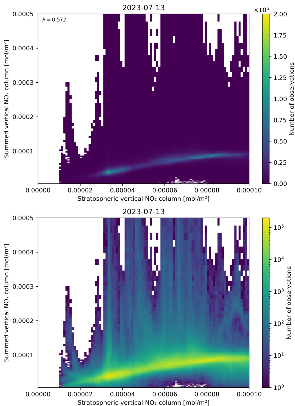
Figure 98: Scatter density plot of “Stratospheric vertical NO 2 column” against “Summed vertical NO 2 column” for 2023-07-13 to 2023-07-14.
