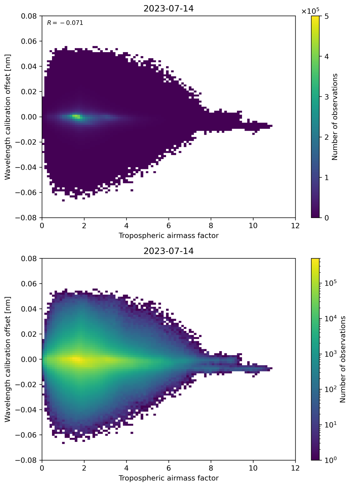
Figure 80: Scatter density plot of “Tropospheric airmass factor” against “Wavelength calibration offset” for 2023-07-14 to 2023-07-15.
