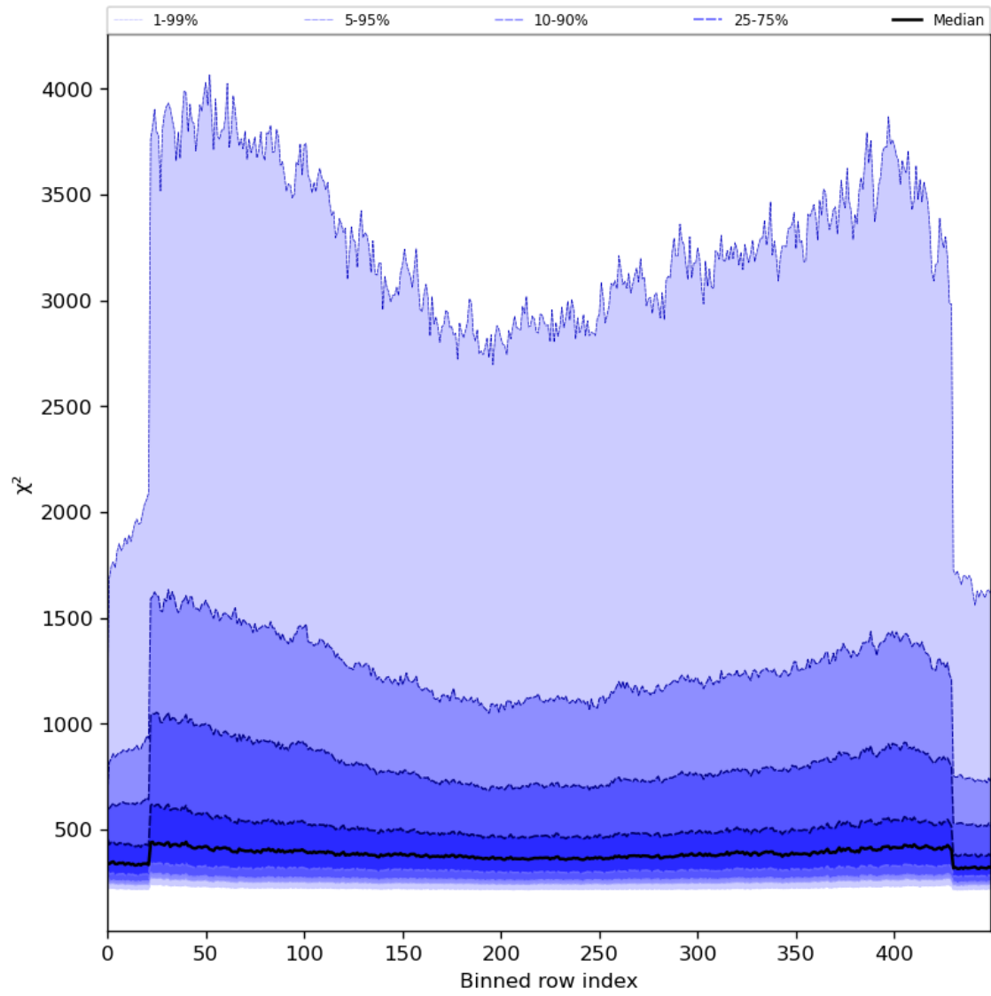
Figure 59: Along track statistics of “ \chi^2 ” for 2023-07-14 to 2023-07-15
