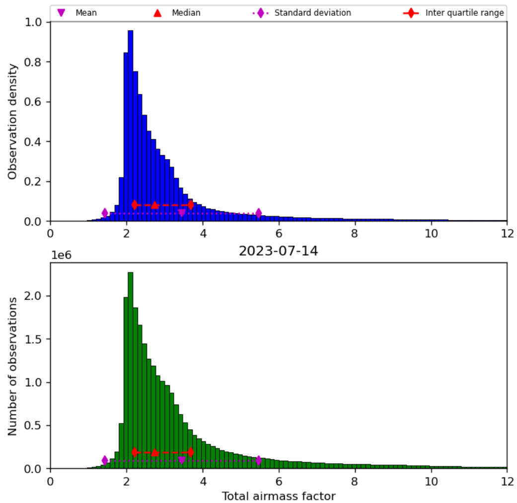
Figure 32: Histogram of “Total airmass factor” for 2023-07-14 to 2023-07-15
