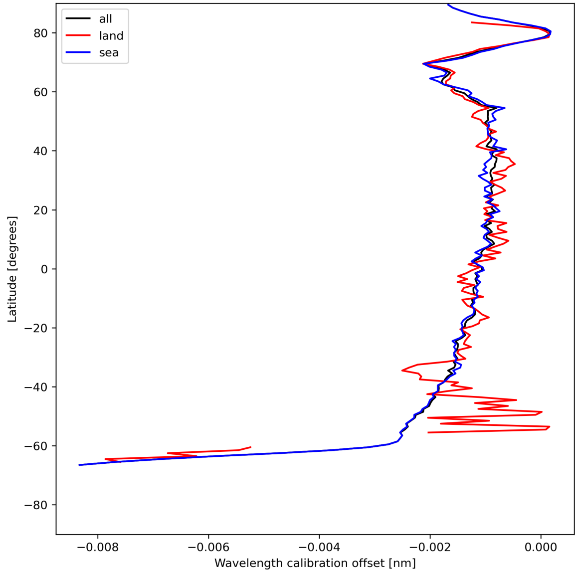
Figure 18: Zonal average of “Wavelength calibration offset” for 2023-07-14 to 2023-07-15.
