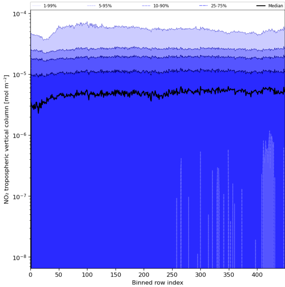
Figure 46: Along track statistics of “NO 2 tropospheric vertical column” for 2023-07-14 to 2023-07-15
