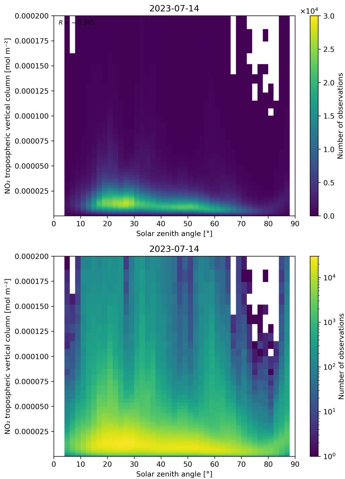
Figure 155: Scatter density plot of “Solar zenith angle” against “NO 2 tropospheric vertical column” for 2023-07-14 to 2023-07-15.
