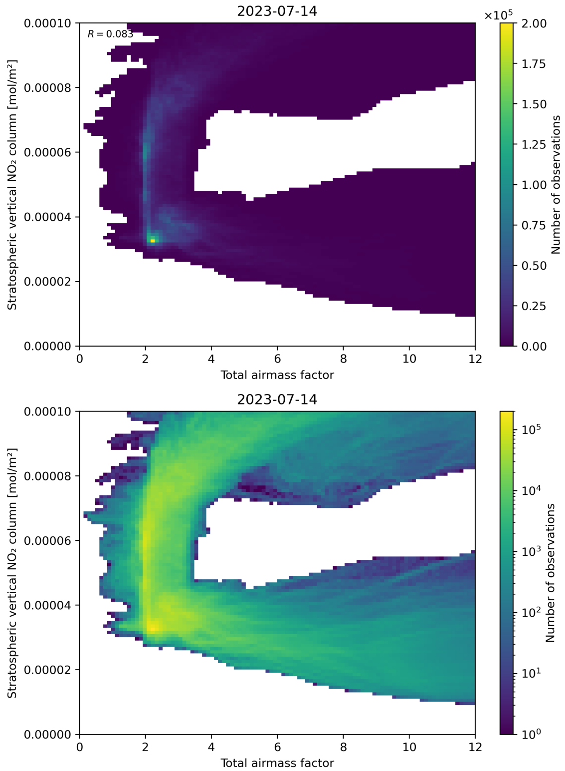
Figure 64: Scatter density plot of “Total airmass factor” against “Stratospheric vertical NO 2 column” for 2023-07-14 to 2023-07-15.
