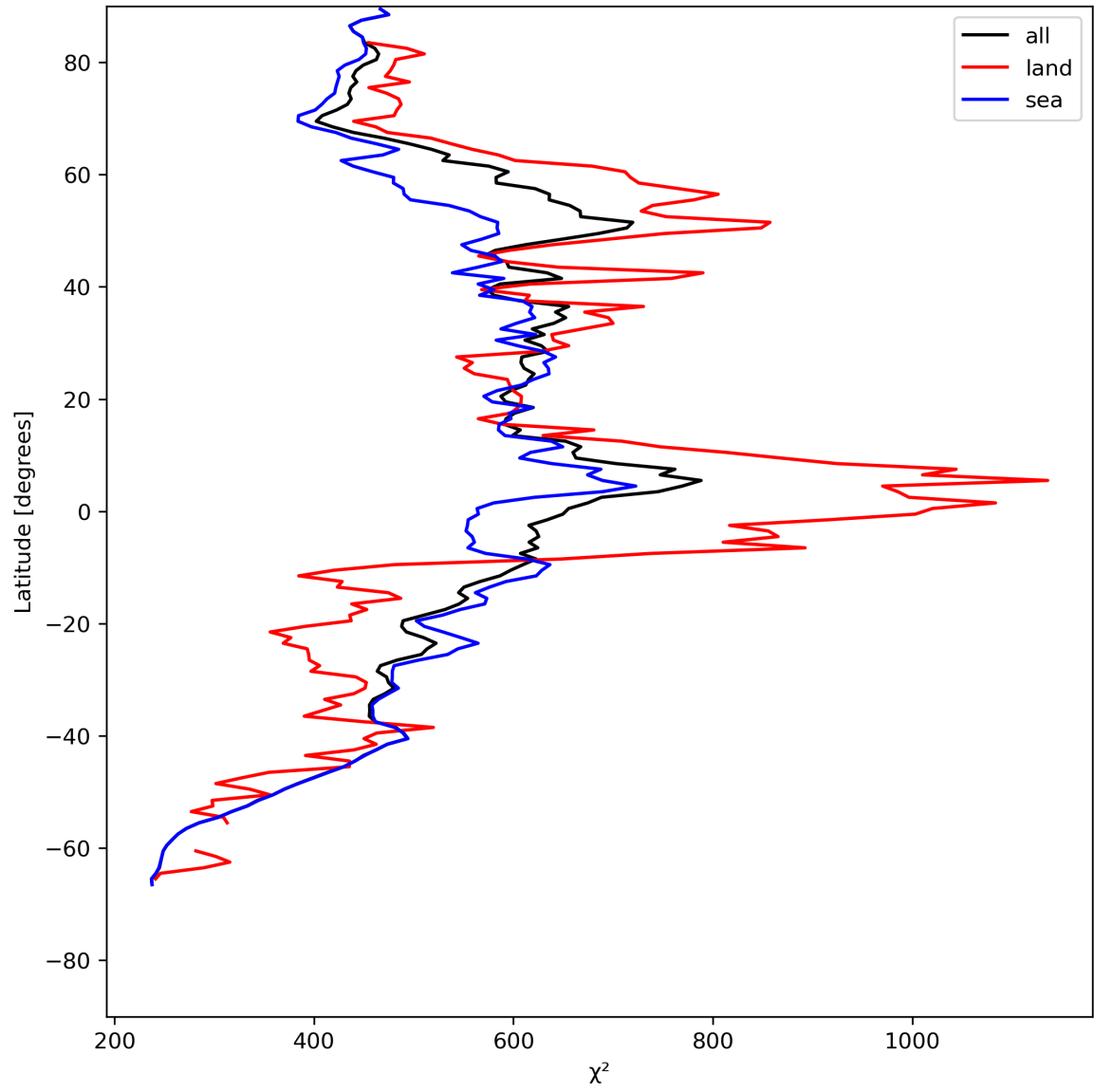
Figure 25: Zonal average of “ \chi^2 ” for 2023-07-14 to 2023-07-15.
