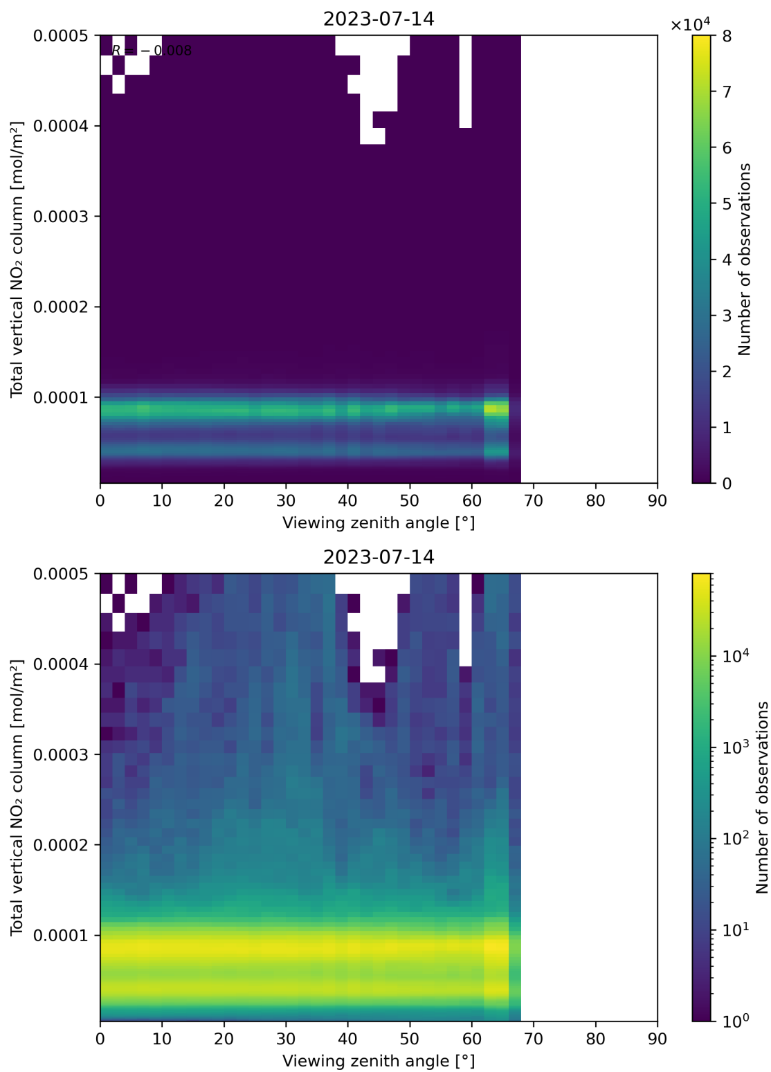
Figure 167: Scatter density plot of “Viewing zenith angle” against “Total vertical NO 2 column” for 2023-07-14 to 2023-07-15.
