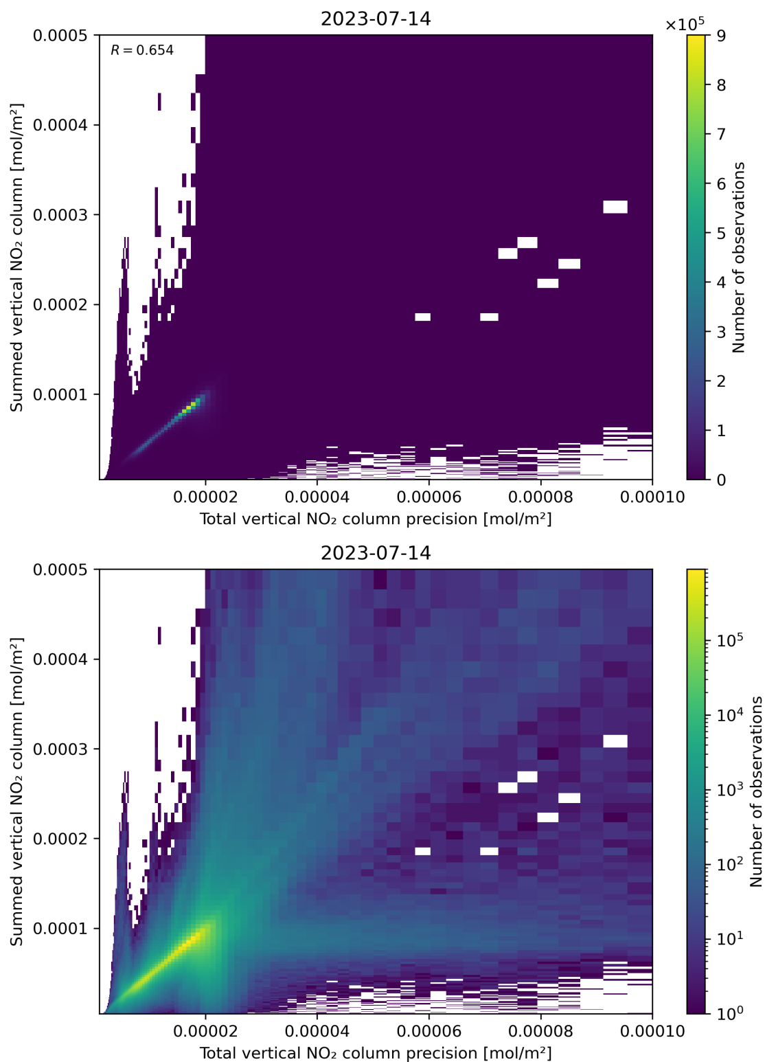
Figure 117: Scatter density plot of “Total vertical NO 2 column precision” against “Summed vertical NO 2 column” for 2023-07-14 to 2023-07-15.
