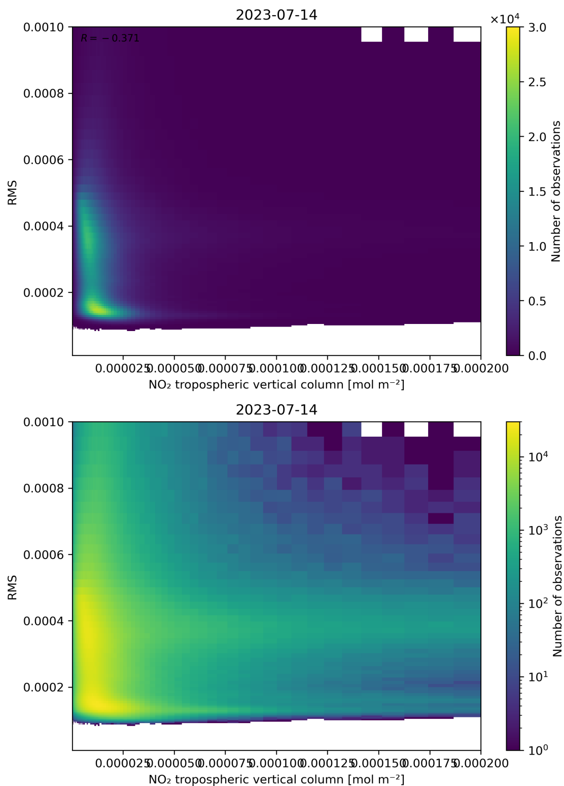
Figure 142: Scatter density plot of “NO 2 tropospheric vertical column” against “RMS” for 2023-07-14 to 2023-07-15.
