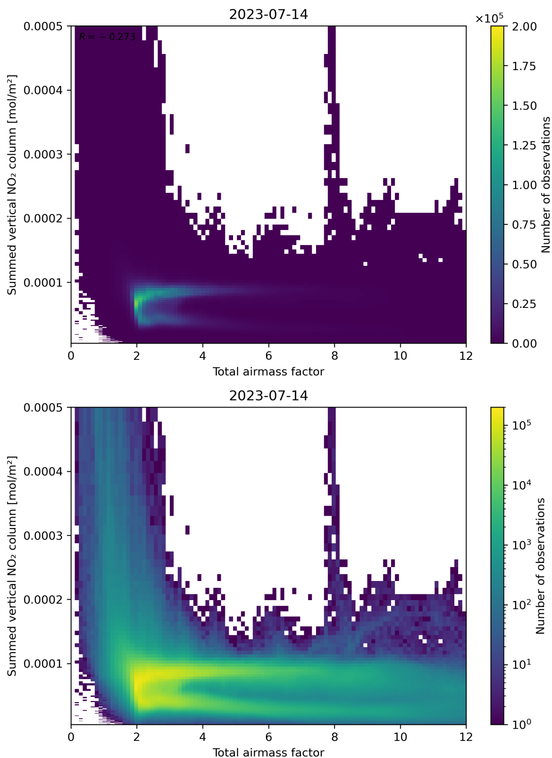
Figure 65: Scatter density plot of “Total airmass factor” against “Summed vertical NO 2 column” for 2023-07-14 to 2023-07-15.
