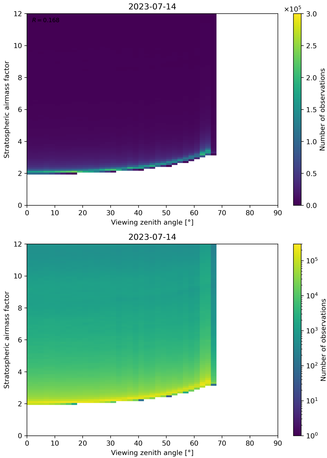
Figure 159: Scatter density plot of “Viewing zenith angle” against “Stratospheric airmass factor” for 2023-07-14 to 2023-07-15.
