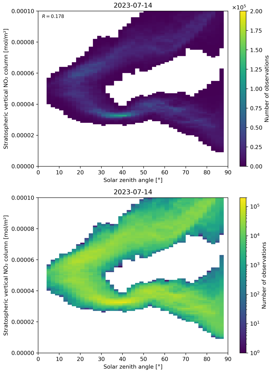
Figure 150: Scatter density plot of “Solar zenith angle” against “Stratospheric vertical NO 2 column” for 2023-07-14 to 2023-07-15.
