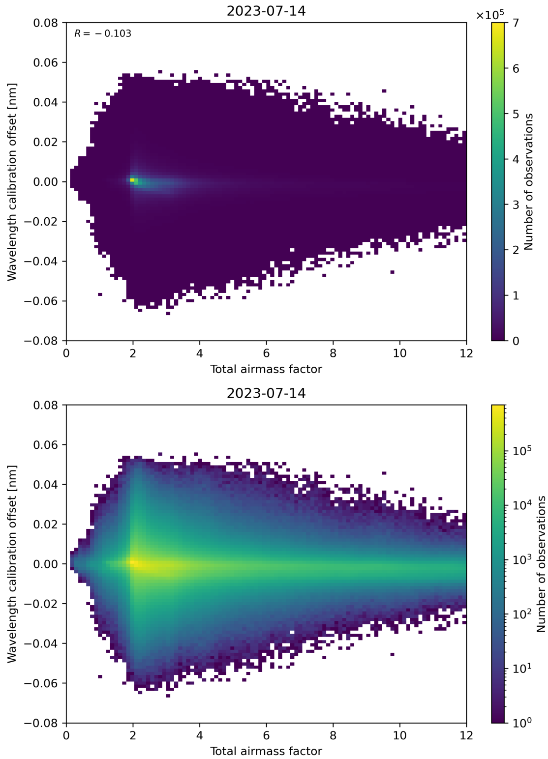
Figure 70: Scatter density plot of “Total airmass factor” against “Wavelength calibration offset” for 2023-07-14 to 2023-07-15.
