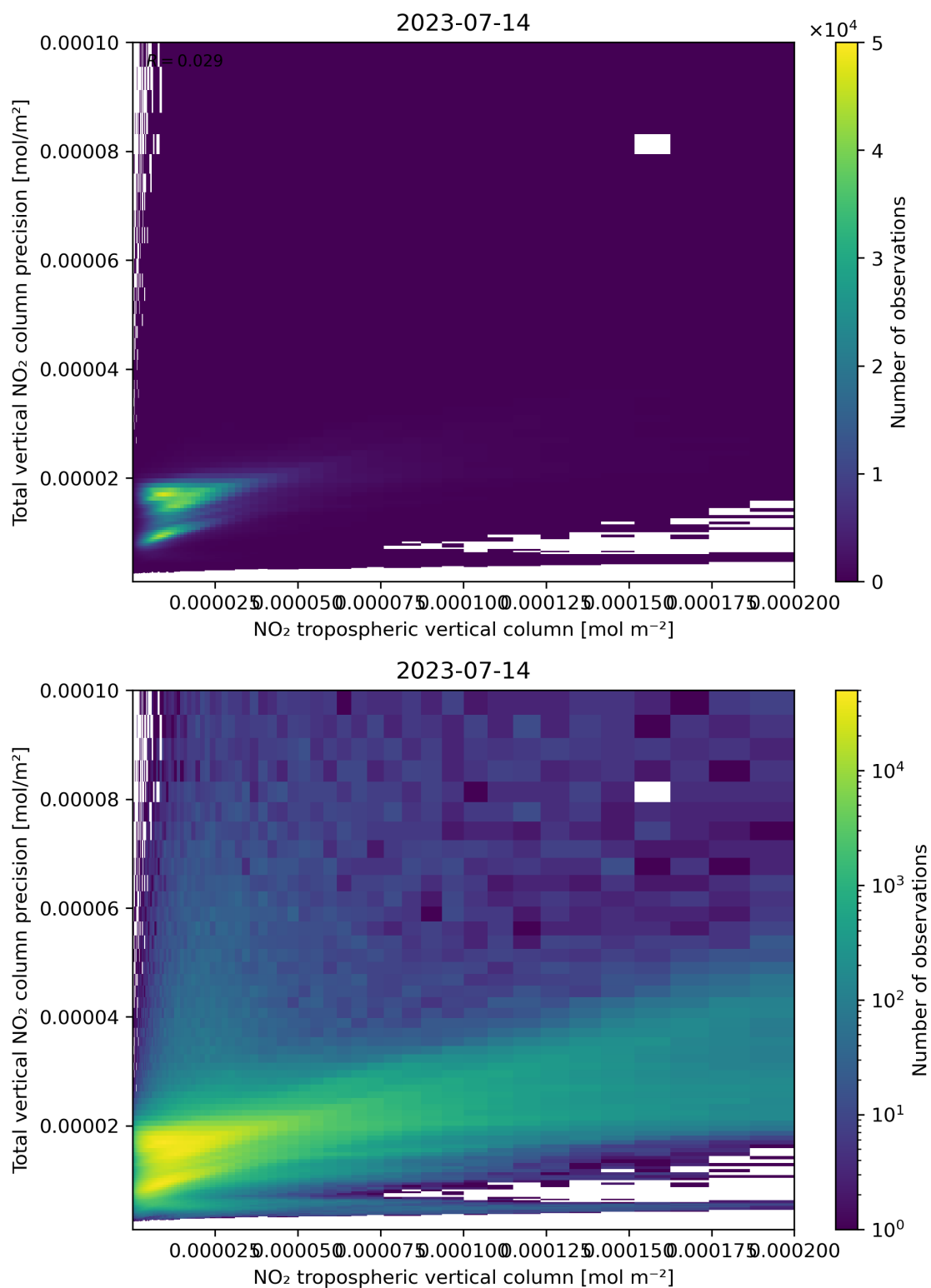
Figure 129: Scatter density plot of “NO 2 tropospheric vertical column” against “Total vertical NO 2 column precision” for 2023-07-14 to 2023-07-15.
