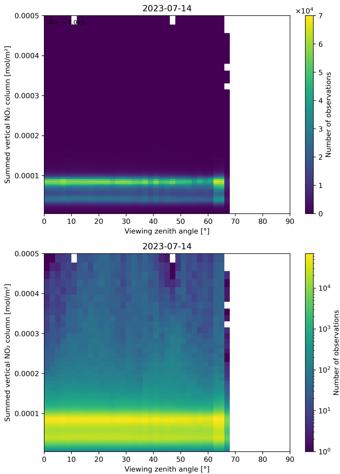
Figure 165: Scatter density plot of “Viewing zenith angle” against “Summed vertical NO 2 column” for 2023-07-14 to 2023-07-15.
