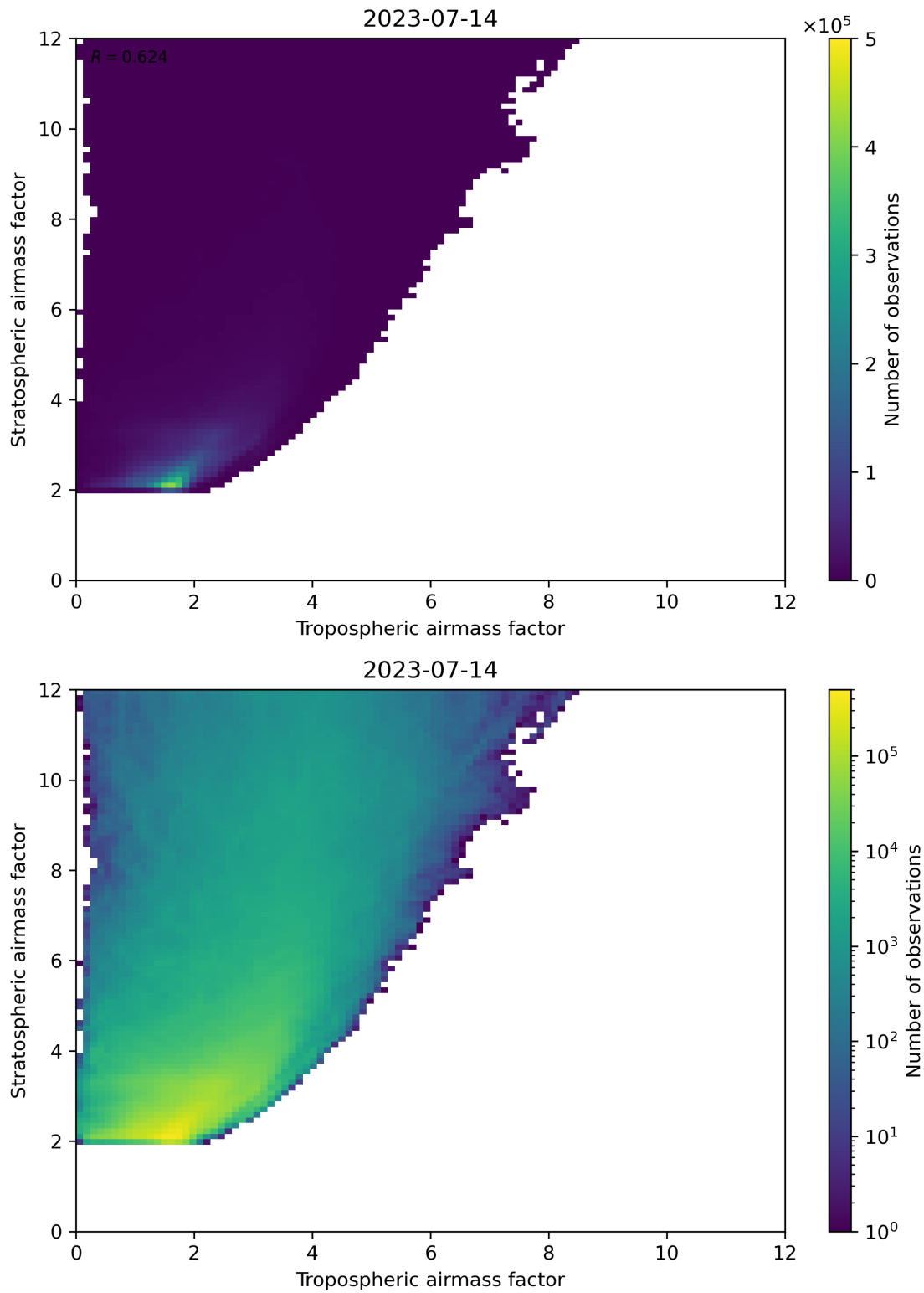
Figure 71: Scatter density plot of “Tropospheric airmass factor” against “Stratospheric airmass factor” for 2023-07-14 to 2023-07-15.
