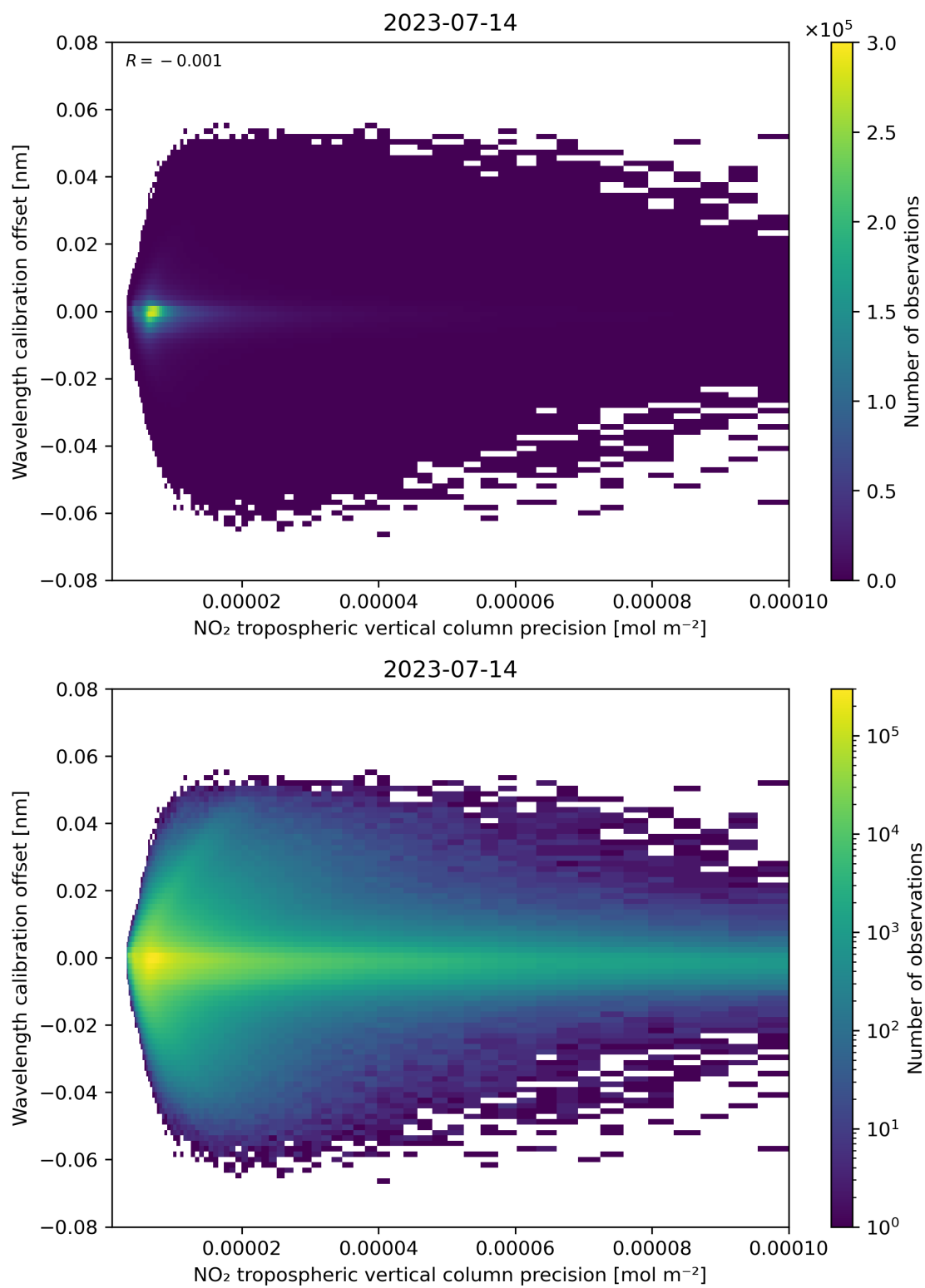
Figure 141: Scatter density plot of “NO 2 tropospheric vertical column precision” against “Wavelength calibration offset” for 2023-07-14 to 2023-07-15.
