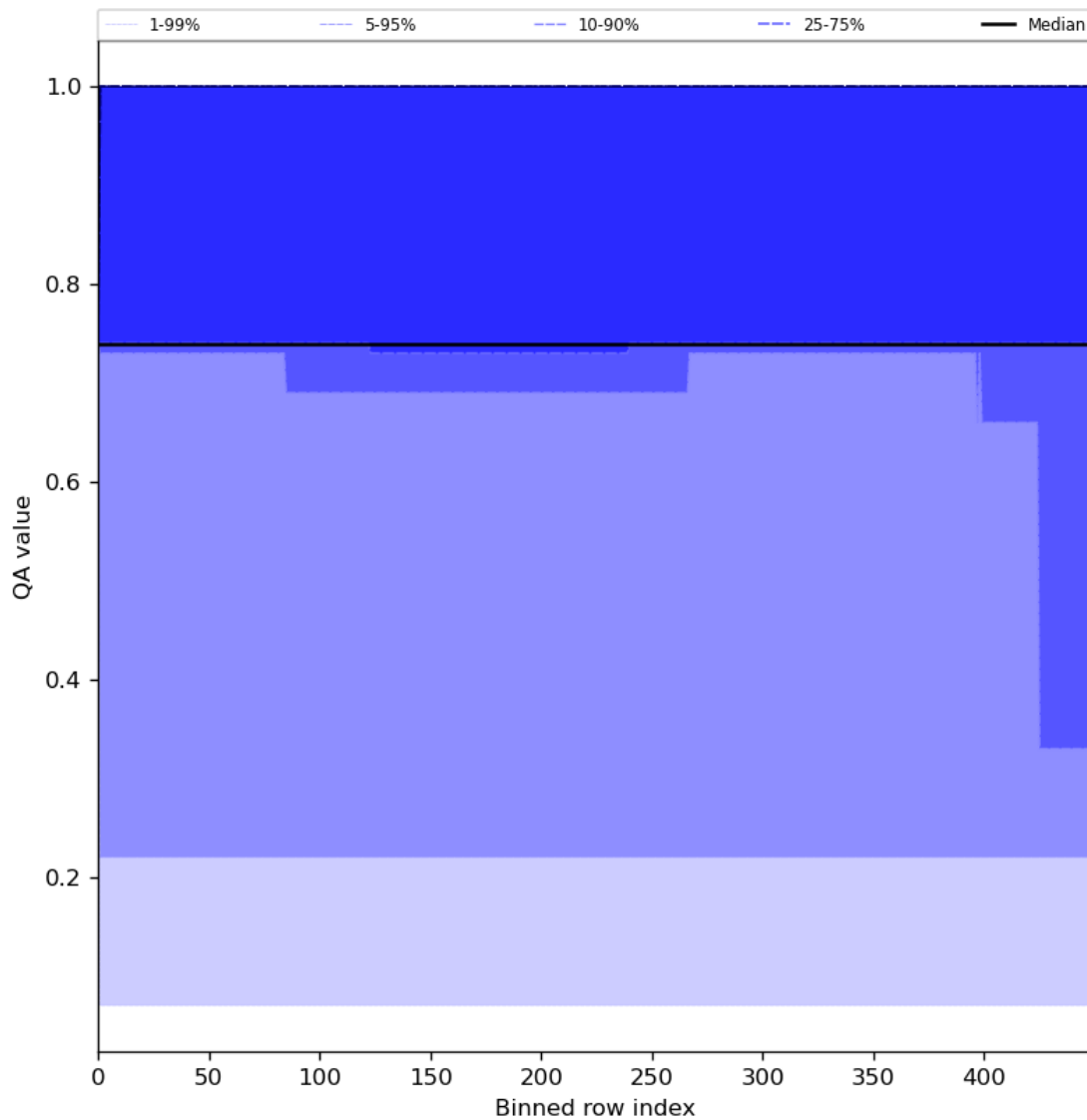
Figure 45: Along track statistics of “QA value” for 2023-07-14 to 2023-07-15
