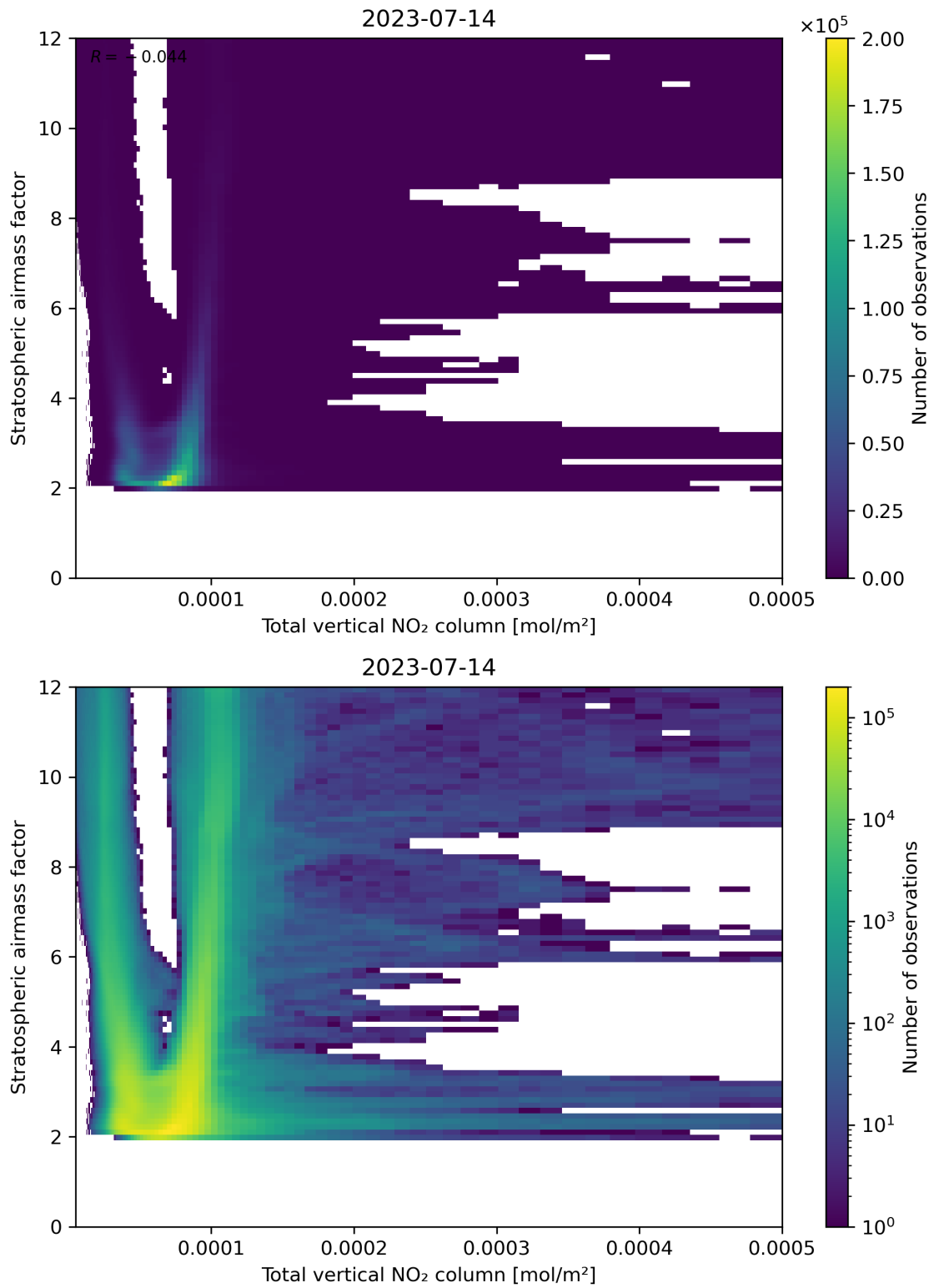
Figure 110: Scatter density plot of “Total vertical NO 2 column” against “Stratospheric airmass factor” for 2023-07-14 to 2023-07-15.
