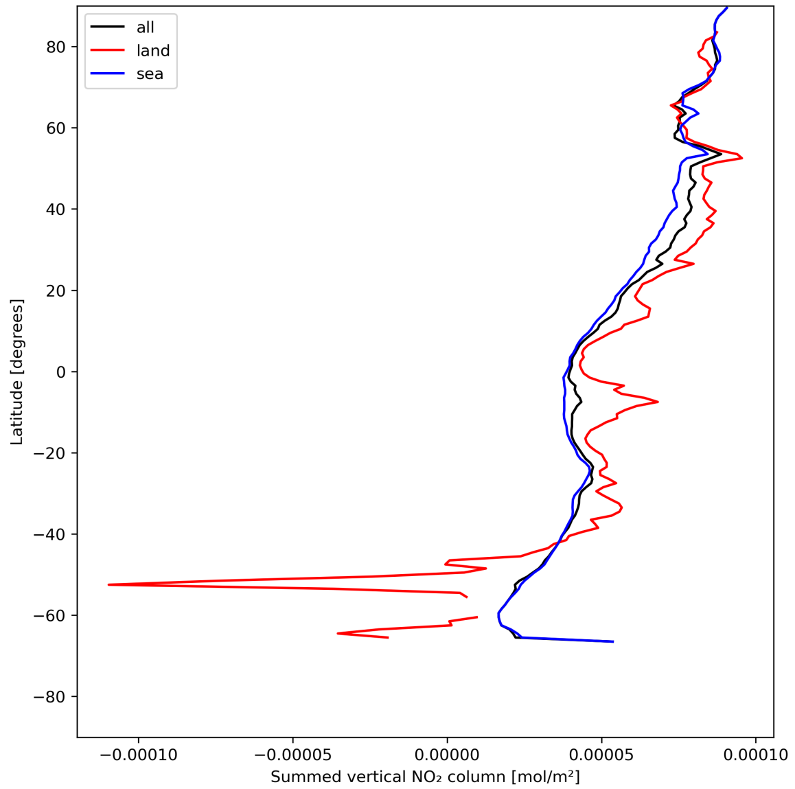
Figure 23: Zonal average of “Summed vertical NO 2 column” for 2023-07-14 to 2023-07-15.
