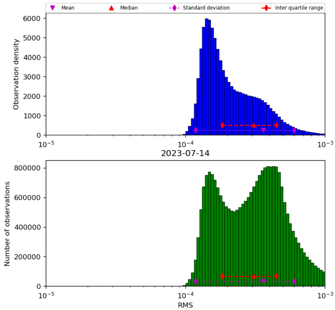
Figure 43: Histogram of “RMS” for 2023-07-14 to 2023-07-15
