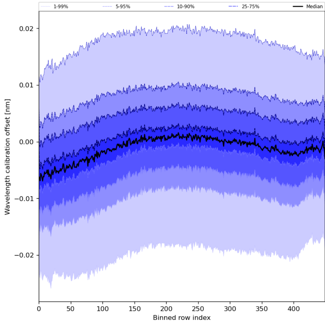
Figure 52: Along track statistics of “Wavelength calibration offset” for 2023-07-14 to 2023-07-15
