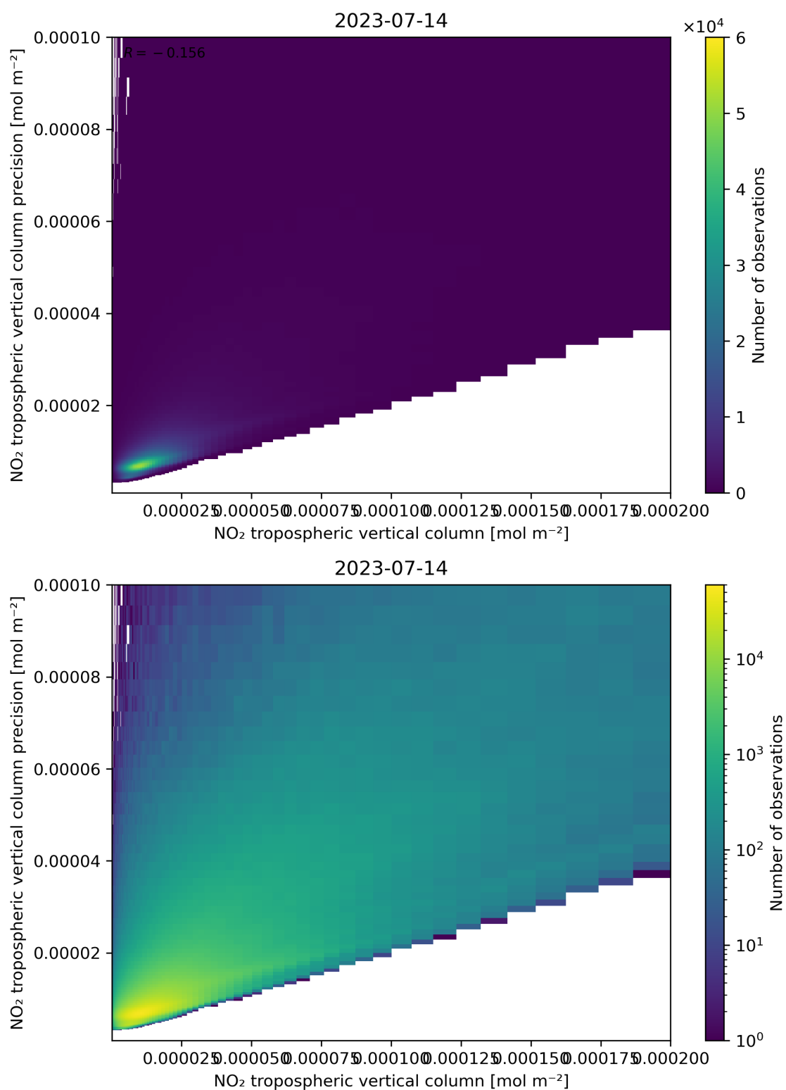
Figure 130: Scatter density plot of “NO 2 tropospheric vertical column” against “NO 2 tropospheric vertical column precision” for 2023-07-14 to 2023-07-15.
