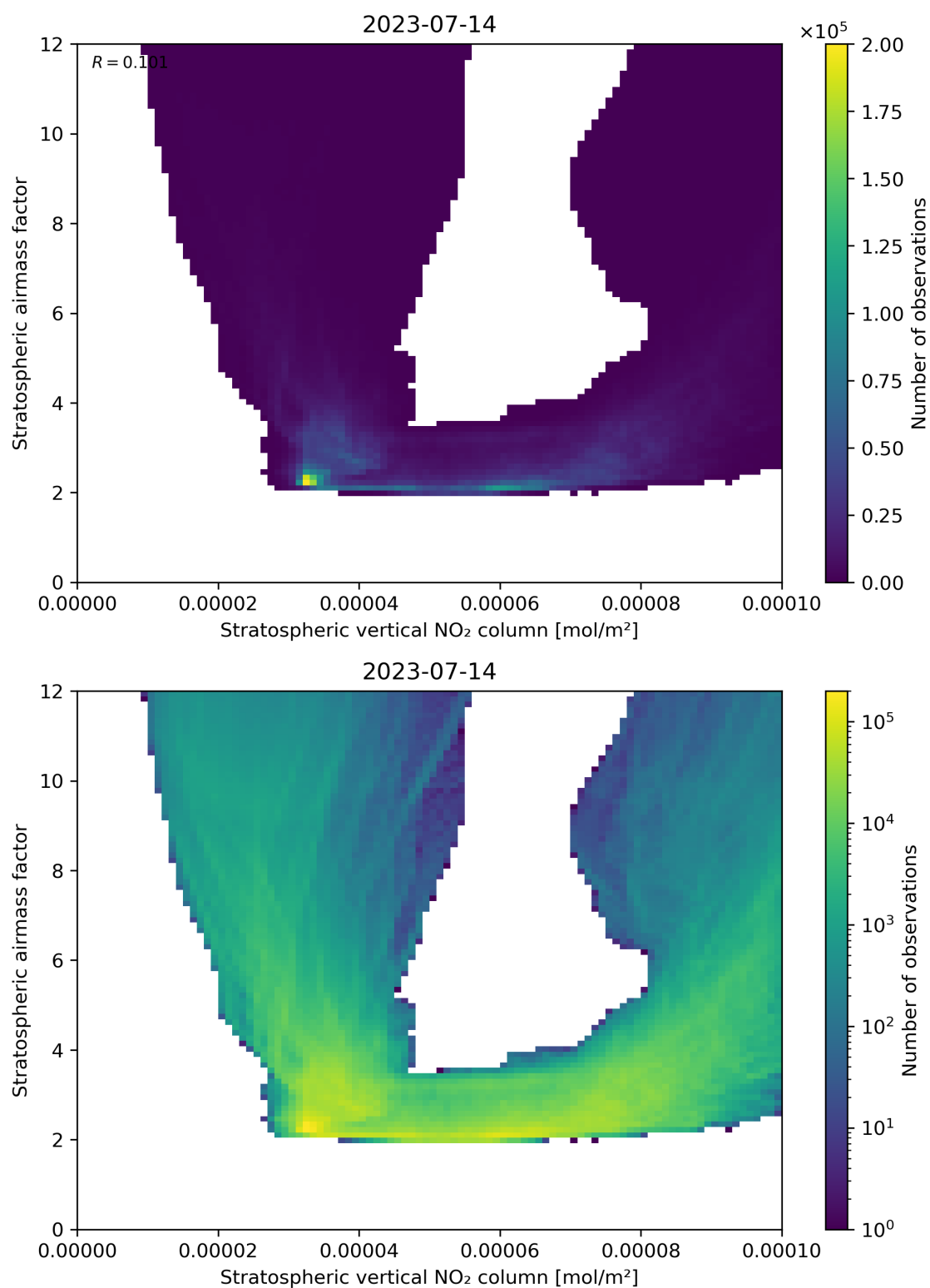
Figure 96: Scatter density plot of “Stratospheric vertical NO 2 column” against “Stratospheric airmass factor” for 2023-07-14 to 2023-07-15.
