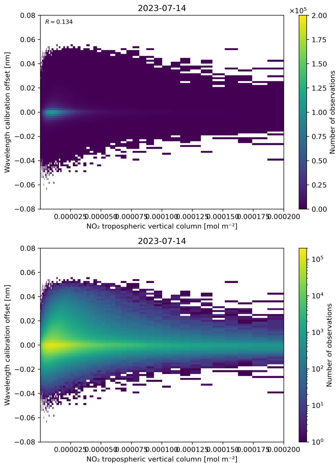
Figure 143: Scatter density plot of “NO 2 tropospheric vertical column” against “Wavelength calibration offset” for 2023-07-14 to 2023-07-15.
