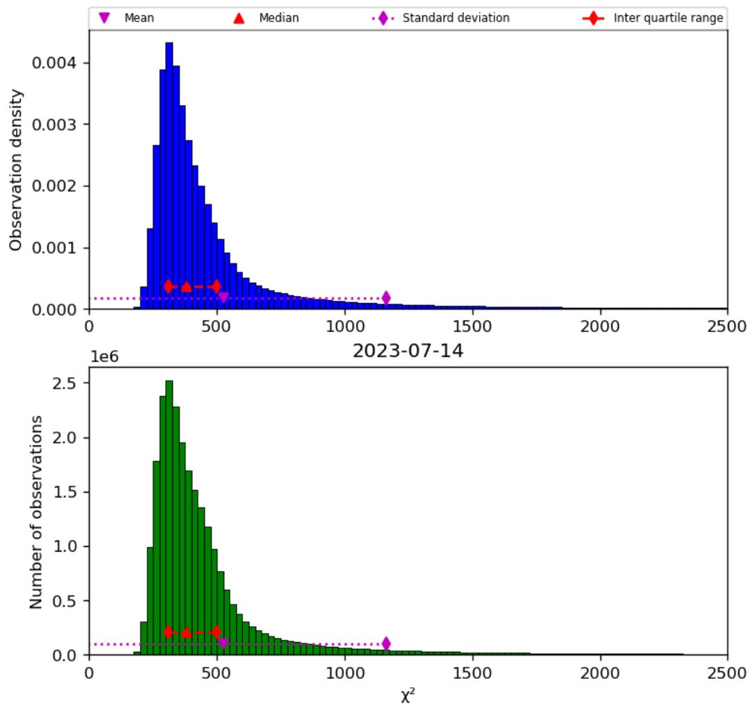
Figure 42: Histogram of “ \chi^2 ” for 2023-07-14 to 2023-07-15
