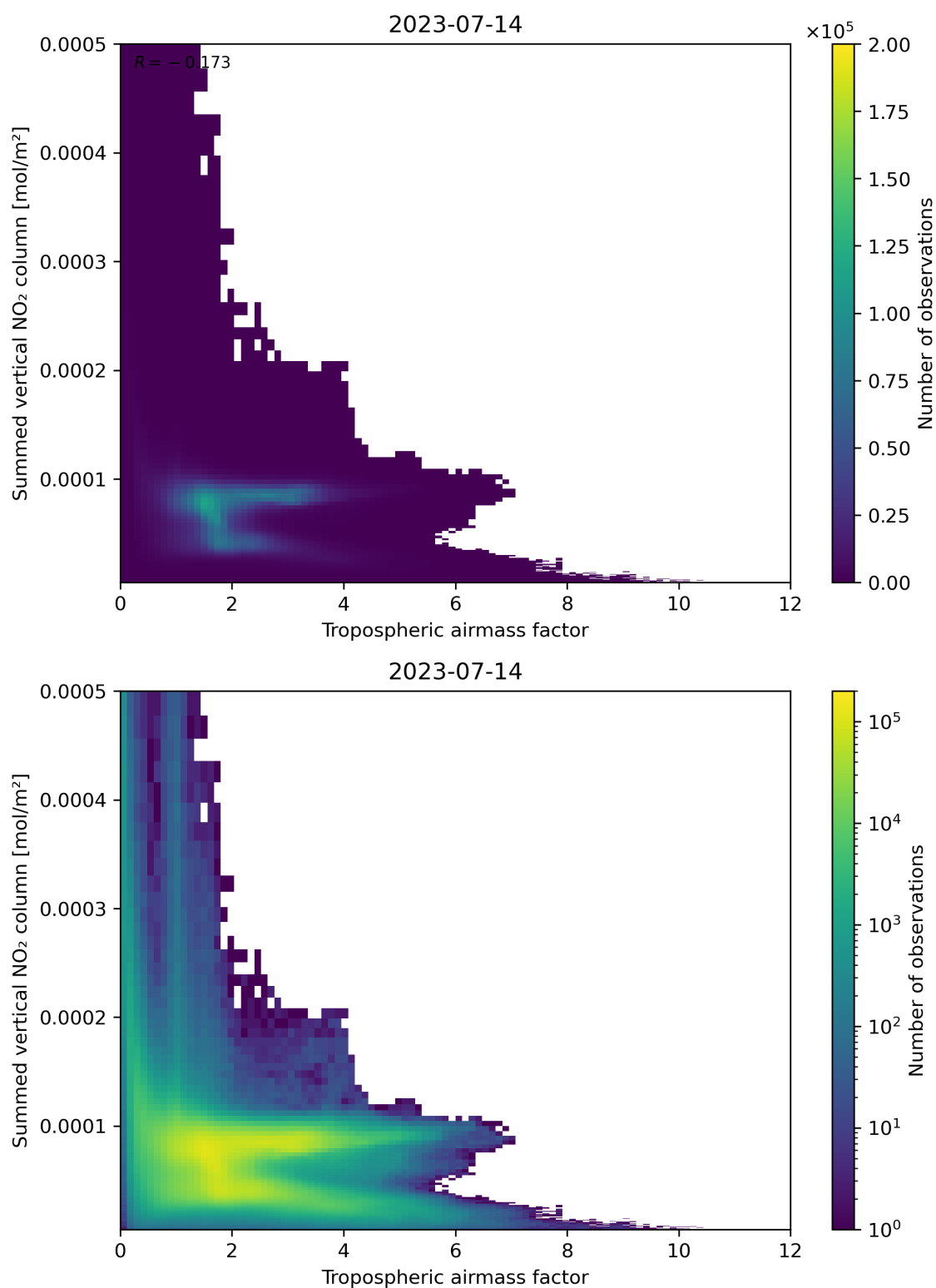
Figure 75: Scatter density plot of “Tropospheric air mass factor” against “Summed vertical NO 2 column” for 2023-07-14 to 2023-07-15.
