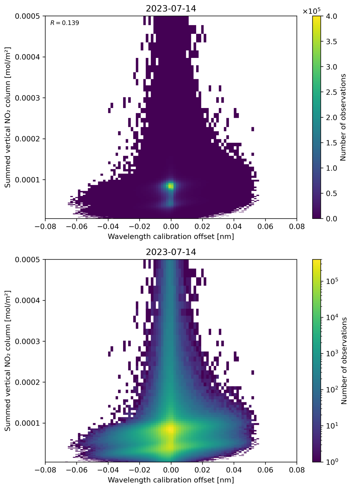
Figure 177: Scatter density plot of “Wavelength calibration offset” against “Summed vertical NO 2 column” for 2023-07-14 to 2023-07-15.
