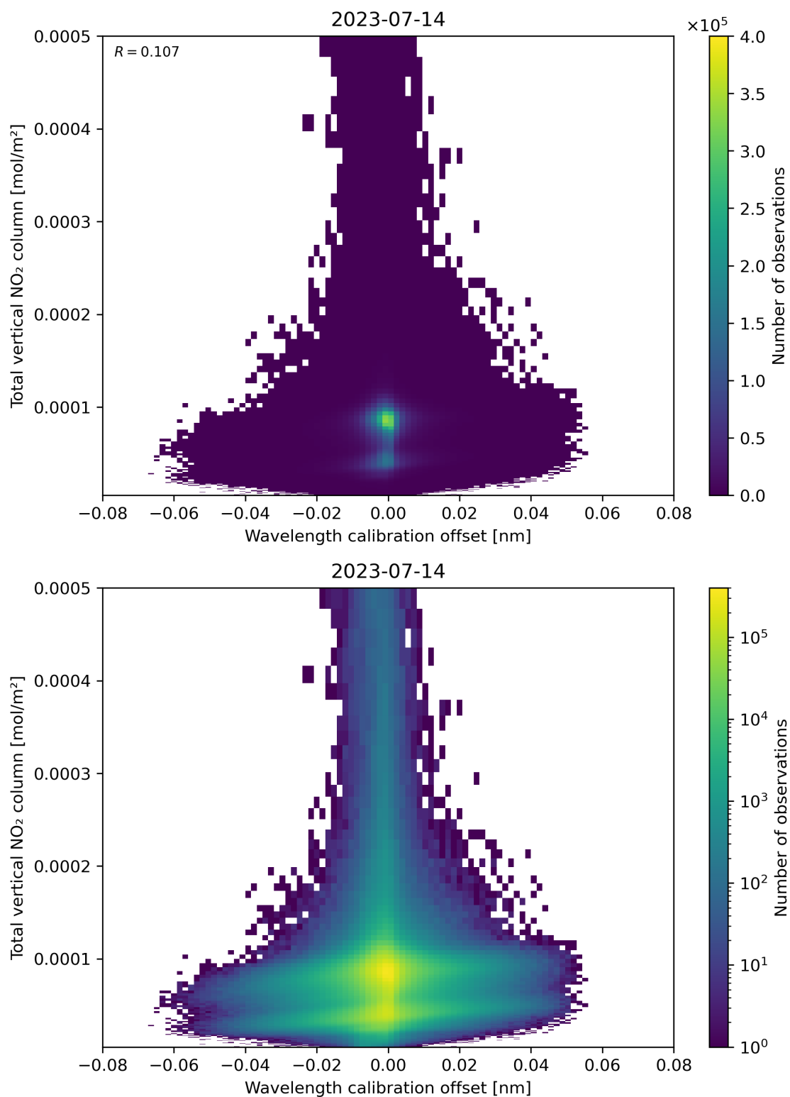
Figure 179: Scatter density plot of “Wavelength calibration offset” against “Total vertical NO 2 column” for 2023-07-14 to 2023-07-15.
