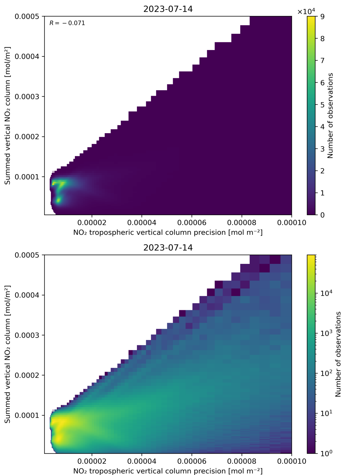
Figure 136: Scatter density plot of “NO 2 tropospheric vertical column precision” against “Summed vertical NO 2 column” for 2023-07-14 to 2023-07-15.
