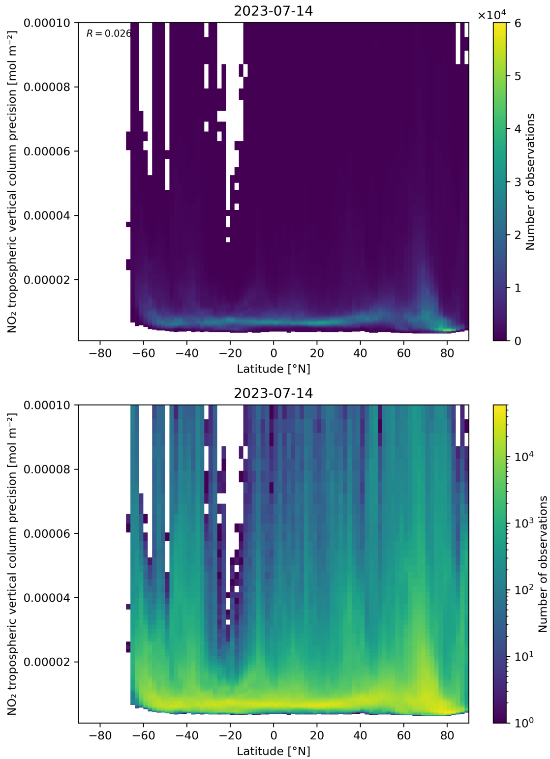
Figure 93: Scatter density plot of “Latitude” against “NO 2 tropospheric vertical column precision” for 2023-07-14 to 2023-07-15.
