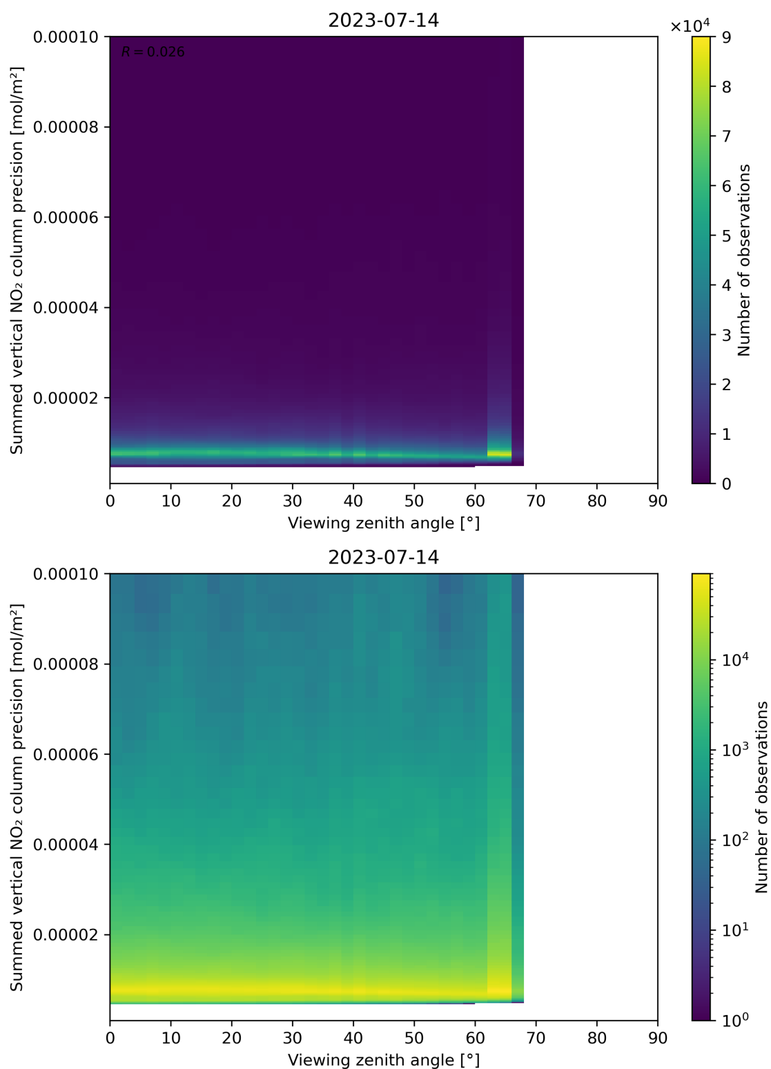
Figure 166: Scatter density plot of “Viewing zenith angle” against “Summed vertical NO 2 column precision” for 2023-07-14 to 2023-07-15.
