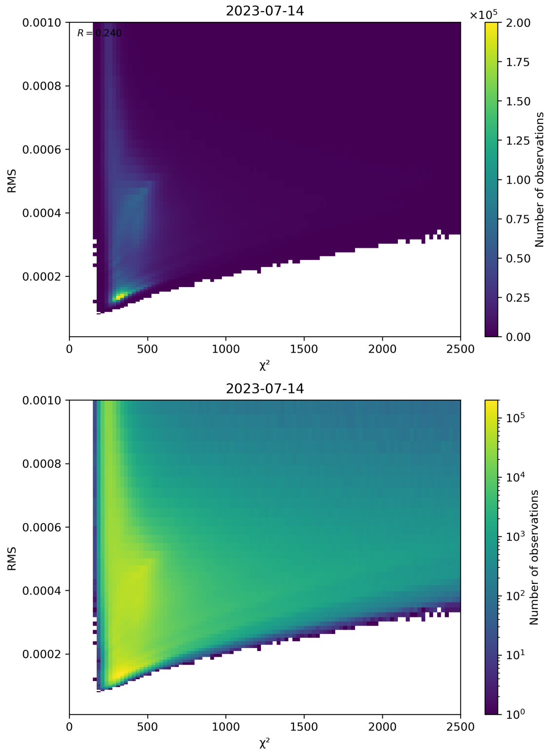
Figure 82: Scatter density plot of “ \chi^2 ” against “RMS” for 2023-07-14 to 2023-07-15.
