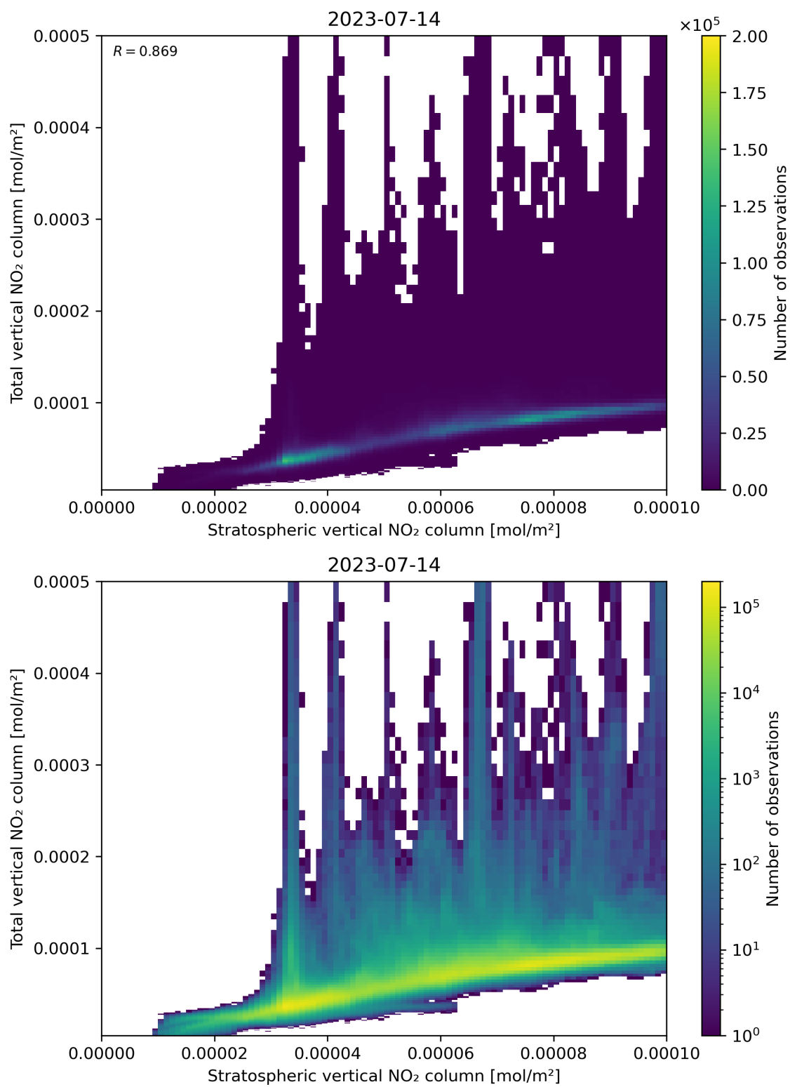
Figure 100: Scatter density plot of “Stratospheric vertical NO 2 column” against “Total vertical NO 2 column” for 2023-07-14 to 2023-07-15.
