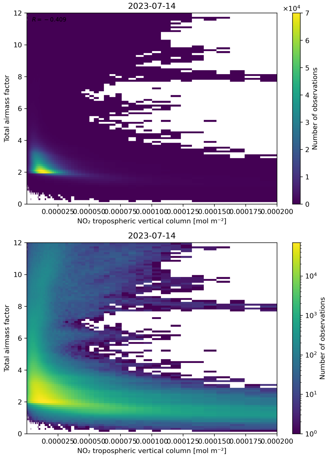
Figure 122: Scatter density plot of “NO 2 tropospheric vertical column” against “Total air mass factor” for 2023-07-14 to 2023-07-15.
