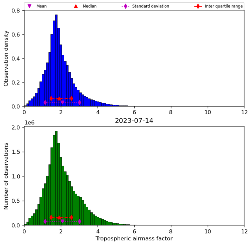
Figure 31: Histogram of “Tropospheric airmass factor” for 2023-07-14 to 2023-07-15
