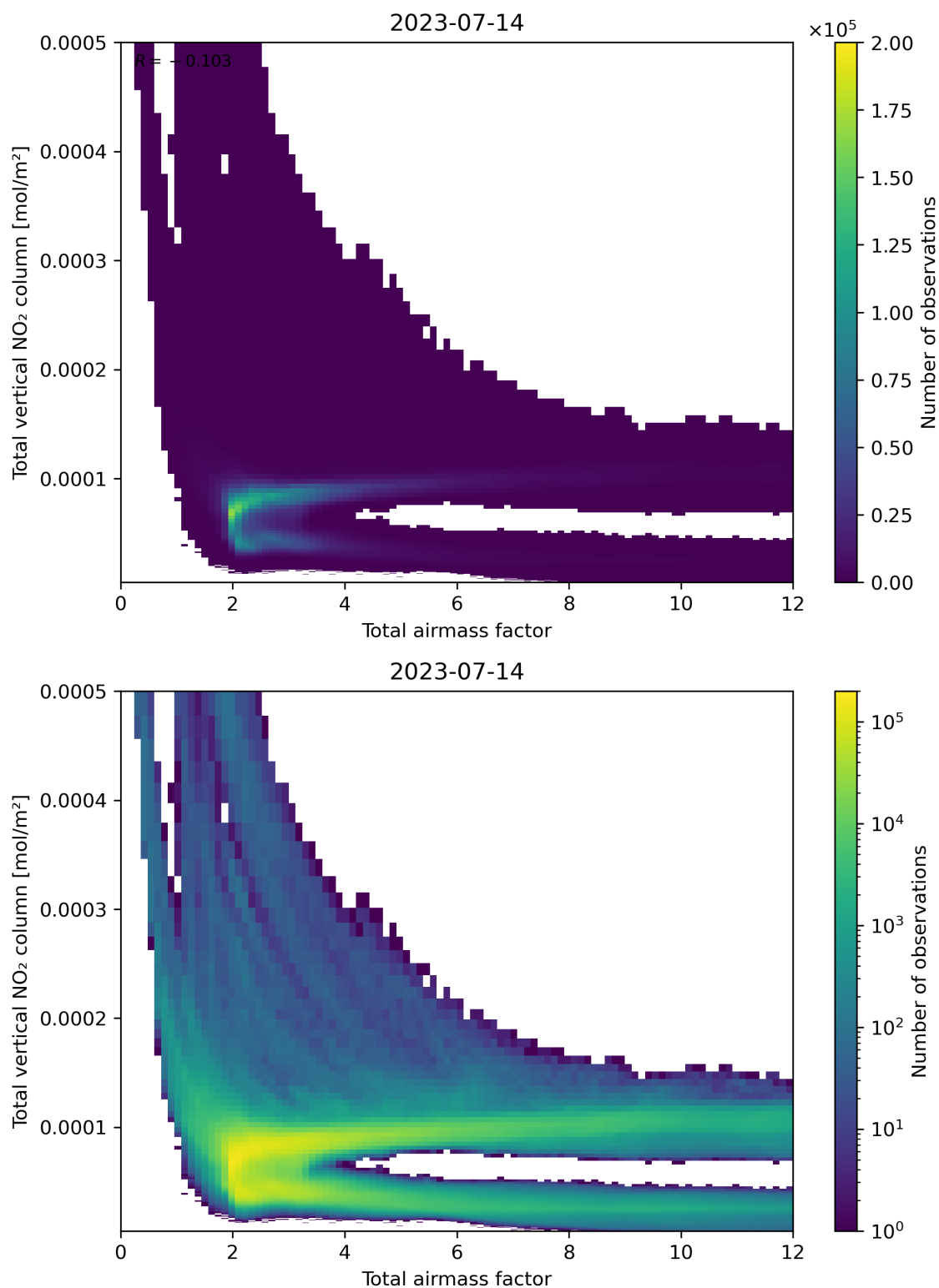
Figure 67: Scatter density plot of “Total airmass factor” against “Total vertical NO 2 column” for 2023-07-14 to 2023-07-15.
