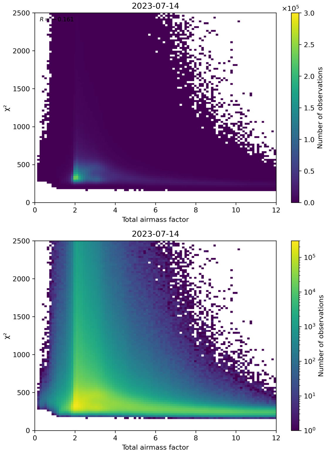
Figure 63: Scatter density plot of “Total airmass factor” against “ \chi^2 ” for 2023-07-14 to 2023-07-15.
