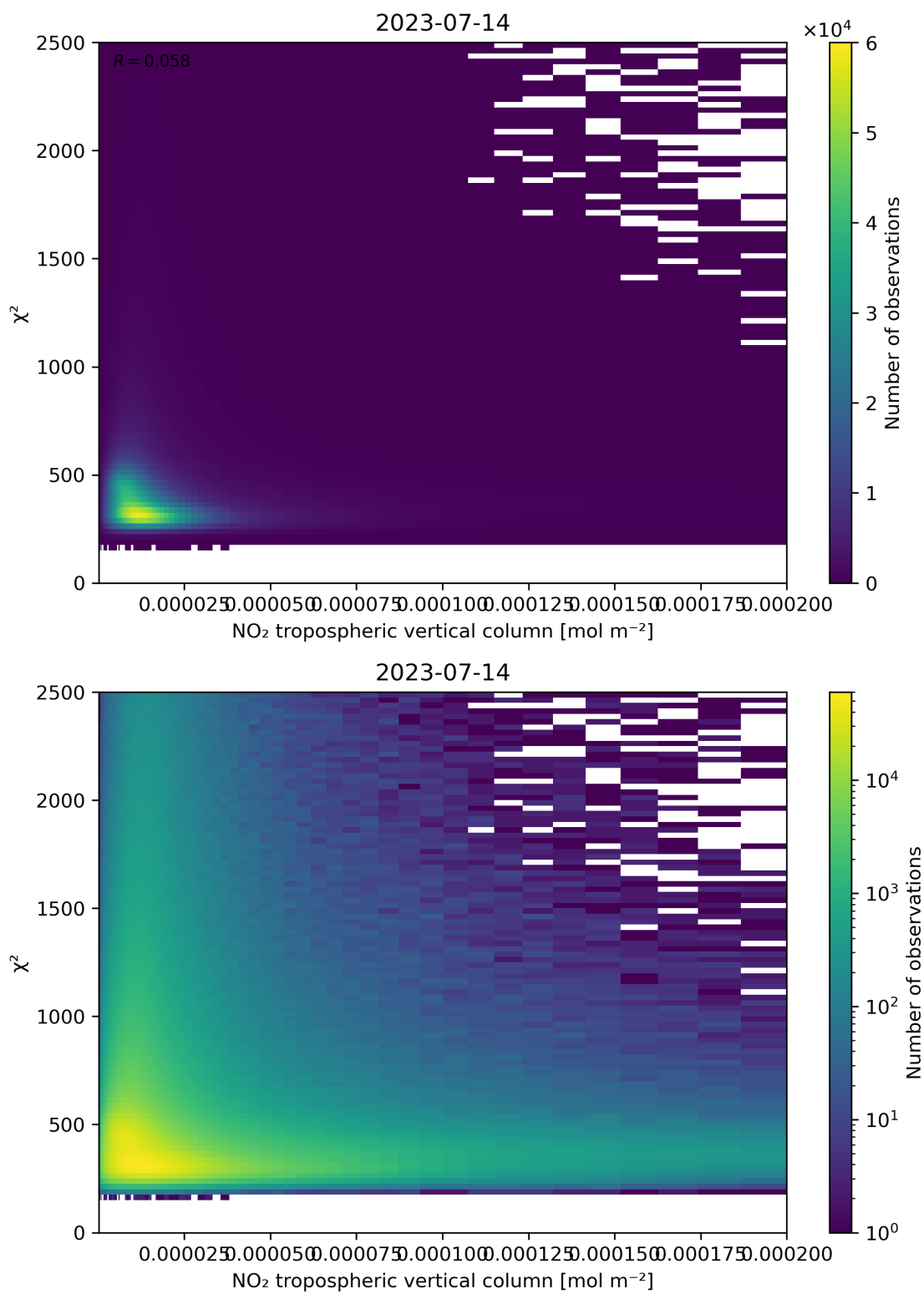
Figure 124: Scatter density plot of “NO 2 tropospheric vertical column” against “ \chi^2 ” for 2023-07-14 to 2023-07-15.
