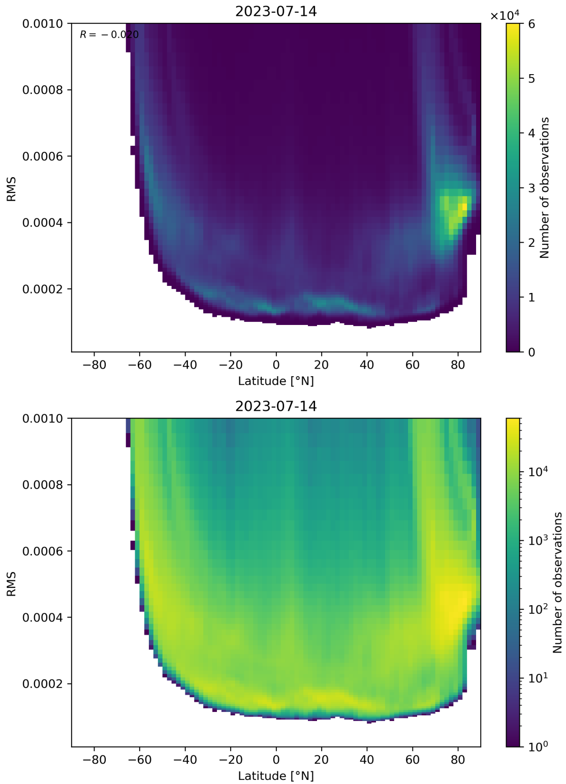
Figure 94: Scatter density plot of “Latitude” against “RMS” for 2023-07-14 to 2023-07-15.
