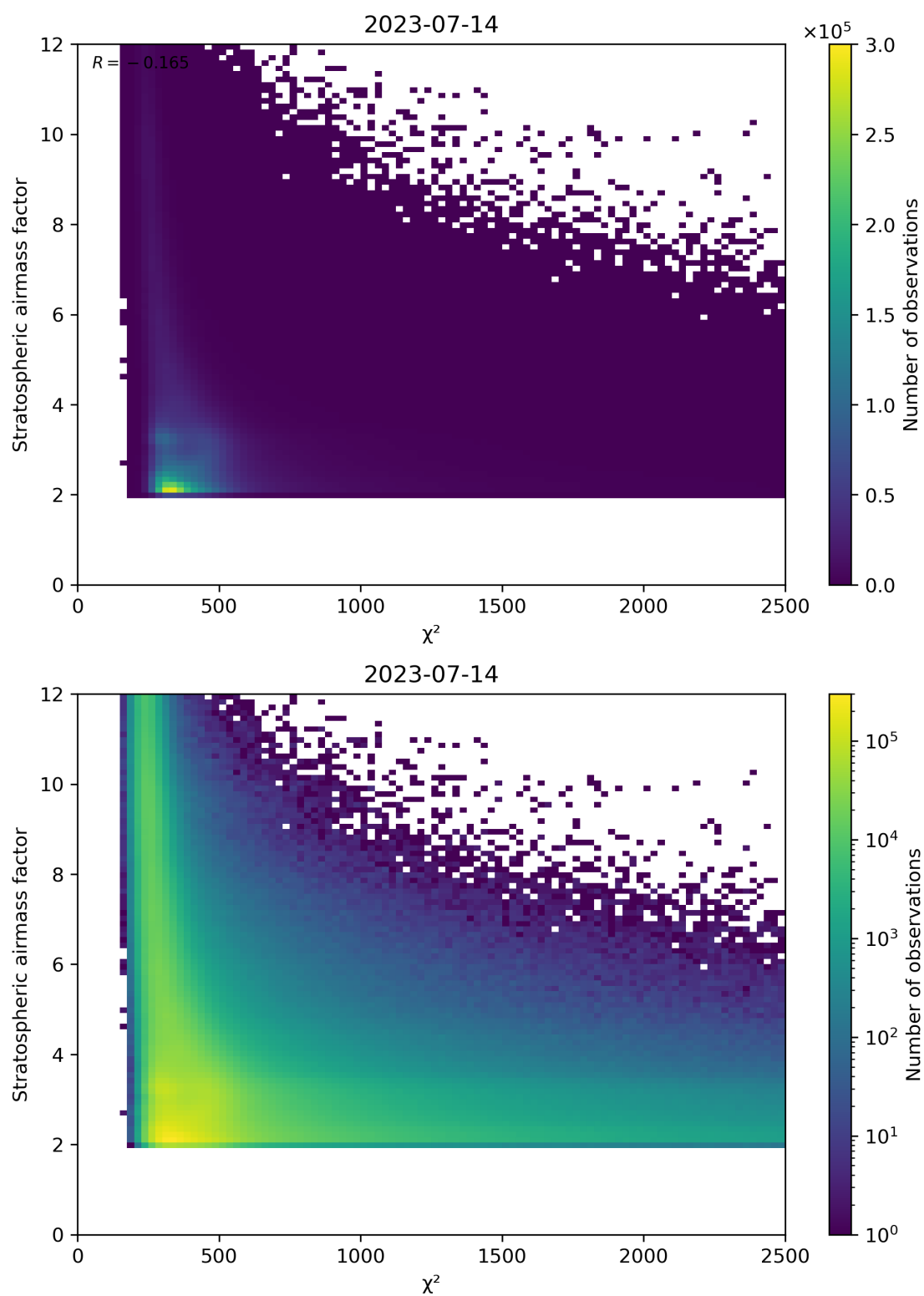
Figure 81: Scatter density plot of " \chi^2 " against "Stratospheric airmass factor" for 2023-07-14 to 2023-07-15.
