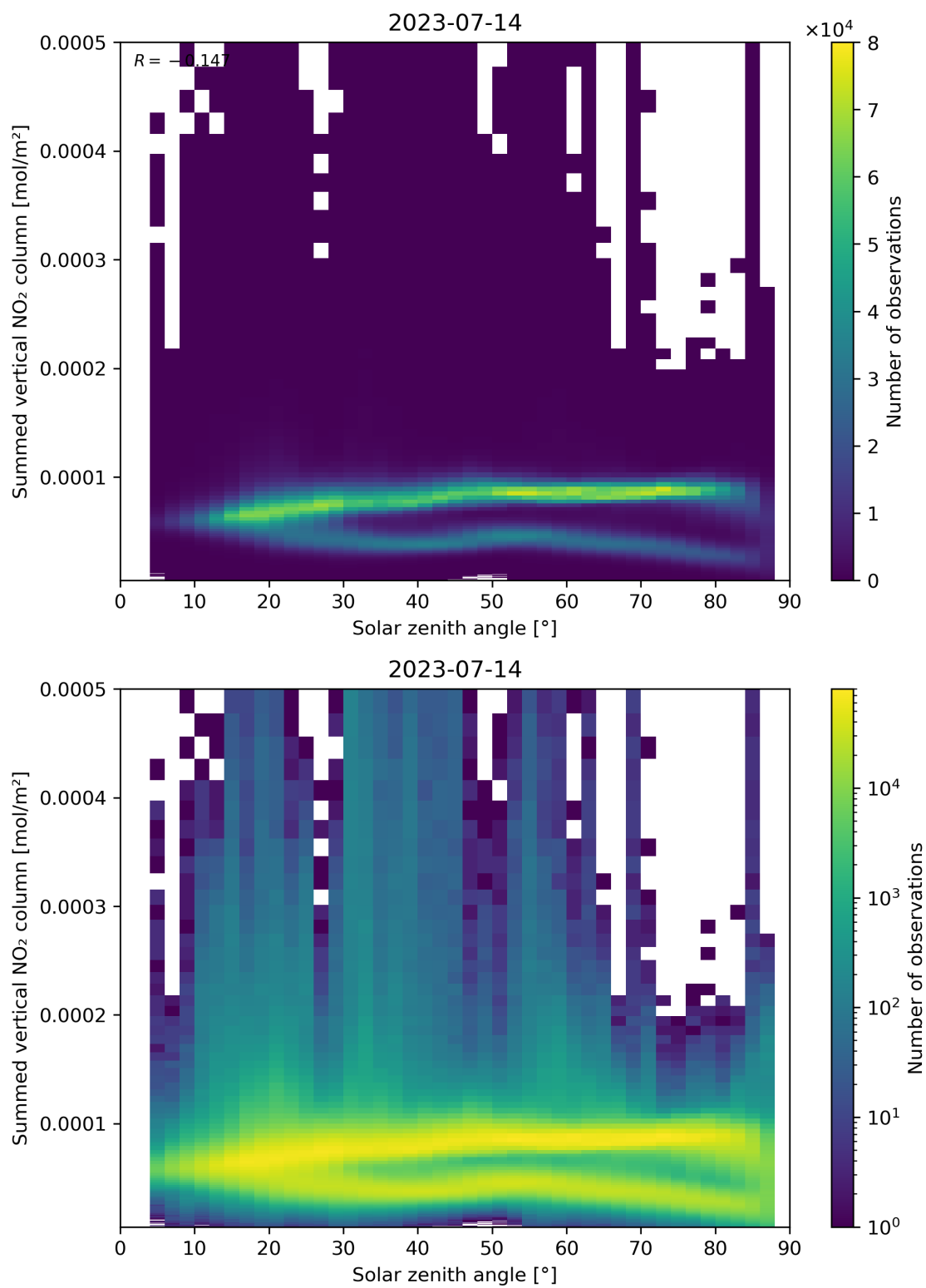
Figure 151: Scatter density plot of “Solar zenith angle” against “Summed vertical NO 2 column” for 2023-07-14 to 2023-07-15.
