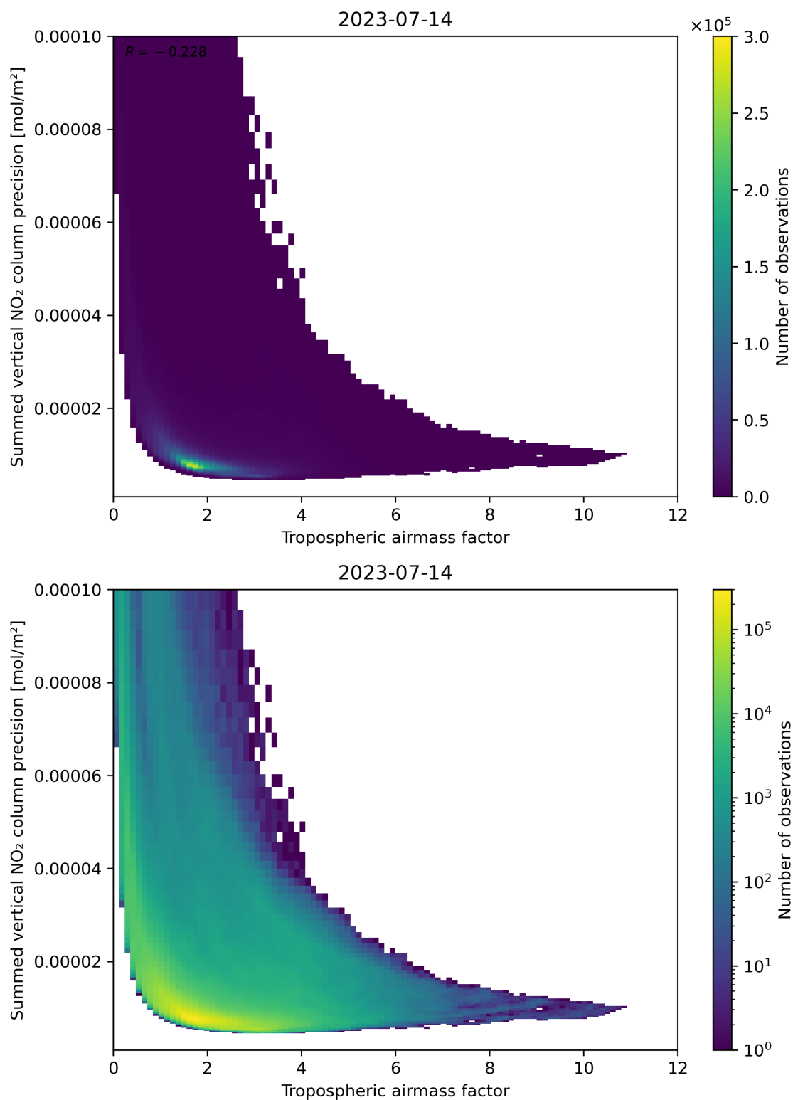
Figure 76: Scatter density plot of “Tropospheric air mass factor” against “Summed vertical NO 2 column precision” for 2023-07-14 to 2023-07-15.
