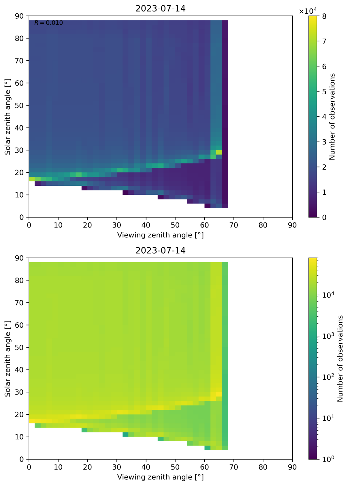
Figure 172: Scatter density plot of “Viewing zenith angle” against “Solar zenith angle” for 2023-07-14 to 2023-07-15.
