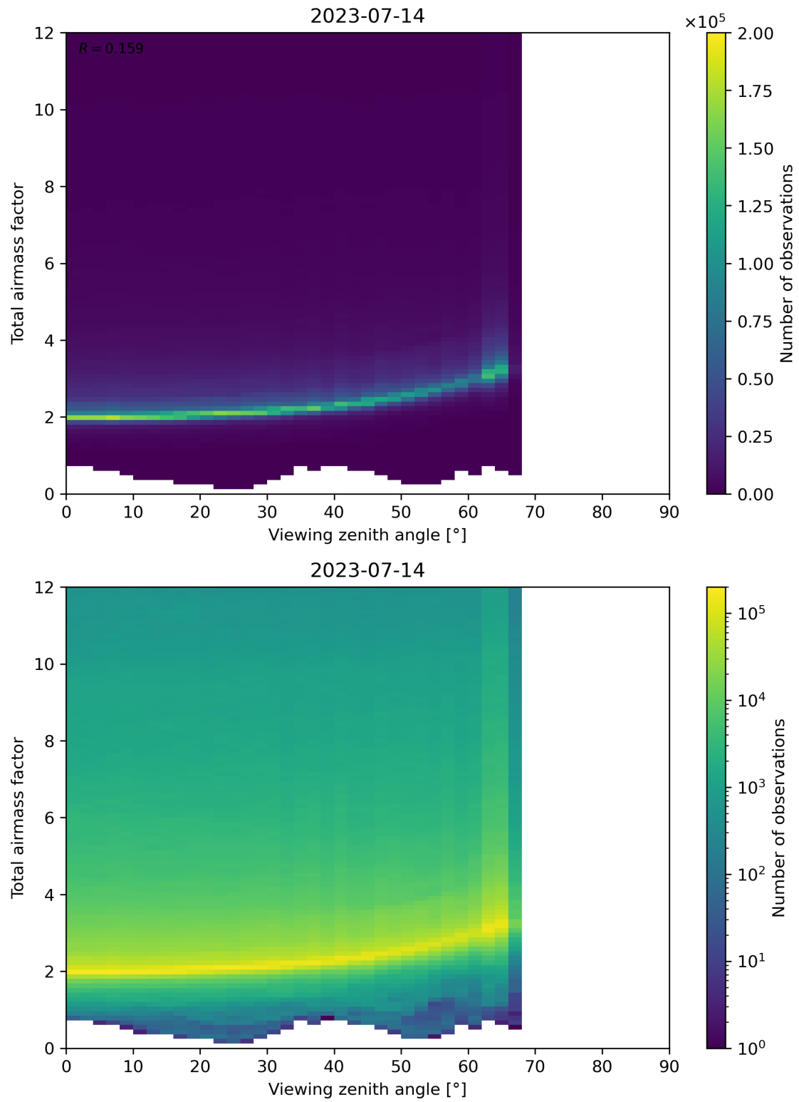
Figure 160: Scatter density plot of “Viewing zenith angle” against “Total airmass factor” for 2023-07-14 to 2023-07-15.
