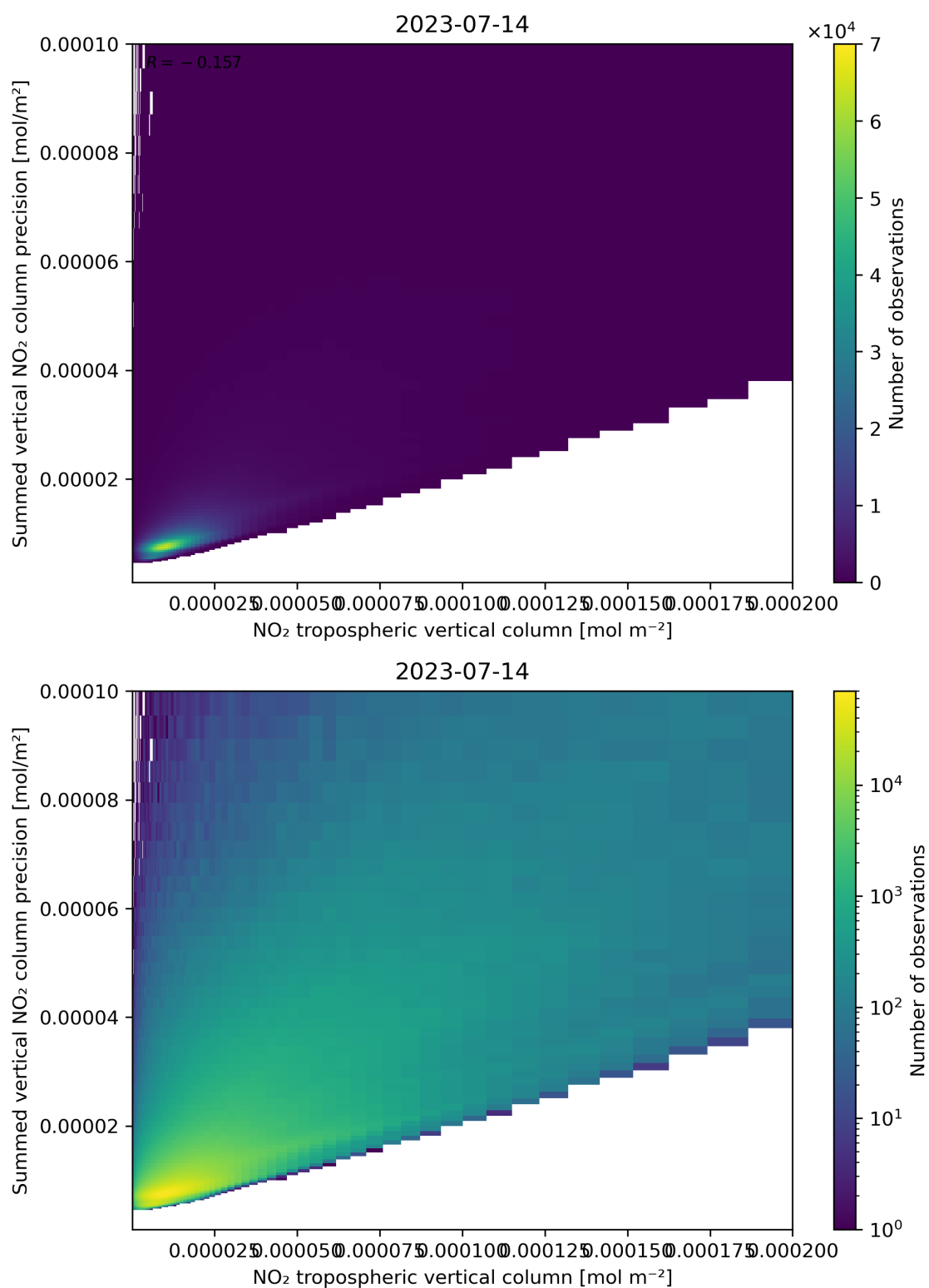
Figure 127: Scatter density plot of “NO 2 tropospheric vertical column” against “Summed vertical NO 2 column precision” for 2023-07-14 to 2023-07-15.
