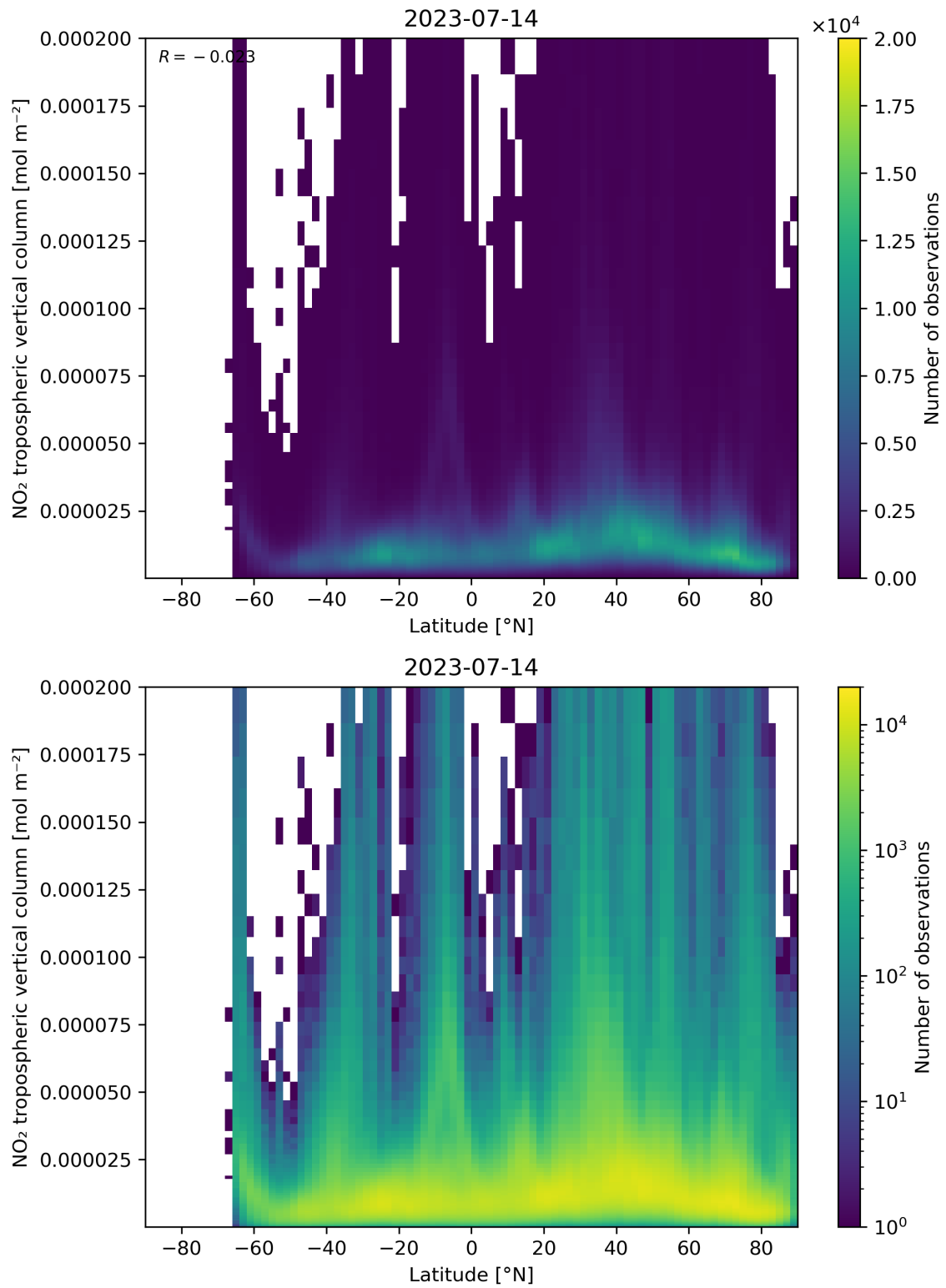
Figure 92: Scatter density plot of “Latitude” against “NO 2 tropospheric vertical column” for 2023-07-14 to 2023-07-15.
