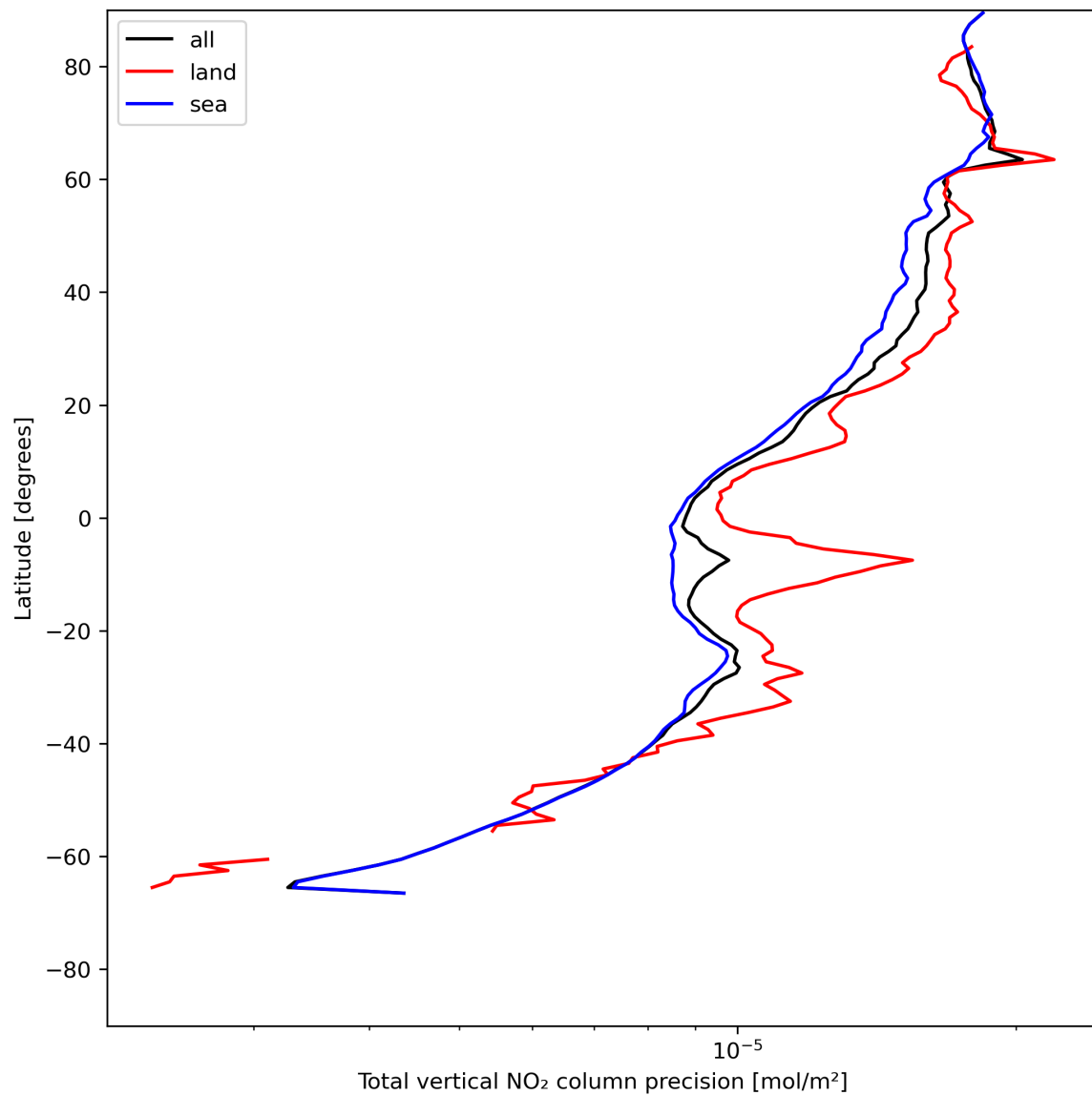
Figure 22: Zonal average of “Total vertical NO 2 column precision” for 2023-07-14 to 2023-07-15.
