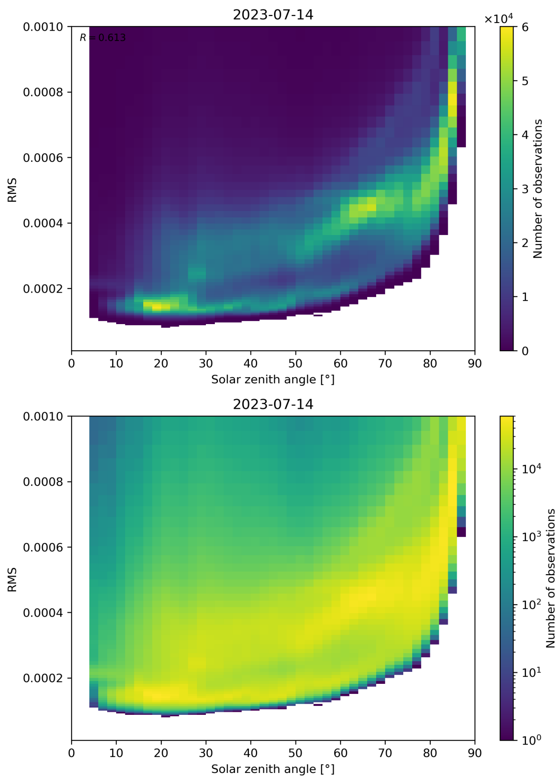
Figure 157: Scatter density plot of “Solar zenith angle” against “RMS” for 2023-07-14 to 2023-07-15.
