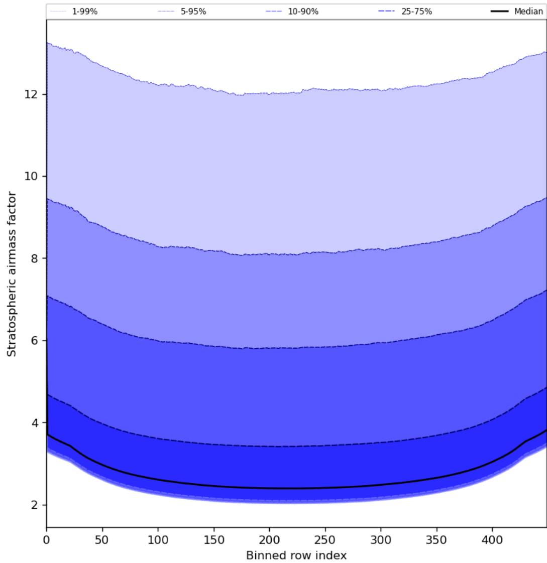
Figure 61: Along track statistics of “Stratospheric airmass factor” for 2023-07-14 to 2023-07-15
