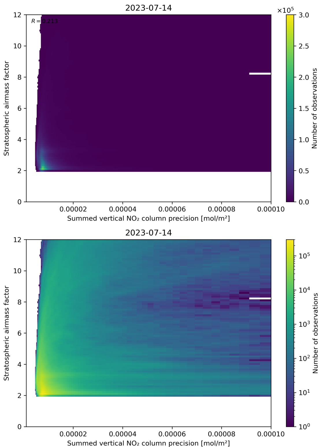
Figure 106: Scatter density plot of “Summed vertical NO 2 column precision” against “Stratospheric airmass factor” for 2023-07-14 to 2023-07-15.
