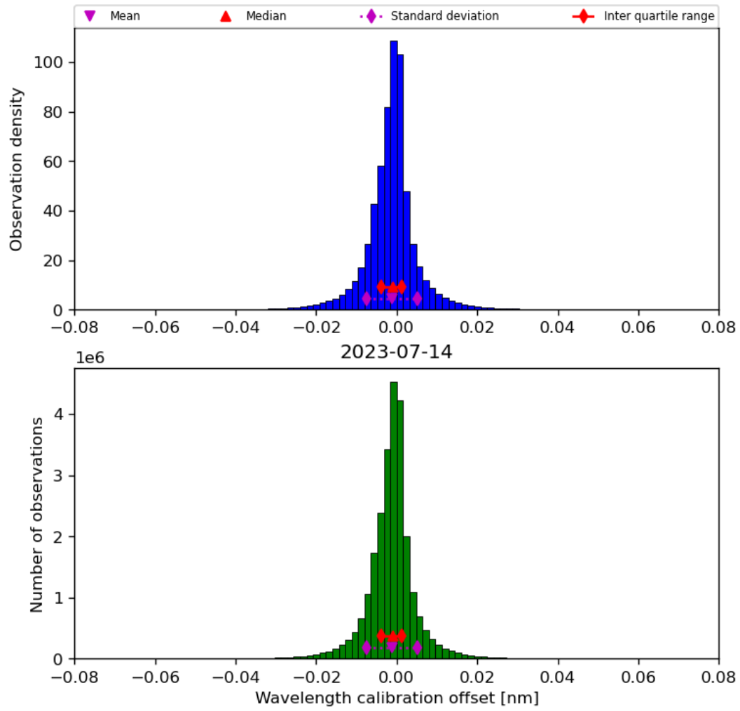
Figure 35: Histogram of “Wavelength calibration offset” for 2023-07-14 to 2023-07-15
