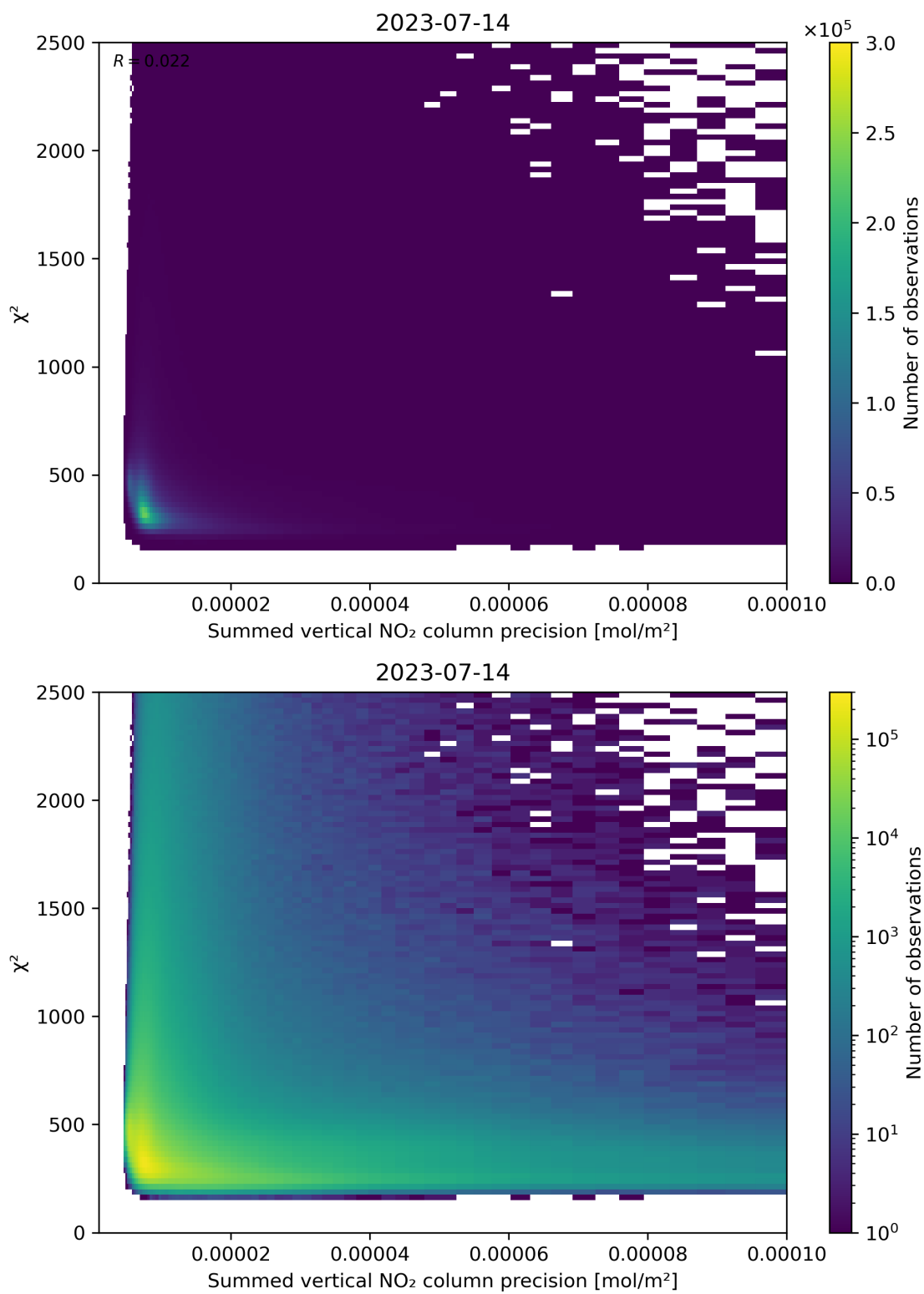
Figure 107: Scatter density plot of “Summed vertical NO 2 column precision” against “ \chi^2 ” for 2023-07-14 to 2023-07-15.
