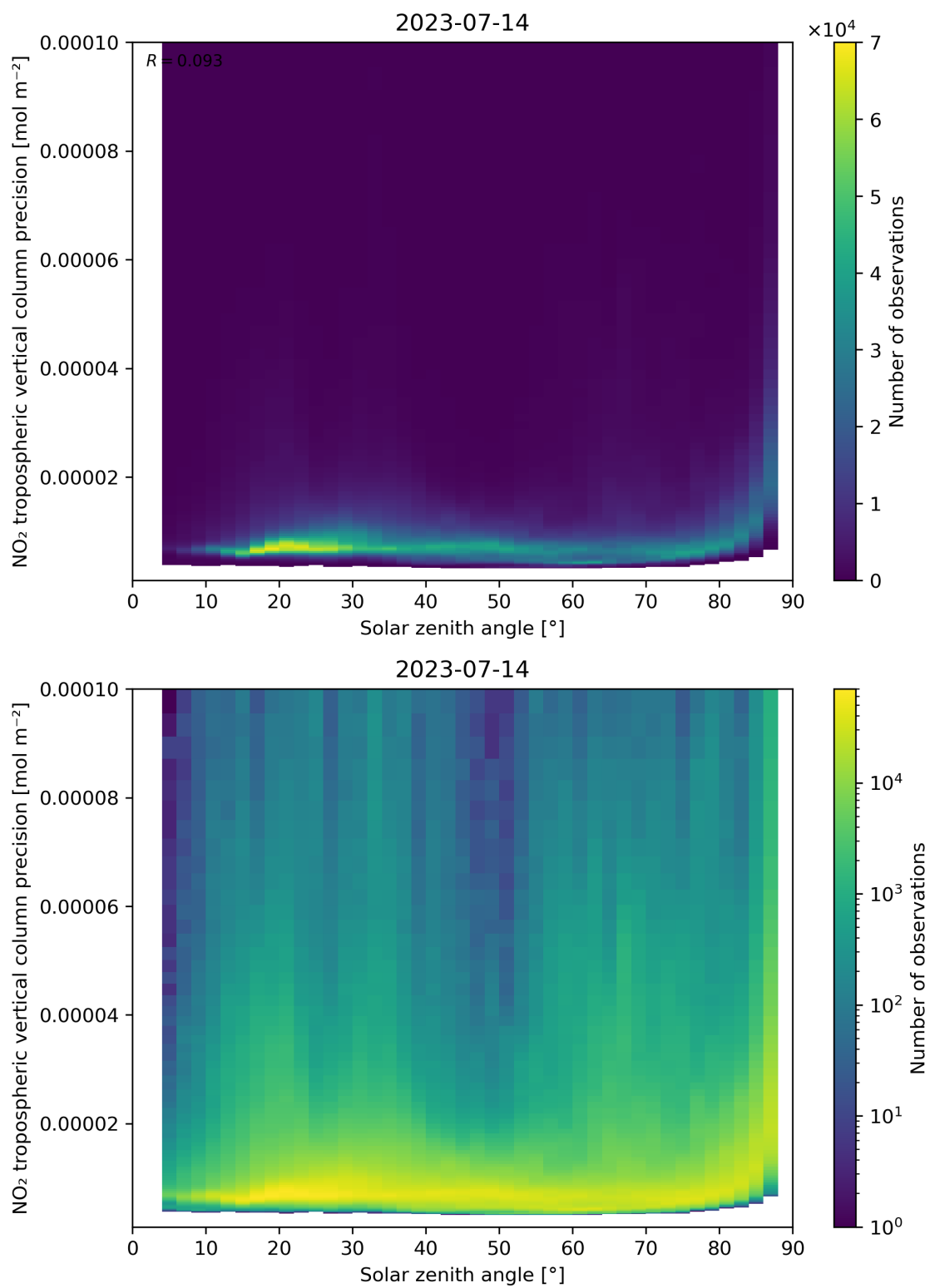
Figure 156: Scatter density plot of “Solar zenith angle” against “NO 2 tropospheric vertical column precision” for 2023-07-14 to 2023-07-15.
