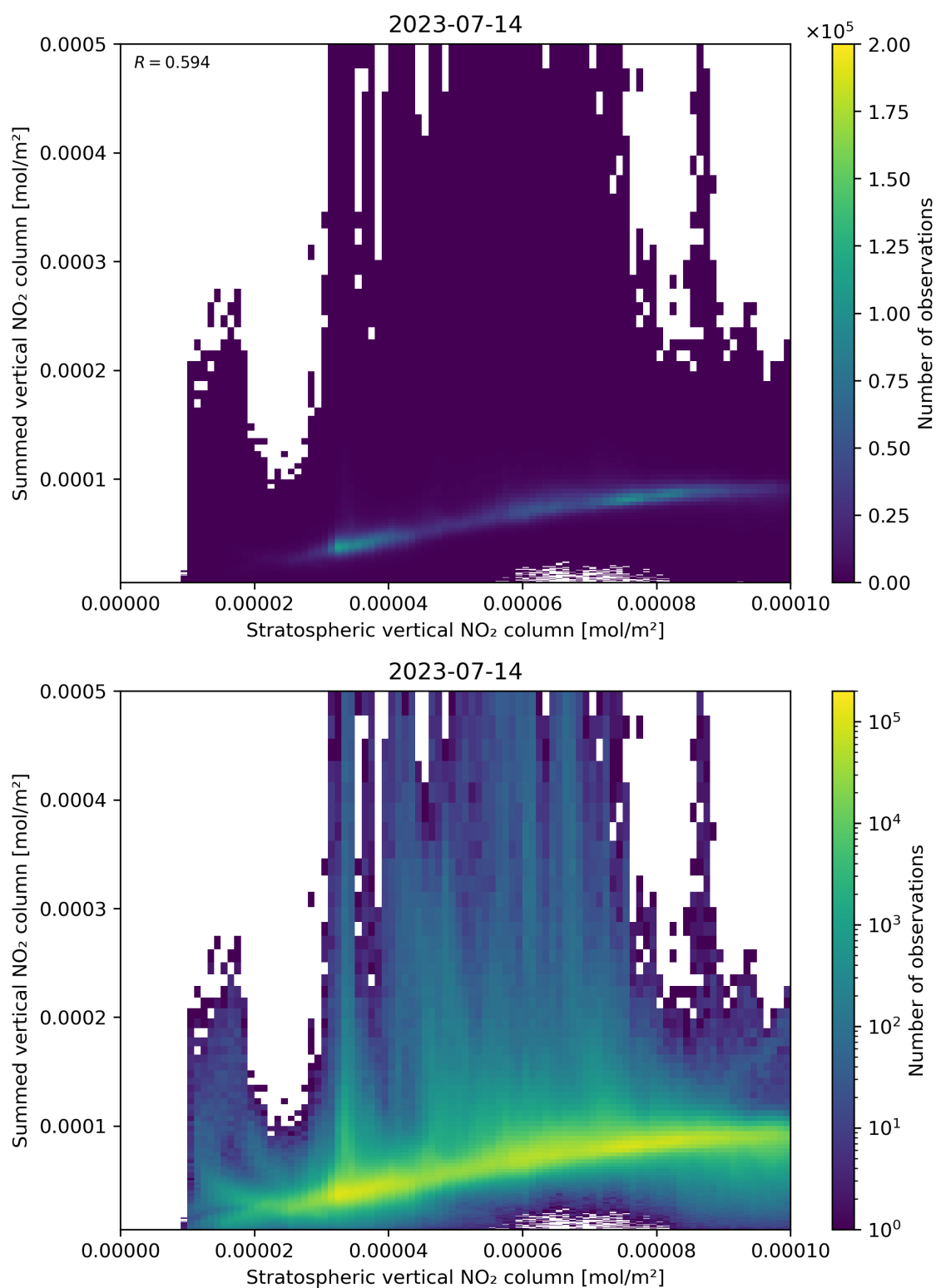
Figure 98: Scatter density plot of “Stratospheric vertical NO 2 column” against “Summed vertical NO 2 column” for 2023-07-14 to 2023-07-15.
