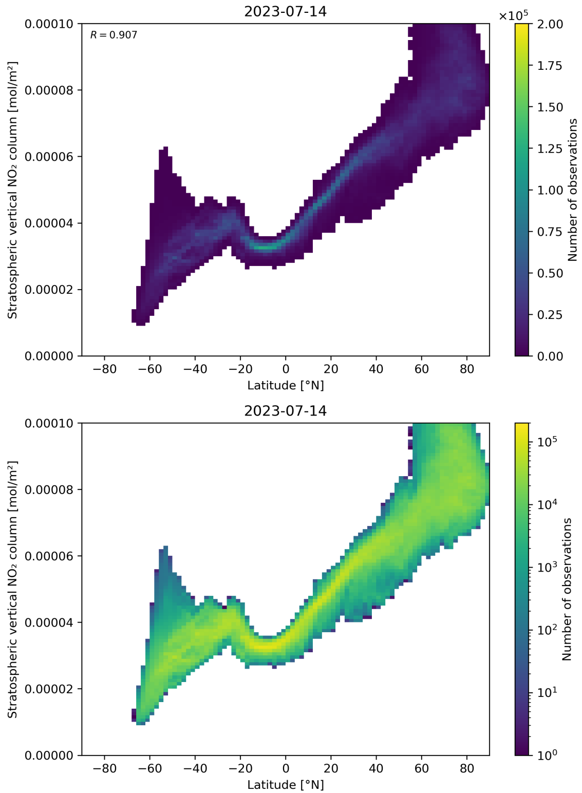
Figure 87: Scatter density plot of “Latitude” against “Stratospheric vertical NO 2 column” for 2023-07-14 to 2023-07-15.
