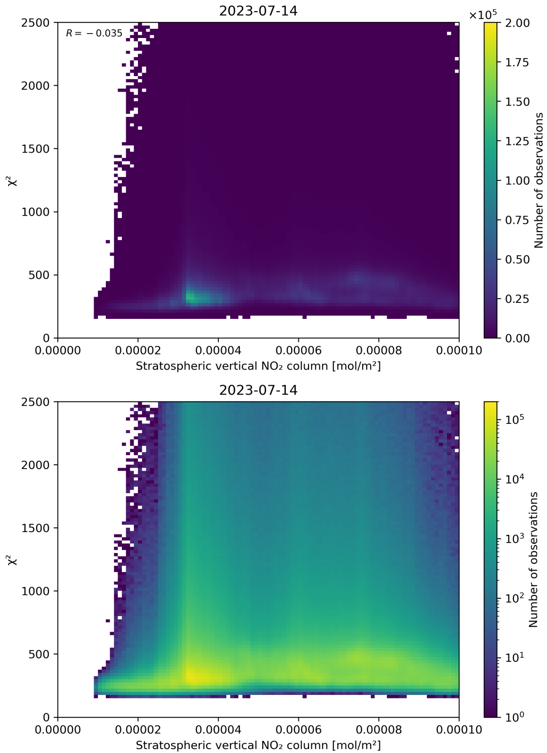
Figure 97: Scatter density plot of “Stratospheric vertical NO 2 column” against “ \chi^2 ” for 2023-07-14 to 2023-07-15.
