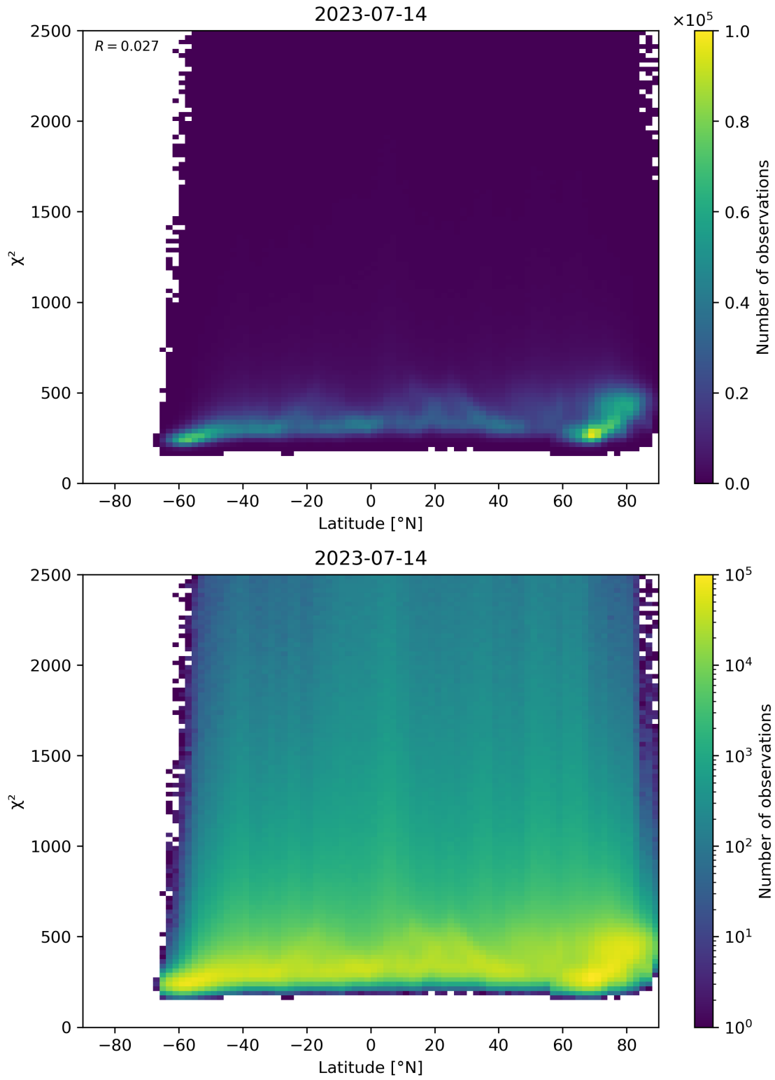
Figure 86: Scatter density plot of “Latitude” against “ \chi^2 ” for 2023-07-14 to 2023-07-15.
