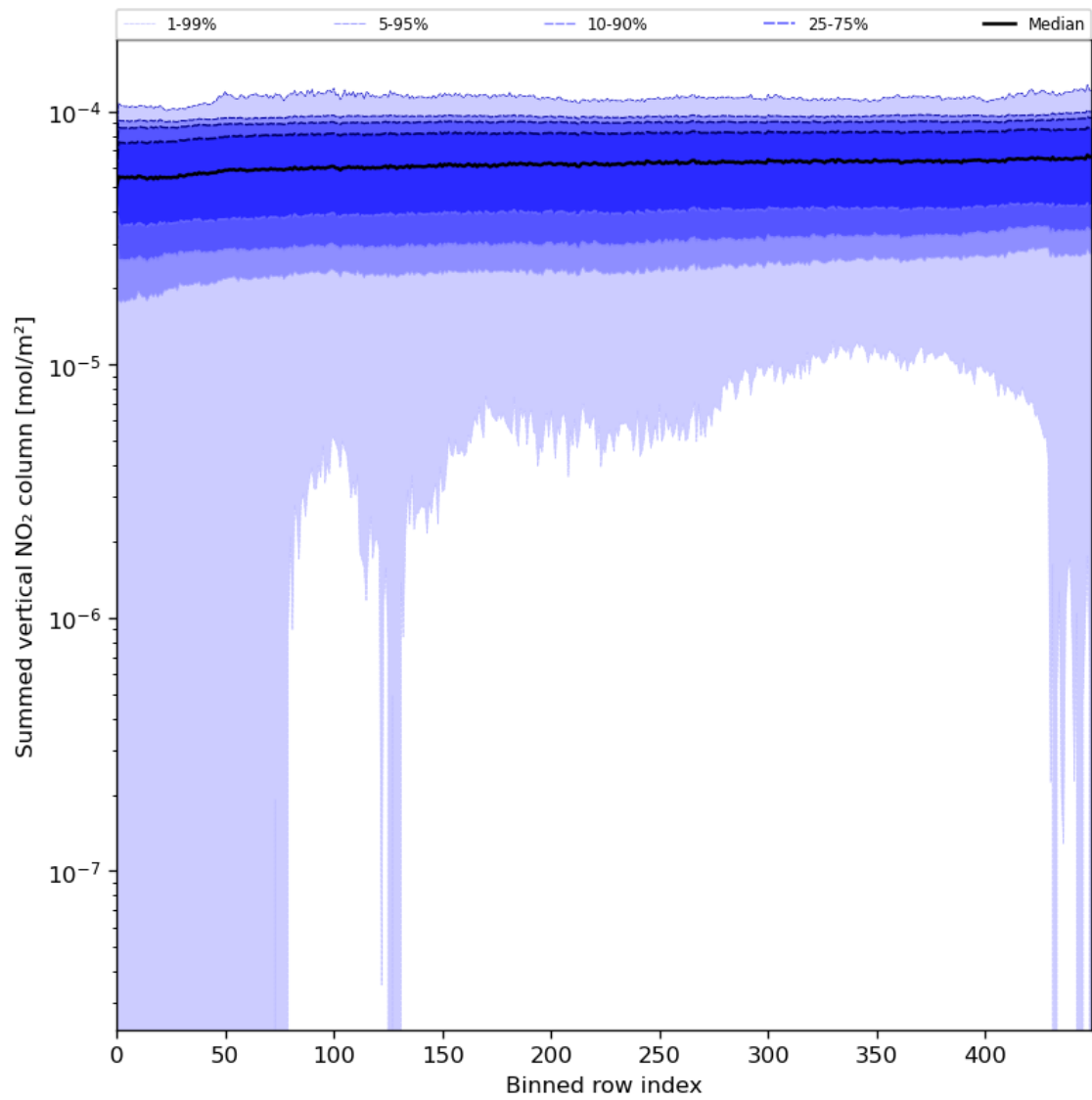
Figure 57: Along track statistics of “Summed vertical NO 2 column” for 2023-07-14 to 2023-07-15
