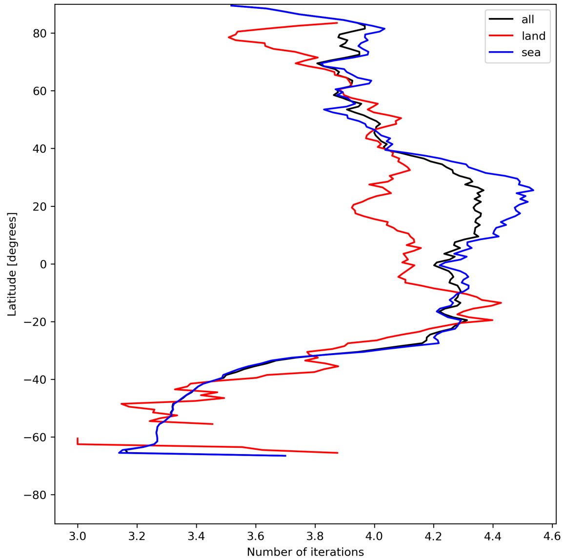
Figure 17: Zonal average of “Number of iterations” for 2023-07-14 to 2023-07-15.
