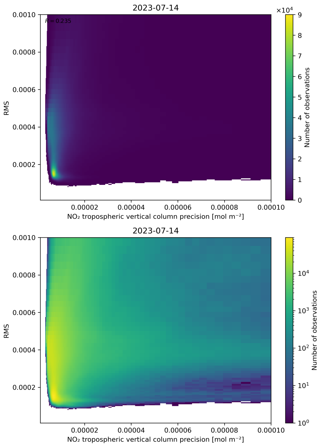
Figure 140: Scatter density plot of “NO 2 tropospheric vertical column precision” against “RMS” for 2023-07-14 to 2023-07-15.
