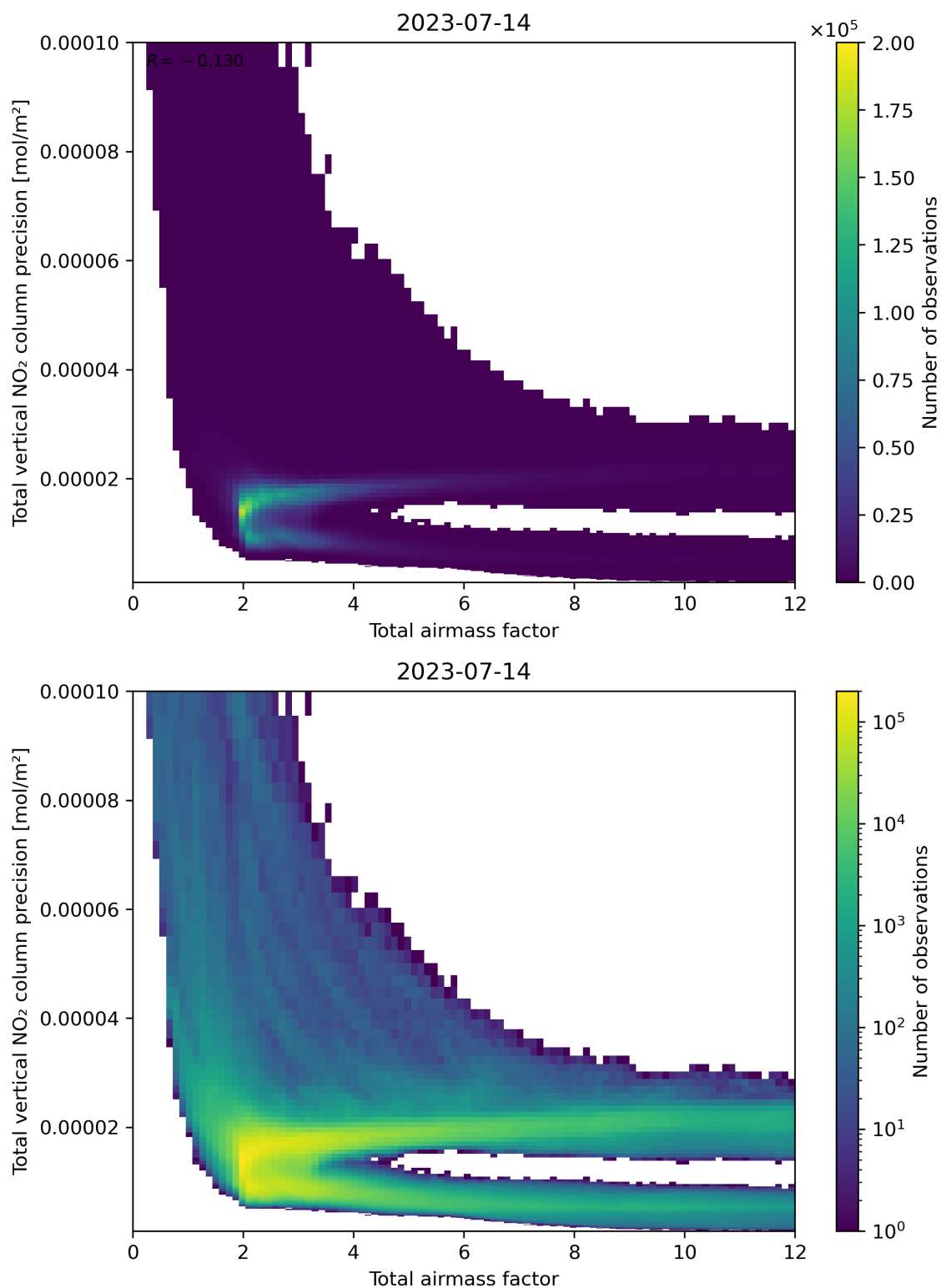
Figure 68: Scatter density plot of “Total airmass factor” against “Total vertical NO 2 column precision” for 2023-07-14 to 2023-07-15.
