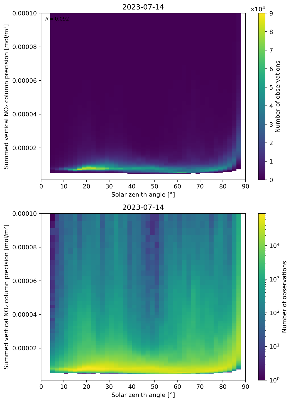
Figure 152: Scatter density plot of “Solar zenith angle” against “Summed vertical NO 2 column precision” for 2023-07-14 to 2023-07-15.
