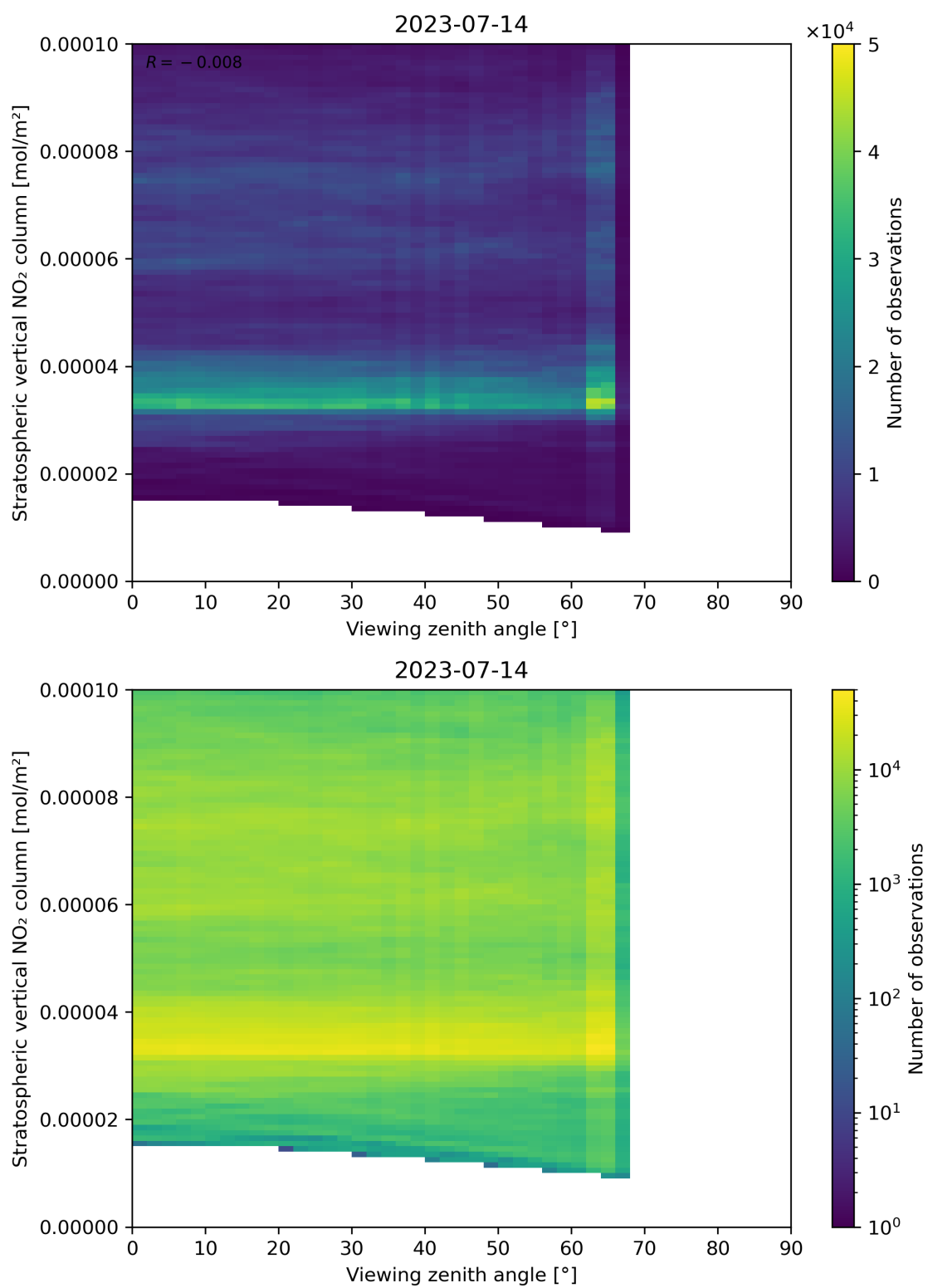
Figure 164: Scatter density plot of “Viewing zenith angle” against “Stratospheric vertical NO 2 column” for 2023-07-14 to 2023-07-15.
