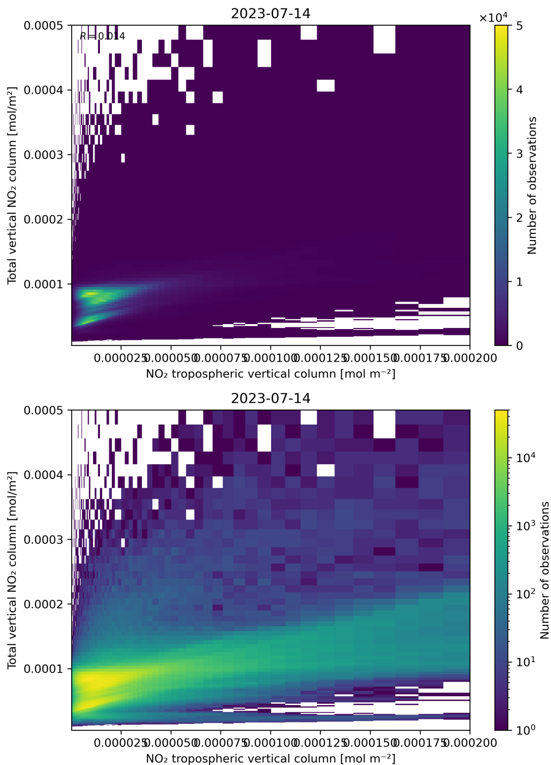
Figure 128: Scatter density plot of “NO 2 tropospheric vertical column” against “Total vertical NO 2 column” for 2023-07-14 to 2023-07-15.
