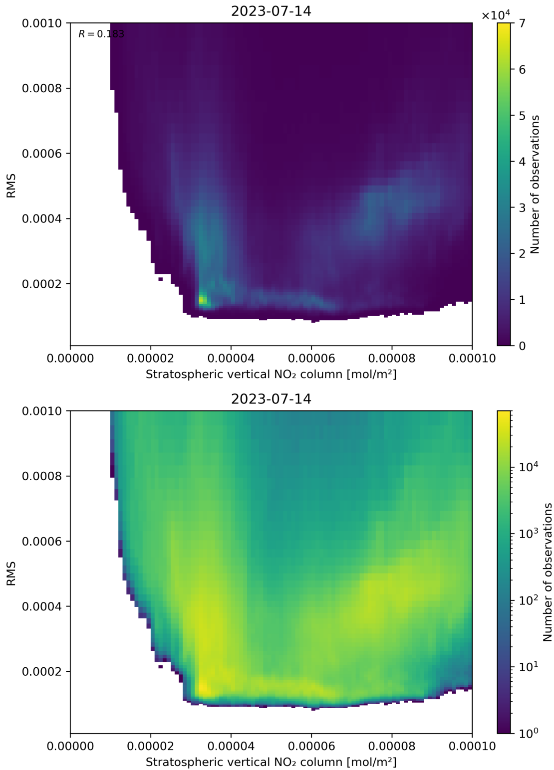
Figure 102: Scatter density plot of “Stratospheric vertical NO 2 column” against “RMS” for 2023-07-14 to 2023-07-15.
