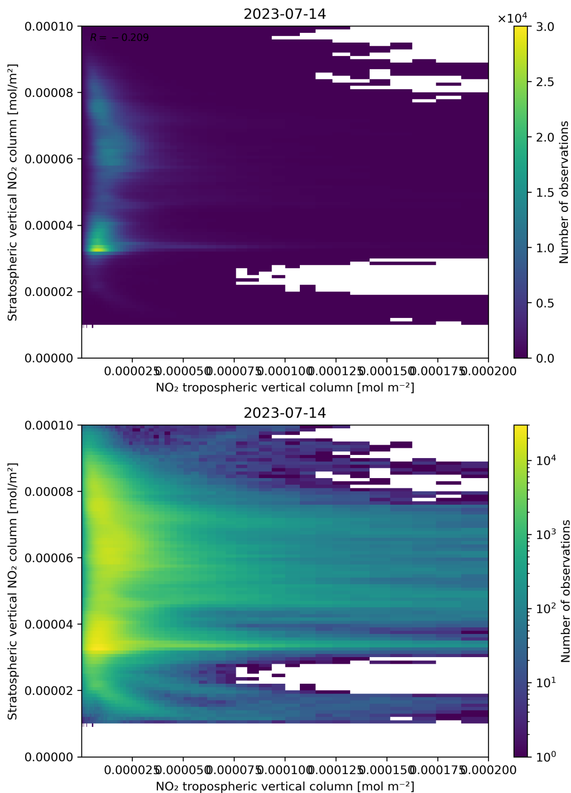
Figure 125: Scatter density plot of “NO 2 tropospheric vertical column” against “Stratospheric vertical NO 2 column” for 2023-07-14 to 2023-07-15.
