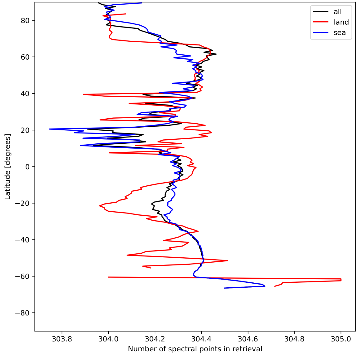
Figure 16: Zonal average of “Number of spectral points in retrieval” for 2023-07-14 to 2023-07-15.
