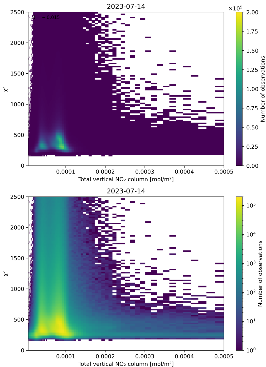
Figure 111: Scatter density plot of “Total vertical NO 2 column” against “ \chi^2 ” for 2023-07-14 to 2023-07-15.
