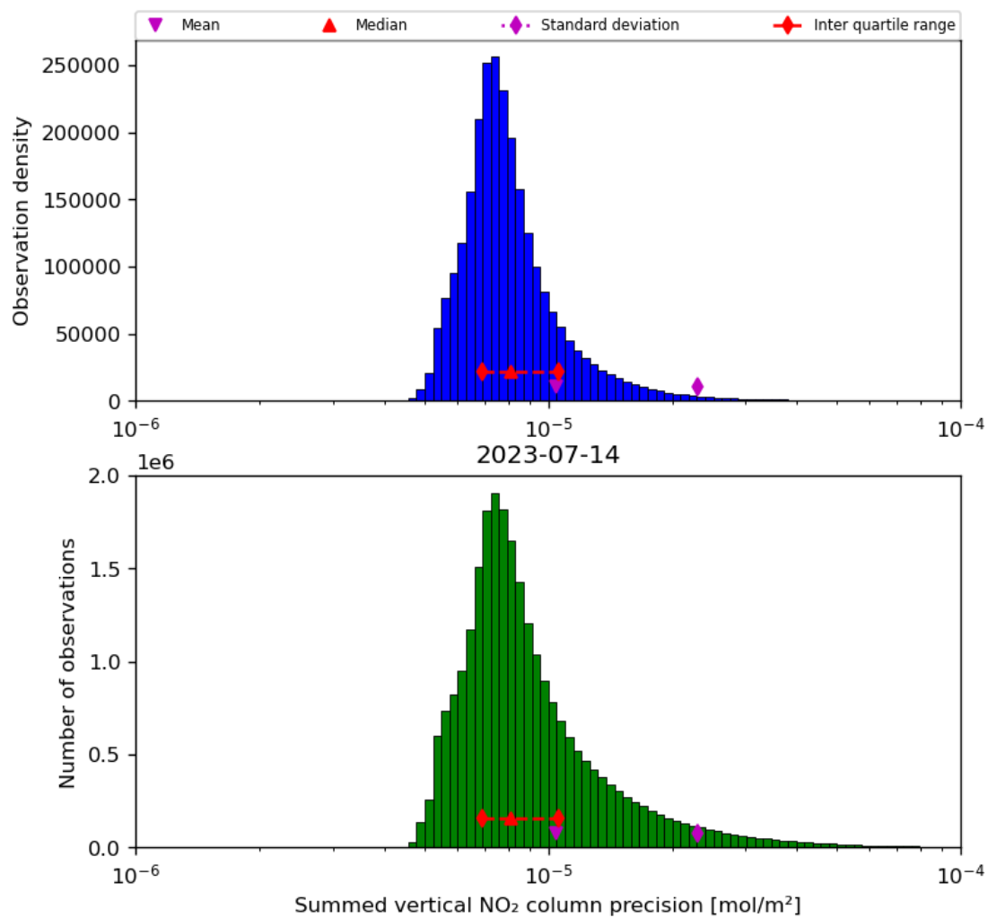
Figure 41: Histogram of "Summed vertical NO 2 column precision" for 2023-07-14 to 2023-07-15
