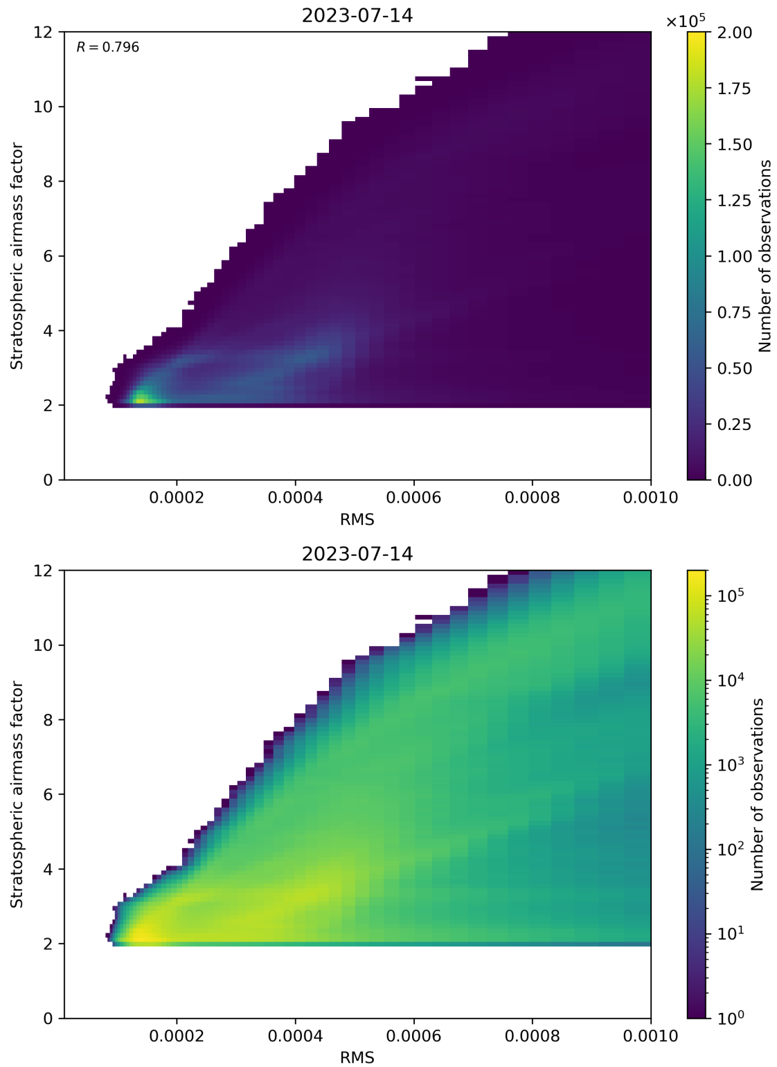
Figure 144: Scatter density plot of “RMS” against “Stratospheric airmass factor” for 2023-07-14 to 2023-07-15.
