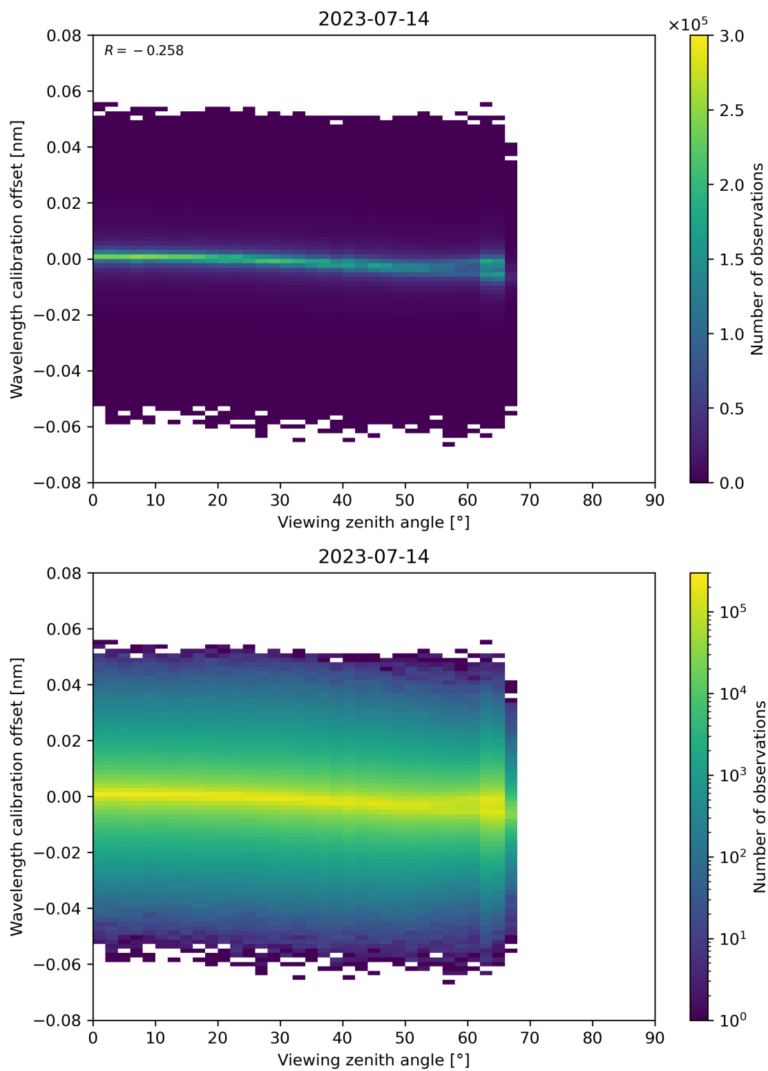
Figure 173: Scatter density plot of “Viewing zenith angle” against “Wavelength calibration offset” for 2023-07-14 to 2023-07-15.
