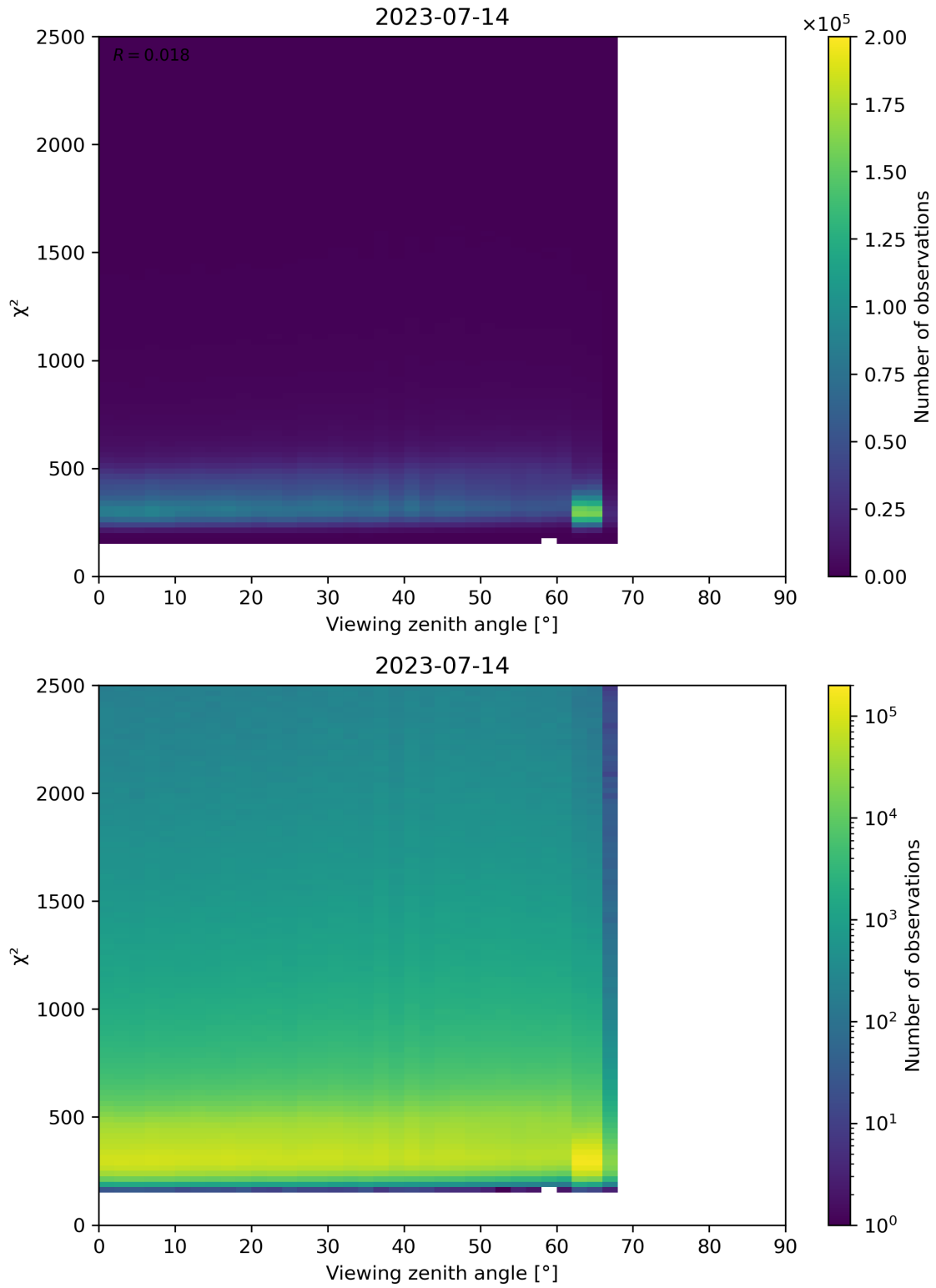
Figure 162: Scatter density plot of “Viewing zenith angle” against “ \chi^2 ” for 2023-07-14 to 2023-07-15.
