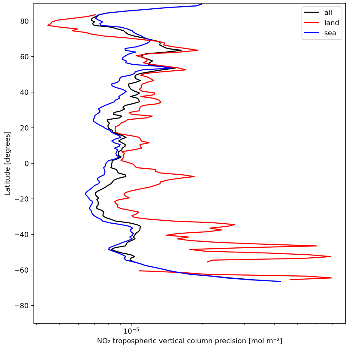
Figure 13: Zonal average of “NO 2 tropospheric vertical column precision” for 2023-07-14 to 2023-07-15.
