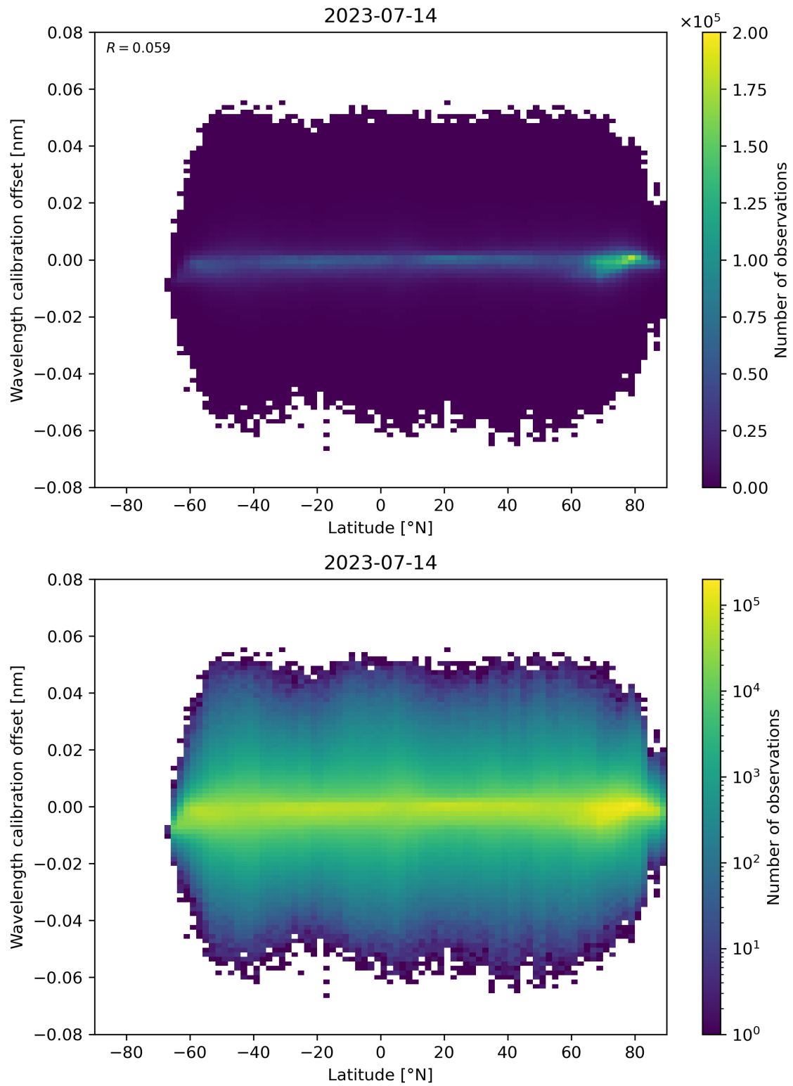
Figure 95: Scatter density plot of “Latitude” against “Wavelength calibration offset” for 2023-07-14 to 2023-07-15.
