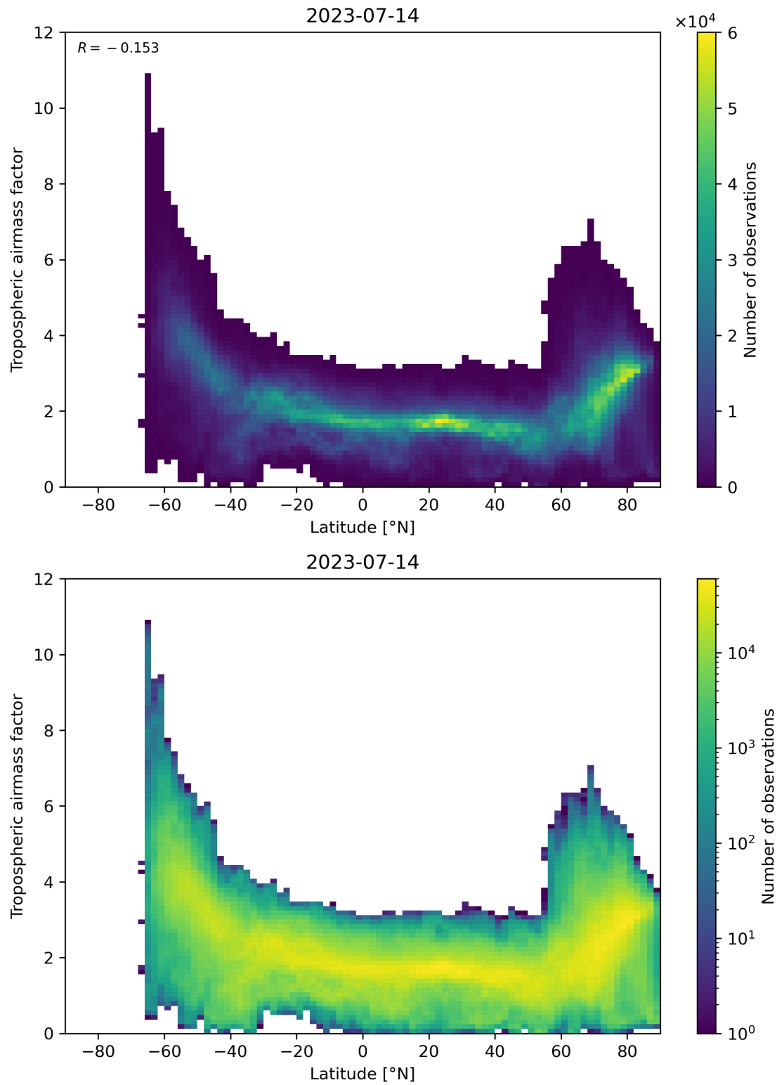
Figure 85: Scatter density plot of “Latitude” against “Tropospheric air mass factor” for 2023-07-14 to 2023-07-15.
