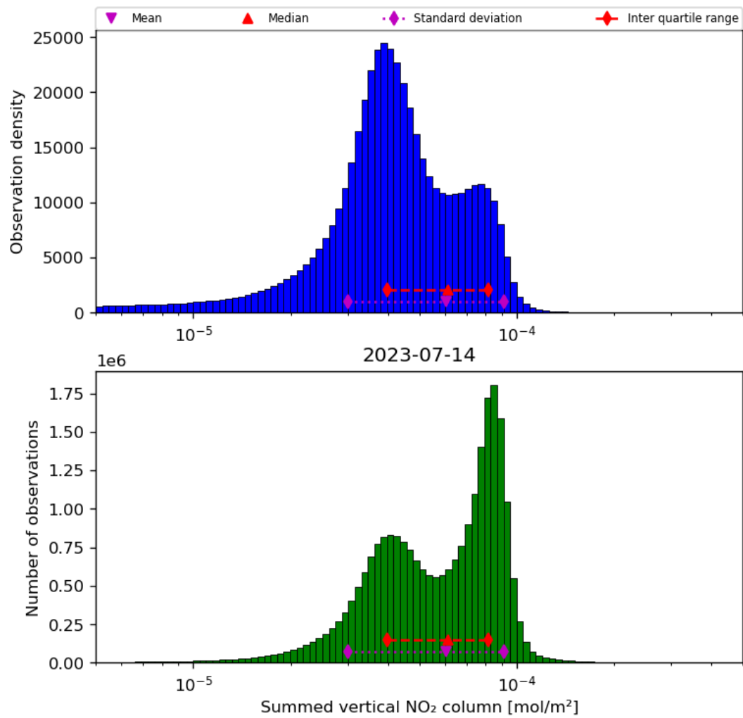
Figure 40: Histogram of “Summed vertical NO 2 column” for 2023-07-14 to 2023-07-15
