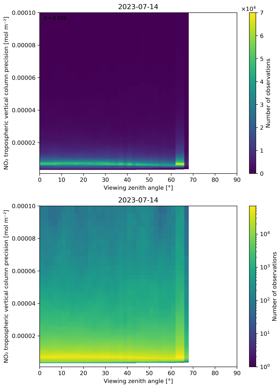
Figure 170: Scatter density plot of “Viewing zenith angle” against “NO 2 tropospheric vertical column precision” for 2023-07-14 to 2023-07-15.
