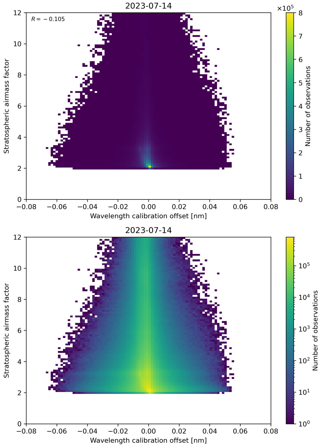
Figure 174: Scatter density plot of “Wavelength calibration offset” against “Stratospheric airmass factor” for 2023-07-14 to 2023-07-15.
