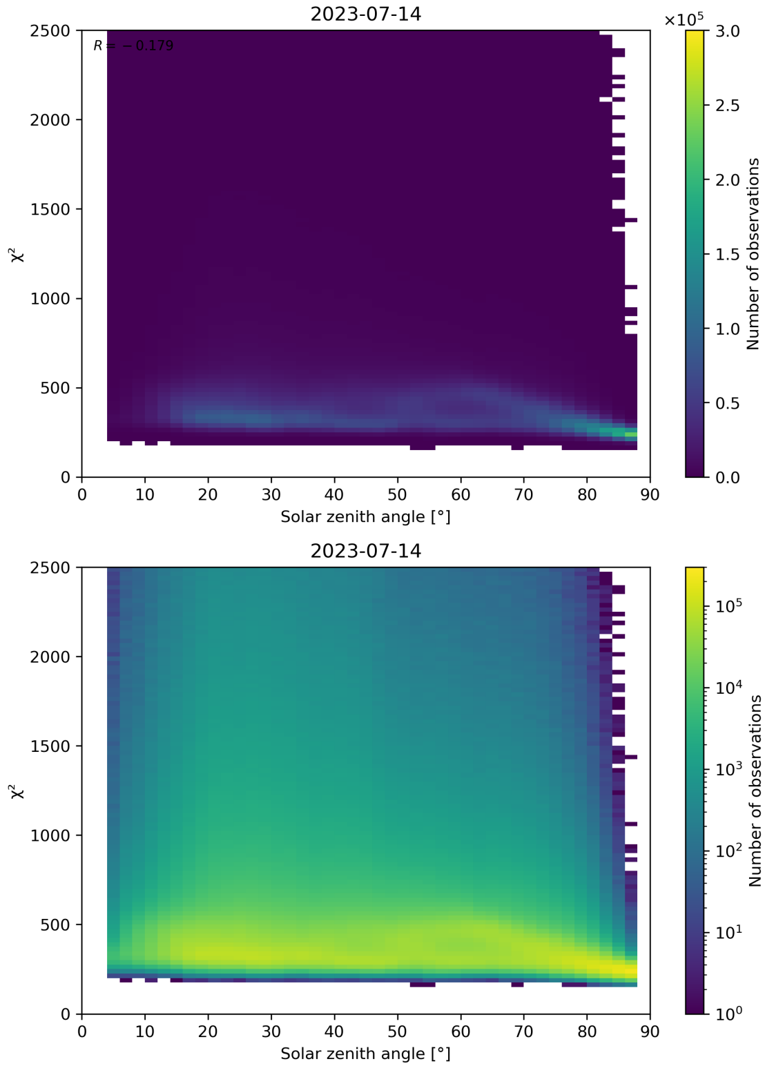
Figure 148: Scatter density plot of “Solar zenith angle” against “ \chi^2 ” for 2023-07-14 to 2023-07-15.
