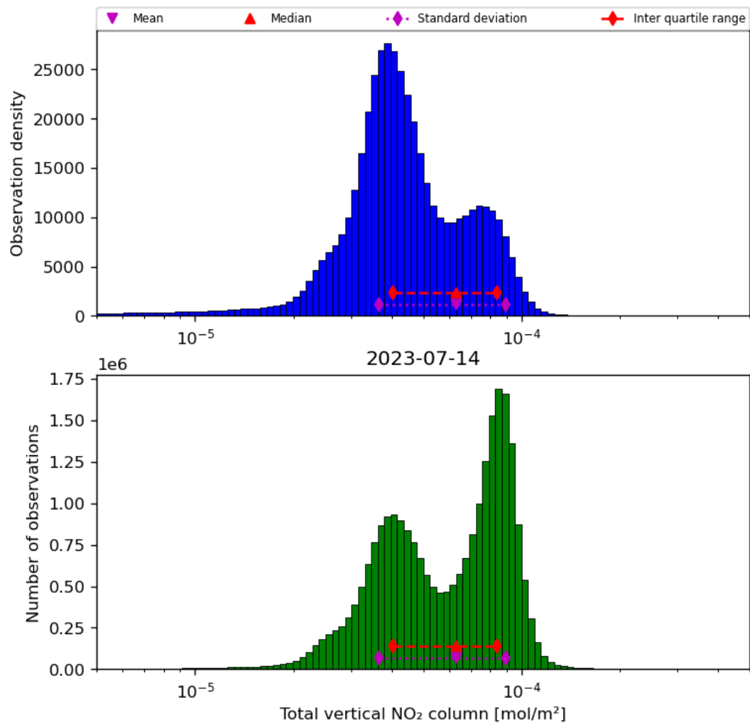
Figure 38: Histogram of “Total vertical NO 2 column” for 2023-07-14 to 2023-07-15
