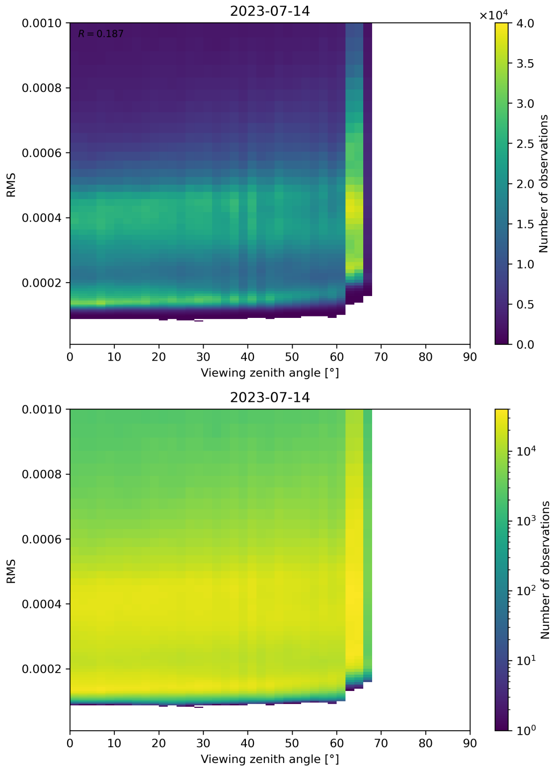
Figure 171: Scatter density plot of “Viewing zenith angle” against “RMS” for 2023-07-14 to 2023-07-15.
