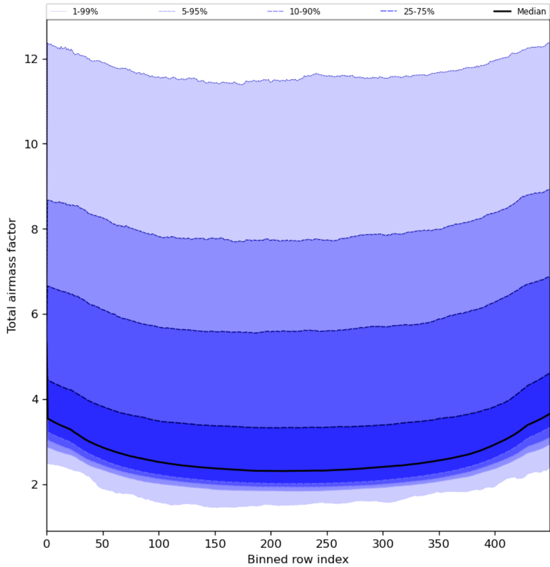
Figure 49: Along track statistics of “Total airmass factor” for 2023-07-14 to 2023-07-15
