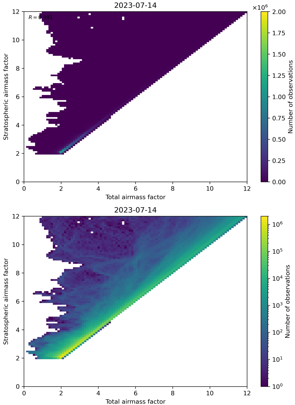
Figure 62: Scatter density plot of “Total airmass factor” against “Stratospheric airmass factor” for 2023-07-14 to 2023-07-15.
