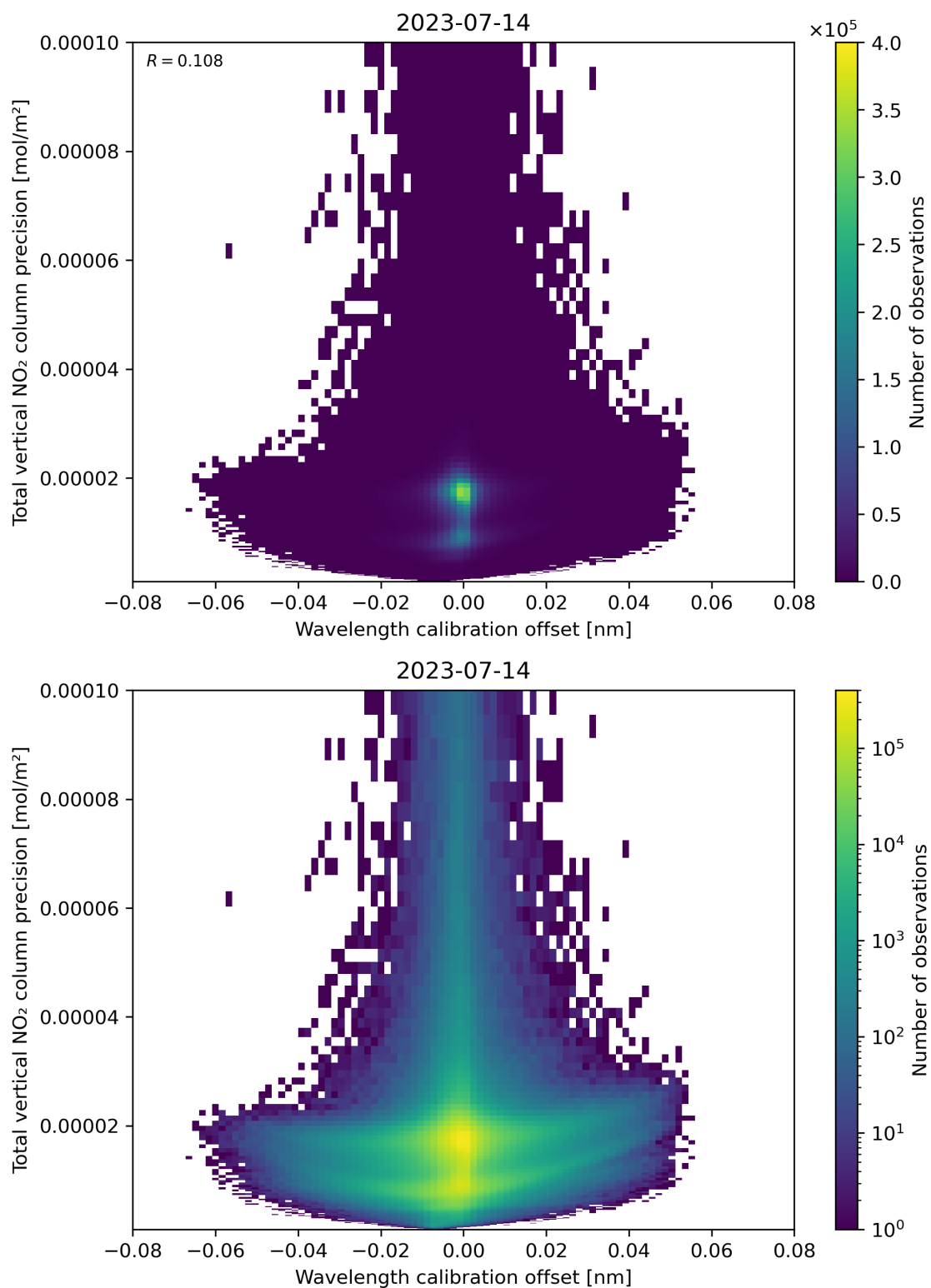
Figure 180: Scatter density plot of “Wavelength calibration offset” against “Total vertical NO 2 column precision” for 2023-07-14 to 2023-07-15.
