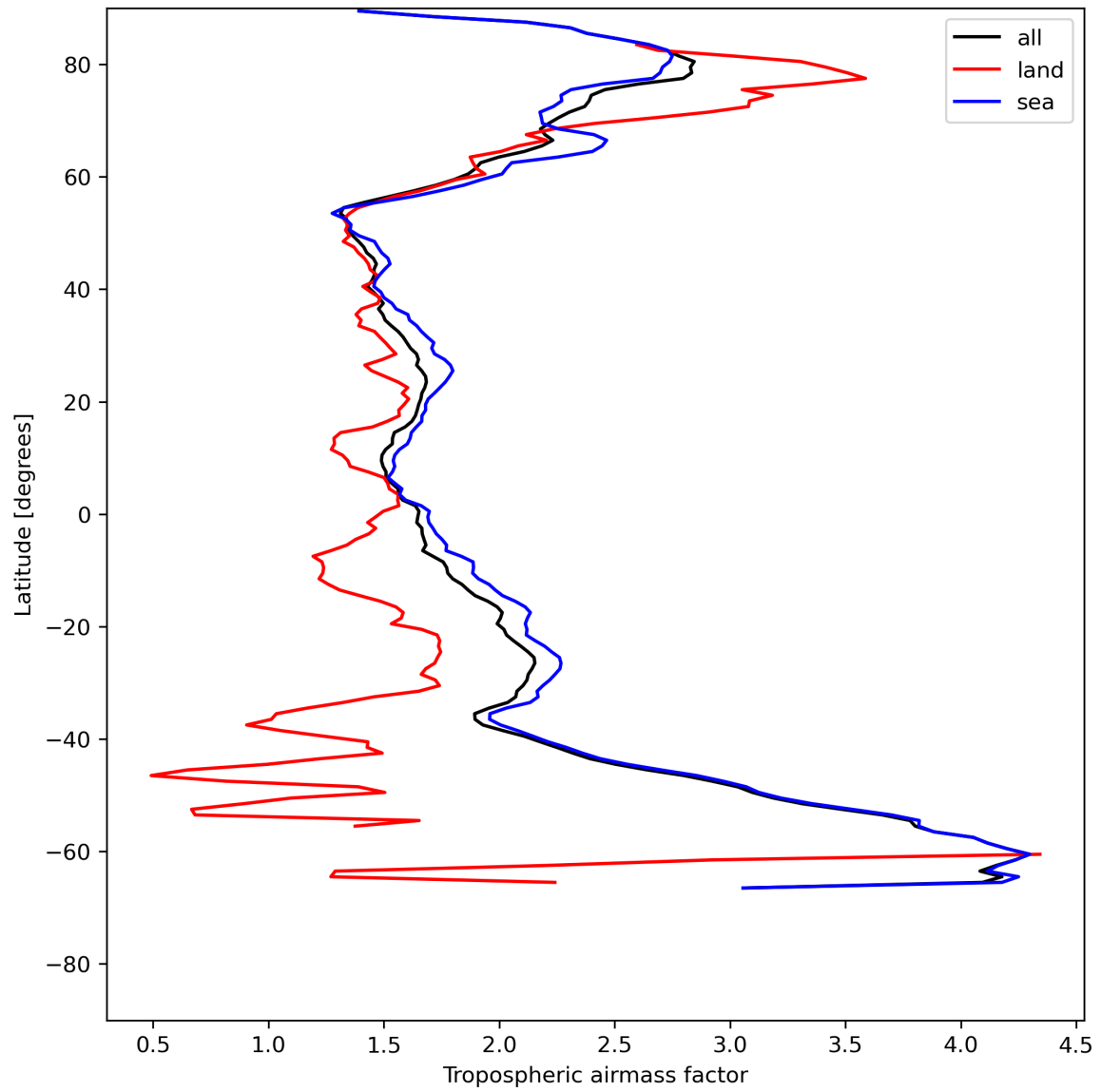
Figure 14: Zonal average of “Tropospheric airmass factor” for 2023-07-14 to 2023-07-15.
