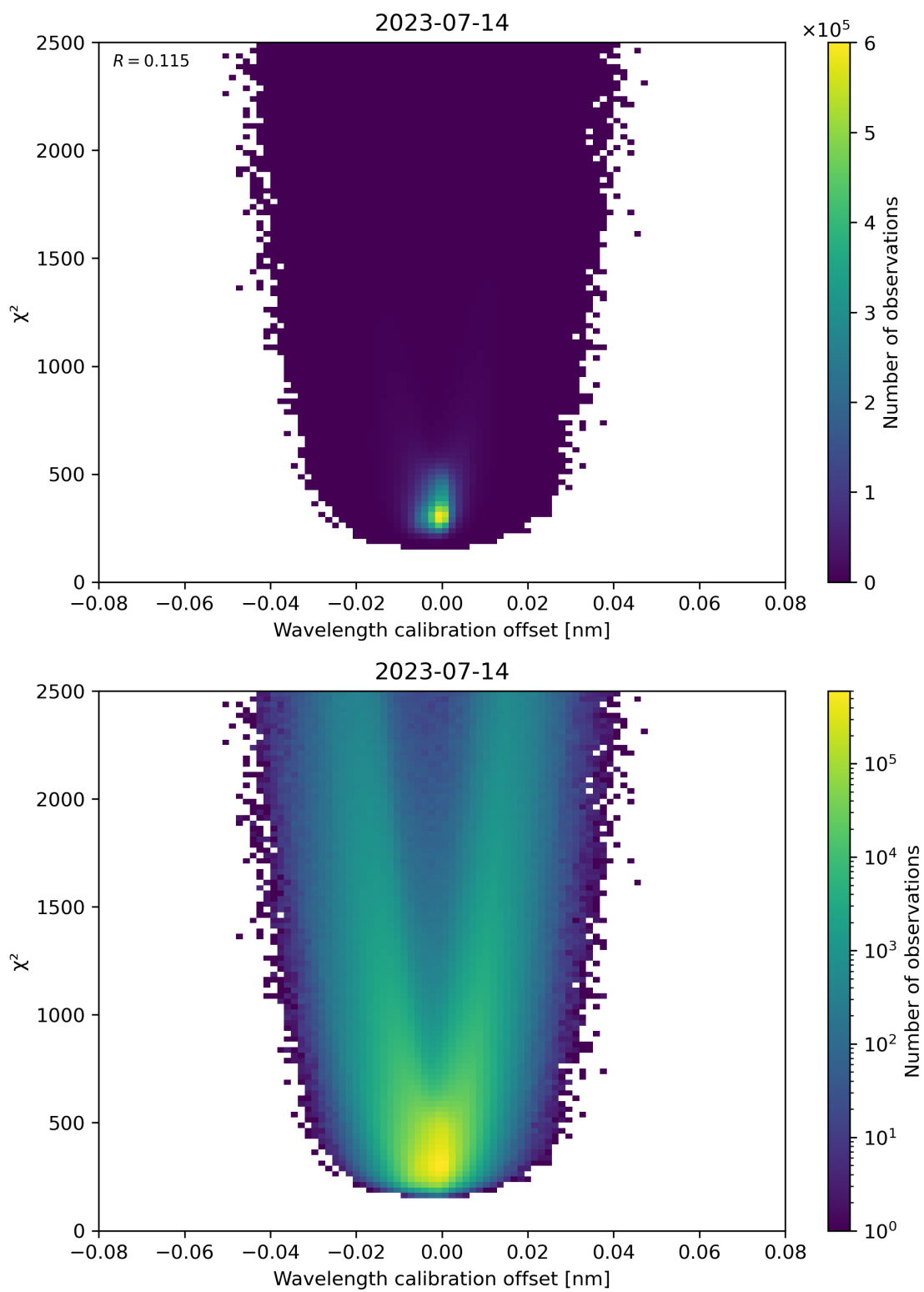
Figure 175: Scatter density plot of “Wavelength calibration offset” against “ \chi^2 ” for 2023-07-14 to 2023-07-15.
