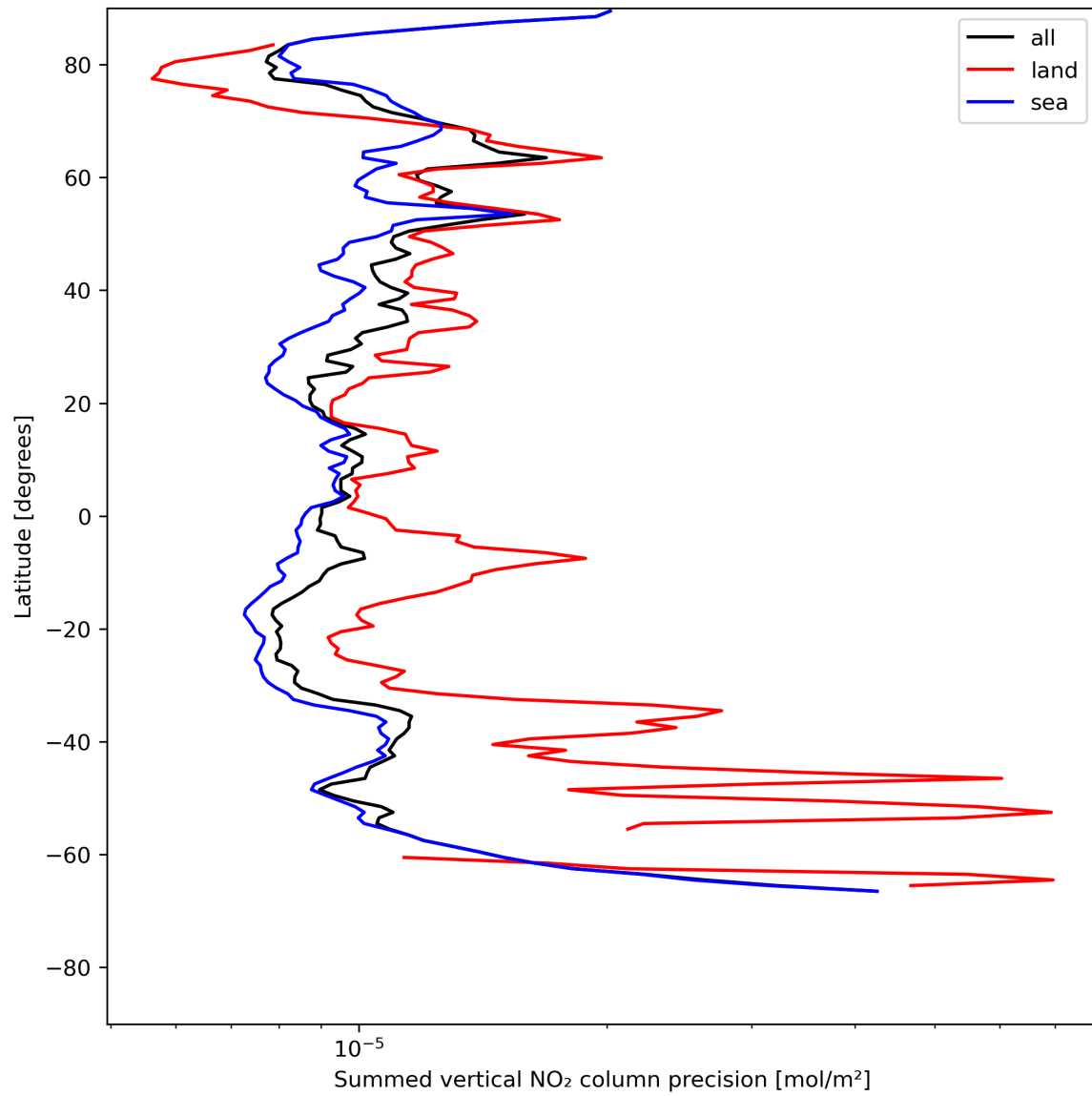
Figure 24: Zonal average of “Summed vertical NO 2 column precision” for 2023-07-14 to 2023-07-15.
