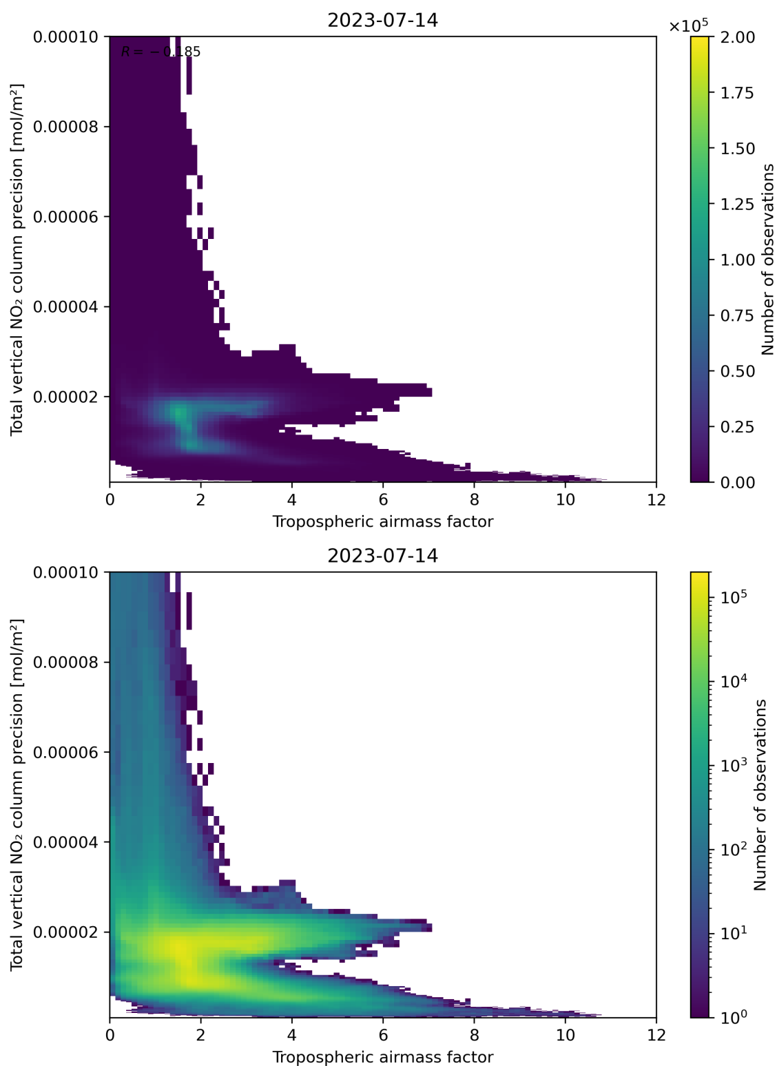
Figure 78: Scatter density plot of “Tropospheric air mass factor” against “Total vertical NO 2 column precision” for 2023-07-14 to 2023-07-15.
