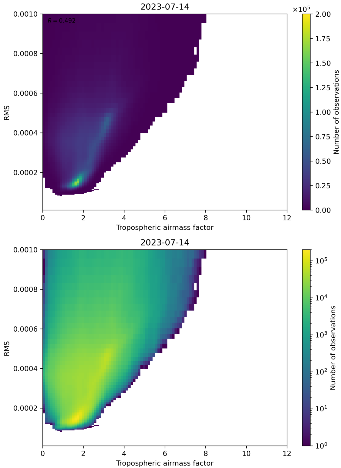
Figure 79: Scatter density plot of “Tropospheric airmass factor” against “RMS” for 2023-07-14 to 2023-07-15.
