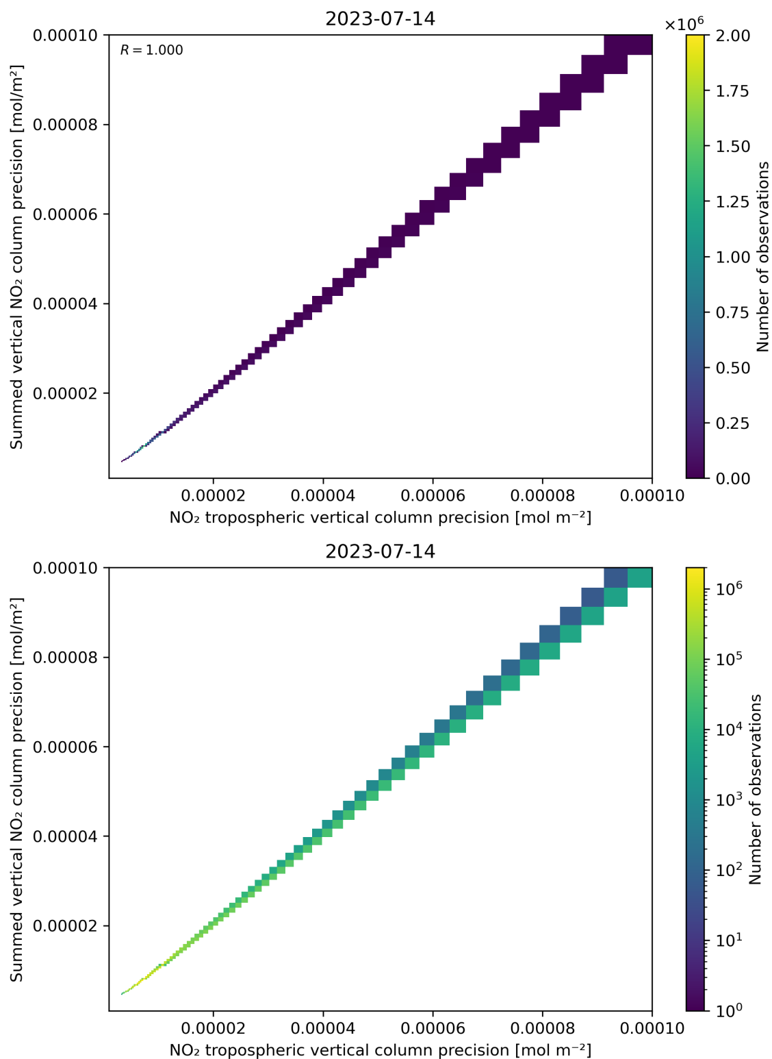
Figure 137: Scatter density plot of “NO 2 tropospheric vertical column precision” against “Summed vertical NO 2 column precision” for 2023-07-14 to 2023-07-15.
