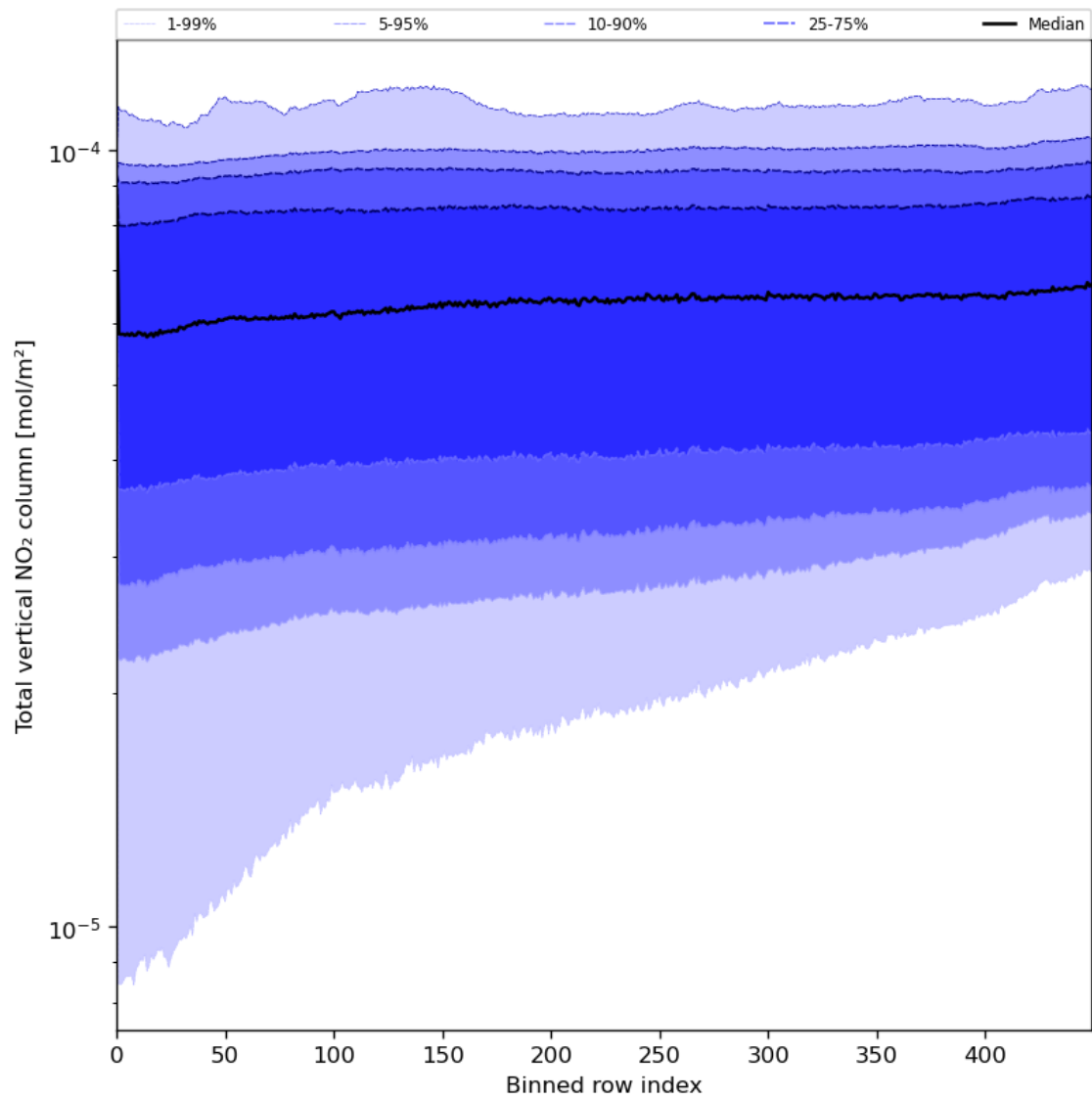
Figure 55: Along track statistics of “Total vertical NO 2 column” for 2023-07-14 to 2023-07-15
