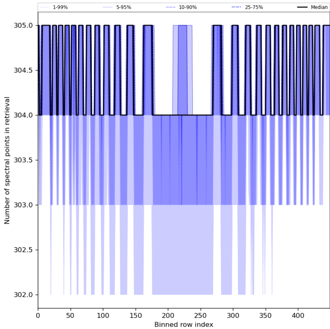
Figure 50: Along track statistics of “Number of spectral points in retrieval” for 2023-07-14 to 2023-07-15
