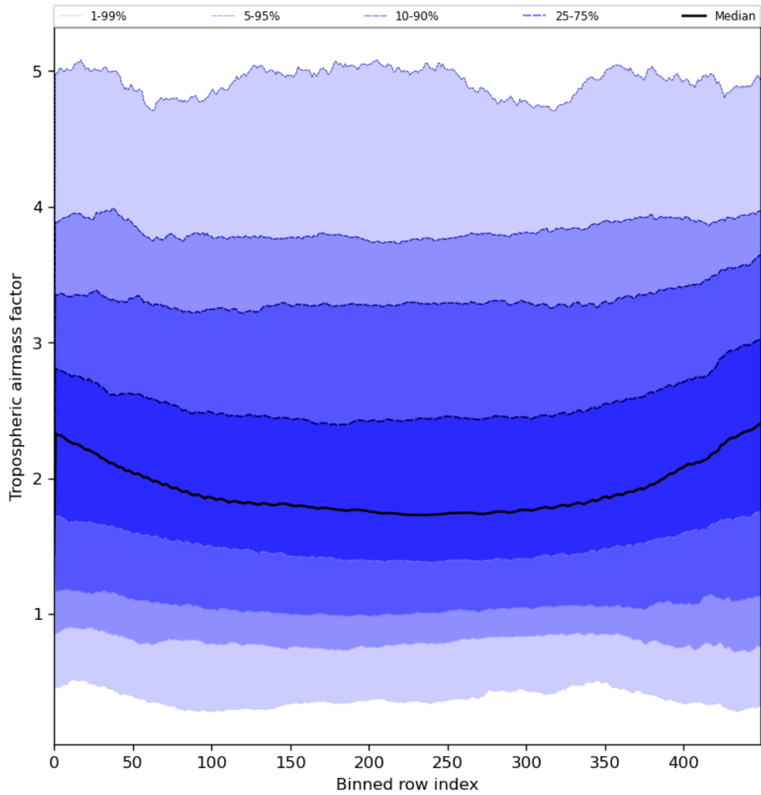
Figure 48: Along track statistics of “Tropospheric airmass factor” for 2023-07-14 to 2023-07-15
