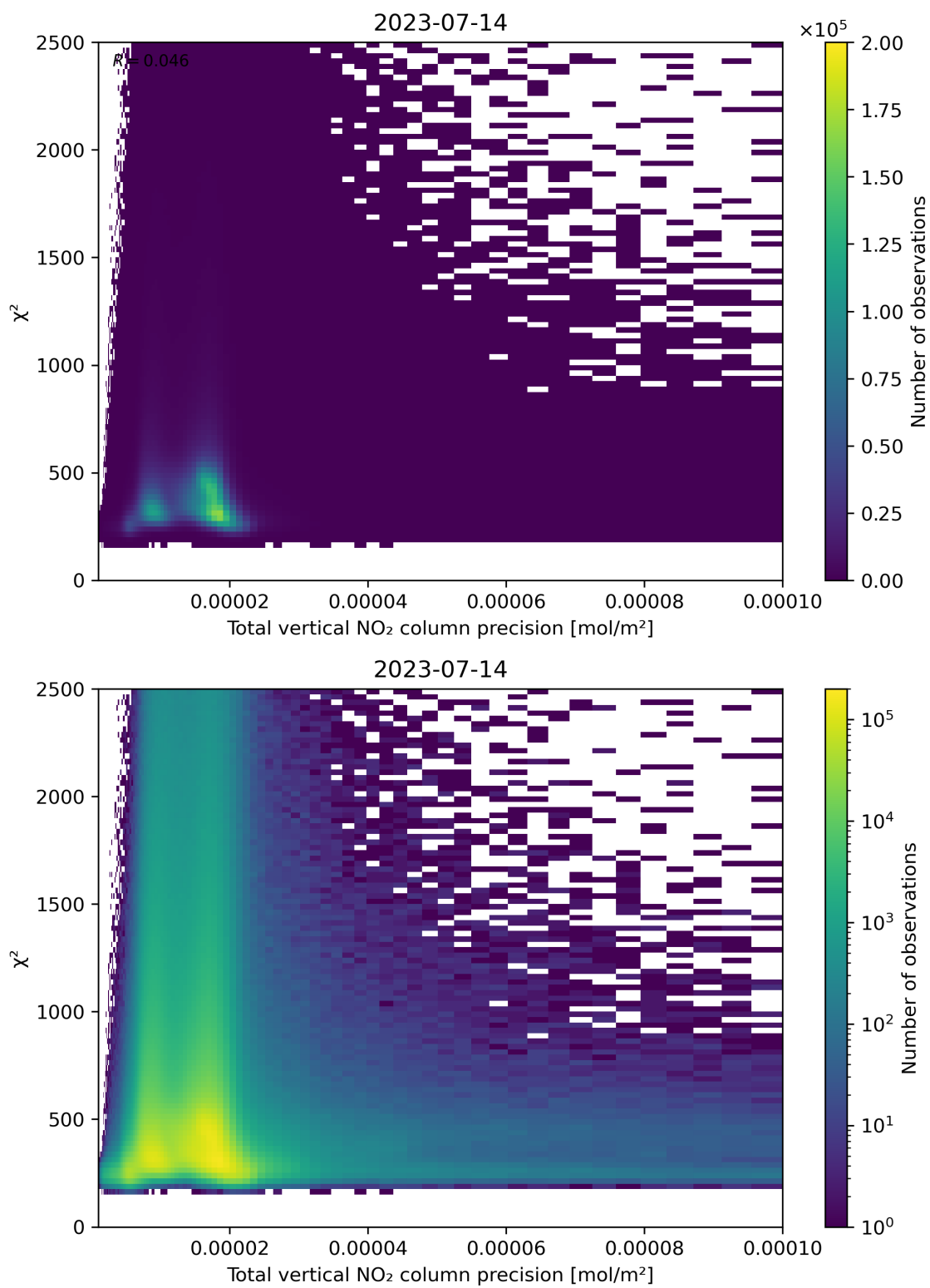
Figure 116: Scatter density plot of “Total vertical NO 2 column precision” against “ \chi^2 ” for 2023-07-14 to 2023-07-15.
