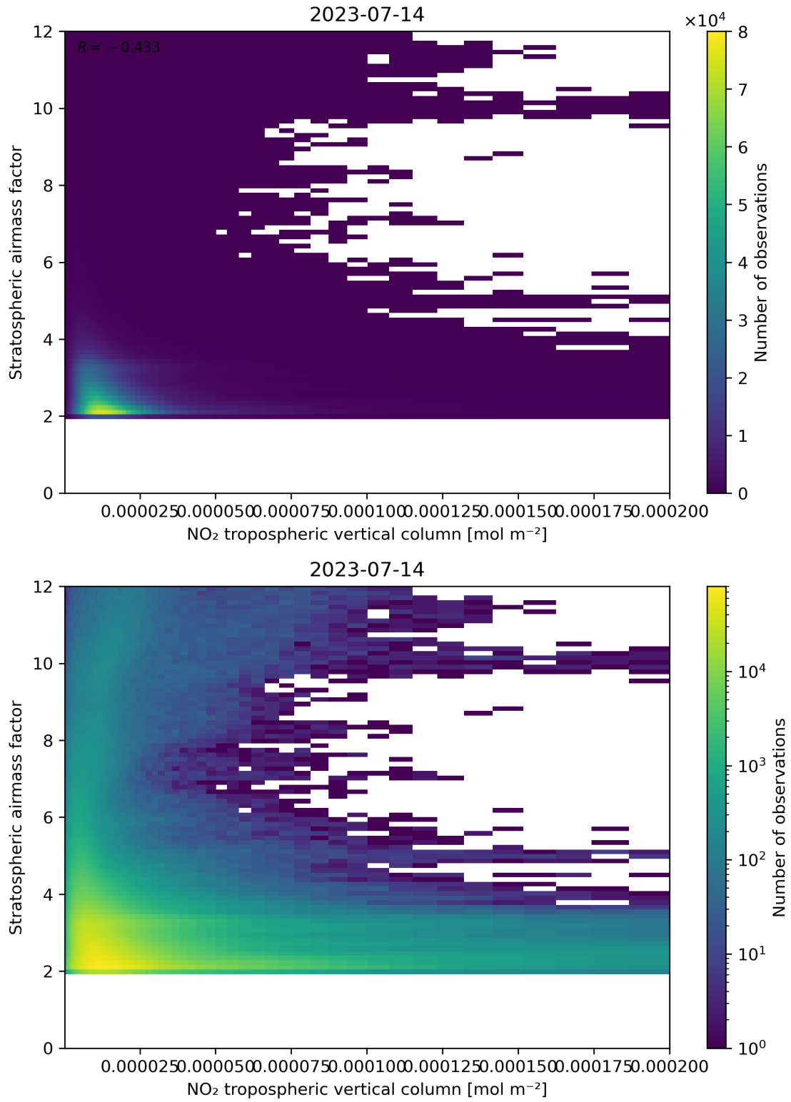
Figure 121: Scatter density plot of “NO 2 tropospheric vertical column” against “Stratospheric air mass factor” for 2023-07-14 to 2023-07-15.
