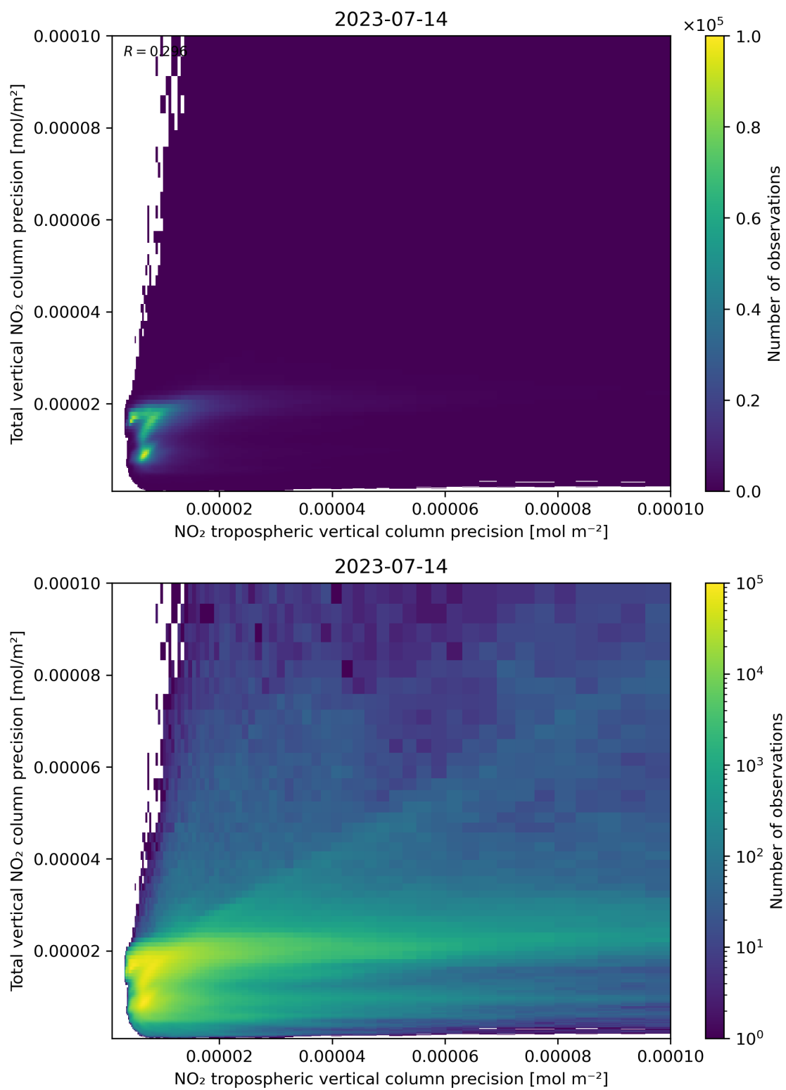
Figure 139: Scatter density plot of “NO 2 tropospheric vertical column precision” against “Total vertical NO 2 column precision” for 2023-07-14 to 2023-07-15.
