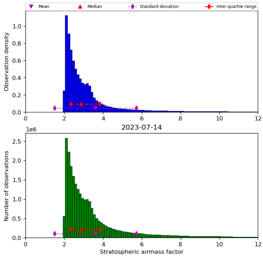
Figure 44: Histogram of "Stratospheric airmass factor" for 2023-07-14 to 2023-07-15
