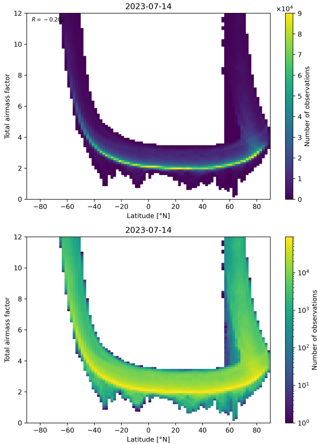
Figure 84: Scatter density plot of “Latitude” against “Total airmass factor” for 2023-07-14 to 2023-07-15.
