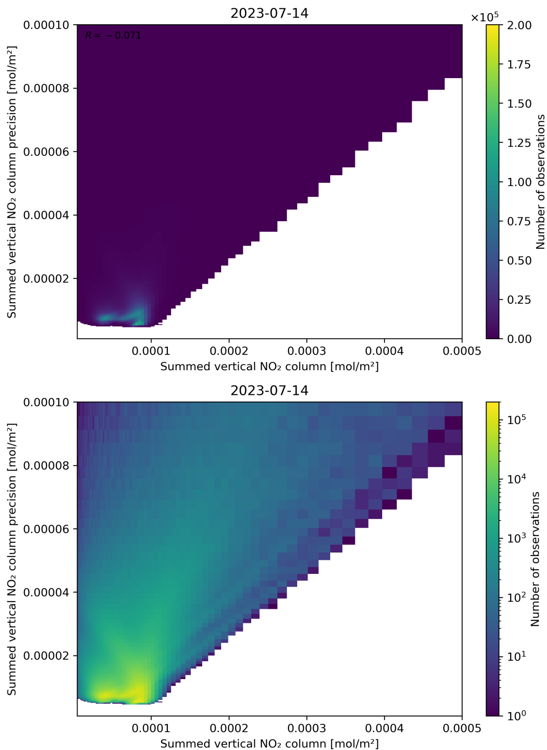
Figure 105: Scatter density plot of “Summed vertical NO 2 column” against “Summed vertical NO 2 column precision” for 2023-07-14 to 2023-07-15.
