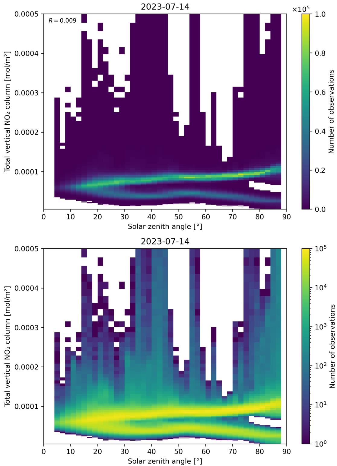
Figure 153: Scatter density plot of “Solar zenith angle” against “Total vertical NO 2 column” for 2023-07-14 to 2023-07-15.
