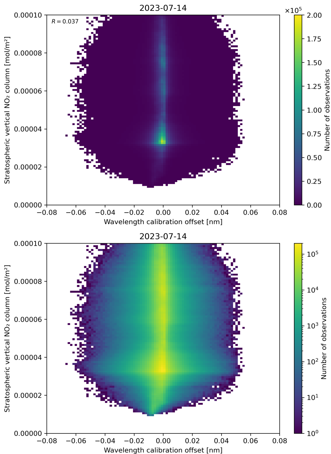
Figure 176: Scatter density plot of “Wavelength calibration offset” against “Stratospheric vertical NO 2 column” for 2023-07-14 to 2023-07-15.
