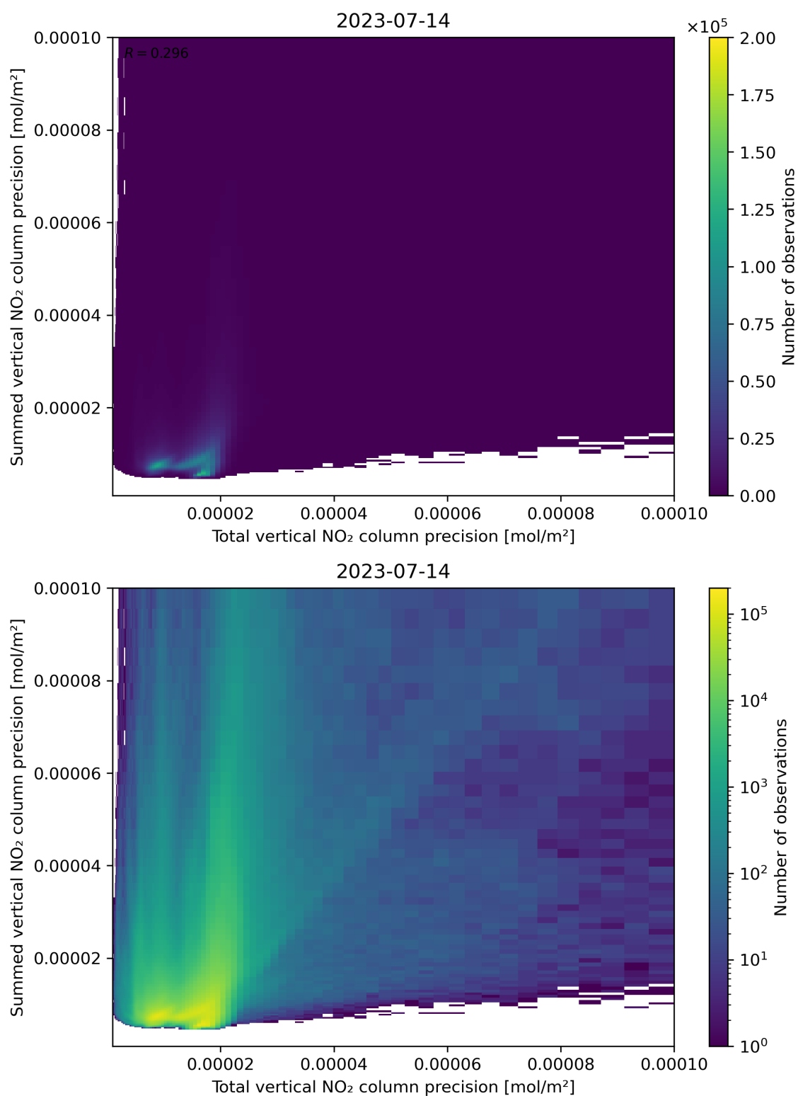
Figure 118: Scatter density plot of “Total vertical NO 2 column precision” against “Summed vertical NO 2 column precision” for 2023-07-14 to 2023-07-15.
