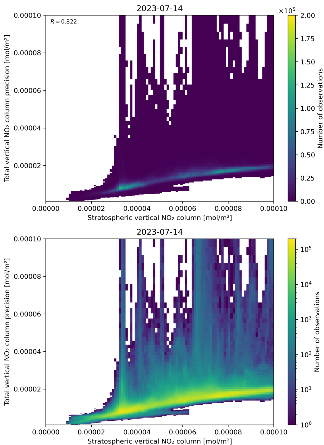
Figure 101: Scatter density plot of “Stratospheric vertical NO 2 column” against “Total vertical NO 2 column precision” for 2023-07-14 to 2023-07-15.
