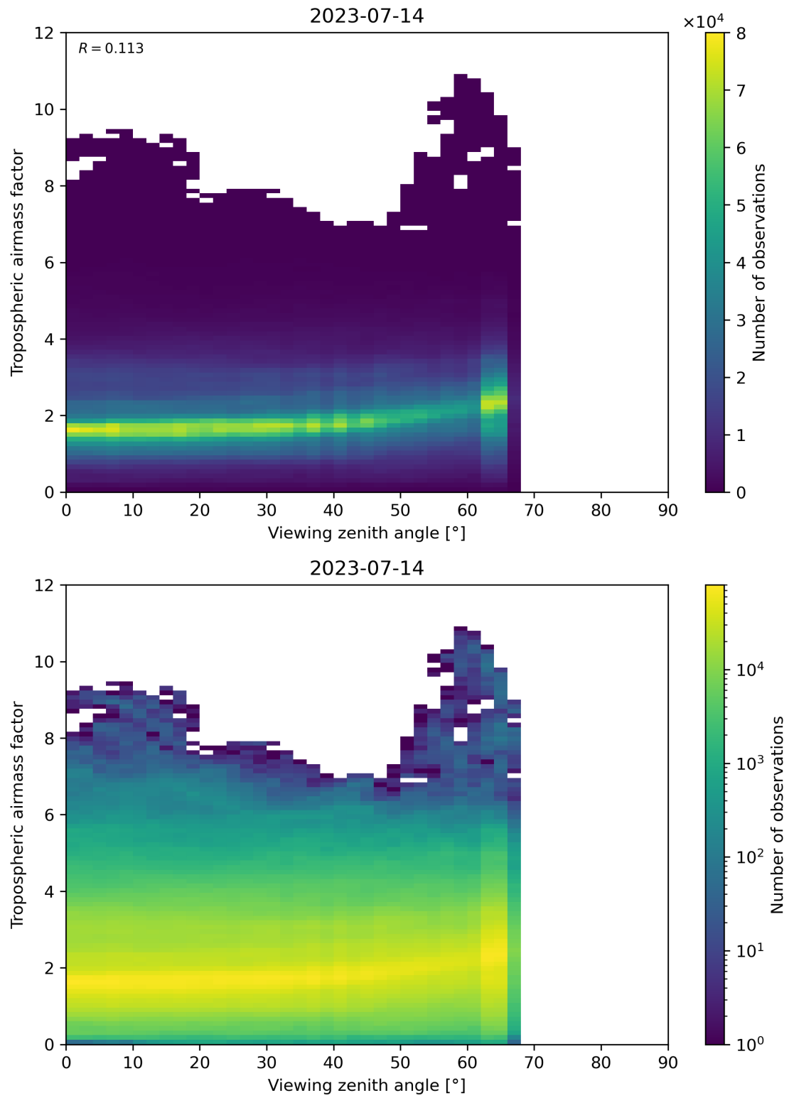
Figure 161: Scatter density plot of “Viewing zenith angle” against “Tropospheric airmass factor” for 2023-07-14 to 2023-07-15.
