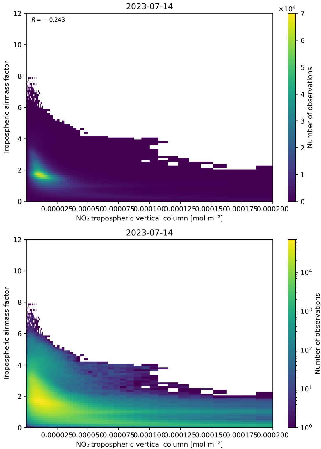
Figure 123: Scatter density plot of “NO 2 tropospheric vertical column” against “Tropospheric air mass factor” for 2023-07-14 to 2023-07-15.
