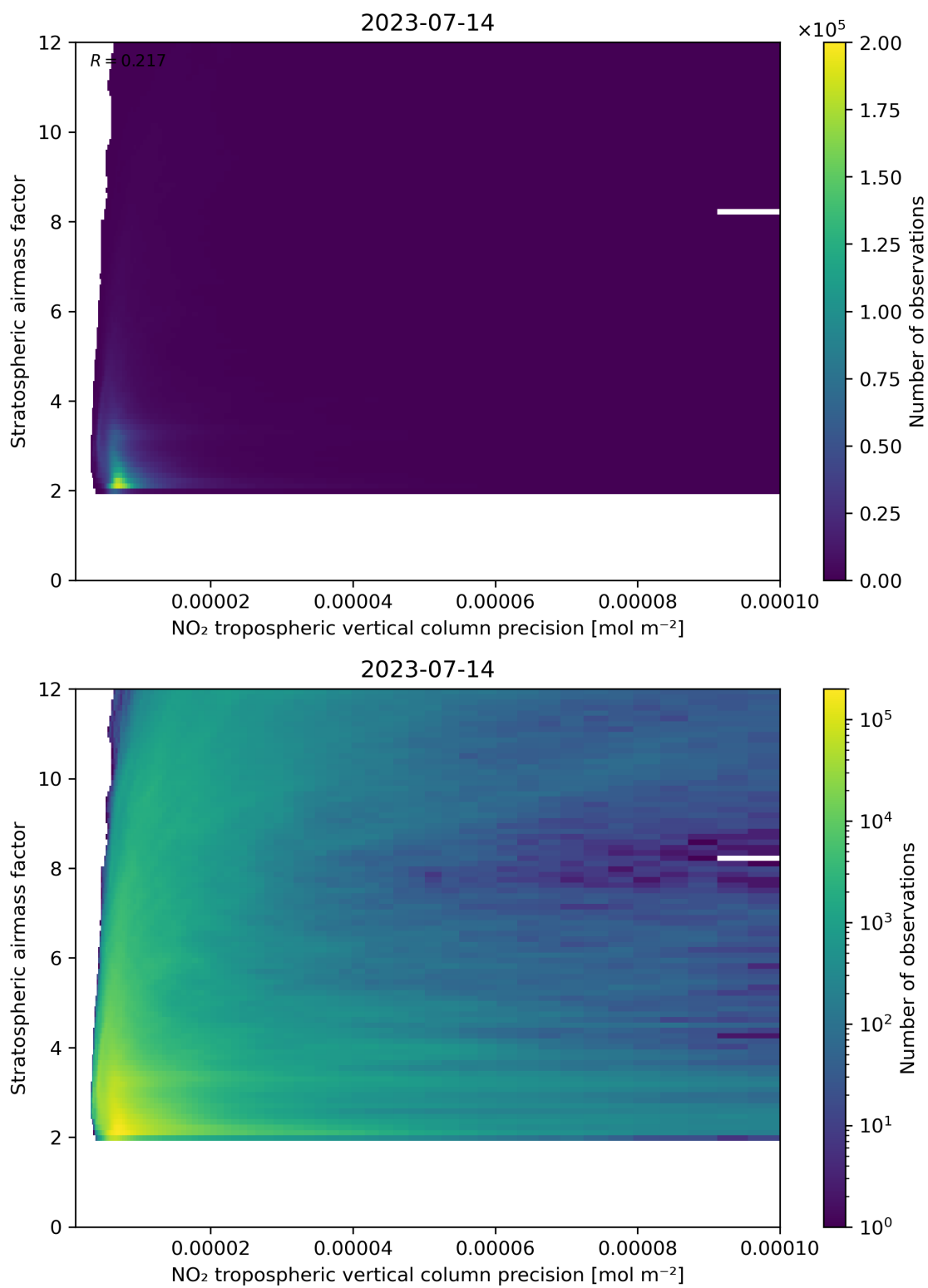
Figure 131: Scatter density plot of “NO 2 tropospheric vertical column precision” against “Stratospheric airmass factor” for 2023-07-14 to 2023-07-15.
