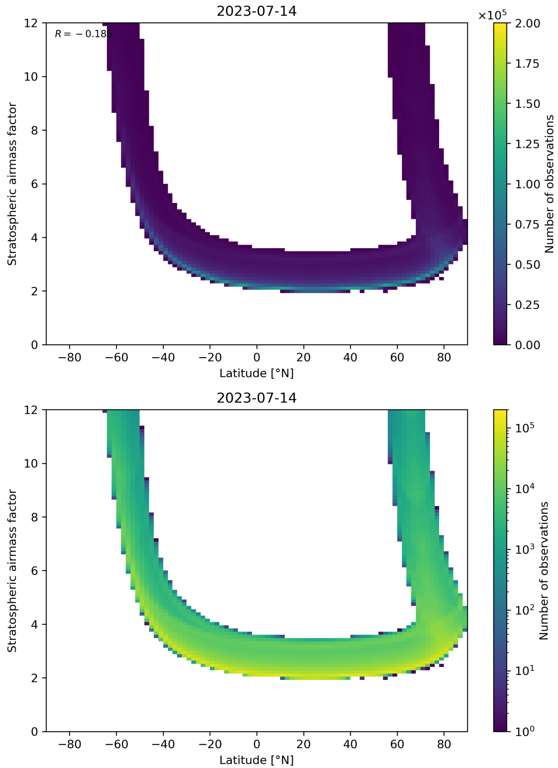
Figure 83: Scatter density plot of “Latitude” against “Stratospheric air mass factor” for 2023-07-14 to 2023-07-15.
