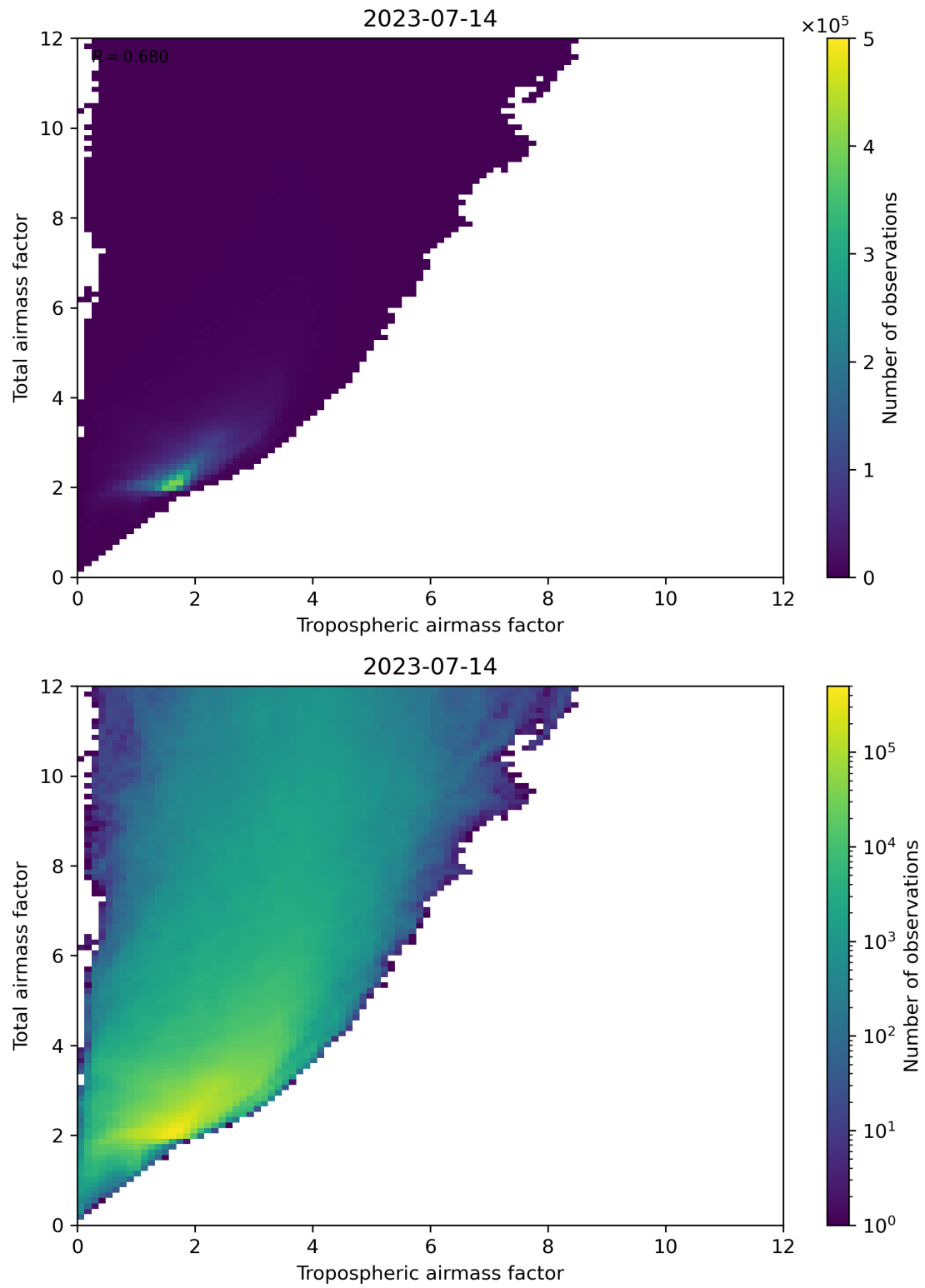
Figure 72: Scatter density plot of “Tropospheric airmass factor” against “Total airmass factor” for 2023-07-14 to 2023-07-15.
