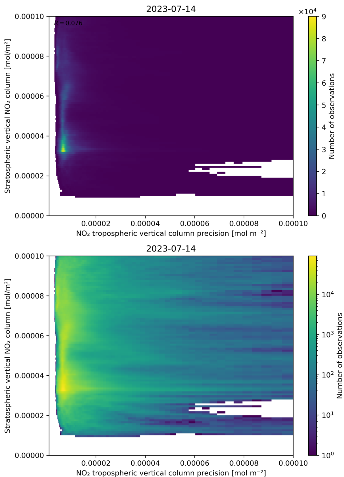
Figure 135: Scatter density plot of “NO 2 tropospheric vertical column precision” against “Stratospheric vertical NO 2 column” for 2023-07-14 to 2023-07-15.
