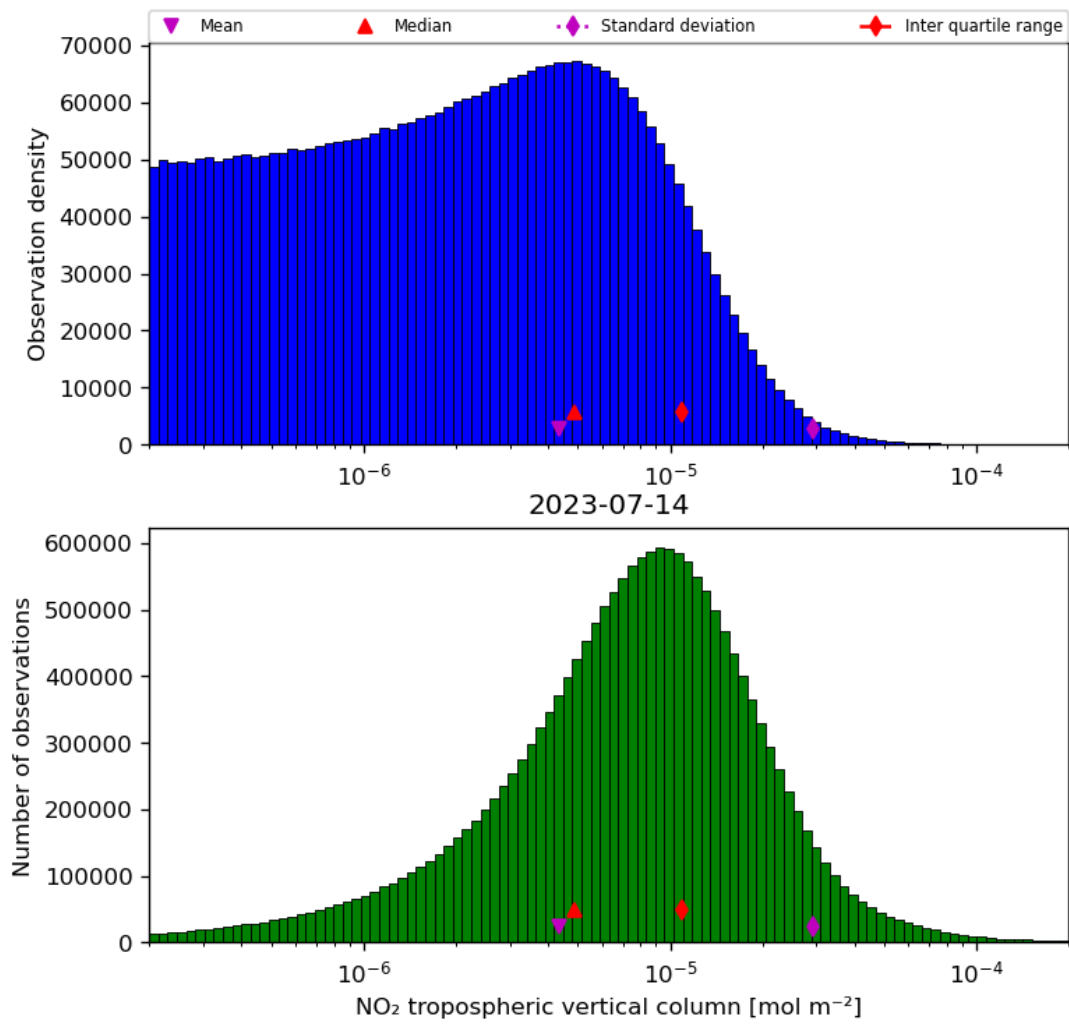
Figure 29: Histogram of “NO 2 tropospheric vertical column” for 2023-07-14 to 2023-07-15
