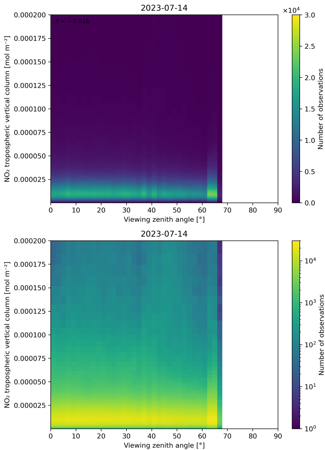
Figure 169: Scatter density plot of “Viewing zenith angle” against “NO 2 tropospheric vertical column” for 2023-07-14 to 2023-07-15.
