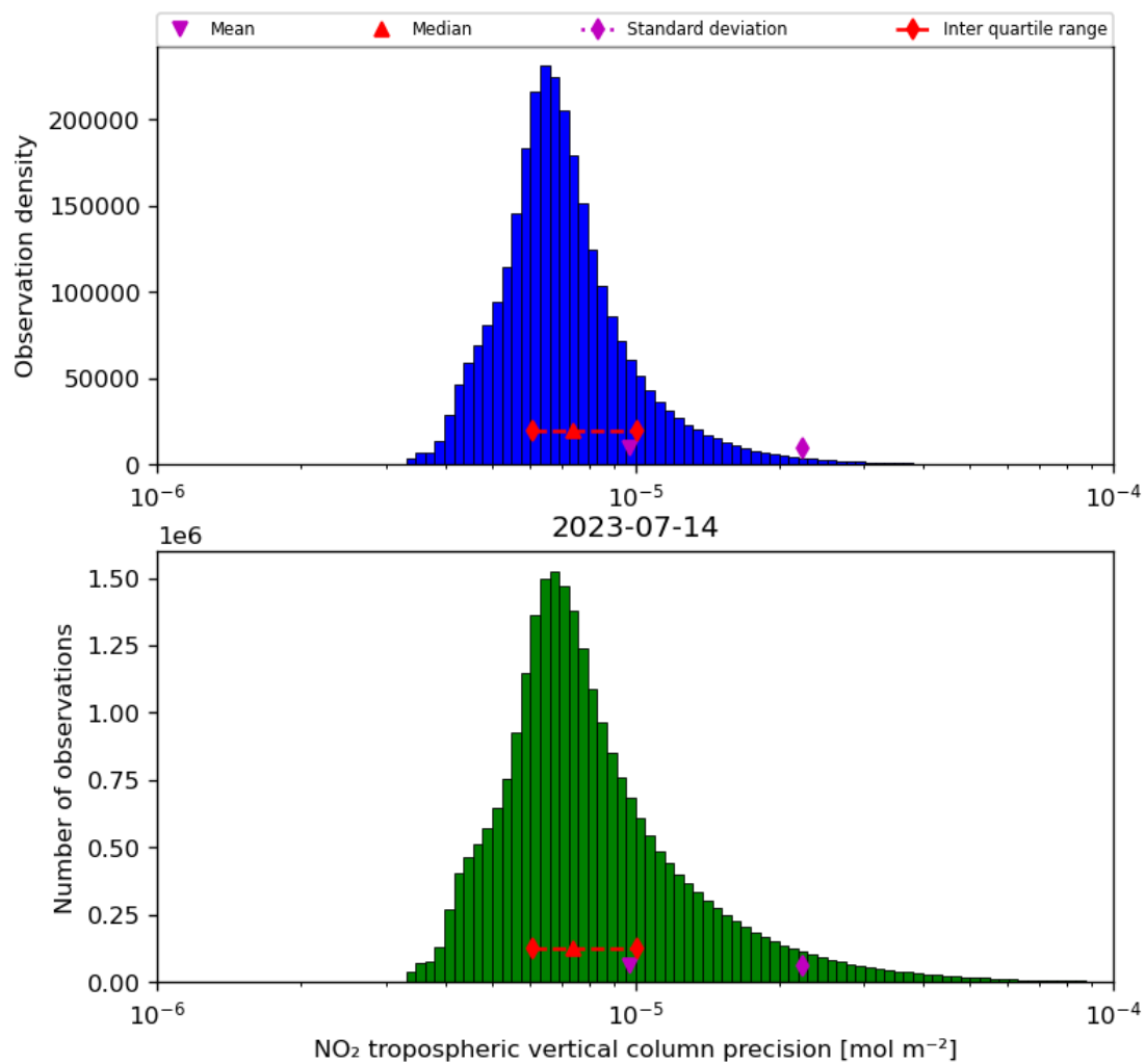
Figure 30: Histogram of “NO 2 tropospheric vertical column precision” for 2023-07-14 to 2023-07-15
