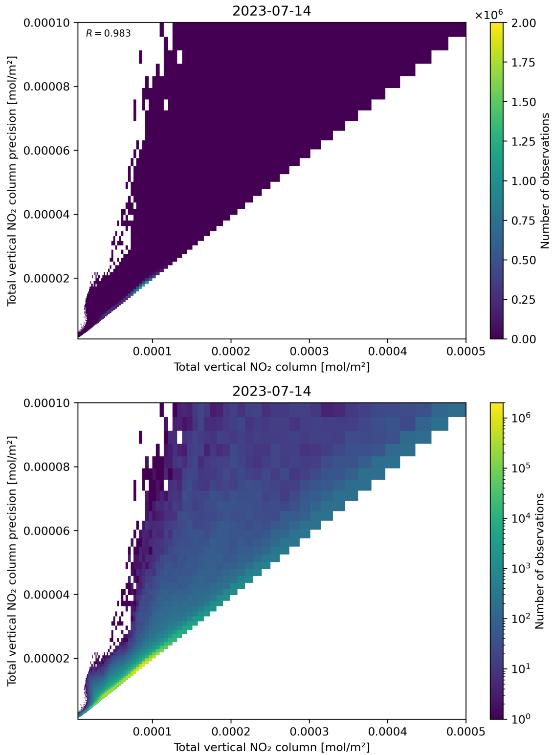
Figure 114: Scatter density plot of “Total vertical NO 2 column” against “Total vertical NO 2 column precision” for 2023-07-14 to 2023-07-15.
