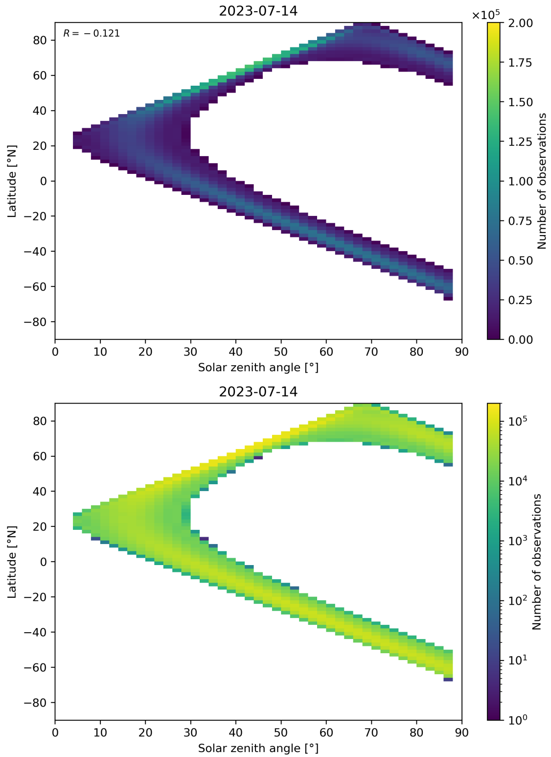
Figure 149: Scatter density plot of “Solar zenith angle” against “Latitude” for 2023-07-14 to 2023-07-15.
