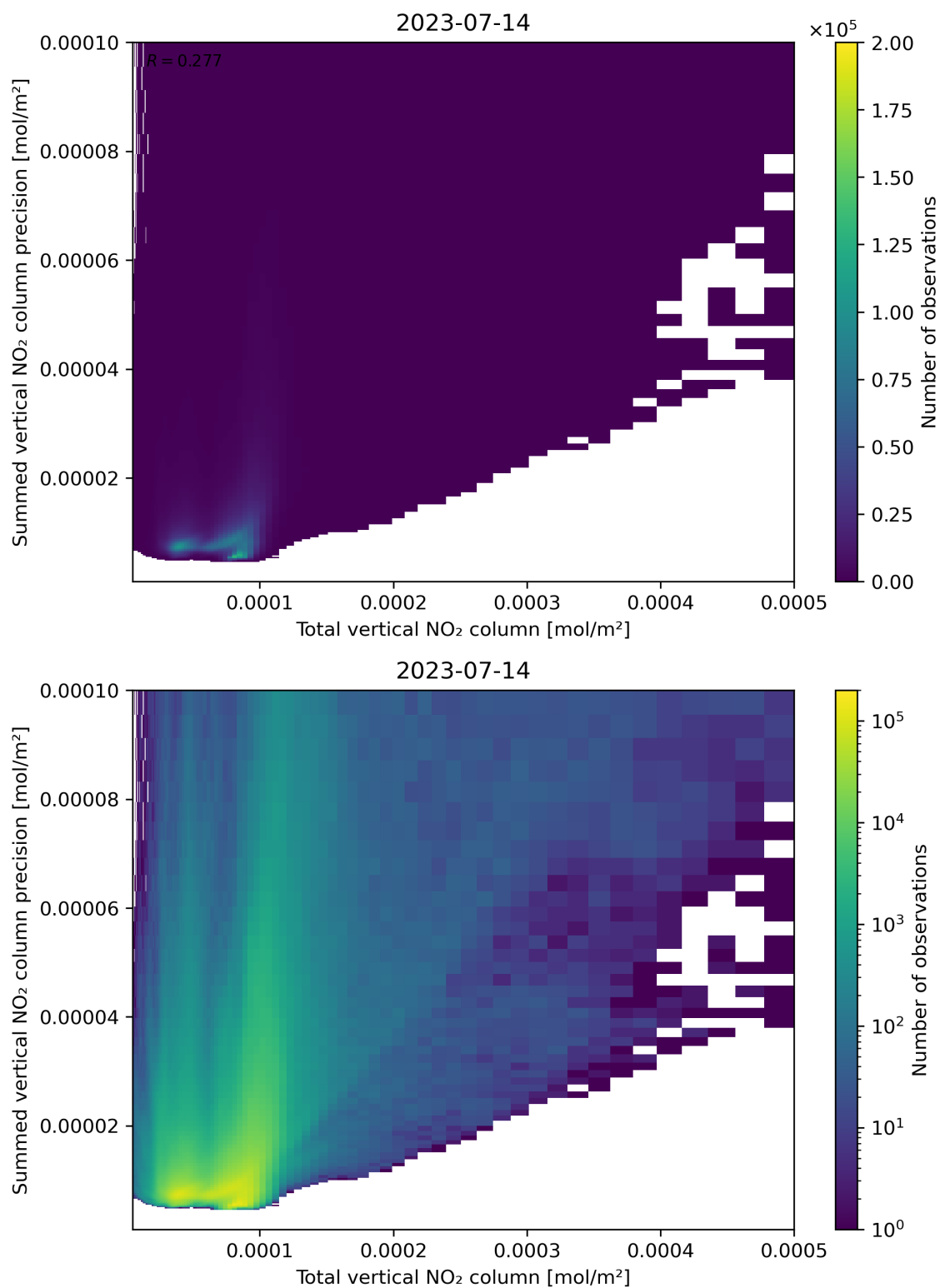
Figure 113: Scatter density plot of “Total vertical NO 2 column” against “Summed vertical NO 2 column precision” for 2023-07-14 to 2023-07-15.
