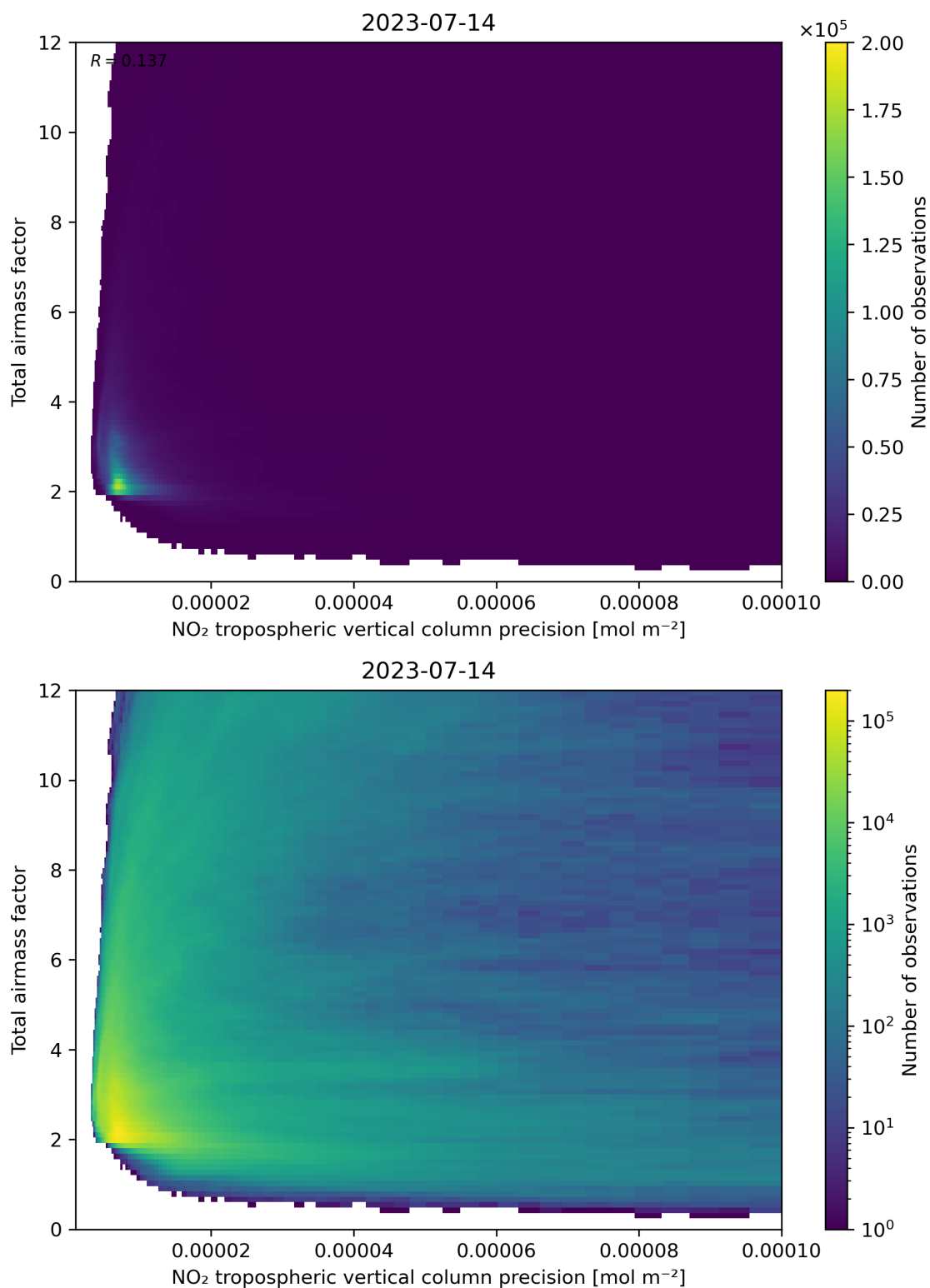
Figure 132: Scatter density plot of “NO 2 tropospheric vertical column precision” against “Total air mass factor” for 2023-07-14 to 2023-07-15.
