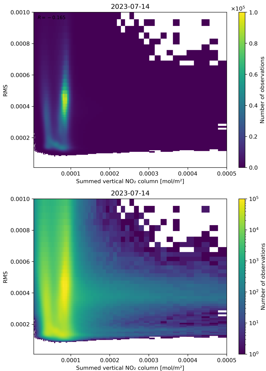
Figure 109: Scatter density plot of “Summed vertical NO 2 column” against “RMS” for 2023-07-14 to 2023-07-15.
