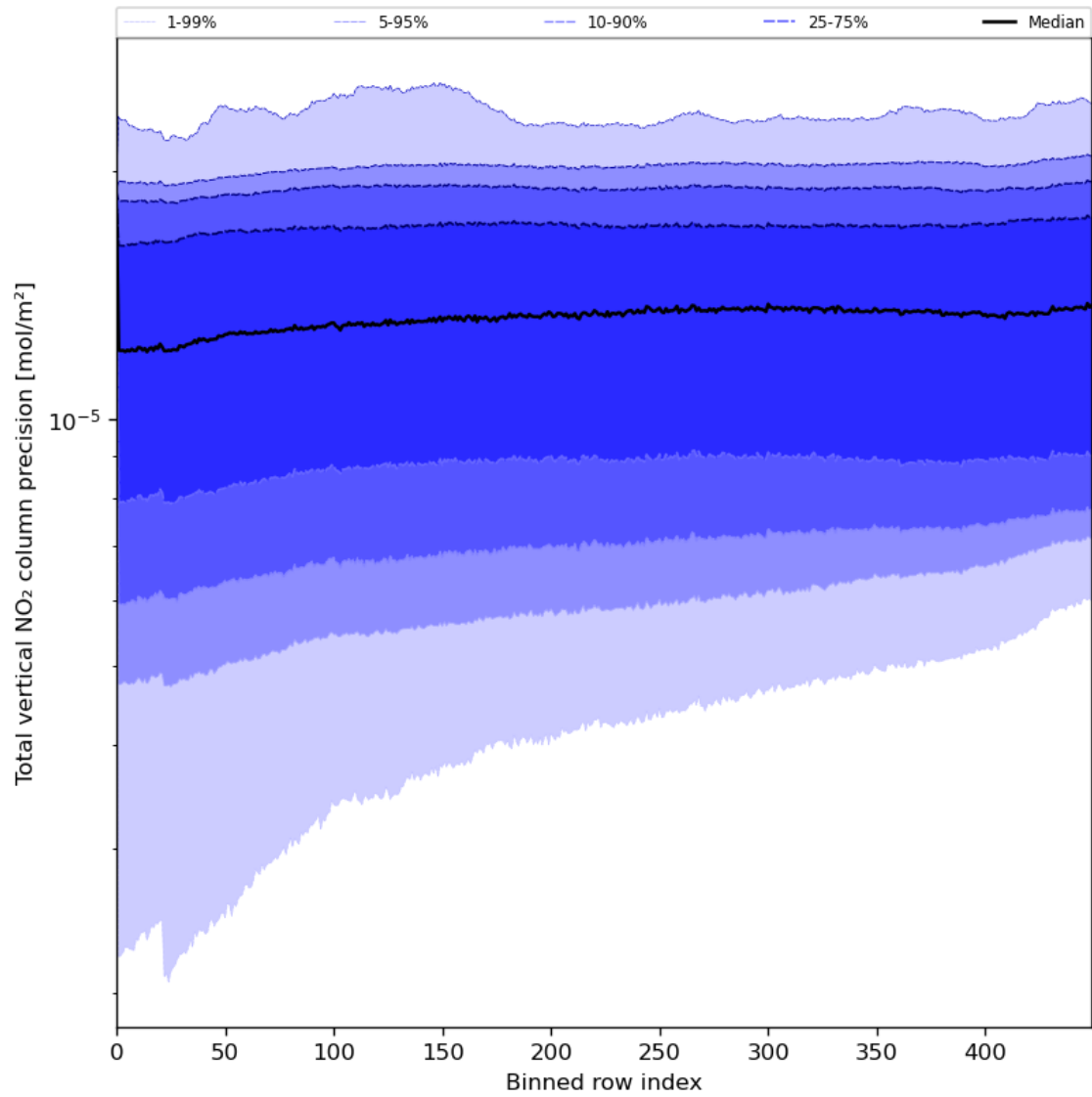
Figure 56: Along track statistics of “Total vertical NO 2 column precision” for 2023-07-14 to 2023-07-15
