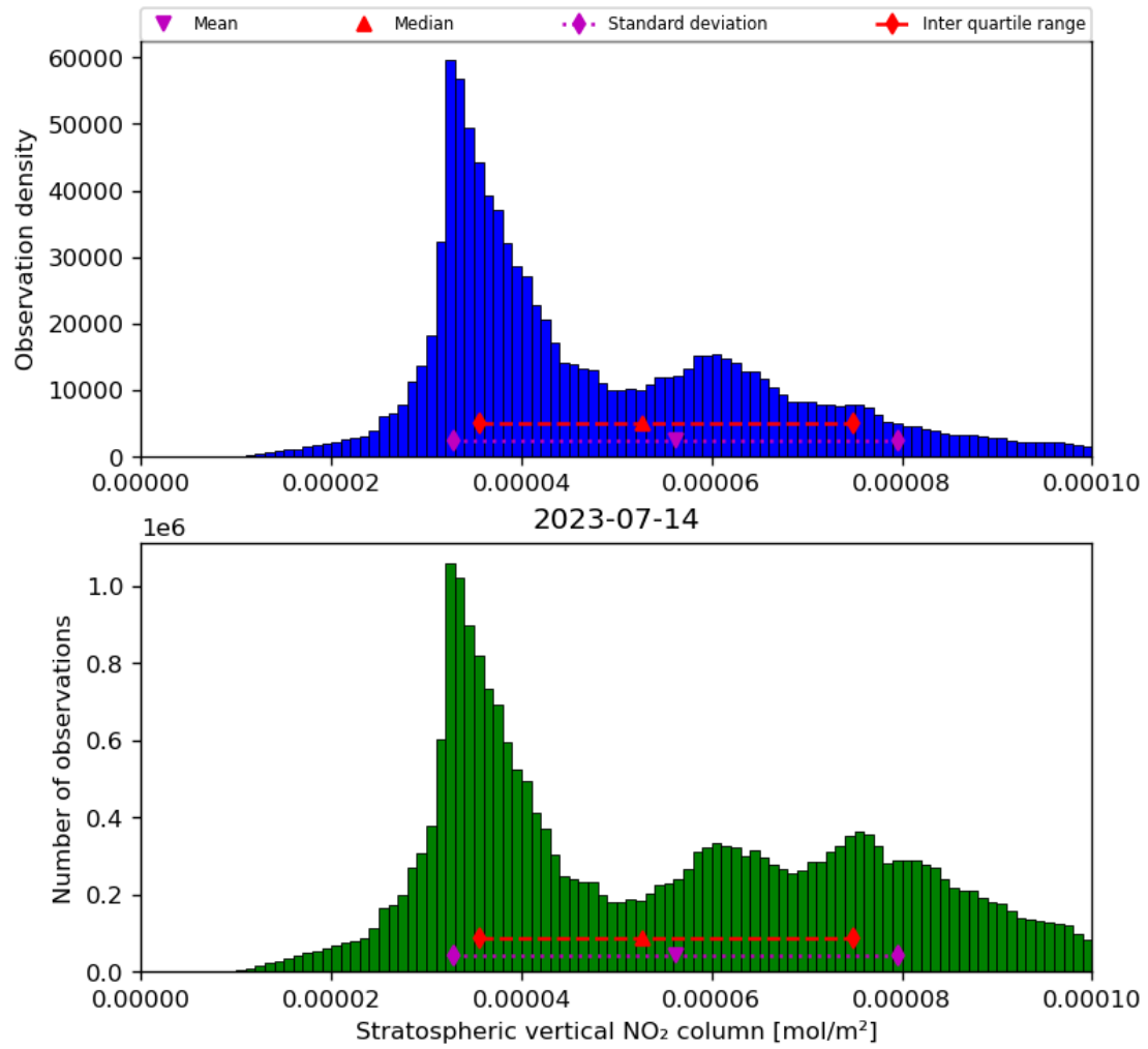
Figure 36: Histogram of “Stratospheric vertical NO 2 column” for 2023-07-14 to 2023-07-15
