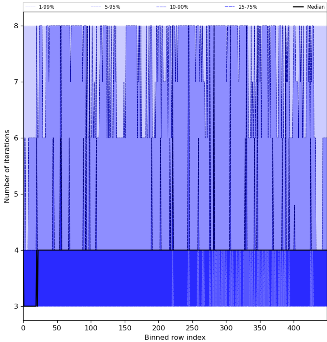
Figure 51: Along track statistics of “Number of iterations” for 2023-07-14 to 2023-07-15
