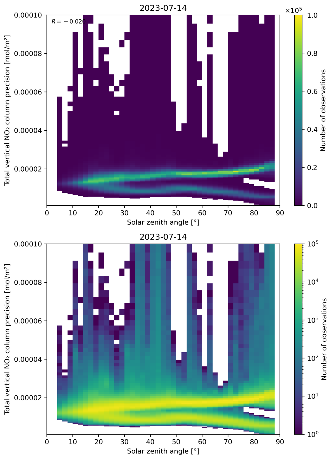
Figure 154: Scatter density plot of “Solar zenith angle” against “Total vertical NO 2 column precision” for 2023-07-14 to 2023-07-15.
