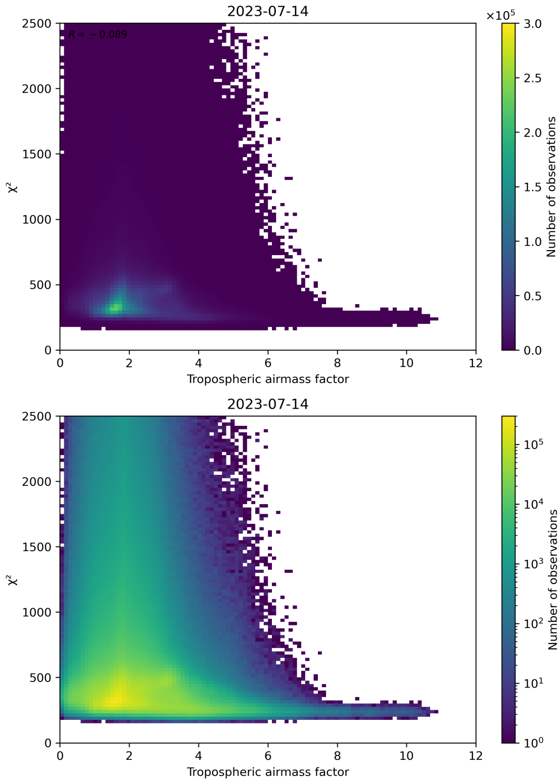
Figure 73: Scatter density plot of “Tropospheric airmass factor” against “ \chi^2 ” for 2023-07-14 to 2023-07-15.
