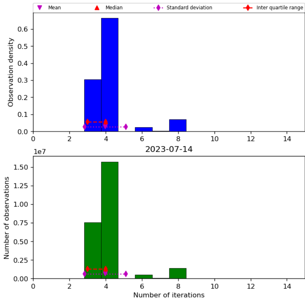
Figure 34: Histogram of “Number of iterations” for 2023-07-14 to 2023-07-15
