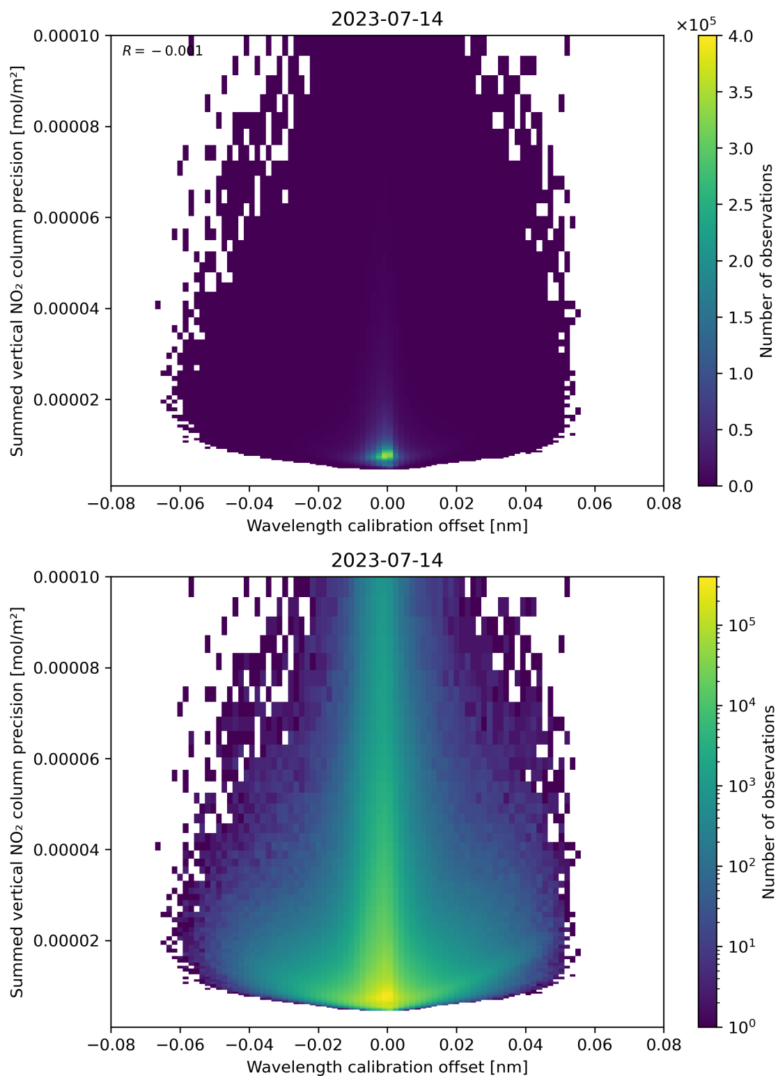
Figure 178: Scatter density plot of “Wavelength calibration offset” against “Summed vertical NO 2 column precision” for 2023-07-14 to 2023-07-15.
