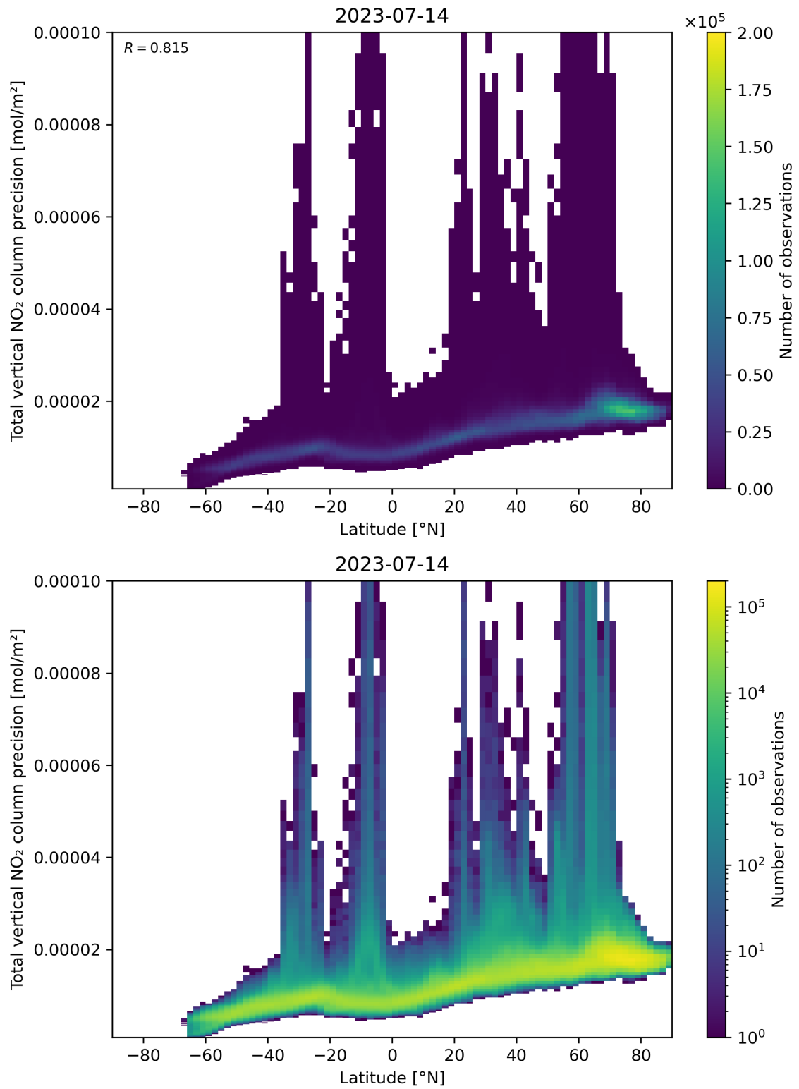
Figure 91: Scatter density plot of “Latitude” against “Total vertical NO 2 column precision” for 2023-07-14 to 2023-07-15.
