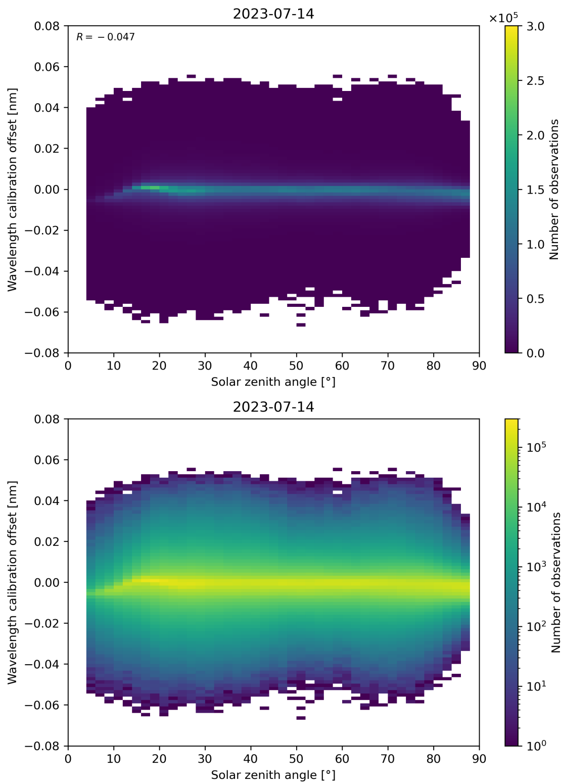
Figure 158: Scatter density plot of “Solar zenith angle” against “Wavelength calibration offset” for 2023-07-14 to 2023-07-15.
