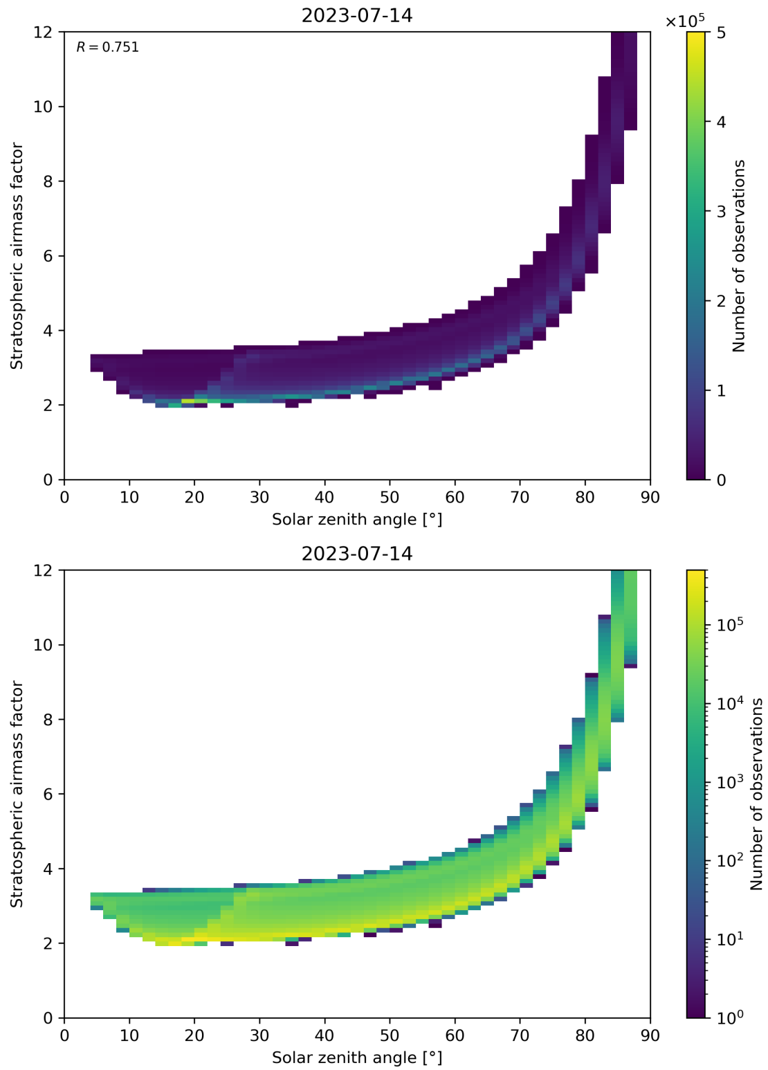
Figure 145: Scatter density plot of “Solar zenith angle” against “Stratospheric airmass factor” for 2023-07-14 to 2023-07-15.
