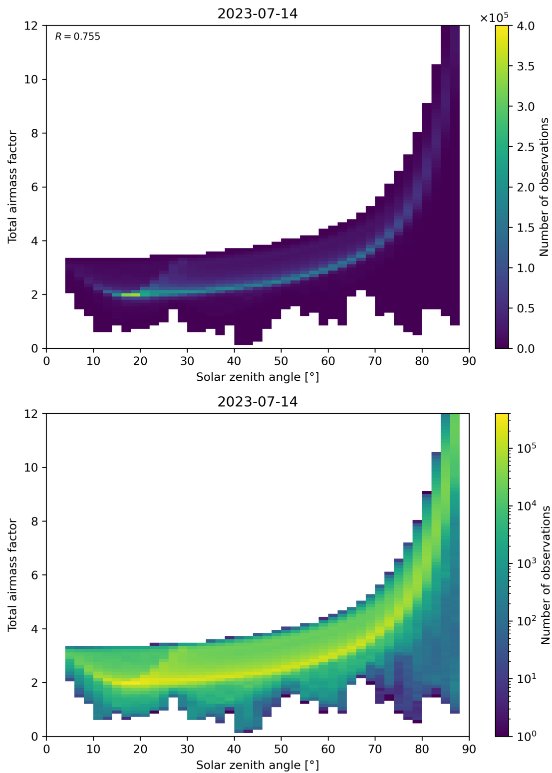
Figure 146: Scatter density plot of “Solar zenith angle” against “Total air mass factor” for 2023-07-14 to 2023-07-15.
