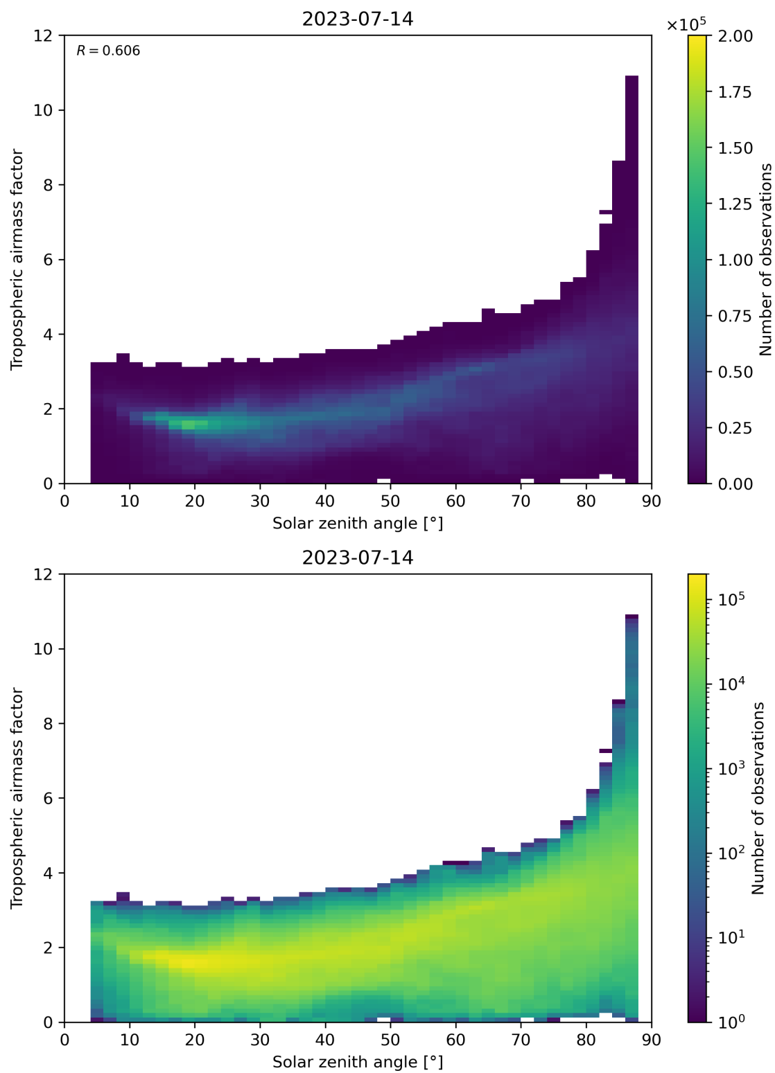
Figure 147: Scatter density plot of “Solar zenith angle” against “Tropospheric airmass factor” for 2023-07-14 to 2023-07-15.
