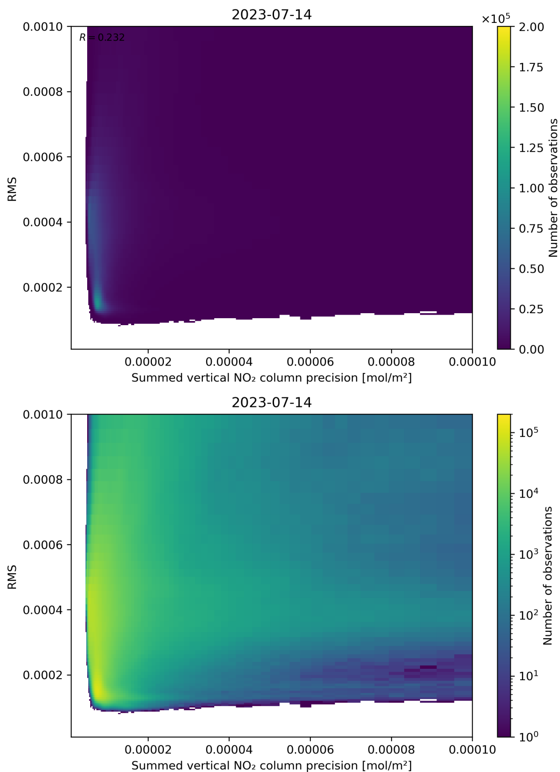
Figure 108: Scatter density plot of “Summed vertical NO 2 column precision” against “RMS” for 2023-07-14 to 2023-07-15.
