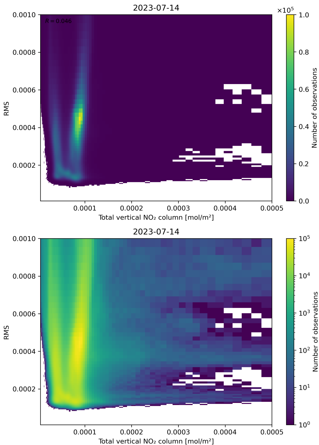
Figure 120: Scatter density plot of “Total vertical NO 2 column” against “RMS” for 2023-07-14 to 2023-07-15.
