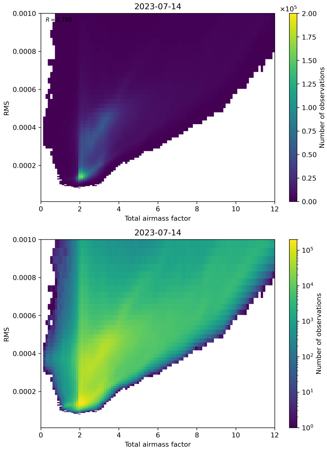
Figure 69: Scatter density plot of “Total airmass factor” against “RMS” for 2023-07-14 to 2023-07-15.
