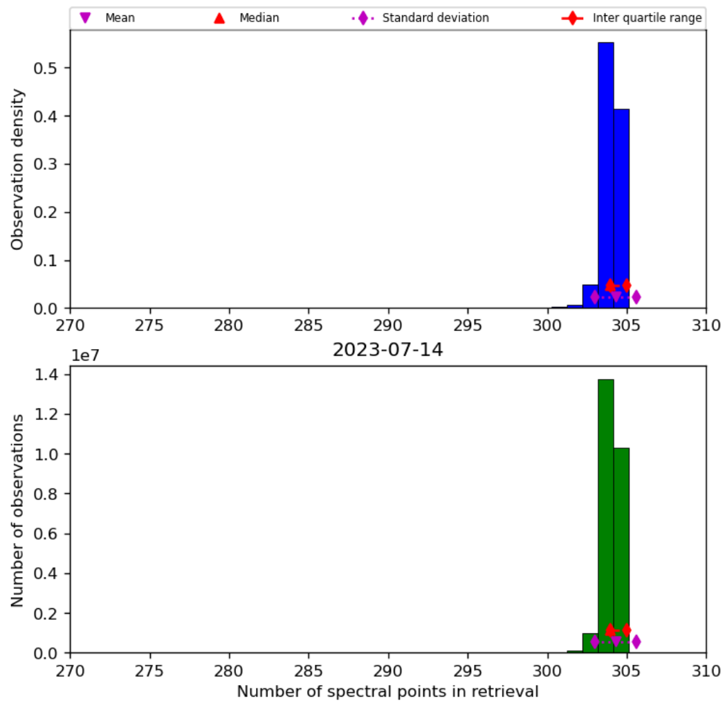
Figure 33: Histogram of “Number of spectral points in retrieval” for 2023-07-14 to 2023-07-15
