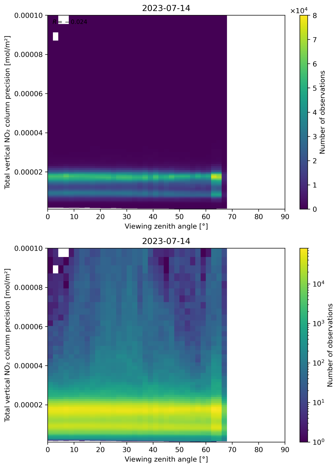
Figure 168: Scatter density plot of “Viewing zenith angle” against “Total vertical NO 2 column precision” for 2023-07-14 to 2023-07-15.
