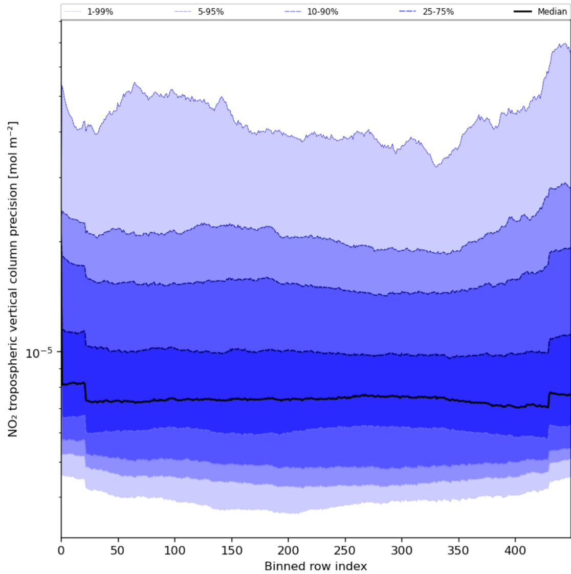
Figure 47: Along track statistics of “NO 2 tropospheric vertical column precision” for 2023-07-14 to 2023-07-15
