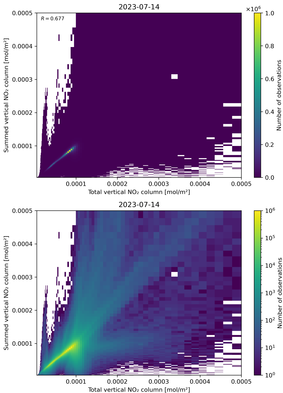
Figure 112: Scatter density plot of “Total vertical NO 2 column” against “Summed vertical NO 2 column” for 2023-07-14 to 2023-07-15.
