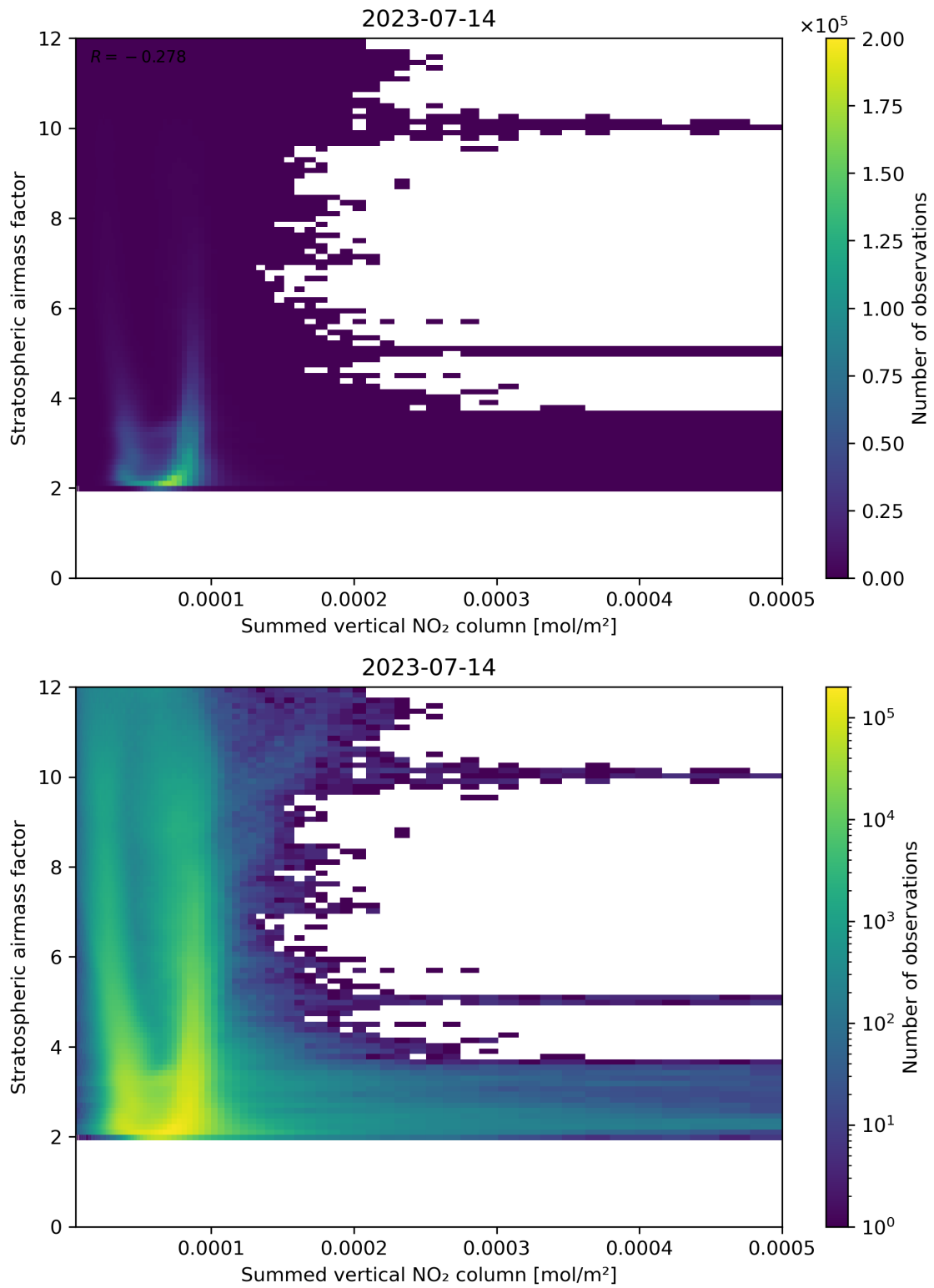
Figure 103: Scatter density plot of “Summed vertical NO 2 column” against “Stratospheric airmass factor” for 2023-07-14 to 2023-07-15.
