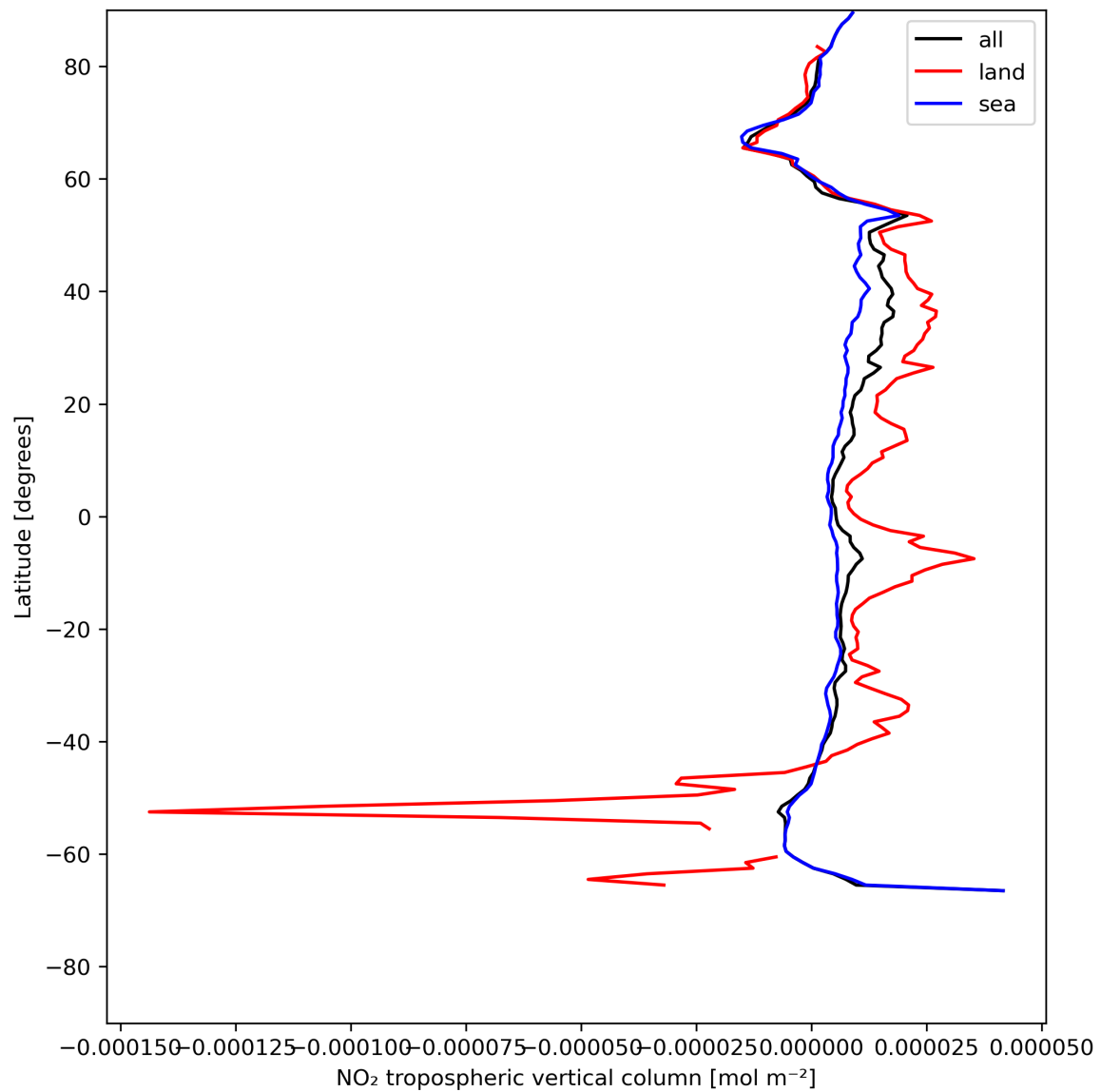
Figure 12: Zonal average of “NO 2 tropospheric vertical column” for 2023-07-14 to 2023-07-15.
