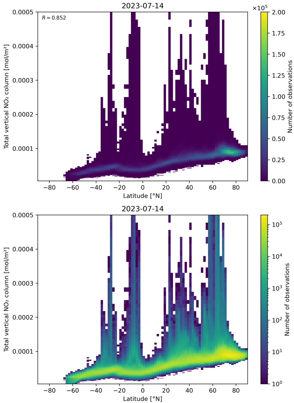
Figure 90: Scatter density plot of “Latitude” against “Total vertical NO 2 column” for 2023-07-14 to 2023-07-15.
