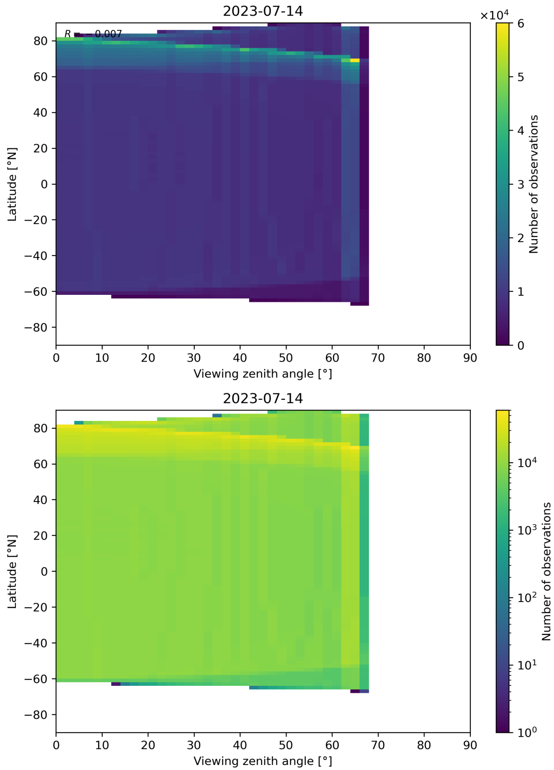
Figure 163: Scatter density plot of “Viewing zenith angle” against “Latitude” for 2023-07-14 to 2023-07-15.
