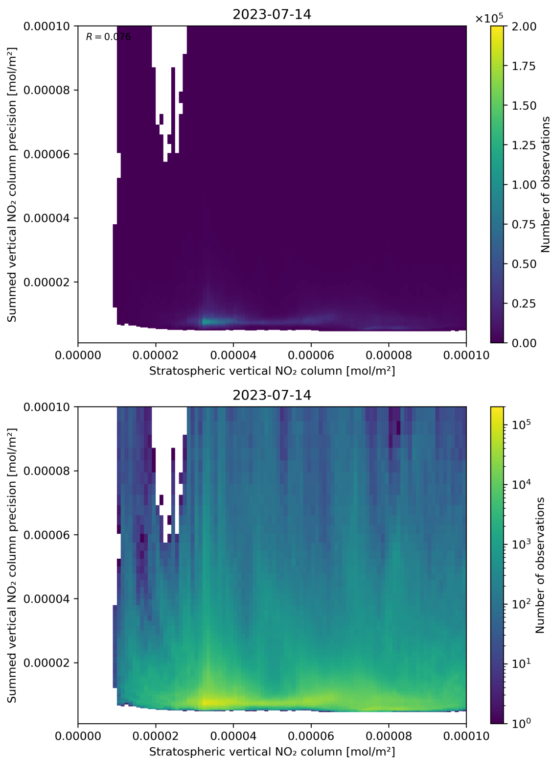
Figure 99: Scatter density plot of “Stratospheric vertical NO 2 column” against “Summed vertical NO 2 column precision” for 2023-07-14 to 2023-07-15.
