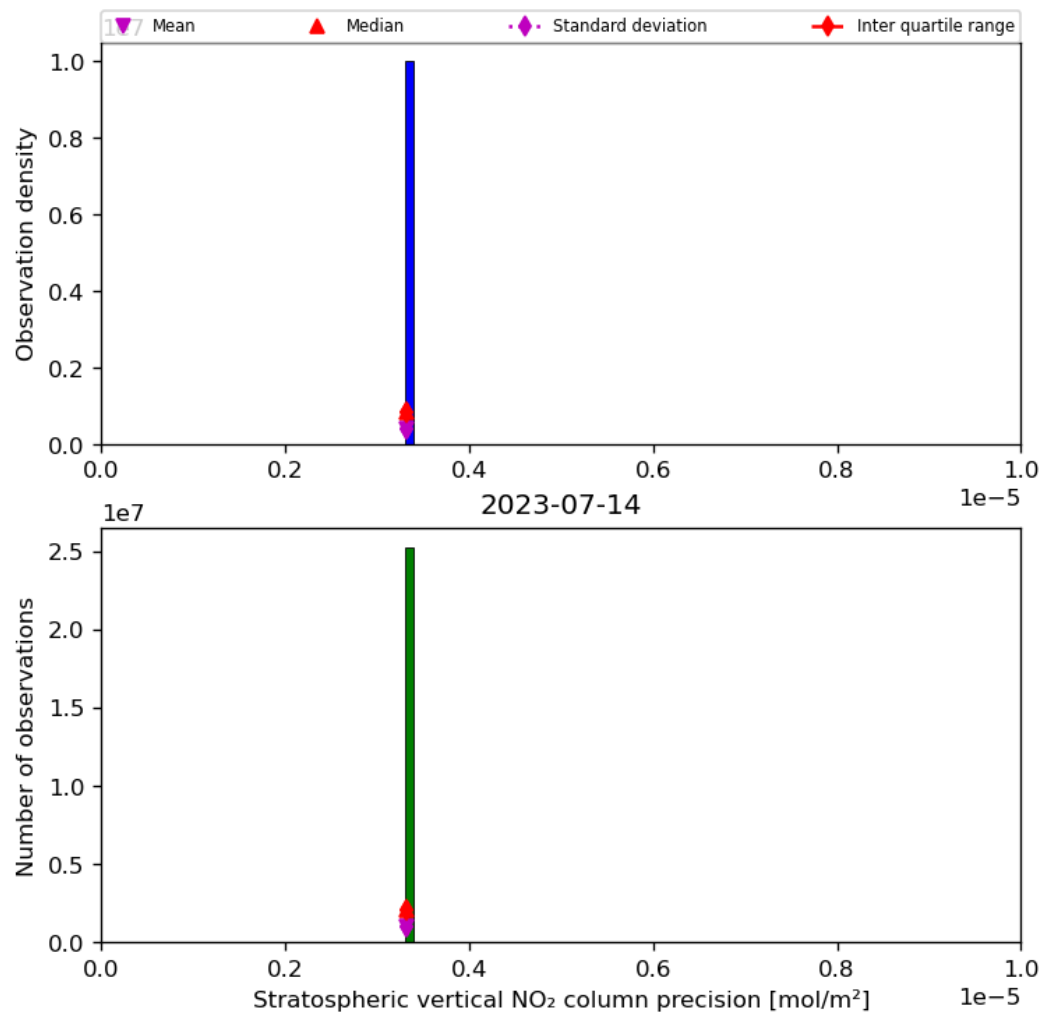
Figure 37: Histogram of “Stratospheric vertical NO 2 column precision” for 2023-07-14 to 2023-07-15
