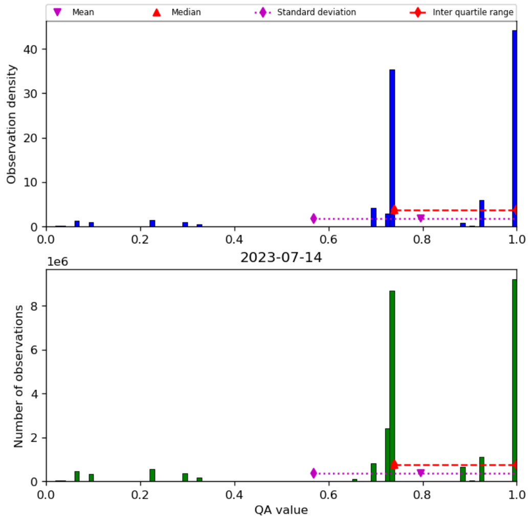
Figure 28: Histogram of “QA value” for 2023-07-14 to 2023-07-15
