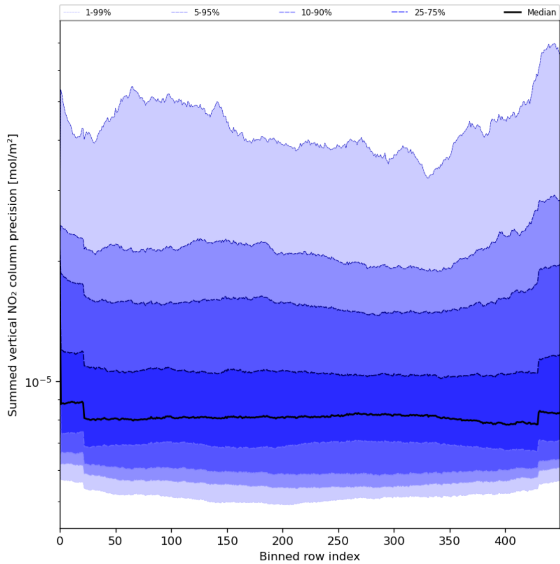
Figure 58: Along track statistics of “Summed vertical NO 2 column precision” for 2023-07-14 to 2023-07-15
