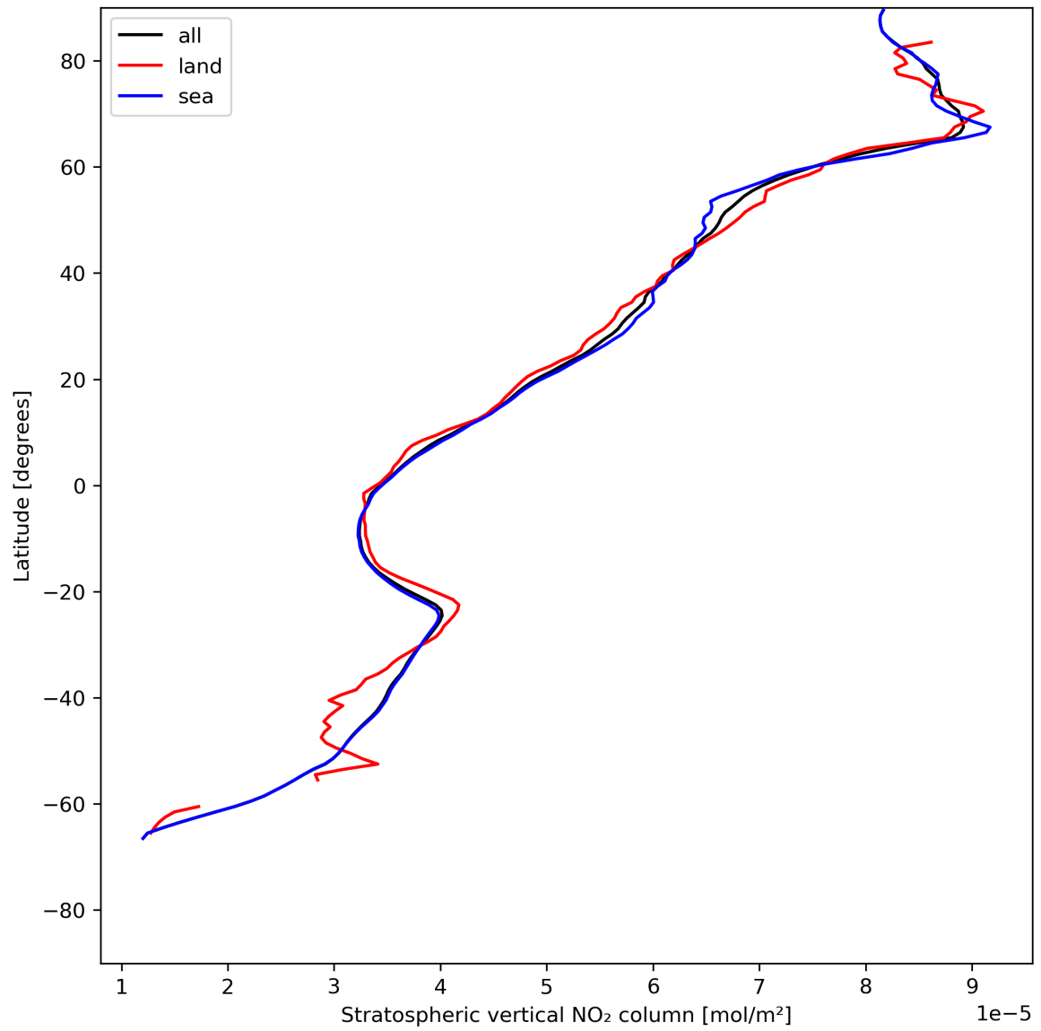
Figure 19: Zonal average of “Stratospheric vertical NO 2 column” for 2023-07-14 to 2023-07-15.
