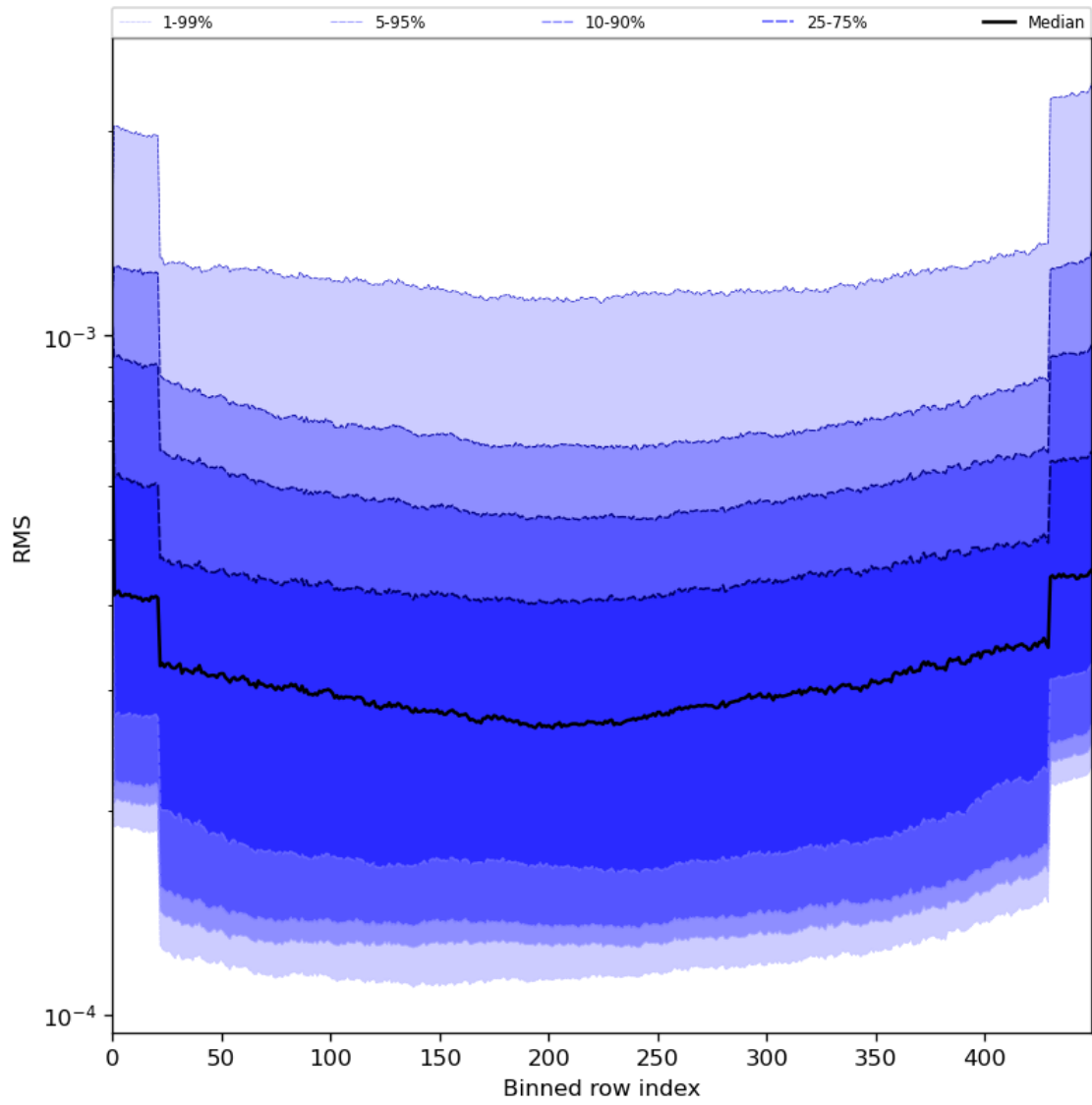
Figure 60: Along track statistics of “RMS” for 2023-07-14 to 2023-07-15
