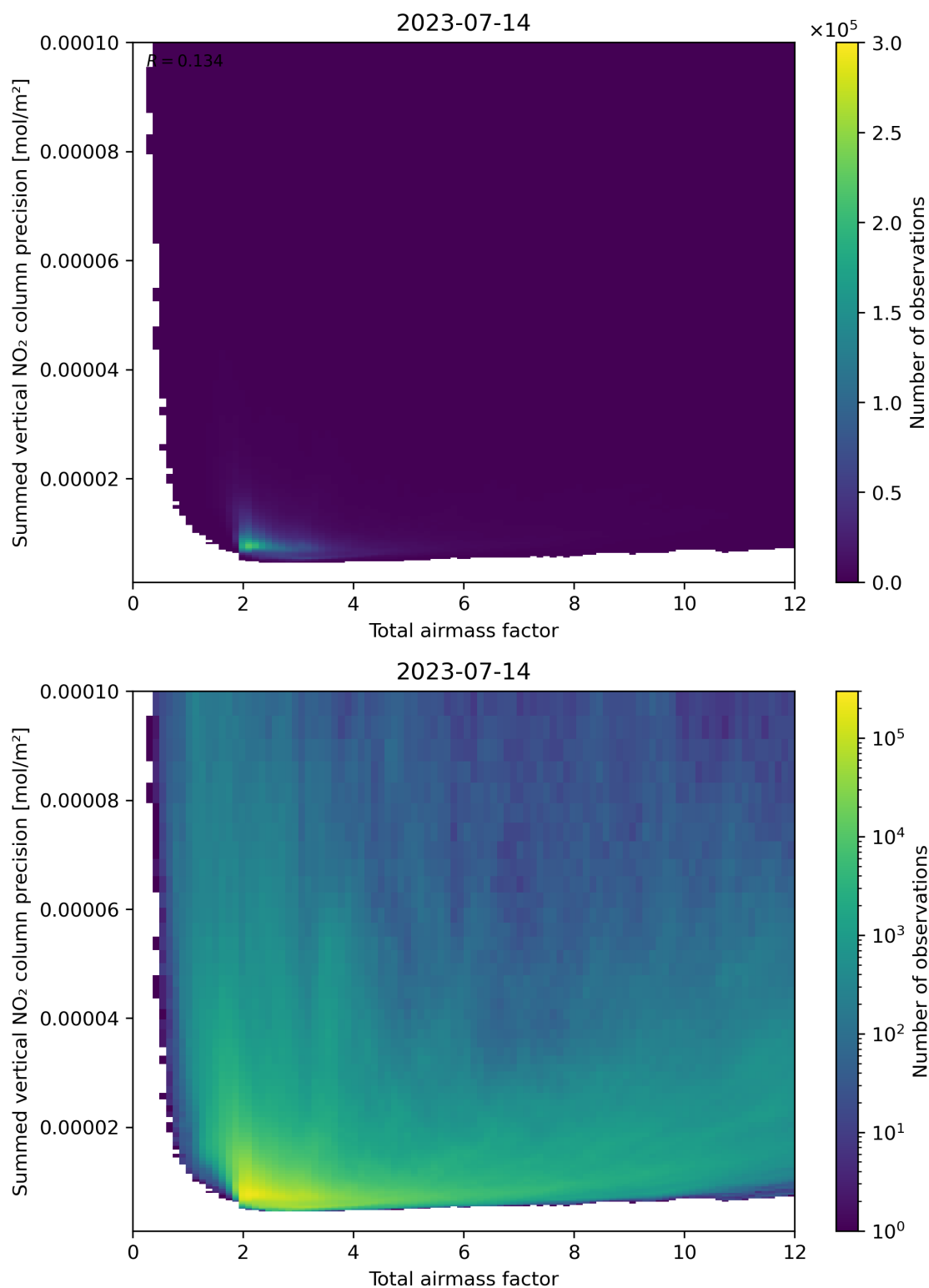
Figure 66: Scatter density plot of “Total airmass factor” against “Summed vertical NO 2 column precision” for 2023-07-14 to 2023-07-15.
