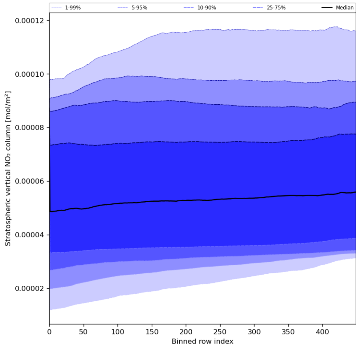
Figure 53: Along track statistics of “Stratospheric vertical NO 2 column” for 2023-07-14 to 2023-07-15
