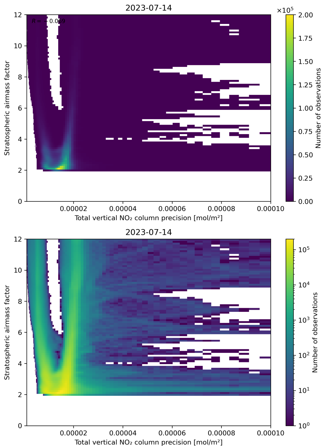
Figure 115: Scatter density plot of “Total vertical NO 2 column precision” against “Stratospheric air mass factor” for 2023-07-14 to 2023-07-15.
