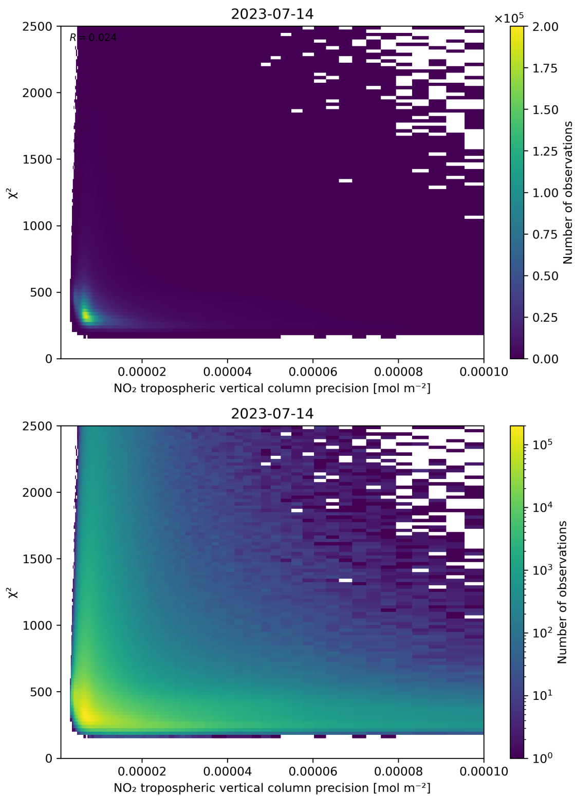
Figure 134: Scatter density plot of “NO 2 tropospheric vertical column precision” against “ \chi^2 ” for 2023-07-14 to 2023-07-15.
