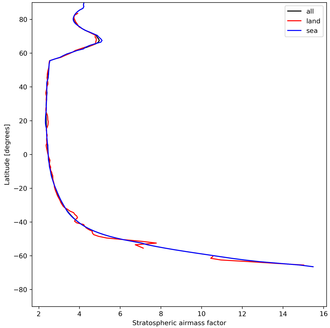
Figure 27: Zonal average of “Stratospheric airmass factor” for 2023-07-14 to 2023-07-15.
