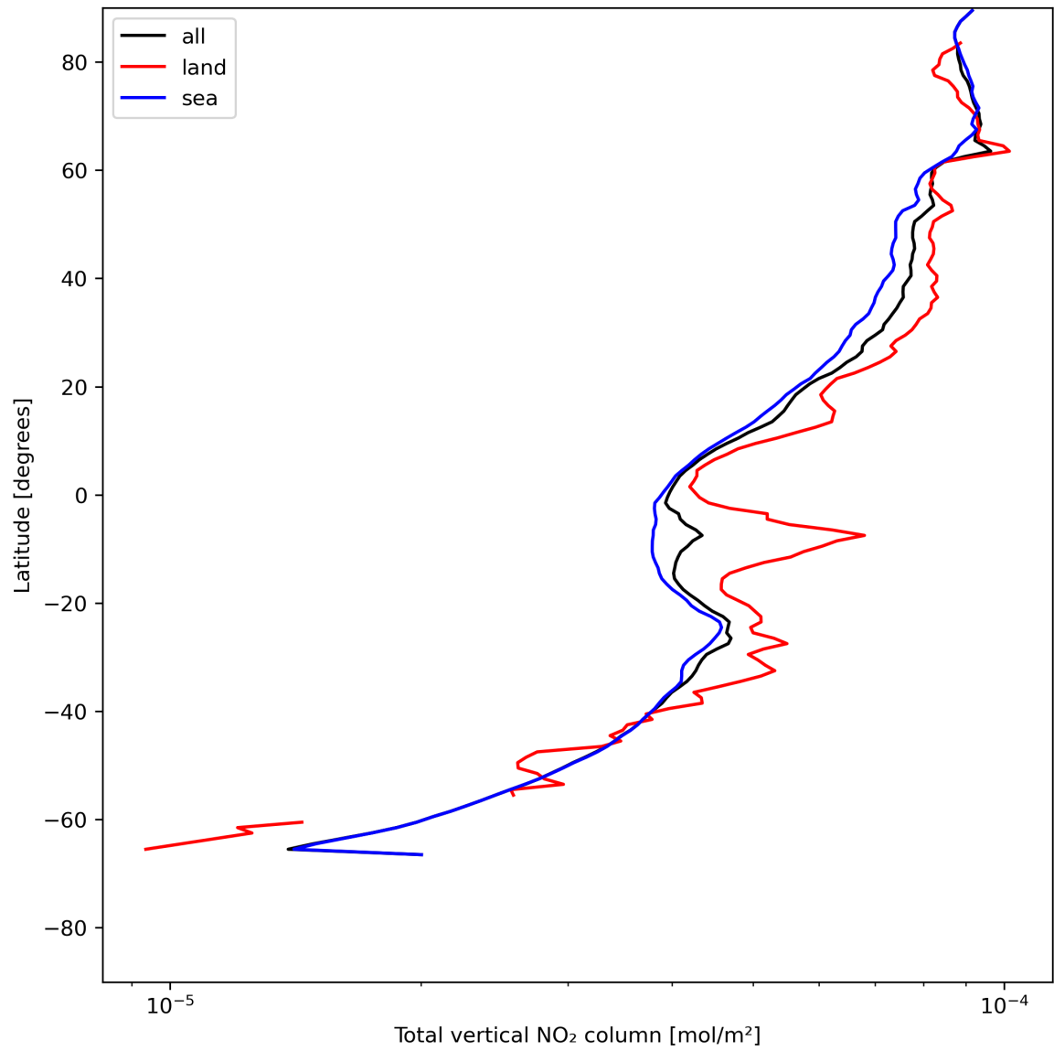
Figure 21: Zonal average of “Total vertical NO 2 column” for 2023-07-14 to 2023-07-15.
