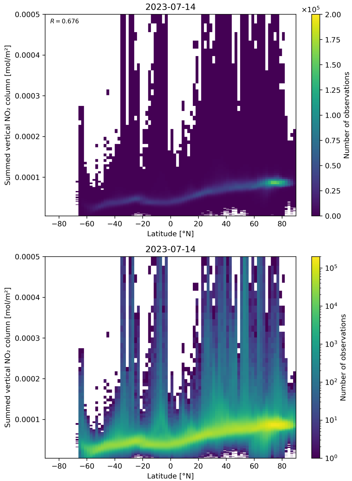
Figure 88: Scatter density plot of “Latitude” against “Summed vertical NO 2 column” for 2023-07-14 to 2023-07-15.
