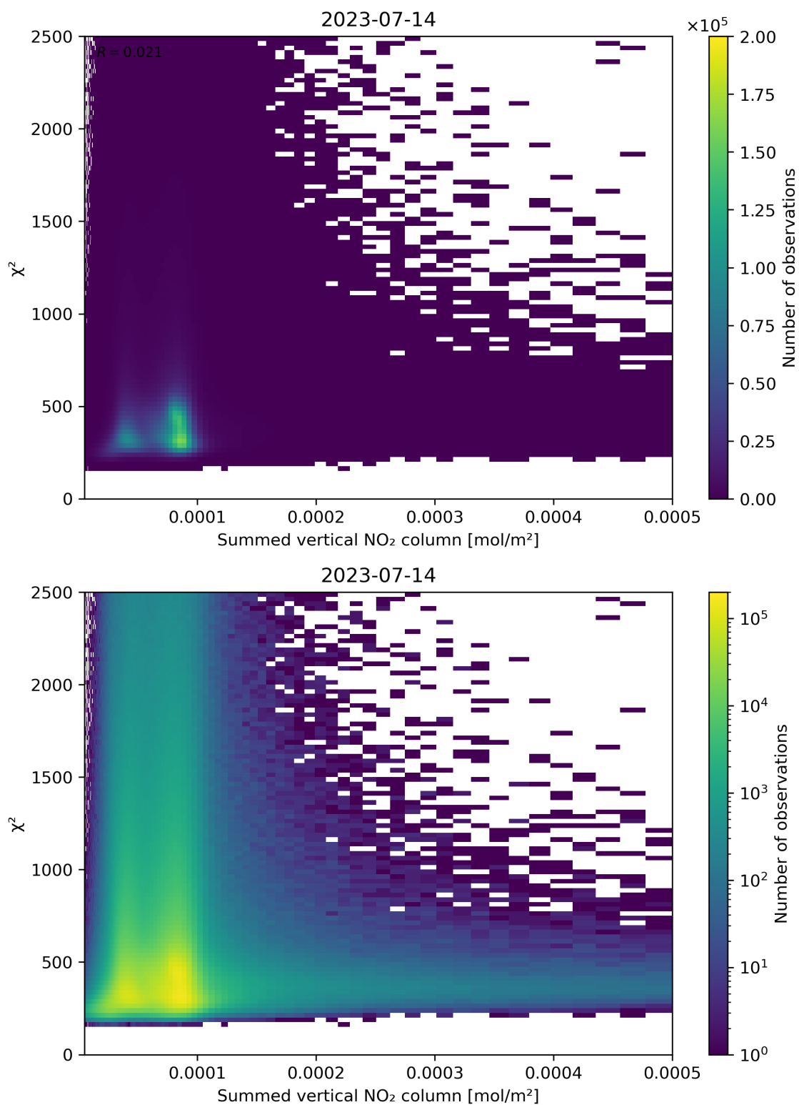
Figure 104: Scatter density plot of “Summed vertical NO 2 column” against “ \chi^2 ” for 2023-07-14 to 2023-07-15.
