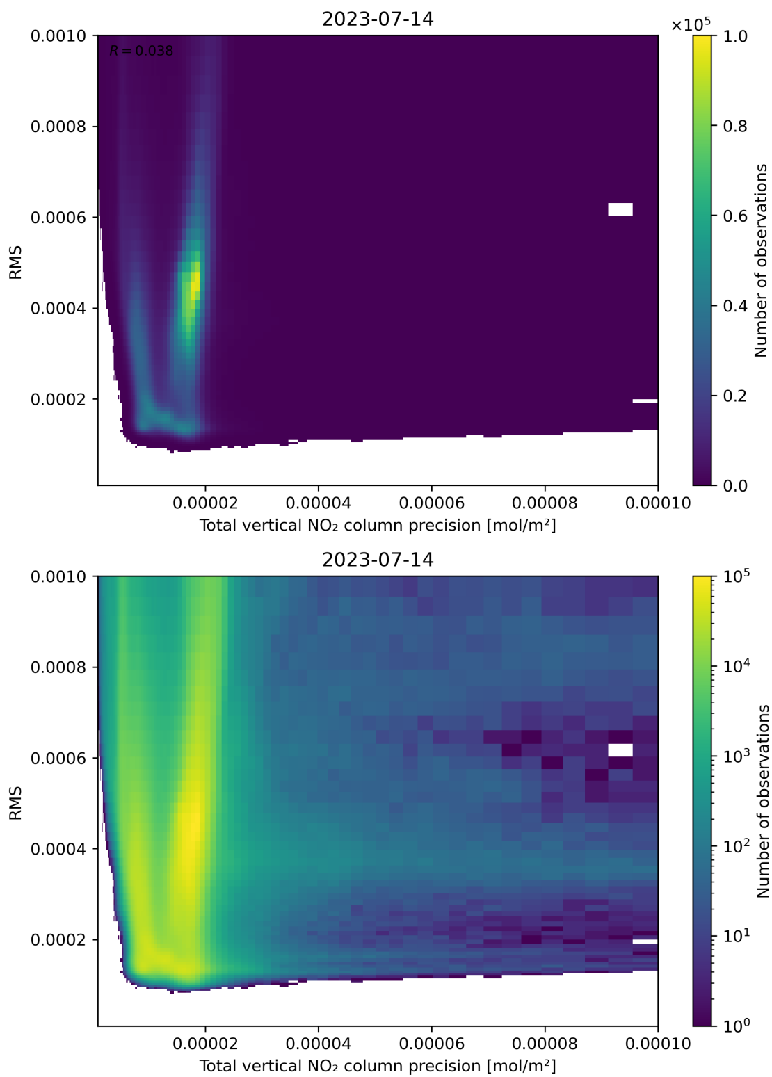
Figure 119: Scatter density plot of “Total vertical NO 2 column precision” against “RMS” for 2023-07-14 to 2023-07-15.
