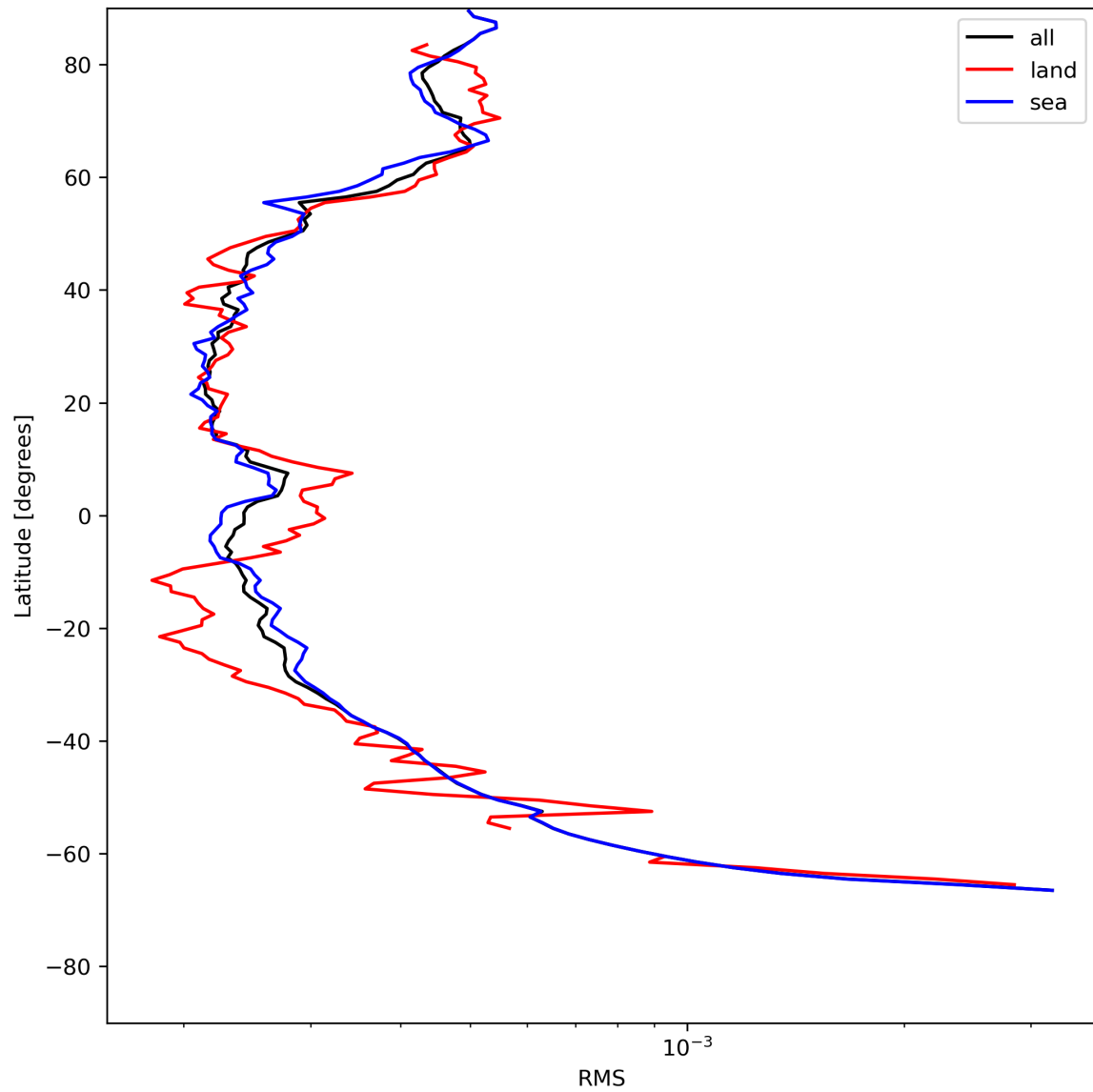
Figure 26: Zonal average of “RMS” for 2023-07-14 to 2023-07-15.
