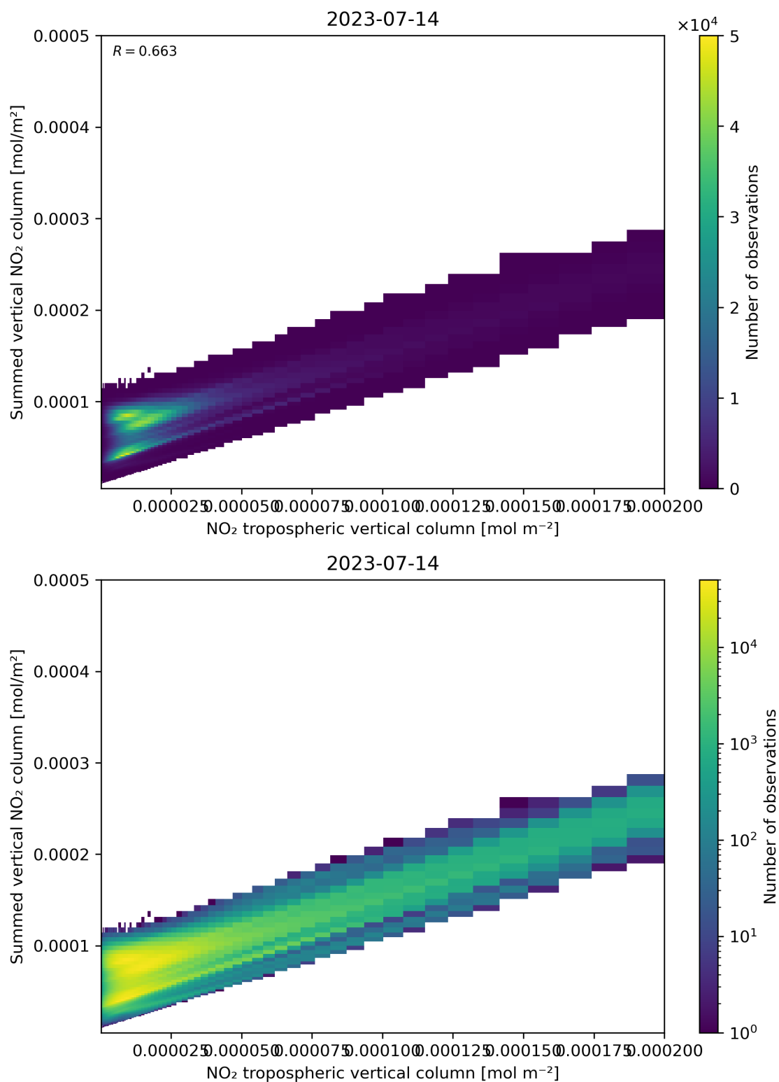
Figure 126: Scatter density plot of “NO 2 tropospheric vertical column” against “Summed vertical NO 2 column” for 2023-07-14 to 2023-07-15.
