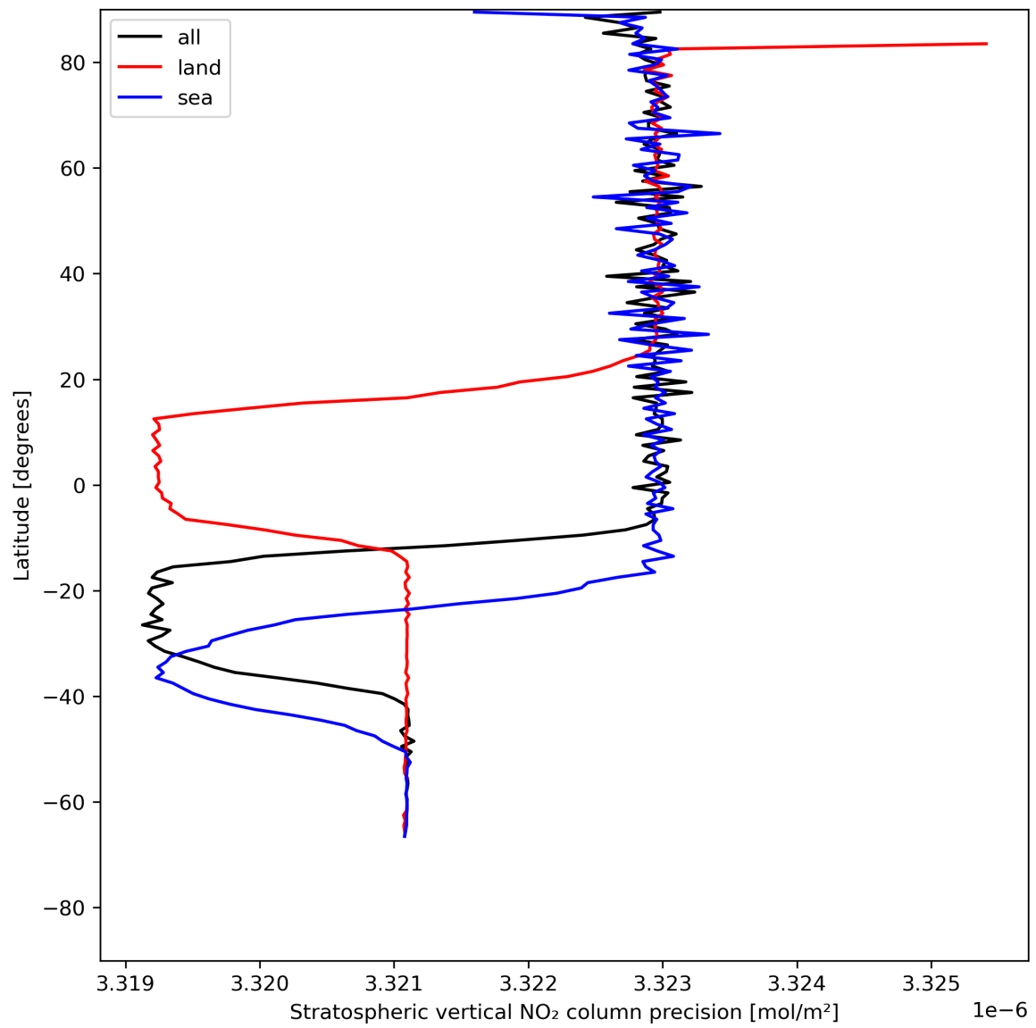
Figure 20: Zonal average of “Stratospheric vertical NO 2 column precision” for 2023-07-14 to 2023-07-15.
