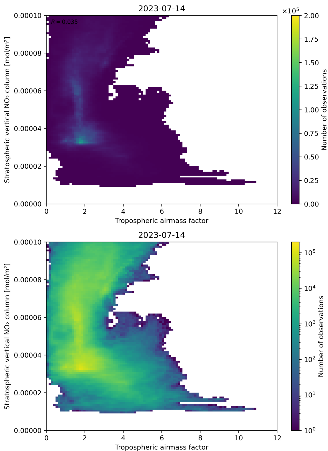
Figure 74: Scatter density plot of “Tropospheric air mass factor” against “Stratospheric vertical NO 2 column” for 2023-07-14 to 2023-07-15.
