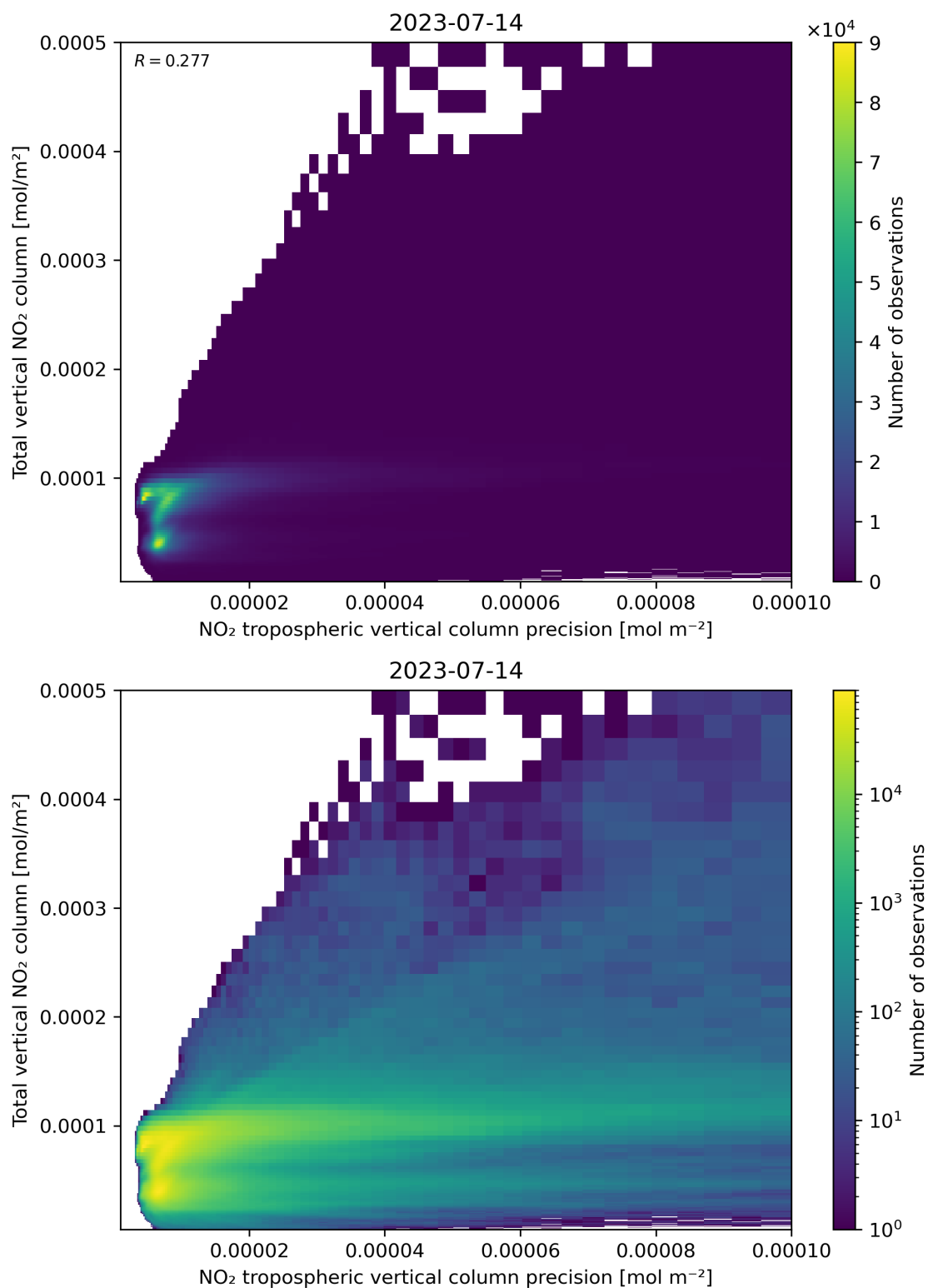
Figure 138: Scatter density plot of “NO 2 tropospheric vertical column precision” against “Total vertical NO 2 column” for 2023-07-14 to 2023-07-15.
