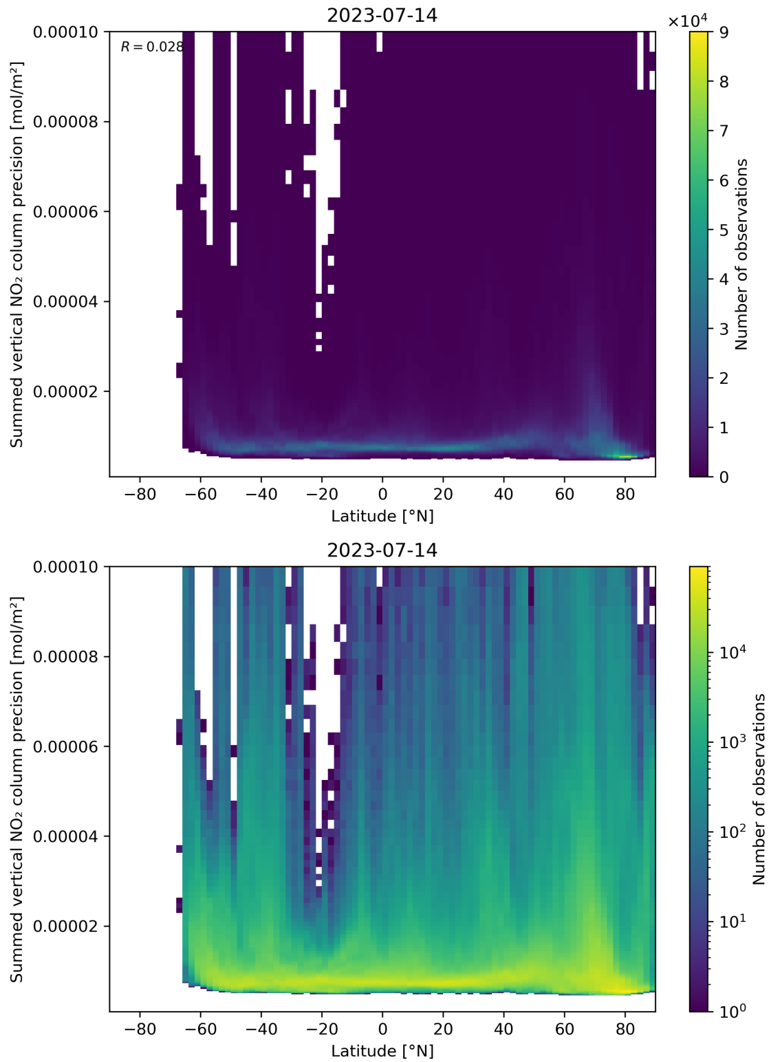
Figure 89: Scatter density plot of “Latitude” against “Summed vertical NO 2 column precision” for 2023-07-14 to 2023-07-15.
