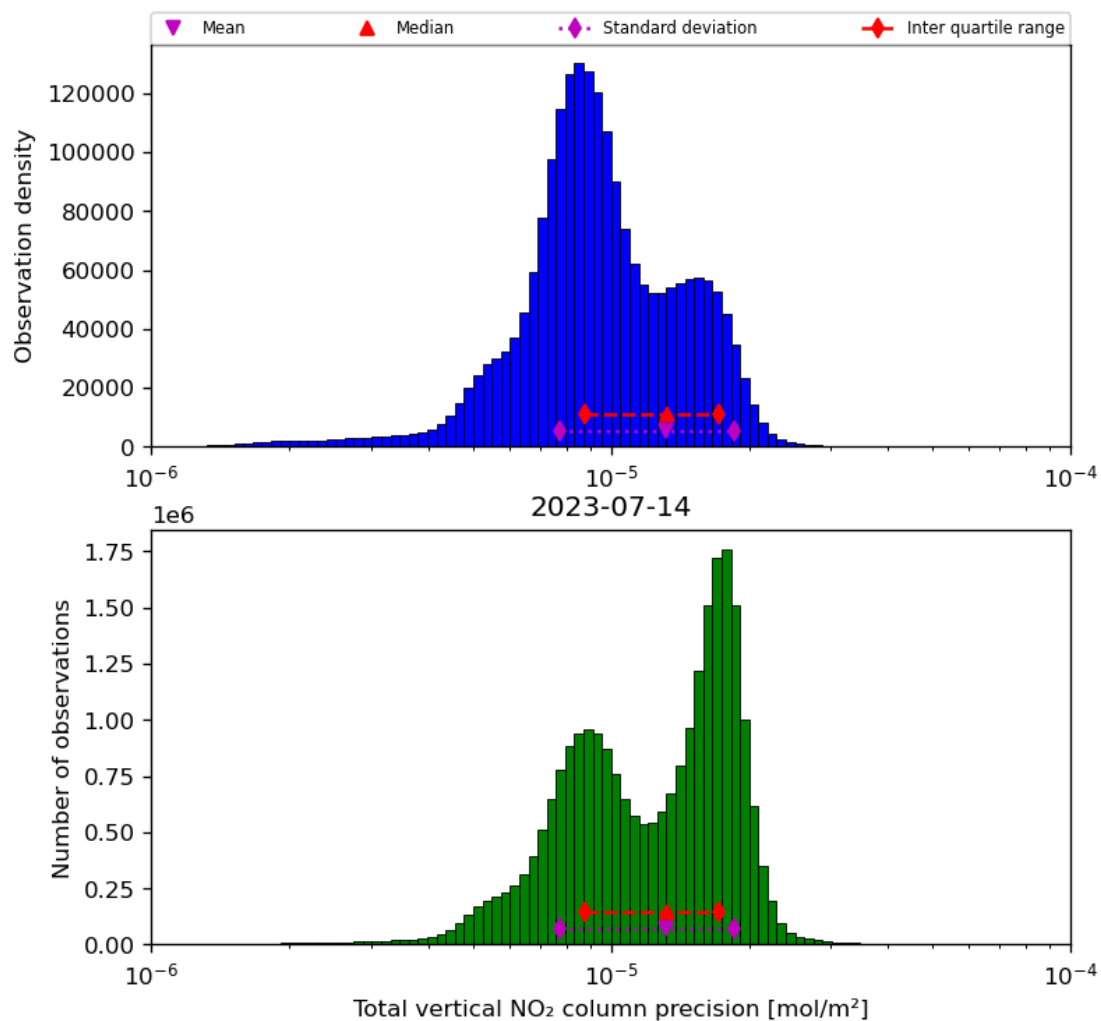
Figure 39: Histogram of “Total vertical NO 2 column precision” for 2023-07-14 to 2023-07-15
