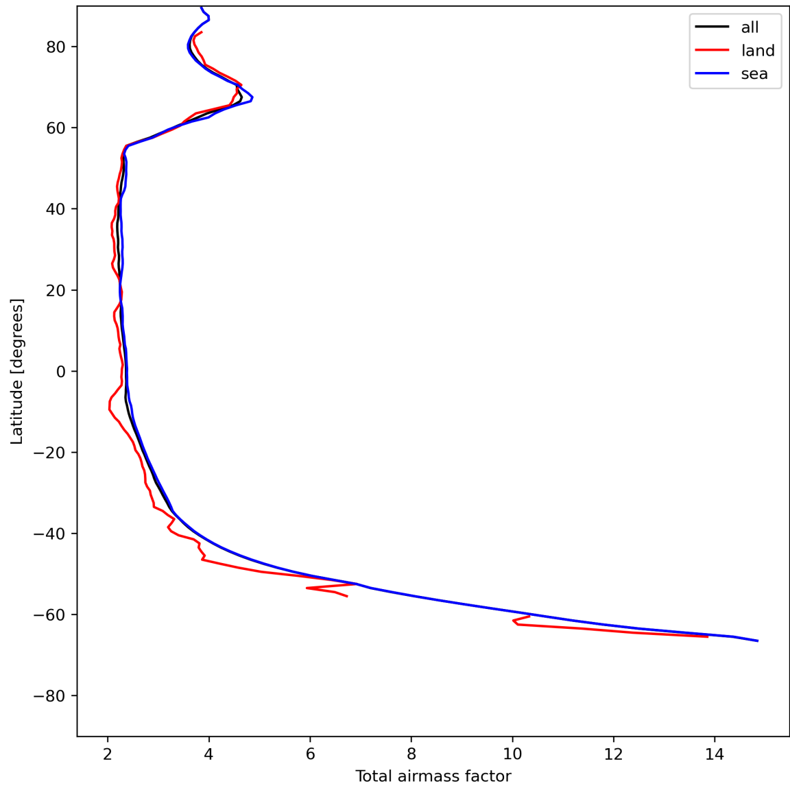
Figure 15: Zonal average of “Total airmass factor” for 2023-07-14 to 2023-07-15.
