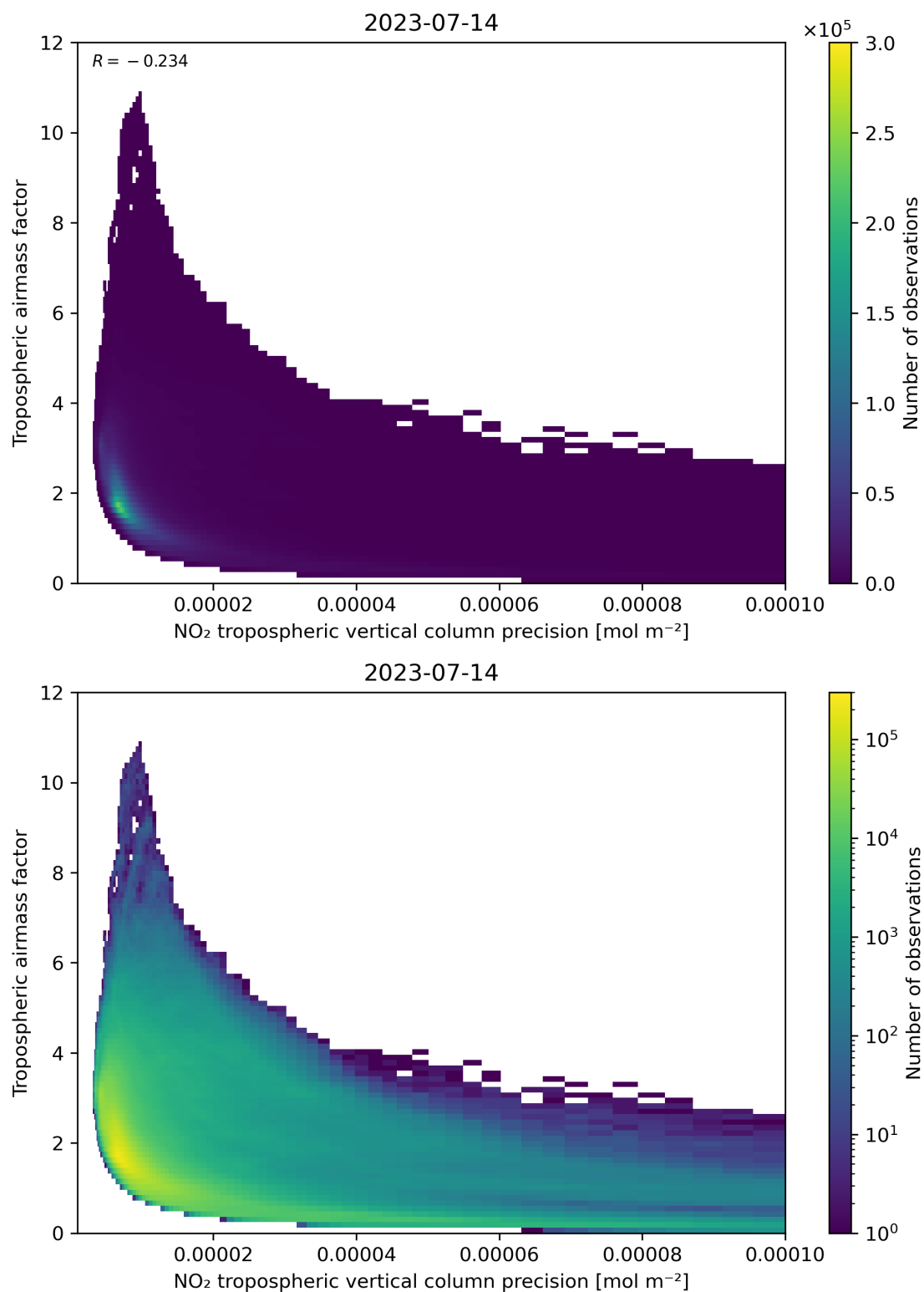
Figure 133: Scatter density plot of “NO 2 tropospheric vertical column precision” against “Tropospheric airmass factor” for 2023-07-14 to 2023-07-15.
