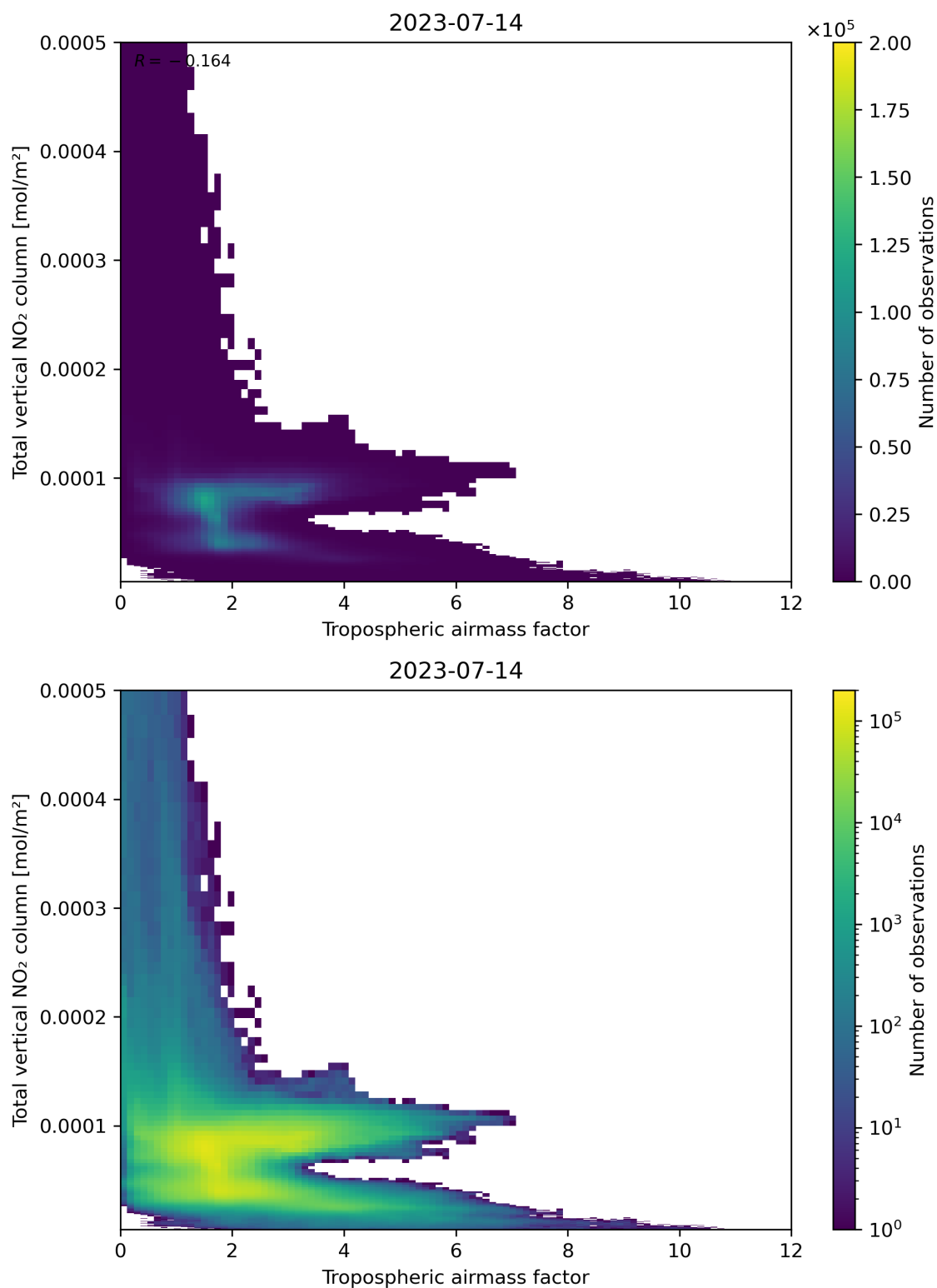
Figure 77: Scatter density plot of “Tropospheric airmass factor” against “Total vertical NO 2 column” for 2023-07-14 to 2023-07-15.
