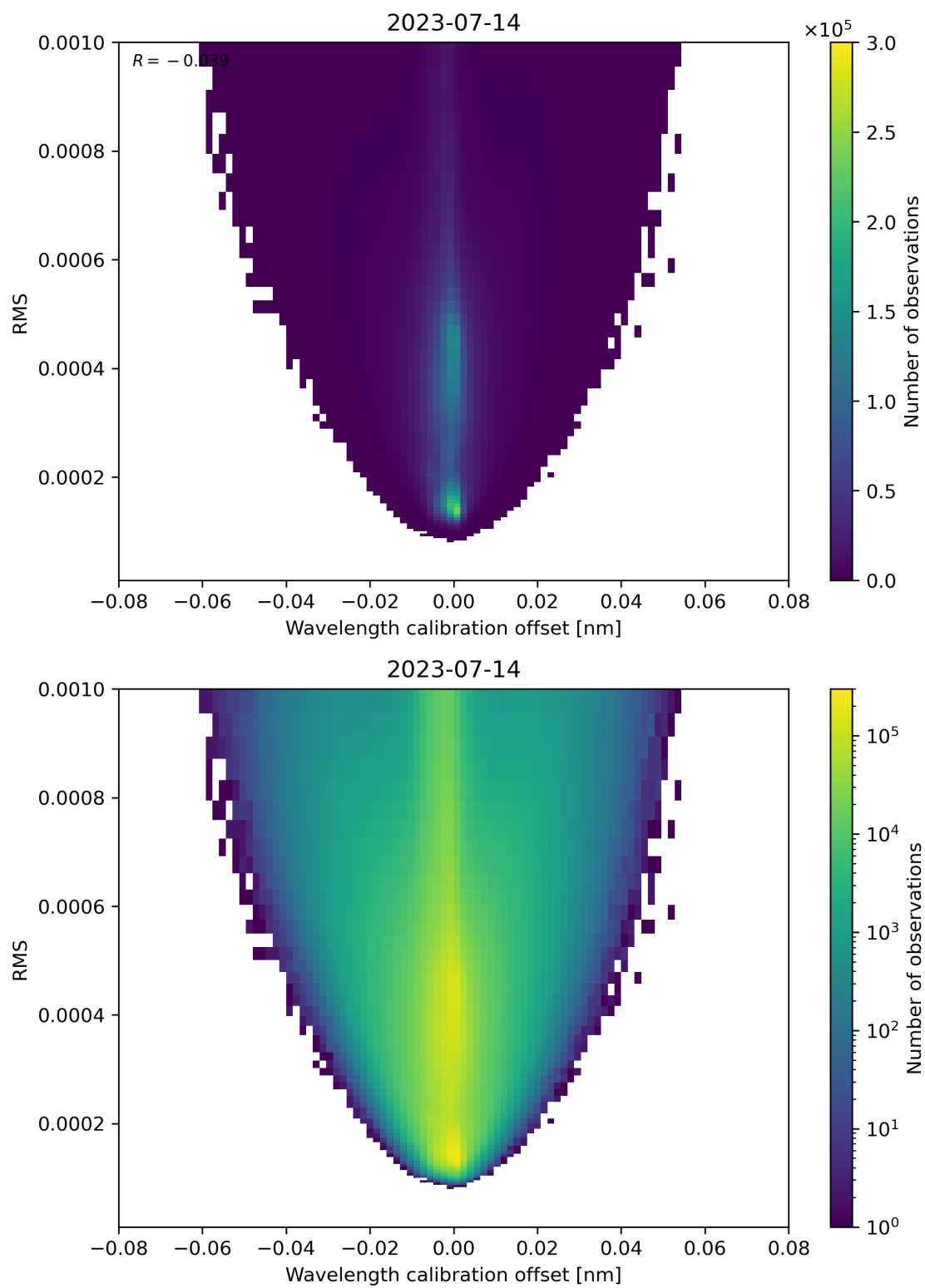
Figure 181: Scatter density plot of “Wavelength calibration offset” against “RMS” for 2023-07-14 to 2023-07-15.
