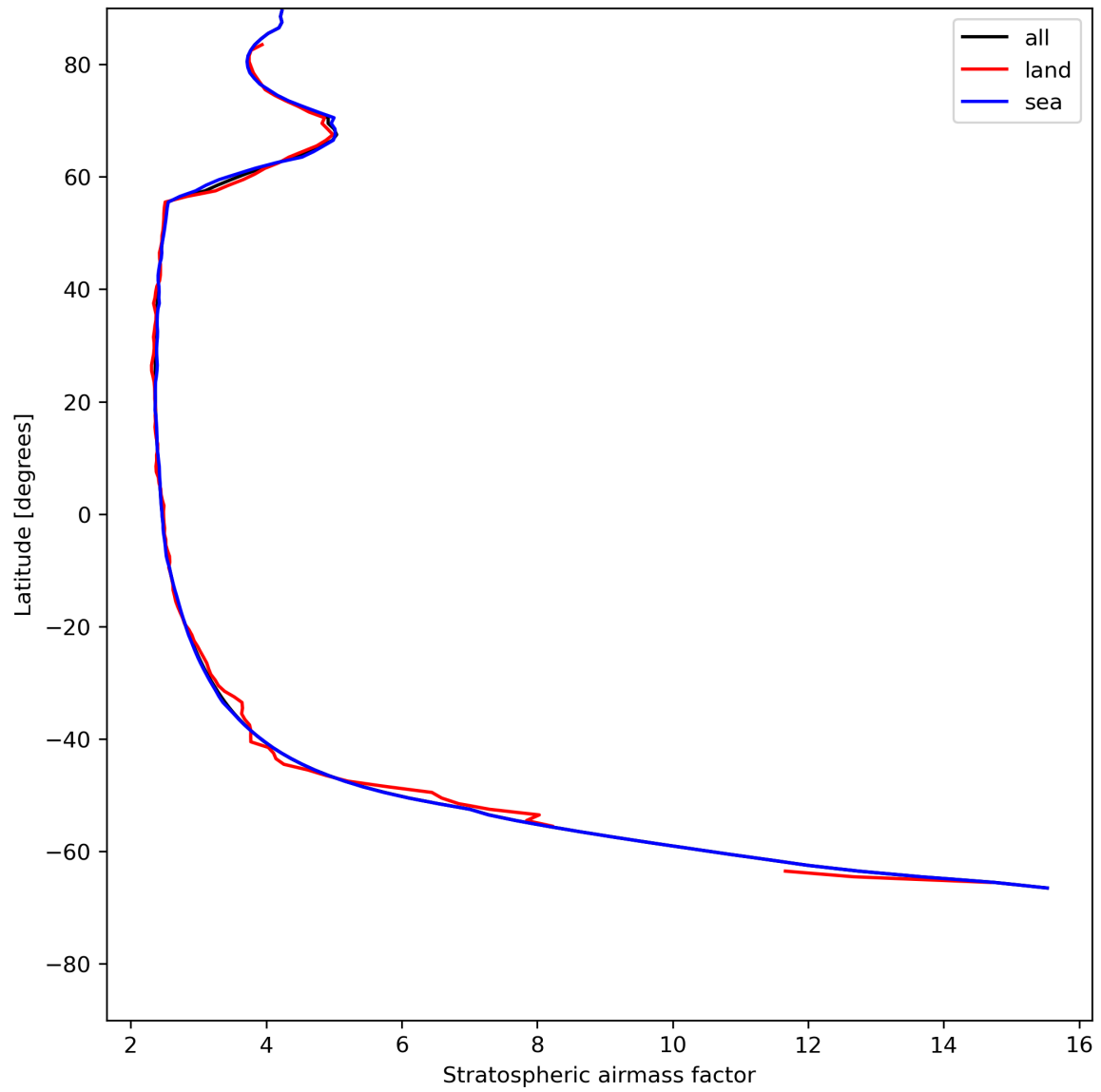
Figure 27: Zonal average of “Stratospheric airmass factor” for 2023-07-14 to 2023-07-16.
