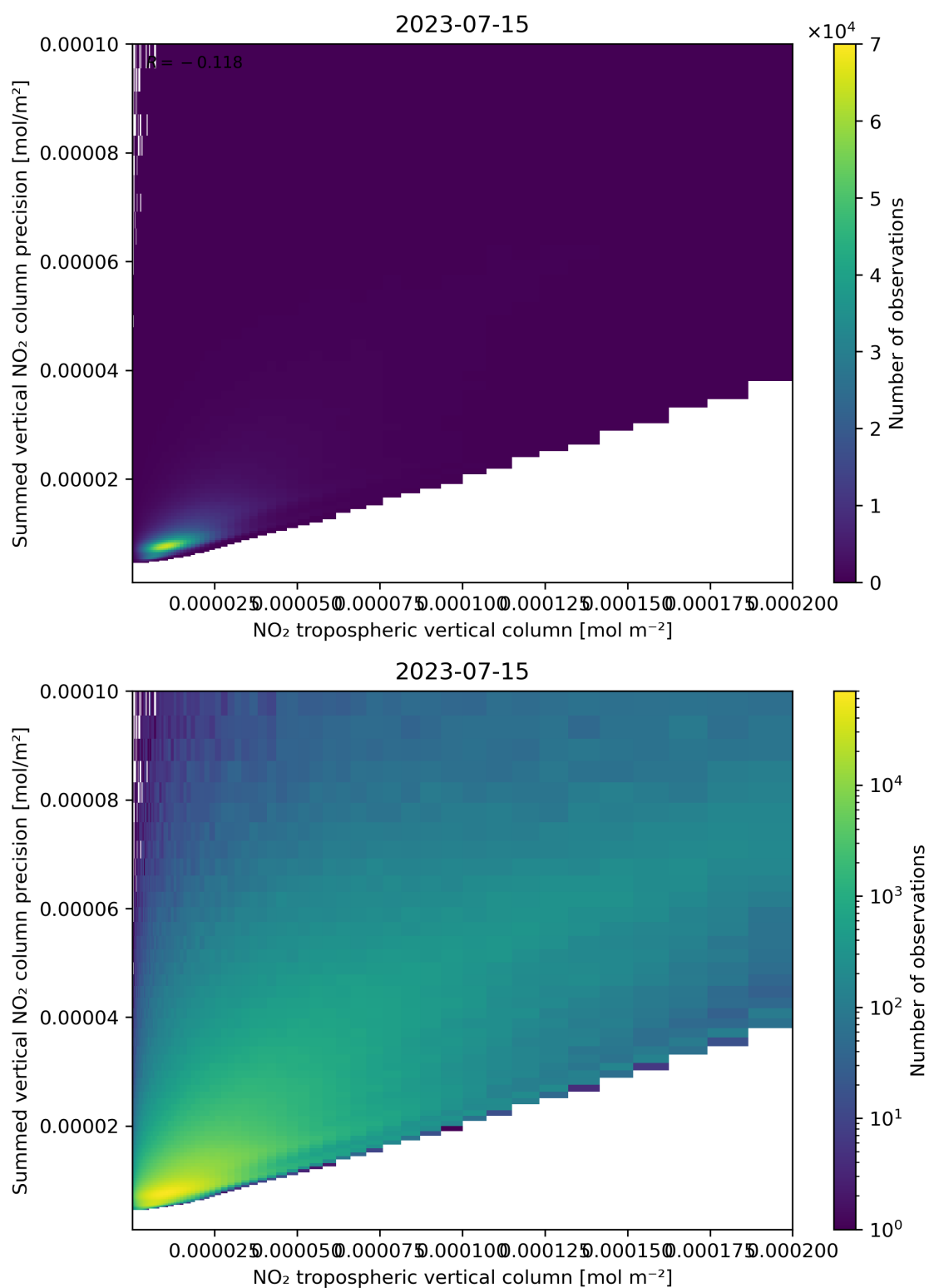
Figure 127: Scatter density plot of “NO 2 tropospheric vertical column” against “Summed vertical NO 2 column precision” for 2023-07-14 to 2023-07-16.
