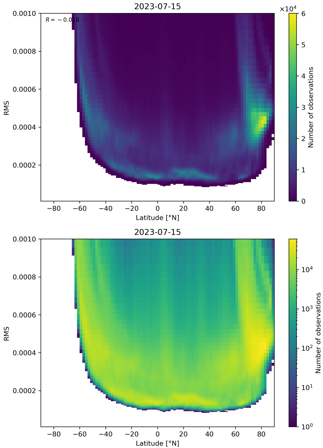
Figure 94: Scatter density plot of “Latitude” against “RMS” for 2023-07-14 to 2023-07-16.
