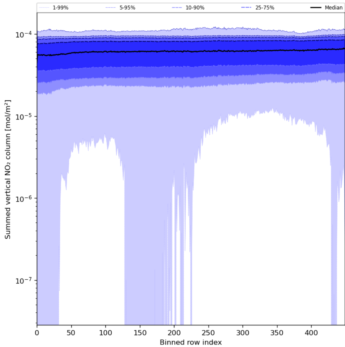
Figure 57: Along track statistics of “Summed vertical NO 2 column” for 2023-07-14 to 2023-07-16
