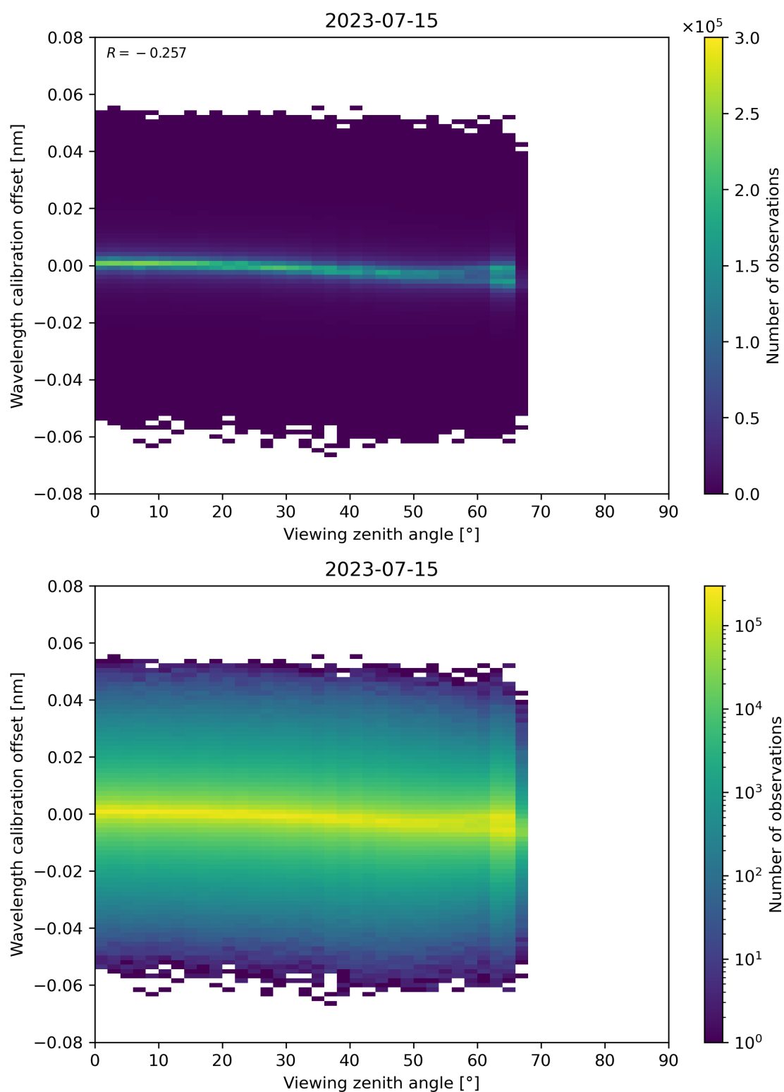
Figure 173: Scatter density plot of “Viewing zenith angle” against “Wavelength calibration offset” for 2023-07-14 to 2023-07-16.
