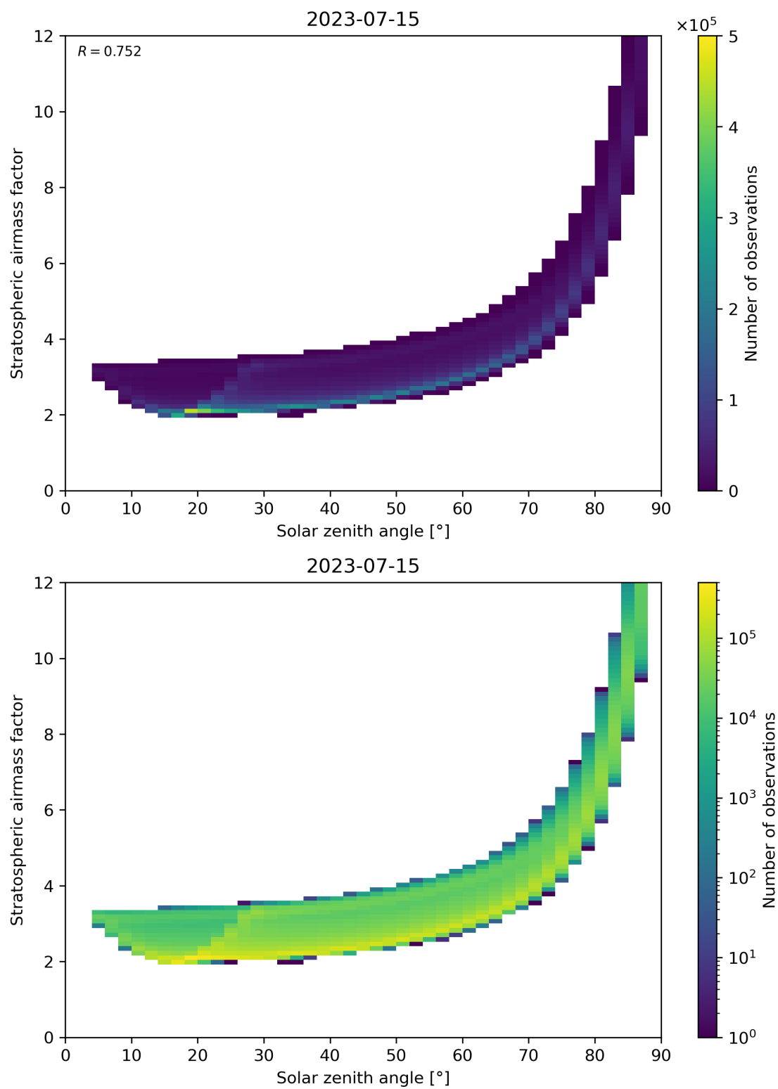
Figure 145: Scatter density plot of “Solar zenith angle” against “Stratospheric airmass factor” for 2023-07-14 to 2023-07-16.
