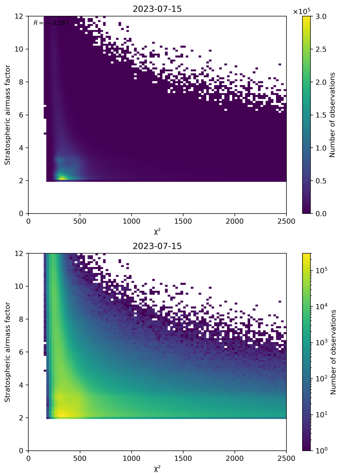
Figure 81: Scatter density plot of “ \chi^2 ” against “Stratospheric airmass factor” for 2023-07-14 to 2023-07-16.
