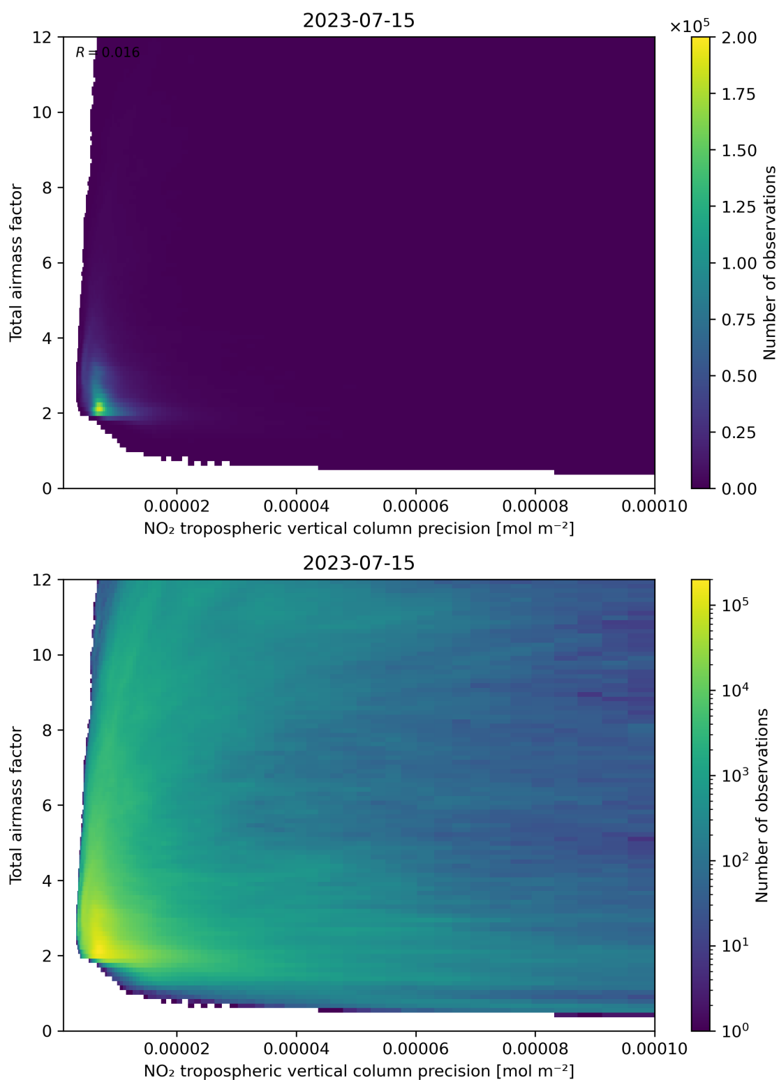
Figure 132: Scatter density plot of “NO 2 tropospheric vertical column precision” against “Total air mass factor” for 2023-07-14 to 2023-07-16.
