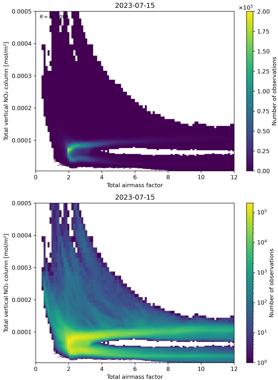
Figure 67: Scatter density plot of “Total airmass factor” against “Total vertical NO 2 column” for 2023-07-14 to 2023-07-16.
