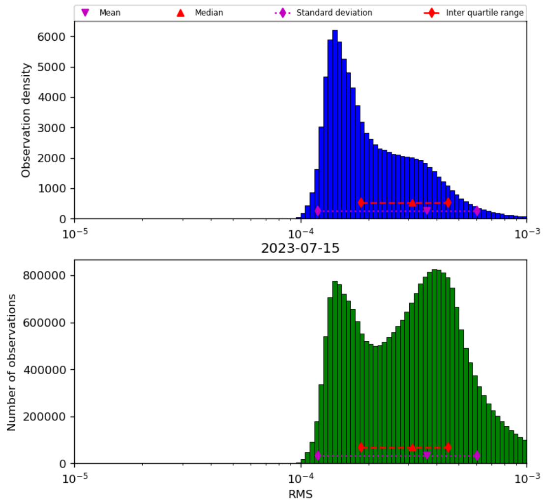
Figure 43: Histogram of “RMS” for 2023-07-14 to 2023-07-16
