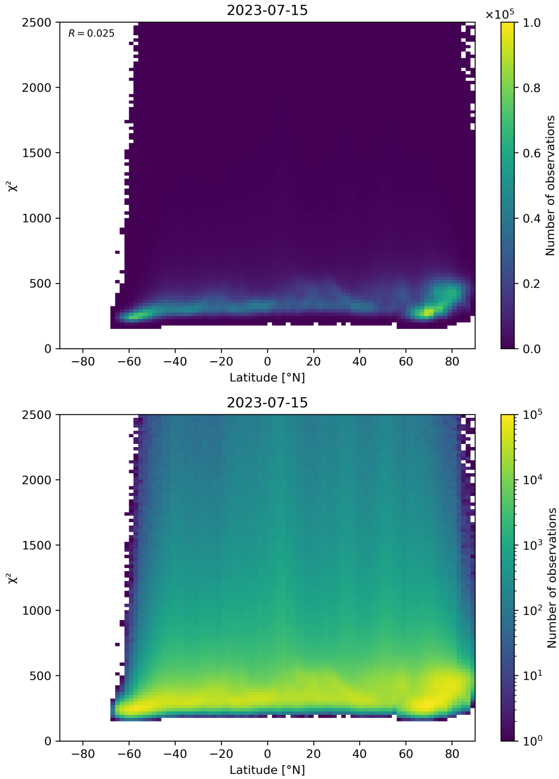
Figure 86: Scatter density plot of “Latitude” against “ \chi^2 ” for 2023-07-14 to 2023-07-16.
