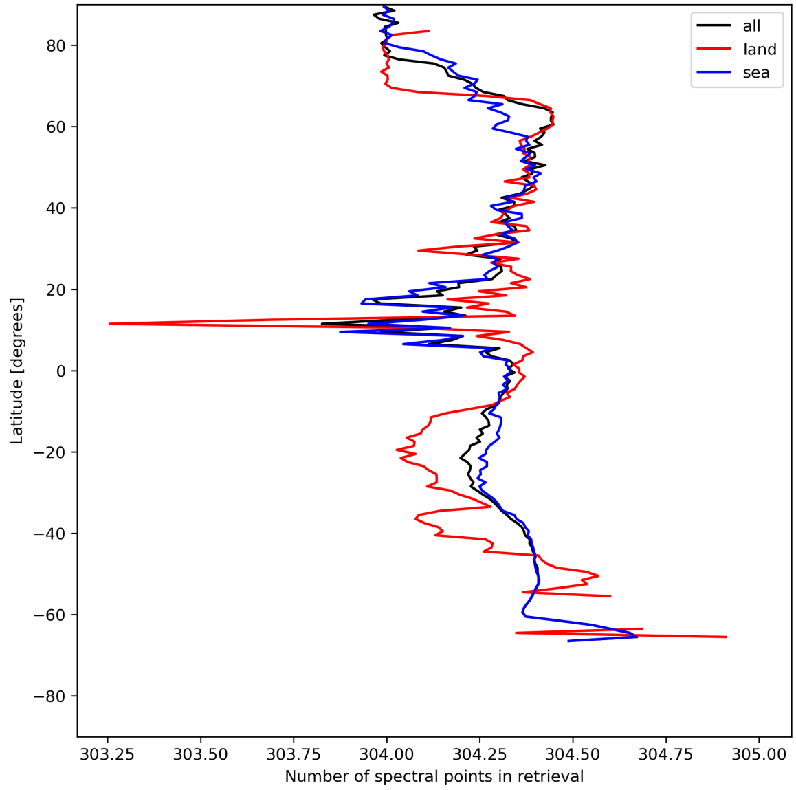
Figure 16: Zonal average of “Number of spectral points in retrieval” for 2023-07-14 to 2023-07-16.
