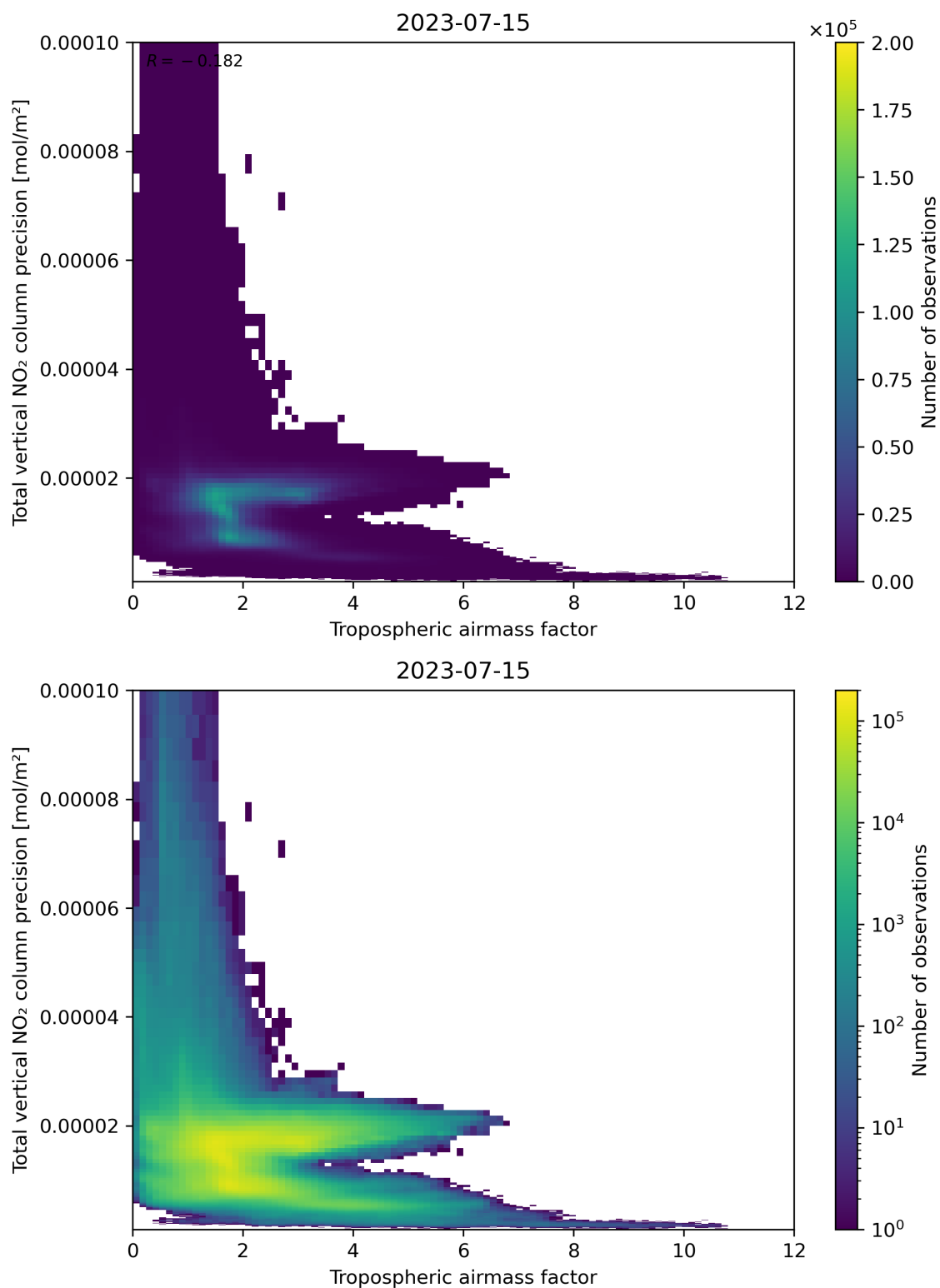
Figure 78: Scatter density plot of “Tropospheric air mass factor” against “Total vertical NO 2 column precision” for 2023-07-14 to 2023-07-16.
