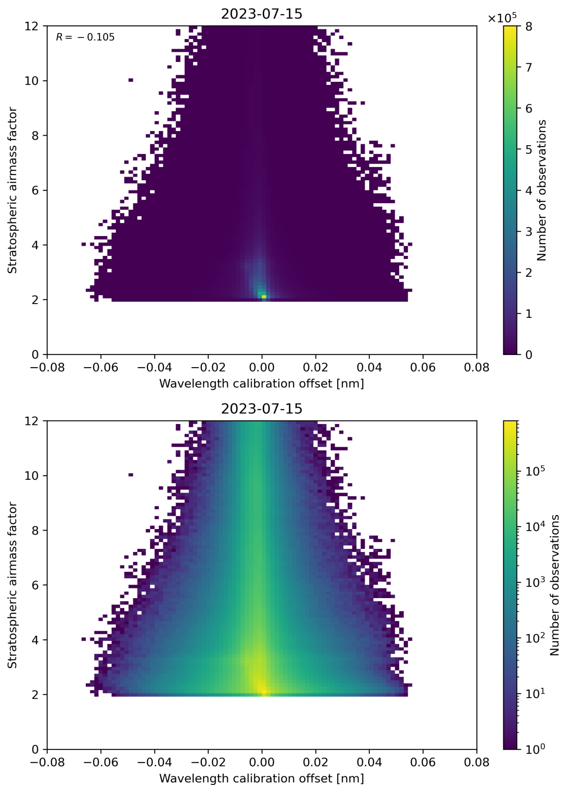
Figure 174: Scatter density plot of “Wavelength calibration offset” against “Stratospheric airmass factor” for 2023-07-14 to 2023-07-16.
