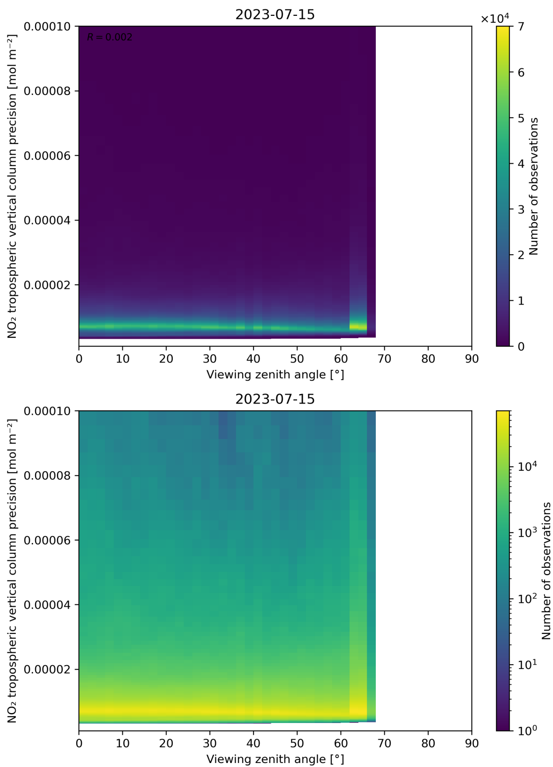
Figure 170: Scatter density plot of “Viewing zenith angle” against “NO 2 tropospheric vertical column precision” for 2023-07-14 to 2023-07-16.
