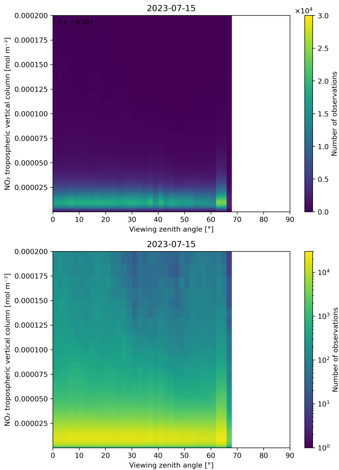
Figure 169: Scatter density plot of “Viewing zenith angle” against “NO 2 tropospheric vertical column” for 2023-07-14 to 2023-07-16.
