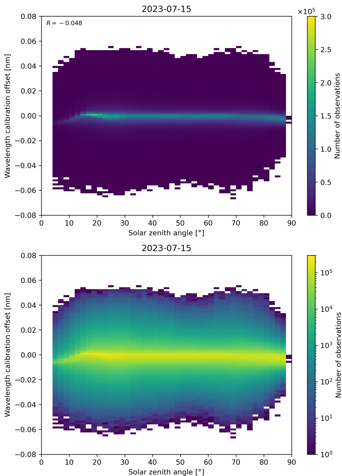
Figure 158: Scatter density plot of “Solar zenith angle” against “Wavelength calibration offset” for 2023-07-14 to 2023-07-16.
