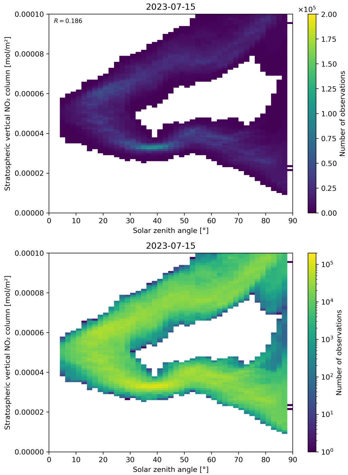
Figure 150: Scatter density plot of “Solar zenith angle” against “Stratospheric vertical NO 2 column” for 2023-07-14 to 2023-07-16.
