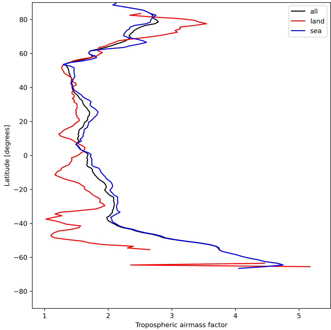
Figure 14: Zonal average of “Tropospheric airmass factor” for 2023-07-14 to 2023-07-16.
