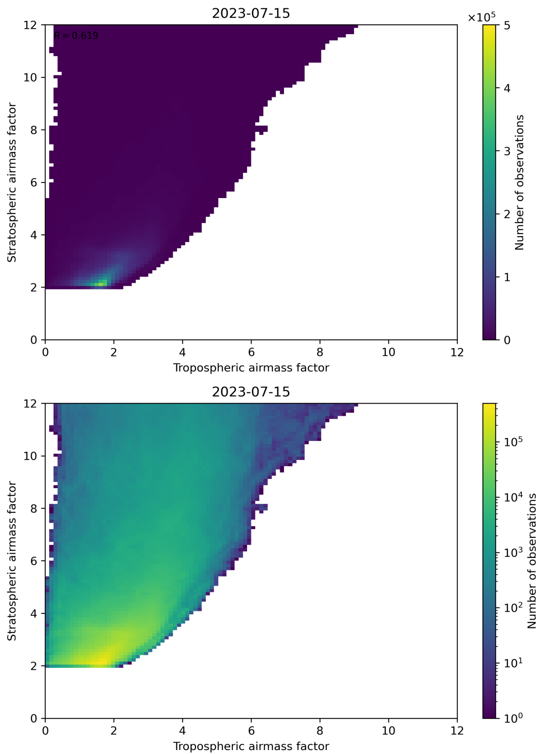
Figure 71: Scatter density plot of “Tropospheric airmass factor” against “Stratospheric airmass factor” for 2023-07-14 to 2023-07-16.
