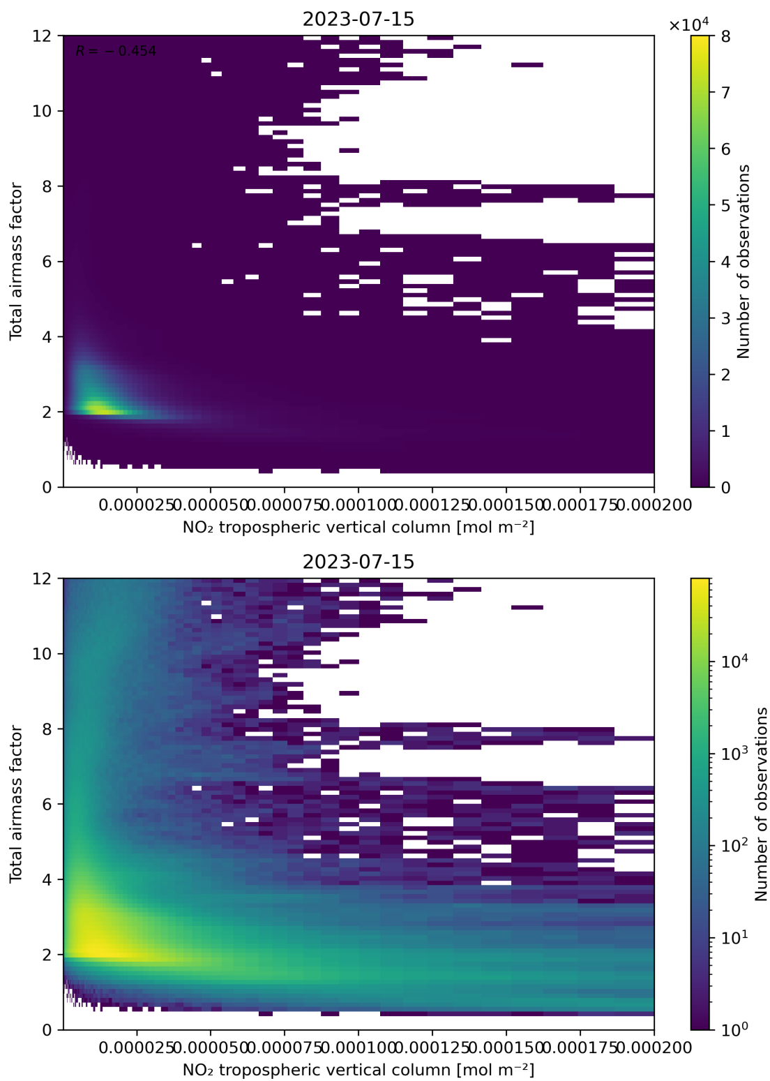
Figure 122: Scatter density plot of “NO 2 tropospheric vertical column” against “Total air mass factor” for 2023-07-14 to 2023-07-16.
