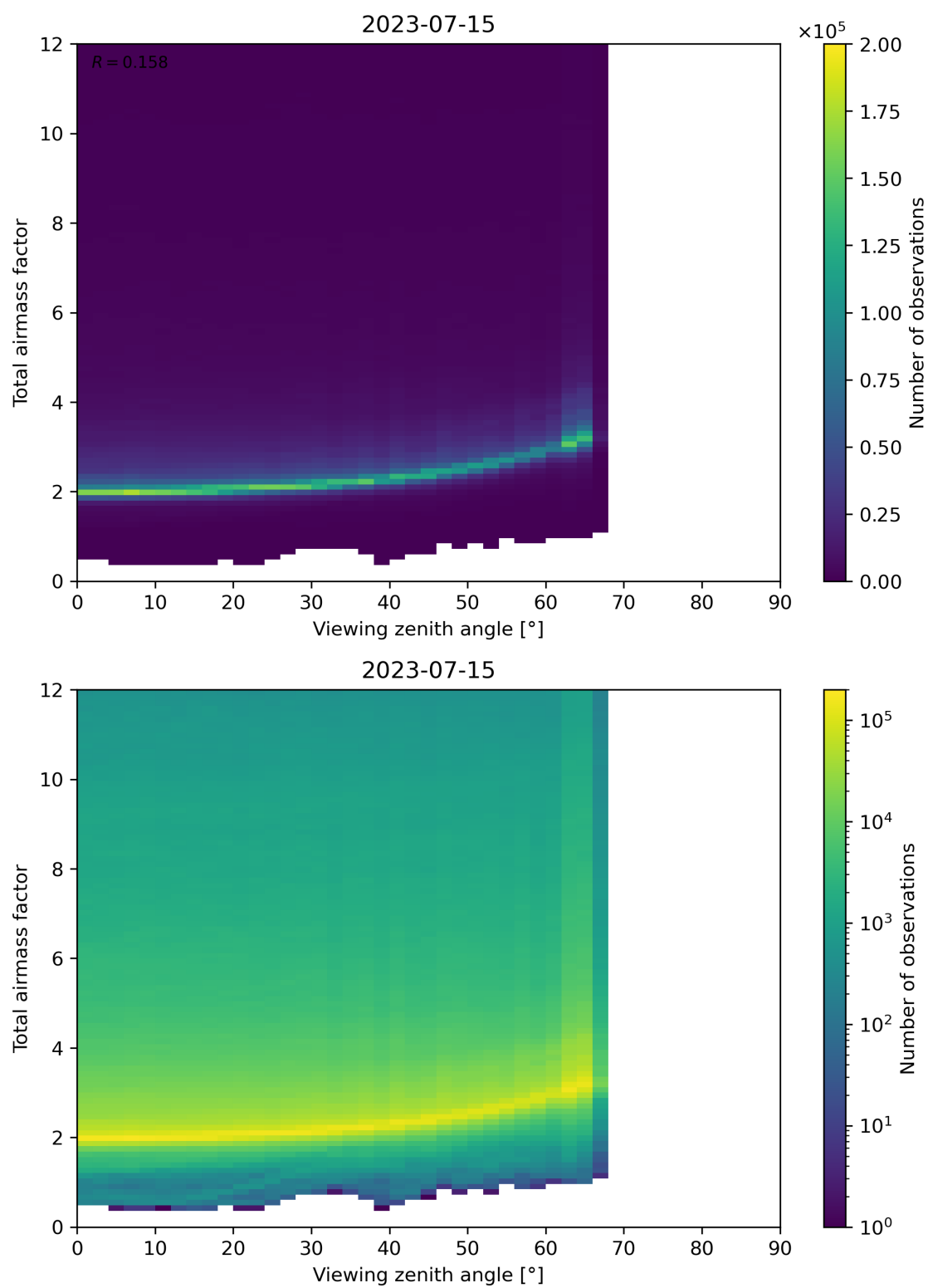
Figure 160: Scatter density plot of “Viewing zenith angle” against “Total airmass factor” for 2023-07-14 to 2023-07-16.
