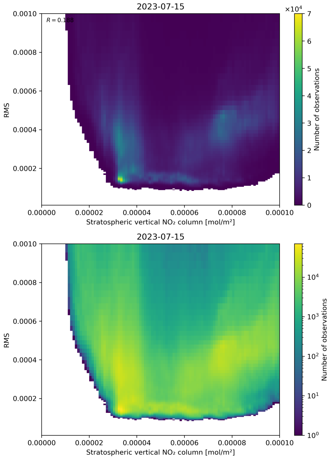
Figure 102: Scatter density plot of “Stratospheric vertical NO 2 column” against “RMS” for 2023-07-14 to 2023-07-16.
