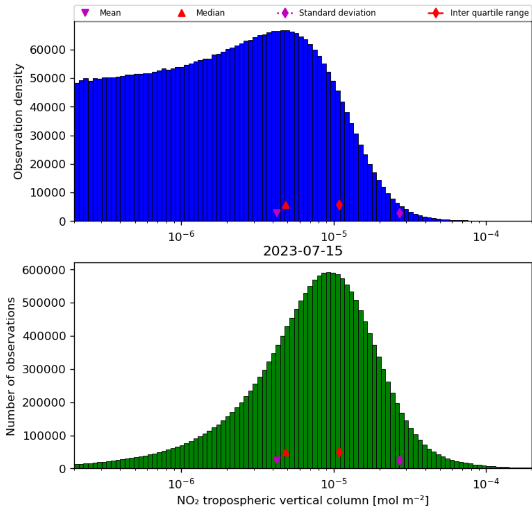
Figure 29: Histogram of “NO 2 tropospheric vertical column” for 2023-07-14 to 2023-07-16
