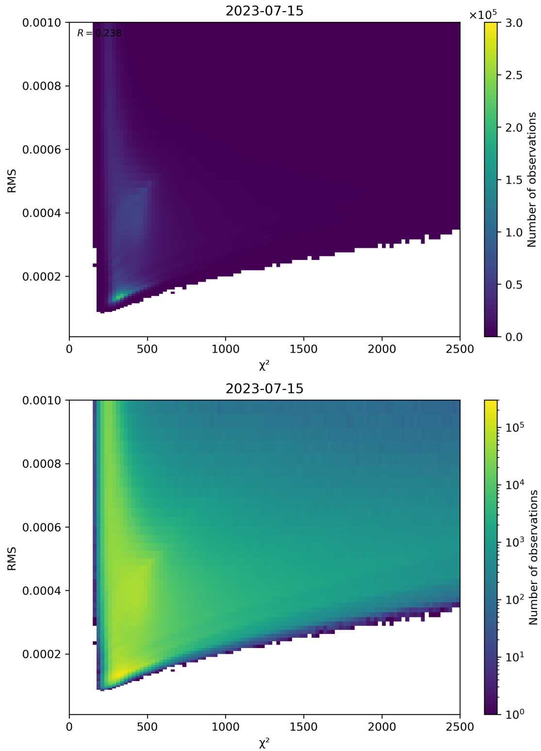
Figure 82: Scatter density plot of “ \chi^2 ” against “RMS” for 2023-07-14 to 2023-07-16.
