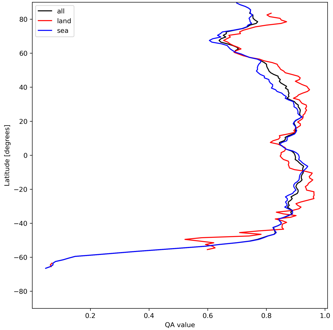
Figure 11: Zonal average of “QA value” for 2023-07-14 to 2023-07-16.
