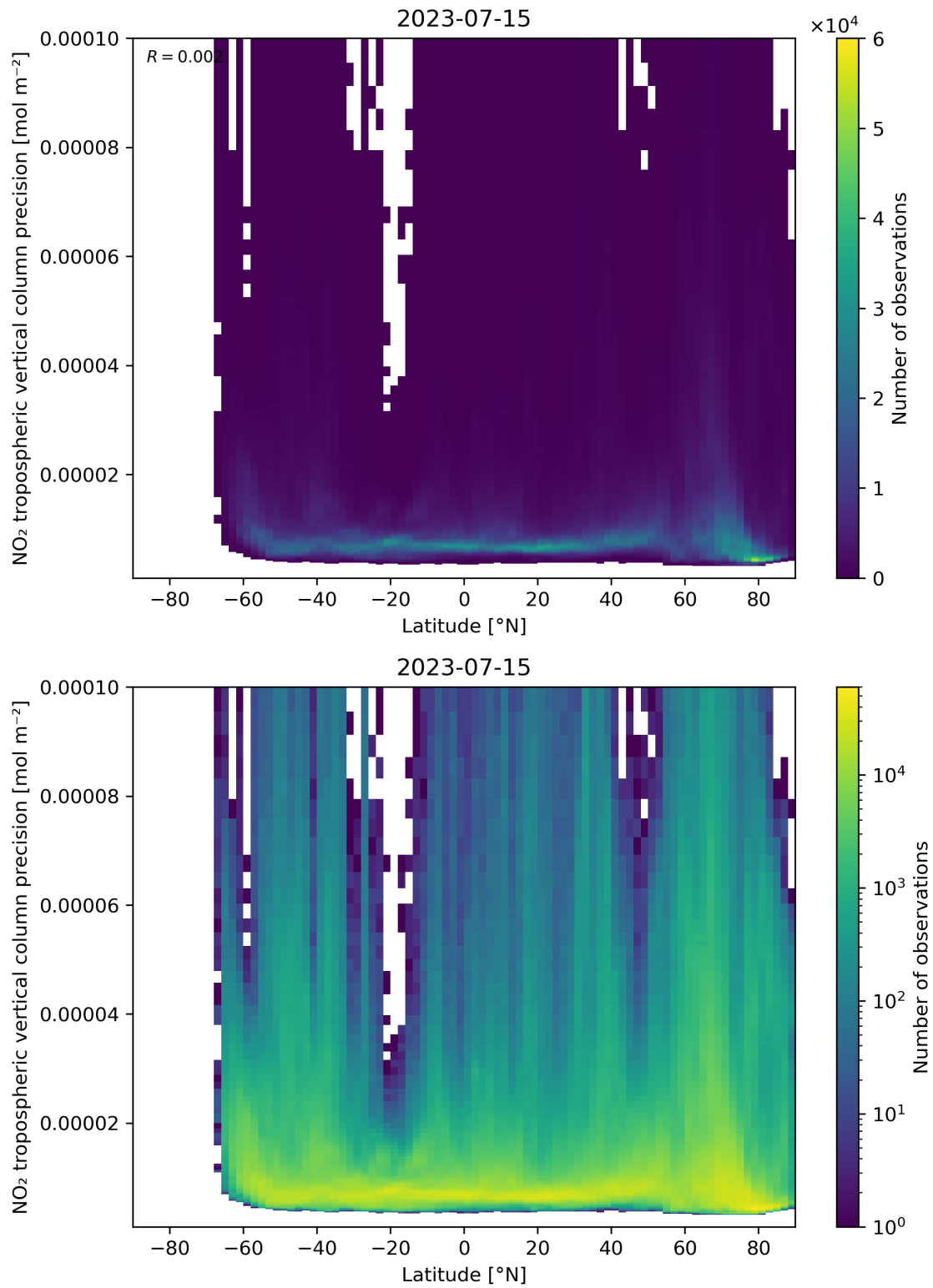
Figure 93: Scatter density plot of “Latitude” against “NO 2 tropospheric vertical column precision” for 2023-07-14 to 2023-07-16.
