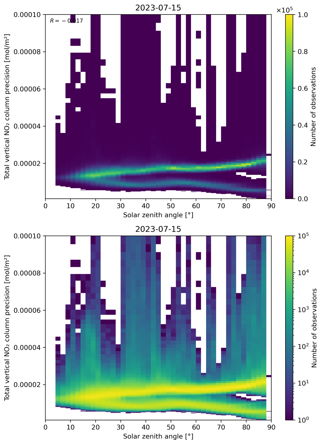
Figure 154: Scatter density plot of “Solar zenith angle” against “Total vertical NO 2 column precision” for 2023-07-14 to 2023-07-16.
