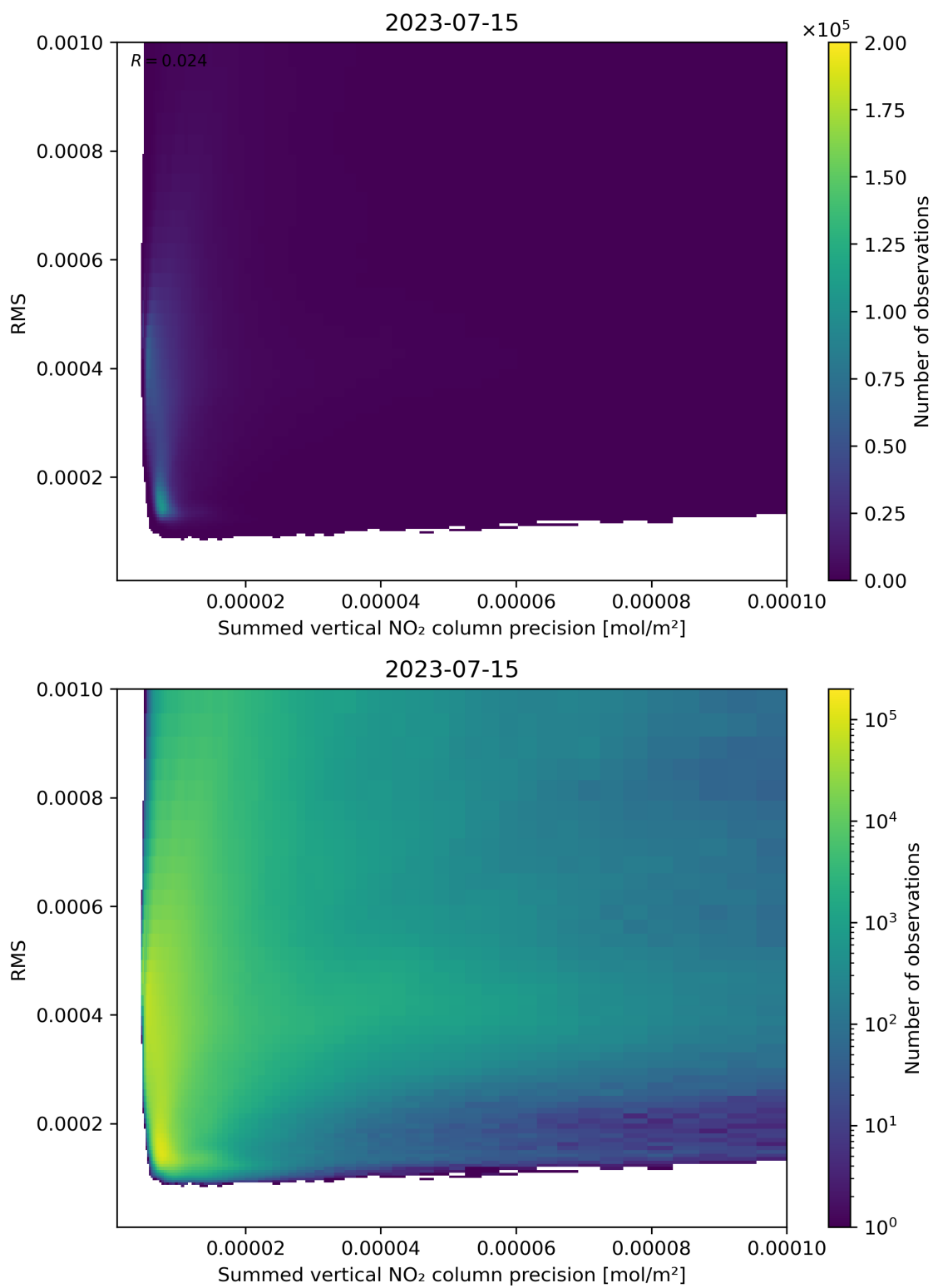
Figure 108: Scatter density plot of “Summed vertical NO 2 column precision” against “RMS” for 2023-07-14 to 2023-07-16.
