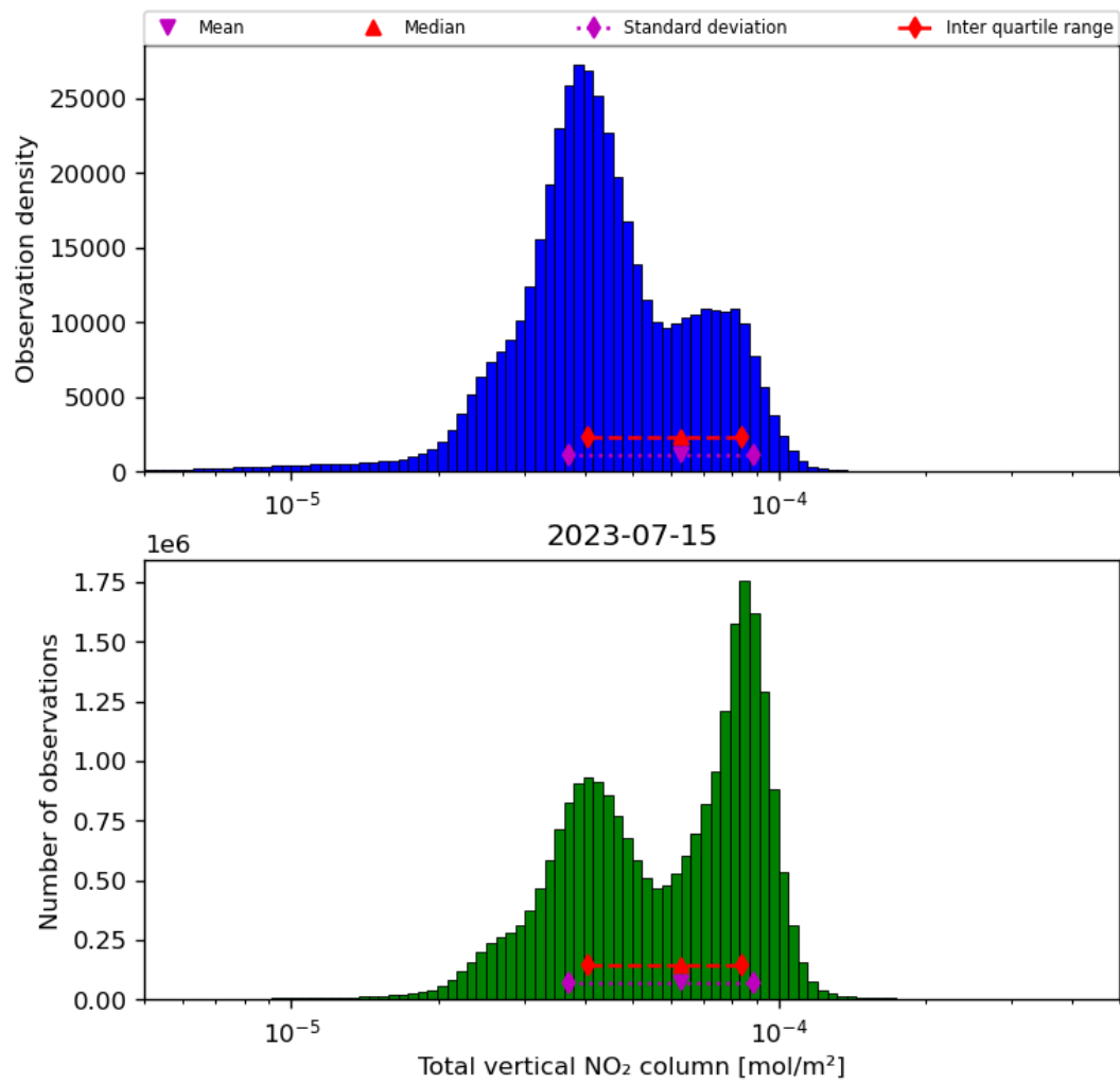
Figure 38: Histogram of “Total vertical NO 2 column” for 2023-07-14 to 2023-07-16
