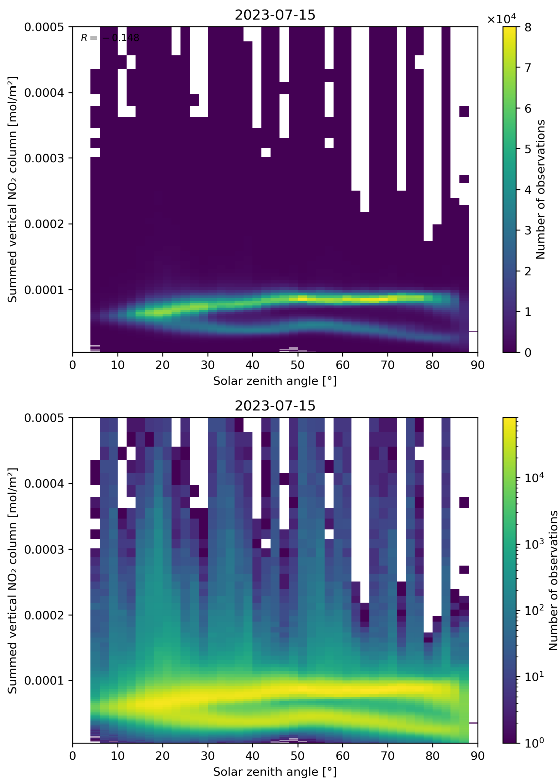
Figure 151: Scatter density plot of “Solar zenith angle” against “Summed vertical NO 2 column” for 2023-07-14 to 2023-07-16.
