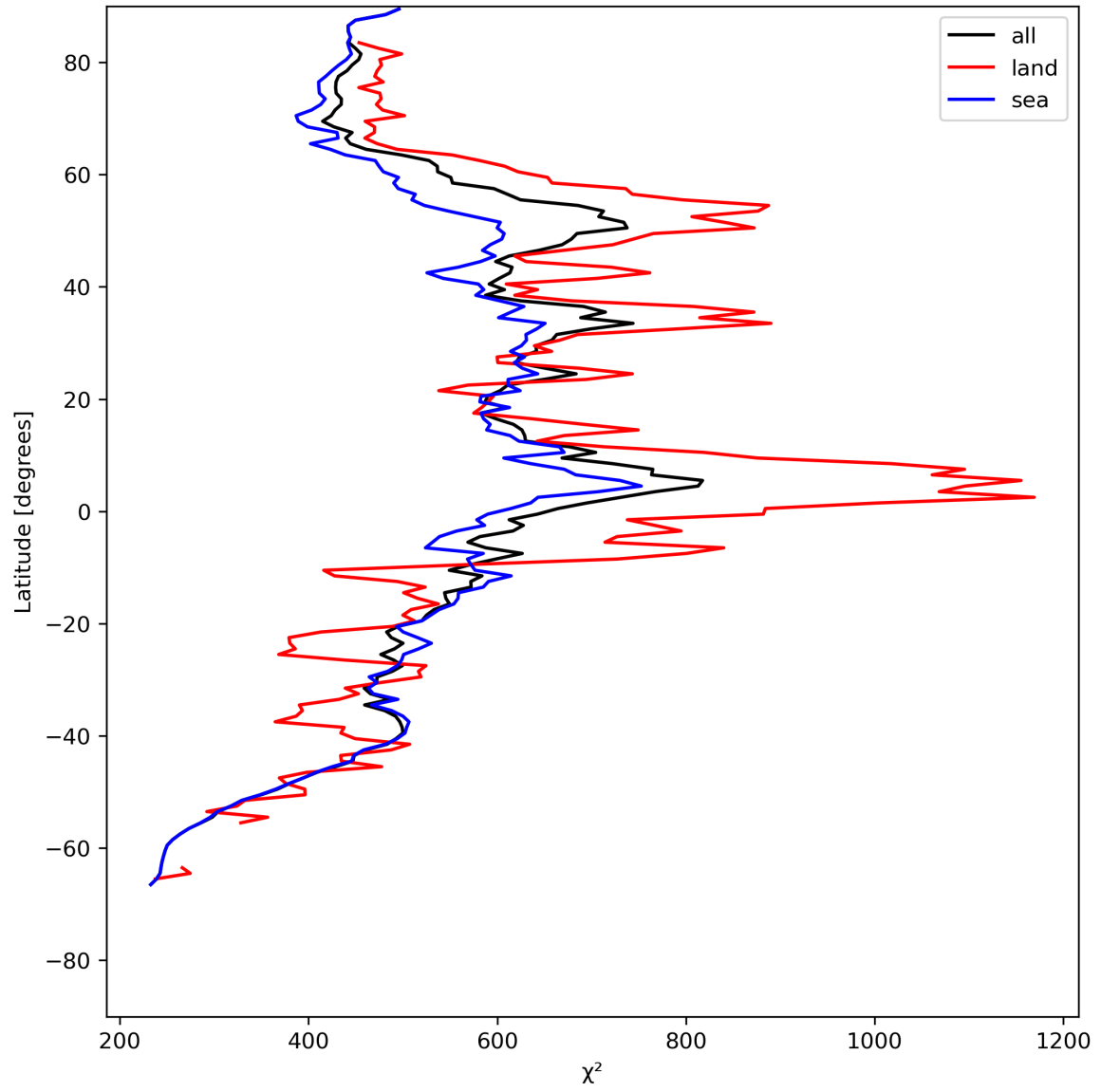
Figure 25: Zonal average of “ \chi^2 ” for 2023-07-14 to 2023-07-16.
