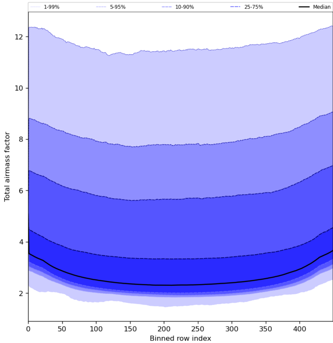
Figure 49: Along track statistics of “Total airmass factor” for 2023-07-14 to 2023-07-16
