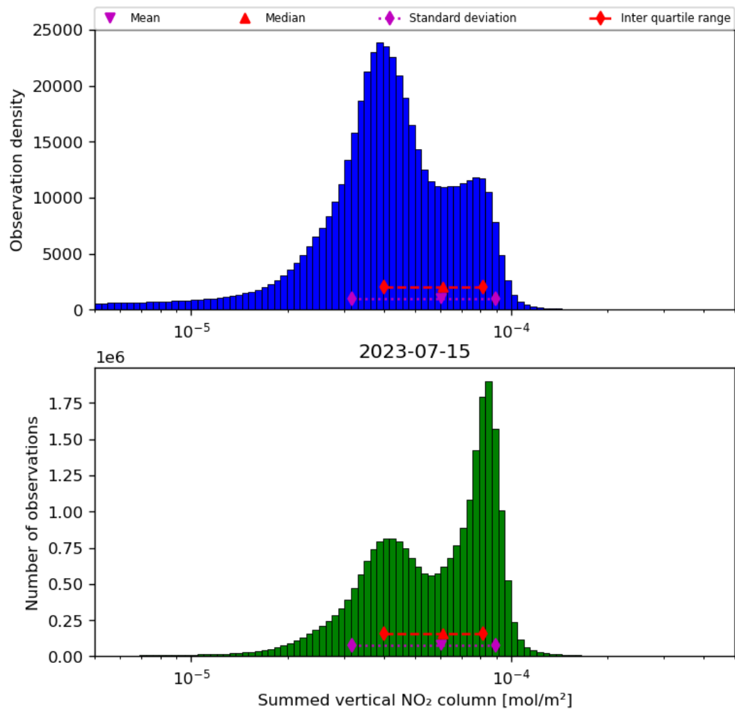
Figure 40: Histogram of “Summed vertical NO 2 column” for 2023-07-14 to 2023-07-16
