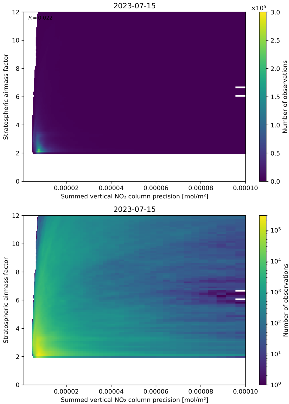
Figure 106: Scatter density plot of “Summed vertical NO 2 column precision” against “Stratospheric airmass factor” for 2023-07-14 to 2023-07-16.
