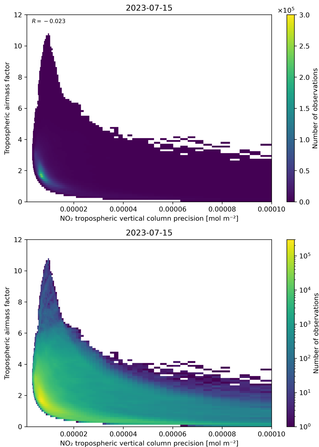
Figure 133: Scatter density plot of “NO 2 tropospheric vertical column precision” against “Tropospheric airmass factor” for 2023-07-14 to 2023-07-16.
