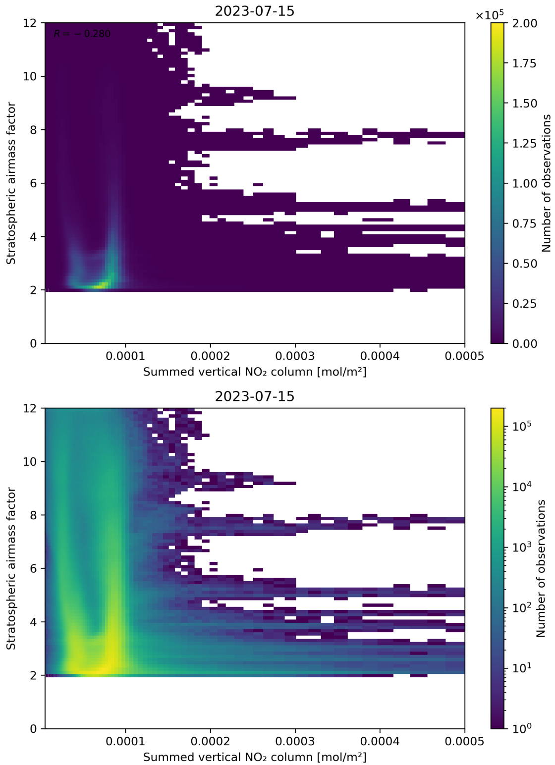
Figure 103: Scatter density plot of “Summed vertical NO 2 column” against “Stratospheric air mass factor” for 2023-07-14 to 2023-07-16.
