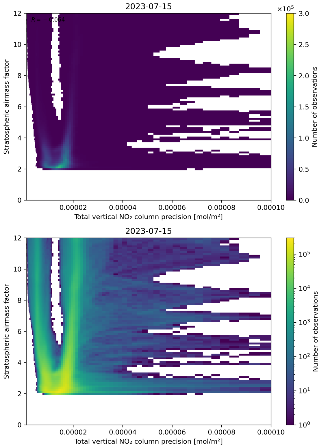
Figure 115: Scatter density plot of “Total vertical NO 2 column precision” against “Stratospheric airmass factor” for 2023-07-14 to 2023-07-16.
