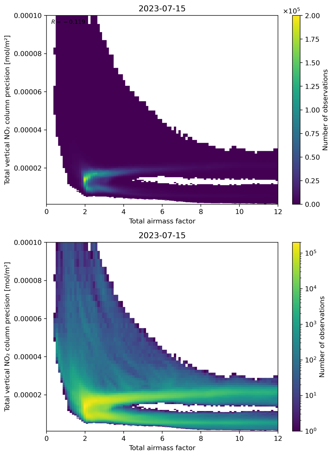
Figure 68: Scatter density plot of “Total airmass factor” against “Total vertical NO 2 column precision” for 2023-07-14 to 2023-07-16.
