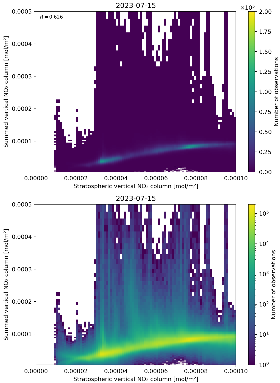
Figure 98: Scatter density plot of “Stratospheric vertical NO 2 column” against “Summed vertical NO 2 column” for 2023-07-14 to 2023-07-16.
