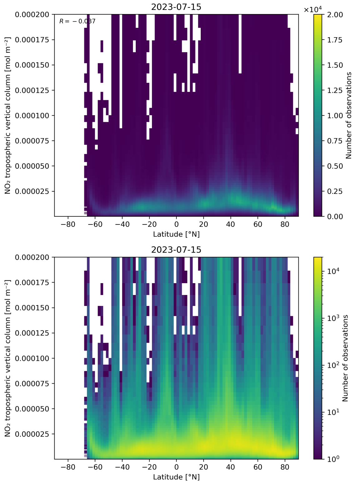
Figure 92: Scatter density plot of “Latitude” against “NO 2 tropospheric vertical column” for 2023-07-14 to 2023-07-16.
