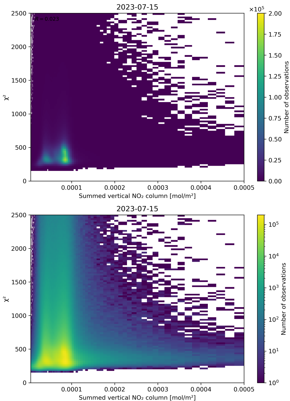
Figure 104: Scatter density plot of “Summed vertical NO 2 column” against “ \chi^2 ” for 2023-07-14 to 2023-07-16.
