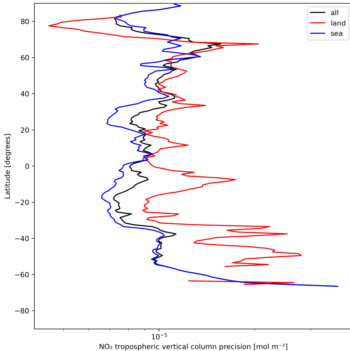
Figure 13: Zonal average of “NO 2 tropospheric vertical column precision” for 2023-07-14 to 2023-07-16.
