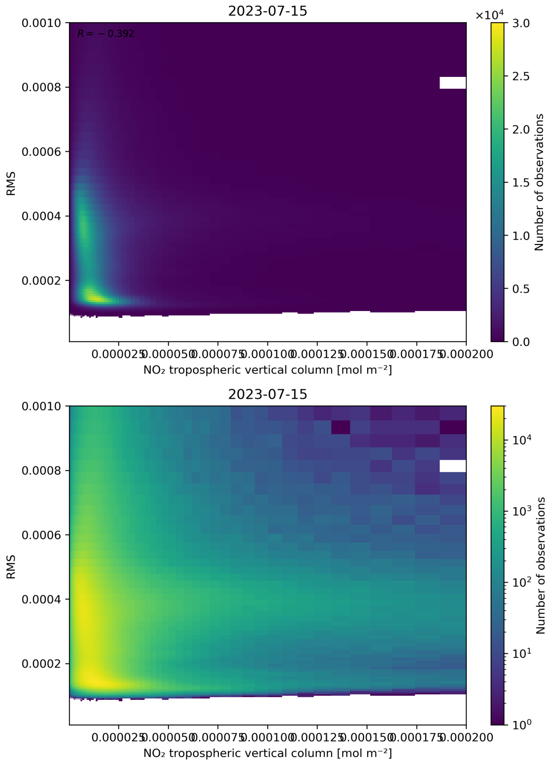
Figure 142: Scatter density plot of “NO 2 tropospheric vertical column” against “RMS” for 2023-07-14 to 2023-07-16.
