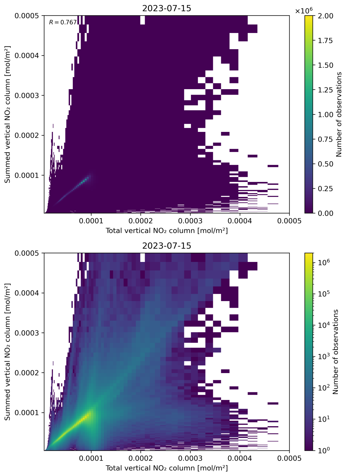
Figure 112: Scatter density plot of “Total vertical NO 2 column” against “Summed vertical NO 2 column” for 2023-07-14 to 2023-07-16.
