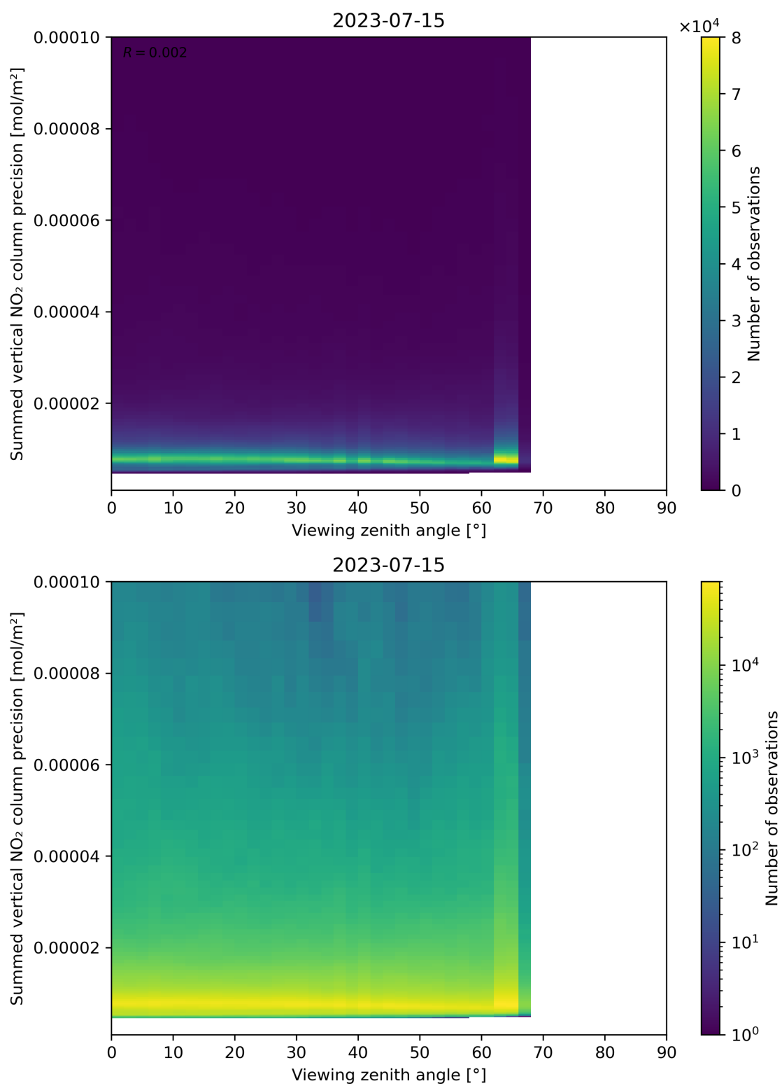
Figure 166: Scatter density plot of “Viewing zenith angle” against “Summed vertical NO 2 column precision” for 2023-07-14 to 2023-07-16.
