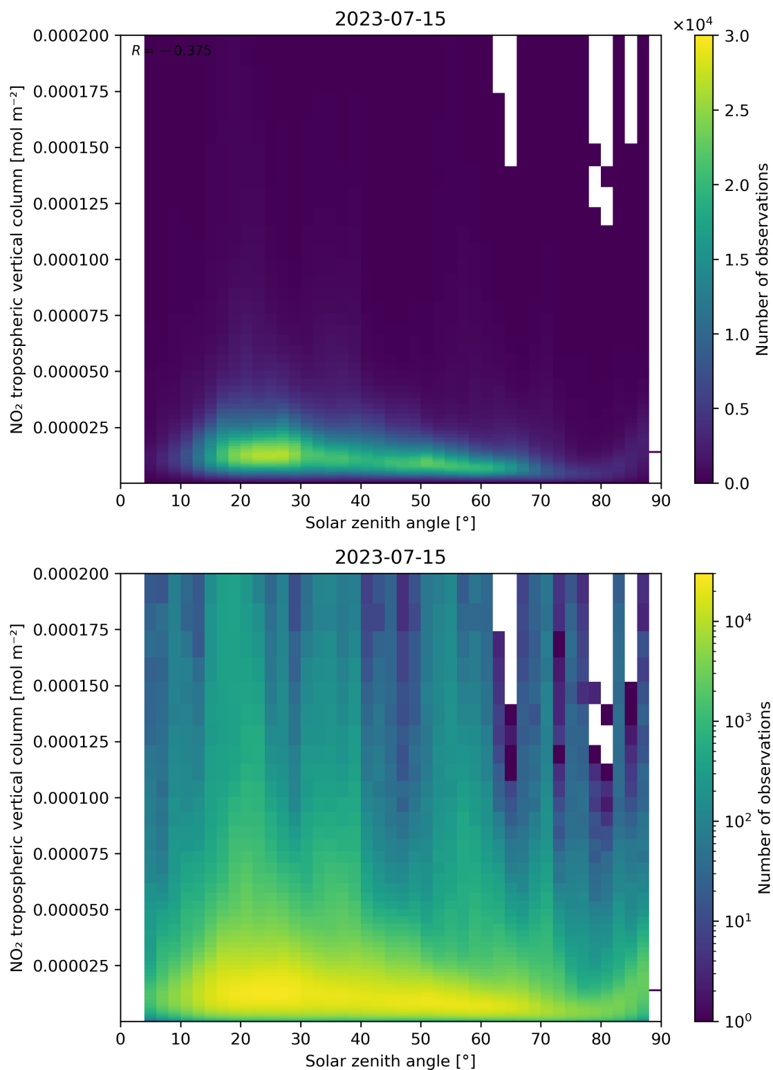
Figure 155: Scatter density plot of “Solar zenith angle” against “NO 2 tropospheric vertical column” for 2023-07-14 to 2023-07-16.
