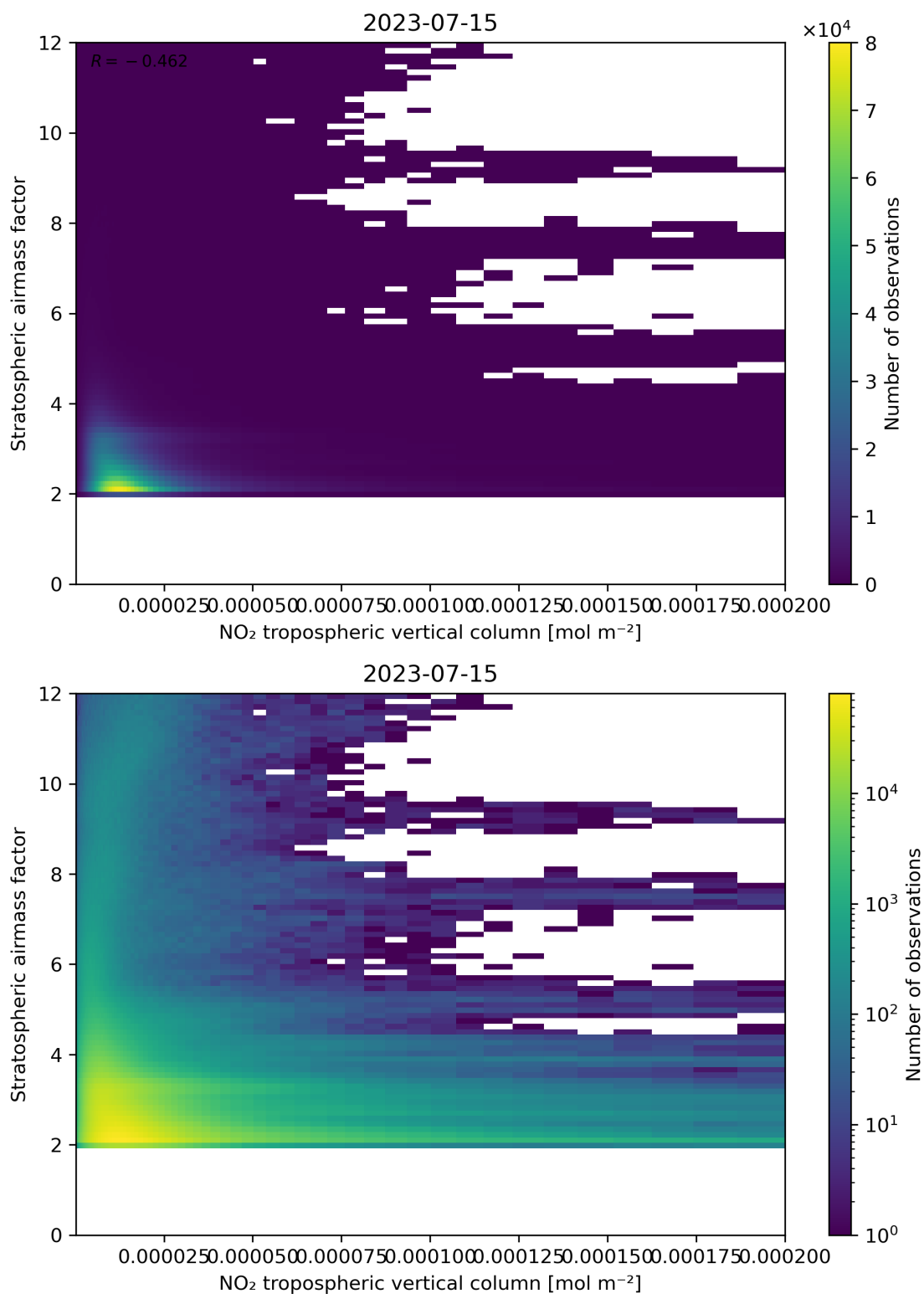
Figure 121: Scatter density plot of “NO 2 tropospheric vertical column” against “Stratospheric air mass factor” for 2023-07-14 to 2023-07-16.
