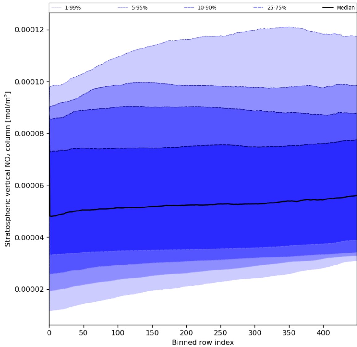
Figure 53: Along track statistics of “Stratospheric vertical NO 2 column” for 2023-07-14 to 2023-07-16
