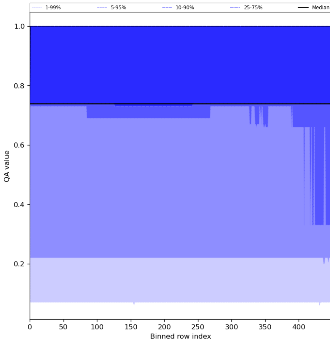
Figure 45: Along track statistics of “QA value” for 2023-07-14 to 2023-07-16
