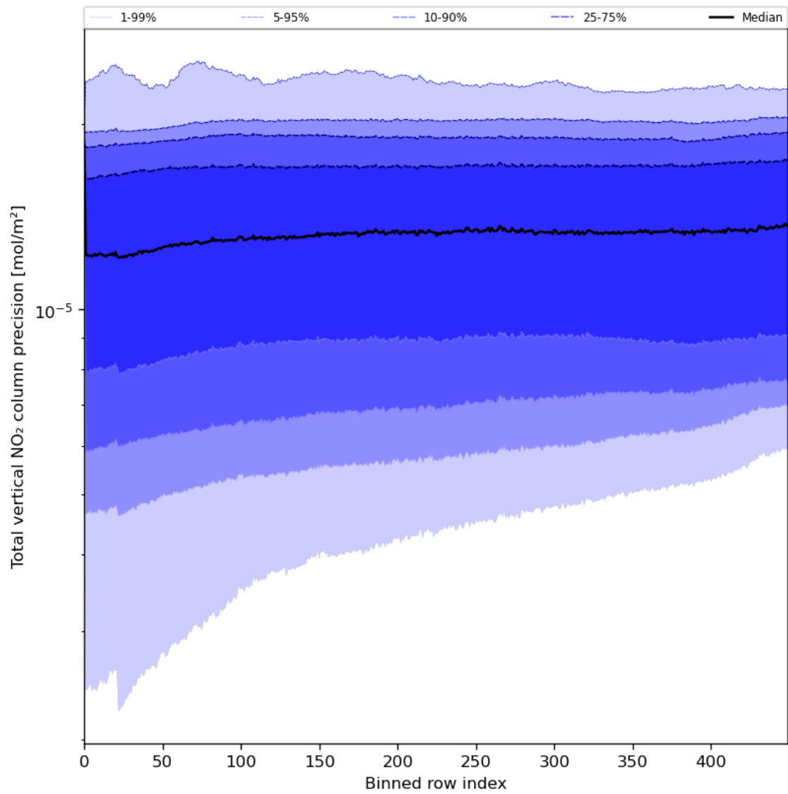
Figure 56: Along track statistics of “Total vertical NO 2 column precision” for 2023-07-14 to 2023-07-16
