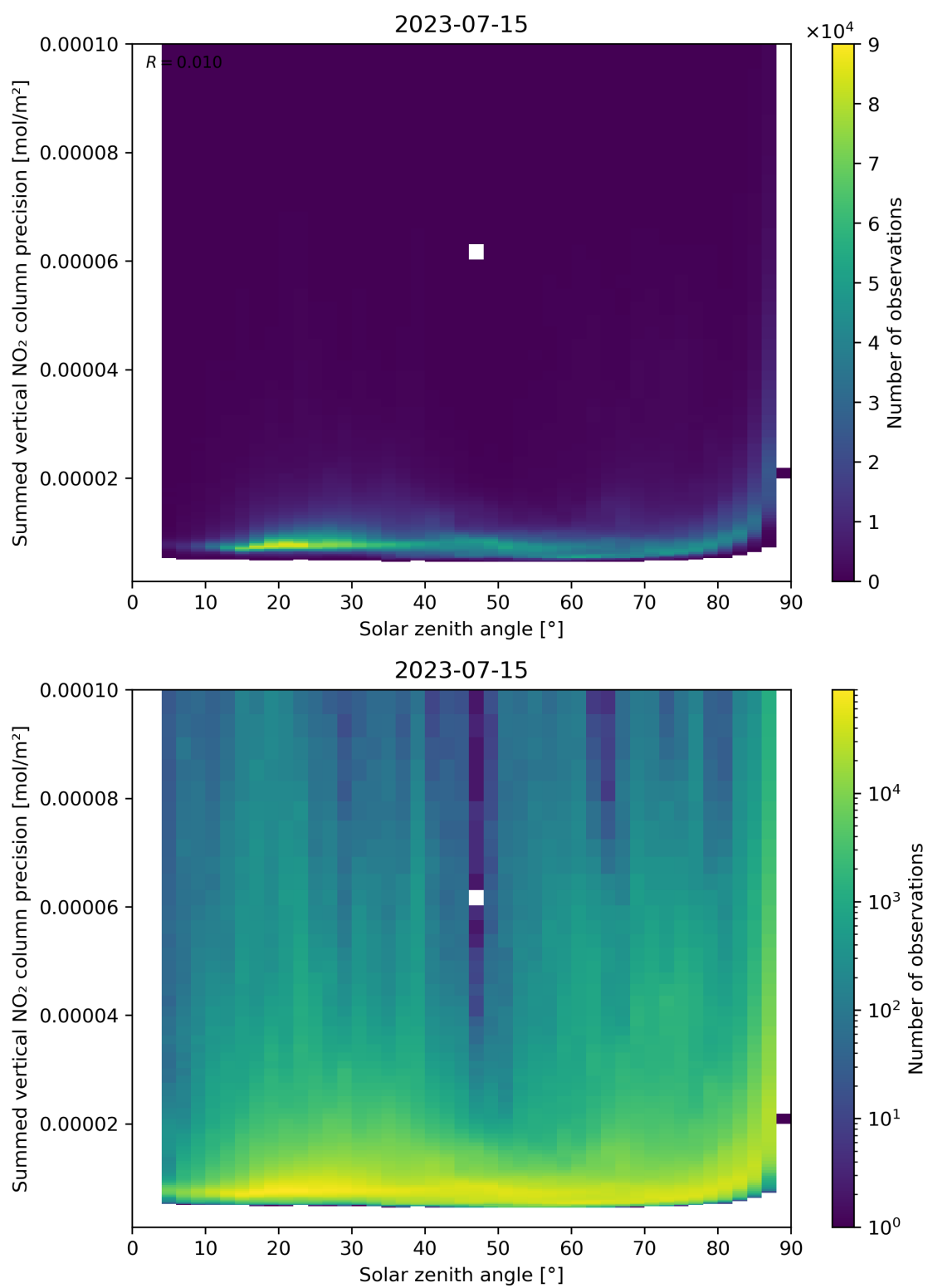
Figure 152: Scatter density plot of “Solar zenith angle” against “Summed vertical NO 2 column precision” for 2023-07-14 to 2023-07-16.
