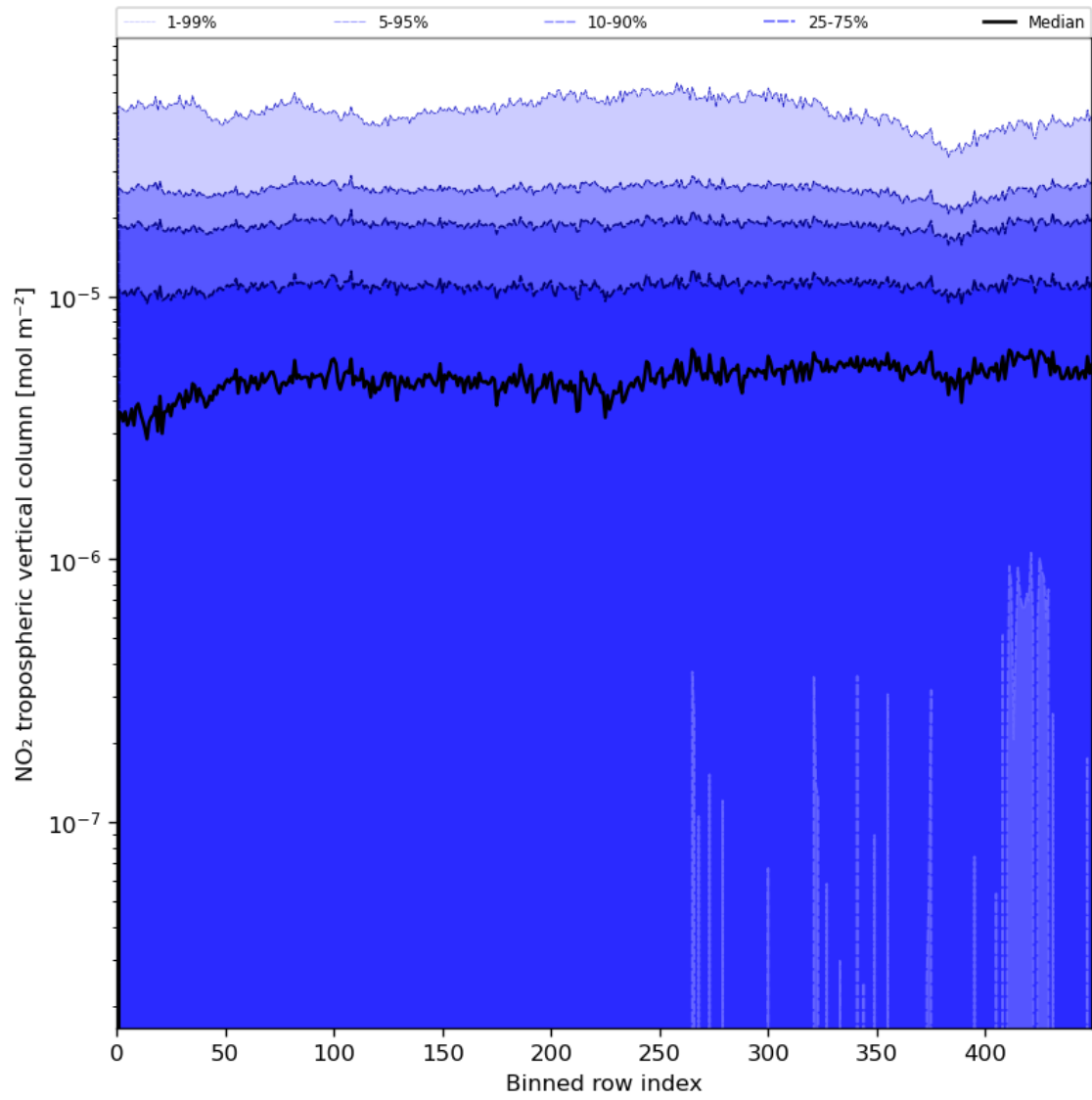
Figure 46: Along track statistics of “NO 2 tropospheric vertical column” for 2023-07-14 to 2023-07-16
