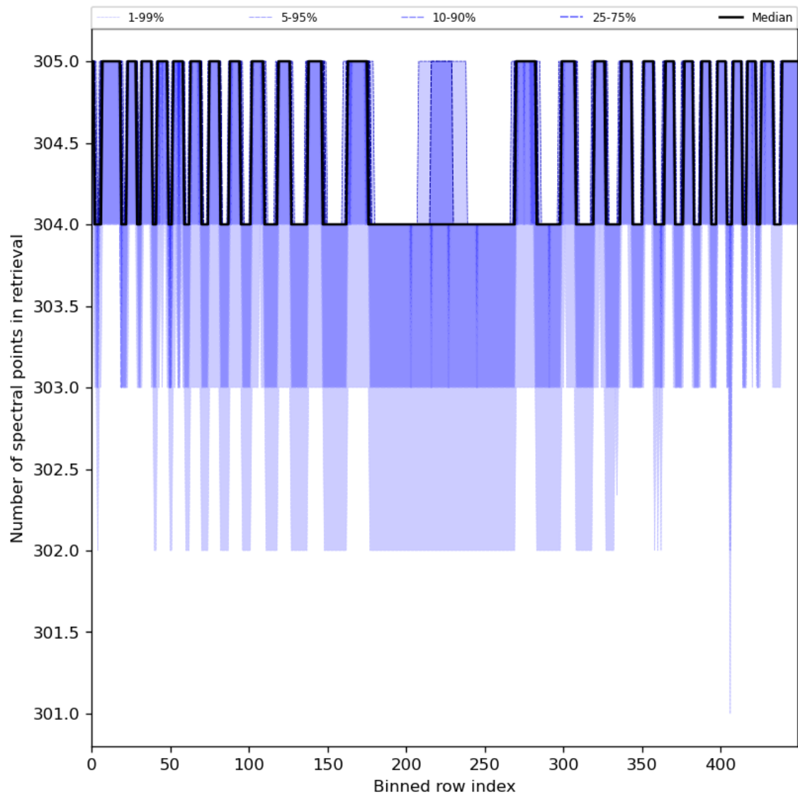
Figure 50: Along track statistics of “Number of spectral points in retrieval” for 2023-07-14 to 2023-07-16
