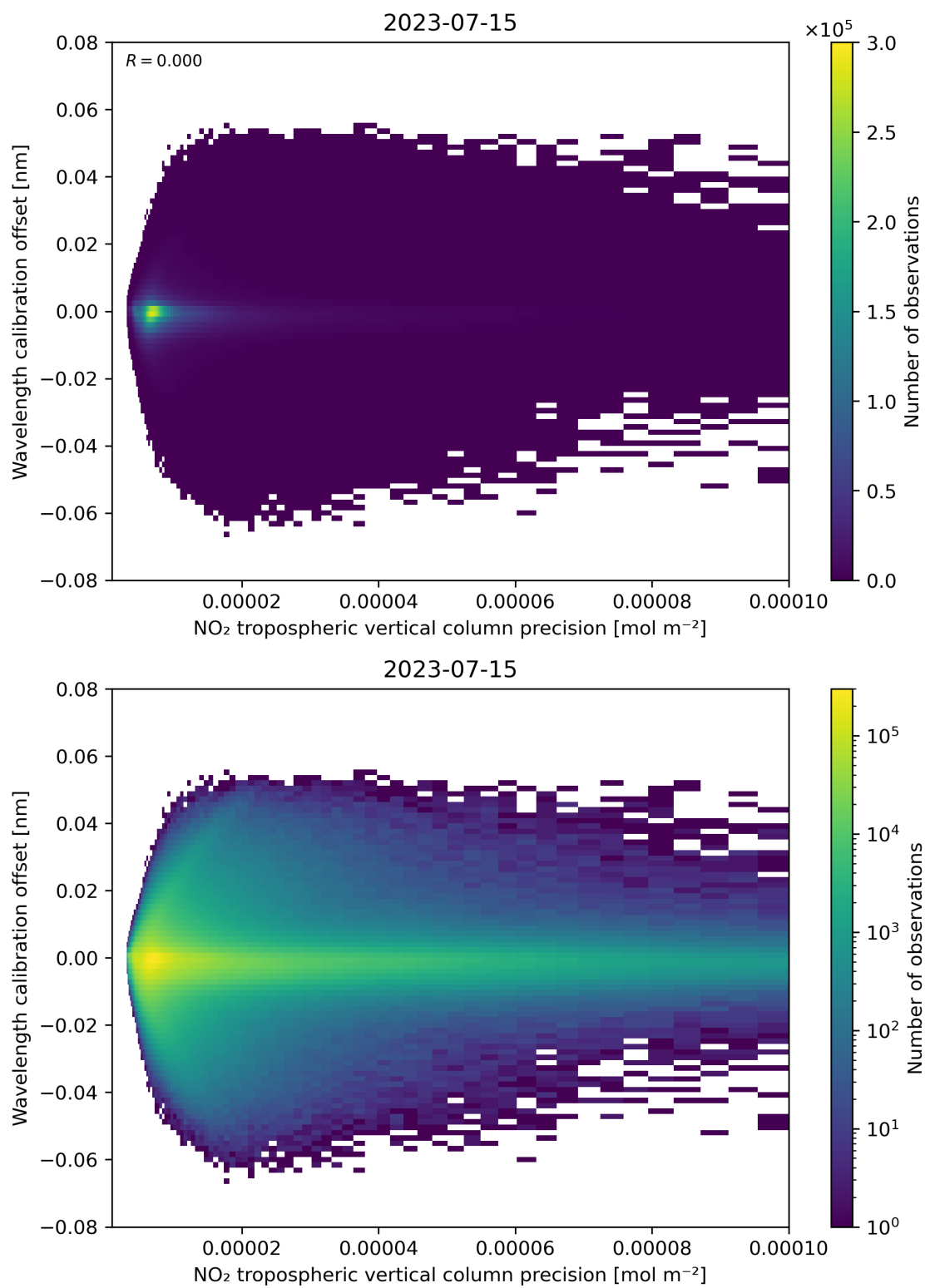
Figure 141: Scatter density plot of “NO 2 tropospheric vertical column precision” against “Wavelength calibration offset” for 2023-07-14 to 2023-07-16.
