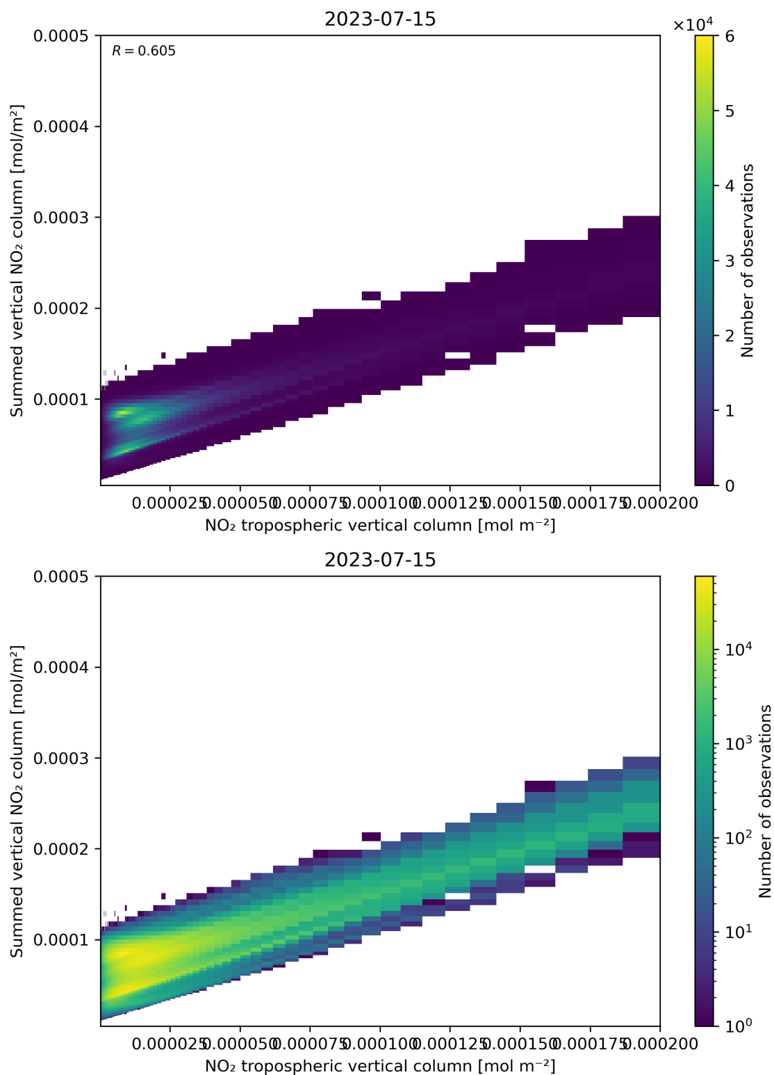
Figure 126: Scatter density plot of “NO 2 tropospheric vertical column” against “Summed vertical NO 2 column” for 2023-07-14 to 2023-07-16.
