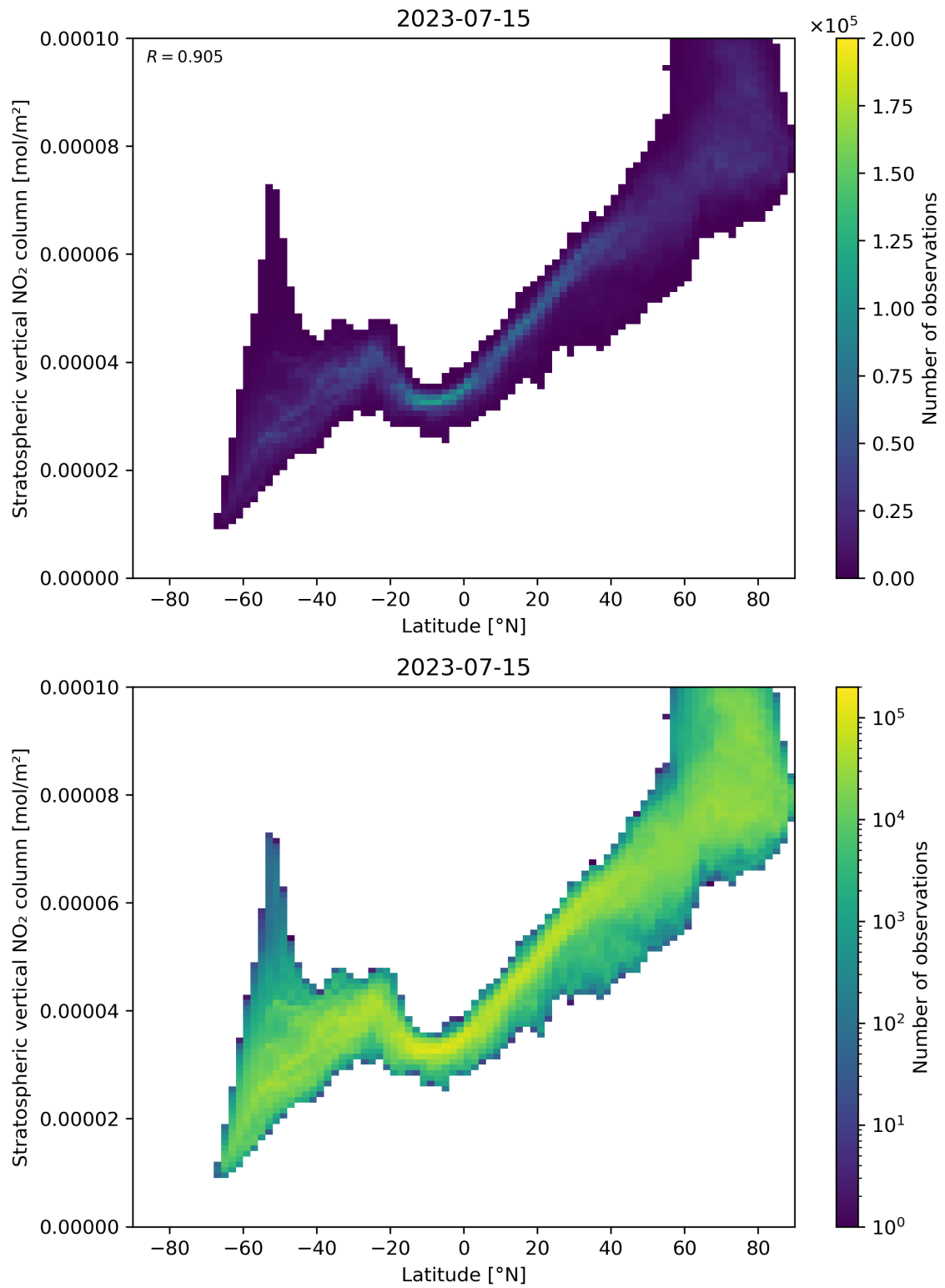
Figure 87: Scatter density plot of “Latitude” against “Stratospheric vertical NO 2 column” for 2023-07-14 to 2023-07-16.
