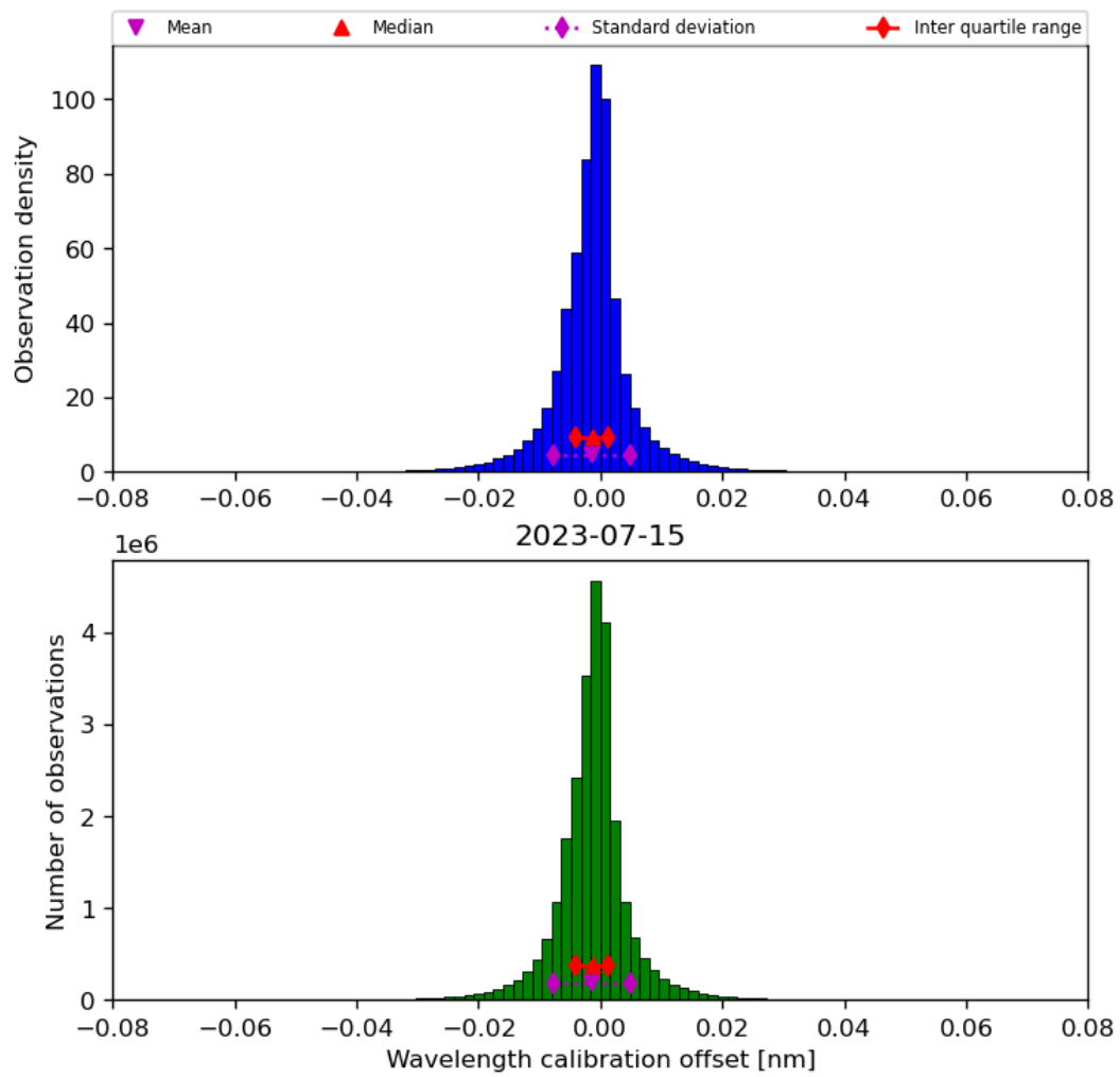
Figure 35: Histogram of “Wavelength calibration offset” for 2023-07-14 to 2023-07-16
