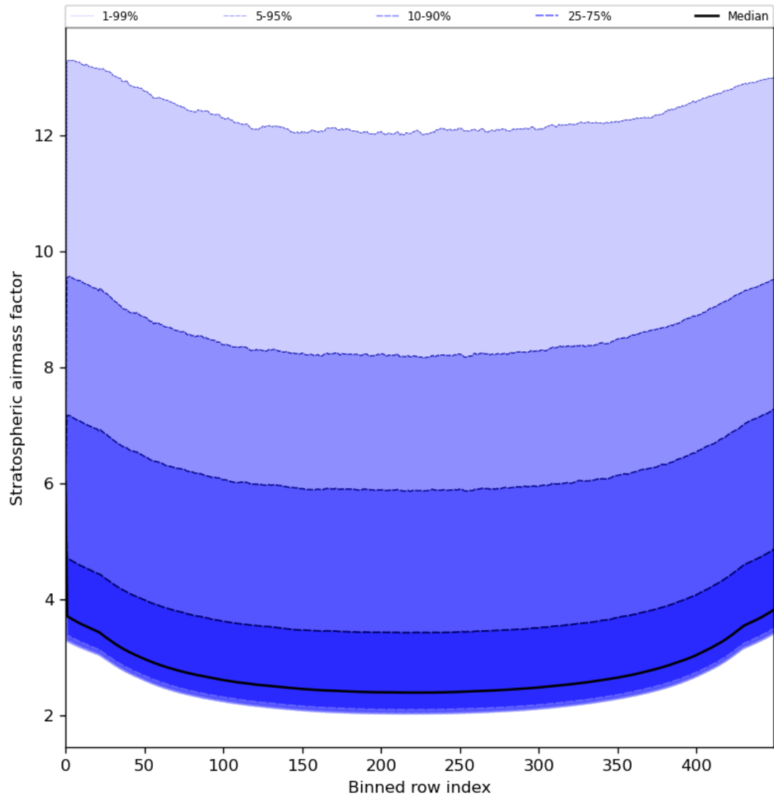
Figure 61: Along track statistics of “Stratospheric airmass factor” for 2023-07-14 to 2023-07-16
