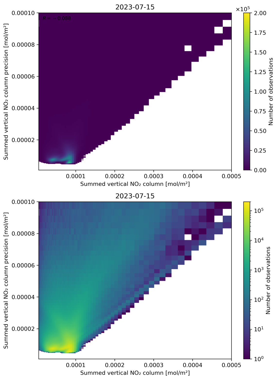
Figure 105: Scatter density plot of “Summed vertical NO 2 column” against “Summed vertical NO 2 column precision” for 2023-07-14 to 2023-07-16.
