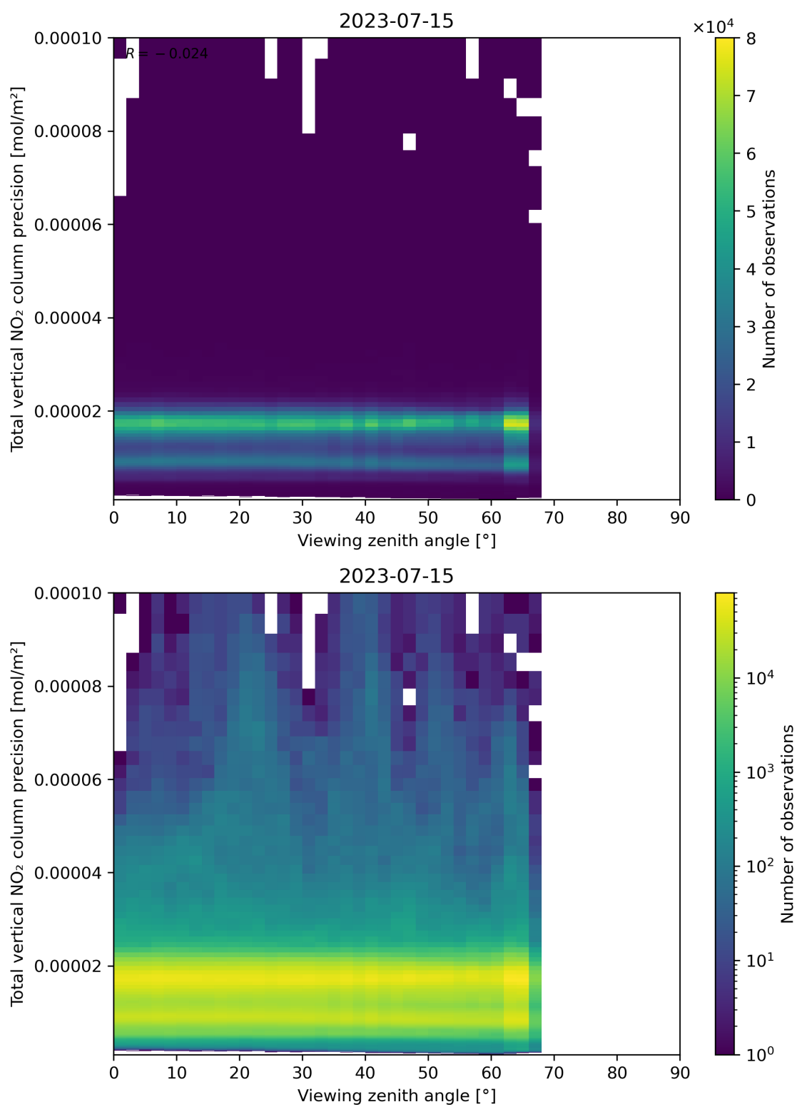
Figure 168: Scatter density plot of “Viewing zenith angle” against “Total vertical NO 2 column precision” for 2023-07-14 to 2023-07-16.
