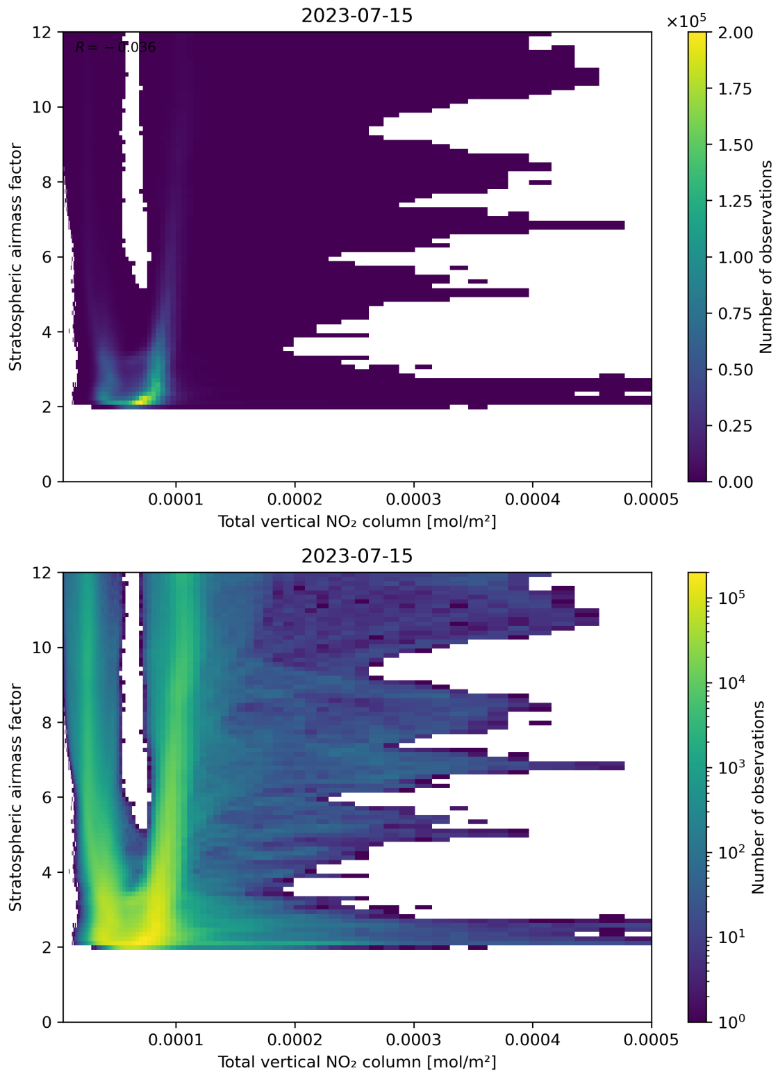
Figure 110: Scatter density plot of “Total vertical NO 2 column” against “Stratospheric airmass factor” for 2023-07-14 to 2023-07-16.
