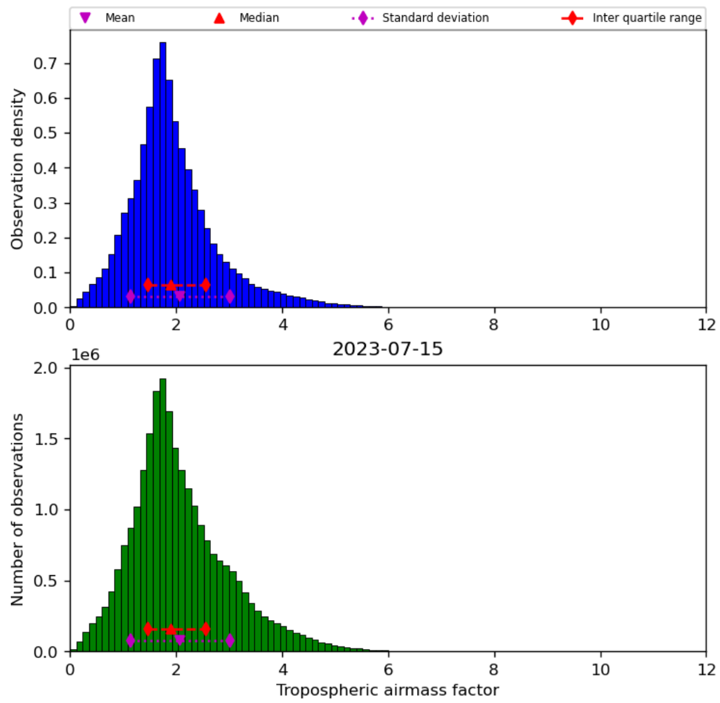
Figure 31: Histogram of “Tropospheric airmass factor” for 2023-07-14 to 2023-07-16
