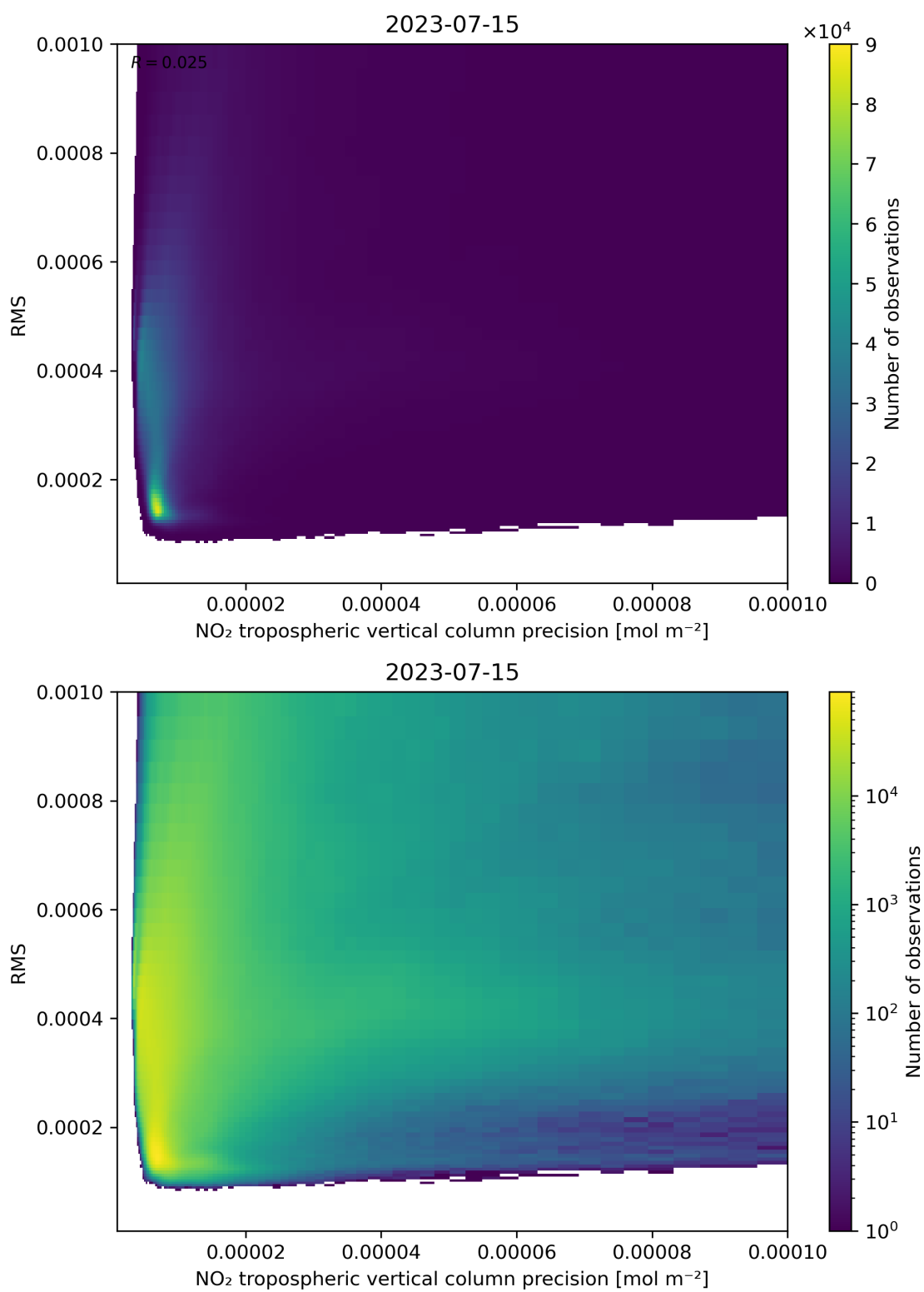
Figure 140: Scatter density plot of “NO 2 tropospheric vertical column precision” against “RMS” for 2023-07-14 to 2023-07-16.
