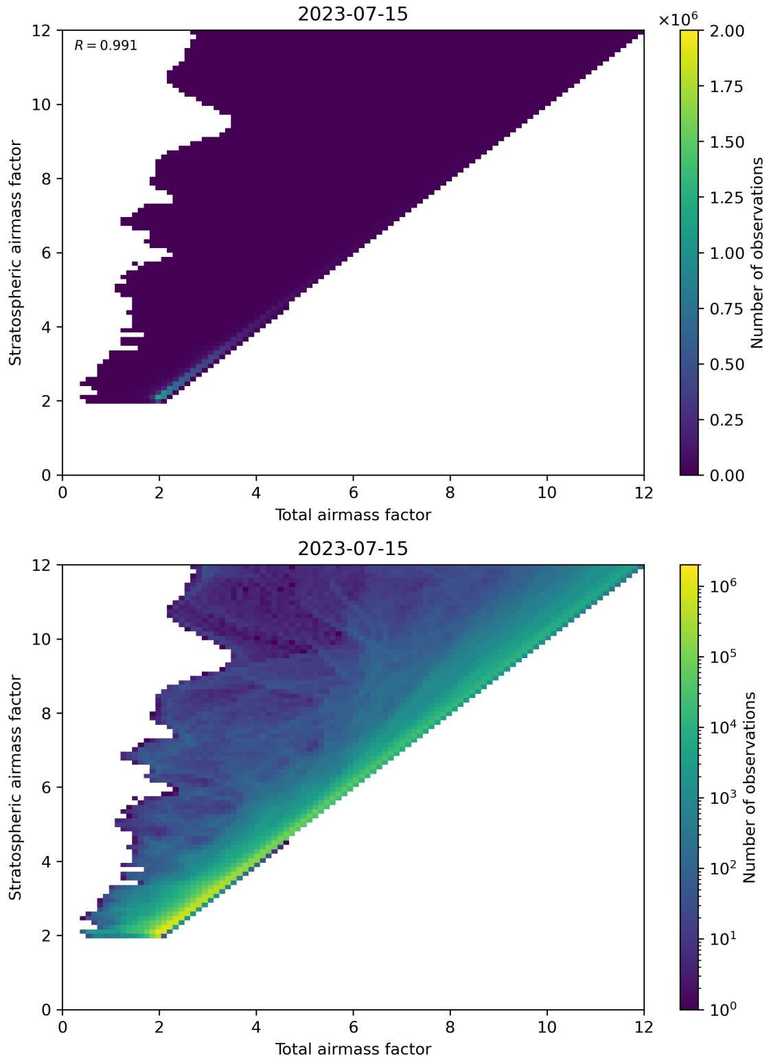
Figure 62: Scatter density plot of “Total airmass factor” against “Stratospheric airmass factor” for 2023-07-14 to 2023-07-16.
