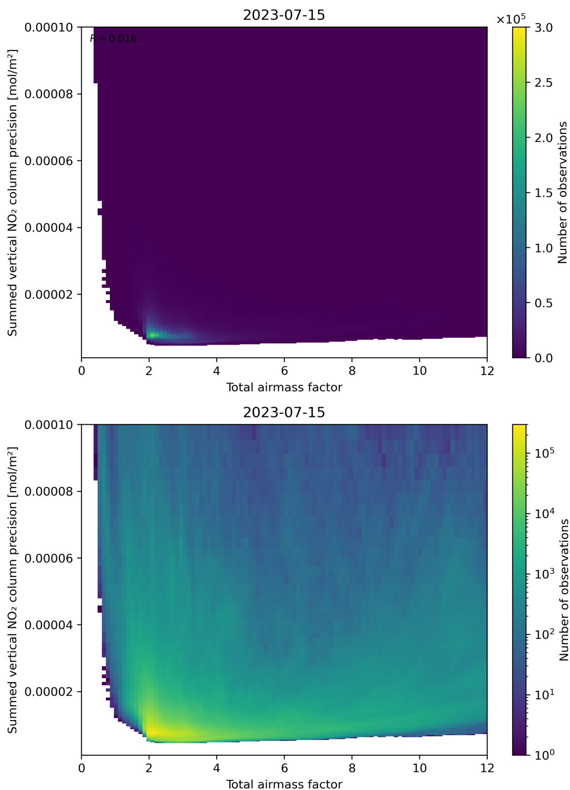
Figure 66: Scatter density plot of “Total airmass factor” against “Summed vertical NO 2 column precision” for 2023-07-14 to 2023-07-16.
