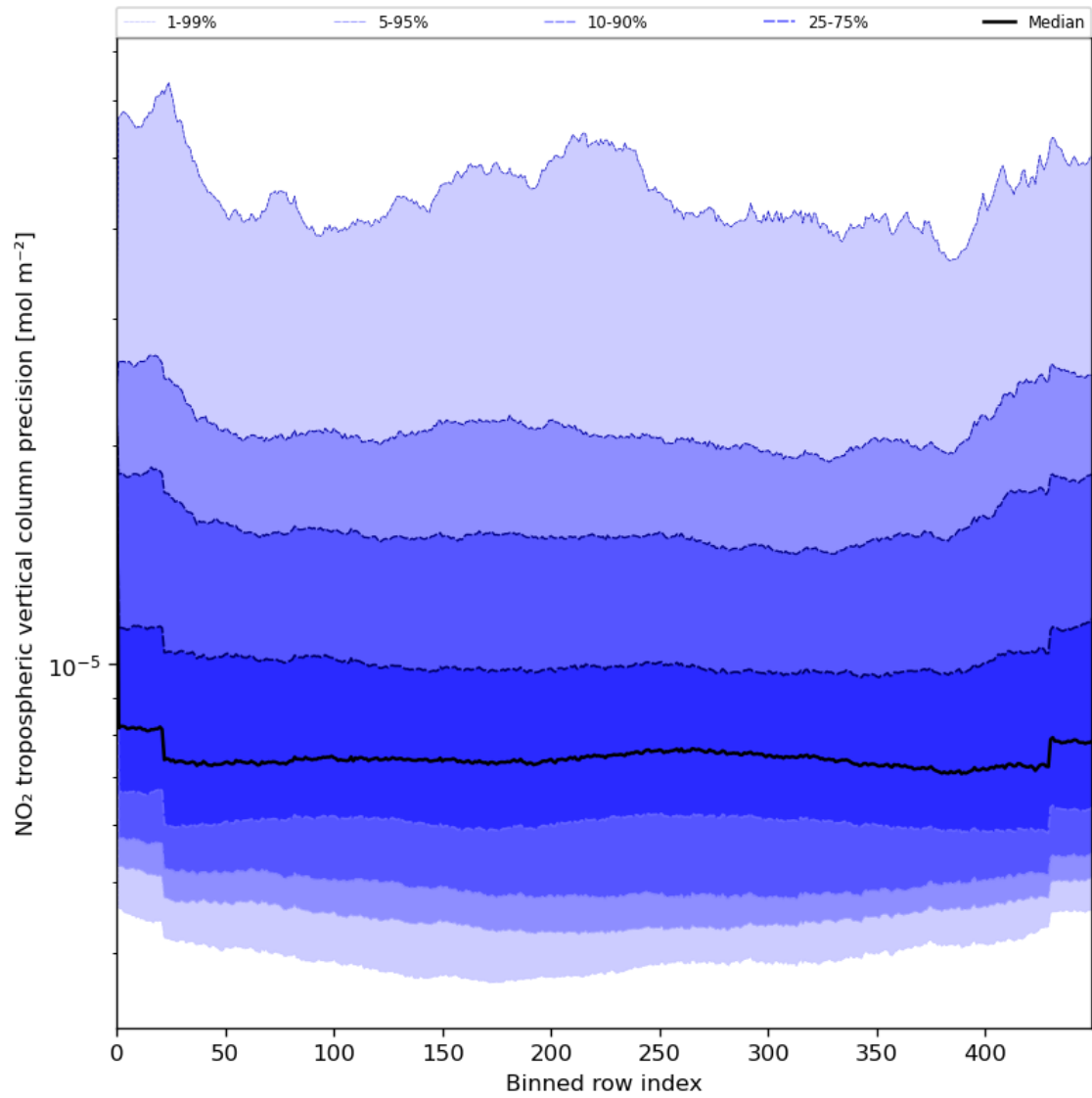
Figure 47: Along track statistics of “NO 2 tropospheric vertical column precision” for 2023-07-14 to 2023-07-16
