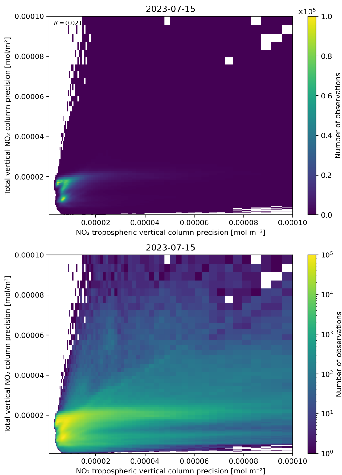
Figure 139: Scatter density plot of “NO 2 tropospheric vertical column precision” against “Total vertical NO 2 column precision” for 2023-07-14 to 2023-07-16.
