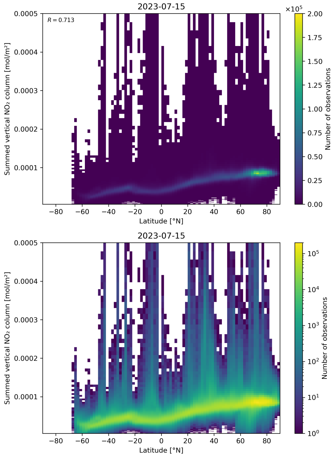
Figure 88: Scatter density plot of “Latitude” against “Summed vertical NO 2 column” for 2023-07-14 to 2023-07-16.
