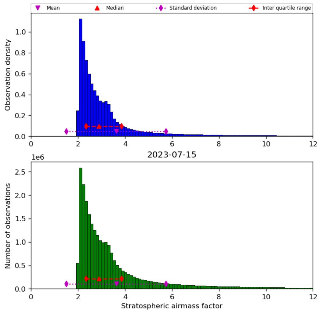
Figure 44: Histogram of “Stratospheric airmass factor” for 2023-07-14 to 2023-07-16
