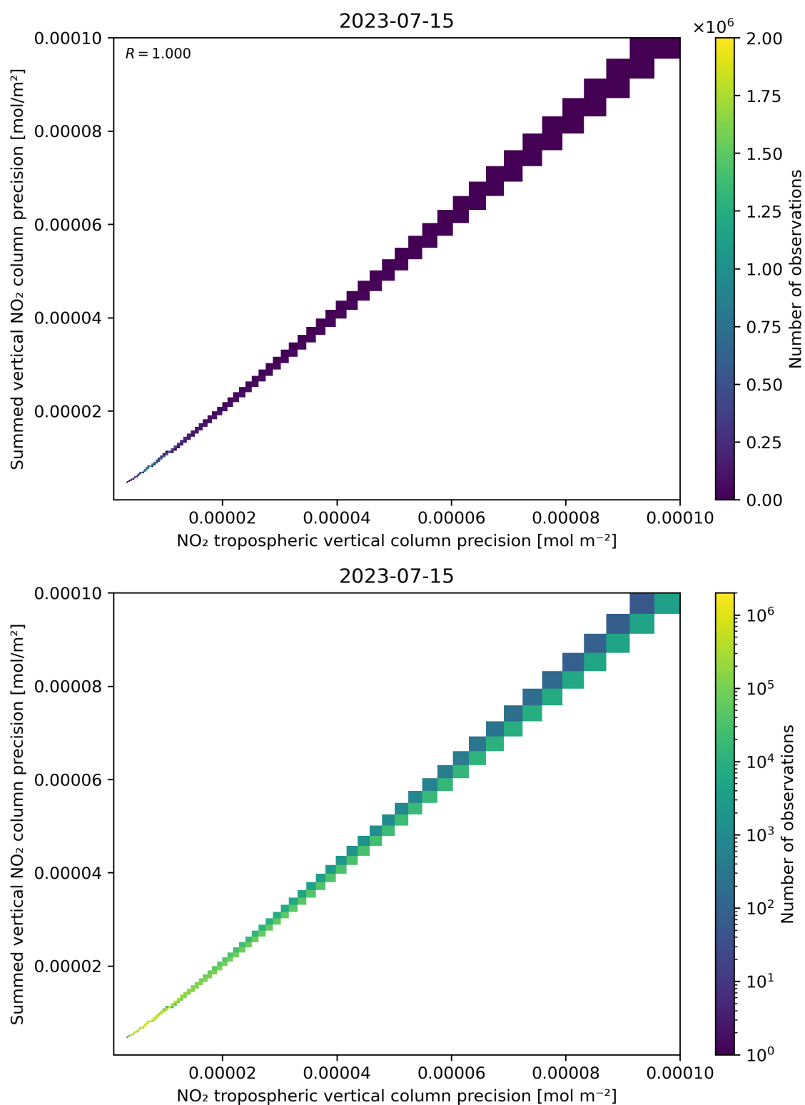
Figure 137: Scatter density plot of “NO 2 tropospheric vertical column precision” against “Summed vertical NO 2 column precision” for 2023-07-14 to 2023-07-16.
