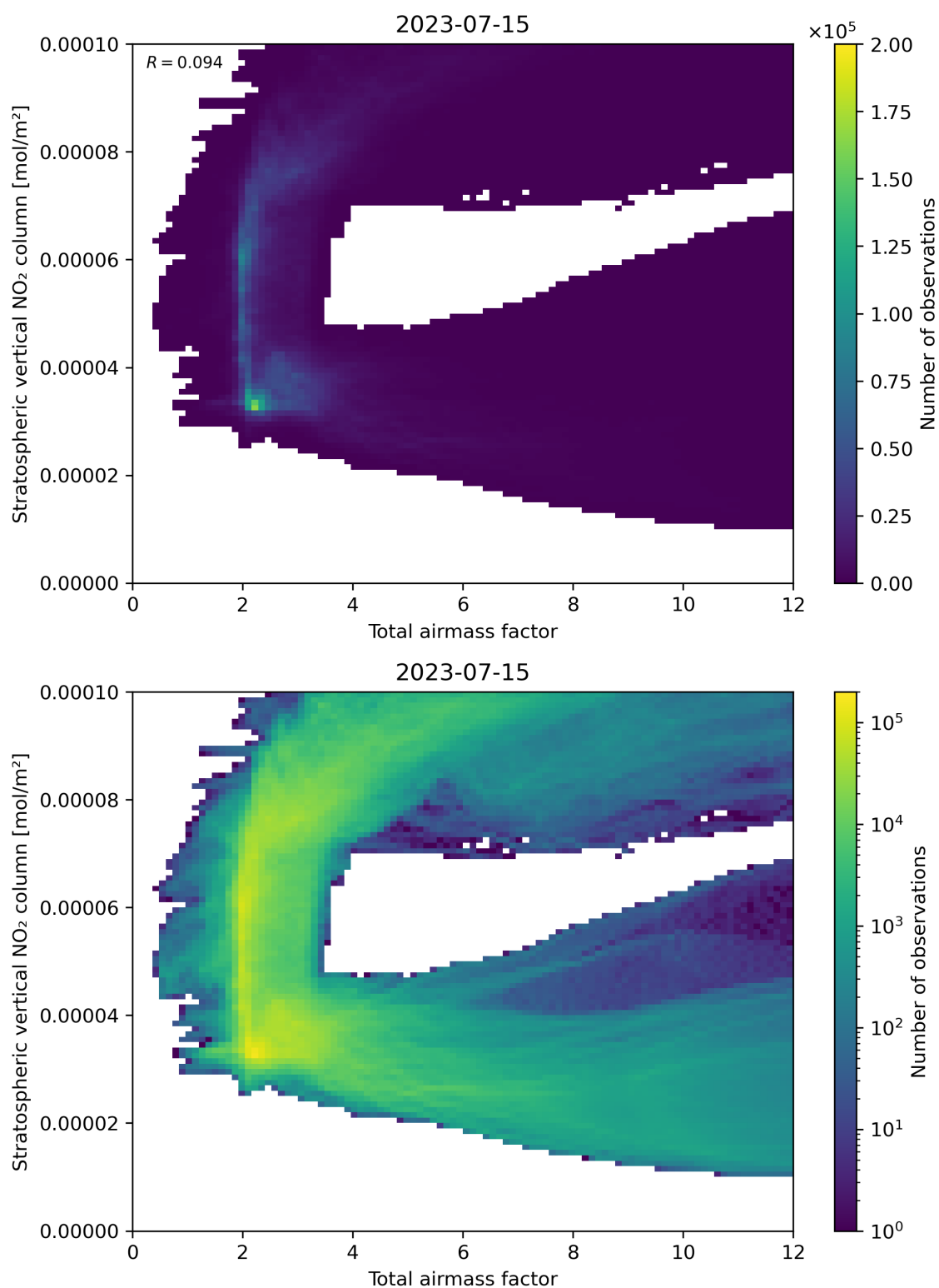
Figure 64: Scatter density plot of “Total airmass factor” against “Stratospheric vertical NO 2 column” for 2023-07-14 to 2023-07-16.
