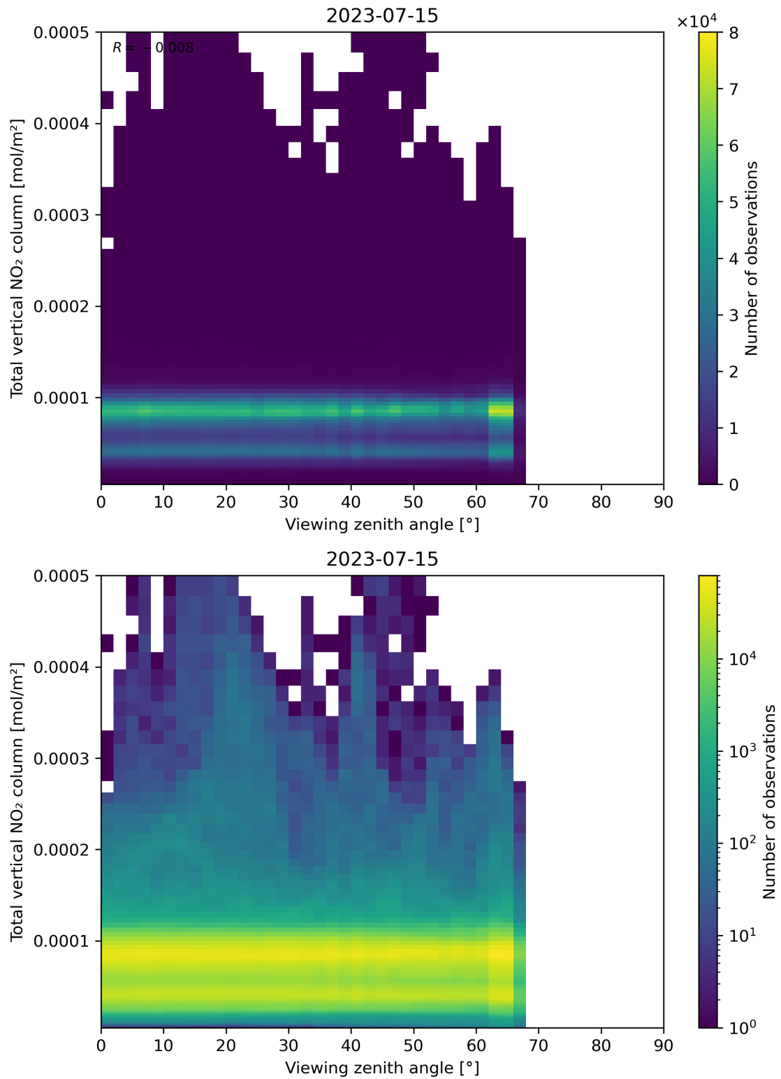
Figure 167: Scatter density plot of “Viewing zenith angle” against “Total vertical NO 2 column” for 2023-07-14 to 2023-07-16.
