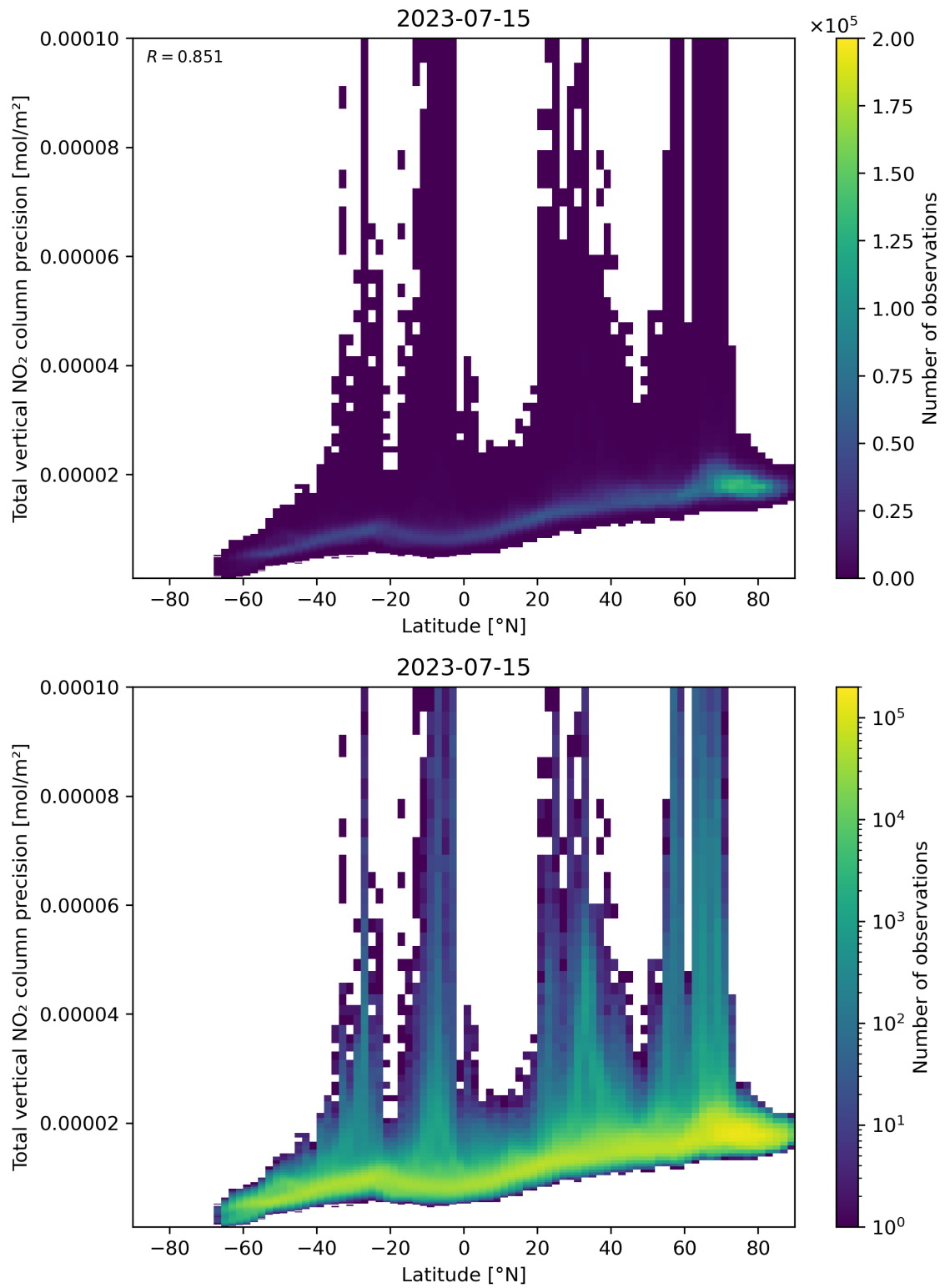
Figure 91: Scatter density plot of “Latitude” against “Total vertical NO 2 column precision” for 2023-07-14 to 2023-07-16.
