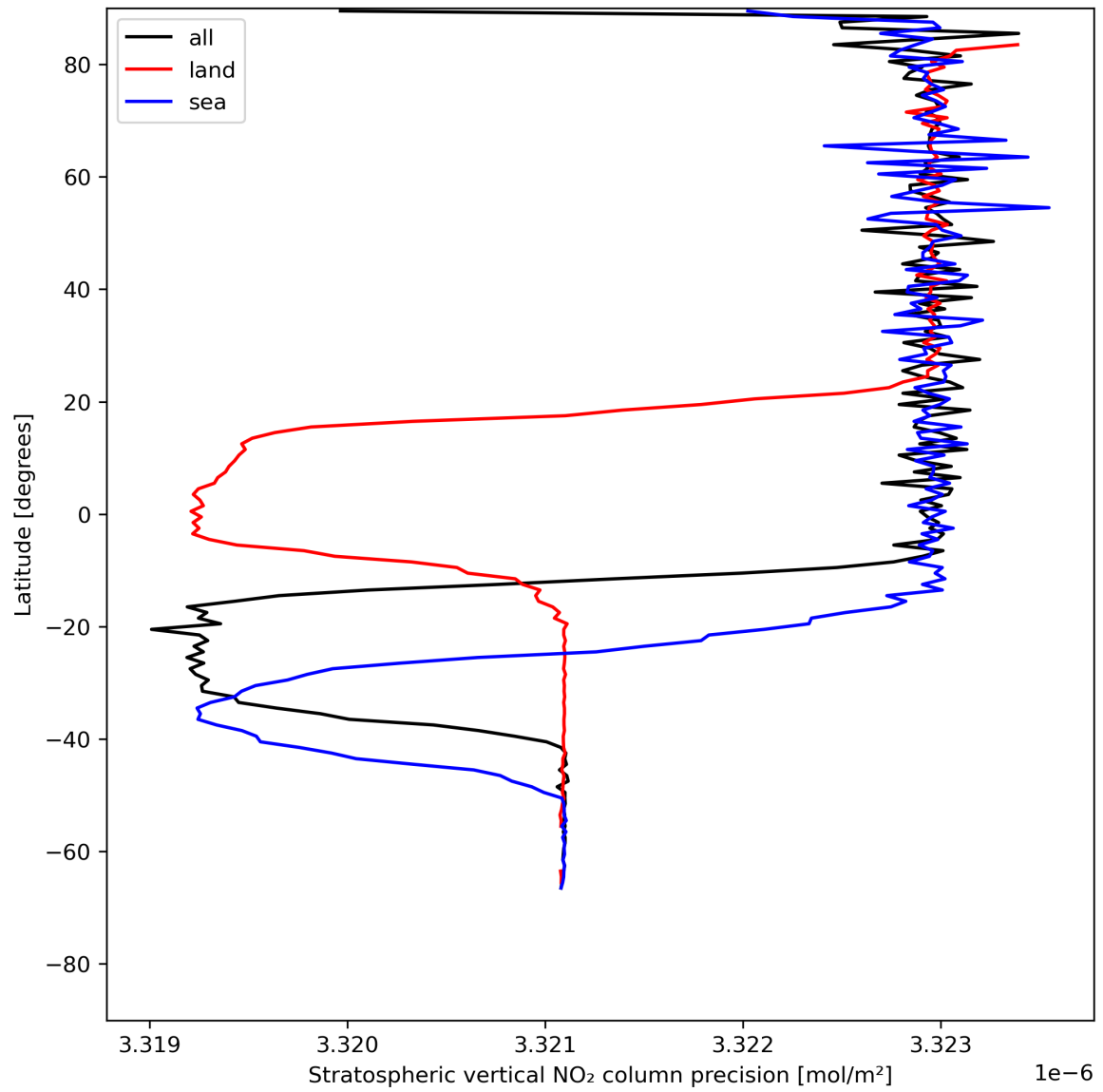
Figure 20: Zonal average of “Stratospheric vertical NO 2 column precision” for 2023-07-14 to 2023-07-16.
