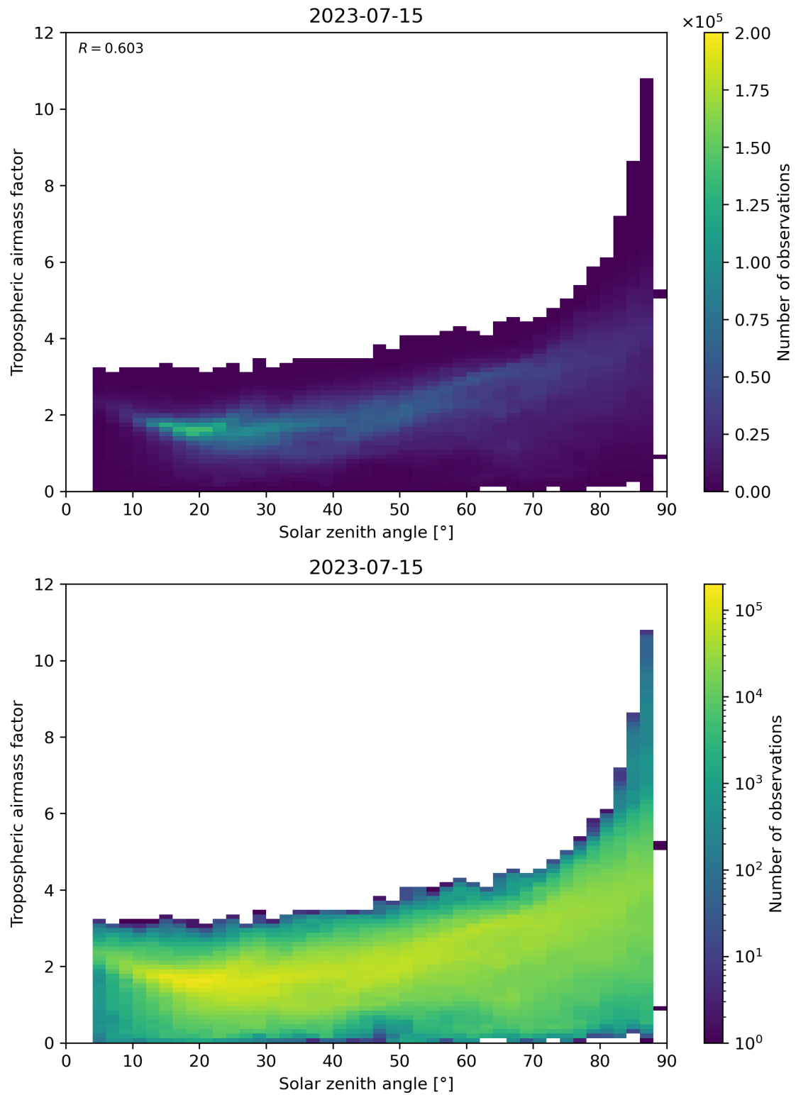
Figure 147: Scatter density plot of “Solar zenith angle” against “Tropospheric airmass factor” for 2023-07-14 to 2023-07-16.
