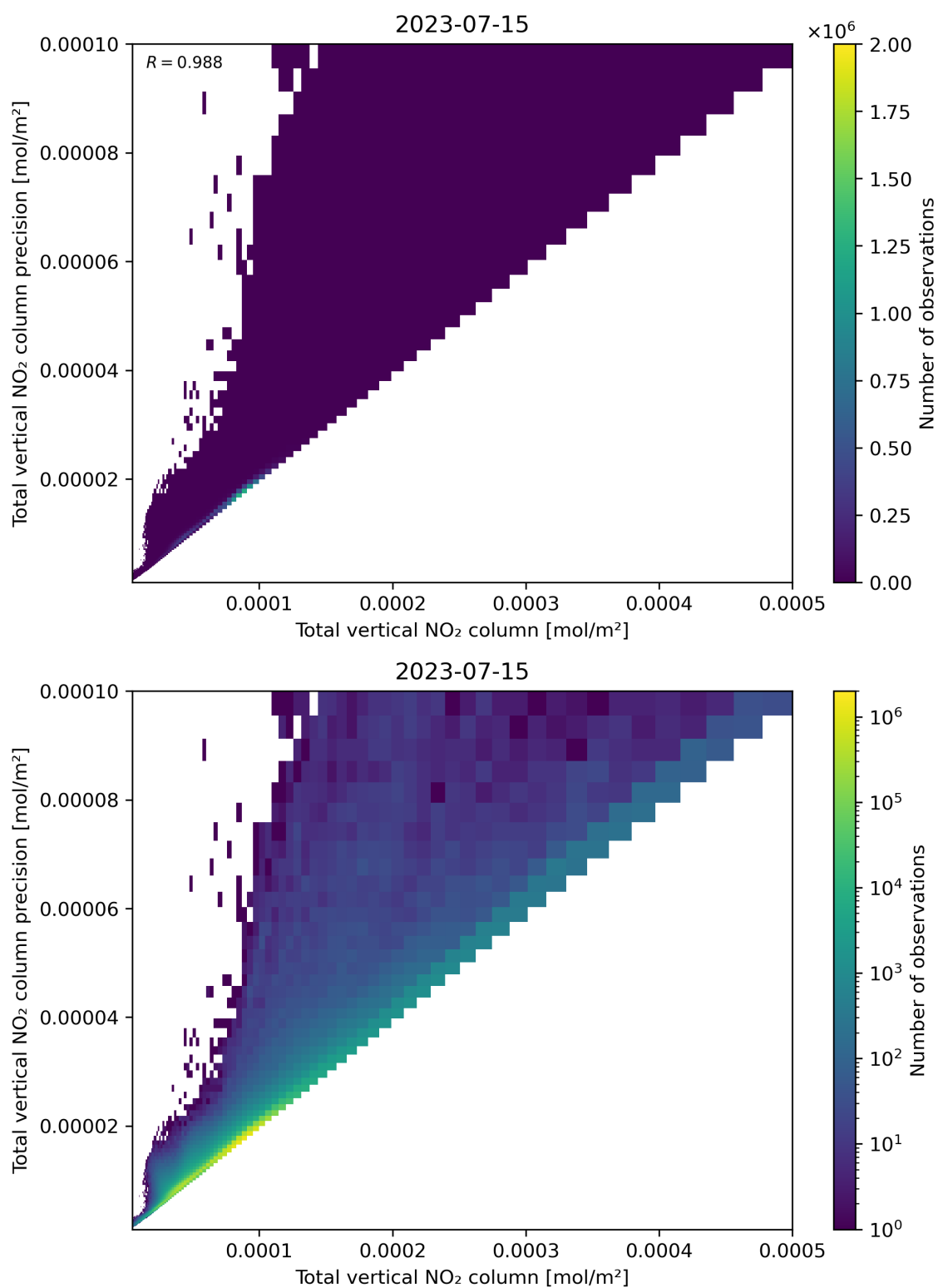
Figure 114: Scatter density plot of “Total vertical NO 2 column” against “Total vertical NO 2 column precision” for 2023-07-14 to 2023-07-16.
