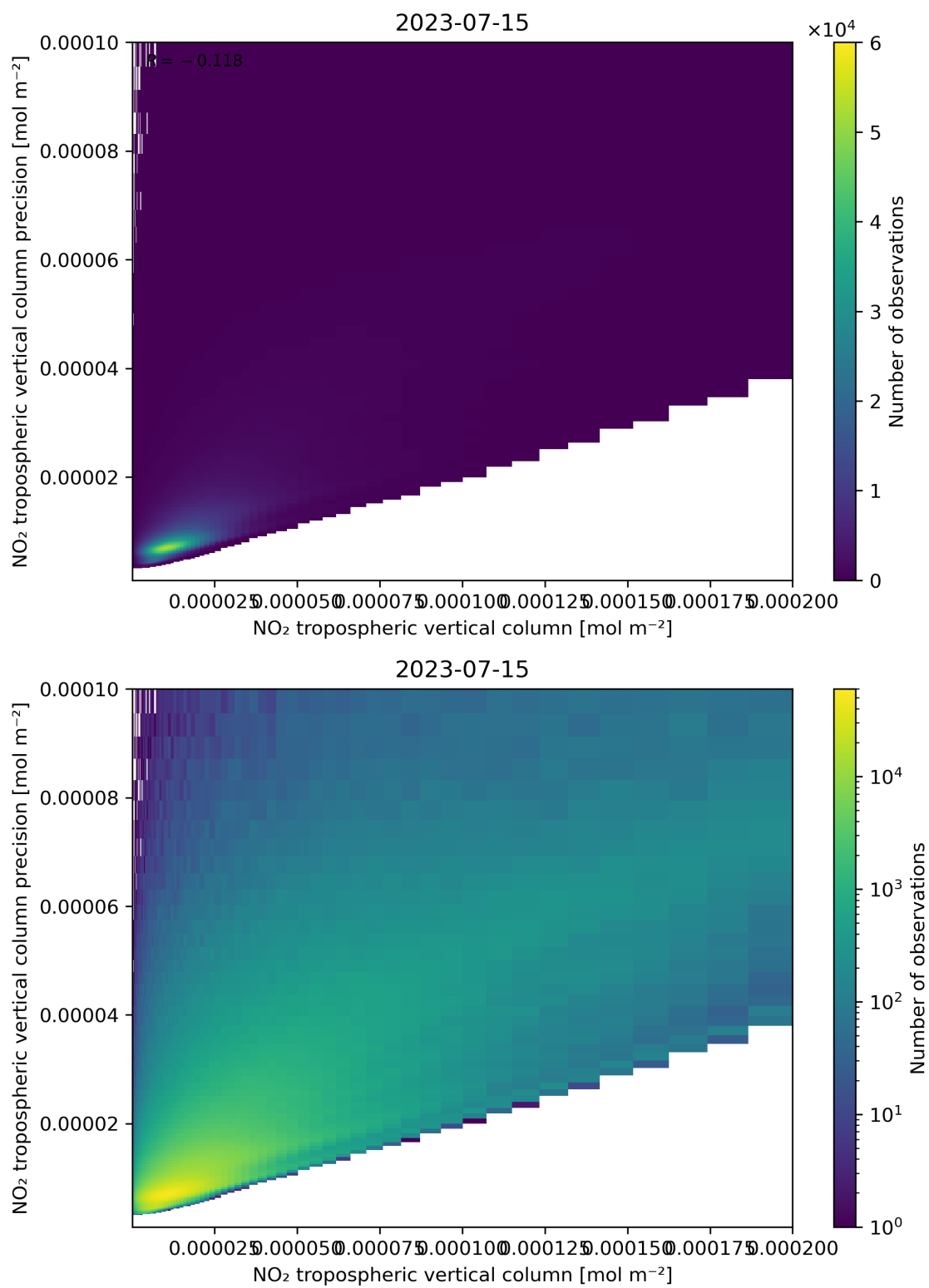
Figure 130: Scatter density plot of “NO 2 tropospheric vertical column” against “NO 2 tropospheric vertical column precision” for 2023-07-14 to 2023-07-16.
