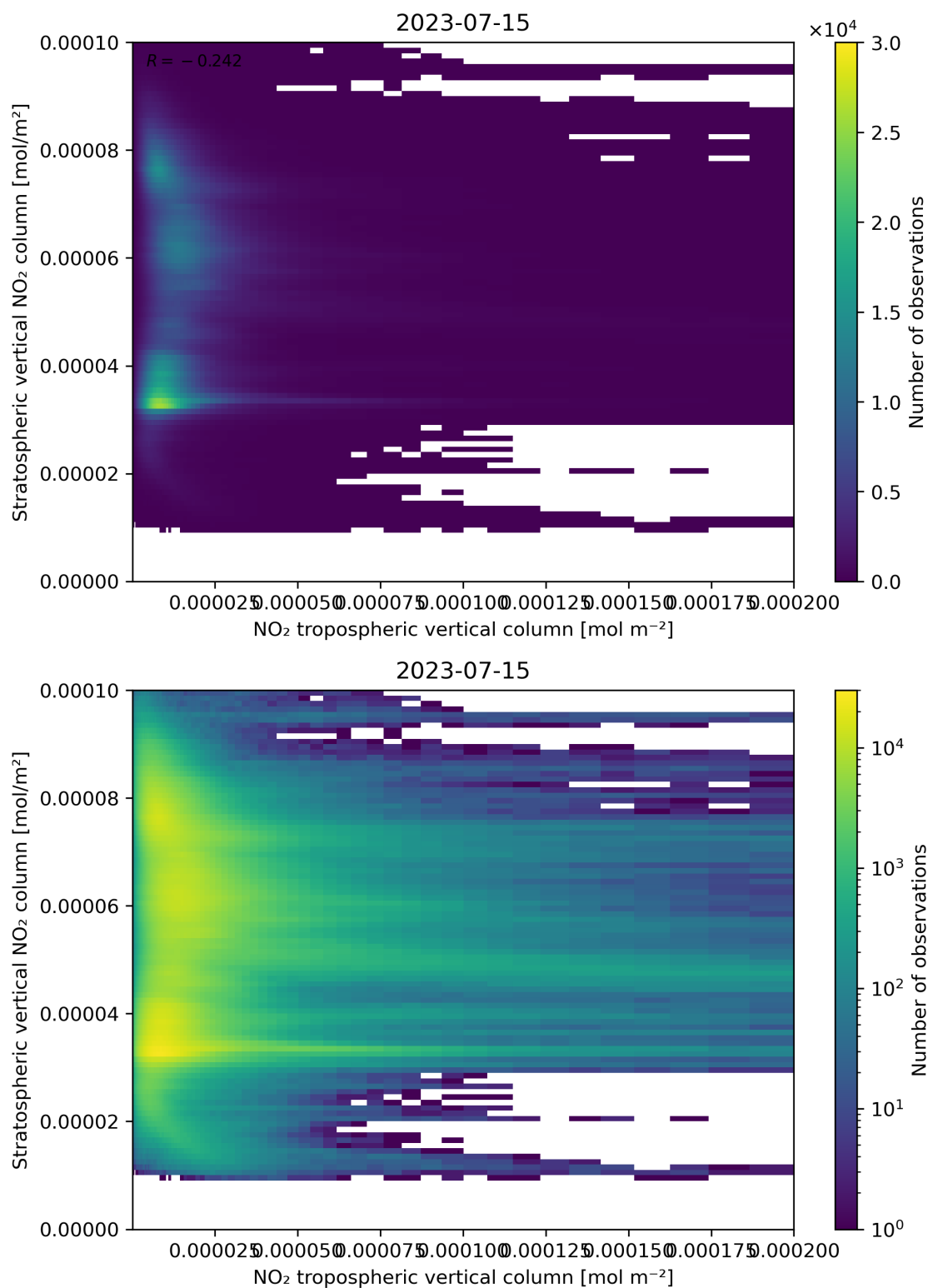
Figure 125: Scatter density plot of “NO 2 tropospheric vertical column” against “Stratospheric vertical NO 2 column” for 2023-07-14 to 2023-07-16.
