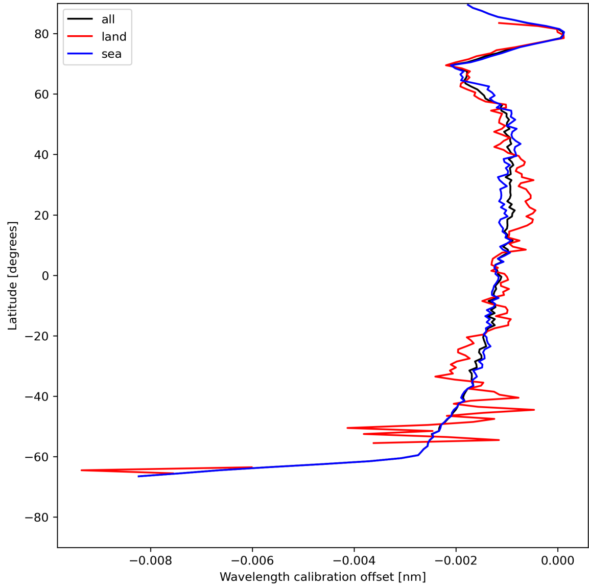
Figure 18: Zonal average of “Wavelength calibration offset” for 2023-07-14 to 2023-07-16.
