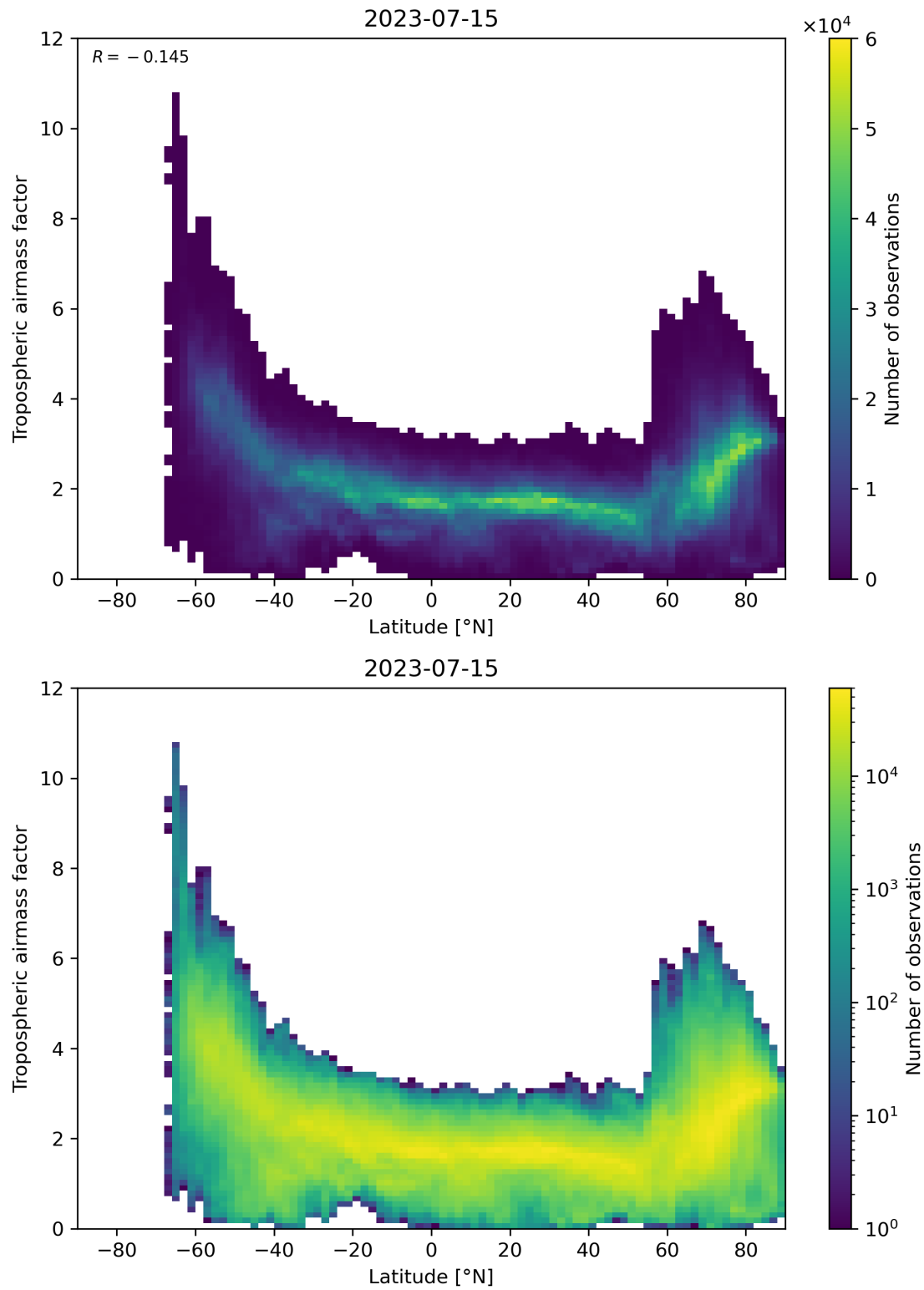
Figure 85: Scatter density plot of “Latitude” against “Tropospheric airmass factor” for 2023-07-14 to 2023-07-16.
