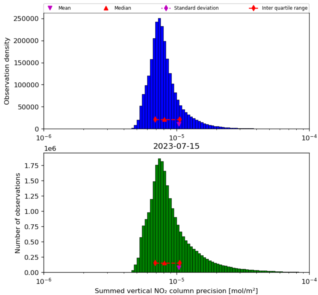
Figure 41: Histogram of “Summed vertical NO 2 column precision” for 2023-07-14 to 2023-07-16
