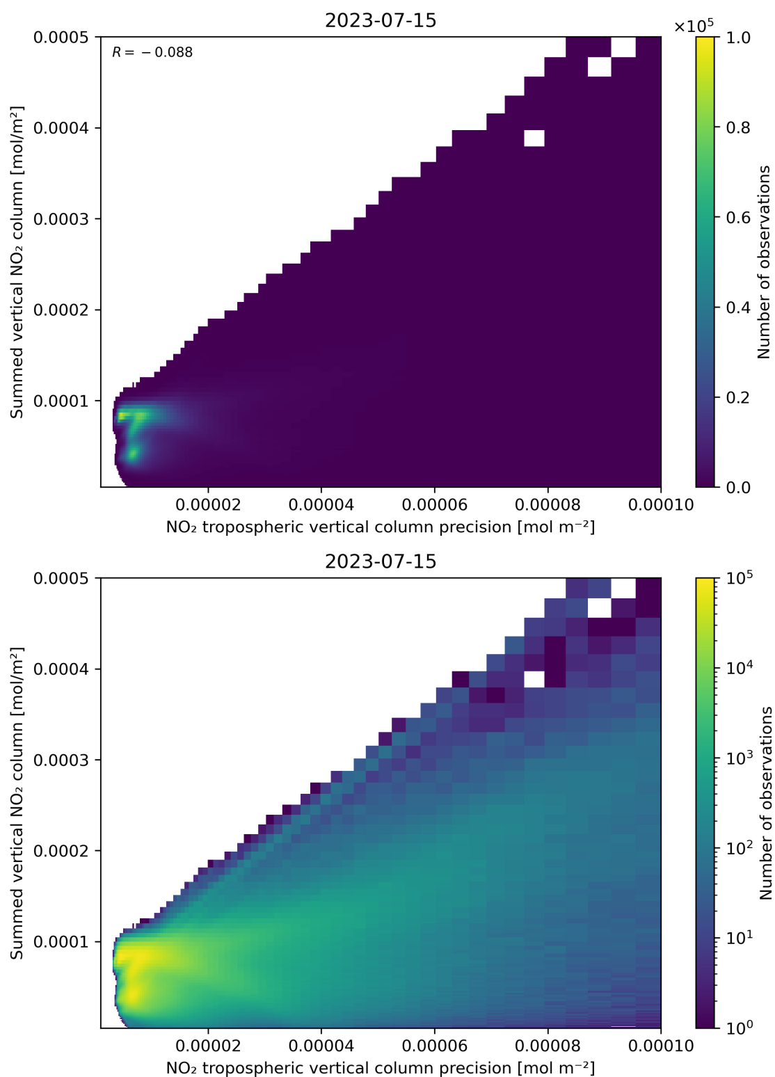
Figure 136: Scatter density plot of “NO 2 tropospheric vertical column precision” against “Summed vertical NO 2 column” for 2023-07-14 to 2023-07-16.
