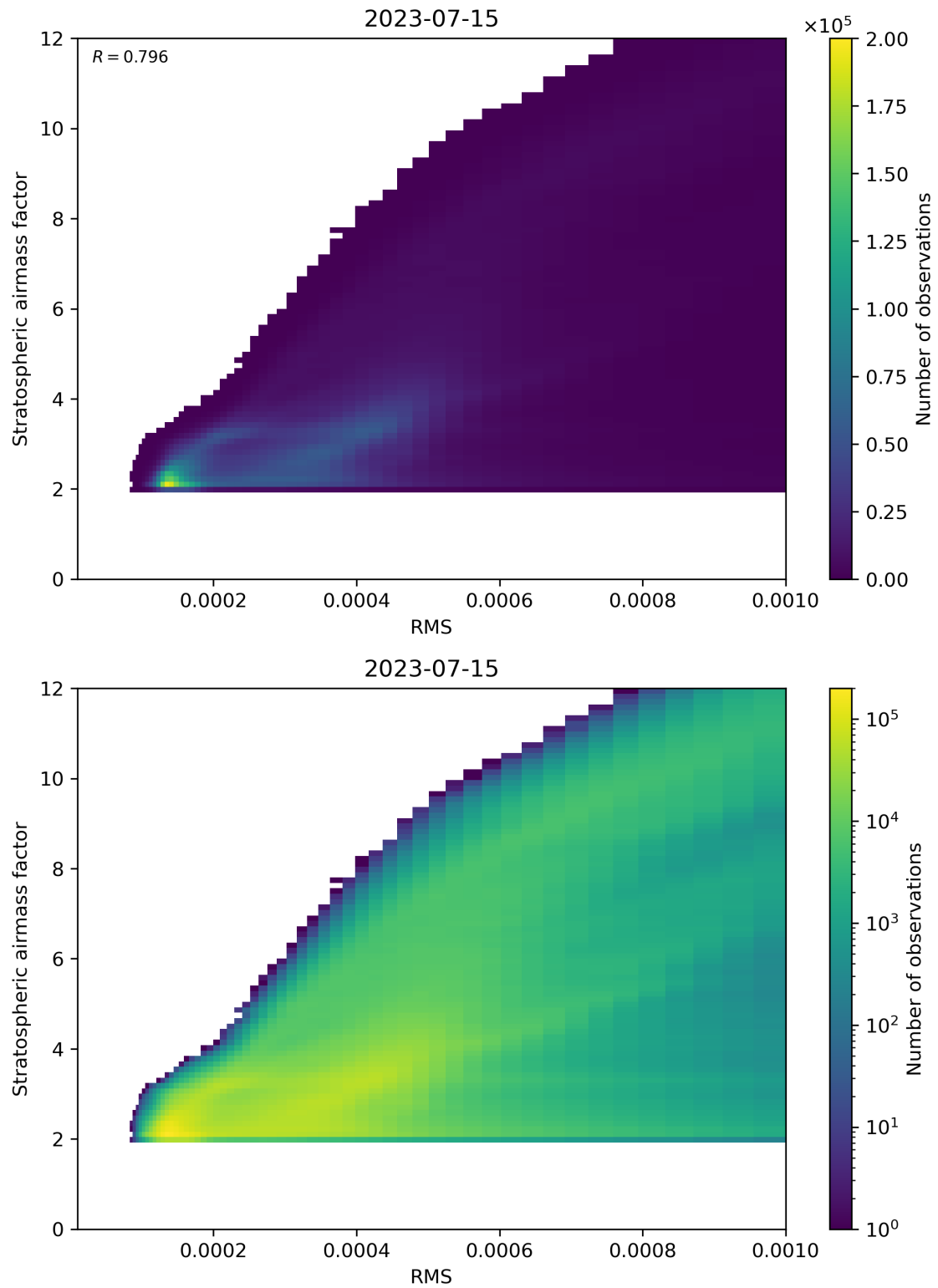
Figure 144: Scatter density plot of “RMS” against “Stratospheric airmass factor” for 2023-07-14 to 2023-07-16.
