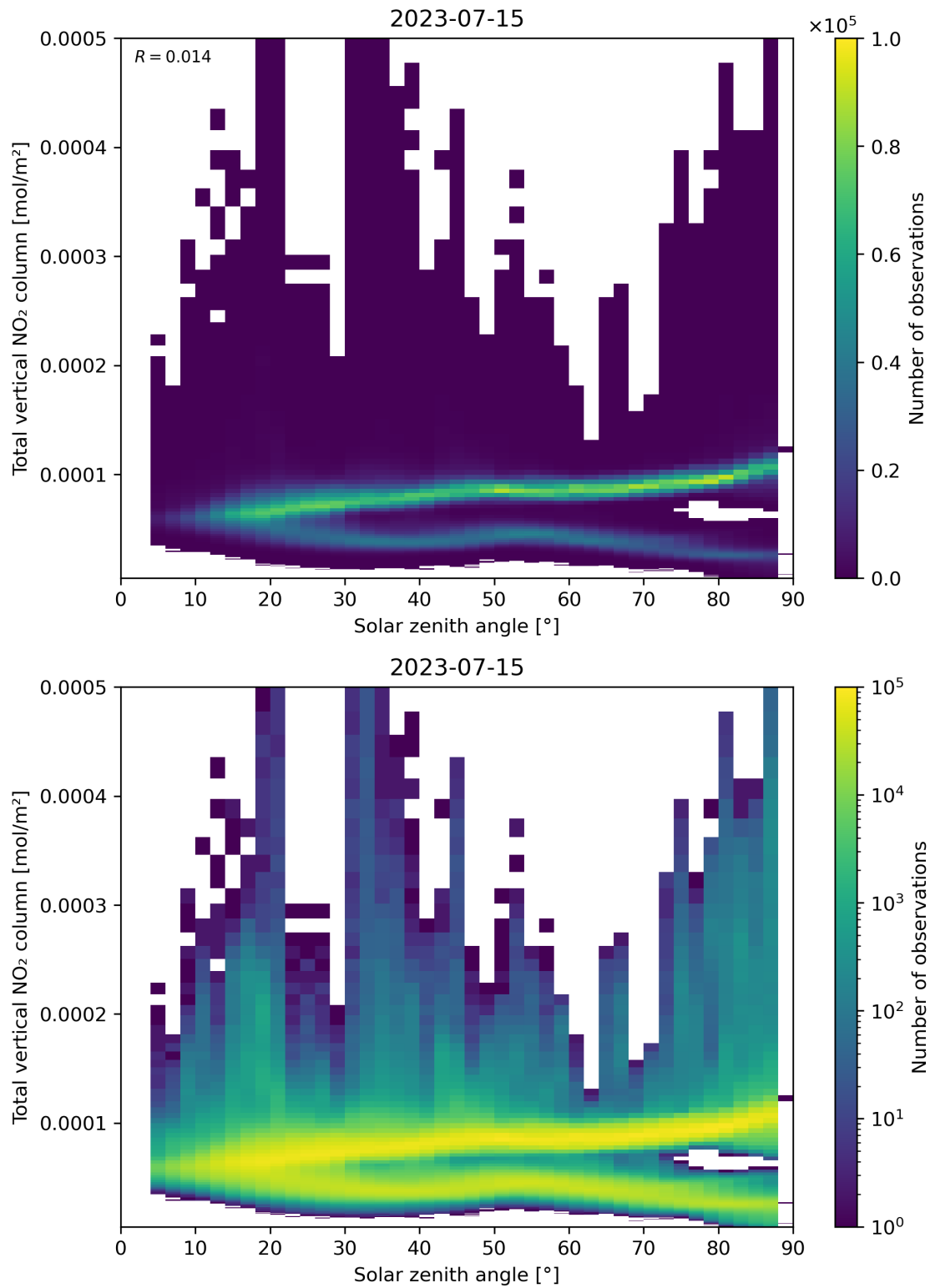
Figure 153: Scatter density plot of “Solar zenith angle” against “Total vertical NO 2 column” for 2023-07-14 to 2023-07-16.
