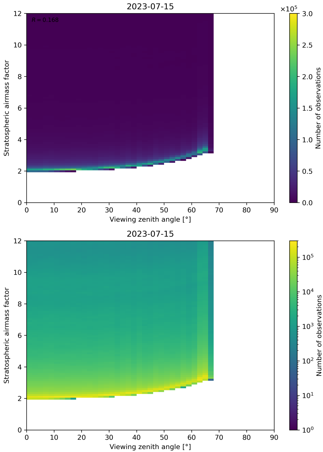
Figure 159: Scatter density plot of “Viewing zenith angle” against “Stratospheric airmass factor” for 2023-07-14 to 2023-07-16.
