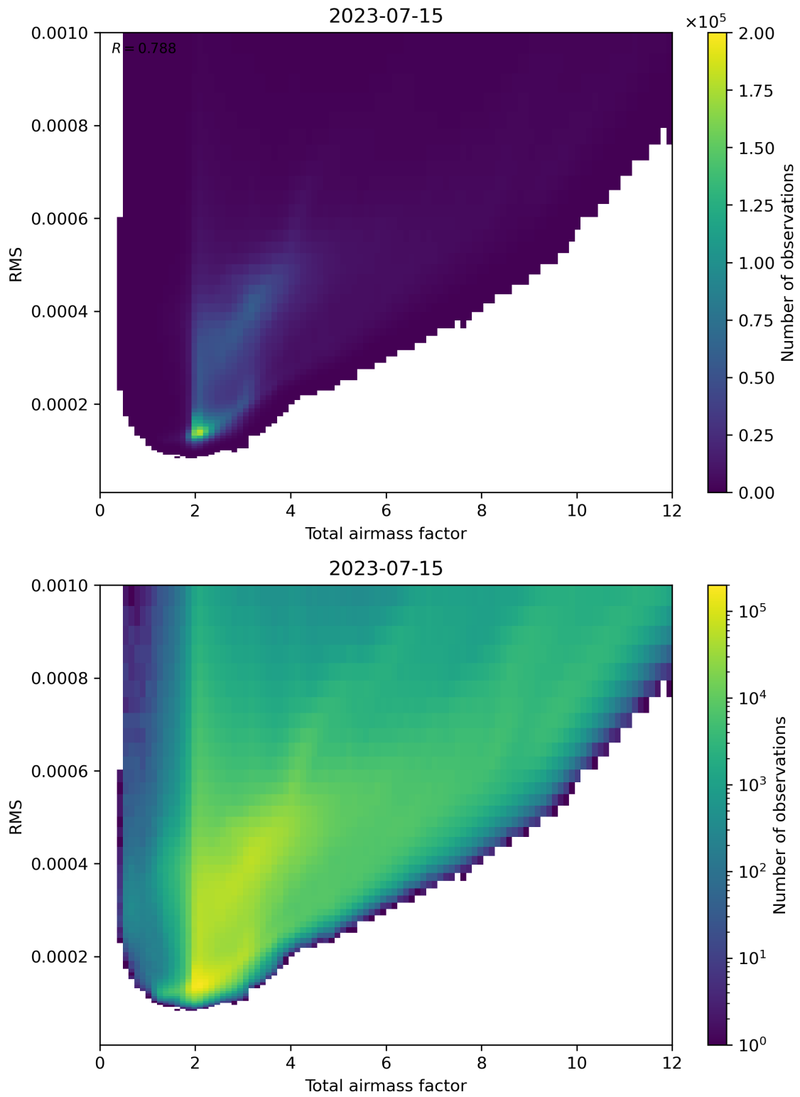
Figure 69: Scatter density plot of “Total airmass factor” against “RMS” for 2023-07-14 to 2023-07-16.
