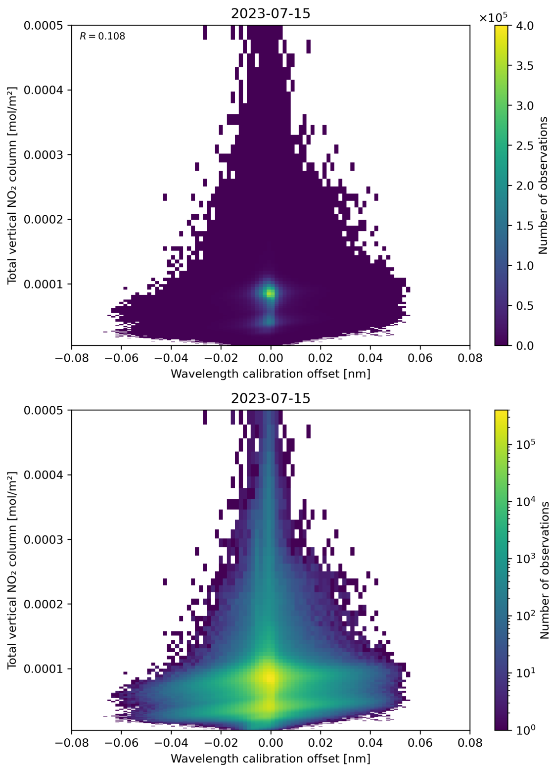
Figure 179: Scatter density plot of “Wavelength calibration offset” against “Total vertical NO 2 column” for 2023-07-14 to 2023-07-16.
