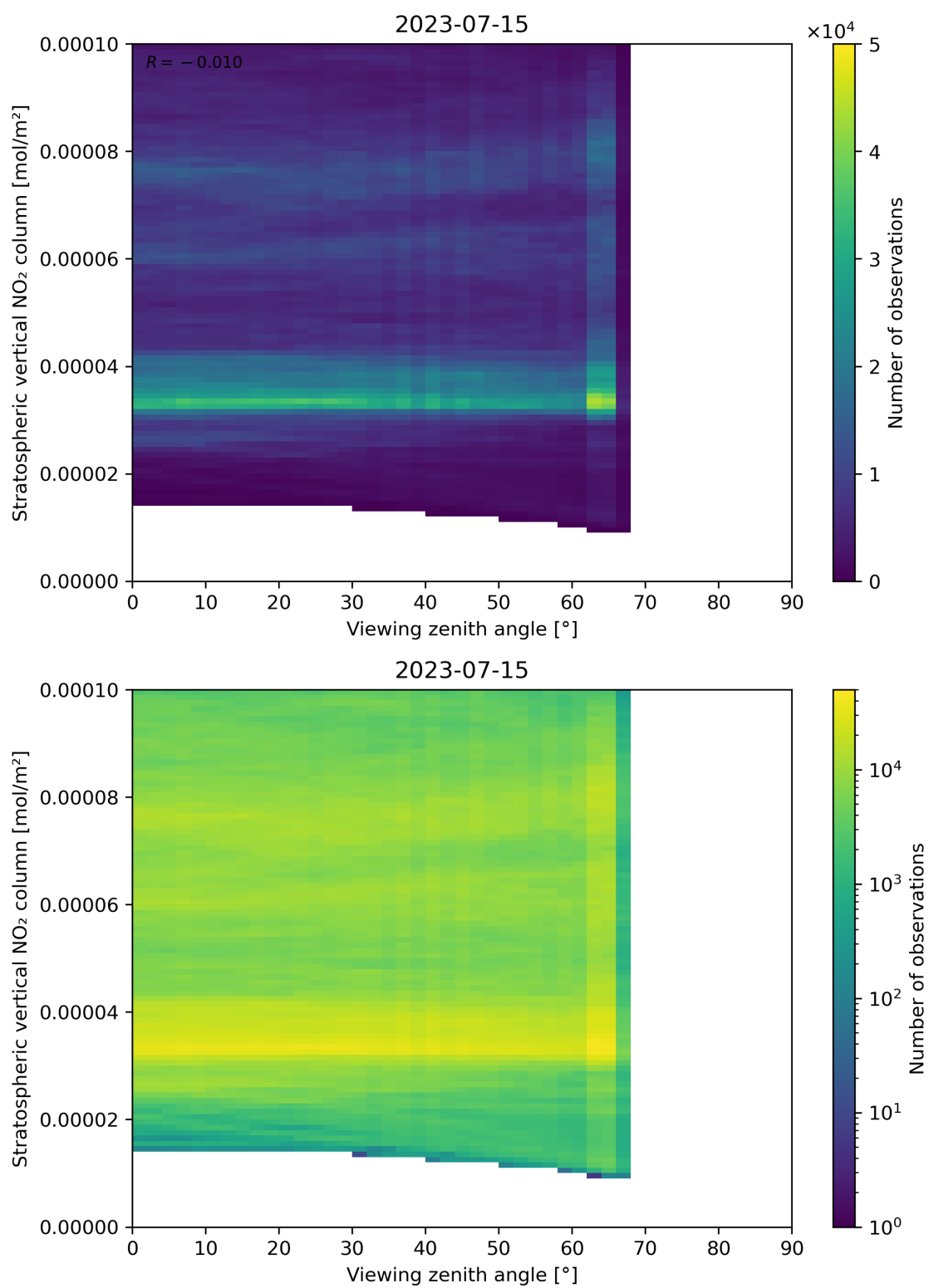
Figure 164: Scatter density plot of “Viewing zenith angle” against “Stratospheric vertical NO 2 column” for 2023-07-14 to 2023-07-16.
