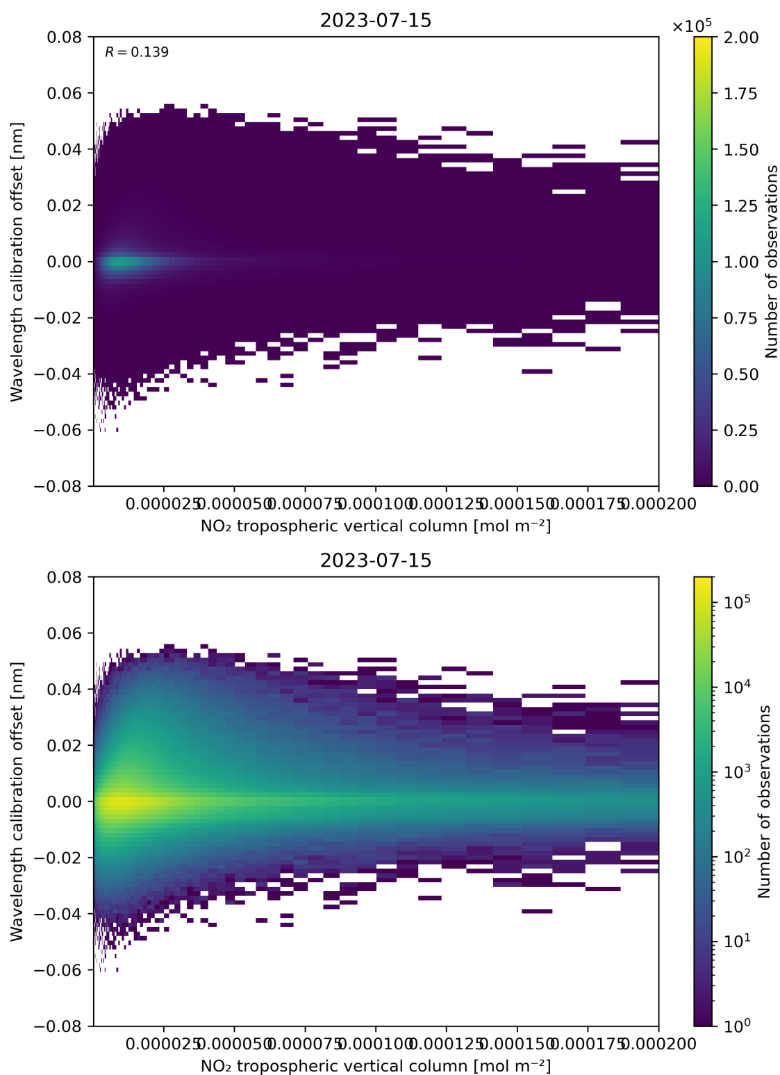
Figure 143: Scatter density plot of “NO 2 tropospheric vertical column” against “Wavelength calibration offset” for 2023-07-14 to 2023-07-16.
