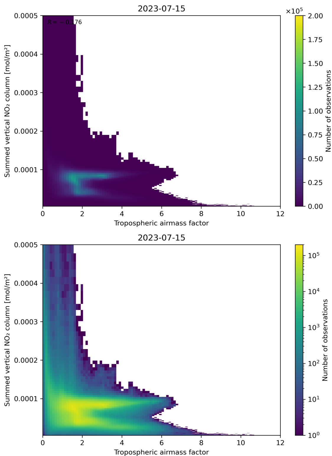
Figure 75: Scatter density plot of “Tropospheric airmass factor” against “Summed vertical NO 2 column” for 2023-07-14 to 2023-07-16.
