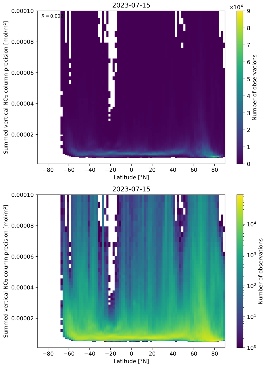
Figure 89: Scatter density plot of “Latitude” against “Summed vertical NO 2 column precision” for 2023-07-14 to 2023-07-16.
