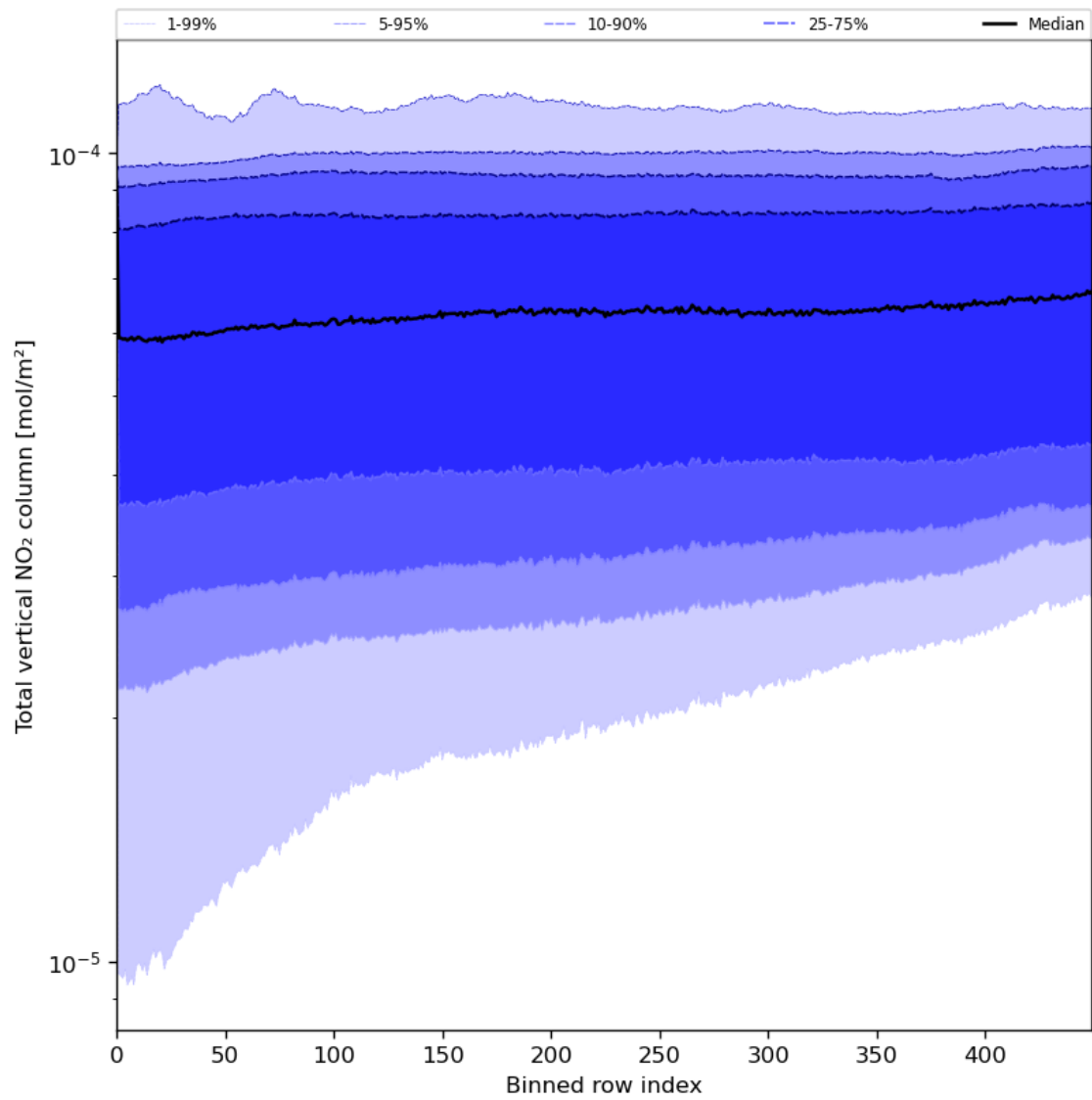
Figure 55: Along track statistics of “Total vertical NO 2 column” for 2023-07-14 to 2023-07-16
