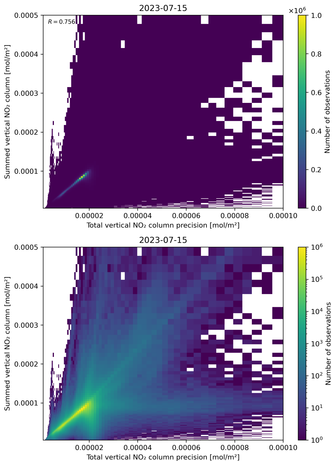
Figure 117: Scatter density plot of “Total vertical NO 2 column precision” against “Summed vertical NO 2 column” for 2023-07-14 to 2023-07-16.
