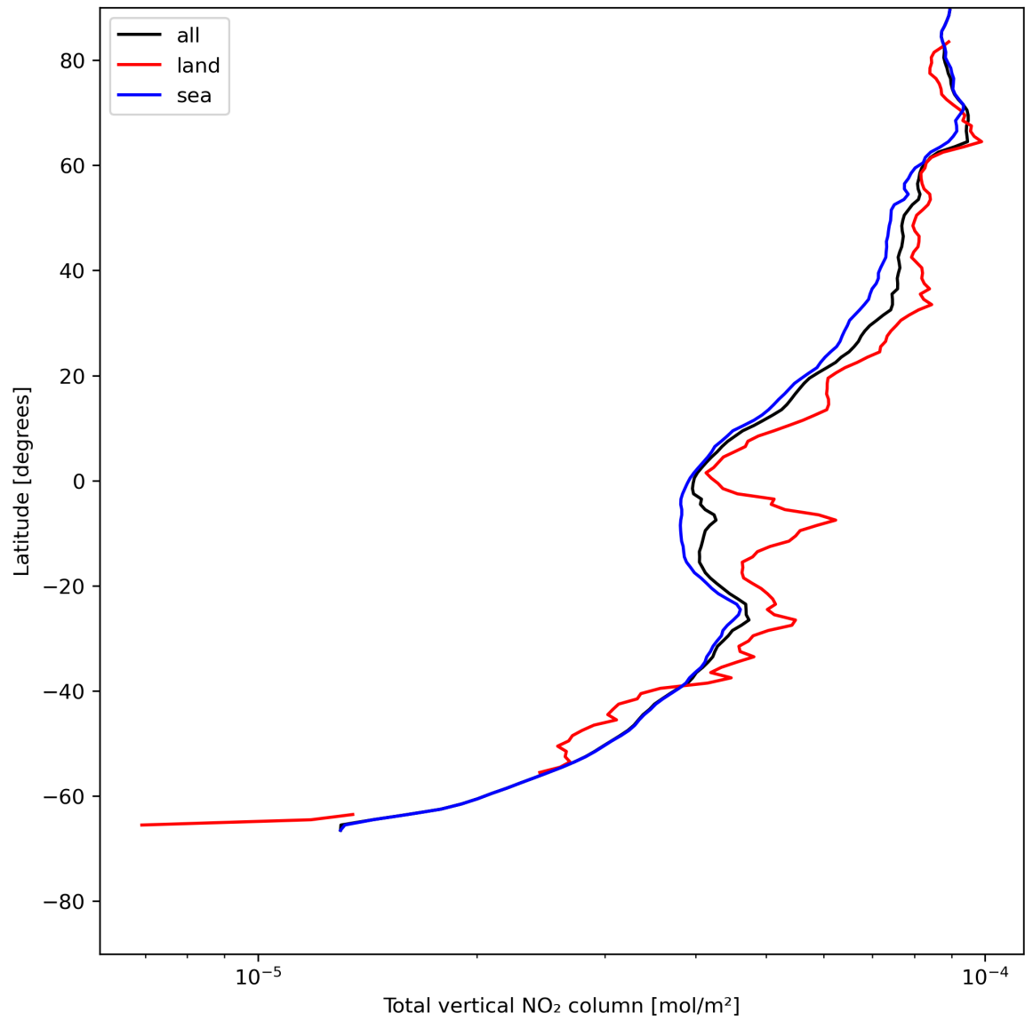
Figure 21: Zonal average of “Total vertical NO 2 column” for 2023-07-14 to 2023-07-16.
