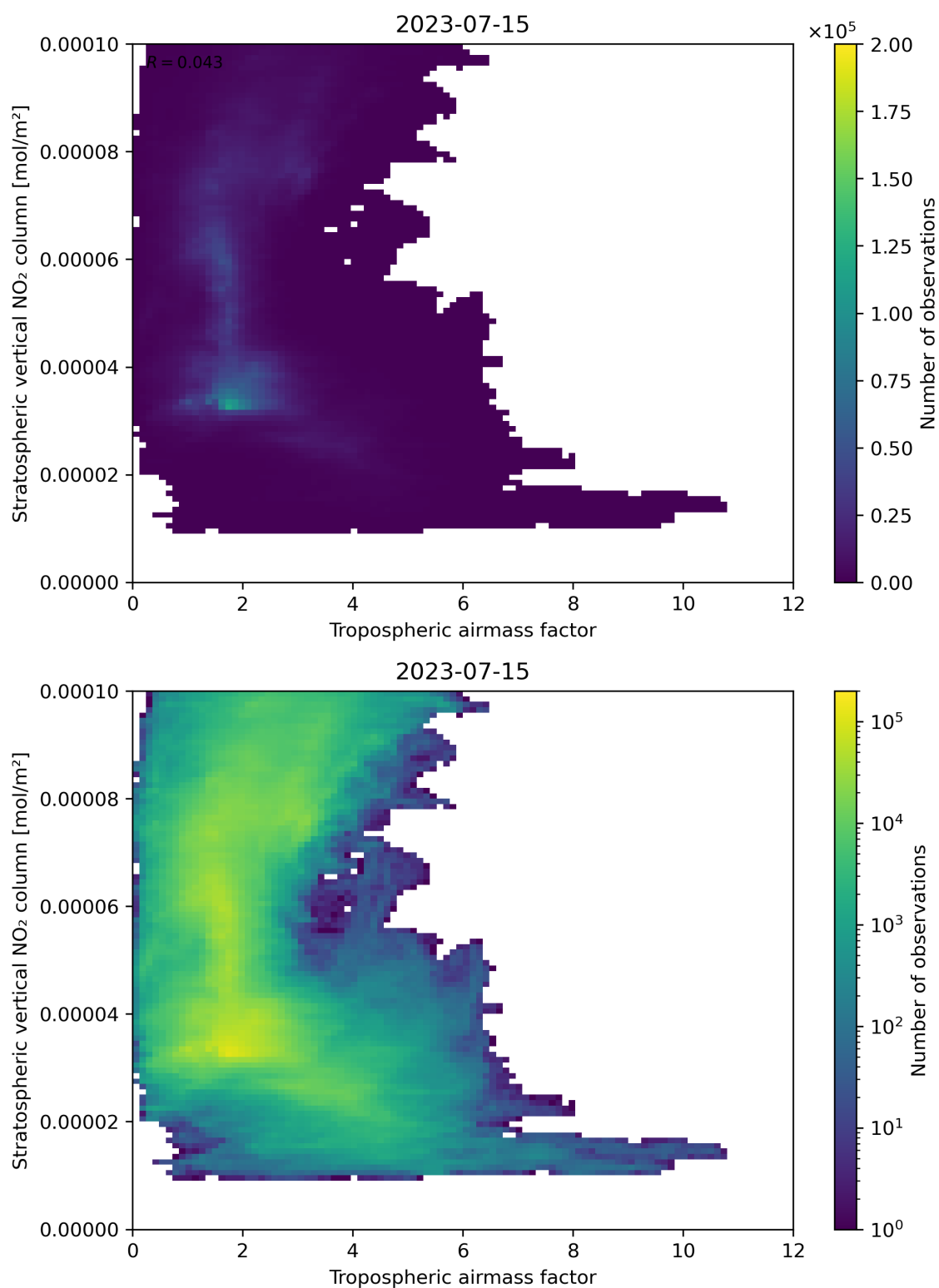
Figure 74: Scatter density plot of “Tropospheric air mass factor” against “Stratospheric vertical NO 2 column” for 2023-07-14 to 2023-07-16.
