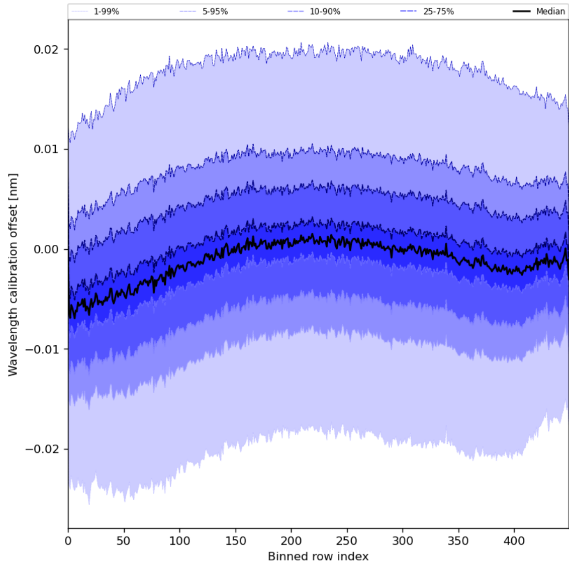
Figure 52: Along track statistics of “Wavelength calibration offset” for 2023-07-14 to 2023-07-16
