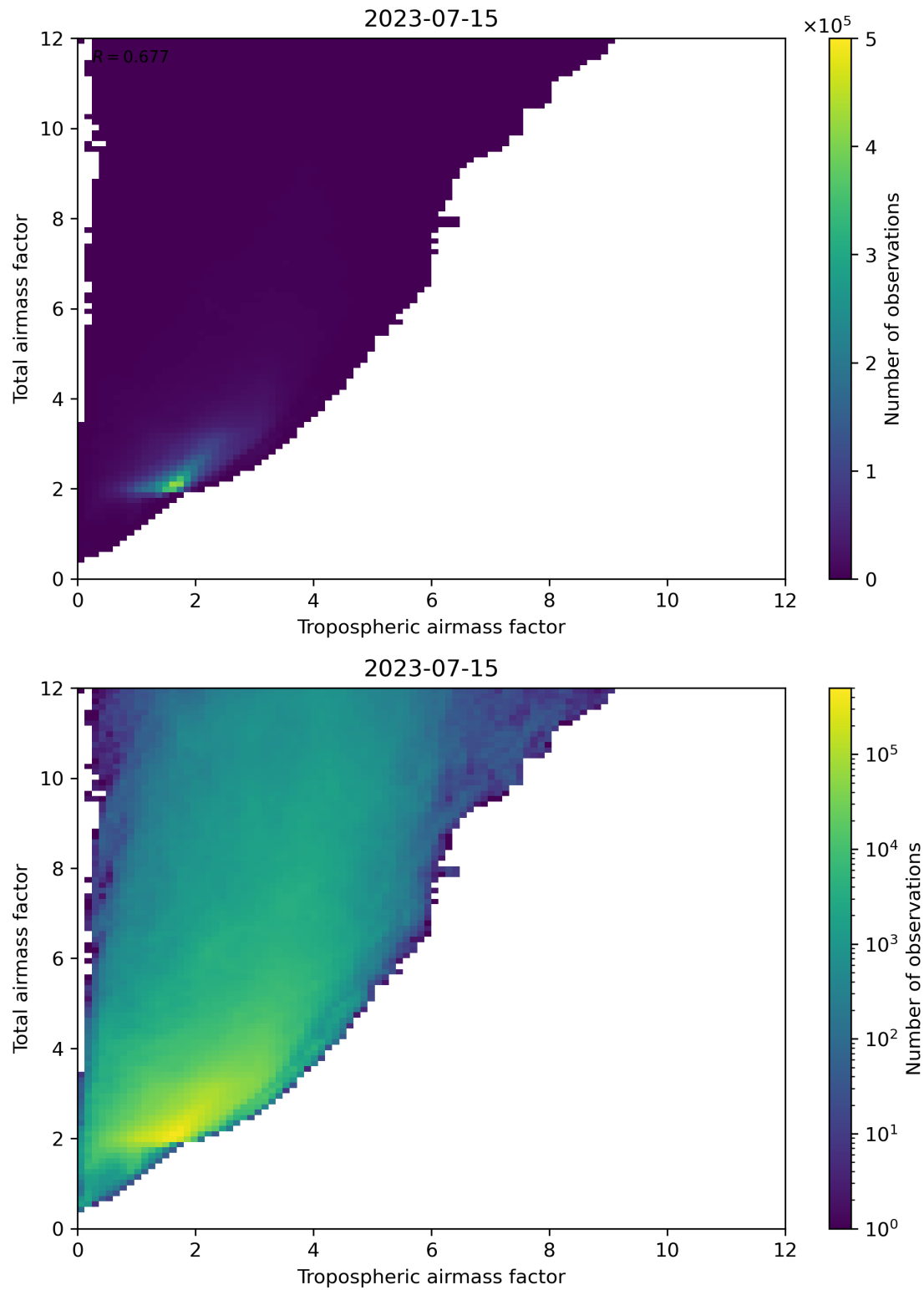
Figure 72: Scatter density plot of “Tropospheric airmass factor” against “Total airmass factor” for 2023-07-14 to 2023-07-16.
