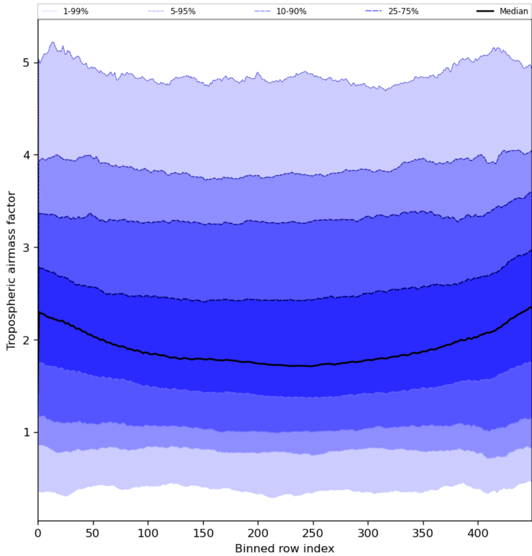
Figure 48: Along track statistics of “Tropospheric air mass factor” for 2023-07-14 to 2023-07-16
