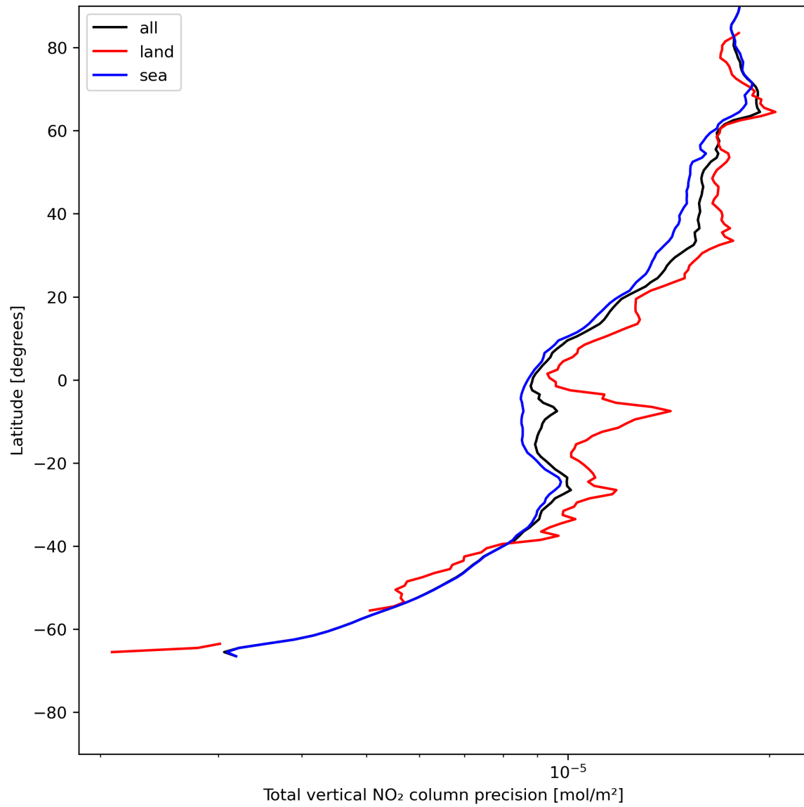
Figure 22: Zonal average of “Total vertical NO 2 column precision” for 2023-07-14 to 2023-07-16.
