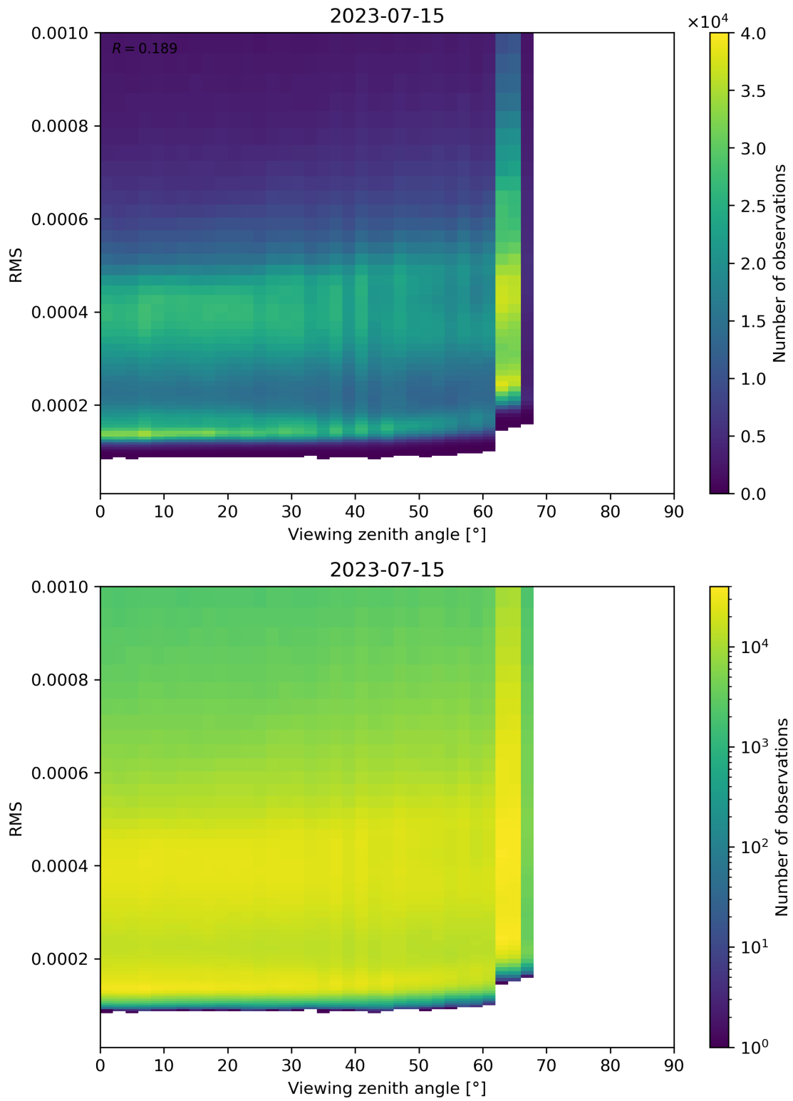
Figure 171: Scatter density plot of “Viewing zenith angle” against “RMS” for 2023-07-14 to 2023-07-16.
