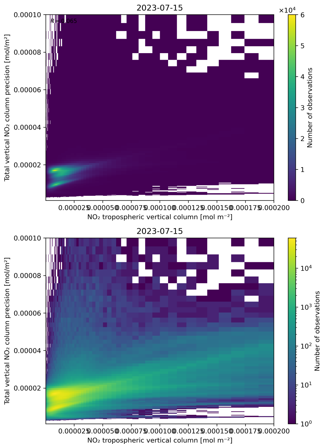
Figure 129: Scatter density plot of “NO 2 tropospheric vertical column” against “Total vertical NO 2 column precision” for 2023-07-14 to 2023-07-16.
