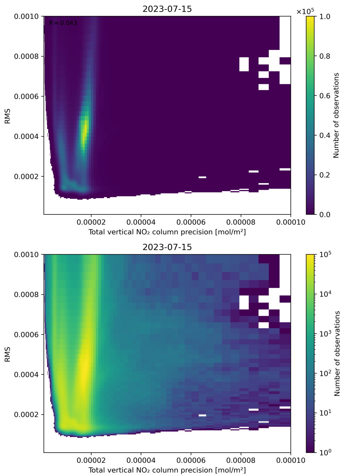
Figure 119: Scatter density plot of “Total vertical NO 2 column precision” against “RMS” for 2023-07-14 to 2023-07-16.
