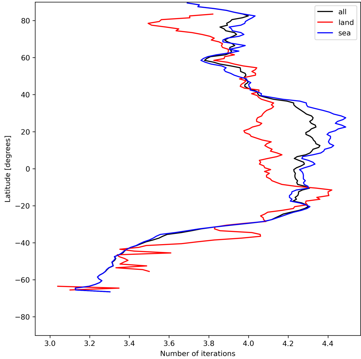
Figure 17: Zonal average of “Number of iterations” for 2023-07-14 to 2023-07-16.
