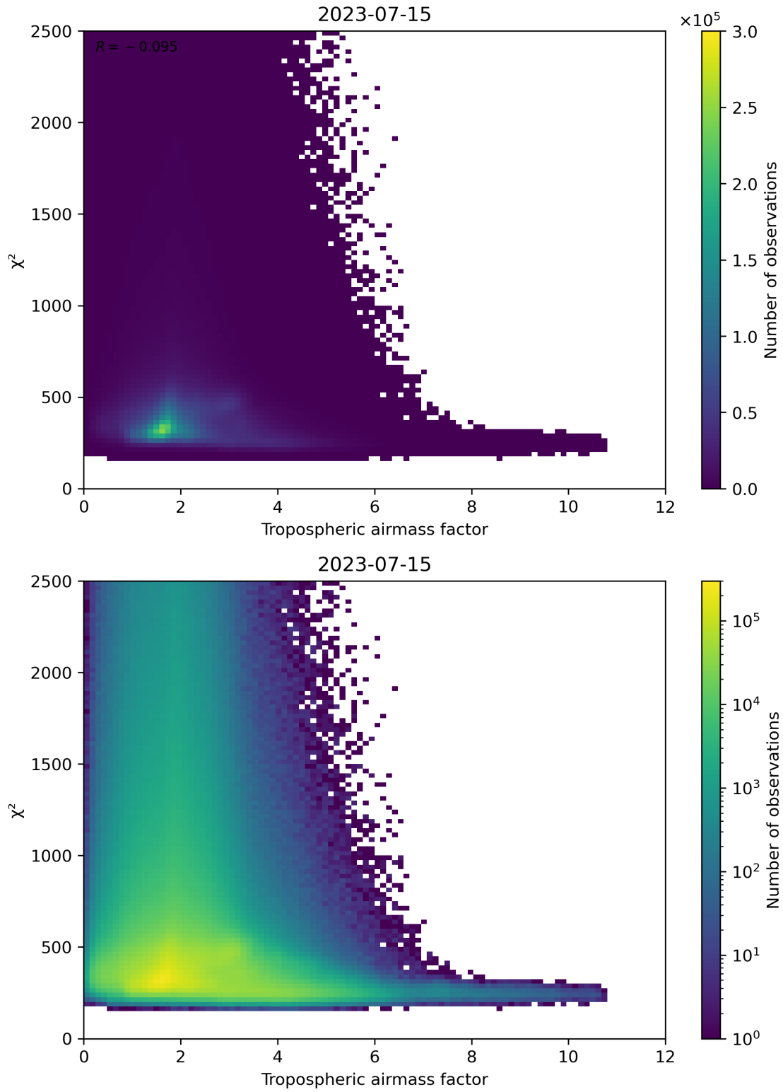
Figure 73: Scatter density plot of “Tropospheric airmass factor” against “ \chi^2 ” for 2023-07-14 to 2023-07-16.
