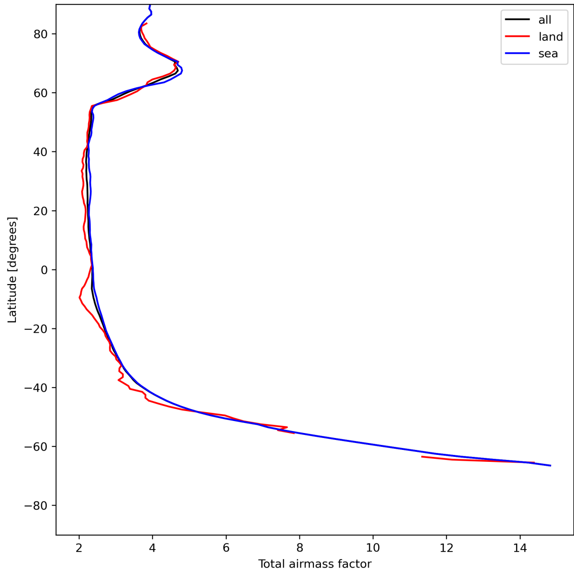
Figure 15: Zonal average of “Total airmass factor” for 2023-07-14 to 2023-07-16.
