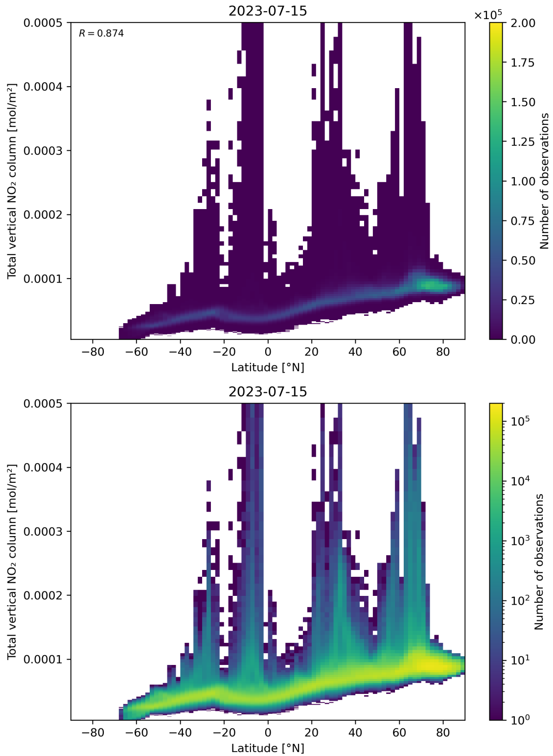
Figure 90: Scatter density plot of “Latitude” against “Total vertical NO 2 column” for 2023-07-14 to 2023-07-16.
