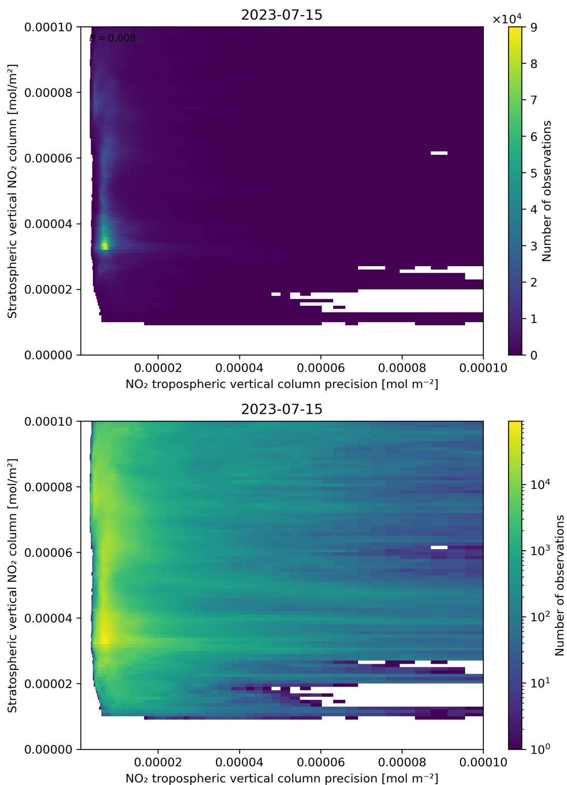
Figure 135: Scatter density plot of “NO 2 tropospheric vertical column precision” against “Stratospheric vertical NO 2 column” for 2023-07-14 to 2023-07-16.
