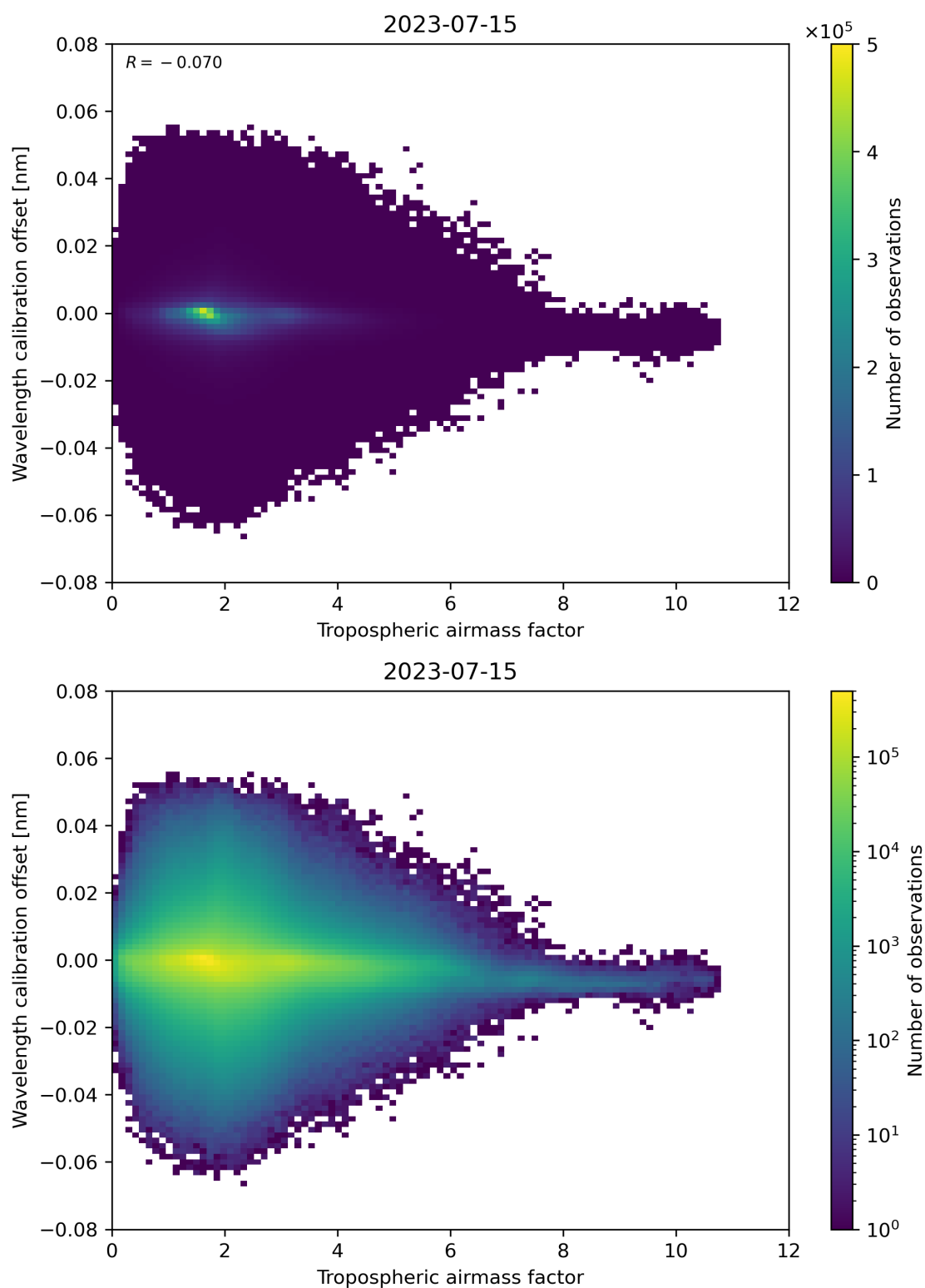
Figure 80: Scatter density plot of “Tropospheric airmass factor” against “Wavelength calibration offset” for 2023-07-14 to 2023-07-16.
