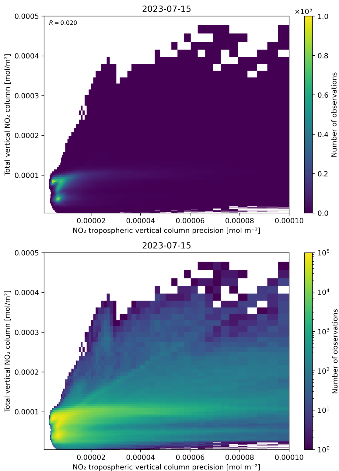
Figure 138: Scatter density plot of “NO 2 tropospheric vertical column precision” against “Total vertical NO 2 column” for 2023-07-14 to 2023-07-16.
