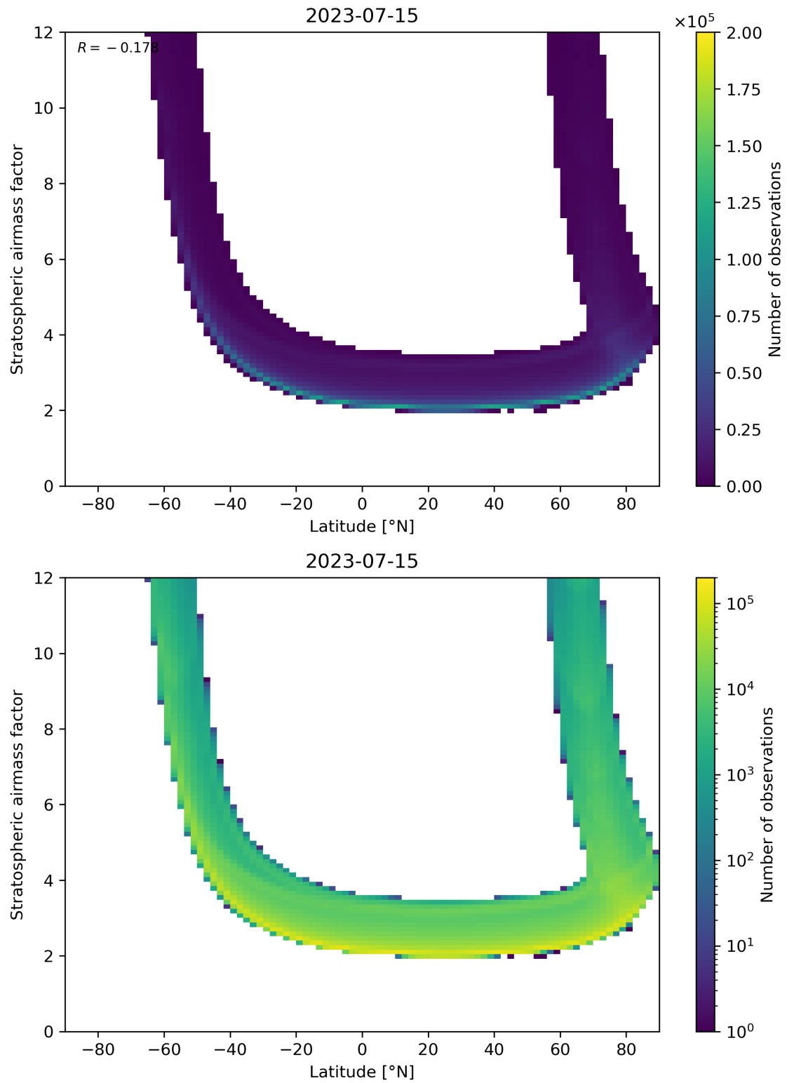
Figure 83: Scatter density plot of “Latitude” against “Stratospheric air mass factor” for 2023-07-14 to 2023-07-16.
