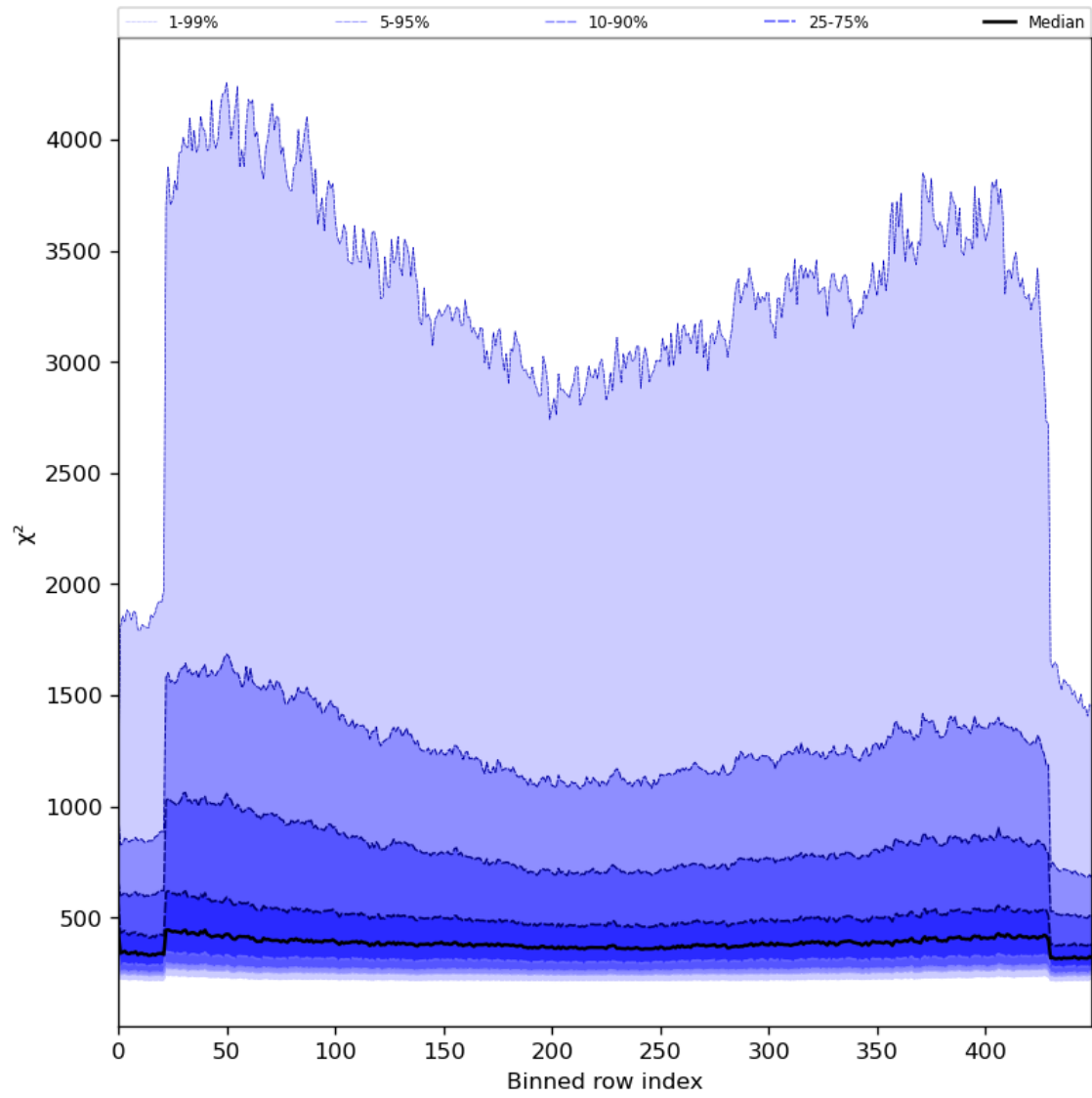
Figure 59: Along track statistics of “ \chi^2 ” for 2023-07-14 to 2023-07-16
