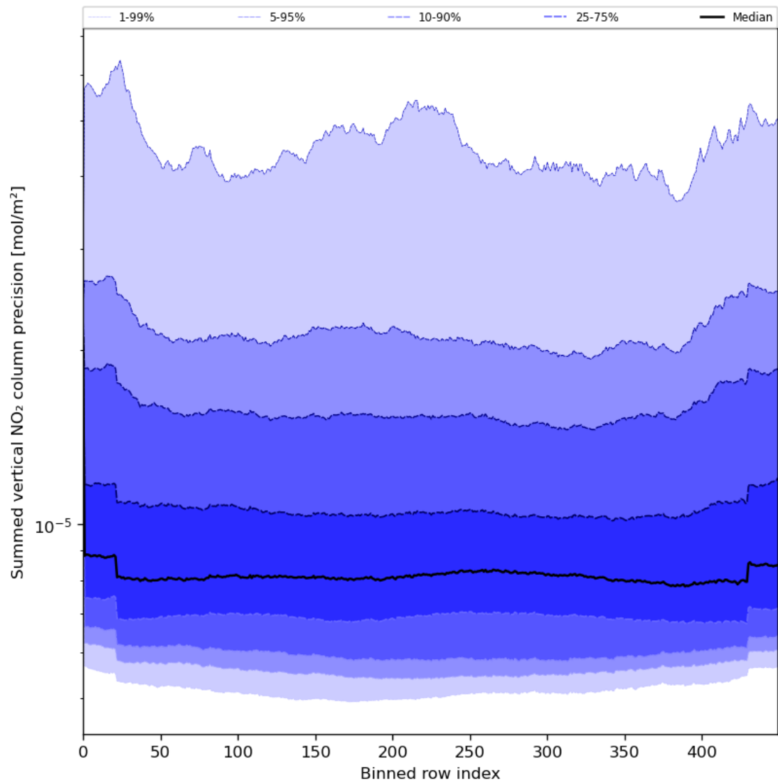
Figure 58: Along track statistics of “Summed vertical NO 2 column precision” for 2023-07-14 to 2023-07-16
