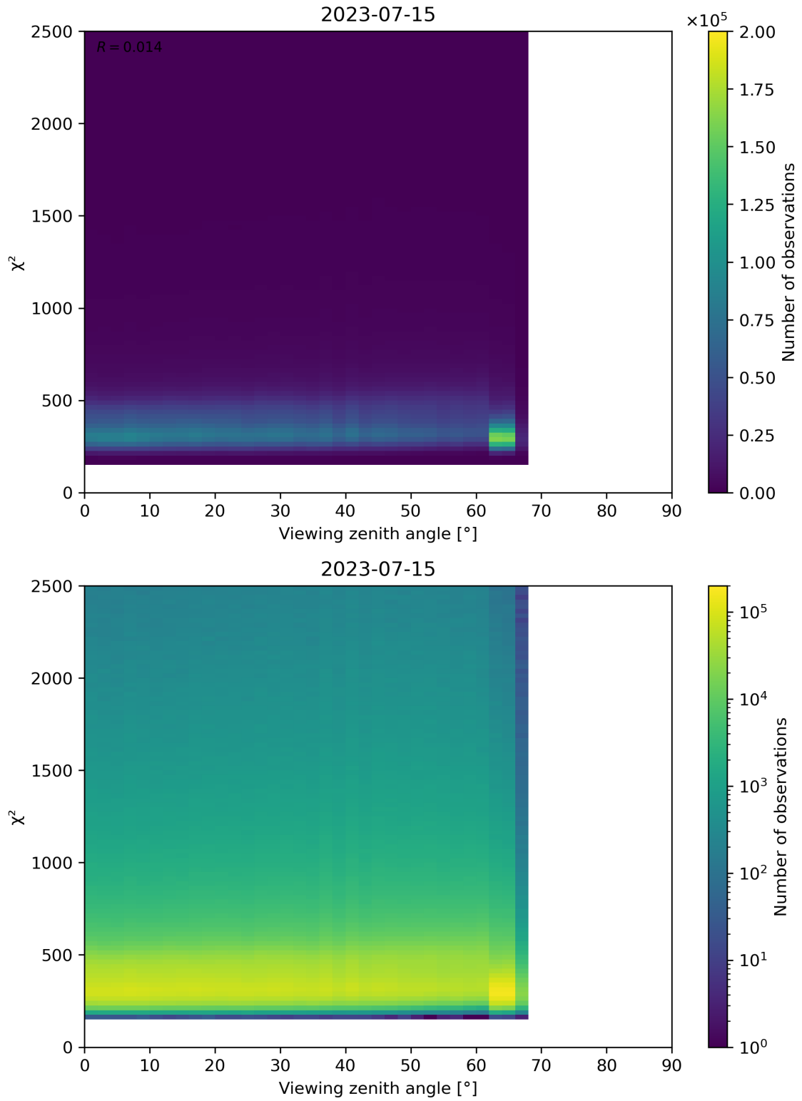
Figure 162: Scatter density plot of “Viewing zenith angle” against “ \chi^2 ” for 2023-07-14 to 2023-07-16.
