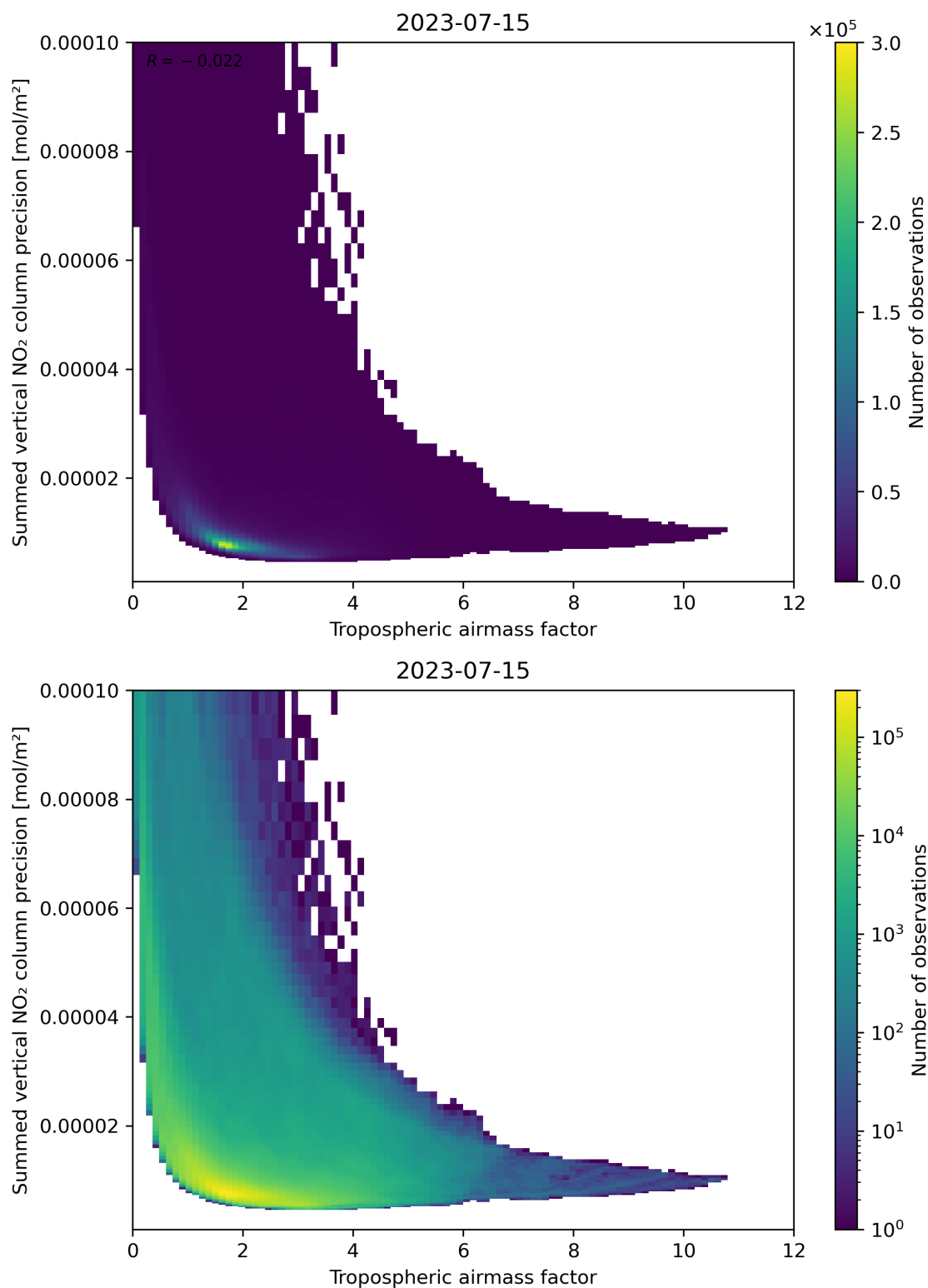
Figure 76: Scatter density plot of “Tropospheric air mass factor” against “Summed vertical NO 2 column precision” for 2023-07-14 to 2023-07-16.
