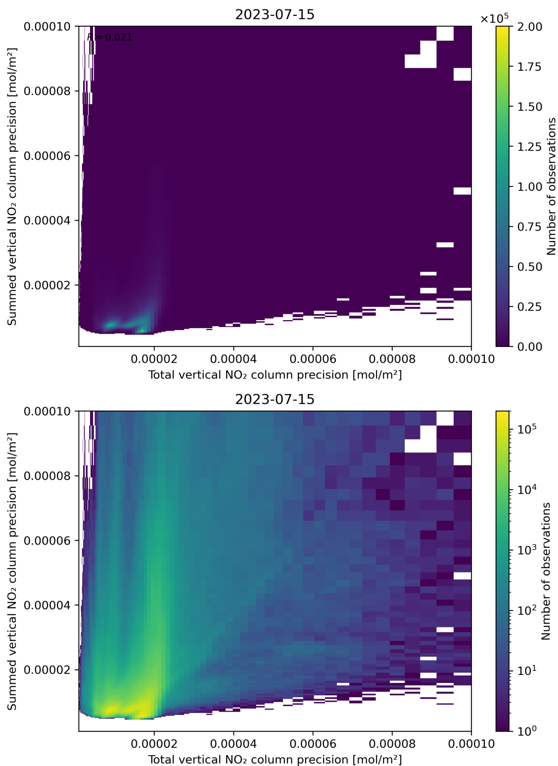
Figure 118: Scatter density plot of “Total vertical NO 2 column precision” against “Summed vertical NO 2 column precision” for 2023-07-14 to 2023-07-16.
