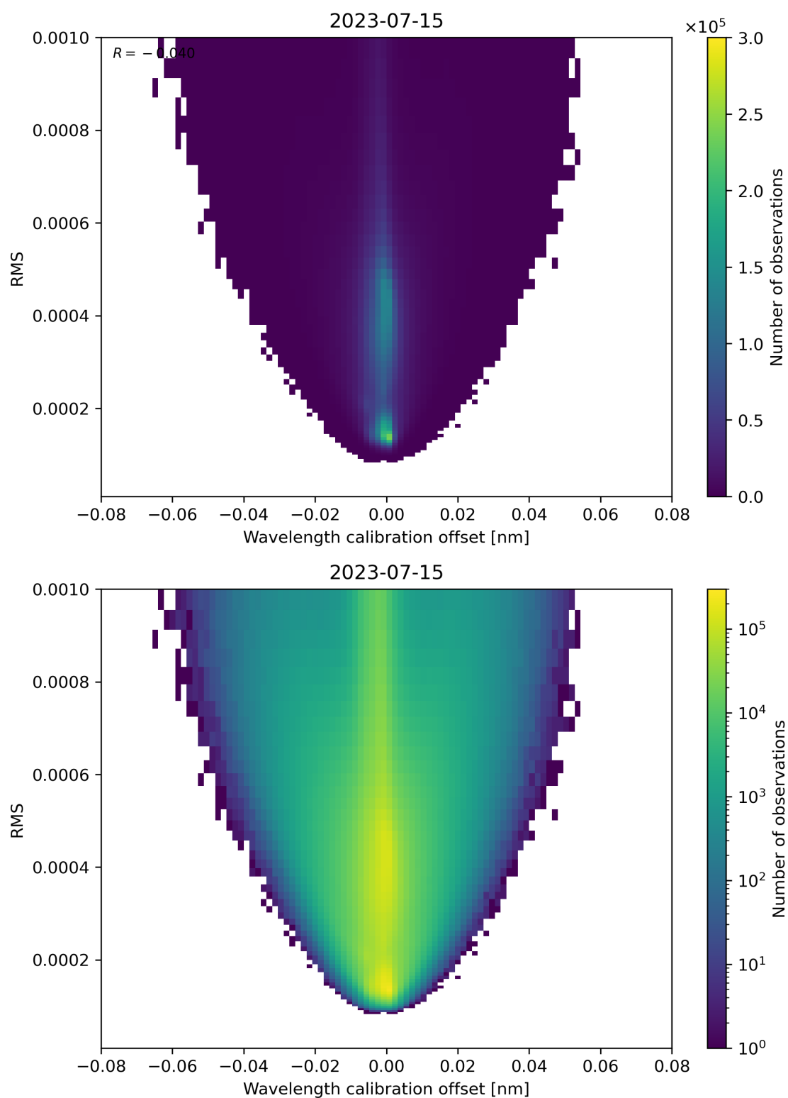
Figure 181: Scatter density plot of “Wavelength calibration offset” against “RMS” for 2023-07-14 to 2023-07-16.
