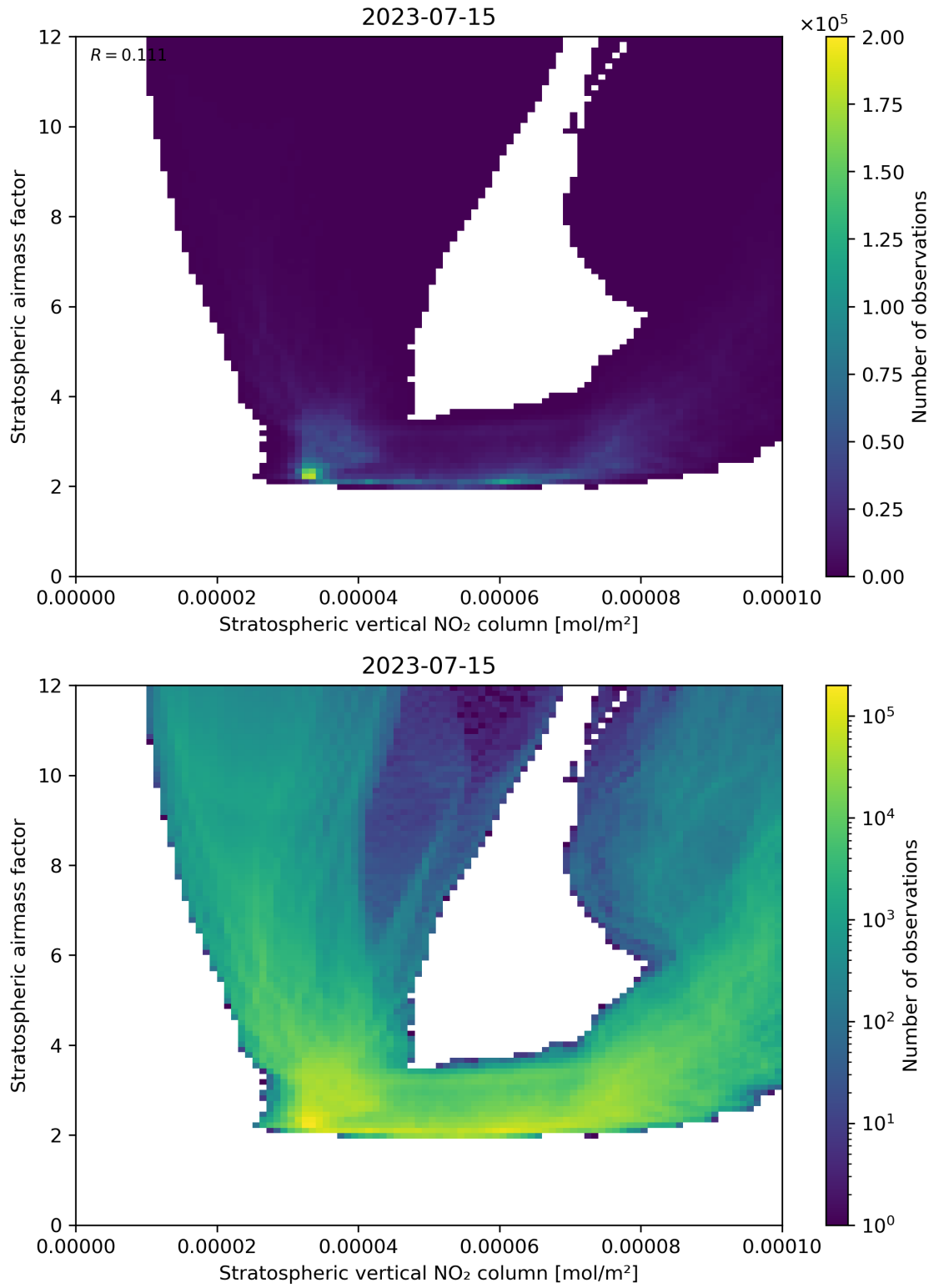
Figure 96: Scatter density plot of “Stratospheric vertical NO 2 column” against “Stratospheric airmass factor” for 2023-07-14 to 2023-07-16.
