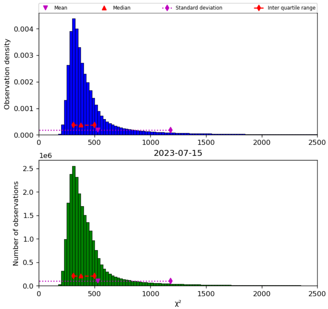
Figure 42: Histogram of “ \chi^2 ” for 2023-07-14 to 2023-07-16
