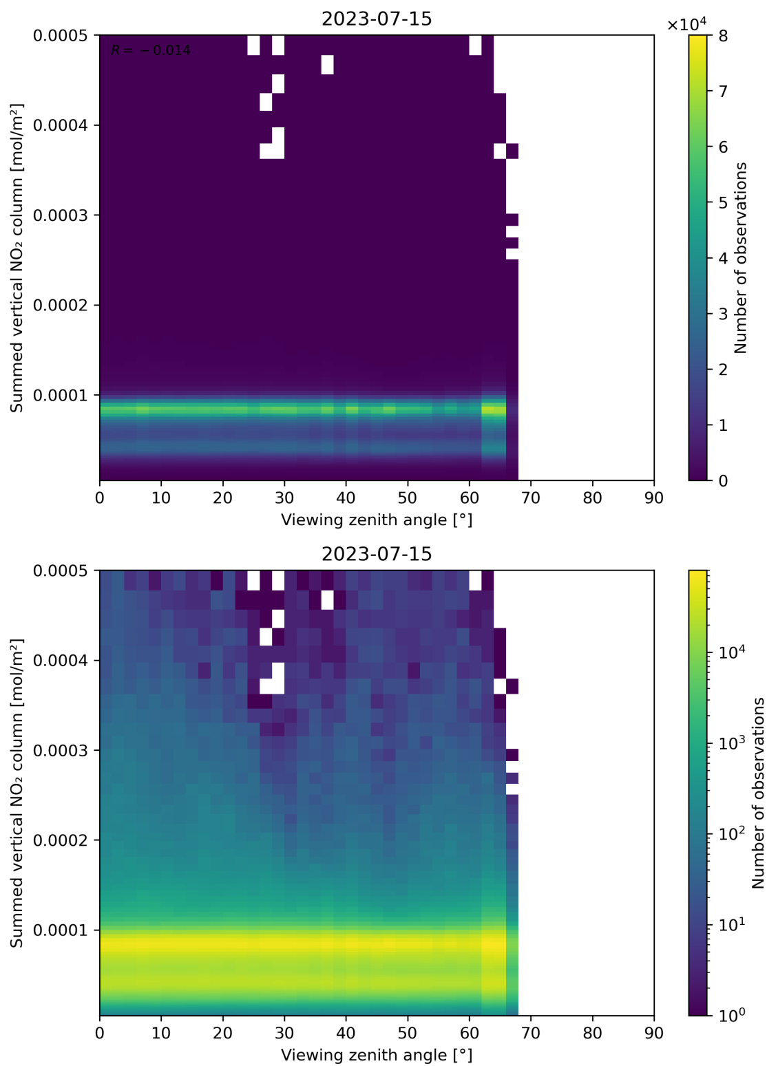
Figure 165: Scatter density plot of “Viewing zenith angle” against “Summed vertical NO 2 column” for 2023-07-14 to 2023-07-16.
