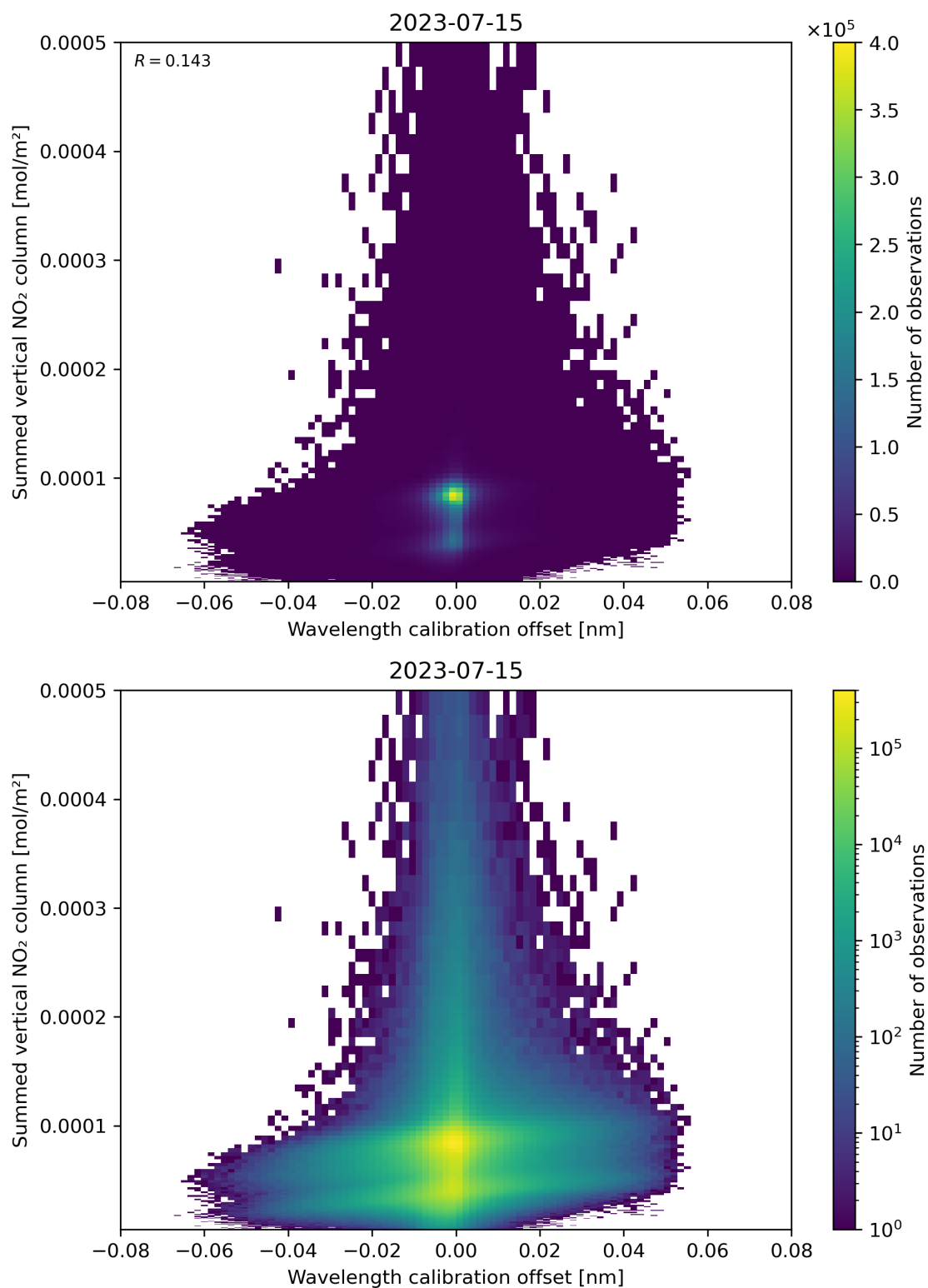
Figure 177: Scatter density plot of “Wavelength calibration offset” against “Summed vertical NO 2 column” for 2023-07-14 to 2023-07-16.
