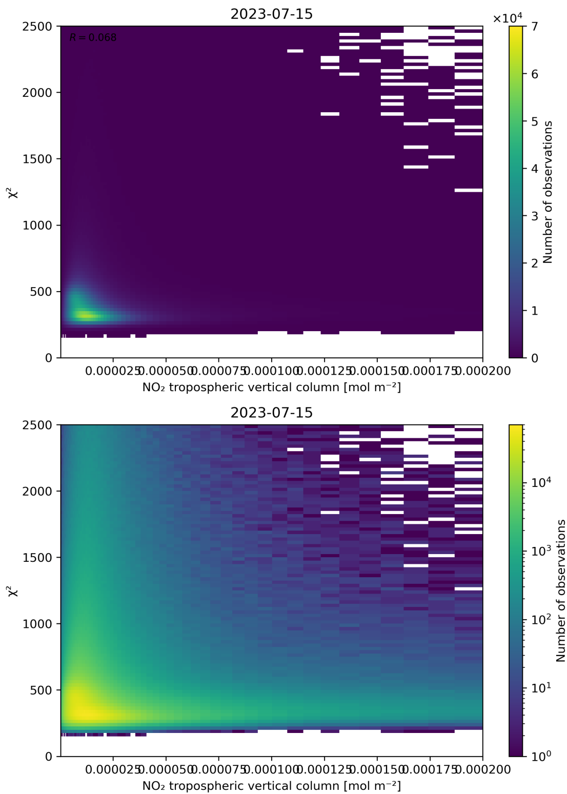
Figure 124: Scatter density plot of “NO 2 tropospheric vertical column” against “ \chi^2 ” for 2023-07-14 to 2023-07-16.
