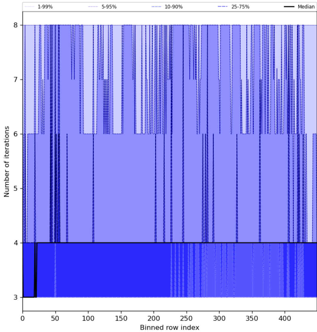
Figure 51: Along track statistics of “Number of iterations” for 2023-07-14 to 2023-07-16
