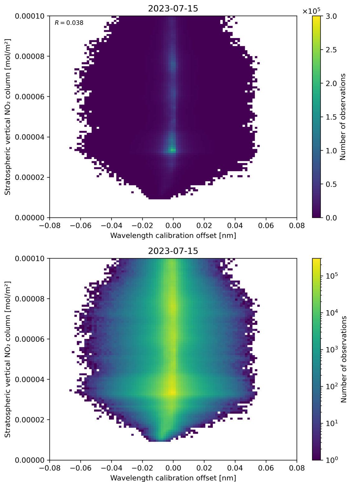
Figure 176: Scatter density plot of “Wavelength calibration offset” against “Stratospheric vertical NO 2 column” for 2023-07-14 to 2023-07-16.
