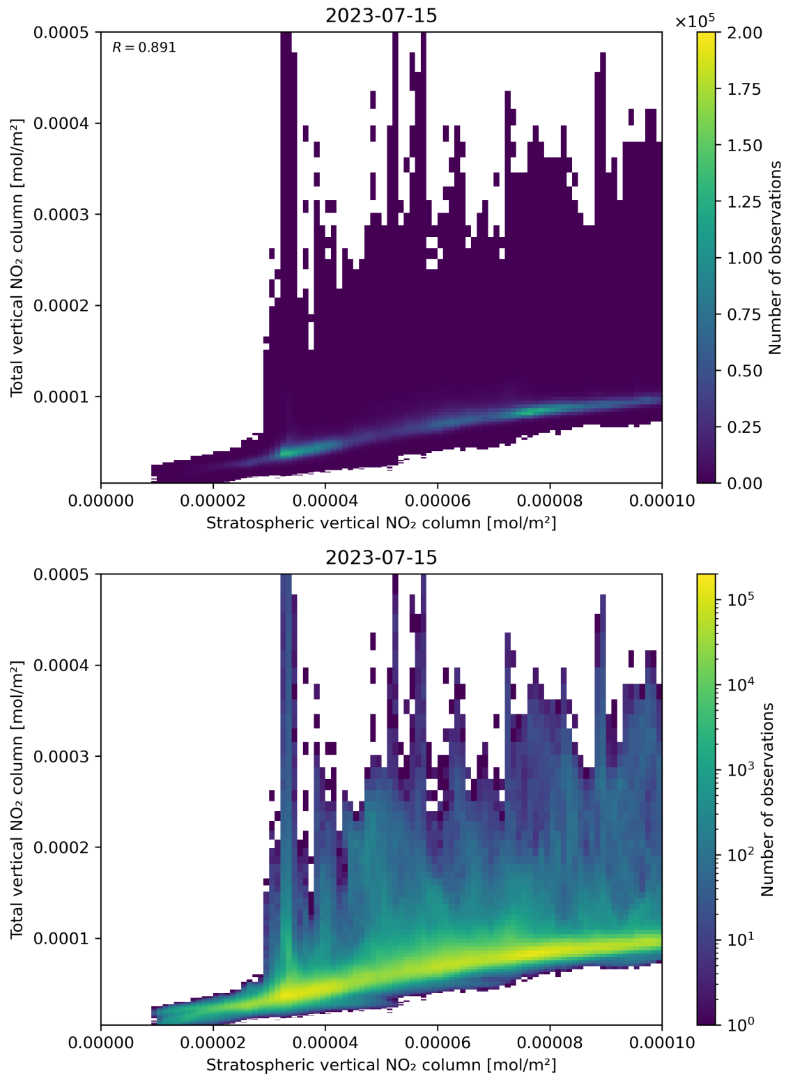
Figure 100: Scatter density plot of “Stratospheric vertical NO 2 column” against “Total vertical NO 2 column” for 2023-07-14 to 2023-07-16.
