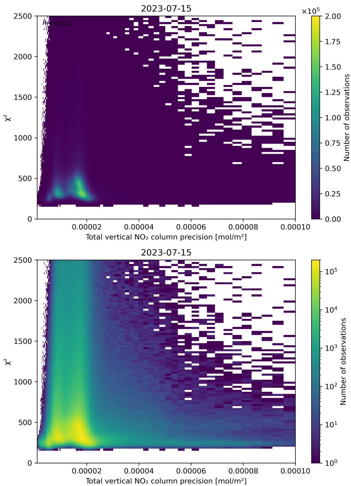
Figure 116: Scatter density plot of “Total vertical NO 2 column precision” against “ \chi^2 ” for 2023-07-14 to 2023-07-16.
