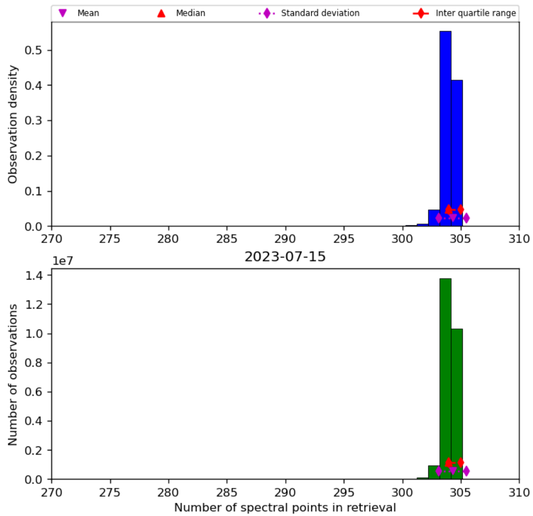
Figure 33: Histogram of “Number of spectral points in retrieval” for 2023-07-14 to 2023-07-16
