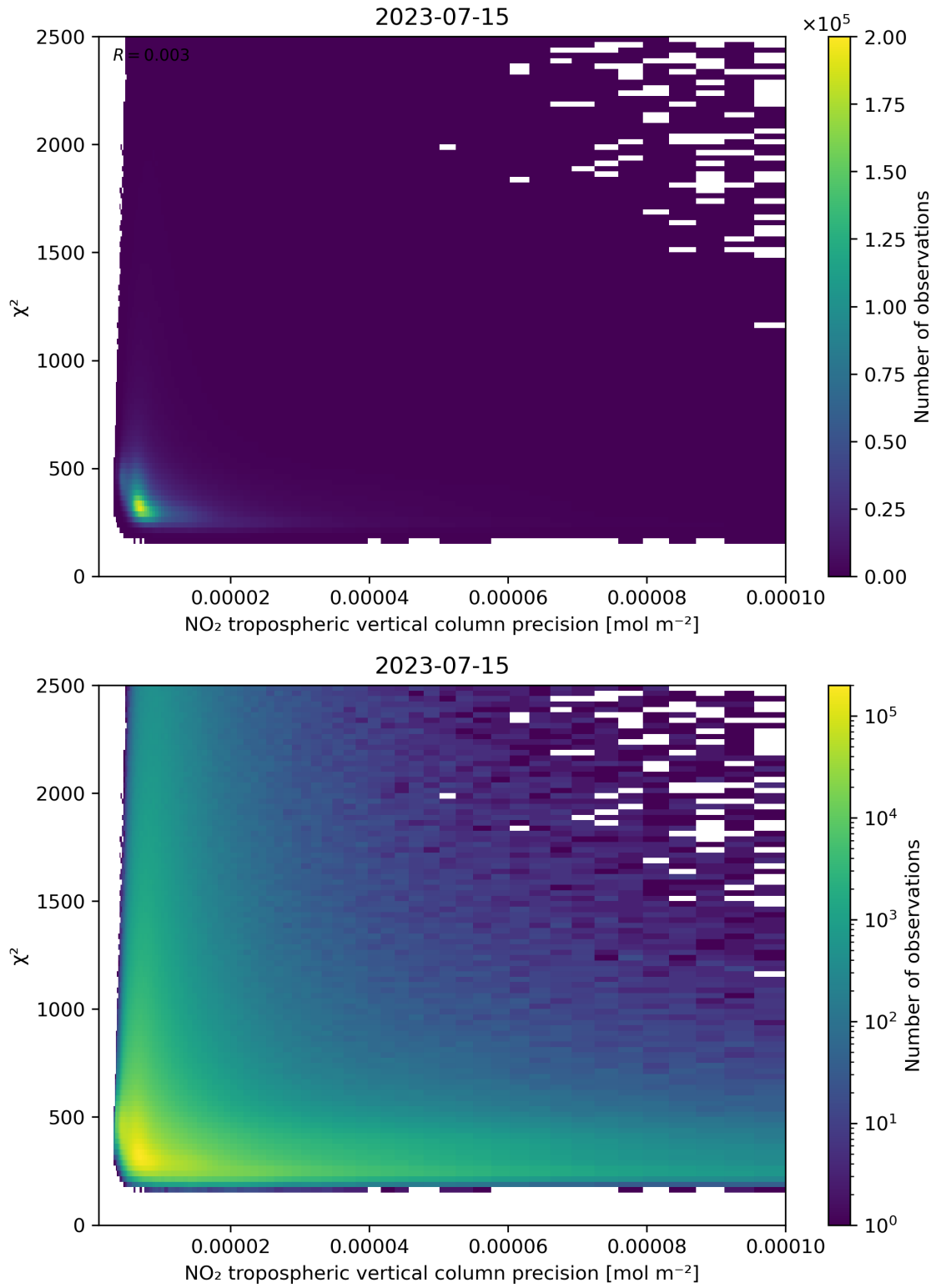
Figure 134: Scatter density plot of “NO 2 tropospheric vertical column precision” against “ \chi^2 ” for 2023-07-14 to 2023-07-16.
