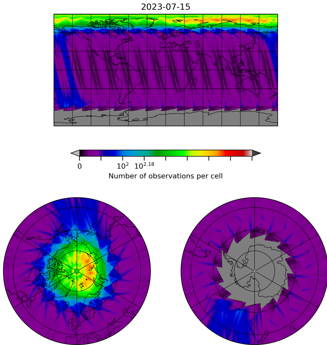
Figure 10: Map of the number of observations for 2023-07-14 to 2023-07-16
