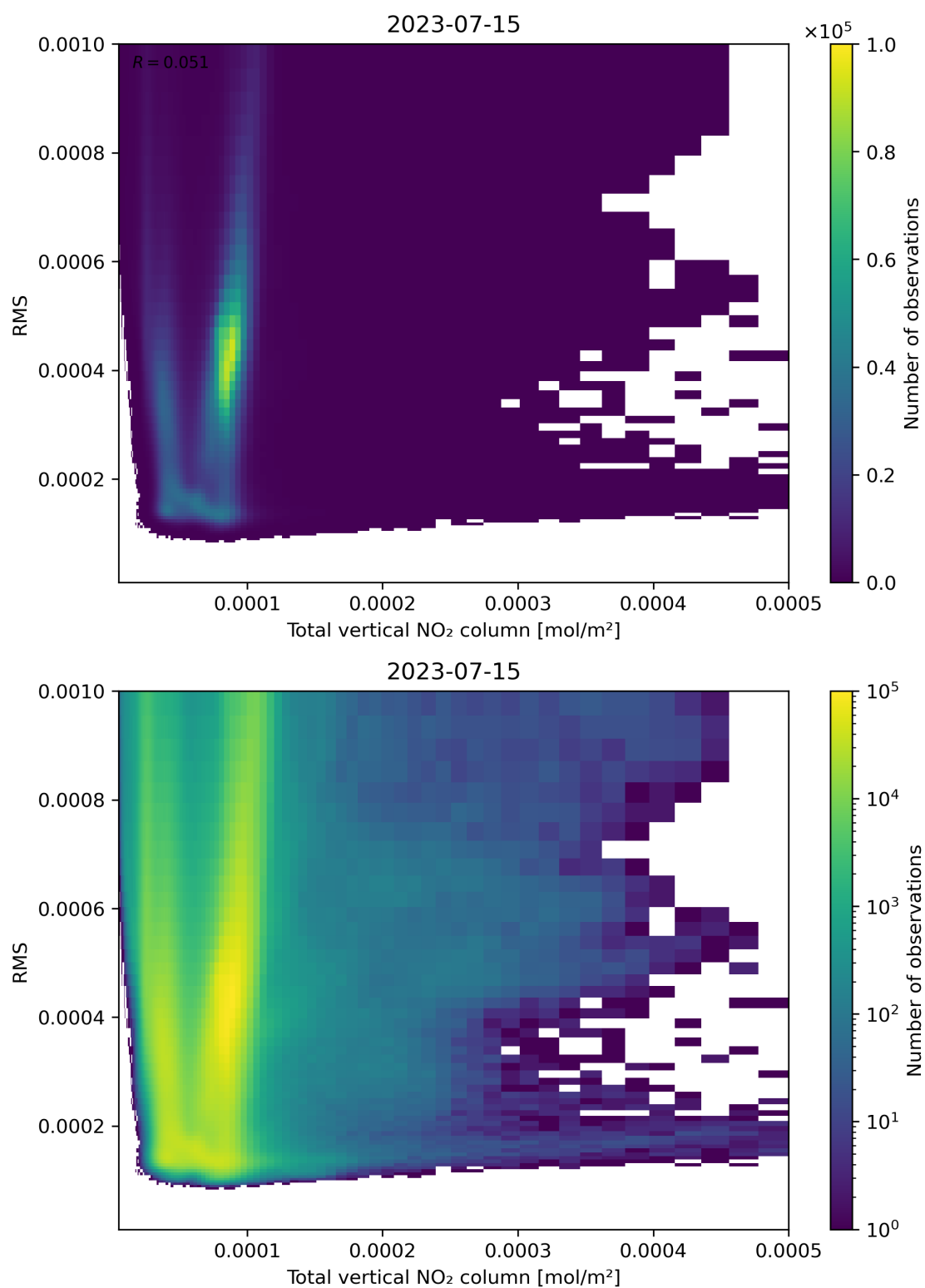
Figure 120: Scatter density plot of “Total vertical NO 2 column” against “RMS” for 2023-07-14 to 2023-07-16.
