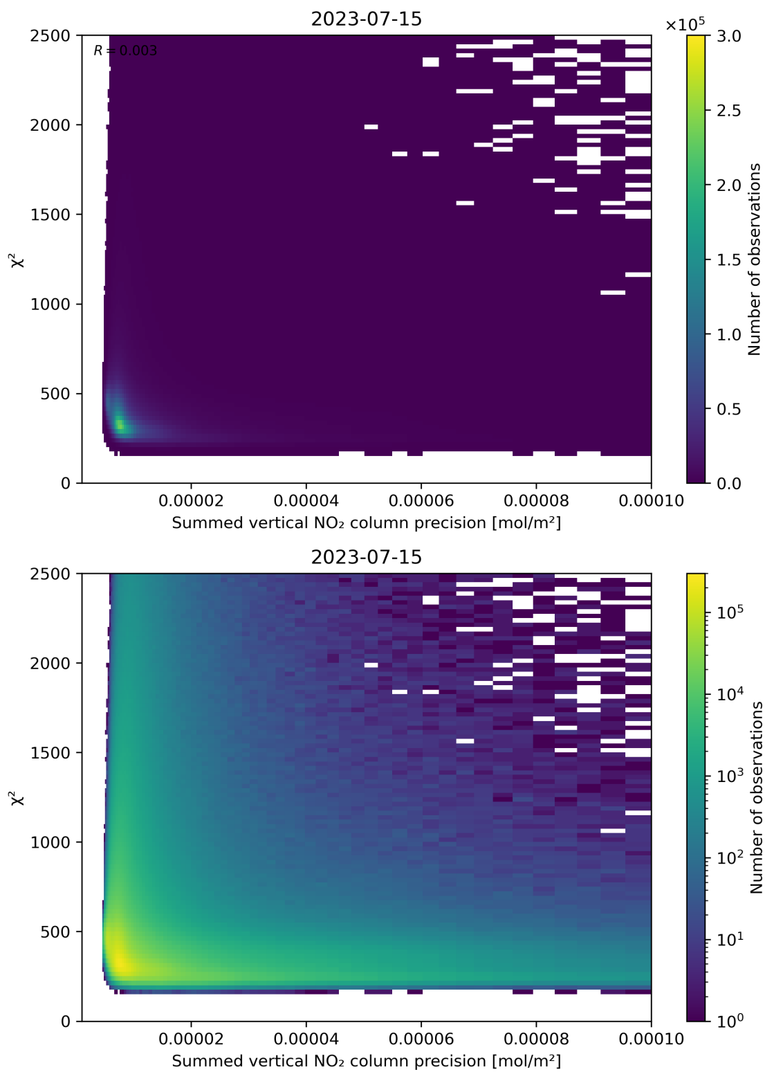
Figure 107: Scatter density plot of “Summed vertical NO 2 column precision” against “ \chi^2 ” for 2023-07-14 to 2023-07-16.
