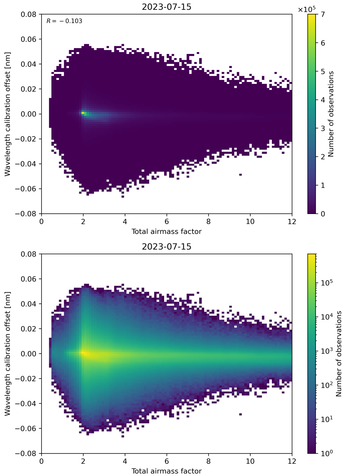
Figure 70: Scatter density plot of “Total airmass factor” against “Wavelength calibration offset” for 2023-07-14 to 2023-07-16.
