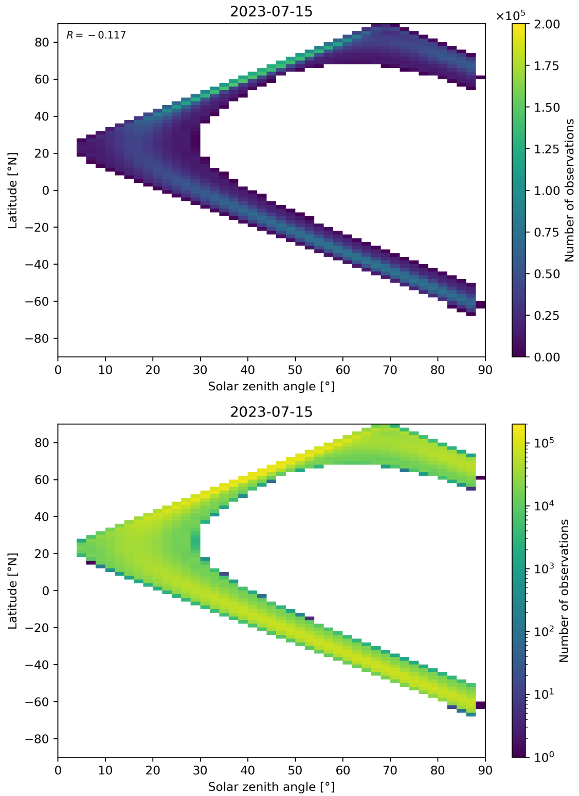
Figure 149: Scatter density plot of “Solar zenith angle” against “Latitude” for 2023-07-14 to 2023-07-16.
