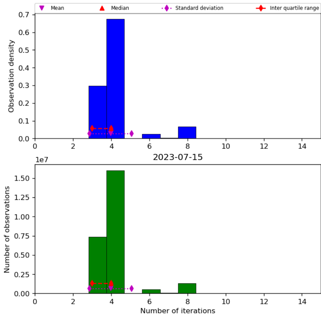
Figure 34: Histogram of “Number of iterations” for 2023-07-14 to 2023-07-16
