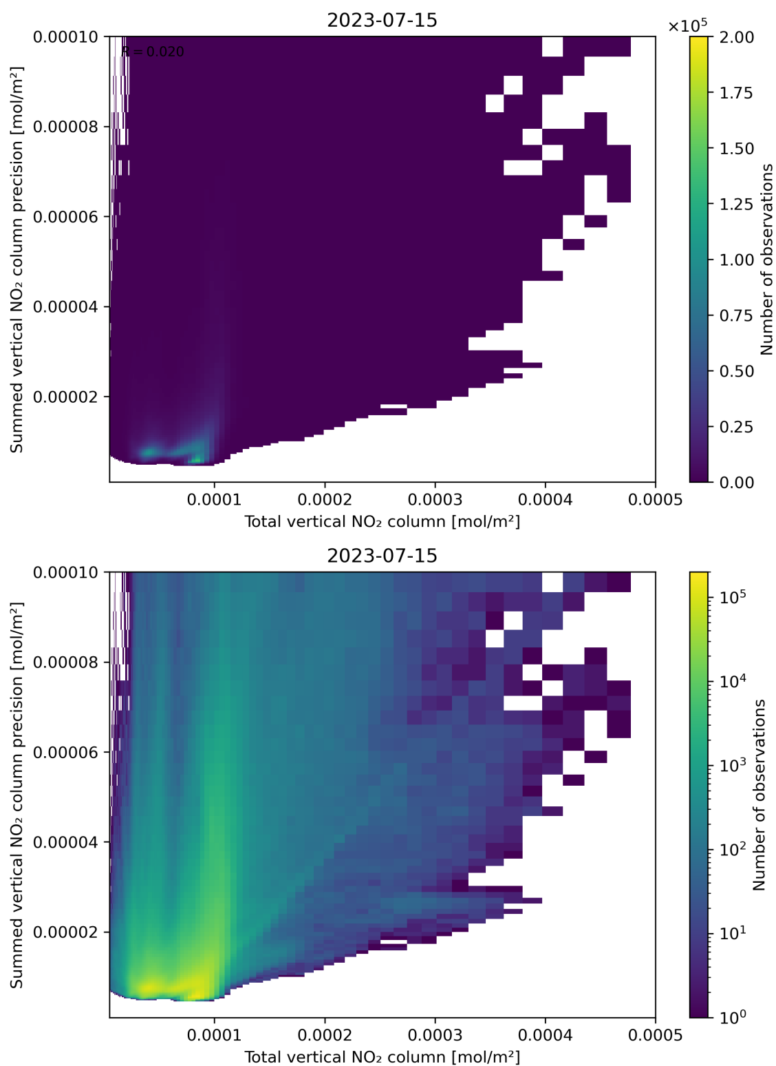
Figure 113: Scatter density plot of “Total vertical NO 2 column” against “Summed vertical NO 2 column precision” for 2023-07-14 to 2023-07-16.
