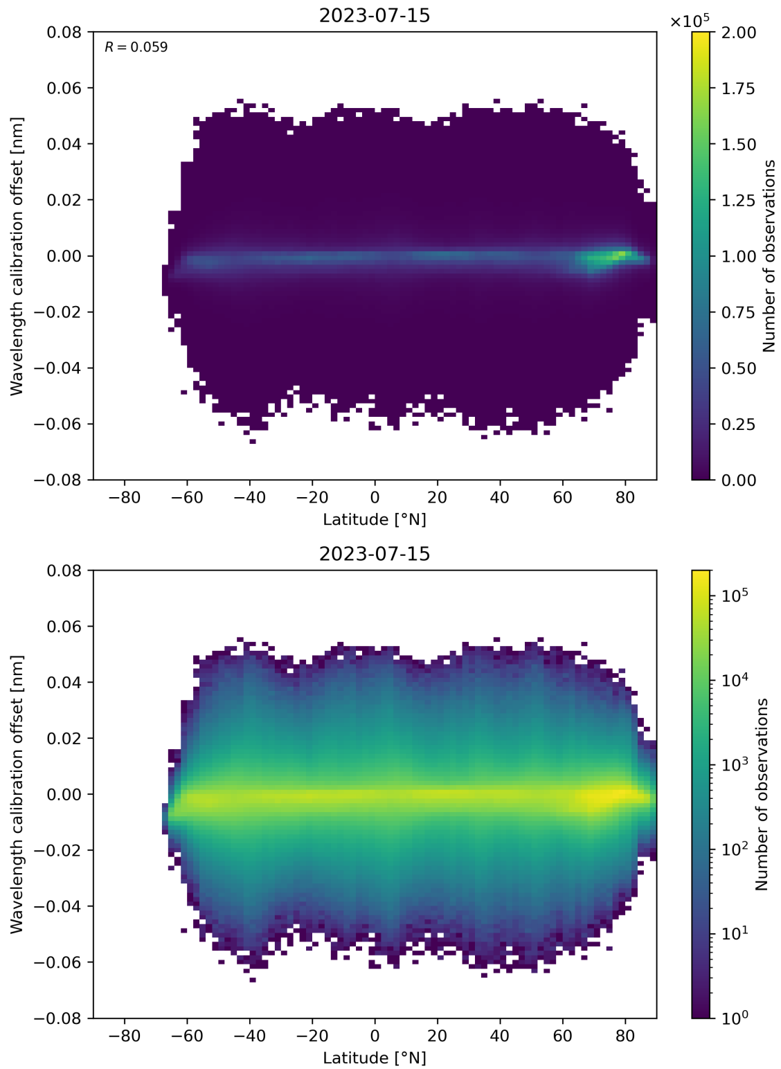
Figure 95: Scatter density plot of “Latitude” against “Wavelength calibration offset” for 2023-07-14 to 2023-07-16.
