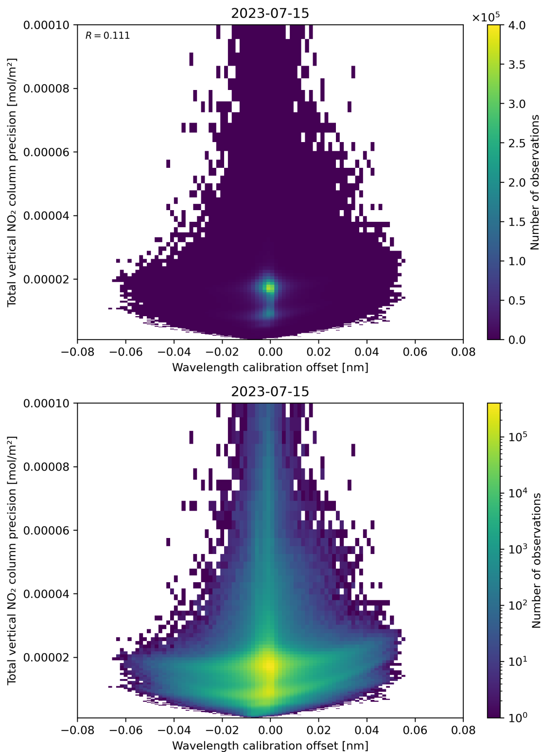
Figure 180: Scatter density plot of “Wavelength calibration offset” against “Total vertical NO 2 column precision” for 2023-07-14 to 2023-07-16.
