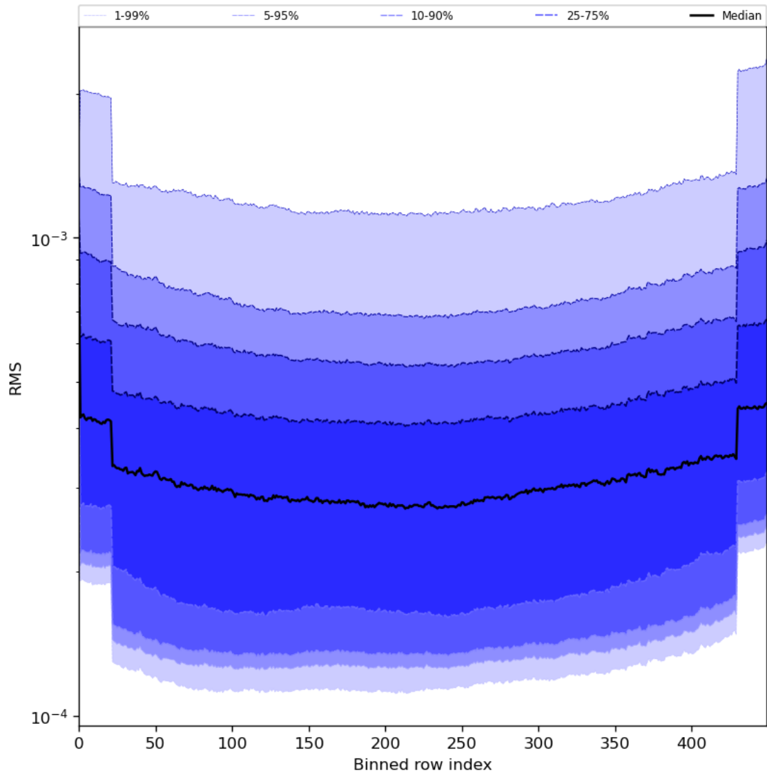
Figure 60: Along track statistics of “RMS” for 2023-07-14 to 2023-07-16
