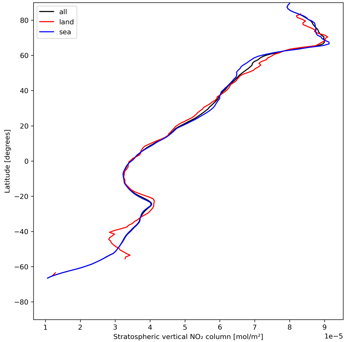
Figure 19: Zonal average of “Stratospheric vertical NO 2 column” for 2023-07-14 to 2023-07-16.
