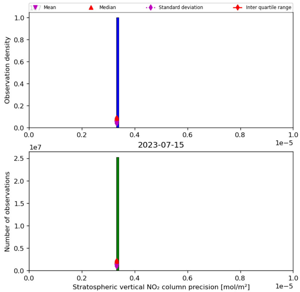
Figure 37: Histogram of “Stratospheric vertical NO 2 column precision” for 2023-07-14 to 2023-07-16
