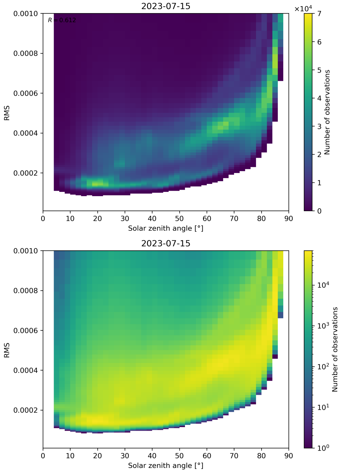
Figure 157: Scatter density plot of “Solar zenith angle” against “RMS” for 2023-07-14 to 2023-07-16.
