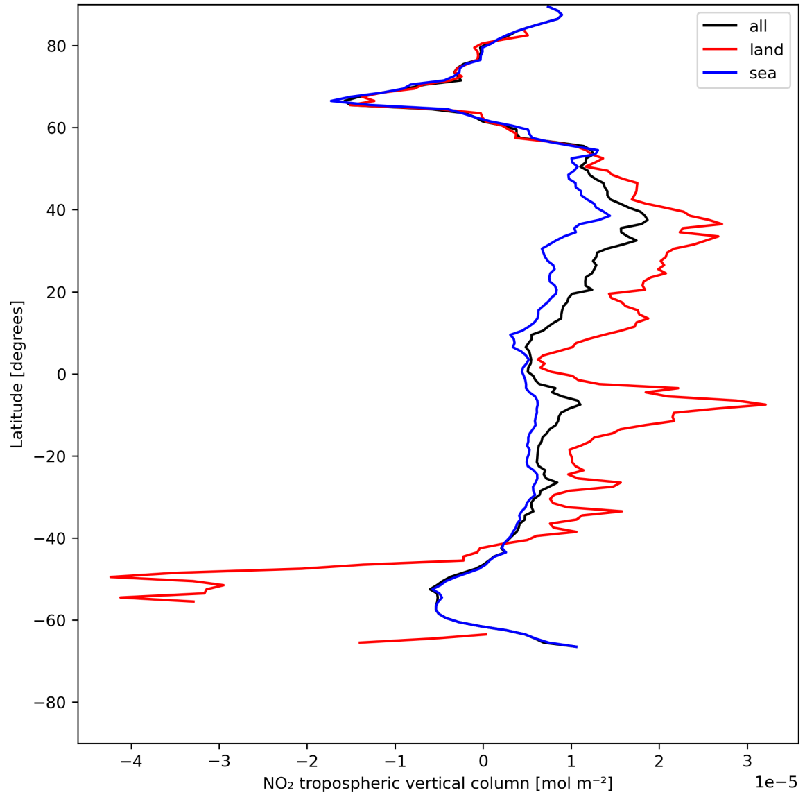
Figure 12: Zonal average of “NO 2 tropospheric vertical column” for 2023-07-14 to 2023-07-16.
