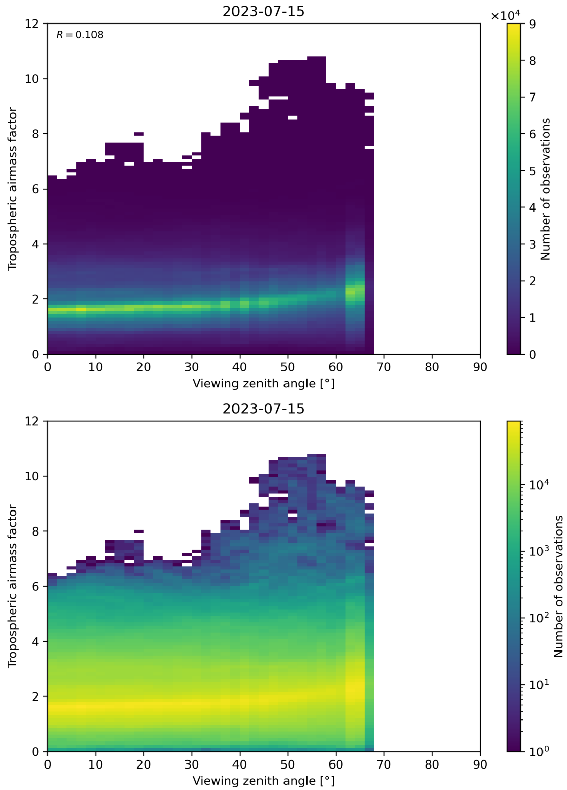
Figure 161: Scatter density plot of “Viewing zenith angle” against “Tropospheric airmass factor” for 2023-07-14 to 2023-07-16.
