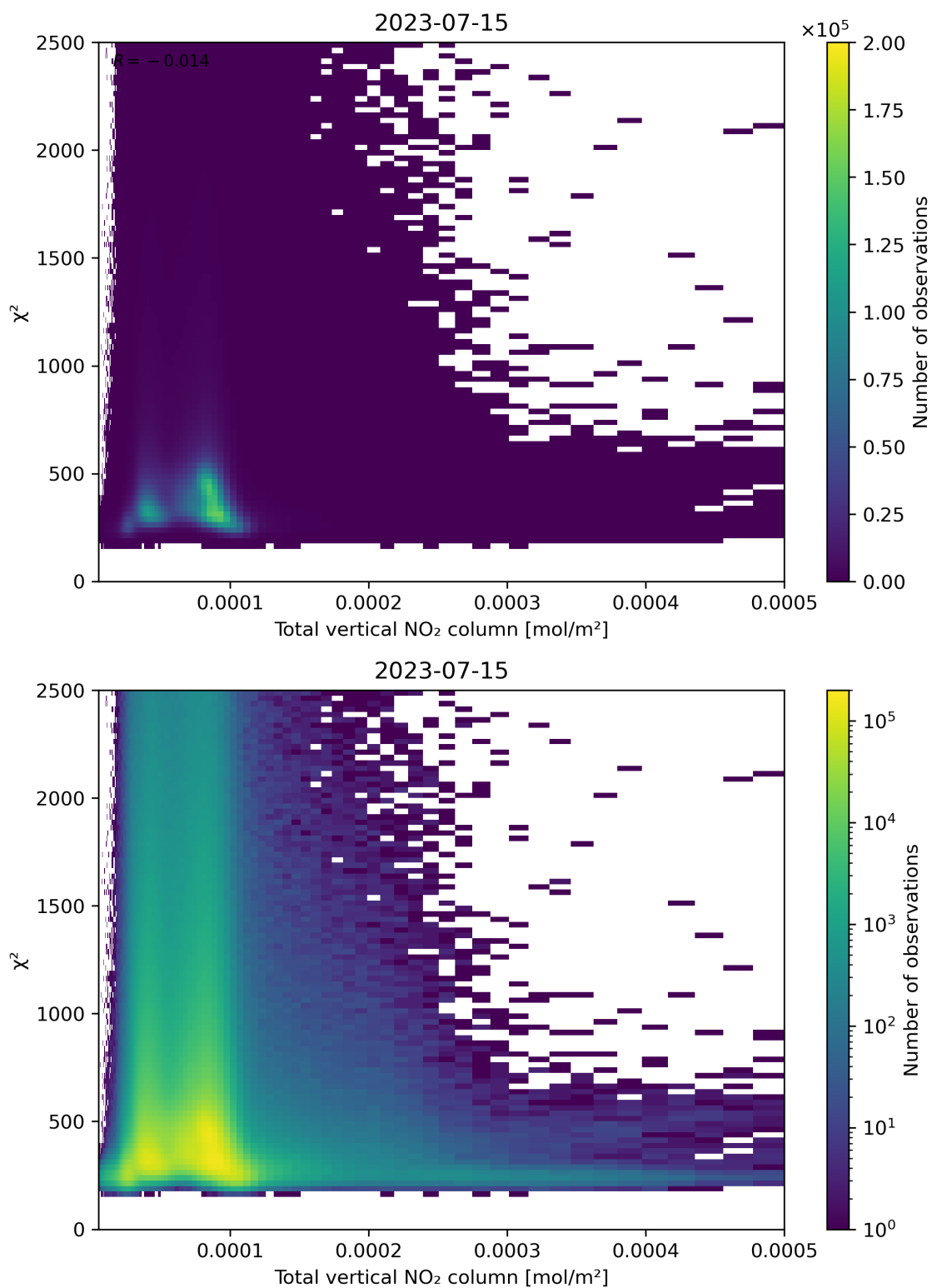
Figure 111: Scatter density plot of “Total vertical NO 2 column” against “ \chi^2 ” for 2023-07-14 to 2023-07-16.
