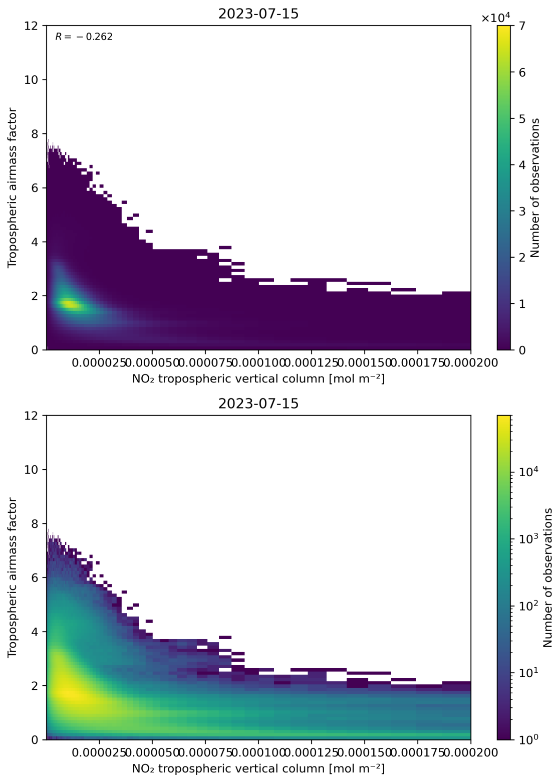
Figure 123: Scatter density plot of “NO 2 tropospheric vertical column” against “Tropospheric air mass factor” for 2023-07-14 to 2023-07-16.
