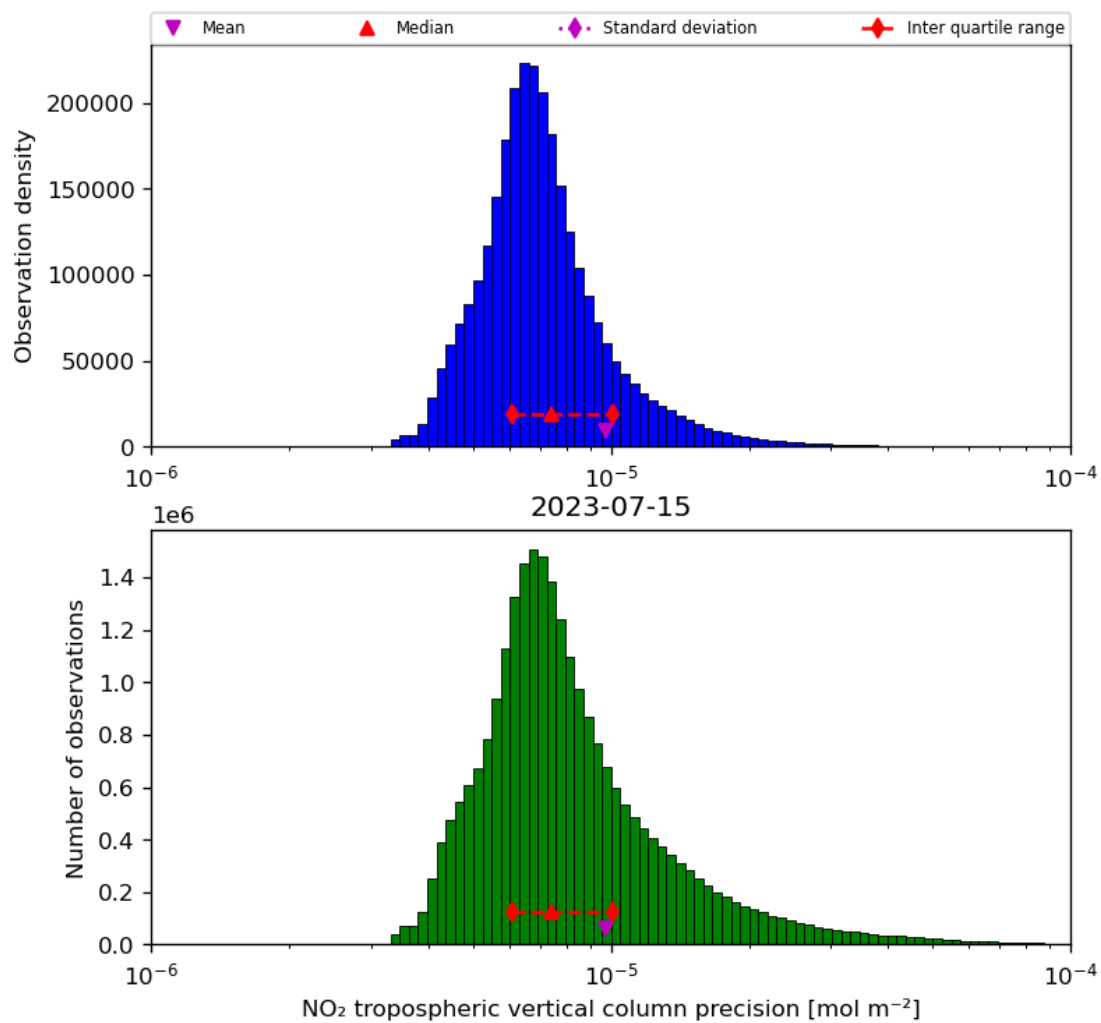
Figure 30: Histogram of “NO 2 tropospheric vertical column precision” for 2023-07-14 to 2023-07-16
