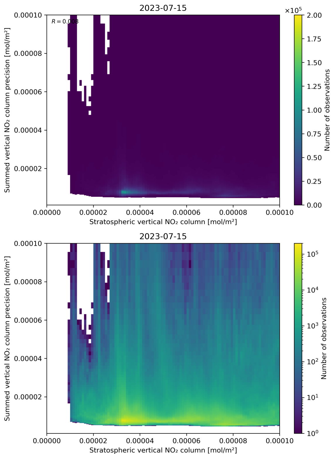
Figure 99: Scatter density plot of “Stratospheric vertical NO 2 column” against “Summed vertical NO 2 column precision” for 2023-07-14 to 2023-07-16.
