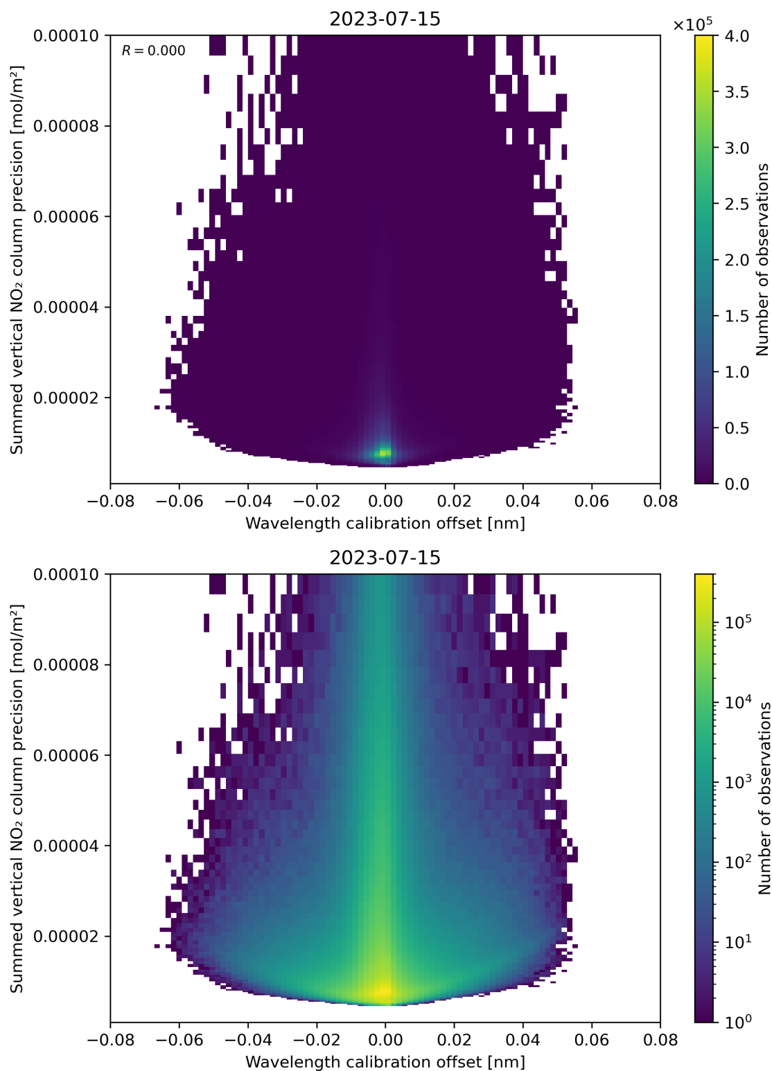
Figure 178: Scatter density plot of “Wavelength calibration offset” against “Summed vertical NO 2 column precision” for 2023-07-14 to 2023-07-16.
