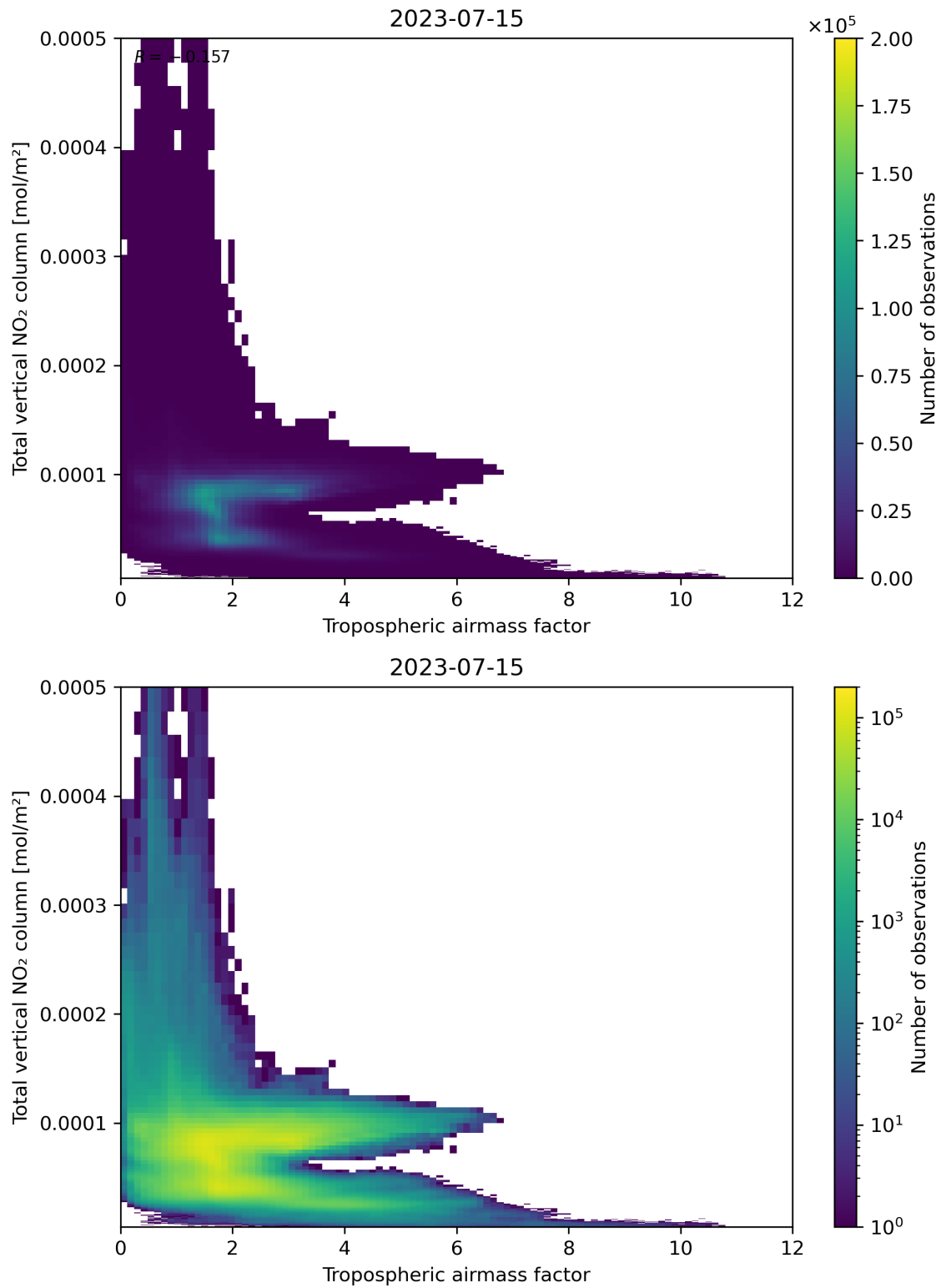
Figure 77: Scatter density plot of “Tropospheric airmass factor” against “Total vertical NO 2 column” for 2023-07-14 to 2023-07-16.
