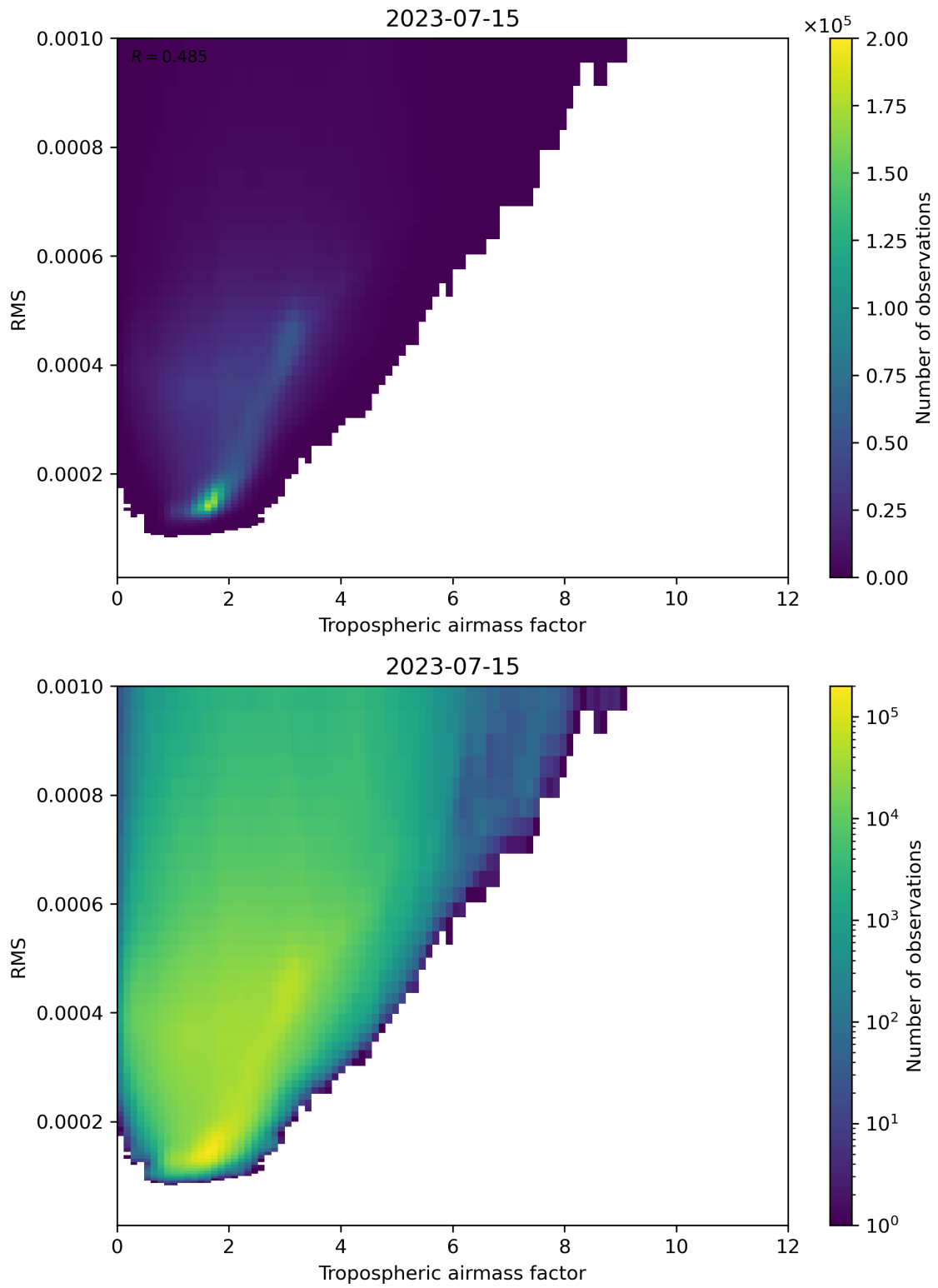
Figure 79: Scatter density plot of “Tropospheric airmass factor” against “RMS” for 2023-07-14 to 2023-07-16.
