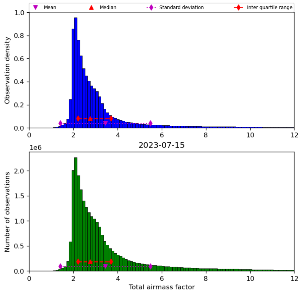
Figure 32: Histogram of “Total airmass factor” for 2023-07-14 to 2023-07-16
