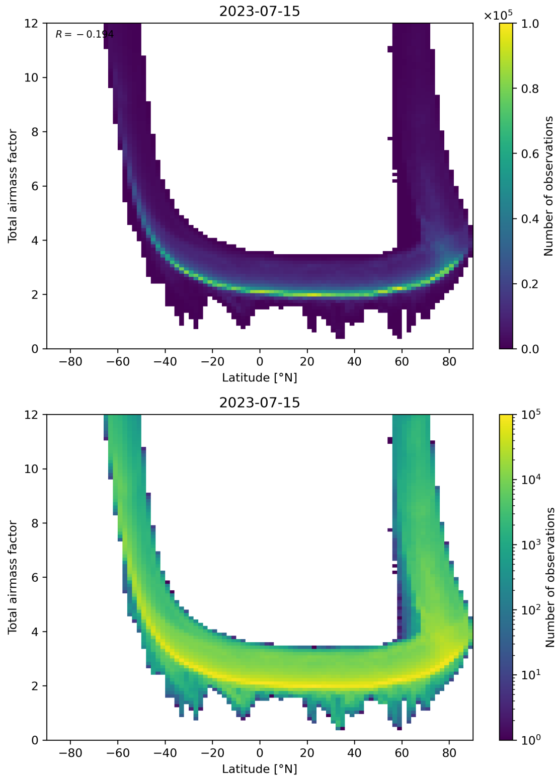
Figure 84: Scatter density plot of “Latitude” against “Total airmass factor” for 2023-07-14 to 2023-07-16.
