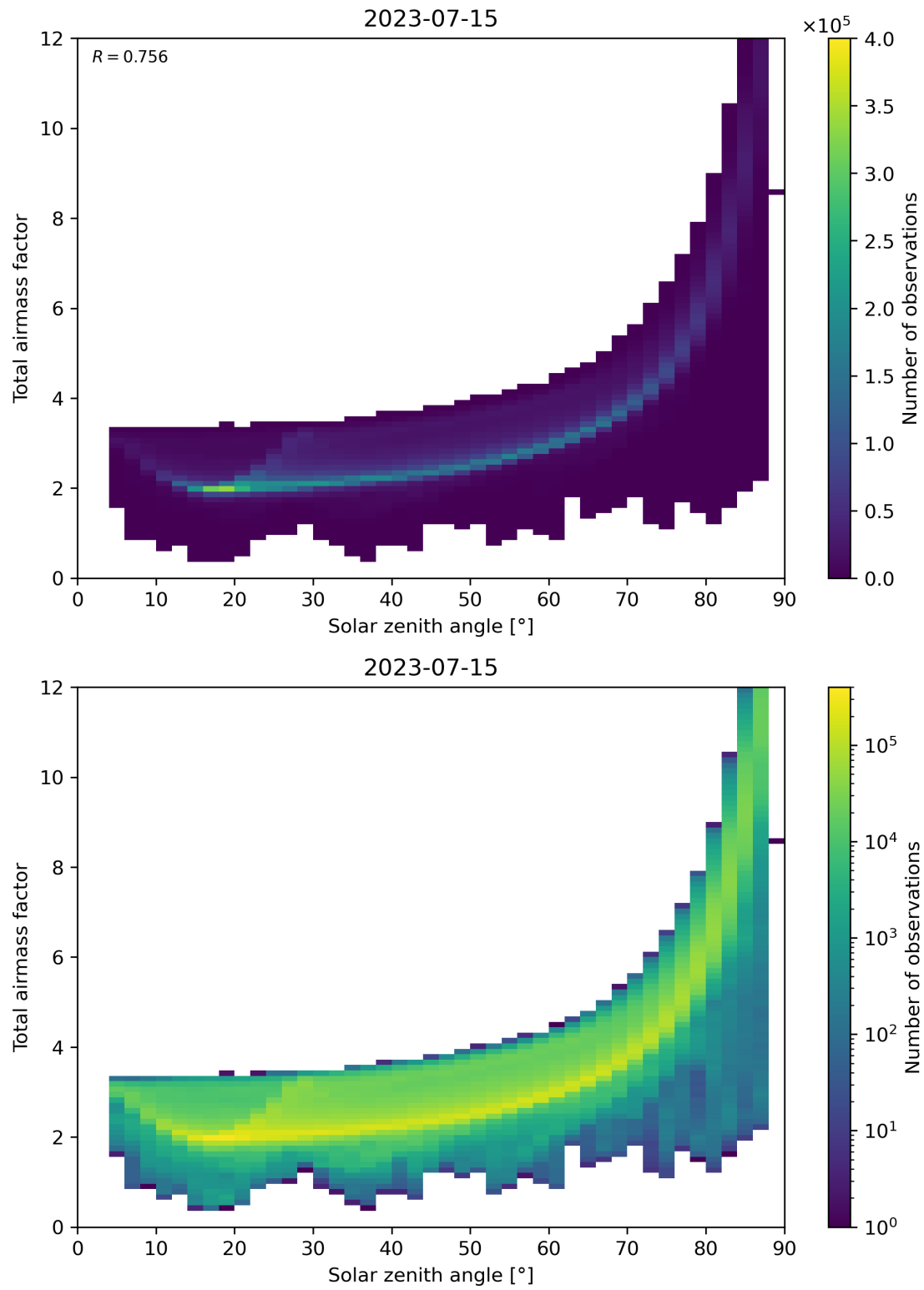
Figure 146: Scatter density plot of “Solar zenith angle” against “Total air mass factor” for 2023-07-14 to 2023-07-16.
