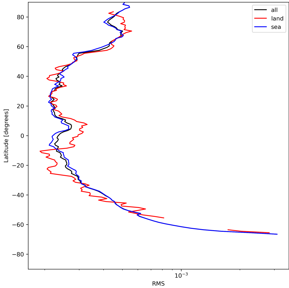
Figure 26: Zonal average of “RMS” for 2023-07-14 to 2023-07-16.
