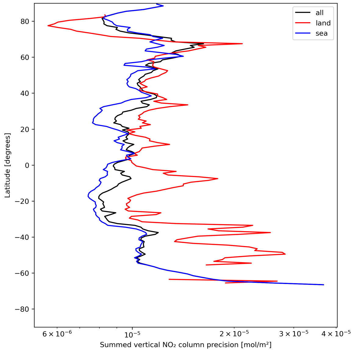
Figure 24: Zonal average of “Summed vertical NO 2 column precision” for 2023-07-14 to 2023-07-16.
