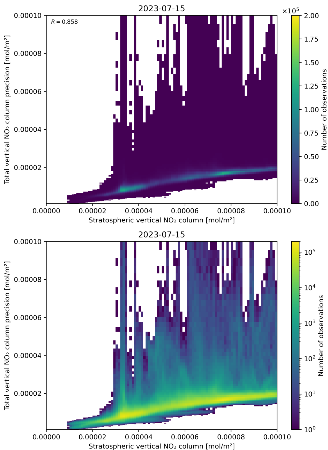
Figure 101: Scatter density plot of “Stratospheric vertical NO 2 column” against “Total vertical NO 2 column precision” for 2023-07-14 to 2023-07-16.
