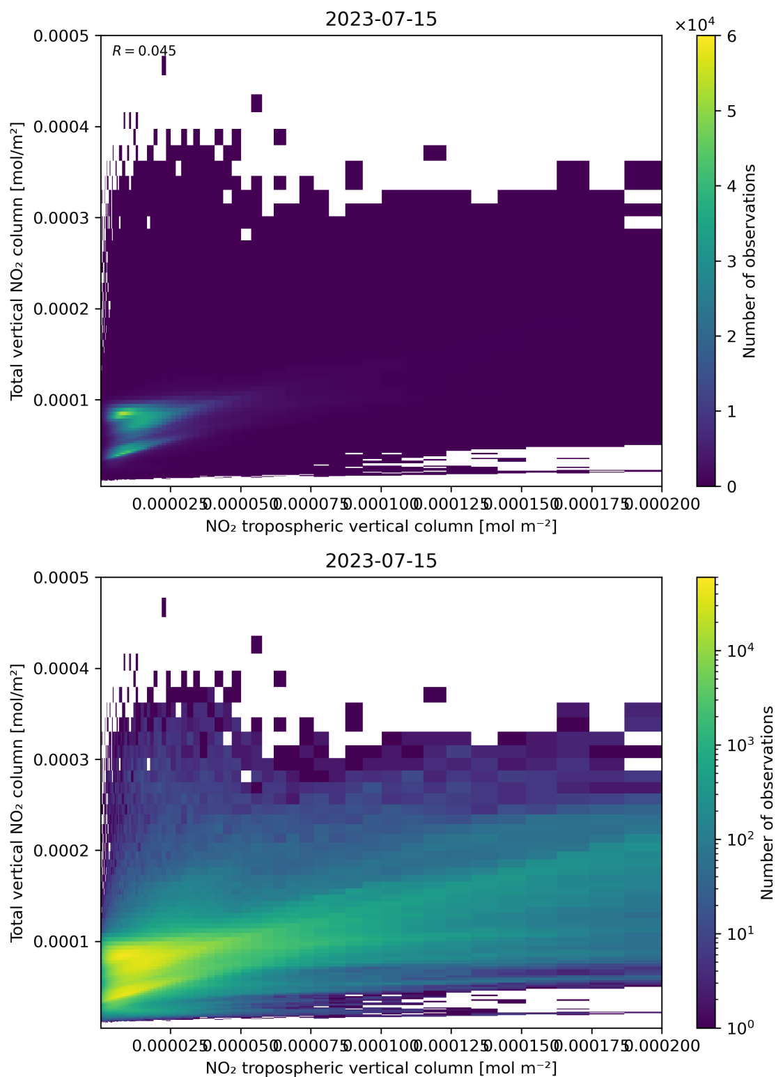
Figure 128: Scatter density plot of “NO 2 tropospheric vertical column” against “Total vertical NO 2 column” for 2023-07-14 to 2023-07-16.
