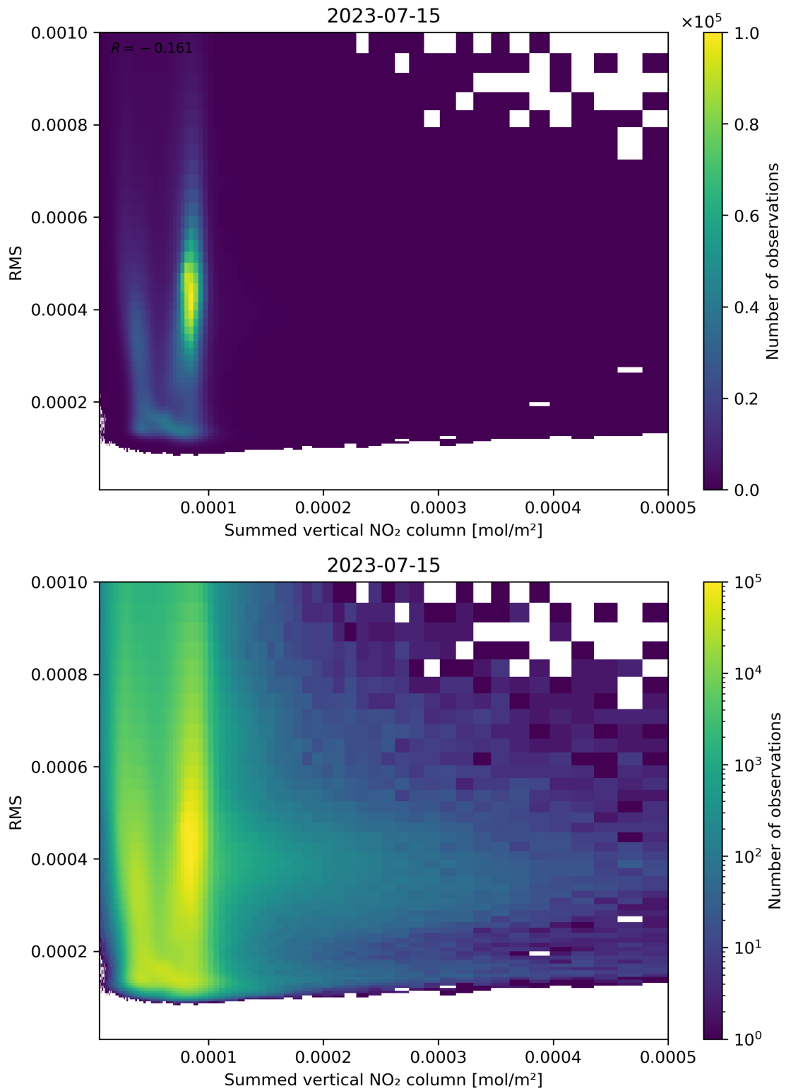
Figure 109: Scatter density plot of “Summed vertical NO 2 column” against “RMS” for 2023-07-14 to 2023-07-16.
