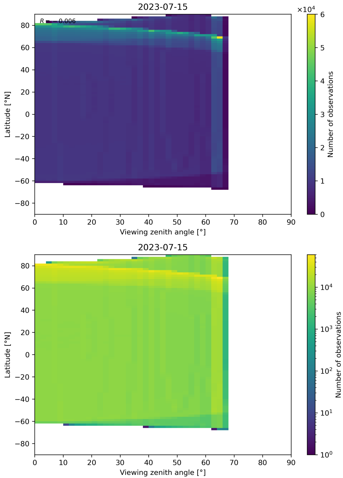
Figure 163: Scatter density plot of “Viewing zenith angle” against “Latitude” for 2023-07-14 to 2023-07-16.
