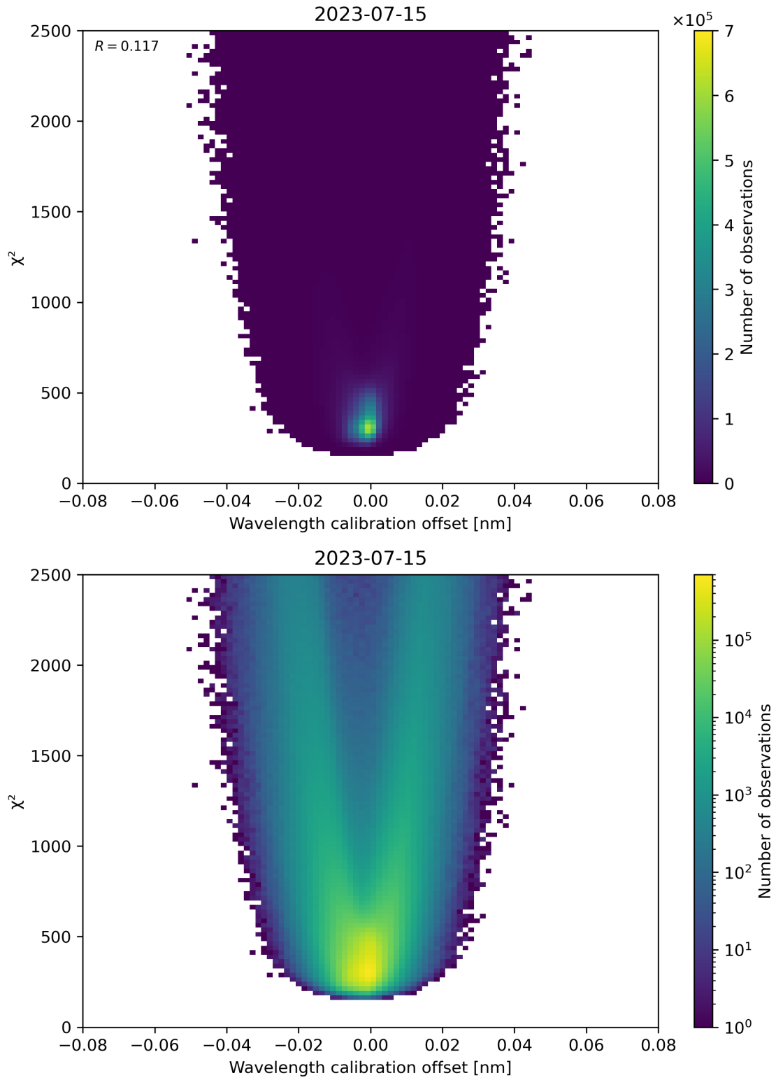
Figure 175: Scatter density plot of “Wavelength calibration offset” against “ \chi^2 ” for 2023-07-14 to 2023-07-16.
