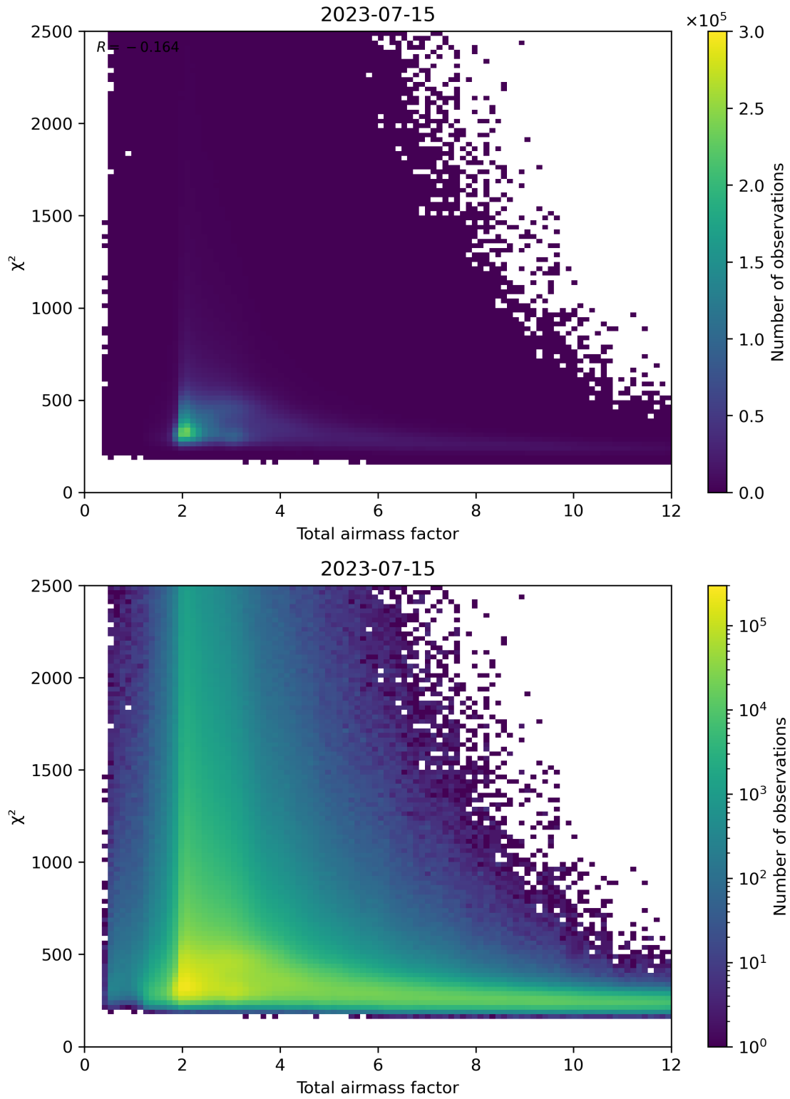
Figure 63: Scatter density plot of “Total airmass factor” against “ \chi^2 ” for 2023-07-14 to 2023-07-16.
