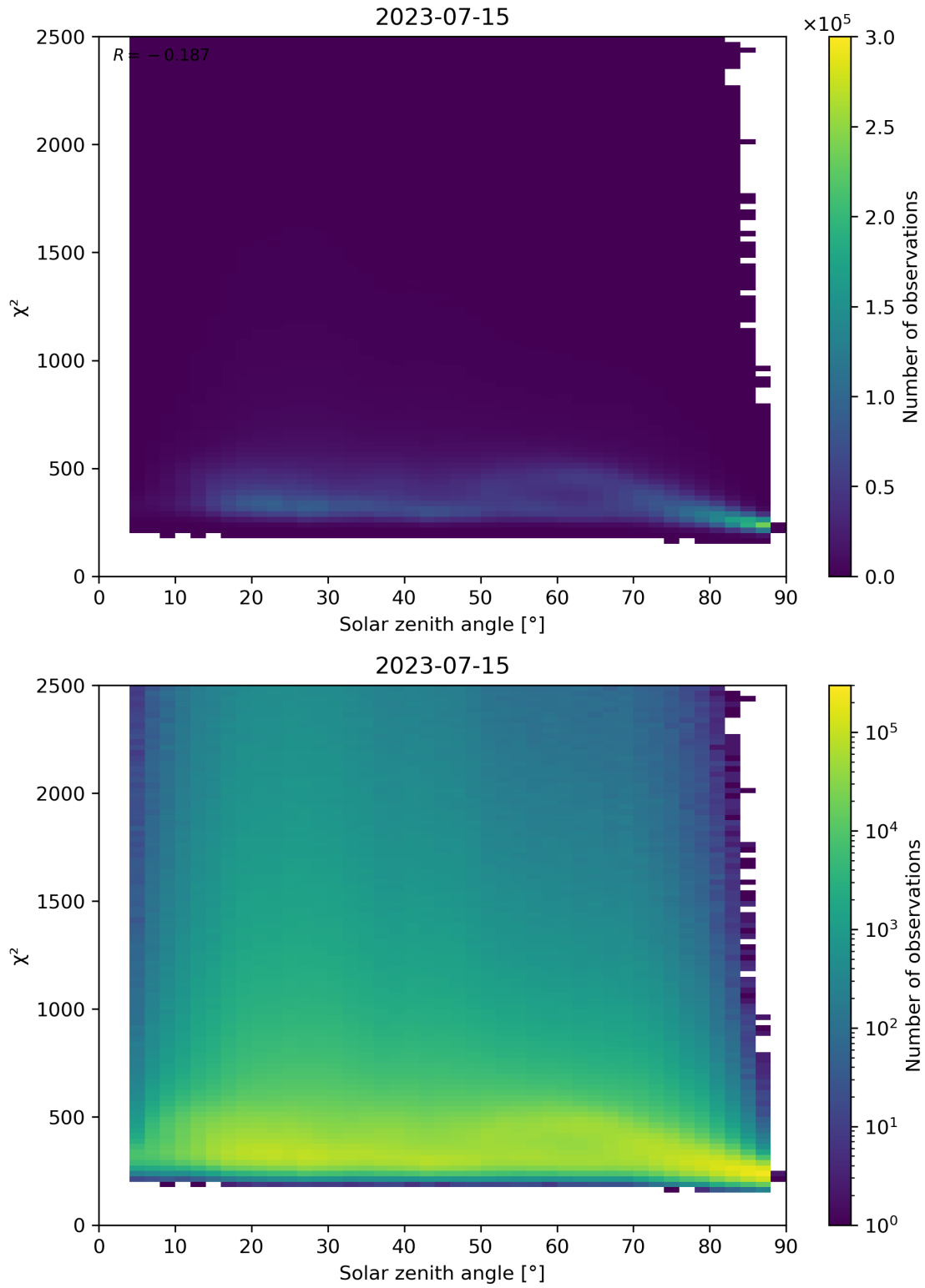
Figure 148: Scatter density plot of “Solar zenith angle” against “ \chi^2 ” for 2023-07-14 to 2023-07-16.
