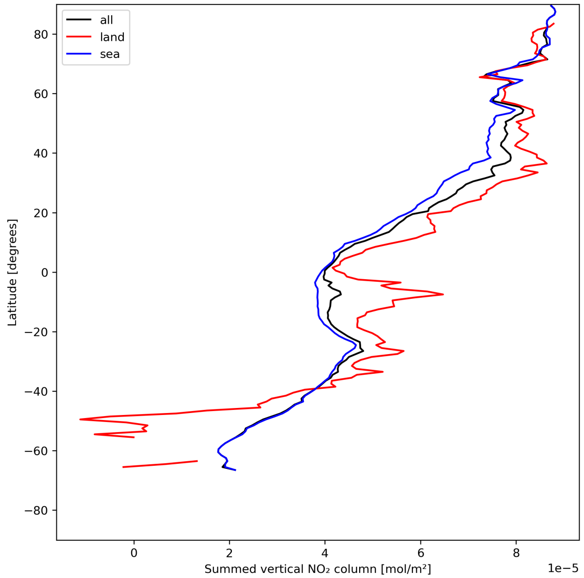
Figure 23: Zonal average of “Summed vertical NO 2 column” for 2023-07-14 to 2023-07-16.
