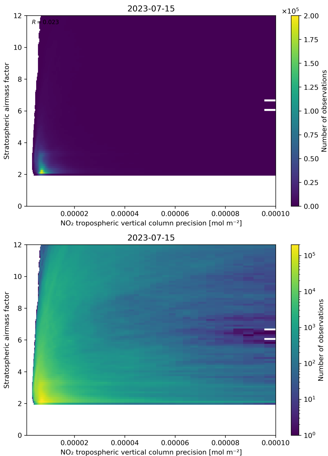
Figure 131: Scatter density plot of “NO 2 tropospheric vertical column precision” against “Stratospheric airmass factor” for 2023-07-14 to 2023-07-16.
