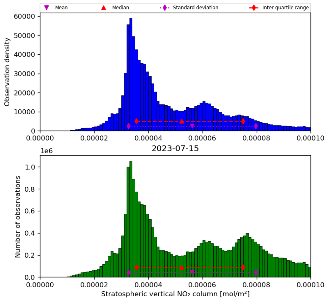
Figure 36: Histogram of “Stratospheric vertical NO 2 column” for 2023-07-14 to 2023-07-16
