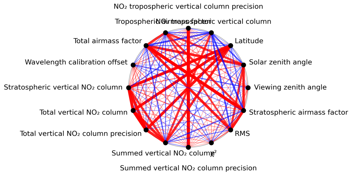
Figure 1: Map of correlation graph for 2023-07-14 to 2023-07-16.
