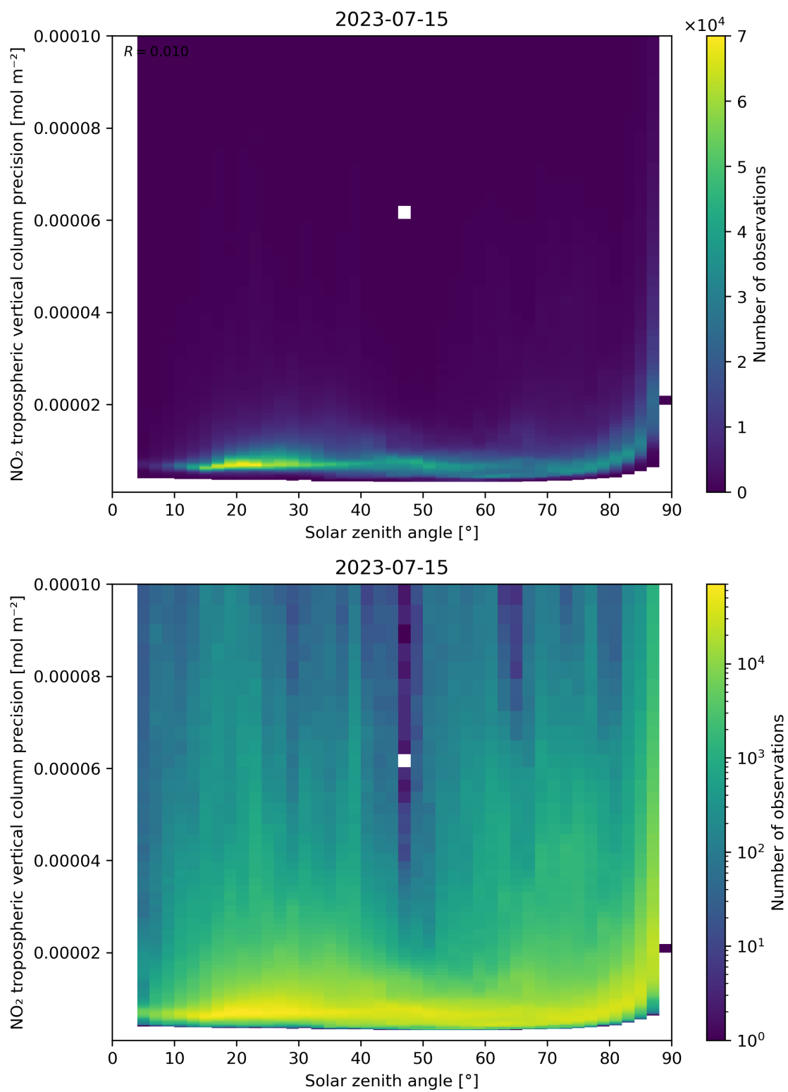
Figure 156: Scatter density plot of “Solar zenith angle” against “NO 2 tropospheric vertical column precision” for 2023-07-14 to 2023-07-16.
