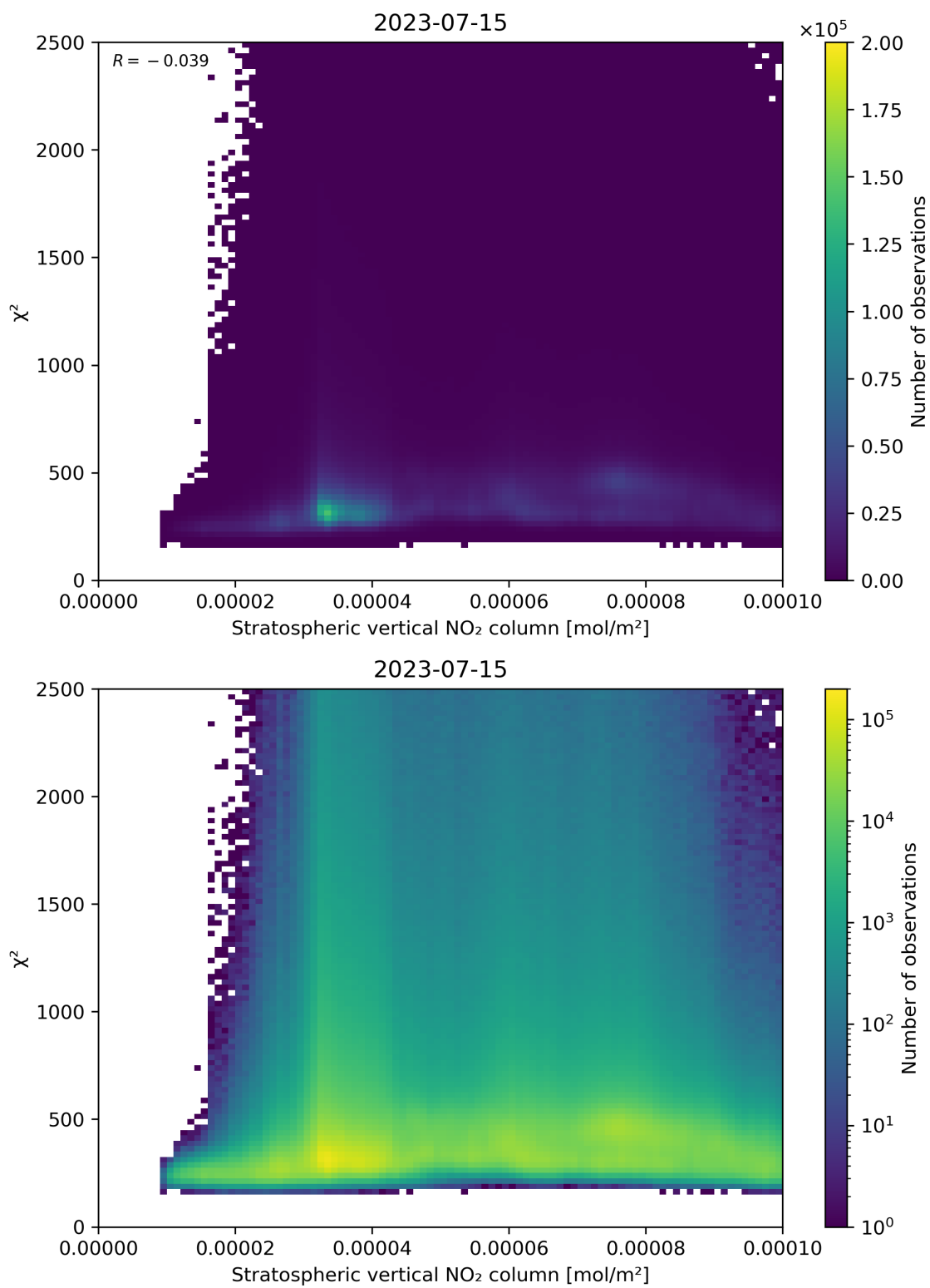
Figure 97: Scatter density plot of “Stratospheric vertical NO 2 column” against “ \chi^2 ” for 2023-07-14 to 2023-07-16.
