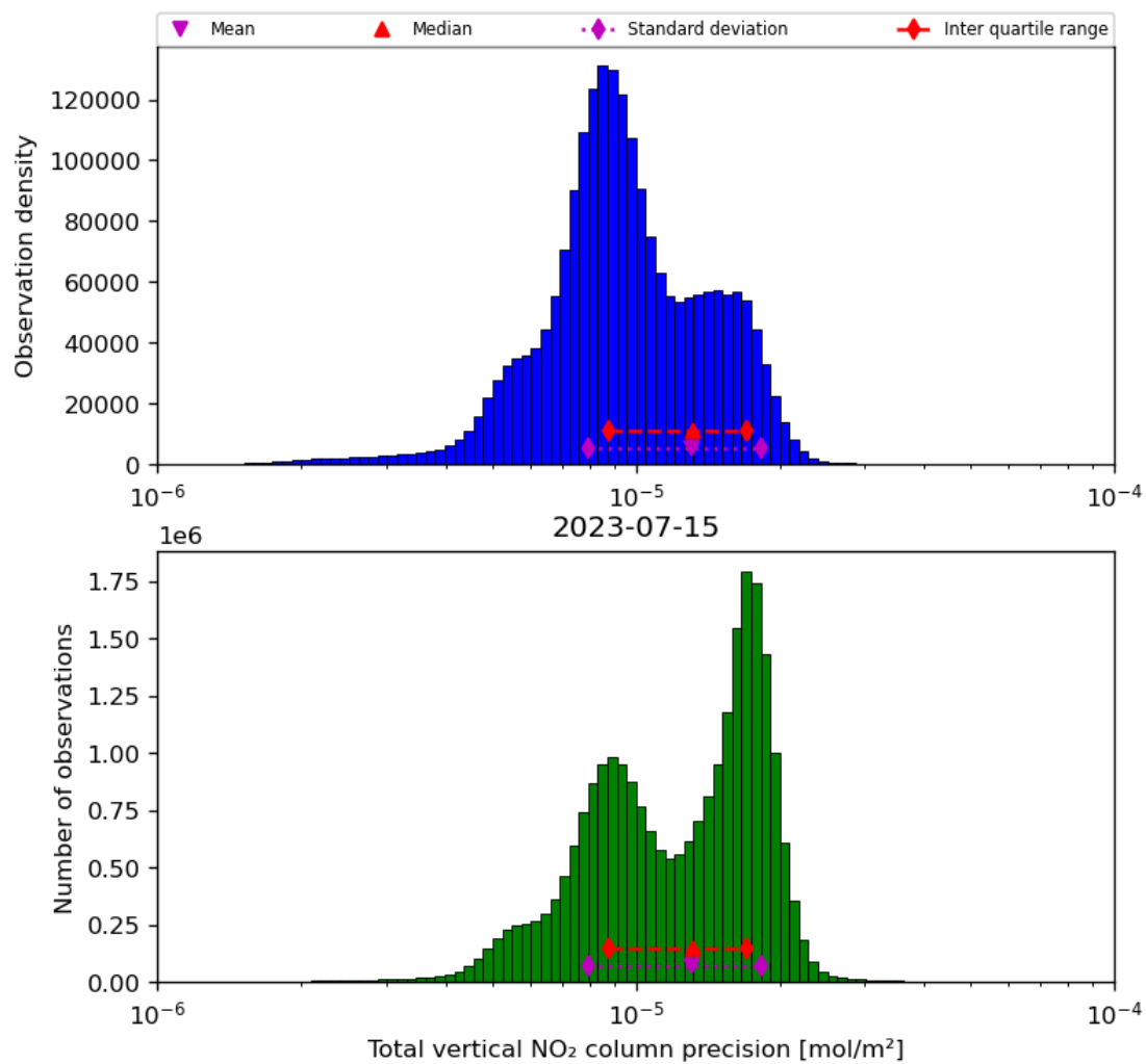
Figure 39: Histogram of “Total vertical NO 2 column precision” for 2023-07-14 to 2023-07-16
