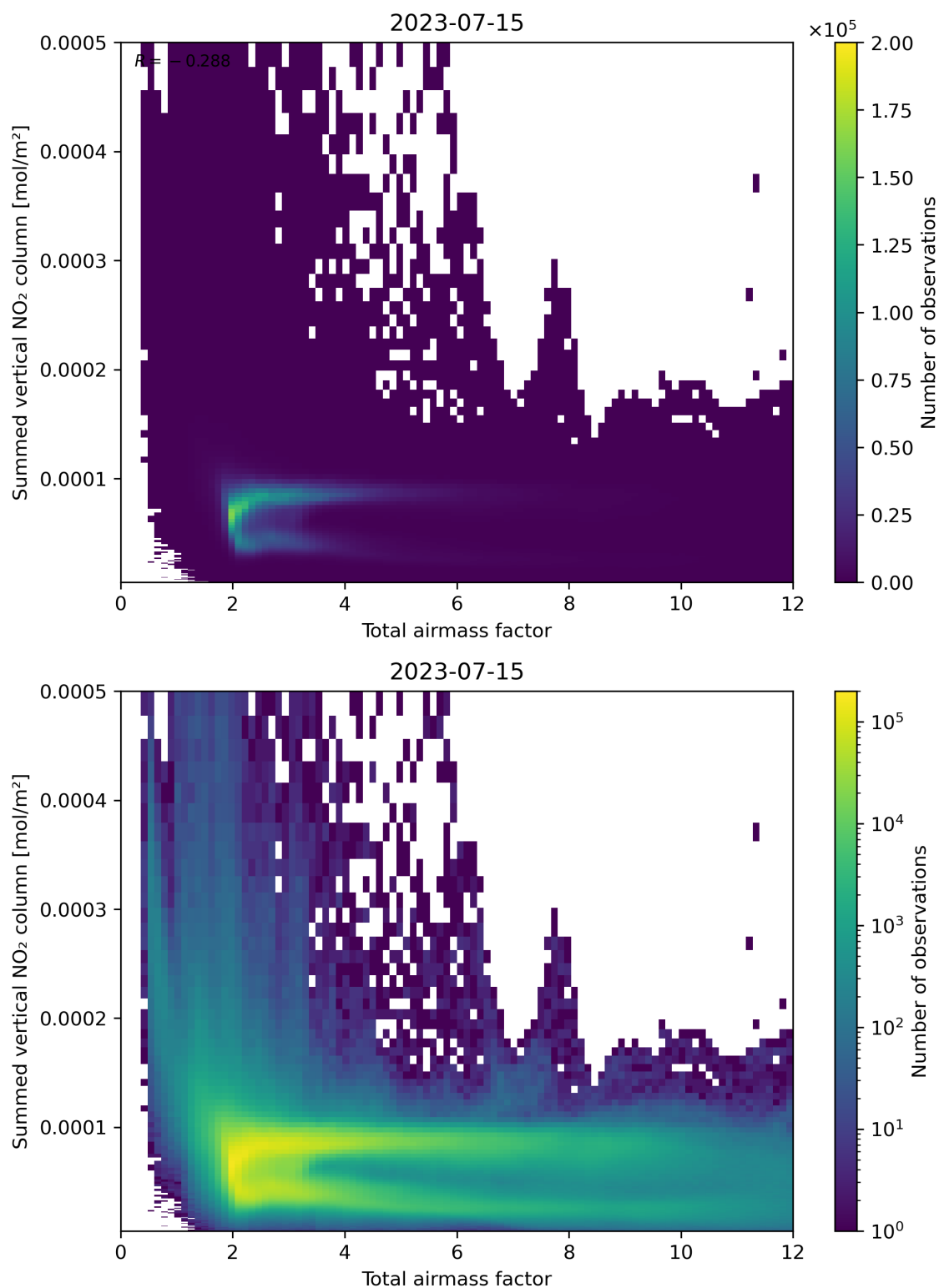
Figure 65: Scatter density plot of “Total airmass factor” against “Summed vertical NO 2 column” for 2023-07-14 to 2023-07-16.
