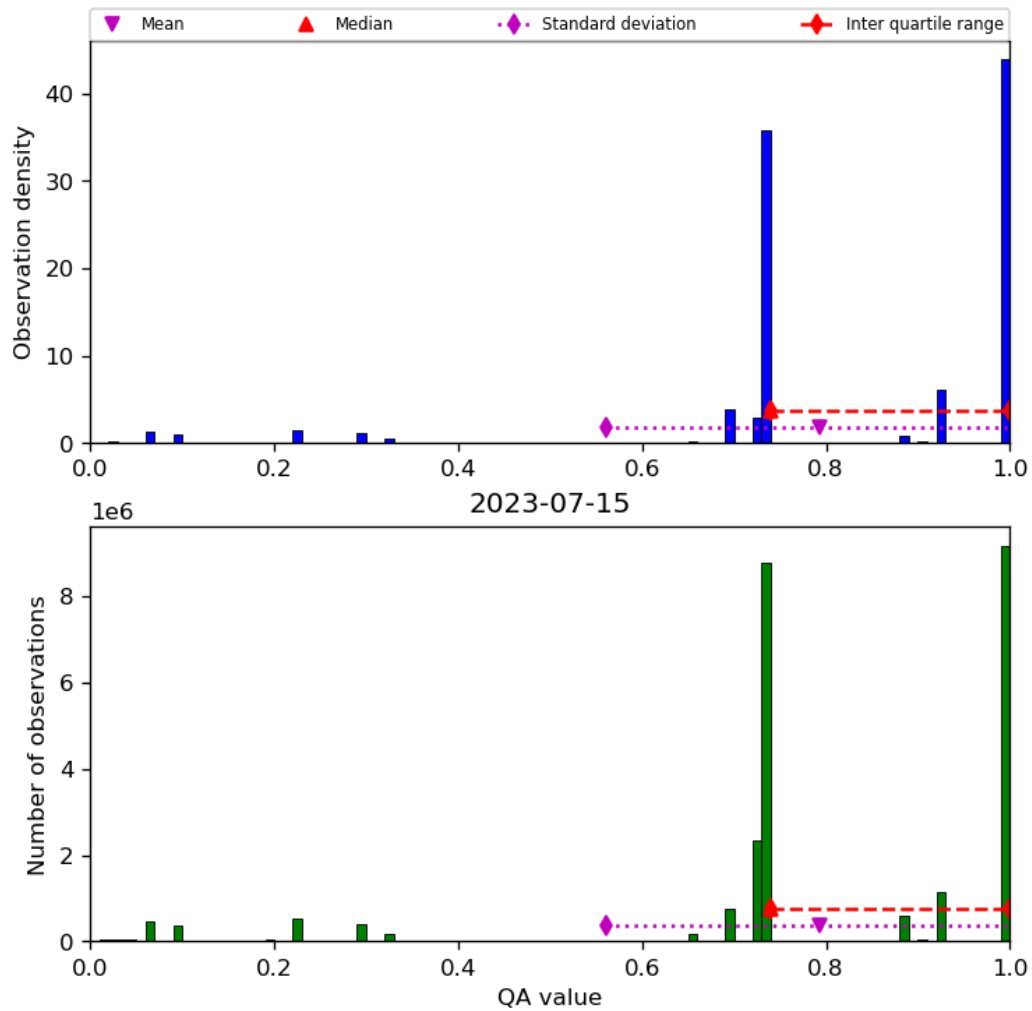
Figure 28: Histogram of “QA value” for 2023-07-14 to 2023-07-16
