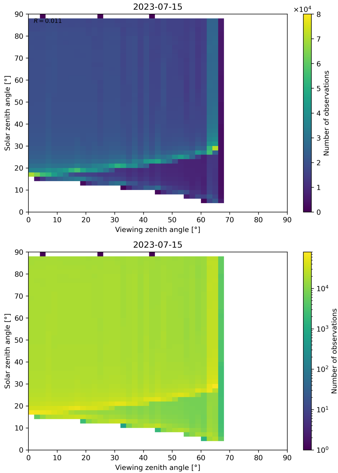
Figure 172: Scatter density plot of “Viewing zenith angle” against “Solar zenith angle” for 2023-07-14 to 2023-07-16.
