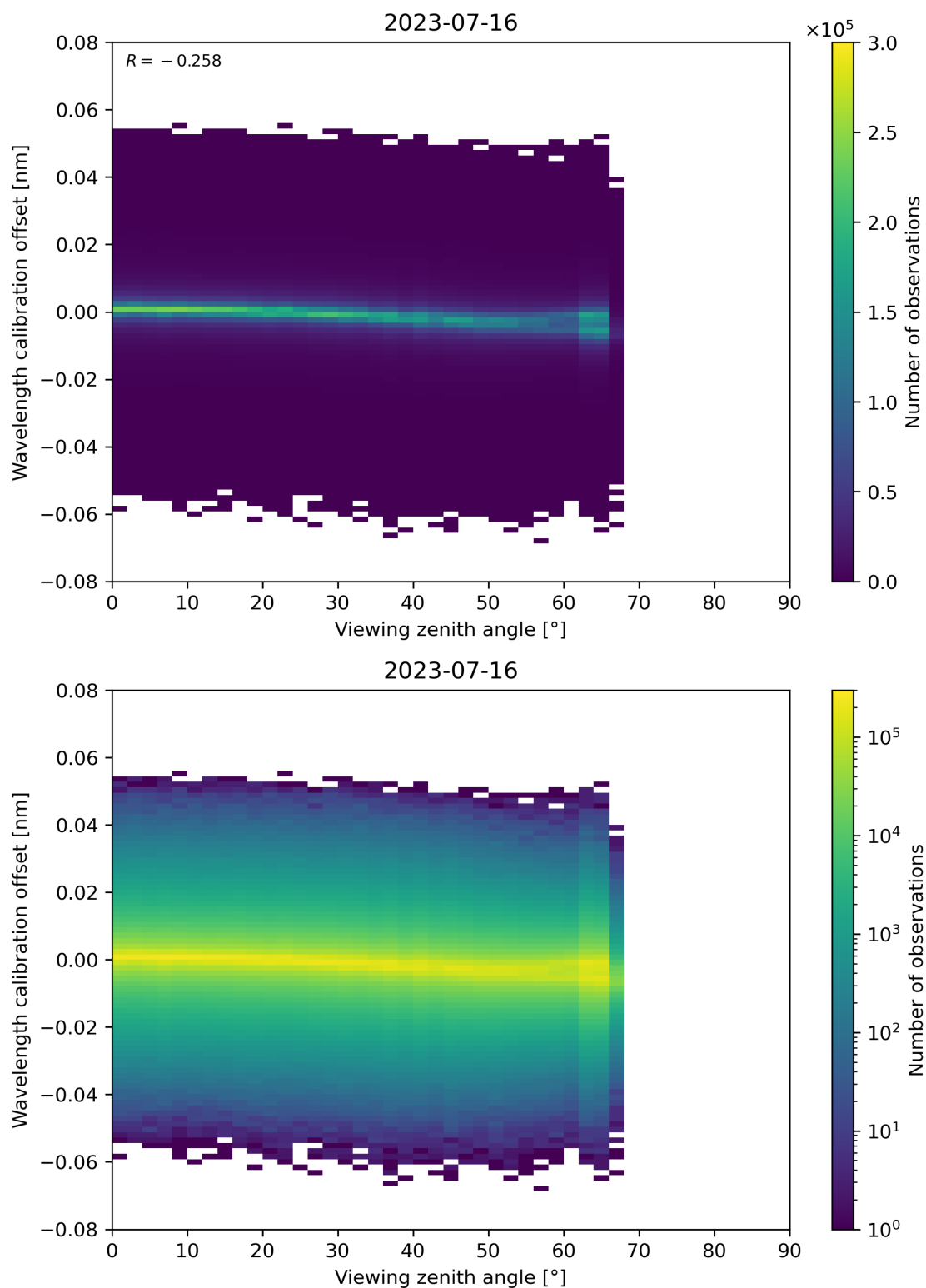
Figure 173: Scatter density plot of “Viewing zenith angle” against “Wavelength calibration offset” for 2023-07-15 to 2023-07-17.
