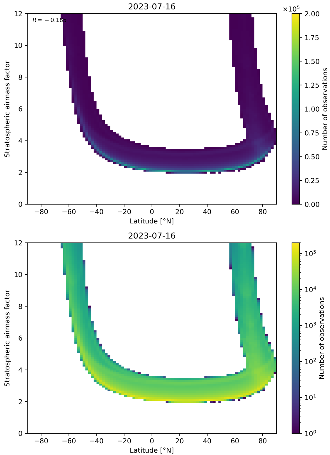
Figure 83: Scatter density plot of “Latitude” against “Stratospheric air mass factor” for 2023-07-15 to 2023-07-17.
