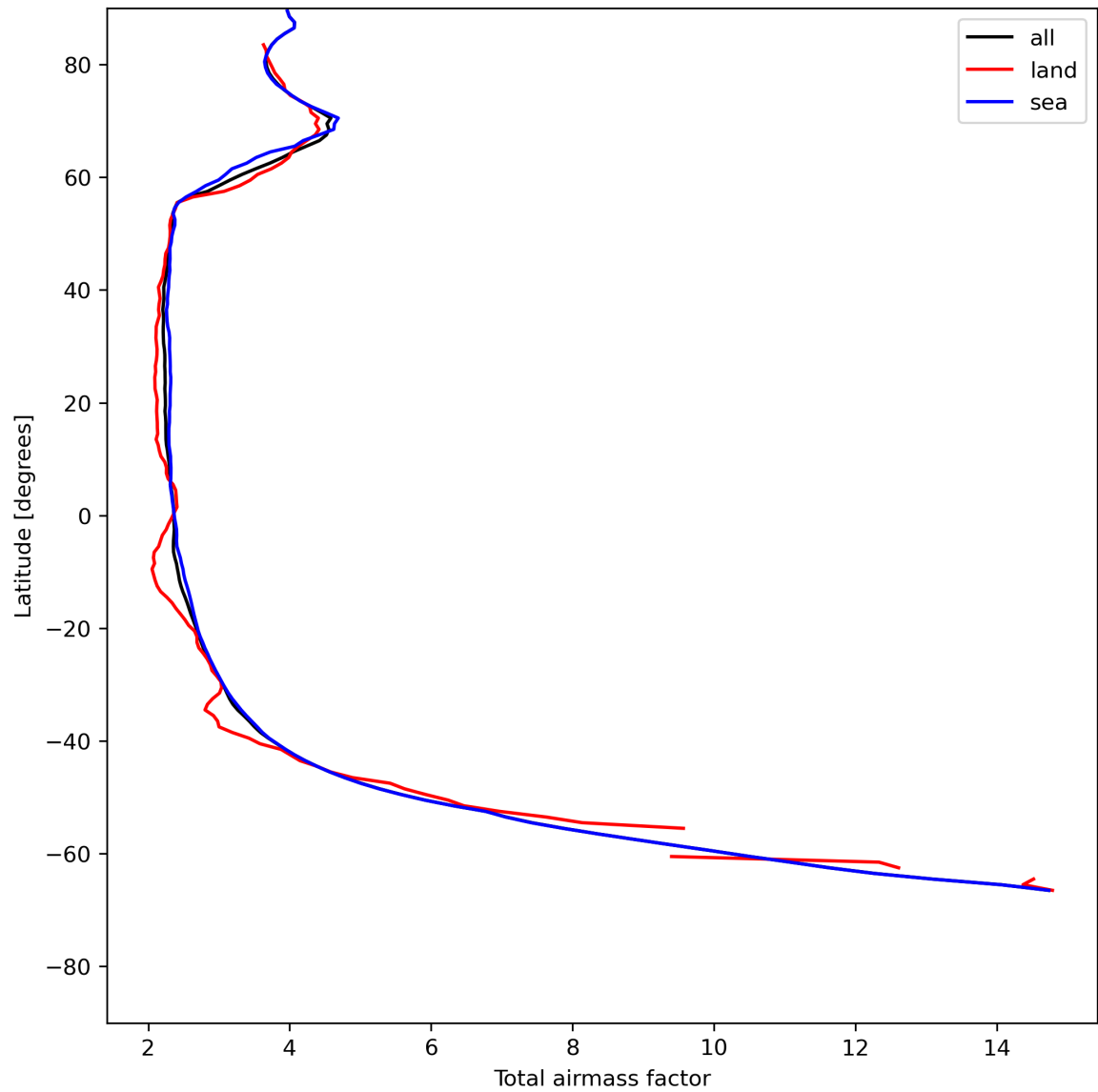
Figure 15: Zonal average of “Total airmass factor” for 2023-07-15 to 2023-07-17.
