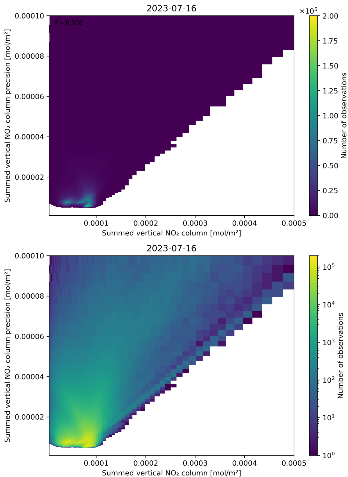
Figure 105: Scatter density plot of “Summed vertical NO 2 column” against “Summed vertical NO 2 column precision” for 2023-07-15 to 2023-07-17.
