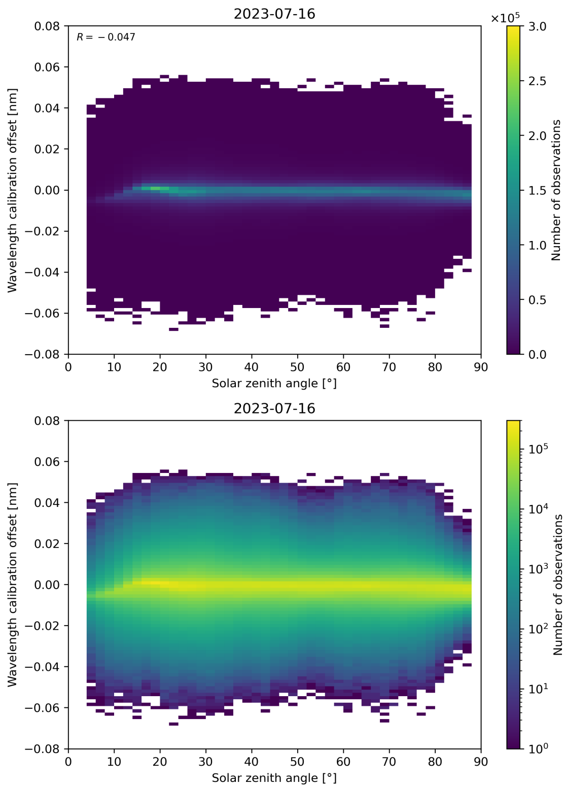
Figure 158: Scatter density plot of “Solar zenith angle” against “Wavelength calibration offset” for 2023-07-15 to 2023-07-17.
