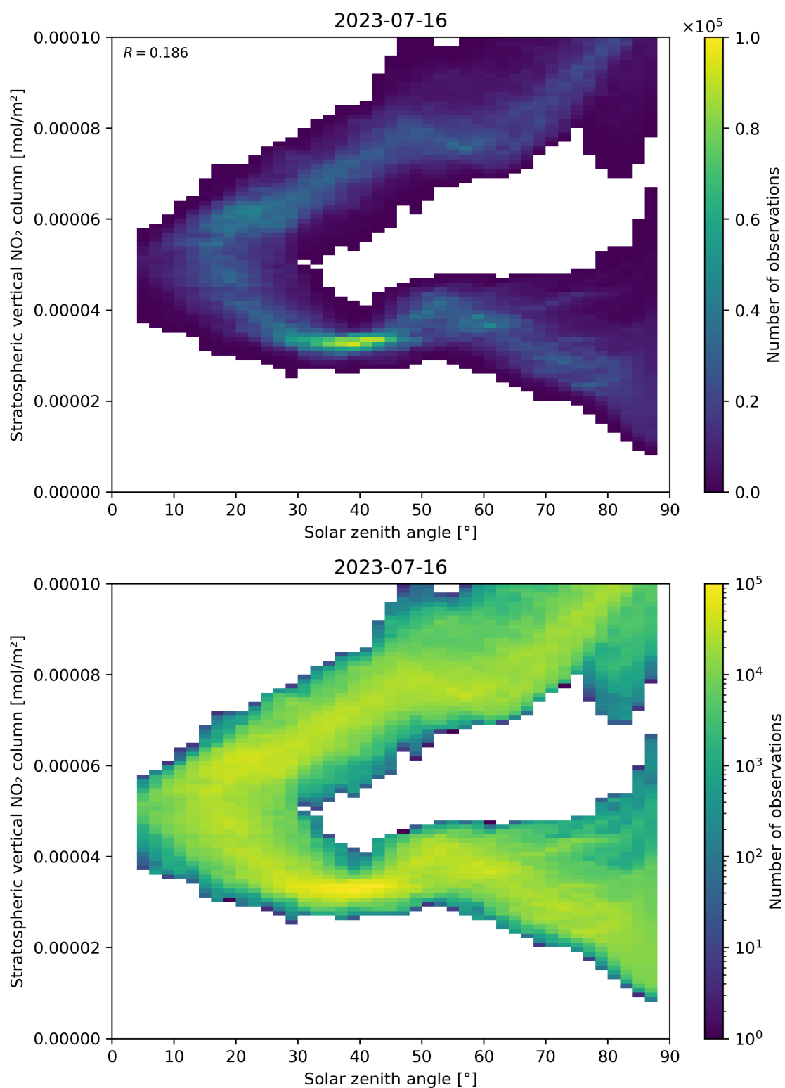
Figure 150: Scatter density plot of “Solar zenith angle” against “Stratospheric vertical NO 2 column” for 2023-07-15 to 2023-07-17.
