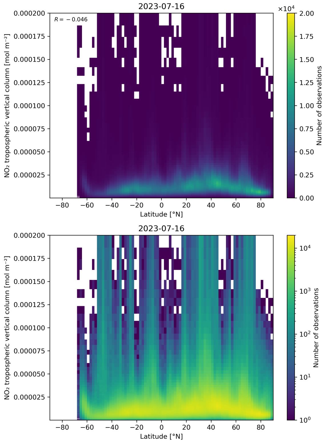
Figure 92: Scatter density plot of “Latitude” against “NO 2 tropospheric vertical column” for 2023-07-15 to 2023-07-17.
