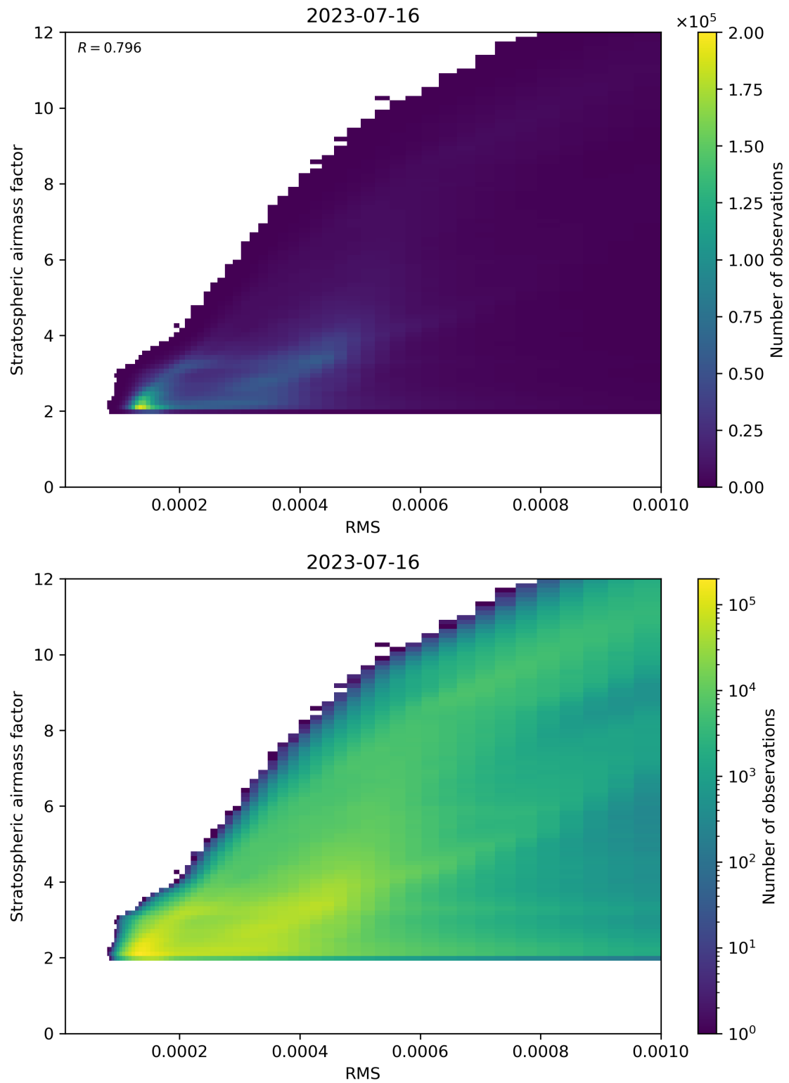
Figure 144: Scatter density plot of “RMS” against “Stratospheric airmass factor” for 2023-07-15 to 2023-07-17.
