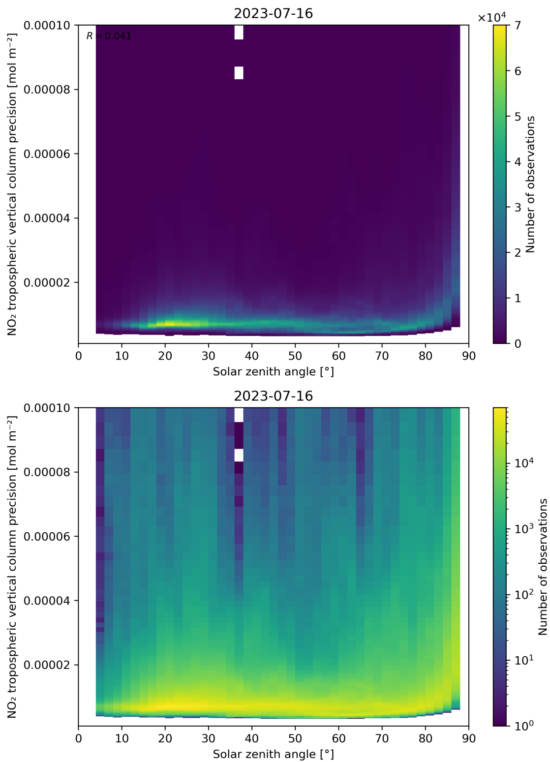
Figure 156: Scatter density plot of “Solar zenith angle” against “NO 2 tropospheric vertical column precision” for 2023-07-15 to 2023-07-17.
