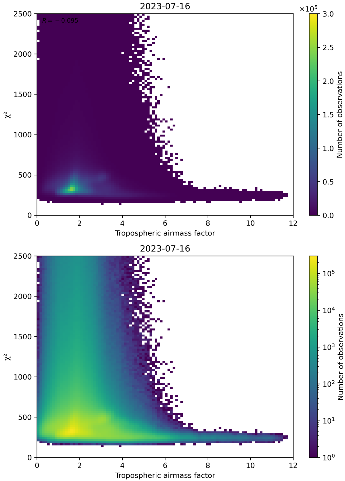
Figure 73: Scatter density plot of “Tropospheric airmass factor” against “ \chi^2 ” for 2023-07-15 to 2023-07-17.
