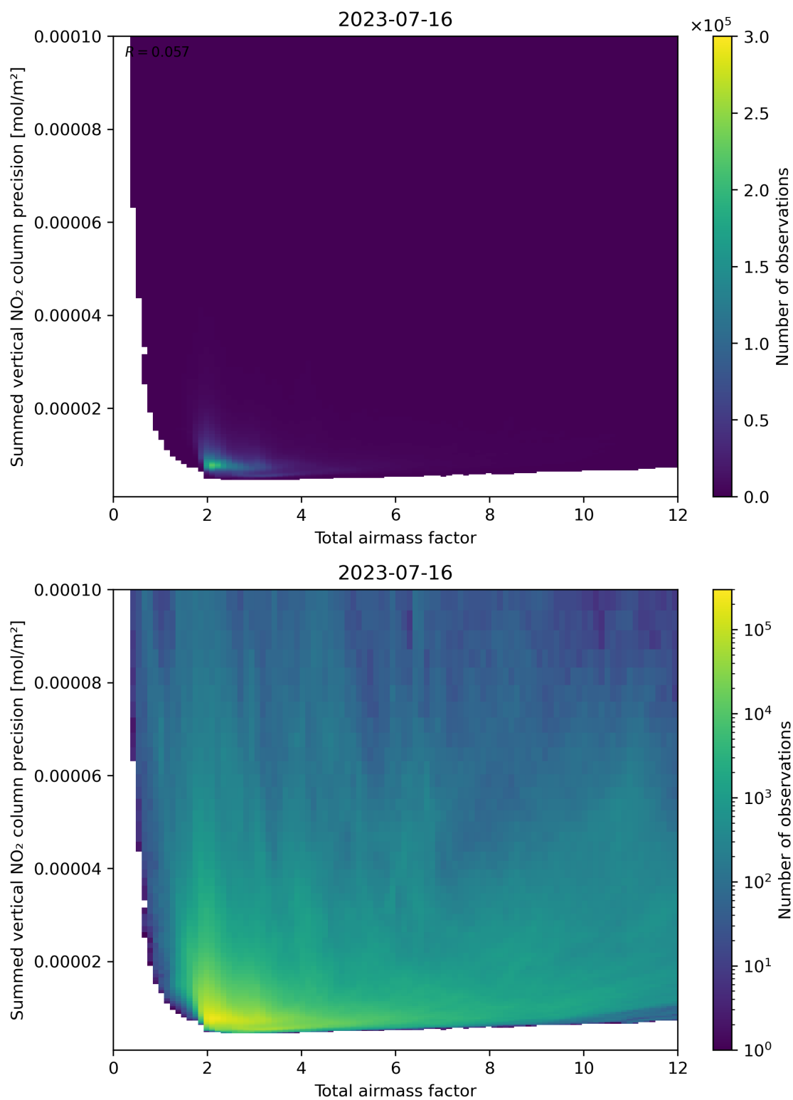
Figure 66: Scatter density plot of “Total airmass factor” against “Summed vertical NO 2 column precision” for 2023-07-15 to 2023-07-17.
