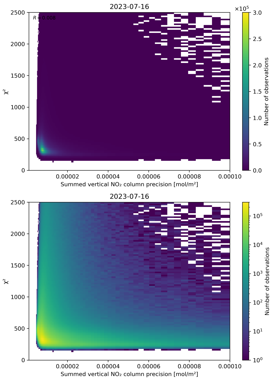
Figure 107: Scatter density plot of “Summed vertical NO 2 column precision” against “ \chi^2 ” for 2023-07-15 to 2023-07-17.
