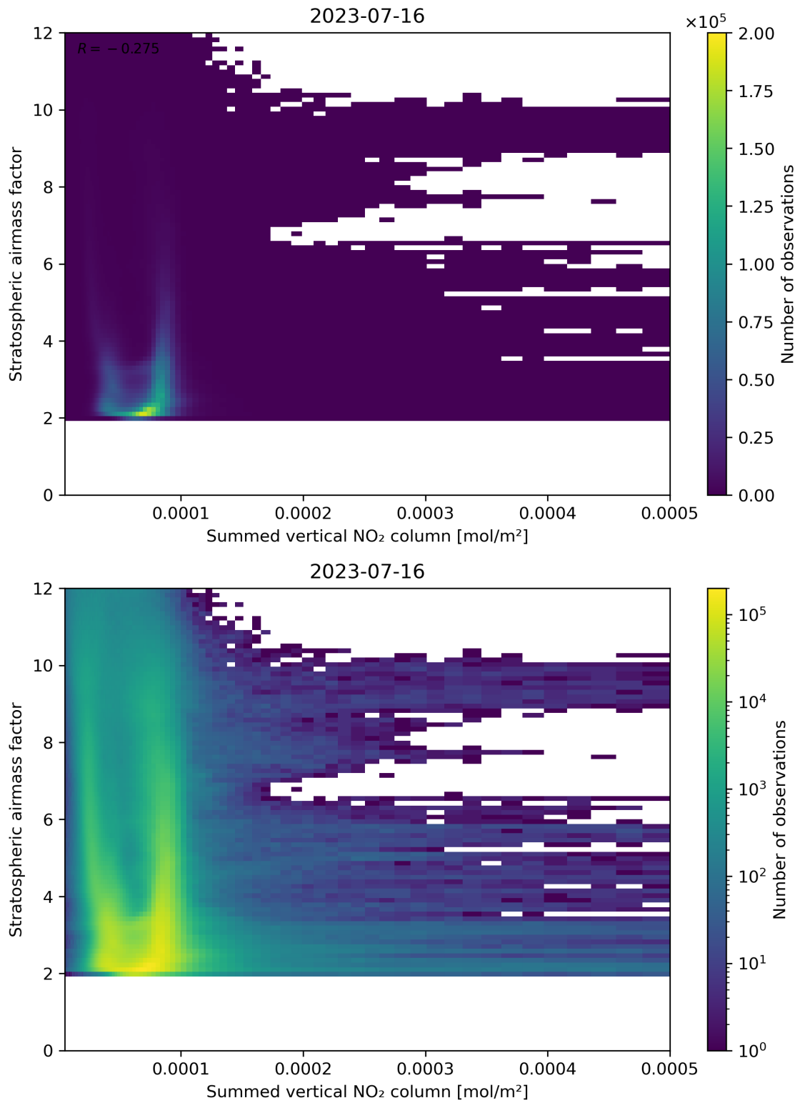
Figure 103: Scatter density plot of “Summed vertical NO 2 column” against “Stratospheric air mass factor” for 2023-07-15 to 2023-07-17.
