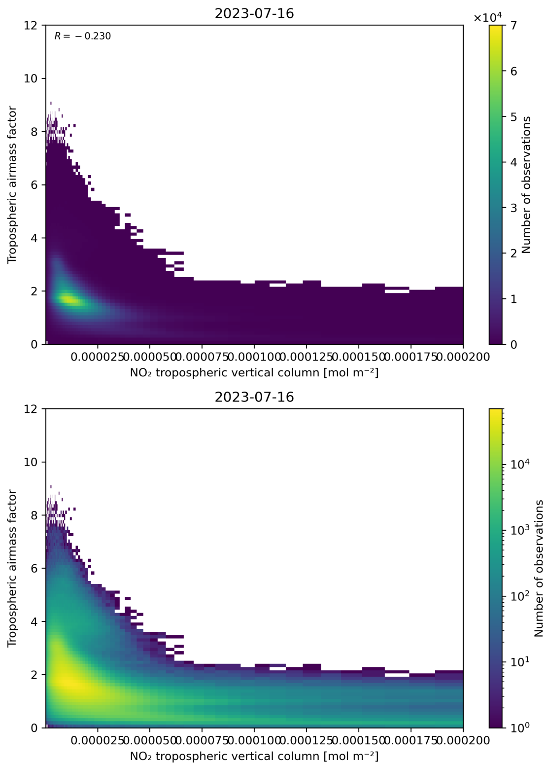
Figure 123: Scatter density plot of “NO 2 tropospheric vertical column” against “Tropospheric air mass factor” for 2023-07-15 to 2023-07-17.
