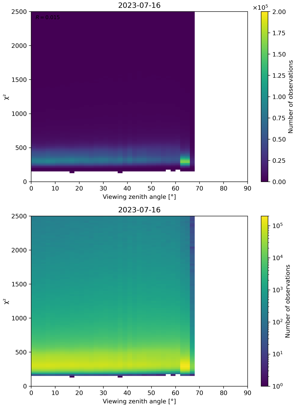
Figure 162: Scatter density plot of “Viewing zenith angle” against “ \chi^2 ” for 2023-07-15 to 2023-07-17.
