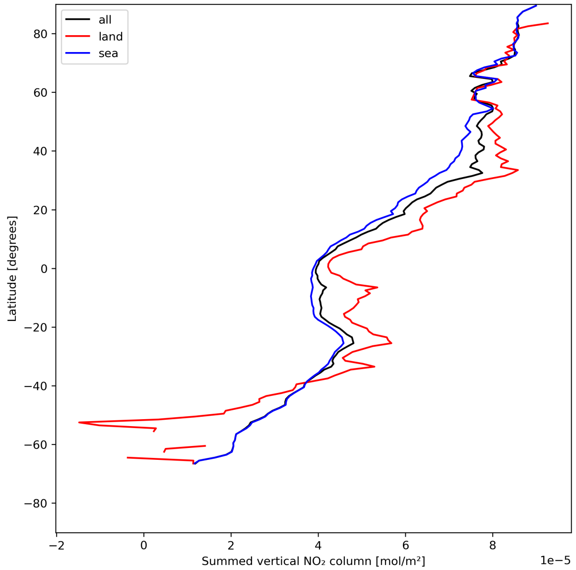
Figure 23: Zonal average of “Summed vertical NO 2 column” for 2023-07-15 to 2023-07-17.
