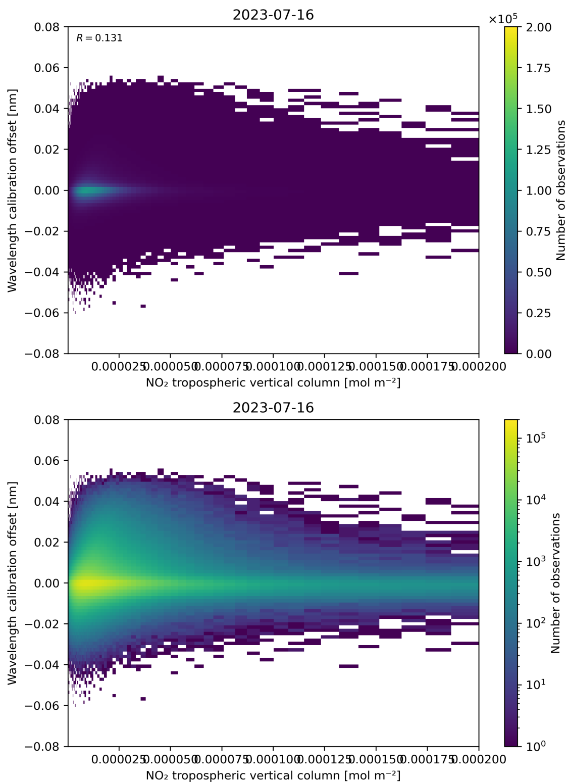
Figure 143: Scatter density plot of “NO 2 tropospheric vertical column” against “Wavelength calibration offset” for 2023-07-15 to 2023-07-17.
