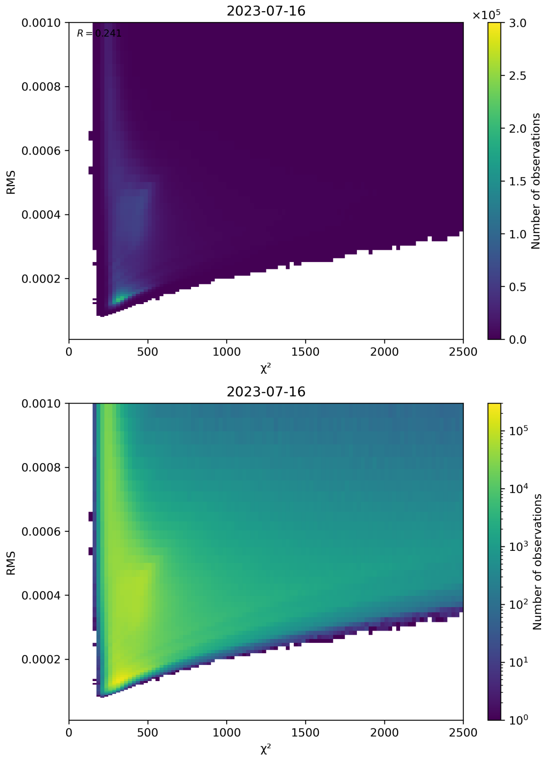
Figure 82: Scatter density plot of “ \chi^2 ” against “RMS” for 2023-07-15 to 2023-07-17.
