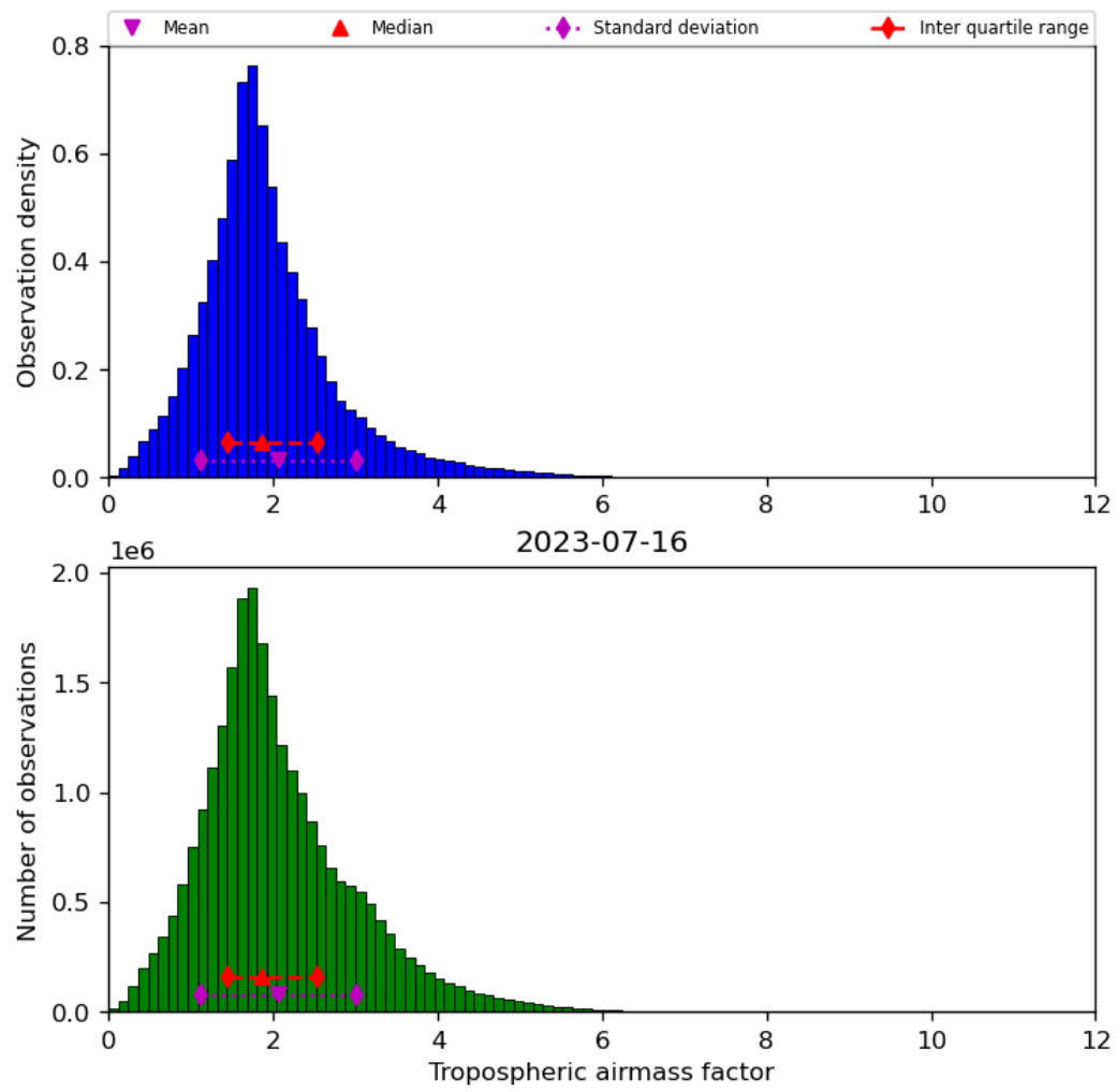
Figure 31: Histogram of “Tropospheric airmass factor” for 2023-07-15 to 2023-07-17
