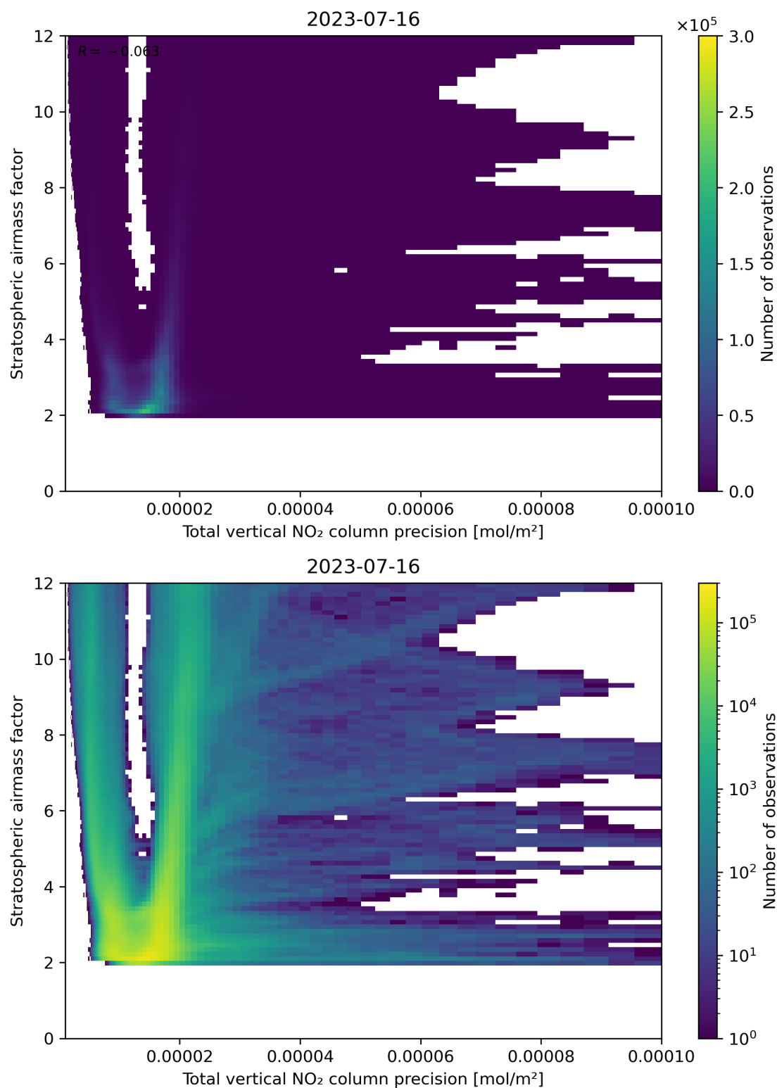
Figure 115: Scatter density plot of “Total vertical NO 2 column precision” against “Stratospheric air mass factor” for 2023-07-15 to 2023-07-17.
