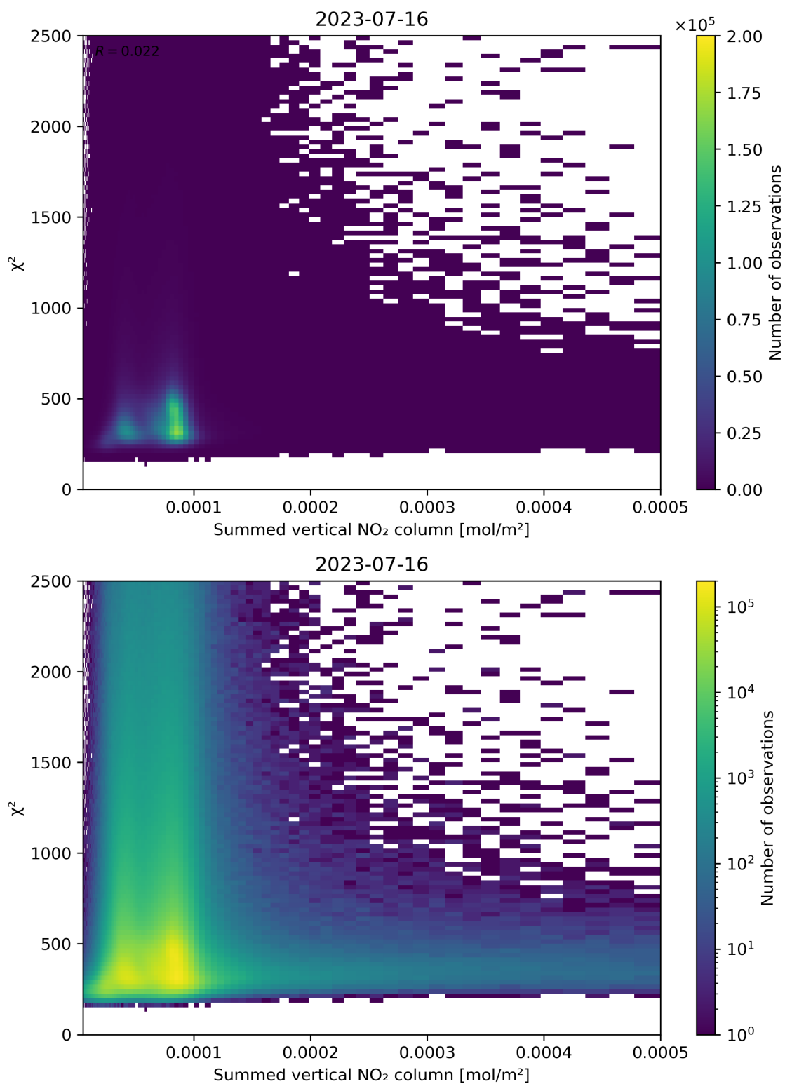
Figure 104: Scatter density plot of “Summed vertical NO 2 column” against “ \chi^2 ” for 2023-07-15 to 2023-07-17.
