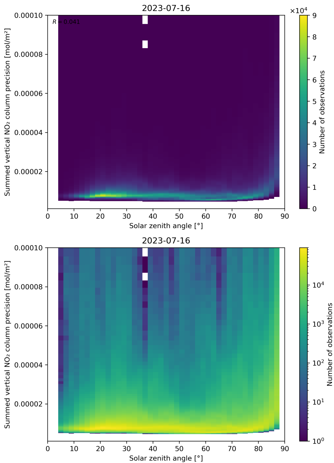
Figure 152: Scatter density plot of “Solar zenith angle” against “Summed vertical NO 2 column precision” for 2023-07-15 to 2023-07-17.
