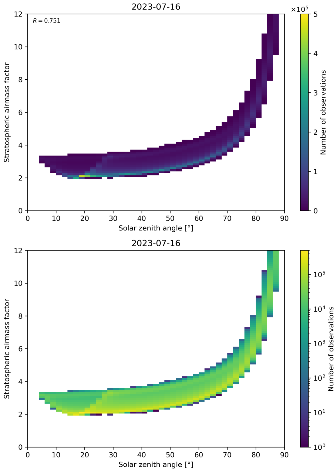
Figure 145: Scatter density plot of “Solar zenith angle” against “Stratospheric airmass factor” for 2023-07-15 to 2023-07-17.
