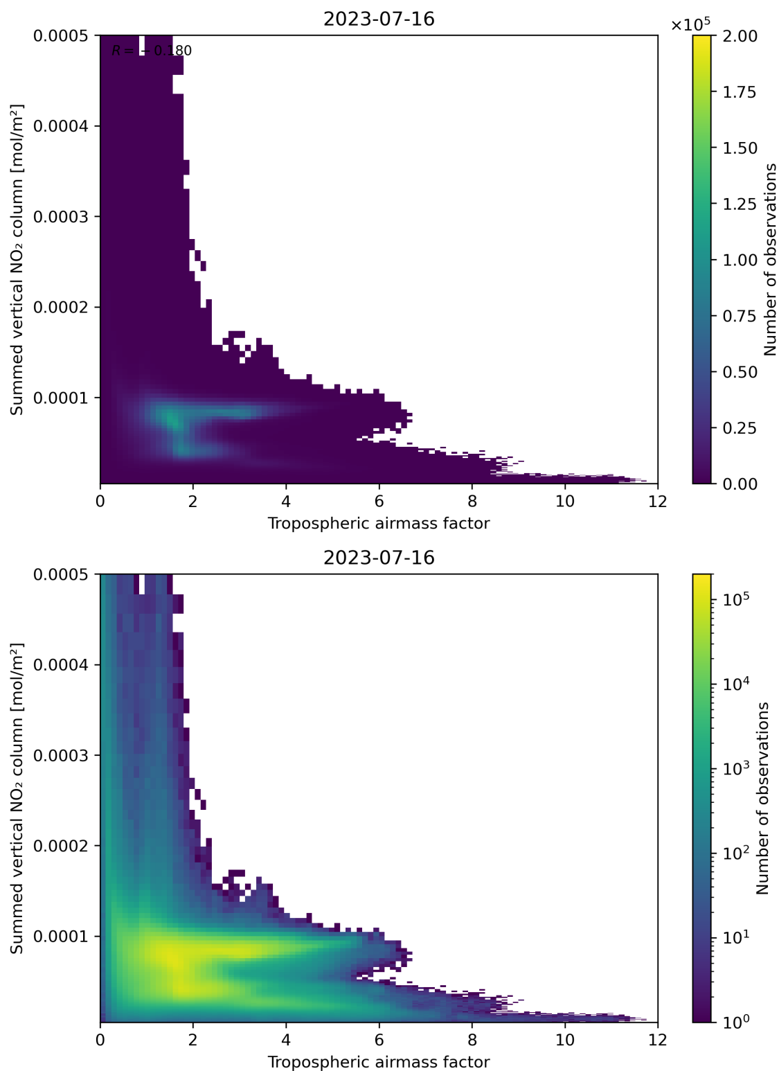
Figure 75: Scatter density plot of “Tropospheric airmass factor” against “Summed vertical NO 2 column” for 2023-07-15 to 2023-07-17.
