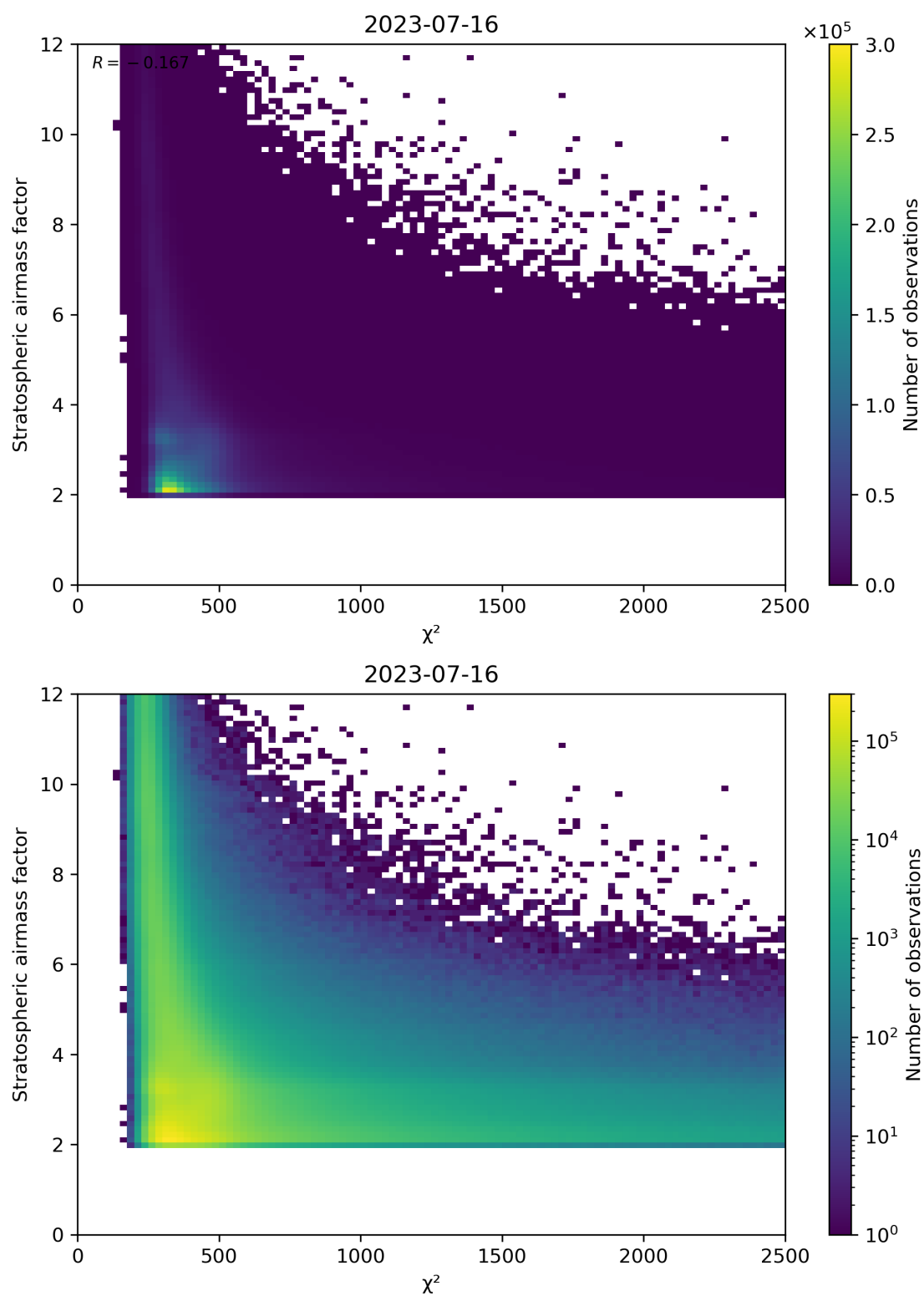
Figure 81: Scatter density plot of “ \chi^2 ” against “Stratospheric airmass factor” for 2023-07-15 to 2023-07-17.
