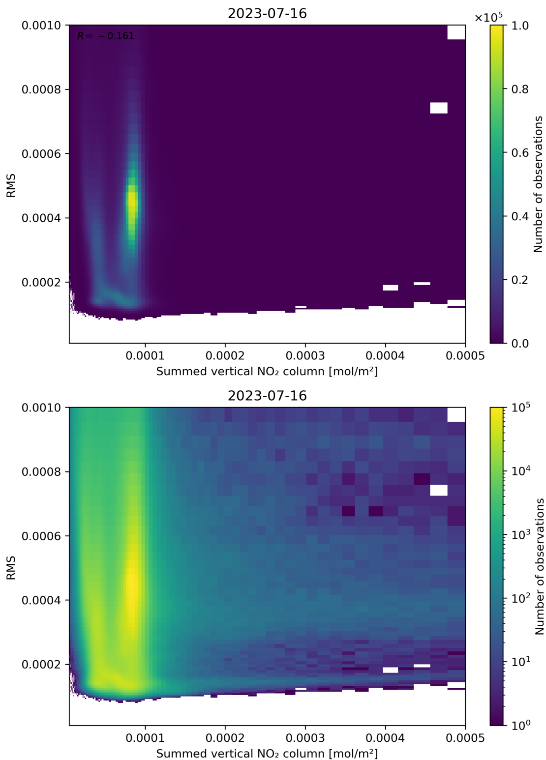
Figure 109: Scatter density plot of “Summed vertical NO 2 column” against “RMS” for 2023-07-15 to 2023-07-17.
