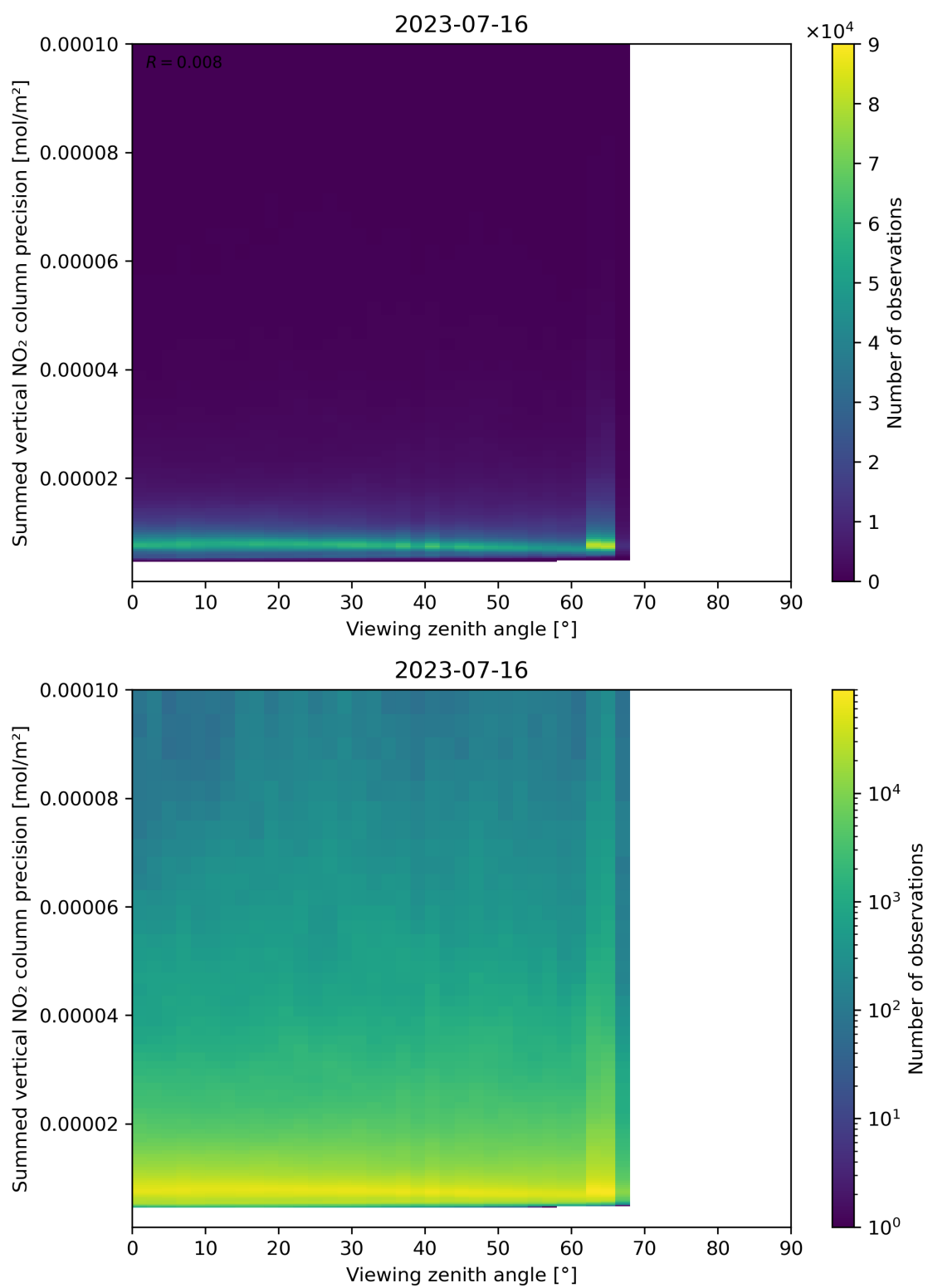
Figure 166: Scatter density plot of “Viewing zenith angle” against “Summed vertical NO 2 column precision” for 2023-07-15 to 2023-07-17.
