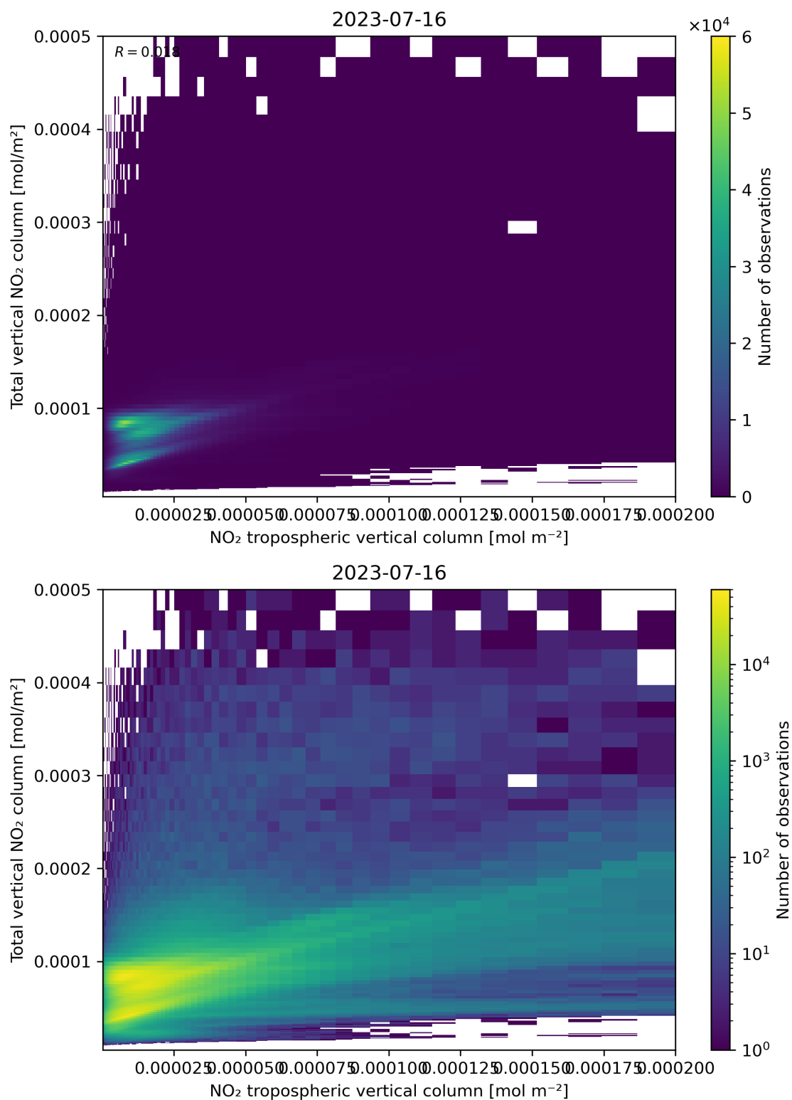
Figure 128: Scatter density plot of “NO 2 tropospheric vertical column” against “Total vertical NO 2 column” for 2023-07-15 to 2023-07-17.
