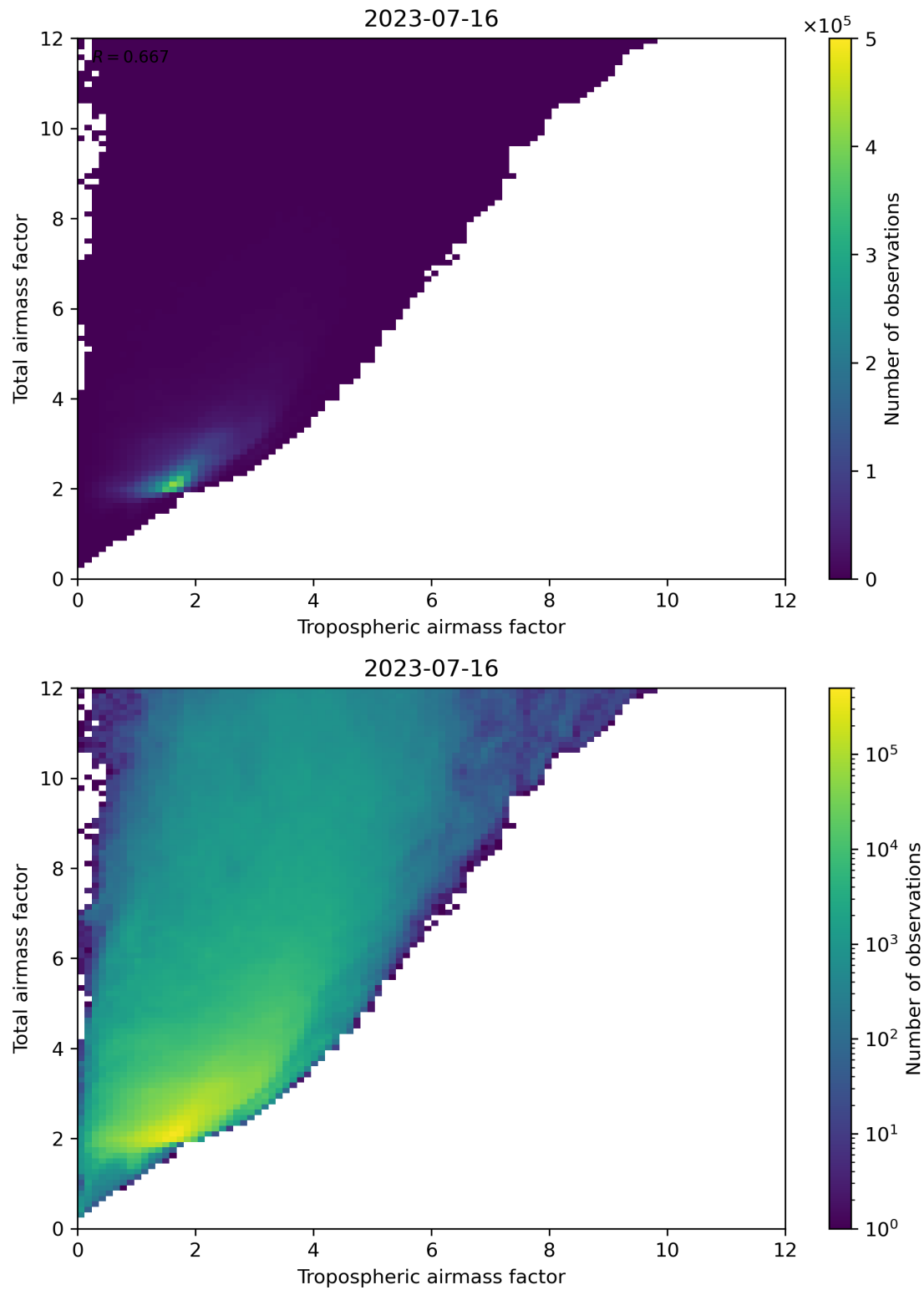
Figure 72: Scatter density plot of “Tropospheric airmass factor” against “Total airmass factor” for 2023-07-15 to 2023-07-17.
