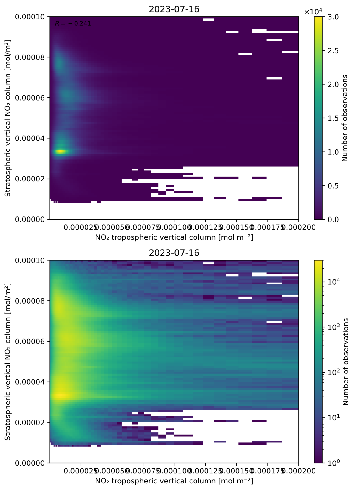
Figure 125: Scatter density plot of “NO 2 tropospheric vertical column” against “Stratospheric vertical NO 2 column” for 2023-07-15 to 2023-07-17.
