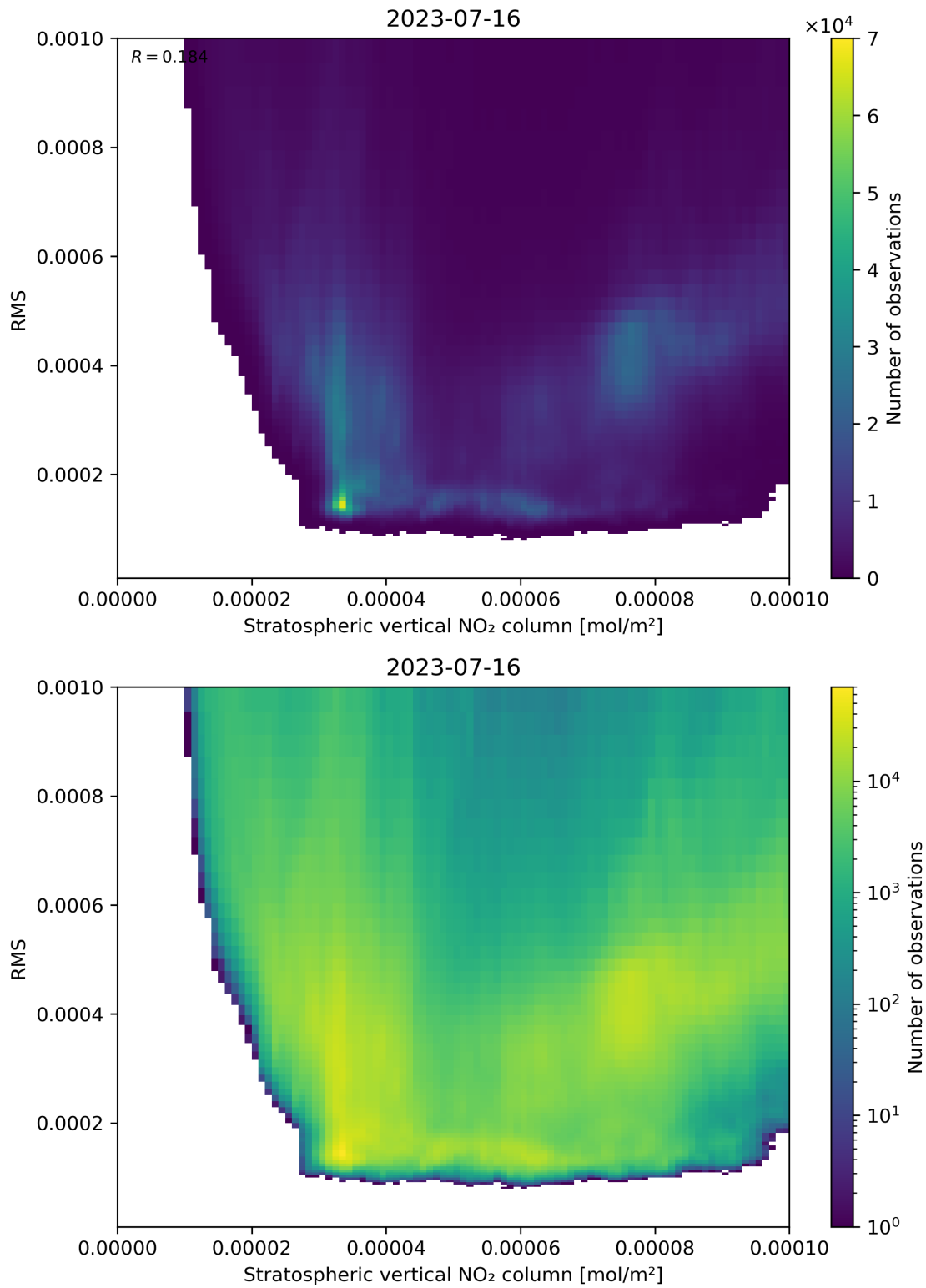
Figure 102: Scatter density plot of “Stratospheric vertical NO 2 column” against “RMS” for 2023-07-15 to 2023-07-17.
