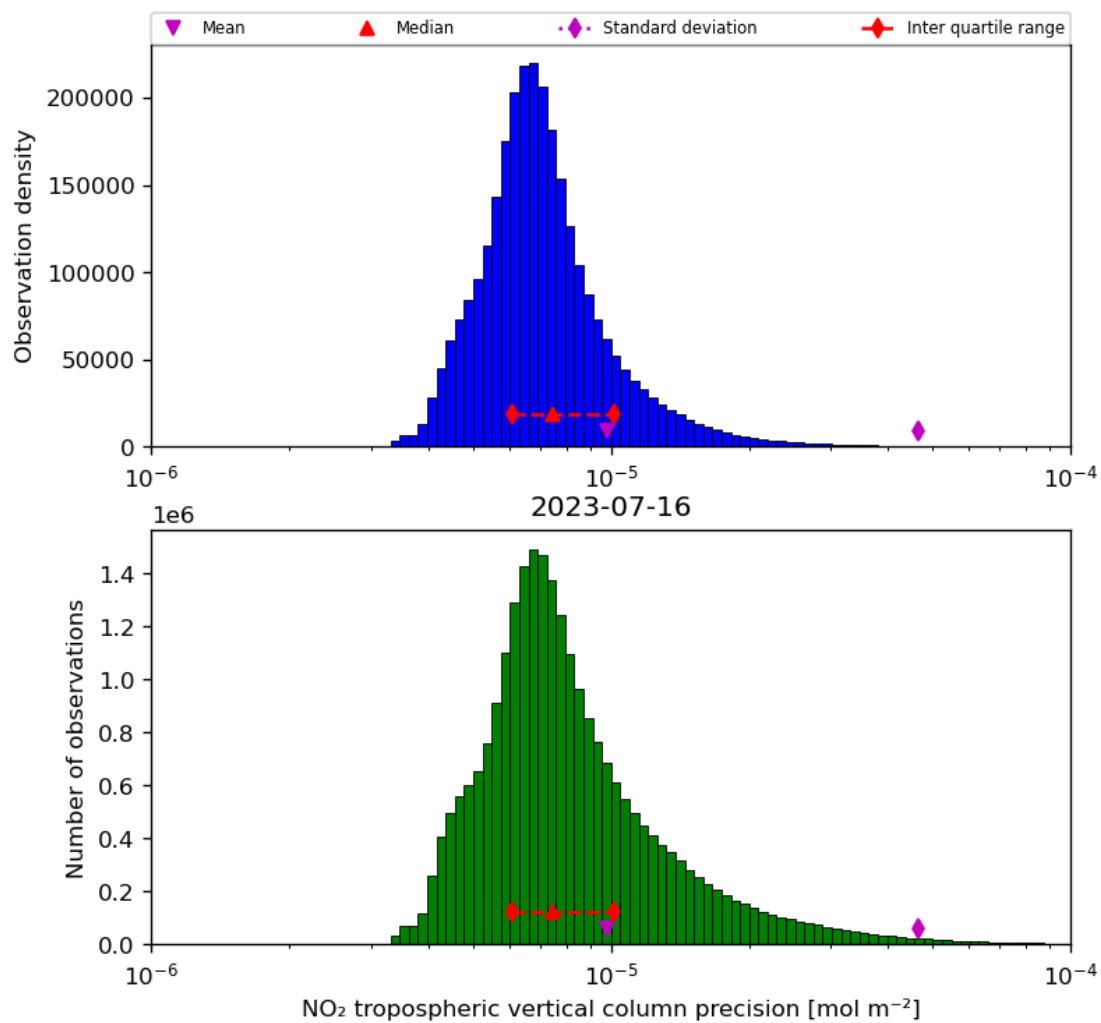
Figure 30: Histogram of “NO 2 tropospheric vertical column precision” for 2023-07-15 to 2023-07-17
