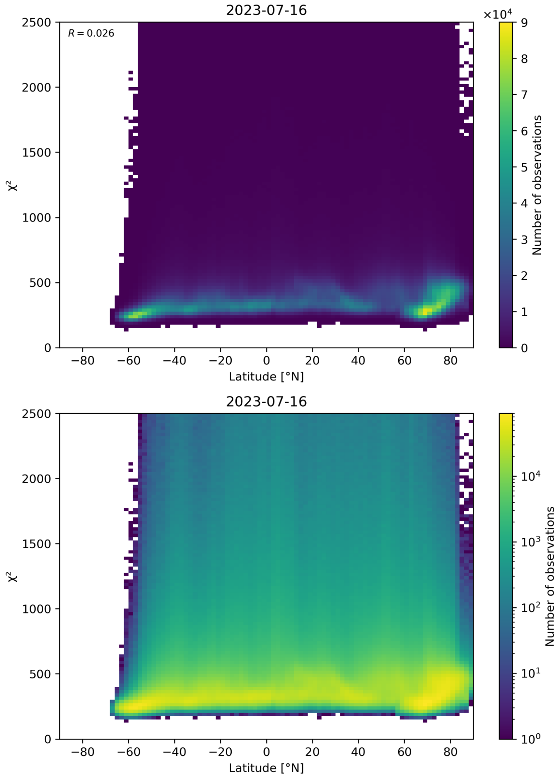
Figure 86: Scatter density plot of “Latitude” against “ \chi^2 ” for 2023-07-15 to 2023-07-17.
