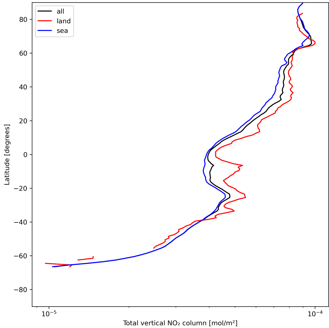
Figure 21: Zonal average of “Total vertical NO 2 column” for 2023-07-15 to 2023-07-17.
