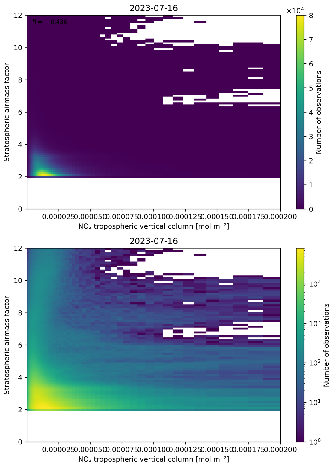
Figure 121: Scatter density plot of “NO 2 tropospheric vertical column” against “Stratospheric air mass factor” for 2023-07-15 to 2023-07-17.
