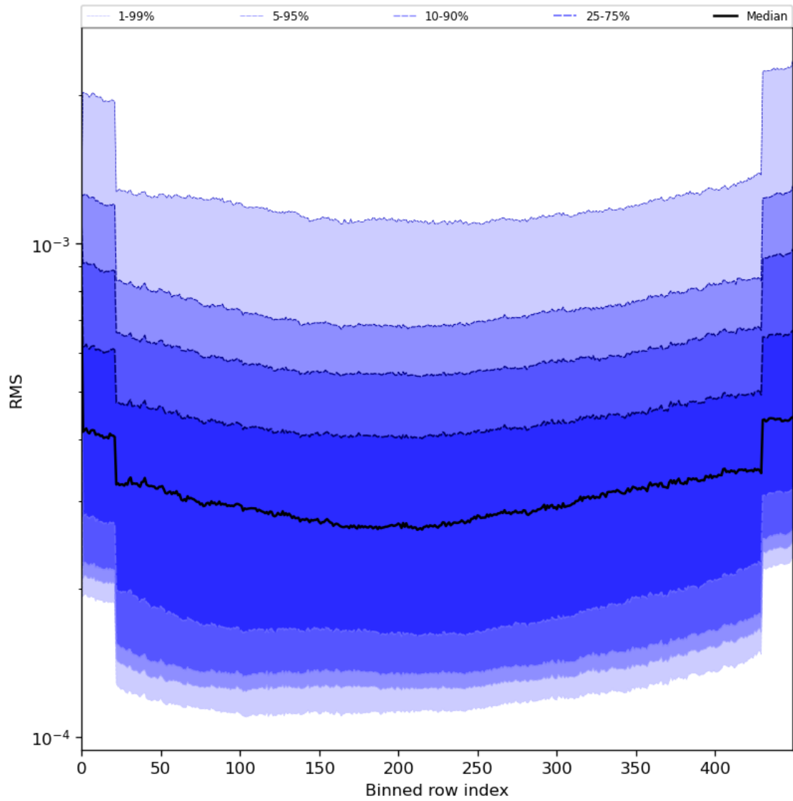
Figure 60: Along track statistics of “RMS” for 2023-07-15 to 2023-07-17
