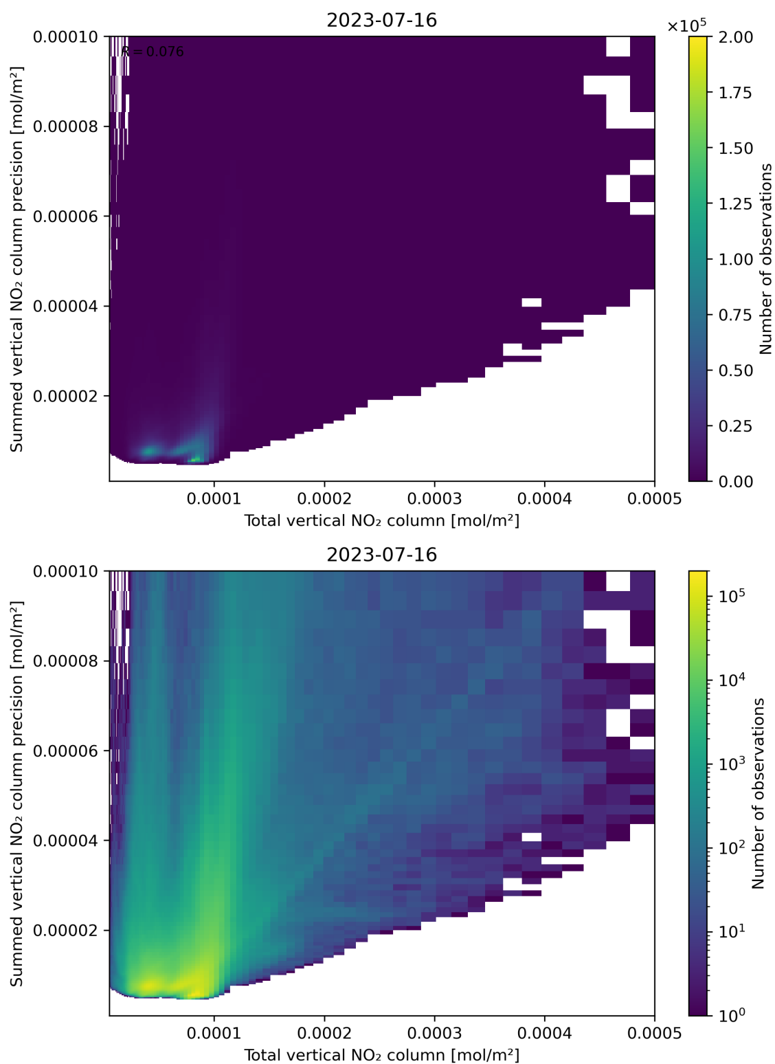
Figure 113: Scatter density plot of “Total vertical NO 2 column” against “Summed vertical NO 2 column precision” for 2023-07-15 to 2023-07-17.
