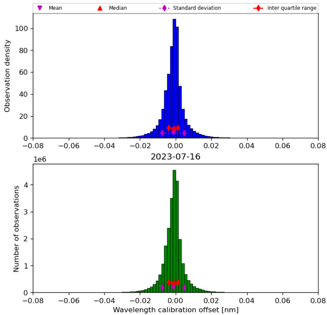
Figure 35: Histogram of “Wavelength calibration offset” for 2023-07-15 to 2023-07-17
