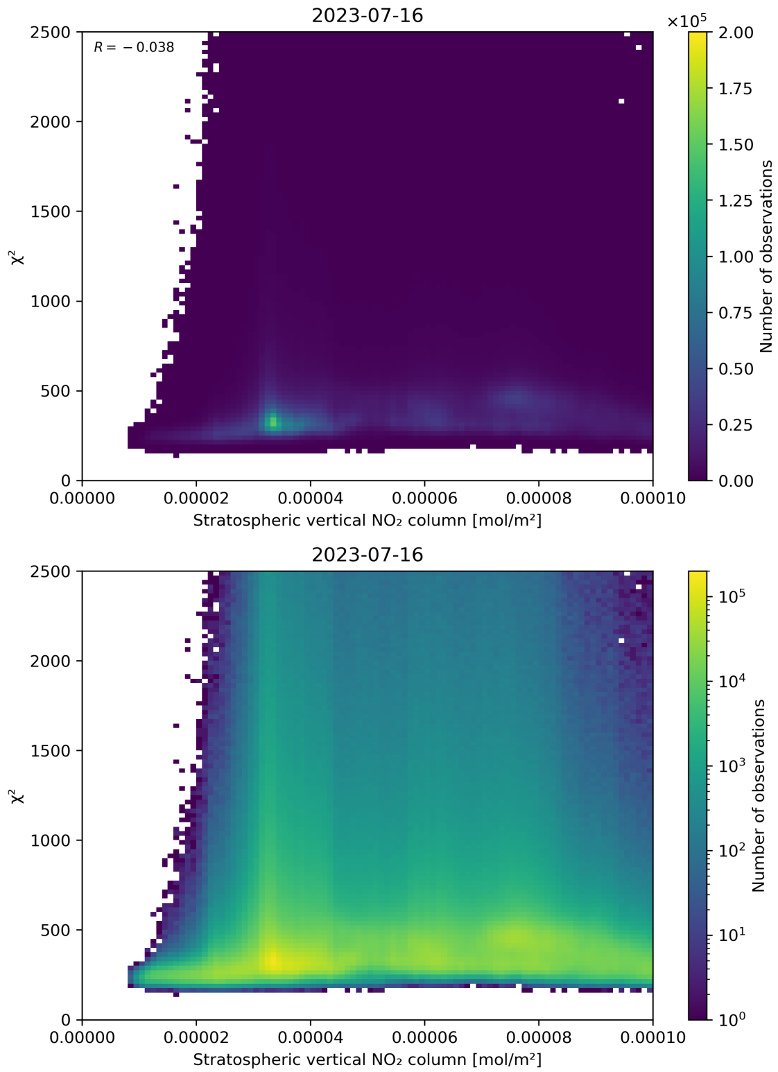
Figure 97: Scatter density plot of “Stratospheric vertical NO 2 column” against “ \chi^2 ” for 2023-07-15 to 2023-07-17.
