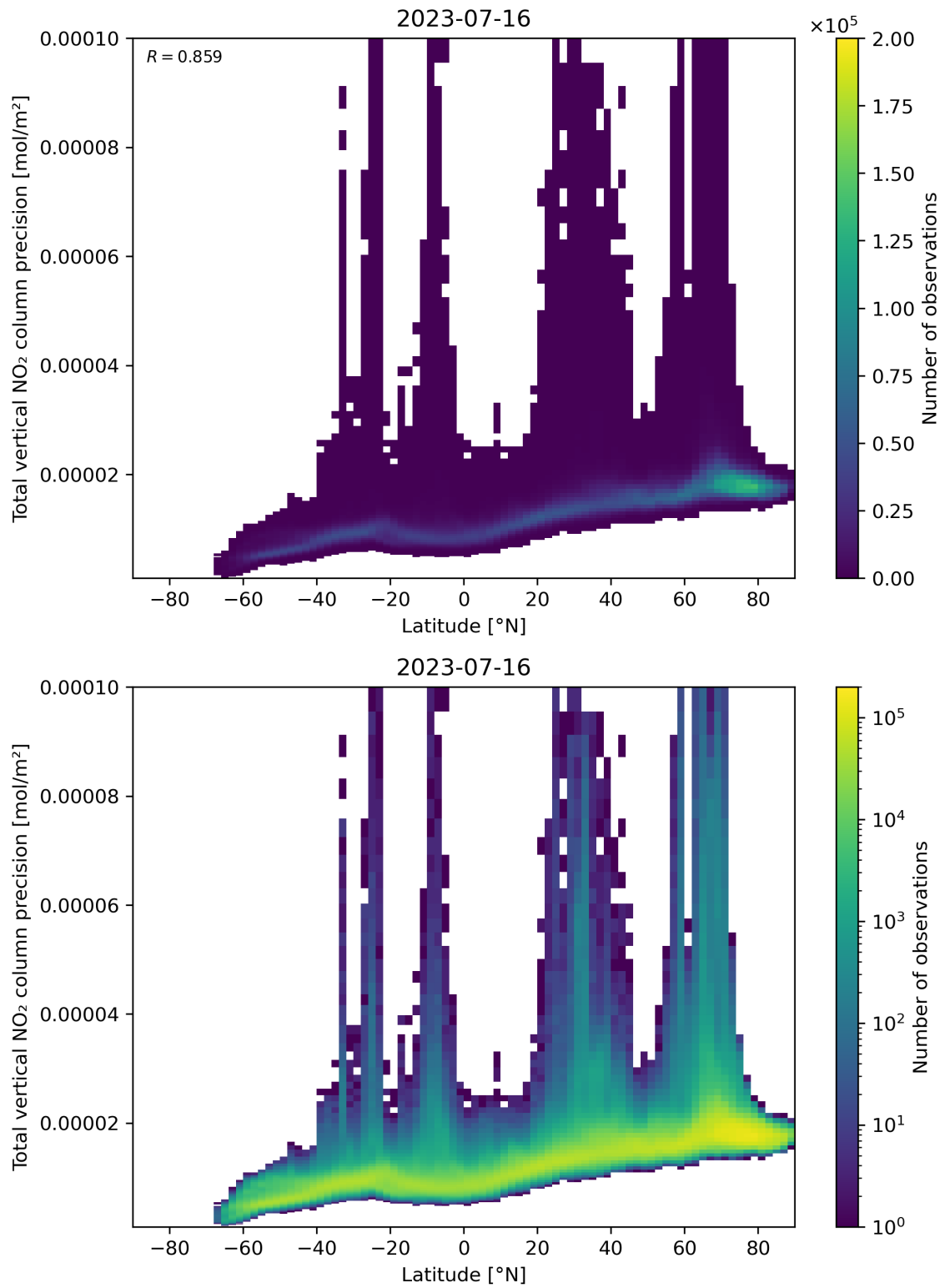
Figure 91: Scatter density plot of “Latitude” against “Total vertical NO 2 column precision” for 2023-07-15 to 2023-07-17.
