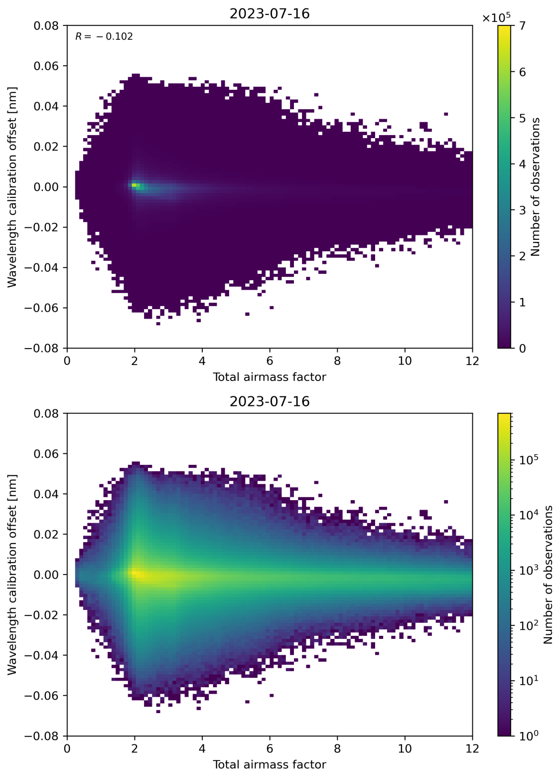
Figure 70: Scatter density plot of “Total airmass factor” against “Wavelength calibration offset” for 2023-07-15 to 2023-07-17.
