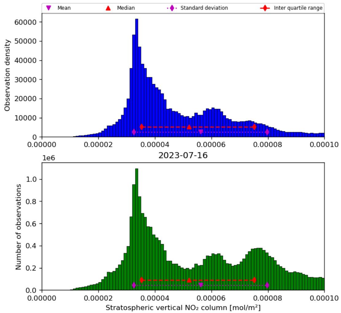
Figure 36: Histogram of “Stratospheric vertical NO 2 column” for 2023-07-15 to 2023-07-17
