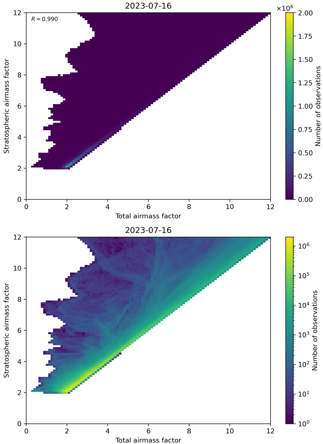
Figure 62: Scatter density plot of “Total airmass factor” against “Stratospheric airmass factor” for 2023-07-15 to 2023-07-17.
