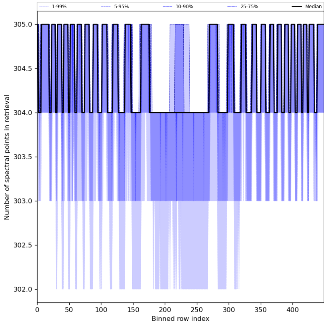
Figure 50: Along track statistics of “Number of spectral points in retrieval” for 2023-07-15 to 2023-07-17
