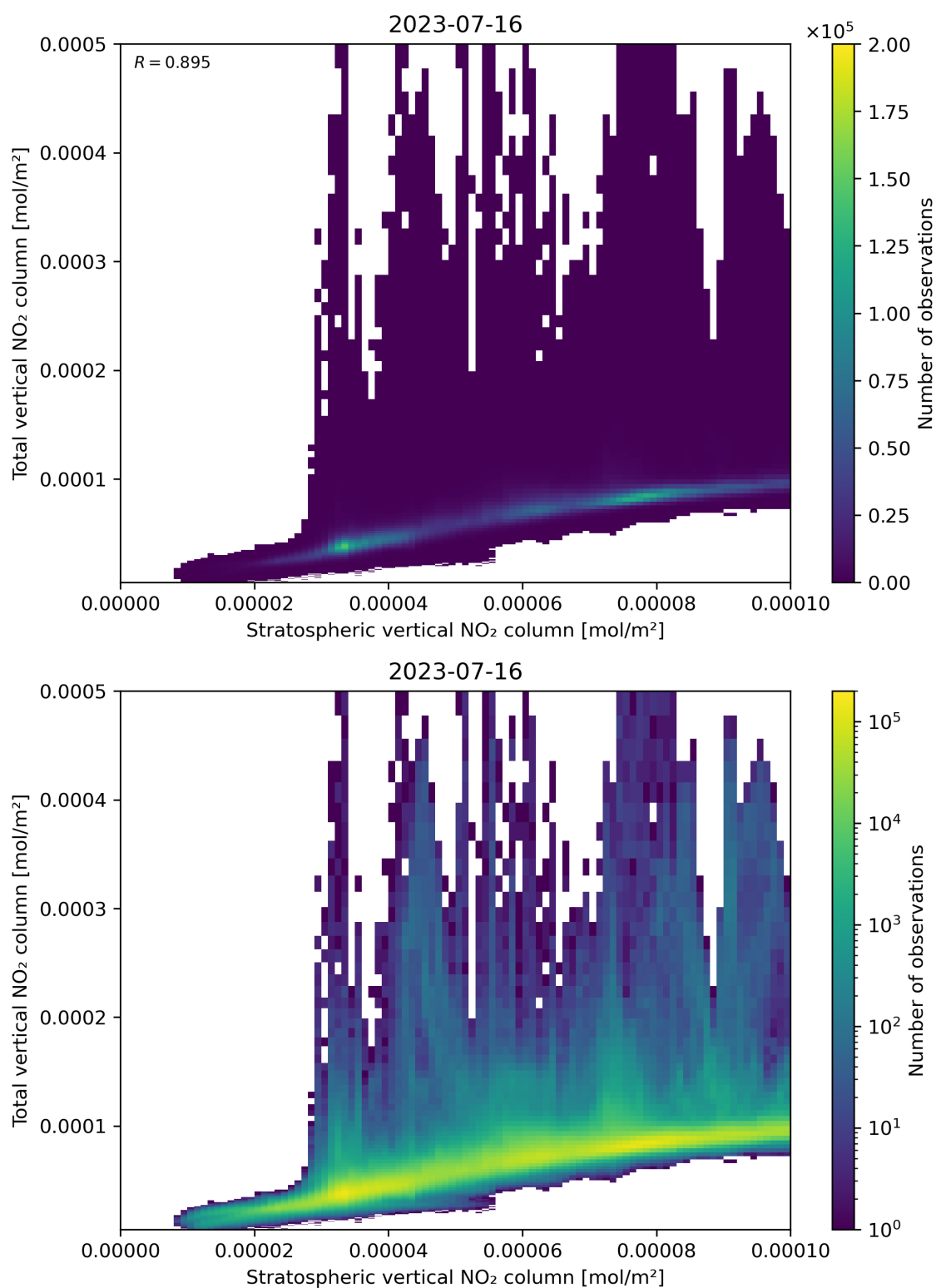
Figure 100: Scatter density plot of “Stratospheric vertical NO 2 column” against “Total vertical NO 2 column” for 2023-07-15 to 2023-07-17.
