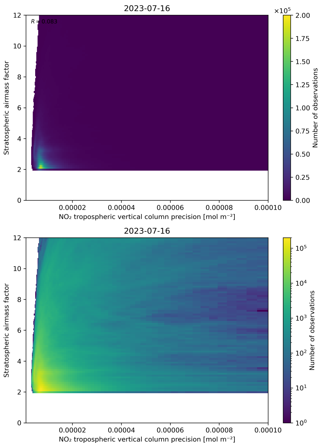
Figure 131: Scatter density plot of “NO 2 tropospheric vertical column precision” against “Stratospheric airmass factor” for 2023-07-15 to 2023-07-17.
