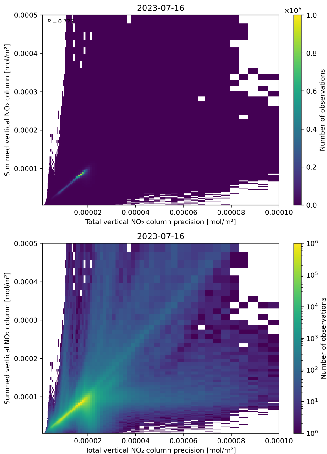
Figure 117: Scatter density plot of “Total vertical NO 2 column precision” against “Summed vertical NO 2 column” for 2023-07-15 to 2023-07-17.
