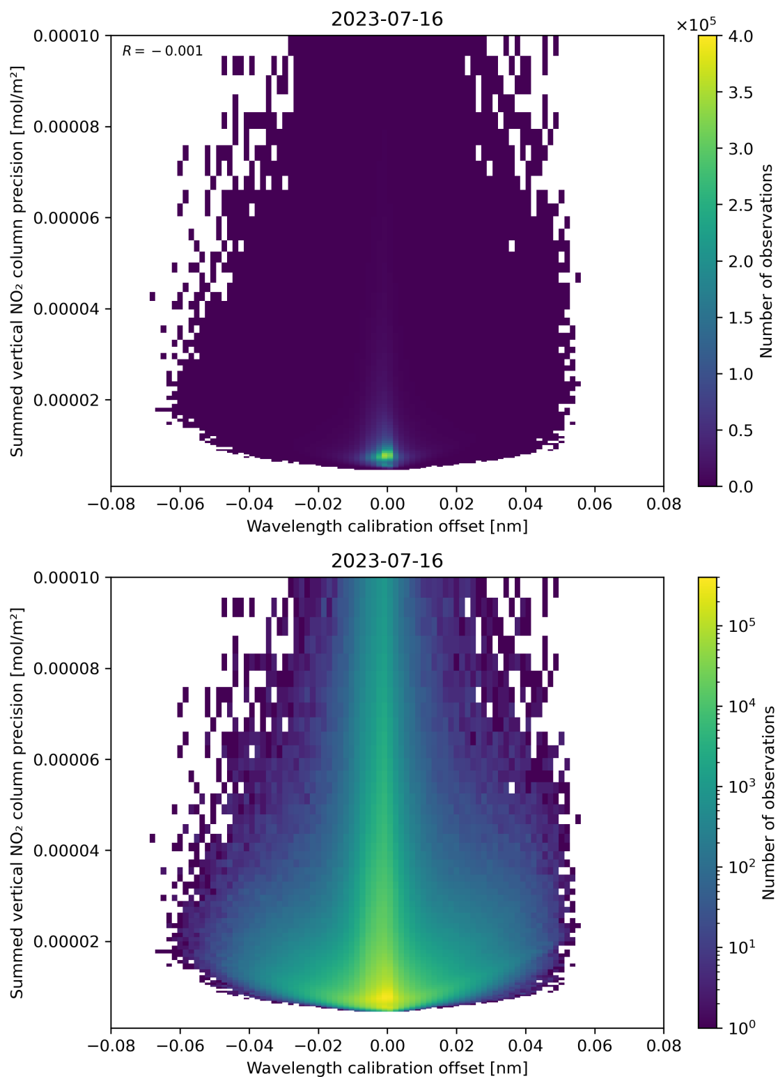
Figure 178: Scatter density plot of “Wavelength calibration offset” against “Summed vertical NO 2 column precision” for 2023-07-15 to 2023-07-17.
