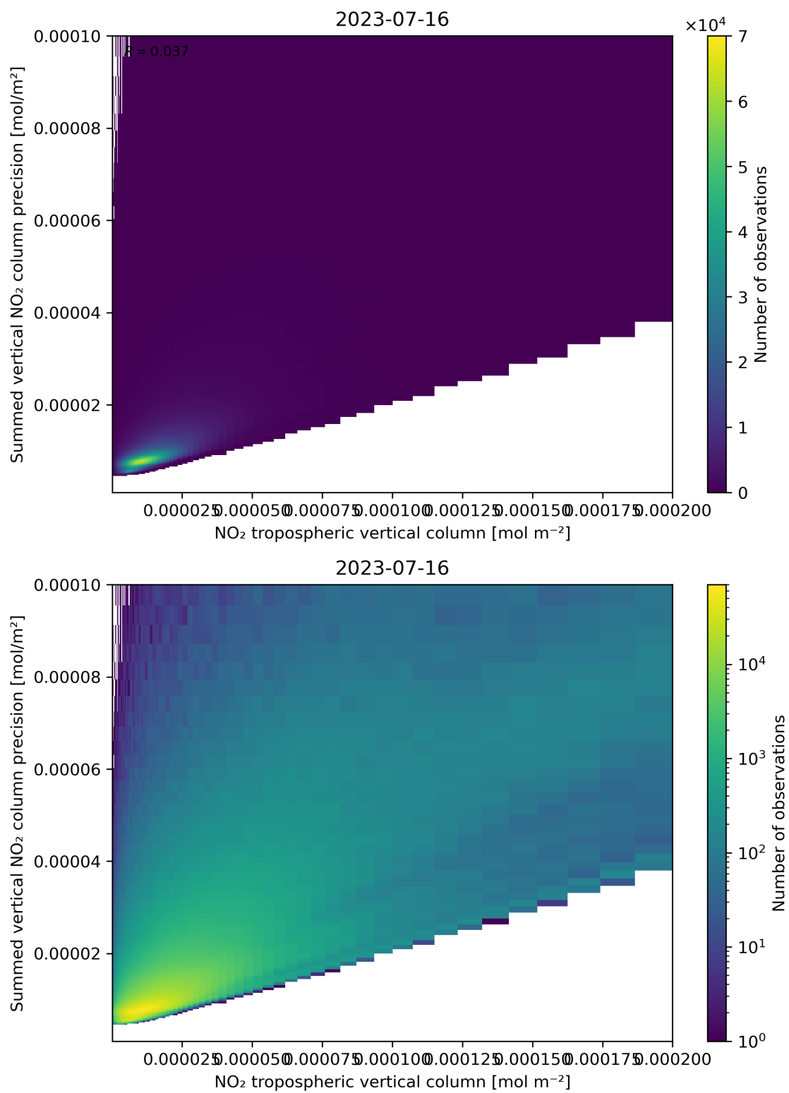
Figure 127: Scatter density plot of “NO 2 tropospheric vertical column” against “Summed vertical NO 2 column precision” for 2023-07-15 to 2023-07-17.
