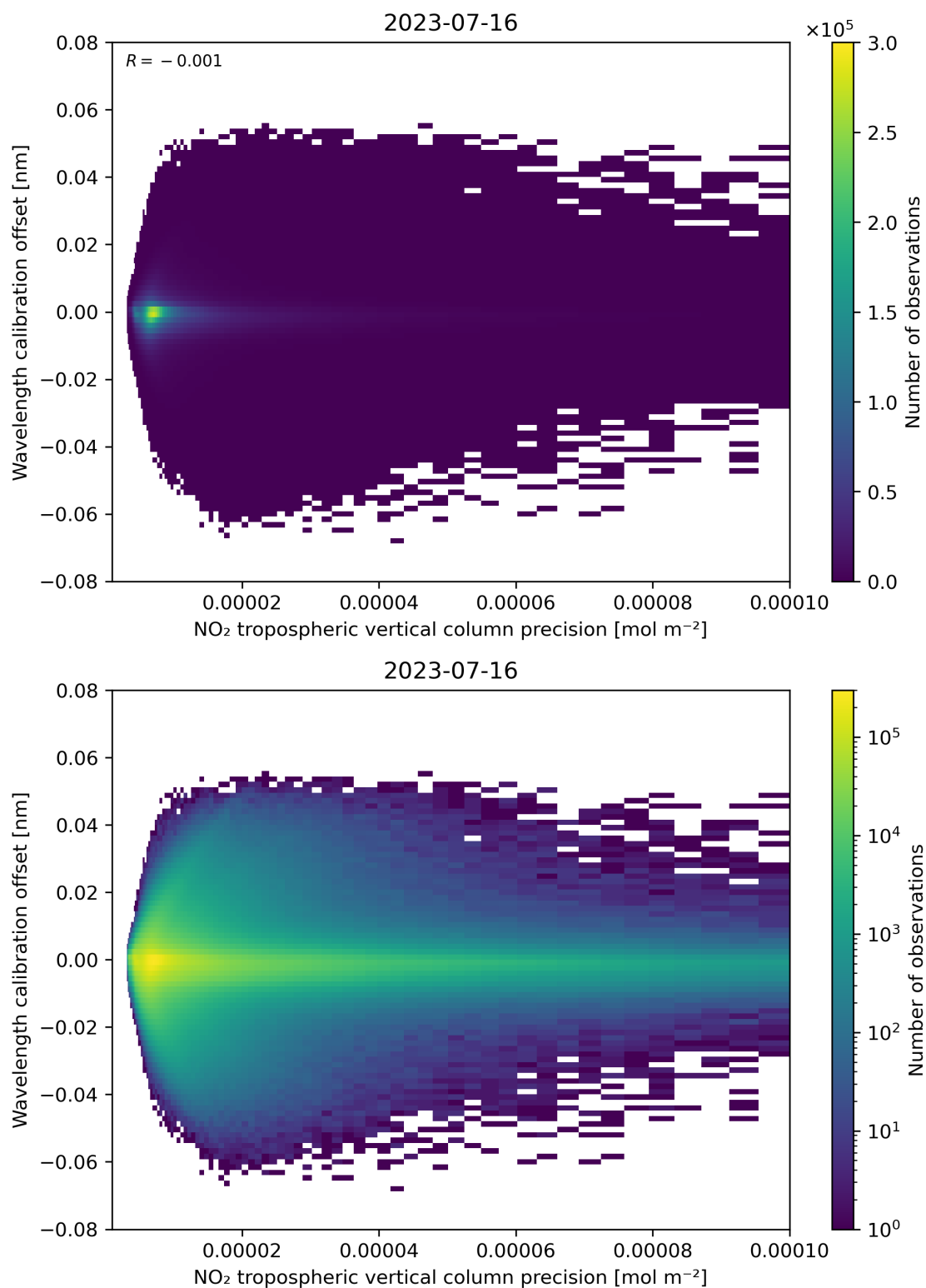
Figure 141: Scatter density plot of “NO 2 tropospheric vertical column precision” against “Wavelength calibration offset” for 2023-07-15 to 2023-07-17.
