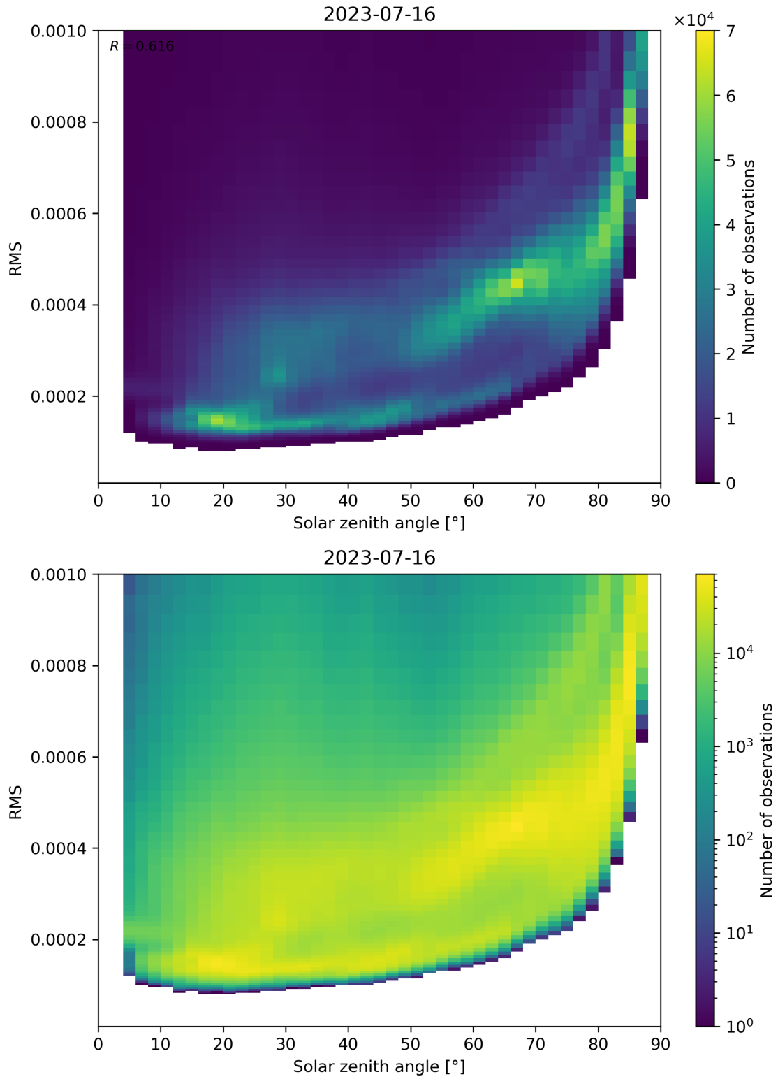
Figure 157: Scatter density plot of “Solar zenith angle” against “RMS” for 2023-07-15 to 2023-07-17.
