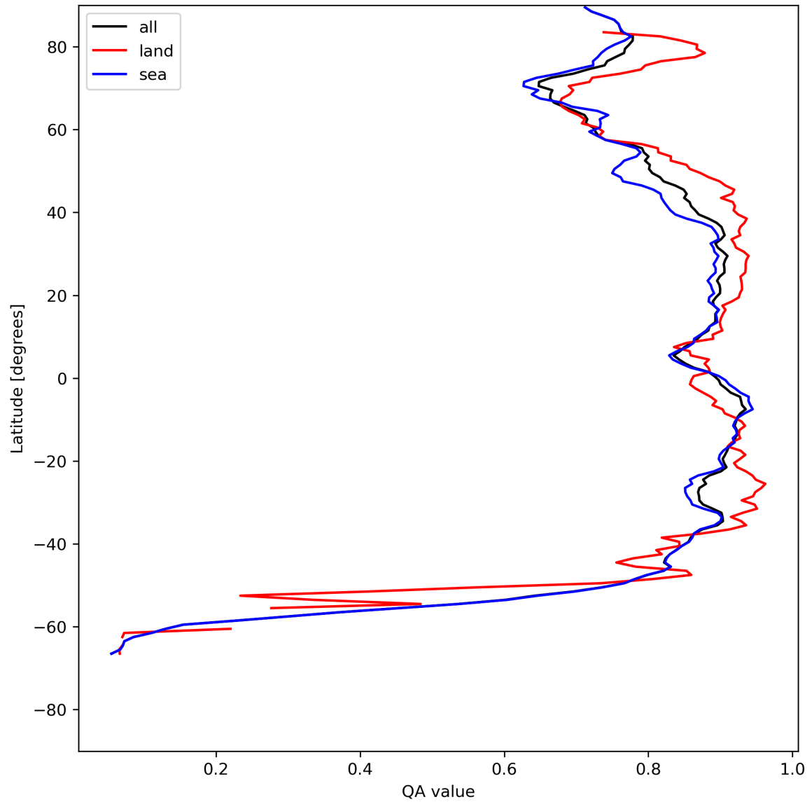
Figure 11: Zonal average of “QA value” for 2023-07-15 to 2023-07-17.
