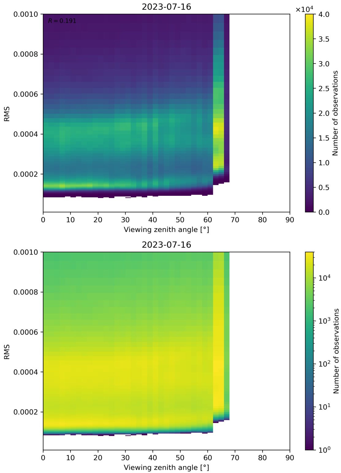
Figure 171: Scatter density plot of “Viewing zenith angle” against “RMS” for 2023-07-15 to 2023-07-17.
