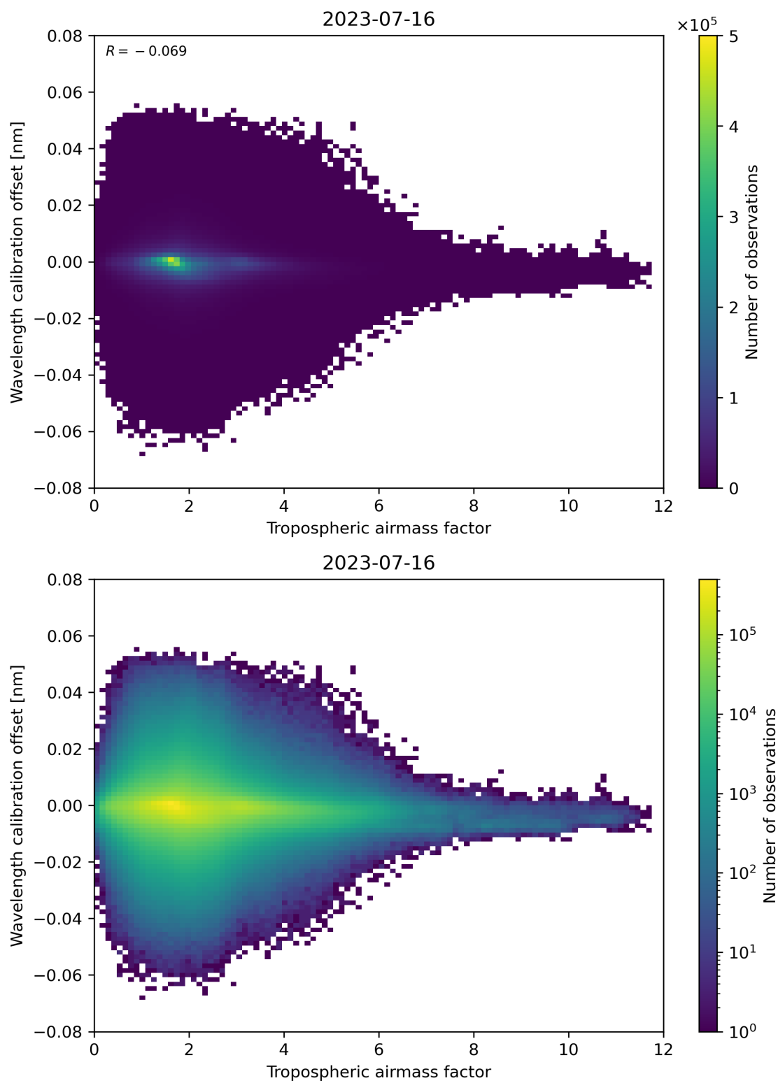
Figure 80: Scatter density plot of “Tropospheric air mass factor” against “Wavelength calibration offset” for 2023-07-15 to 2023-07-17.
