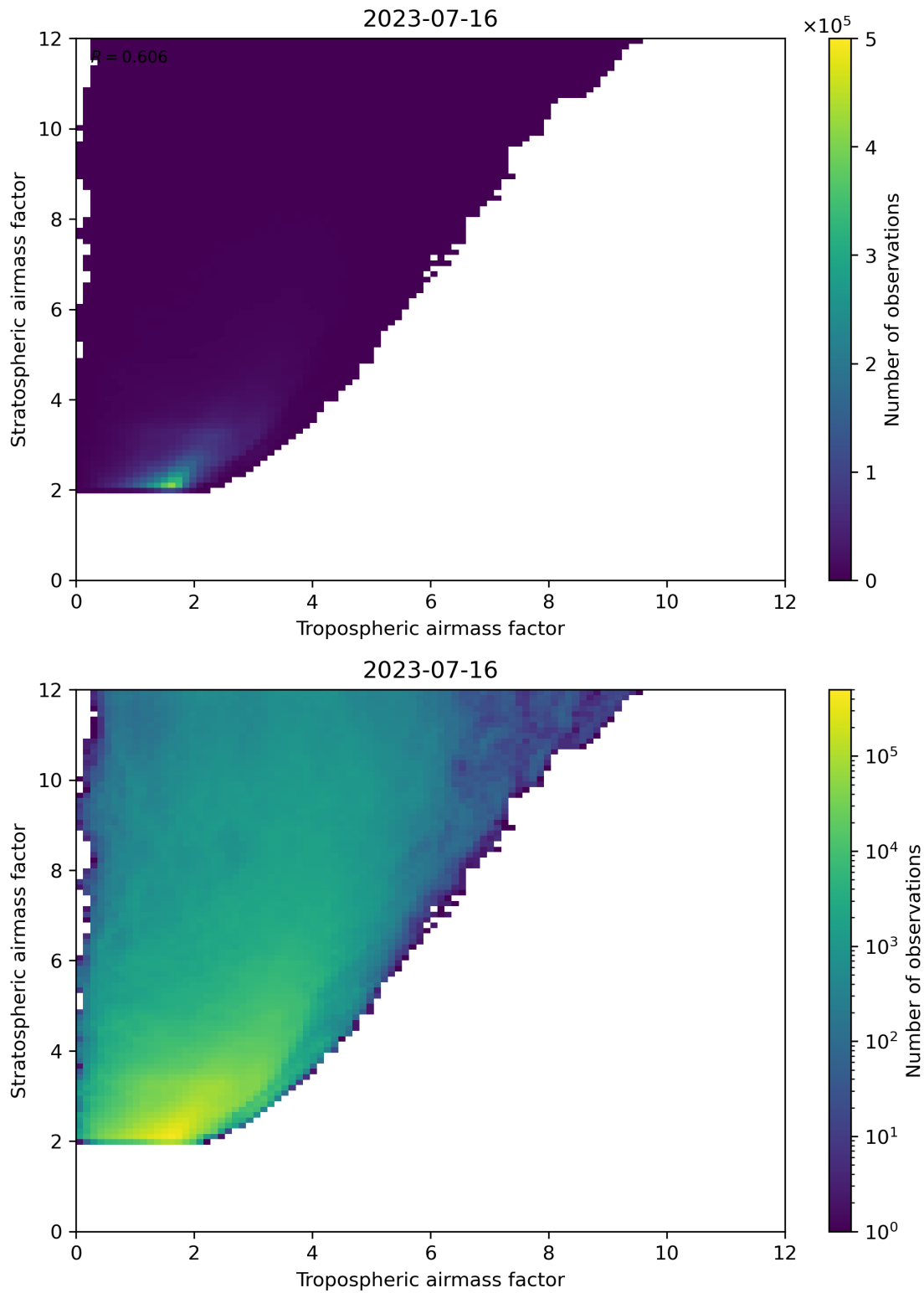
Figure 71: Scatter density plot of “Tropospheric airmass factor” against “Stratospheric airmass factor” for 2023-07-15 to 2023-07-17.
