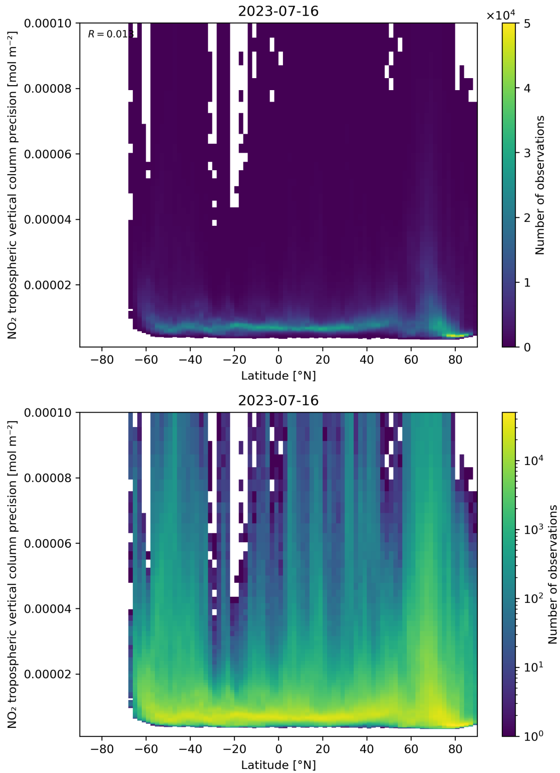
Figure 93: Scatter density plot of “Latitude” against “NO 2 tropospheric vertical column precision” for 2023-07-15 to 2023-07-17.
