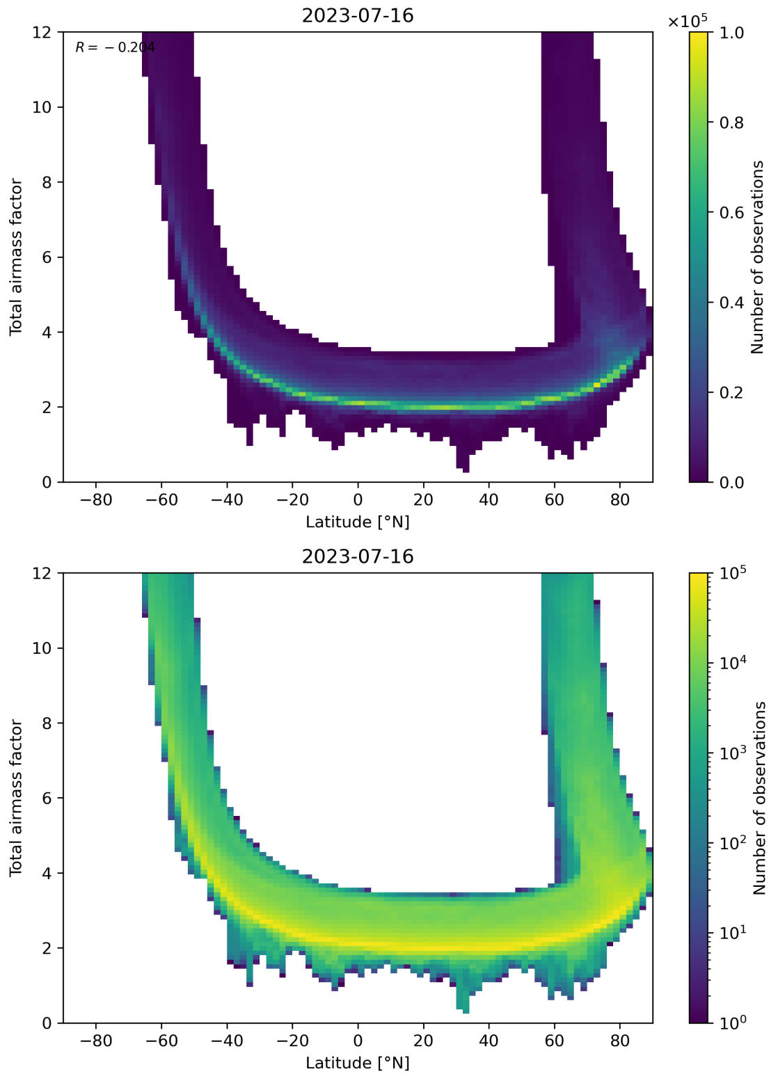
Figure 84: Scatter density plot of “Latitude” against “Total airmass factor” for 2023-07-15 to 2023-07-17.
