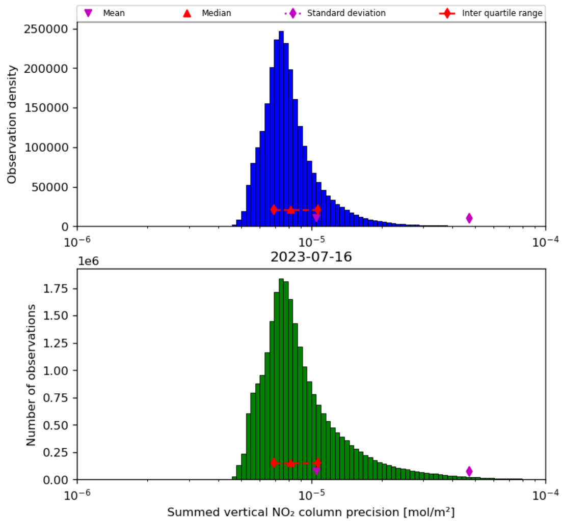
Figure 41: Histogram of "Summed vertical NO 2 column precision" for 2023-07-15 to 2023-07-17
