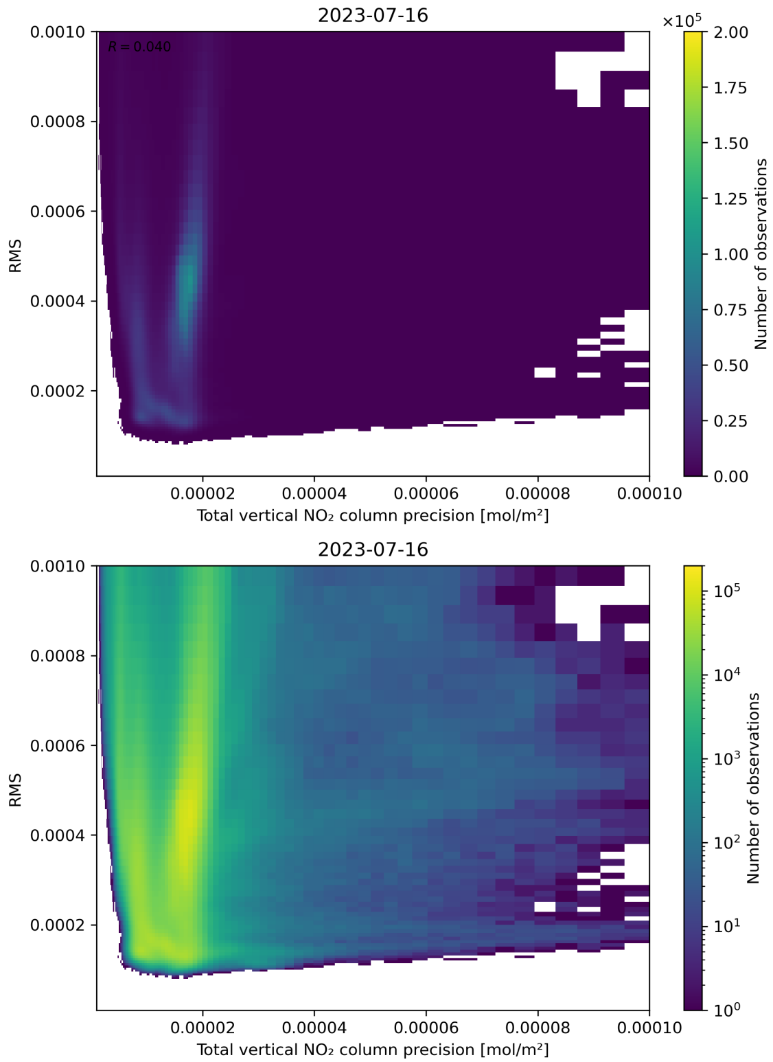
Figure 119: Scatter density plot of “Total vertical NO 2 column precision” against “RMS” for 2023-07-15 to 2023-07-17.
