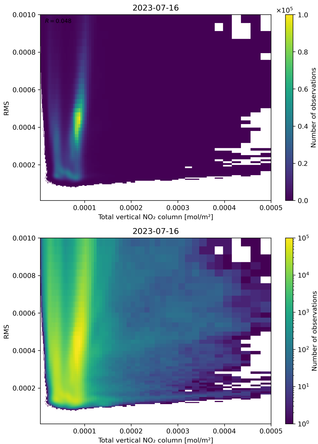
Figure 120: Scatter density plot of “Total vertical NO 2 column” against “RMS” for 2023-07-15 to 2023-07-17.
