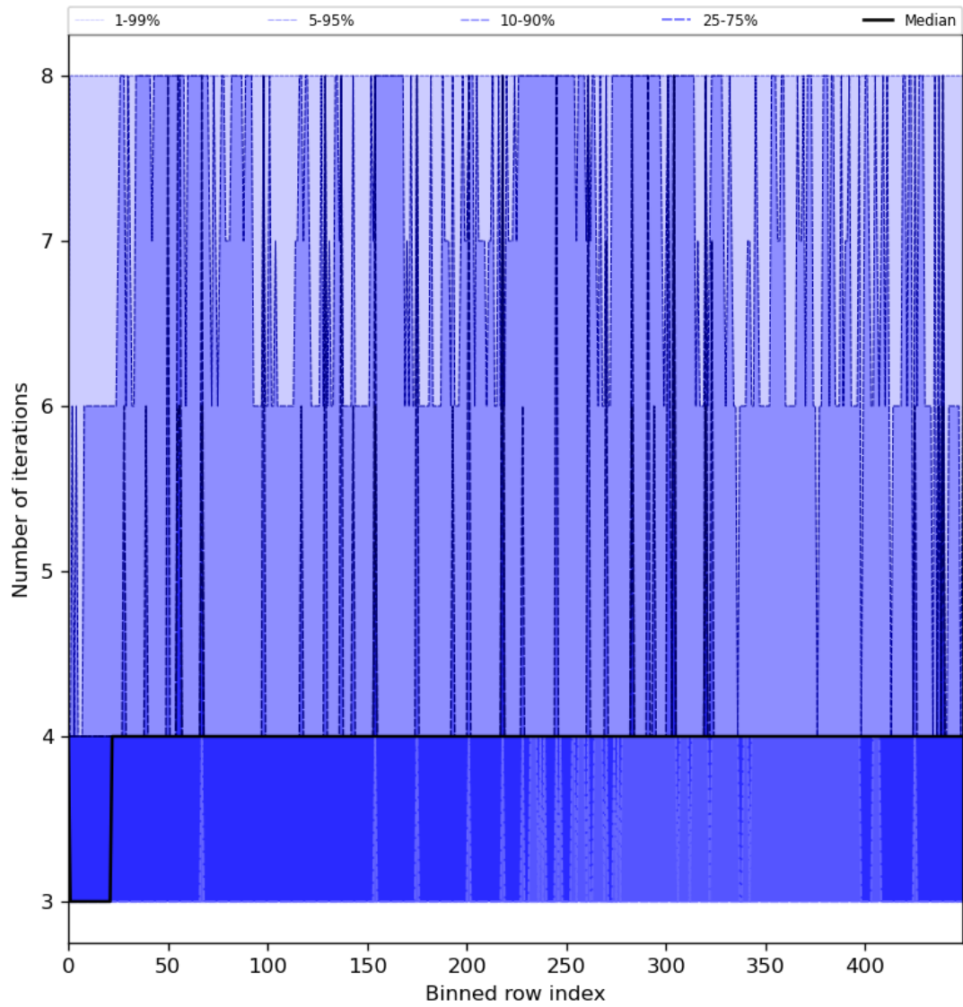
Figure 51: Along track statistics of “Number of iterations” for 2023-07-15 to 2023-07-17
