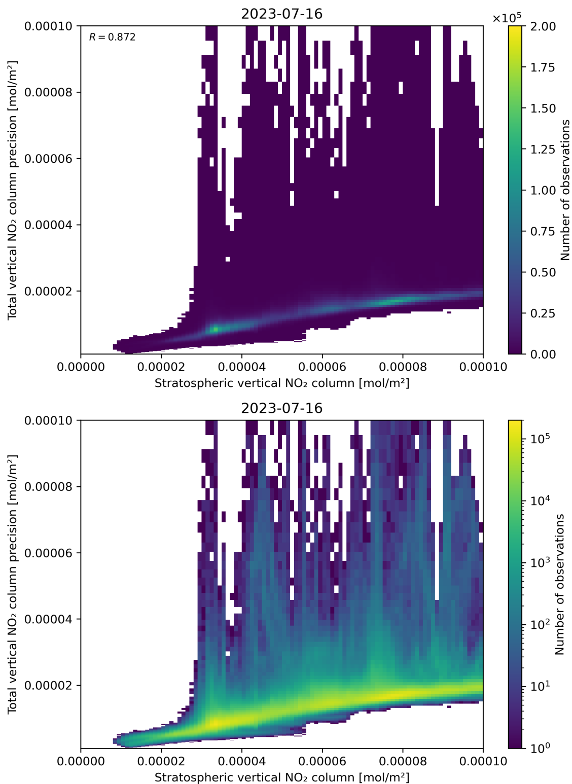
Figure 101: Scatter density plot of “Stratospheric vertical NO 2 column” against “Total vertical NO 2 column precision” for 2023-07-15 to 2023-07-17.
