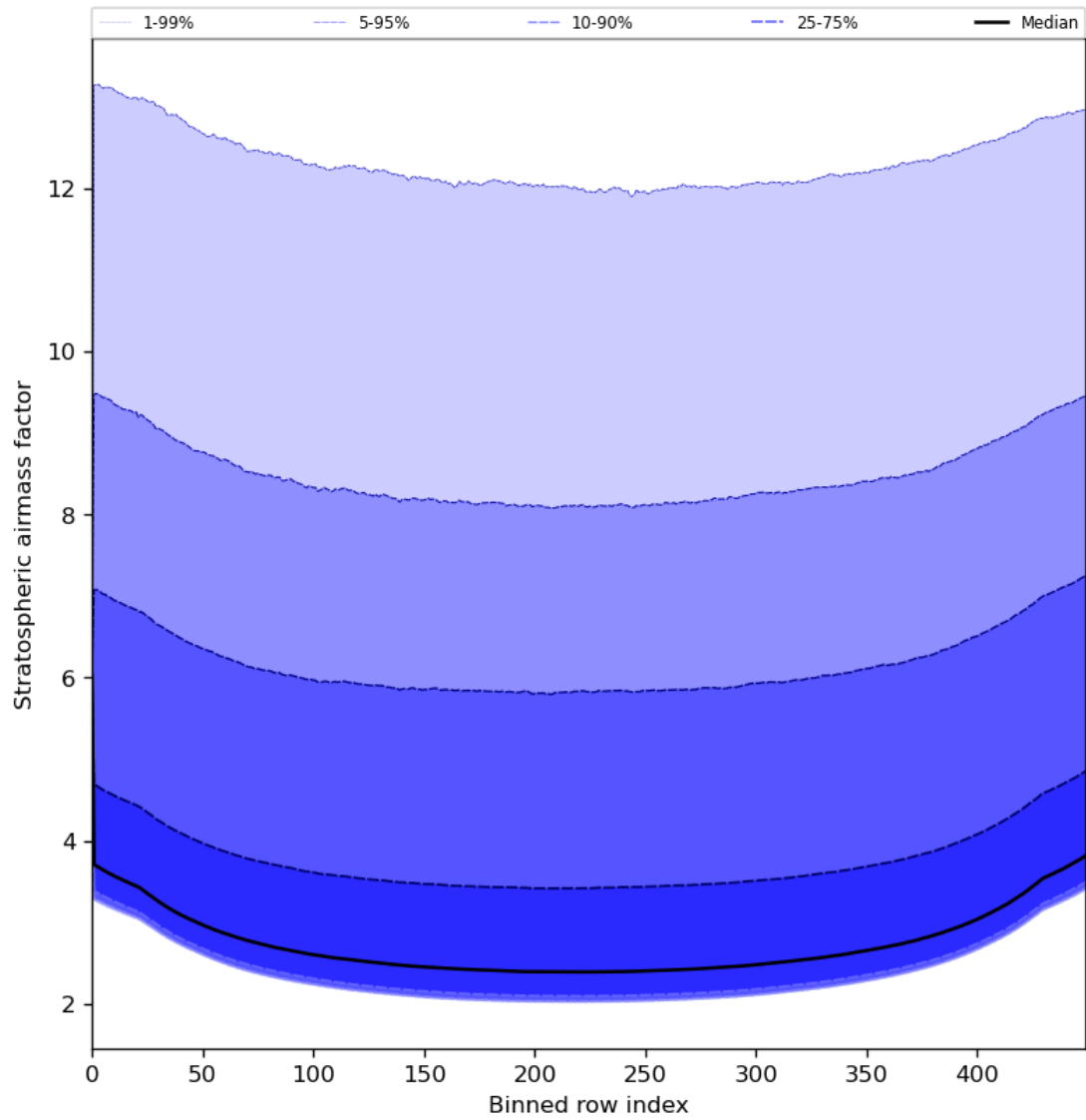
Figure 61: Along track statistics of “Stratospheric airmass factor” for 2023-07-15 to 2023-07-17
