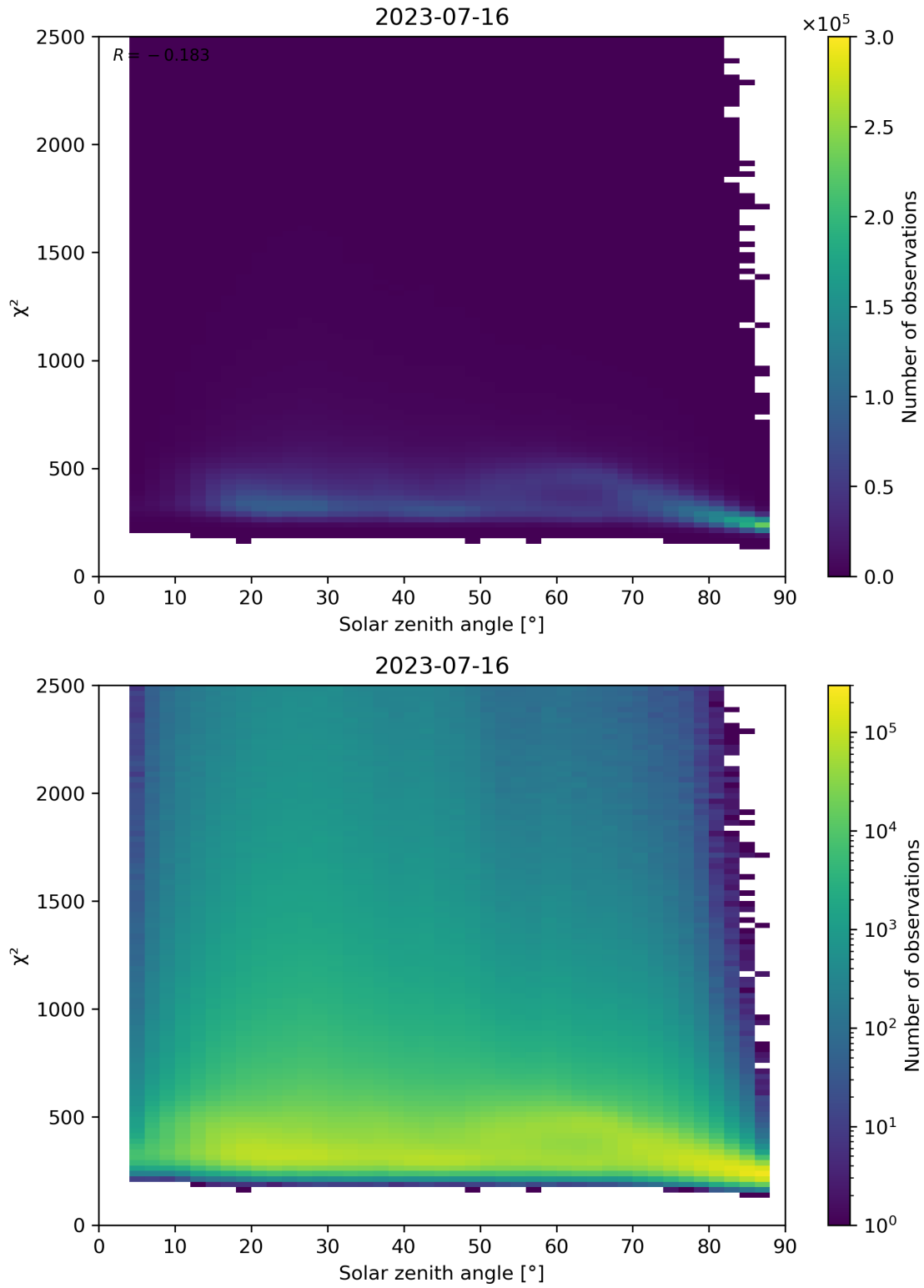
Figure 148: Scatter density plot of “Solar zenith angle” against “ \chi^2 ” for 2023-07-15 to 2023-07-17.
