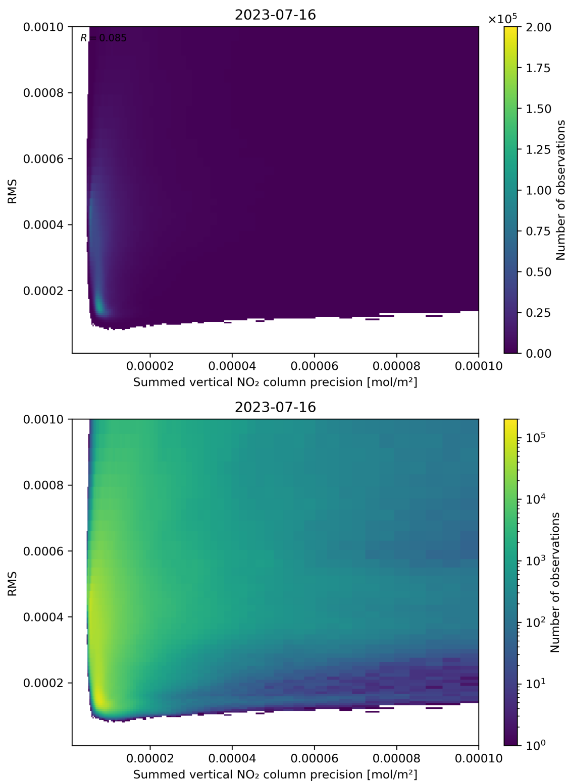
Figure 108: Scatter density plot of “Summed vertical NO 2 column precision” against “RMS” for 2023-07-15 to 2023-07-17.
