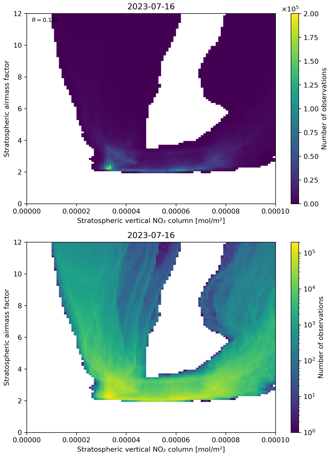
Figure 96: Scatter density plot of “Stratospheric vertical NO 2 column” against “Stratospheric airmass factor” for 2023-07-15 to 2023-07-17.
