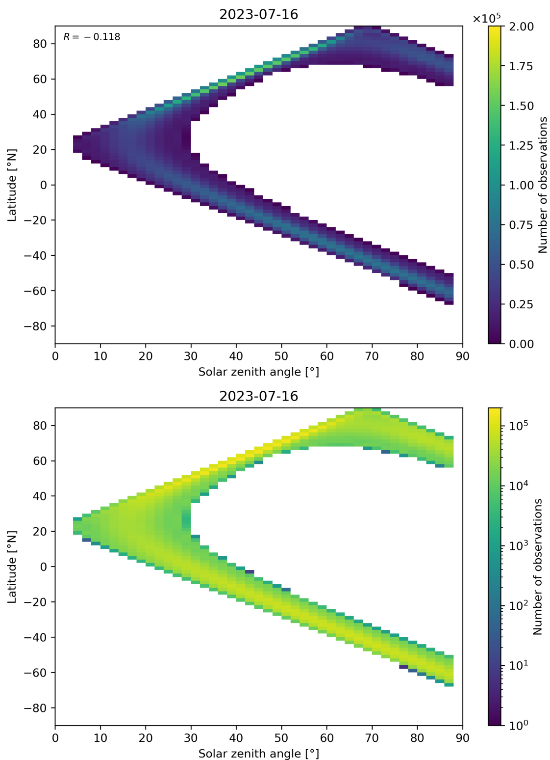
Figure 149: Scatter density plot of “Solar zenith angle” against “Latitude” for 2023-07-15 to 2023-07-17.
