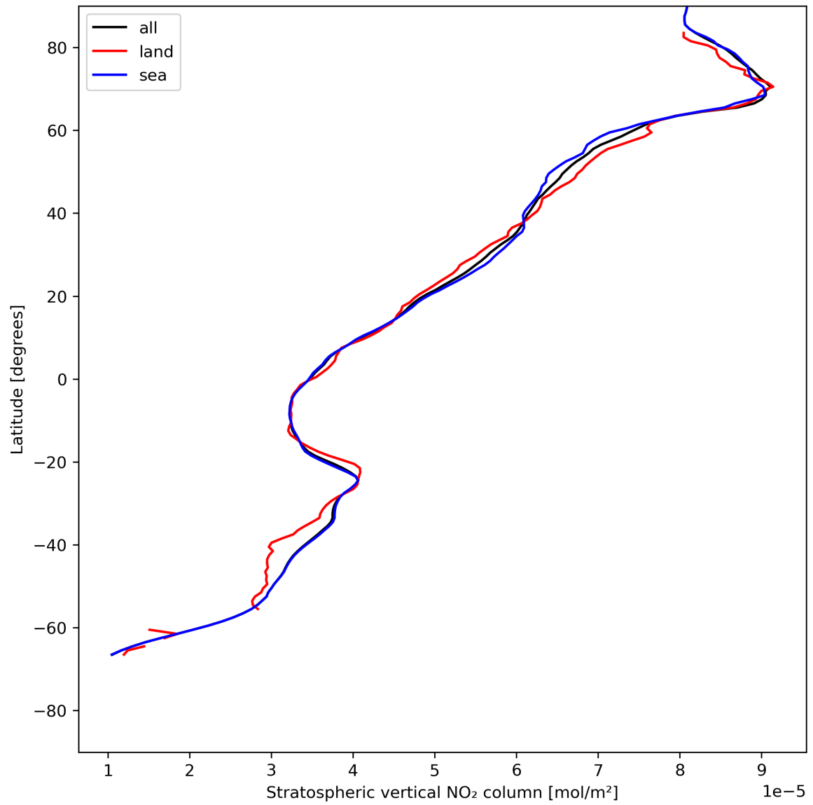
Figure 19: Zonal average of “Stratospheric vertical NO 2 column” for 2023-07-15 to 2023-07-17.
