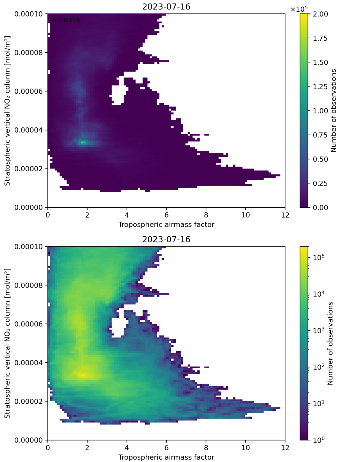
Figure 74: Scatter density plot of “Tropospheric air mass factor” against “Stratospheric vertical NO 2 column” for 2023-07-15 to 2023-07-17.
