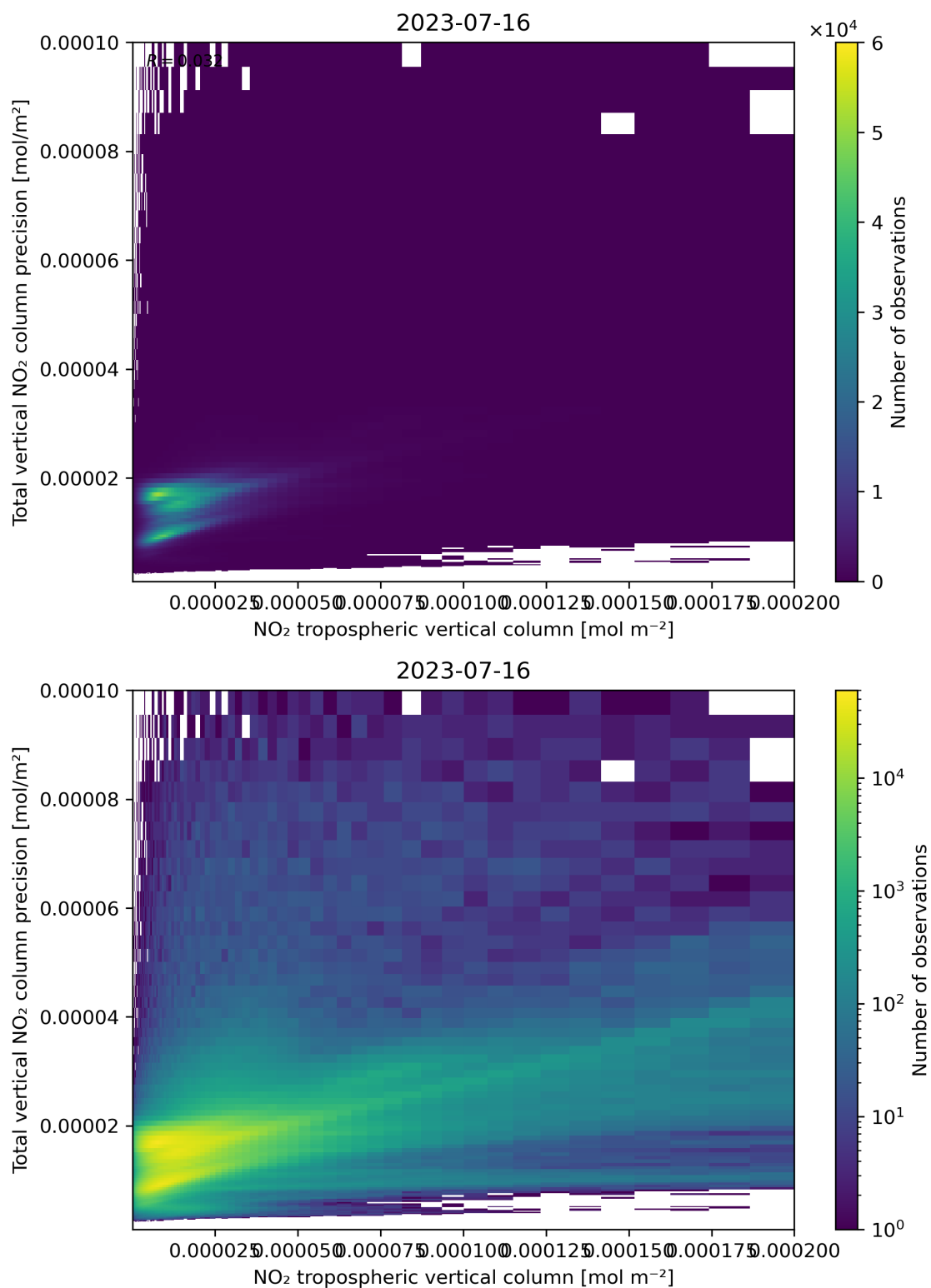
Figure 129: Scatter density plot of “NO 2 tropospheric vertical column” against “Total vertical NO 2 column precision” for 2023-07-15 to 2023-07-17.
