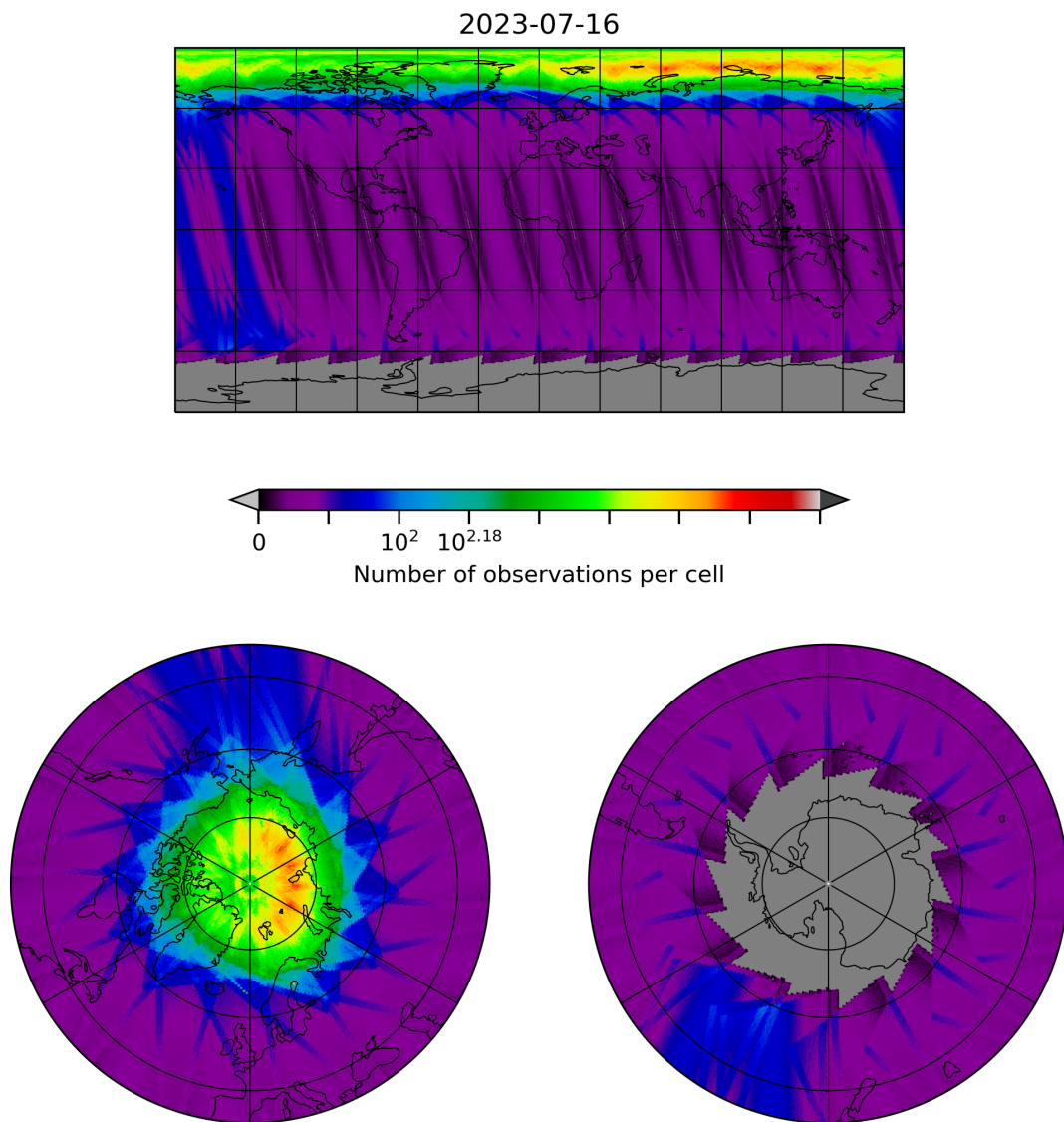
Figure 10: Map of the number of observations for 2023-07-15 to 2023-07-17
