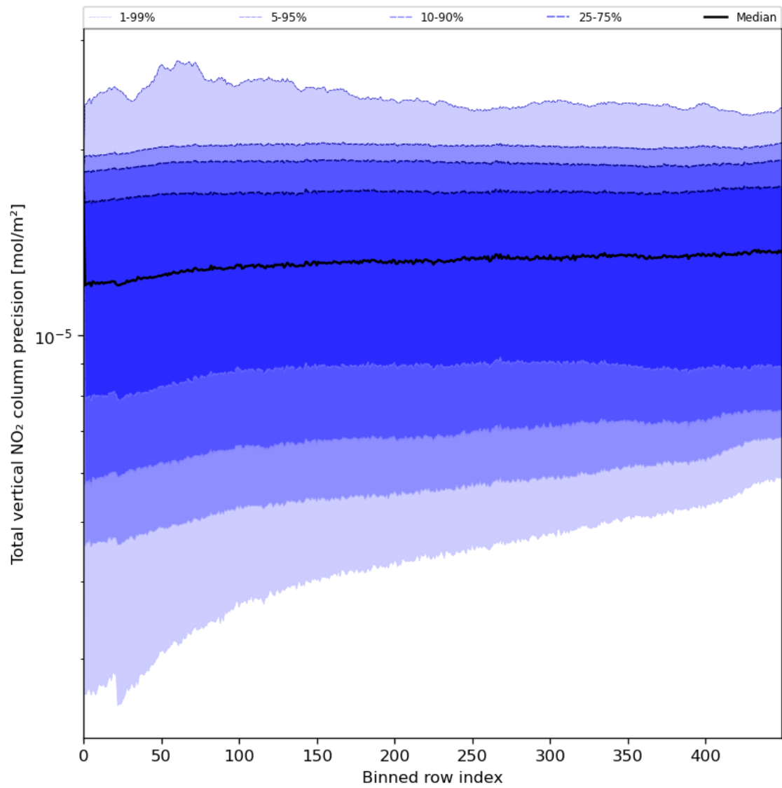
Figure 56: Along track statistics of “Total vertical NO 2 column precision” for 2023-07-15 to 2023-07-17
