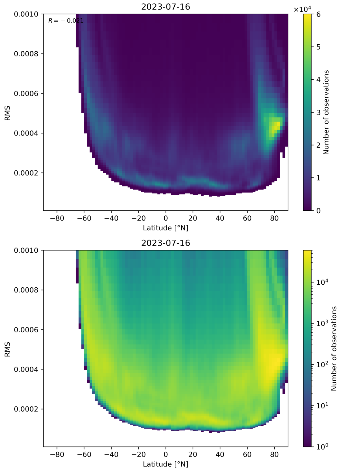
Figure 94: Scatter density plot of “Latitude” against “RMS” for 2023-07-15 to 2023-07-17.
