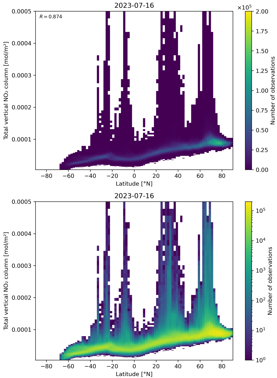
Figure 90: Scatter density plot of “Latitude” against “Total vertical NO 2 column” for 2023-07-15 to 2023-07-17.
