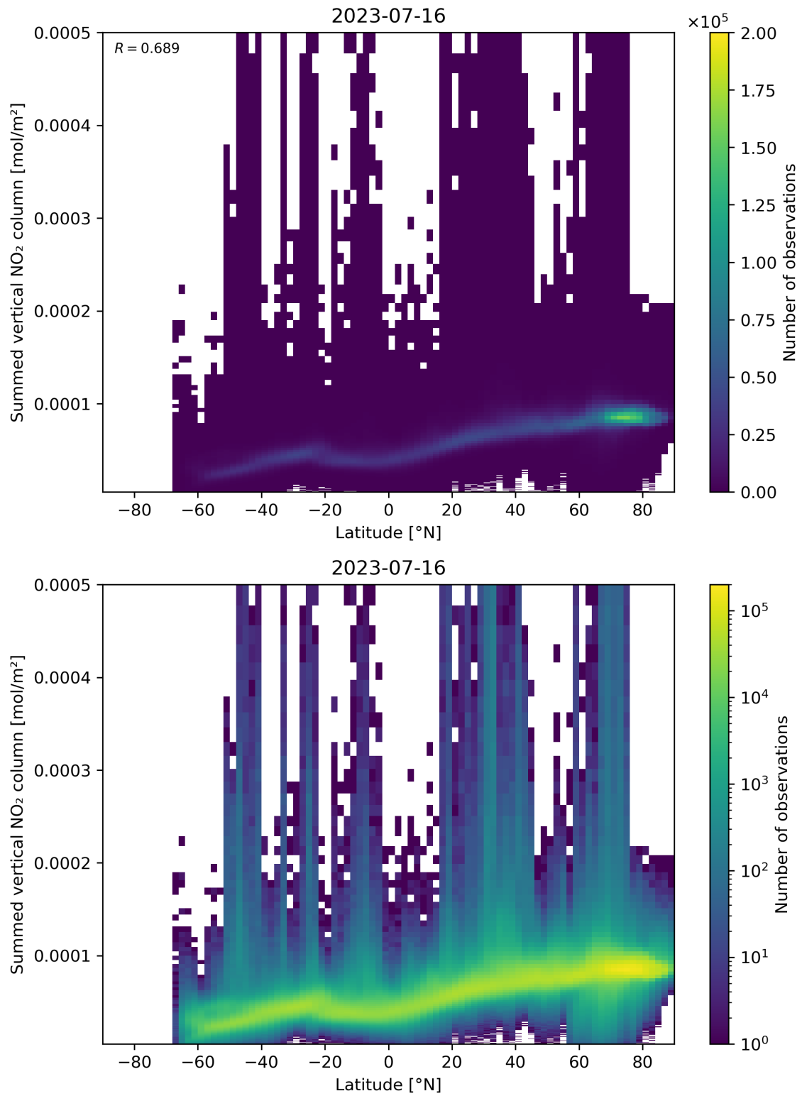
Figure 88: Scatter density plot of “Latitude” against “Summed vertical NO 2 column” for 2023-07-15 to 2023-07-17.
