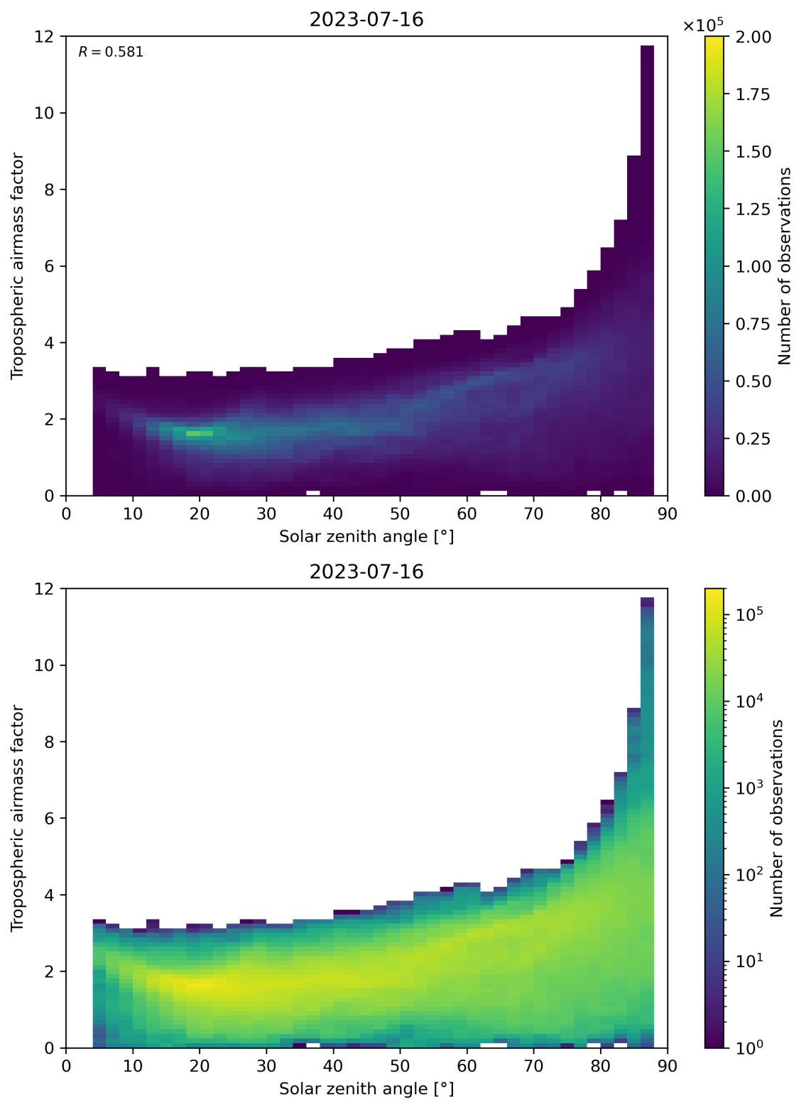
Figure 147: Scatter density plot of “Solar zenith angle” against “Tropospheric airmass factor” for 2023-07-15 to 2023-07-17.
