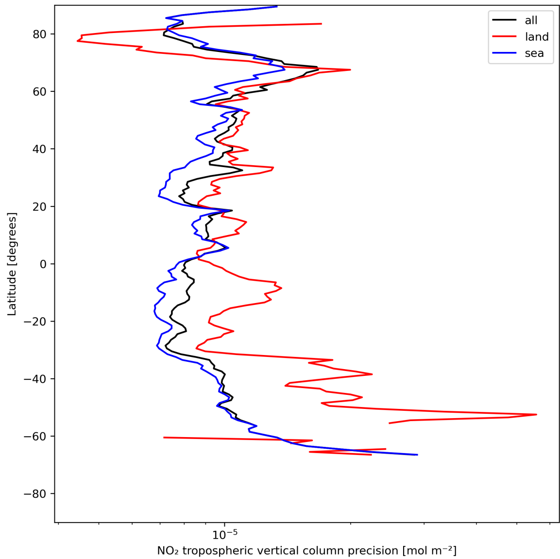
Figure 13: Zonal average of "NO 2 tropospheric vertical column precision" for 2023-07-15 to 2023-07-17.
