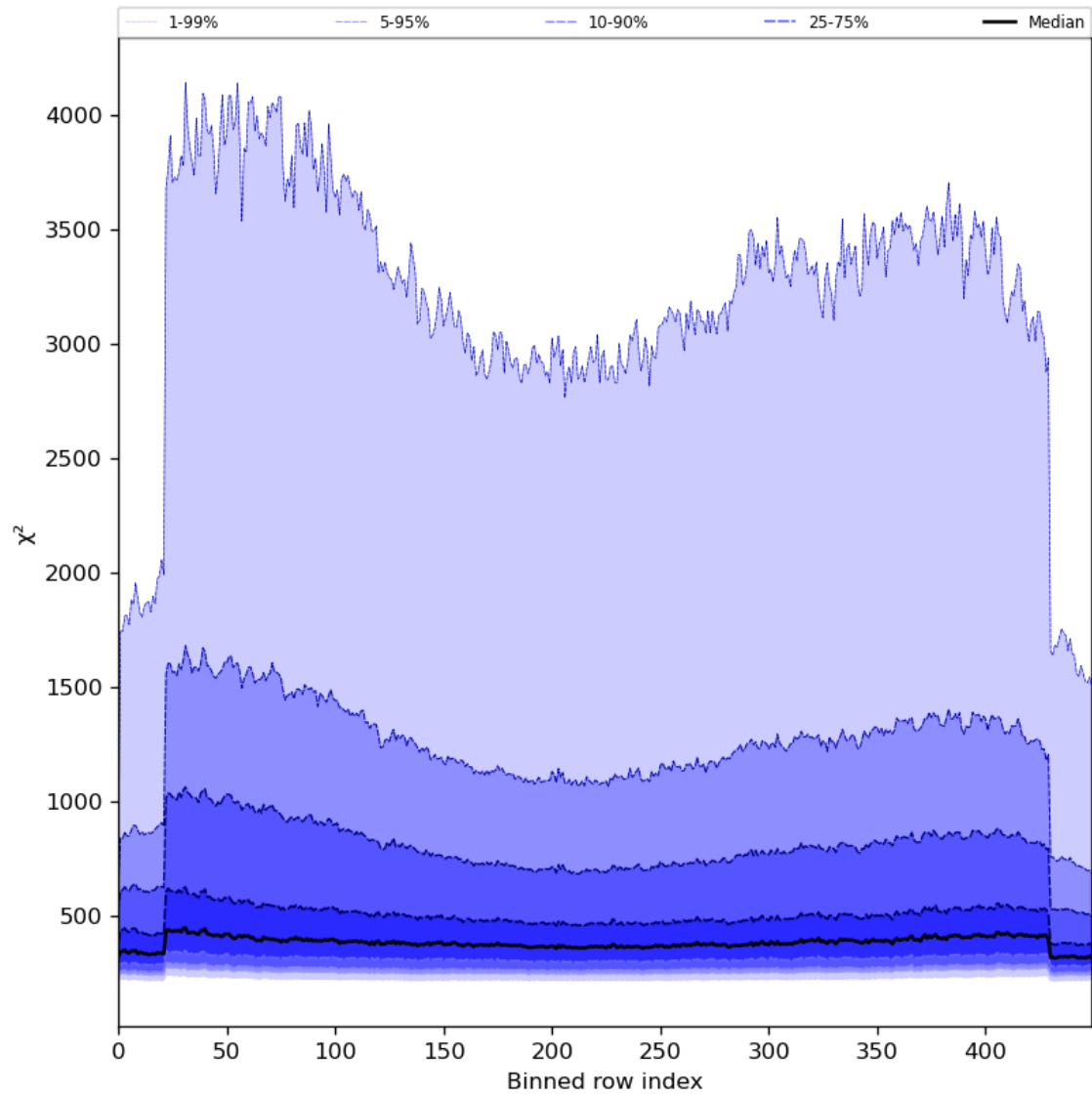
Figure 59: Along track statistics of “ \chi^2 ” for 2023-07-15 to 2023-07-17
