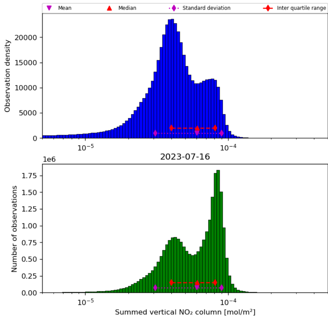
Figure 40: Histogram of “Summed vertical NO 2 column” for 2023-07-15 to 2023-07-17
