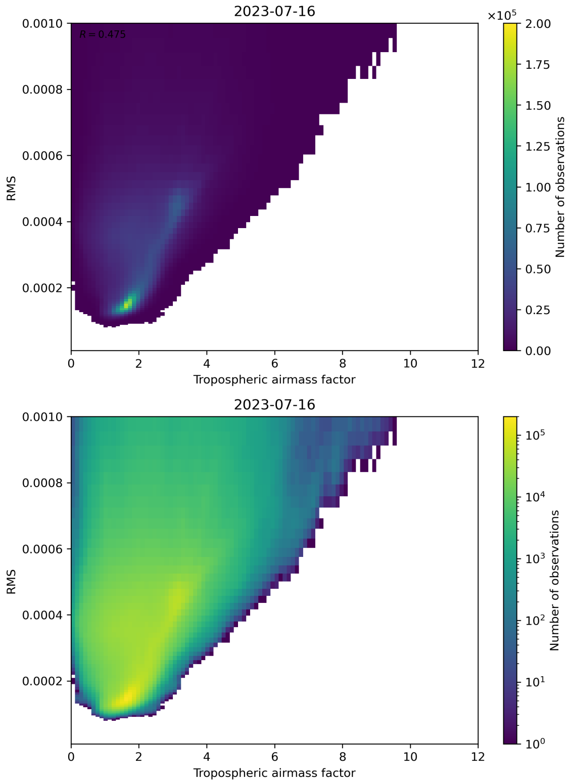
Figure 79: Scatter density plot of “Tropospheric airmass factor” against “RMS” for 2023-07-15 to 2023-07-17.
