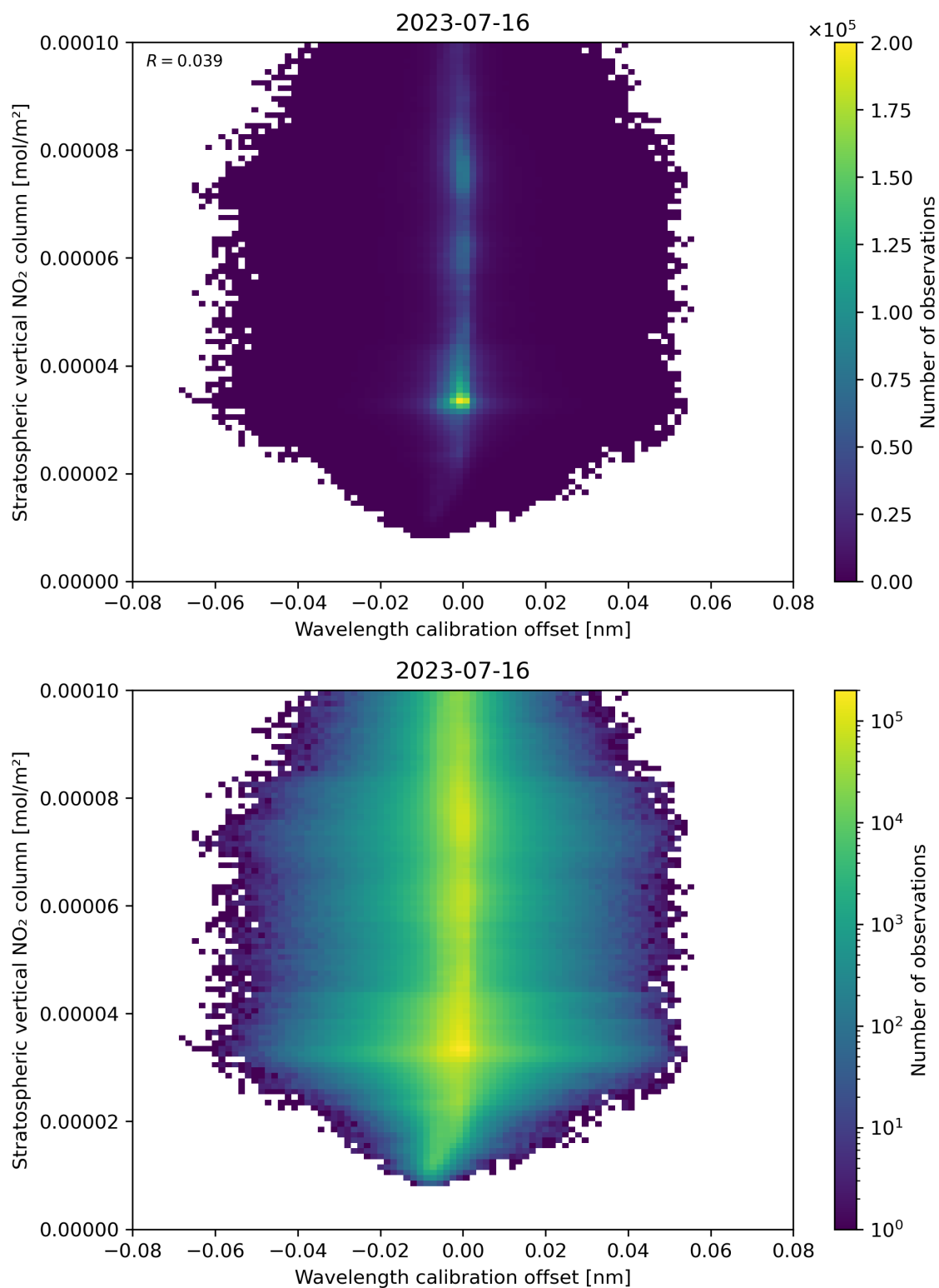
Figure 176: Scatter density plot of “Wavelength calibration offset” against “Stratospheric vertical NO 2 column” for 2023-07-15 to 2023-07-17.
