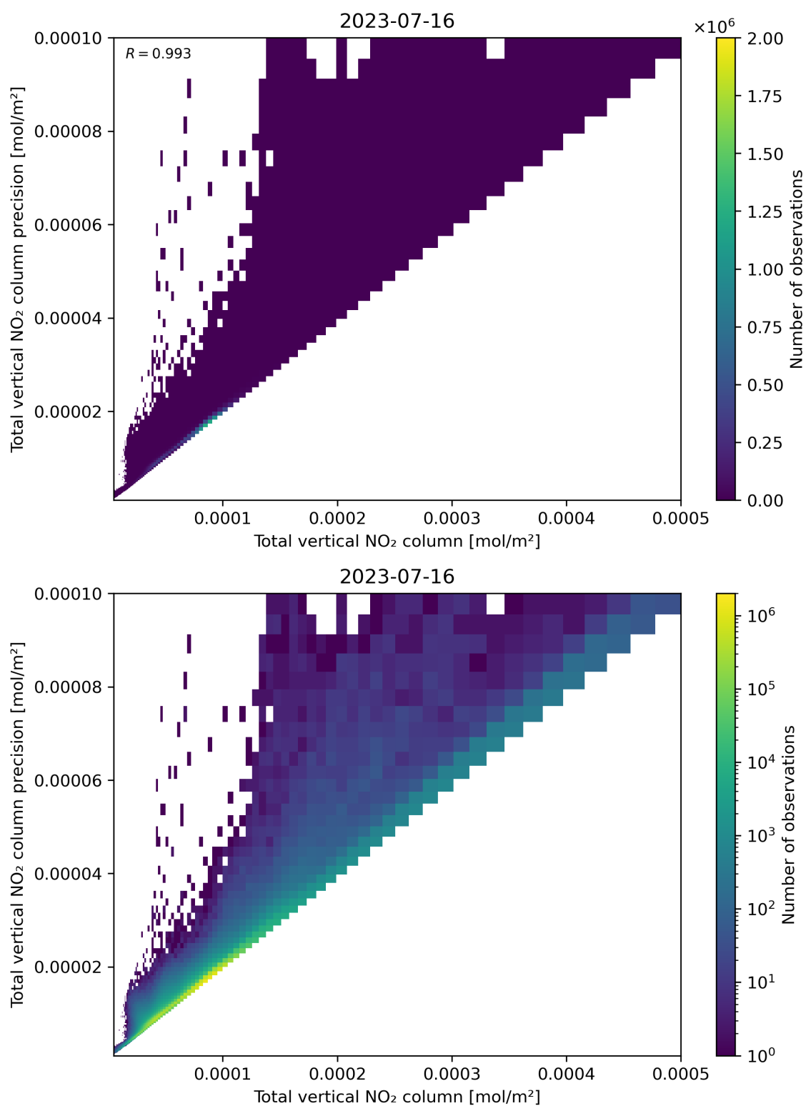
Figure 114: Scatter density plot of “Total vertical NO 2 column” against “Total vertical NO 2 column precision” for 2023-07-15 to 2023-07-17.
