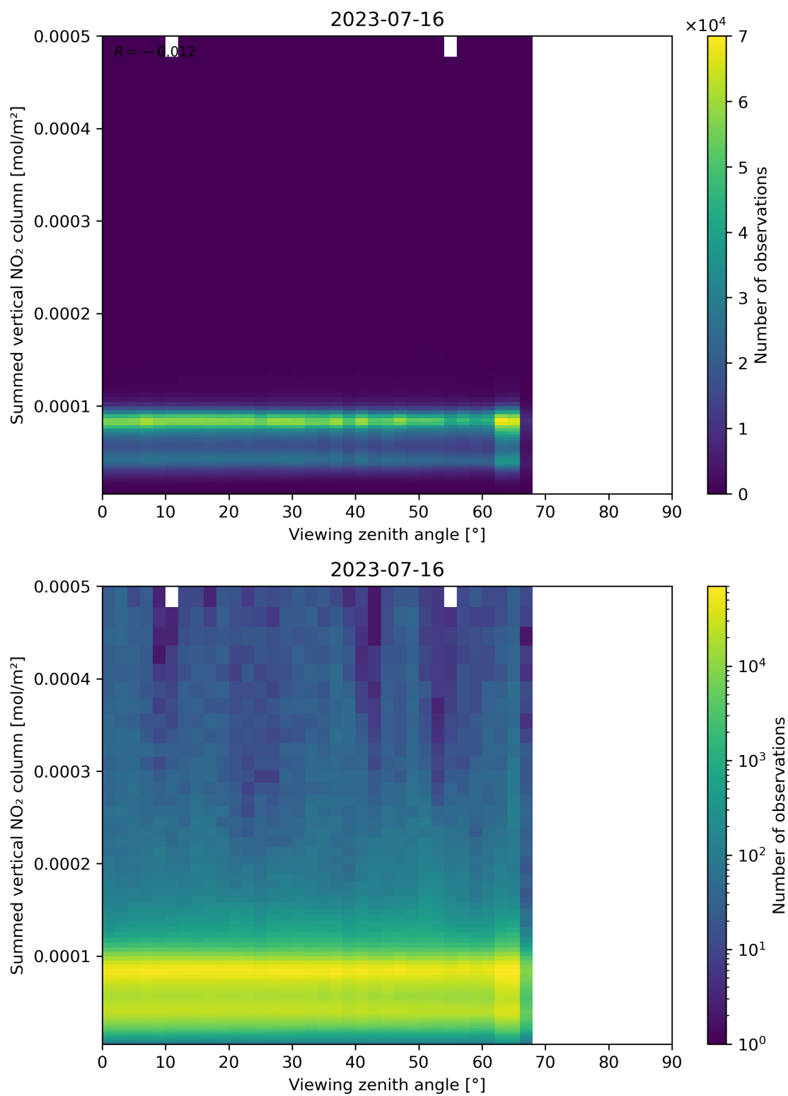
Figure 165: Scatter density plot of “Viewing zenith angle” against “Summed vertical NO 2 column” for 2023-07-15 to 2023-07-17.
