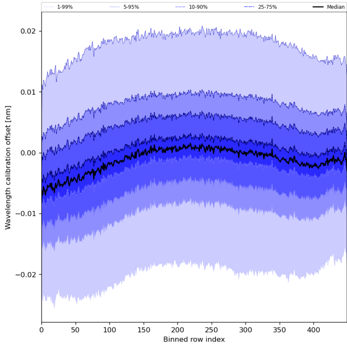
Figure 52: Along track statistics of “Wavelength calibration offset” for 2023-07-15 to 2023-07-17
