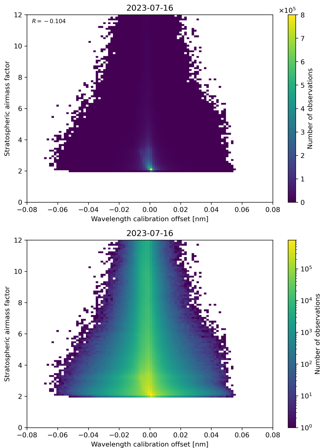
Figure 174: Scatter density plot of “Wavelength calibration offset” against “Stratospheric airmass factor” for 2023-07-15 to 2023-07-17.
