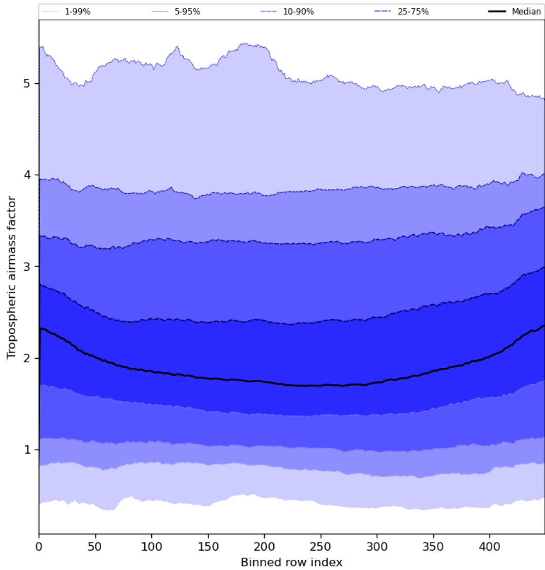
Figure 48: Along track statistics of “Tropospheric airmass factor” for 2023-07-15 to 2023-07-17
