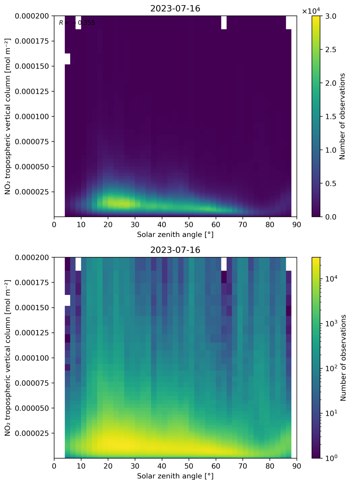
Figure 155: Scatter density plot of “Solar zenith angle” against “NO 2 tropospheric vertical column” for 2023-07-15 to 2023-07-17.
