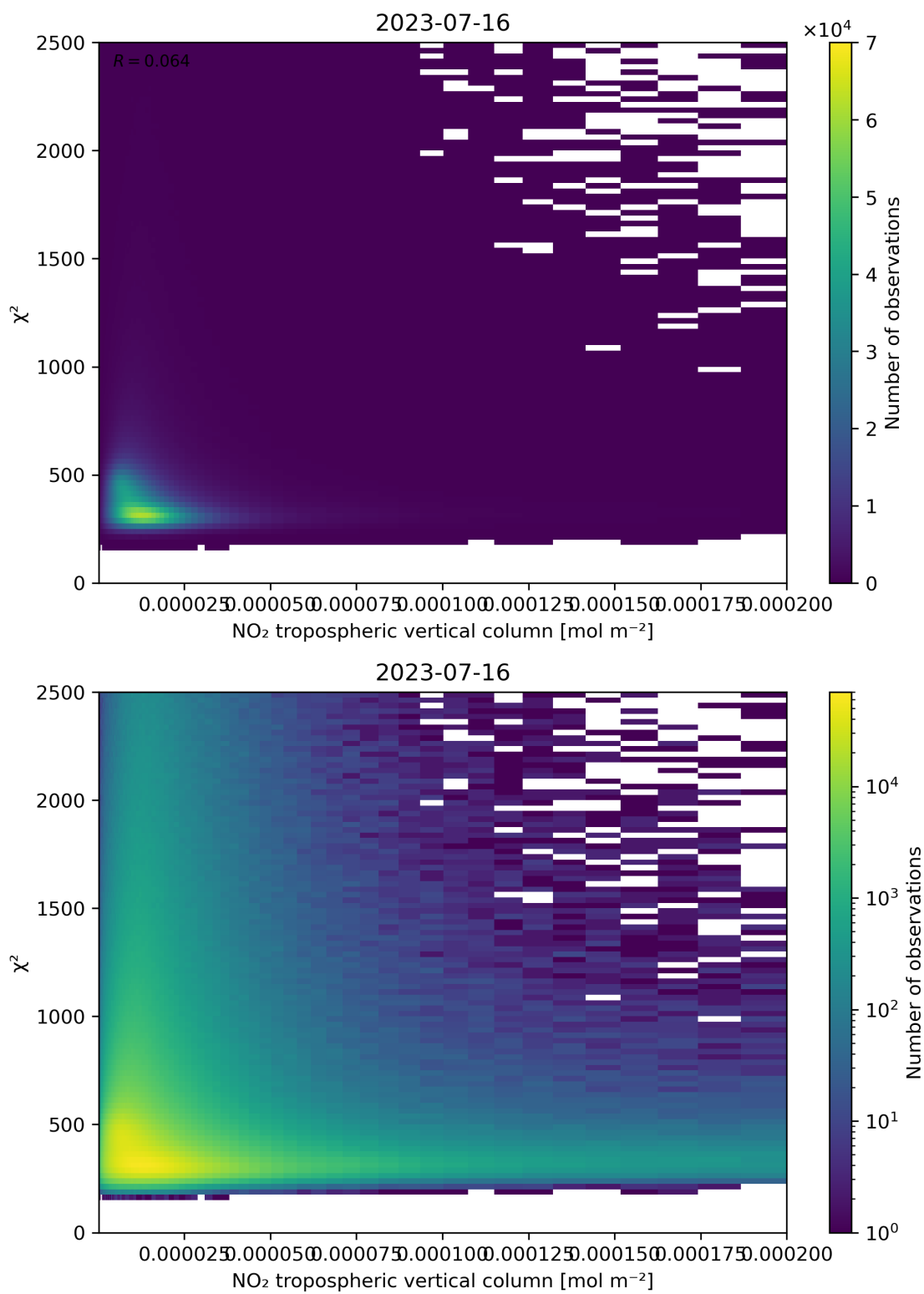
Figure 124: Scatter density plot of “NO 2 tropospheric vertical column” against “ \chi^2 ” for 2023-07-15 to 2023-07-17.
