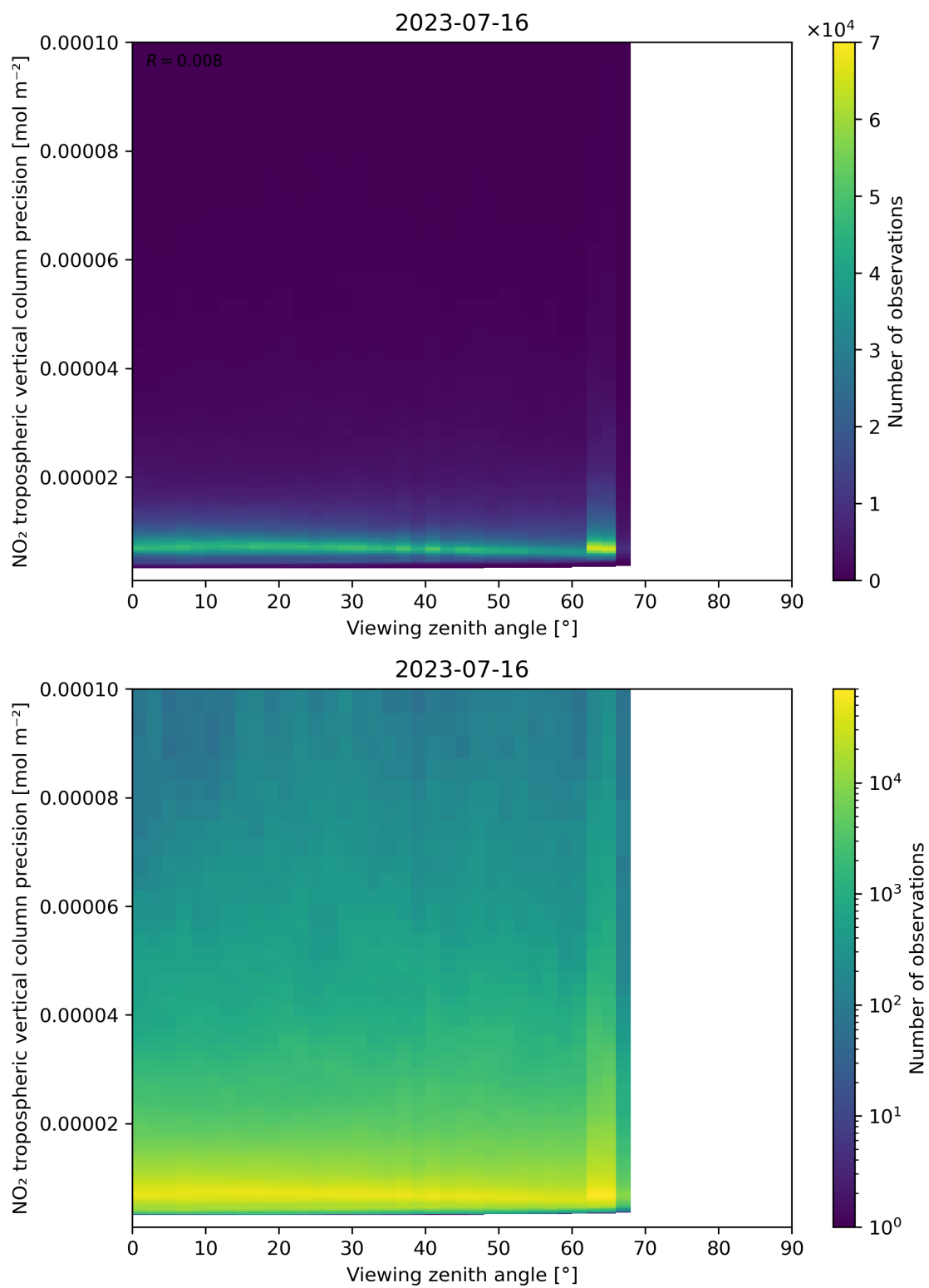
Figure 170: Scatter density plot of “Viewing zenith angle” against “NO 2 tropospheric vertical column precision” for 2023-07-15 to 2023-07-17.
