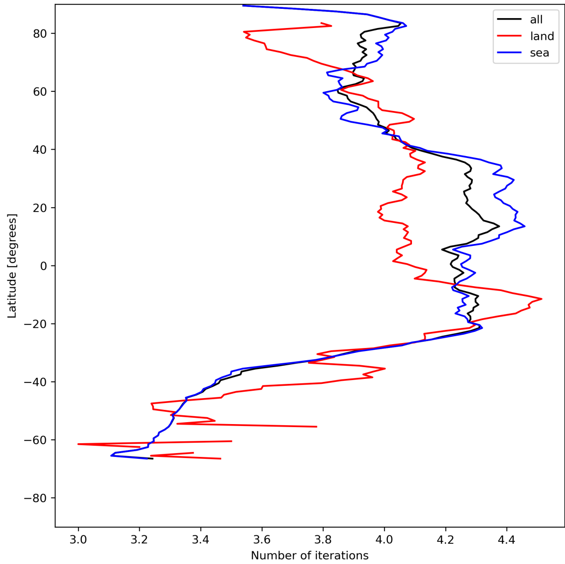
Figure 17: Zonal average of “Number of iterations” for 2023-07-15 to 2023-07-17.
