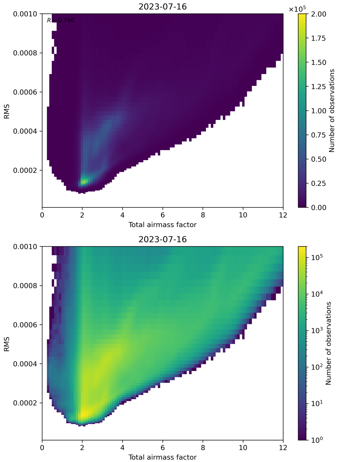
Figure 69: Scatter density plot of “Total airmass factor” against “RMS” for 2023-07-15 to 2023-07-17.
