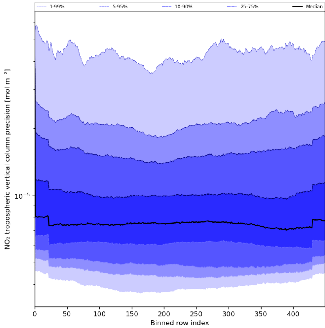
Figure 47: Along track statistics of “NO 2 tropospheric vertical column precision” for 2023-07-15 to 2023-07-17
