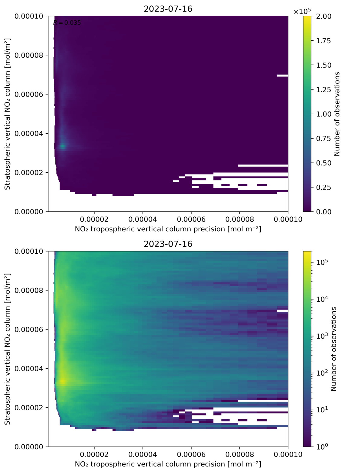
Figure 135: Scatter density plot of “NO 2 tropospheric vertical column precision” against “Stratospheric vertical NO 2 column” for 2023-07-15 to 2023-07-17.
