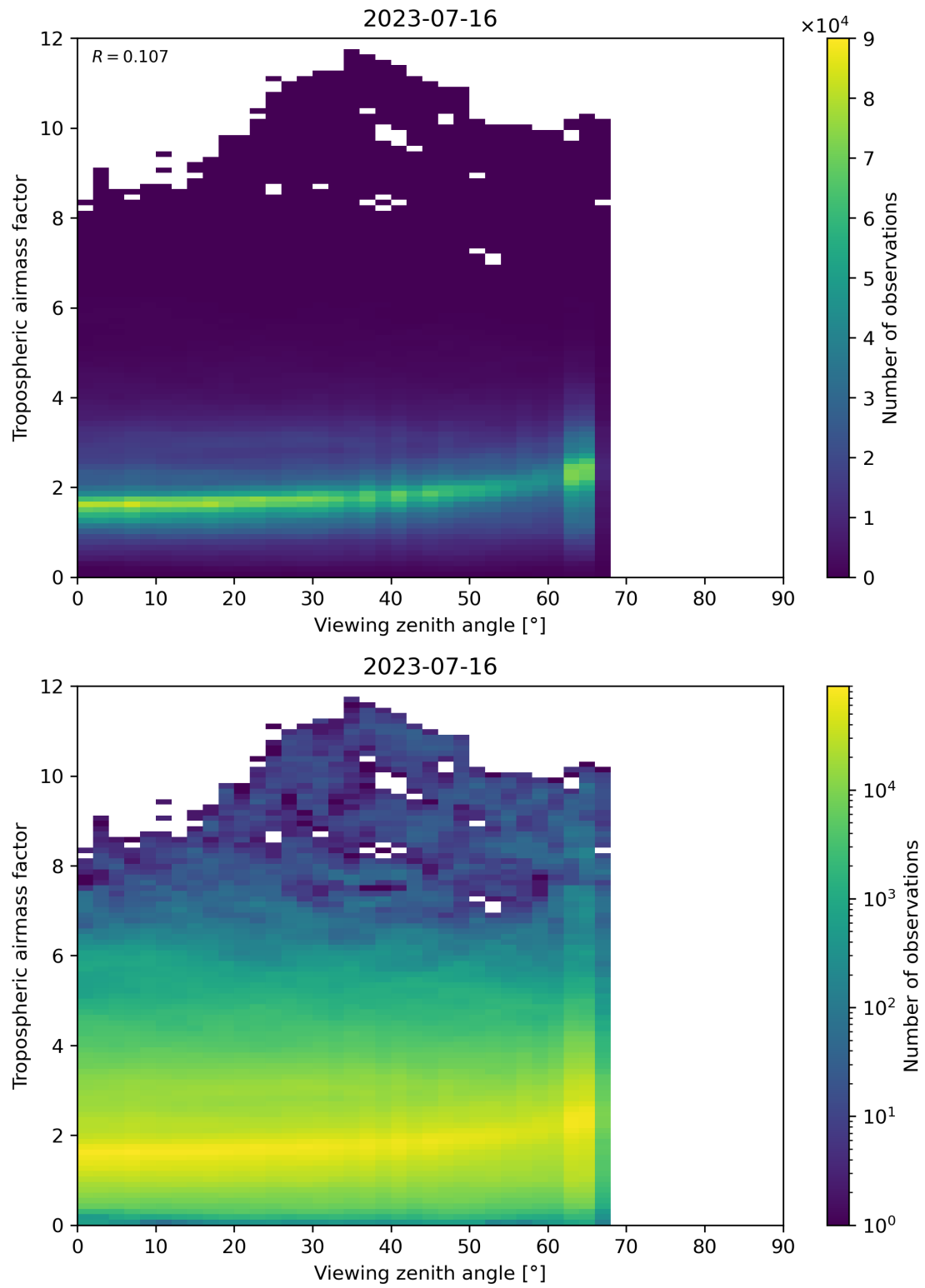
Figure 161: Scatter density plot of “Viewing zenith angle” against “Tropospheric airmass factor” for 2023-07-15 to 2023-07-17.
