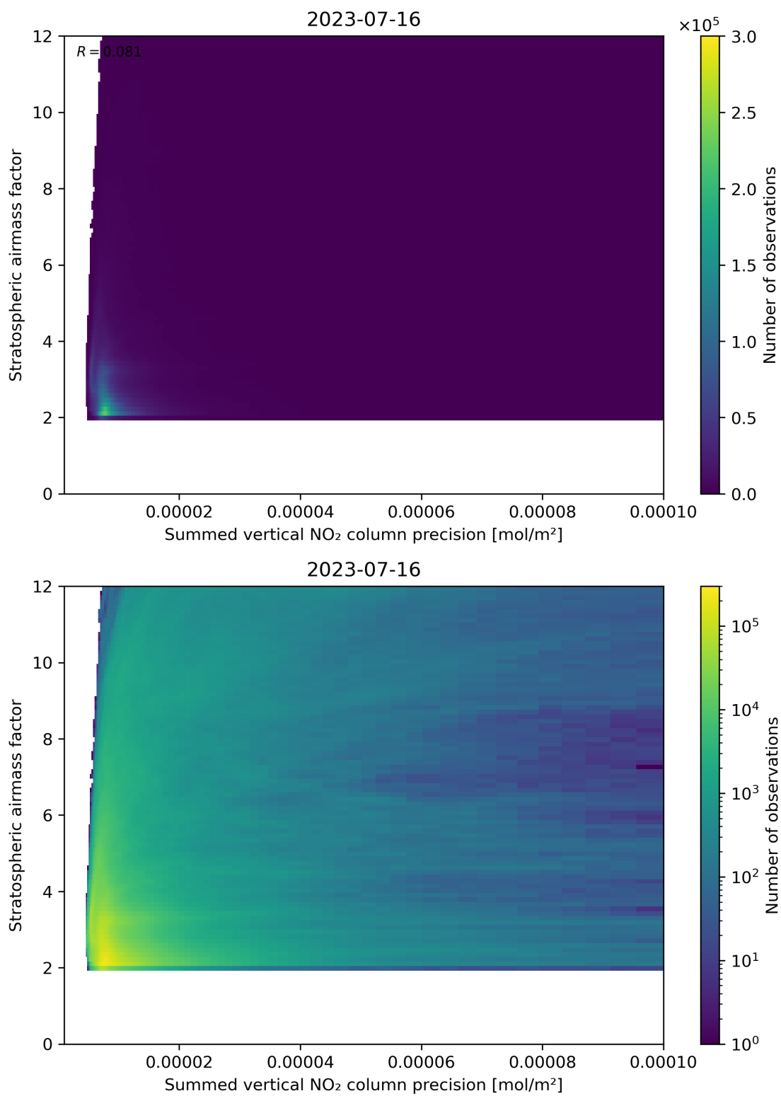
Figure 106: Scatter density plot of “Summed vertical NO 2 column precision” against “Stratospheric airmass factor” for 2023-07-15 to 2023-07-17.
