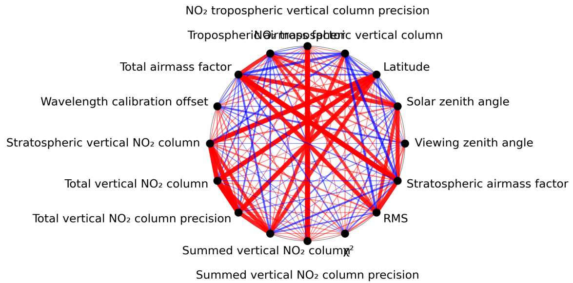
Figure 1: Map of correlation graph for 2023-07-15 to 2023-07-17.
