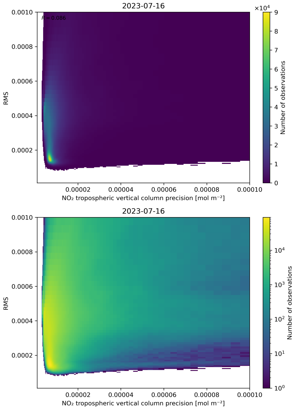
Figure 140: Scatter density plot of “NO 2 tropospheric vertical column precision” against “RMS” for 2023-07-15 to 2023-07-17.
