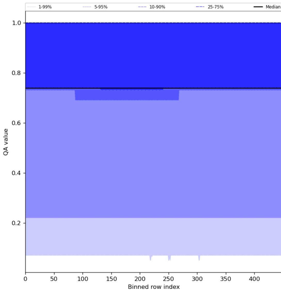
Figure 45: Along track statistics of “QA value” for 2023-07-15 to 2023-07-17
