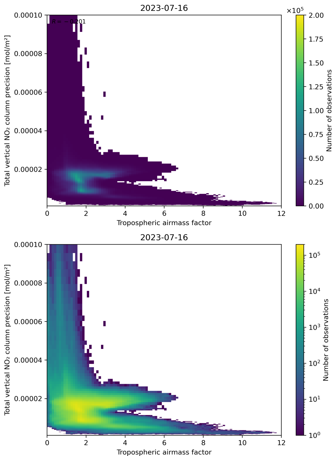
Figure 78: Scatter density plot of “Tropospheric air mass factor” against “Total vertical NO 2 column precision” for 2023-07-15 to 2023-07-17.
