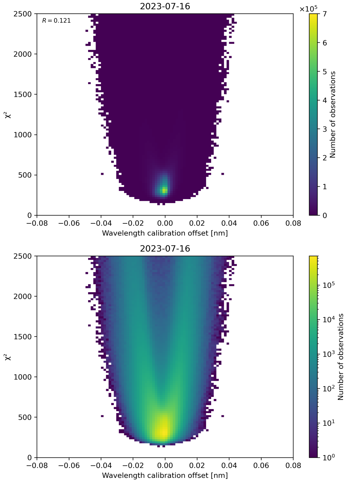
Figure 175: Scatter density plot of “Wavelength calibration offset” against “ \chi^2 ” for 2023-07-15 to 2023-07-17.
