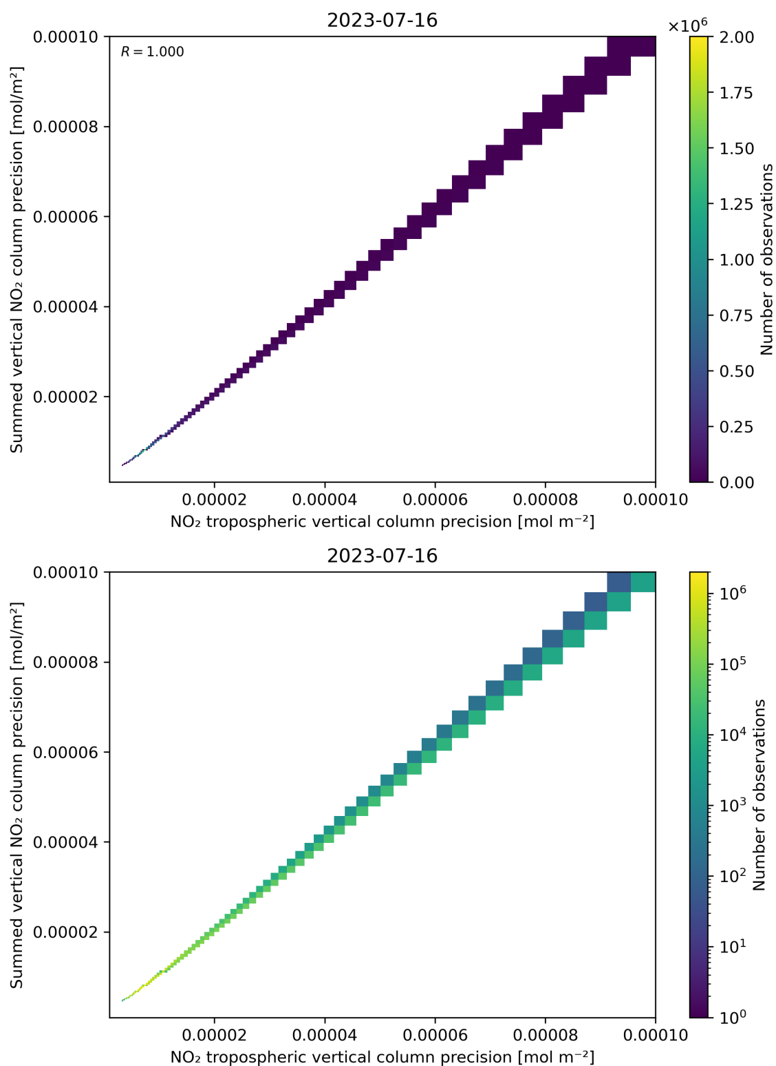
Figure 137: Scatter density plot of “NO 2 tropospheric vertical column precision” against “Summed vertical NO 2 column precision” for 2023-07-15 to 2023-07-17.
