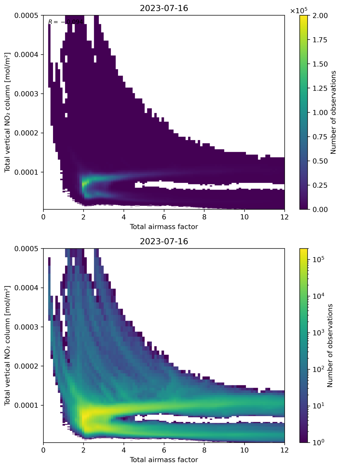
Figure 67: Scatter density plot of “Total airmass factor” against “Total vertical NO 2 column” for 2023-07-15 to 2023-07-17.
