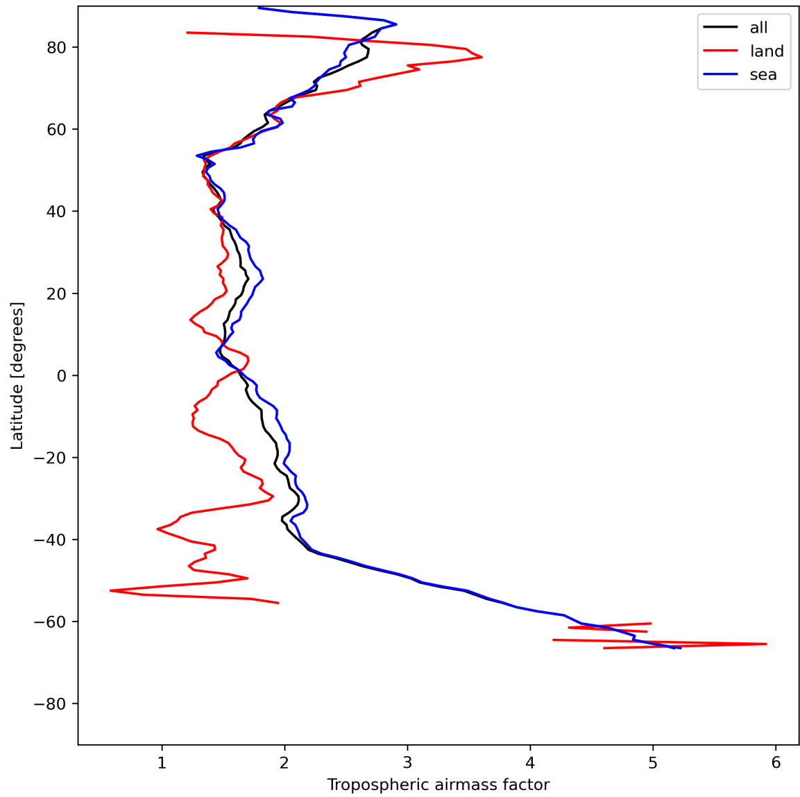
Figure 14: Zonal average of “Tropospheric airmass factor” for 2023-07-15 to 2023-07-17.
