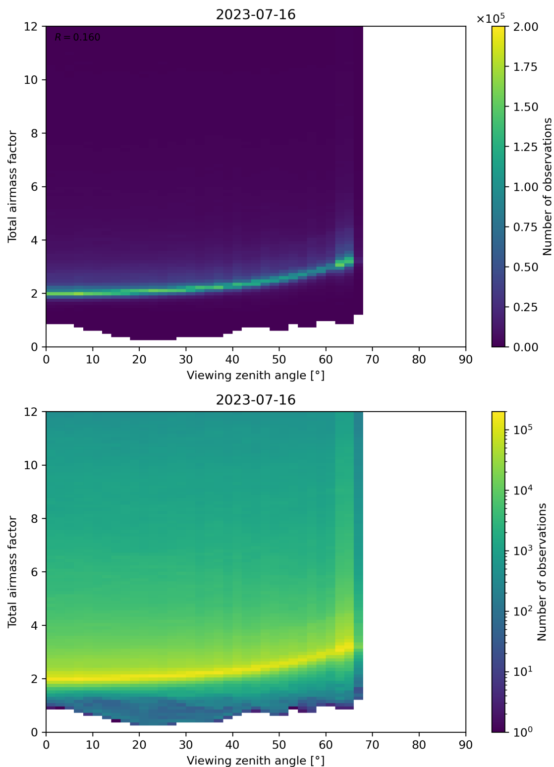
Figure 160: Scatter density plot of “Viewing zenith angle” against “Total airmass factor” for 2023-07-15 to 2023-07-17.
