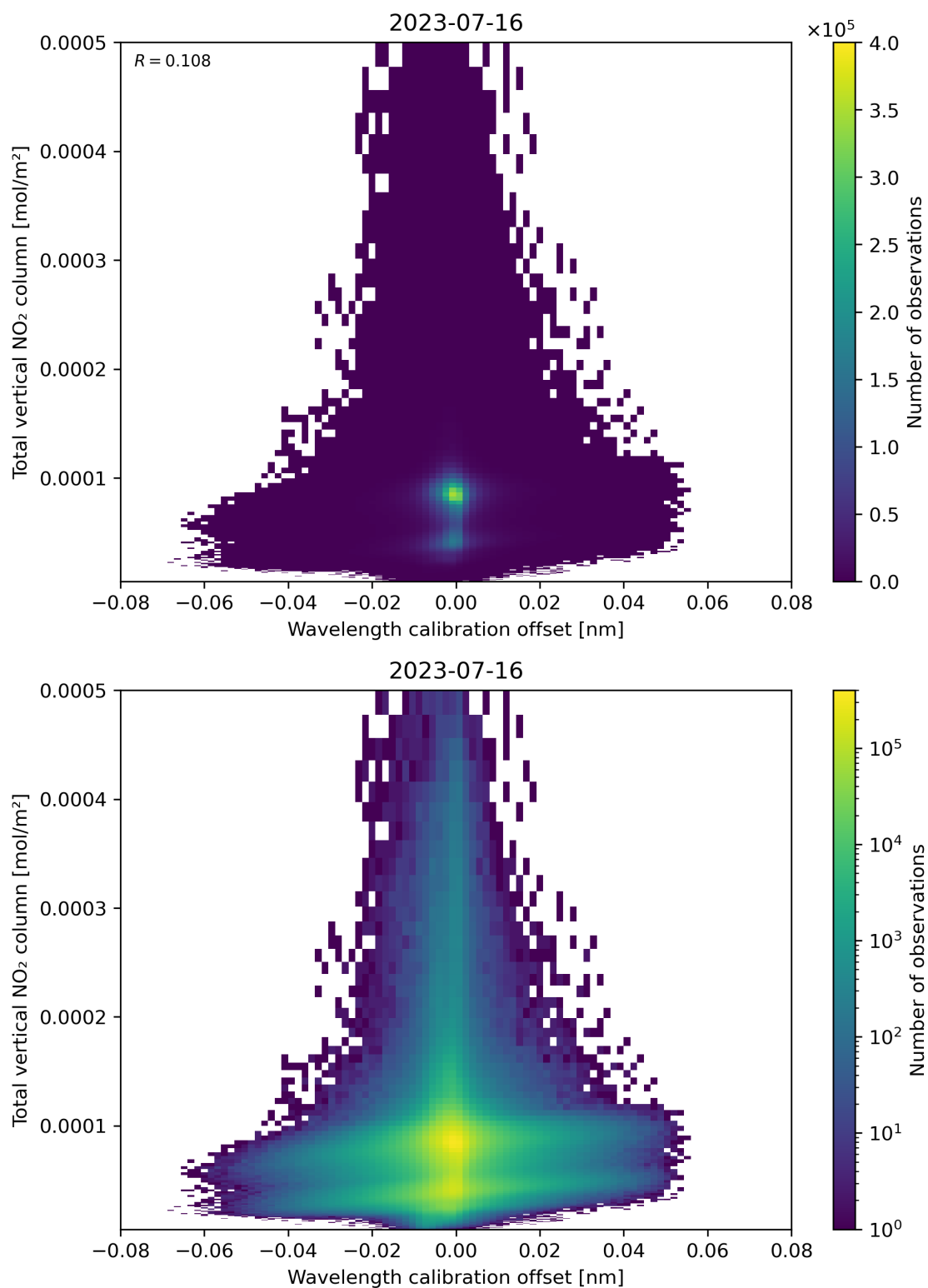
Figure 179: Scatter density plot of “Wavelength calibration offset” against “Total vertical NO 2 column” for 2023-07-15 to 2023-07-17.
