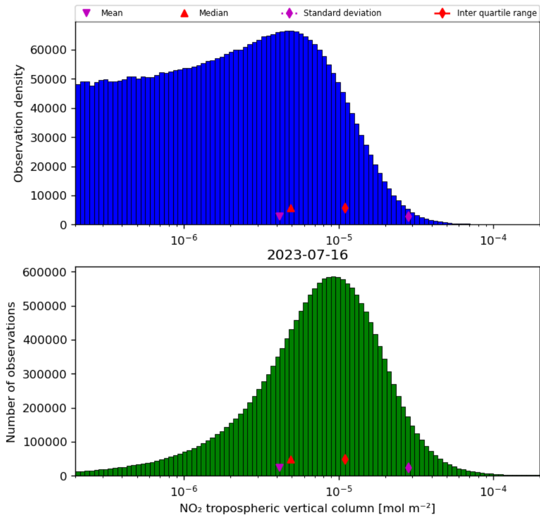
Figure 29: Histogram of “NO 2 tropospheric vertical column” for 2023-07-15 to 2023-07-17
