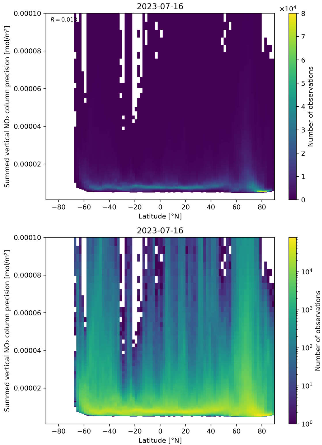
Figure 89: Scatter density plot of “Latitude” against “Summed vertical NO 2 column precision” for 2023-07-15 to 2023-07-17.
