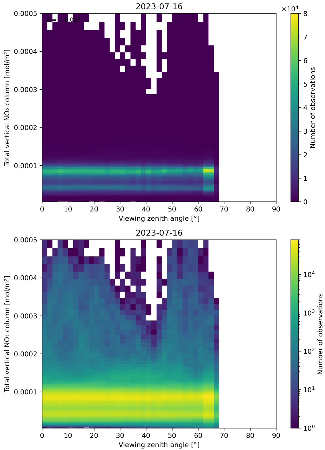
Figure 167: Scatter density plot of “Viewing zenith angle” against “Total vertical NO 2 column” for 2023-07-15 to 2023-07-17.
