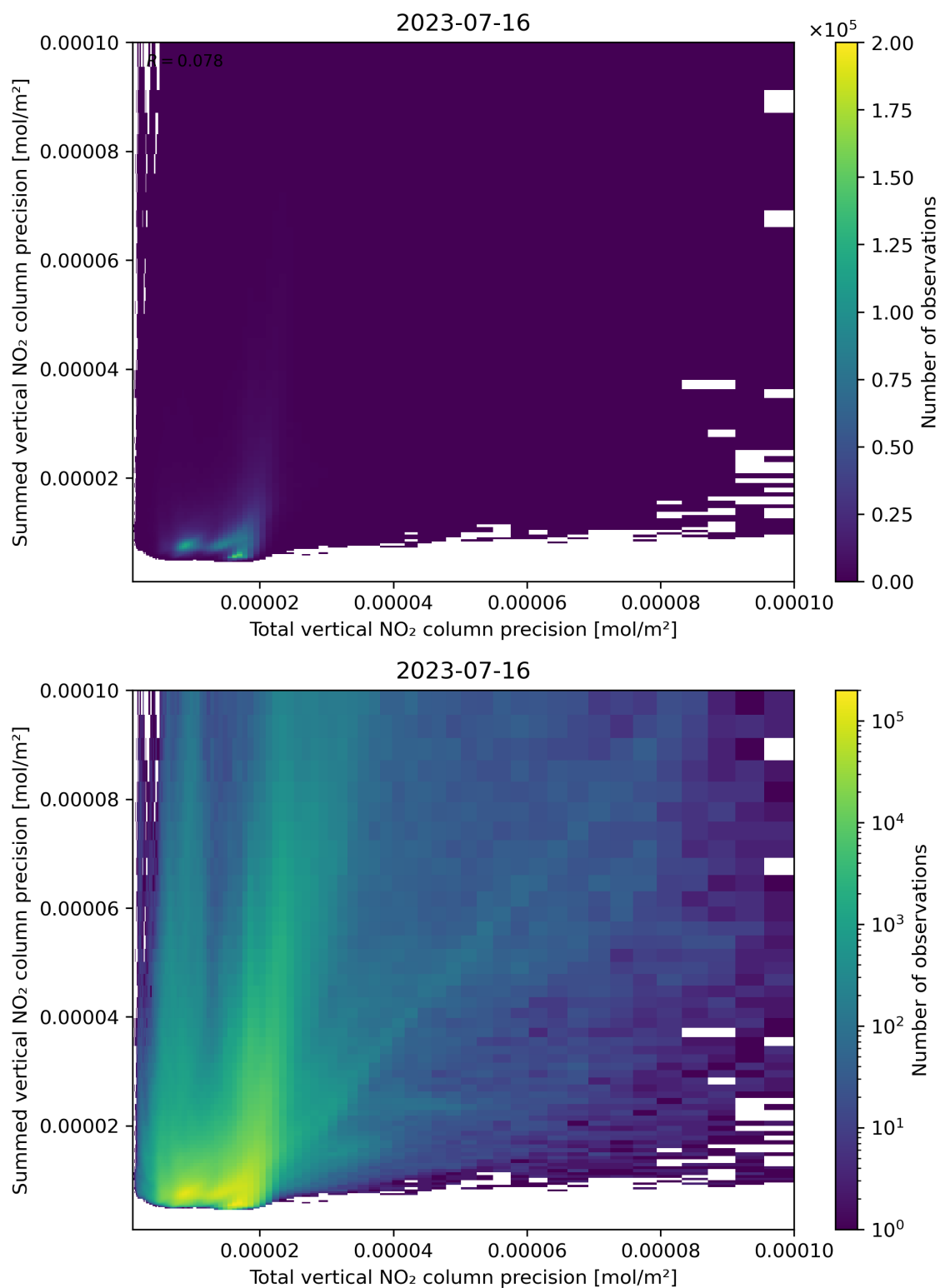
Figure 118: Scatter density plot of “Total vertical NO 2 column precision” against “Summed vertical NO 2 column precision” for 2023-07-15 to 2023-07-17.
