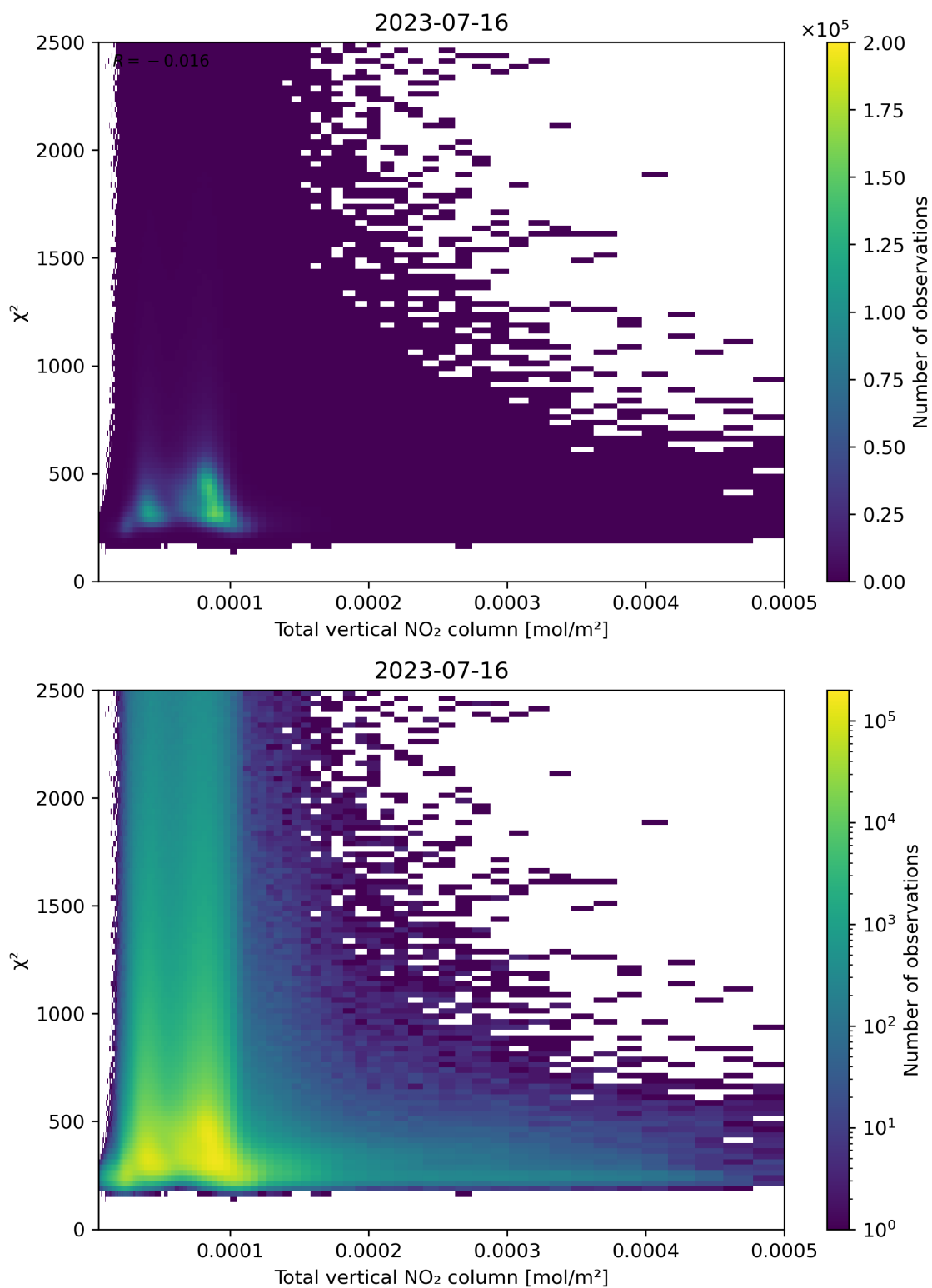
Figure 111: Scatter density plot of “Total vertical NO 2 column” against “ \chi^2 ” for 2023-07-15 to 2023-07-17.
