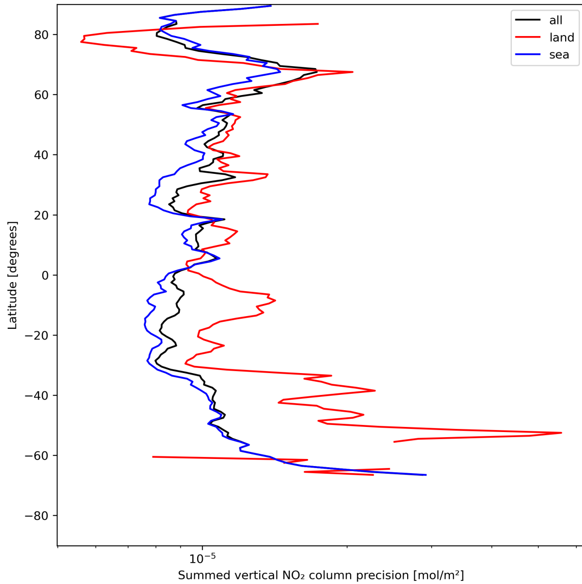
Figure 24: Zonal average of “Summed vertical NO 2 column precision” for 2023-07-15 to 2023-07-17.
