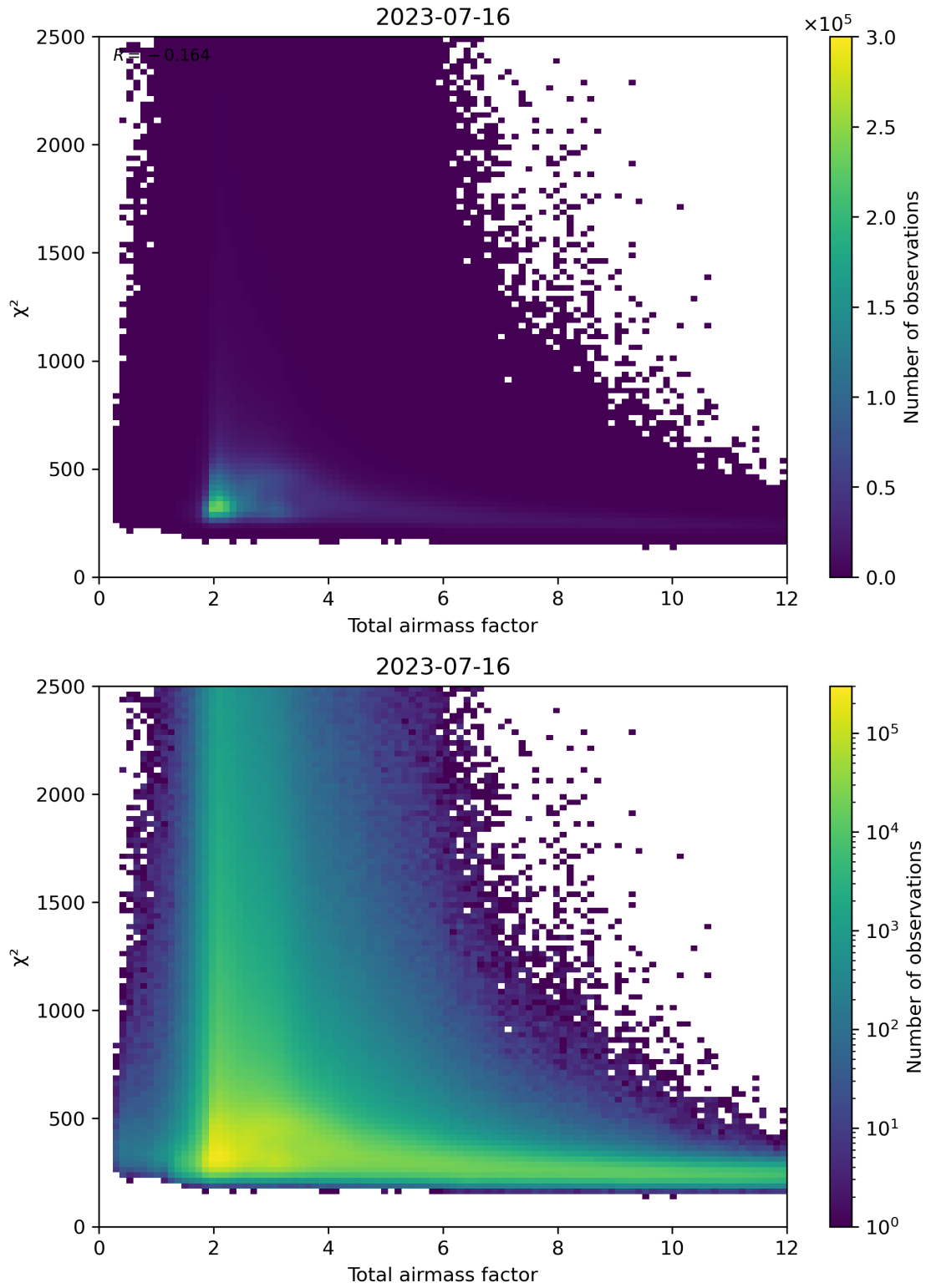
Figure 63: Scatter density plot of “Total airmass factor” against “ \chi^2 ” for 2023-07-15 to 2023-07-17.
