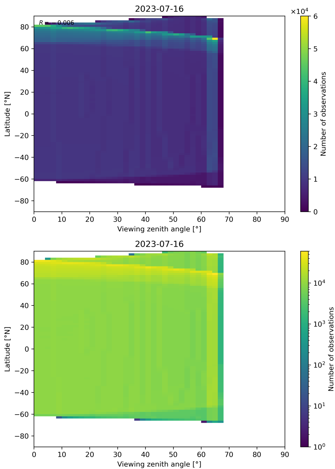
Figure 163: Scatter density plot of “Viewing zenith angle” against “Latitude” for 2023-07-15 to 2023-07-17.
