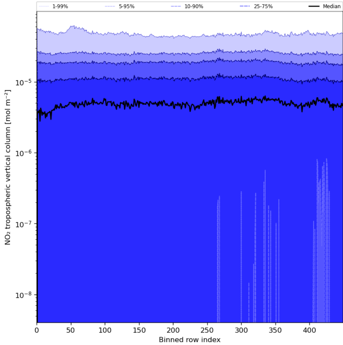
Figure 46: Along track statistics of "NO 2 tropospheric vertical column" for 2023-07-15 to 2023-07-17
