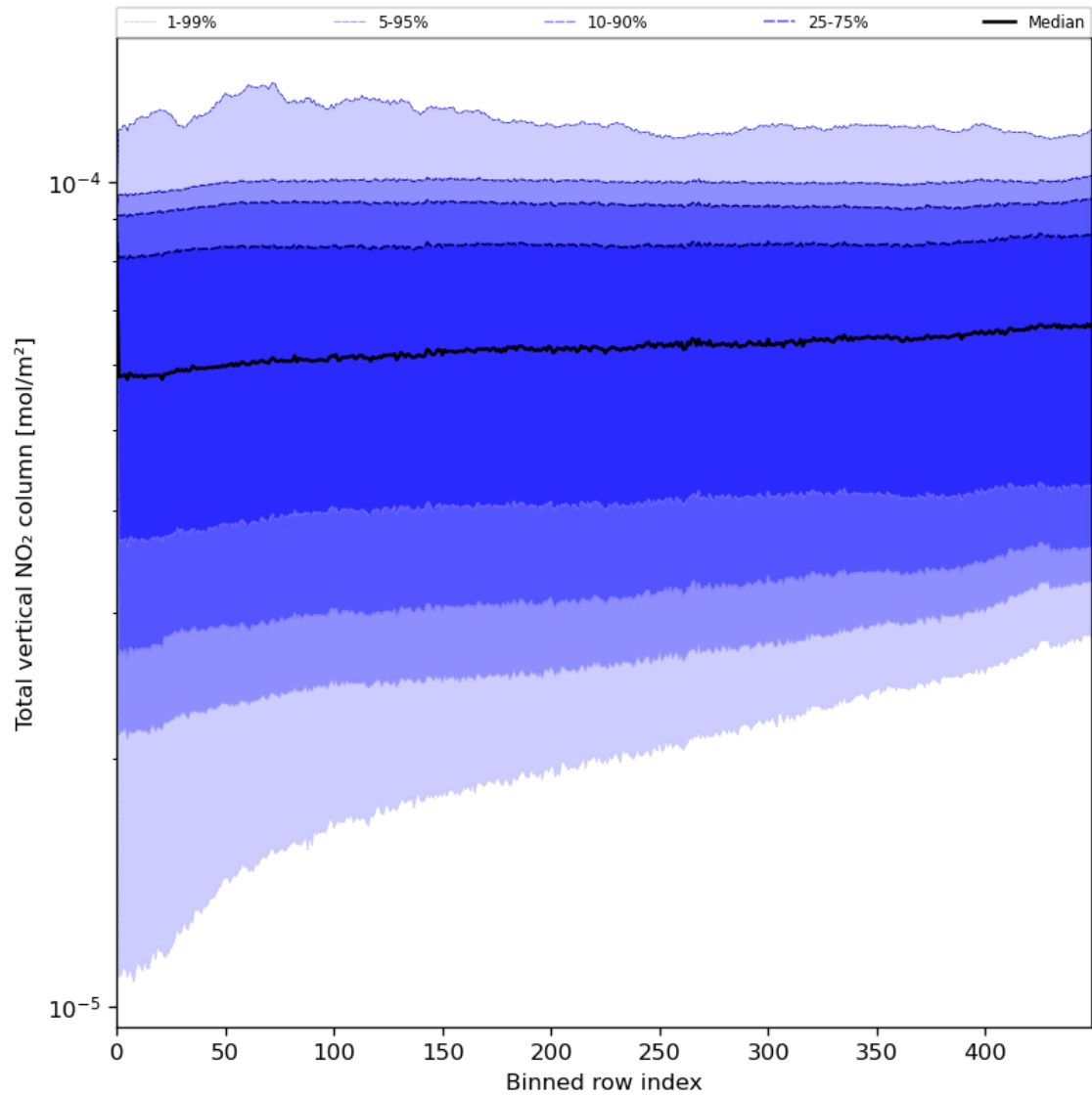
Figure 55: Along track statistics of “Total vertical NO 2 column” for 2023-07-15 to 2023-07-17
