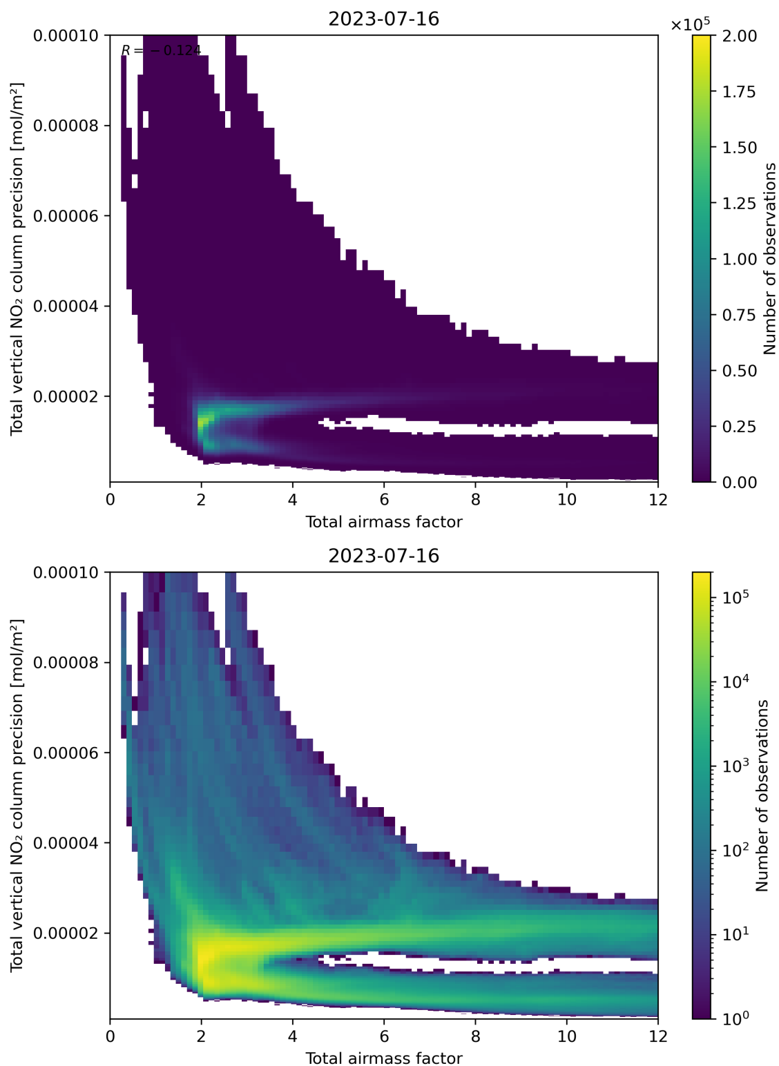
Figure 68: Scatter density plot of “Total airmass factor” against “Total vertical NO 2 column precision” for 2023-07-15 to 2023-07-17.
