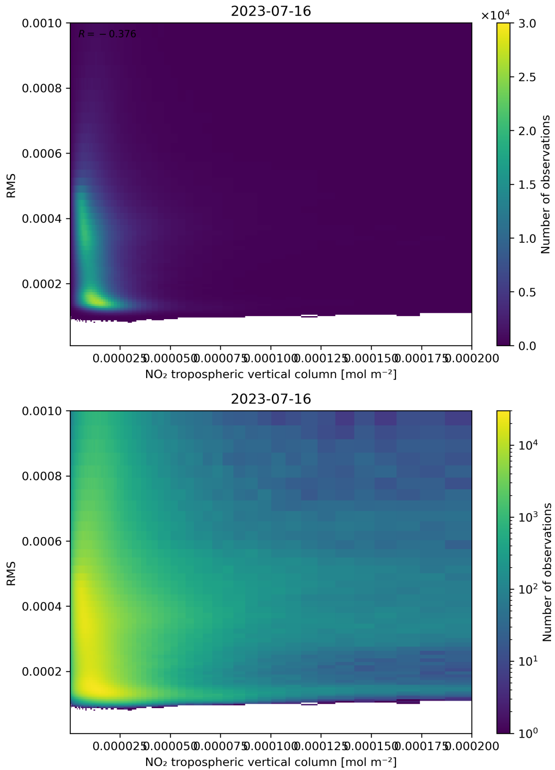
Figure 142: Scatter density plot of “NO 2 tropospheric vertical column” against “RMS” for 2023-07-15 to 2023-07-17.
