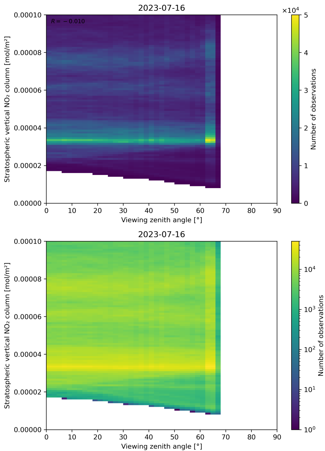
Figure 164: Scatter density plot of “Viewing zenith angle” against “Stratospheric vertical NO 2 column” for 2023-07-15 to 2023-07-17.
