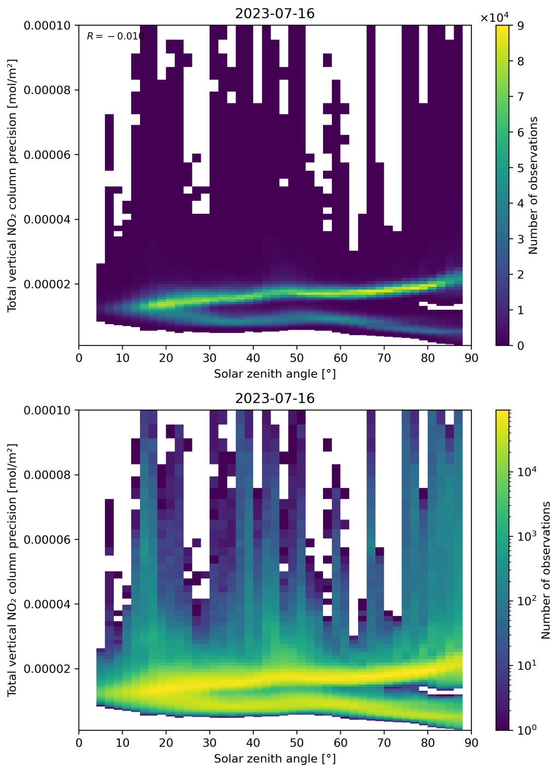
Figure 154: Scatter density plot of “Solar zenith angle” against “Total vertical NO 2 column precision” for 2023-07-15 to 2023-07-17.
