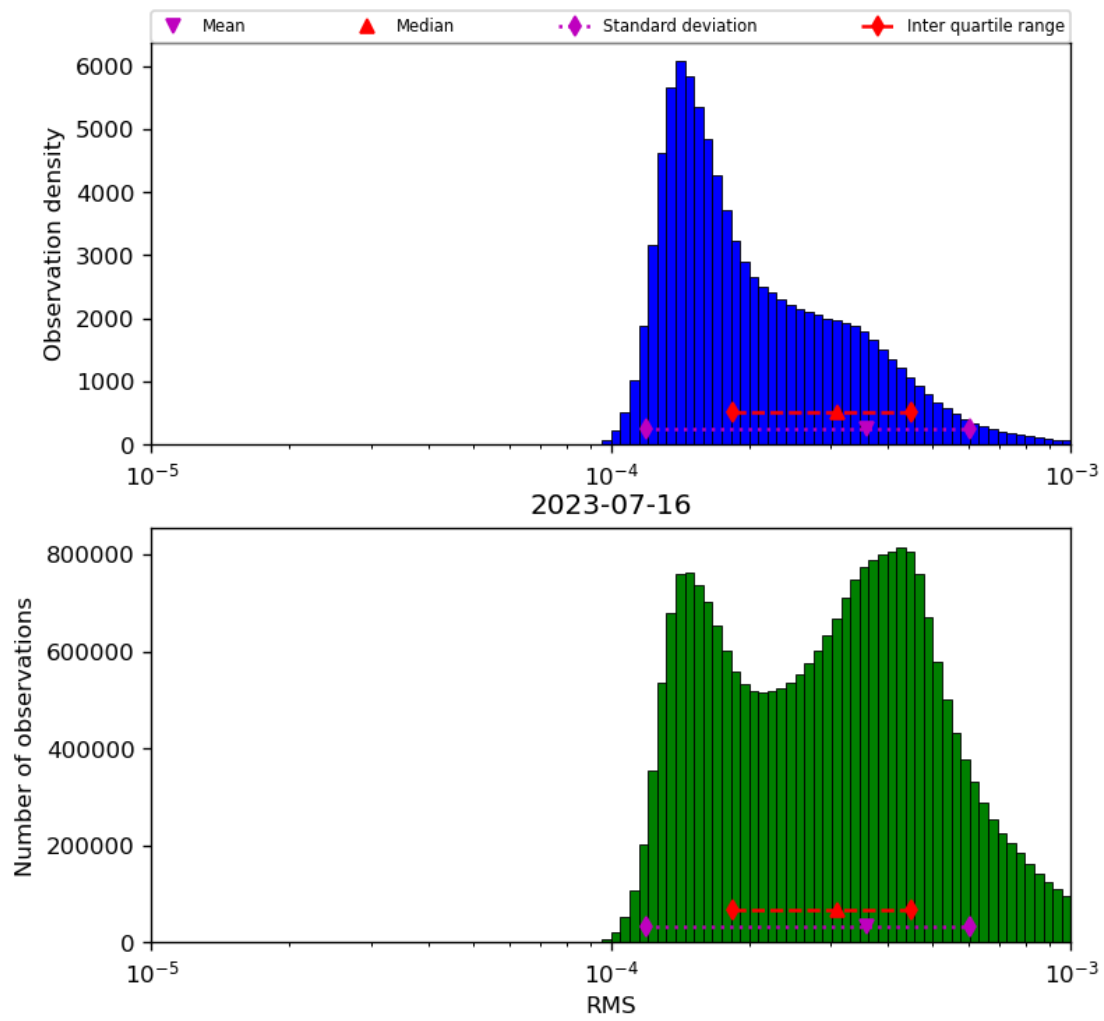
Figure 43: Histogram of “RMS” for 2023-07-15 to 2023-07-17
