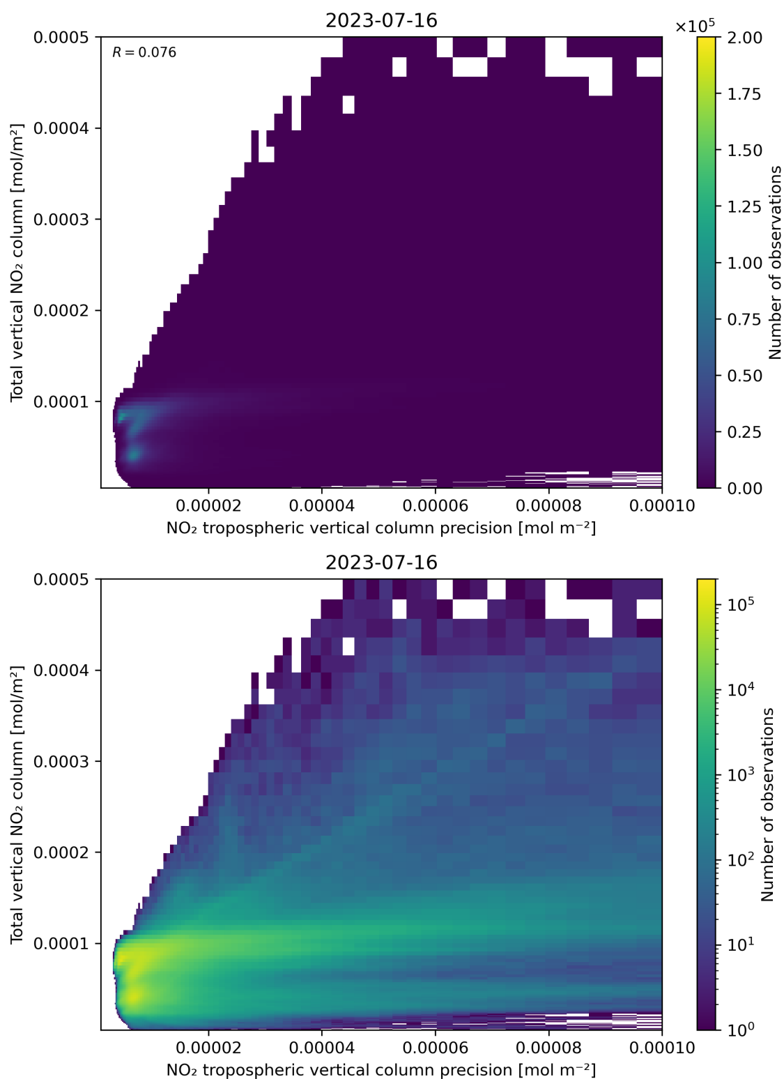
Figure 138: Scatter density plot of “NO 2 tropospheric vertical column precision” against “Total vertical NO 2 column” for 2023-07-15 to 2023-07-17.
