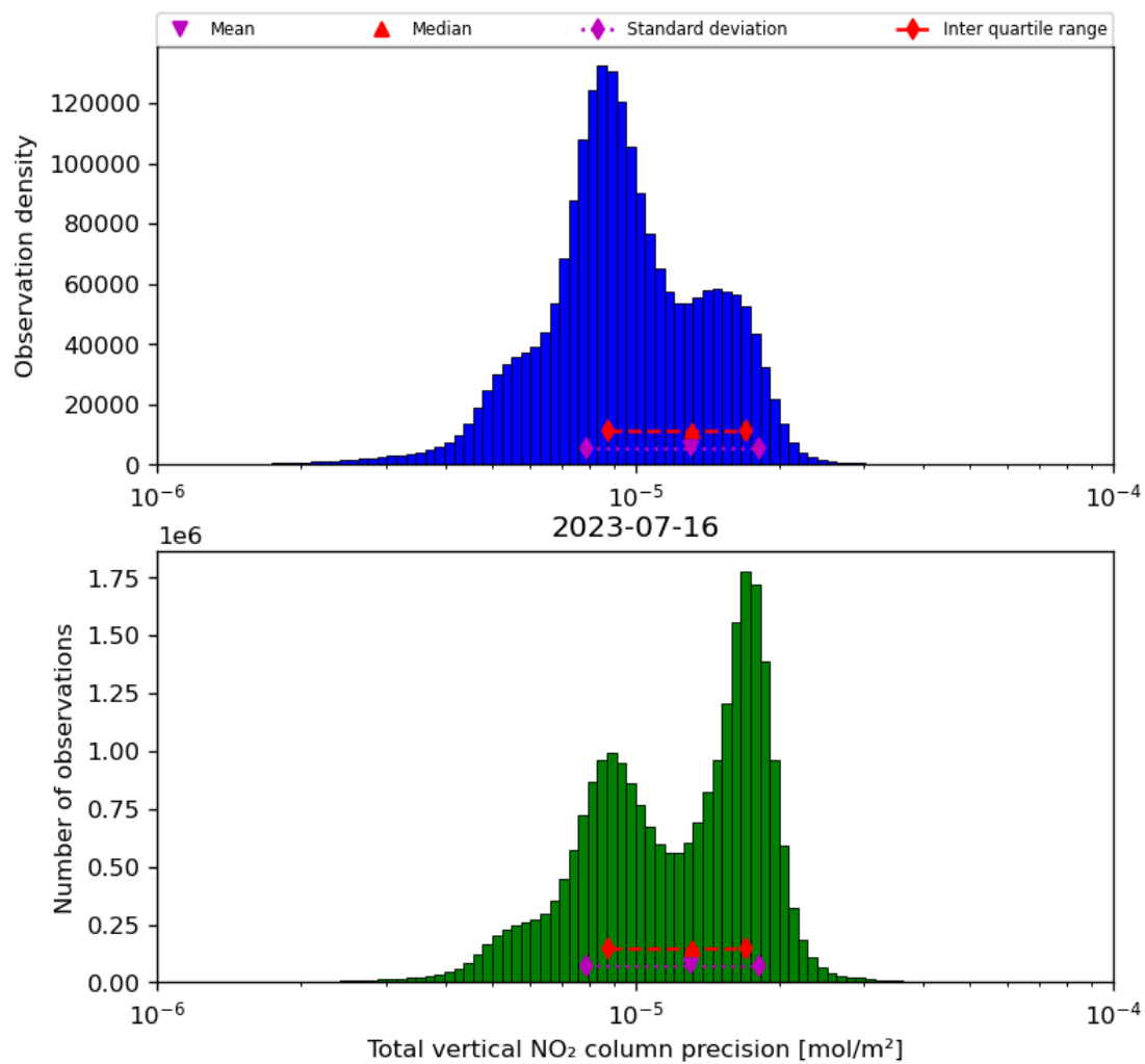
Figure 39: Histogram of “Total vertical NO 2 column precision” for 2023-07-15 to 2023-07-17
