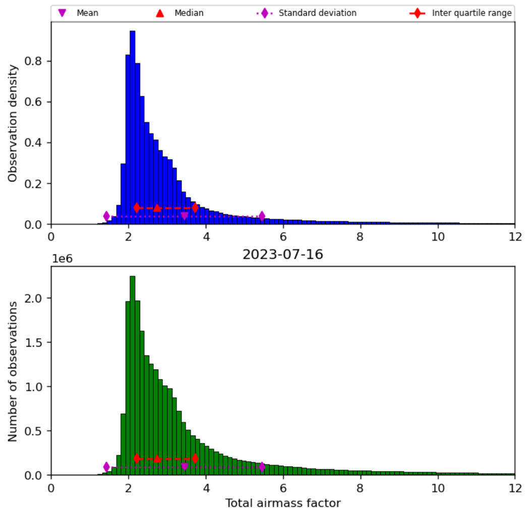
Figure 32: Histogram of “Total airmass factor” for 2023-07-15 to 2023-07-17
