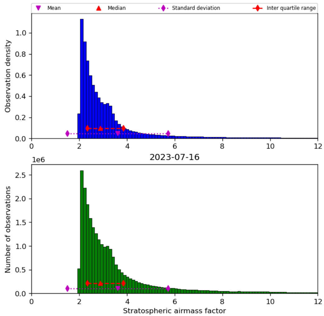
Figure 44: Histogram of “Stratospheric airmass factor” for 2023-07-15 to 2023-07-17
