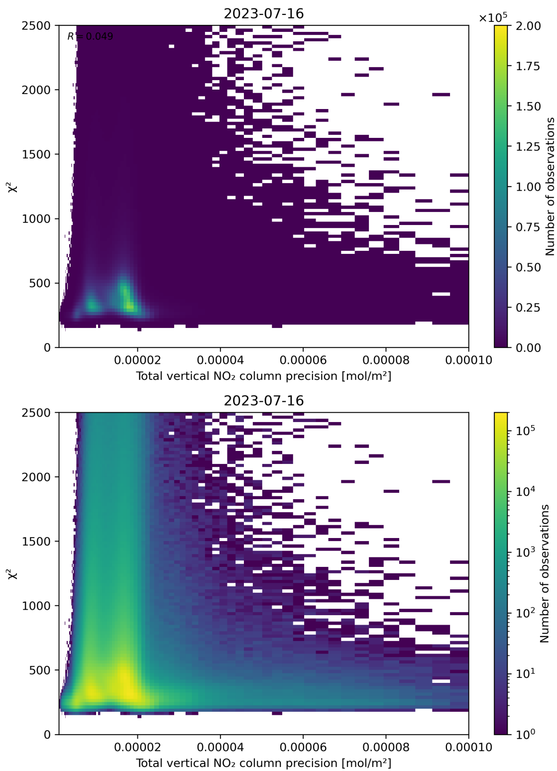
Figure 116: Scatter density plot of “Total vertical NO 2 column precision” against “ \chi^2 ” for 2023-07-15 to 2023-07-17.
