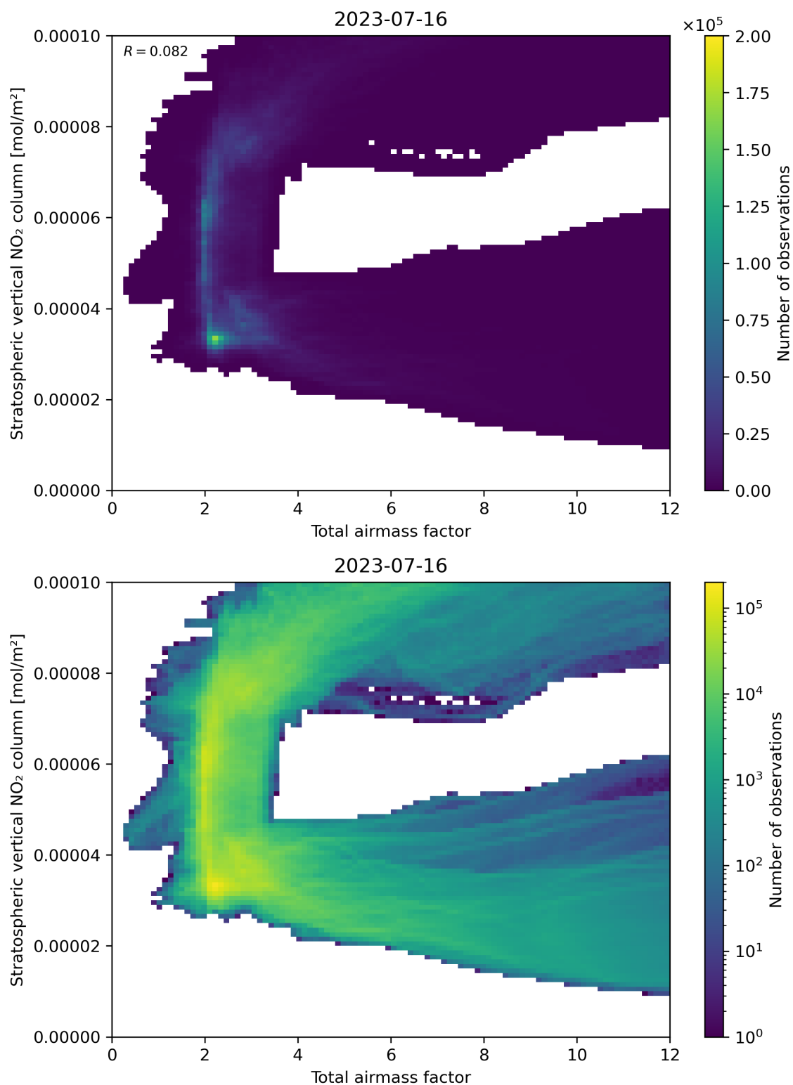
Figure 64: Scatter density plot of “Total airmass factor” against “Stratospheric vertical \text{NO}_2 column” for 2023-07-15 to 2023-07-17.
