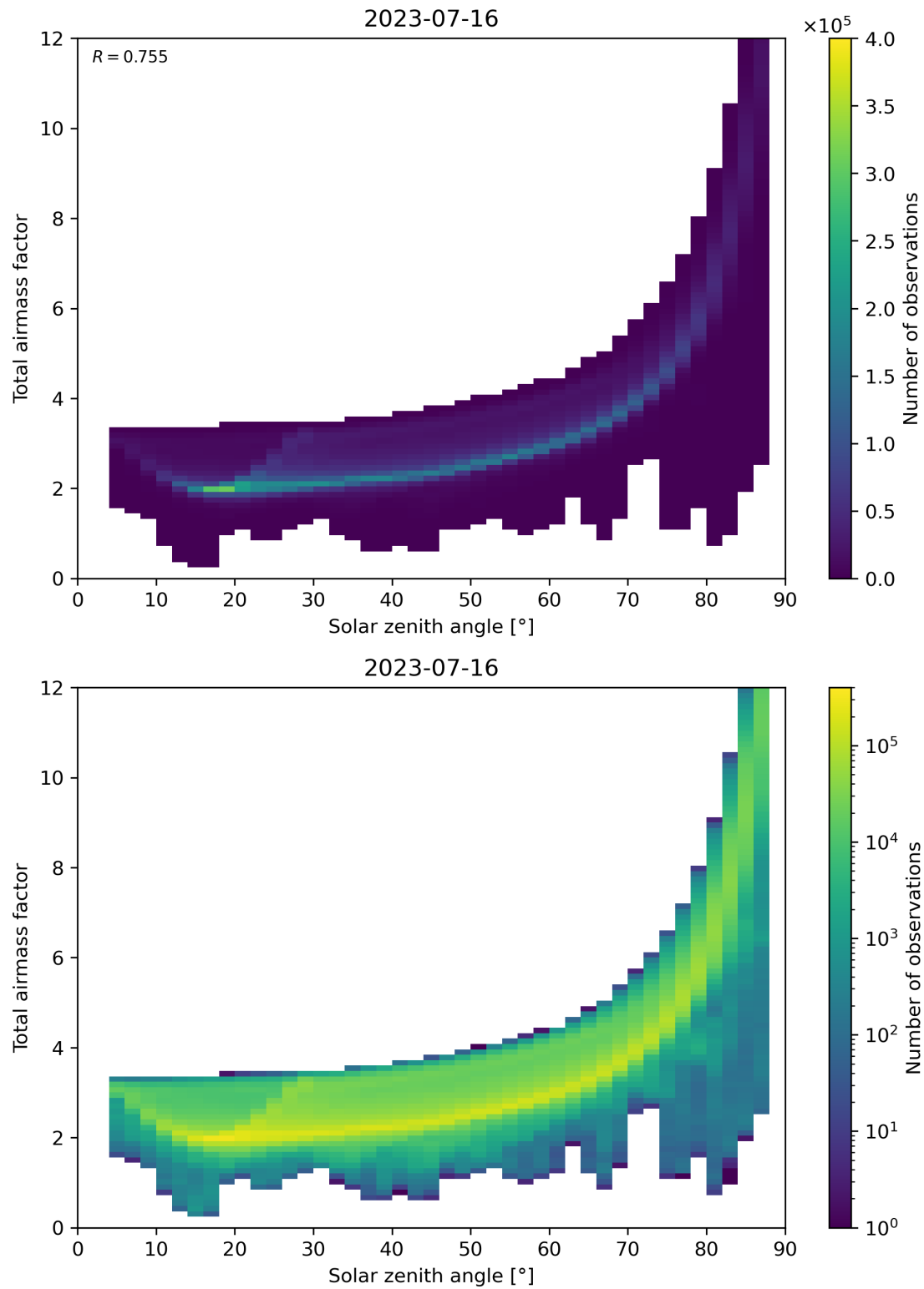
Figure 146: Scatter density plot of “Solar zenith angle” against “Total air mass factor” for 2023-07-15 to 2023-07-17.
