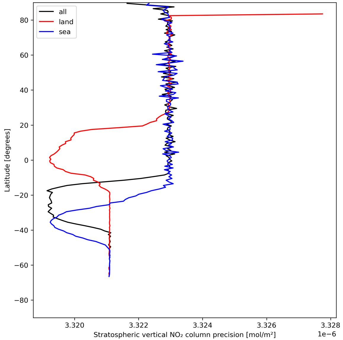
Figure 20: Zonal average of “Stratospheric vertical NO 2 column precision” for 2023-07-15 to 2023-07-17.
