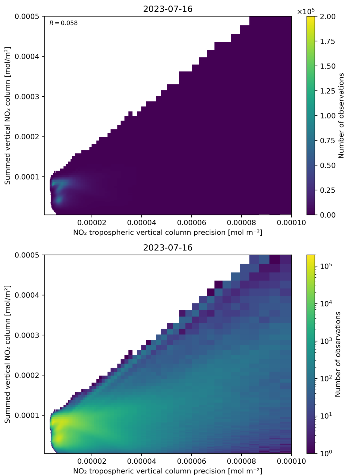
Figure 136: Scatter density plot of “NO 2 tropospheric vertical column precision” against “Summed vertical NO 2 column” for 2023-07-15 to 2023-07-17.
