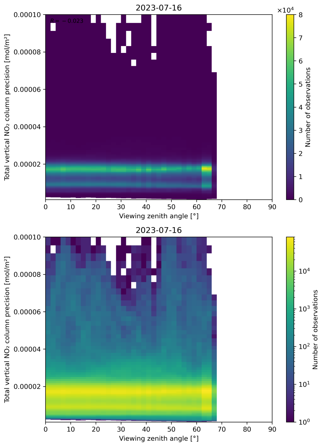
Figure 168: Scatter density plot of “Viewing zenith angle” against “Total vertical NO 2 column precision” for 2023-07-15 to 2023-07-17.
