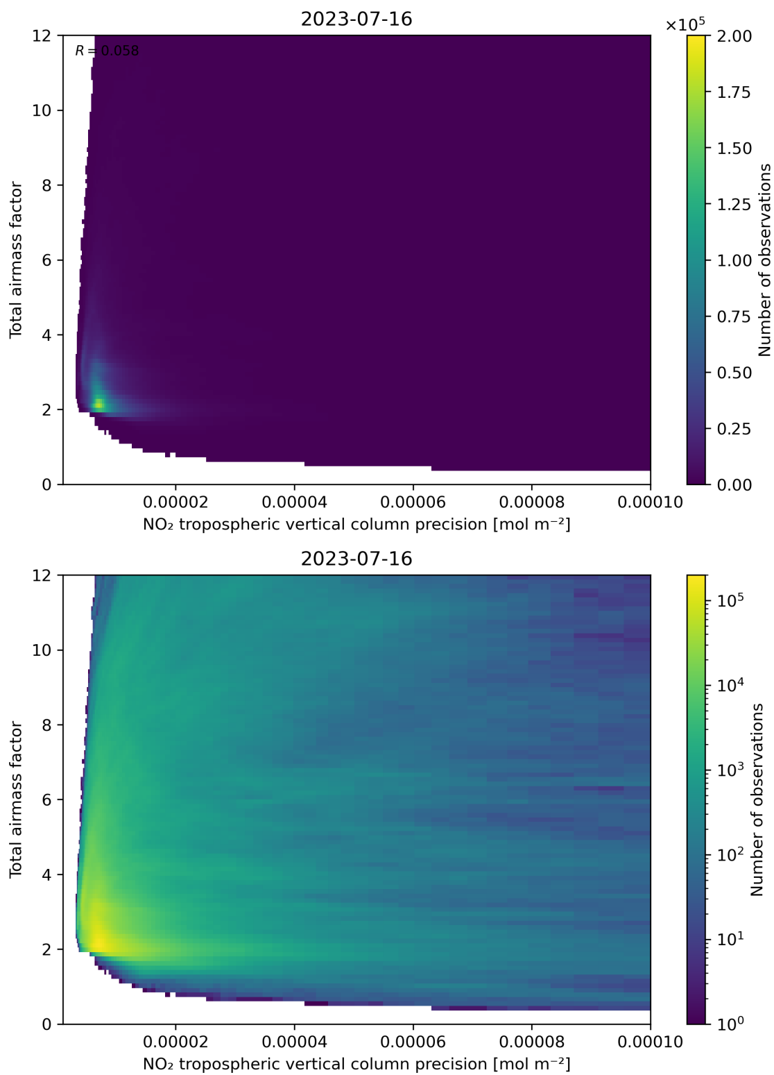
Figure 132: Scatter density plot of “NO 2 tropospheric vertical column precision” against “Total air mass factor” for 2023-07-15 to 2023-07-17.
