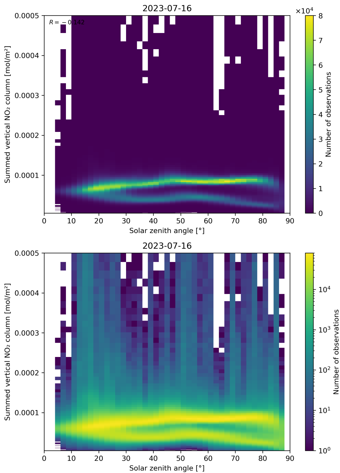
Figure 151: Scatter density plot of “Solar zenith angle” against “Summed vertical NO 2 column” for 2023-07-15 to 2023-07-17.
