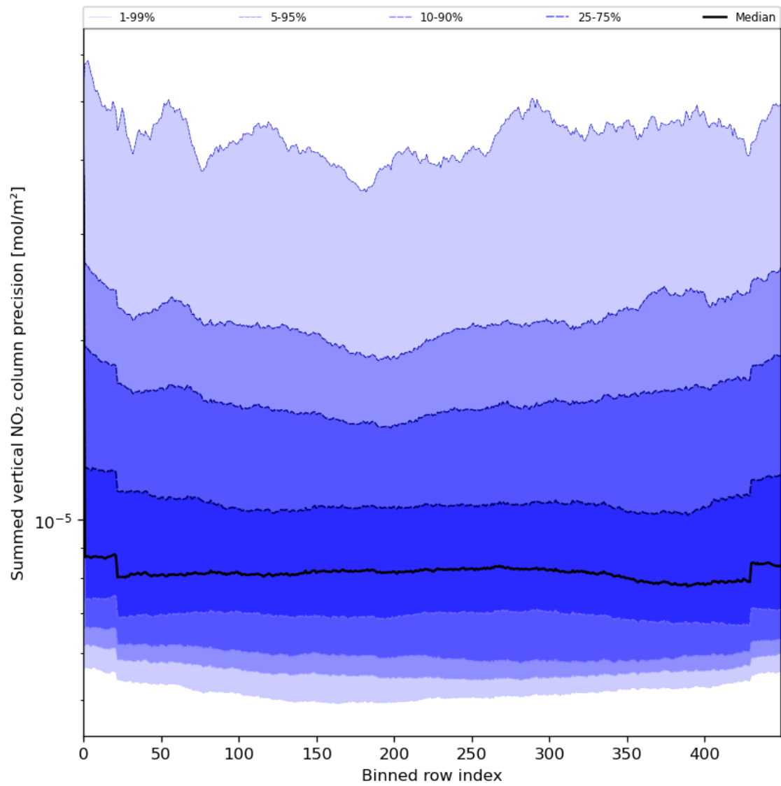
Figure 58: Along track statistics of “Summed vertical NO 2 column precision” for 2023-07-15 to 2023-07-17
