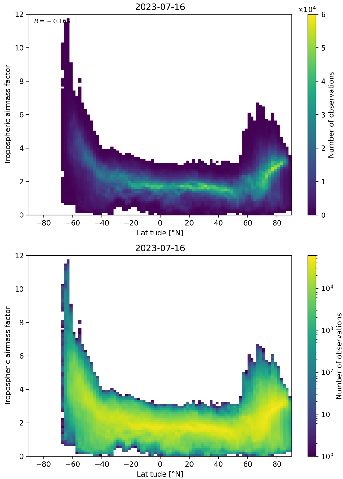
Figure 85: Scatter density plot of “Latitude” against “Tropospheric airmass factor” for 2023-07-15 to 2023-07-17.
