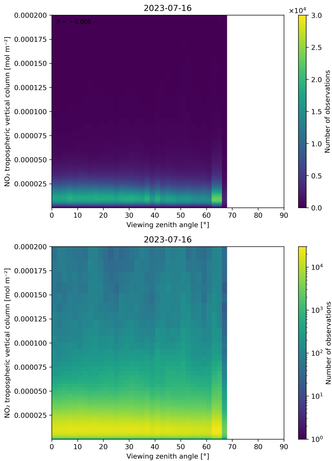
Figure 169: Scatter density plot of “Viewing zenith angle” against “NO 2 tropospheric vertical column” for 2023-07-15 to 2023-07-17.
