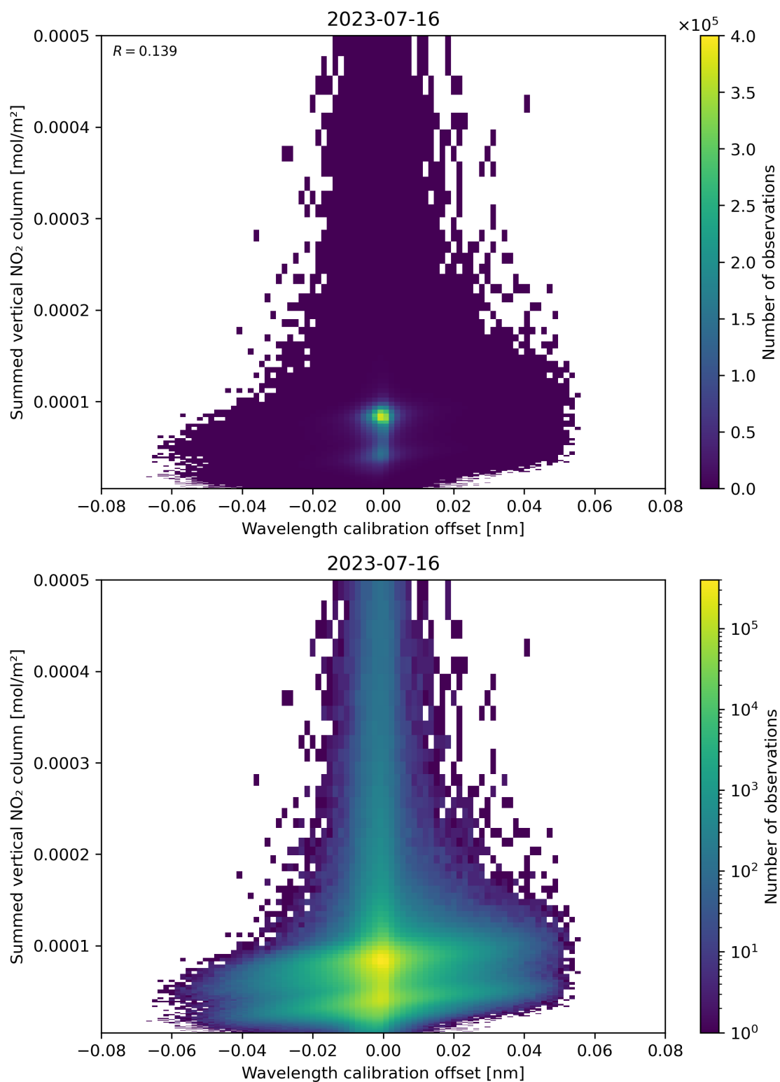
Figure 177: Scatter density plot of “Wavelength calibration offset” against “Summed vertical NO 2 column” for 2023-07-15 to 2023-07-17.
