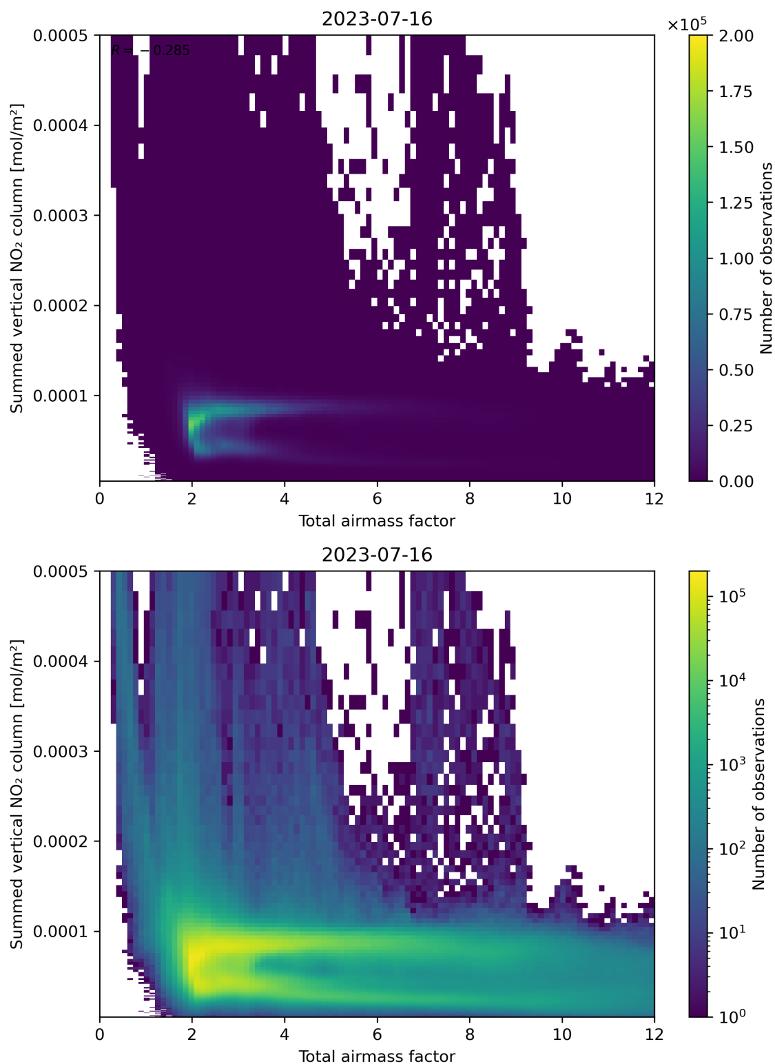
Figure 65: Scatter density plot of “Total airmass factor” against “Summed vertical NO 2 column” for 2023-07-15 to 2023-07-17.
