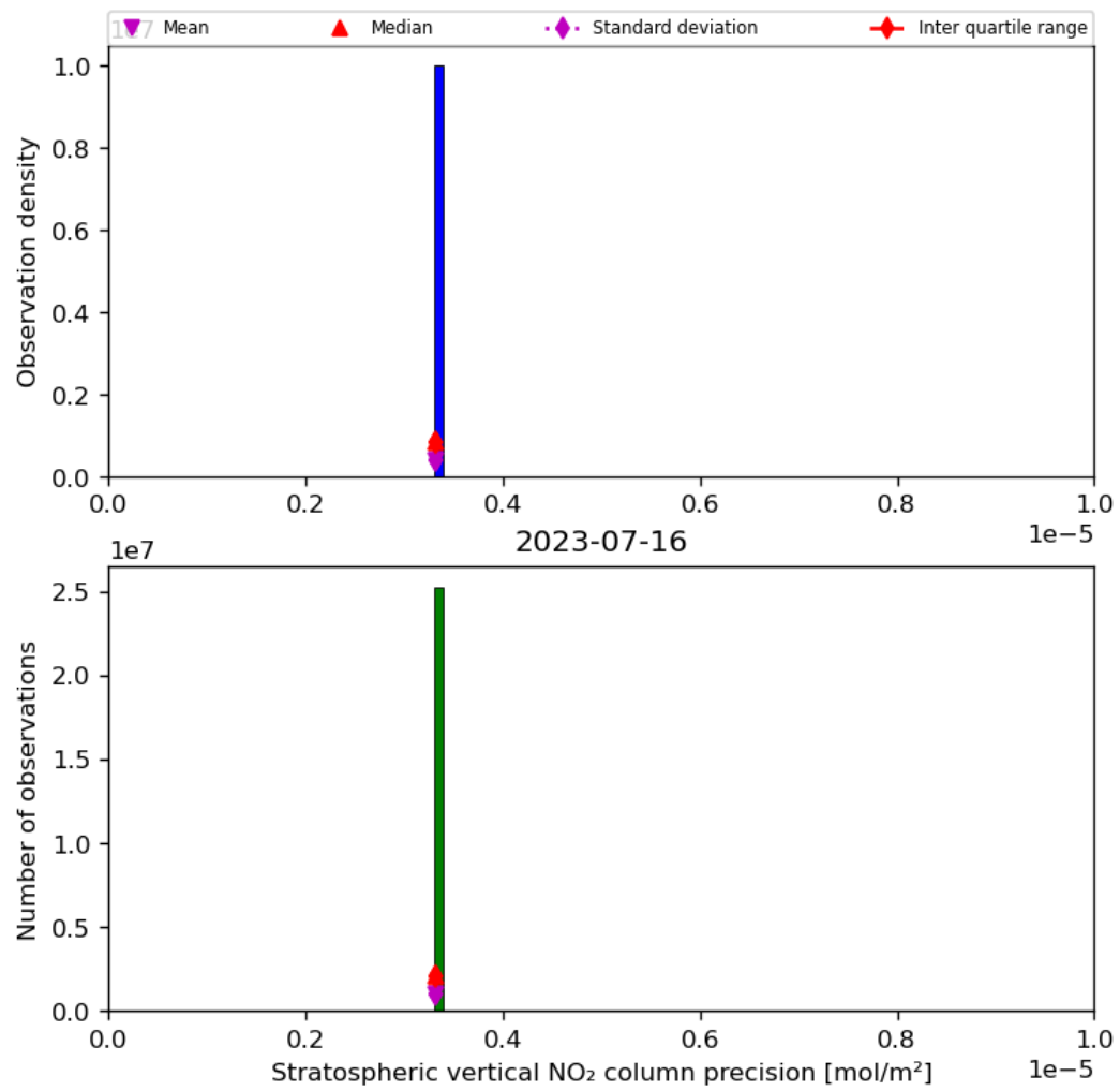
Figure 37: Histogram of “Stratospheric vertical NO 2 column precision” for 2023-07-15 to 2023-07-17
