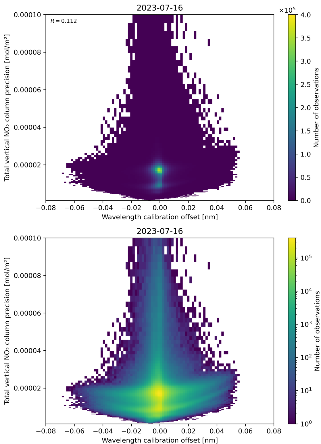
Figure 180: Scatter density plot of “Wavelength calibration offset” against “Total vertical NO 2 column precision” for 2023-07-15 to 2023-07-17.
