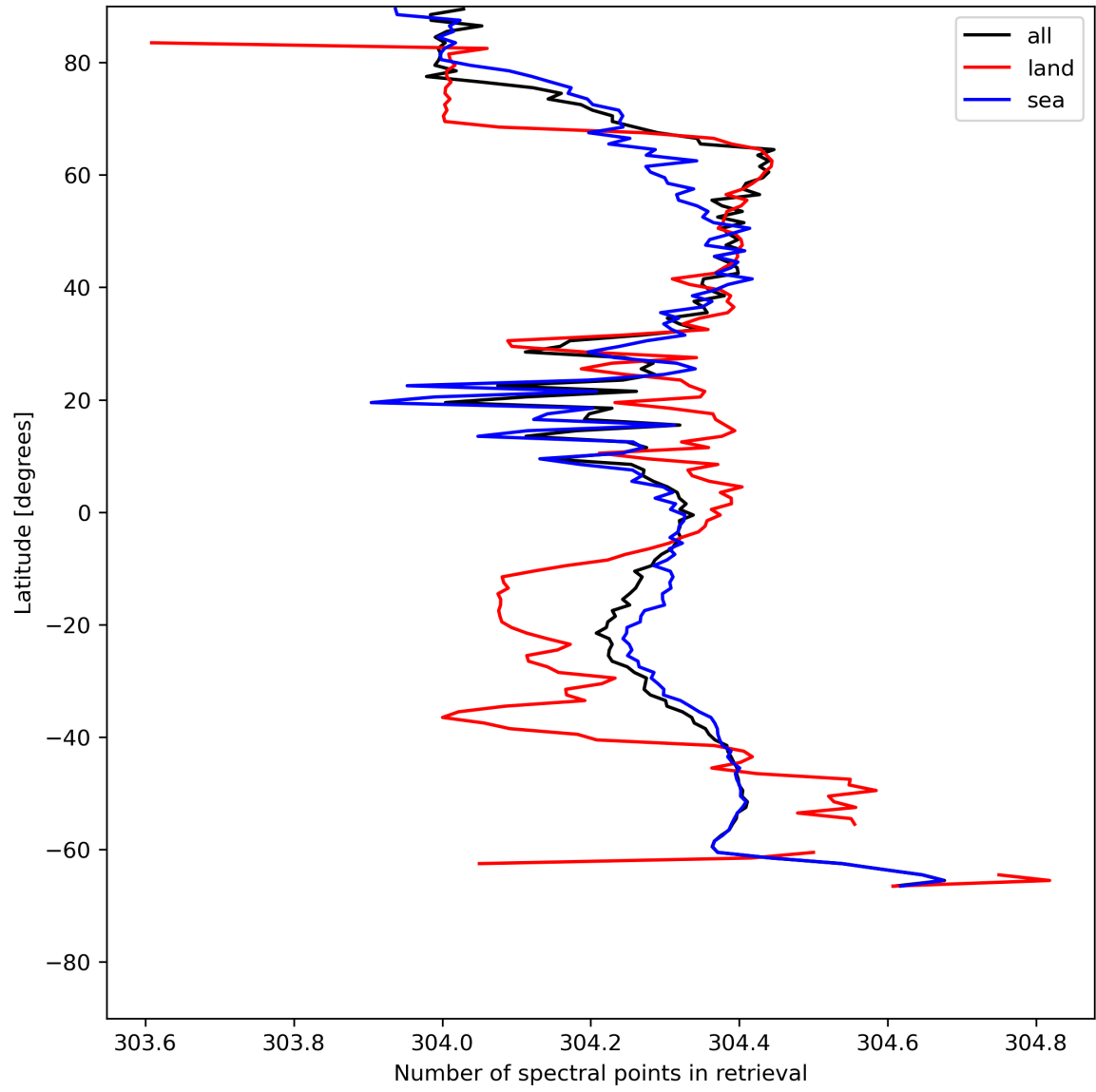
Figure 16: Zonal average of “Number of spectral points in retrieval” for 2023-07-15 to 2023-07-17.
