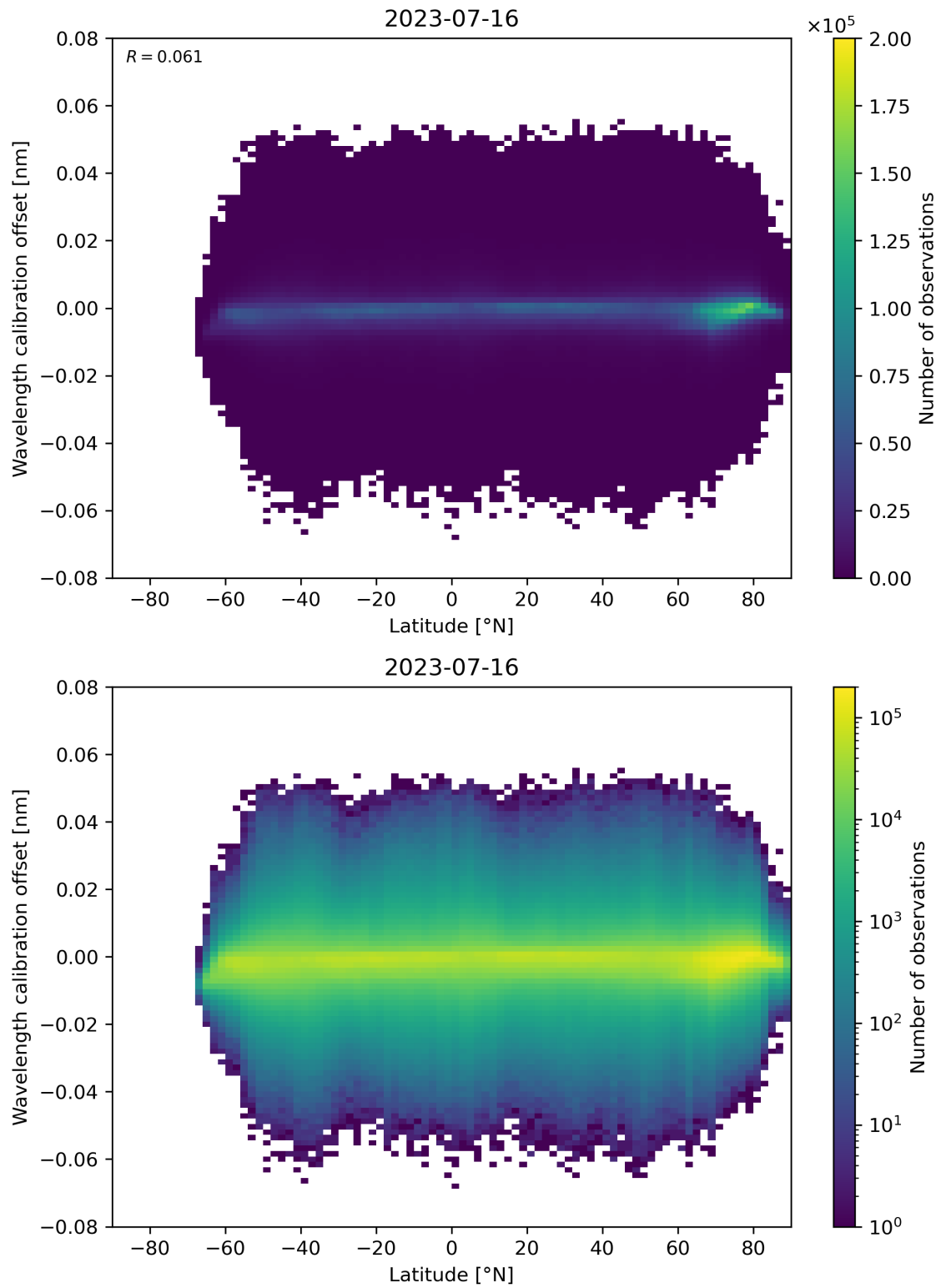
Figure 95: Scatter density plot of “Latitude” against “Wavelength calibration offset” for 2023-07-15 to 2023-07-17.
