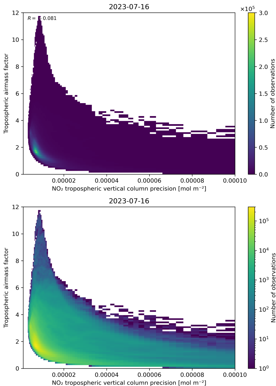
Figure 133: Scatter density plot of “NO 2 tropospheric vertical column precision” against “Tropospheric airmass factor” for 2023-07-15 to 2023-07-17.
