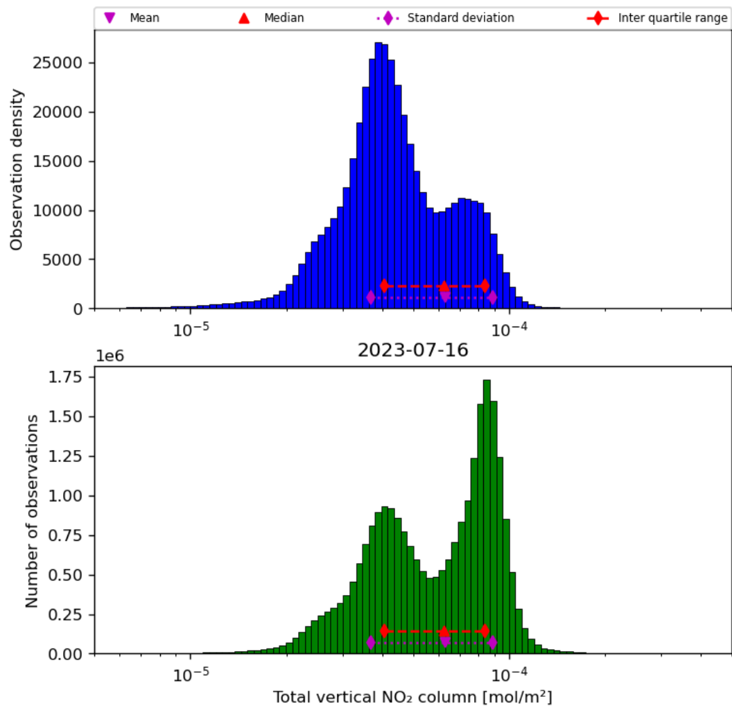
Figure 38: Histogram of “Total vertical NO 2 column” for 2023-07-15 to 2023-07-17
