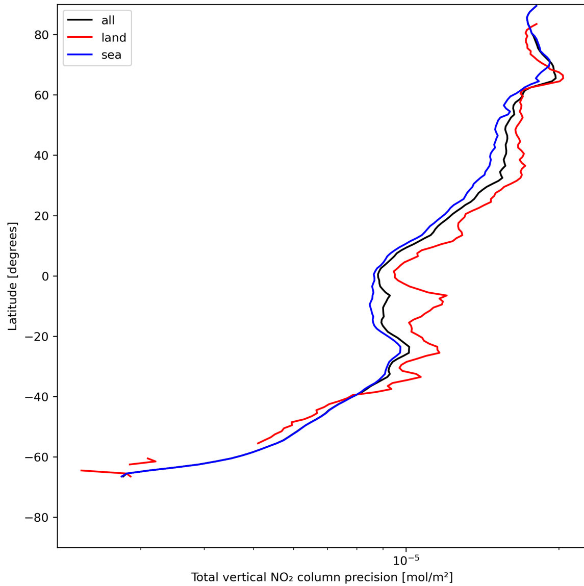
Figure 22: Zonal average of “Total vertical NO 2 column precision” for 2023-07-15 to 2023-07-17.
