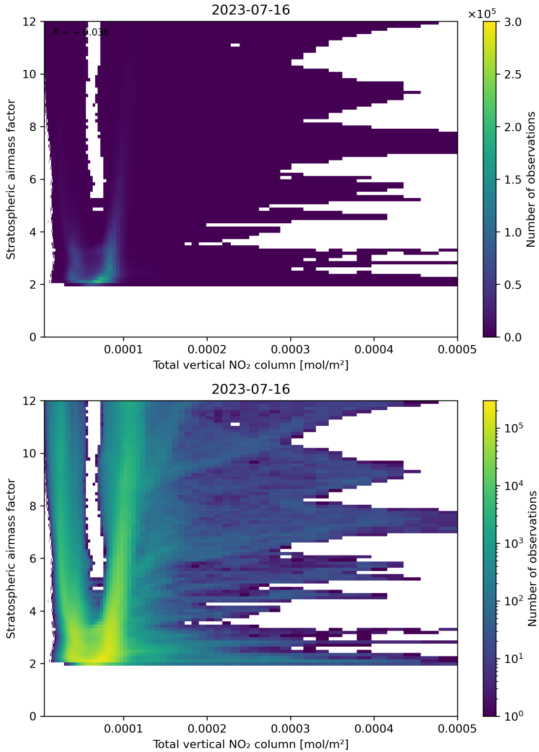
Figure 110: Scatter density plot of “Total vertical NO 2 column” against “Stratospheric airmass factor” for 2023-07-15 to 2023-07-17.
