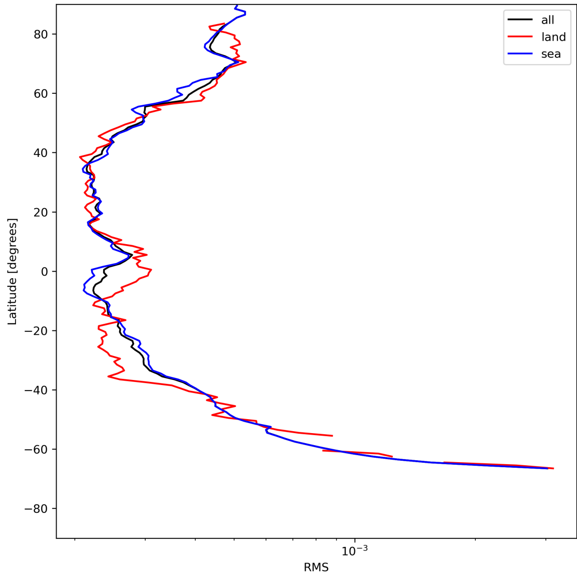
Figure 26: Zonal average of “RMS” for 2023-07-15 to 2023-07-17.
