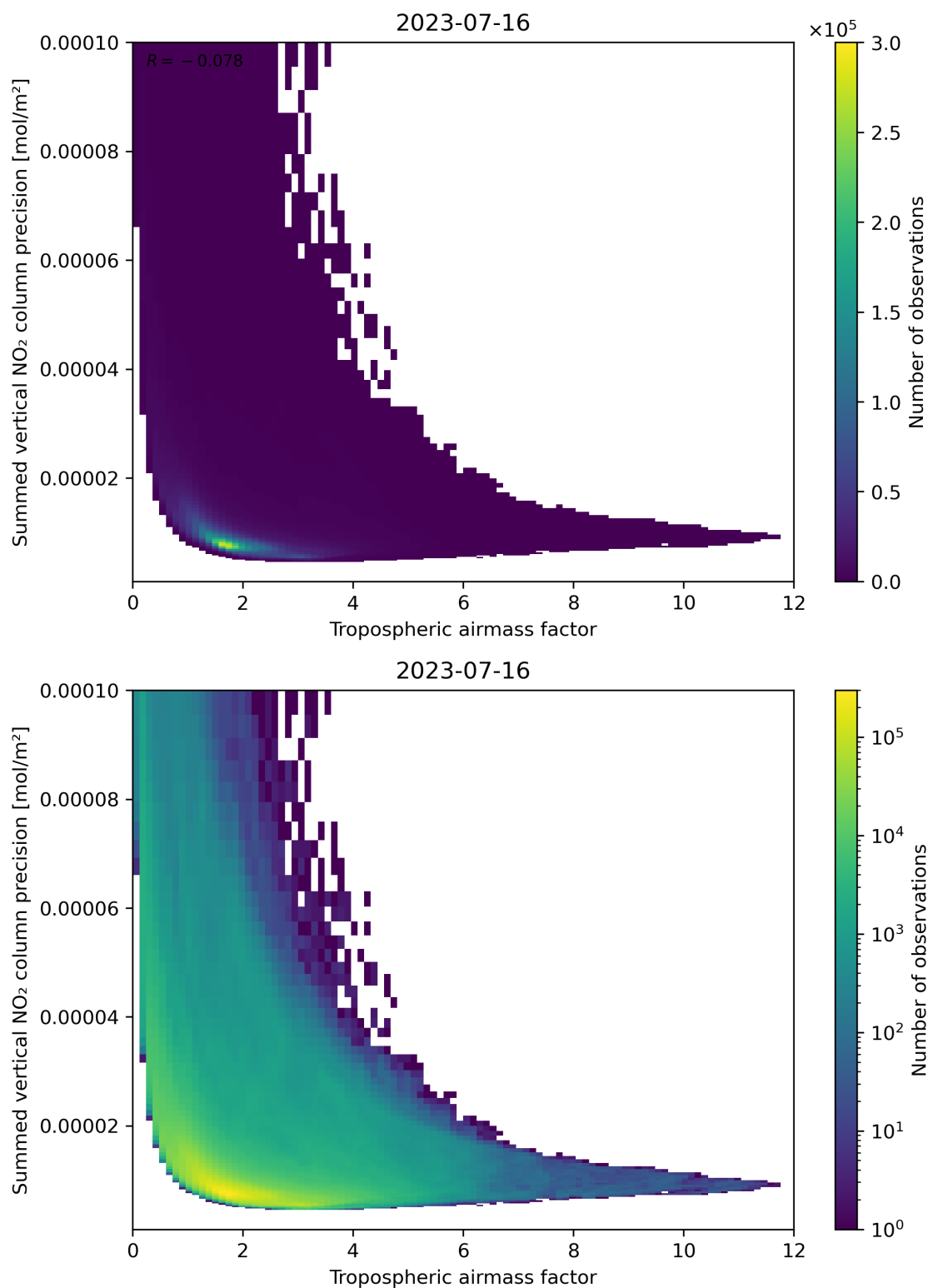
Figure 76: Scatter density plot of “Tropospheric air mass factor” against “Summed vertical NO 2 column precision” for 2023-07-15 to 2023-07-17.
