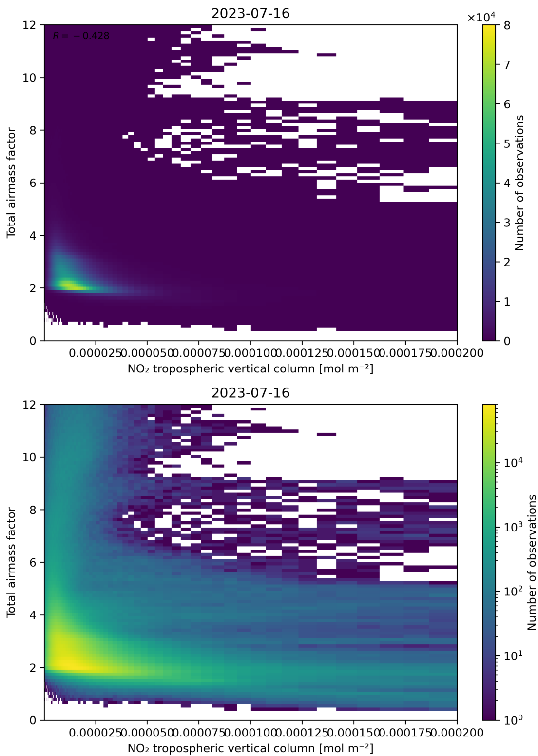
Figure 122: Scatter density plot of “NO 2 tropospheric vertical column” against “Total air mass factor” for 2023-07-15 to 2023-07-17.
