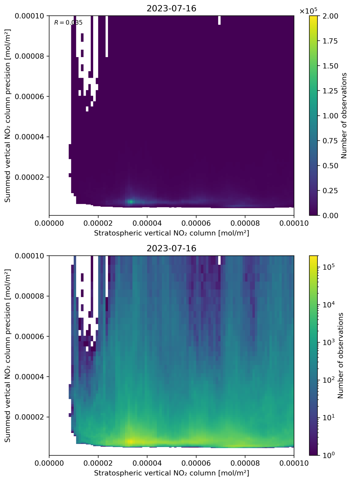
Figure 99: Scatter density plot of “Stratospheric vertical NO 2 column” against “Summed vertical NO 2 column precision” for 2023-07-15 to 2023-07-17.
