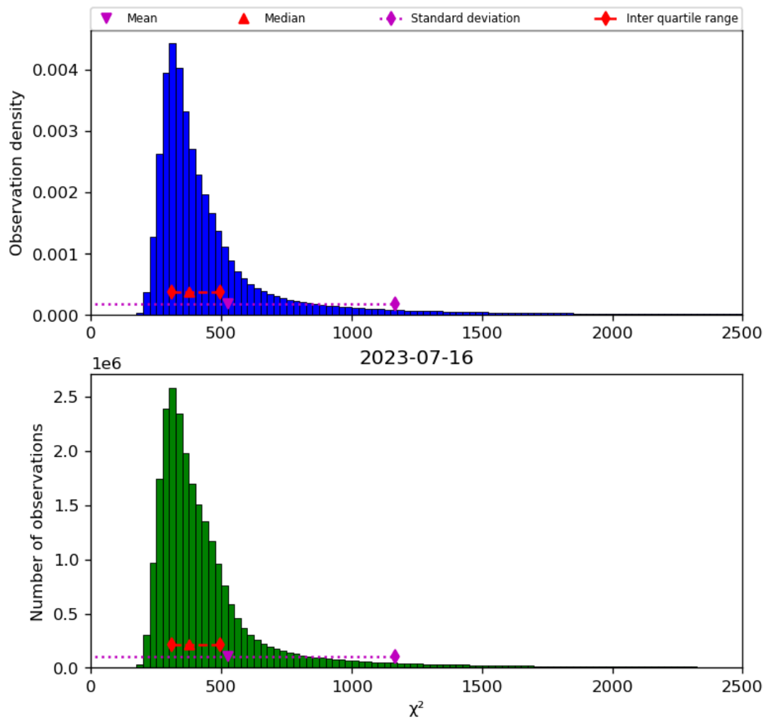
Figure 42: Histogram of “ \chi^2 ” for 2023-07-15 to 2023-07-17
