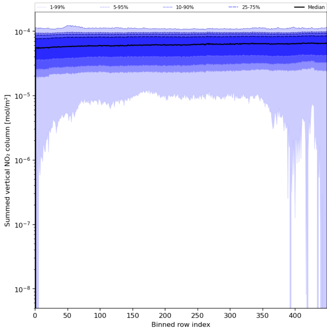
Figure 57: Along track statistics of “Summed vertical NO 2 column” for 2023-07-15 to 2023-07-17
