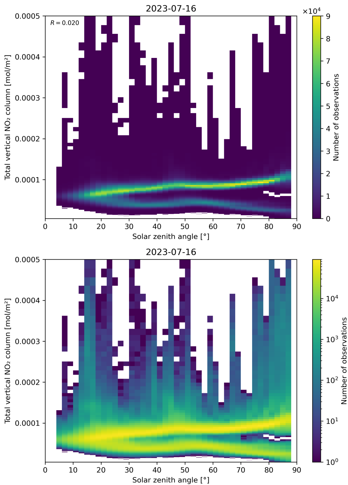
Figure 153: Scatter density plot of “Solar zenith angle” against “Total vertical NO 2 column” for 2023-07-15 to 2023-07-17.
