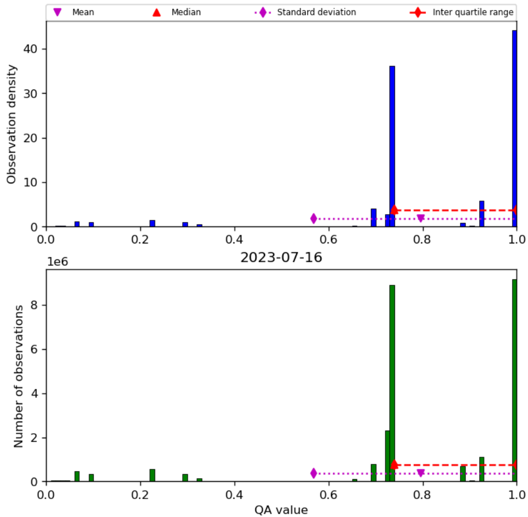
Figure 28: Histogram of “QA value” for 2023-07-15 to 2023-07-17
