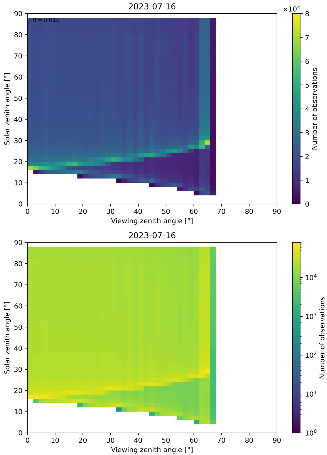
Figure 172: Scatter density plot of “Viewing zenith angle” against “Solar zenith angle” for 2023-07-15 to 2023-07-17.
