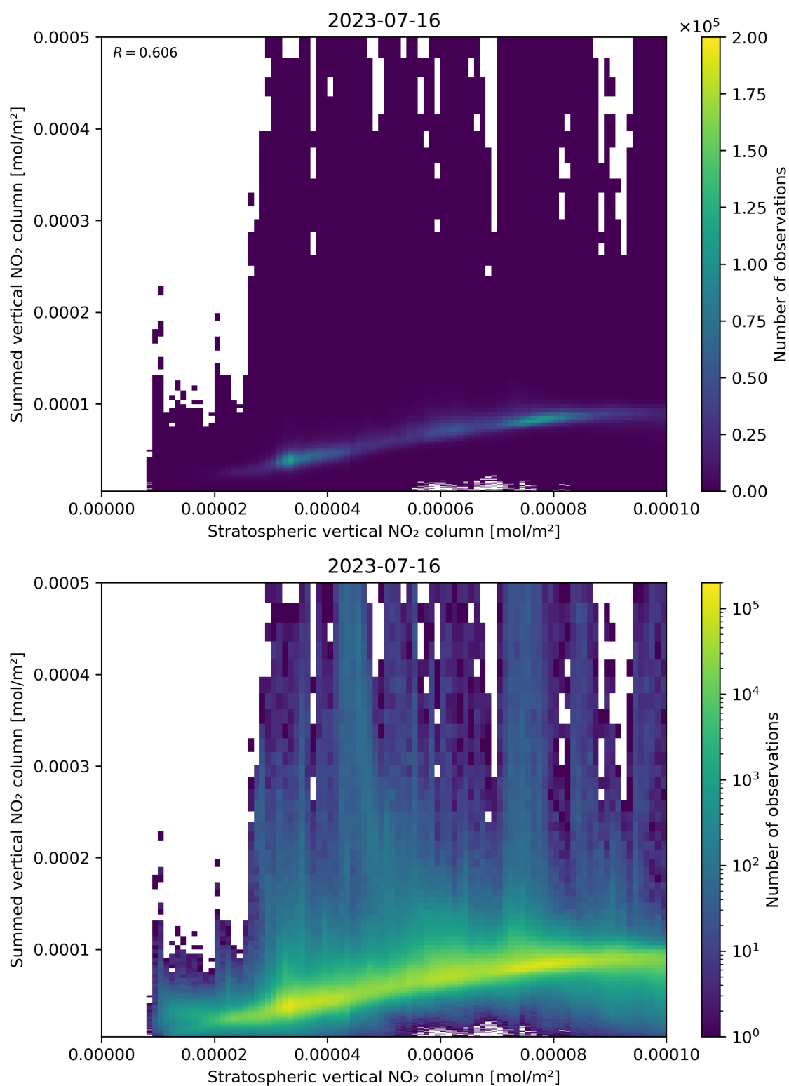
Figure 98: Scatter density plot of “Stratospheric vertical NO 2 column” against “Summed vertical NO 2 column” for 2023-07-15 to 2023-07-17.
