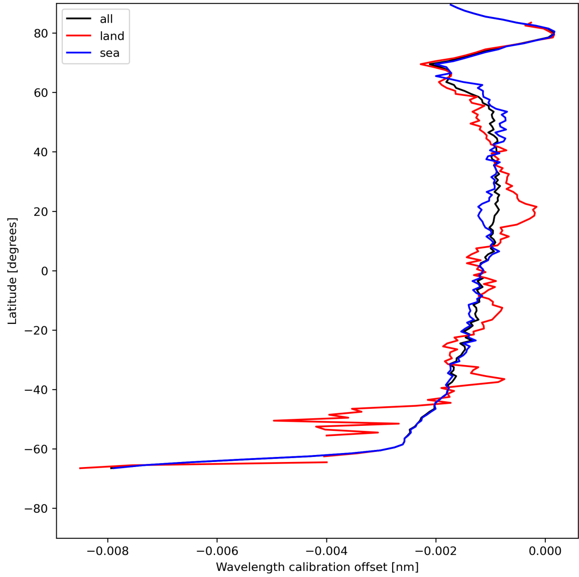
Figure 18: Zonal average of “Wavelength calibration offset” for 2023-07-15 to 2023-07-17.
