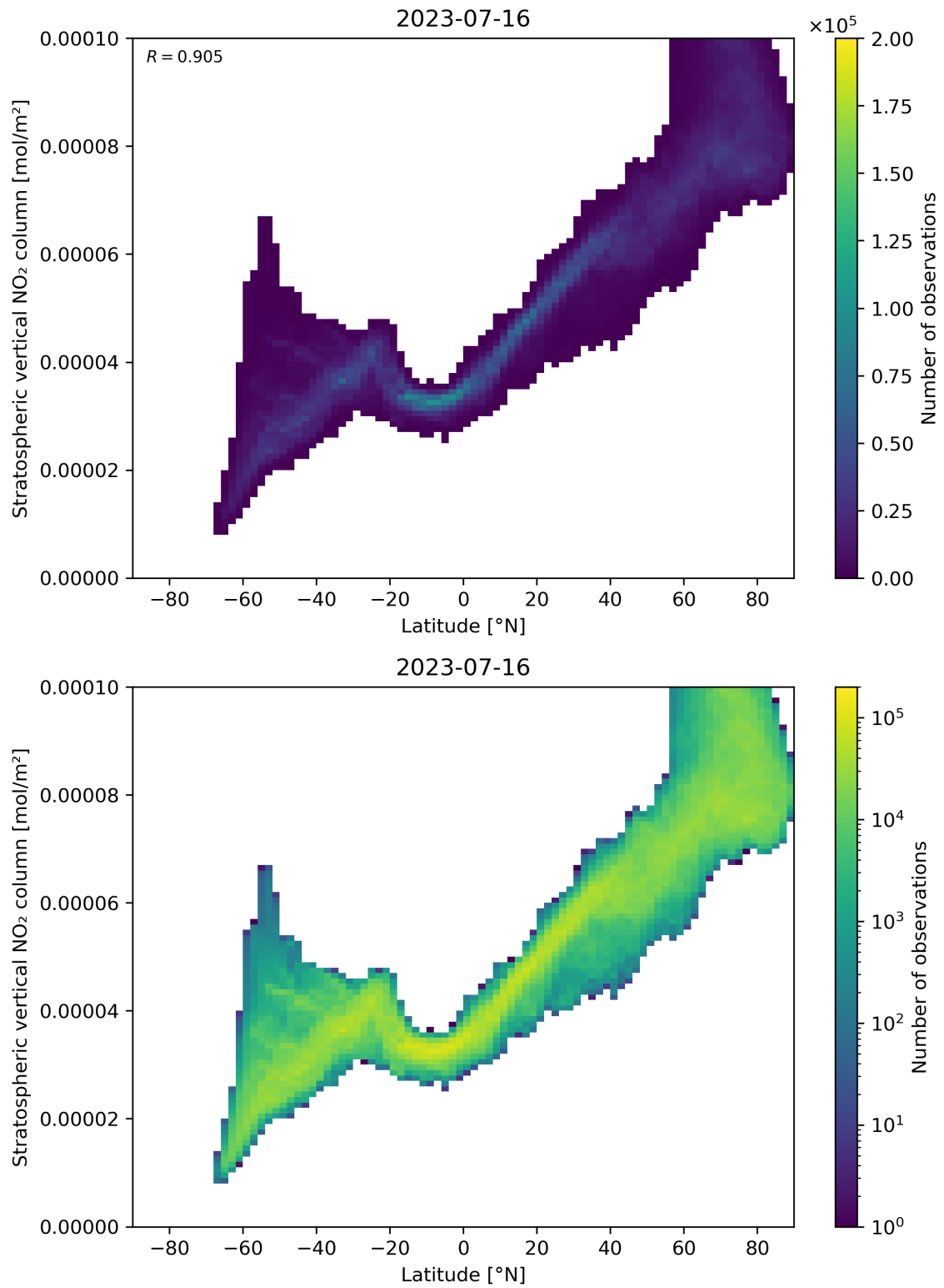
Figure 87: Scatter density plot of “Latitude” against “Stratospheric vertical NO 2 column” for 2023-07-15 to 2023-07-17.
