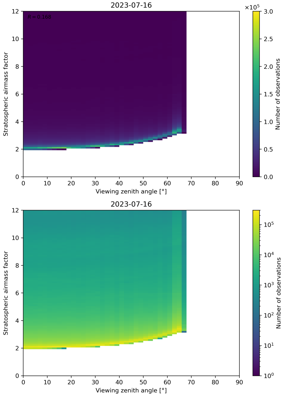
Figure 159: Scatter density plot of “Viewing zenith angle” against “Stratospheric airmass factor” for 2023-07-15 to 2023-07-17.
