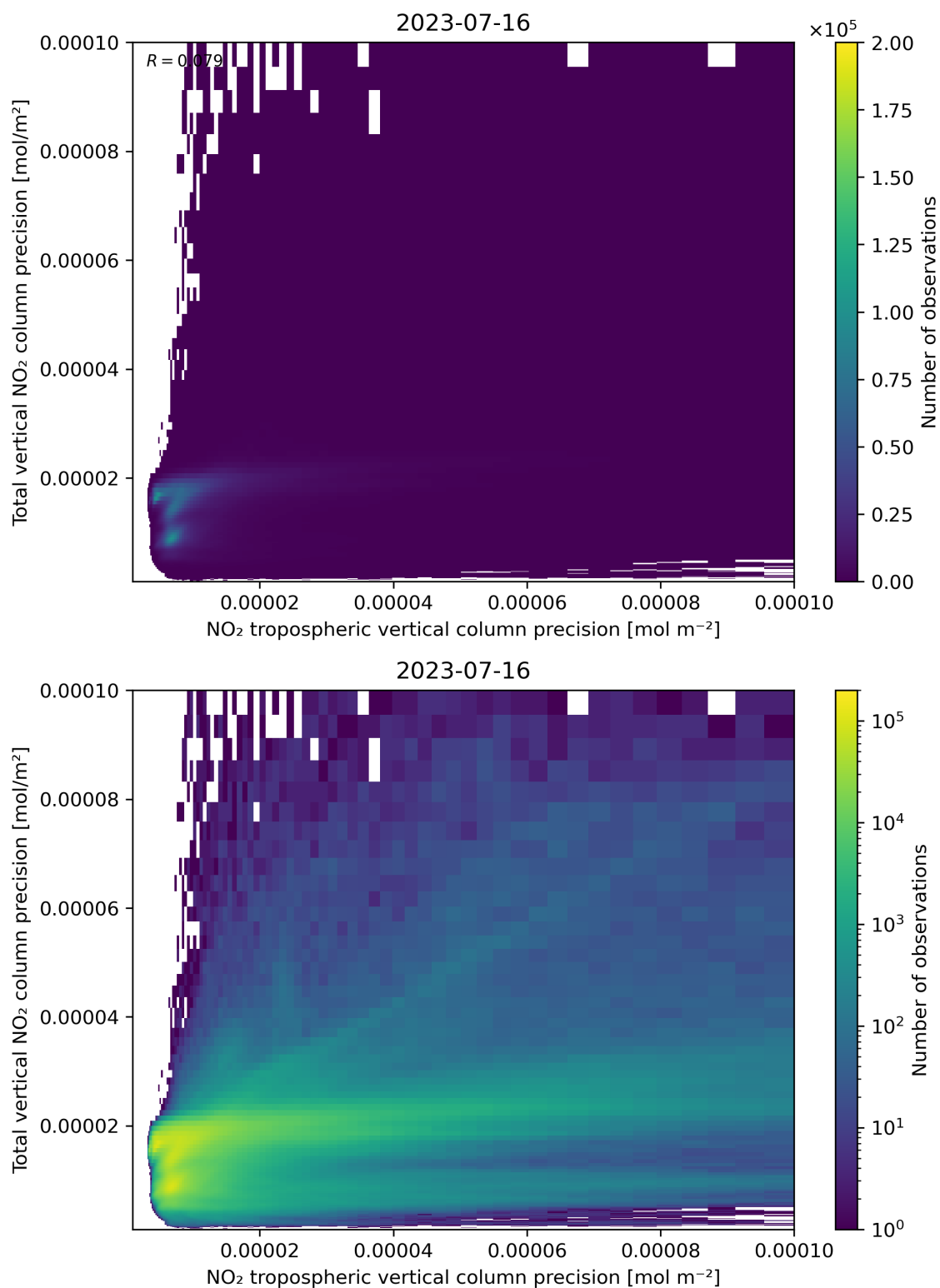
Figure 139: Scatter density plot of “NO 2 tropospheric vertical column precision” against “Total vertical NO 2 column precision” for 2023-07-15 to 2023-07-17.
