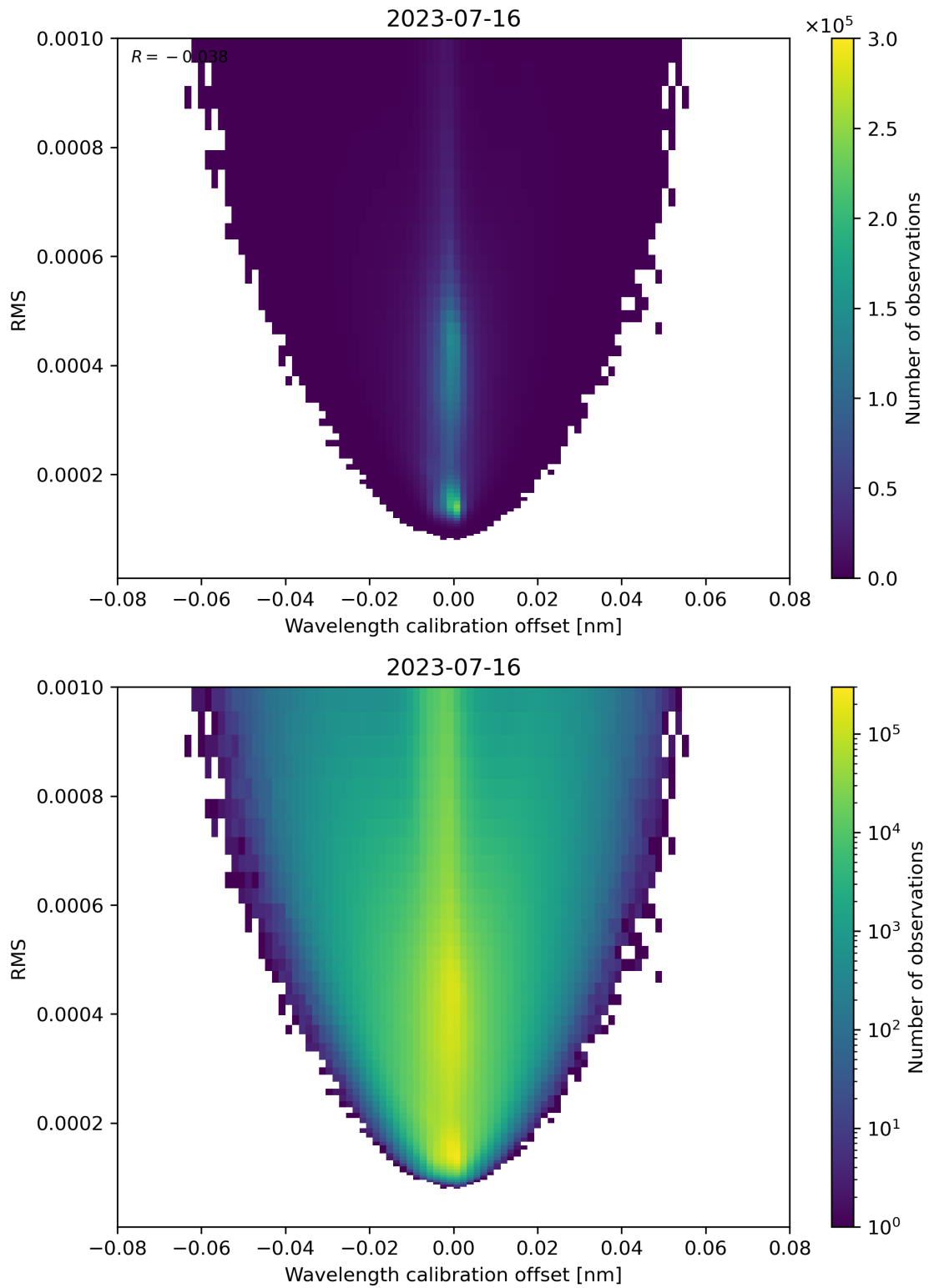
Figure 181: Scatter density plot of “Wavelength calibration offset” against “RMS” for 2023-07-15 to 2023-07-17.
