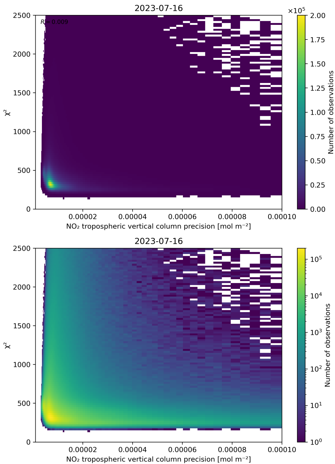
Figure 134: Scatter density plot of “NO 2 tropospheric vertical column precision” against “ \chi^2 ” for 2023-07-15 to 2023-07-17.
