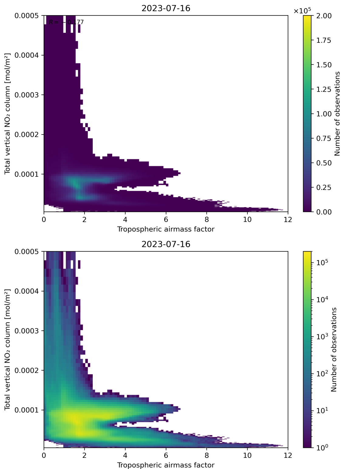
Figure 77: Scatter density plot of “Tropospheric airmass factor” against “Total vertical NO 2 column” for 2023-07-15 to 2023-07-17.
