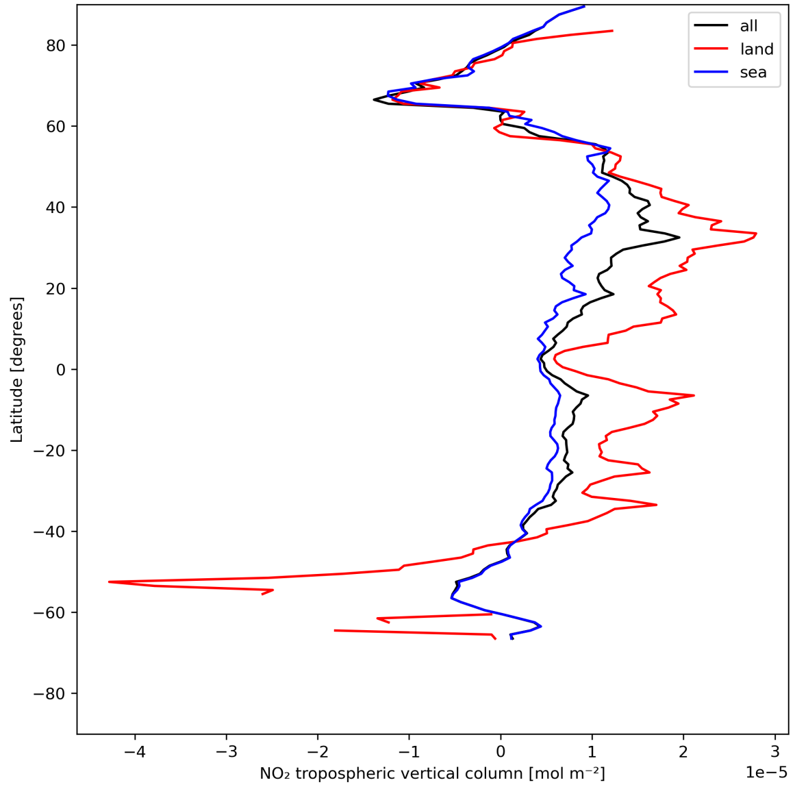
Figure 12: Zonal average of “NO 2 tropospheric vertical column” for 2023-07-15 to 2023-07-17.
