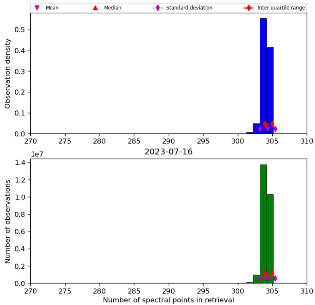
Figure 33: Histogram of “Number of spectral points in retrieval” for 2023-07-15 to 2023-07-17
