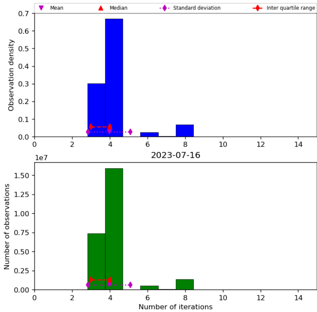
Figure 34: Histogram of “Number of iterations” for 2023-07-15 to 2023-07-17
