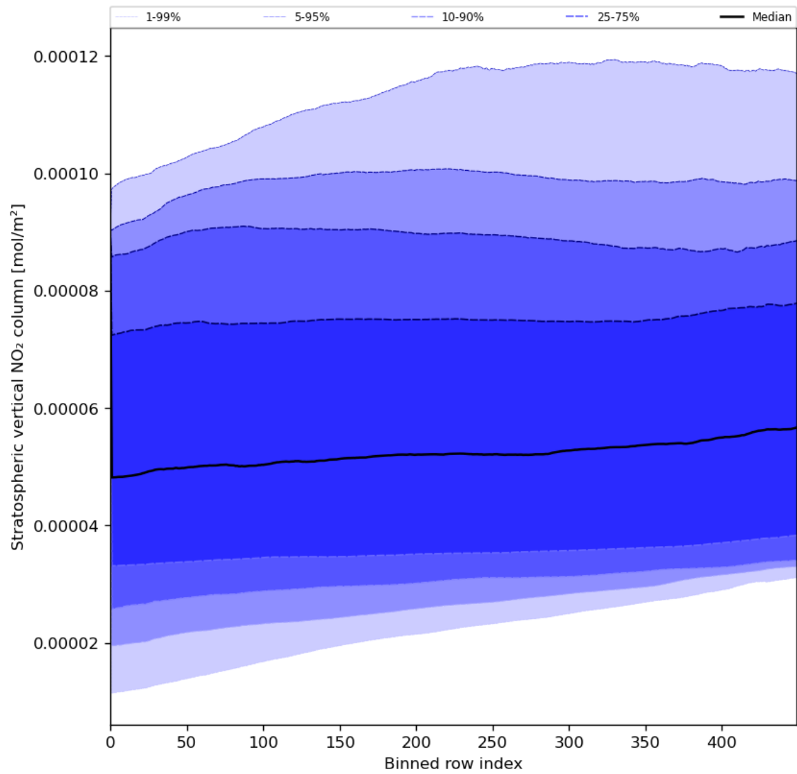
Figure 53: Along track statistics of “Stratospheric vertical NO 2 column” for 2023-07-15 to 2023-07-17
