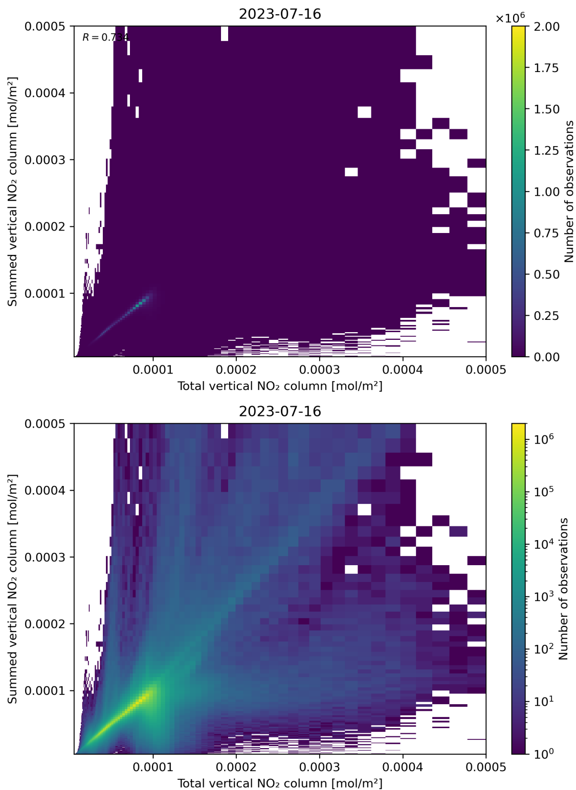
Figure 112: Scatter density plot of “Total vertical NO 2 column” against “Summed vertical NO 2 column” for 2023-07-15 to 2023-07-17.
