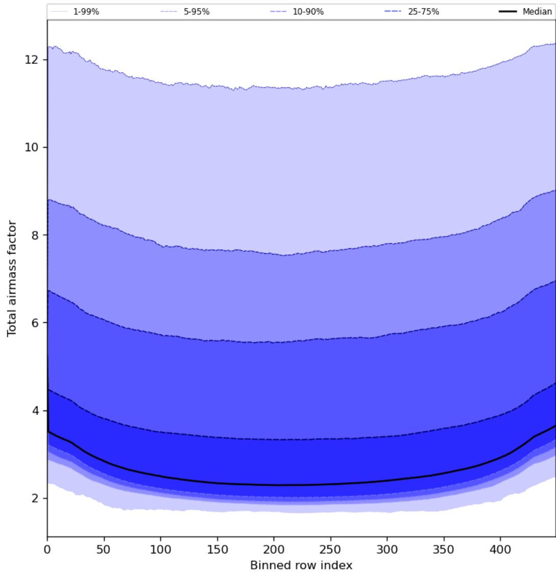
Figure 49: Along track statistics of “Total airmass factor” for 2023-07-15 to 2023-07-17
