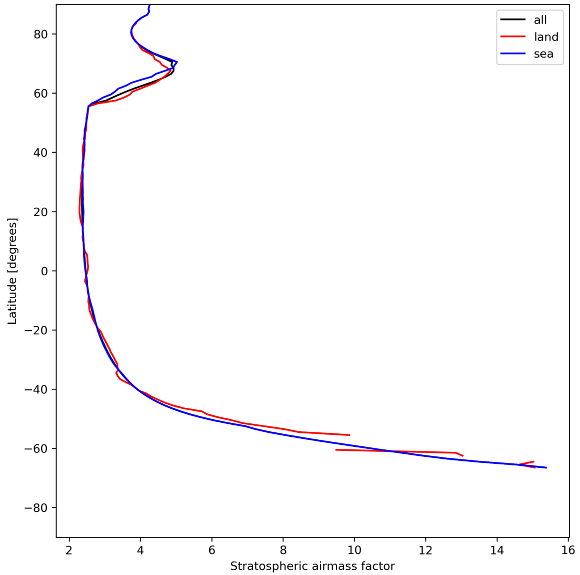
Figure 27: Zonal average of “Stratospheric airmass factor” for 2023-07-15 to 2023-07-17.
