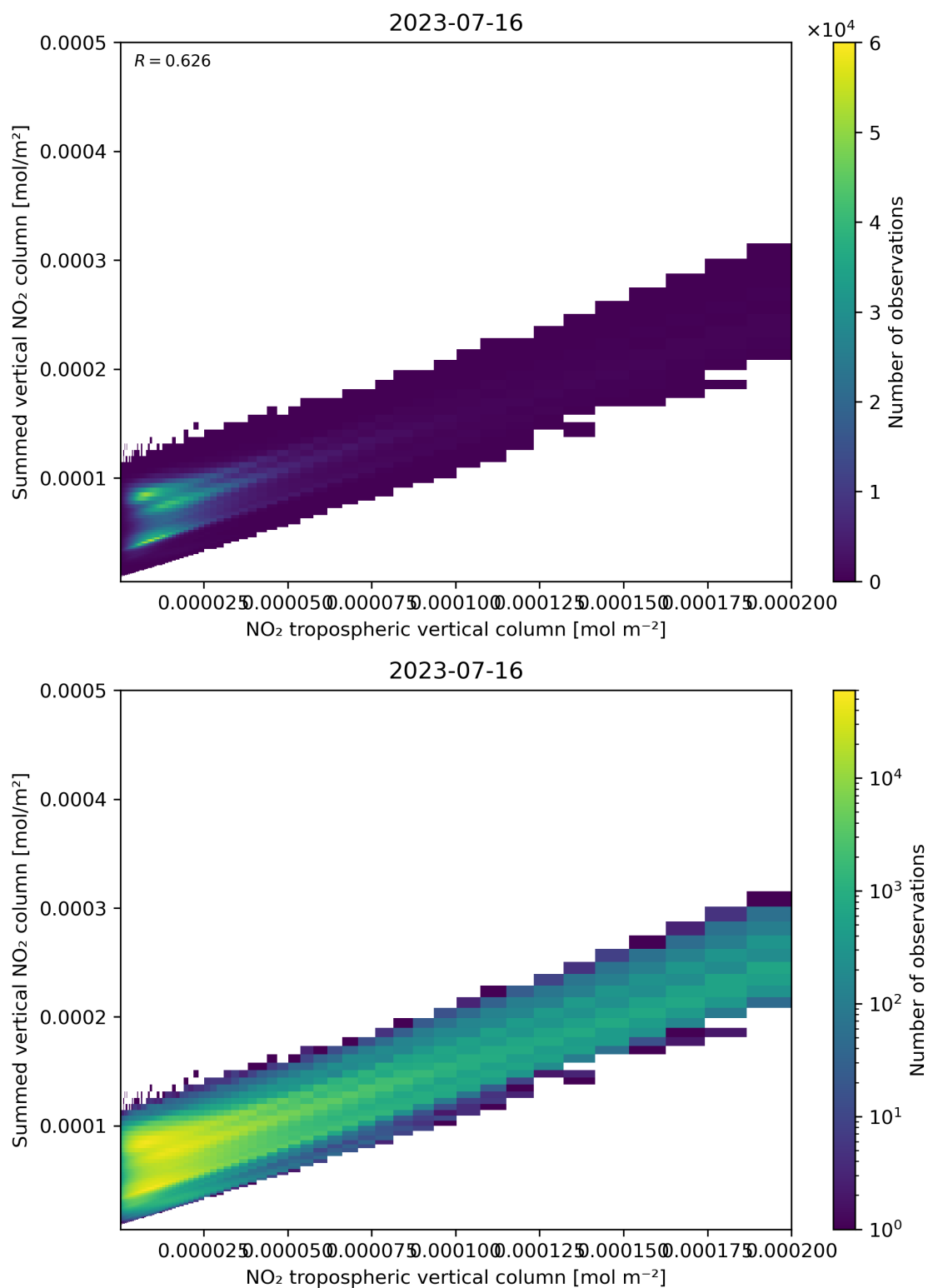
Figure 126: Scatter density plot of “NO 2 tropospheric vertical column” against “Summed vertical NO 2 column” for 2023-07-15 to 2023-07-17.
