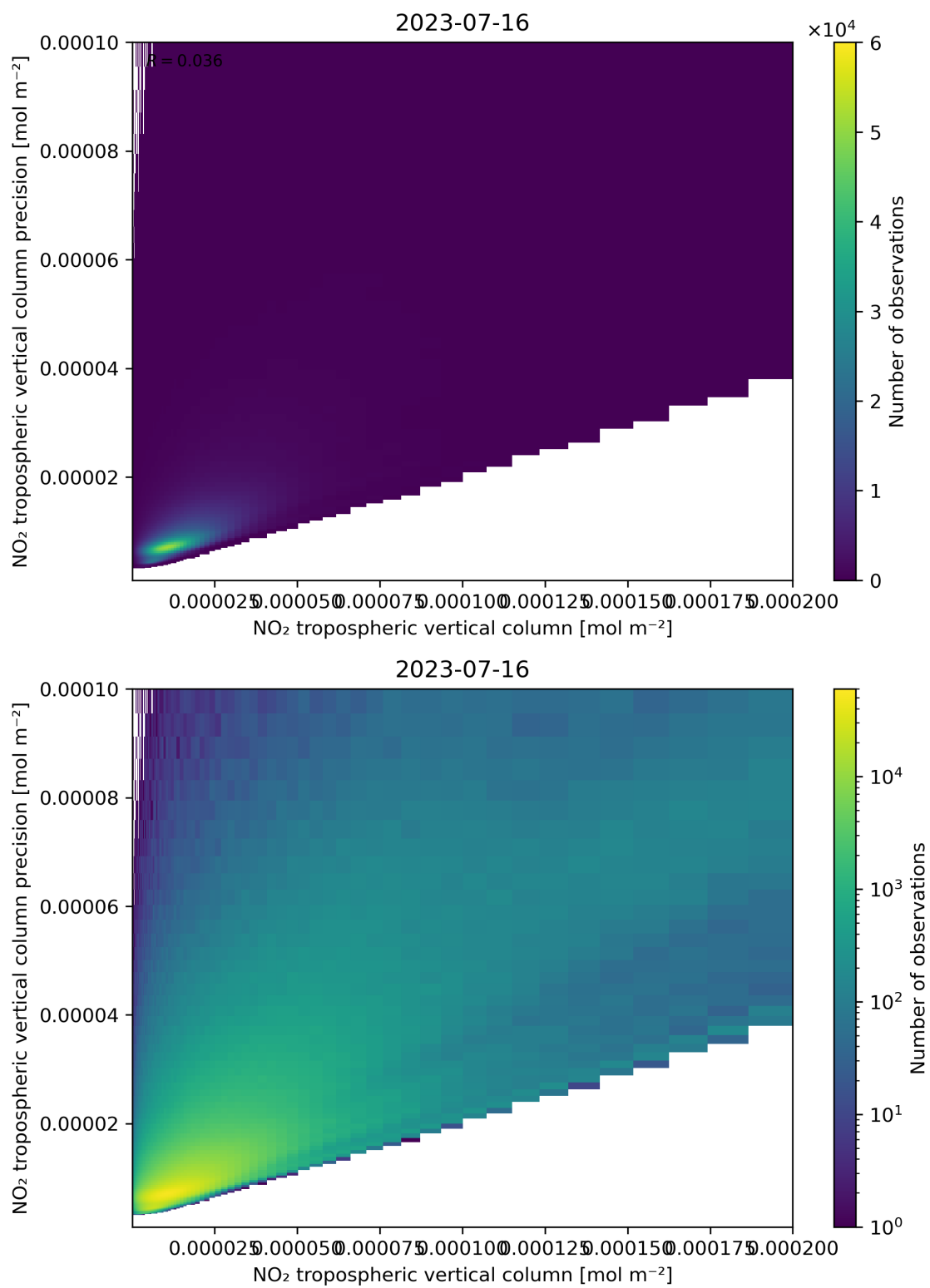
Figure 130: Scatter density plot of “NO 2 tropospheric vertical column” against “NO 2 tropospheric vertical column precision” for 2023-07-15 to 2023-07-17.
