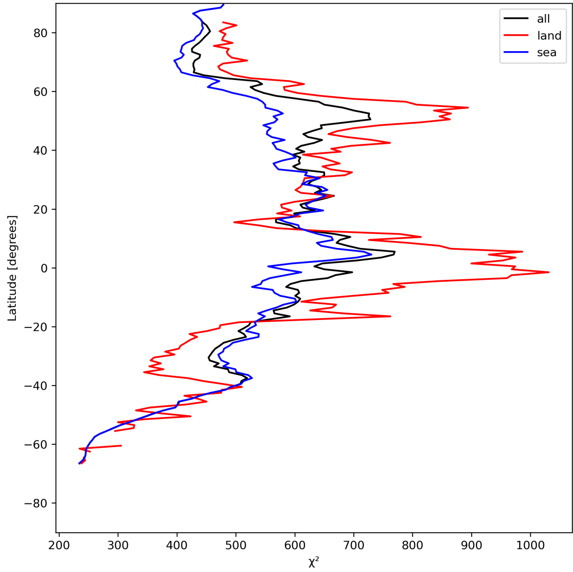
Figure 25: Zonal average of “ \chi^2 ” for 2023-07-15 to 2023-07-17.
