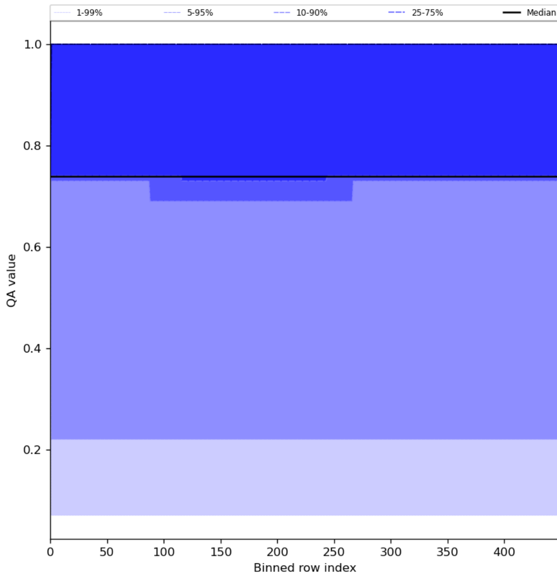
Figure 45: Along track statistics of “QA value” for 2023-07-16 to 2023-07-18
