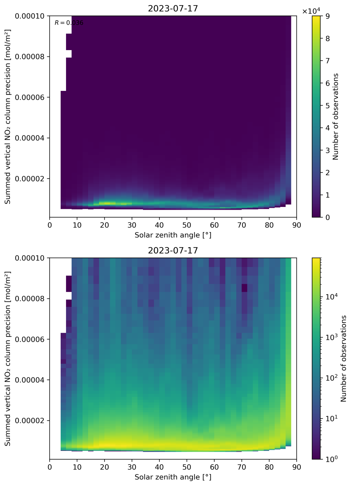
Figure 152: Scatter density plot of “Solar zenith angle” against “Summed vertical NO 2 column precision” for 2023-07-16 to 2023-07-18.
