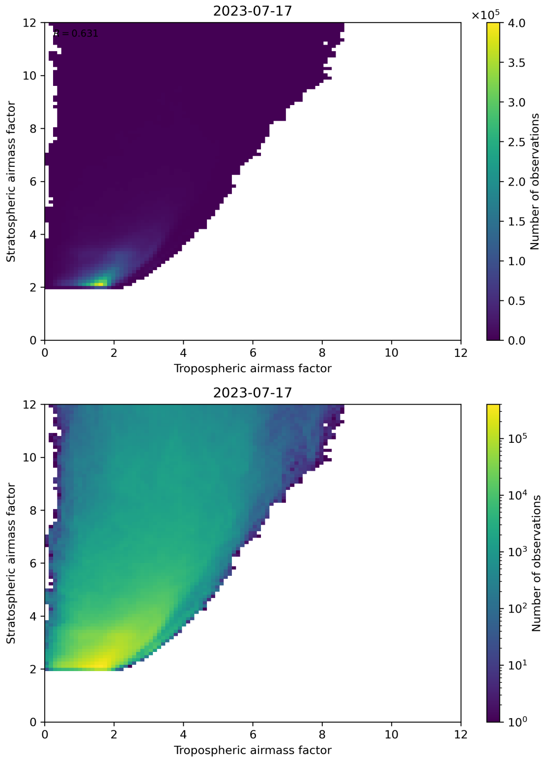
Figure 71: Scatter density plot of “Tropospheric airmass factor” against “Stratospheric airmass factor” for 2023-07-16 to 2023-07-18.
