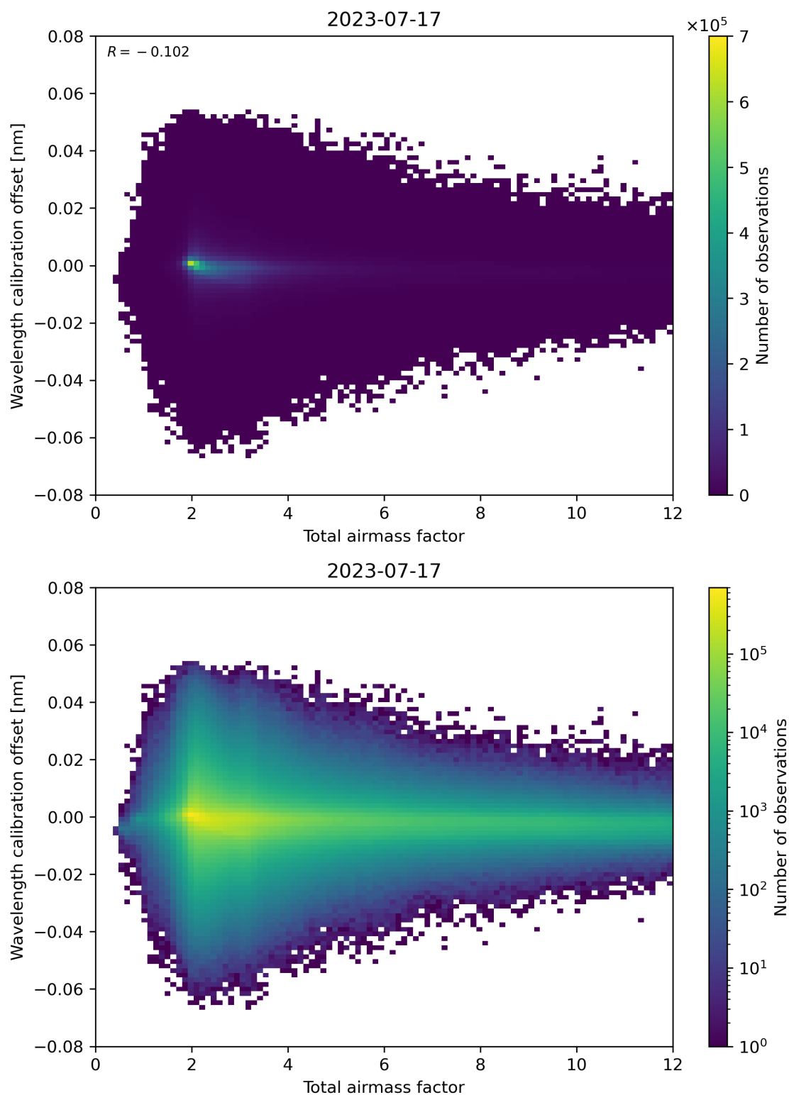
Figure 70: Scatter density plot of “Total airmass factor” against “Wavelength calibration offset” for 2023-07-16 to 2023-07-18.
