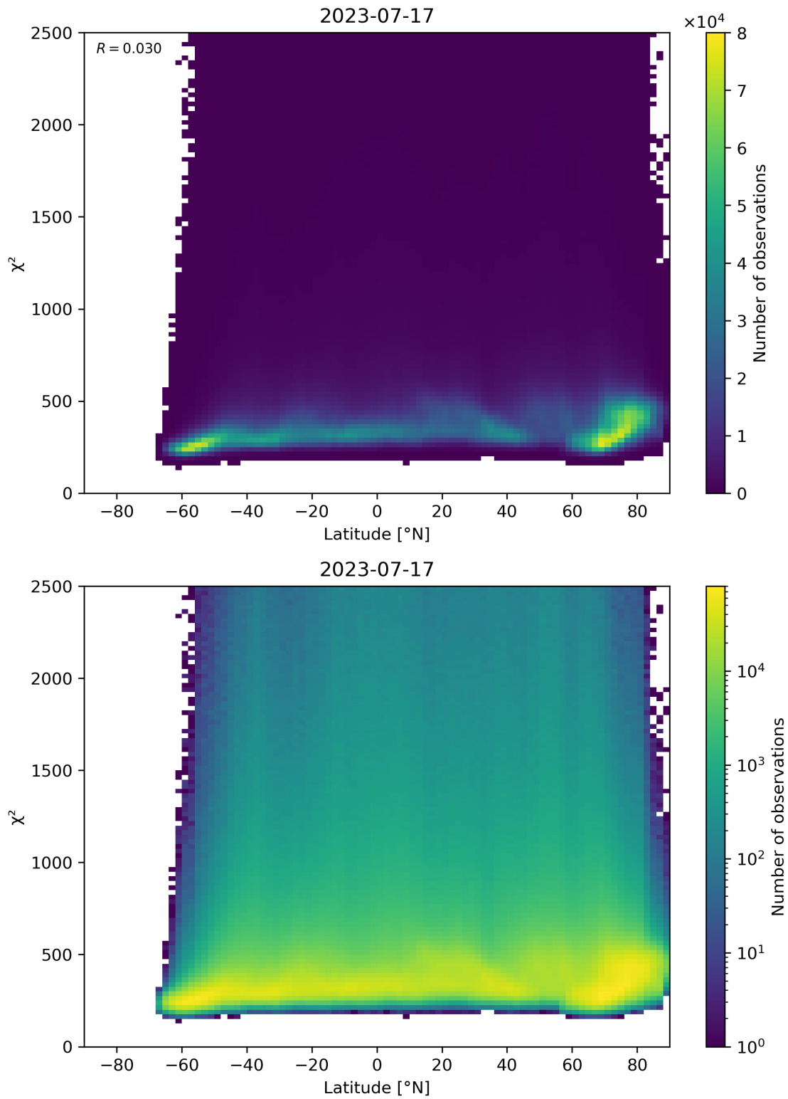
Figure 86: Scatter density plot of “Latitude” against “ \chi^2 ” for 2023-07-16 to 2023-07-18.
