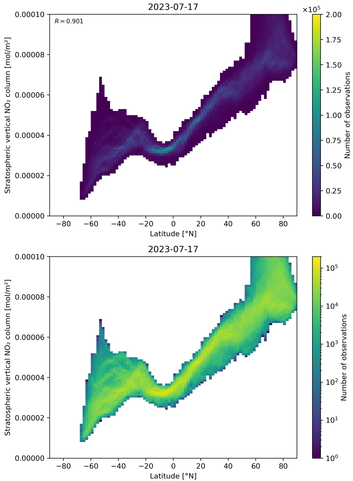
Figure 87: Scatter density plot of “Latitude” against “Stratospheric vertical \text{NO}_2 column” for 2023-07-16 to 2023-07-18.
