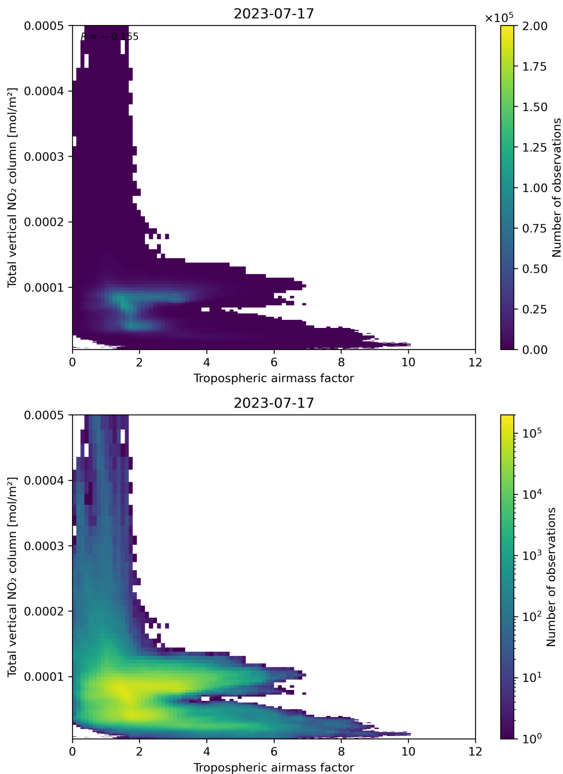
Figure 77: Scatter density plot of “Tropospheric airmass factor” against “Total vertical NO 2 column” for 2023-07-16 to 2023-07-18.
