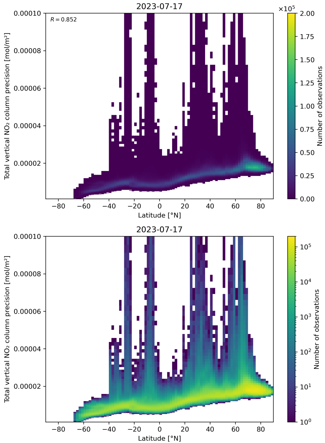
Figure 91: Scatter density plot of “Latitude” against “Total vertical NO 2 column precision” for 2023-07-16 to 2023-07-18.
