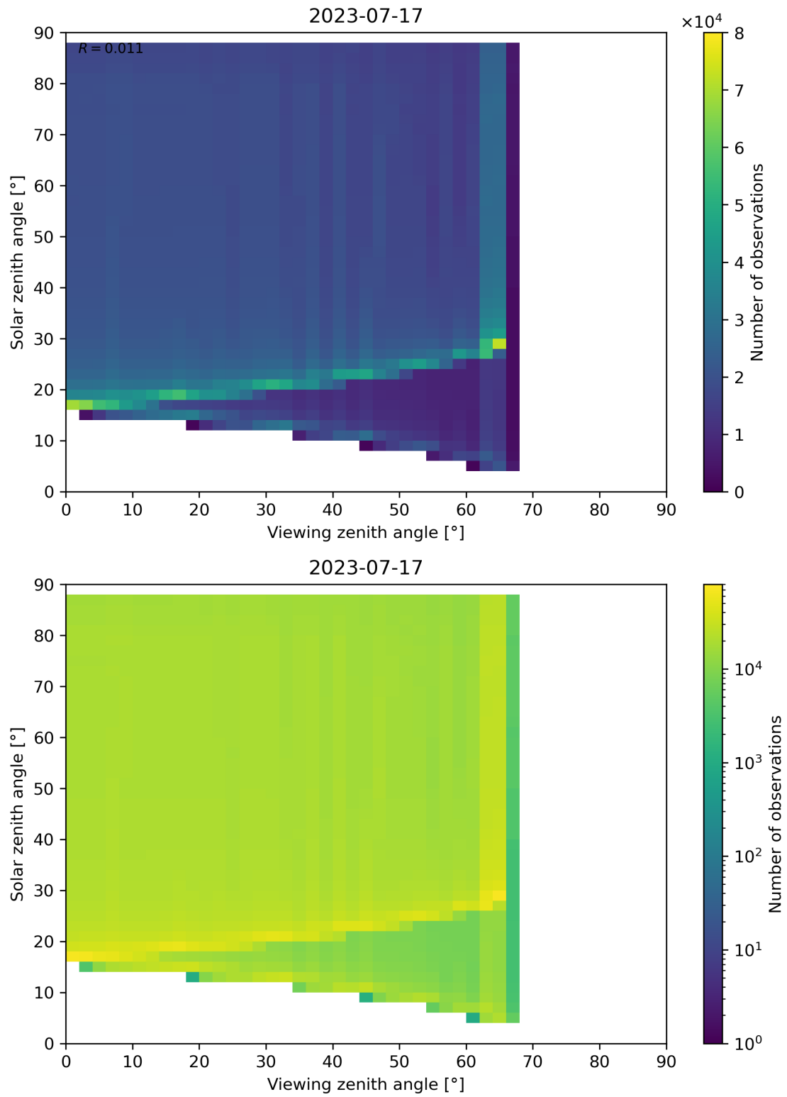
Figure 172: Scatter density plot of “Viewing zenith angle” against “Solar zenith angle” for 2023-07-16 to 2023-07-18.
