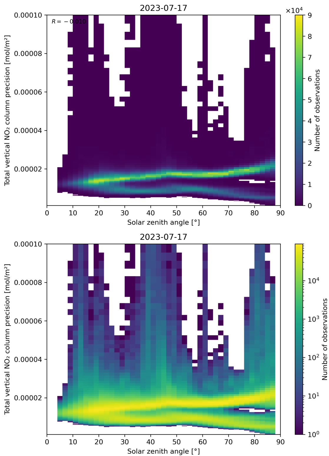
Figure 154: Scatter density plot of “Solar zenith angle” against “Total vertical NO 2 column precision” for 2023-07-16 to 2023-07-18.
