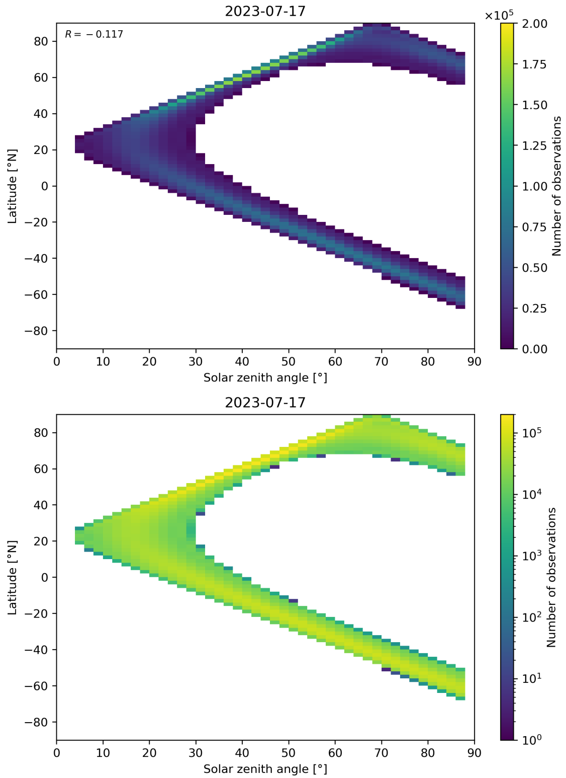
Figure 149: Scatter density plot of “Solar zenith angle” against “Latitude” for 2023-07-16 to 2023-07-18.
