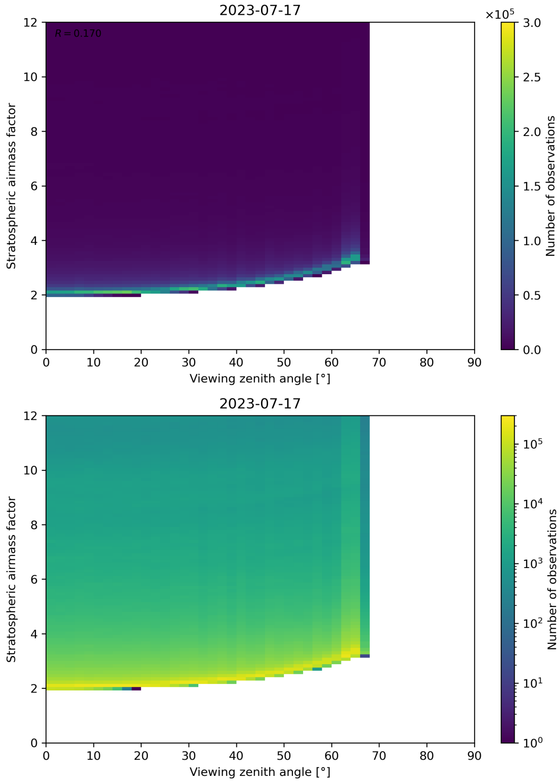
Figure 159: Scatter density plot of “Viewing zenith angle” against “Stratospheric airmass factor” for 2023-07-16 to 2023-07-18.
