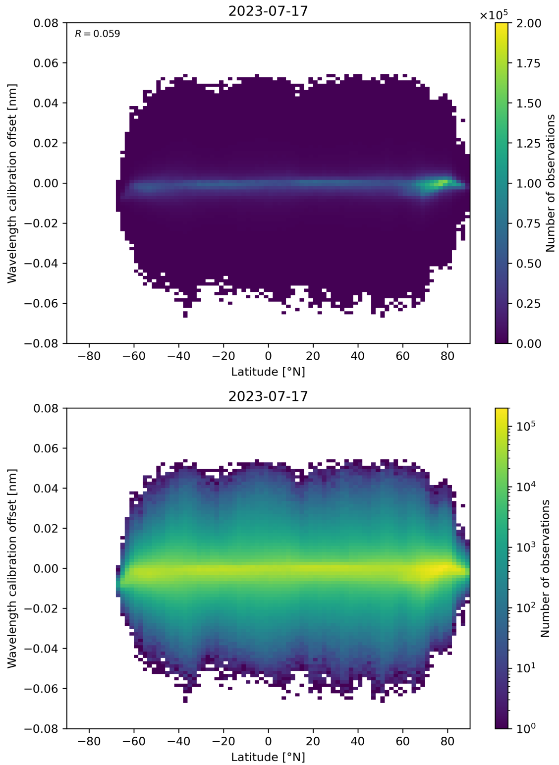
Figure 95: Scatter density plot of “Latitude” against “Wavelength calibration offset” for 2023-07-16 to 2023-07-18.
