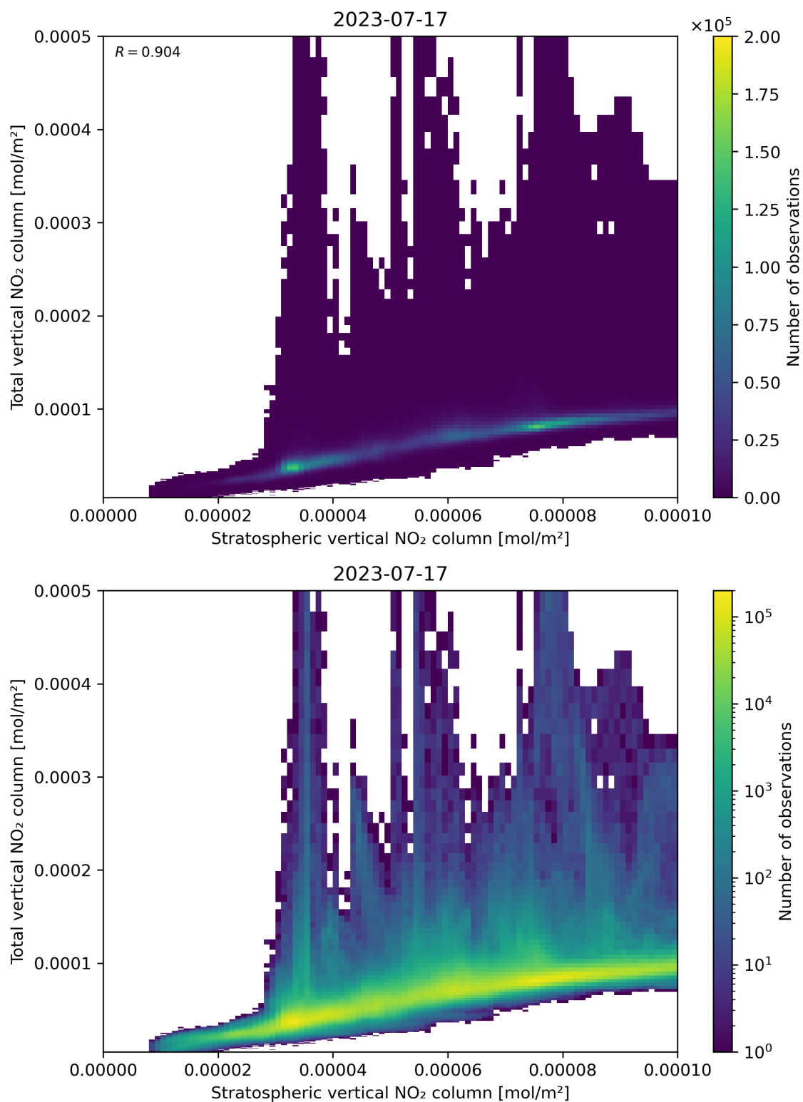
Figure 100: Scatter density plot of “Stratospheric vertical NO 2 column” against “Total vertical NO 2 column” for 2023-07-16 to 2023-07-18.
