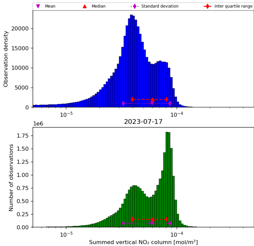
Figure 40: Histogram of “Summed vertical NO 2 column” for 2023-07-16 to 2023-07-18
