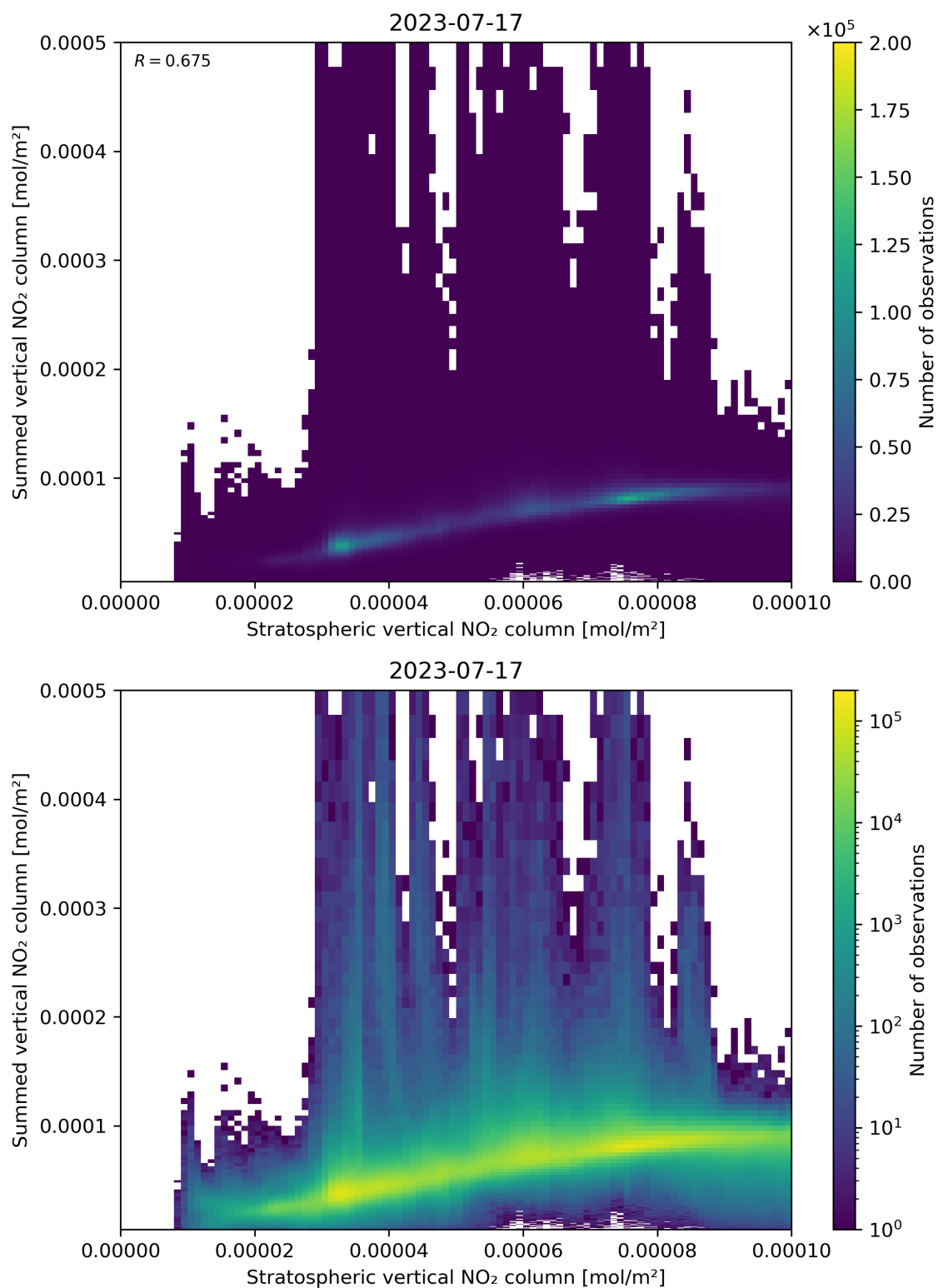
Figure 98: Scatter density plot of “Stratospheric vertical NO 2 column” against “Summed vertical NO 2 column” for 2023-07-16 to 2023-07-18.
