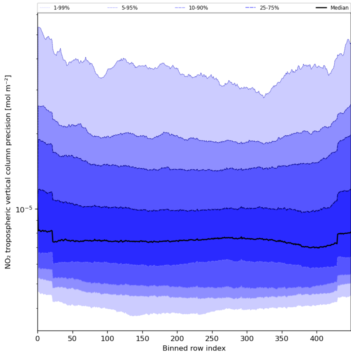
Figure 47: Along track statistics of “NO 2 tropospheric vertical column precision” for 2023-07-16 to 2023-07-18
