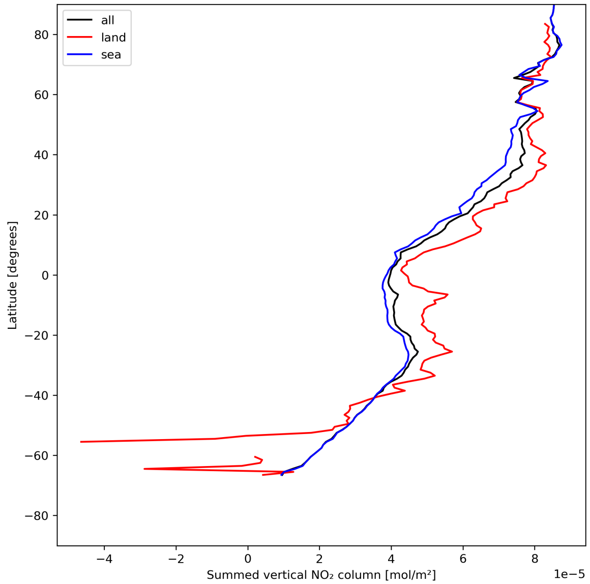
Figure 23: Zonal average of “Summed vertical NO 2 column” for 2023-07-16 to 2023-07-18.
