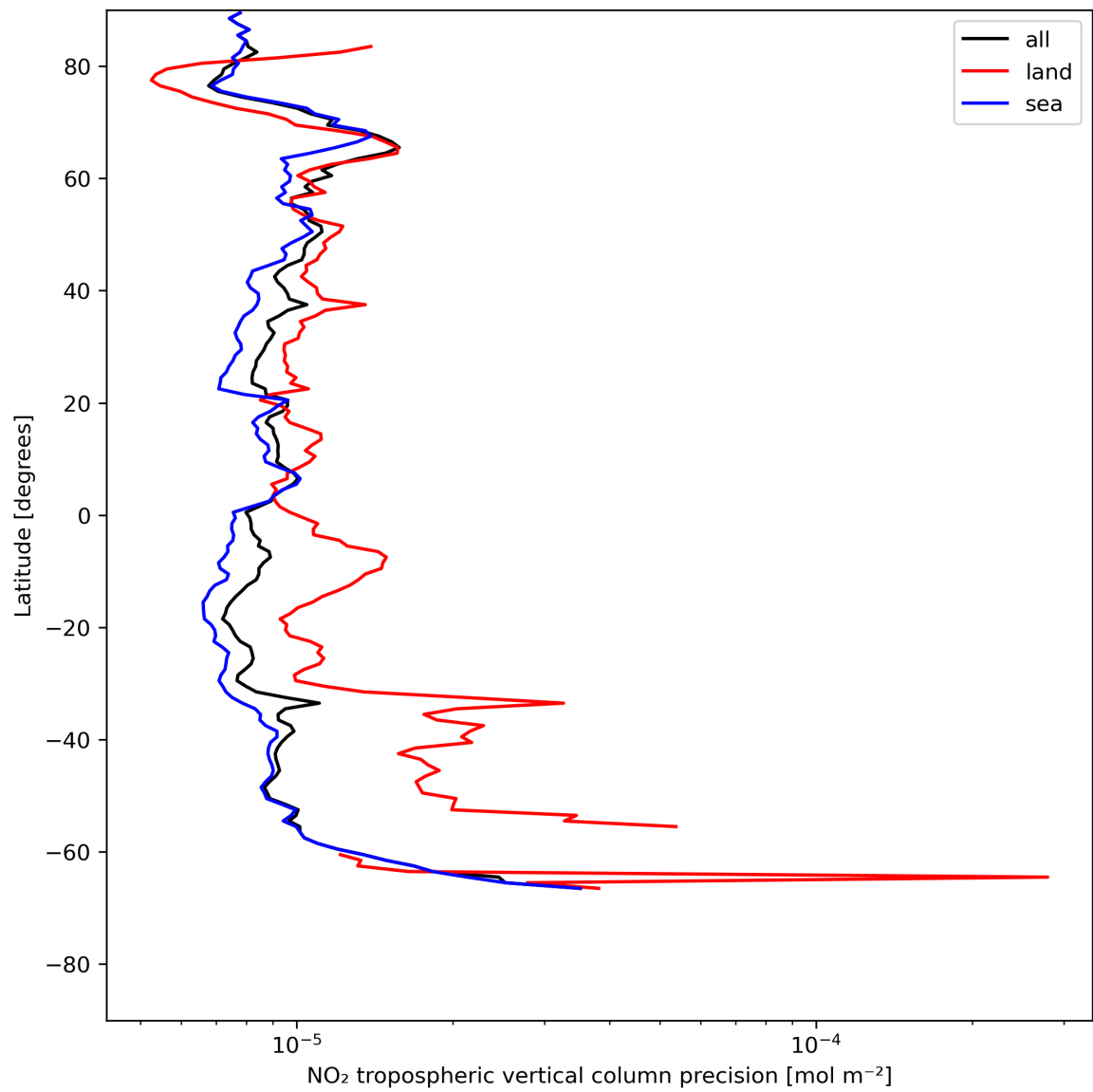
Figure 13: Zonal average of “NO 2 tropospheric vertical column precision” for 2023-07-16 to 2023-07-18.
