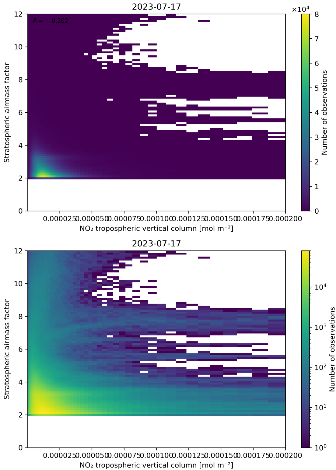
Figure 121: Scatter density plot of “NO 2 tropospheric vertical column” against “Stratospheric air mass factor” for 2023-07-16 to 2023-07-18.
