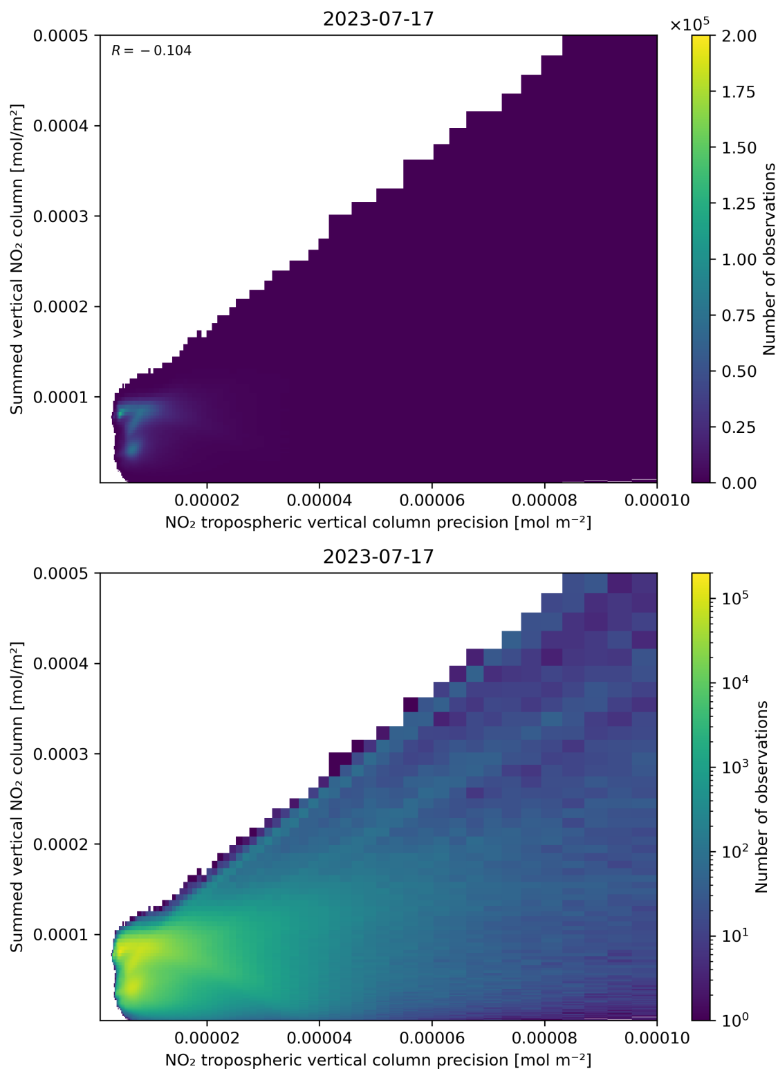
Figure 136: Scatter density plot of “NO 2 tropospheric vertical column precision” against “Summed vertical NO 2 column” for 2023-07-16 to 2023-07-18.
