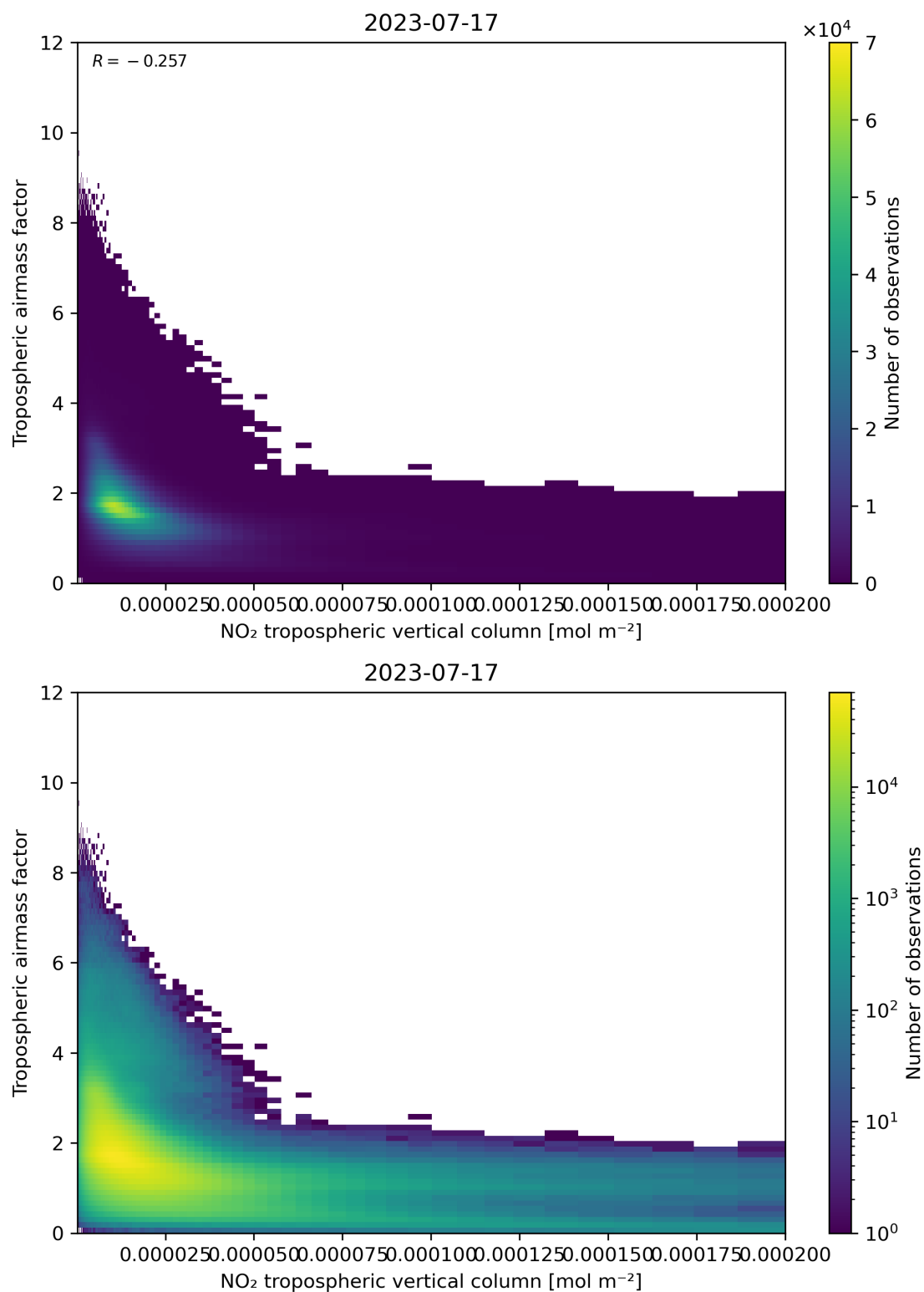
Figure 123: Scatter density plot of “NO 2 tropospheric vertical column” against “Tropospheric air mass factor” for 2023-07-16 to 2023-07-18.
