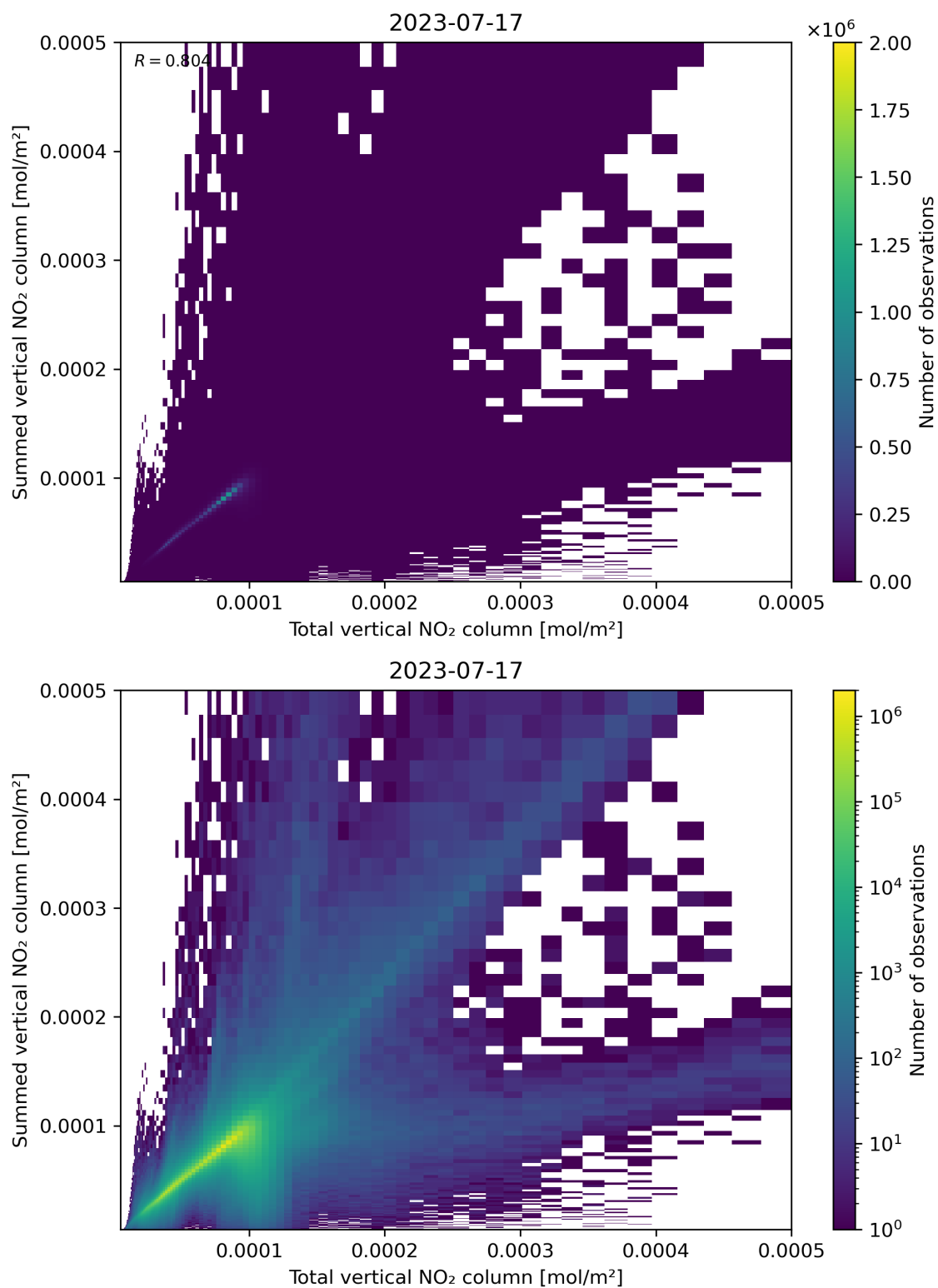
Figure 112: Scatter density plot of “Total vertical NO 2 column” against “Summed vertical NO 2 column” for 2023-07-16 to 2023-07-18.
