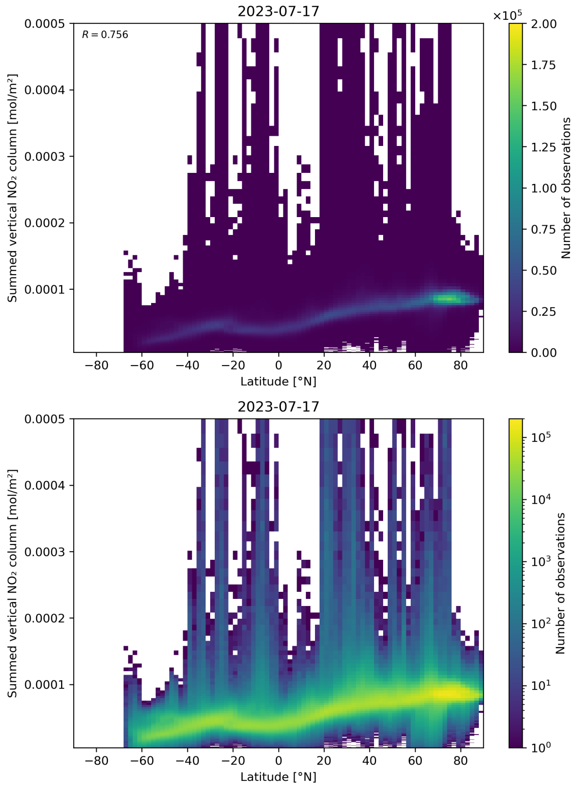
Figure 88: Scatter density plot of “Latitude” against “Summed vertical NO 2 column” for 2023-07-16 to 2023-07-18.
