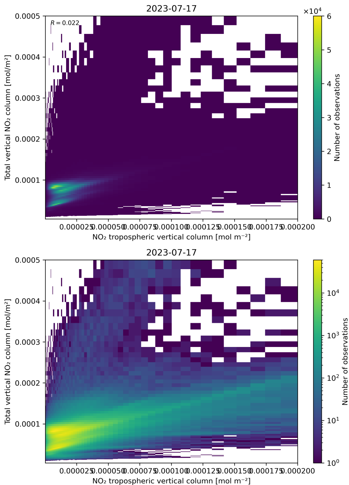
Figure 128: Scatter density plot of “NO 2 tropospheric vertical column” against “Total vertical NO 2 column” for 2023-07-16 to 2023-07-18.
