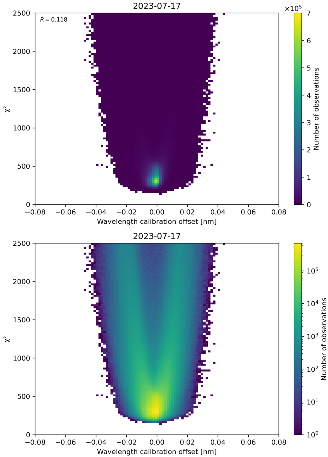
Figure 175: Scatter density plot of “Wavelength calibration offset” against “ \chi^2 ” for 2023-07-16 to 2023-07-18.
