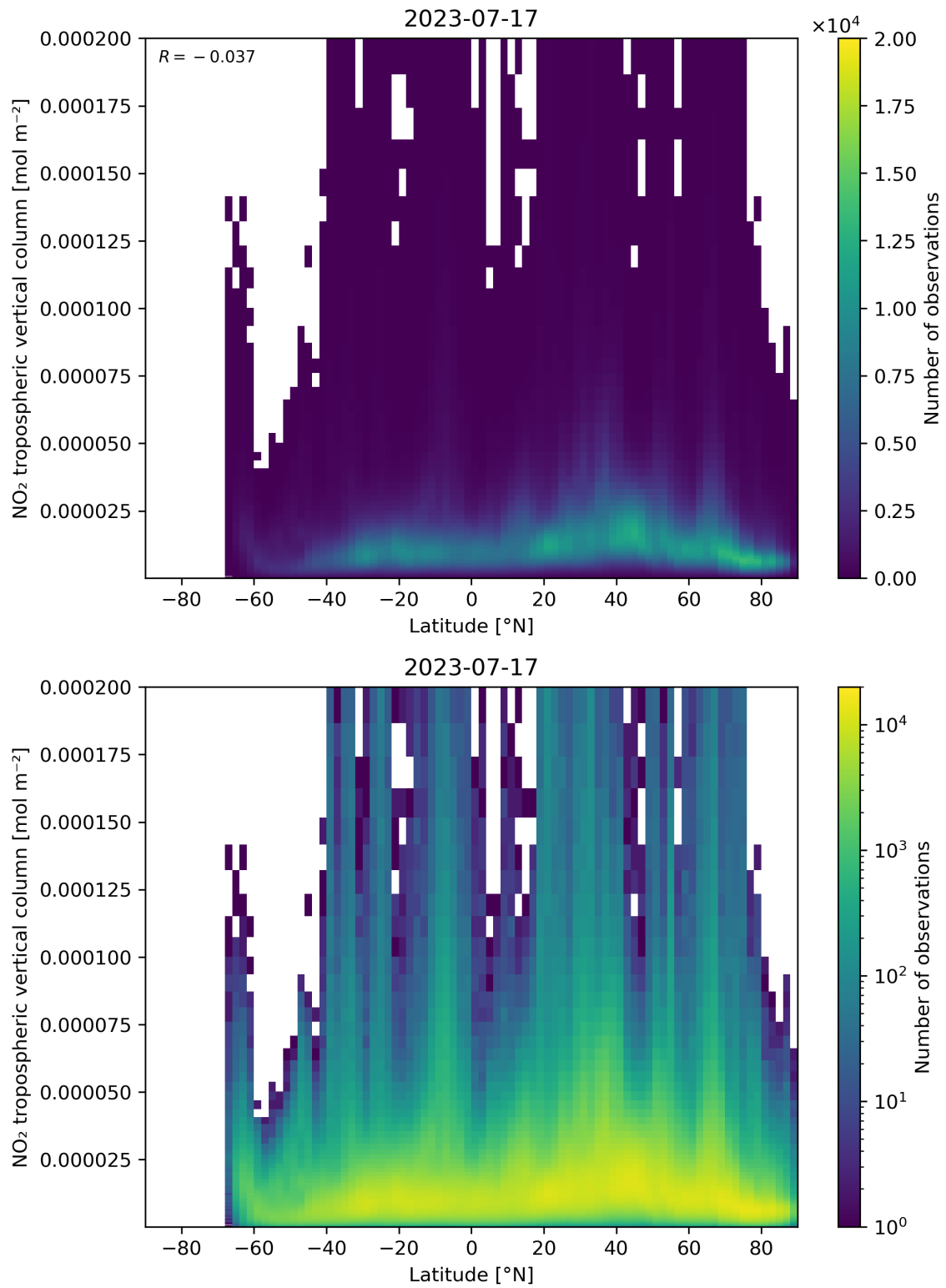
Figure 92: Scatter density plot of “Latitude” against “NO 2 tropospheric vertical column” for 2023-07-16 to 2023-07-18.
