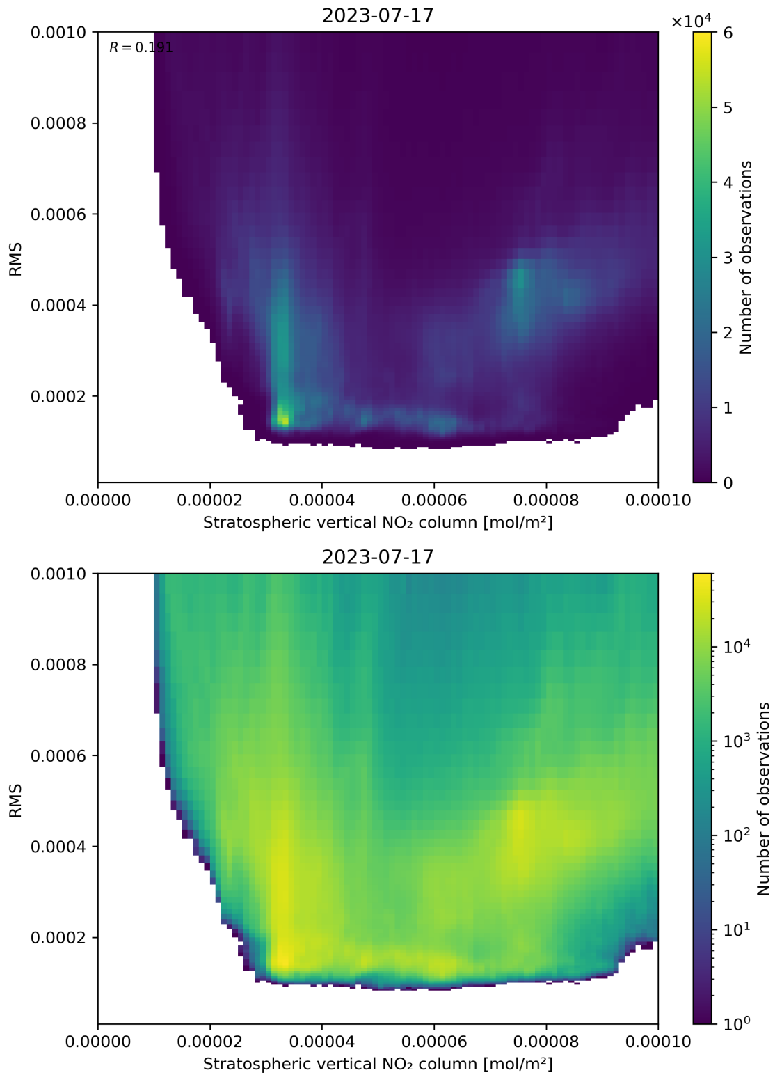
Figure 102: Scatter density plot of “Stratospheric vertical NO 2 column” against “RMS” for 2023-07-16 to 2023-07-18.
