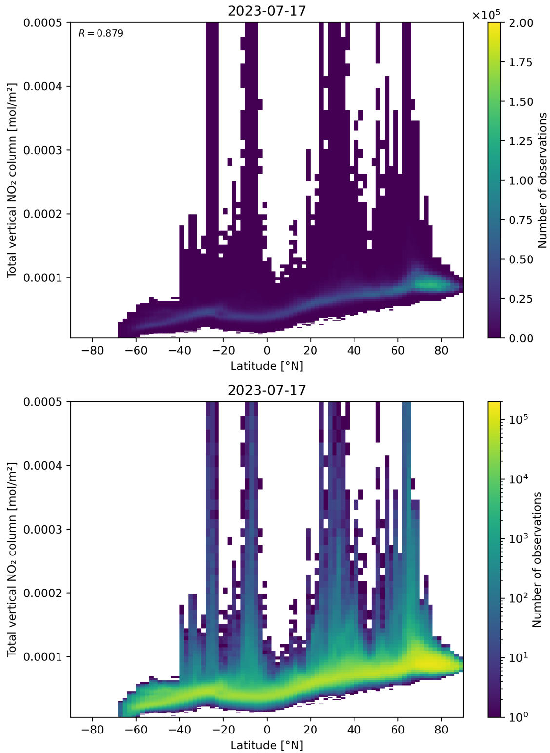
Figure 90: Scatter density plot of “Latitude” against “Total vertical NO 2 column” for 2023-07-16 to 2023-07-18.
