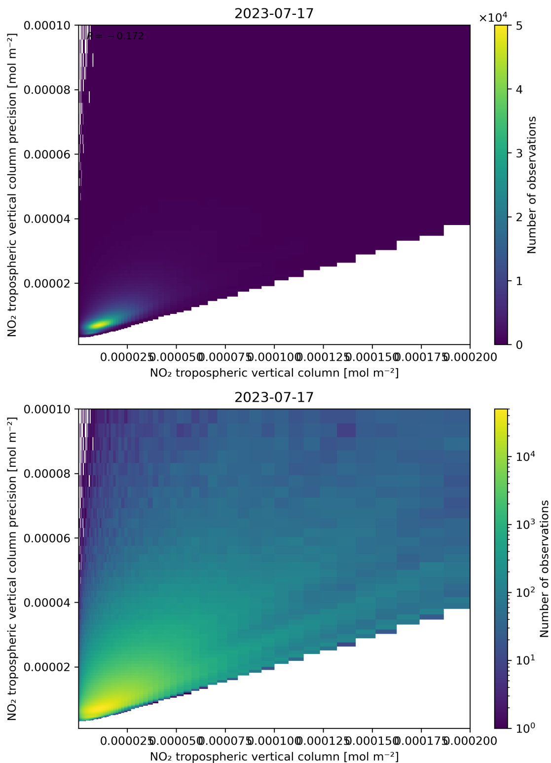
Figure 130: Scatter density plot of “NO 2 tropospheric vertical column” against “NO 2 tropospheric vertical column precision” for 2023-07-16 to 2023-07-18.
