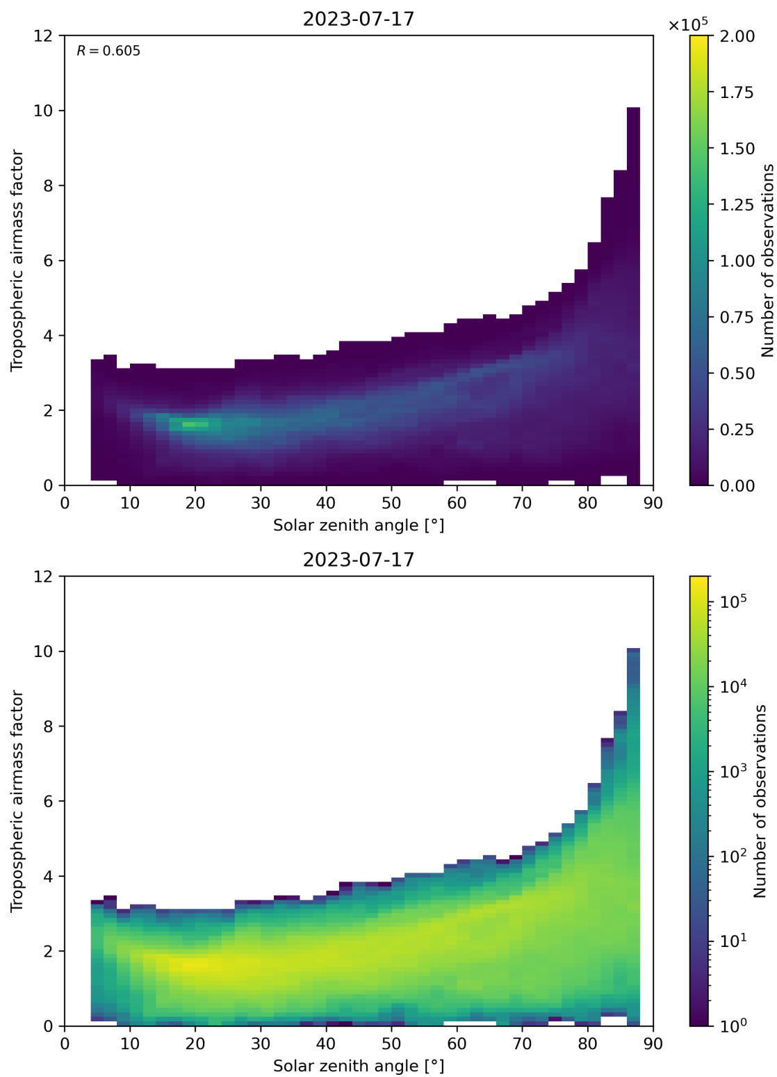
Figure 147: Scatter density plot of “Solar zenith angle” against “Tropospheric airmass factor” for 2023-07-16 to 2023-07-18.
