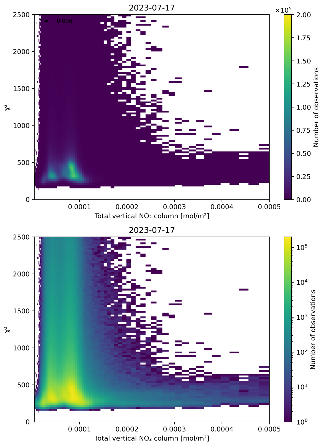
Figure 111: Scatter density plot of “Total vertical NO 2 column” against “ \chi^2 ” for 2023-07-16 to 2023-07-18.
