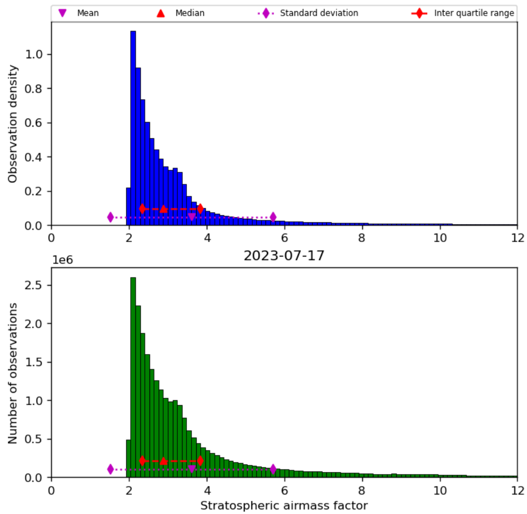
Figure 44: Histogram of “Stratospheric airmass factor” for 2023-07-16 to 2023-07-18
