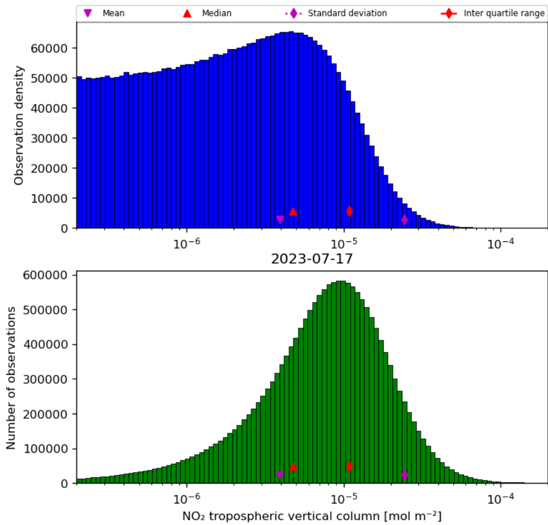
Figure 29: Histogram of “NO 2 tropospheric vertical column” for 2023-07-16 to 2023-07-18
