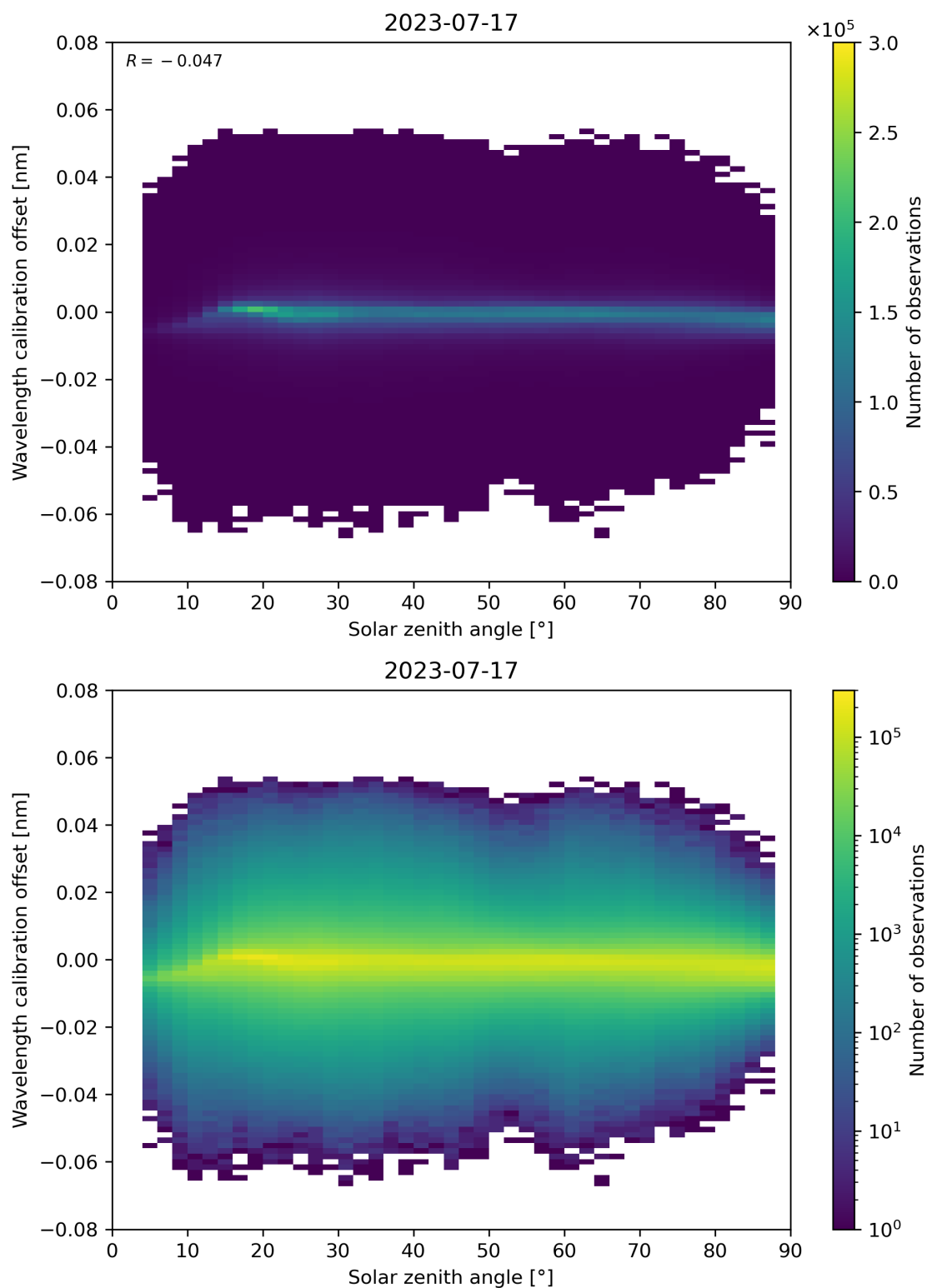
Figure 158: Scatter density plot of “Solar zenith angle” against “Wavelength calibration offset” for 2023-07-16 to 2023-07-18.
