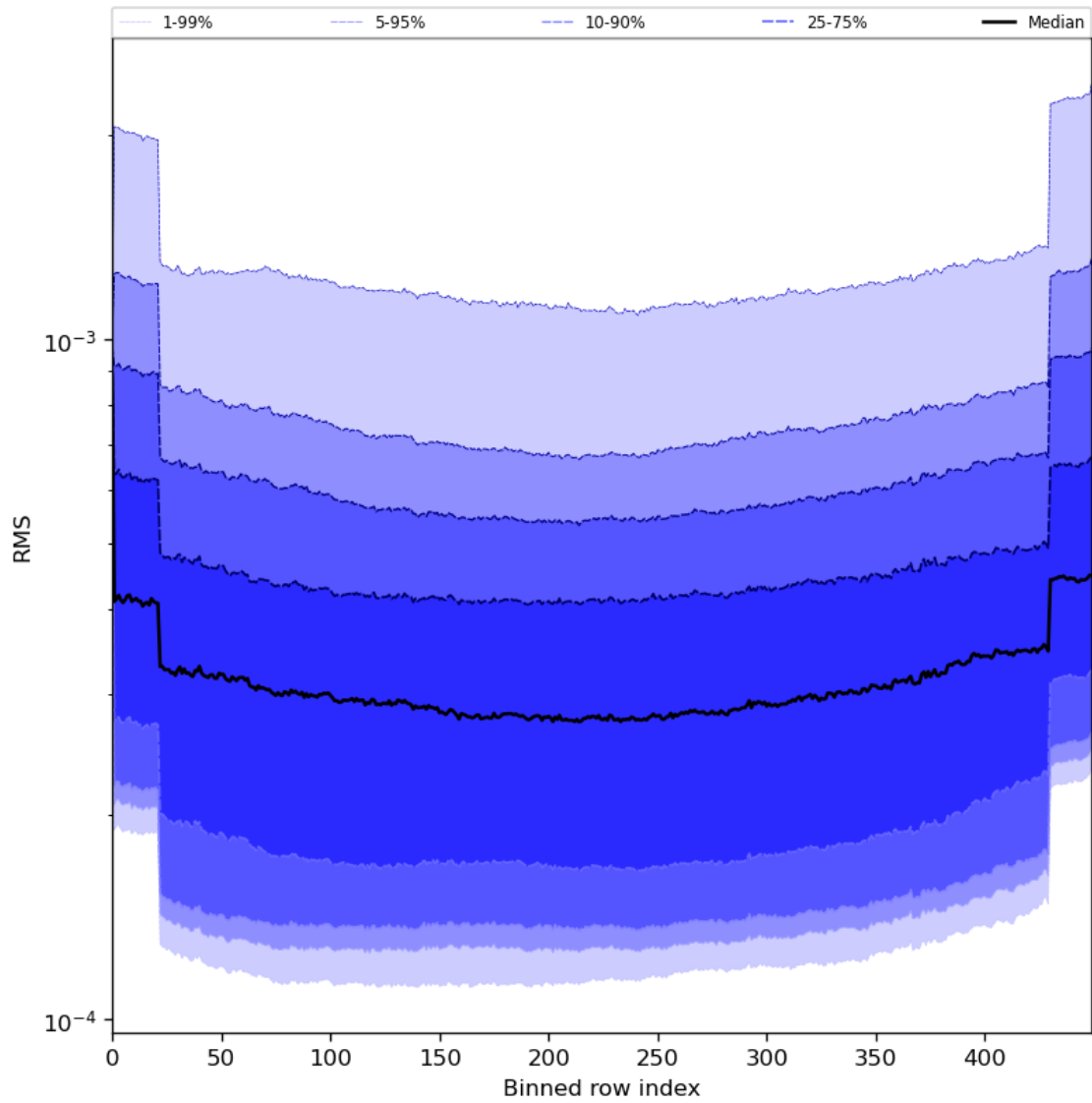
Figure 60: Along track statistics of “RMS” for 2023-07-16 to 2023-07-18
