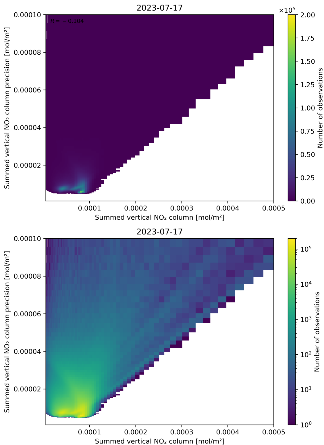
Figure 105: Scatter density plot of “Summed vertical NO 2 column” against “Summed vertical NO 2 column precision” for 2023-07-16 to 2023-07-18.
