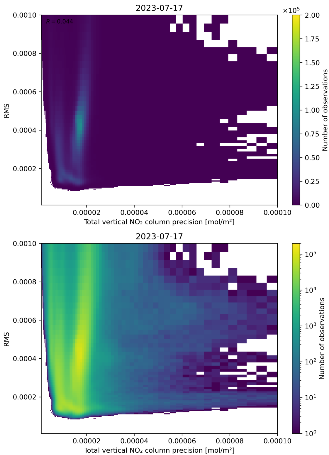
Figure 119: Scatter density plot of “Total vertical NO 2 column precision” against “RMS” for 2023-07-16 to 2023-07-18.
