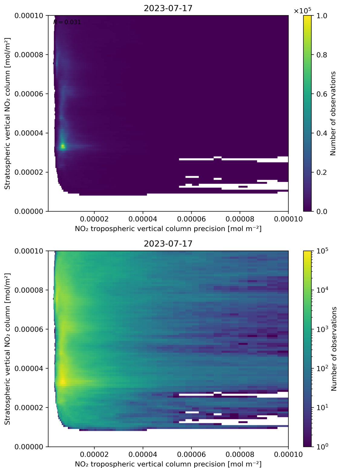
Figure 135: Scatter density plot of “NO 2 tropospheric vertical column precision” against “Stratospheric vertical NO 2 column” for 2023-07-16 to 2023-07-18.
