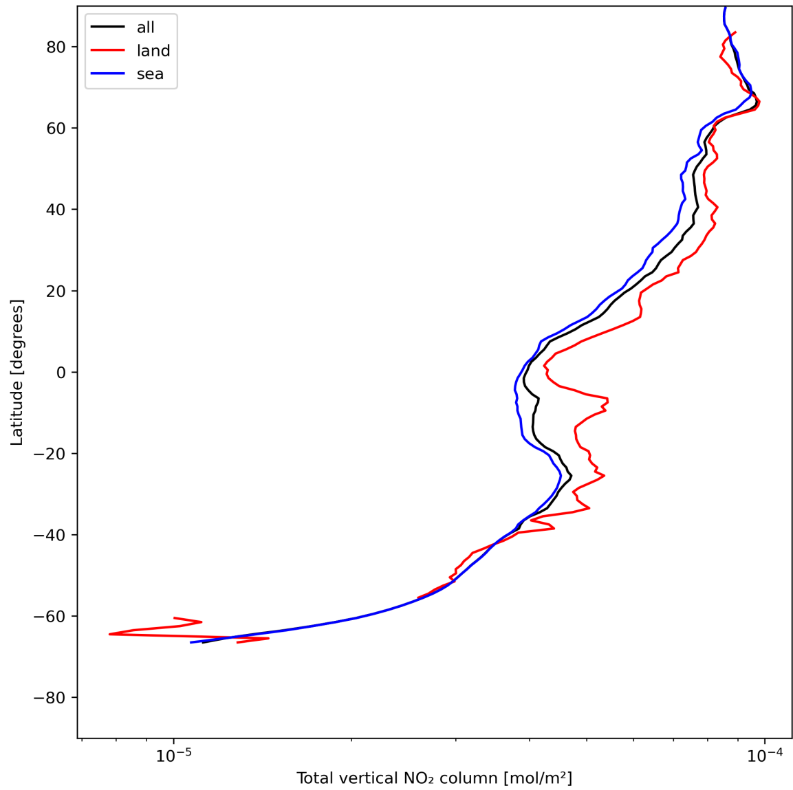
Figure 21: Zonal average of “Total vertical NO 2 column” for 2023-07-16 to 2023-07-18.
