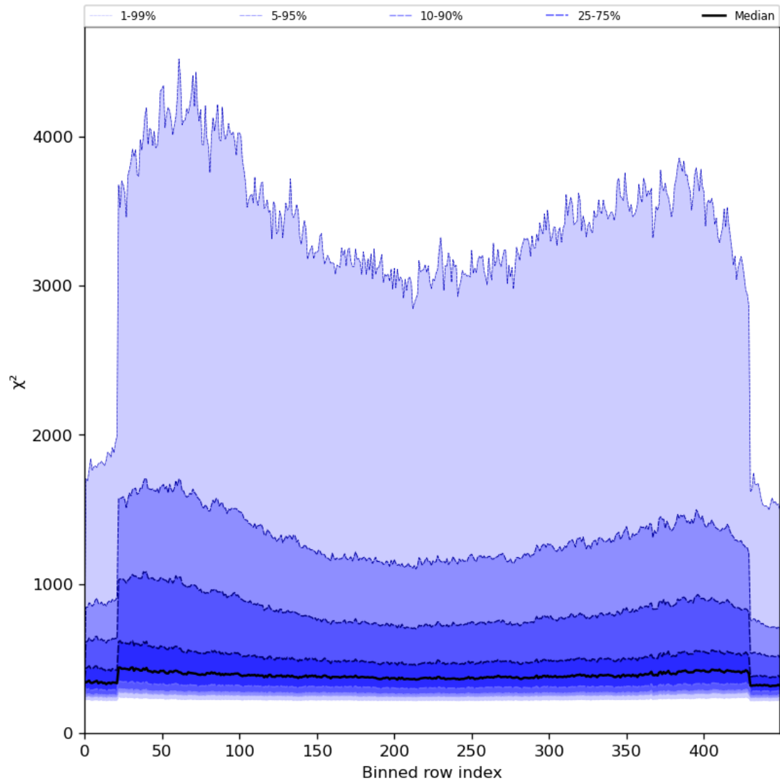
Figure 59: Along track statistics of “ \chi^2 ” for 2023-07-16 to 2023-07-18
