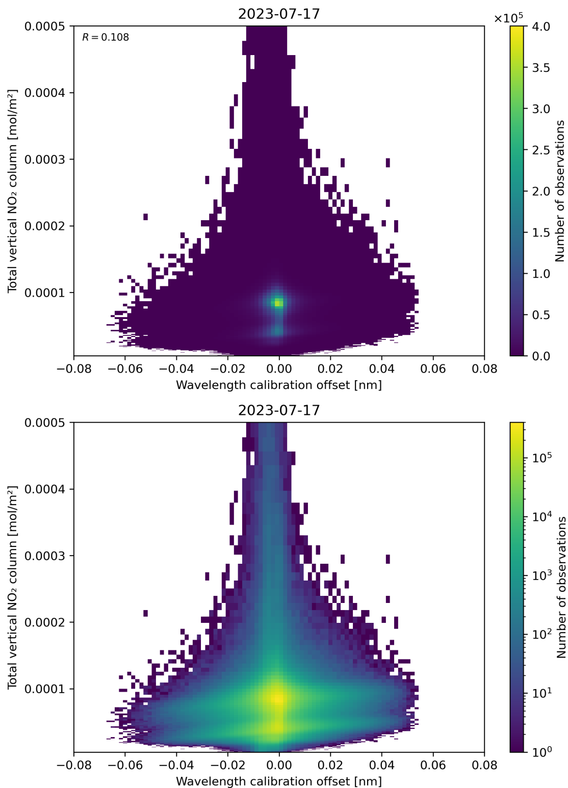
Figure 179: Scatter density plot of “Wavelength calibration offset” against “Total vertical NO 2 column” for 2023-07-16 to 2023-07-18.
