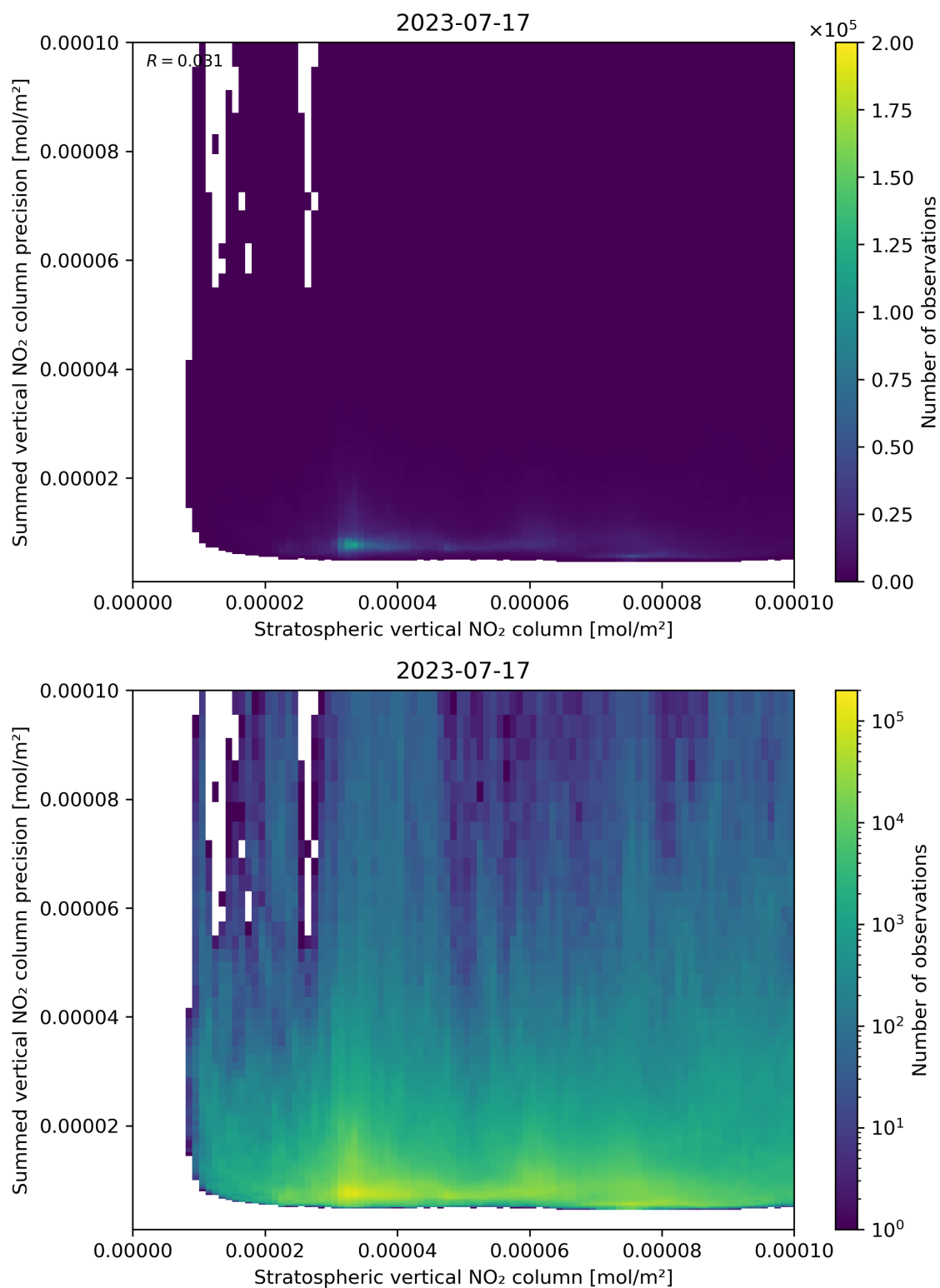
Figure 99: Scatter density plot of “Stratospheric vertical NO 2 column” against “Summed vertical NO 2 column precision” for 2023-07-16 to 2023-07-18.
