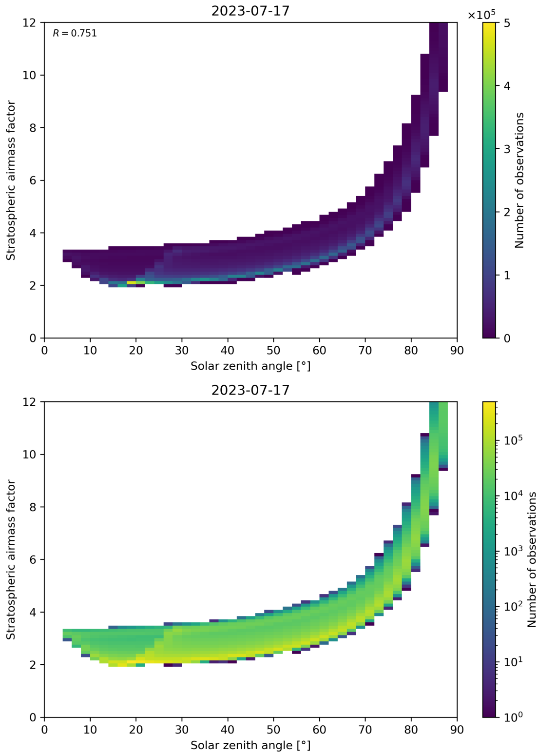
Figure 145: Scatter density plot of “Solar zenith angle” against “Stratospheric airmass factor” for 2023-07-16 to 2023-07-18.
