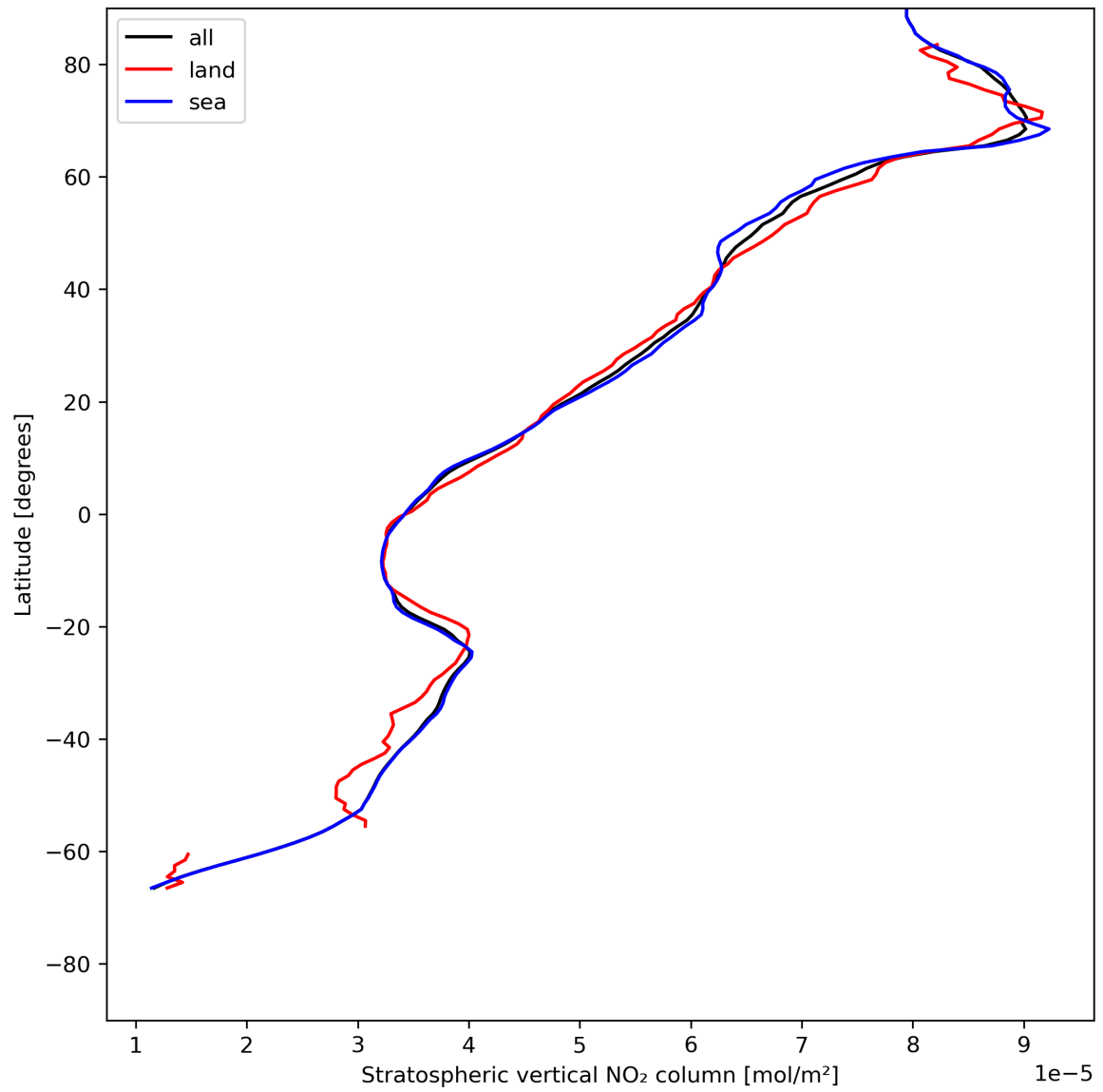
Figure 19: Zonal average of “Stratospheric vertical NO 2 column” for 2023-07-16 to 2023-07-18.
