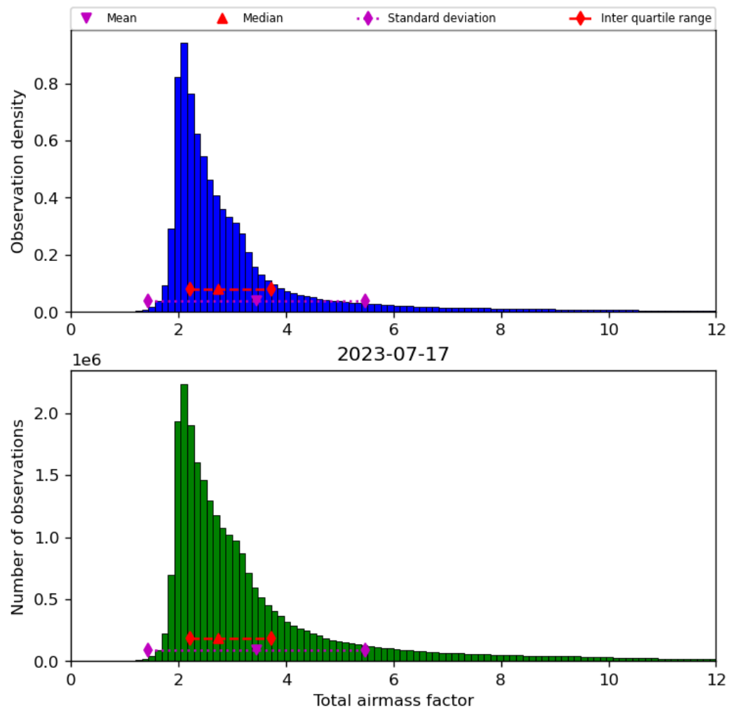
Figure 32: Histogram of “Total airmass factor” for 2023-07-16 to 2023-07-18
