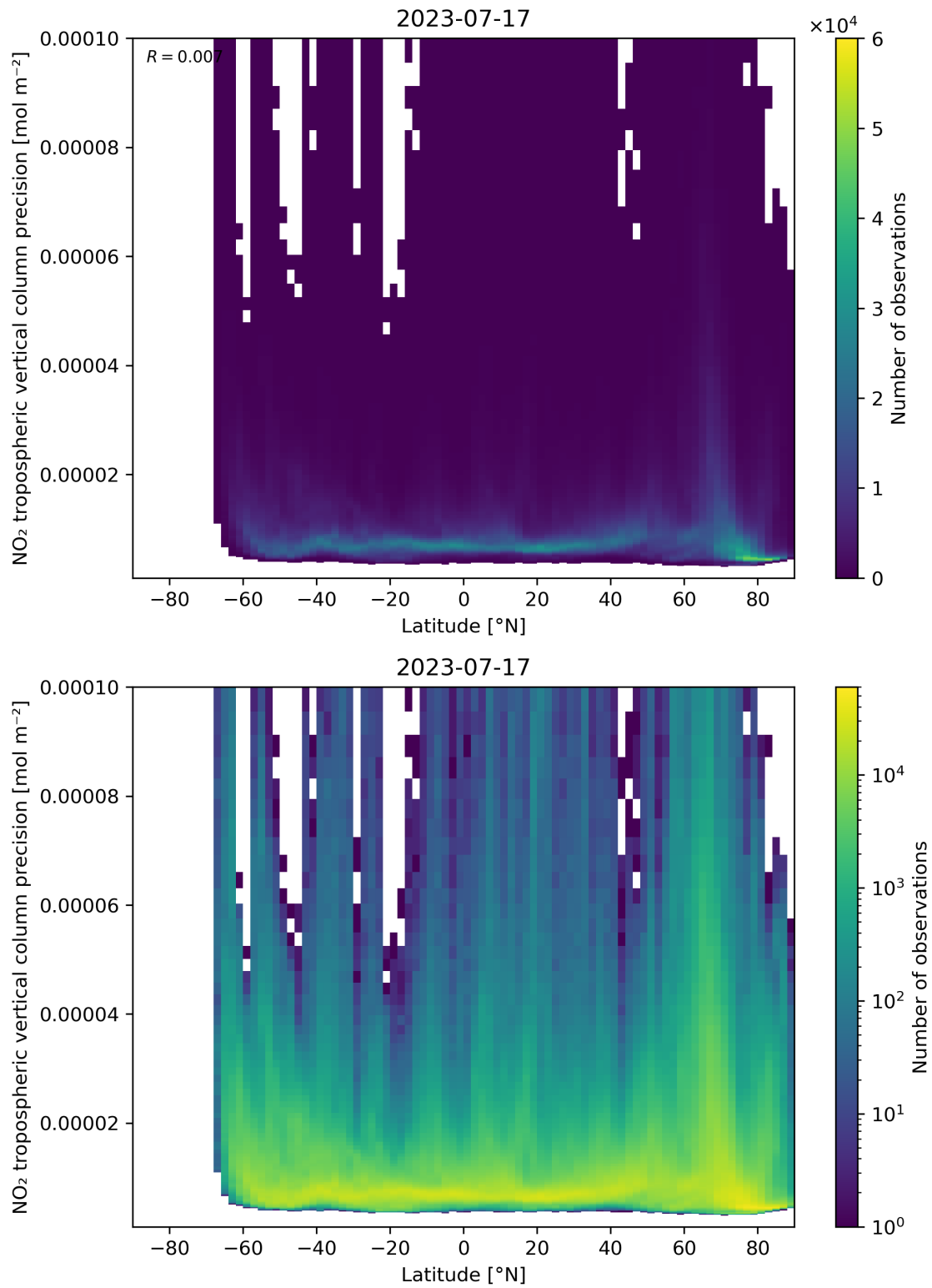
Figure 93: Scatter density plot of “Latitude” against “NO 2 tropospheric vertical column precision” for 2023-07-16 to 2023-07-18.
