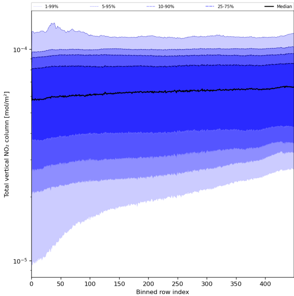
Figure 55: Along track statistics of “Total vertical NO 2 column” for 2023-07-16 to 2023-07-18
