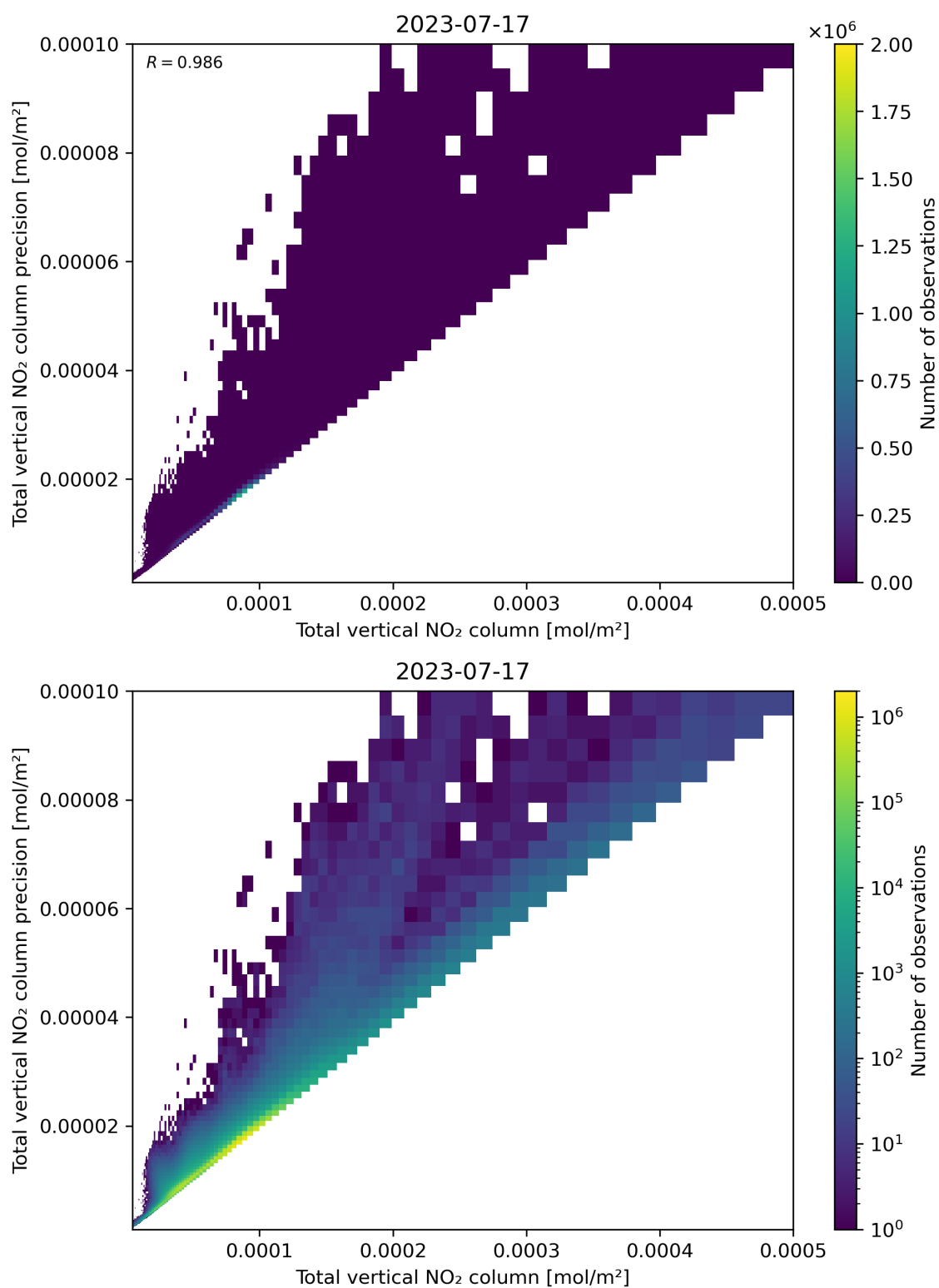
Figure 114: Scatter density plot of “Total vertical NO 2 column” against “Total vertical NO 2 column precision” for 2023-07-16 to 2023-07-18.
