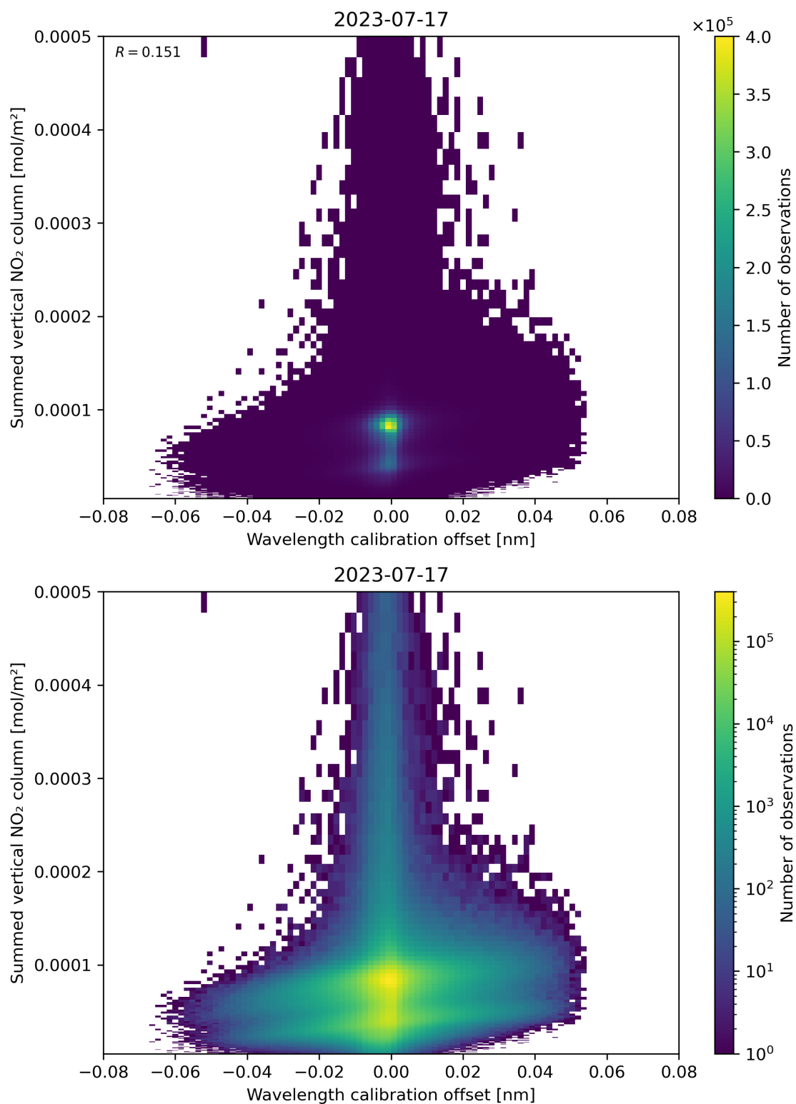
Figure 177: Scatter density plot of “Wavelength calibration offset” against “Summed vertical NO 2 column” for 2023-07-16 to 2023-07-18.
