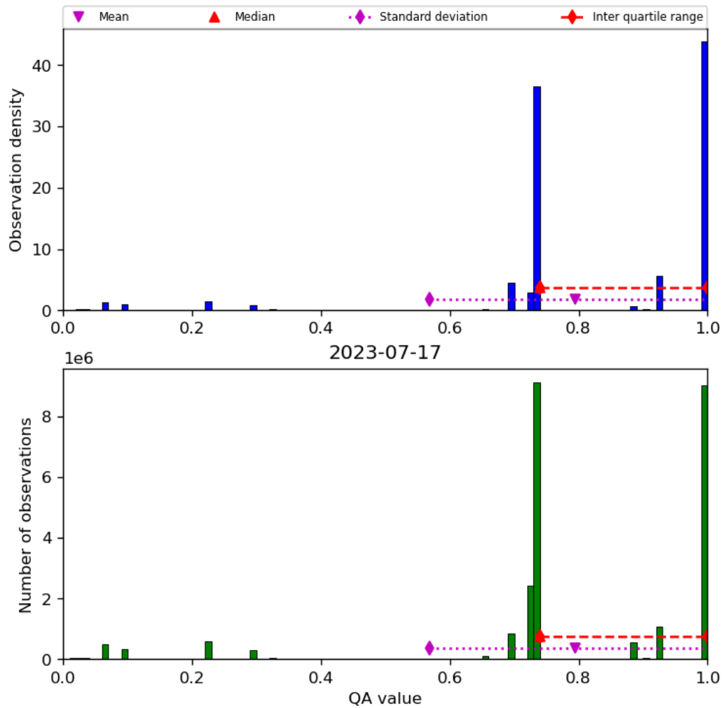
Figure 28: Histogram of “QA value” for 2023-07-16 to 2023-07-18
