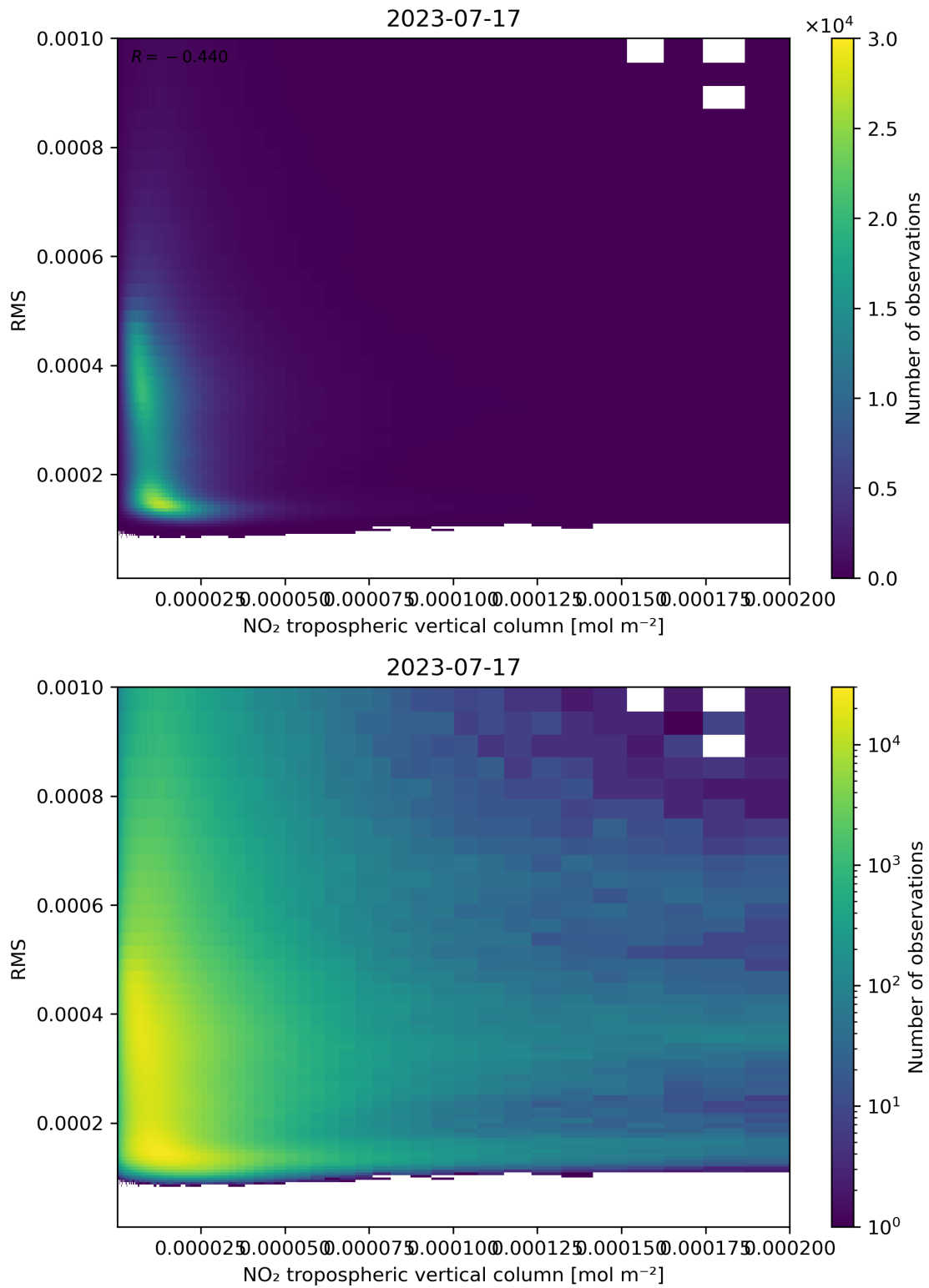
Figure 142: Scatter density plot of “NO 2 tropospheric vertical column” against “RMS” for 2023-07-16 to 2023-07-18.
