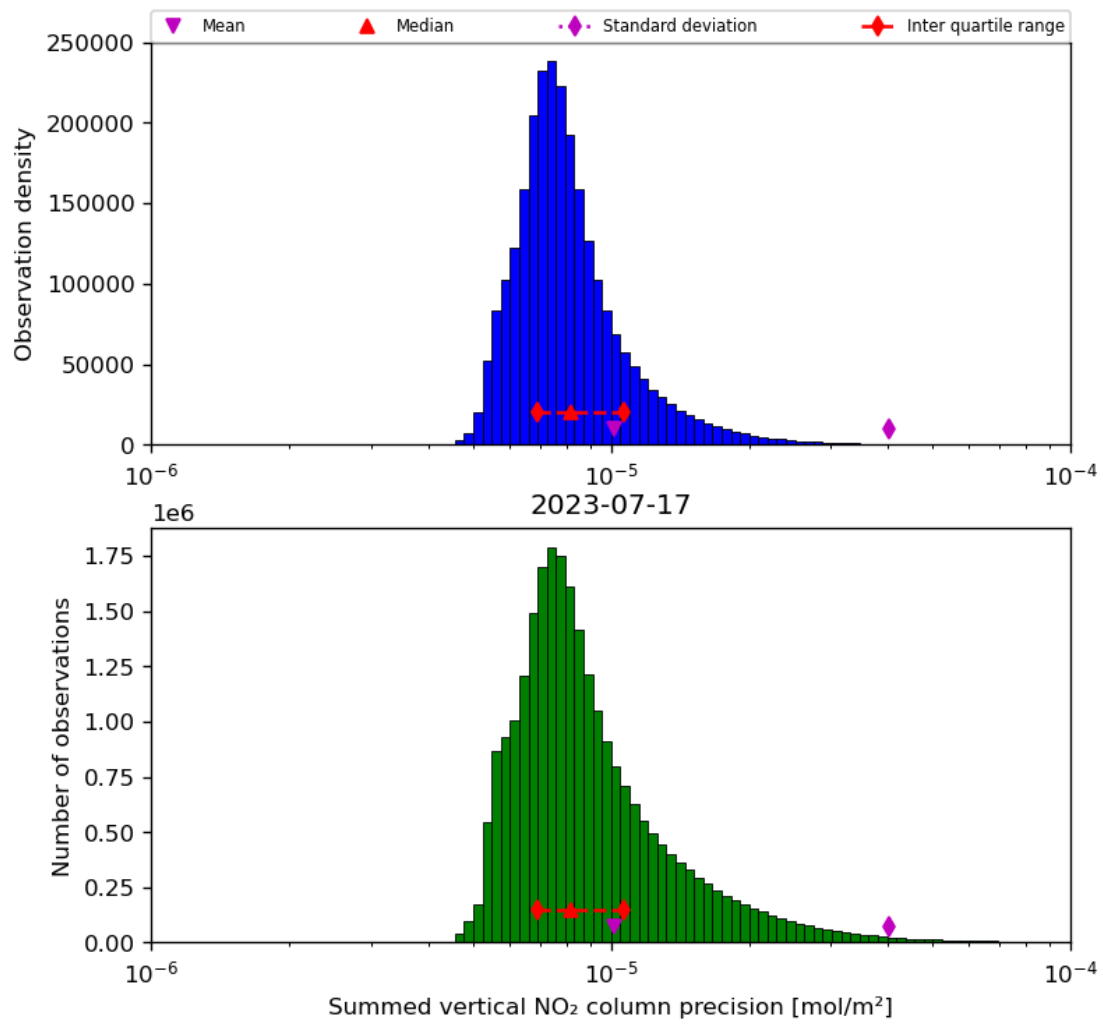
Figure 41: Histogram of “Summed vertical NO 2 column precision” for 2023-07-16 to 2023-07-18
