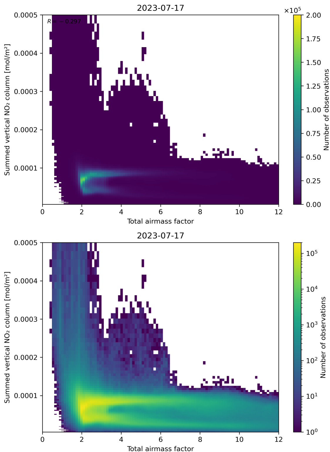
Figure 65: Scatter density plot of “Total airmass factor” against “Summed vertical NO 2 column” for 2023-07-16 to 2023-07-18.
