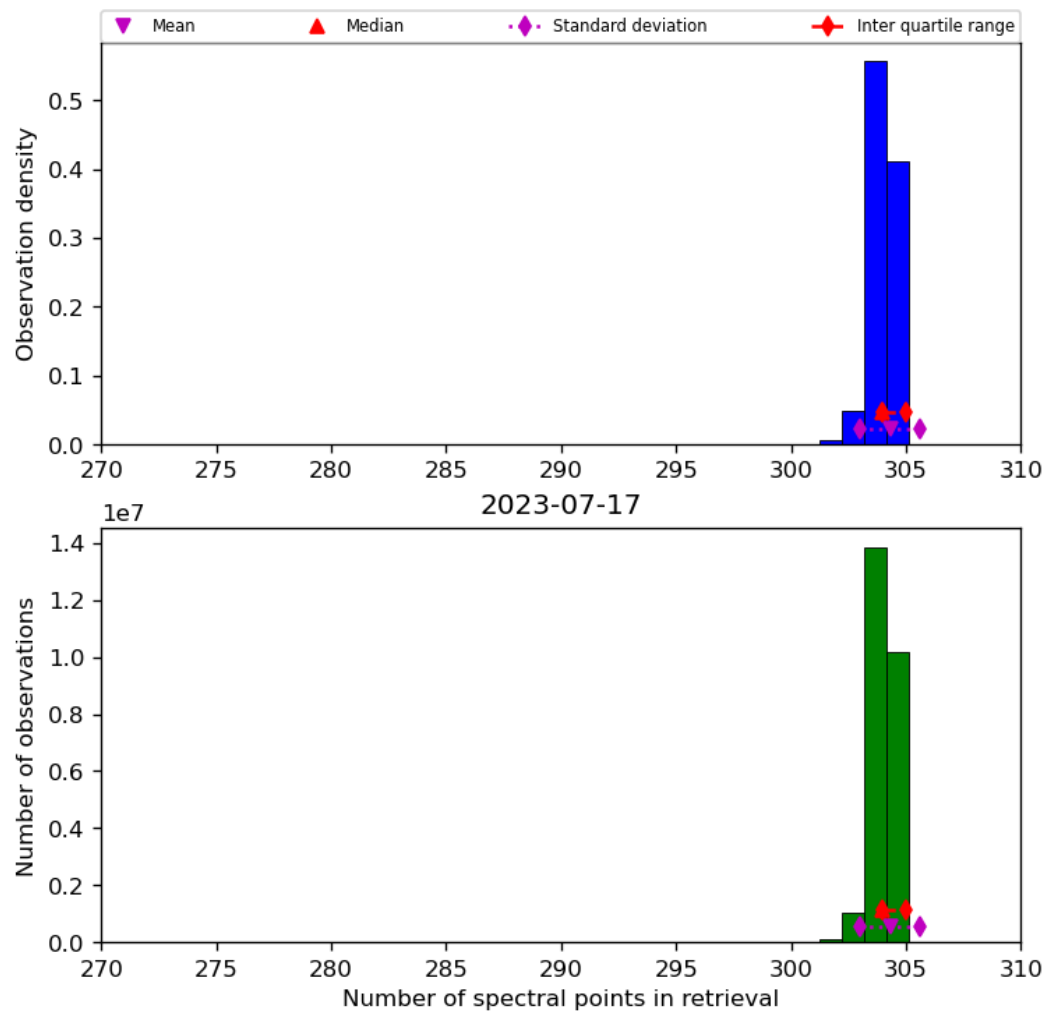
Figure 33: Histogram of “Number of spectral points in retrieval” for 2023-07-16 to 2023-07-18
