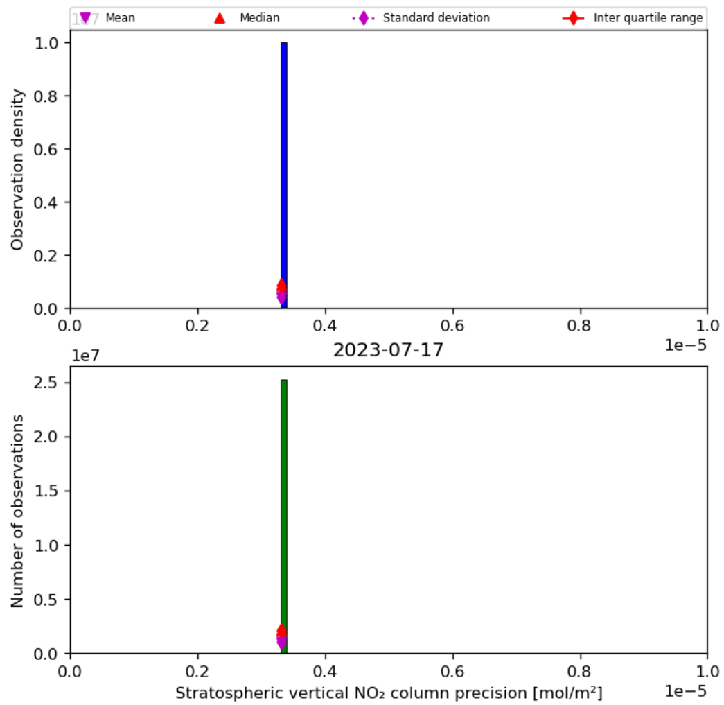
Figure 37: Histogram of “Stratospheric vertical NO 2 column precision” for 2023-07-16 to 2023-07-18
