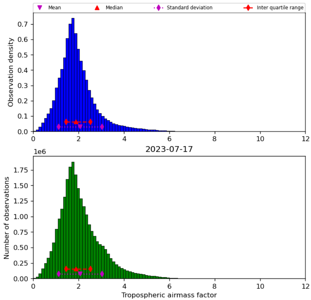
Figure 31: Histogram of “Tropospheric airmass factor” for 2023-07-16 to 2023-07-18
