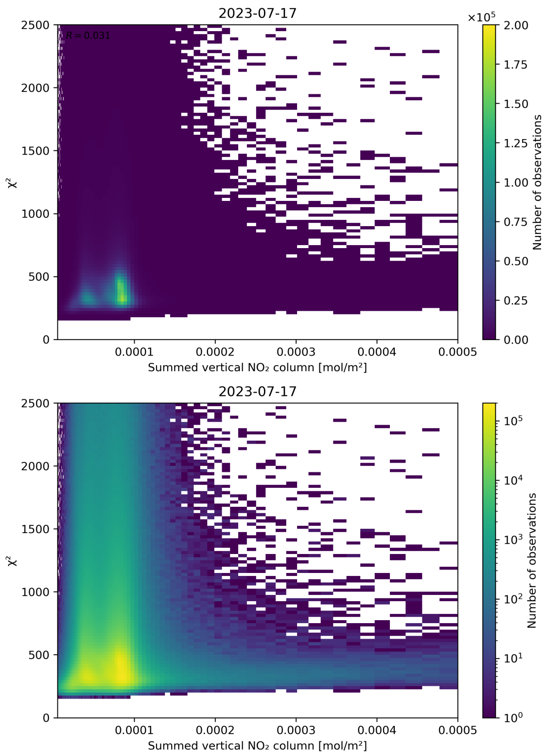
Figure 104: Scatter density plot of “Summed vertical NO 2 column” against “ \chi^2 ” for 2023-07-16 to 2023-07-18.
