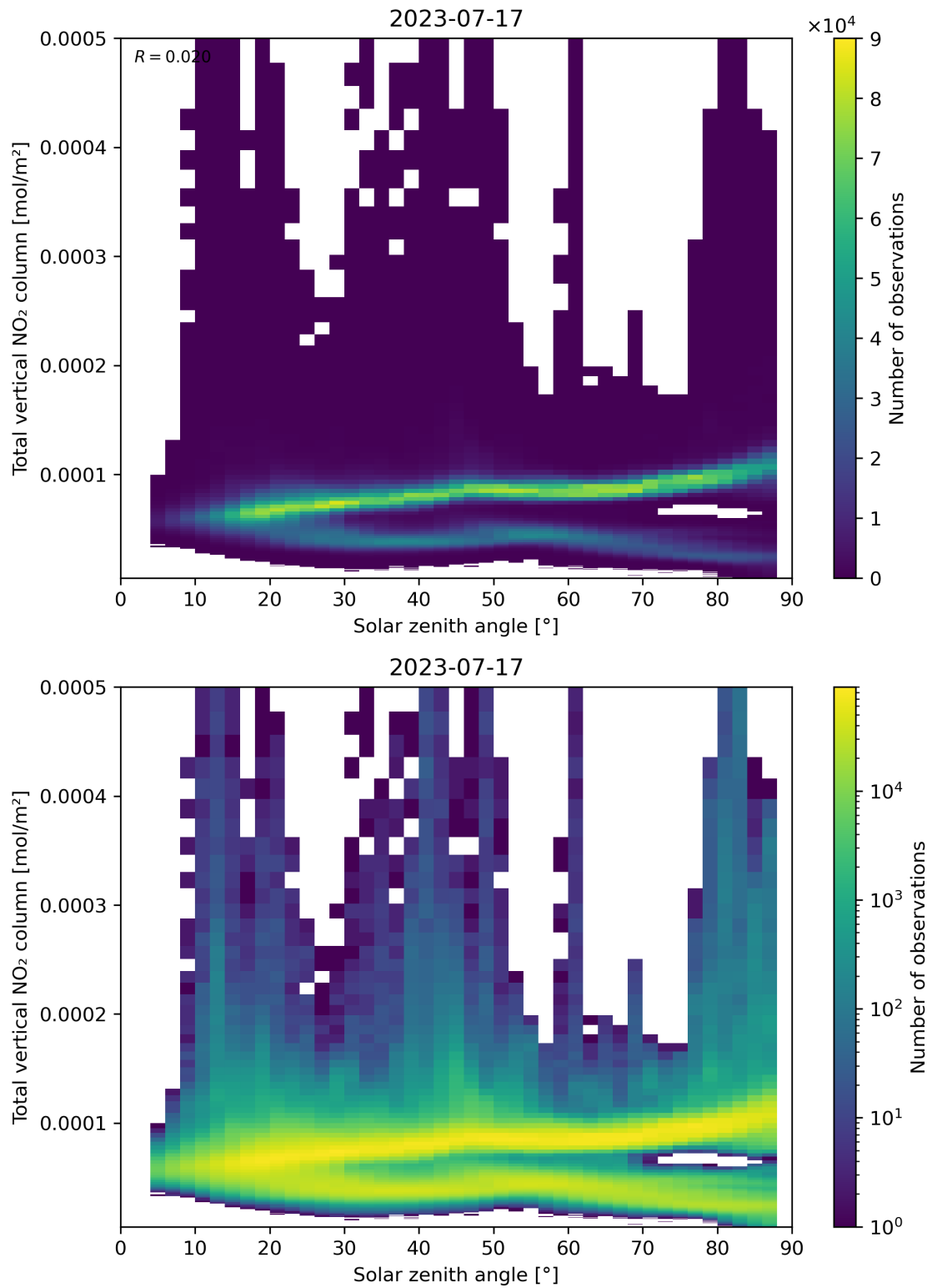
Figure 153: Scatter density plot of “Solar zenith angle” against “Total vertical NO 2 column” for 2023-07-16 to 2023-07-18.
