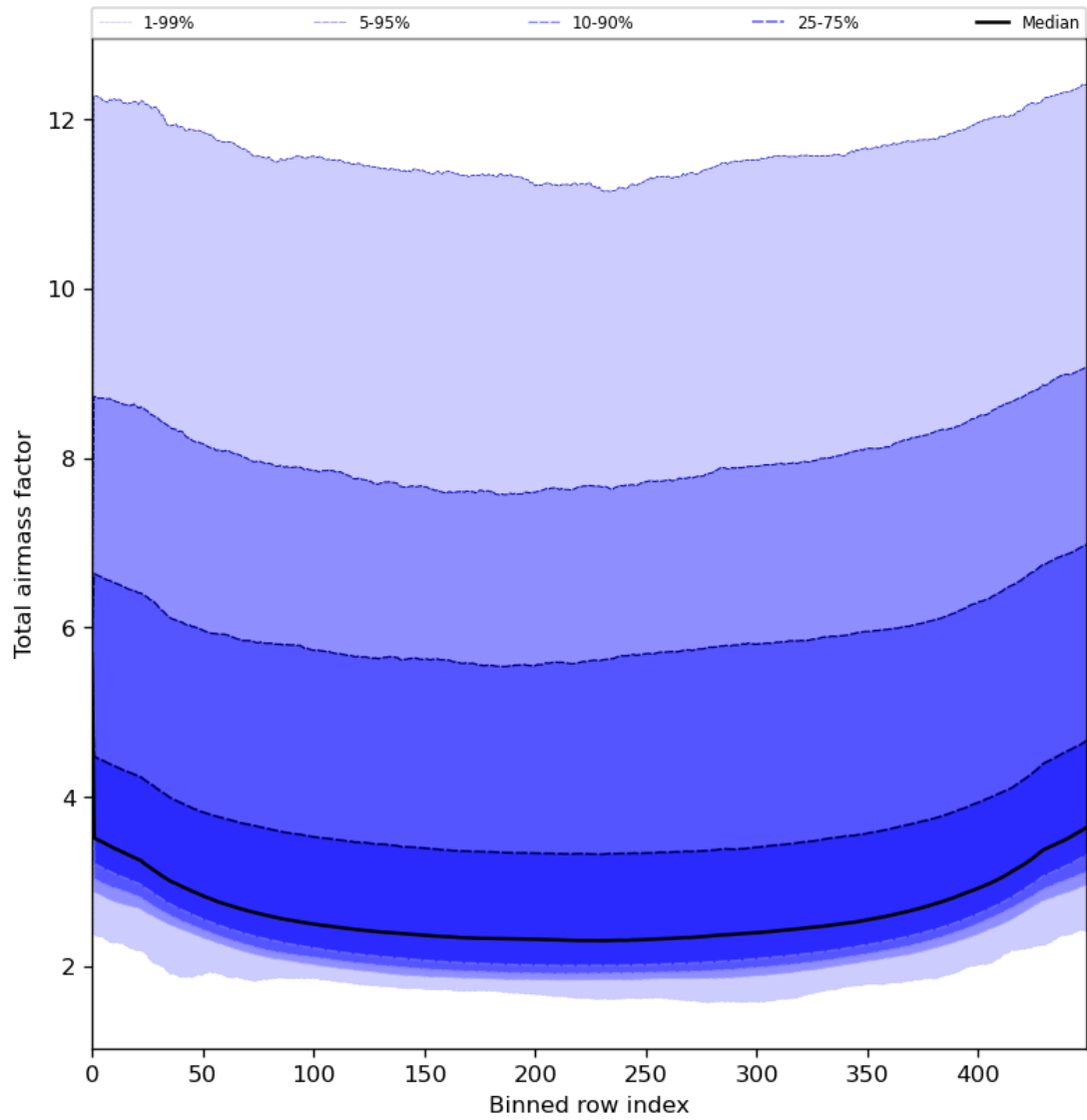
Figure 49: Along track statistics of “Total airmass factor” for 2023-07-16 to 2023-07-18
