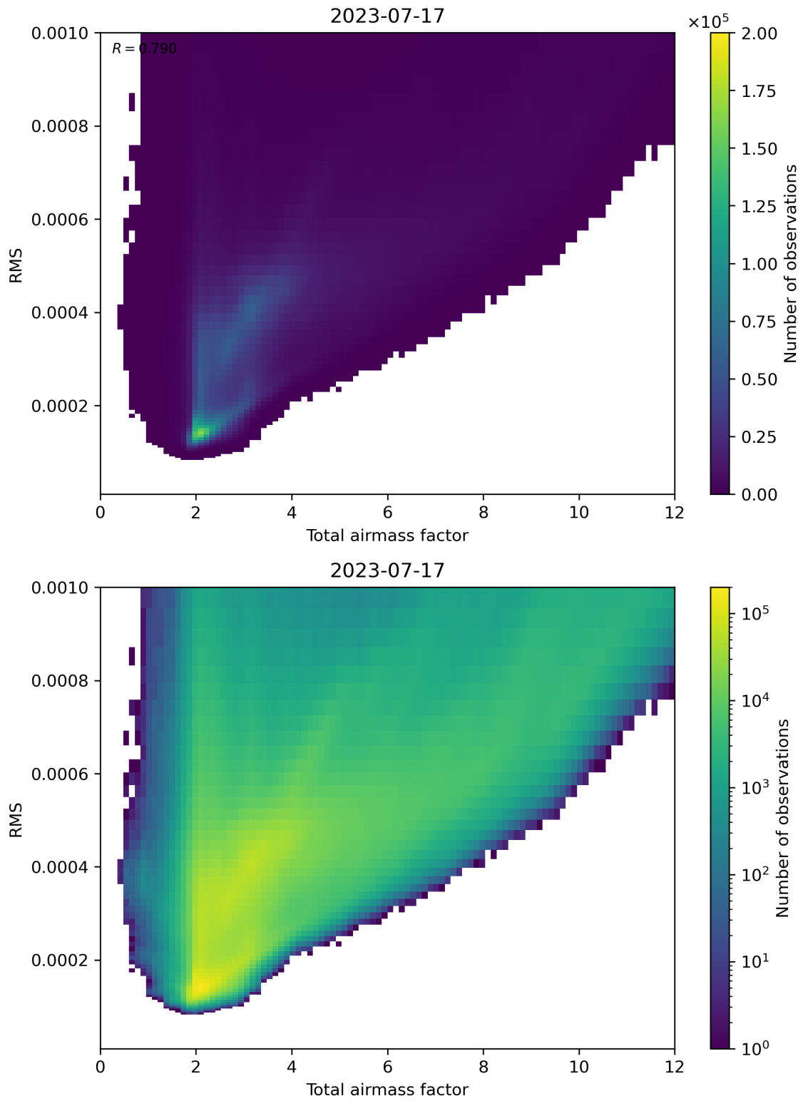
Figure 69: Scatter density plot of “Total airmass factor” against “RMS” for 2023-07-16 to 2023-07-18.
