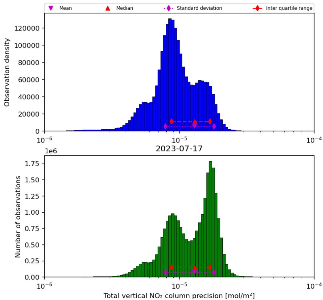
Figure 39: Histogram of “Total vertical NO 2 column precision” for 2023-07-16 to 2023-07-18
