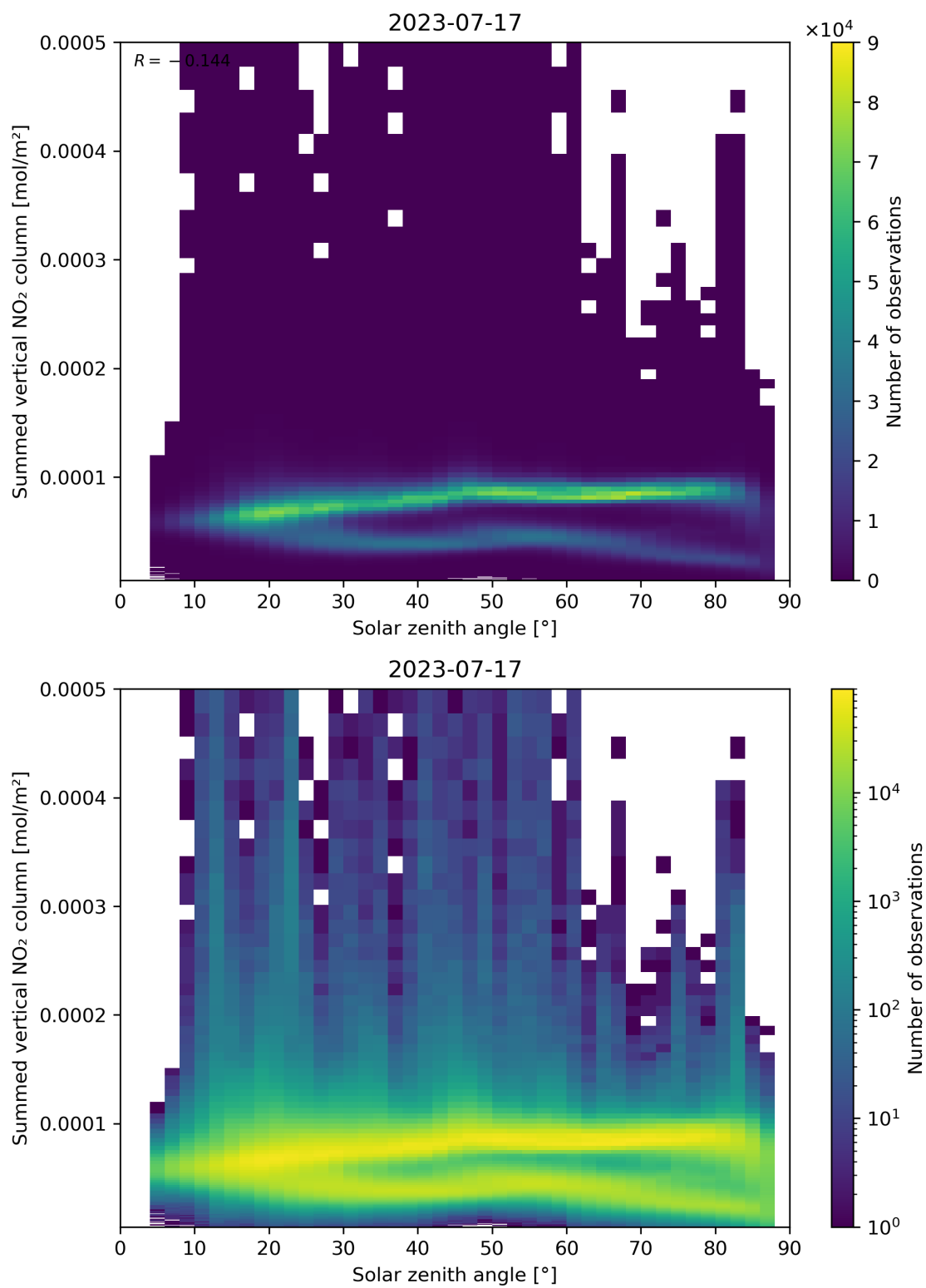
Figure 151: Scatter density plot of “Solar zenith angle” against “Summed vertical NO 2 column” for 2023-07-16 to 2023-07-18.
