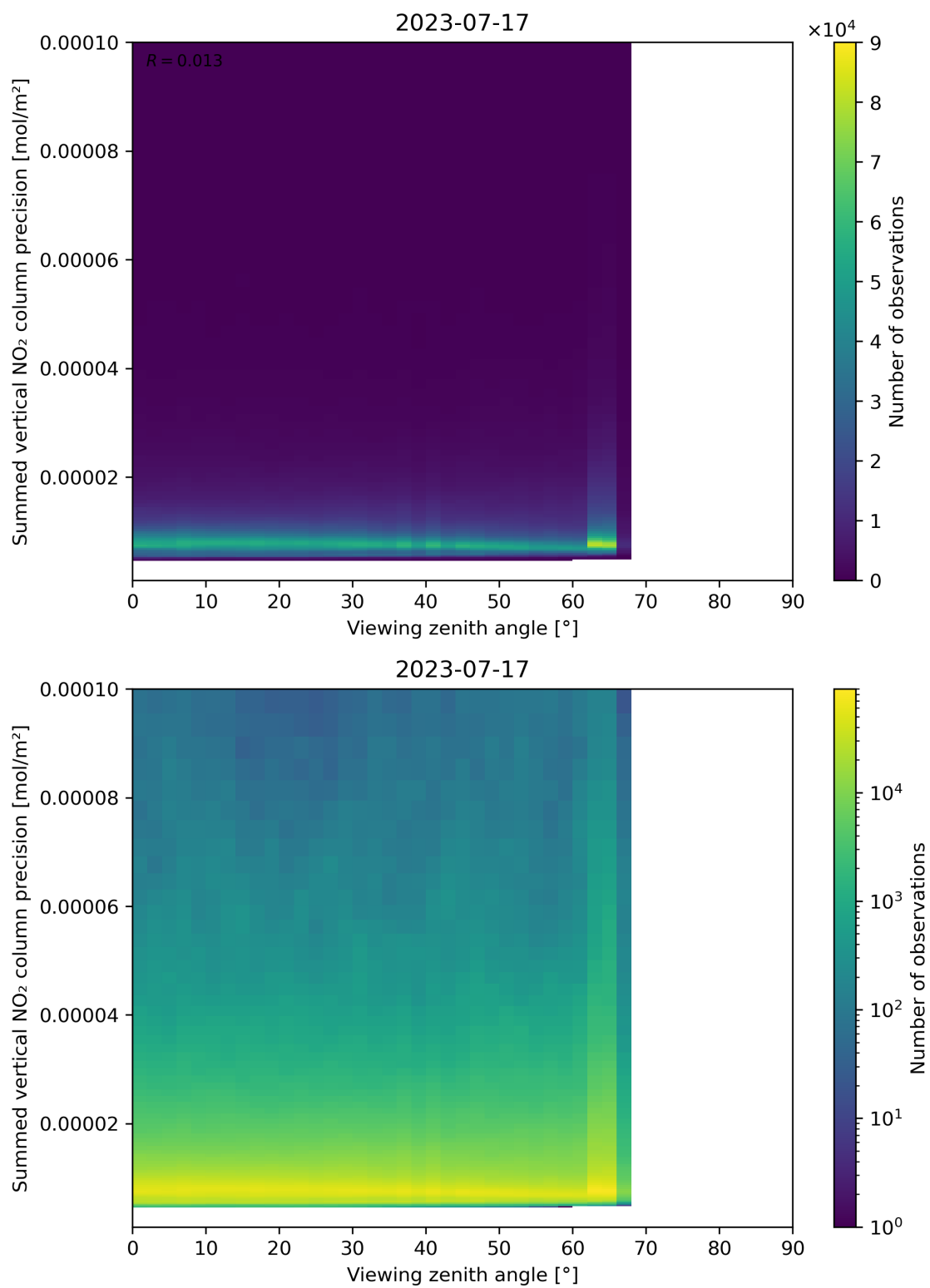
Figure 166: Scatter density plot of “Viewing zenith angle” against “Summed vertical NO 2 column precision” for 2023-07-16 to 2023-07-18.
