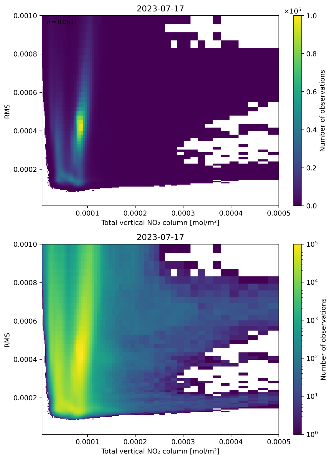
Figure 120: Scatter density plot of “Total vertical NO 2 column” against “RMS” for 2023-07-16 to 2023-07-18.
