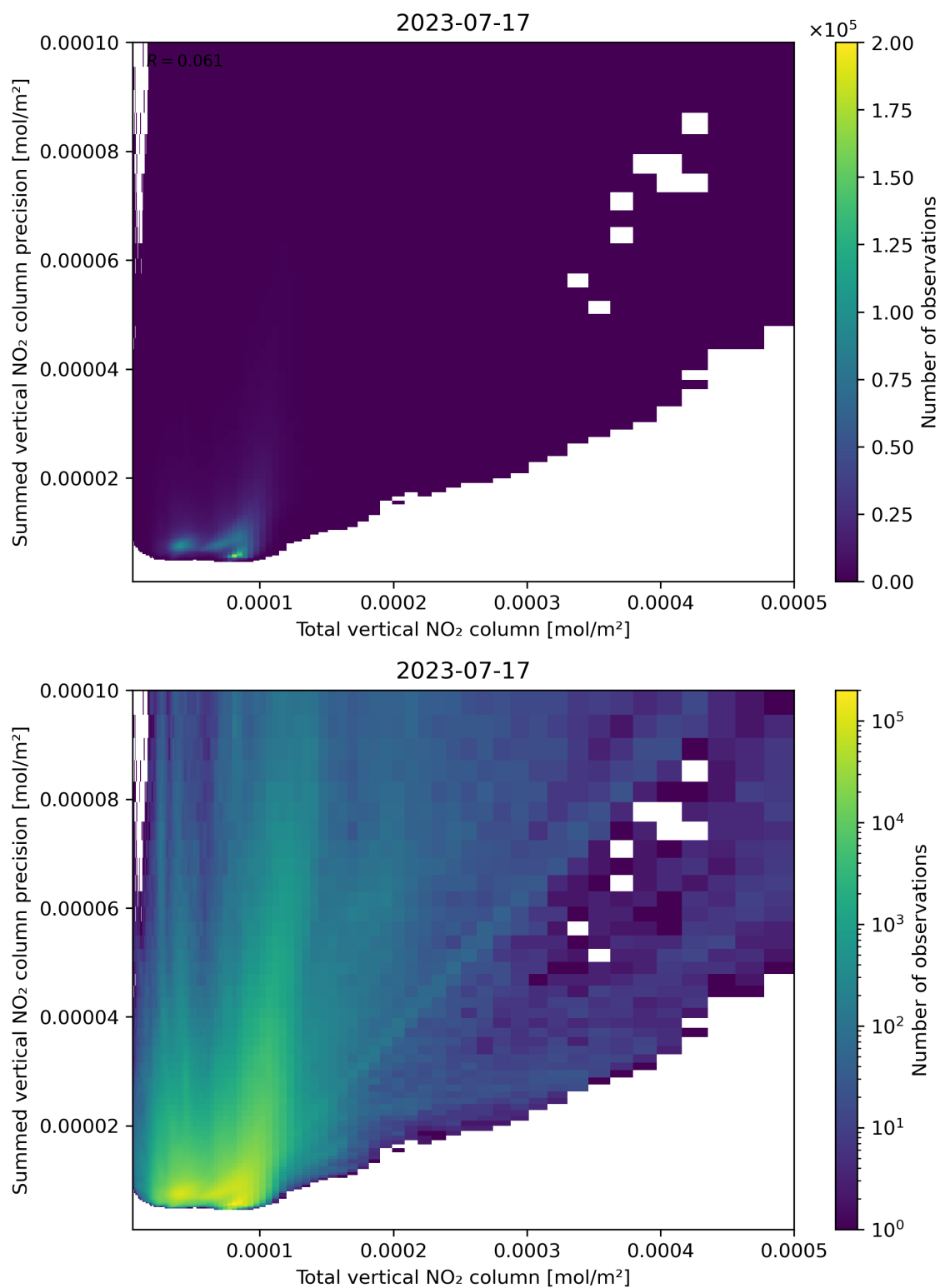
Figure 113: Scatter density plot of “Total vertical NO 2 column” against “Summed vertical NO 2 column precision” for 2023-07-16 to 2023-07-18.
