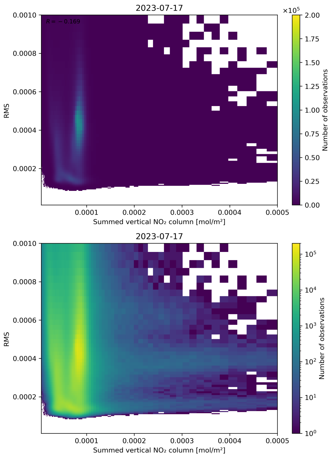
Figure 109: Scatter density plot of “Summed vertical NO 2 column” against “RMS” for 2023-07-16 to 2023-07-18.
