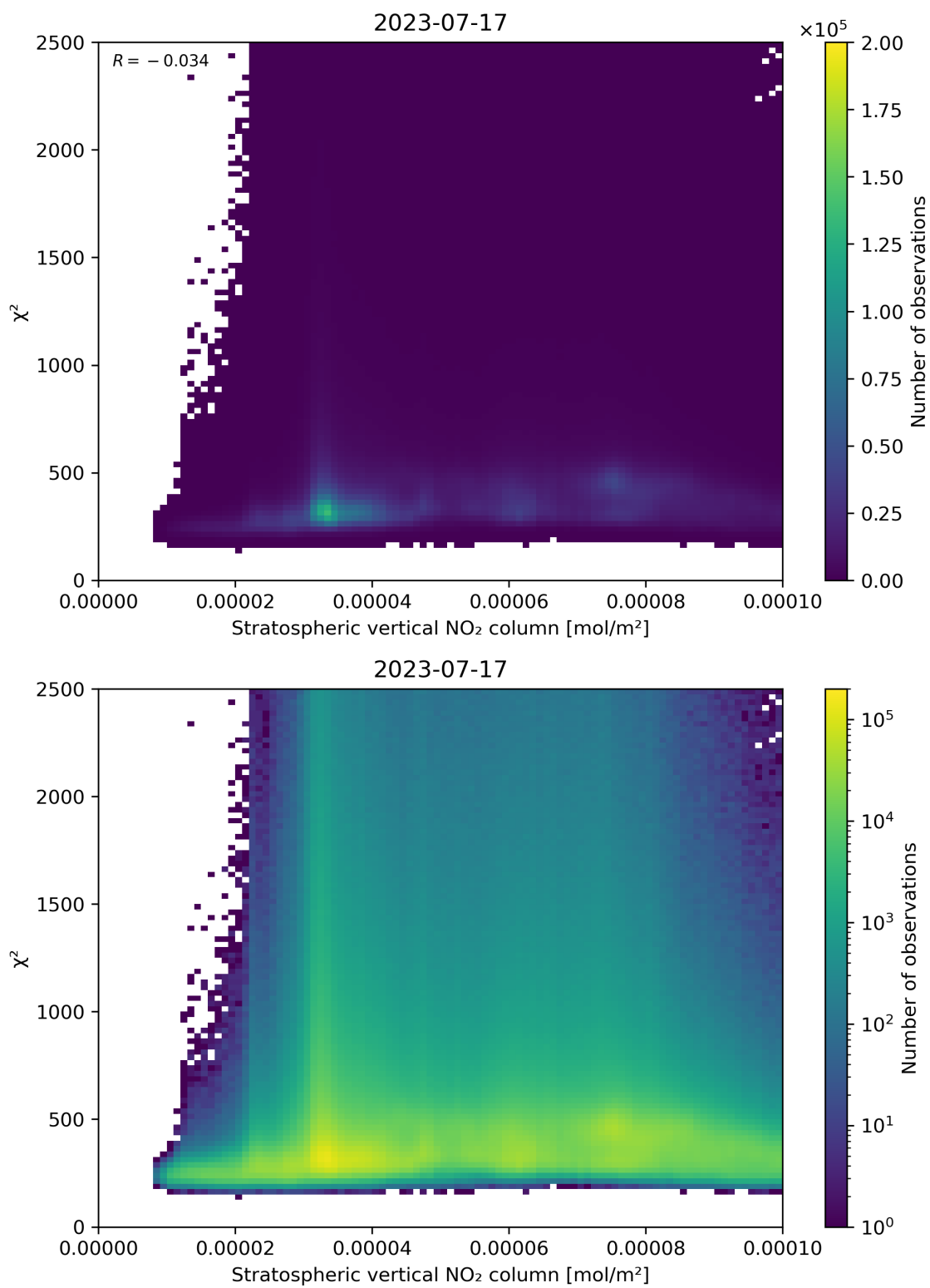
Figure 97: Scatter density plot of “Stratospheric vertical NO 2 column” against “ \chi^2 ” for 2023-07-16 to 2023-07-18.
