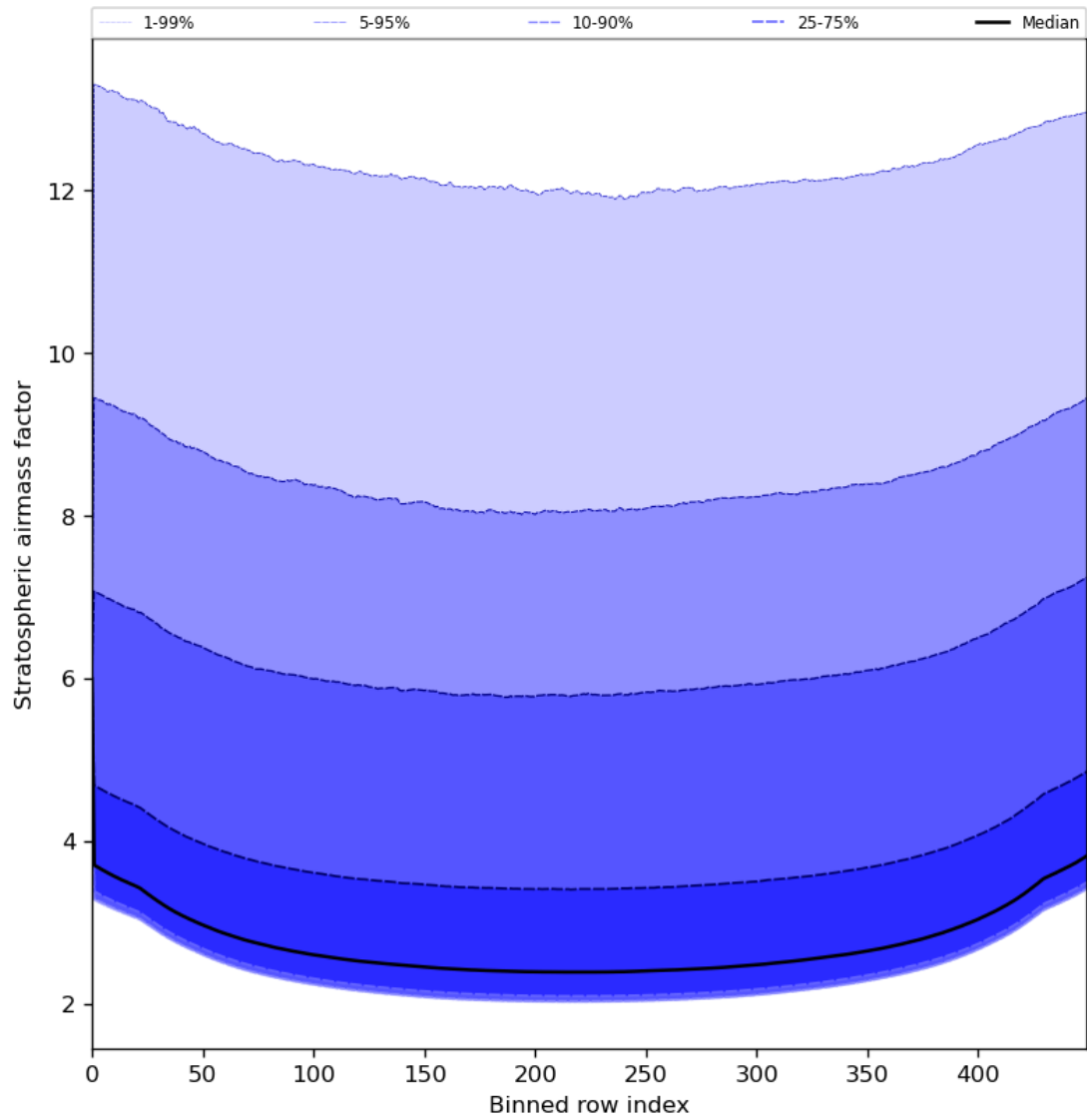
Figure 61: Along track statistics of “Stratospheric airmass factor” for 2023-07-16 to 2023-07-18
