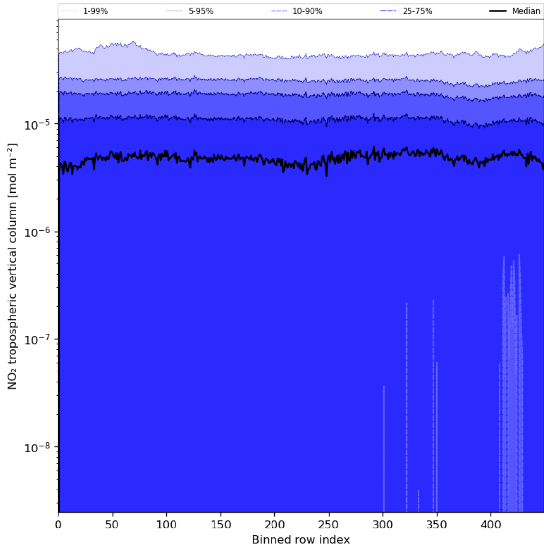
Figure 46: Along track statistics of “NO 2 tropospheric vertical column” for 2023-07-16 to 2023-07-18
