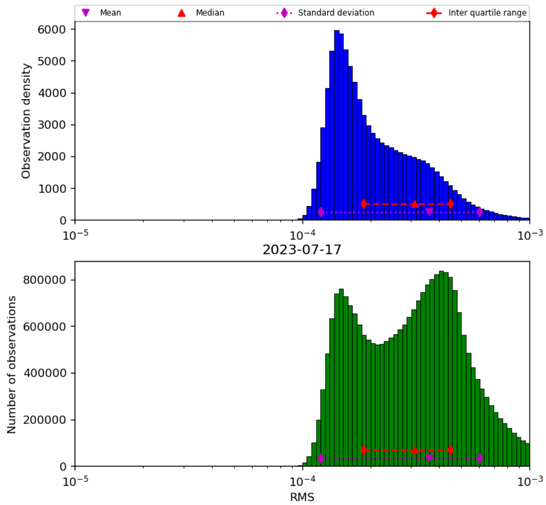
Figure 43: Histogram of “RMS” for 2023-07-16 to 2023-07-18
