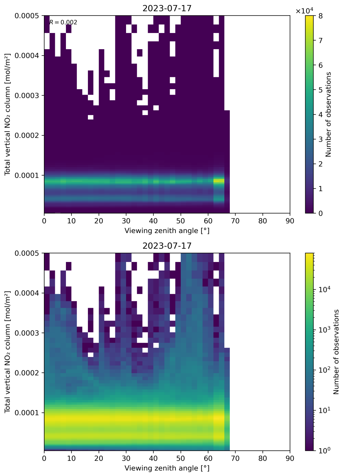
Figure 167: Scatter density plot of “Viewing zenith angle” against “Total vertical NO 2 column” for 2023-07-16 to 2023-07-18.
