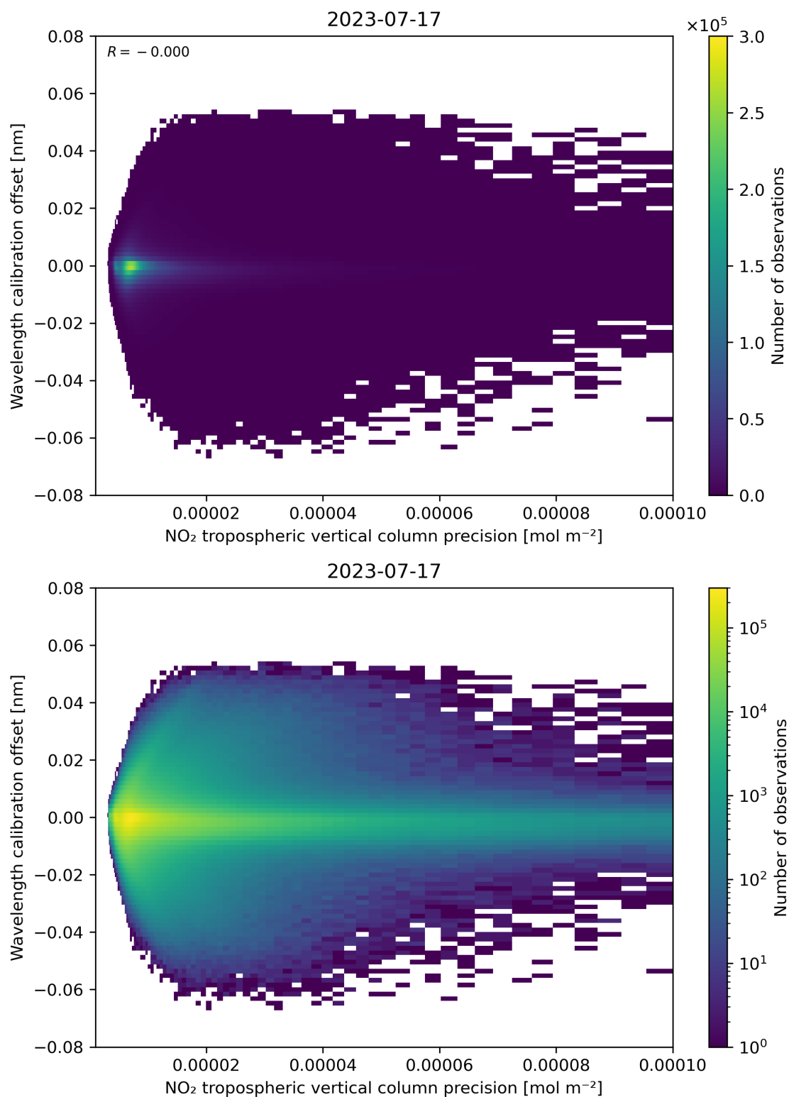
Figure 141: Scatter density plot of “NO 2 tropospheric vertical column precision” against “Wavelength calibration offset” for 2023-07-16 to 2023-07-18.
