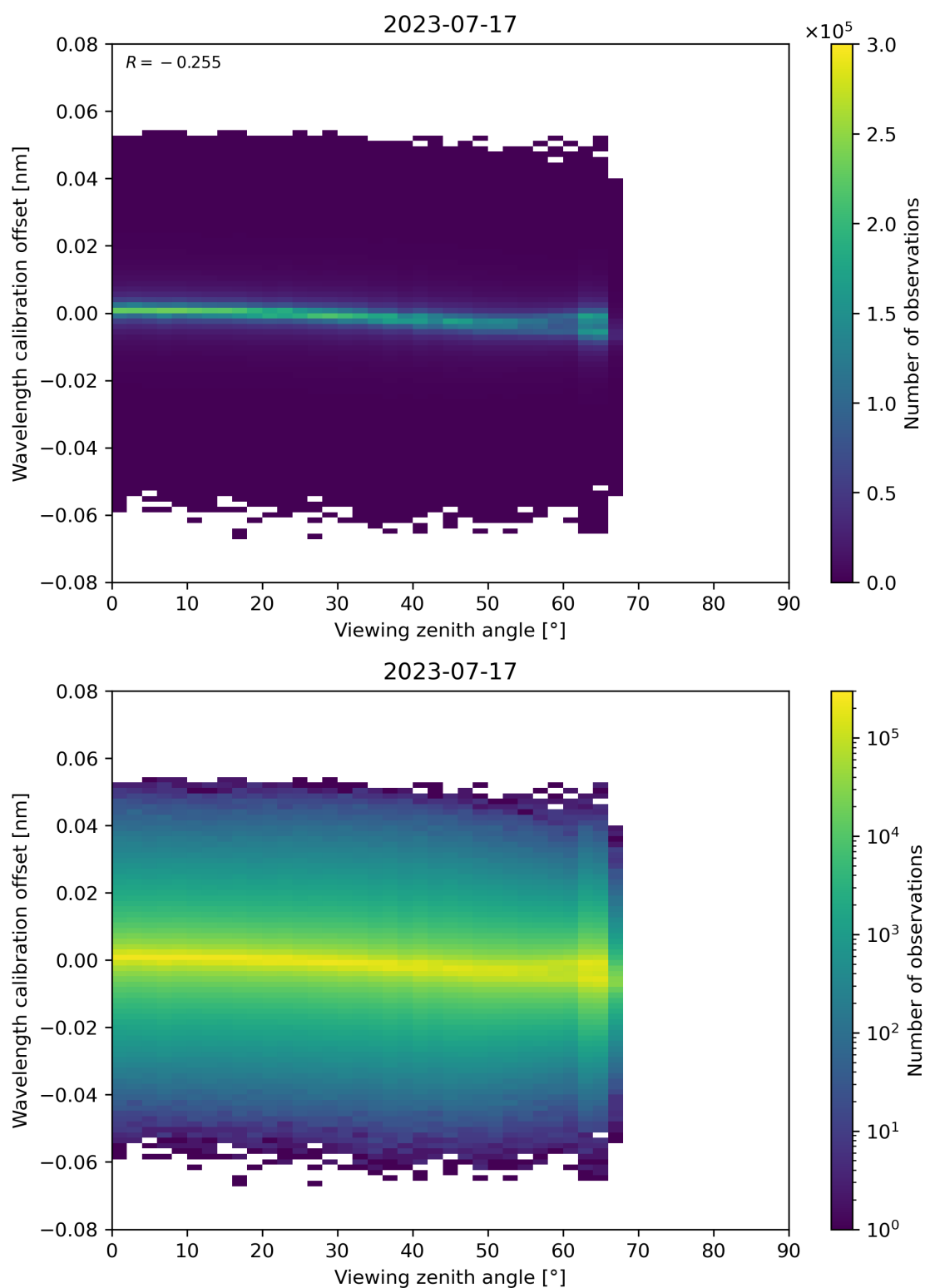
Figure 173: Scatter density plot of “Viewing zenith angle” against “Wavelength calibration offset” for 2023-07-16 to 2023-07-18.
