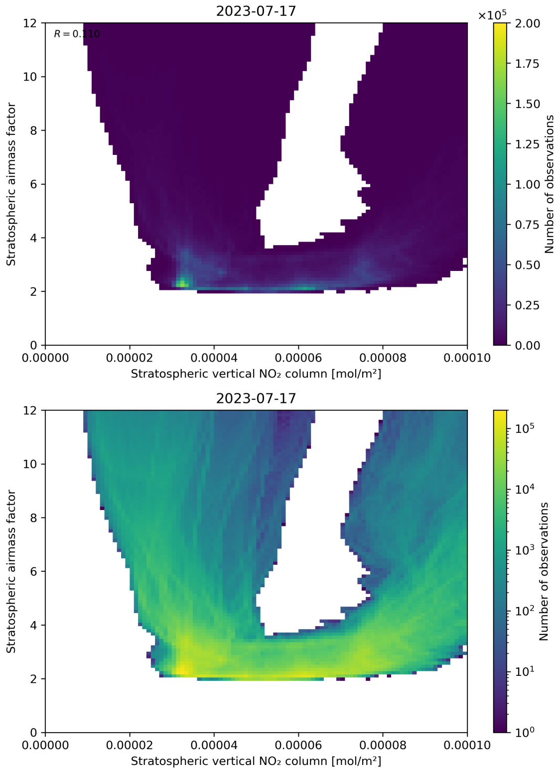
Figure 96: Scatter density plot of “Stratospheric vertical NO 2 column” against “Stratospheric airmass factor” for 2023-07-16 to 2023-07-18.
