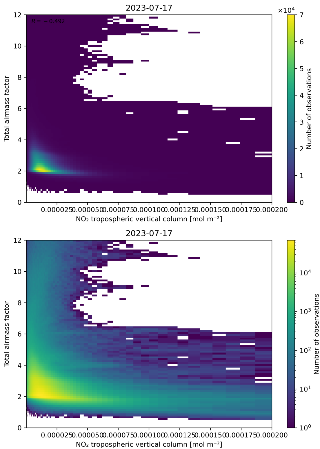
Figure 122: Scatter density plot of “NO 2 tropospheric vertical column” against “Total air mass factor” for 2023-07-16 to 2023-07-18.
