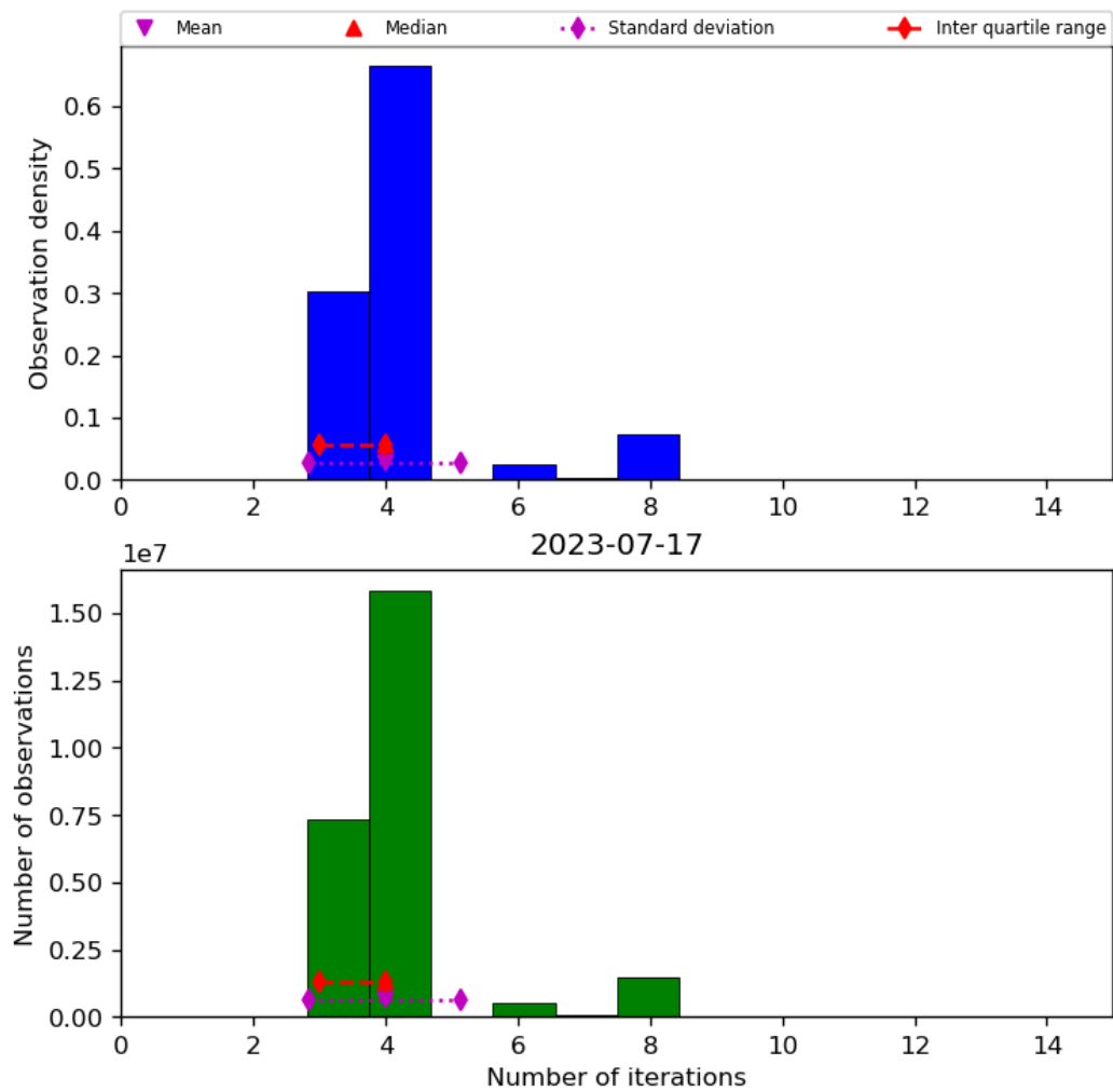
Figure 34: Histogram of “Number of iterations” for 2023-07-16 to 2023-07-18
