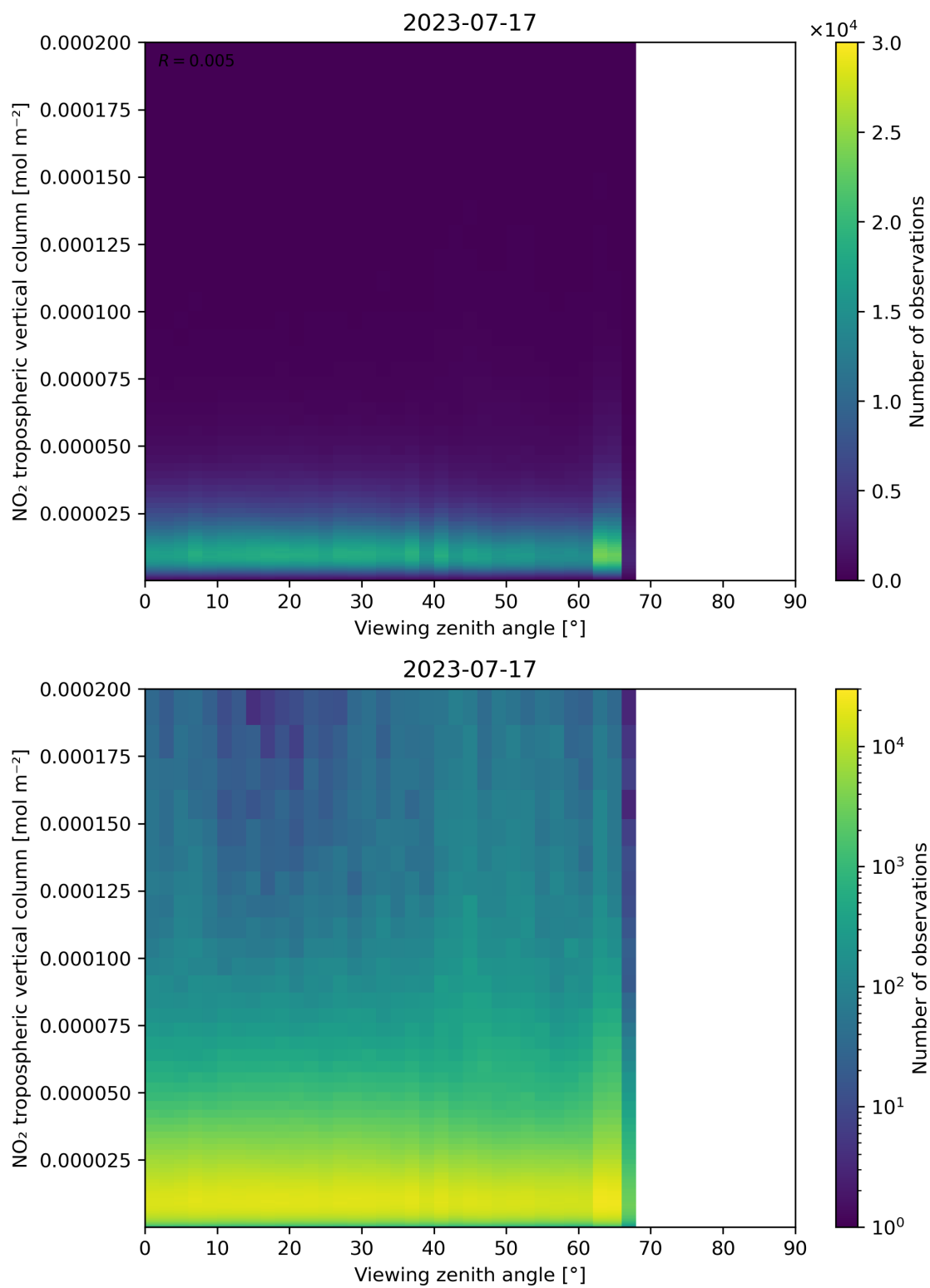
Figure 169: Scatter density plot of “Viewing zenith angle” against “NO 2 tropospheric vertical column” for 2023-07-16 to 2023-07-18.
