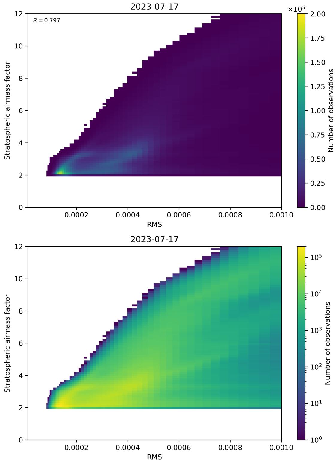
Figure 144: Scatter density plot of “RMS” against “Stratospheric airmass factor” for 2023-07-16 to 2023-07-18.
