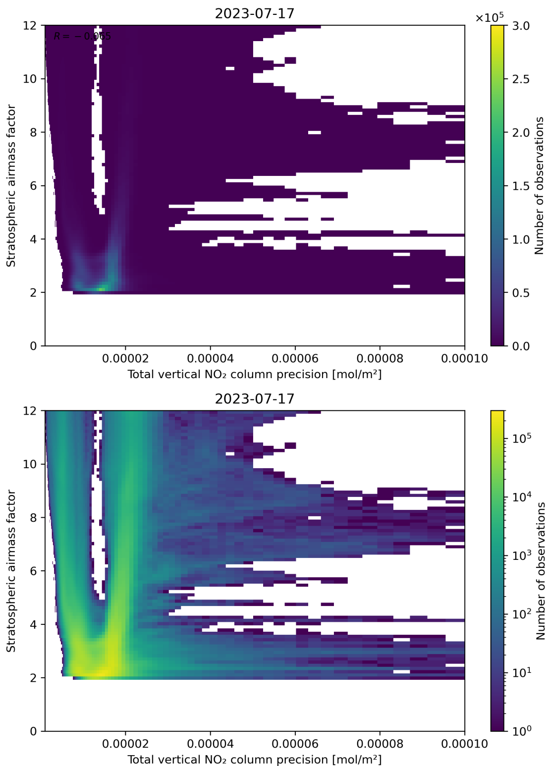
Figure 115: Scatter density plot of “Total vertical NO 2 column precision” against “Stratospheric air mass factor” for 2023-07-16 to 2023-07-18.
