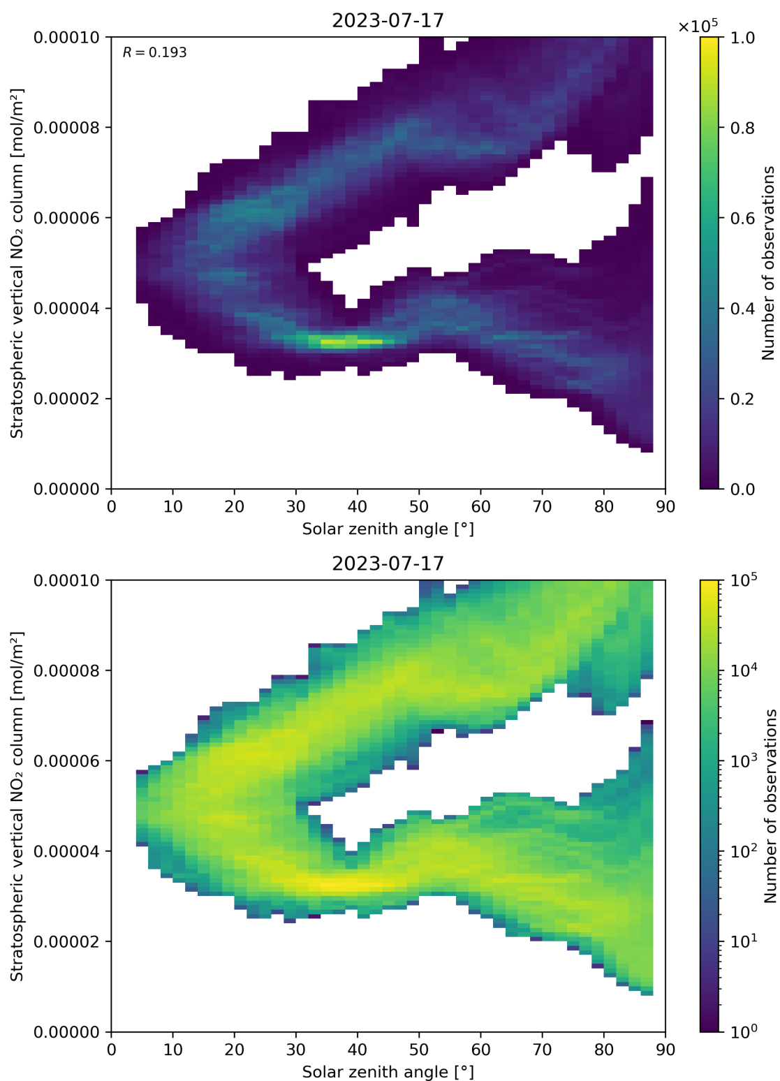
Figure 150: Scatter density plot of “Solar zenith angle” against “Stratospheric vertical NO 2 column” for 2023-07-16 to 2023-07-18.
