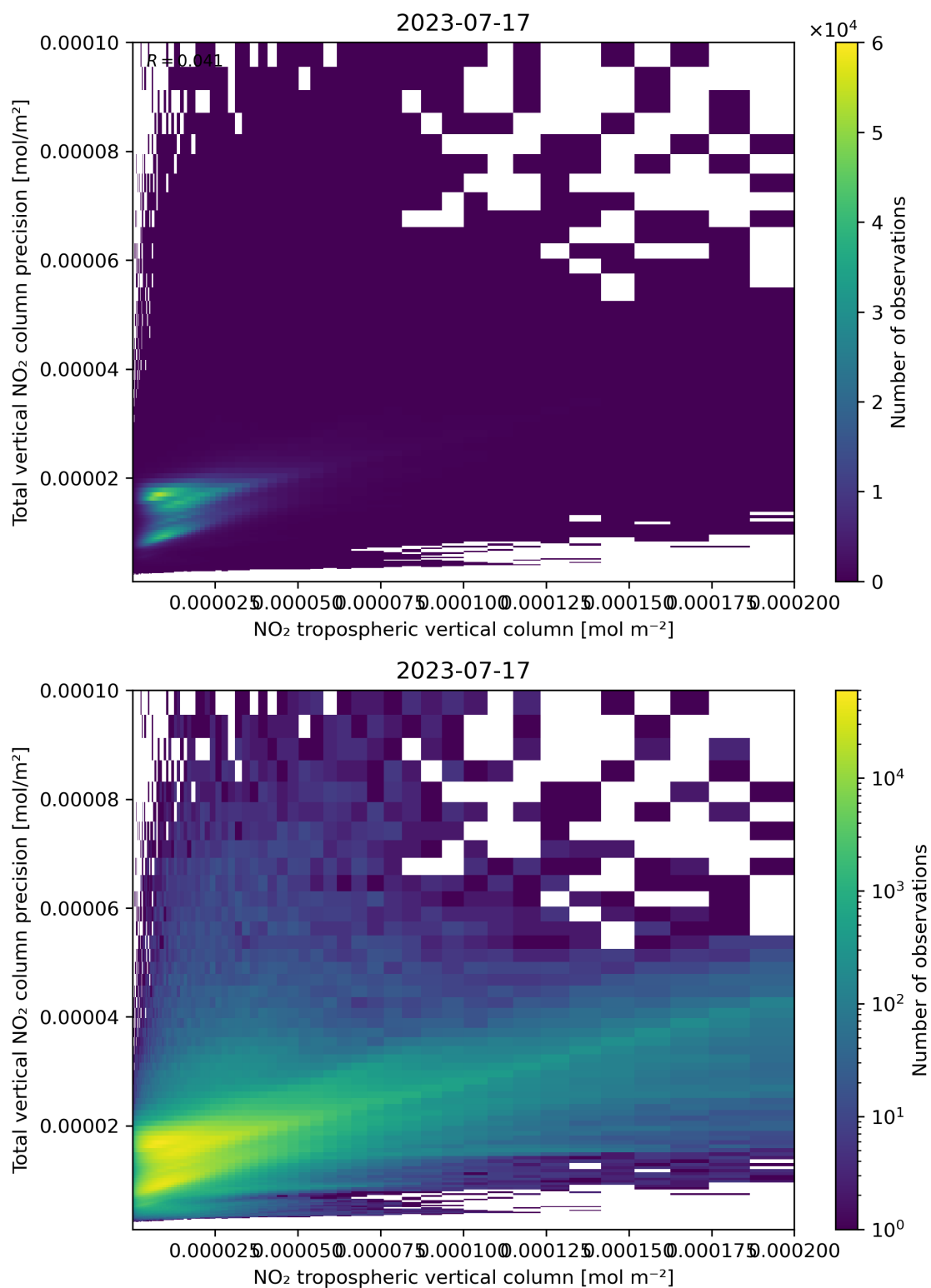
Figure 129: Scatter density plot of “NO 2 tropospheric vertical column” against “Total vertical NO 2 column precision” for 2023-07-16 to 2023-07-18.
