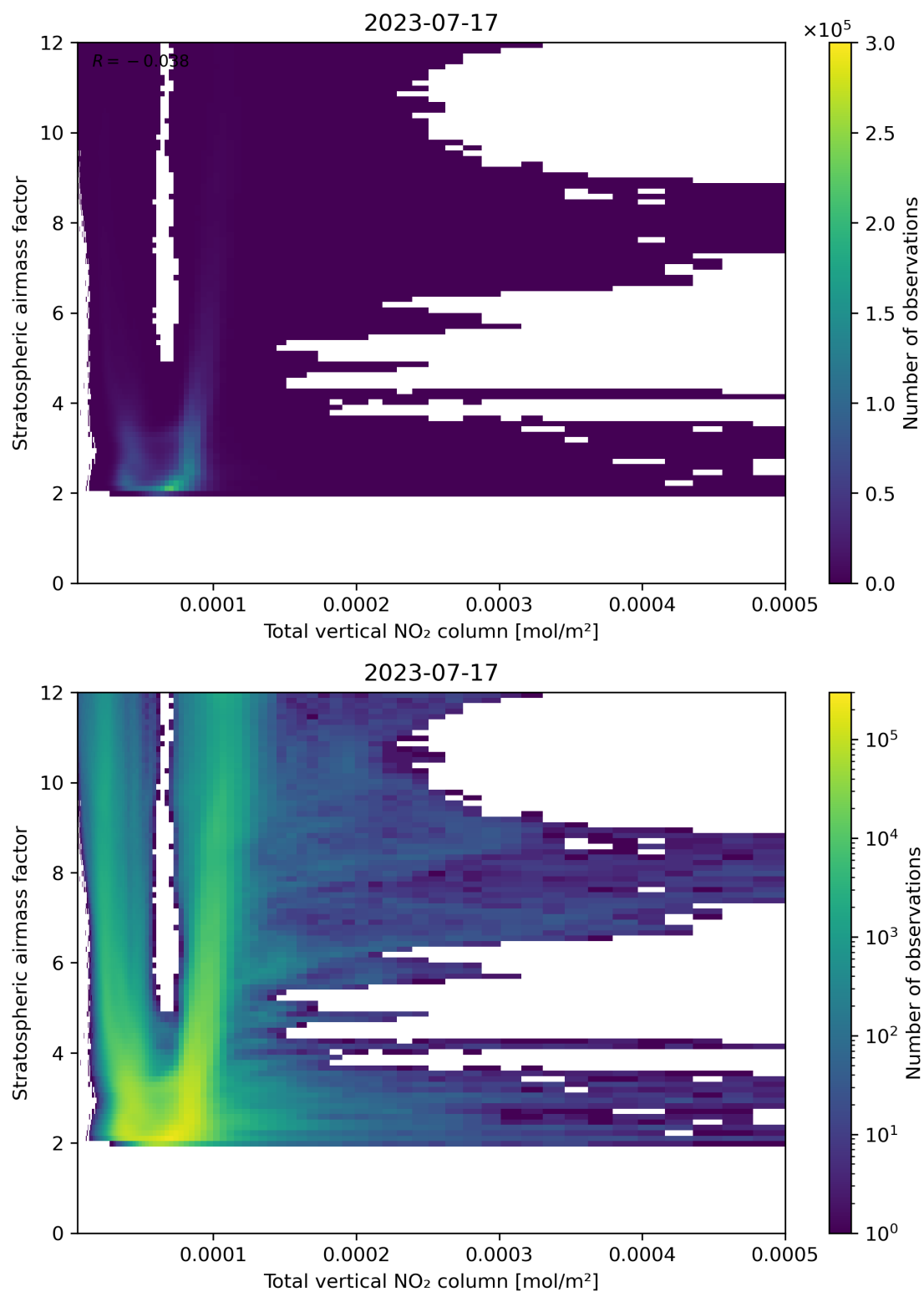
Figure 110: Scatter density plot of “Total vertical NO 2 column” against “Stratospheric air mass factor” for 2023-07-16 to 2023-07-18.
