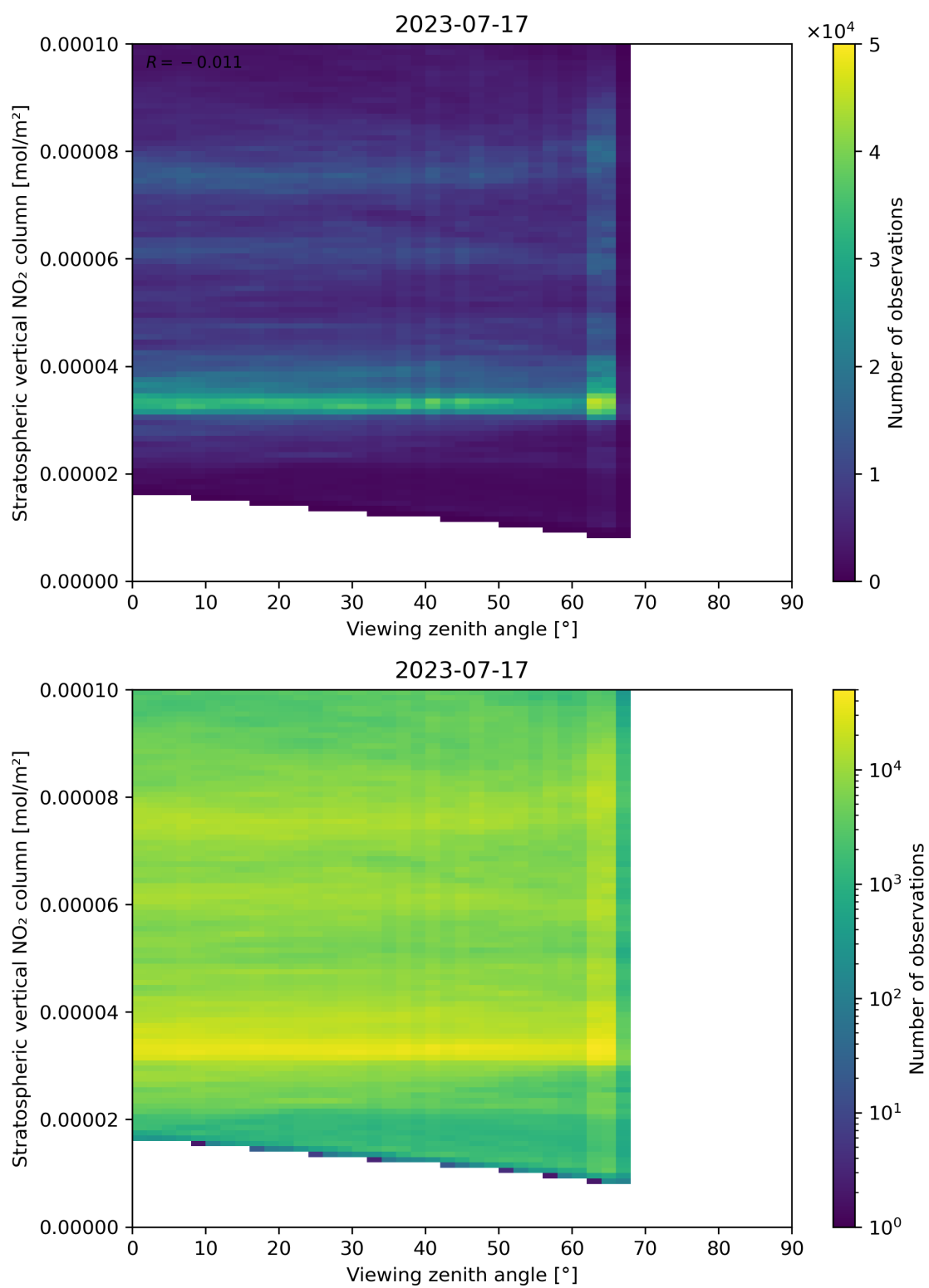
Figure 164: Scatter density plot of “Viewing zenith angle” against “Stratospheric vertical NO 2 column” for 2023-07-16 to 2023-07-18.
