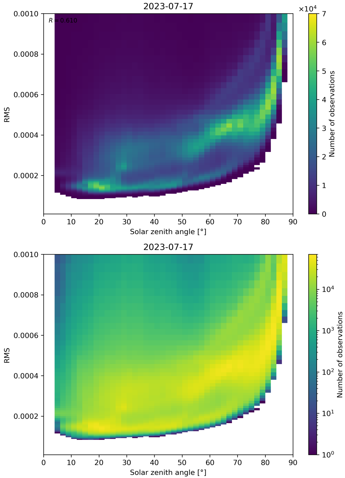
Figure 157: Scatter density plot of “Solar zenith angle” against “RMS” for 2023-07-16 to 2023-07-18.
