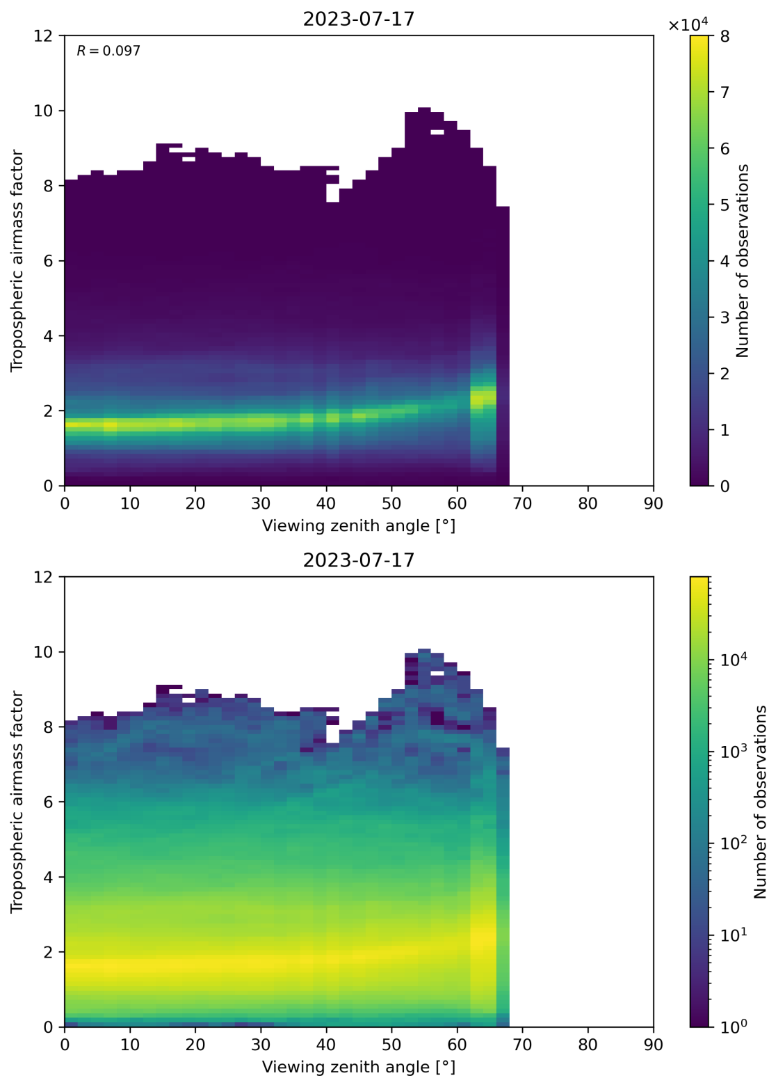
Figure 161: Scatter density plot of “Viewing zenith angle” against “Tropospheric airmass factor” for 2023-07-16 to 2023-07-18.
