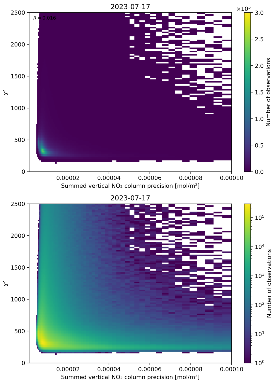
Figure 107: Scatter density plot of “Summed vertical NO 2 column precision” against “ \chi^2 ” for 2023-07-16 to 2023-07-18.
