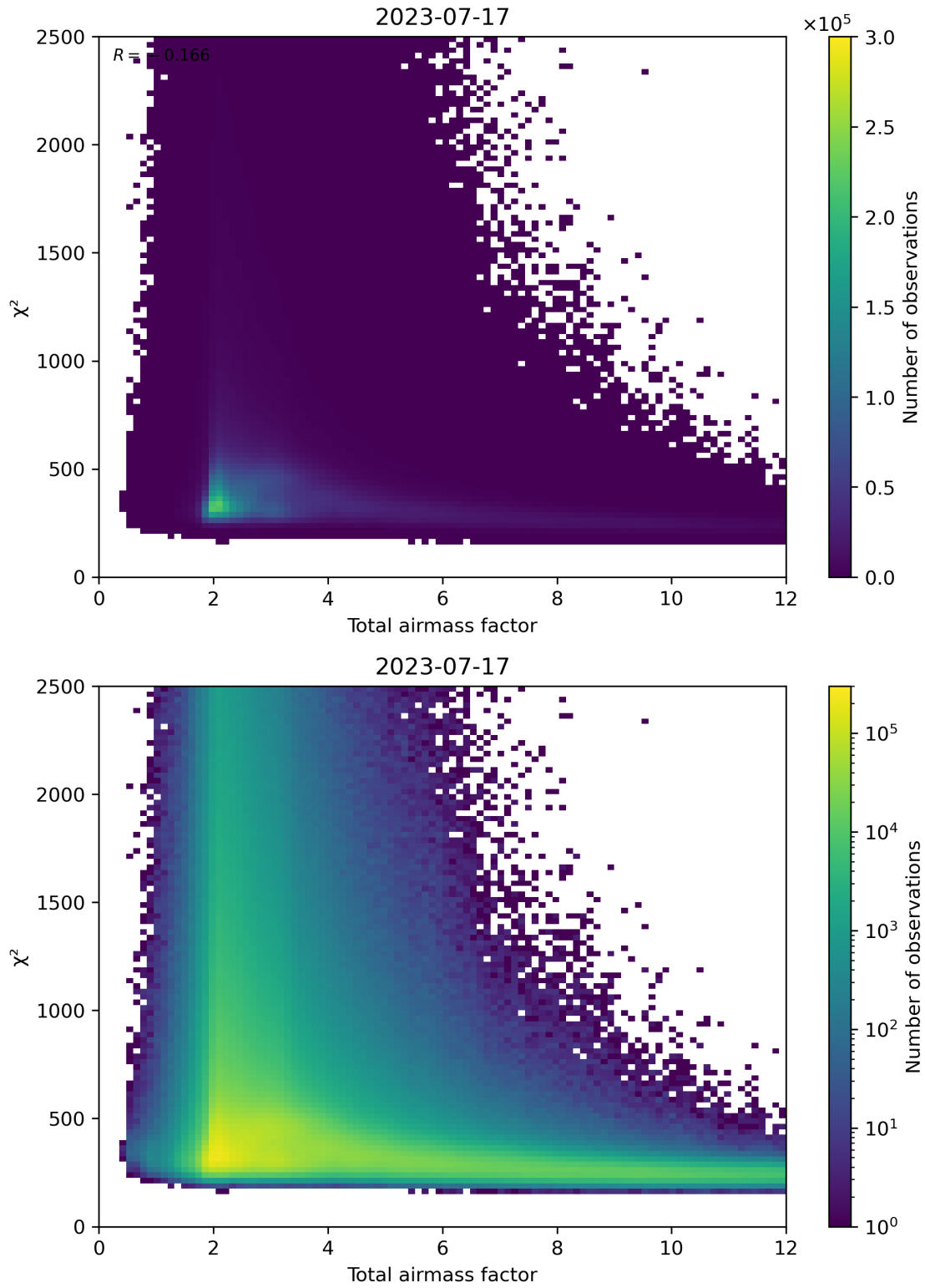
Figure 63: Scatter density plot of “Total airmass factor” against “ \chi^2 ” for 2023-07-16 to 2023-07-18.
