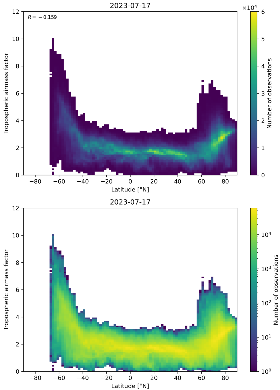
Figure 85: Scatter density plot of “Latitude” against “Tropospheric air mass factor” for 2023-07-16 to 2023-07-18.
