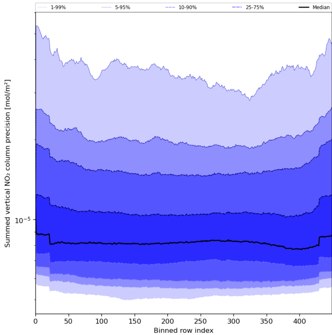
Figure 58: Along track statistics of “Summed vertical NO 2 column precision” for 2023-07-16 to 2023-07-18
