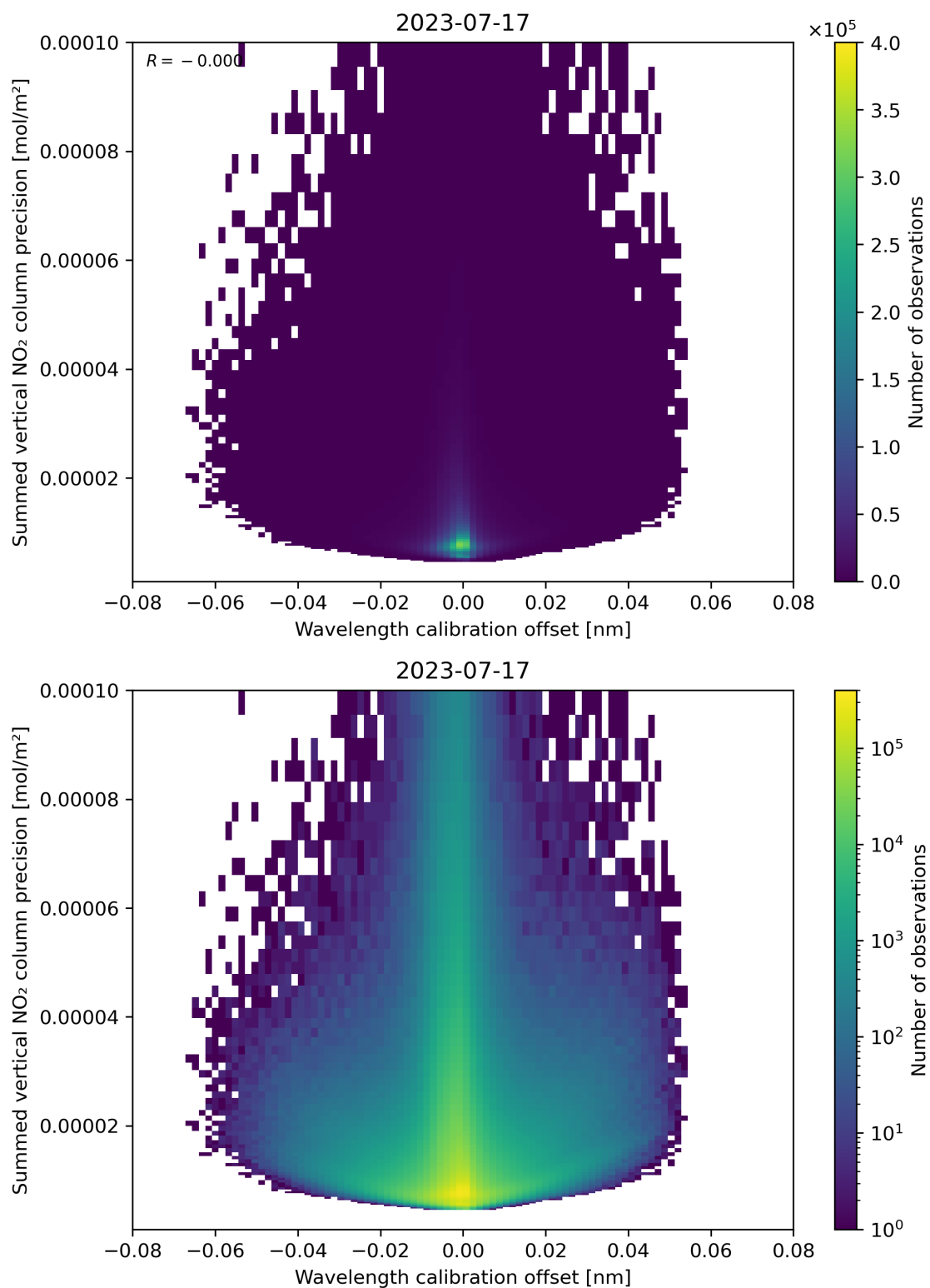
Figure 178: Scatter density plot of “Wavelength calibration offset” against “Summed vertical NO 2 column precision” for 2023-07-16 to 2023-07-18.
