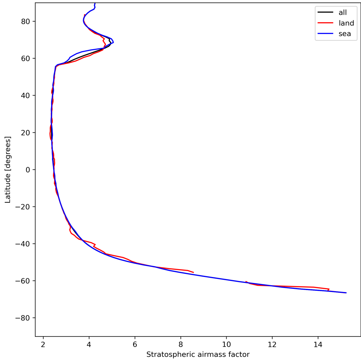
Figure 27: Zonal average of “Stratospheric airmass factor” for 2023-07-16 to 2023-07-18.
