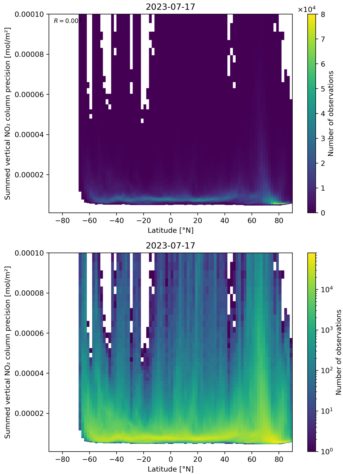
Figure 89: Scatter density plot of “Latitude” against “Summed vertical NO 2 column precision” for 2023-07-16 to 2023-07-18.
