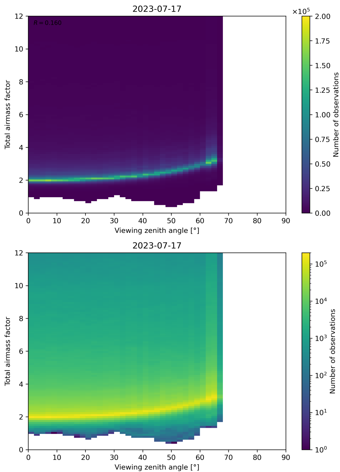
Figure 160: Scatter density plot of “Viewing zenith angle” against “Total airmass factor” for 2023-07-16 to 2023-07-18.
