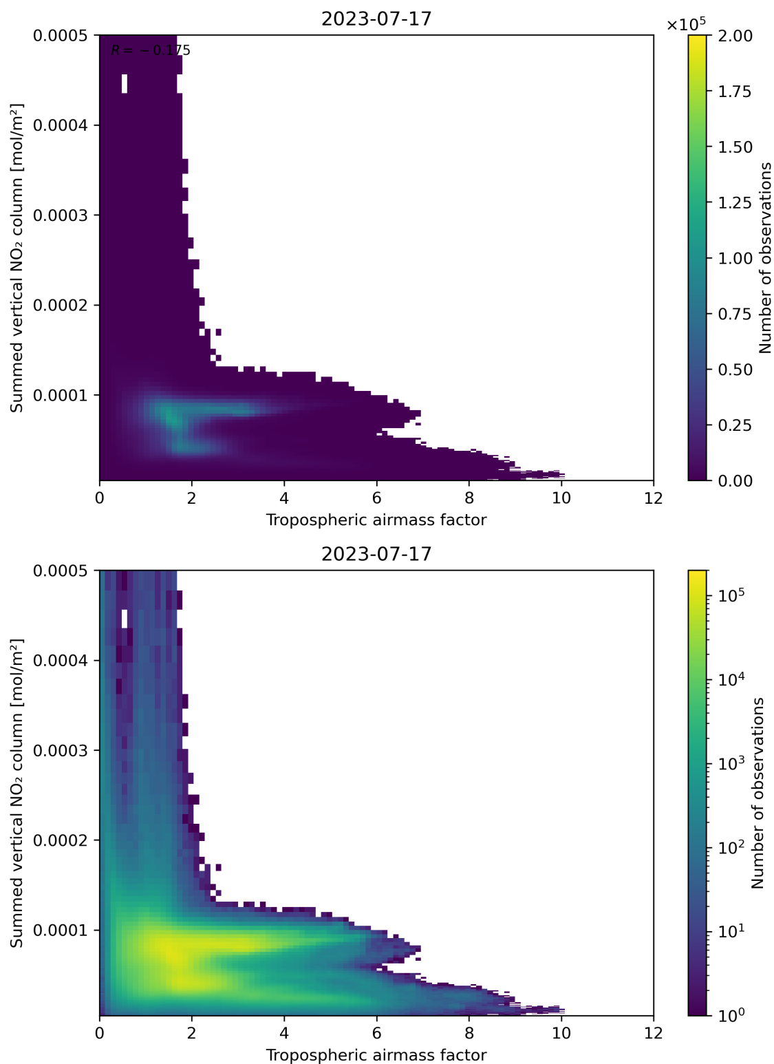
Figure 75: Scatter density plot of “Tropospheric airmass factor” against “Summed vertical NO 2 column” for 2023-07-16 to 2023-07-18.
