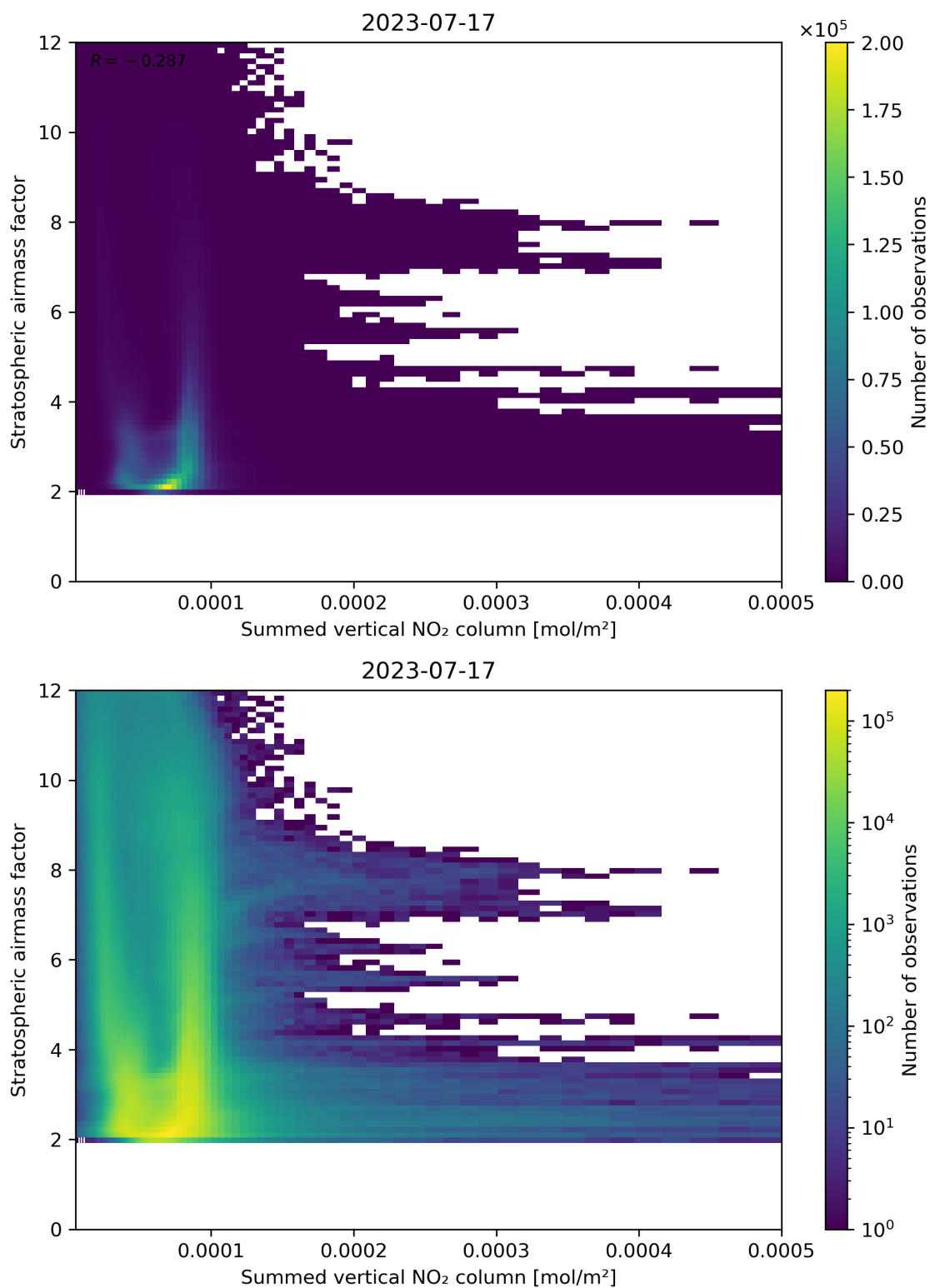
Figure 103: Scatter density plot of “Summed vertical NO 2 column” against “Stratospheric air mass factor” for 2023-07-16 to 2023-07-18.
