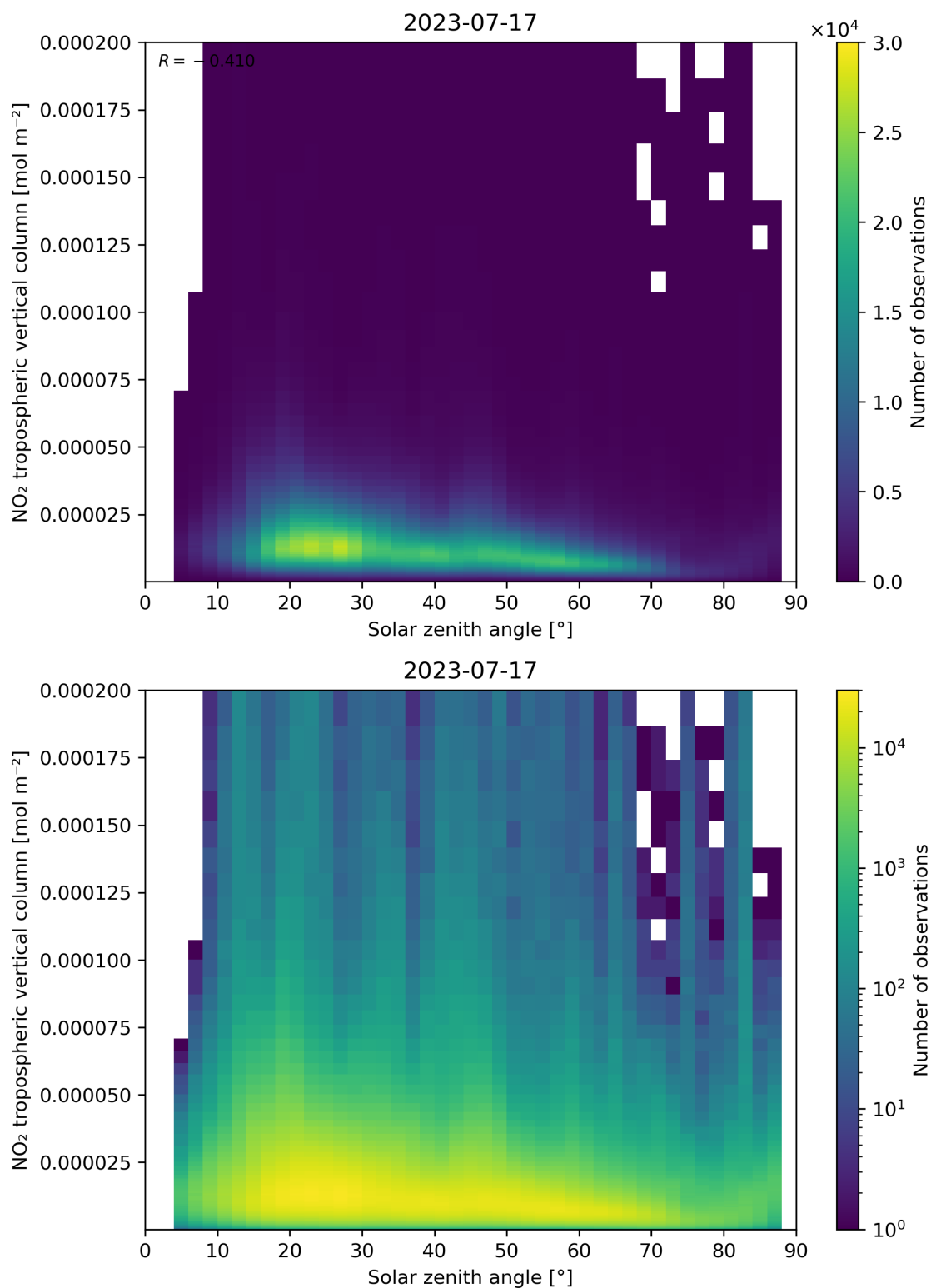
Figure 155: Scatter density plot of “Solar zenith angle” against “NO 2 tropospheric vertical column” for 2023-07-16 to 2023-07-18.
