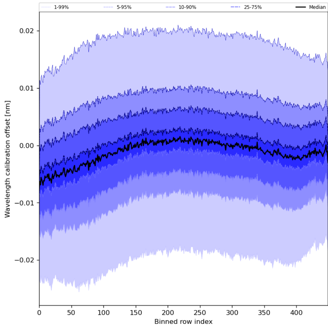
Figure 52: Along track statistics of “Wavelength calibration offset” for 2023-07-16 to 2023-07-18
