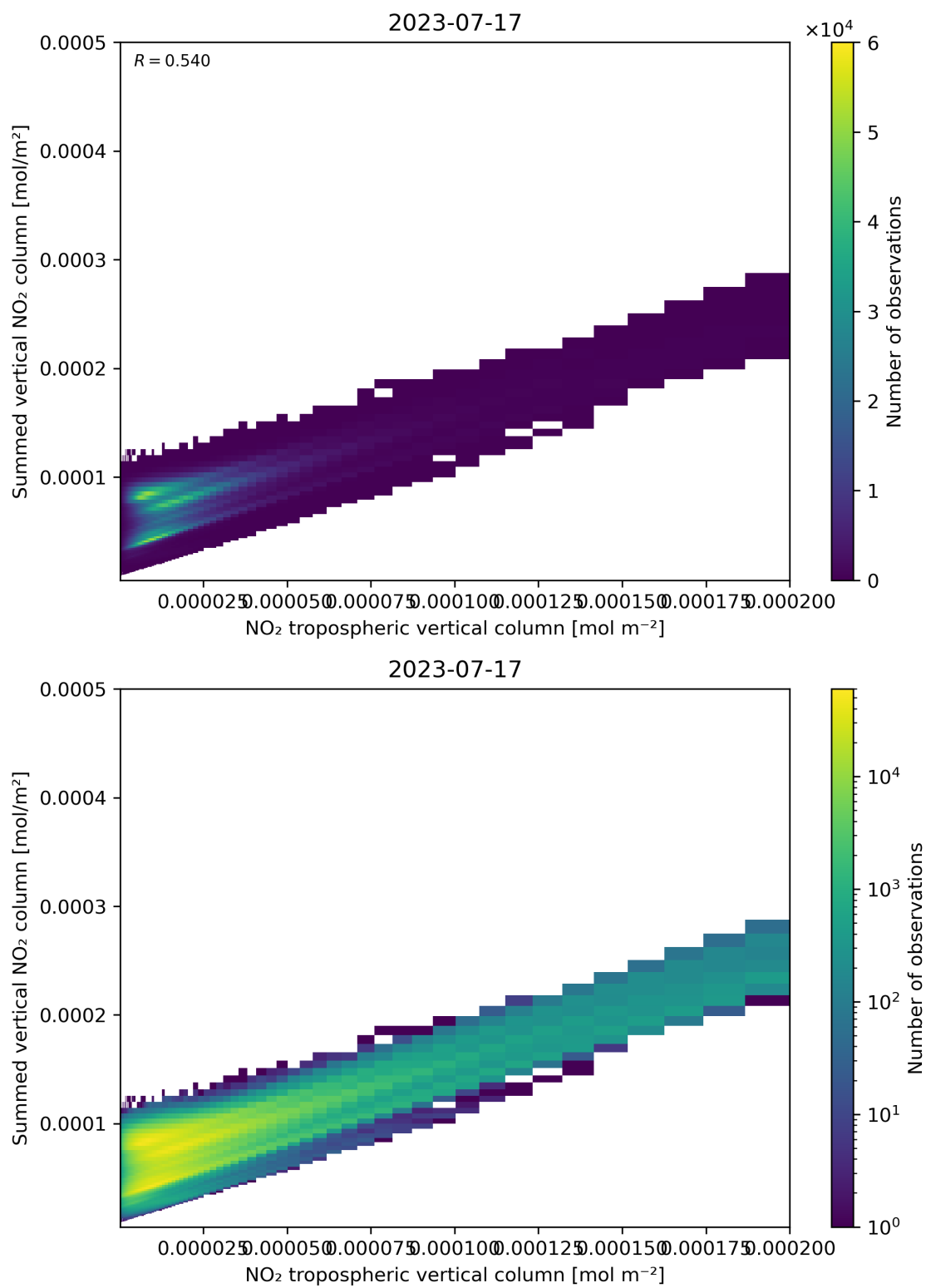
Figure 126: Scatter density plot of “NO 2 tropospheric vertical column” against “Summed vertical NO 2 column” for 2023-07-16 to 2023-07-18.
