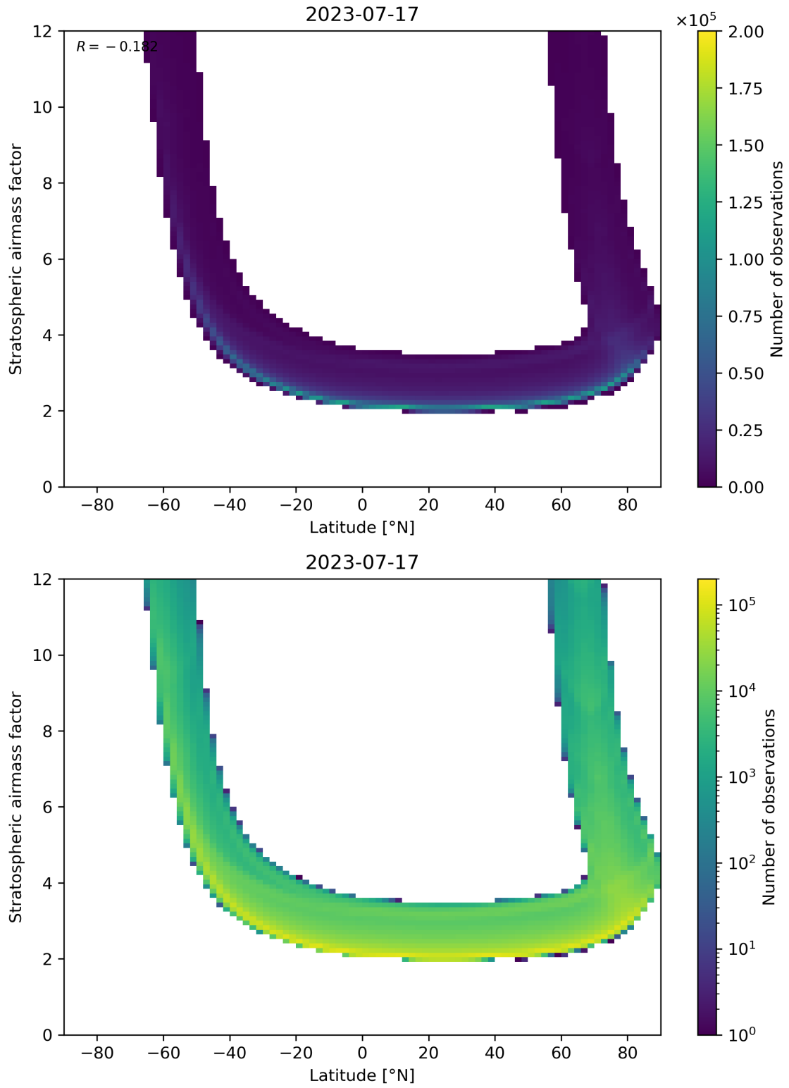
Figure 83: Scatter density plot of “Latitude” against “Stratospheric air mass factor” for 2023-07-16 to 2023-07-18.
