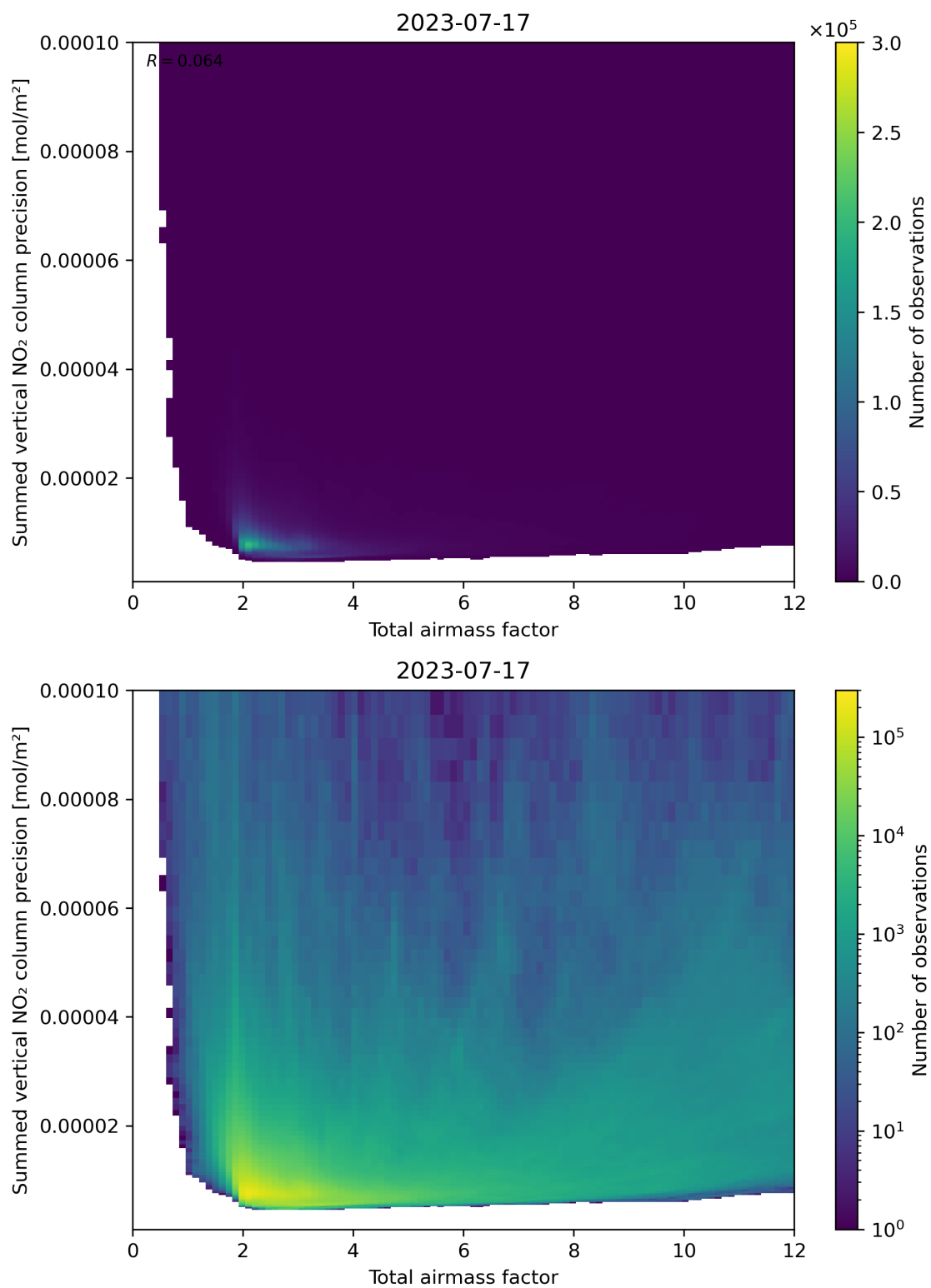
Figure 66: Scatter density plot of “Total airmass factor” against “Summed vertical NO 2 column precision” for 2023-07-16 to 2023-07-18.
