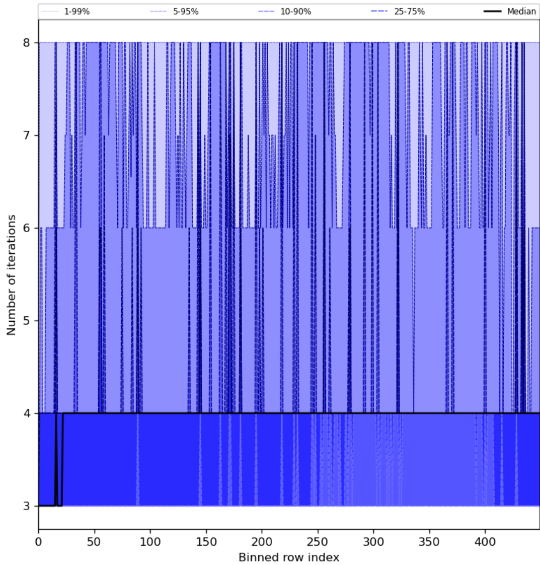
Figure 51: Along track statistics of “Number of iterations” for 2023-07-16 to 2023-07-18
