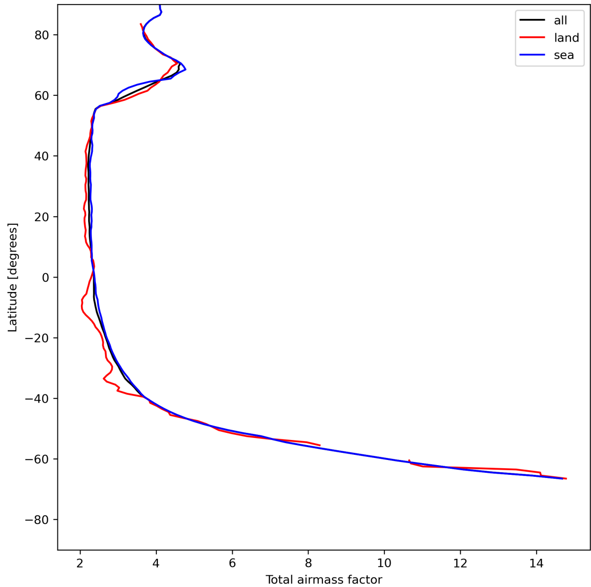
Figure 15: Zonal average of “Total airmass factor” for 2023-07-16 to 2023-07-18.
