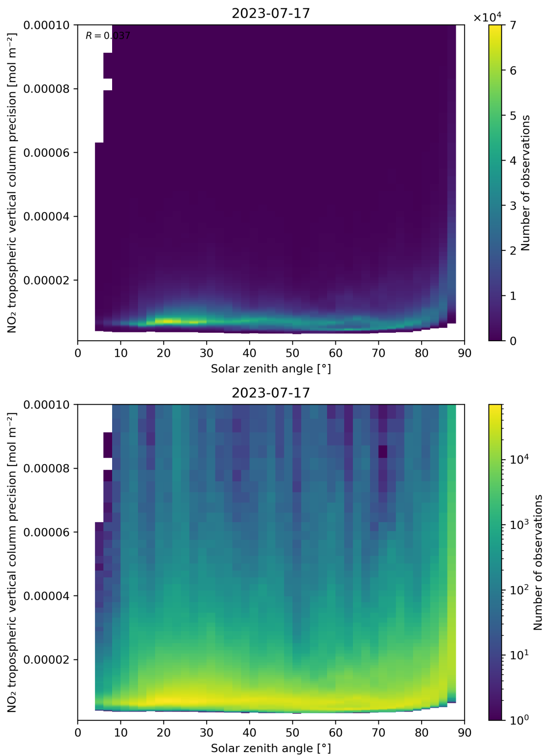
Figure 156: Scatter density plot of “Solar zenith angle” against “NO 2 tropospheric vertical column precision” for 2023-07-16 to 2023-07-18.
