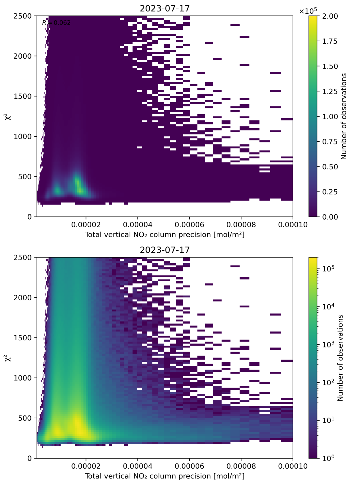
Figure 116: Scatter density plot of “Total vertical NO 2 column precision” against “ \chi^2 ” for 2023-07-16 to 2023-07-18.
