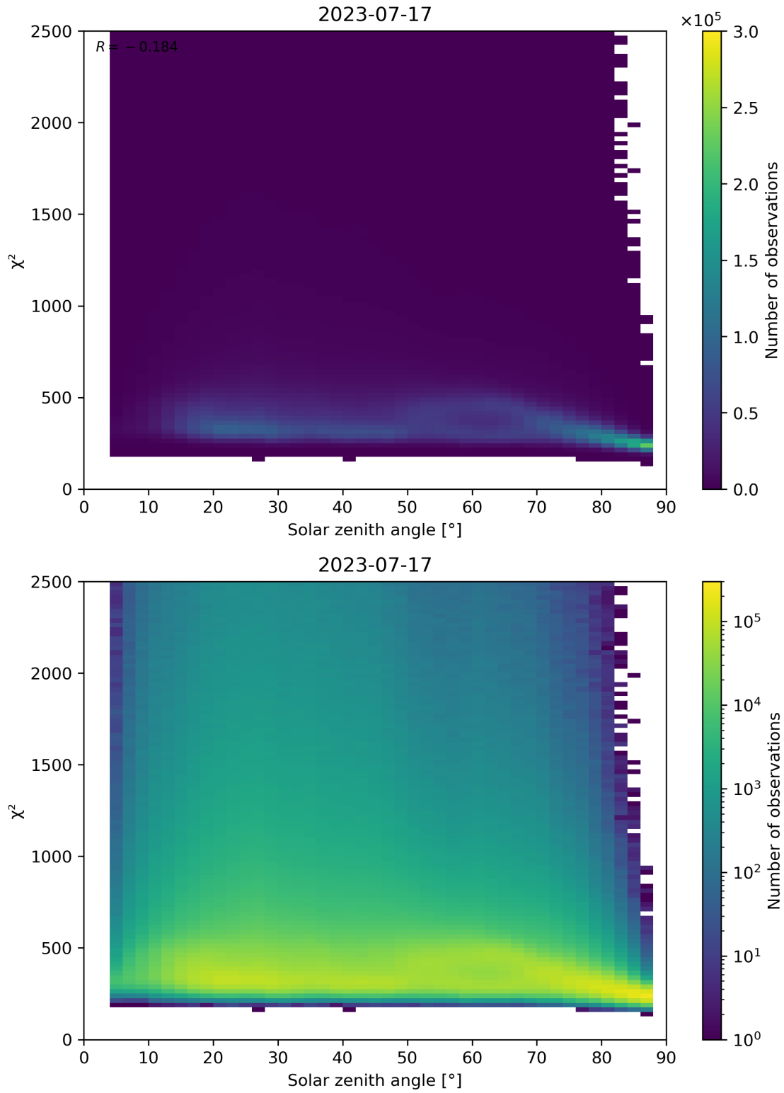
Figure 148: Scatter density plot of “Solar zenith angle” against “ \chi^2 ” for 2023-07-16 to 2023-07-18.
