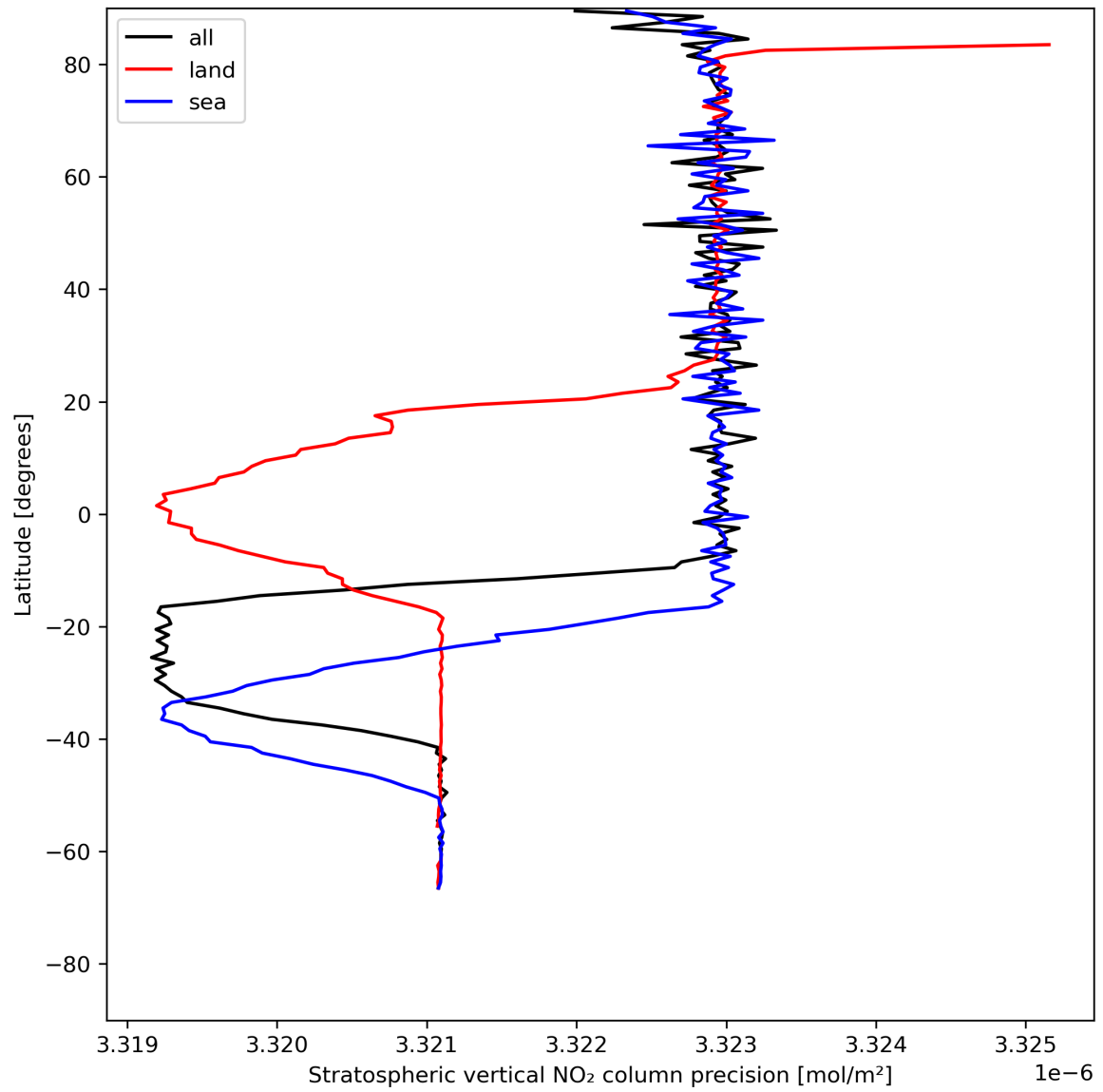
Figure 20: Zonal average of “Stratospheric vertical NO 2 column precision” for 2023-07-16 to 2023-07-18.
