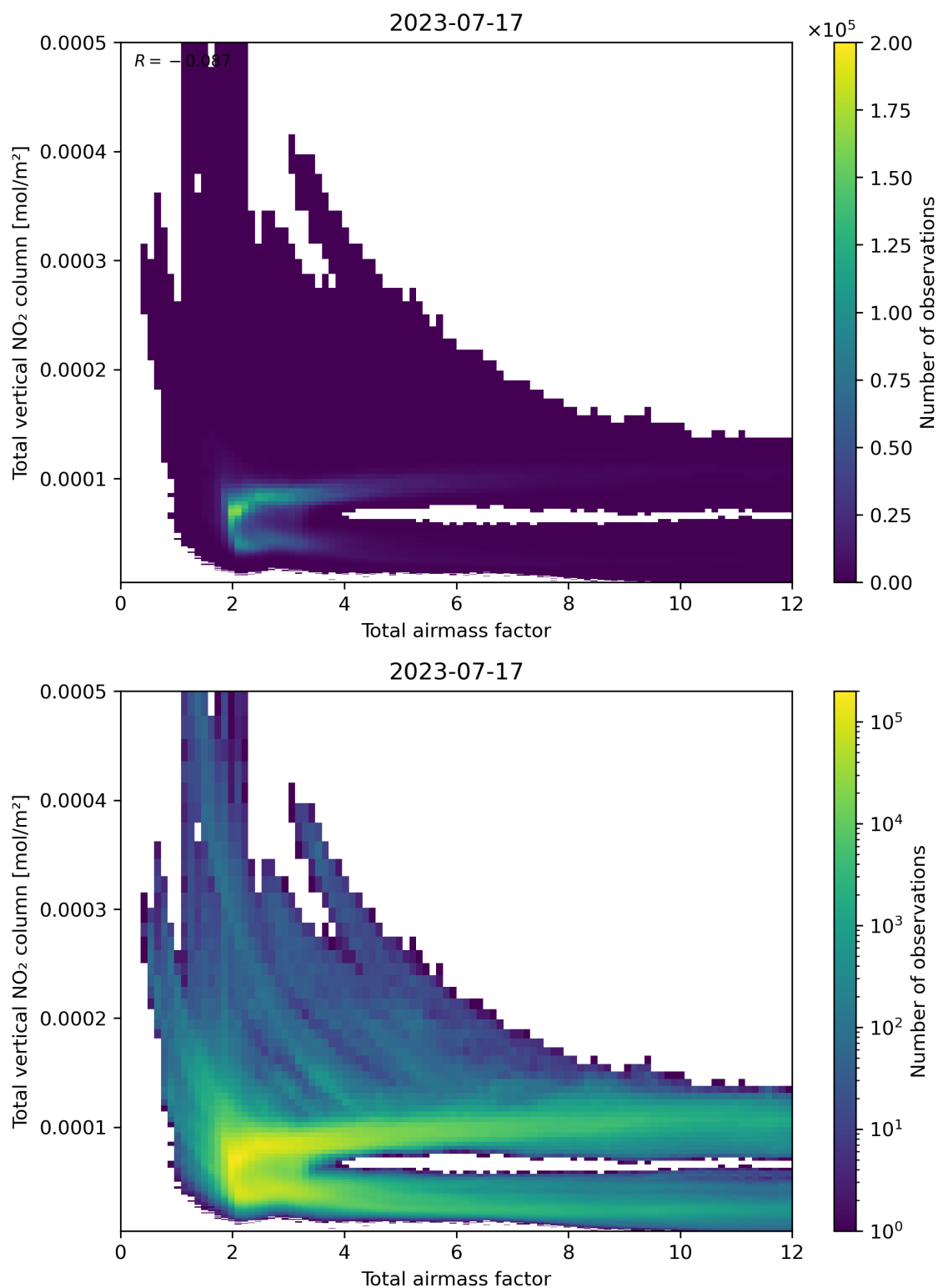
Figure 67: Scatter density plot of “Total airmass factor” against “Total vertical NO 2 column” for 2023-07-16 to 2023-07-18.
