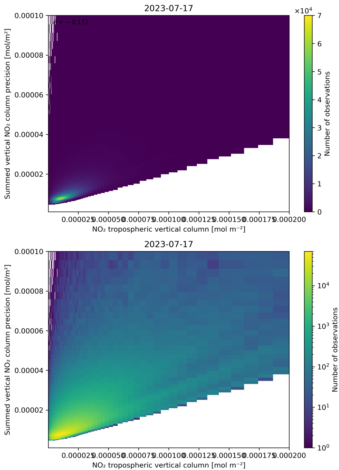
Figure 127: Scatter density plot of “NO 2 tropospheric vertical column” against “Summed vertical NO 2 column precision” for 2023-07-16 to 2023-07-18.
