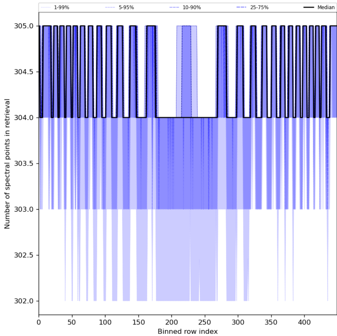
Figure 50: Along track statistics of “Number of spectral points in retrieval” for 2023-07-16 to 2023-07-18
