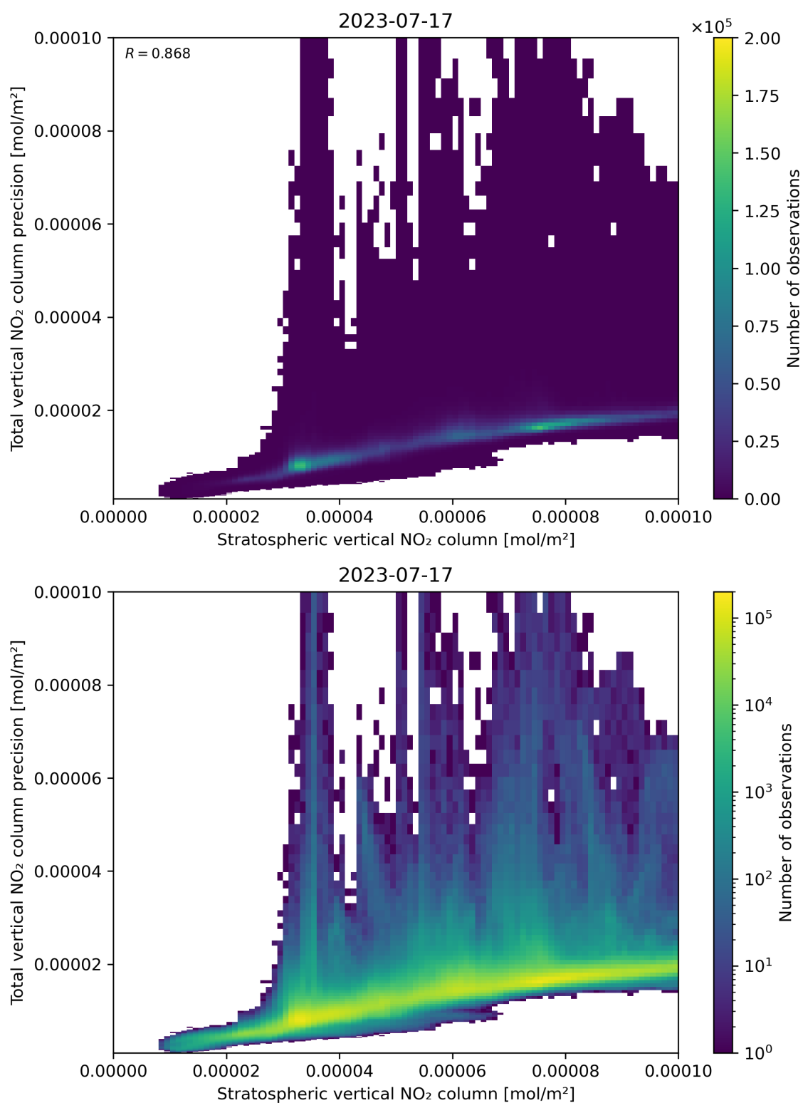
Figure 101: Scatter density plot of “Stratospheric vertical NO 2 column” against “Total vertical NO 2 column precision” for 2023-07-16 to 2023-07-18.
