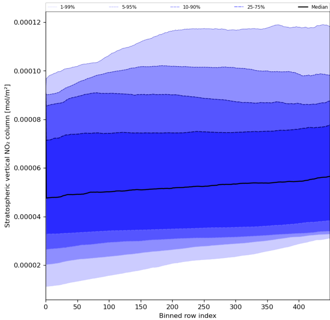
Figure 53: Along track statistics of “Stratospheric vertical NO 2 column” for 2023-07-16 to 2023-07-18
