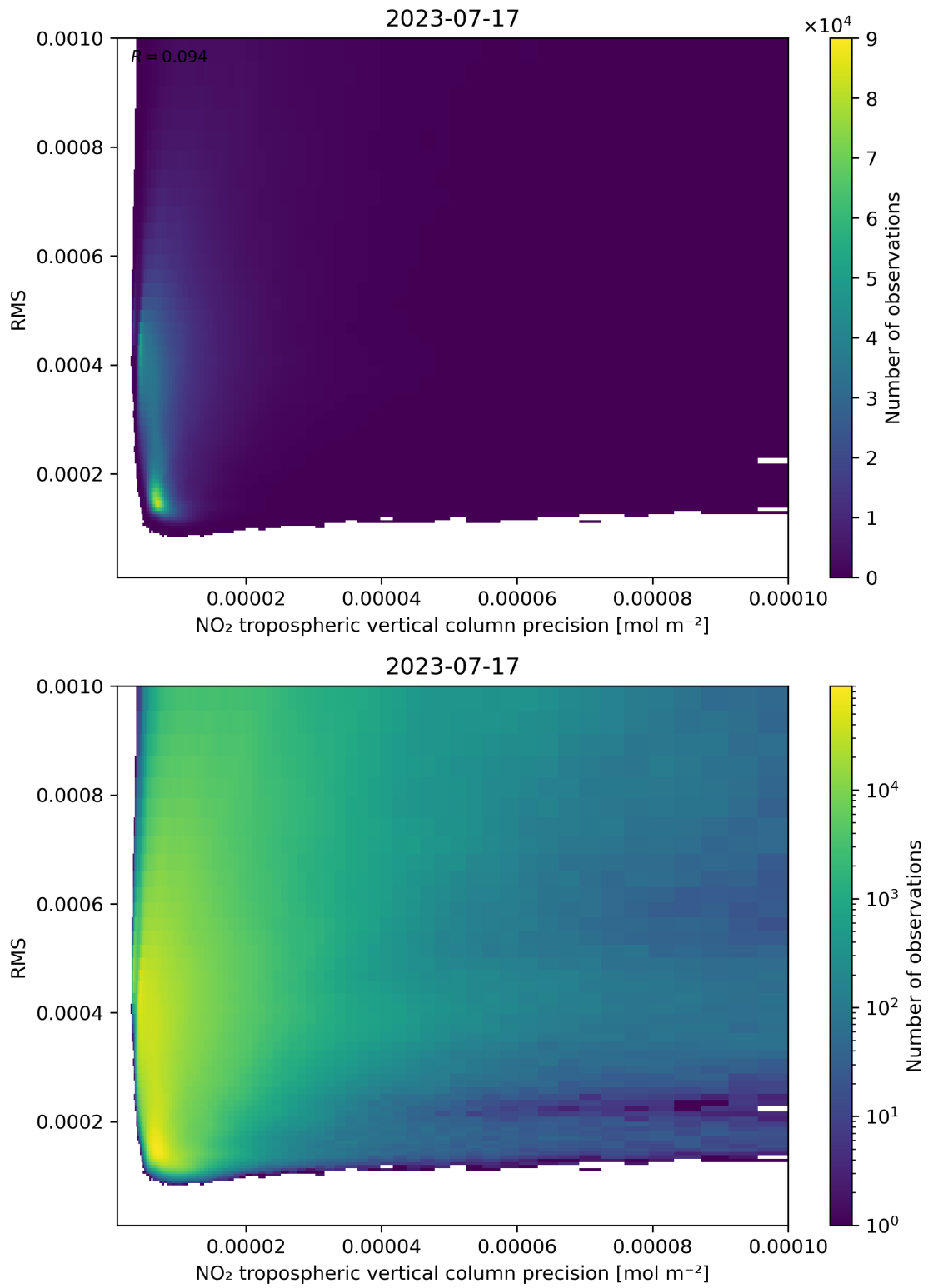
Figure 140: Scatter density plot of “NO 2 tropospheric vertical column precision” against “RMS” for 2023-07-16 to 2023-07-18.
