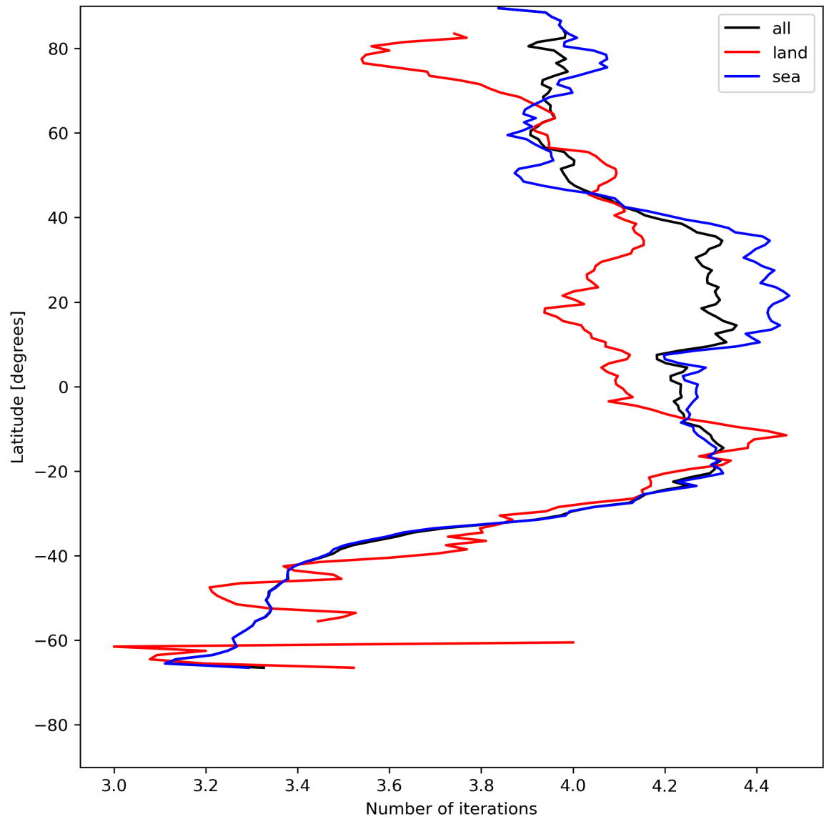
Figure 17: Zonal average of “Number of iterations” for 2023-07-16 to 2023-07-18.
