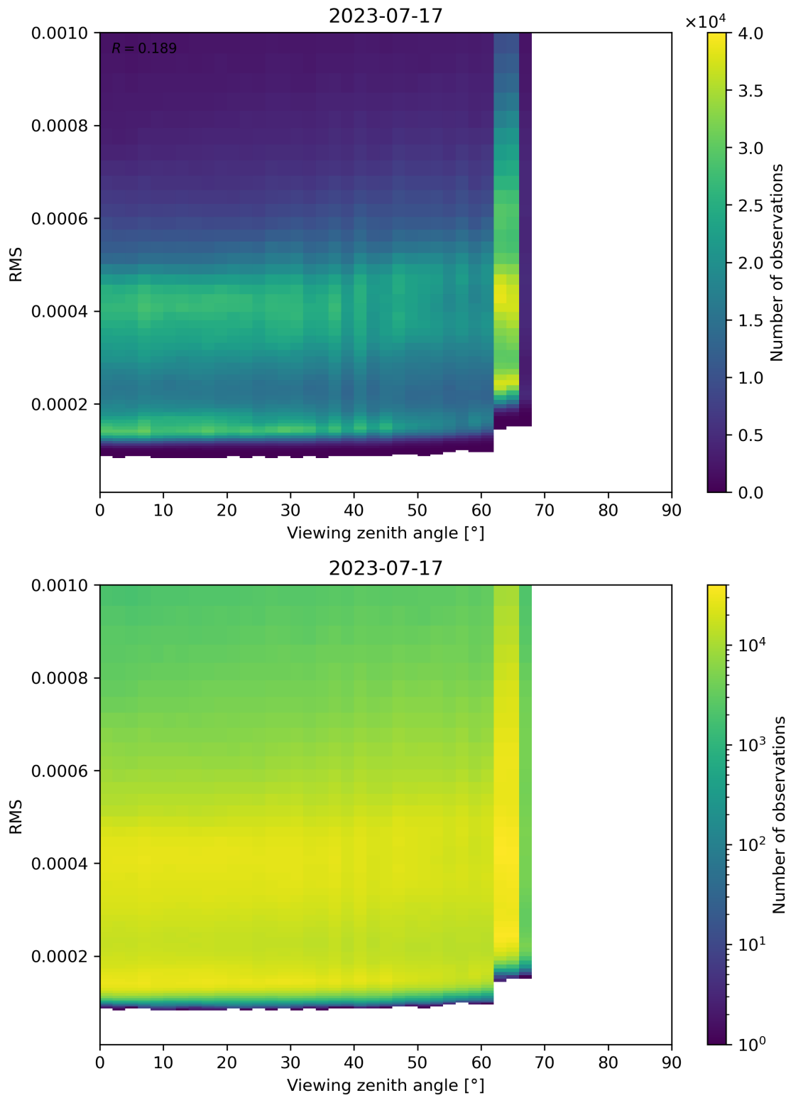
Figure 171: Scatter density plot of “Viewing zenith angle” against “RMS” for 2023-07-16 to 2023-07-18.
