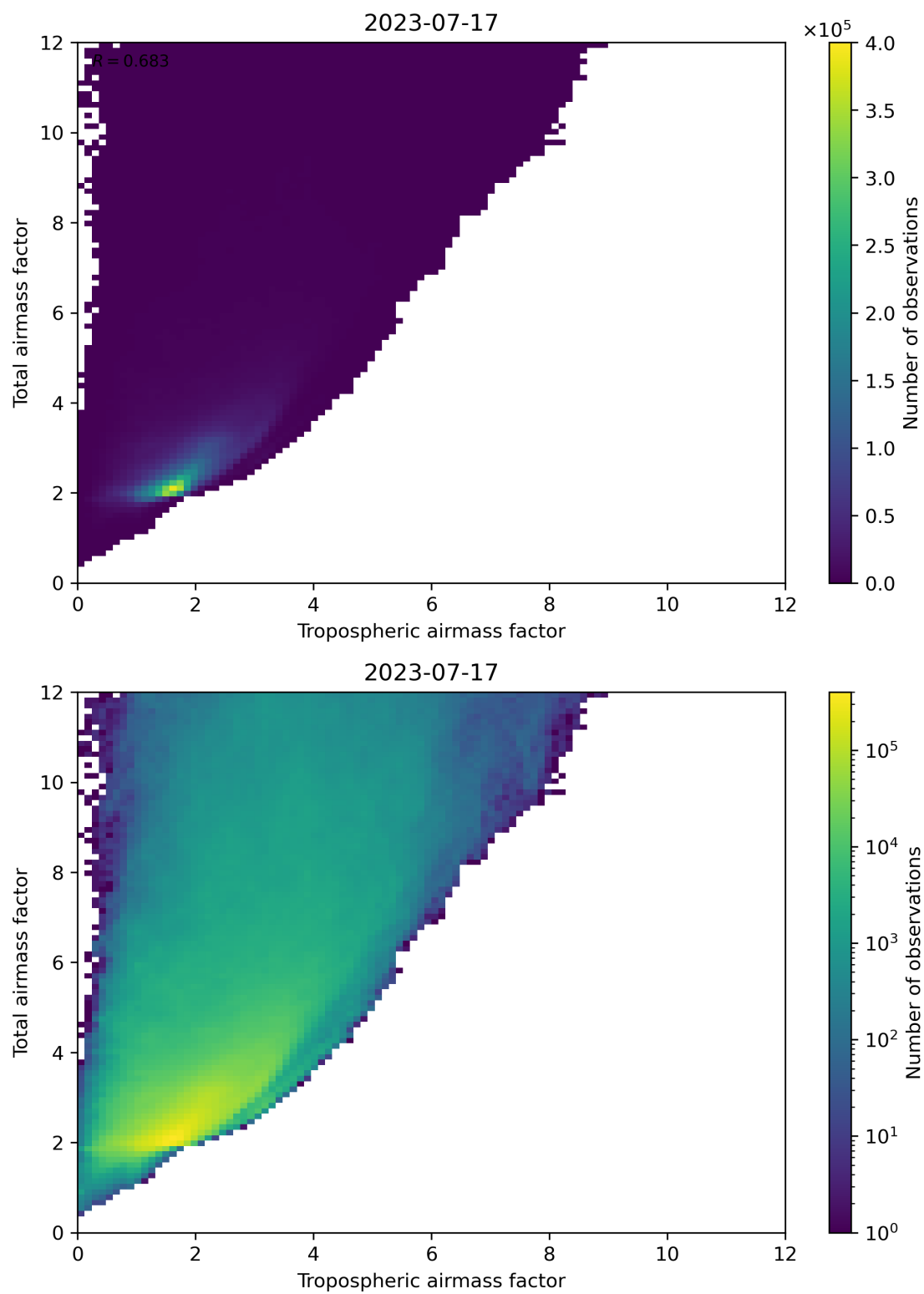
Figure 72: Scatter density plot of “Tropospheric airmass factor” against “Total airmass factor” for 2023-07-16 to 2023-07-18.
