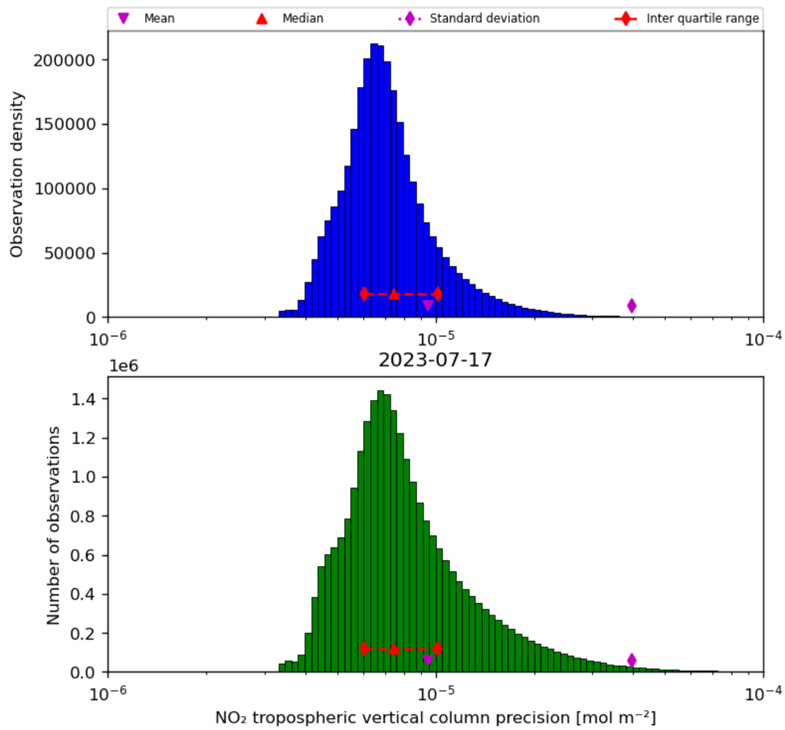
Figure 30: Histogram of “NO 2 tropospheric vertical column precision” for 2023-07-16 to 2023-07-18
