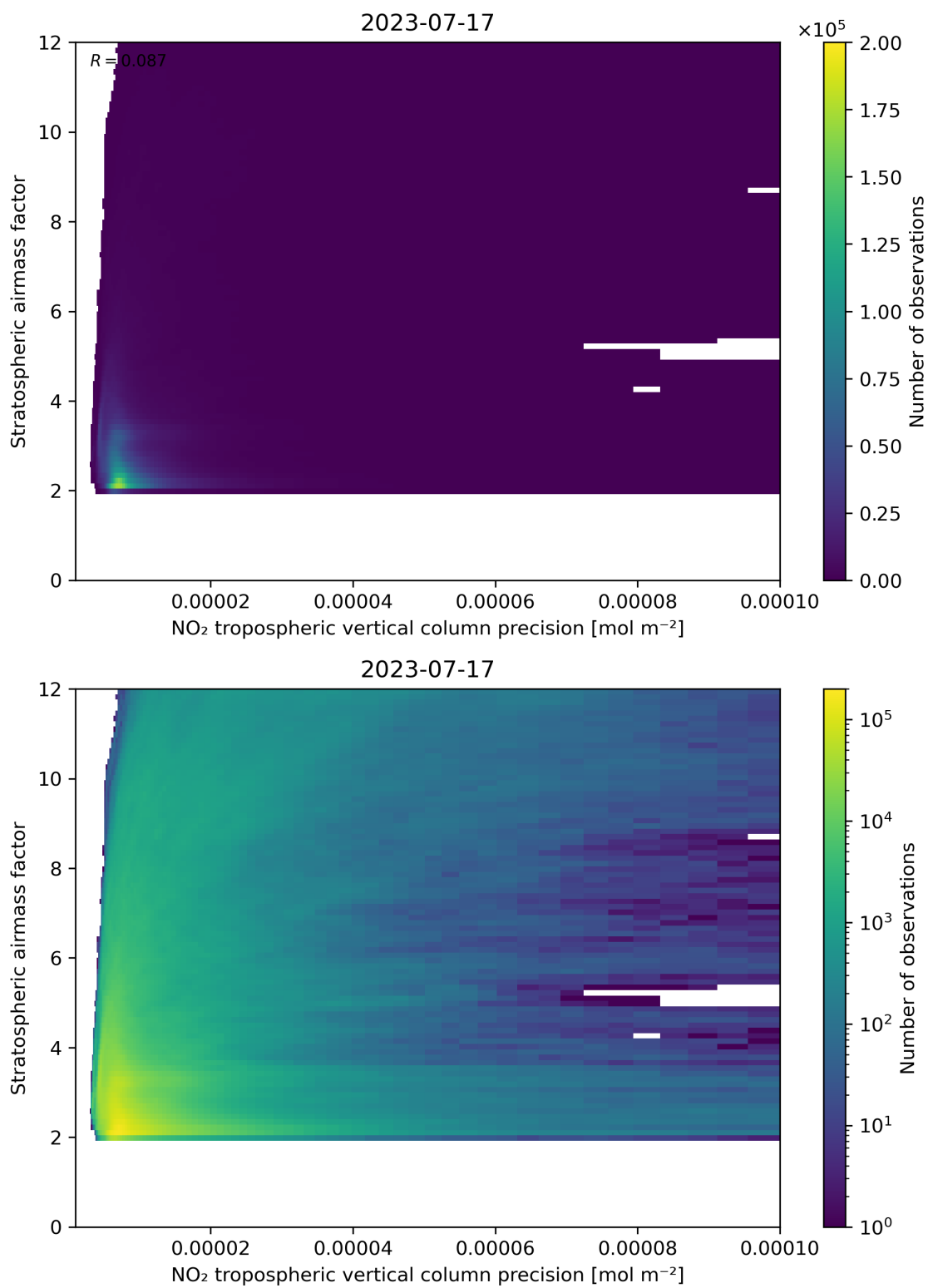
Figure 131: Scatter density plot of “NO 2 tropospheric vertical column precision” against “Stratospheric airmass factor” for 2023-07-16 to 2023-07-18.
