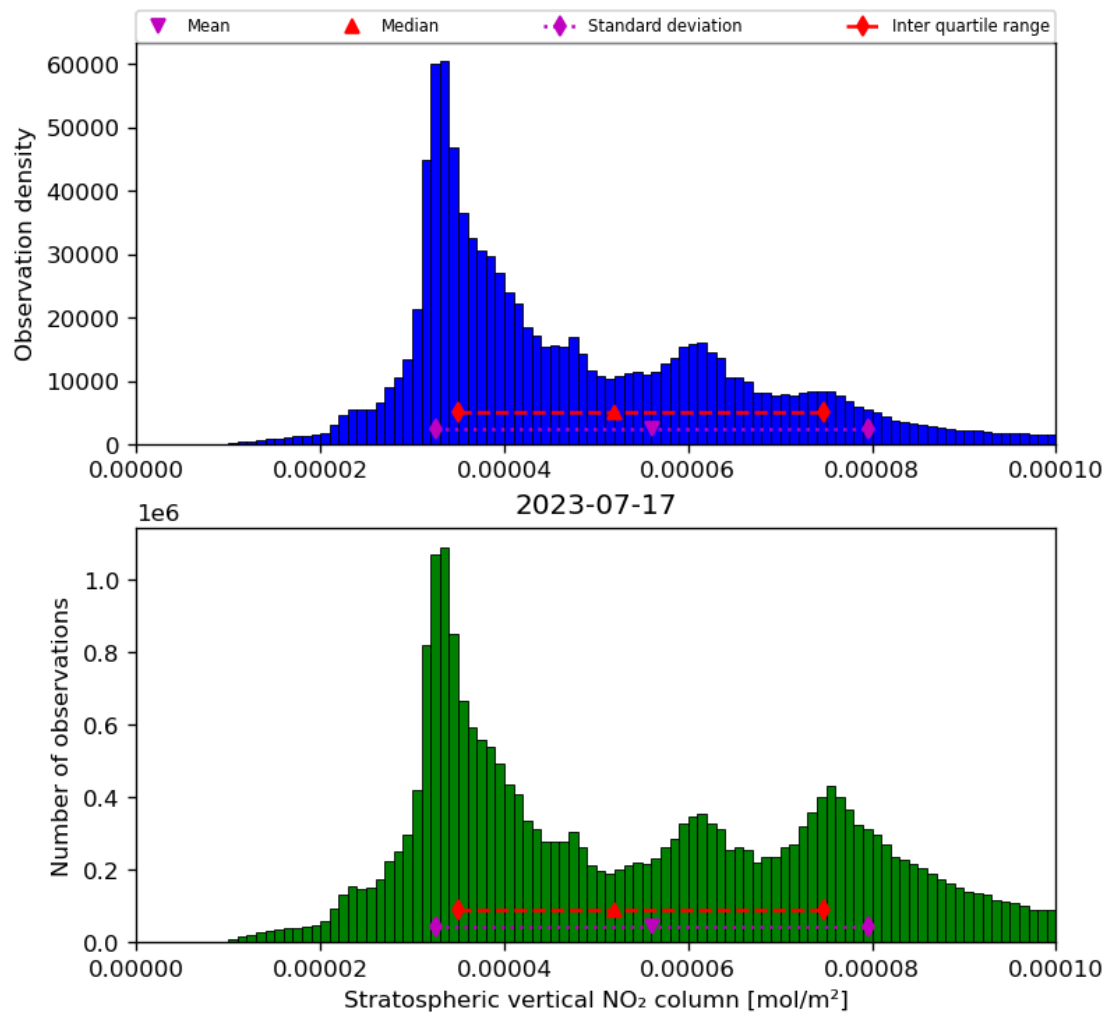
Figure 36: Histogram of “Stratospheric vertical NO 2 column” for 2023-07-16 to 2023-07-18
