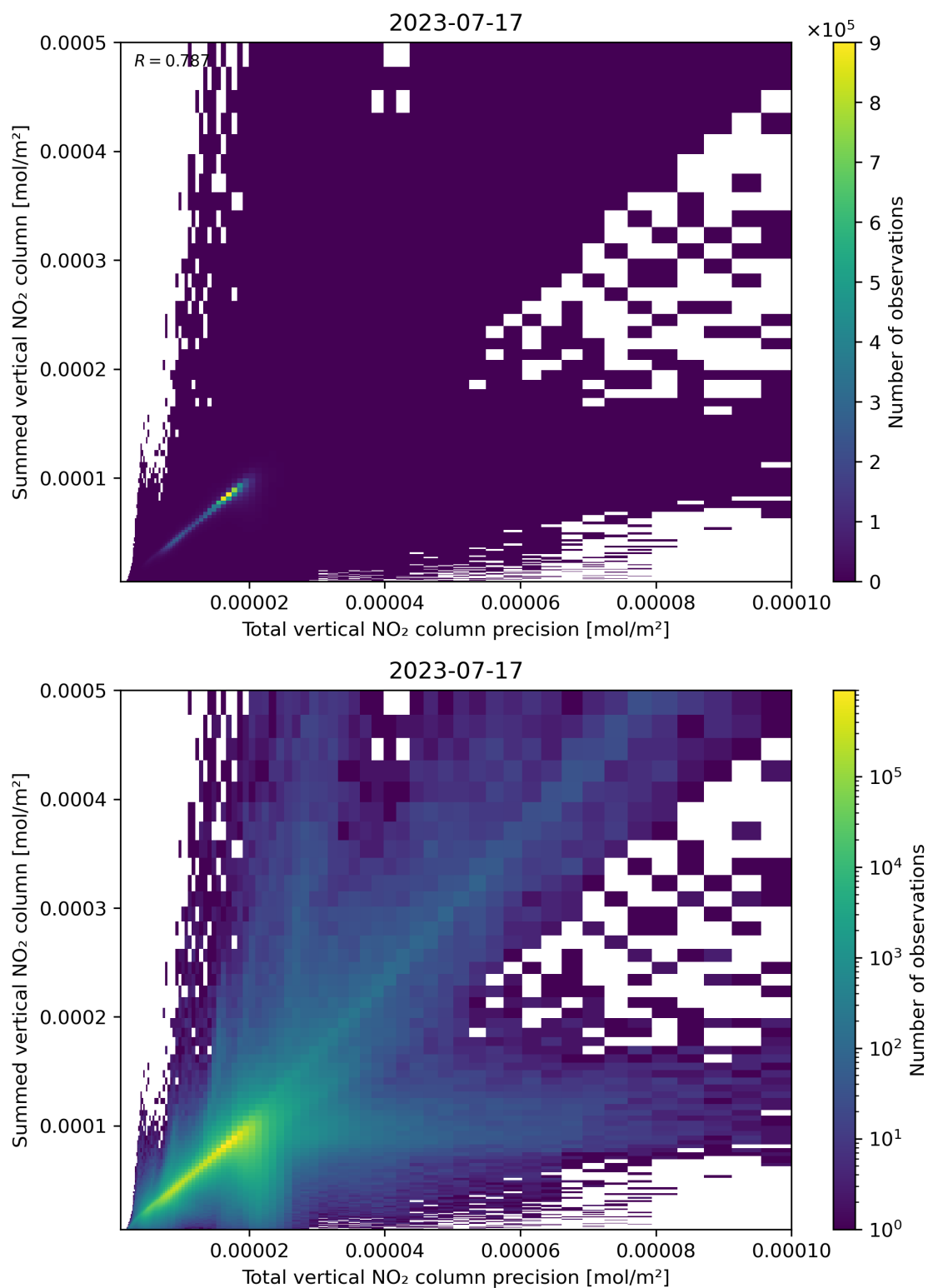
Figure 117: Scatter density plot of “Total vertical NO 2 column precision” against “Summed vertical NO 2 column” for 2023-07-16 to 2023-07-18.
