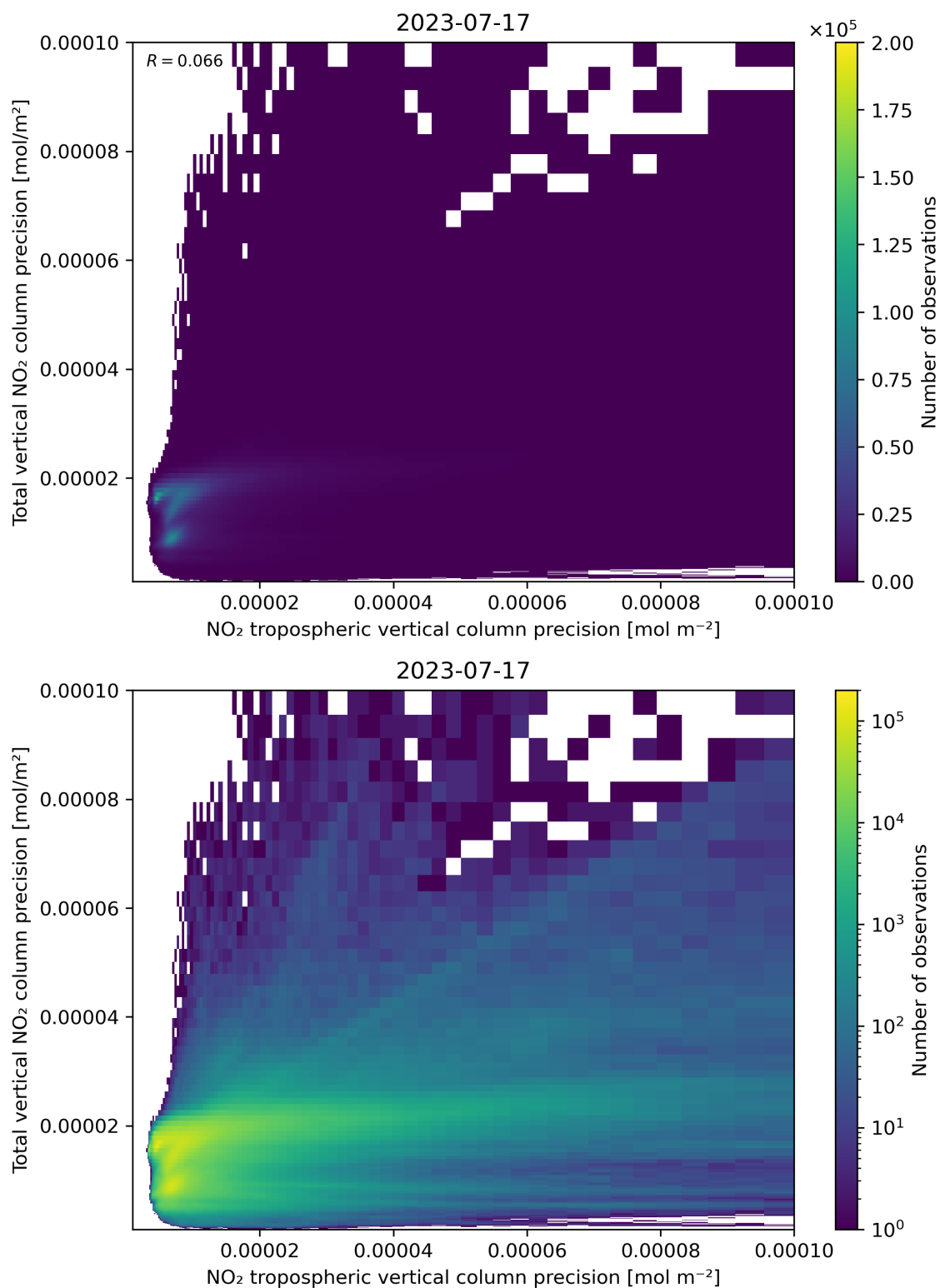
Figure 139: Scatter density plot of “NO 2 tropospheric vertical column precision” against “Total vertical NO 2 column precision” for 2023-07-16 to 2023-07-18.
