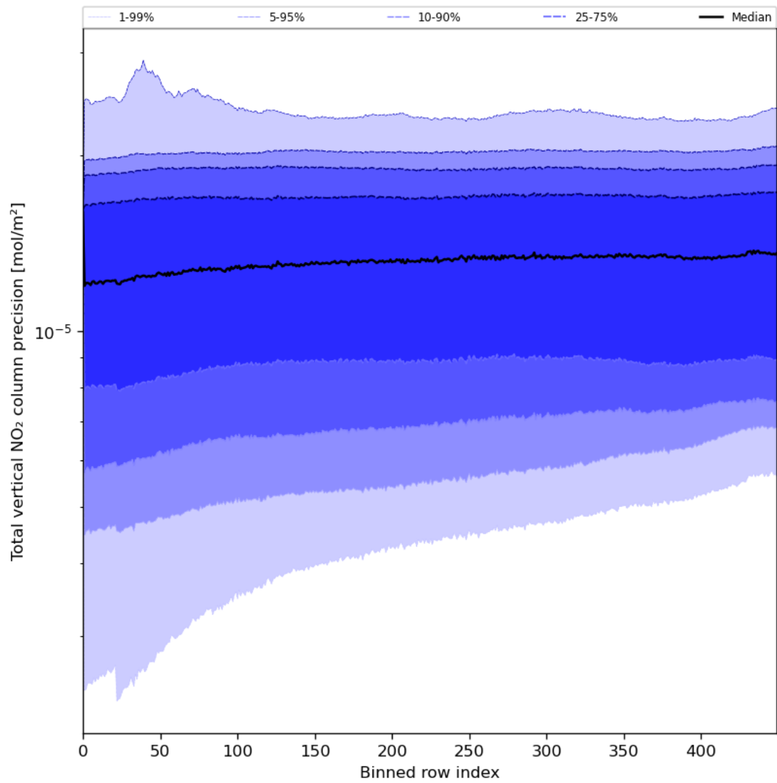
Figure 56: Along track statistics of “Total vertical NO 2 column precision” for 2023-07-16 to 2023-07-18
