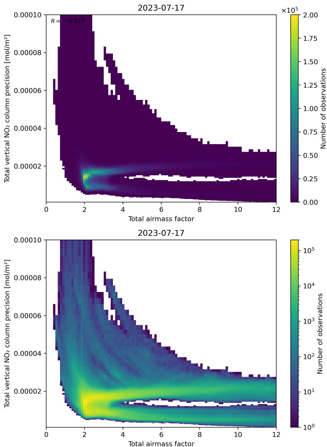
Figure 68: Scatter density plot of “Total airmass factor” against “Total vertical NO 2 column precision” for 2023-07-16 to 2023-07-18.
