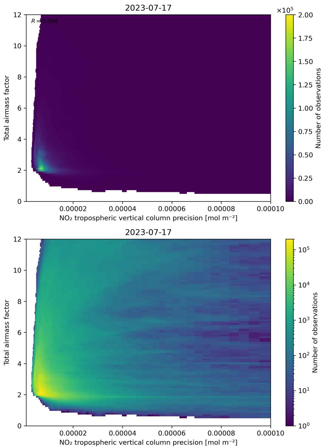
Figure 132: Scatter density plot of “NO 2 tropospheric vertical column precision” against “Total air mass factor” for 2023-07-16 to 2023-07-18.
