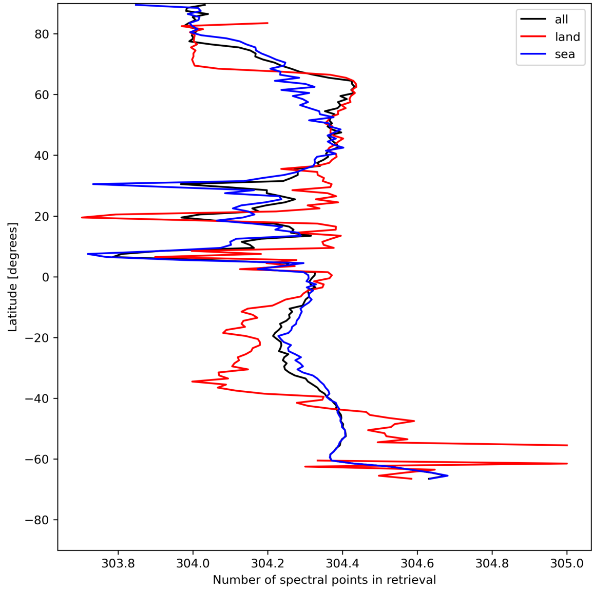
Figure 16: Zonal average of “Number of spectral points in retrieval” for 2023-07-16 to 2023-07-18.
