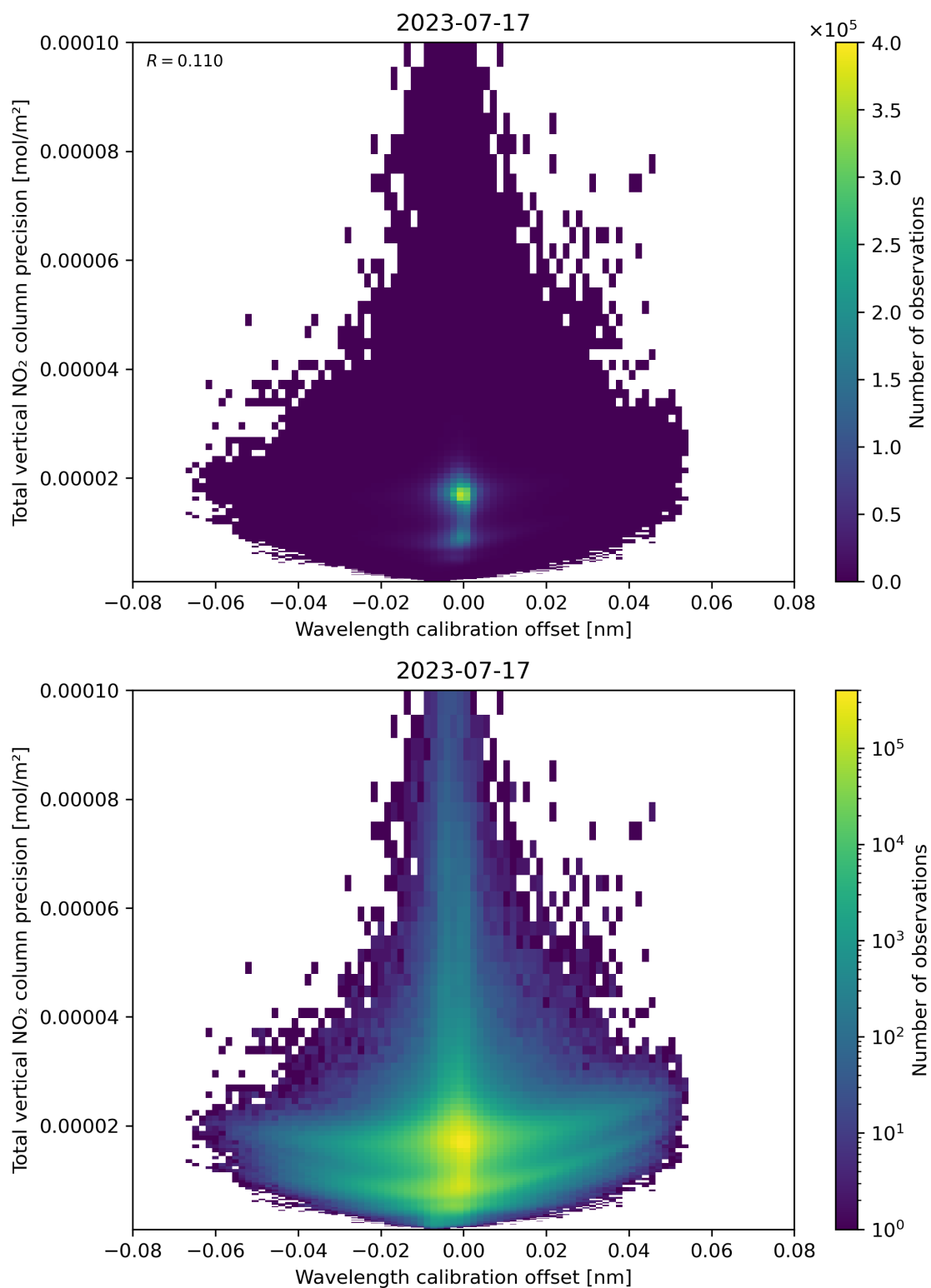
Figure 180: Scatter density plot of “Wavelength calibration offset” against “Total vertical NO 2 column precision” for 2023-07-16 to 2023-07-18.
