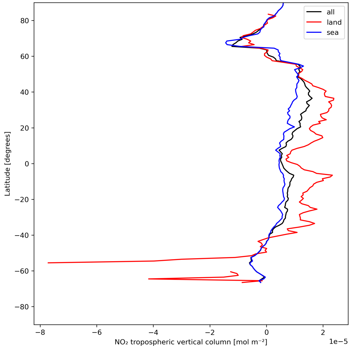
Figure 12: Zonal average of “NO 2 tropospheric vertical column” for 2023-07-16 to 2023-07-18.
