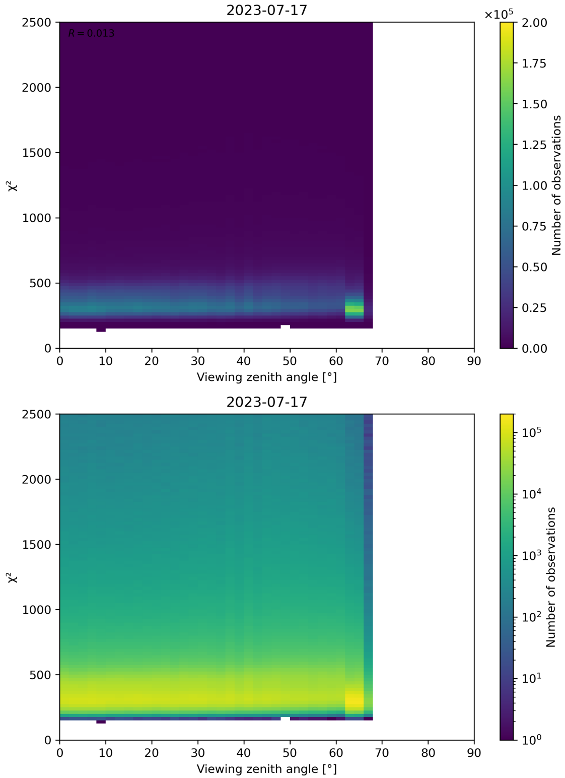
Figure 162: Scatter density plot of “Viewing zenith angle” against “ \chi^2 ” for 2023-07-16 to 2023-07-18.
