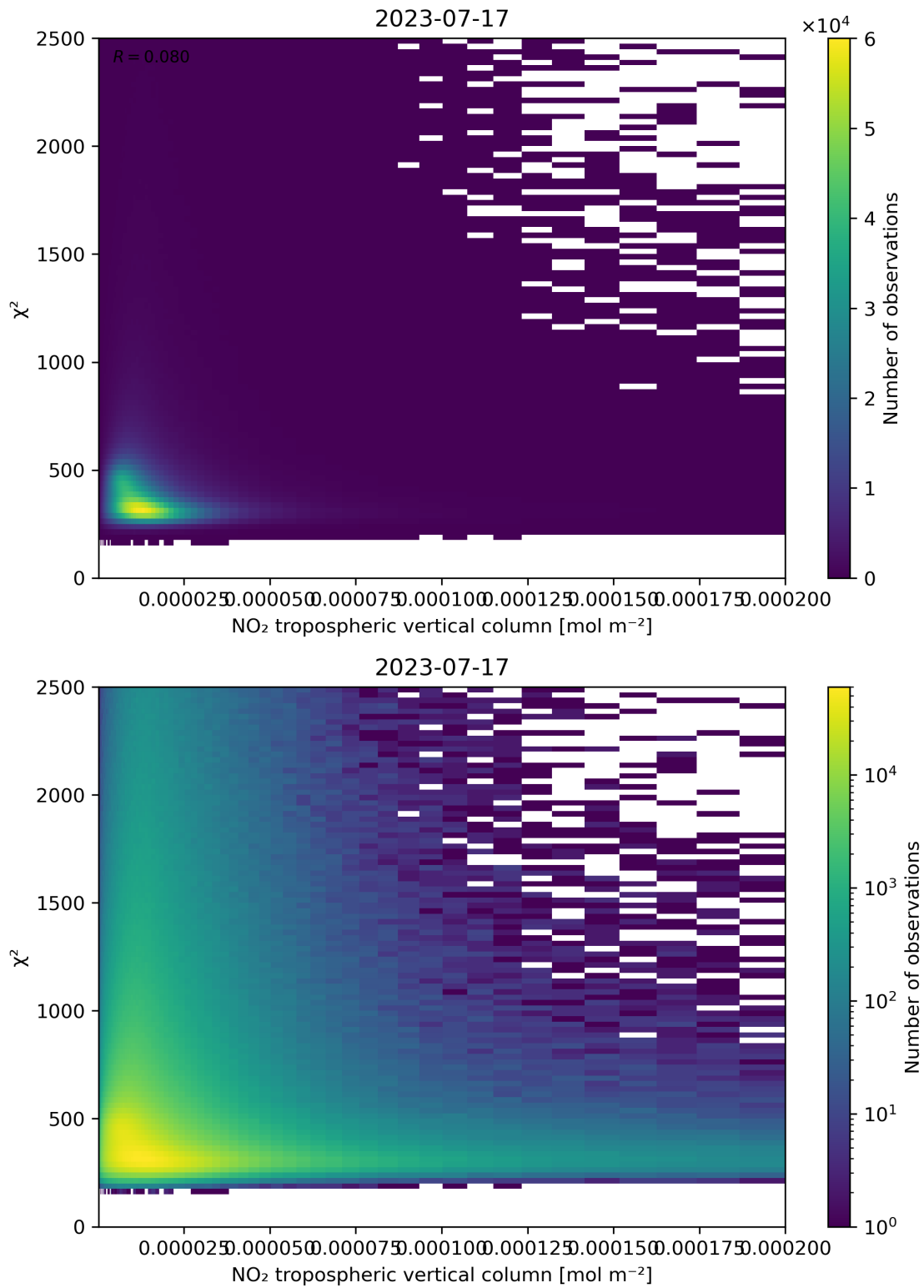
Figure 124: Scatter density plot of “NO 2 tropospheric vertical column” against “ \chi^2 ” for 2023-07-16 to 2023-07-18.
