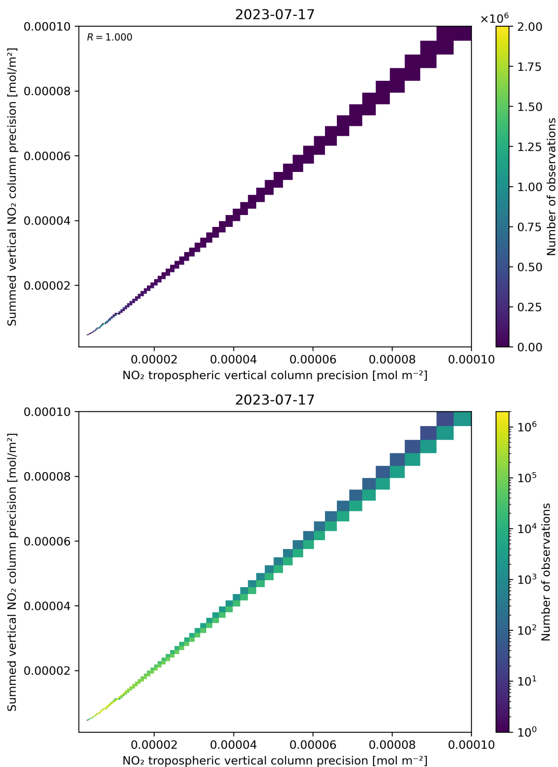
Figure 137: Scatter density plot of “NO 2 tropospheric vertical column precision” against “Summed vertical NO 2 column precision” for 2023-07-16 to 2023-07-18.
