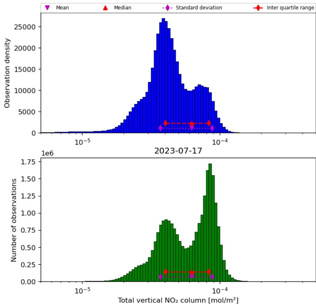
Figure 38: Histogram of “Total vertical NO 2 column” for 2023-07-16 to 2023-07-18
