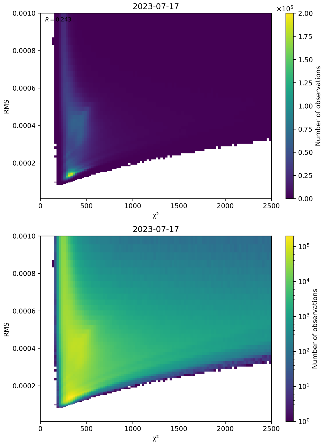
Figure 82: Scatter density plot of “ \chi^2 ” against “RMS” for 2023-07-16 to 2023-07-18.
