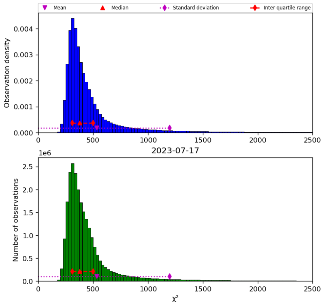
Figure 42: Histogram of “ \chi^2 ” for 2023-07-16 to 2023-07-18
