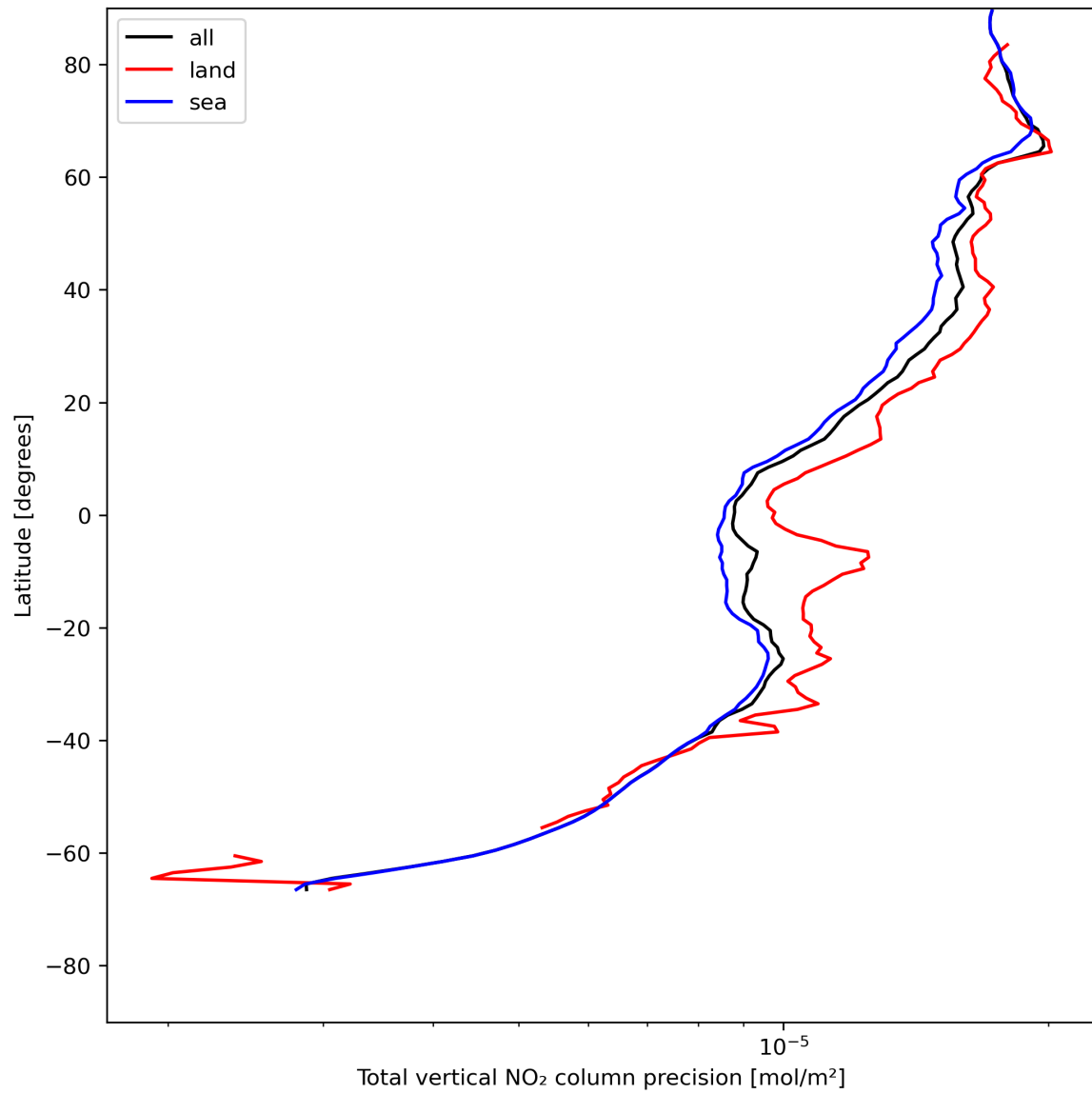
Figure 22: Zonal average of “Total vertical NO 2 column precision” for 2023-07-16 to 2023-07-18.
