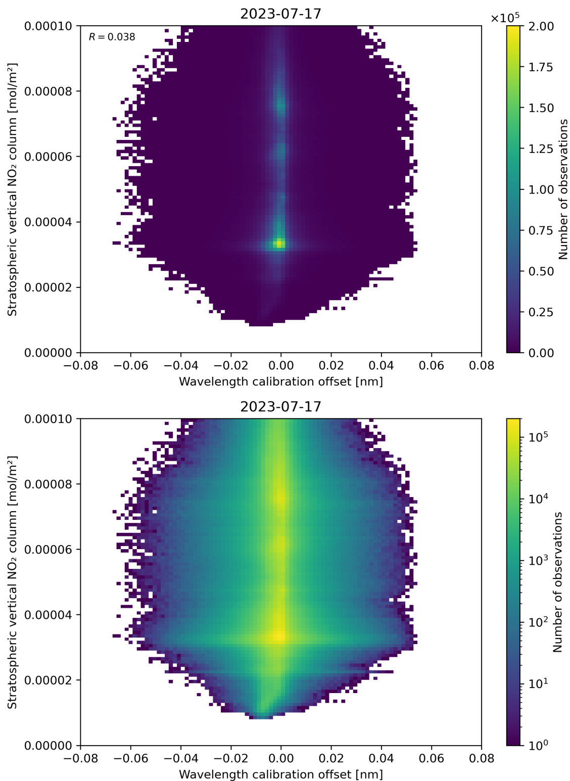
Figure 176: Scatter density plot of “Wavelength calibration offset” against “Stratospheric vertical NO 2 column” for 2023-07-16 to 2023-07-18.
