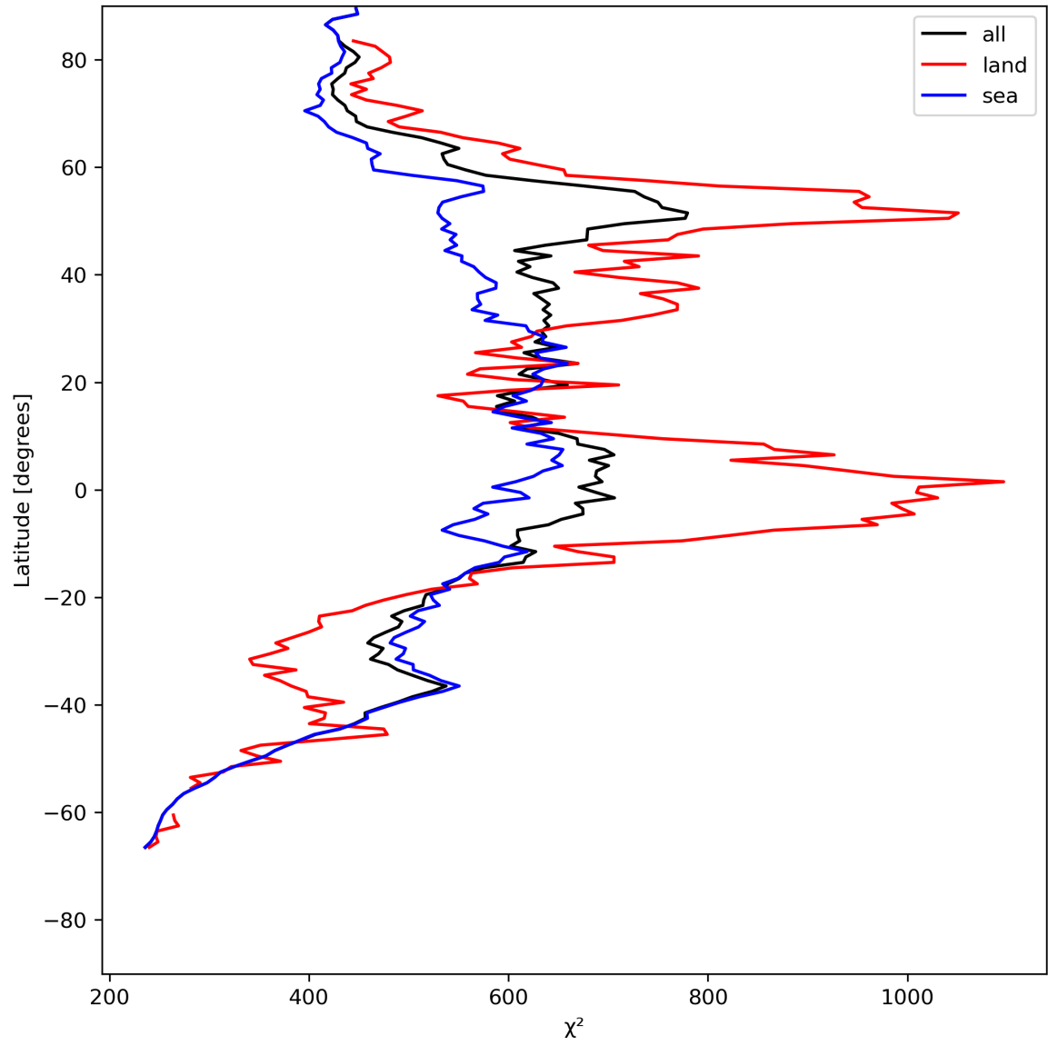
Figure 25: Zonal average of “ \chi^2 ” for 2023-07-16 to 2023-07-18.
