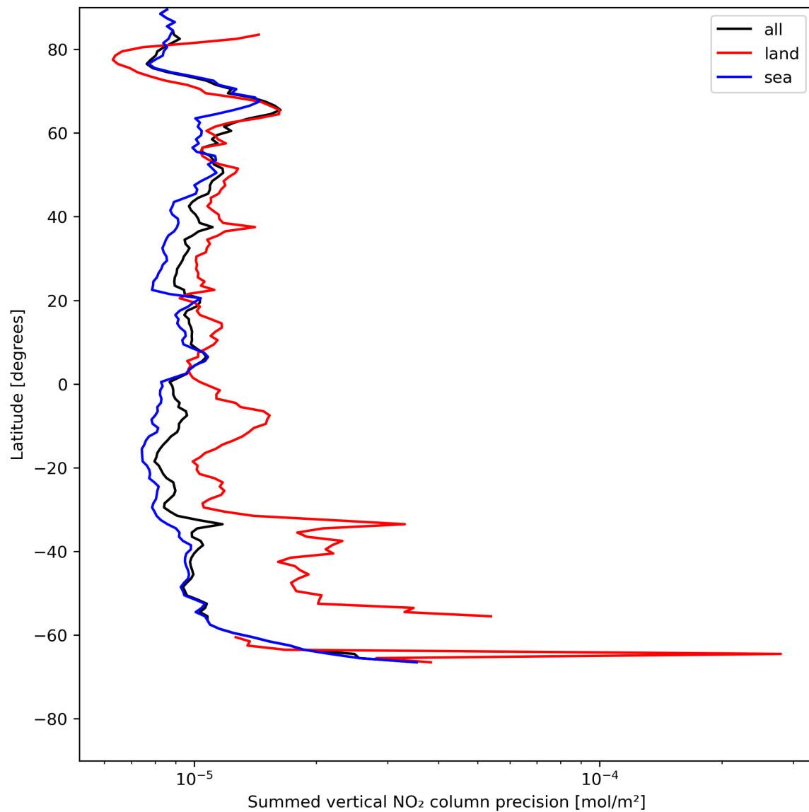
Figure 24: Zonal average of “Summed vertical NO 2 column precision” for 2023-07-16 to 2023-07-18.
