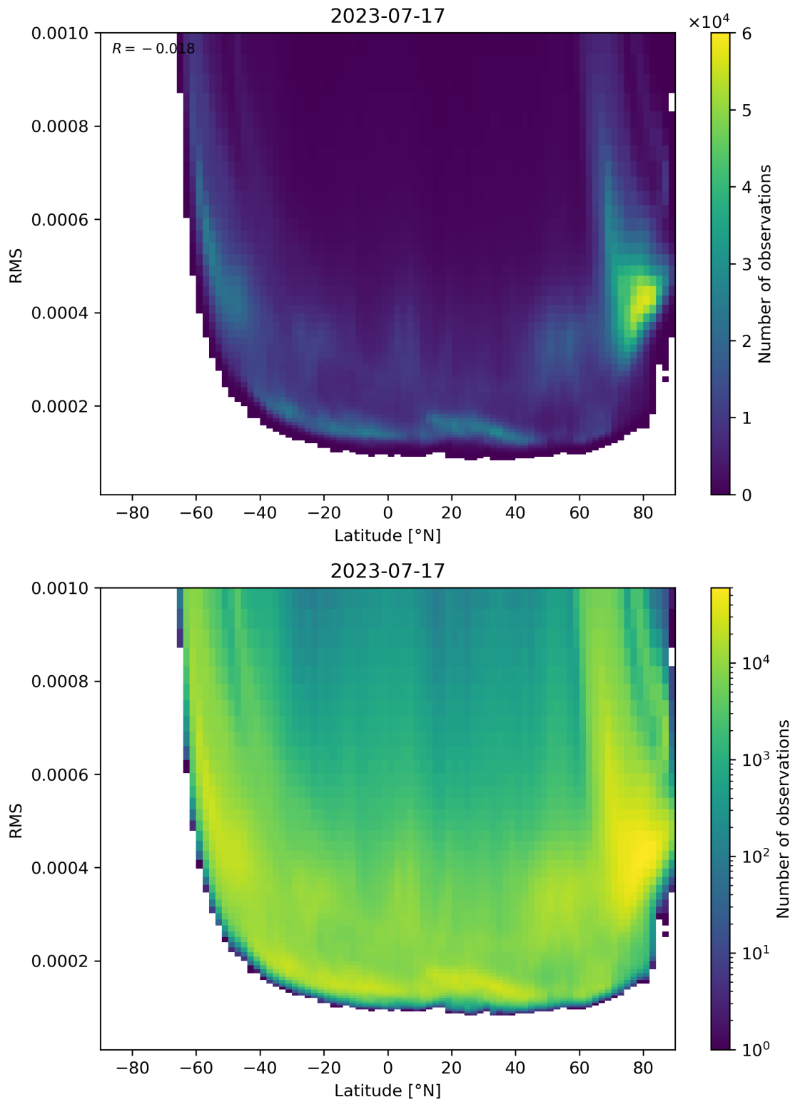
Figure 94: Scatter density plot of “Latitude” against “RMS” for 2023-07-16 to 2023-07-18.
