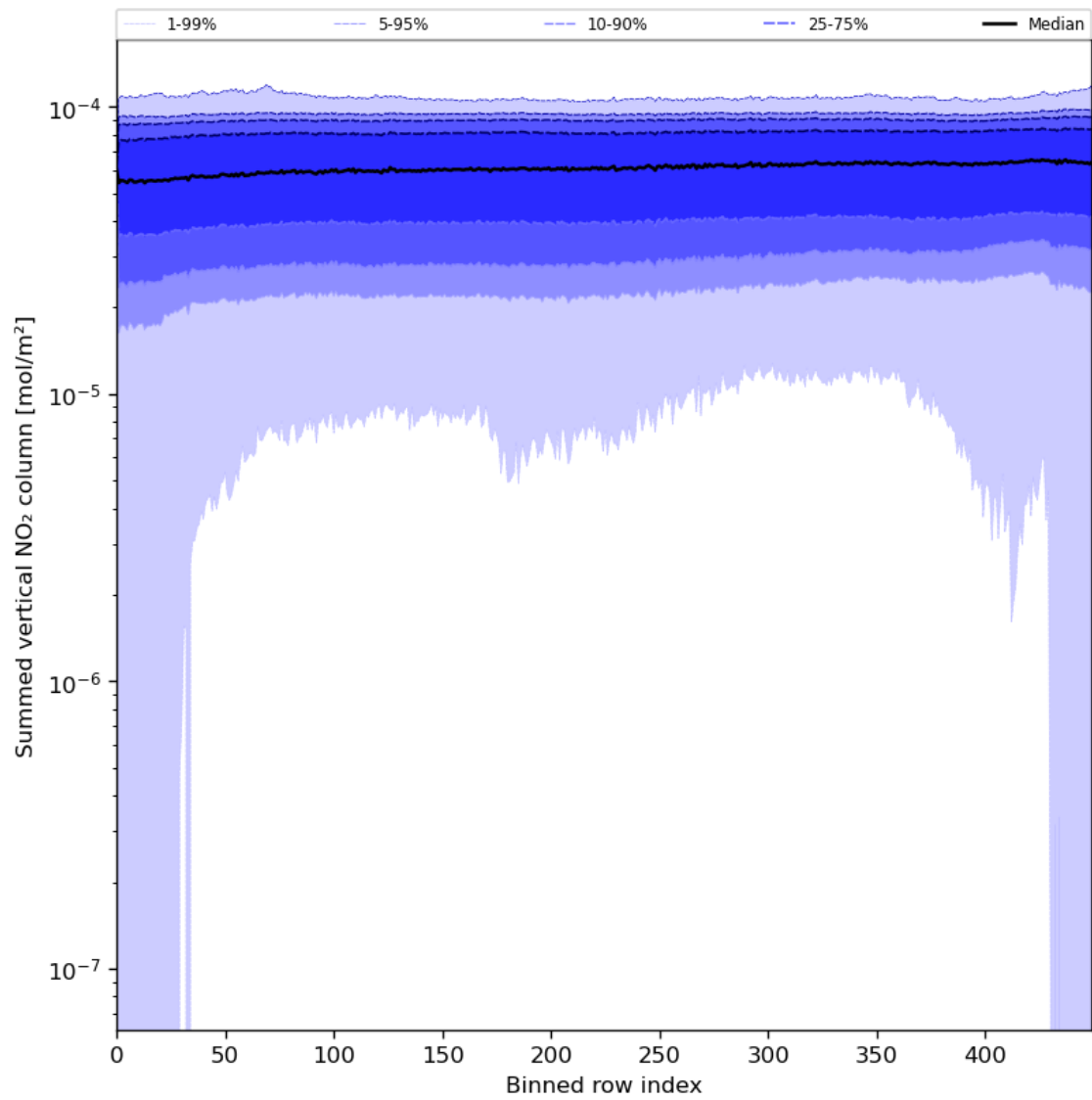
Figure 57: Along track statistics of “Summed vertical NO 2 column” for 2023-07-16 to 2023-07-18
