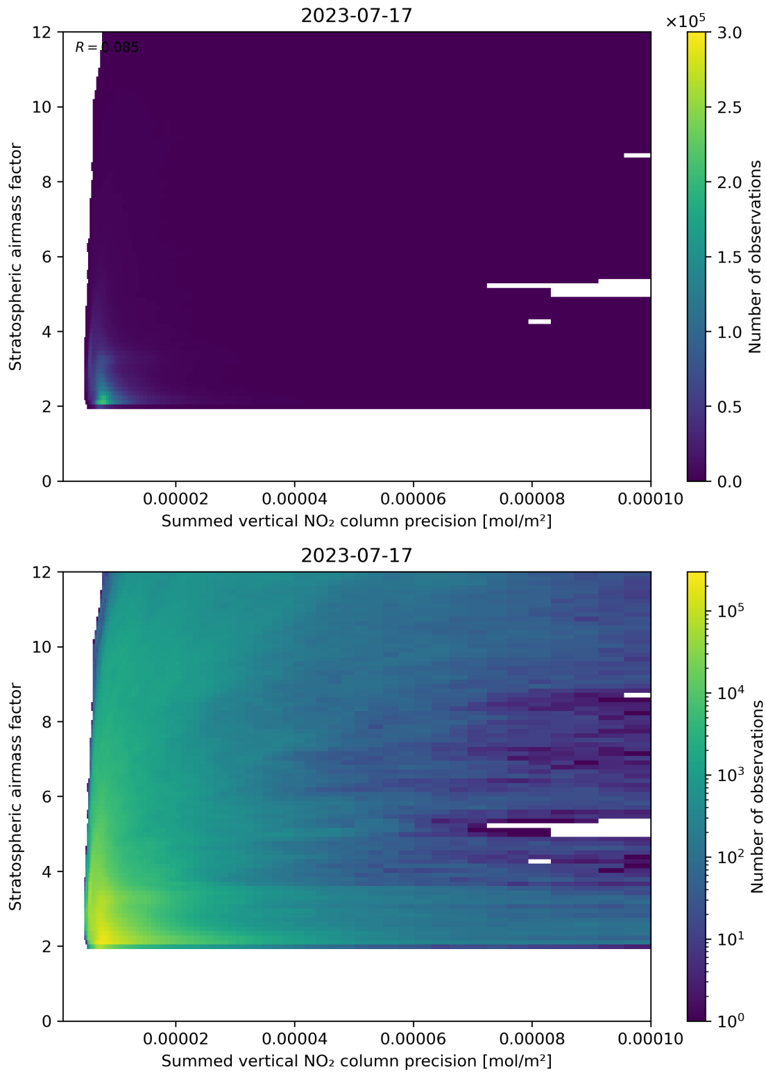
Figure 106: Scatter density plot of “Summed vertical NO 2 column precision” against “Stratospheric airmass factor” for 2023-07-16 to 2023-07-18.
