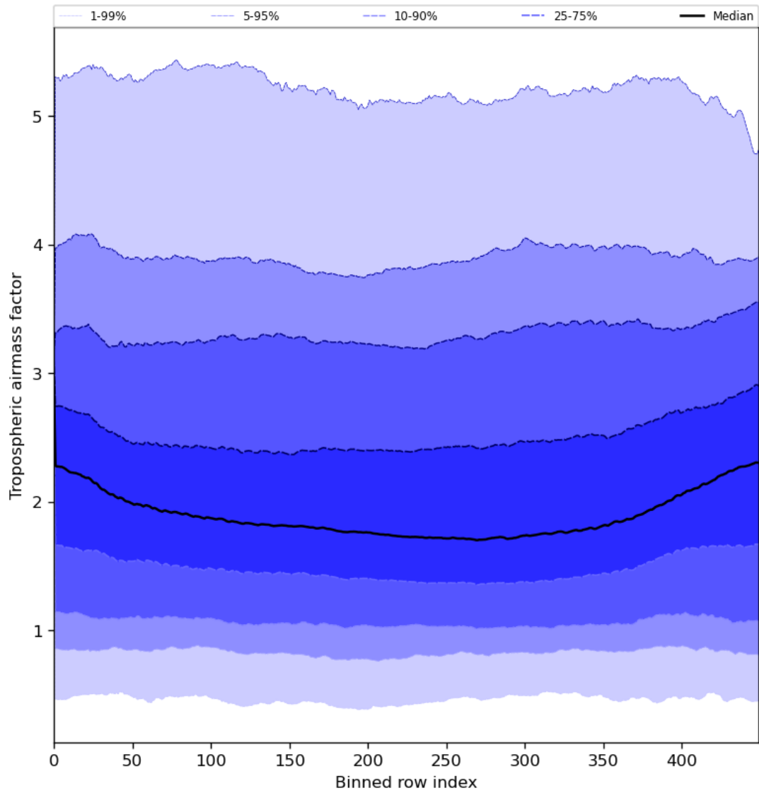
Figure 48: Along track statistics of “Tropospheric airmass factor” for 2023-07-16 to 2023-07-18
