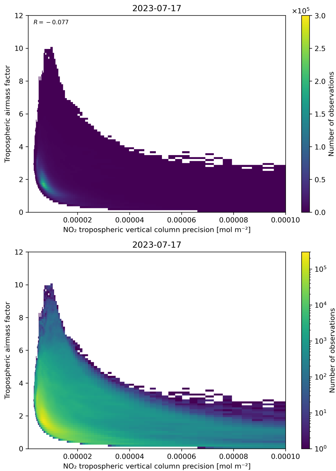
Figure 133: Scatter density plot of “NO 2 tropospheric vertical column precision” against “Tropospheric airmass factor” for 2023-07-16 to 2023-07-18.
