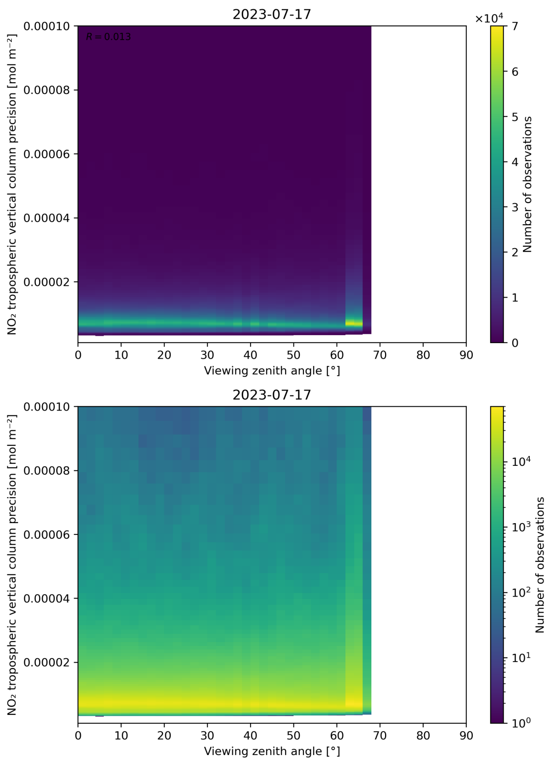
Figure 170: Scatter density plot of “Viewing zenith angle” against “NO 2 tropospheric vertical column precision” for 2023-07-16 to 2023-07-18.
