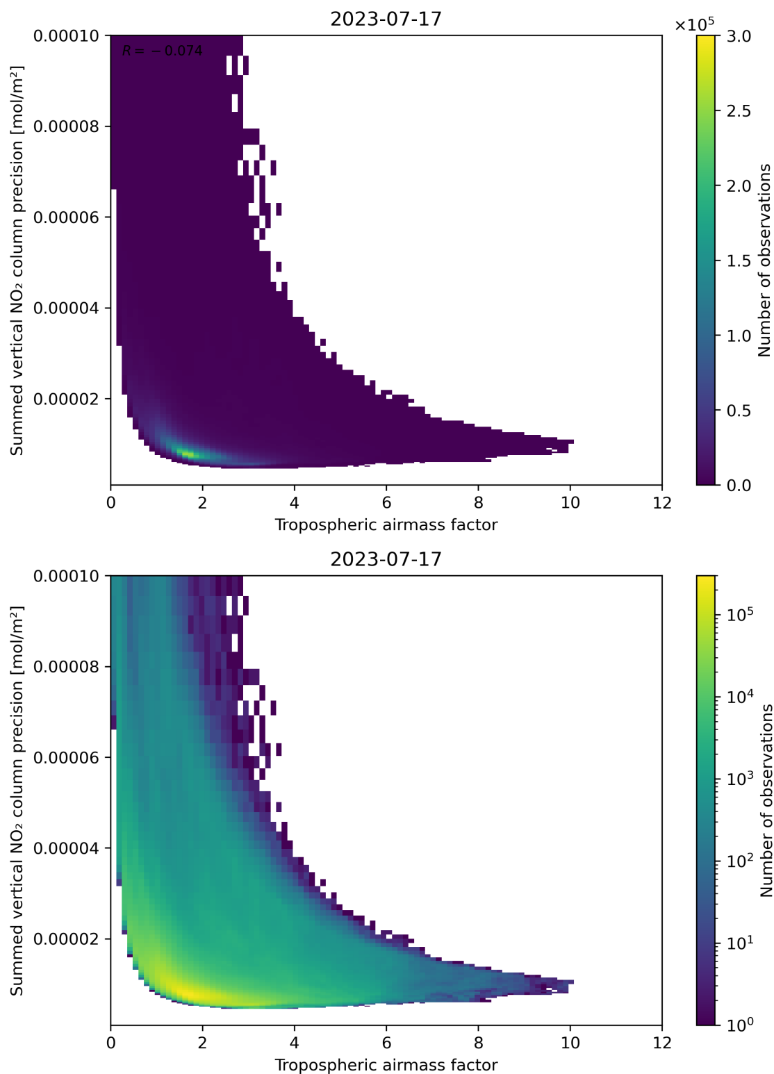
Figure 76: Scatter density plot of “Tropospheric air mass factor” against “Summed vertical NO 2 column precision” for 2023-07-16 to 2023-07-18.
