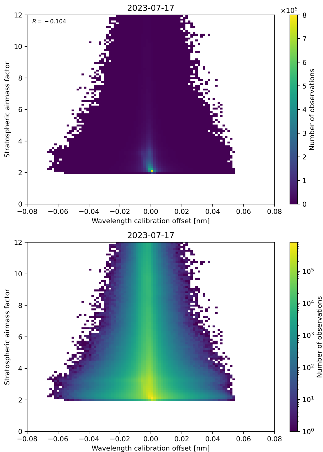
Figure 174: Scatter density plot of “Wavelength calibration offset” against “Stratospheric airmass factor” for 2023-07-16 to 2023-07-18.
