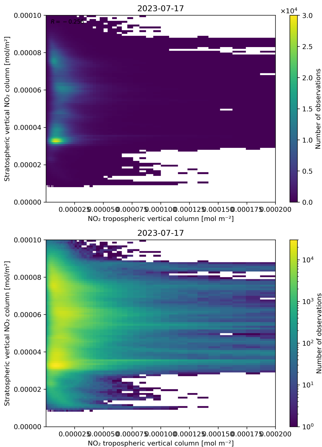
Figure 125: Scatter density plot of “NO 2 tropospheric vertical column” against “Stratospheric vertical NO 2 column” for 2023-07-16 to 2023-07-18.
