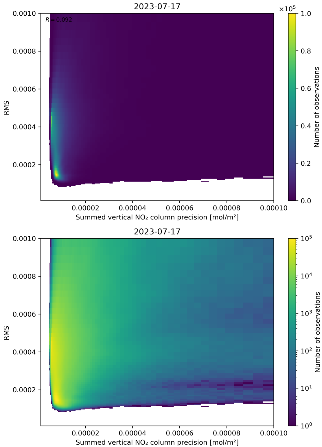
Figure 108: Scatter density plot of “Summed vertical NO 2 column precision” against “RMS” for 2023-07-16 to 2023-07-18.
