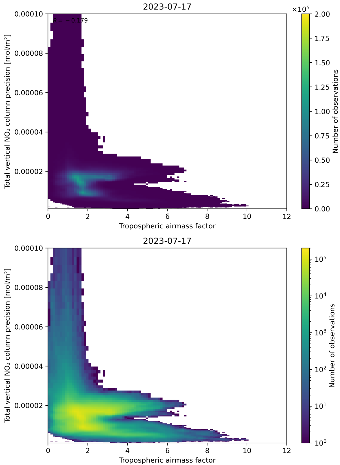
Figure 78: Scatter density plot of “Tropospheric airmass factor” against “Total vertical NO 2 column precision” for 2023-07-16 to 2023-07-18.
