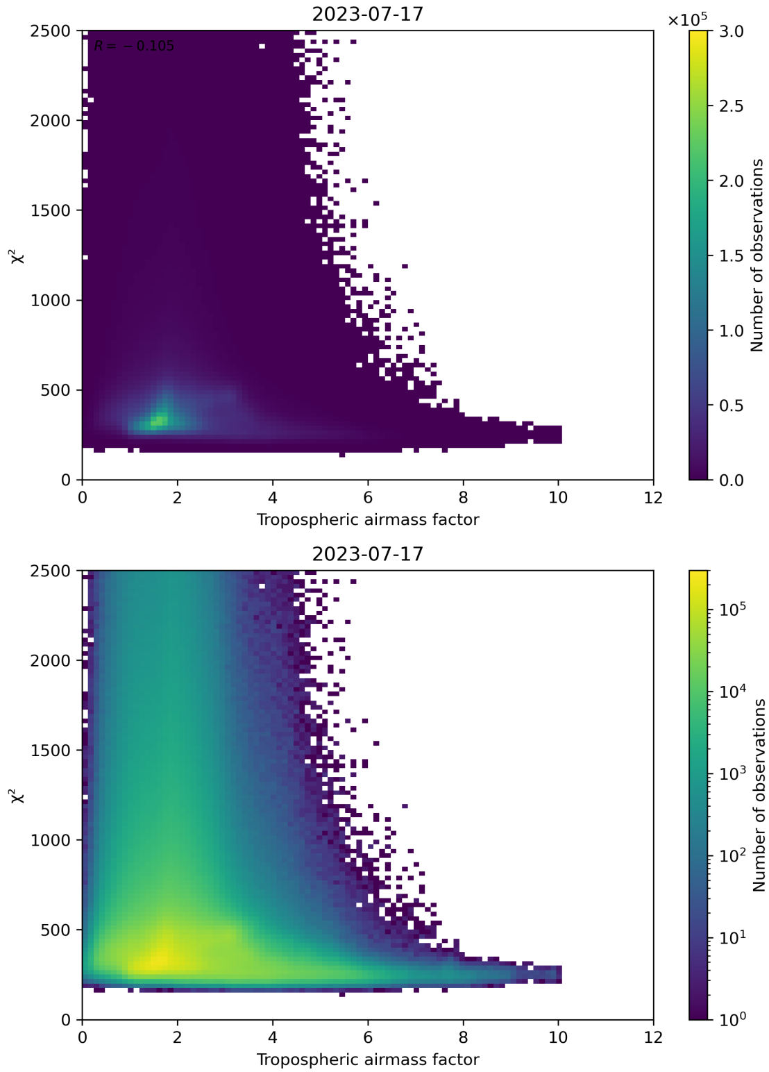
Figure 73: Scatter density plot of “Tropospheric airmass factor” against “ \chi^2 ” for 2023-07-16 to 2023-07-18.
