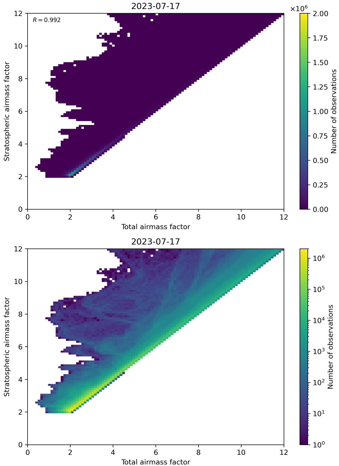
Figure 62: Scatter density plot of “Total airmass factor” against “Stratospheric airmass factor” for 2023-07-16 to 2023-07-18.
