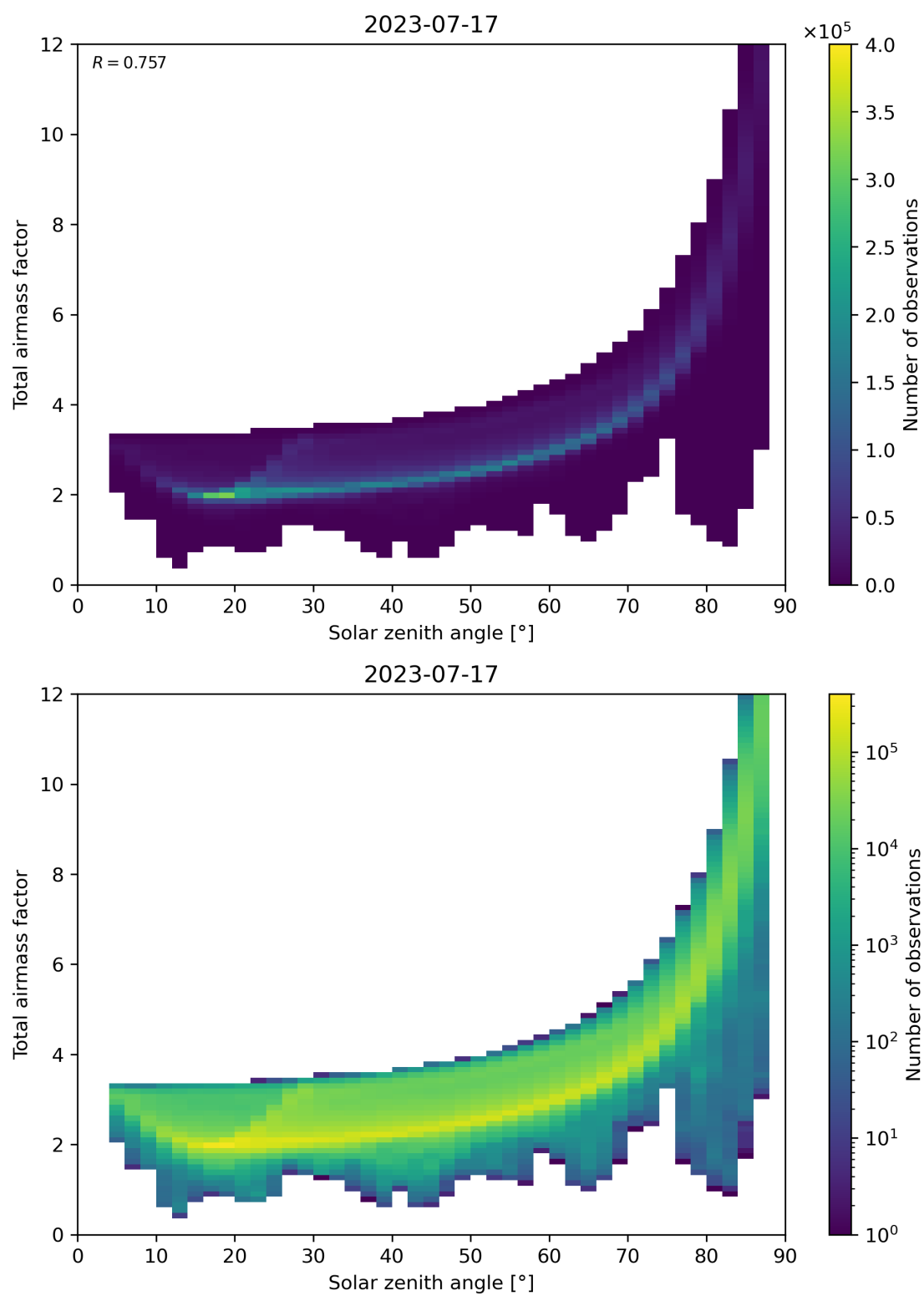
Figure 146: Scatter density plot of “Solar zenith angle” against “Total air mass factor” for 2023-07-16 to 2023-07-18.
