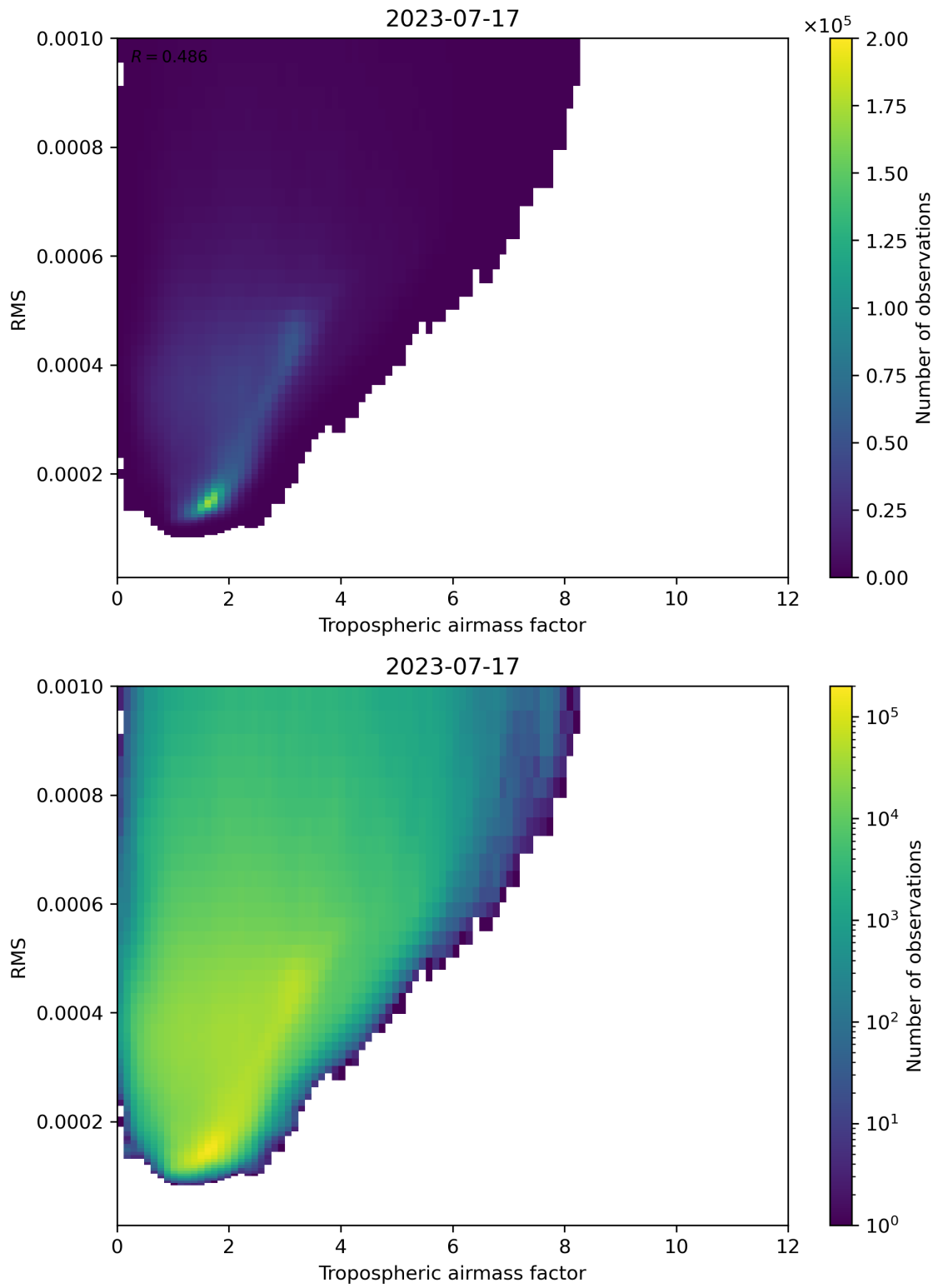
Figure 79: Scatter density plot of “Tropospheric airmass factor” against “RMS” for 2023-07-16 to 2023-07-18.
