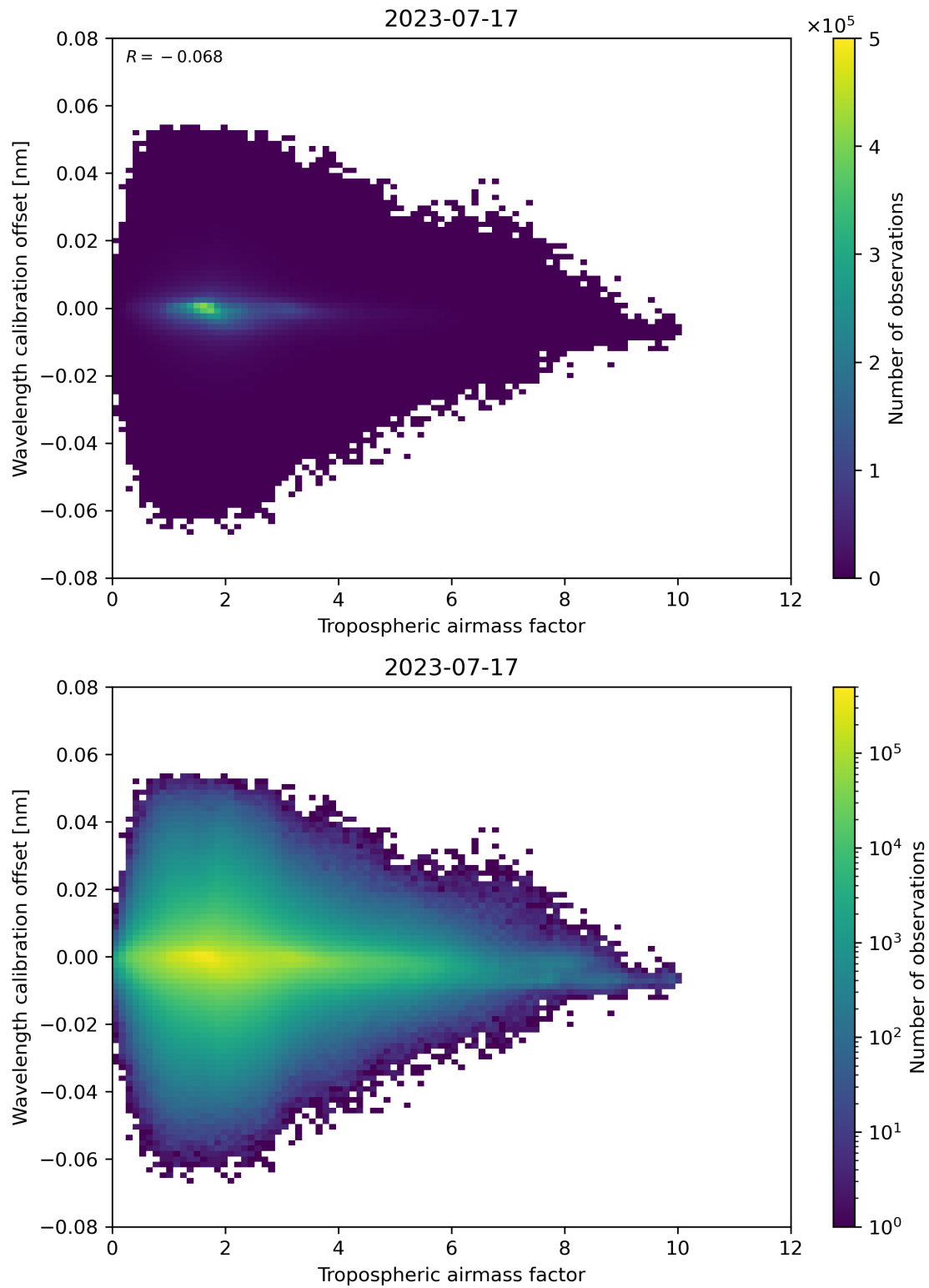
Figure 80: Scatter density plot of “Tropospheric air mass factor” against “Wavelength calibration offset” for 2023-07-16 to 2023-07-18.
