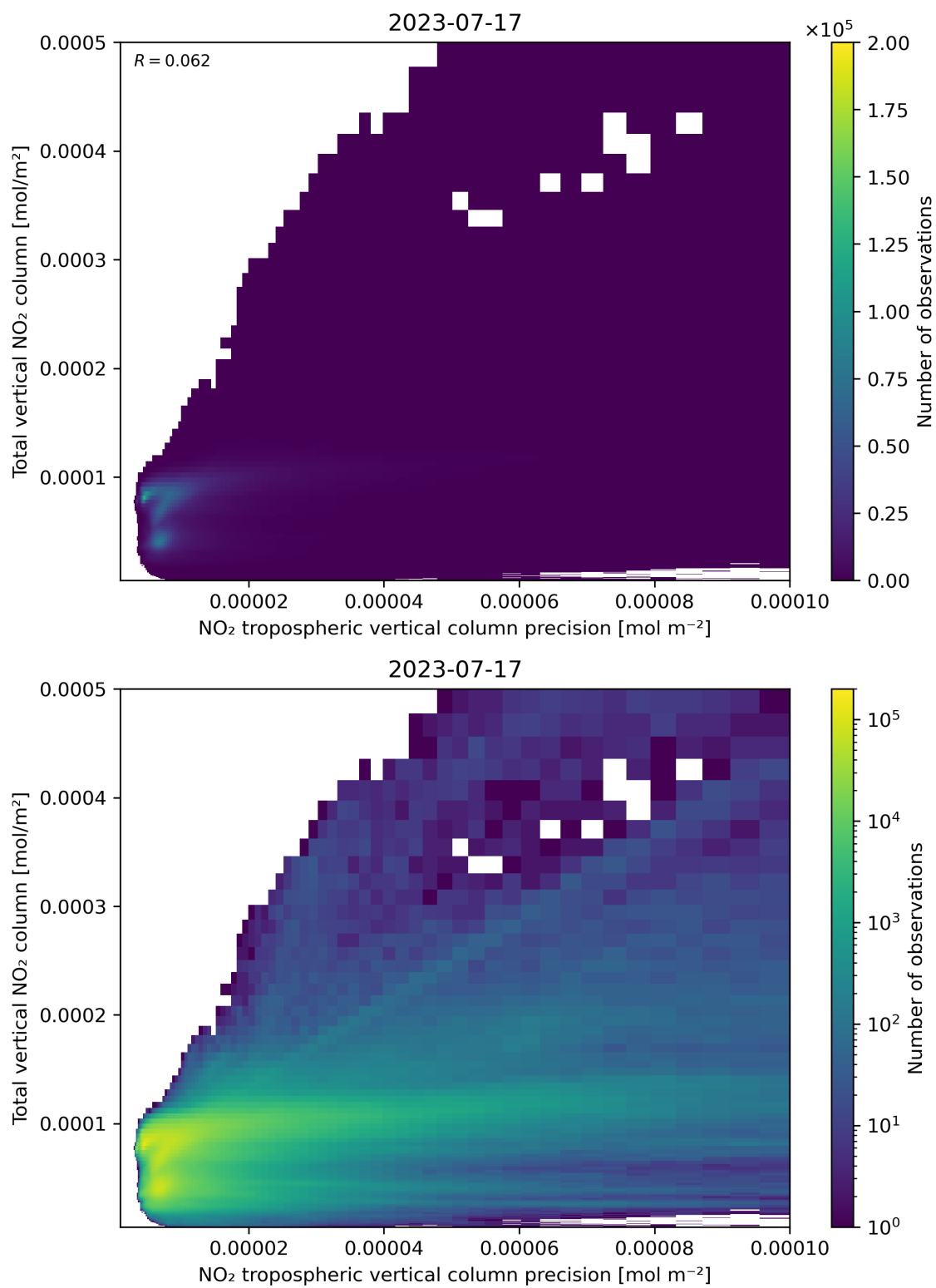
Figure 138: Scatter density plot of “NO 2 tropospheric vertical column precision” against “Total vertical NO 2 column” for 2023-07-16 to 2023-07-18.
