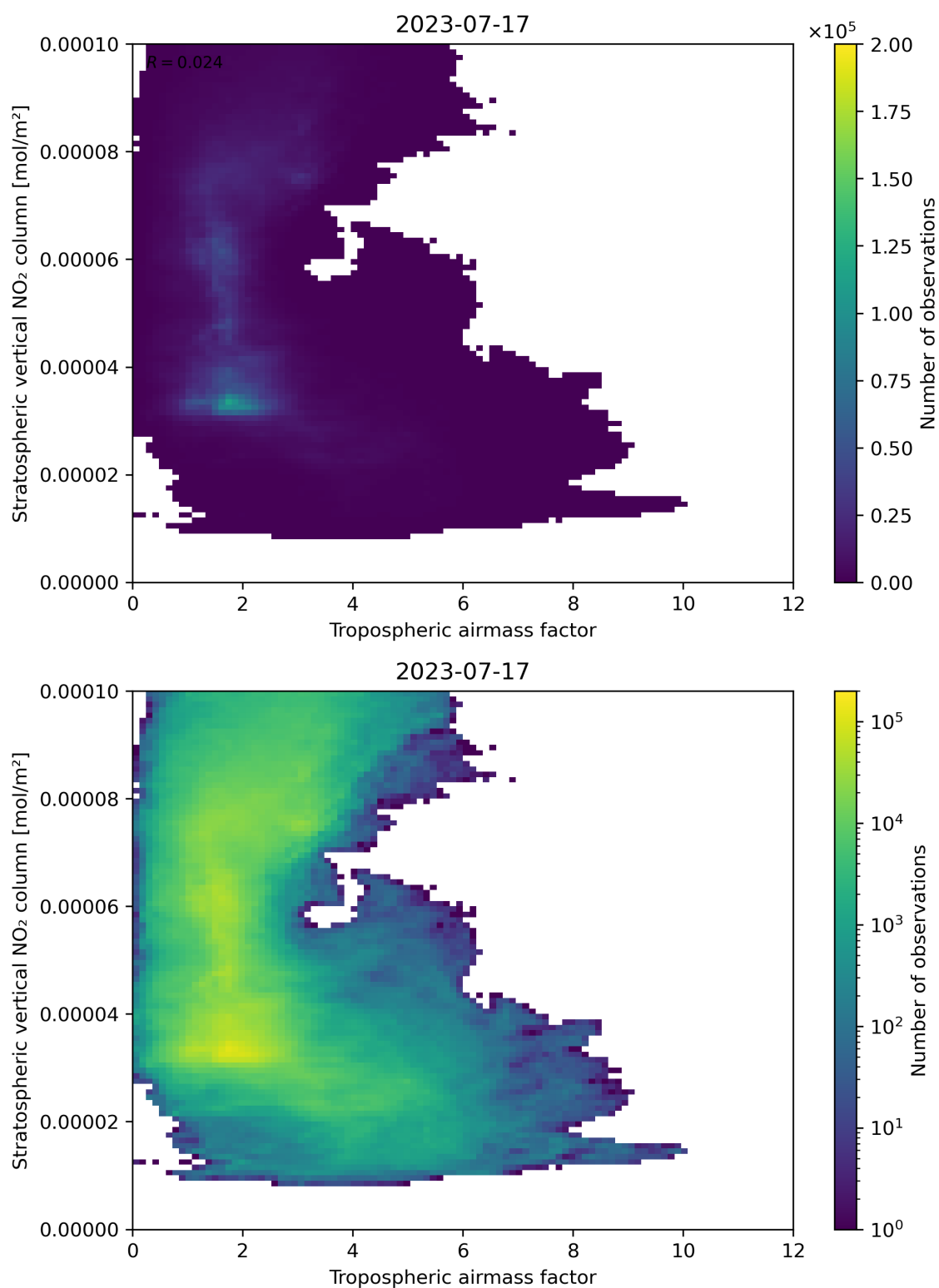
Figure 74: Scatter density plot of “Tropospheric airmass factor” against “Stratospheric vertical NO 2 column” for 2023-07-16 to 2023-07-18.
