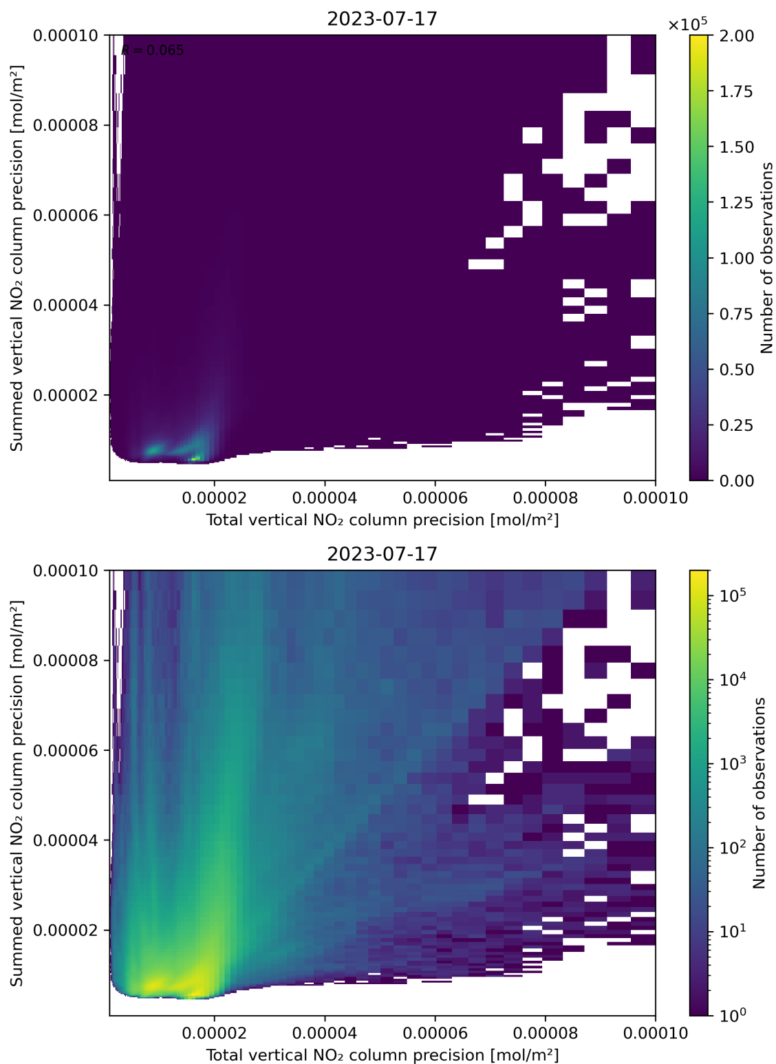
Figure 118: Scatter density plot of “Total vertical NO 2 column precision” against “Summed vertical NO 2 column precision” for 2023-07-16 to 2023-07-18.
