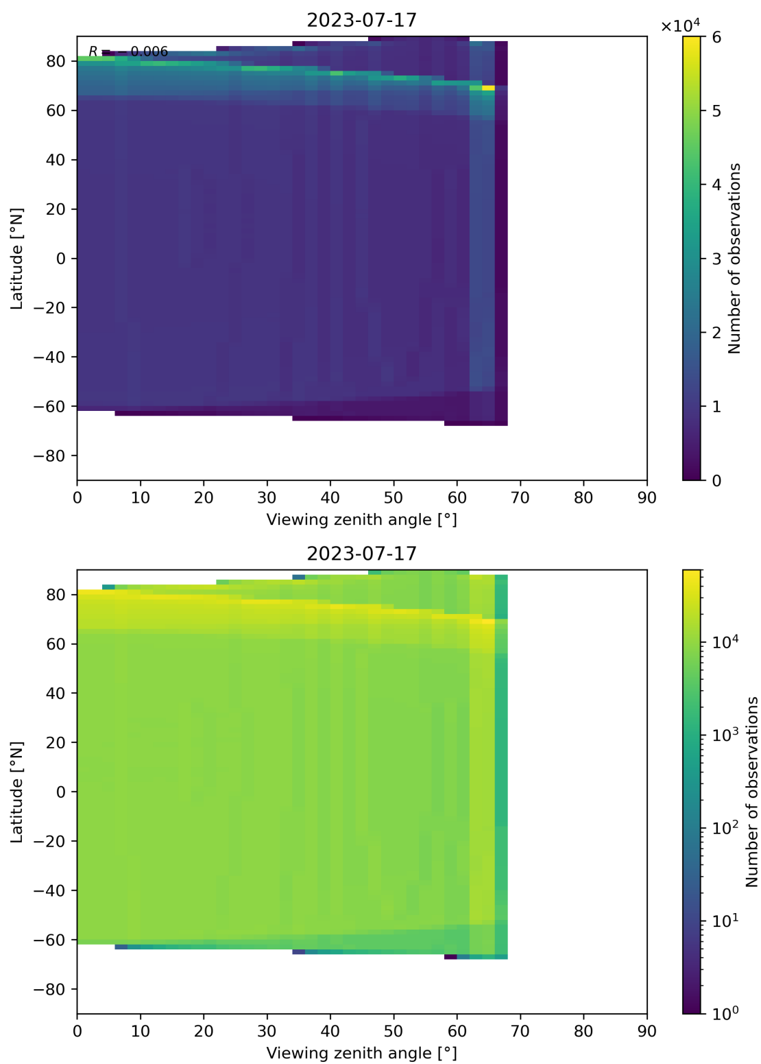
Figure 163: Scatter density plot of “Viewing zenith angle” against “Latitude” for 2023-07-16 to 2023-07-18.
