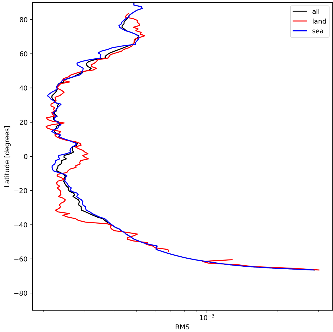
Figure 26: Zonal average of “RMS” for 2023-07-16 to 2023-07-18.
