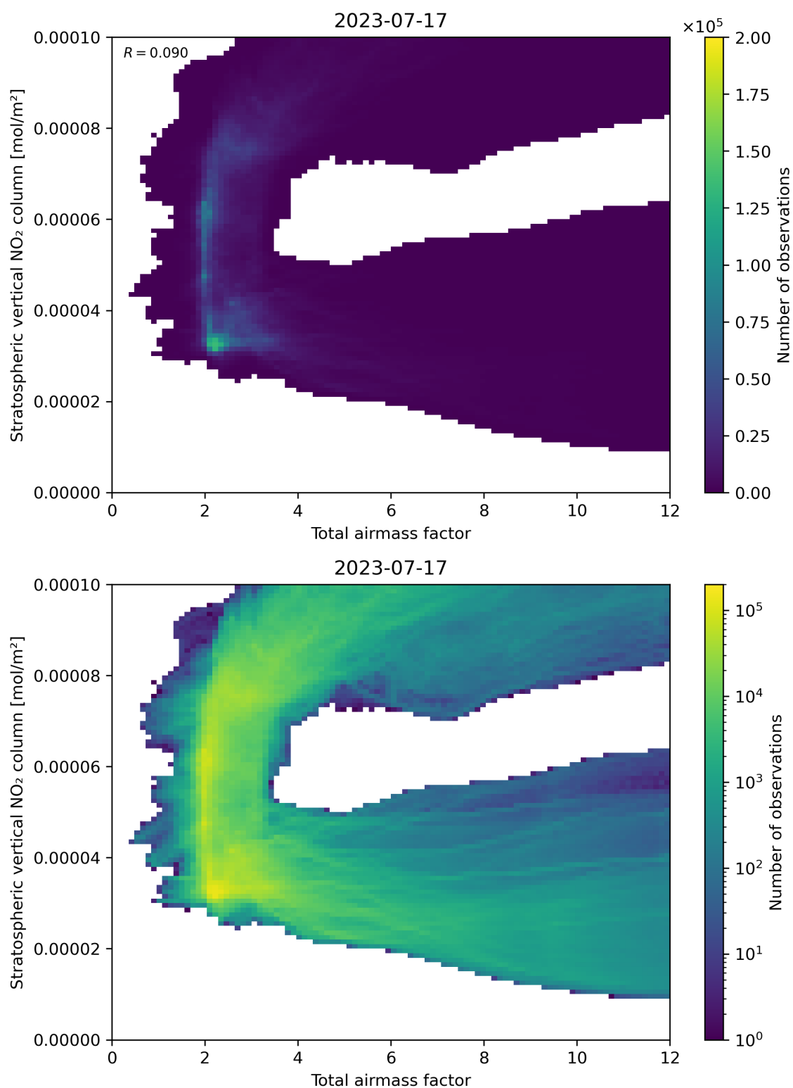
Figure 64: Scatter density plot of “Total airmass factor” against “Stratospheric vertical NO 2 column” for 2023-07-16 to 2023-07-18.
