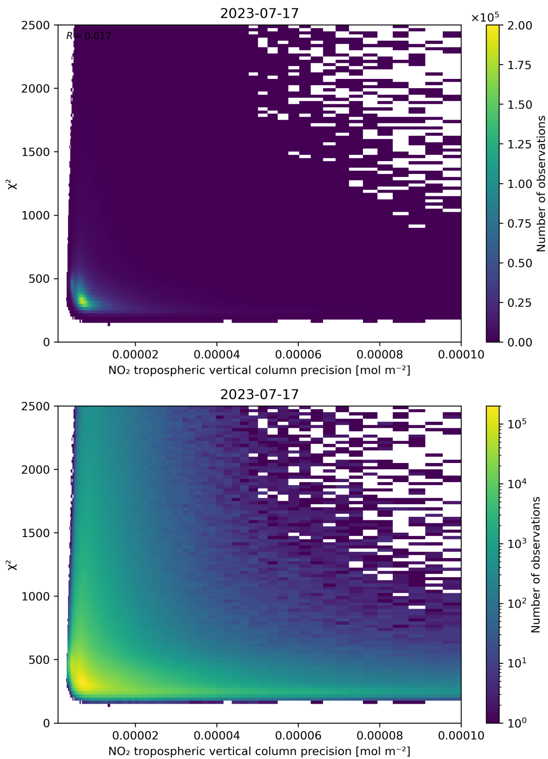
Figure 134: Scatter density plot of “NO 2 tropospheric vertical column precision” against “ \chi^2 ” for 2023-07-16 to 2023-07-18.
