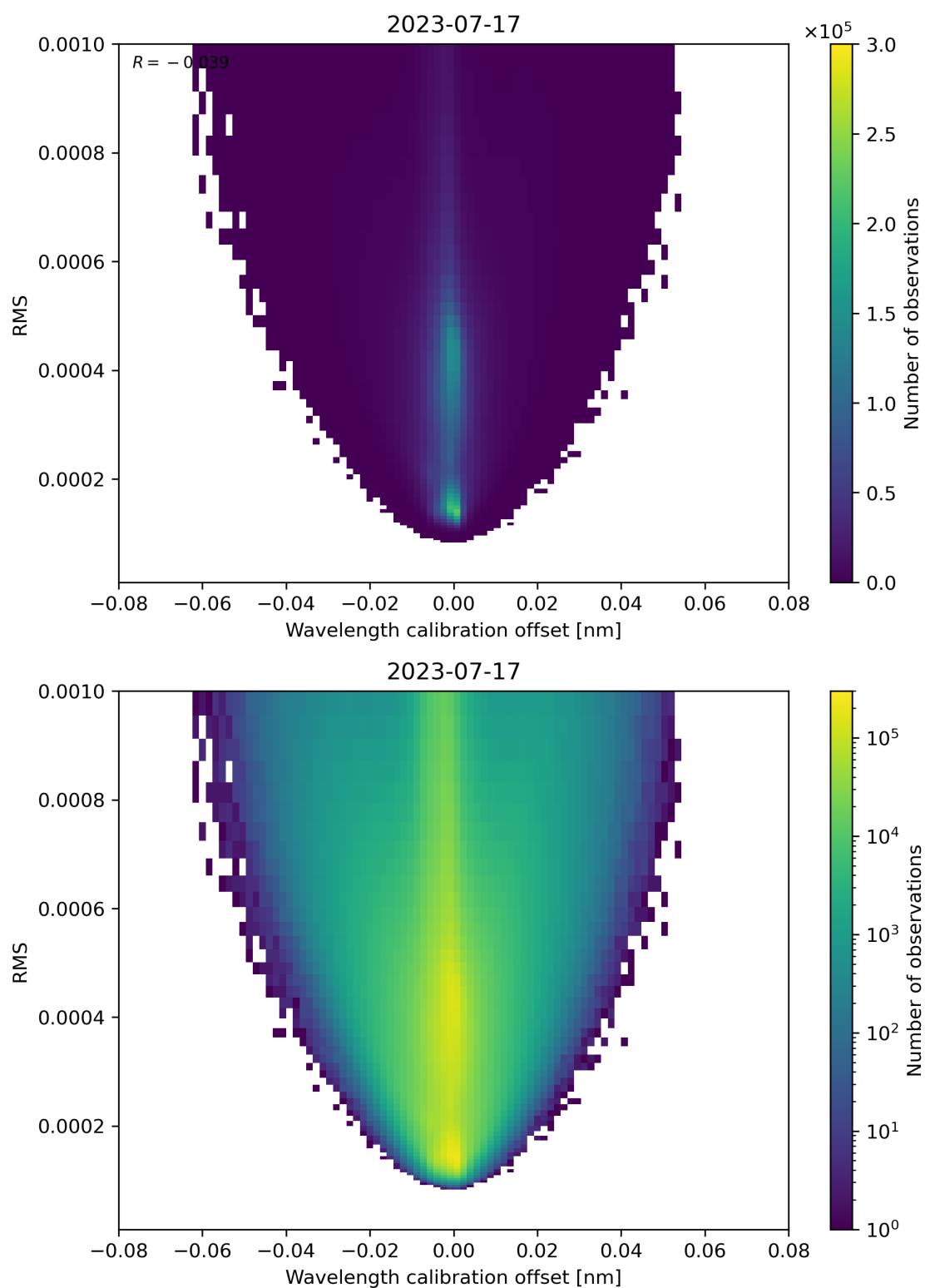
Figure 181: Scatter density plot of “Wavelength calibration offset” against “RMS” for 2023-07-16 to 2023-07-18.
