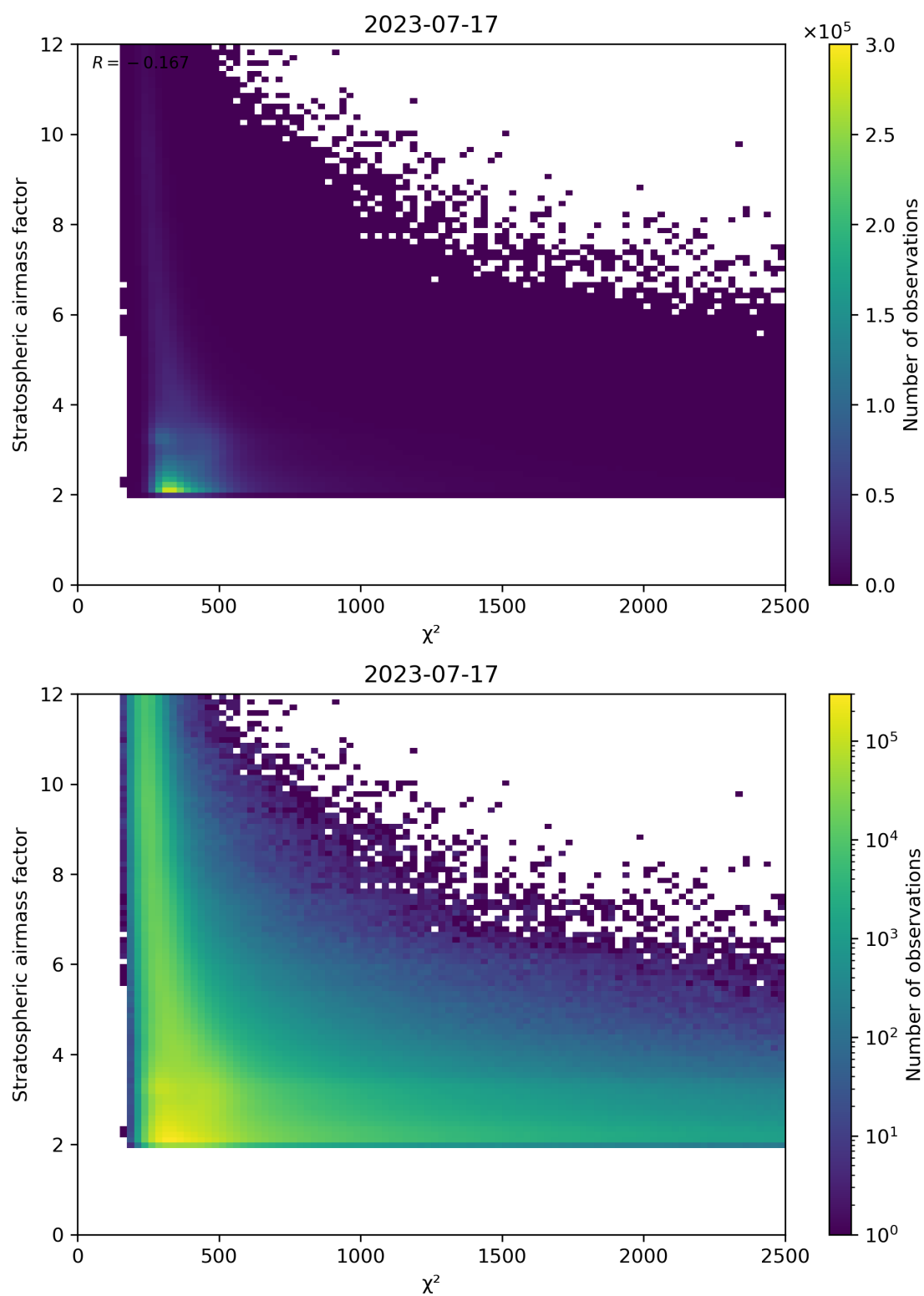
Figure 81: Scatter density plot of “ \chi^2 ” against “Stratospheric airmass factor” for 2023-07-16 to 2023-07-18.
