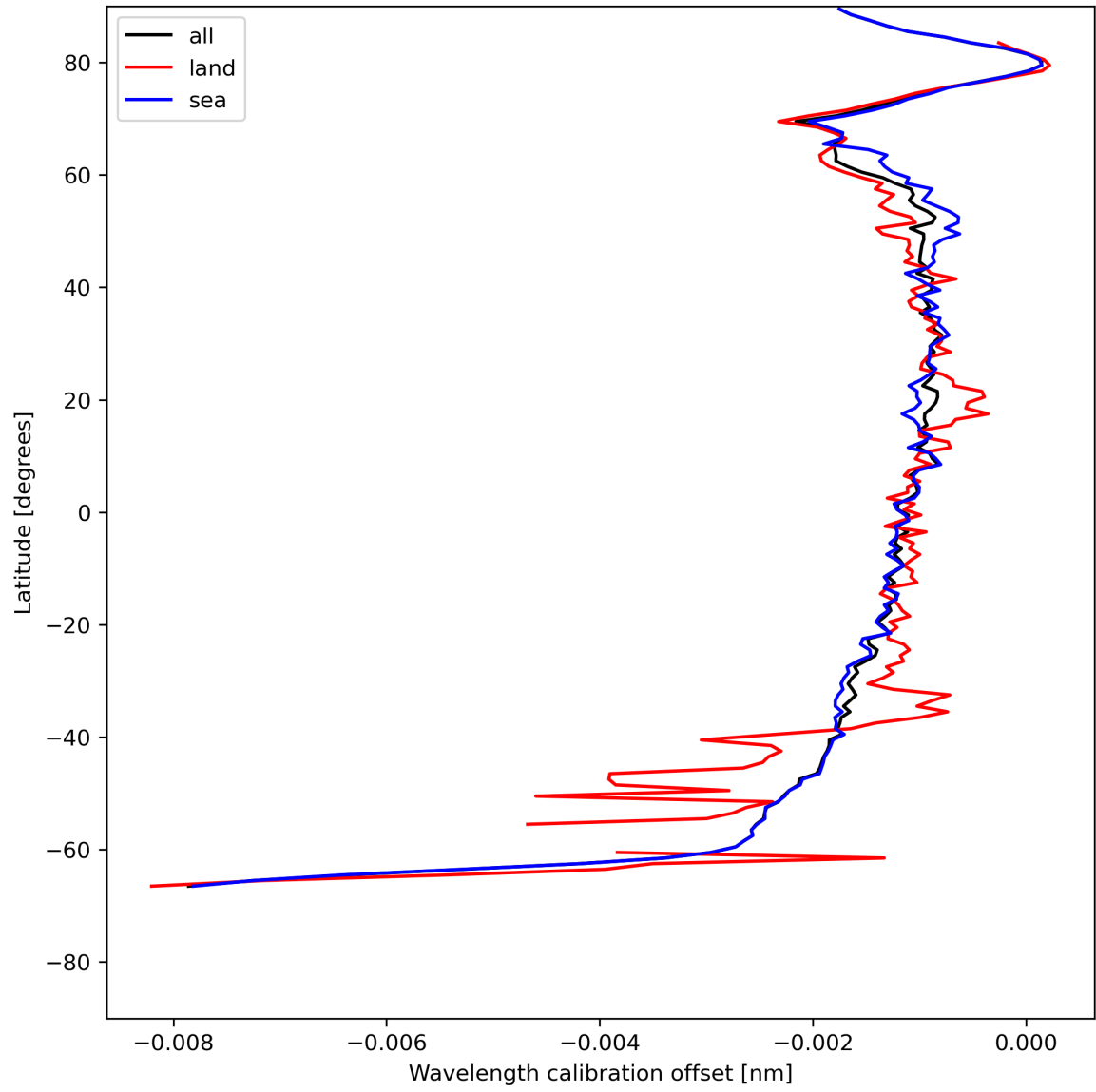
Figure 18: Zonal average of “Wavelength calibration offset” for 2023-07-16 to 2023-07-18.
