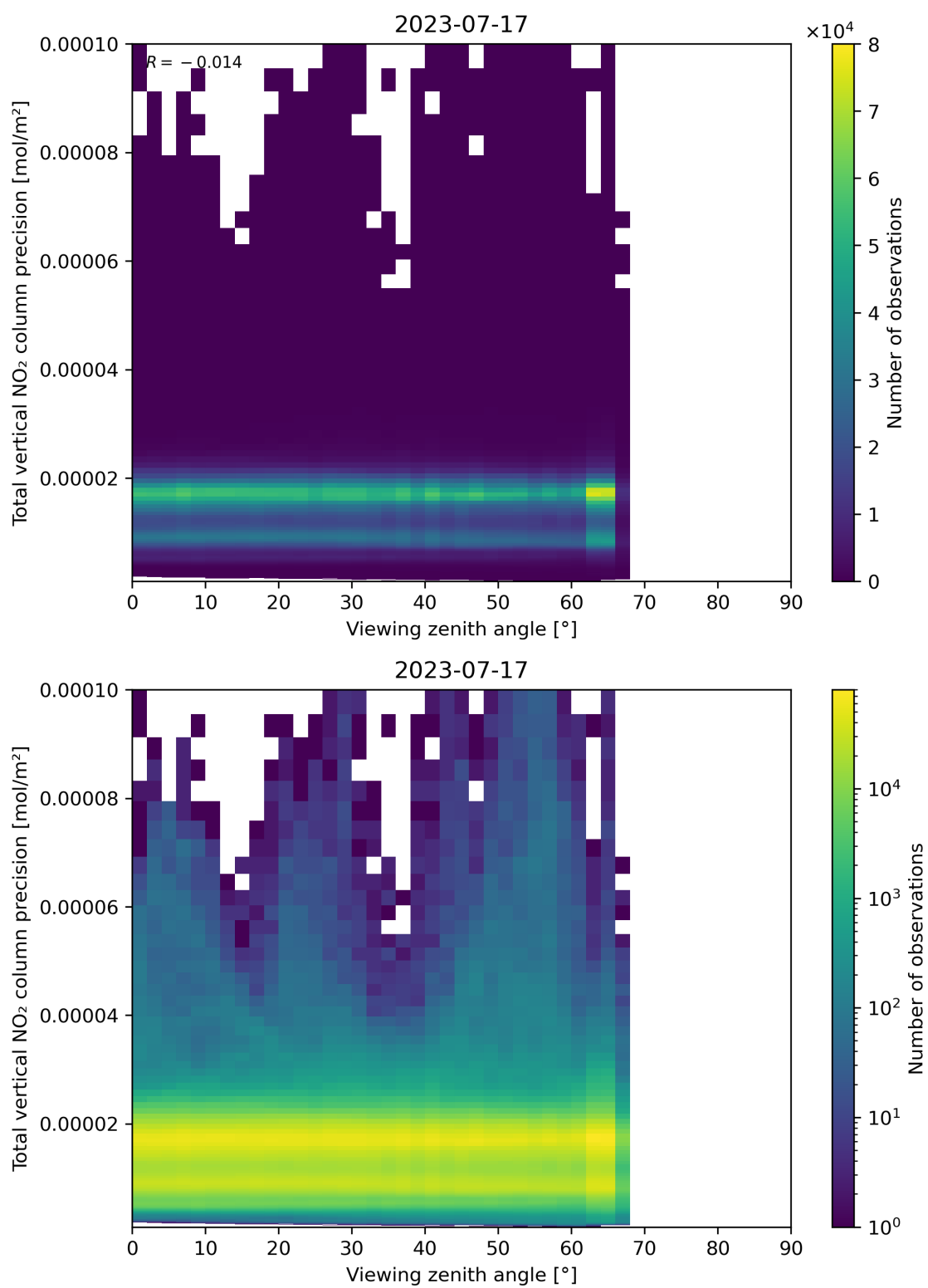
Figure 168: Scatter density plot of “Viewing zenith angle” against “Total vertical NO 2 column precision” for 2023-07-16 to 2023-07-18.
