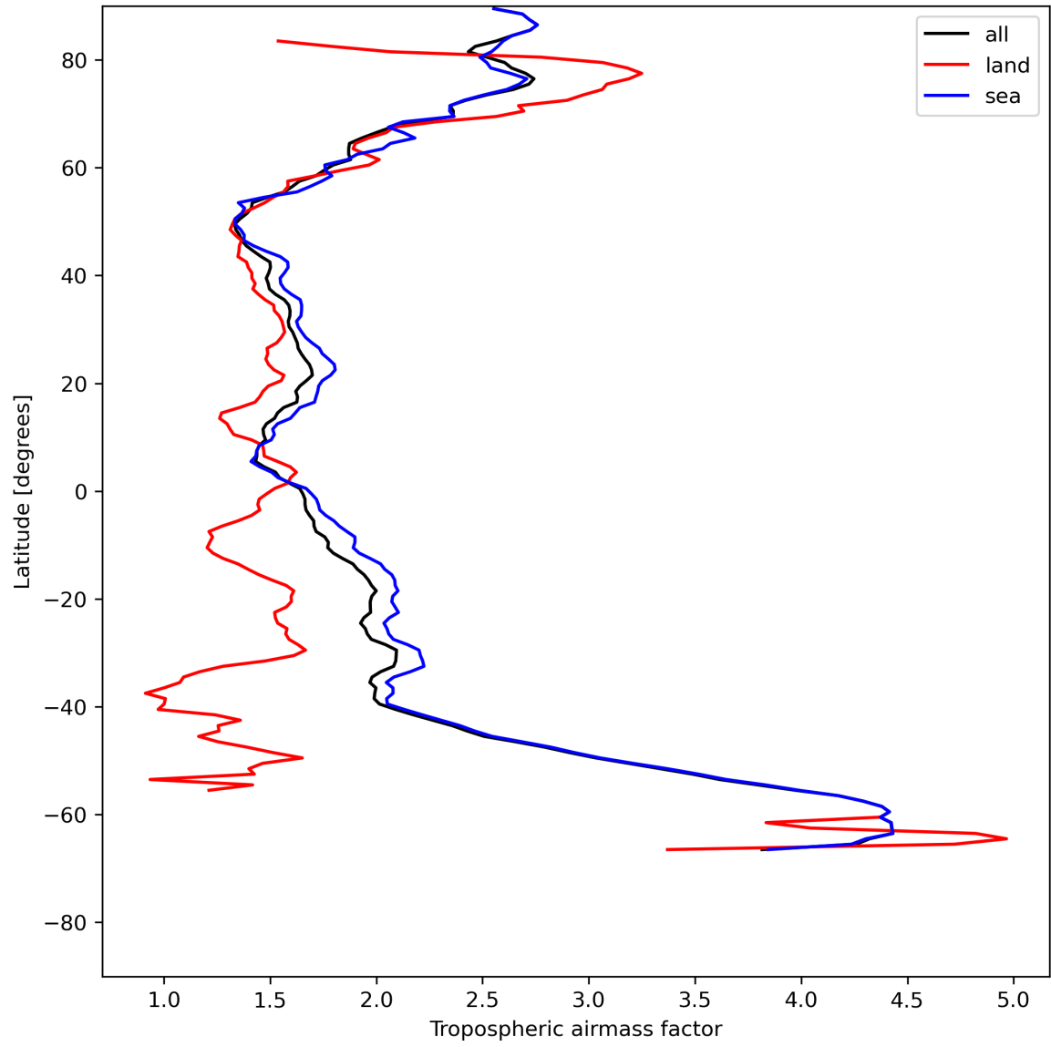
Figure 14: Zonal average of “Tropospheric airmass factor” for 2023-07-16 to 2023-07-18.
