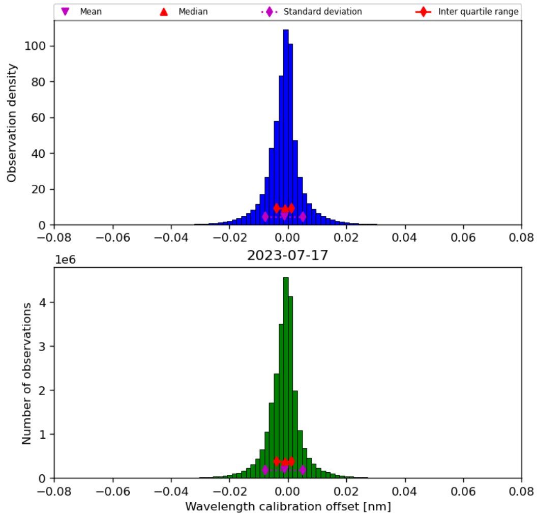
Figure 35: Histogram of “Wavelength calibration offset” for 2023-07-16 to 2023-07-18
