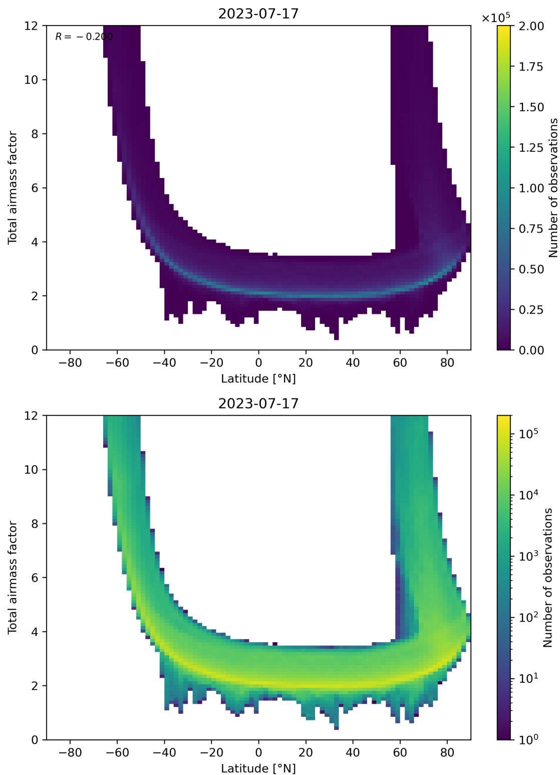
Figure 84: Scatter density plot of “Latitude” against “Total airmass factor” for 2023-07-16 to 2023-07-18.
