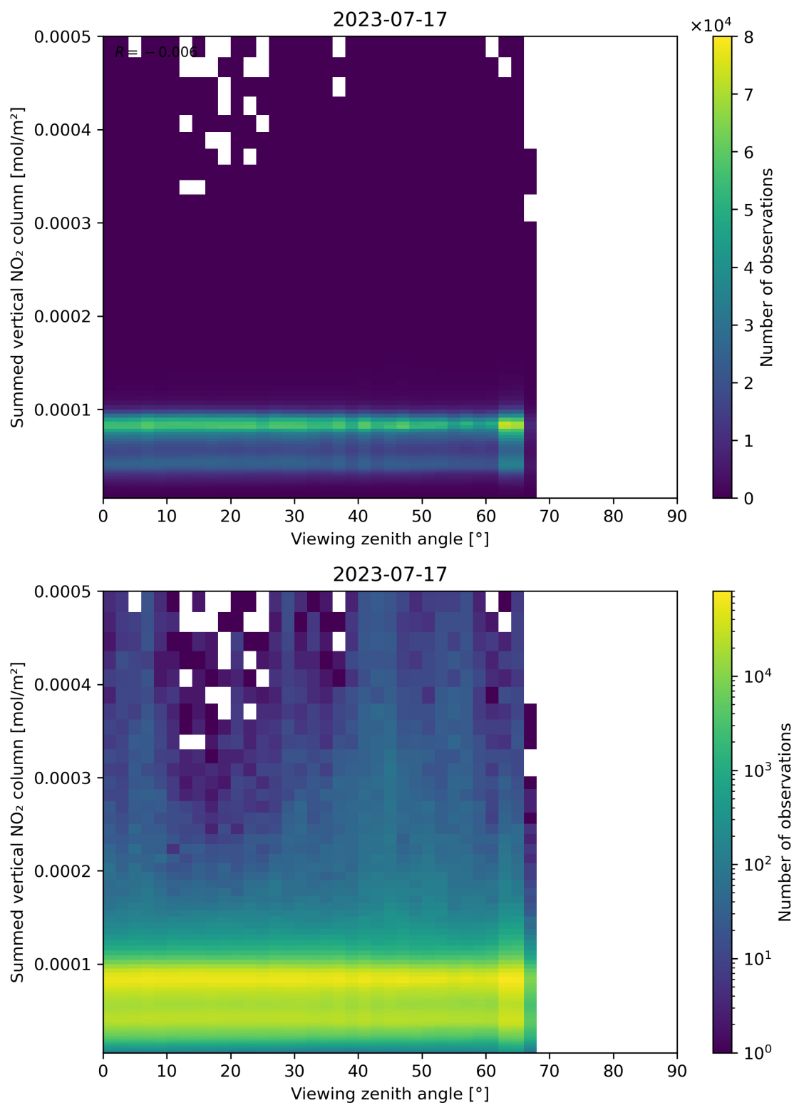
Figure 165: Scatter density plot of “Viewing zenith angle” against “Summed vertical NO 2 column” for 2023-07-16 to 2023-07-18.
