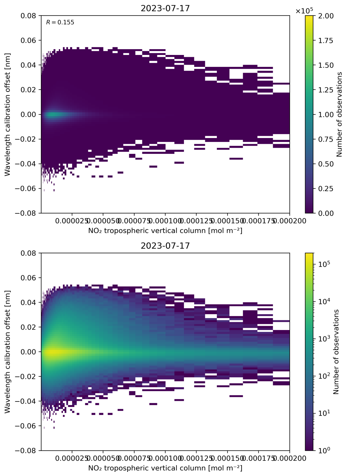
Figure 143: Scatter density plot of “NO 2 tropospheric vertical column” against “Wavelength calibration offset” for 2023-07-16 to 2023-07-18.
