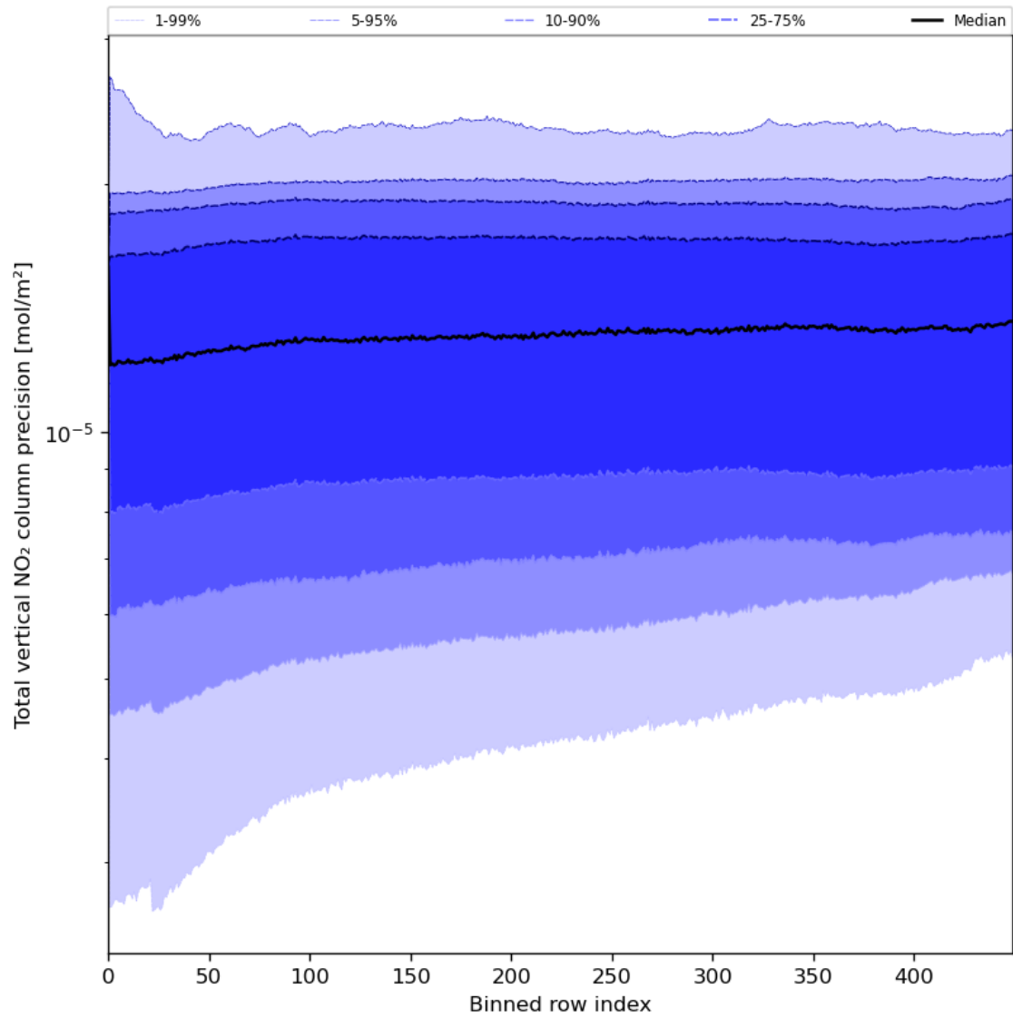
Figure 56: Along track statistics of “Total vertical NO 2 column precision” for 2023-07-19 to 2023-07-20
