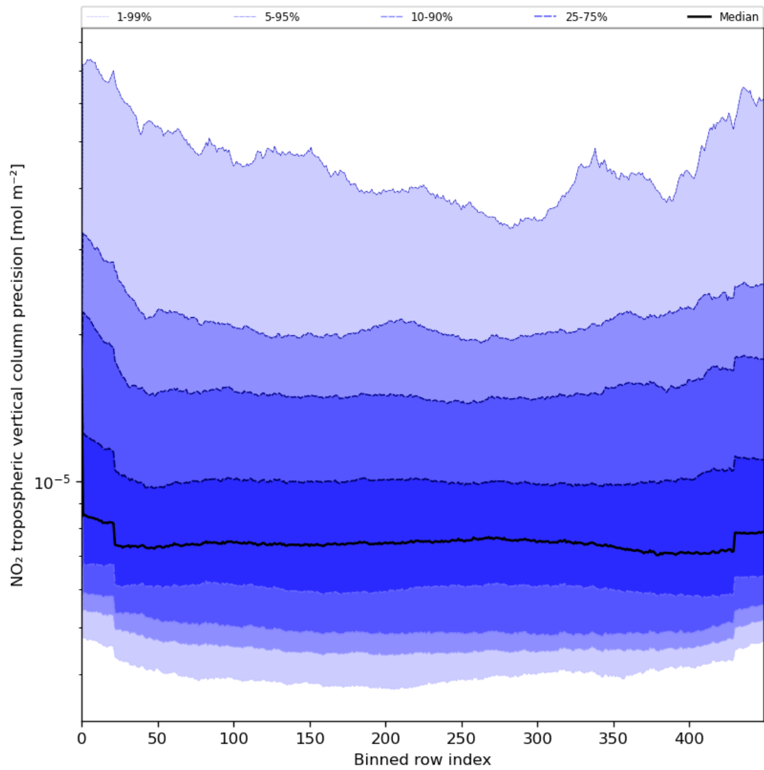
Figure 47: Along track statistics of “NO 2 tropospheric vertical column precision” for 2023-07-19 to 2023-07-20
