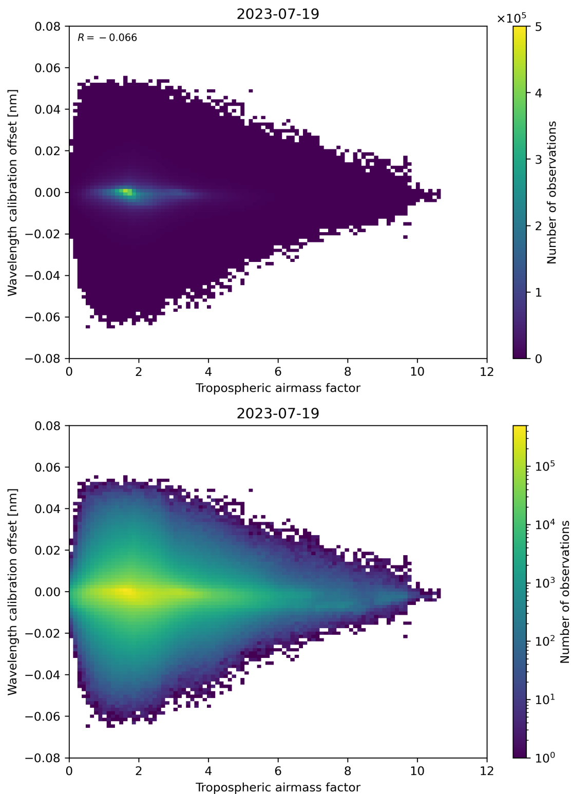
Figure 80: Scatter density plot of “Tropospheric air mass factor” against “Wavelength calibration offset” for 2023-07-19 to 2023-07-20.
