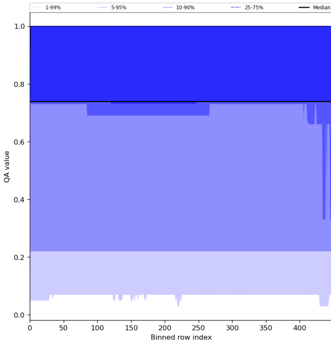
Figure 45: Along track statistics of “QA value” for 2023-07-19 to 2023-07-20
