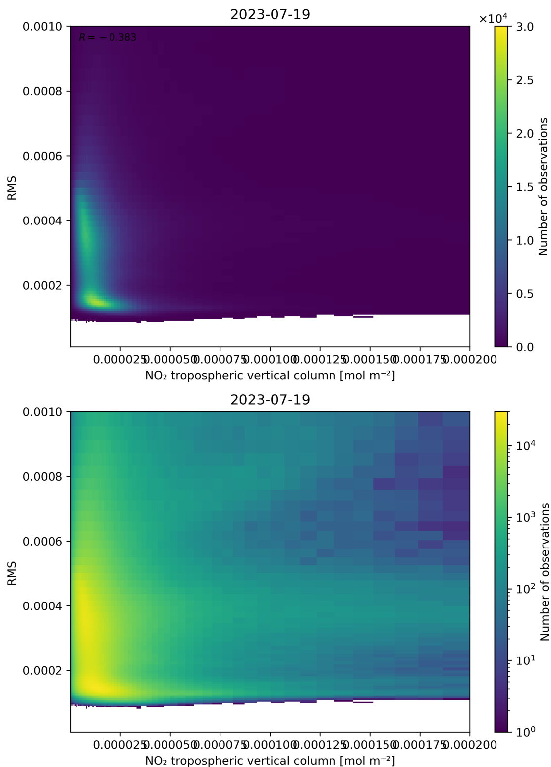
Figure 142: Scatter density plot of “NO 2 tropospheric vertical column” against “RMS” for 2023-07-19 to 2023-07-20.
