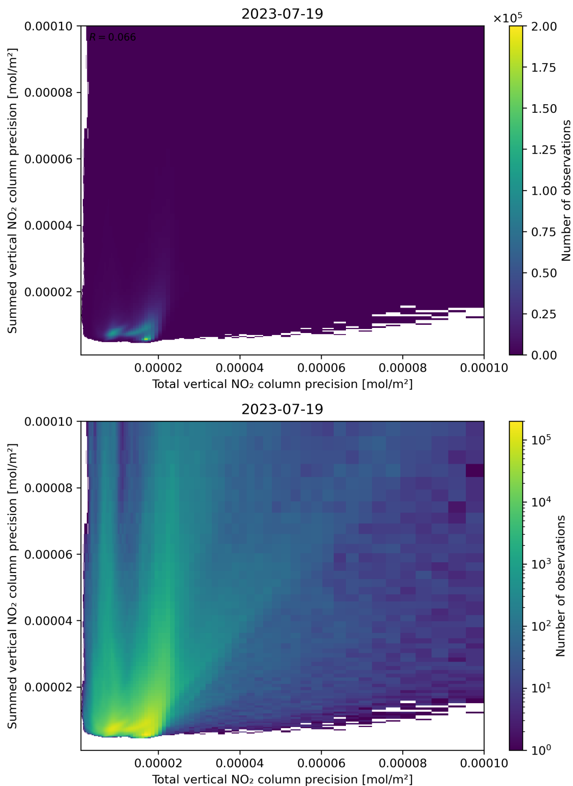
Figure 118: Scatter density plot of “Total vertical NO 2 column precision” against “Summed vertical NO 2 column precision” for 2023-07-19 to 2023-07-20.
