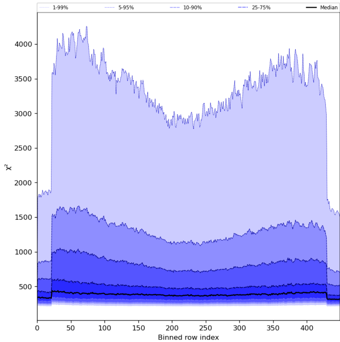
Figure 59: Along track statistics of “ \chi^2 ” for 2023-07-19 to 2023-07-20
