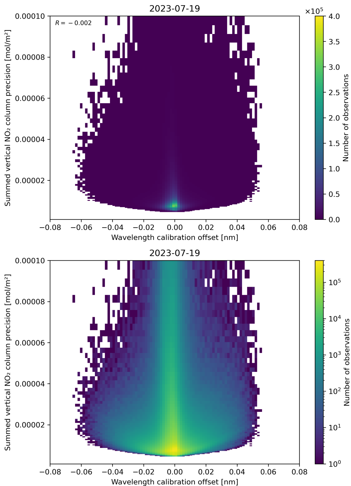
Figure 178: Scatter density plot of “Wavelength calibration offset” against “Summed vertical NO 2 column precision” for 2023-07-19 to 2023-07-20.
