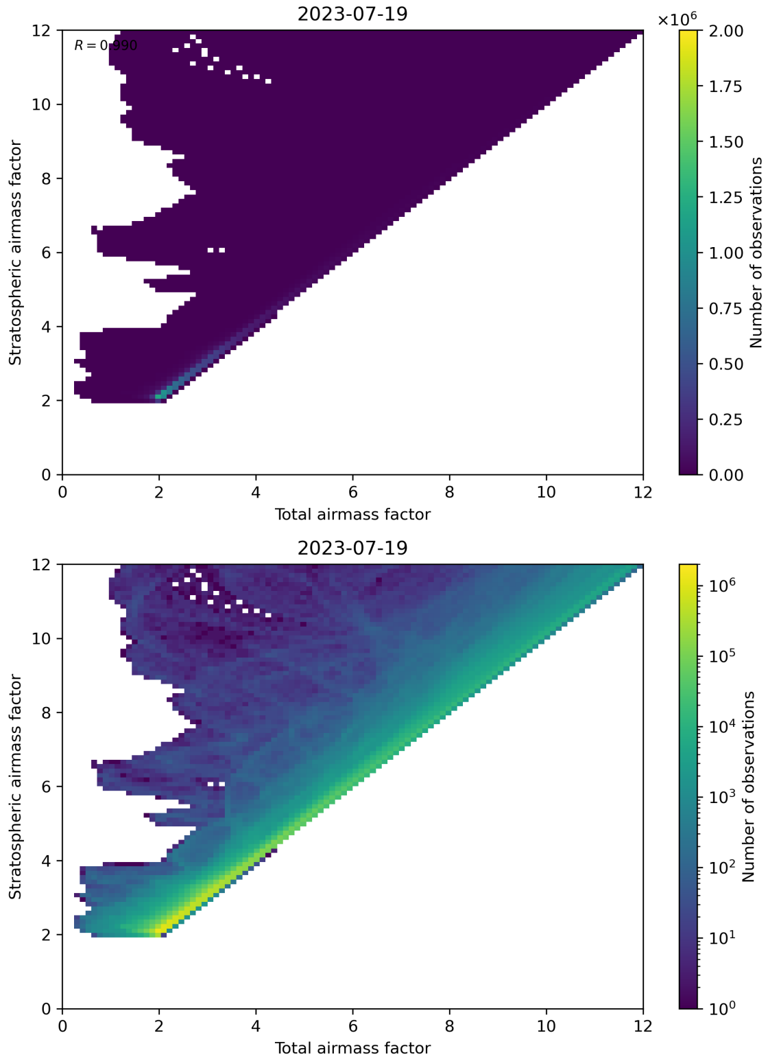
Figure 62: Scatter density plot of “Total airmass factor” against “Stratospheric airmass factor” for 2023-07-19 to 2023-07-20.
