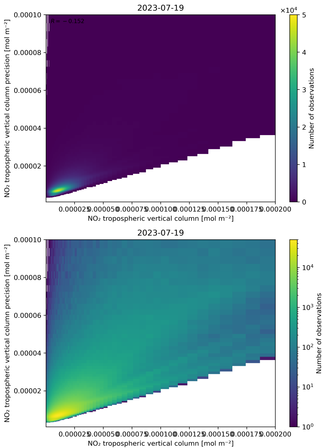
Figure 130: Scatter density plot of “NO 2 tropospheric vertical column” against “NO 2 tropospheric vertical column precision” for 2023-07-19 to 2023-07-20.
