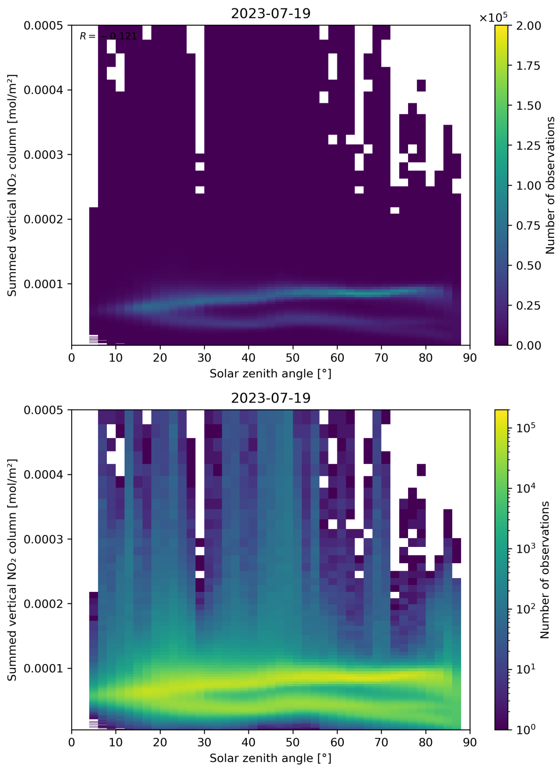
Figure 151: Scatter density plot of “Solar zenith angle” against “Summed vertical NO 2 column” for 2023-07-19 to 2023-07-20.
