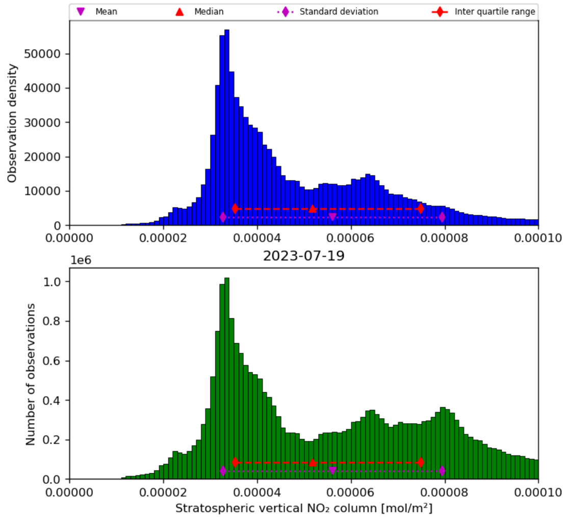
Figure 36: Histogram of “Stratospheric vertical NO 2 column” for 2023-07-19 to 2023-07-20
