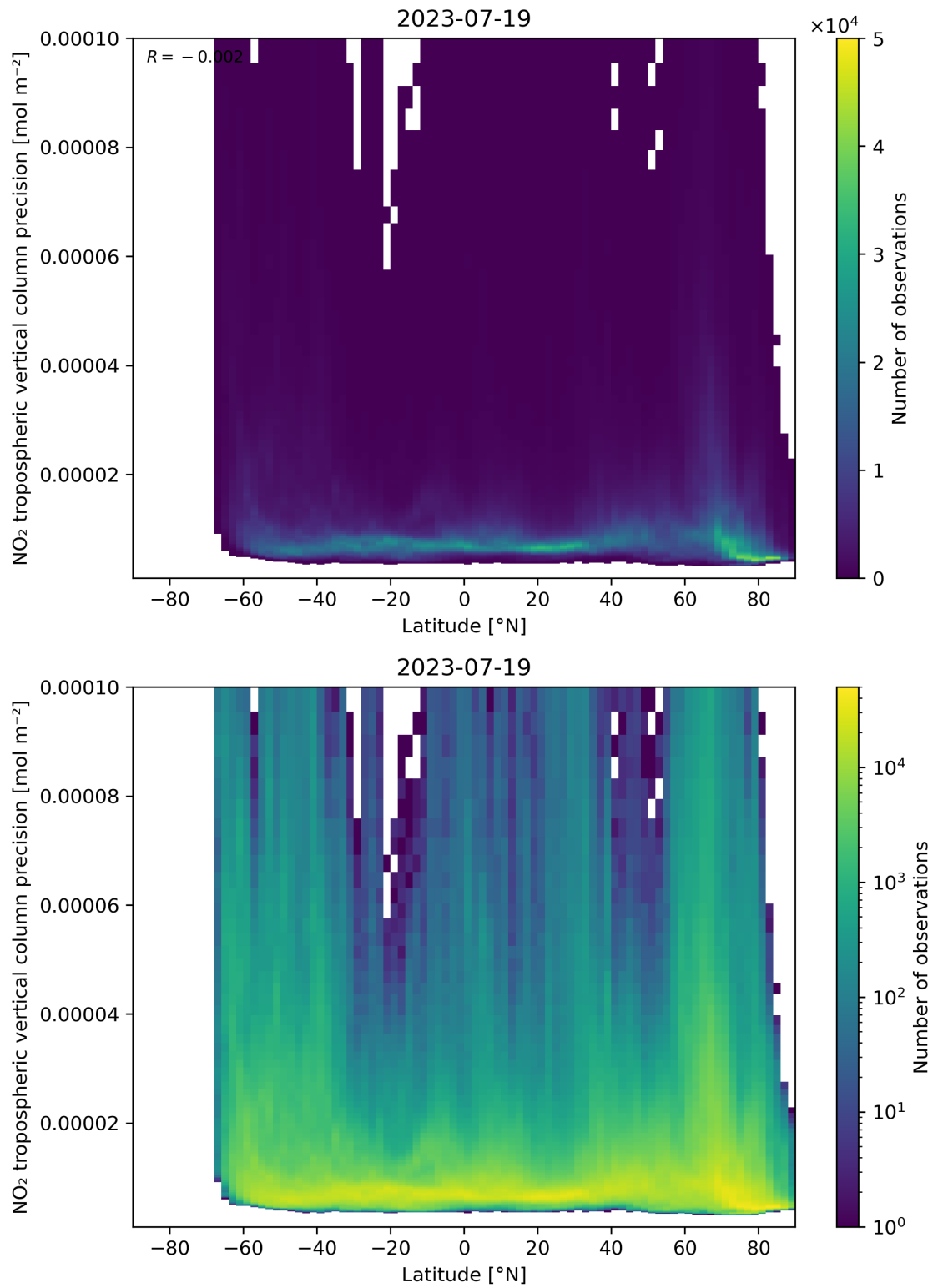
Figure 93: Scatter density plot of “Latitude” against “NO 2 tropospheric vertical column precision” for 2023-07-19 to 2023-07-20.
