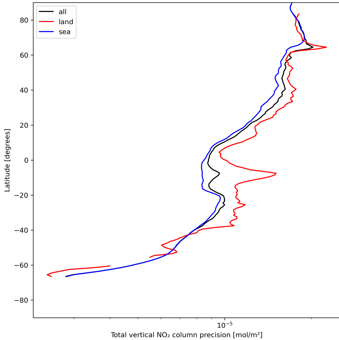
Figure 22: Zonal average of “Total vertical NO 2 column precision” for 2023-07-19 to 2023-07-20.
