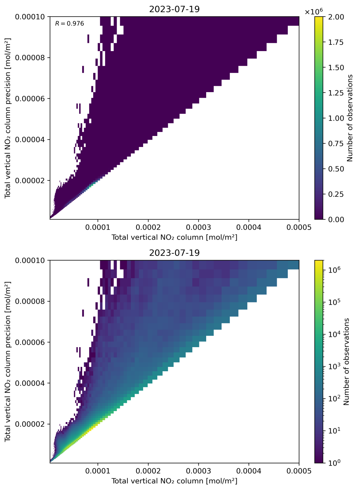
Figure 114: Scatter density plot of “Total vertical NO 2 column” against “Total vertical NO 2 column precision” for 2023-07-19 to 2023-07-20.
