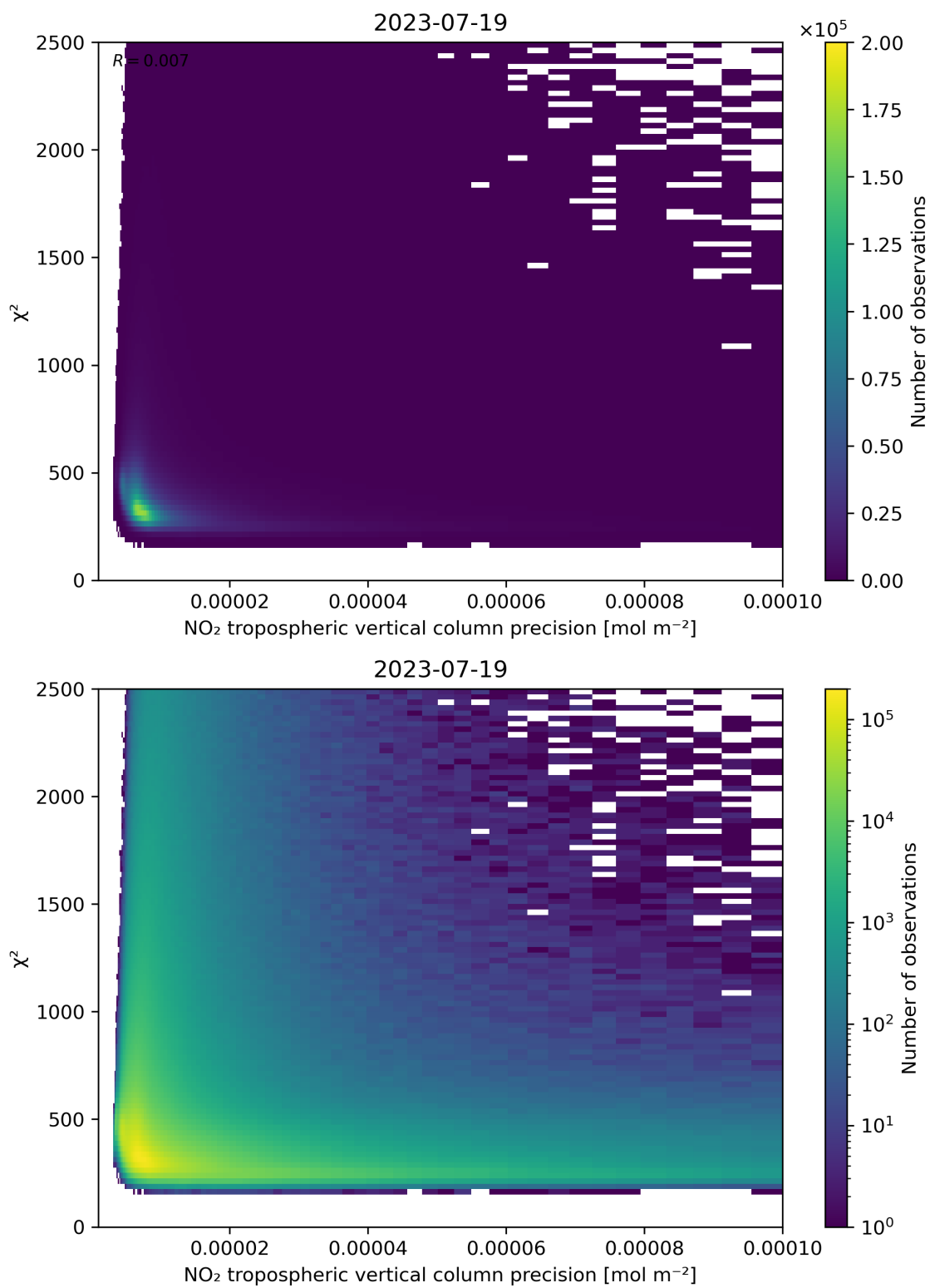
Figure 134: Scatter density plot of “NO 2 tropospheric vertical column precision” against “ \chi^2 ” for 2023-07-19 to 2023-07-20.
