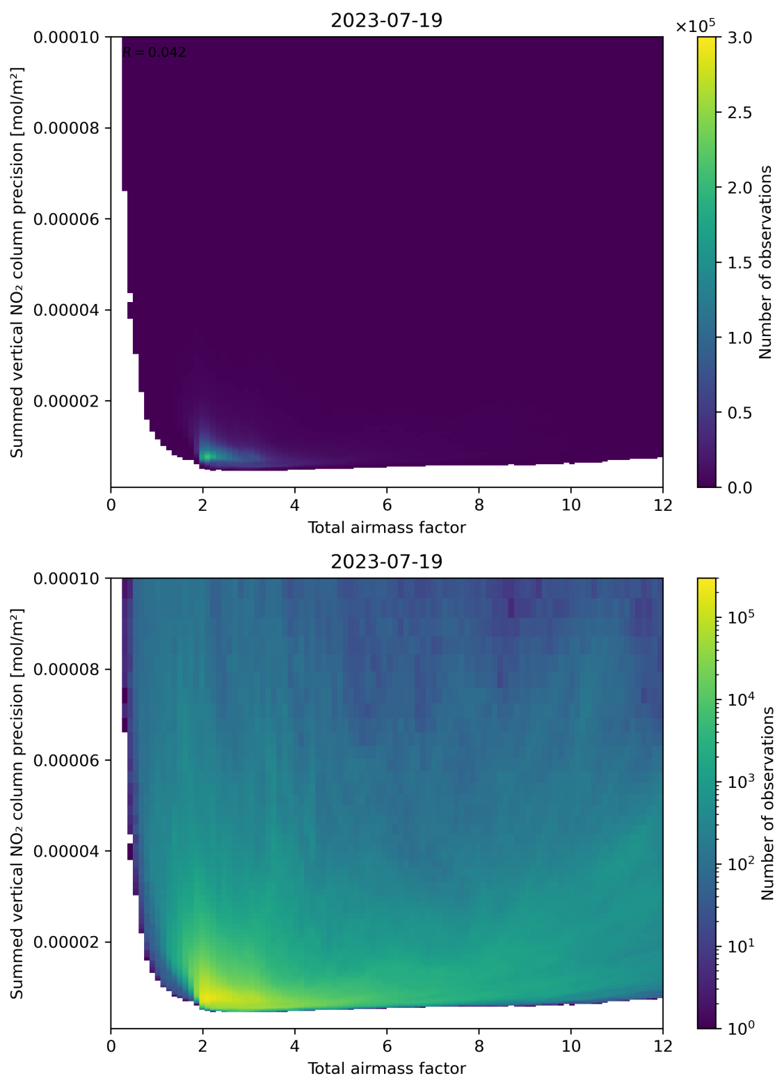
Figure 66: Scatter density plot of “Total airmass factor” against “Summed vertical NO 2 column precision” for 2023-07-19 to 2023-07-20.
