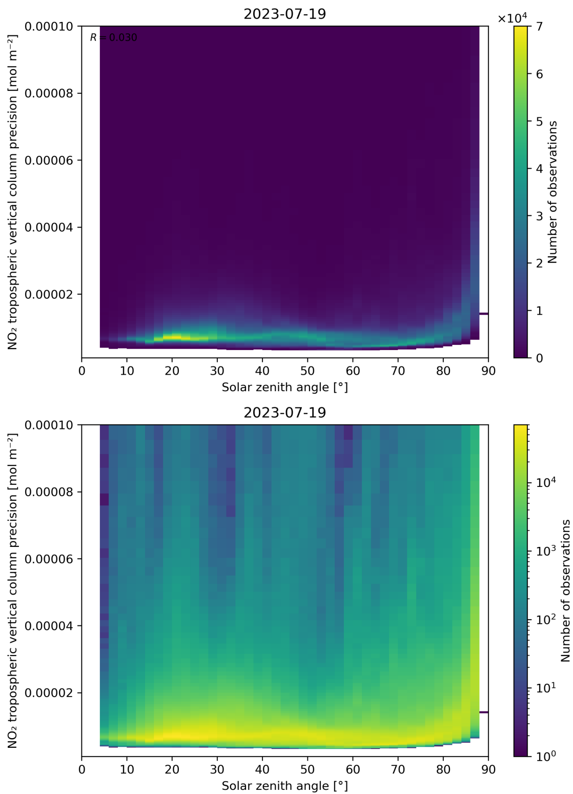
Figure 156: Scatter density plot of “Solar zenith angle” against “NO 2 tropospheric vertical column precision” for 2023-07-19 to 2023-07-20.
