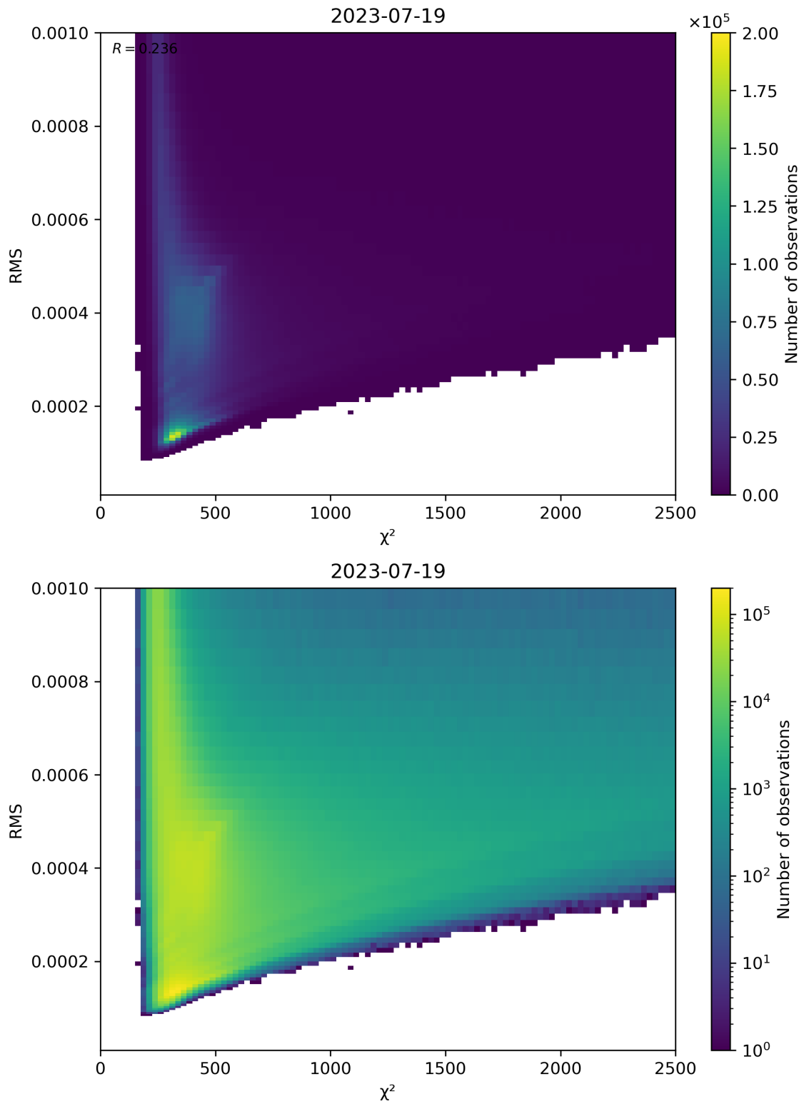
Figure 82: Scatter density plot of “ \chi^2 ” against “RMS” for 2023-07-19 to 2023-07-20.
