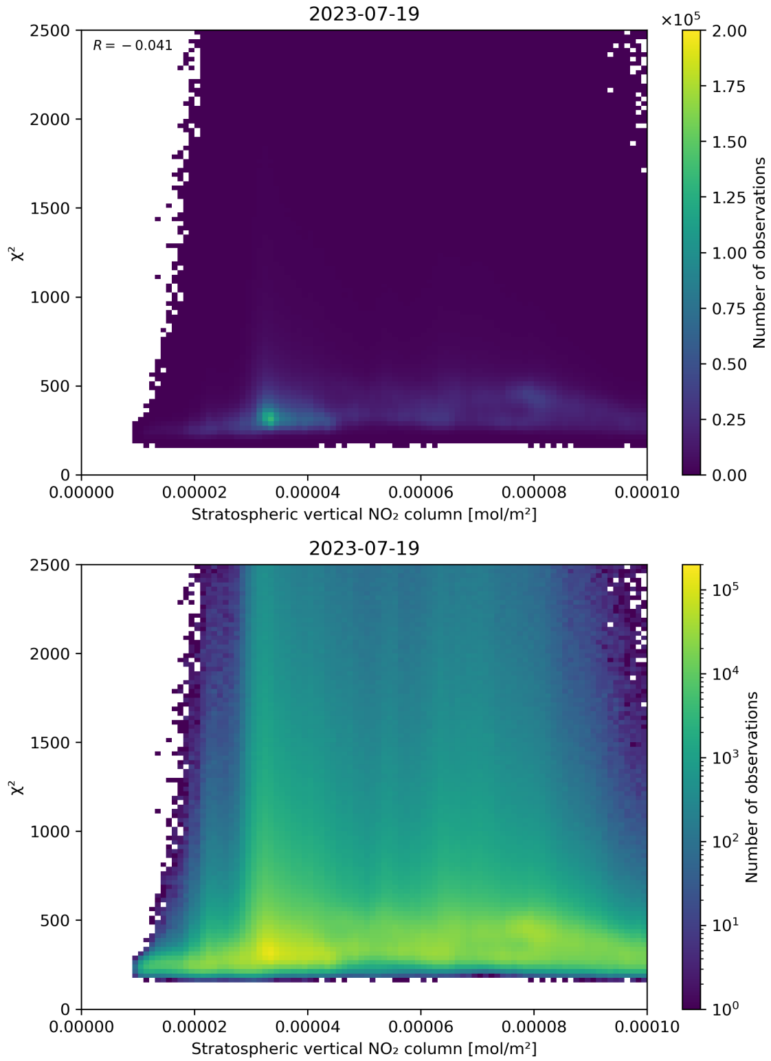
Figure 97: Scatter density plot of “Stratospheric vertical NO 2 column” against “ \chi^2 ” for 2023-07-19 to 2023-07-20.
