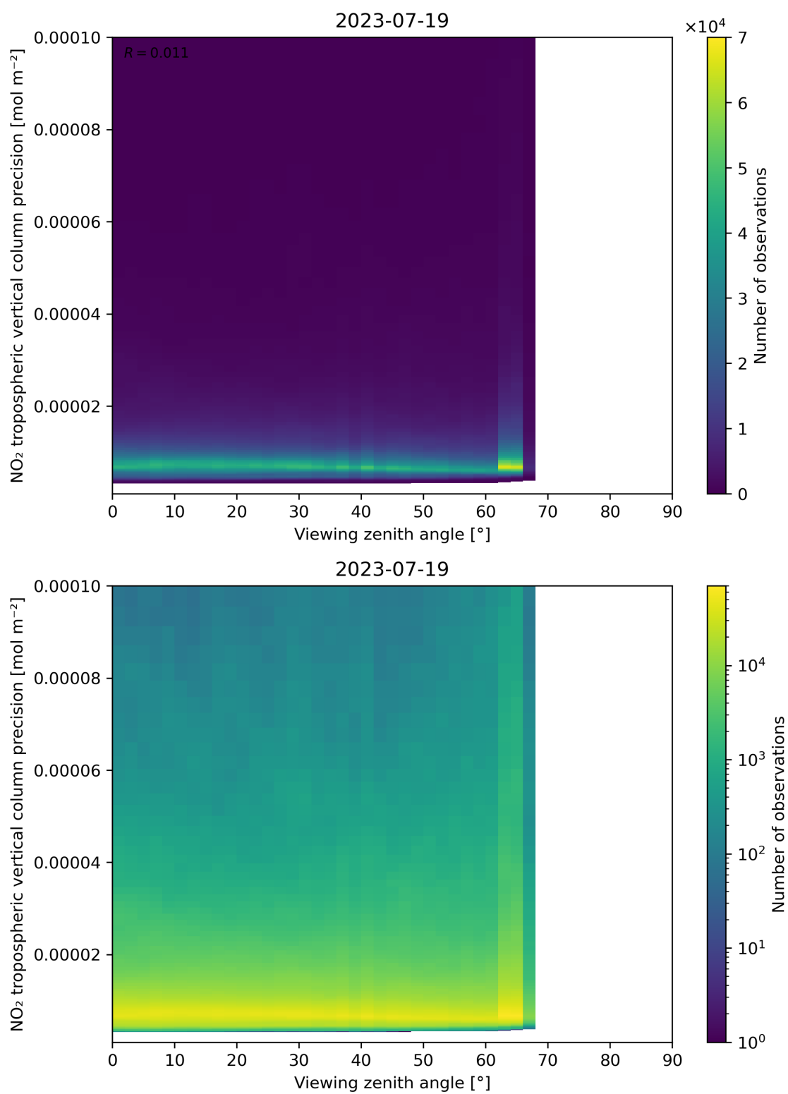
Figure 170: Scatter density plot of “Viewing zenith angle” against “NO 2 tropospheric vertical column precision” for 2023-07-19 to 2023-07-20.
