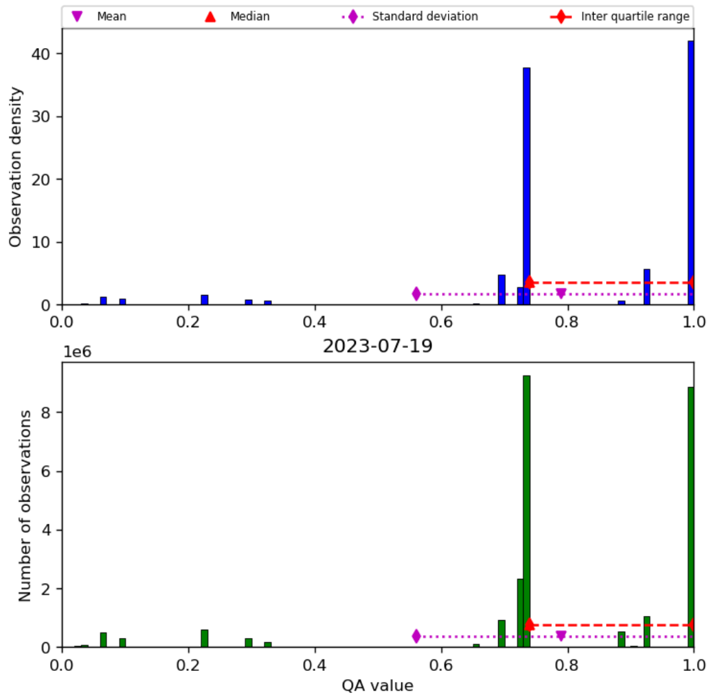
Figure 28: Histogram of “QA value” for 2023-07-19 to 2023-07-20
