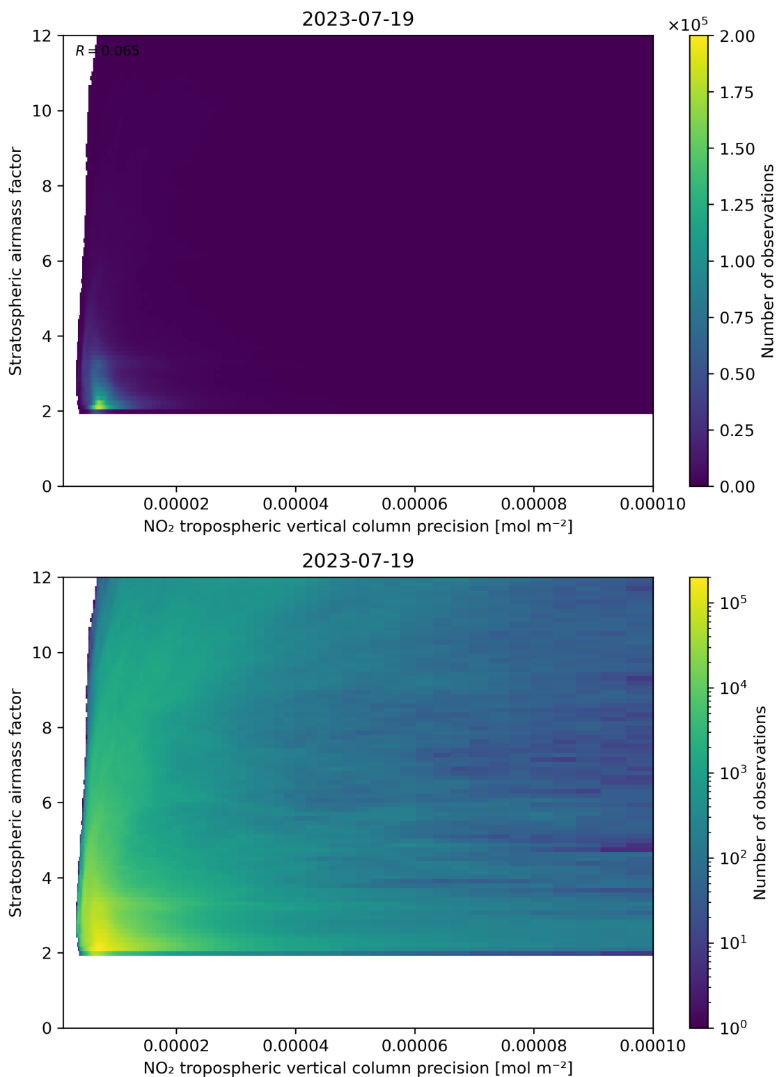
Figure 131: Scatter density plot of “NO 2 tropospheric vertical column precision” against “Stratospheric airmass factor” for 2023-07-19 to 2023-07-20.
