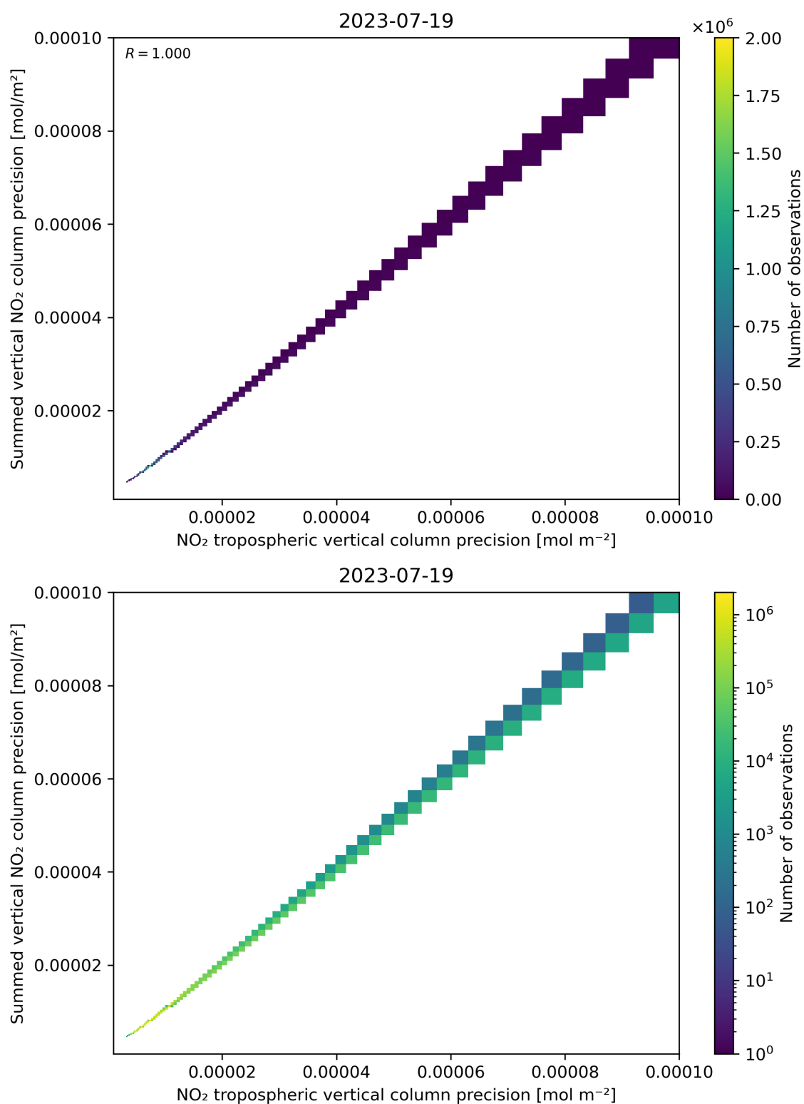
Figure 137: Scatter density plot of “NO 2 tropospheric vertical column precision” against “Summed vertical NO 2 column precision” for 2023-07-19 to 2023-07-20.
