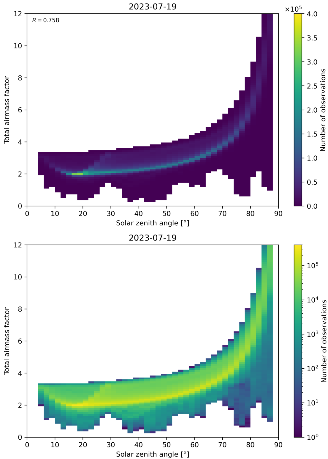
Figure 146: Scatter density plot of “Solar zenith angle” against “Total air mass factor” for 2023-07-19 to 2023-07-20.
