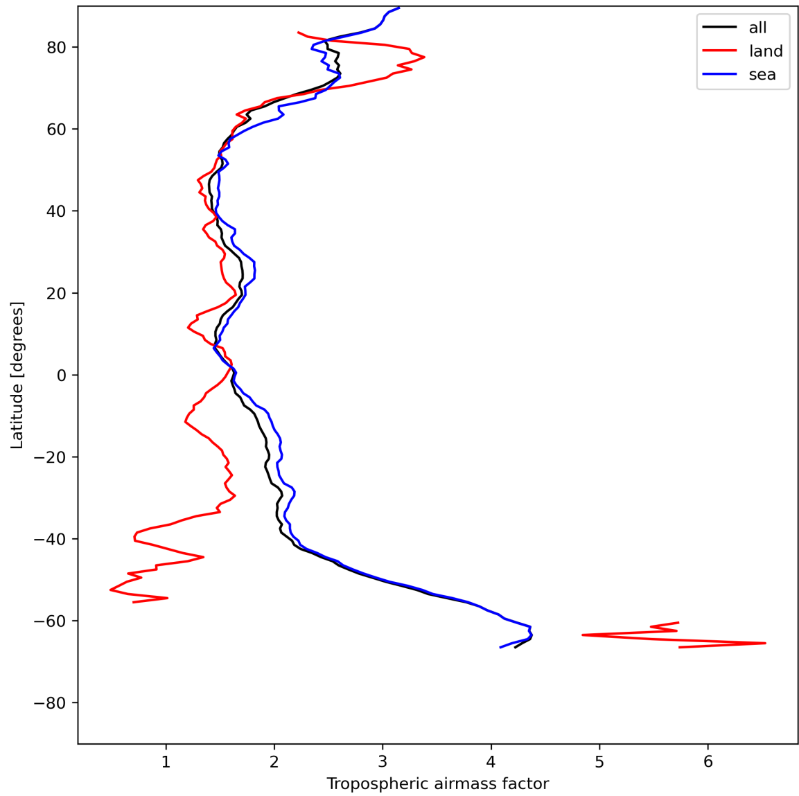
Figure 14: Zonal average of “Tropospheric airmass factor” for 2023-07-19 to 2023-07-20.
