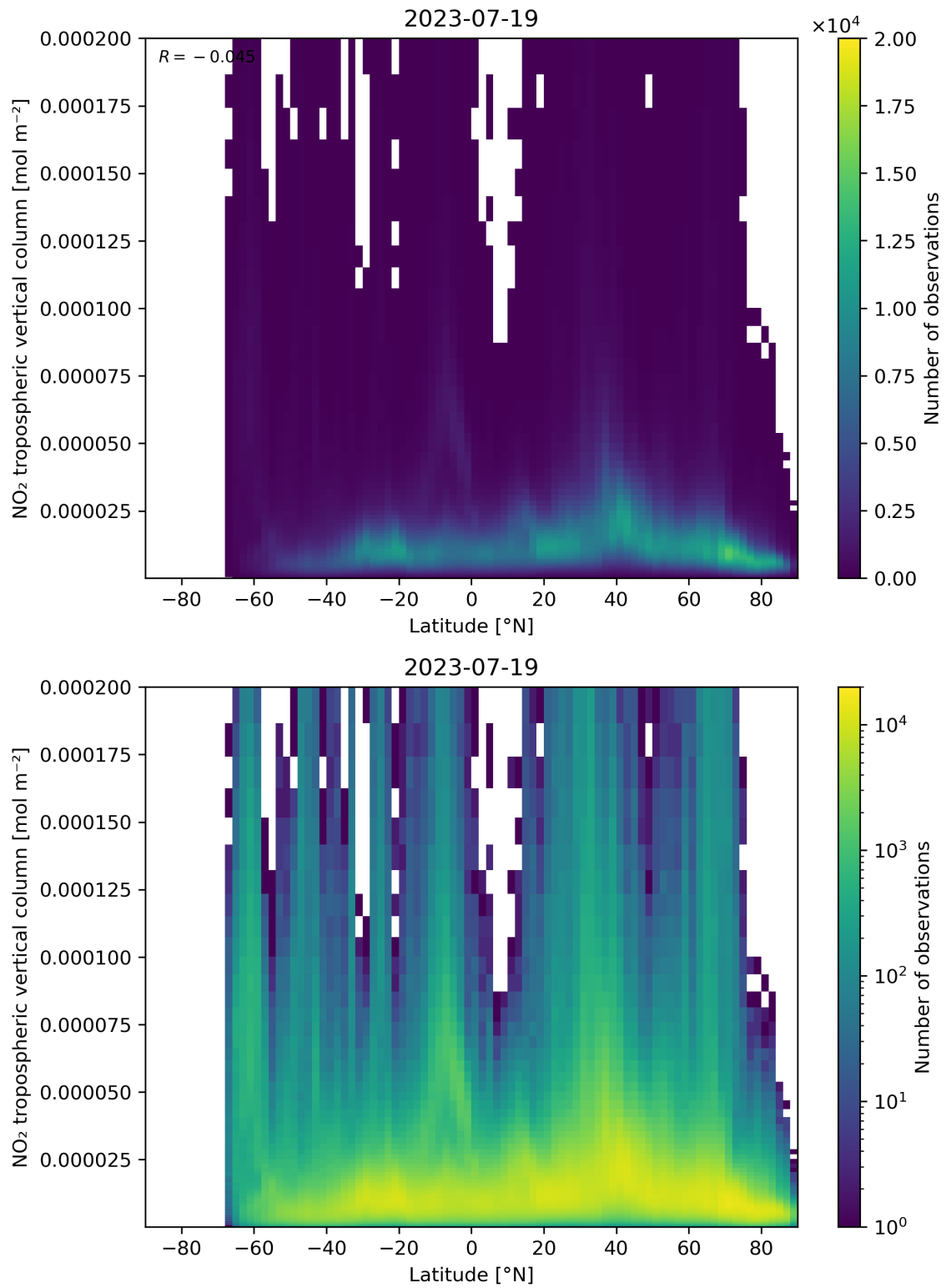
Figure 92: Scatter density plot of “Latitude” against “NO 2 tropospheric vertical column” for 2023-07-19 to 2023-07-20.
