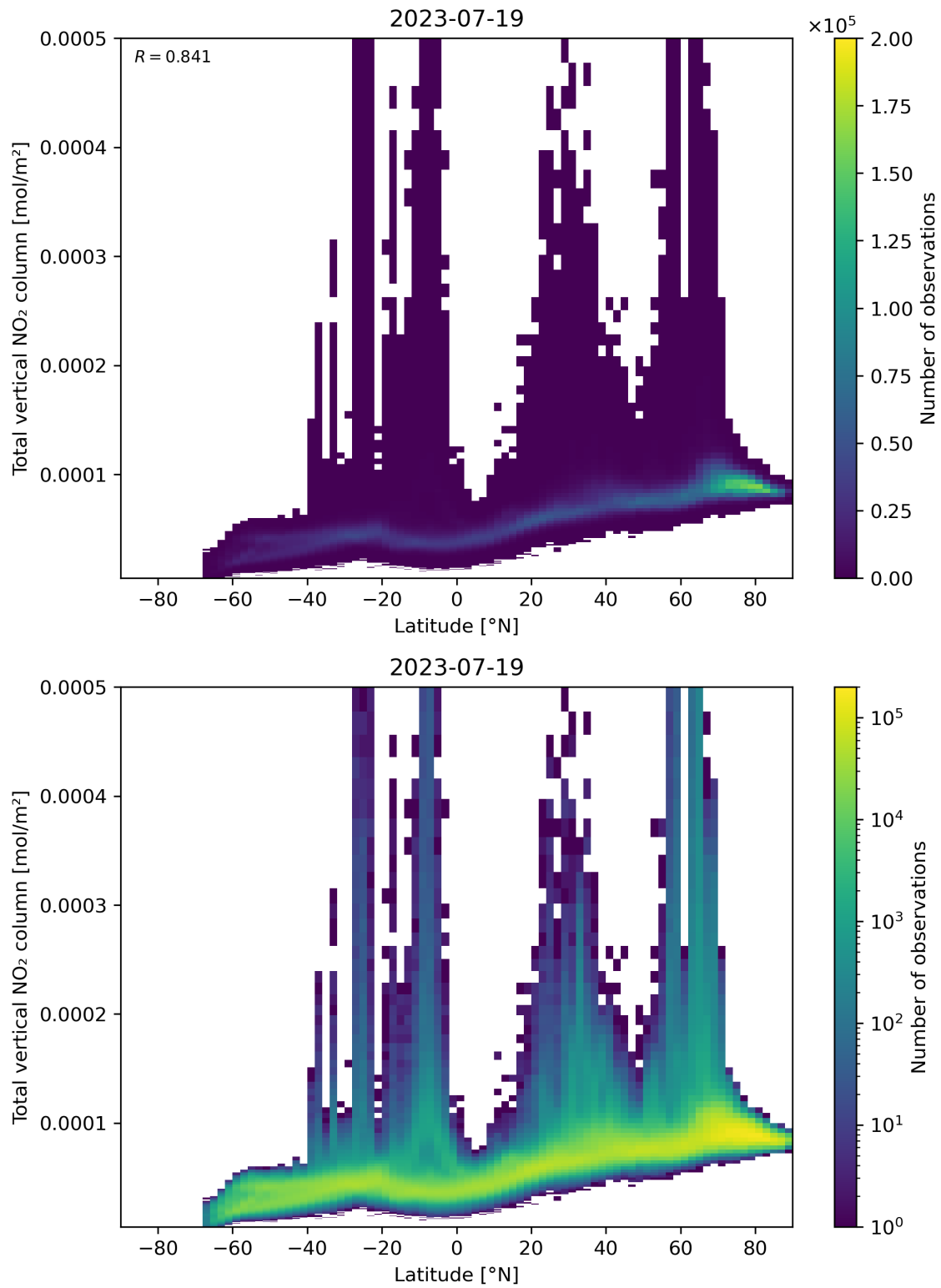
Figure 90: Scatter density plot of “Latitude” against “Total vertical NO 2 column” for 2023-07-19 to 2023-07-20.
