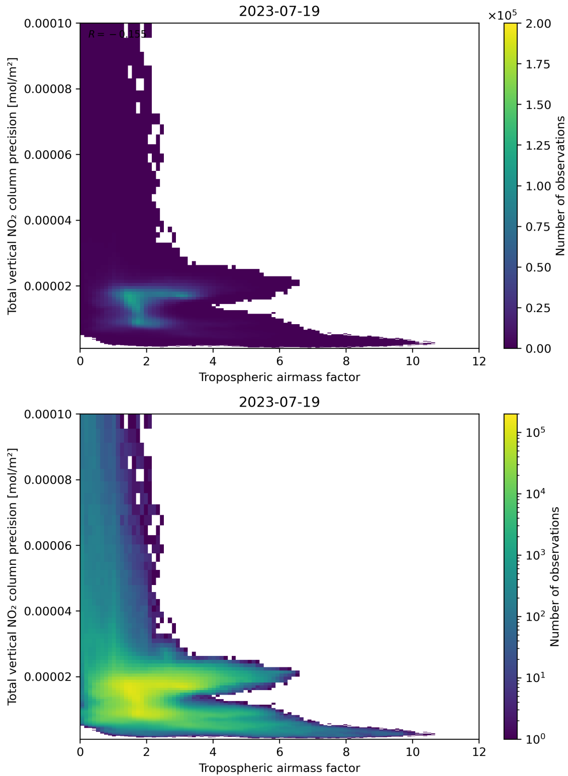
Figure 78: Scatter density plot of “Tropospheric air mass factor” against “Total vertical NO 2 column precision” for 2023-07-19 to 2023-07-20.
