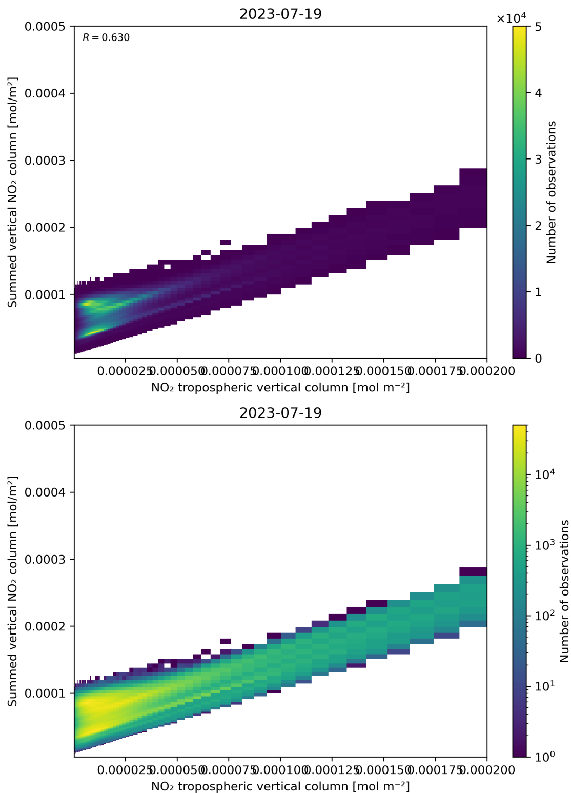
Figure 126: Scatter density plot of “NO 2 tropospheric vertical column” against “Summed vertical NO 2 column” for 2023-07-19 to 2023-07-20.
