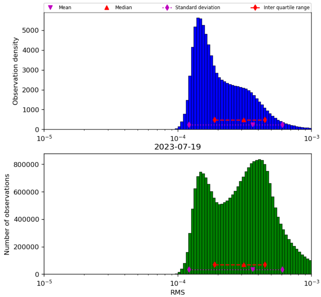
Figure 43: Histogram of “RMS” for 2023-07-19 to 2023-07-20
