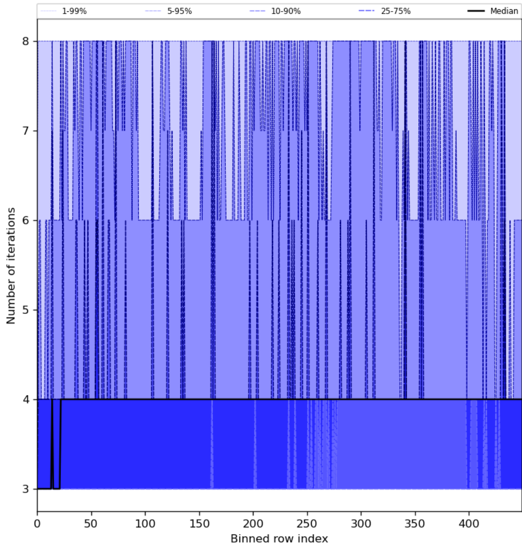
Figure 51: Along track statistics of “Number of iterations” for 2023-07-19 to 2023-07-20
