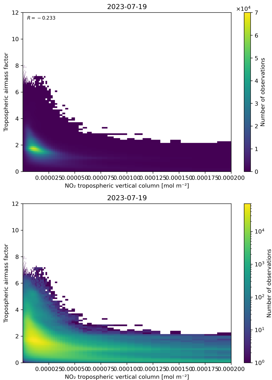
Figure 123: Scatter density plot of “NO 2 tropospheric vertical column” against “Tropospheric air mass factor” for 2023-07-19 to 2023-07-20.
