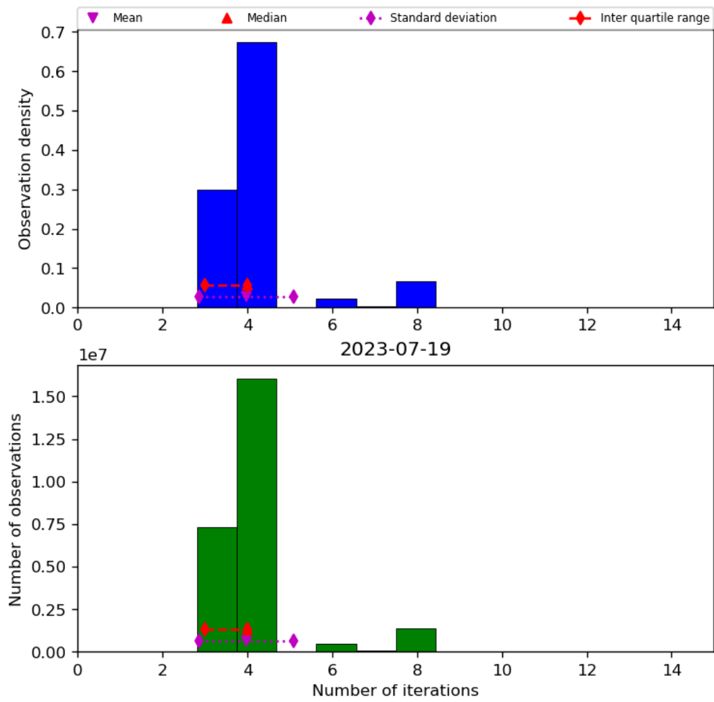
Figure 34: Histogram of “Number of iterations” for 2023-07-19 to 2023-07-20
