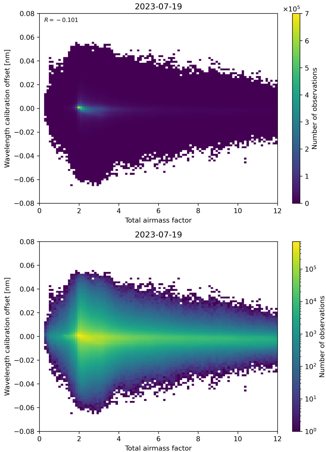
Figure 70: Scatter density plot of “Total airmass factor” against “Wavelength calibration offset” for 2023-07-19 to 2023-07-20.
