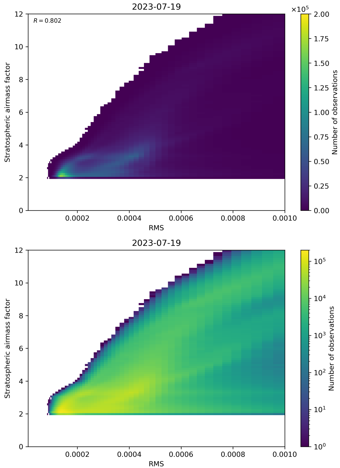
Figure 144: Scatter density plot of “RMS” against “Stratospheric airmass factor” for 2023-07-19 to 2023-07-20.
