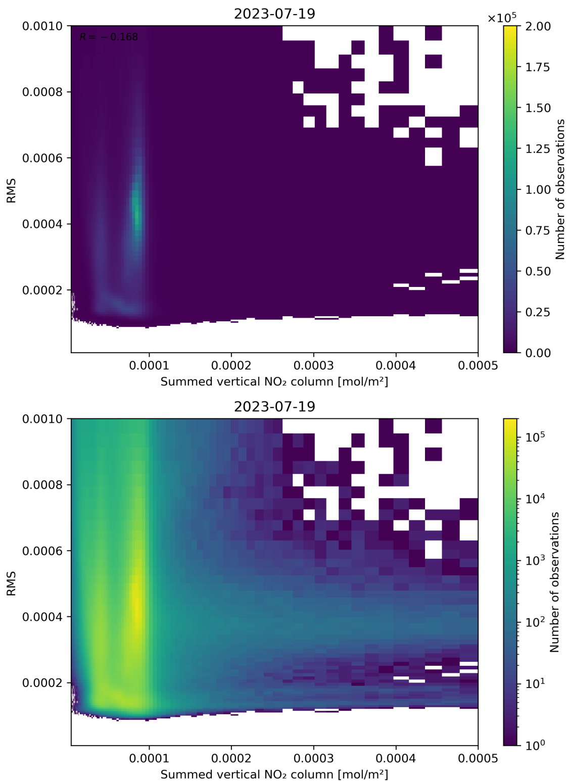
Figure 109: Scatter density plot of “Summed vertical NO 2 column” against “RMS” for 2023-07-19 to 2023-07-20.
