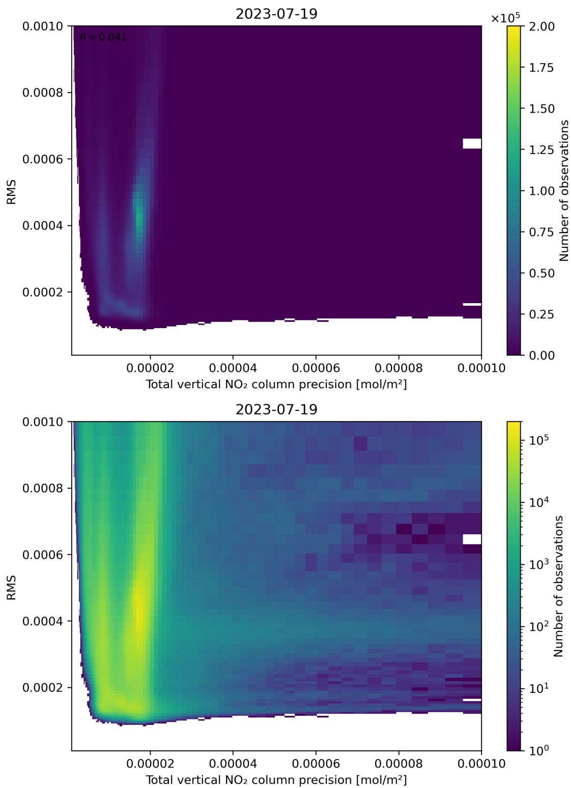
Figure 119: Scatter density plot of “Total vertical NO 2 column precision” against “RMS” for 2023-07-19 to 2023-07-20.
