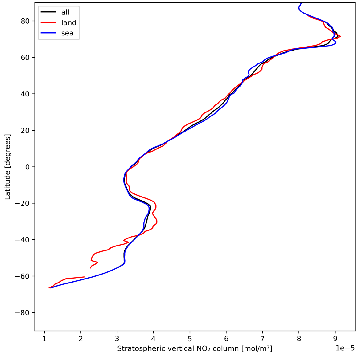
Figure 19: Zonal average of “Stratospheric vertical NO 2 column” for 2023-07-19 to 2023-07-20.
