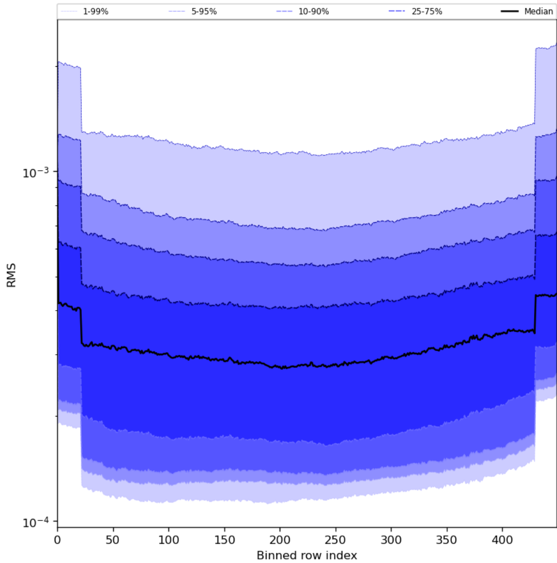
Figure 60: Along track statistics of “RMS” for 2023-07-19 to 2023-07-20
