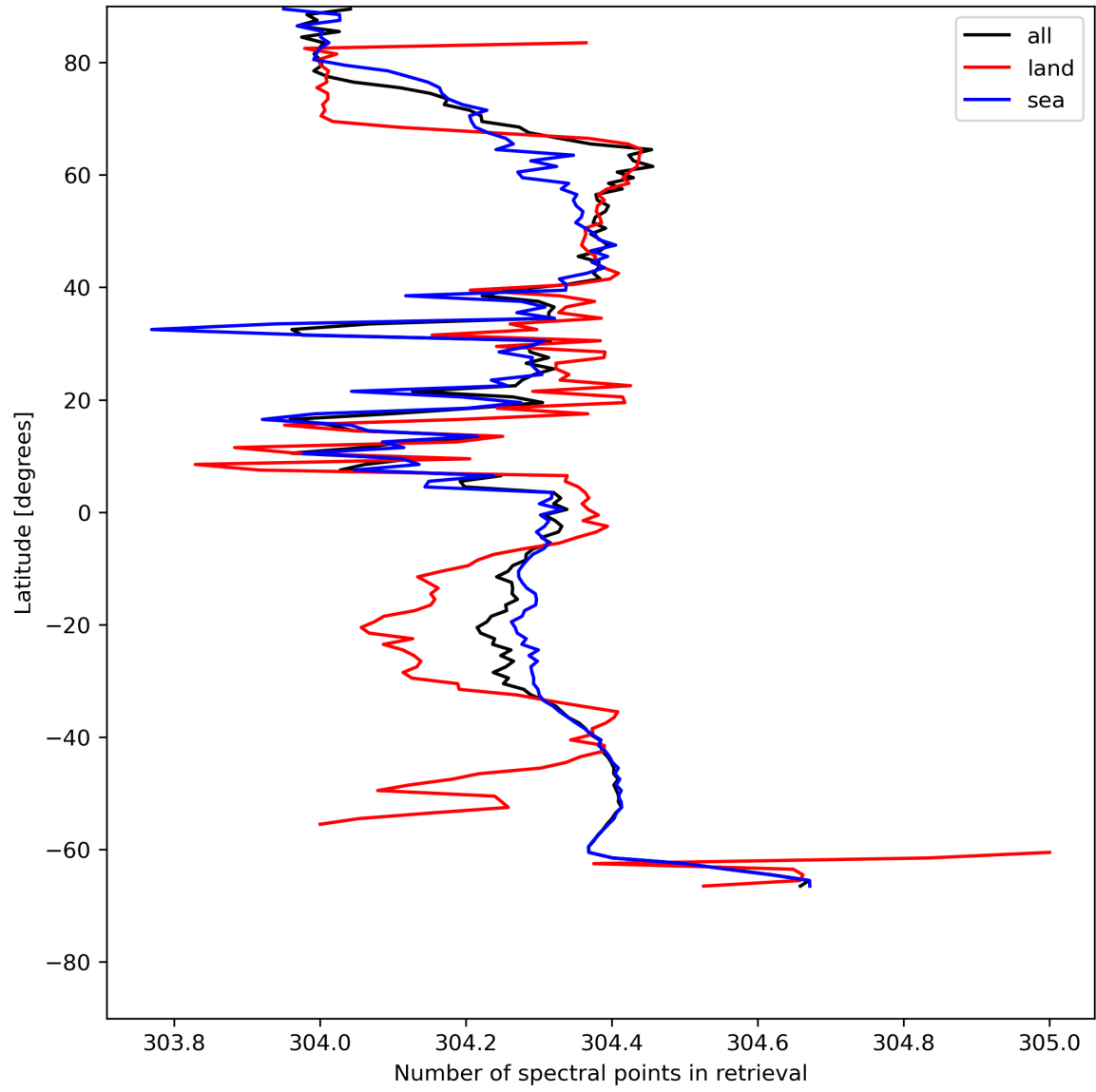
Figure 16: Zonal average of “Number of spectral points in retrieval” for 2023-07-19 to 2023-07-20.
