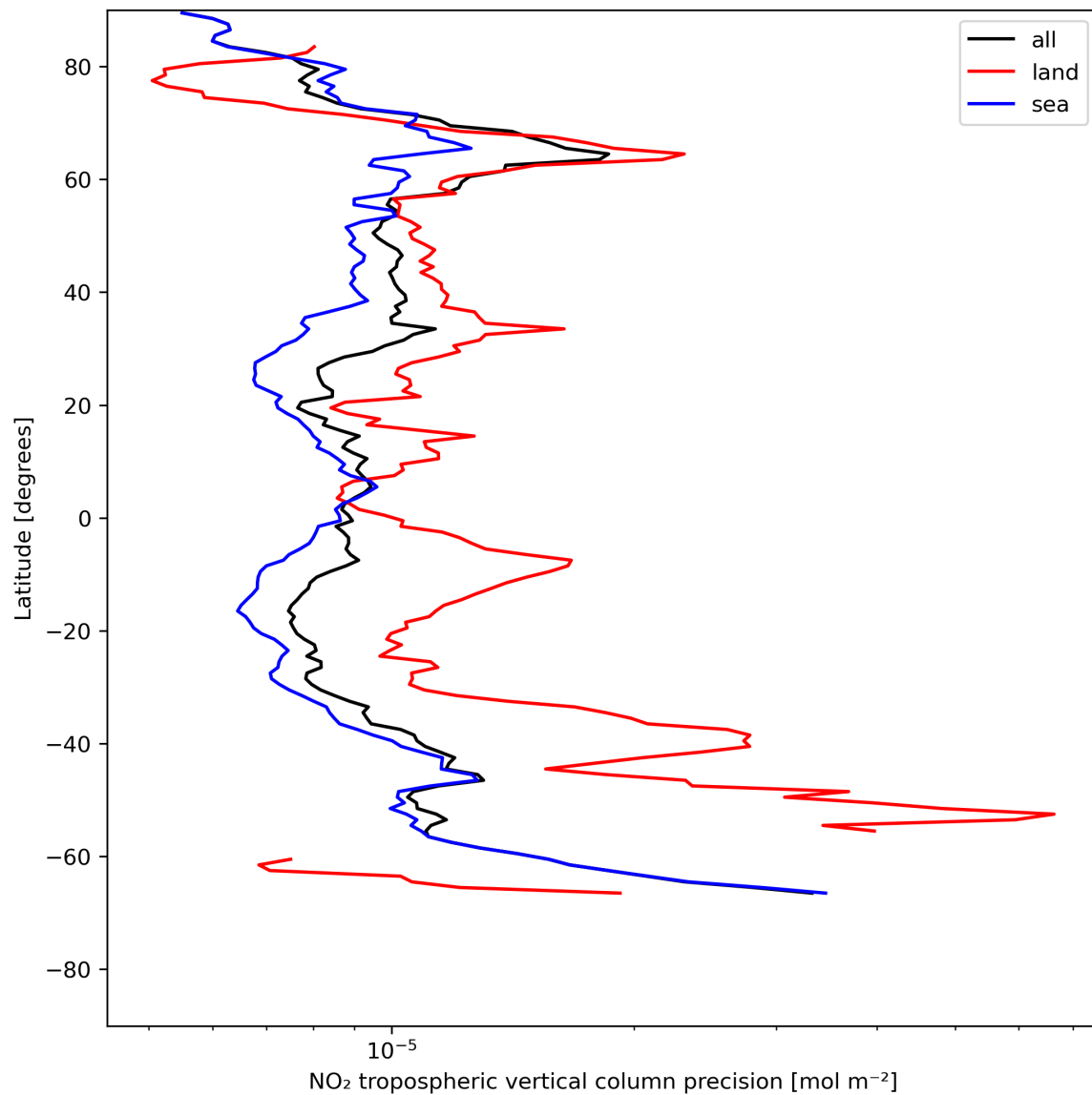
Figure 13: Zonal average of “NO 2 tropospheric vertical column precision” for 2023-07-19 to 2023-07-20.
