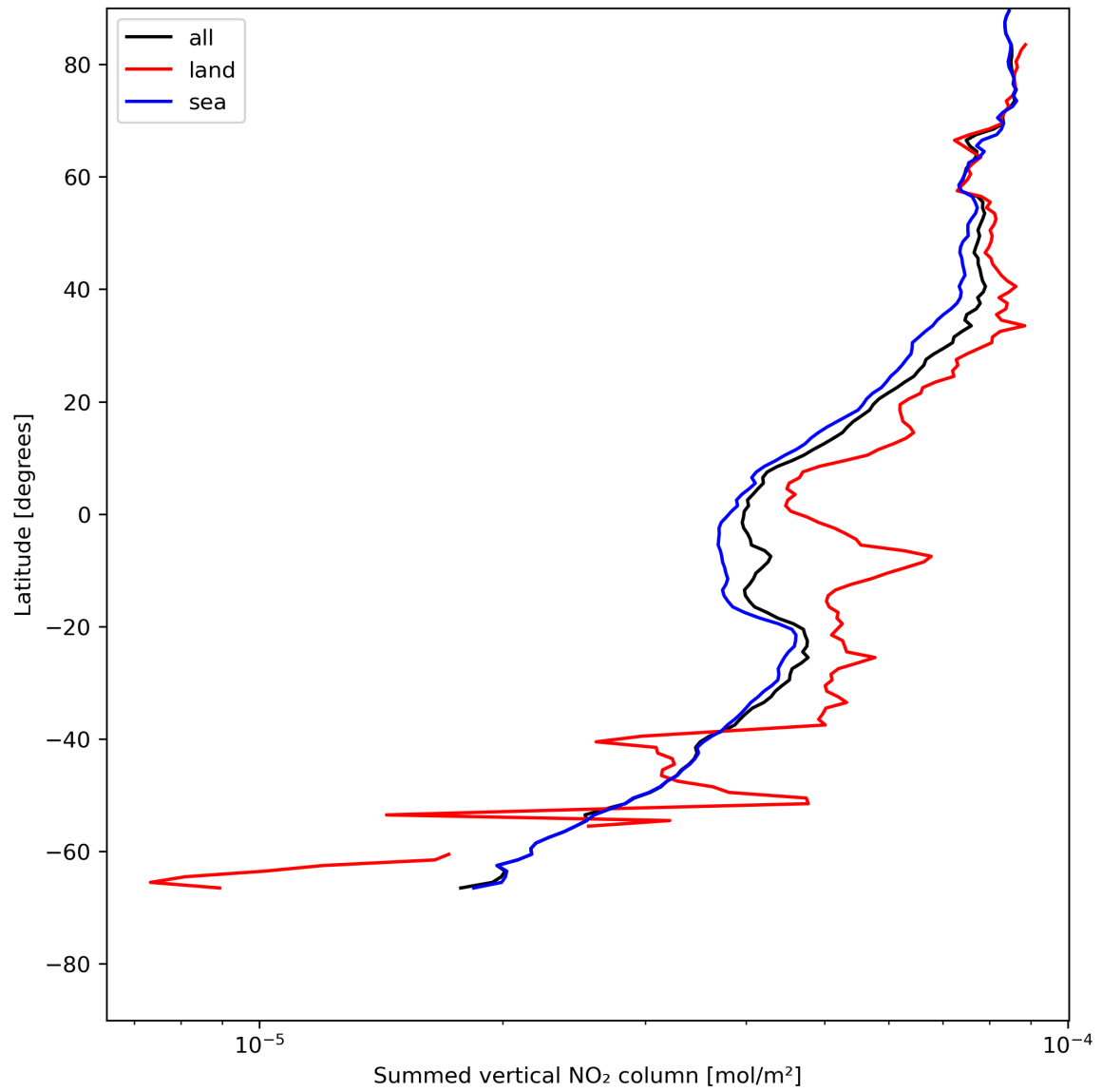
Figure 23: Zonal average of “Summed vertical NO 2 column” for 2023-07-19 to 2023-07-20.
