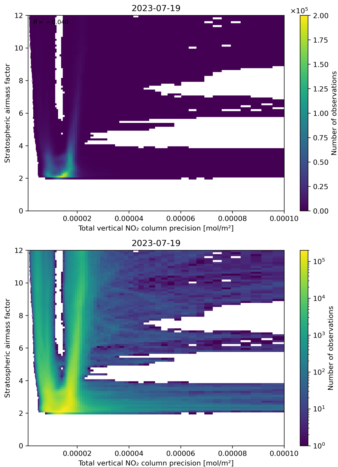
Figure 115: Scatter density plot of “Total vertical NO 2 column precision” against “Stratospheric air mass factor” for 2023-07-19 to 2023-07-20.
