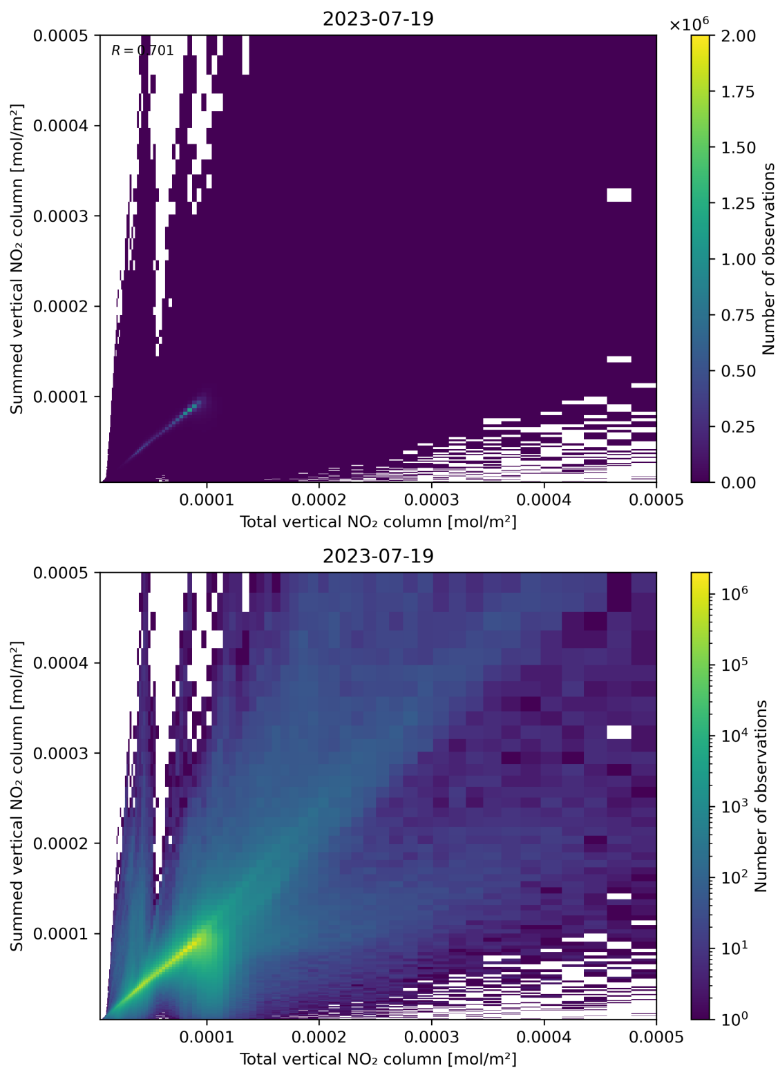
Figure 112: Scatter density plot of “Total vertical NO 2 column” against “Summed vertical NO 2 column” for 2023-07-19 to 2023-07-20.
