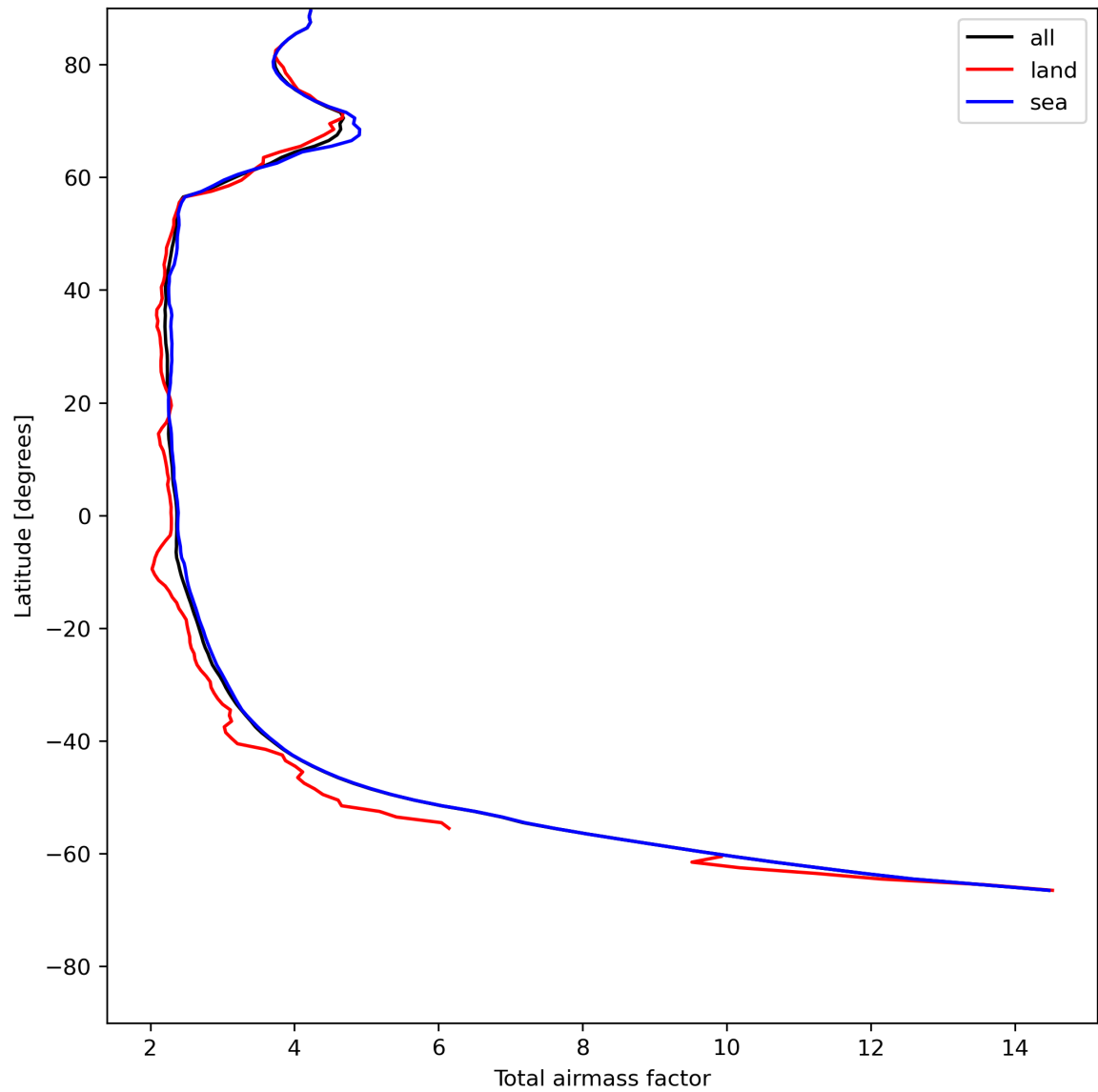
Figure 15: Zonal average of “Total airmass factor” for 2023-07-19 to 2023-07-20.
