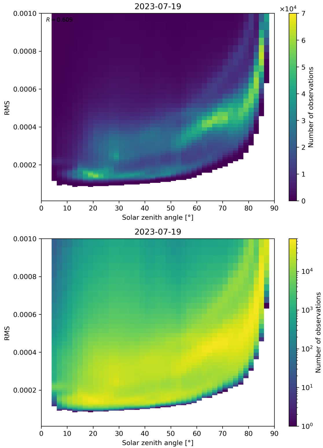
Figure 157: Scatter density plot of “Solar zenith angle” against “RMS” for 2023-07-19 to 2023-07-20.
