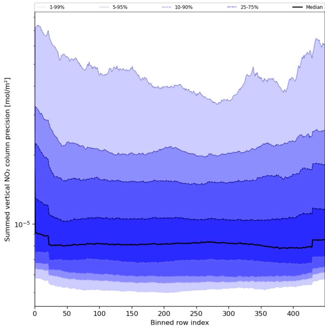
Figure 58: Along track statistics of “Summed vertical NO 2 column precision” for 2023-07-19 to 2023-07-20
