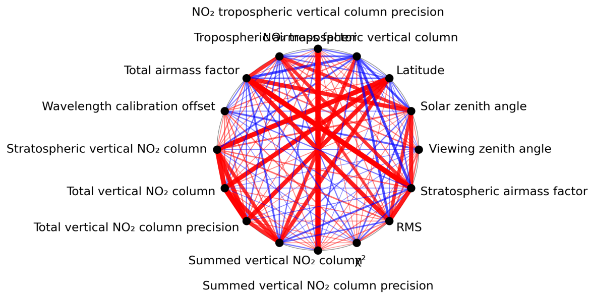
Figure 1: Map of correlation graph for 2023-07-19 to 2023-07-20.
