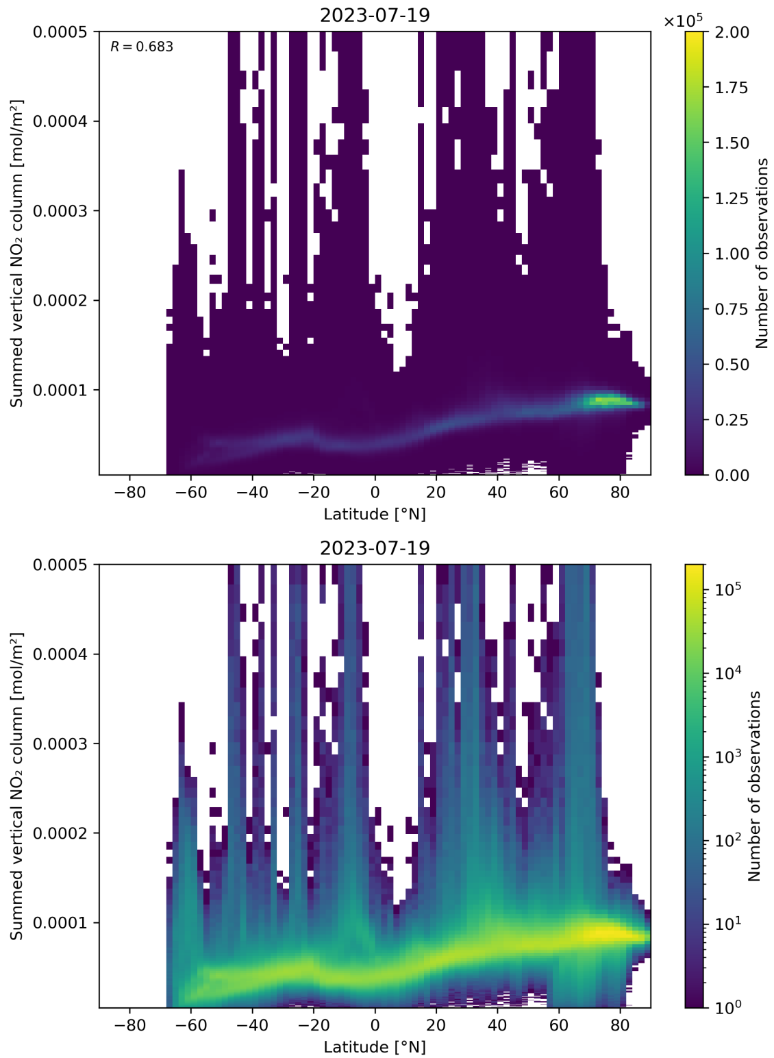
Figure 88: Scatter density plot of “Latitude” against “Summed vertical NO 2 column” for 2023-07-19 to 2023-07-20.
