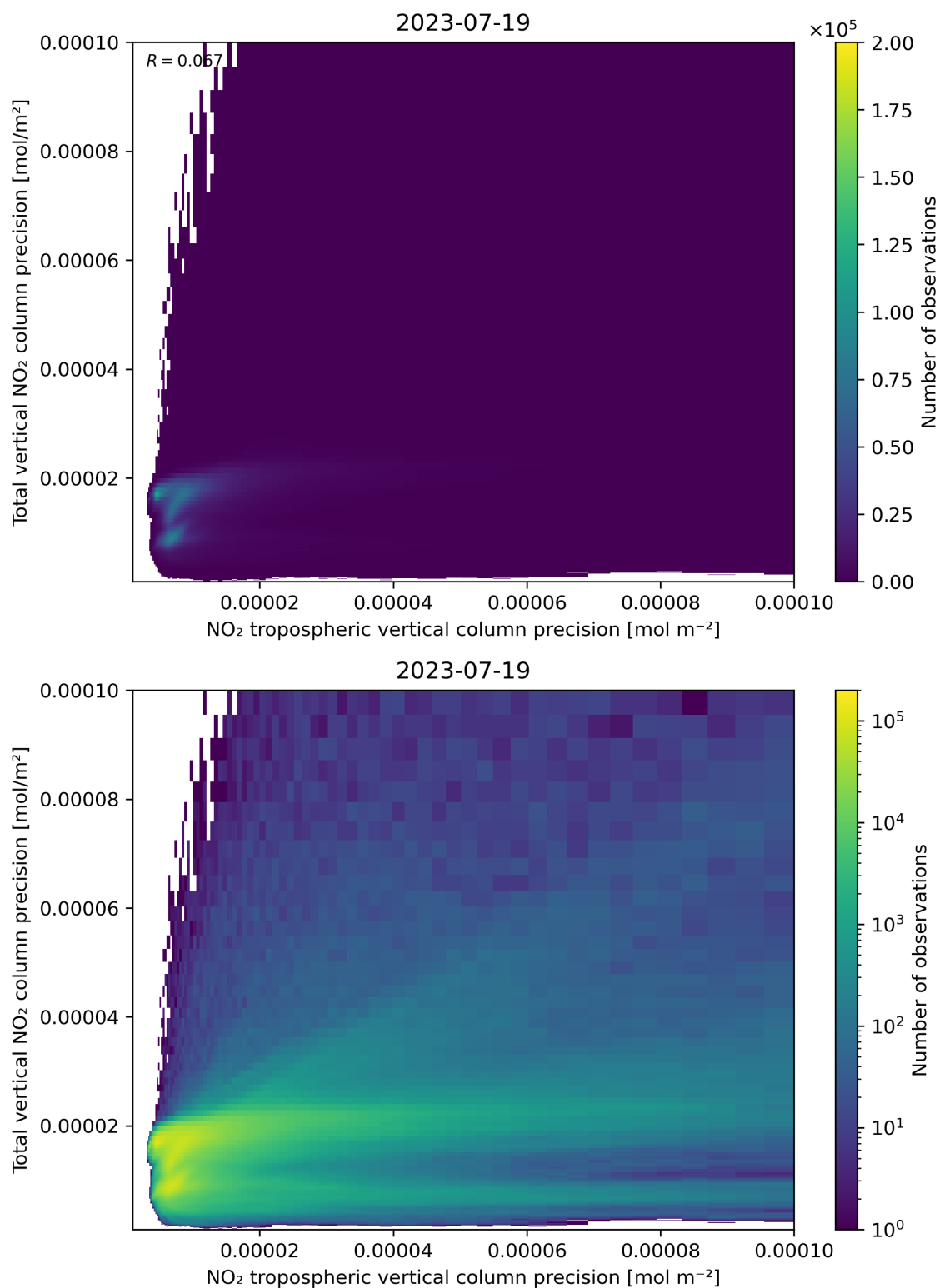
Figure 139: Scatter density plot of “NO 2 tropospheric vertical column precision” against “Total vertical NO 2 column precision” for 2023-07-19 to 2023-07-20.
