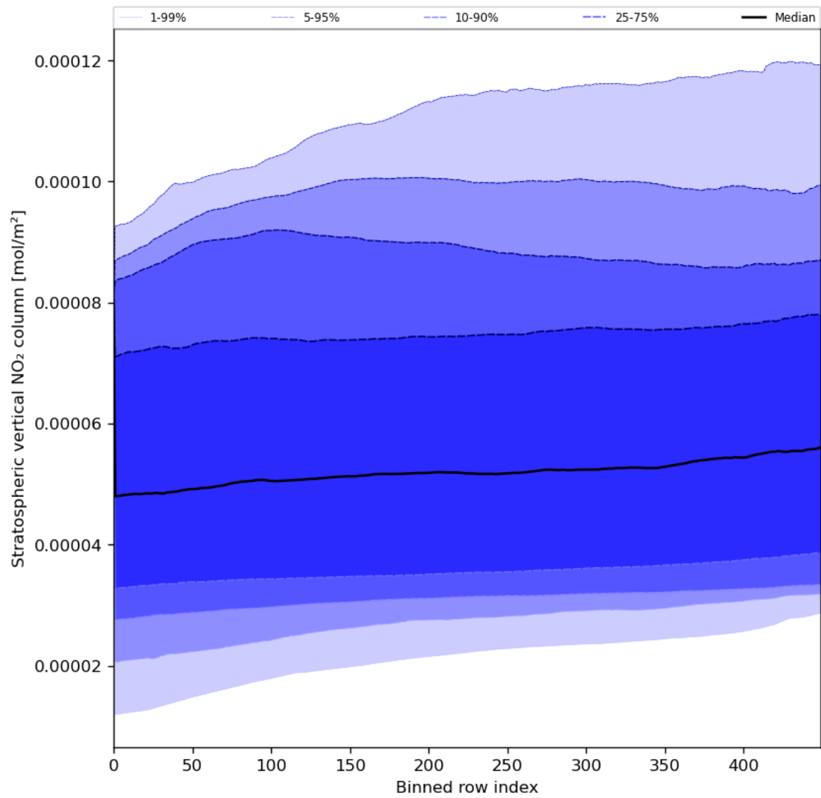
Figure 53: Along track statistics of “Stratospheric vertical NO 2 column” for 2023-07-19 to 2023-07-20
