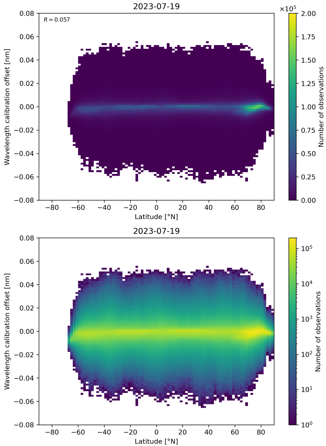
Figure 95: Scatter density plot of “Latitude” against “Wavelength calibration offset” for 2023-07-19 to 2023-07-20.
