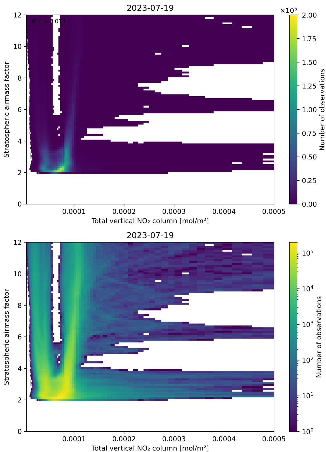
Figure 110: Scatter density plot of “Total vertical NO 2 column” against “Stratospheric air mass factor” for 2023-07-19 to 2023-07-20.
