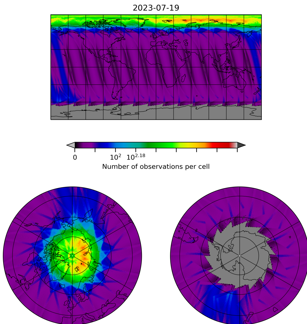
Figure 10: Map of the number of observations for 2023-07-19 to 2023-07-20
