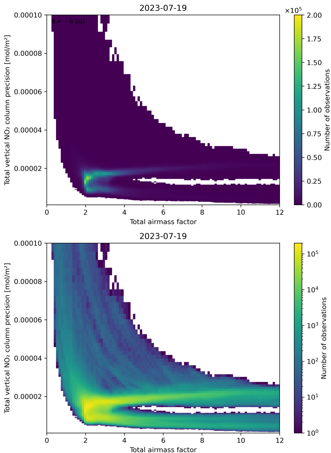
Figure 68: Scatter density plot of “Total airmass factor” against “Total vertical NO 2 column precision” for 2023-07-19 to 2023-07-20.
