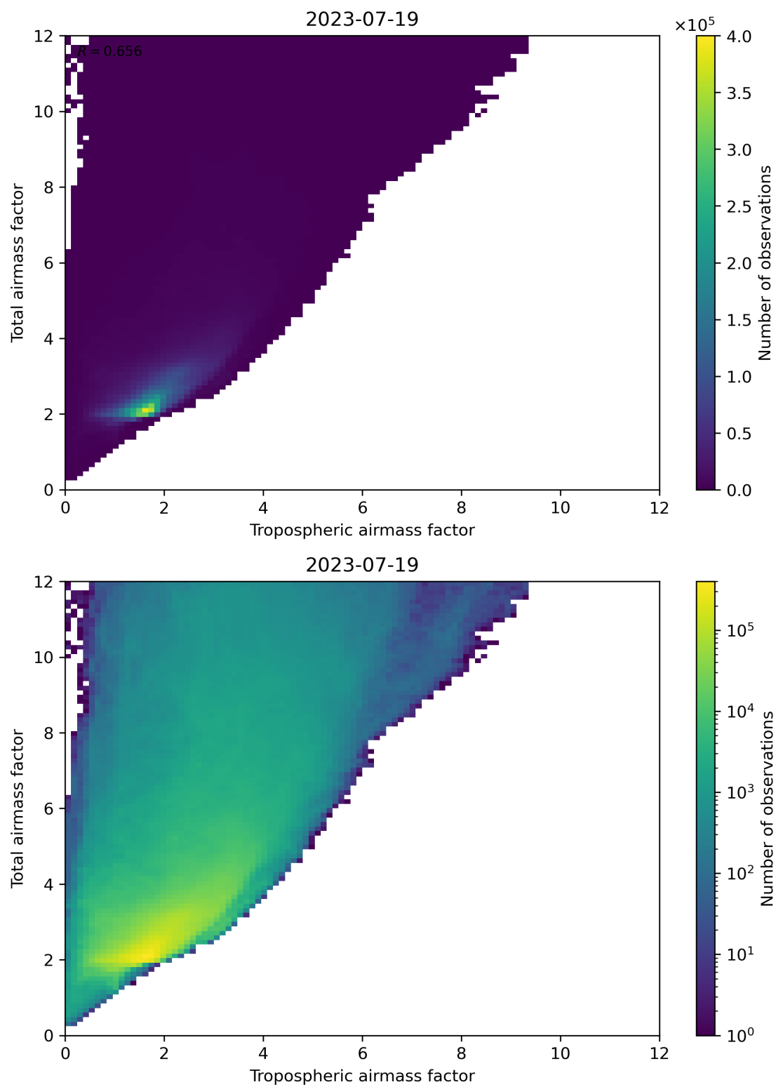
Figure 72: Scatter density plot of “Tropospheric airmass factor” against “Total airmass factor” for 2023-07-19 to 2023-07-20.
