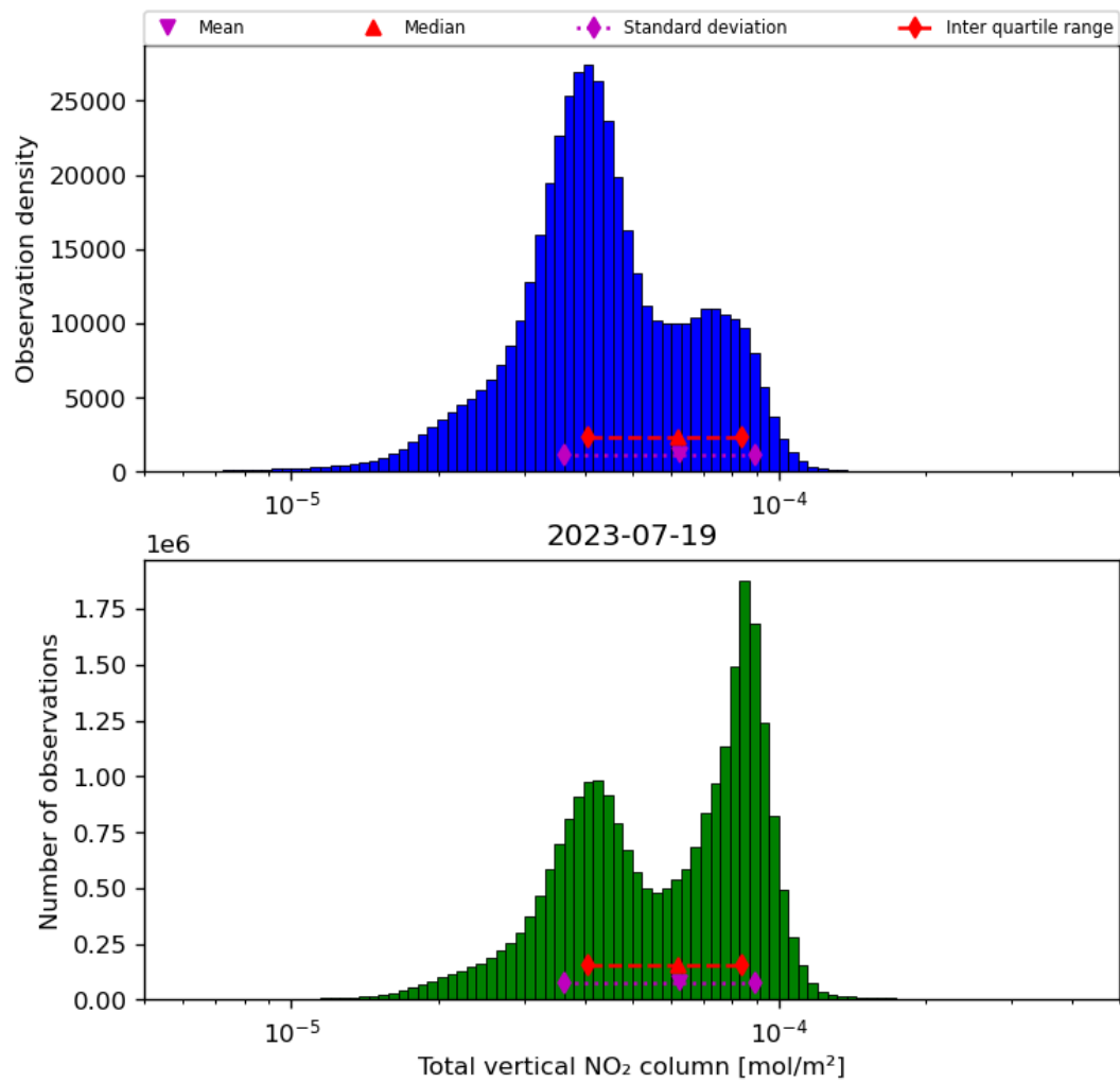
Figure 38: Histogram of “Total vertical NO 2 column” for 2023-07-19 to 2023-07-20
