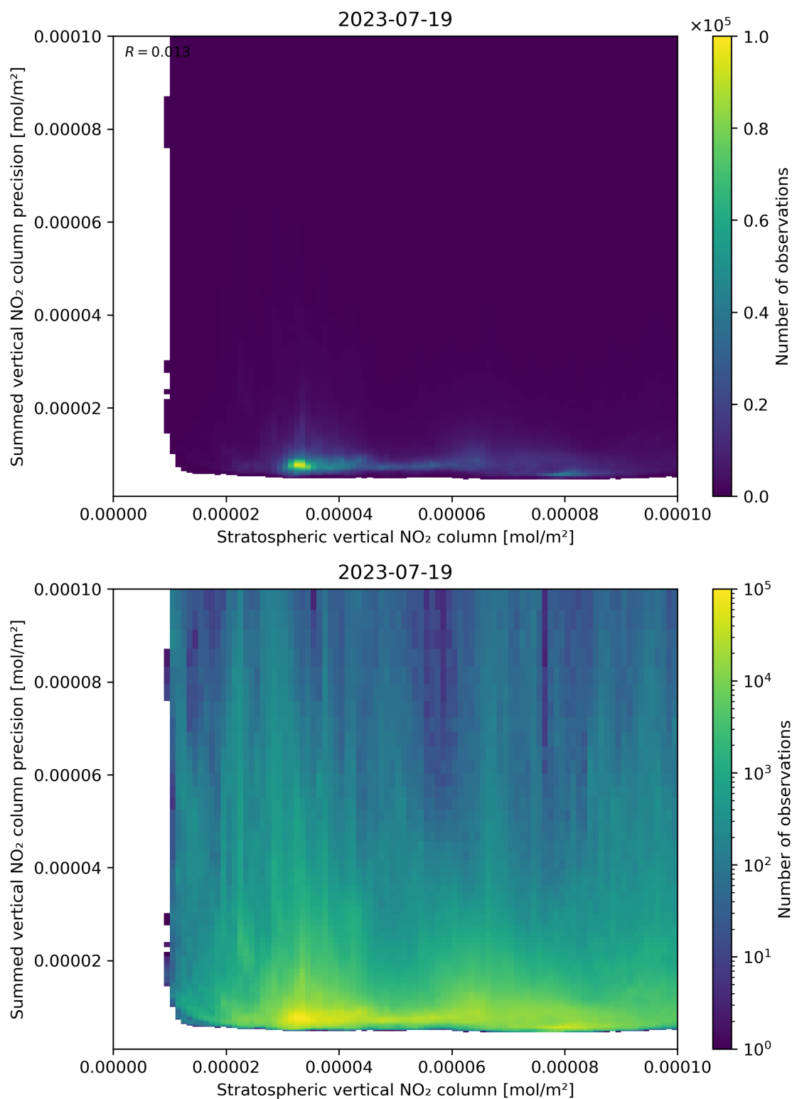
Figure 99: Scatter density plot of “Stratospheric vertical NO 2 column” against “Summed vertical NO 2 column precision” for 2023-07-19 to 2023-07-20.
