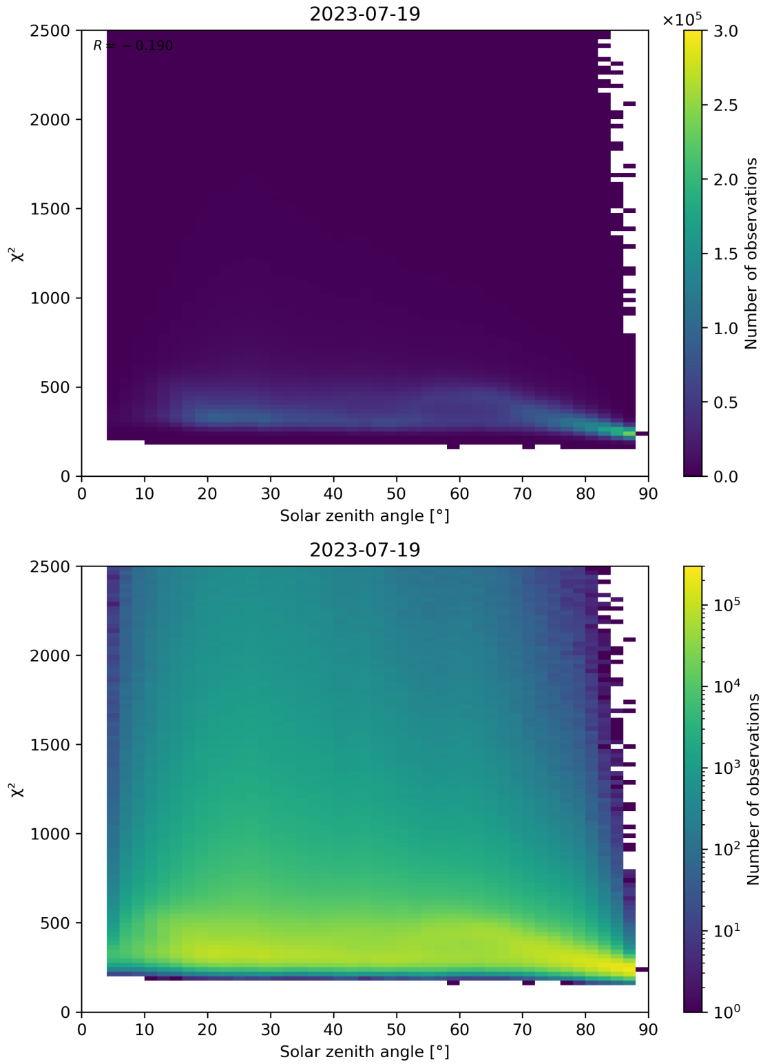
Figure 148: Scatter density plot of “Solar zenith angle” against “ \chi^2 ” for 2023-07-19 to 2023-07-20.
