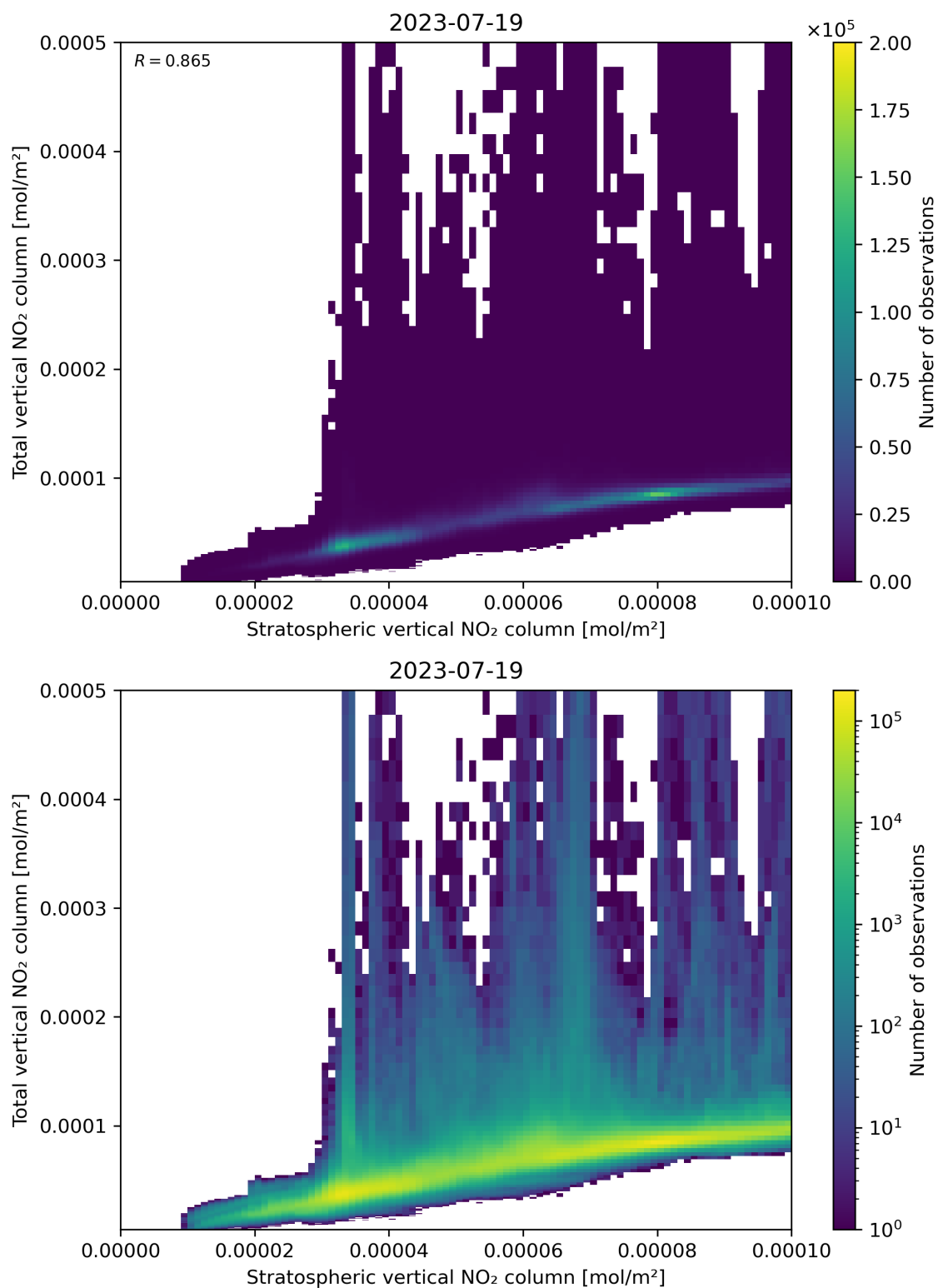
Figure 100: Scatter density plot of “Stratospheric vertical NO 2 column” against “Total vertical NO 2 column” for 2023-07-19 to 2023-07-20.
