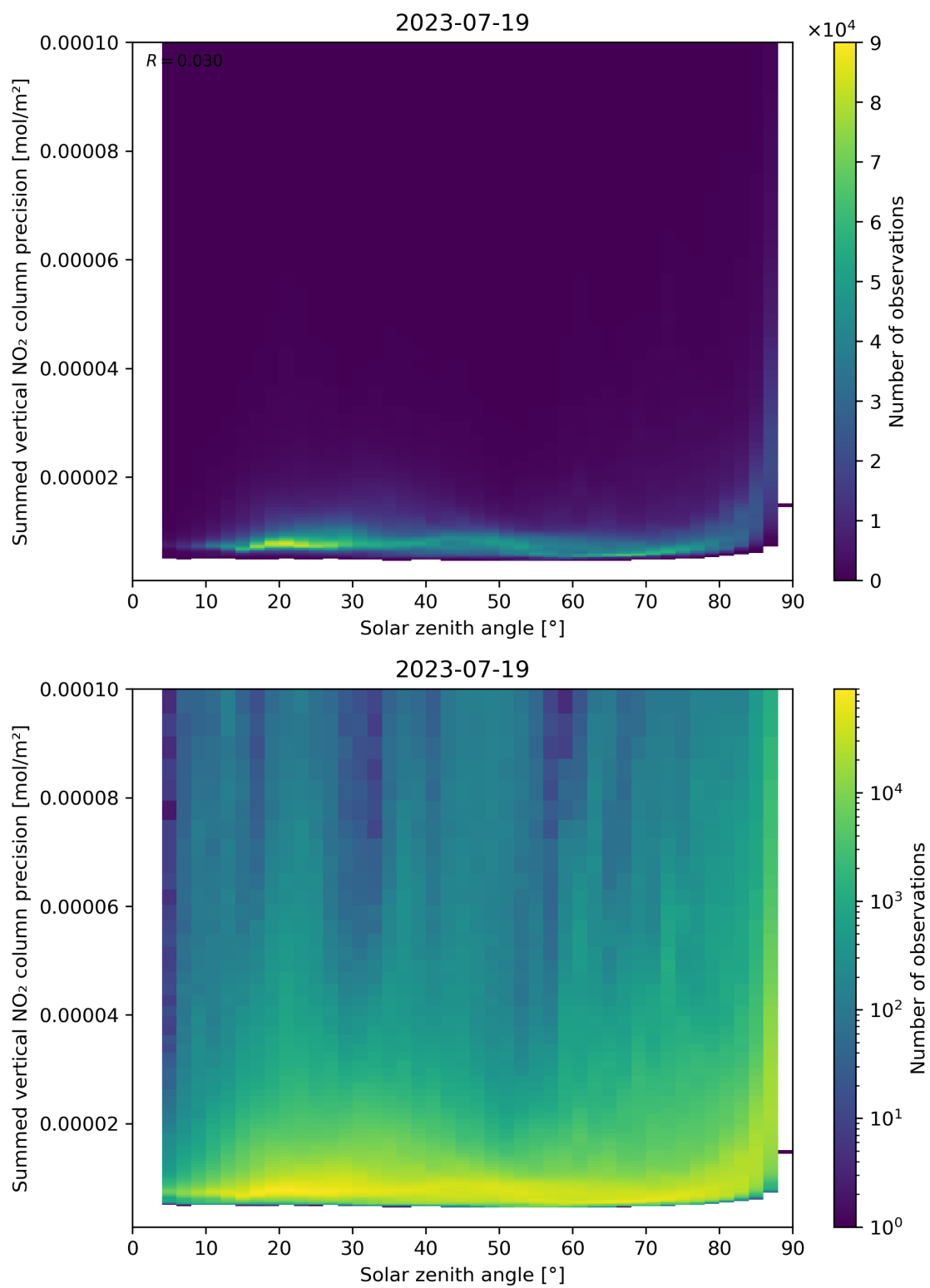
Figure 152: Scatter density plot of “Solar zenith angle” against “Summed vertical NO 2 column precision” for 2023-07-19 to 2023-07-20.
