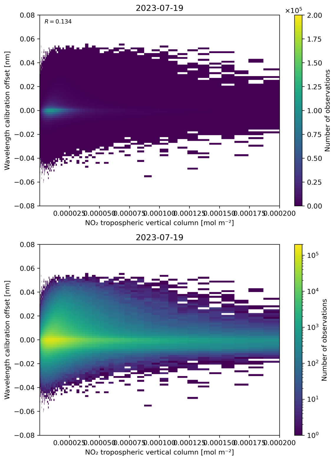
Figure 143: Scatter density plot of “NO 2 tropospheric vertical column” against “Wavelength calibration offset” for 2023-07-19 to 2023-07-20.
