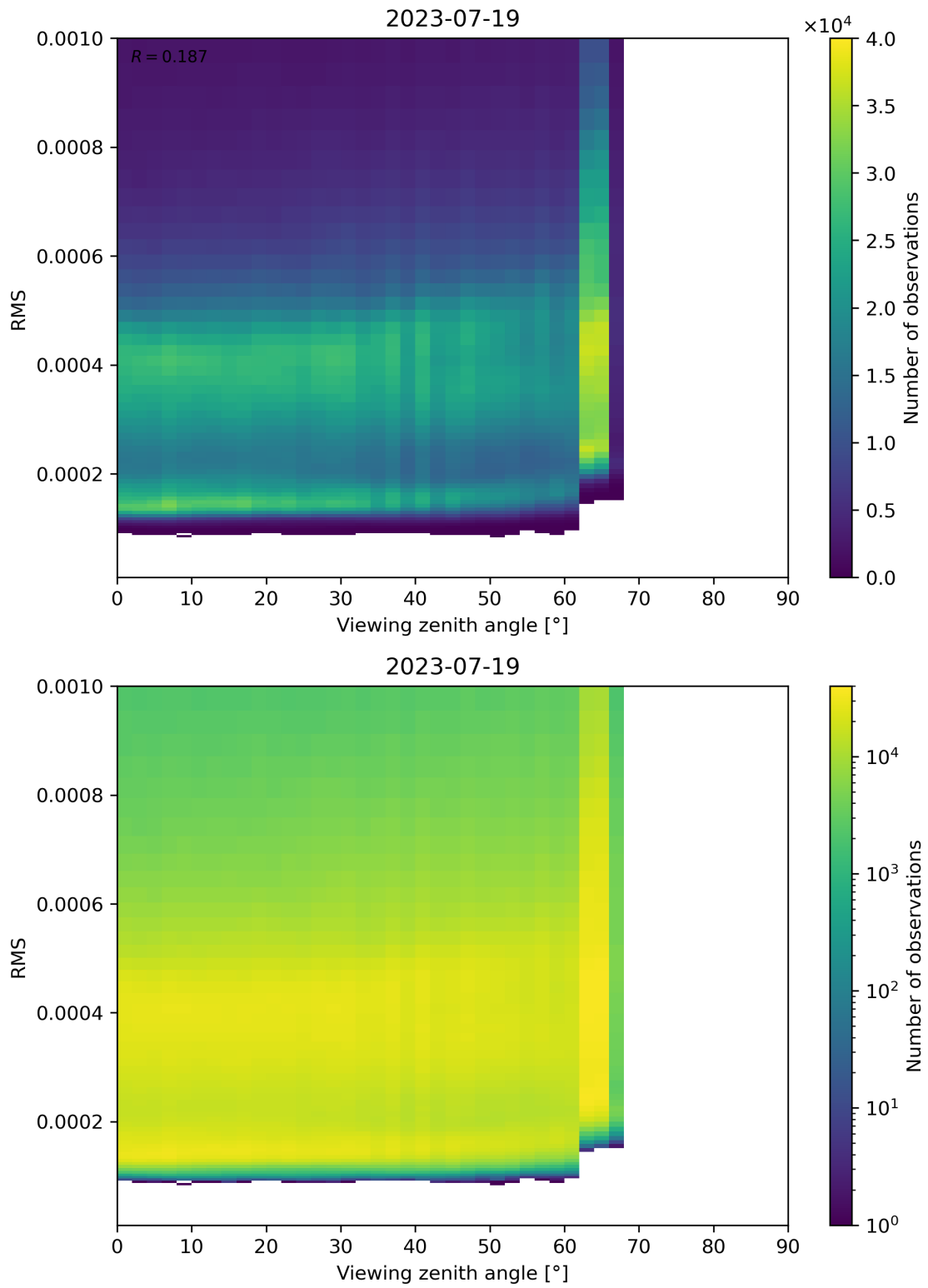
Figure 171: Scatter density plot of “Viewing zenith angle” against “RMS” for 2023-07-19 to 2023-07-20.
