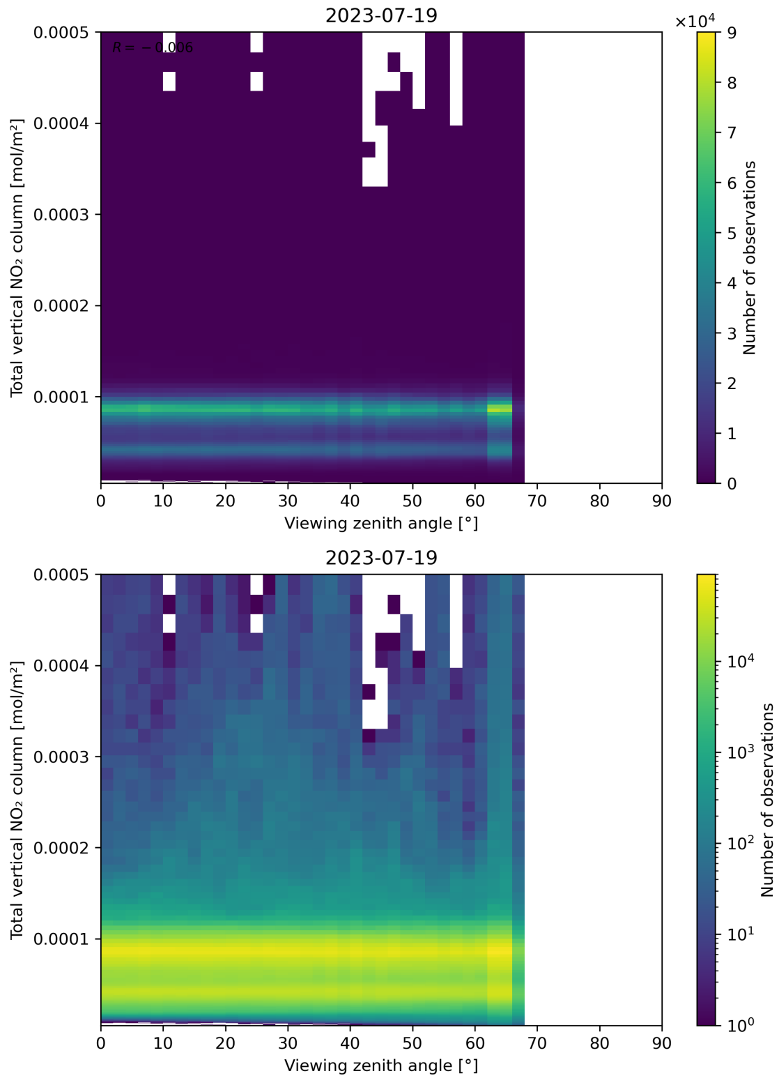
Figure 167: Scatter density plot of “Viewing zenith angle” against “Total vertical NO 2 column” for 2023-07-19 to 2023-07-20.
