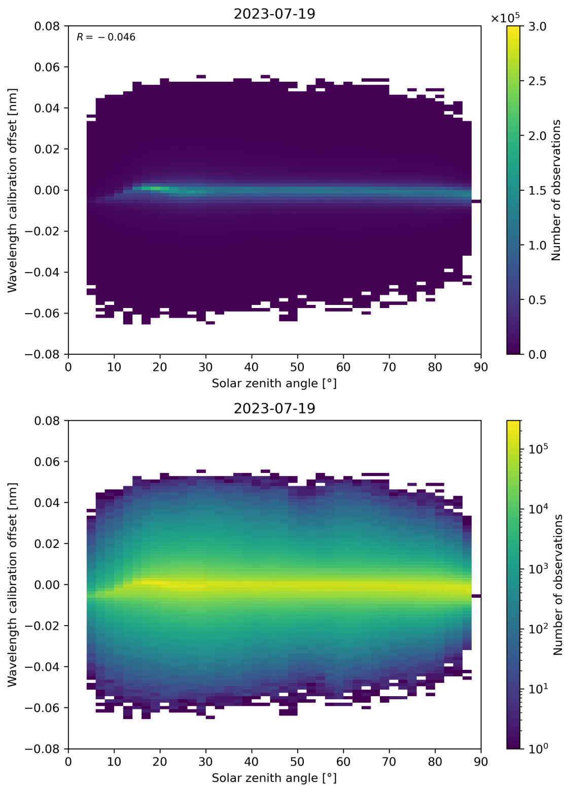
Figure 158: Scatter density plot of “Solar zenith angle” against “Wavelength calibration offset” for 2023-07-19 to 2023-07-20.
