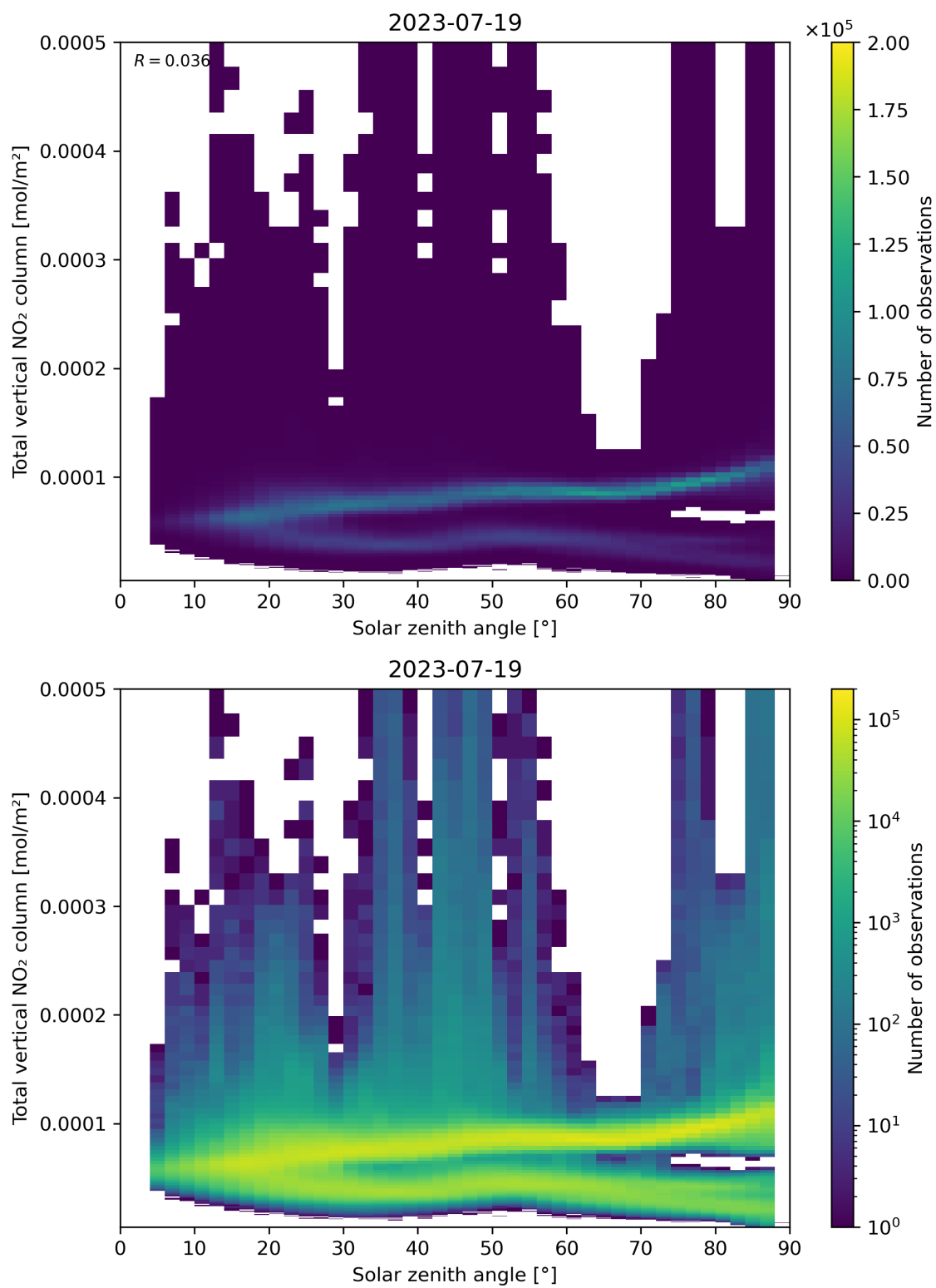
Figure 153: Scatter density plot of “Solar zenith angle” against “Total vertical NO 2 column” for 2023-07-19 to 2023-07-20.
