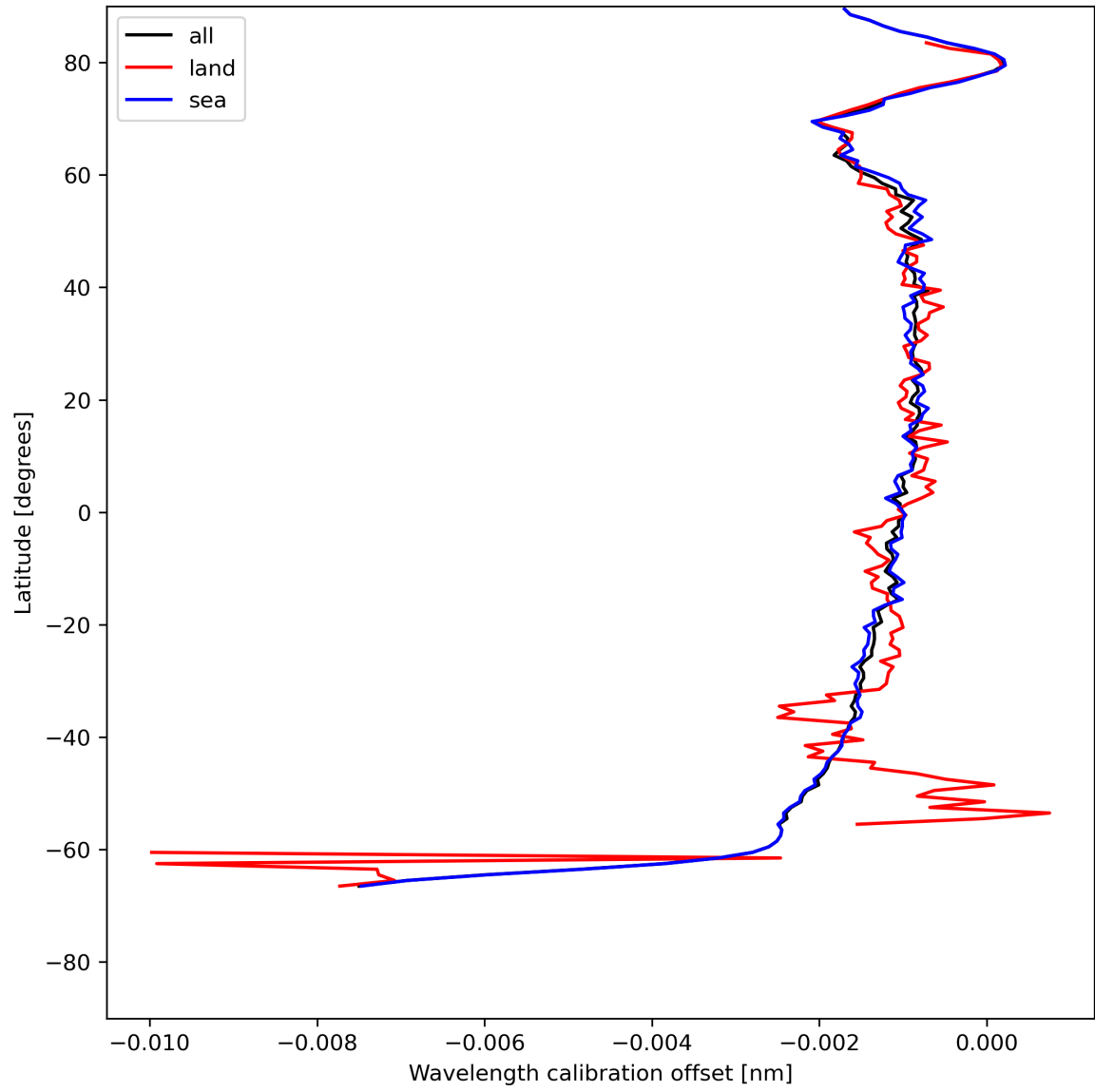
Figure 18: Zonal average of “Wavelength calibration offset” for 2023-07-19 to 2023-07-20.
