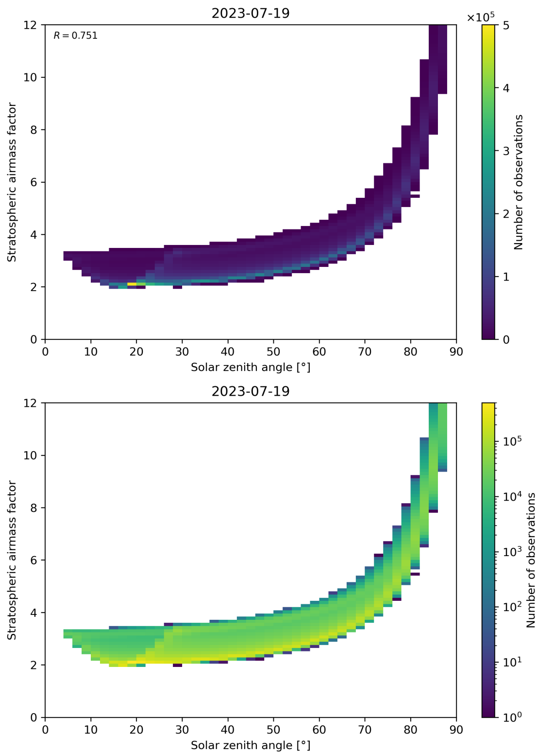
Figure 145: Scatter density plot of “Solar zenith angle” against “Stratospheric airmass factor” for 2023-07-19 to 2023-07-20.
