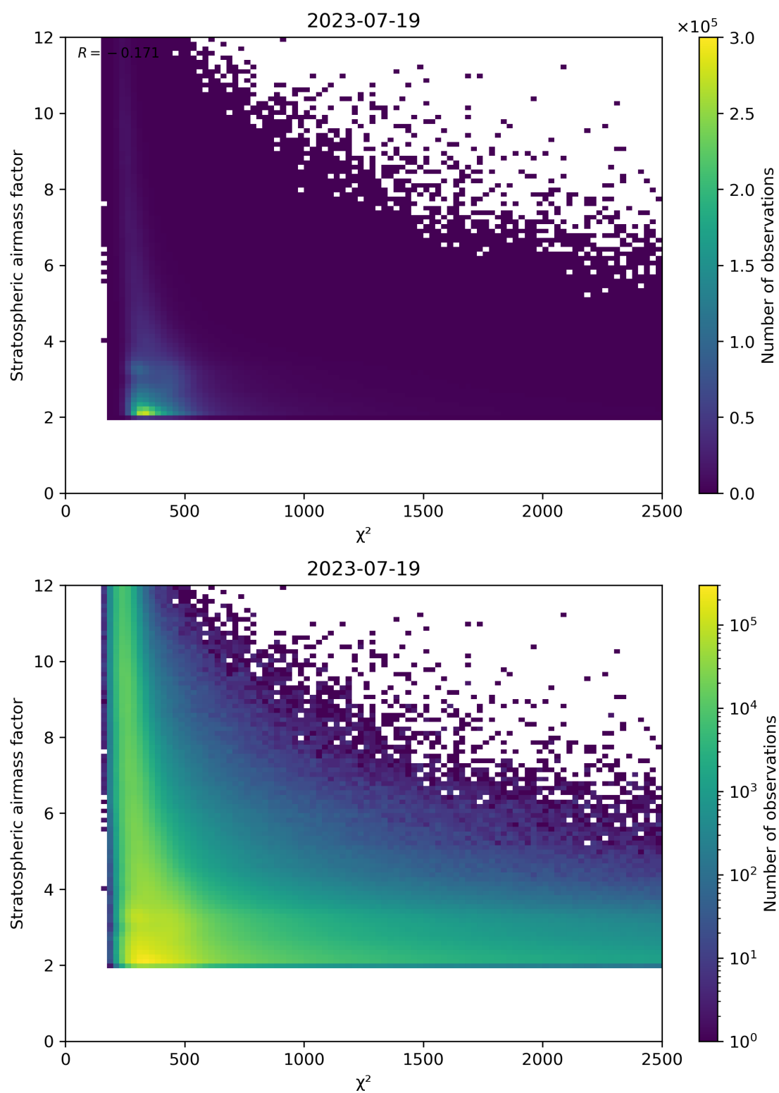
Figure 81: Scatter density plot of “ \chi^2 ” against “Stratospheric air mass factor” for 2023-07-19 to 2023-07-20.
