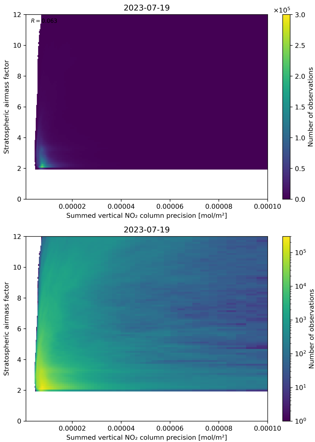
Figure 106: Scatter density plot of “Summed vertical NO 2 column precision” against “Stratospheric airmass factor” for 2023-07-19 to 2023-07-20.
