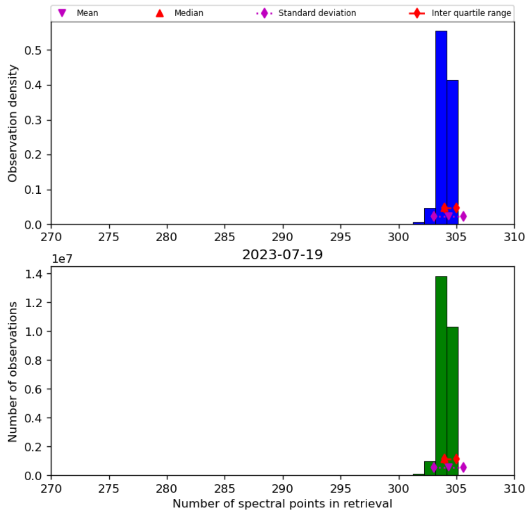
Figure 33: Histogram of “Number of spectral points in retrieval” for 2023-07-19 to 2023-07-20
