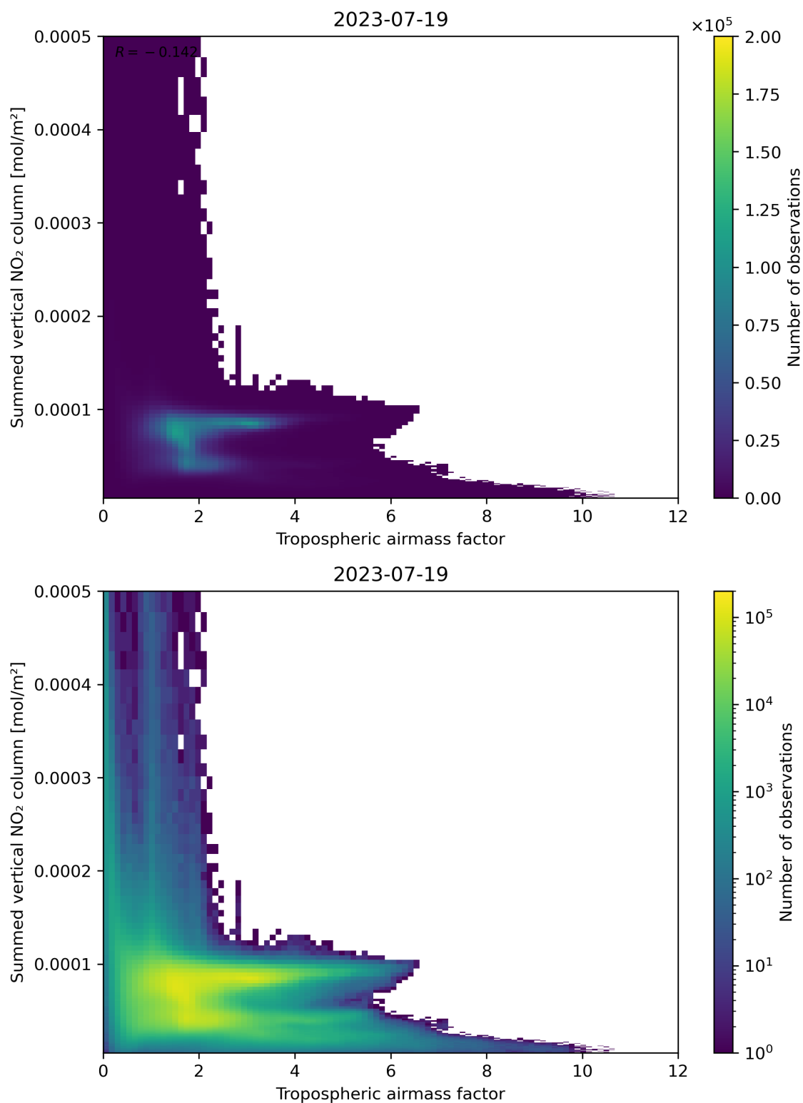
Figure 75: Scatter density plot of “Tropospheric air mass factor” against “Summed vertical NO 2 column” for 2023-07-19 to 2023-07-20.
