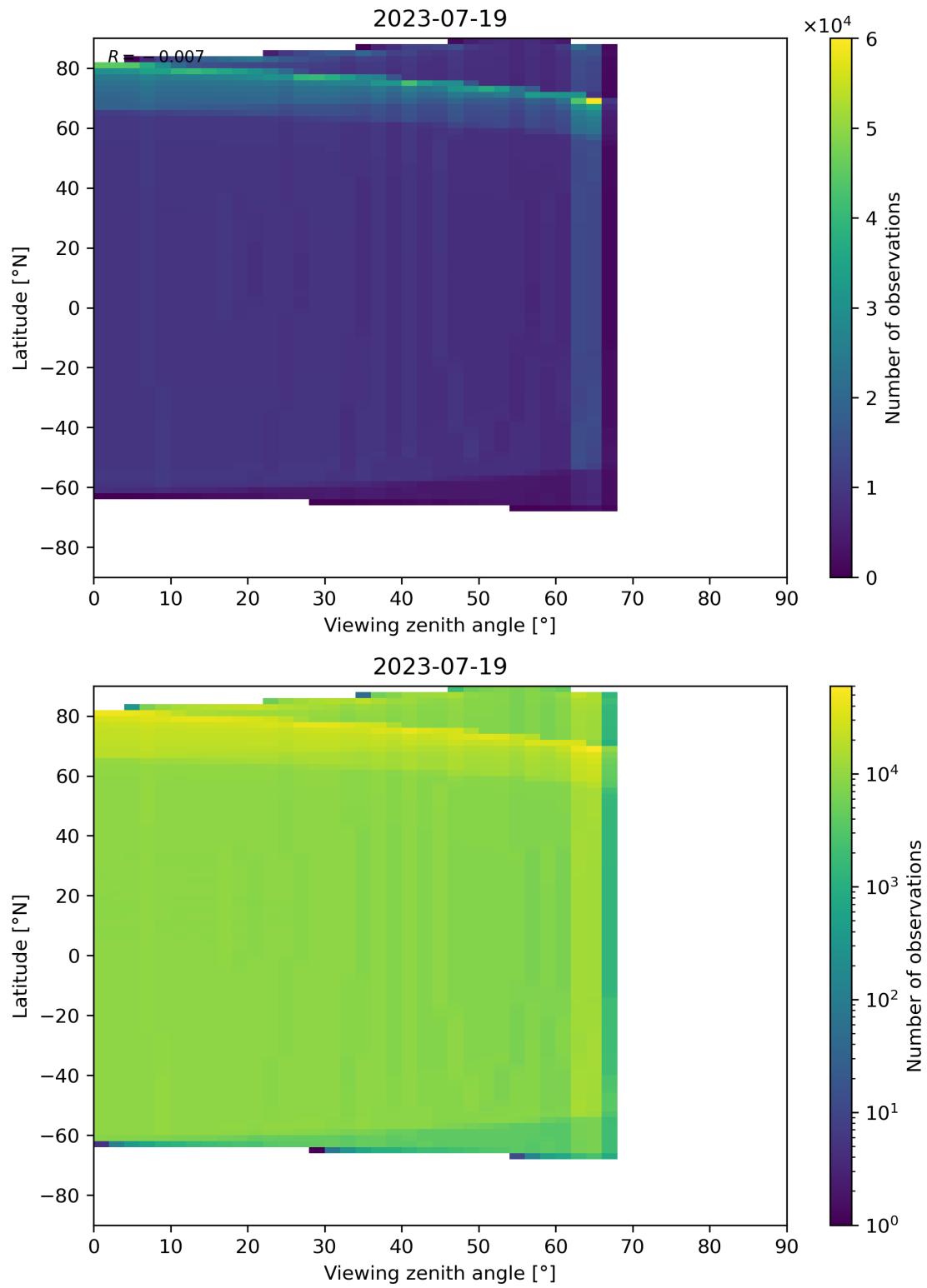
Figure 163: Scatter density plot of “Viewing zenith angle” against “Latitude” for 2023-07-19 to 2023-07-20.
