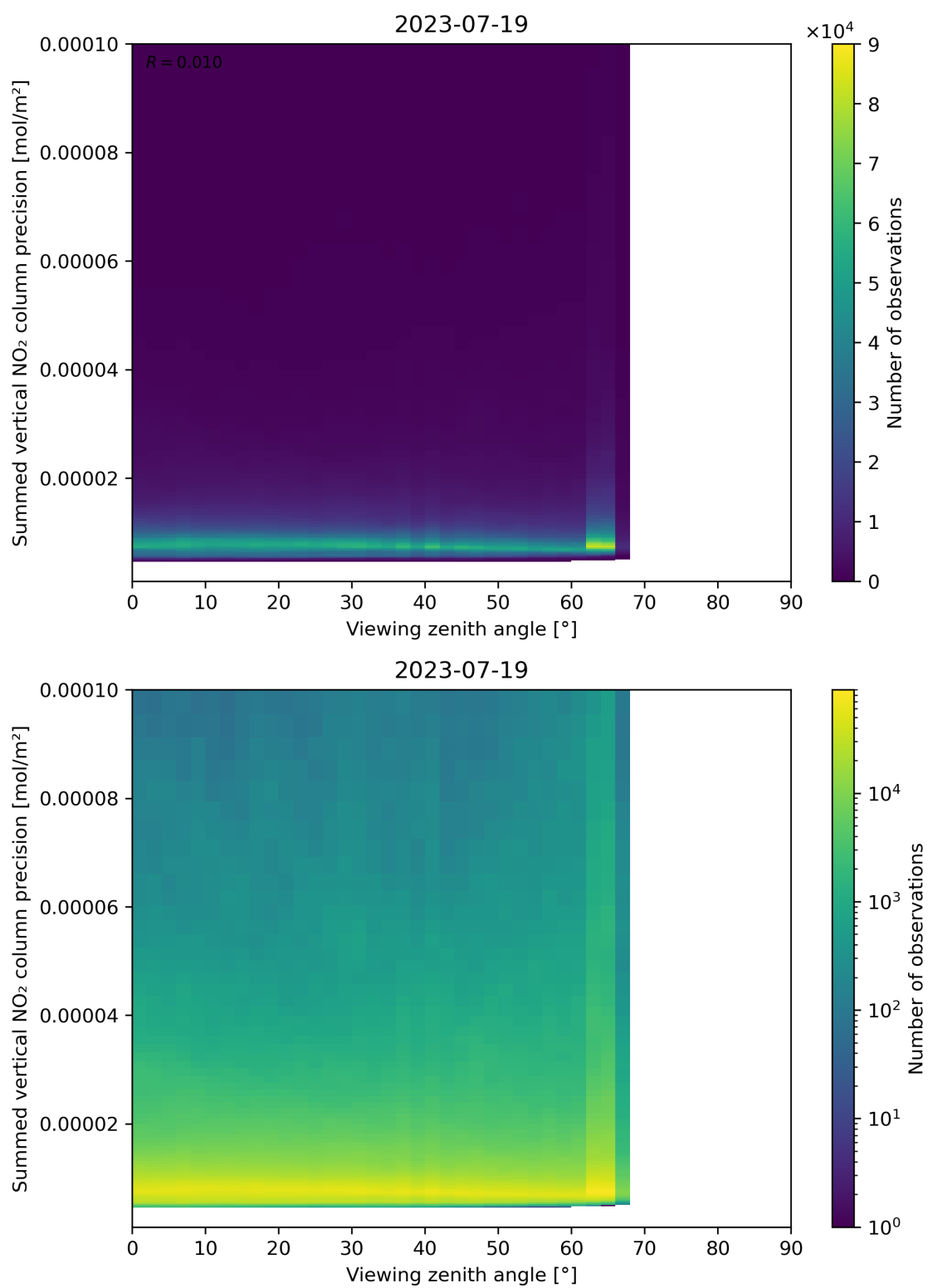
Figure 166: Scatter density plot of “Viewing zenith angle” against “Summed vertical NO 2 column precision” for 2023-07-19 to 2023-07-20.
