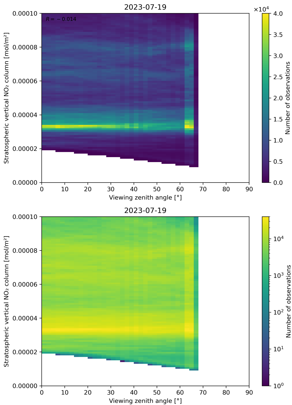
Figure 164: Scatter density plot of “Viewing zenith angle” against “Stratospheric vertical NO 2 column” for 2023-07-19 to 2023-07-20.
