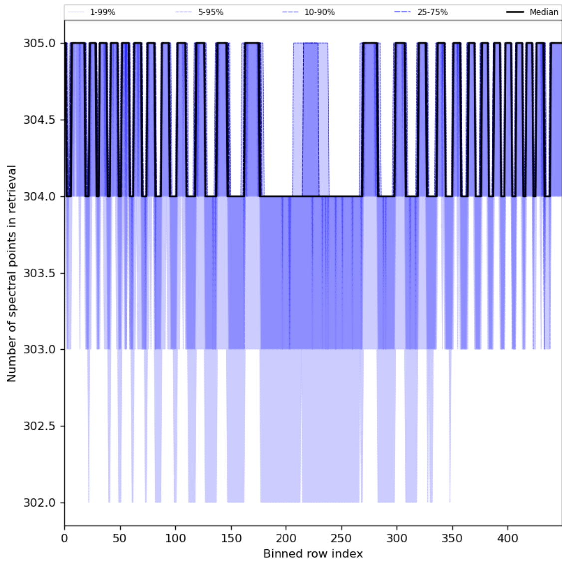
Figure 50: Along track statistics of “Number of spectral points in retrieval” for 2023-07-19 to 2023-07-20
