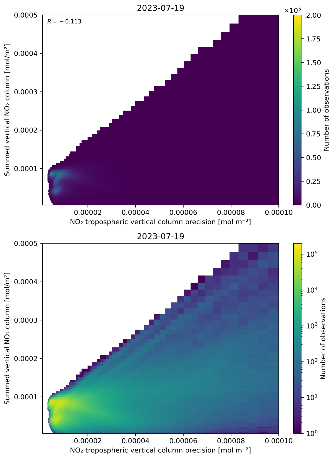
Figure 136: Scatter density plot of “NO 2 tropospheric vertical column precision” against “Summed vertical NO 2 column” for 2023-07-19 to 2023-07-20.
