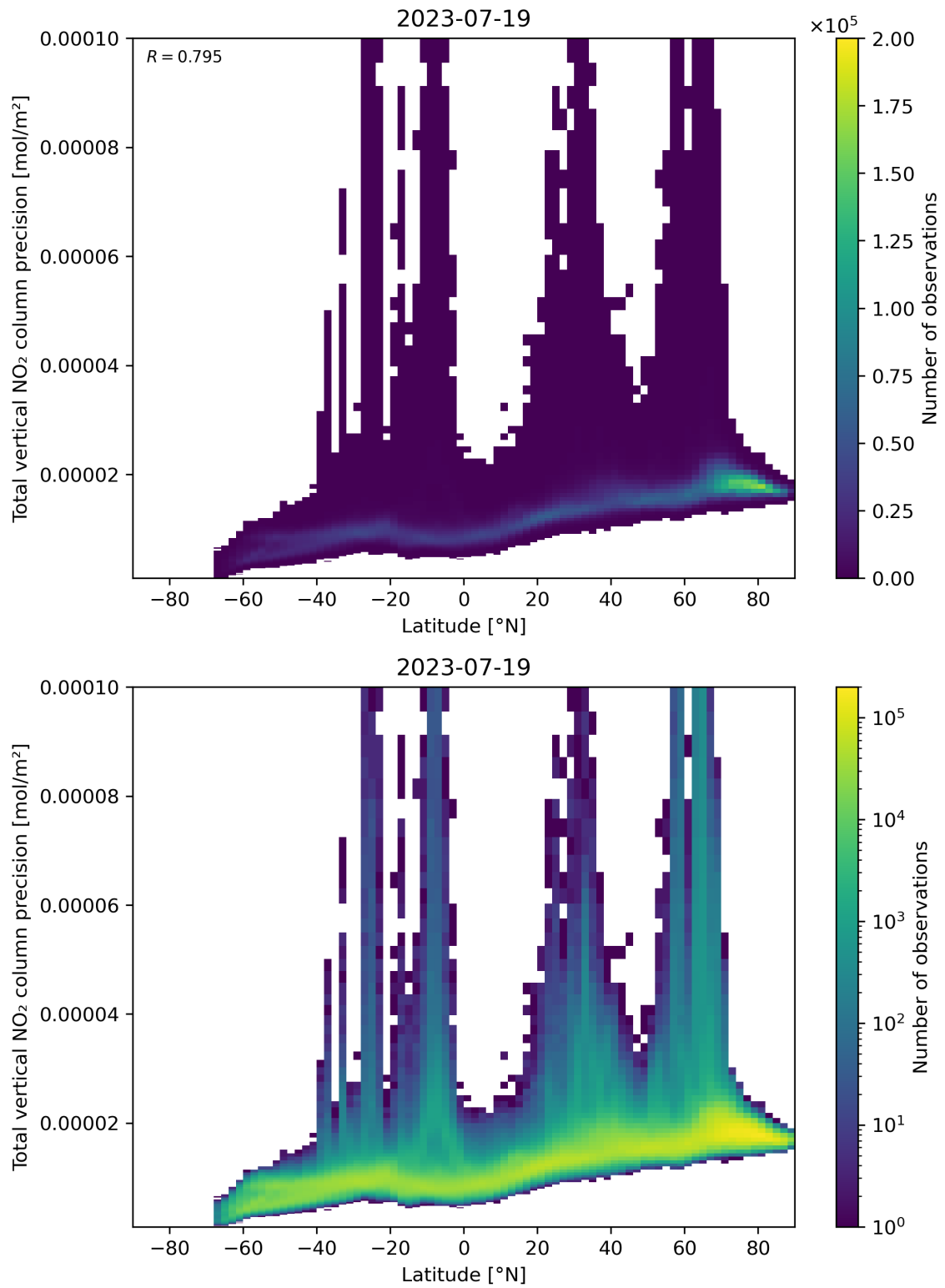
Figure 91: Scatter density plot of “Latitude” against “Total vertical NO 2 column precision” for 2023-07-19 to 2023-07-20.
