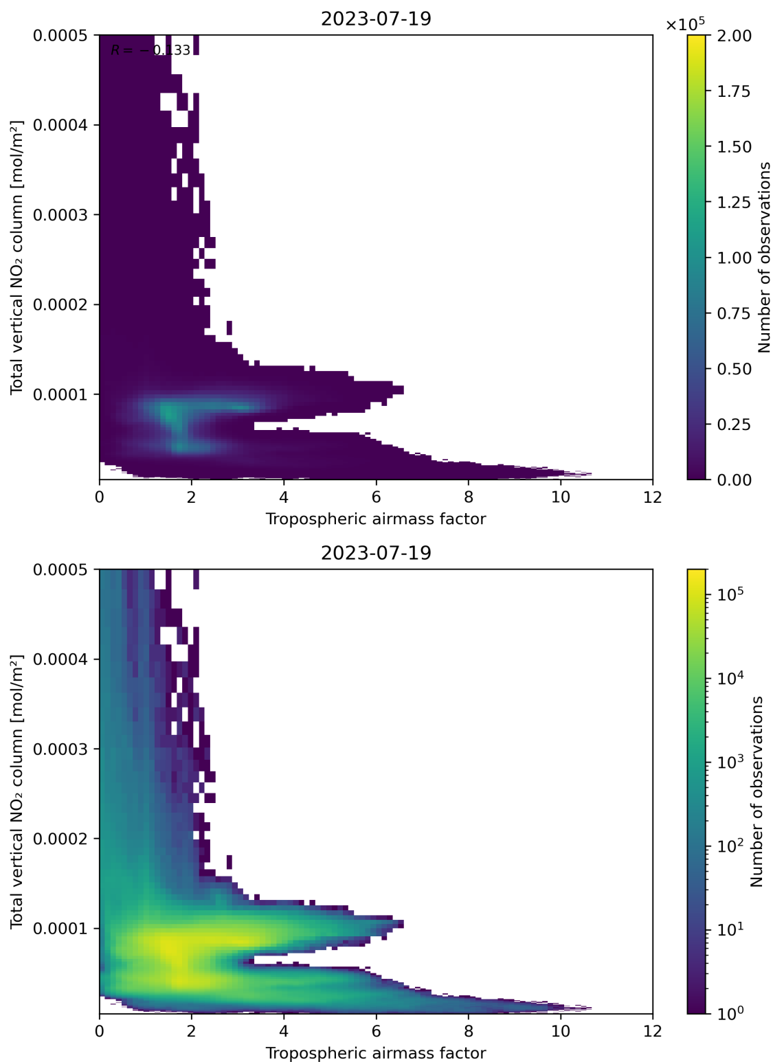
Figure 77: Scatter density plot of “Tropospheric airmass factor” against “Total vertical NO 2 column” for 2023-07-19 to 2023-07-20.
