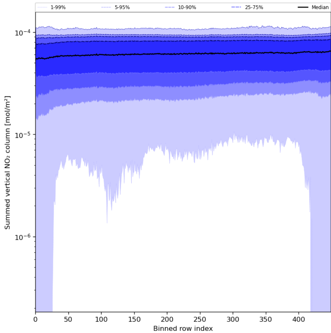
Figure 57: Along track statistics of “Summed vertical NO 2 column” for 2023-07-19 to 2023-07-20
