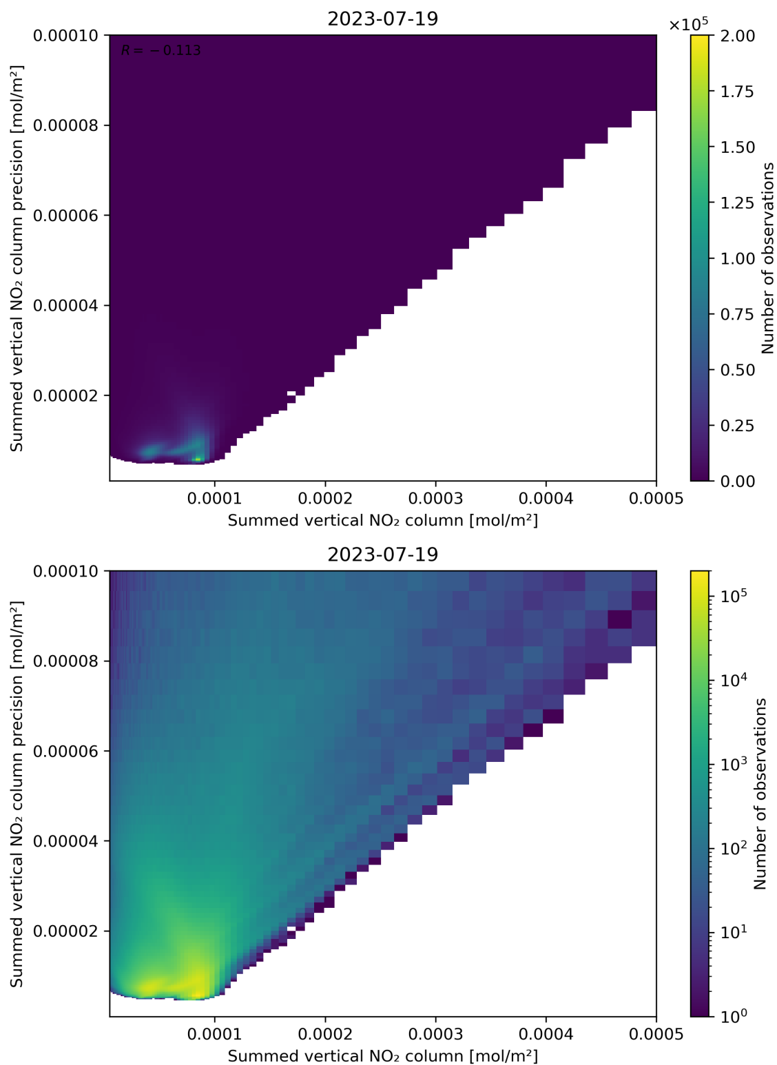
Figure 105: Scatter density plot of “Summed vertical NO 2 column” against “Summed vertical NO 2 column precision” for 2023-07-19 to 2023-07-20.
