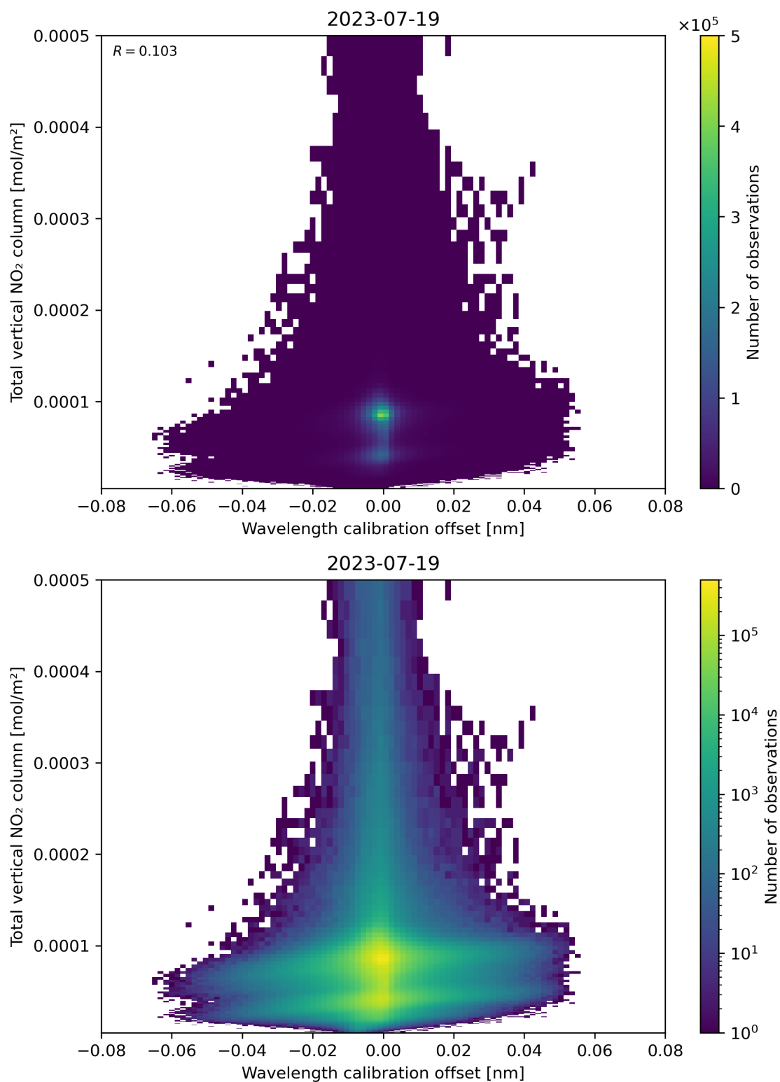
Figure 179: Scatter density plot of “Wavelength calibration offset” against “Total vertical NO 2 column” for 2023-07-19 to 2023-07-20.
