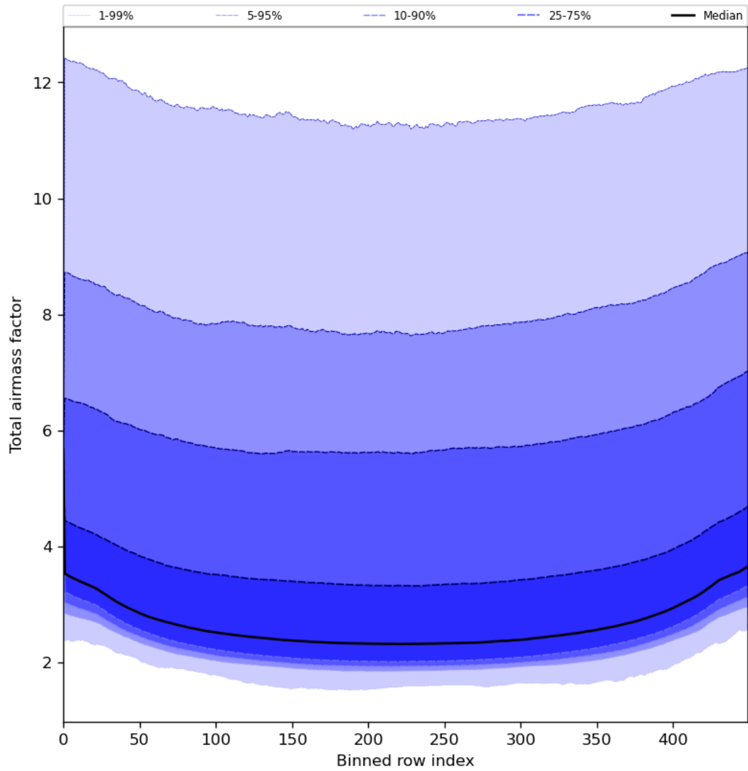
Figure 49: Along track statistics of “Total airmass factor” for 2023-07-19 to 2023-07-20
