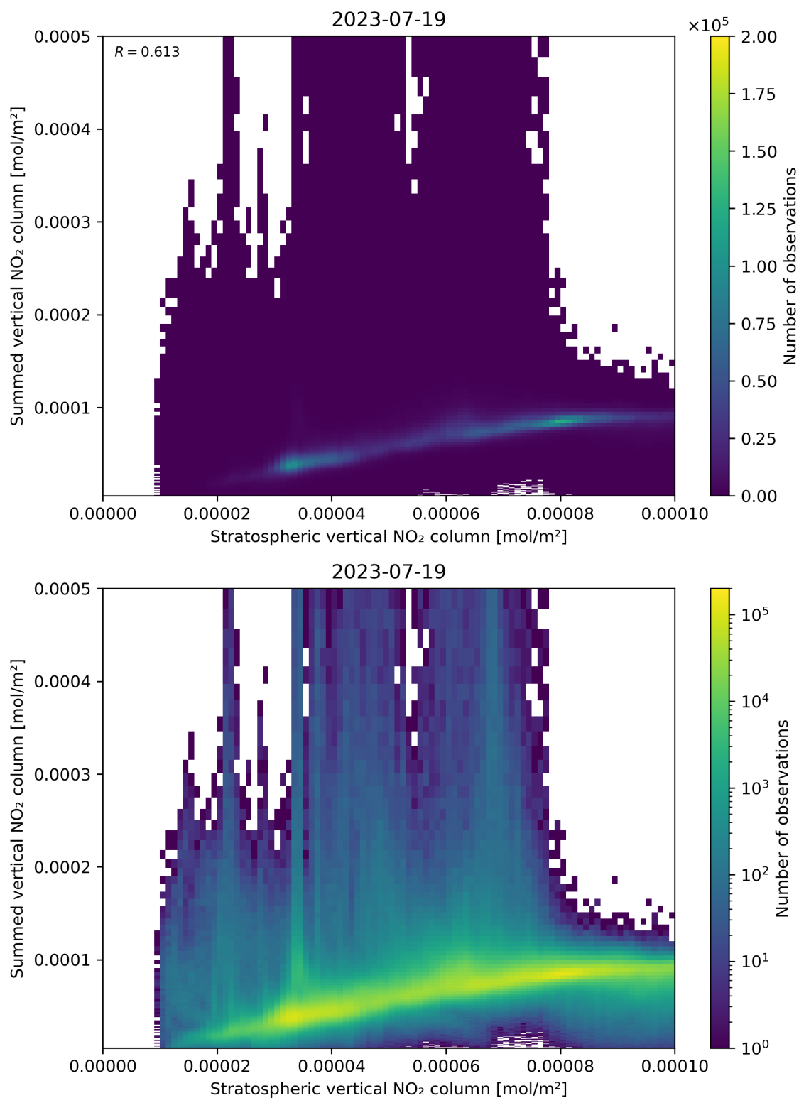
Figure 98: Scatter density plot of “Stratospheric vertical NO 2 column” against “Summed vertical NO 2 column” for 2023-07-19 to 2023-07-20.
