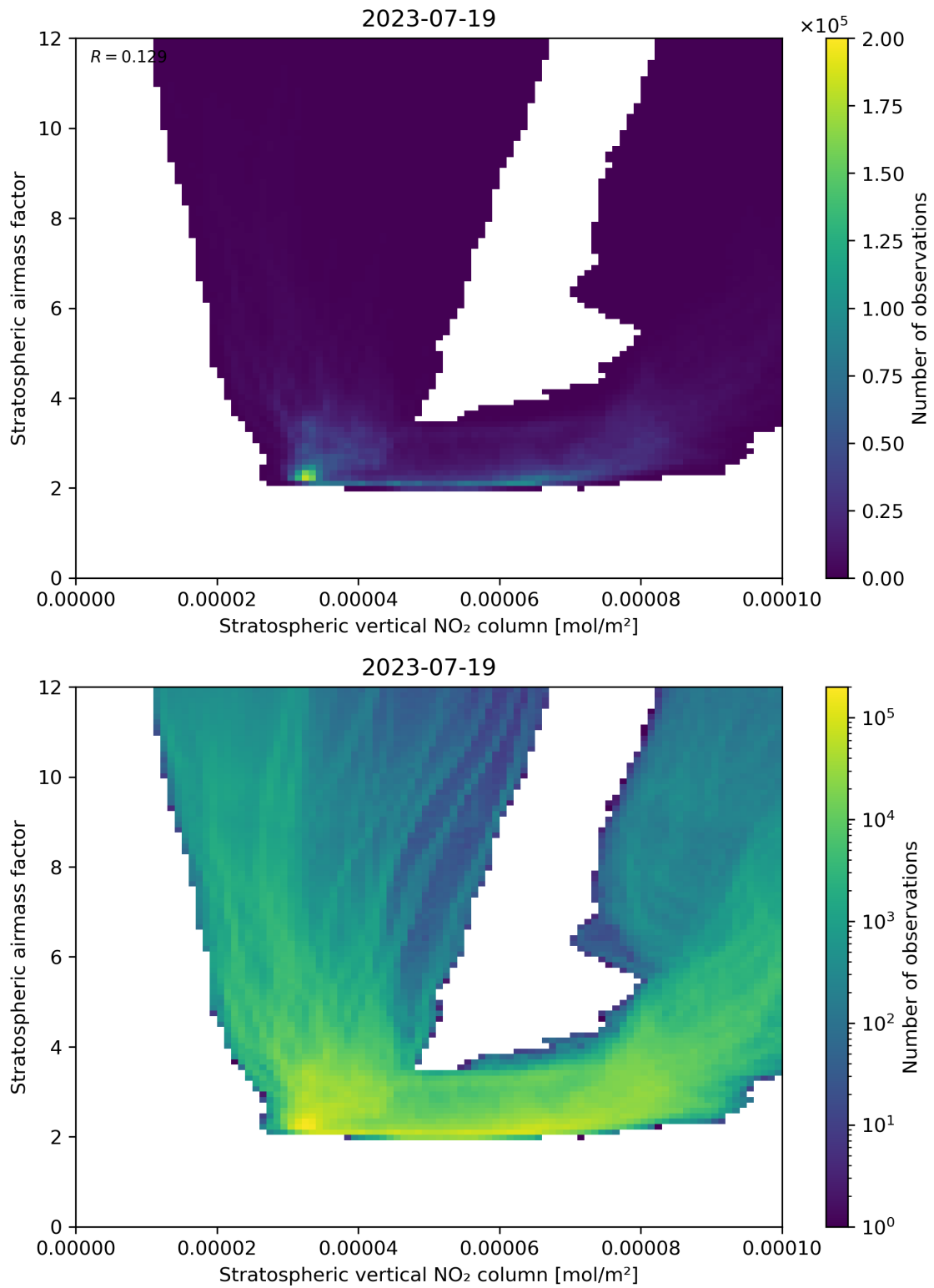
Figure 96: Scatter density plot of “Stratospheric vertical NO 2 column” against “Stratospheric airmass factor” for 2023-07-19 to 2023-07-20.
