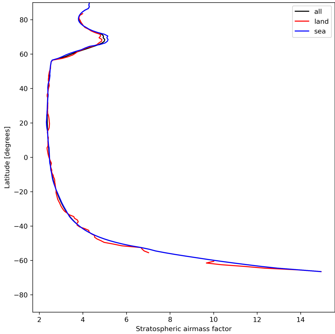
Figure 27: Zonal average of “Stratospheric air mass factor” for 2023-07-19 to 2023-07-20.
