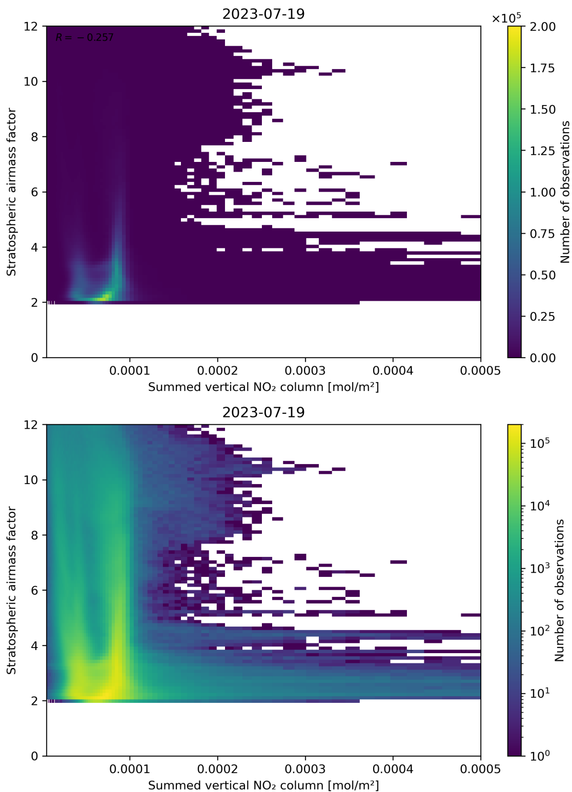
Figure 103: Scatter density plot of “Summed vertical NO 2 column” against “Stratospheric air mass factor” for 2023-07-19 to 2023-07-20.
