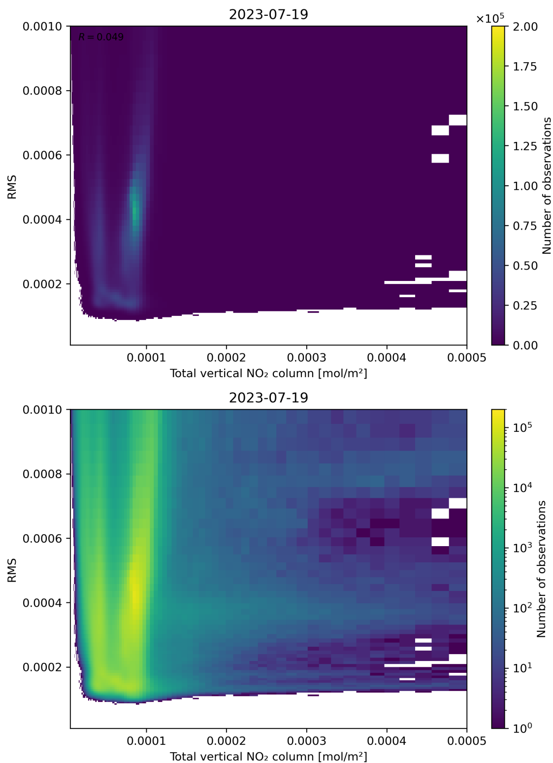
Figure 120: Scatter density plot of “Total vertical NO 2 column” against “RMS” for 2023-07-19 to 2023-07-20.
