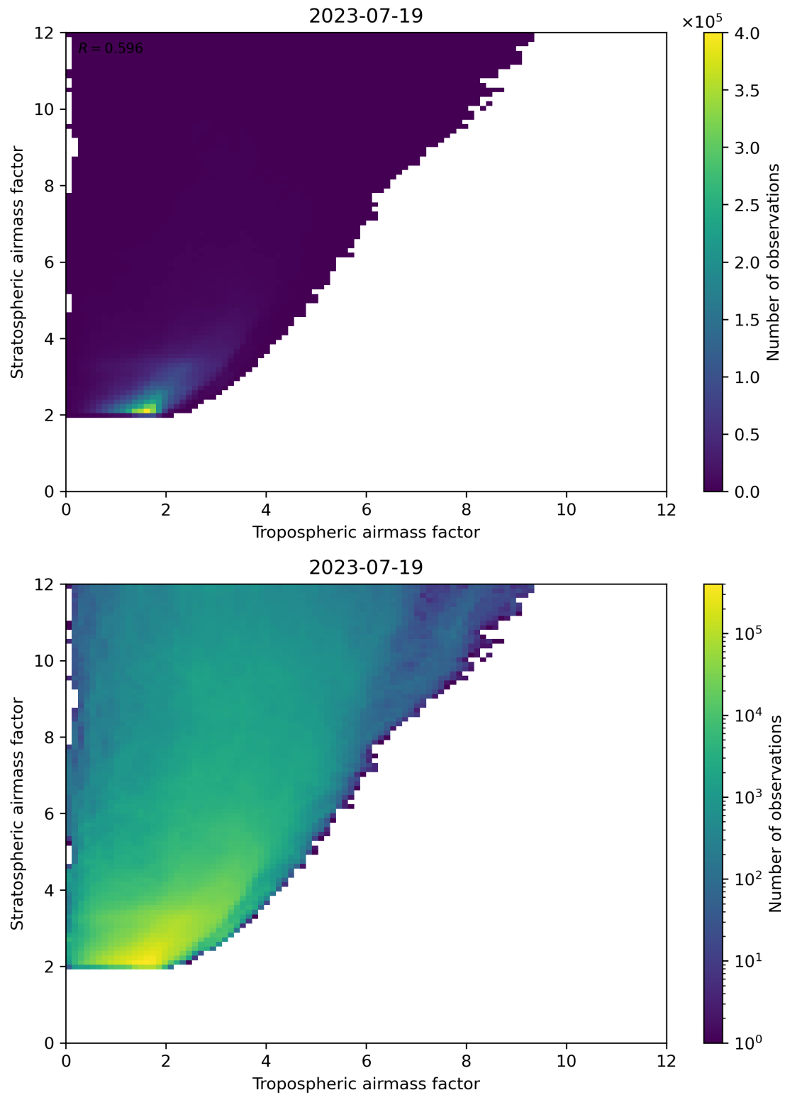
Figure 71: Scatter density plot of “Tropospheric airmass factor” against “Stratospheric airmass factor” for 2023-07-19 to 2023-07-20.
