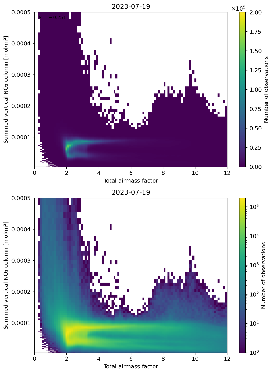
Figure 65: Scatter density plot of “Total airmass factor” against “Summed vertical NO 2 column” for 2023-07-19 to 2023-07-20.
