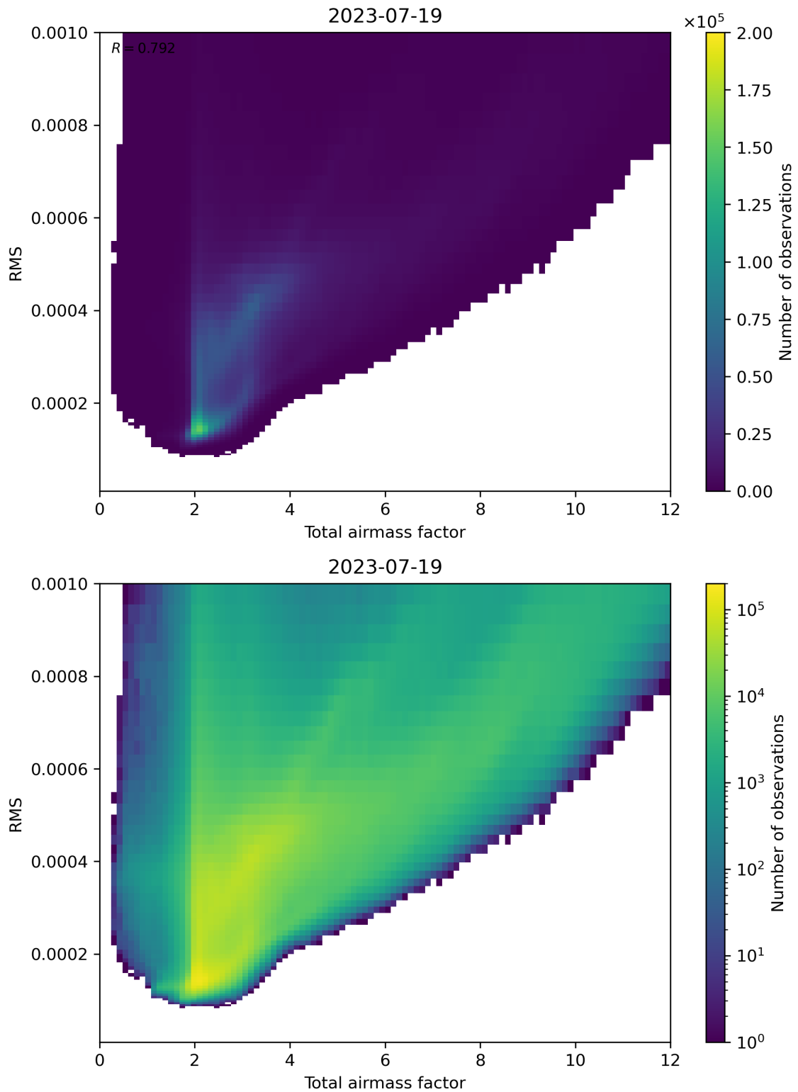
Figure 69: Scatter density plot of “Total airmass factor” against “RMS” for 2023-07-19 to 2023-07-20.
