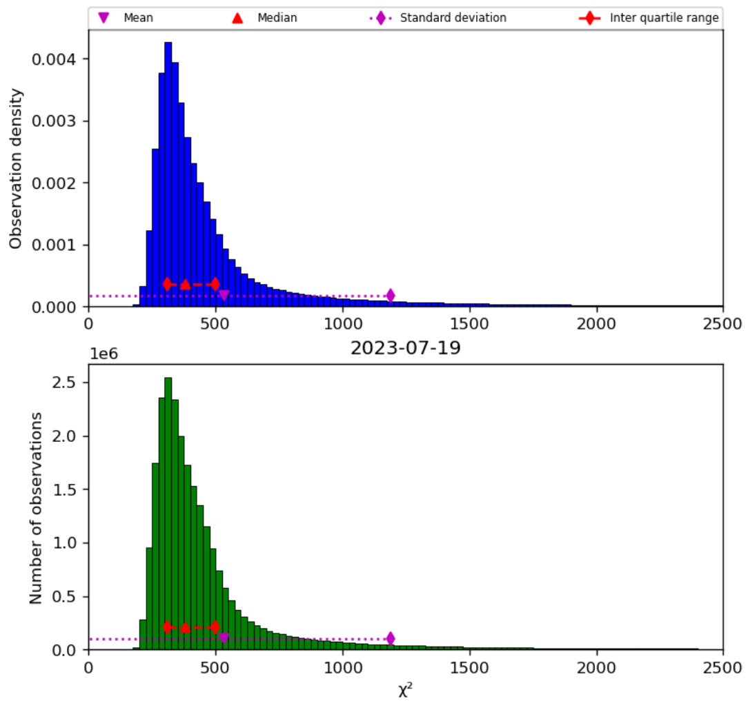
Figure 42: Histogram of “ \chi^2 ” for 2023-07-19 to 2023-07-20
