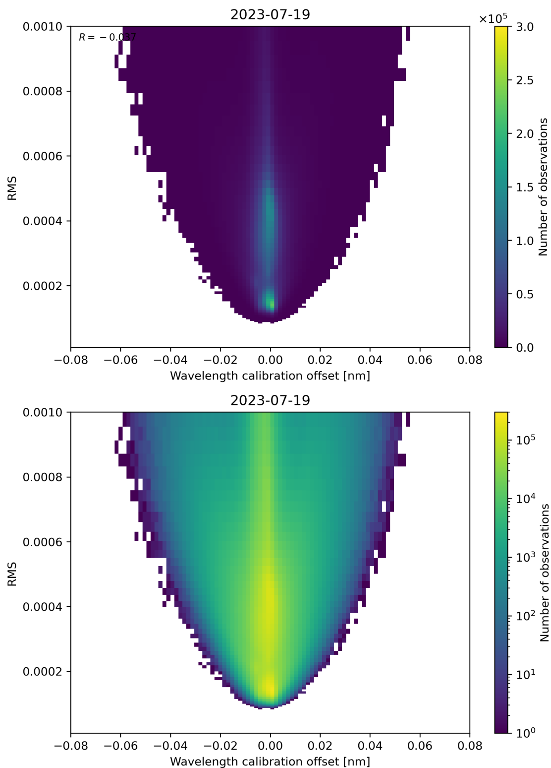
Figure 181: Scatter density plot of “Wavelength calibration offset” against “RMS” for 2023-07-19 to 2023-07-20.
