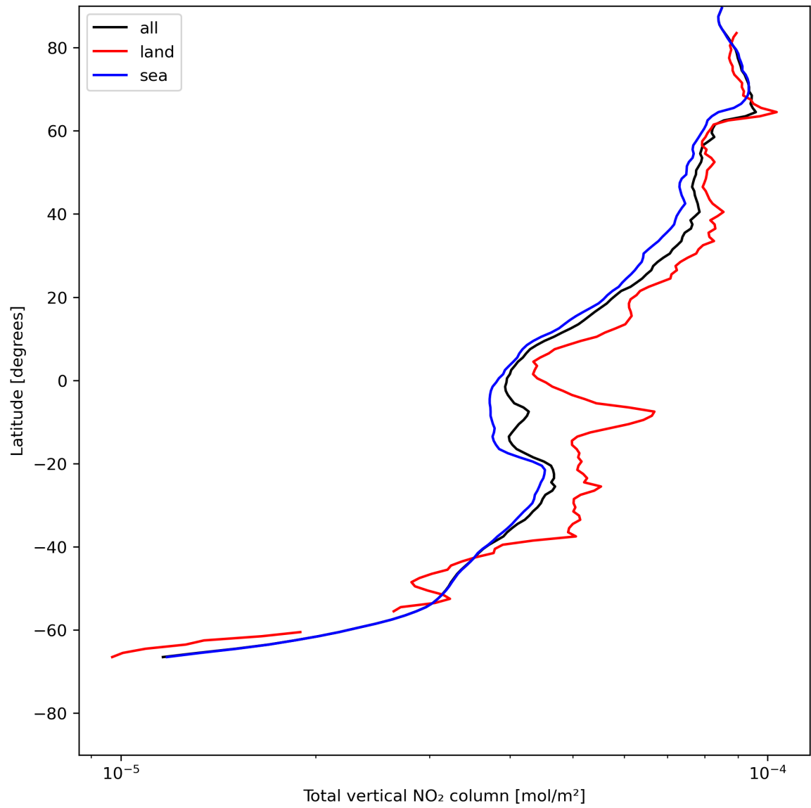
Figure 21: Zonal average of “Total vertical NO 2 column” for 2023-07-19 to 2023-07-20.
