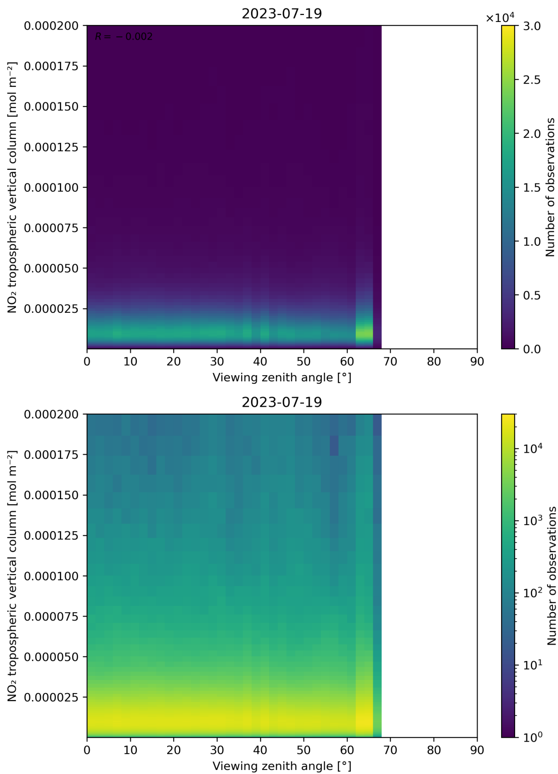
Figure 169: Scatter density plot of “Viewing zenith angle” against “NO 2 tropospheric vertical column” for 2023-07-19 to 2023-07-20.
