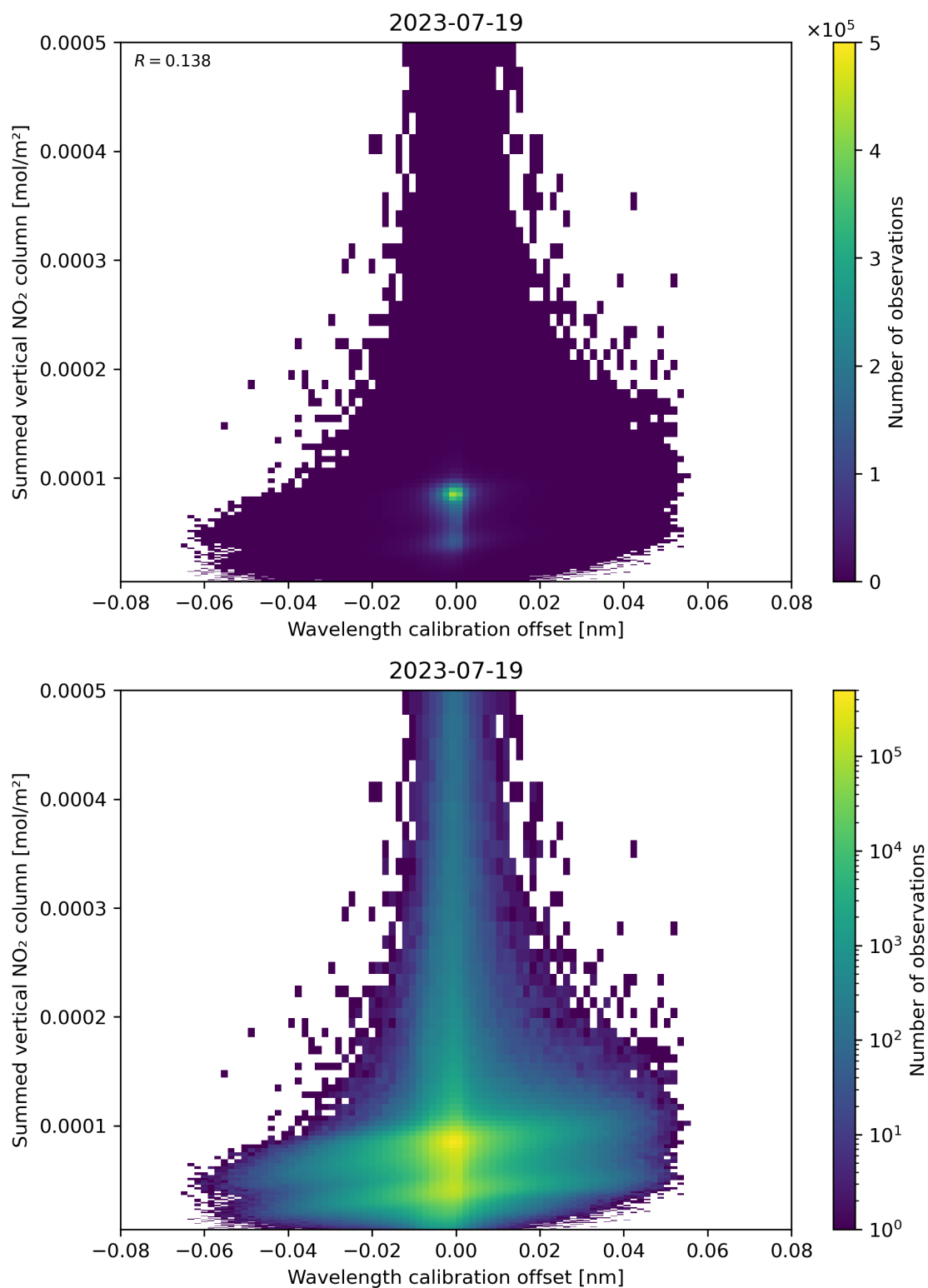
Figure 177: Scatter density plot of “Wavelength calibration offset” against “Summed vertical NO 2 column” for 2023-07-19 to 2023-07-20.
