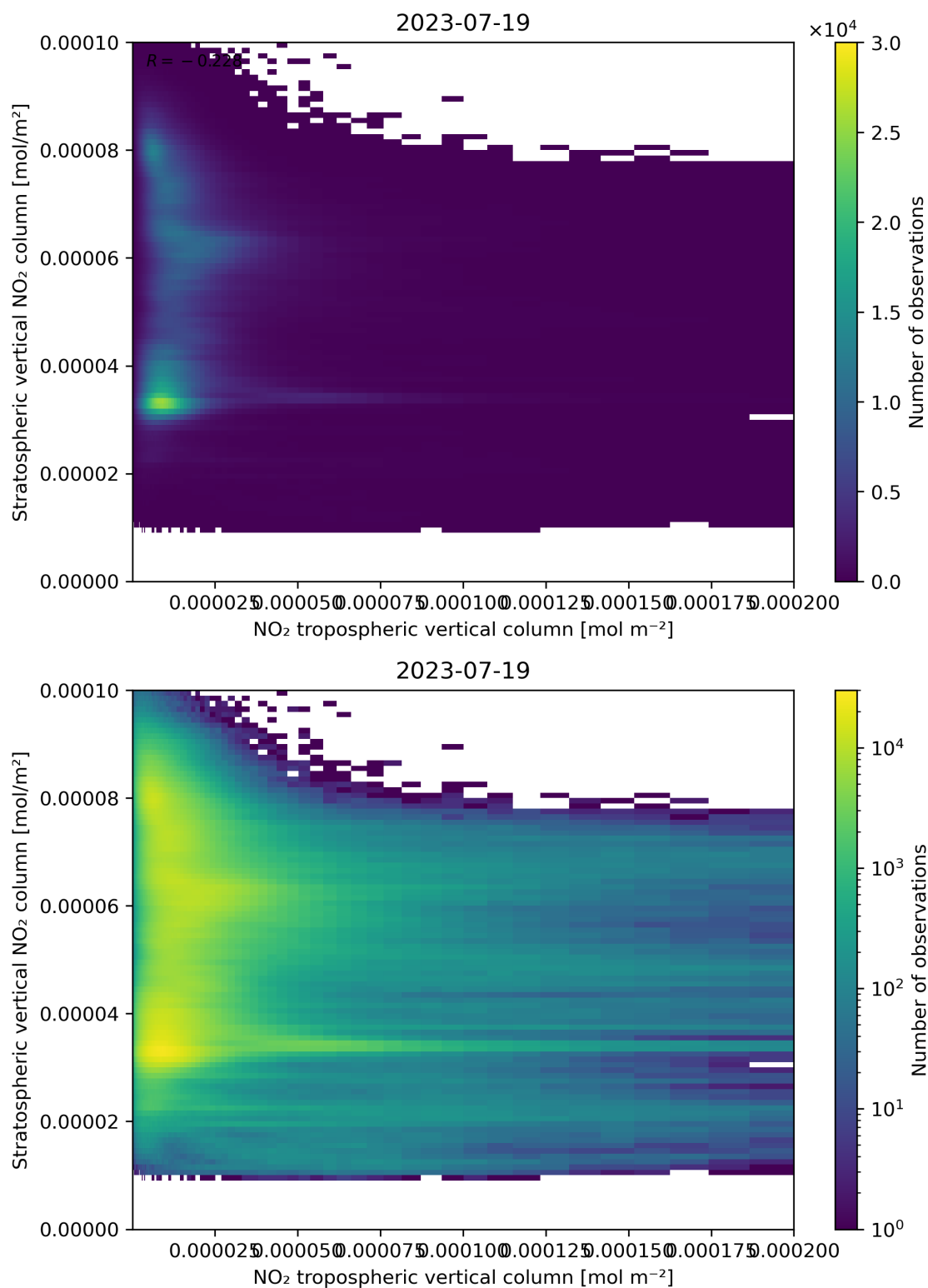
Figure 125: Scatter density plot of “NO 2 tropospheric vertical column” against “Stratospheric vertical NO 2 column” for 2023-07-19 to 2023-07-20.
