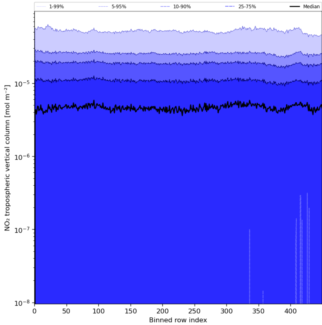
Figure 46: Along track statistics of “NO 2 tropospheric vertical column” for 2023-07-19 to 2023-07-20
