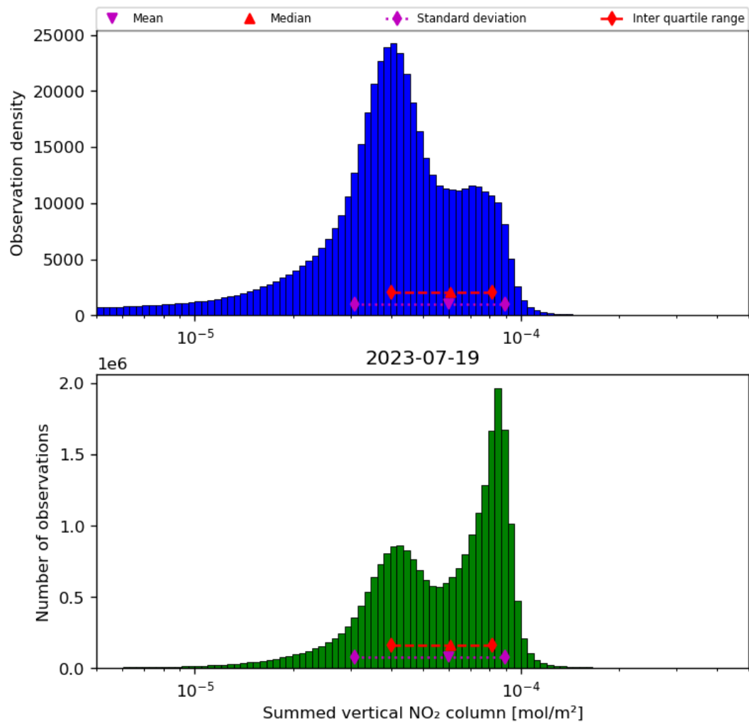
Figure 40: Histogram of "Summed vertical NO 2 column" for 2023-07-19 to 2023-07-20
