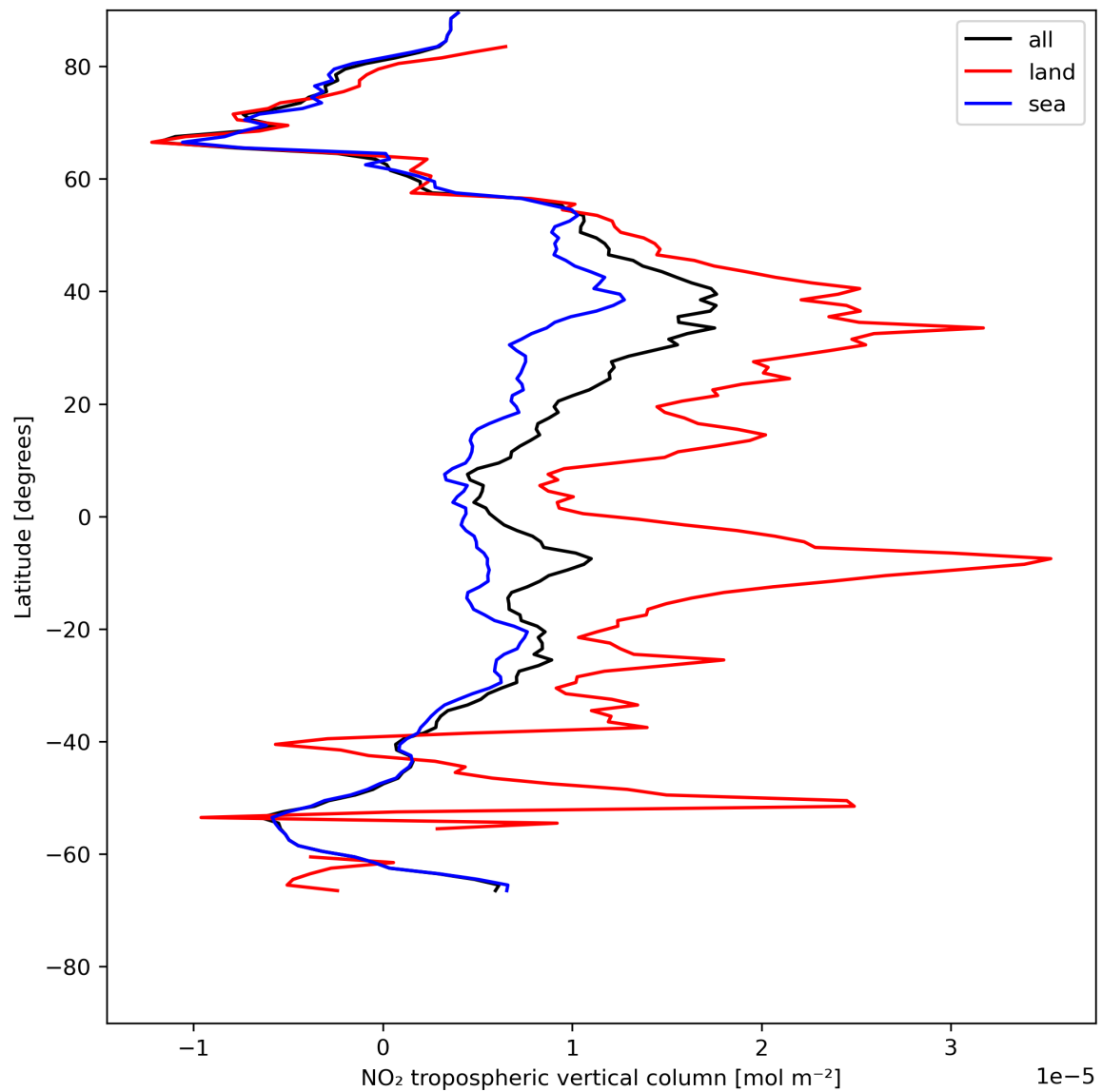
Figure 12: Zonal average of “NO 2 tropospheric vertical column” for 2023-07-19 to 2023-07-20.
