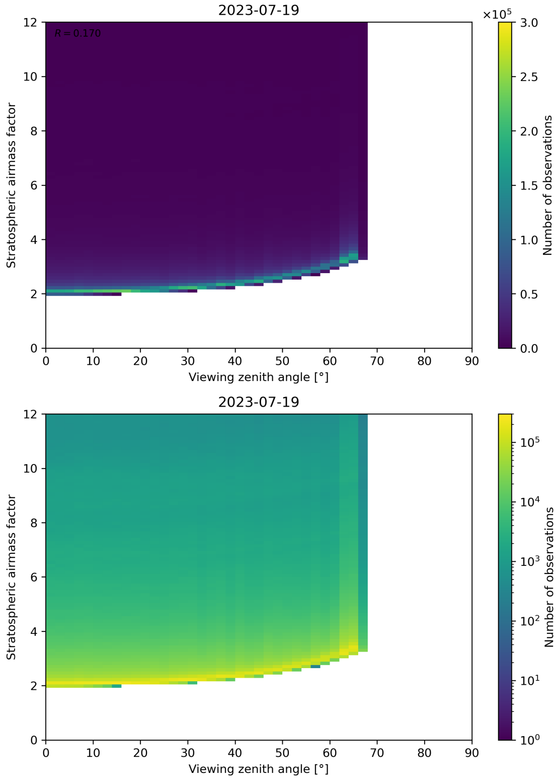
Figure 159: Scatter density plot of “Viewing zenith angle” against “Stratospheric airmass factor” for 2023-07-19 to 2023-07-20.
