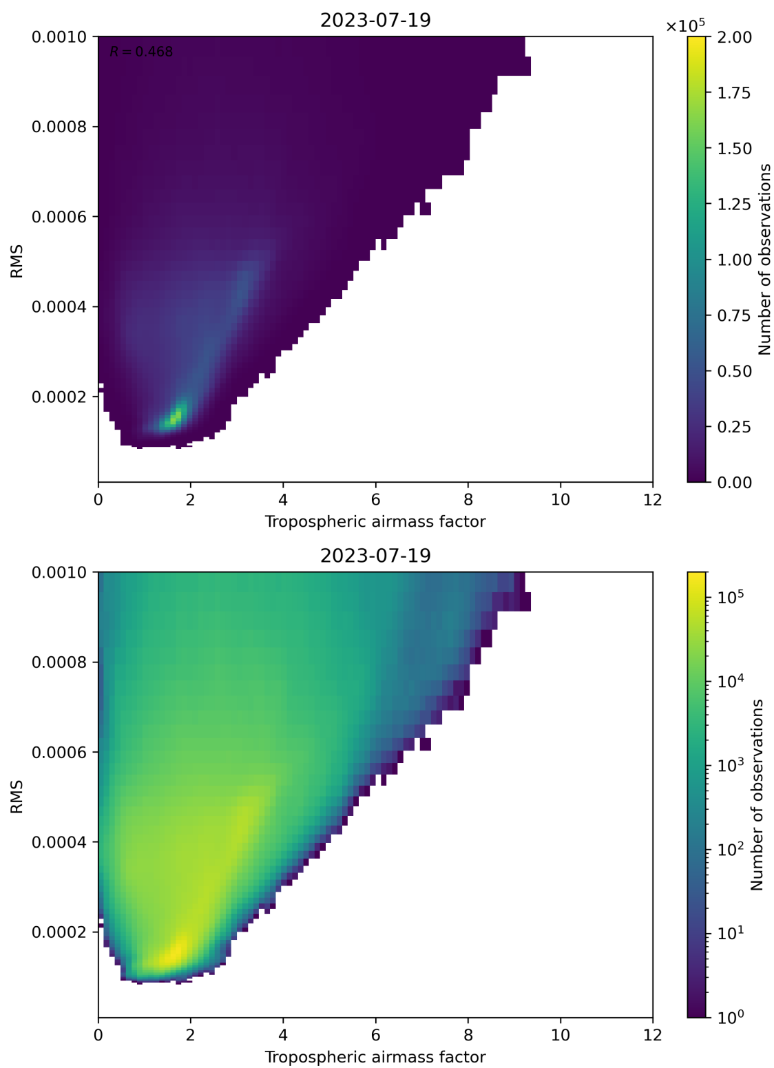
Figure 79: Scatter density plot of “Tropospheric airmass factor” against “RMS” for 2023-07-19 to 2023-07-20.
