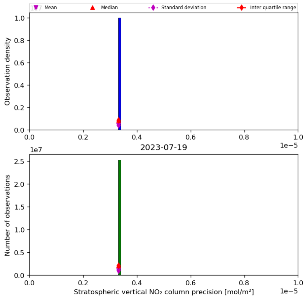
Figure 37: Histogram of “Stratospheric vertical NO 2 column precision” for 2023-07-19 to 2023-07-20
