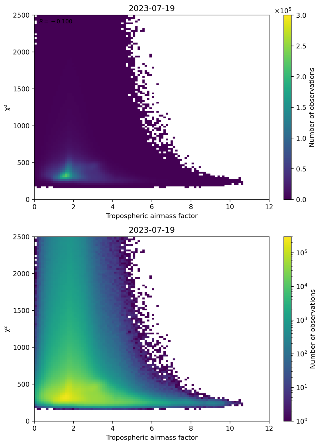
Figure 73: Scatter density plot of “Tropospheric airmass factor” against “ \chi^2 ” for 2023-07-19 to 2023-07-20.
