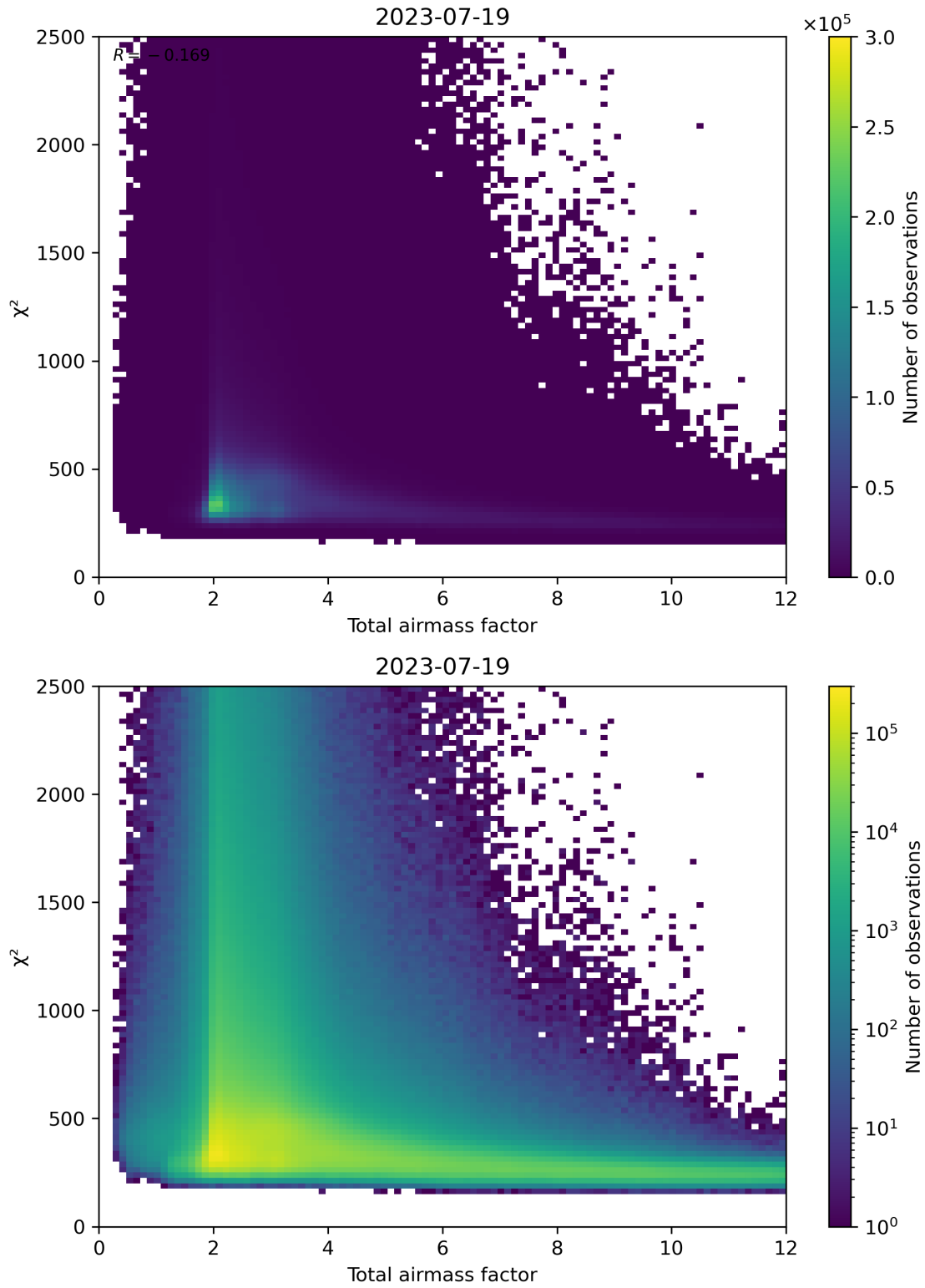
Figure 63: Scatter density plot of “Total airmass factor” against “ \chi^2 ” for 2023-07-19 to 2023-07-20.
