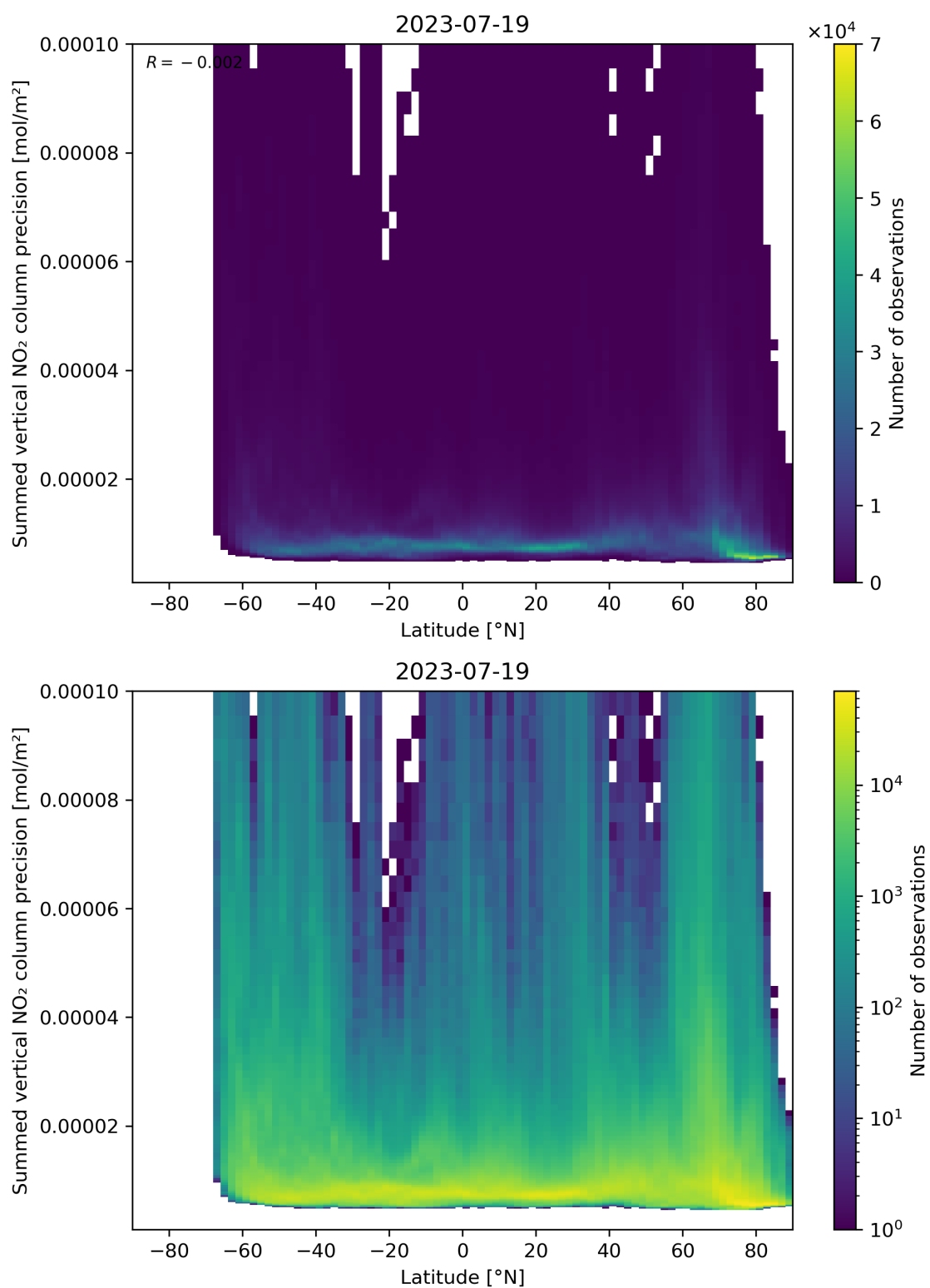
Figure 89: Scatter density plot of “Latitude” against “Summed vertical NO 2 column precision” for 2023-07-19 to 2023-07-20.
