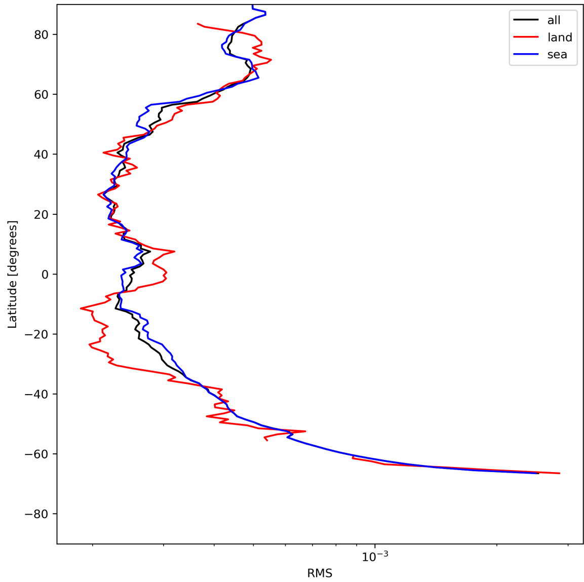
Figure 26: Zonal average of “RMS” for 2023-07-19 to 2023-07-20.
