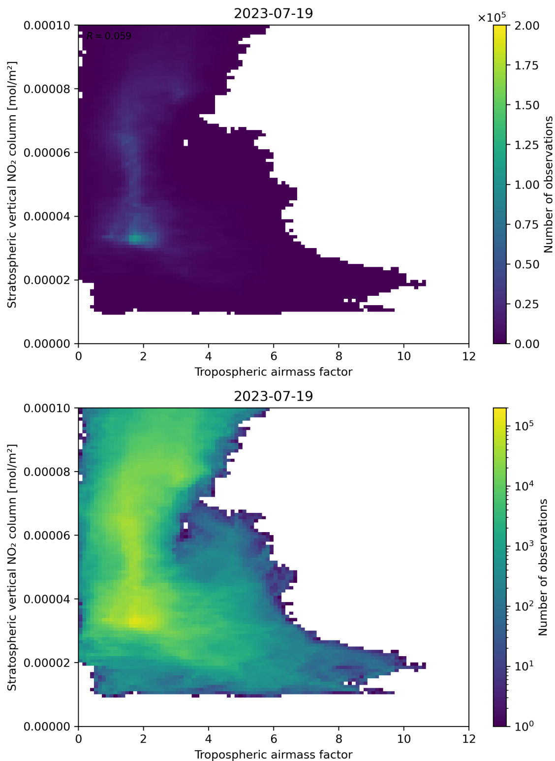
Figure 74: Scatter density plot of “Tropospheric air mass factor” against “Stratospheric vertical NO 2 column” for 2023-07-19 to 2023-07-20.
