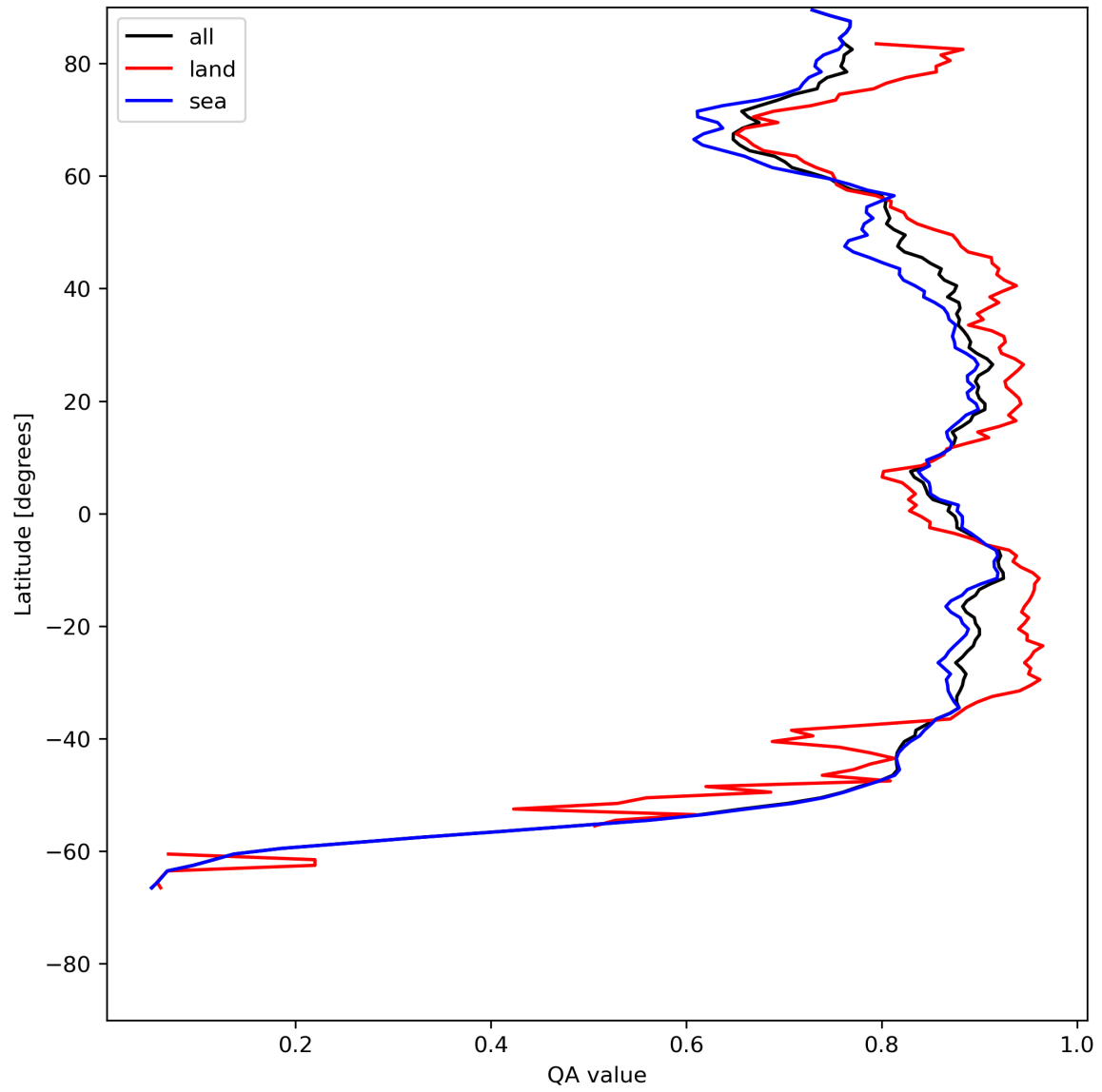
Figure 11: Zonal average of “QA value” for 2023-07-19 to 2023-07-20.
