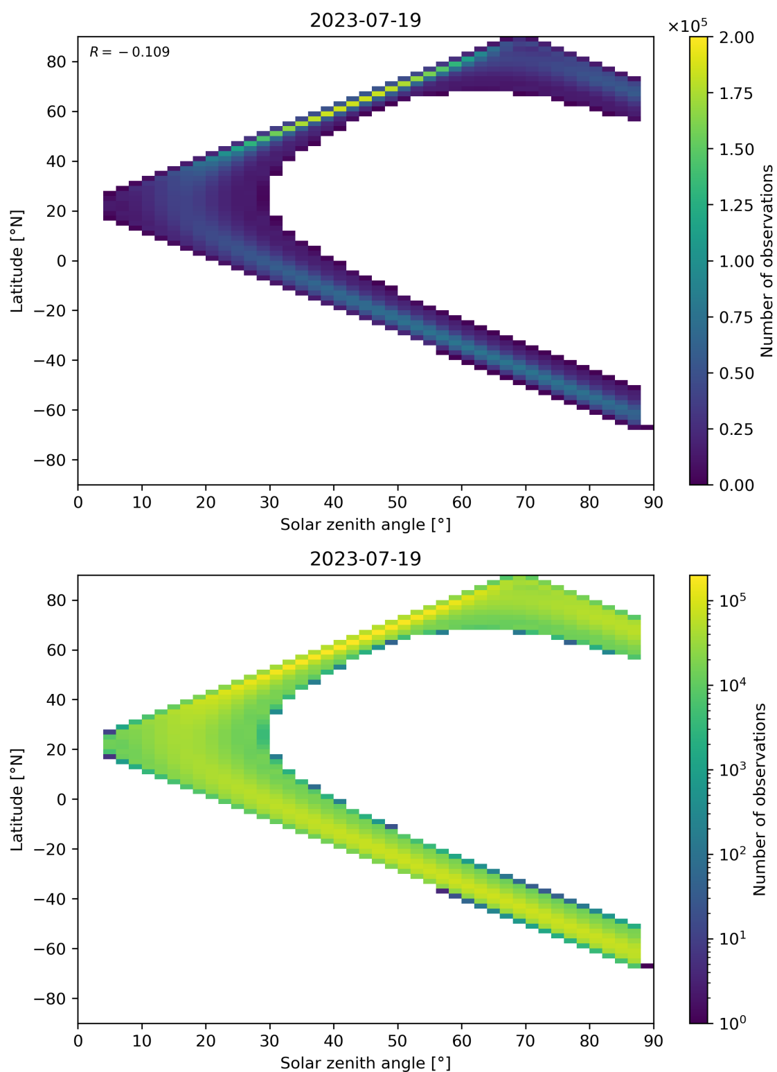
Figure 149: Scatter density plot of “Solar zenith angle” against “Latitude” for 2023-07-19 to 2023-07-20.
