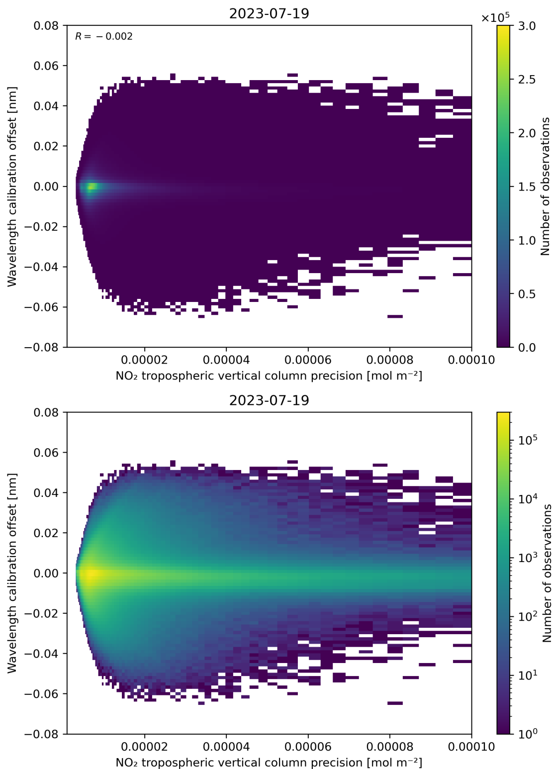
Figure 141: Scatter density plot of “NO 2 tropospheric vertical column precision” against “Wavelength calibration offset” for 2023-07-19 to 2023-07-20.
