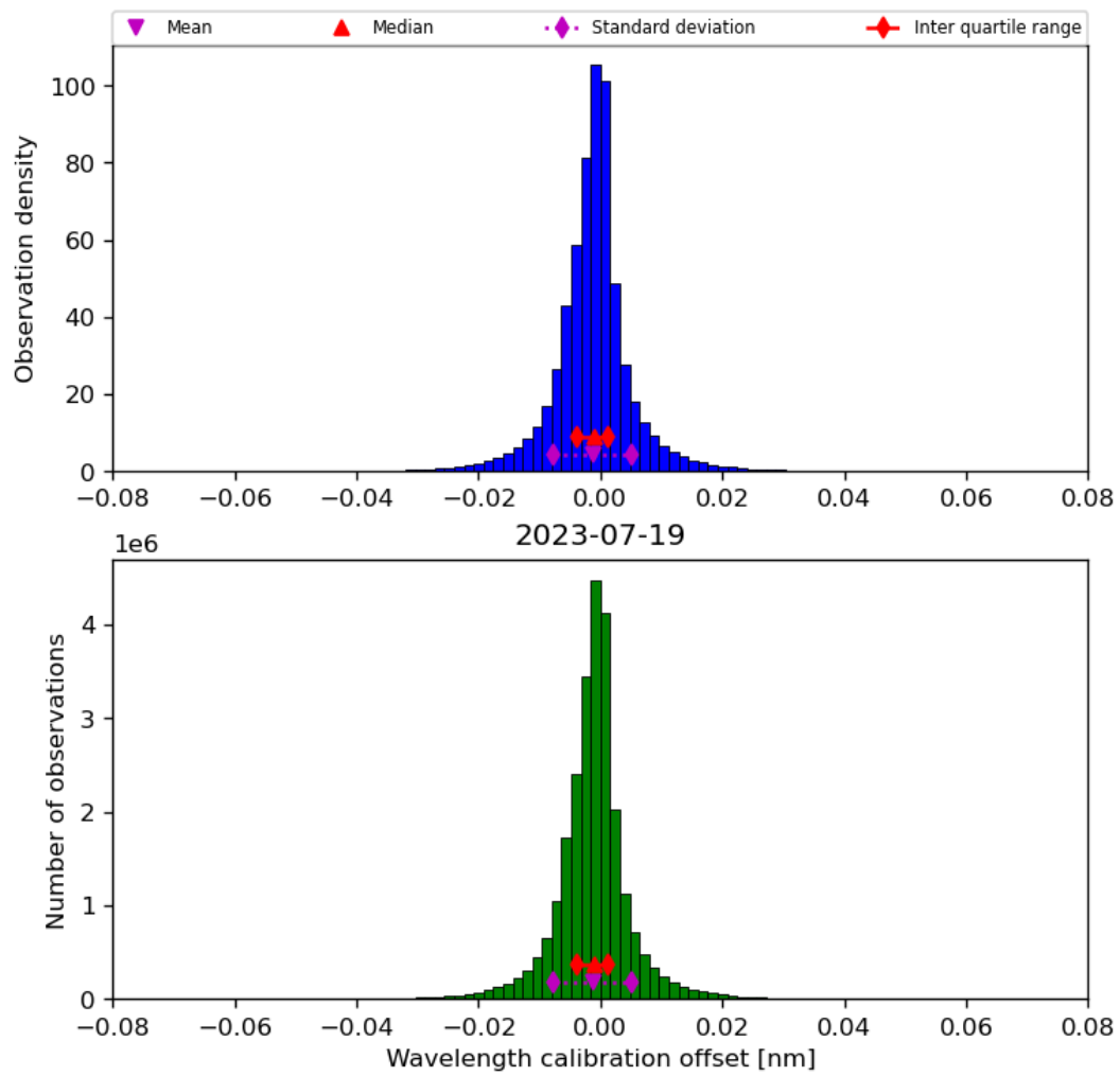
Figure 35: Histogram of “Wavelength calibration offset” for 2023-07-19 to 2023-07-20
