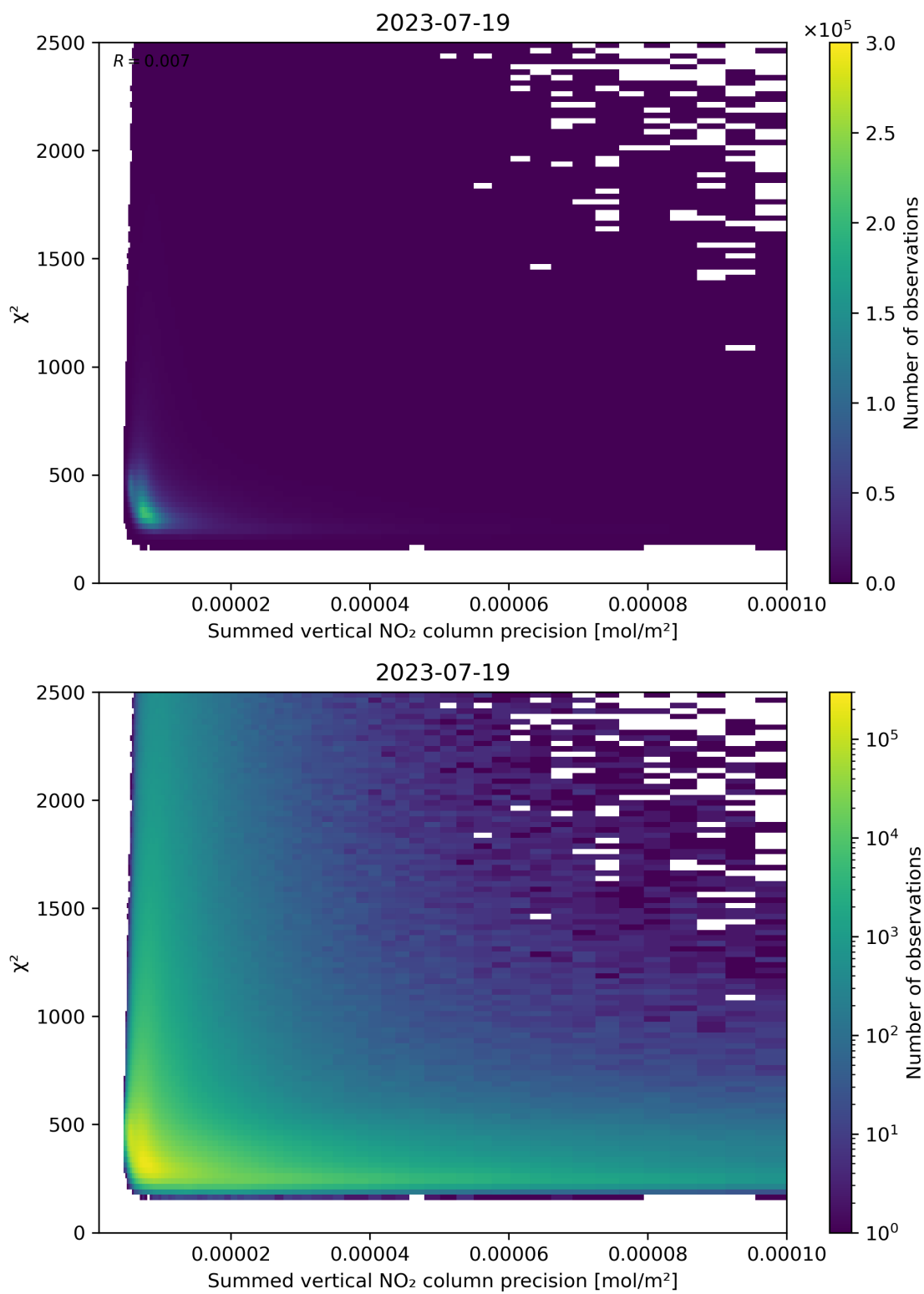
Figure 107: Scatter density plot of “Summed vertical NO 2 column precision” against “ \chi^2 ” for 2023-07-19 to 2023-07-20.
