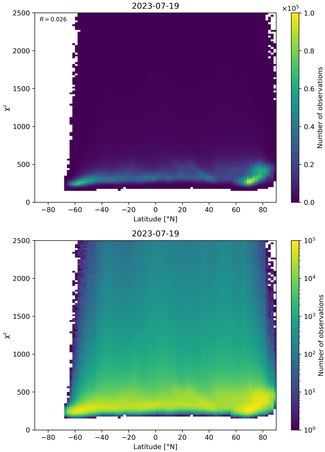
Figure 86: Scatter density plot of “Latitude” against “ \chi^2 ” for 2023-07-19 to 2023-07-20.
