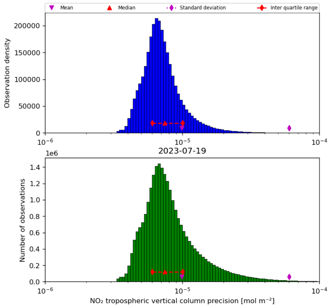
Figure 30: Histogram of “NO 2 tropospheric vertical column precision” for 2023-07-19 to 2023-07-20
