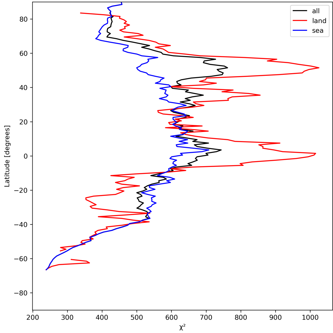
Figure 25: Zonal average of “ \chi^2 ” for 2023-07-19 to 2023-07-20.
