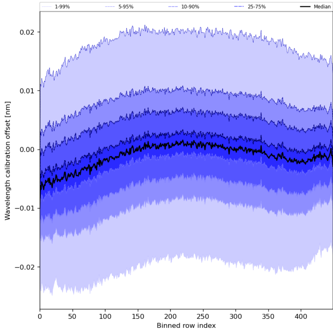
Figure 52: Along track statistics of “Wavelength calibration offset” for 2023-07-19 to 2023-07-20
