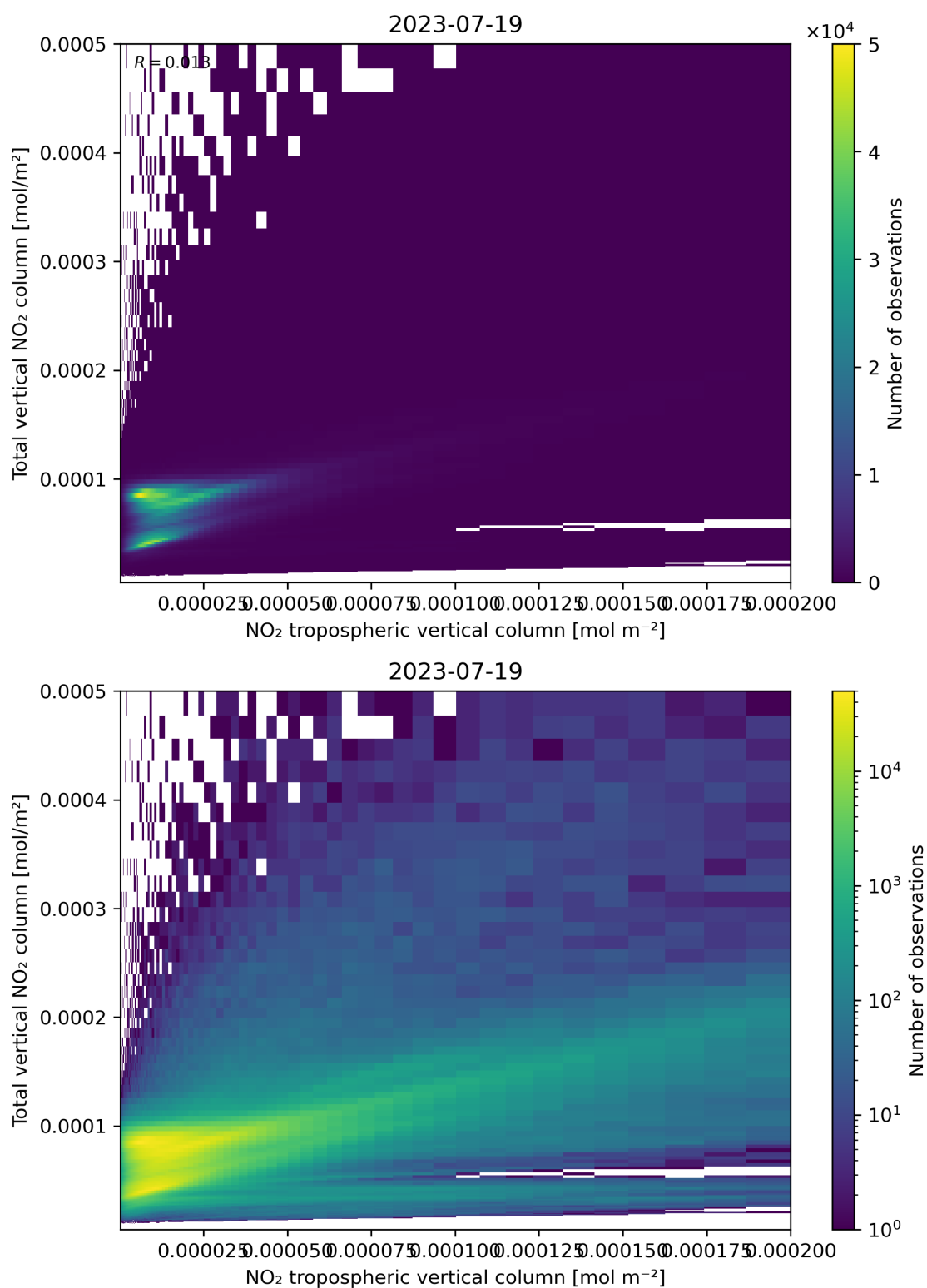
Figure 128: Scatter density plot of “NO 2 tropospheric vertical column” against “Total vertical NO 2 column” for 2023-07-19 to 2023-07-20.
