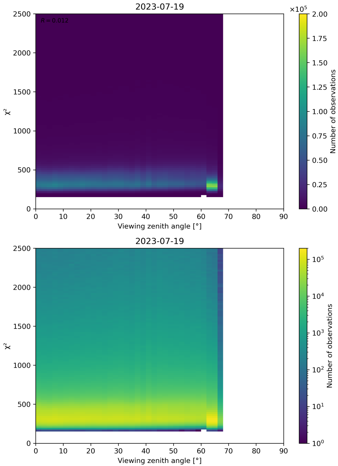
Figure 162: Scatter density plot of “Viewing zenith angle” against “ \chi^2 ” for 2023-07-19 to 2023-07-20.
