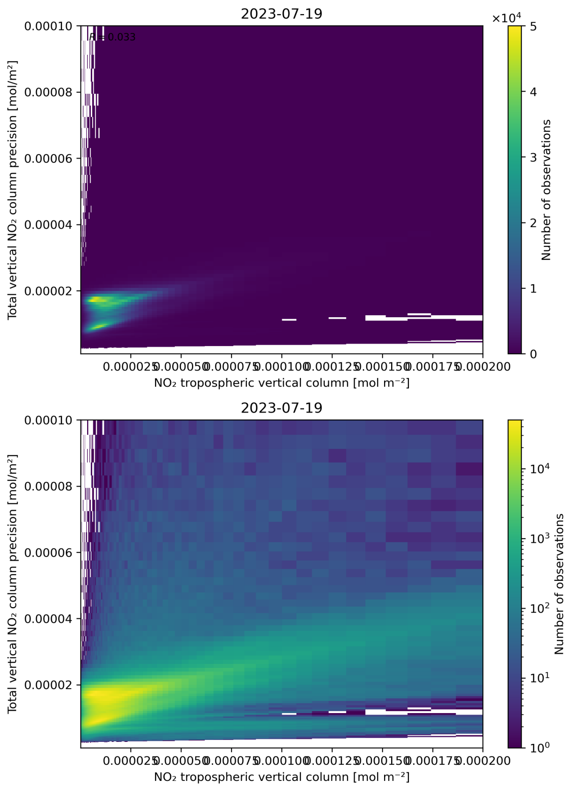
Figure 129: Scatter density plot of “NO 2 tropospheric vertical column” against “Total vertical NO 2 column precision” for 2023-07-19 to 2023-07-20.
