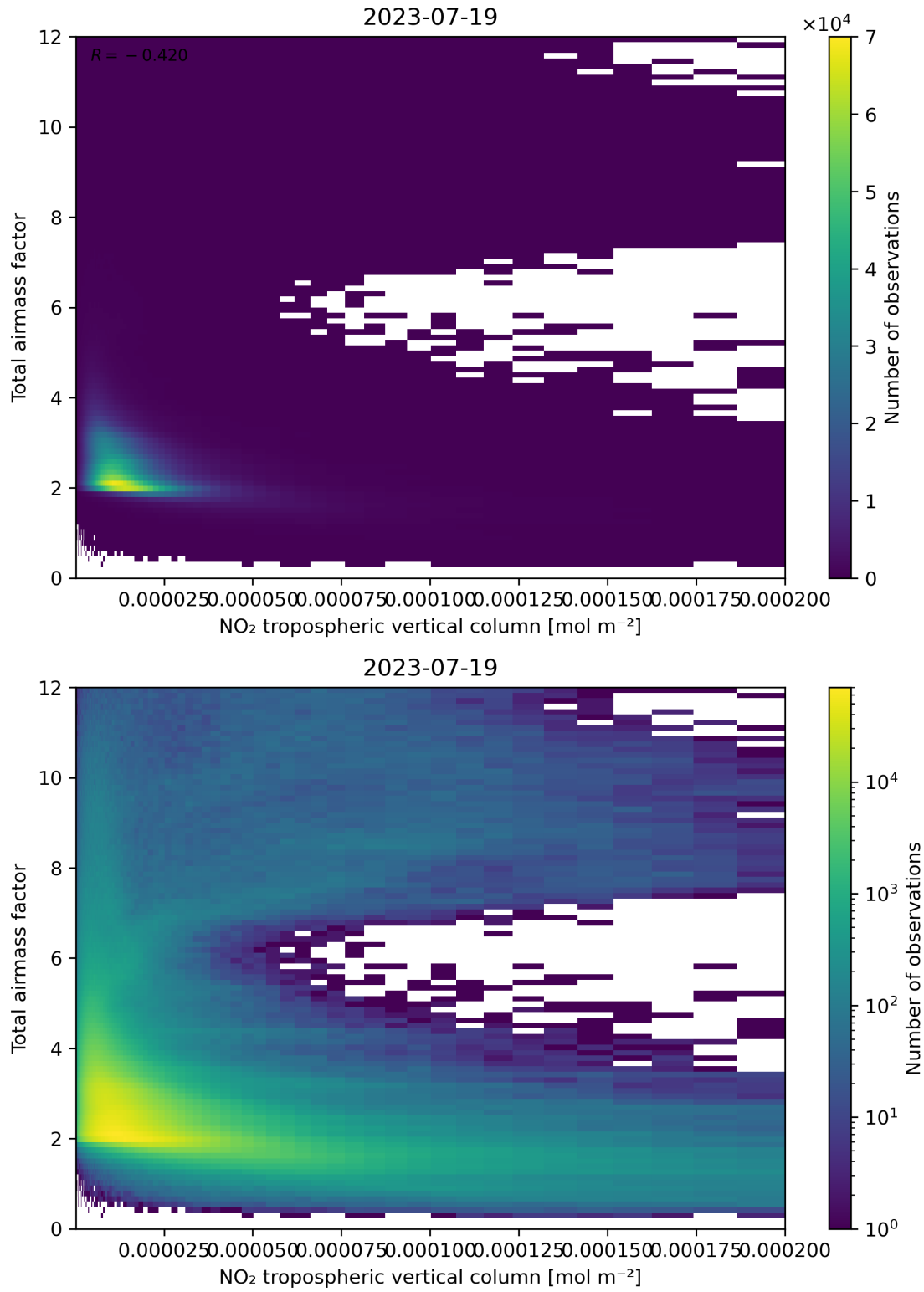
Figure 122: Scatter density plot of “NO 2 tropospheric vertical column” against “Total air mass factor” for 2023-07-19 to 2023-07-20.
