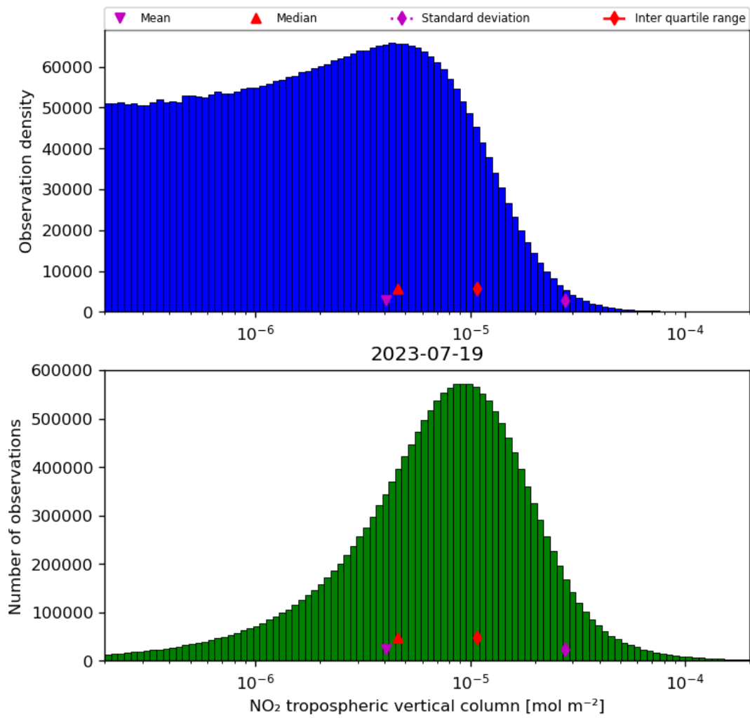
Figure 29: Histogram of “NO 2 tropospheric vertical column” for 2023-07-19 to 2023-07-20
