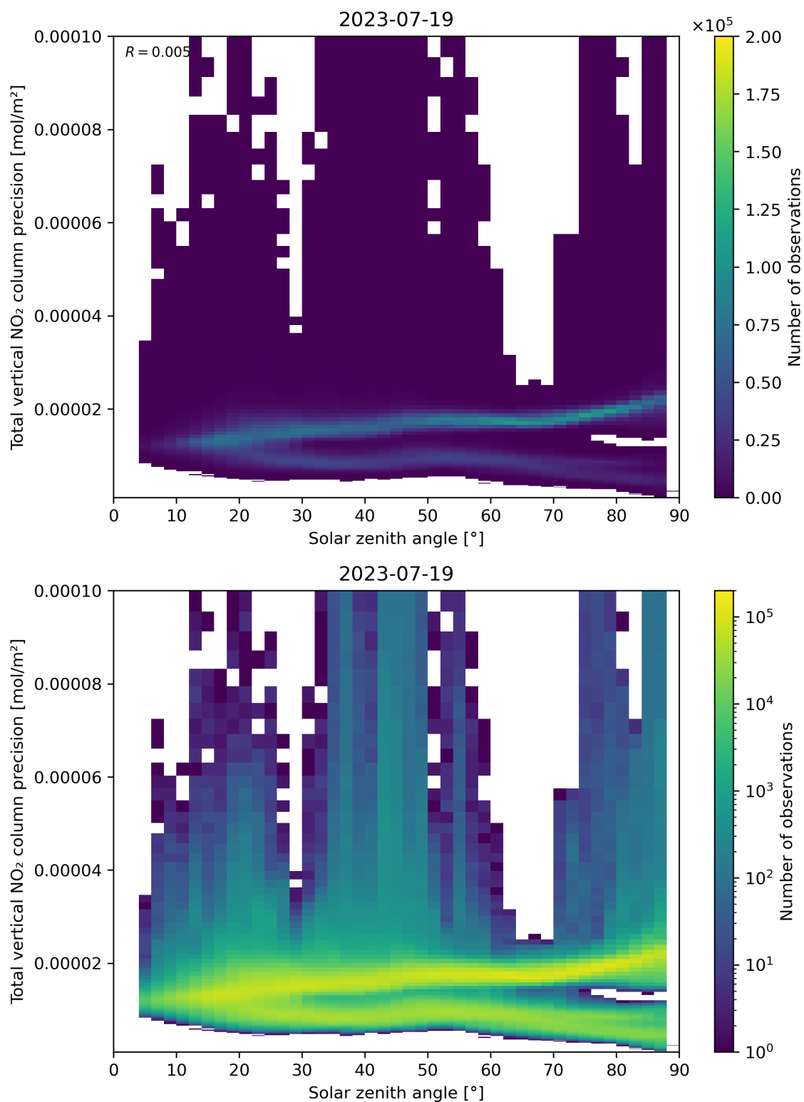
Figure 154: Scatter density plot of “Solar zenith angle” against “Total vertical NO 2 column precision” for 2023-07-19 to 2023-07-20.
