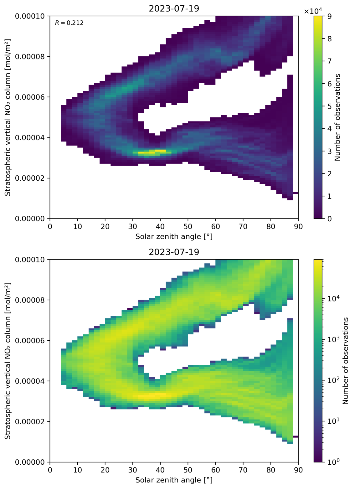
Figure 150: Scatter density plot of “Solar zenith angle” against “Stratospheric vertical NO 2 column” for 2023-07-19 to 2023-07-20.
