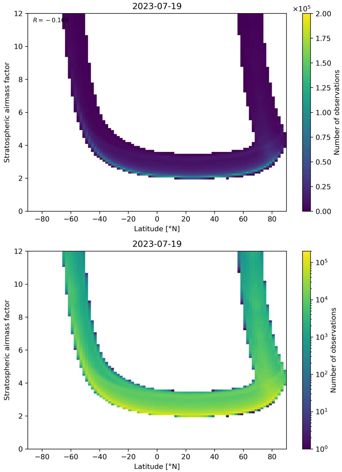
Figure 83: Scatter density plot of “Latitude” against “Stratospheric air mass factor” for 2023-07-19 to 2023-07-20.
