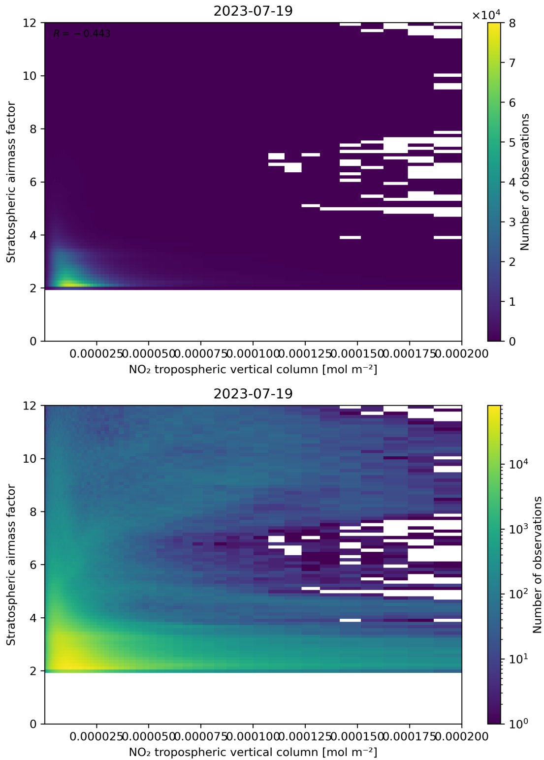
Figure 121: Scatter density plot of “NO 2 tropospheric vertical column” against “Stratospheric air mass factor” for 2023-07-19 to 2023-07-20.
