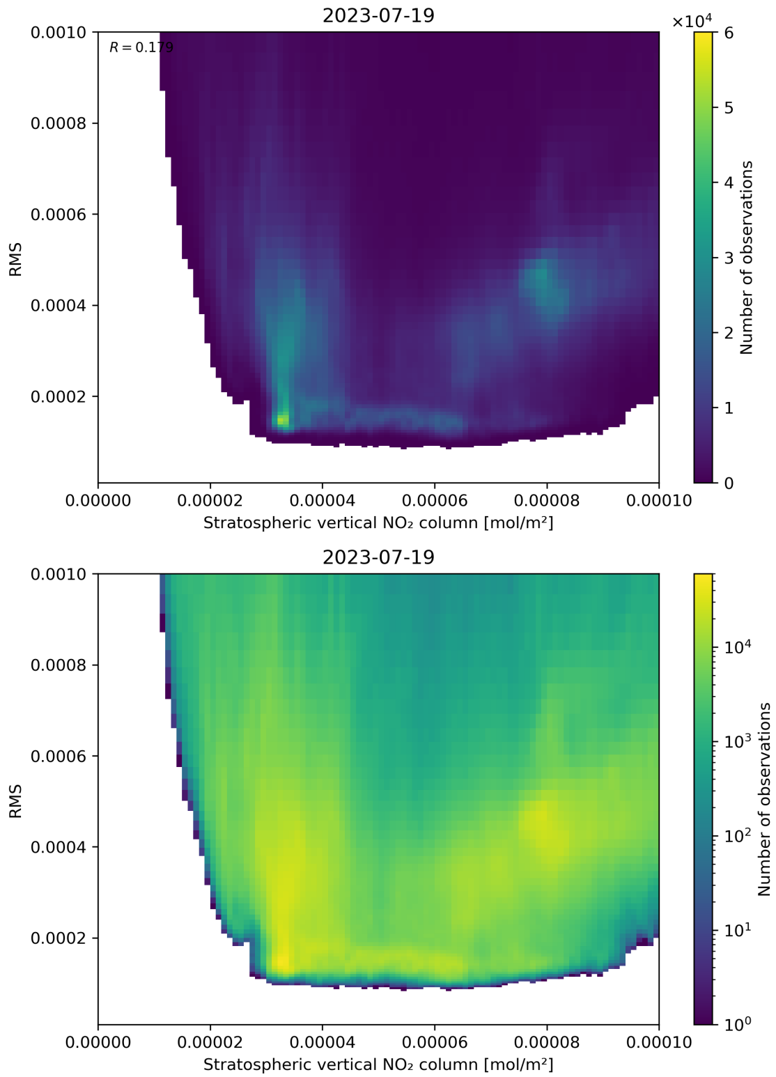
Figure 102: Scatter density plot of “Stratospheric vertical NO 2 column” against “RMS” for 2023-07-19 to 2023-07-20.
