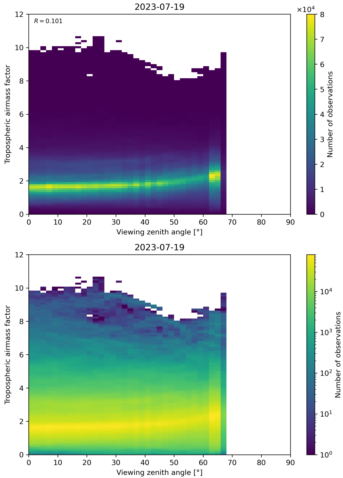
Figure 161: Scatter density plot of “Viewing zenith angle” against “Tropospheric airmass factor” for 2023-07-19 to 2023-07-20.
