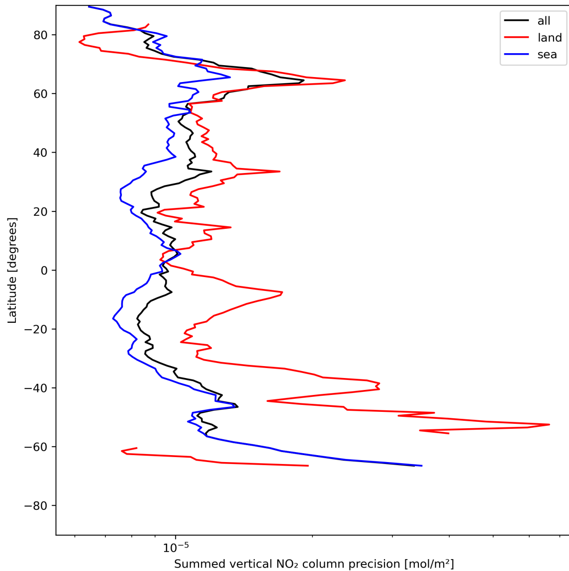
Figure 24: Zonal average of “Summed vertical NO 2 column precision” for 2023-07-19 to 2023-07-20.
