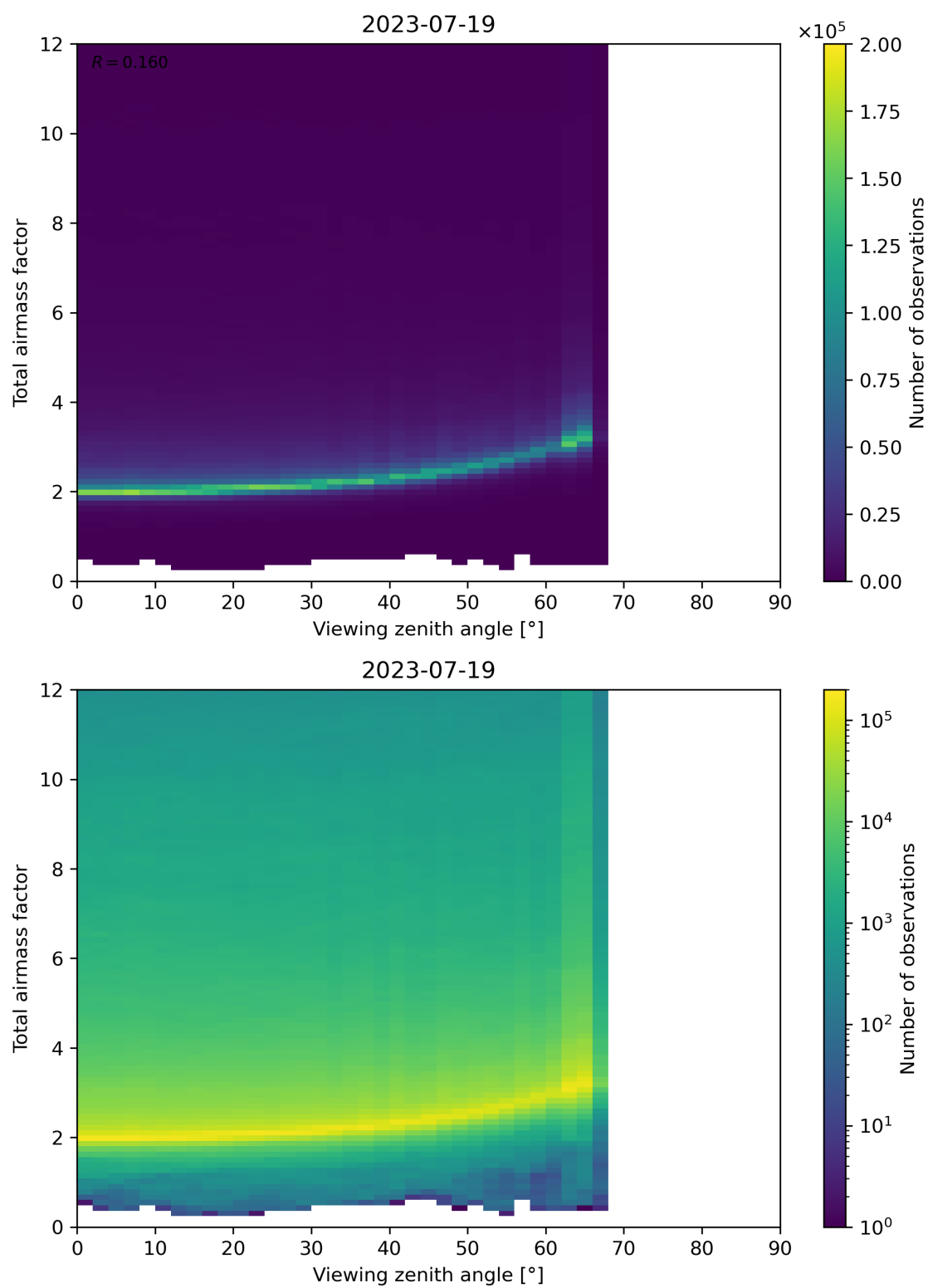
Figure 160: Scatter density plot of “Viewing zenith angle” against “Total airmass factor” for 2023-07-19 to 2023-07-20.
