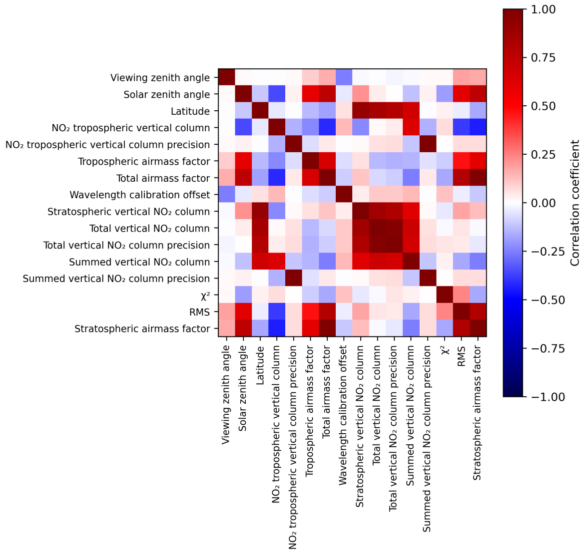
Figure 2: Map of correlation matrix for 2023-07-19 to 2023-07-20.
