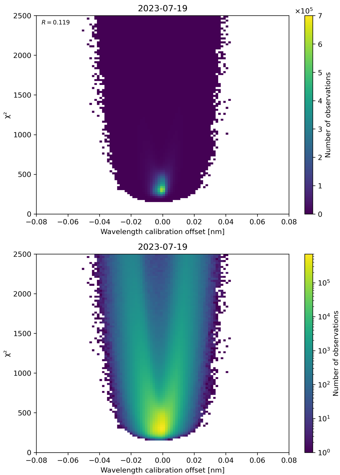
Figure 175: Scatter density plot of “Wavelength calibration offset” against “ \chi^2 ” for 2023-07-19 to 2023-07-20.
