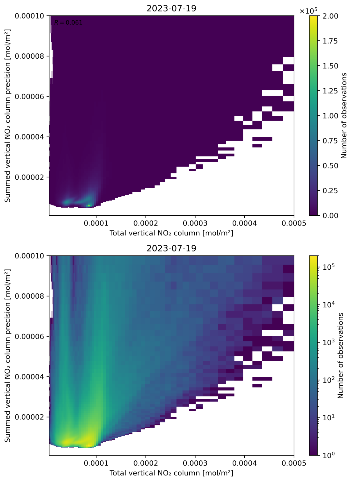
Figure 113: Scatter density plot of “Total vertical NO 2 column” against “Summed vertical NO 2 column precision” for 2023-07-19 to 2023-07-20.
