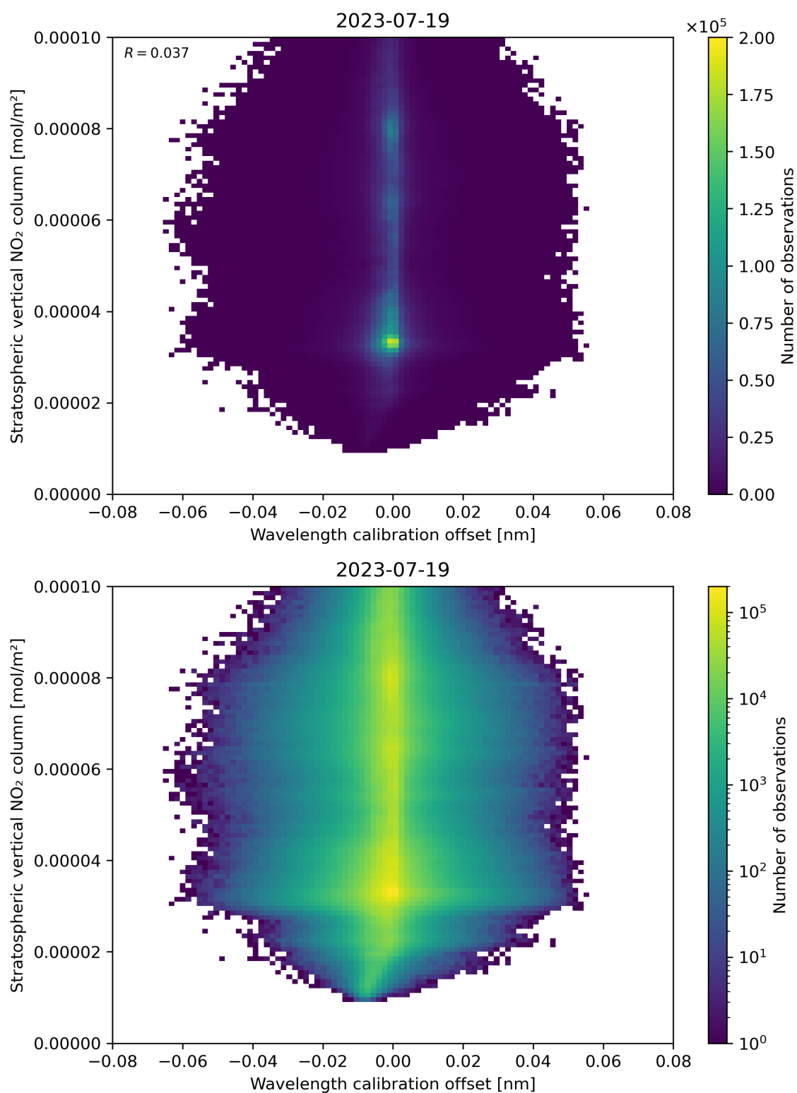
Figure 176: Scatter density plot of “Wavelength calibration offset” against “Stratospheric vertical NO 2 column” for 2023-07-19 to 2023-07-20.
