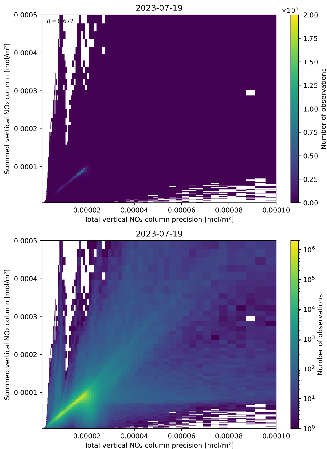
Figure 117: Scatter density plot of “Total vertical NO 2 column precision” against “Summed vertical NO 2 column” for 2023-07-19 to 2023-07-20.
