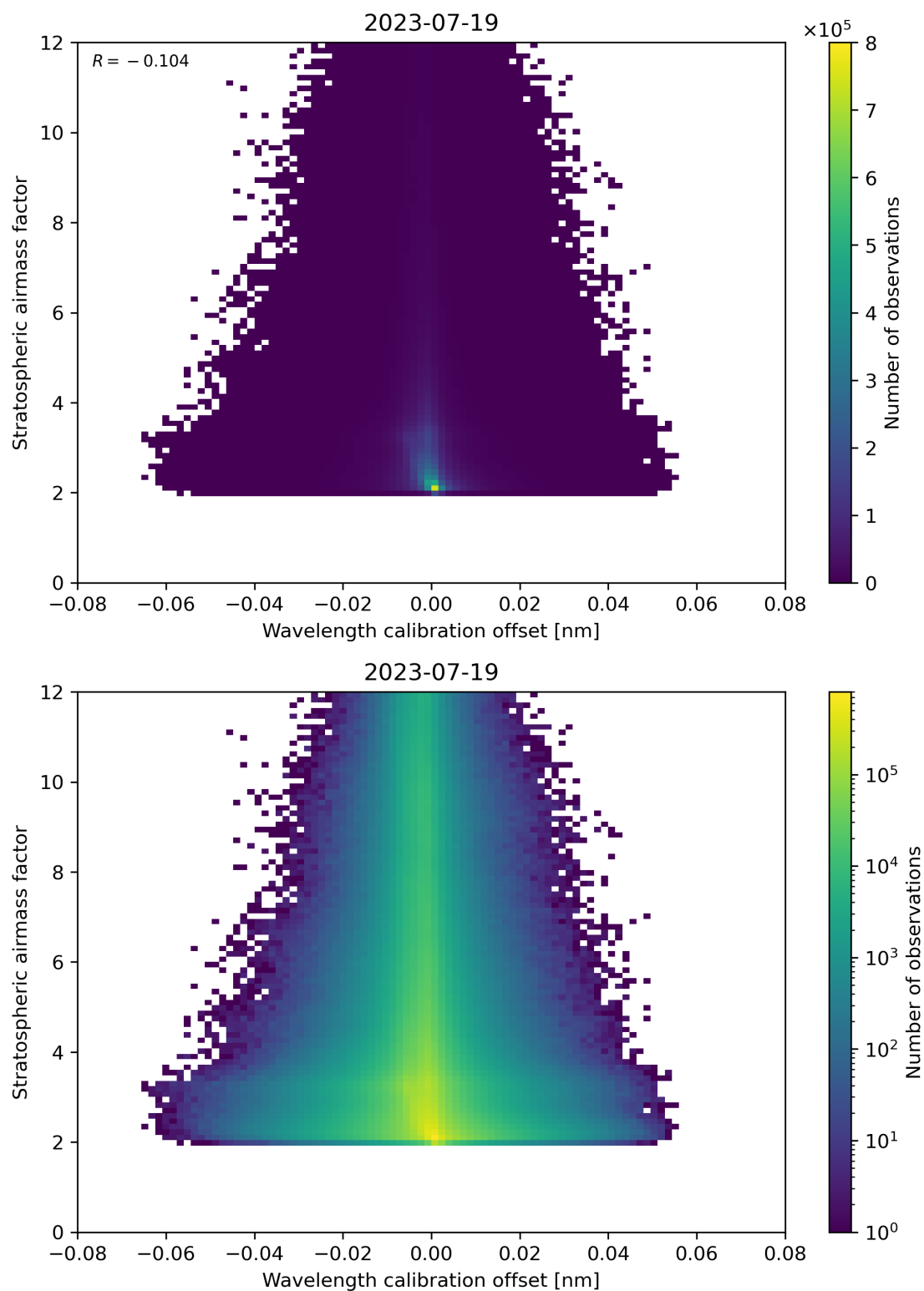
Figure 174: Scatter density plot of “Wavelength calibration offset” against “Stratospheric air mass factor” for 2023-07-19 to 2023-07-20.
