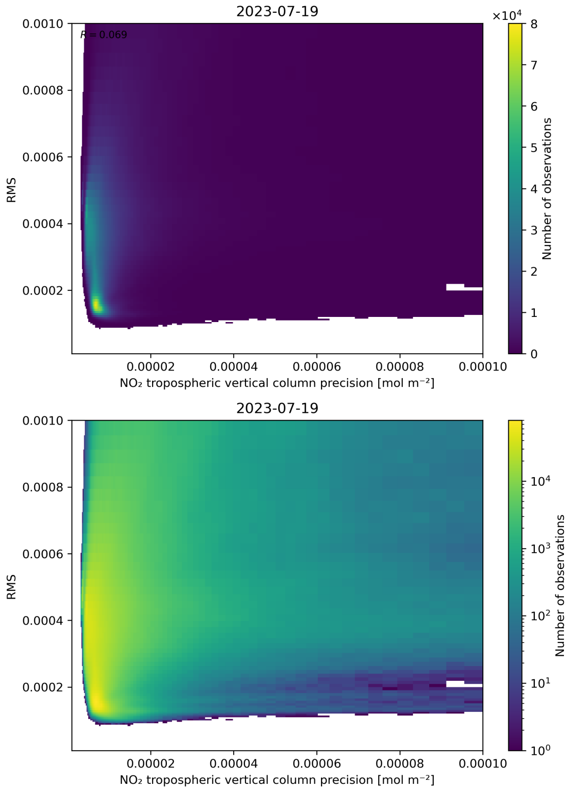
Figure 140: Scatter density plot of “NO 2 tropospheric vertical column precision” against “RMS” for 2023-07-19 to 2023-07-20.
