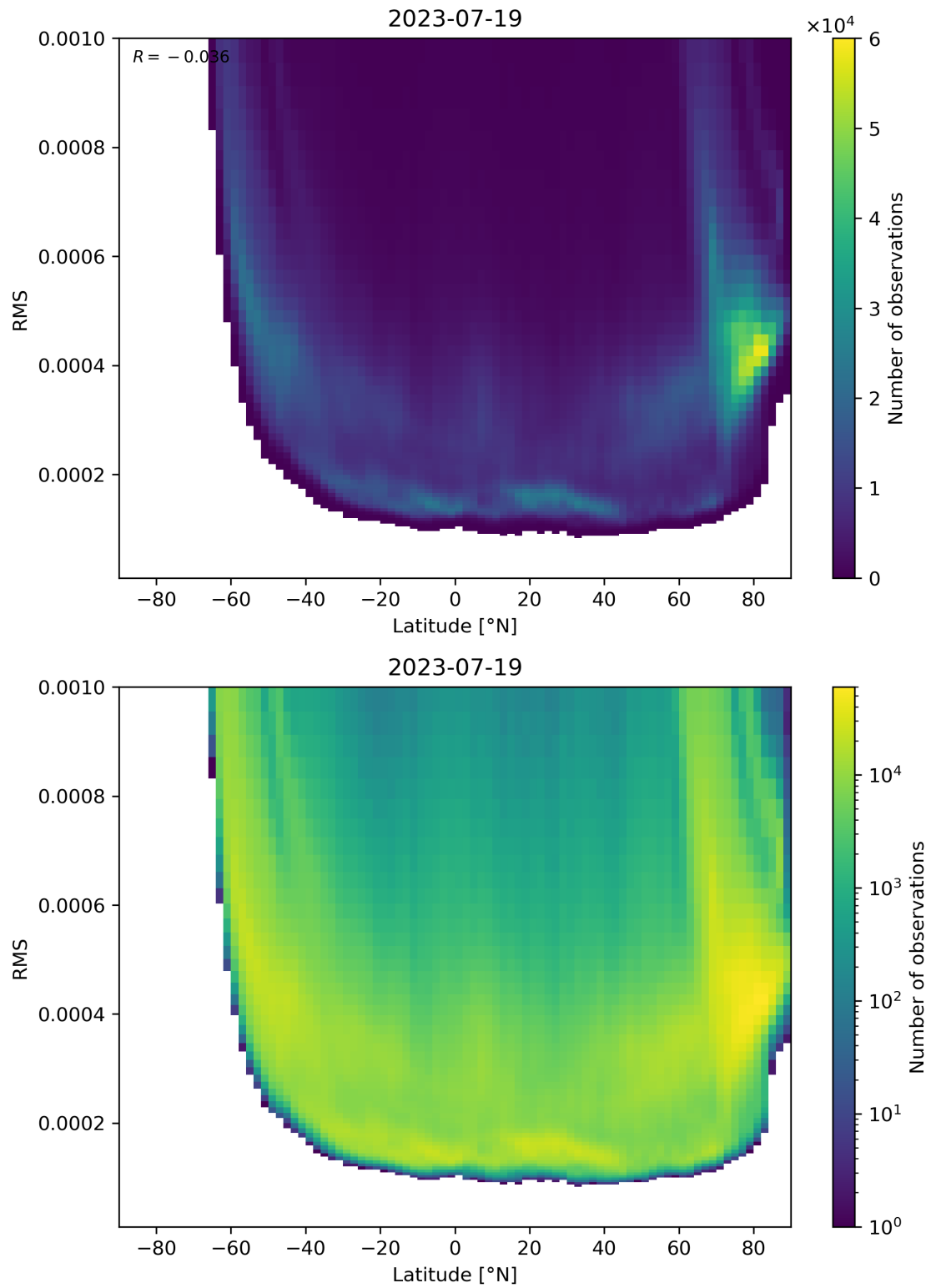
Figure 94: Scatter density plot of “Latitude” against “RMS” for 2023-07-19 to 2023-07-20.
