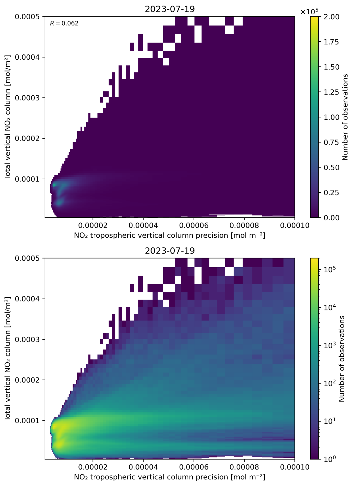
Figure 138: Scatter density plot of “NO 2 tropospheric vertical column precision” against “Total vertical NO 2 column” for 2023-07-19 to 2023-07-20.
