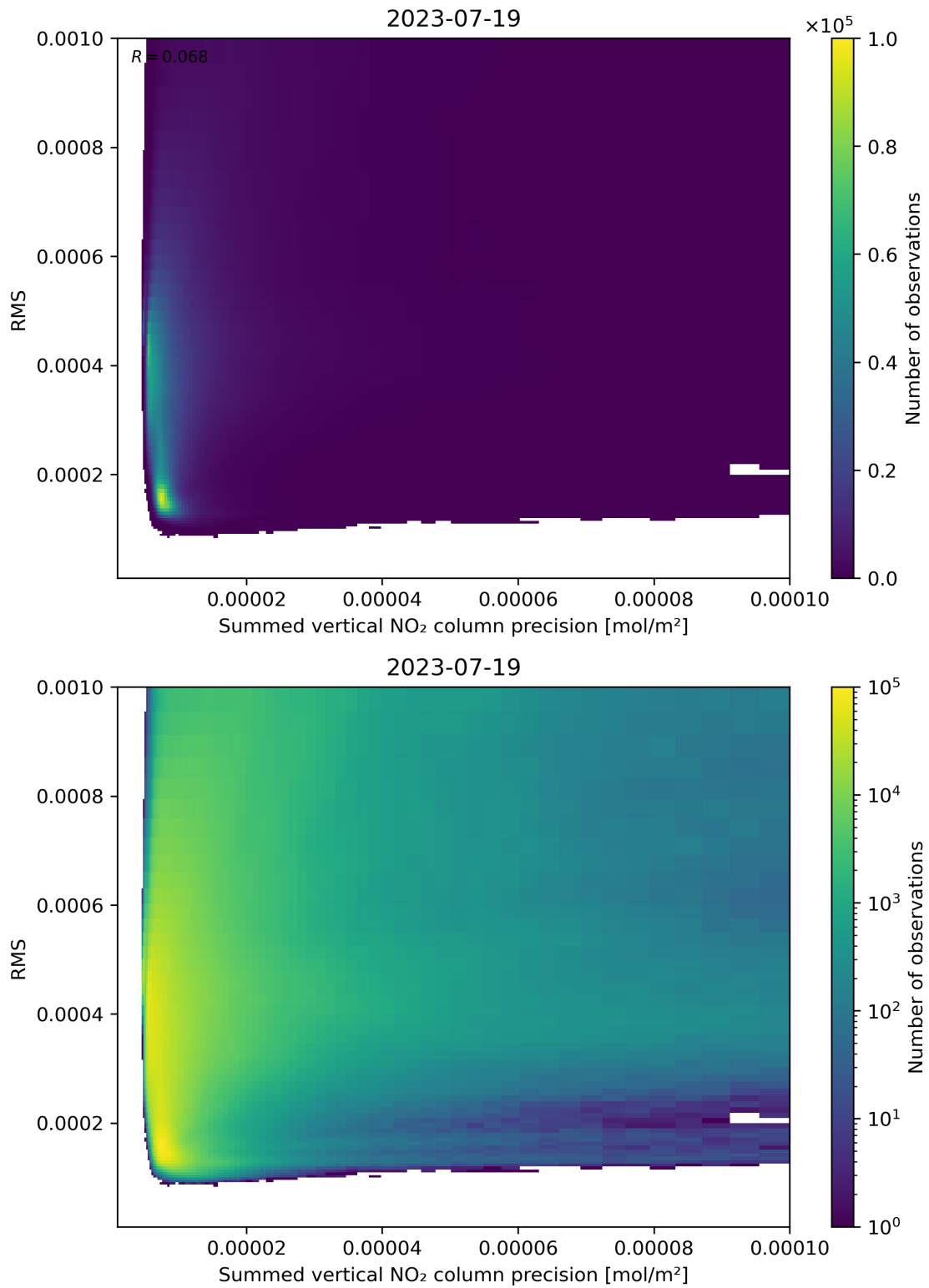
Figure 108: Scatter density plot of “Summed vertical NO 2 column precision” against “RMS” for 2023-07-19 to 2023-07-20.
