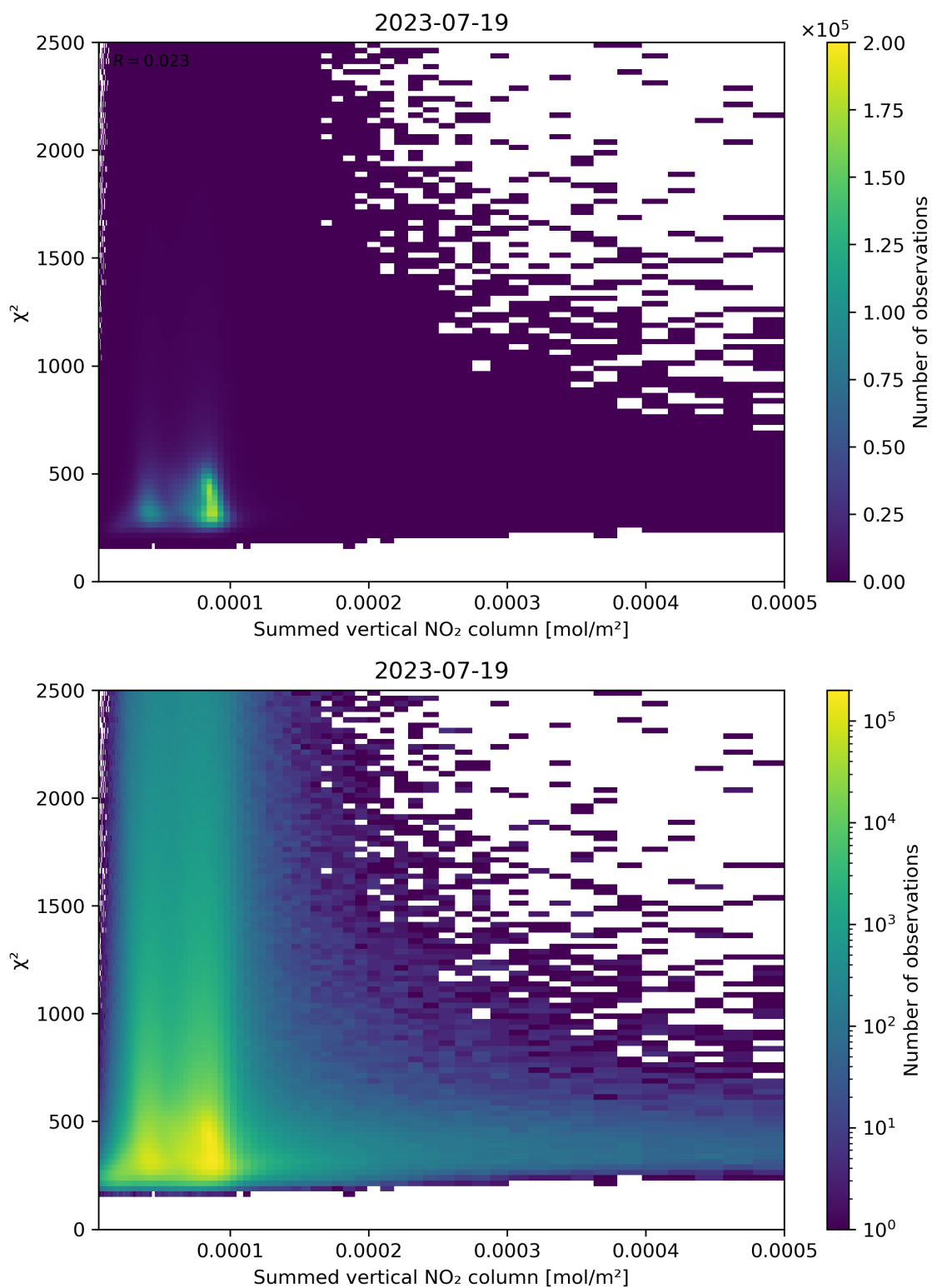
Figure 104: Scatter density plot of “Summed vertical NO 2 column” against “ \chi^2 ” for 2023-07-19 to 2023-07-20.
