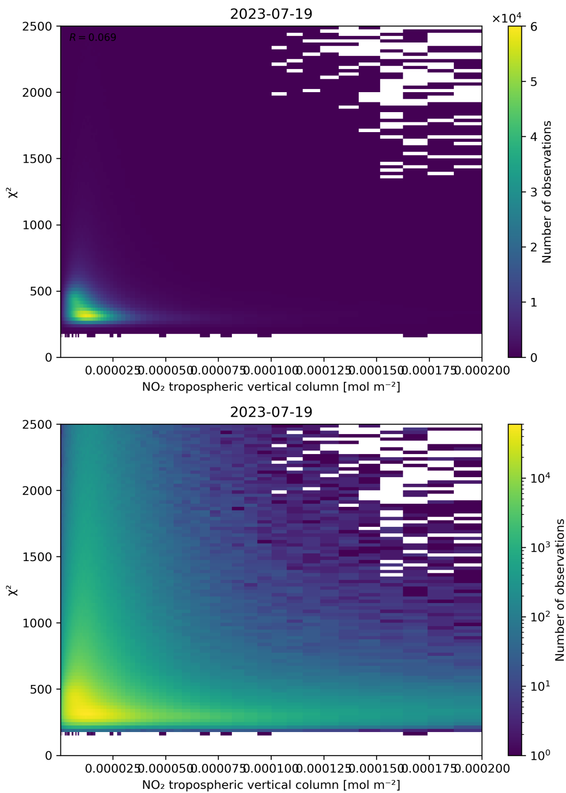
Figure 124: Scatter density plot of “NO 2 tropospheric vertical column” against “ \chi^2 ” for 2023-07-19 to 2023-07-20.
