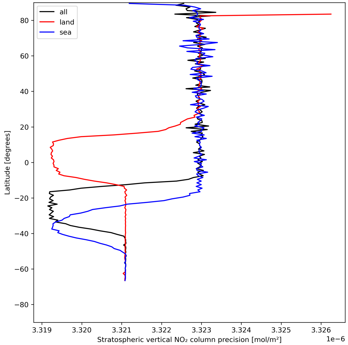
Figure 20: Zonal average of “Stratospheric vertical NO 2 column precision” for 2023-07-19 to 2023-07-20.
