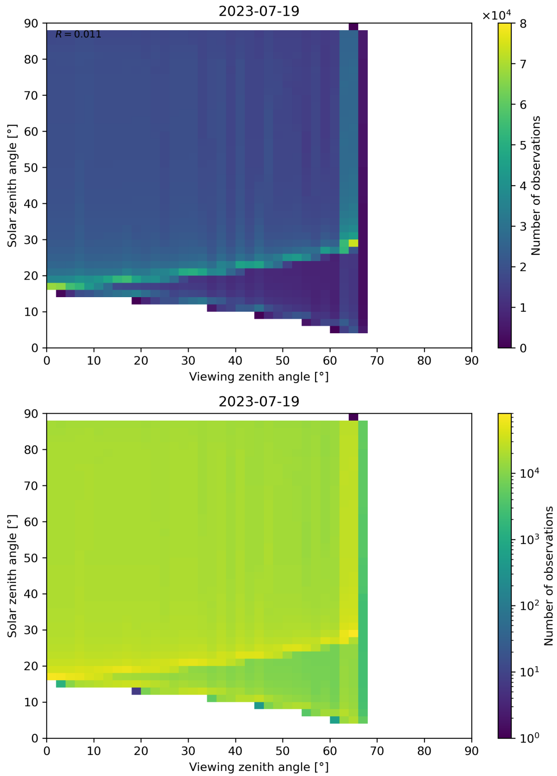
Figure 172: Scatter density plot of “Viewing zenith angle” against “Solar zenith angle” for 2023-07-19 to 2023-07-20.
