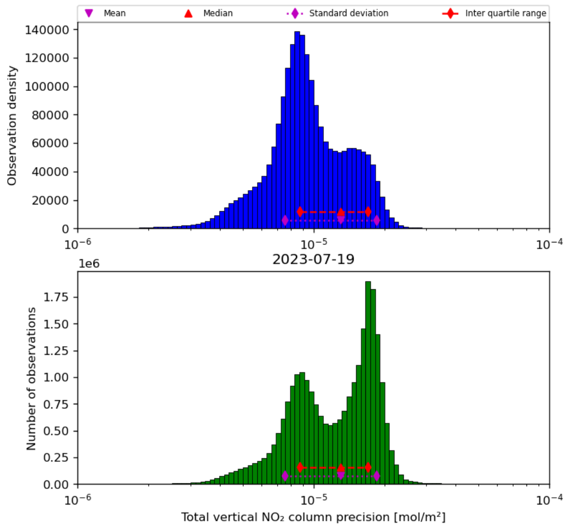
Figure 39: Histogram of “Total vertical NO 2 column precision” for 2023-07-19 to 2023-07-20
