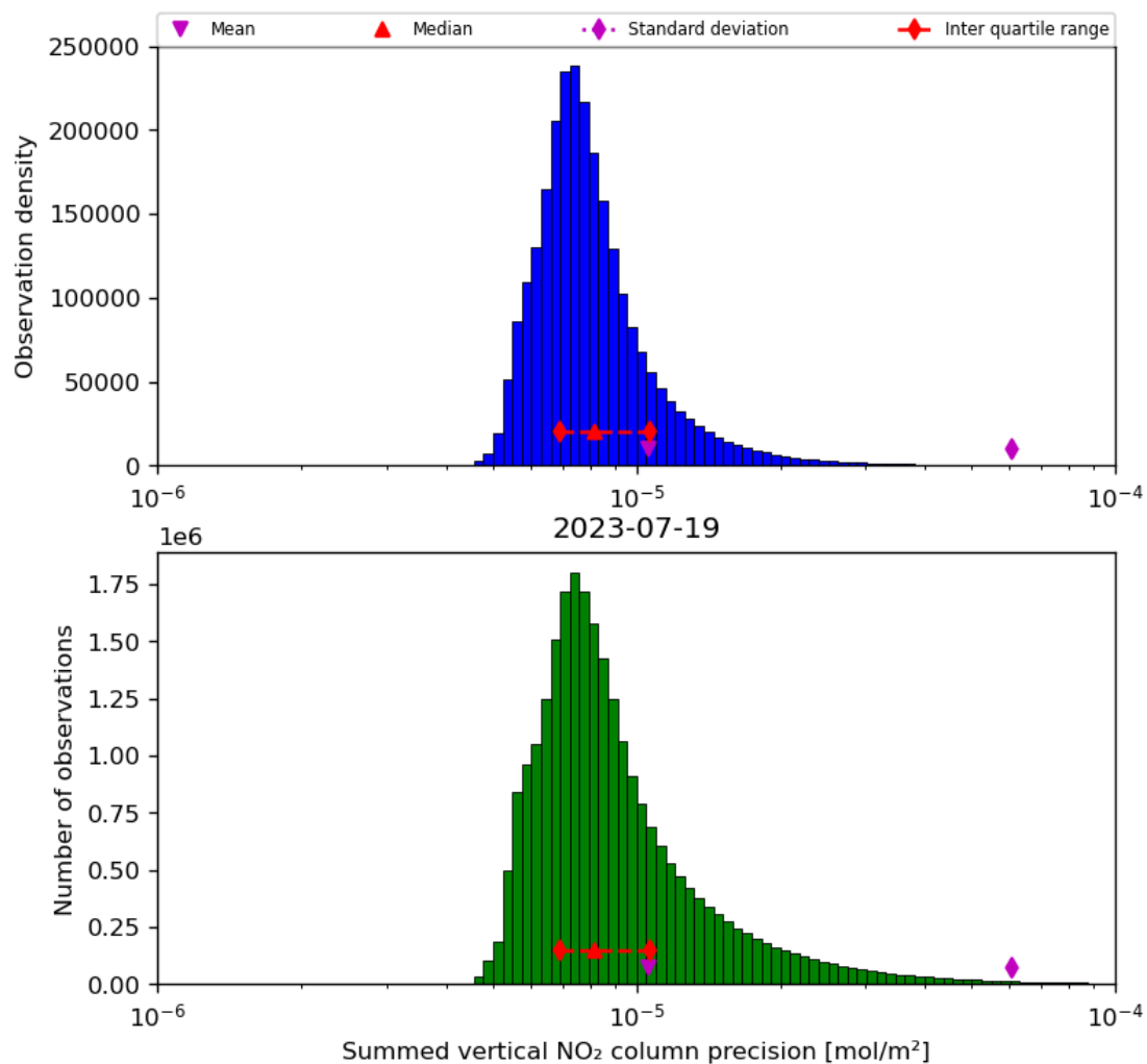
Figure 41: Histogram of "Summed vertical NO 2 column precision" for 2023-07-19 to 2023-07-20
