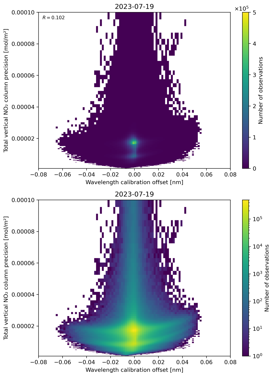
Figure 180: Scatter density plot of “Wavelength calibration offset” against “Total vertical NO 2 column precision” for 2023-07-19 to 2023-07-20.
