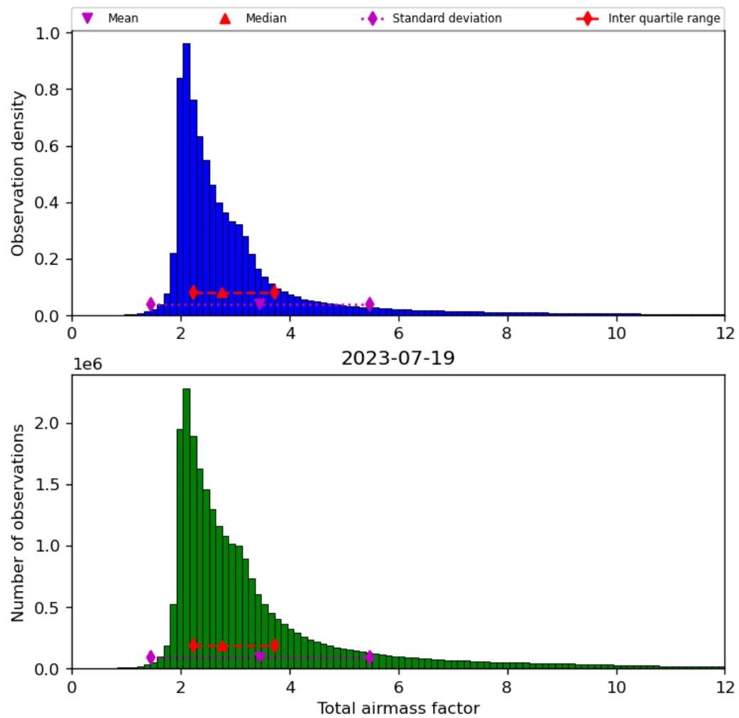
Figure 32: Histogram of “Total airmass factor” for 2023-07-19 to 2023-07-20
