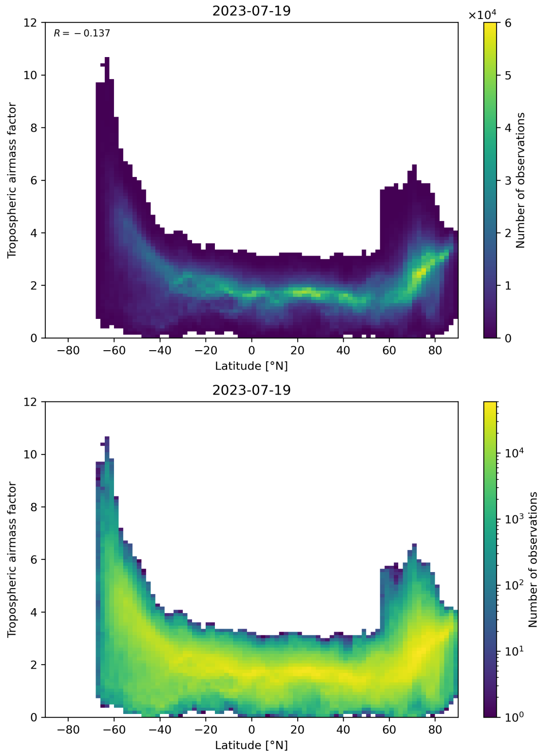
Figure 85: Scatter density plot of “Latitude” against “Tropospheric air mass factor” for 2023-07-19 to 2023-07-20.
