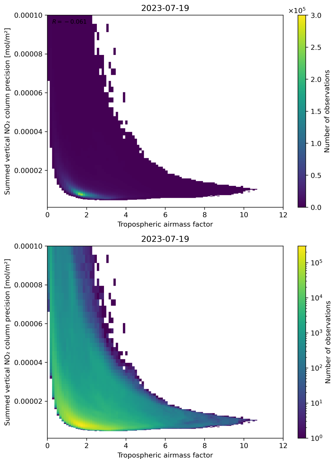
Figure 76: Scatter density plot of “Tropospheric air mass factor” against “Summed vertical NO 2 column precision” for 2023-07-19 to 2023-07-20.
