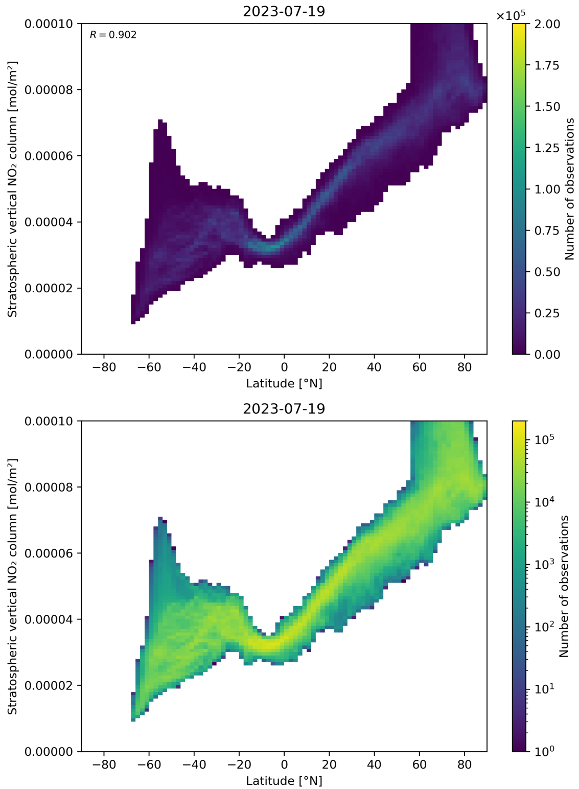
Figure 87: Scatter density plot of “Latitude” against “Stratospheric vertical NO 2 column” for 2023-07-19 to 2023-07-20.
