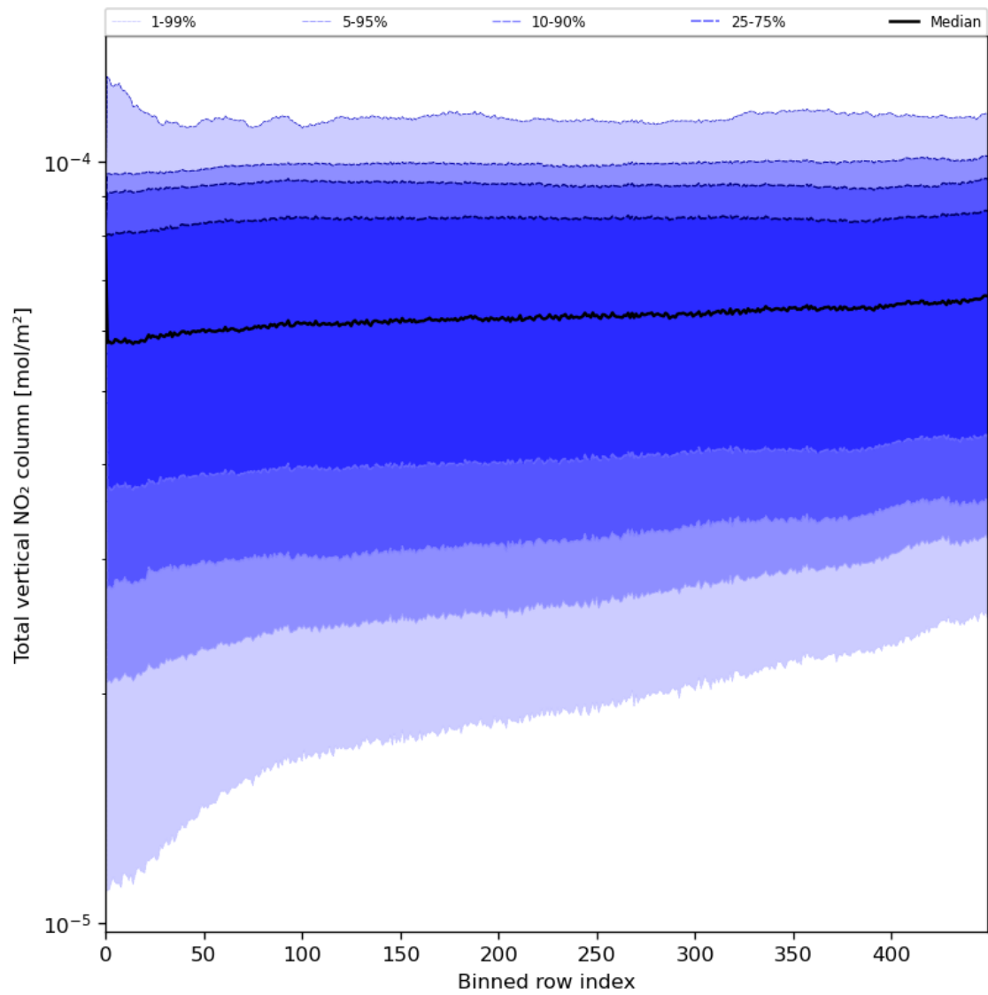
Figure 55: Along track statistics of “Total vertical NO 2 column” for 2023-07-19 to 2023-07-20
