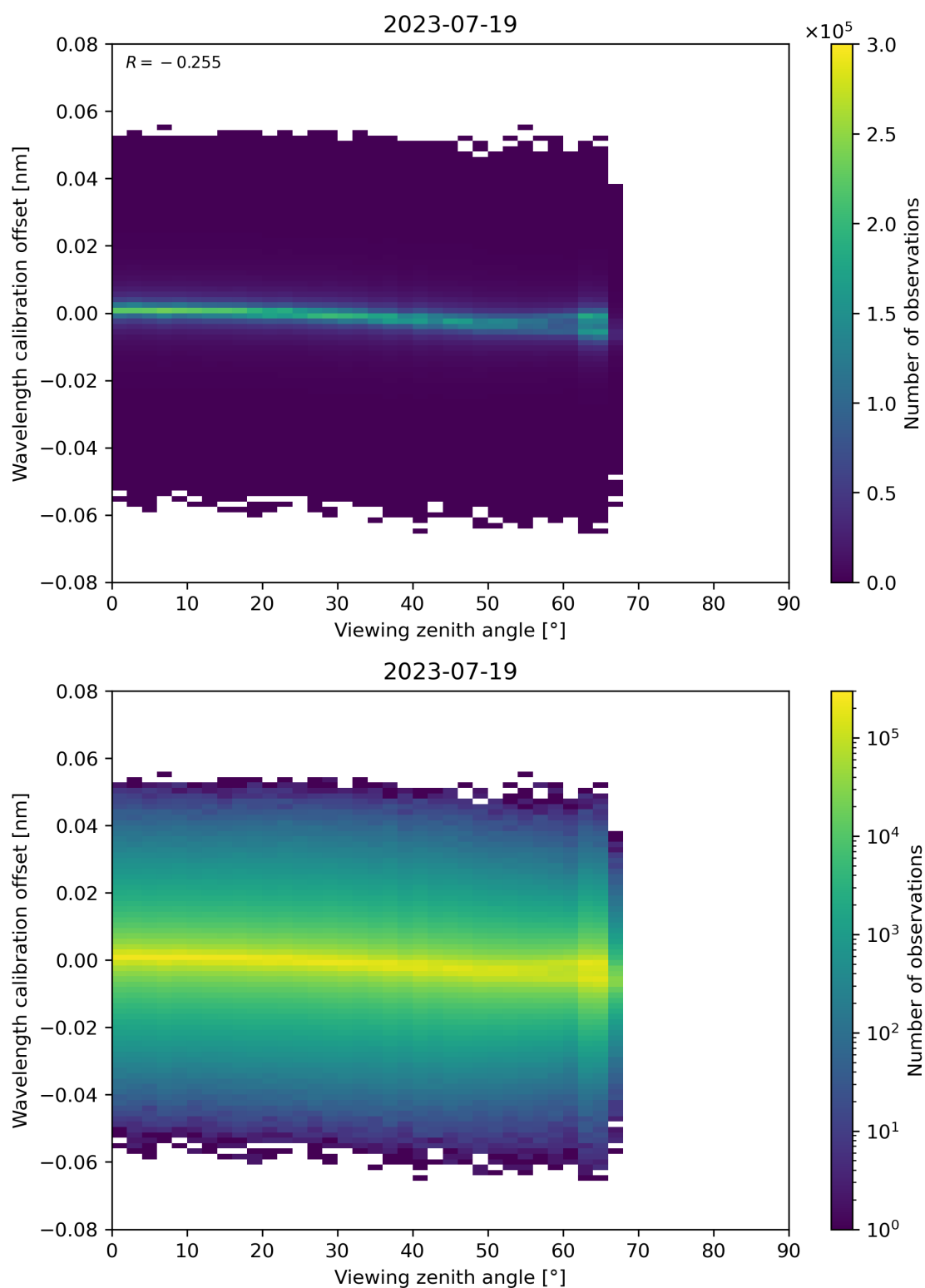
Figure 173: Scatter density plot of “Viewing zenith angle” against “Wavelength calibration offset” for 2023-07-19 to 2023-07-20.
