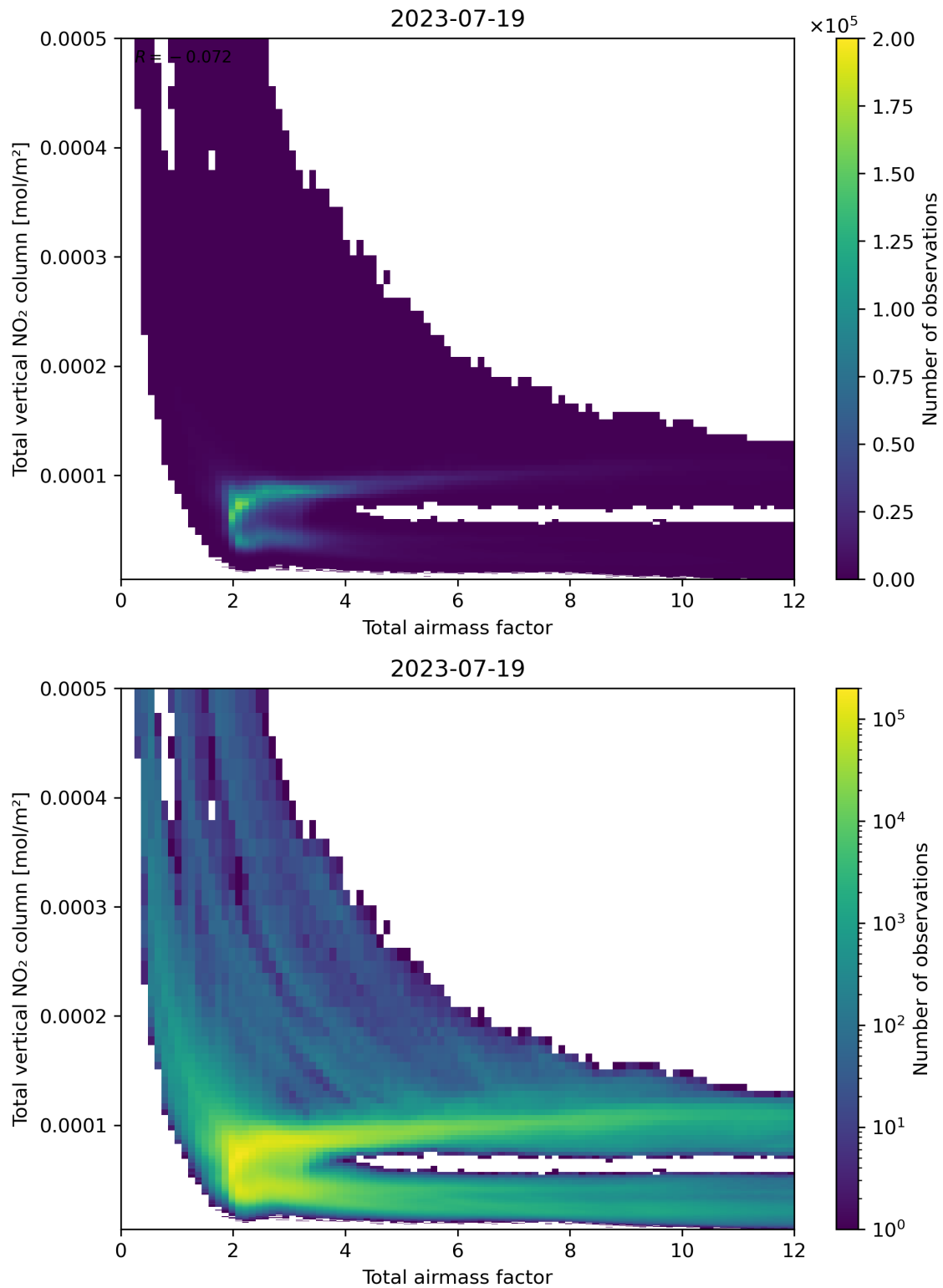
Figure 67: Scatter density plot of “Total airmass factor” against “Total vertical NO 2 column” for 2023-07-19 to 2023-07-20.
