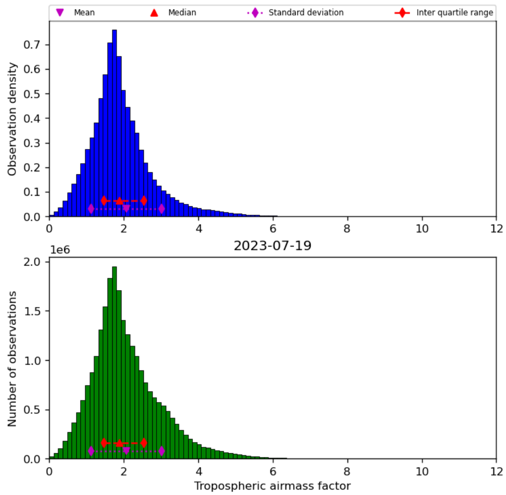
Figure 31: Histogram of “Tropospheric airmass factor” for 2023-07-19 to 2023-07-20
