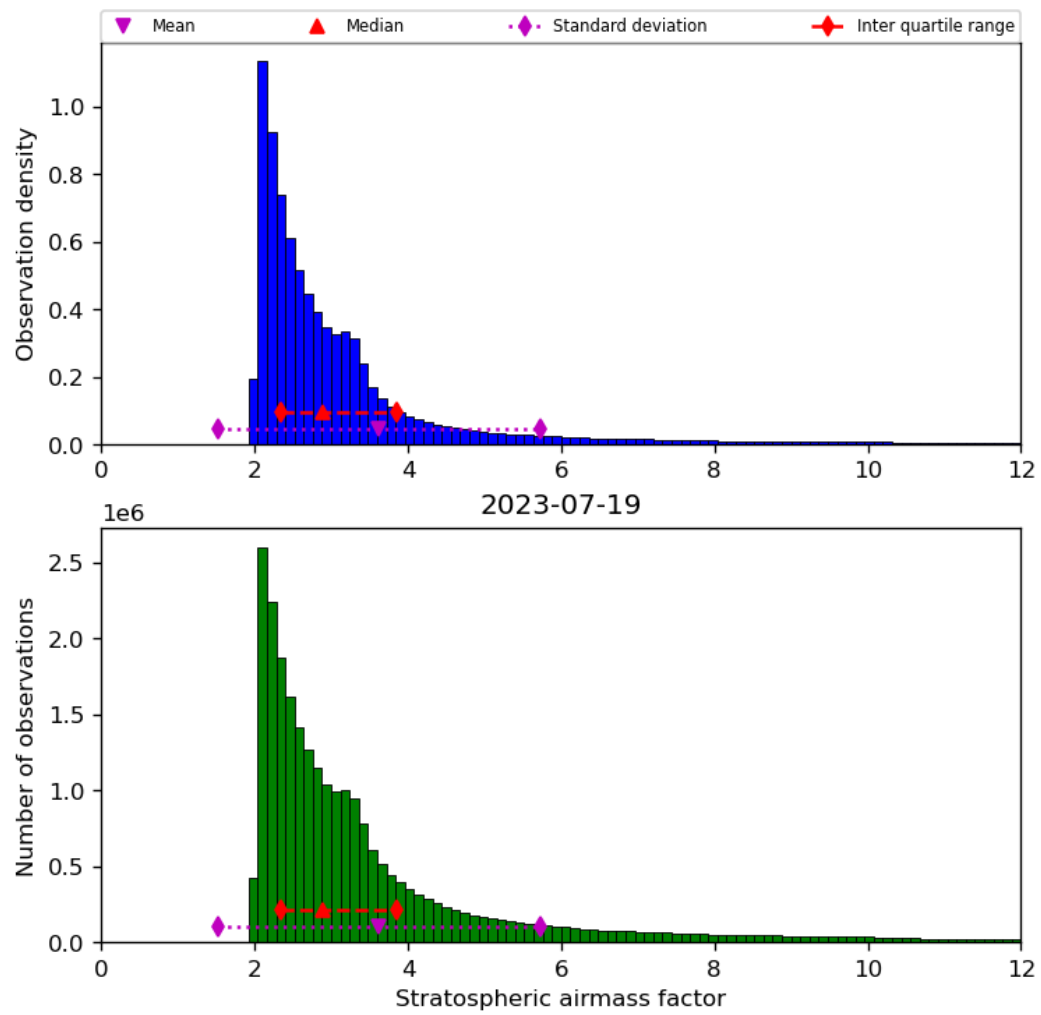
Figure 44: Histogram of “Stratospheric airmass factor” for 2023-07-19 to 2023-07-20
