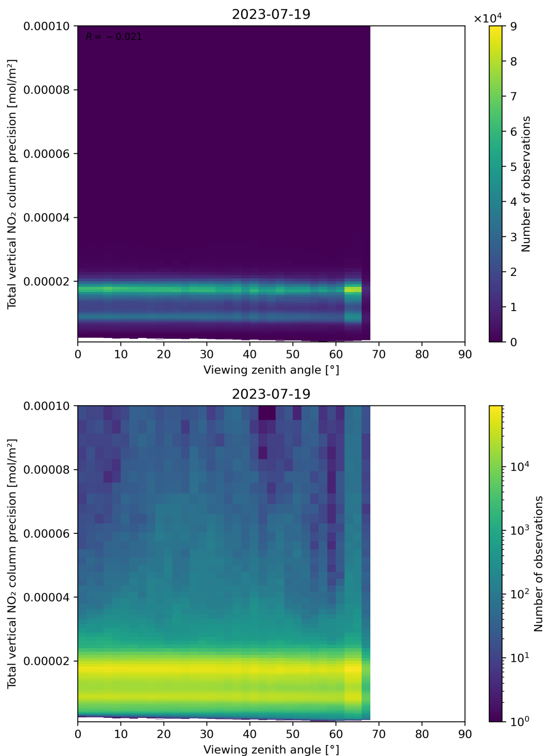
Figure 168: Scatter density plot of “Viewing zenith angle” against “Total vertical NO 2 column precision” for 2023-07-19 to 2023-07-20.
