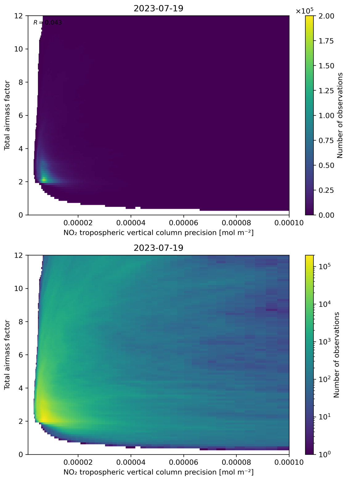
Figure 132: Scatter density plot of “NO 2 tropospheric vertical column precision” against “Total air mass factor” for 2023-07-19 to 2023-07-20.
