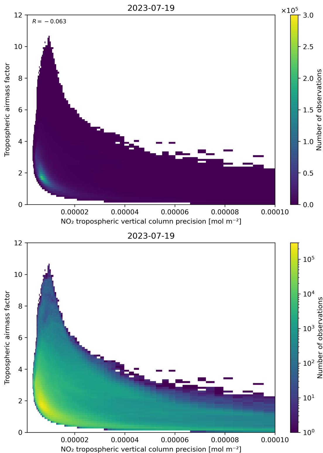
Figure 133: Scatter density plot of “NO 2 tropospheric vertical column precision” against “Tropospheric airmass factor” for 2023-07-19 to 2023-07-20.
