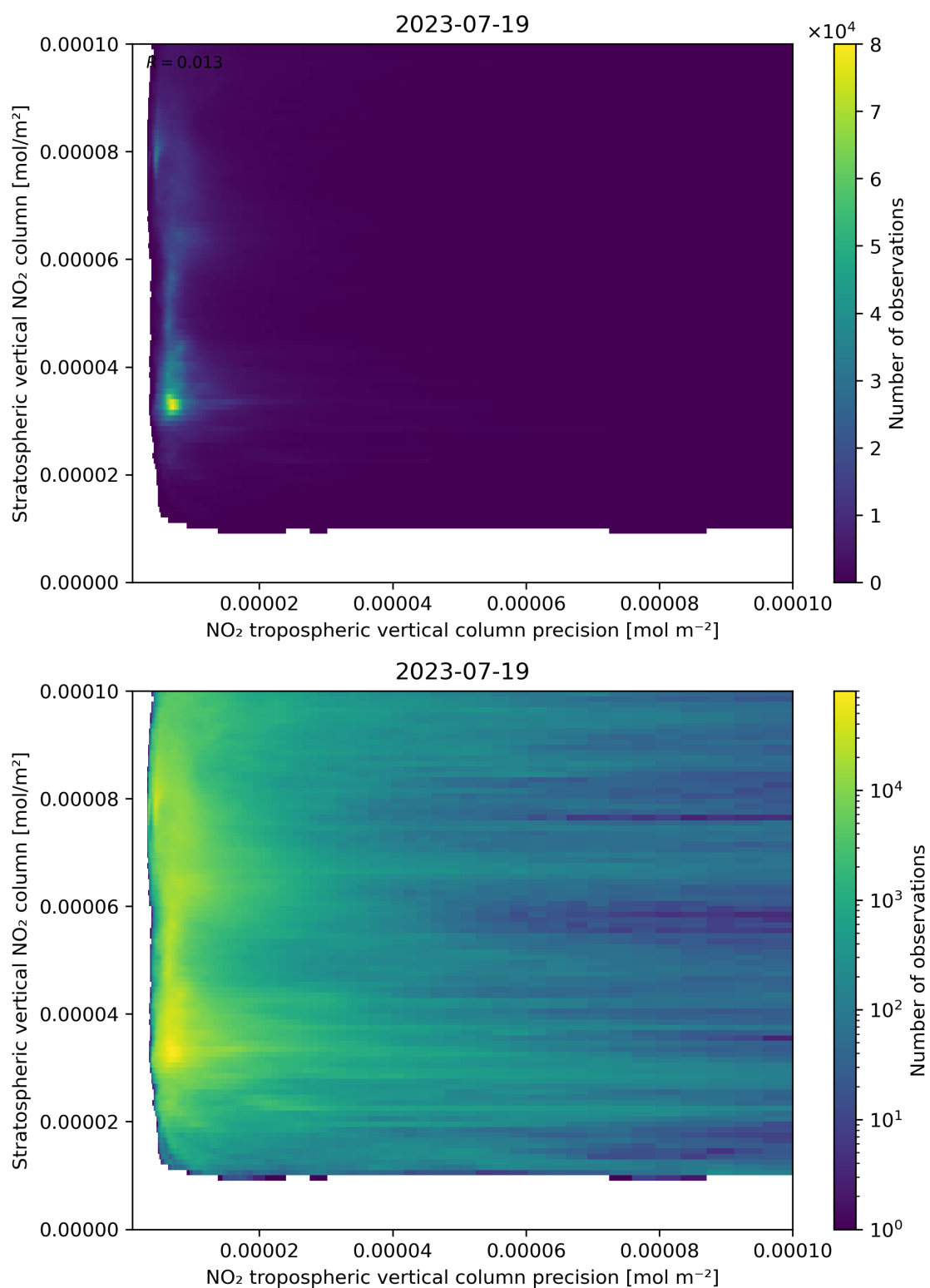
Figure 135: Scatter density plot of “NO 2 tropospheric vertical column precision” against “Stratospheric vertical NO 2 column” for 2023-07-19 to 2023-07-20.
