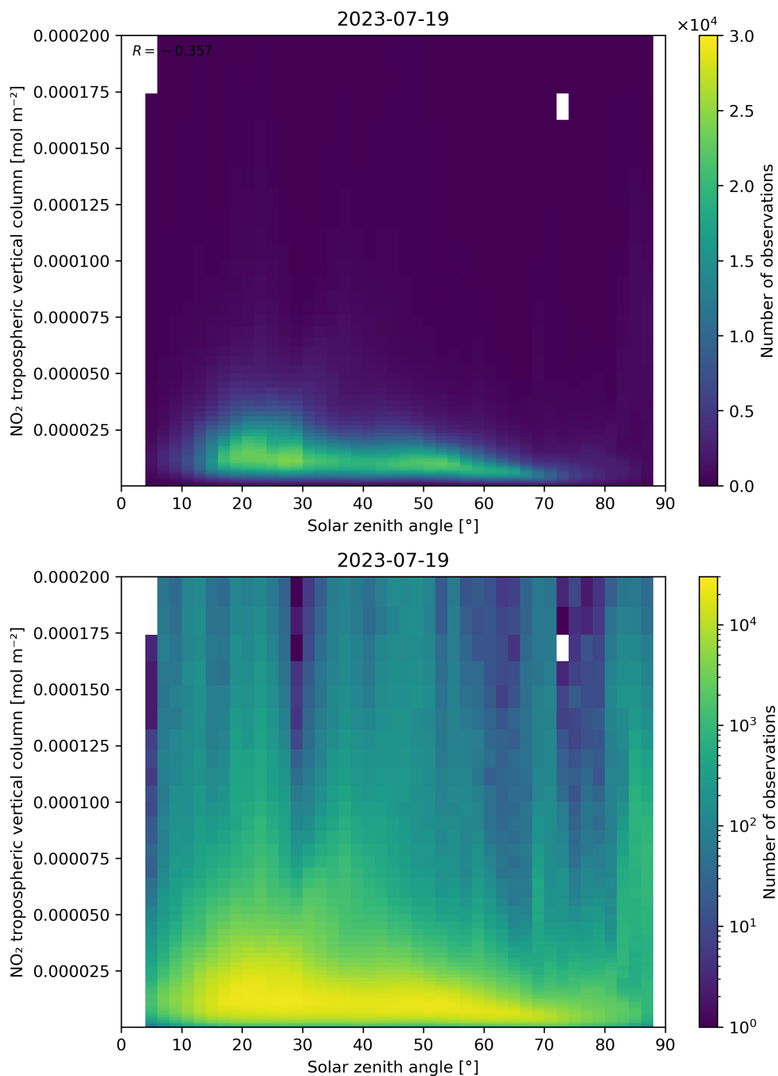
Figure 155: Scatter density plot of “Solar zenith angle” against “NO 2 tropospheric vertical column” for 2023-07-19 to 2023-07-20.
