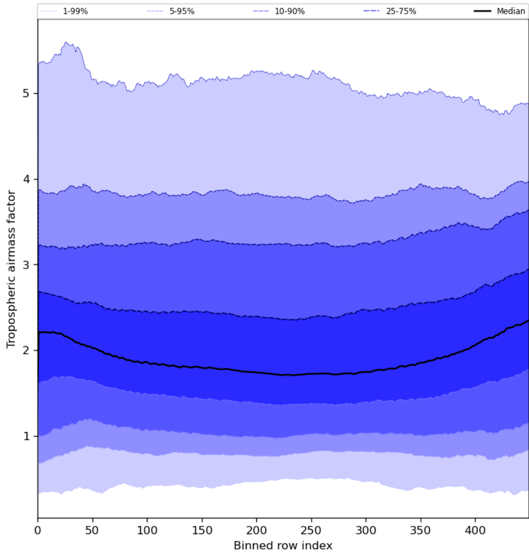
Figure 48: Along track statistics of “Tropospheric airmass factor” for 2023-07-19 to 2023-07-20
