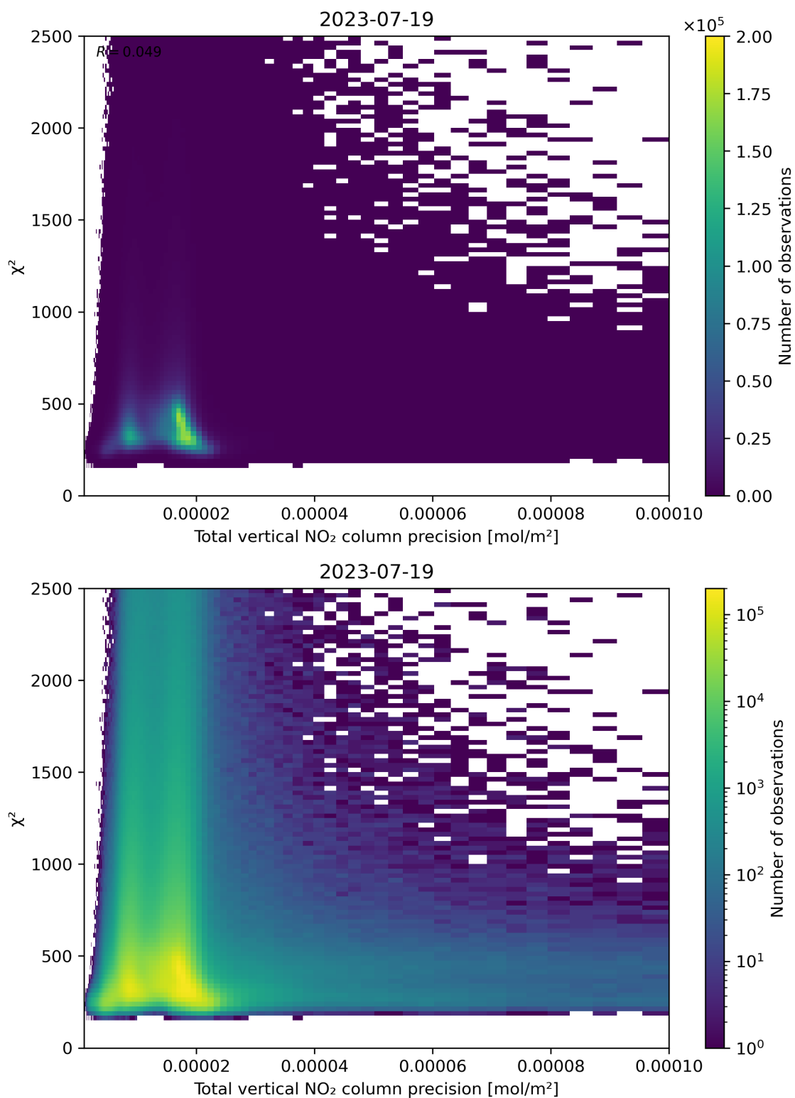
Figure 116: Scatter density plot of “Total vertical NO 2 column precision” against “ \chi^2 ” for 2023-07-19 to 2023-07-20.
