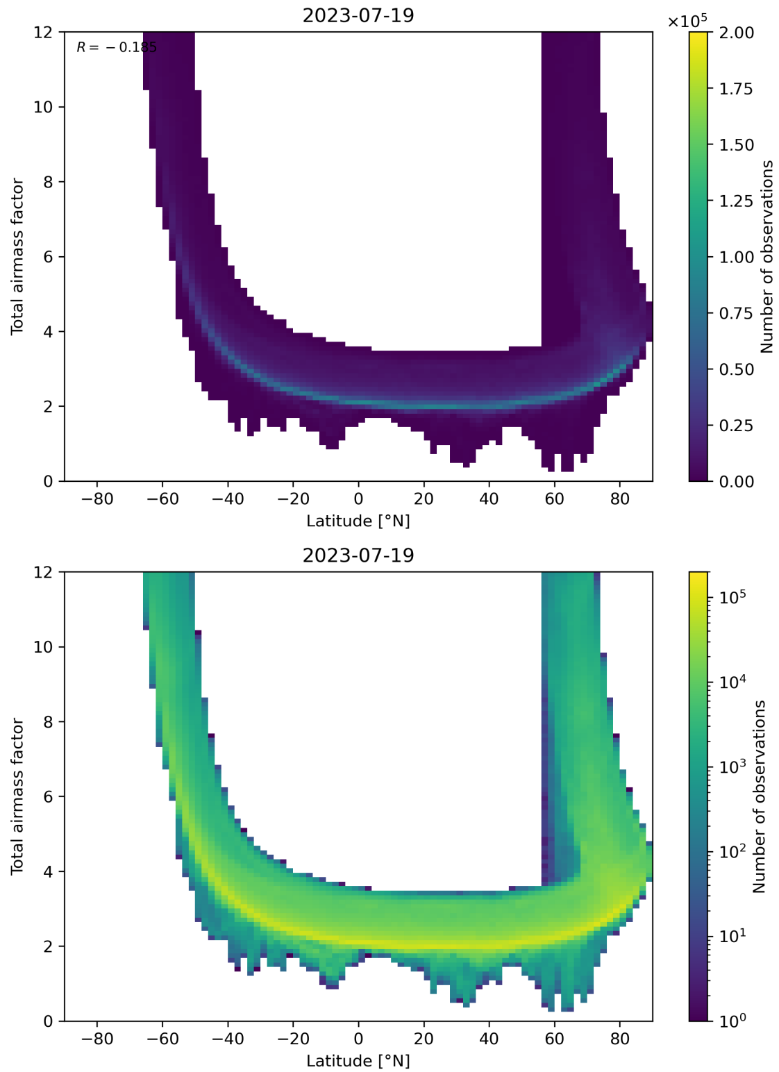
Figure 84: Scatter density plot of “Latitude” against “Total airmass factor” for 2023-07-19 to 2023-07-20.
