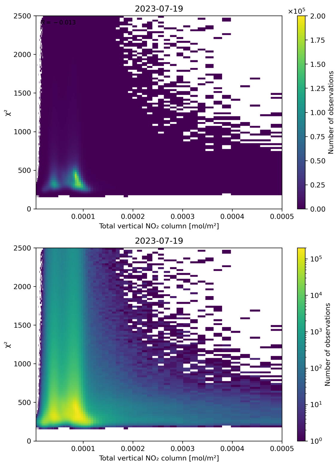
Figure 111: Scatter density plot of “Total vertical NO 2 column” against “ \chi^2 ” for 2023-07-19 to 2023-07-20.
