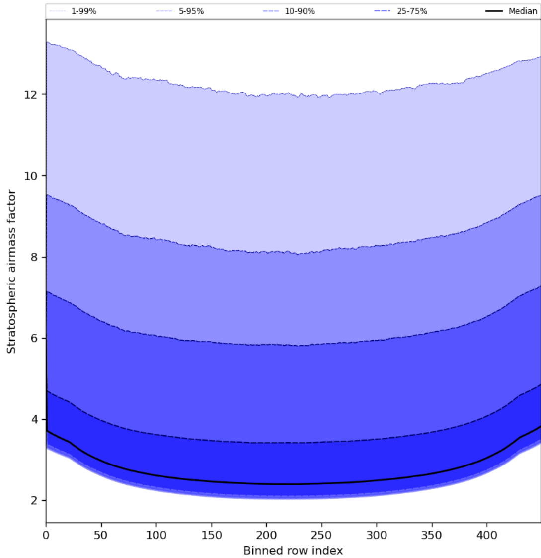
Figure 61: Along track statistics of “Stratospheric airmass factor” for 2023-07-19 to 2023-07-20
