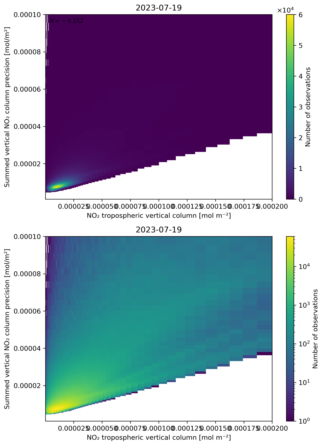
Figure 127: Scatter density plot of “NO 2 tropospheric vertical column” against “Summed vertical NO 2 column precision” for 2023-07-19 to 2023-07-20.
