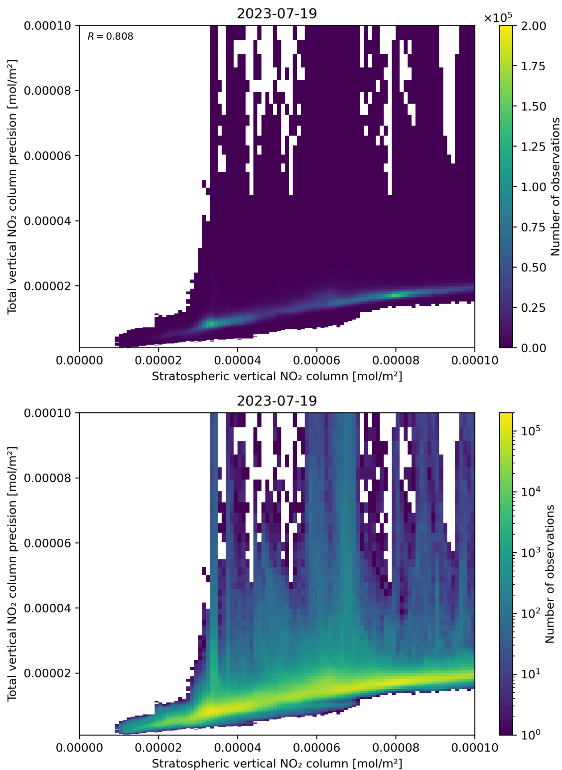
Figure 101: Scatter density plot of “Stratospheric vertical NO 2 column” against “Total vertical NO 2 column precision” for 2023-07-19 to 2023-07-20.
