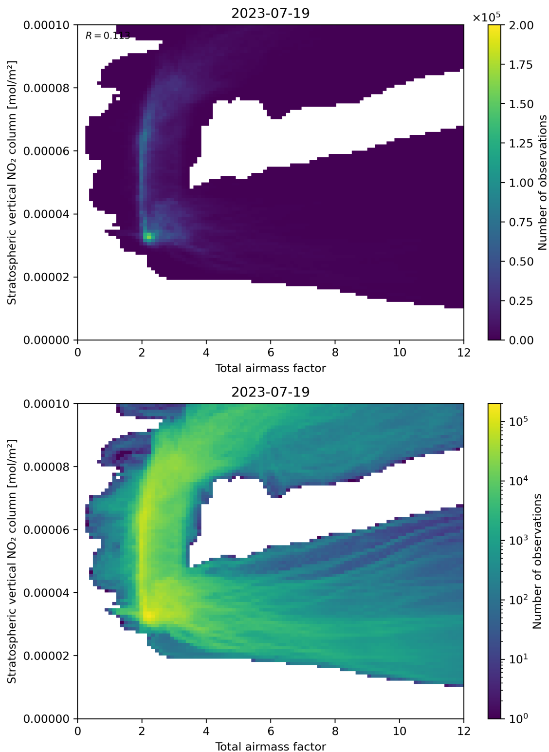
Figure 64: Scatter density plot of “Total airmass factor” against “Stratospheric vertical NO 2 column” for 2023-07-19 to 2023-07-20.
