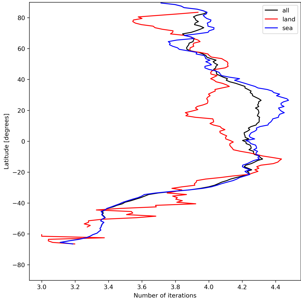
Figure 17: Zonal average of “Number of iterations” for 2023-07-19 to 2023-07-20.
