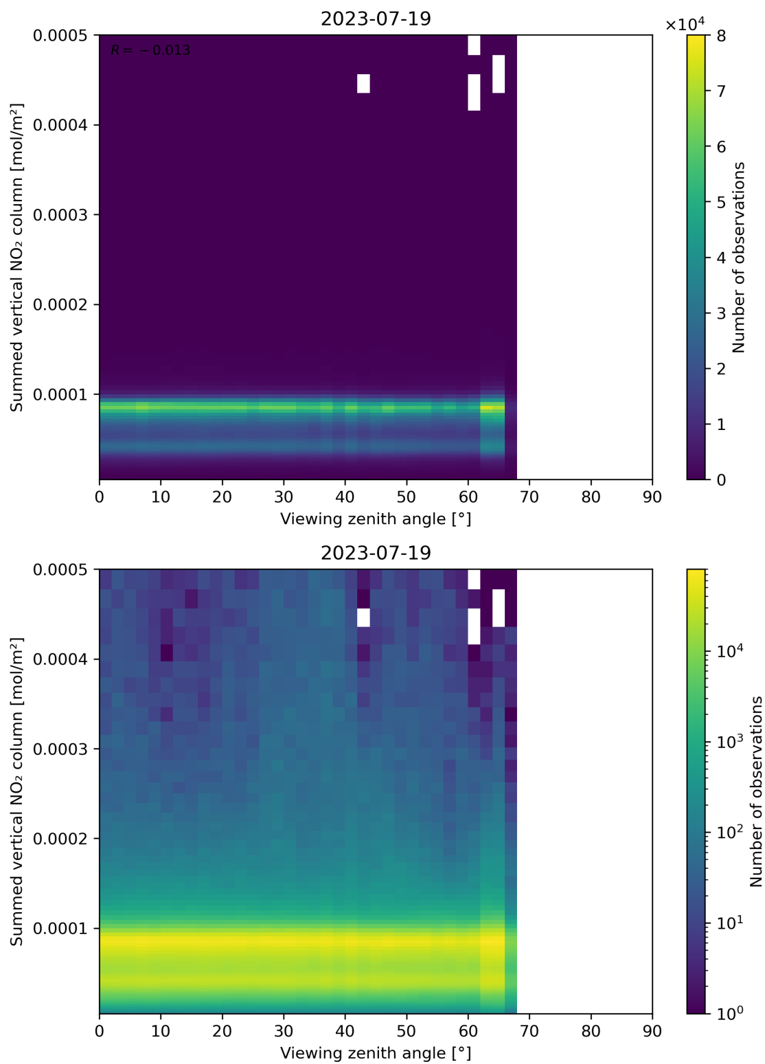
Figure 165: Scatter density plot of “Viewing zenith angle” against “Summed vertical NO 2 column” for 2023-07-19 to 2023-07-20.
