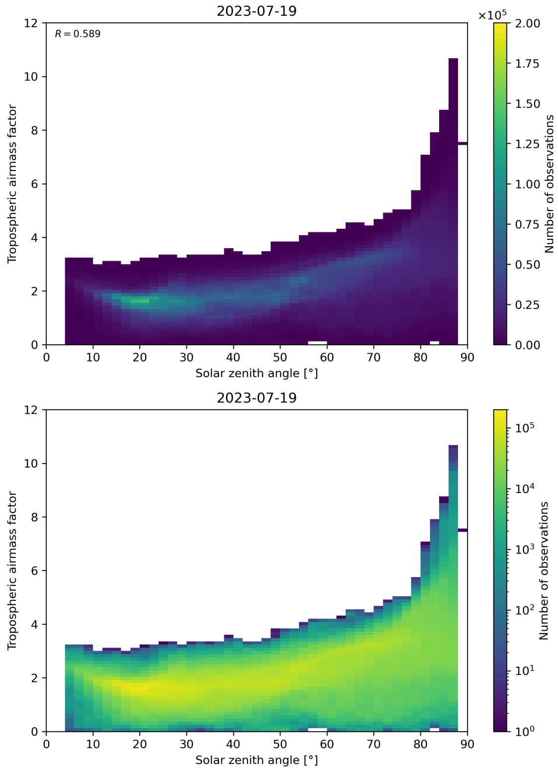
Figure 147: Scatter density plot of “Solar zenith angle” against “Tropospheric airmass factor” for 2023-07-19 to 2023-07-20.
