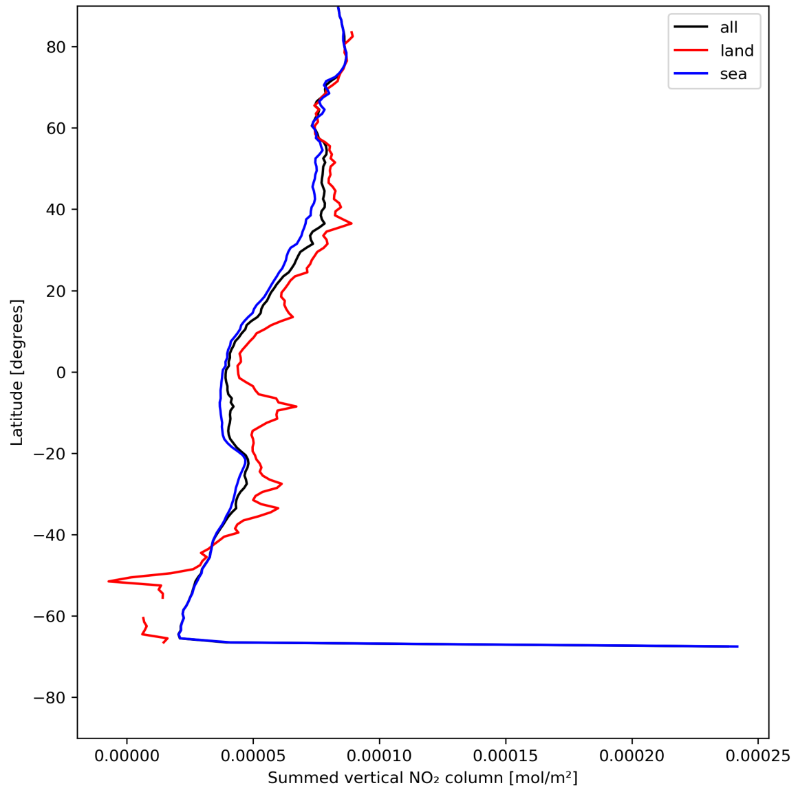
Figure 23: Zonal average of “Summed vertical NO 2 column” for 2023-07-19 to 2023-07-21.
