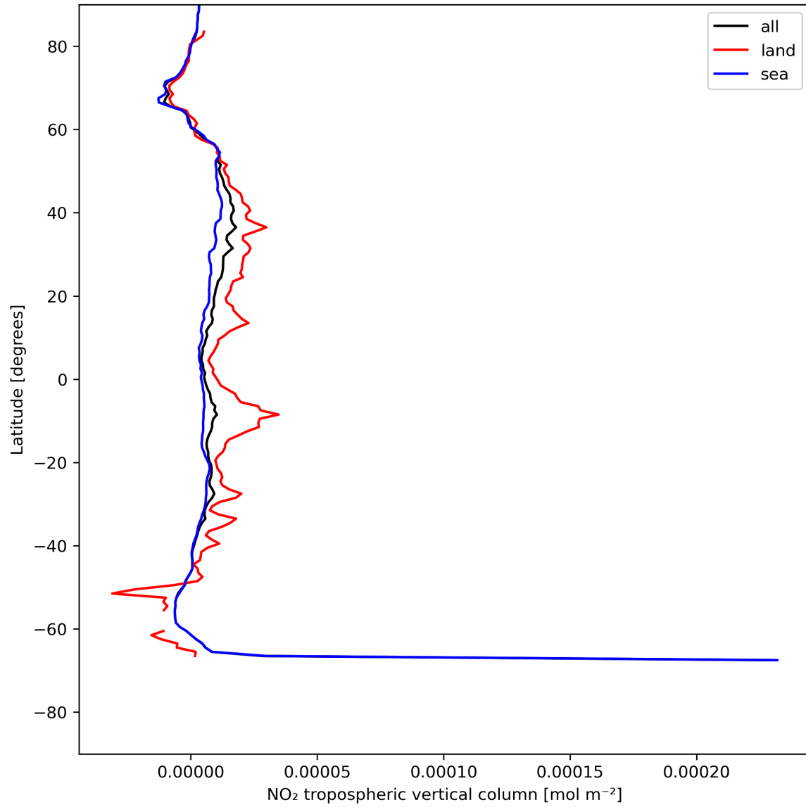
Figure 12: Zonal average of “NO 2 tropospheric vertical column” for 2023-07-19 to 2023-07-21.
