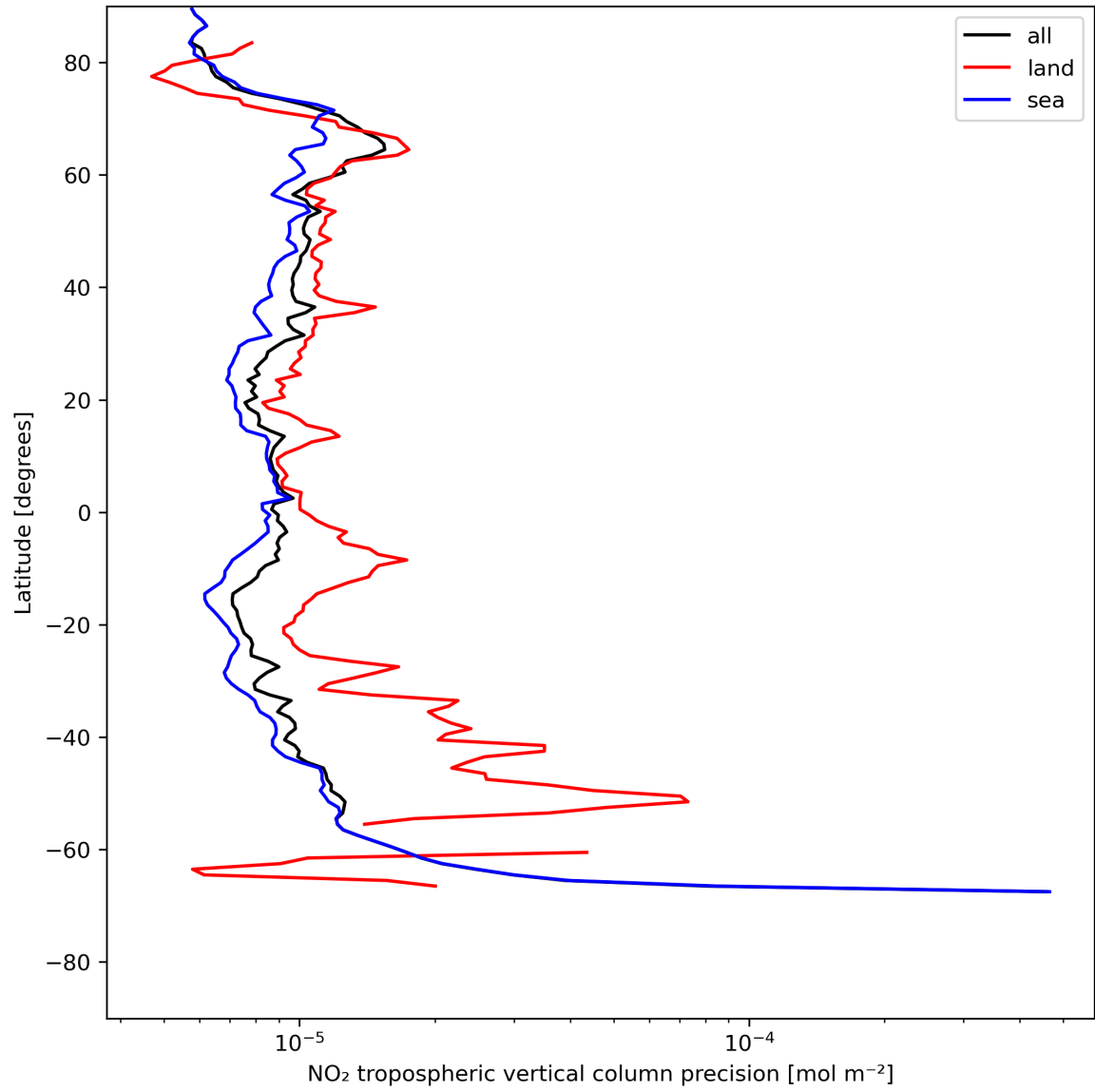
Figure 13: Zonal average of “NO 2 tropospheric vertical column precision” for 2023-07-19 to 2023-07-21.
