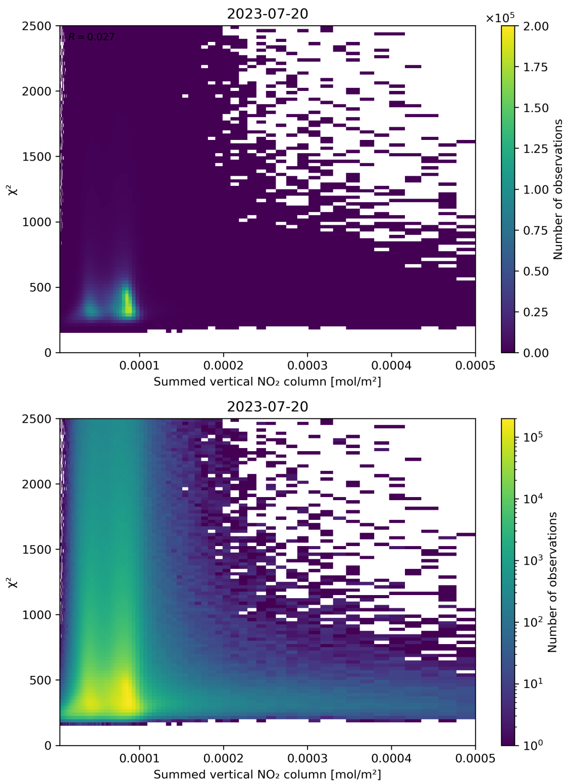
Figure 104: Scatter density plot of “Summed vertical NO 2 column” against “ \chi^2 ” for 2023-07-19 to 2023-07-21.
