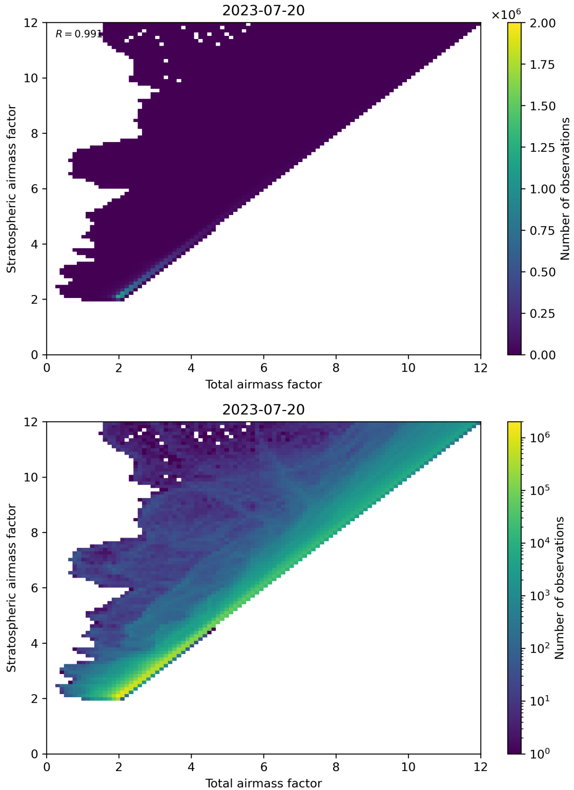
Figure 62: Scatter density plot of “Total airmass factor” against “Stratospheric airmass factor” for 2023-07-19 to 2023-07-21.
