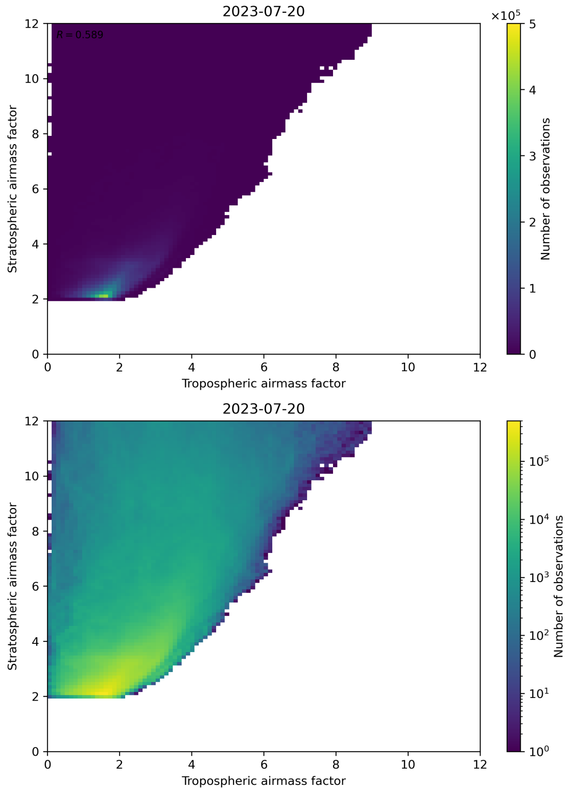
Figure 71: Scatter density plot of “Tropospheric airmass factor” against “Stratospheric airmass factor” for 2023-07-19 to 2023-07-21.
