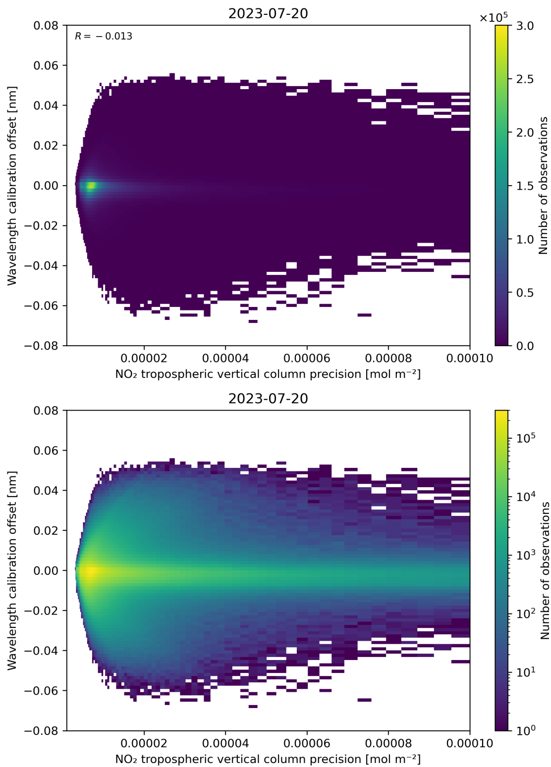
Figure 141: Scatter density plot of “NO 2 tropospheric vertical column precision” against “Wavelength calibration offset” for 2023-07-19 to 2023-07-21.
