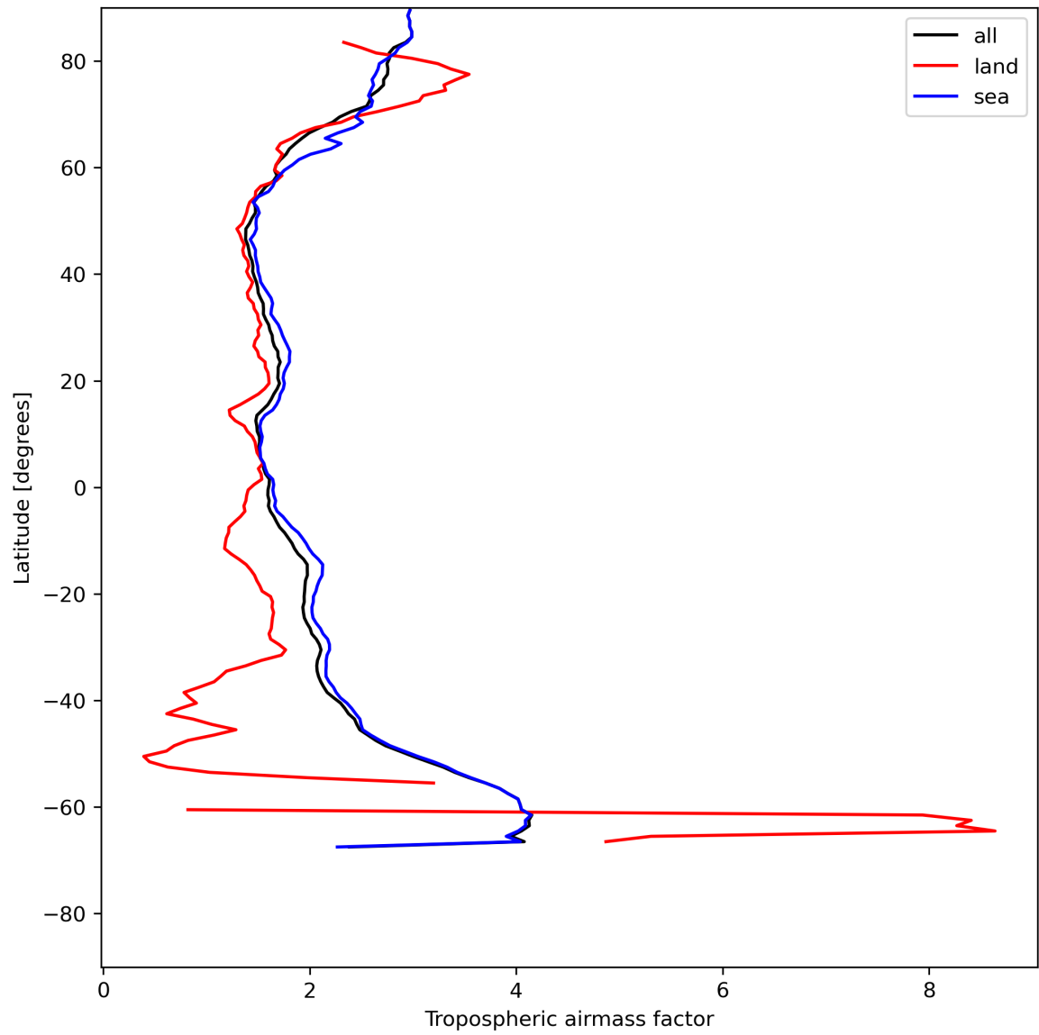
Figure 14: Zonal average of “Tropospheric airmass factor” for 2023-07-19 to 2023-07-21.
