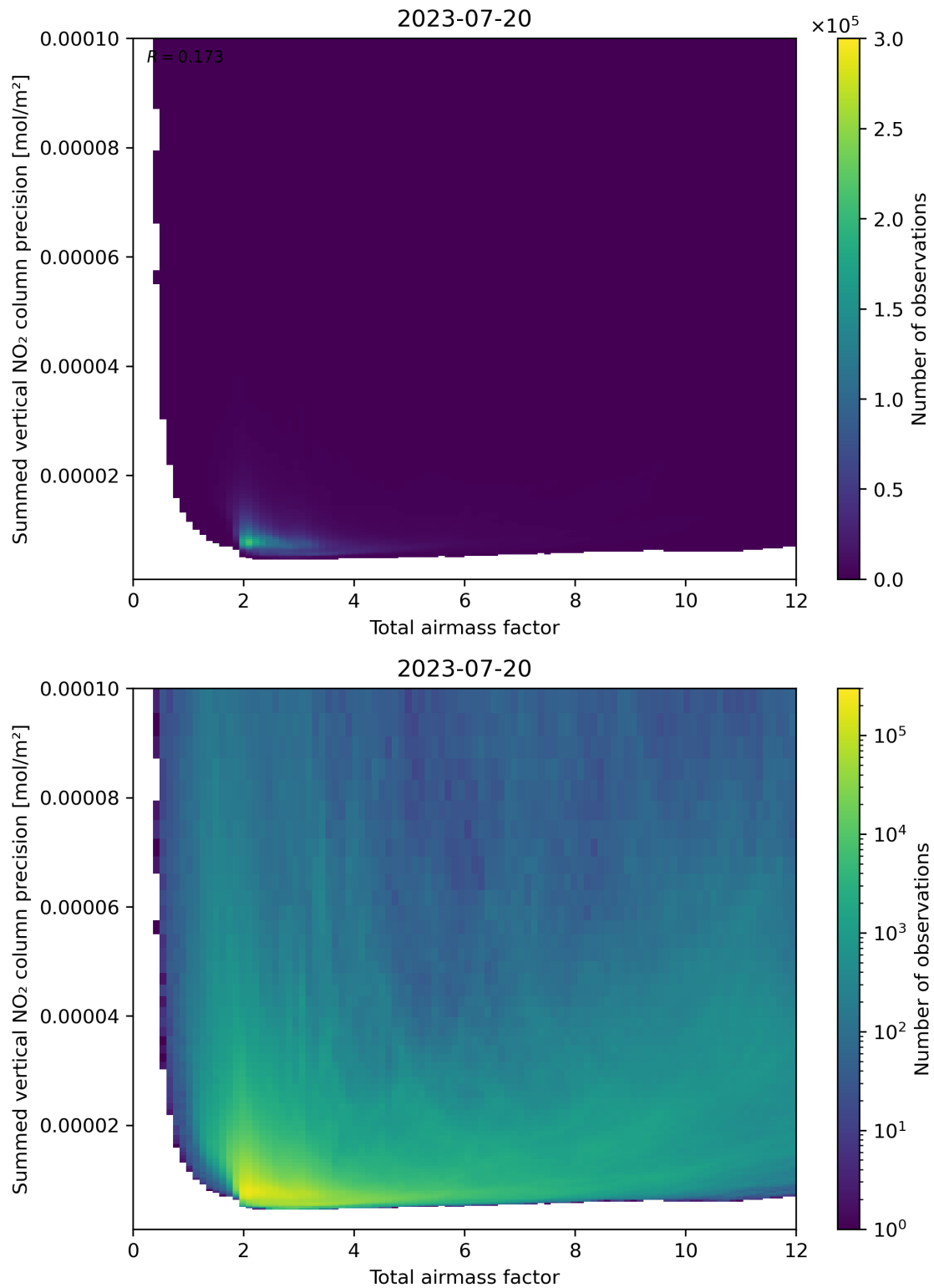
Figure 66: Scatter density plot of “Total airmass factor” against “Summed vertical NO 2 column precision” for 2023-07-19 to 2023-07-21.
