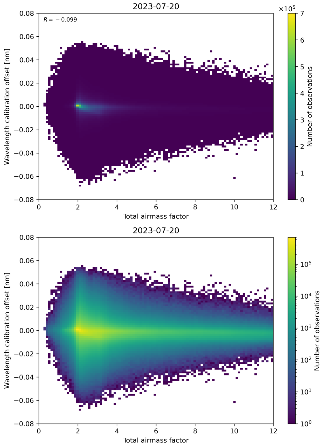
Figure 70: Scatter density plot of “Total airmass factor” against “Wavelength calibration offset” for 2023-07-19 to 2023-07-21.
