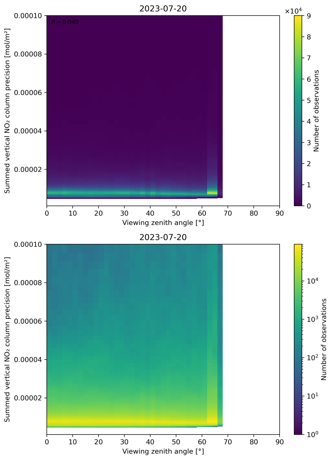
Figure 166: Scatter density plot of “Viewing zenith angle” against “Summed vertical NO 2 column precision” for 2023-07-19 to 2023-07-21.
