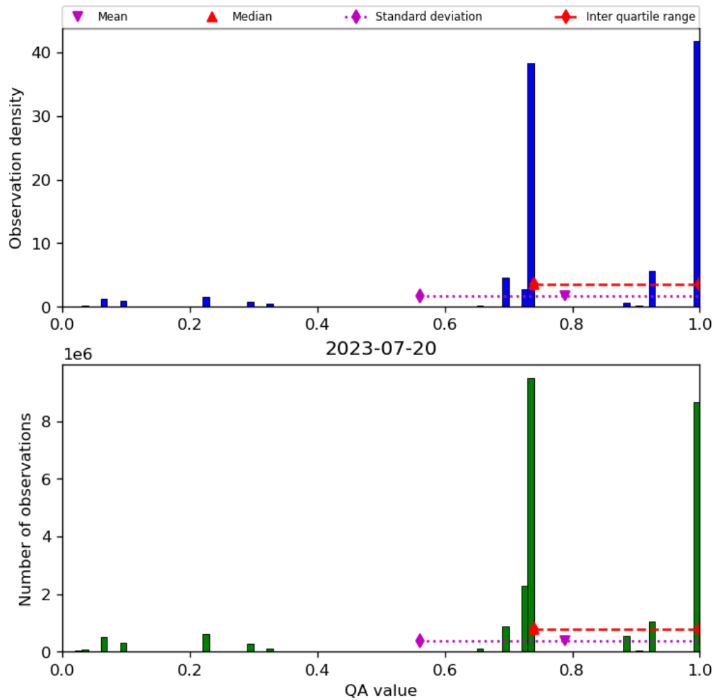
Figure 28: Histogram of “QA value” for 2023-07-19 to 2023-07-21
