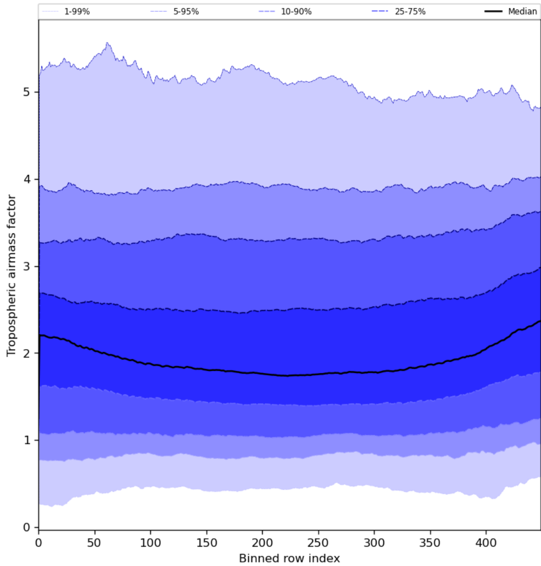
Figure 48: Along track statistics of “Tropospheric airmass factor” for 2023-07-19 to 2023-07-21
