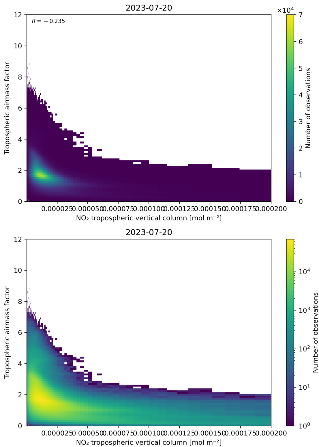
Figure 123: Scatter density plot of “NO 2 tropospheric vertical column” against “Tropospheric air mass factor” for 2023-07-19 to 2023-07-21.
