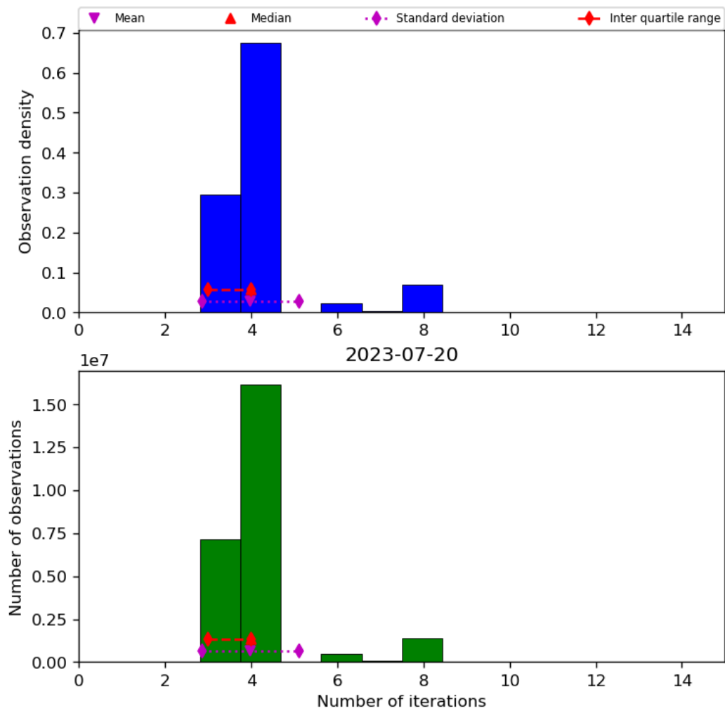
Figure 34: Histogram of “Number of iterations” for 2023-07-19 to 2023-07-21
