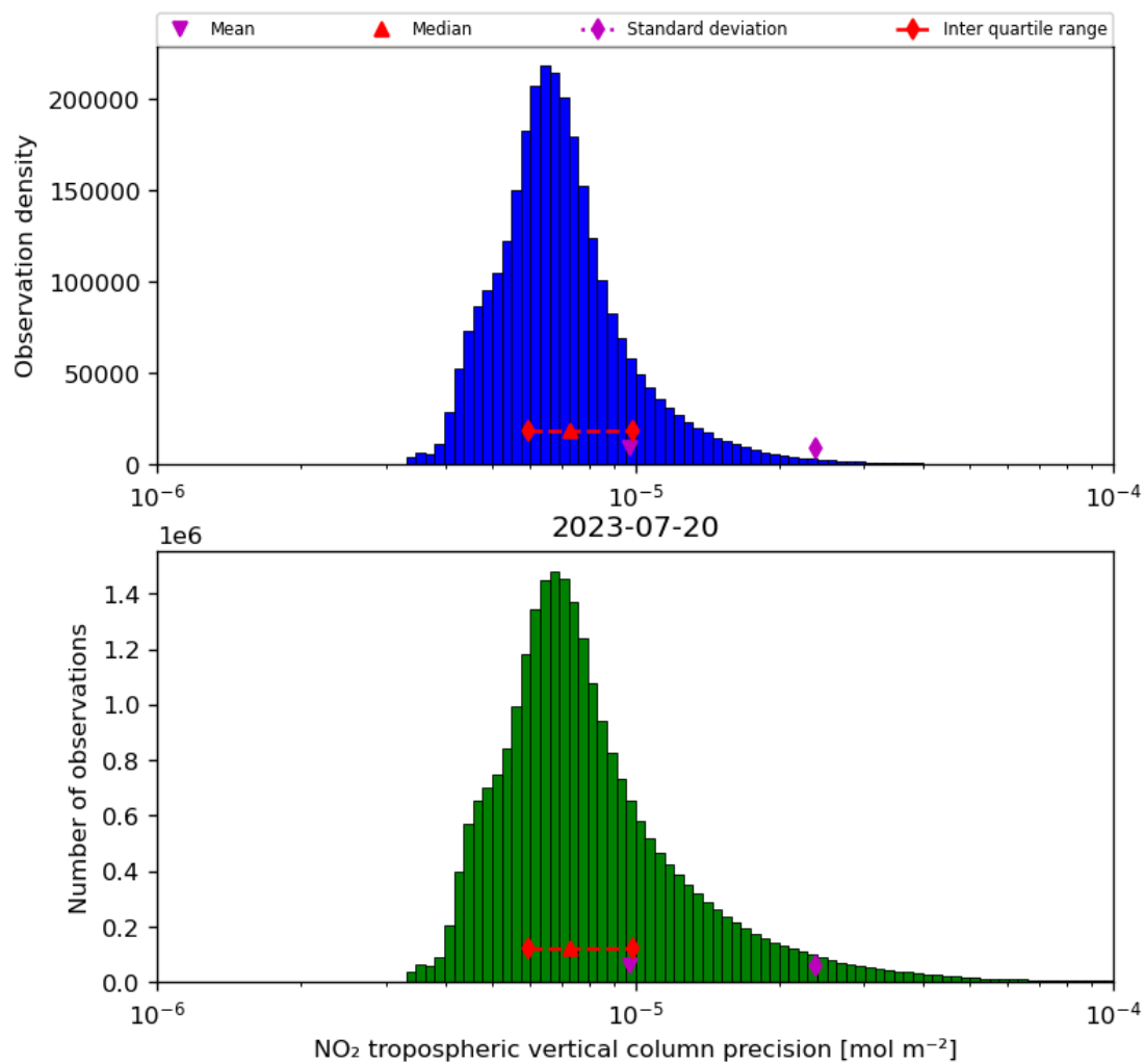
Figure 30: Histogram of “NO 2 tropospheric vertical column precision” for 2023-07-19 to 2023-07-21
