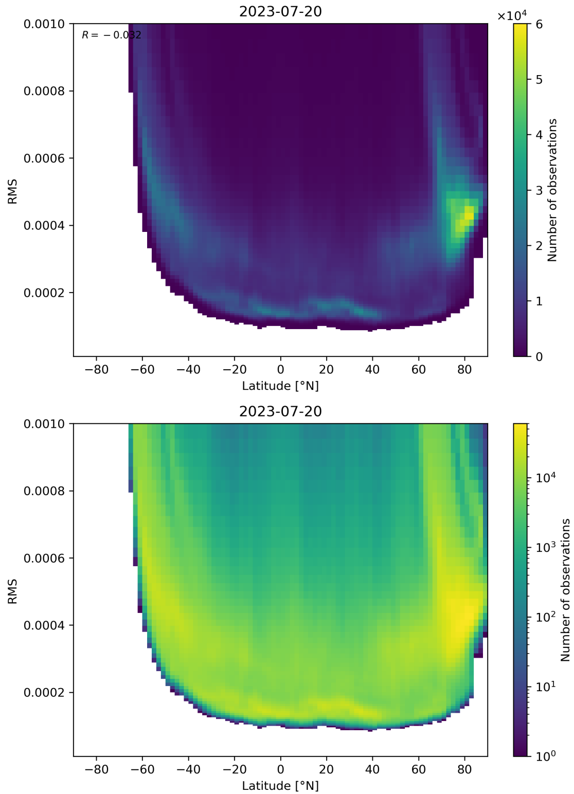
Figure 94: Scatter density plot of “Latitude” against “RMS” for 2023-07-19 to 2023-07-21.
