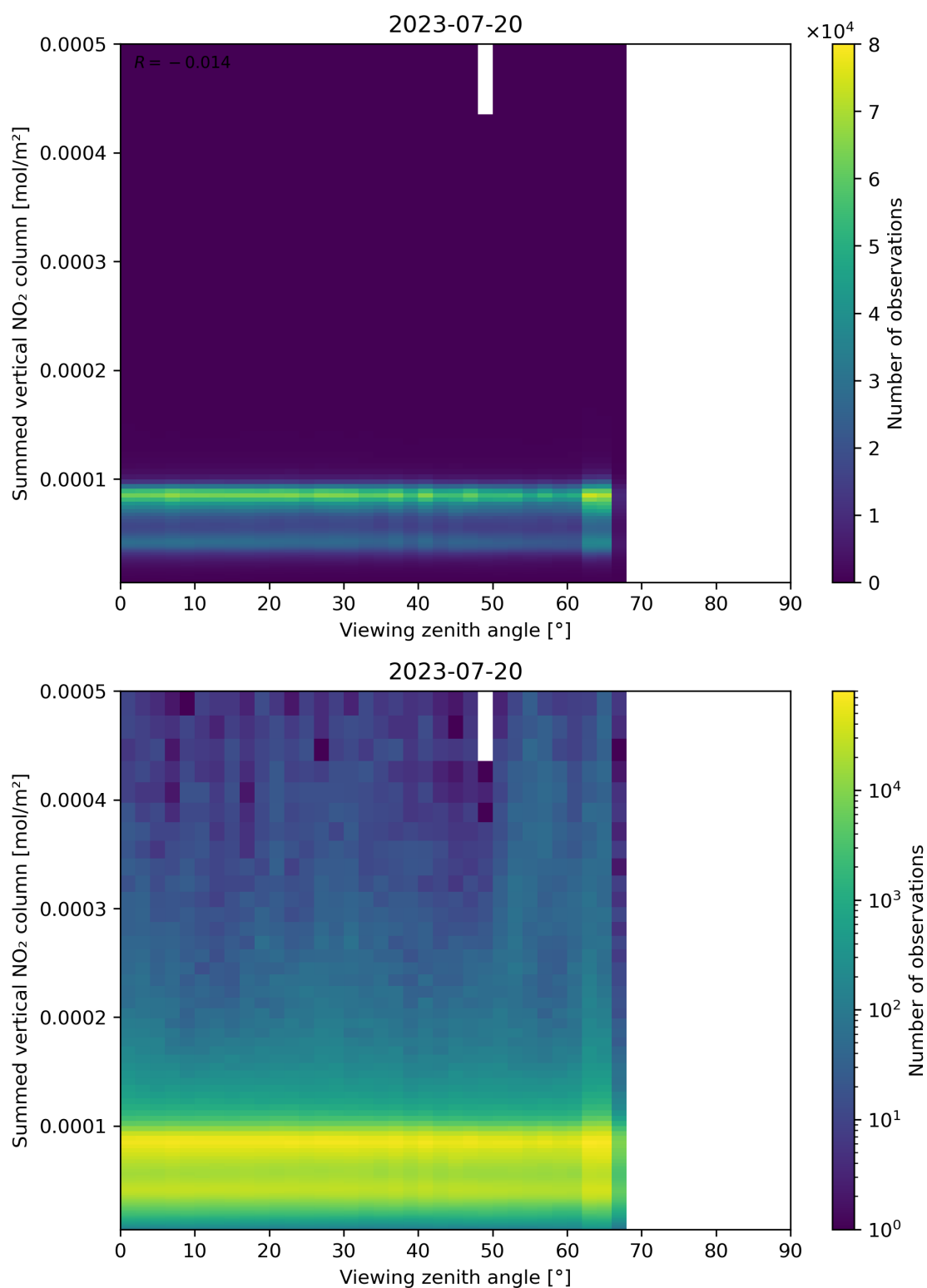
Figure 165: Scatter density plot of “Viewing zenith angle” against “Summed vertical NO 2 column” for 2023-07-19 to 2023-07-21.
