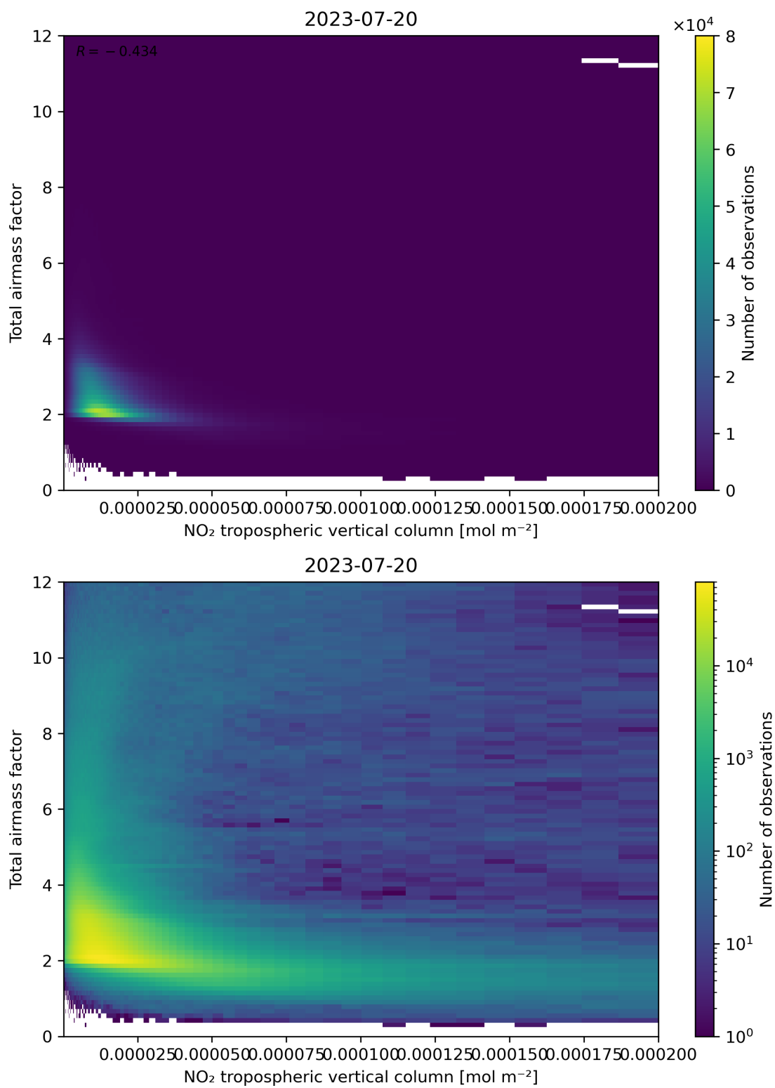
Figure 122: Scatter density plot of “NO 2 tropospheric vertical column” against “Total air mass factor” for 2023-07-19 to 2023-07-21.
