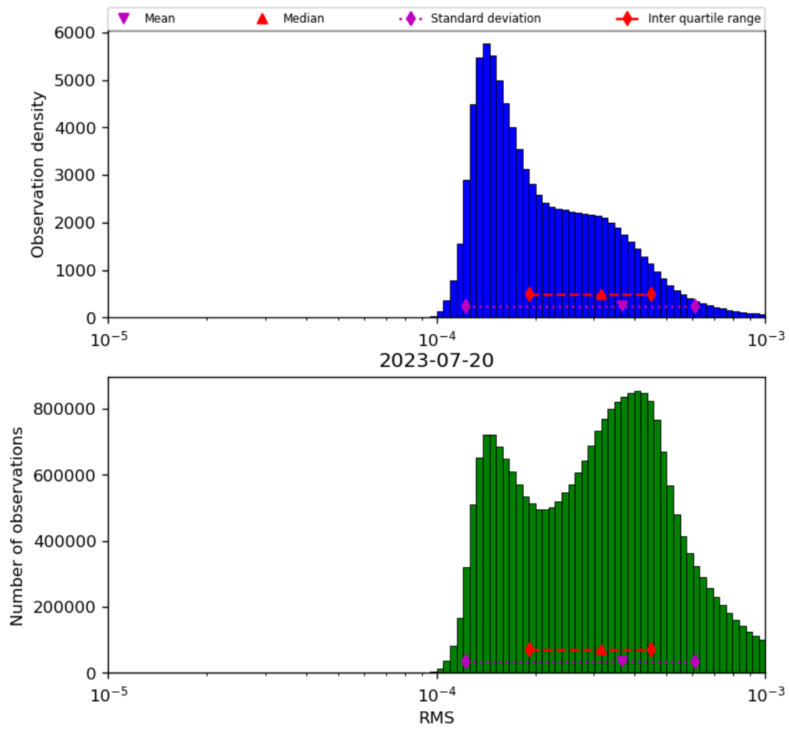
Figure 43: Histogram of “RMS” for 2023-07-19 to 2023-07-21
