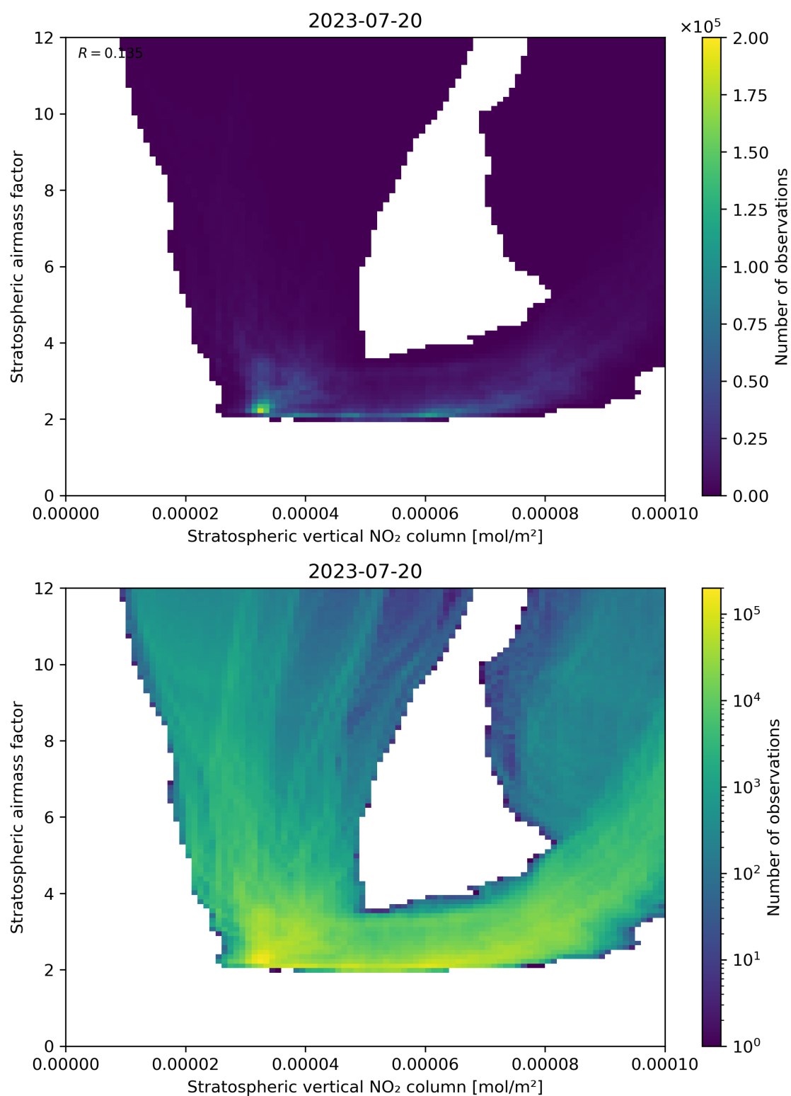
Figure 96: Scatter density plot of “Stratospheric vertical NO 2 column” against “Stratospheric airmass factor” for 2023-07-19 to 2023-07-21.
