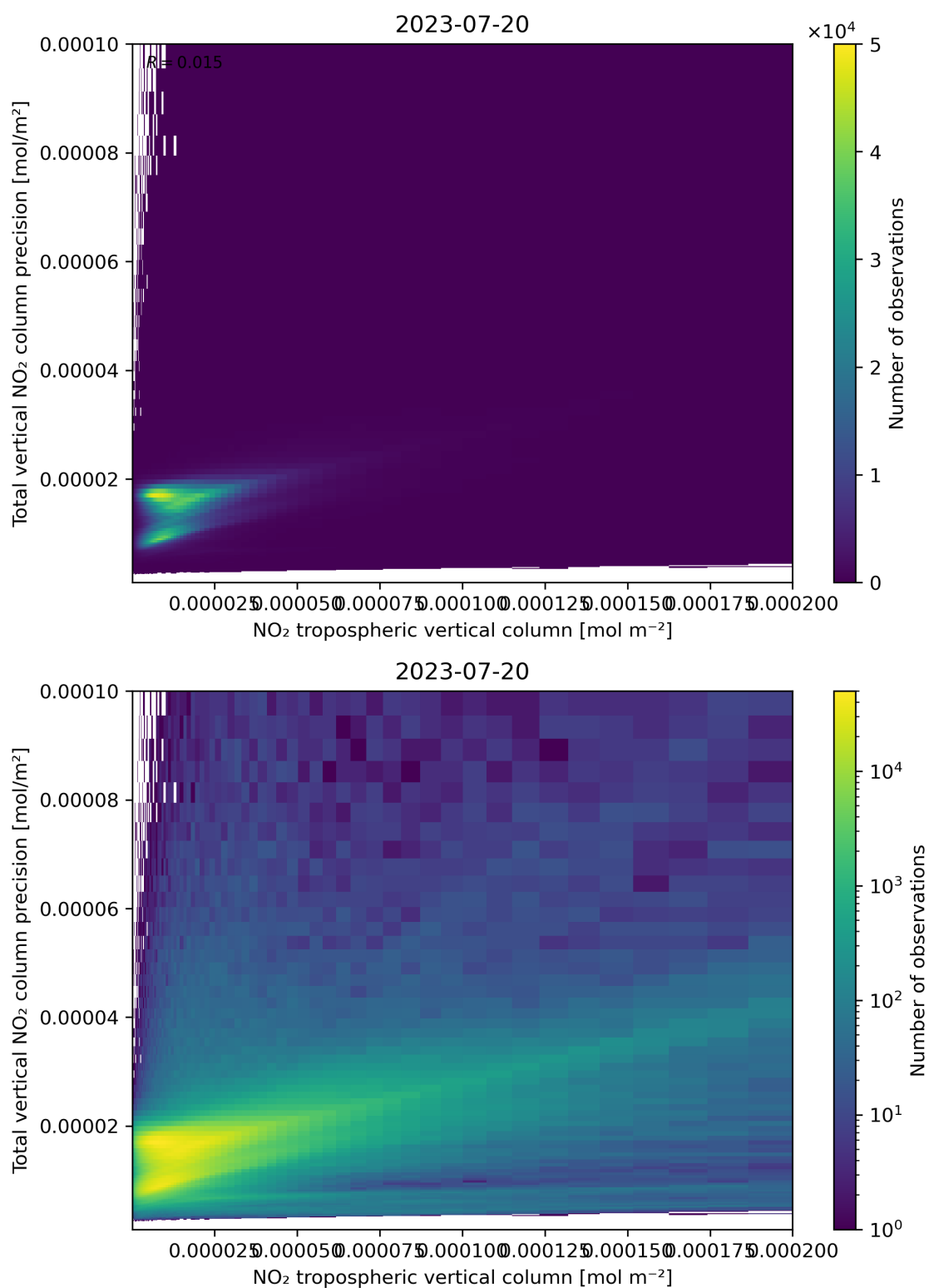
Figure 129: Scatter density plot of “NO 2 tropospheric vertical column” against “Total vertical NO 2 column precision” for 2023-07-19 to 2023-07-21.
