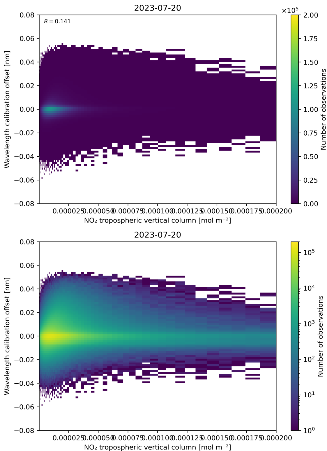
Figure 143: Scatter density plot of “NO 2 tropospheric vertical column” against “Wavelength calibration offset” for 2023-07-19 to 2023-07-21.
