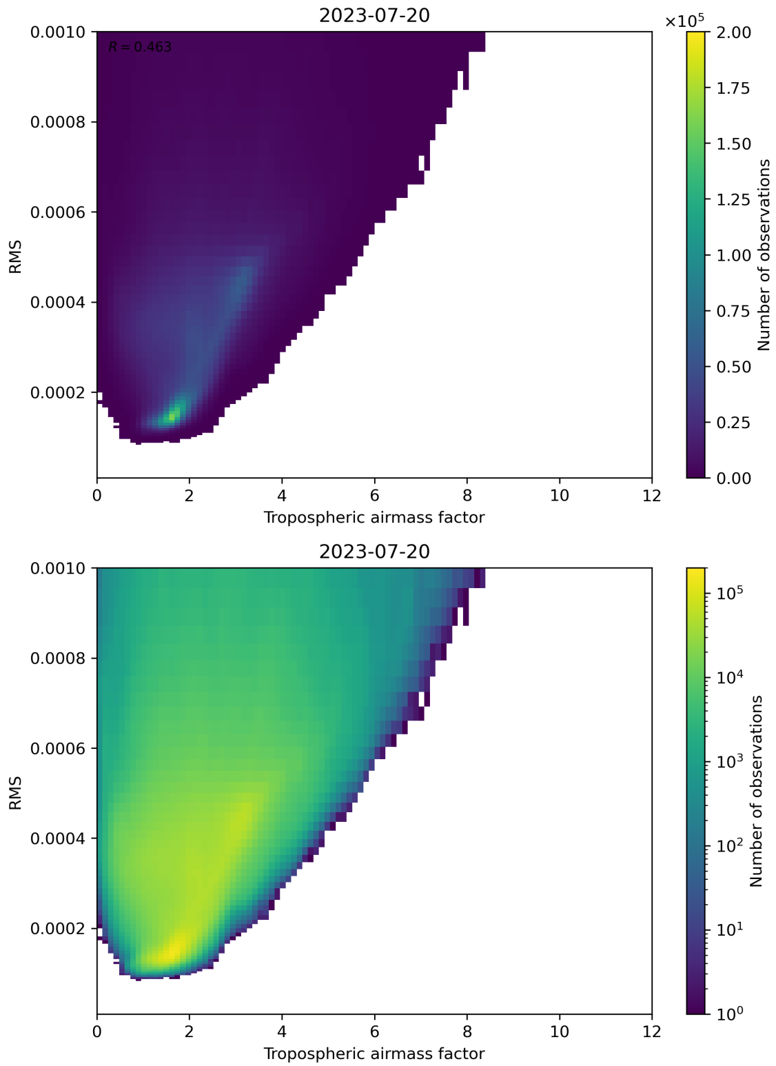
Figure 79: Scatter density plot of “Tropospheric airmass factor” against “RMS” for 2023-07-19 to 2023-07-21.
