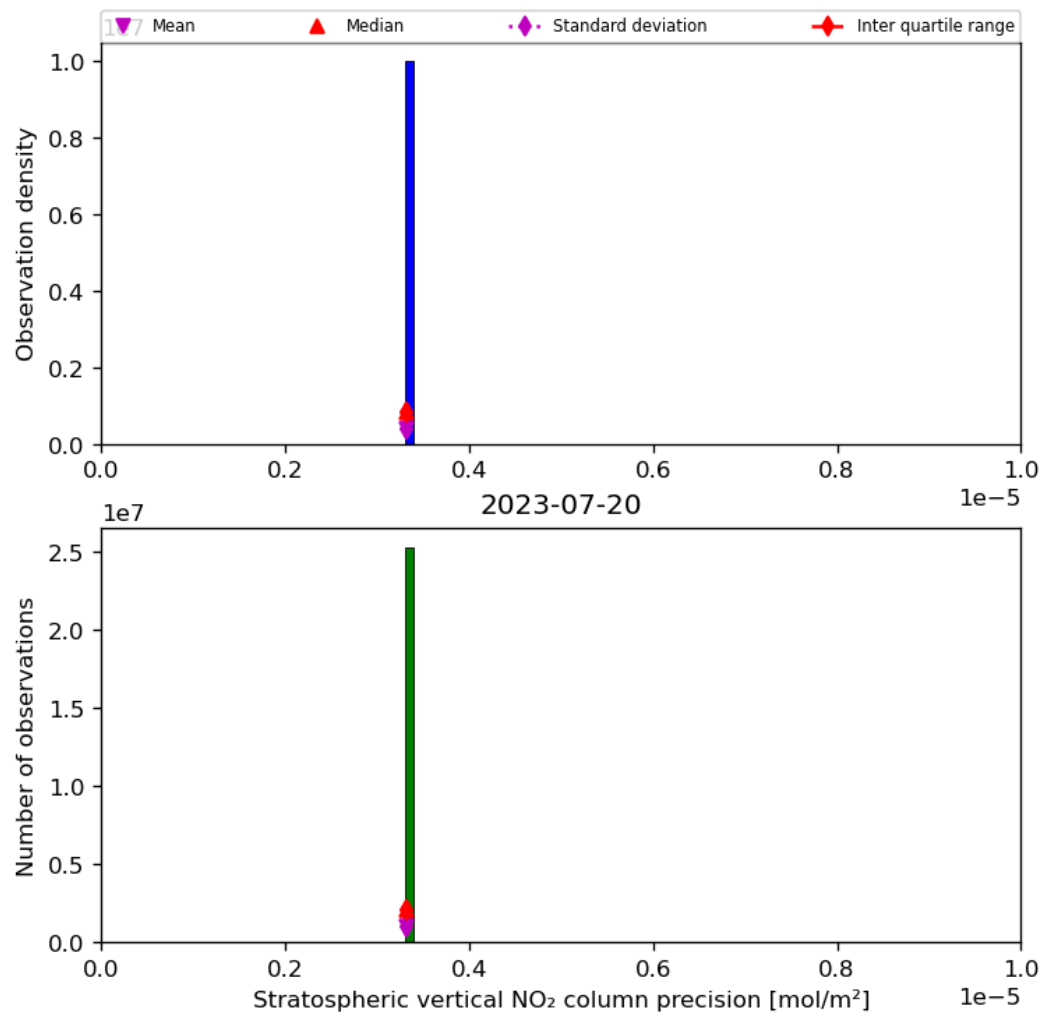
Figure 37: Histogram of “Stratospheric vertical NO 2 column precision” for 2023-07-19 to 2023-07-21
