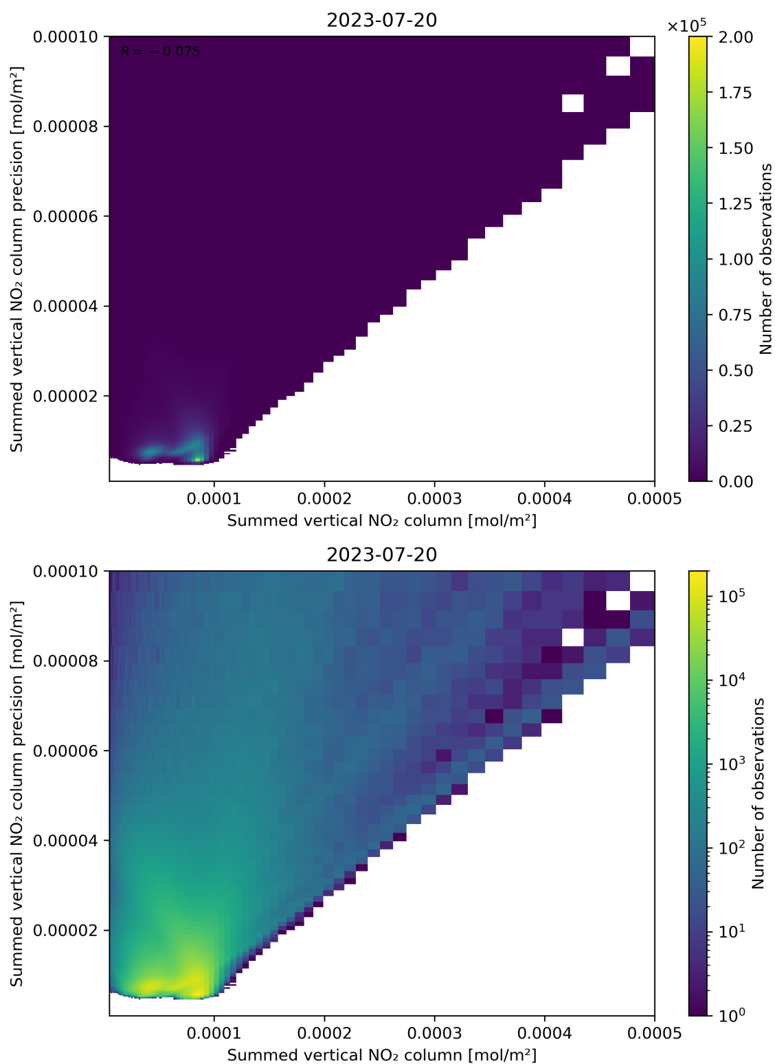
Figure 105: Scatter density plot of “Summed vertical NO 2 column” against “Summed vertical NO 2 column precision” for 2023-07-19 to 2023-07-21.
