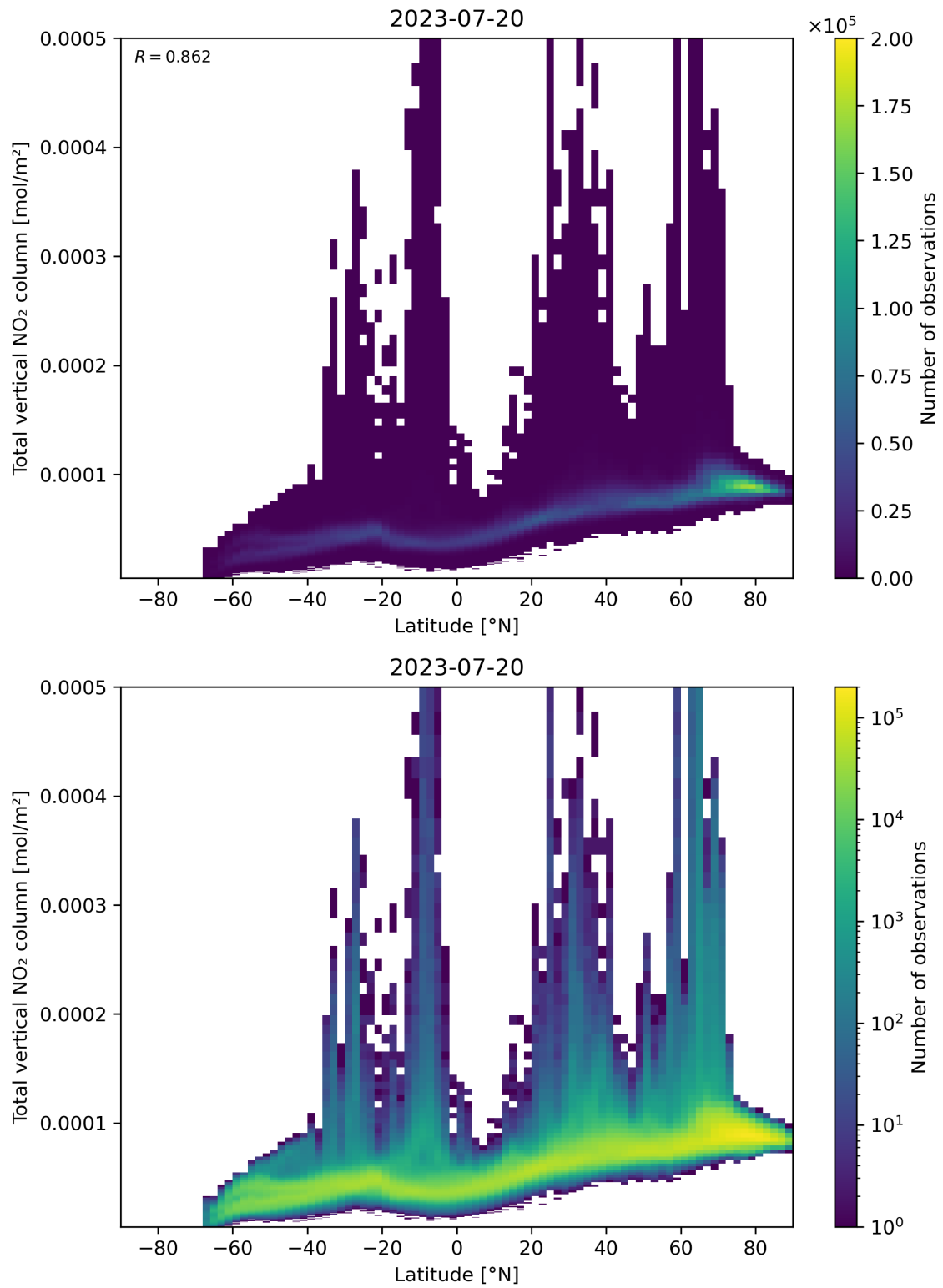
Figure 90: Scatter density plot of “Latitude” against “Total vertical NO 2 column” for 2023-07-19 to 2023-07-21.
