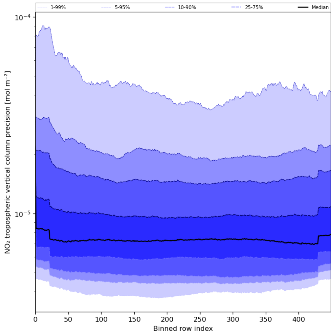
Figure 47: Along track statistics of “NO 2 tropospheric vertical column precision” for 2023-07-19 to 2023-07-21
