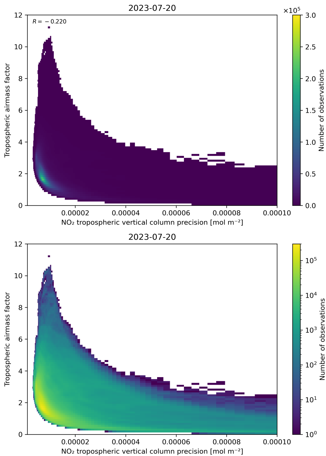
Figure 133: Scatter density plot of “NO 2 tropospheric vertical column precision” against “Tropospheric airmass factor” for 2023-07-19 to 2023-07-21.
