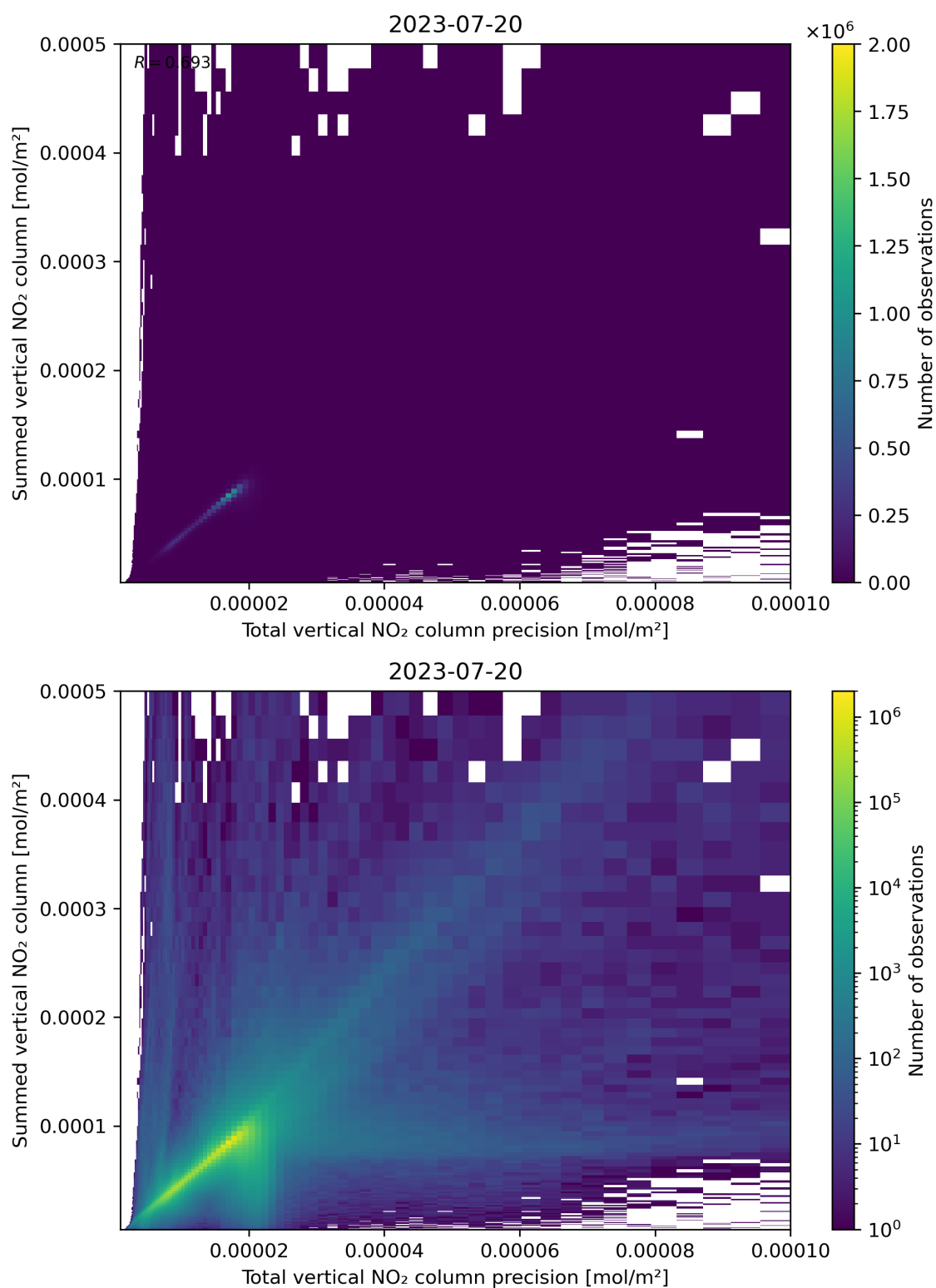
Figure 117: Scatter density plot of “Total vertical NO 2 column precision” against “Summed vertical NO 2 column” for 2023-07-19 to 2023-07-21.
