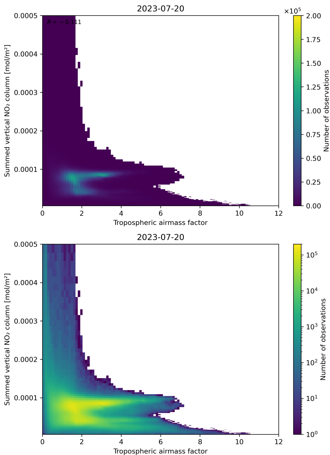
Figure 75: Scatter density plot of “Tropospheric airmass factor” against “Summed vertical NO 2 column” for 2023-07-19 to 2023-07-21.
