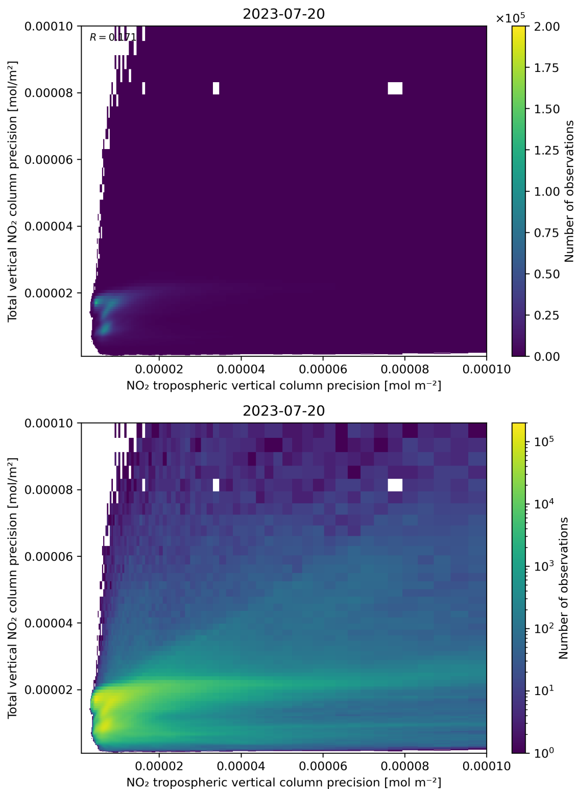
Figure 139: Scatter density plot of “NO 2 tropospheric vertical column precision” against “Total vertical NO 2 column precision” for 2023-07-19 to 2023-07-21.
