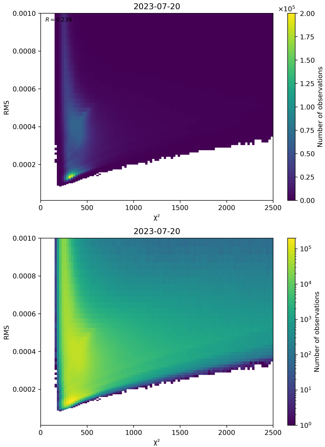
Figure 82: Scatter density plot of “ \chi^2 ” against “RMS” for 2023-07-19 to 2023-07-21.
