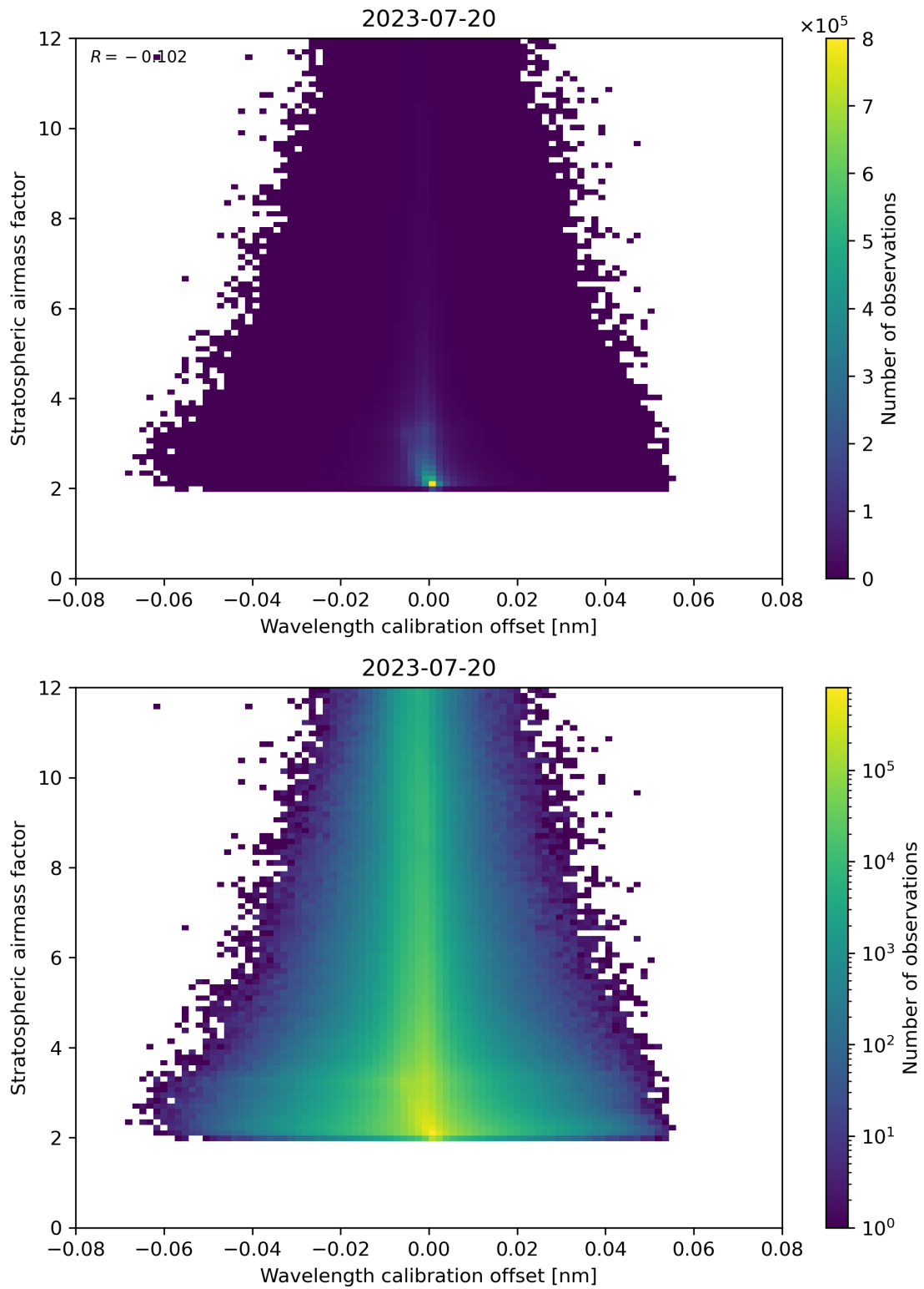
Figure 174: Scatter density plot of “Wavelength calibration offset” against “Stratospheric airmass factor” for 2023-07-19 to 2023-07-21.
