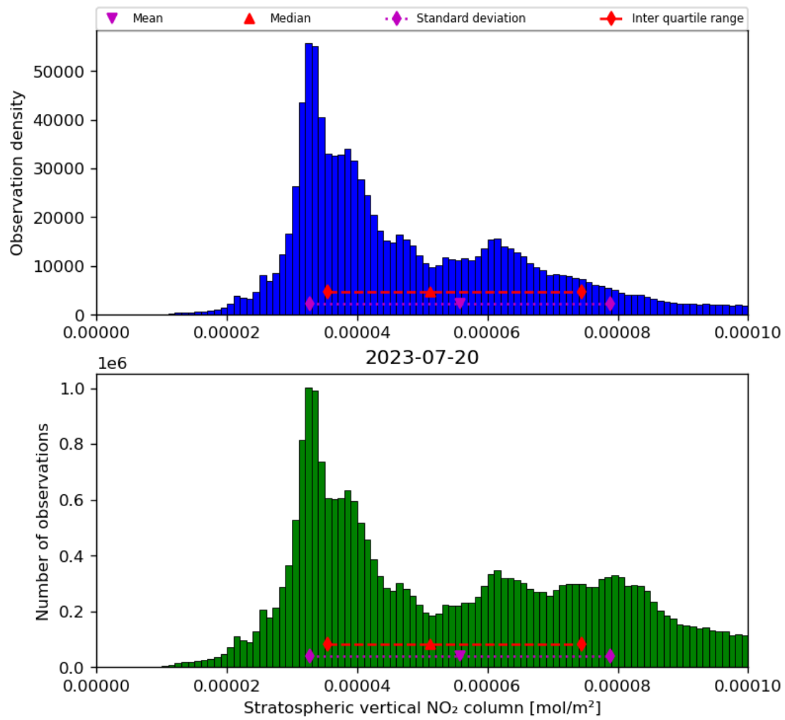
Figure 36: Histogram of “Stratospheric vertical NO 2 column” for 2023-07-19 to 2023-07-21
