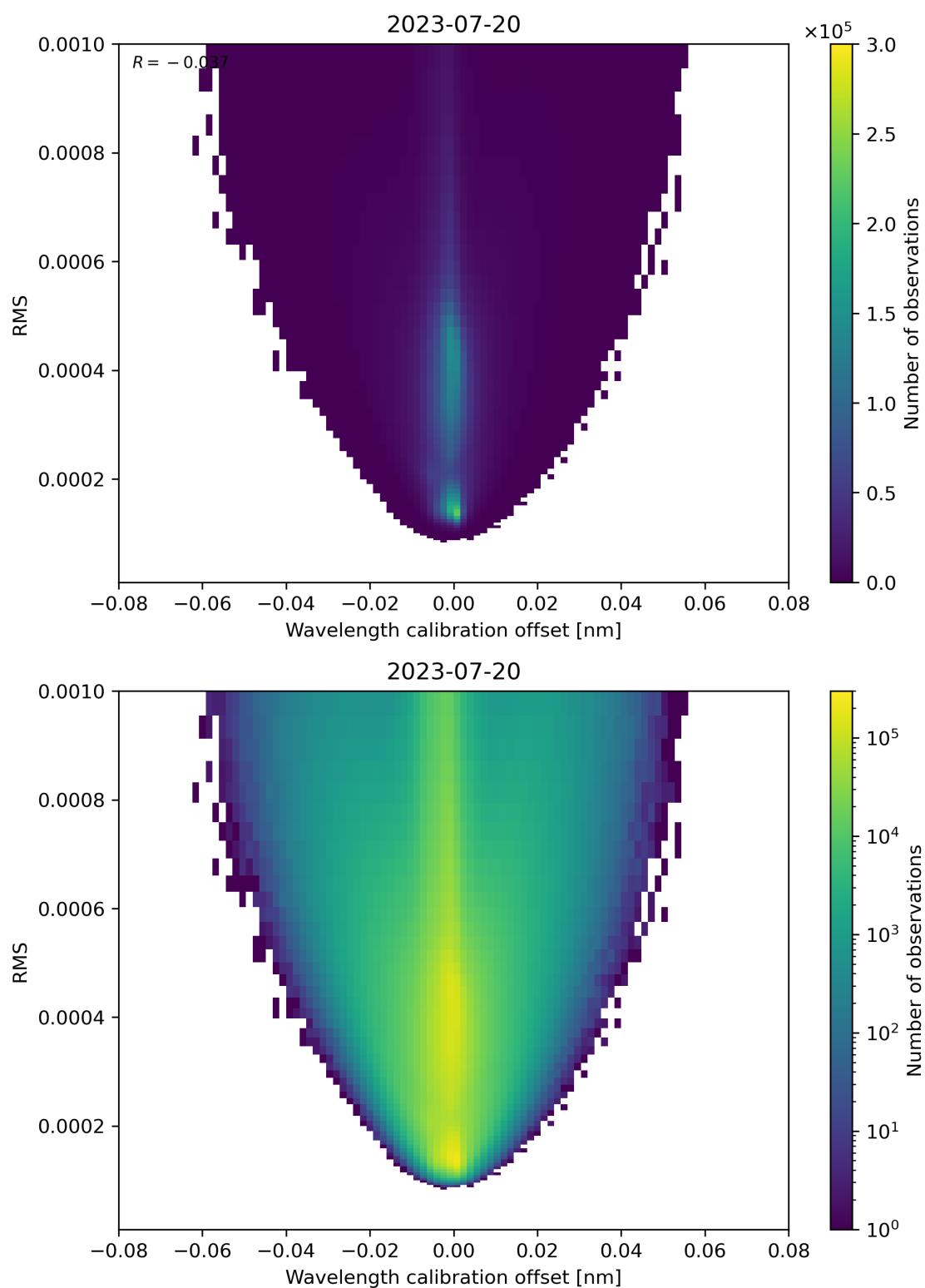
Figure 181: Scatter density plot of “Wavelength calibration offset” against “RMS” for 2023-07-19 to 2023-07-21.
