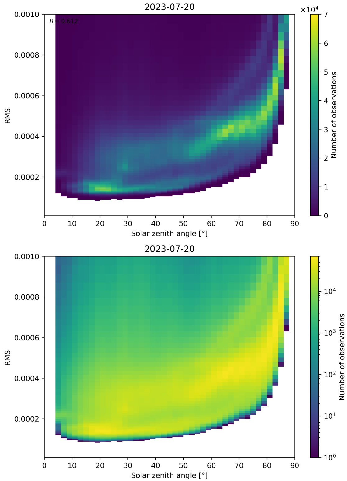
Figure 157: Scatter density plot of “Solar zenith angle” against “RMS” for 2023-07-19 to 2023-07-21.
