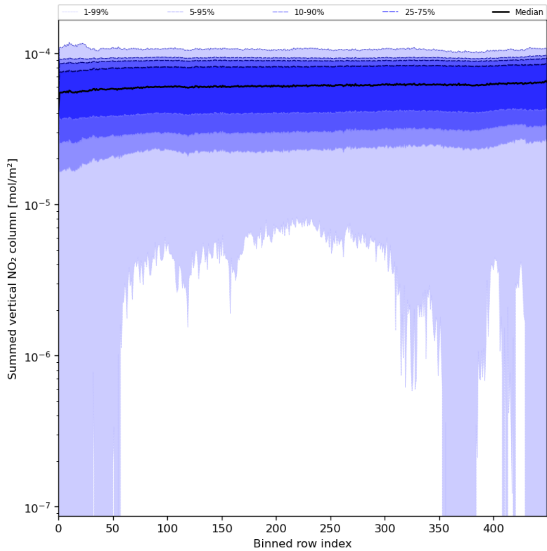
Figure 57: Along track statistics of “Summed vertical NO 2 column” for 2023-07-19 to 2023-07-21
