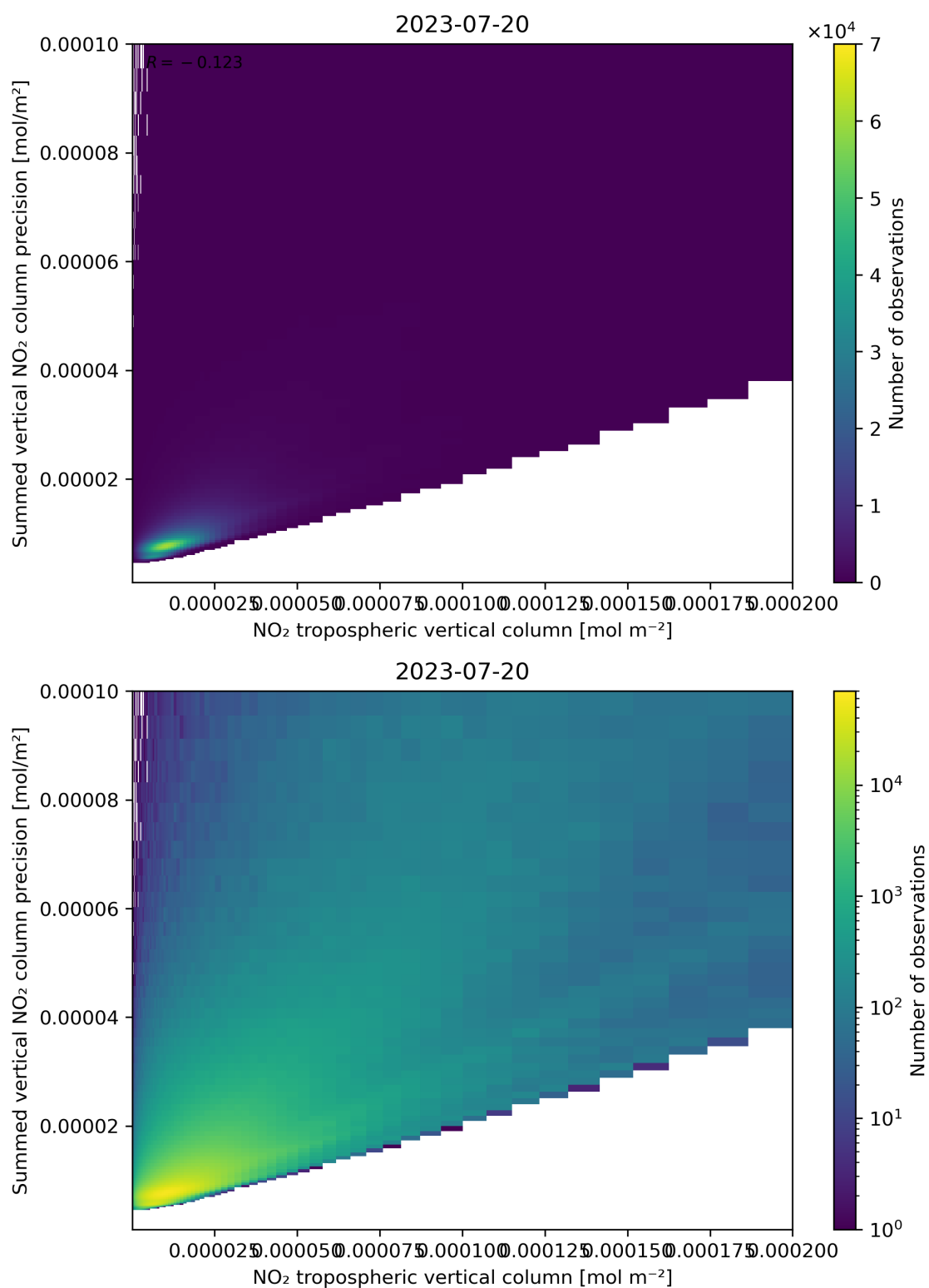
Figure 127: Scatter density plot of “NO 2 tropospheric vertical column” against “Summed vertical NO 2 column precision” for 2023-07-19 to 2023-07-21.
