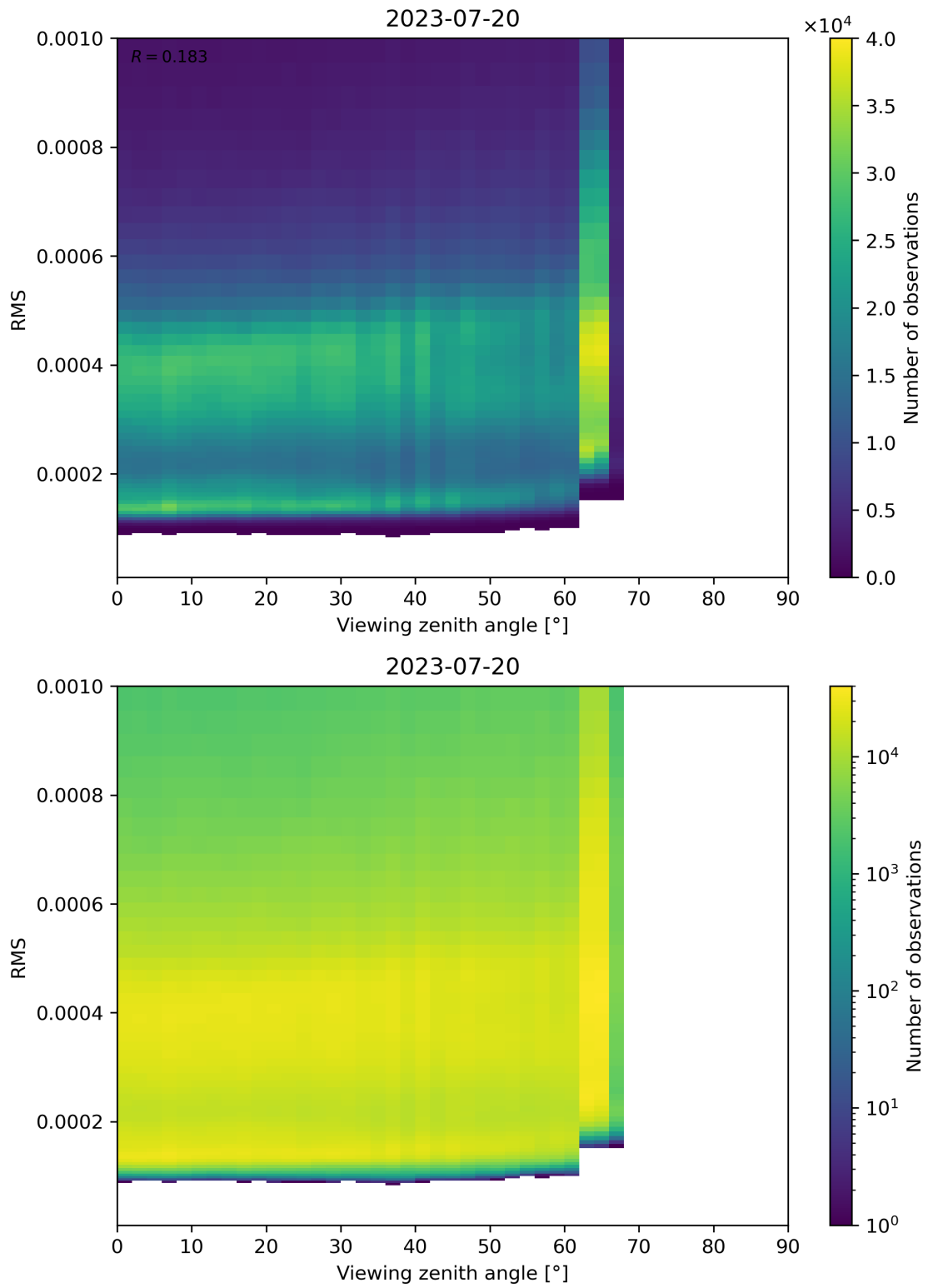
Figure 171: Scatter density plot of “Viewing zenith angle” against “RMS” for 2023-07-19 to 2023-07-21.
