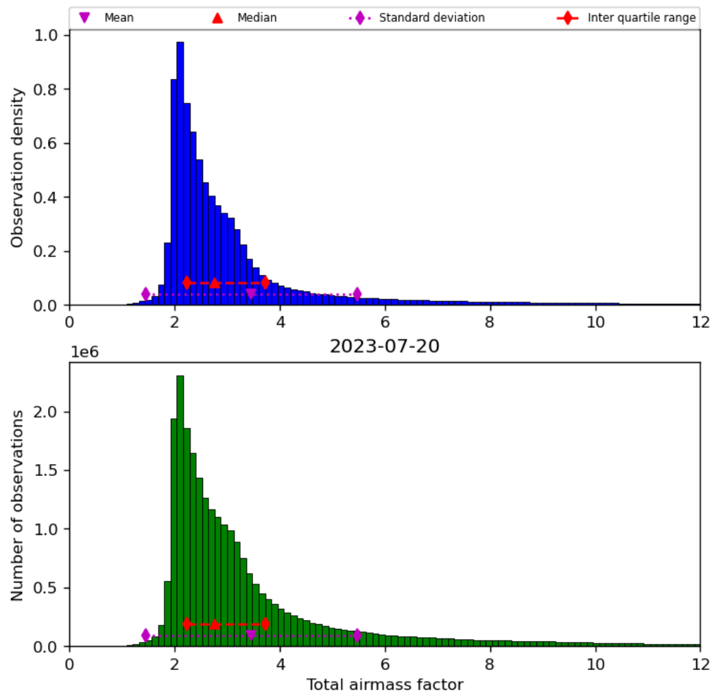
Figure 32: Histogram of “Total airmass factor” for 2023-07-19 to 2023-07-21
