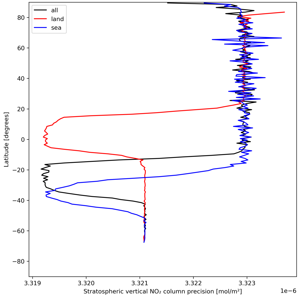
Figure 20: Zonal average of “Stratospheric vertical NO 2 column precision” for 2023-07-19 to 2023-07-21.
