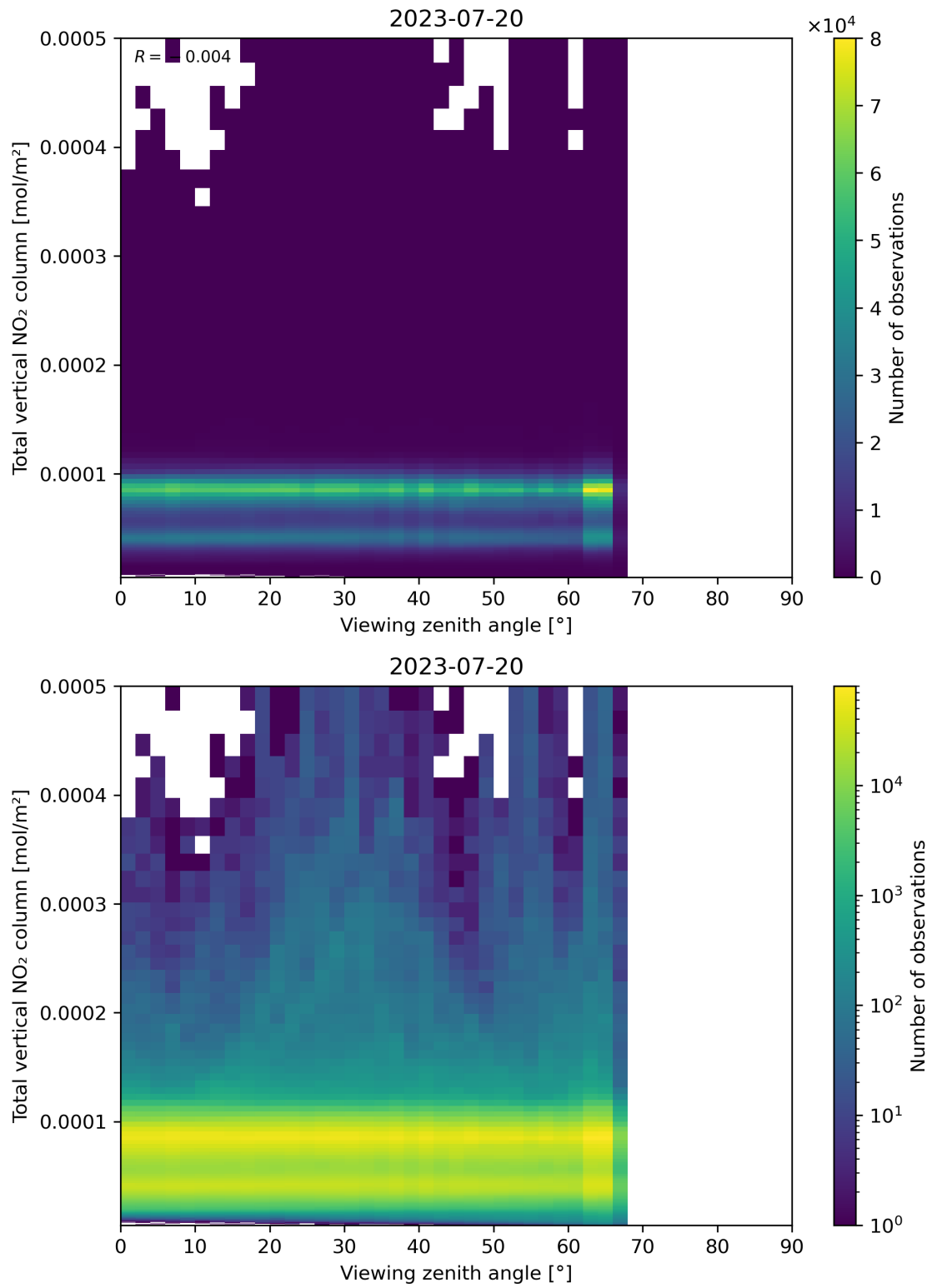
Figure 167: Scatter density plot of “Viewing zenith angle” against “Total vertical NO 2 column” for 2023-07-19 to 2023-07-21.
