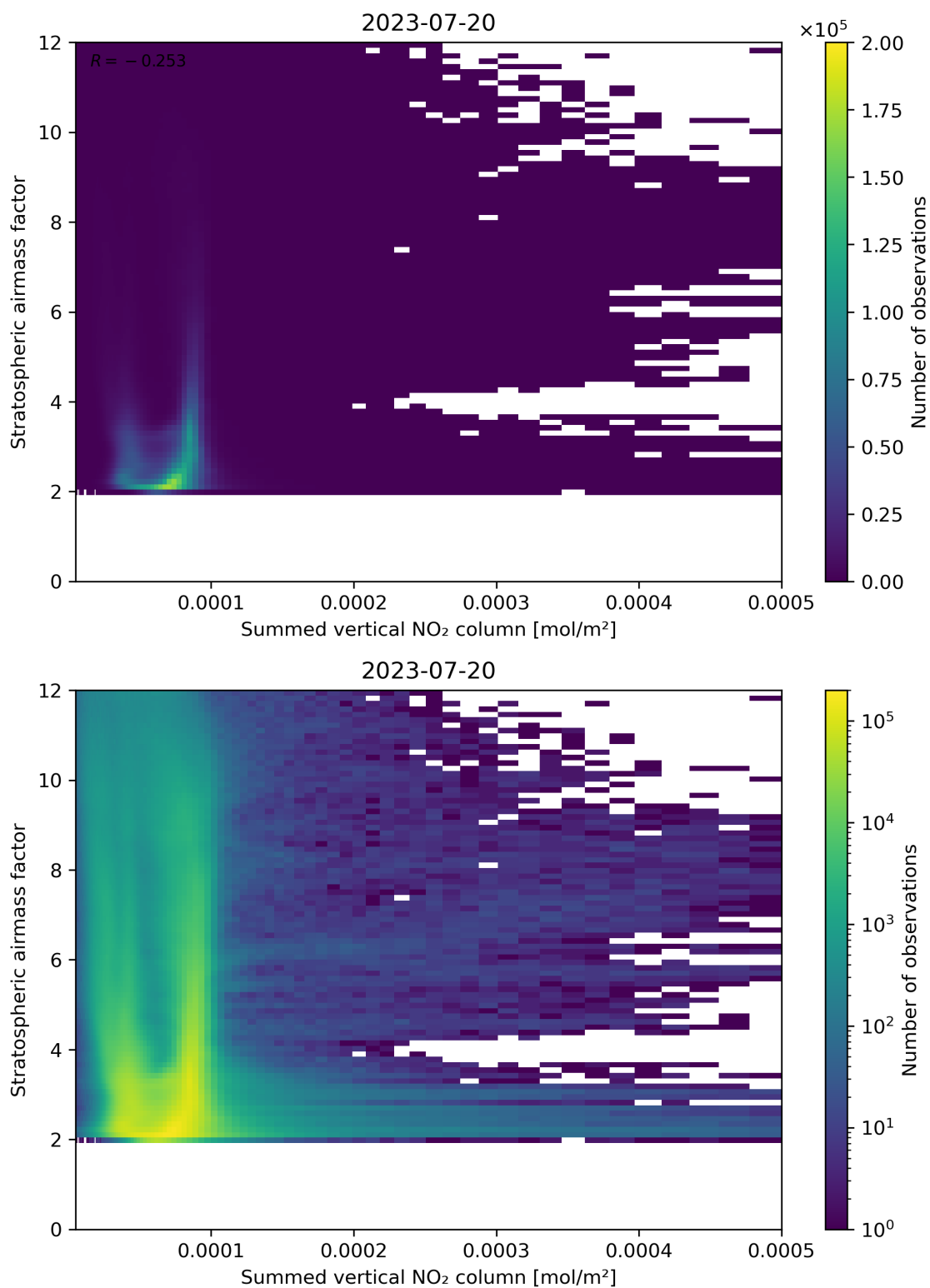
Figure 103: Scatter density plot of “Summed vertical NO 2 column” against “Stratospheric air mass factor” for 2023-07-19 to 2023-07-21.
