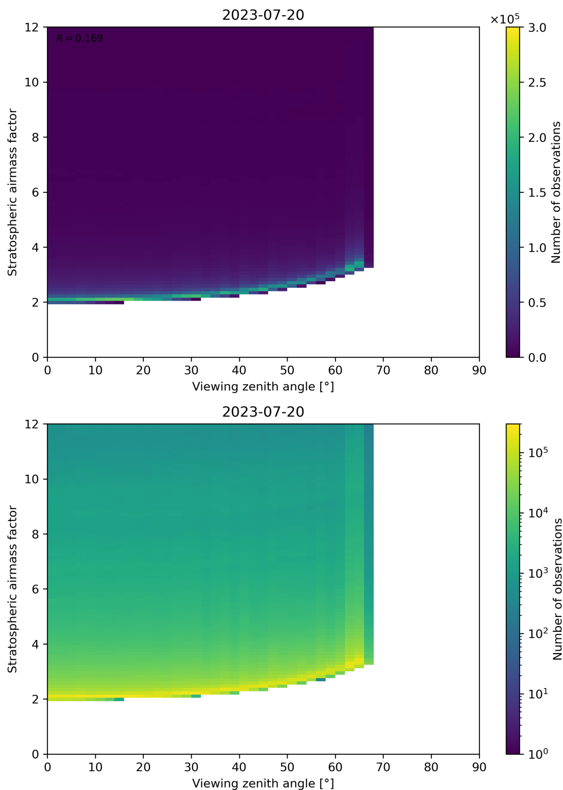
Figure 159: Scatter density plot of “Viewing zenith angle” against “Stratospheric airmass factor” for 2023-07-19 to 2023-07-21.
