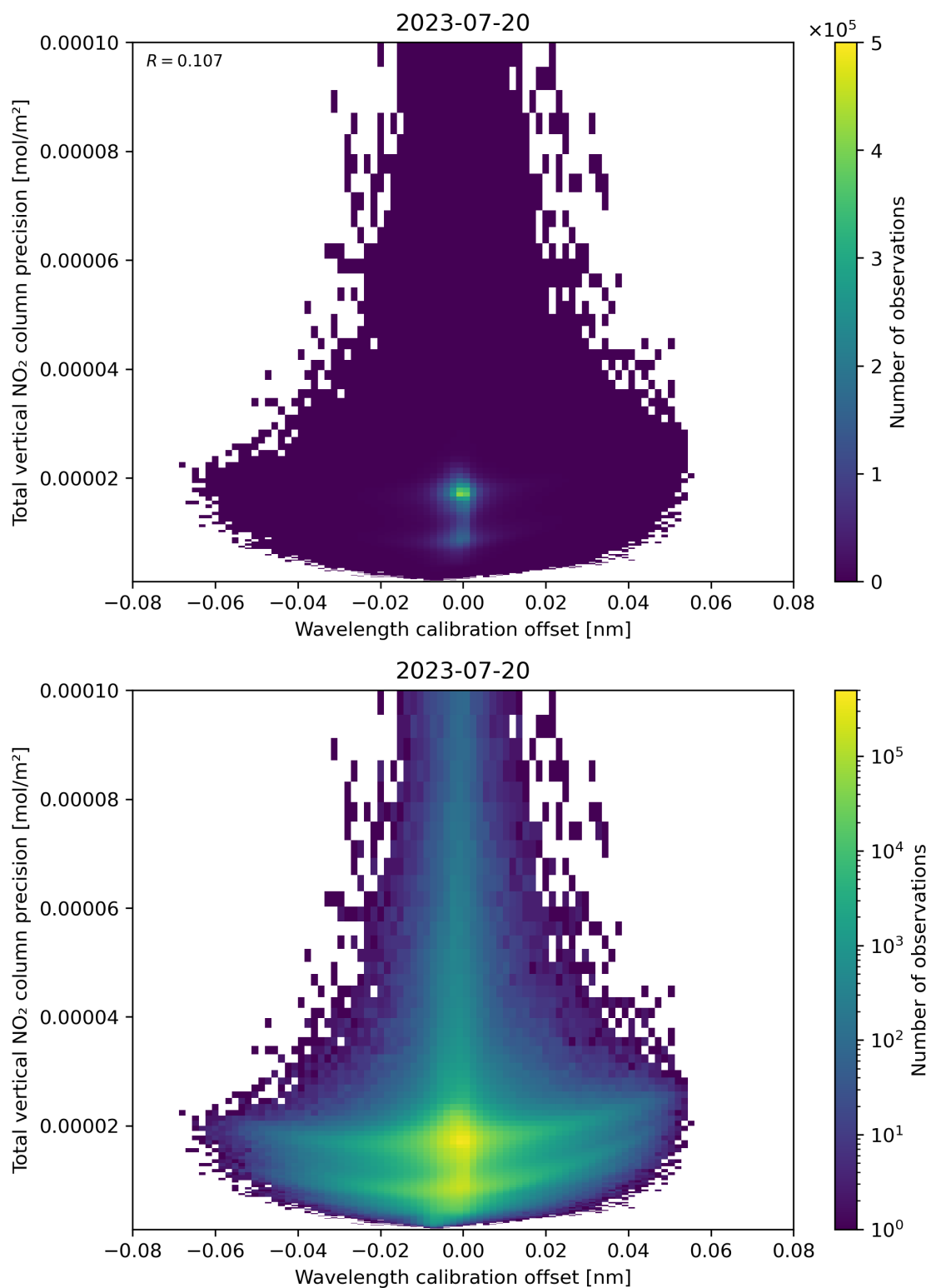
Figure 180: Scatter density plot of “Wavelength calibration offset” against “Total vertical NO 2 column precision” for 2023-07-19 to 2023-07-21.
