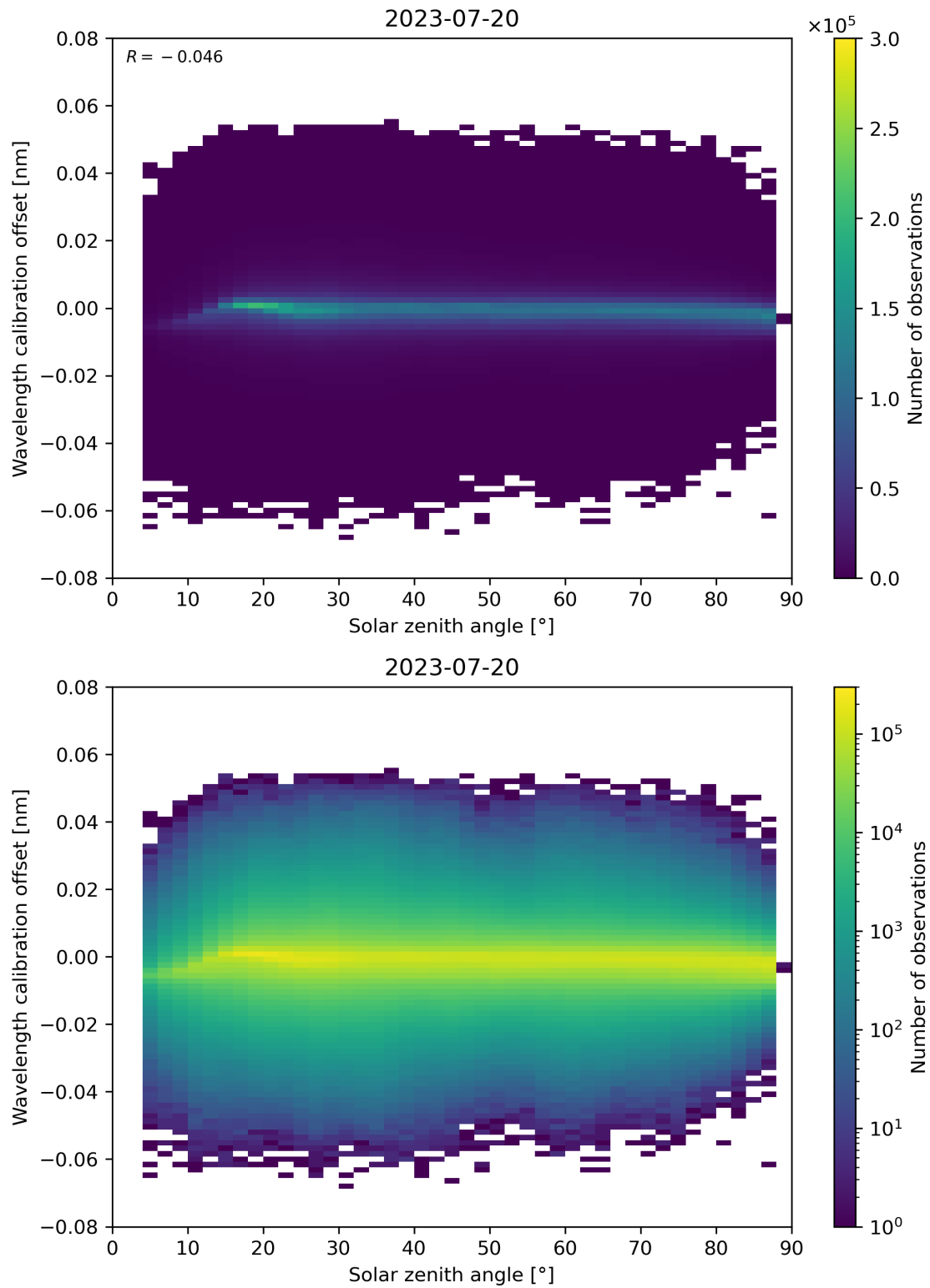
Figure 158: Scatter density plot of “Solar zenith angle” against “Wavelength calibration offset” for 2023-07-19 to 2023-07-21.
