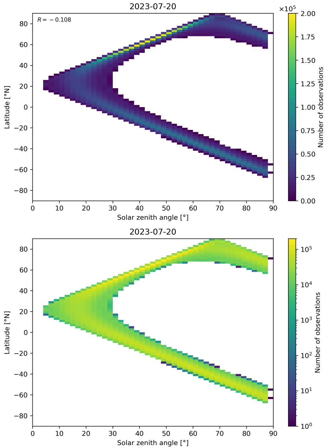
Figure 149: Scatter density plot of “Solar zenith angle” against “Latitude” for 2023-07-19 to 2023-07-21.
