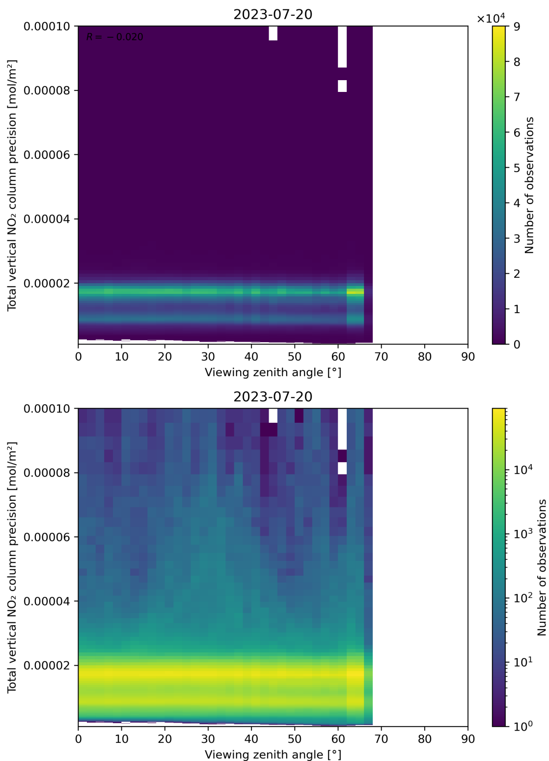
Figure 168: Scatter density plot of “Viewing zenith angle” against “Total vertical NO 2 column precision” for 2023-07-19 to 2023-07-21.
