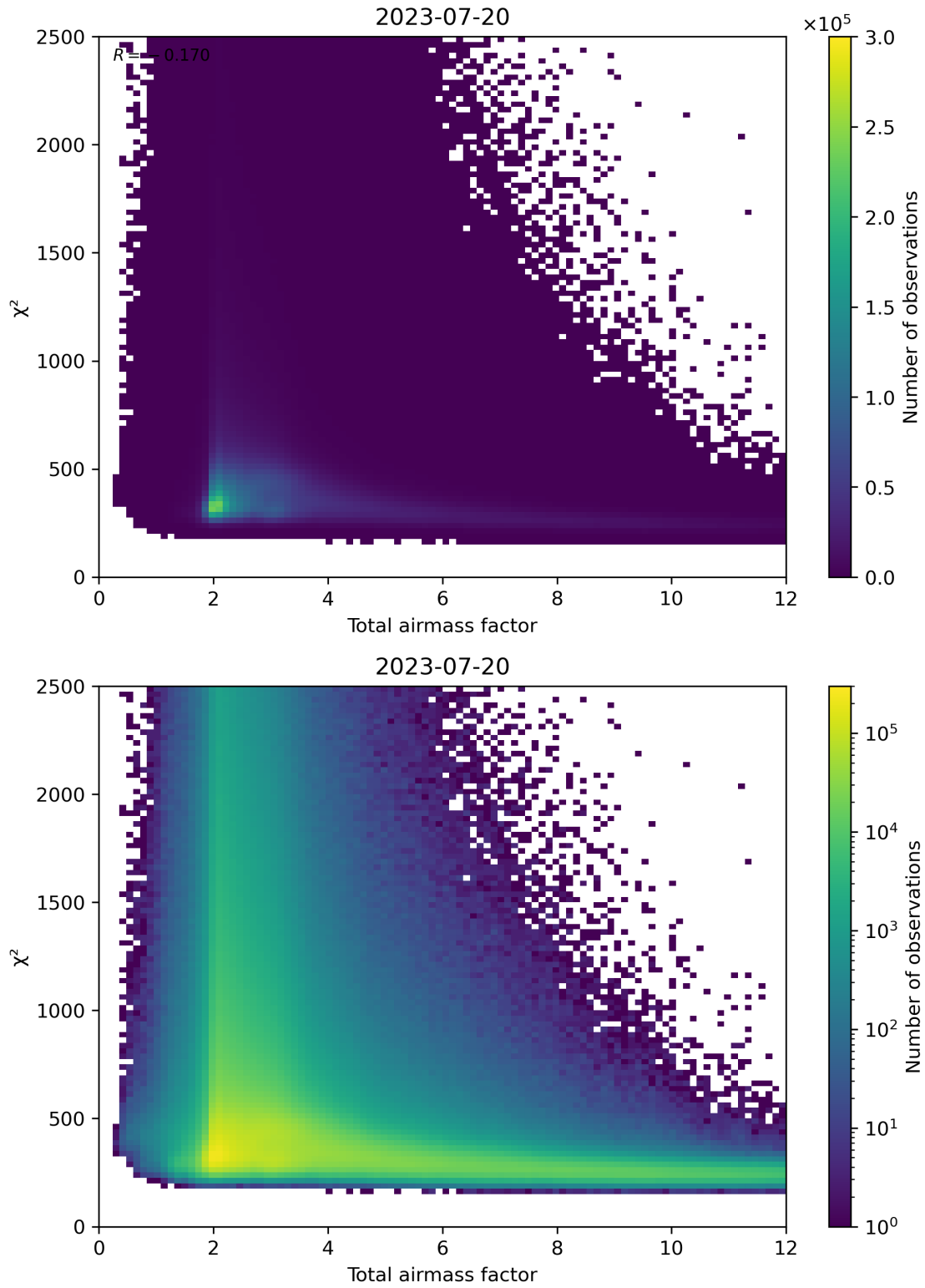
Figure 63: Scatter density plot of “Total airmass factor” against “ \chi^2 ” for 2023-07-19 to 2023-07-21.
