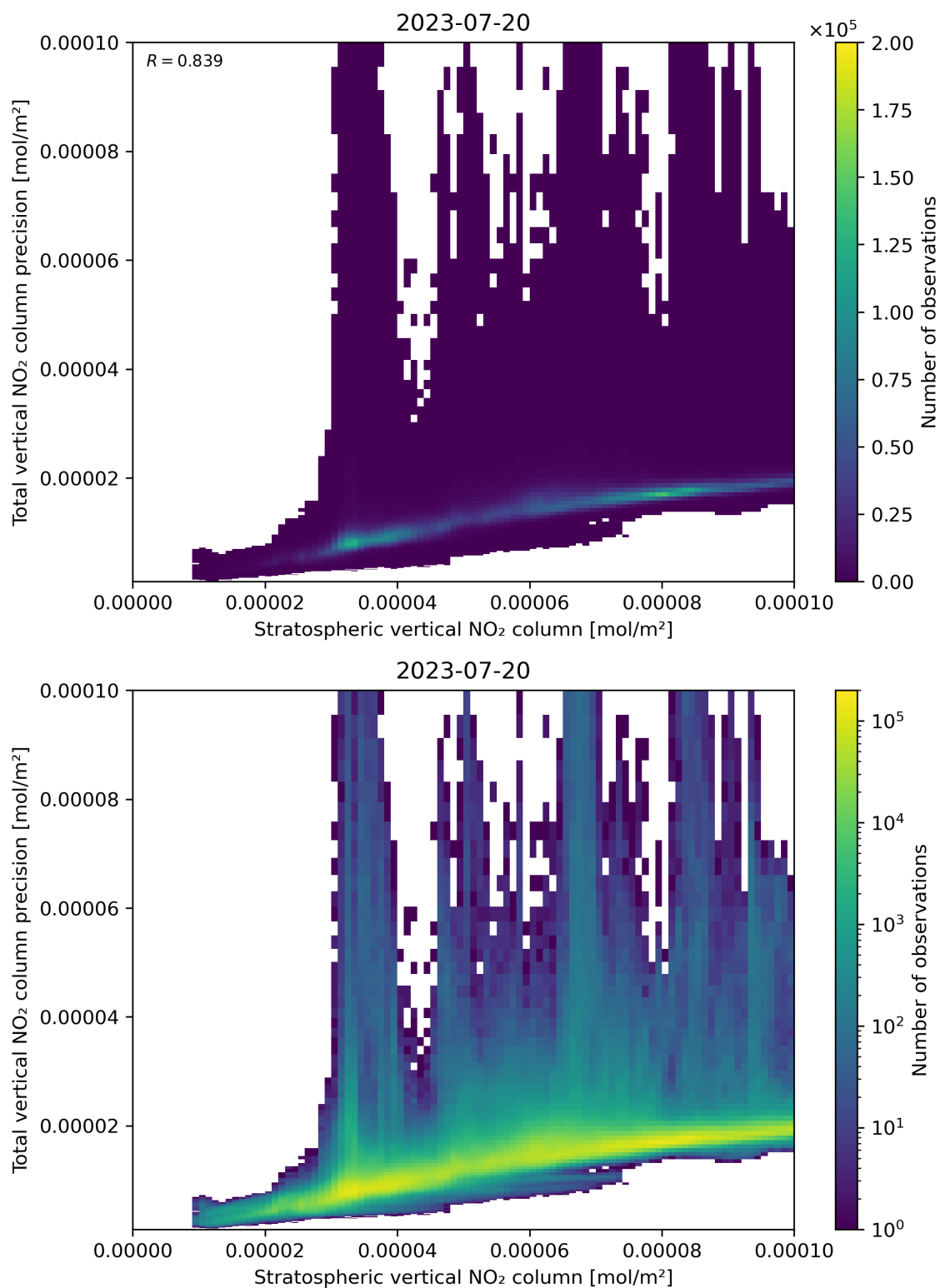
Figure 101: Scatter density plot of “Stratospheric vertical NO 2 column” against “Total vertical NO 2 column precision” for 2023-07-19 to 2023-07-21.
