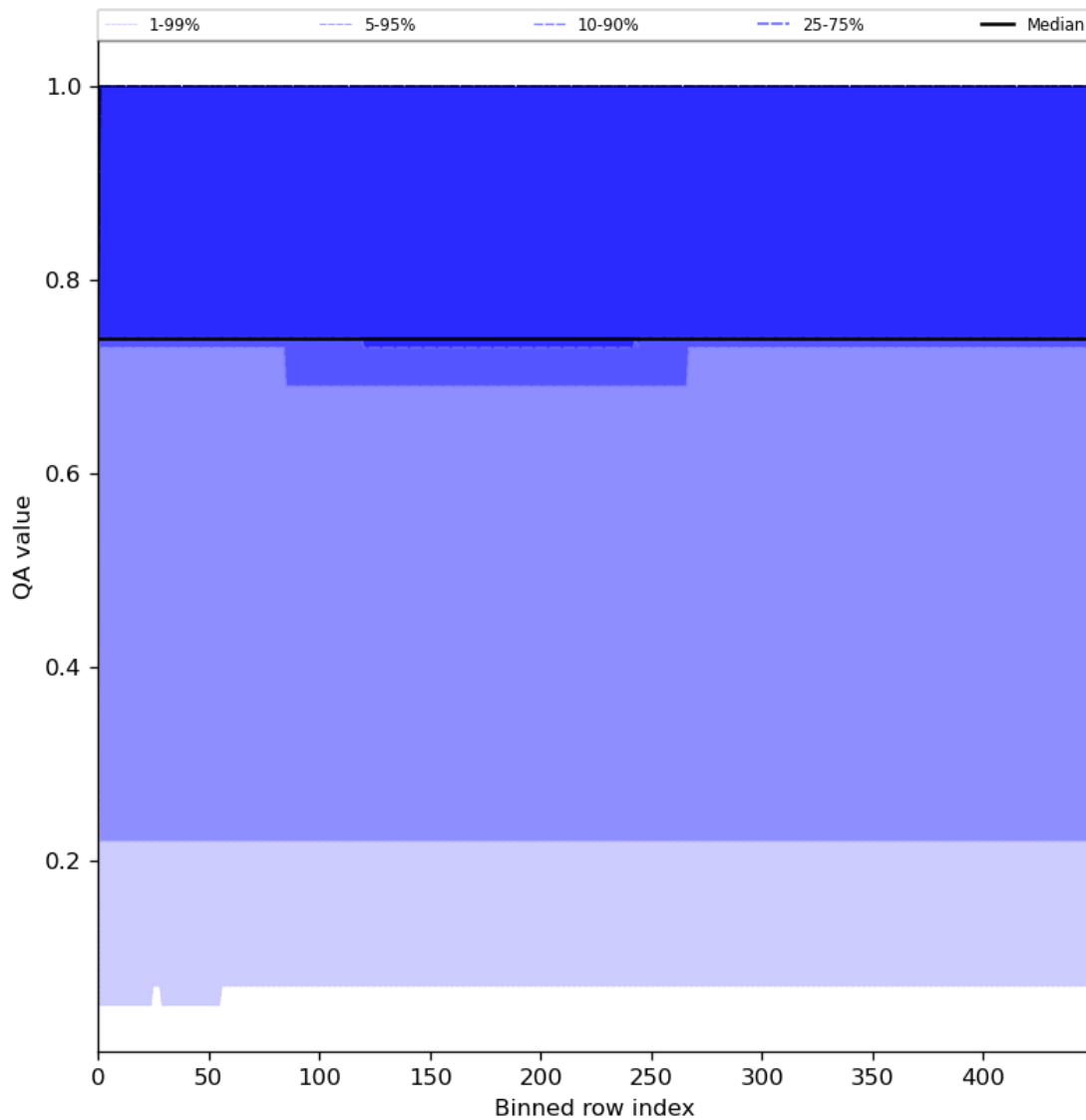
Figure 45: Along track statistics of “QA value” for 2023-07-19 to 2023-07-21
