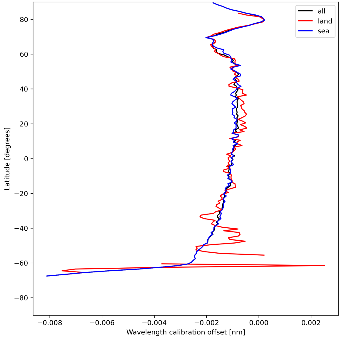
Figure 18: Zonal average of “Wavelength calibration offset” for 2023-07-19 to 2023-07-21.
