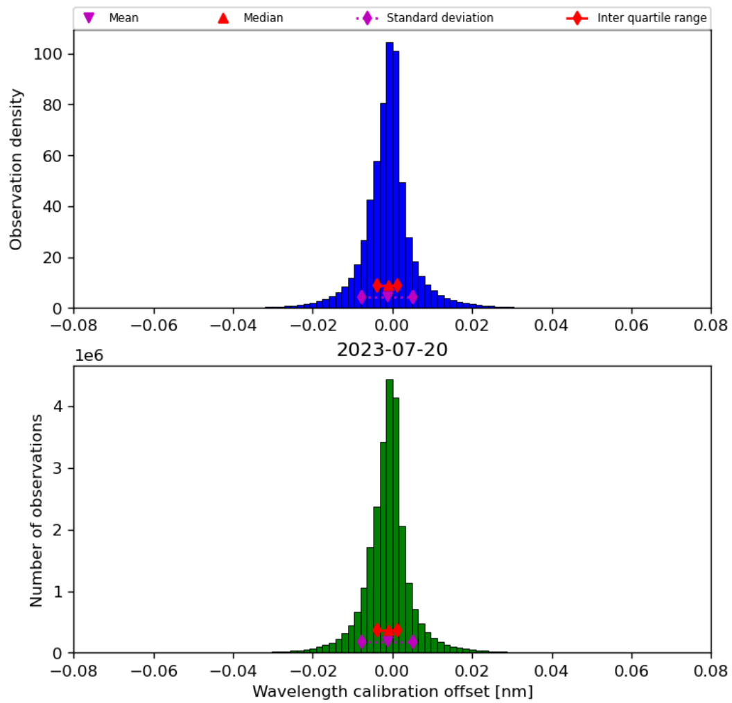
Figure 35: Histogram of “Wavelength calibration offset” for 2023-07-19 to 2023-07-21
