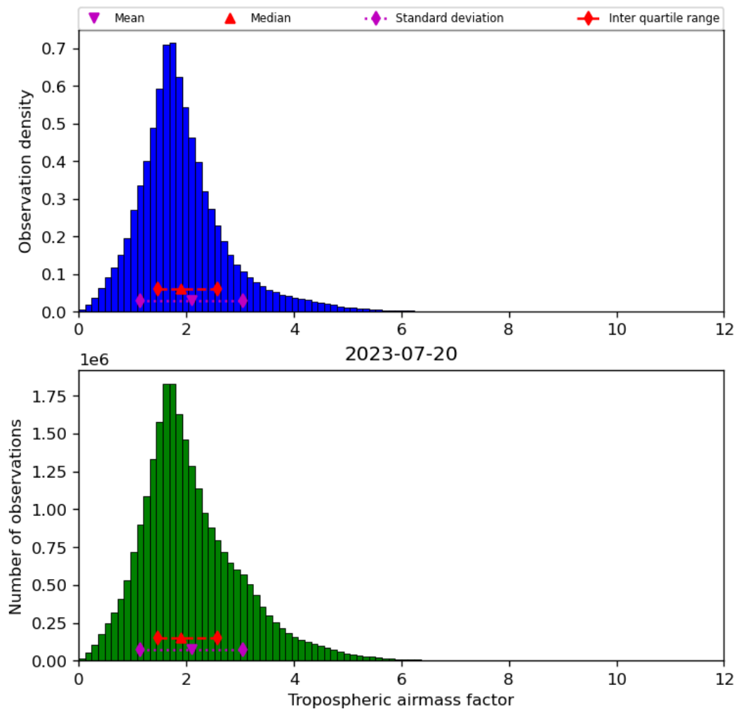
Figure 31: Histogram of “Tropospheric airmass factor” for 2023-07-19 to 2023-07-21
