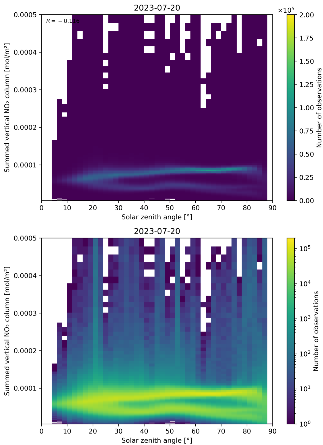
Figure 151: Scatter density plot of “Solar zenith angle” against “Summed vertical NO 2 column” for 2023-07-19 to 2023-07-21.
