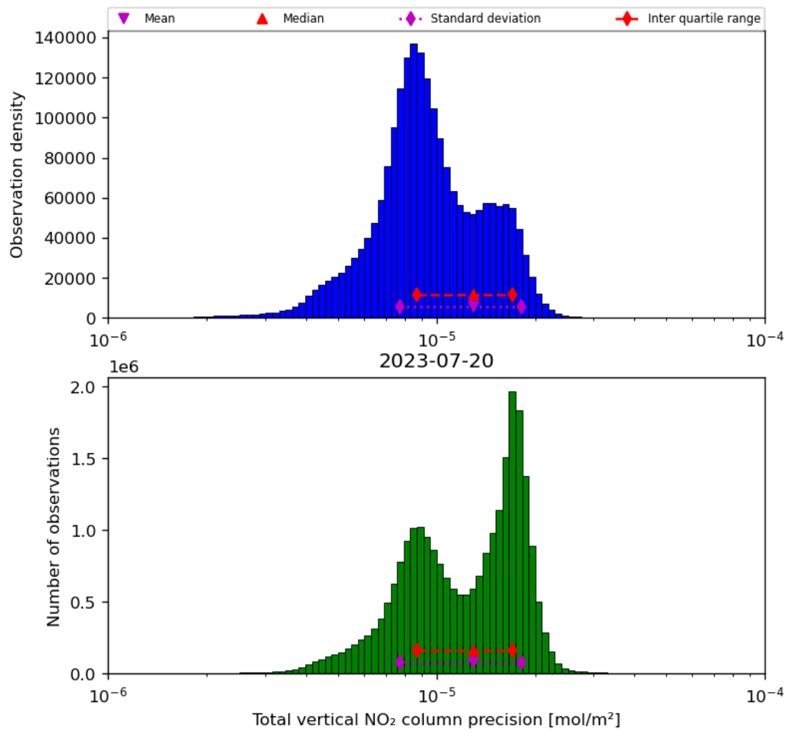
Figure 39: Histogram of “Total vertical NO 2 column precision” for 2023-07-19 to 2023-07-21
