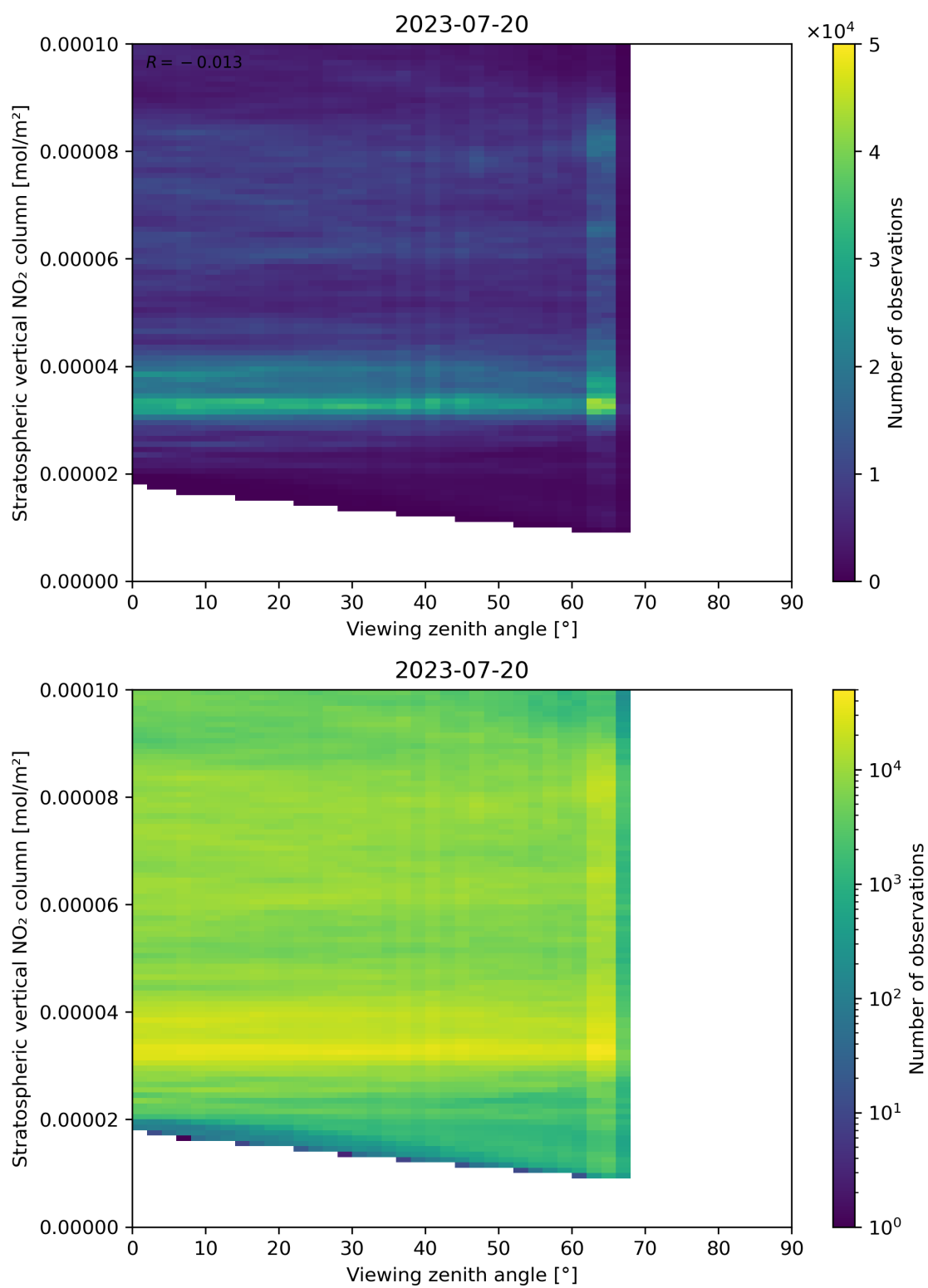
Figure 164: Scatter density plot of “Viewing zenith angle” against “Stratospheric vertical NO 2 column” for 2023-07-19 to 2023-07-21.
