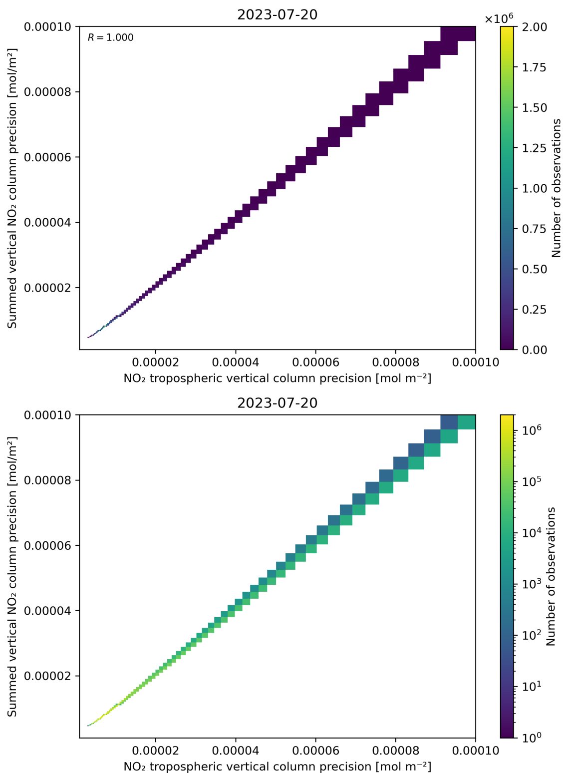
Figure 137: Scatter density plot of “NO 2 tropospheric vertical column precision” against “Summed vertical NO 2 column precision” for 2023-07-19 to 2023-07-21.
