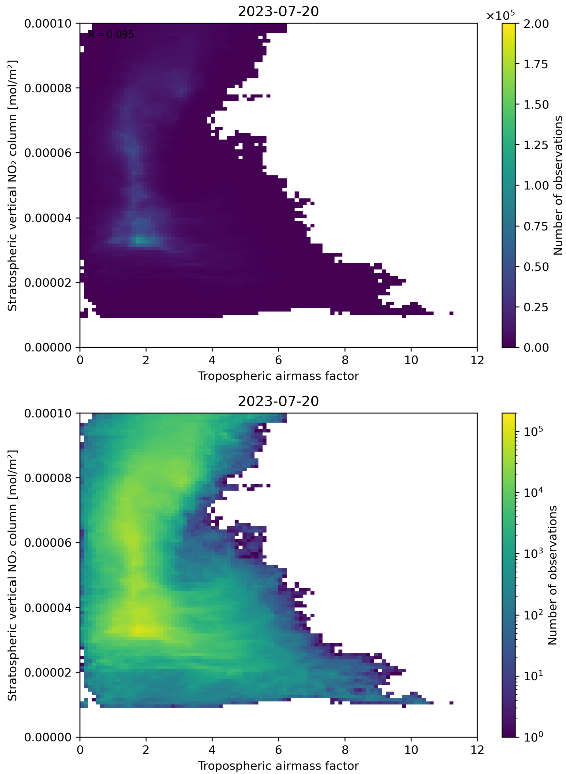
Figure 74: Scatter density plot of “Tropospheric airmass factor” against “Stratospheric vertical NO 2 column” for 2023-07-19 to 2023-07-21.
