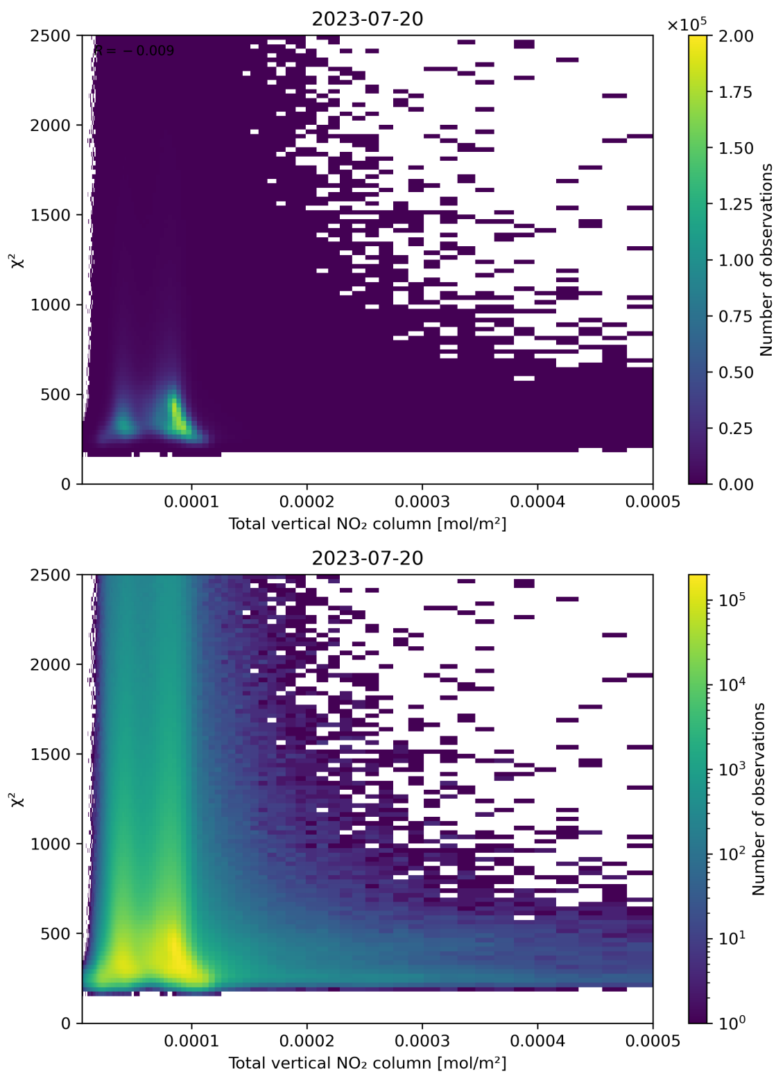
Figure 111: Scatter density plot of “Total vertical NO 2 column” against “ \chi^2 ” for 2023-07-19 to 2023-07-21.
