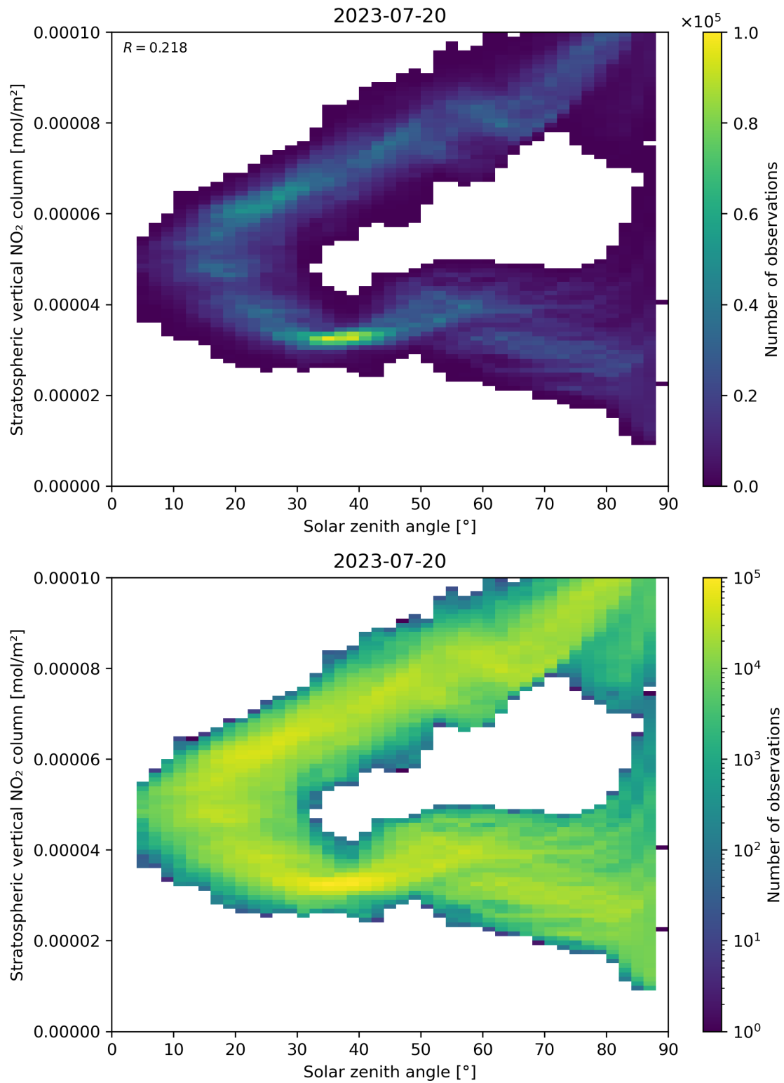
Figure 150: Scatter density plot of “Solar zenith angle” against “Stratospheric vertical NO 2 column” for 2023-07-19 to 2023-07-21.
