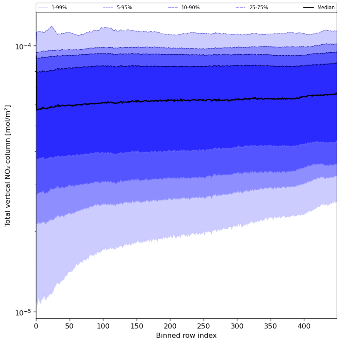
Figure 55: Along track statistics of “Total vertical NO 2 column” for 2023-07-19 to 2023-07-21
