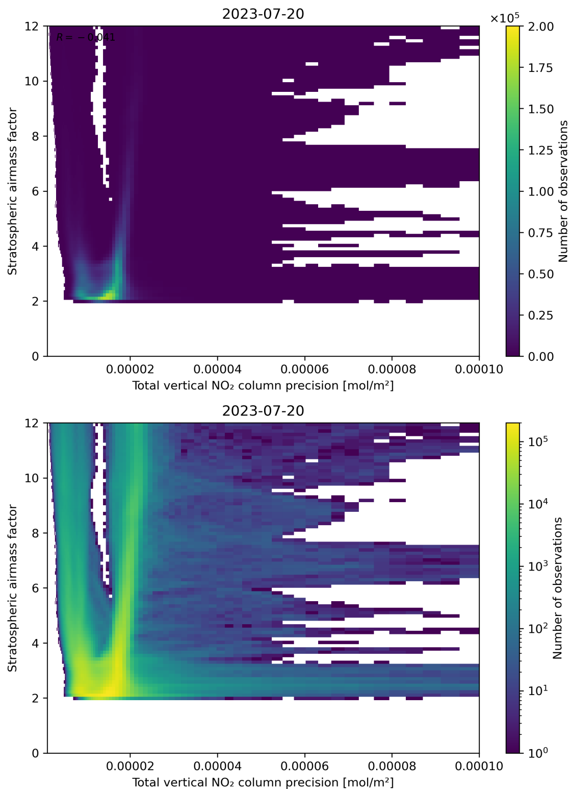
Figure 115: Scatter density plot of “Total vertical NO 2 column precision” against “Stratospheric air mass factor” for 2023-07-19 to 2023-07-21.
