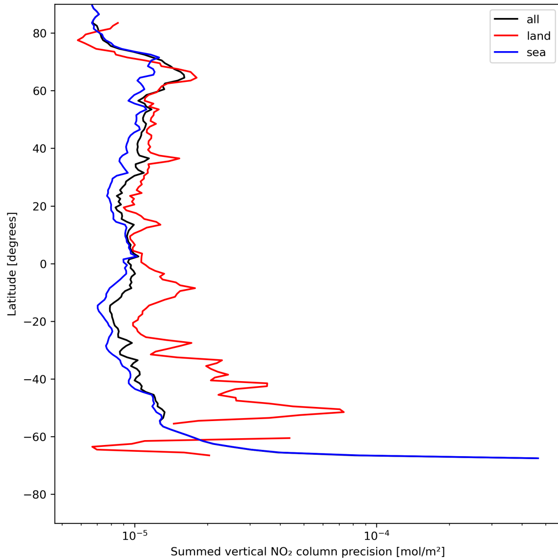
Figure 24: Zonal average of “Summed vertical NO 2 column precision” for 2023-07-19 to 2023-07-21.
