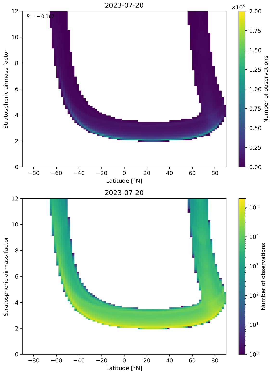
Figure 83: Scatter density plot of “Latitude” against “Stratospheric air mass factor” for 2023-07-19 to 2023-07-21.
