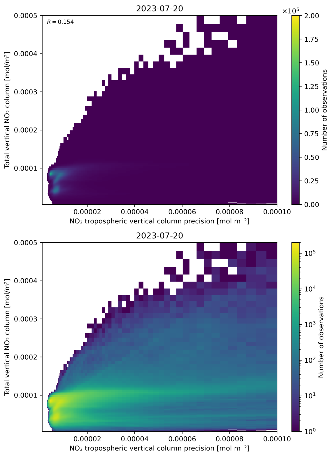
Figure 138: Scatter density plot of “NO 2 tropospheric vertical column precision” against “Total vertical NO 2 column” for 2023-07-19 to 2023-07-21.
