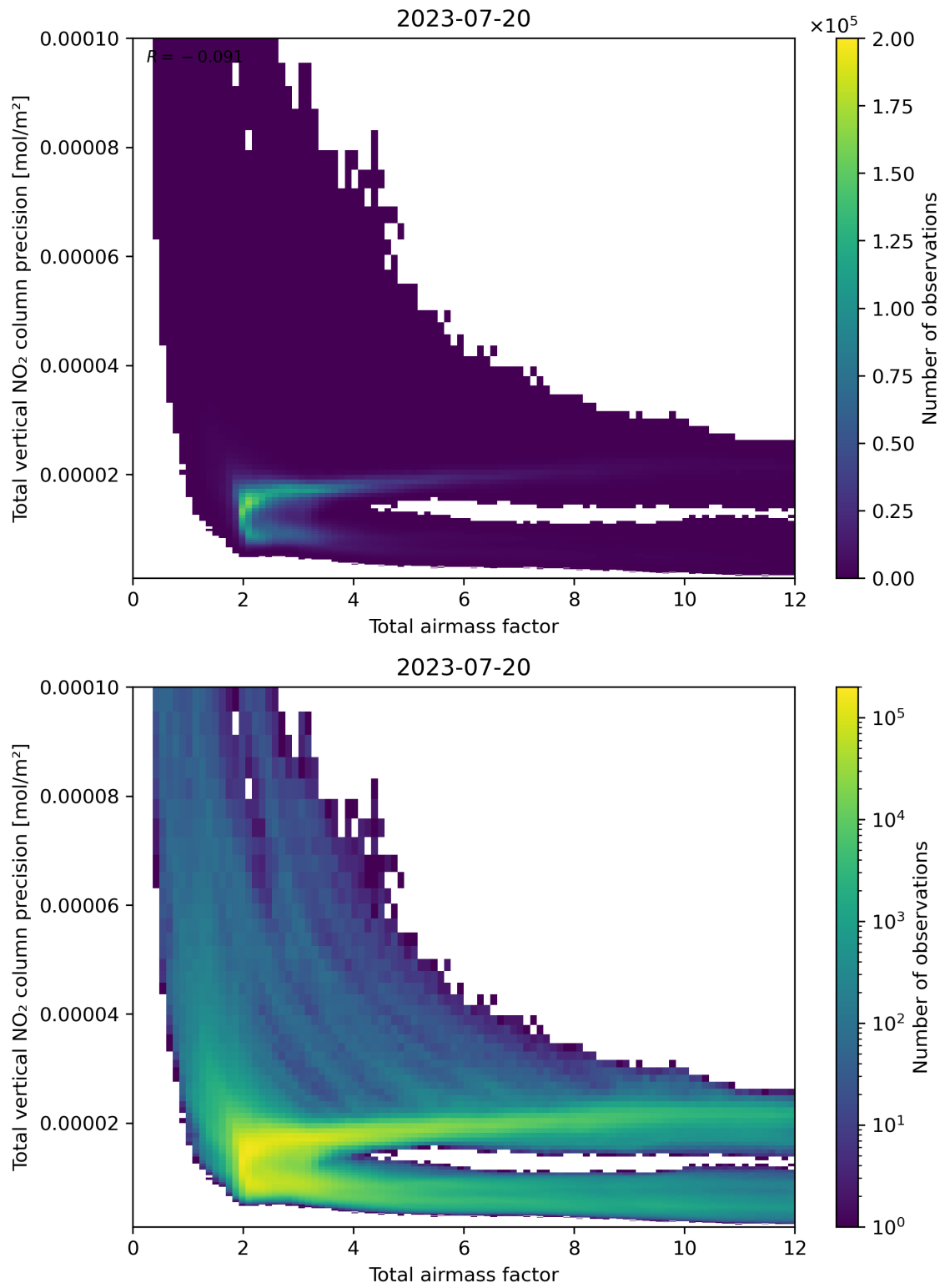
Figure 68: Scatter density plot of “Total airmass factor” against “Total vertical NO 2 column precision” for 2023-07-19 to 2023-07-21.
