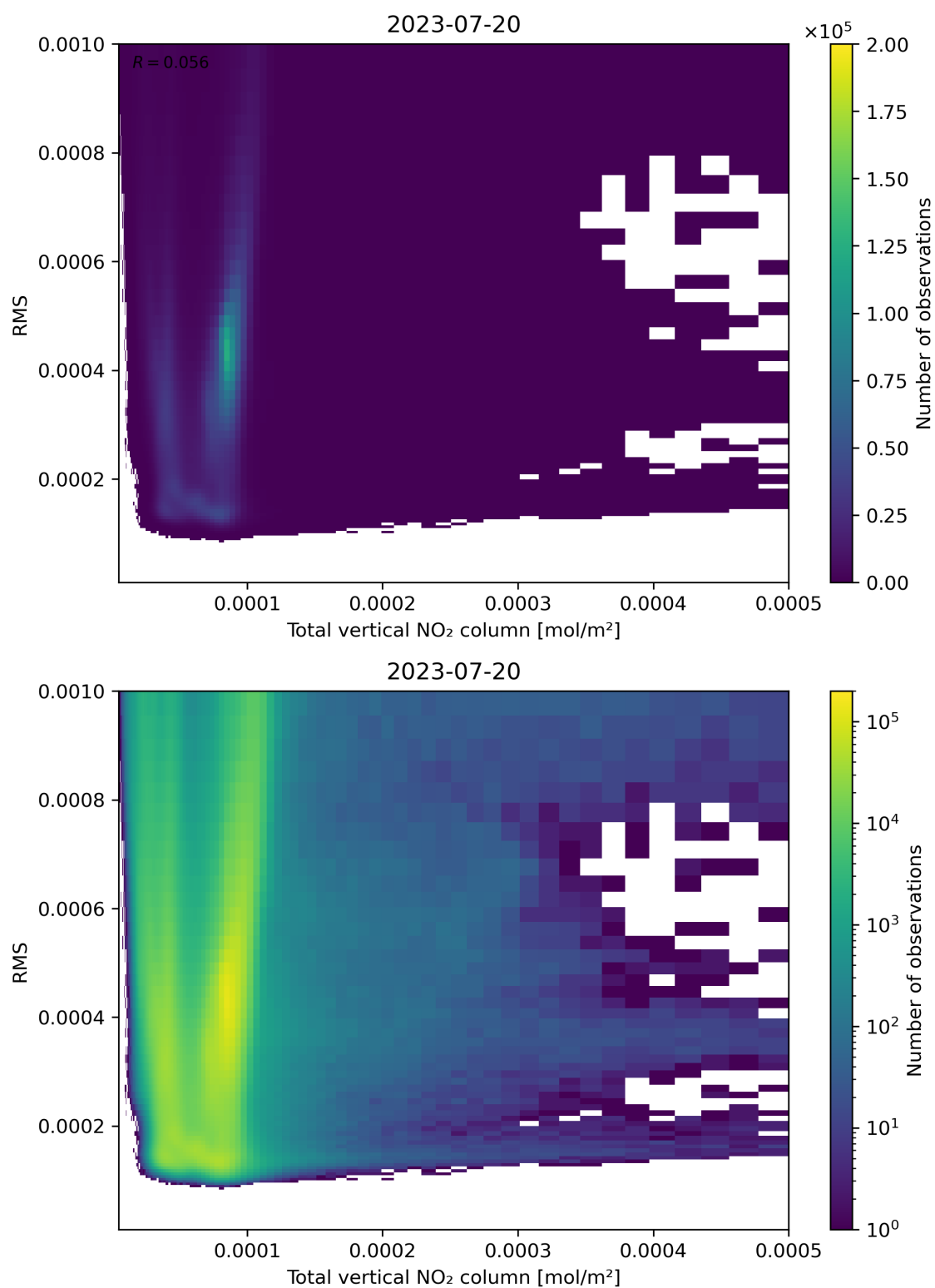
Figure 120: Scatter density plot of “Total vertical NO 2 column” against “RMS” for 2023-07-19 to 2023-07-21.
