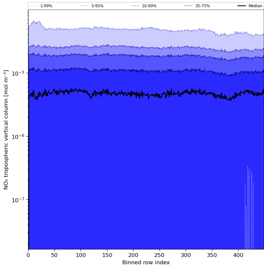
Figure 46: Along track statistics of “NO 2 tropospheric vertical column” for 2023-07-19 to 2023-07-21
