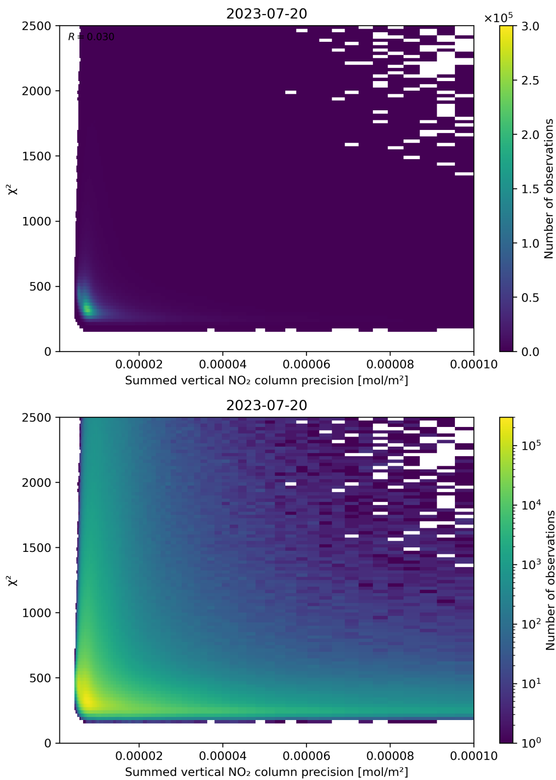
Figure 107: Scatter density plot of “Summed vertical NO 2 column precision” against “ \chi^2 ” for 2023-07-19 to 2023-07-21.
