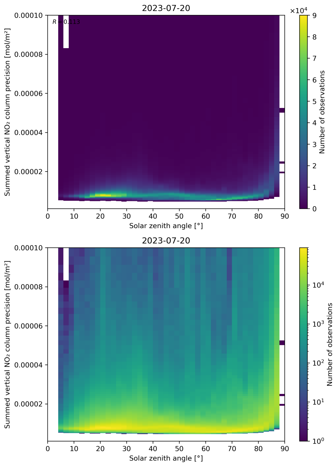
Figure 152: Scatter density plot of “Solar zenith angle” against “Summed vertical NO 2 column precision” for 2023-07-19 to 2023-07-21.
