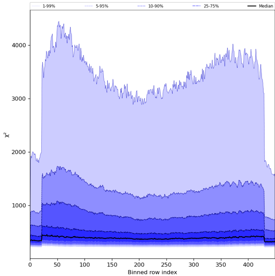
Figure 59: Along track statistics of “ \chi^2 ” for 2023-07-19 to 2023-07-21
