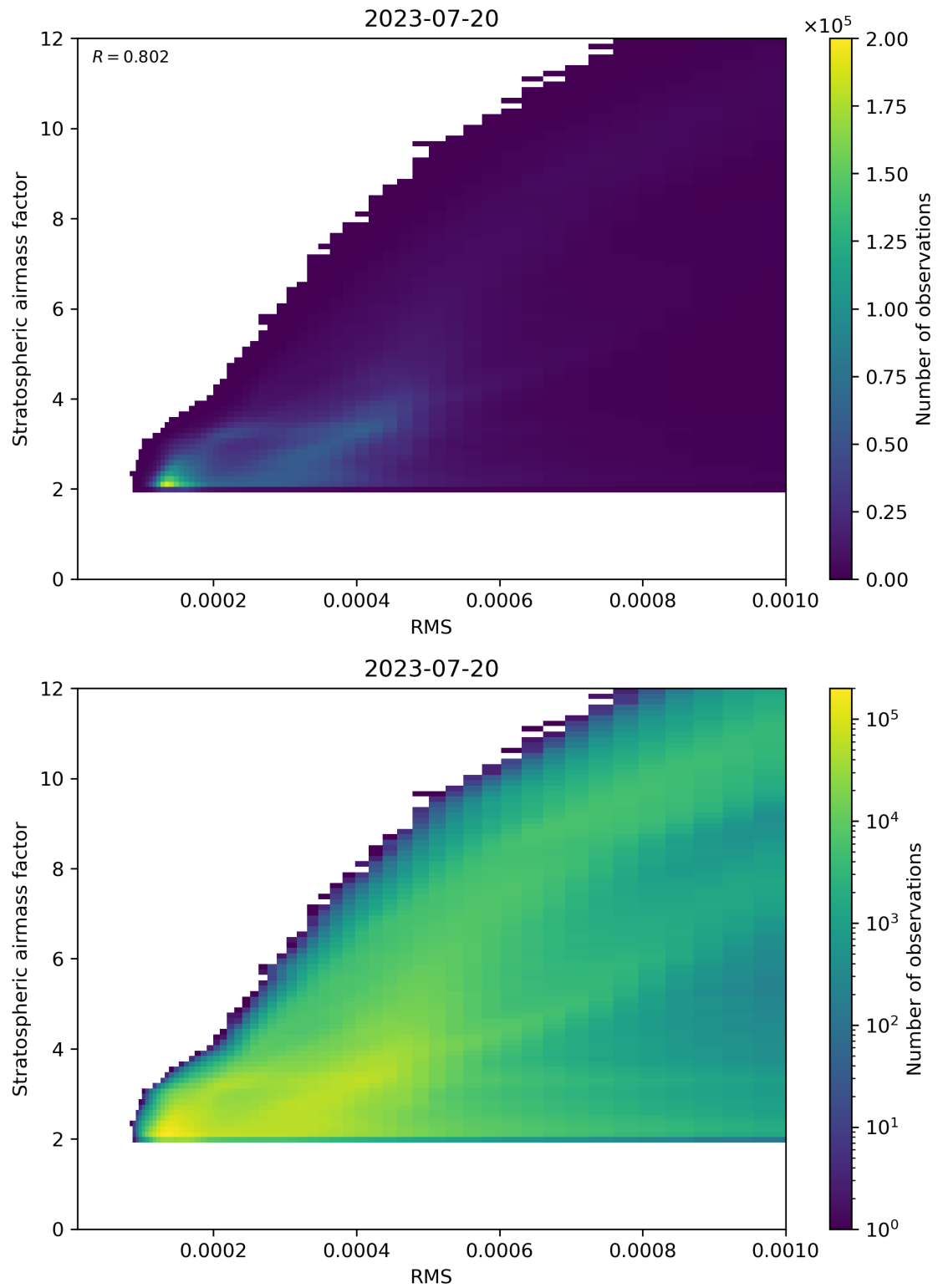
Figure 144: Scatter density plot of “RMS” against “Stratospheric airmass factor” for 2023-07-19 to 2023-07-21.
