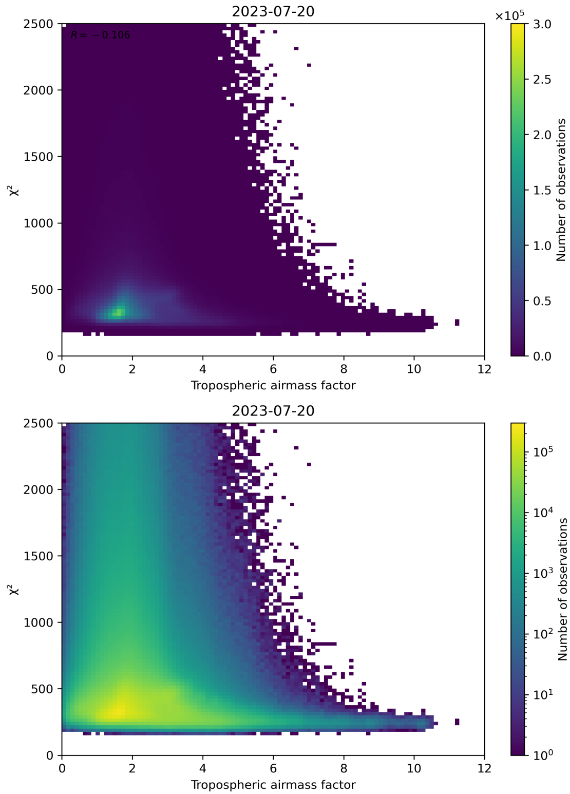
Figure 73: Scatter density plot of “Tropospheric airmass factor” against “ \chi^2 ” for 2023-07-19 to 2023-07-21.
