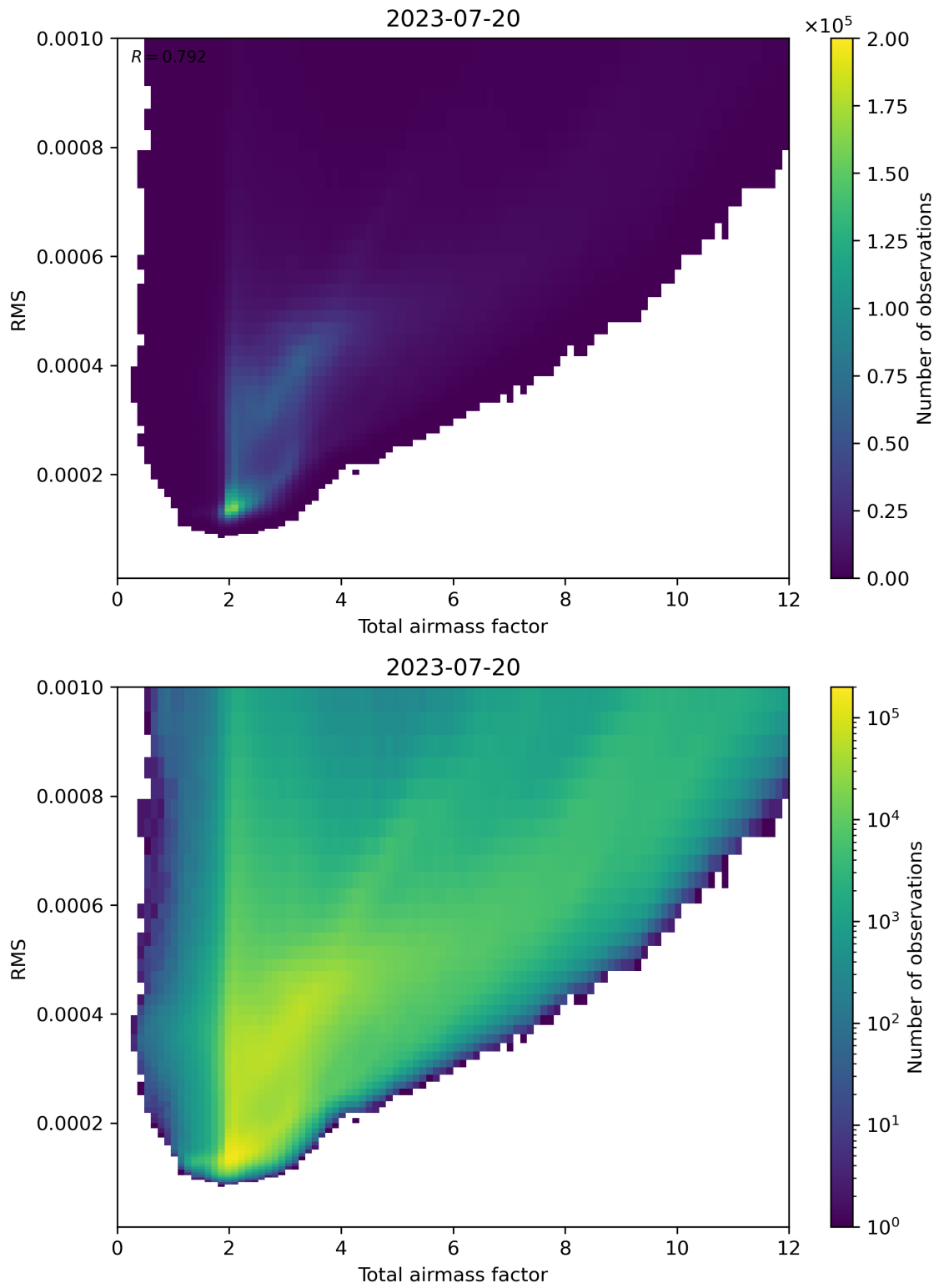
Figure 69: Scatter density plot of “Total airmass factor” against “RMS” for 2023-07-19 to 2023-07-21.
