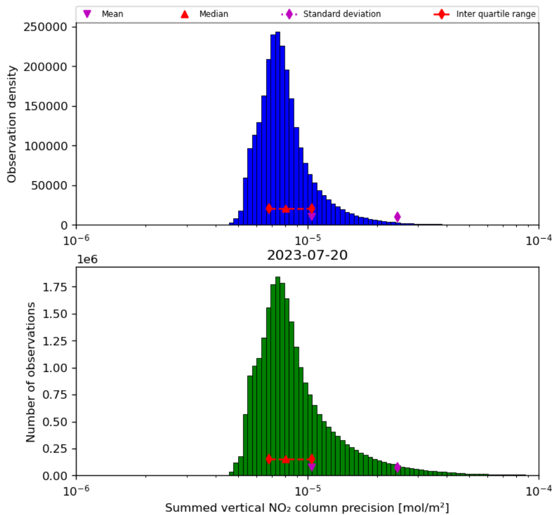
Figure 41: Histogram of "Summed vertical NO 2 column precision" for 2023-07-19 to 2023-07-21
