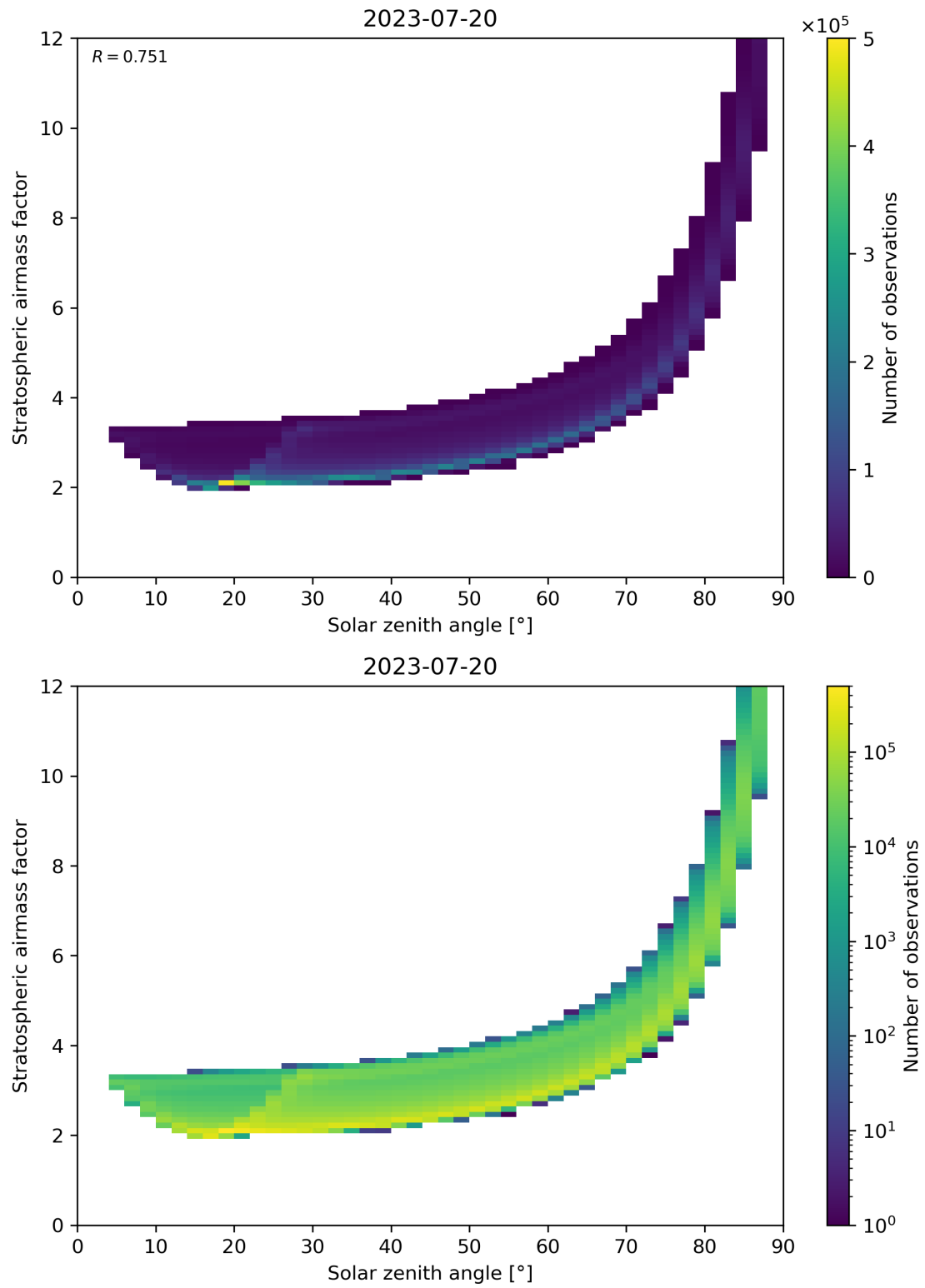
Figure 145: Scatter density plot of “Solar zenith angle” against “Stratospheric airmass factor” for 2023-07-19 to 2023-07-21.
