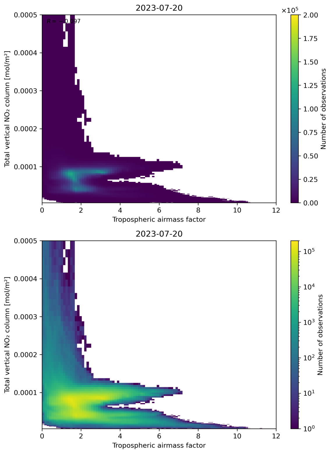
Figure 77: Scatter density plot of “Tropospheric airmass factor” against “Total vertical NO 2 column” for 2023-07-19 to 2023-07-21.
