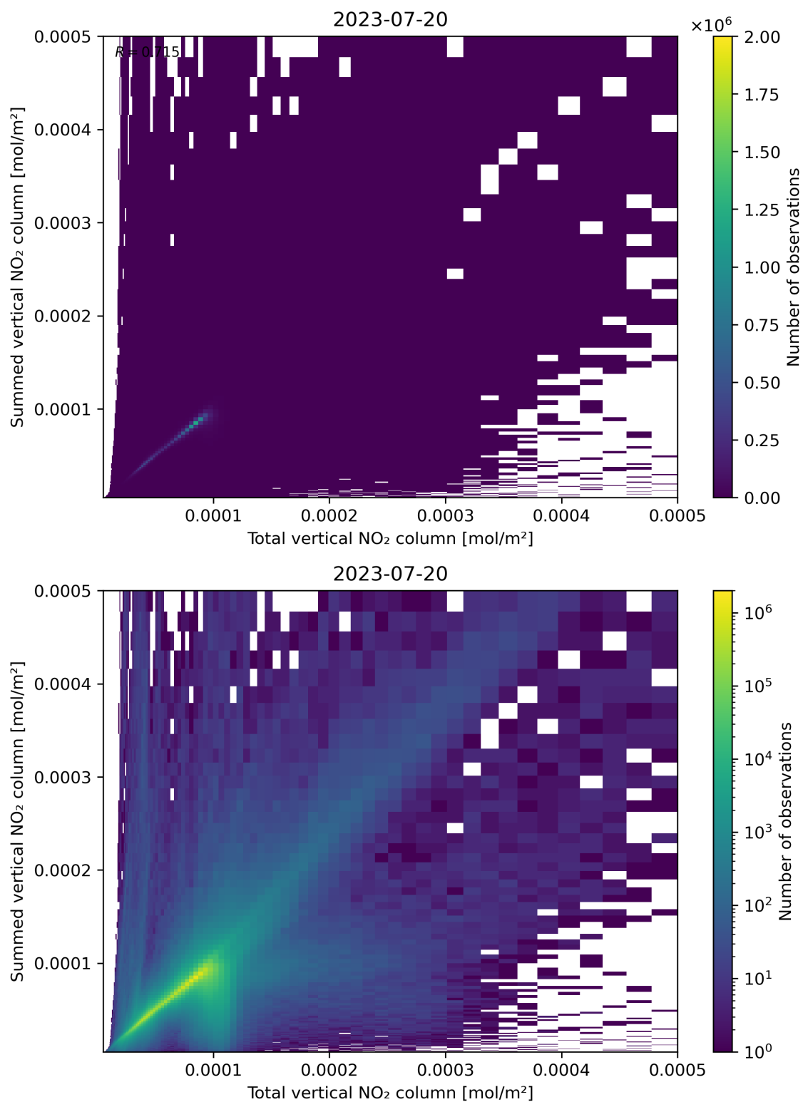
Figure 112: Scatter density plot of “Total vertical NO 2 column” against “Summed vertical NO 2 column” for 2023-07-19 to 2023-07-21.
