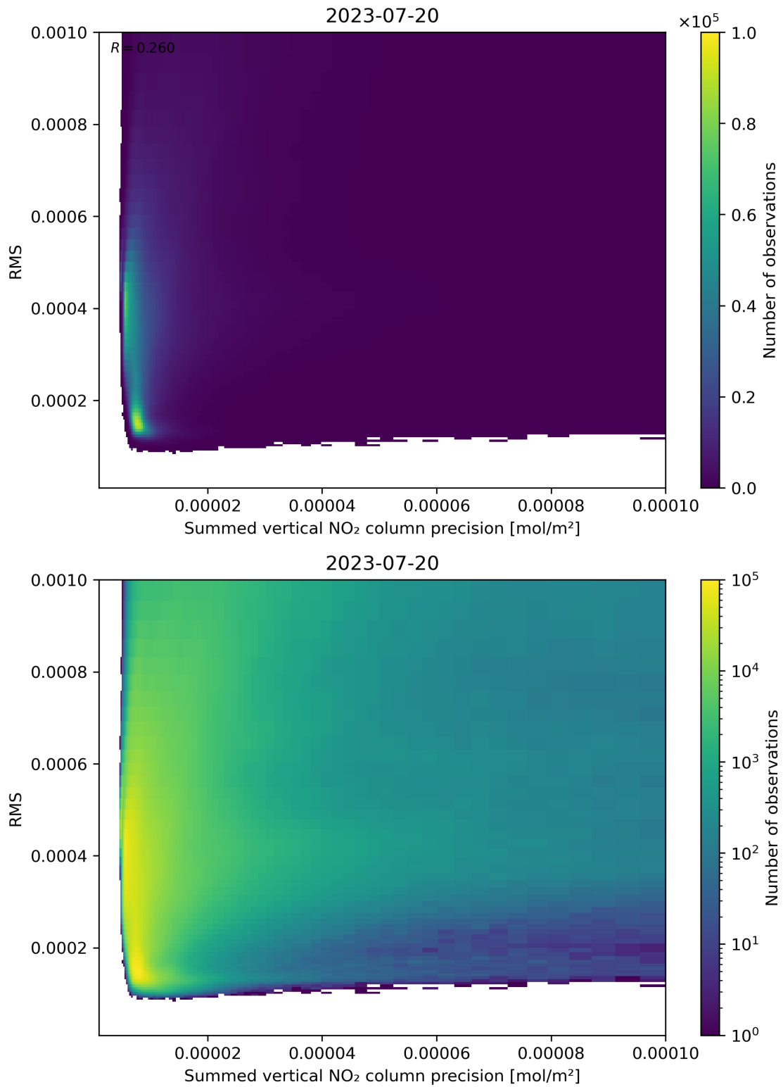
Figure 108: Scatter density plot of “Summed vertical NO 2 column precision” against “RMS” for 2023-07-19 to 2023-07-21.
