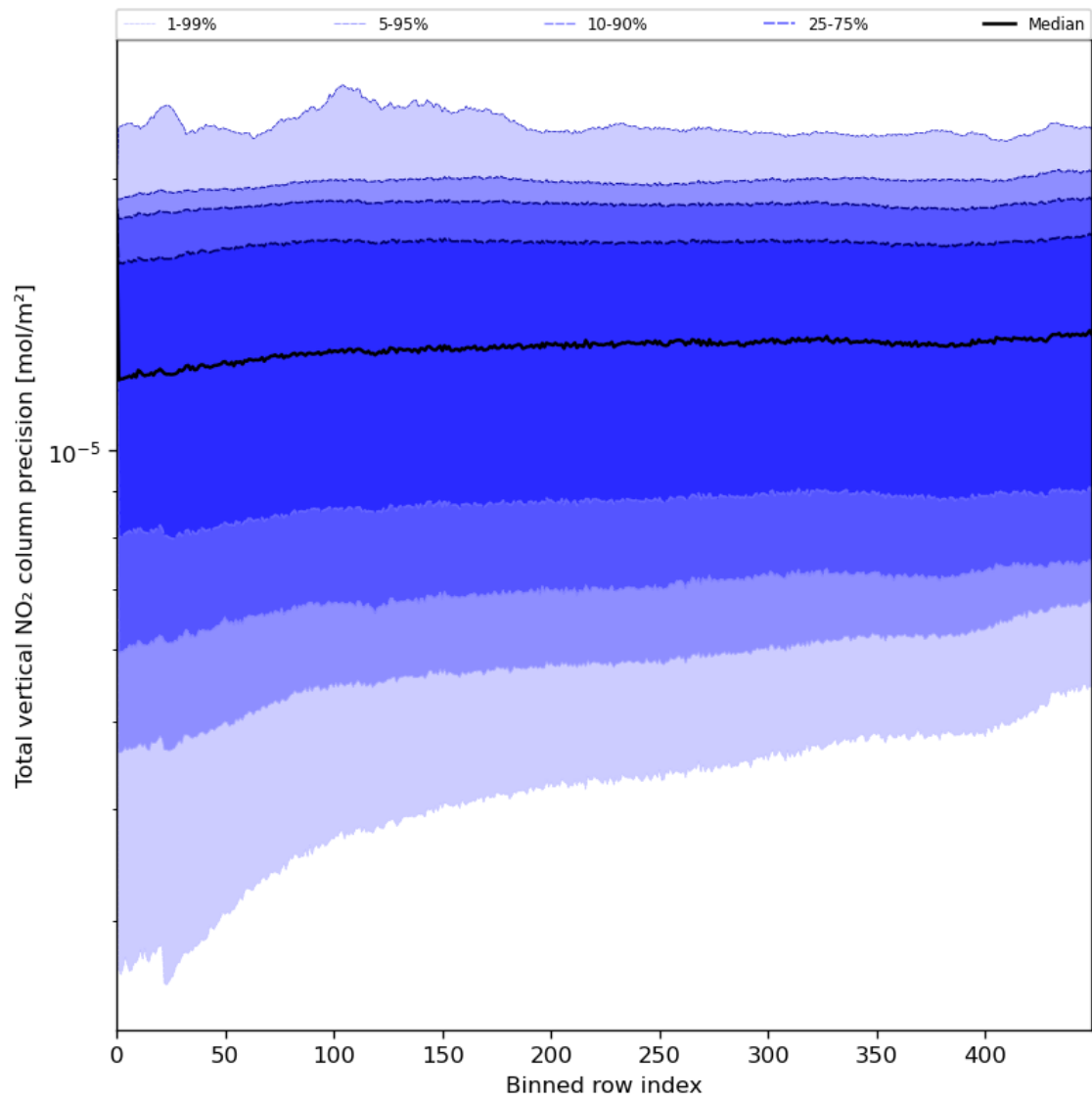
Figure 56: Along track statistics of “Total vertical NO 2 column precision” for 2023-07-19 to 2023-07-21
