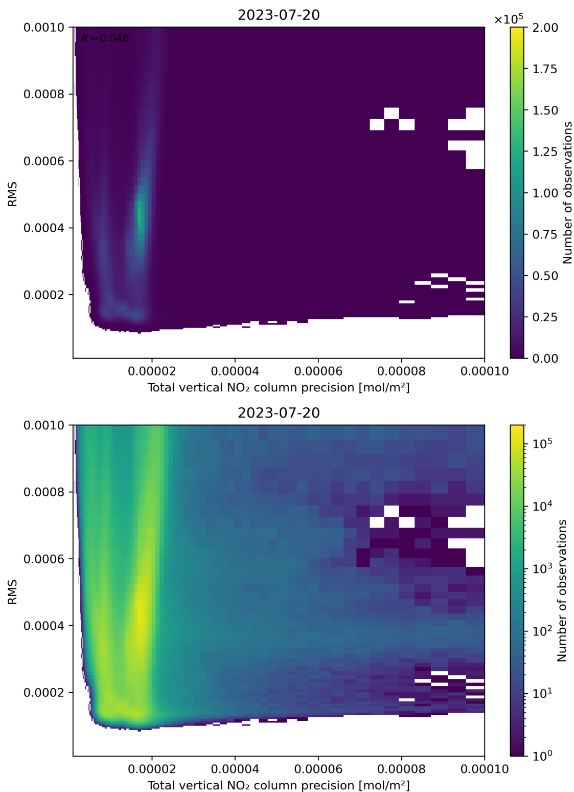
Figure 119: Scatter density plot of “Total vertical NO 2 column precision” against “RMS” for 2023-07-19 to 2023-07-21.
