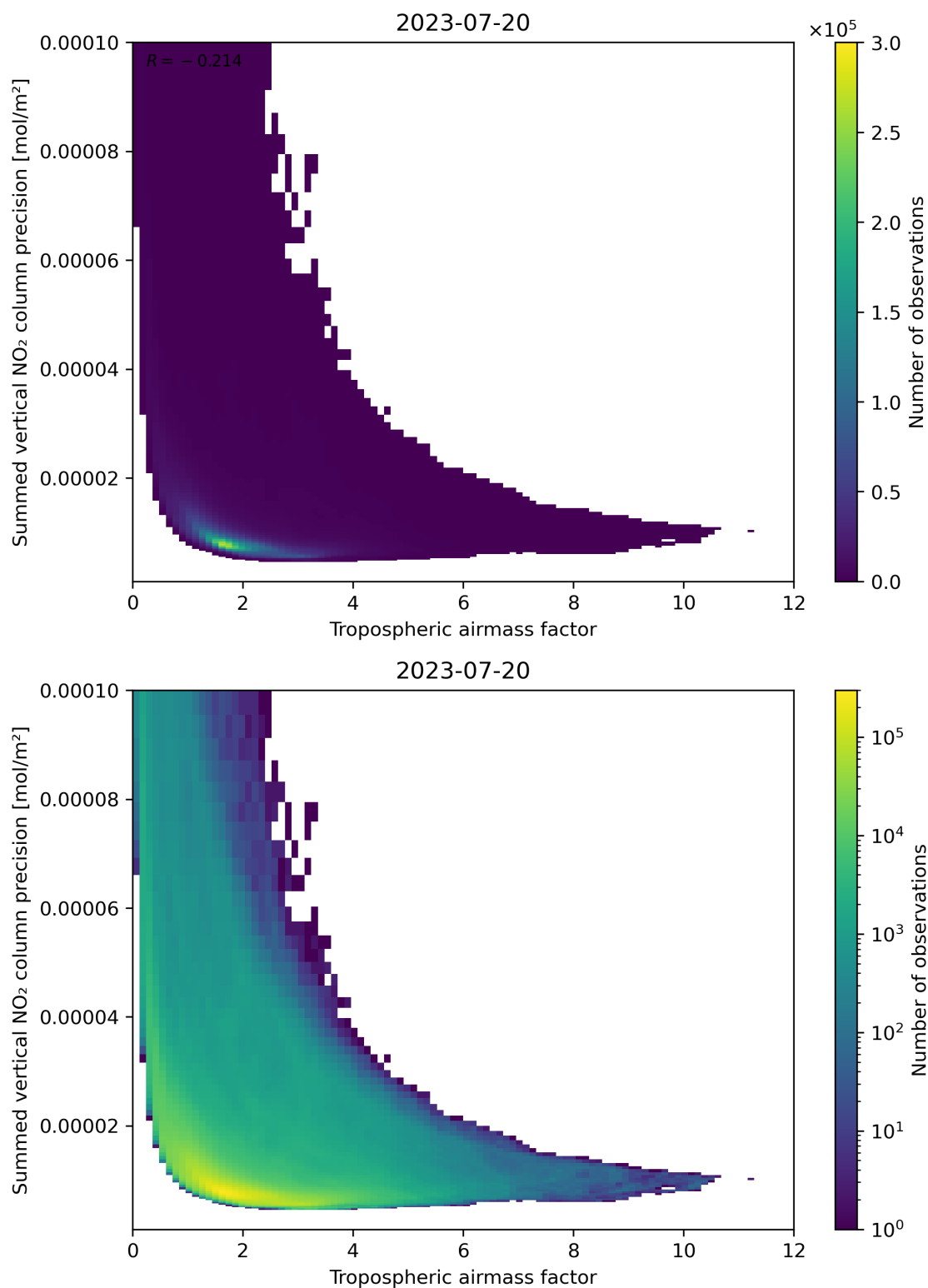
Figure 76: Scatter density plot of “Tropospheric air mass factor” against “Summed vertical NO 2 column precision” for 2023-07-19 to 2023-07-21.
