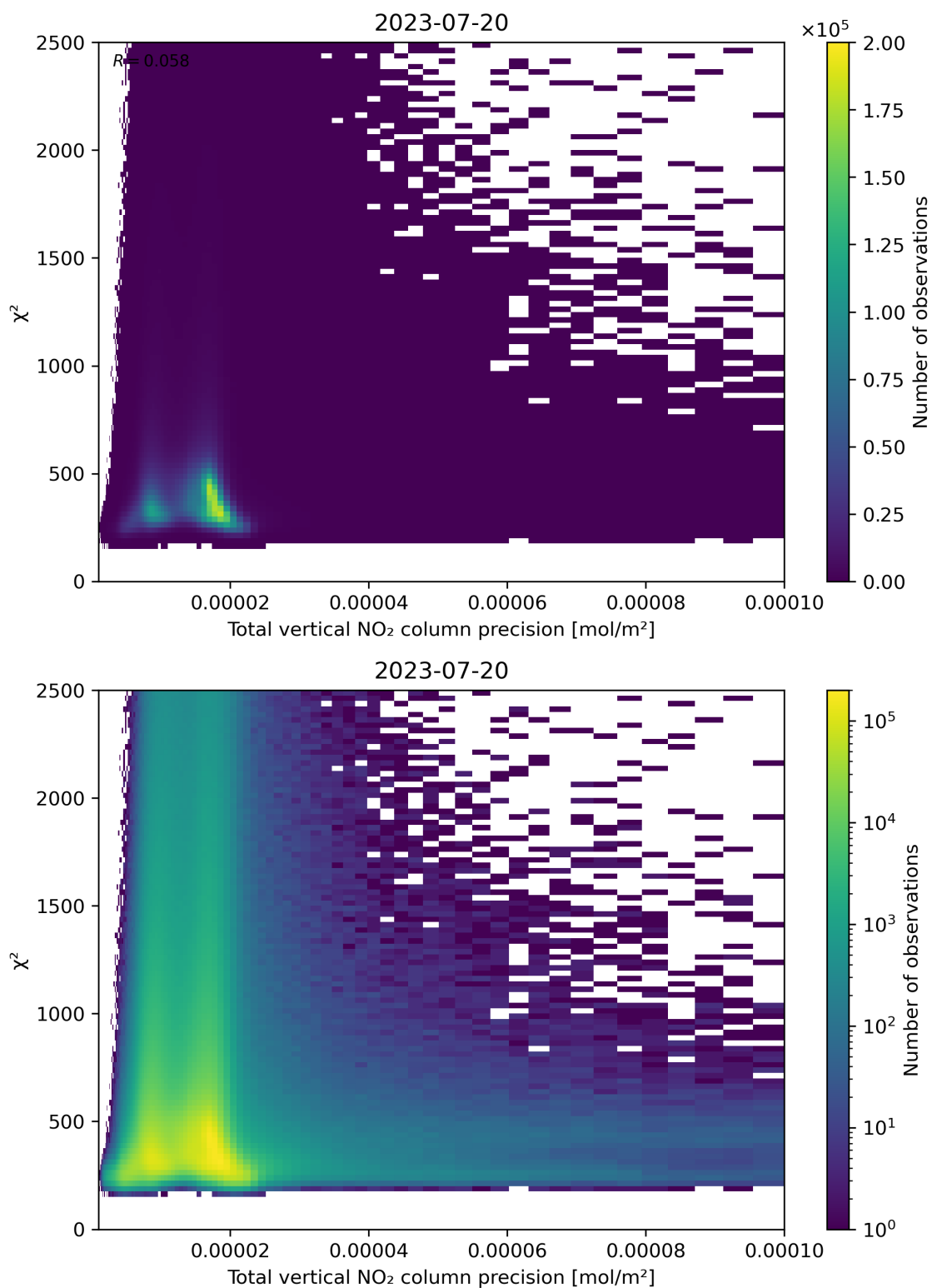
Figure 116: Scatter density plot of “Total vertical NO 2 column precision” against “ \chi^2 ” for 2023-07-19 to 2023-07-21.
