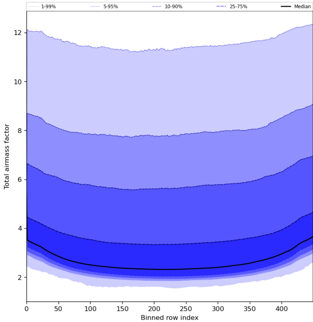
Figure 49: Along track statistics of “Total airmass factor” for 2023-07-19 to 2023-07-21
