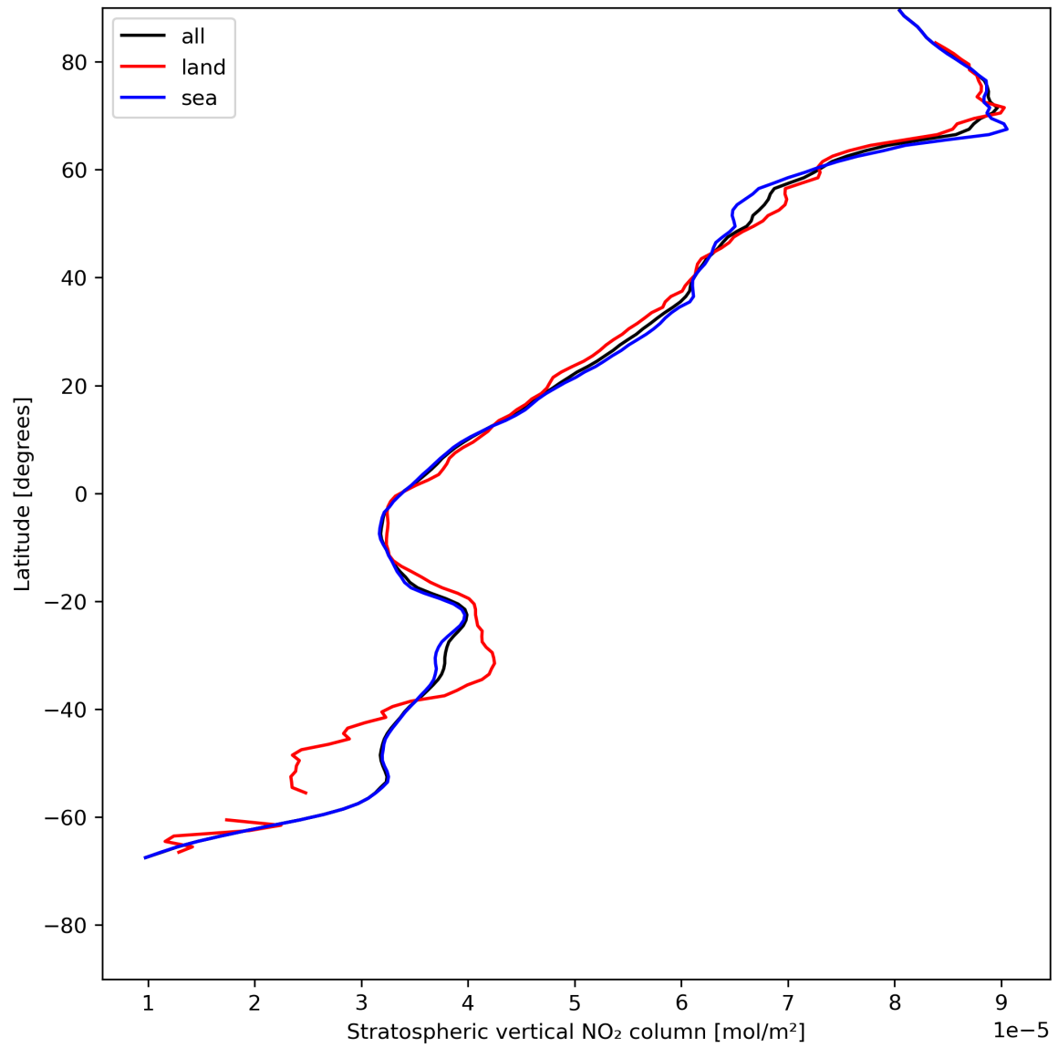
Figure 19: Zonal average of “Stratospheric vertical NO 2 column” for 2023-07-19 to 2023-07-21.
