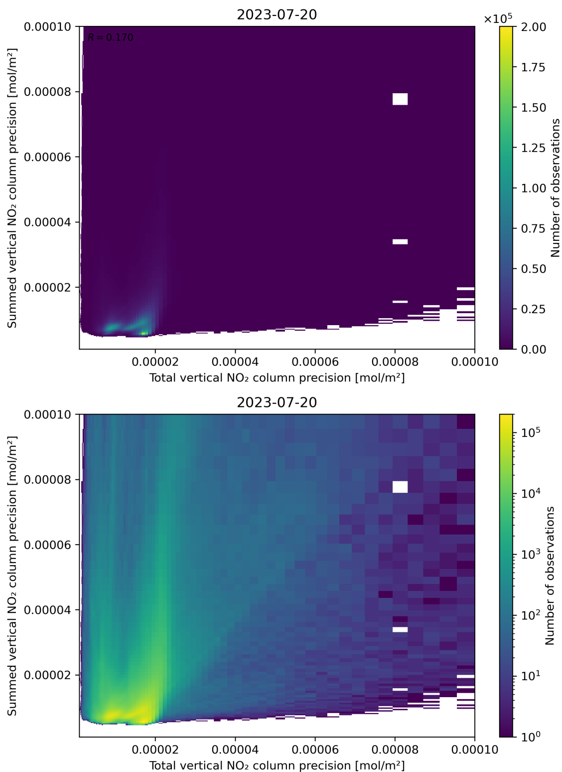
Figure 118: Scatter density plot of “Total vertical NO 2 column precision” against “Summed vertical NO 2 column precision” for 2023-07-19 to 2023-07-21.
