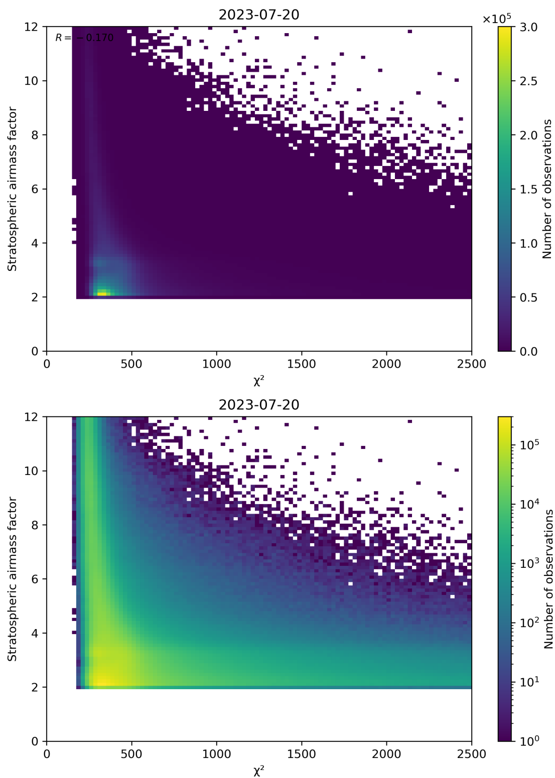
Figure 81: Scatter density plot of “ \chi^2 ” against “Stratospheric airmass factor” for 2023-07-19 to 2023-07-21.
