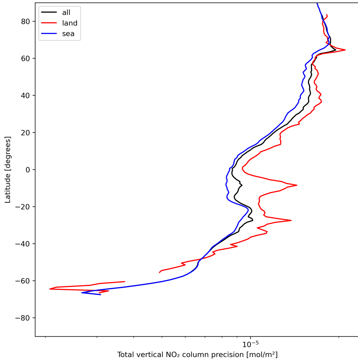
Figure 22: Zonal average of “Total vertical NO 2 column precision” for 2023-07-19 to 2023-07-21.
