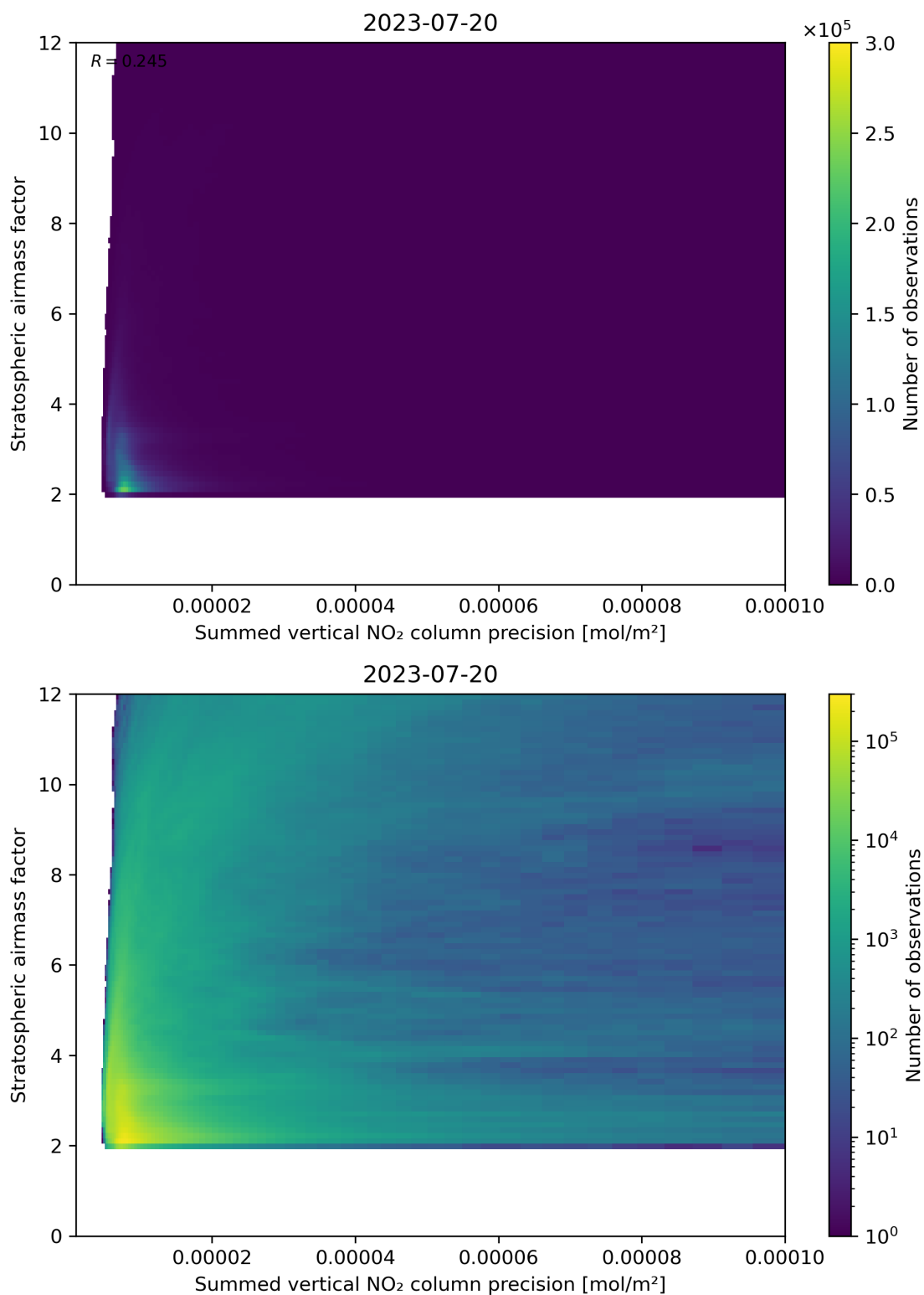
Figure 106: Scatter density plot of “Summed vertical NO 2 column precision” against “Stratospheric airmass factor” for 2023-07-19 to 2023-07-21.
