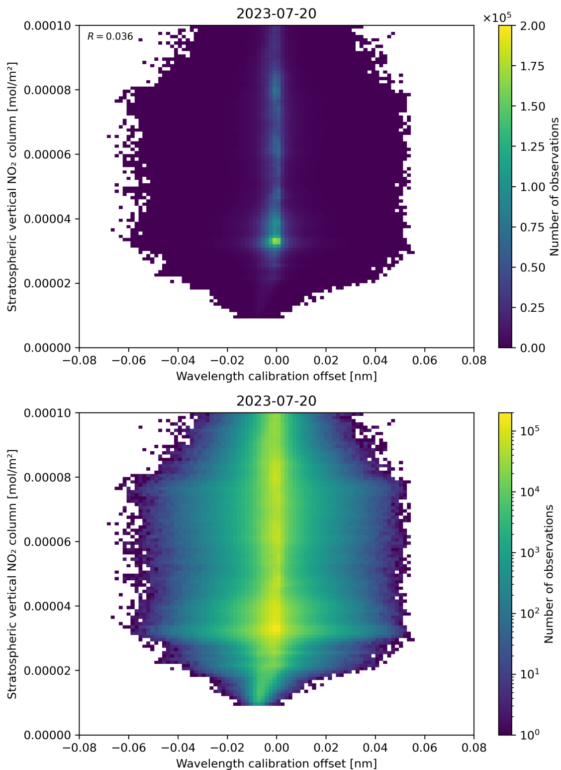
Figure 176: Scatter density plot of “Wavelength calibration offset” against “Stratospheric vertical NO 2 column” for 2023-07-19 to 2023-07-21.
