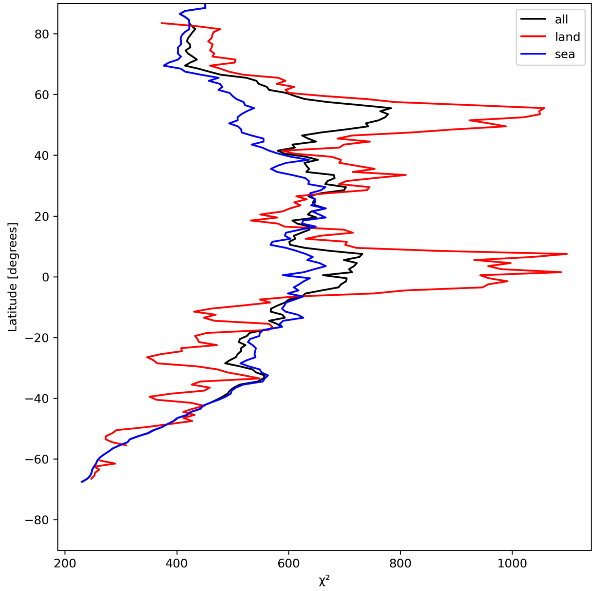
Figure 25: Zonal average of “ \chi^2 ” for 2023-07-19 to 2023-07-21.
