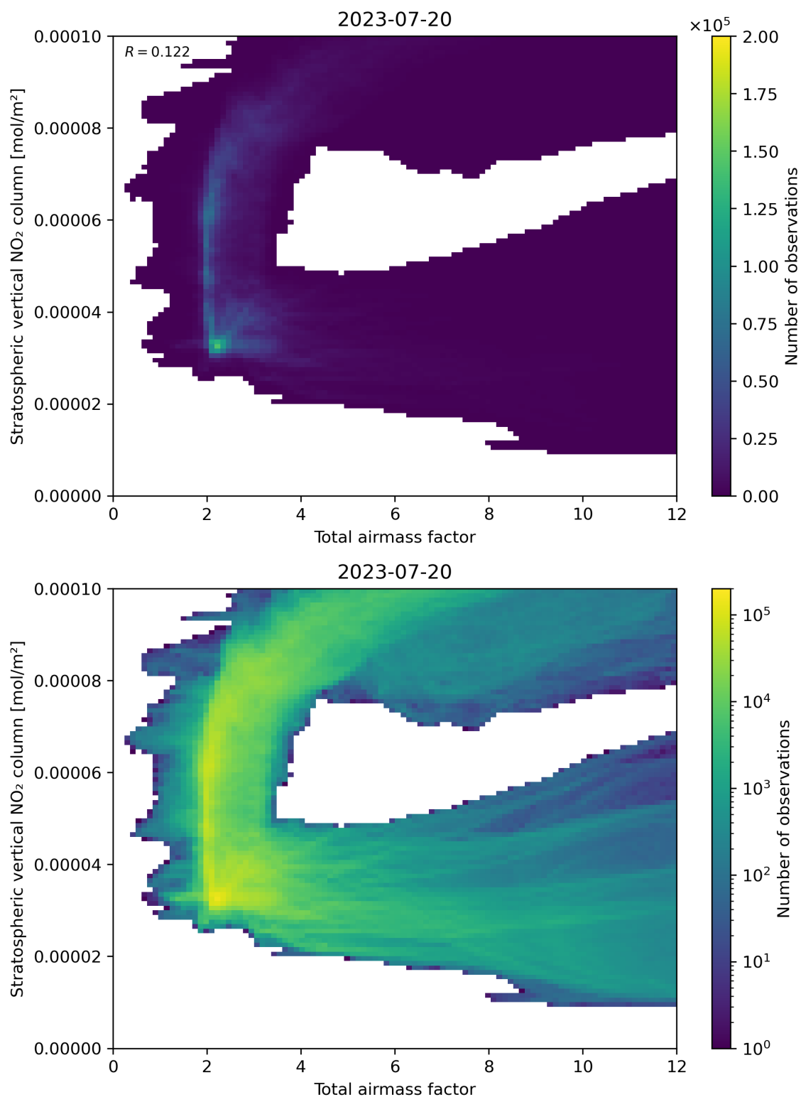
Figure 64: Scatter density plot of “Total airmass factor” against “Stratospheric vertical \text{NO}_2 column” for 2023-07-19 to 2023-07-21.
