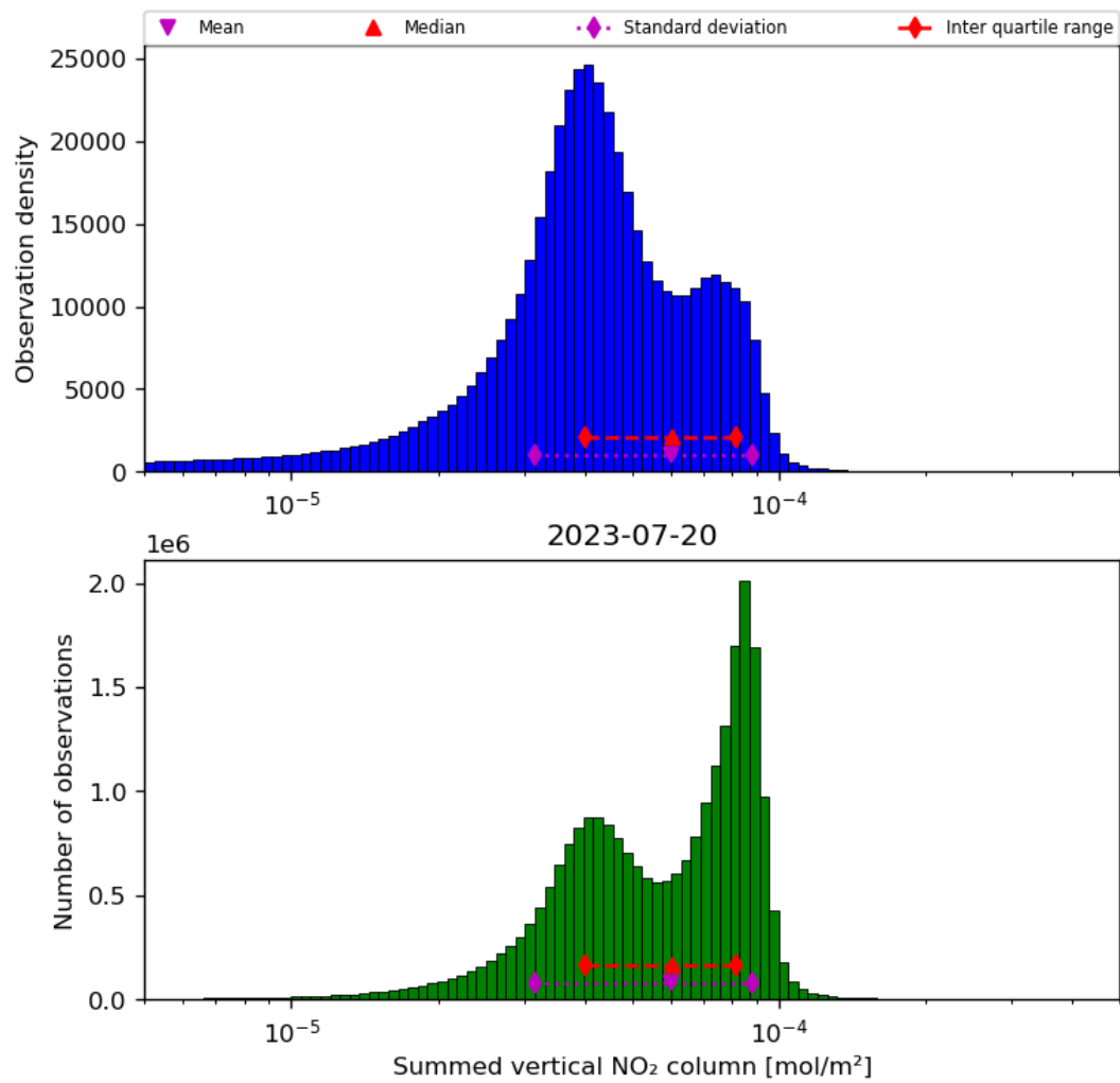
Figure 40: Histogram of “Summed vertical NO 2 column” for 2023-07-19 to 2023-07-21
