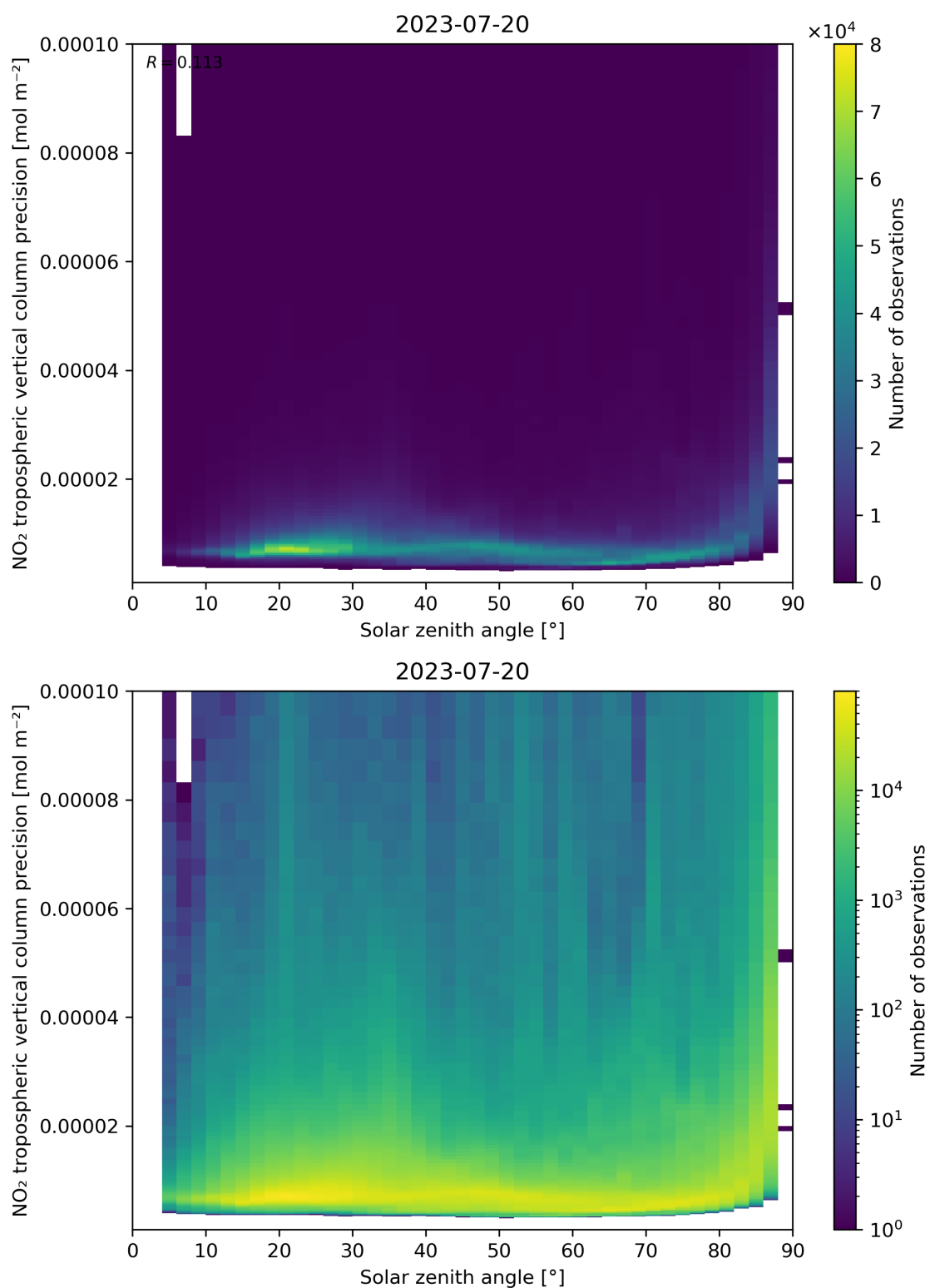
Figure 156: Scatter density plot of “Solar zenith angle” against “NO 2 tropospheric vertical column precision” for 2023-07-19 to 2023-07-21.
