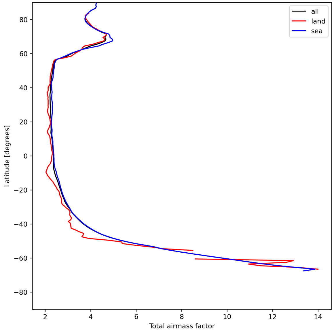
Figure 15: Zonal average of “Total airmass factor” for 2023-07-19 to 2023-07-21.
