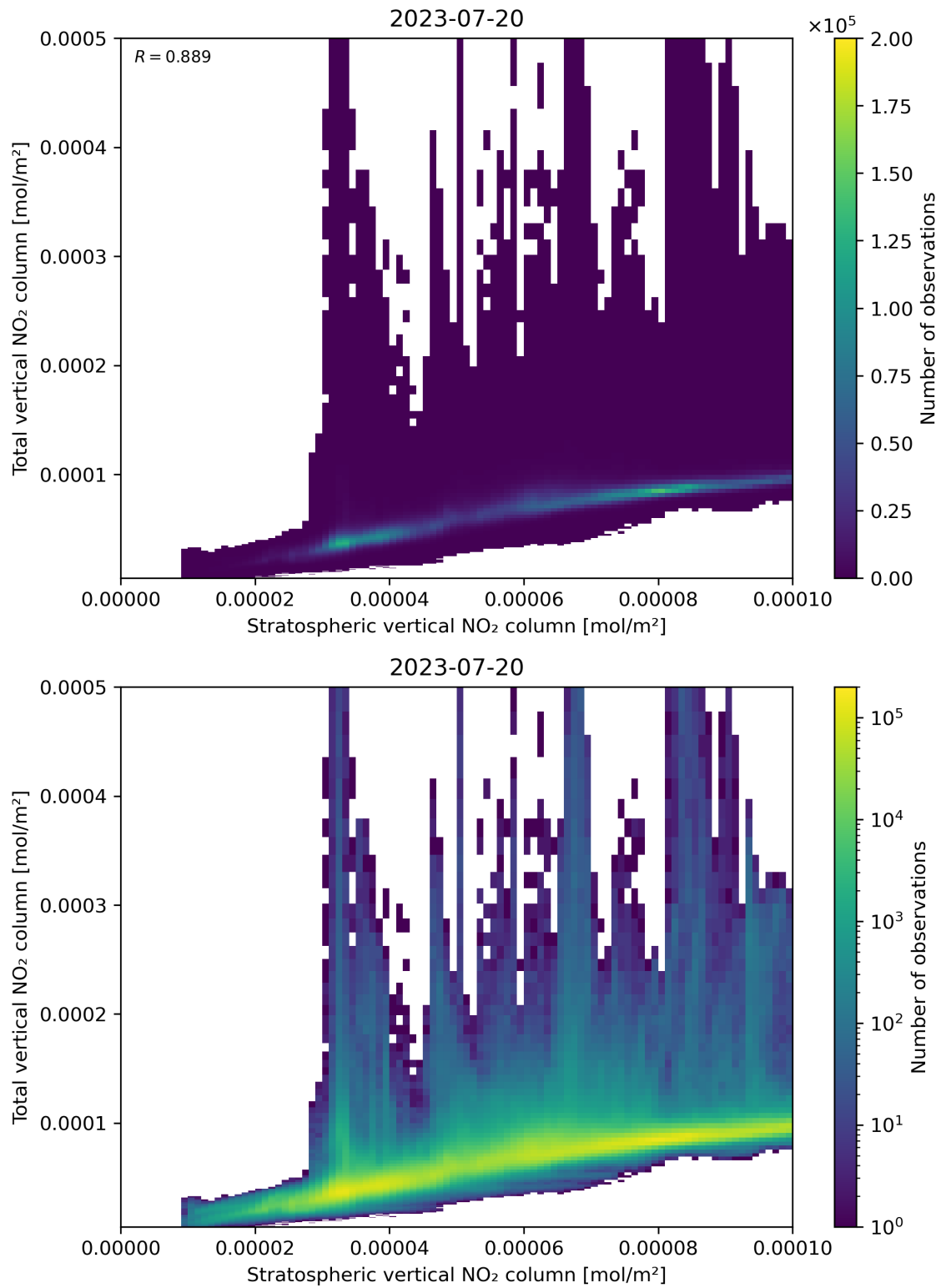
Figure 100: Scatter density plot of “Stratospheric vertical NO 2 column” against “Total vertical NO 2 column” for 2023-07-19 to 2023-07-21.
