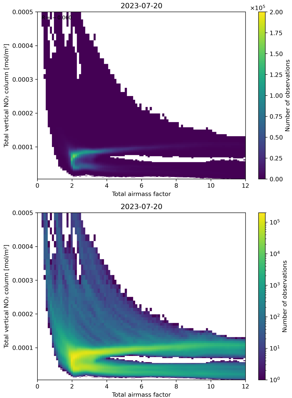
Figure 67: Scatter density plot of “Total airmass factor” against “Total vertical NO 2 column” for 2023-07-19 to 2023-07-21.
