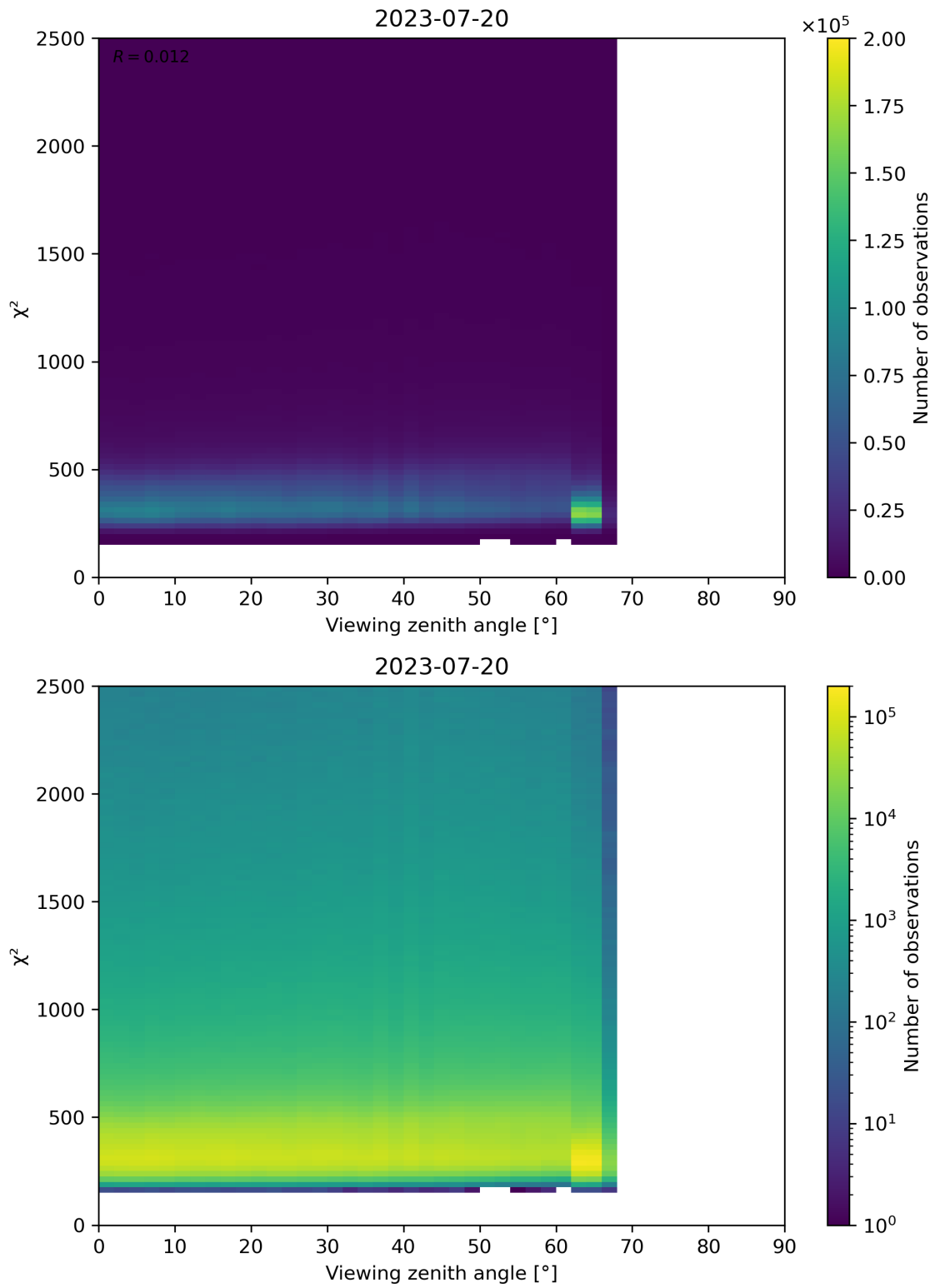
Figure 162: Scatter density plot of “Viewing zenith angle” against “ \chi^2 ” for 2023-07-19 to 2023-07-21.
