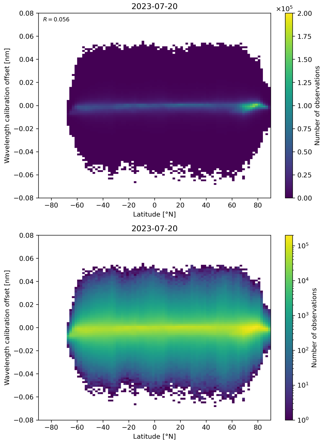
Figure 95: Scatter density plot of “Latitude” against “Wavelength calibration offset” for 2023-07-19 to 2023-07-21.
