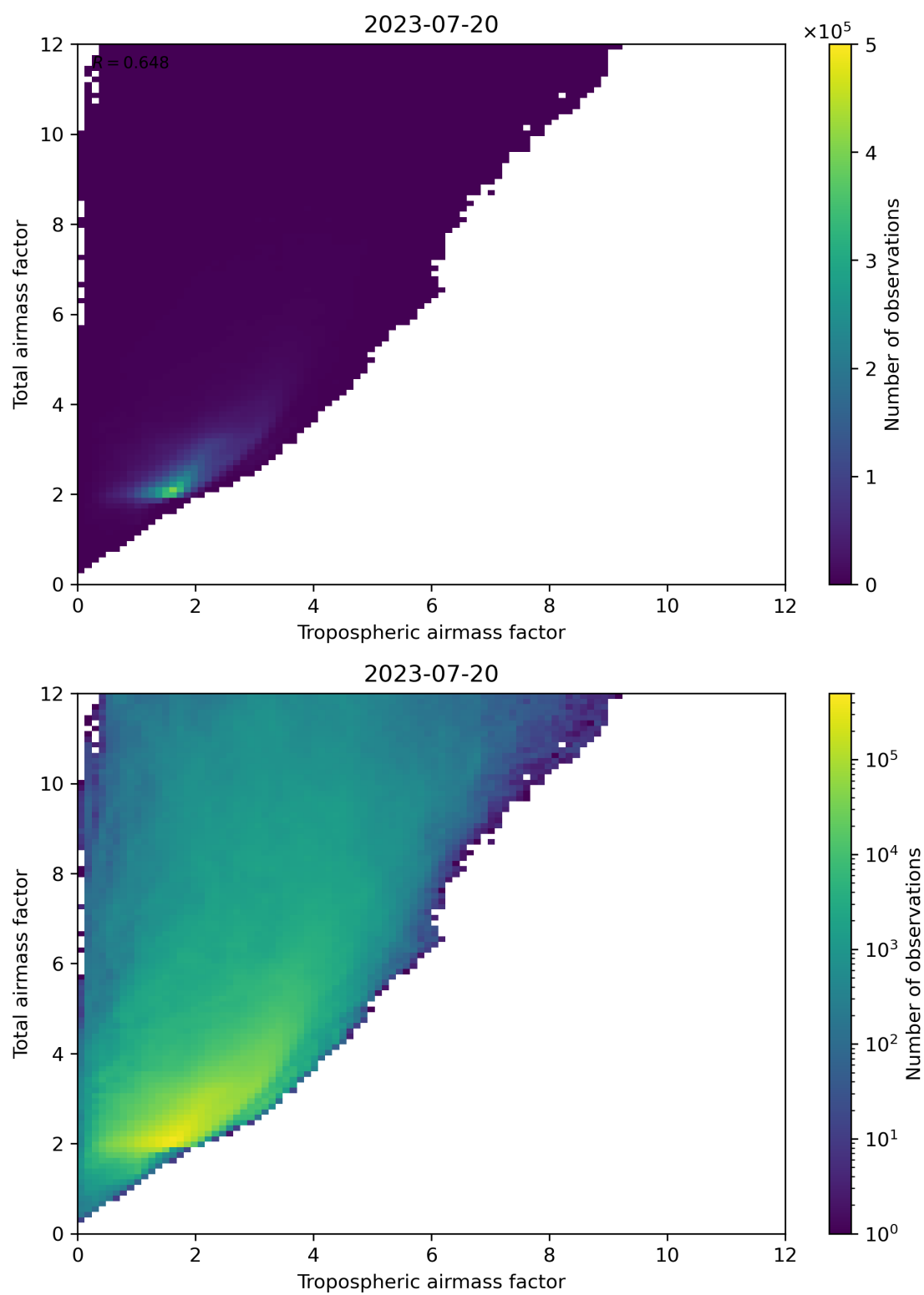
Figure 72: Scatter density plot of “Tropospheric airmass factor” against “Total airmass factor” for 2023-07-19 to 2023-07-21.
