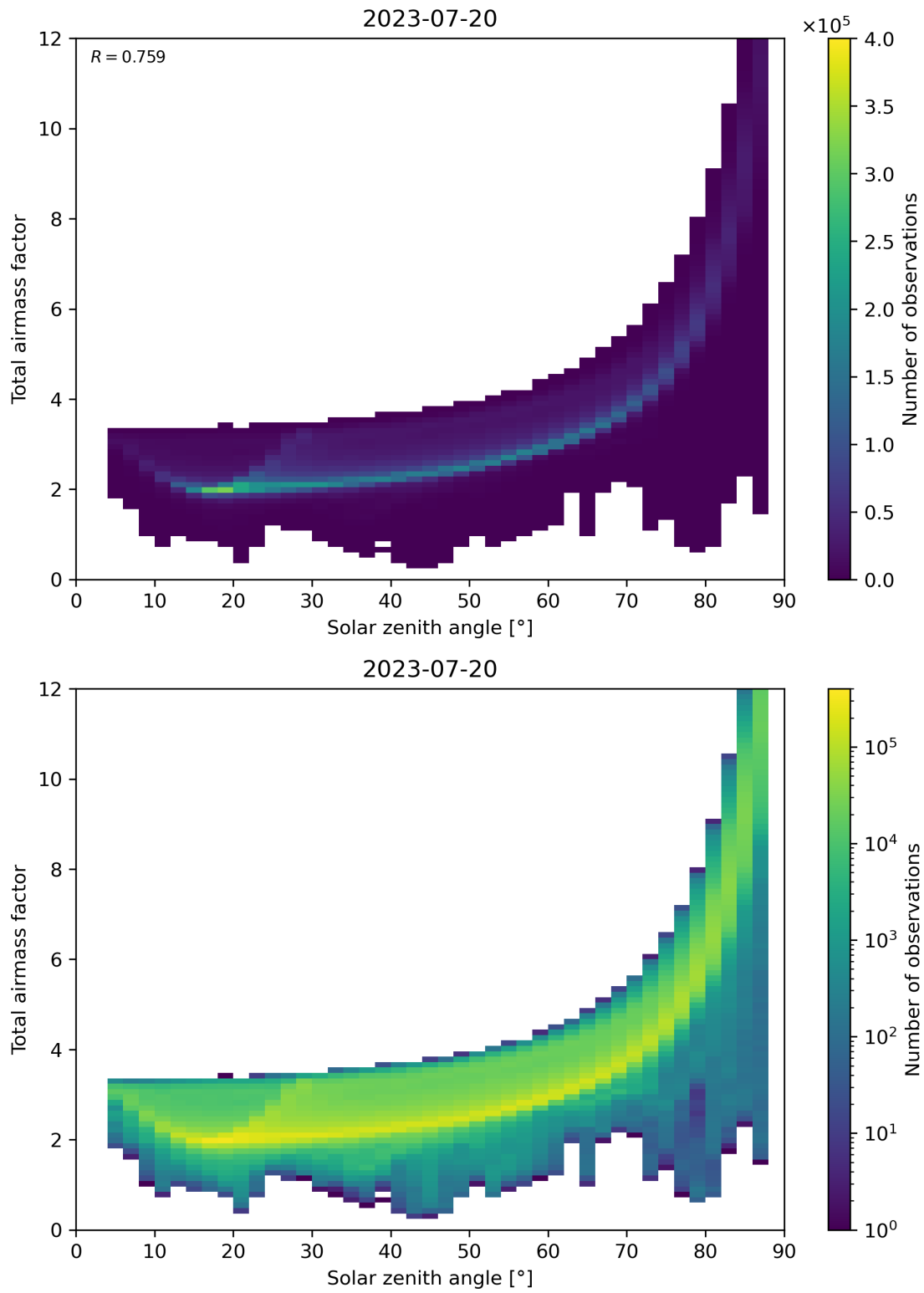
Figure 146: Scatter density plot of “Solar zenith angle” against “Total air mass factor” for 2023-07-19 to 2023-07-21.
