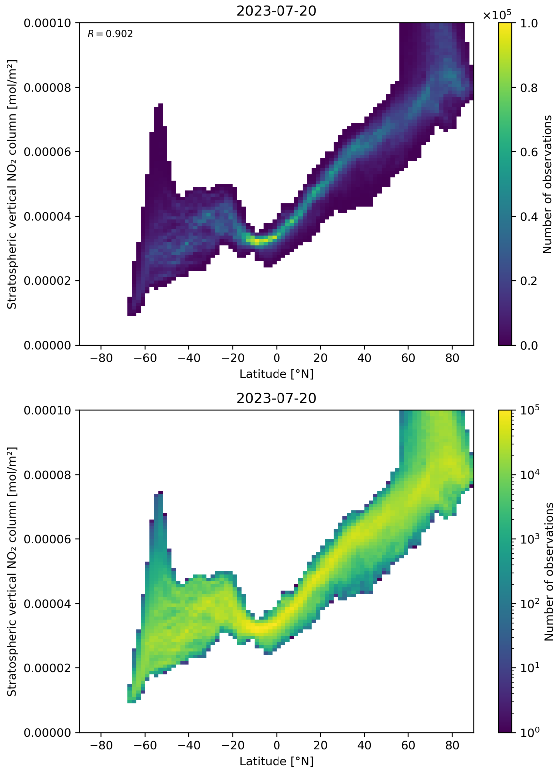
Figure 87: Scatter density plot of “Latitude” against “Stratospheric vertical NO 2 column” for 2023-07-19 to 2023-07-21.
