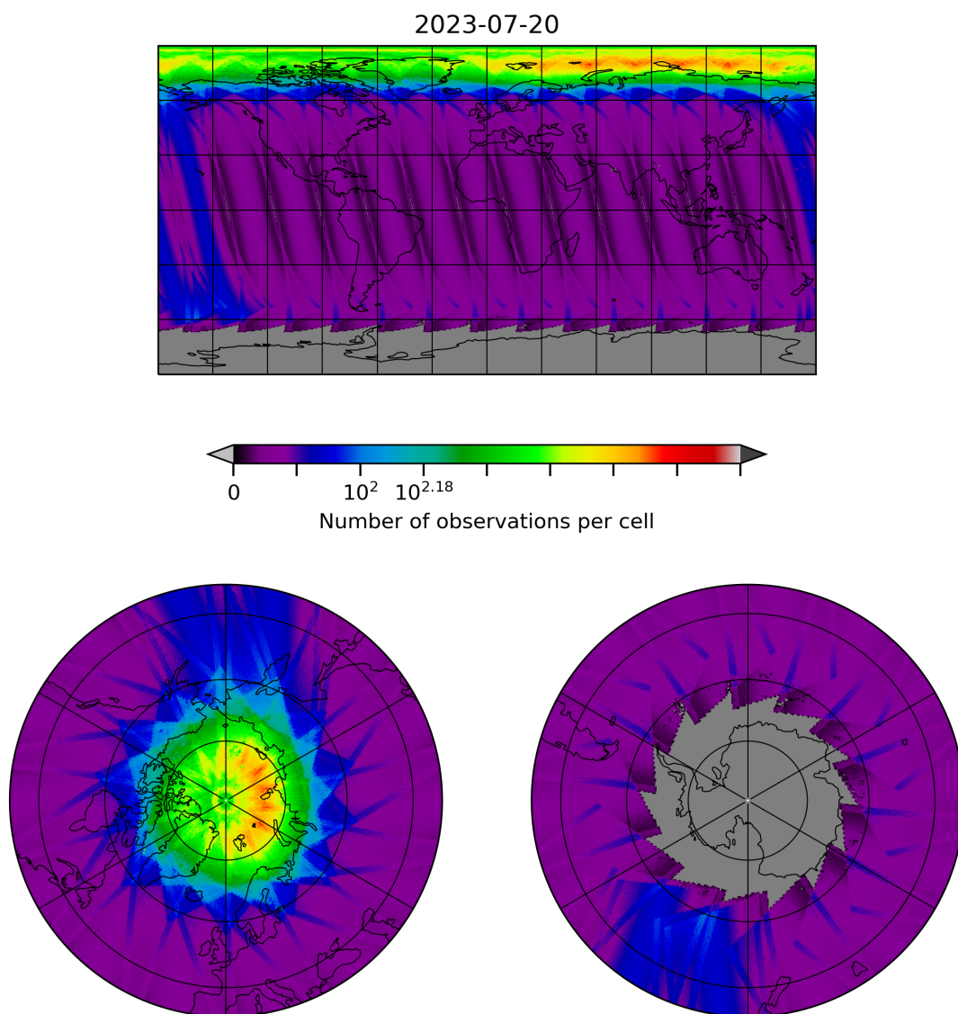
Figure 10: Map of the number of observations for 2023-07-19 to 2023-07-21
