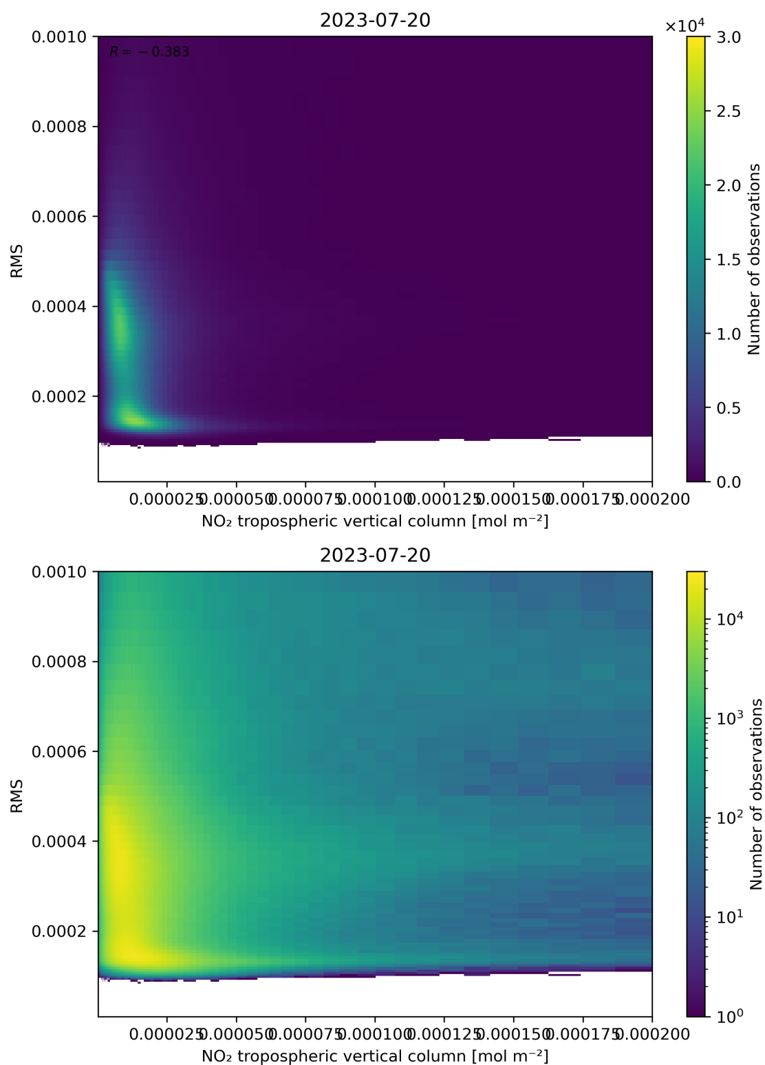
Figure 142: Scatter density plot of “NO 2 tropospheric vertical column” against “RMS” for 2023-07-19 to 2023-07-21.
