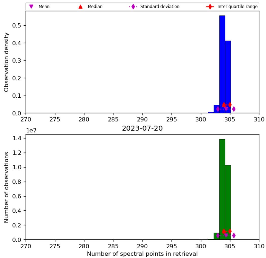
Figure 33: Histogram of “Number of spectral points in retrieval” for 2023-07-19 to 2023-07-21
