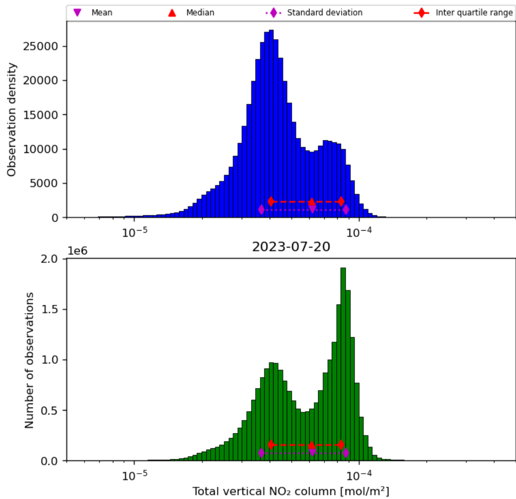
Figure 38: Histogram of “Total vertical NO 2 column” for 2023-07-19 to 2023-07-21
