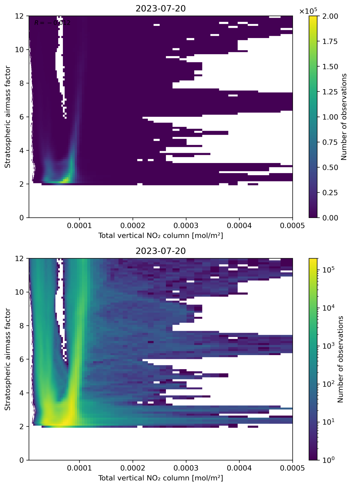
Figure 110: Scatter density plot of “Total vertical NO 2 column” against “Stratospheric airmass factor” for 2023-07-19 to 2023-07-21.
