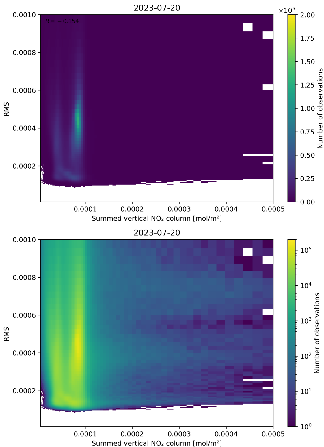
Figure 109: Scatter density plot of “Summed vertical NO 2 column” against “RMS” for 2023-07-19 to 2023-07-21.
