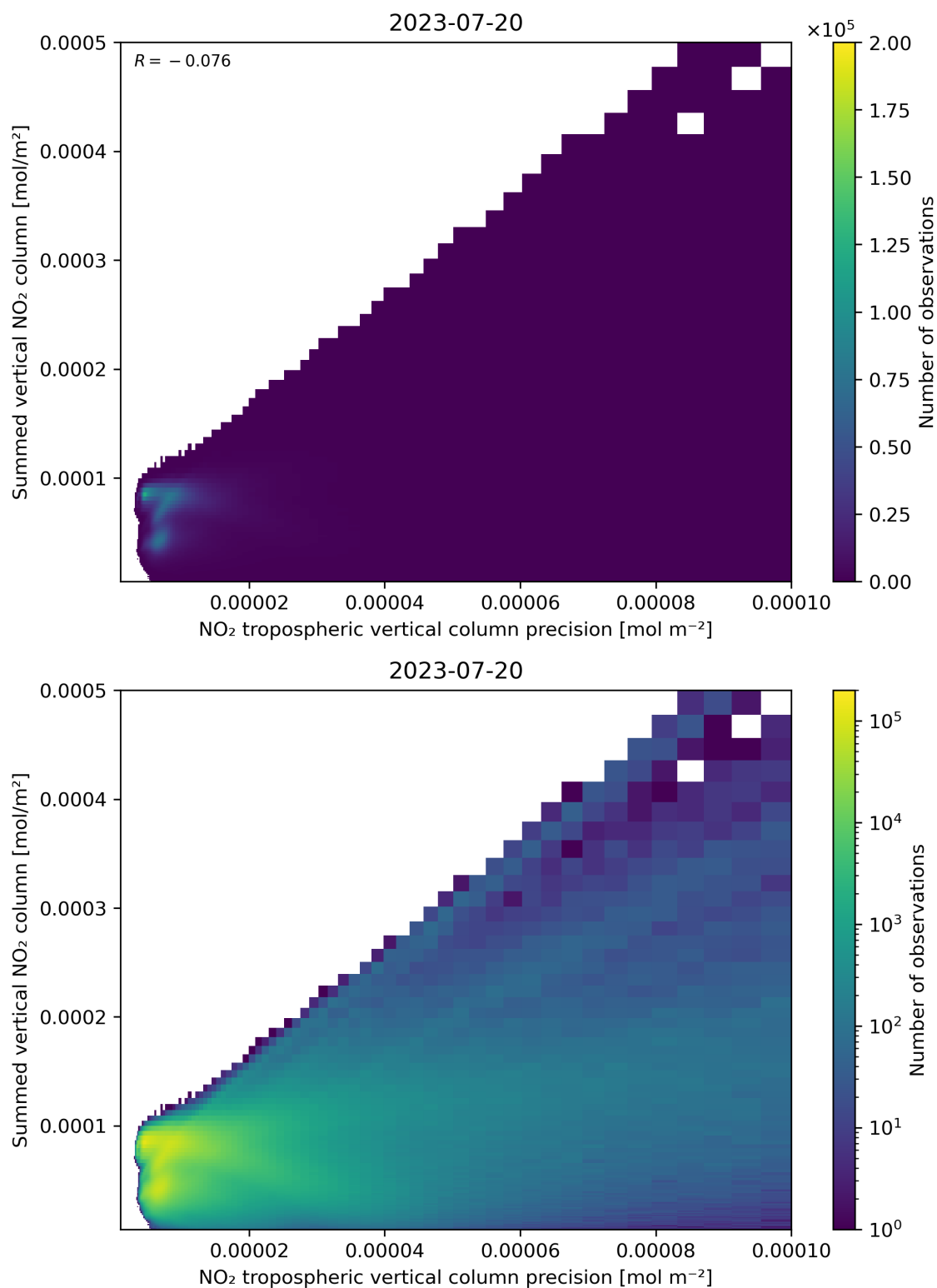
Figure 136: Scatter density plot of “NO 2 tropospheric vertical column precision” against “Summed vertical NO 2 column” for 2023-07-19 to 2023-07-21.
