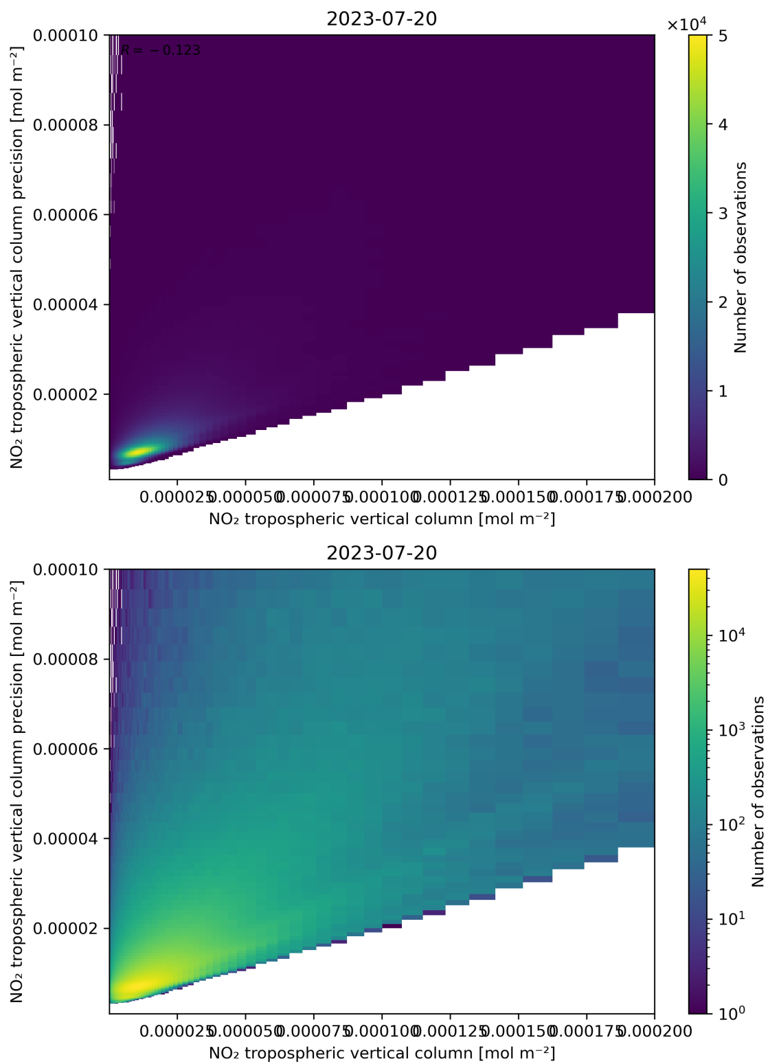
Figure 130: Scatter density plot of “NO 2 tropospheric vertical column” against “NO 2 tropospheric vertical column precision” for 2023-07-19 to 2023-07-21.
