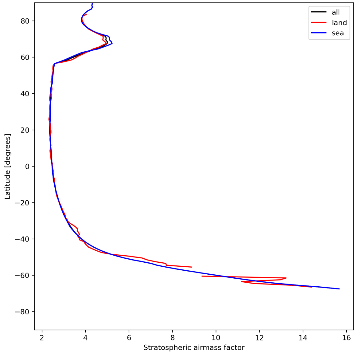
Figure 27: Zonal average of “Stratospheric air mass factor” for 2023-07-19 to 2023-07-21.
