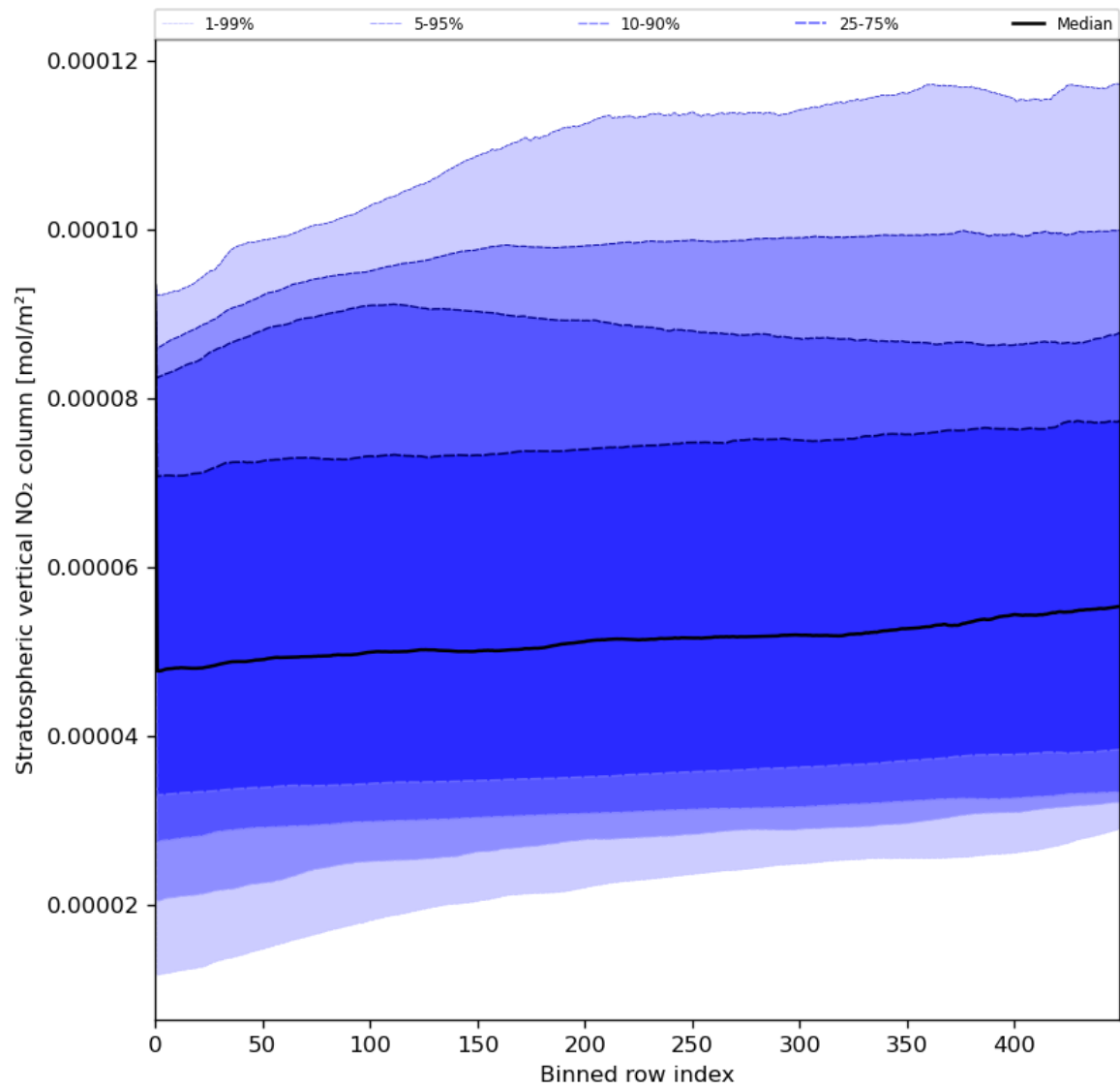
Figure 53: Along track statistics of “Stratospheric vertical NO 2 column” for 2023-07-19 to 2023-07-21
