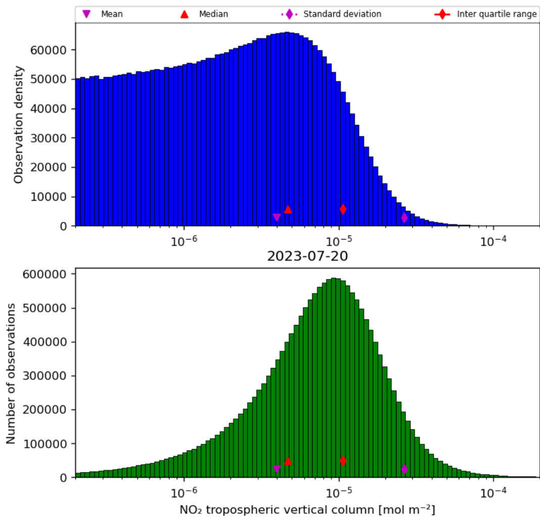
Figure 29: Histogram of “NO 2 tropospheric vertical column” for 2023-07-19 to 2023-07-21
