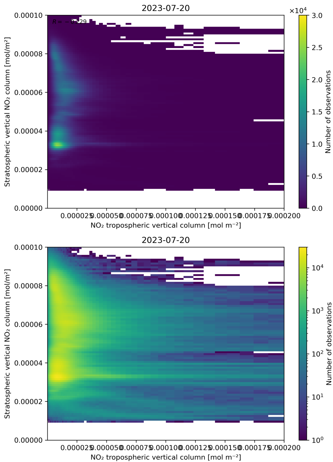
Figure 125: Scatter density plot of “NO 2 tropospheric vertical column” against “Stratospheric vertical NO 2 column” for 2023-07-19 to 2023-07-21.
