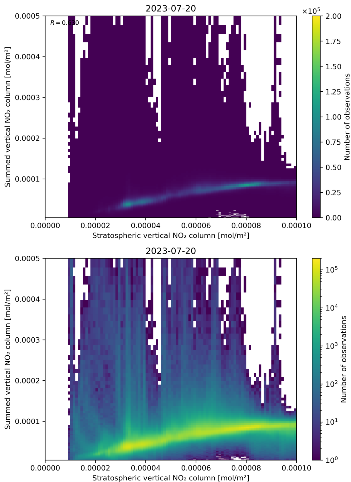
Figure 98: Scatter density plot of “Stratospheric vertical NO 2 column” against “Summed vertical NO 2 column” for 2023-07-19 to 2023-07-21.
