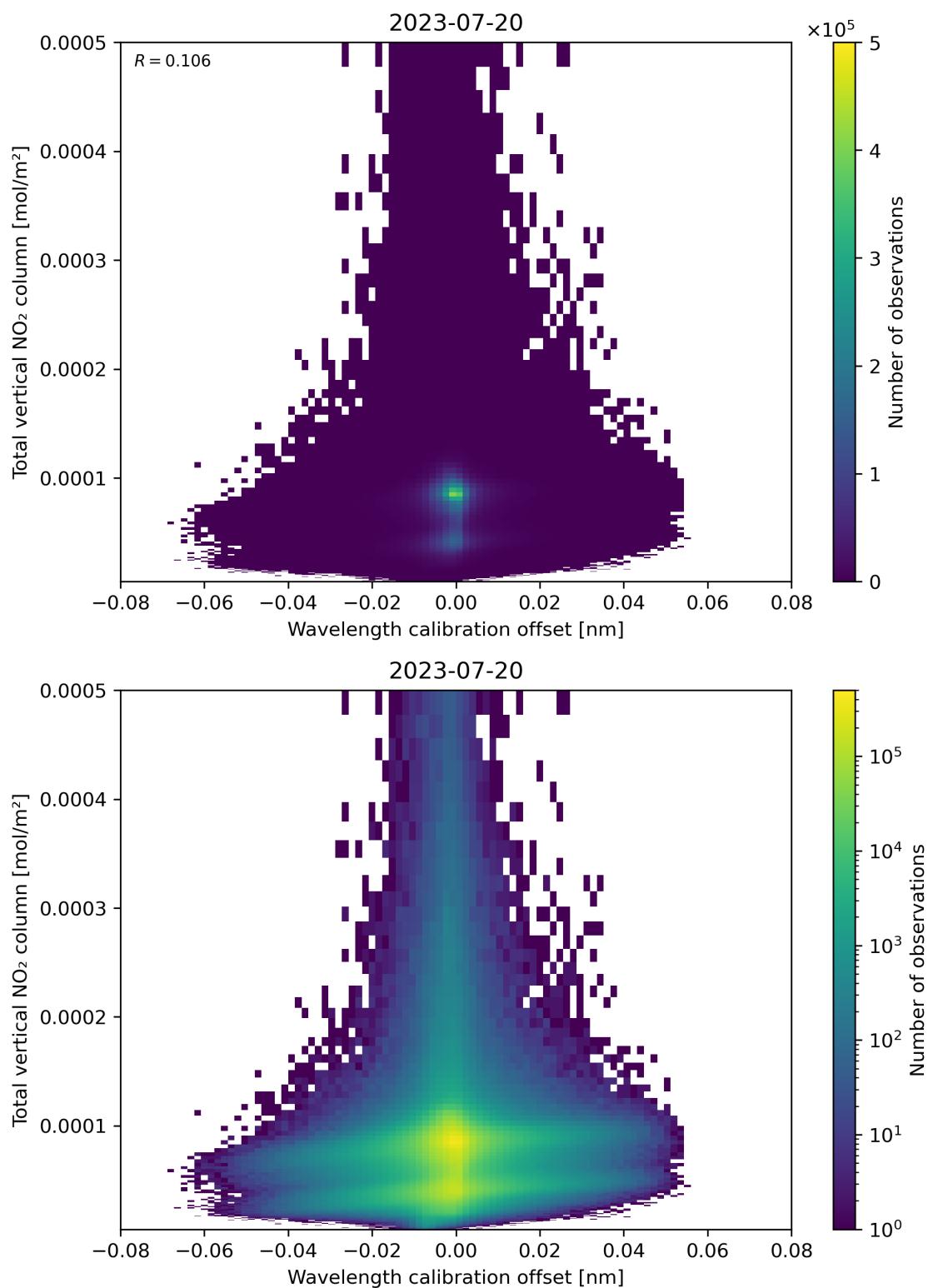
Figure 179: Scatter density plot of “Wavelength calibration offset” against “Total vertical NO 2 column” for 2023-07-19 to 2023-07-21.
