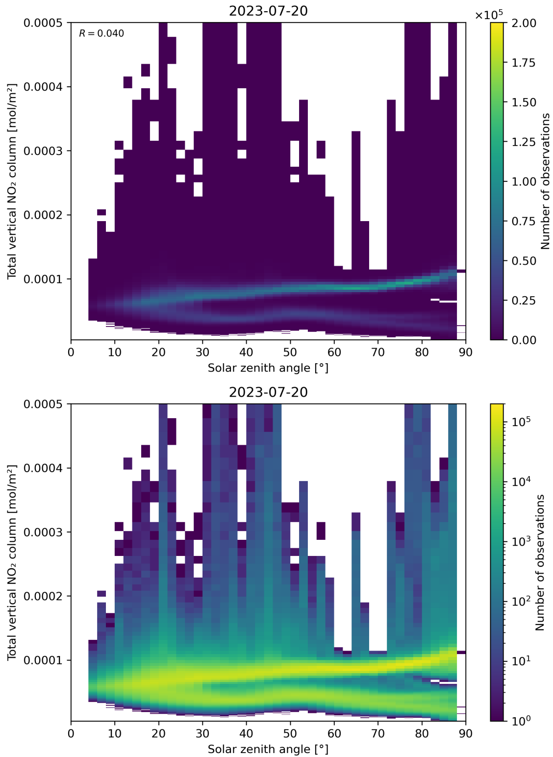
Figure 153: Scatter density plot of “Solar zenith angle” against “Total vertical \text{NO}_2 column” for 2023-07-19 to 2023-07-21.
