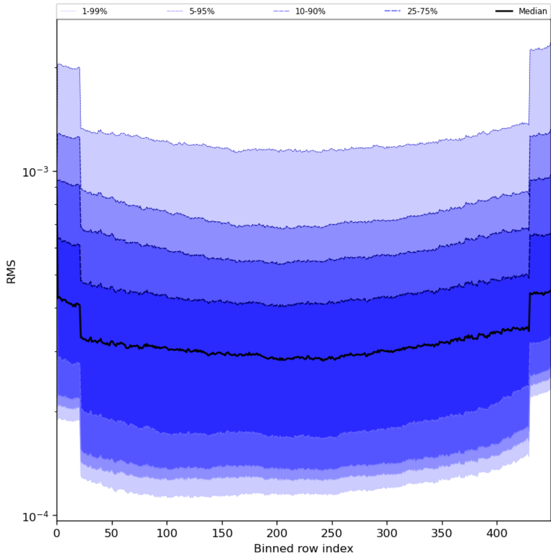
Figure 60: Along track statistics of “RMS” for 2023-07-19 to 2023-07-21
