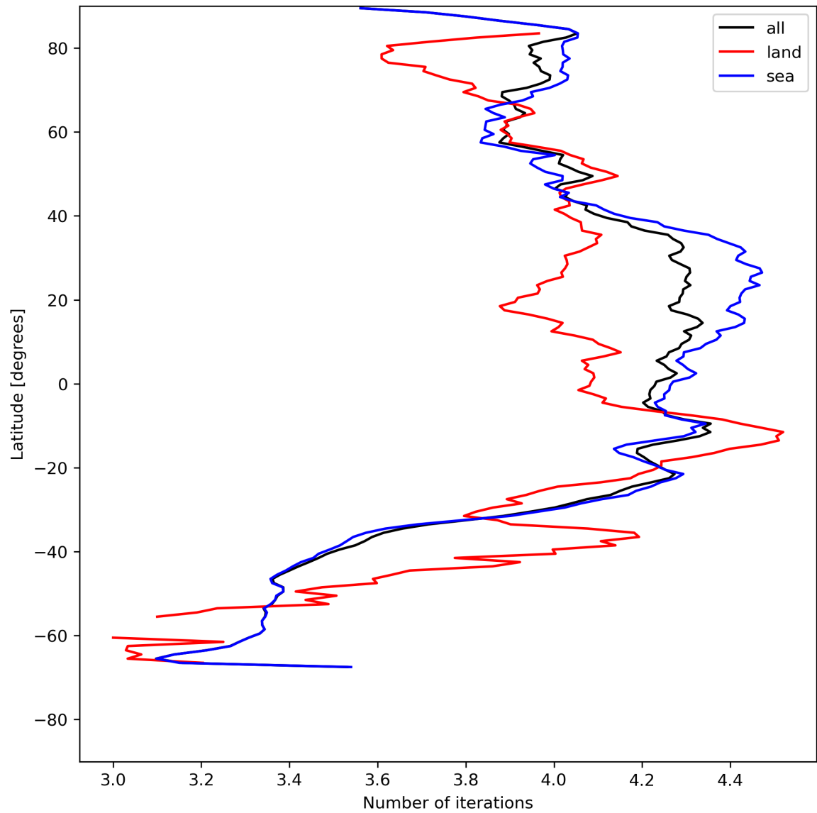
Figure 17: Zonal average of “Number of iterations” for 2023-07-19 to 2023-07-21.
