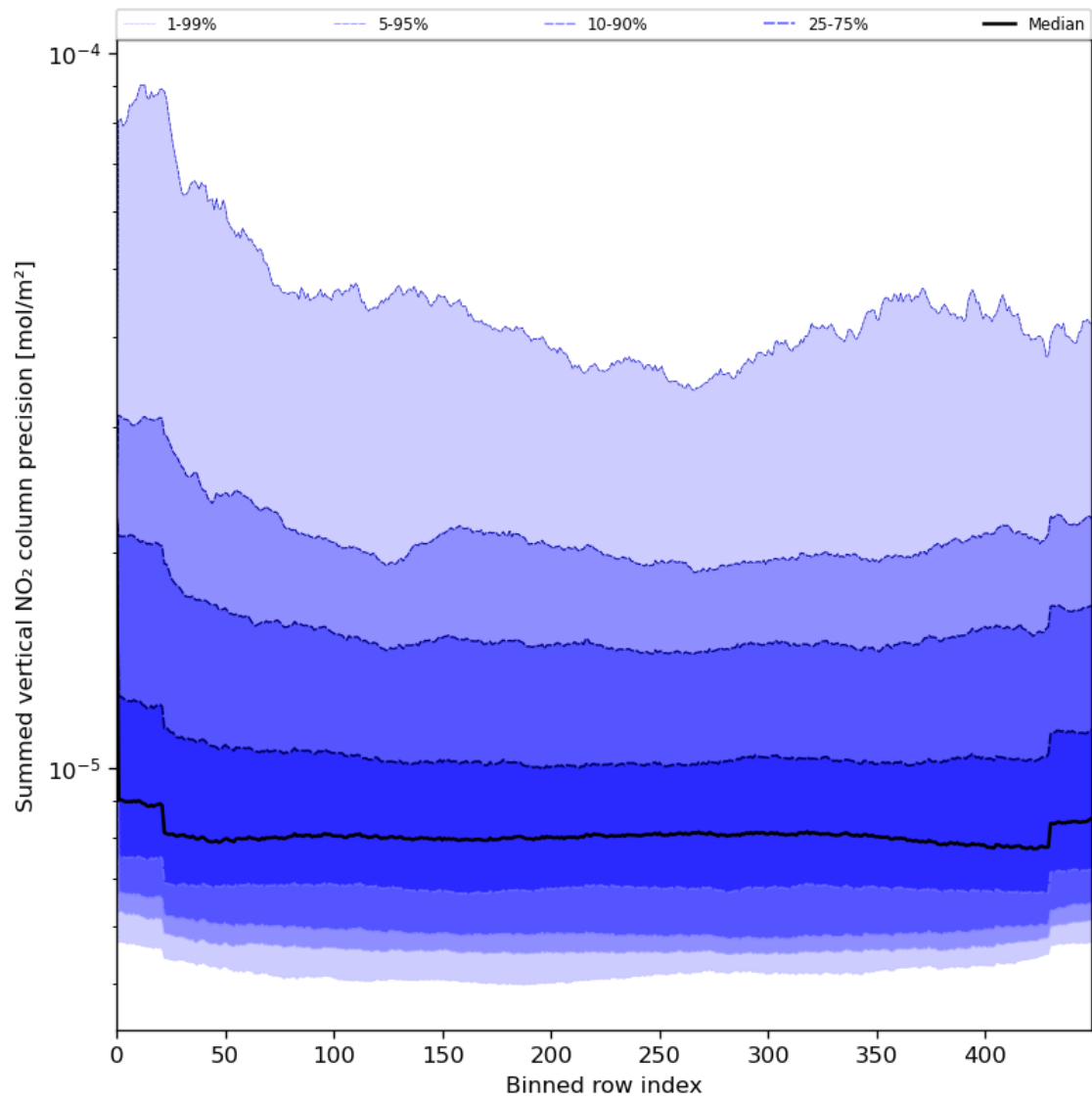
Figure 58: Along track statistics of “Summed vertical NO 2 column precision” for 2023-07-19 to 2023-07-21
