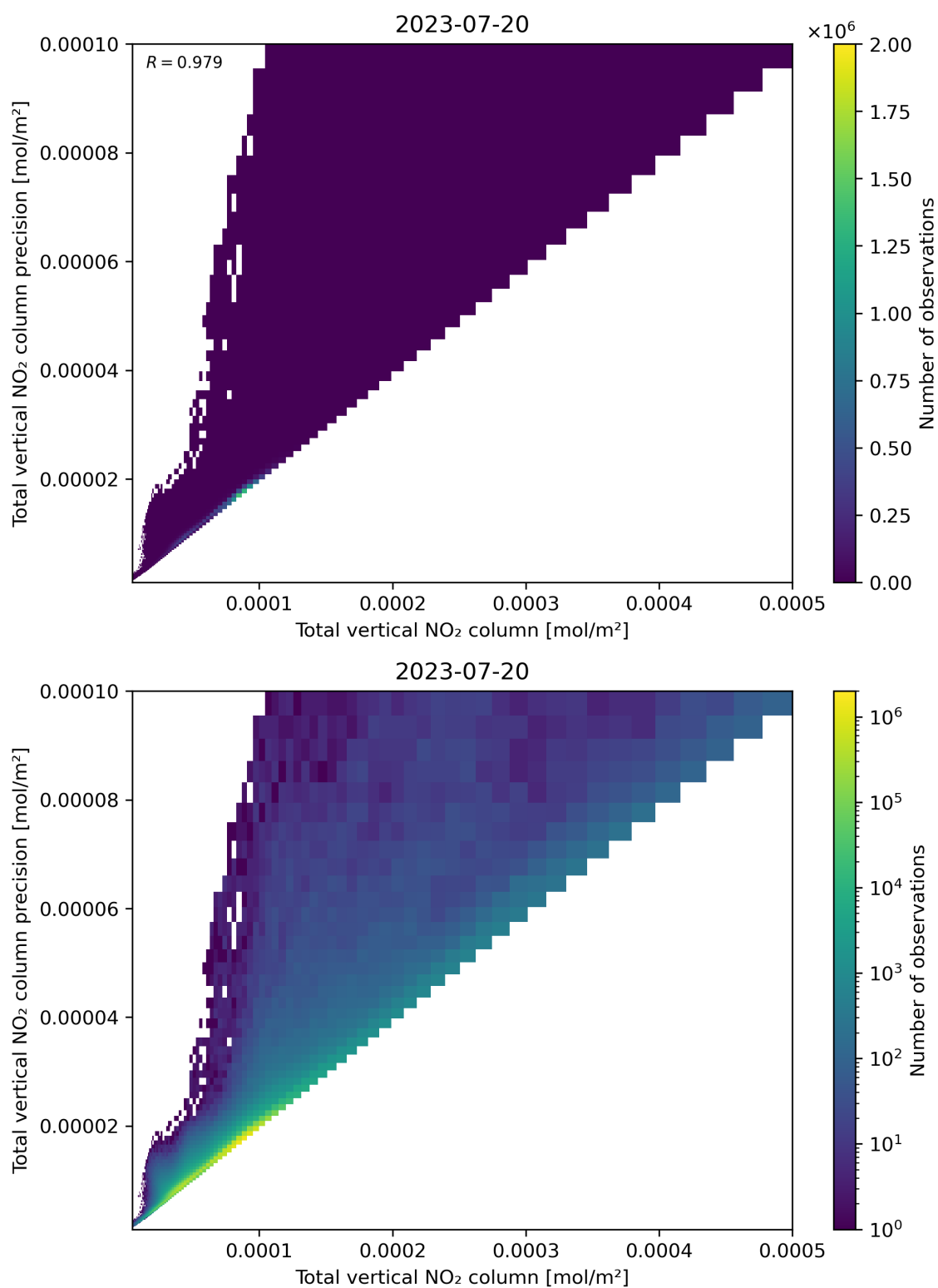
Figure 114: Scatter density plot of “Total vertical NO 2 column” against “Total vertical NO 2 column precision” for 2023-07-19 to 2023-07-21.
