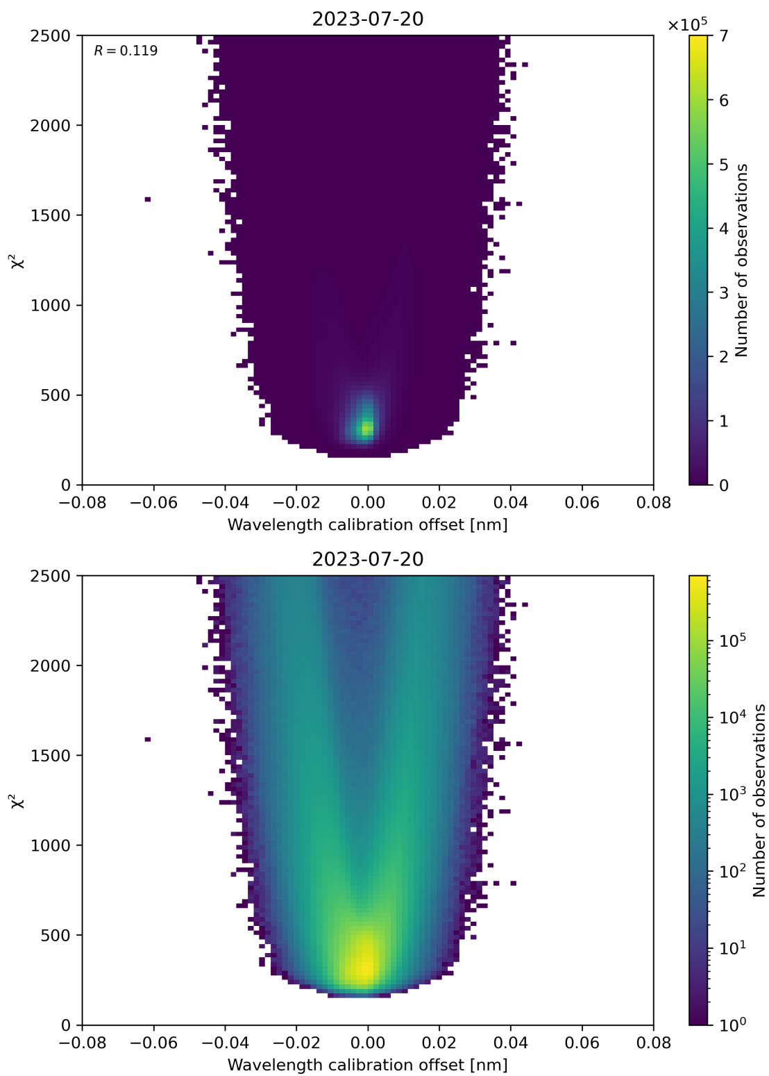
Figure 175: Scatter density plot of “Wavelength calibration offset” against “ \chi^2 ” for 2023-07-19 to 2023-07-21.
