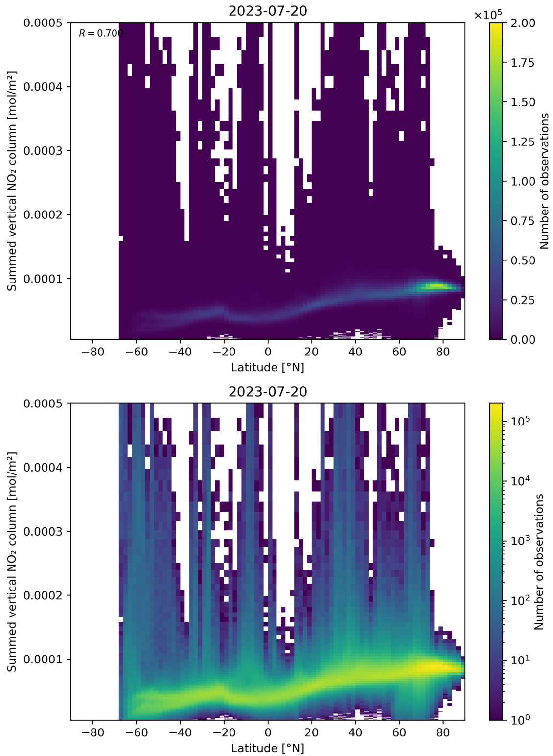
Figure 88: Scatter density plot of “Latitude” against “Summed vertical NO 2 column” for 2023-07-19 to 2023-07-21.
