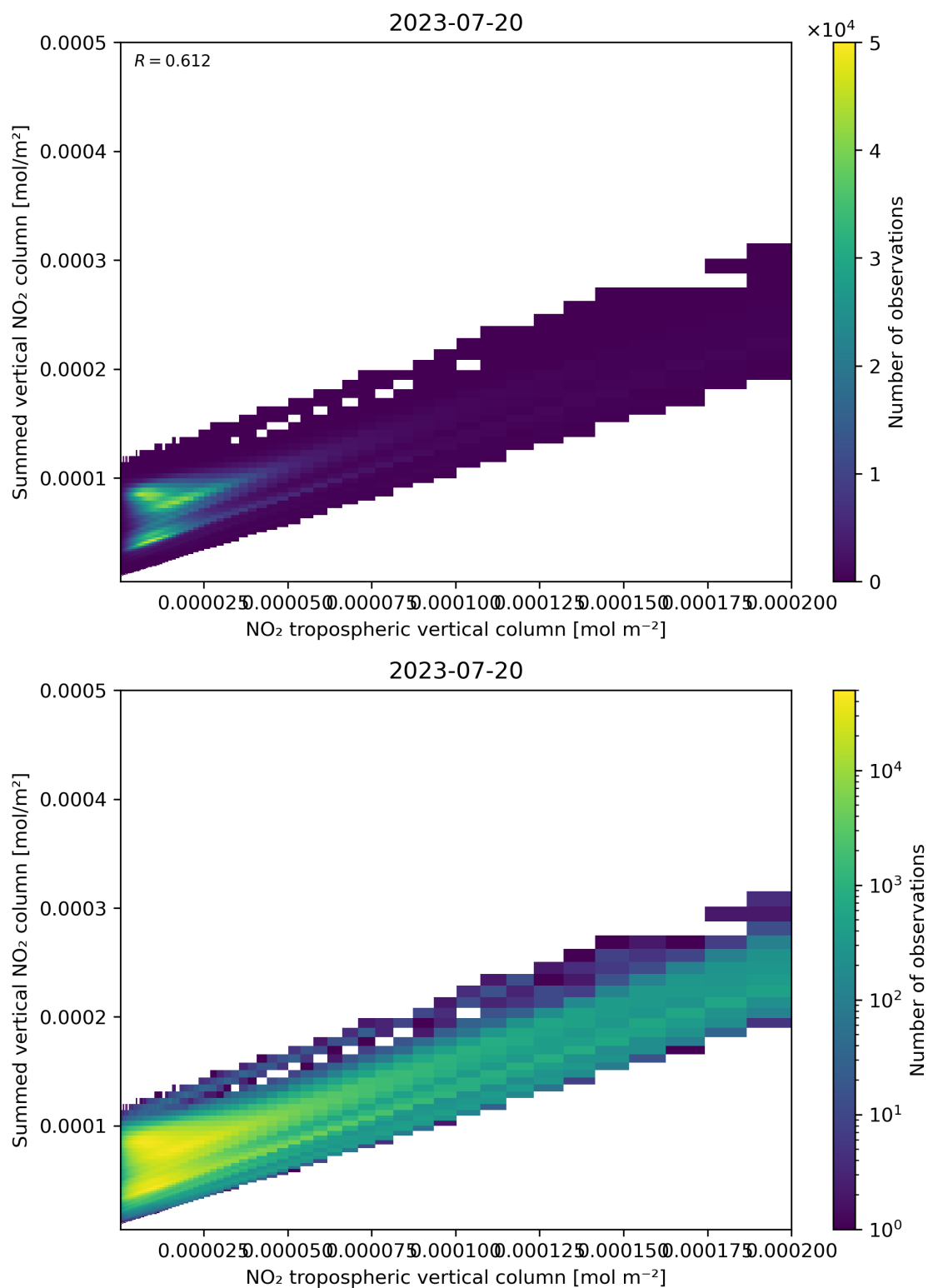
Figure 126: Scatter density plot of “NO 2 tropospheric vertical column” against “Summed vertical NO 2 column” for 2023-07-19 to 2023-07-21.
