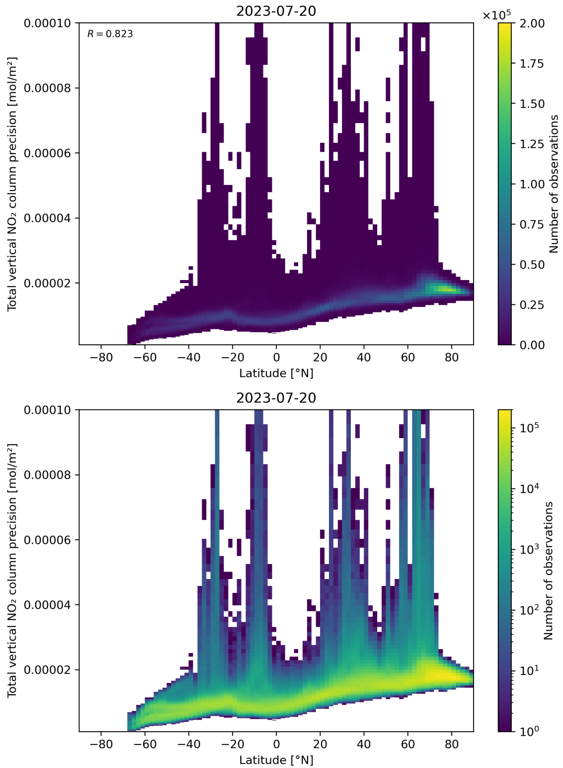
Figure 91: Scatter density plot of “Latitude” against “Total vertical NO 2 column precision” for 2023-07-19 to 2023-07-21.
