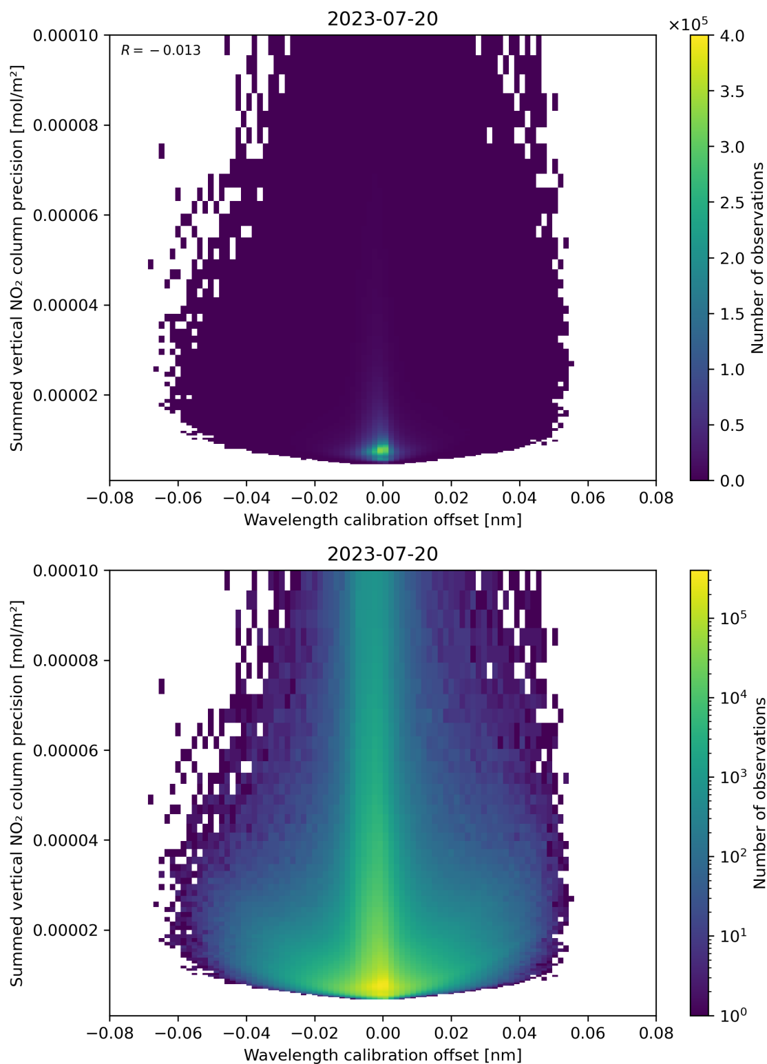
Figure 178: Scatter density plot of “Wavelength calibration offset” against “Summed vertical NO 2 column precision” for 2023-07-19 to 2023-07-21.
