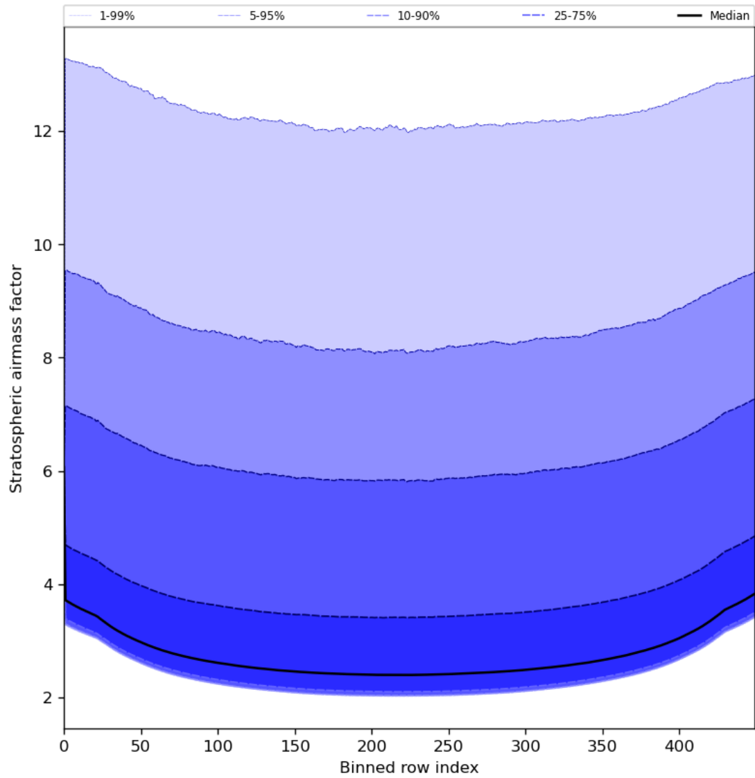
Figure 61: Along track statistics of “Stratospheric airmass factor” for 2023-07-19 to 2023-07-21
