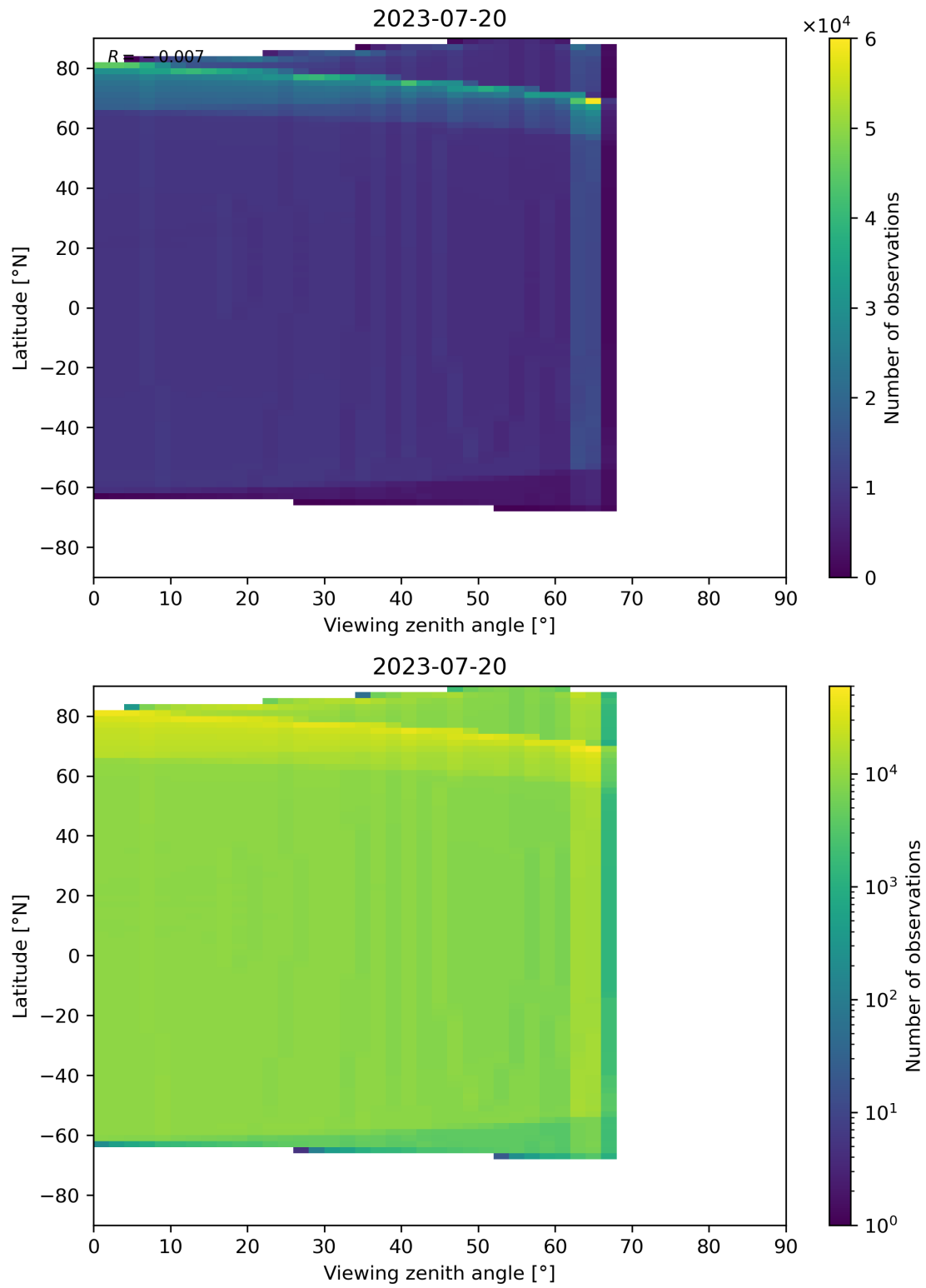
Figure 163: Scatter density plot of “Viewing zenith angle” against “Latitude” for 2023-07-19 to 2023-07-21.
