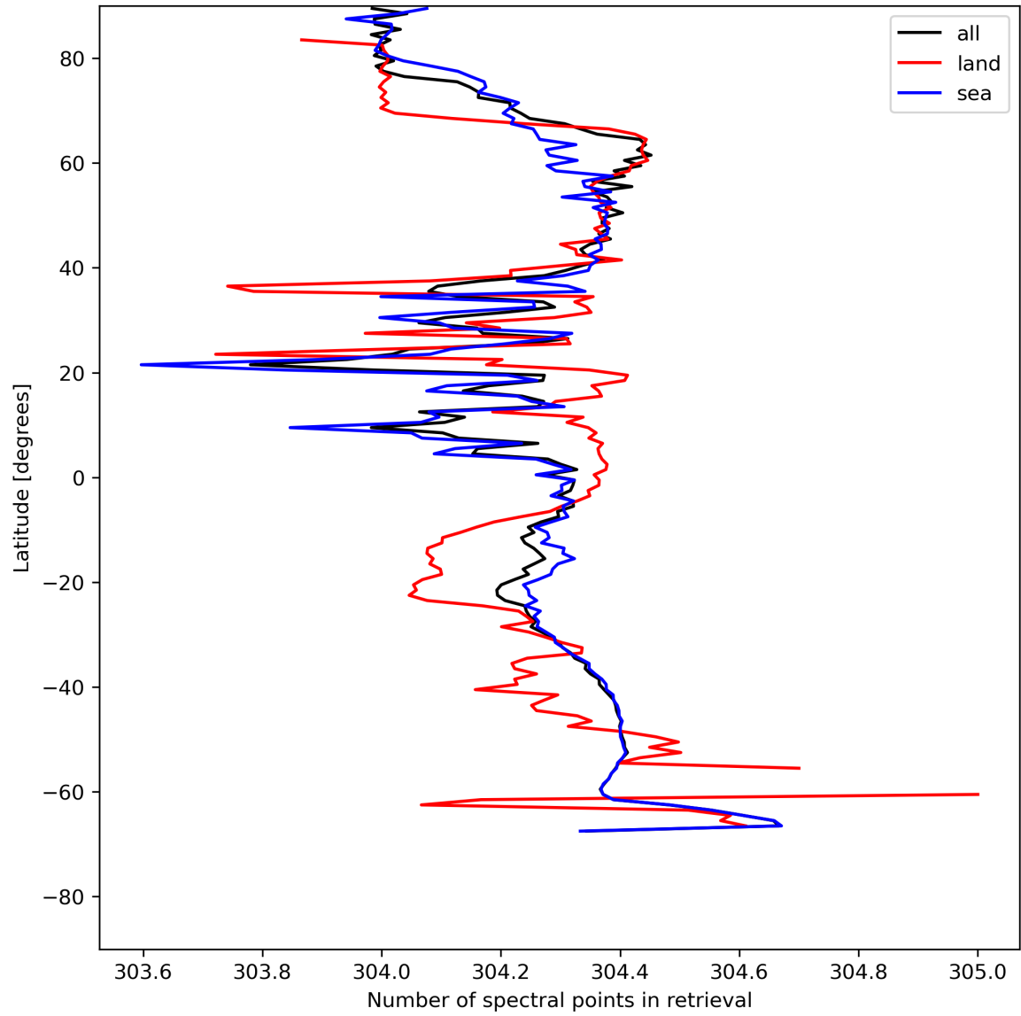
Figure 16: Zonal average of “Number of spectral points in retrieval” for 2023-07-19 to 2023-07-21.
