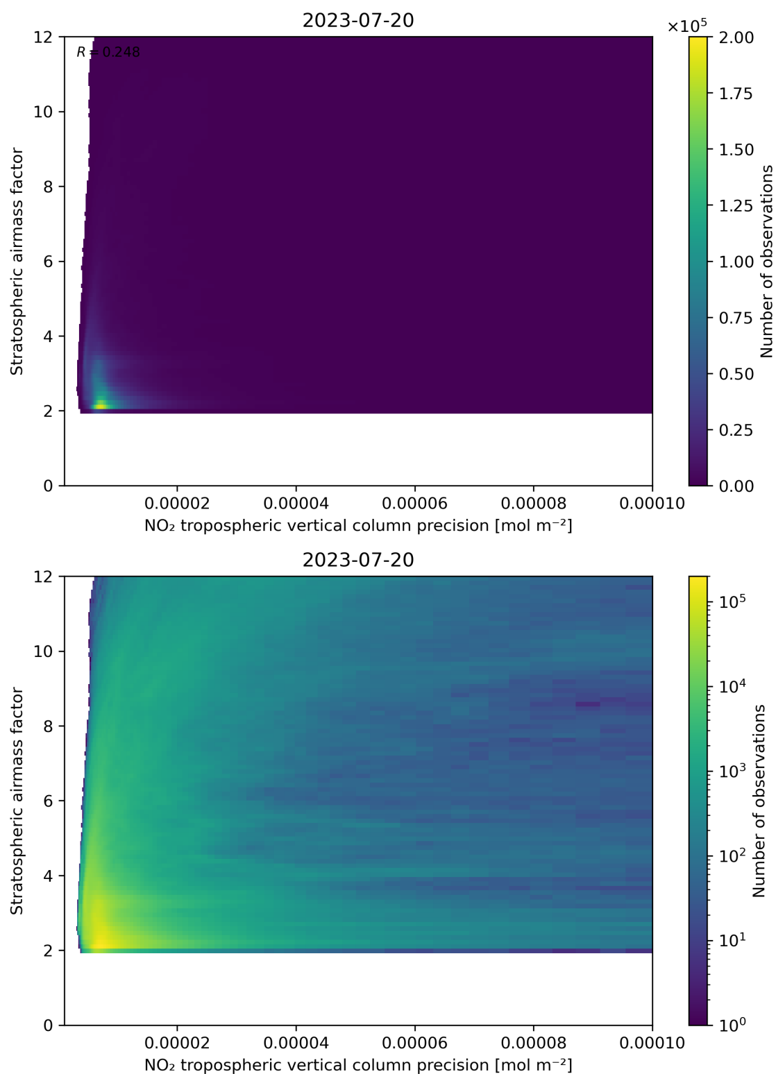
Figure 131: Scatter density plot of “NO 2 tropospheric vertical column precision” against “Stratospheric airmass factor” for 2023-07-19 to 2023-07-21.
