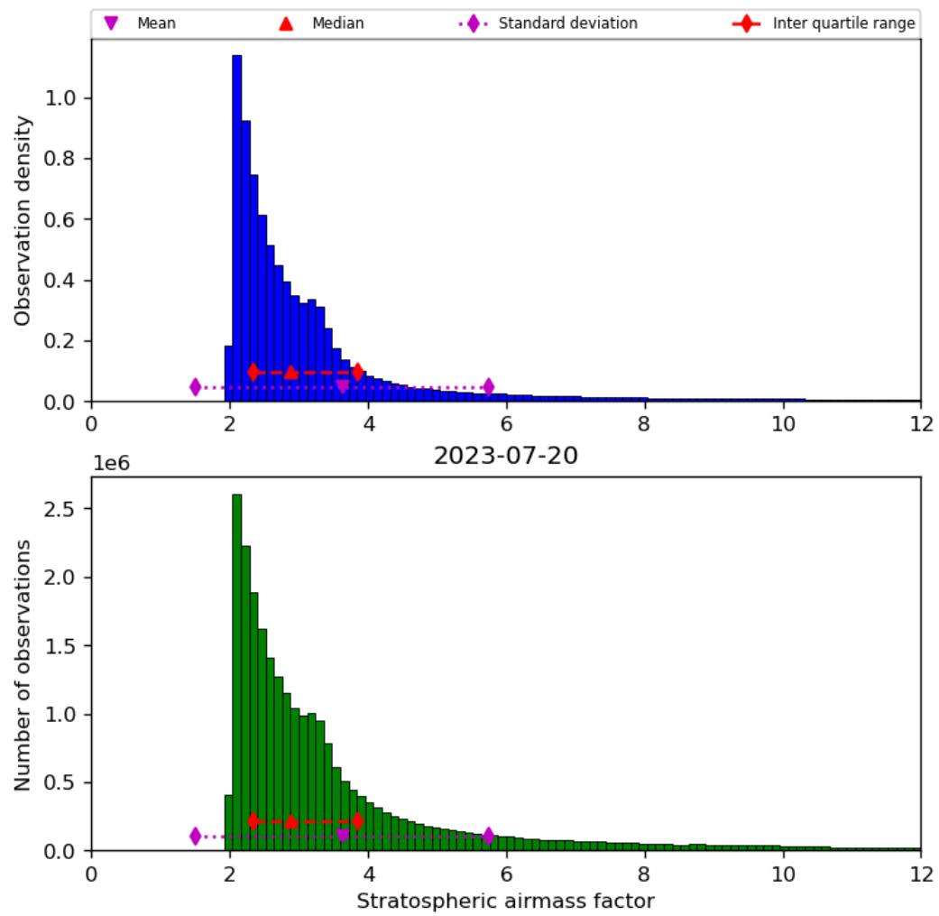
Figure 44: Histogram of “Stratospheric airmass factor” for 2023-07-19 to 2023-07-21
