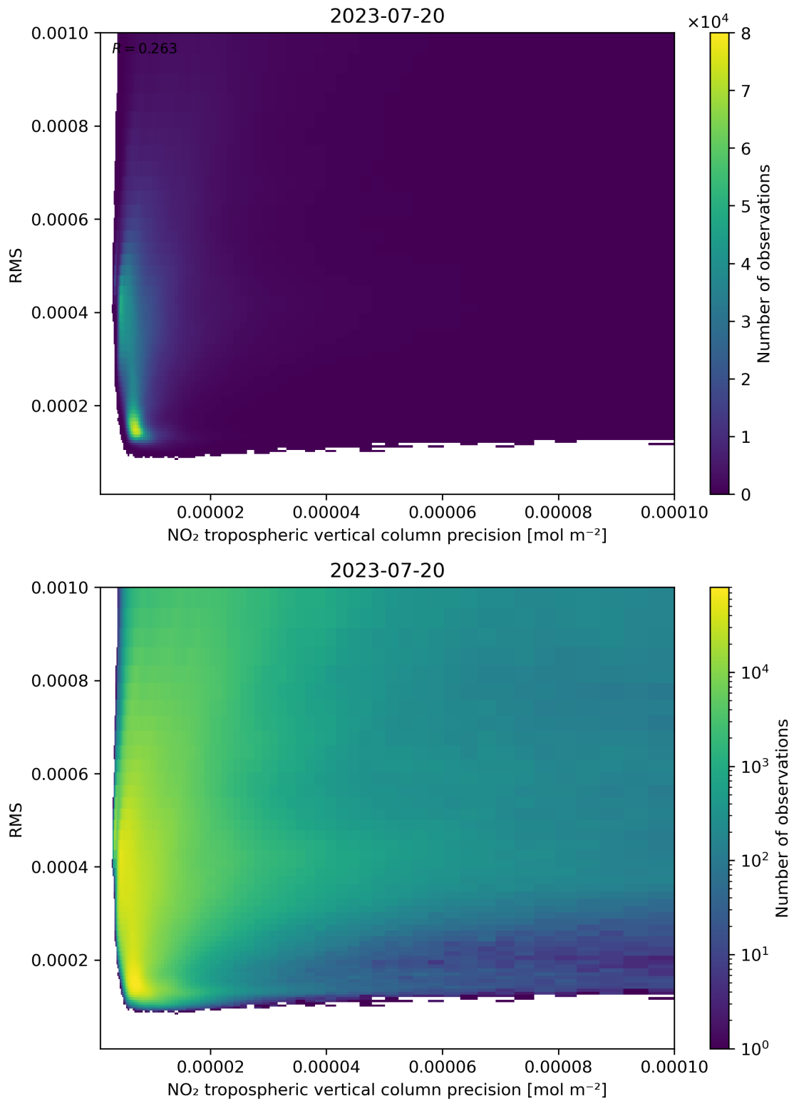
Figure 140: Scatter density plot of “NO 2 tropospheric vertical column precision” against “RMS” for 2023-07-19 to 2023-07-21.
