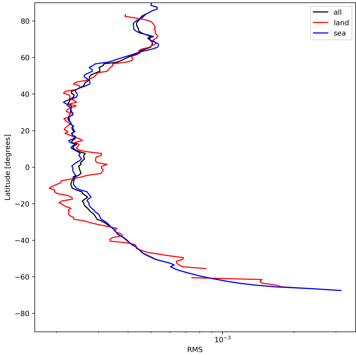
Figure 26: Zonal average of “RMS” for 2023-07-19 to 2023-07-21.
