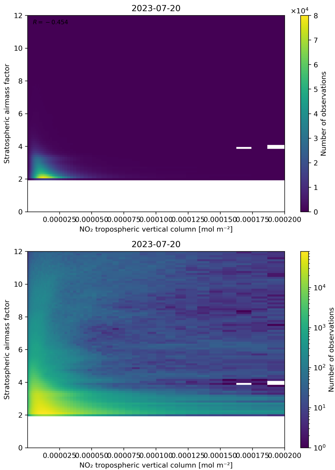
Figure 121: Scatter density plot of “NO 2 tropospheric vertical column” against “Stratospheric air mass factor” for 2023-07-19 to 2023-07-21.
