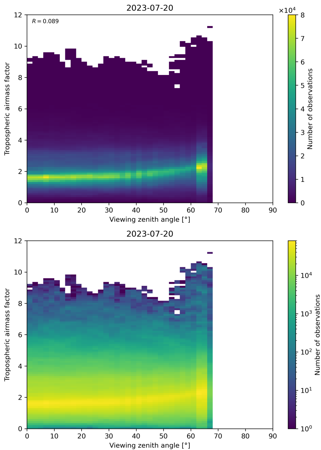
Figure 161: Scatter density plot of “Viewing zenith angle” against “Tropospheric airmass factor” for 2023-07-19 to 2023-07-21.
