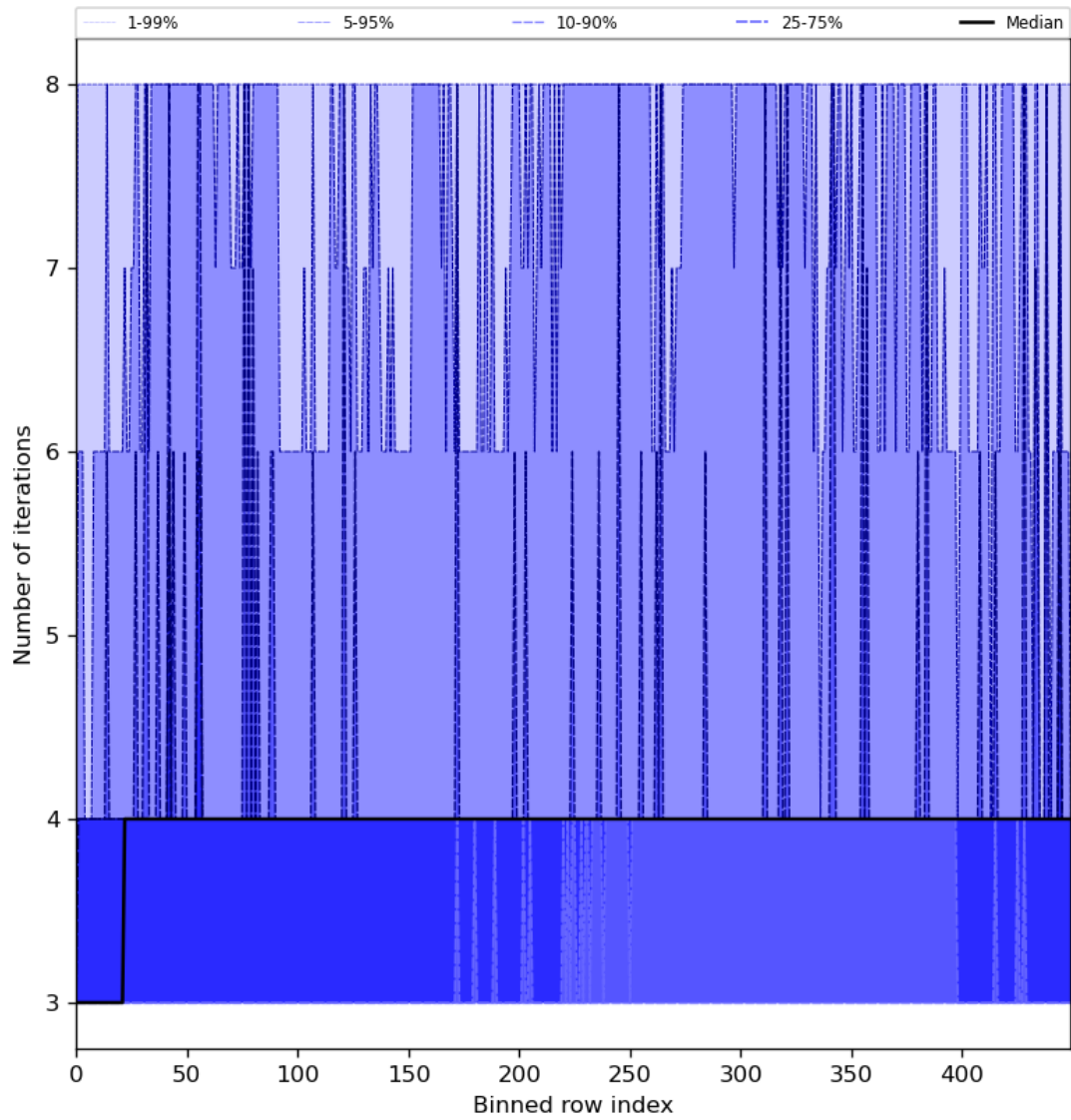
Figure 51: Along track statistics of “Number of iterations” for 2023-07-19 to 2023-07-21
