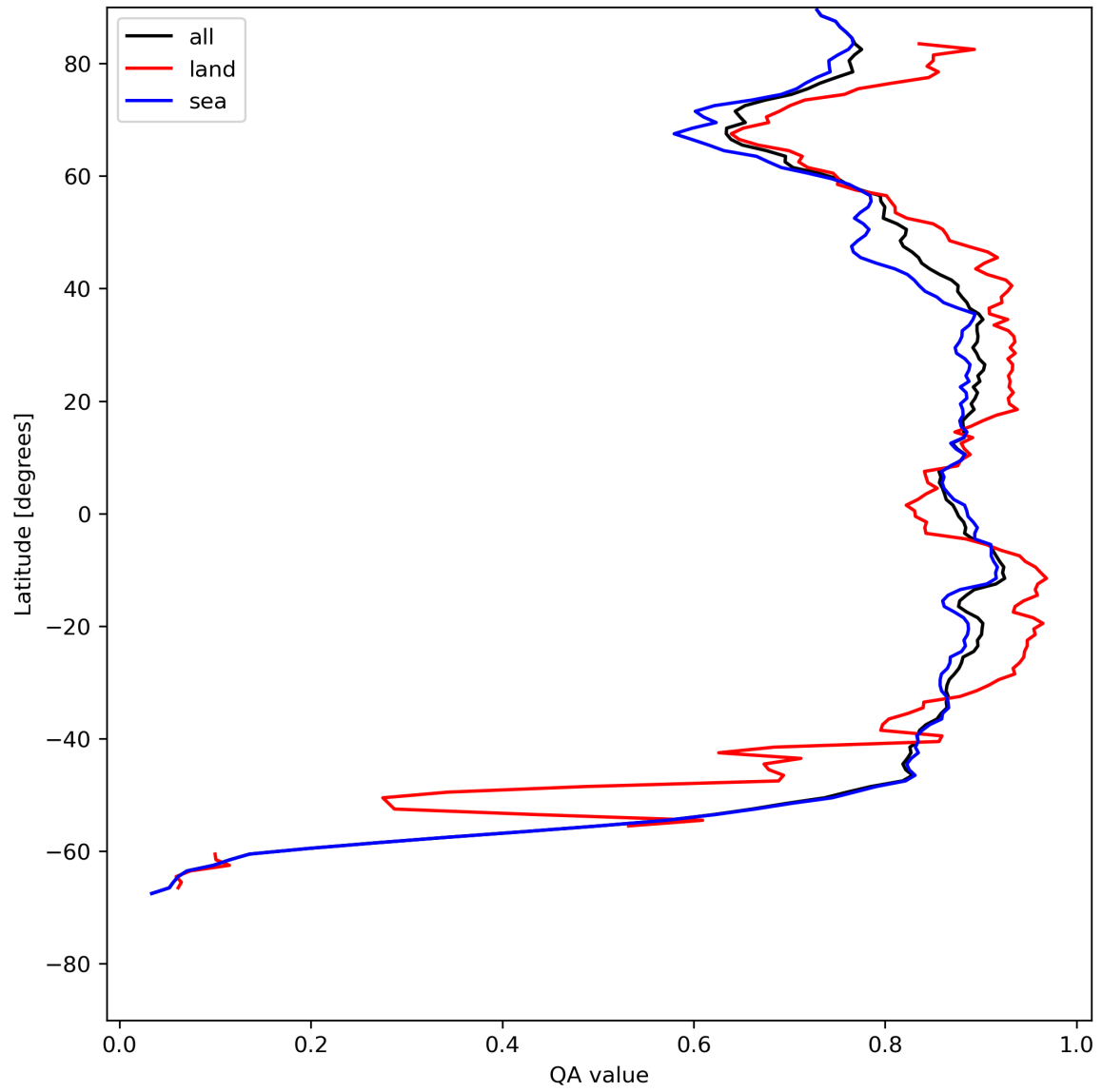
Figure 11: Zonal average of “QA value” for 2023-07-19 to 2023-07-21.
