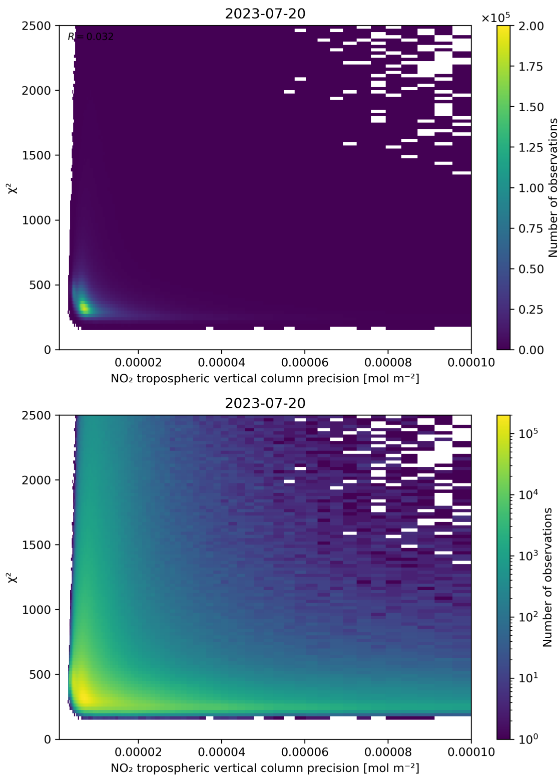
Figure 134: Scatter density plot of “NO 2 tropospheric vertical column precision” against “ \chi^2 ” for 2023-07-19 to 2023-07-21.
