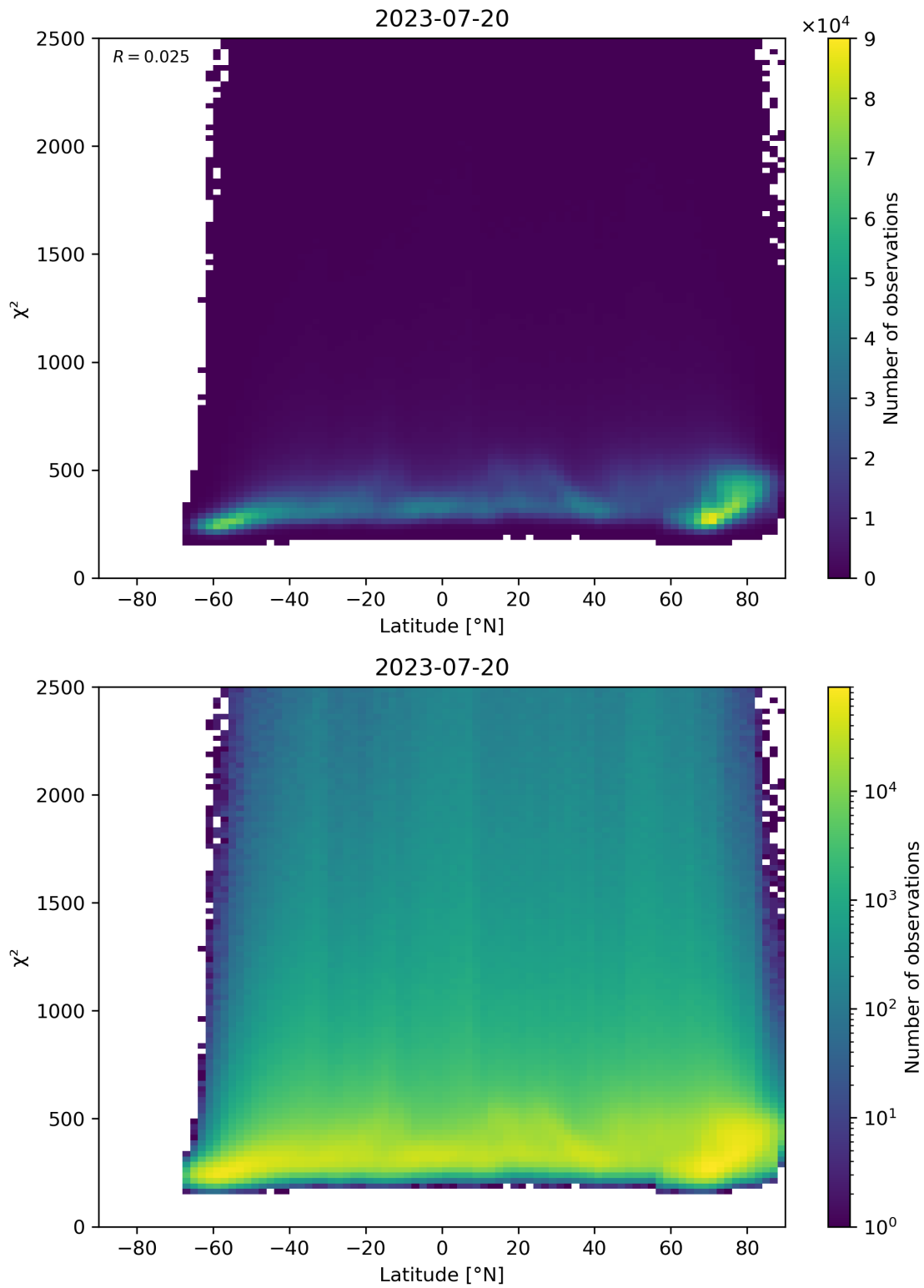
Figure 86: Scatter density plot of “Latitude” against “ \chi^2 ” for 2023-07-19 to 2023-07-21.
