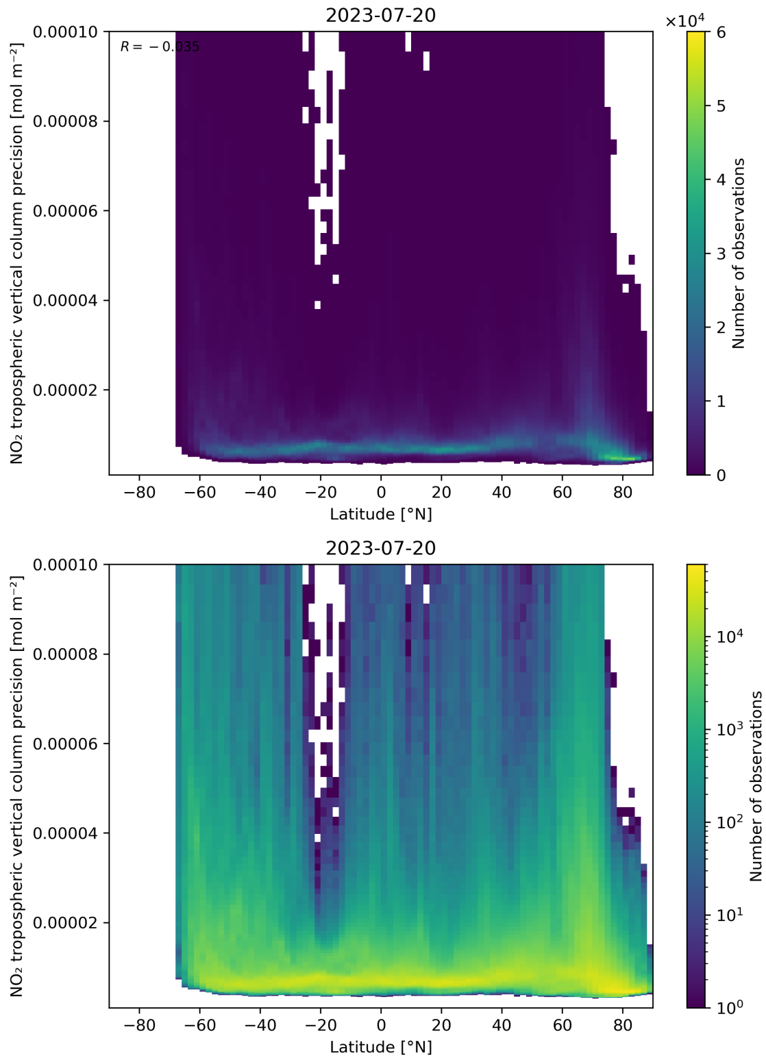
Figure 93: Scatter density plot of “Latitude” against “NO 2 tropospheric vertical column precision” for 2023-07-19 to 2023-07-21.
