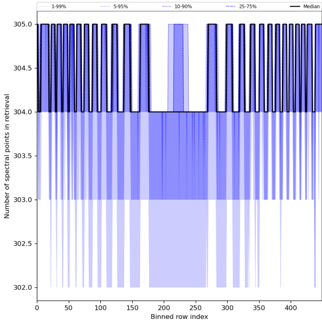
Figure 50: Along track statistics of “Number of spectral points in retrieval” for 2023-07-19 to 2023-07-21
