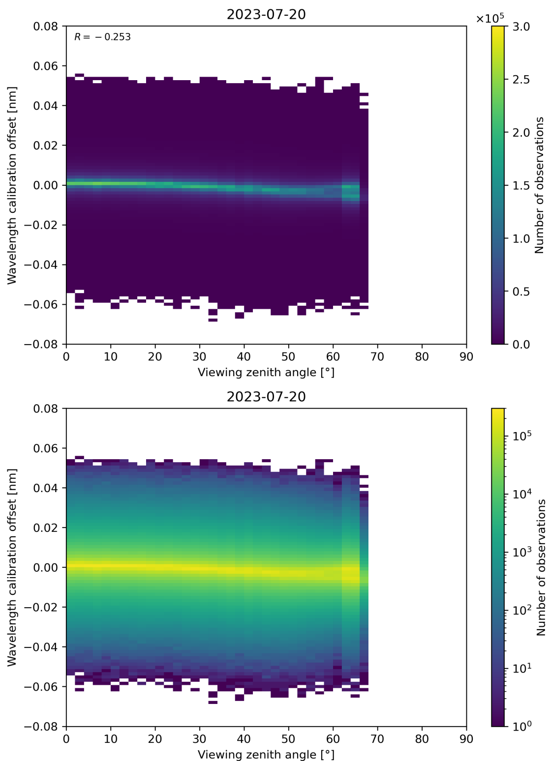
Figure 173: Scatter density plot of “Viewing zenith angle” against “Wavelength calibration offset” for 2023-07-19 to 2023-07-21.
