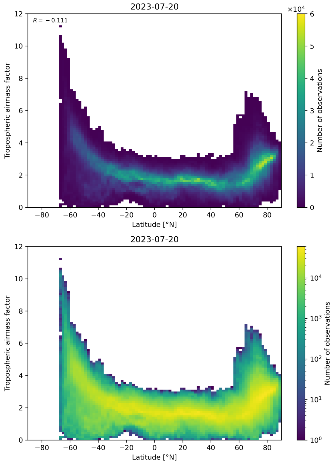
Figure 85: Scatter density plot of “Latitude” against “Tropospheric air mass factor” for 2023-07-19 to 2023-07-21.
