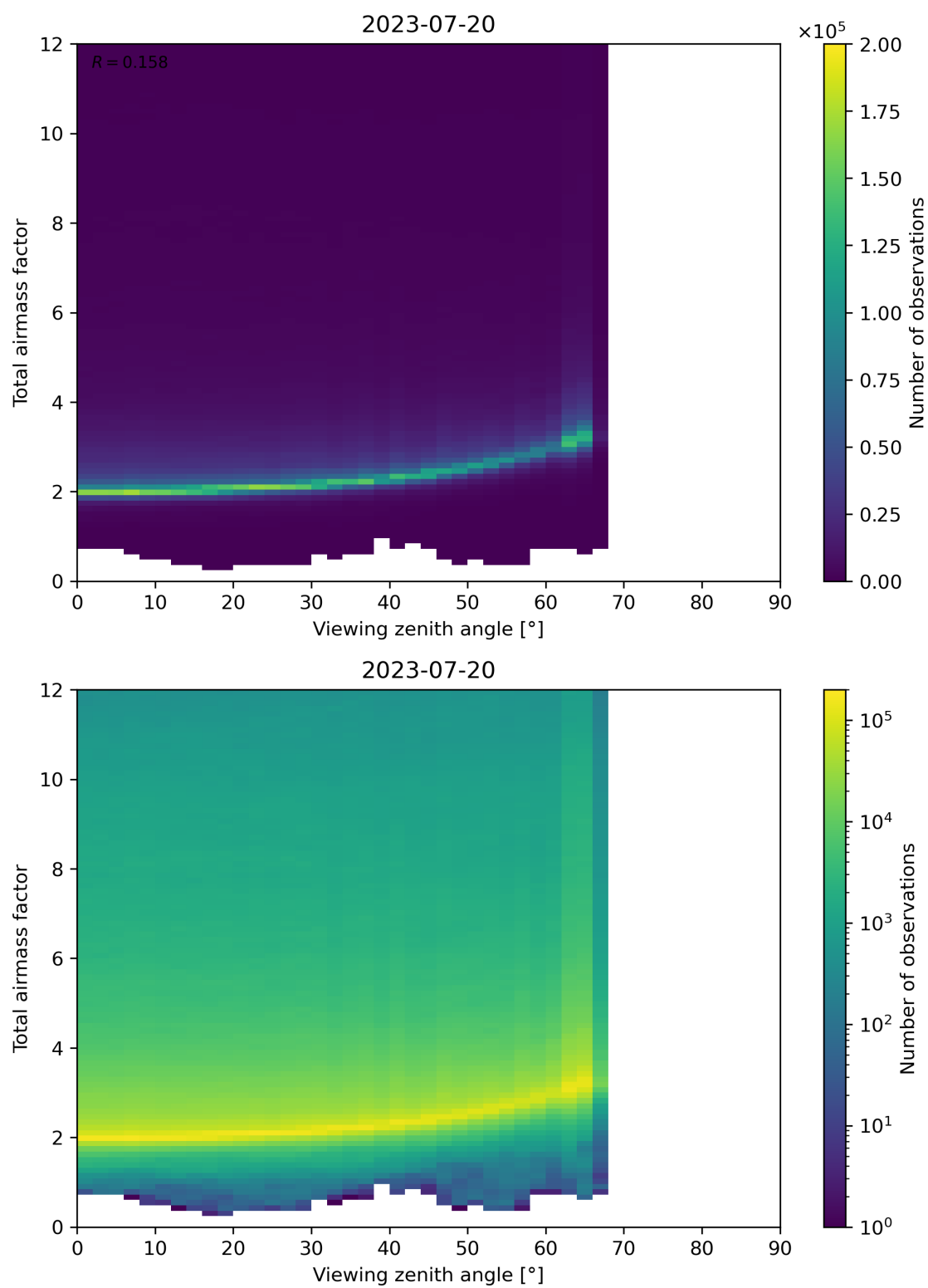
Figure 160: Scatter density plot of “Viewing zenith angle” against “Total airmass factor” for 2023-07-19 to 2023-07-21.
