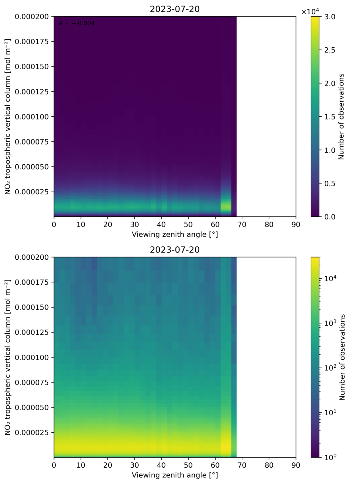
Figure 169: Scatter density plot of “Viewing zenith angle” against “NO 2 tropospheric vertical column” for 2023-07-19 to 2023-07-21.
