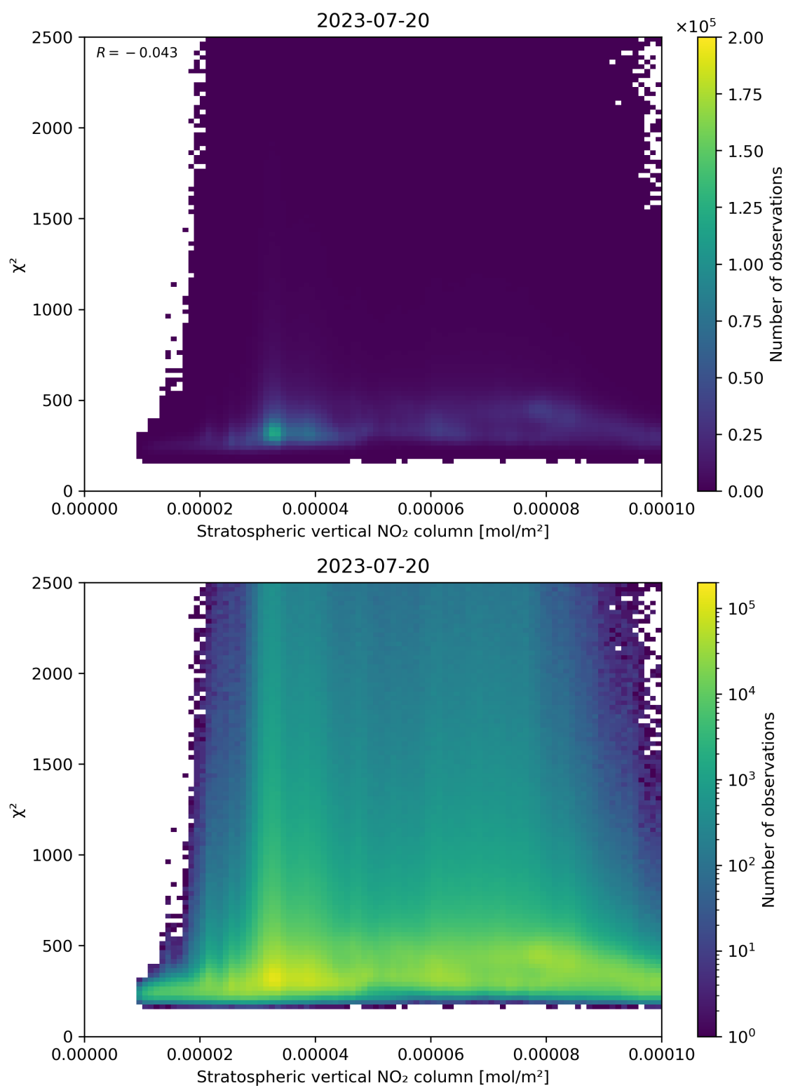
Figure 97: Scatter density plot of “Stratospheric vertical NO 2 column” against “ \chi^2 ” for 2023-07-19 to 2023-07-21.
