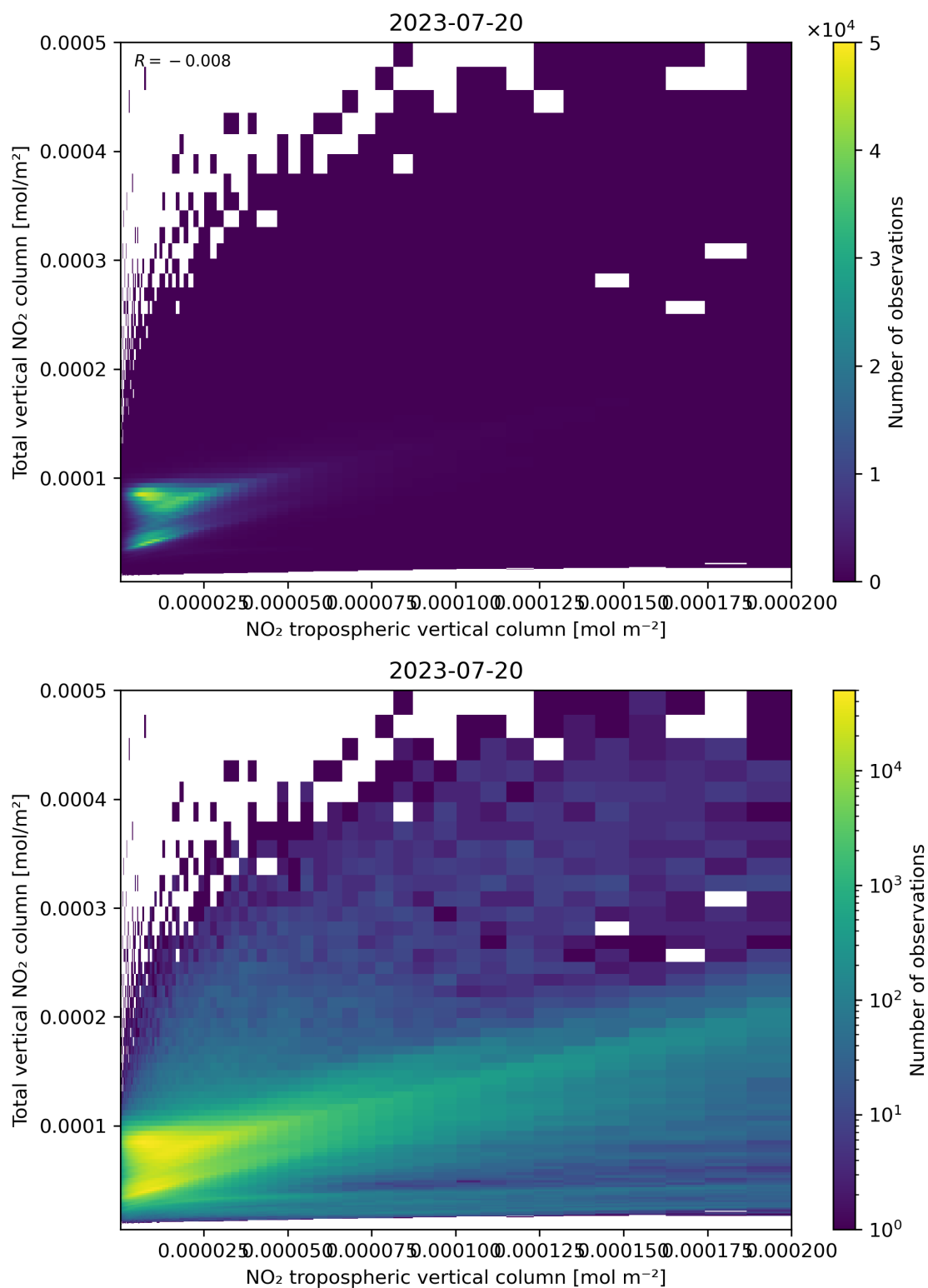
Figure 128: Scatter density plot of “NO 2 tropospheric vertical column” against “Total vertical NO 2 column” for 2023-07-19 to 2023-07-21.
