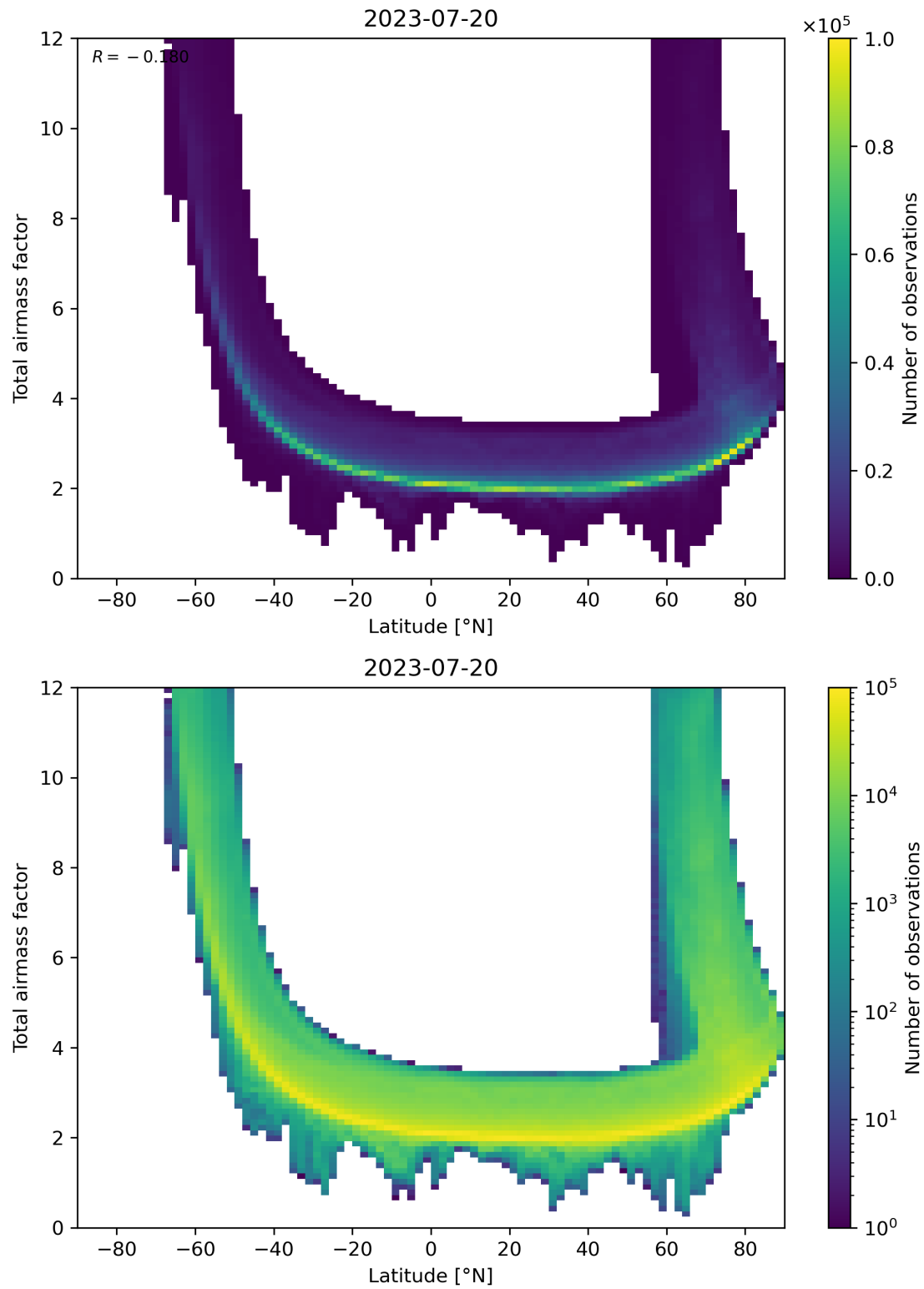
Figure 84: Scatter density plot of “Latitude” against “Total airmass factor” for 2023-07-19 to 2023-07-21.
