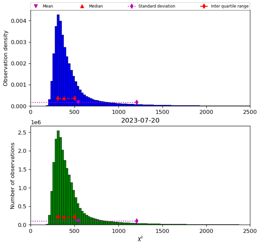
Figure 42: Histogram of “ \chi^2 ” for 2023-07-19 to 2023-07-21
