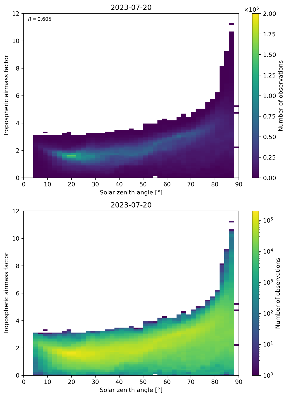
Figure 147: Scatter density plot of “Solar zenith angle” against “Tropospheric airmass factor” for 2023-07-19 to 2023-07-21.
