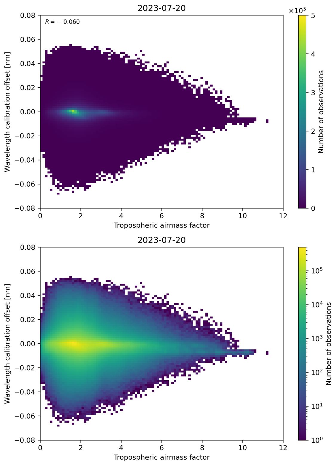
Figure 80: Scatter density plot of “Tropospheric airmass factor” against “Wavelength calibration offset” for 2023-07-19 to 2023-07-21.
