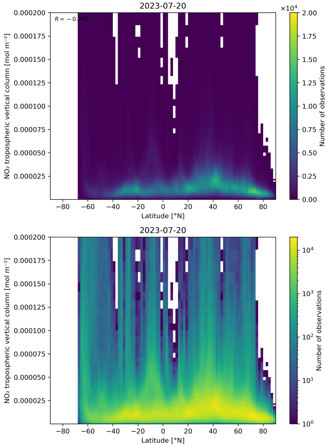
Figure 92: Scatter density plot of “Latitude” against “NO 2 tropospheric vertical column” for 2023-07-19 to 2023-07-21.
