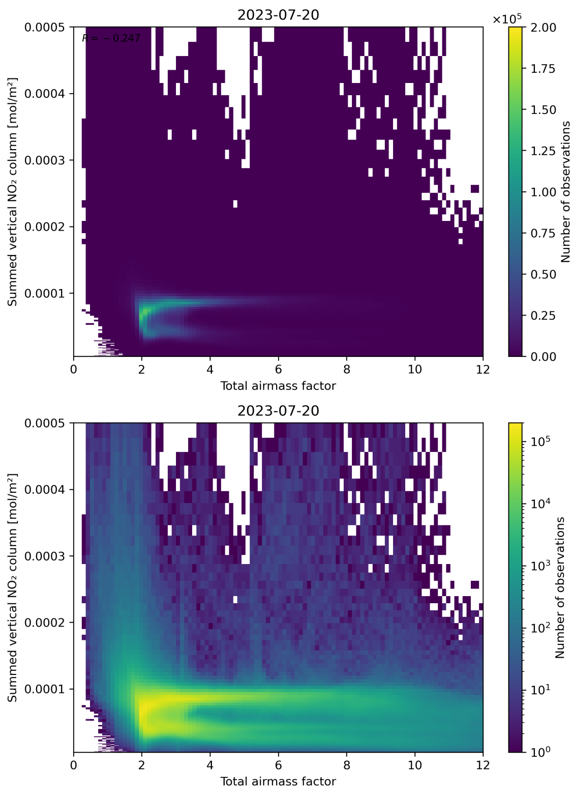
Figure 65: Scatter density plot of “Total airmass factor” against “Summed vertical NO 2 column” for 2023-07-19 to 2023-07-21.
