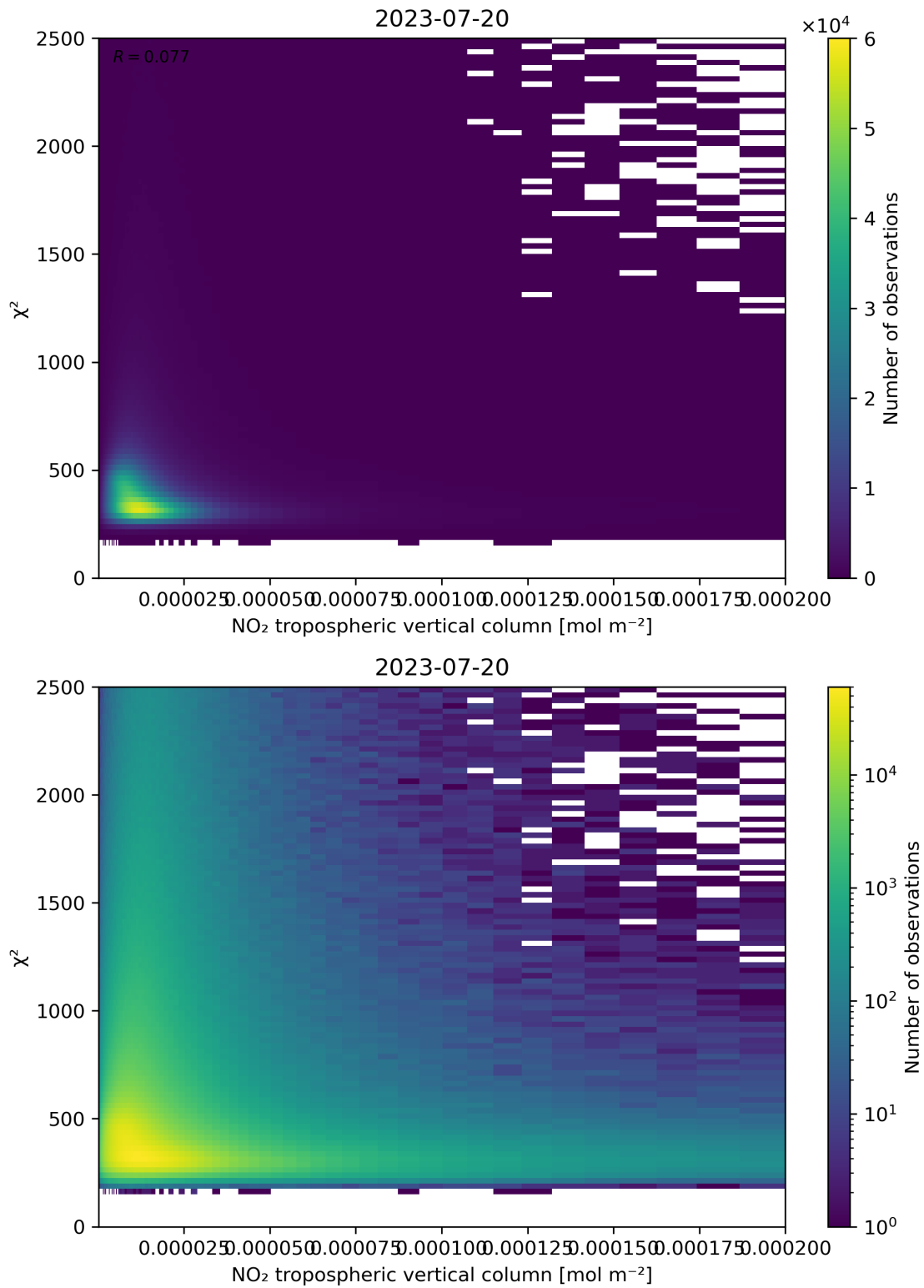
Figure 124: Scatter density plot of “NO 2 tropospheric vertical column” against “ \chi^2 ” for 2023-07-19 to 2023-07-21.
