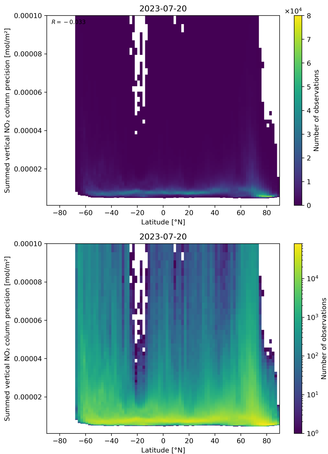
Figure 89: Scatter density plot of “Latitude” against “Summed vertical NO 2 column precision” for 2023-07-19 to 2023-07-21.
