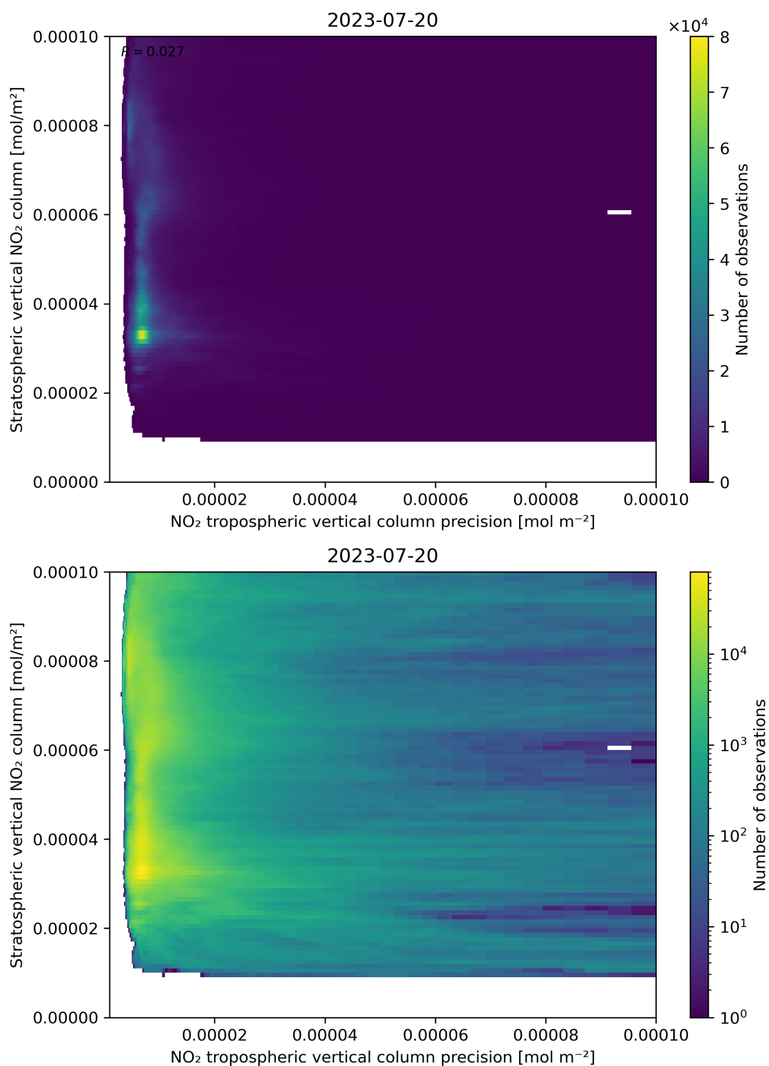
Figure 135: Scatter density plot of “NO 2 tropospheric vertical column precision” against “Stratospheric vertical NO 2 column” for 2023-07-19 to 2023-07-21.
