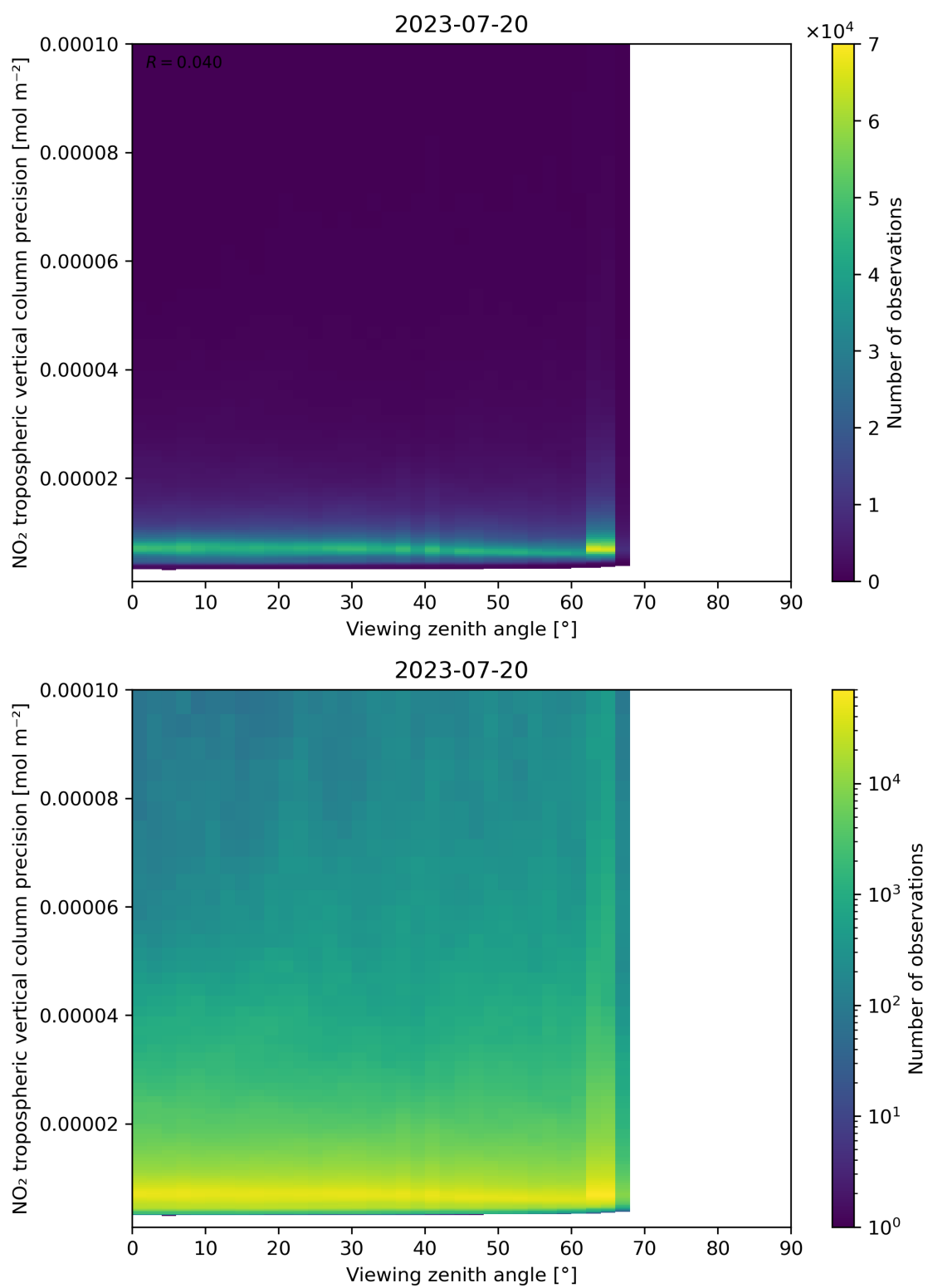
Figure 170: Scatter density plot of “Viewing zenith angle” against “NO 2 tropospheric vertical column precision” for 2023-07-19 to 2023-07-21.
