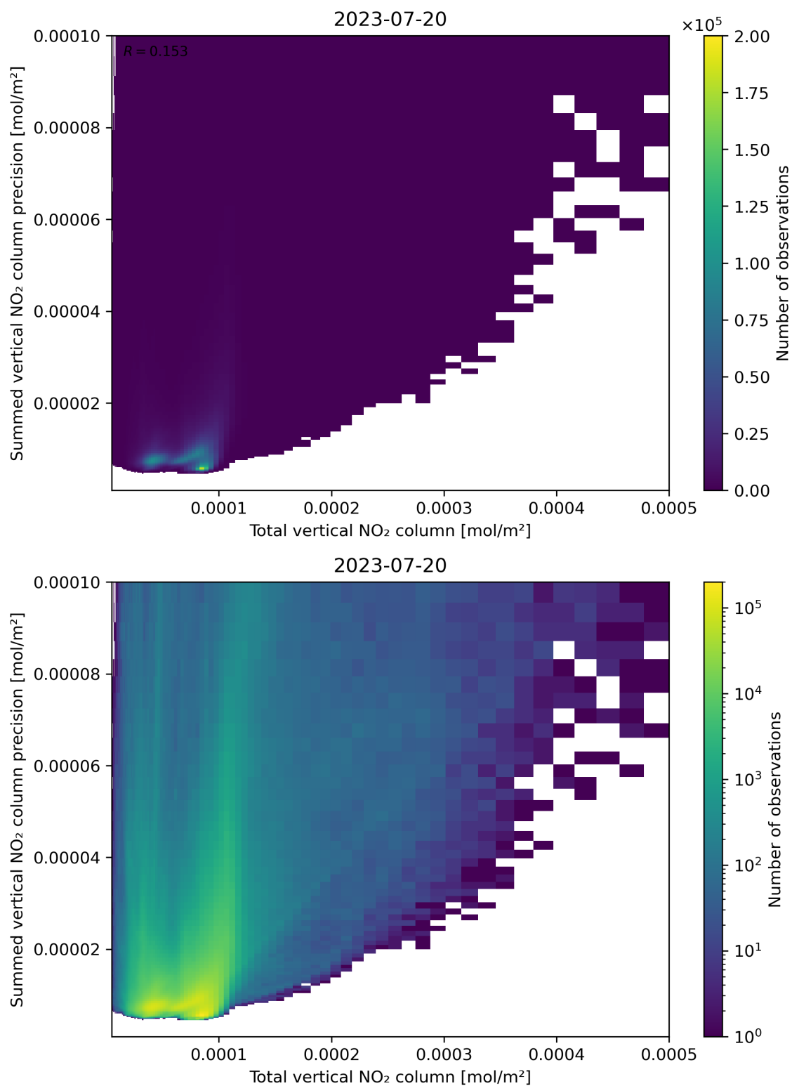
Figure 113: Scatter density plot of “Total vertical NO 2 column” against “Summed vertical NO 2 column precision” for 2023-07-19 to 2023-07-21.
