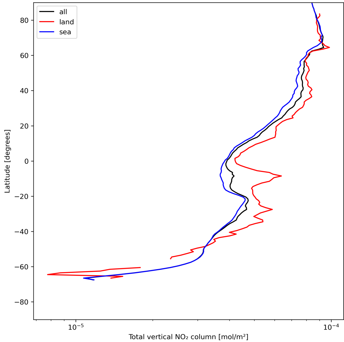
Figure 21: Zonal average of “Total vertical NO 2 column” for 2023-07-19 to 2023-07-21.
