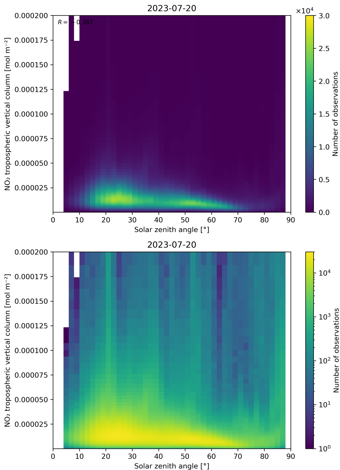
Figure 155: Scatter density plot of “Solar zenith angle” against “NO 2 tropospheric vertical column” for 2023-07-19 to 2023-07-21.
