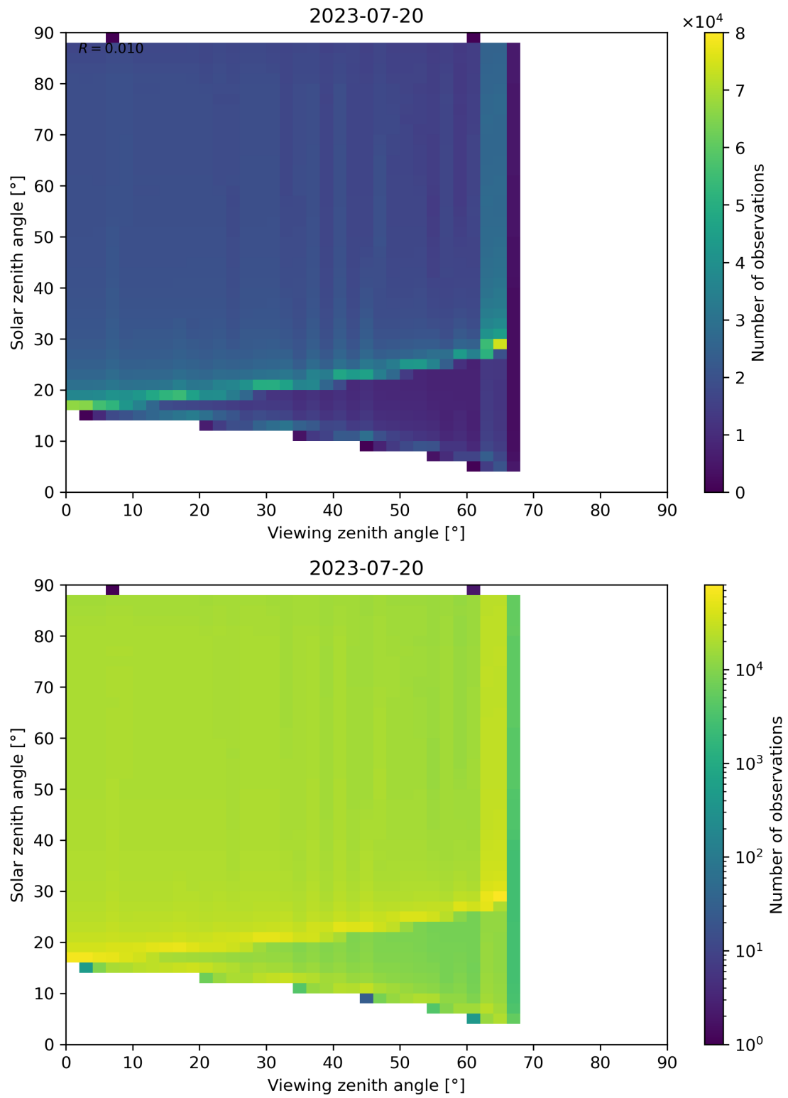
Figure 172: Scatter density plot of “Viewing zenith angle” against “Solar zenith angle” for 2023-07-19 to 2023-07-21.
