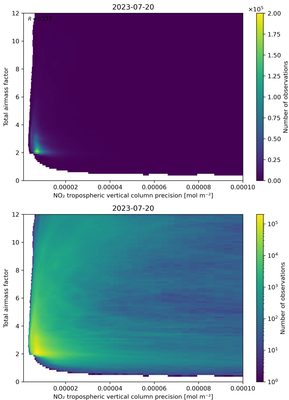
Figure 132: Scatter density plot of “NO 2 tropospheric vertical column precision” against “Total airmass factor” for 2023-07-19 to 2023-07-21.
