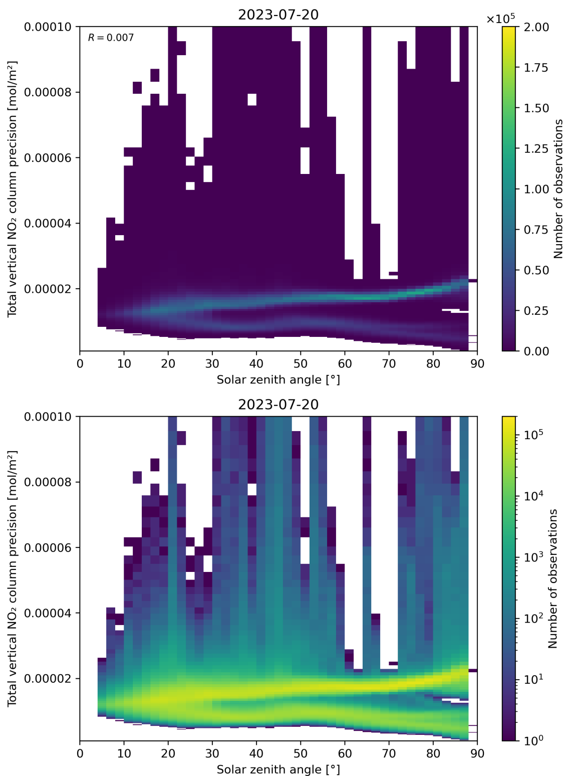
Figure 154: Scatter density plot of “Solar zenith angle” against “Total vertical NO 2 column precision” for 2023-07-19 to 2023-07-21.
