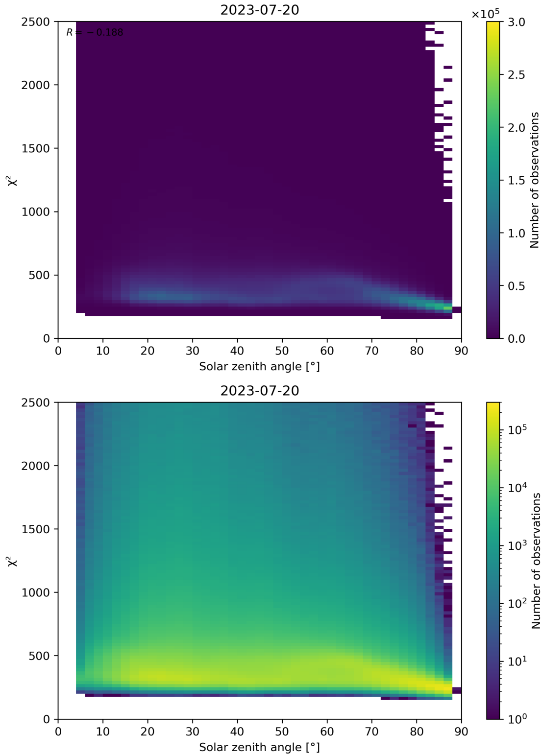
Figure 148: Scatter density plot of “Solar zenith angle” against “ \chi^2 ” for 2023-07-19 to 2023-07-21.
