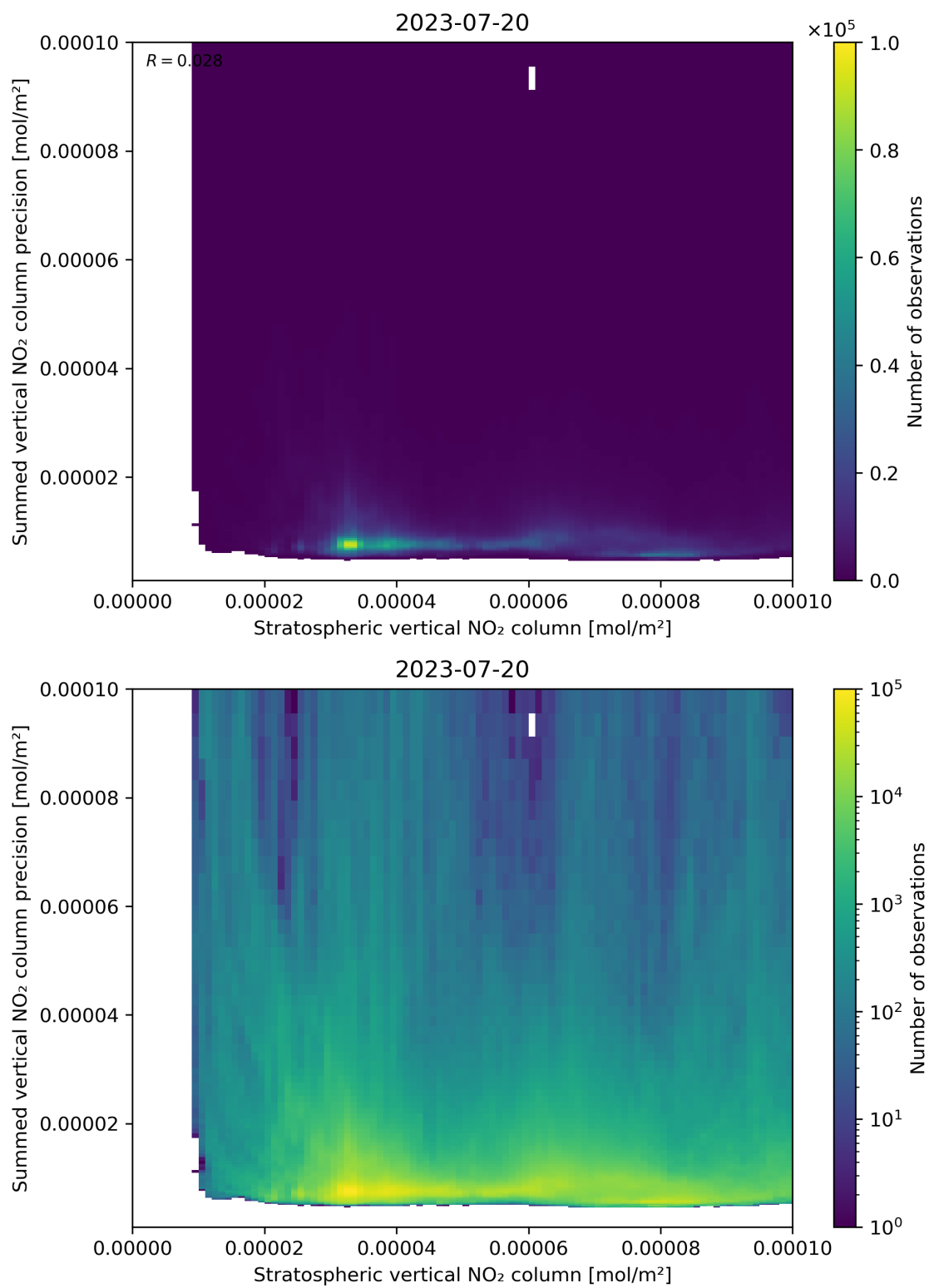
Figure 99: Scatter density plot of “Stratospheric vertical NO 2 column” against “Summed vertical NO 2 column precision” for 2023-07-19 to 2023-07-21.
