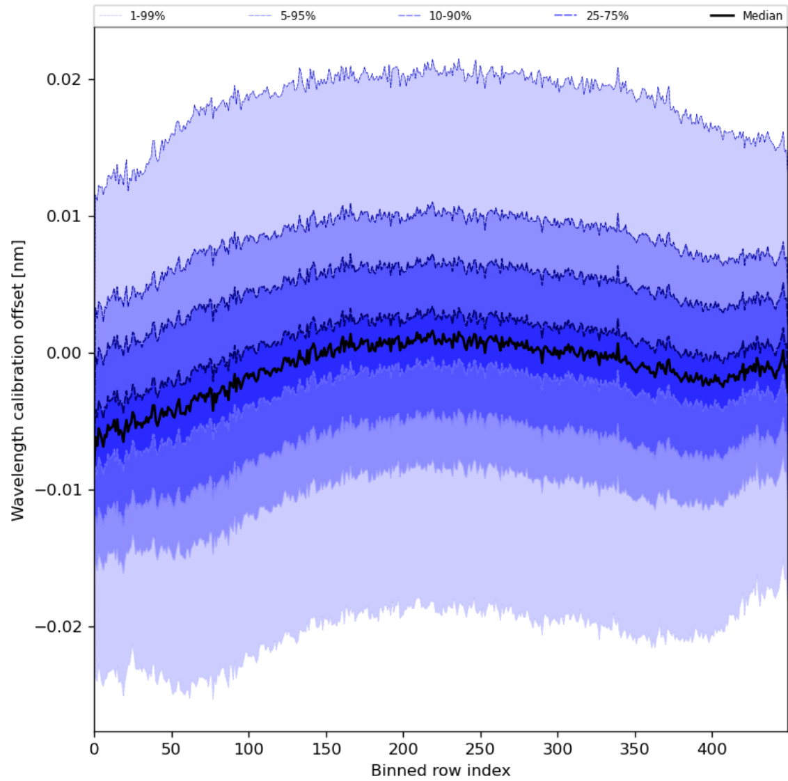
Figure 52: Along track statistics of “Wavelength calibration offset” for 2023-07-19 to 2023-07-21
