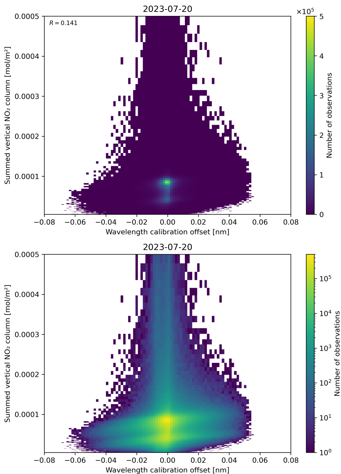
Figure 177: Scatter density plot of “Wavelength calibration offset” against “Summed vertical NO 2 column” for 2023-07-19 to 2023-07-21.
