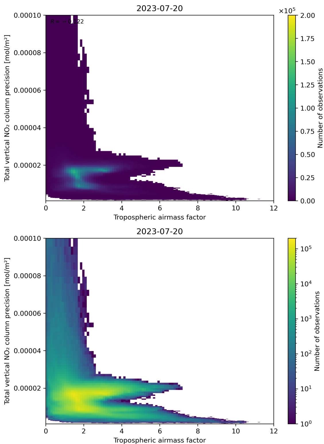
Figure 78: Scatter density plot of “Tropospheric airmass factor” against “Total vertical NO 2 column precision” for 2023-07-19 to 2023-07-21.
