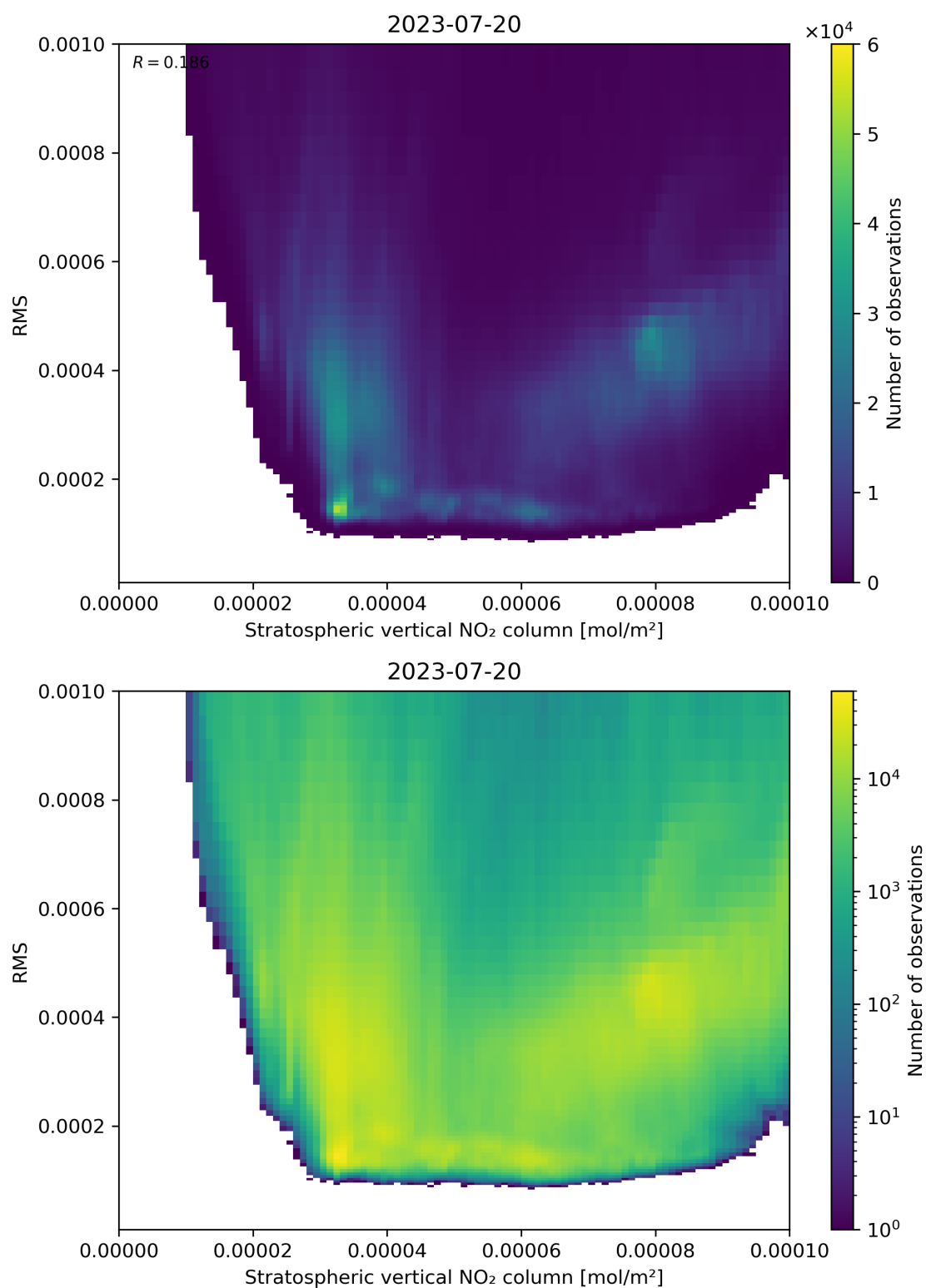
Figure 102: Scatter density plot of “Stratospheric vertical NO 2 column” against “RMS” for 2023-07-19 to 2023-07-21.
