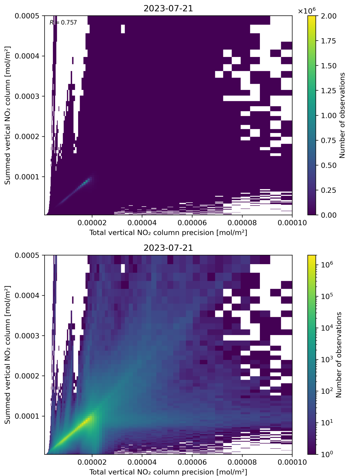
Figure 117: Scatter density plot of “Total vertical NO 2 column precision” against “Summed vertical NO 2 column” for 2023-07-20 to 2023-07-22.
