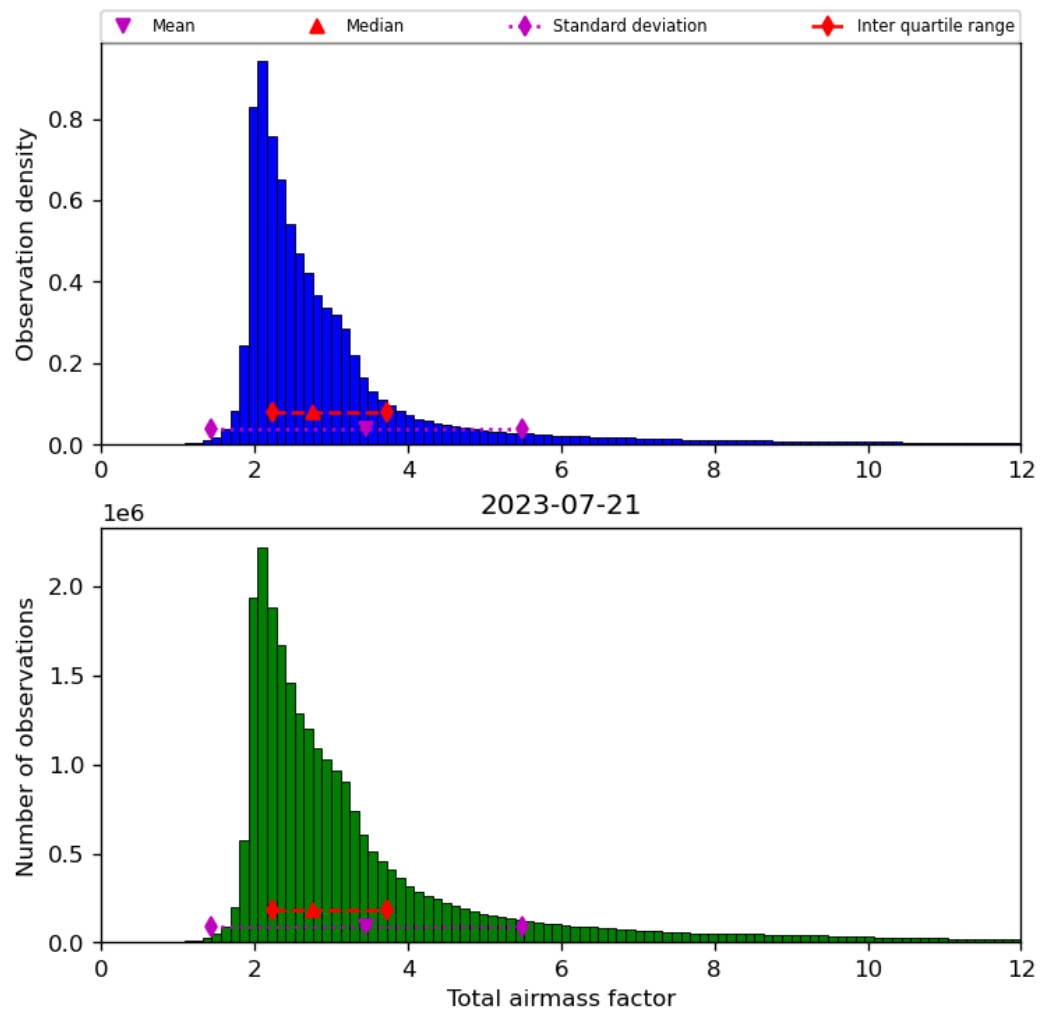
Figure 32: Histogram of “Total airmass factor” for 2023-07-20 to 2023-07-22
