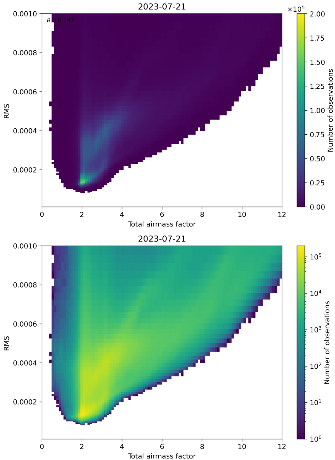
Figure 69: Scatter density plot of “Total airmass factor” against “RMS” for 2023-07-20 to 2023-07-22.
