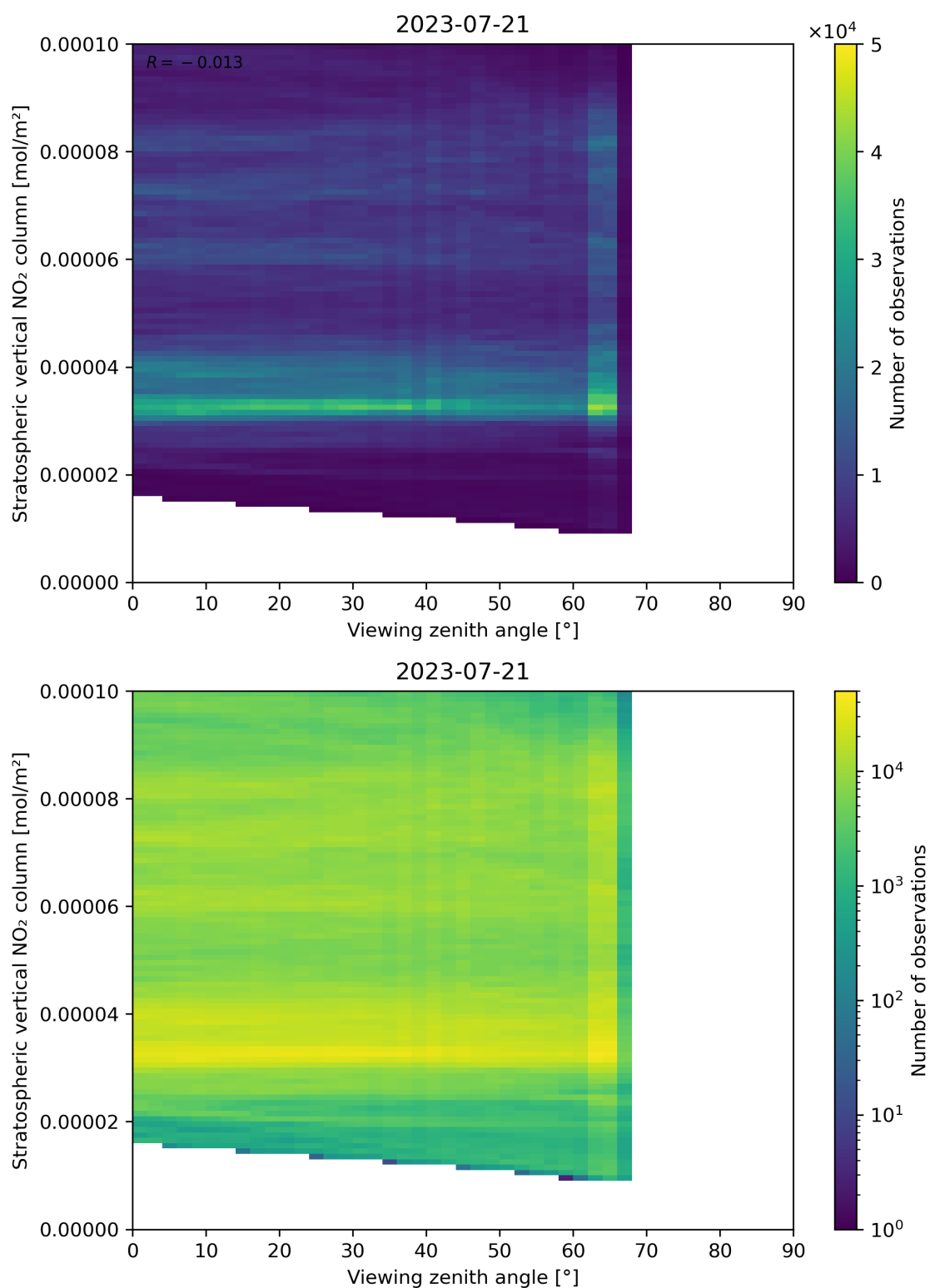
Figure 164: Scatter density plot of “Viewing zenith angle” against “Stratospheric vertical NO 2 column” for 2023-07-20 to 2023-07-22.
