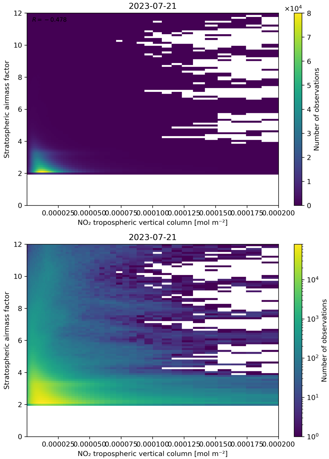
Figure 121: Scatter density plot of “NO 2 tropospheric vertical column” against “Stratospheric air mass factor” for 2023-07-20 to 2023-07-22.
