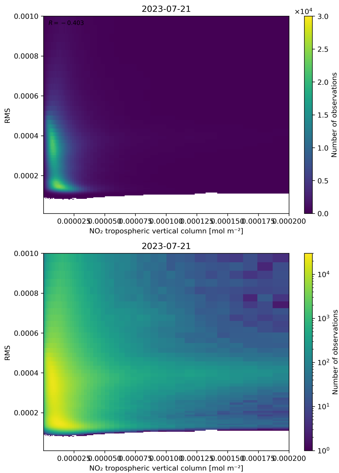
Figure 142: Scatter density plot of “NO 2 tropospheric vertical column” against “RMS” for 2023-07-20 to 2023-07-22.
