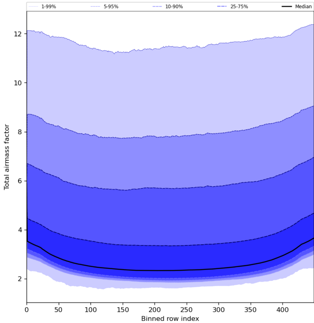
Figure 49: Along track statistics of “Total airmass factor” for 2023-07-20 to 2023-07-22
