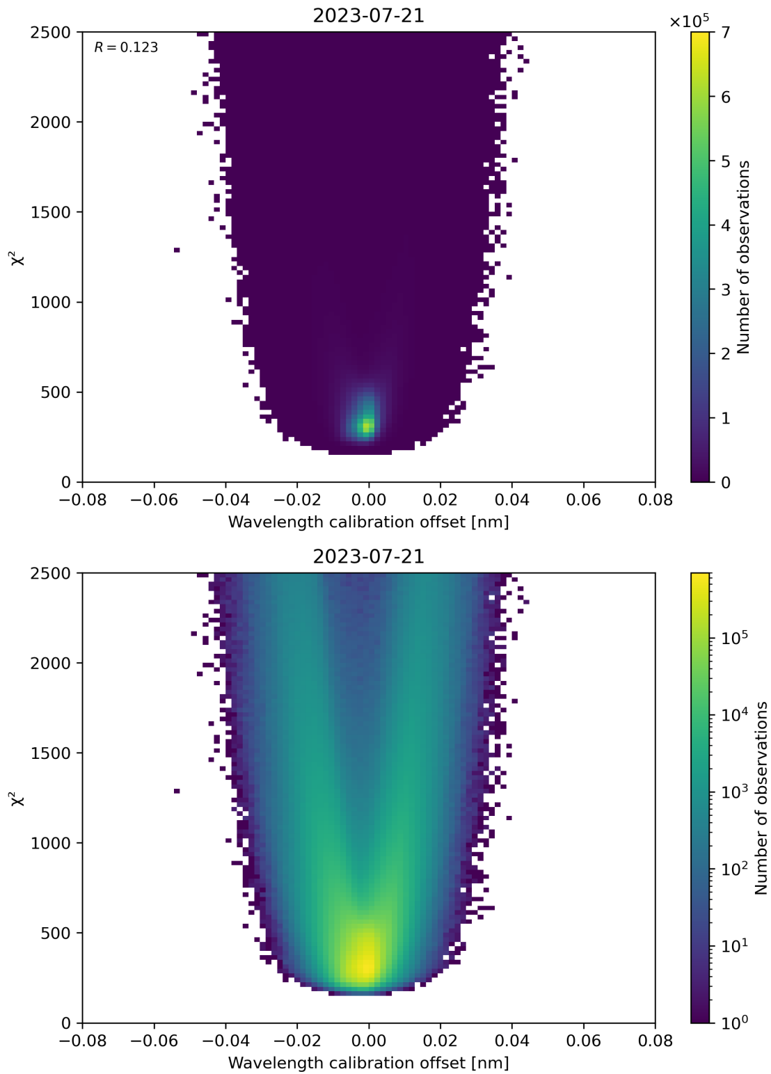
Figure 175: Scatter density plot of “Wavelength calibration offset” against “ \chi^2 ” for 2023-07-20 to 2023-07-22.
