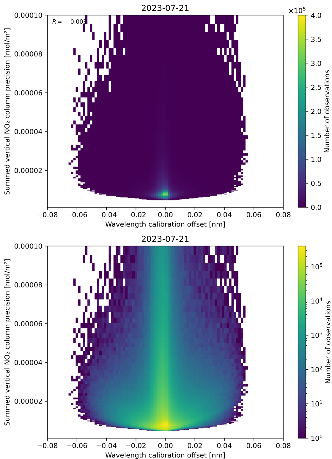
Figure 178: Scatter density plot of “Wavelength calibration offset” against “Summed vertical NO 2 column precision” for 2023-07-20 to 2023-07-22.
