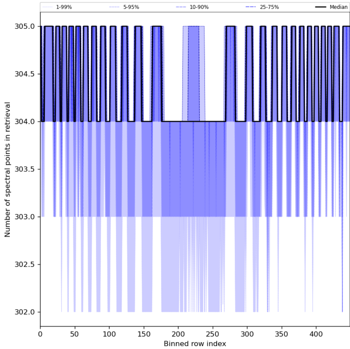
Figure 50: Along track statistics of “Number of spectral points in retrieval” for 2023-07-20 to 2023-07-22
