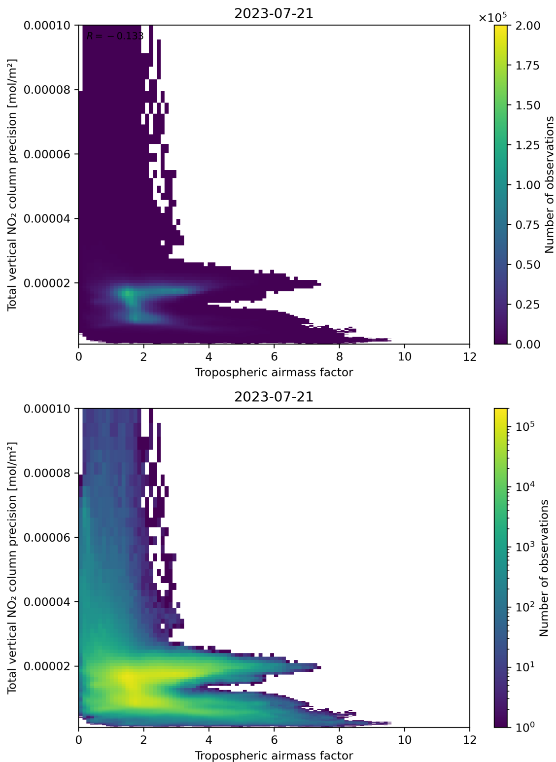
Figure 78: Scatter density plot of “Tropospheric air mass factor” against “Total vertical NO 2 column precision” for 2023-07-20 to 2023-07-22.
