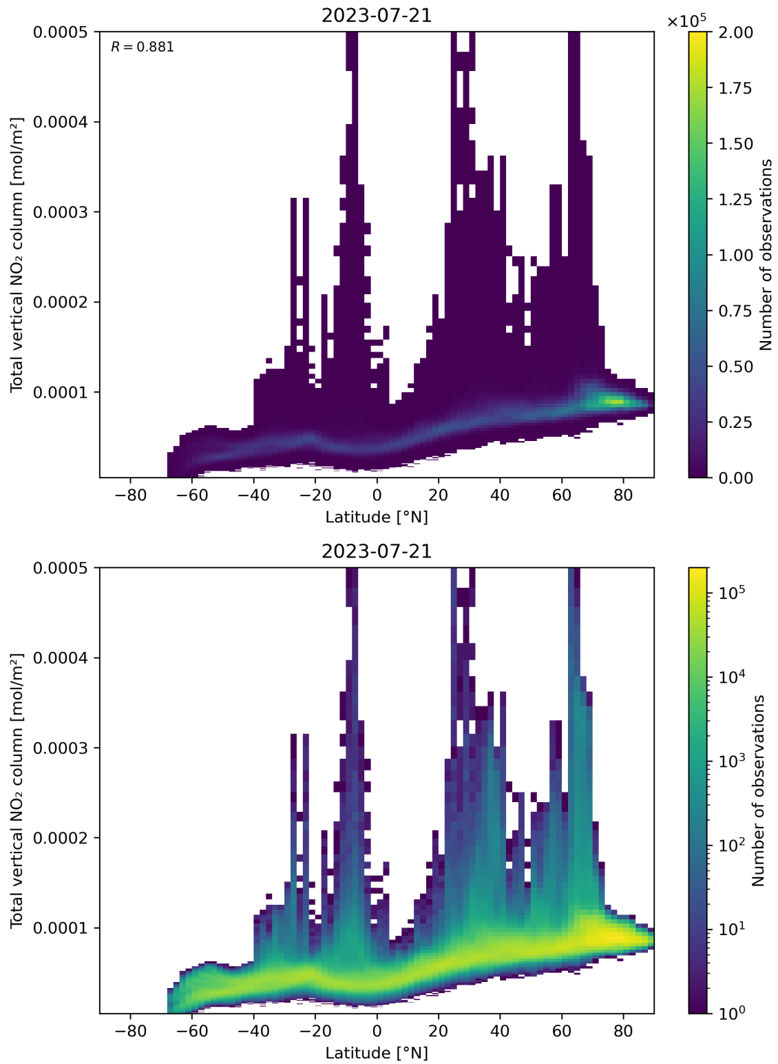
Figure 90: Scatter density plot of “Latitude” against “Total vertical NO 2 column” for 2023-07-20 to 2023-07-22.
