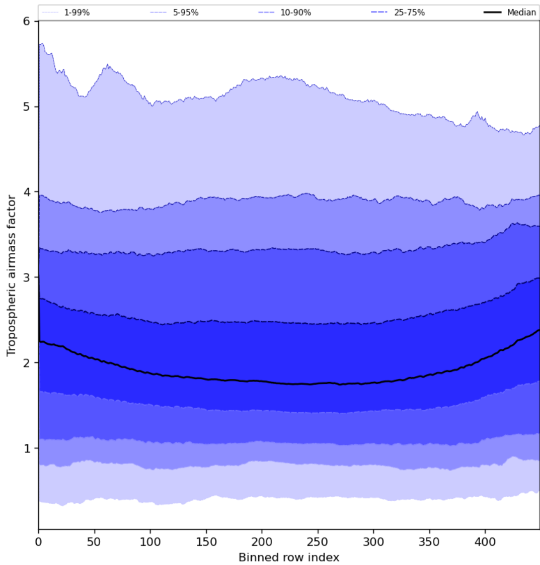
Figure 48: Along track statistics of “Tropospheric airmass factor” for 2023-07-20 to 2023-07-22
