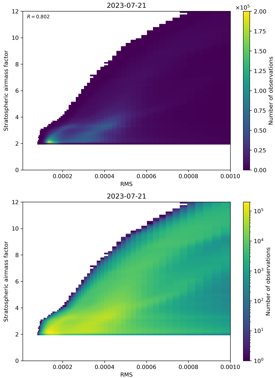
Figure 144: Scatter density plot of “RMS” against “Stratospheric airmass factor” for 2023-07-20 to 2023-07-22.
