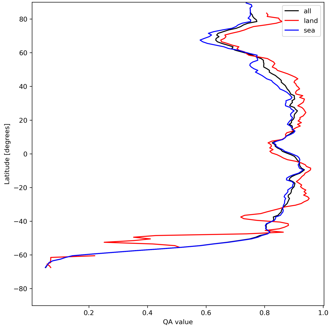
Figure 11: Zonal average of “QA value” for 2023-07-20 to 2023-07-22.
