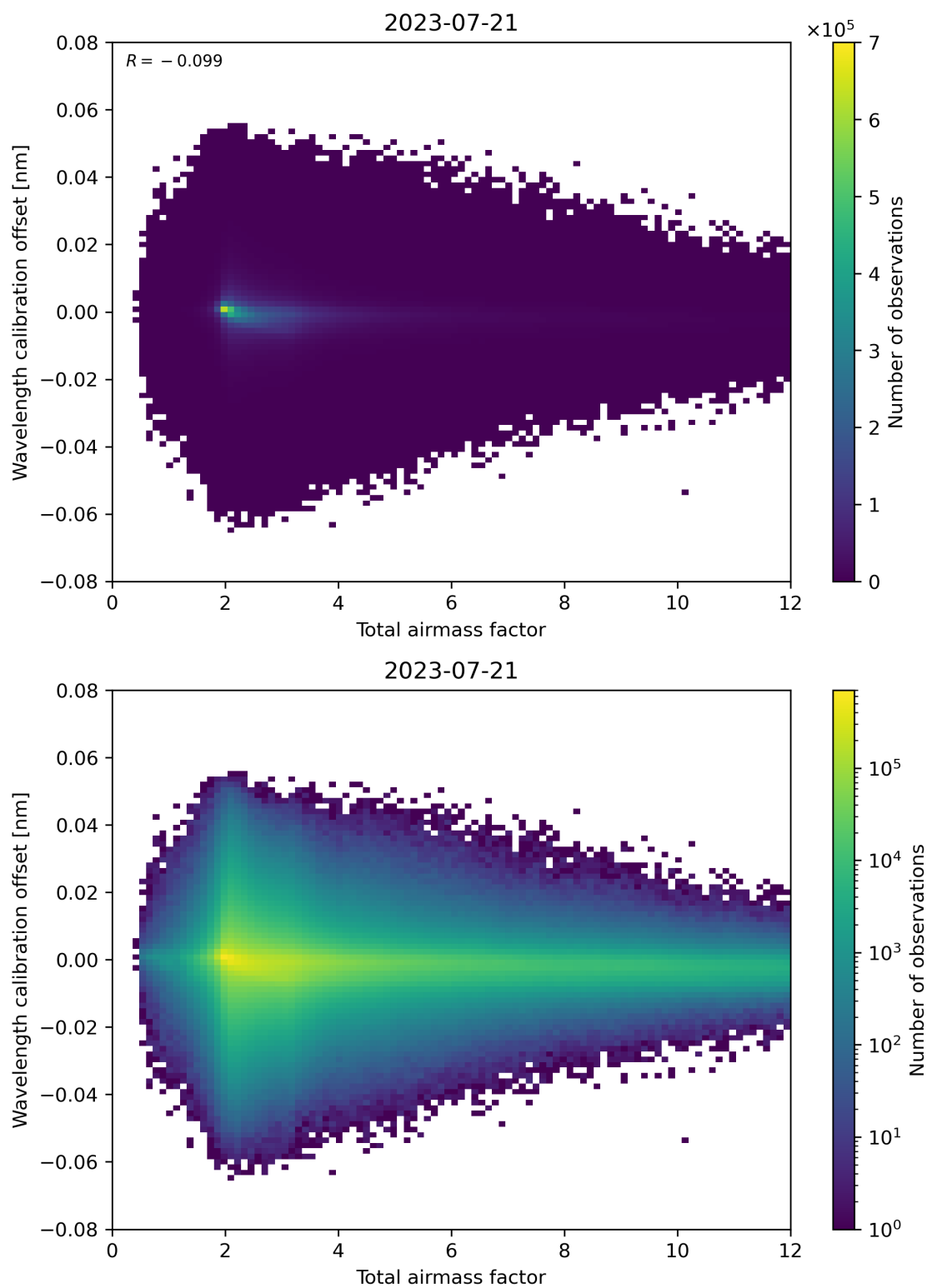
Figure 70: Scatter density plot of “Total airmass factor” against “Wavelength calibration offset” for 2023-07-20 to 2023-07-22.
