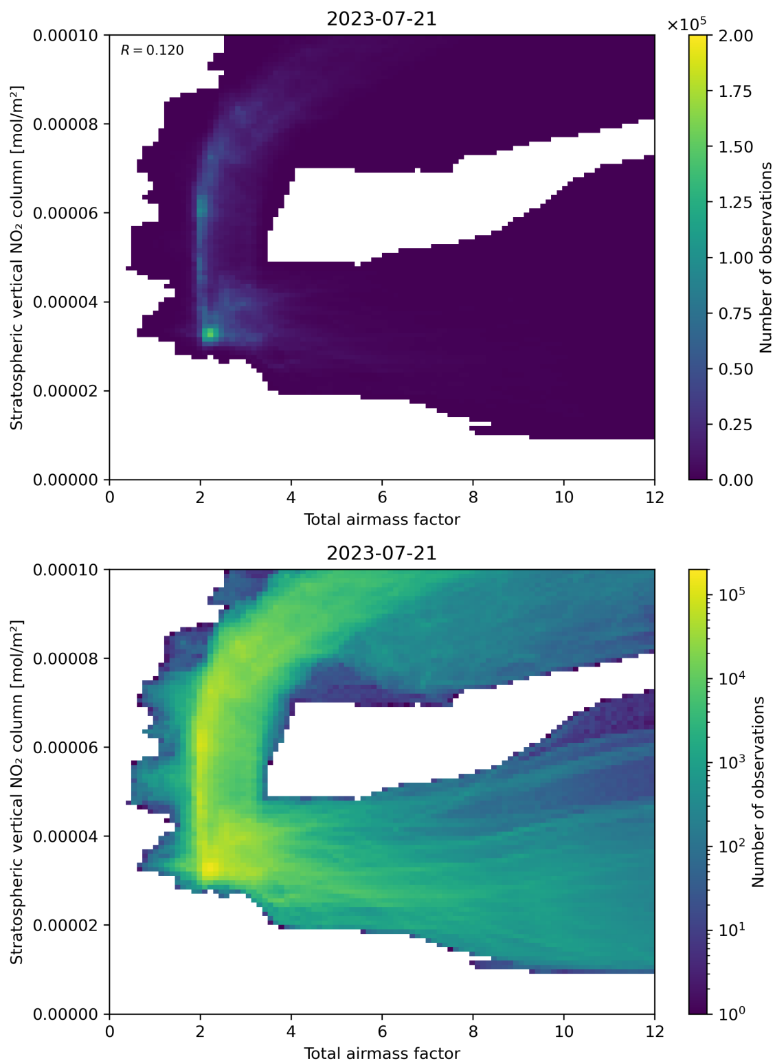
Figure 64: Scatter density plot of “Total airmass factor” against “Stratospheric vertical NO 2 column” for 2023-07-20 to 2023-07-22.
