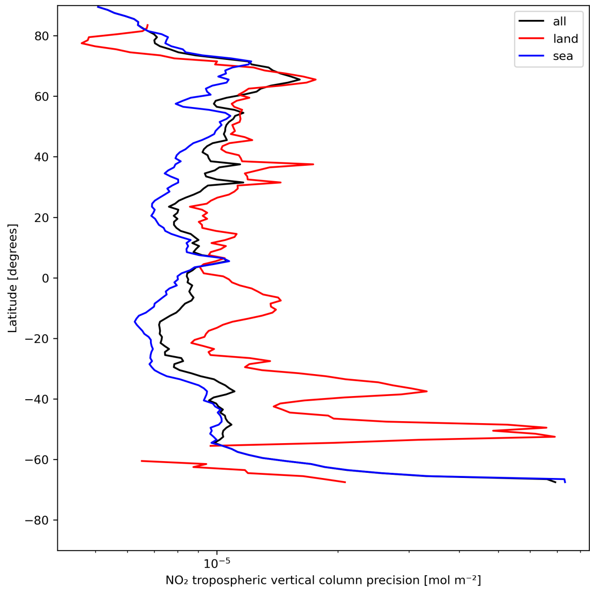
Figure 13: Zonal average of "NO 2 tropospheric vertical column precision" for 2023-07-20 to 2023-07-22.
