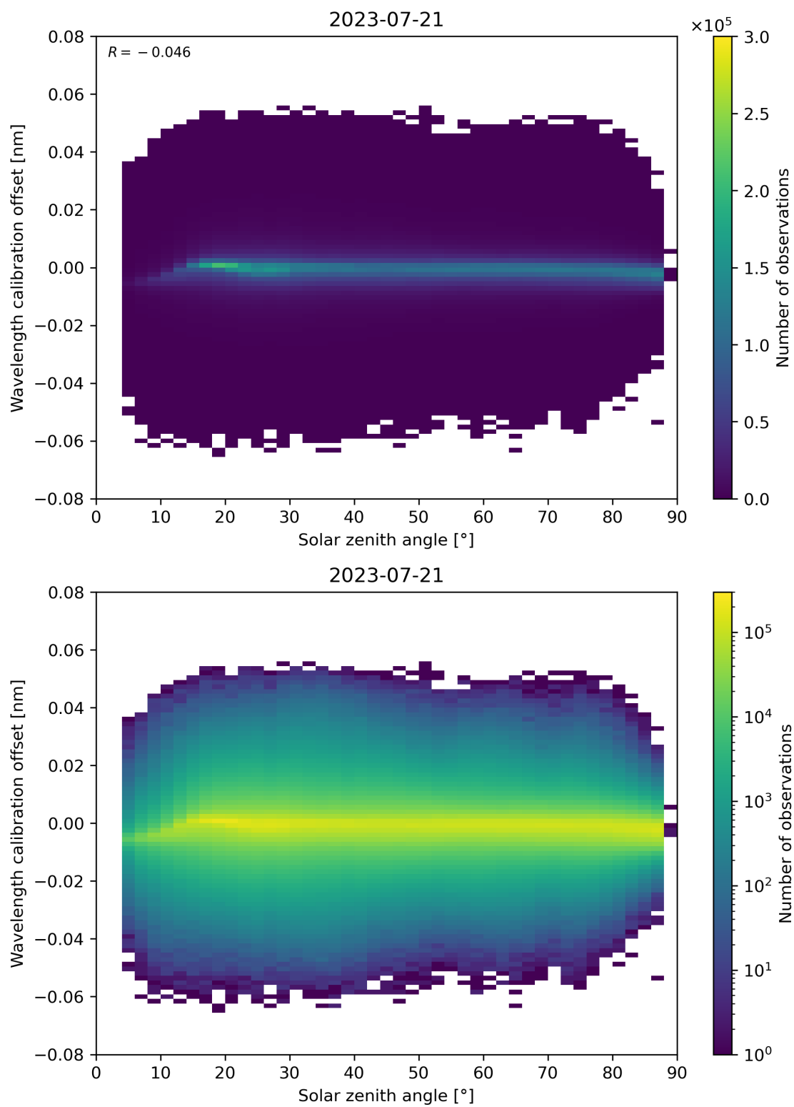
Figure 158: Scatter density plot of “Solar zenith angle” against “Wavelength calibration offset” for 2023-07-20 to 2023-07-22.
