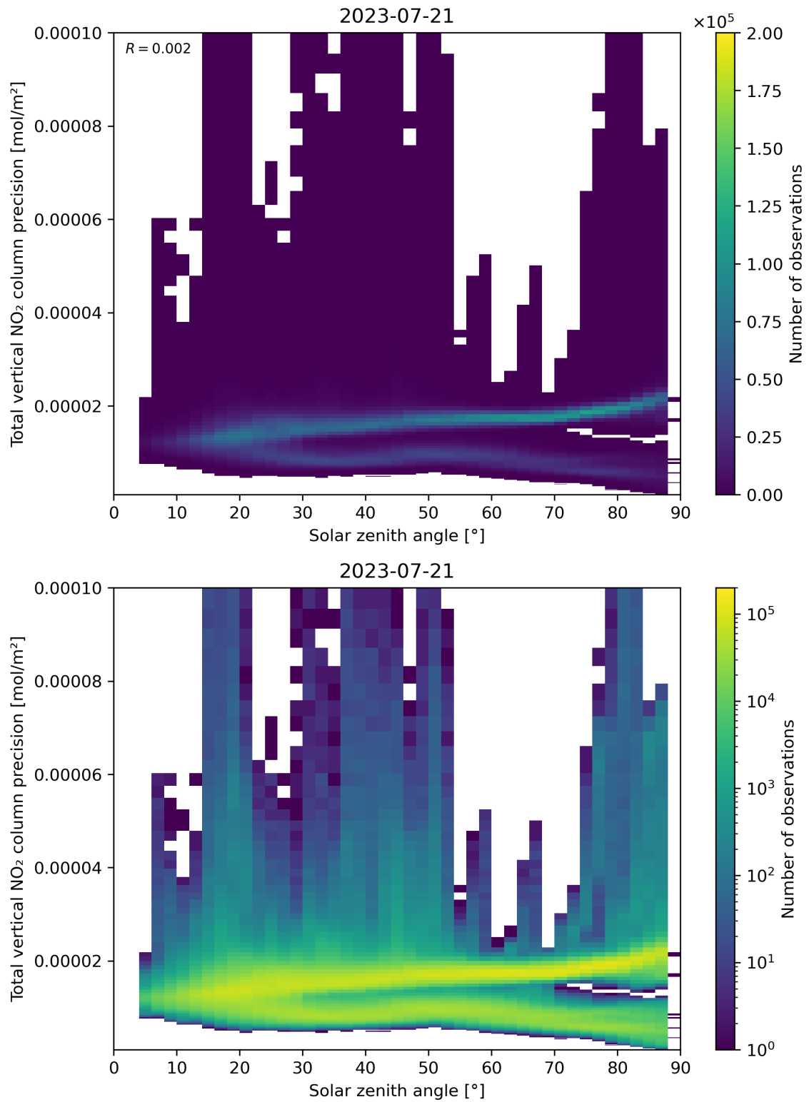
Figure 154: Scatter density plot of “Solar zenith angle” against “Total vertical NO 2 column precision” for 2023-07-20 to 2023-07-22.
