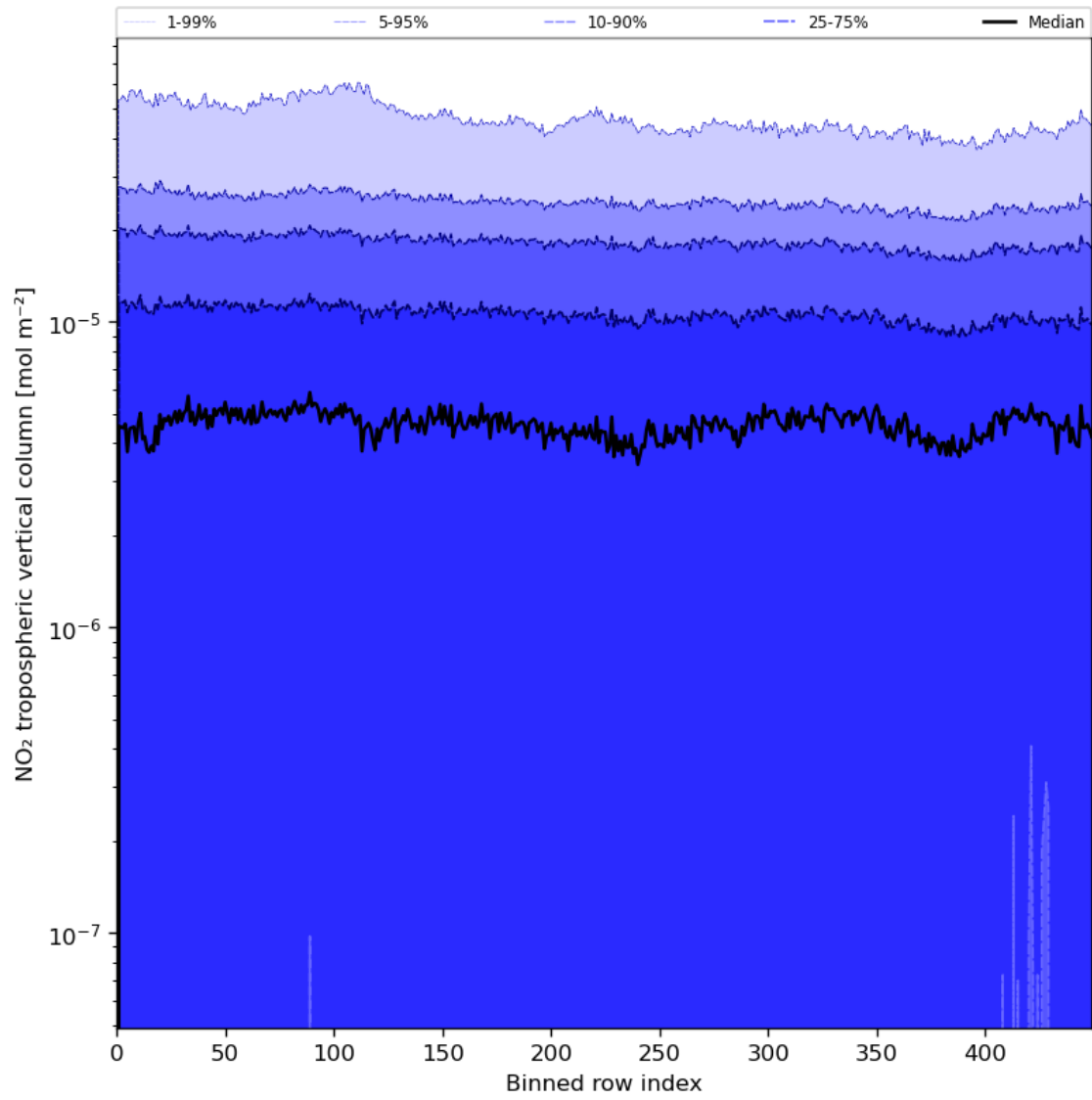
Figure 46: Along track statistics of “NO 2 tropospheric vertical column” for 2023-07-20 to 2023-07-22
