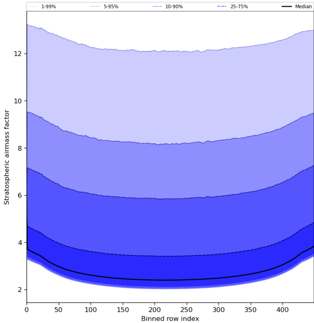
Figure 61: Along track statistics of “Stratospheric airmass factor” for 2023-07-20 to 2023-07-22
