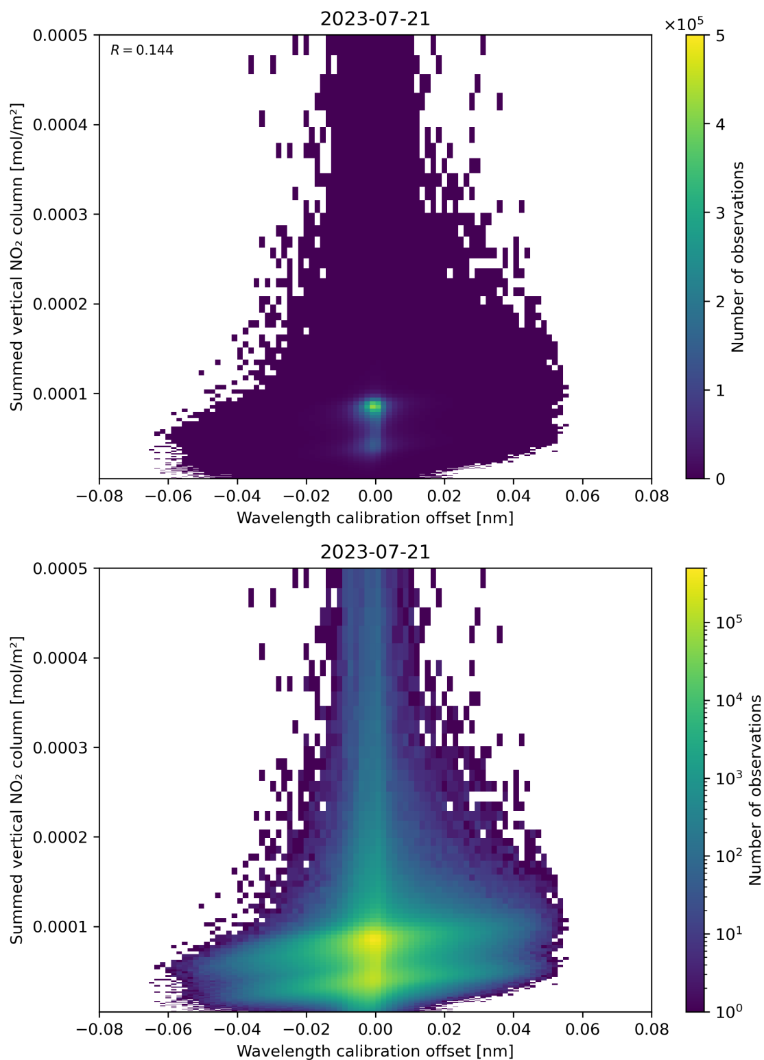
Figure 177: Scatter density plot of “Wavelength calibration offset” against “Summed vertical NO 2 column” for 2023-07-20 to 2023-07-22.
