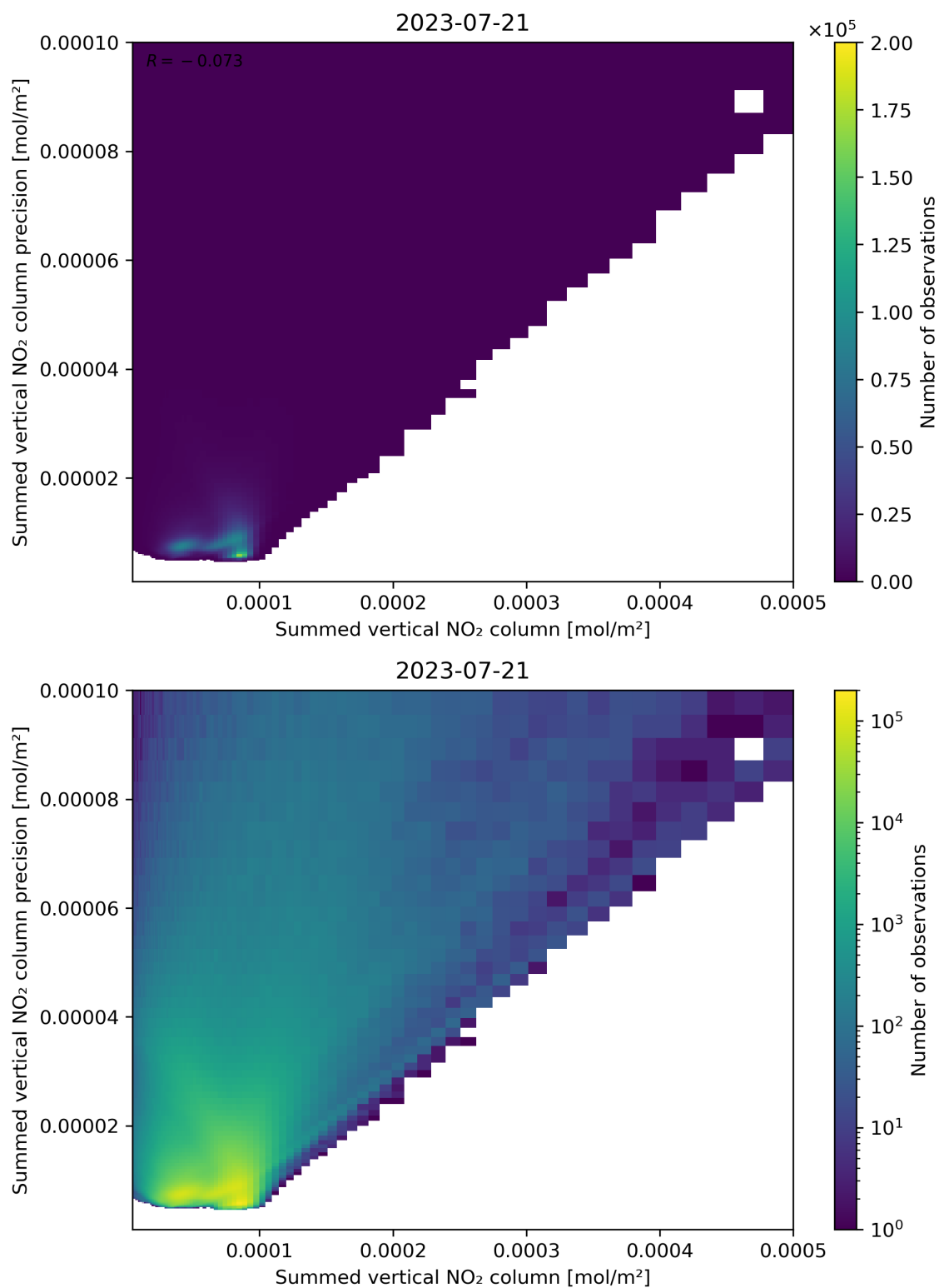
Figure 105: Scatter density plot of “Summed vertical NO 2 column” against “Summed vertical NO 2 column precision” for 2023-07-20 to 2023-07-22.
