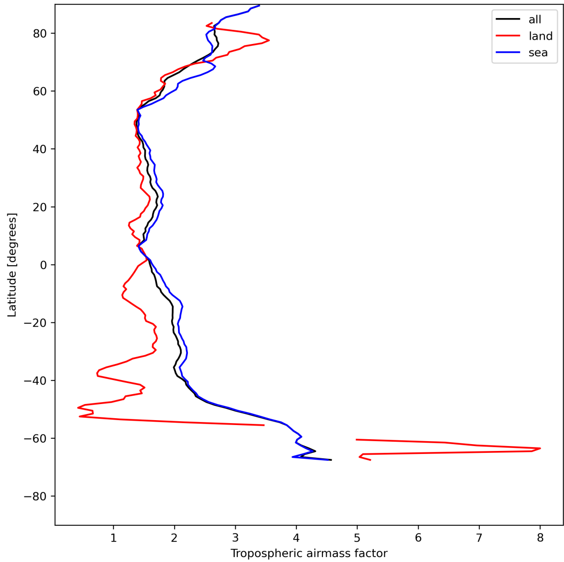
Figure 14: Zonal average of “Tropospheric air mass factor” for 2023-07-20 to 2023-07-22.
