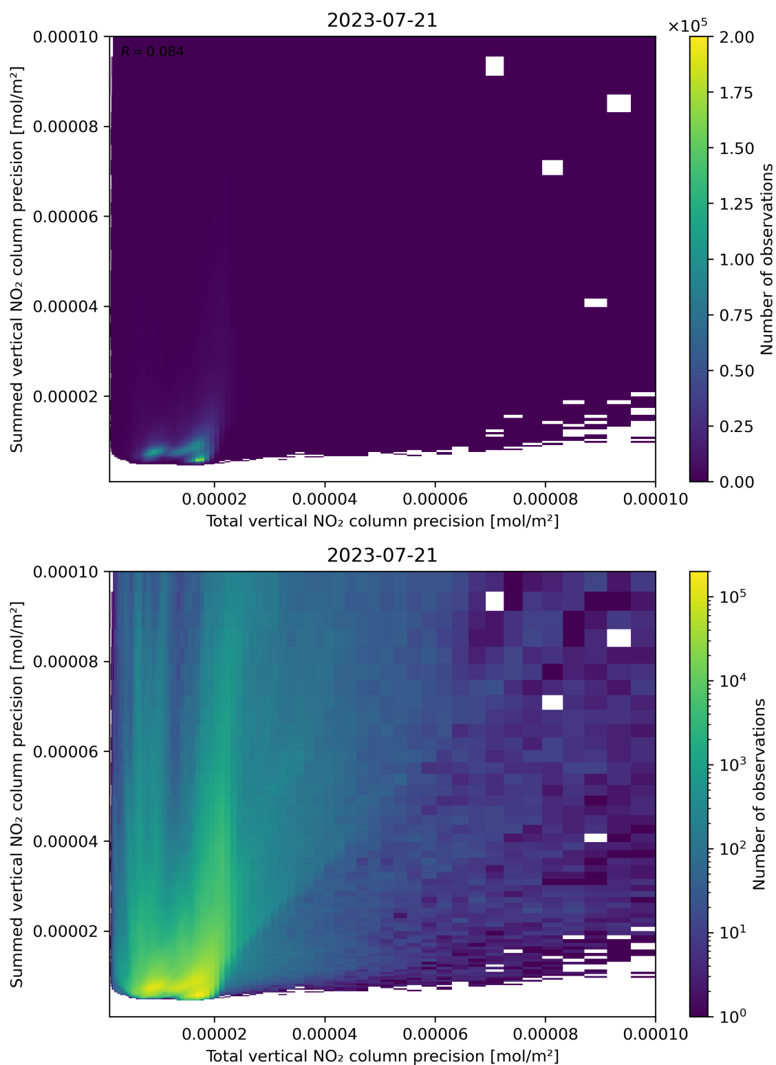
Figure 118: Scatter density plot of “Total vertical NO 2 column precision” against “Summed vertical NO 2 column precision” for 2023-07-20 to 2023-07-22.
