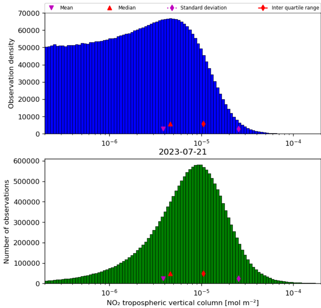
Figure 29: Histogram of “NO 2 tropospheric vertical column” for 2023-07-20 to 2023-07-22
