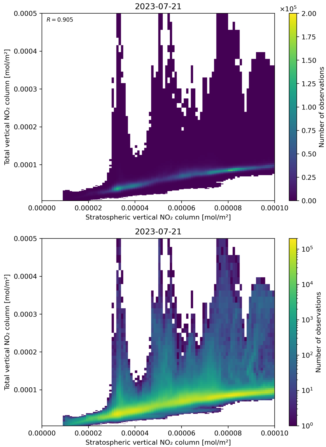
Figure 100: Scatter density plot of “Stratospheric vertical NO 2 column” against “Total vertical NO 2 column” for 2023-07-20 to 2023-07-22.
