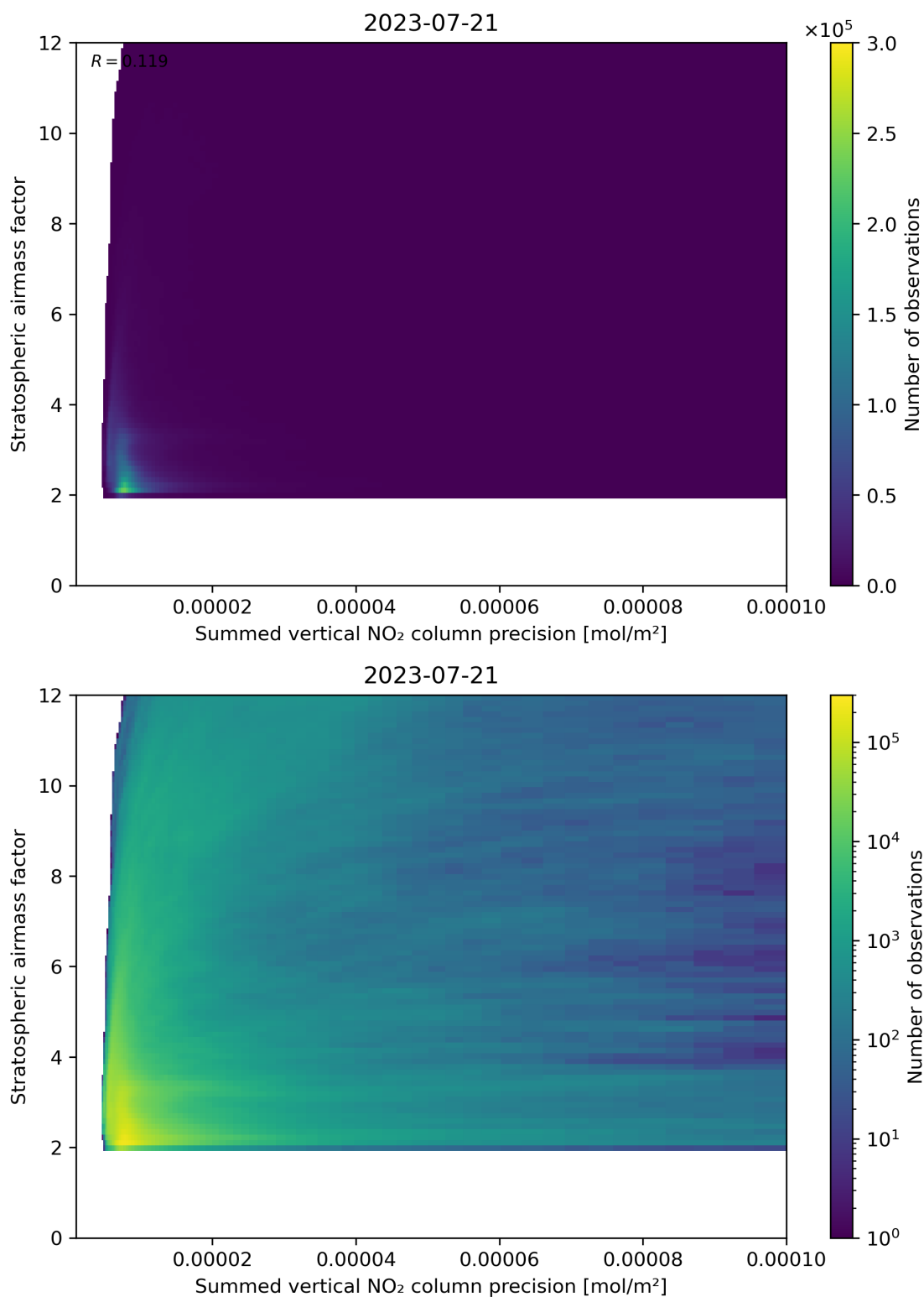
Figure 106: Scatter density plot of “Summed vertical NO 2 column precision” against “Stratospheric airmass factor” for 2023-07-20 to 2023-07-22.
