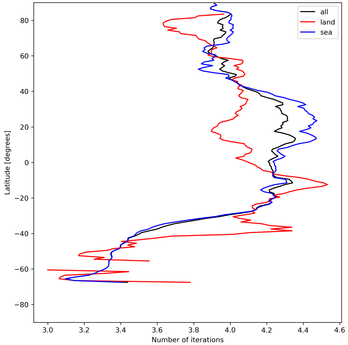
Figure 17: Zonal average of “Number of iterations” for 2023-07-20 to 2023-07-22.
