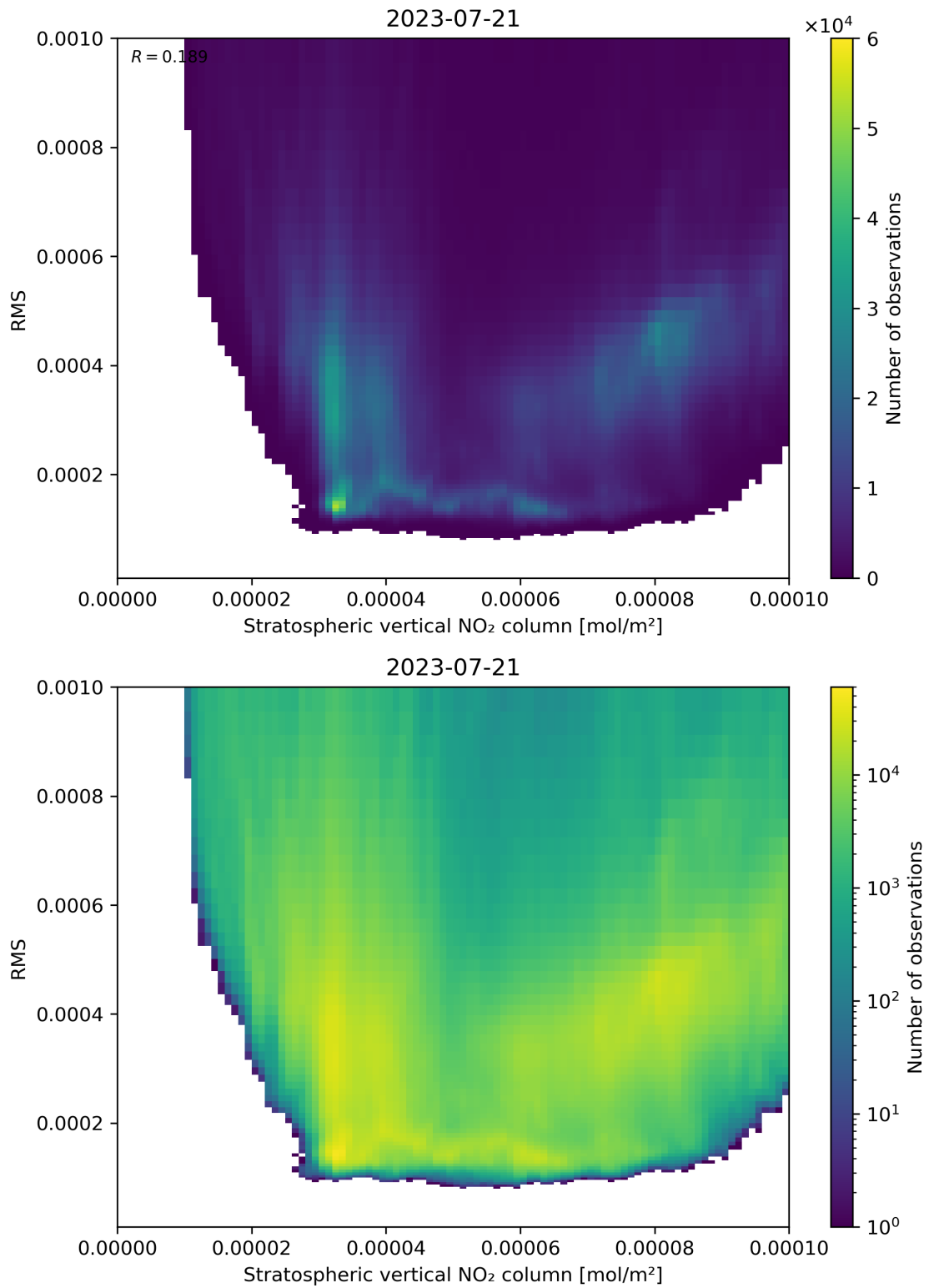
Figure 102: Scatter density plot of “Stratospheric vertical NO 2 column” against “RMS” for 2023-07-20 to 2023-07-22.
