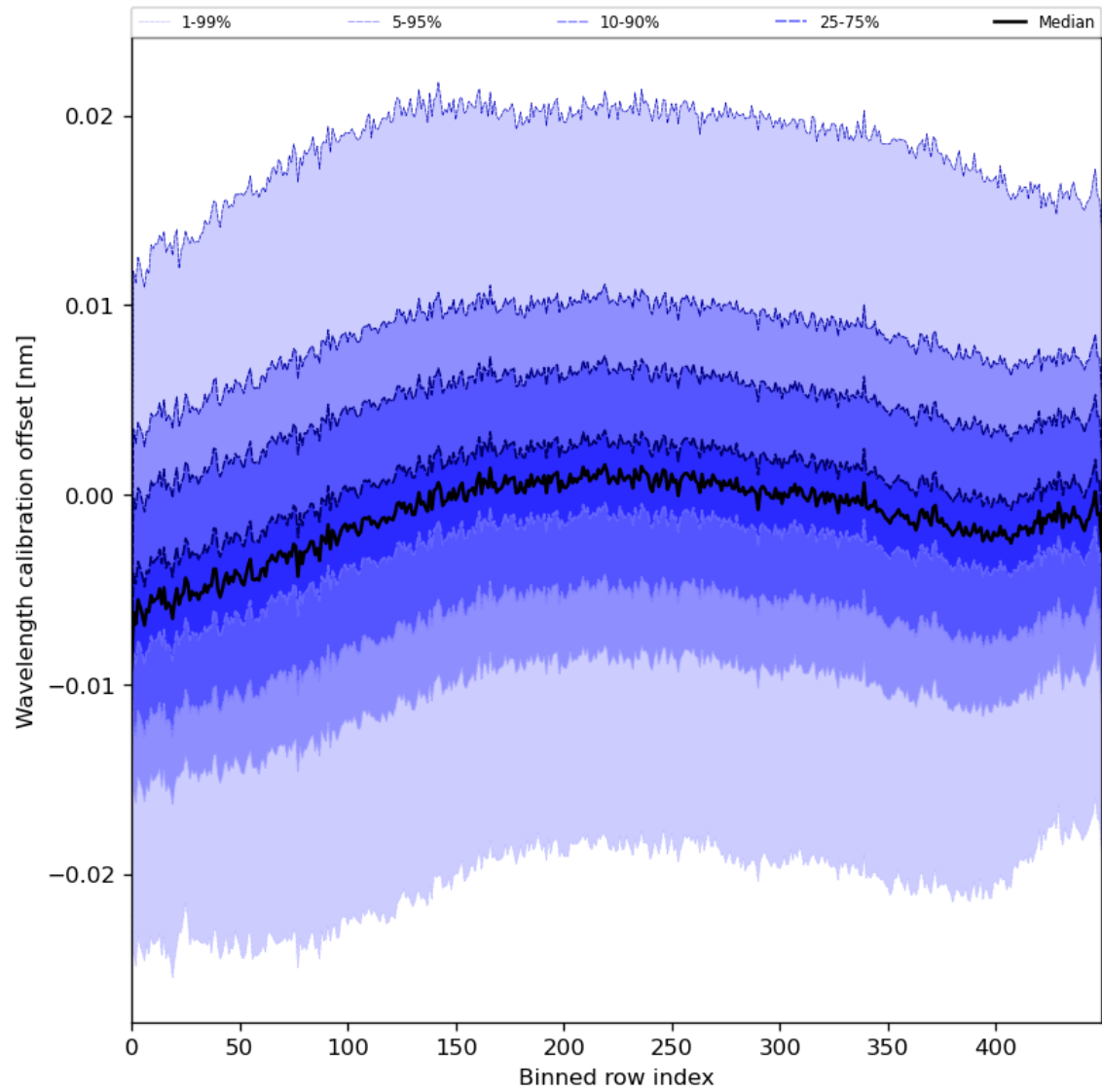
Figure 52: Along track statistics of “Wavelength calibration offset” for 2023-07-20 to 2023-07-22
