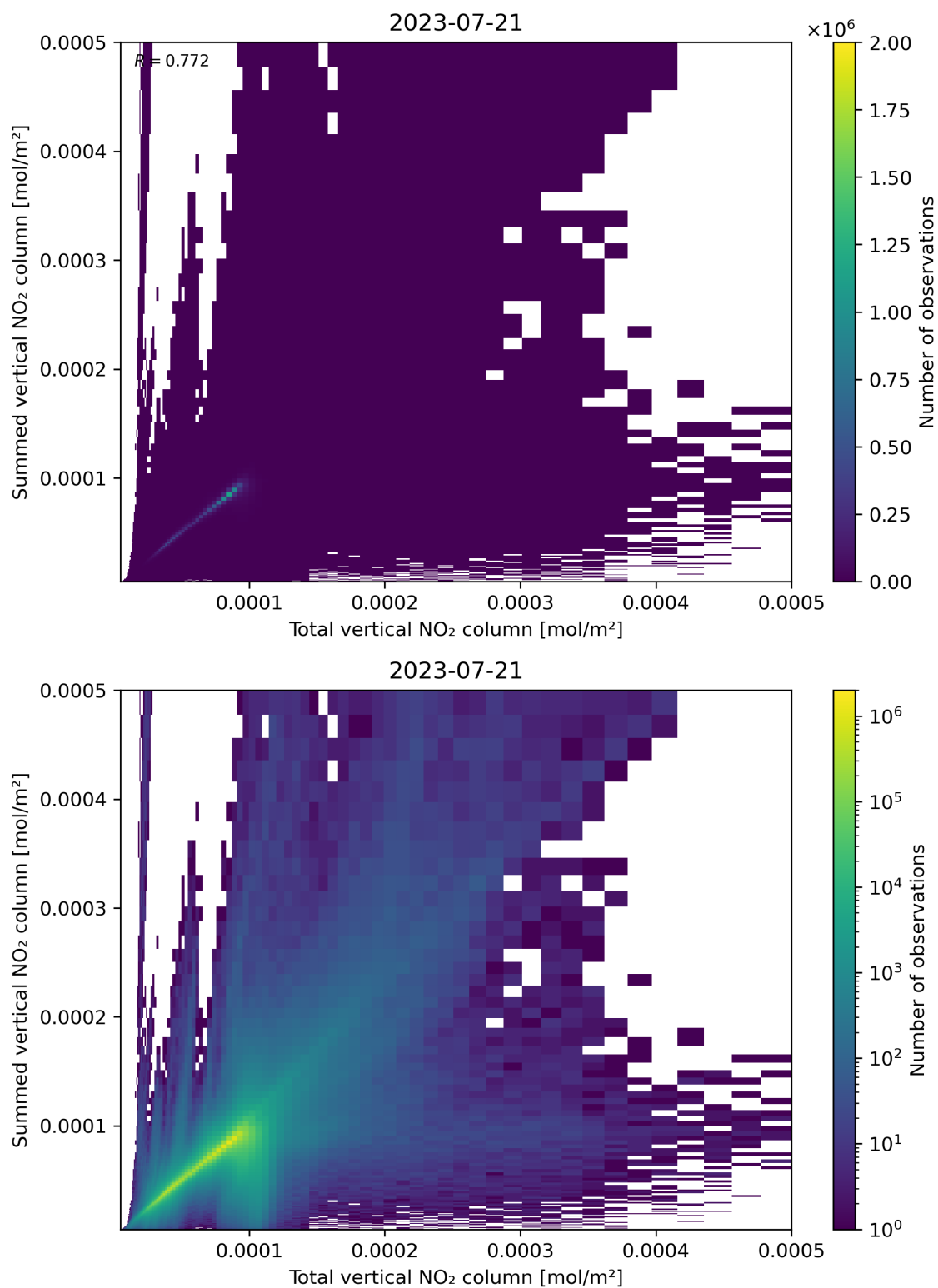
Figure 112: Scatter density plot of “Total vertical NO 2 column” against “Summed vertical NO 2 column” for 2023-07-20 to 2023-07-22.
