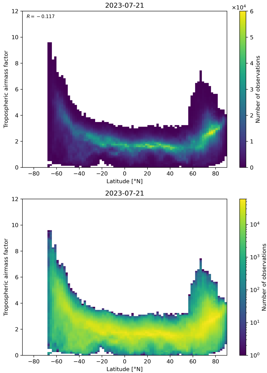
Figure 85: Scatter density plot of “Latitude” against “Tropospheric air mass factor” for 2023-07-20 to 2023-07-22.
