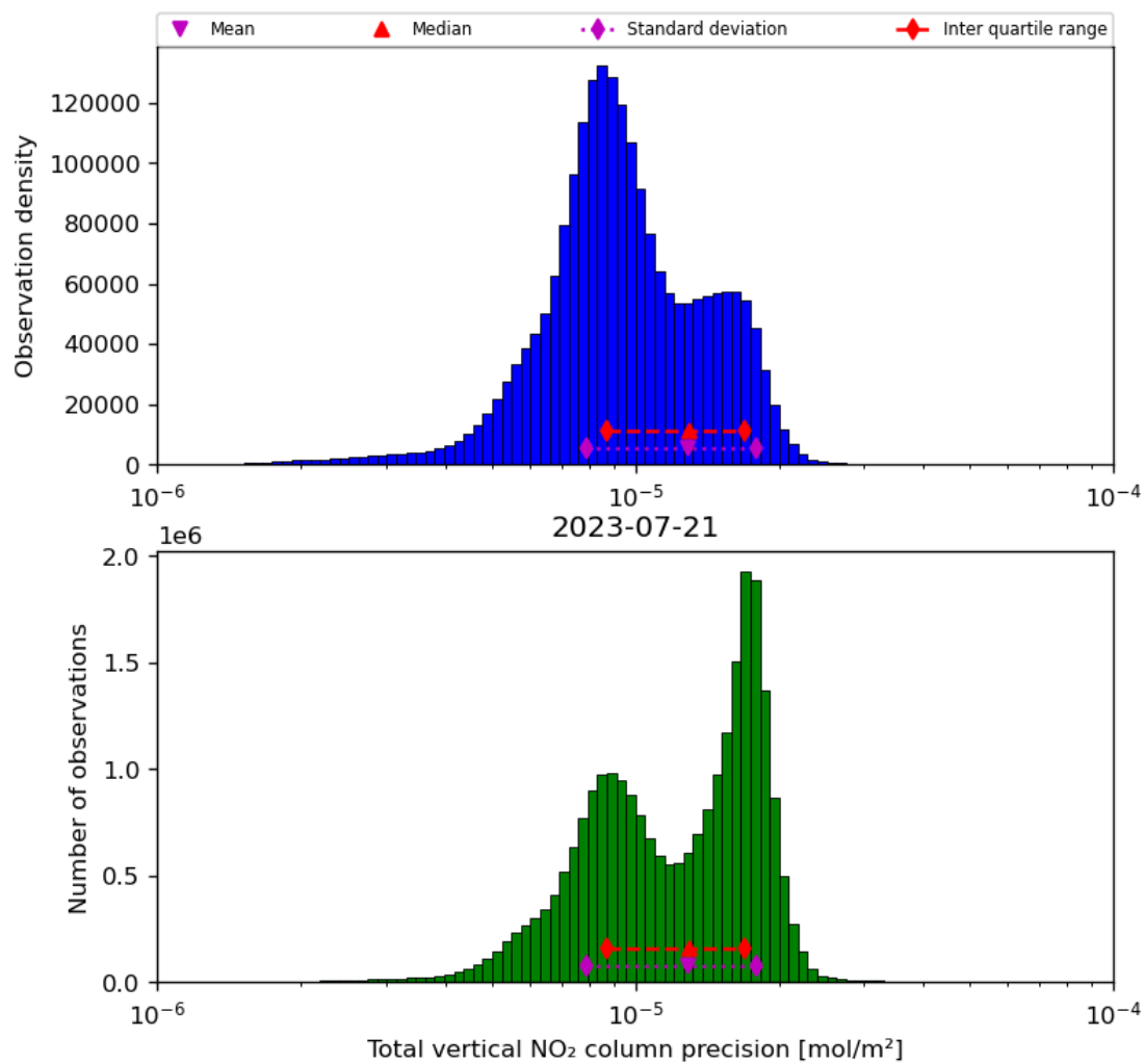
Figure 39: Histogram of “Total vertical NO 2 column precision” for 2023-07-20 to 2023-07-22
