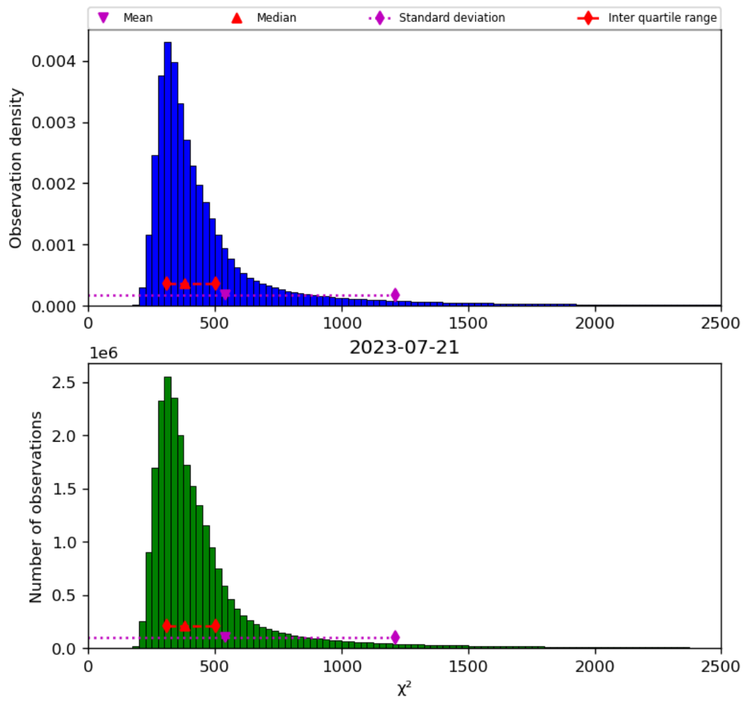
Figure 42: Histogram of “ \chi^2 ” for 2023-07-20 to 2023-07-22
