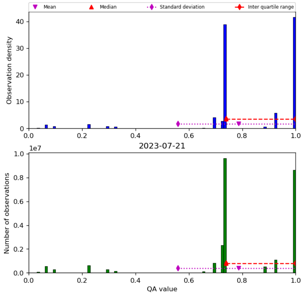
Figure 28: Histogram of “QA value” for 2023-07-20 to 2023-07-22
