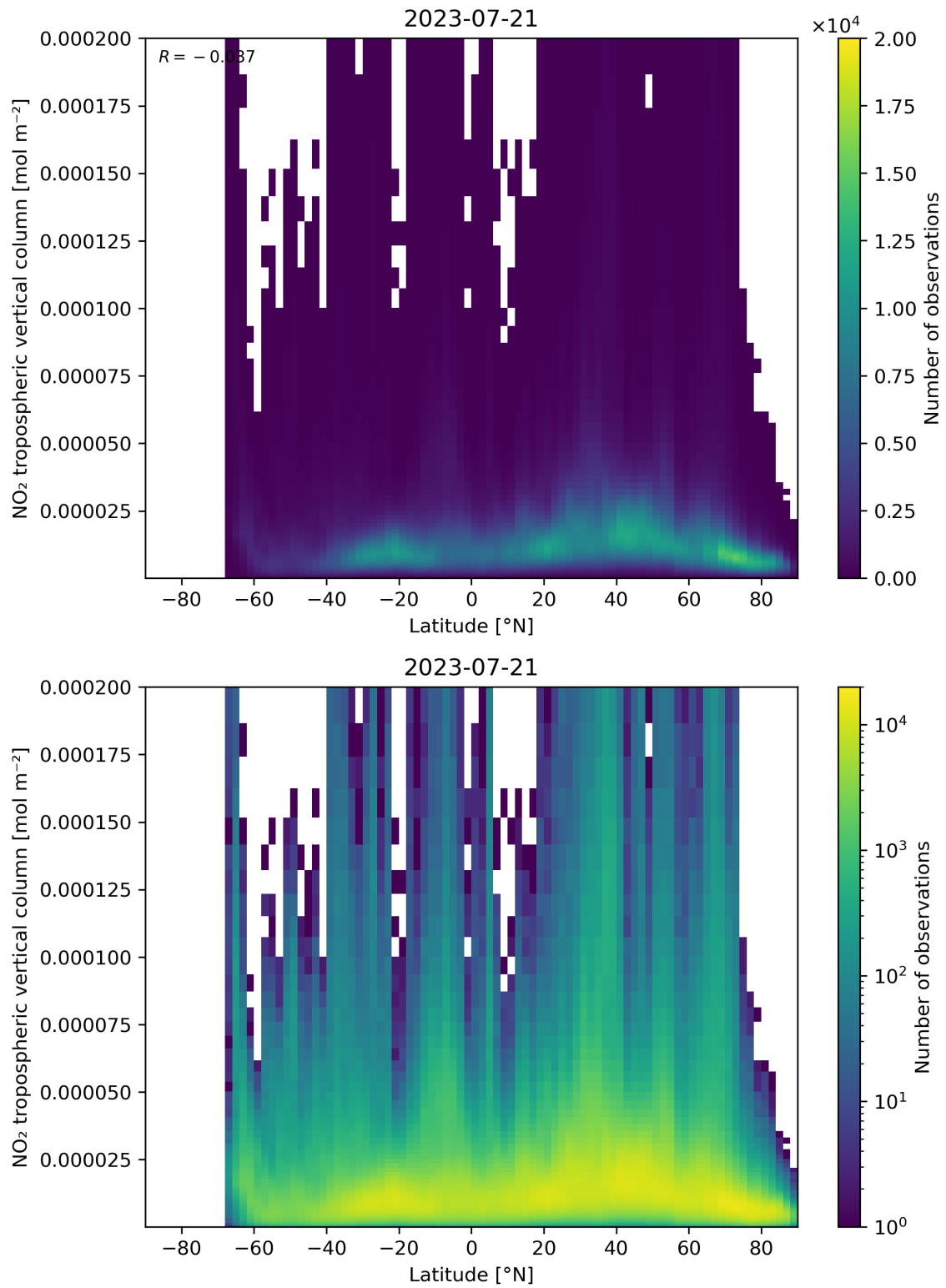
Figure 92: Scatter density plot of “Latitude” against “NO 2 tropospheric vertical column” for 2023-07-20 to 2023-07-22.
