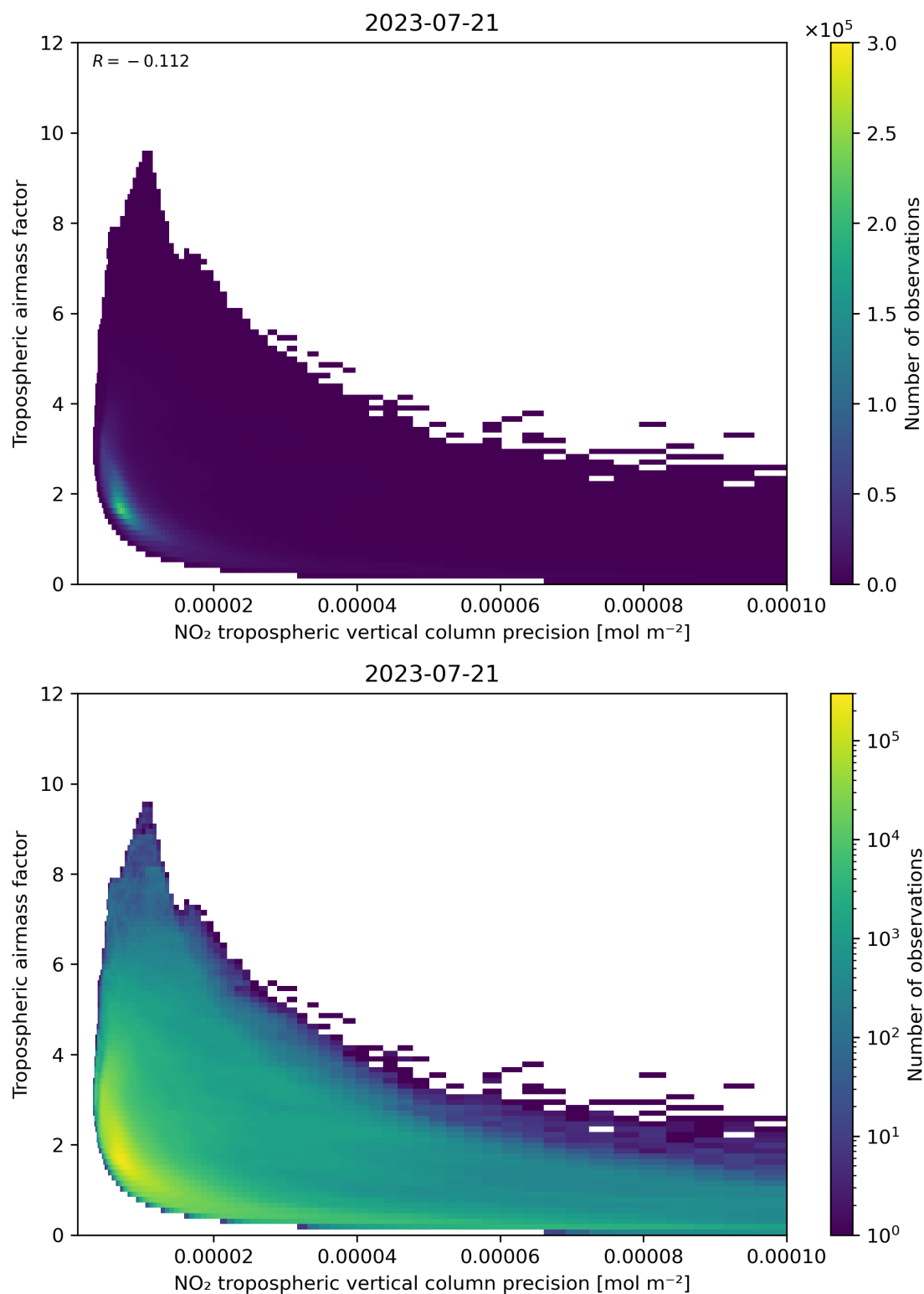
Figure 133: Scatter density plot of “NO 2 tropospheric vertical column precision” against “Tropospheric airmass factor” for 2023-07-20 to 2023-07-22.
