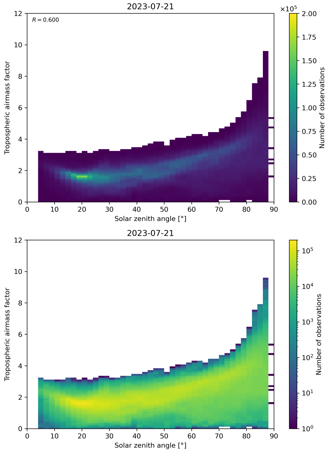
Figure 147: Scatter density plot of “Solar zenith angle” against “Tropospheric airmass factor” for 2023-07-20 to 2023-07-22.
