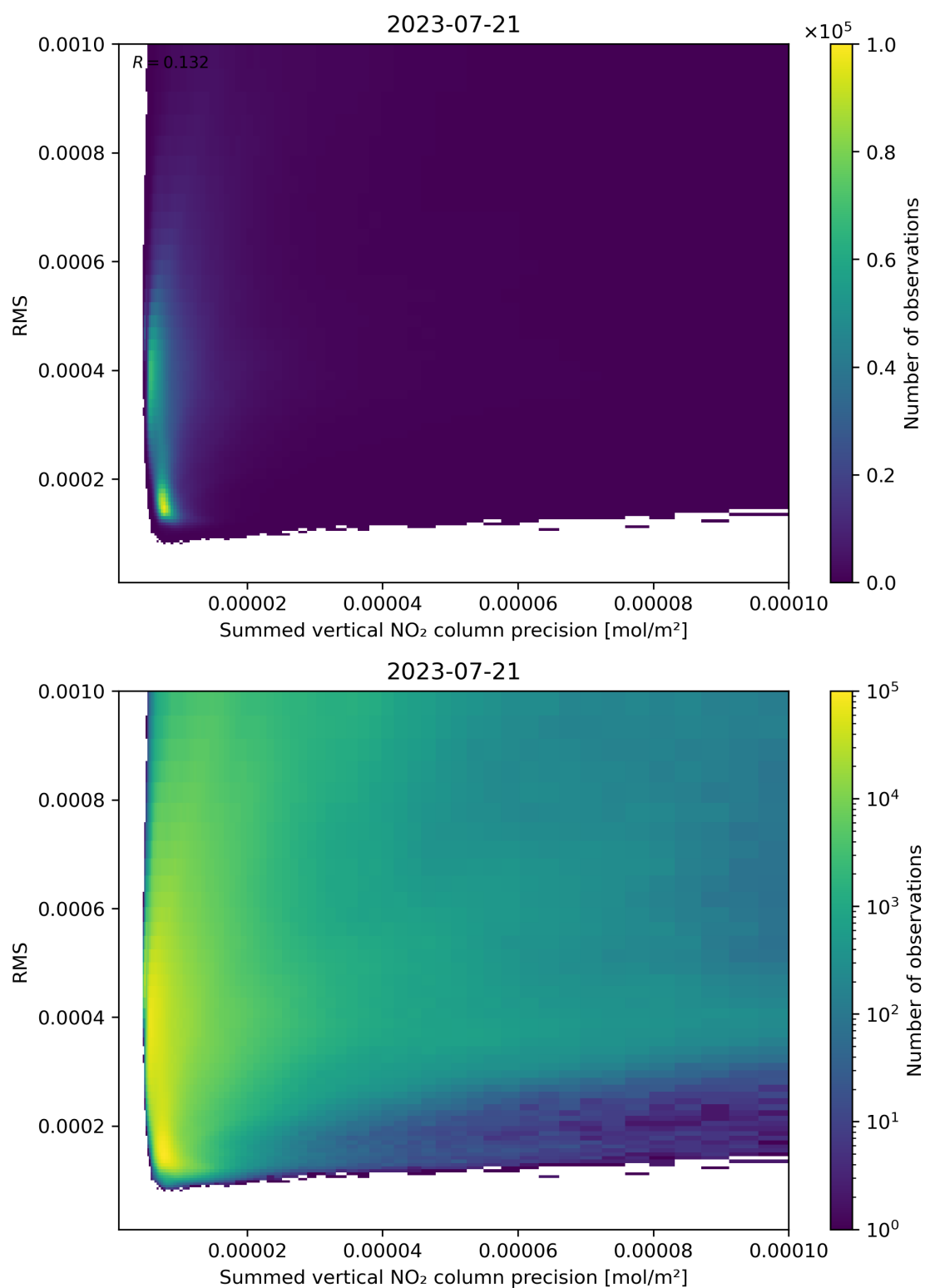
Figure 108: Scatter density plot of “Summed vertical NO 2 column precision” against “RMS” for 2023-07-20 to 2023-07-22.
