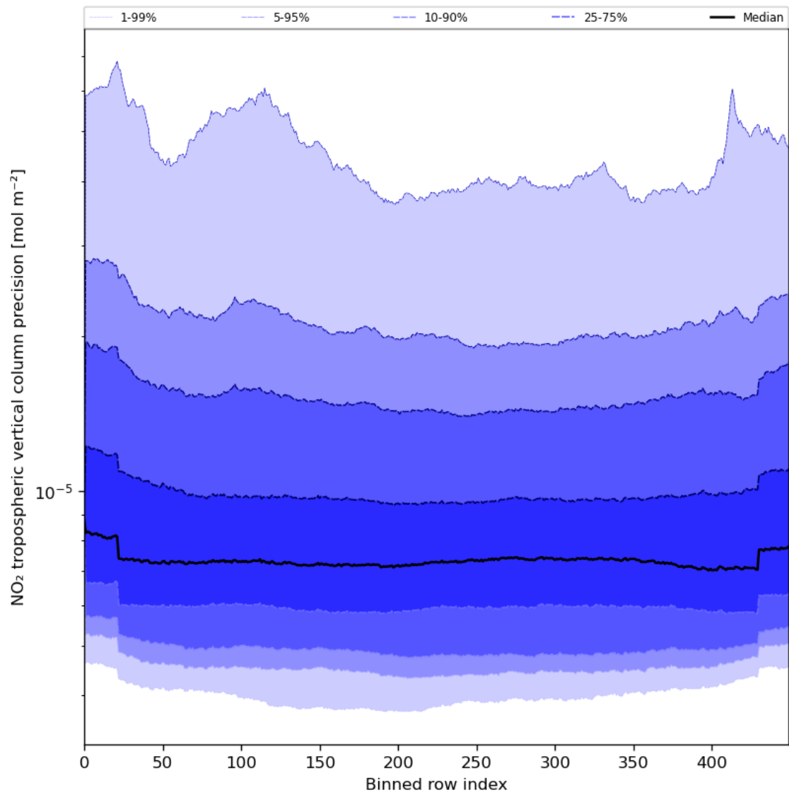
Figure 47: Along track statistics of “NO 2 tropospheric vertical column precision” for 2023-07-20 to 2023-07-22
