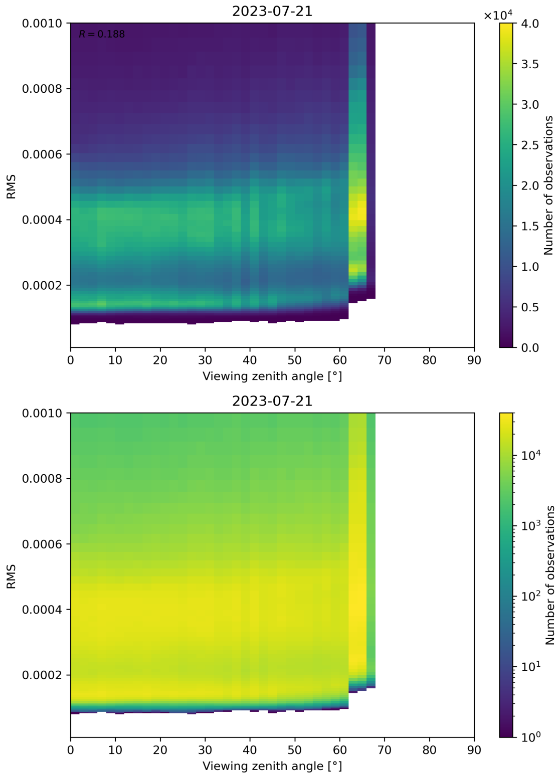
Figure 171: Scatter density plot of “Viewing zenith angle” against “RMS” for 2023-07-20 to 2023-07-22.
