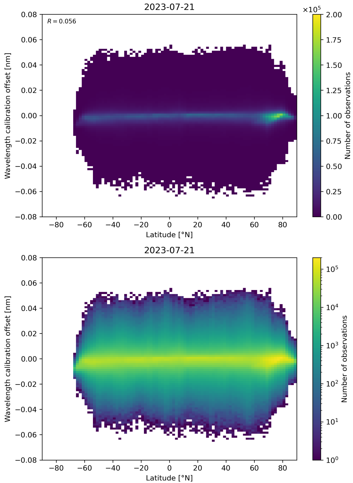
Figure 95: Scatter density plot of “Latitude” against “Wavelength calibration offset” for 2023-07-20 to 2023-07-22.
