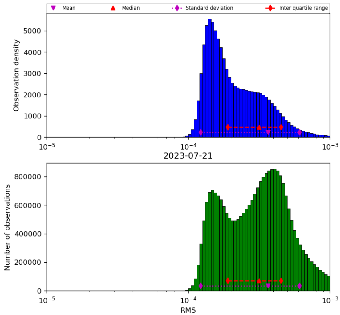
Figure 43: Histogram of “RMS” for 2023-07-20 to 2023-07-22
