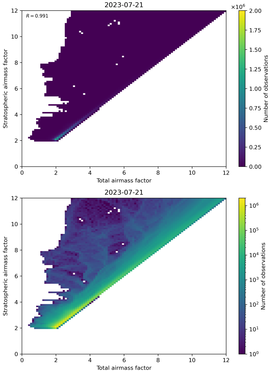
Figure 62: Scatter density plot of “Total airmass factor” against “Stratospheric airmass factor” for 2023-07-20 to 2023-07-22.
