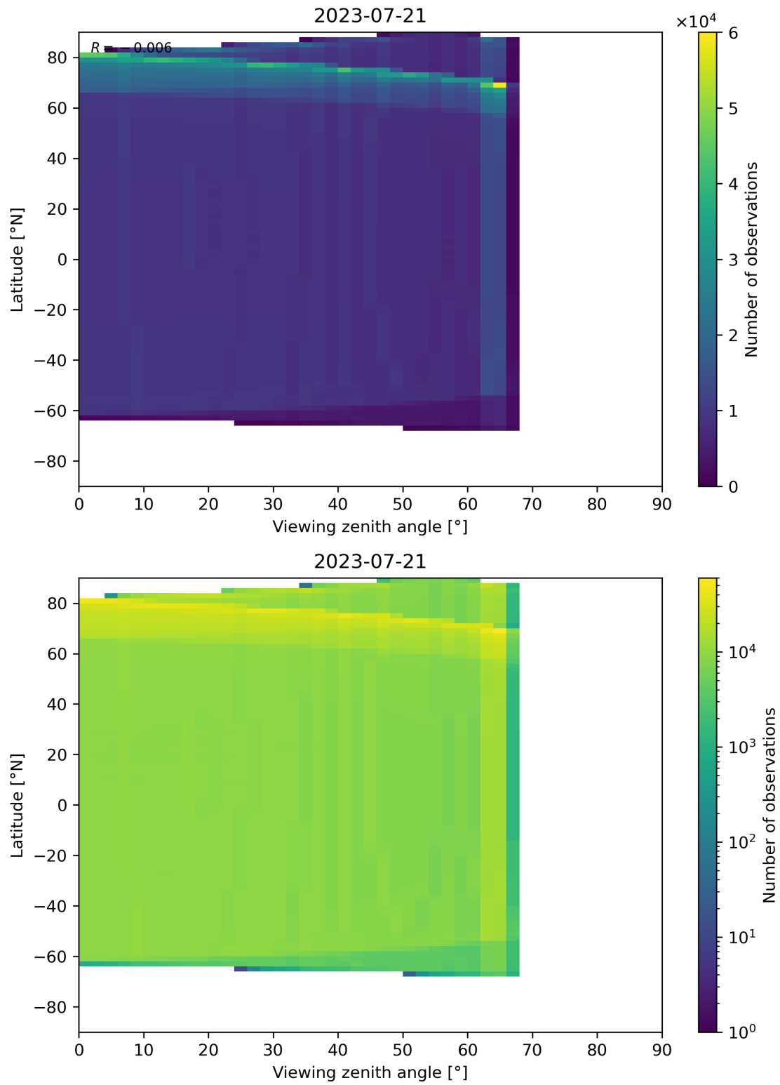
Figure 163: Scatter density plot of “Viewing zenith angle” against “Latitude” for 2023-07-20 to 2023-07-22.
