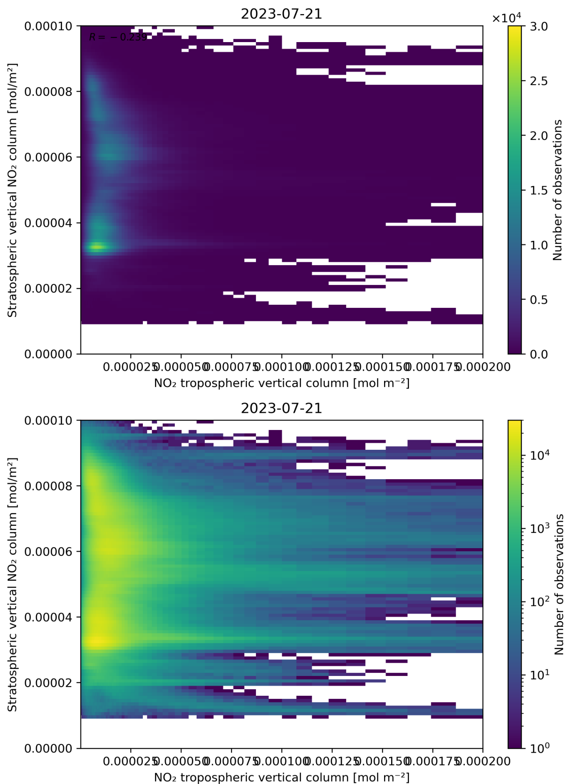
Figure 125: Scatter density plot of “NO 2 tropospheric vertical column” against “Stratospheric vertical NO 2 column” for 2023-07-20 to 2023-07-22.
