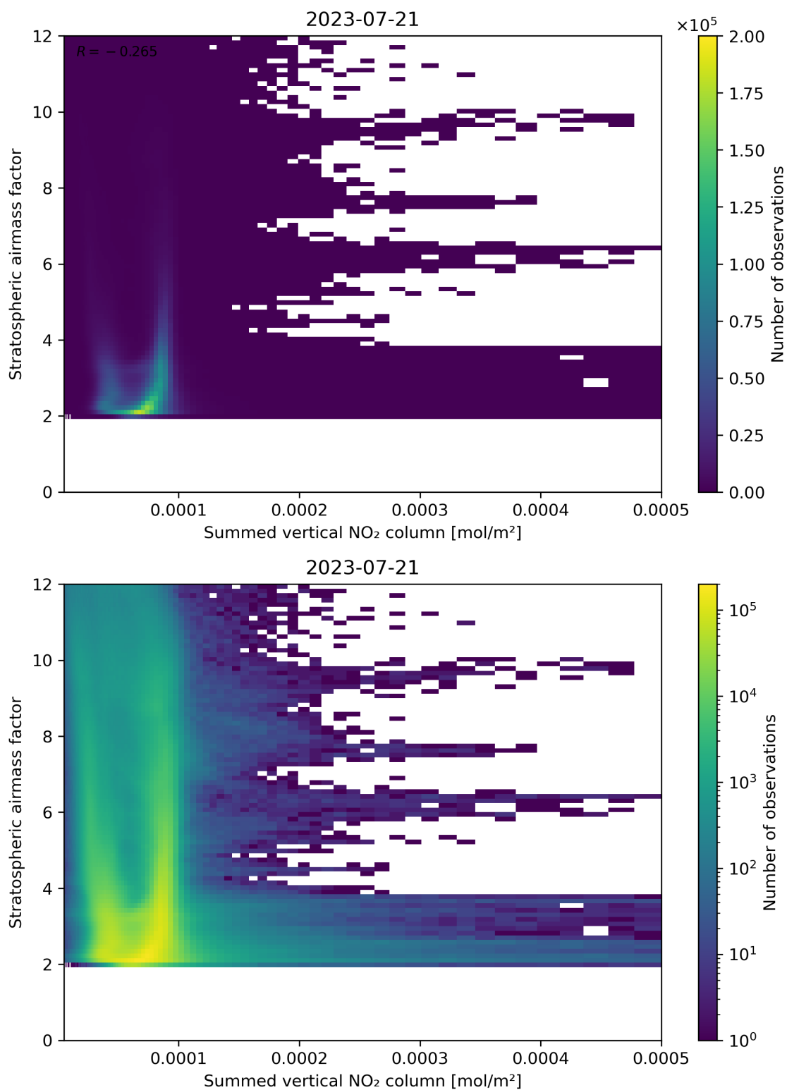
Figure 103: Scatter density plot of “Summed vertical NO 2 column” against “Stratospheric air mass factor” for 2023-07-20 to 2023-07-22.
