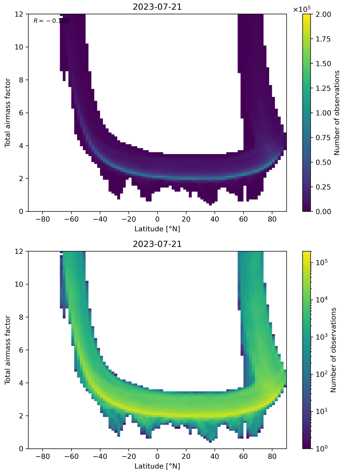
Figure 84: Scatter density plot of “Latitude” against “Total airmass factor” for 2023-07-20 to 2023-07-22.
