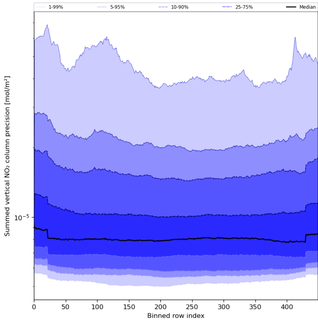
Figure 58: Along track statistics of “Summed vertical NO 2 column precision” for 2023-07-20 to 2023-07-22
