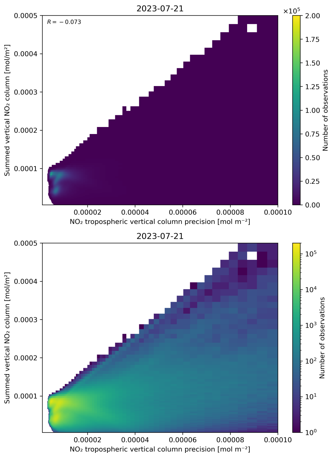
Figure 136: Scatter density plot of “NO 2 tropospheric vertical column precision” against “Summed vertical NO 2 column” for 2023-07-20 to 2023-07-22.
