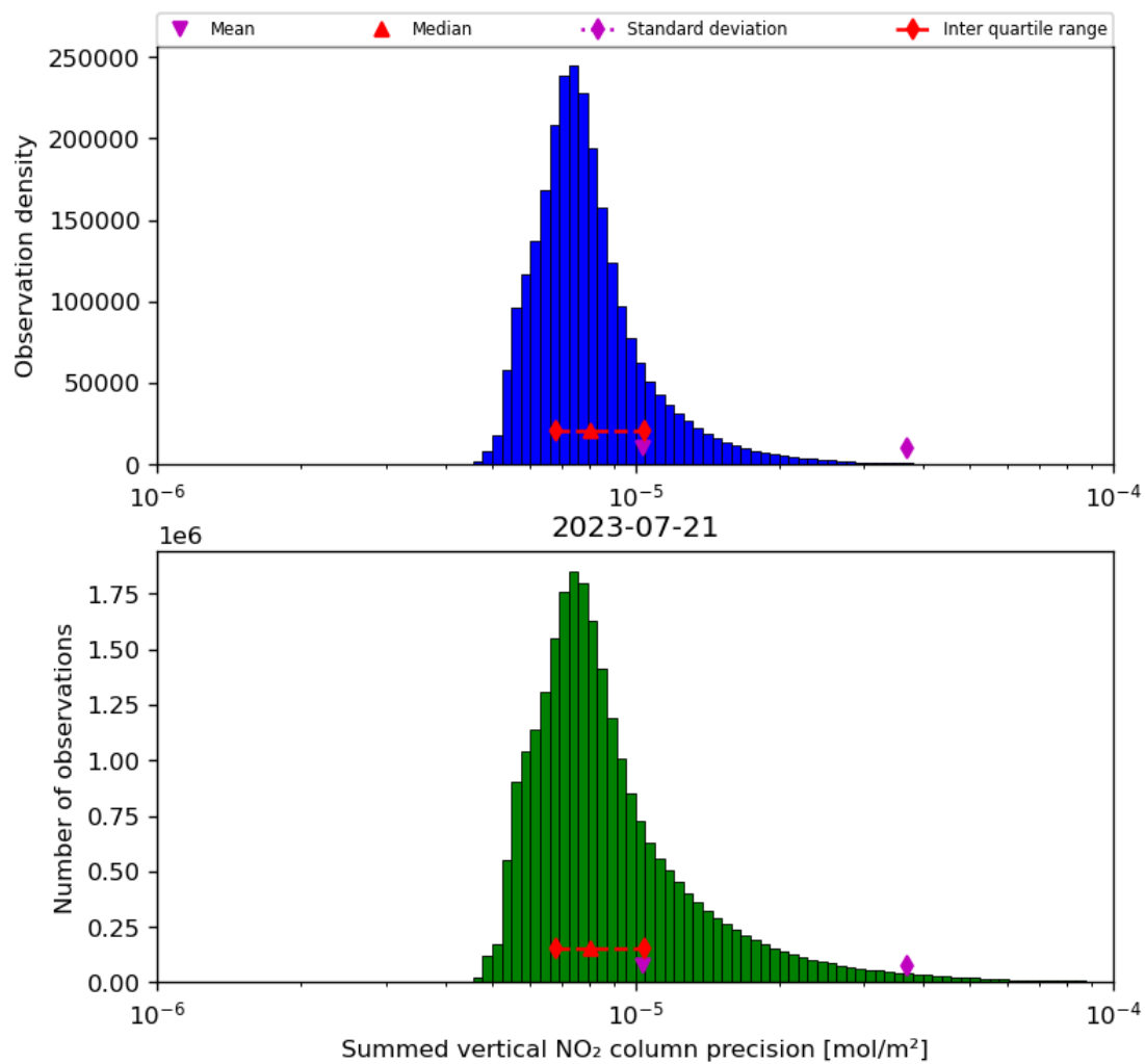
Figure 41: Histogram of "Summed vertical NO 2 column precision" for 2023-07-20 to 2023-07-22
