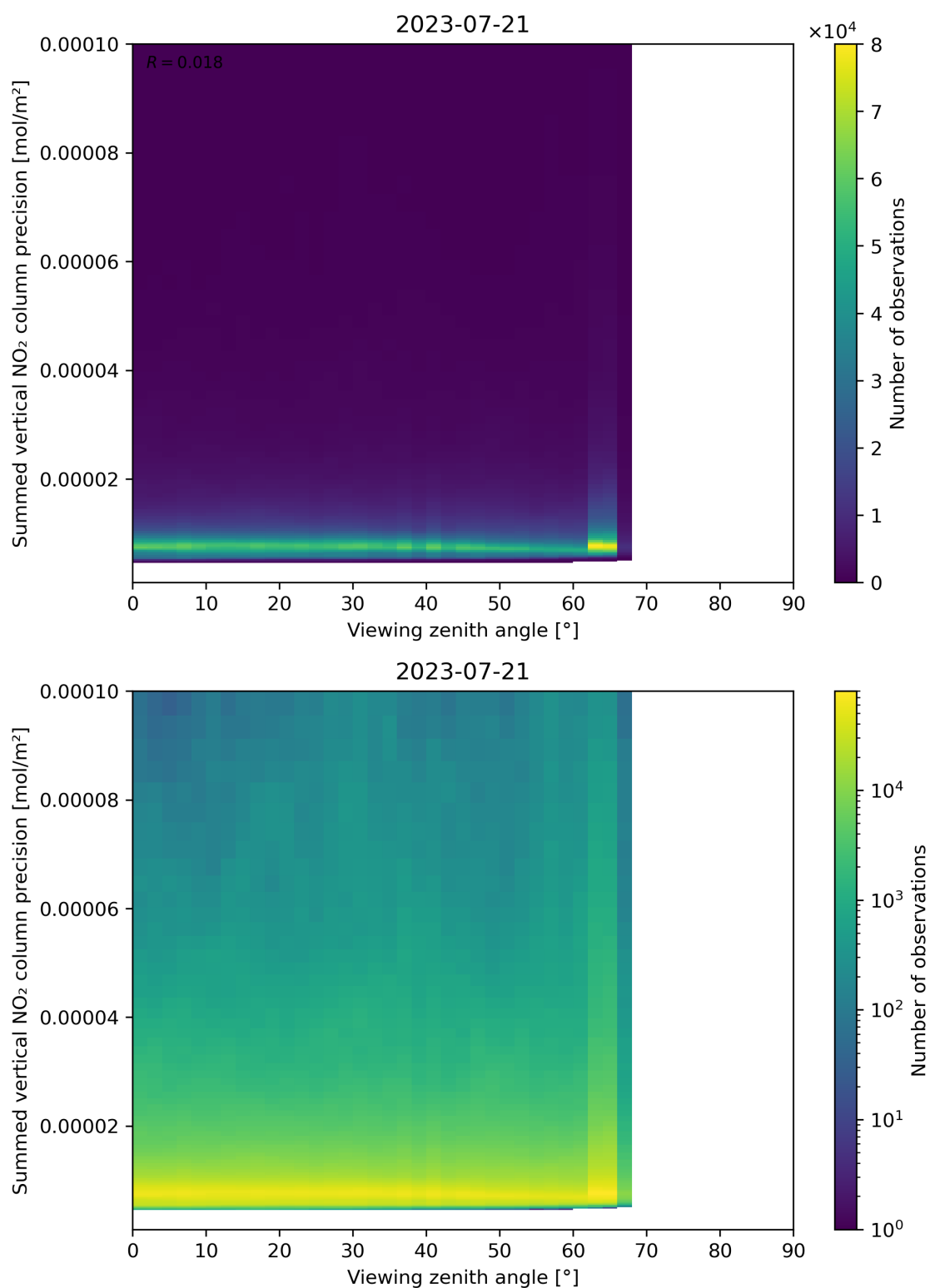
Figure 166: Scatter density plot of “Viewing zenith angle” against “Summed vertical NO 2 column precision” for 2023-07-20 to 2023-07-22.
