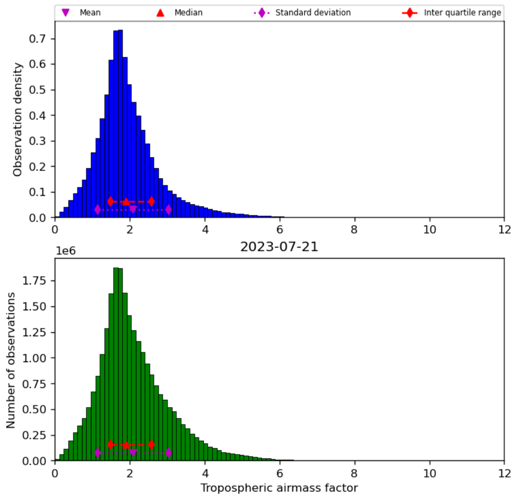
Figure 31: Histogram of “Tropospheric airmass factor” for 2023-07-20 to 2023-07-22
