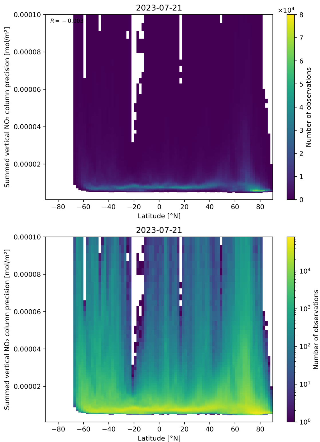
Figure 89: Scatter density plot of “Latitude” against “Summed vertical NO 2 column precision” for 2023-07-20 to 2023-07-22.
