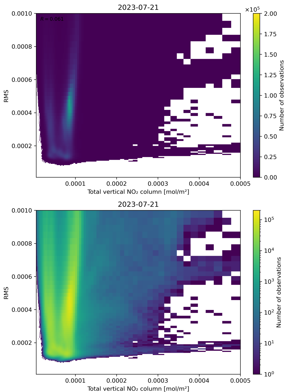
Figure 120: Scatter density plot of “Total vertical NO 2 column” against “RMS” for 2023-07-20 to 2023-07-22.
