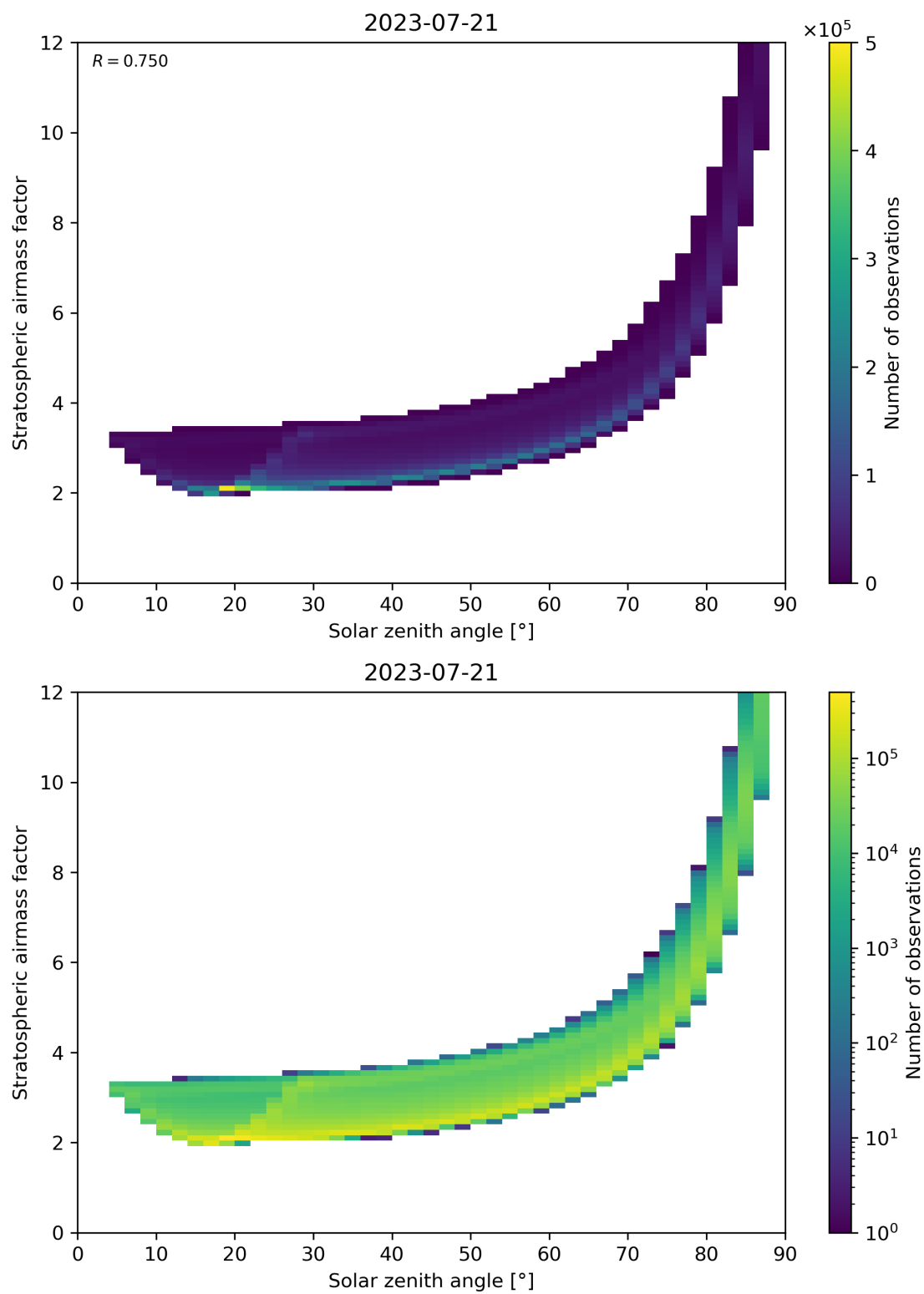
Figure 145: Scatter density plot of “Solar zenith angle” against “Stratospheric airmass factor” for 2023-07-20 to 2023-07-22.
