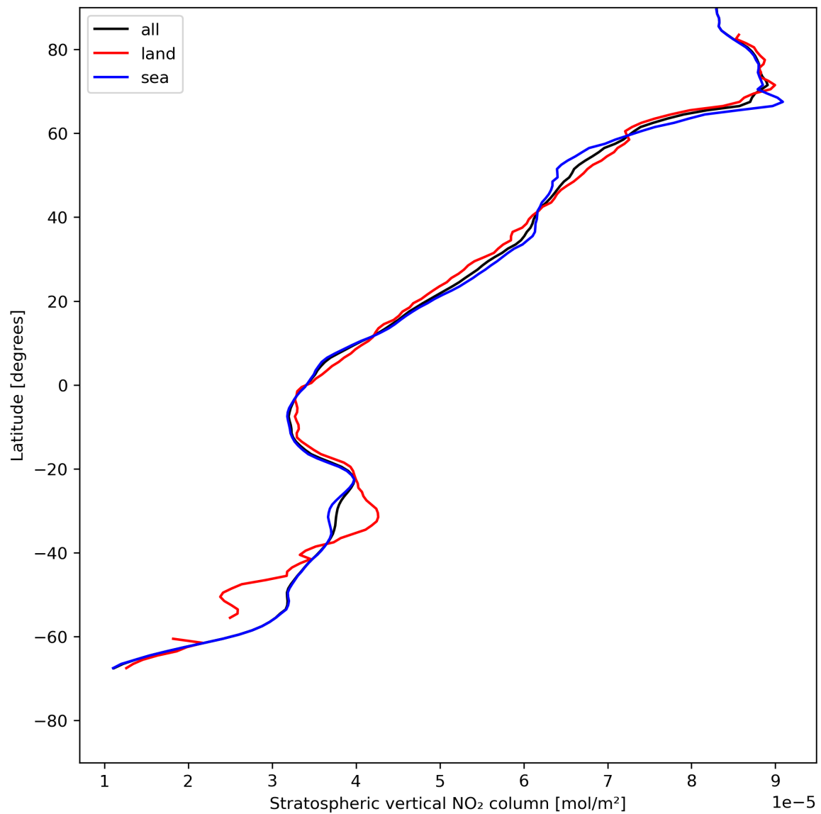
Figure 19: Zonal average of “Stratospheric vertical NO 2 column” for 2023-07-20 to 2023-07-22.
