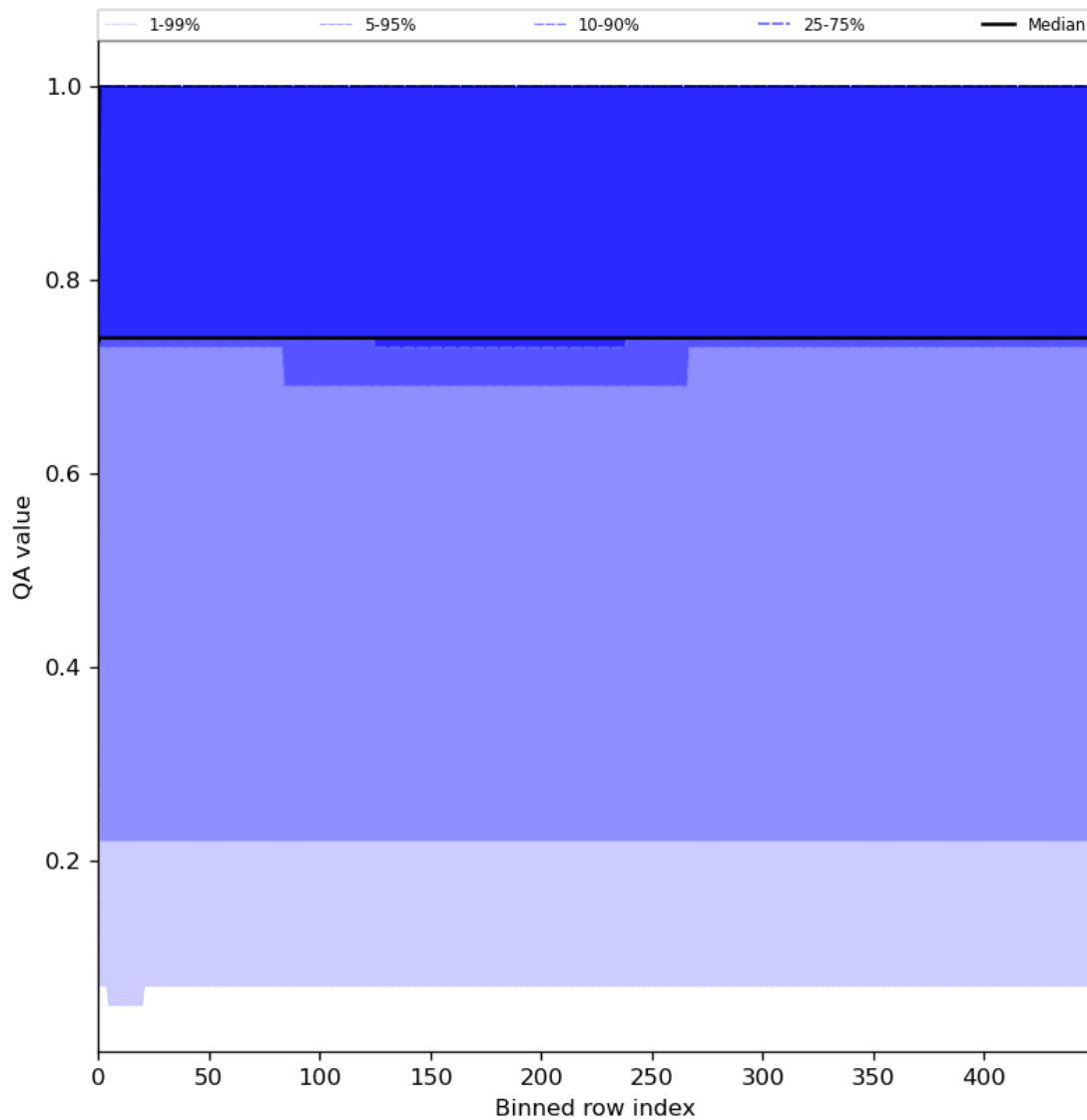
Figure 45: Along track statistics of “QA value” for 2023-07-20 to 2023-07-22
