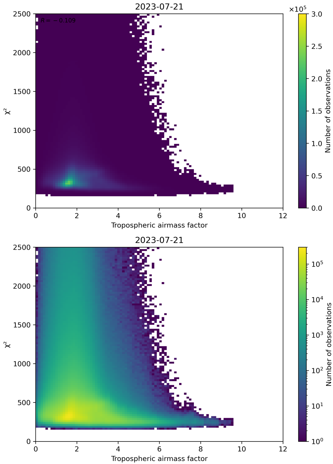
Figure 73: Scatter density plot of “Tropospheric airmass factor” against “ \chi^2 ” for 2023-07-20 to 2023-07-22.
