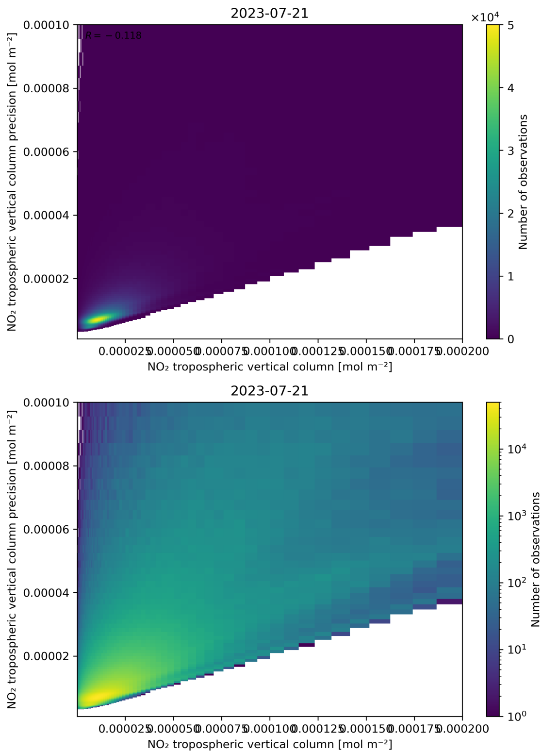
Figure 130: Scatter density plot of “NO 2 tropospheric vertical column” against “NO 2 tropospheric vertical column precision” for 2023-07-20 to 2023-07-22.
