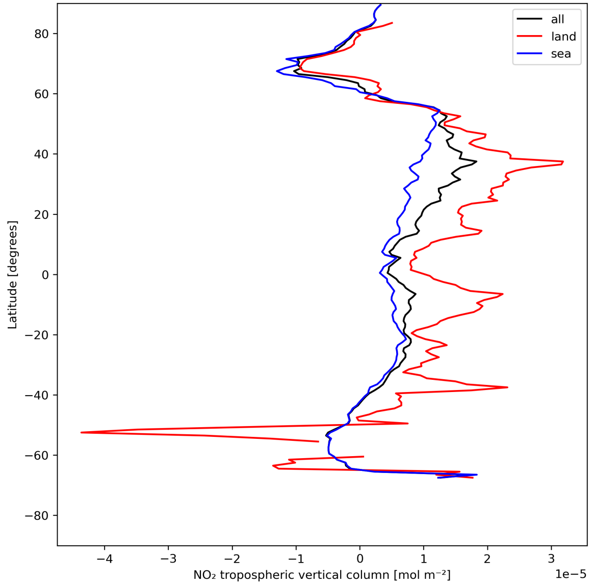
Figure 12: Zonal average of “NO 2 tropospheric vertical column” for 2023-07-20 to 2023-07-22.
