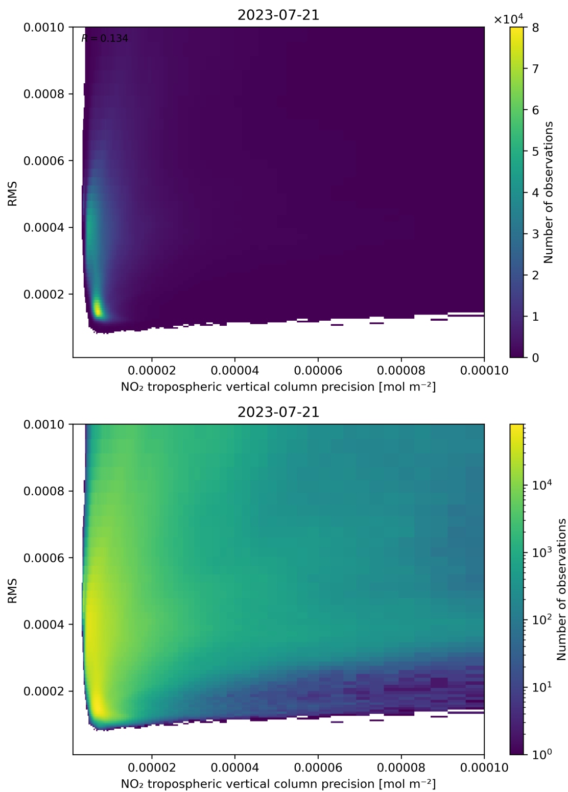
Figure 140: Scatter density plot of “NO 2 tropospheric vertical column precision” against “RMS” for 2023-07-20 to 2023-07-22.
