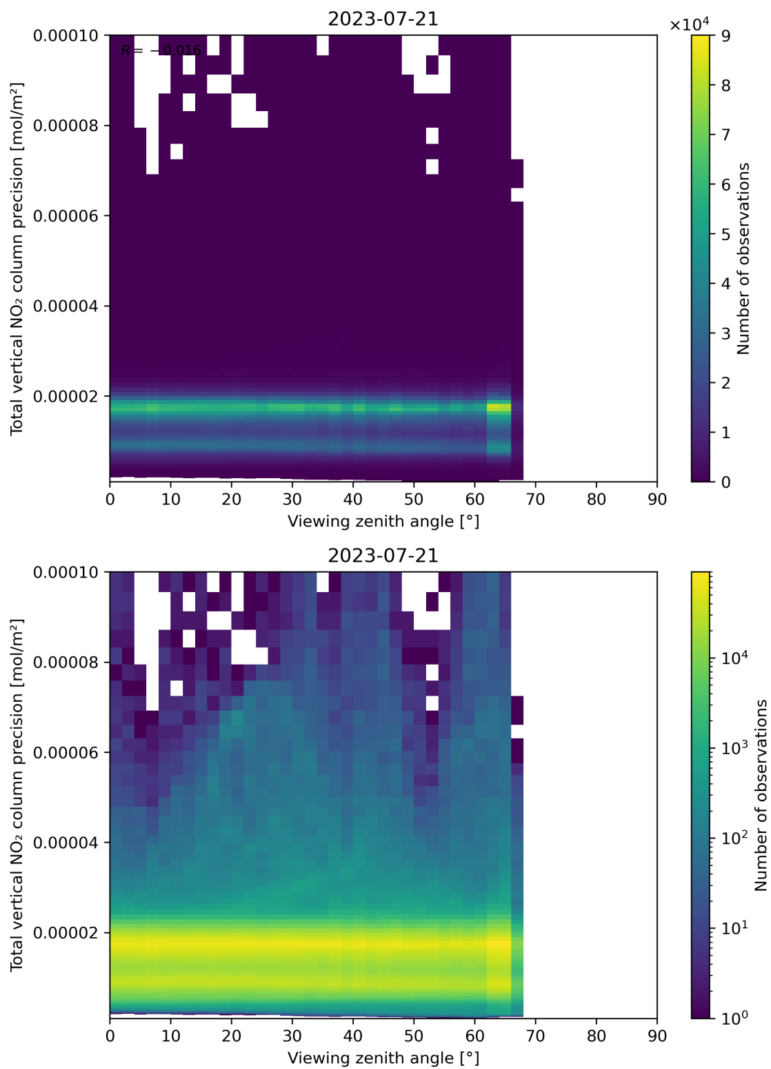
Figure 168: Scatter density plot of “Viewing zenith angle” against “Total vertical NO 2 column precision” for 2023-07-20 to 2023-07-22.
