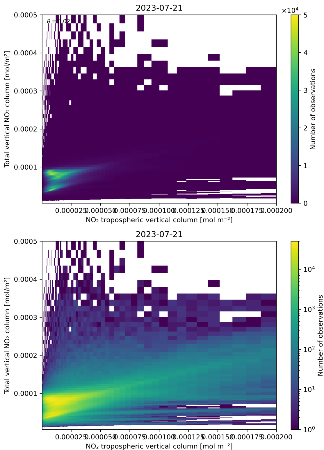
Figure 128: Scatter density plot of “NO 2 tropospheric vertical column” against “Total vertical NO 2 column” for 2023-07-20 to 2023-07-22.
