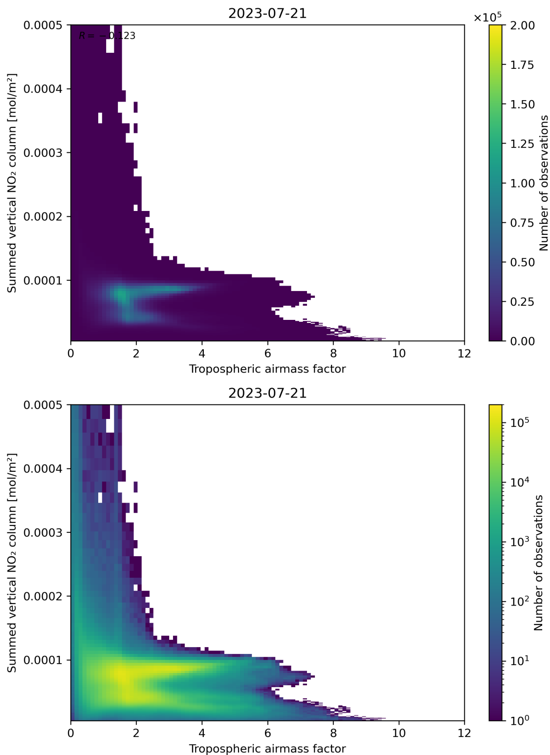
Figure 75: Scatter density plot of “Tropospheric airmass factor” against “Summed vertical NO 2 column” for 2023-07-20 to 2023-07-22.
