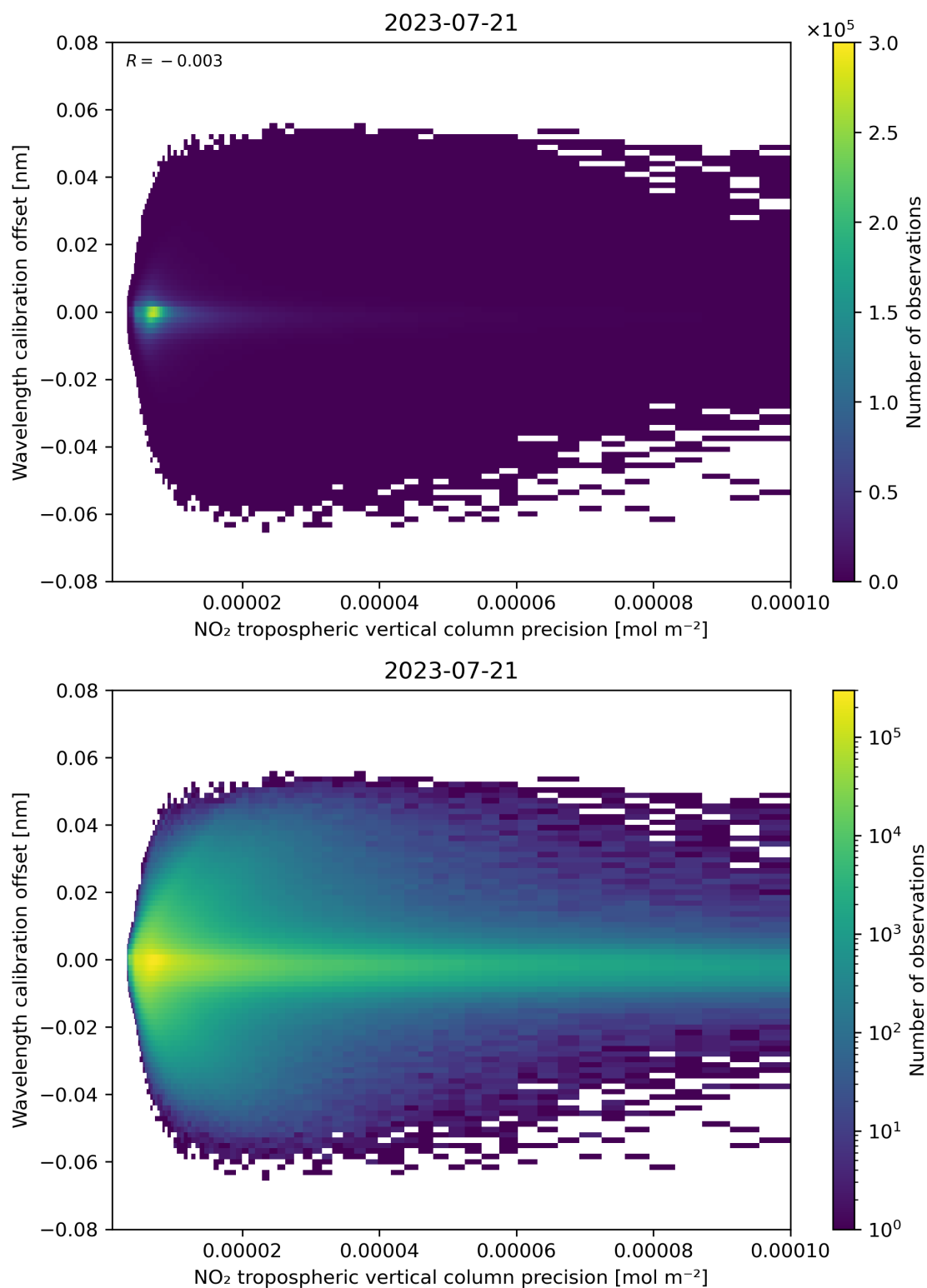
Figure 141: Scatter density plot of “NO 2 tropospheric vertical column precision” against “Wavelength calibration offset” for 2023-07-20 to 2023-07-22.
