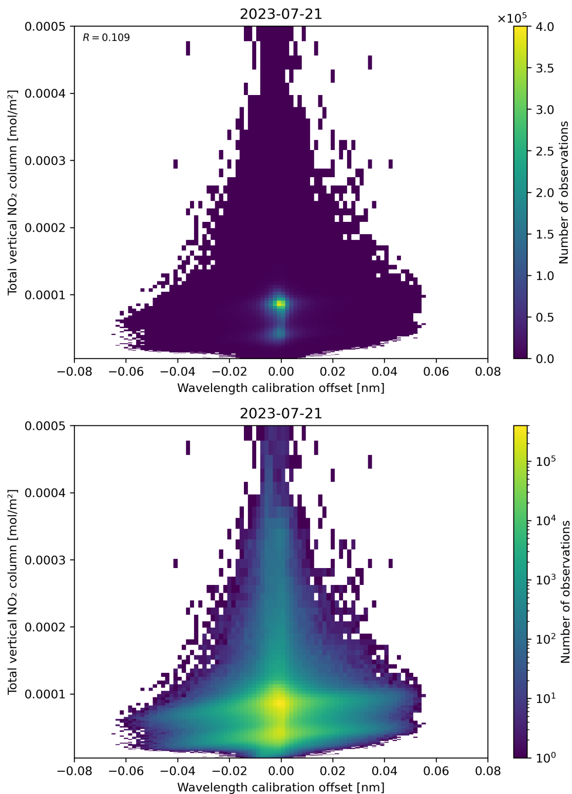
Figure 179: Scatter density plot of “Wavelength calibration offset” against “Total vertical NO 2 column” for 2023-07-20 to 2023-07-22.
