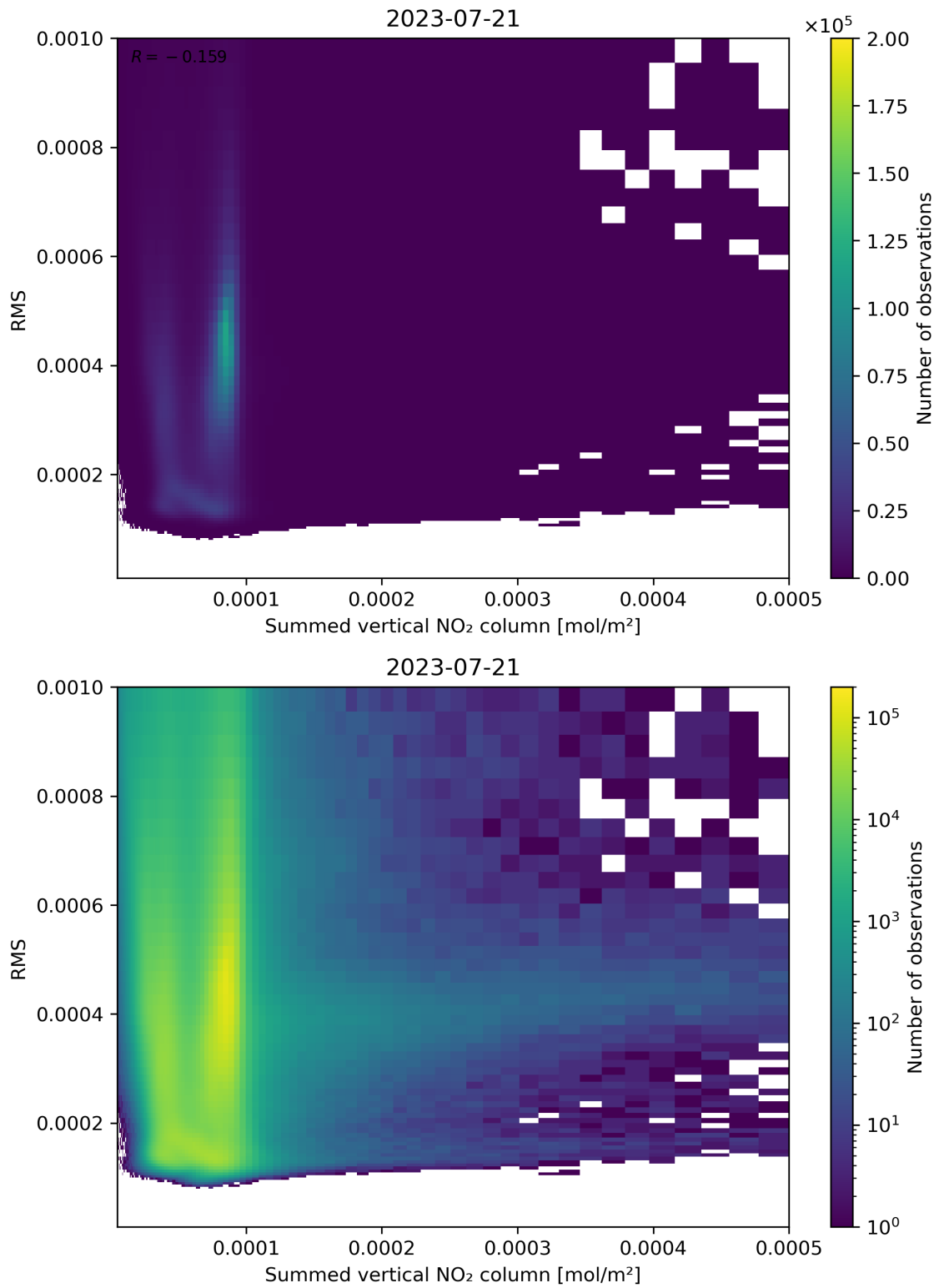
Figure 109: Scatter density plot of “Summed vertical NO 2 column” against “RMS” for 2023-07-20 to 2023-07-22.
