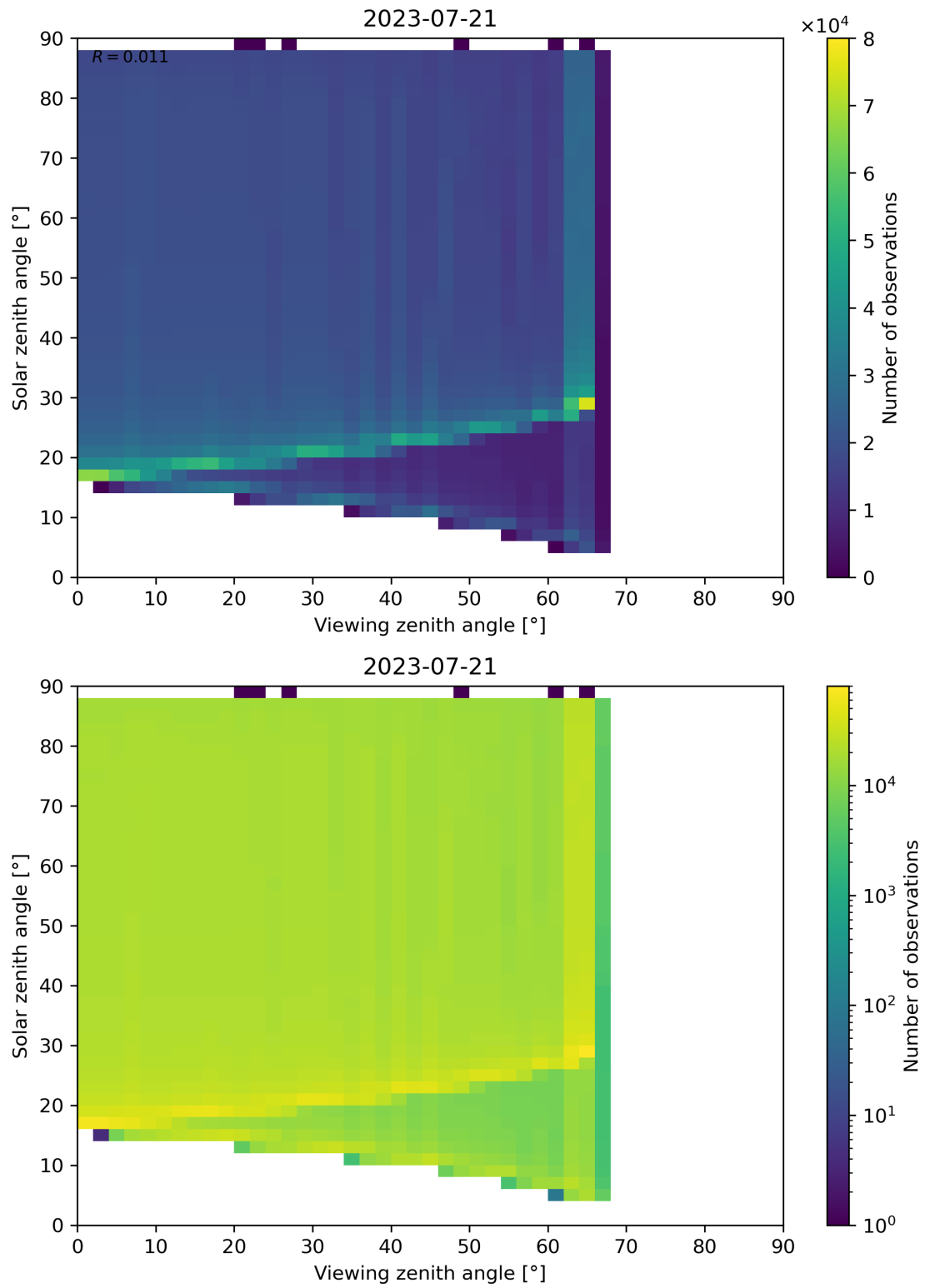
Figure 172: Scatter density plot of “Viewing zenith angle” against “Solar zenith angle” for 2023-07-20 to 2023-07-22.
