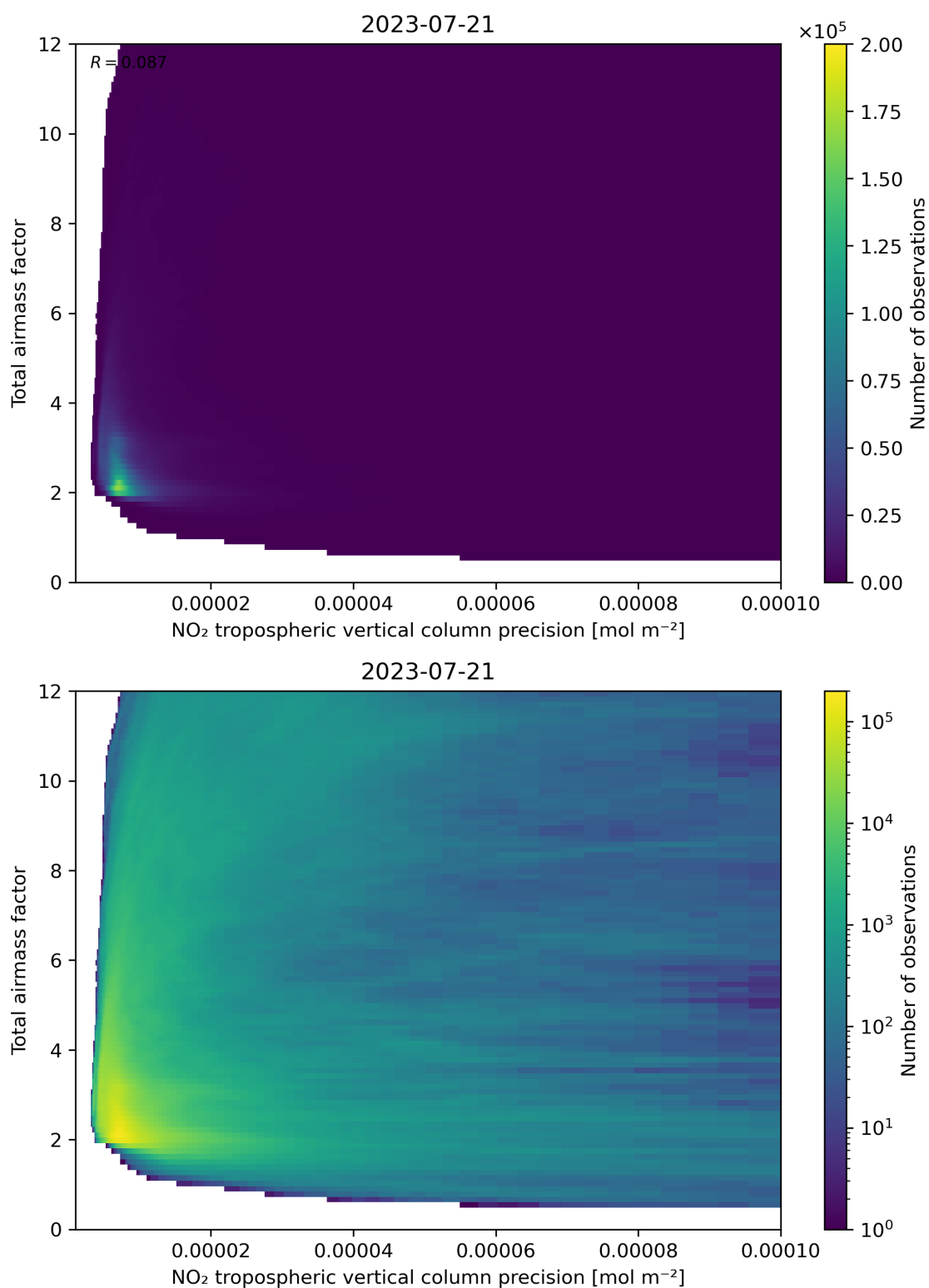
Figure 132: Scatter density plot of “NO 2 tropospheric vertical column precision” against “Total air mass factor” for 2023-07-20 to 2023-07-22.
