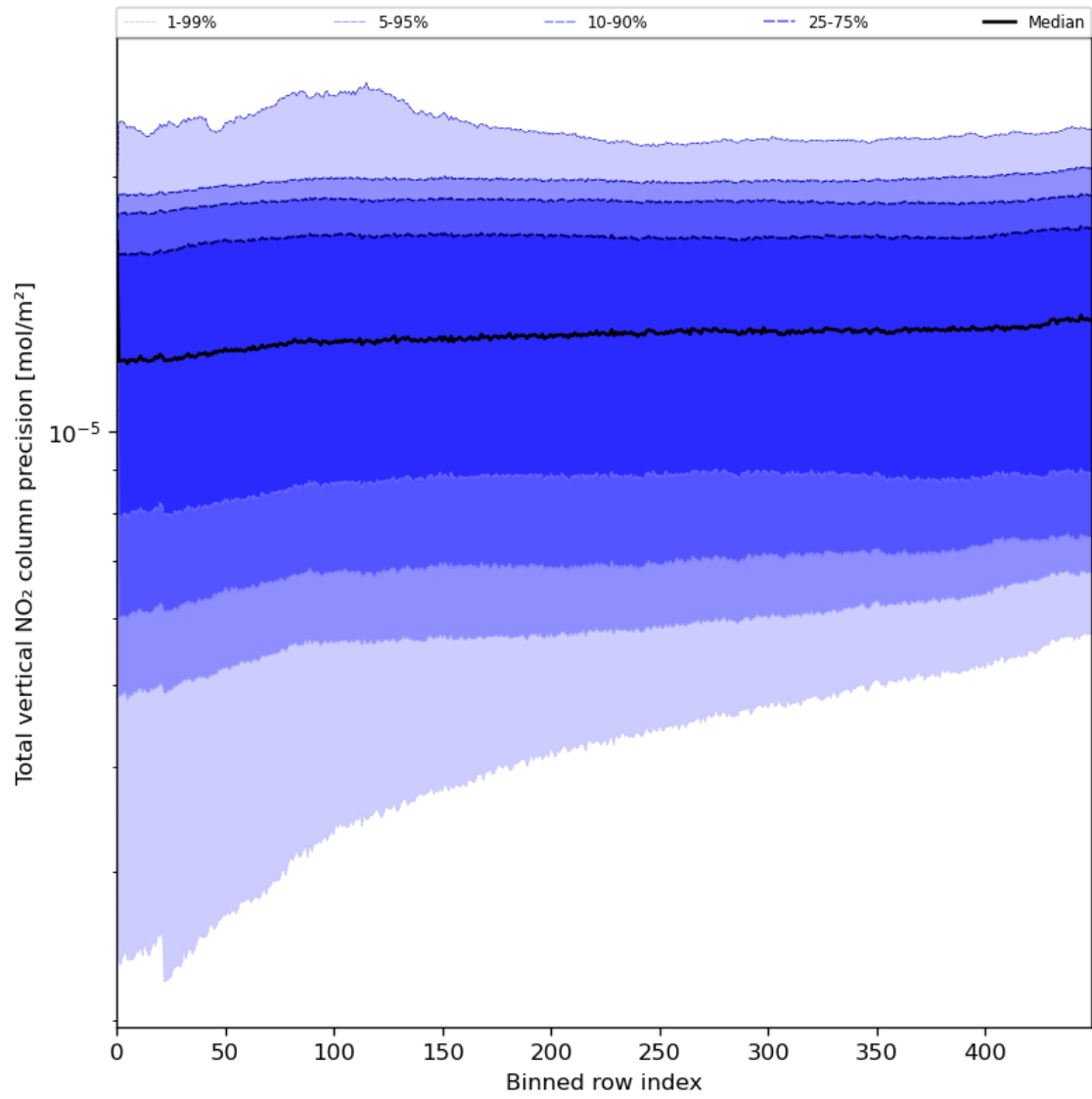
Figure 56: Along track statistics of “Total vertical NO 2 column precision” for 2023-07-20 to 2023-07-22
