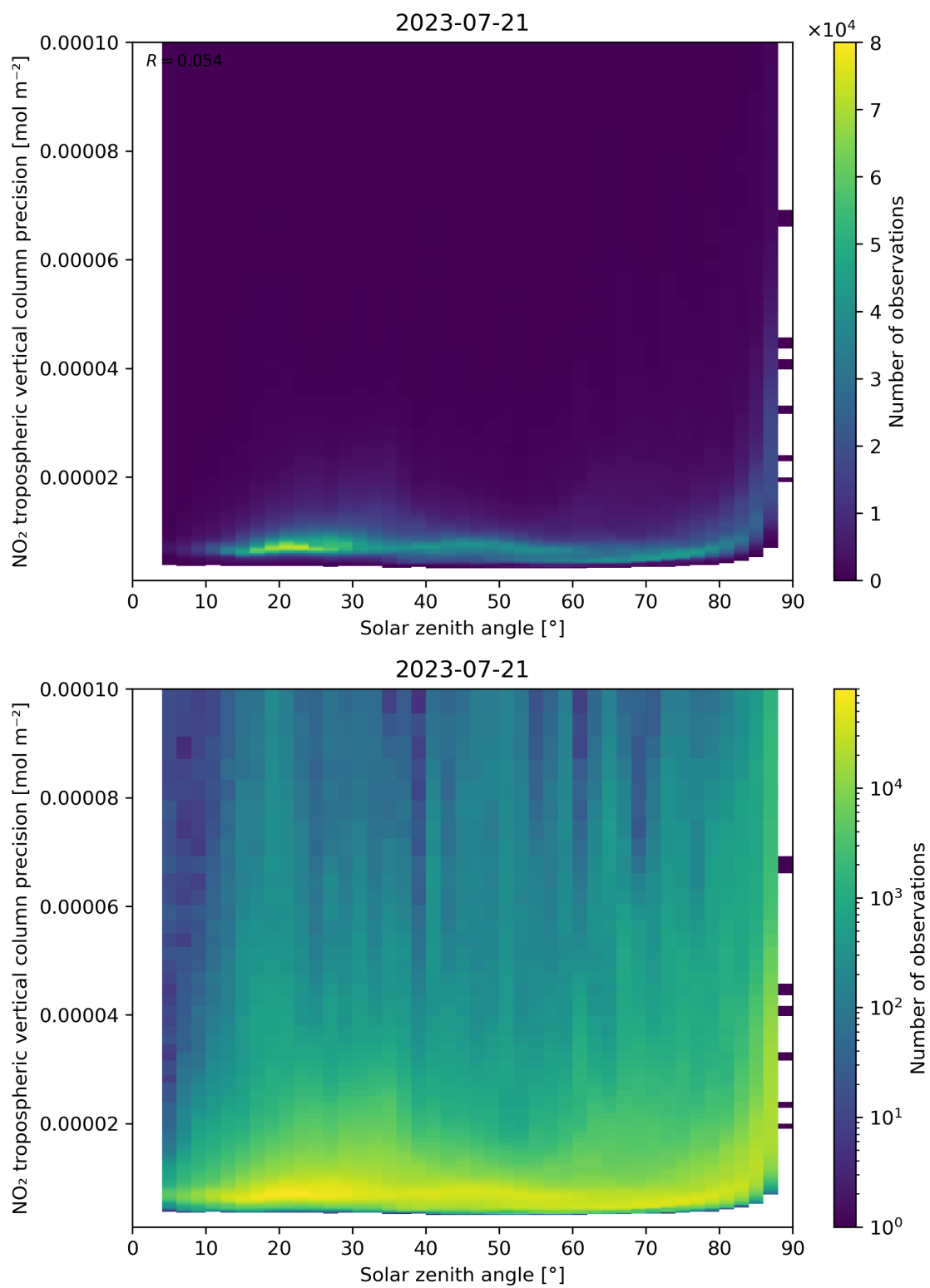
Figure 156: Scatter density plot of “Solar zenith angle” against “NO 2 tropospheric vertical column precision” for 2023-07-20 to 2023-07-22.
