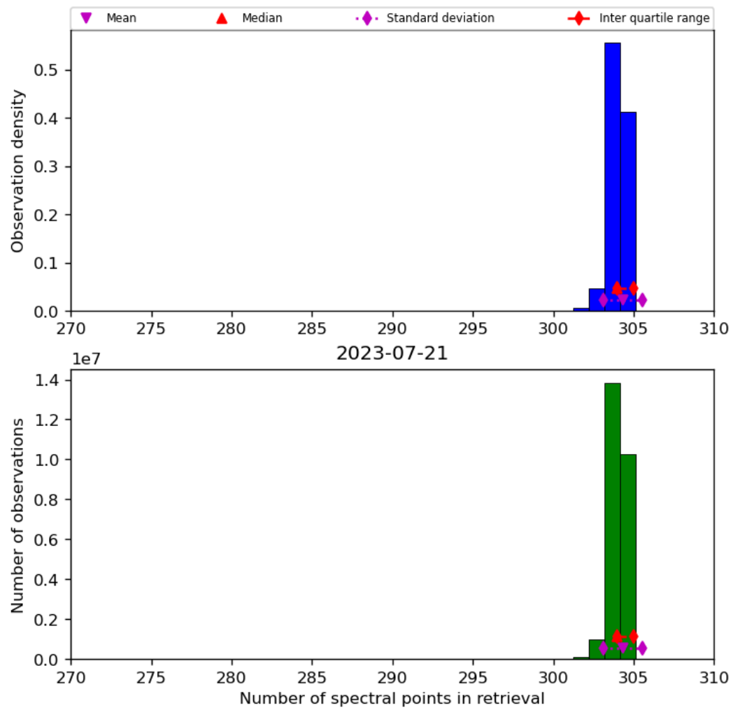
Figure 33: Histogram of “Number of spectral points in retrieval” for 2023-07-20 to 2023-07-22
