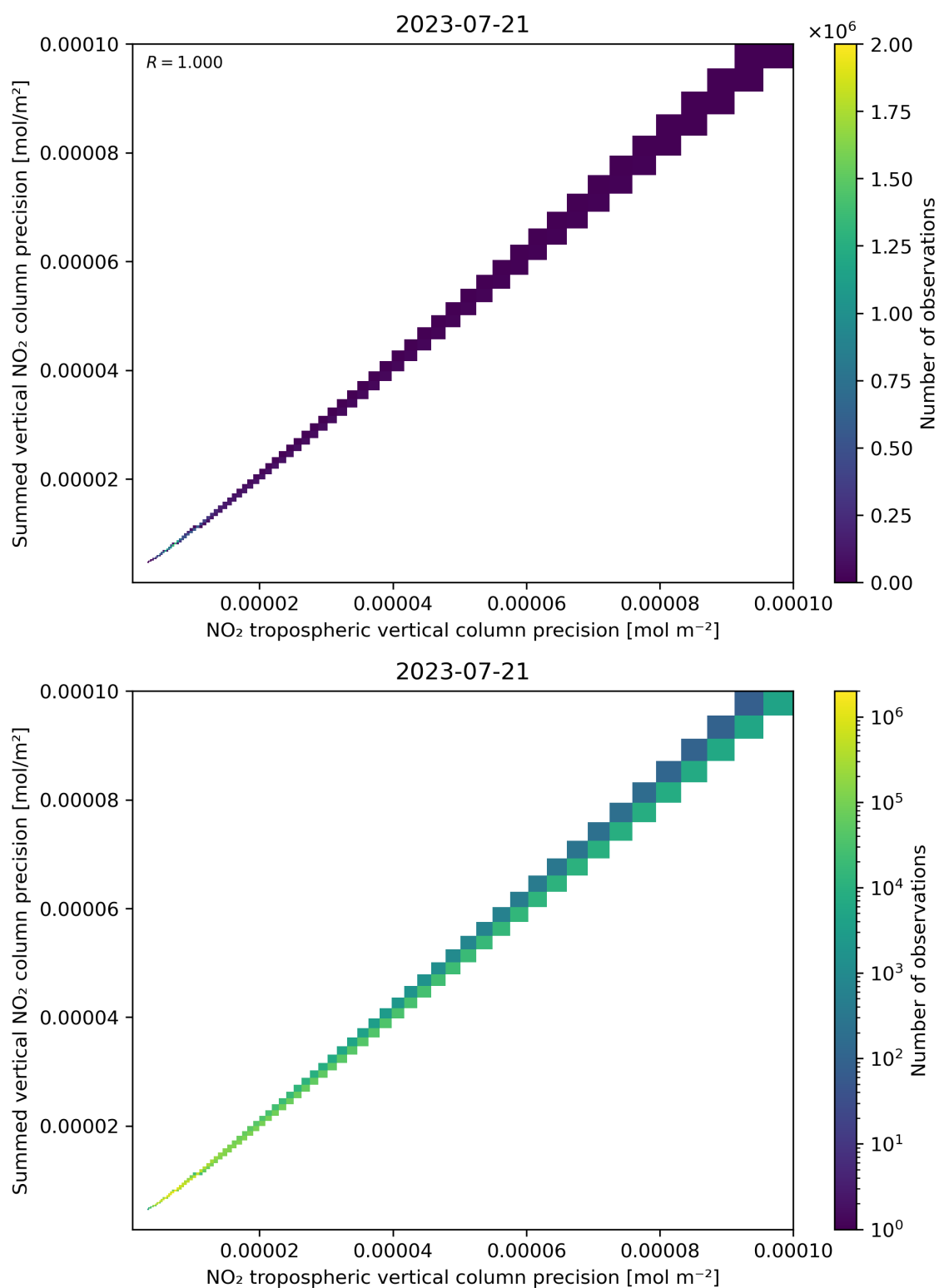
Figure 137: Scatter density plot of “NO 2 tropospheric vertical column precision” against “Summed vertical NO 2 column precision” for 2023-07-20 to 2023-07-22.
