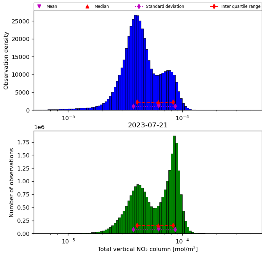
Figure 38: Histogram of “Total vertical NO 2 column” for 2023-07-20 to 2023-07-22
