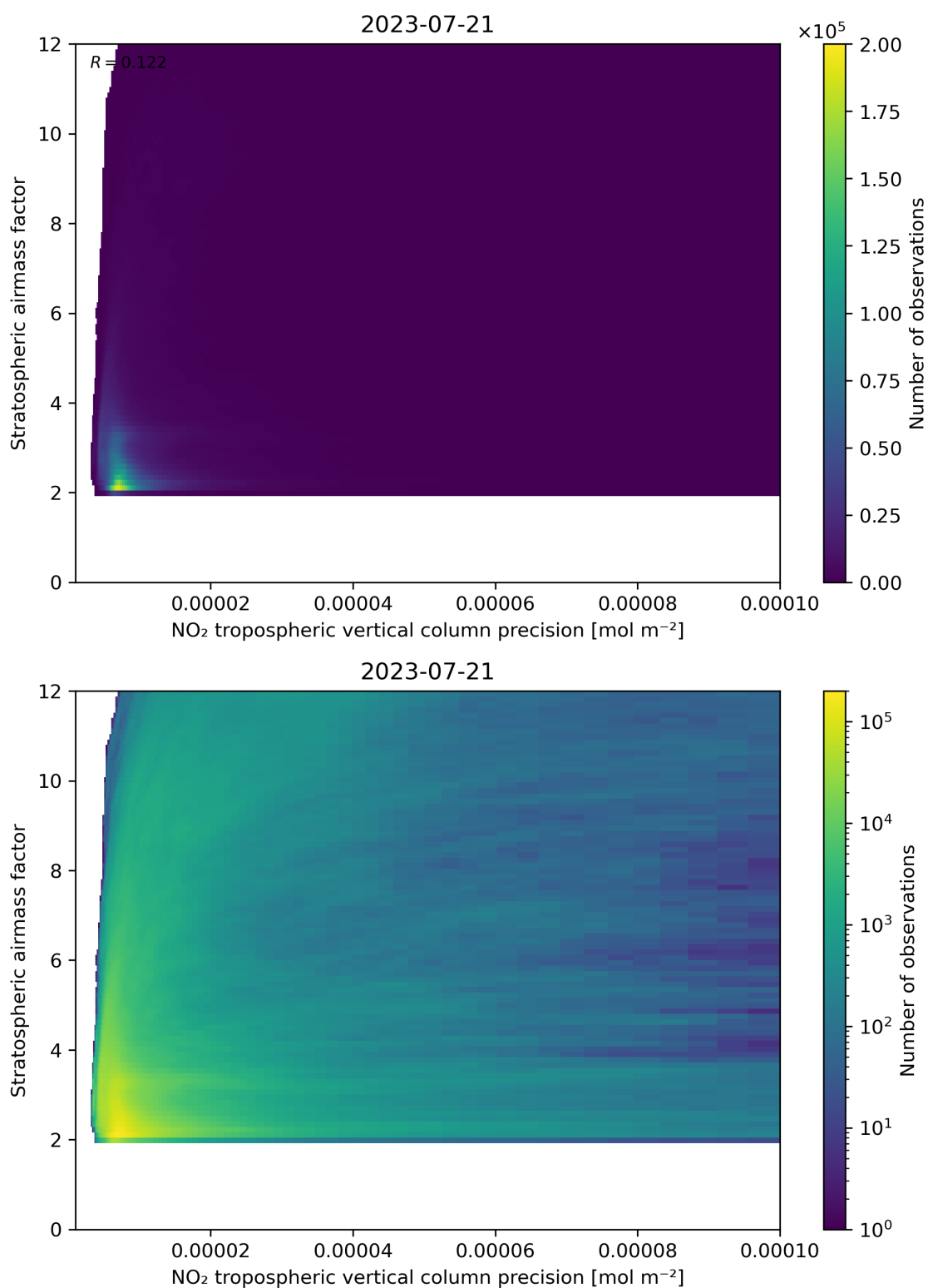
Figure 131: Scatter density plot of “NO 2 tropospheric vertical column precision” against “Stratospheric airmass factor” for 2023-07-20 to 2023-07-22.
