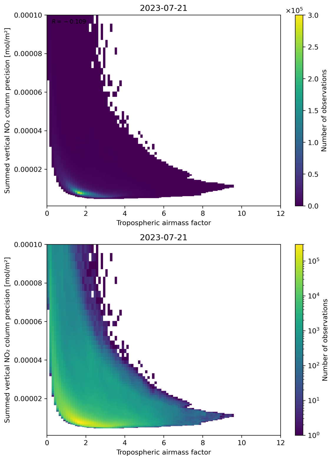
Figure 76: Scatter density plot of “Tropospheric air mass factor” against “Summed vertical NO 2 column precision” for 2023-07-20 to 2023-07-22.
