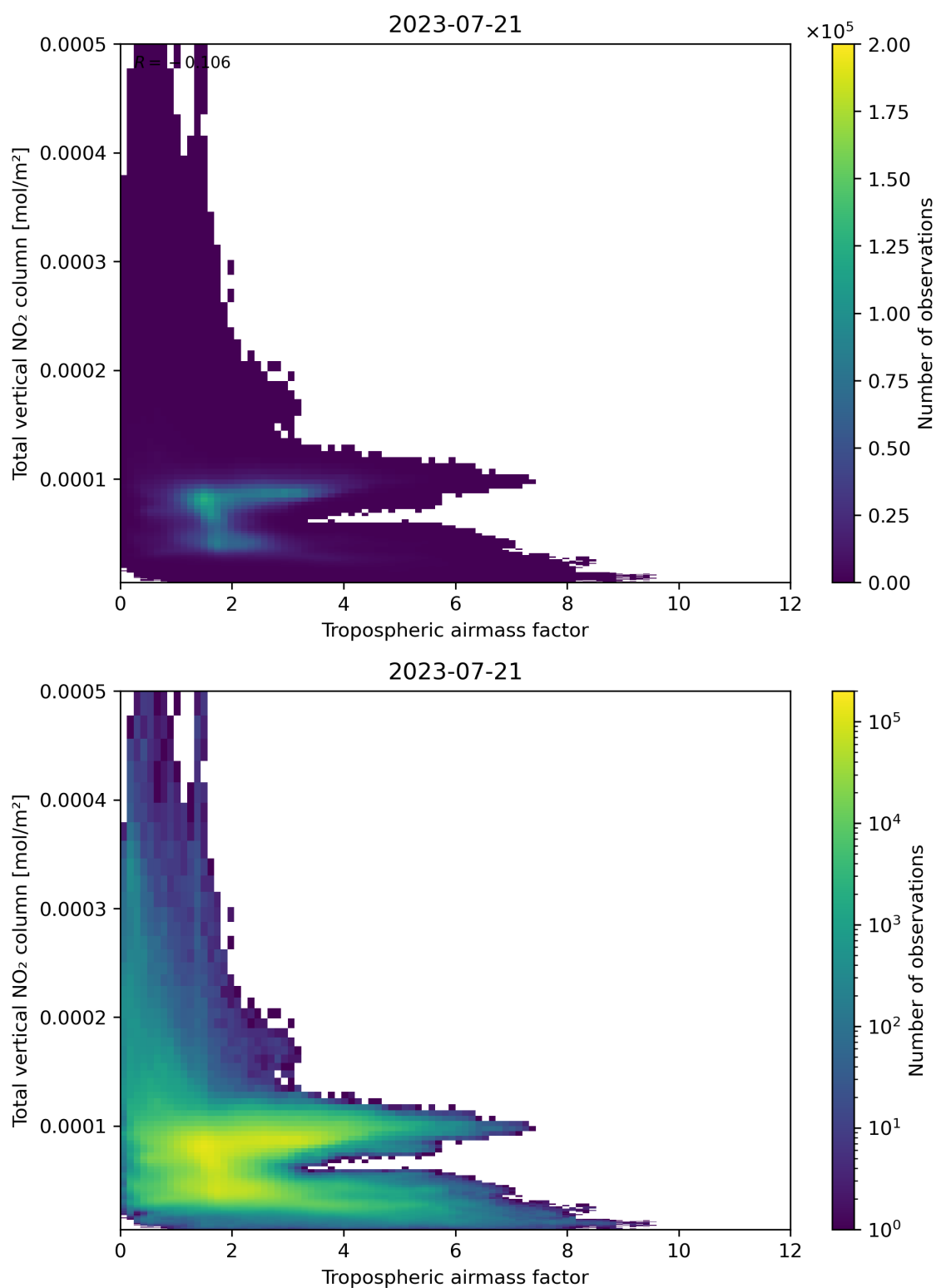
Figure 77: Scatter density plot of “Tropospheric airmass factor” against “Total vertical NO 2 column” for 2023-07-20 to 2023-07-22.
