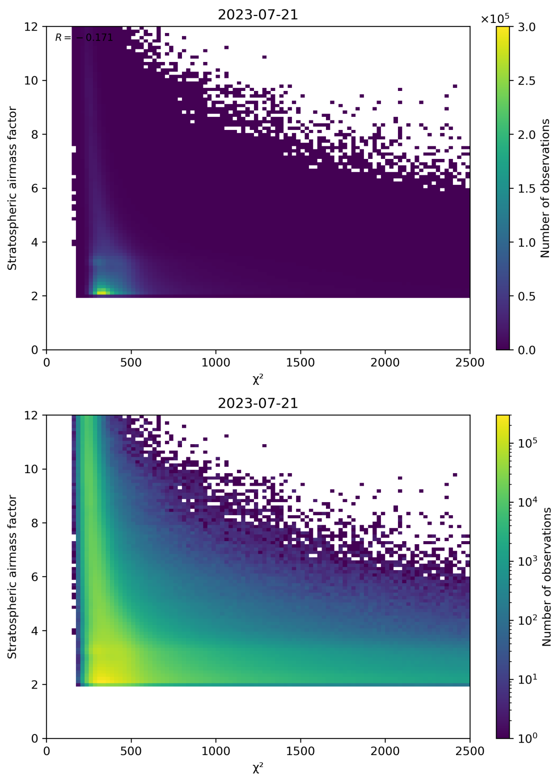
Figure 81: Scatter density plot of “ \chi^2 ” against “Stratospheric airmass factor” for 2023-07-20 to 2023-07-22.
