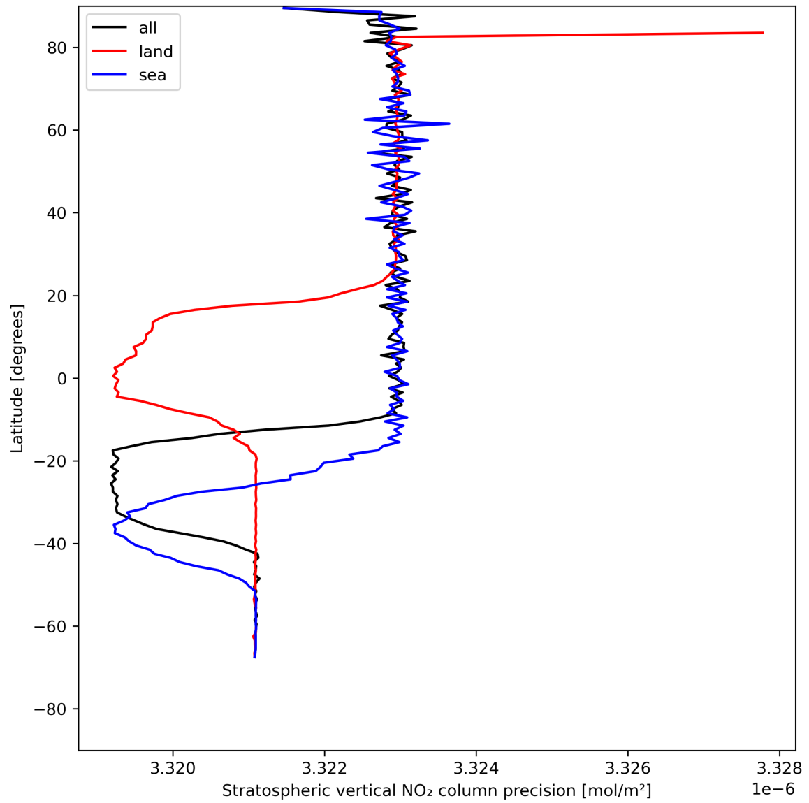
Figure 20: Zonal average of “Stratospheric vertical NO 2 column precision” for 2023-07-20 to 2023-07-22.
