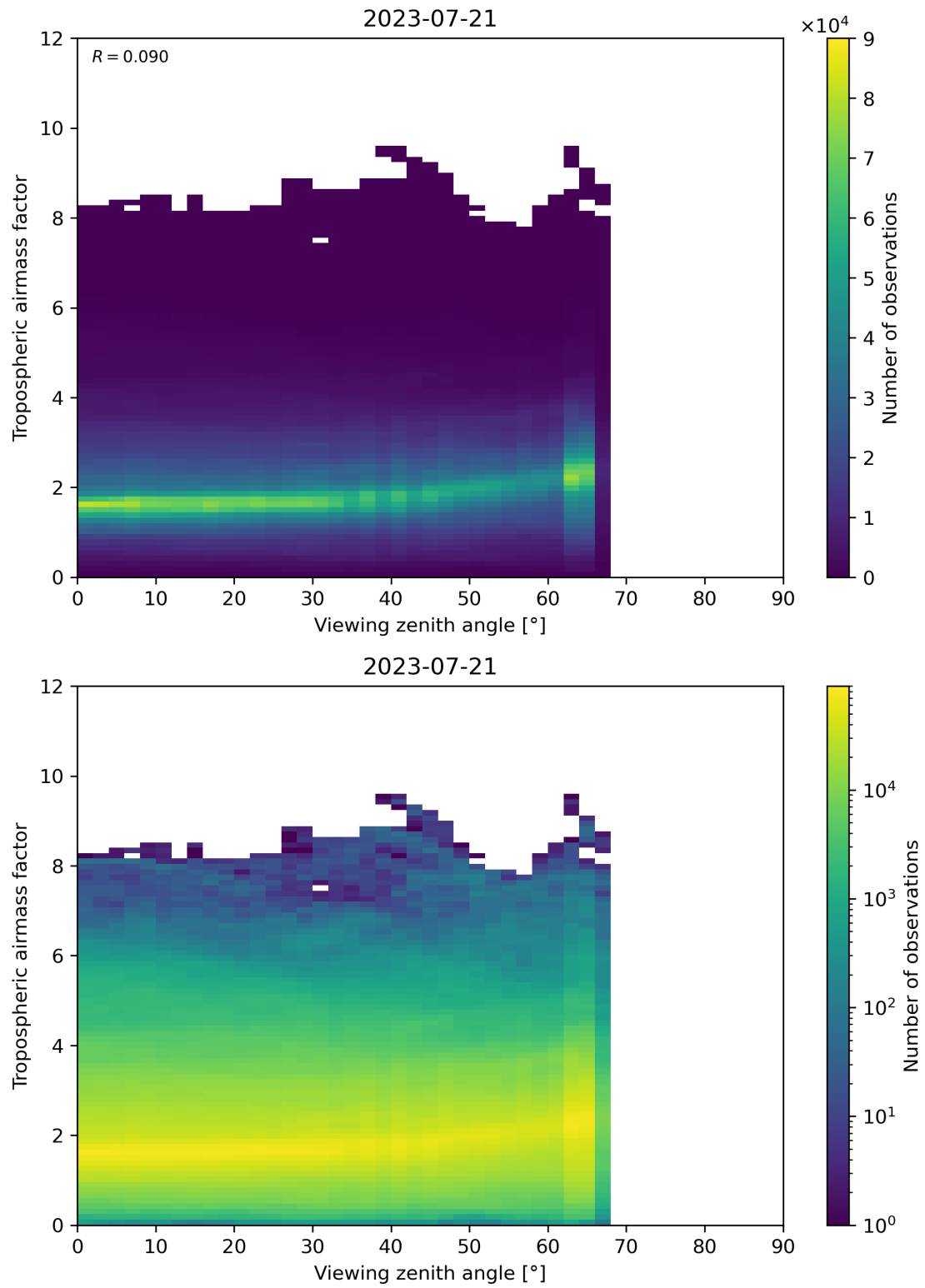
Figure 161: Scatter density plot of “Viewing zenith angle” against “Tropospheric airmass factor” for 2023-07-20 to 2023-07-22.
