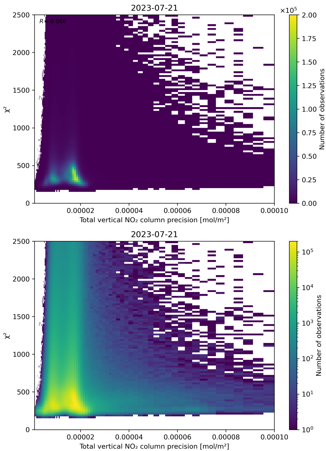
Figure 116: Scatter density plot of “Total vertical NO 2 column precision” against “ \chi^2 ” for 2023-07-20 to 2023-07-22.
