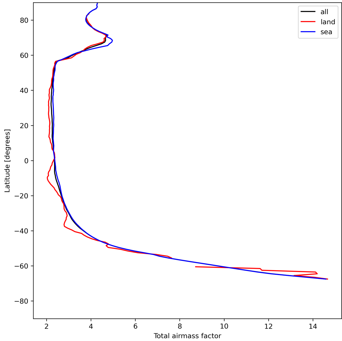
Figure 15: Zonal average of “Total airmass factor” for 2023-07-20 to 2023-07-22.
