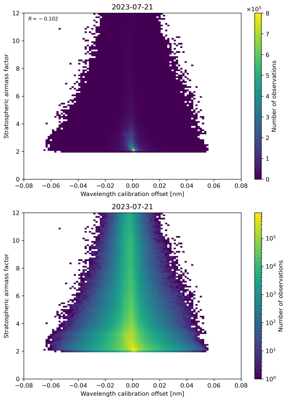
Figure 174: Scatter density plot of “Wavelength calibration offset” against “Stratospheric air mass factor” for 2023-07-20 to 2023-07-22.
