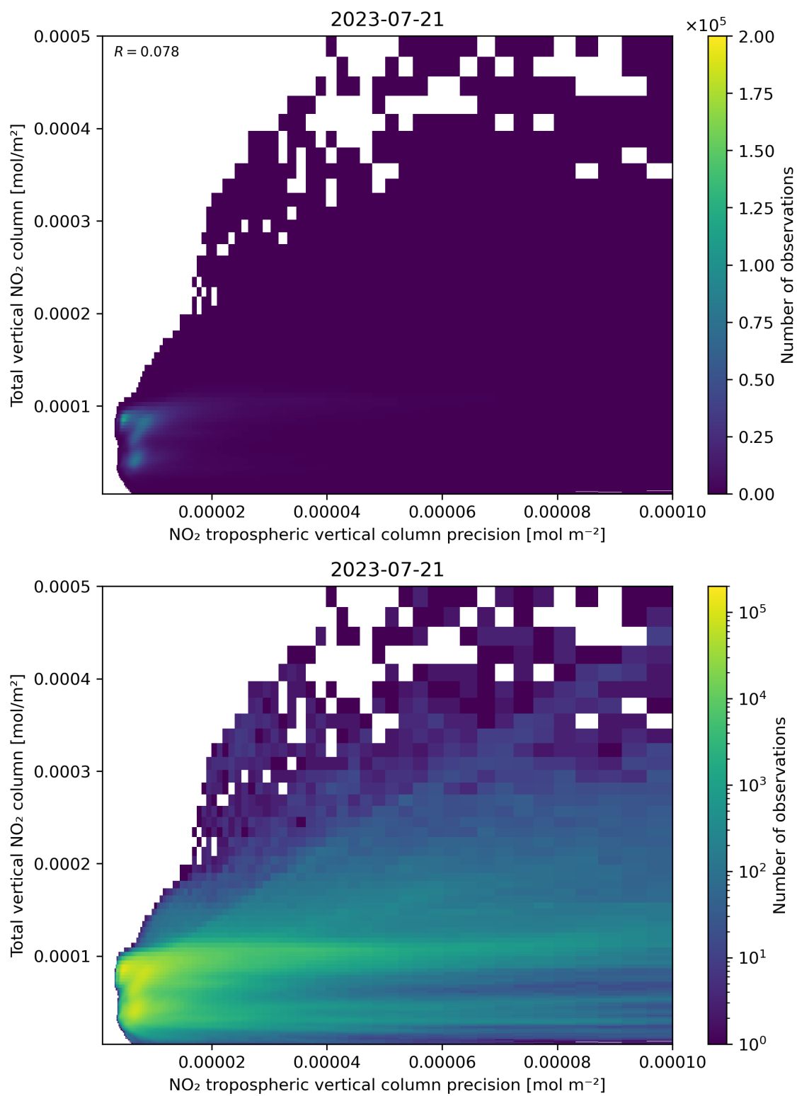
Figure 138: Scatter density plot of “NO 2 tropospheric vertical column precision” against “Total vertical NO 2 column” for 2023-07-20 to 2023-07-22.
