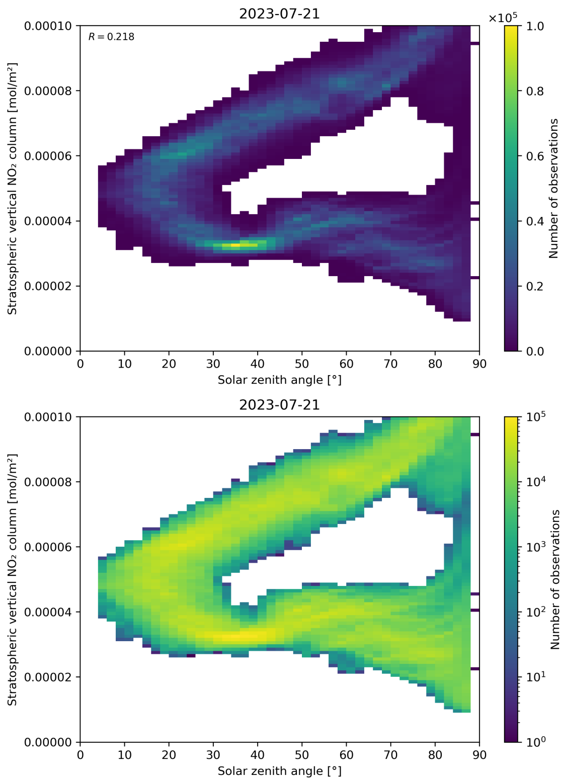
Figure 150: Scatter density plot of “Solar zenith angle” against “Stratospheric vertical NO 2 column” for 2023-07-20 to 2023-07-22.
