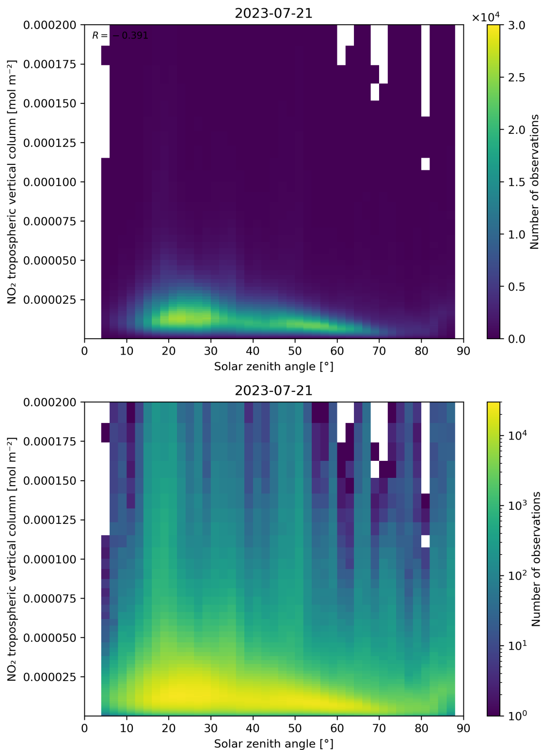
Figure 155: Scatter density plot of “Solar zenith angle” against “NO 2 tropospheric vertical column” for 2023-07-20 to 2023-07-22.
