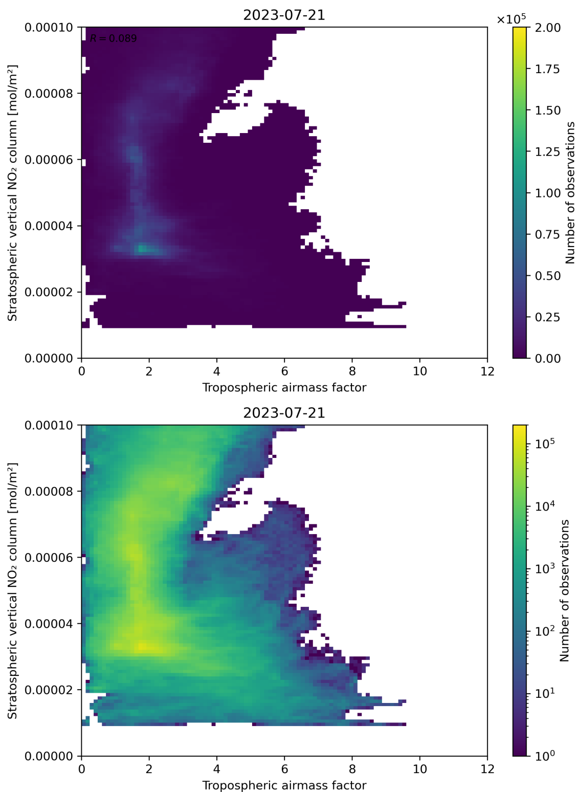
Figure 74: Scatter density plot of “Tropospheric air mass factor” against “Stratospheric vertical NO 2 column” for 2023-07-20 to 2023-07-22.
