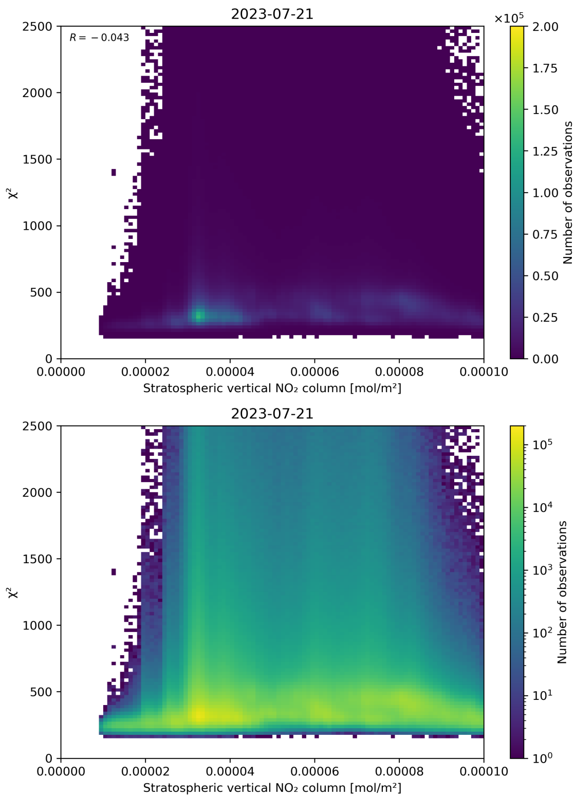
Figure 97: Scatter density plot of “Stratospheric vertical NO 2 column” against “ \chi^2 ” for 2023-07-20 to 2023-07-22.
