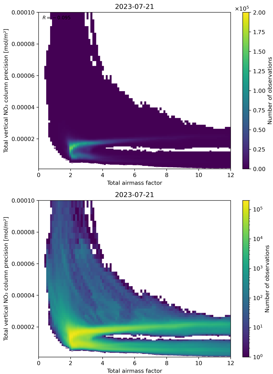
Figure 68: Scatter density plot of “Total airmass factor” against “Total vertical NO 2 column precision” for 2023-07-20 to 2023-07-22.
