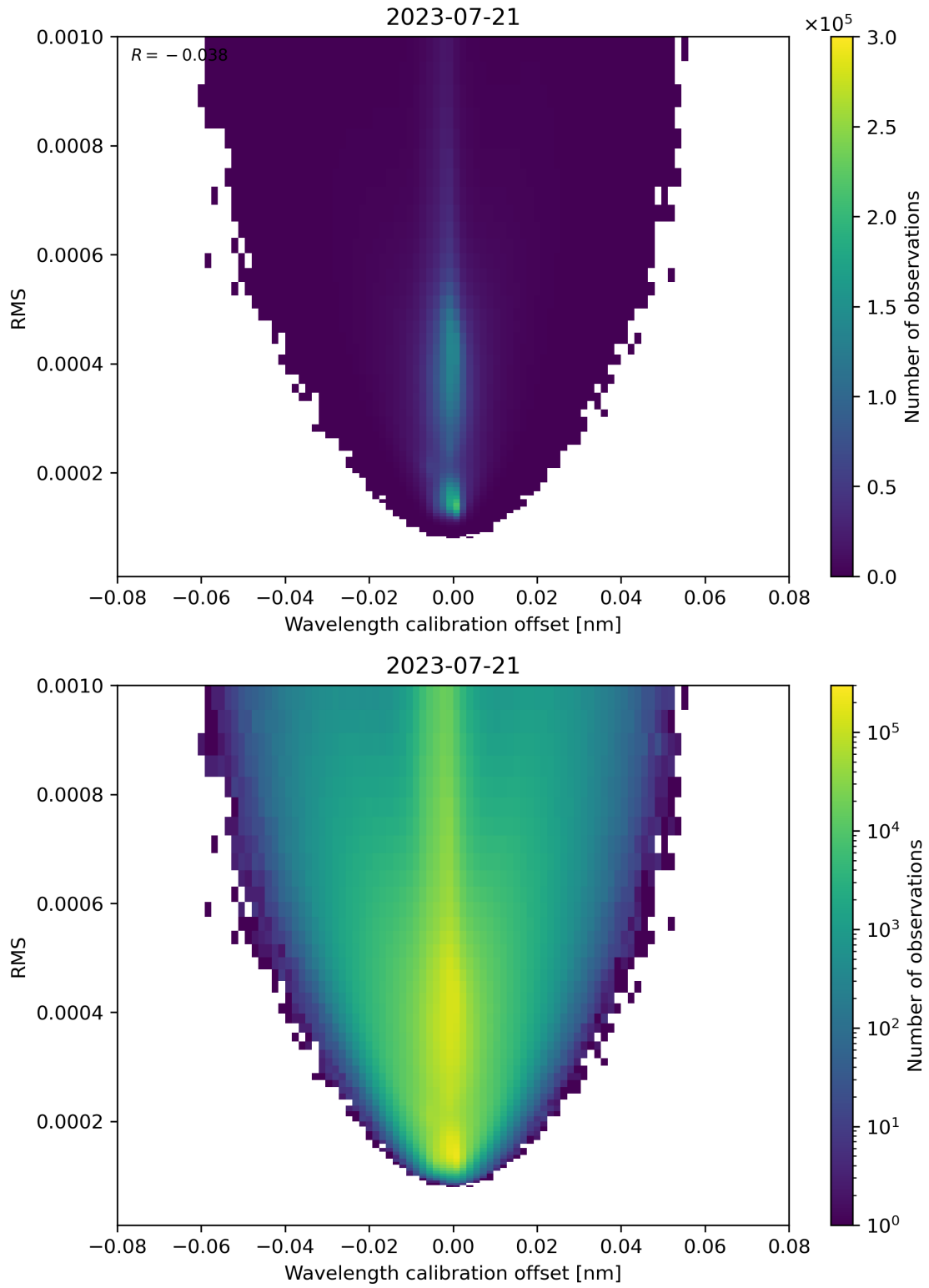
Figure 181: Scatter density plot of “Wavelength calibration offset” against “RMS” for 2023-07-20 to 2023-07-22.
