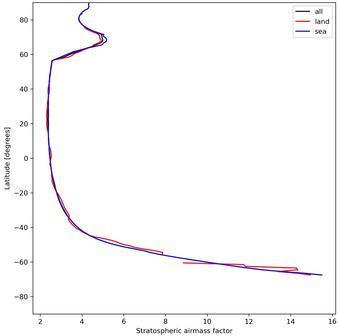
Figure 27: Zonal average of “Stratospheric airmass factor” for 2023-07-20 to 2023-07-22.
