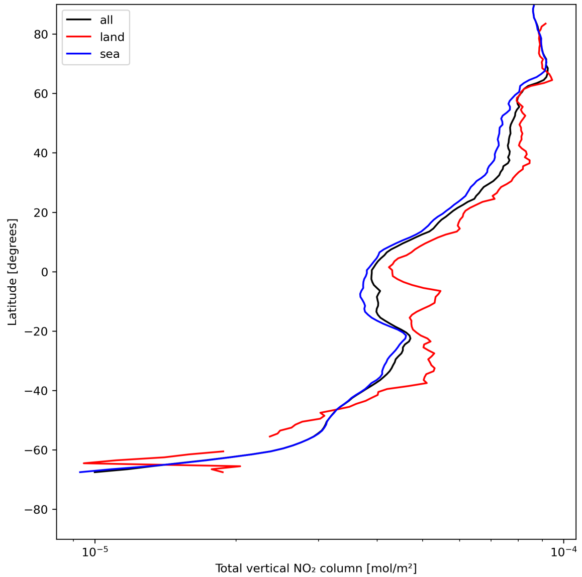
Figure 21: Zonal average of “Total vertical NO 2 column” for 2023-07-20 to 2023-07-22.
