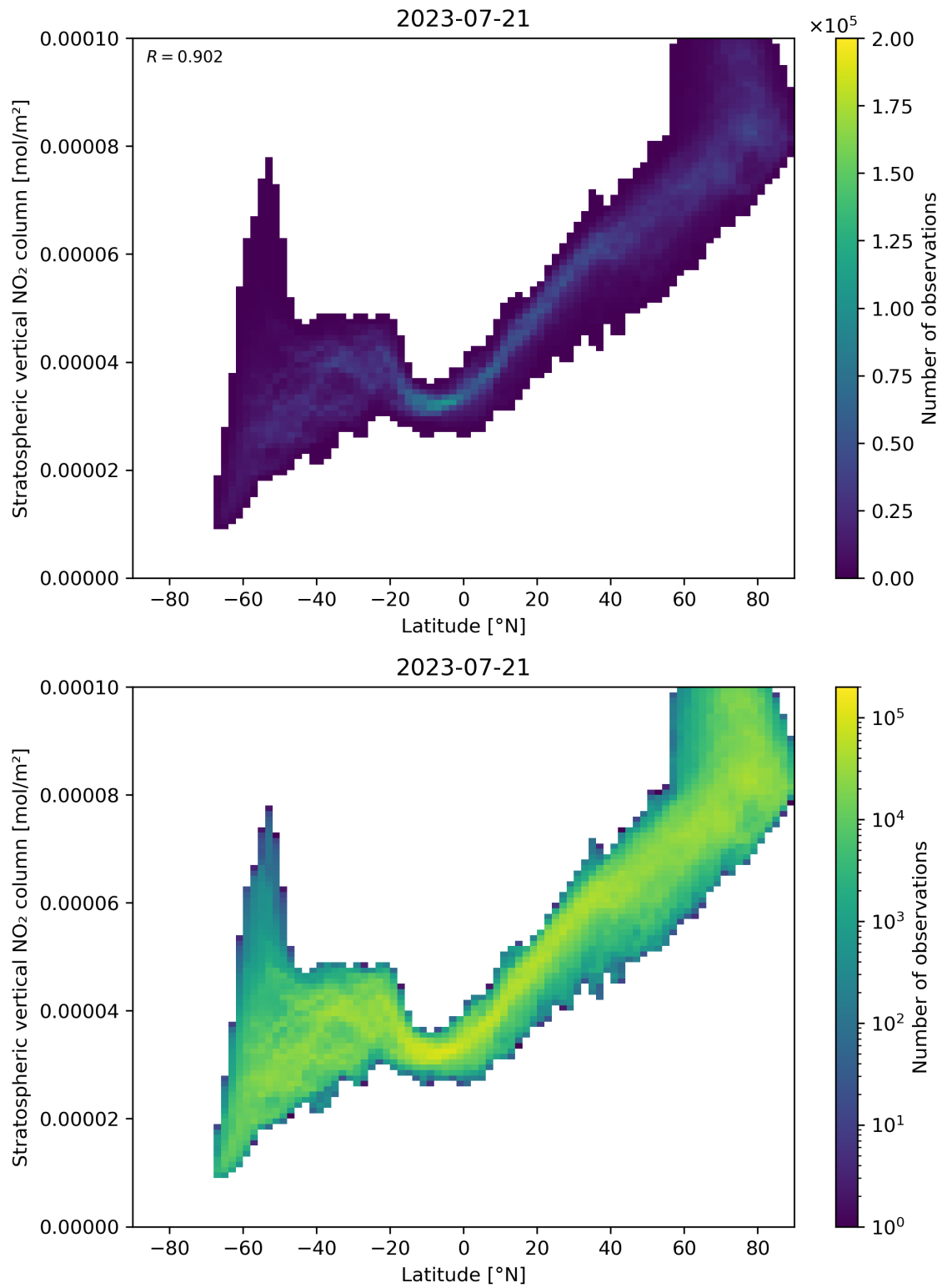
Figure 87: Scatter density plot of “Latitude” against “Stratospheric vertical NO 2 column” for 2023-07-20 to 2023-07-22.
