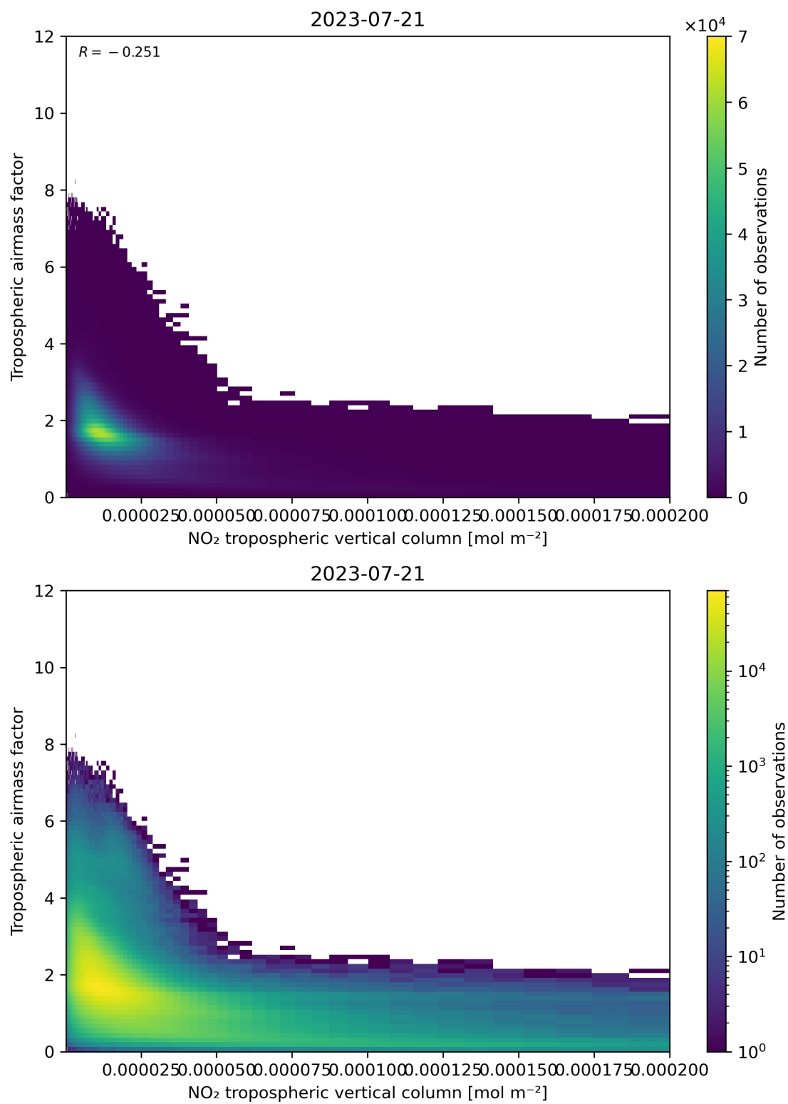
Figure 123: Scatter density plot of “NO 2 tropospheric vertical column” against “Tropospheric air mass factor” for 2023-07-20 to 2023-07-22.
