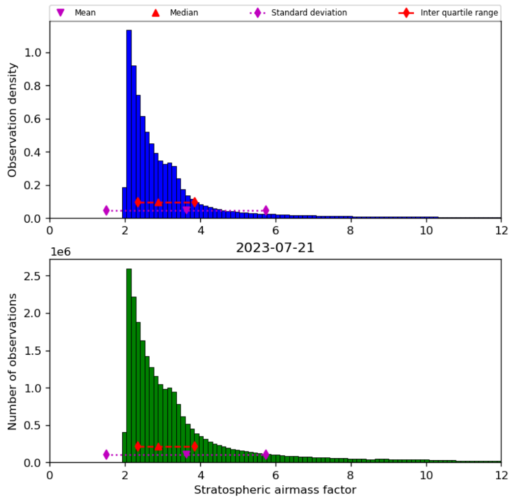
Figure 44: Histogram of “Stratospheric airmass factor” for 2023-07-20 to 2023-07-22
