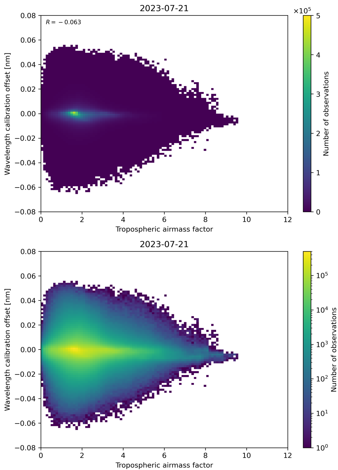
Figure 80: Scatter density plot of “Tropospheric airmass factor” against “Wavelength calibration offset” for 2023-07-20 to 2023-07-22.
