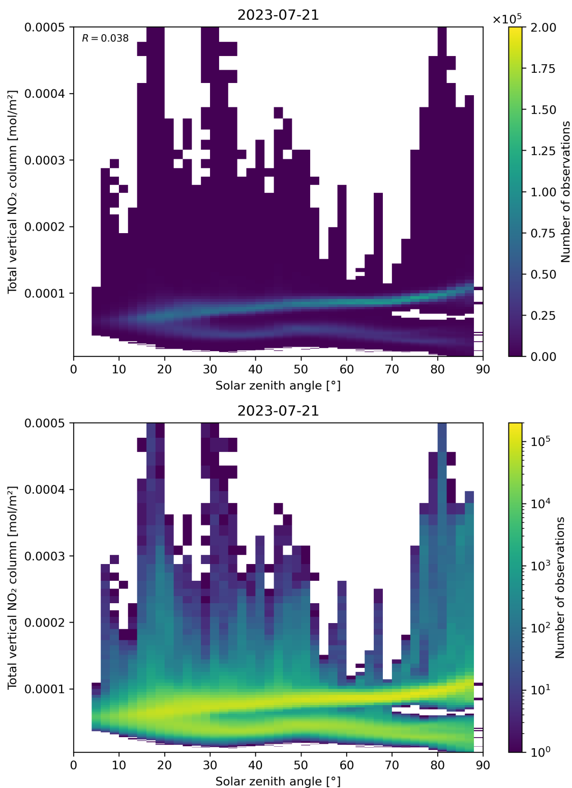
Figure 153: Scatter density plot of “Solar zenith angle” against “Total vertical NO 2 column” for 2023-07-20 to 2023-07-22.
