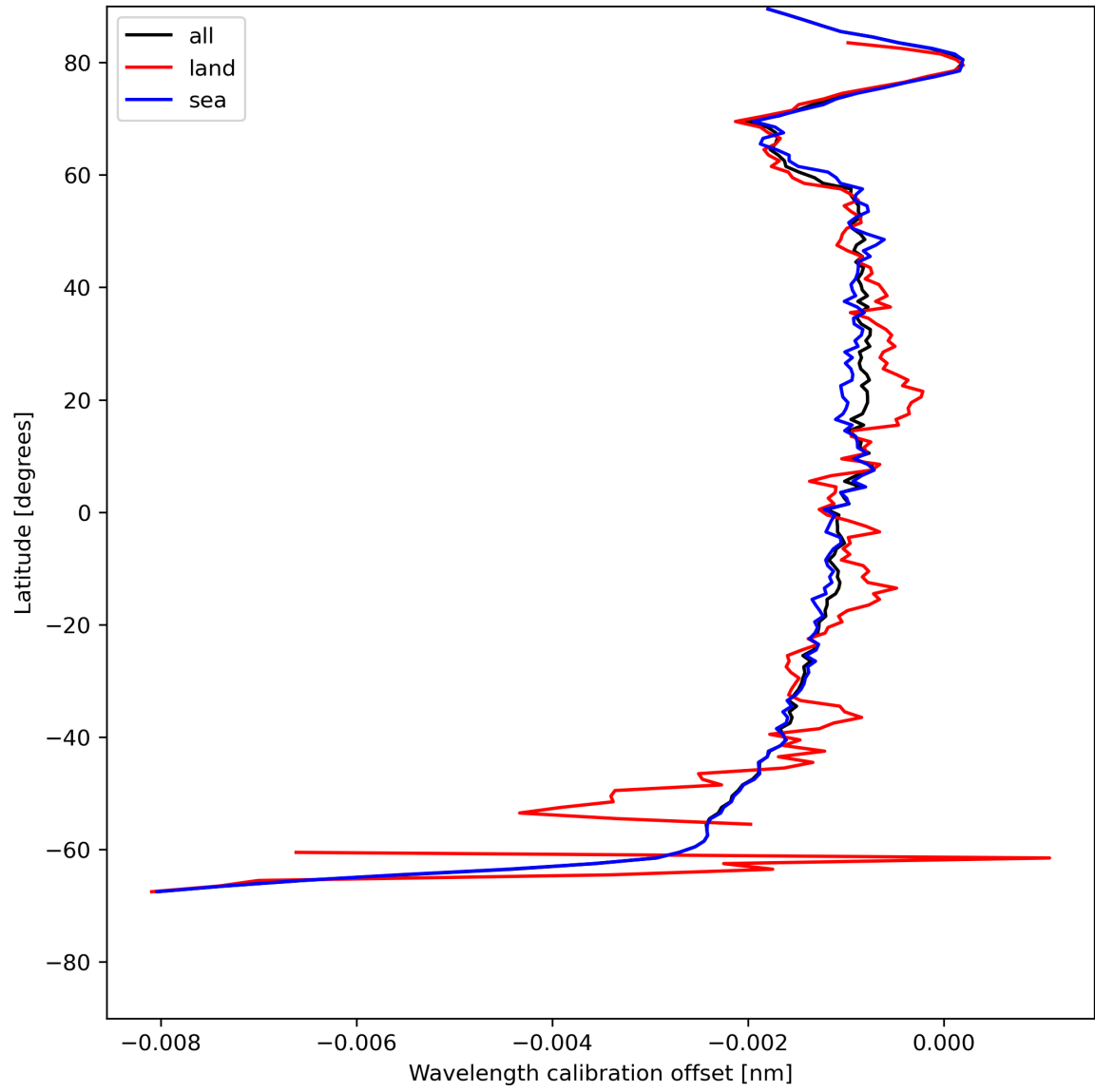
Figure 18: Zonal average of “Wavelength calibration offset” for 2023-07-20 to 2023-07-22.
