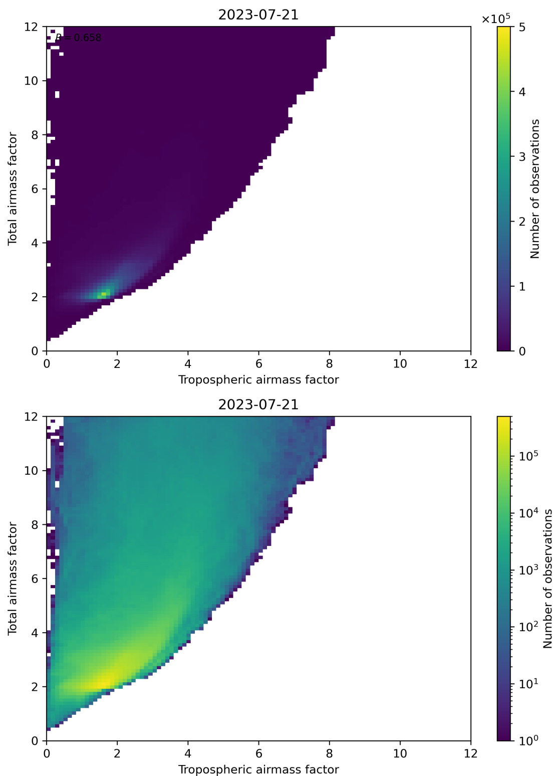
Figure 72: Scatter density plot of “Tropospheric airmass factor” against “Total airmass factor” for 2023-07-20 to 2023-07-22.
