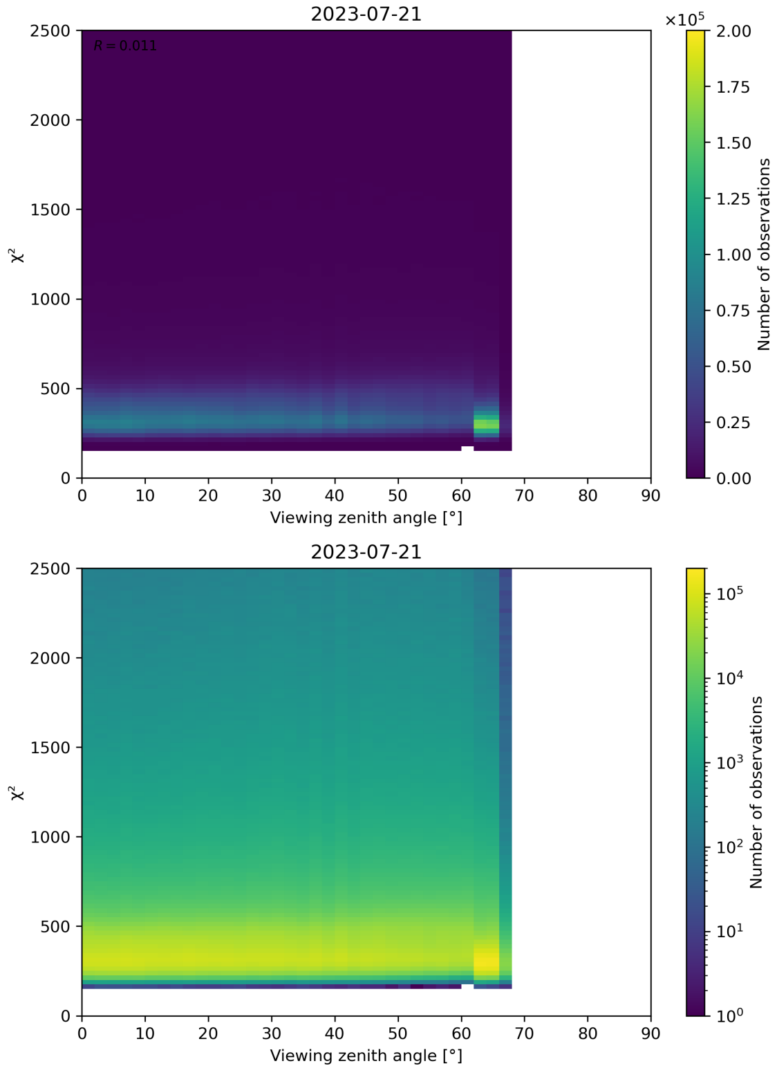
Figure 162: Scatter density plot of “Viewing zenith angle” against “ \chi^2 ” for 2023-07-20 to 2023-07-22.
