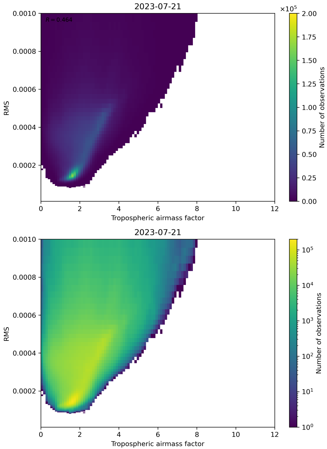
Figure 79: Scatter density plot of “Tropospheric airmass factor” against “RMS” for 2023-07-20 to 2023-07-22.
