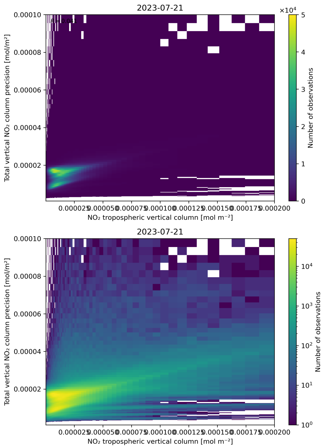
Figure 129: Scatter density plot of “NO 2 tropospheric vertical column” against “Total vertical NO 2 column precision” for 2023-07-20 to 2023-07-22.
