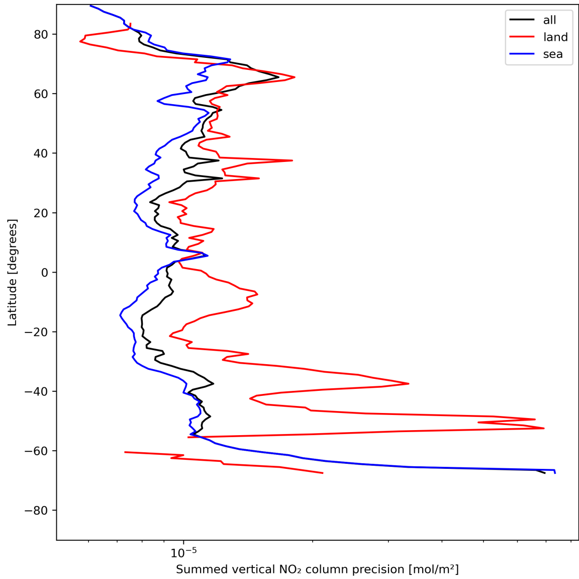
Figure 24: Zonal average of “Summed vertical NO 2 column precision” for 2023-07-20 to 2023-07-22.
