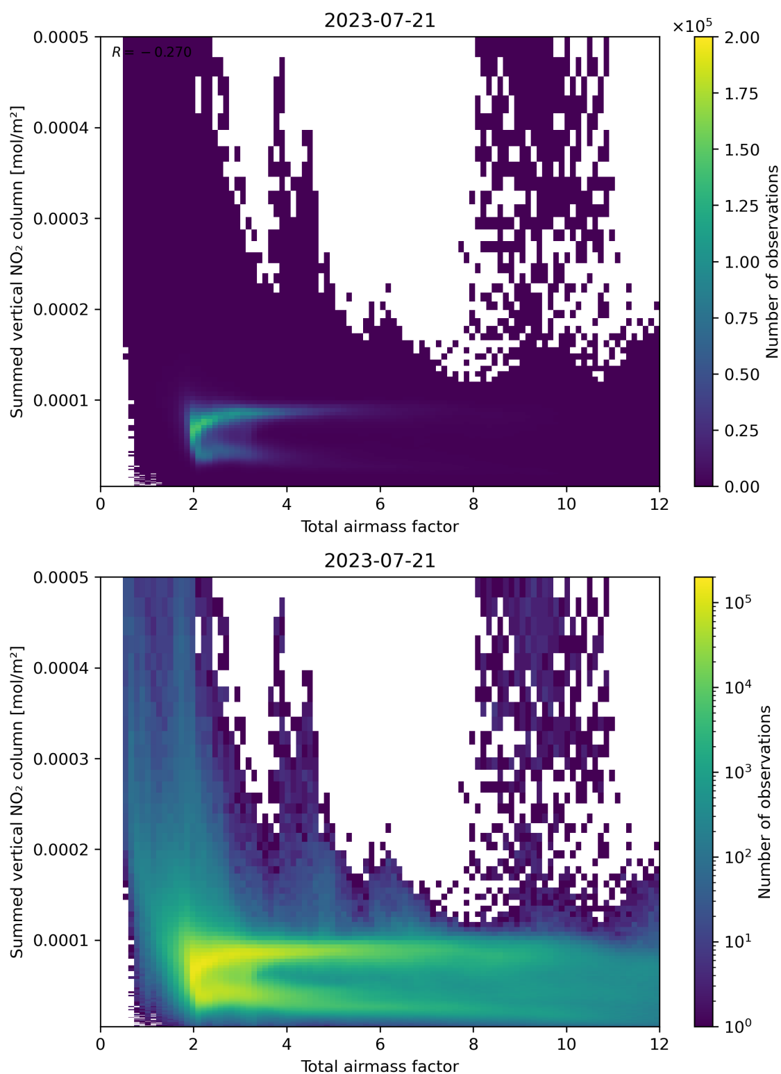
Figure 65: Scatter density plot of “Total airmass factor” against “Summed vertical NO 2 column” for 2023-07-20 to 2023-07-22.
