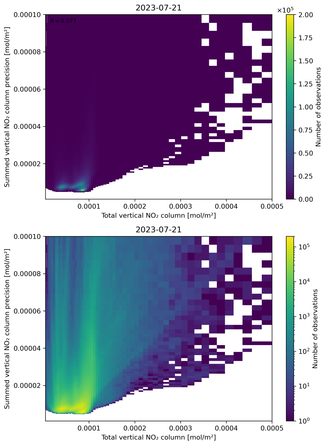
Figure 113: Scatter density plot of “Total vertical NO 2 column” against “Summed vertical NO 2 column precision” for 2023-07-20 to 2023-07-22.
