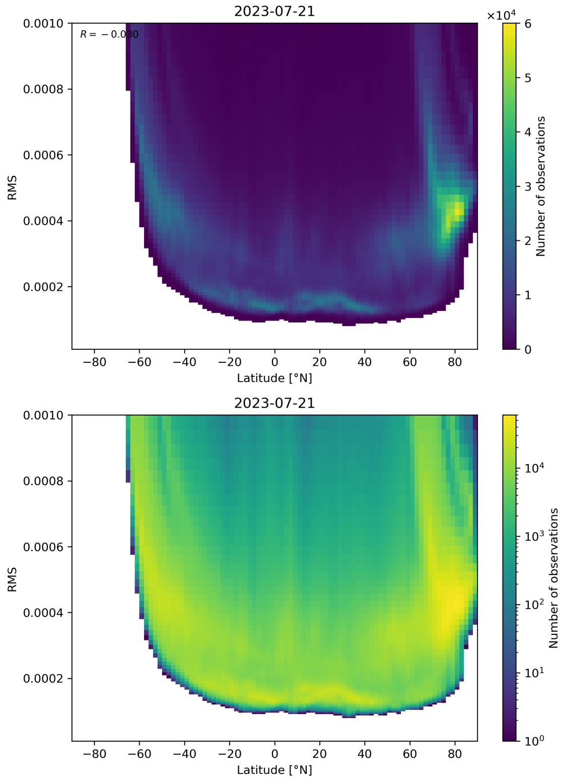
Figure 94: Scatter density plot of “Latitude” against “RMS” for 2023-07-20 to 2023-07-22.
