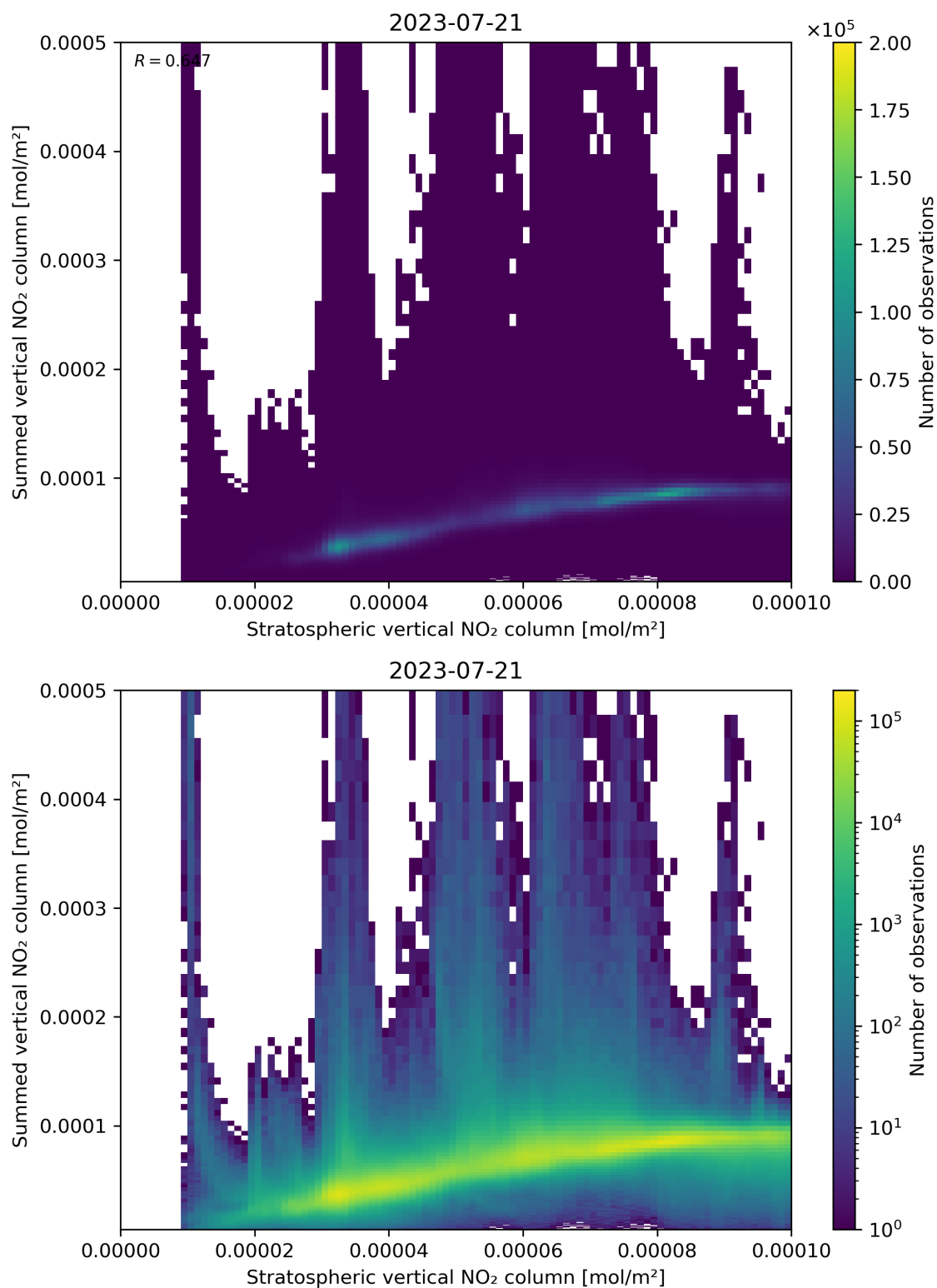
Figure 98: Scatter density plot of “Stratospheric vertical NO 2 column” against “Summed vertical NO 2 column” for 2023-07-20 to 2023-07-22.
