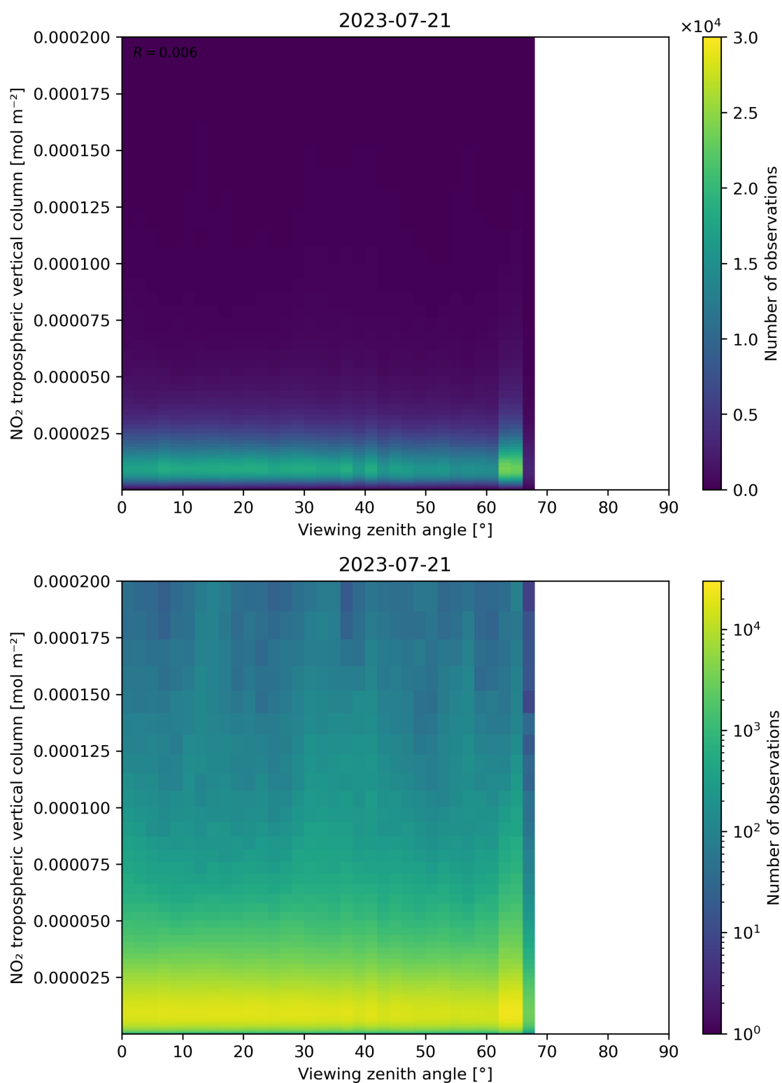
Figure 169: Scatter density plot of “Viewing zenith angle” against “NO 2 tropospheric vertical column” for 2023-07-20 to 2023-07-22.
