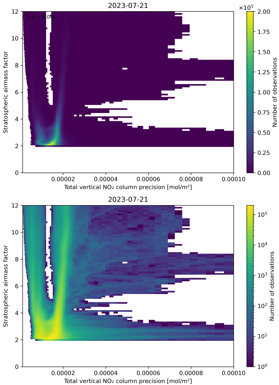
Figure 115: Scatter density plot of “Total vertical NO 2 column precision” against “Stratospheric air mass factor” for 2023-07-20 to 2023-07-22.
