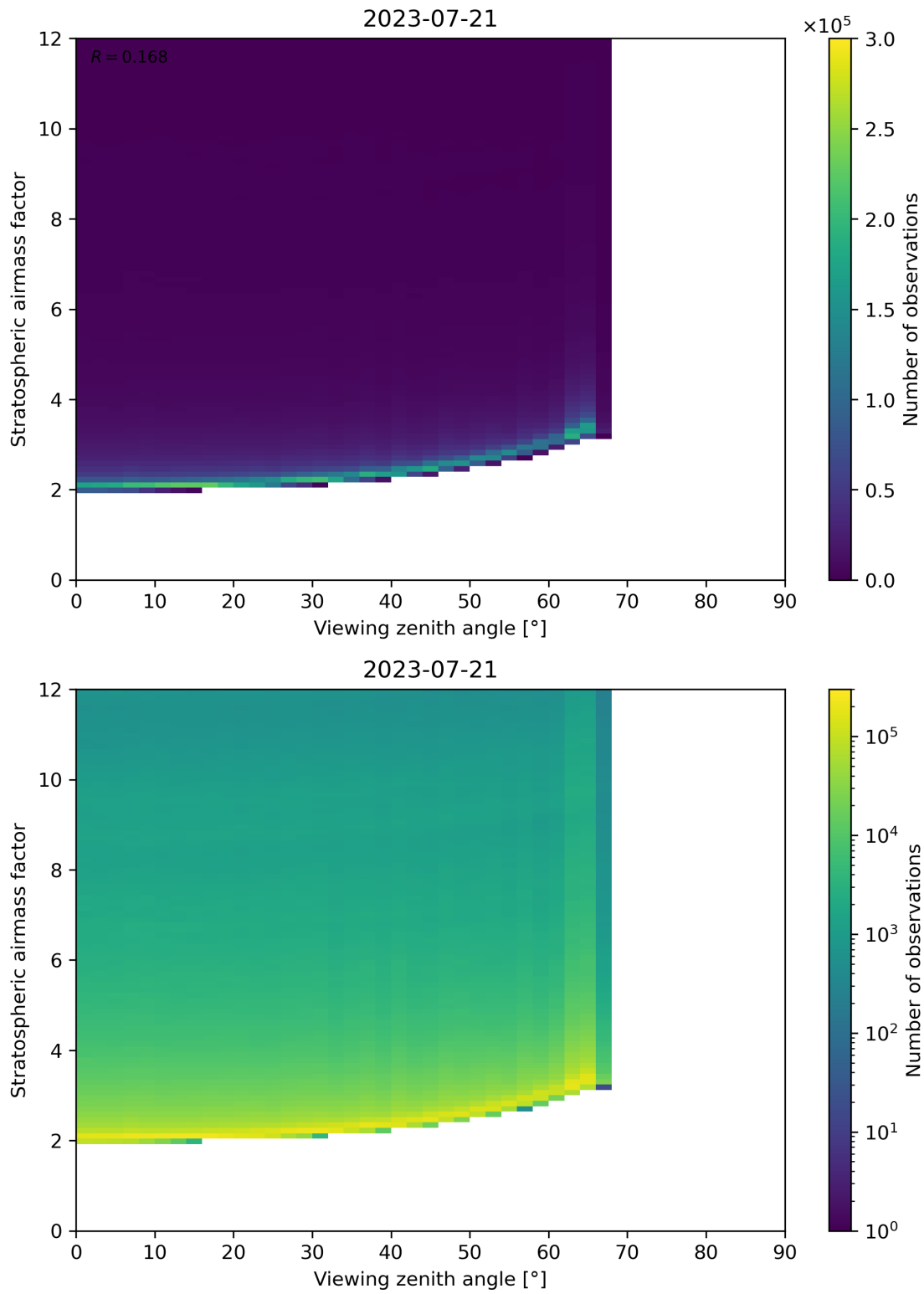
Figure 159: Scatter density plot of “Viewing zenith angle” against “Stratospheric airmass factor” for 2023-07-20 to 2023-07-22.
