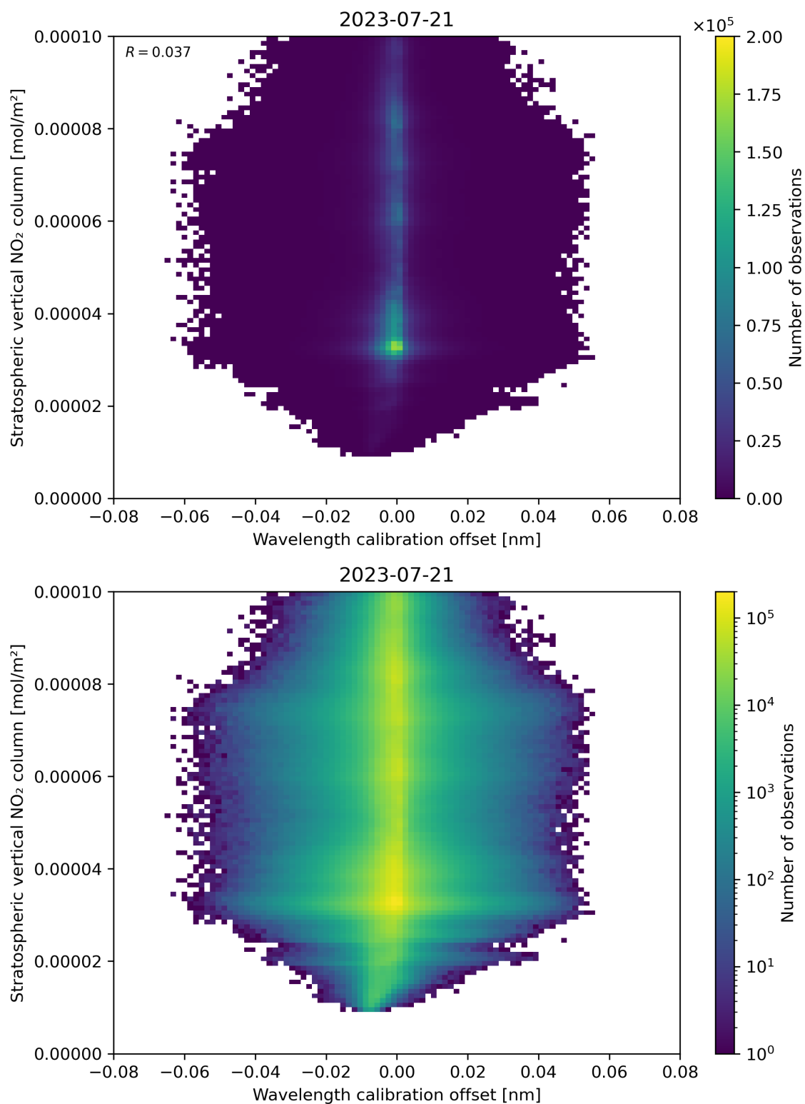
Figure 176: Scatter density plot of “Wavelength calibration offset” against “Stratospheric vertical NO 2 column” for 2023-07-20 to 2023-07-22.
