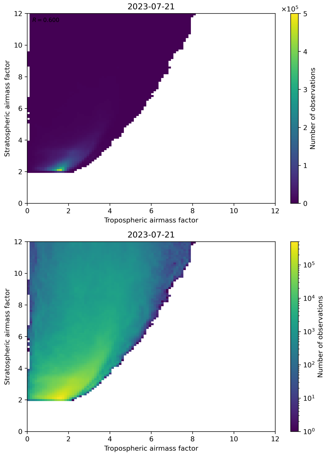
Figure 71: Scatter density plot of “Tropospheric airmass factor” against “Stratospheric airmass factor” for 2023-07-20 to 2023-07-22.
