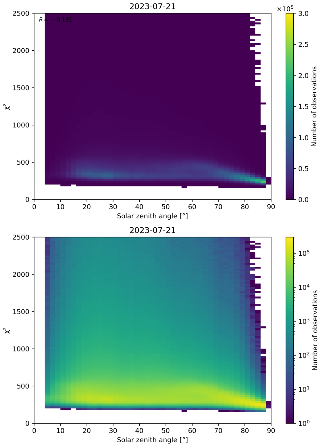
Figure 148: Scatter density plot of “Solar zenith angle” against “ \chi^2 ” for 2023-07-20 to 2023-07-22.
