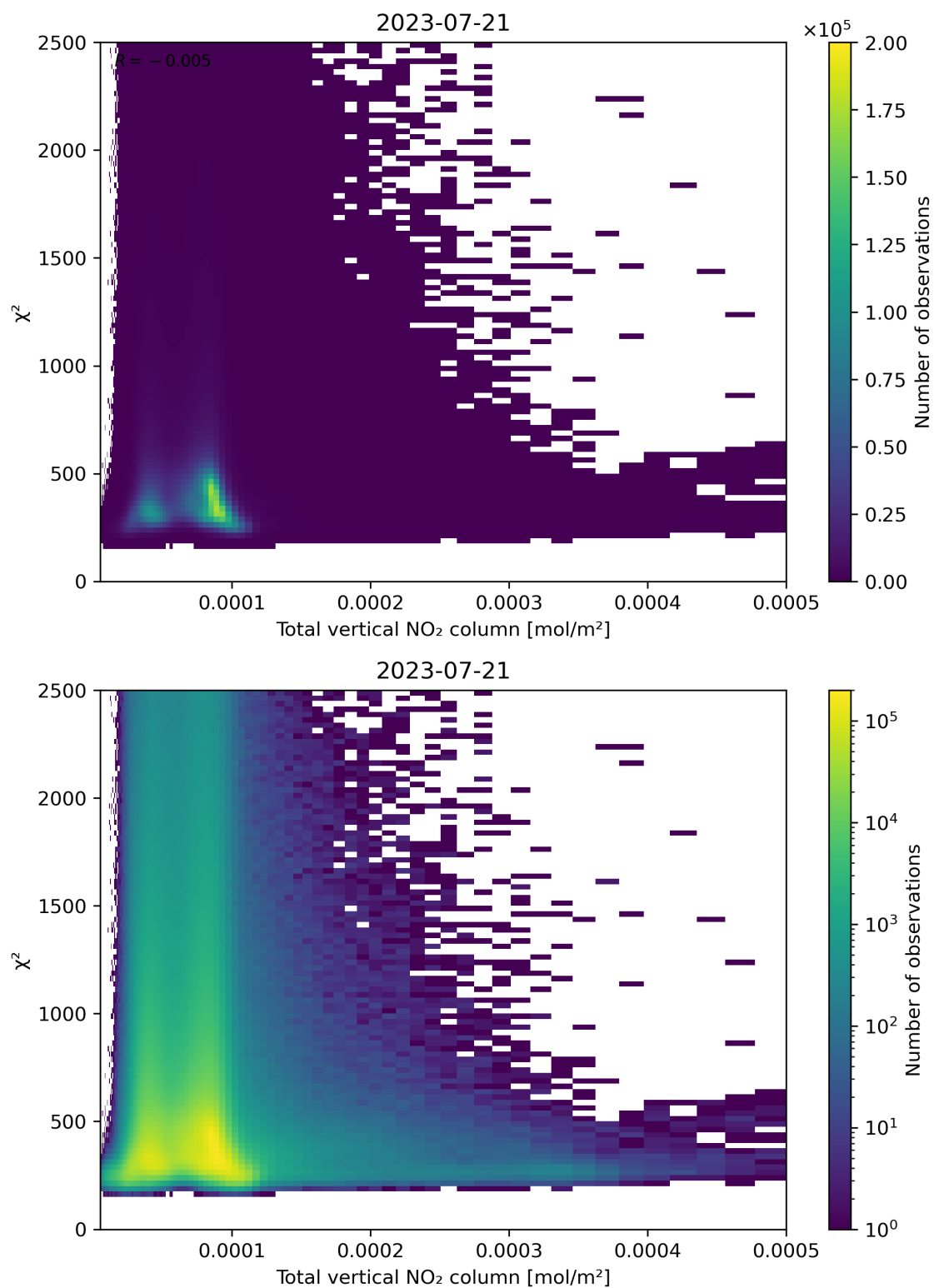
Figure 111: Scatter density plot of “Total vertical NO 2 column” against “ \chi^2 ” for 2023-07-20 to 2023-07-22.
