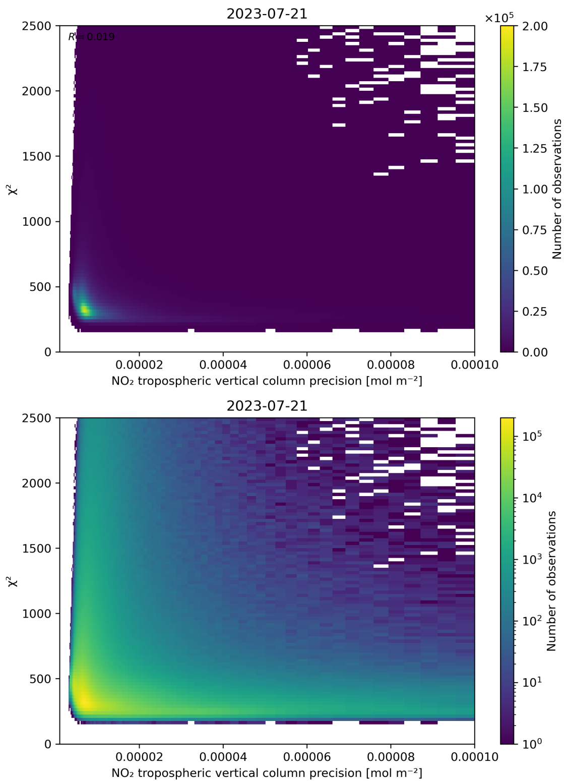
Figure 134: Scatter density plot of “NO 2 tropospheric vertical column precision” against “ \chi^2 ” for 2023-07-20 to 2023-07-22.
