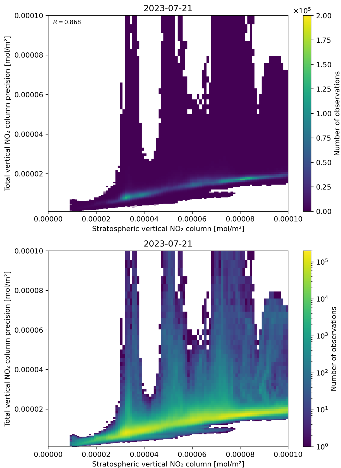
Figure 101: Scatter density plot of “Stratospheric vertical NO 2 column” against “Total vertical NO 2 column precision” for 2023-07-20 to 2023-07-22.
