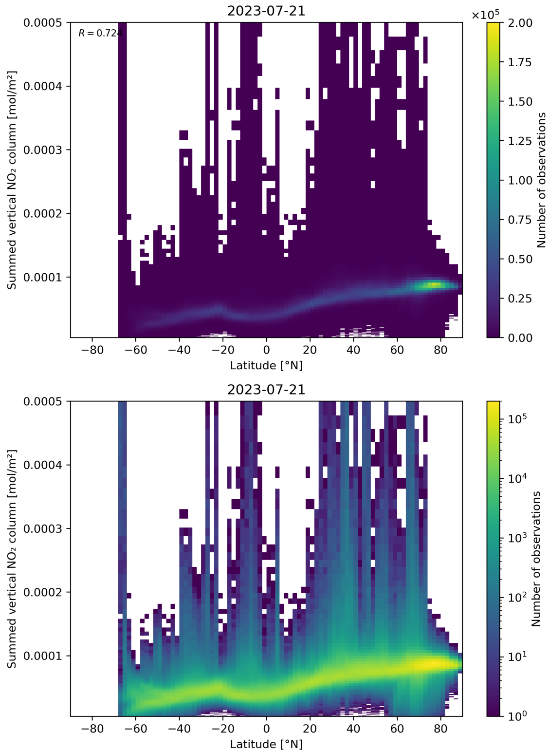
Figure 88: Scatter density plot of “Latitude” against “Summed vertical NO 2 column” for 2023-07-20 to 2023-07-22.
