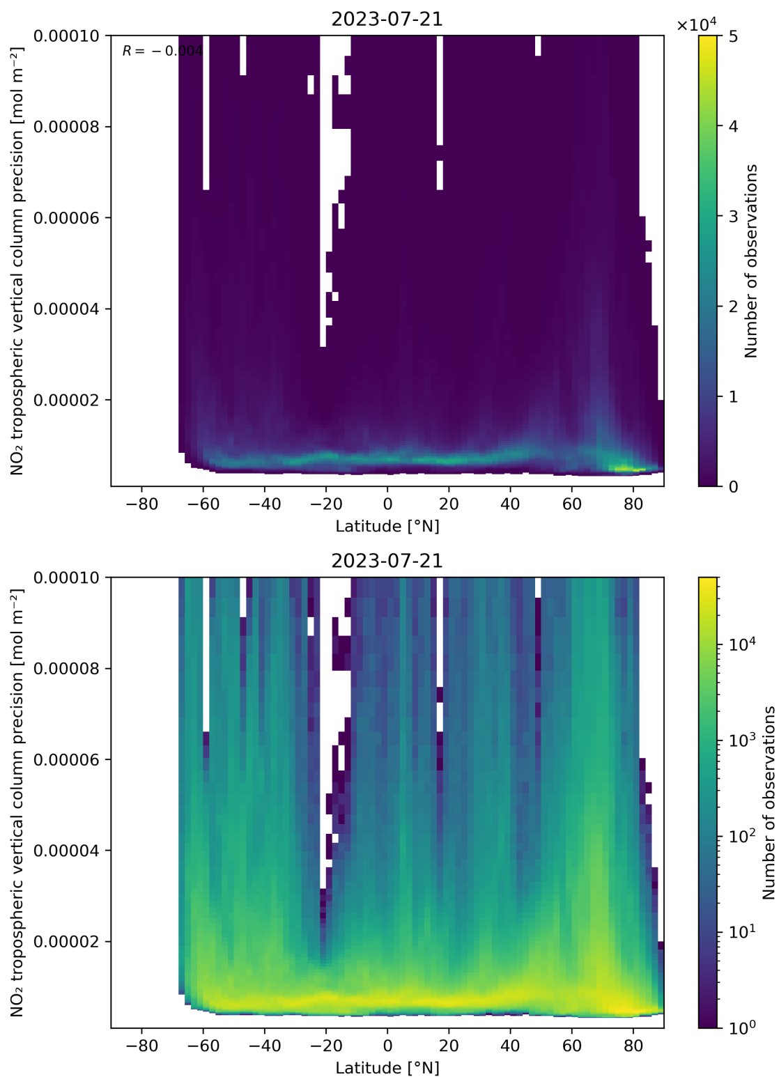
Figure 93: Scatter density plot of “Latitude” against “NO 2 tropospheric vertical column precision” for 2023-07-20 to 2023-07-22.
