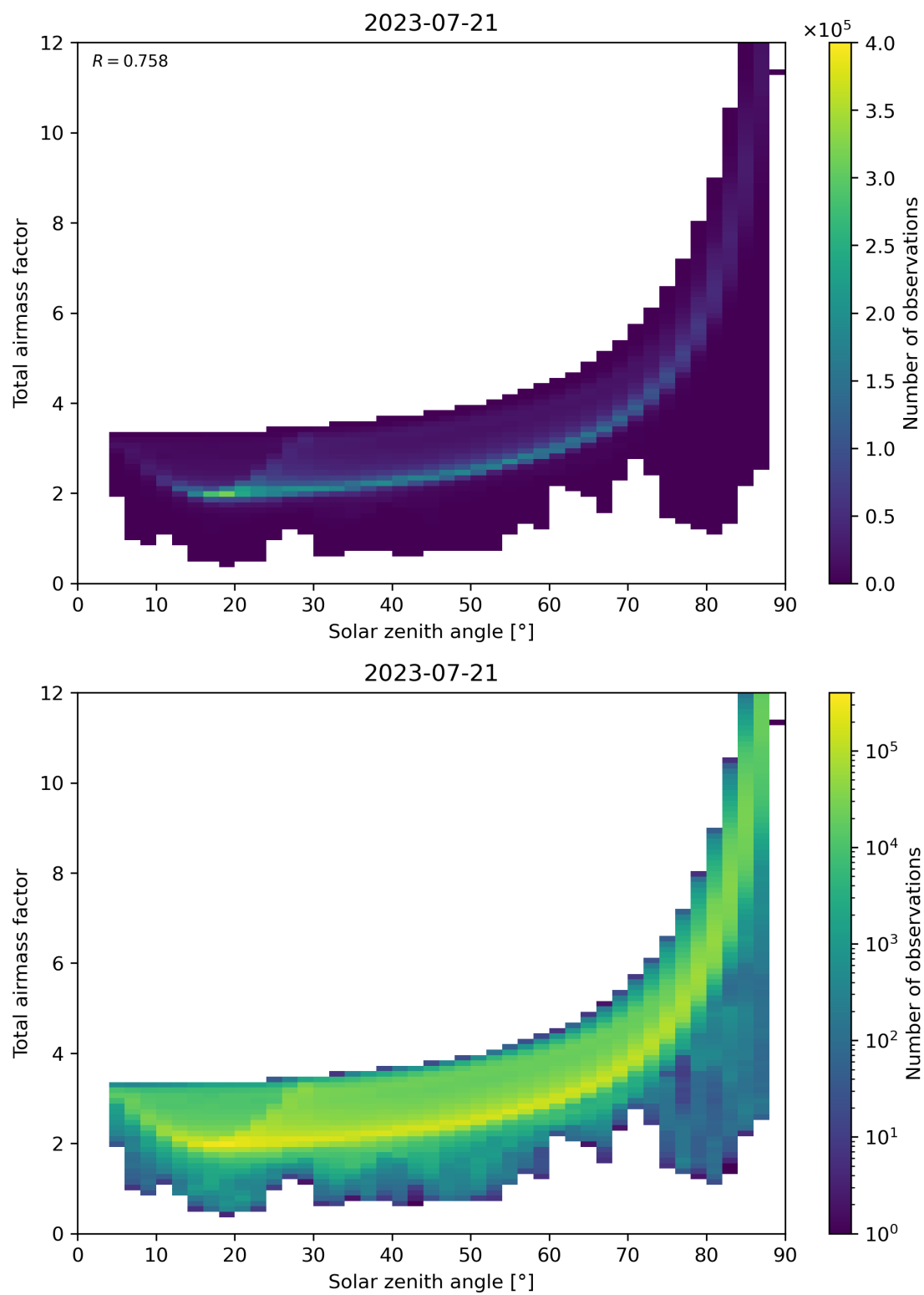
Figure 146: Scatter density plot of “Solar zenith angle” against “Total air mass factor” for 2023-07-20 to 2023-07-22.
