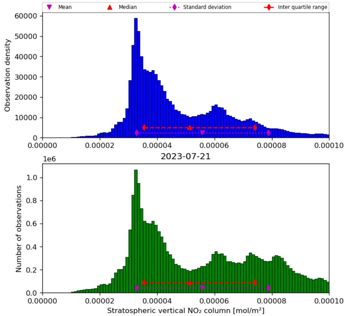
Figure 36: Histogram of “Stratospheric vertical NO 2 column” for 2023-07-20 to 2023-07-22
