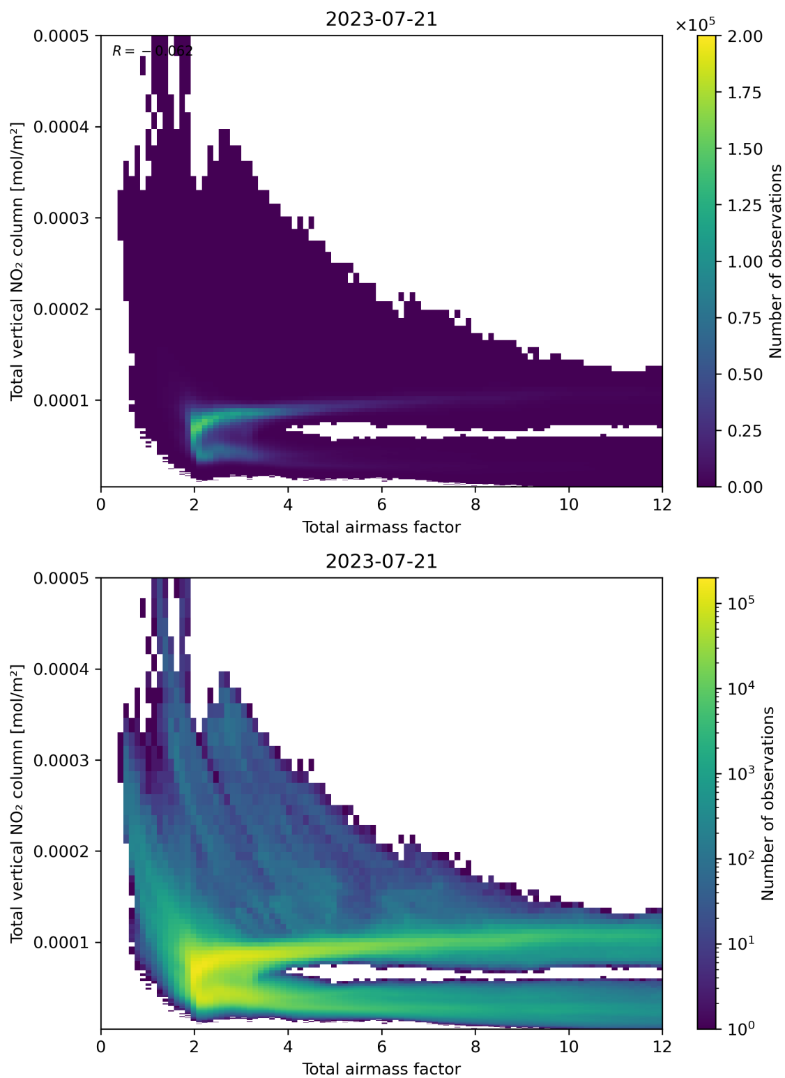
Figure 67: Scatter density plot of “Total airmass factor” against “Total vertical NO 2 column” for 2023-07-20 to 2023-07-22.
