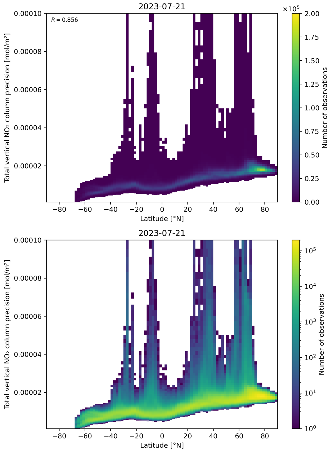
Figure 91: Scatter density plot of “Latitude” against “Total vertical NO 2 column precision” for 2023-07-20 to 2023-07-22.
