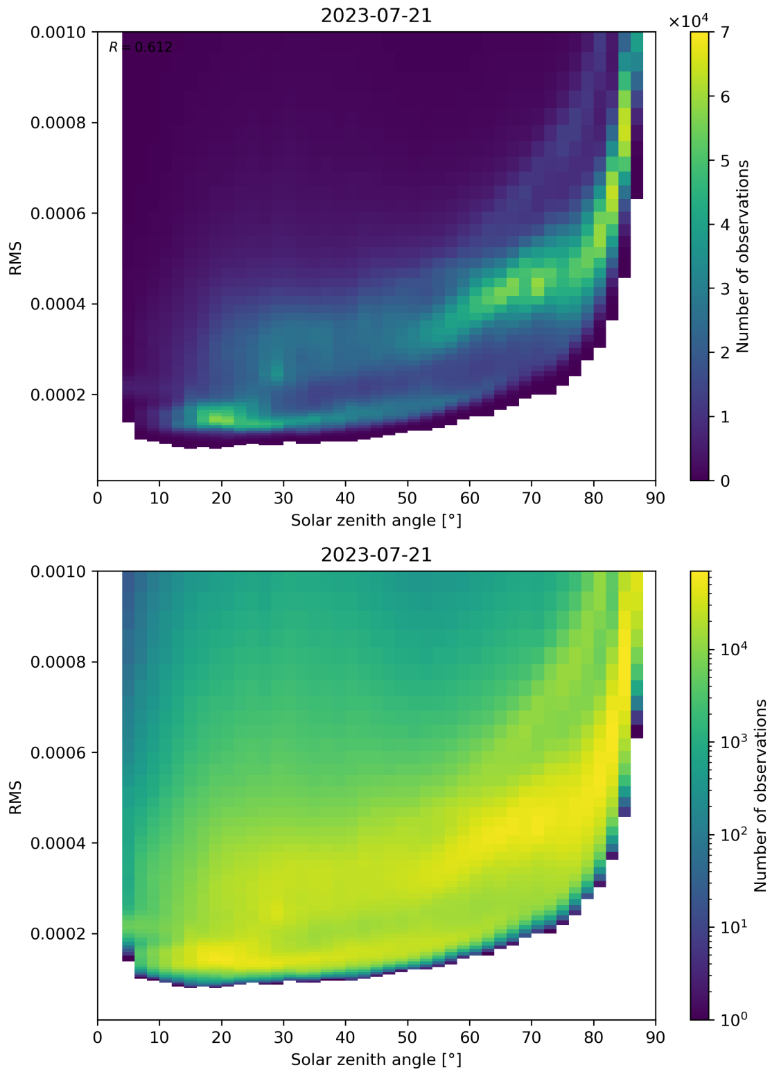
Figure 157: Scatter density plot of “Solar zenith angle” against “RMS” for 2023-07-20 to 2023-07-22.
