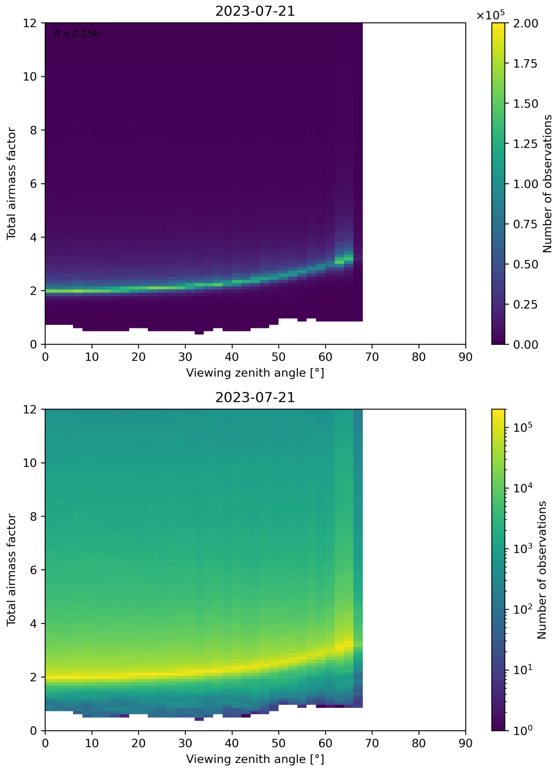
Figure 160: Scatter density plot of “Viewing zenith angle” against “Total airmass factor” for 2023-07-20 to 2023-07-22.
