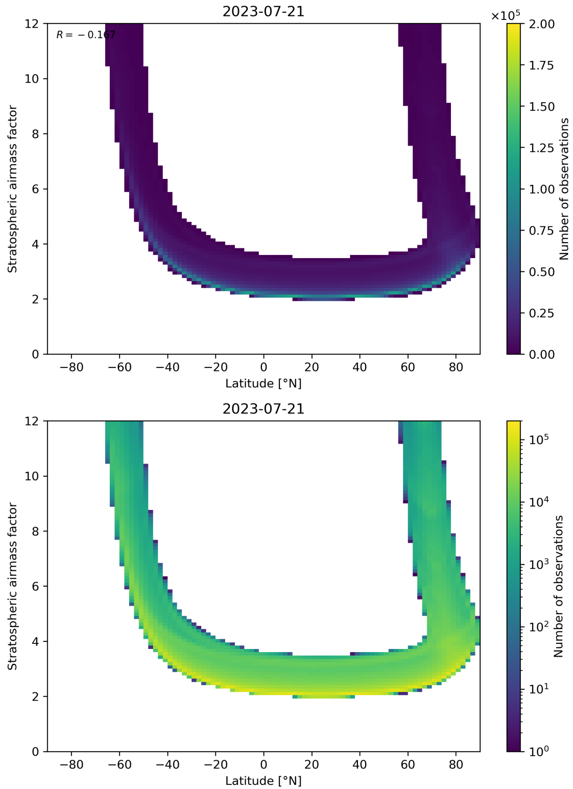
Figure 83: Scatter density plot of “Latitude” against “Stratospheric air mass factor” for 2023-07-20 to 2023-07-22.
