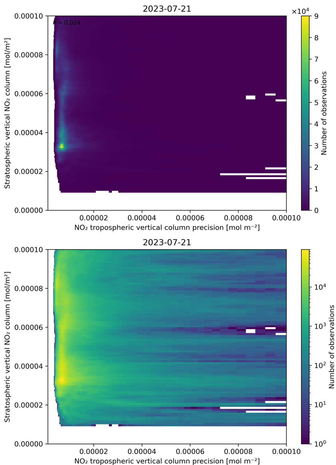
Figure 135: Scatter density plot of “NO 2 tropospheric vertical column precision” against “Stratospheric vertical NO 2 column” for 2023-07-20 to 2023-07-22.
