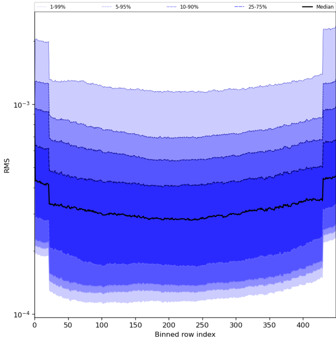
Figure 60: Along track statistics of “RMS” for 2023-07-20 to 2023-07-22
