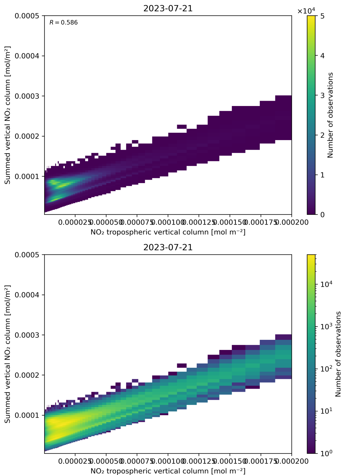
Figure 126: Scatter density plot of “NO 2 tropospheric vertical column” against “Summed vertical NO 2 column” for 2023-07-20 to 2023-07-22.
