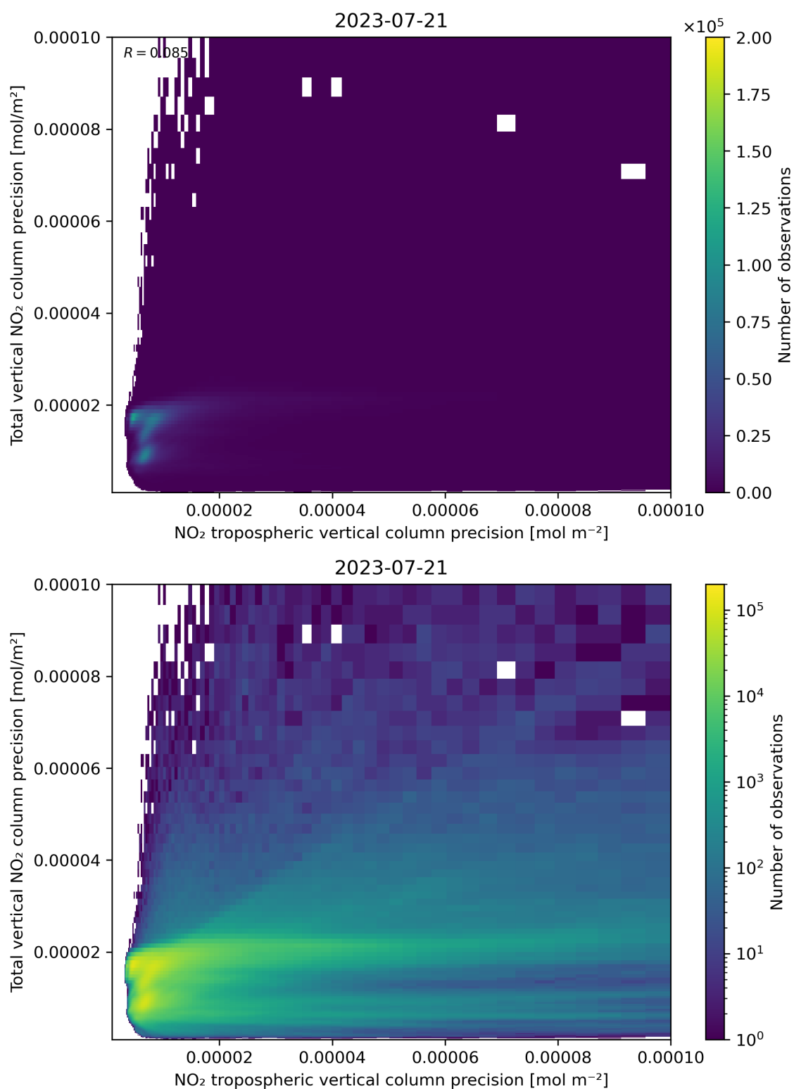
Figure 139: Scatter density plot of “NO 2 tropospheric vertical column precision” against “Total vertical NO 2 column precision” for 2023-07-20 to 2023-07-22.
