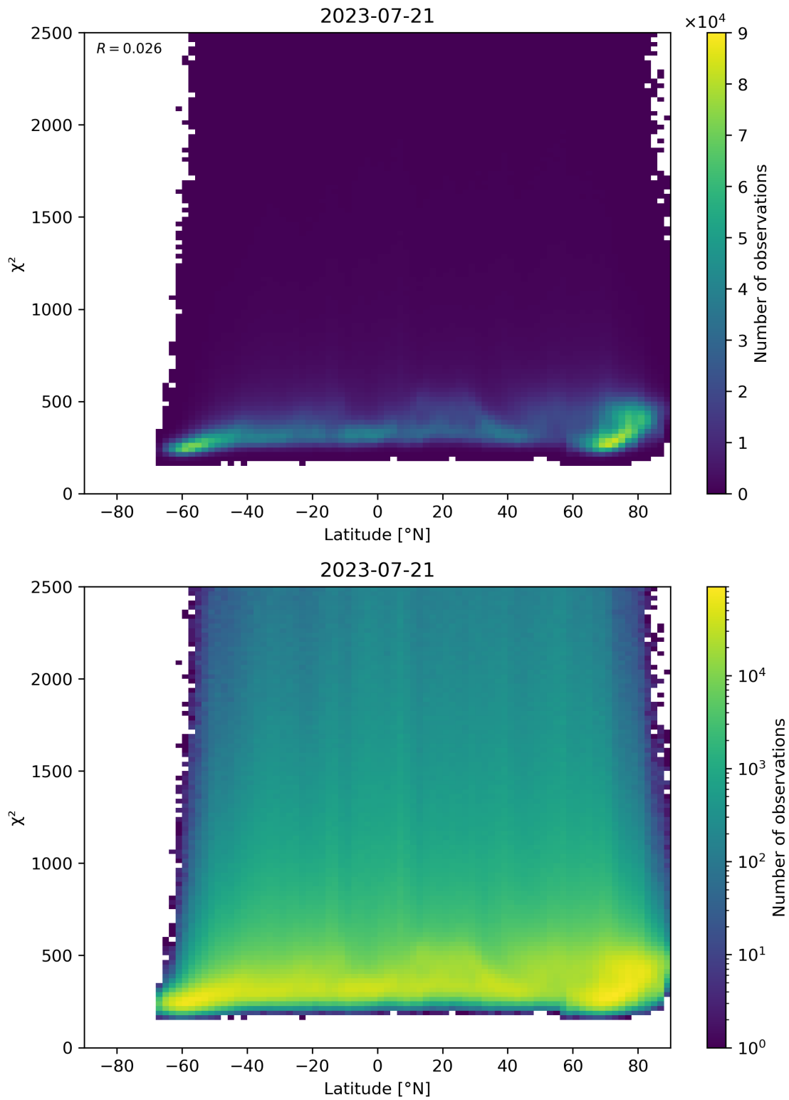
Figure 86: Scatter density plot of “Latitude” against “ \chi^2 ” for 2023-07-20 to 2023-07-22.
