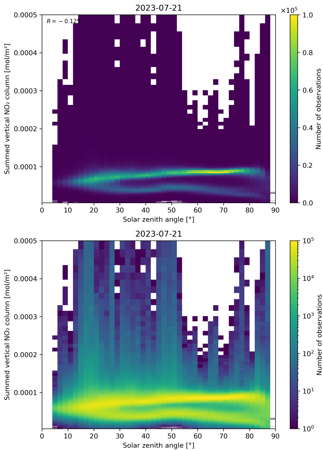
Figure 151: Scatter density plot of “Solar zenith angle” against “Summed vertical NO 2 column” for 2023-07-20 to 2023-07-22.
