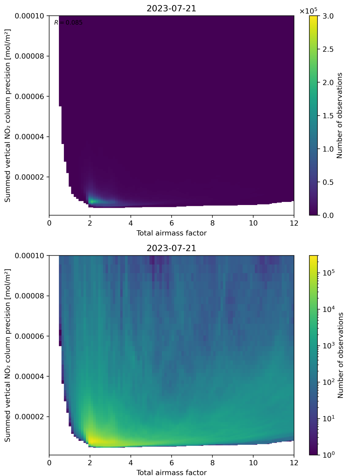
Figure 66: Scatter density plot of “Total airmass factor” against “Summed vertical NO 2 column precision” for 2023-07-20 to 2023-07-22.
