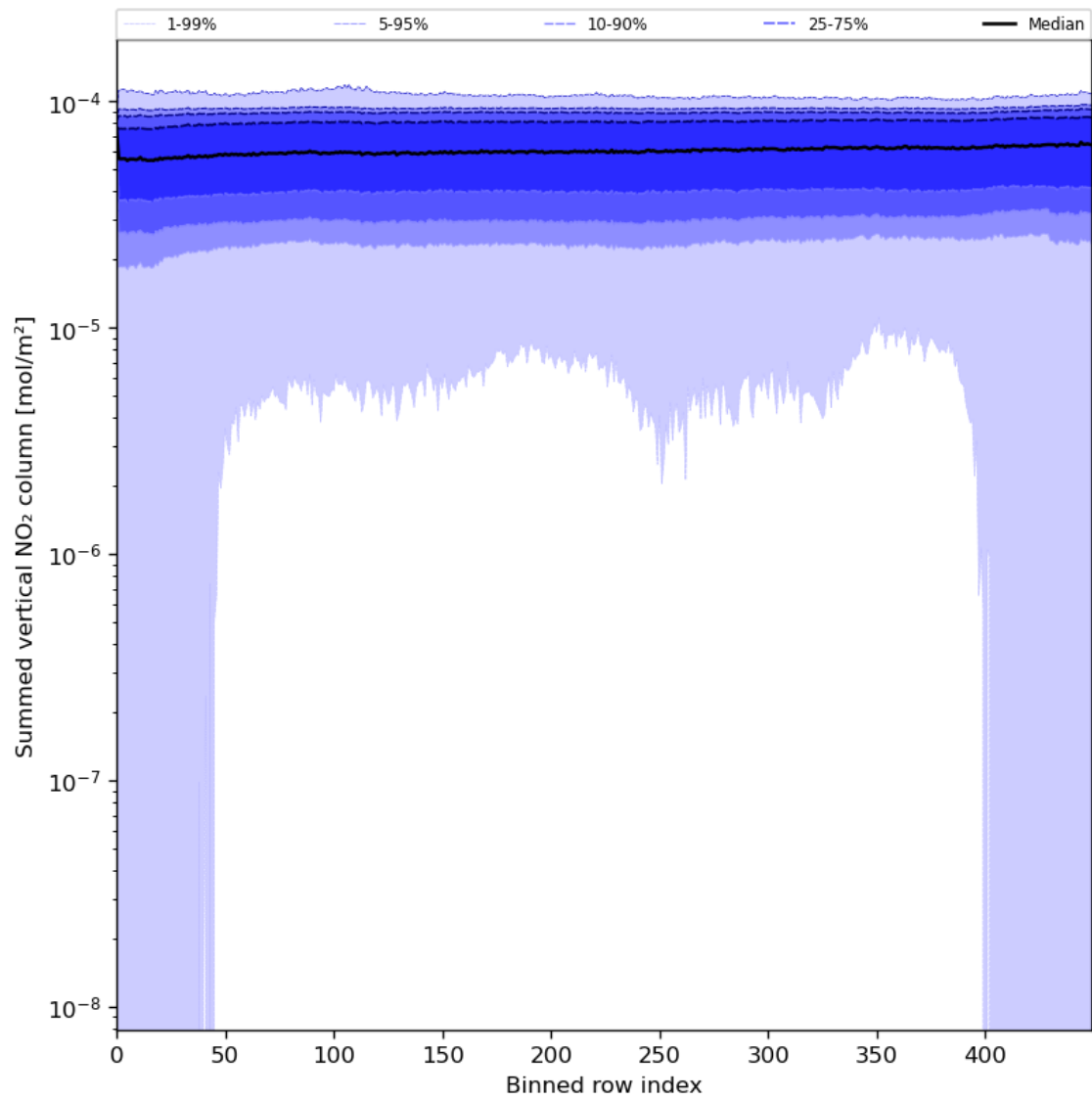
Figure 57: Along track statistics of “Summed vertical NO 2 column” for 2023-07-20 to 2023-07-22
