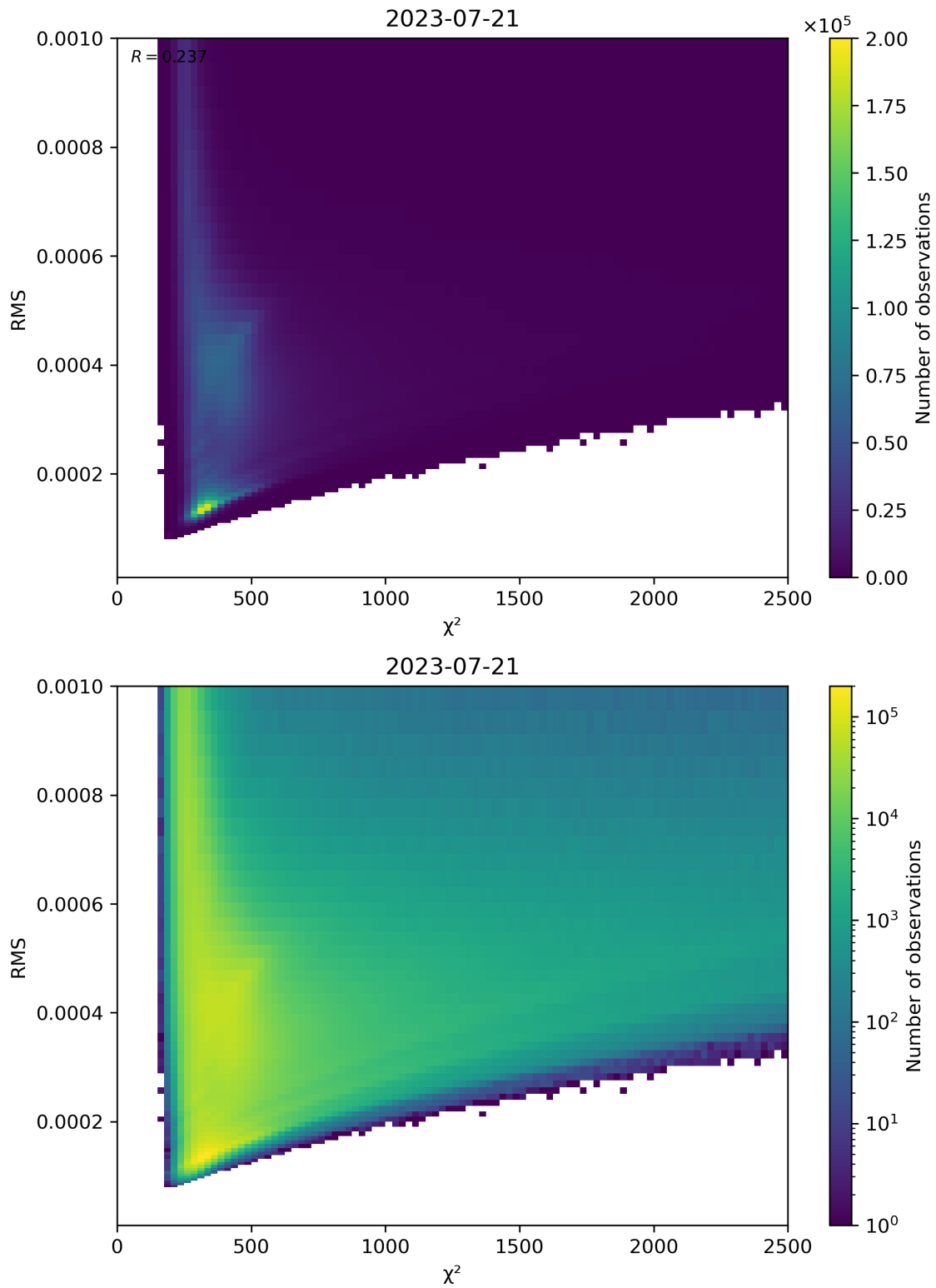
Figure 82: Scatter density plot of “ \chi^2 ” against “RMS” for 2023-07-20 to 2023-07-22.
