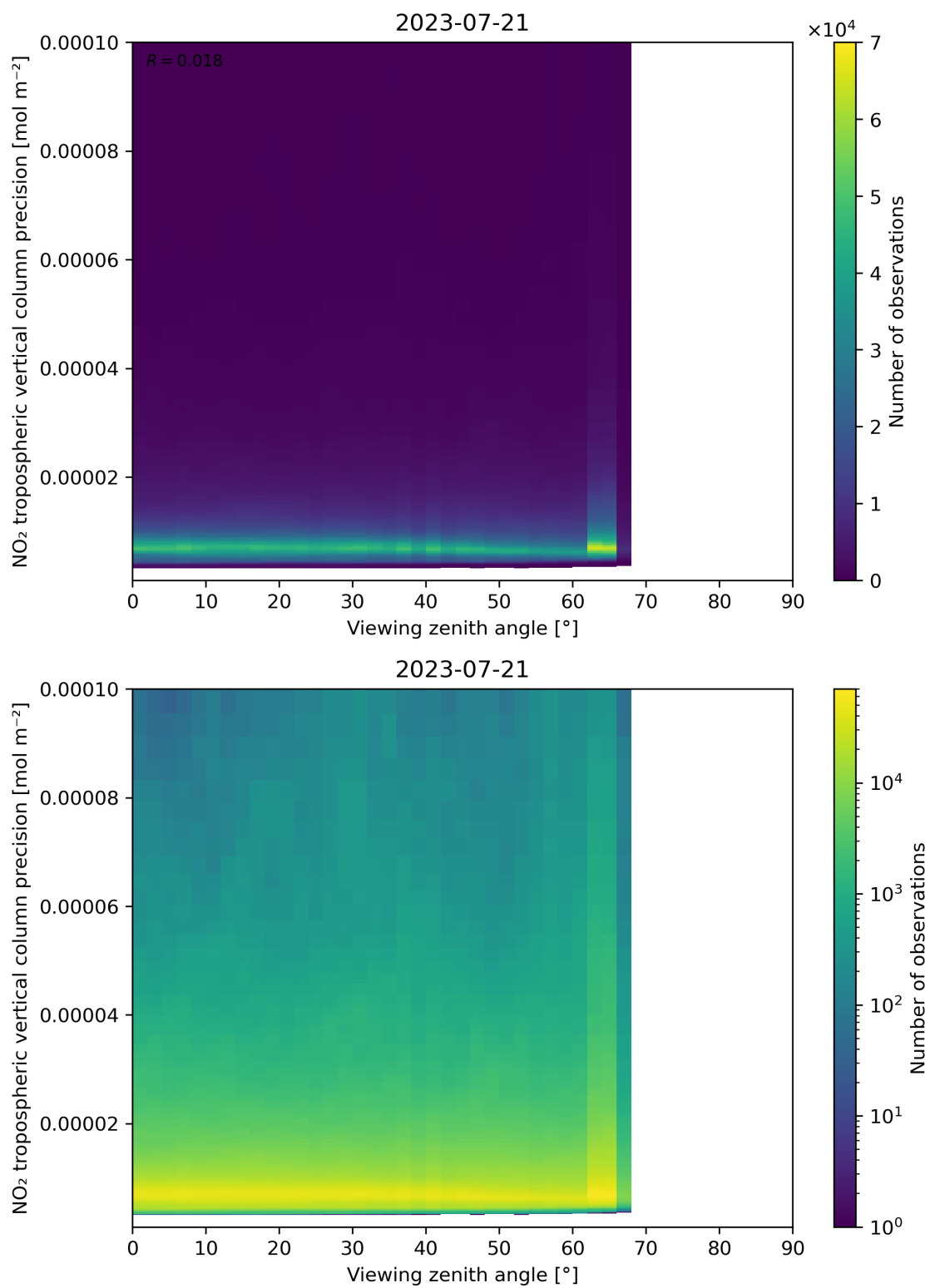
Figure 170: Scatter density plot of “Viewing zenith angle” against “NO 2 tropospheric vertical column precision” for 2023-07-20 to 2023-07-22.
