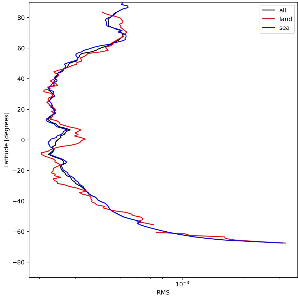
Figure 26: Zonal average of “RMS” for 2023-07-20 to 2023-07-22.
