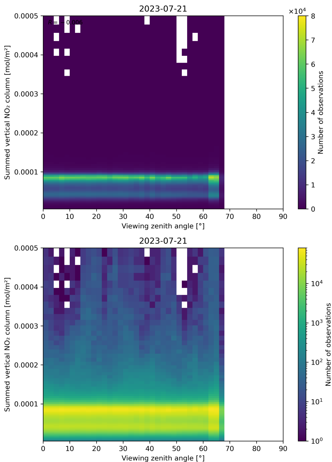
Figure 165: Scatter density plot of “Viewing zenith angle” against “Summed vertical NO 2 column” for 2023-07-20 to 2023-07-22.
