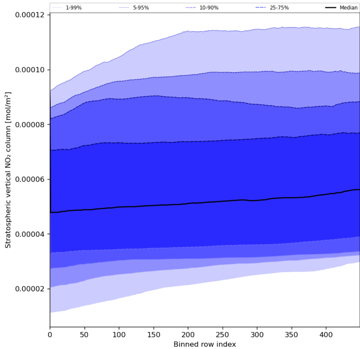
Figure 53: Along track statistics of “Stratospheric vertical NO 2 column” for 2023-07-20 to 2023-07-22
