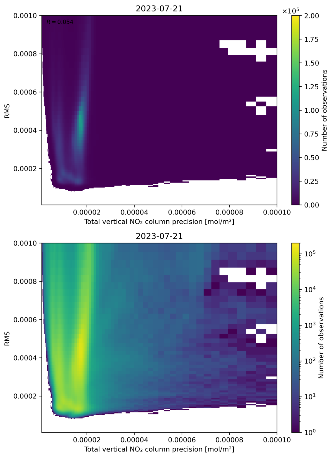
Figure 119: Scatter density plot of “Total vertical NO 2 column precision” against “RMS” for 2023-07-20 to 2023-07-22.
