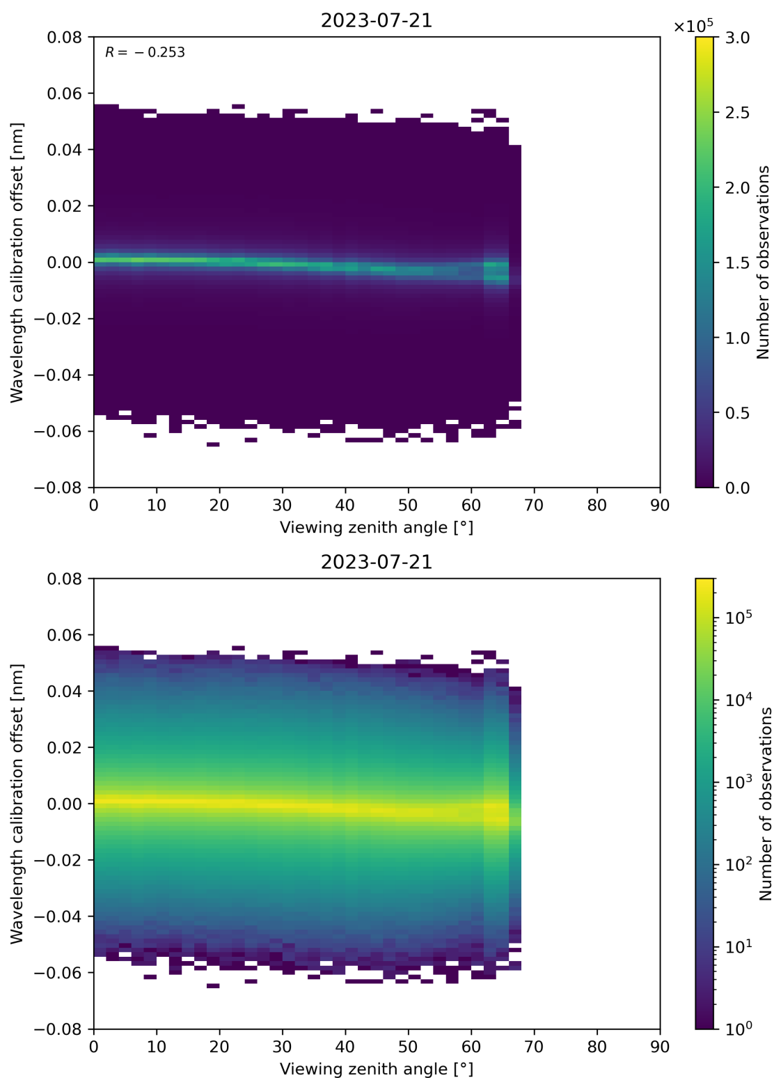
Figure 173: Scatter density plot of “Viewing zenith angle” against “Wavelength calibration offset” for 2023-07-20 to 2023-07-22.
