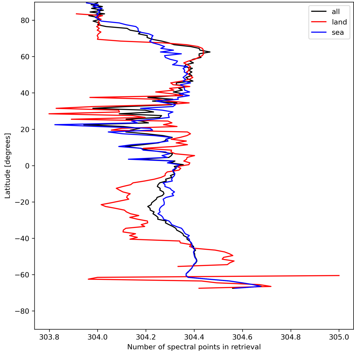
Figure 16: Zonal average of “Number of spectral points in retrieval” for 2023-07-20 to 2023-07-22.
