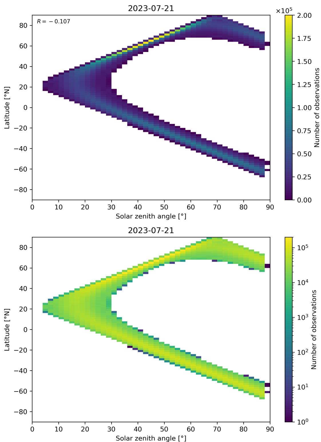
Figure 149: Scatter density plot of “Solar zenith angle” against “Latitude” for 2023-07-20 to 2023-07-22.
