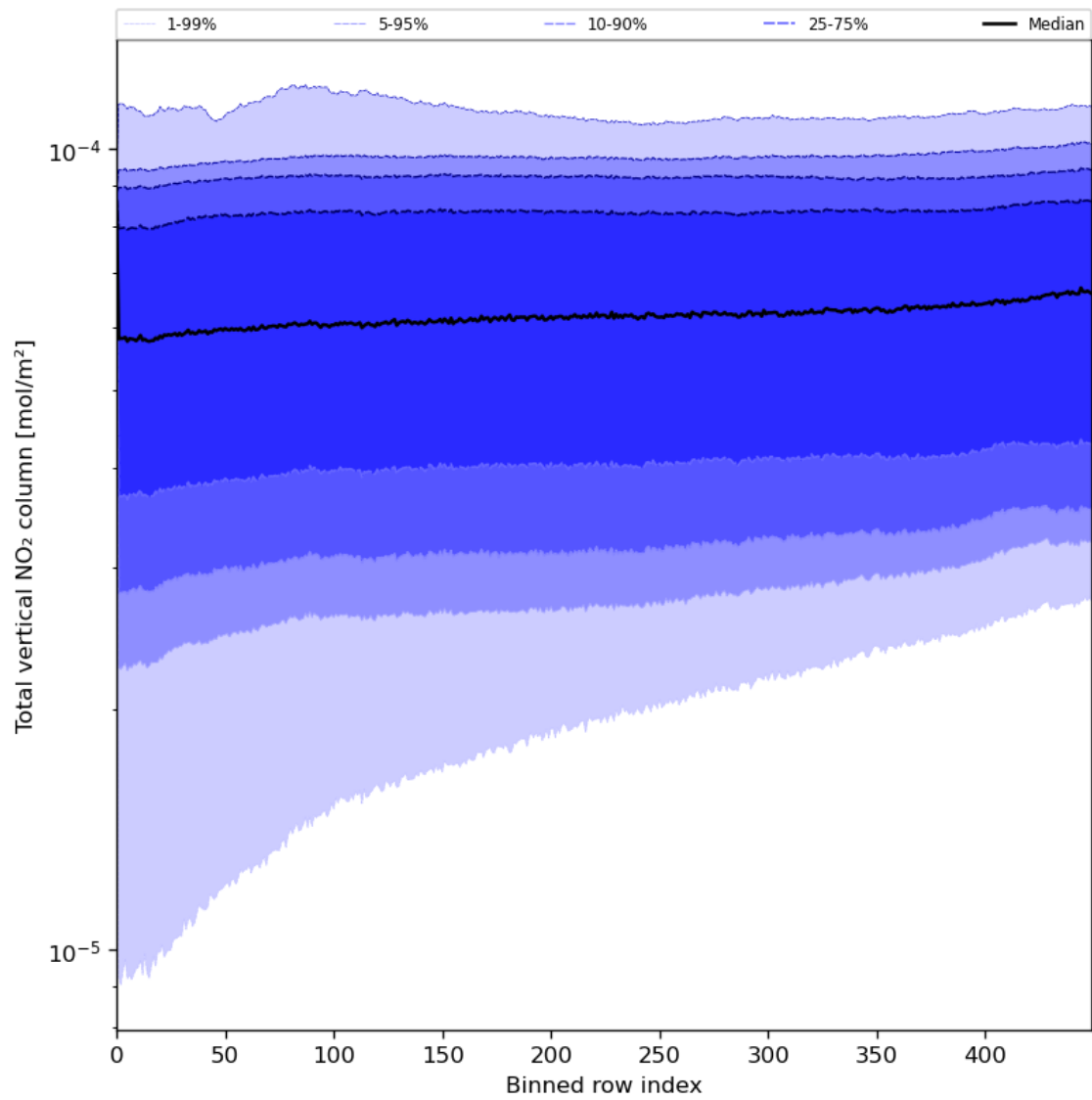
Figure 55: Along track statistics of “Total vertical NO 2 column” for 2023-07-20 to 2023-07-22
