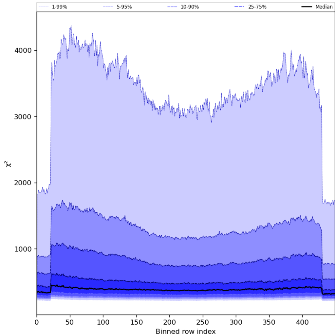
Figure 59: Along track statistics of “ \chi^2 ” for 2023-07-20 to 2023-07-22
