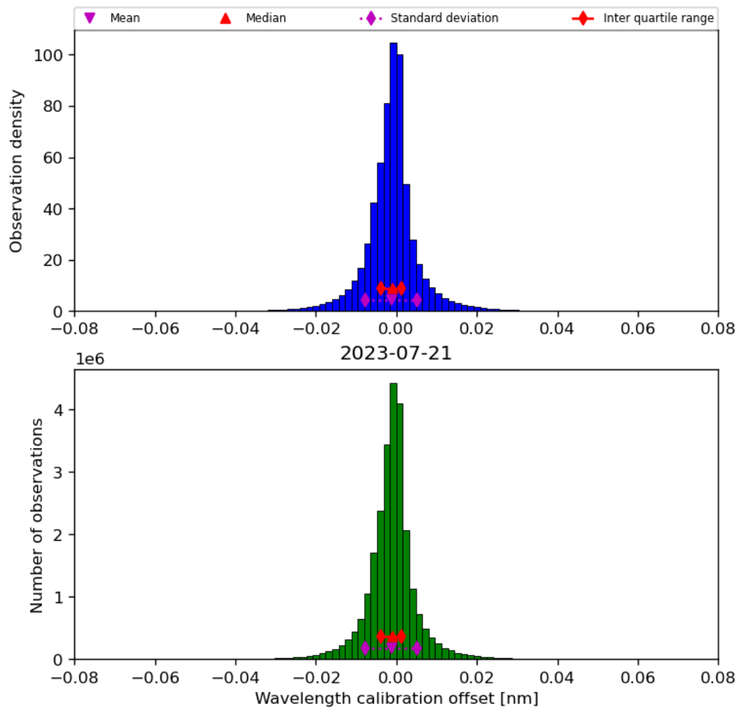
Figure 35: Histogram of “Wavelength calibration offset” for 2023-07-20 to 2023-07-22
