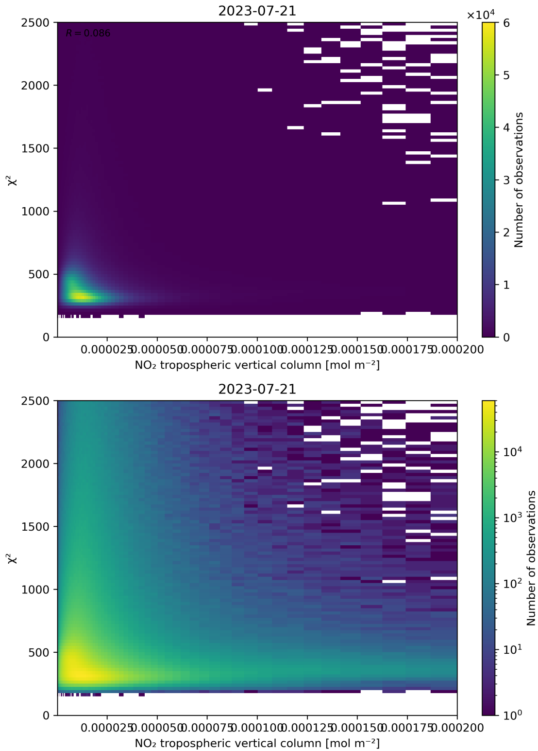
Figure 124: Scatter density plot of “NO 2 tropospheric vertical column” against “ \chi^2 ” for 2023-07-20 to 2023-07-22.
