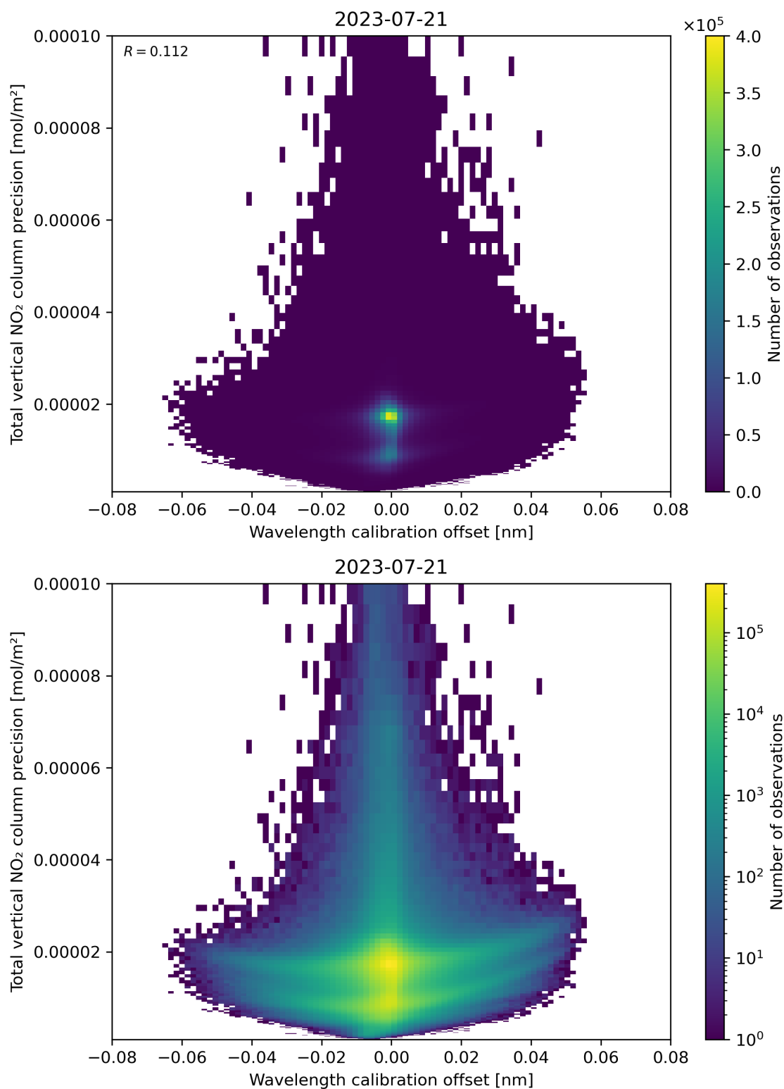
Figure 180: Scatter density plot of “Wavelength calibration offset” against “Total vertical NO 2 column precision” for 2023-07-20 to 2023-07-22.
