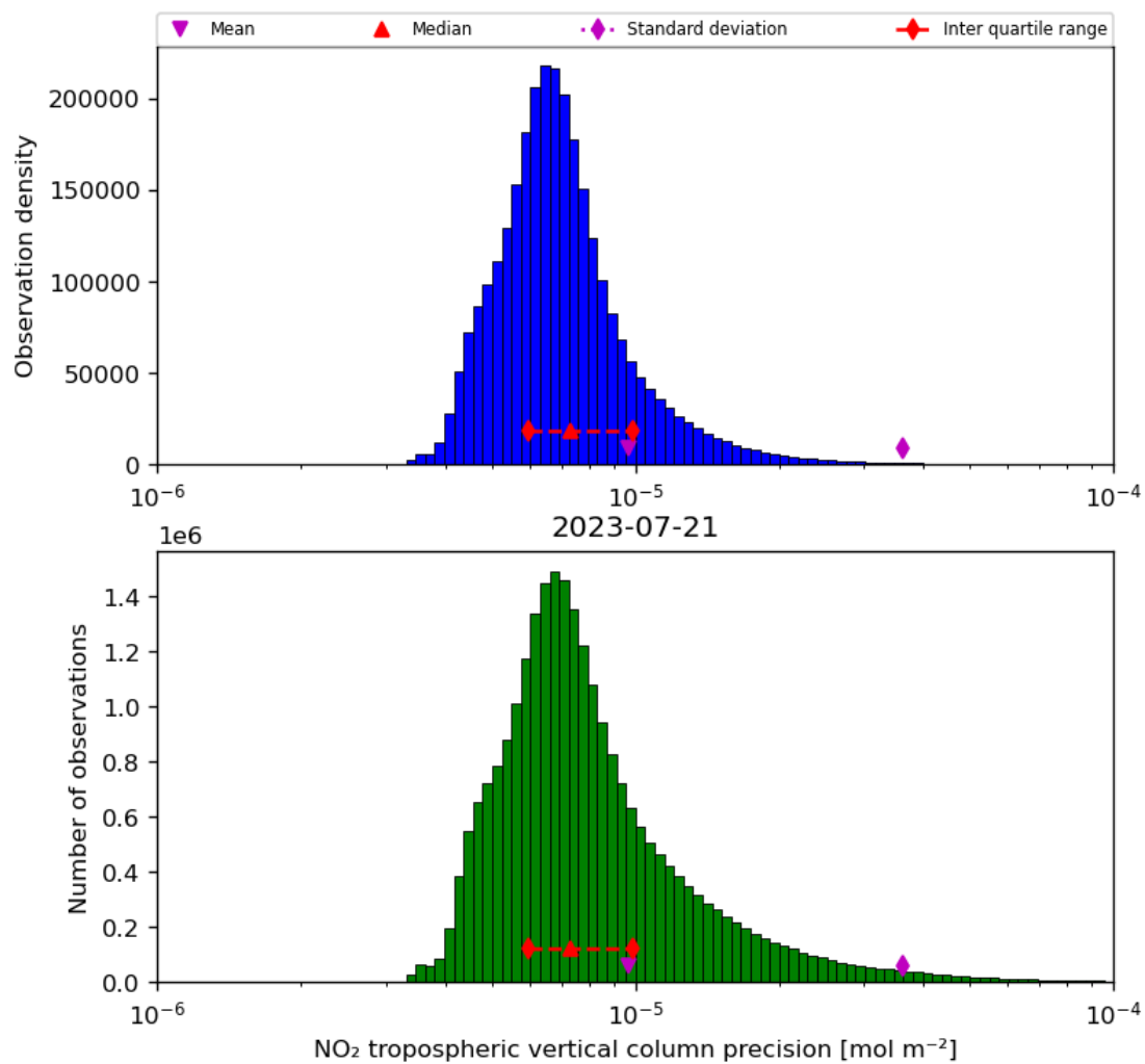
Figure 30: Histogram of “NO 2 tropospheric vertical column precision” for 2023-07-20 to 2023-07-22
