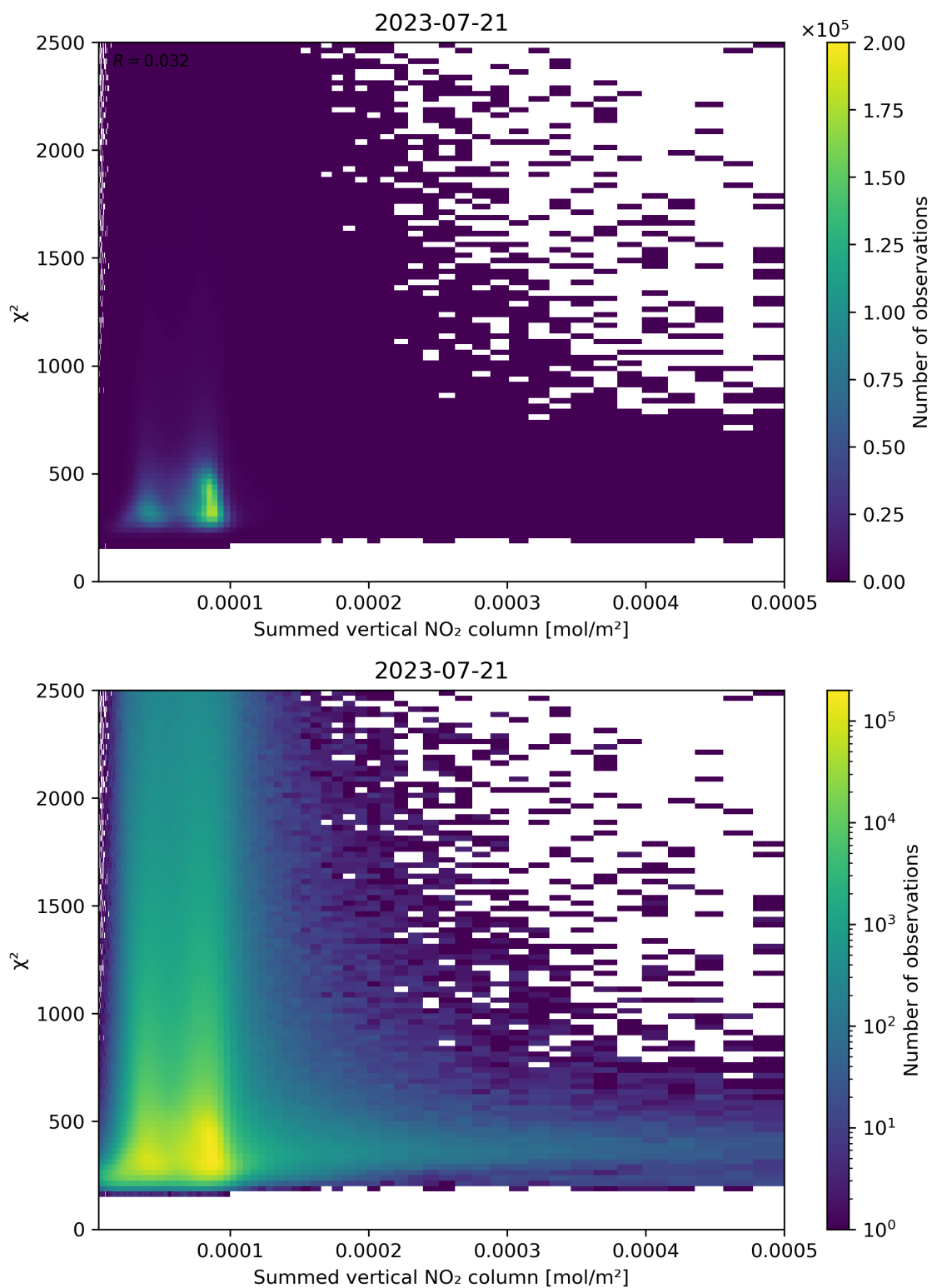
Figure 104: Scatter density plot of “Summed vertical NO 2 column” against “ \chi^2 ” for 2023-07-20 to 2023-07-22.
