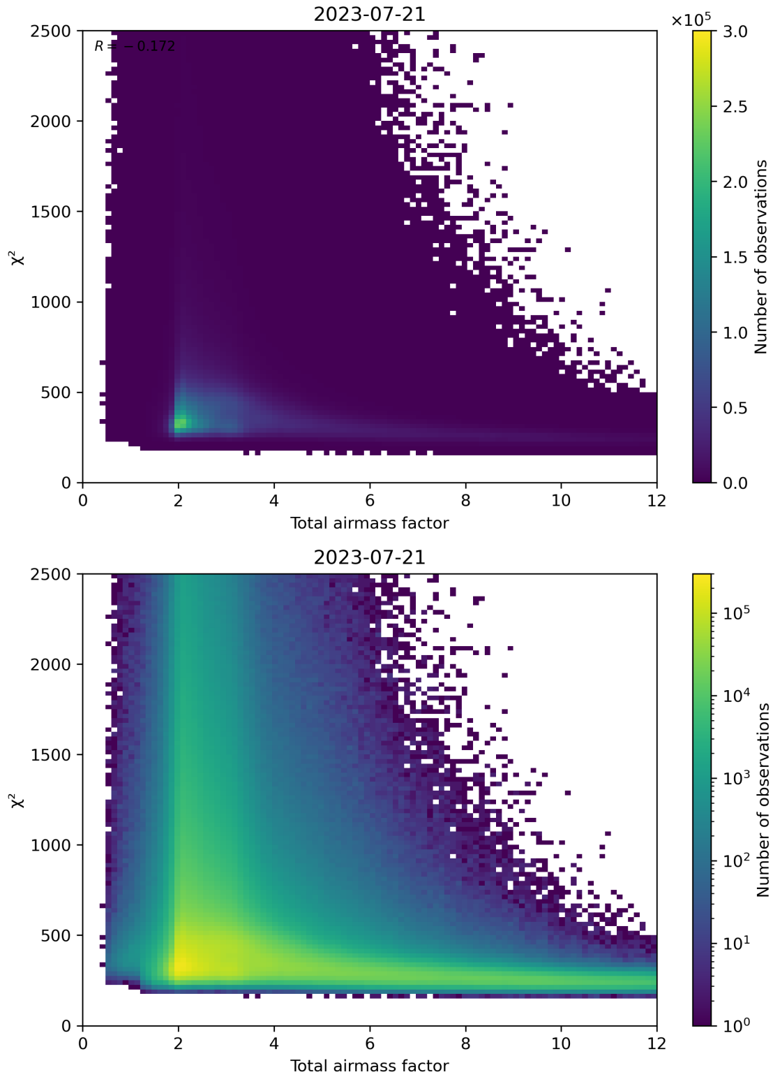
Figure 63: Scatter density plot of “Total airmass factor” against “ \chi^2 ” for 2023-07-20 to 2023-07-22.
