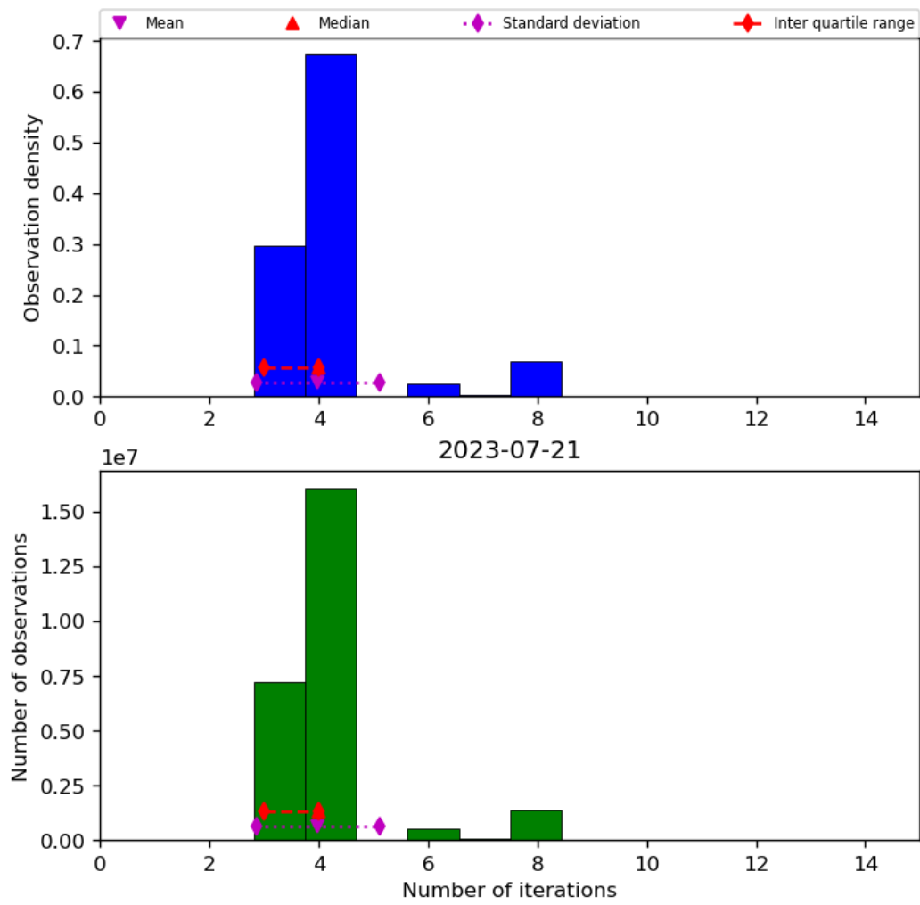
Figure 34: Histogram of “Number of iterations” for 2023-07-20 to 2023-07-22
