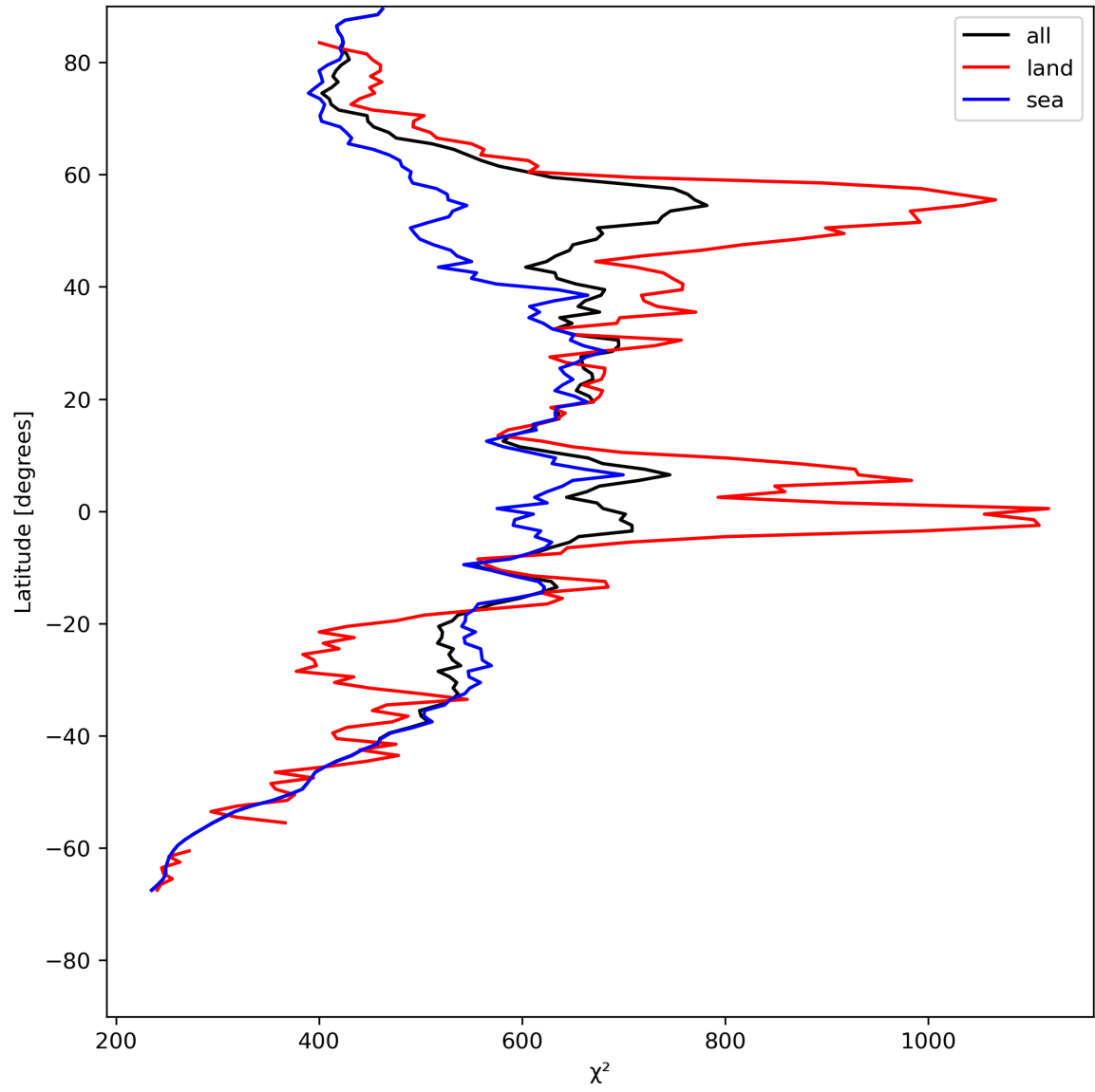
Figure 25: Zonal average of “ \chi^2 ” for 2023-07-20 to 2023-07-22.
