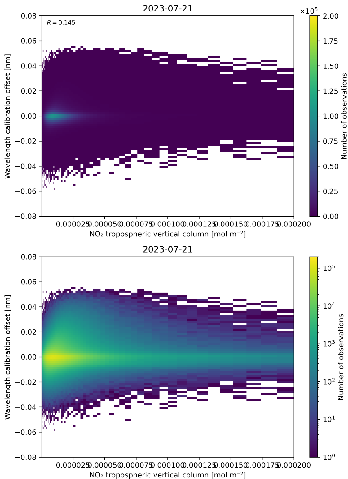
Figure 143: Scatter density plot of “NO 2 tropospheric vertical column” against “Wavelength calibration offset” for 2023-07-20 to 2023-07-22.
