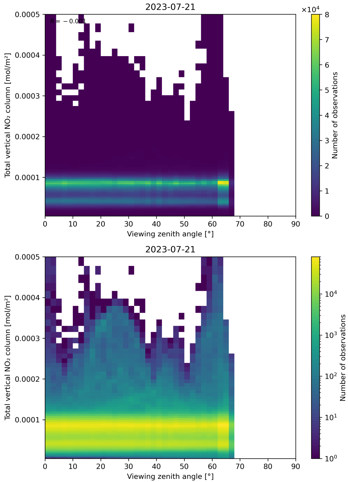
Figure 167: Scatter density plot of “Viewing zenith angle” against “Total vertical NO 2 column” for 2023-07-20 to 2023-07-22.
