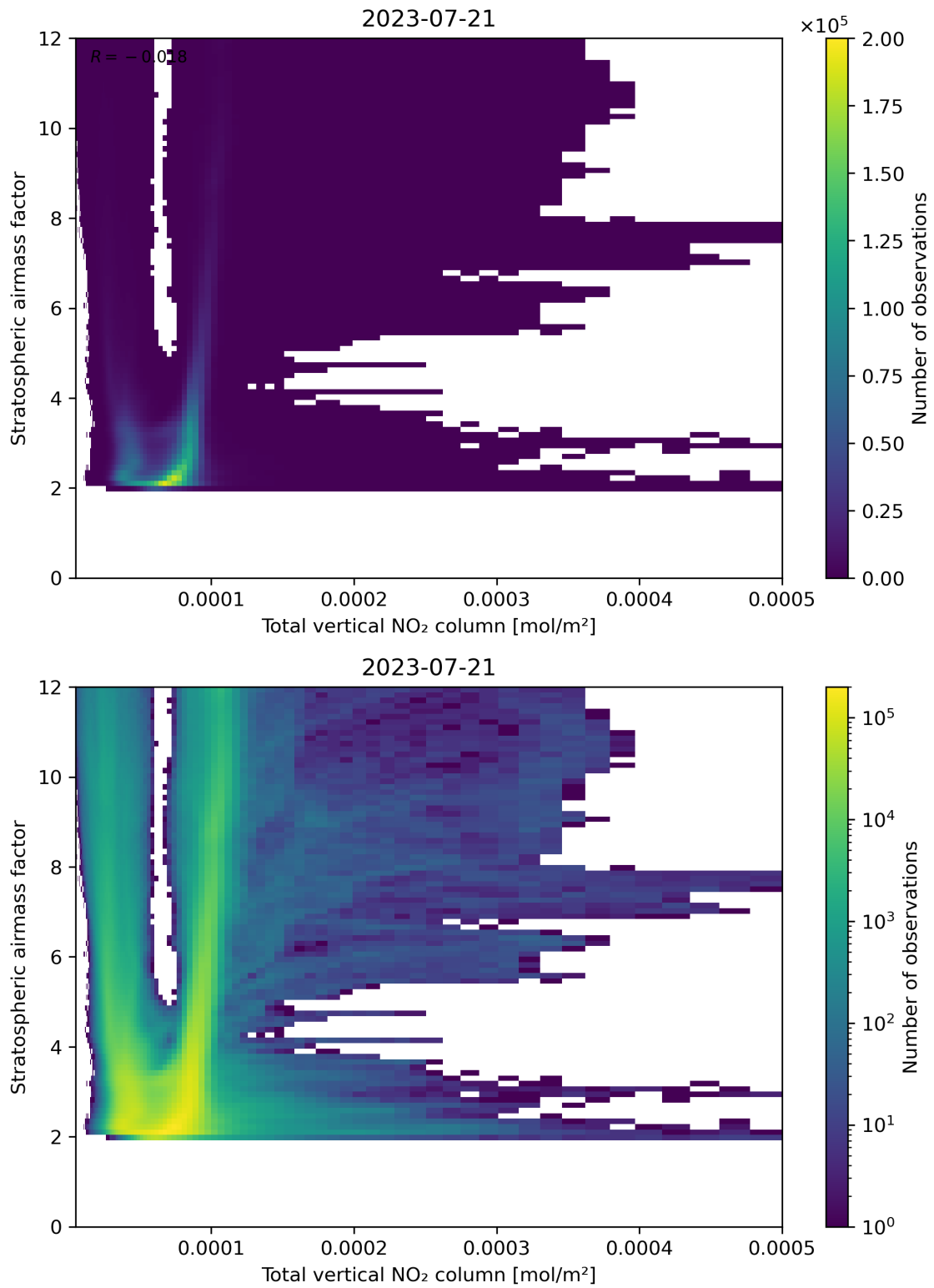
Figure 110: Scatter density plot of “Total vertical NO 2 column” against “Stratospheric airmass factor” for 2023-07-20 to 2023-07-22.
