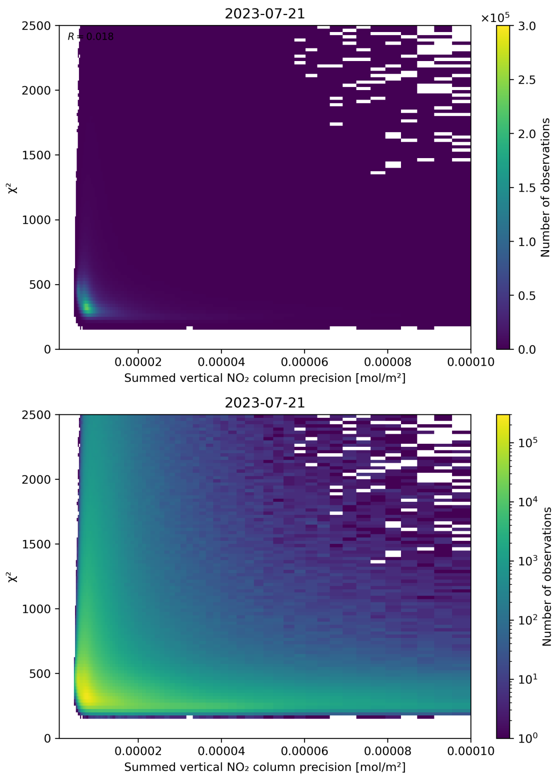
Figure 107: Scatter density plot of “Summed vertical NO 2 column precision” against “ \chi^2 ” for 2023-07-20 to 2023-07-22.
