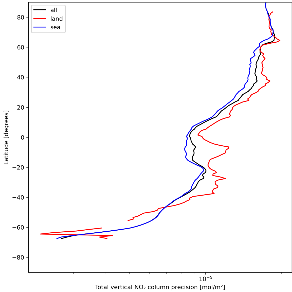
Figure 22: Zonal average of “Total vertical NO 2 column precision” for 2023-07-20 to 2023-07-22.
