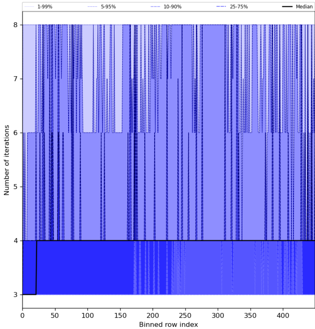
Figure 51: Along track statistics of “Number of iterations” for 2023-07-20 to 2023-07-22
