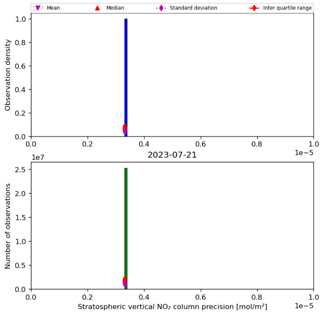
Figure 37: Histogram of “Stratospheric vertical NO 2 column precision” for 2023-07-20 to 2023-07-22
