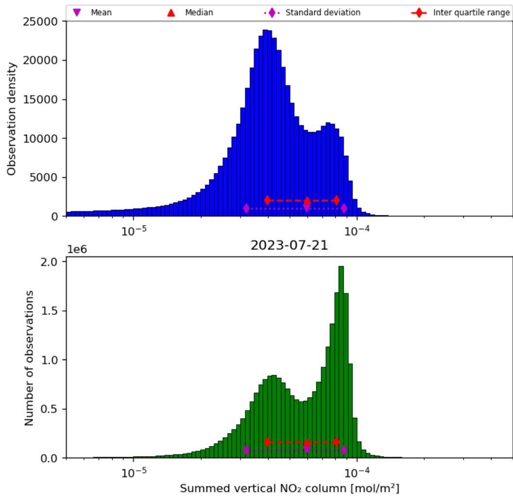
Figure 40: Histogram of “Summed vertical NO 2 column” for 2023-07-20 to 2023-07-22
