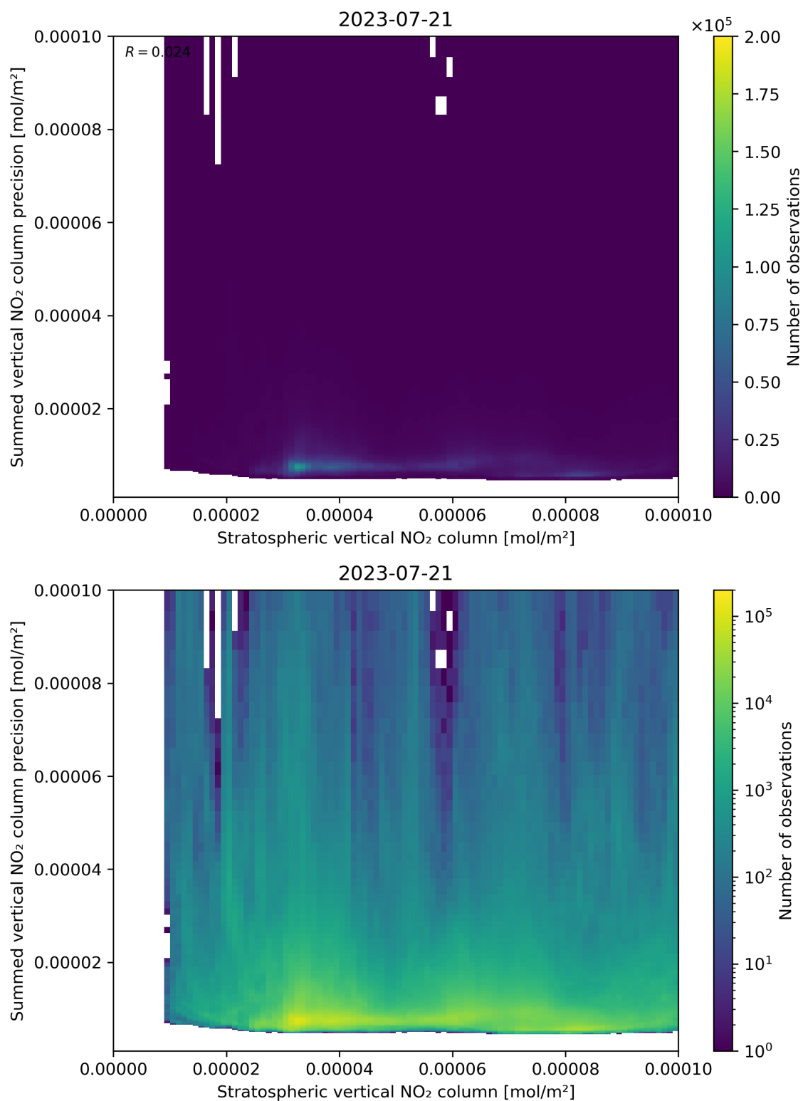
Figure 99: Scatter density plot of “Stratospheric vertical NO 2 column” against “Summed vertical NO 2 column precision” for 2023-07-20 to 2023-07-22.
