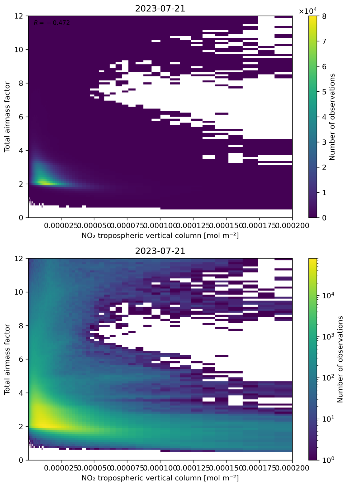
Figure 122: Scatter density plot of “NO 2 tropospheric vertical column” against “Total air mass factor” for 2023-07-20 to 2023-07-22.
