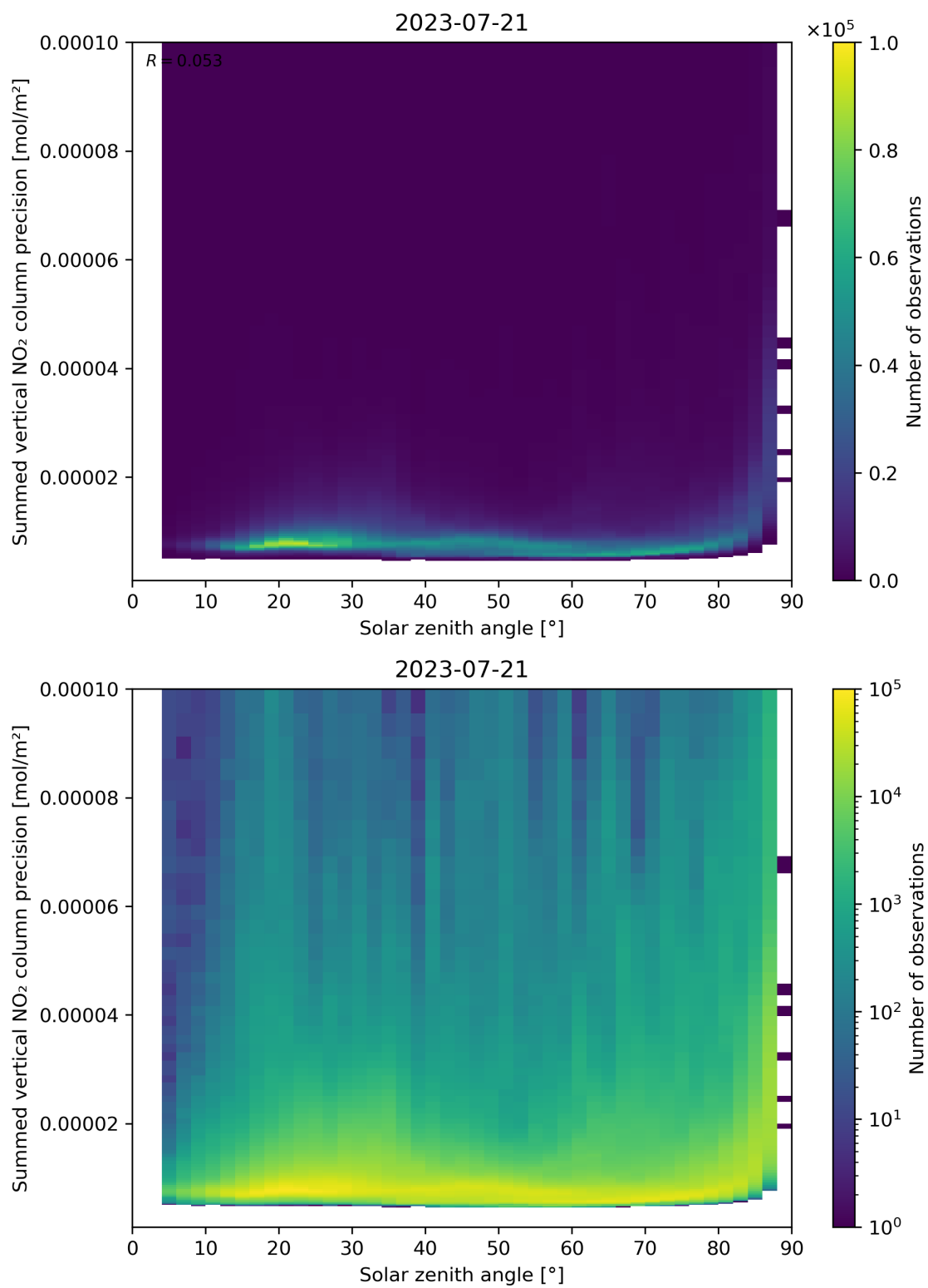
Figure 152: Scatter density plot of “Solar zenith angle” against “Summed vertical NO 2 column precision” for 2023-07-20 to 2023-07-22.
