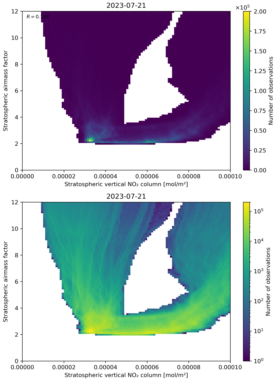
Figure 96: Scatter density plot of “Stratospheric vertical NO 2 column” against “Stratospheric airmass factor” for 2023-07-20 to 2023-07-22.
