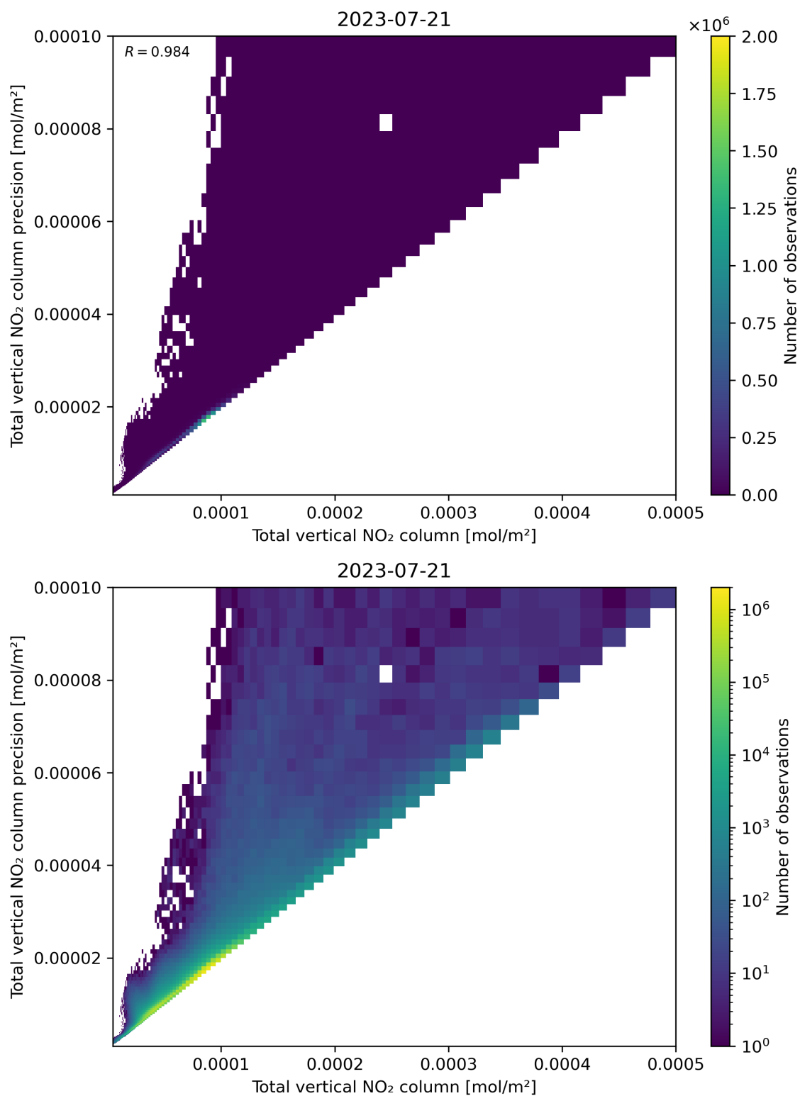
Figure 114: Scatter density plot of “Total vertical NO 2 column” against “Total vertical NO 2 column precision” for 2023-07-20 to 2023-07-22.
