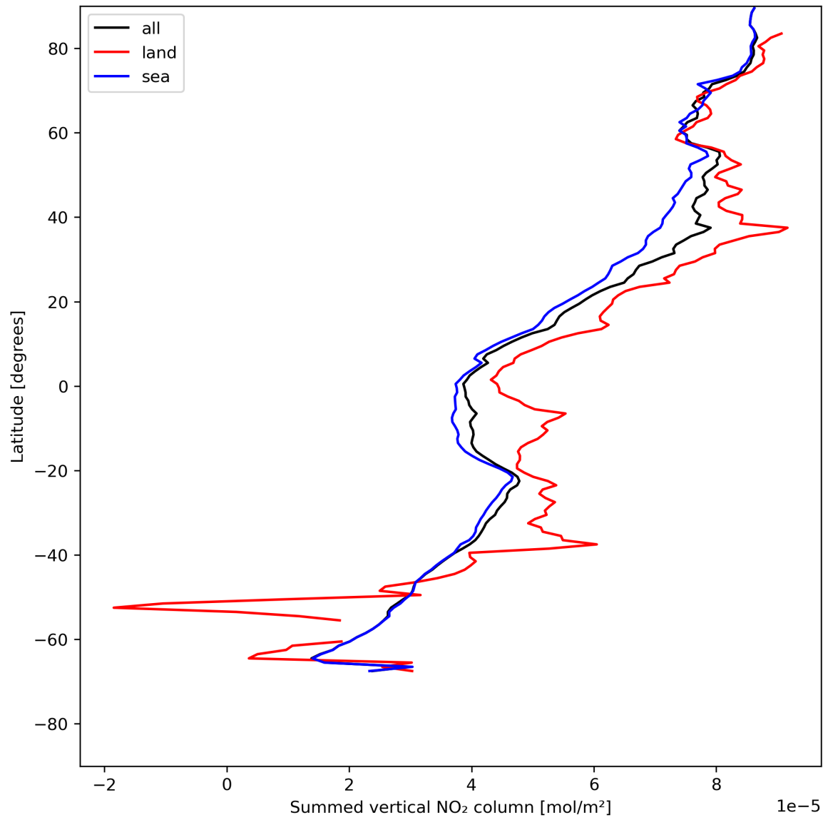
Figure 23: Zonal average of “Summed vertical NO 2 column” for 2023-07-20 to 2023-07-22.
