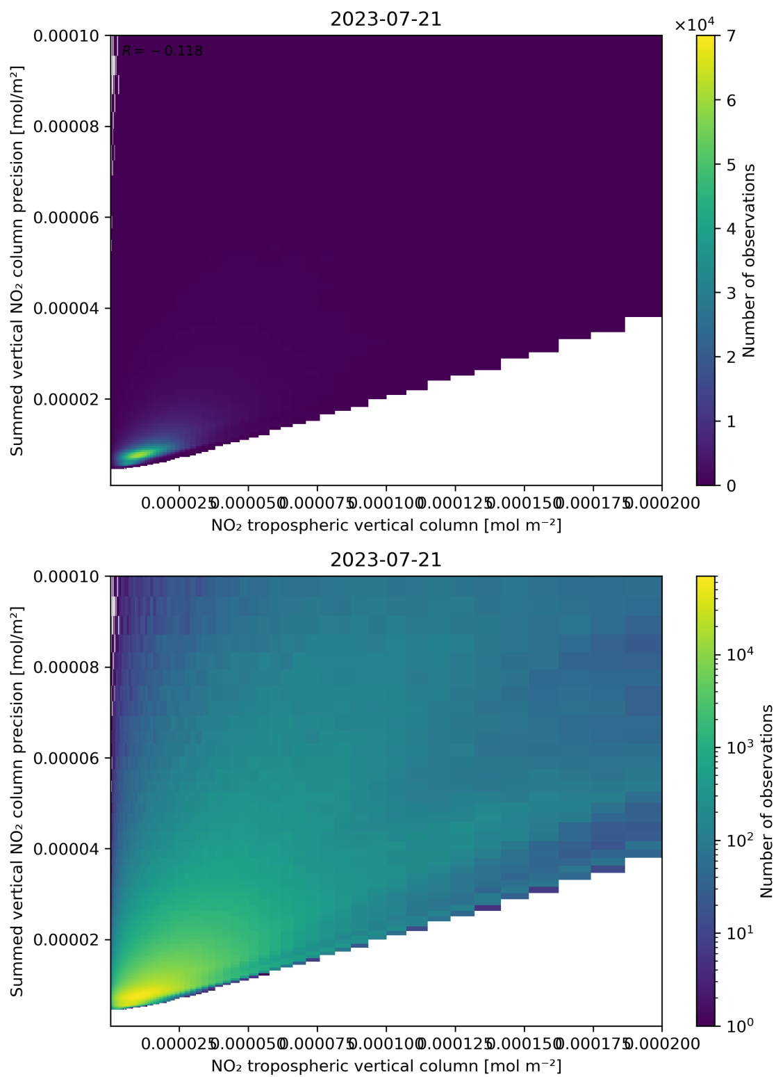
Figure 127: Scatter density plot of “NO 2 tropospheric vertical column” against “Summed vertical NO 2 column precision” for 2023-07-20 to 2023-07-22.
