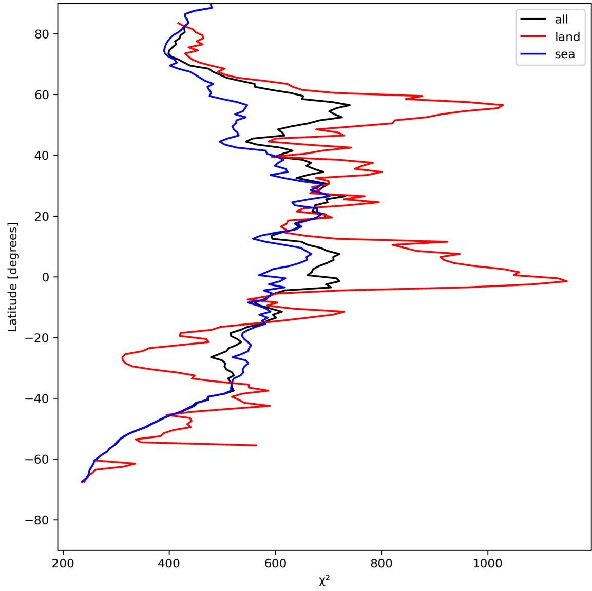
Figure 25: Zonal average of “ \chi^2 ” for 2023-07-21 to 2023-07-23.
