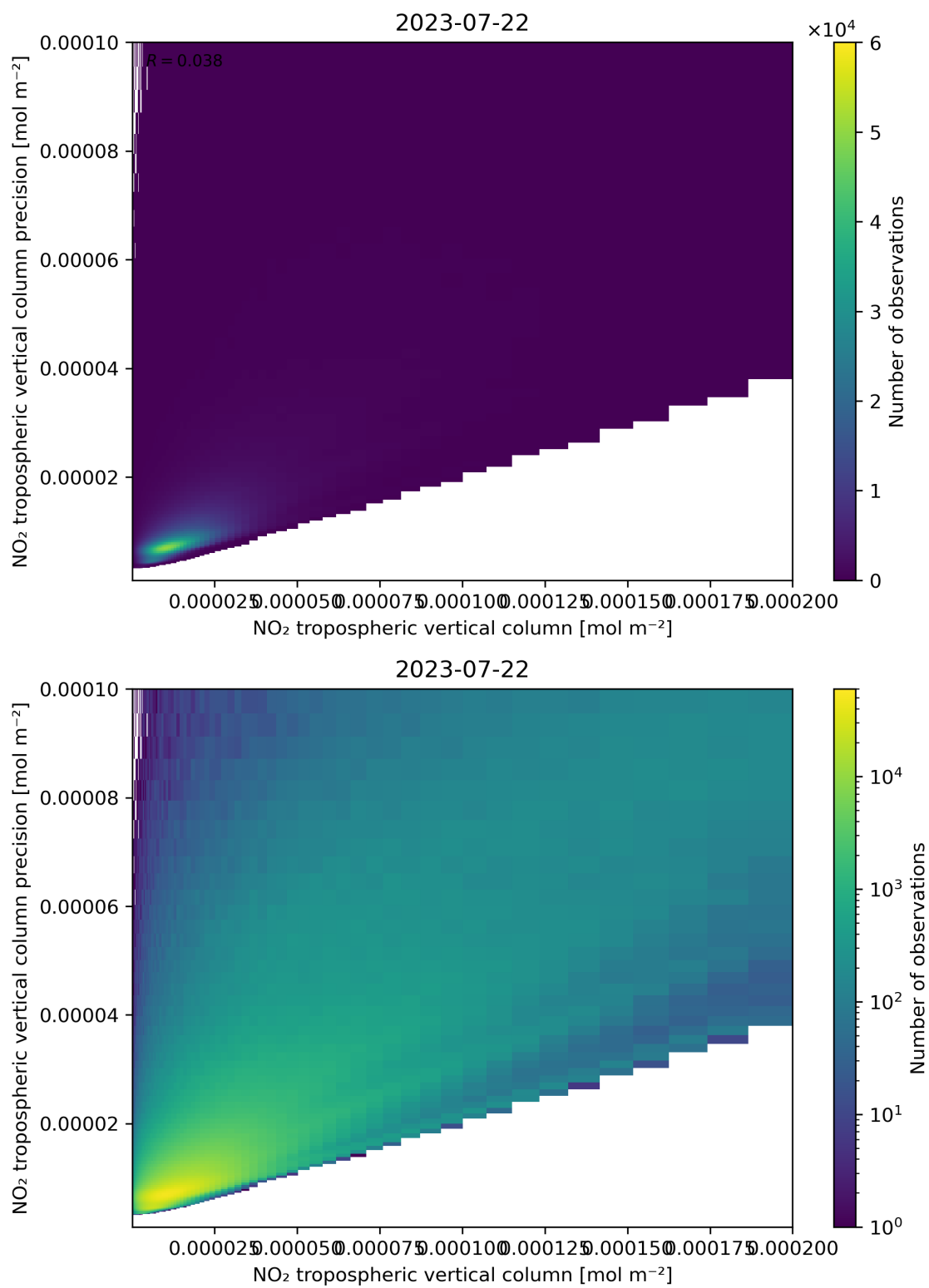
Figure 130: Scatter density plot of “NO 2 tropospheric vertical column” against “NO 2 tropospheric vertical column precision” for 2023-07-21 to 2023-07-23.
