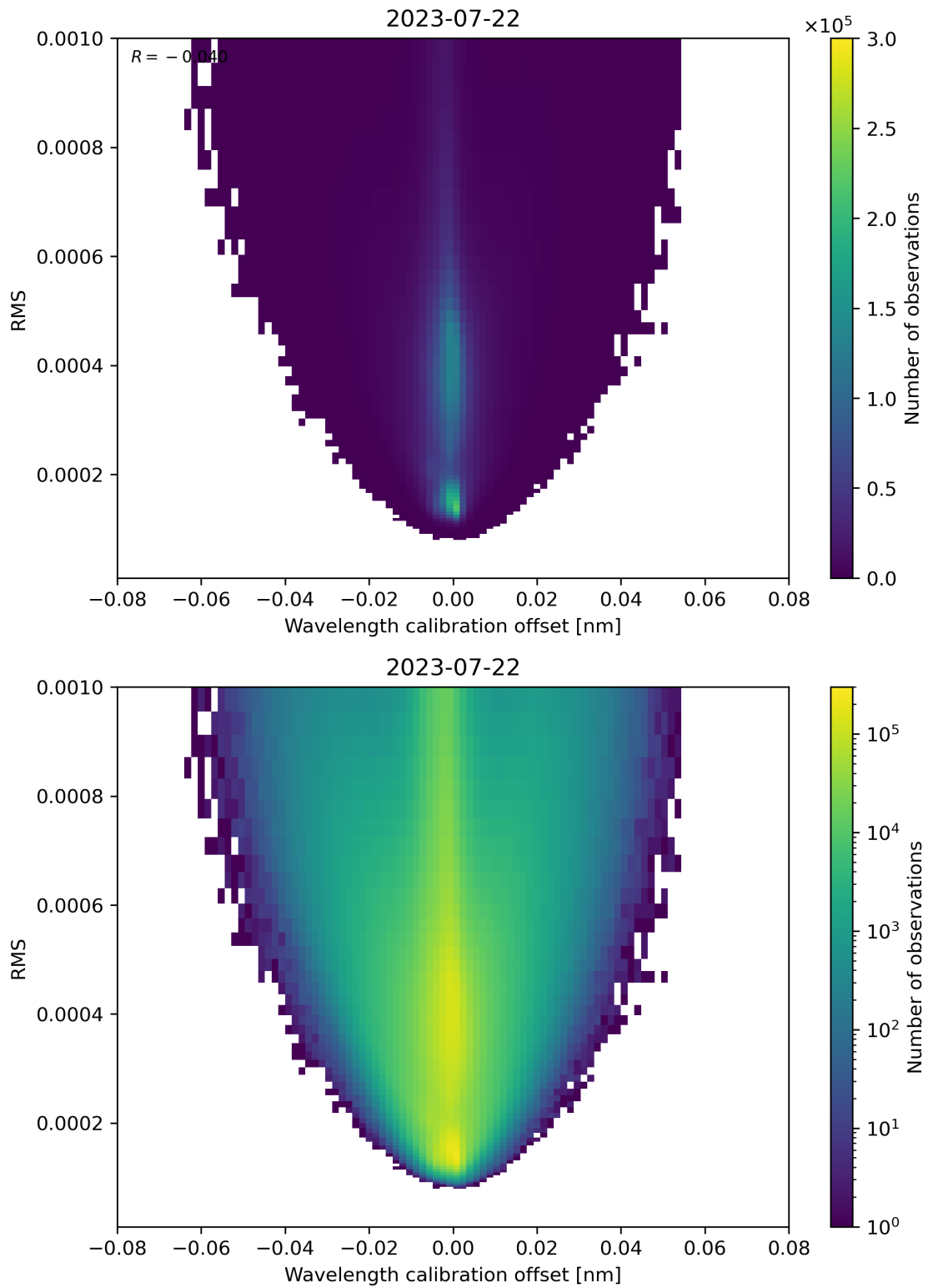
Figure 181: Scatter density plot of “Wavelength calibration offset” against “RMS” for 2023-07-21 to 2023-07-23.
