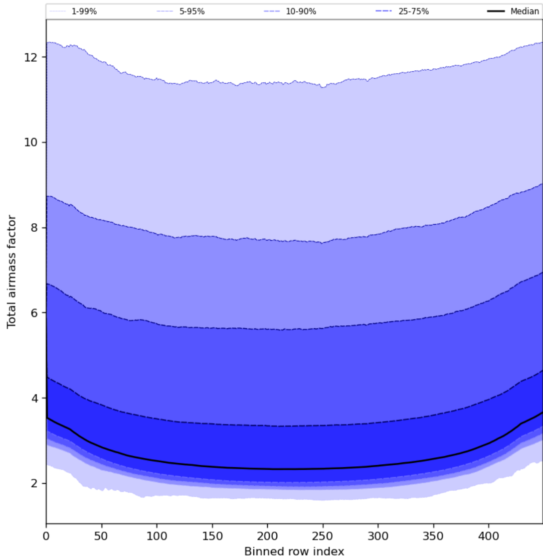
Figure 49: Along track statistics of “Total airmass factor” for 2023-07-21 to 2023-07-23
