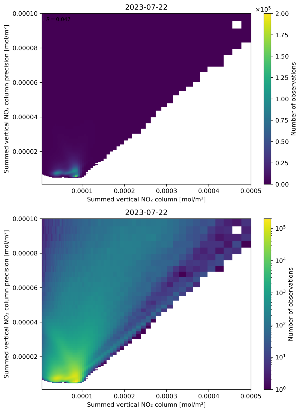
Figure 105: Scatter density plot of “Summed vertical NO 2 column” against “Summed vertical NO 2 column precision” for 2023-07-21 to 2023-07-23.
