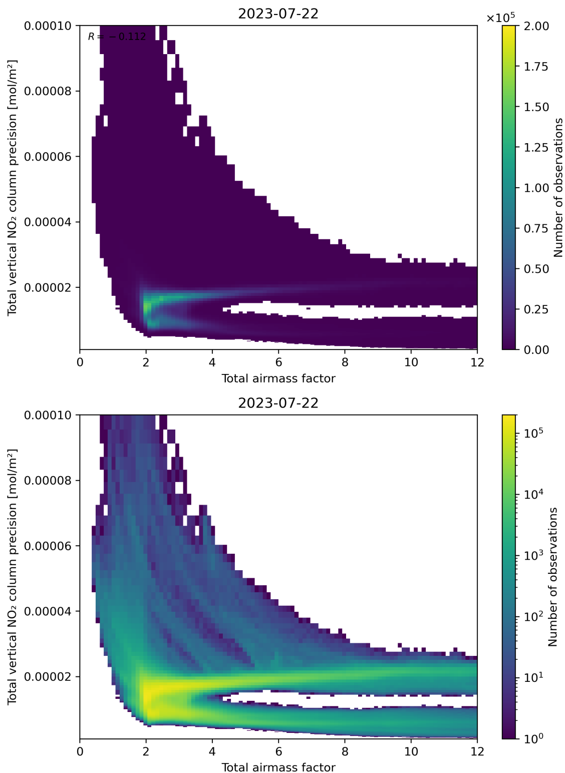
Figure 68: Scatter density plot of “Total airmass factor” against “Total vertical NO 2 column precision” for 2023-07-21 to 2023-07-23.
