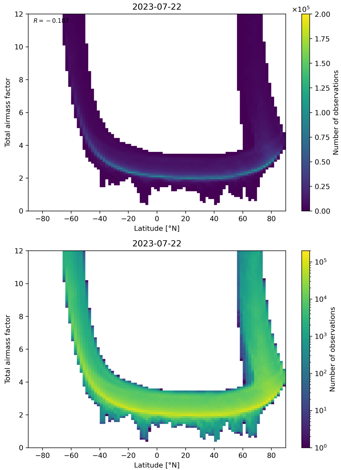
Figure 84: Scatter density plot of “Latitude” against “Total airmass factor” for 2023-07-21 to 2023-07-23.
