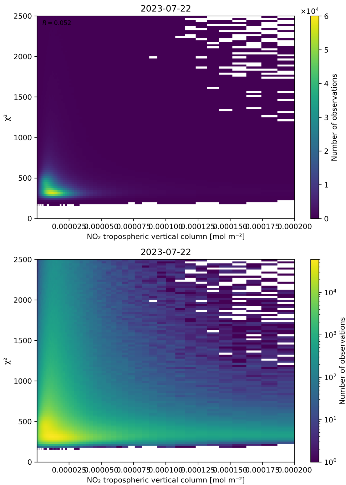
Figure 124: Scatter density plot of “NO 2 tropospheric vertical column” against “ \chi^2 ” for 2023-07-21 to 2023-07-23.
