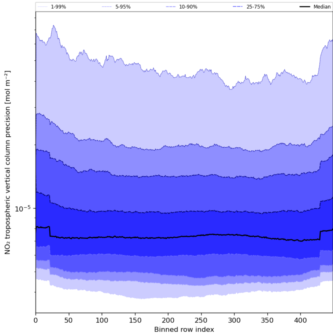
Figure 47: Along track statistics of “NO 2 tropospheric vertical column precision” for 2023-07-21 to 2023-07-23
