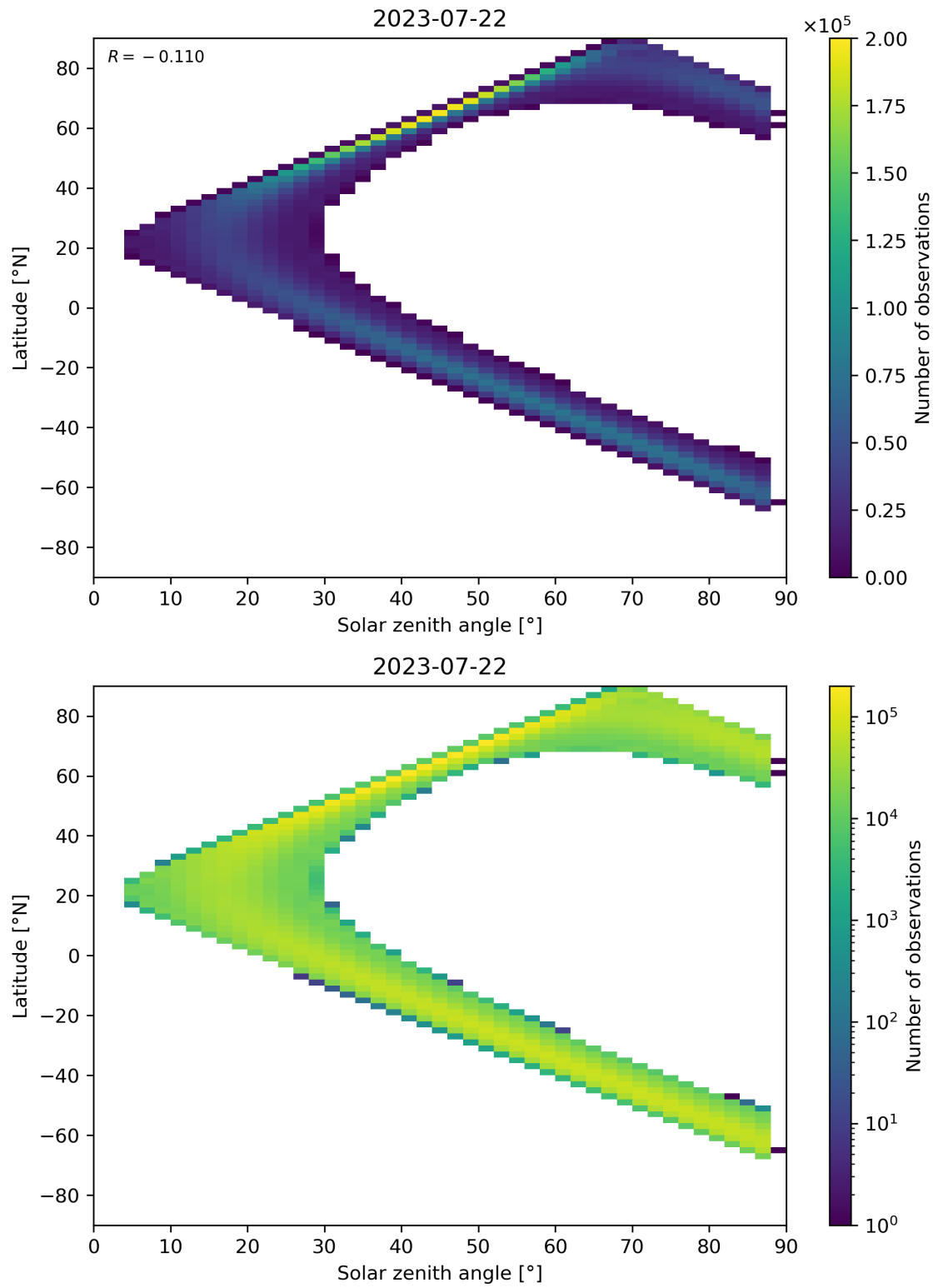
Figure 149: Scatter density plot of “Solar zenith angle” against “Latitude” for 2023-07-21 to 2023-07-23.
