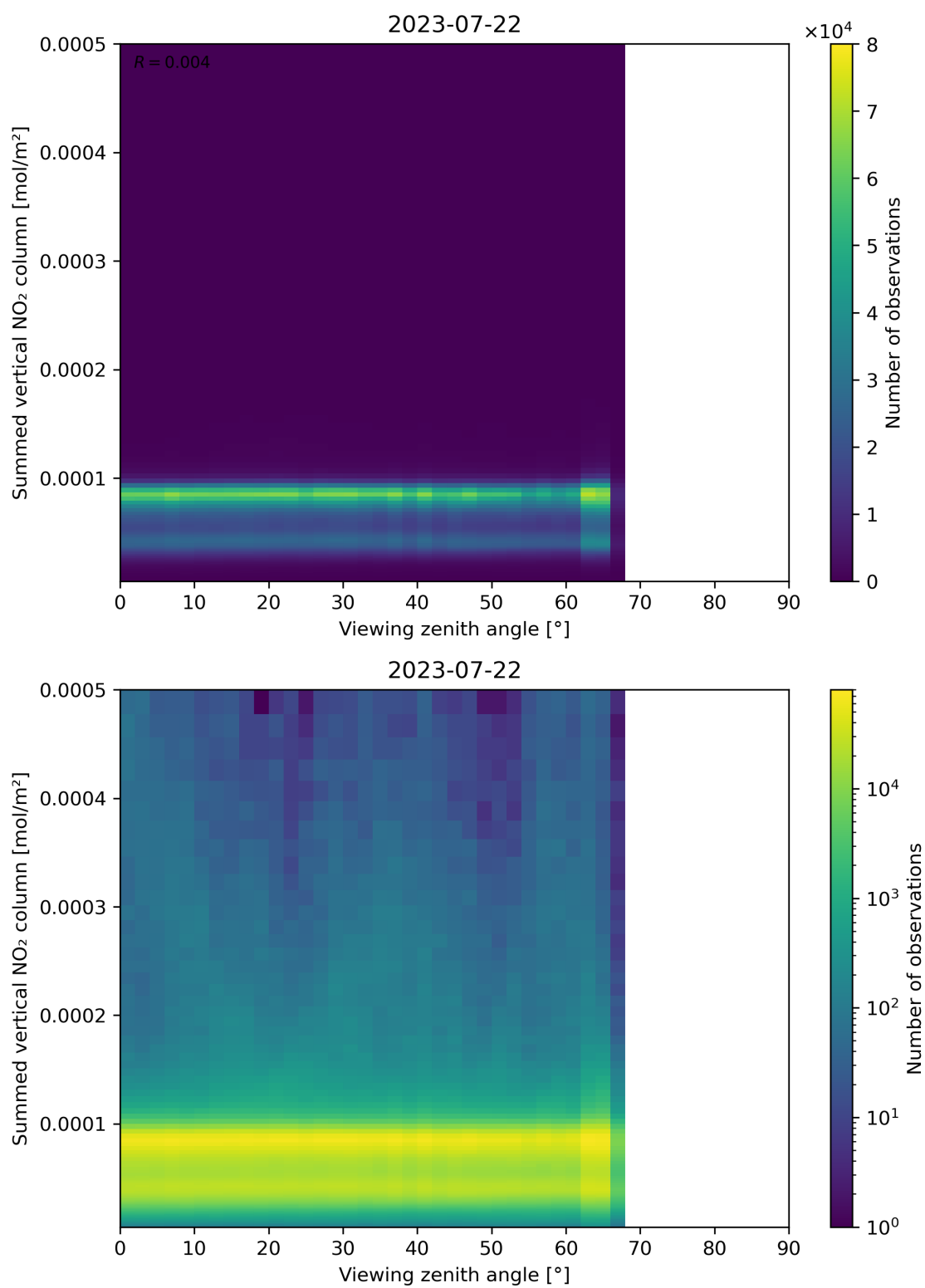
Figure 165: Scatter density plot of “Viewing zenith angle” against “Summed vertical NO 2 column” for 2023-07-21 to 2023-07-23.
