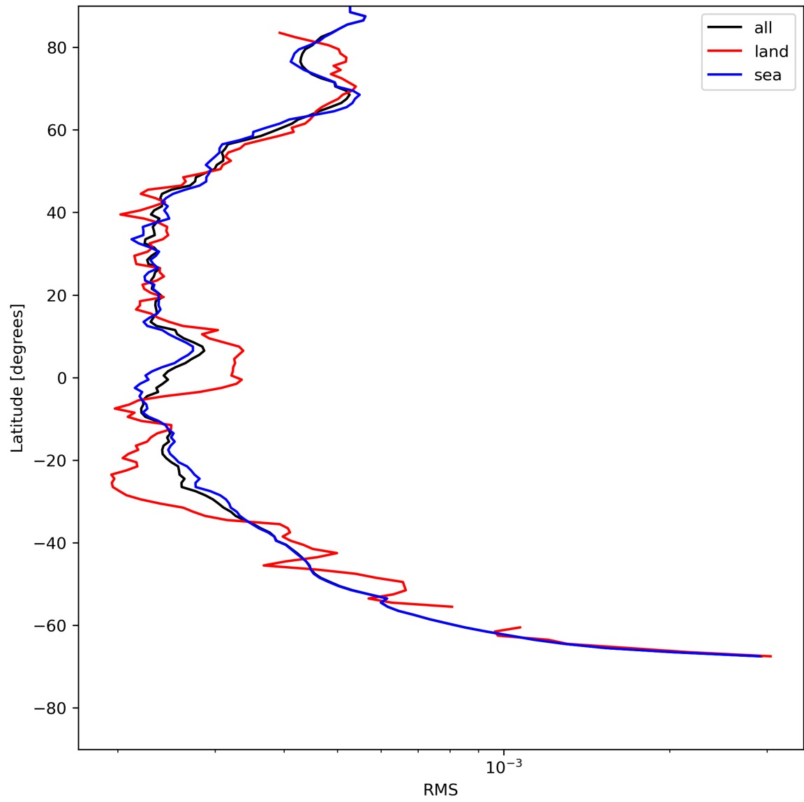
Figure 26: Zonal average of “RMS” for 2023-07-21 to 2023-07-23.
