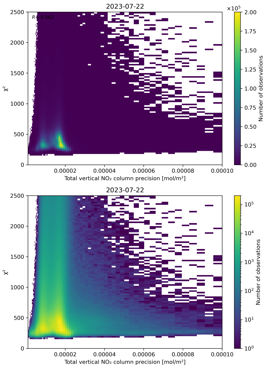
Figure 116: Scatter density plot of “Total vertical NO 2 column precision” against “ \chi^2 ” for 2023-07-21 to 2023-07-23.
