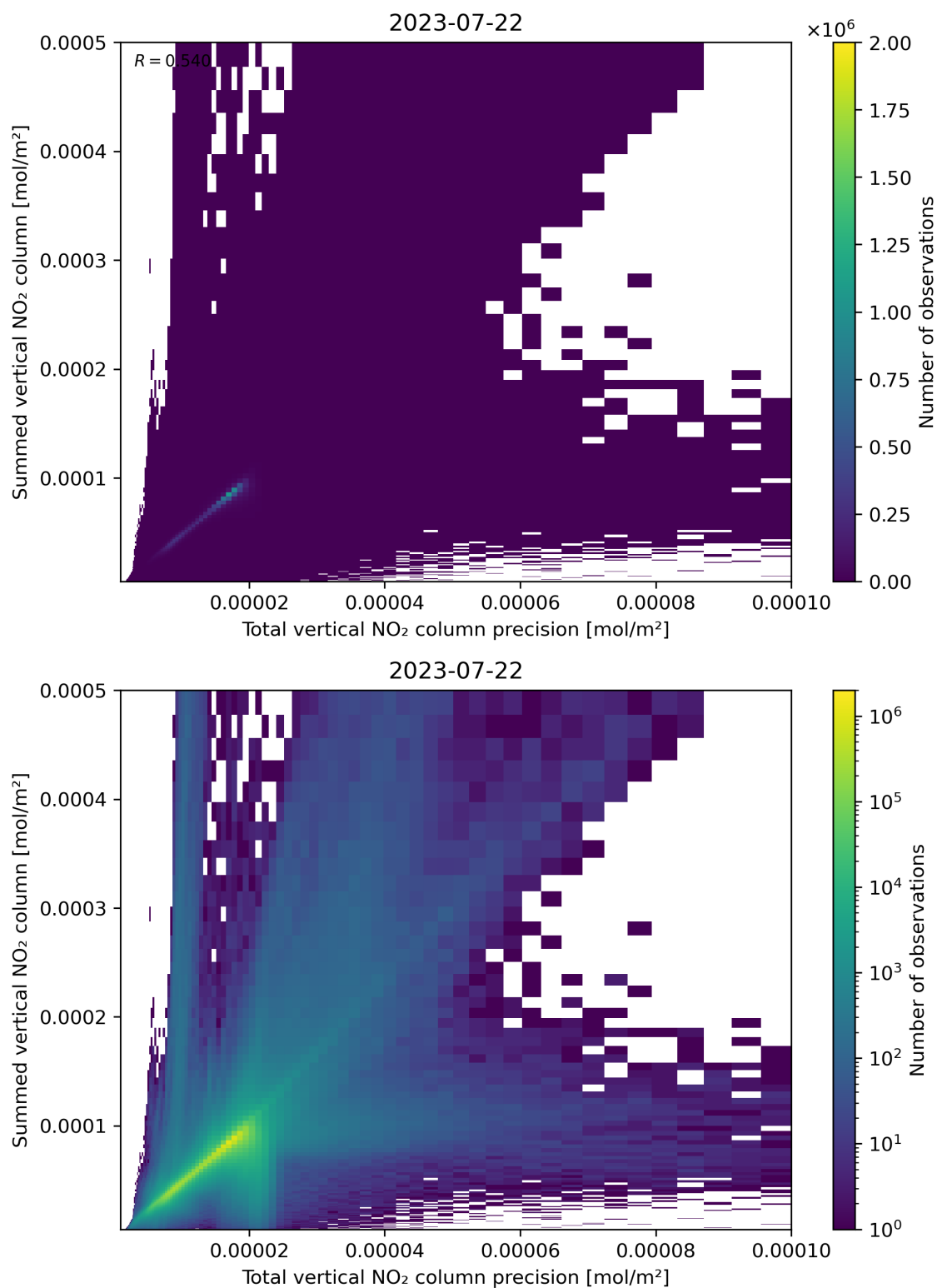
Figure 117: Scatter density plot of “Total vertical NO 2 column precision” against “Summed vertical NO 2 column” for 2023-07-21 to 2023-07-23.
