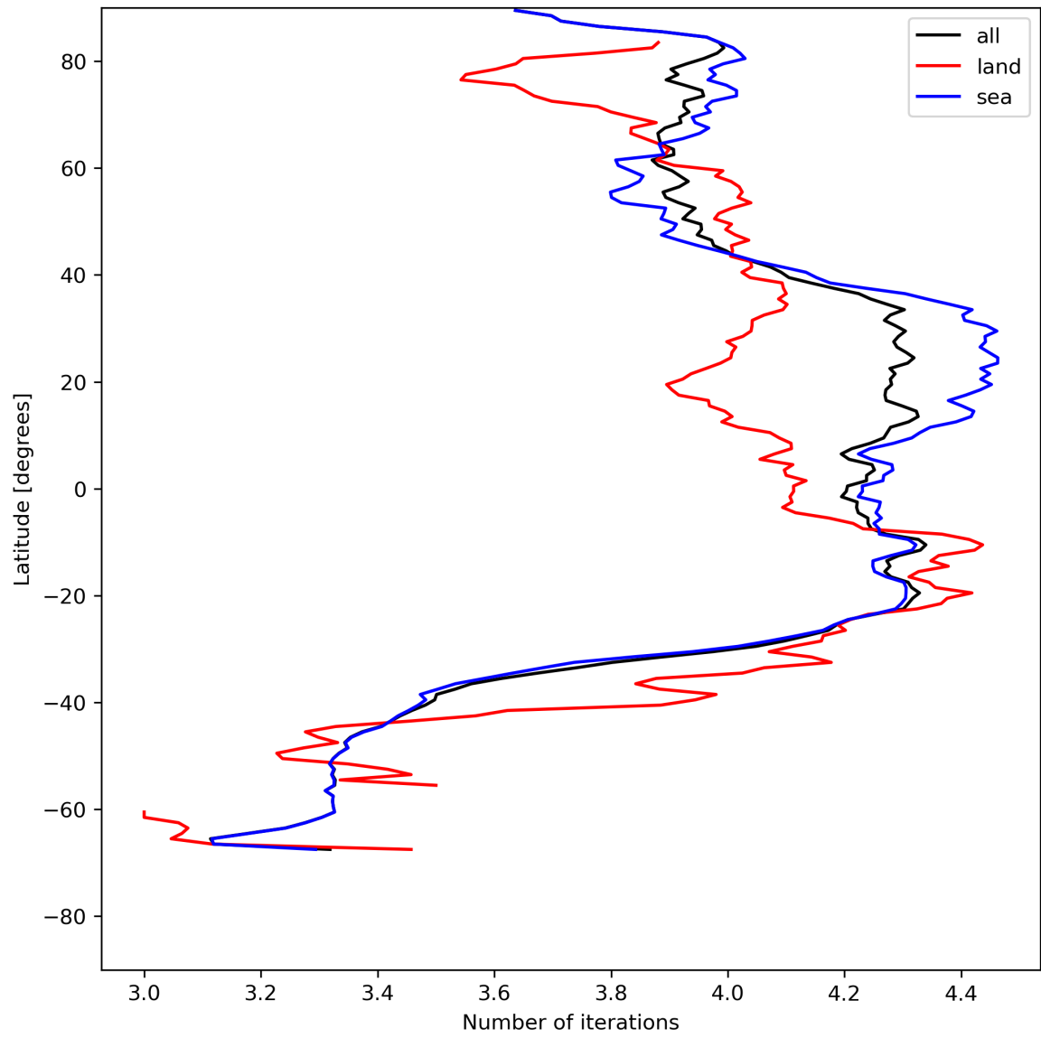
Figure 17: Zonal average of “Number of iterations” for 2023-07-21 to 2023-07-23.
