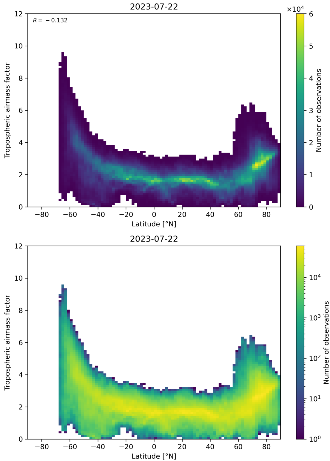
Figure 85: Scatter density plot of “Latitude” against “Tropospheric airmass factor” for 2023-07-21 to 2023-07-23.
