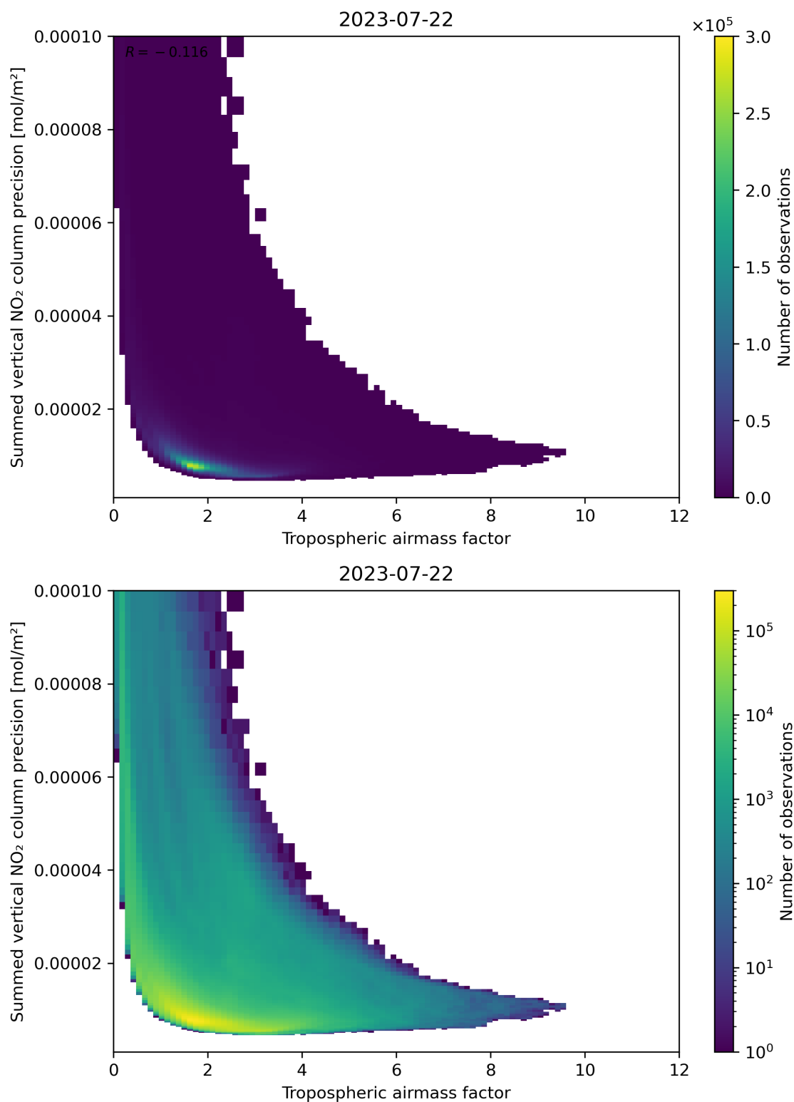
Figure 76: Scatter density plot of “Tropospheric air mass factor” against “Summed vertical NO 2 column precision” for 2023-07-21 to 2023-07-23.
