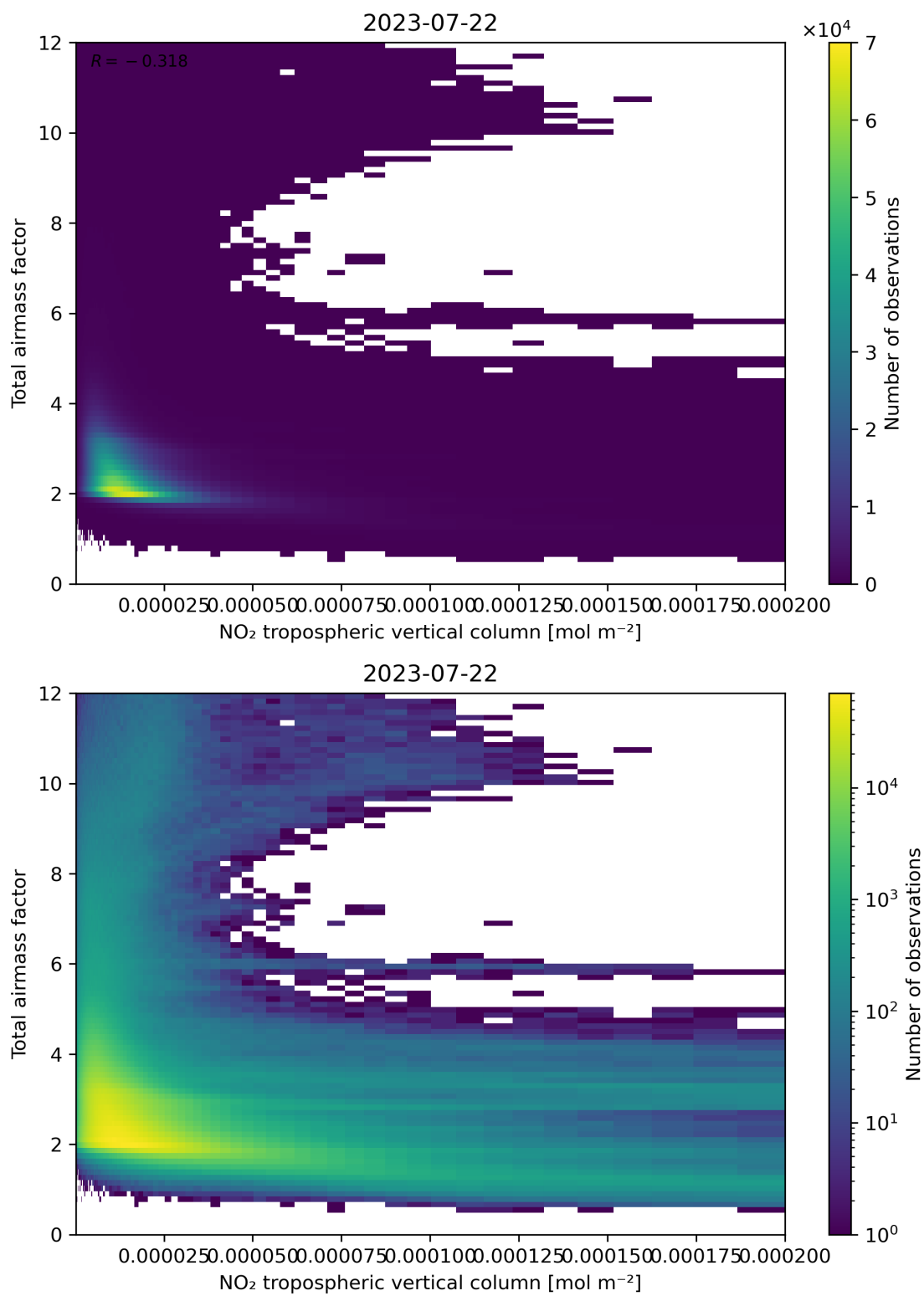
Figure 122: Scatter density plot of “NO 2 tropospheric vertical column” against “Total air mass factor” for 2023-07-21 to 2023-07-23.
