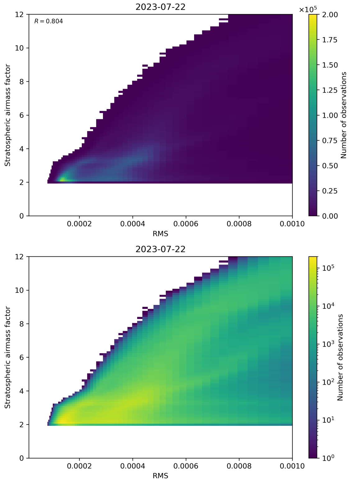
Figure 144: Scatter density plot of “RMS” against “Stratospheric airmass factor” for 2023-07-21 to 2023-07-23.
