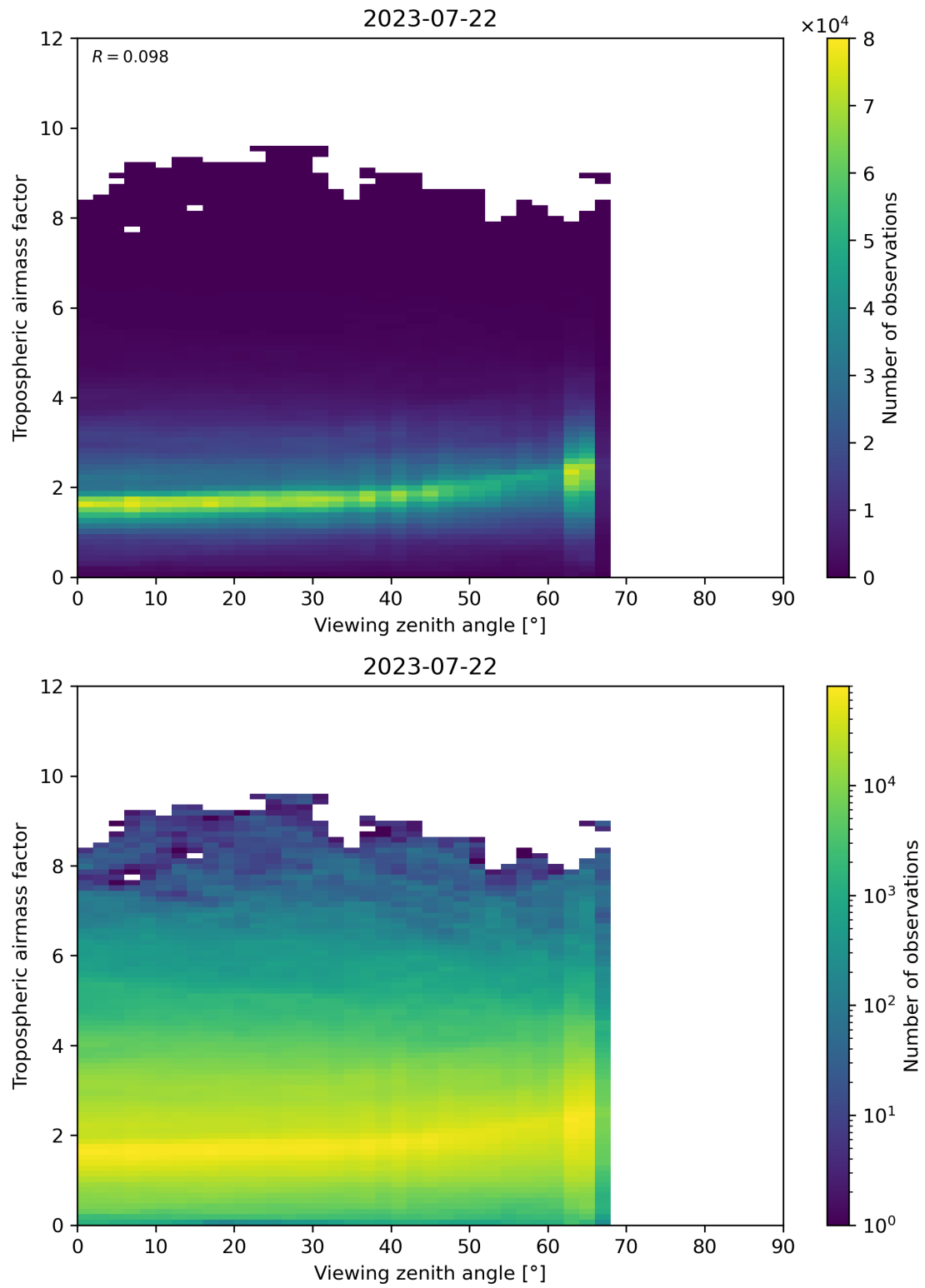
Figure 161: Scatter density plot of “Viewing zenith angle” against “Tropospheric airmass factor” for 2023-07-21 to 2023-07-23.
