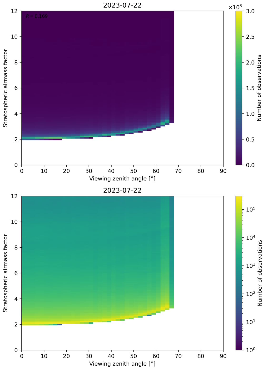
Figure 159: Scatter density plot of “Viewing zenith angle” against “Stratospheric airmass factor” for 2023-07-21 to 2023-07-23.
