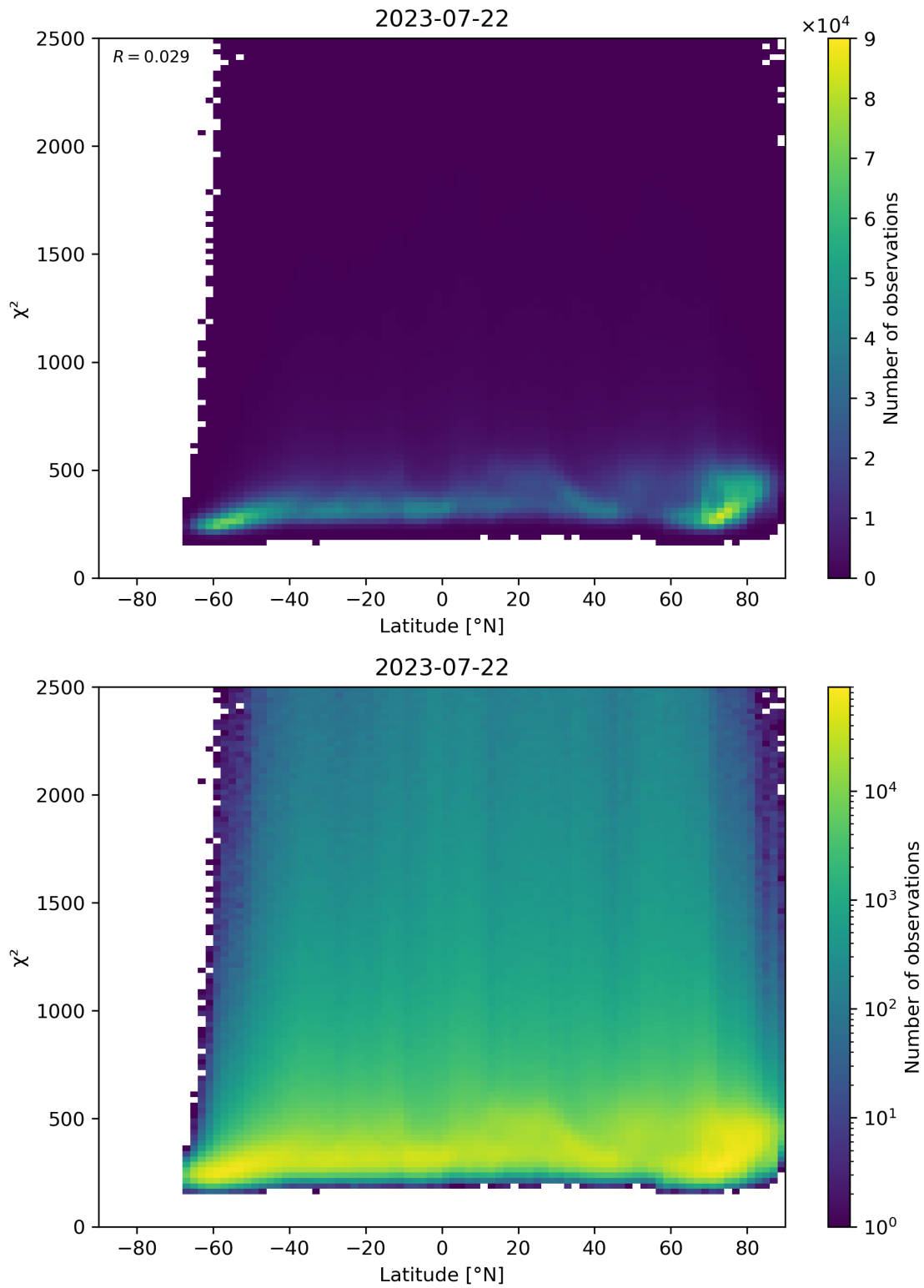
Figure 86: Scatter density plot of “Latitude” against “ \chi^2 ” for 2023-07-21 to 2023-07-23.
