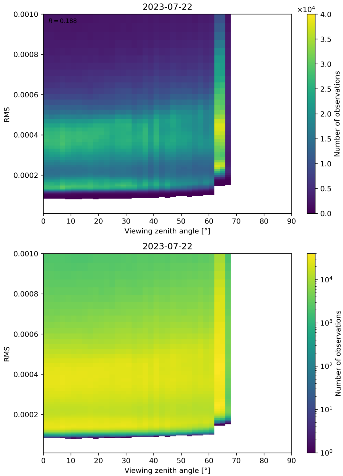
Figure 171: Scatter density plot of “Viewing zenith angle” against “RMS” for 2023-07-21 to 2023-07-23.
