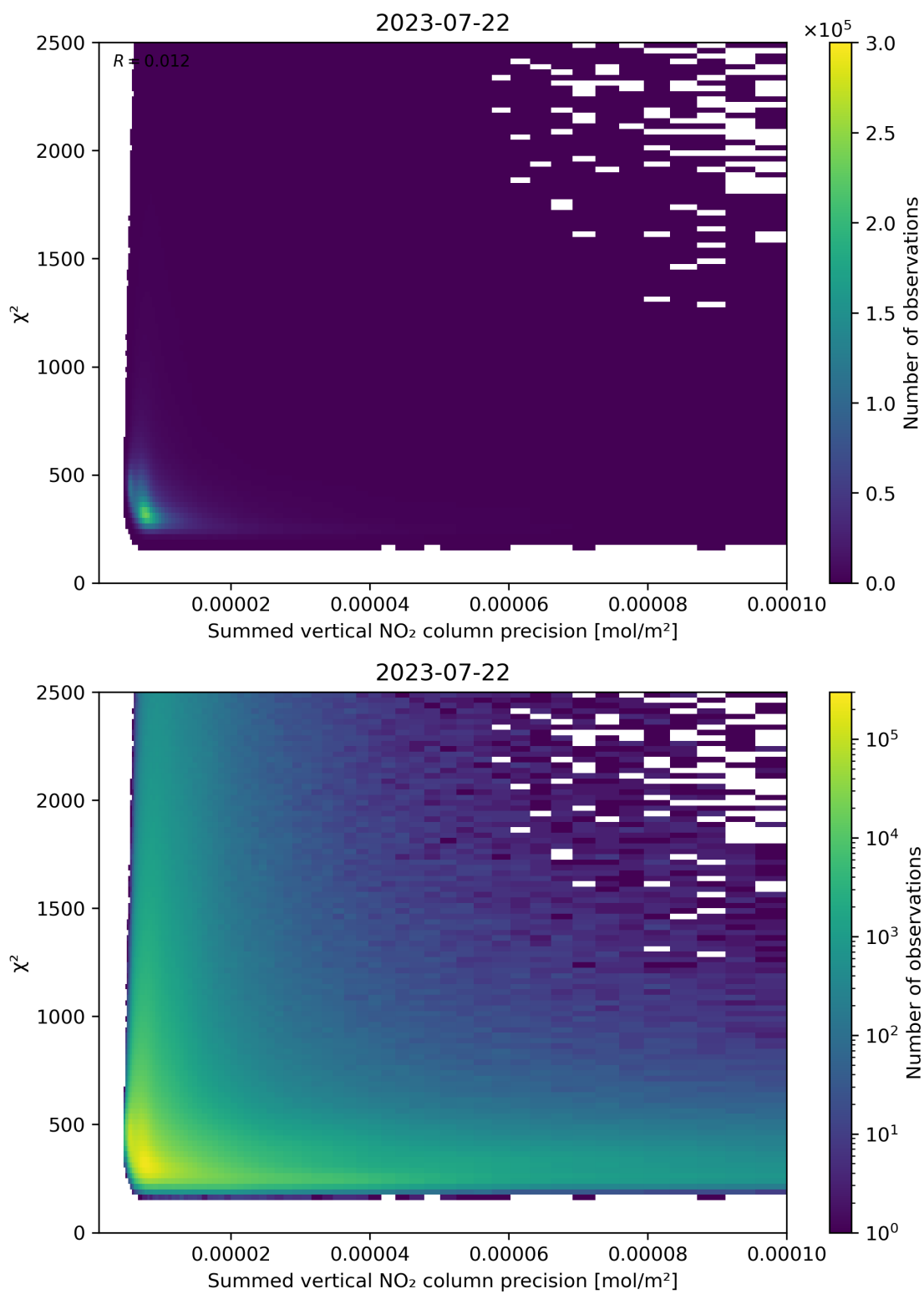
Figure 107: Scatter density plot of “Summed vertical NO 2 column precision” against “ \chi^2 ” for 2023-07-21 to 2023-07-23.
