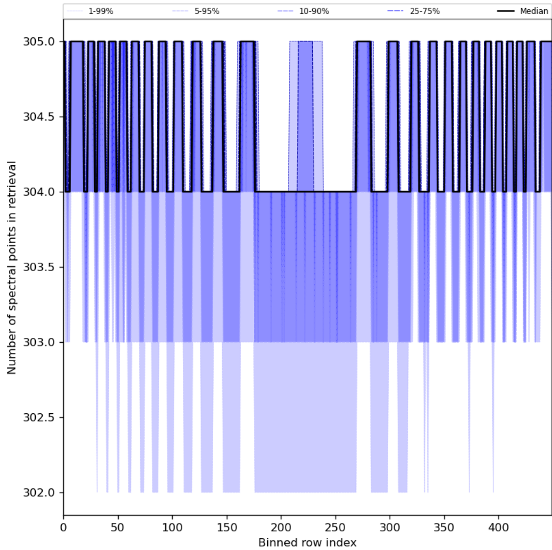
Figure 50: Along track statistics of “Number of spectral points in retrieval” for 2023-07-21 to 2023-07-23
