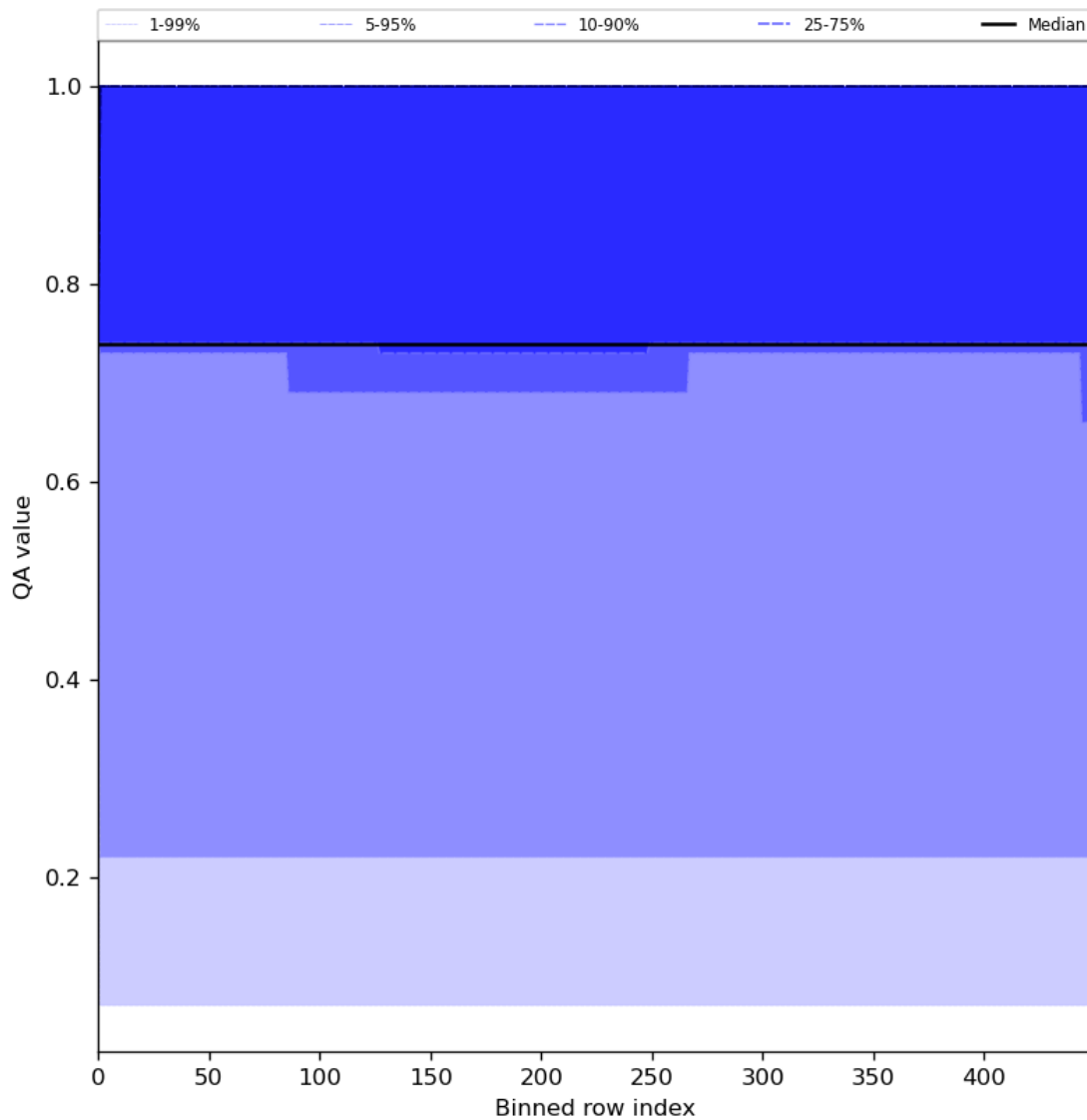
Figure 45: Along track statistics of “QA value” for 2023-07-21 to 2023-07-23
