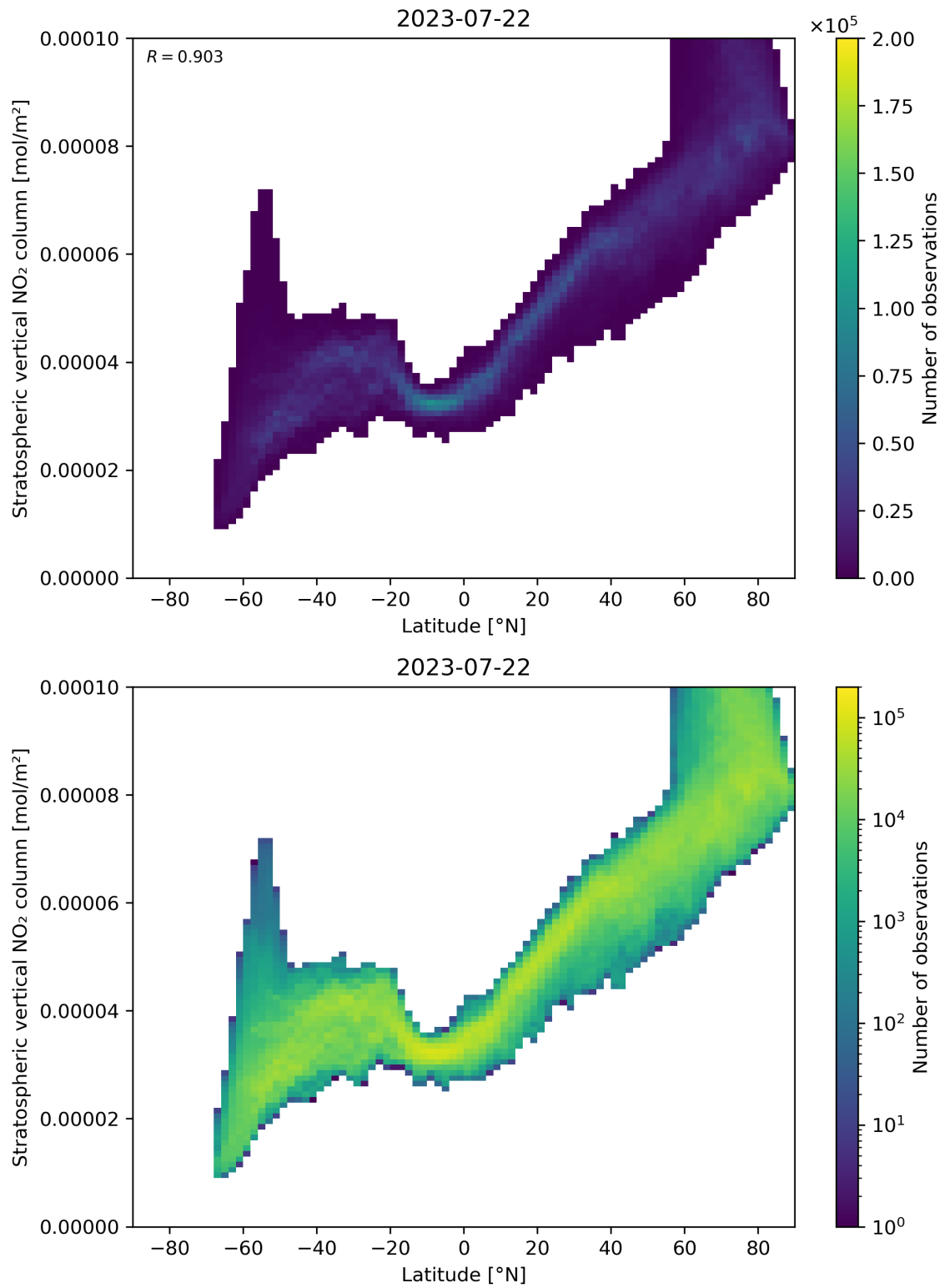
Figure 87: Scatter density plot of “Latitude” against “Stratospheric vertical NO 2 column” for 2023-07-21 to 2023-07-23.
