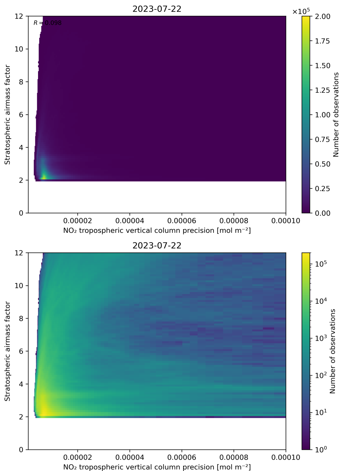
Figure 131: Scatter density plot of “NO 2 tropospheric vertical column precision” against “Stratospheric airmass factor” for 2023-07-21 to 2023-07-23.
