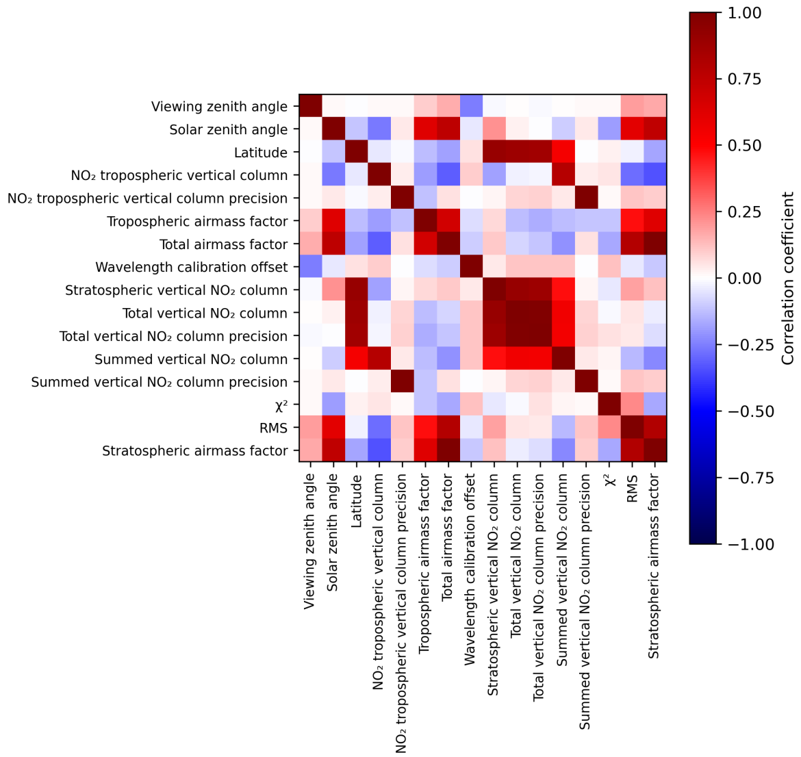
Figure 2: Map of correlation matrix for 2023-07-21 to 2023-07-23.
