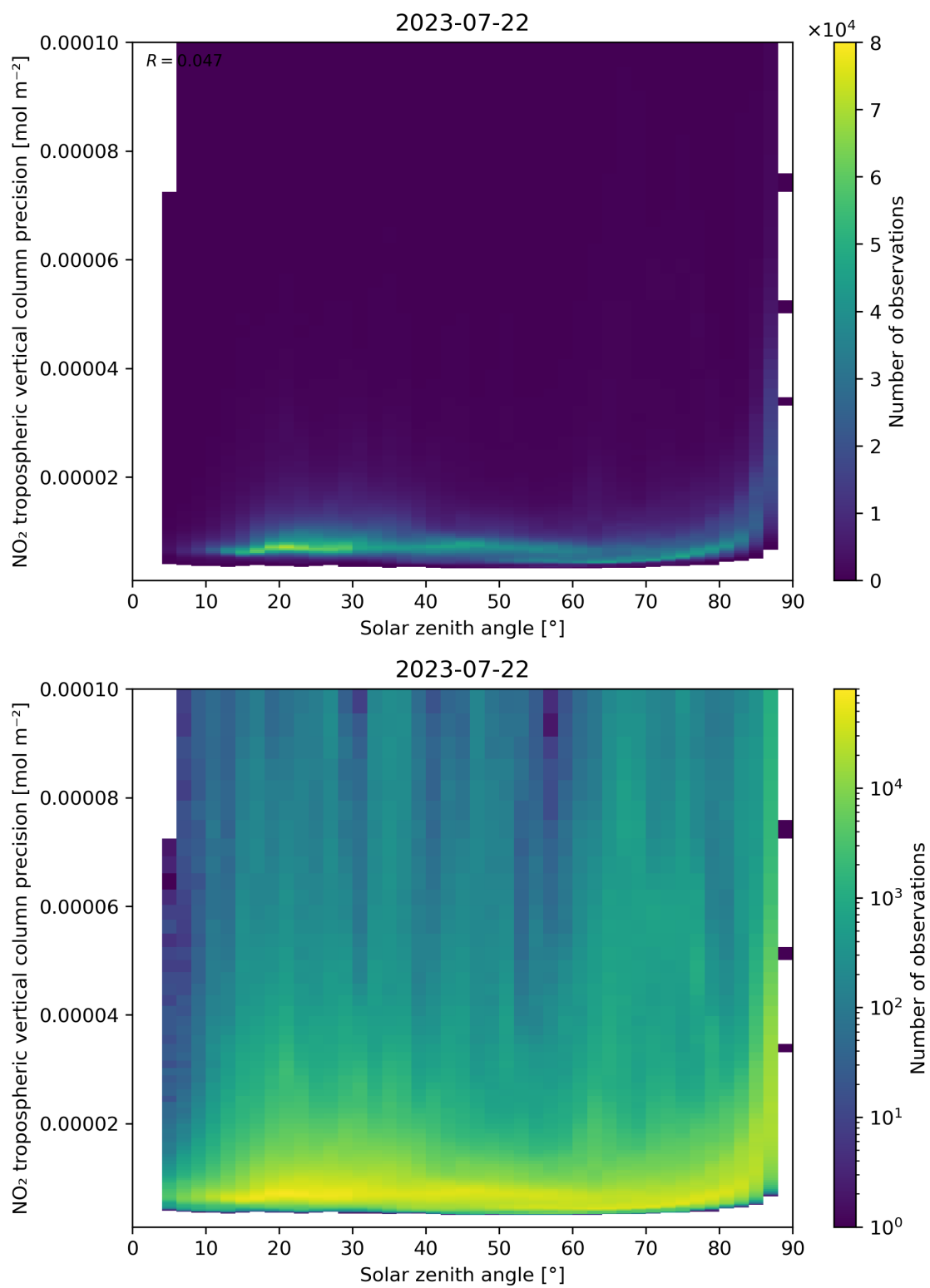
Figure 156: Scatter density plot of “Solar zenith angle” against “NO 2 tropospheric vertical column precision” for 2023-07-21 to 2023-07-23.
