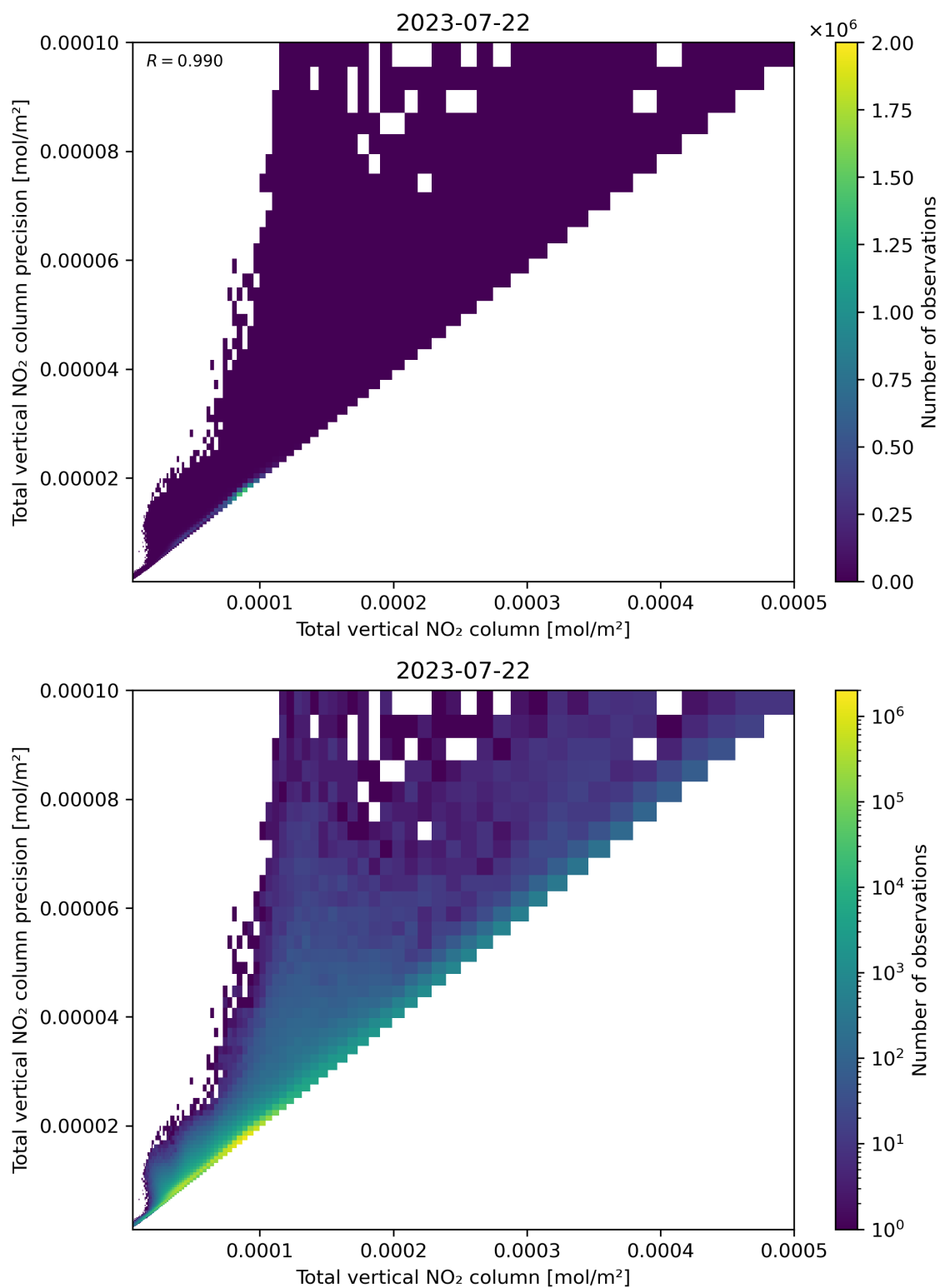
Figure 114: Scatter density plot of “Total vertical NO 2 column” against “Total vertical NO 2 column precision” for 2023-07-21 to 2023-07-23.
