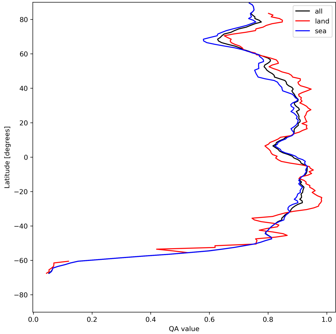
Figure 11: Zonal average of “QA value” for 2023-07-21 to 2023-07-23.
