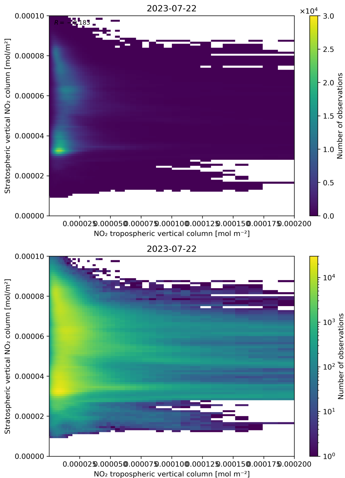
Figure 125: Scatter density plot of “NO 2 tropospheric vertical column” against “Stratospheric vertical NO 2 column” for 2023-07-21 to 2023-07-23.
