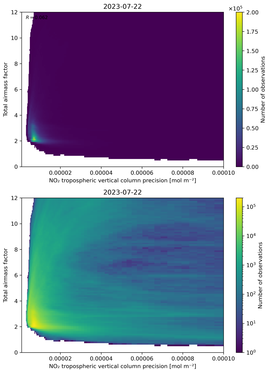
Figure 132: Scatter density plot of “NO 2 tropospheric vertical column precision” against “Total air mass factor” for 2023-07-21 to 2023-07-23.
