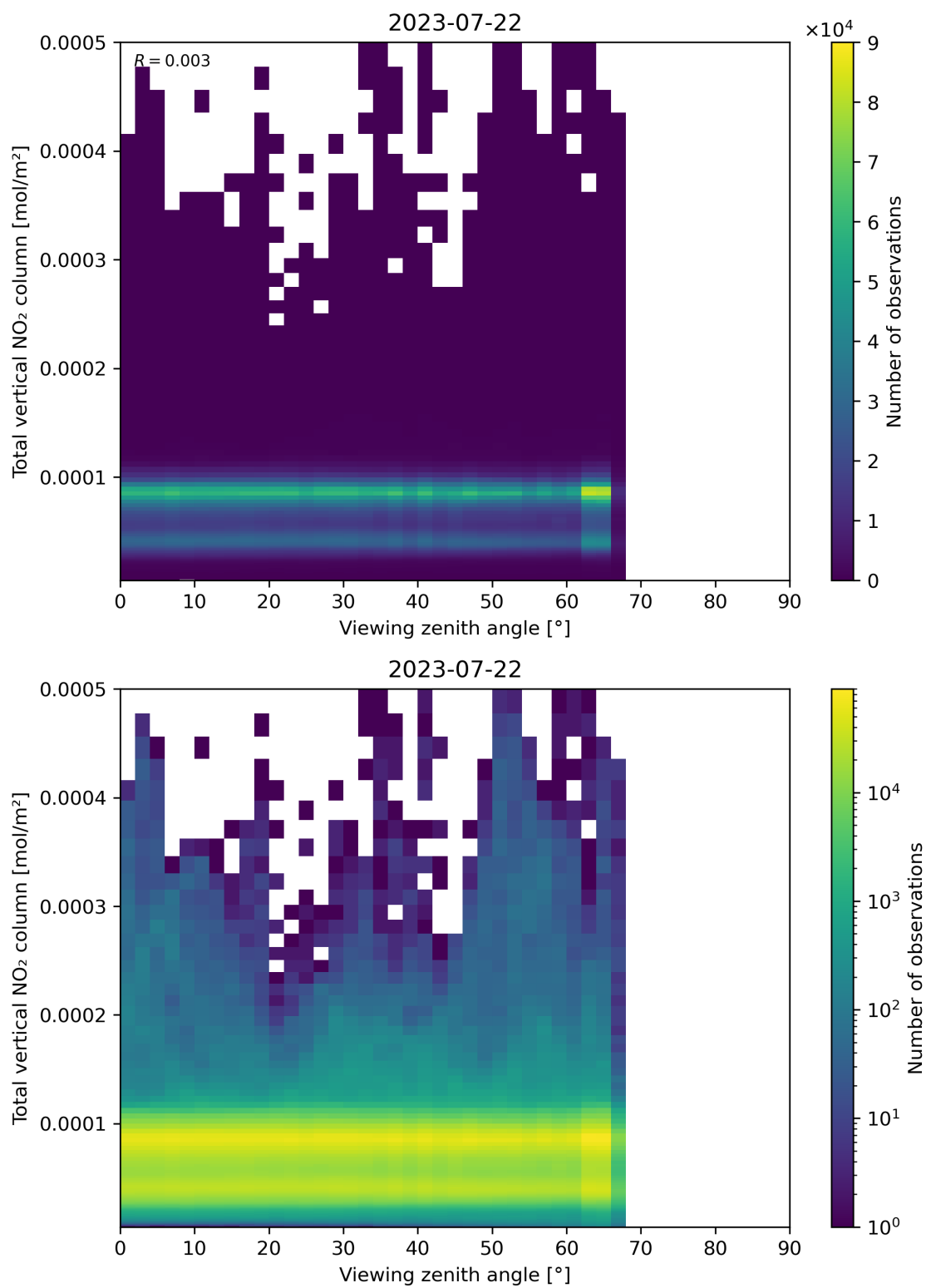
Figure 167: Scatter density plot of “Viewing zenith angle” against “Total vertical NO 2 column” for 2023-07-21 to 2023-07-23.
