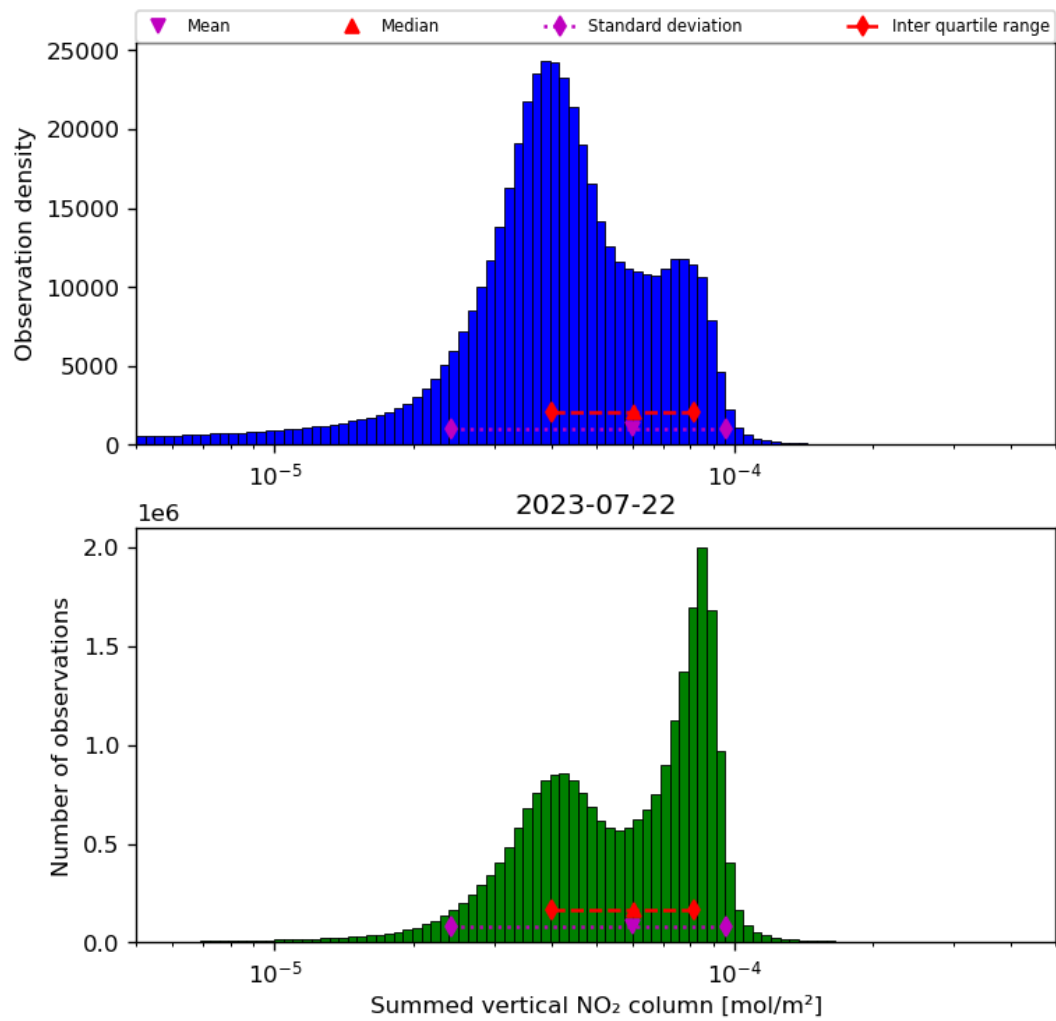
Figure 40: Histogram of “Summed vertical NO 2 column” for 2023-07-21 to 2023-07-23
