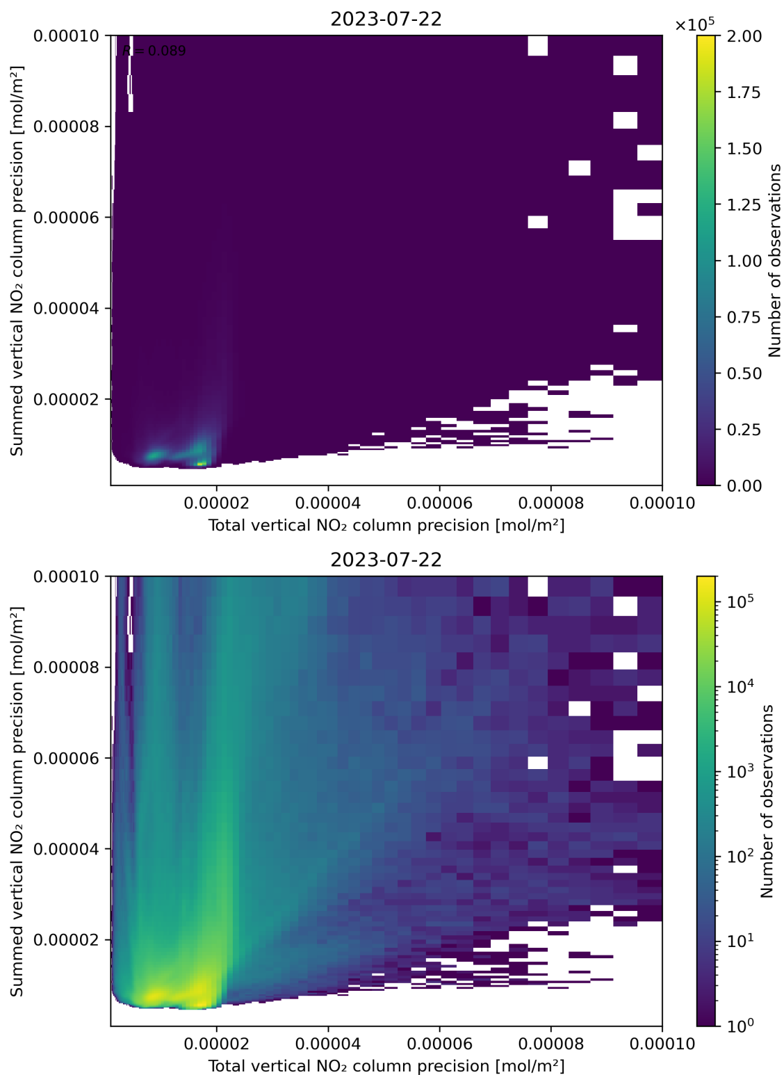
Figure 118: Scatter density plot of “Total vertical NO 2 column precision” against “Summed vertical NO 2 column precision” for 2023-07-21 to 2023-07-23.
