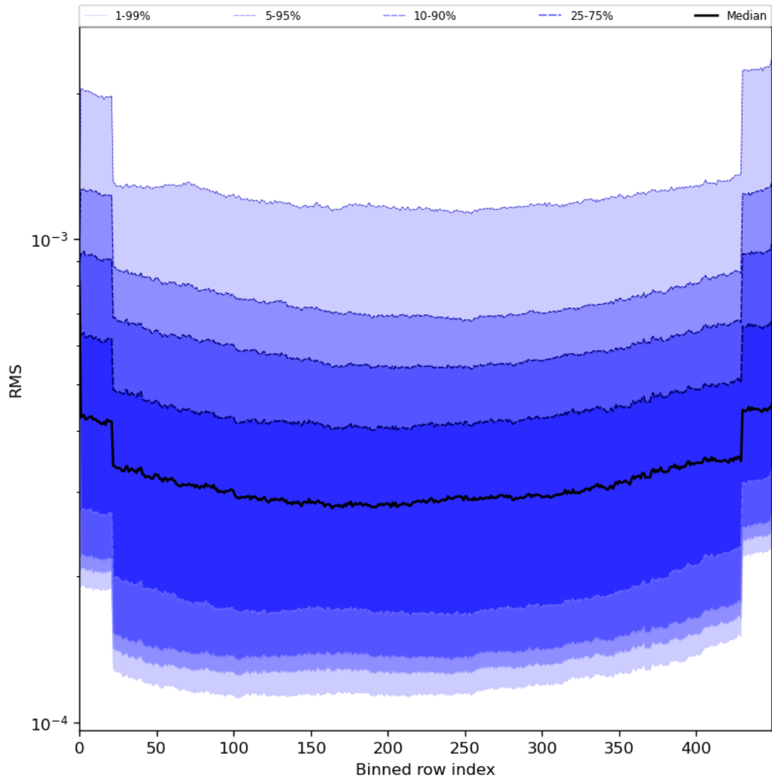
Figure 60: Along track statistics of “RMS” for 2023-07-21 to 2023-07-23
