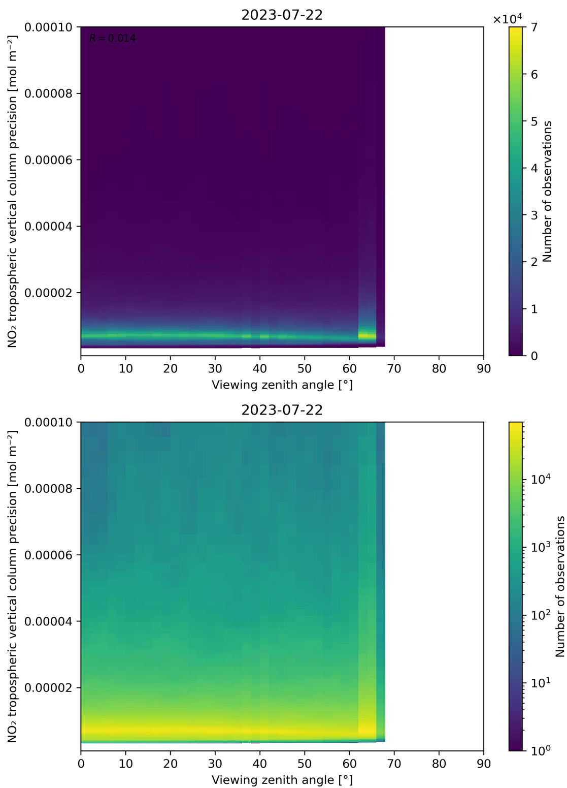
Figure 170: Scatter density plot of “Viewing zenith angle” against “NO 2 tropospheric vertical column precision” for 2023-07-21 to 2023-07-23.
