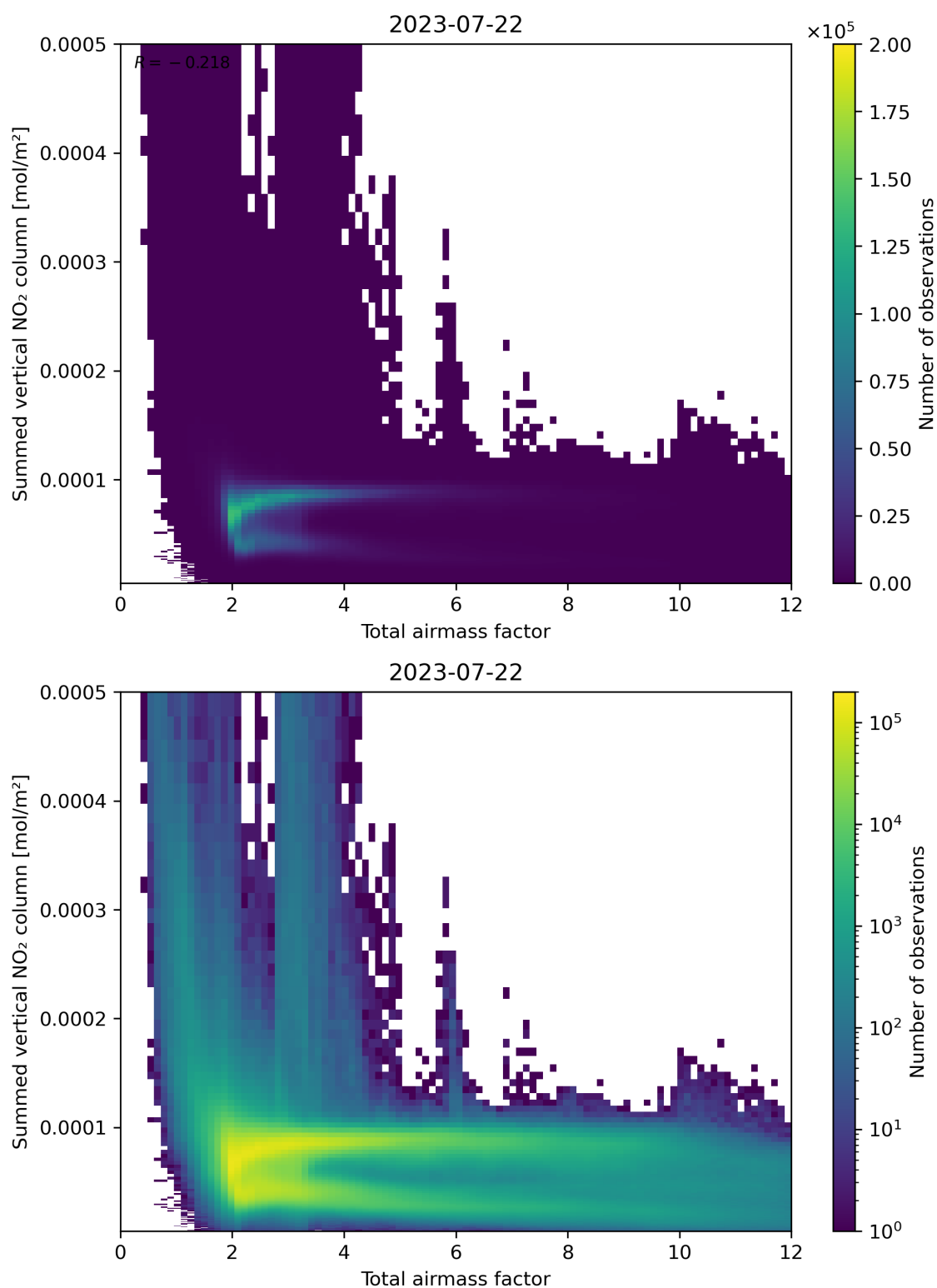
Figure 65: Scatter density plot of “Total airmass factor” against “Summed vertical NO 2 column” for 2023-07-21 to 2023-07-23.
