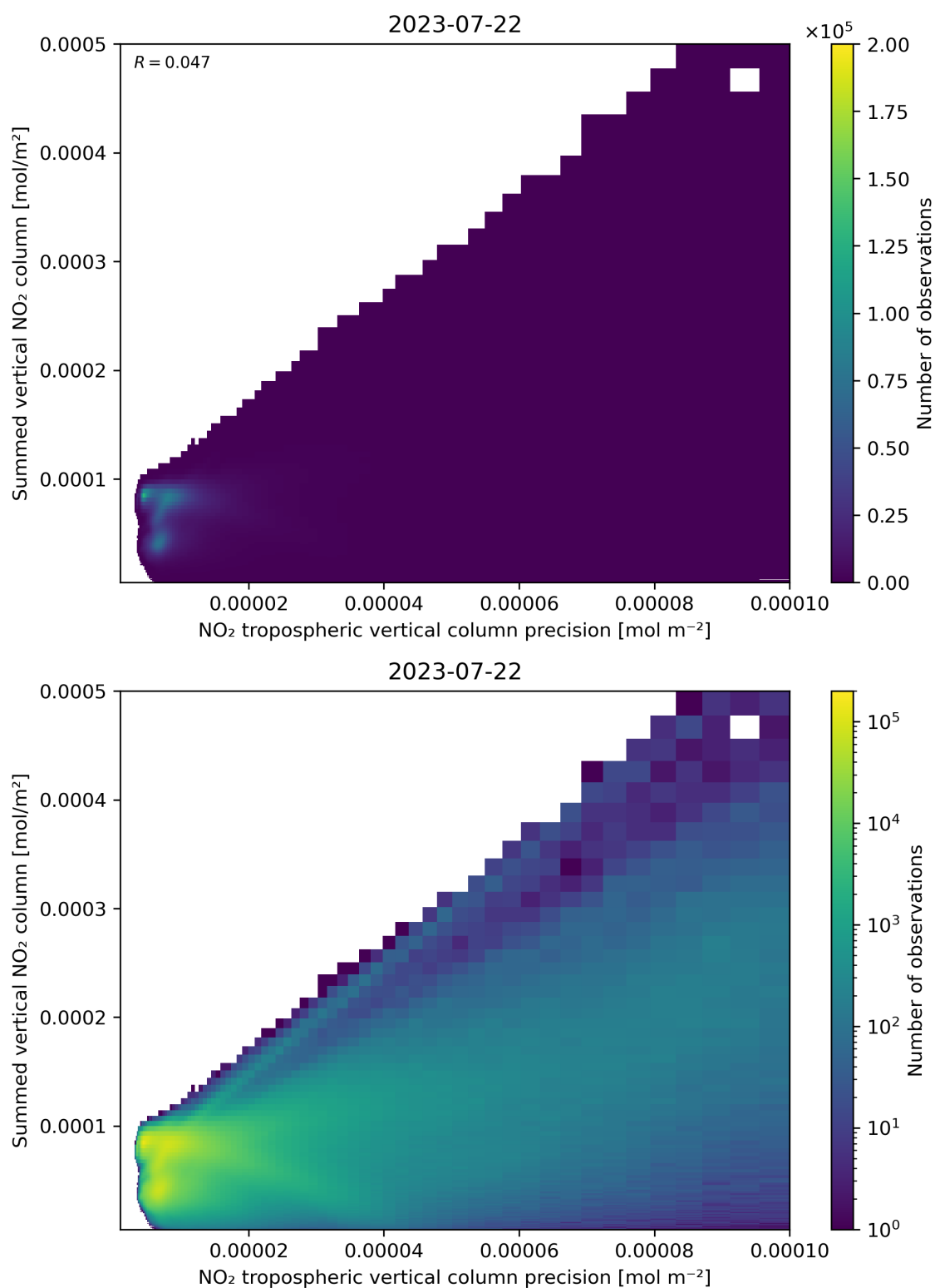
Figure 136: Scatter density plot of “NO 2 tropospheric vertical column precision” against “Summed vertical NO 2 column” for 2023-07-21 to 2023-07-23.
