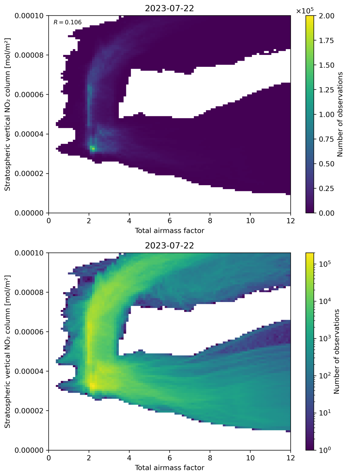
Figure 64: Scatter density plot of “Total airmass factor” against “Stratospheric vertical NO 2 column” for 2023-07-21 to 2023-07-23.
