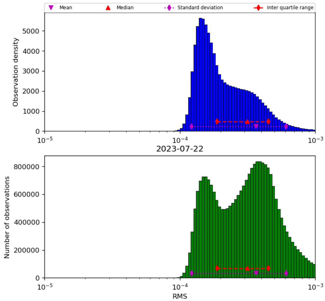
Figure 43: Histogram of “RMS” for 2023-07-21 to 2023-07-23
