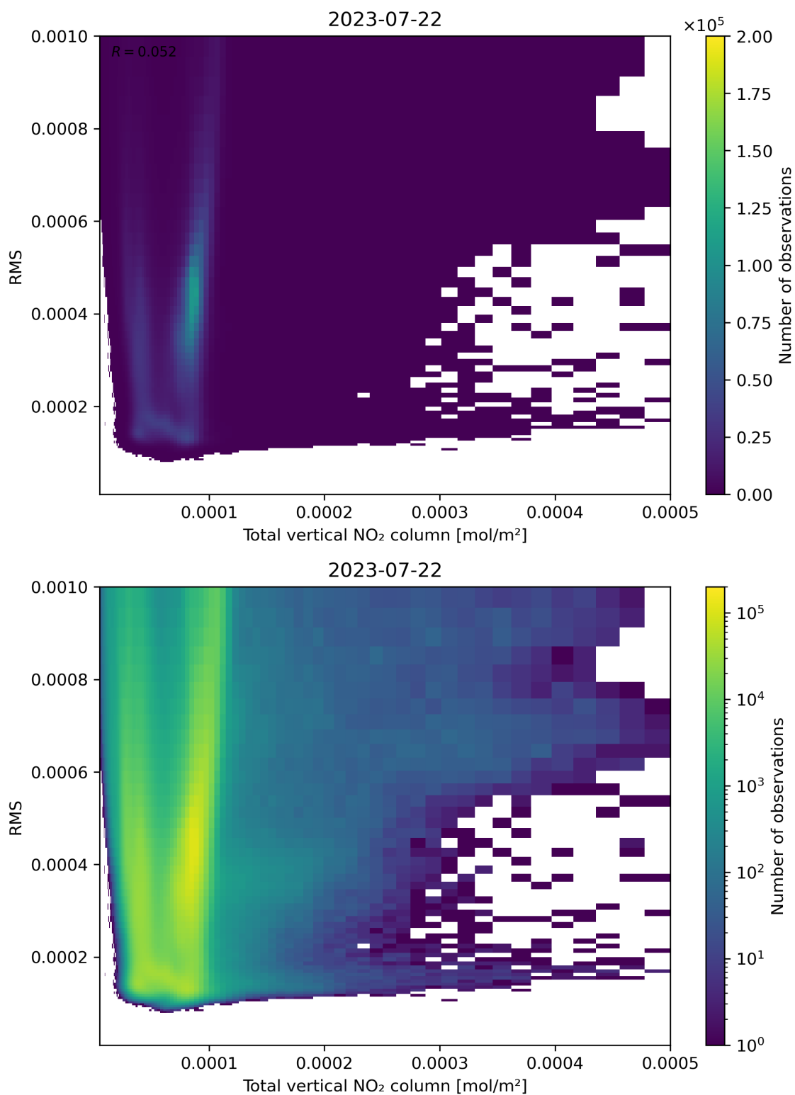
Figure 120: Scatter density plot of “Total vertical NO 2 column” against “RMS” for 2023-07-21 to 2023-07-23.
