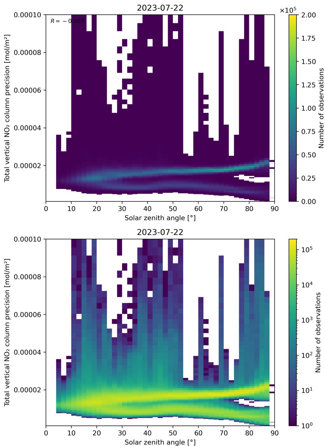
Figure 154: Scatter density plot of “Solar zenith angle” against “Total vertical NO 2 column precision” for 2023-07-21 to 2023-07-23.
