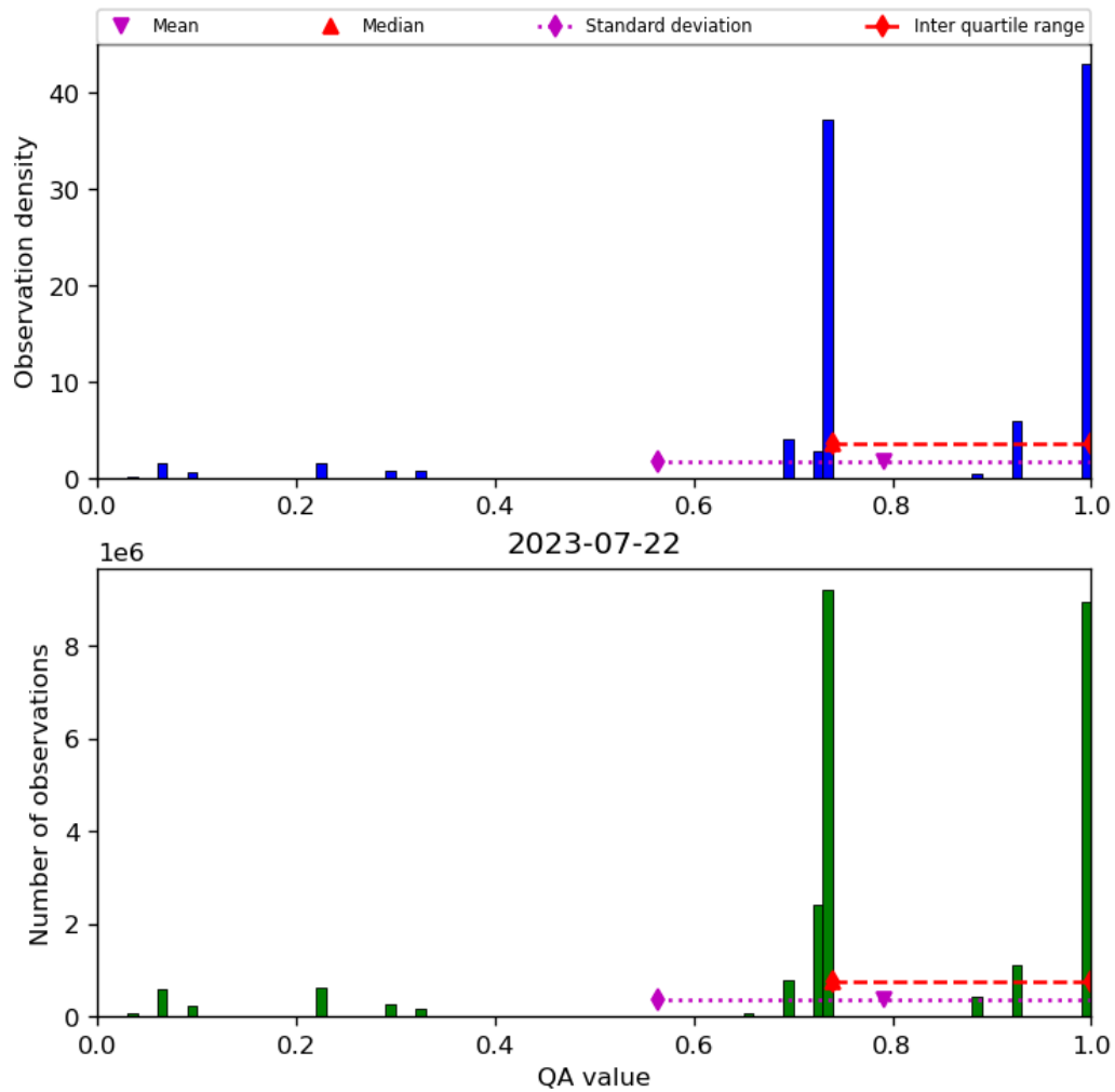
Figure 28: Histogram of “QA value” for 2023-07-21 to 2023-07-23
