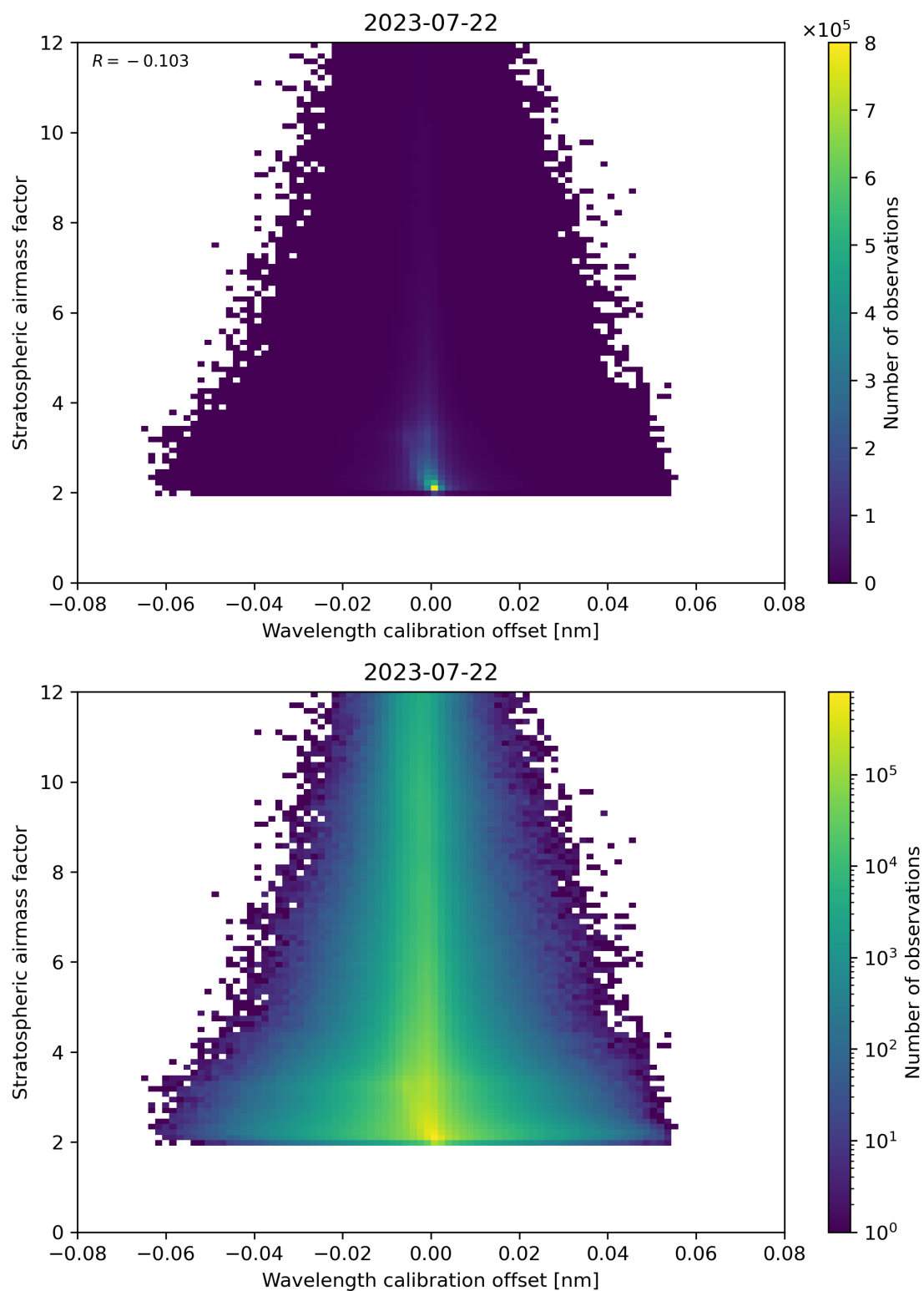
Figure 174: Scatter density plot of “Wavelength calibration offset” against “Stratospheric air mass factor” for 2023-07-21 to 2023-07-23.
