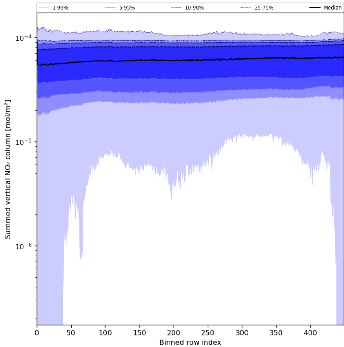
Figure 57: Along track statistics of “Summed vertical NO 2 column” for 2023-07-21 to 2023-07-23
