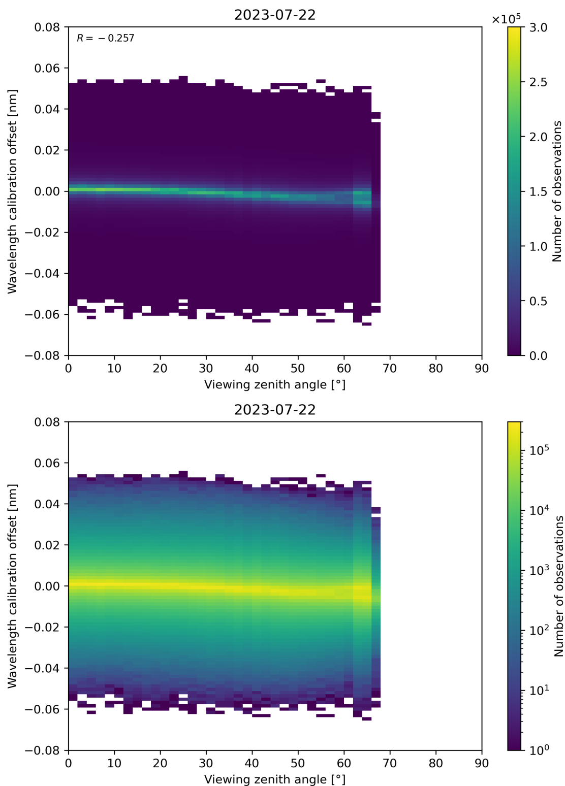
Figure 173: Scatter density plot of “Viewing zenith angle” against “Wavelength calibration offset” for 2023-07-21 to 2023-07-23.
