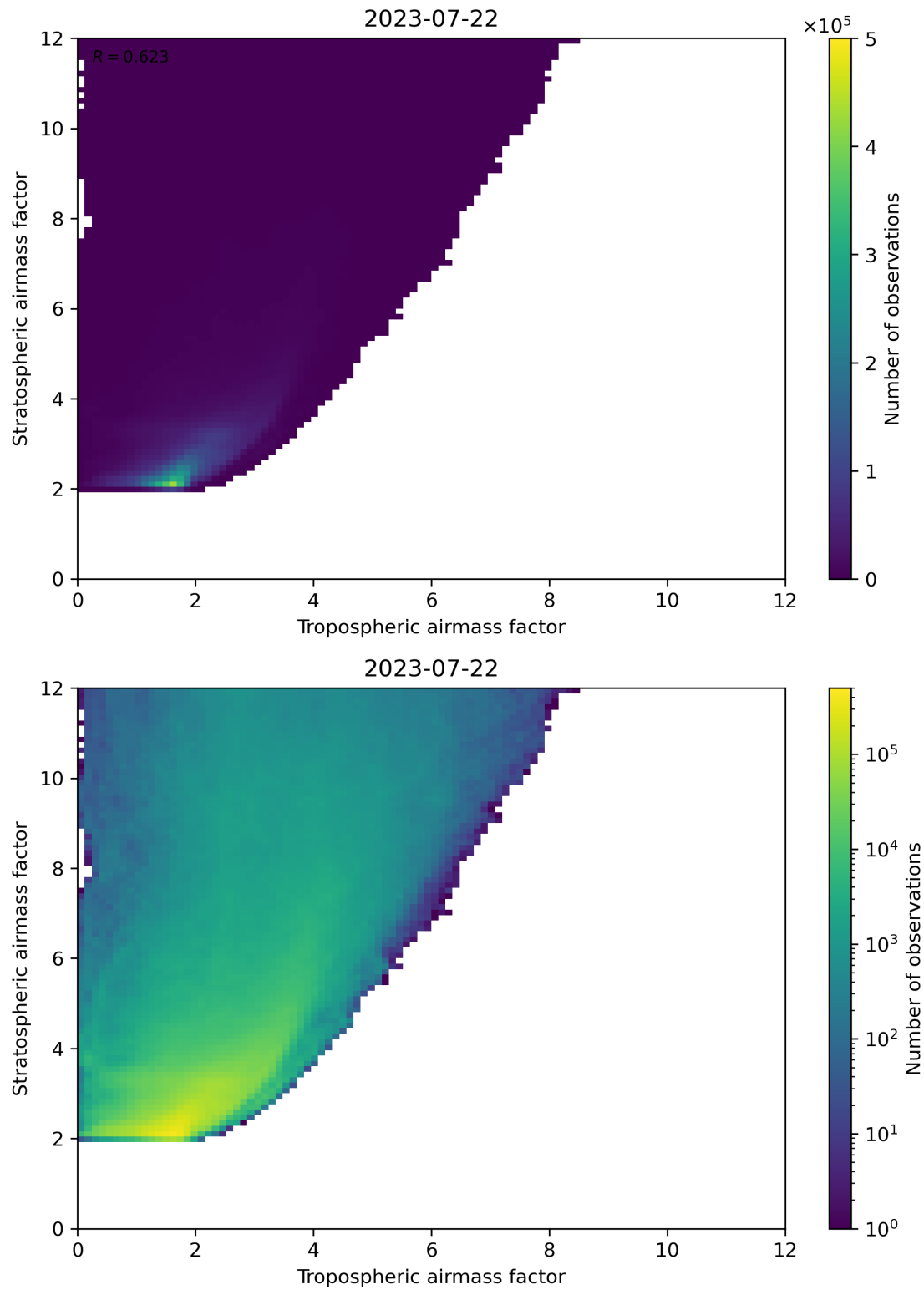
Figure 71: Scatter density plot of “Tropospheric airmass factor” against “Stratospheric airmass factor” for 2023-07-21 to 2023-07-23.
