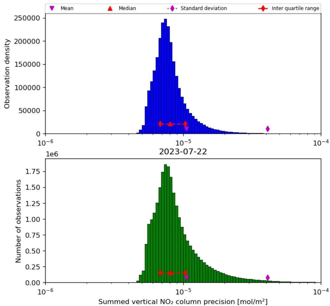
Figure 41: Histogram of "Summed vertical NO 2 column precision" for 2023-07-21 to 2023-07-23
