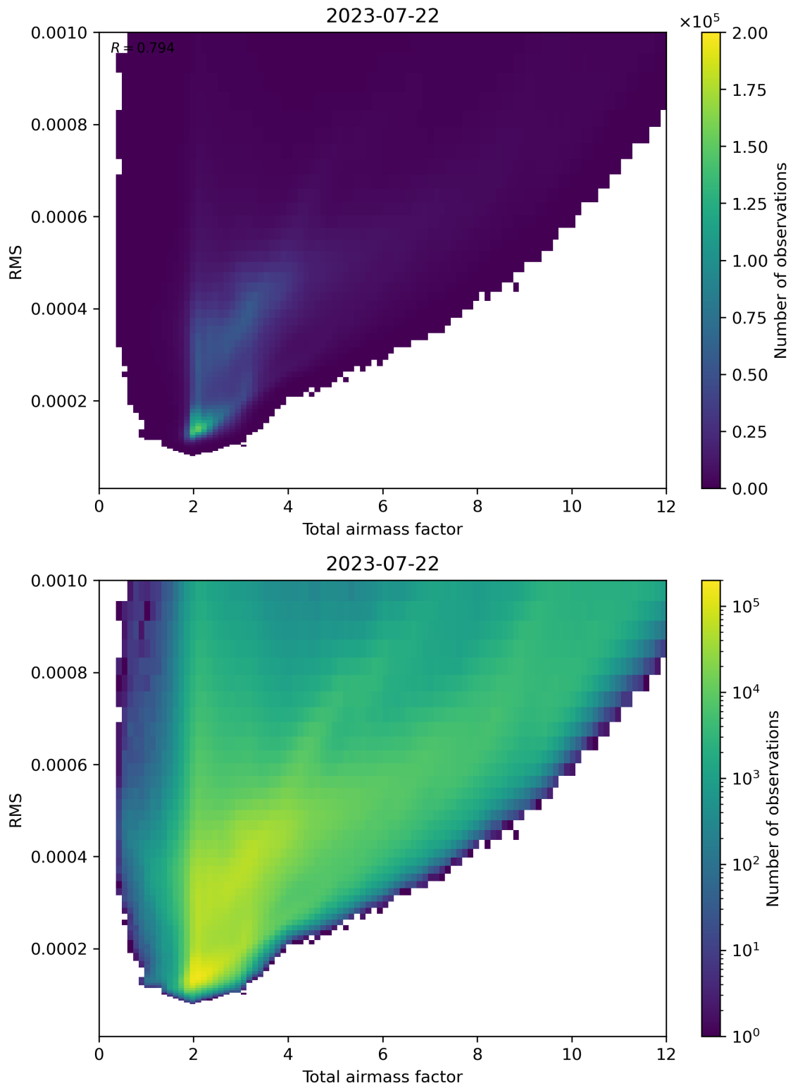
Figure 69: Scatter density plot of “Total airmass factor” against “RMS” for 2023-07-21 to 2023-07-23.
