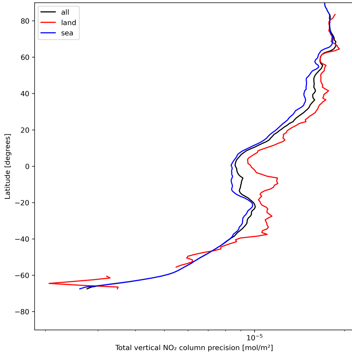
Figure 22: Zonal average of “Total vertical NO 2 column precision” for 2023-07-21 to 2023-07-23.
