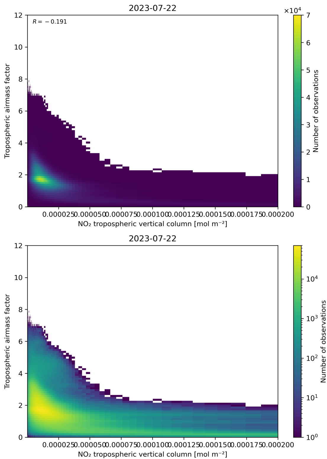
Figure 123: Scatter density plot of “NO 2 tropospheric vertical column” against “Tropospheric airmass factor” for 2023-07-21 to 2023-07-23.
