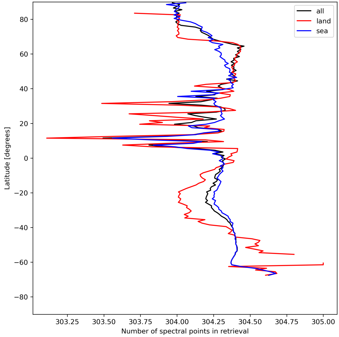
Figure 16: Zonal average of “Number of spectral points in retrieval” for 2023-07-21 to 2023-07-23.
