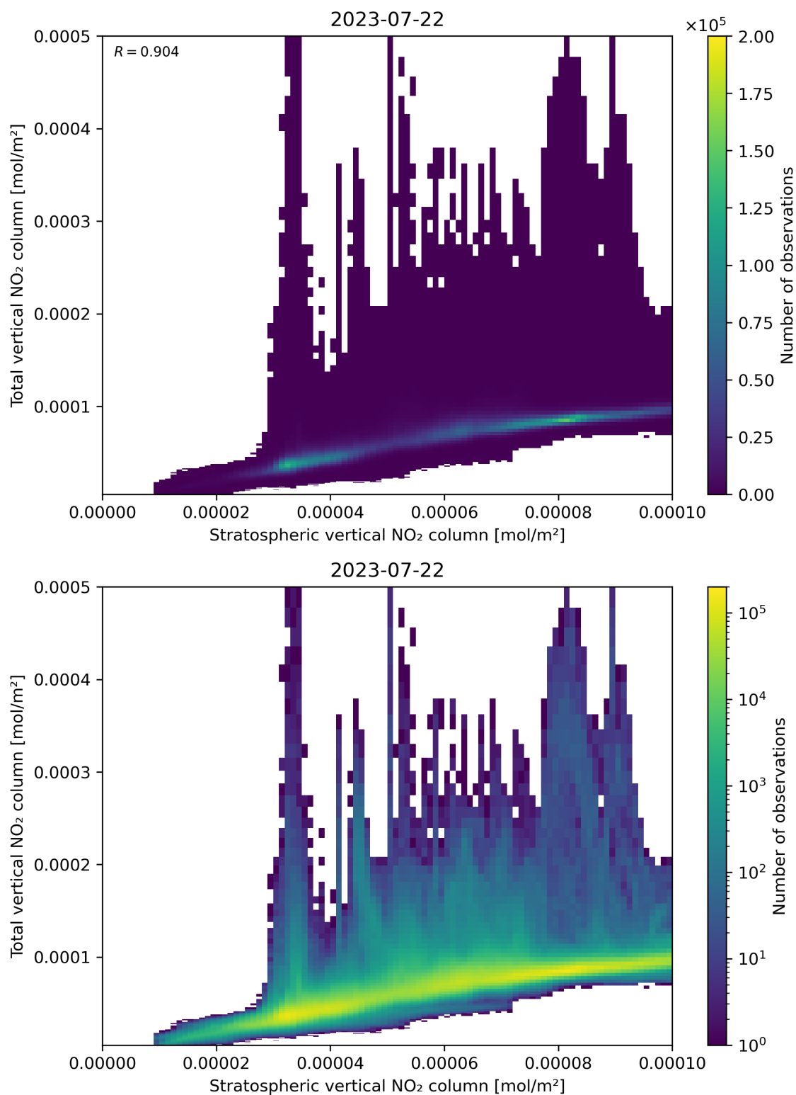
Figure 100: Scatter density plot of “Stratospheric vertical NO 2 column” against “Total vertical NO 2 column” for 2023-07-21 to 2023-07-23.
