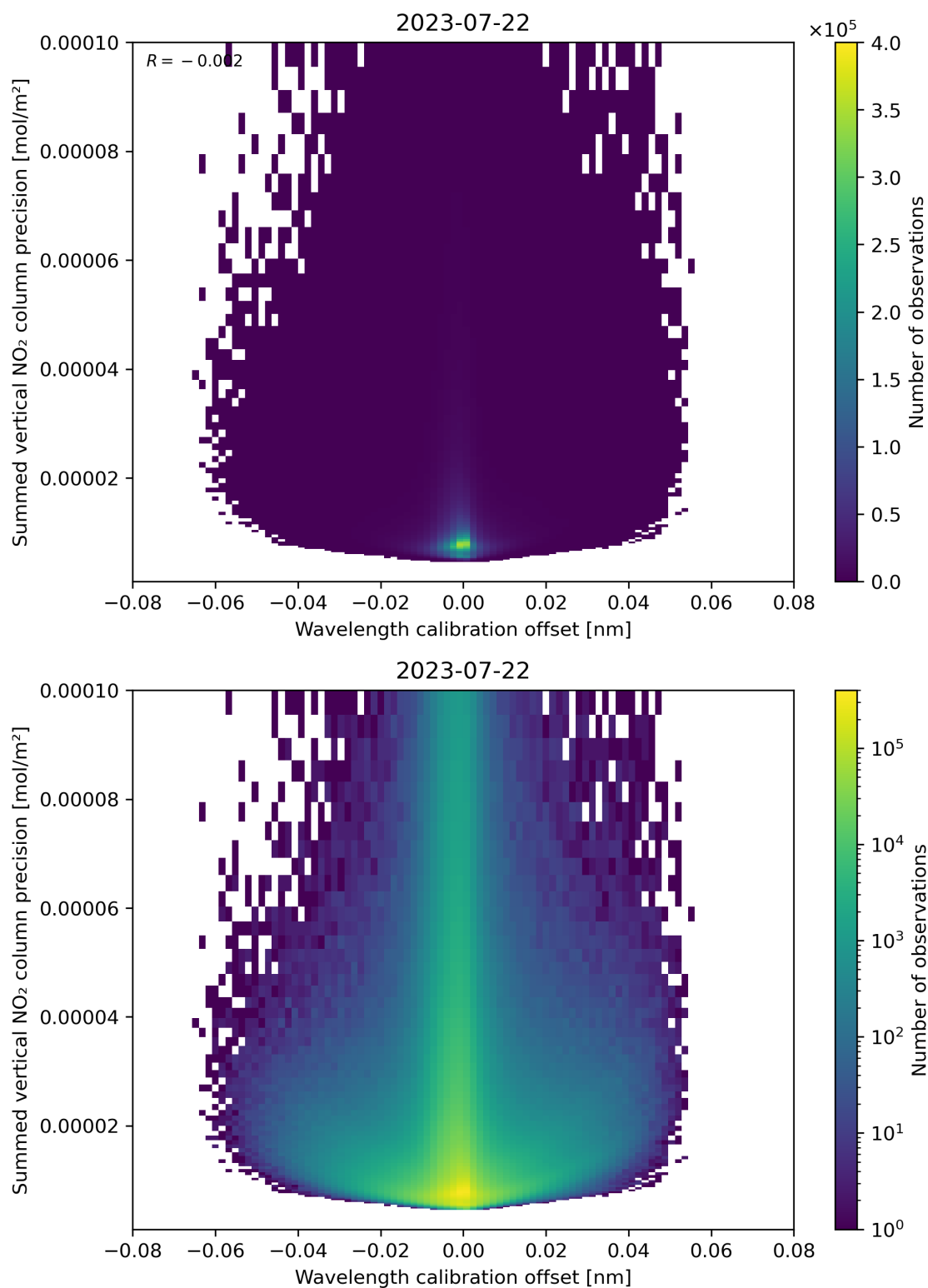
Figure 178: Scatter density plot of “Wavelength calibration offset” against “Summed vertical NO 2 column precision” for 2023-07-21 to 2023-07-23.
