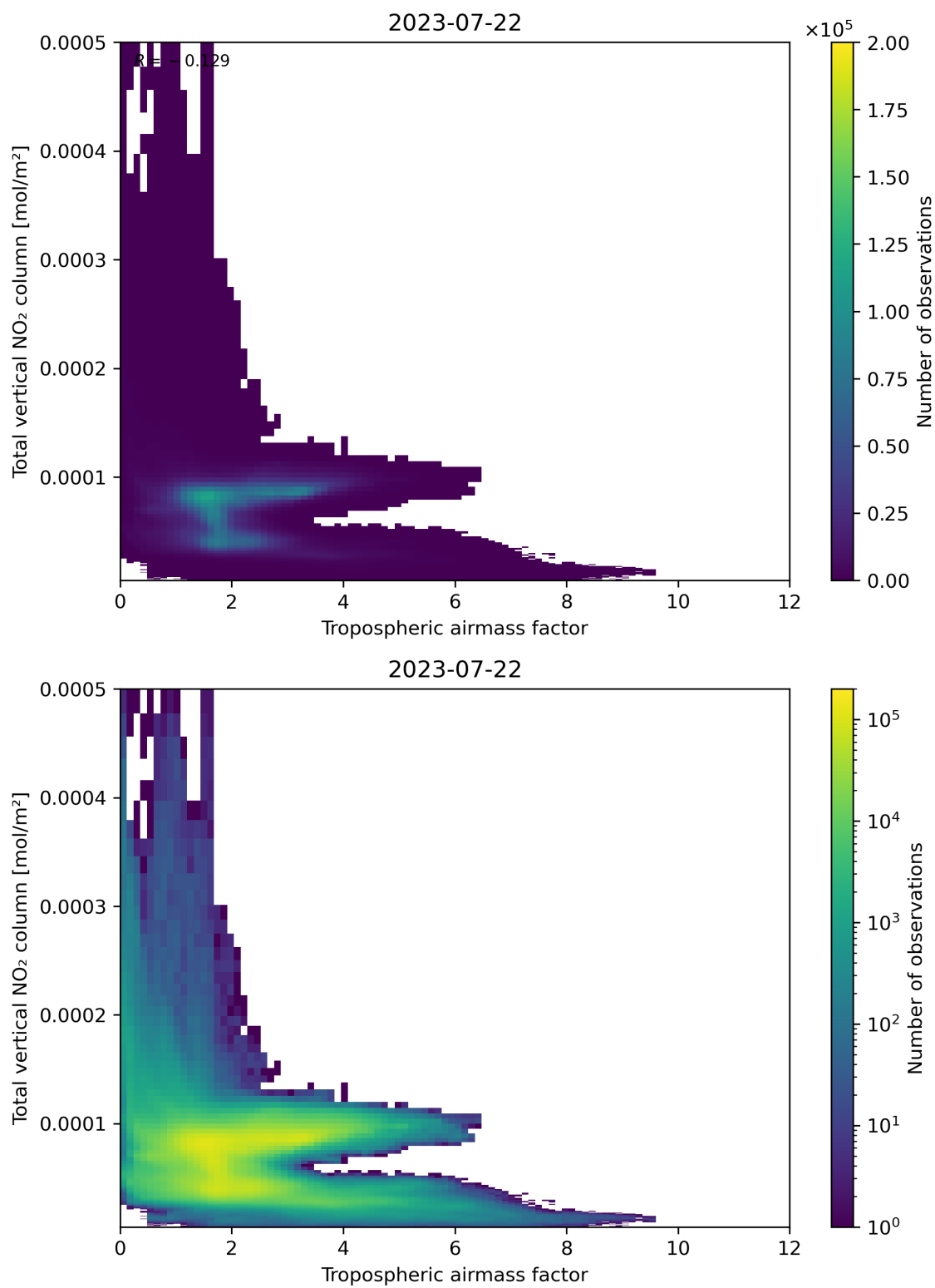
Figure 77: Scatter density plot of “Tropospheric airmass factor” against “Total vertical NO 2 column” for 2023-07-21 to 2023-07-23.
