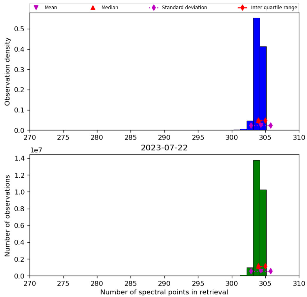
Figure 33: Histogram of “Number of spectral points in retrieval” for 2023-07-21 to 2023-07-23
