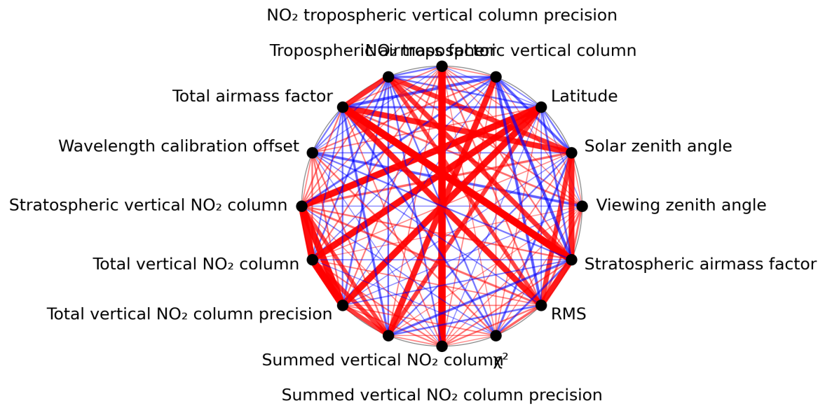
Figure 1: Map of correlation graph for 2023-07-21 to 2023-07-23.
