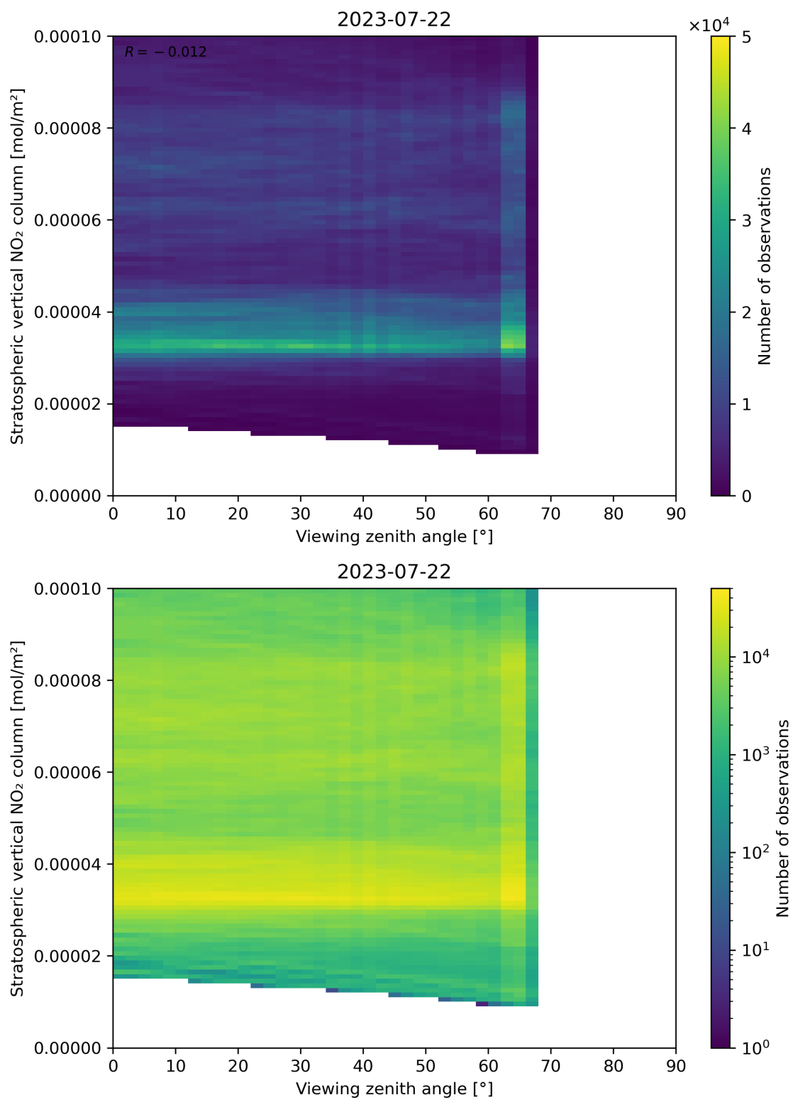
Figure 164: Scatter density plot of “Viewing zenith angle” against “Stratospheric vertical NO 2 column” for 2023-07-21 to 2023-07-23.
