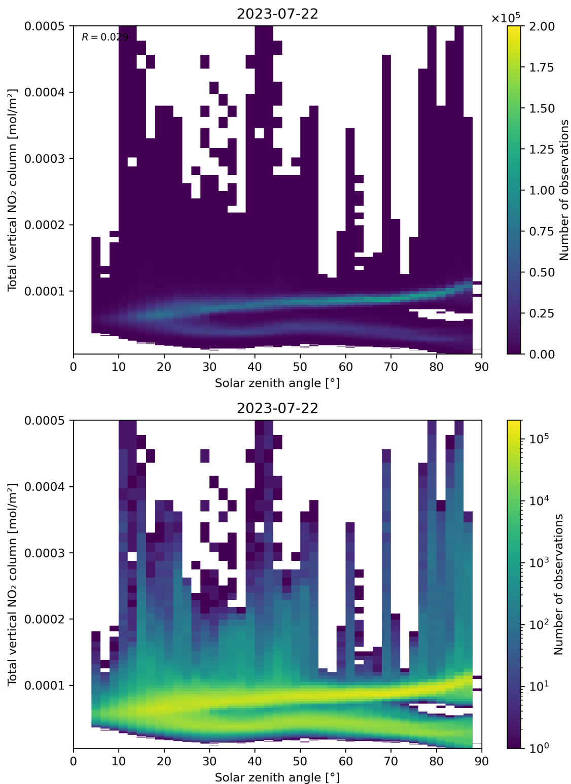
Figure 153: Scatter density plot of “Solar zenith angle” against “Total vertical NO 2 column” for 2023-07-21 to 2023-07-23.
