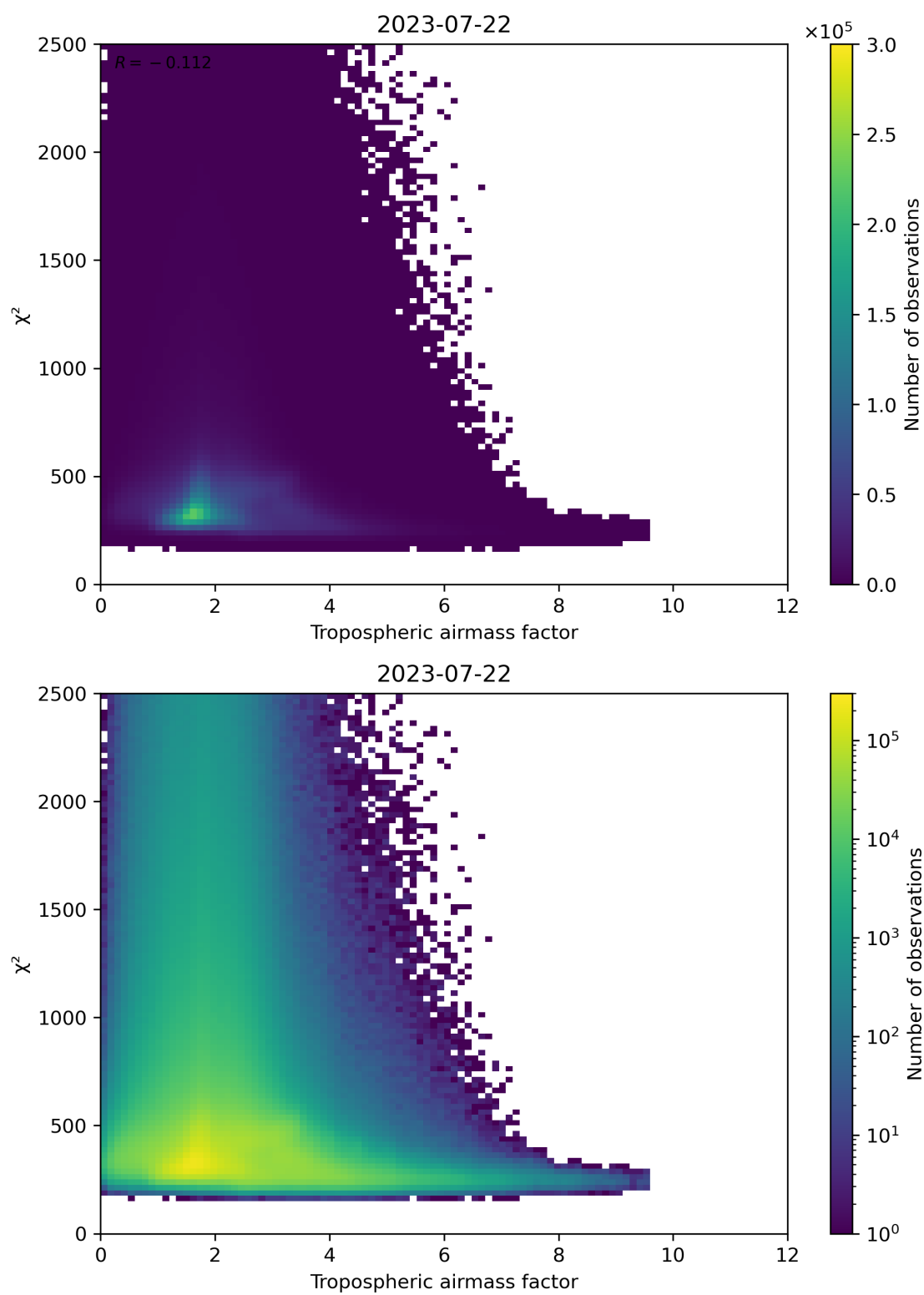
Figure 73: Scatter density plot of “Tropospheric airmass factor” against “ \chi^2 ” for 2023-07-21 to 2023-07-23.
