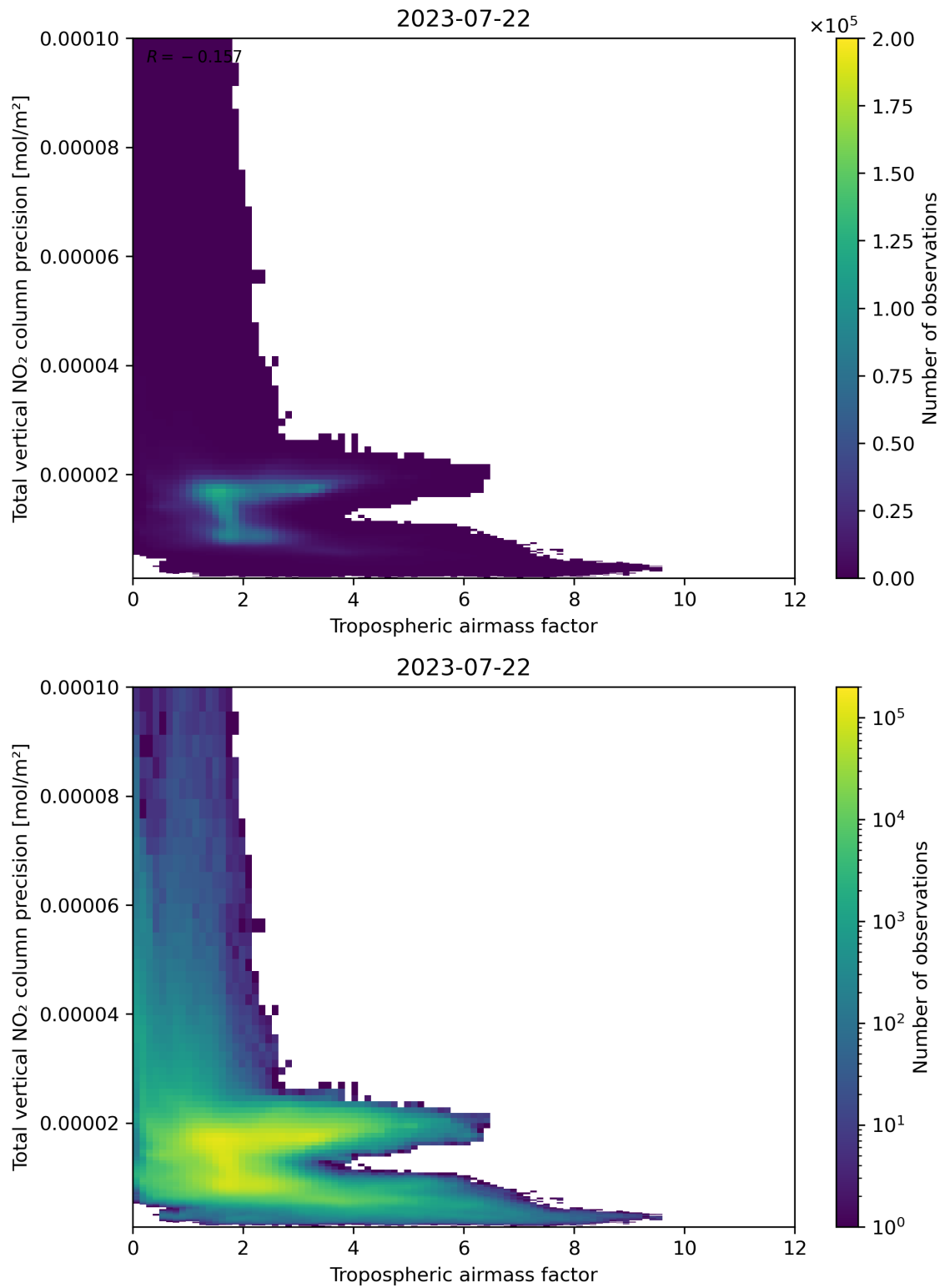
Figure 78: Scatter density plot of “Tropospheric air mass factor” against “Total vertical NO 2 column precision” for 2023-07-21 to 2023-07-23.
