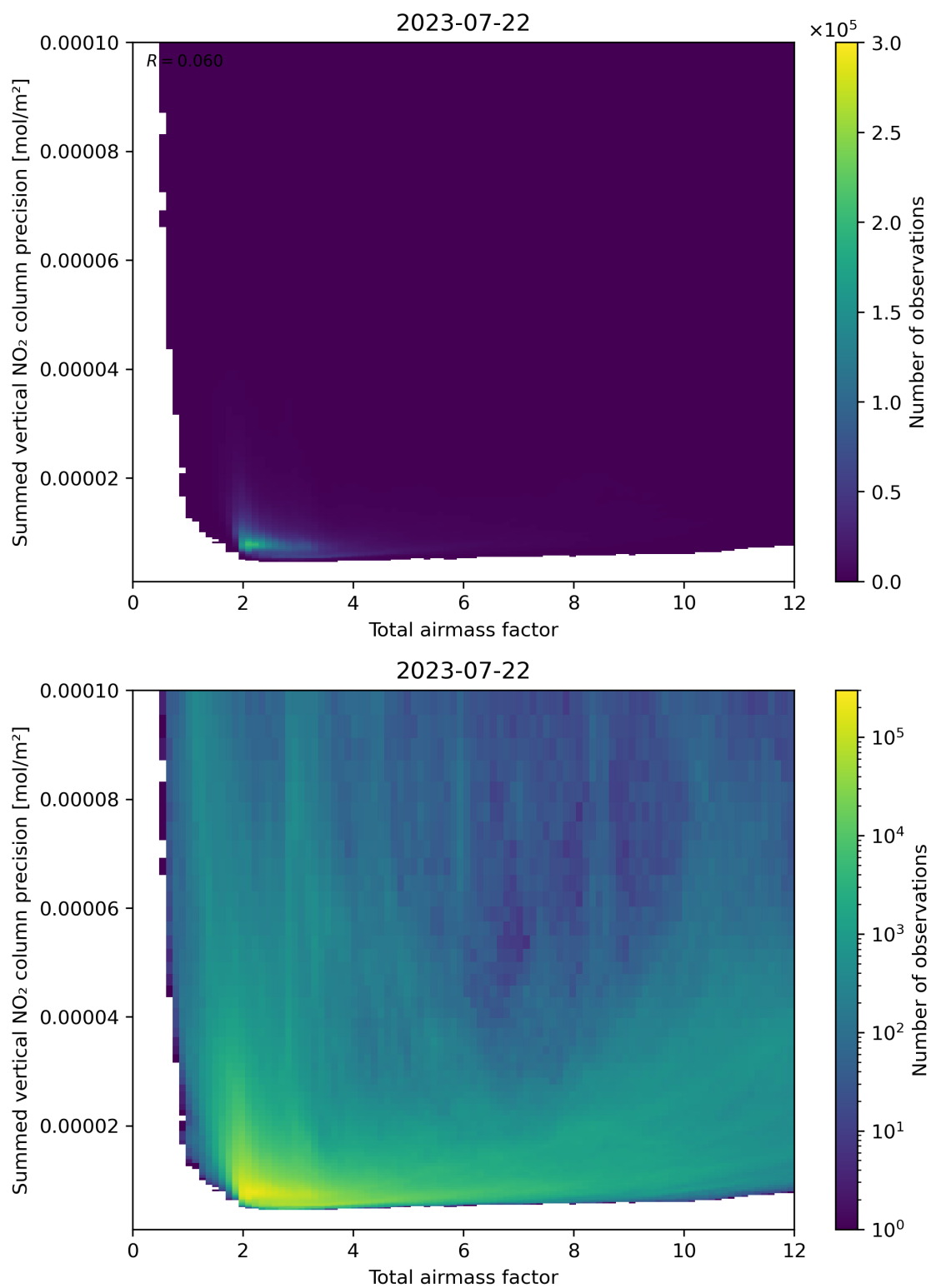
Figure 66: Scatter density plot of “Total airmass factor” against “Summed vertical NO 2 column precision” for 2023-07-21 to 2023-07-23.
