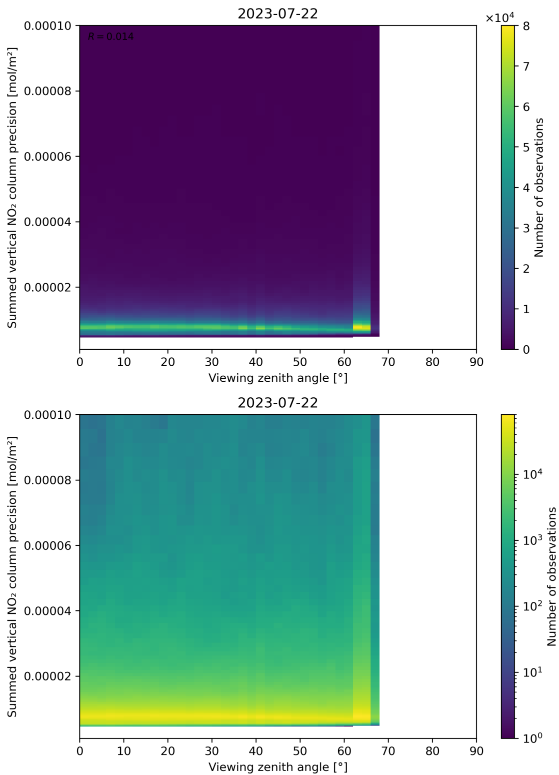
Figure 166: Scatter density plot of “Viewing zenith angle” against “Summed vertical NO 2 column precision” for 2023-07-21 to 2023-07-23.
