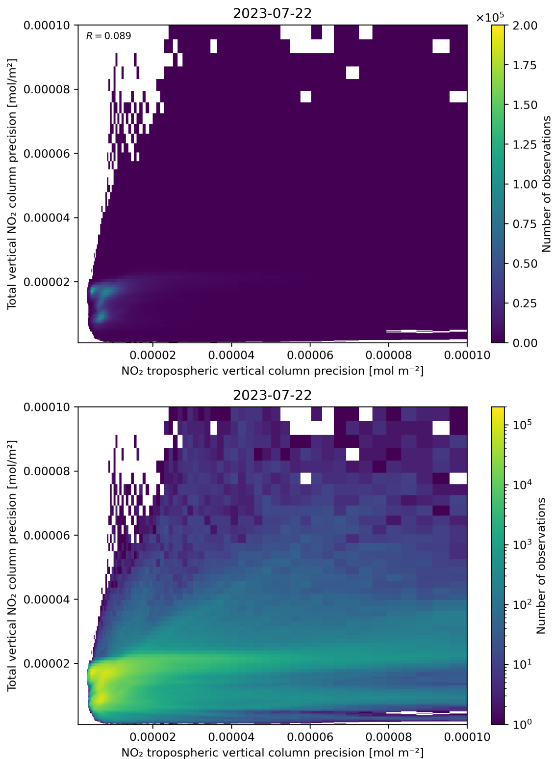
Figure 139: Scatter density plot of “NO 2 tropospheric vertical column precision” against “Total vertical NO 2 column precision” for 2023-07-21 to 2023-07-23.
