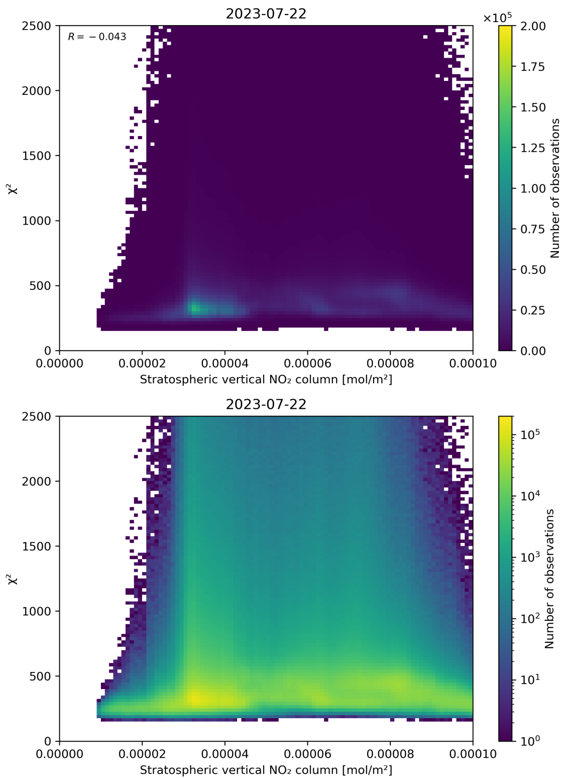
Figure 97: Scatter density plot of “Stratospheric vertical NO 2 column” against “ \chi^2 ” for 2023-07-21 to 2023-07-23.
