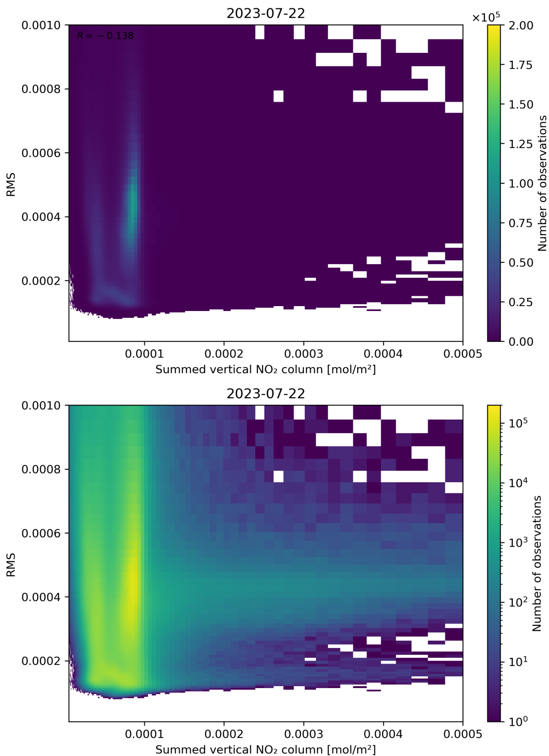
Figure 109: Scatter density plot of “Summed vertical NO 2 column” against “RMS” for 2023-07-21 to 2023-07-23.
