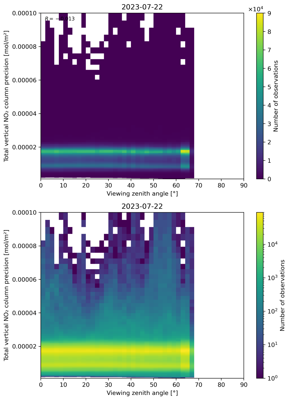
Figure 168: Scatter density plot of “Viewing zenith angle” against “Total vertical NO 2 column precision” for 2023-07-21 to 2023-07-23.
