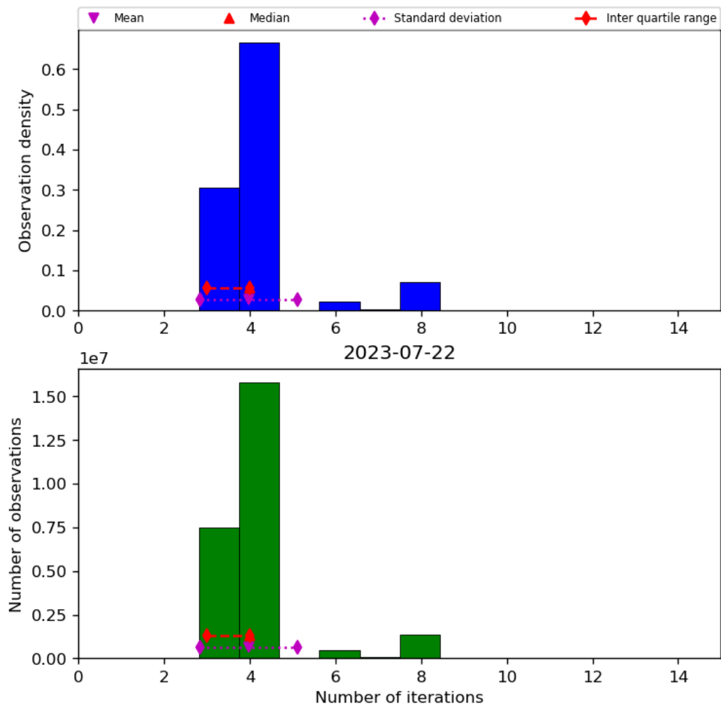
Figure 34: Histogram of “Number of iterations” for 2023-07-21 to 2023-07-23
