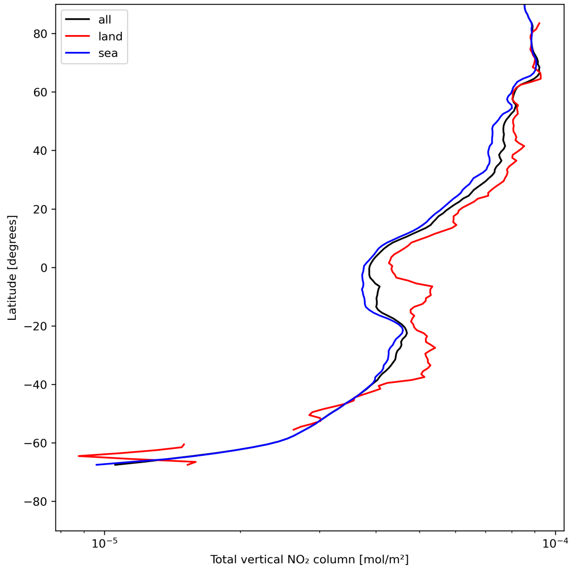
Figure 21: Zonal average of “Total vertical NO 2 column” for 2023-07-21 to 2023-07-23.
