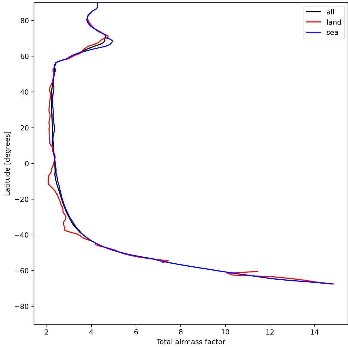
Figure 15: Zonal average of “Total airmass factor” for 2023-07-21 to 2023-07-23.
