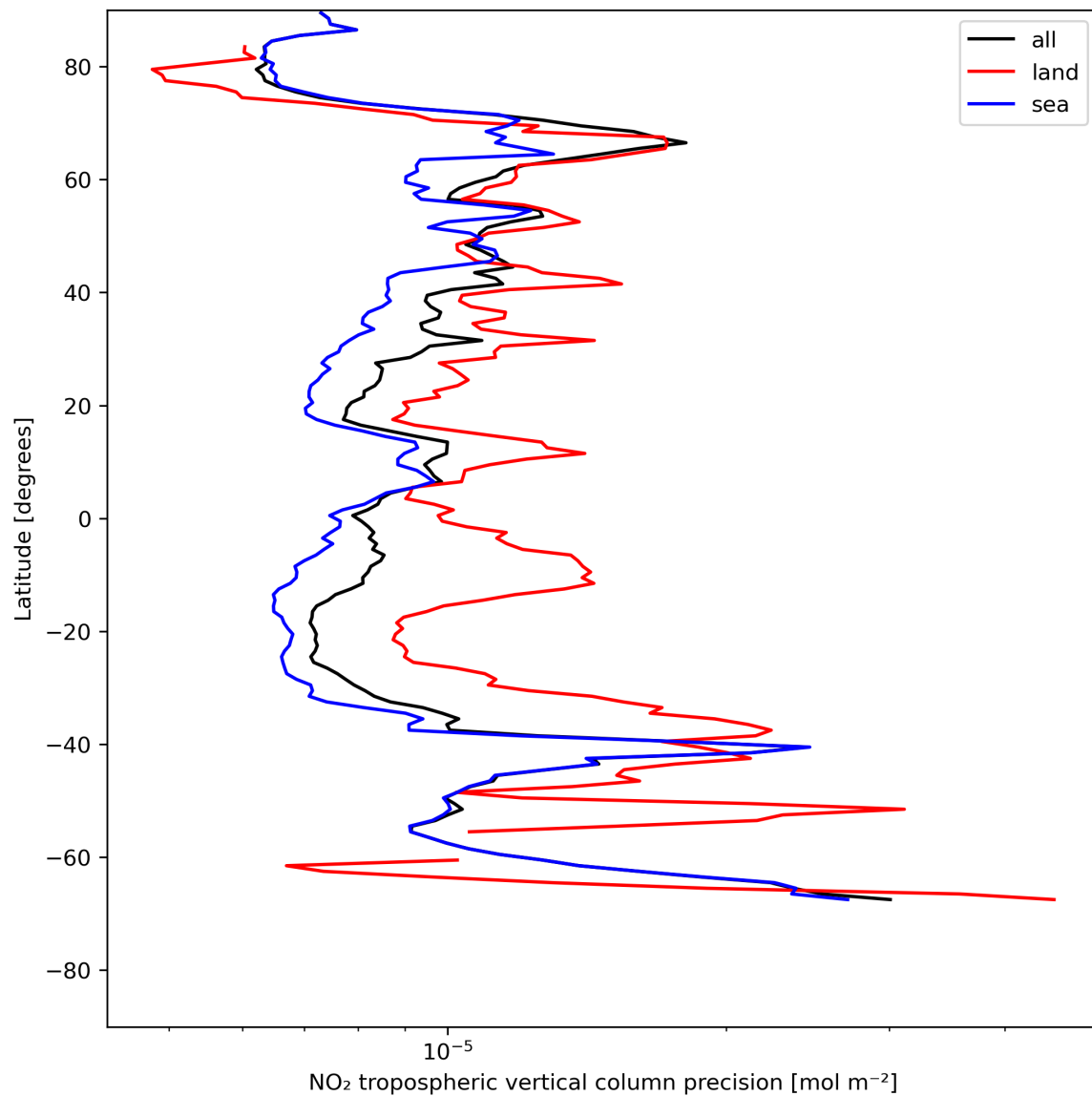
Figure 13: Zonal average of “NO 2 tropospheric vertical column precision” for 2023-07-21 to 2023-07-23.
