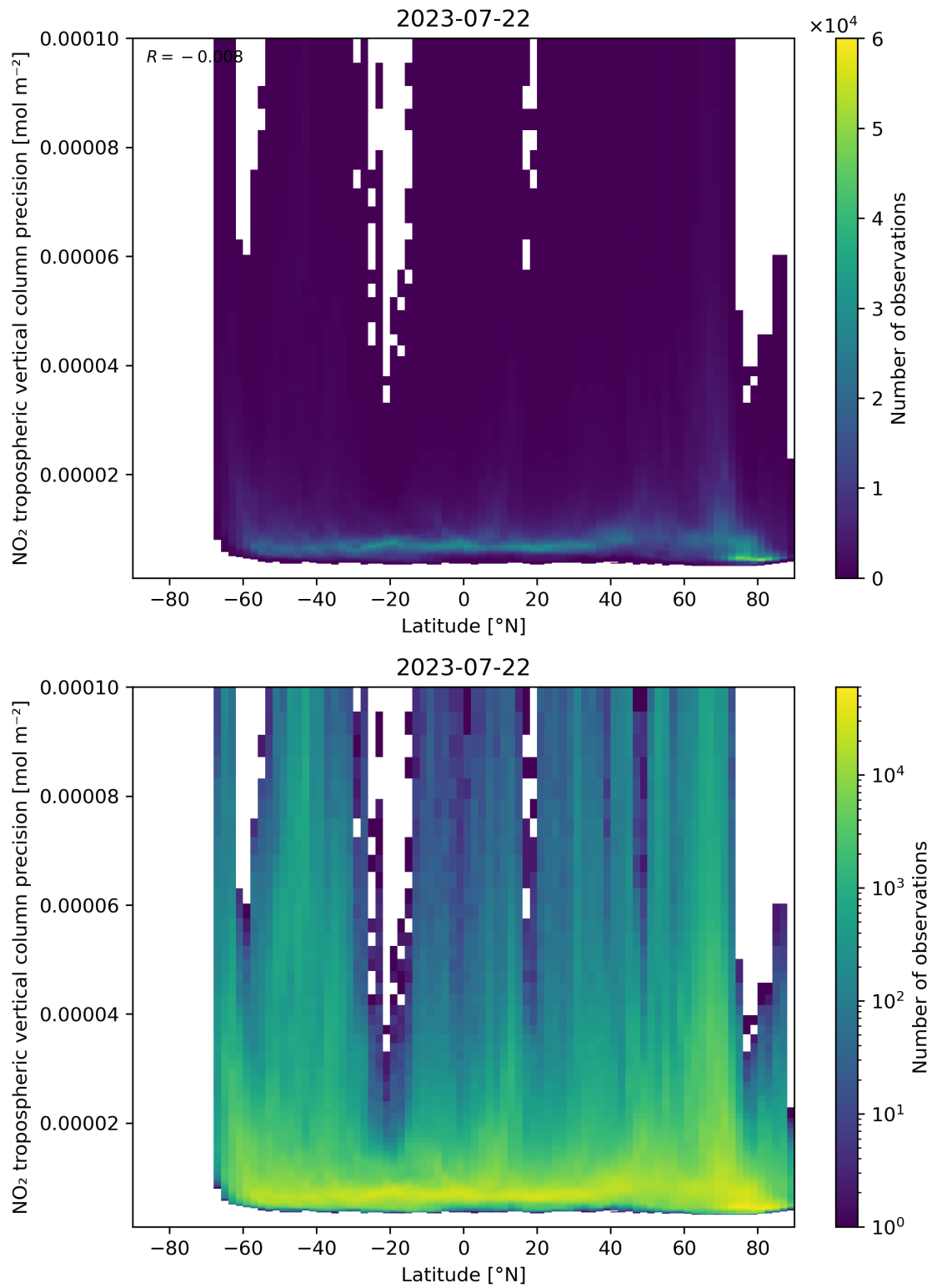
Figure 93: Scatter density plot of “Latitude” against “NO 2 tropospheric vertical column precision” for 2023-07-21 to 2023-07-23.
