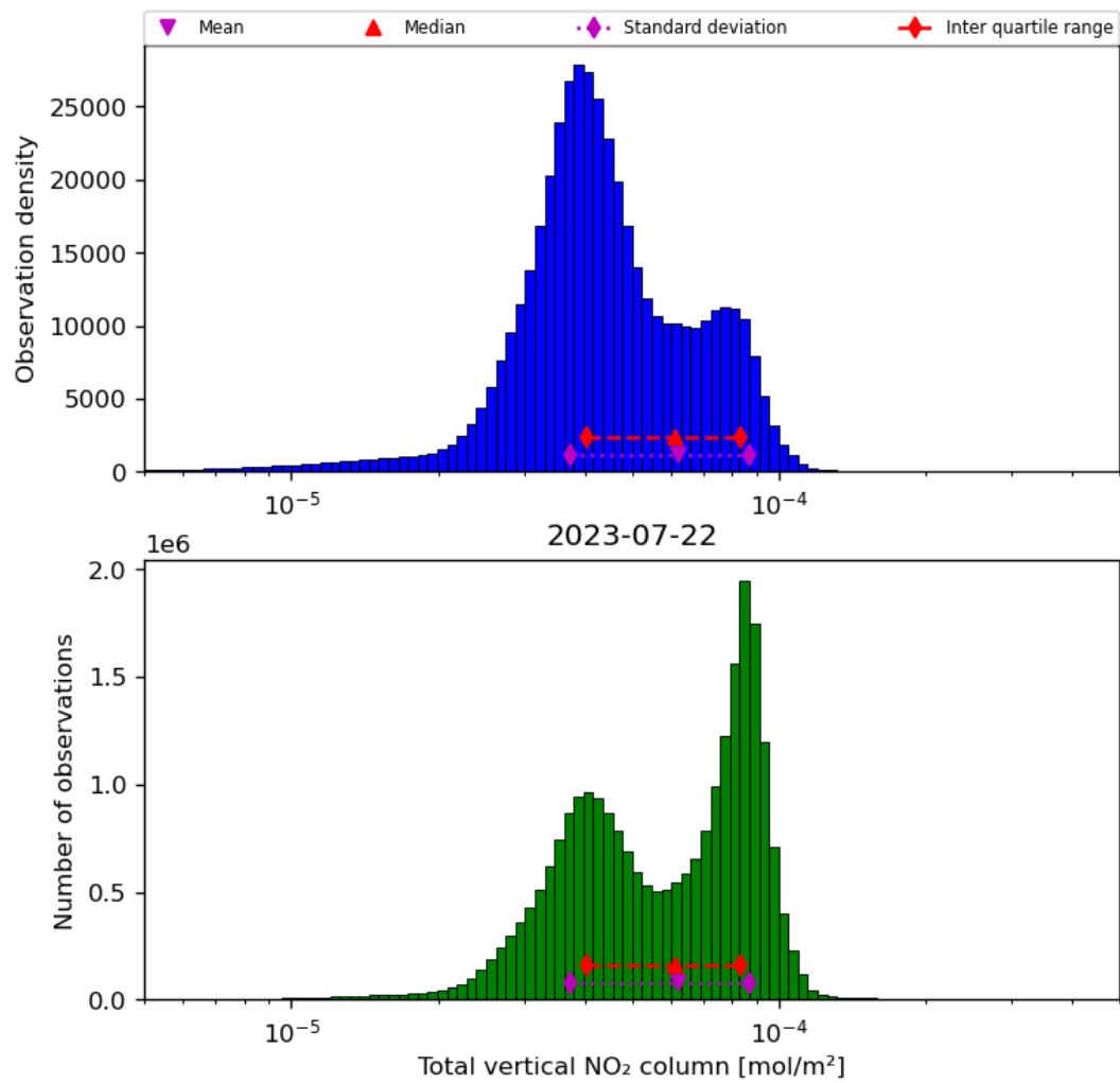
Figure 38: Histogram of “Total vertical NO 2 column” for 2023-07-21 to 2023-07-23
