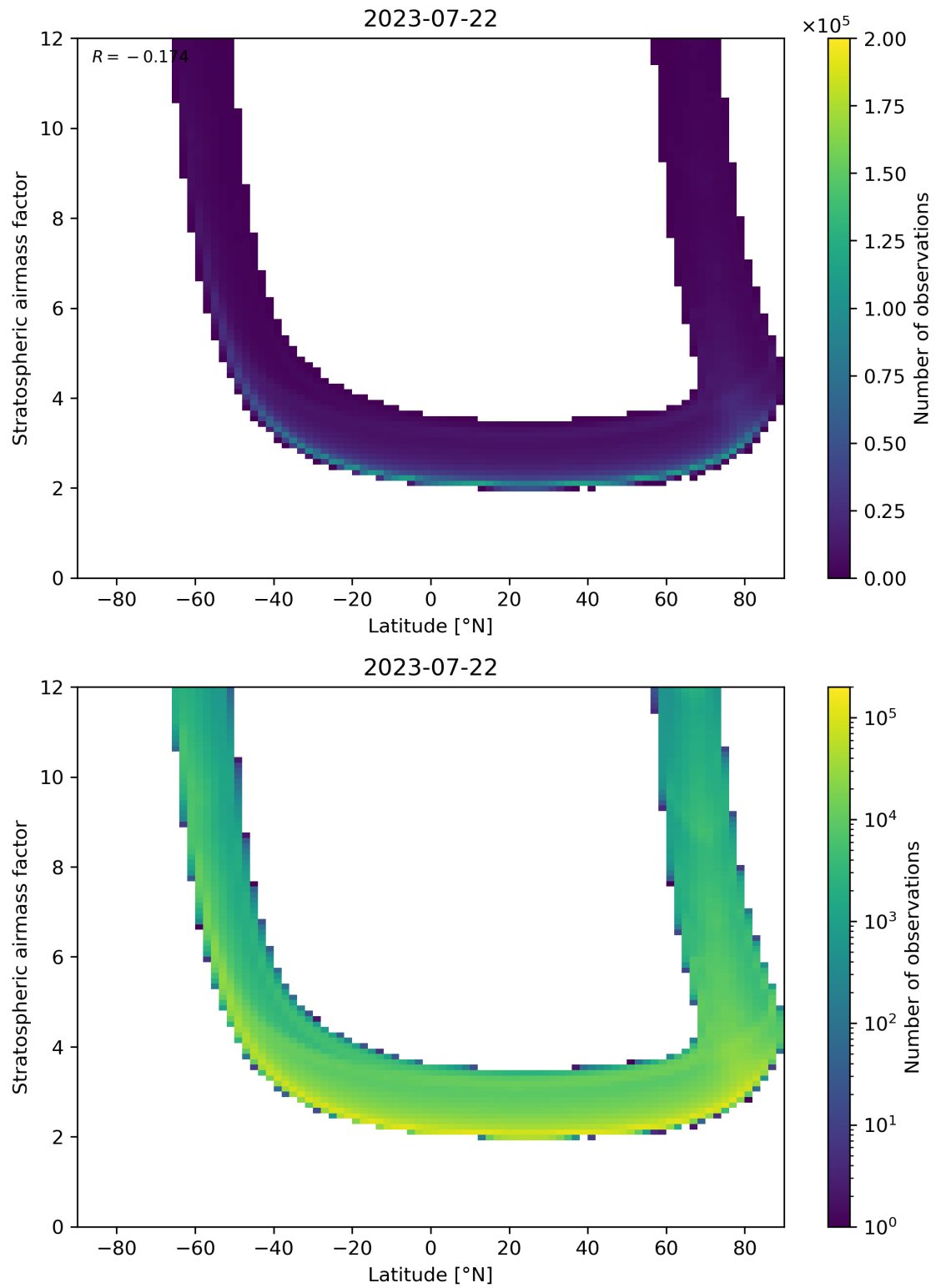
Figure 83: Scatter density plot of “Latitude” against “Stratospheric airmass factor” for 2023-07-21 to 2023-07-23.
