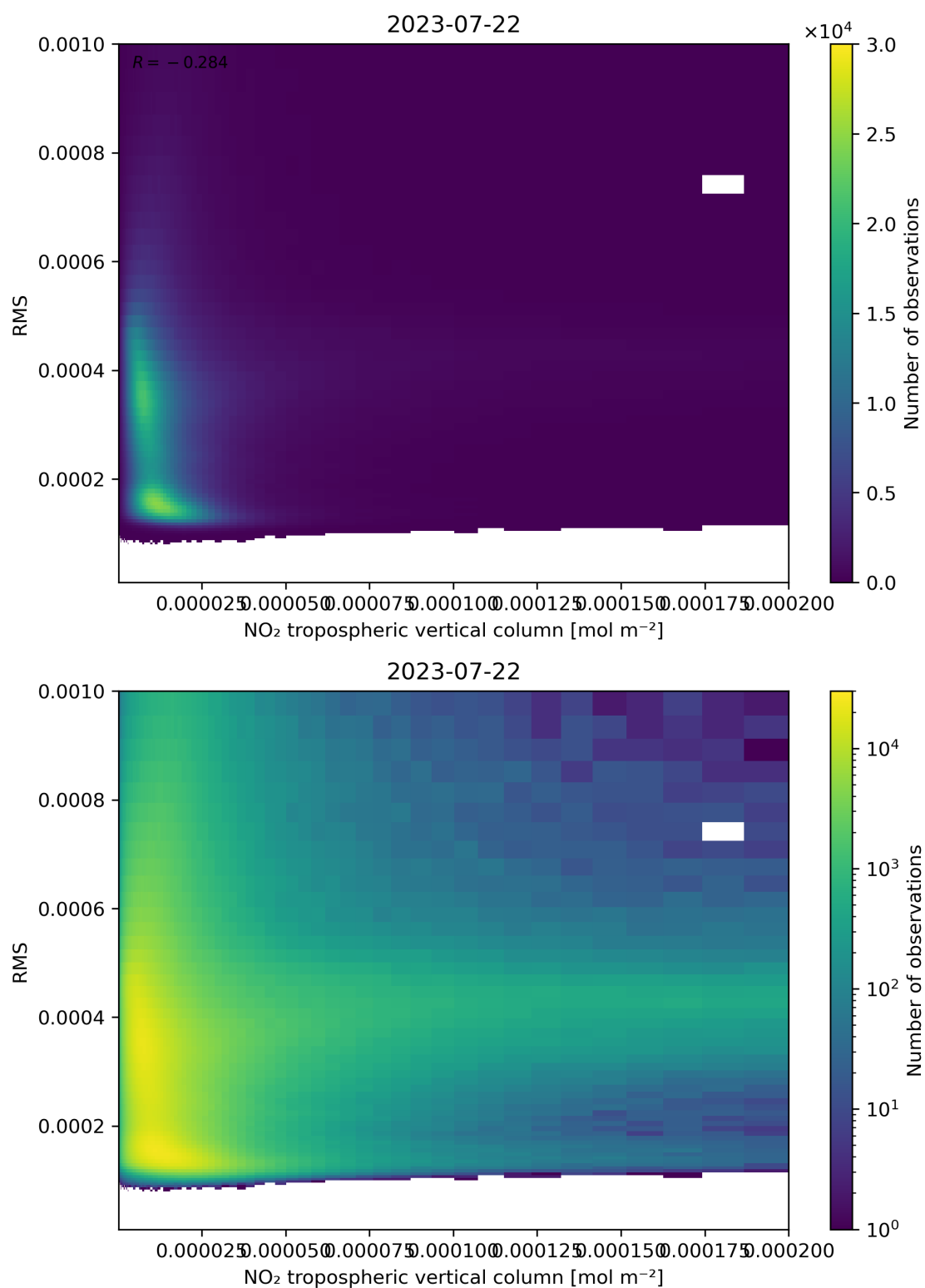
Figure 142: Scatter density plot of “NO 2 tropospheric vertical column” against “RMS” for 2023-07-21 to 2023-07-23.
