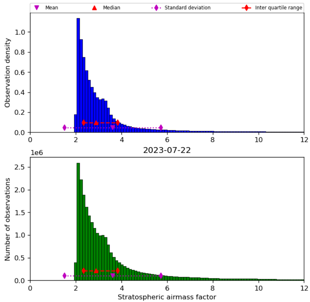
Figure 44: Histogram of “Stratospheric airmass factor” for 2023-07-21 to 2023-07-23
