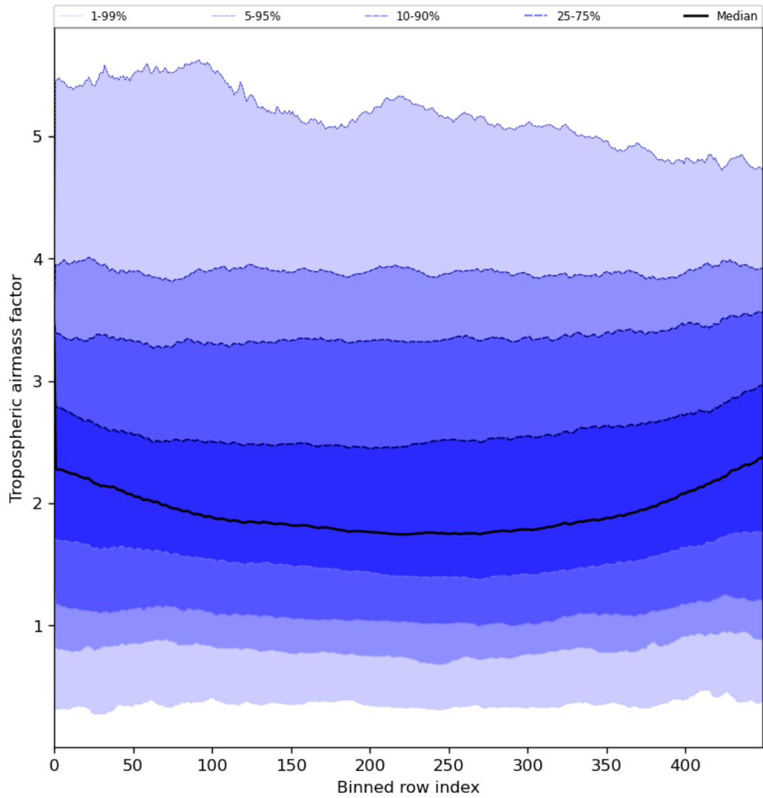
Figure 48: Along track statistics of “Tropospheric airmass factor” for 2023-07-21 to 2023-07-23
