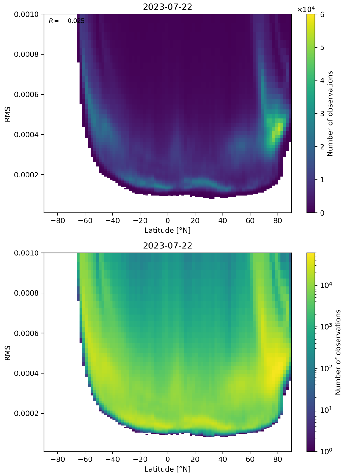
Figure 94: Scatter density plot of “Latitude” against “RMS” for 2023-07-21 to 2023-07-23.
