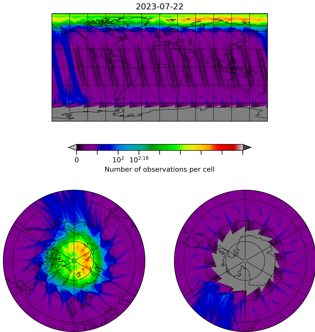
Figure 10: Map of the number of observations for 2023-07-21 to 2023-07-23
