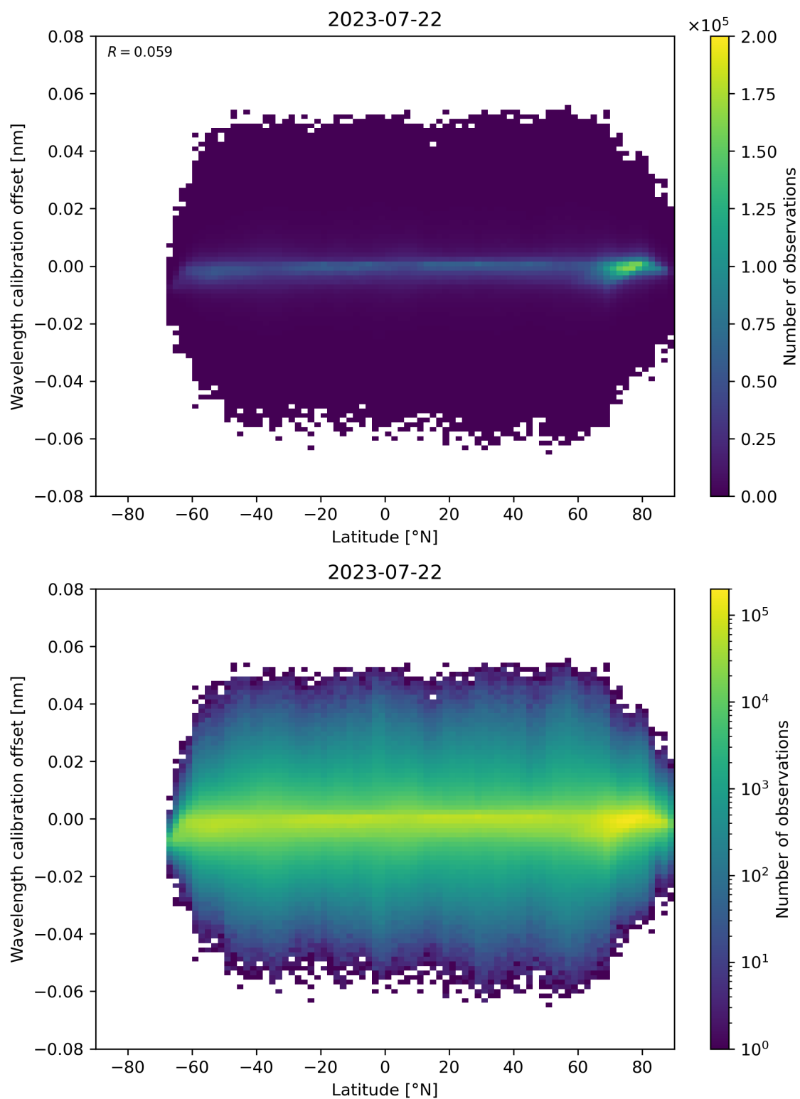
Figure 95: Scatter density plot of “Latitude” against “Wavelength calibration offset” for 2023-07-21 to 2023-07-23.
