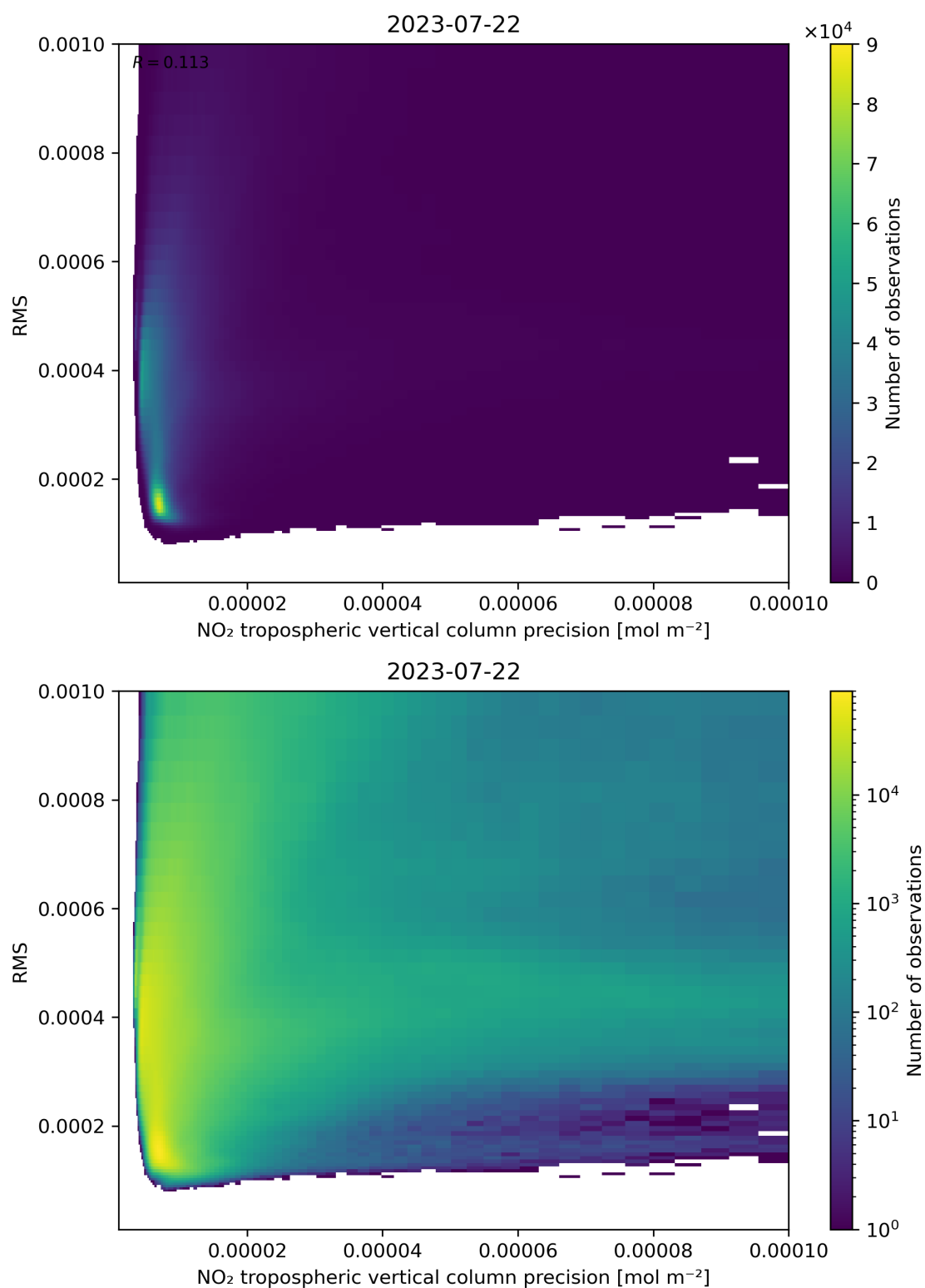
Figure 140: Scatter density plot of “NO 2 tropospheric vertical column precision” against “RMS” for 2023-07-21 to 2023-07-23.
