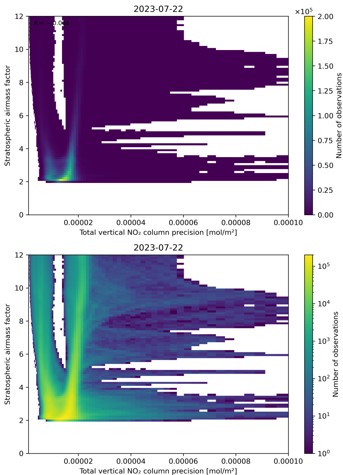
Figure 115: Scatter density plot of “Total vertical NO 2 column precision” against “Stratospheric airmass factor” for 2023-07-21 to 2023-07-23.
