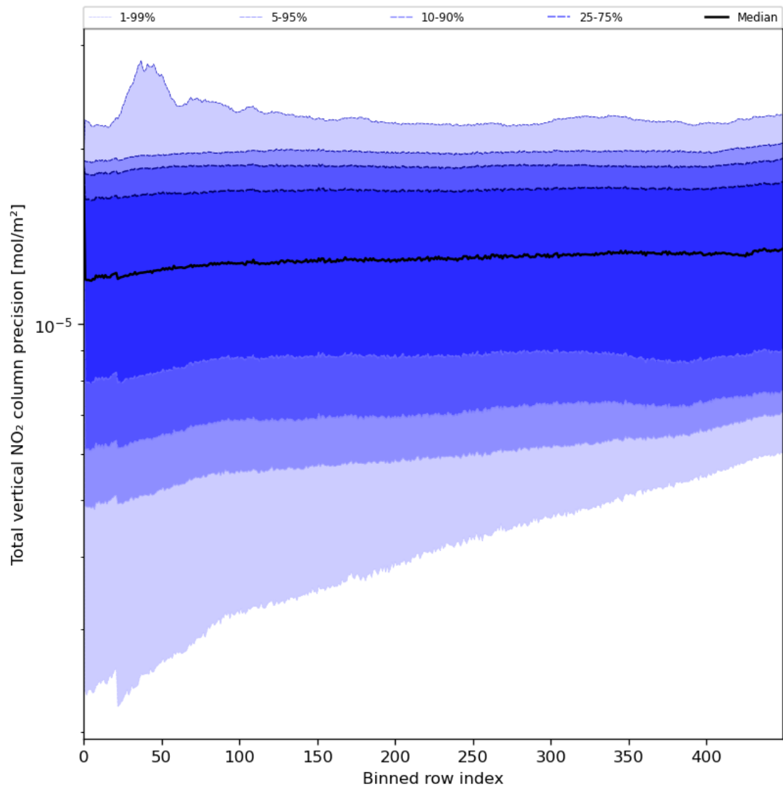
Figure 56: Along track statistics of “Total vertical NO 2 column precision” for 2023-07-21 to 2023-07-23
