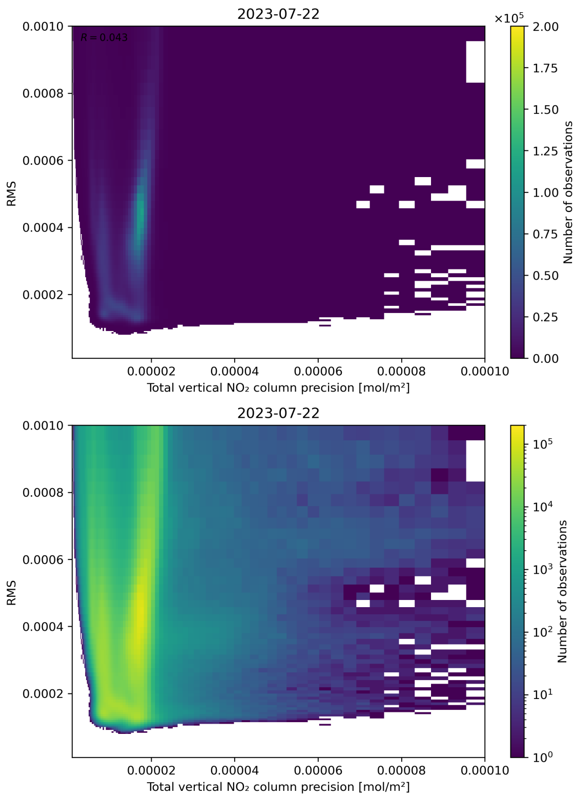
Figure 119: Scatter density plot of “Total vertical NO 2 column precision” against “RMS” for 2023-07-21 to 2023-07-23.
