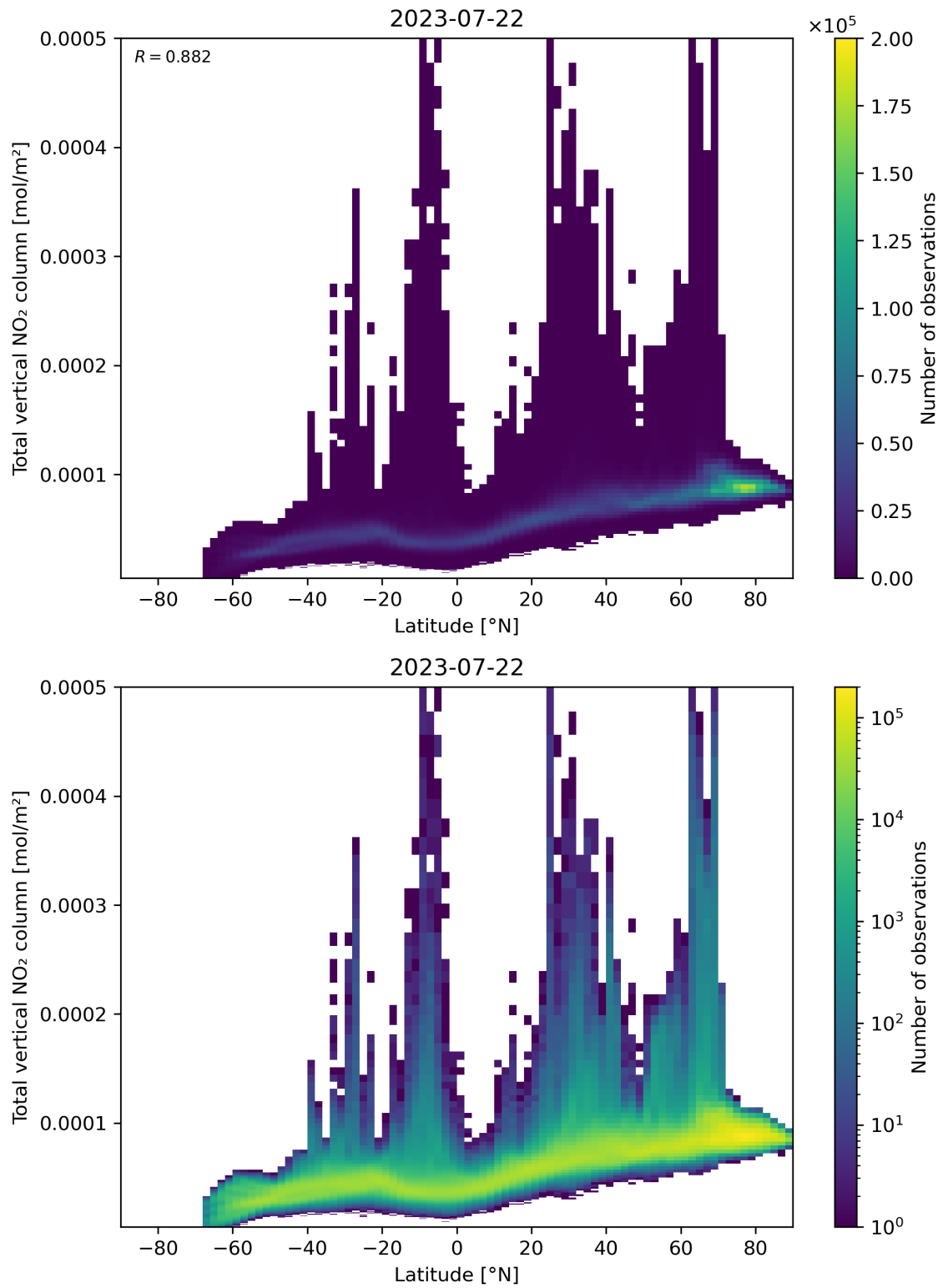
Figure 90: Scatter density plot of “Latitude” against “Total vertical NO 2 column” for 2023-07-21 to 2023-07-23.
