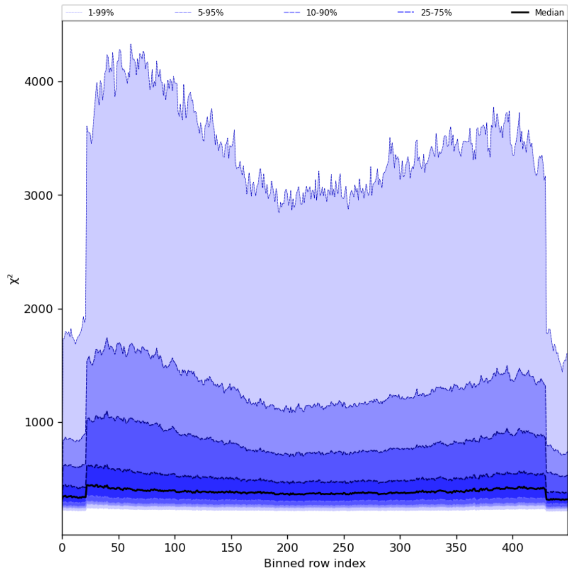
Figure 59: Along track statistics of “ \chi^2 ” for 2023-07-21 to 2023-07-23
