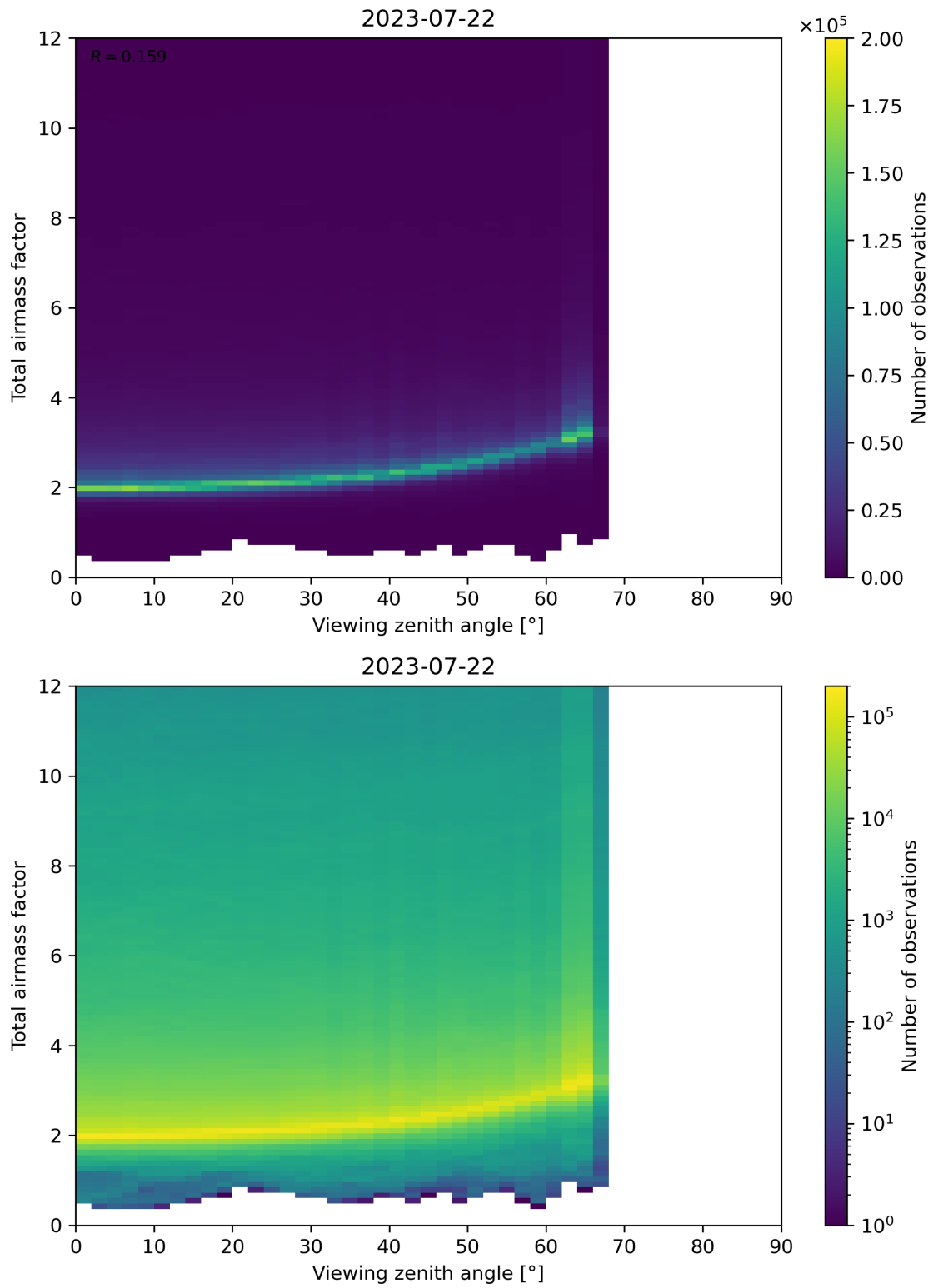
Figure 160: Scatter density plot of “Viewing zenith angle” against “Total airmass factor” for 2023-07-21 to 2023-07-23.
