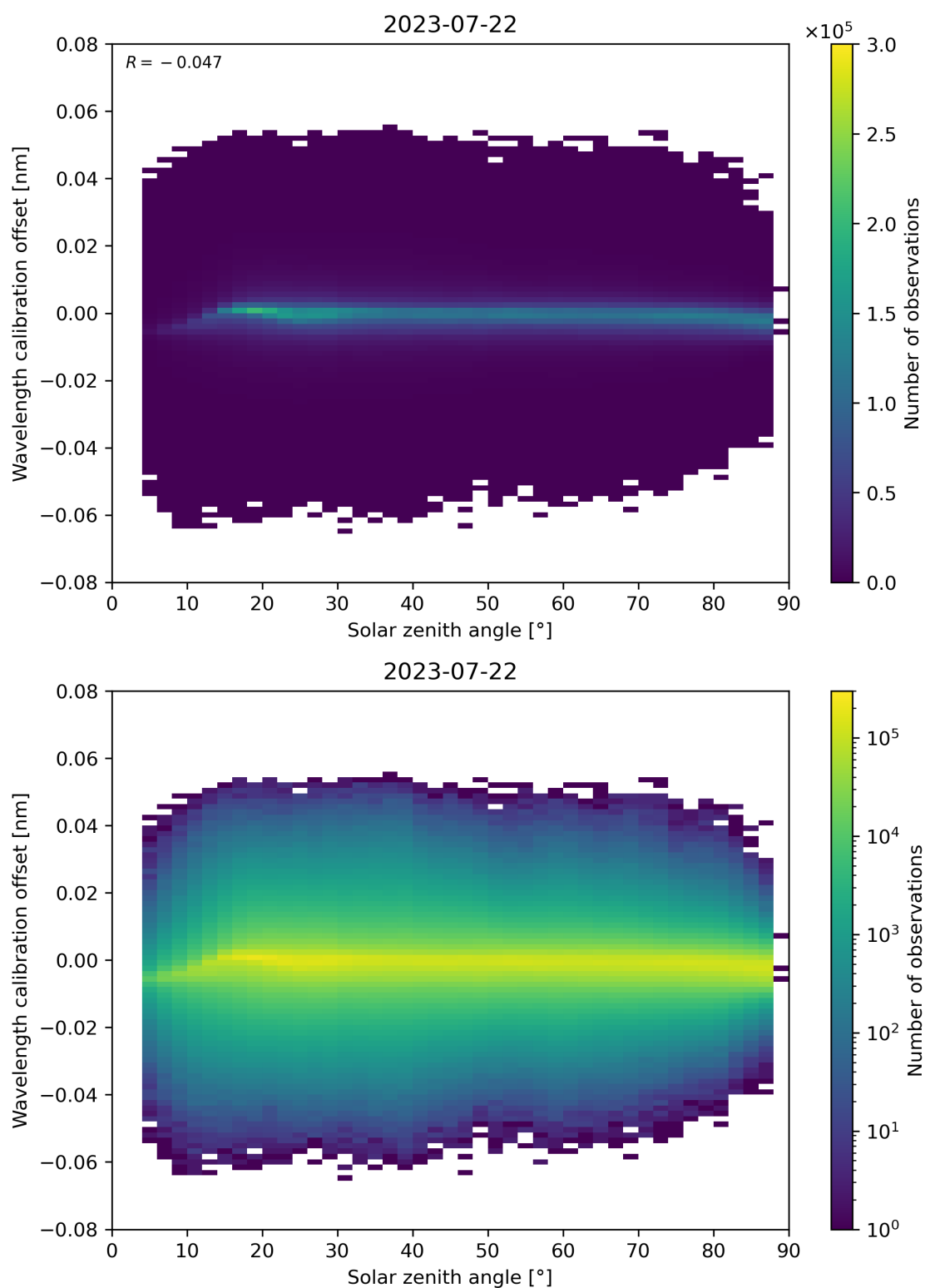
Figure 158: Scatter density plot of “Solar zenith angle” against “Wavelength calibration offset” for 2023-07-21 to 2023-07-23.
