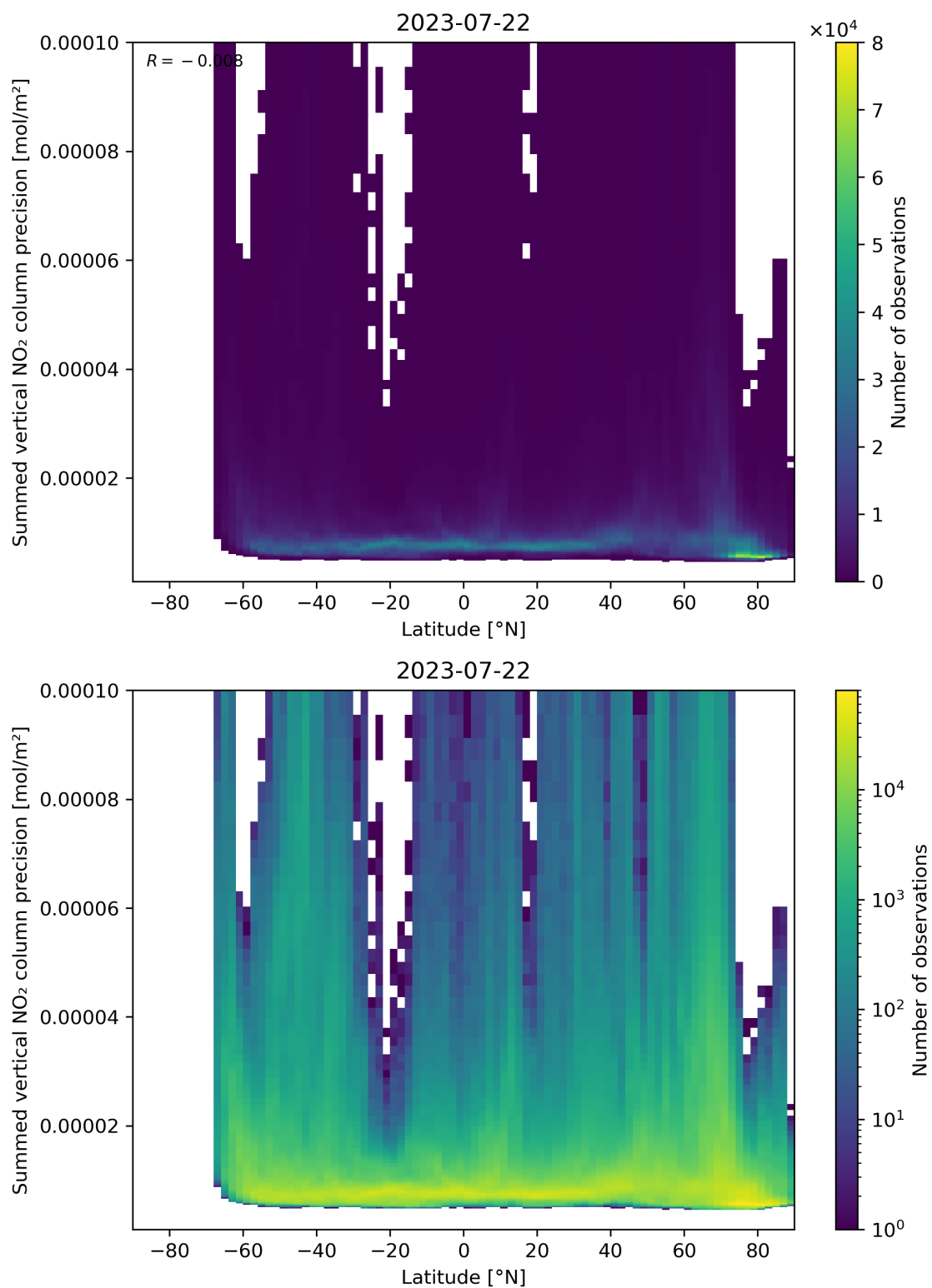
Figure 89: Scatter density plot of “Latitude” against “Summed vertical NO 2 column precision” for 2023-07-21 to 2023-07-23.
