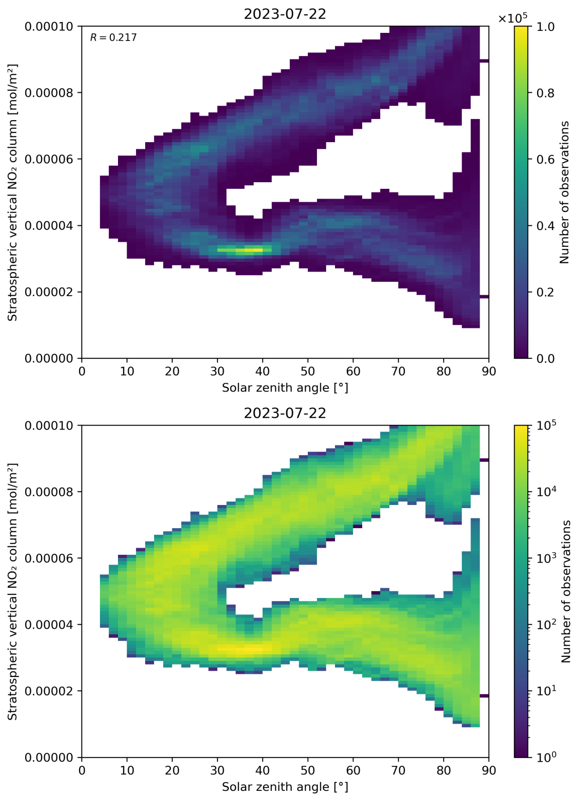
Figure 150: Scatter density plot of “Solar zenith angle” against “Stratospheric vertical NO 2 column” for 2023-07-21 to 2023-07-23.
