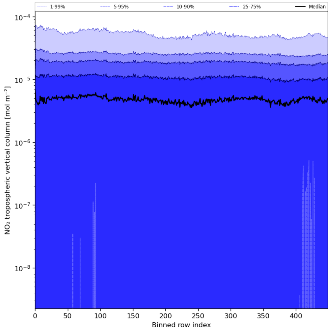
Figure 46: Along track statistics of “NO 2 tropospheric vertical column” for 2023-07-21 to 2023-07-23
