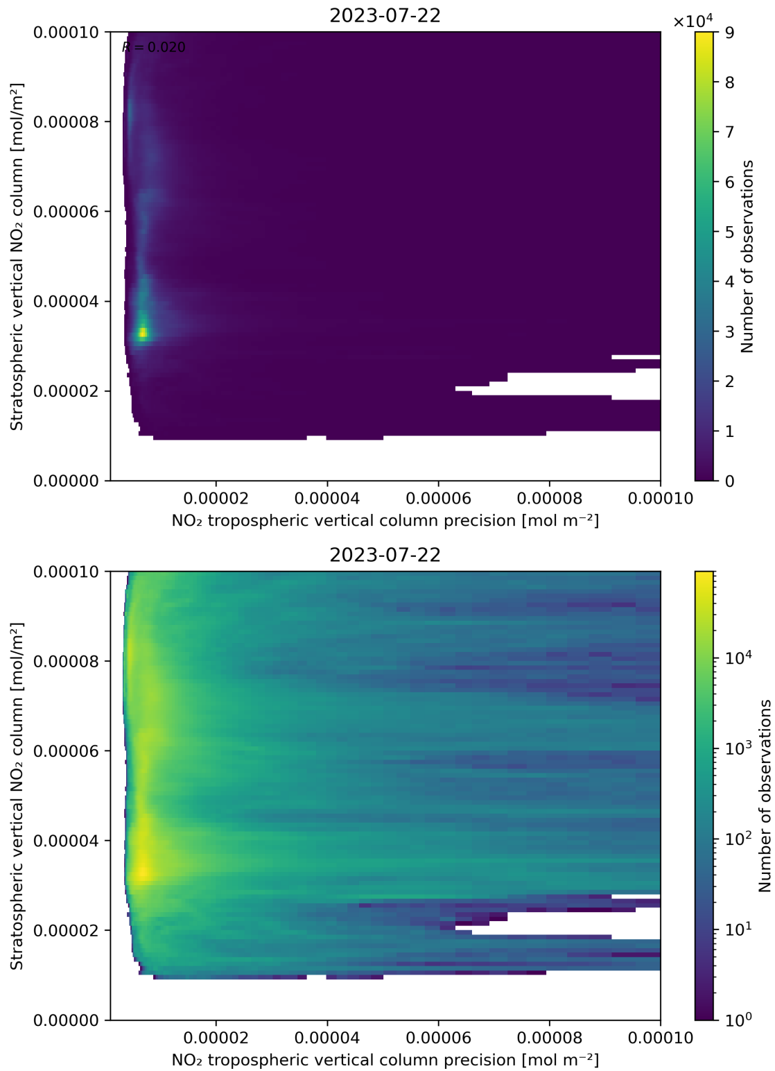
Figure 135: Scatter density plot of “NO 2 tropospheric vertical column precision” against “Stratospheric vertical NO 2 column” for 2023-07-21 to 2023-07-23.
