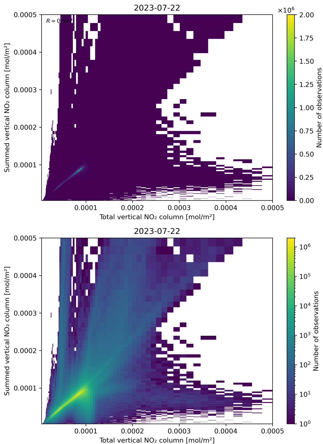
Figure 112: Scatter density plot of “Total vertical NO 2 column” against “Summed vertical NO 2 column” for 2023-07-21 to 2023-07-23.
