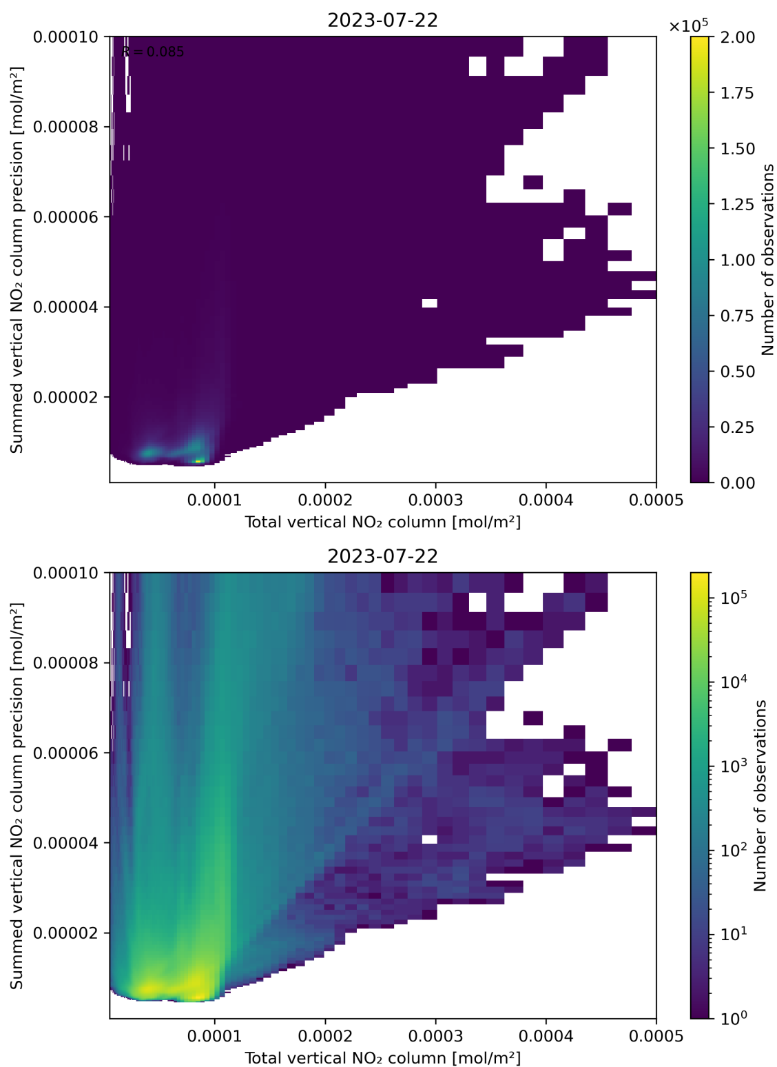
Figure 113: Scatter density plot of “Total vertical NO 2 column” against “Summed vertical NO 2 column precision” for 2023-07-21 to 2023-07-23.
