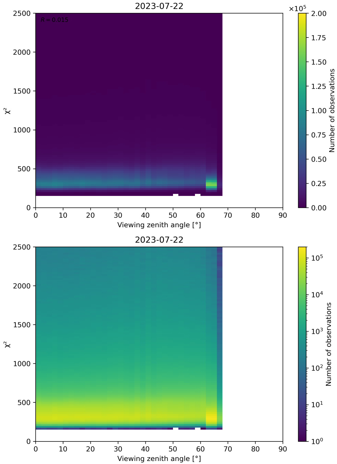
Figure 162: Scatter density plot of “Viewing zenith angle” against “ \chi^2 ” for 2023-07-21 to 2023-07-23.
