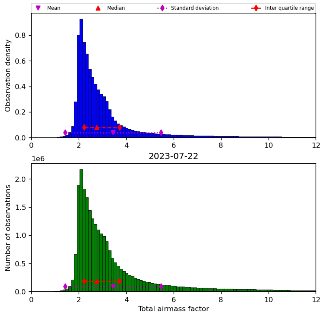
Figure 32: Histogram of “Total airmass factor” for 2023-07-21 to 2023-07-23
