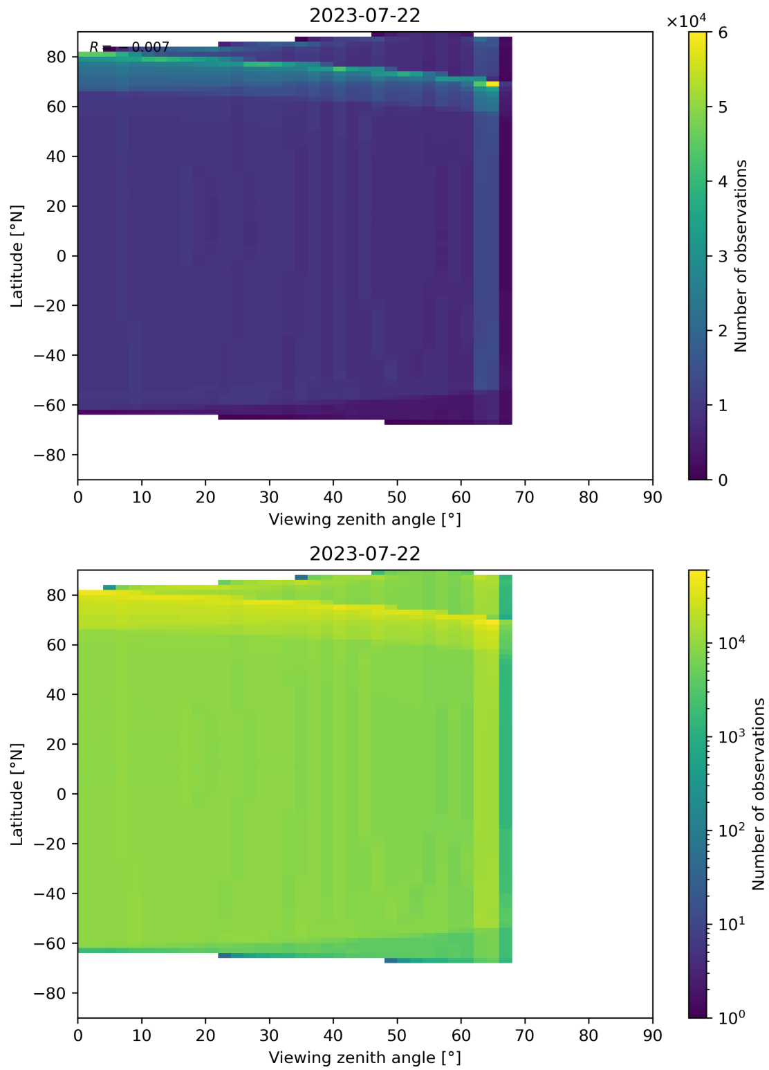
Figure 163: Scatter density plot of “Viewing zenith angle” against “Latitude” for 2023-07-21 to 2023-07-23.
