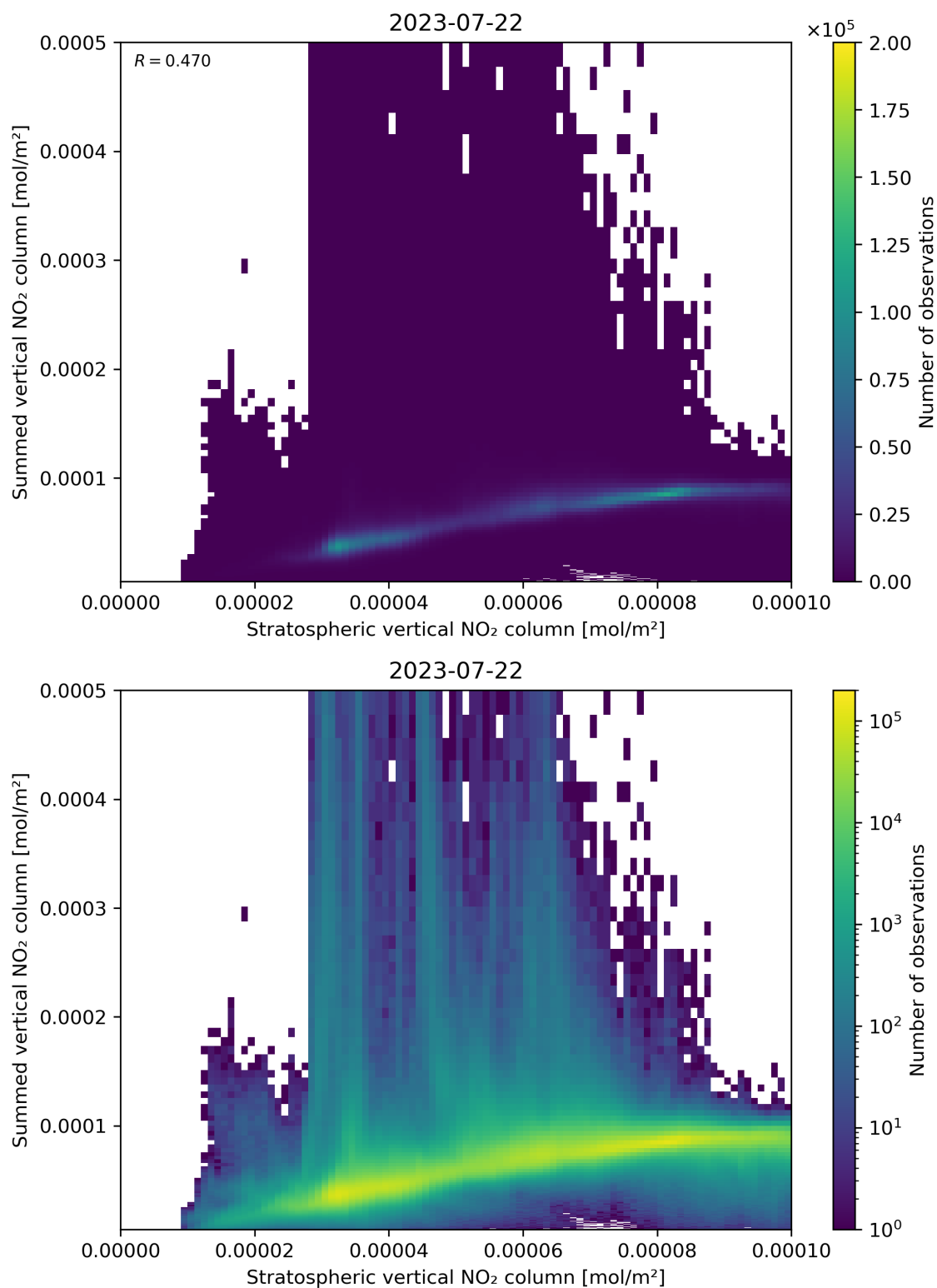
Figure 98: Scatter density plot of “Stratospheric vertical NO 2 column” against “Summed vertical NO 2 column” for 2023-07-21 to 2023-07-23.
