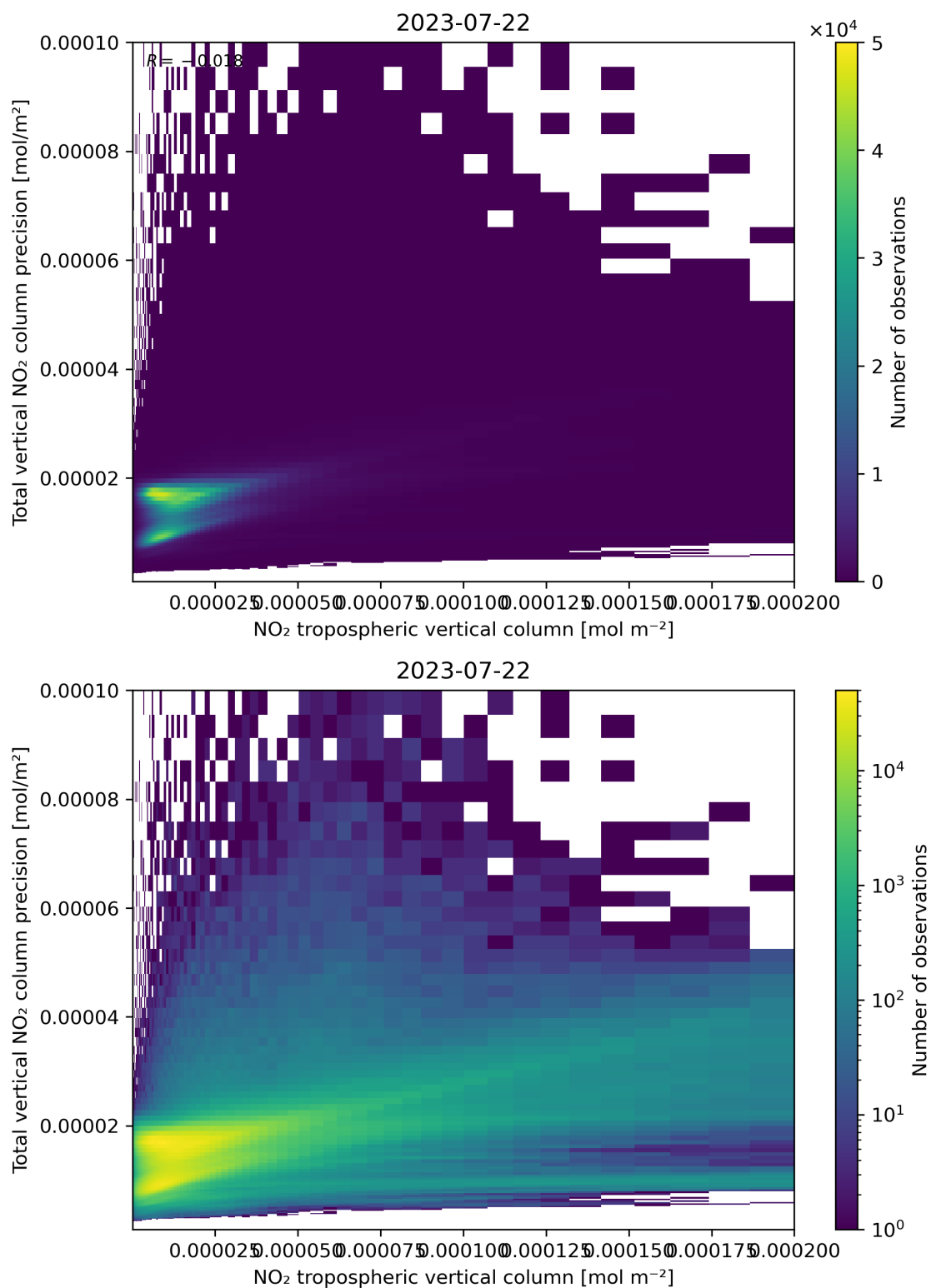
Figure 129: Scatter density plot of “NO 2 tropospheric vertical column” against “Total vertical NO 2 column precision” for 2023-07-21 to 2023-07-23.
