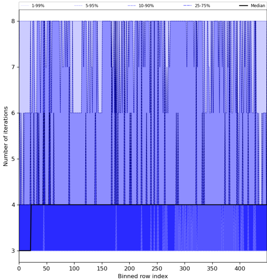
Figure 51: Along track statistics of “Number of iterations” for 2023-07-21 to 2023-07-23
