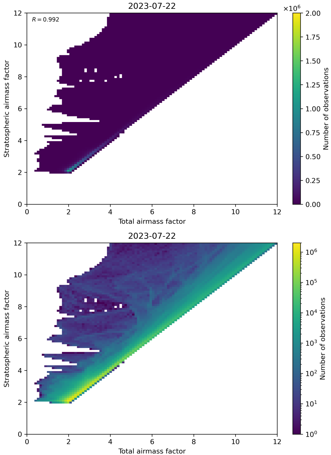
Figure 62: Scatter density plot of “Total airmass factor” against “Stratospheric airmass factor” for 2023-07-21 to 2023-07-23.
