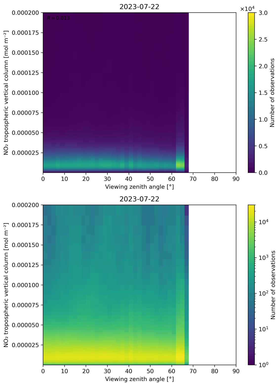
Figure 169: Scatter density plot of “Viewing zenith angle” against “NO 2 tropospheric vertical column” for 2023-07-21 to 2023-07-23.
