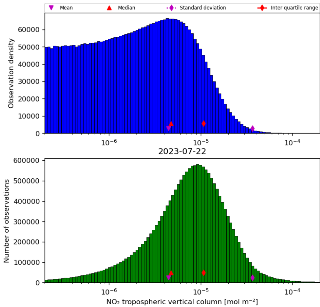
Figure 29: Histogram of “NO 2 tropospheric vertical column” for 2023-07-21 to 2023-07-23
