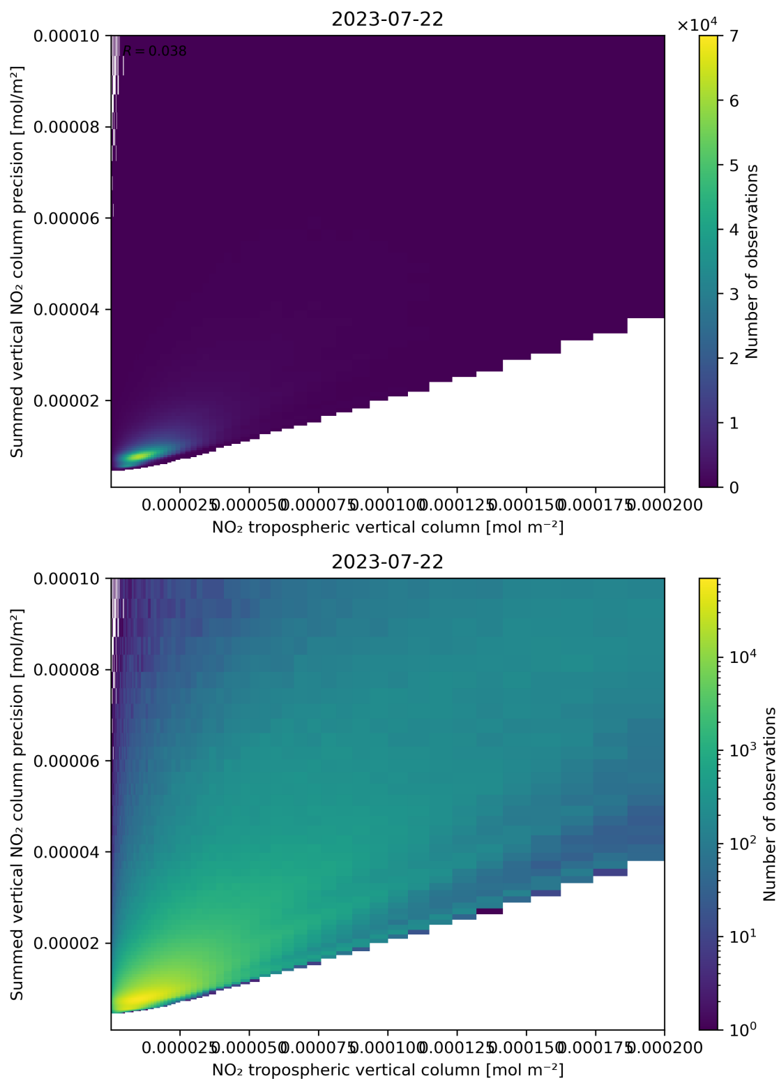
Figure 127: Scatter density plot of “NO 2 tropospheric vertical column” against “Summed vertical NO 2 column precision” for 2023-07-21 to 2023-07-23.
