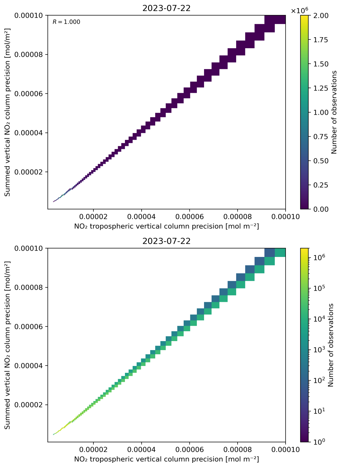
Figure 137: Scatter density plot of “NO 2 tropospheric vertical column precision” against “Summed vertical NO 2 column precision” for 2023-07-21 to 2023-07-23.
