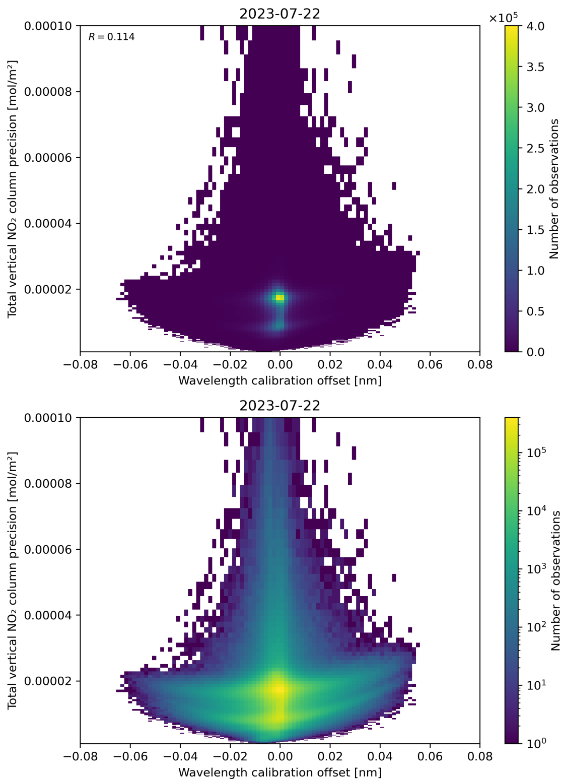
Figure 180: Scatter density plot of “Wavelength calibration offset” against “Total vertical NO 2 column precision” for 2023-07-21 to 2023-07-23.
