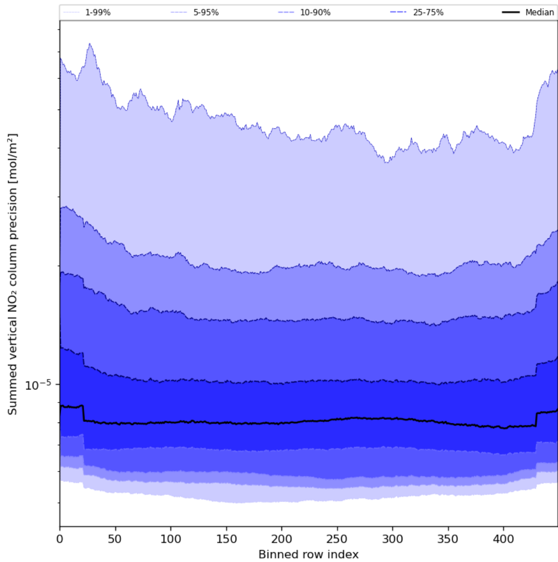
Figure 58: Along track statistics of “Summed vertical NO 2 column precision” for 2023-07-21 to 2023-07-23
