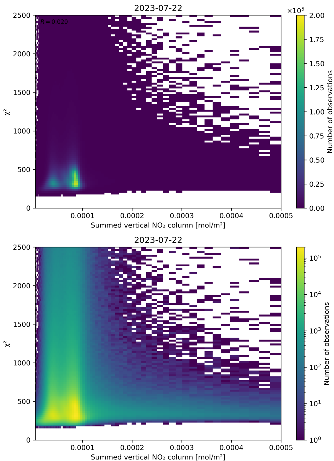
Figure 104: Scatter density plot of “Summed vertical NO 2 column” against “ \chi^2 ” for 2023-07-21 to 2023-07-23.
