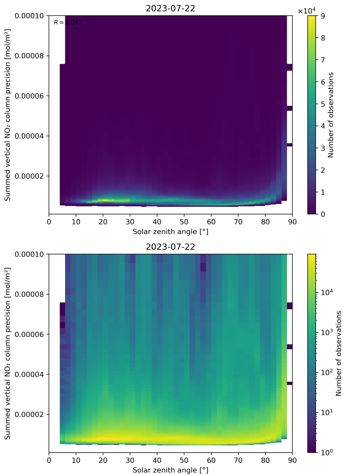
Figure 152: Scatter density plot of “Solar zenith angle” against “Summed vertical NO 2 column precision” for 2023-07-21 to 2023-07-23.
