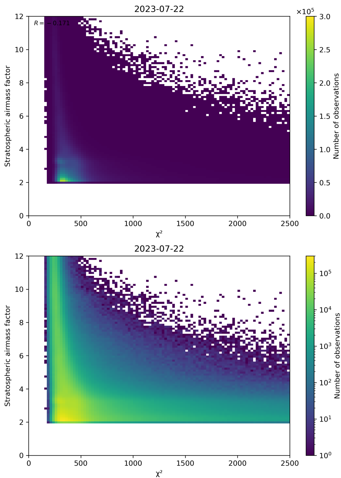
Figure 81: Scatter density plot of “ \chi^2 ” against “Stratospheric airmass factor” for 2023-07-21 to 2023-07-23.
