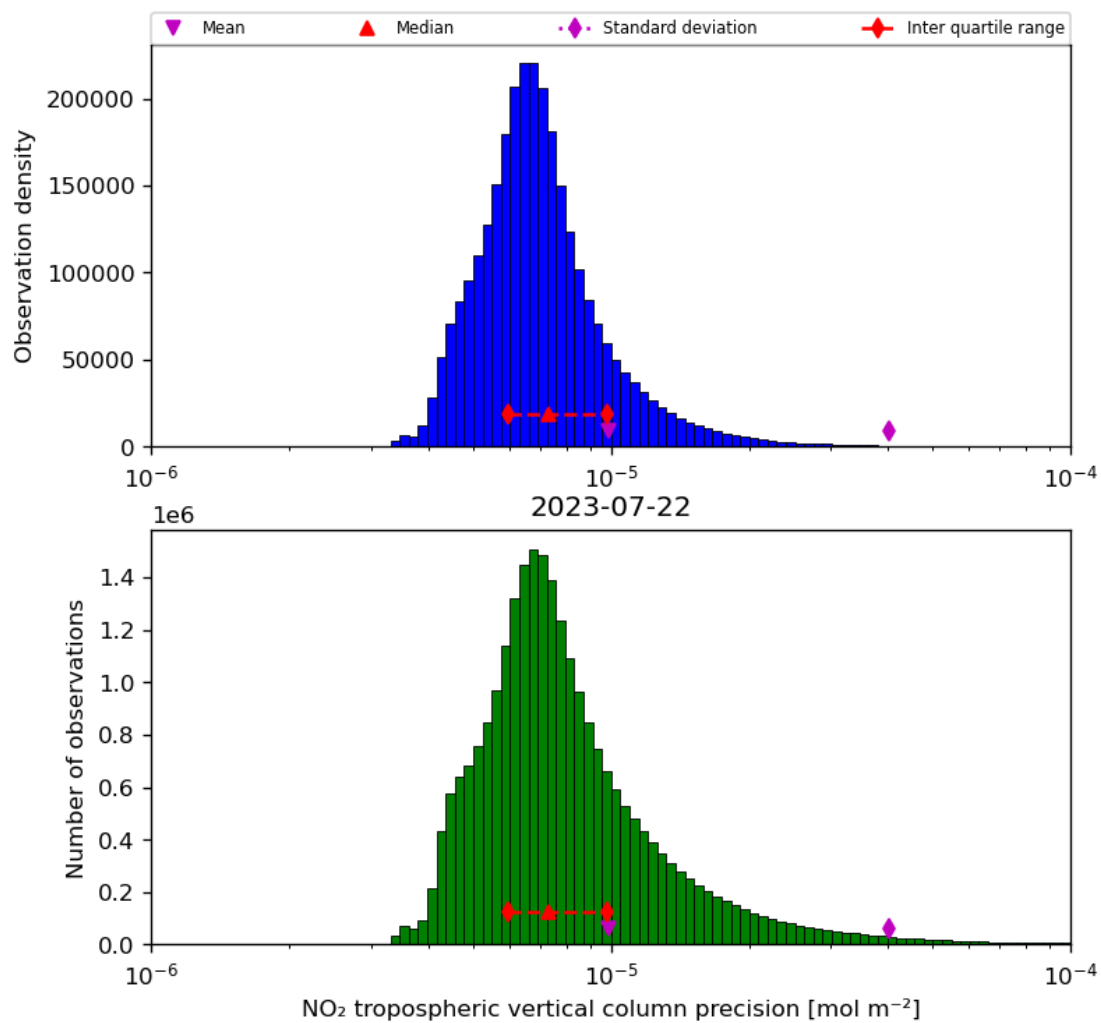
Figure 30: Histogram of “NO 2 tropospheric vertical column precision” for 2023-07-21 to 2023-07-23
