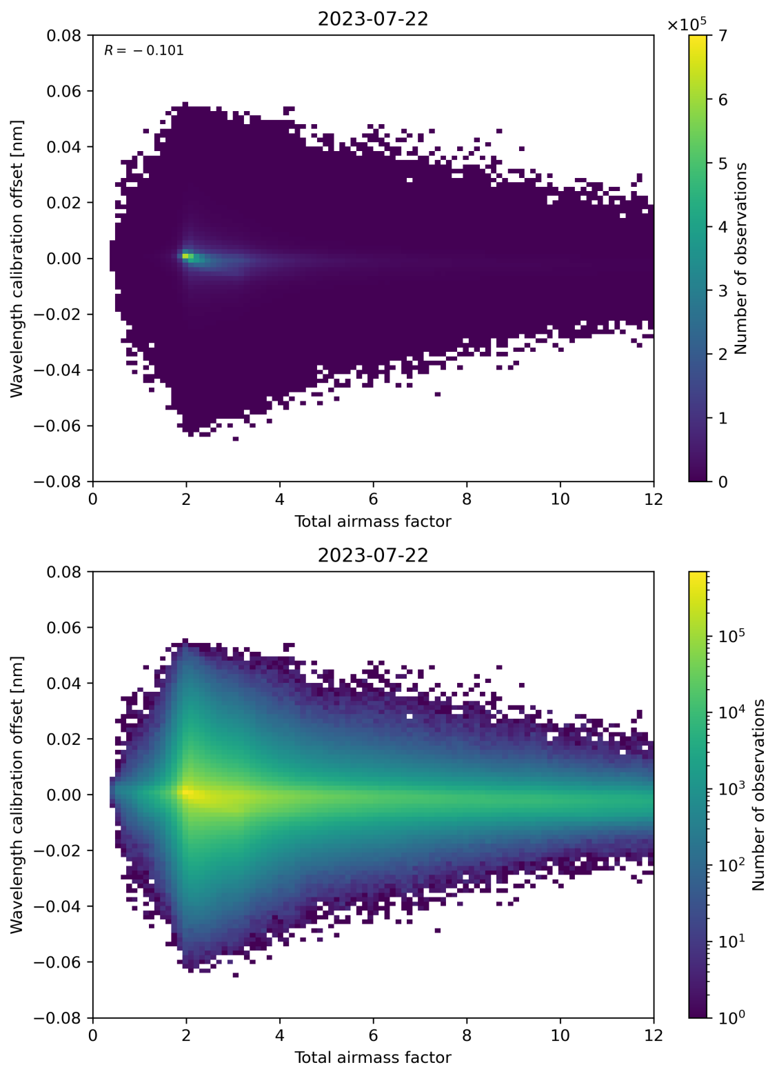
Figure 70: Scatter density plot of “Total airmass factor” against “Wavelength calibration offset” for 2023-07-21 to 2023-07-23.
