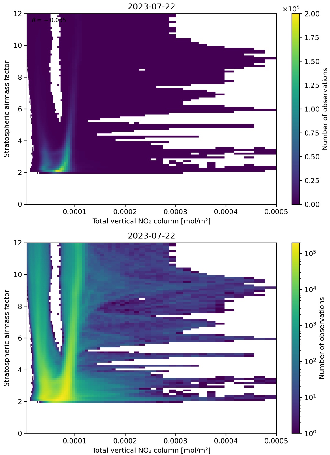
Figure 110: Scatter density plot of “Total vertical NO 2 column” against “Stratospheric airmass factor” for 2023-07-21 to 2023-07-23.
