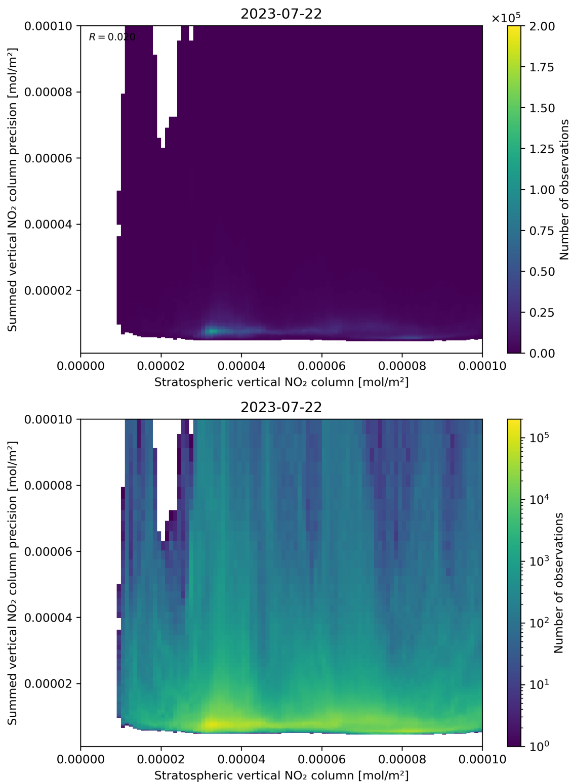
Figure 99: Scatter density plot of “Stratospheric vertical NO 2 column” against “Summed vertical NO 2 column precision” for 2023-07-21 to 2023-07-23.
