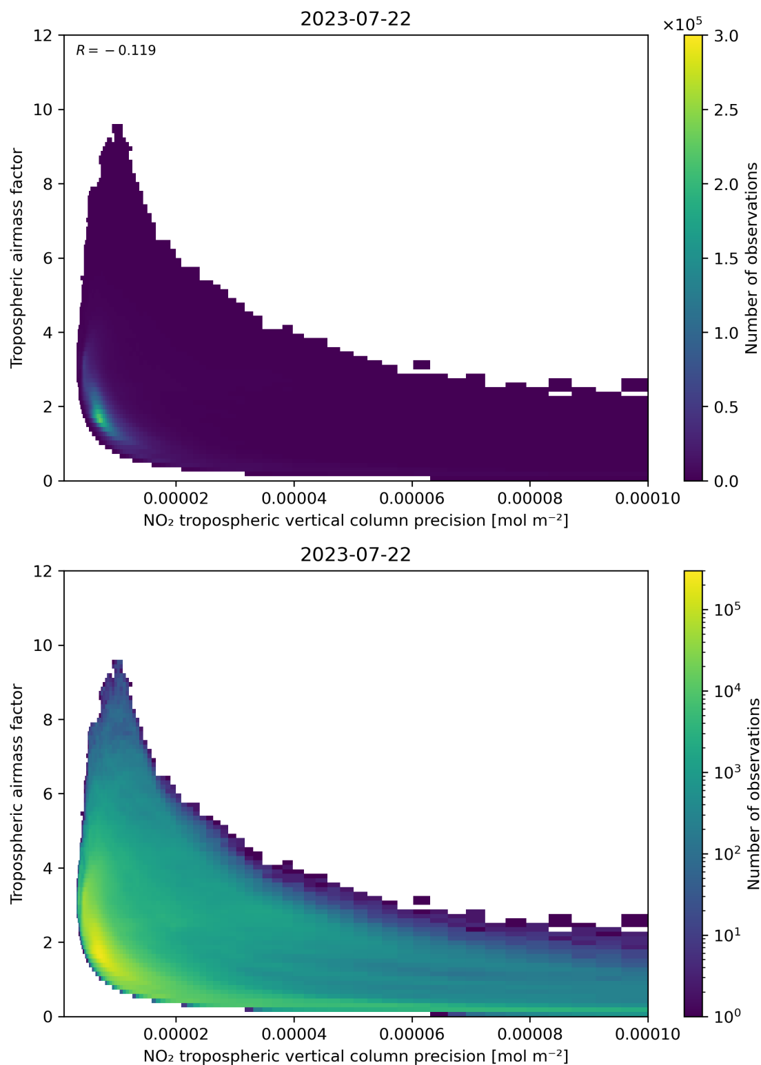
Figure 133: Scatter density plot of “NO 2 tropospheric vertical column precision” against “Tropospheric airmass factor” for 2023-07-21 to 2023-07-23.
