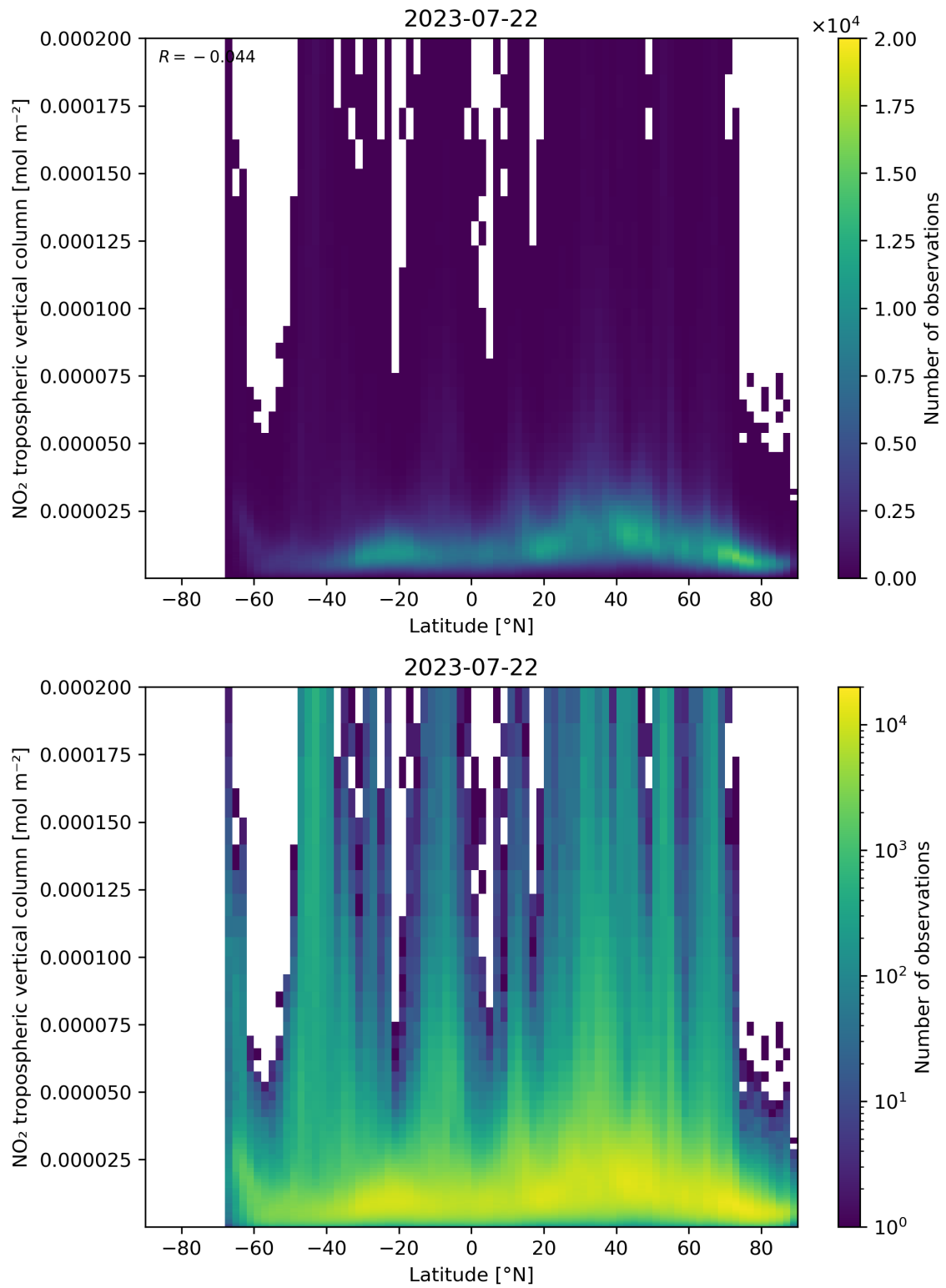
Figure 92: Scatter density plot of “Latitude” against “NO 2 tropospheric vertical column” for 2023-07-21 to 2023-07-23.
