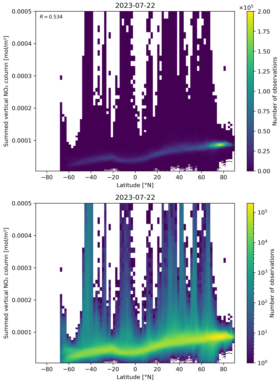
Figure 88: Scatter density plot of “Latitude” against “Summed vertical NO 2 column” for 2023-07-21 to 2023-07-23.
