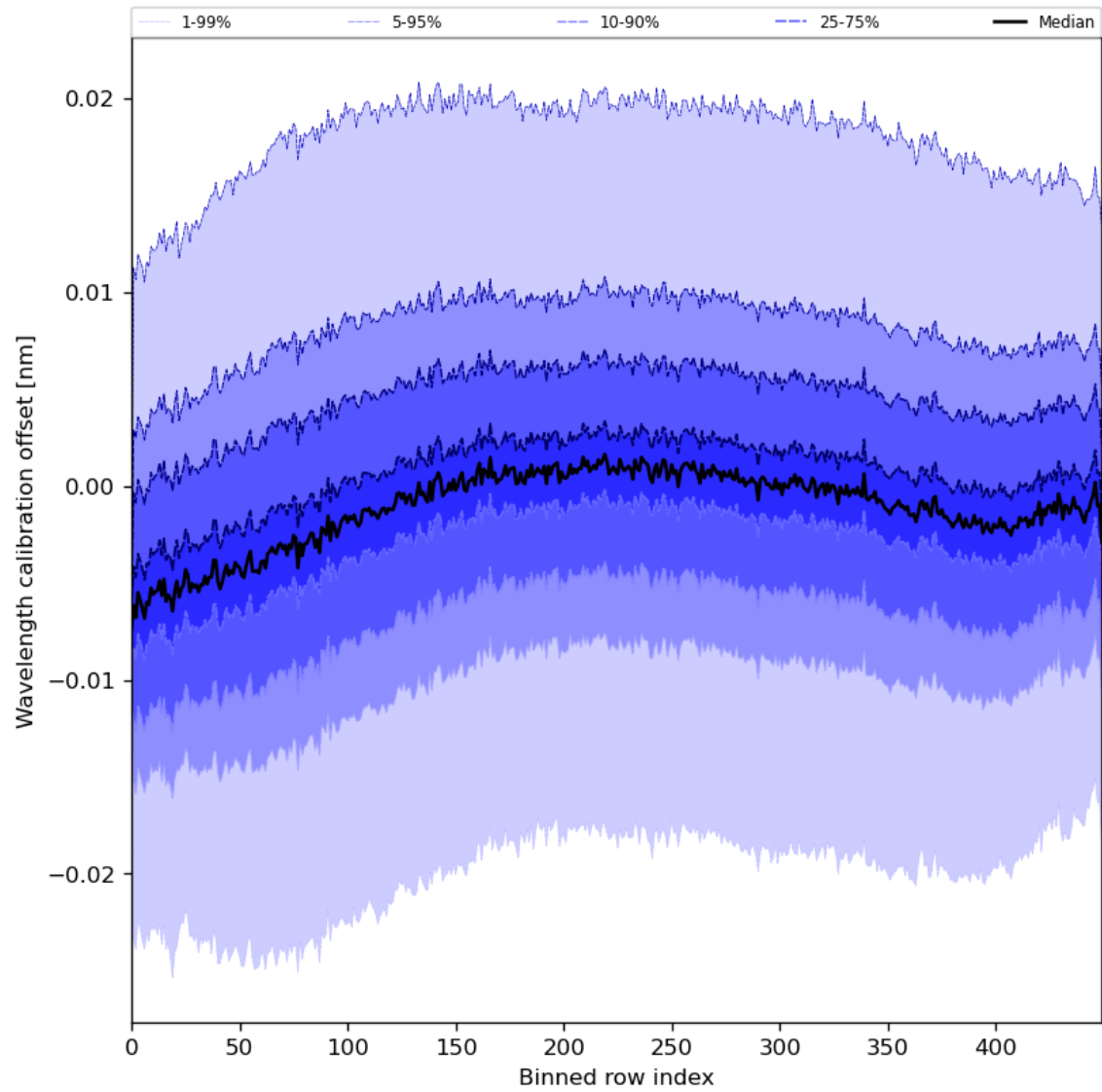
Figure 52: Along track statistics of “Wavelength calibration offset” for 2023-07-21 to 2023-07-23
