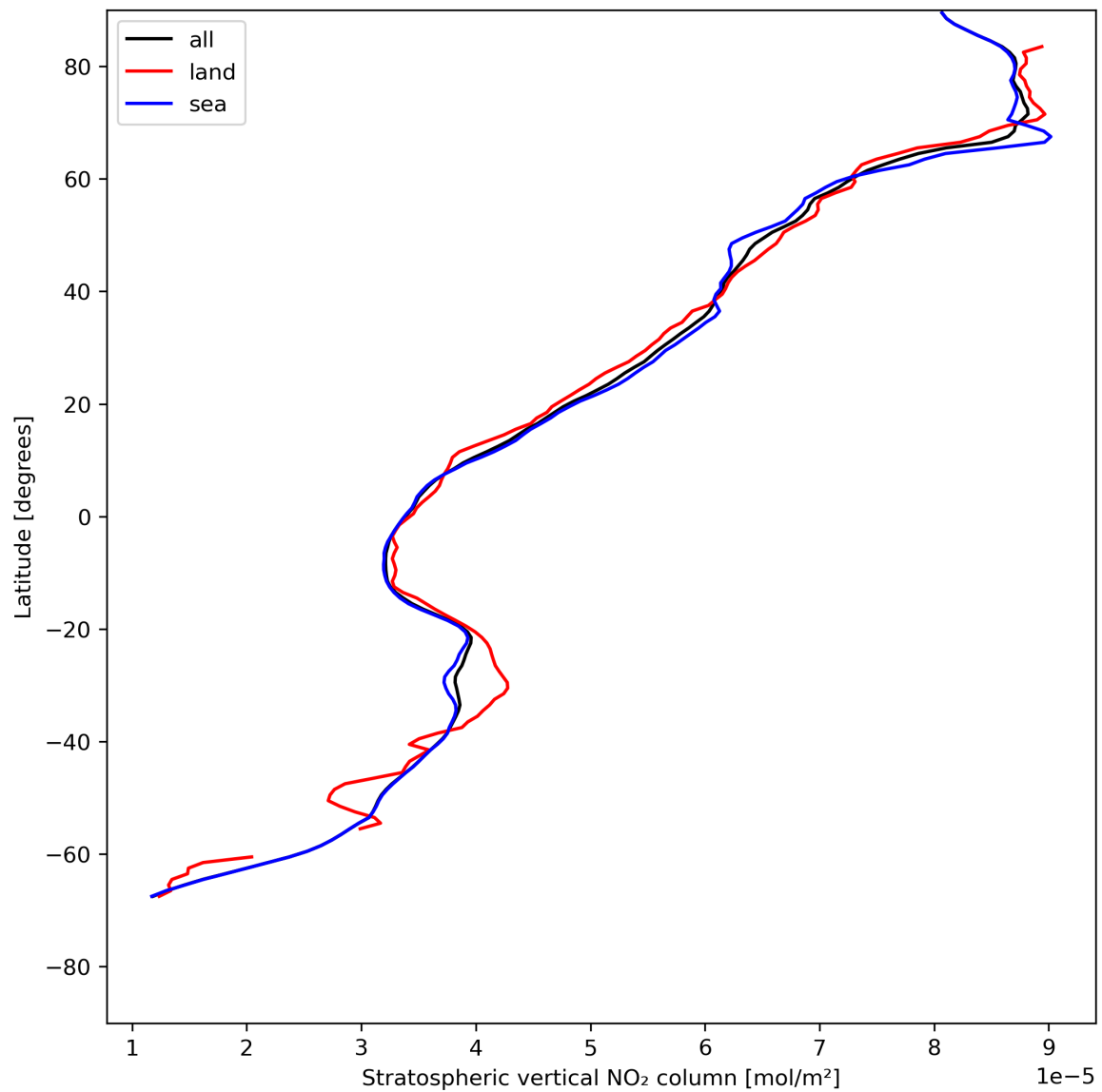
Figure 19: Zonal average of “Stratospheric vertical NO 2 column” for 2023-07-21 to 2023-07-23.
