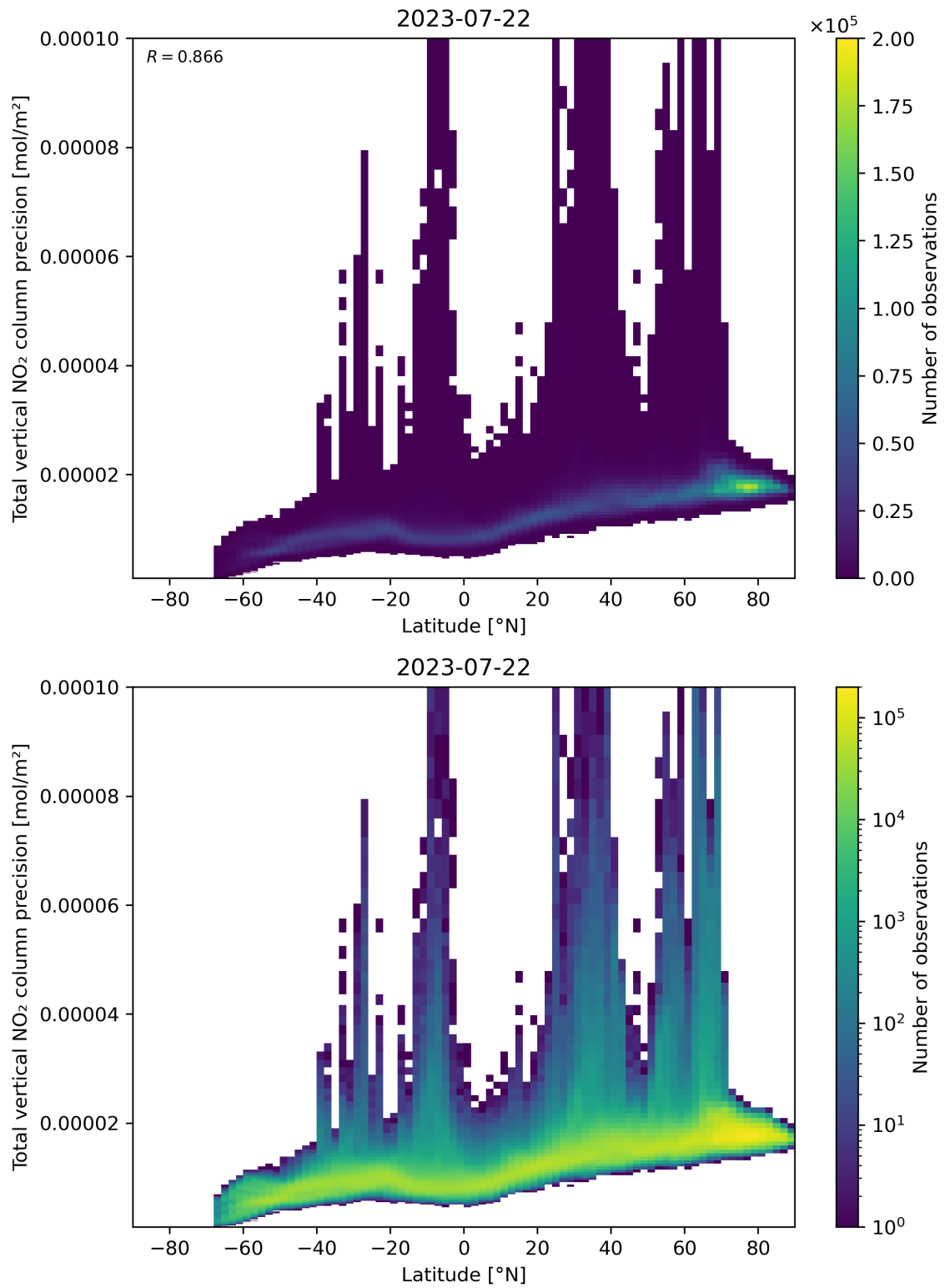
Figure 91: Scatter density plot of “Latitude” against “Total vertical NO 2 column precision” for 2023-07-21 to 2023-07-23.
