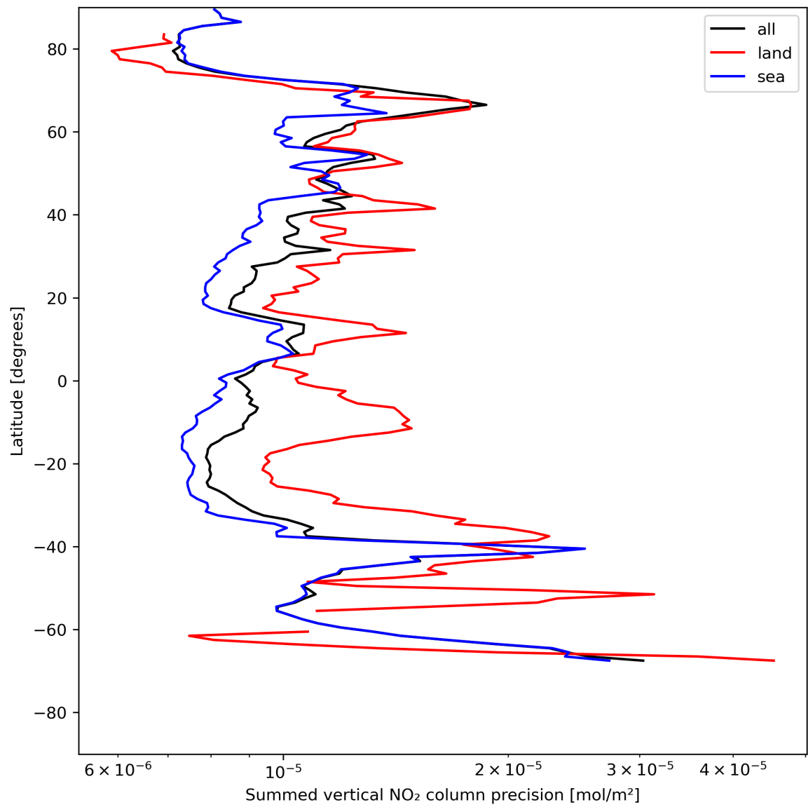
Figure 24: Zonal average of “Summed vertical NO 2 column precision” for 2023-07-21 to 2023-07-23.
