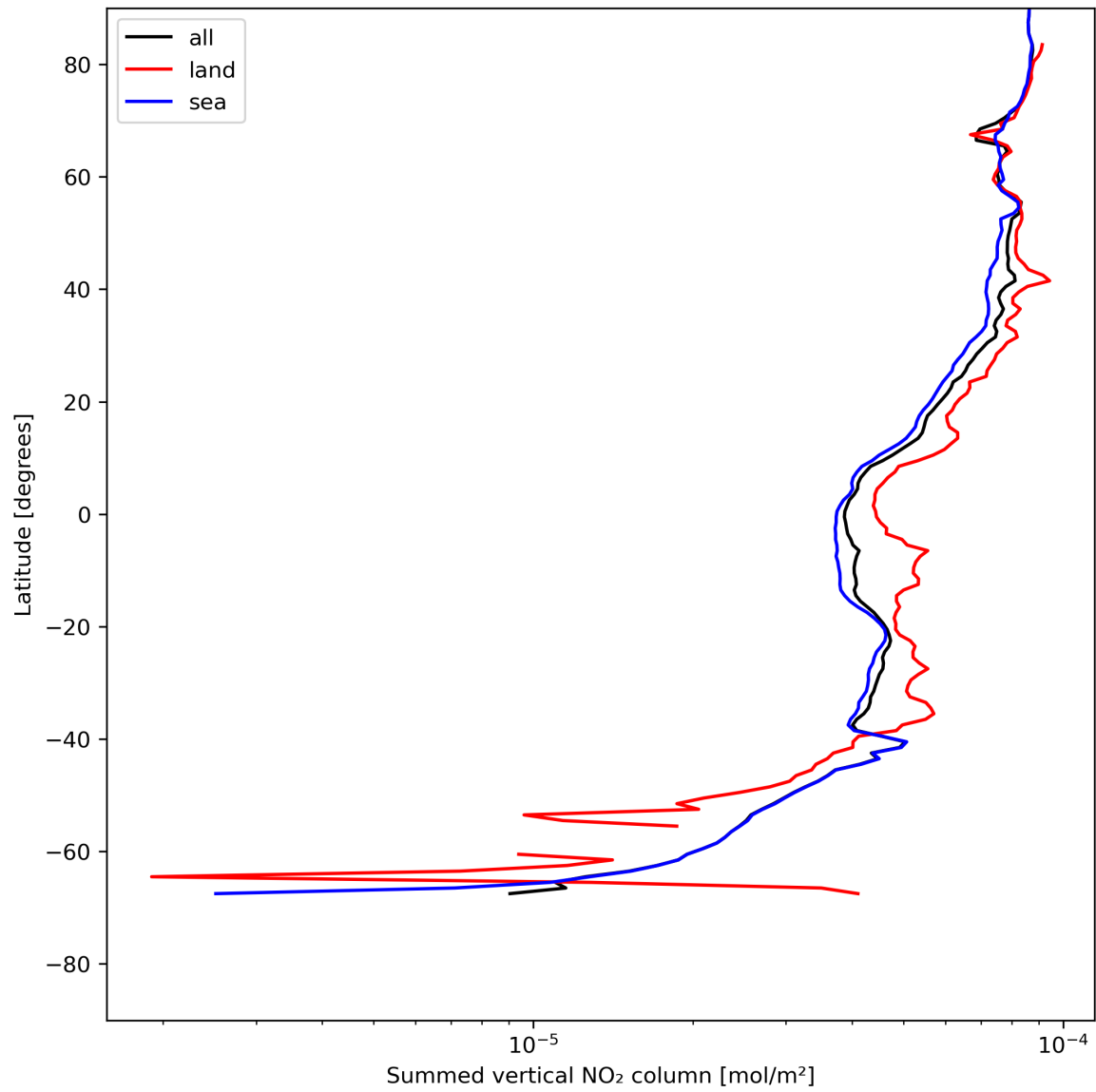
Figure 23: Zonal average of “Summed vertical NO 2 column” for 2023-07-21 to 2023-07-23.
