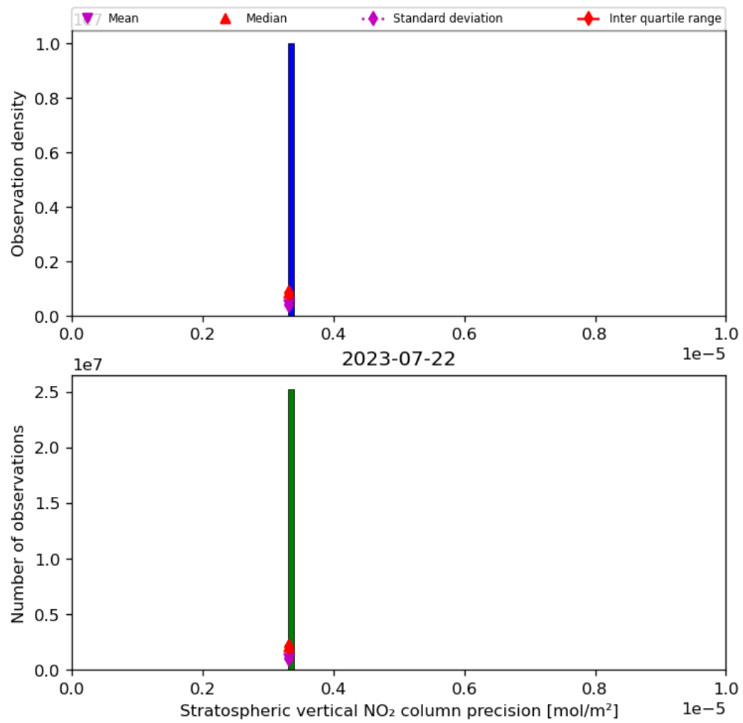
Figure 37: Histogram of “Stratospheric vertical NO 2 column precision” for 2023-07-21 to 2023-07-23
