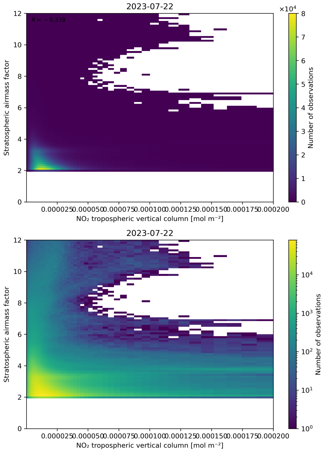
Figure 121: Scatter density plot of “NO 2 tropospheric vertical column” against “Stratospheric air mass factor” for 2023-07-21 to 2023-07-23.
