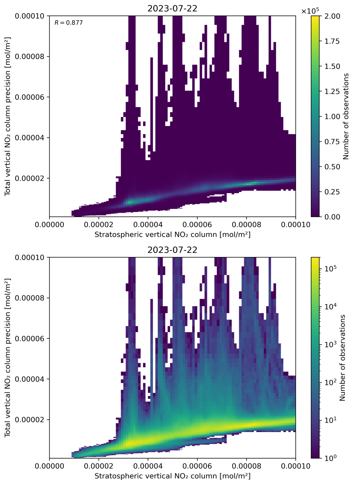
Figure 101: Scatter density plot of “Stratospheric vertical NO 2 column” against “Total vertical NO 2 column precision” for 2023-07-21 to 2023-07-23.
