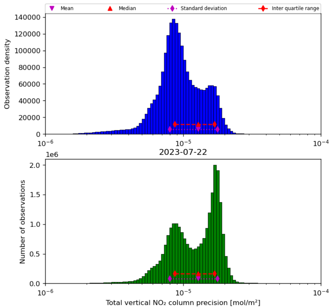
Figure 39: Histogram of “Total vertical NO 2 column precision” for 2023-07-21 to 2023-07-23
