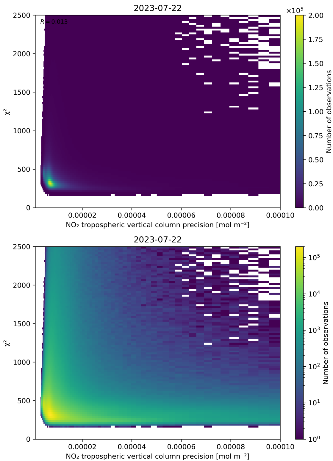
Figure 134: Scatter density plot of “NO 2 tropospheric vertical column precision” against “ \chi^2 ” for 2023-07-21 to 2023-07-23.
