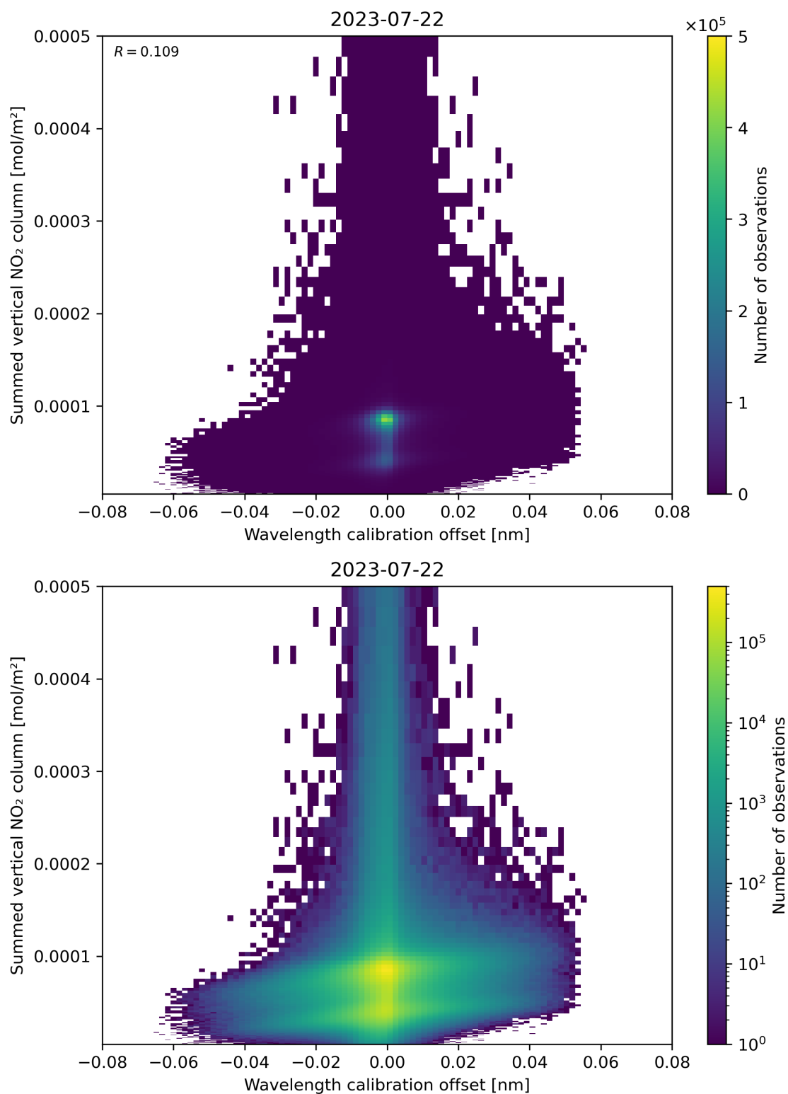
Figure 177: Scatter density plot of “Wavelength calibration offset” against “Summed vertical NO 2 column” for 2023-07-21 to 2023-07-23.
