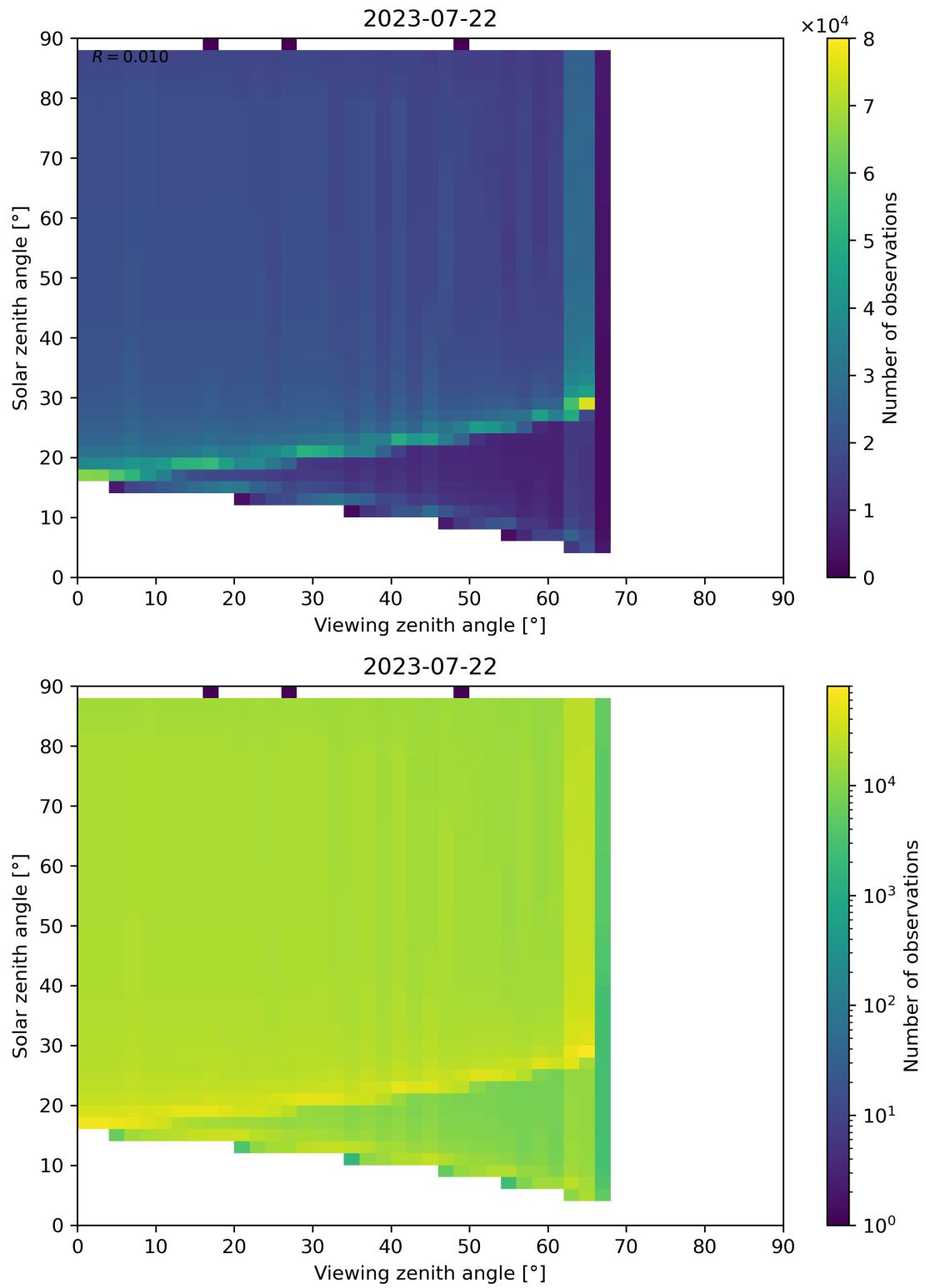
Figure 172: Scatter density plot of “Viewing zenith angle” against “Solar zenith angle” for 2023-07-21 to 2023-07-23.
