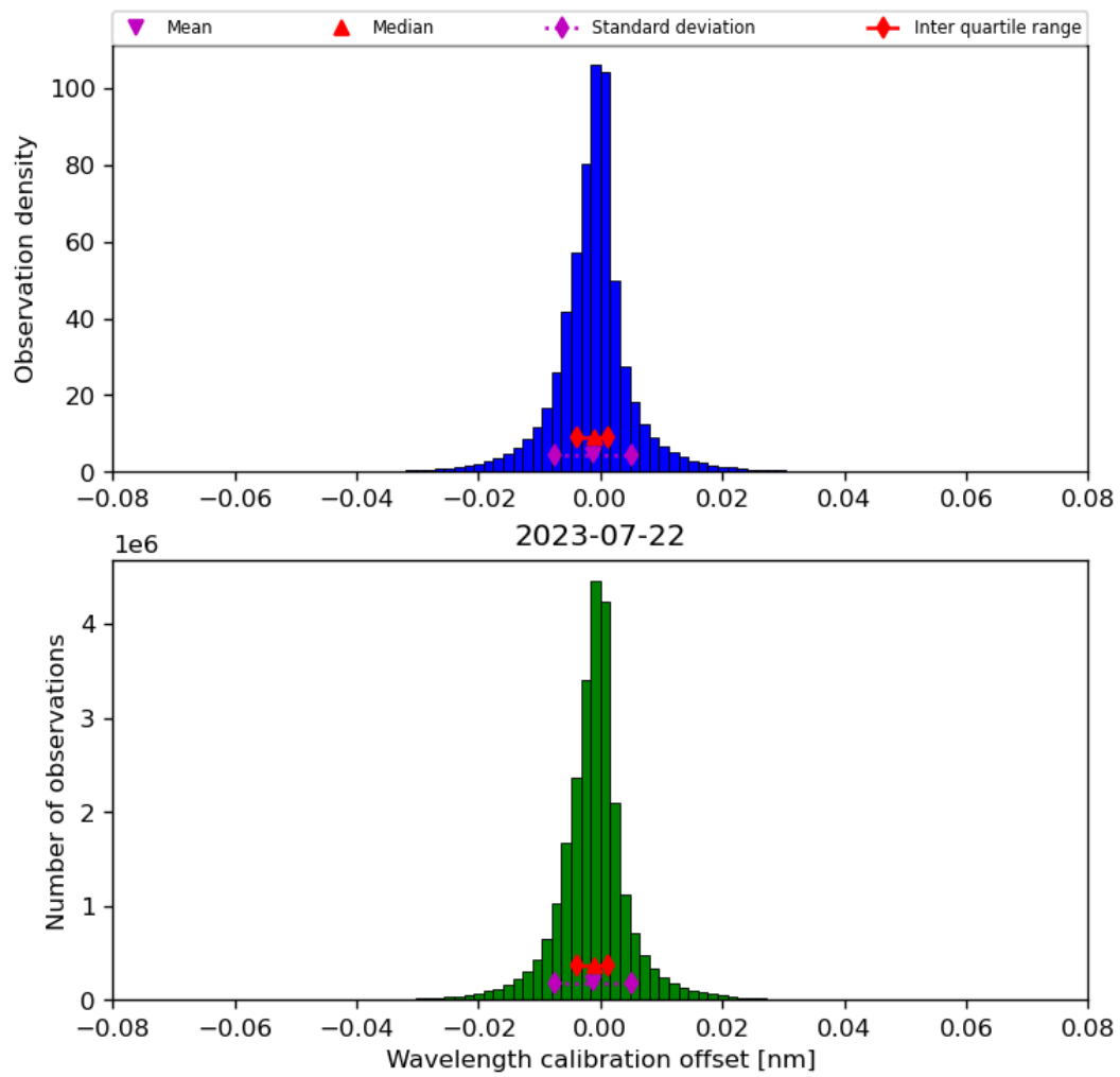
Figure 35: Histogram of “Wavelength calibration offset” for 2023-07-21 to 2023-07-23
