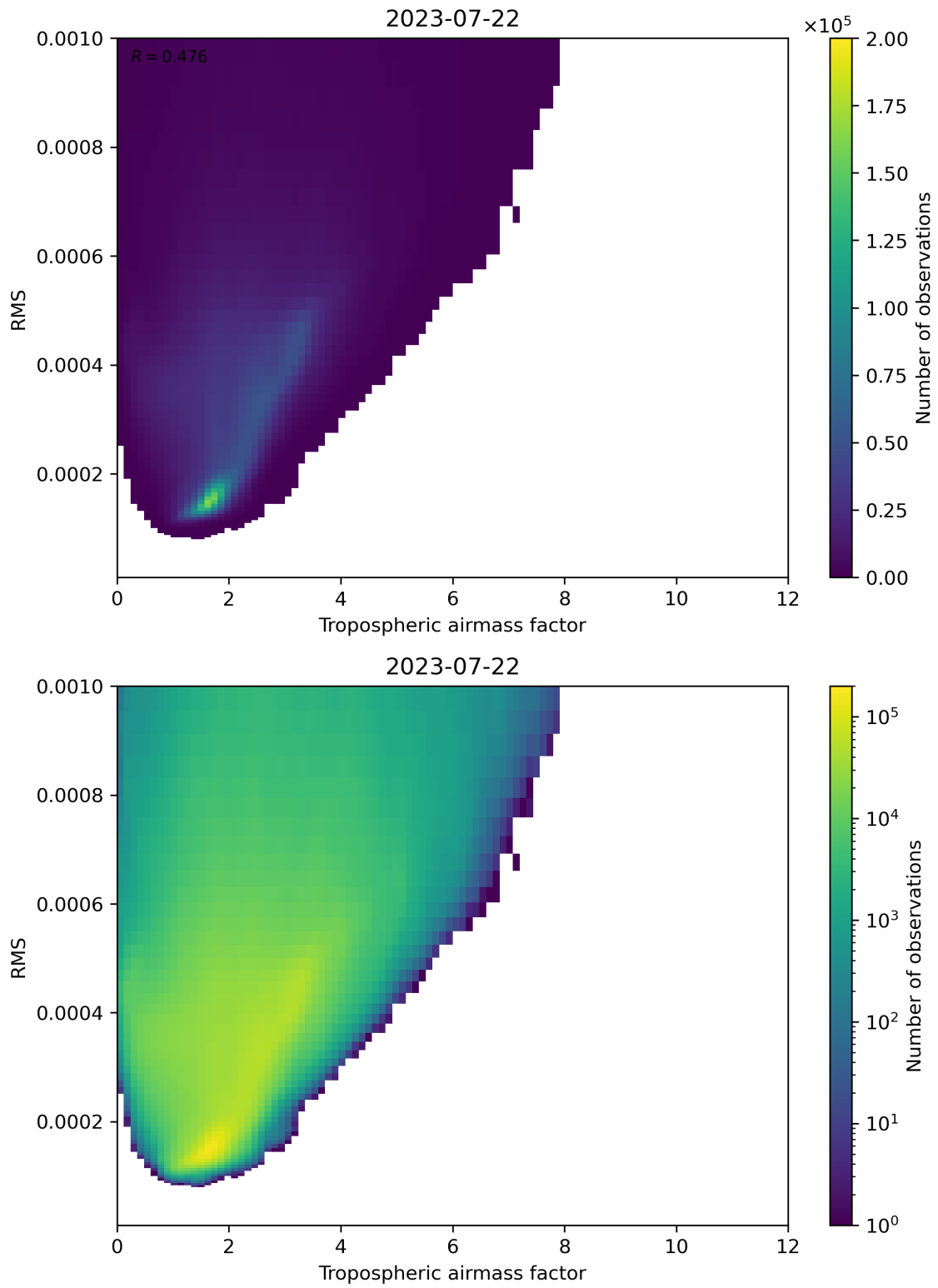
Figure 79: Scatter density plot of “Tropospheric airmass factor” against “RMS” for 2023-07-21 to 2023-07-23.
