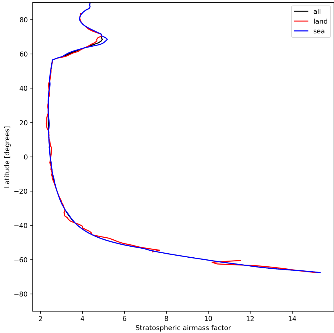
Figure 27: Zonal average of “Stratospheric airmass factor” for 2023-07-21 to 2023-07-23.
