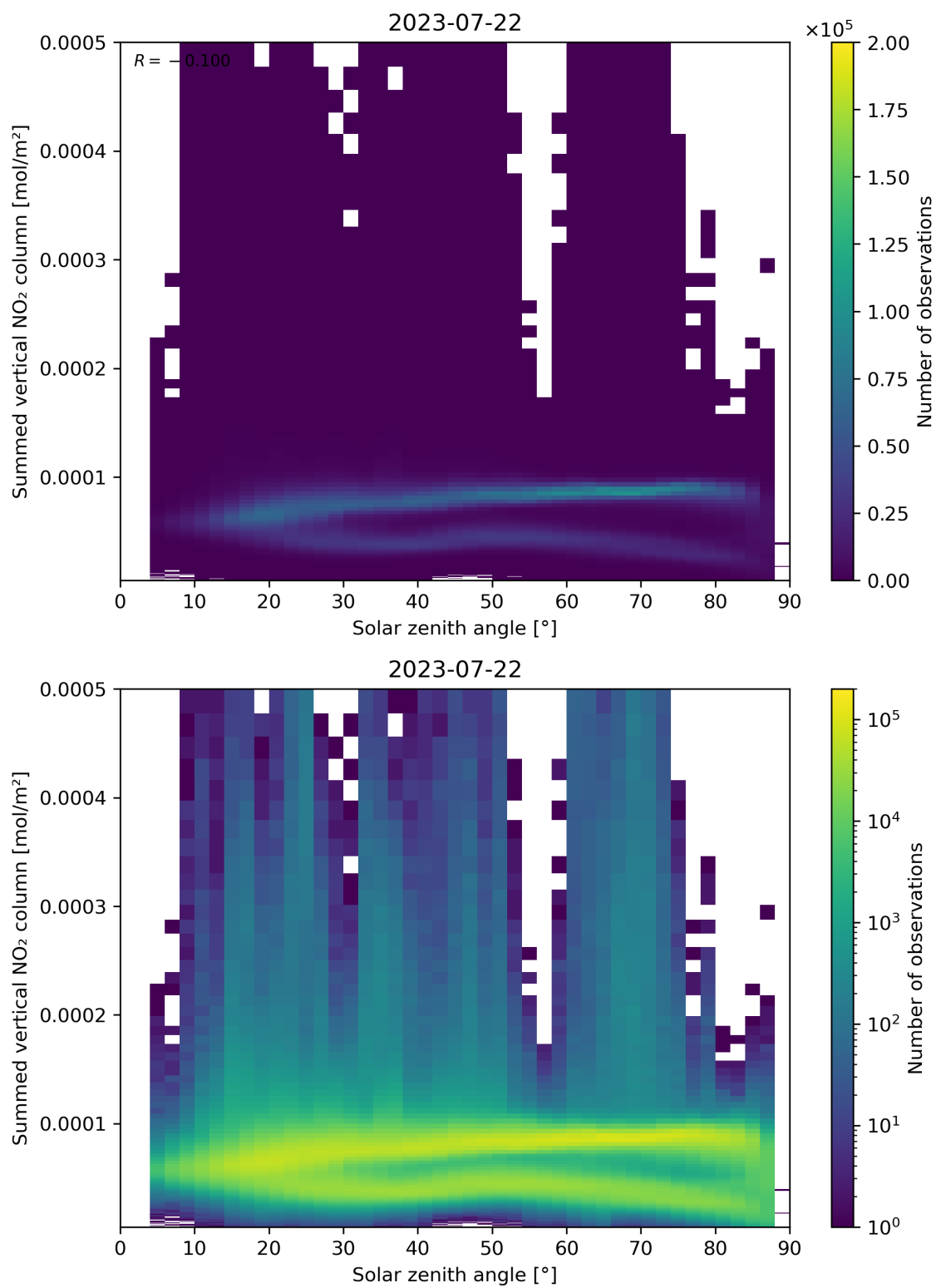
Figure 151: Scatter density plot of “Solar zenith angle” against “Summed vertical NO 2 column” for 2023-07-21 to 2023-07-23.
