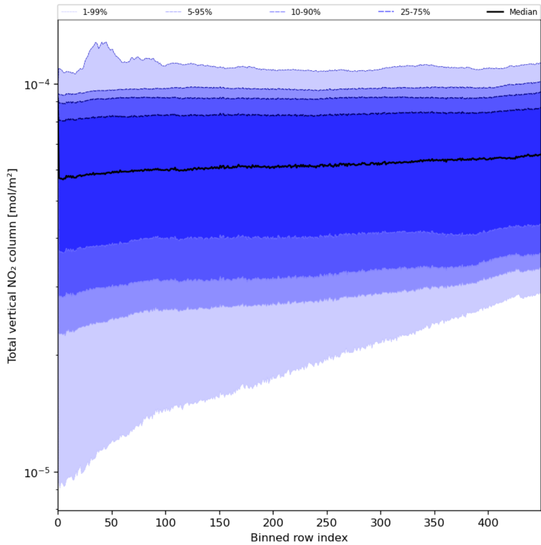
Figure 55: Along track statistics of “Total vertical NO 2 column” for 2023-07-21 to 2023-07-23
