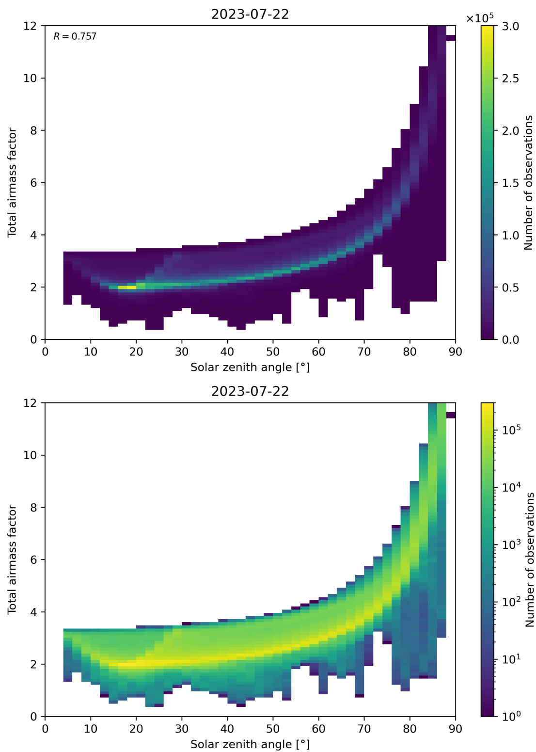
Figure 146: Scatter density plot of “Solar zenith angle” against “Total air mass factor” for 2023-07-21 to 2023-07-23.
