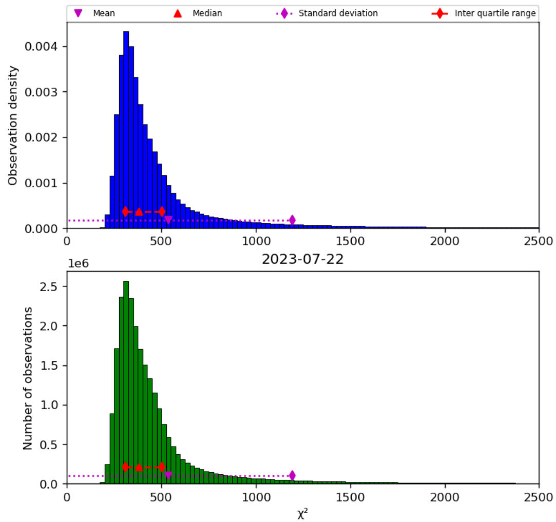
Figure 42: Histogram of “ \chi^2 ” for 2023-07-21 to 2023-07-23
