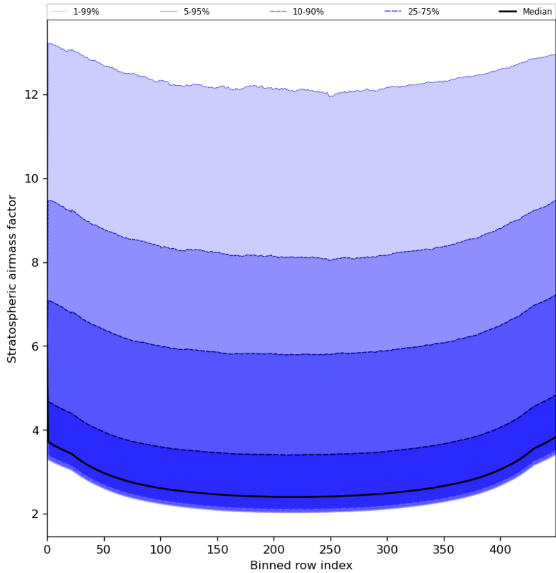
Figure 61: Along track statistics of “Stratospheric airmass factor” for 2023-07-21 to 2023-07-23
