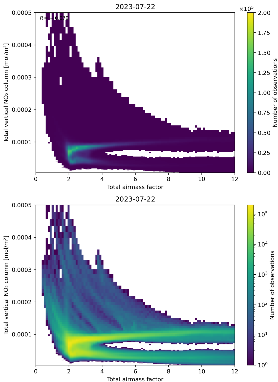
Figure 67: Scatter density plot of “Total airmass factor” against “Total vertical NO 2 column” for 2023-07-21 to 2023-07-23.
