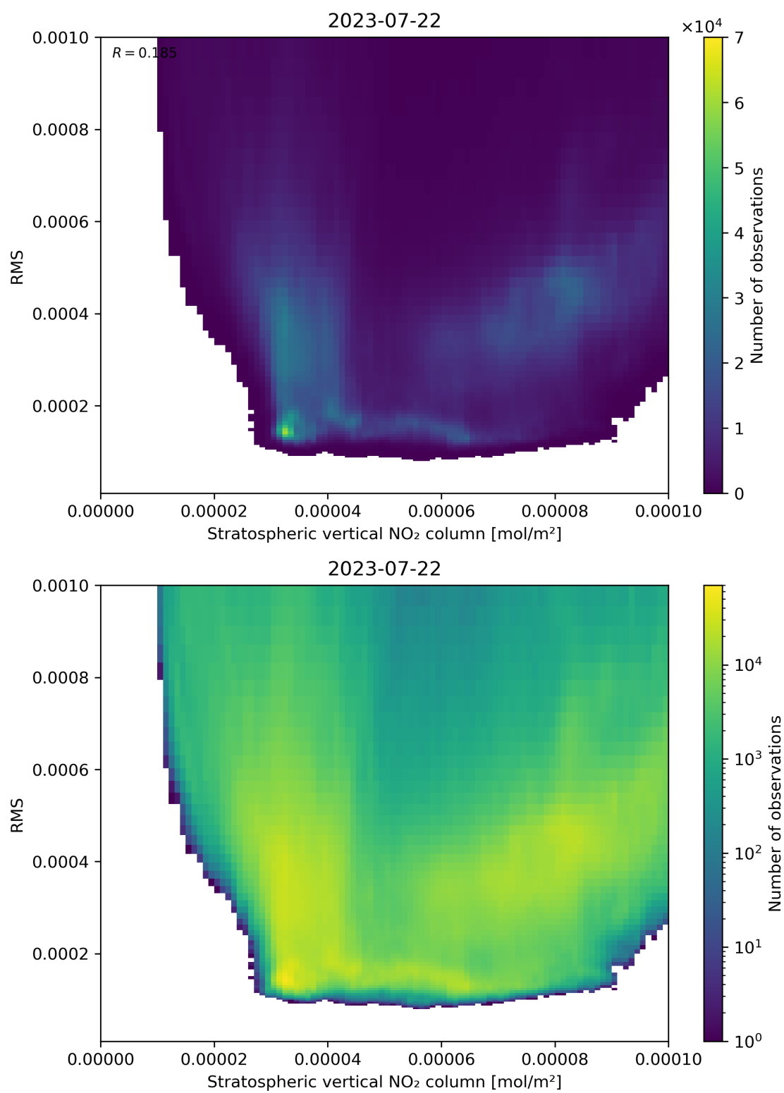
Figure 102: Scatter density plot of “Stratospheric vertical NO 2 column” against “RMS” for 2023-07-21 to 2023-07-23.
