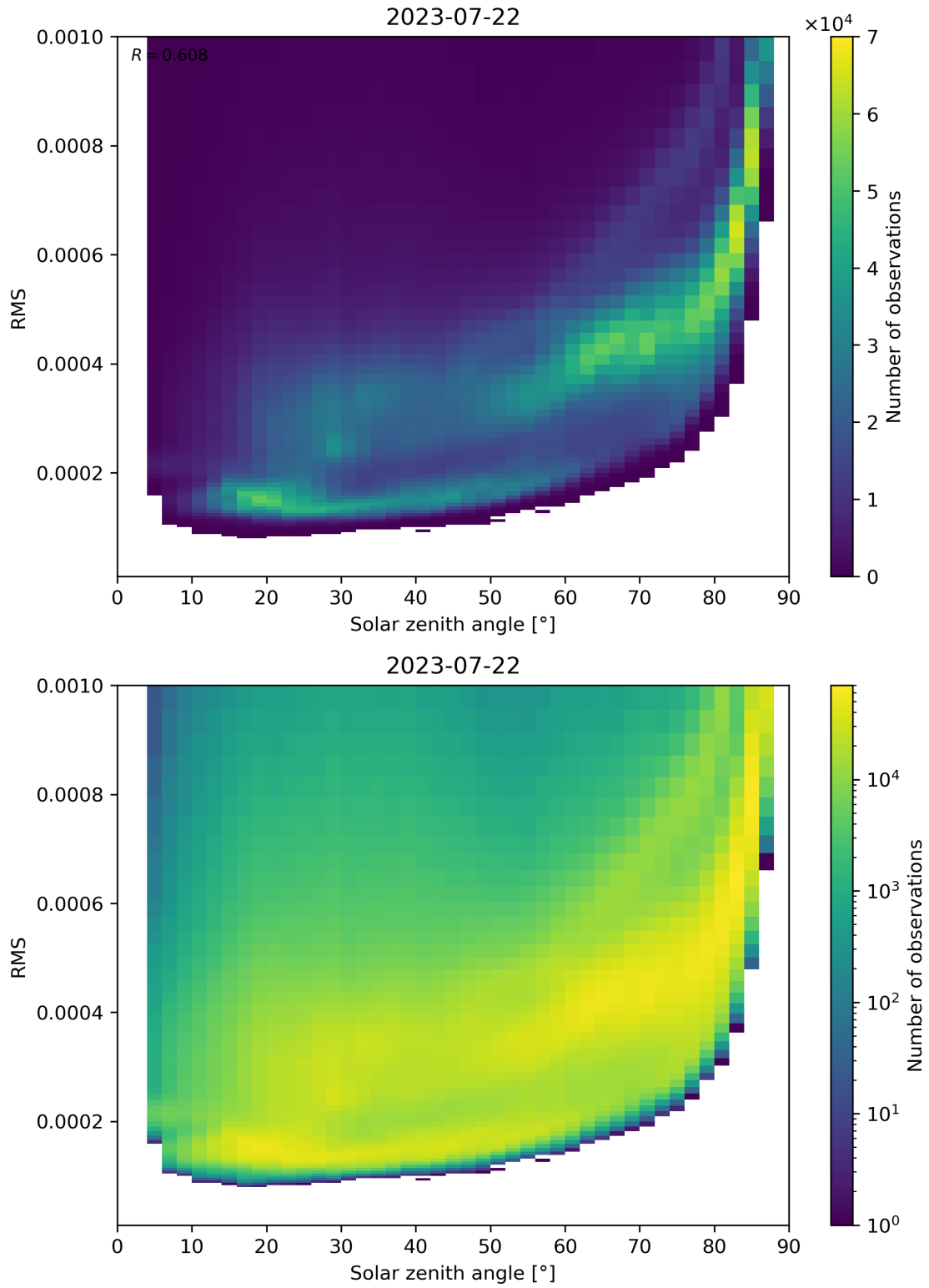
Figure 157: Scatter density plot of “Solar zenith angle” against “RMS” for 2023-07-21 to 2023-07-23.
