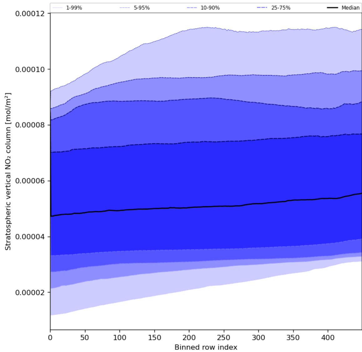
Figure 53: Along track statistics of “Stratospheric vertical NO 2 column” for 2023-07-21 to 2023-07-23
