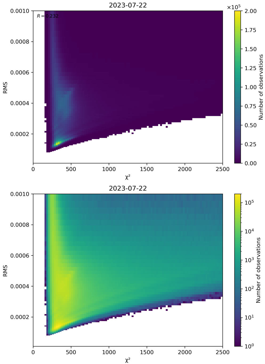
Figure 82: Scatter density plot of “ \chi^2 ” against “RMS” for 2023-07-21 to 2023-07-23.
