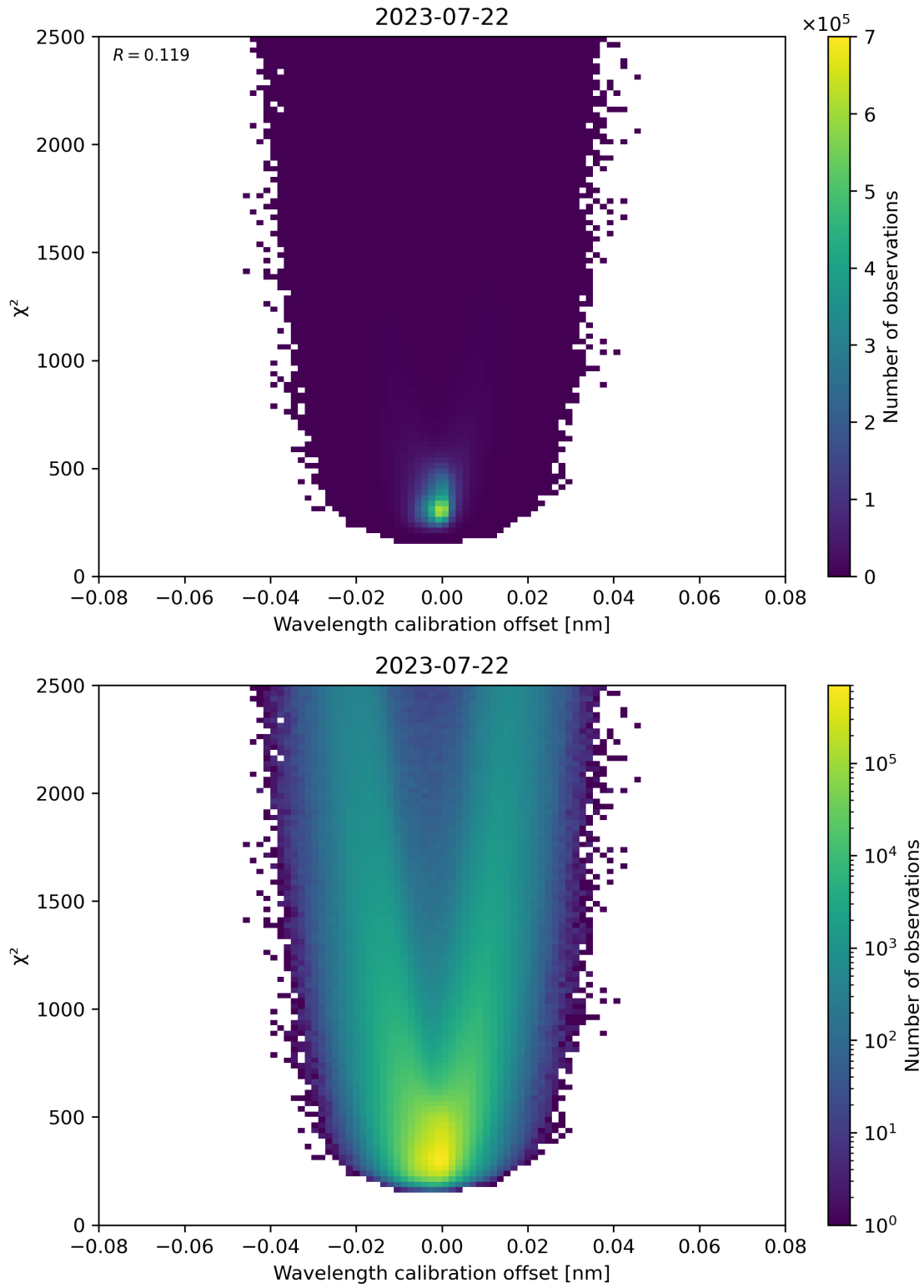
Figure 175: Scatter density plot of “Wavelength calibration offset” against “ \chi^2 ” for 2023-07-21 to 2023-07-23.
