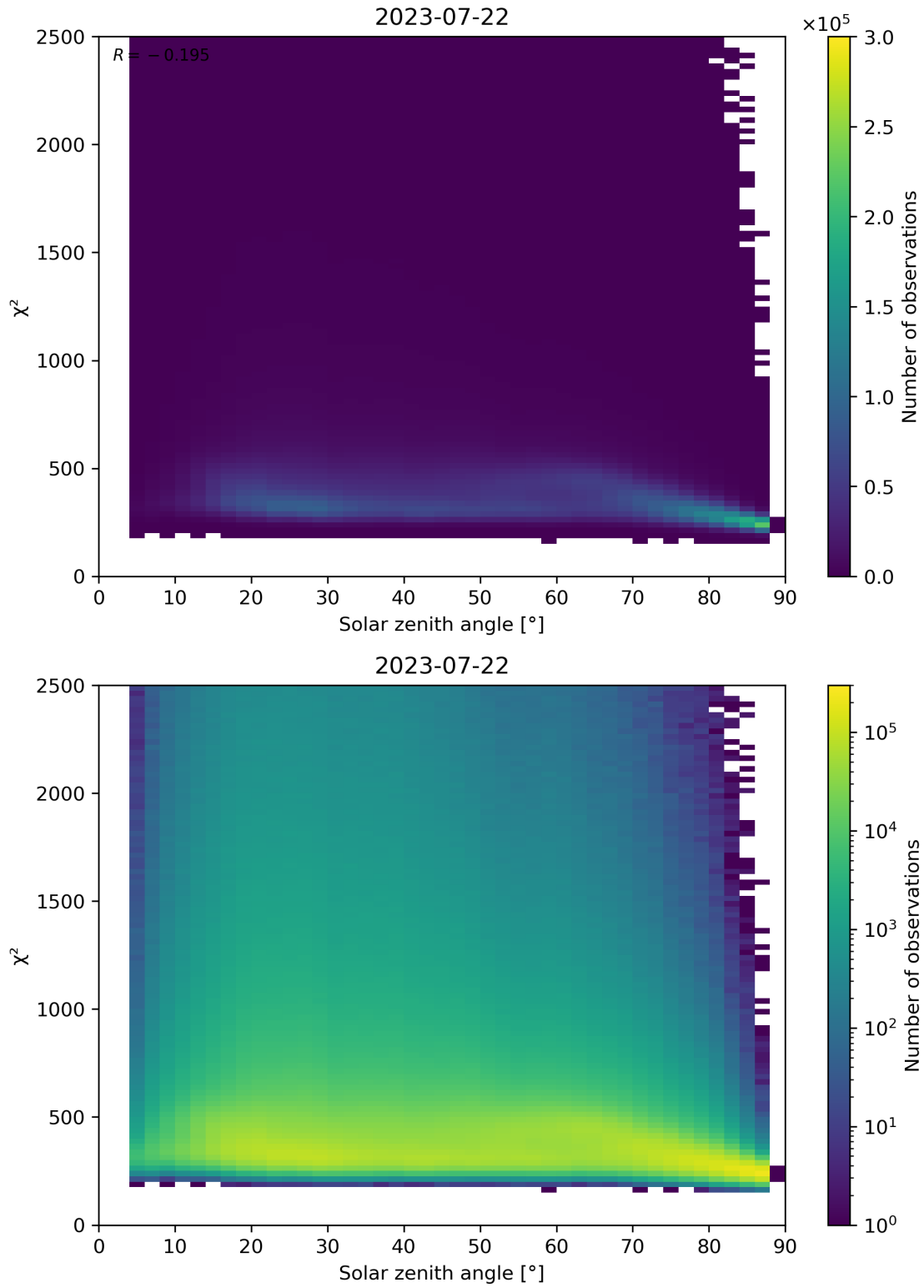
Figure 148: Scatter density plot of “Solar zenith angle” against “ \chi^2 ” for 2023-07-21 to 2023-07-23.
