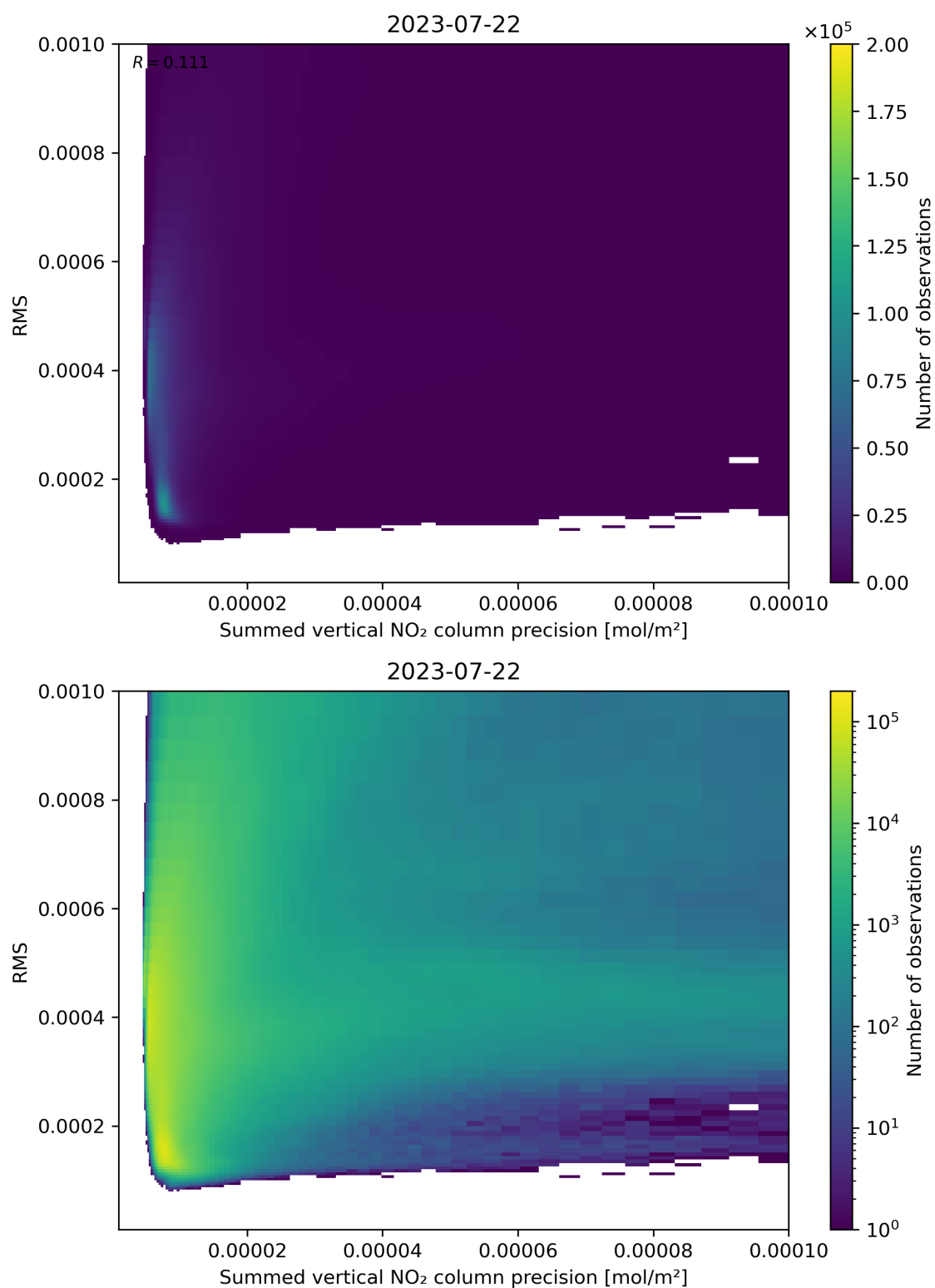
Figure 108: Scatter density plot of “Summed vertical NO 2 column precision” against “RMS” for 2023-07-21 to 2023-07-23.
