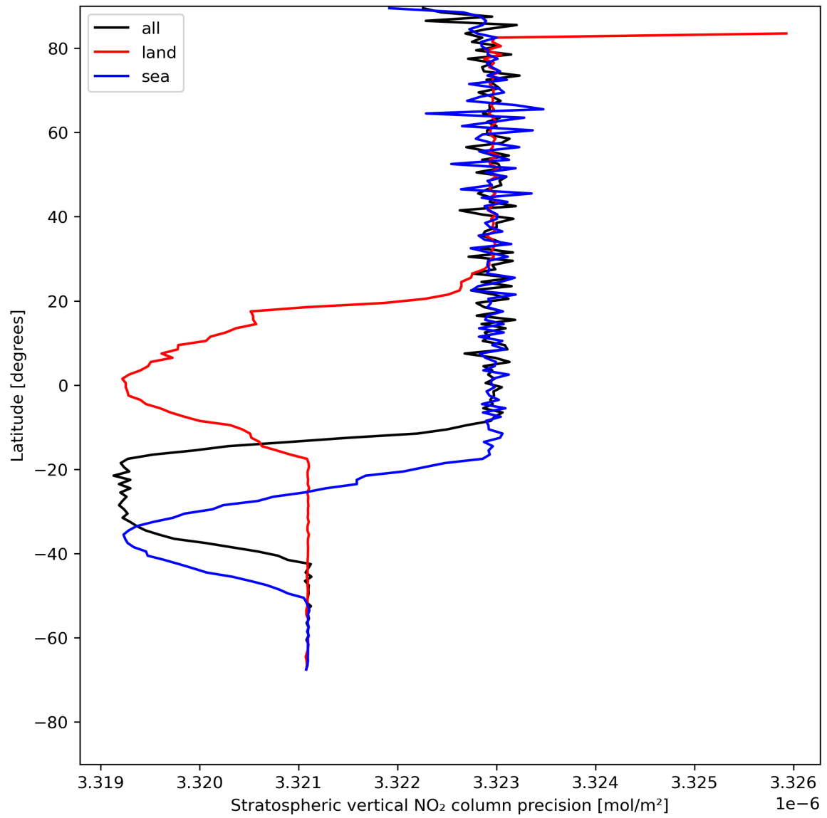
Figure 20: Zonal average of “Stratospheric vertical NO 2 column precision” for 2023-07-21 to 2023-07-23.
