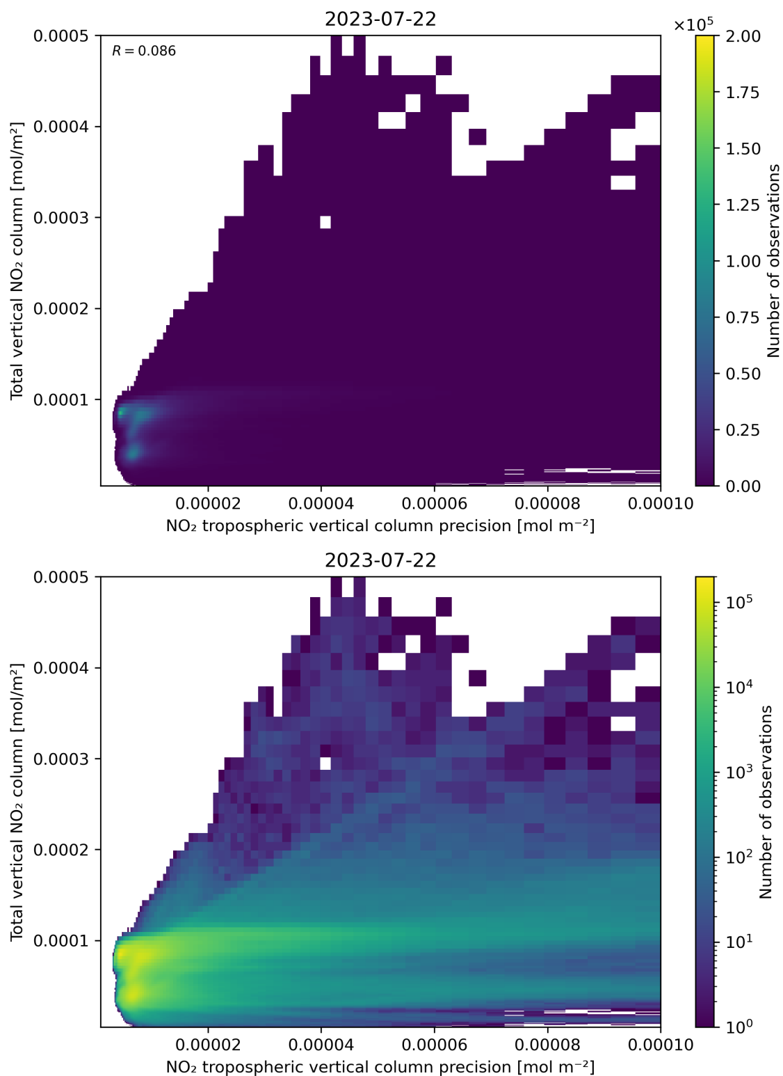
Figure 138: Scatter density plot of “NO 2 tropospheric vertical column precision” against “Total vertical NO 2 column” for 2023-07-21 to 2023-07-23.
