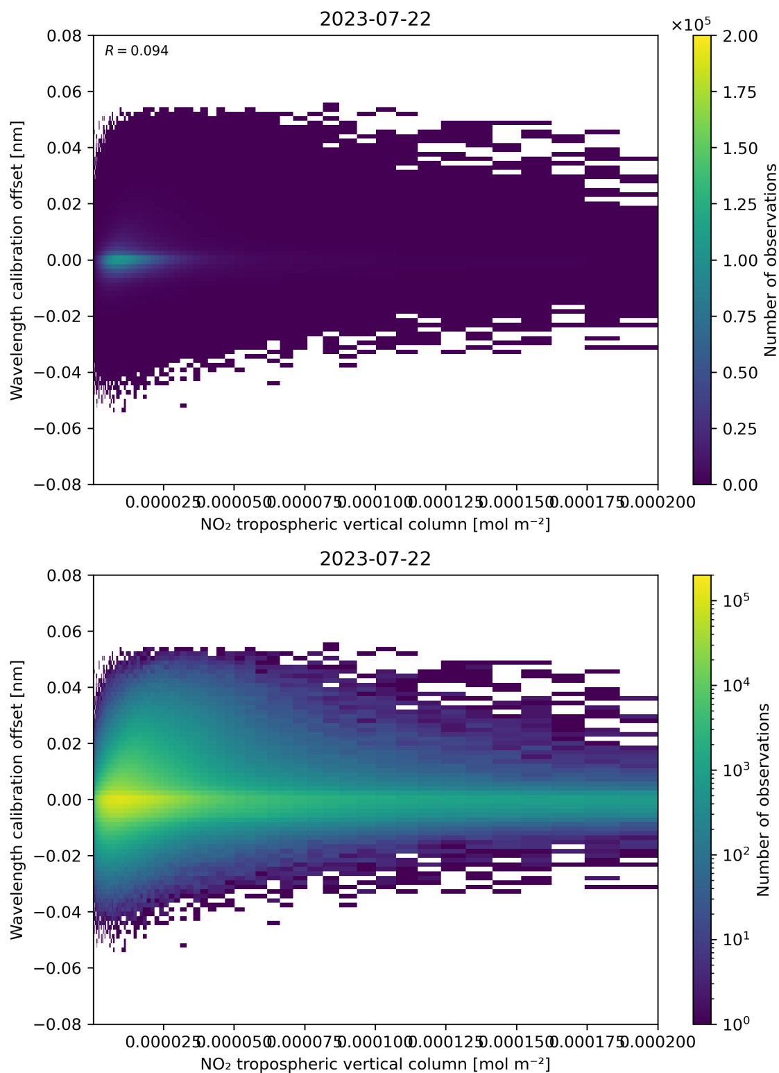
Figure 143: Scatter density plot of “NO 2 tropospheric vertical column” against “Wavelength calibration offset” for 2023-07-21 to 2023-07-23.
