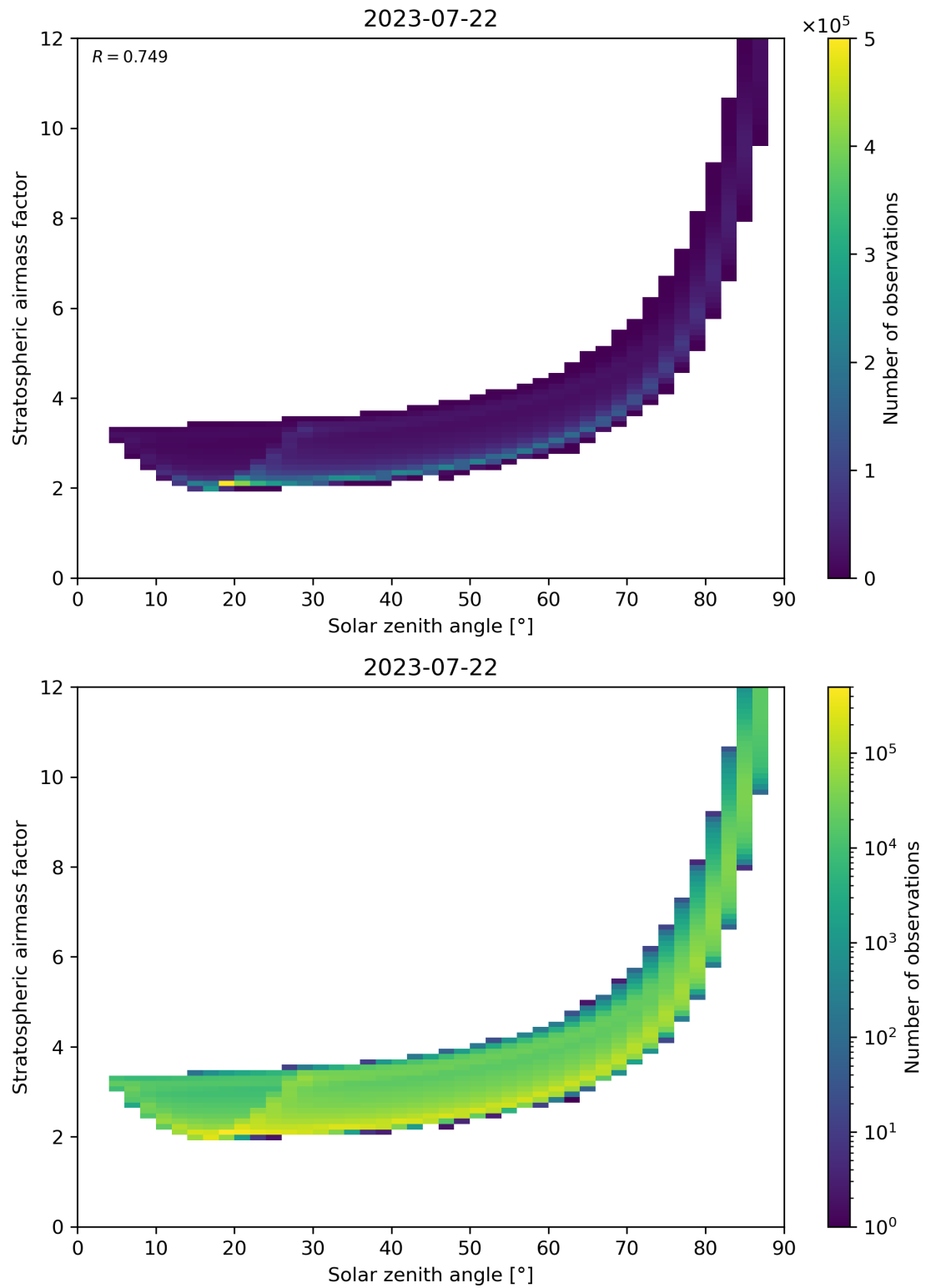
Figure 145: Scatter density plot of “Solar zenith angle” against “Stratospheric airmass factor” for 2023-07-21 to 2023-07-23.
