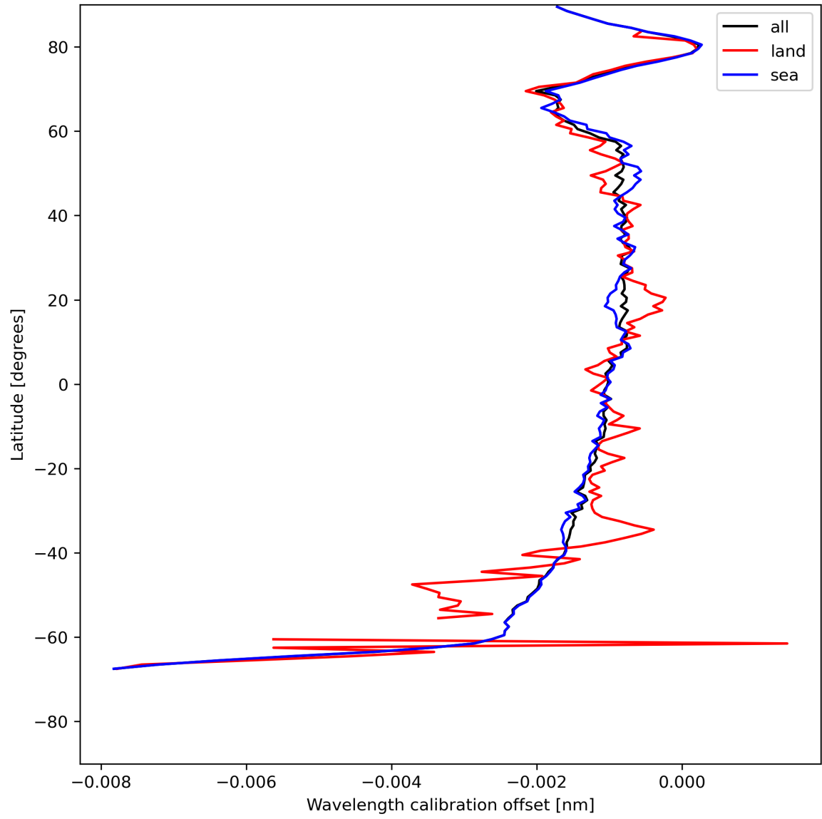
Figure 18: Zonal average of “Wavelength calibration offset” for 2023-07-21 to 2023-07-23.
