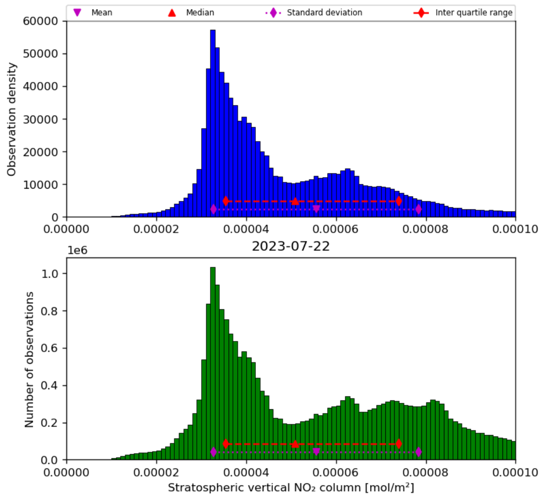
Figure 36: Histogram of “Stratospheric vertical NO 2 column” for 2023-07-21 to 2023-07-23
