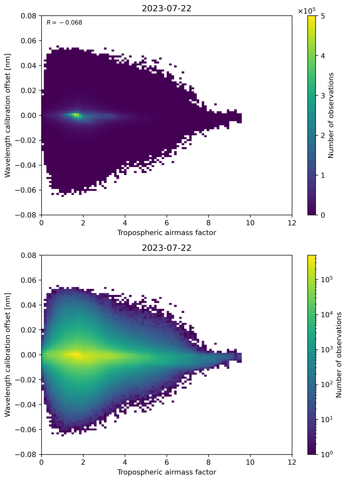
Figure 80: Scatter density plot of “Tropospheric air mass factor” against “Wavelength calibration offset” for 2023-07-21 to 2023-07-23.
