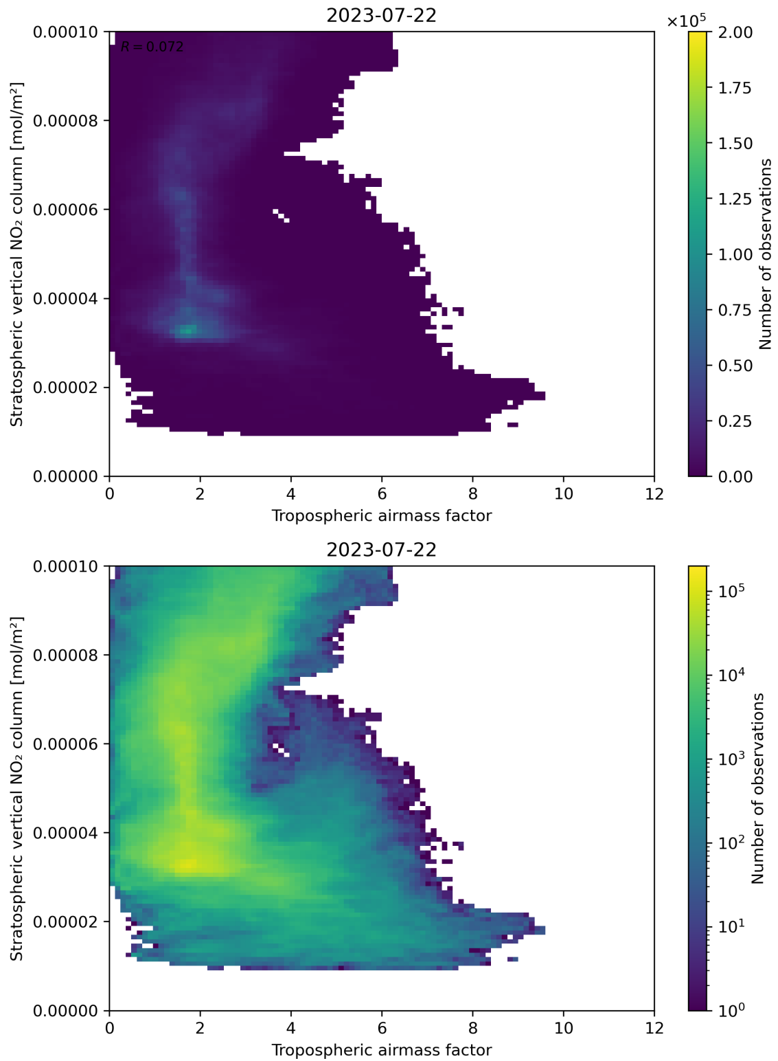
Figure 74: Scatter density plot of “Tropospheric air mass factor” against “Stratospheric vertical NO 2 column” for 2023-07-21 to 2023-07-23.
