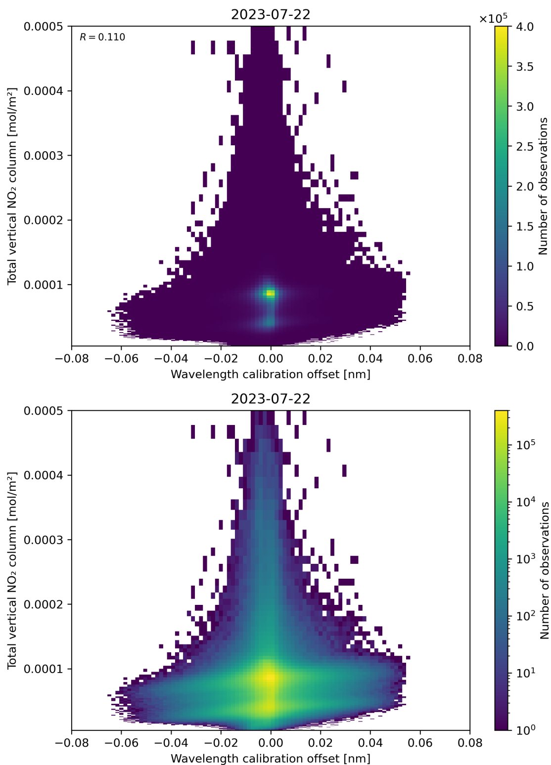
Figure 179: Scatter density plot of “Wavelength calibration offset” against “Total vertical NO 2 column” for 2023-07-21 to 2023-07-23.
