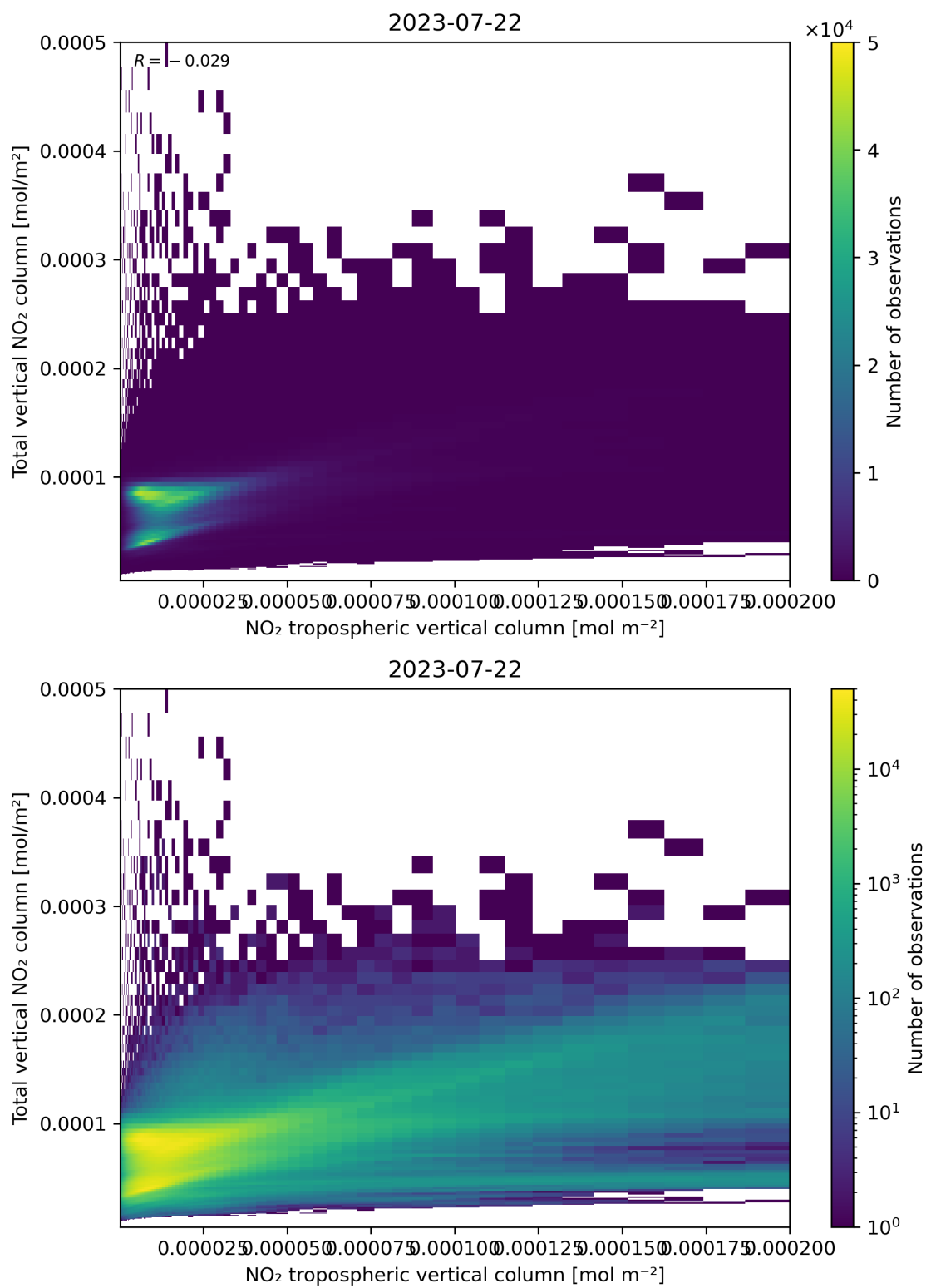
Figure 128: Scatter density plot of “NO 2 tropospheric vertical column” against “Total vertical NO 2 column” for 2023-07-21 to 2023-07-23.
