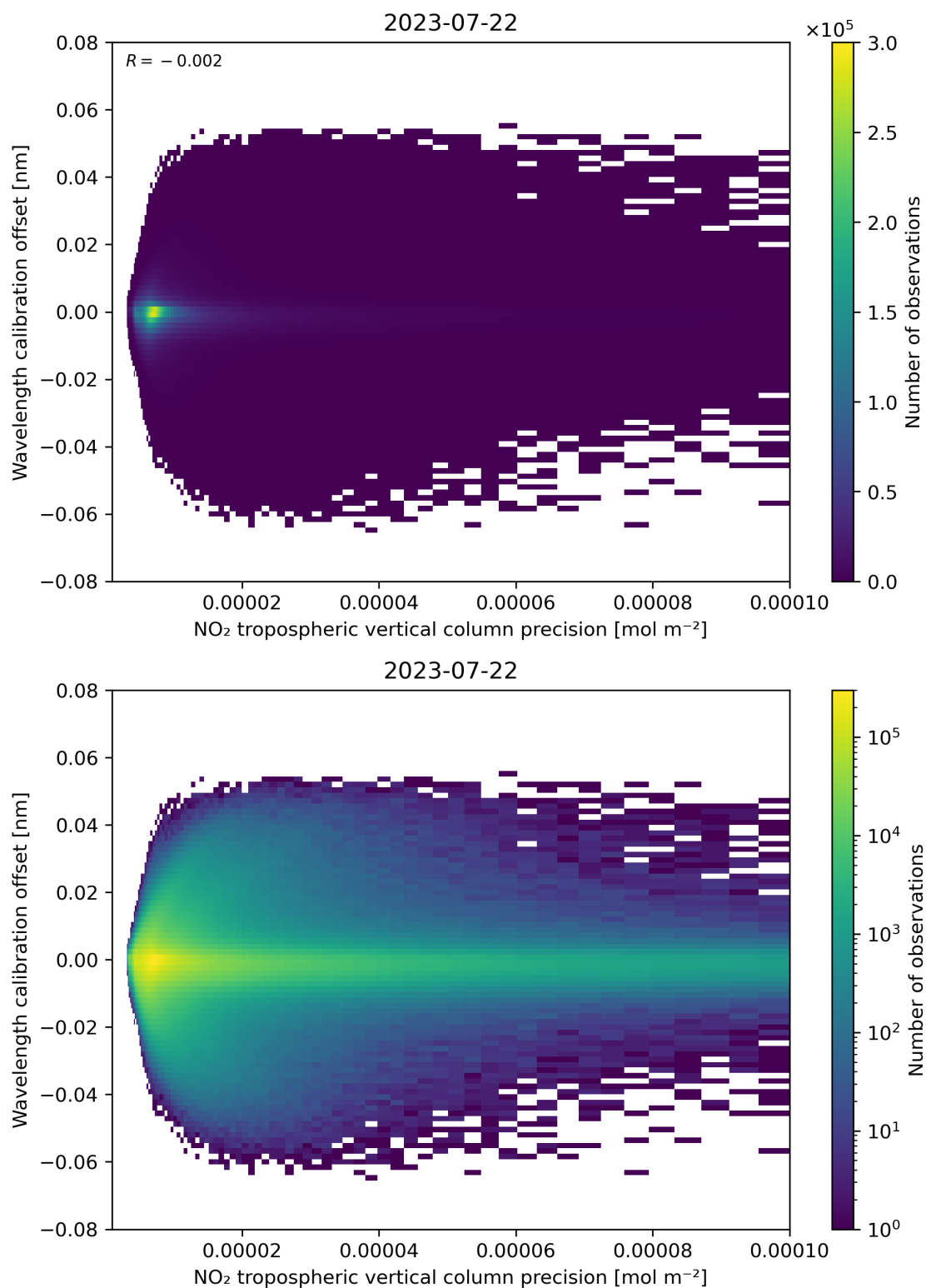
Figure 141: Scatter density plot of “NO 2 tropospheric vertical column precision” against “Wavelength calibration offset” for 2023-07-21 to 2023-07-23.
