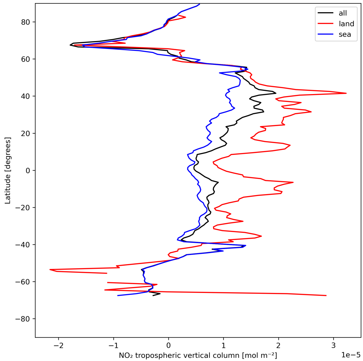
Figure 12: Zonal average of “NO 2 tropospheric vertical column” for 2023-07-21 to 2023-07-23.
