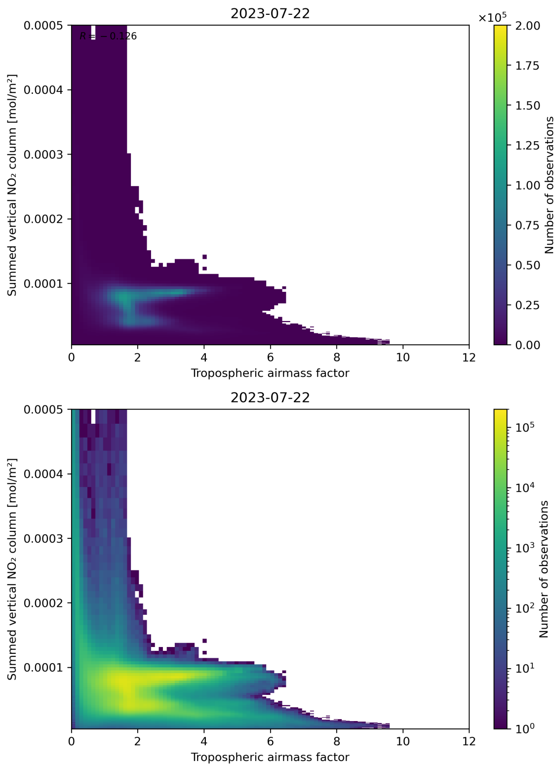
Figure 75: Scatter density plot of “Tropospheric airmass factor” against “Summed vertical NO 2 column” for 2023-07-21 to 2023-07-23.
