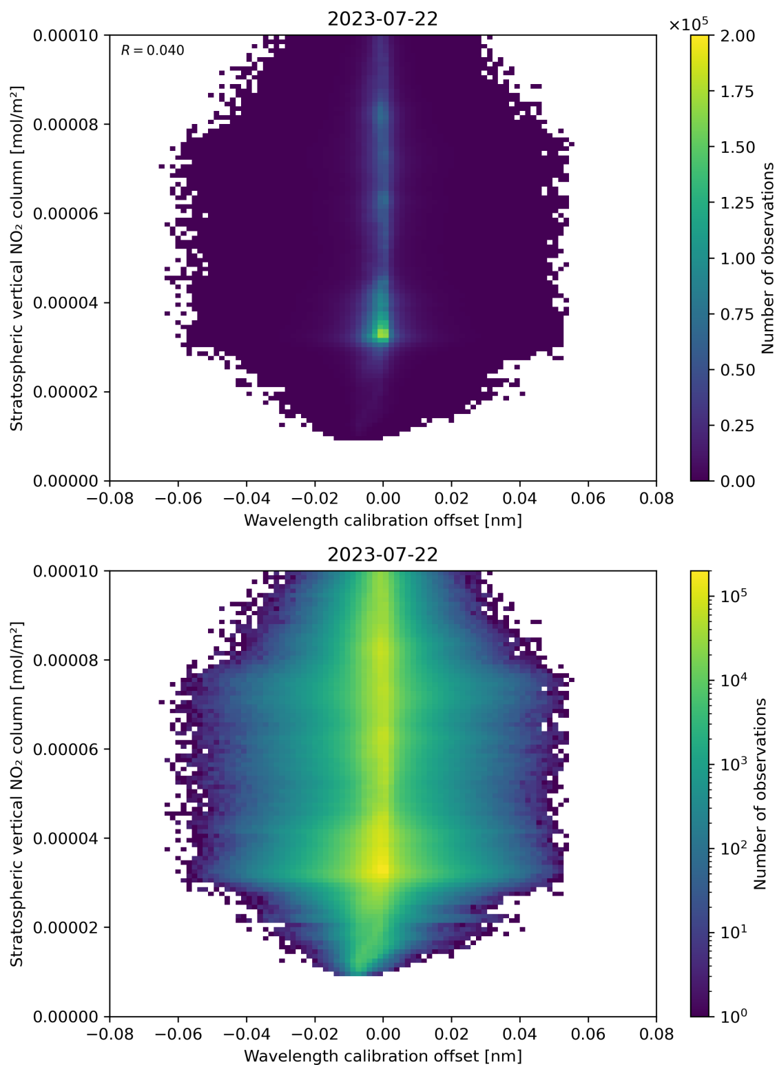
Figure 176: Scatter density plot of “Wavelength calibration offset” against “Stratospheric vertical NO 2 column” for 2023-07-21 to 2023-07-23.
