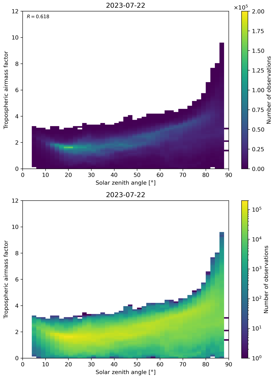
Figure 147: Scatter density plot of “Solar zenith angle” against “Tropospheric airmass factor” for 2023-07-21 to 2023-07-23.
