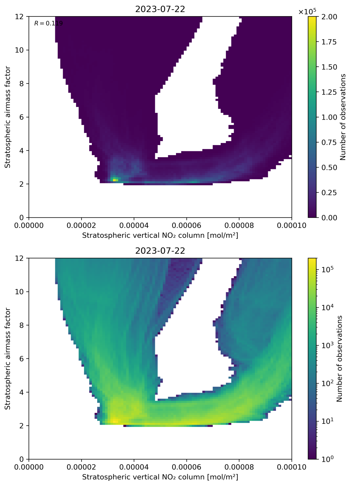
Figure 96: Scatter density plot of “Stratospheric vertical NO 2 column” against “Stratospheric airmass factor” for 2023-07-21 to 2023-07-23.
