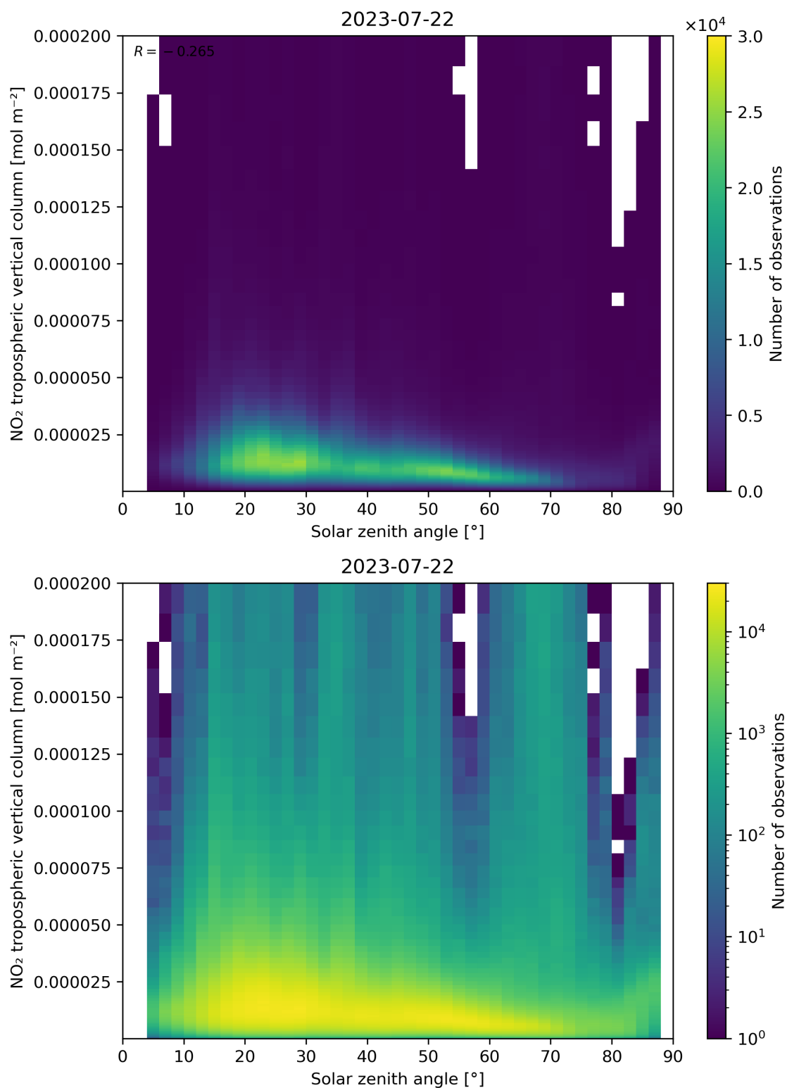
Figure 155: Scatter density plot of “Solar zenith angle” against “NO 2 tropospheric vertical column” for 2023-07-21 to 2023-07-23.
