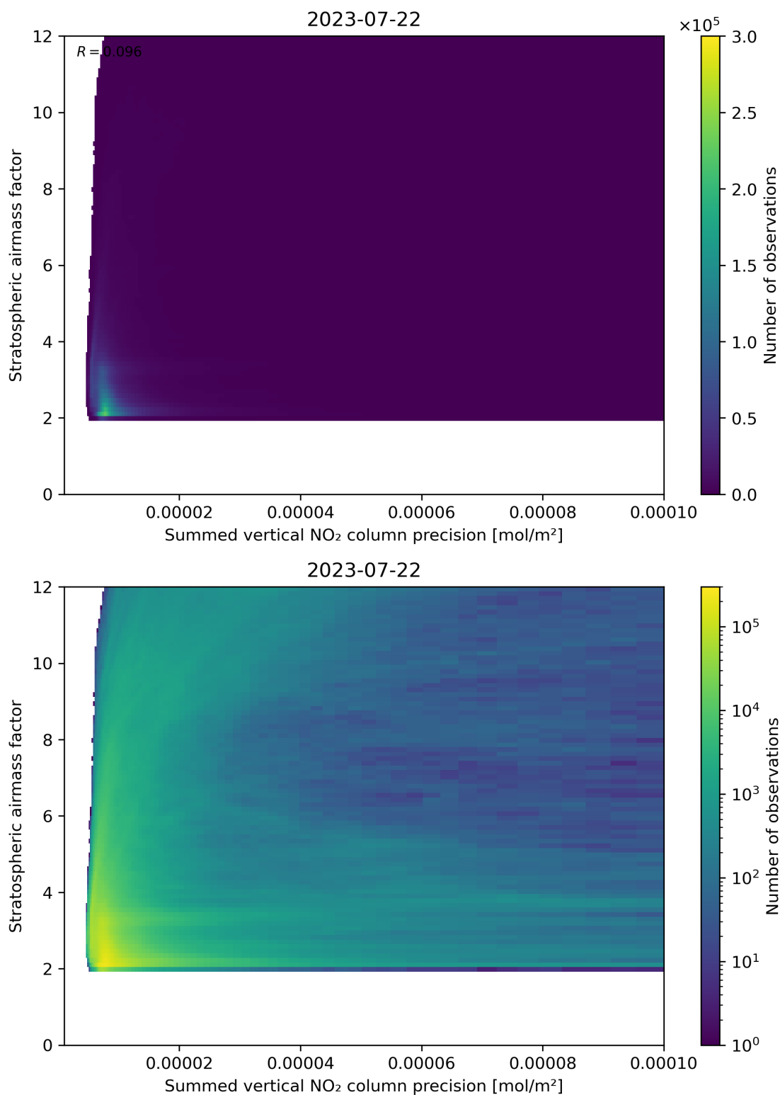
Figure 106: Scatter density plot of “Summed vertical NO 2 column precision” against “Stratospheric airmass factor” for 2023-07-21 to 2023-07-23.
