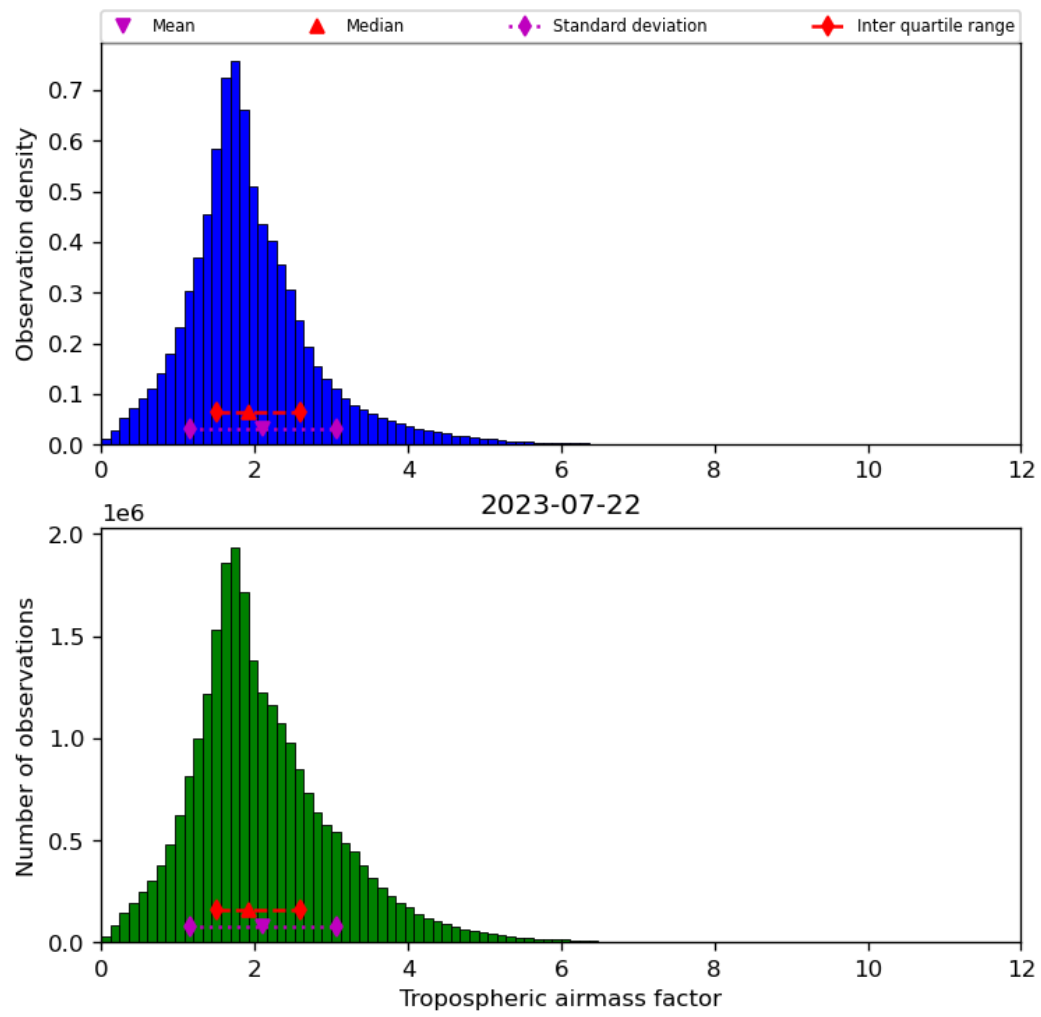
Figure 31: Histogram of “Tropospheric airmass factor” for 2023-07-21 to 2023-07-23
