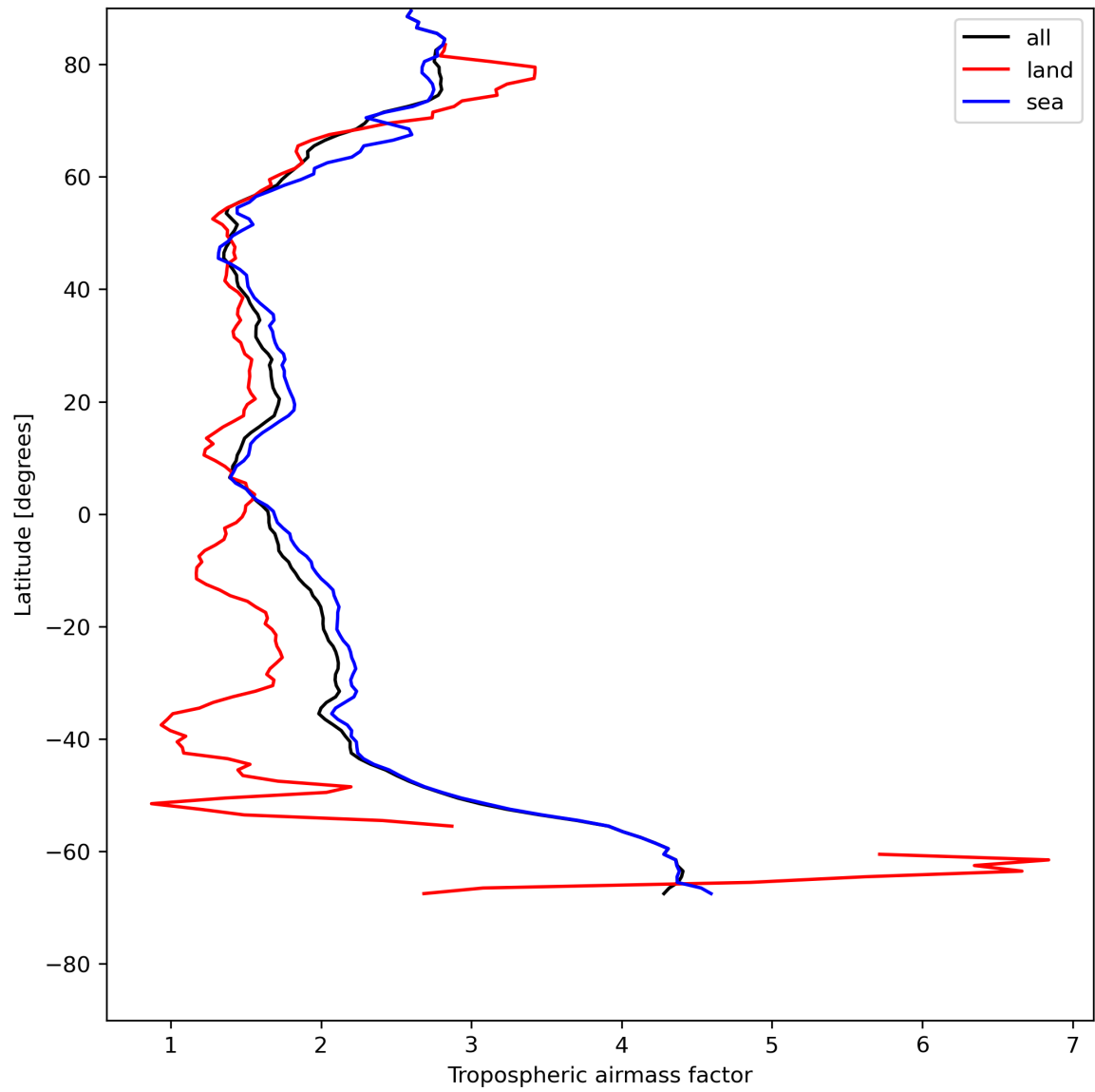
Figure 14: Zonal average of “Tropospheric airmass factor” for 2023-07-21 to 2023-07-23.
