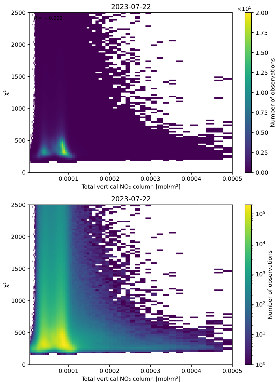
Figure 111: Scatter density plot of “Total vertical NO 2 column” against “ \chi^2 ” for 2023-07-21 to 2023-07-23.
