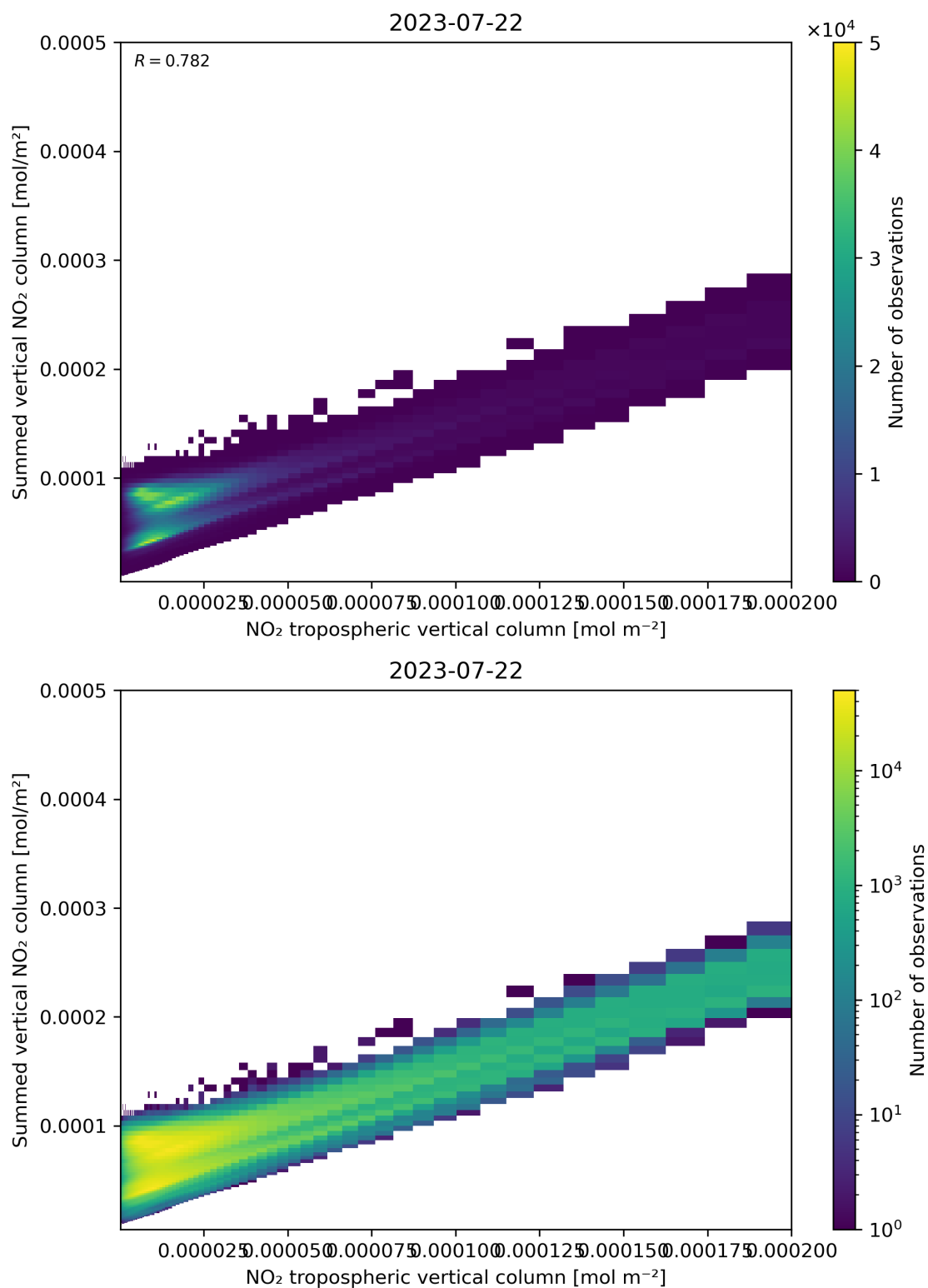
Figure 126: Scatter density plot of “NO 2 tropospheric vertical column” against “Summed vertical NO 2 column” for 2023-07-21 to 2023-07-23.
