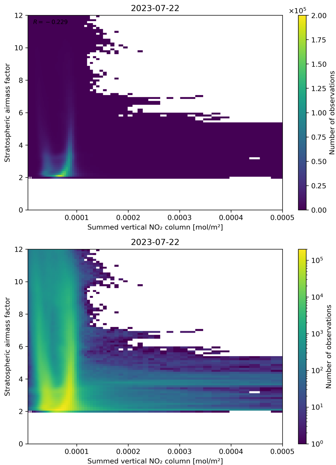
Figure 103: Scatter density plot of “Summed vertical NO 2 column” against “Stratospheric airmass factor” for 2023-07-21 to 2023-07-23.
