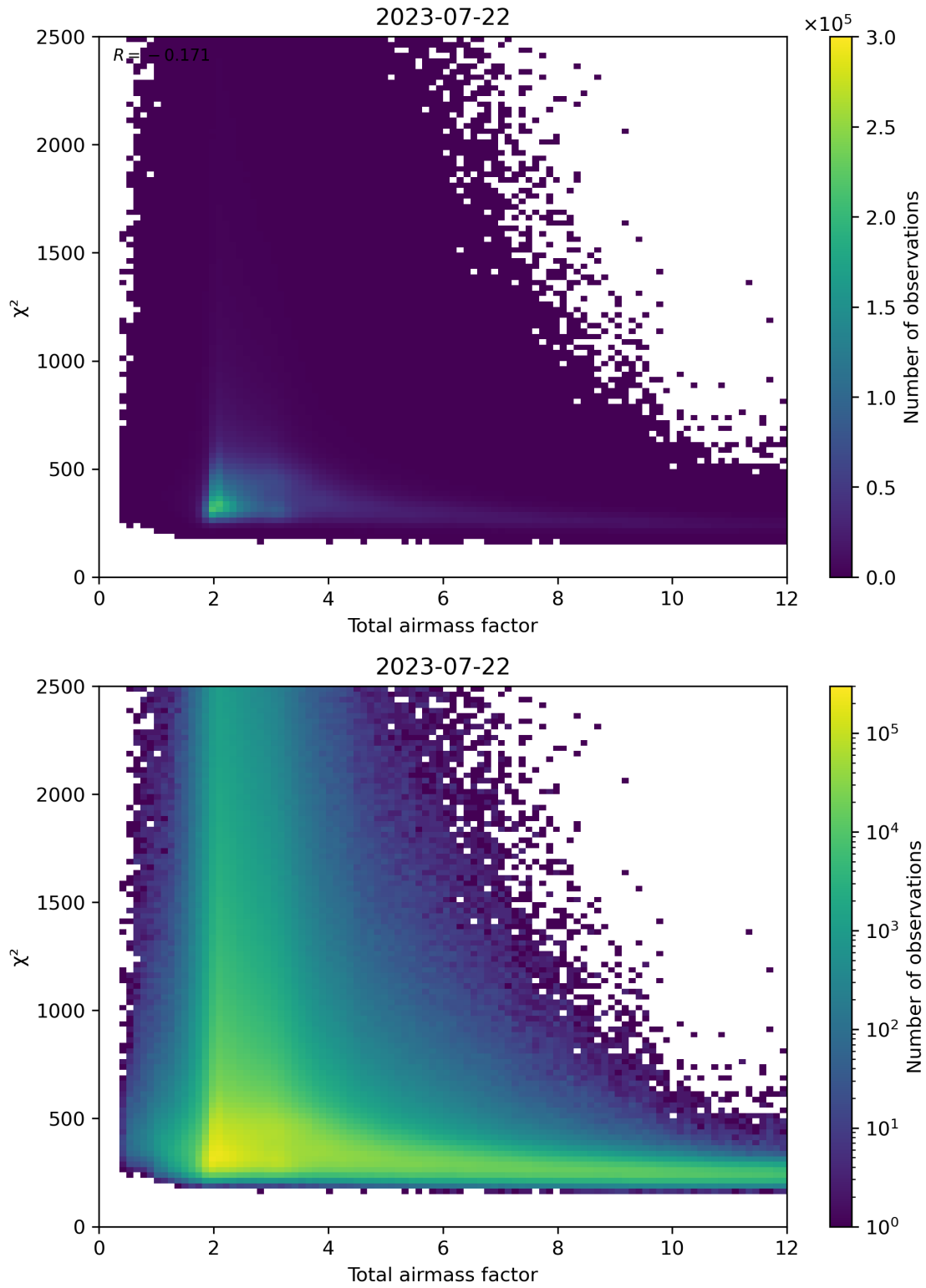
Figure 63: Scatter density plot of “Total airmass factor” against “ \chi^2 ” for 2023-07-21 to 2023-07-23.
