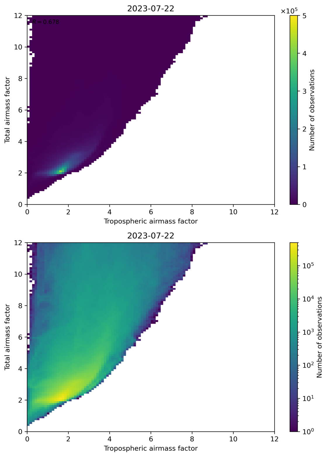
Figure 72: Scatter density plot of “Tropospheric airmass factor” against “Total airmass factor” for 2023-07-21 to 2023-07-23.
