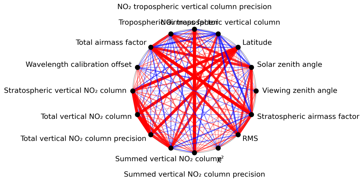
Figure 1: Map of correlation graph for 2023-07-22 to 2023-07-24.
