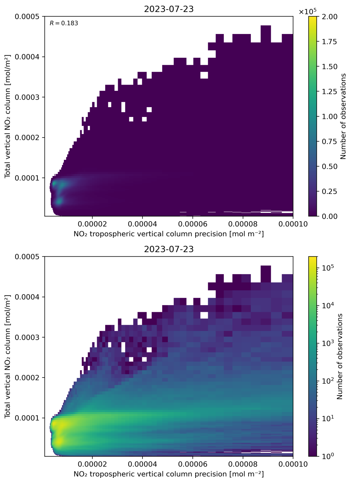
Figure 138: Scatter density plot of “NO 2 tropospheric vertical column precision” against “Total vertical NO 2 column” for 2023-07-22 to 2023-07-24.
