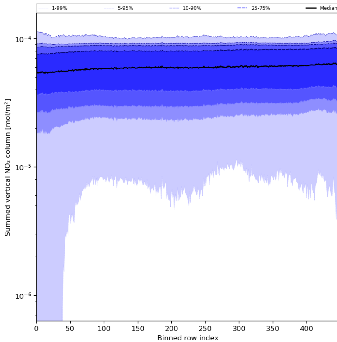
Figure 57: Along track statistics of “Summed vertical NO 2 column” for 2023-07-22 to 2023-07-24
