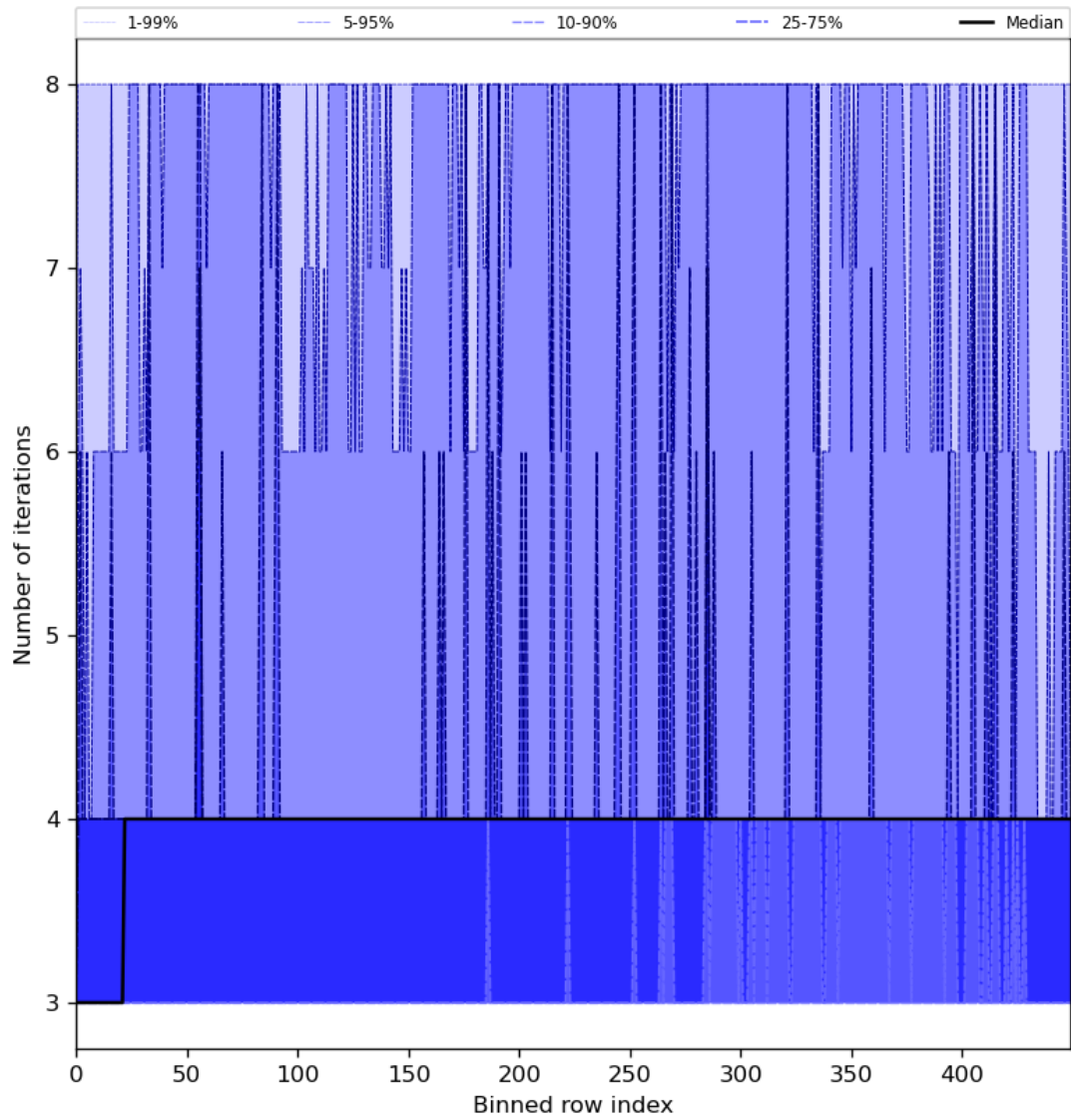
Figure 51: Along track statistics of “Number of iterations” for 2023-07-22 to 2023-07-24
