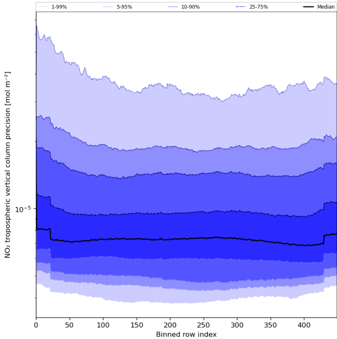
Figure 47: Along track statistics of “NO 2 tropospheric vertical column precision” for 2023-07-22 to 2023-07-24
