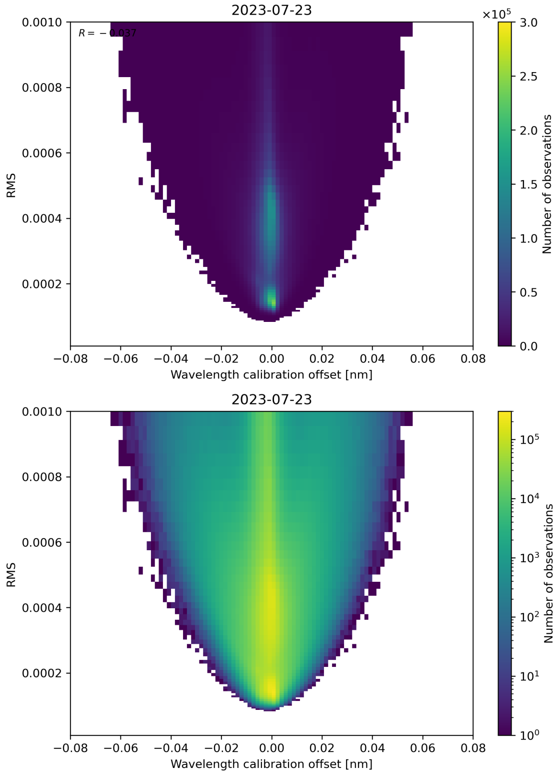
Figure 181: Scatter density plot of “Wavelength calibration offset” against “RMS” for 2023-07-22 to 2023-07-24.
