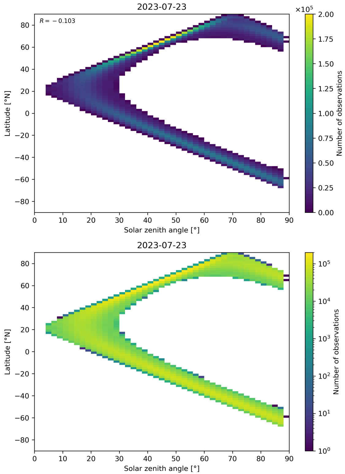
Figure 149: Scatter density plot of “Solar zenith angle” against “Latitude” for 2023-07-22 to 2023-07-24.
