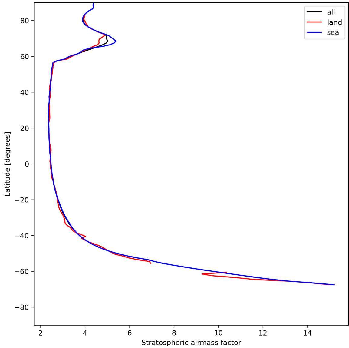
Figure 27: Zonal average of “Stratospheric airmass factor” for 2023-07-22 to 2023-07-24.
