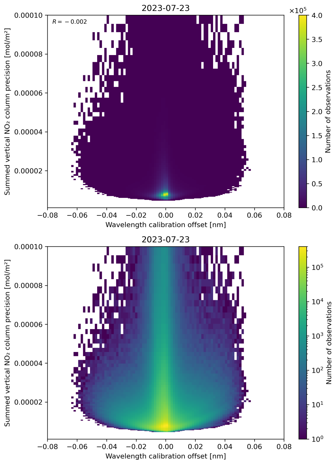
Figure 178: Scatter density plot of “Wavelength calibration offset” against “Summed vertical NO 2 column precision” for 2023-07-22 to 2023-07-24.
