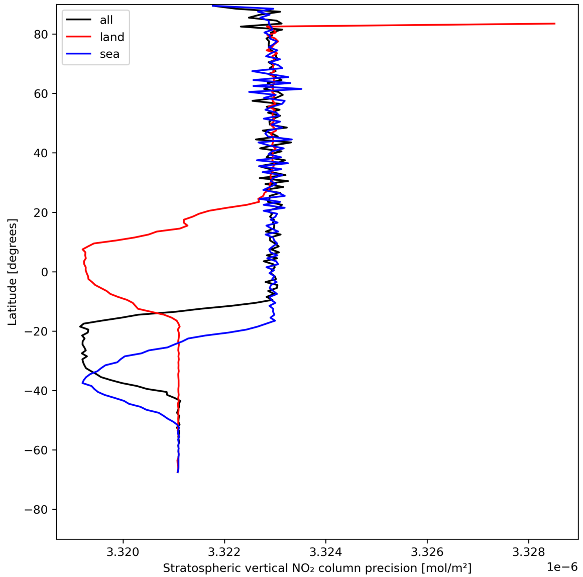
Figure 20: Zonal average of “Stratospheric vertical NO 2 column precision” for 2023-07-22 to 2023-07-24.
