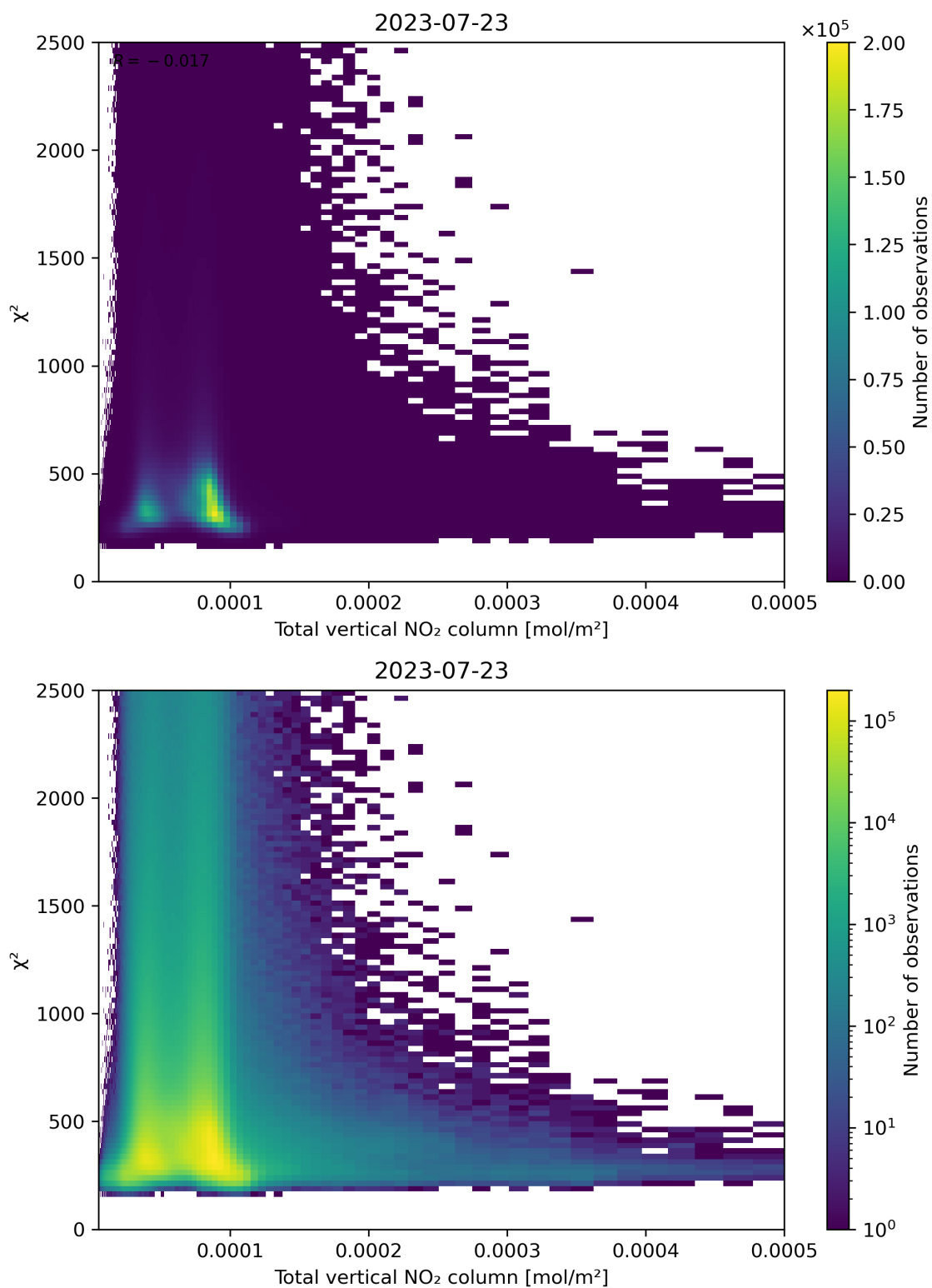
Figure 111: Scatter density plot of “Total vertical NO 2 column” against “ \chi^2 ” for 2023-07-22 to 2023-07-24.
