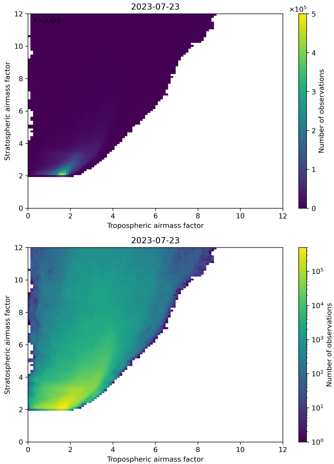
Figure 71: Scatter density plot of “Tropospheric airmass factor” against “Stratospheric airmass factor” for 2023-07-22 to 2023-07-24.
