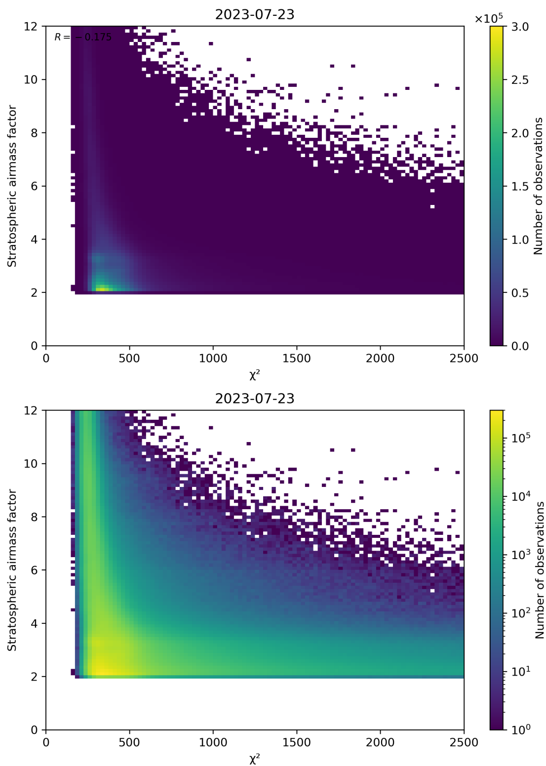
Figure 81: Scatter density plot of “ \chi^2 ” against “Stratospheric airmass factor” for 2023-07-22 to 2023-07-24.
