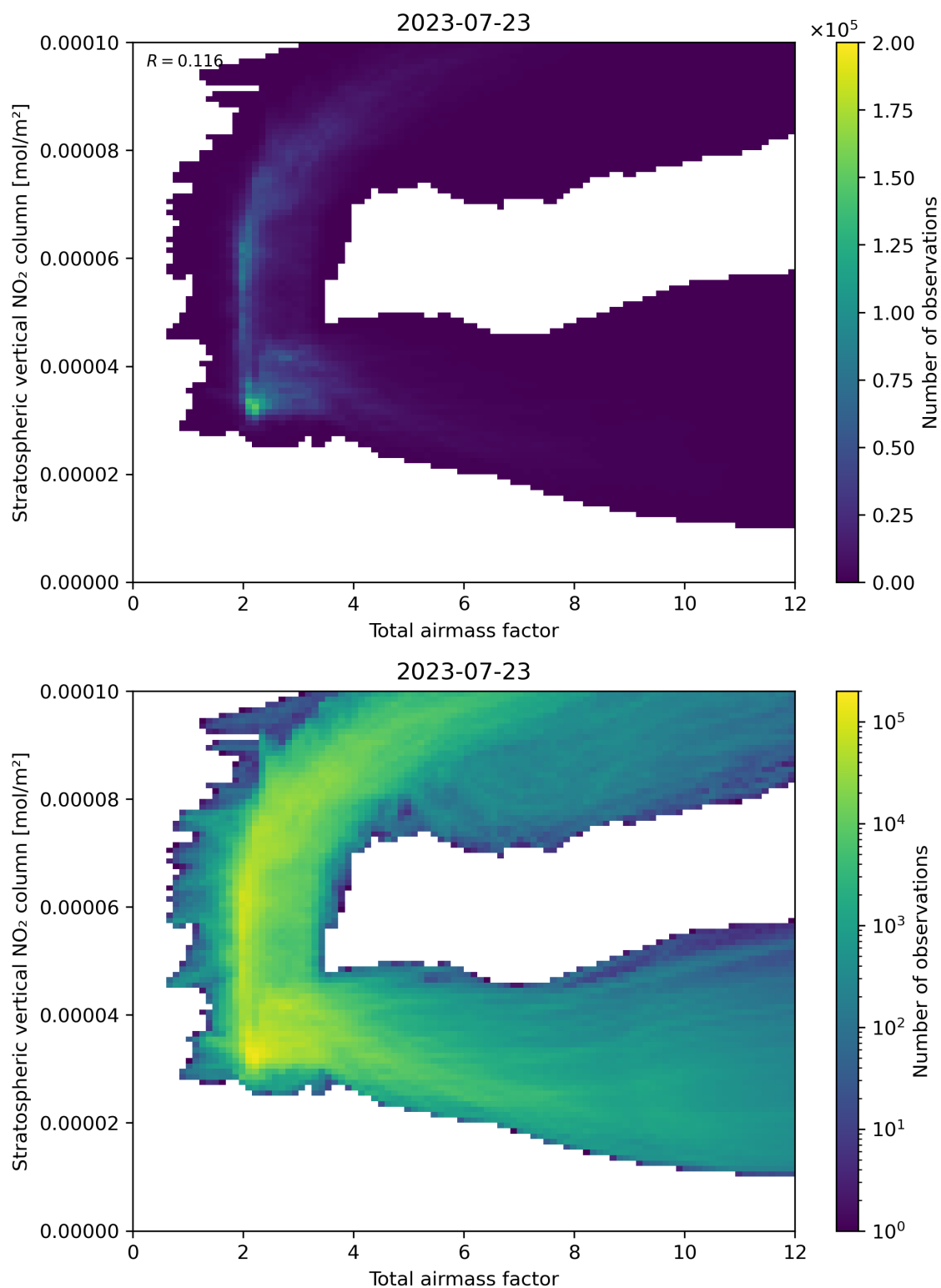
Figure 64: Scatter density plot of “Total airmass factor” against “Stratospheric vertical \text{NO}_2 column” for 2023-07-22 to 2023-07-24.
