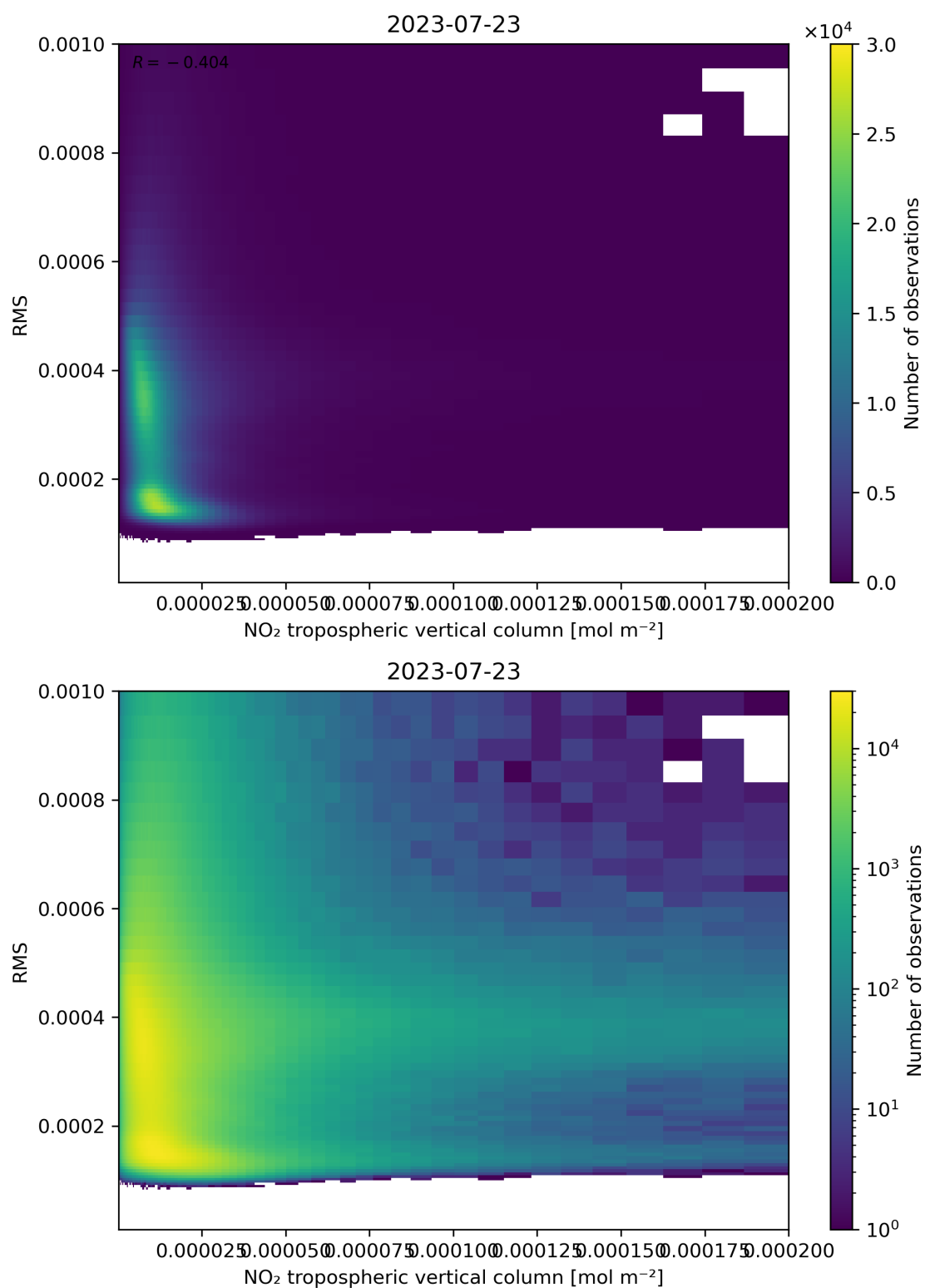
Figure 142: Scatter density plot of “NO 2 tropospheric vertical column” against “RMS” for 2023-07-22 to 2023-07-24.
