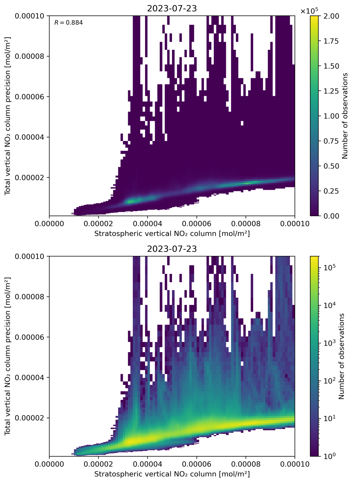
Figure 101: Scatter density plot of “Stratospheric vertical NO 2 column” against “Total vertical NO 2 column precision” for 2023-07-22 to 2023-07-24.
