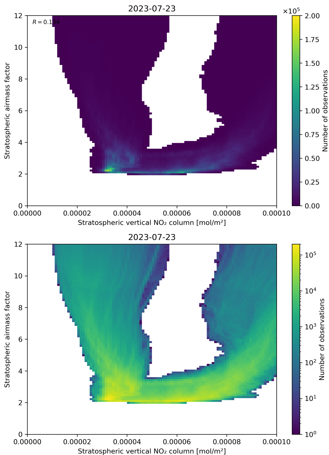
Figure 96: Scatter density plot of “Stratospheric vertical NO 2 column” against “Stratospheric airmass factor” for 2023-07-22 to 2023-07-24.
