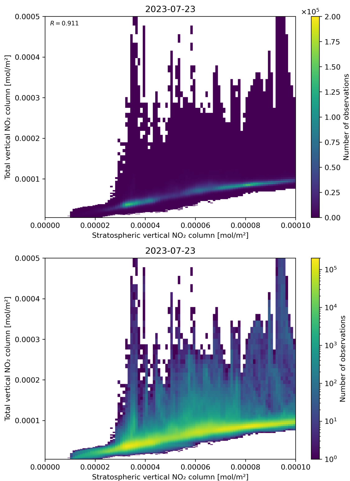
Figure 100: Scatter density plot of “Stratospheric vertical NO 2 column” against “Total vertical NO 2 column” for 2023-07-22 to 2023-07-24.
