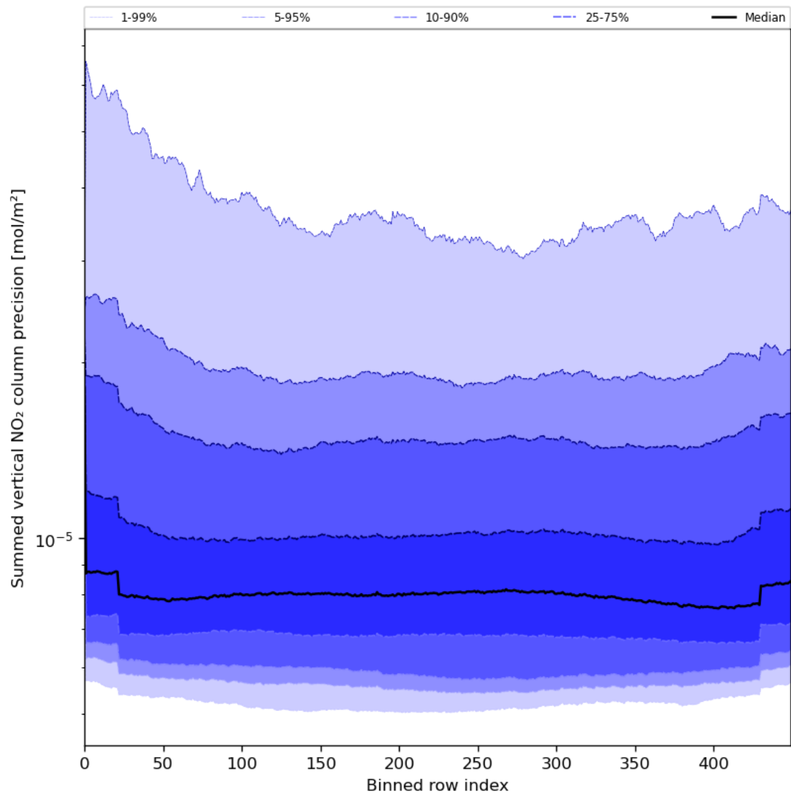
Figure 58: Along track statistics of “Summed vertical NO 2 column precision” for 2023-07-22 to 2023-07-24
