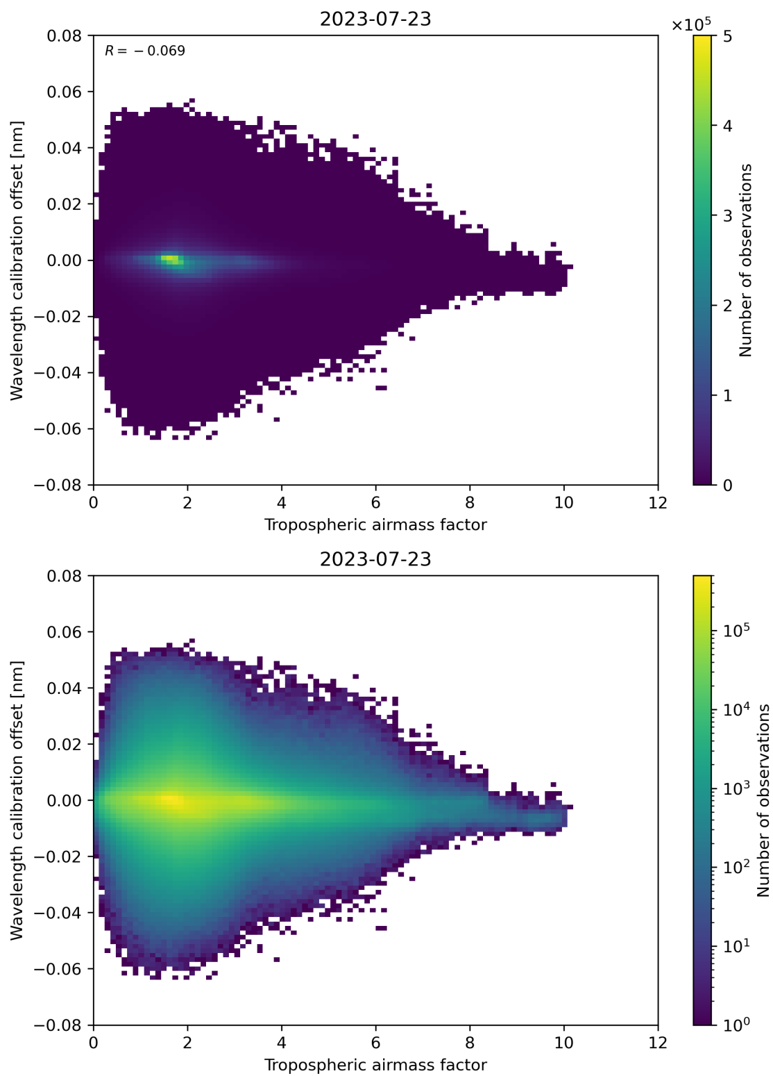
Figure 80: Scatter density plot of “Tropospheric airmass factor” against “Wavelength calibration offset” for 2023-07-22 to 2023-07-24.
