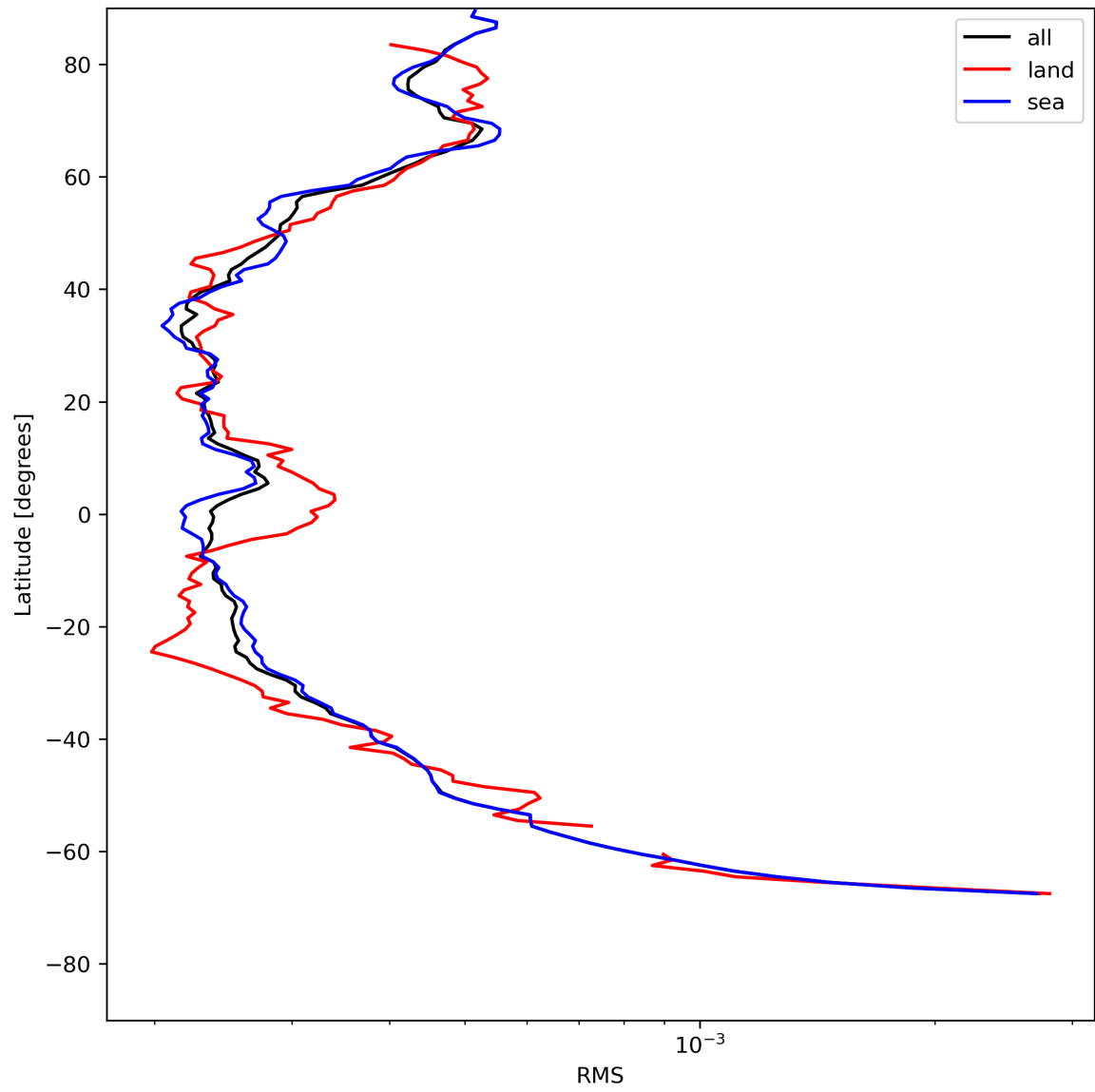
Figure 26: Zonal average of “RMS” for 2023-07-22 to 2023-07-24.
