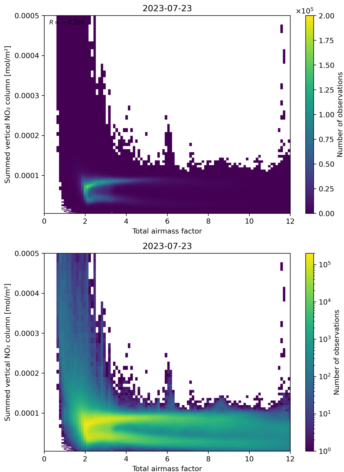
Figure 65: Scatter density plot of “Total airmass factor” against “Summed vertical NO 2 column” for 2023-07-22 to 2023-07-24.
