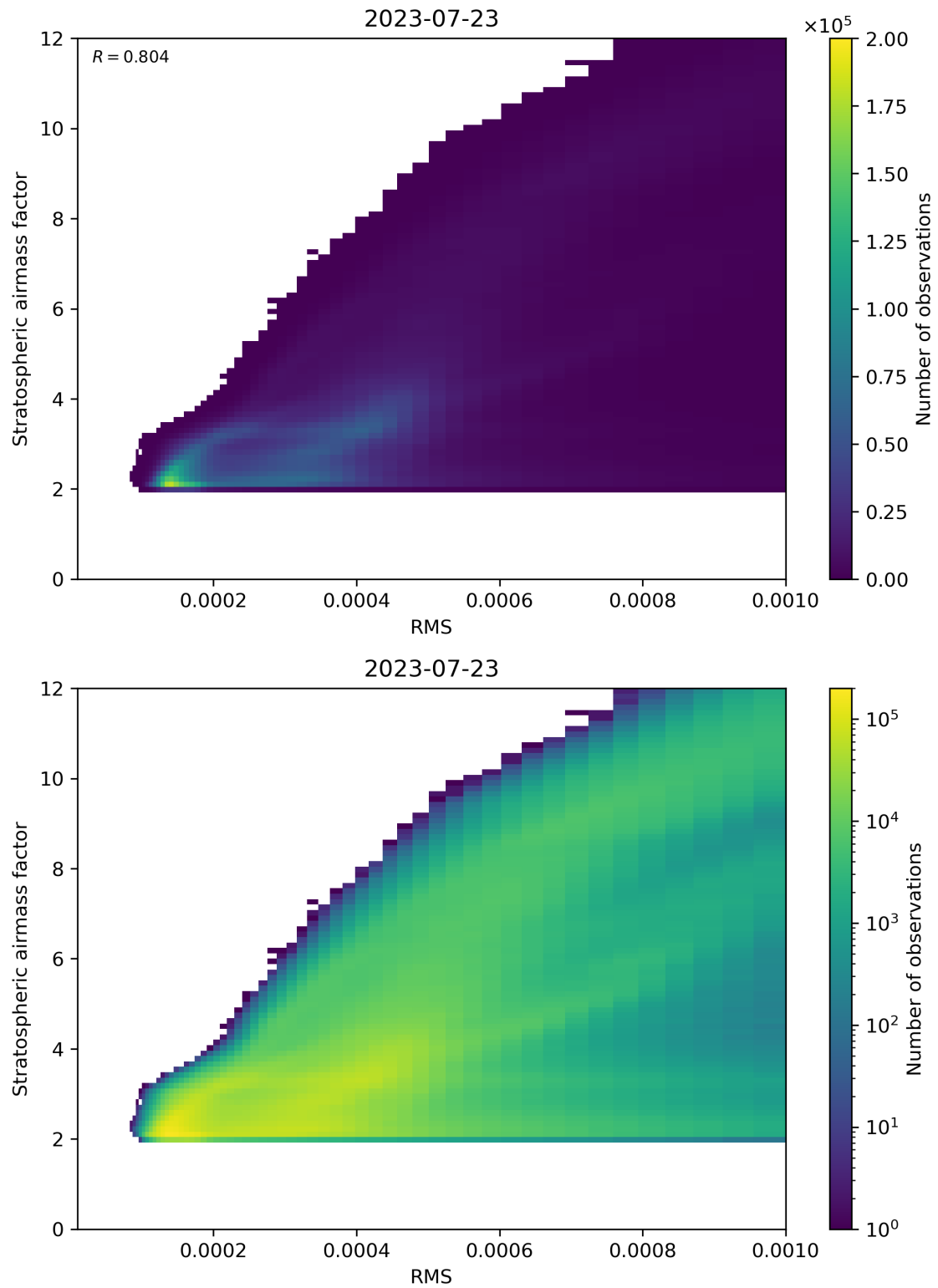
Figure 144: Scatter density plot of “RMS” against “Stratospheric airmass factor” for 2023-07-22 to 2023-07-24.
