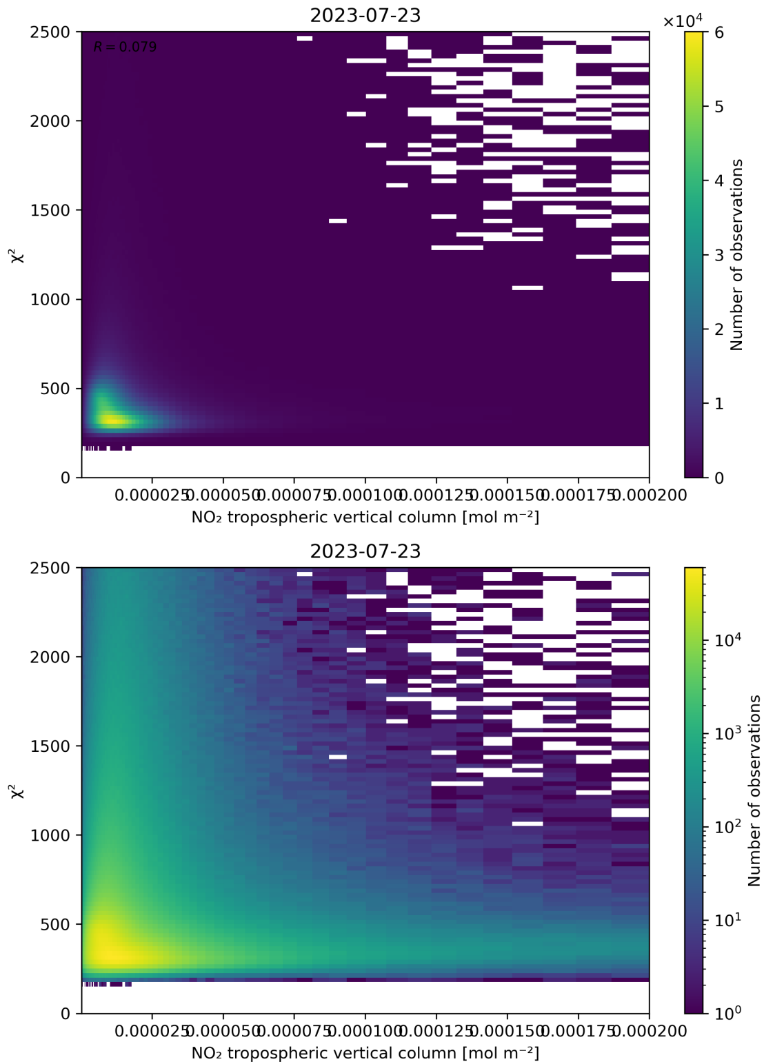
Figure 124: Scatter density plot of “NO 2 tropospheric vertical column” against “ \chi^2 ” for 2023-07-22 to 2023-07-24.
