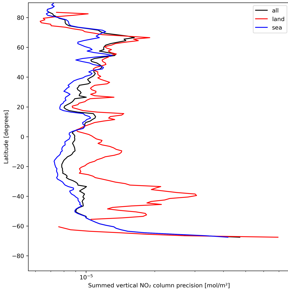
Figure 24: Zonal average of “Summed vertical NO 2 column precision” for 2023-07-22 to 2023-07-24.
