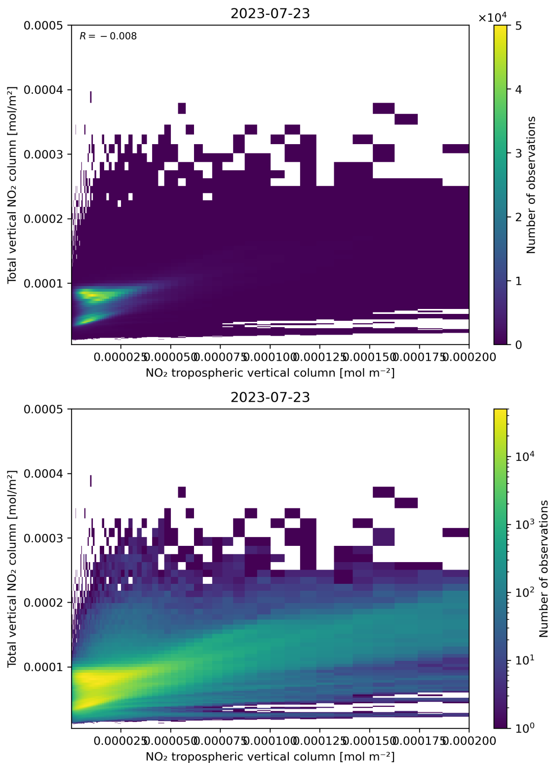
Figure 128: Scatter density plot of “NO 2 tropospheric vertical column” against “Total vertical NO 2 column” for 2023-07-22 to 2023-07-24.
