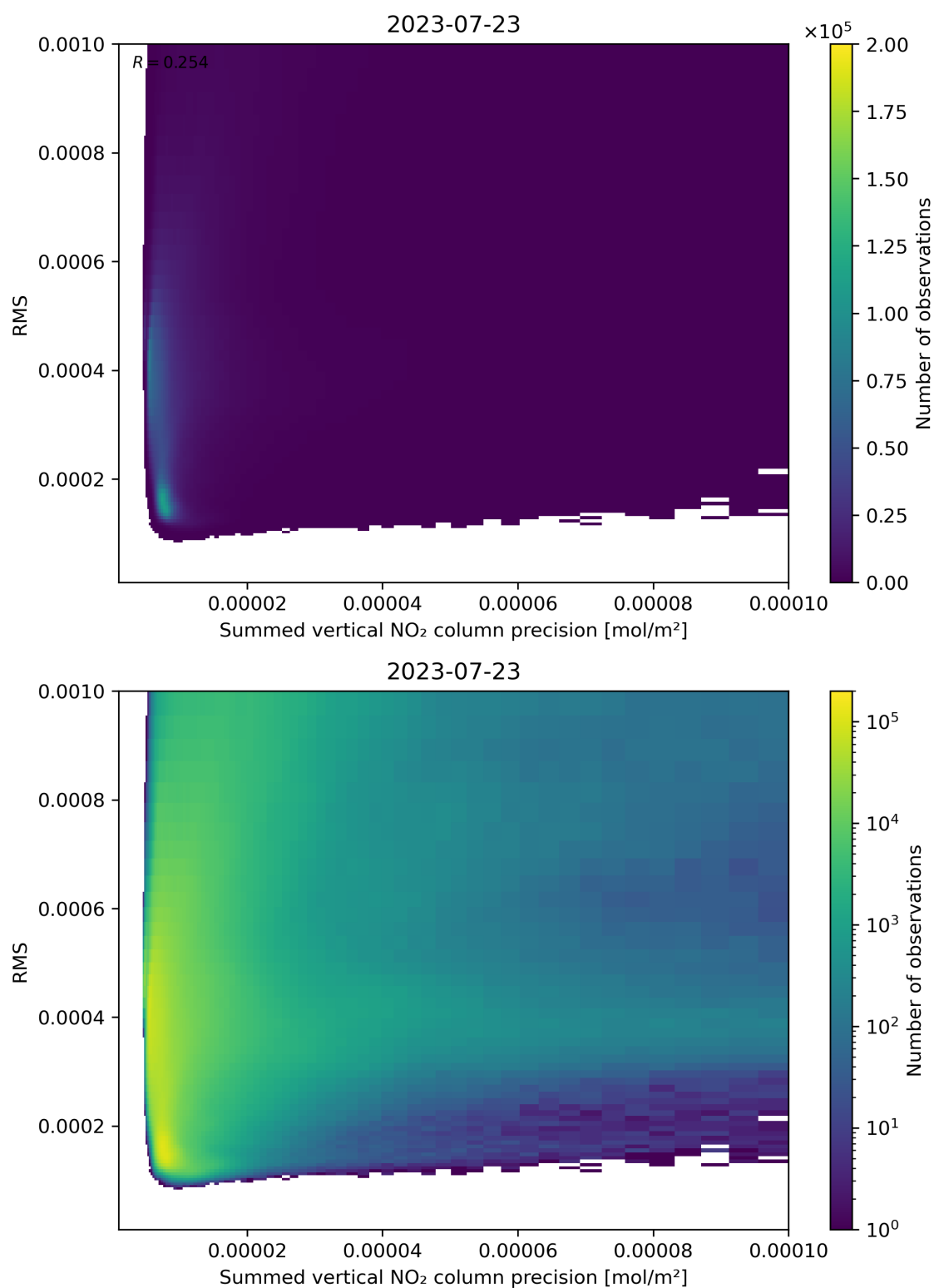
Figure 108: Scatter density plot of “Summed vertical NO 2 column precision” against “RMS” for 2023-07-22 to 2023-07-24.
