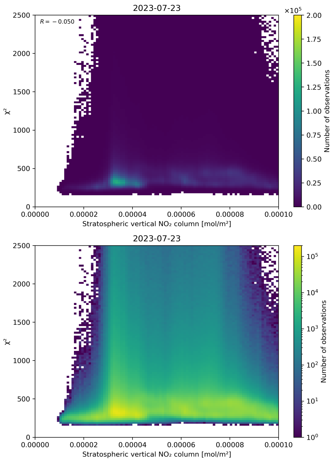
Figure 97: Scatter density plot of “Stratospheric vertical NO 2 column” against “ \chi^2 ” for 2023-07-22 to 2023-07-24.
