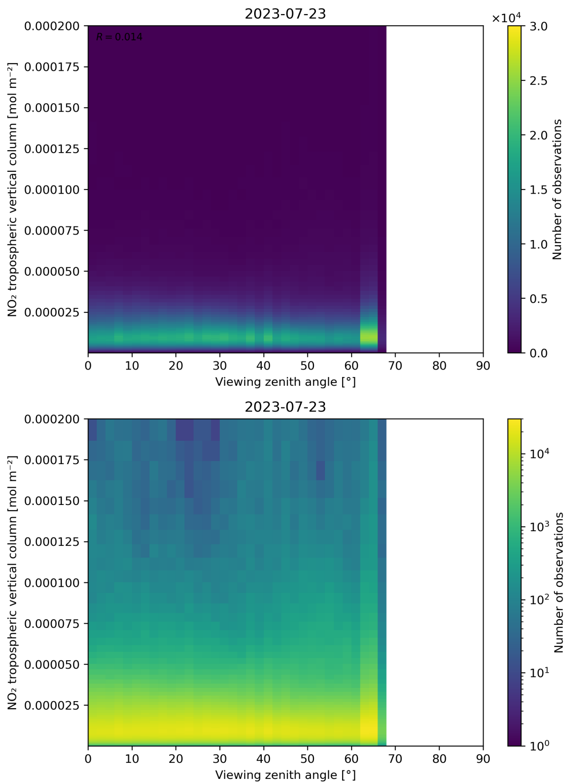
Figure 169: Scatter density plot of “Viewing zenith angle” against “NO 2 tropospheric vertical column” for 2023-07-22 to 2023-07-24.
