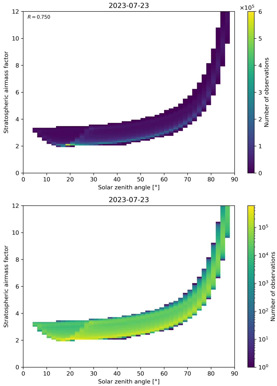
Figure 145: Scatter density plot of “Solar zenith angle” against “Stratospheric airmass factor” for 2023-07-22 to 2023-07-24.
