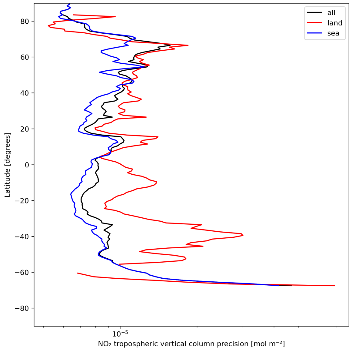
Figure 13: Zonal average of “NO 2 tropospheric vertical column precision” for 2023-07-22 to 2023-07-24.
