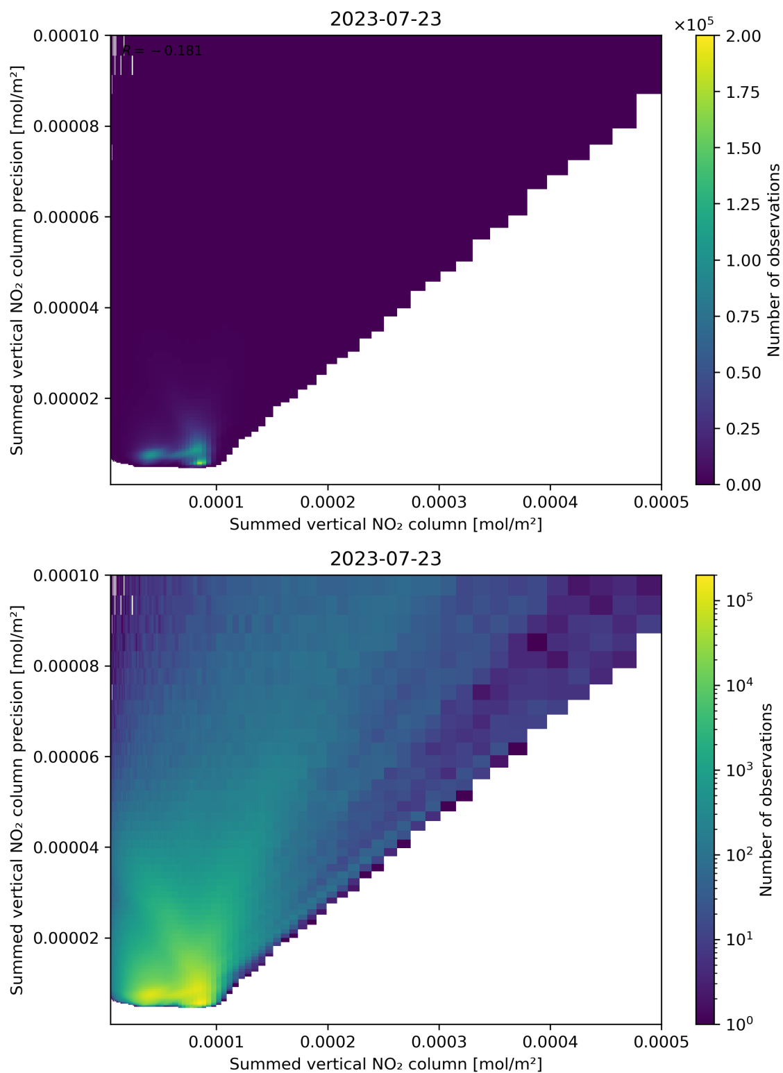
Figure 105: Scatter density plot of “Summed vertical NO 2 column” against “Summed vertical NO 2 column precision” for 2023-07-22 to 2023-07-24.
