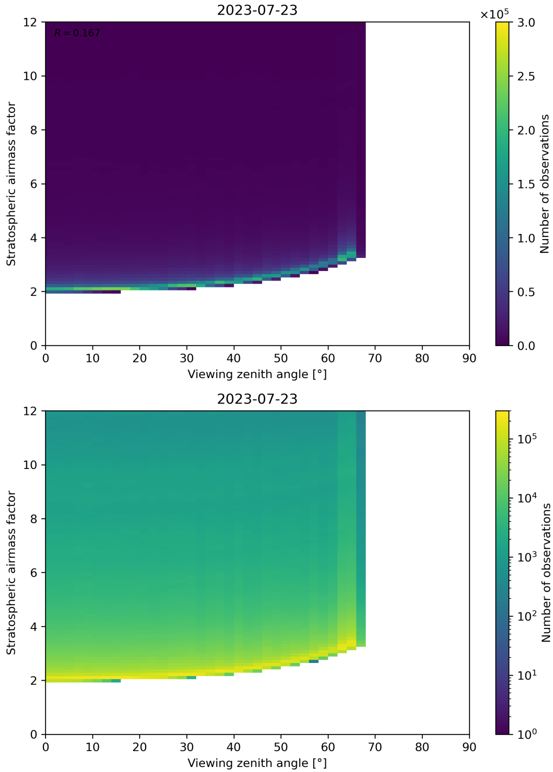
Figure 159: Scatter density plot of “Viewing zenith angle” against “Stratospheric airmass factor” for 2023-07-22 to 2023-07-24.
