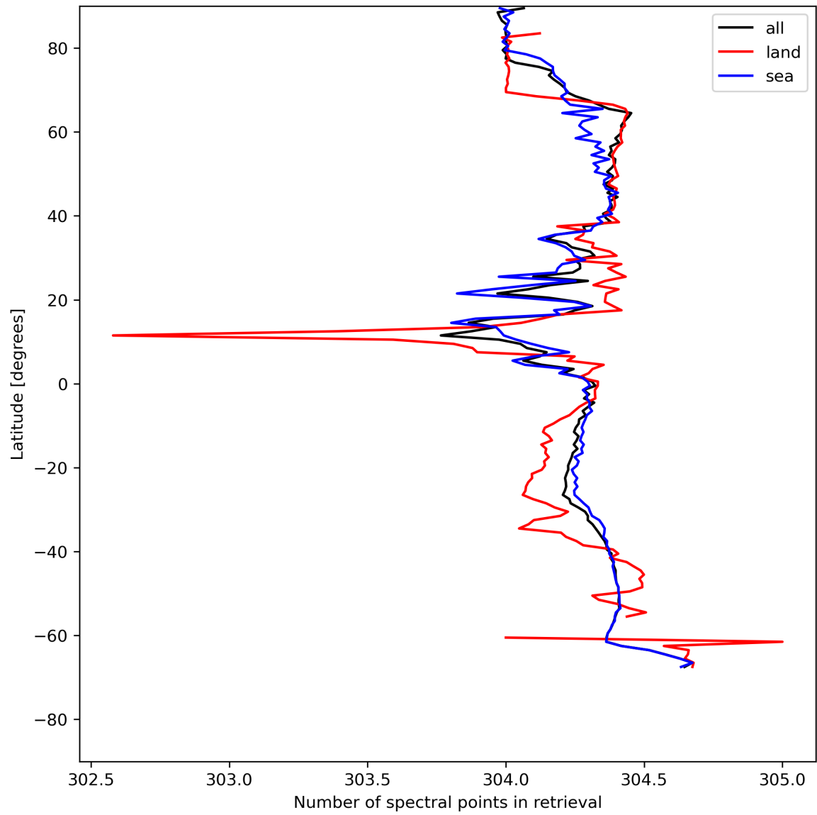
Figure 16: Zonal average of “Number of spectral points in retrieval” for 2023-07-22 to 2023-07-24.
