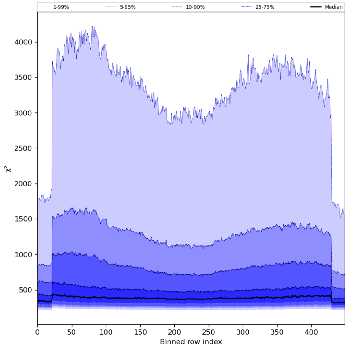
Figure 59: Along track statistics of “ \chi^2 ” for 2023-07-22 to 2023-07-24
