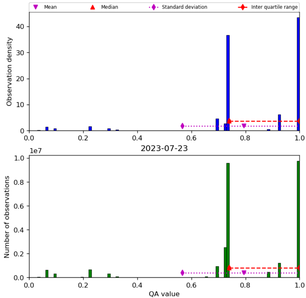
Figure 28: Histogram of “QA value” for 2023-07-22 to 2023-07-24
