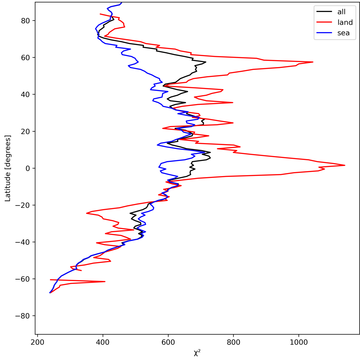
Figure 25: Zonal average of “ \chi^2 ” for 2023-07-22 to 2023-07-24.
