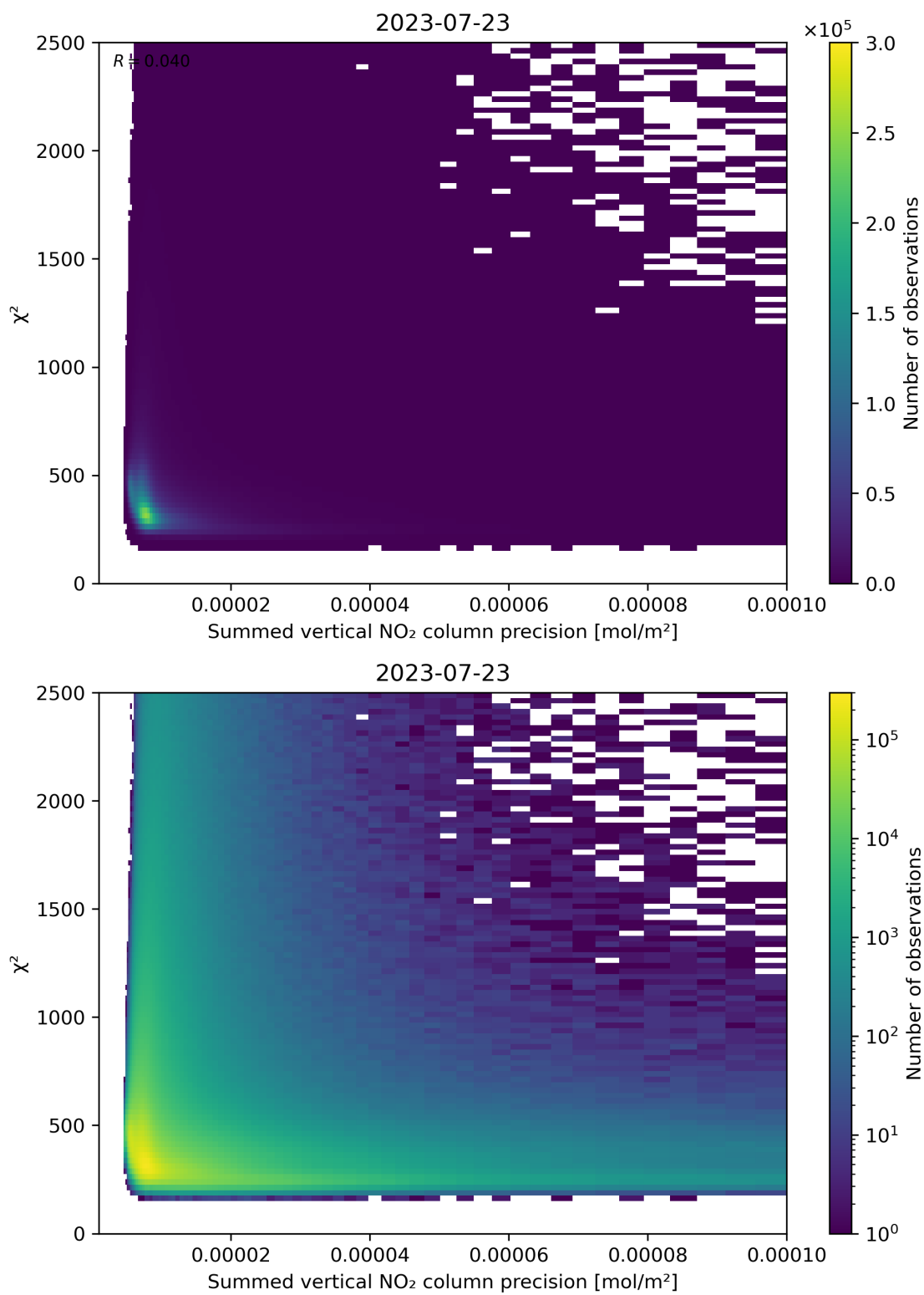
Figure 107: Scatter density plot of “Summed vertical NO 2 column precision” against “ \chi^2 ” for 2023-07-22 to 2023-07-24.
