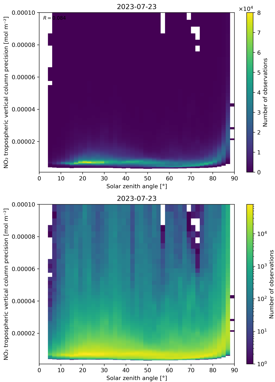
Figure 156: Scatter density plot of “Solar zenith angle” against “NO 2 tropospheric vertical column precision” for 2023-07-22 to 2023-07-24.
