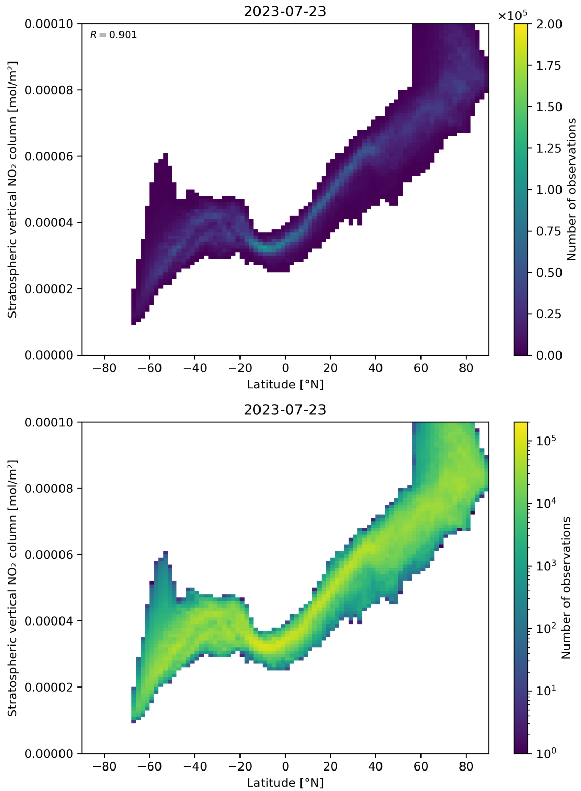
Figure 87: Scatter density plot of “Latitude” against “Stratospheric vertical \text{NO}_2 column” for 2023-07-22 to 2023-07-24.
