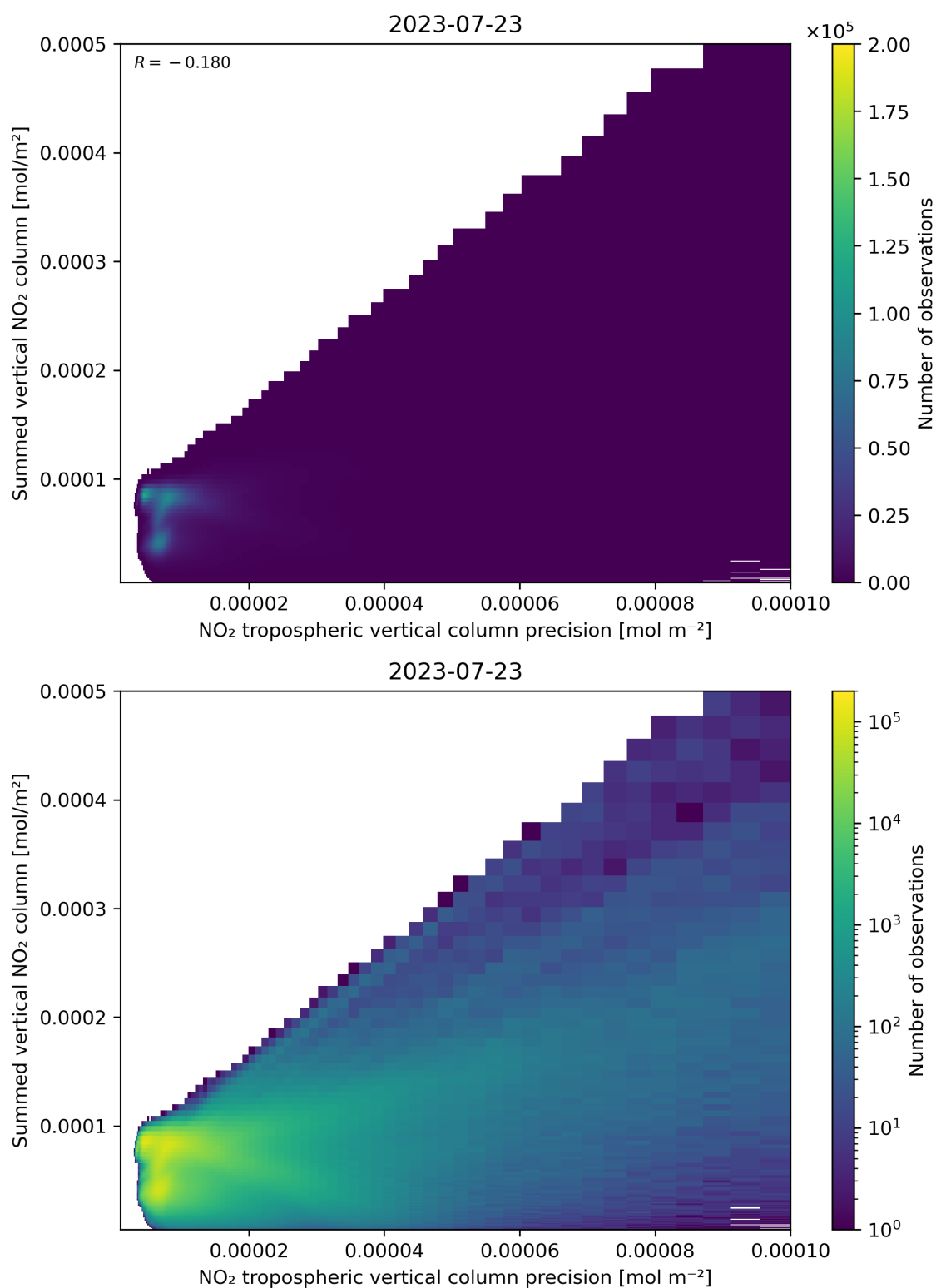
Figure 136: Scatter density plot of “NO 2 tropospheric vertical column precision” against “Summed vertical NO 2 column” for 2023-07-22 to 2023-07-24.
