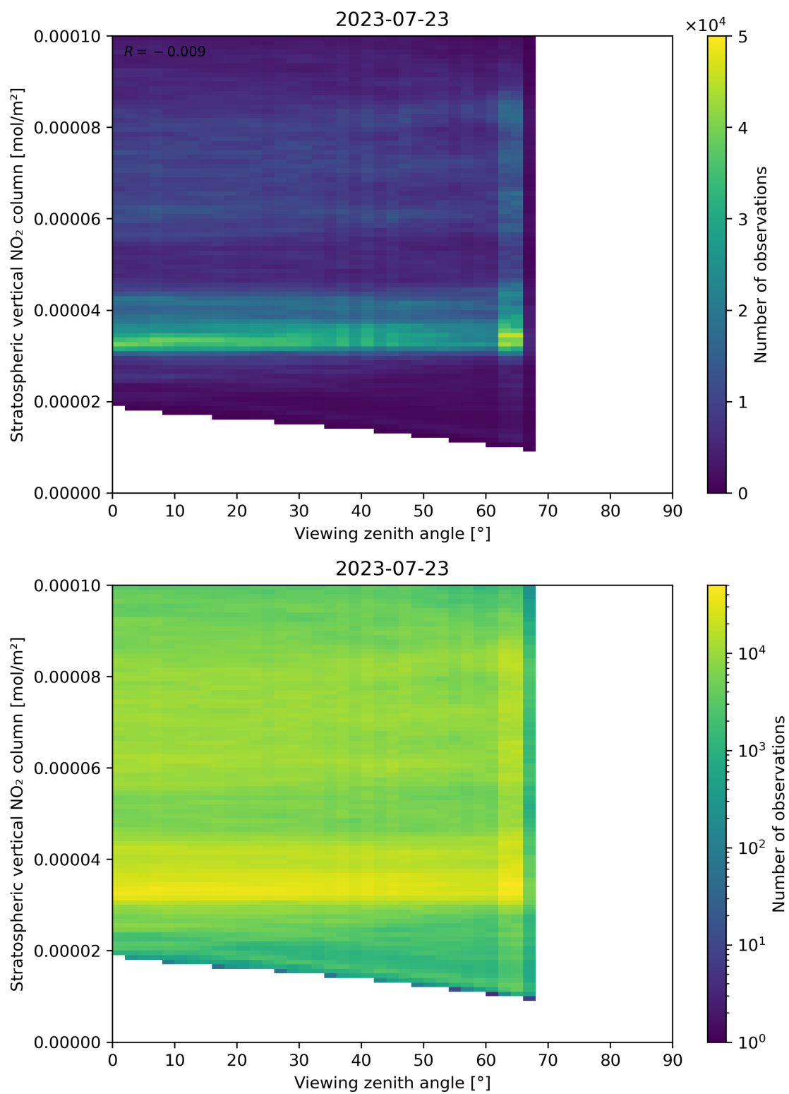
Figure 164: Scatter density plot of “Viewing zenith angle” against “Stratospheric vertical NO 2 column” for 2023-07-22 to 2023-07-24.
