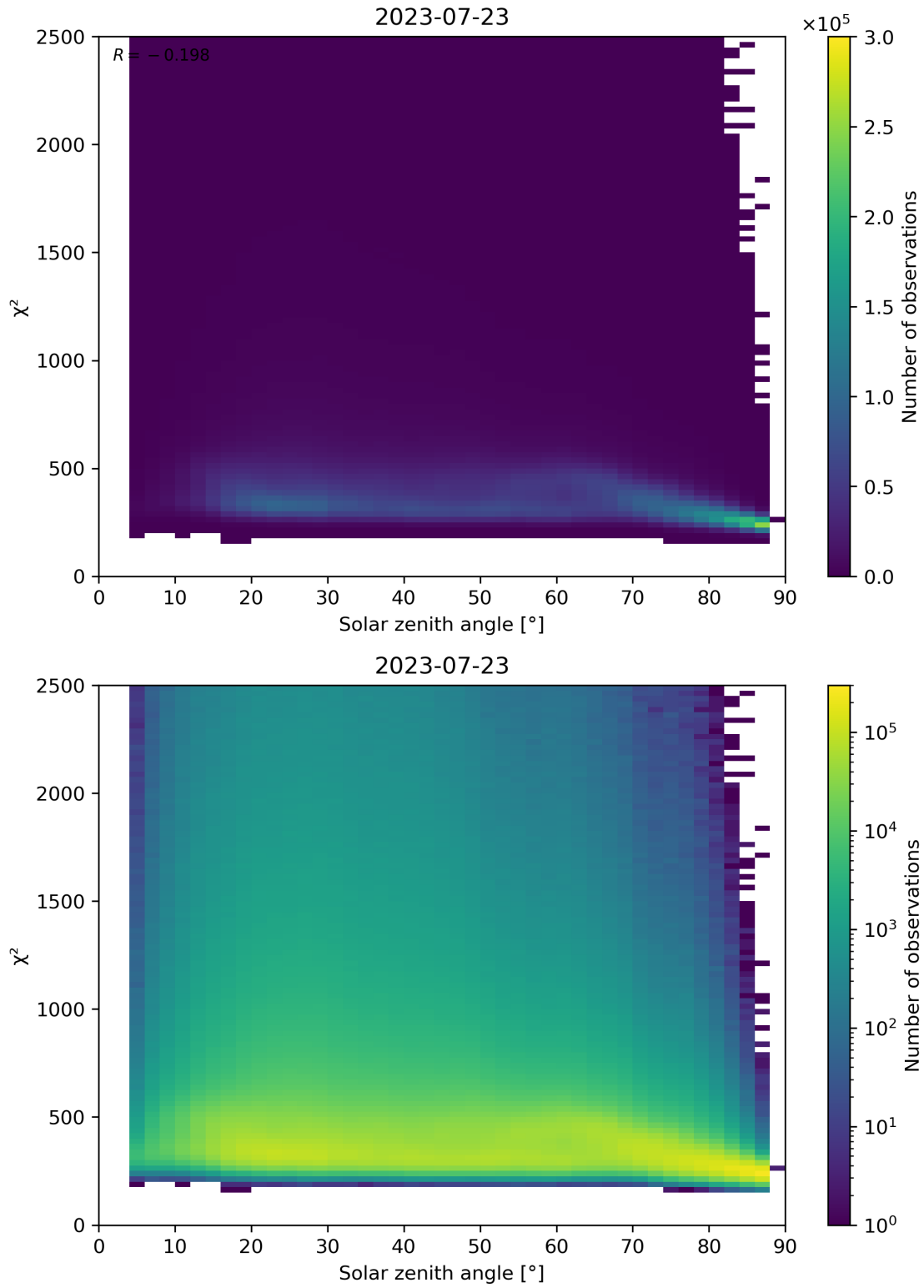
Figure 148: Scatter density plot of “Solar zenith angle” against “ \chi^2 ” for 2023-07-22 to 2023-07-24.
