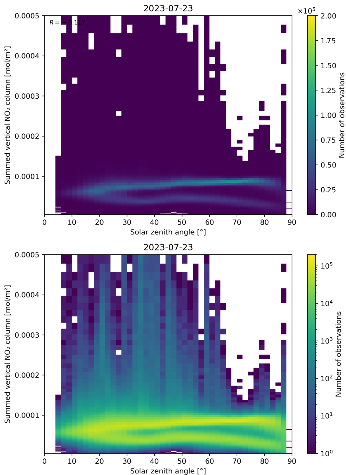
Figure 151: Scatter density plot of “Solar zenith angle” against “Summed vertical NO 2 column” for 2023-07-22 to 2023-07-24.
