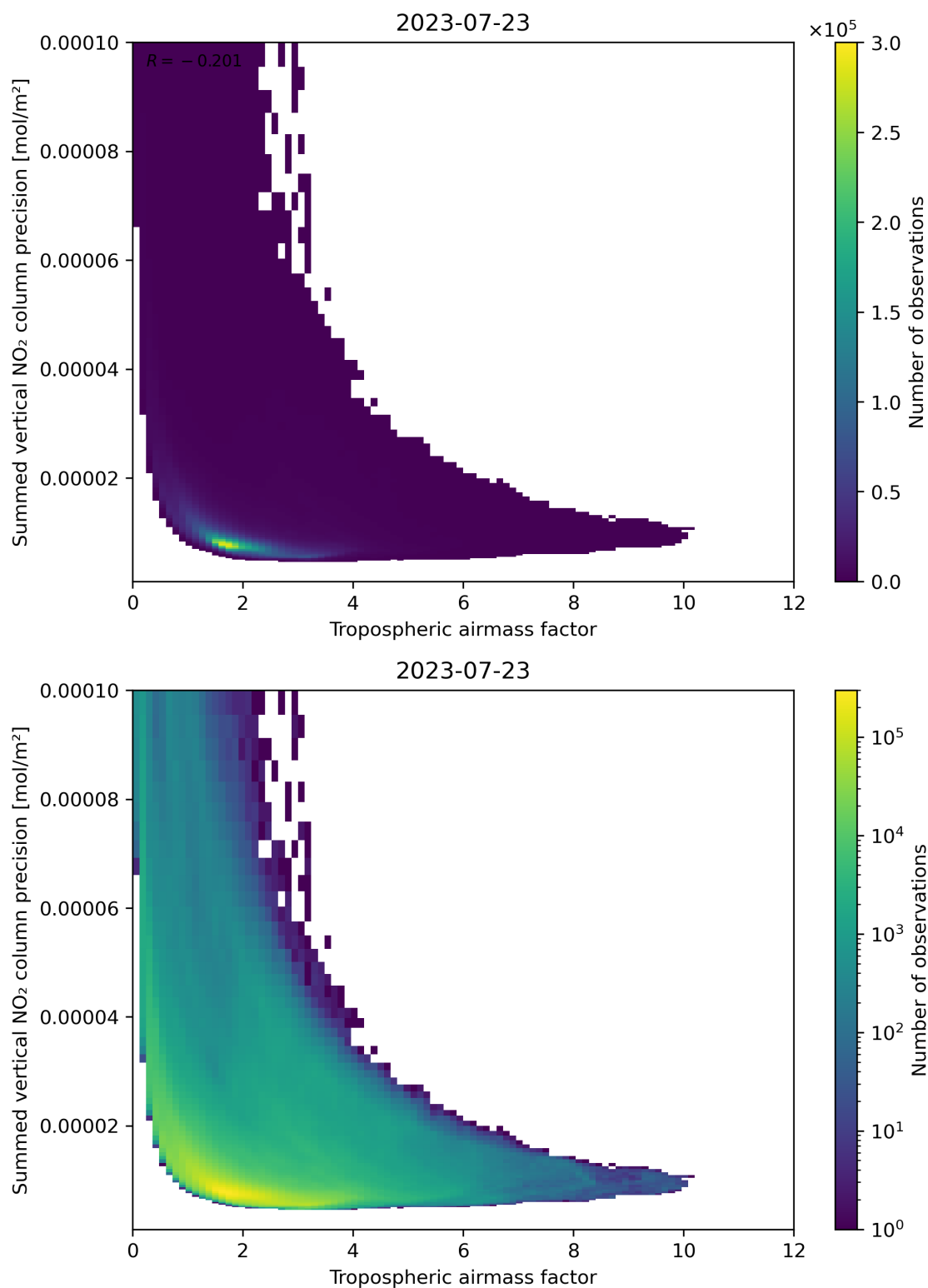
Figure 76: Scatter density plot of “Tropospheric air mass factor” against “Summed vertical NO 2 column precision” for 2023-07-22 to 2023-07-24.
