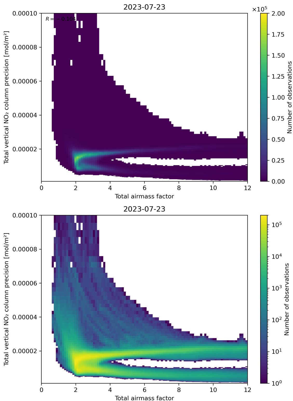
Figure 68: Scatter density plot of “Total airmass factor” against “Total vertical NO 2 column precision” for 2023-07-22 to 2023-07-24.
