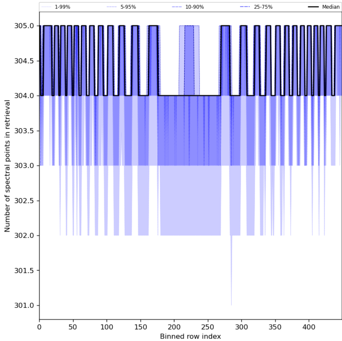
Figure 50: Along track statistics of “Number of spectral points in retrieval” for 2023-07-22 to 2023-07-24
