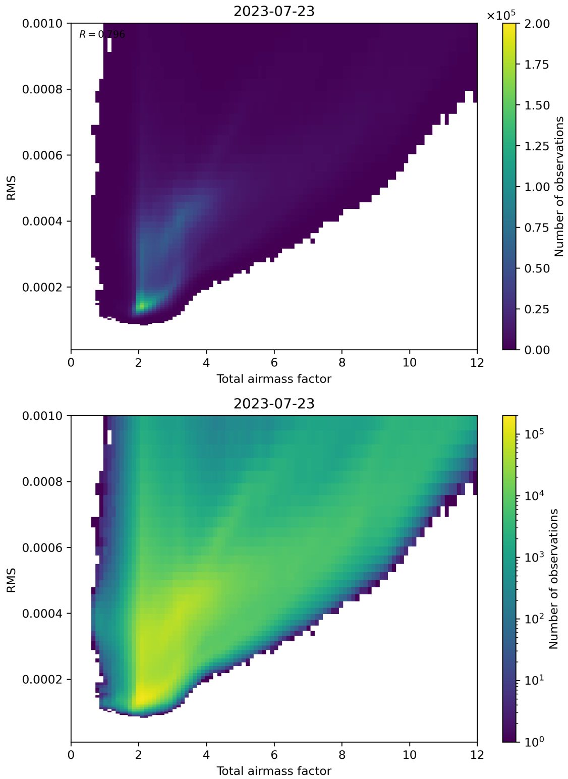
Figure 69: Scatter density plot of “Total airmass factor” against “RMS” for 2023-07-22 to 2023-07-24.
