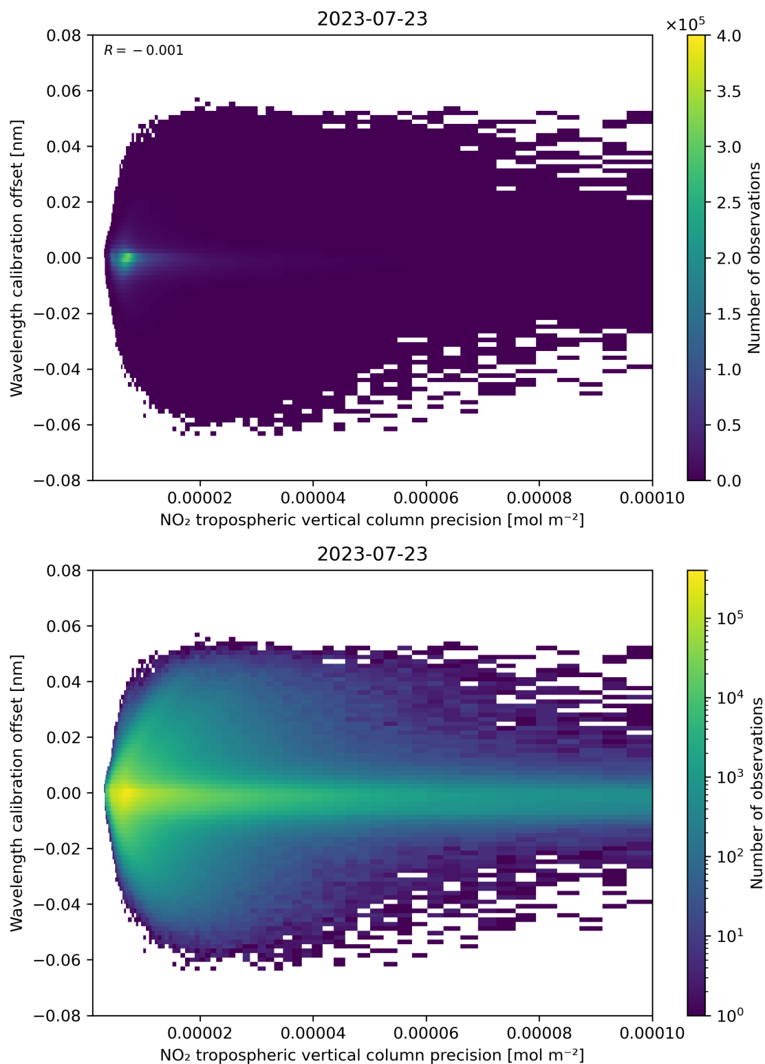
Figure 141: Scatter density plot of “NO 2 tropospheric vertical column precision” against “Wavelength calibration offset” for 2023-07-22 to 2023-07-24.
