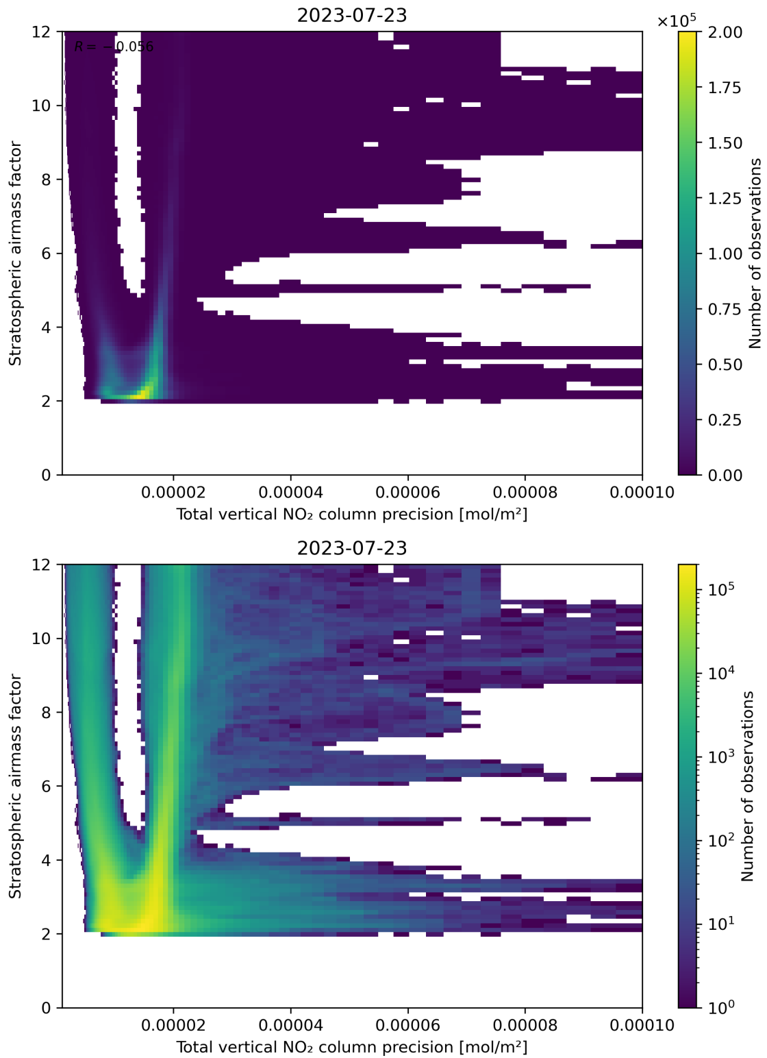
Figure 115: Scatter density plot of “Total vertical NO 2 column precision” against “Stratospheric air mass factor” for 2023-07-22 to 2023-07-24.
