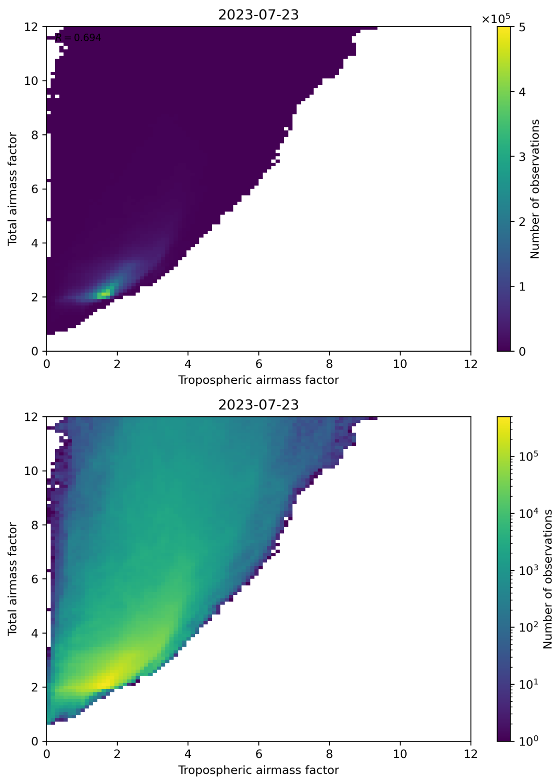
Figure 72: Scatter density plot of “Tropospheric airmass factor” against “Total airmass factor” for 2023-07-22 to 2023-07-24.
