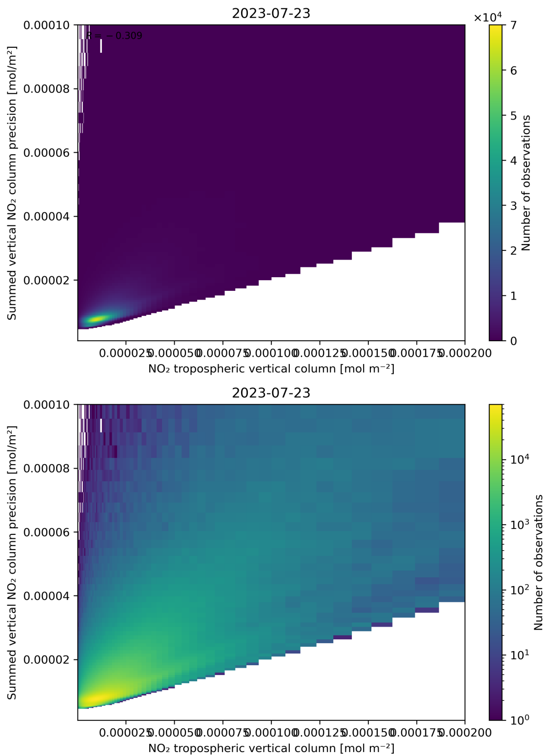
Figure 127: Scatter density plot of “NO 2 tropospheric vertical column” against “Summed vertical NO 2 column precision” for 2023-07-22 to 2023-07-24.
