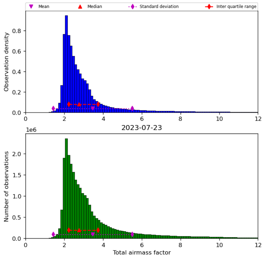
Figure 32: Histogram of “Total airmass factor” for 2023-07-22 to 2023-07-24
