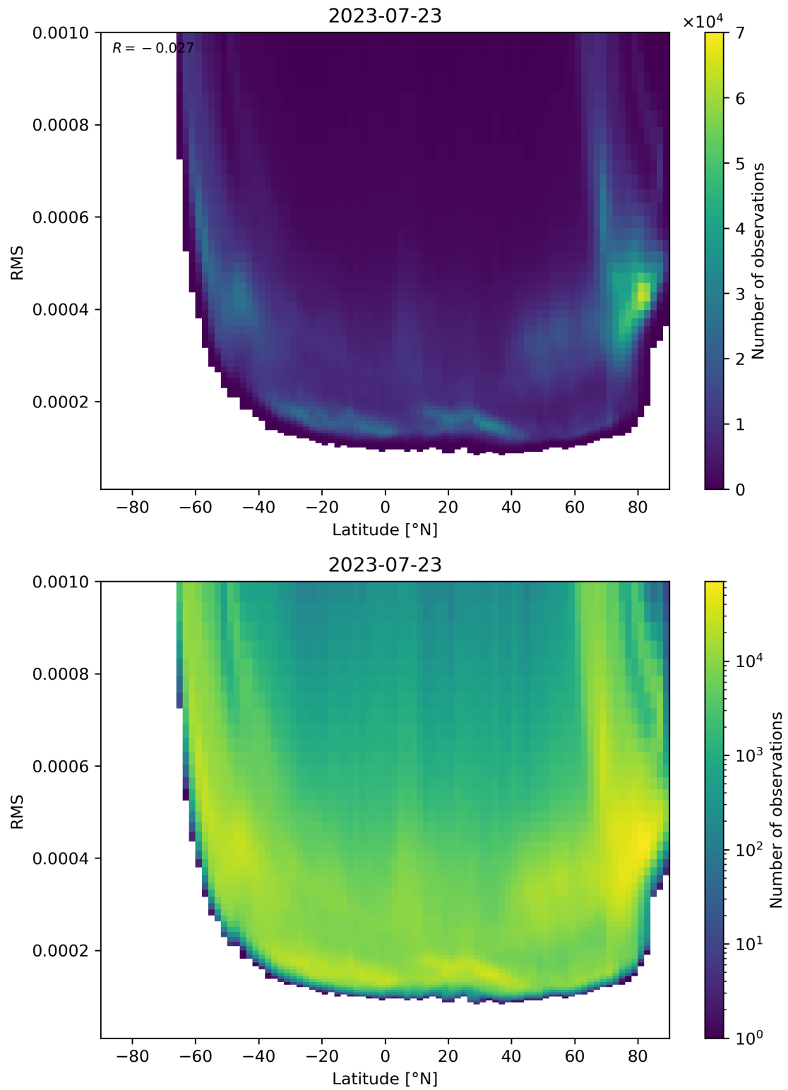
Figure 94: Scatter density plot of “Latitude” against “RMS” for 2023-07-22 to 2023-07-24.
