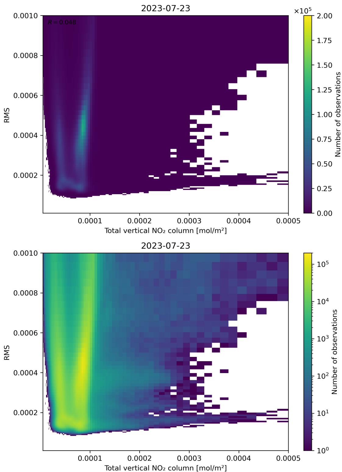
Figure 120: Scatter density plot of “Total vertical NO 2 column” against “RMS” for 2023-07-22 to 2023-07-24.
