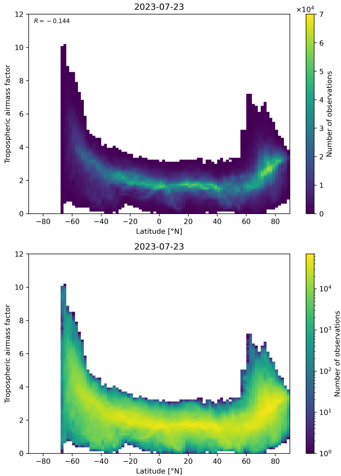
Figure 85: Scatter density plot of “Latitude” against “Tropospheric air mass factor” for 2023-07-22 to 2023-07-24.
