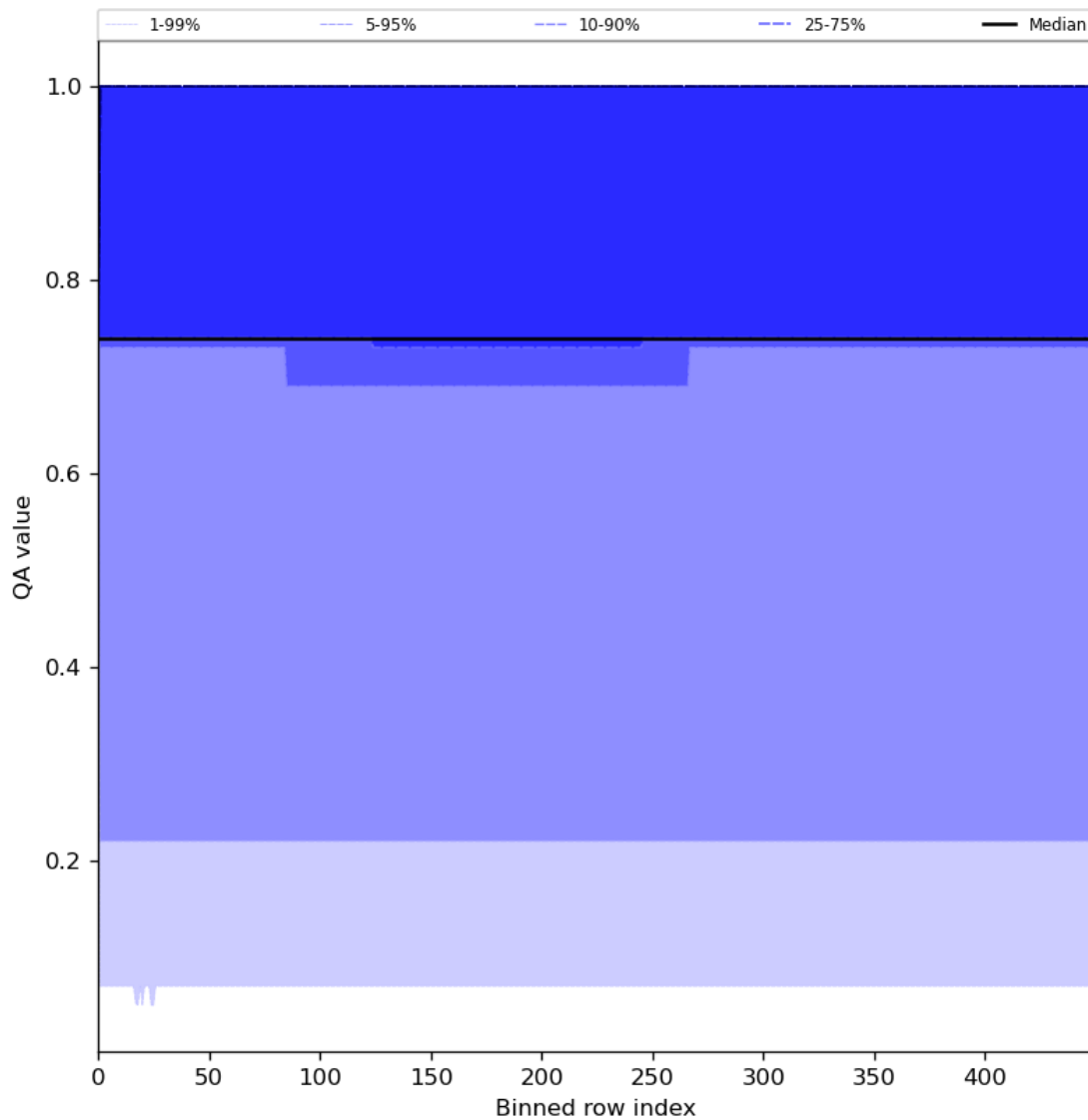
Figure 45: Along track statistics of “QA value” for 2023-07-22 to 2023-07-24
