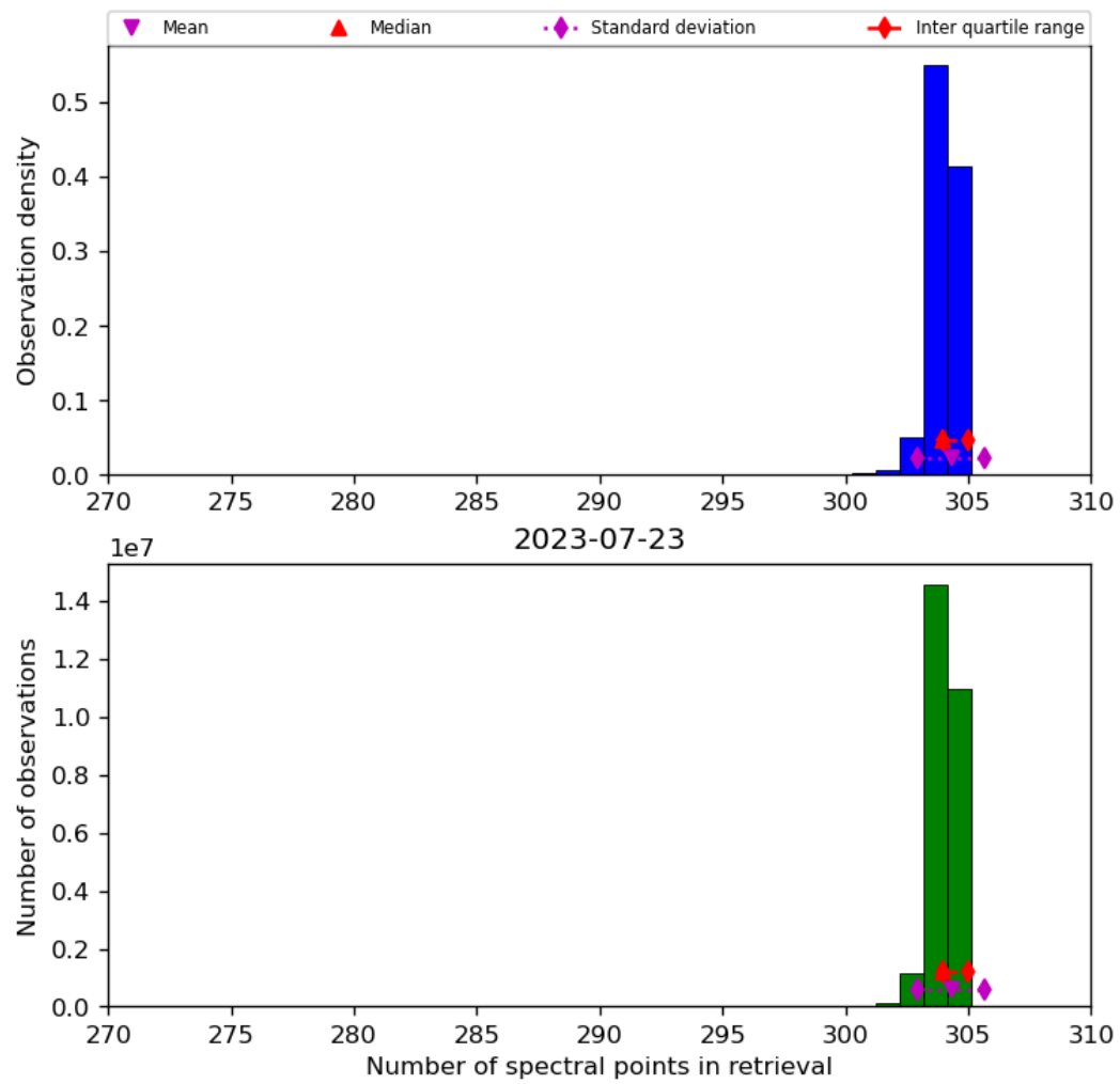
Figure 33: Histogram of “Number of spectral points in retrieval” for 2023-07-22 to 2023-07-24
