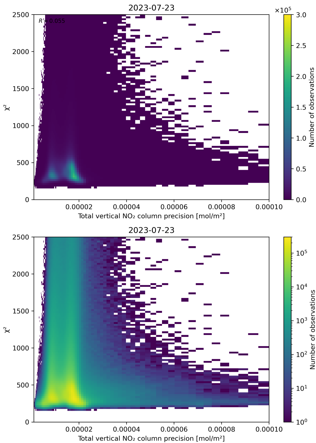
Figure 116: Scatter density plot of “Total vertical NO 2 column precision” against “ \chi^2 ” for 2023-07-22 to 2023-07-24.
