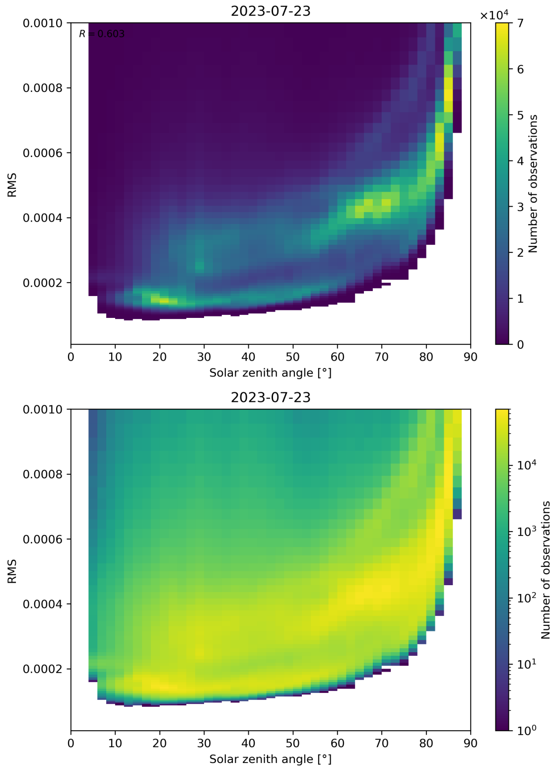
Figure 157: Scatter density plot of “Solar zenith angle” against “RMS” for 2023-07-22 to 2023-07-24.
