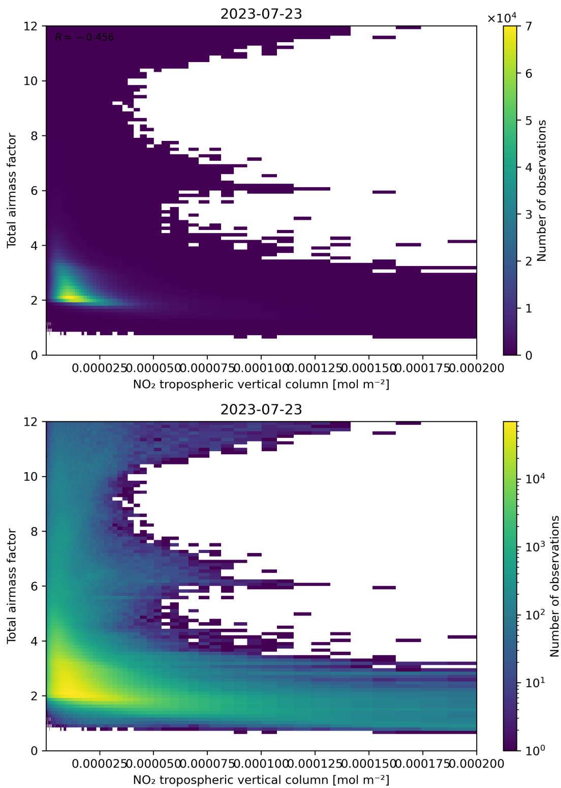
Figure 122: Scatter density plot of “NO 2 tropospheric vertical column” against “Total air mass factor” for 2023-07-22 to 2023-07-24.
