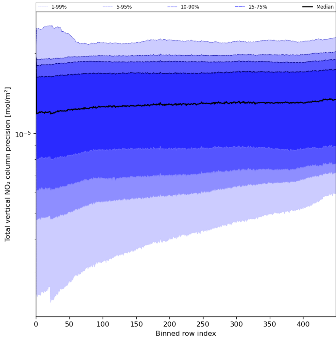
Figure 56: Along track statistics of “Total vertical NO 2 column precision” for 2023-07-22 to 2023-07-24
