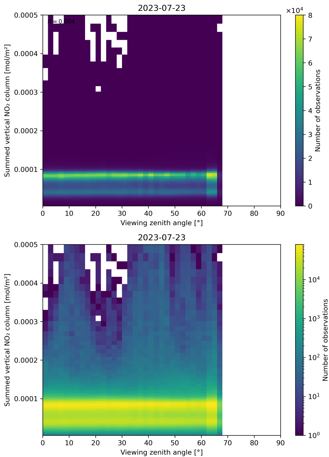
Figure 165: Scatter density plot of “Viewing zenith angle” against “Summed vertical NO 2 column” for 2023-07-22 to 2023-07-24.
