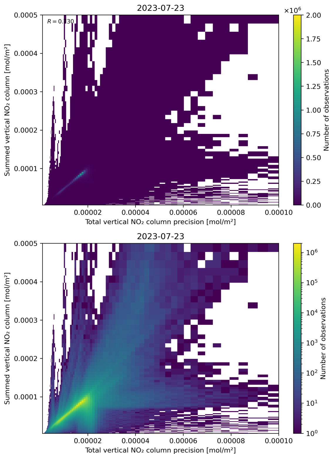
Figure 117: Scatter density plot of “Total vertical NO 2 column precision” against “Summed vertical NO 2 column” for 2023-07-22 to 2023-07-24.
