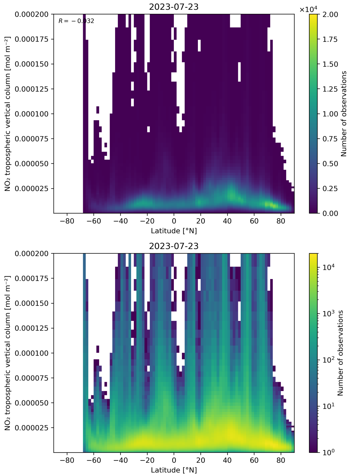
Figure 92: Scatter density plot of “Latitude” against “NO 2 tropospheric vertical column” for 2023-07-22 to 2023-07-24.
