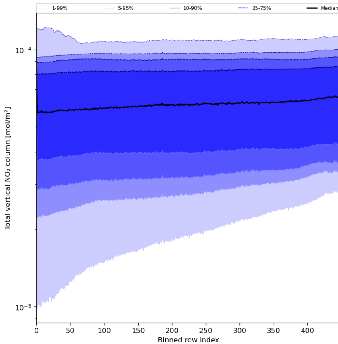
Figure 55: Along track statistics of “Total vertical NO 2 column” for 2023-07-22 to 2023-07-24
