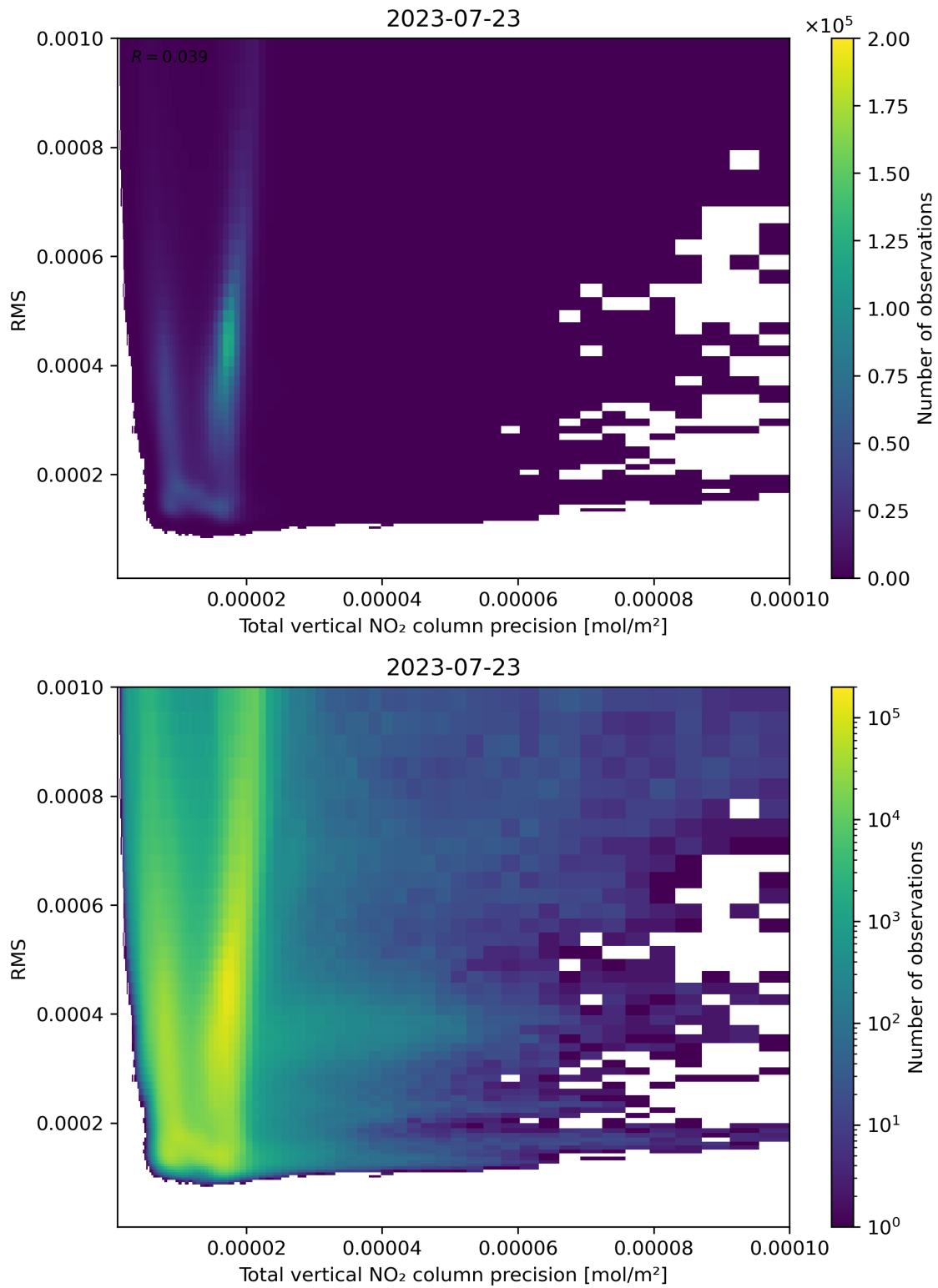
Figure 119: Scatter density plot of “Total vertical NO 2 column precision” against “RMS” for 2023-07-22 to 2023-07-24.
