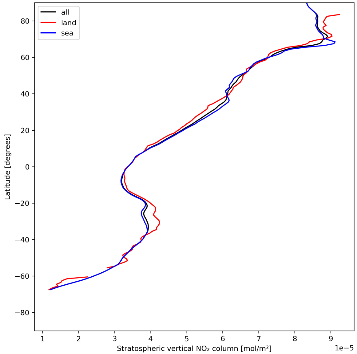
Figure 19: Zonal average of “Stratospheric vertical NO 2 column” for 2023-07-22 to 2023-07-24.
