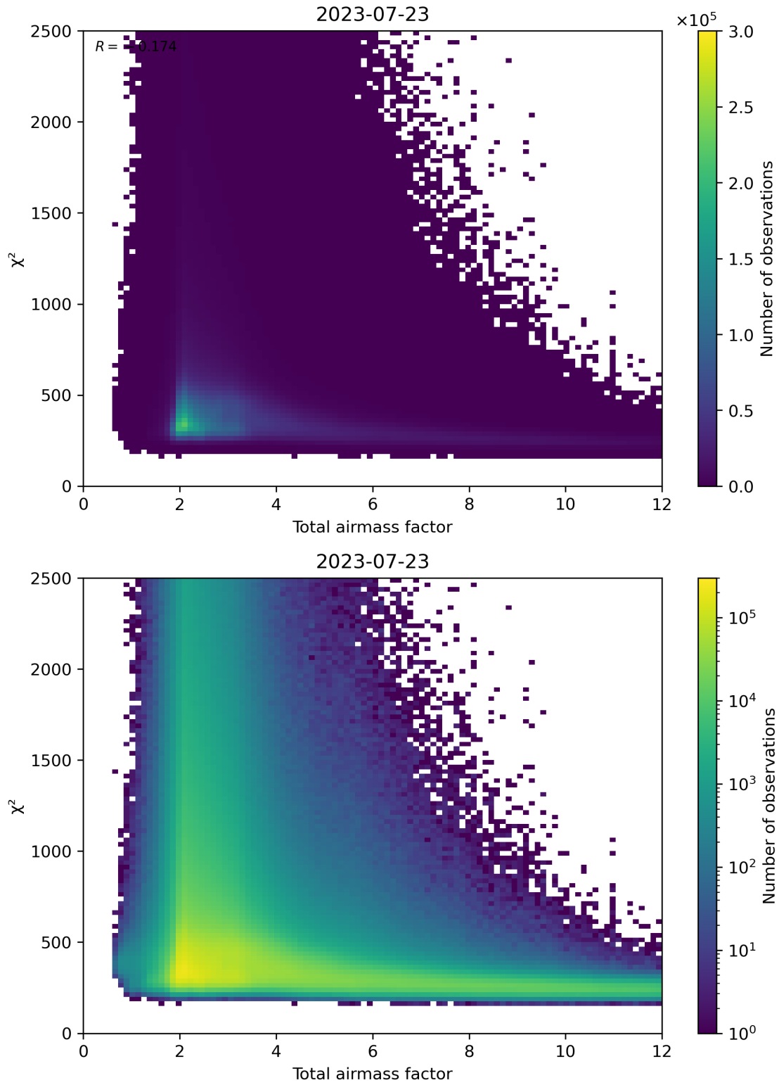
Figure 63: Scatter density plot of “Total airmass factor” against “ \chi^2 ” for 2023-07-22 to 2023-07-24.
