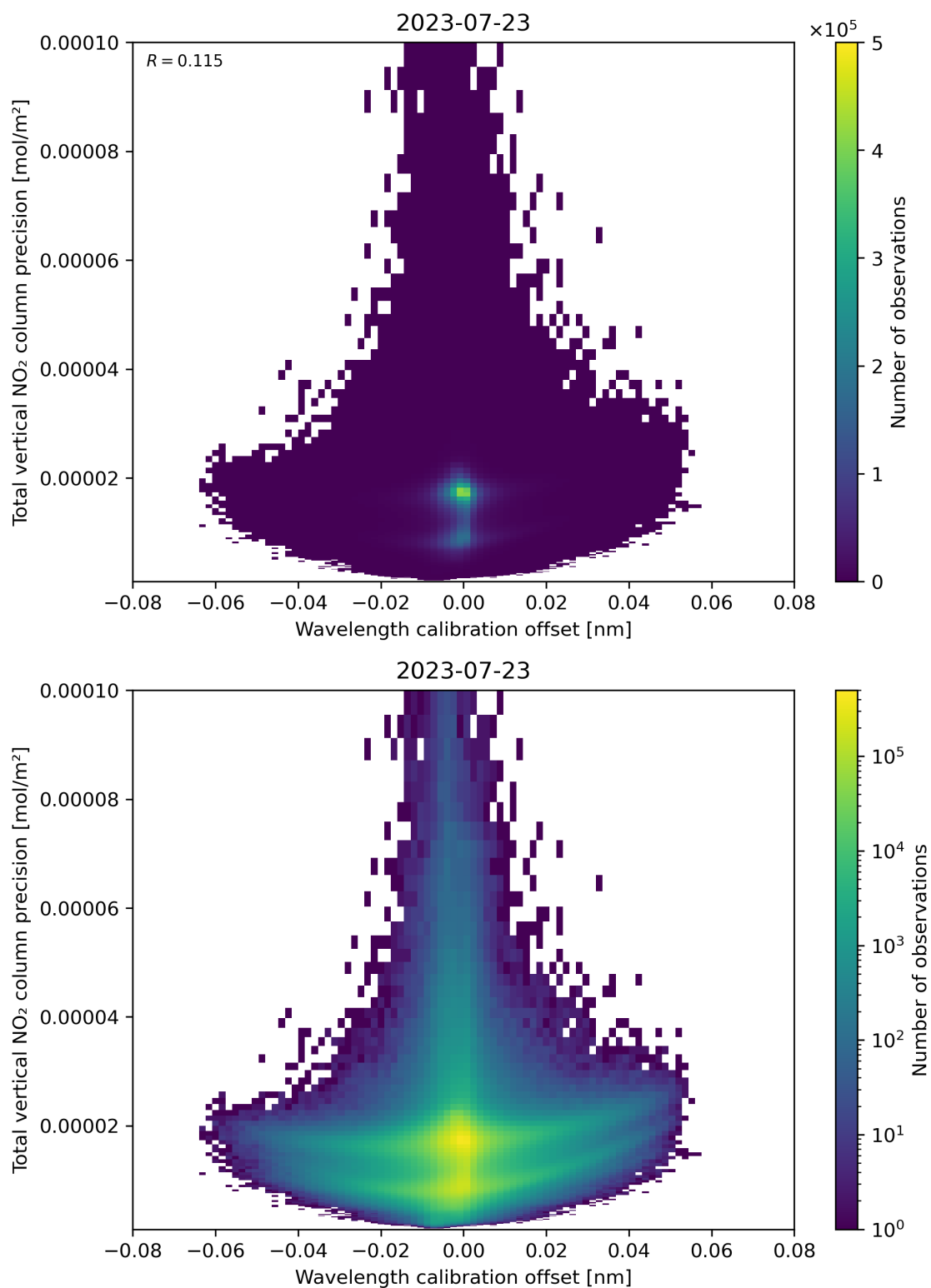
Figure 180: Scatter density plot of “Wavelength calibration offset” against “Total vertical NO 2 column precision” for 2023-07-22 to 2023-07-24.
