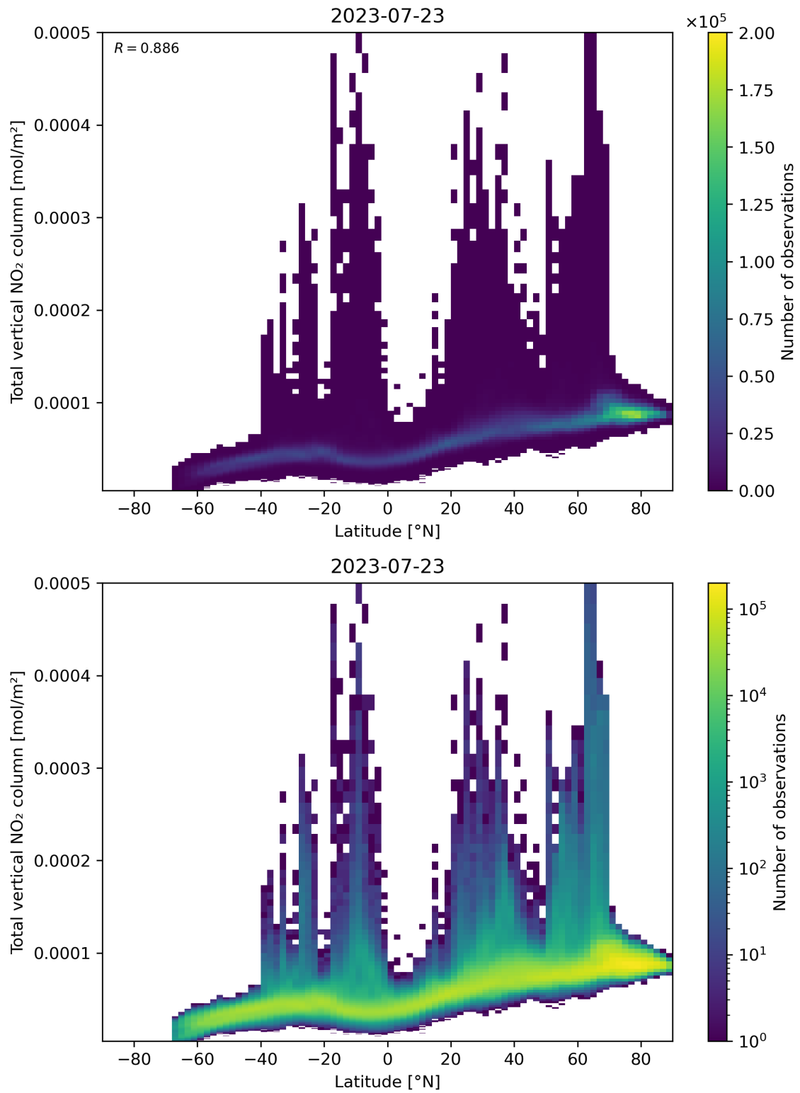
Figure 90: Scatter density plot of “Latitude” against “Total vertical NO 2 column” for 2023-07-22 to 2023-07-24.
