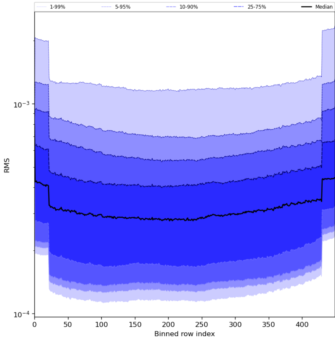
Figure 60: Along track statistics of “RMS” for 2023-07-22 to 2023-07-24
