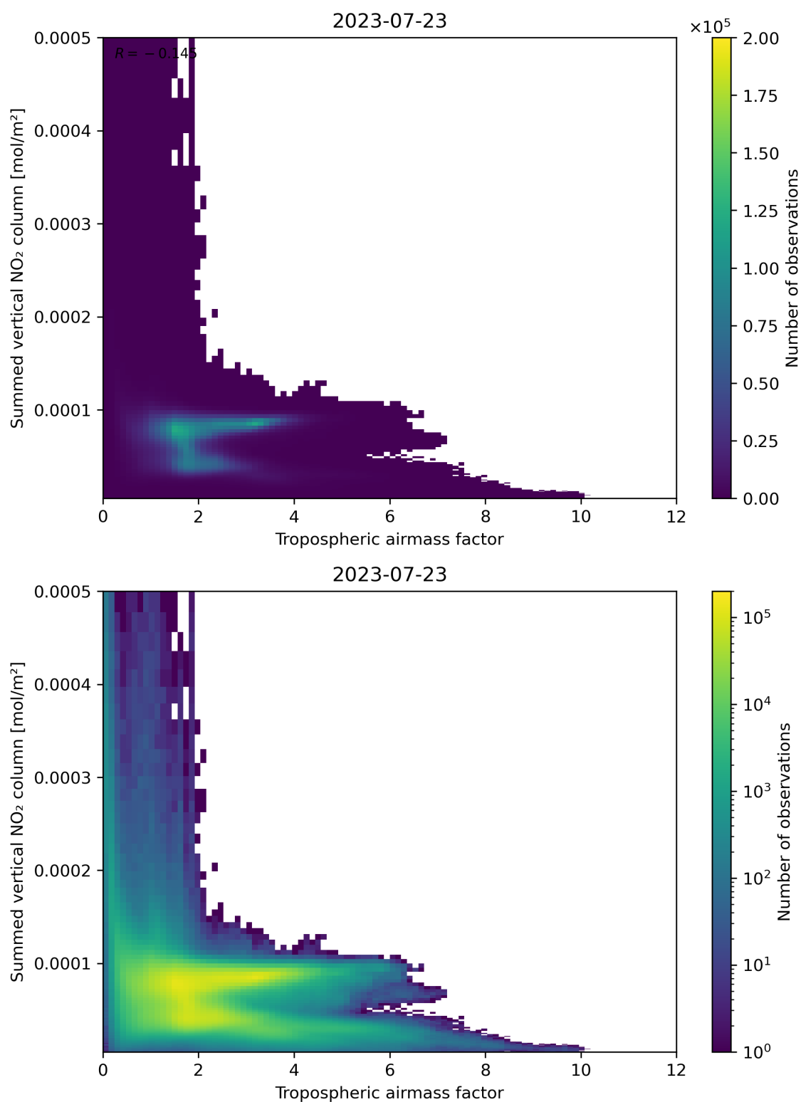
Figure 75: Scatter density plot of “Tropospheric airmass factor” against “Summed vertical NO 2 column” for 2023-07-22 to 2023-07-24.
