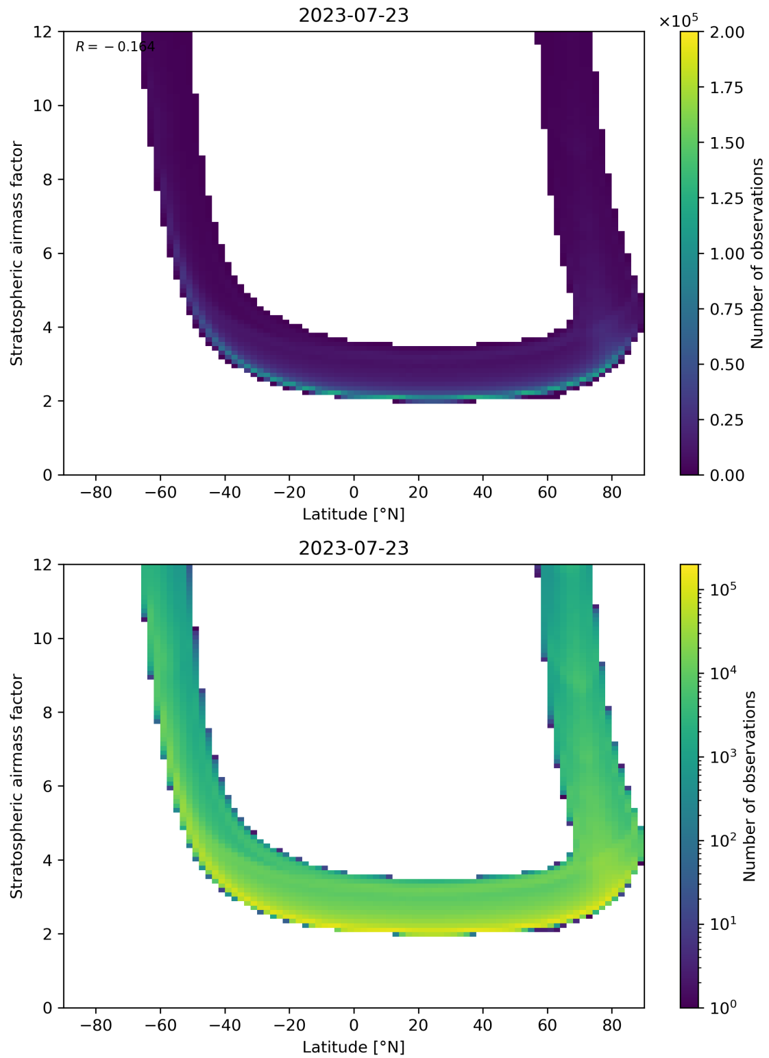
Figure 83: Scatter density plot of “Latitude” against “Stratospheric air mass factor” for 2023-07-22 to 2023-07-24.
