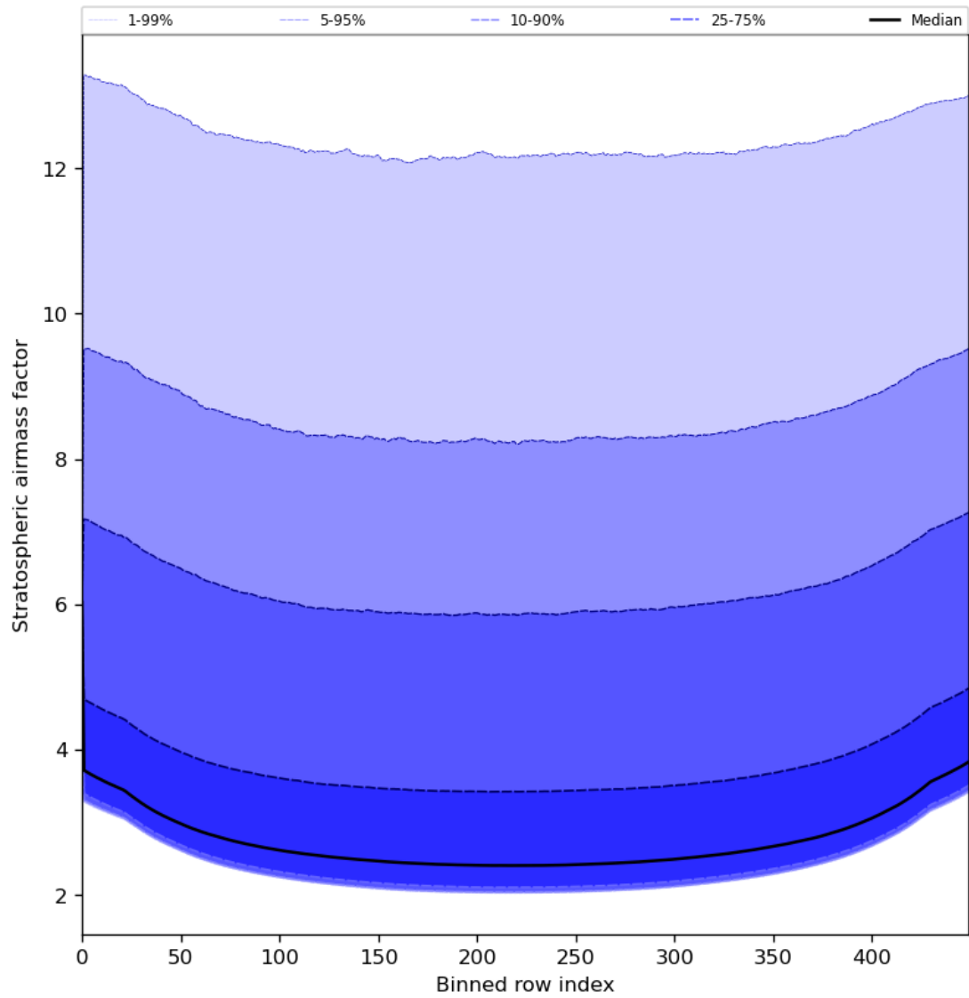
Figure 61: Along track statistics of “Stratospheric airmass factor” for 2023-07-22 to 2023-07-24
