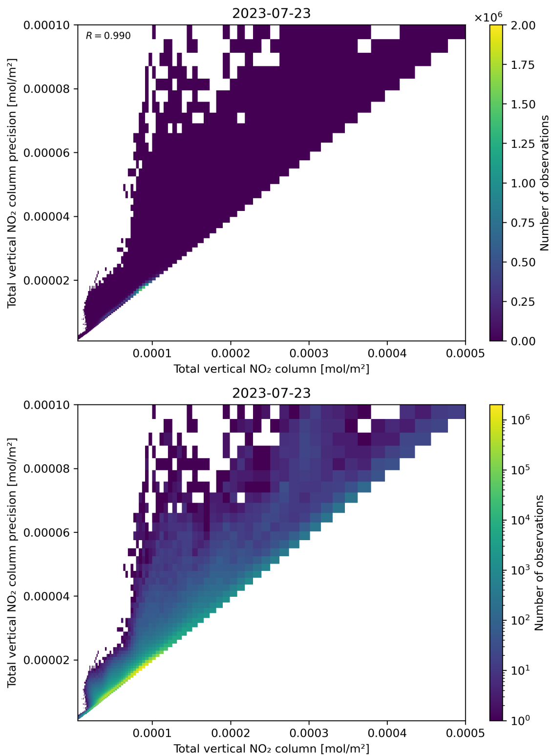
Figure 114: Scatter density plot of “Total vertical NO 2 column” against “Total vertical NO 2 column precision” for 2023-07-22 to 2023-07-24.
