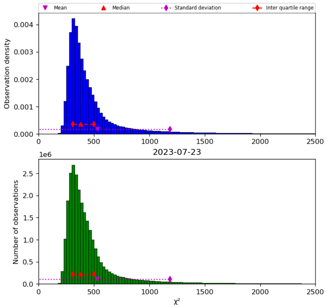
Figure 42: Histogram of “ \chi^2 ” for 2023-07-22 to 2023-07-24
