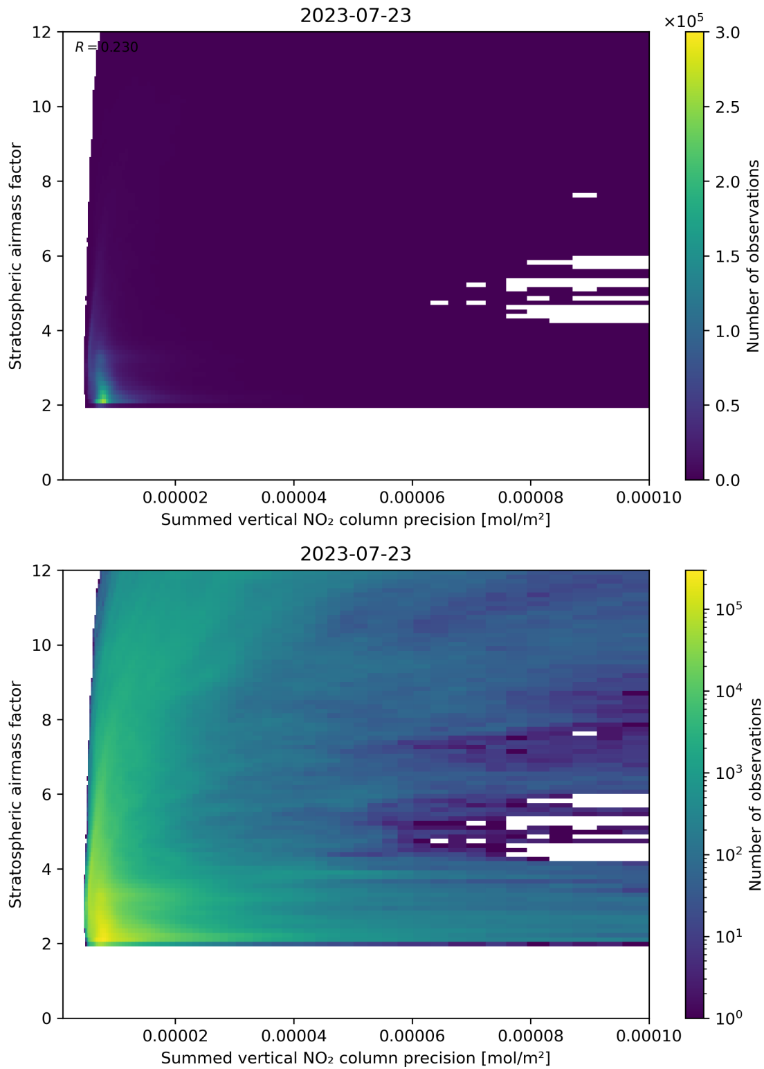
Figure 106: Scatter density plot of “Summed vertical NO 2 column precision” against “Stratospheric airmass factor” for 2023-07-22 to 2023-07-24.
