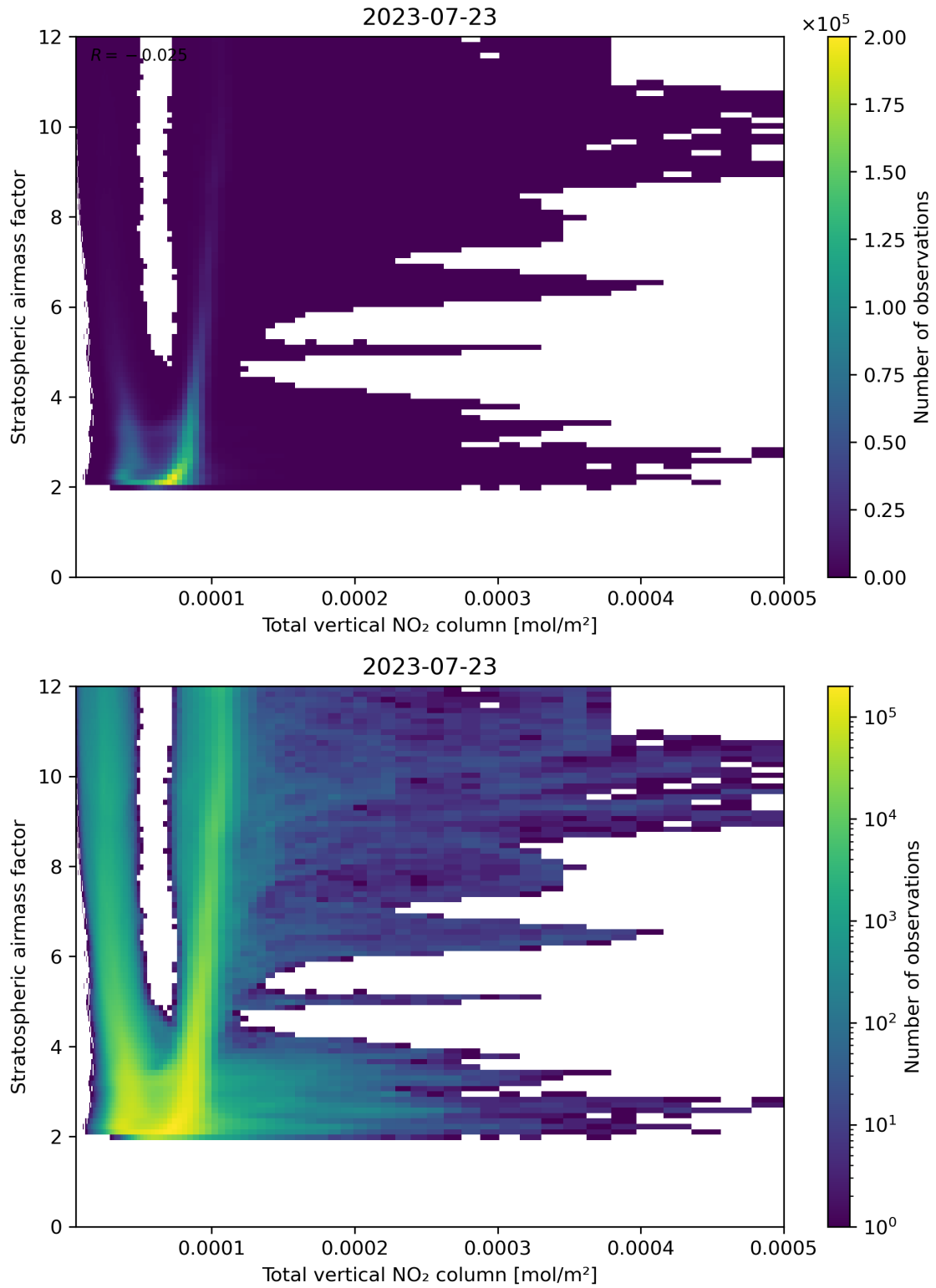
Figure 110: Scatter density plot of “Total vertical NO 2 column” against “Stratospheric airmass factor” for 2023-07-22 to 2023-07-24.
