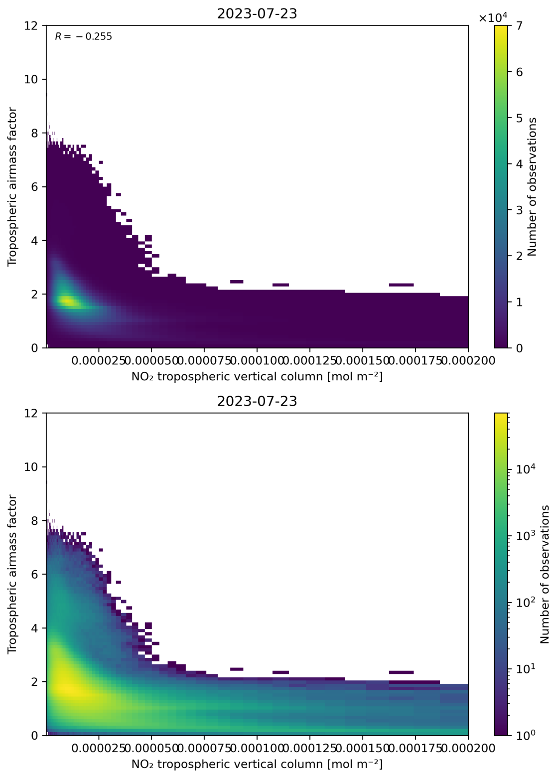
Figure 123: Scatter density plot of “NO 2 tropospheric vertical column” against “Tropospheric airmass factor” for 2023-07-22 to 2023-07-24.
