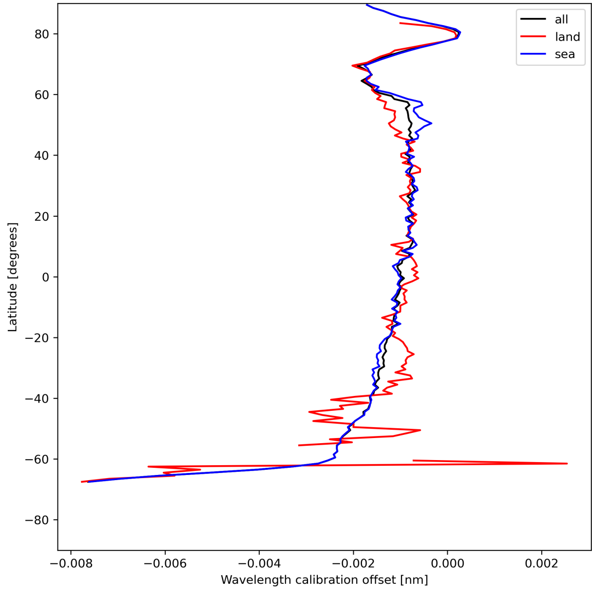
Figure 18: Zonal average of “Wavelength calibration offset” for 2023-07-22 to 2023-07-24.
