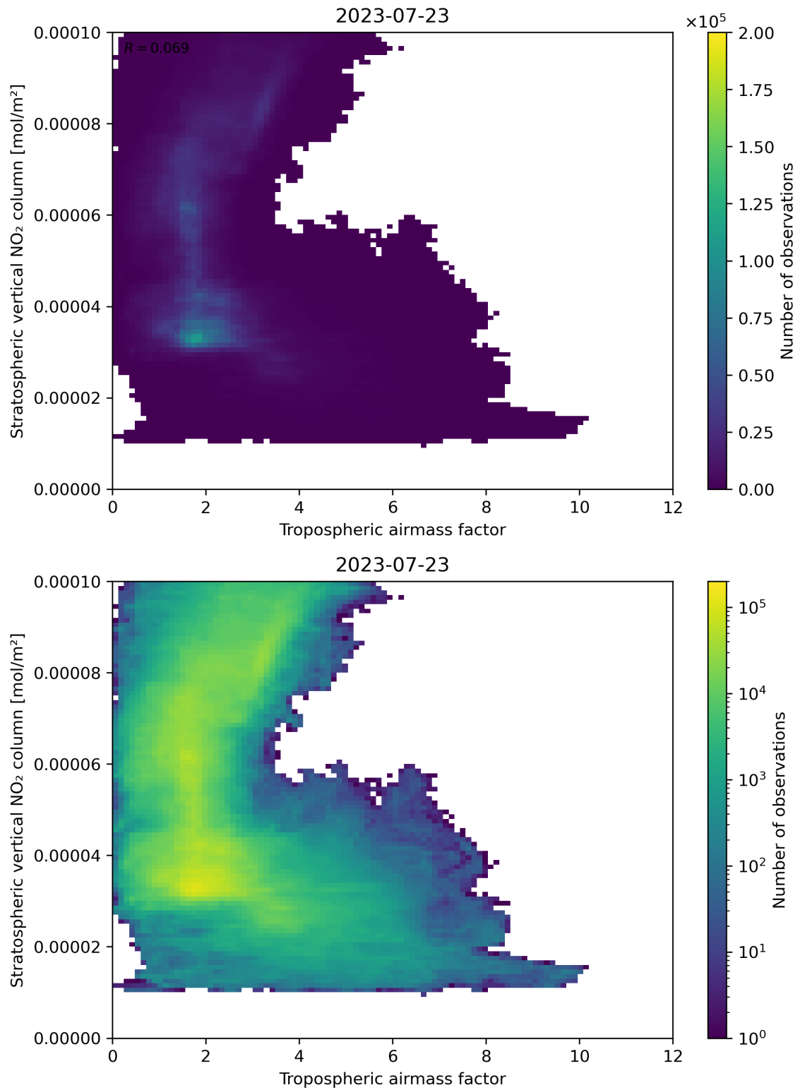
Figure 74: Scatter density plot of “Tropospheric airmass factor” against “Stratospheric vertical NO 2 column” for 2023-07-22 to 2023-07-24.
