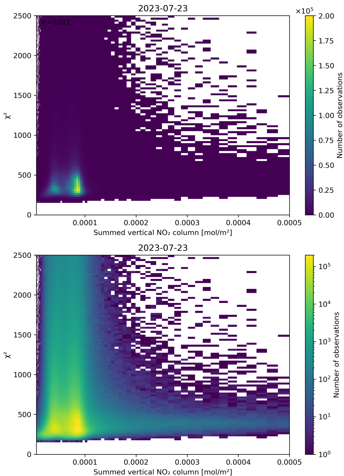
Figure 104: Scatter density plot of “Summed vertical NO 2 column” against “ \chi^2 ” for 2023-07-22 to 2023-07-24.
