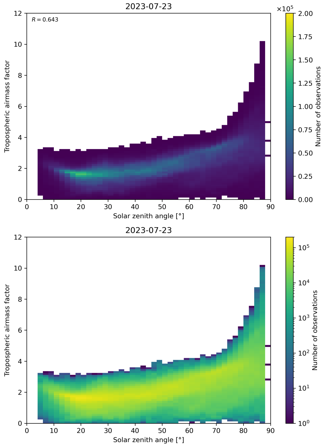
Figure 147: Scatter density plot of “Solar zenith angle” against “Tropospheric airmass factor” for 2023-07-22 to 2023-07-24.
