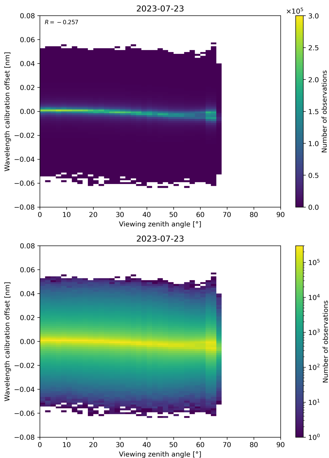
Figure 173: Scatter density plot of “Viewing zenith angle” against “Wavelength calibration offset” for 2023-07-22 to 2023-07-24.
