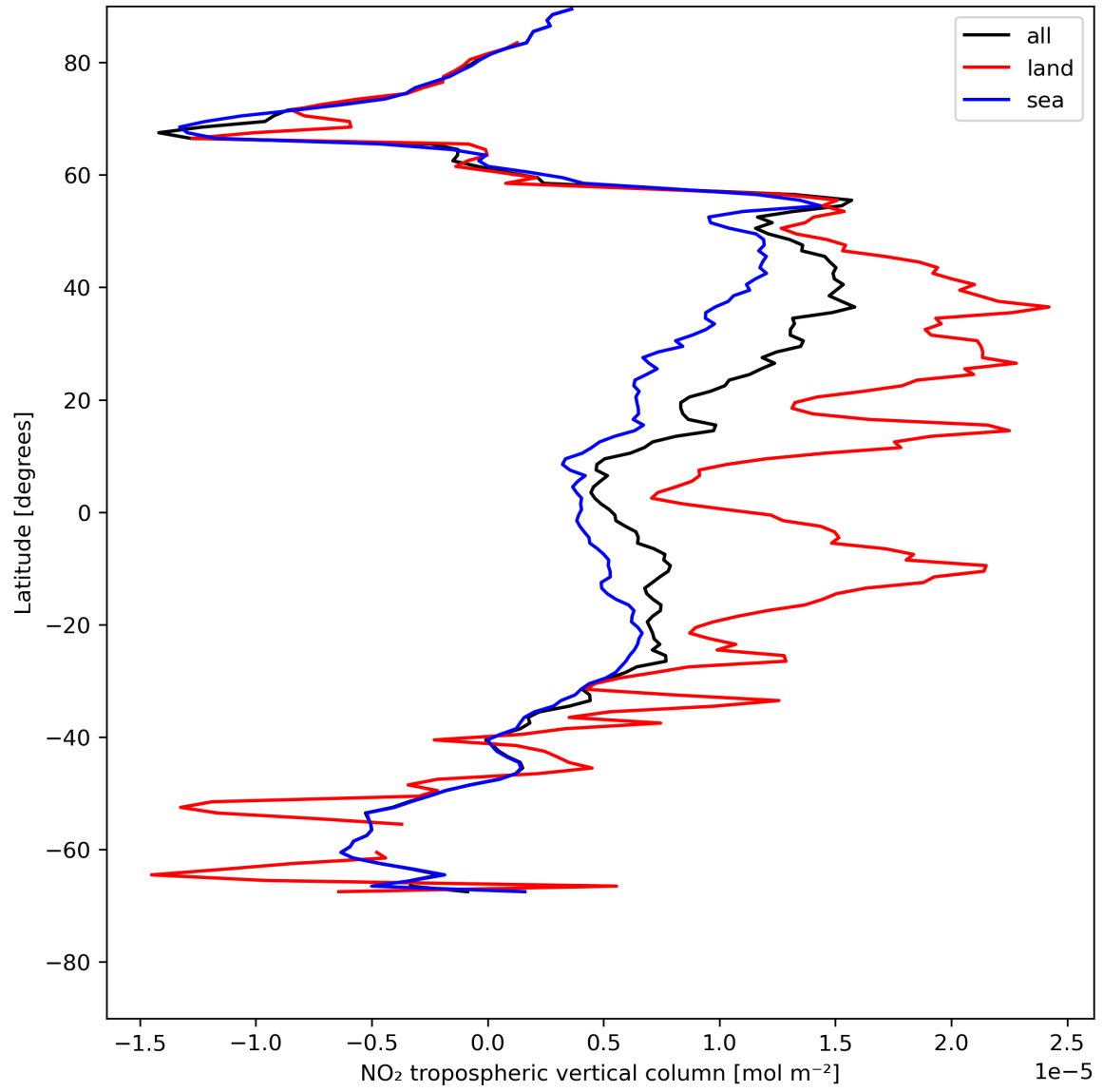
Figure 12: Zonal average of “NO 2 tropospheric vertical column” for 2023-07-22 to 2023-07-24.
