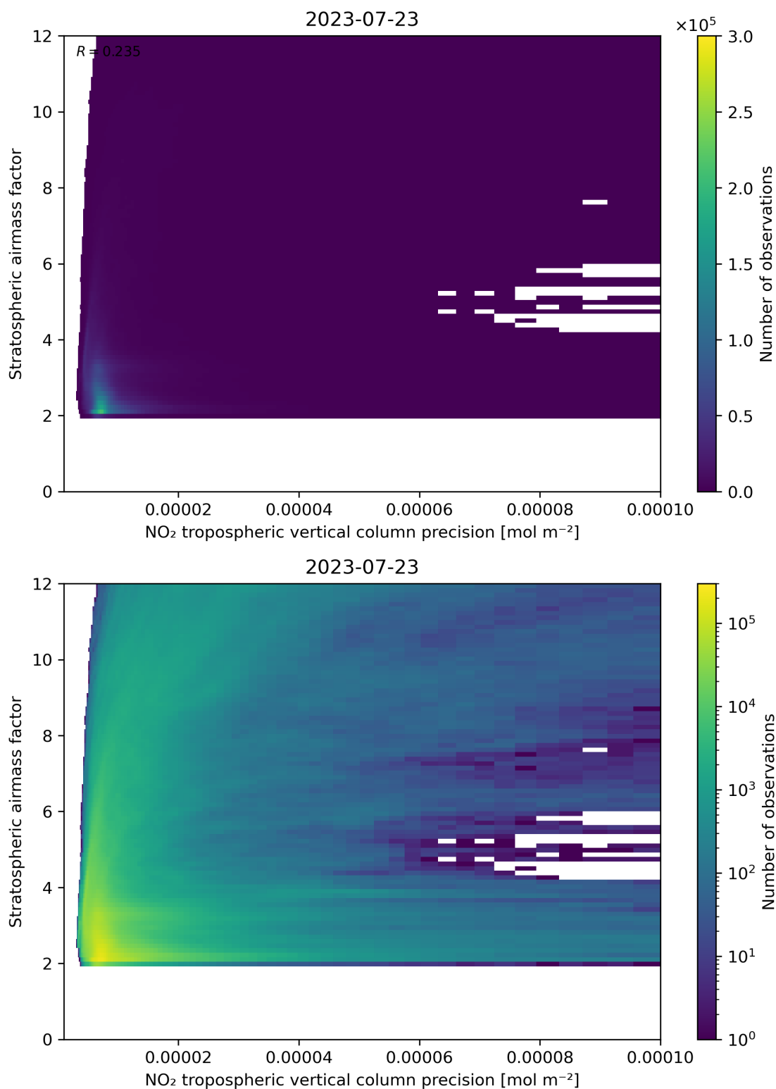
Figure 131: Scatter density plot of “NO 2 tropospheric vertical column precision” against “Stratospheric airmass factor” for 2023-07-22 to 2023-07-24.
