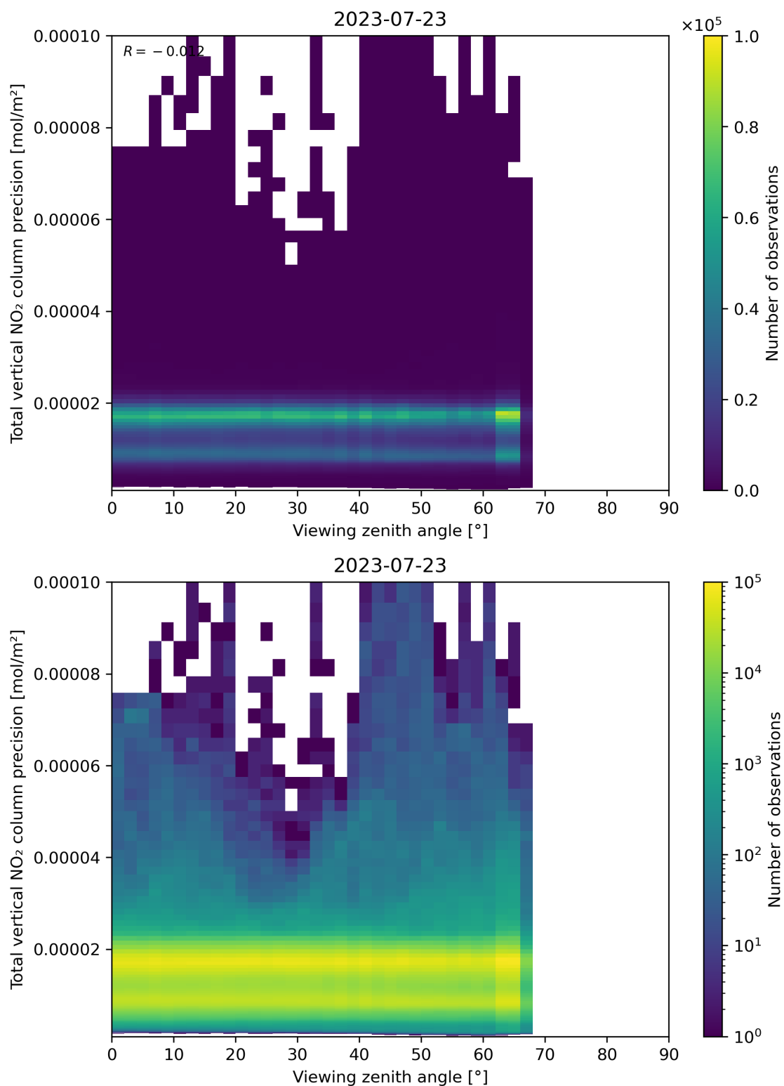
Figure 168: Scatter density plot of “Viewing zenith angle” against “Total vertical NO 2 column precision” for 2023-07-22 to 2023-07-24.
