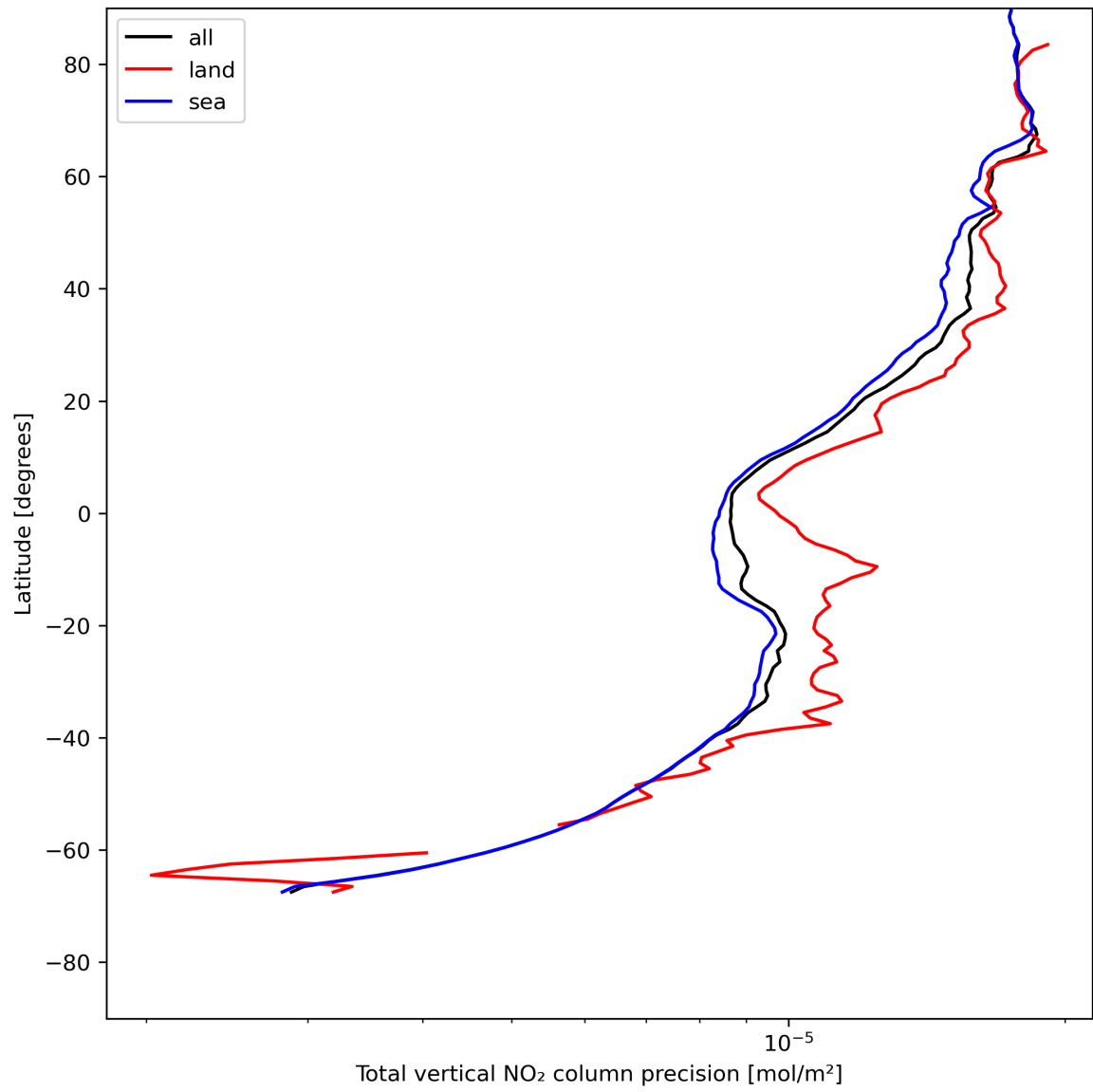
Figure 22: Zonal average of “Total vertical NO 2 column precision” for 2023-07-22 to 2023-07-24.
