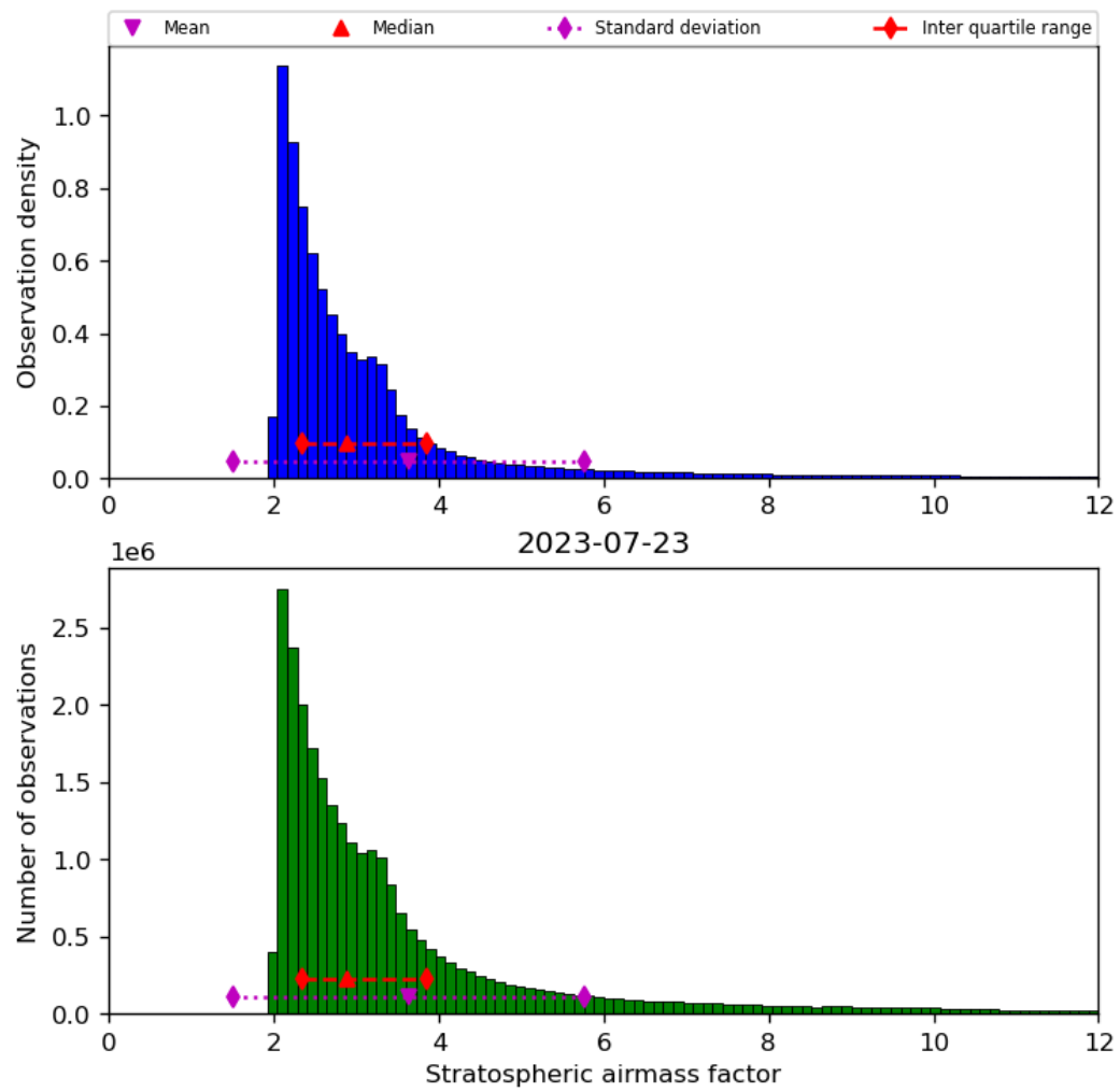
Figure 44: Histogram of “Stratospheric airmass factor” for 2023-07-22 to 2023-07-24
