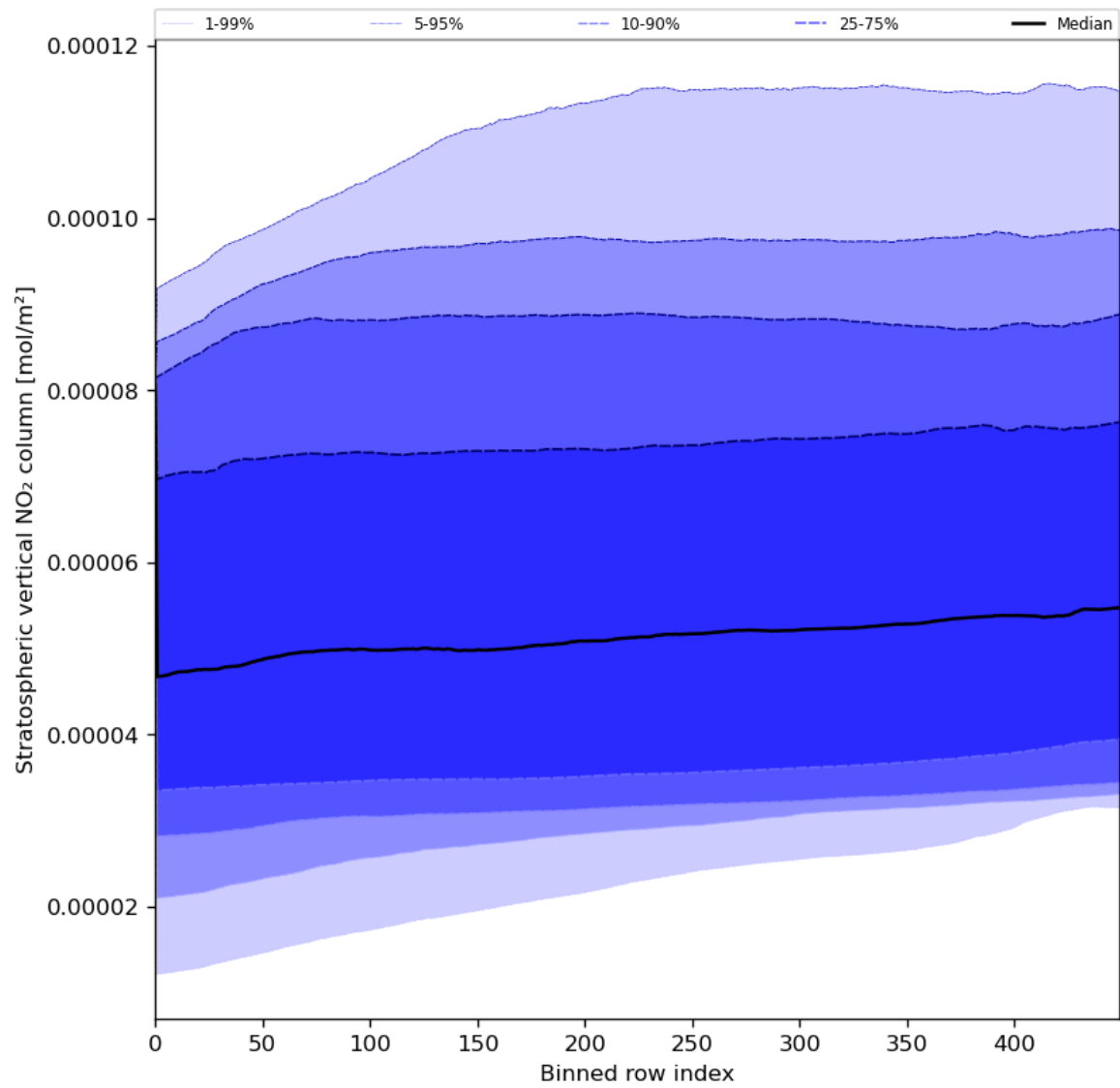
Figure 53: Along track statistics of “Stratospheric vertical NO 2 column” for 2023-07-22 to 2023-07-24
