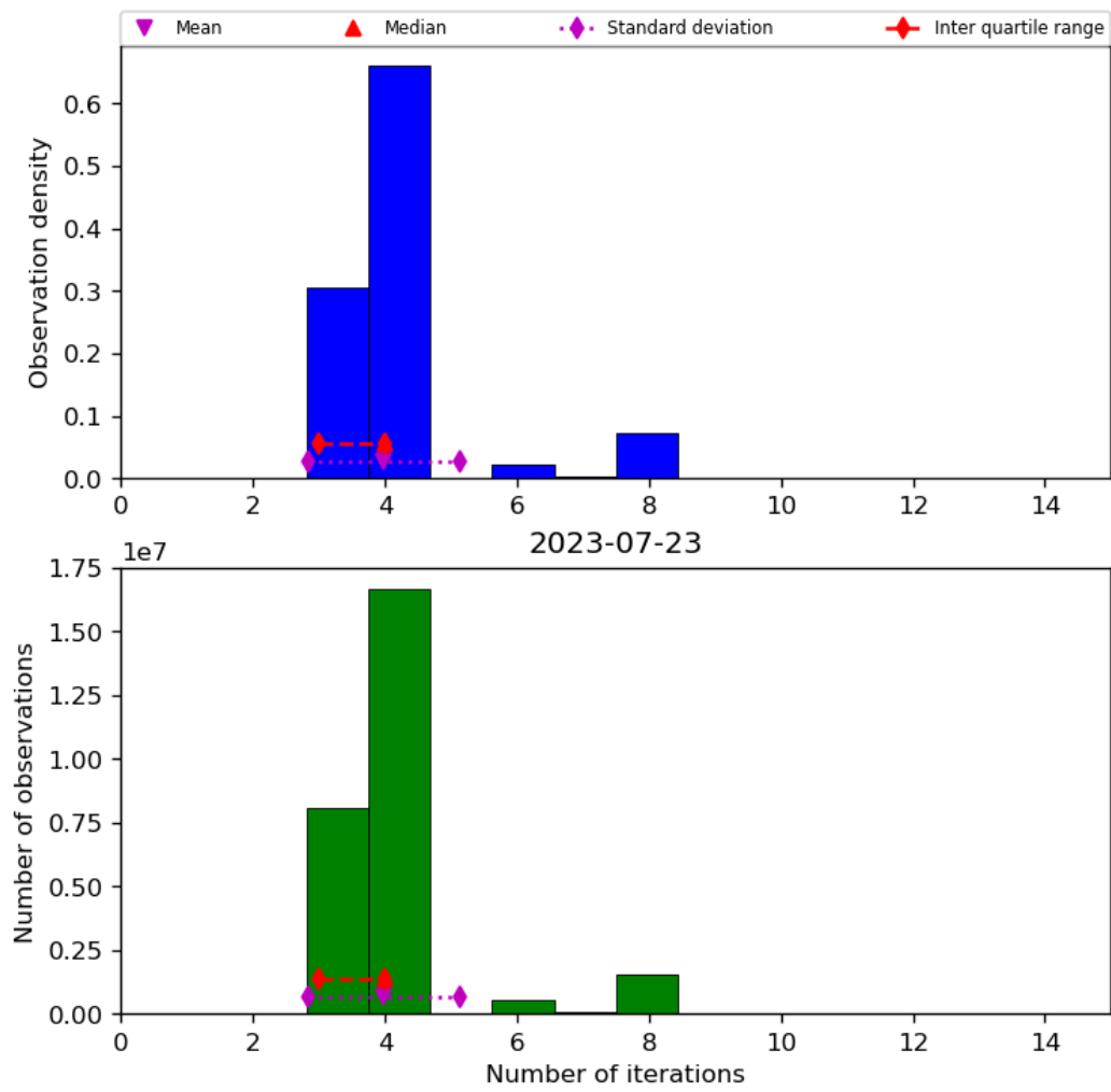
Figure 34: Histogram of “Number of iterations” for 2023-07-22 to 2023-07-24
