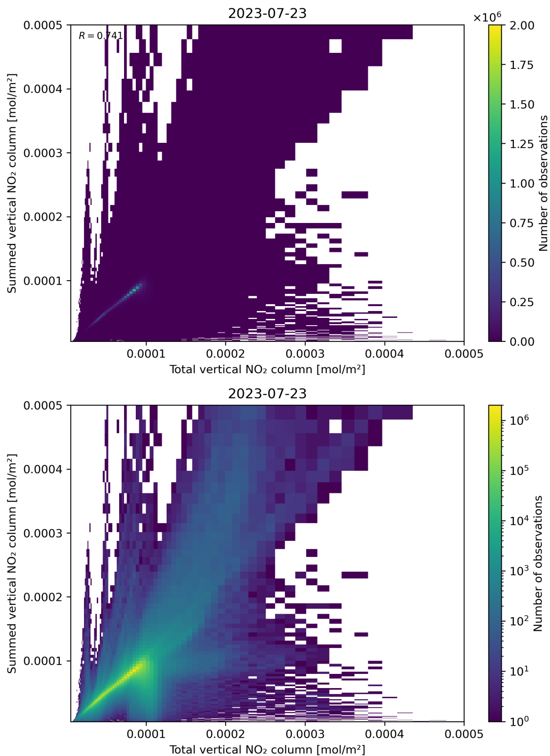
Figure 112: Scatter density plot of “Total vertical NO 2 column” against “Summed vertical NO 2 column” for 2023-07-22 to 2023-07-24.
