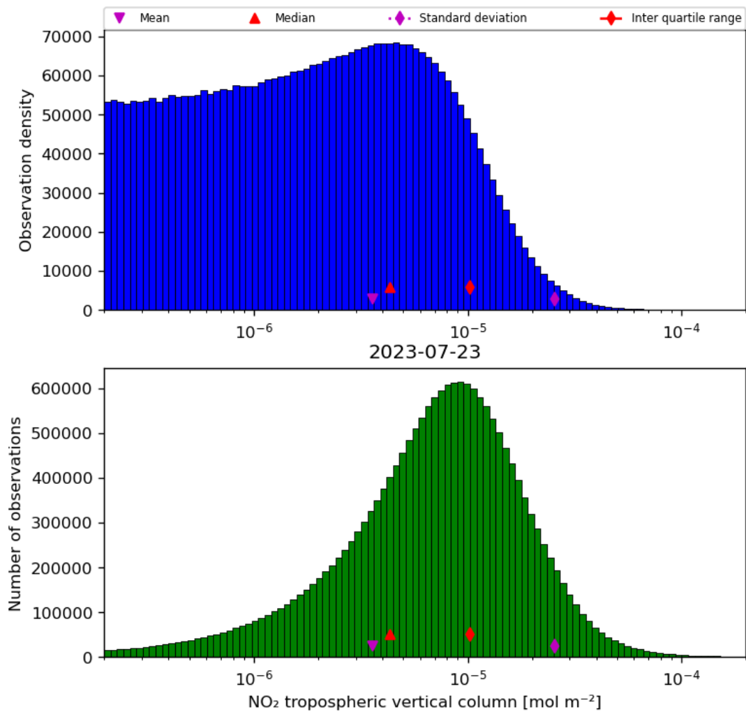
Figure 29: Histogram of “NO 2 tropospheric vertical column” for 2023-07-22 to 2023-07-24
