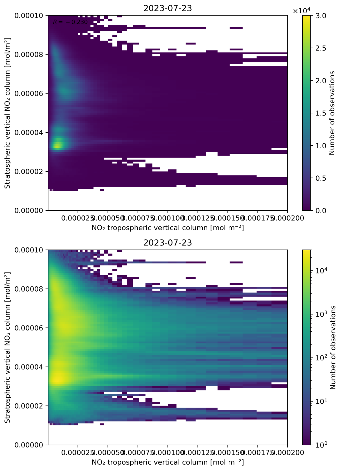
Figure 125: Scatter density plot of “NO 2 tropospheric vertical column” against “Stratospheric vertical NO 2 column” for 2023-07-22 to 2023-07-24.
