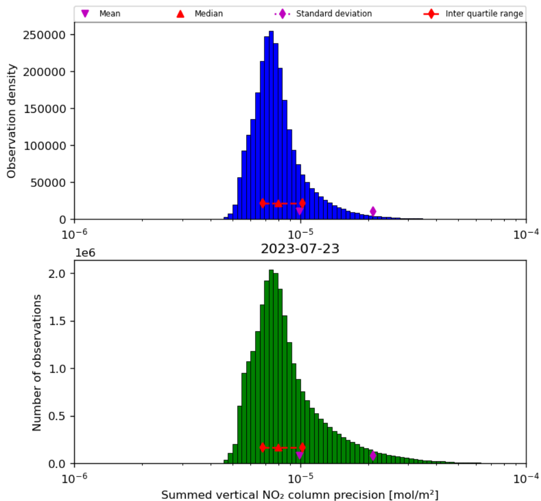
Figure 41: Histogram of “Summed vertical NO 2 column precision” for 2023-07-22 to 2023-07-24
