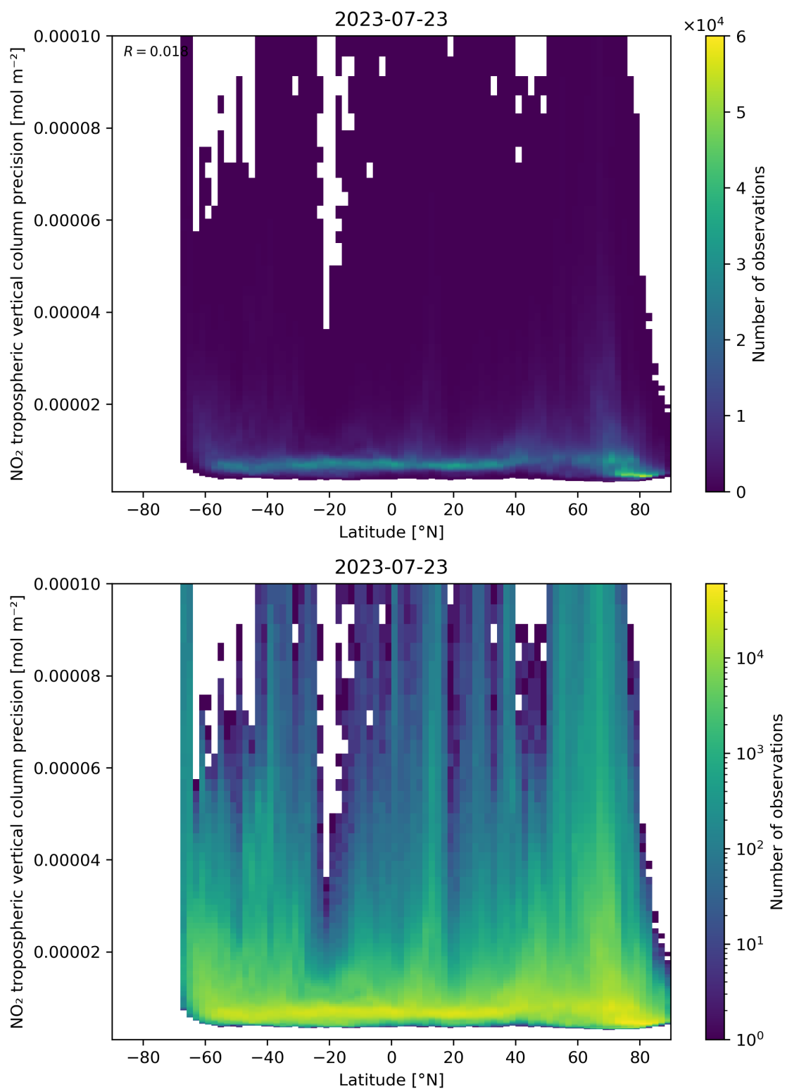
Figure 93: Scatter density plot of “Latitude” against “NO 2 tropospheric vertical column precision” for 2023-07-22 to 2023-07-24.
