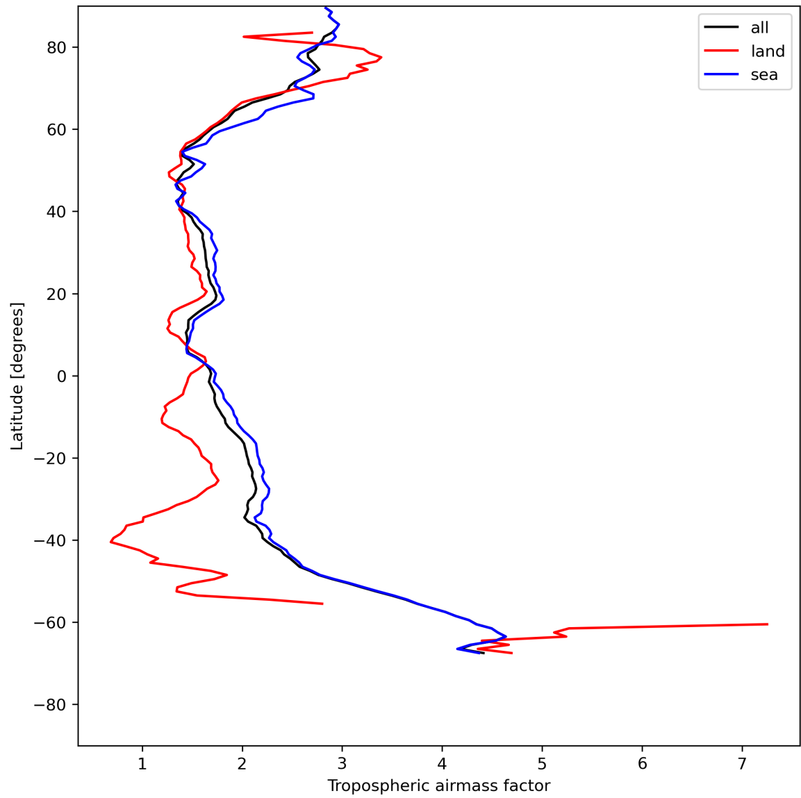
Figure 14: Zonal average of “Tropospheric air mass factor” for 2023-07-22 to 2023-07-24.
