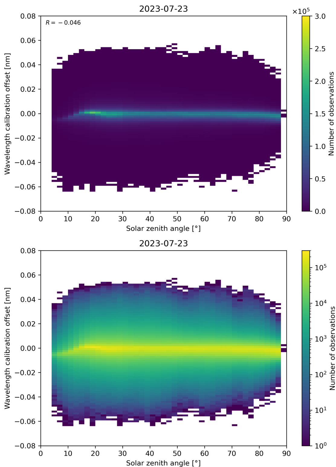
Figure 158: Scatter density plot of “Solar zenith angle” against “Wavelength calibration offset” for 2023-07-22 to 2023-07-24.
