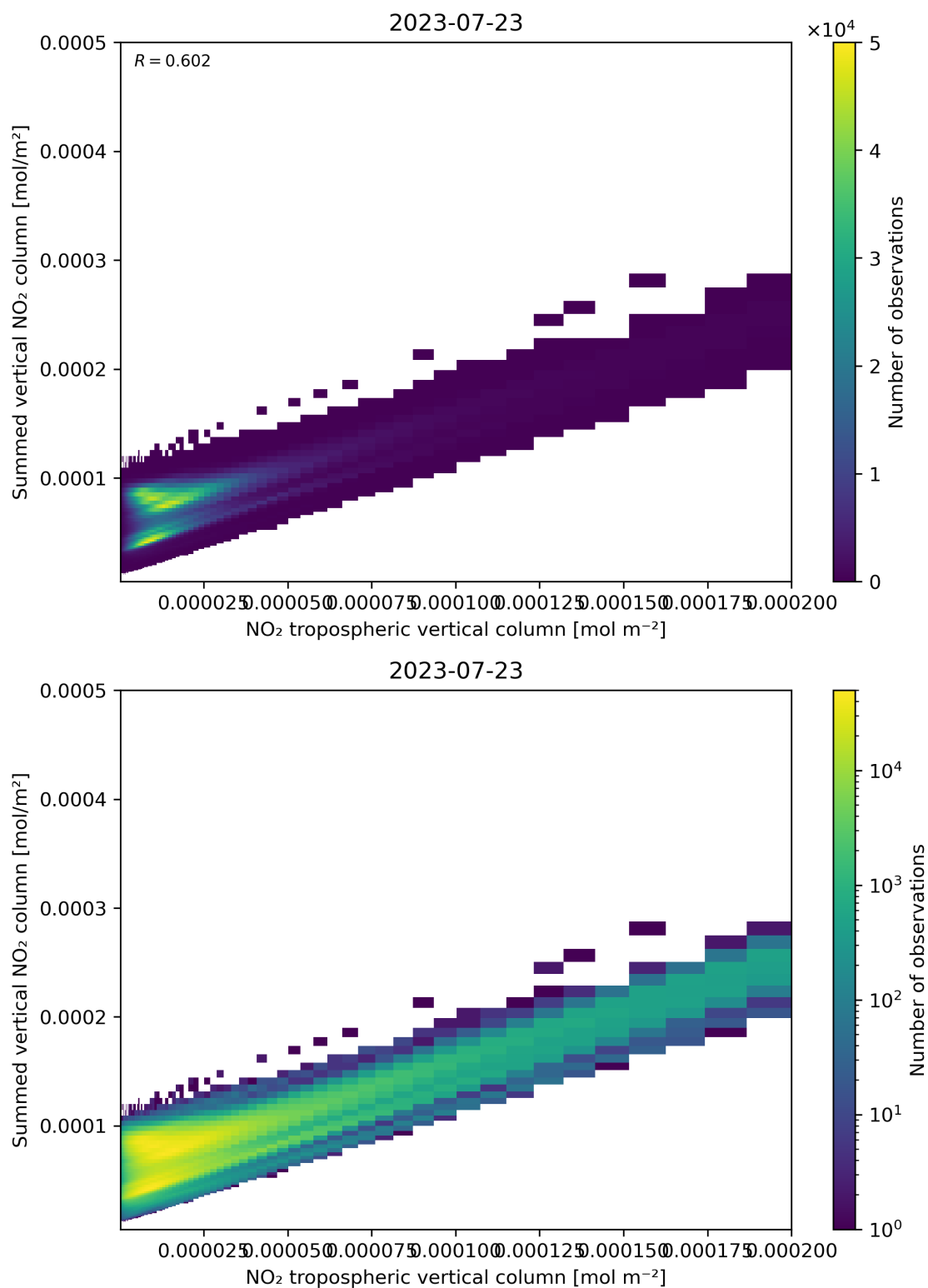
Figure 126: Scatter density plot of “NO 2 tropospheric vertical column” against “Summed vertical NO 2 column” for 2023-07-22 to 2023-07-24.
