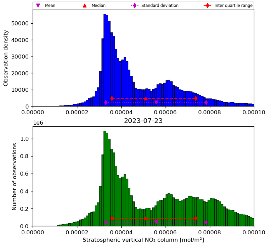
Figure 36: Histogram of “Stratospheric vertical NO 2 column” for 2023-07-22 to 2023-07-24
