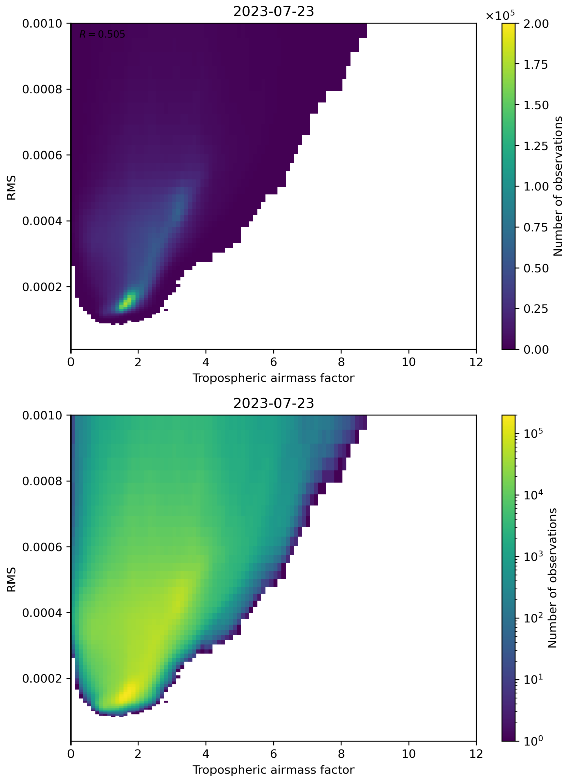
Figure 79: Scatter density plot of “Tropospheric airmass factor” against “RMS” for 2023-07-22 to 2023-07-24.
