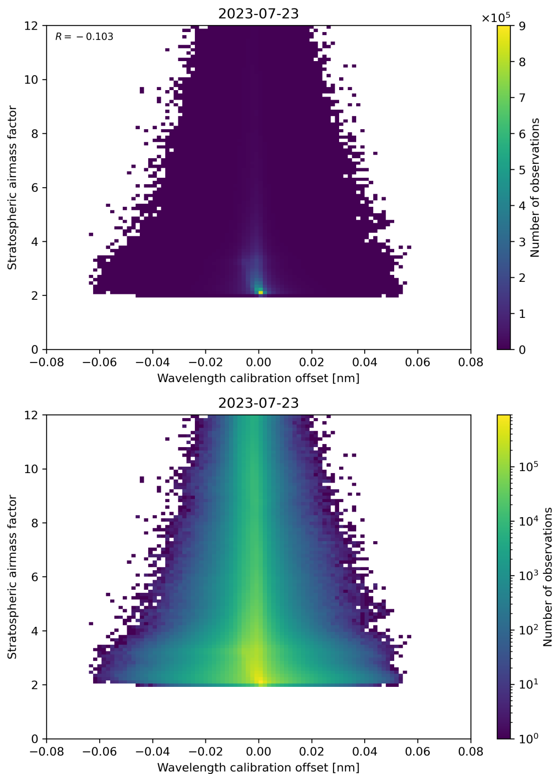
Figure 174: Scatter density plot of “Wavelength calibration offset” against “Stratospheric airmass factor” for 2023-07-22 to 2023-07-24.
