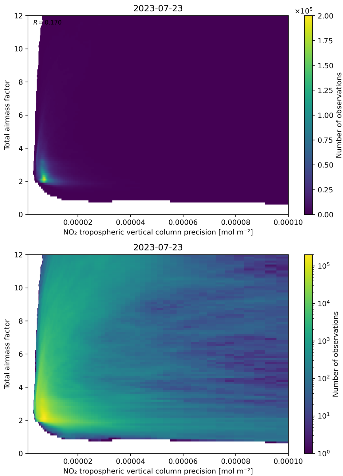
Figure 132: Scatter density plot of “NO 2 tropospheric vertical column precision” against “Total air mass factor” for 2023-07-22 to 2023-07-24.
