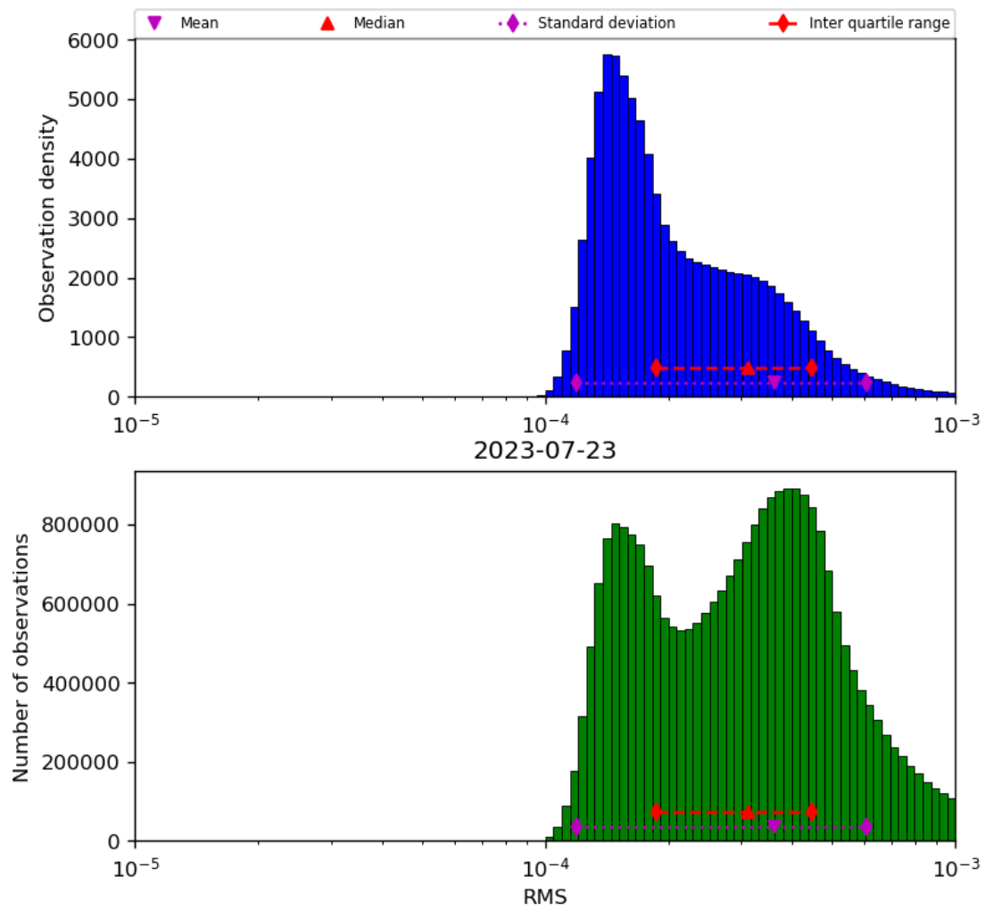
Figure 43: Histogram of “RMS” for 2023-07-22 to 2023-07-24
