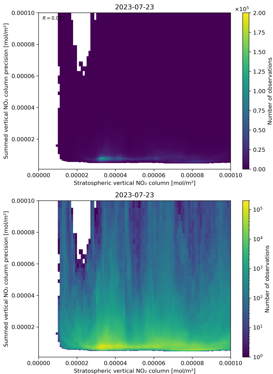
Figure 99: Scatter density plot of “Stratospheric vertical NO 2 column” against “Summed vertical NO 2 column precision” for 2023-07-22 to 2023-07-24.
