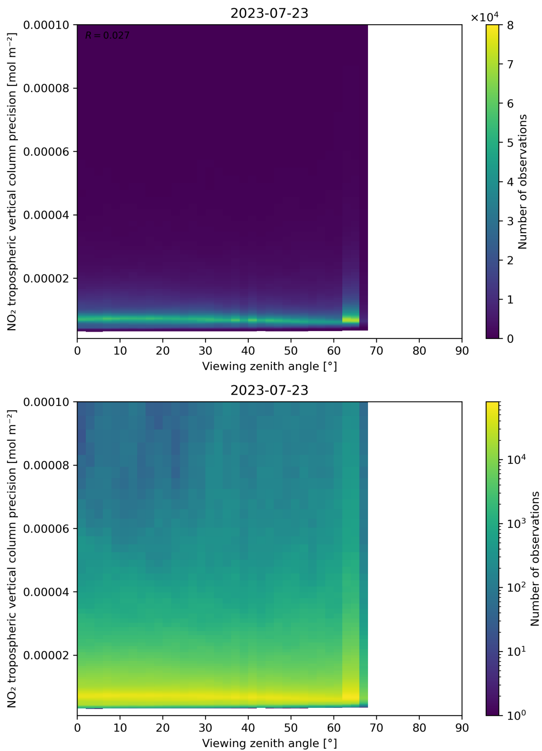
Figure 170: Scatter density plot of “Viewing zenith angle” against “NO 2 tropospheric vertical column precision” for 2023-07-22 to 2023-07-24.
