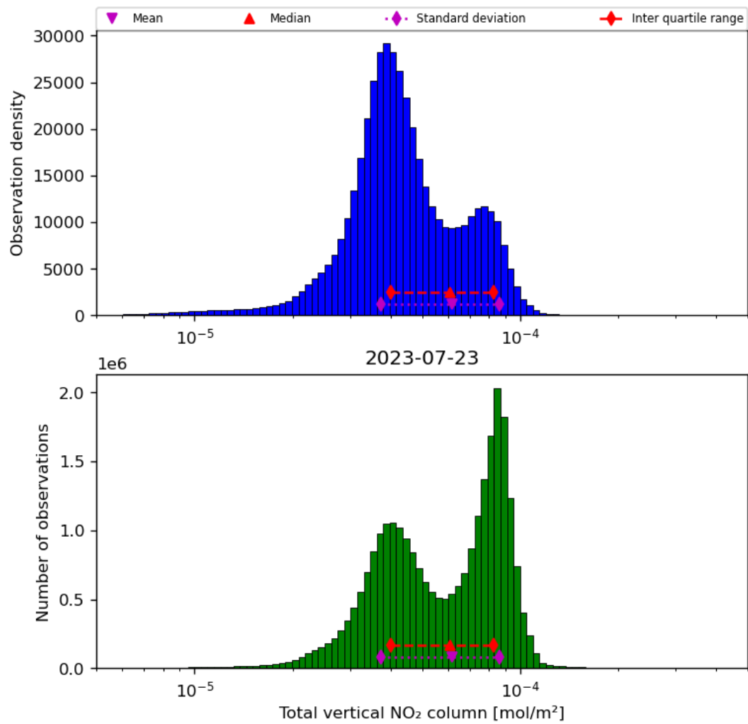
Figure 38: Histogram of “Total vertical NO 2 column” for 2023-07-22 to 2023-07-24
