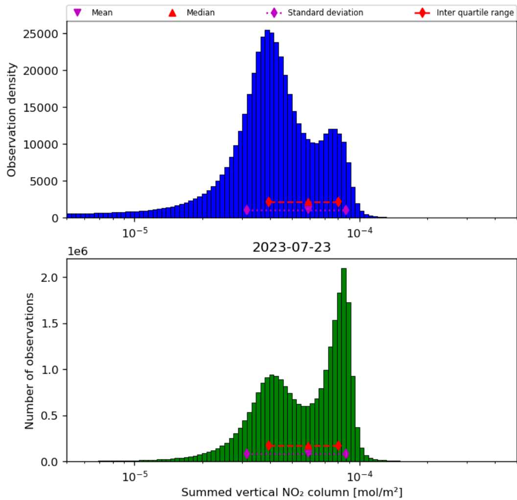
Figure 40: Histogram of “Summed vertical NO 2 column” for 2023-07-22 to 2023-07-24
