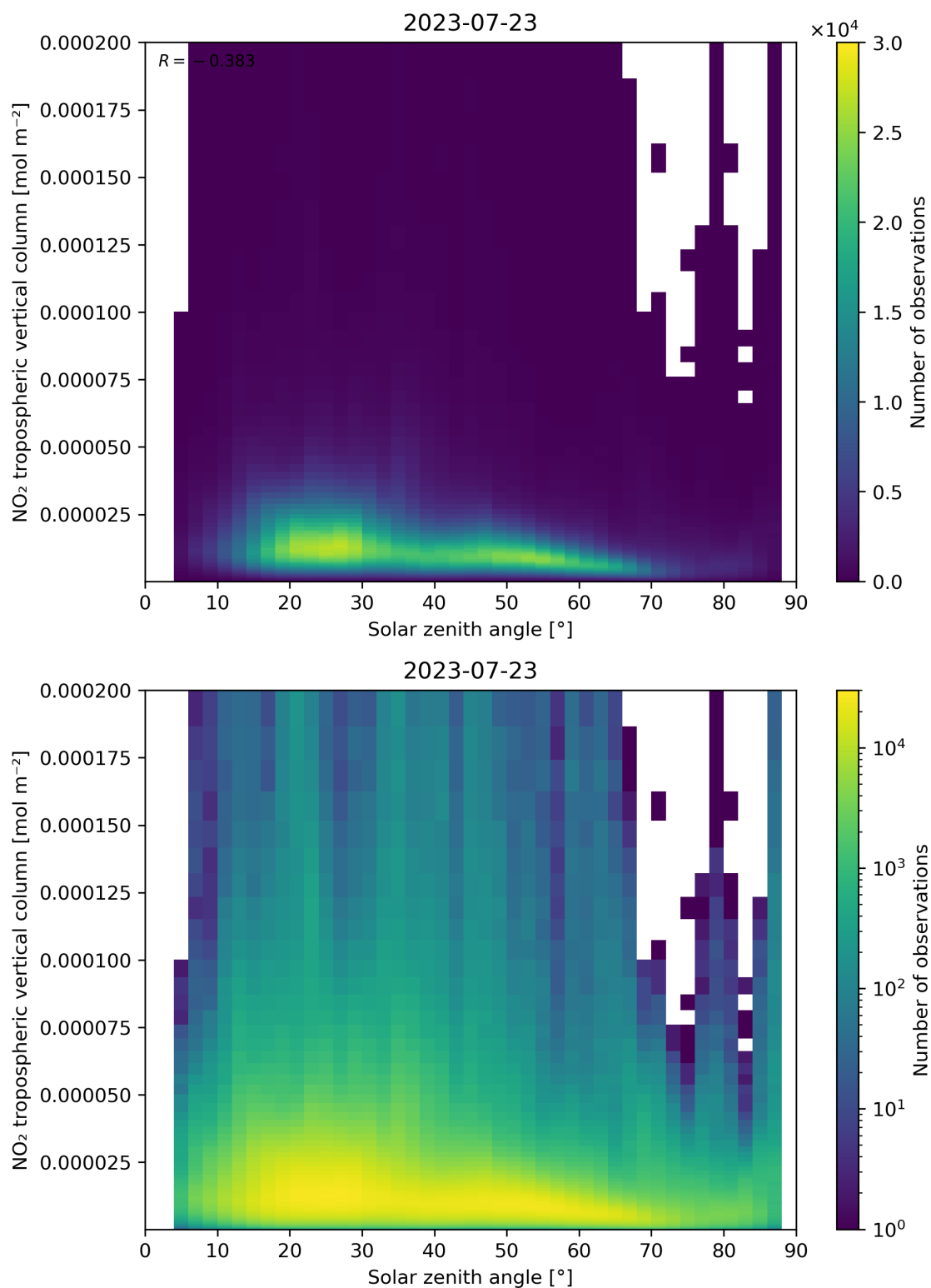
Figure 155: Scatter density plot of “Solar zenith angle” against “NO 2 tropospheric vertical column” for 2023-07-22 to 2023-07-24.
