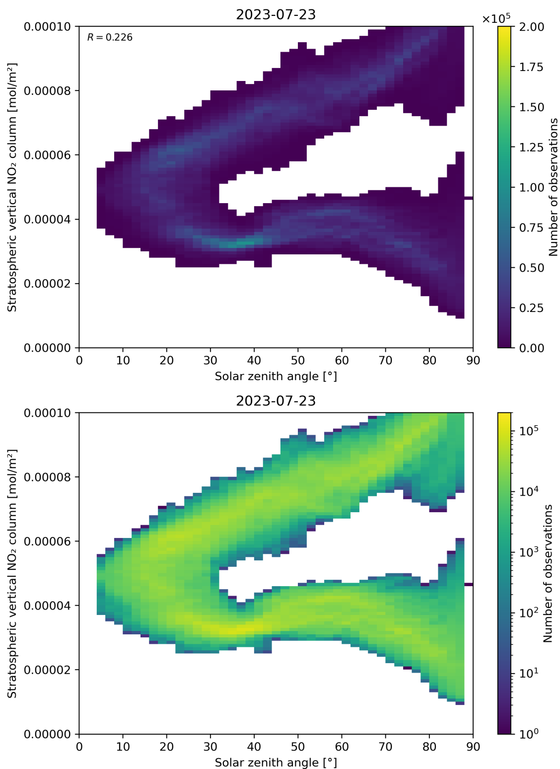
Figure 150: Scatter density plot of “Solar zenith angle” against “Stratospheric vertical NO 2 column” for 2023-07-22 to 2023-07-24.
