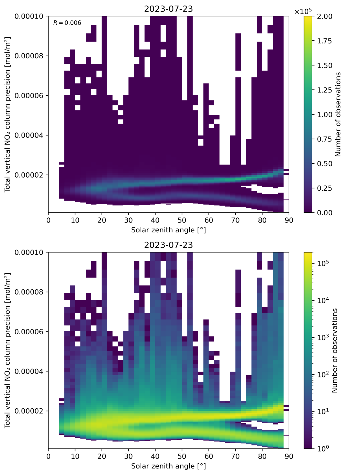
Figure 154: Scatter density plot of “Solar zenith angle” against “Total vertical NO 2 column precision” for 2023-07-22 to 2023-07-24.
