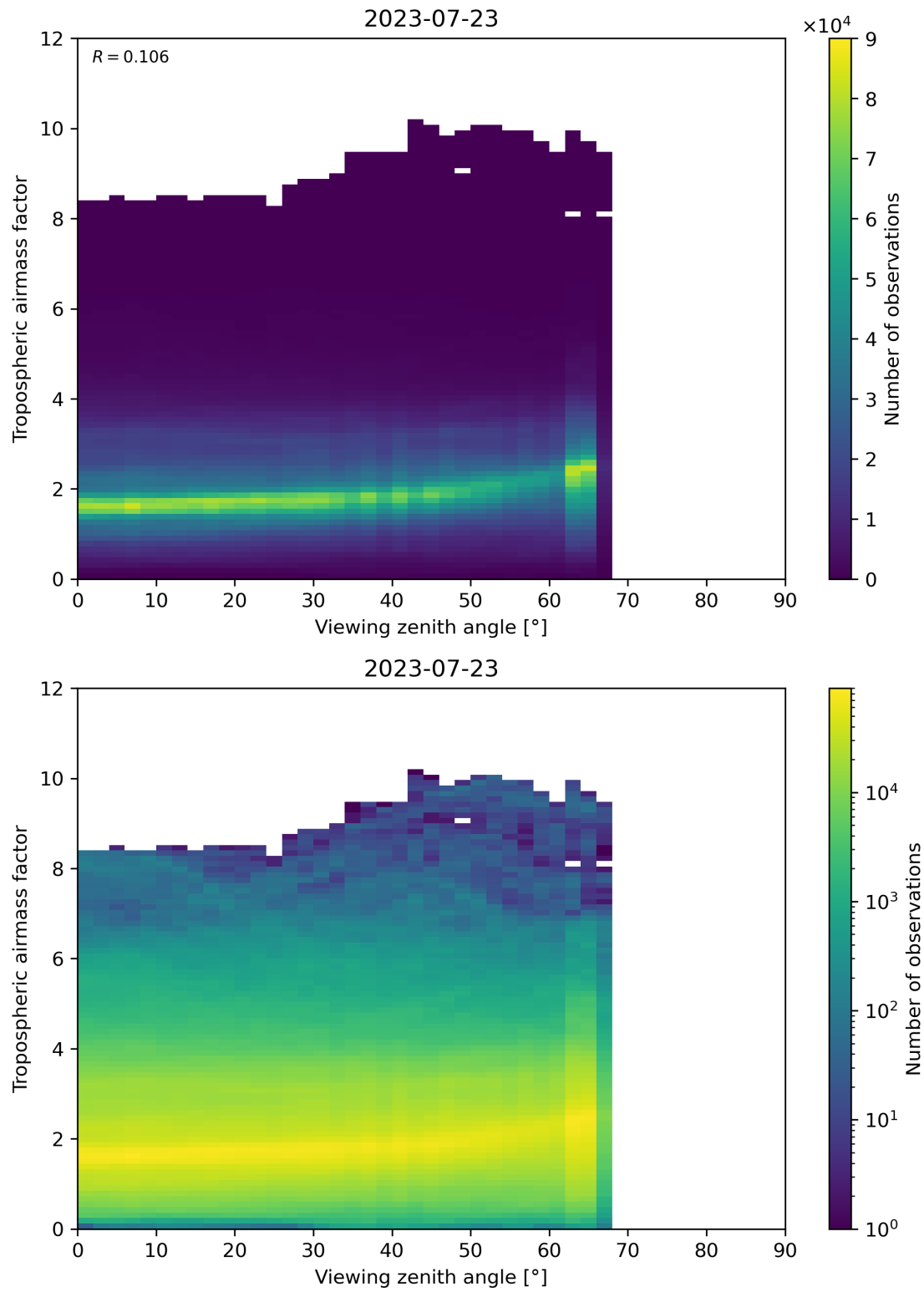
Figure 161: Scatter density plot of “Viewing zenith angle” against “Tropospheric airmass factor” for 2023-07-22 to 2023-07-24.
