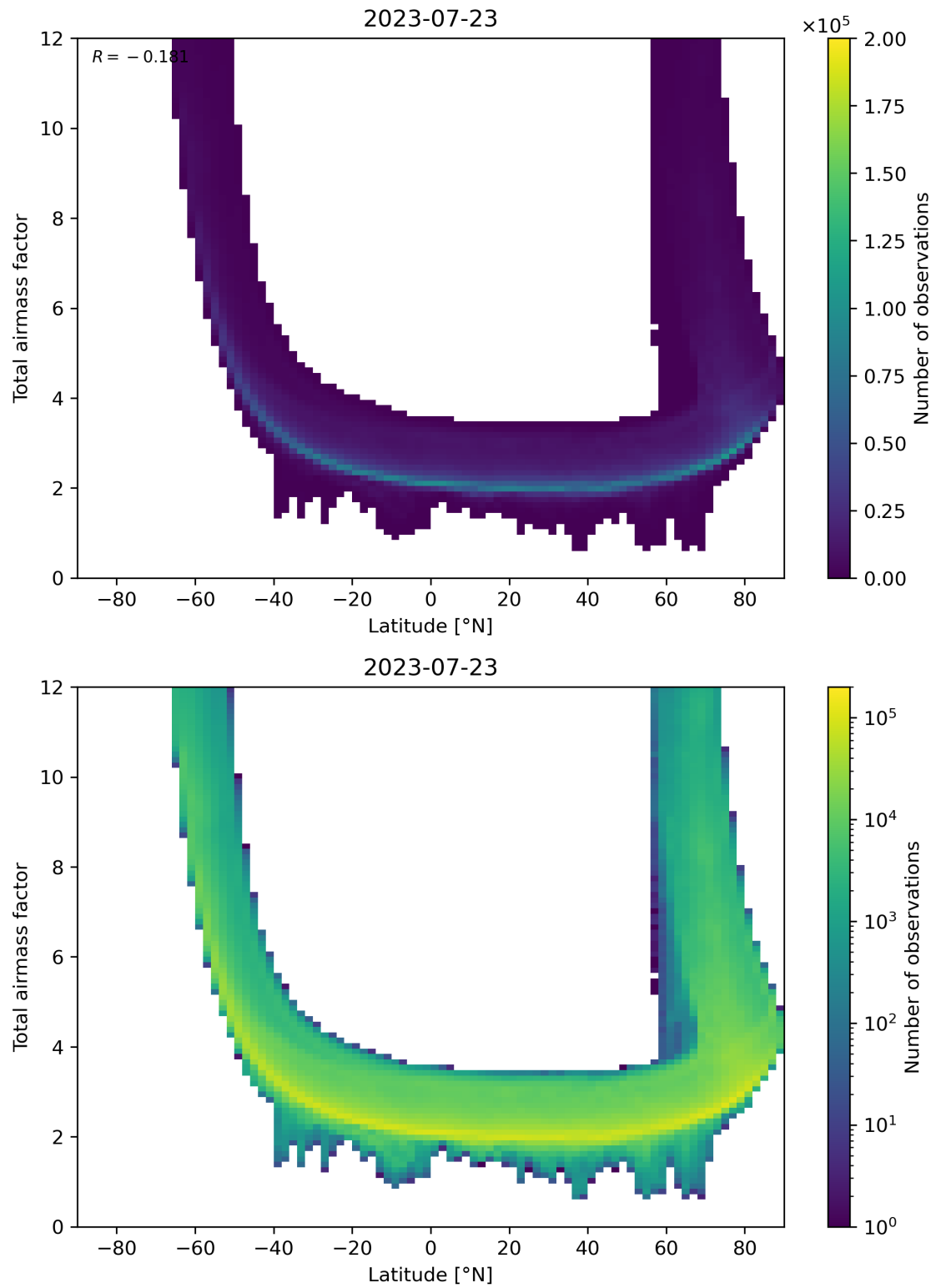
Figure 84: Scatter density plot of “Latitude” against “Total airmass factor” for 2023-07-22 to 2023-07-24.
