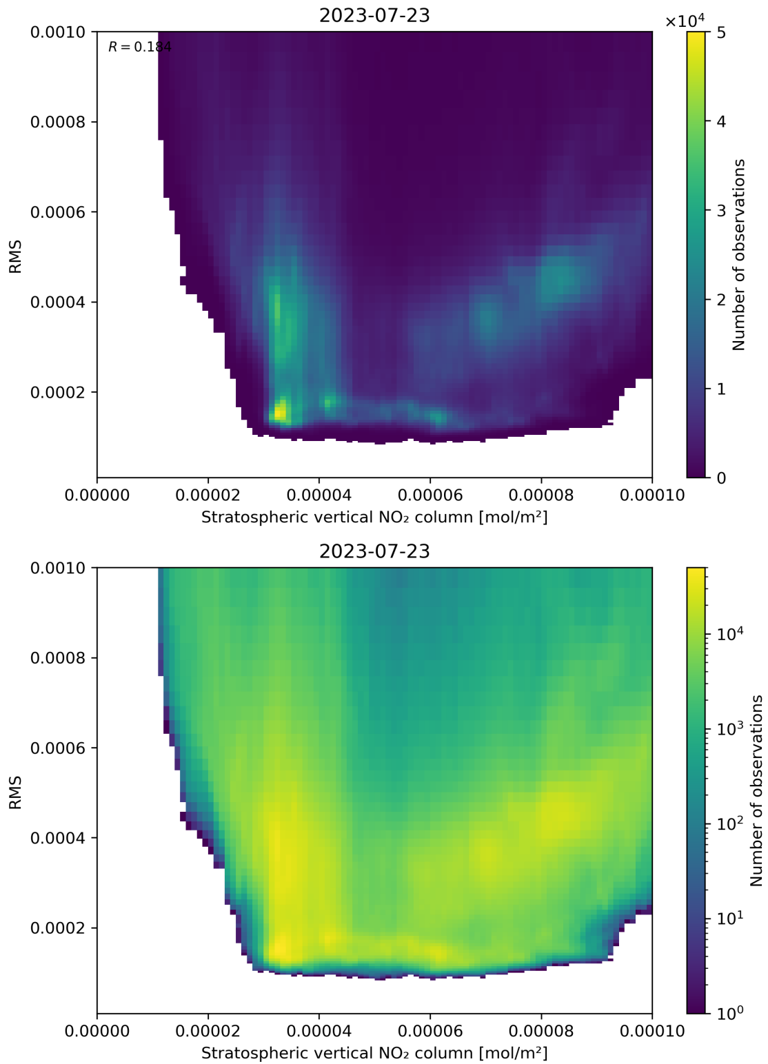
Figure 102: Scatter density plot of “Stratospheric vertical NO 2 column” against “RMS” for 2023-07-22 to 2023-07-24.
