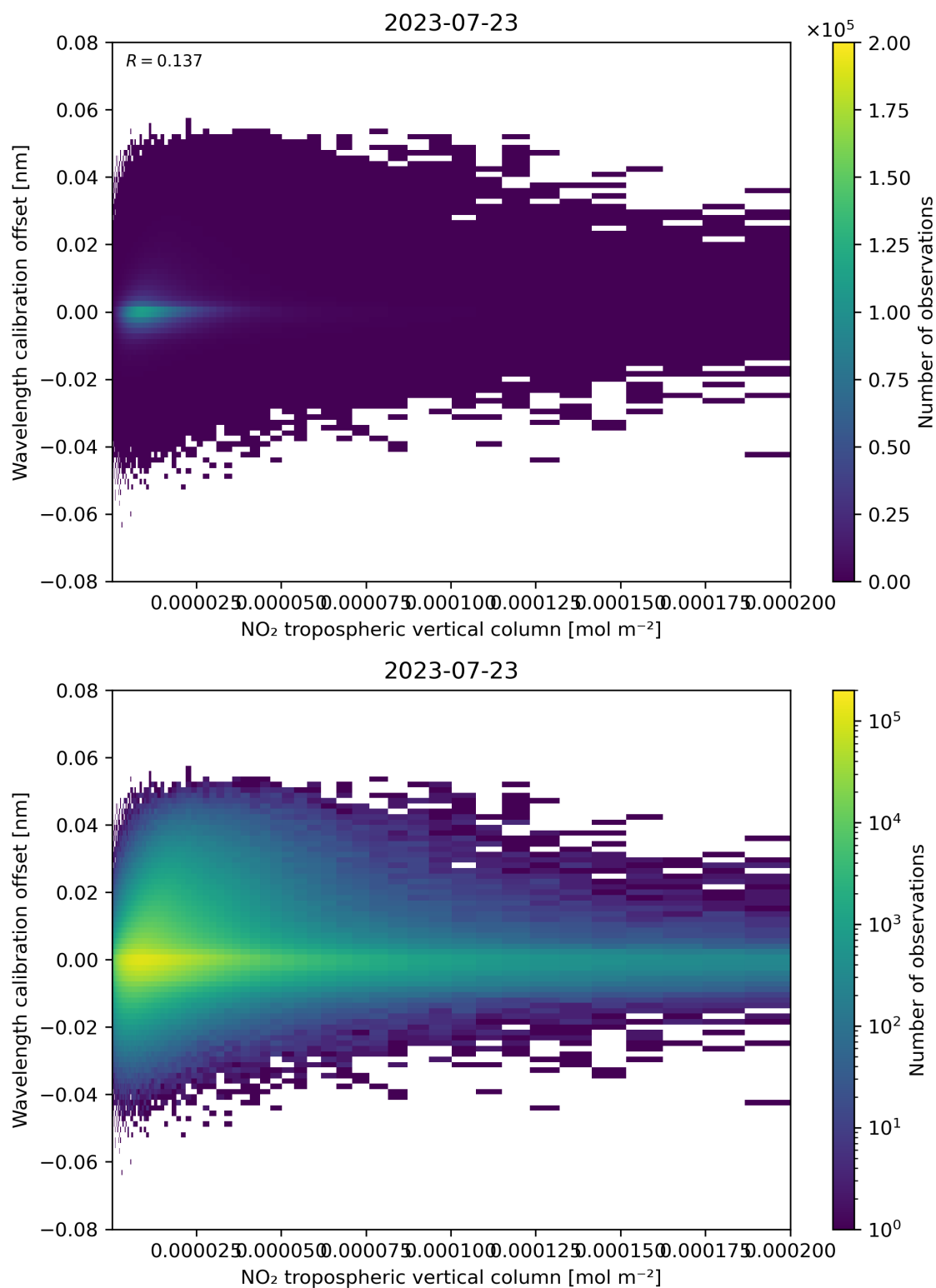
Figure 143: Scatter density plot of “NO 2 tropospheric vertical column” against “Wavelength calibration offset” for 2023-07-22 to 2023-07-24.
