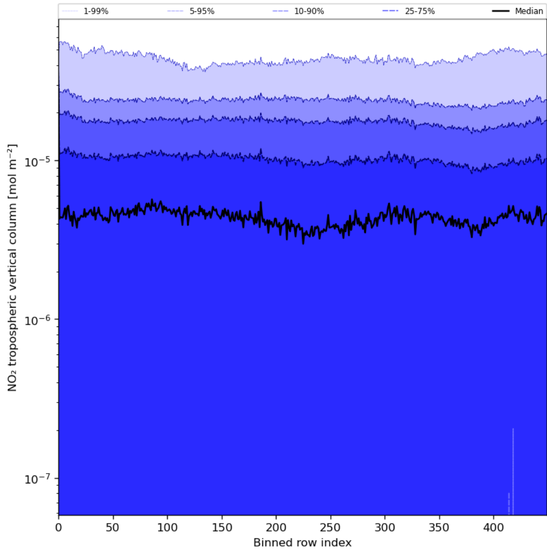
Figure 46: Along track statistics of “NO 2 tropospheric vertical column” for 2023-07-22 to 2023-07-24
