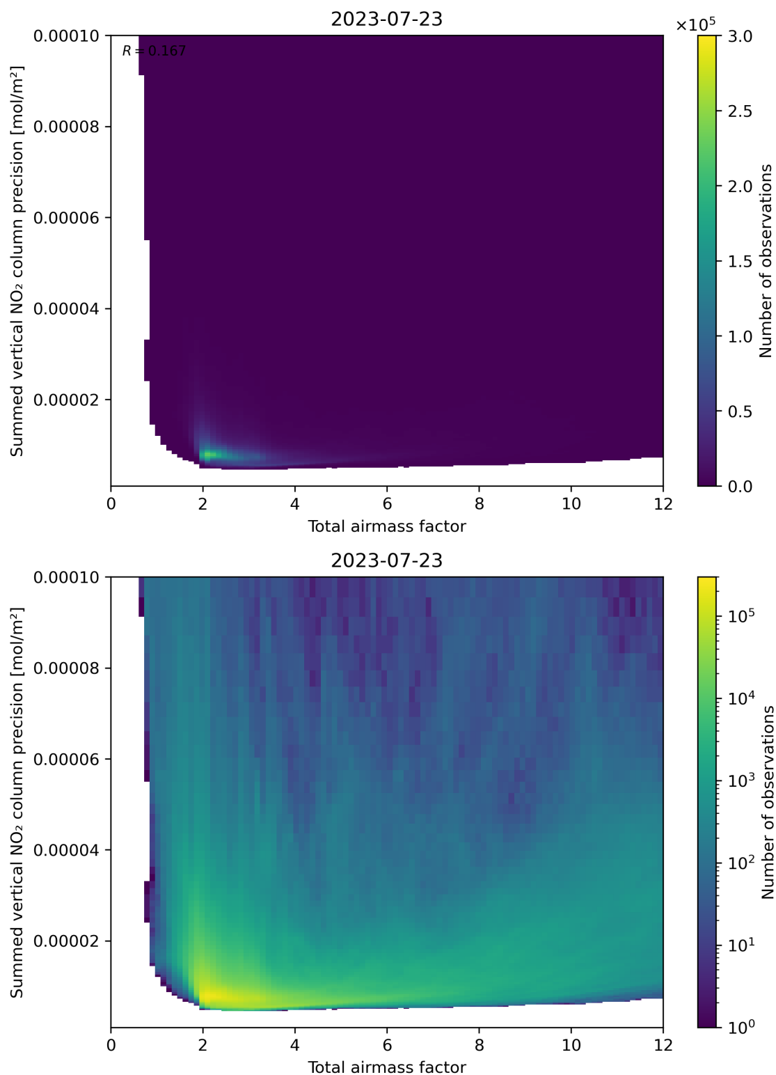
Figure 66: Scatter density plot of “Total airmass factor” against “Summed vertical NO 2 column precision” for 2023-07-22 to 2023-07-24.
