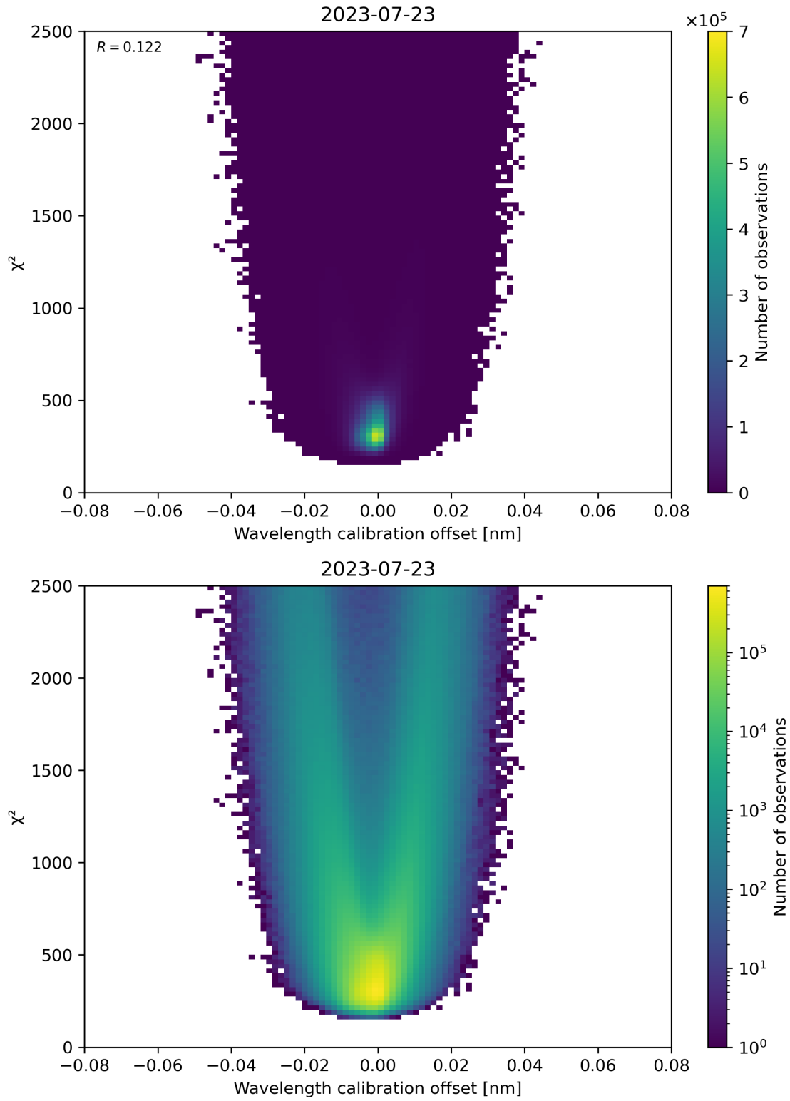
Figure 175: Scatter density plot of “Wavelength calibration offset” against “ \chi^2 ” for 2023-07-22 to 2023-07-24.
