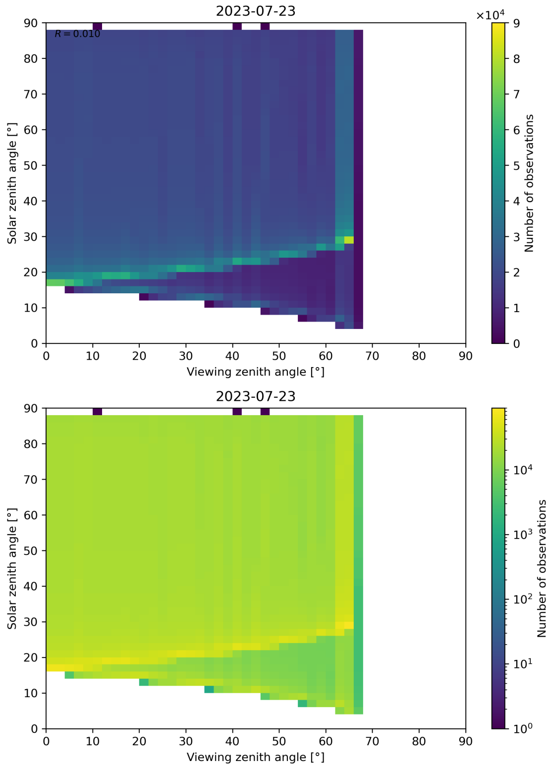
Figure 172: Scatter density plot of “Viewing zenith angle” against “Solar zenith angle” for 2023-07-22 to 2023-07-24.
