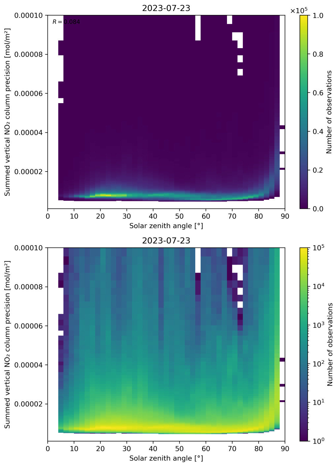
Figure 152: Scatter density plot of “Solar zenith angle” against “Summed vertical NO 2 column precision” for 2023-07-22 to 2023-07-24.
