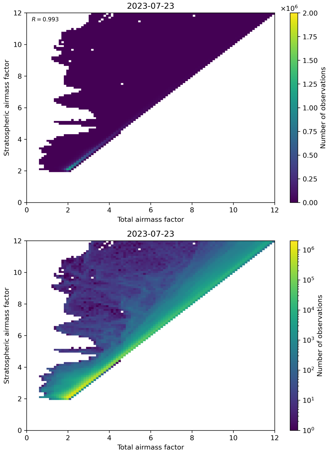
Figure 62: Scatter density plot of “Total air mass factor” against “Stratospheric air mass factor” for 2023-07-22 to 2023-07-24.
