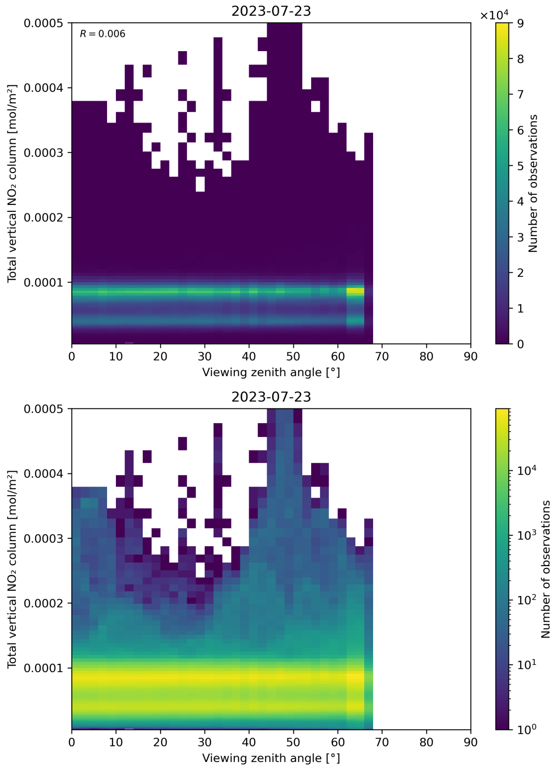
Figure 167: Scatter density plot of “Viewing zenith angle” against “Total vertical NO 2 column” for 2023-07-22 to 2023-07-24.
