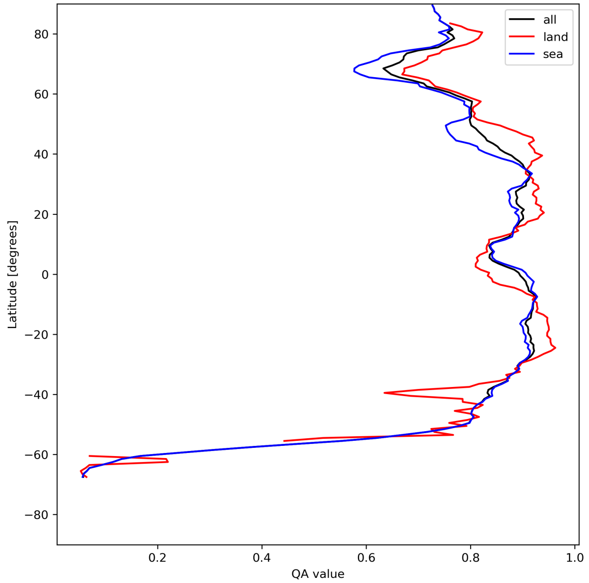
Figure 11: Zonal average of “QA value” for 2023-07-22 to 2023-07-24.
