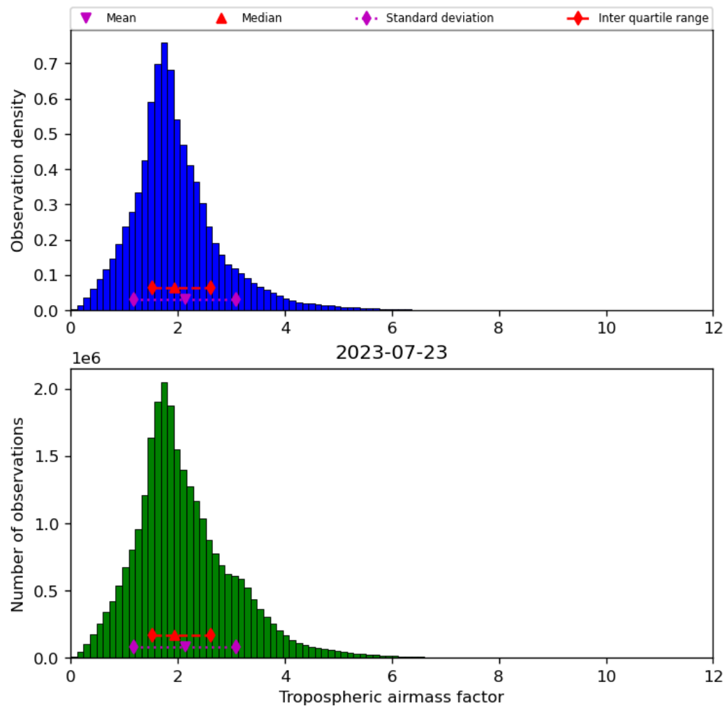
Figure 31: Histogram of “Tropospheric airmass factor” for 2023-07-22 to 2023-07-24
