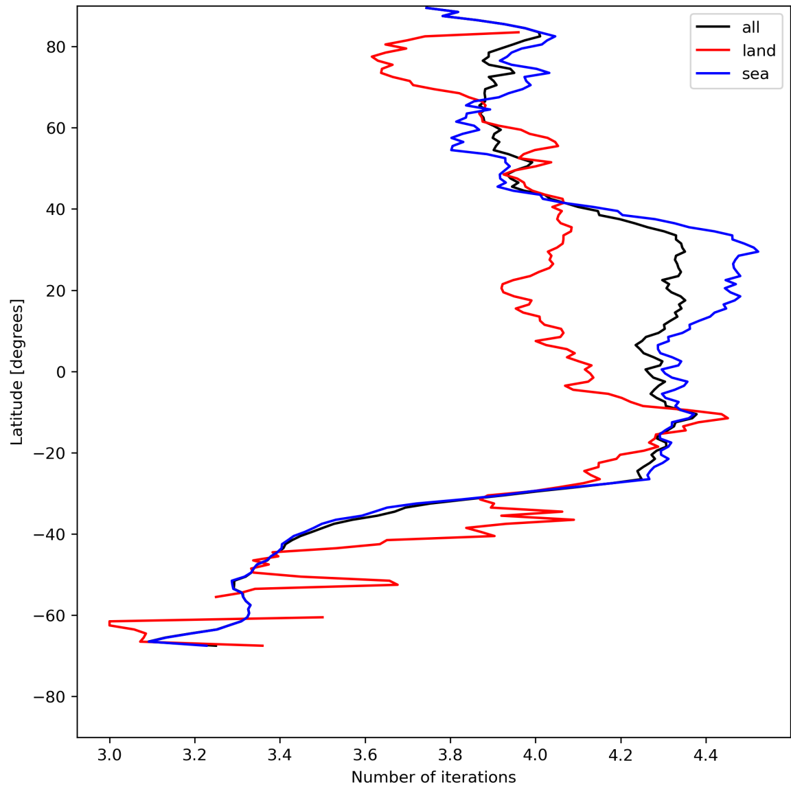
Figure 17: Zonal average of “Number of iterations” for 2023-07-22 to 2023-07-24.
