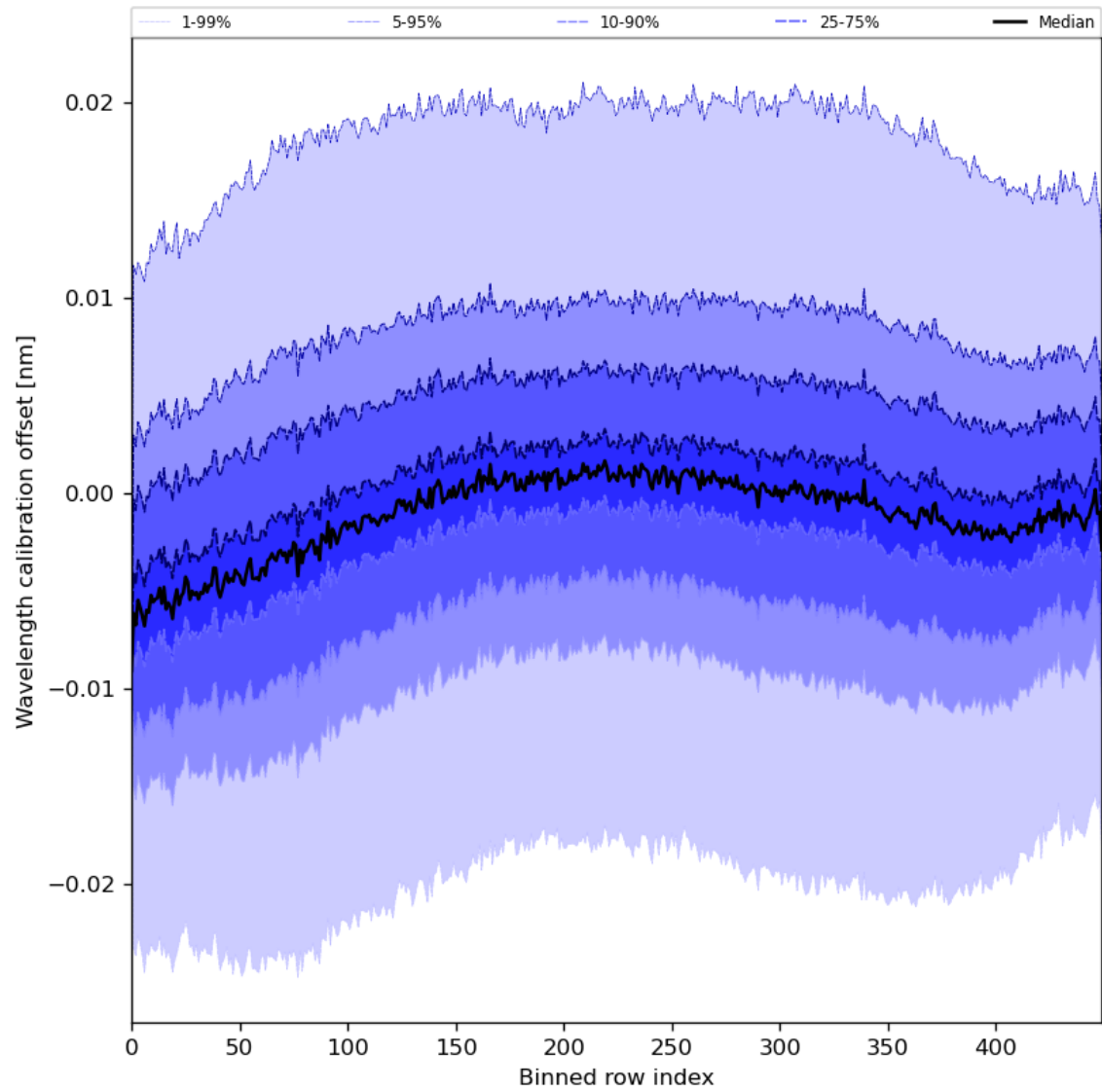
Figure 52: Along track statistics of “Wavelength calibration offset” for 2023-07-22 to 2023-07-24
