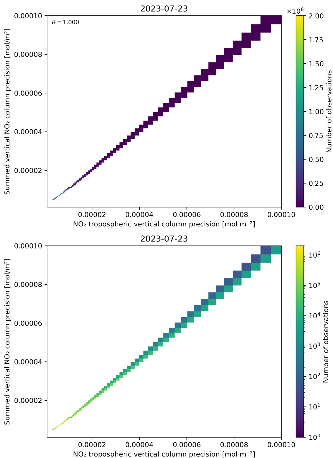
Figure 137: Scatter density plot of “NO 2 tropospheric vertical column precision” against “Summed vertical NO 2 column precision” for 2023-07-22 to 2023-07-24.
