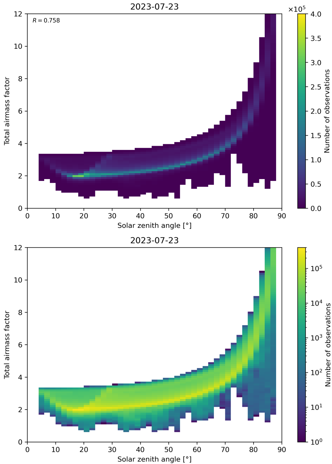
Figure 146: Scatter density plot of “Solar zenith angle” against “Total air mass factor” for 2023-07-22 to 2023-07-24.
