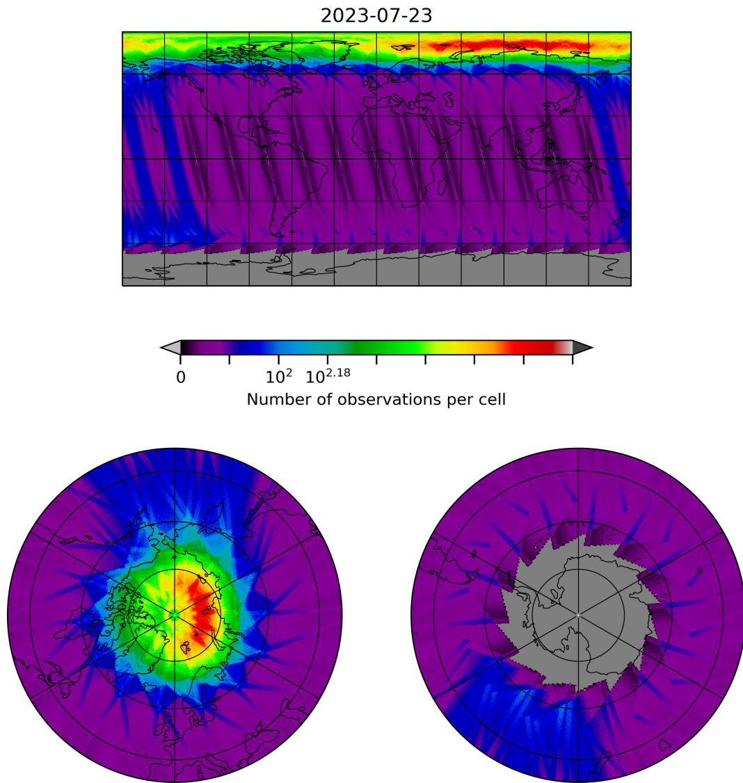
Figure 10: Map of the number of observations for 2023-07-22 to 2023-07-24
