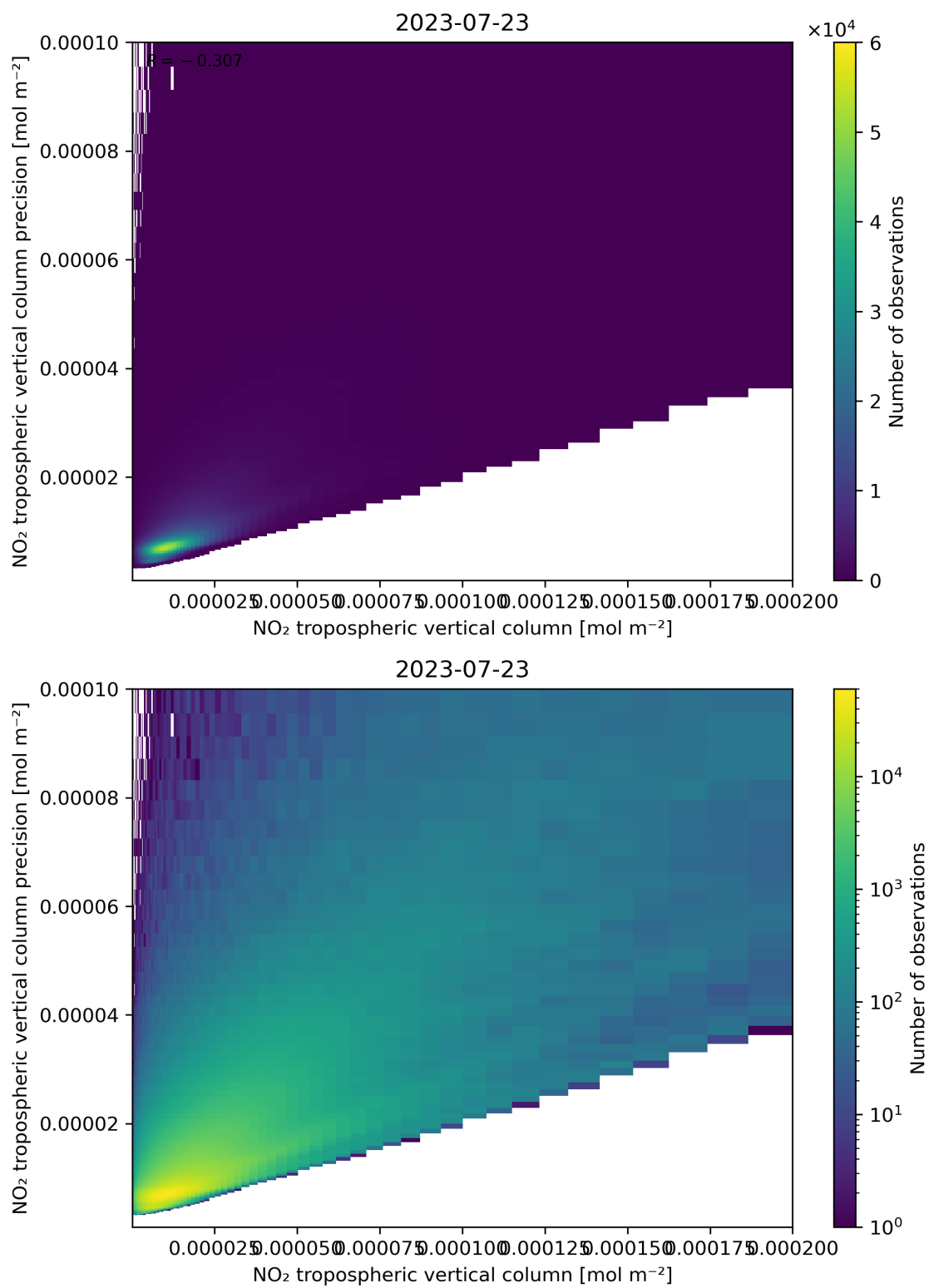
Figure 130: Scatter density plot of “NO 2 tropospheric vertical column” against “NO 2 tropospheric vertical column precision” for 2023-07-22 to 2023-07-24.
