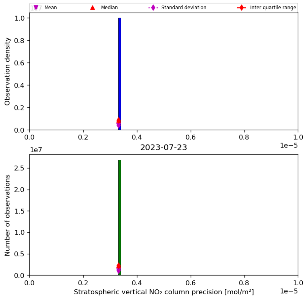
Figure 37: Histogram of “Stratospheric vertical NO 2 column precision” for 2023-07-22 to 2023-07-24
