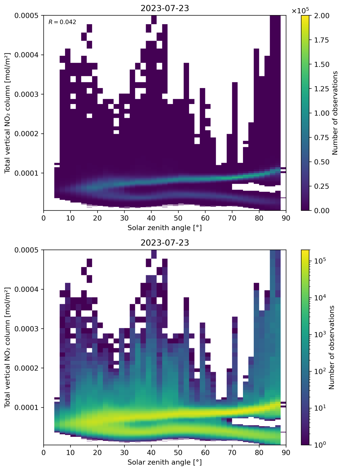
Figure 153: Scatter density plot of “Solar zenith angle” against “Total vertical \text{NO}_2 column” for 2023-07-22 to 2023-07-24.
