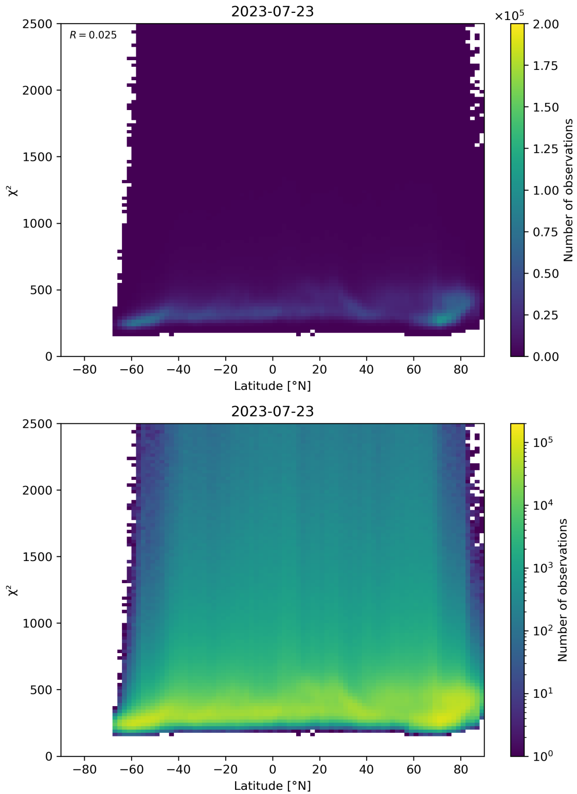
Figure 86: Scatter density plot of “Latitude” against “ \chi^2 ” for 2023-07-22 to 2023-07-24.
