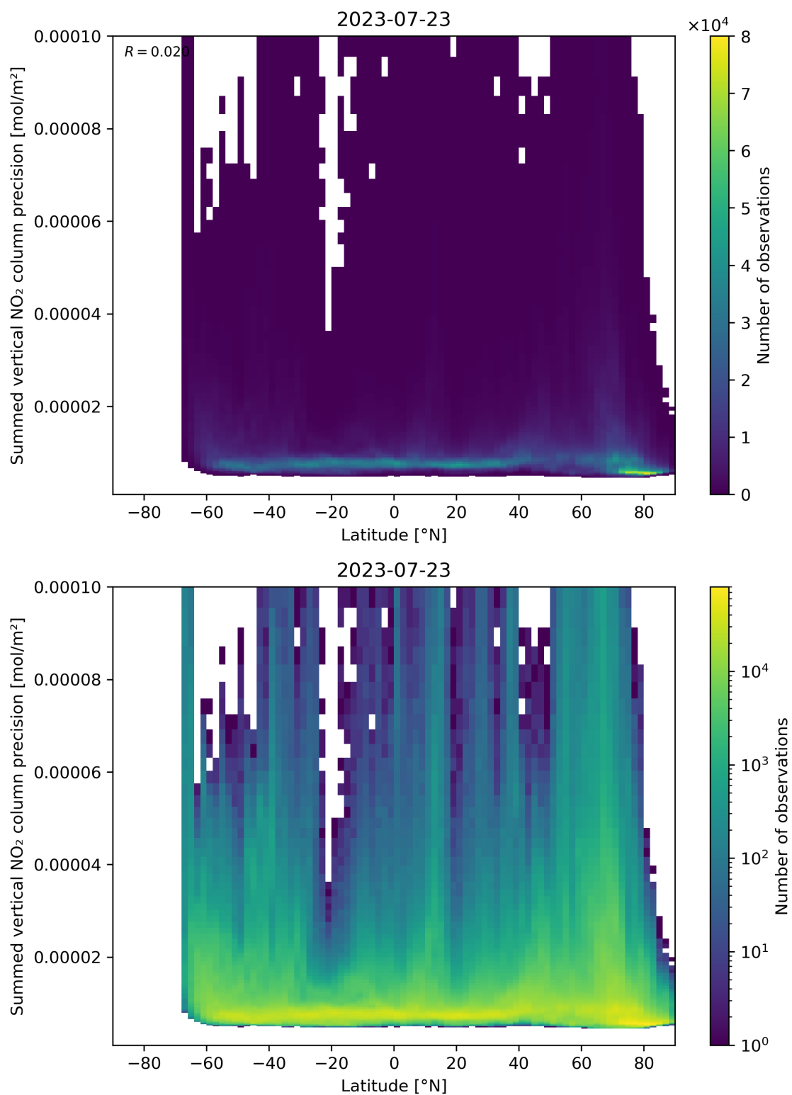
Figure 89: Scatter density plot of “Latitude” against “Summed vertical NO 2 column precision” for 2023-07-22 to 2023-07-24.
