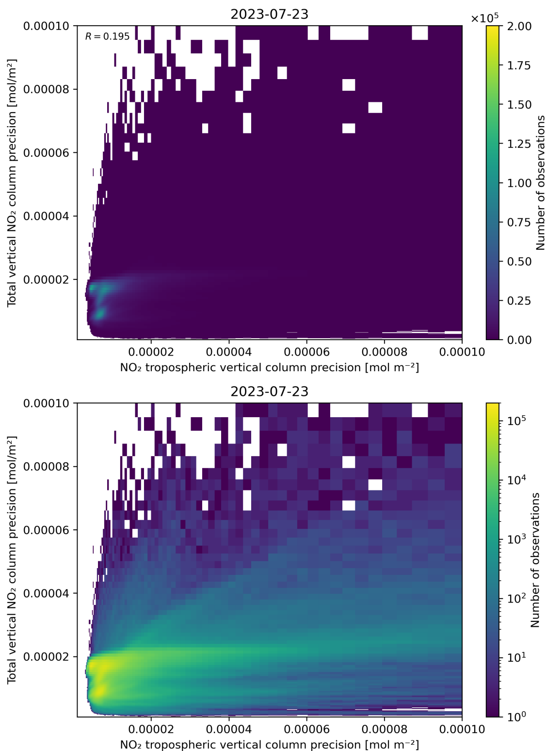
Figure 139: Scatter density plot of “NO 2 tropospheric vertical column precision” against “Total vertical NO 2 column precision” for 2023-07-22 to 2023-07-24.
