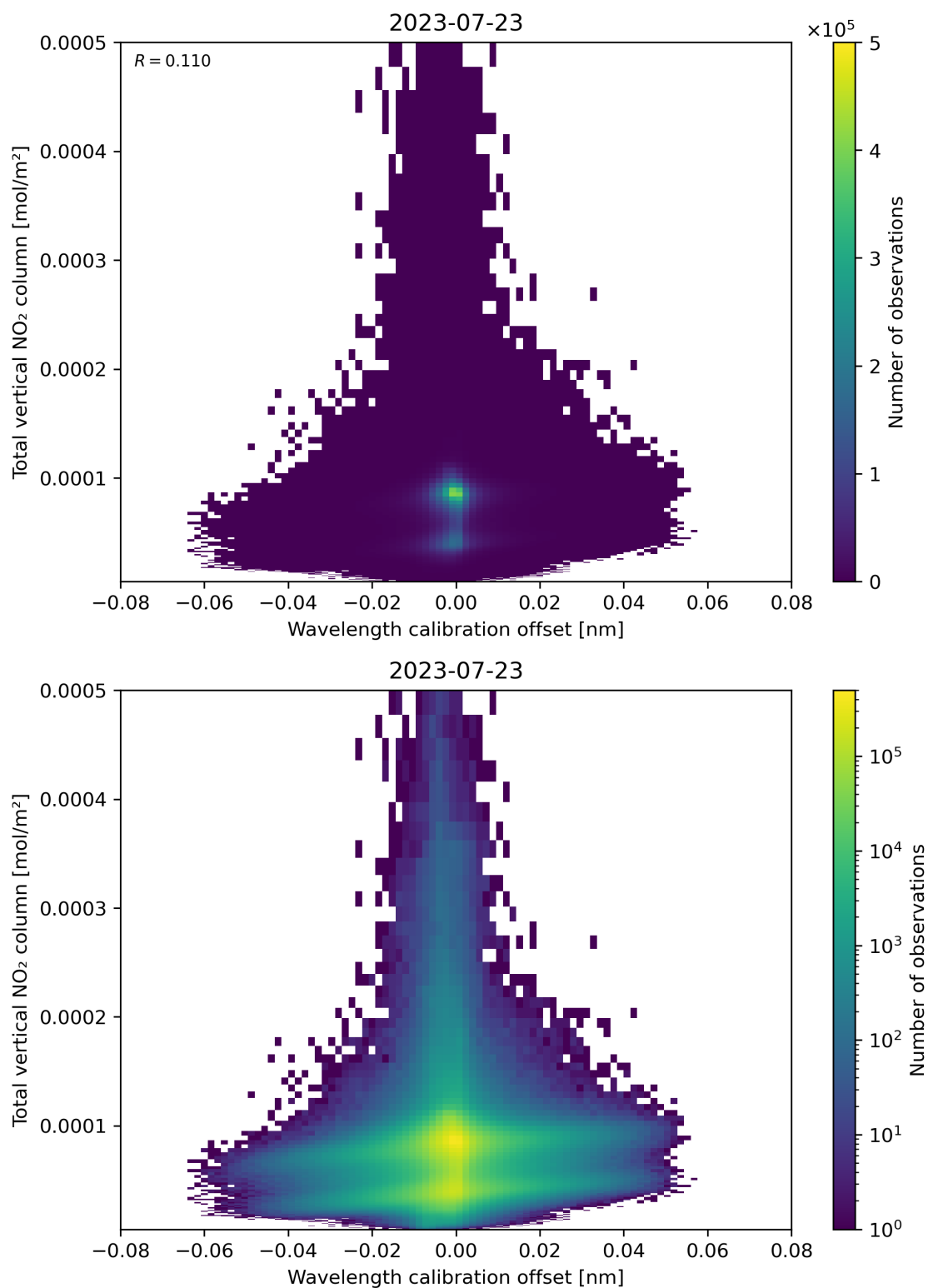
Figure 179: Scatter density plot of “Wavelength calibration offset” against “Total vertical NO 2 column” for 2023-07-22 to 2023-07-24.
