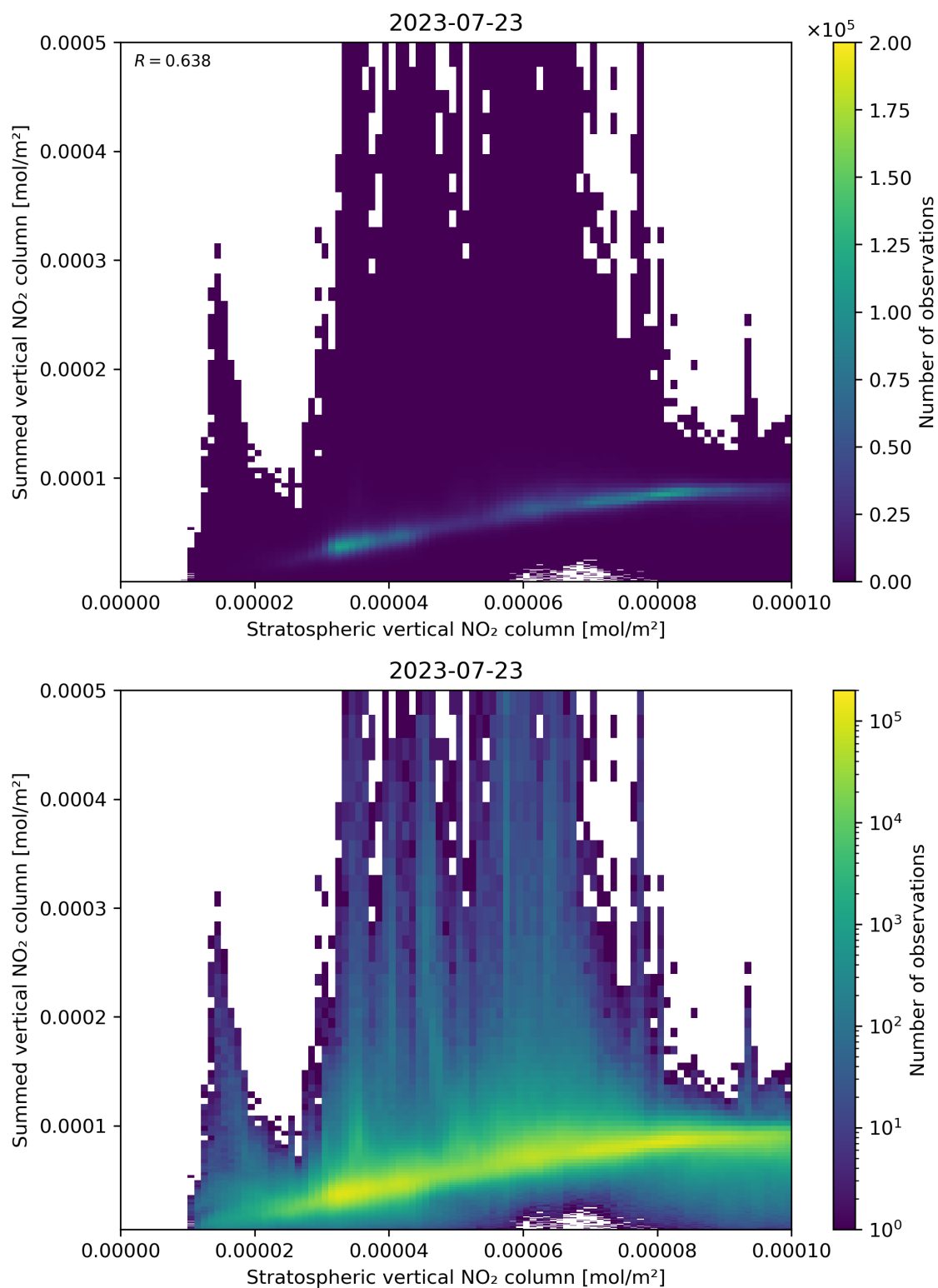
Figure 98: Scatter density plot of “Stratospheric vertical NO 2 column” against “Summed vertical NO 2 column” for 2023-07-22 to 2023-07-24.
