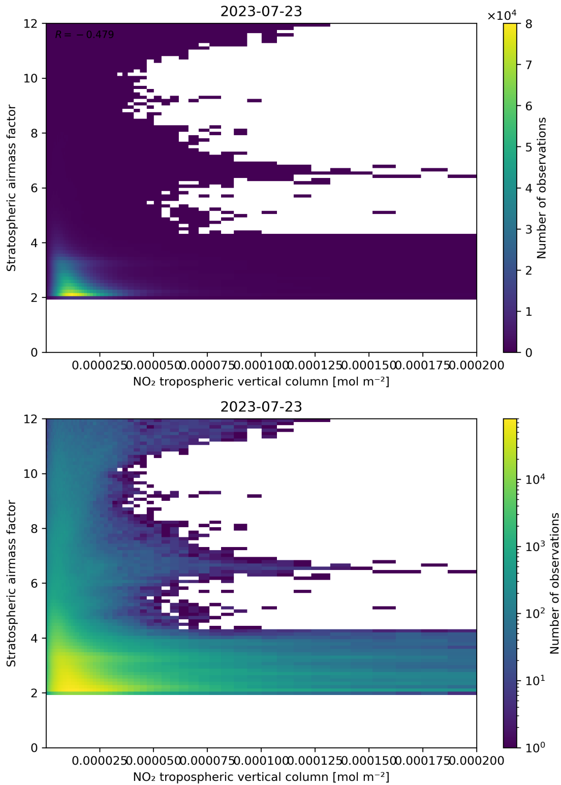
Figure 121: Scatter density plot of “NO 2 tropospheric vertical column” against “Stratospheric air mass factor” for 2023-07-22 to 2023-07-24.
