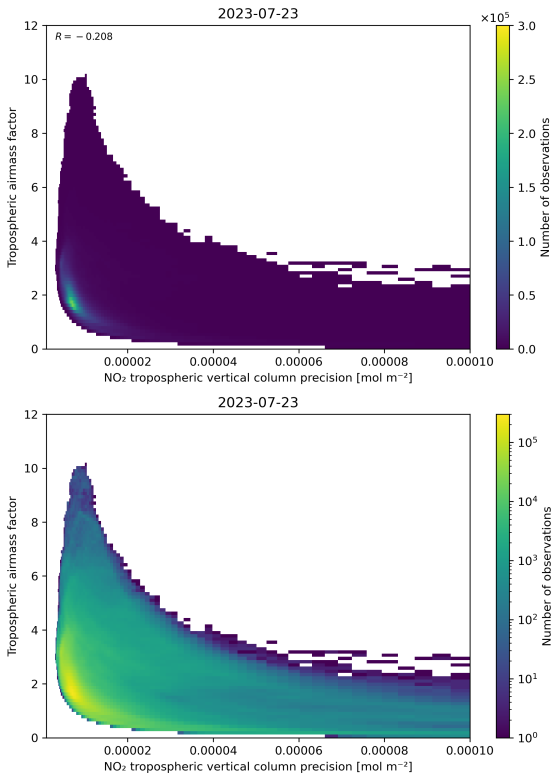
Figure 133: Scatter density plot of “NO 2 tropospheric vertical column precision” against “Tropospheric airmass factor” for 2023-07-22 to 2023-07-24.
