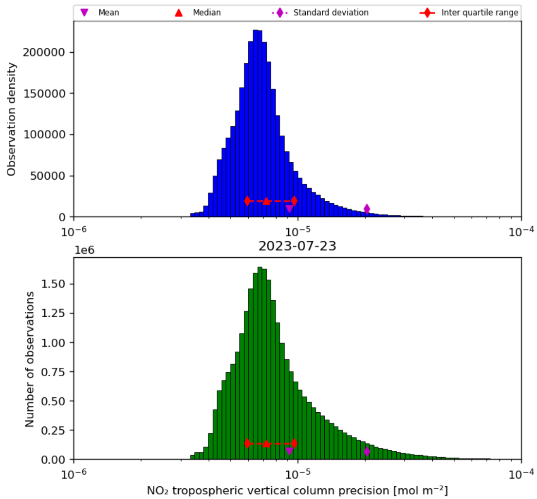
Figure 30: Histogram of “NO 2 tropospheric vertical column precision” for 2023-07-22 to 2023-07-24
