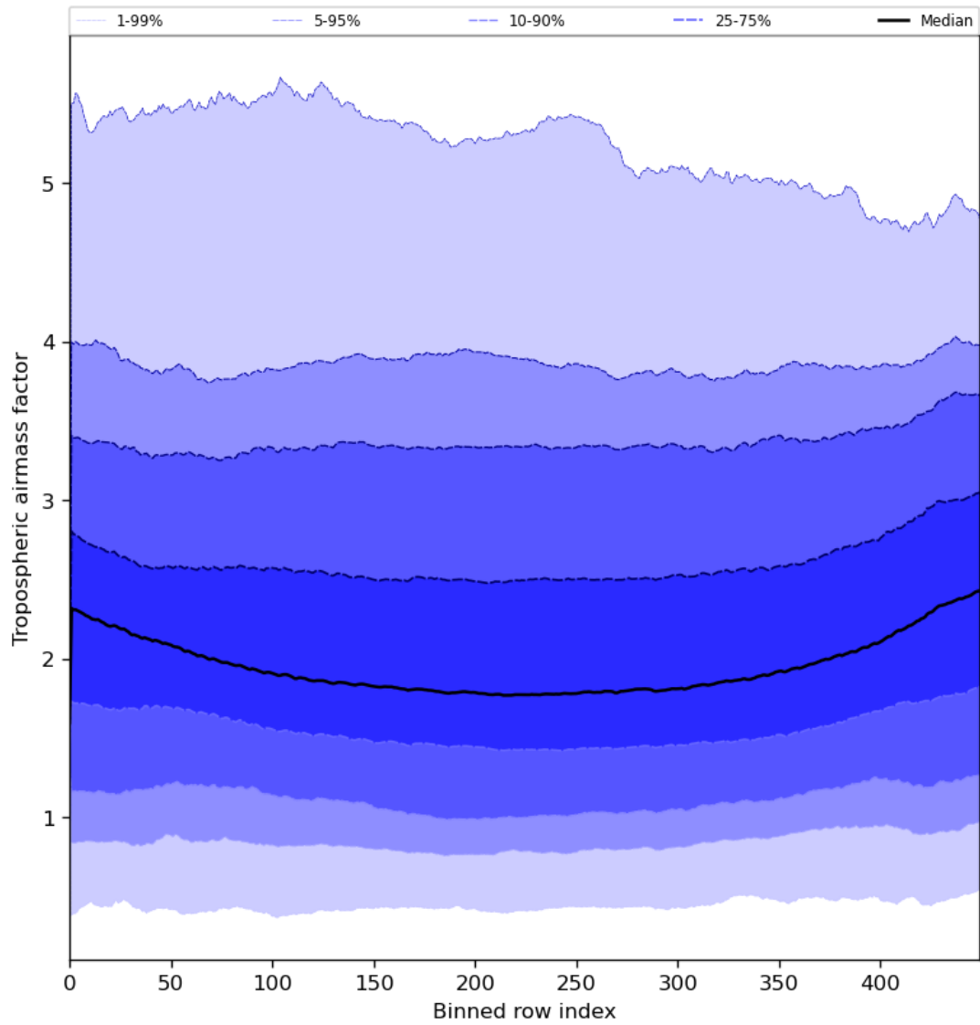
Figure 48: Along track statistics of “Tropospheric air mass factor” for 2023-07-22 to 2023-07-24
