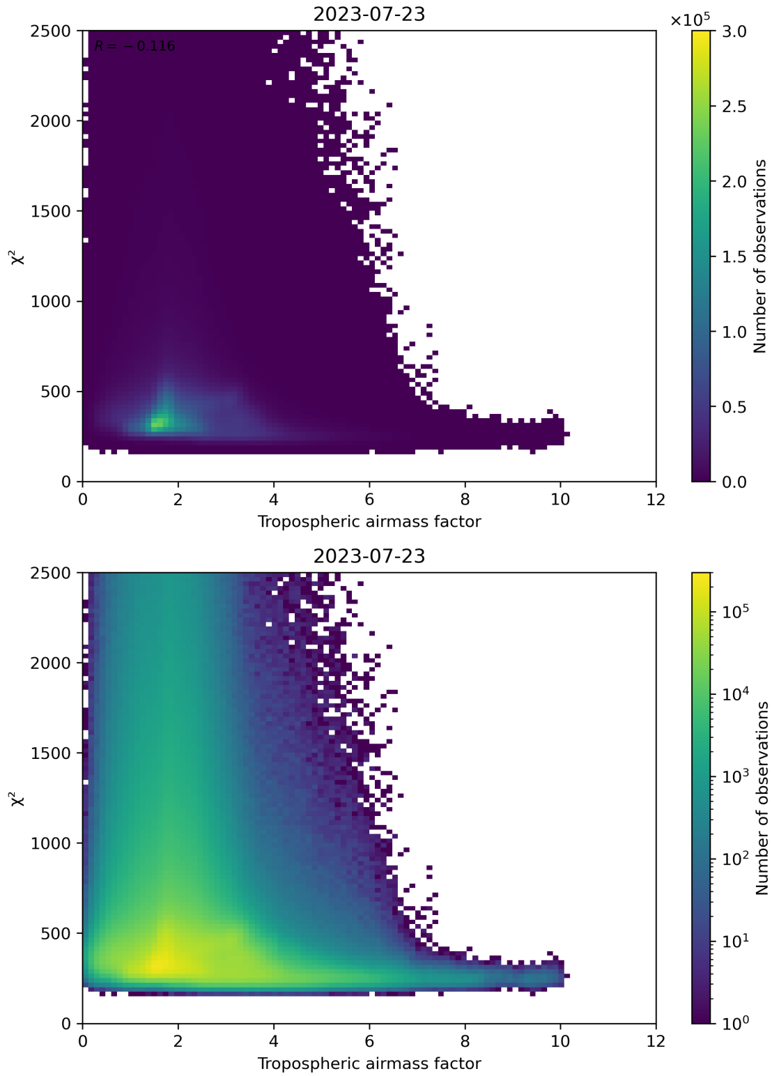
Figure 73: Scatter density plot of “Tropospheric airmass factor” against “ \chi^2 ” for 2023-07-22 to 2023-07-24.
