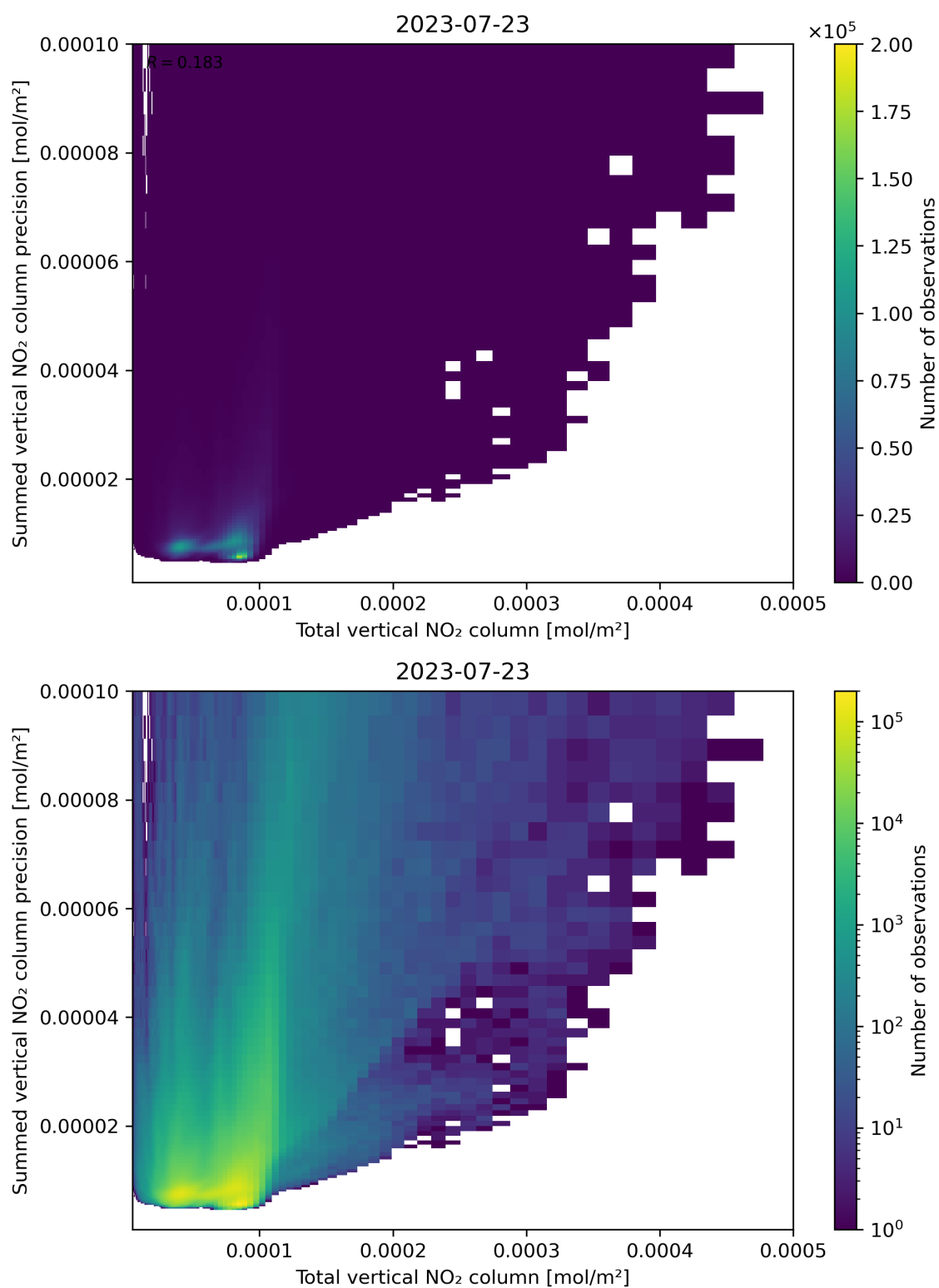
Figure 113: Scatter density plot of “Total vertical NO 2 column” against “Summed vertical NO 2 column precision” for 2023-07-22 to 2023-07-24.
