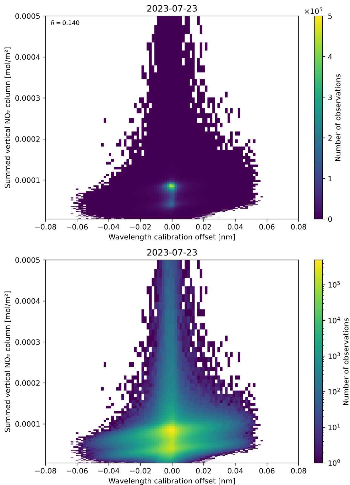
Figure 177: Scatter density plot of “Wavelength calibration offset” against “Summed vertical NO 2 column” for 2023-07-22 to 2023-07-24.
