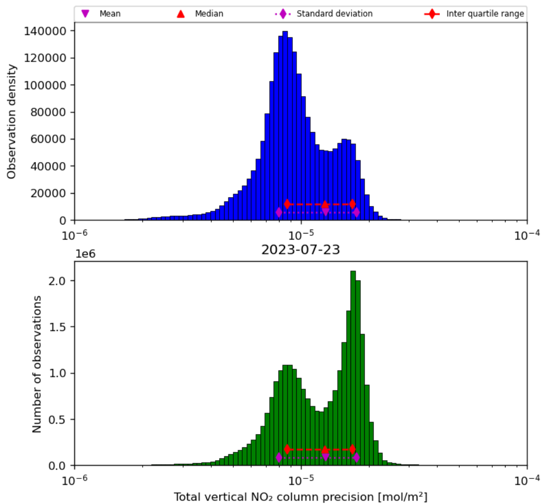
Figure 39: Histogram of "Total vertical NO 2 column precision" for 2023-07-22 to 2023-07-24
