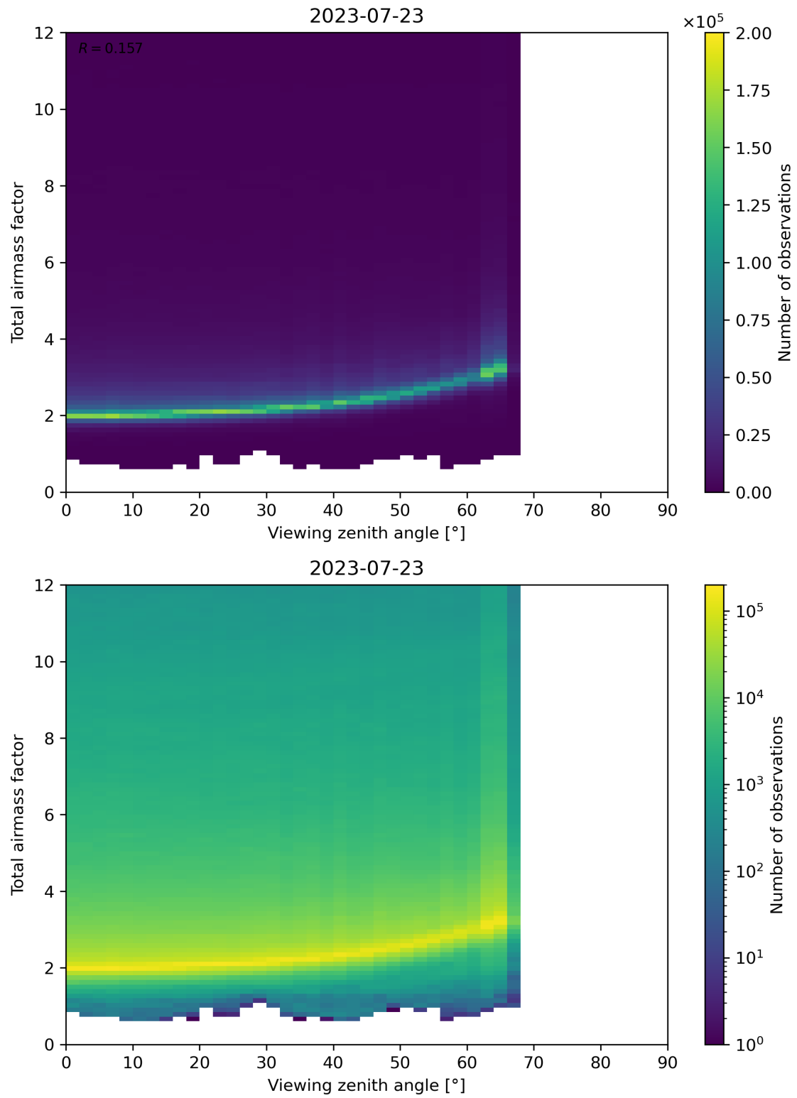
Figure 160: Scatter density plot of “Viewing zenith angle” against “Total airmass factor” for 2023-07-22 to 2023-07-24.
