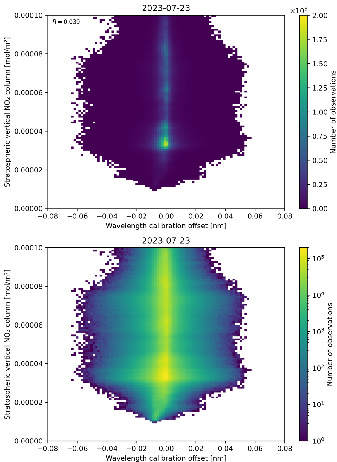
Figure 176: Scatter density plot of “Wavelength calibration offset” against “Stratospheric vertical NO 2 column” for 2023-07-22 to 2023-07-24.
