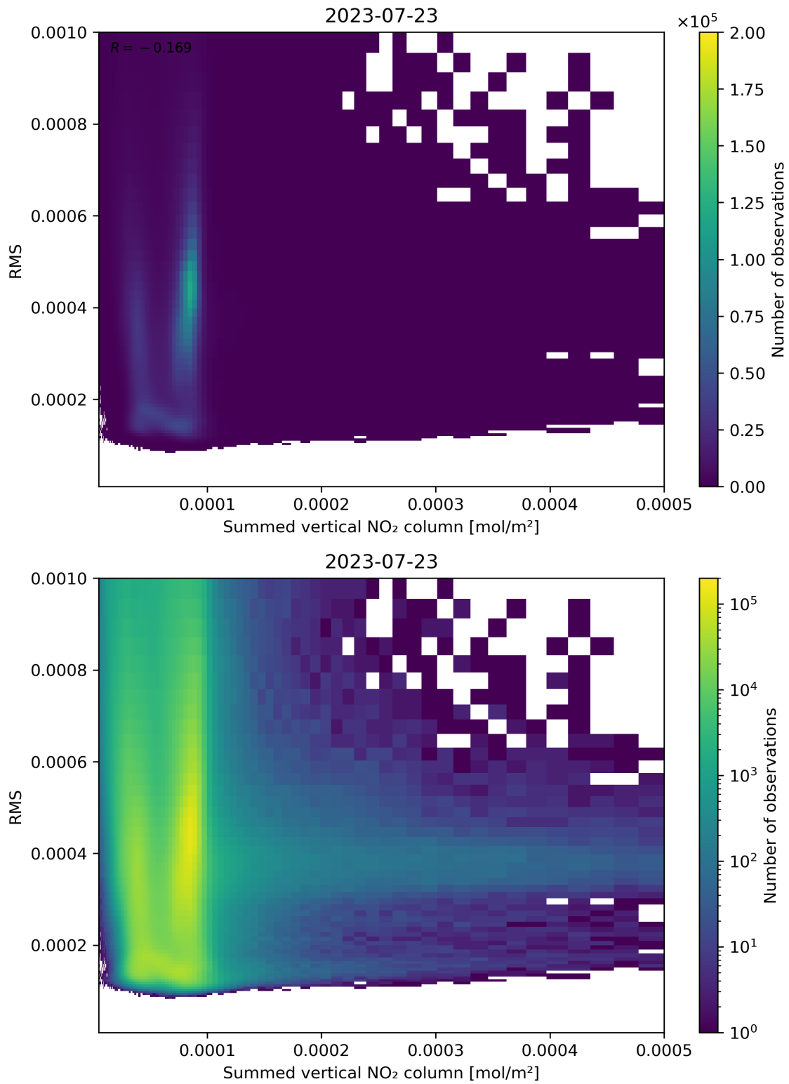
Figure 109: Scatter density plot of “Summed vertical NO 2 column” against “RMS” for 2023-07-22 to 2023-07-24.
