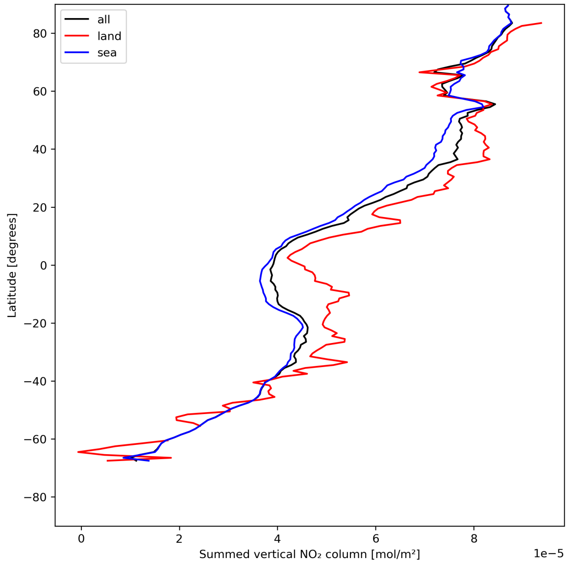
Figure 23: Zonal average of “Summed vertical NO 2 column” for 2023-07-22 to 2023-07-24.
