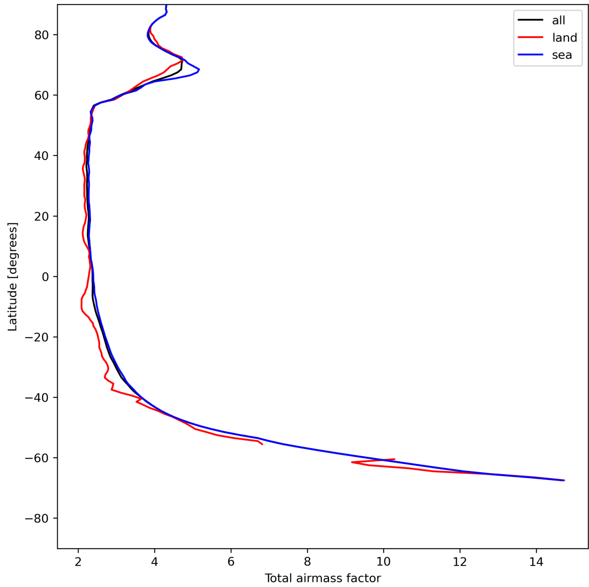
Figure 15: Zonal average of “Total airmass factor” for 2023-07-22 to 2023-07-24.
