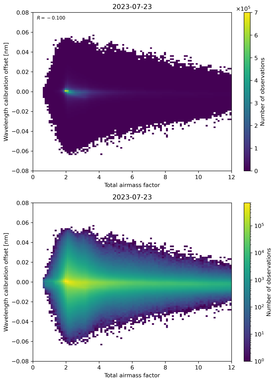
Figure 70: Scatter density plot of “Total airmass factor” against “Wavelength calibration offset” for 2023-07-22 to 2023-07-24.
