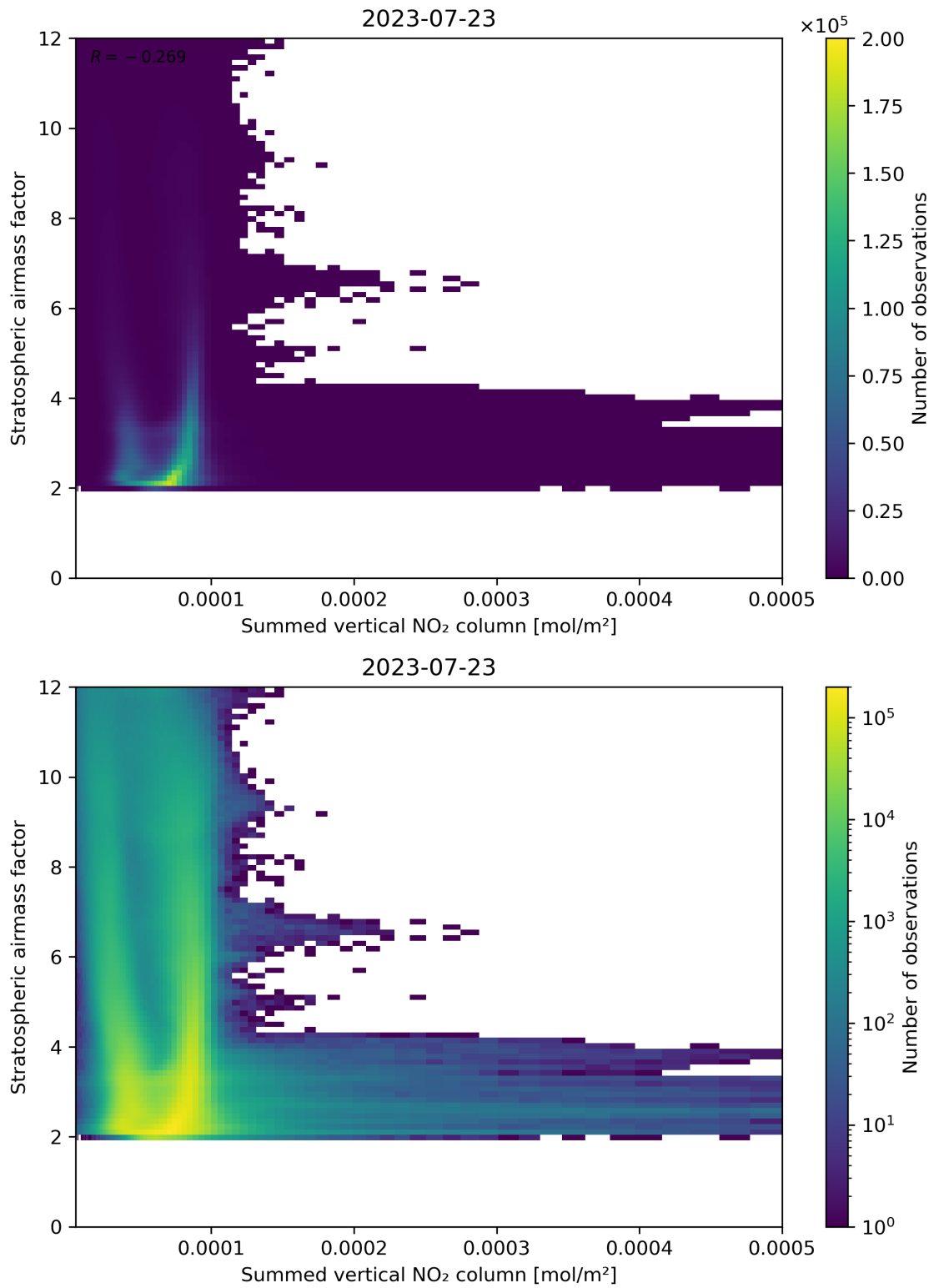
Figure 103: Scatter density plot of “Summed vertical NO 2 column” against “Stratospheric airmass factor” for 2023-07-22 to 2023-07-24.
