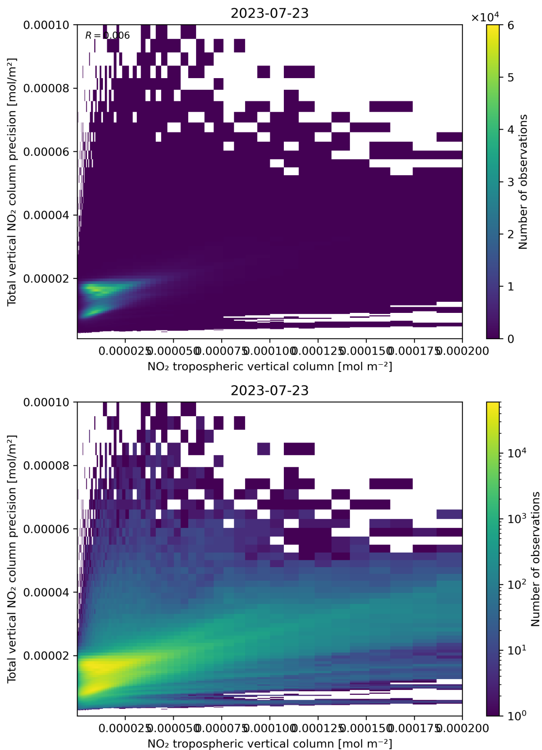
Figure 129: Scatter density plot of “NO 2 tropospheric vertical column” against “Total vertical NO 2 column precision” for 2023-07-22 to 2023-07-24.
