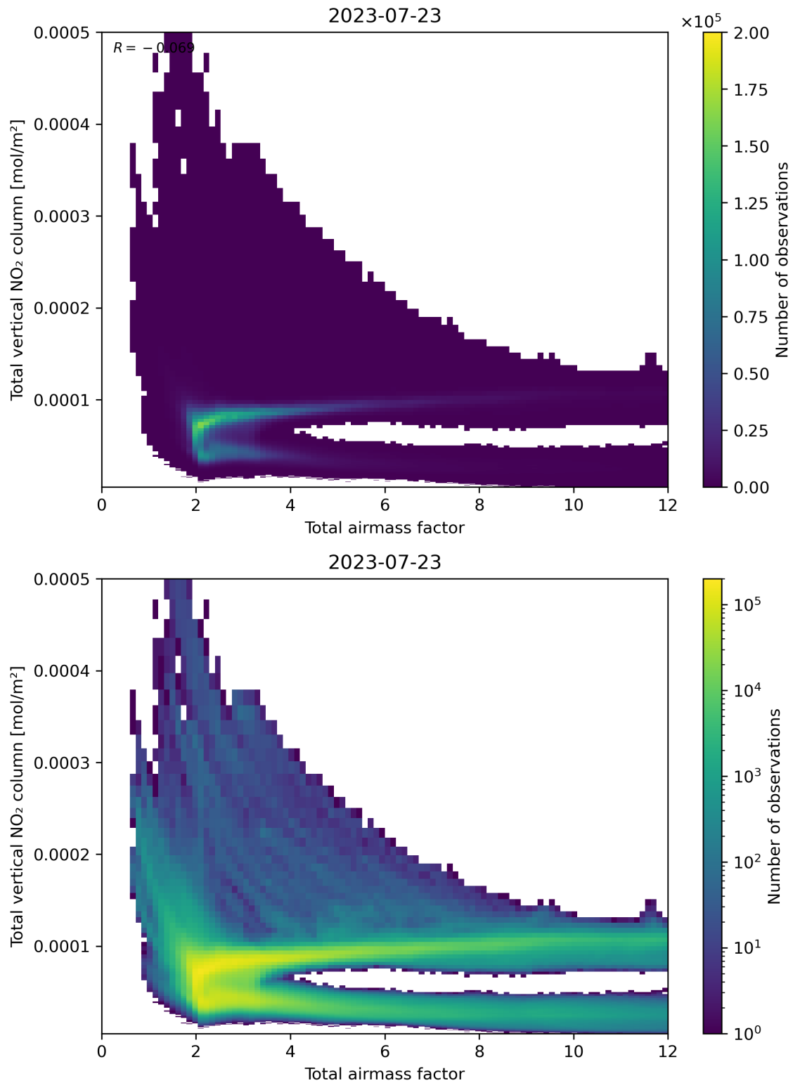
Figure 67: Scatter density plot of “Total airmass factor” against “Total vertical NO 2 column” for 2023-07-22 to 2023-07-24.
