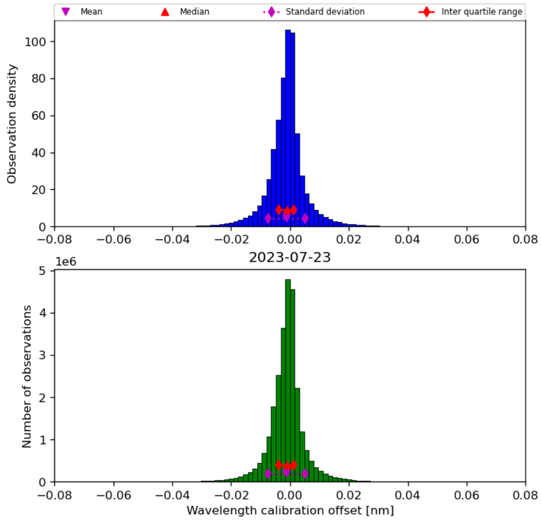
Figure 35: Histogram of “Wavelength calibration offset” for 2023-07-22 to 2023-07-24
