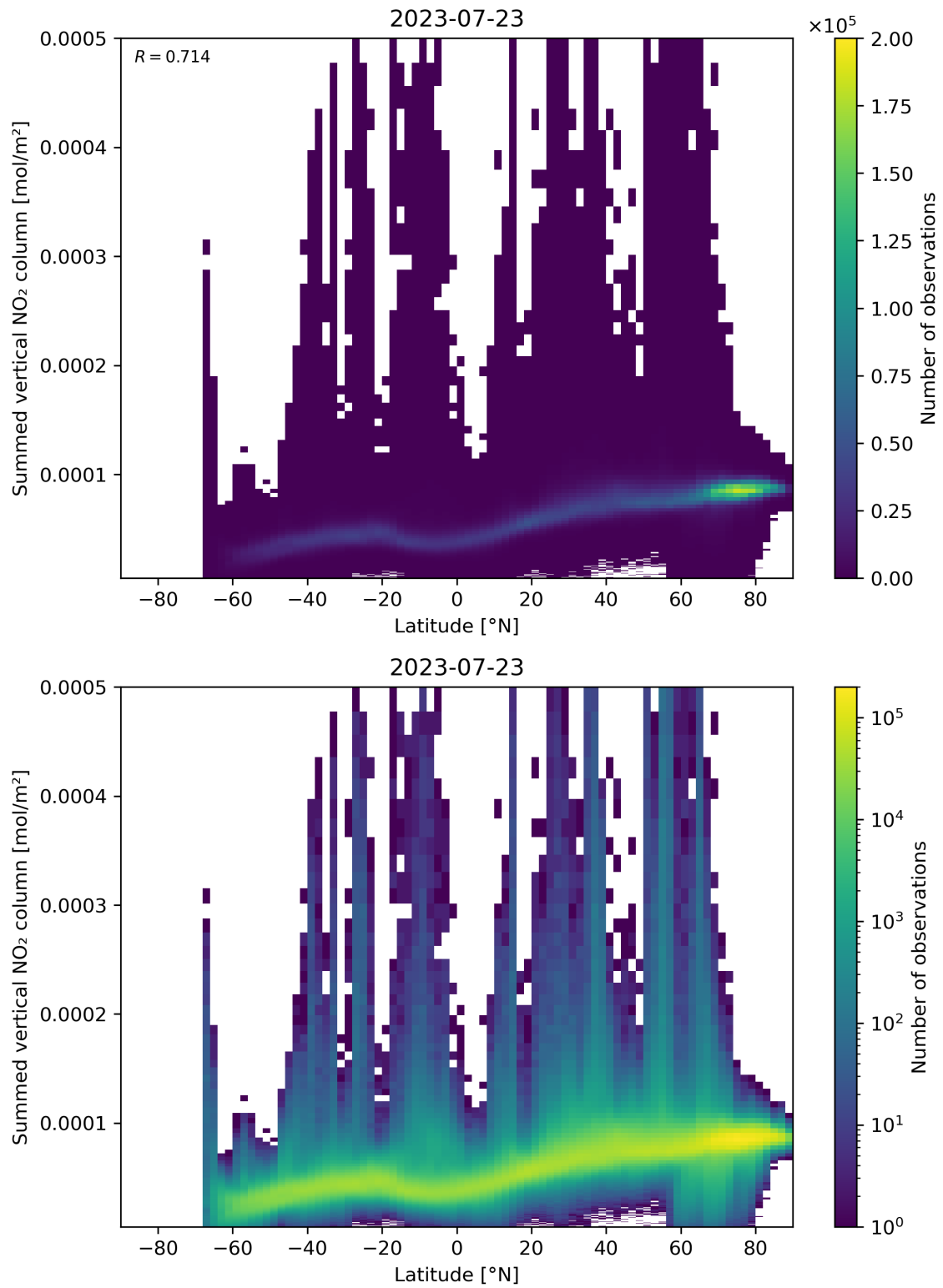
Figure 88: Scatter density plot of “Latitude” against “Summed vertical NO 2 column” for 2023-07-22 to 2023-07-24.
