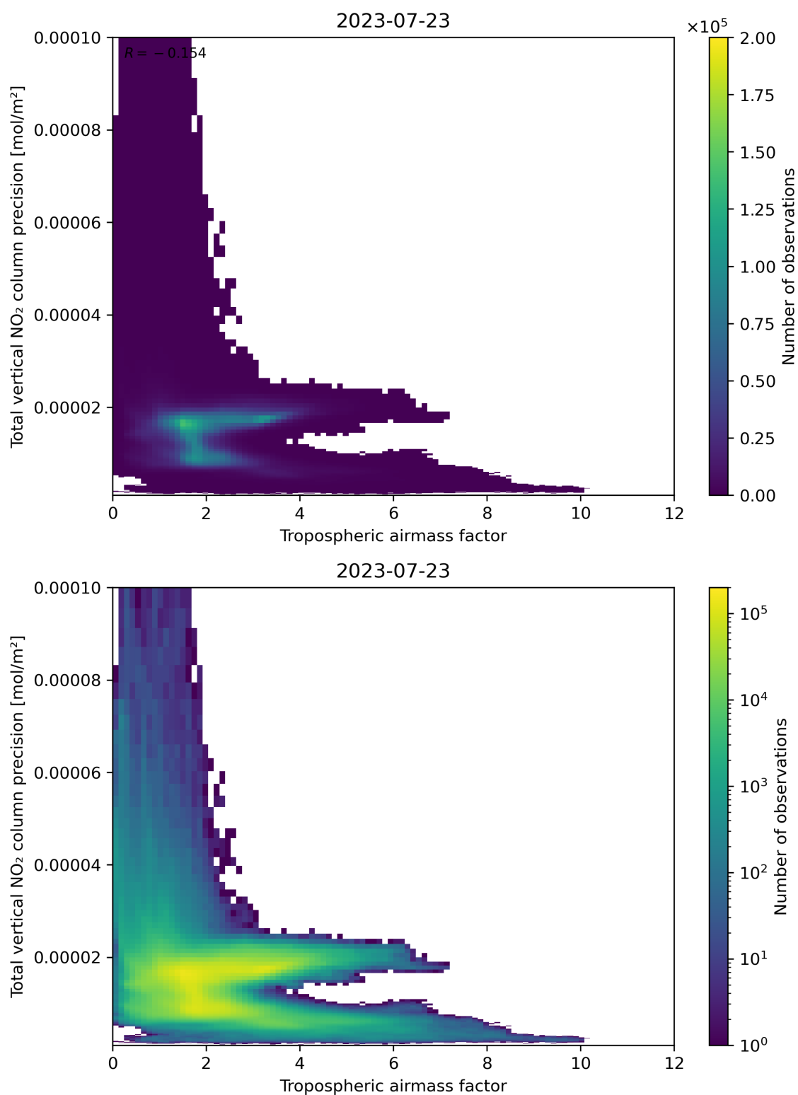
Figure 78: Scatter density plot of “Tropospheric air mass factor” against “Total vertical NO 2 column precision” for 2023-07-22 to 2023-07-24.
