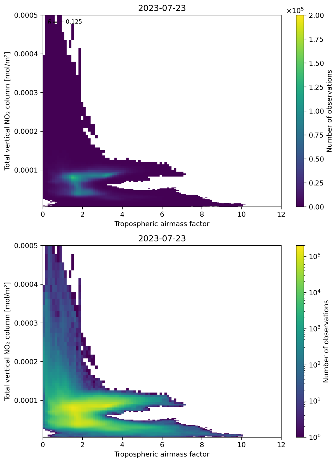
Figure 77: Scatter density plot of “Tropospheric airmass factor” against “Total vertical NO 2 column” for 2023-07-22 to 2023-07-24.
