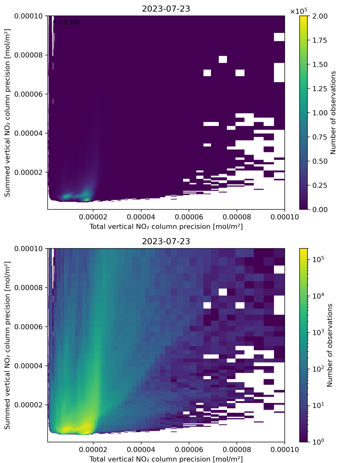
Figure 118: Scatter density plot of “Total vertical NO 2 column precision” against “Summed vertical NO 2 column precision” for 2023-07-22 to 2023-07-24.
