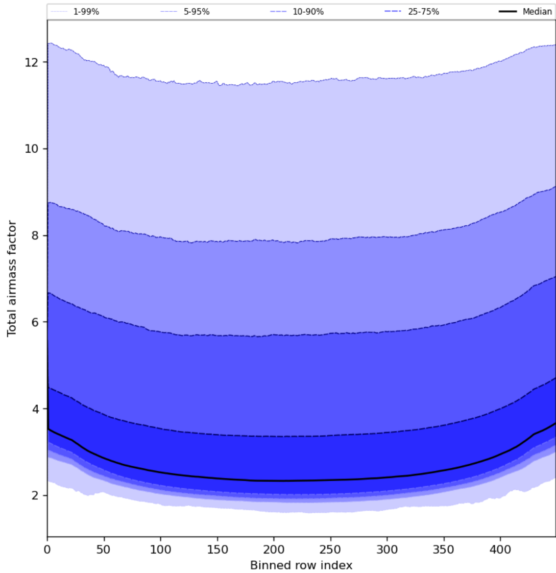
Figure 49: Along track statistics of “Total airmass factor” for 2023-07-22 to 2023-07-24
