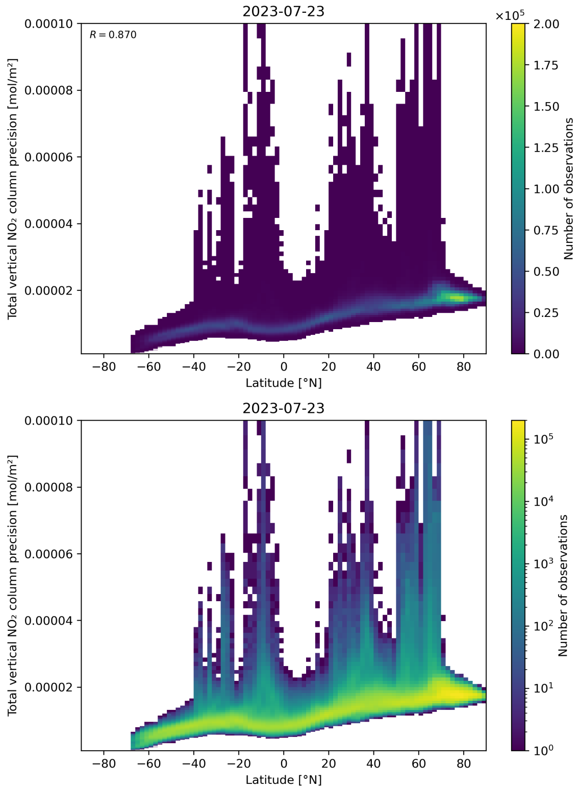
Figure 91: Scatter density plot of “Latitude” against “Total vertical NO 2 column precision” for 2023-07-22 to 2023-07-24.
