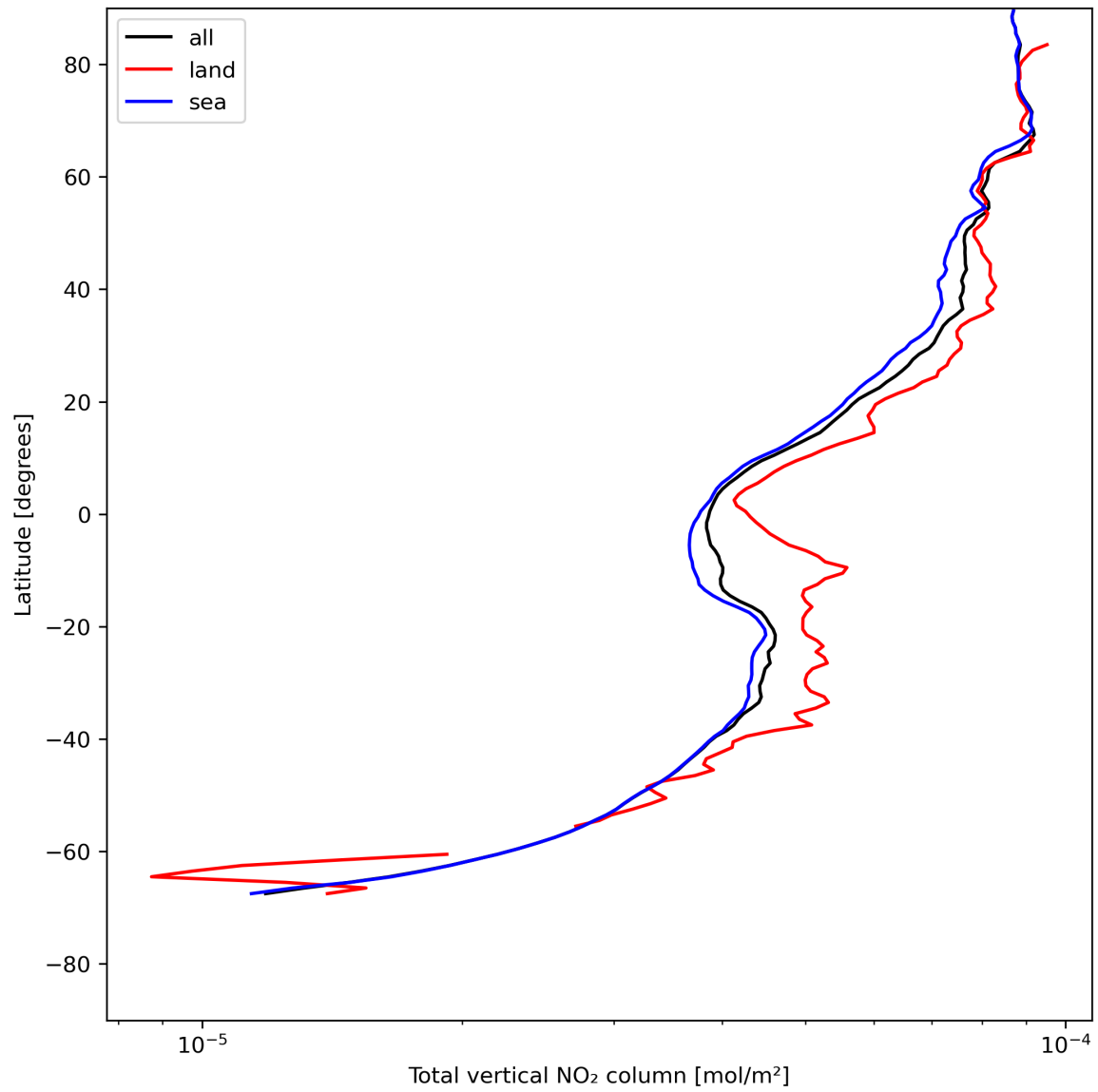
Figure 21: Zonal average of “Total vertical NO 2 column” for 2023-07-22 to 2023-07-24.
