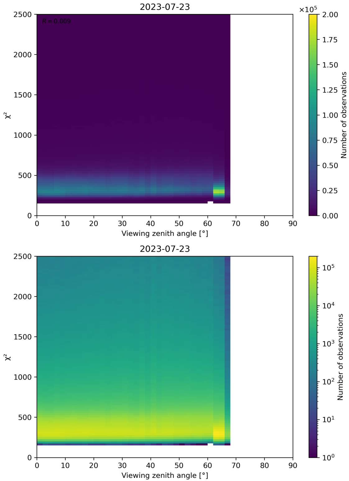
Figure 162: Scatter density plot of “Viewing zenith angle” against “ \chi^2 ” for 2023-07-22 to 2023-07-24.
