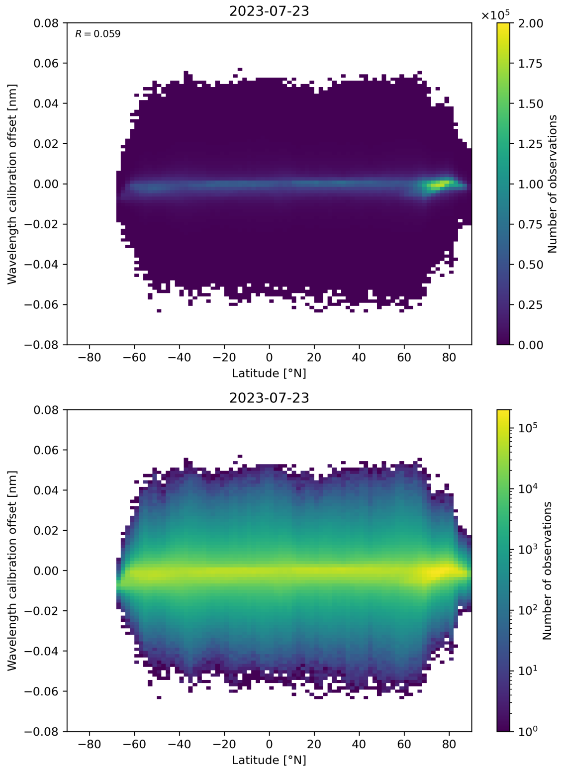
Figure 95: Scatter density plot of “Latitude” against “Wavelength calibration offset” for 2023-07-22 to 2023-07-24.
