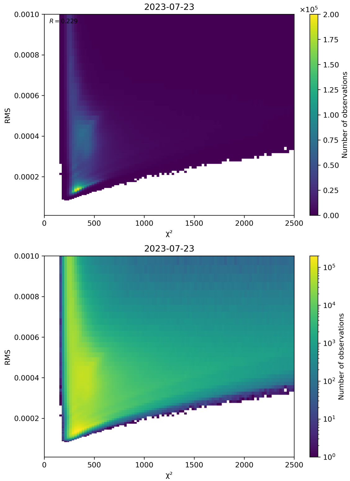
Figure 82: Scatter density plot of “ \chi^2 ” against “RMS” for 2023-07-22 to 2023-07-24.
