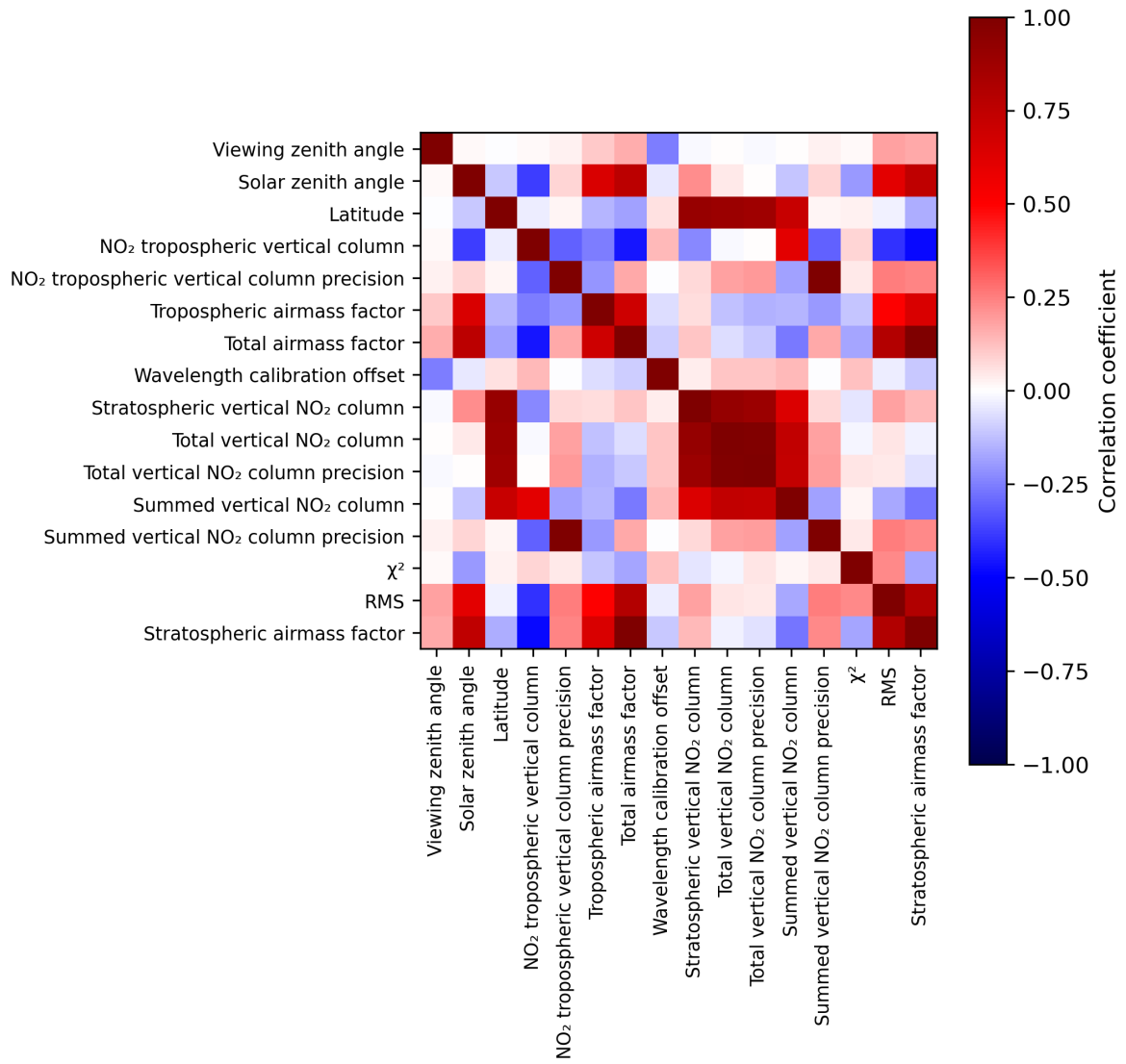
Figure 2: Map of correlation matrix for 2023-07-22 to 2023-07-24.
