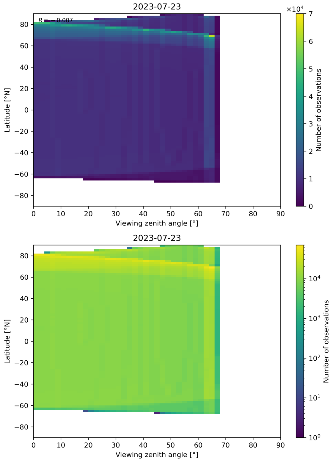
Figure 163: Scatter density plot of “Viewing zenith angle” against “Latitude” for 2023-07-22 to 2023-07-24.
