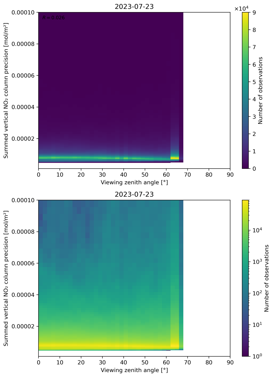
Figure 166: Scatter density plot of “Viewing zenith angle” against “Summed vertical NO 2 column precision” for 2023-07-22 to 2023-07-24.
