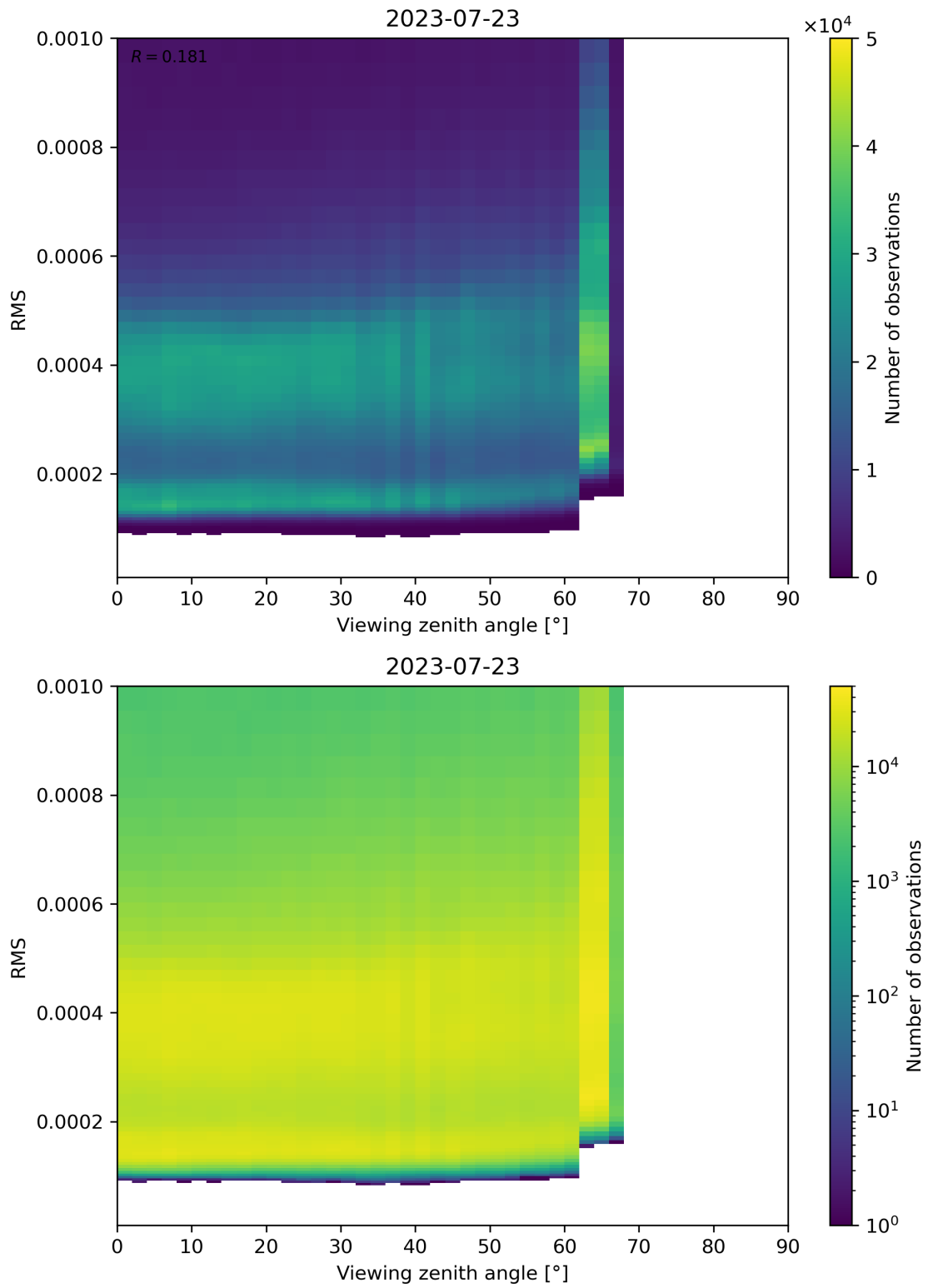
Figure 171: Scatter density plot of “Viewing zenith angle” against “RMS” for 2023-07-22 to 2023-07-24.
