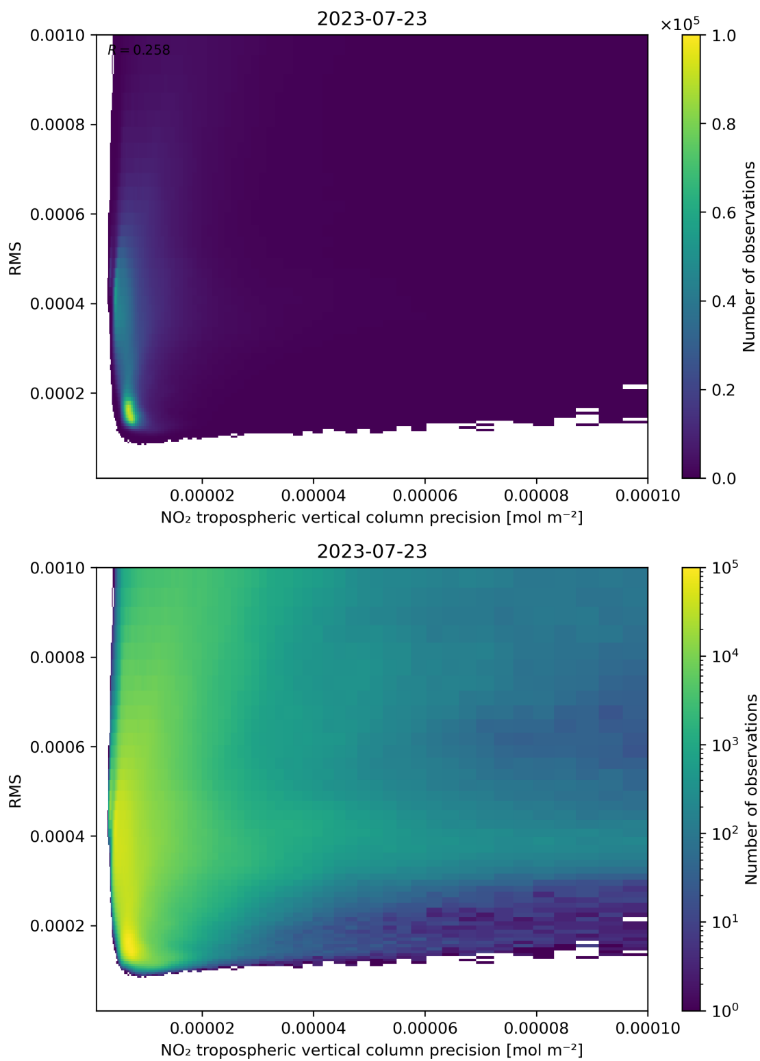
Figure 140: Scatter density plot of “NO 2 tropospheric vertical column precision” against “RMS” for 2023-07-22 to 2023-07-24.
