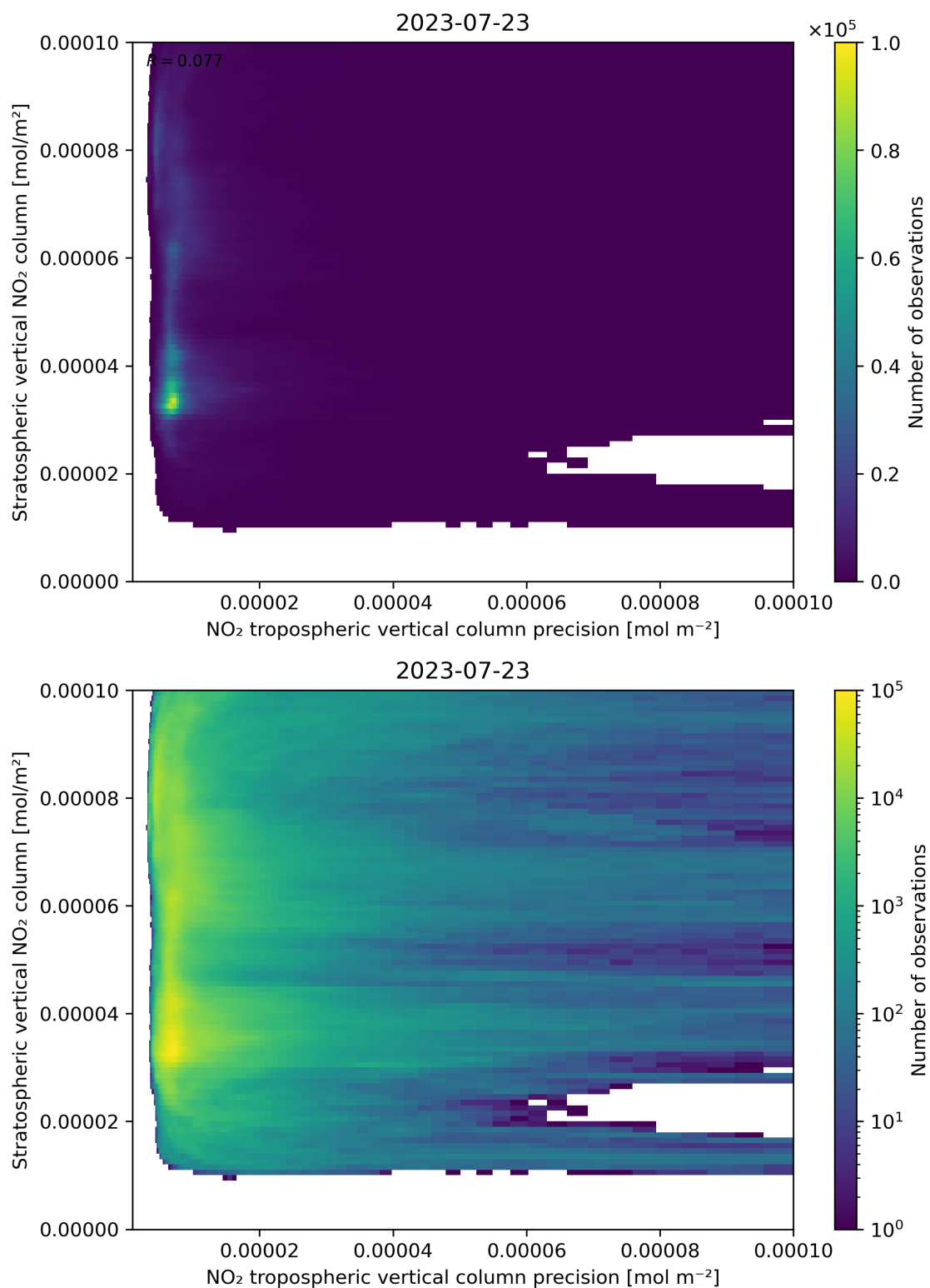
Figure 135: Scatter density plot of “NO 2 tropospheric vertical column precision” against “Stratospheric vertical NO 2 column” for 2023-07-22 to 2023-07-24.
