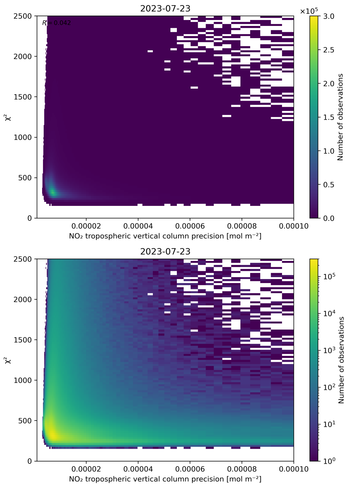
Figure 134: Scatter density plot of “NO 2 tropospheric vertical column precision” against “ \chi^2 ” for 2023-07-22 to 2023-07-24.
