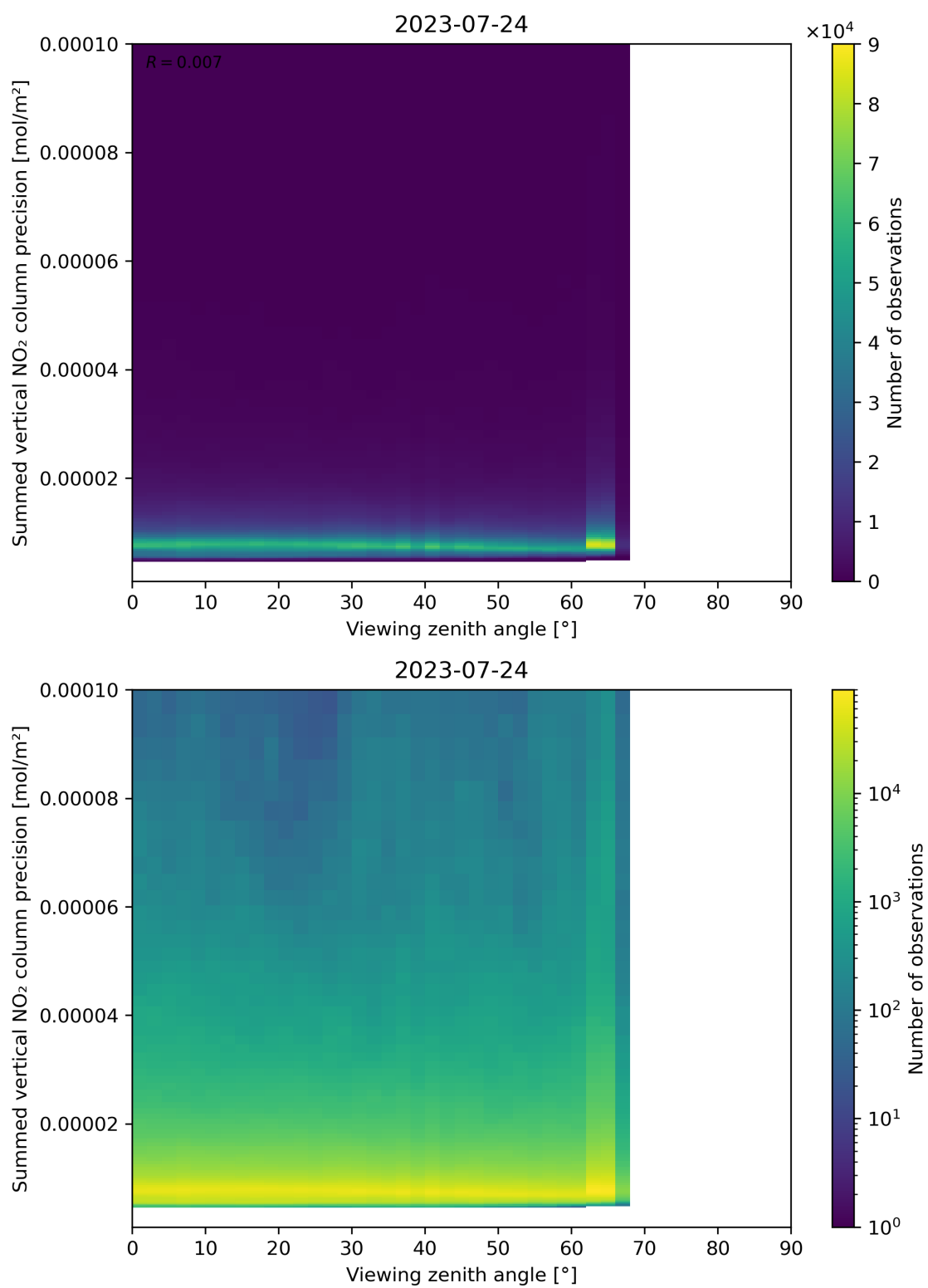
Figure 166: Scatter density plot of “Viewing zenith angle” against “Summed vertical NO 2 column precision” for 2023-07-24 to 2023-07-25.
