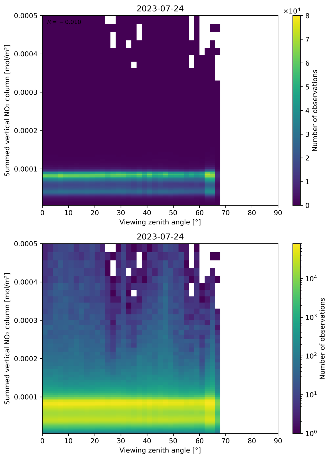
Figure 165: Scatter density plot of “Viewing zenith angle” against “Summed vertical NO 2 column” for 2023-07-24 to 2023-07-25.
