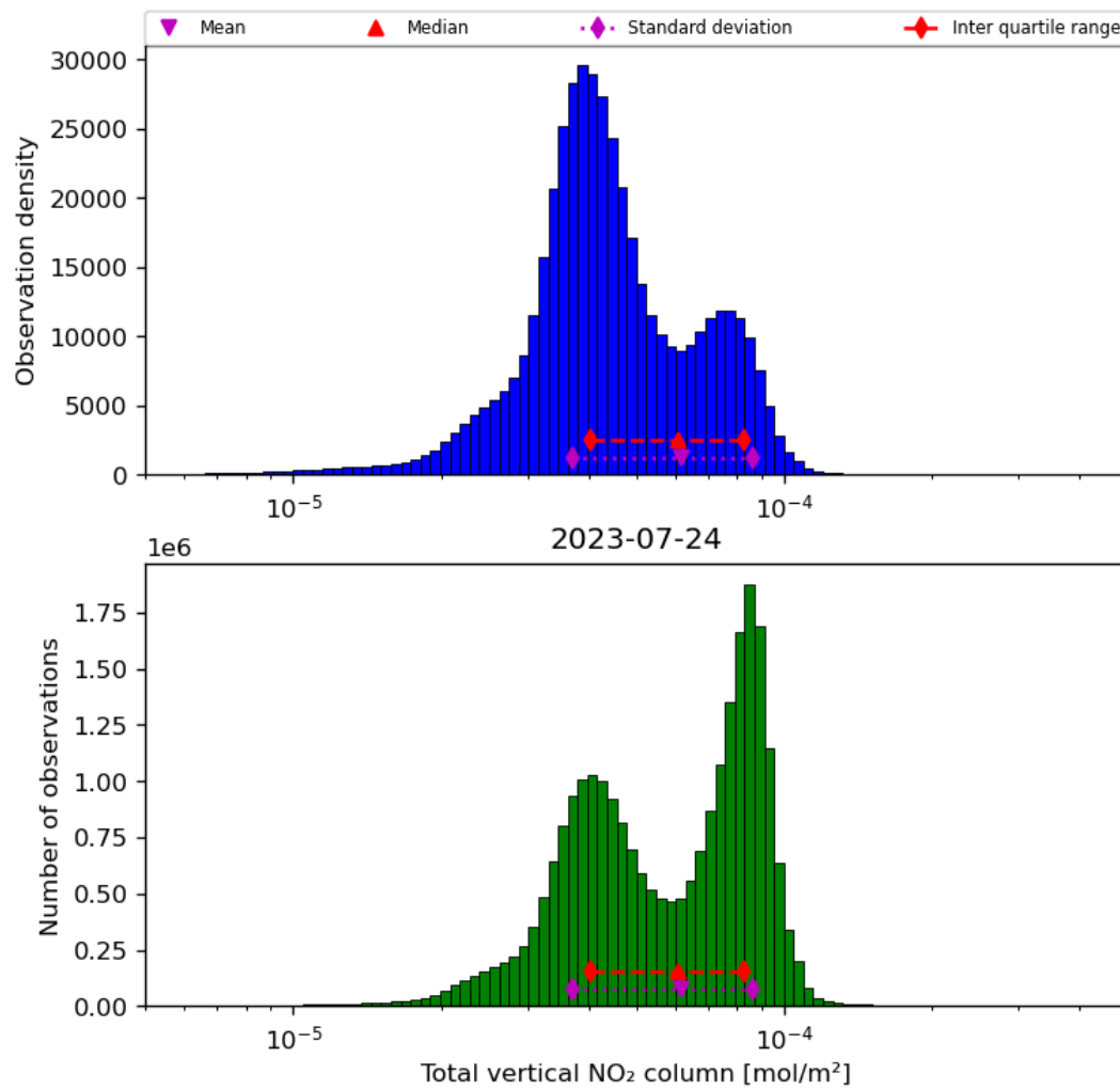
Figure 38: Histogram of “Total vertical NO 2 column” for 2023-07-24 to 2023-07-25
