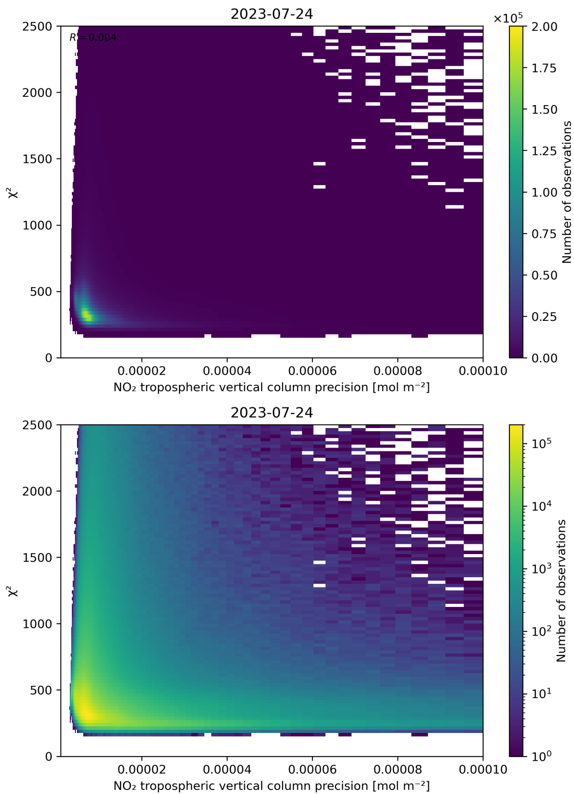
Figure 134: Scatter density plot of “NO 2 tropospheric vertical column precision” against “ \chi^2 ” for 2023-07-24 to 2023-07-25.
