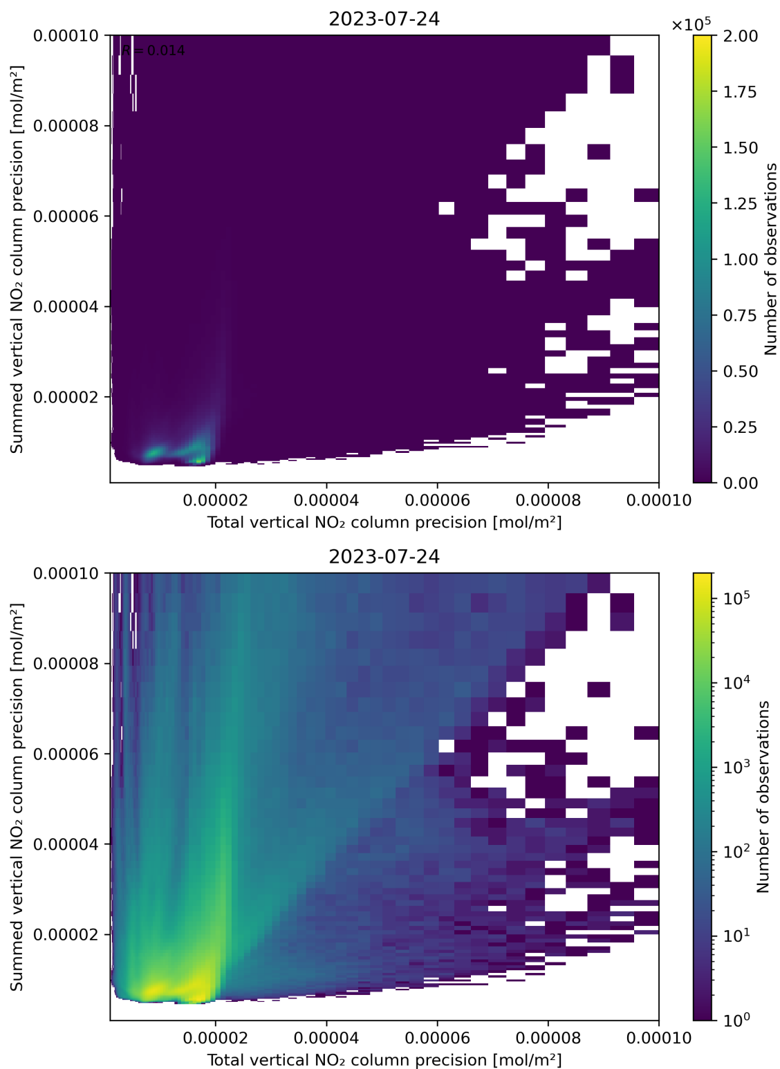
Figure 118: Scatter density plot of “Total vertical NO 2 column precision” against “Summed vertical NO 2 column precision” for 2023-07-24 to 2023-07-25.
