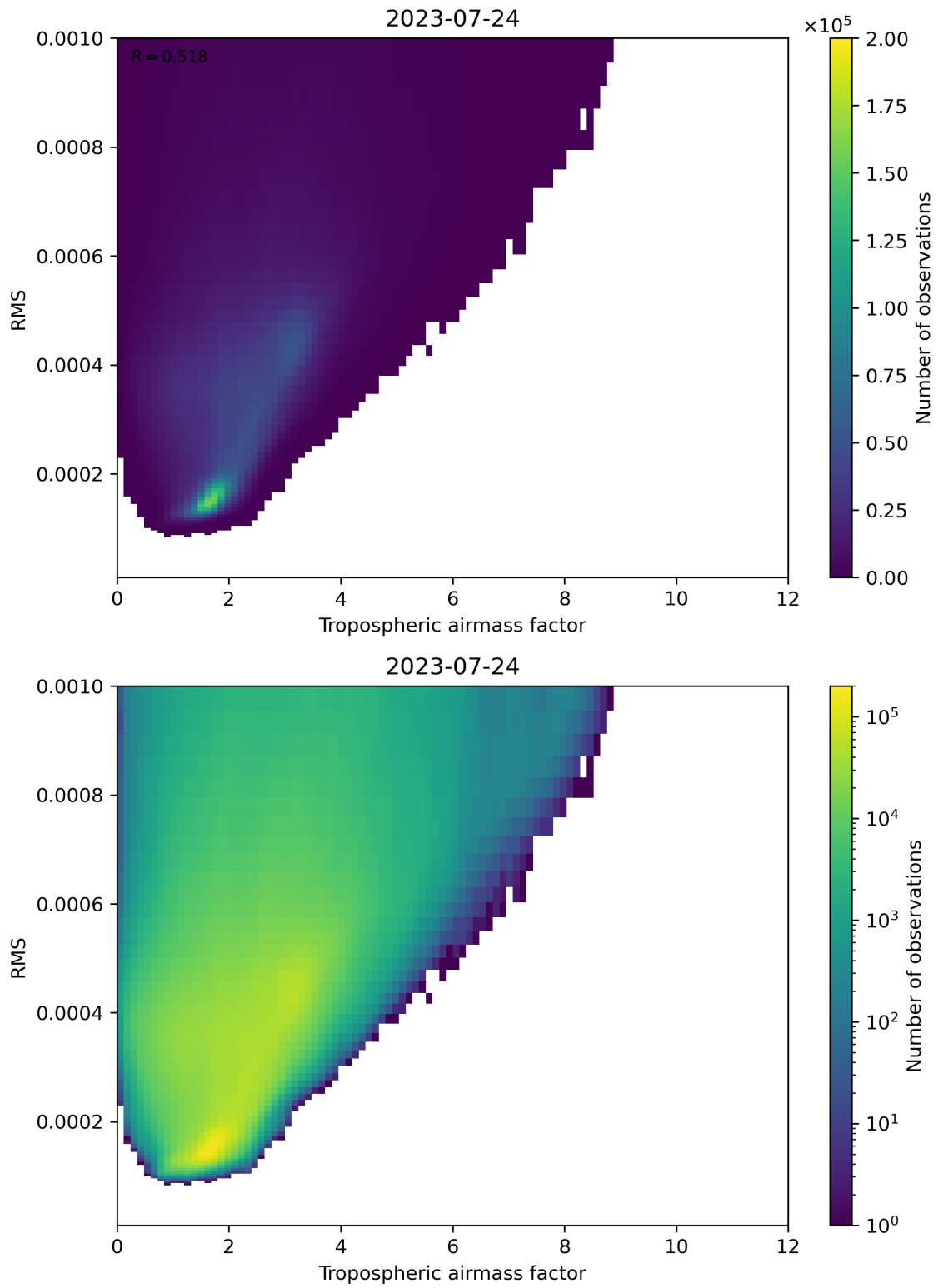
Figure 79: Scatter density plot of “Tropospheric airmass factor” against “RMS” for 2023-07-24 to 2023-07-25.
