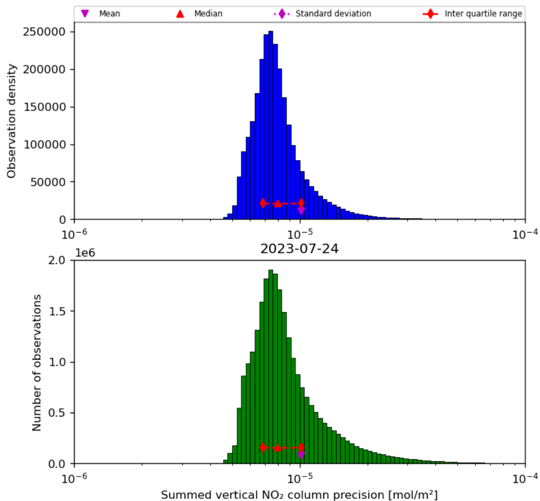
Figure 41: Histogram of “Summed vertical NO 2 column precision” for 2023-07-24 to 2023-07-25
