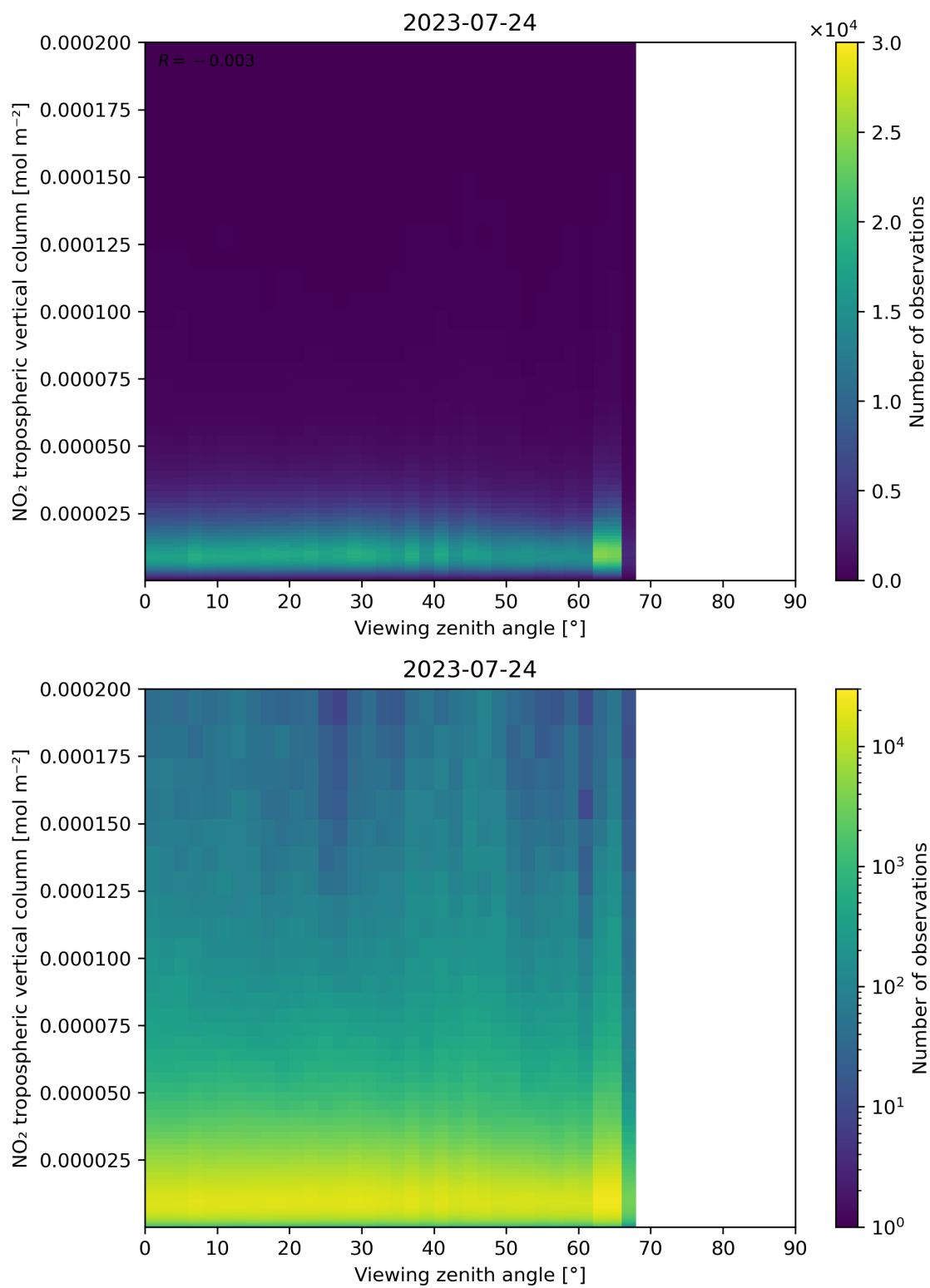
Figure 169: Scatter density plot of “Viewing zenith angle” against “NO 2 tropospheric vertical column” for 2023-07-24 to 2023-07-25.
