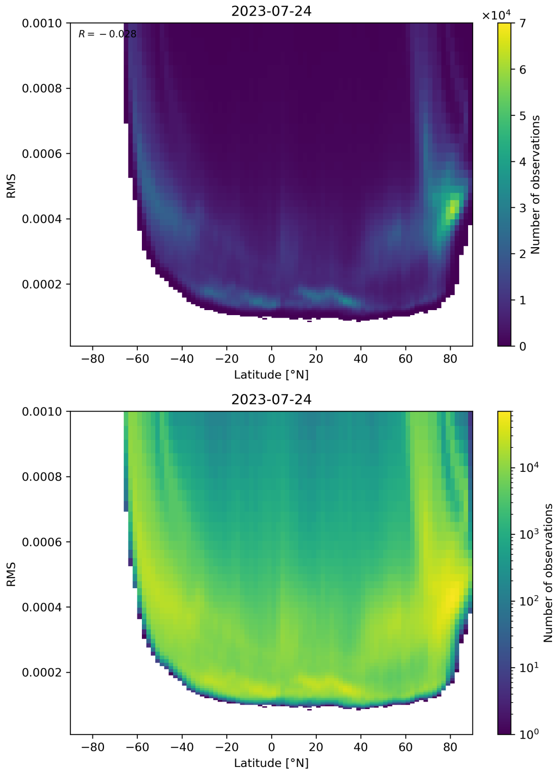
Figure 94: Scatter density plot of “Latitude” against “RMS” for 2023-07-24 to 2023-07-25.
