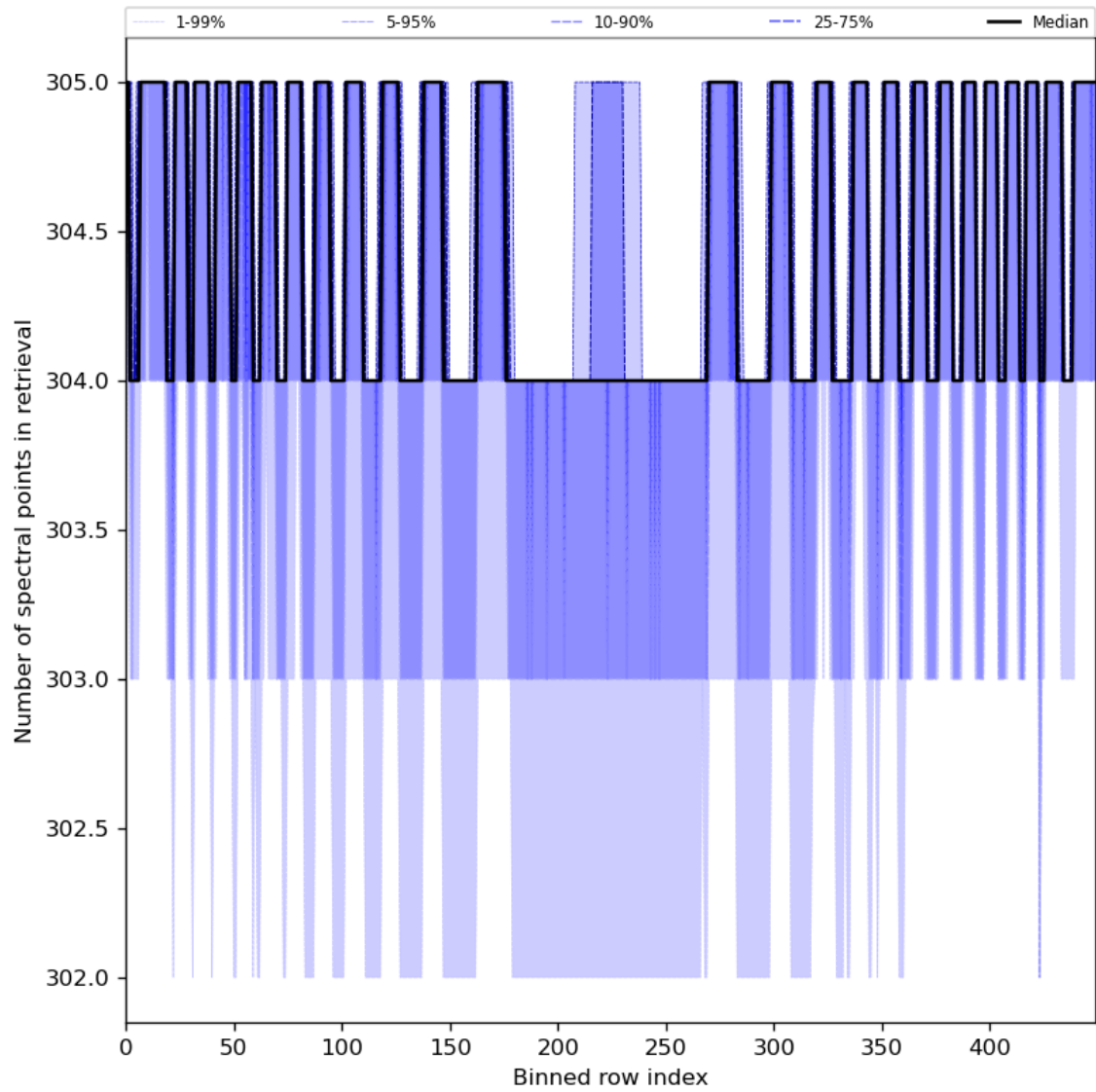
Figure 50: Along track statistics of “Number of spectral points in retrieval” for 2023-07-24 to 2023-07-25
