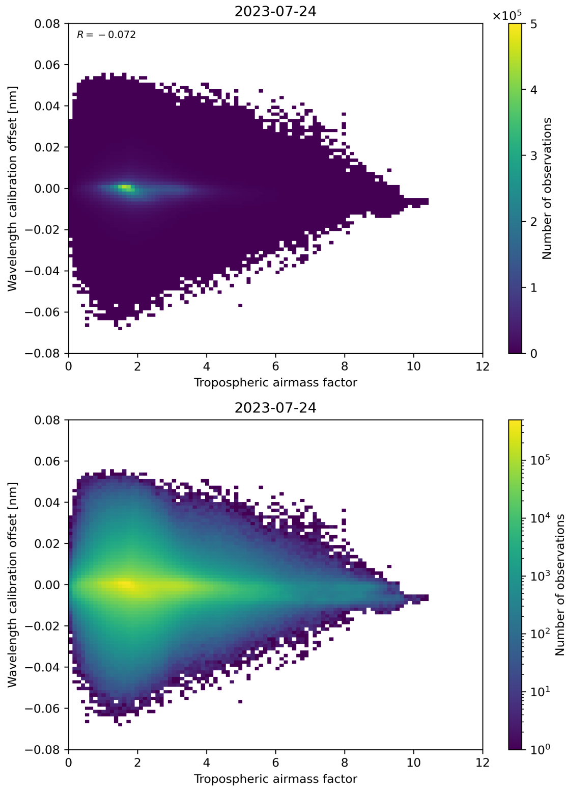
Figure 80: Scatter density plot of “Tropospheric air mass factor” against “Wavelength calibration offset” for 2023-07-24 to 2023-07-25.
