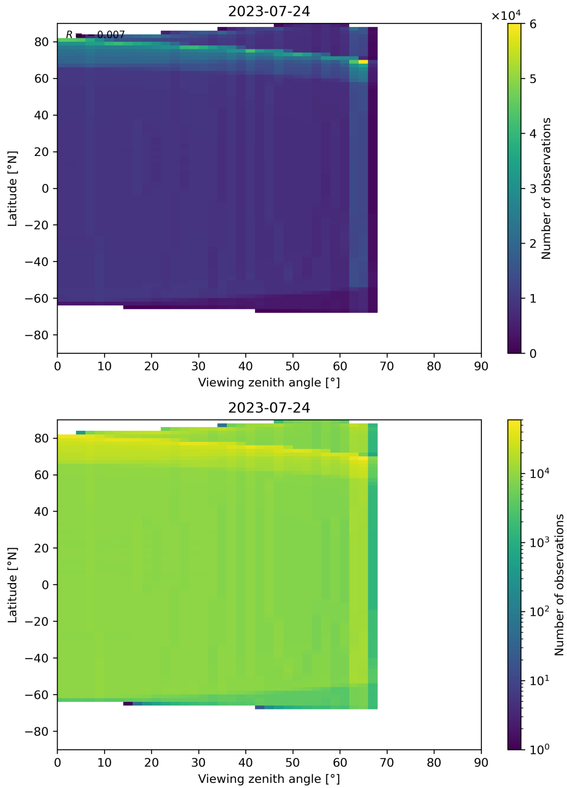
Figure 163: Scatter density plot of “Viewing zenith angle” against “Latitude” for 2023-07-24 to 2023-07-25.
