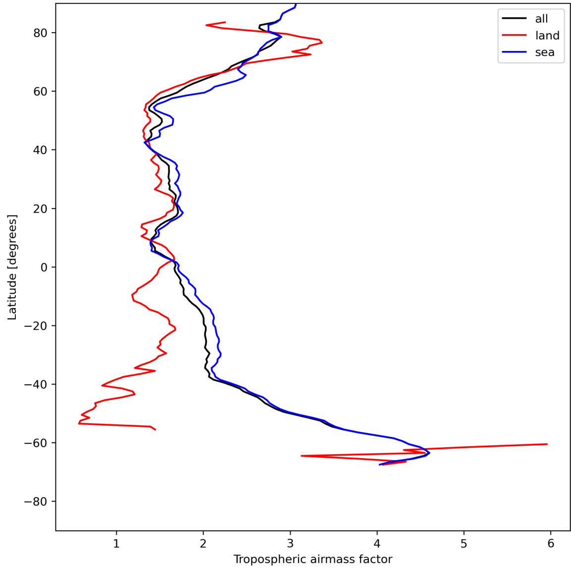
Figure 14: Zonal average of “Tropospheric air mass factor” for 2023-07-24 to 2023-07-25.
