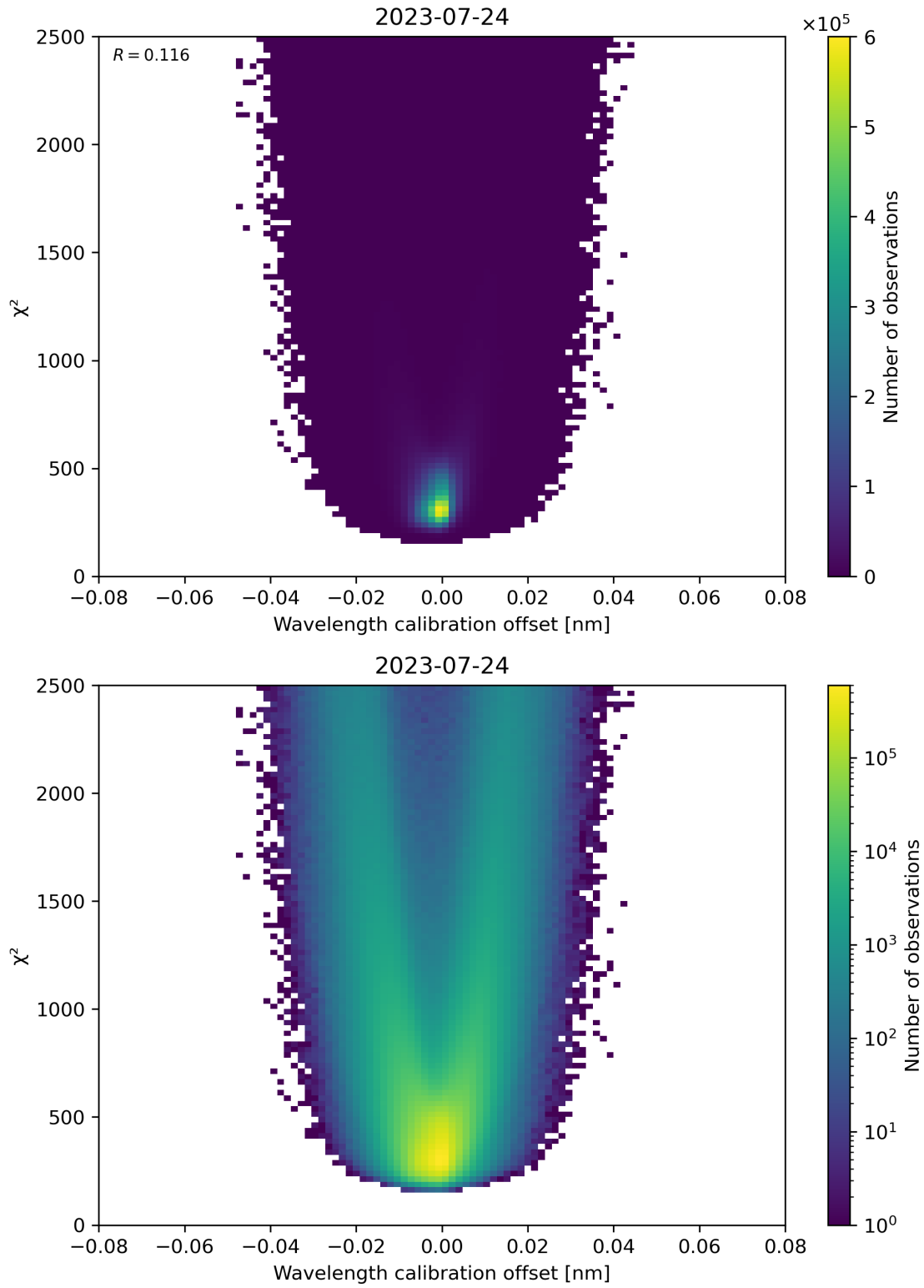
Figure 175: Scatter density plot of “Wavelength calibration offset” against “ \chi^2 ” for 2023-07-24 to 2023-07-25.
