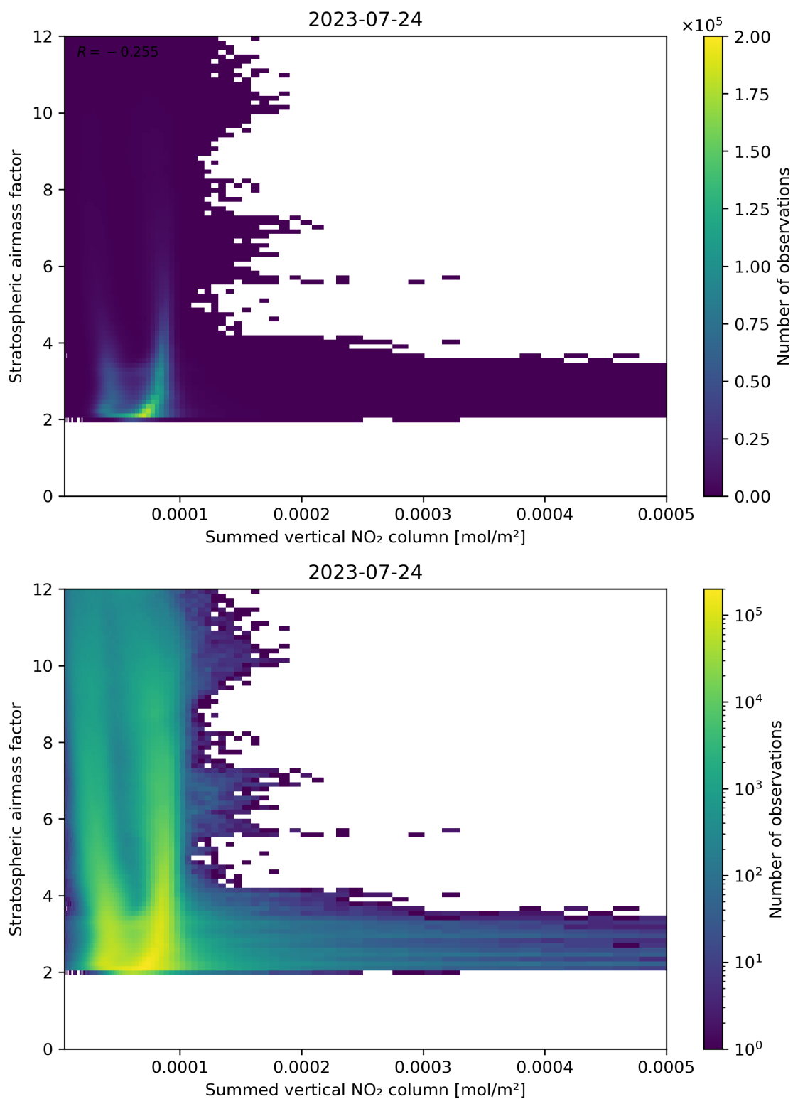
Figure 103: Scatter density plot of “Summed vertical NO 2 column” against “Stratospheric air mass factor” for 2023-07-24 to 2023-07-25.
