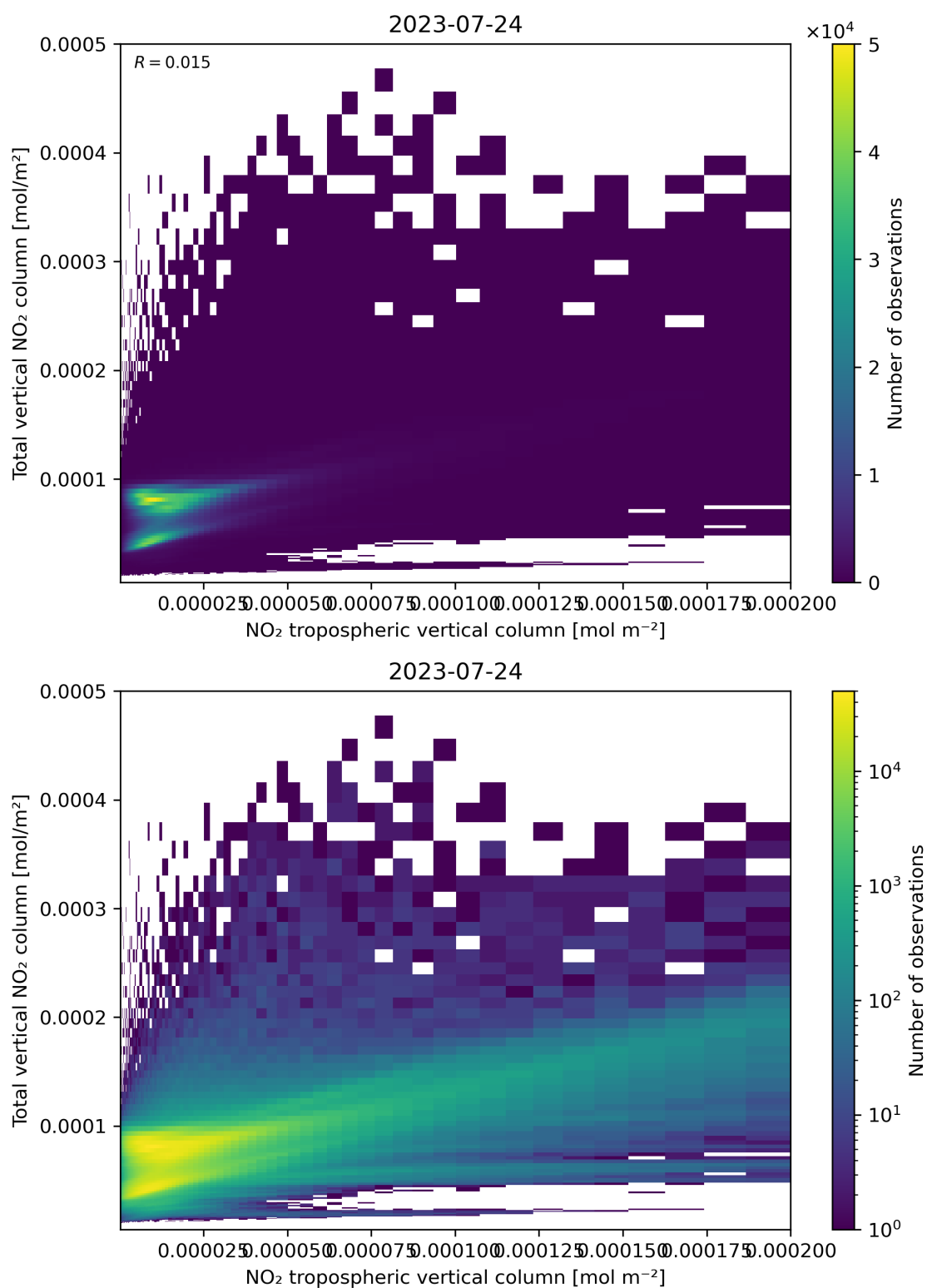
Figure 128: Scatter density plot of “NO 2 tropospheric vertical column” against “Total vertical NO 2 column” for 2023-07-24 to 2023-07-25.
