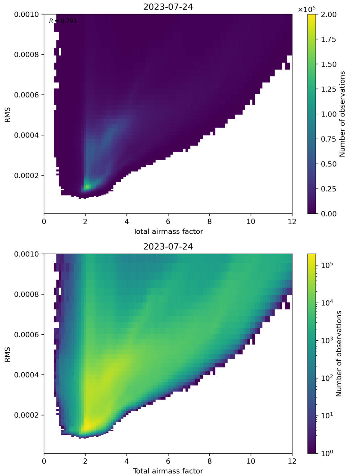
Figure 69: Scatter density plot of “Total airmass factor” against “RMS” for 2023-07-24 to 2023-07-25.
