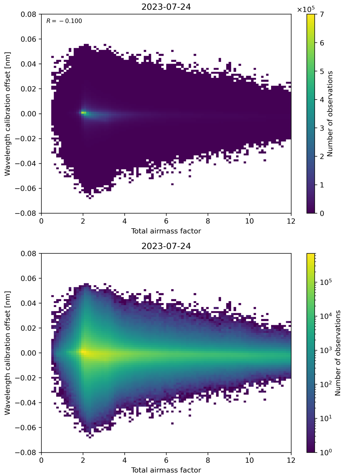
Figure 70: Scatter density plot of “Total airmass factor” against “Wavelength calibration offset” for 2023-07-24 to 2023-07-25.
