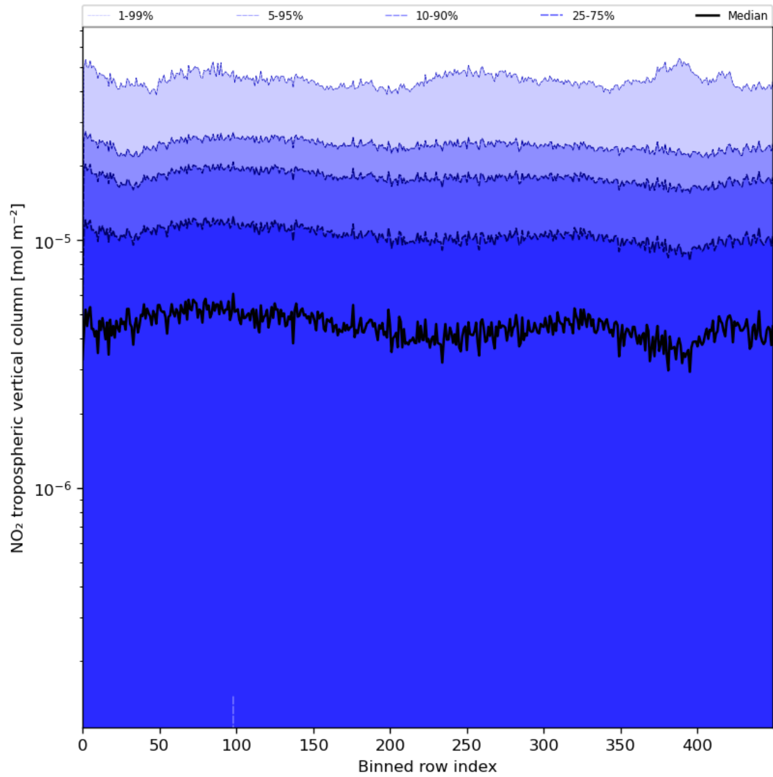
Figure 46: Along track statistics of “NO 2 tropospheric vertical column” for 2023-07-24 to 2023-07-25
