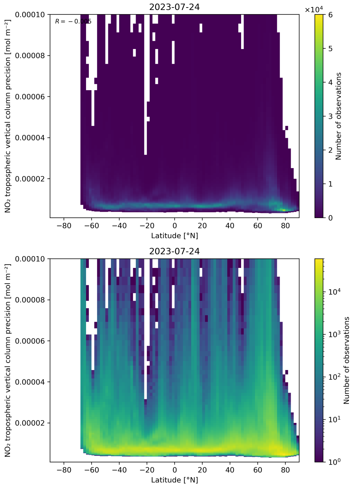
Figure 93: Scatter density plot of “Latitude” against “NO 2 tropospheric vertical column precision” for 2023-07-24 to 2023-07-25.
