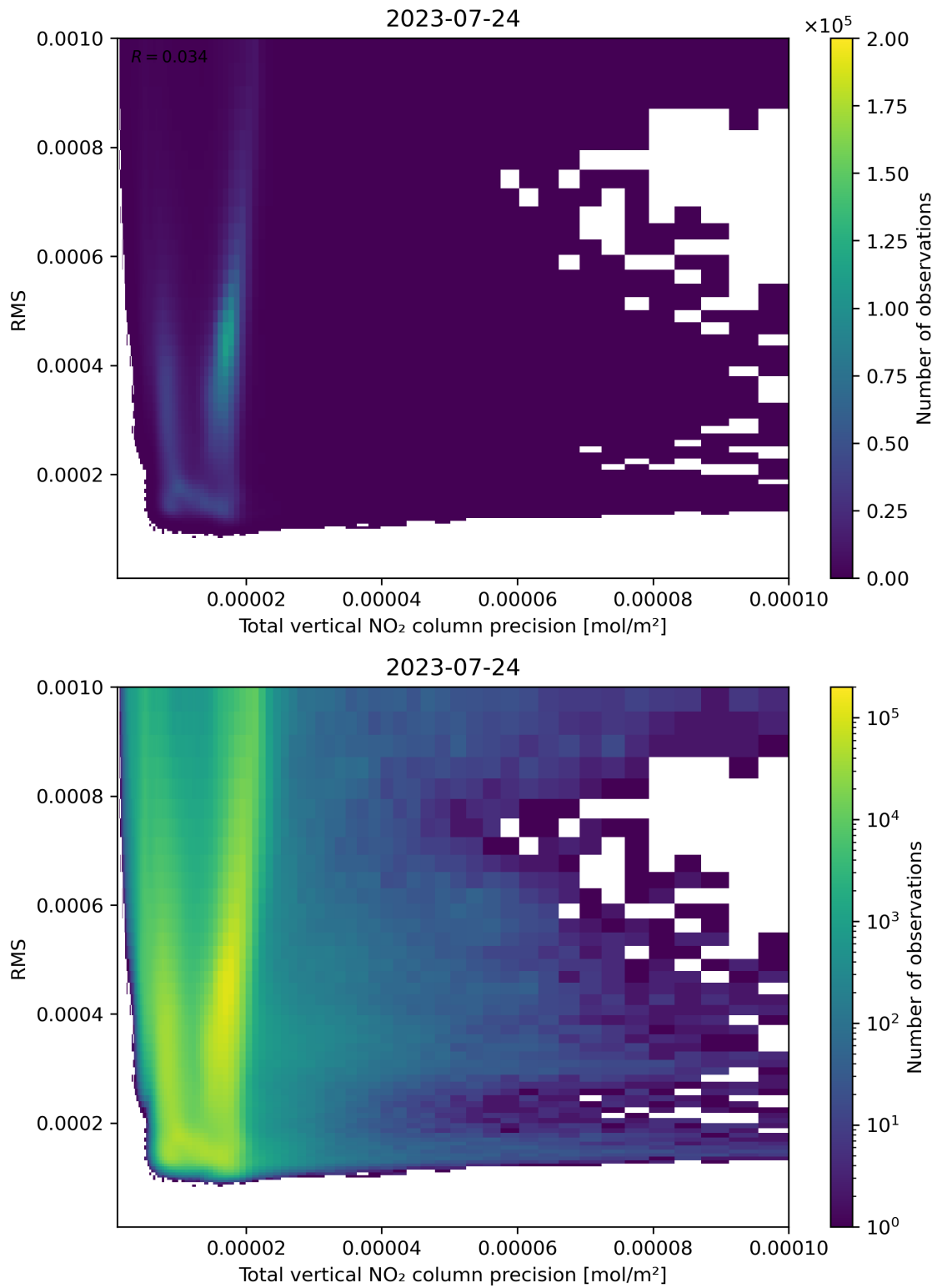
Figure 119: Scatter density plot of “Total vertical NO 2 column precision” against “RMS” for 2023-07-24 to 2023-07-25.
