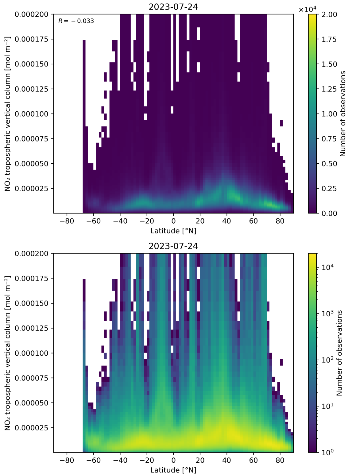
Figure 92: Scatter density plot of “Latitude” against “NO 2 tropospheric vertical column” for 2023-07-24 to 2023-07-25.
