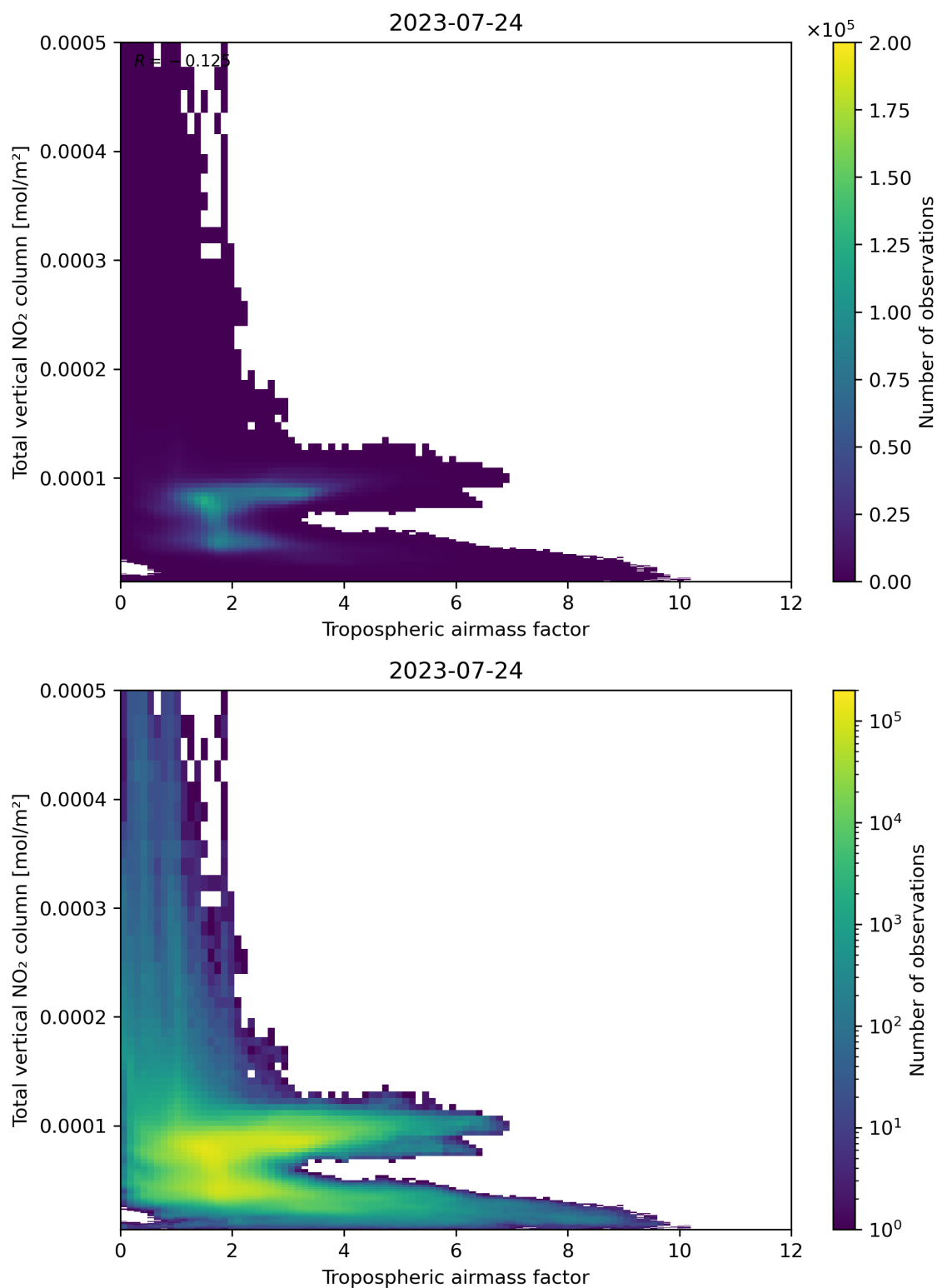
Figure 77: Scatter density plot of “Tropospheric airmass factor” against “Total vertical NO 2 column” for 2023-07-24 to 2023-07-25.
