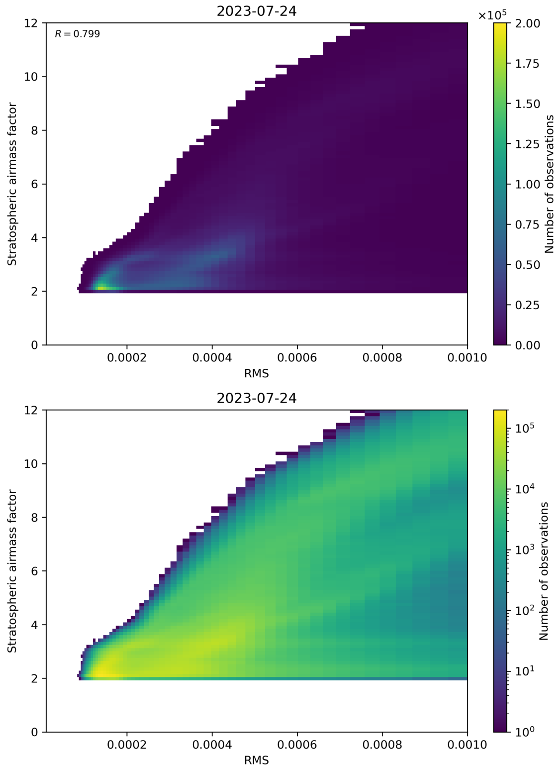
Figure 144: Scatter density plot of “RMS” against “Stratospheric airmass factor” for 2023-07-24 to 2023-07-25.
