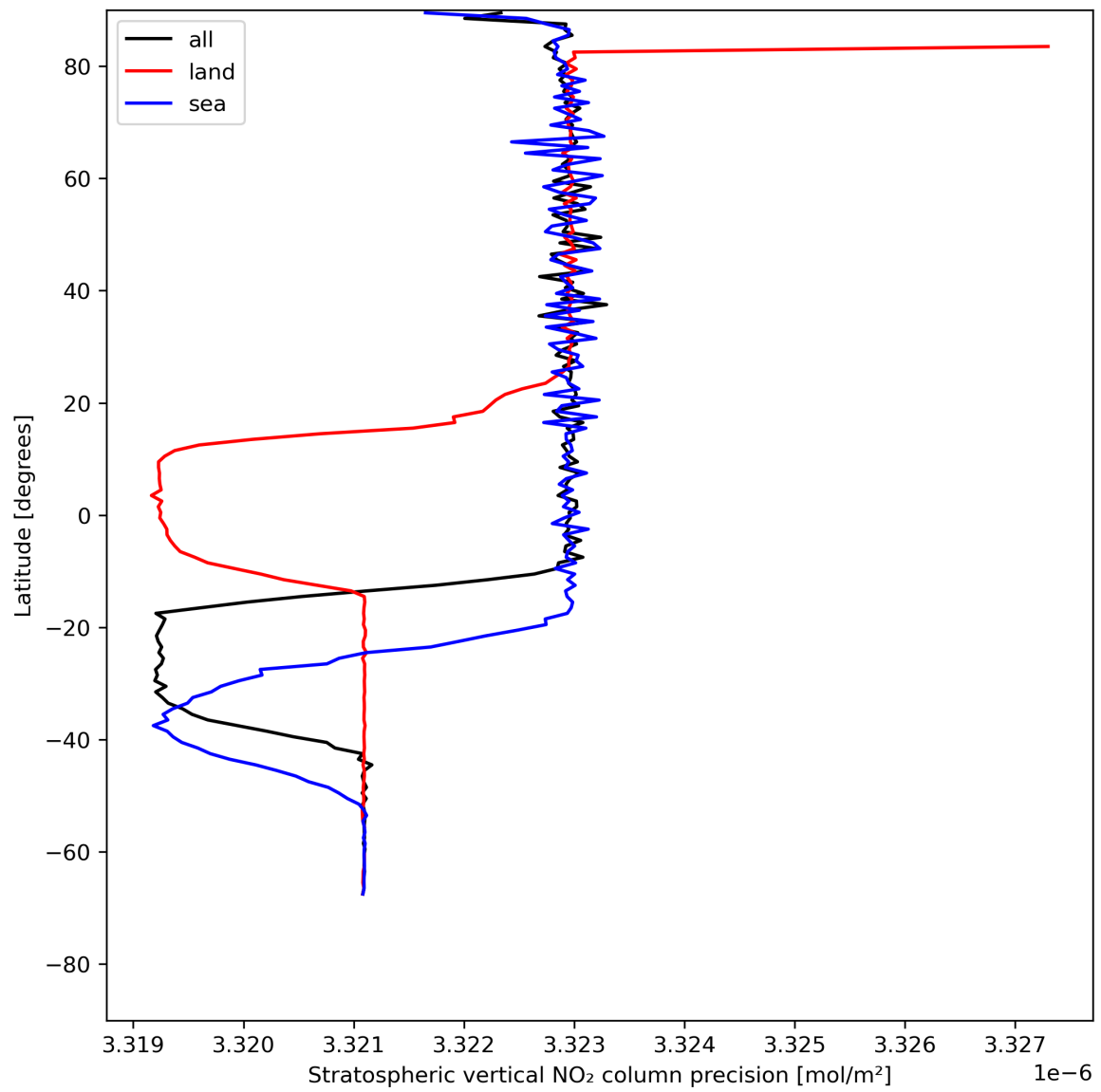
Figure 20: Zonal average of “Stratospheric vertical NO 2 column precision” for 2023-07-24 to 2023-07-25.
