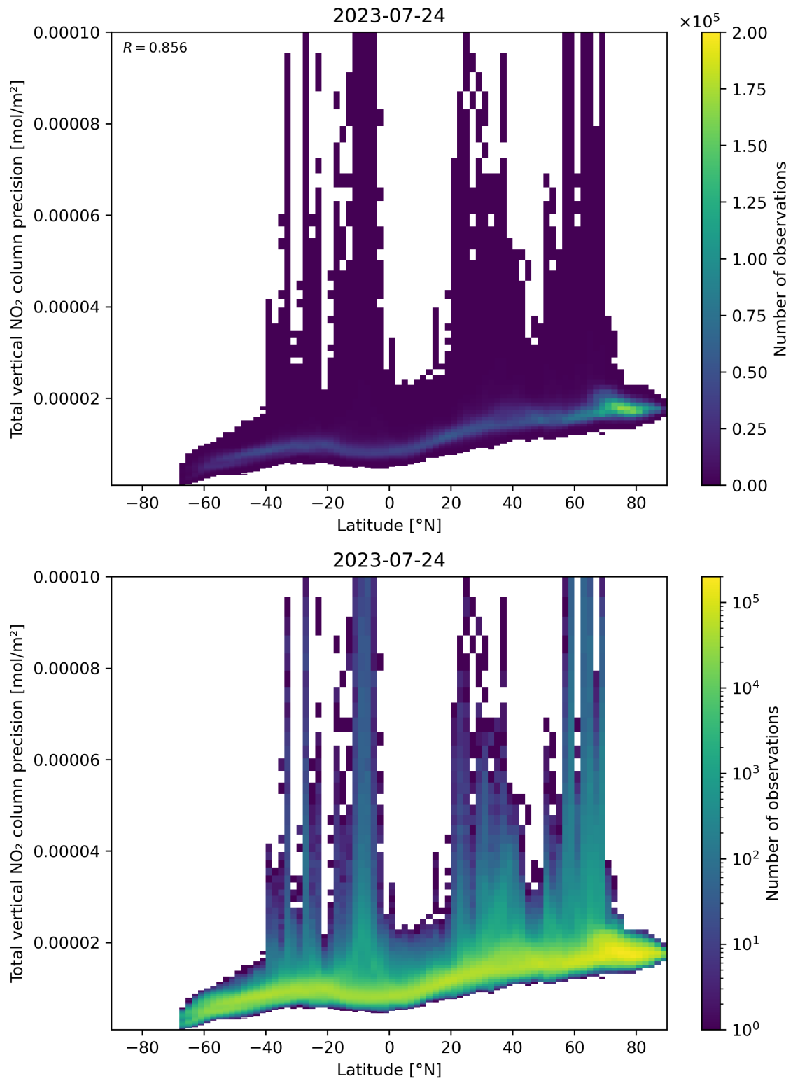
Figure 91: Scatter density plot of “Latitude” against “Total vertical NO 2 column precision” for 2023-07-24 to 2023-07-25.
