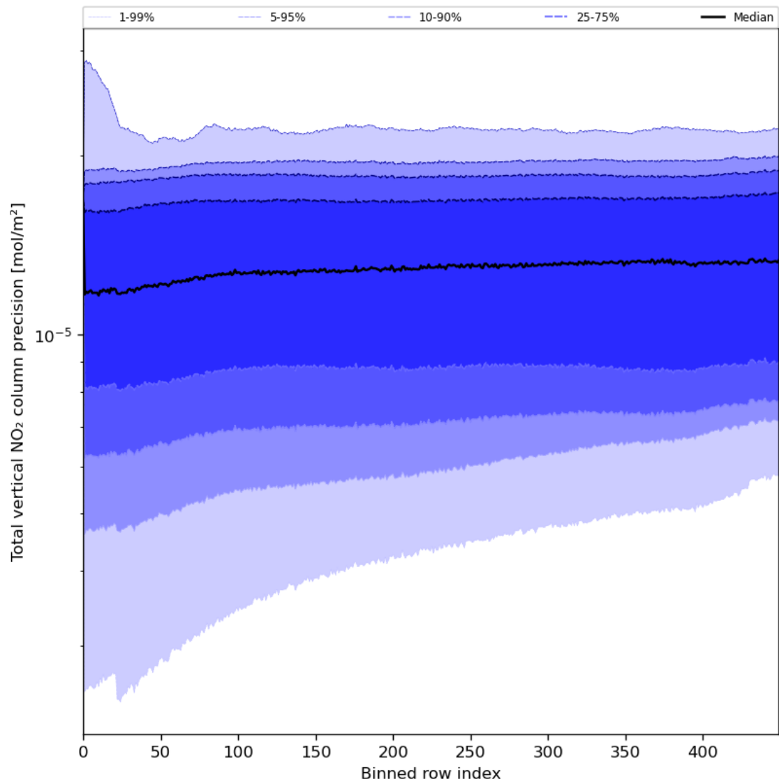
Figure 56: Along track statistics of “Total vertical NO 2 column precision” for 2023-07-24 to 2023-07-25
