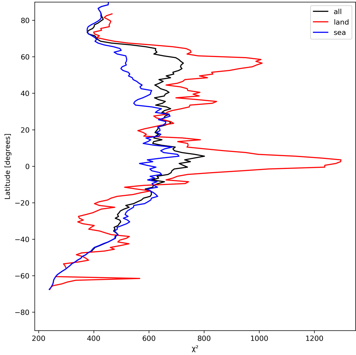
Figure 25: Zonal average of “ \chi^2 ” for 2023-07-24 to 2023-07-25.
