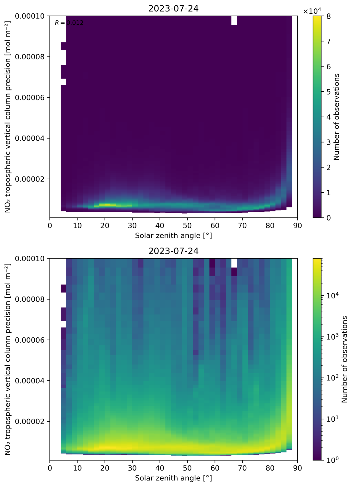
Figure 156: Scatter density plot of “Solar zenith angle” against “NO 2 tropospheric vertical column precision” for 2023-07-24 to 2023-07-25.
