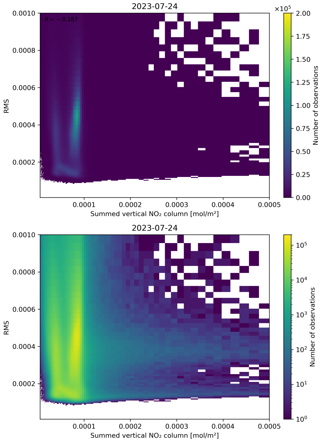
Figure 109: Scatter density plot of “Summed vertical NO 2 column” against “RMS” for 2023-07-24 to 2023-07-25.
