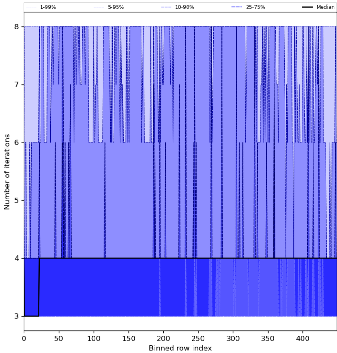
Figure 51: Along track statistics of “Number of iterations” for 2023-07-24 to 2023-07-25
