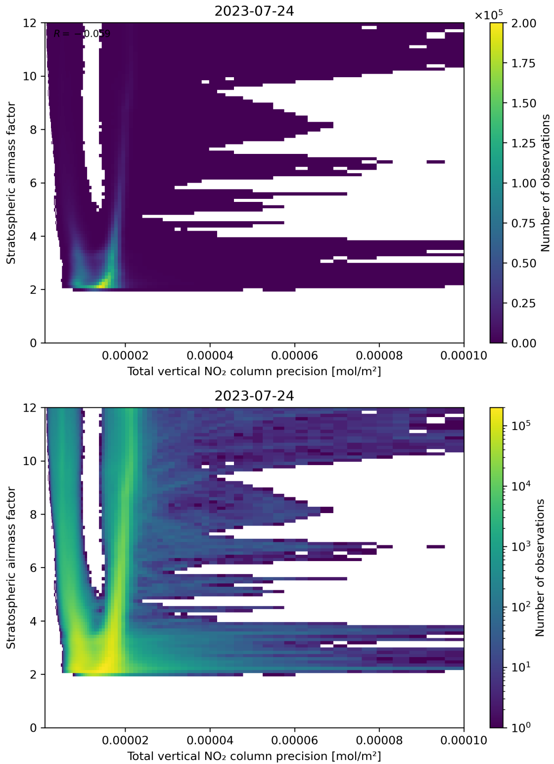
Figure 115: Scatter density plot of “Total vertical NO 2 column precision” against “Stratospheric air mass factor” for 2023-07-24 to 2023-07-25.
