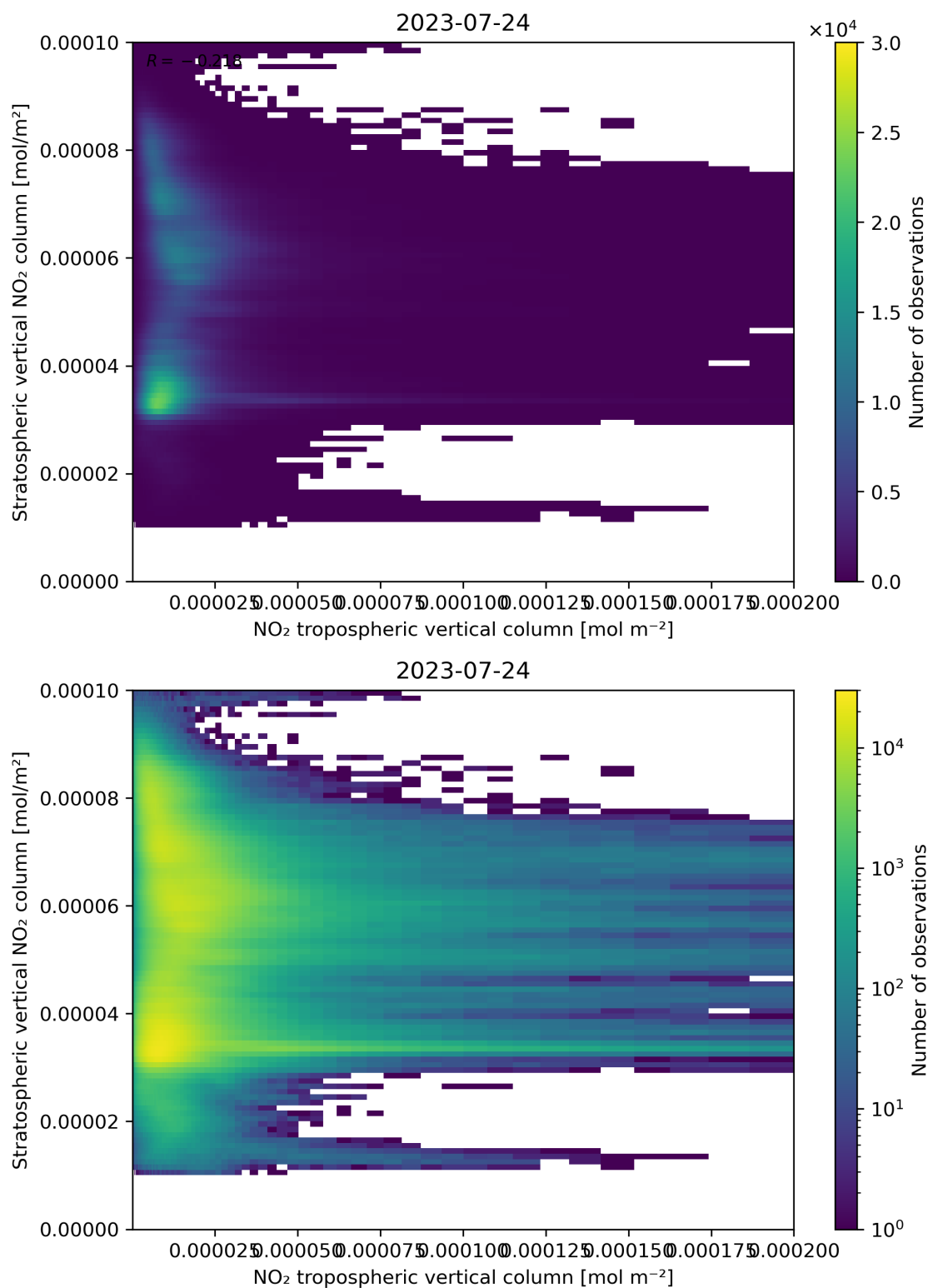
Figure 125: Scatter density plot of “NO 2 tropospheric vertical column” against “Stratospheric vertical NO 2 column” for 2023-07-24 to 2023-07-25.
