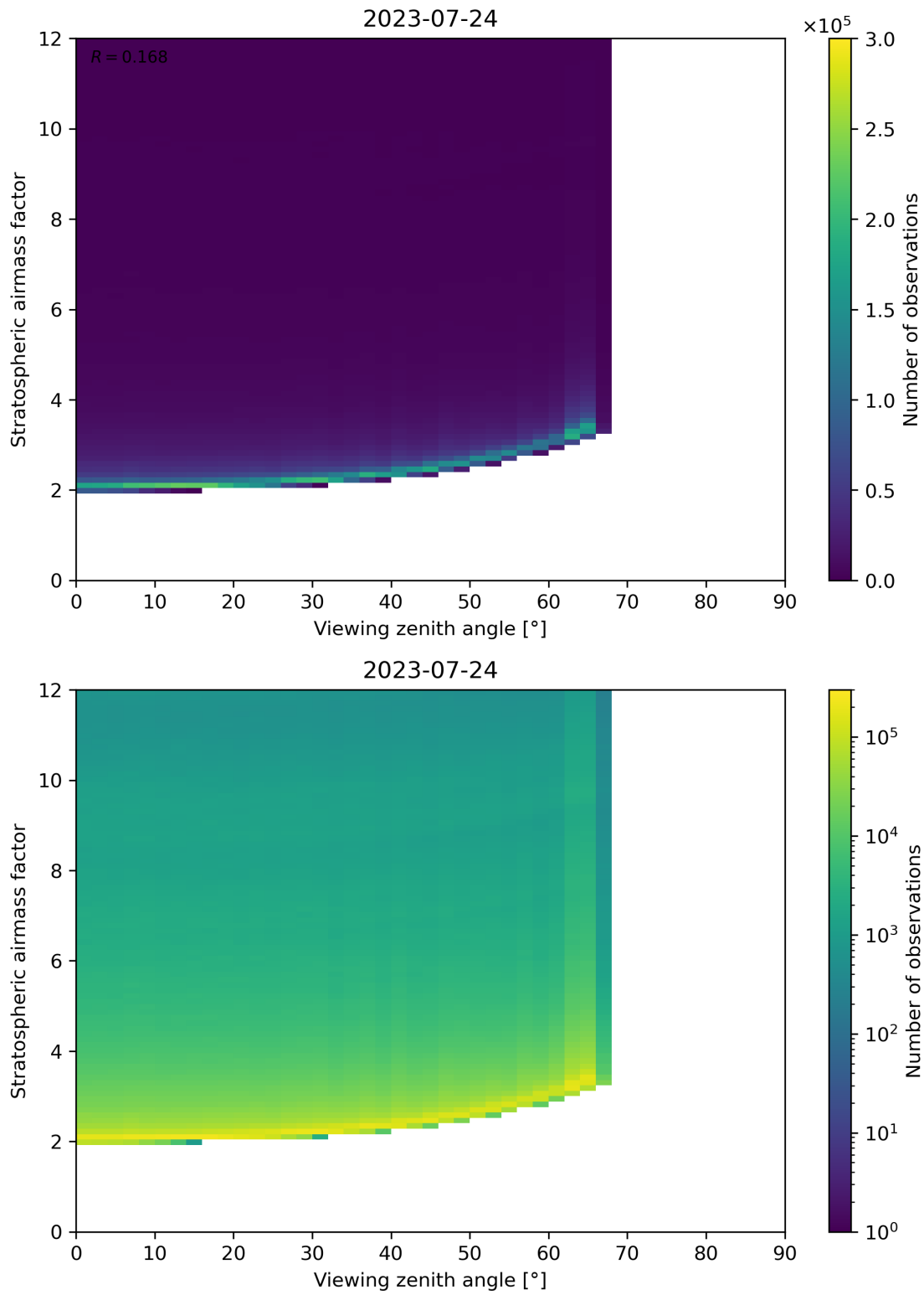
Figure 159: Scatter density plot of “Viewing zenith angle” against “Stratospheric airmass factor” for 2023-07-24 to 2023-07-25.
