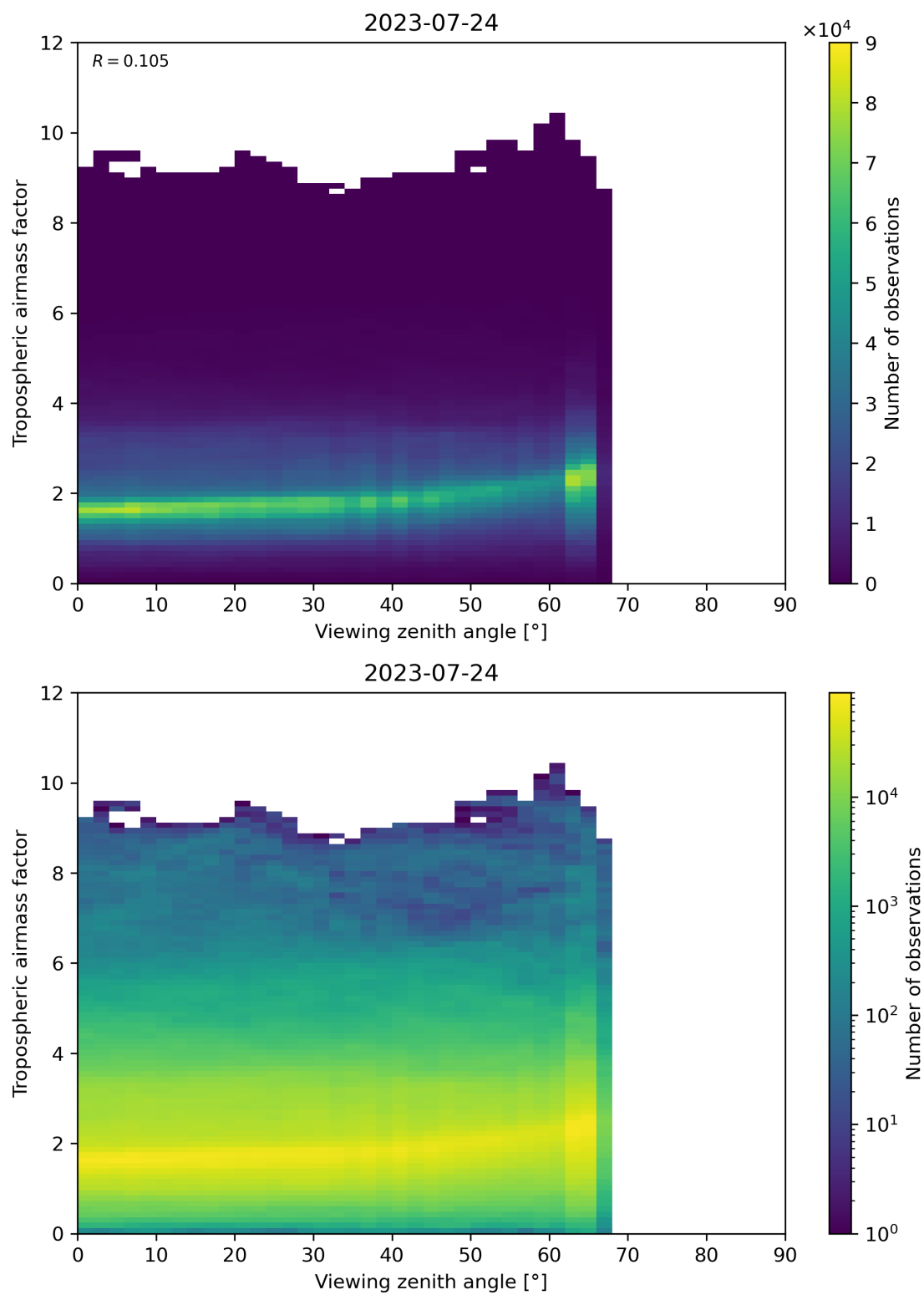
Figure 161: Scatter density plot of “Viewing zenith angle” against “Tropospheric airmass factor” for 2023-07-24 to 2023-07-25.
