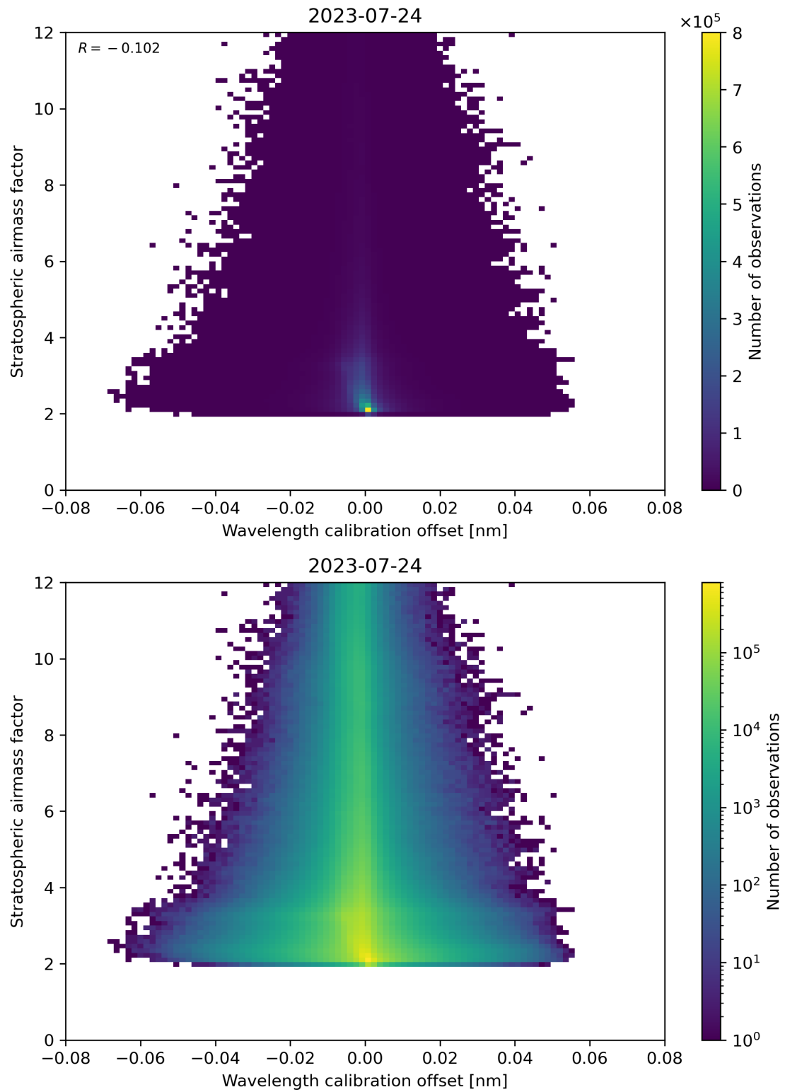
Figure 174: Scatter density plot of “Wavelength calibration offset” against “Stratospheric air mass factor” for 2023-07-24 to 2023-07-25.
