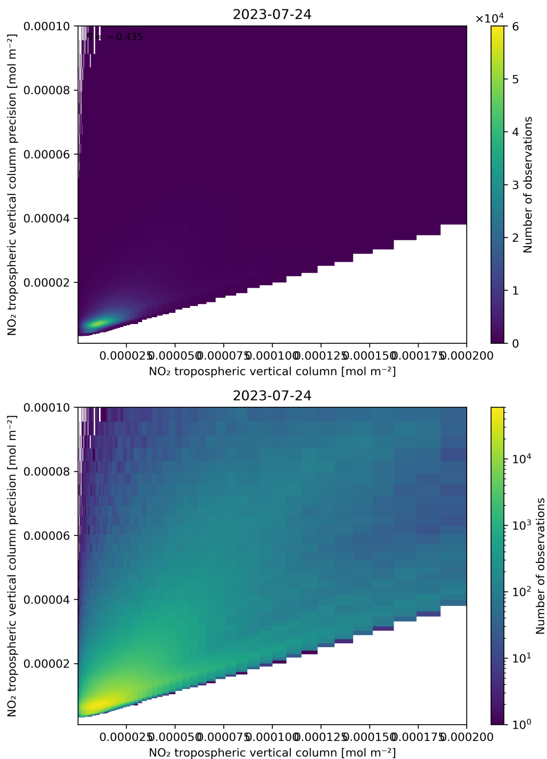
Figure 130: Scatter density plot of “NO 2 tropospheric vertical column” against “NO 2 tropospheric vertical column precision” for 2023-07-24 to 2023-07-25.
