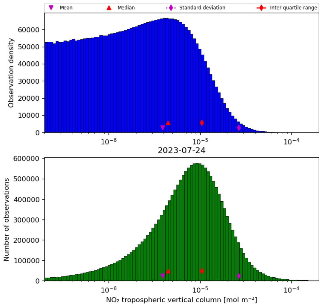
Figure 29: Histogram of “NO 2 tropospheric vertical column” for 2023-07-24 to 2023-07-25
