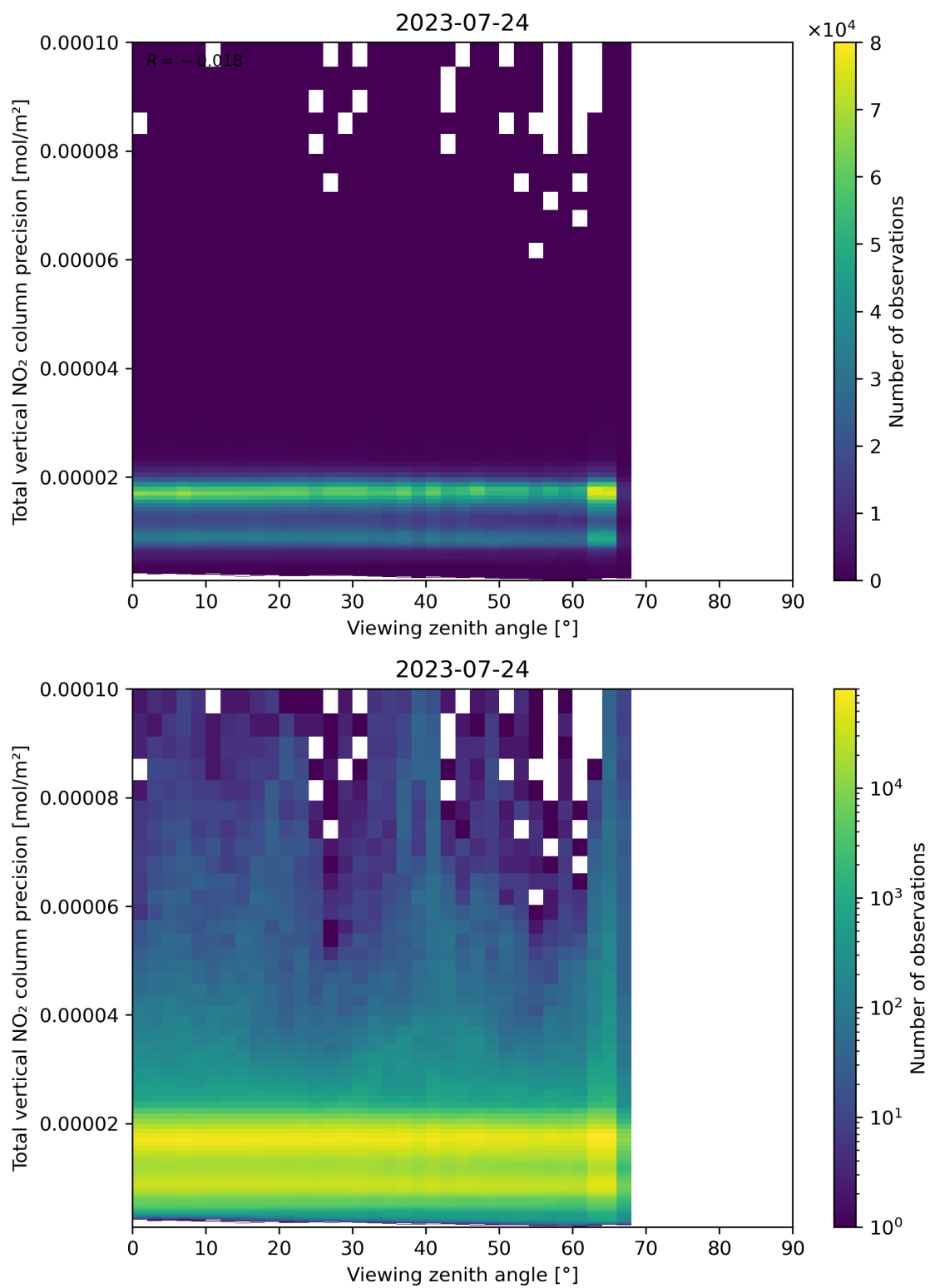
Figure 168: Scatter density plot of “Viewing zenith angle” against “Total vertical NO 2 column precision” for 2023-07-24 to 2023-07-25.
