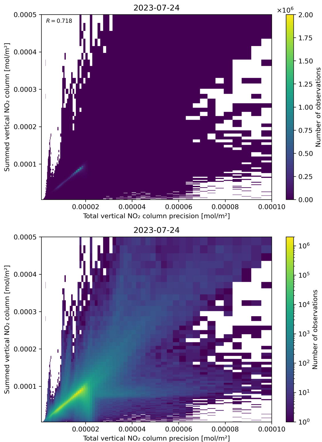
Figure 117: Scatter density plot of “Total vertical NO 2 column precision” against “Summed vertical NO 2 column” for 2023-07-24 to 2023-07-25.
