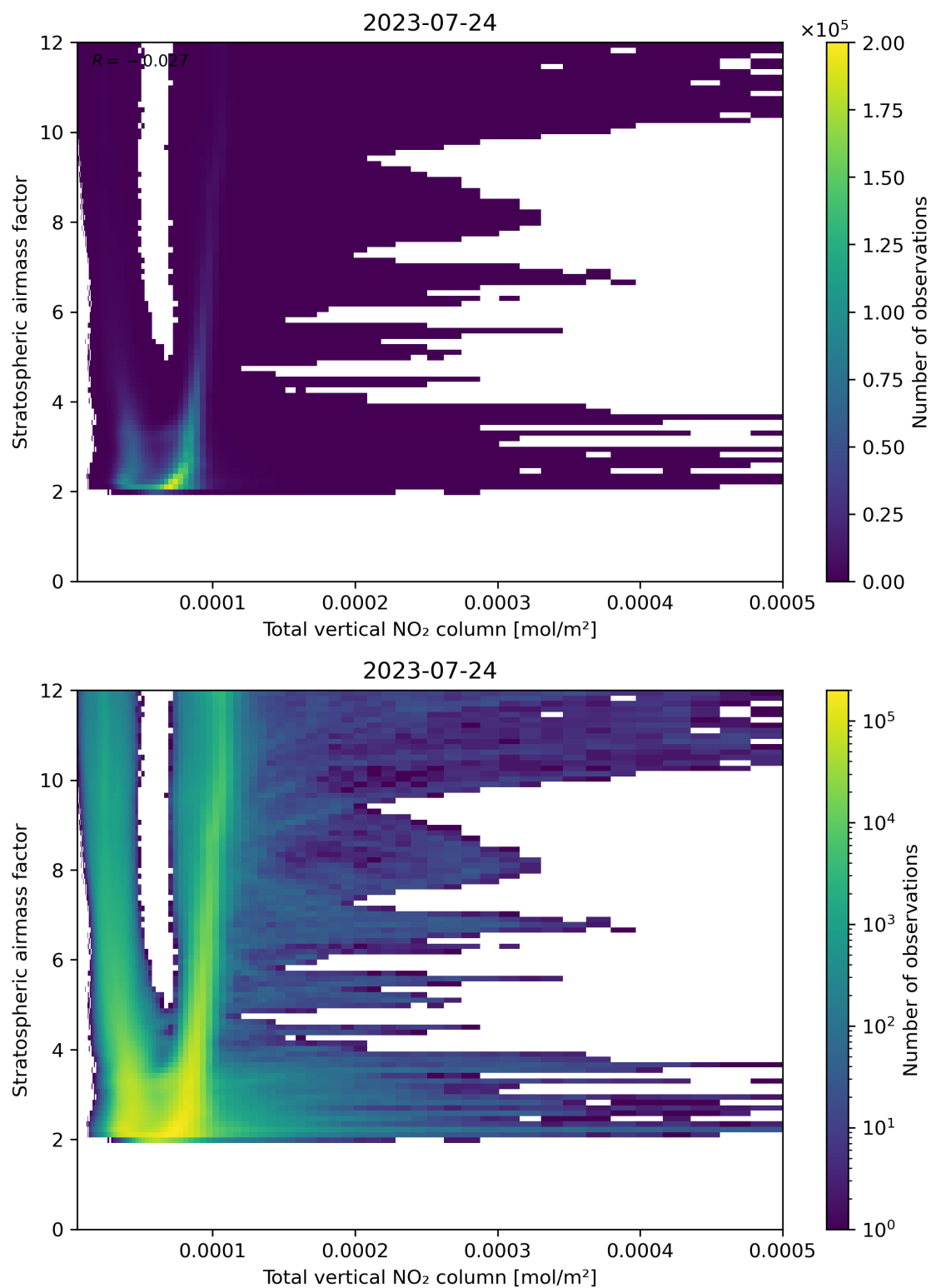
Figure 110: Scatter density plot of “Total vertical NO 2 column” against “Stratospheric airmass factor” for 2023-07-24 to 2023-07-25.
