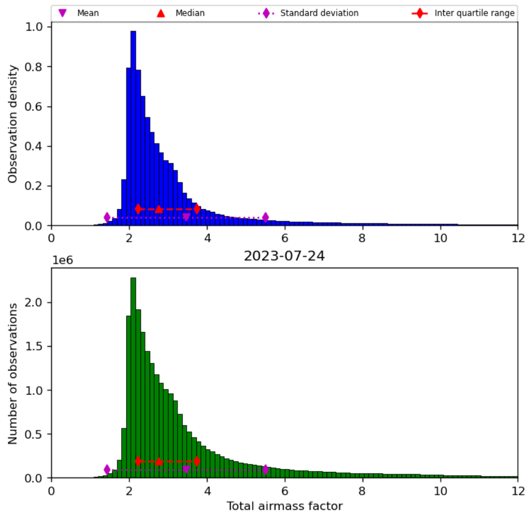
Figure 32: Histogram of “Total airmass factor” for 2023-07-24 to 2023-07-25
