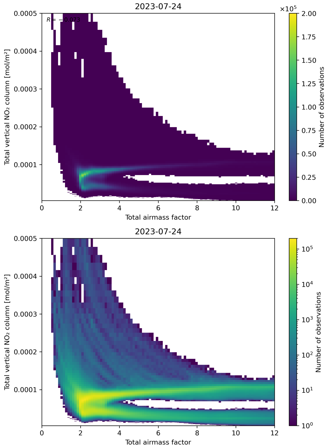
Figure 67: Scatter density plot of “Total airmass factor” against “Total vertical NO 2 column” for 2023-07-24 to 2023-07-25.
