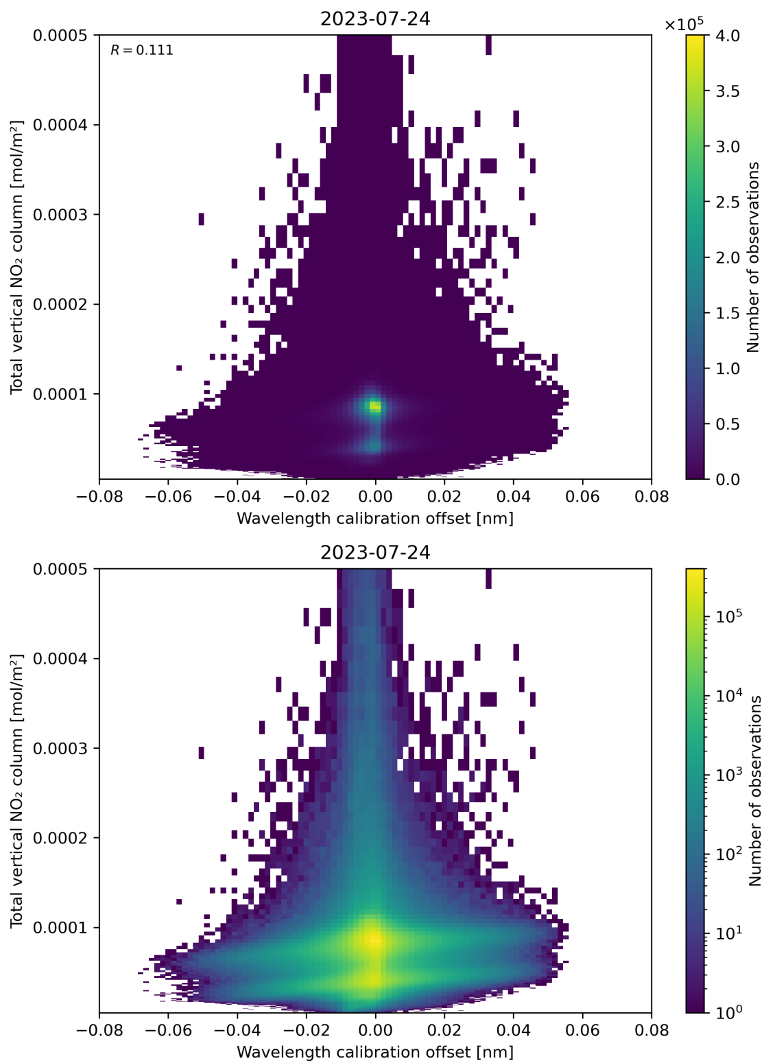
Figure 179: Scatter density plot of “Wavelength calibration offset” against “Total vertical NO 2 column” for 2023-07-24 to 2023-07-25.
