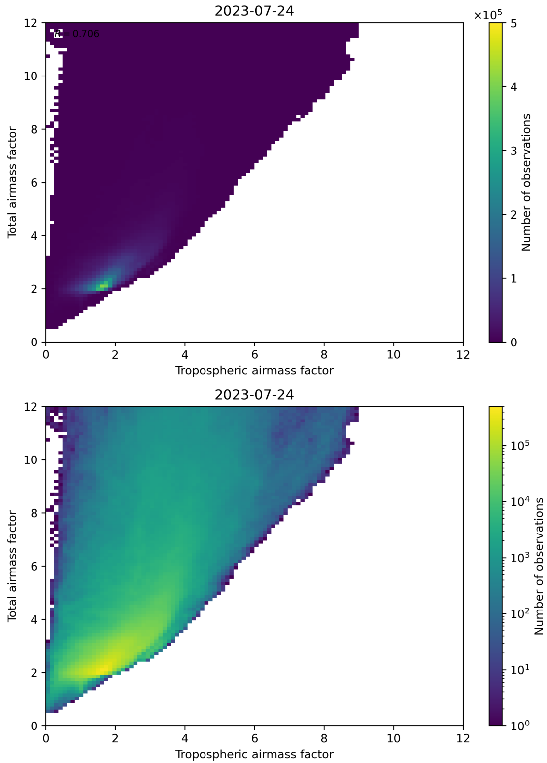
Figure 72: Scatter density plot of “Tropospheric airmass factor” against “Total airmass factor” for 2023-07-24 to 2023-07-25.
