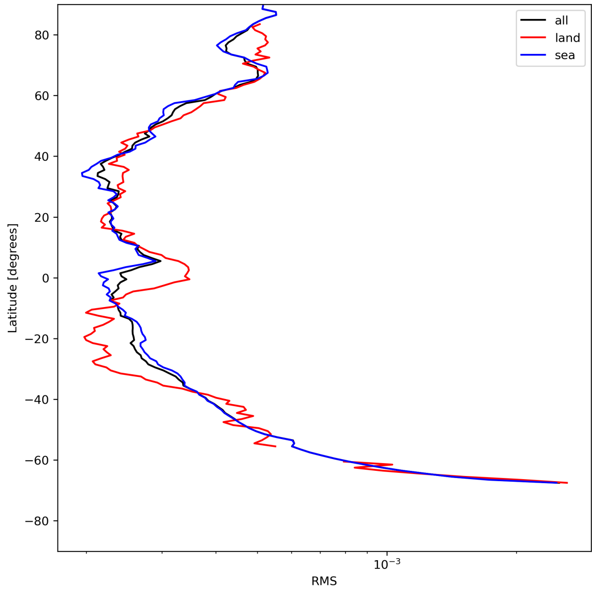
Figure 26: Zonal average of “RMS” for 2023-07-24 to 2023-07-25.
