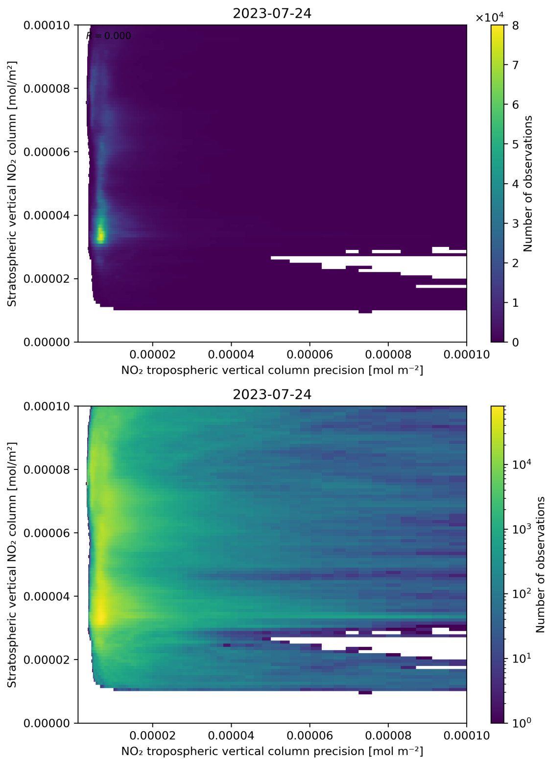
Figure 135: Scatter density plot of “NO 2 tropospheric vertical column precision” against “Stratospheric vertical NO 2 column” for 2023-07-24 to 2023-07-25.
