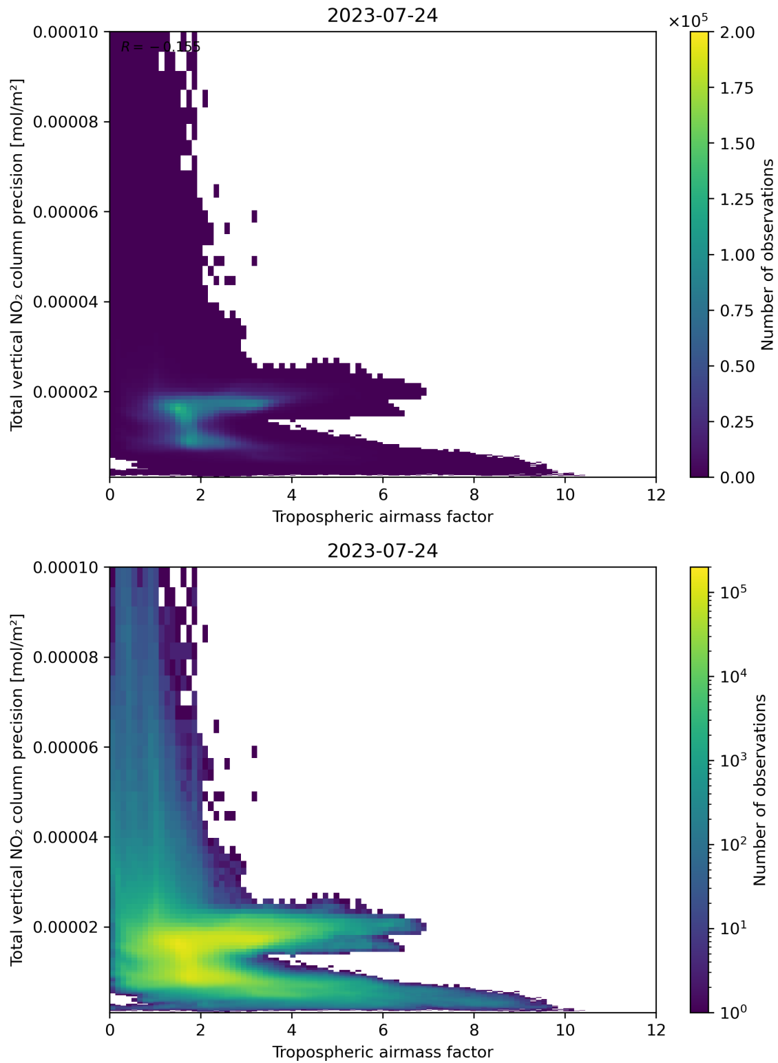
Figure 78: Scatter density plot of “Tropospheric air mass factor” against “Total vertical NO 2 column precision” for 2023-07-24 to 2023-07-25.
