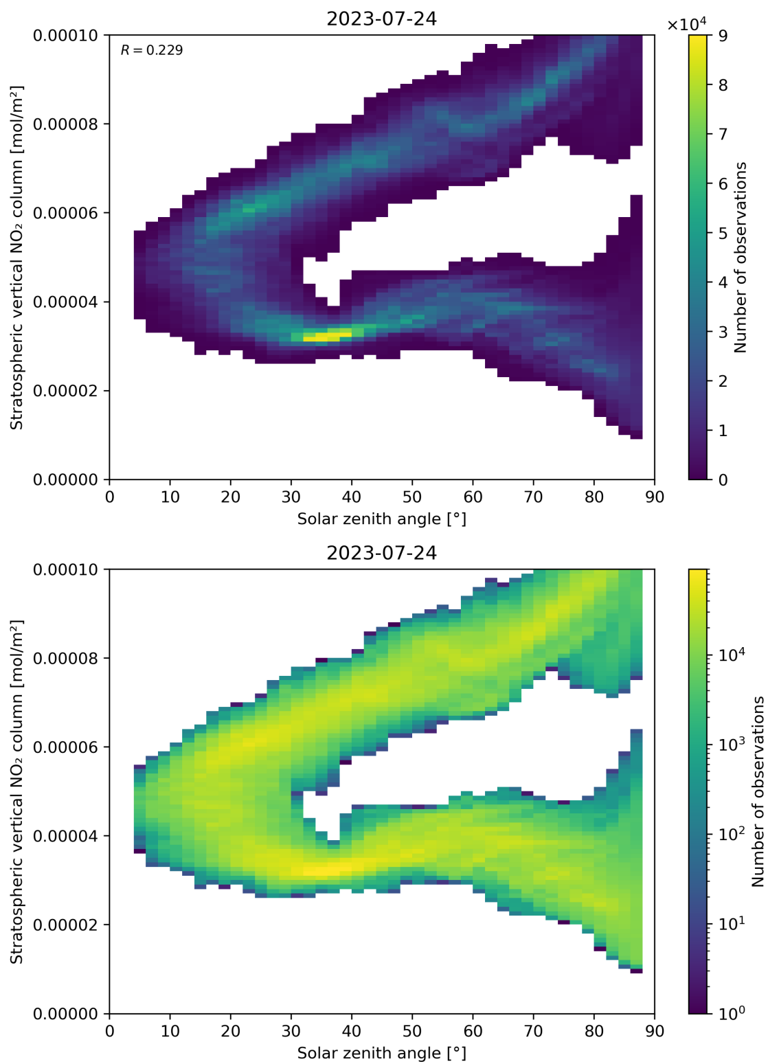
Figure 150: Scatter density plot of “Solar zenith angle” against “Stratospheric vertical \text{NO}_2 column” for 2023-07-24 to 2023-07-25.
