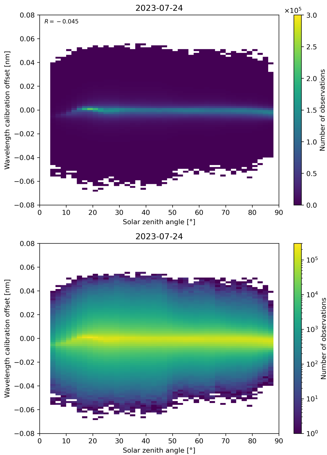
Figure 158: Scatter density plot of “Solar zenith angle” against “Wavelength calibration offset” for 2023-07-24 to 2023-07-25.
