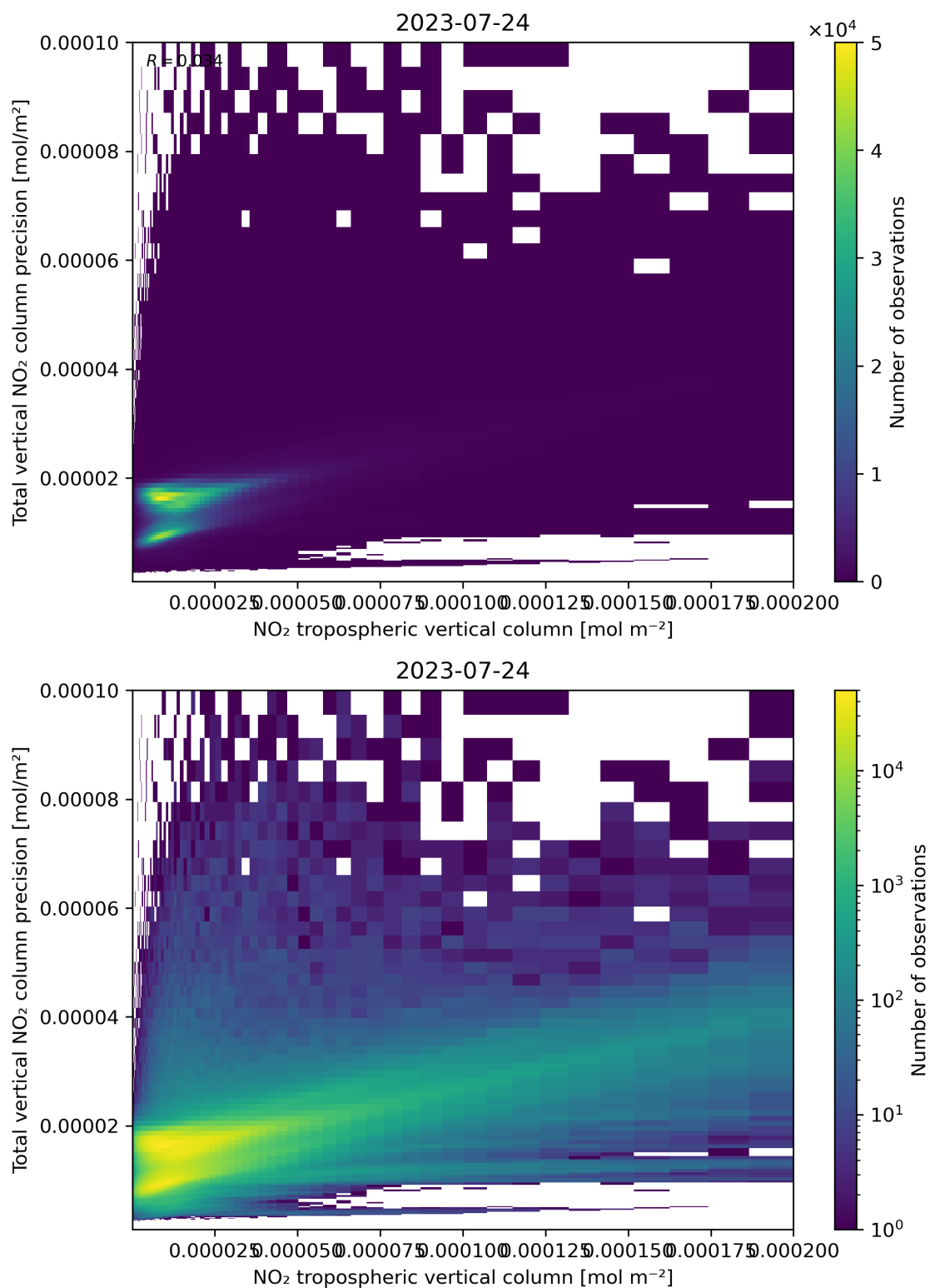
Figure 129: Scatter density plot of “NO 2 tropospheric vertical column” against “Total vertical NO 2 column precision” for 2023-07-24 to 2023-07-25.
