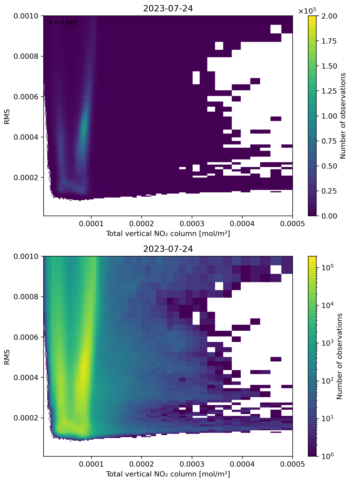
Figure 120: Scatter density plot of “Total vertical NO 2 column” against “RMS” for 2023-07-24 to 2023-07-25.
