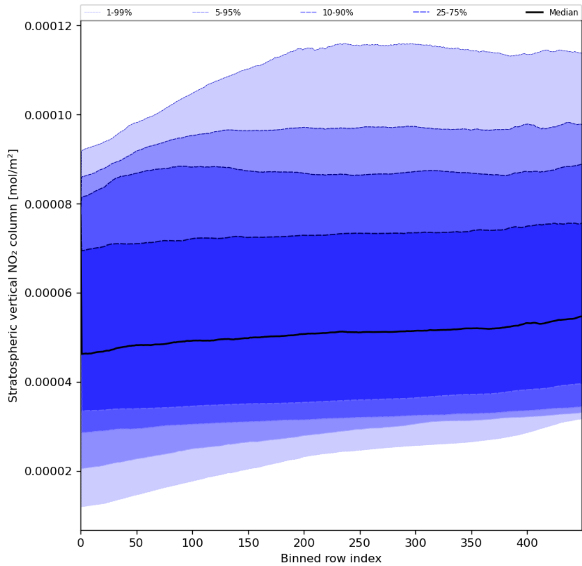
Figure 53: Along track statistics of “Stratospheric vertical NO 2 column” for 2023-07-24 to 2023-07-25
