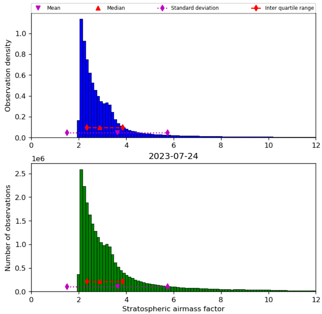
Figure 44: Histogram of “Stratospheric airmass factor” for 2023-07-24 to 2023-07-25
