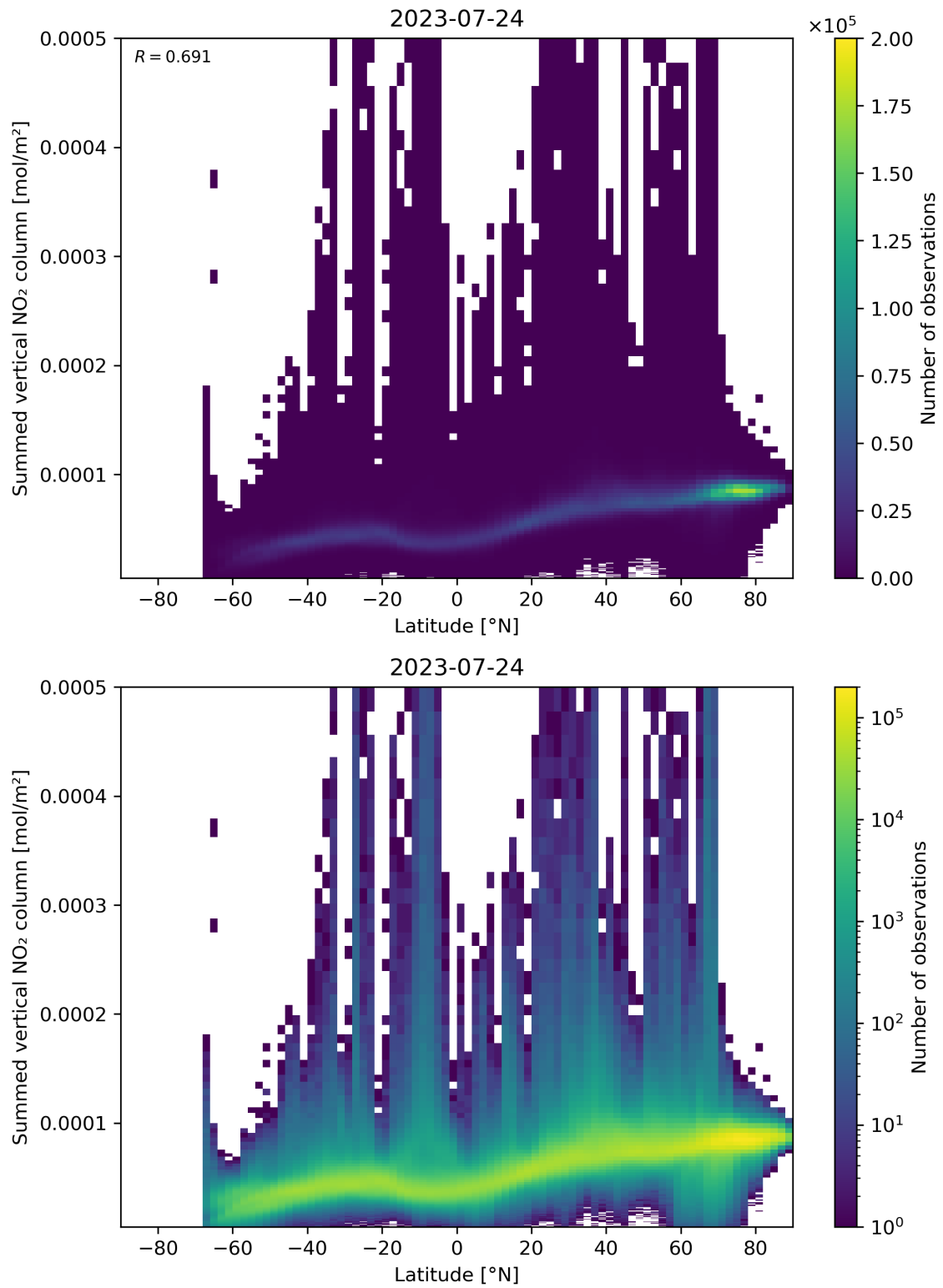
Figure 88: Scatter density plot of “Latitude” against “Summed vertical NO 2 column” for 2023-07-24 to 2023-07-25.
