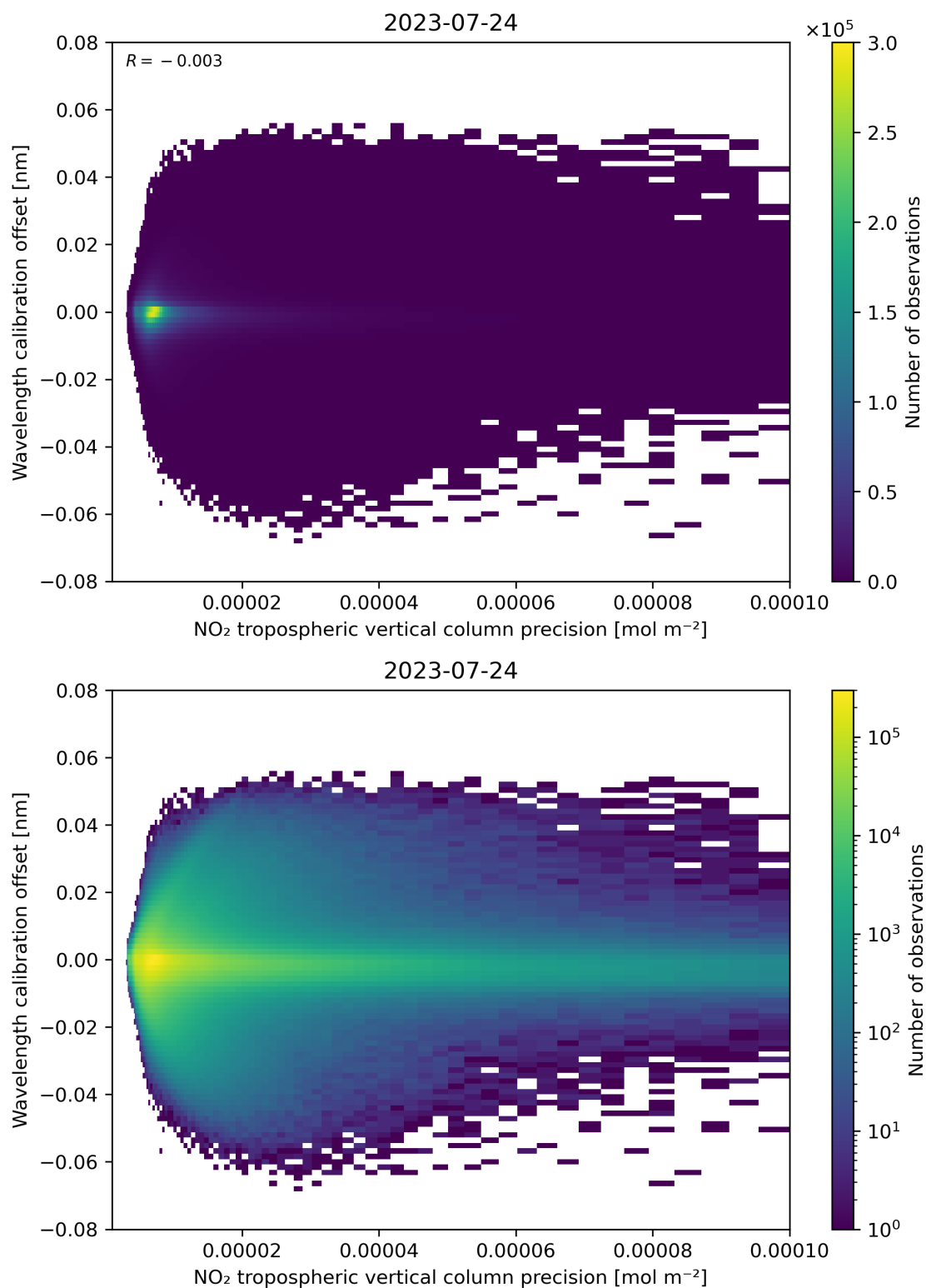
Figure 141: Scatter density plot of “NO 2 tropospheric vertical column precision” against “Wavelength calibration offset” for 2023-07-24 to 2023-07-25.
