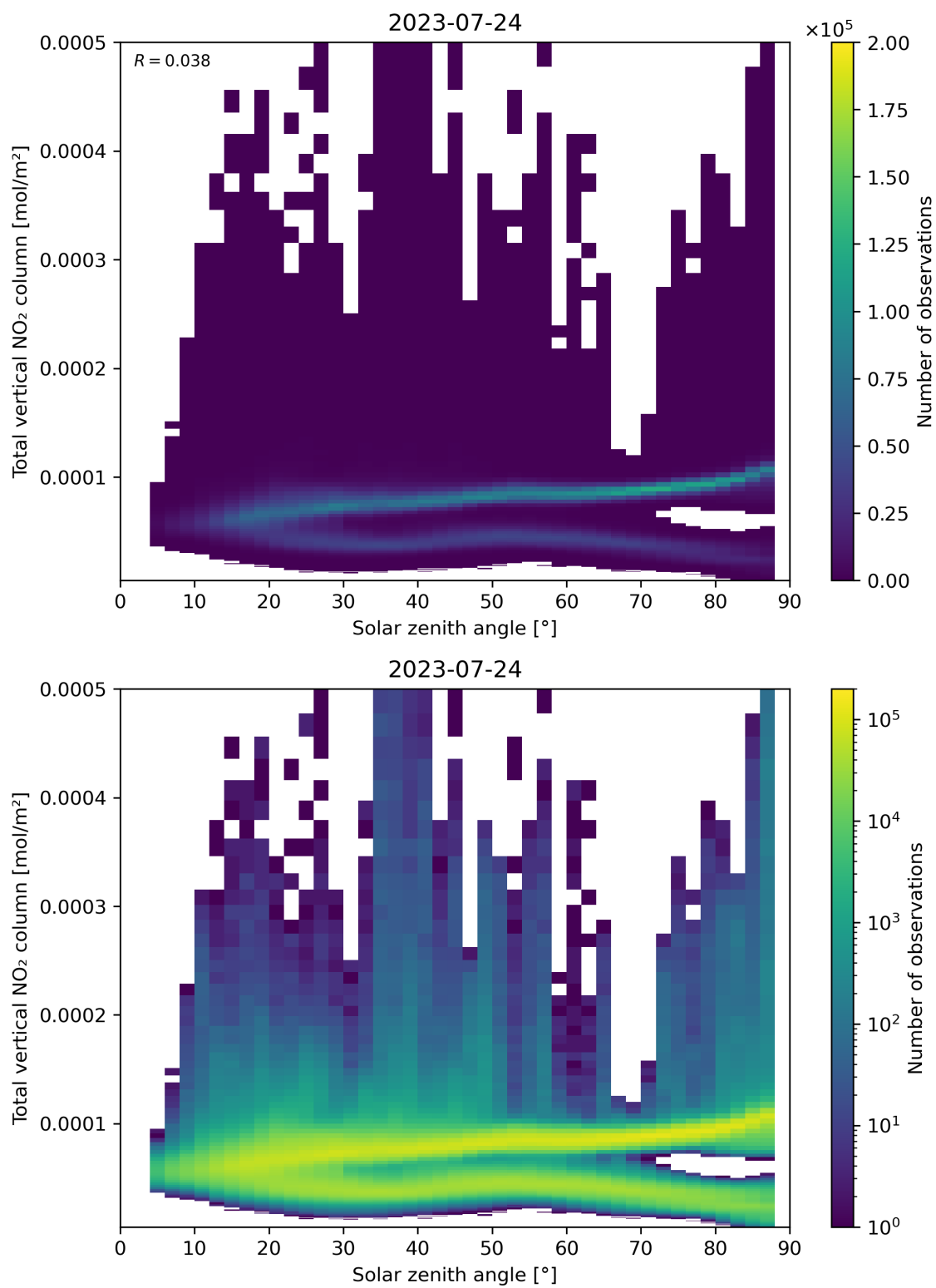
Figure 153: Scatter density plot of “Solar zenith angle” against “Total vertical NO 2 column” for 2023-07-24 to 2023-07-25.
