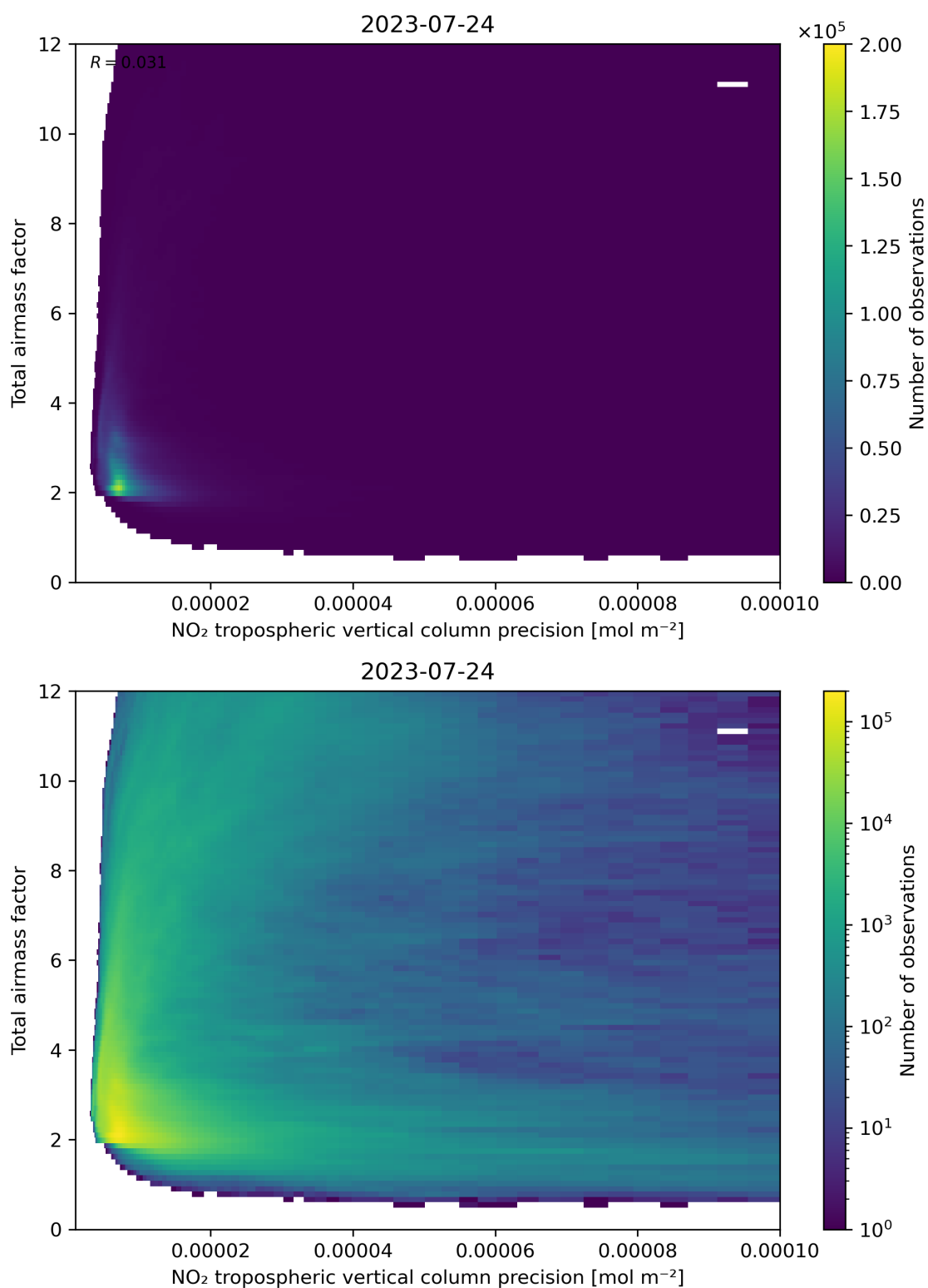
Figure 132: Scatter density plot of “NO 2 tropospheric vertical column precision” against “Total air mass factor” for 2023-07-24 to 2023-07-25.
