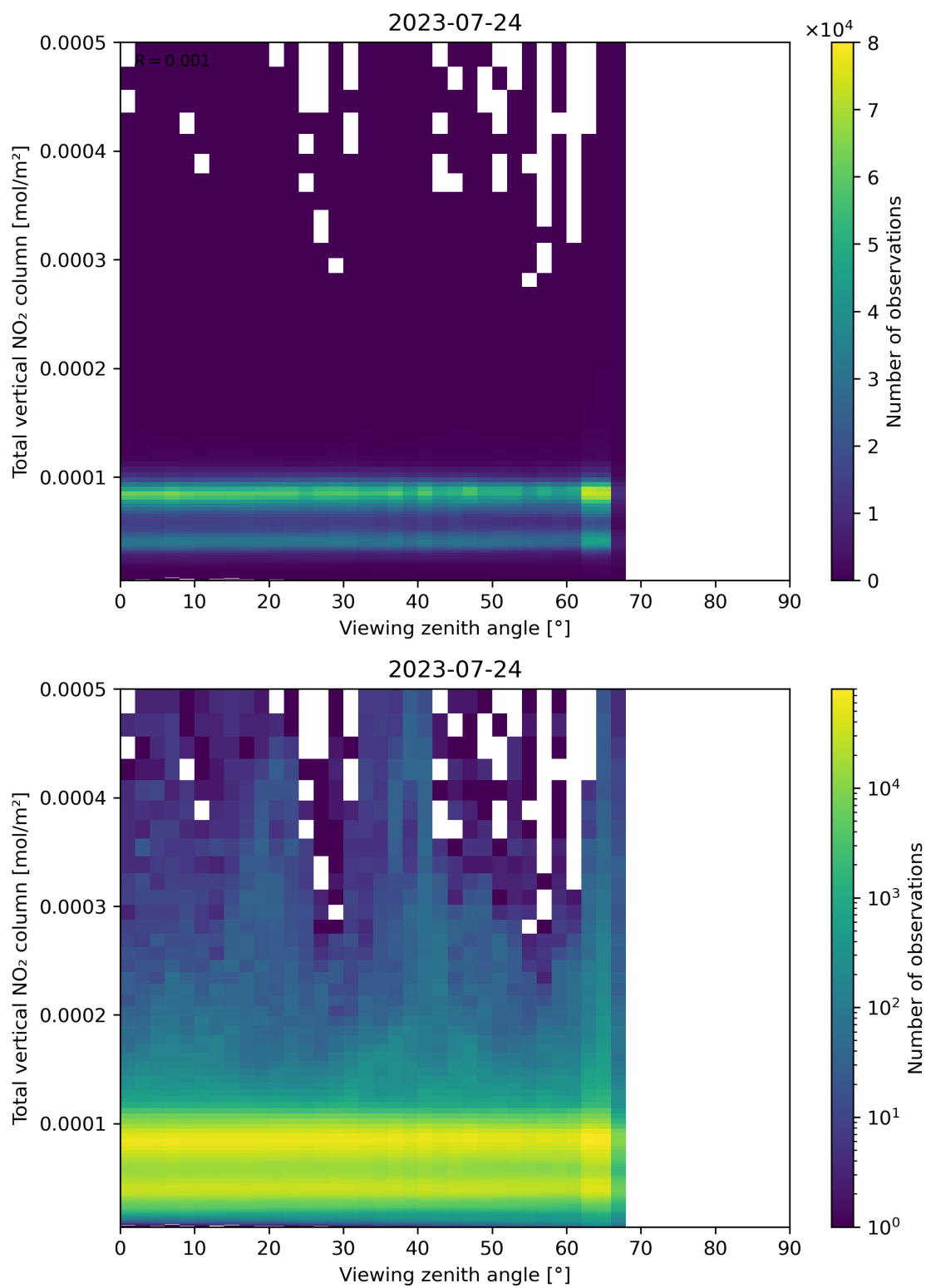
Figure 167: Scatter density plot of “Viewing zenith angle” against “Total vertical NO 2 column” for 2023-07-24 to 2023-07-25.
