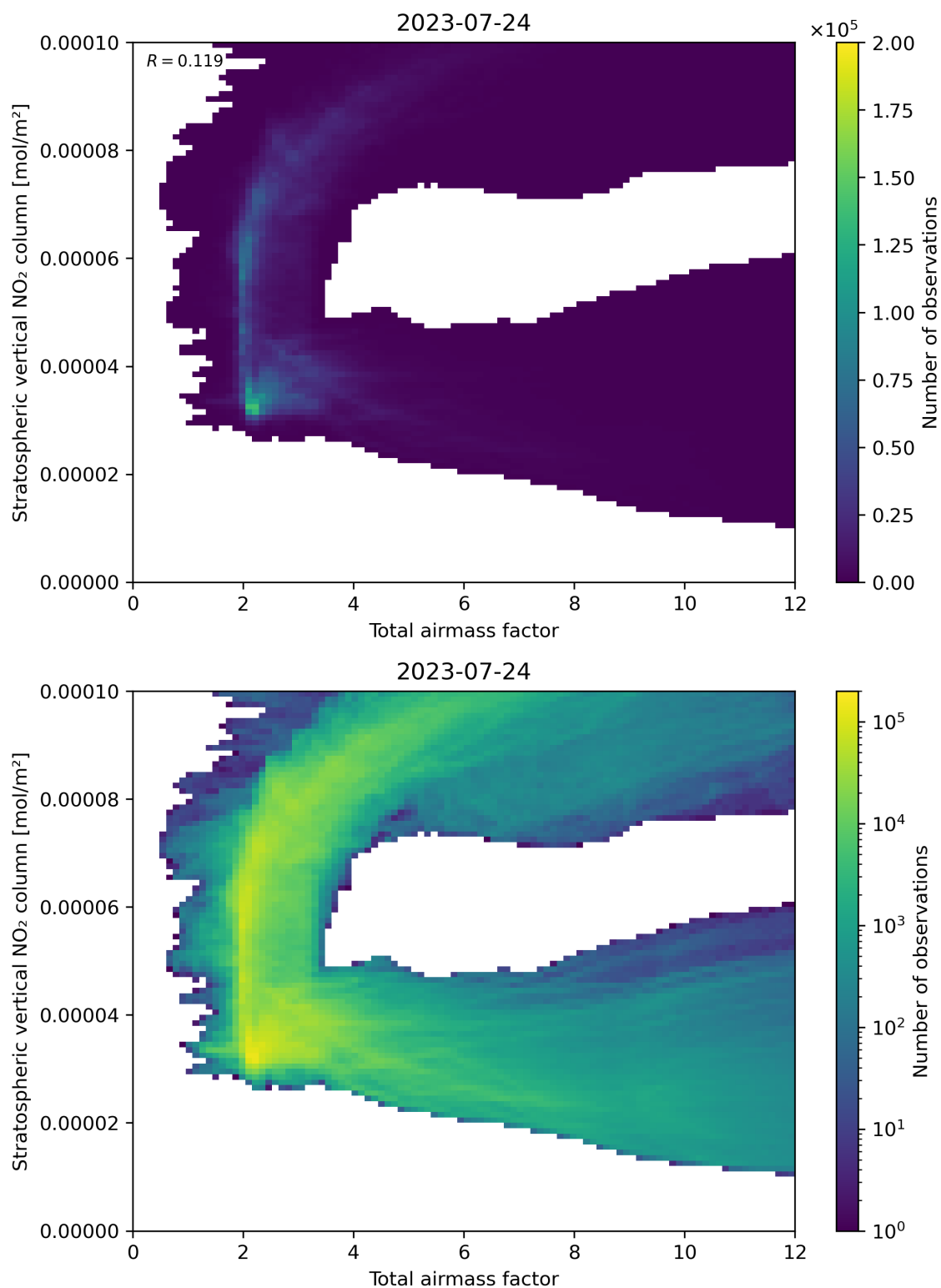
Figure 64: Scatter density plot of “Total airmass factor” against “Stratospheric vertical \text{NO}_2 column” for 2023-07-24 to 2023-07-25.
