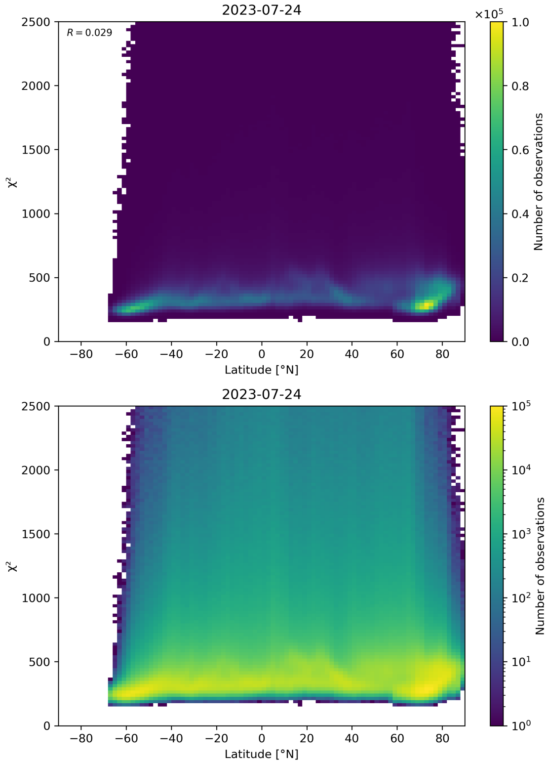
Figure 86: Scatter density plot of “Latitude” against “ \chi^2 ” for 2023-07-24 to 2023-07-25.
