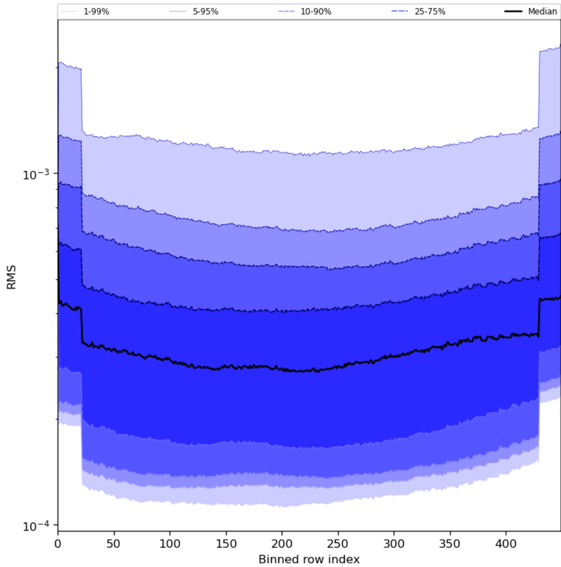
Figure 60: Along track statistics of “RMS” for 2023-07-24 to 2023-07-25
