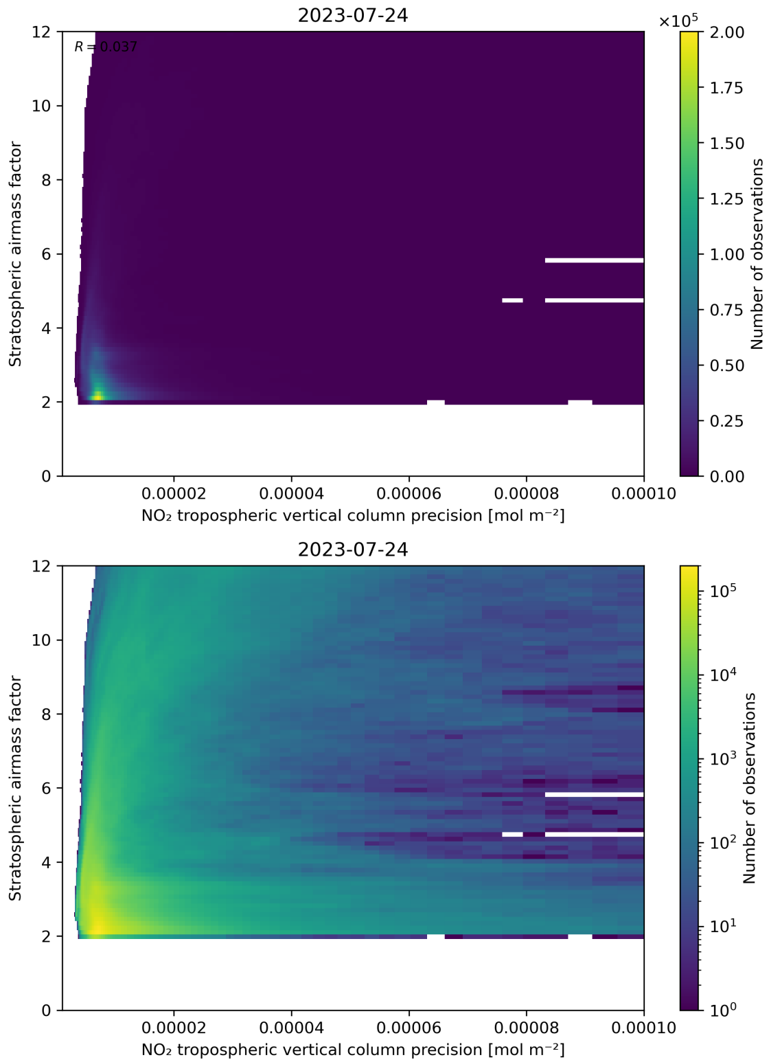
Figure 131: Scatter density plot of “NO 2 tropospheric vertical column precision” against “Stratospheric airmass factor” for 2023-07-24 to 2023-07-25.
