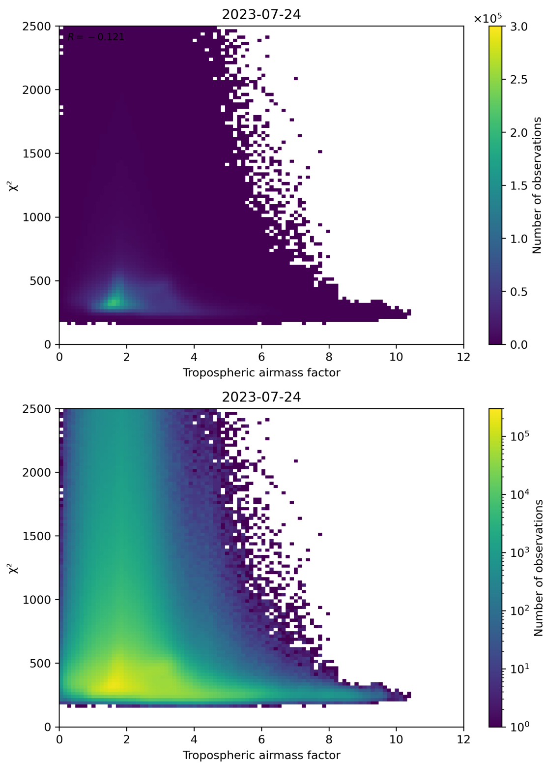
Figure 73: Scatter density plot of “Tropospheric airmass factor” against “ \chi^2 ” for 2023-07-24 to 2023-07-25.
