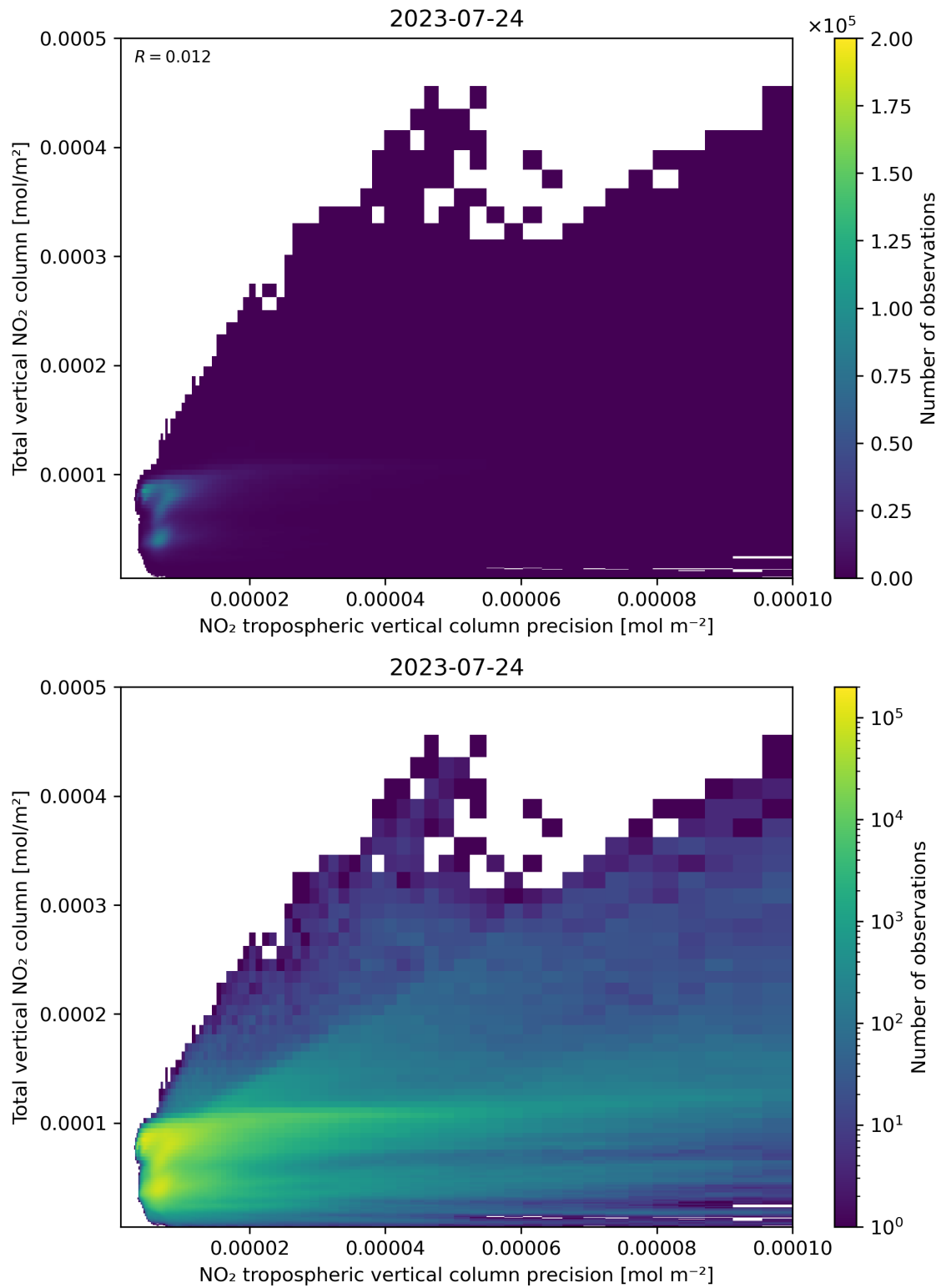
Figure 138: Scatter density plot of “NO 2 tropospheric vertical column precision” against “Total vertical NO 2 column” for 2023-07-24 to 2023-07-25.
