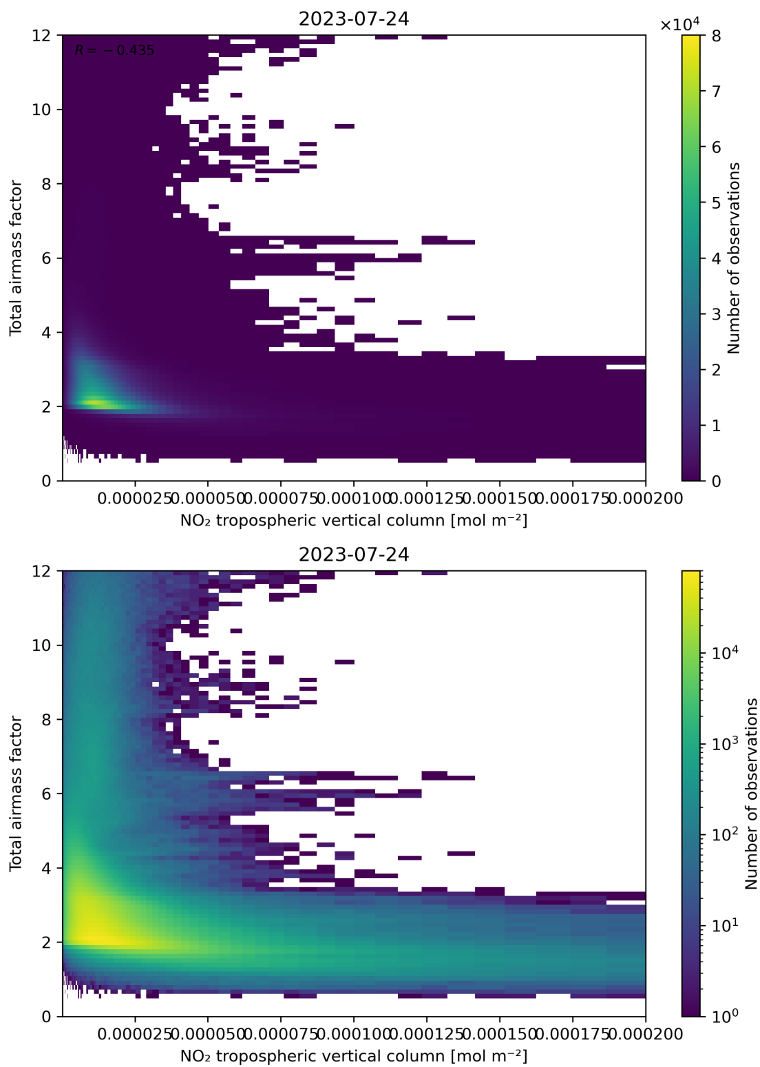
Figure 122: Scatter density plot of “NO 2 tropospheric vertical column” against “Total air mass factor” for 2023-07-24 to 2023-07-25.
