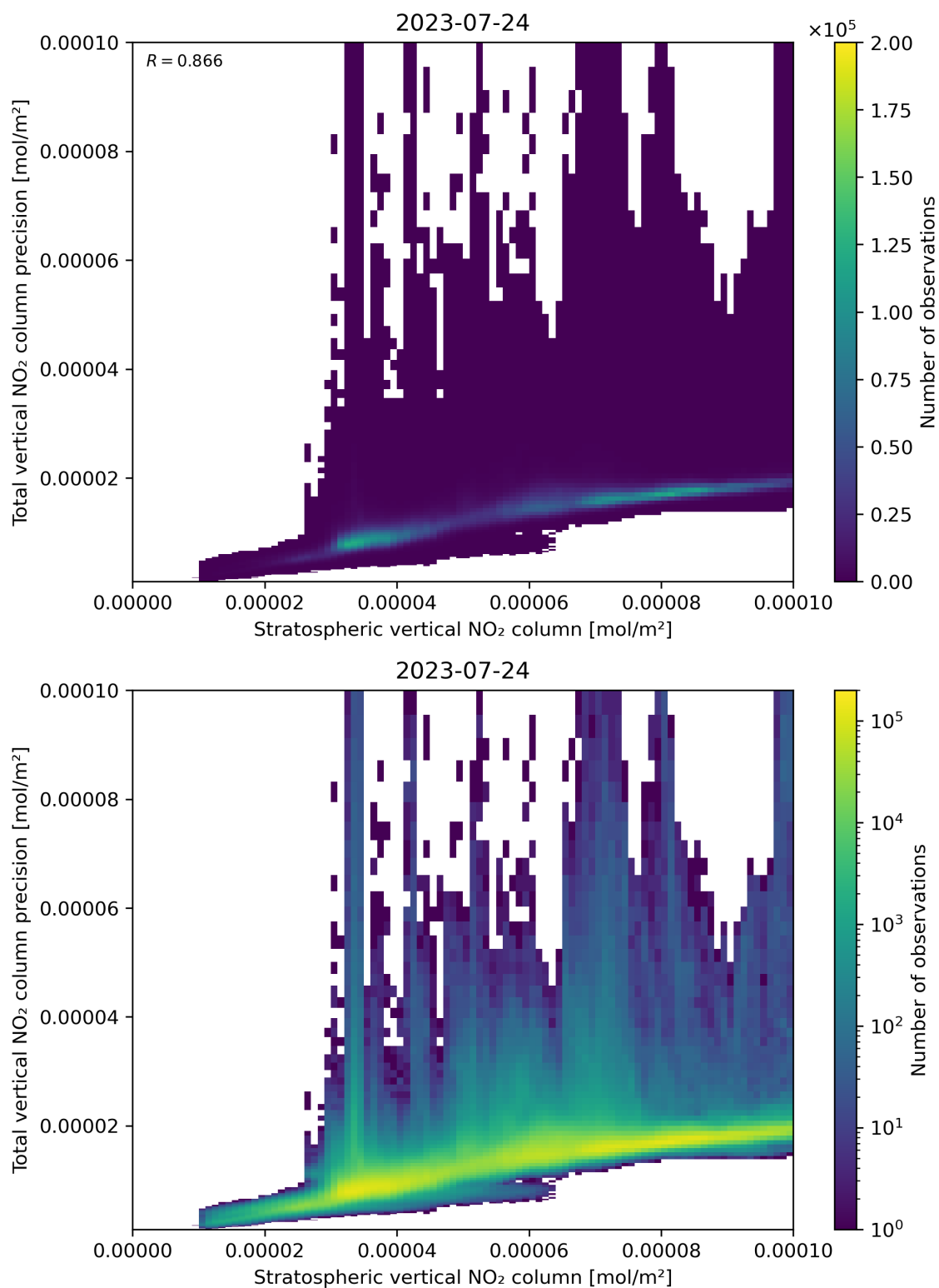
Figure 101: Scatter density plot of “Stratospheric vertical NO 2 column” against “Total vertical NO 2 column precision” for 2023-07-24 to 2023-07-25.
