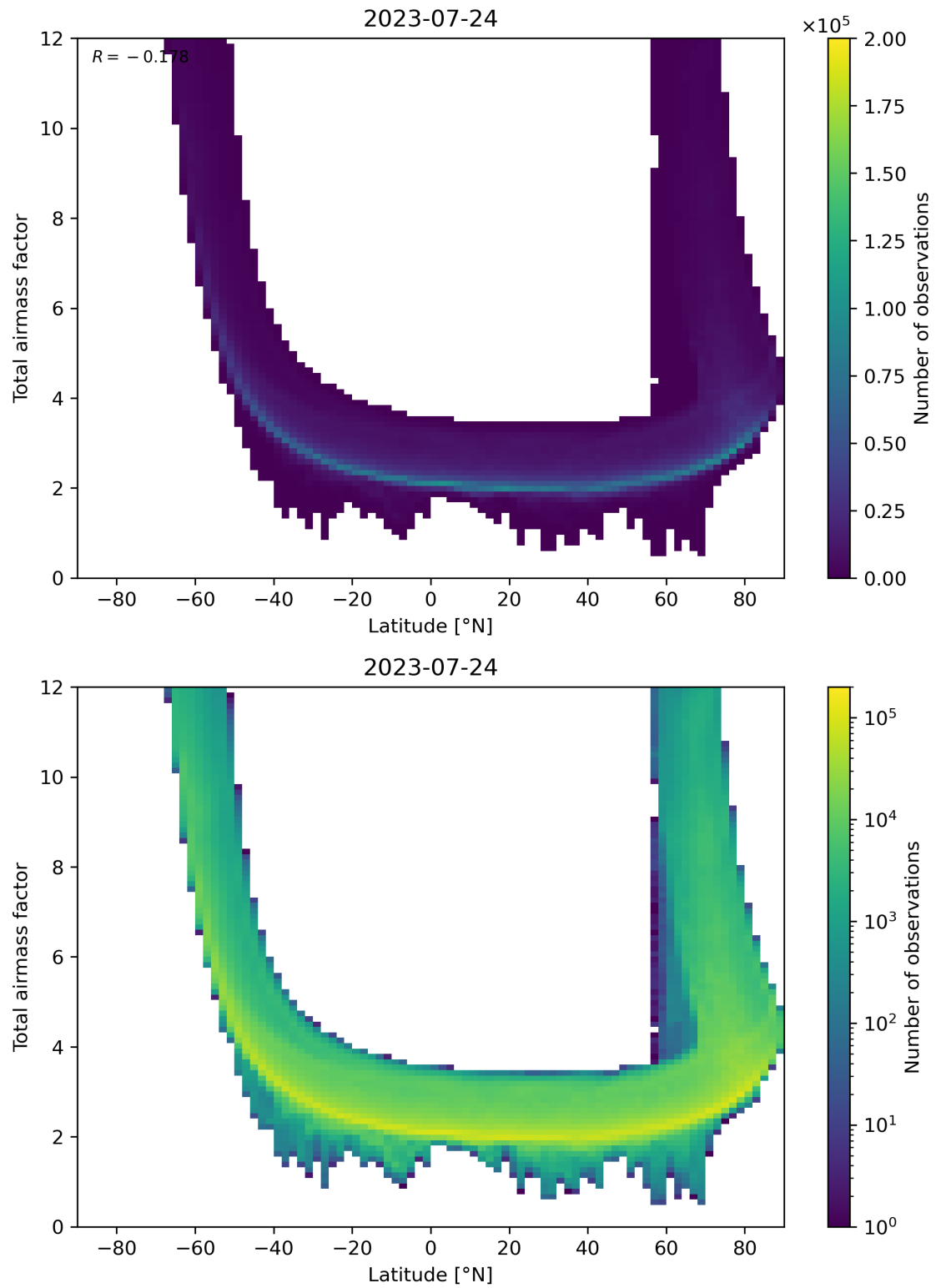
Figure 84: Scatter density plot of “Latitude” against “Total airmass factor” for 2023-07-24 to 2023-07-25.
