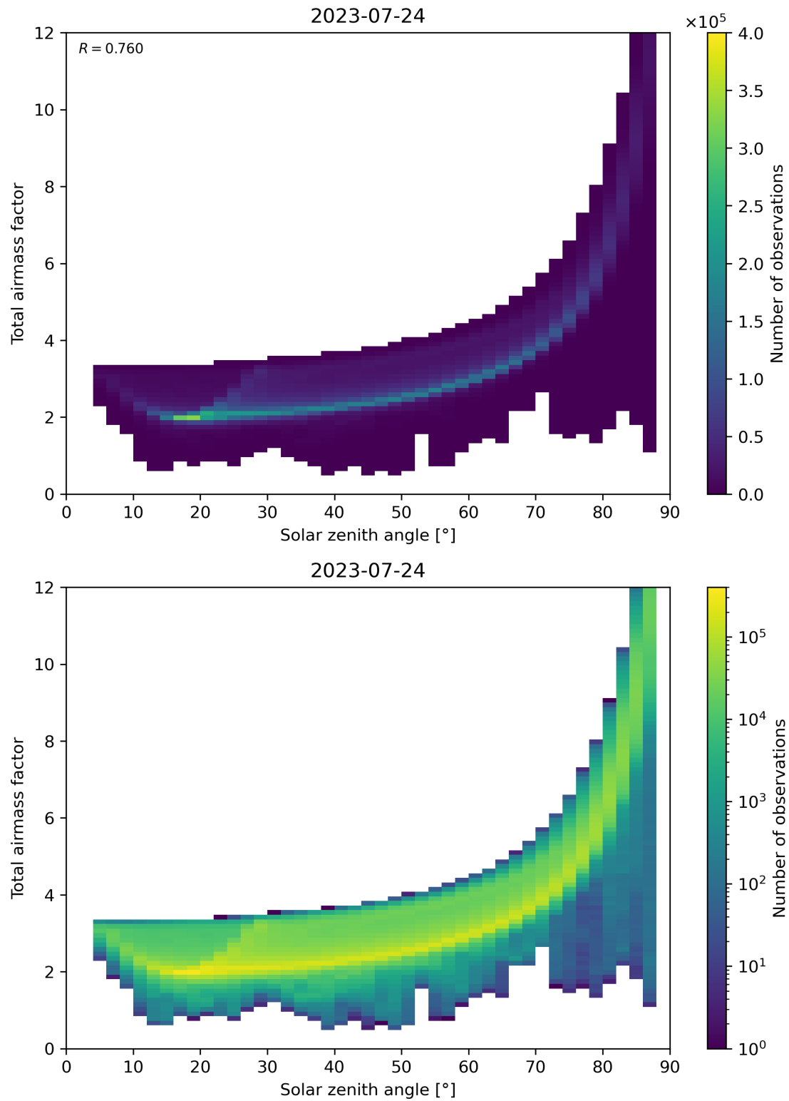
Figure 146: Scatter density plot of “Solar zenith angle” against “Total air mass factor” for 2023-07-24 to 2023-07-25.
