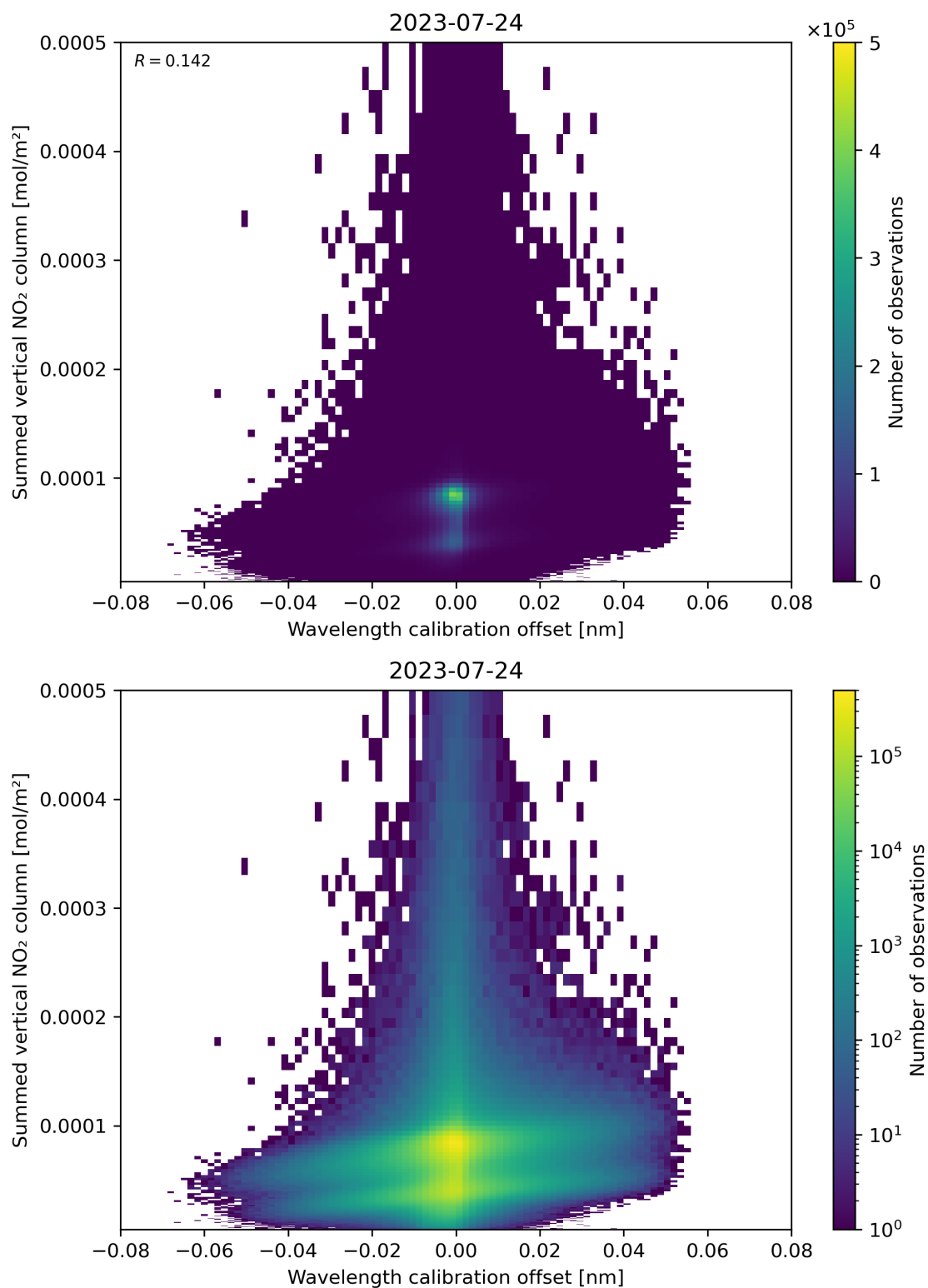
Figure 177: Scatter density plot of “Wavelength calibration offset” against “Summed vertical NO 2 column” for 2023-07-24 to 2023-07-25.
