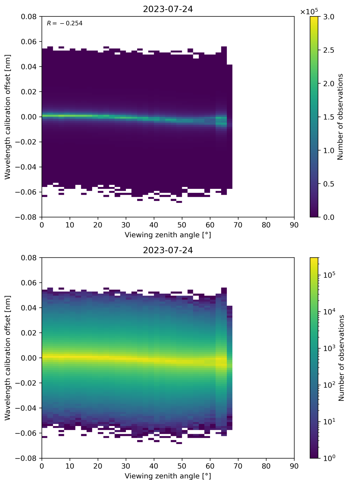
Figure 173: Scatter density plot of “Viewing zenith angle” against “Wavelength calibration offset” for 2023-07-24 to 2023-07-25.
