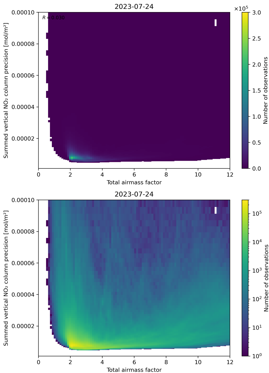
Figure 66: Scatter density plot of “Total airmass factor” against “Summed vertical NO 2 column precision” for 2023-07-24 to 2023-07-25.
