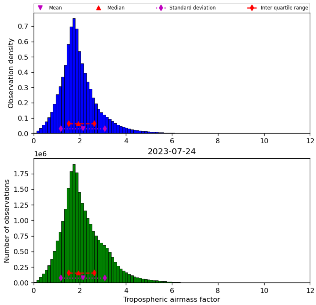
Figure 31: Histogram of “Tropospheric airmass factor” for 2023-07-24 to 2023-07-25
