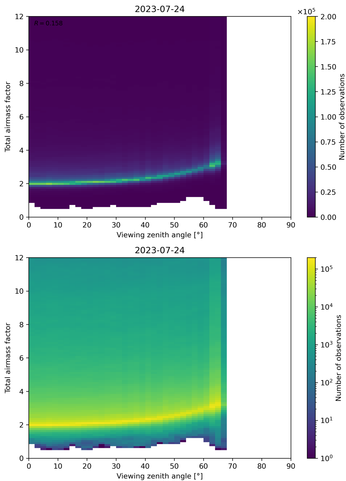
Figure 160: Scatter density plot of “Viewing zenith angle” against “Total airmass factor” for 2023-07-24 to 2023-07-25.
