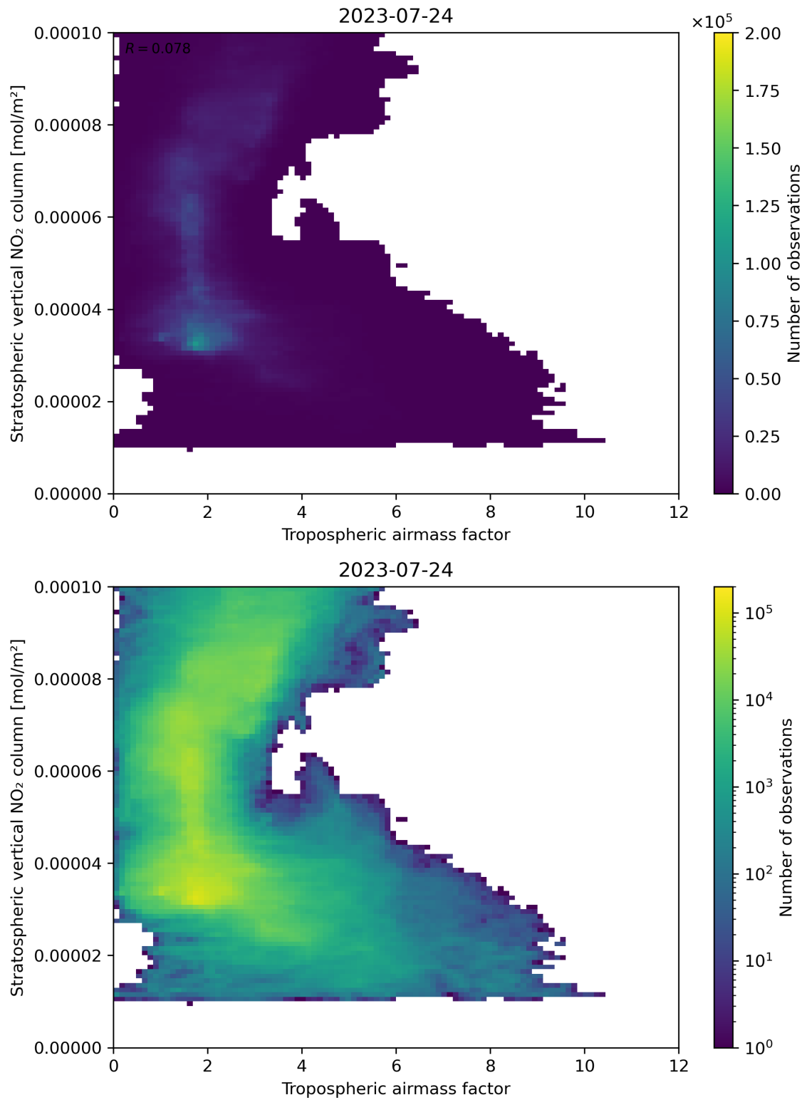
Figure 74: Scatter density plot of “Tropospheric air mass factor” against “Stratospheric vertical \text{NO}_2 column” for 2023-07-24 to 2023-07-25.
