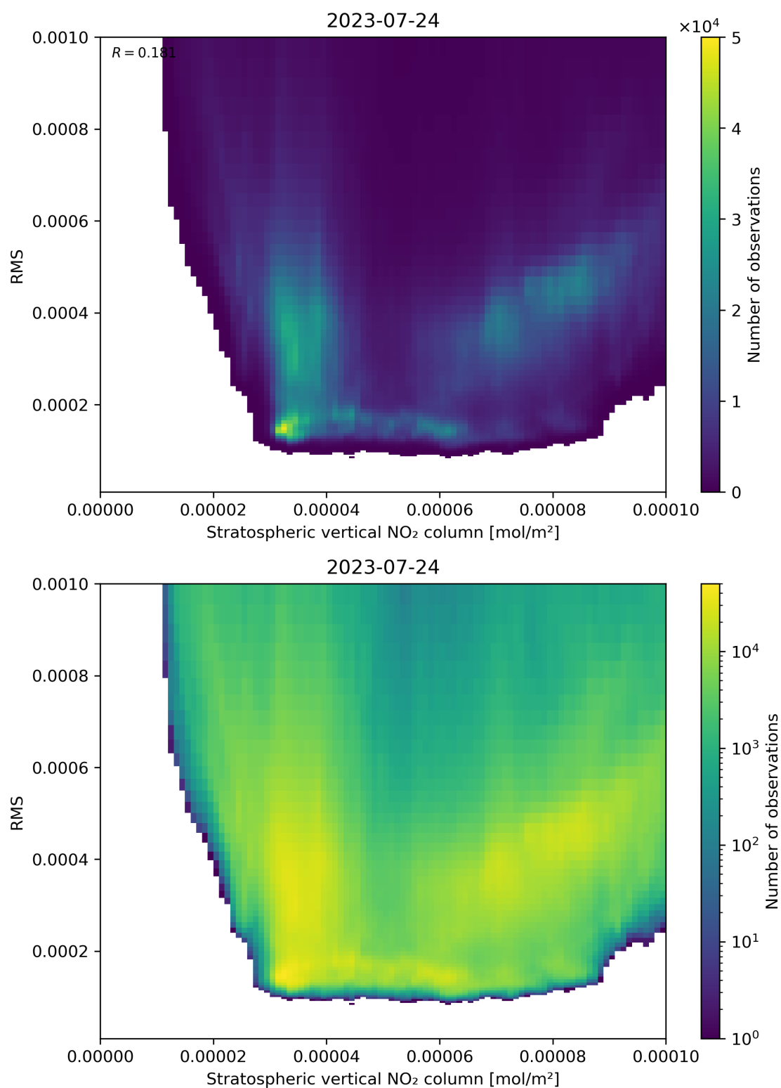
Figure 102: Scatter density plot of “Stratospheric vertical NO 2 column” against “RMS” for 2023-07-24 to 2023-07-25.
