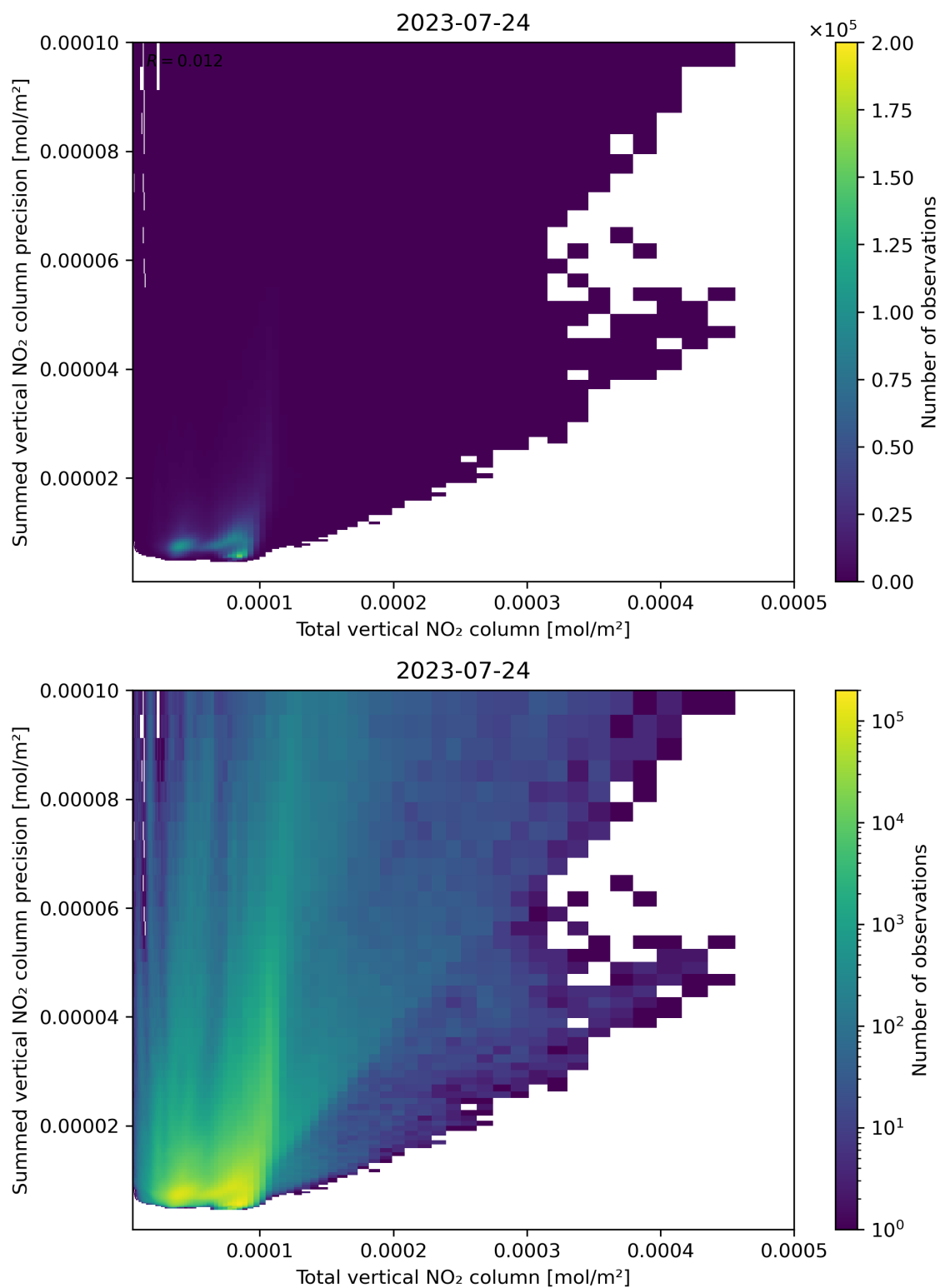
Figure 113: Scatter density plot of “Total vertical NO 2 column” against “Summed vertical NO 2 column precision” for 2023-07-24 to 2023-07-25.
