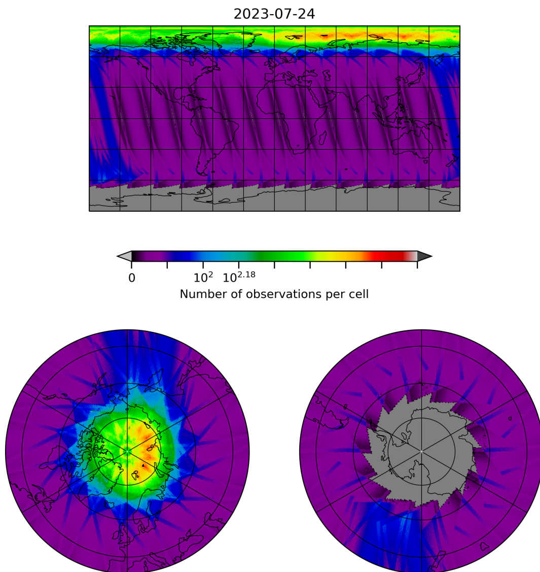
Figure 10: Map of the number of observations for 2023-07-24 to 2023-07-25
