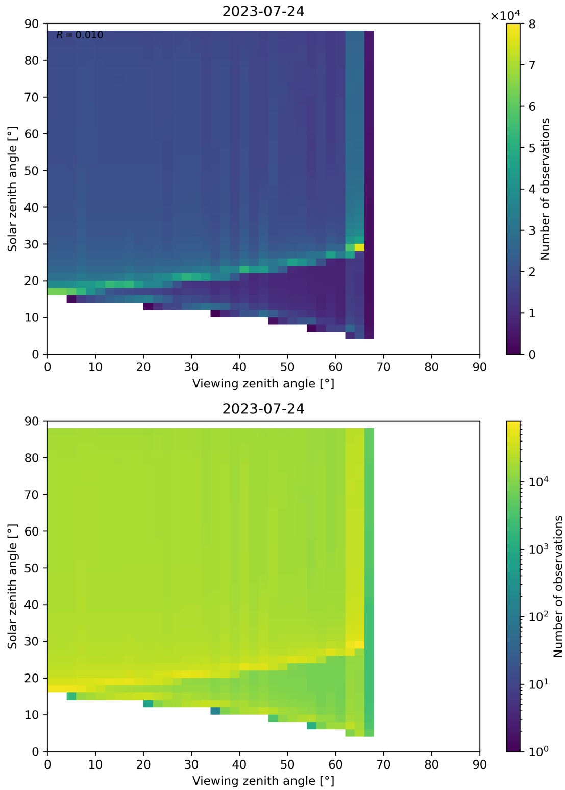
Figure 172: Scatter density plot of “Viewing zenith angle” against “Solar zenith angle” for 2023-07-24 to 2023-07-25.
