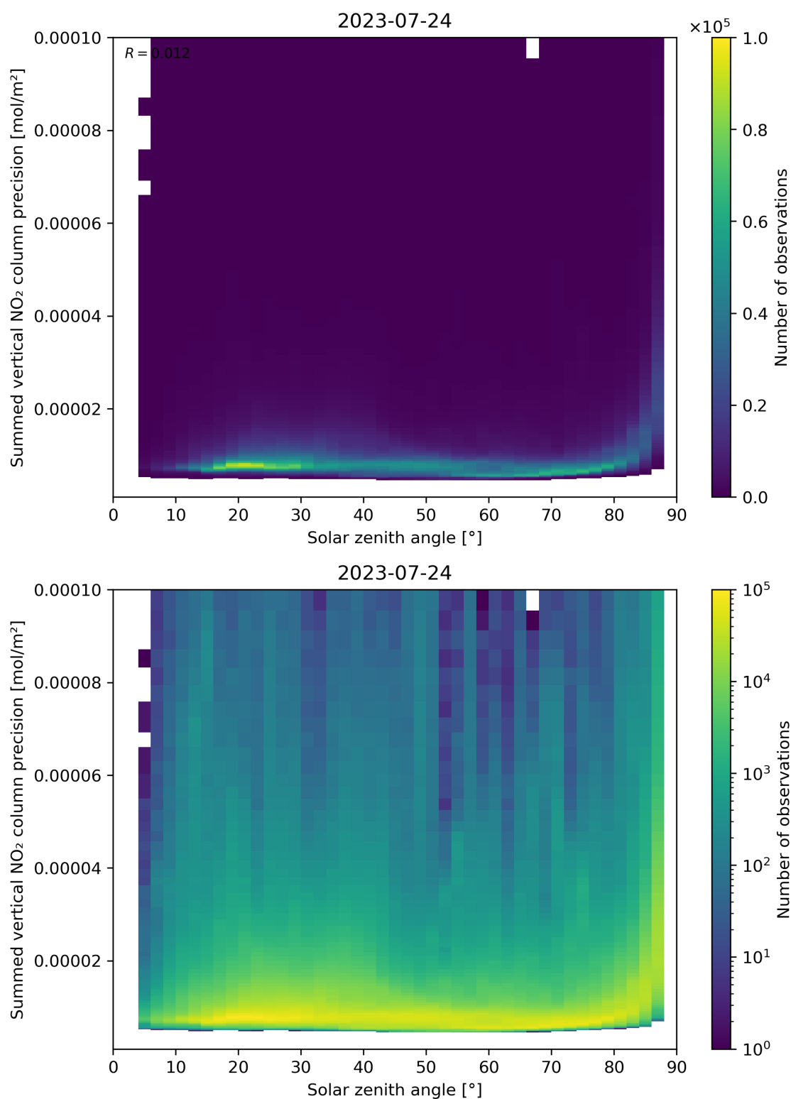
Figure 152: Scatter density plot of “Solar zenith angle” against “Summed vertical NO 2 column precision” for 2023-07-24 to 2023-07-25.
