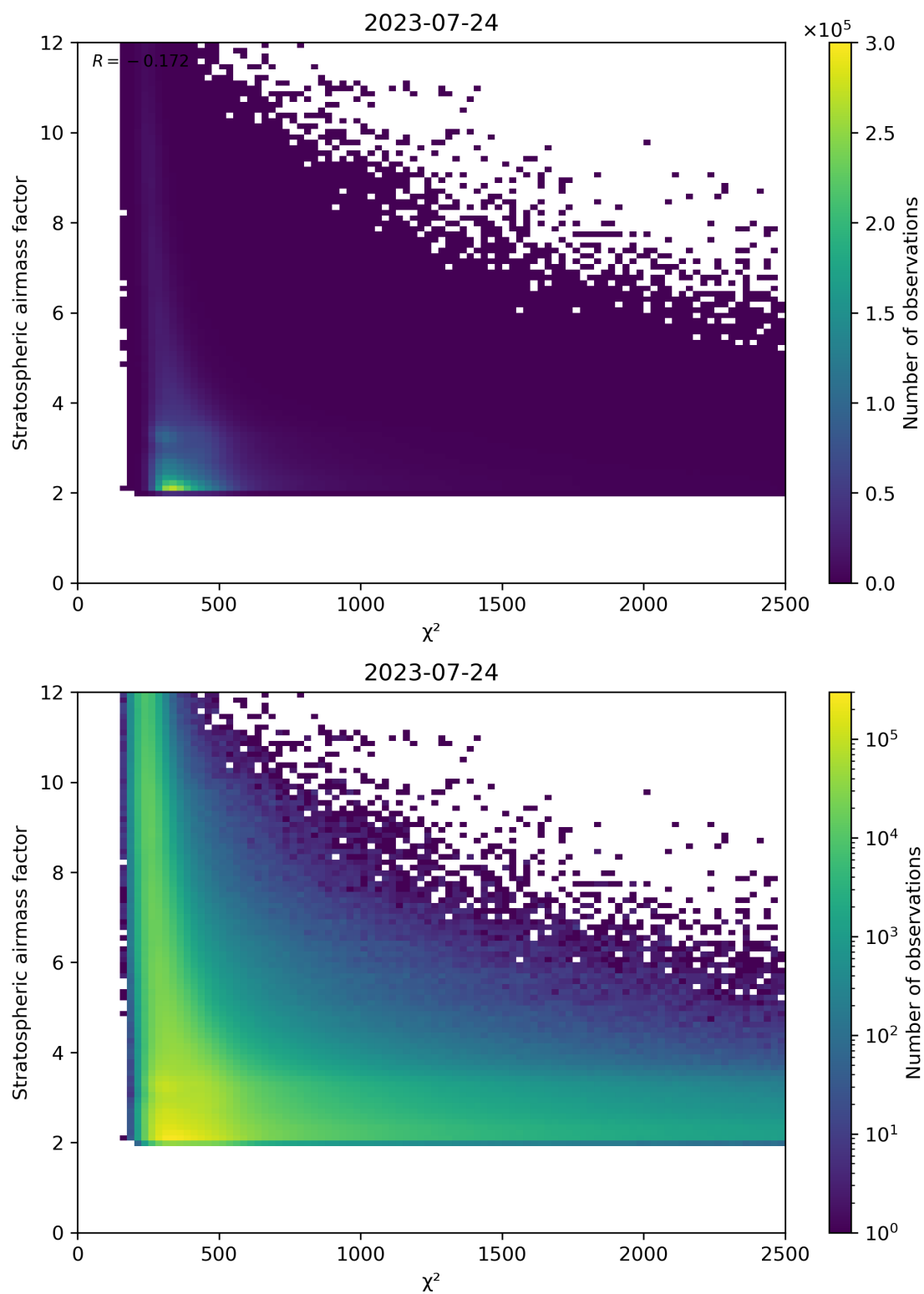
Figure 81: Scatter density plot of “ \chi^2 ” against “Stratospheric airmass factor” for 2023-07-24 to 2023-07-25.
