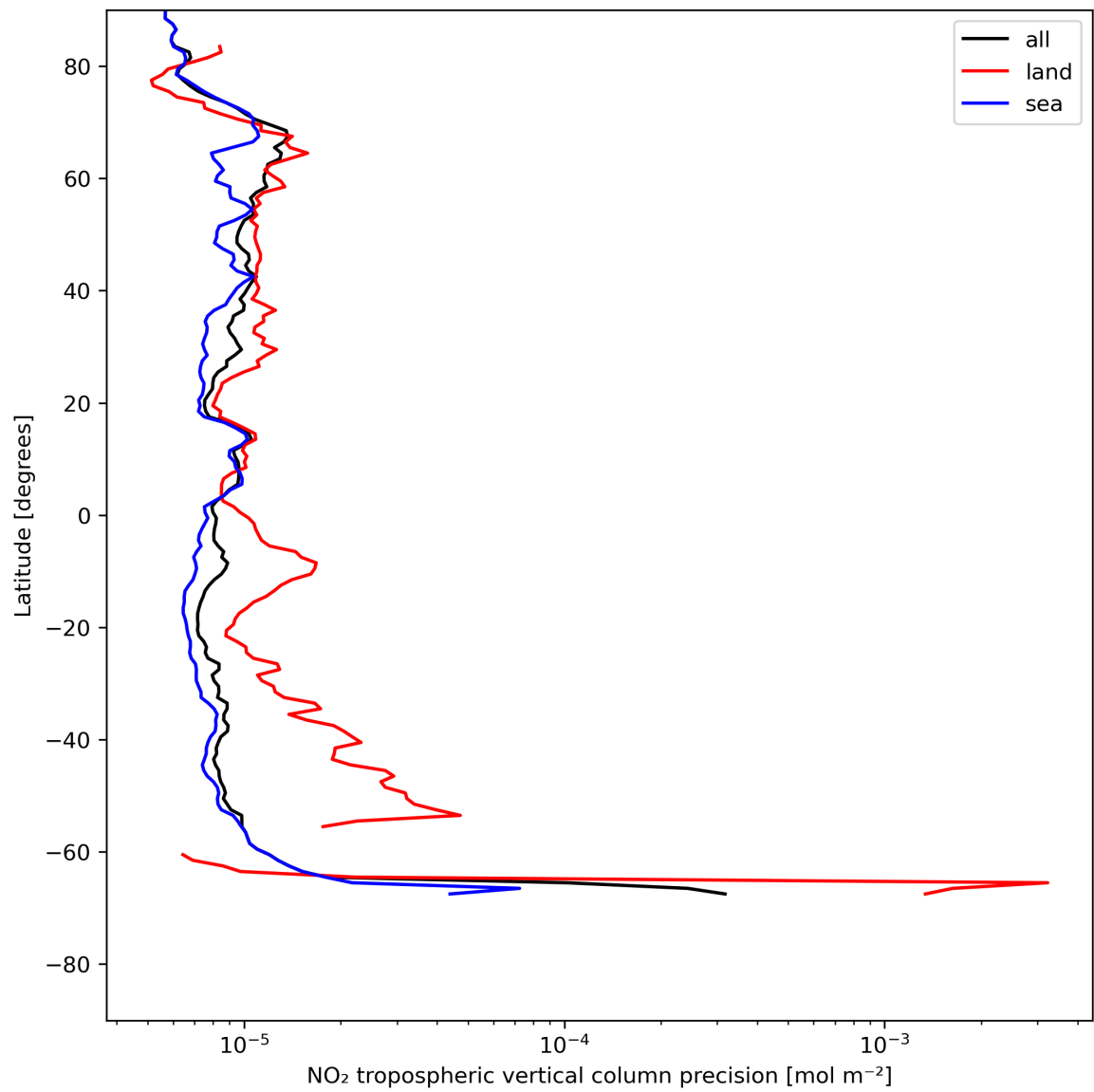
Figure 13: Zonal average of “NO 2 tropospheric vertical column precision” for 2023-07-24 to 2023-07-25.
