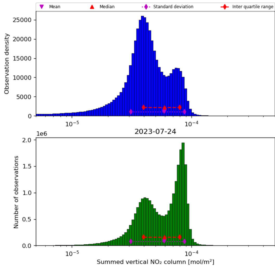
Figure 40: Histogram of “Summed vertical NO 2 column” for 2023-07-24 to 2023-07-25
