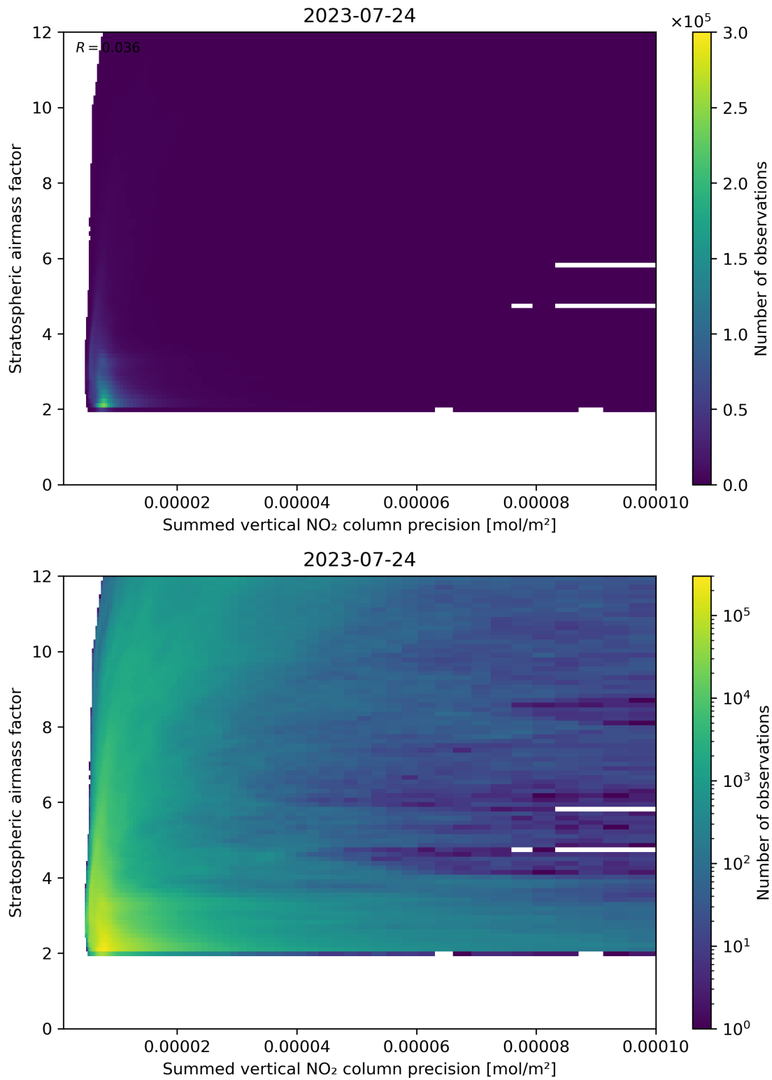
Figure 106: Scatter density plot of “Summed vertical NO 2 column precision” against “Stratospheric airmass factor” for 2023-07-24 to 2023-07-25.
