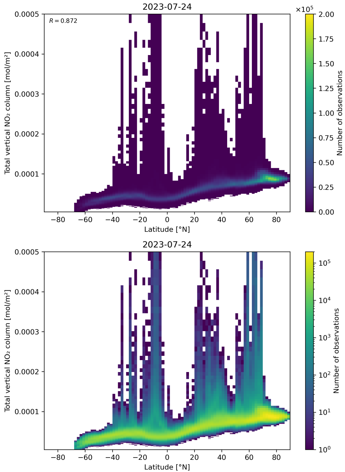
Figure 90: Scatter density plot of “Latitude” against “Total vertical NO 2 column” for 2023-07-24 to 2023-07-25.
