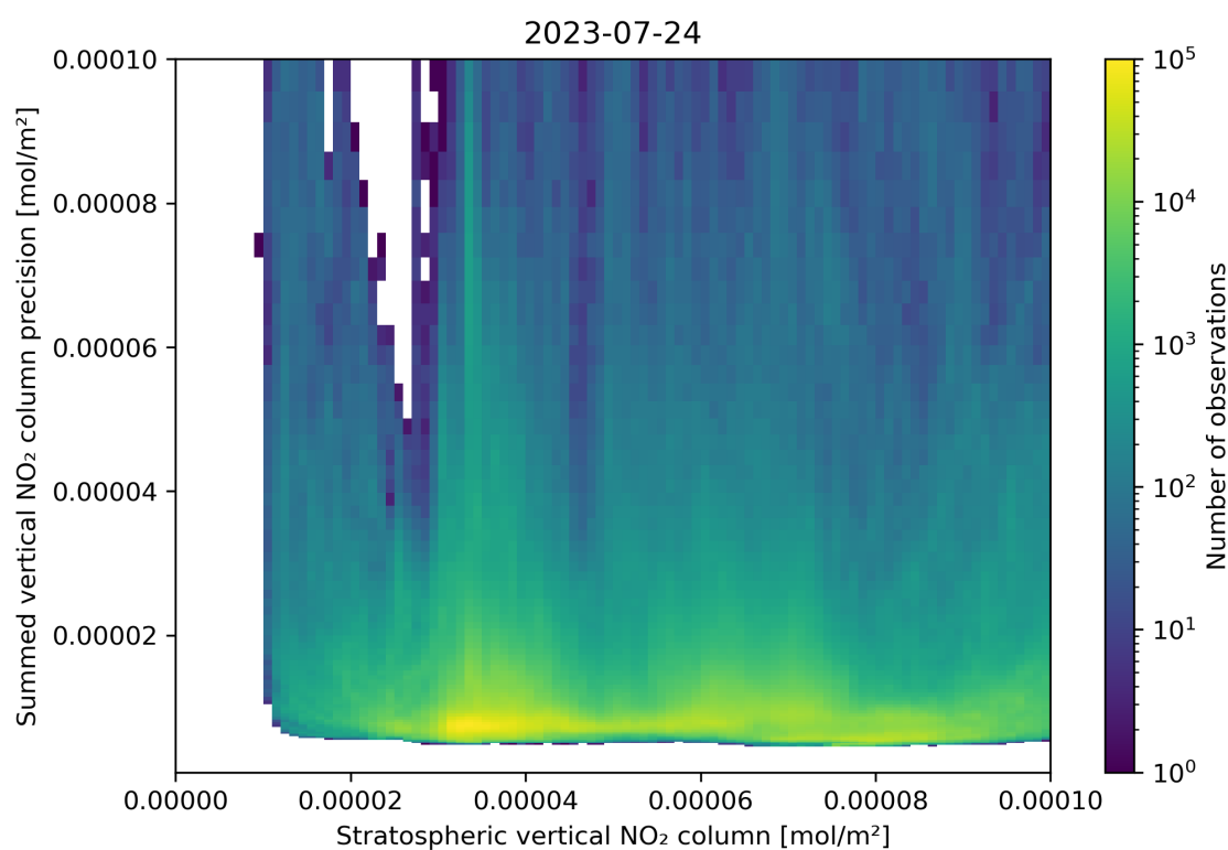
Figure 99: Scatter density plot of “Stratospheric vertical NO 2 column” against “Summed vertical NO 2 column precision” for 2023-07-24 to 2023-07-25.
