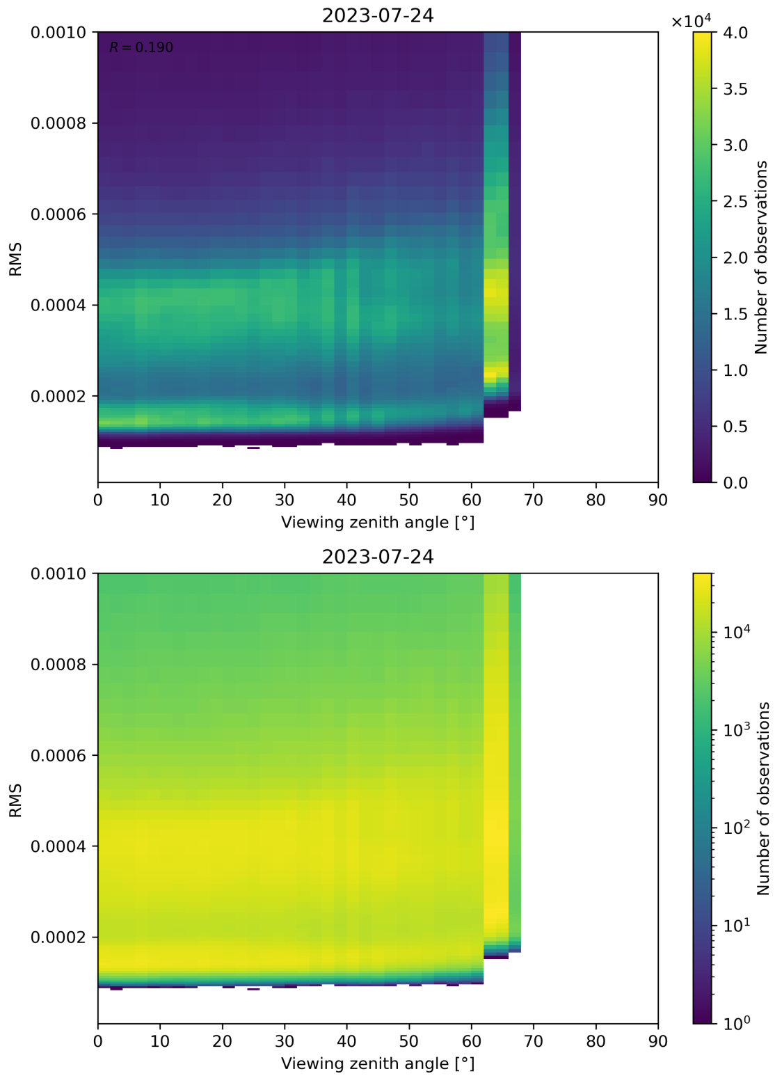
Figure 171: Scatter density plot of “Viewing zenith angle” against “RMS” for 2023-07-24 to 2023-07-25.
