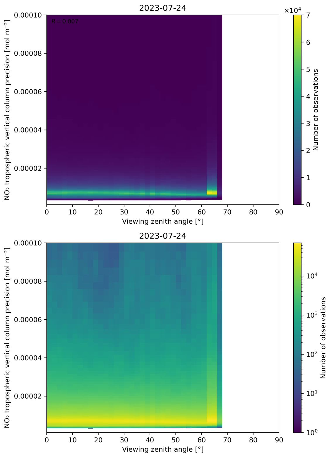
Figure 170: Scatter density plot of “Viewing zenith angle” against “NO 2 tropospheric vertical column precision” for 2023-07-24 to 2023-07-25.
