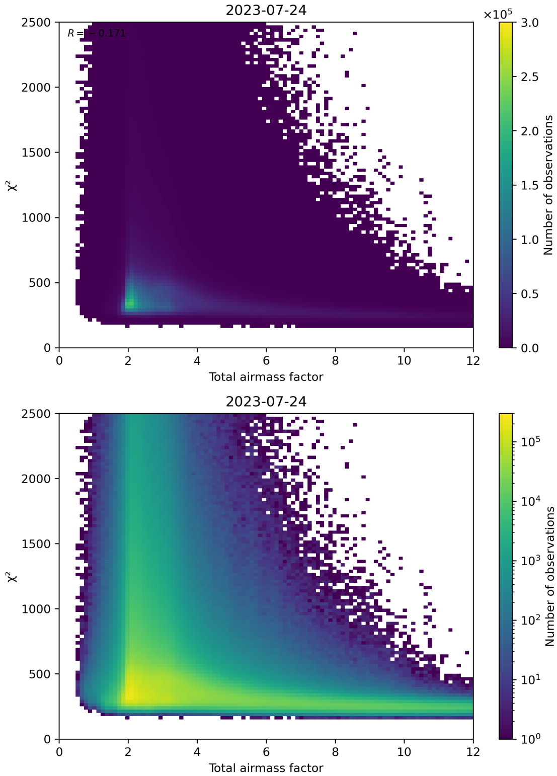
Figure 63: Scatter density plot of “Total airmass factor” against “ \chi^2 ” for 2023-07-24 to 2023-07-25.
