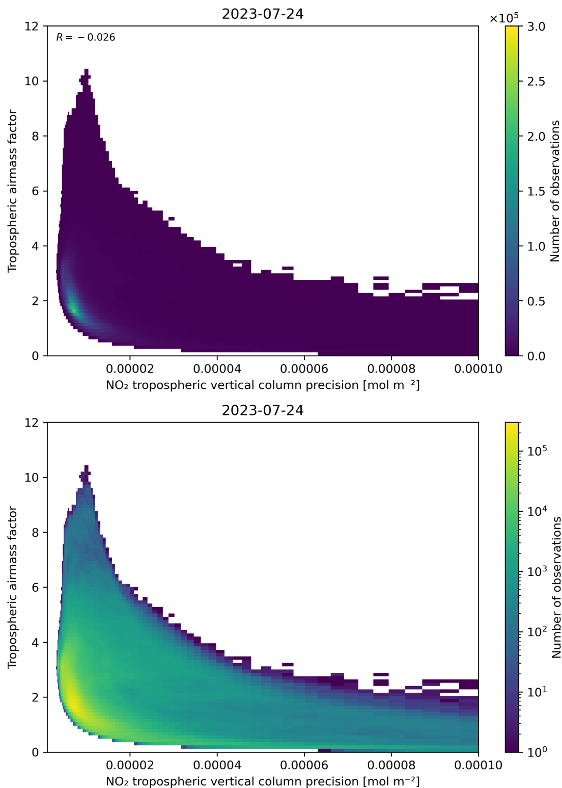
Figure 133: Scatter density plot of “NO 2 tropospheric vertical column precision” against “Tropospheric airmass factor” for 2023-07-24 to 2023-07-25.
