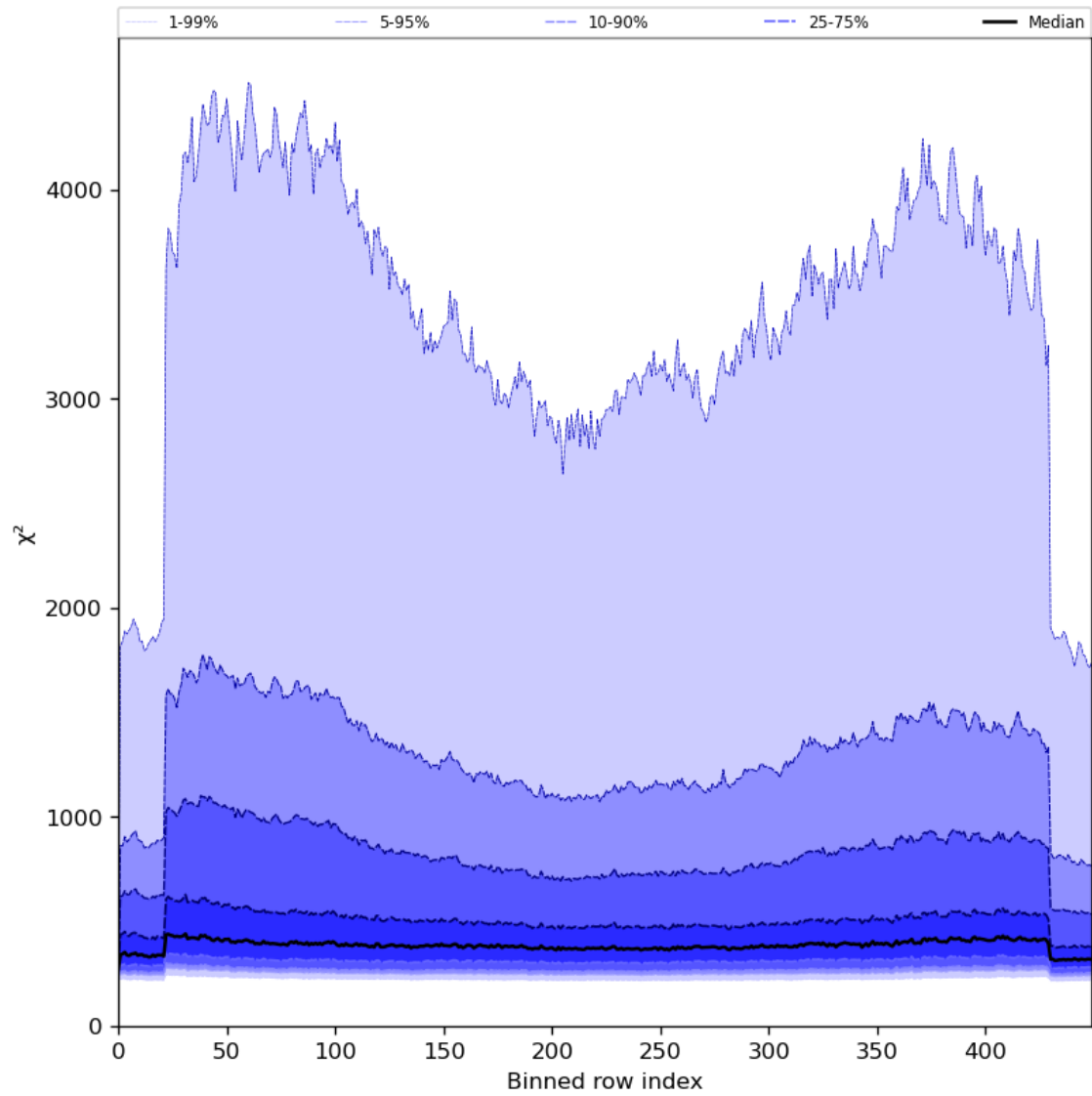
Figure 59: Along track statistics of “ \chi^2 ” for 2023-07-24 to 2023-07-25
