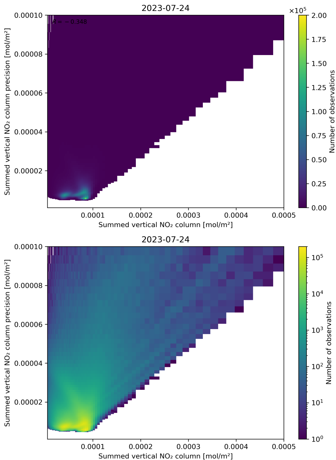
Figure 105: Scatter density plot of “Summed vertical NO 2 column” against “Summed vertical NO 2 column precision” for 2023-07-24 to 2023-07-25.
