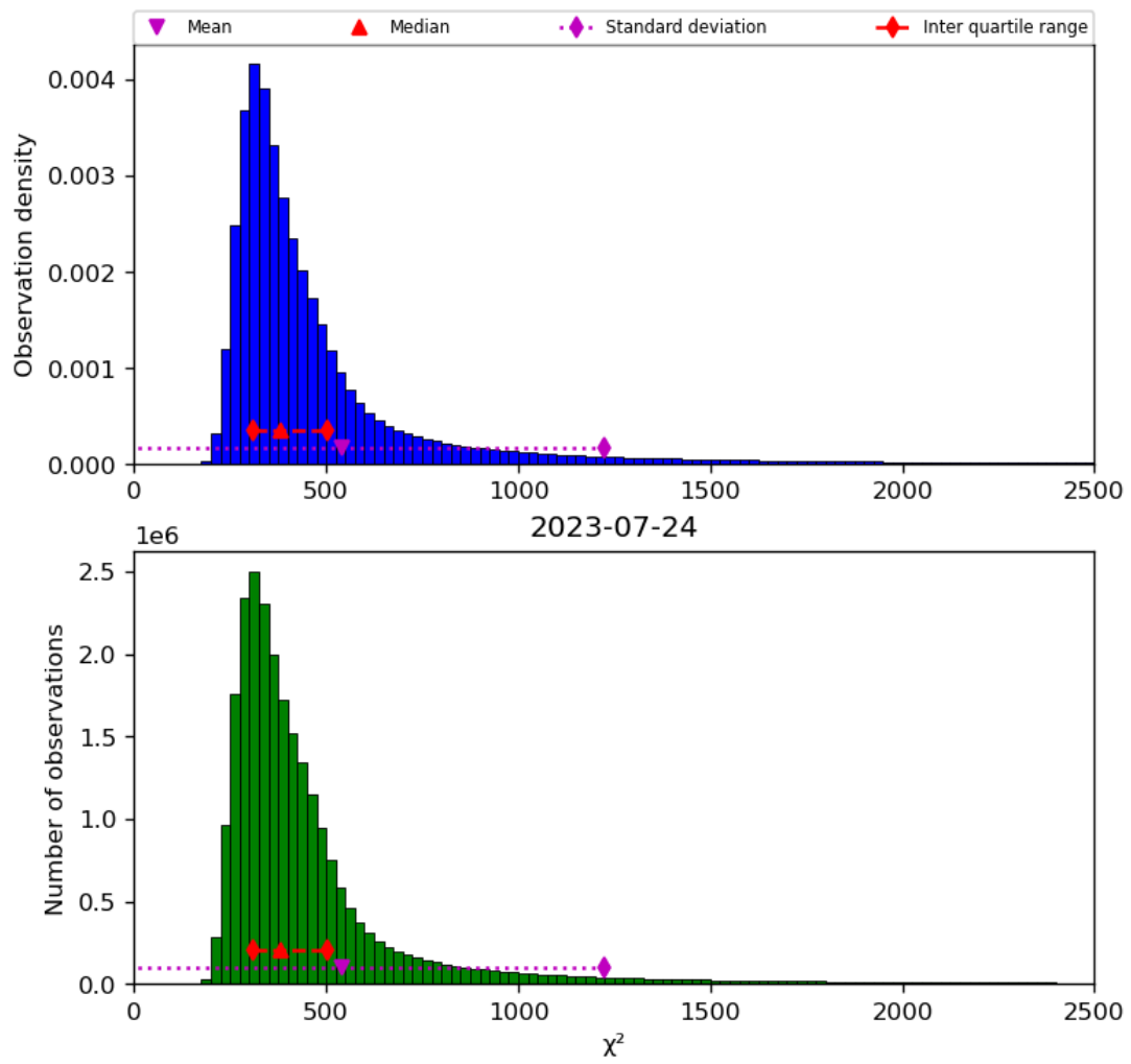
Figure 42: Histogram of " \chi^2 " for 2023-07-24 to 2023-07-25
