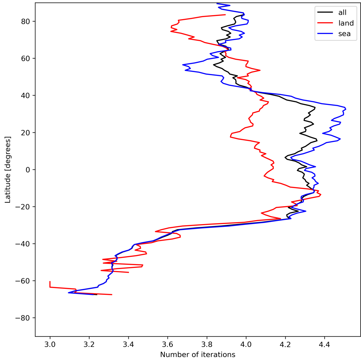
Figure 17: Zonal average of “Number of iterations” for 2023-07-24 to 2023-07-25.
