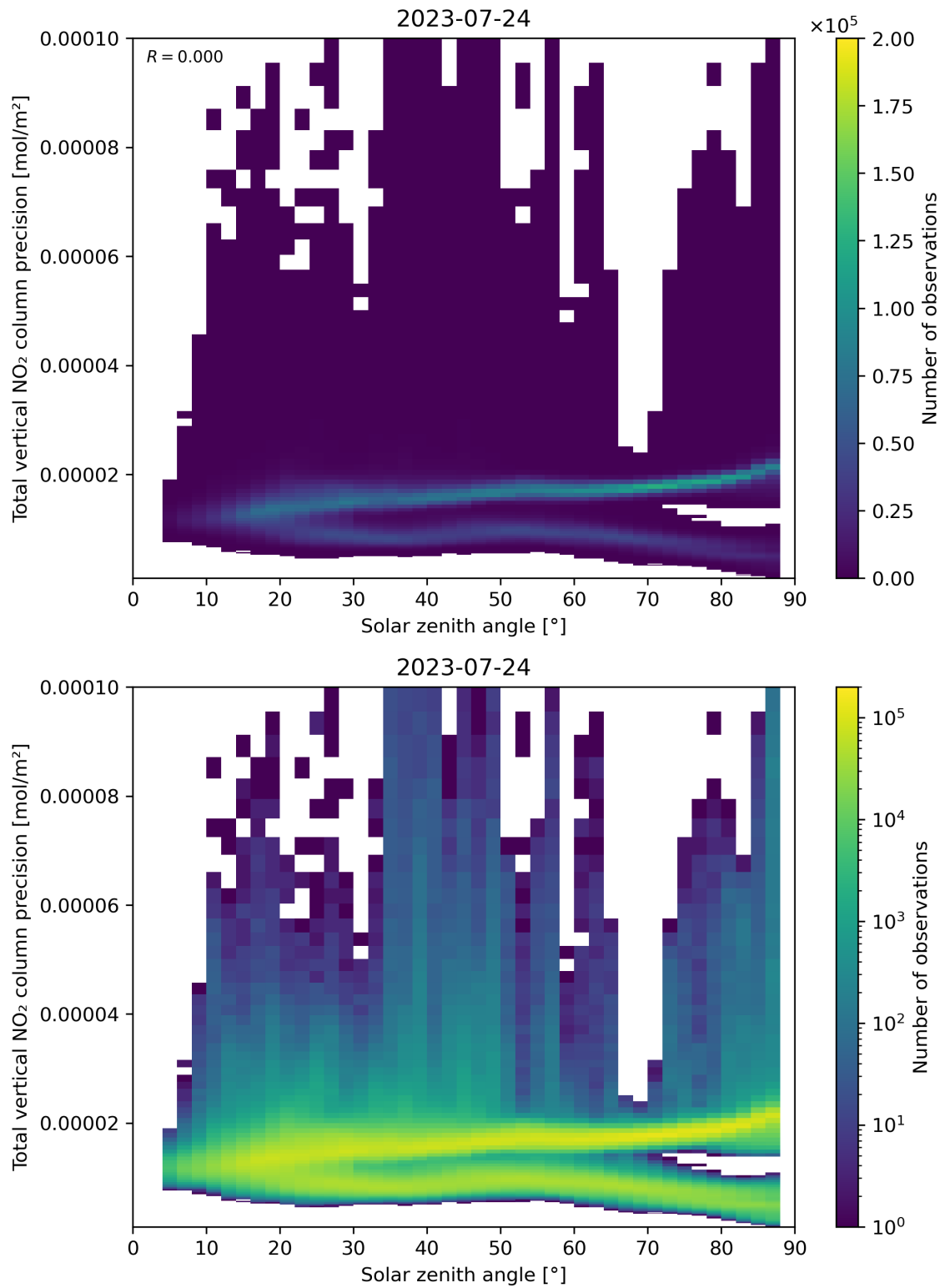
Figure 154: Scatter density plot of “Solar zenith angle” against “Total vertical NO 2 column precision” for 2023-07-24 to 2023-07-25.
