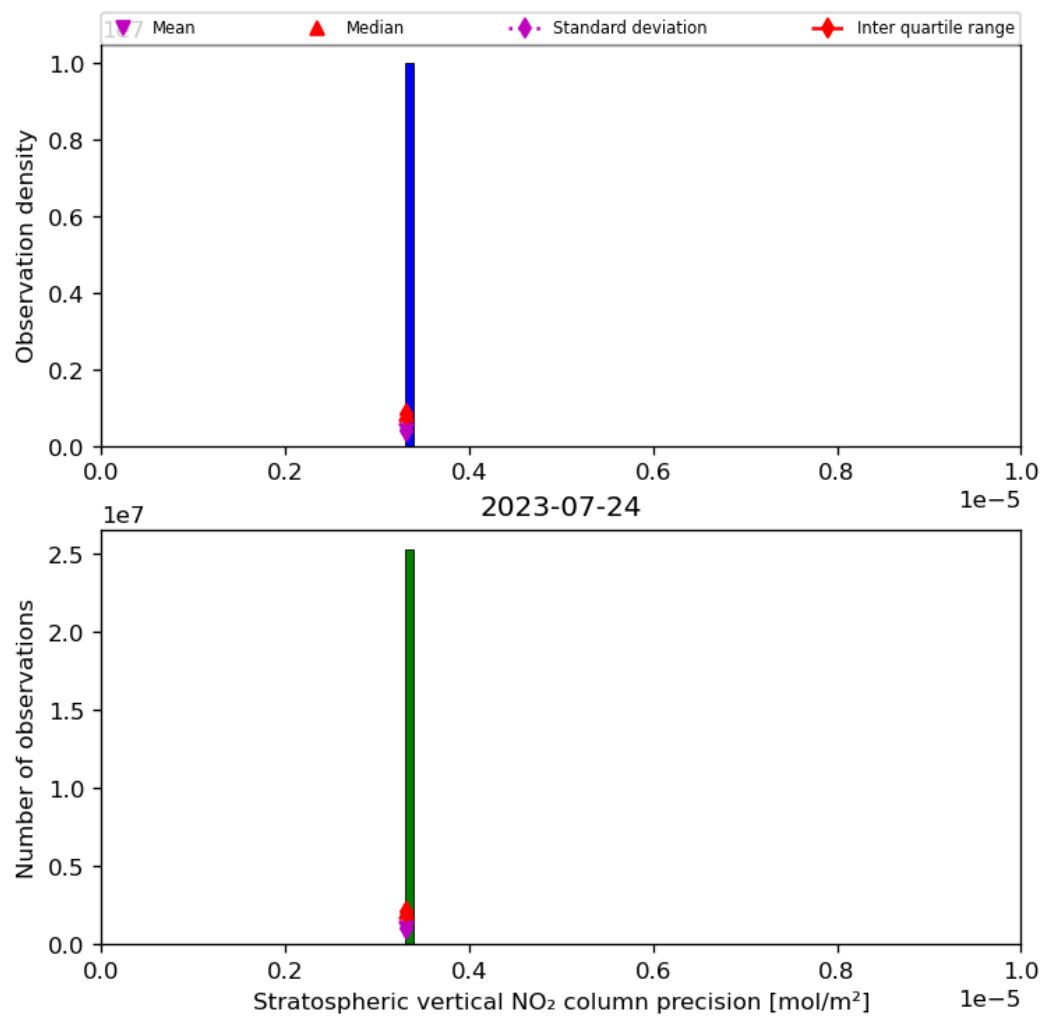
Figure 37: Histogram of “Stratospheric vertical NO 2 column precision” for 2023-07-24 to 2023-07-25
