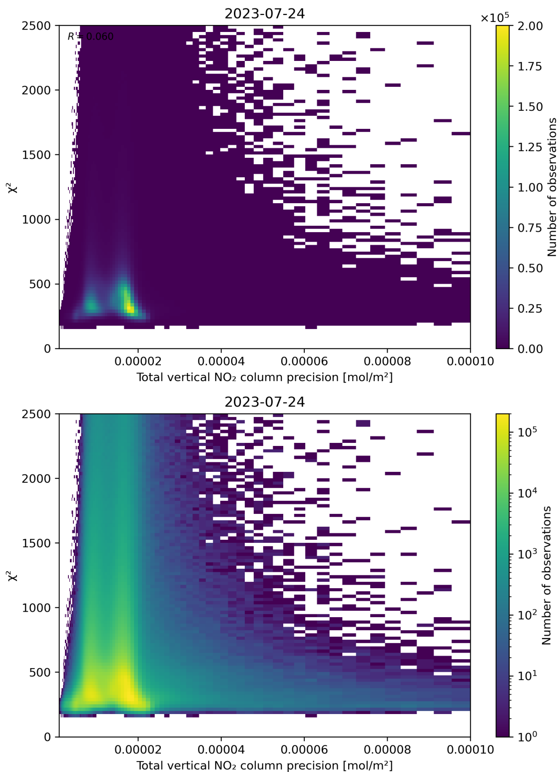
Figure 116: Scatter density plot of “Total vertical NO 2 column precision” against “ \chi^2 ” for 2023-07-24 to 2023-07-25.
