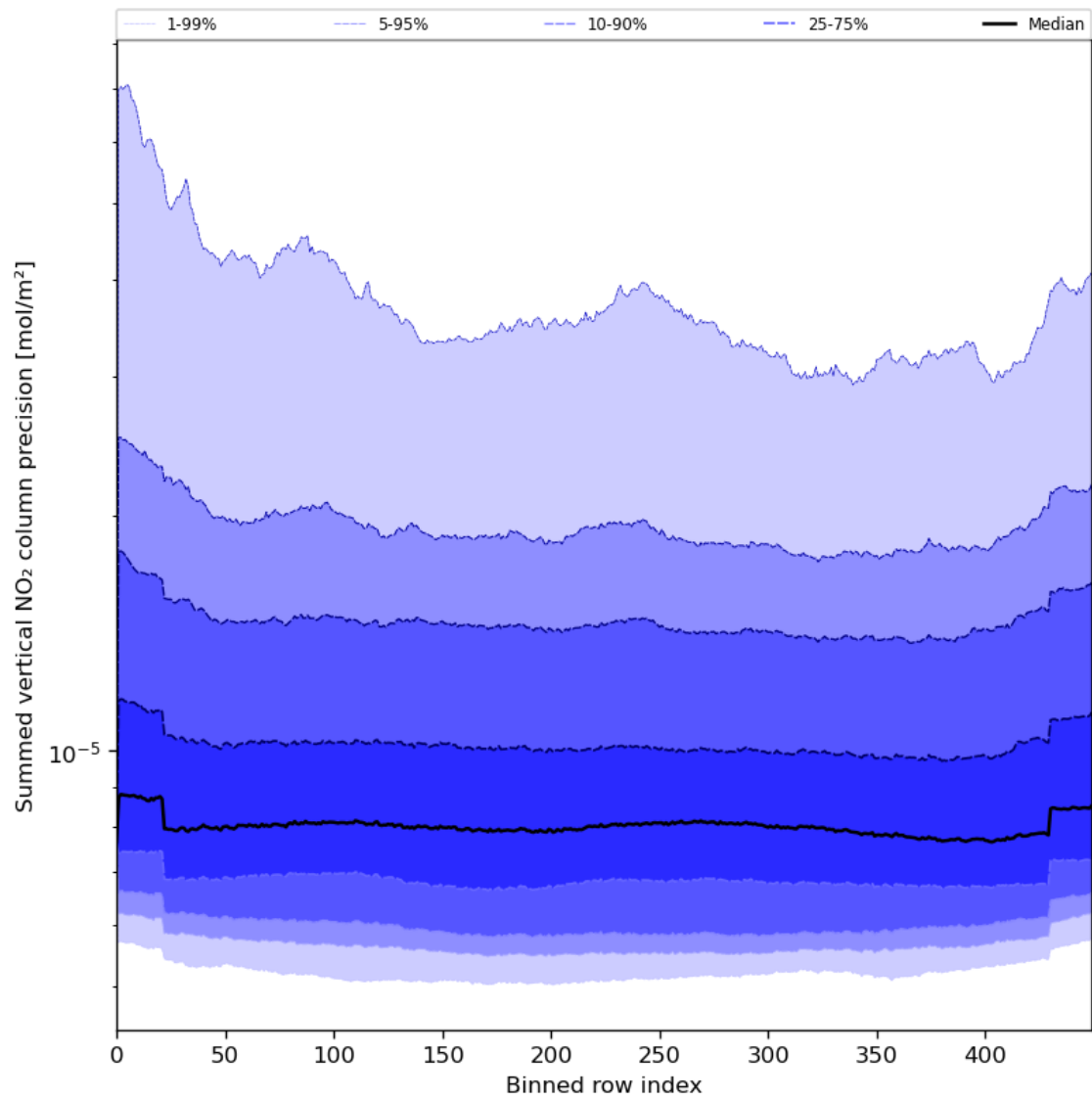
Figure 58: Along track statistics of “Summed vertical NO 2 column precision” for 2023-07-24 to 2023-07-25
