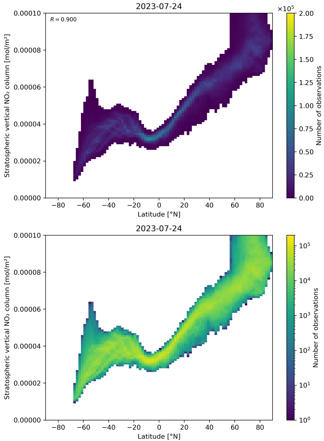
Figure 87: Scatter density plot of “Latitude” against “Stratospheric vertical \text{NO}_2 column” for 2023-07-24 to 2023-07-25.
