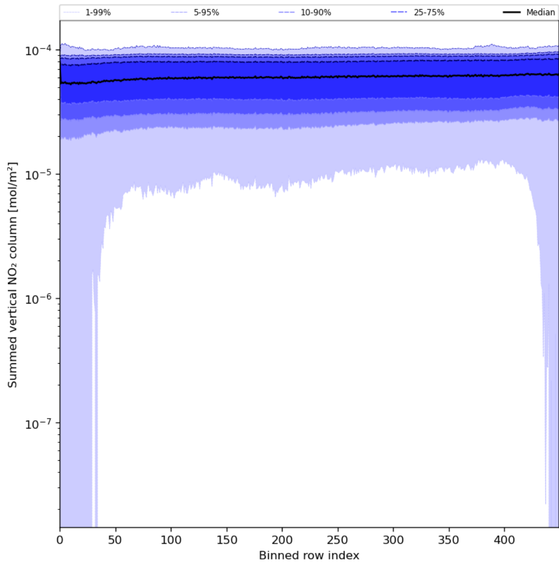
Figure 57: Along track statistics of “Summed vertical NO 2 column” for 2023-07-24 to 2023-07-25
