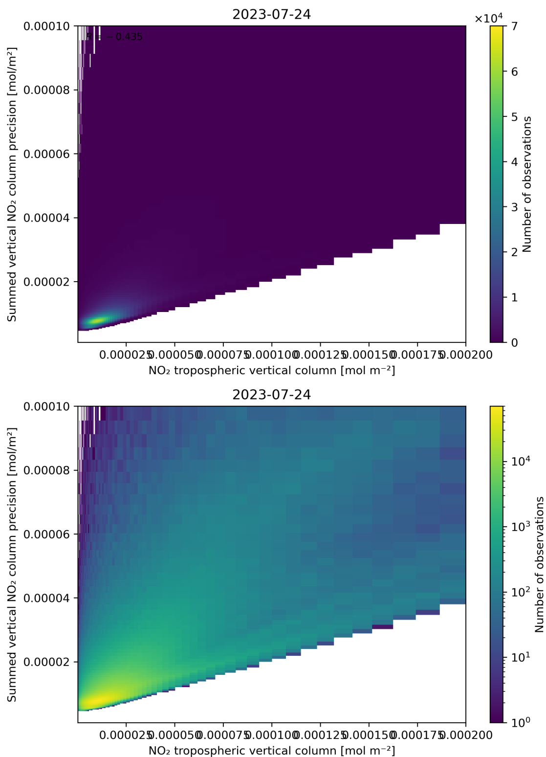
Figure 127: Scatter density plot of “NO 2 tropospheric vertical column” against “Summed vertical NO 2 column precision” for 2023-07-24 to 2023-07-25.
