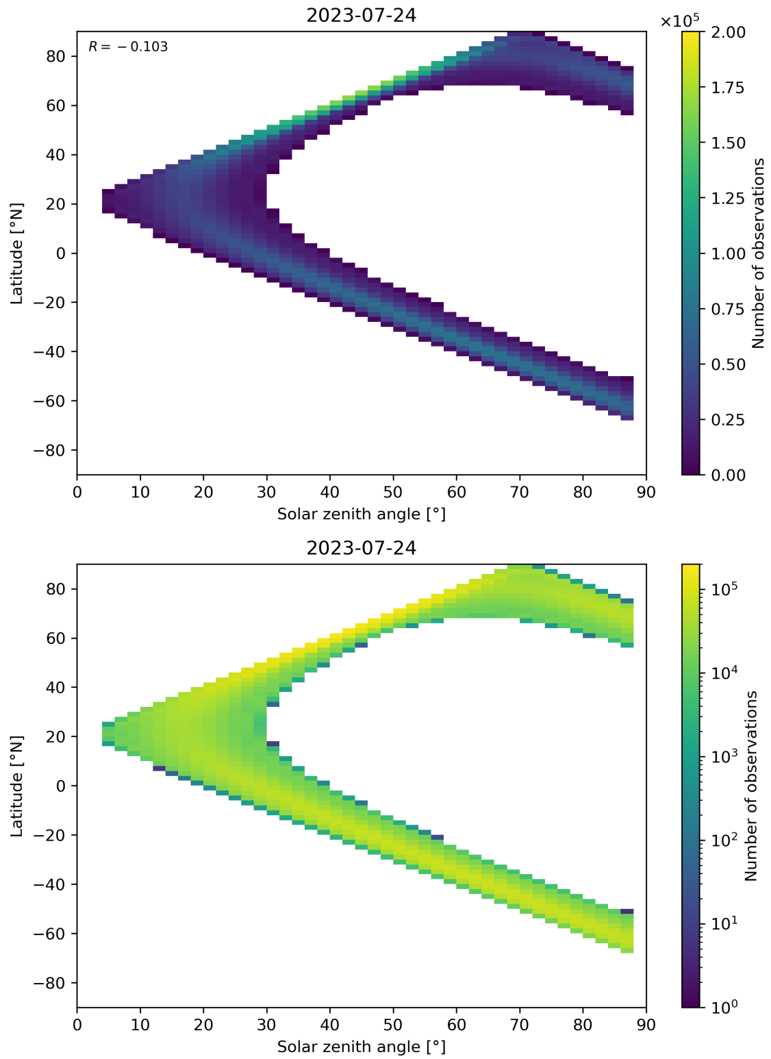
Figure 149: Scatter density plot of “Solar zenith angle” against “Latitude” for 2023-07-24 to 2023-07-25.
