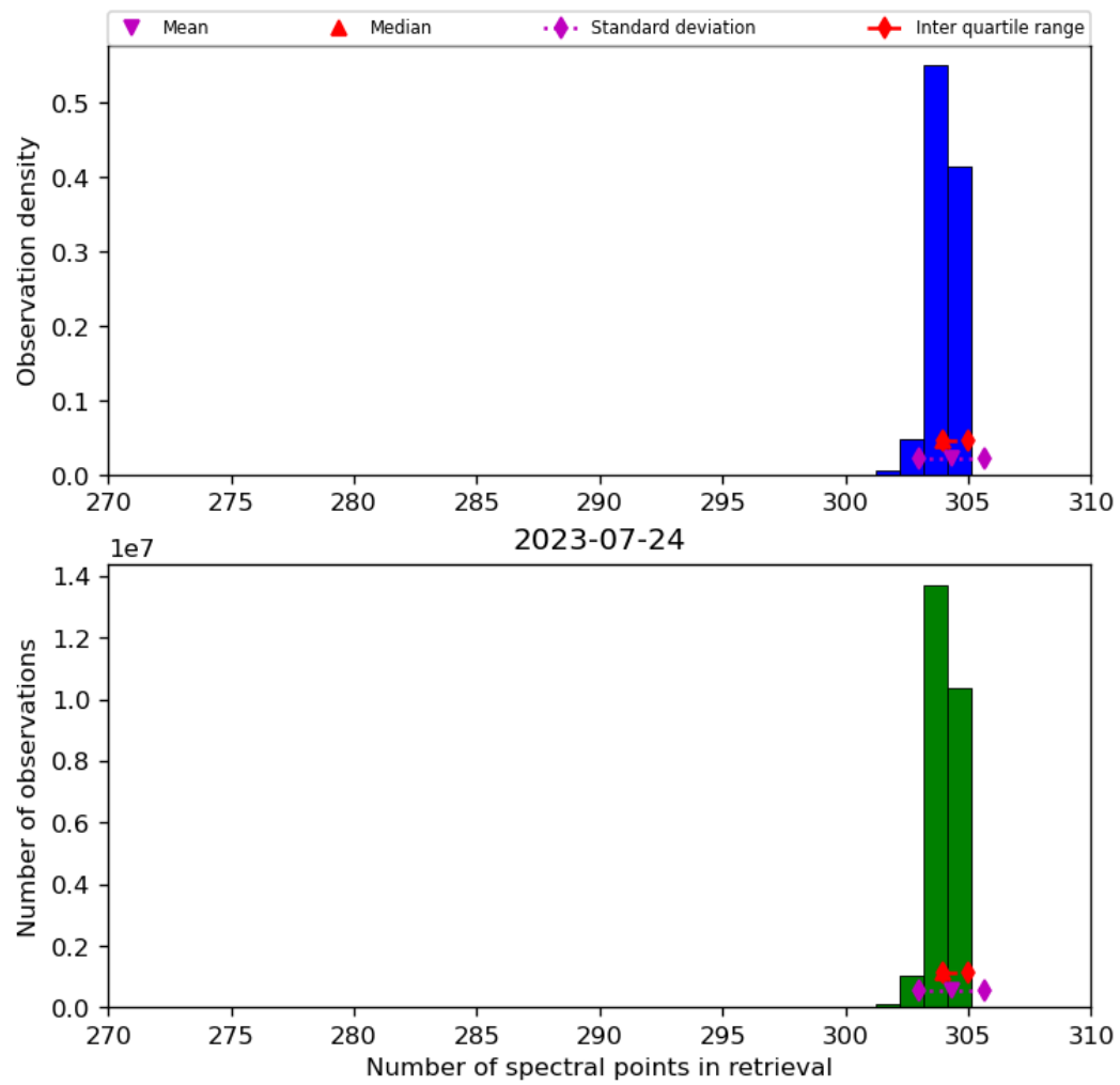
Figure 33: Histogram of “Number of spectral points in retrieval” for 2023-07-24 to 2023-07-25
