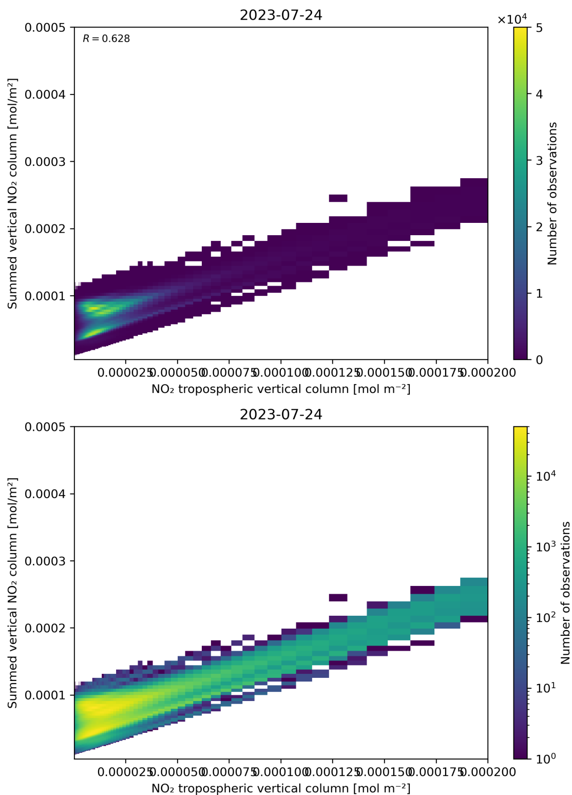
Figure 126: Scatter density plot of “NO 2 tropospheric vertical column” against “Summed vertical NO 2 column” for 2023-07-24 to 2023-07-25.
