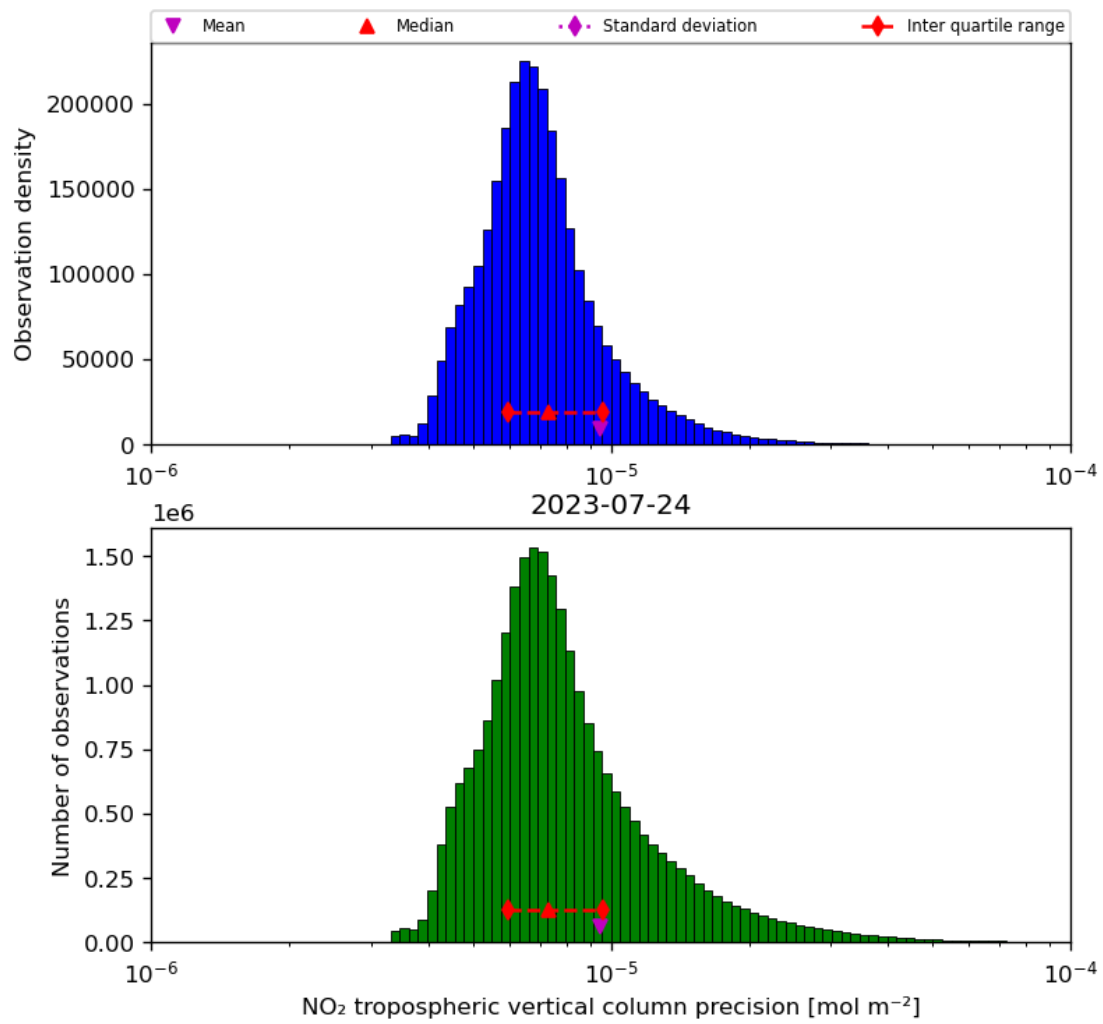
Figure 30: Histogram of “NO 2 tropospheric vertical column precision” for 2023-07-24 to 2023-07-25
