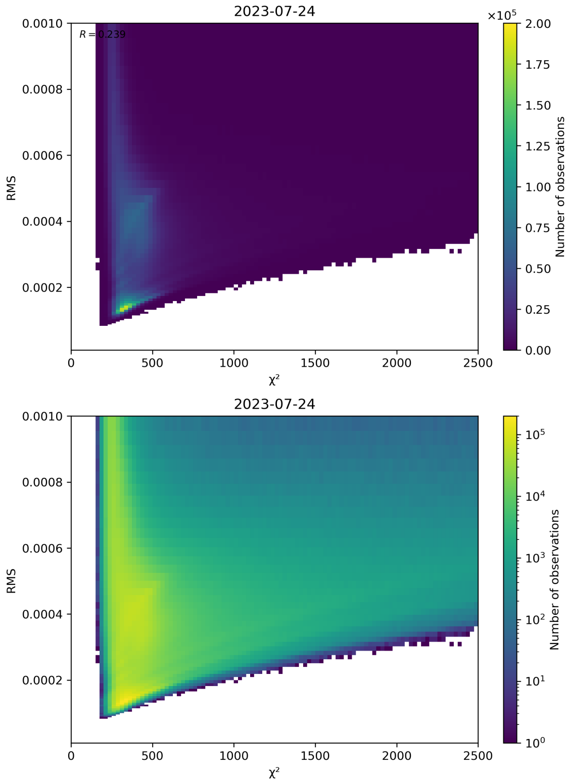
Figure 82: Scatter density plot of “ \chi^2 ” against “RMS” for 2023-07-24 to 2023-07-25.
