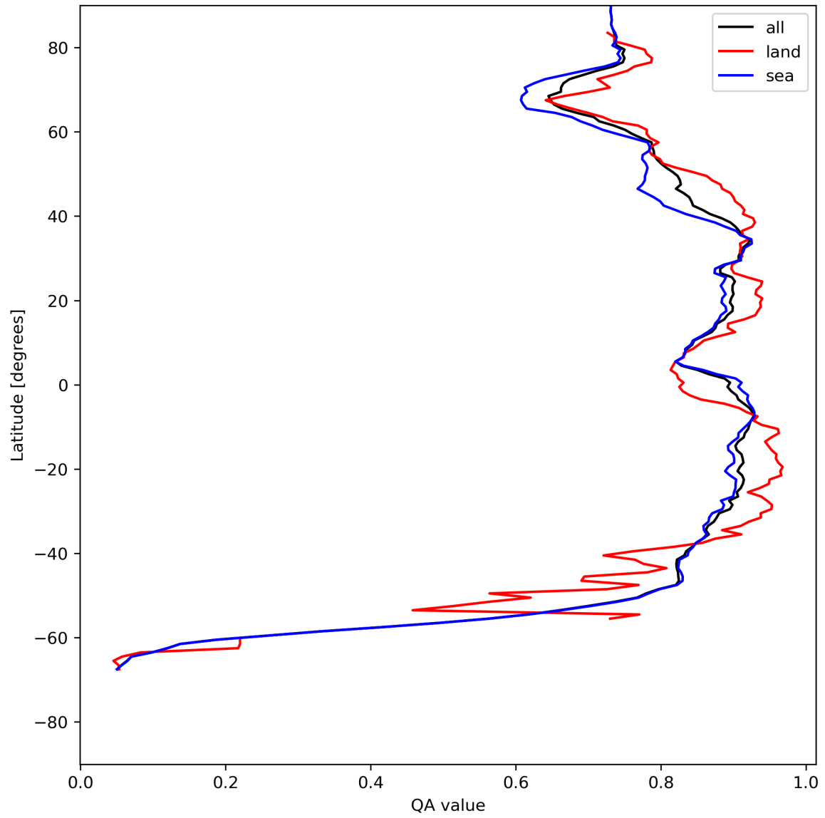
Figure 11: Zonal average of “QA value” for 2023-07-24 to 2023-07-25.
