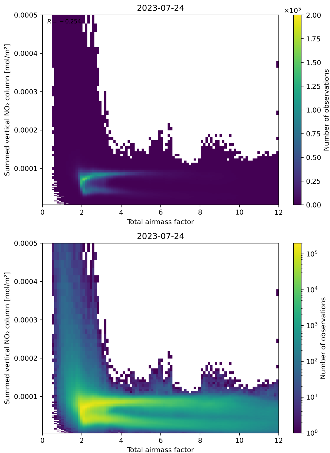
Figure 65: Scatter density plot of “Total airmass factor” against “Summed vertical NO 2 column” for 2023-07-24 to 2023-07-25.
