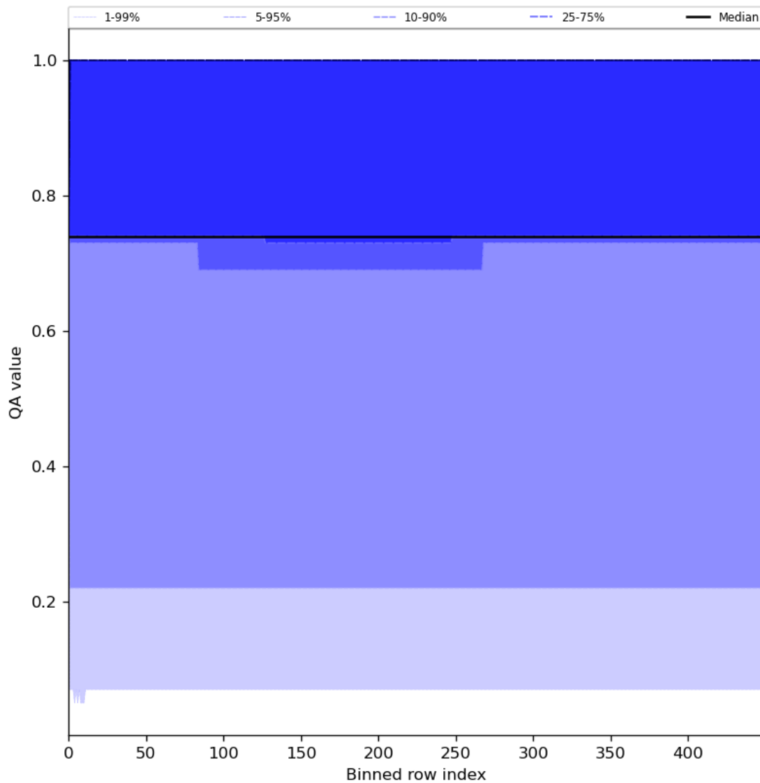
Figure 45: Along track statistics of “QA value” for 2023-07-24 to 2023-07-25
