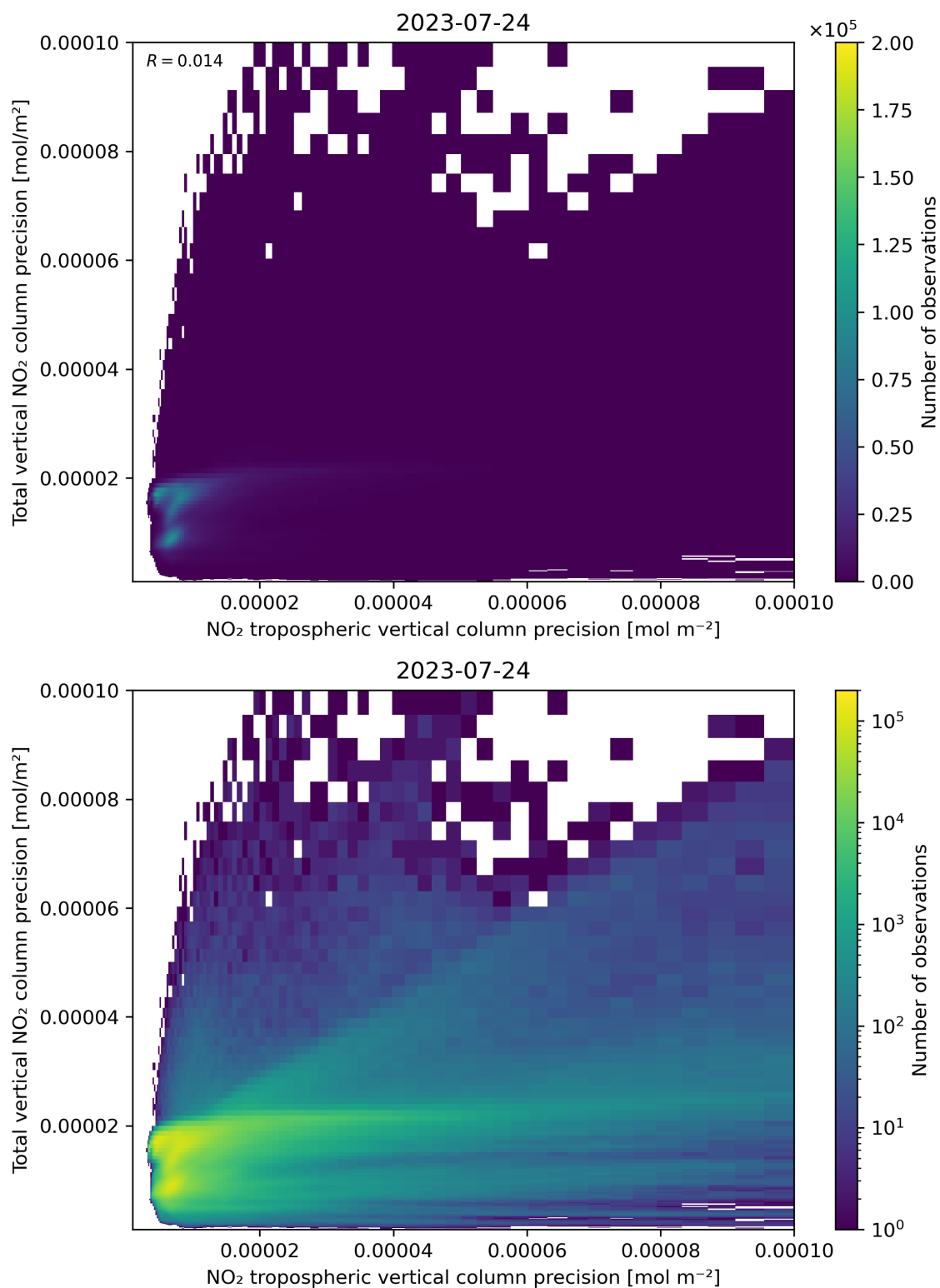
Figure 139: Scatter density plot of “NO 2 tropospheric vertical column precision” against “Total vertical NO 2 column precision” for 2023-07-24 to 2023-07-25.
