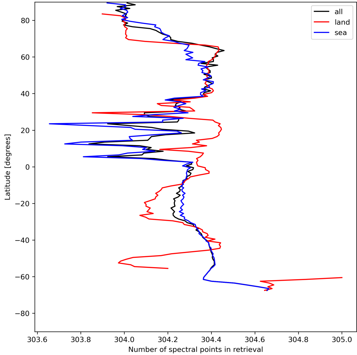
Figure 16: Zonal average of “Number of spectral points in retrieval” for 2023-07-24 to 2023-07-25.
