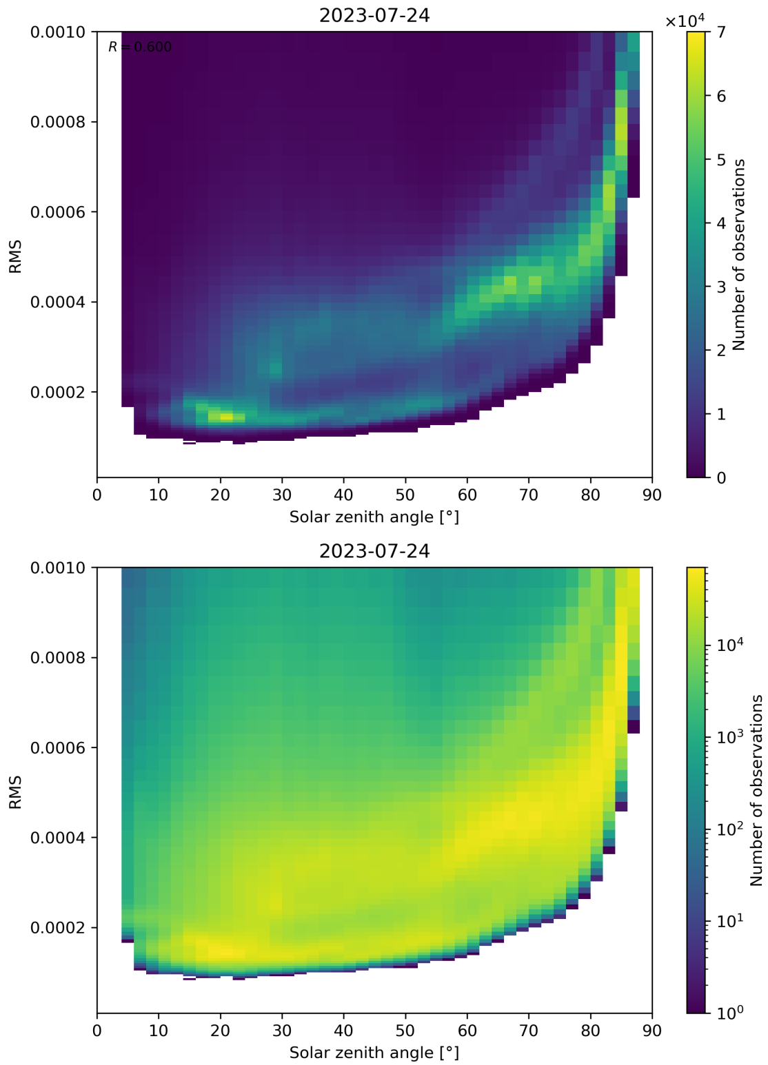
Figure 157: Scatter density plot of “Solar zenith angle” against “RMS” for 2023-07-24 to 2023-07-25.
