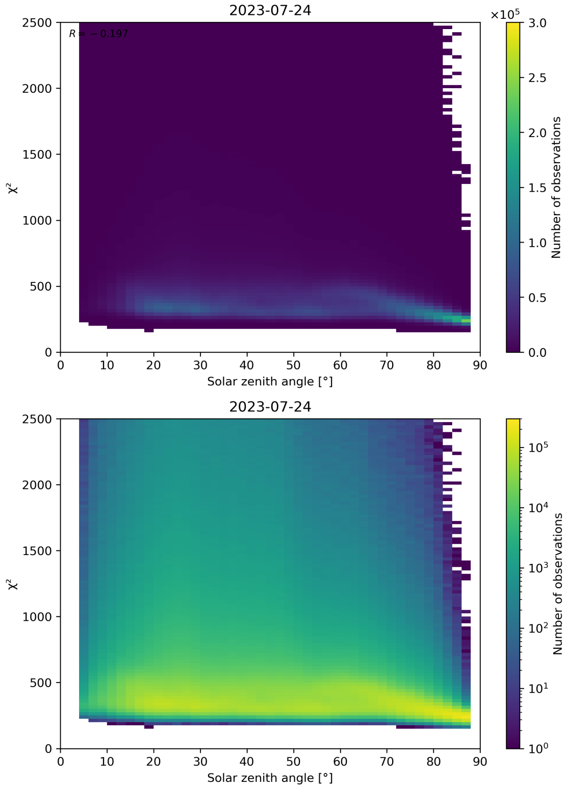
Figure 148: Scatter density plot of “Solar zenith angle” against “ \chi^2 ” for 2023-07-24 to 2023-07-25.
