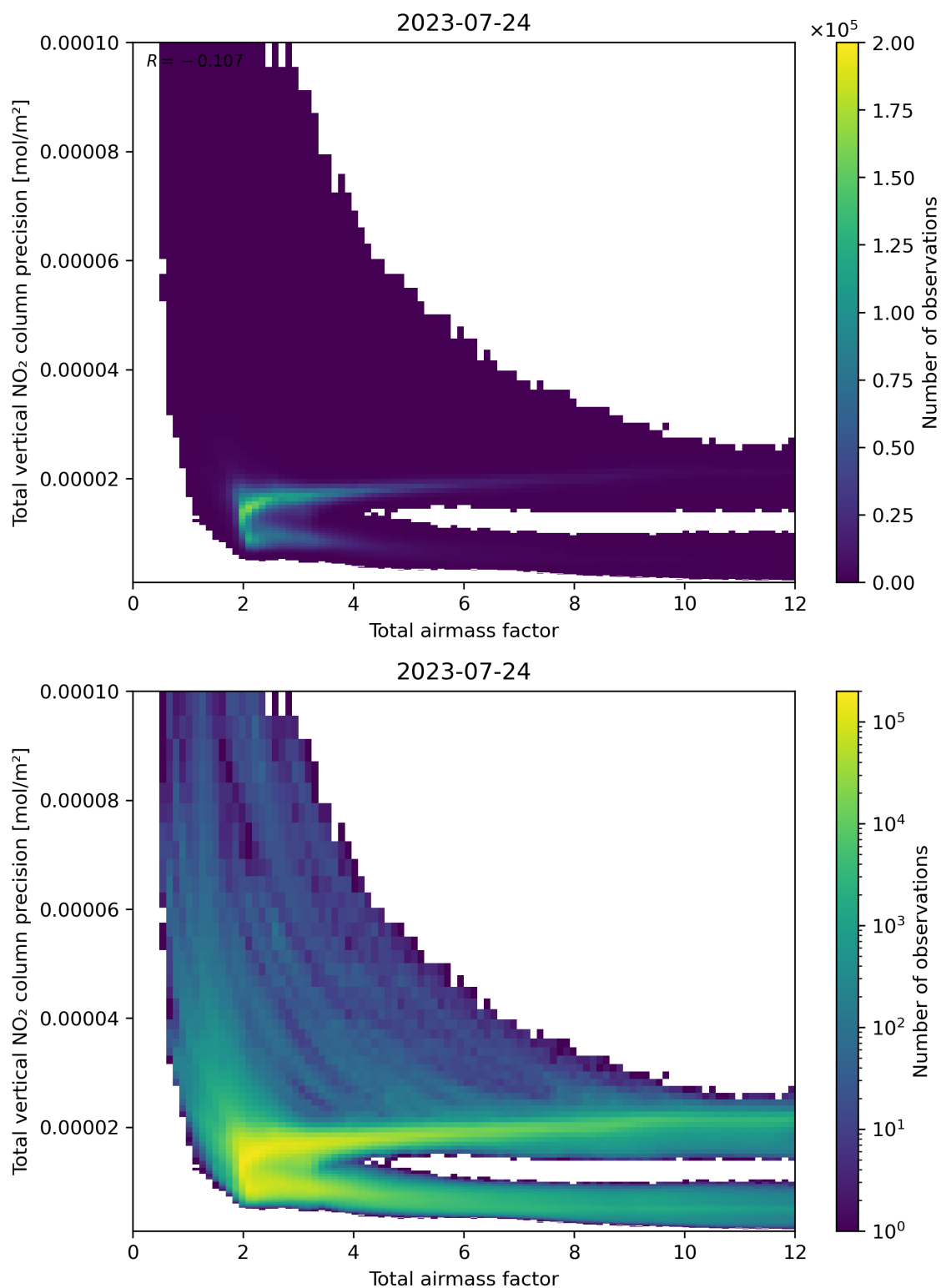
Figure 68: Scatter density plot of “Total airmass factor” against “Total vertical NO 2 column precision” for 2023-07-24 to 2023-07-25.
