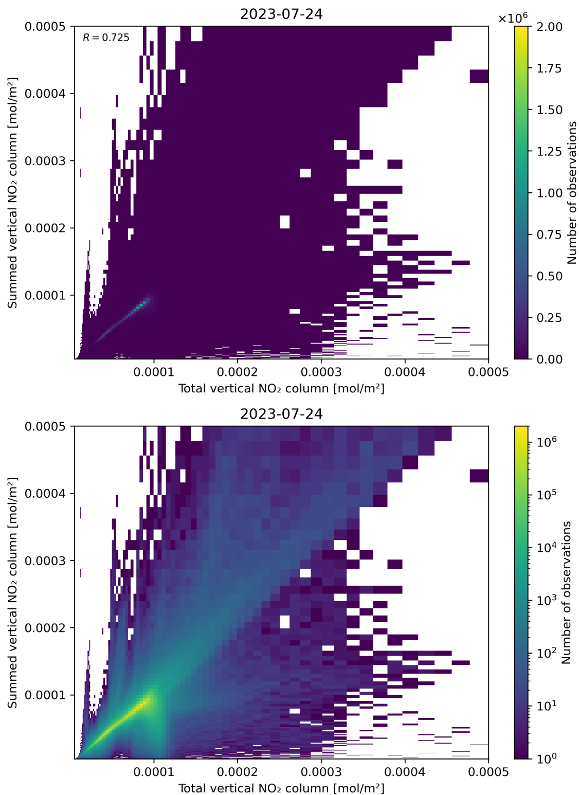
Figure 112: Scatter density plot of “Total vertical NO 2 column” against “Summed vertical NO 2 column” for 2023-07-24 to 2023-07-25.
