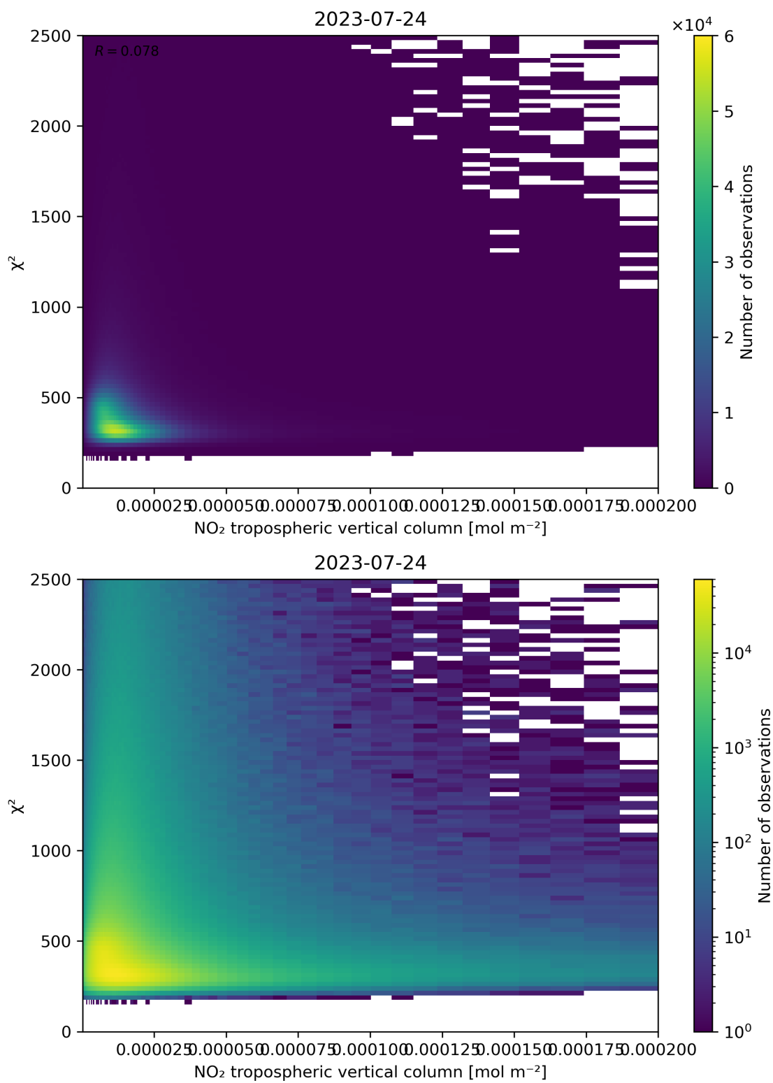
Figure 124: Scatter density plot of “NO 2 tropospheric vertical column” against “ \chi^2 ” for 2023-07-24 to 2023-07-25.
