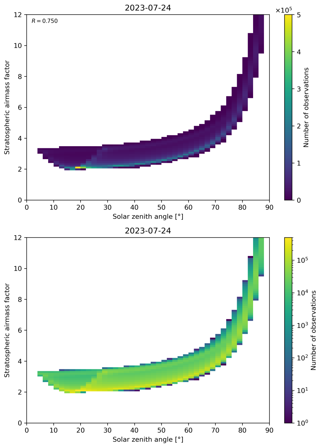
Figure 145: Scatter density plot of “Solar zenith angle” against “Stratospheric airmass factor” for 2023-07-24 to 2023-07-25.
