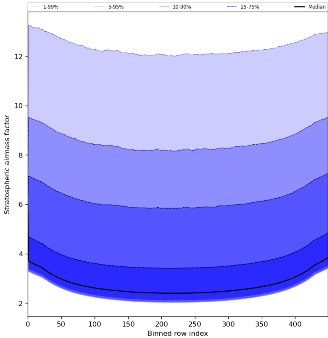
Figure 61: Along track statistics of “Stratospheric airmass factor” for 2023-07-24 to 2023-07-25
