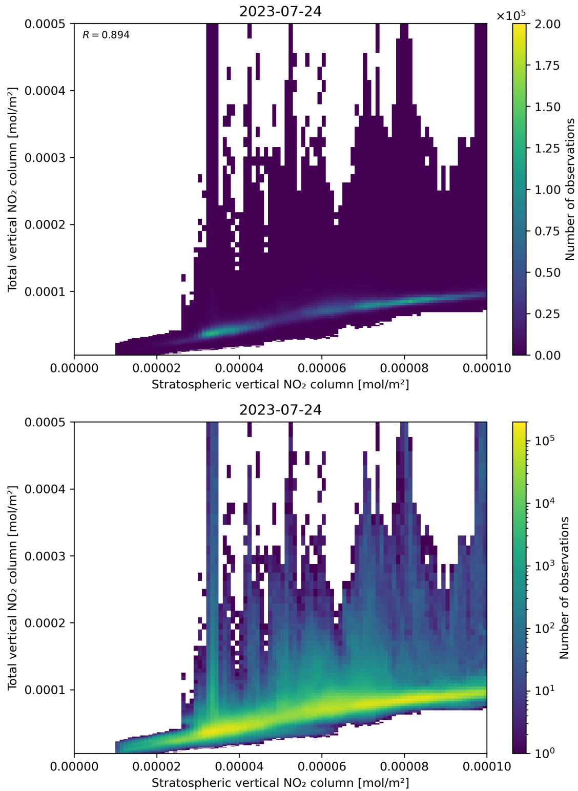
Figure 100: Scatter density plot of “Stratospheric vertical NO 2 column” against “Total vertical NO 2 column” for 2023-07-24 to 2023-07-25.
