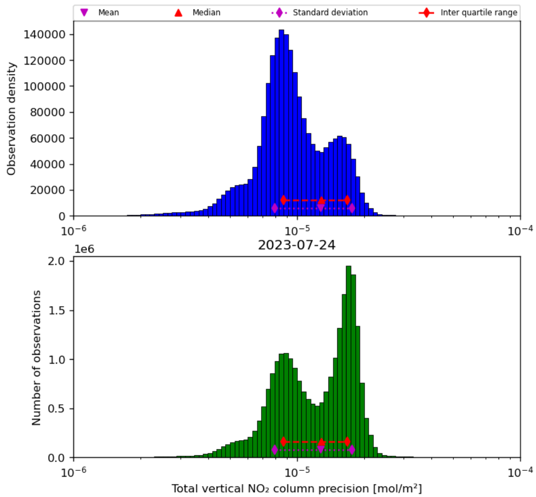
Figure 39: Histogram of “Total vertical NO 2 column precision” for 2023-07-24 to 2023-07-25
