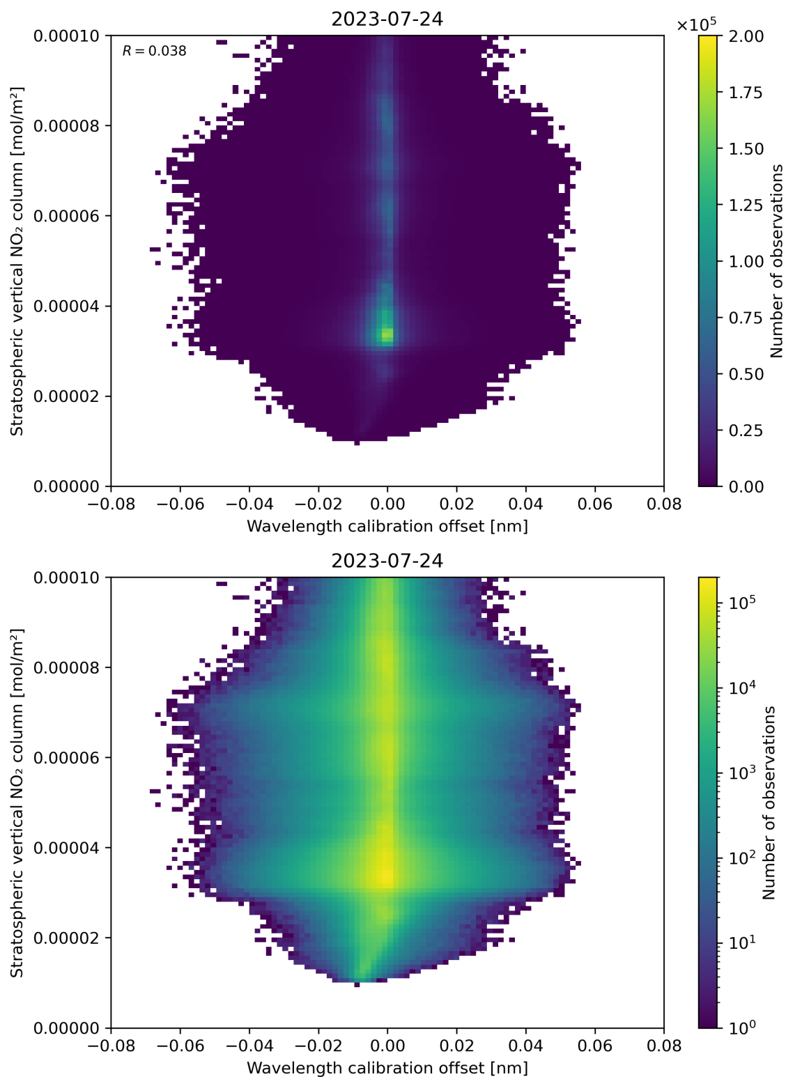
Figure 176: Scatter density plot of “Wavelength calibration offset” against “Stratospheric vertical NO 2 column” for 2023-07-24 to 2023-07-25.
