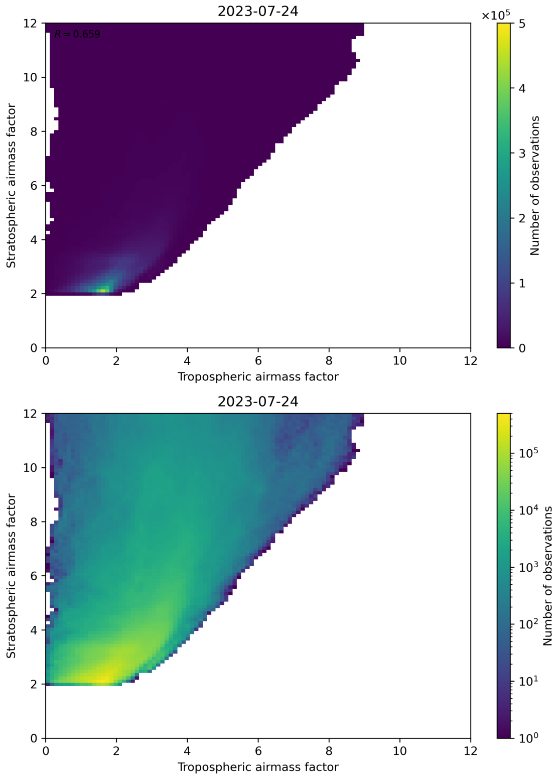
Figure 71: Scatter density plot of “Tropospheric airmass factor” against “Stratospheric airmass factor” for 2023-07-24 to 2023-07-25.
