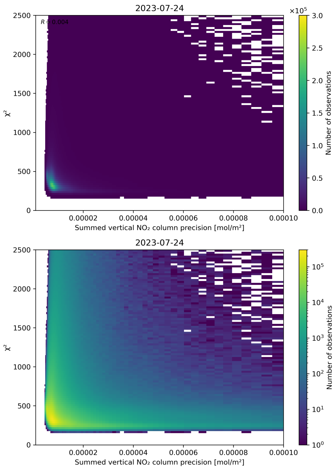
Figure 107: Scatter density plot of “Summed vertical NO 2 column precision” against “ \chi^2 ” for 2023-07-24 to 2023-07-25.
