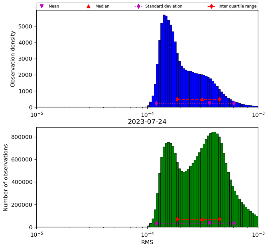
Figure 43: Histogram of “RMS” for 2023-07-24 to 2023-07-25
