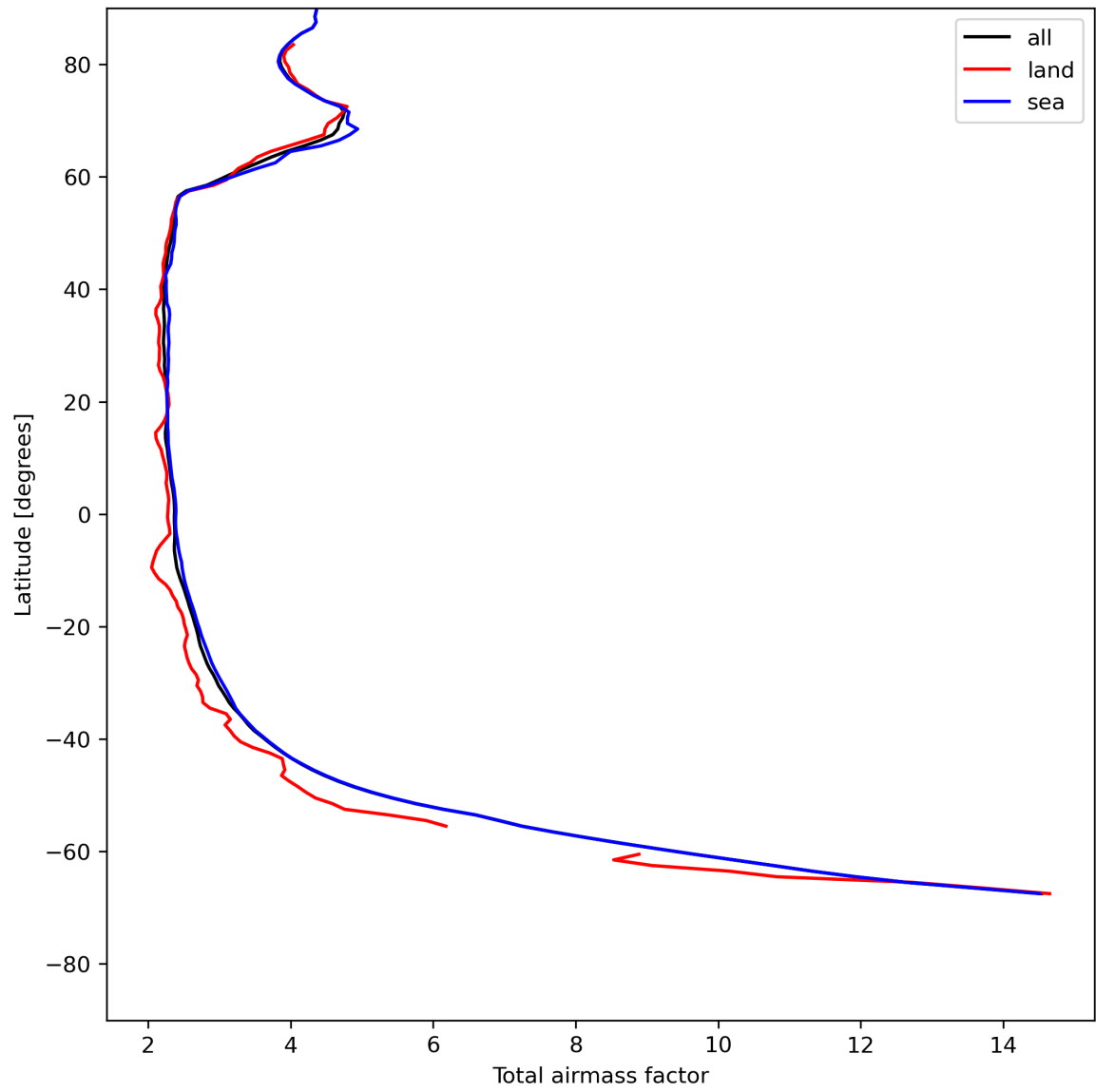
Figure 15: Zonal average of “Total airmass factor” for 2023-07-24 to 2023-07-25.
