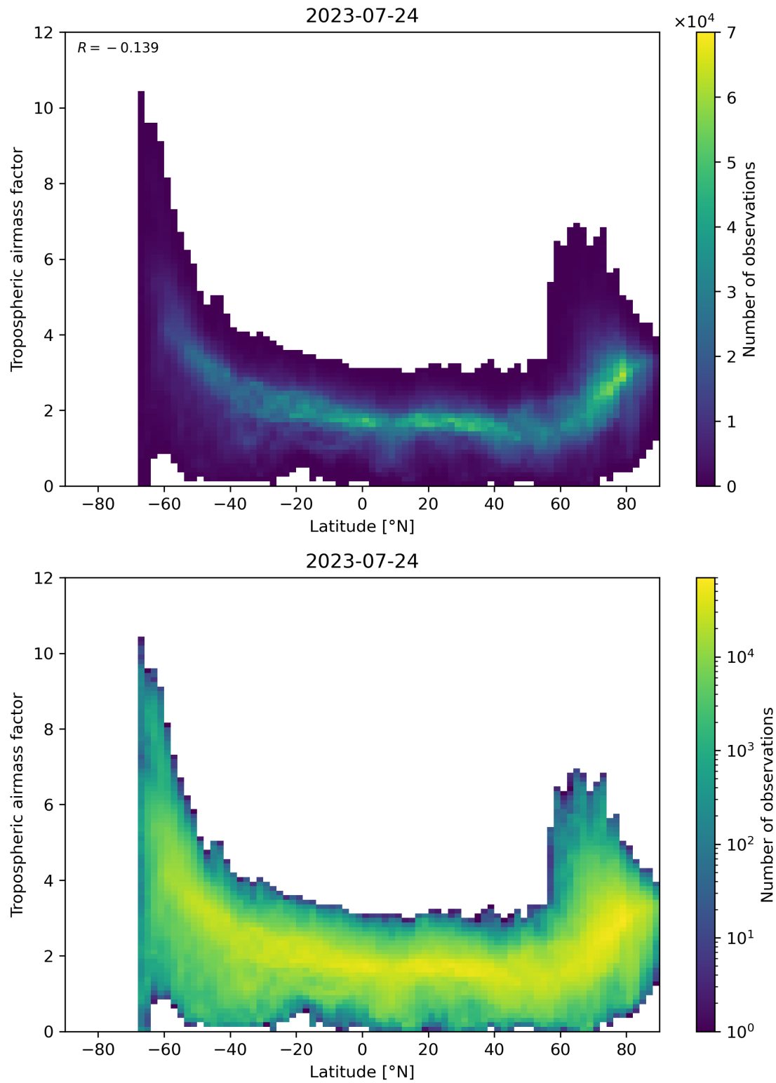
Figure 85: Scatter density plot of “Latitude” against “Tropospheric airmass factor” for 2023-07-24 to 2023-07-25.
