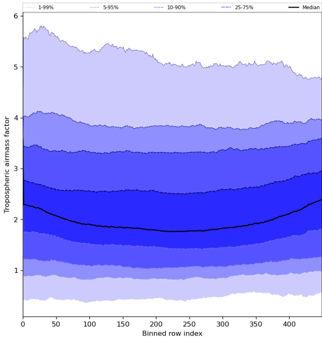
Figure 48: Along track statistics of “Tropospheric airmass factor” for 2023-07-24 to 2023-07-25
