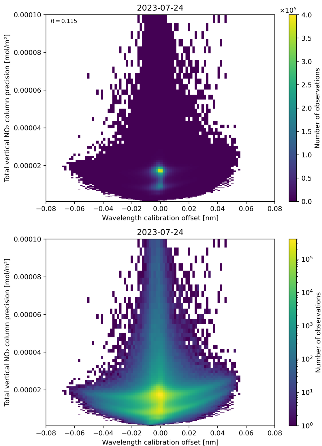
Figure 180: Scatter density plot of “Wavelength calibration offset” against “Total vertical NO 2 column precision” for 2023-07-24 to 2023-07-25.
