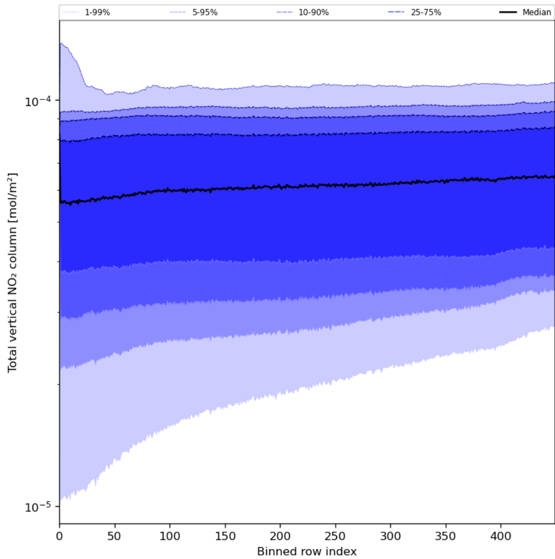
Figure 55: Along track statistics of “Total vertical NO 2 column” for 2023-07-24 to 2023-07-25
