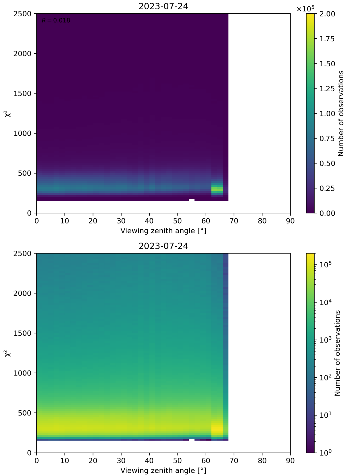
Figure 162: Scatter density plot of “Viewing zenith angle” against “ \chi^2 ” for 2023-07-24 to 2023-07-25.
