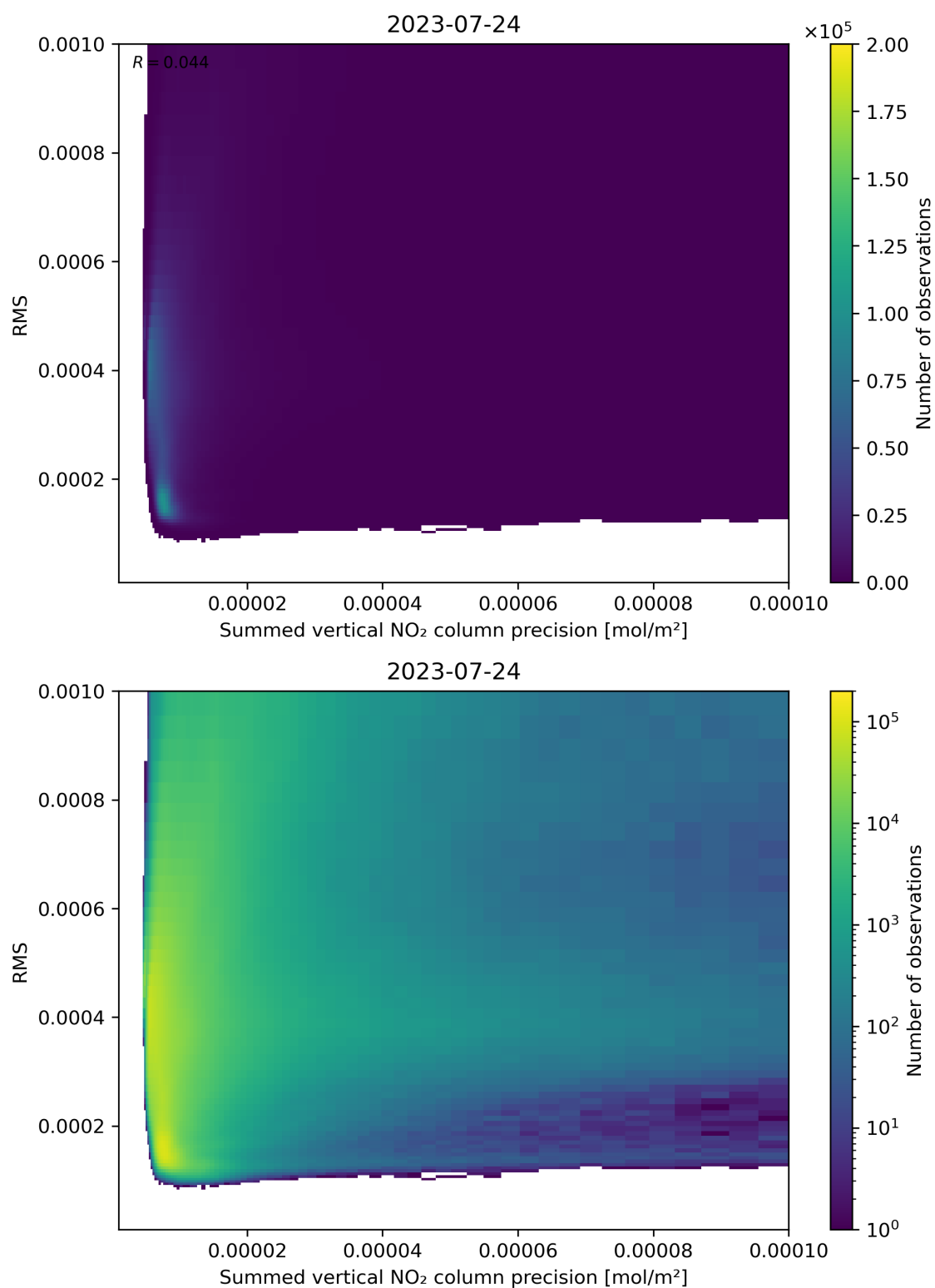
Figure 108: Scatter density plot of “Summed vertical NO 2 column precision” against “RMS” for 2023-07-24 to 2023-07-25.
