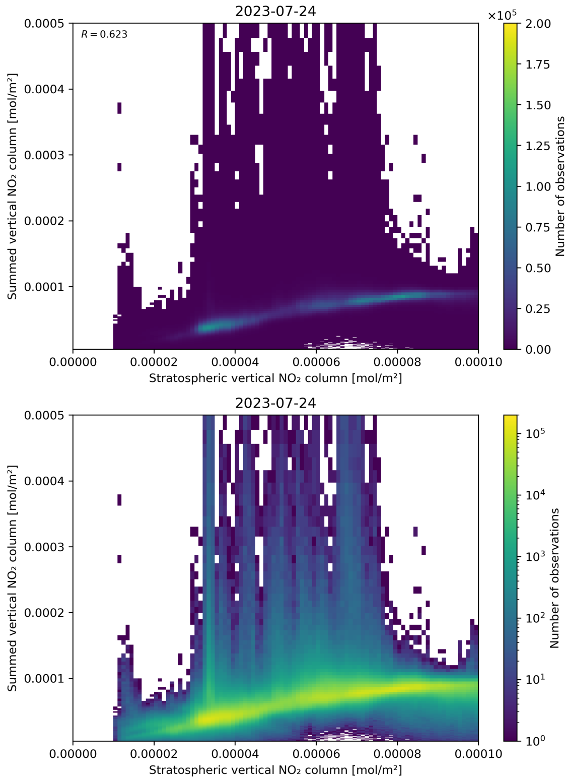
Figure 98: Scatter density plot of “Stratospheric vertical NO 2 column” against “Summed vertical NO 2 column” for 2023-07-24 to 2023-07-25.
