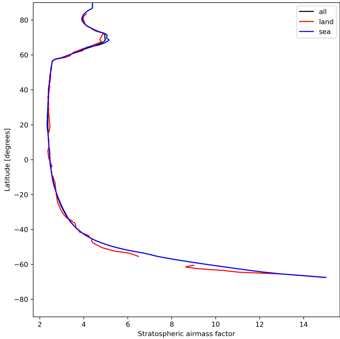
Figure 27: Zonal average of “Stratospheric air mass factor” for 2023-07-24 to 2023-07-25.
