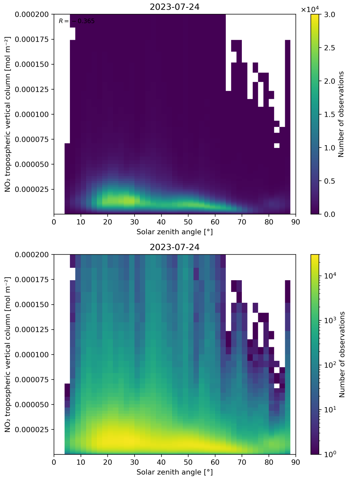
Figure 155: Scatter density plot of “Solar zenith angle” against “NO 2 tropospheric vertical column” for 2023-07-24 to 2023-07-25.
