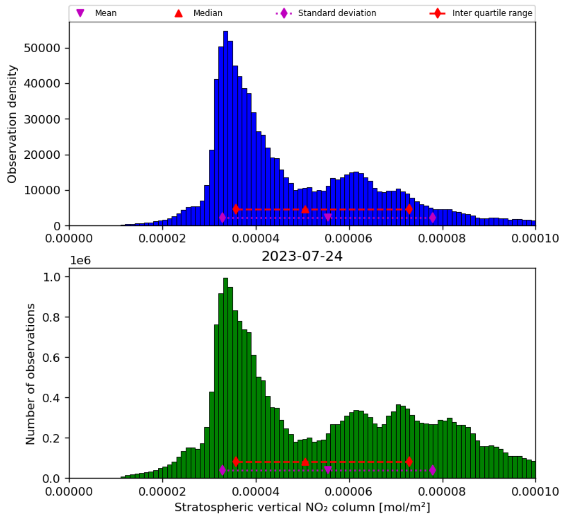
Figure 36: Histogram of “Stratospheric vertical NO 2 column” for 2023-07-24 to 2023-07-25
