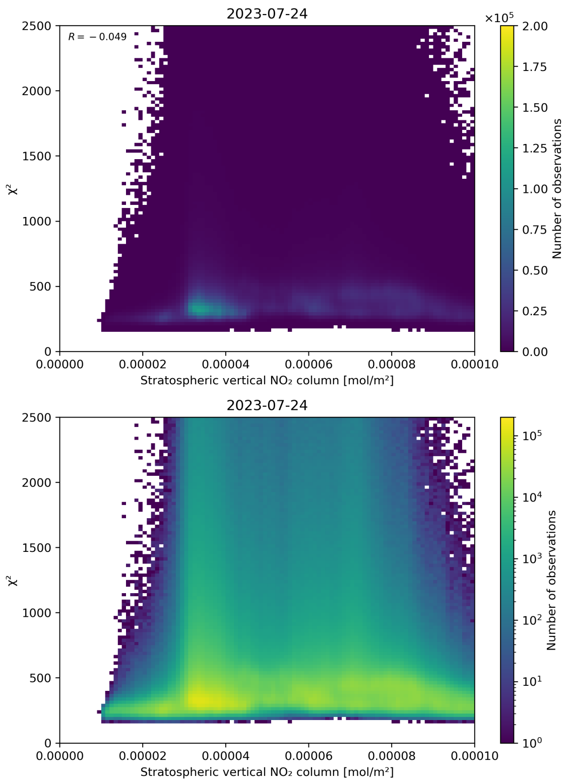
Figure 97: Scatter density plot of “Stratospheric vertical NO 2 column” against “ \chi^2 ” for 2023-07-24 to 2023-07-25.
