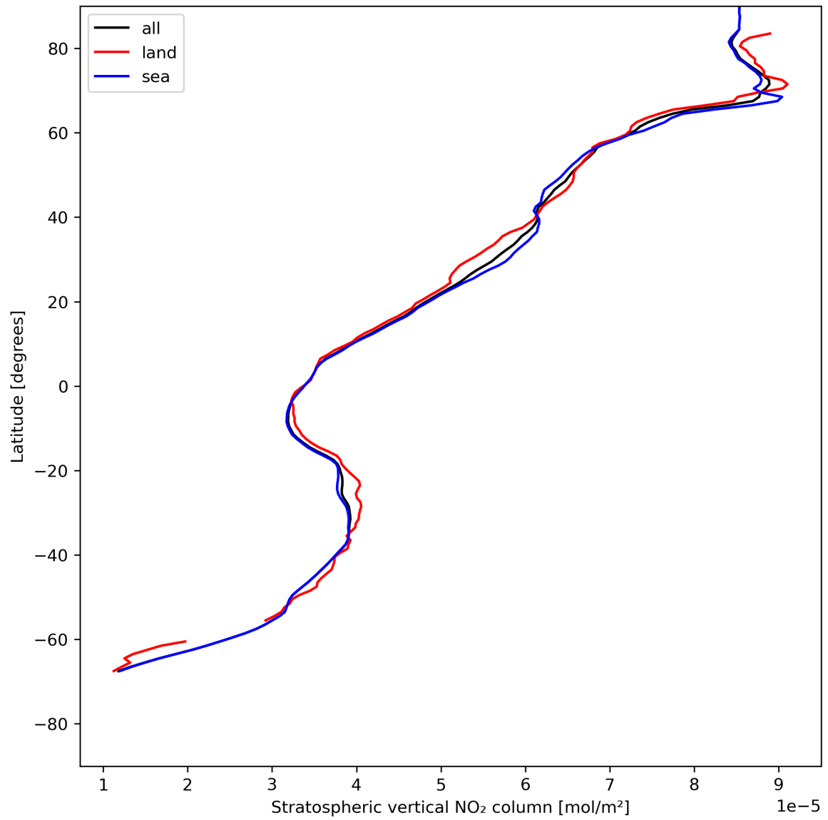
Figure 19: Zonal average of “Stratospheric vertical NO 2 column” for 2023-07-24 to 2023-07-25.
