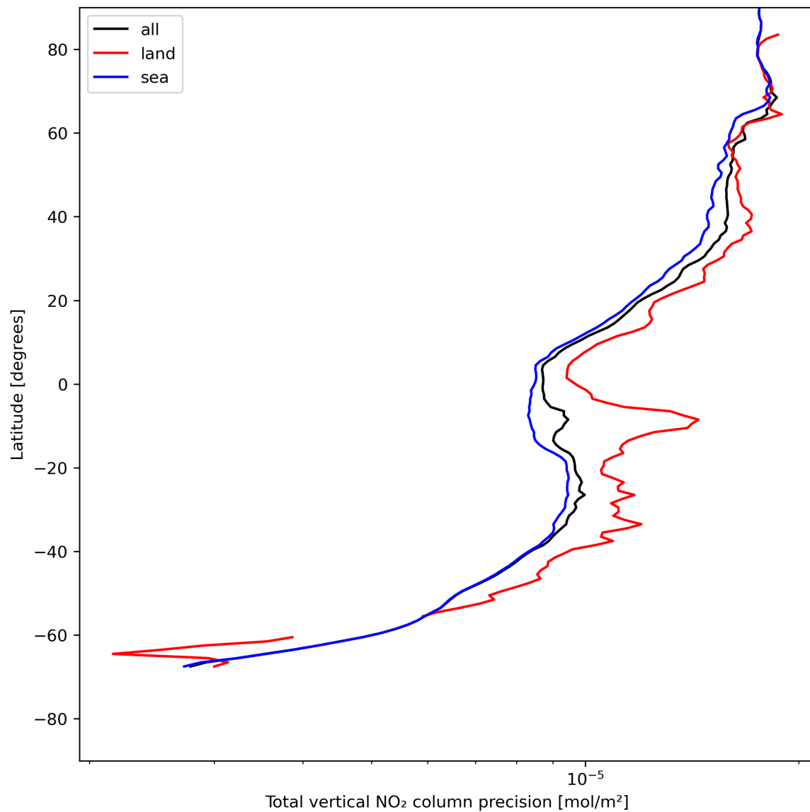
Figure 22: Zonal average of “Total vertical NO 2 column precision” for 2023-07-24 to 2023-07-25.
