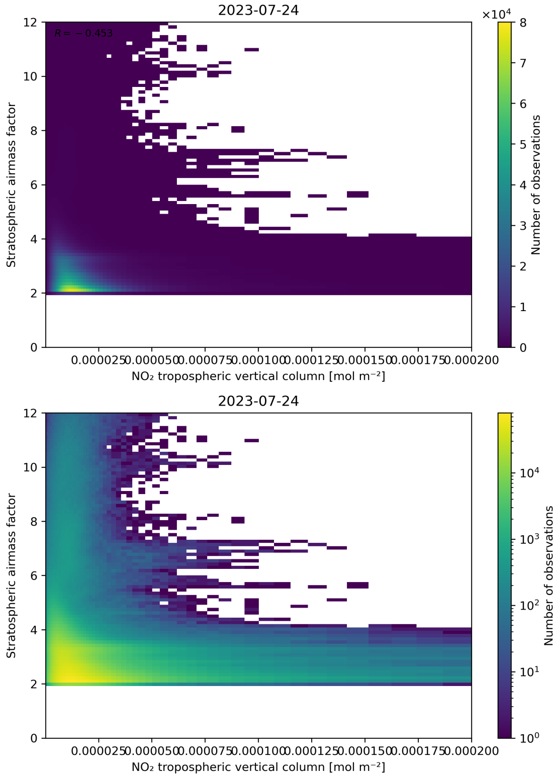
Figure 121: Scatter density plot of “NO 2 tropospheric vertical column” against “Stratospheric air mass factor” for 2023-07-24 to 2023-07-25.
