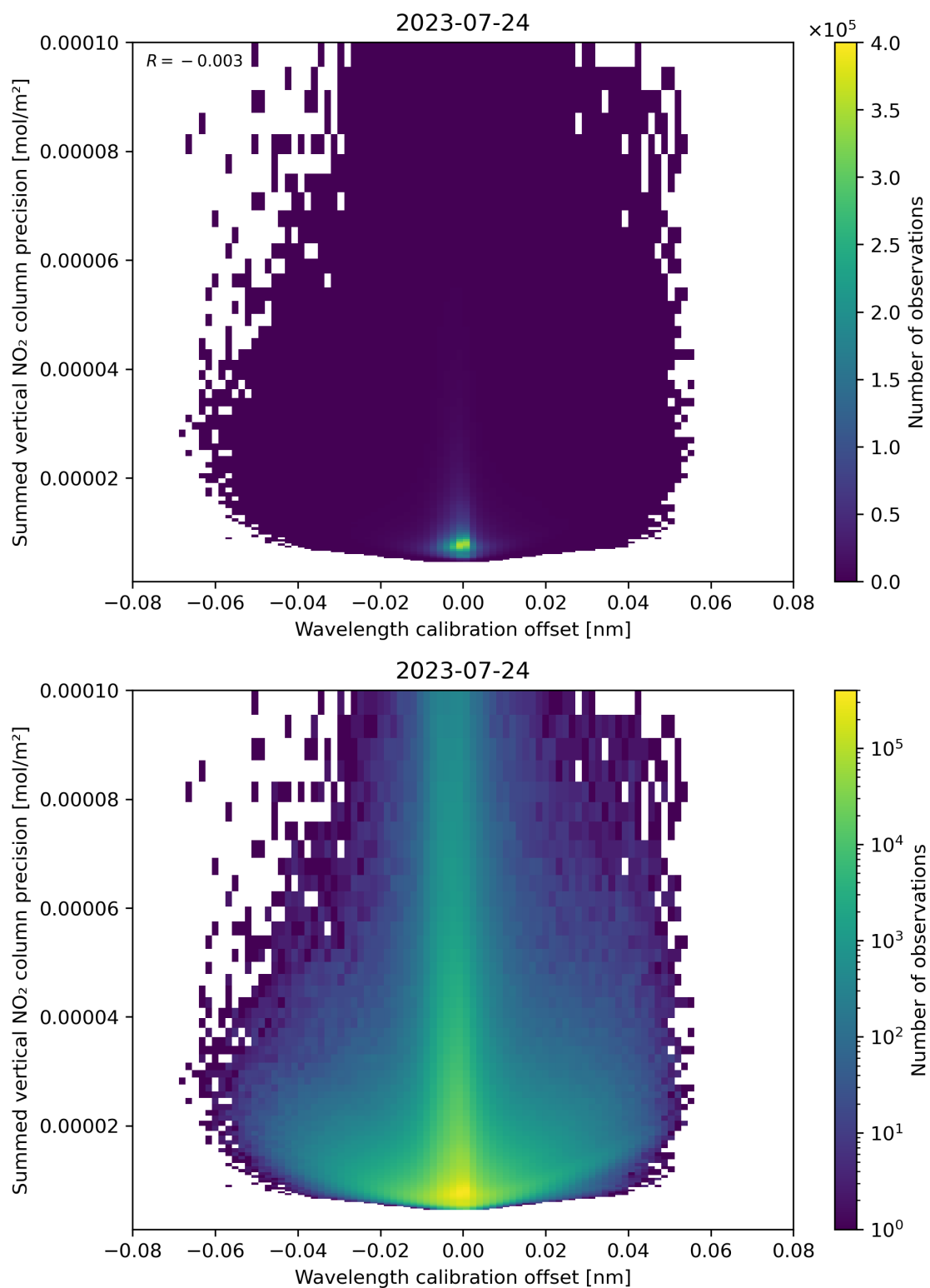
Figure 178: Scatter density plot of “Wavelength calibration offset” against “Summed vertical NO 2 column precision” for 2023-07-24 to 2023-07-25.
