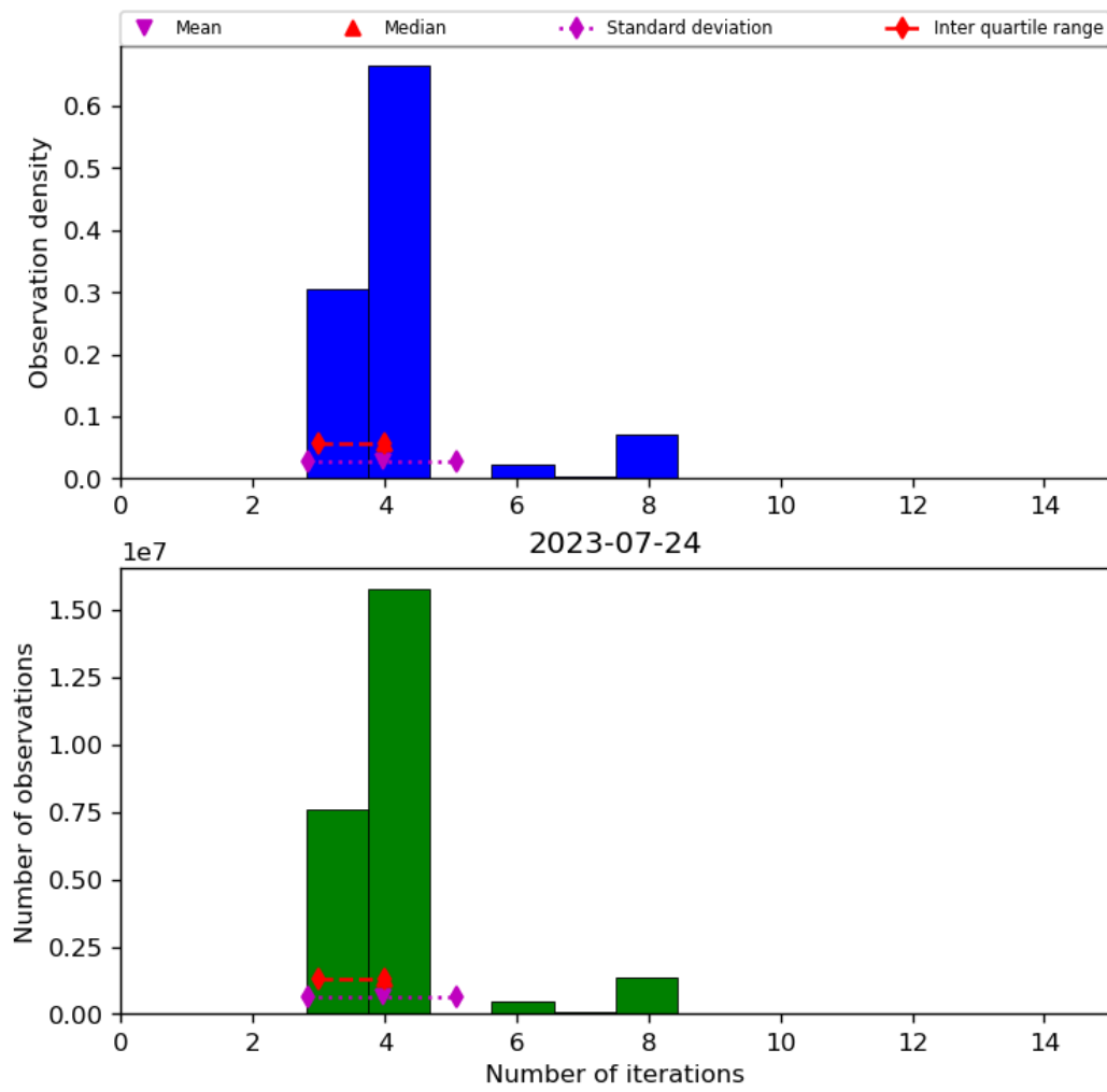
Figure 34: Histogram of “Number of iterations” for 2023-07-24 to 2023-07-25
