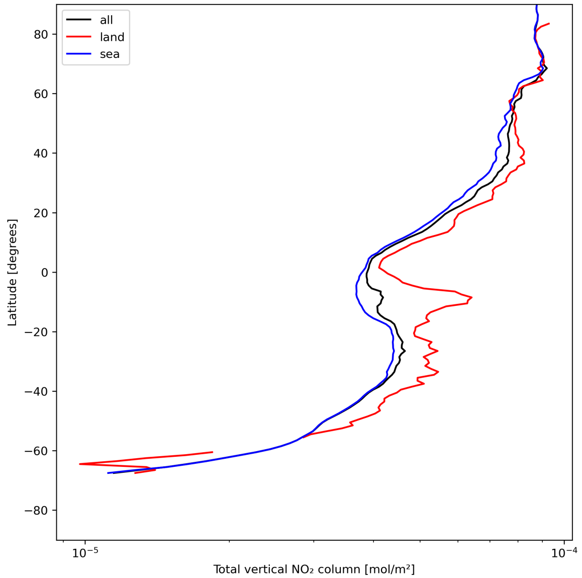
Figure 21: Zonal average of “Total vertical NO 2 column” for 2023-07-24 to 2023-07-25.
