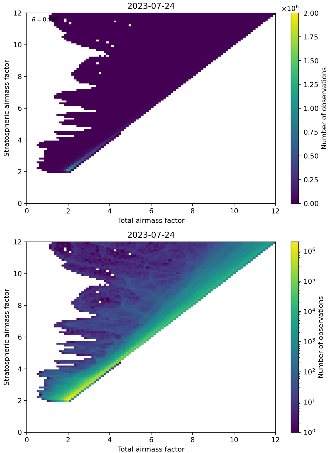
Figure 62: Scatter density plot of “Total airmass factor” against “Stratospheric airmass factor” for 2023-07-24 to 2023-07-25.
