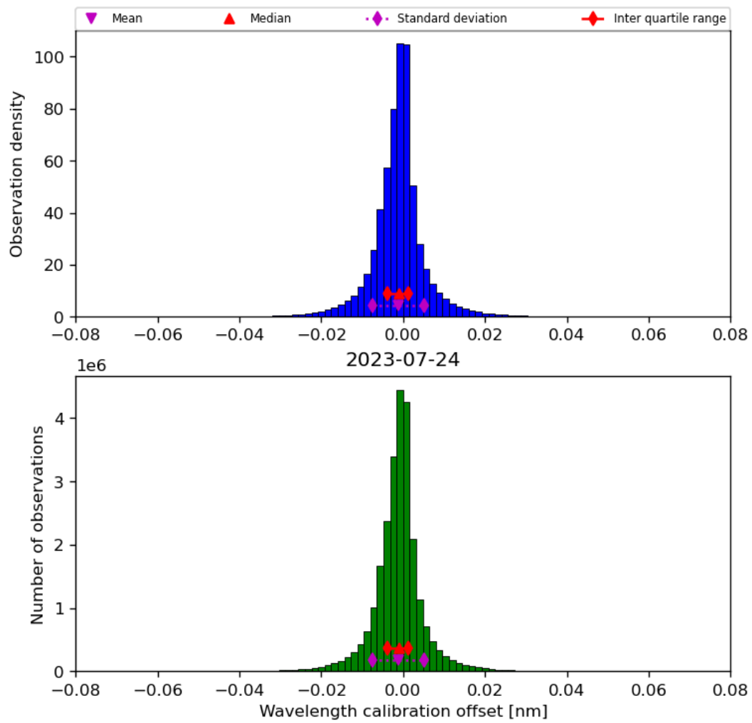
Figure 35: Histogram of “Wavelength calibration offset” for 2023-07-24 to 2023-07-25
