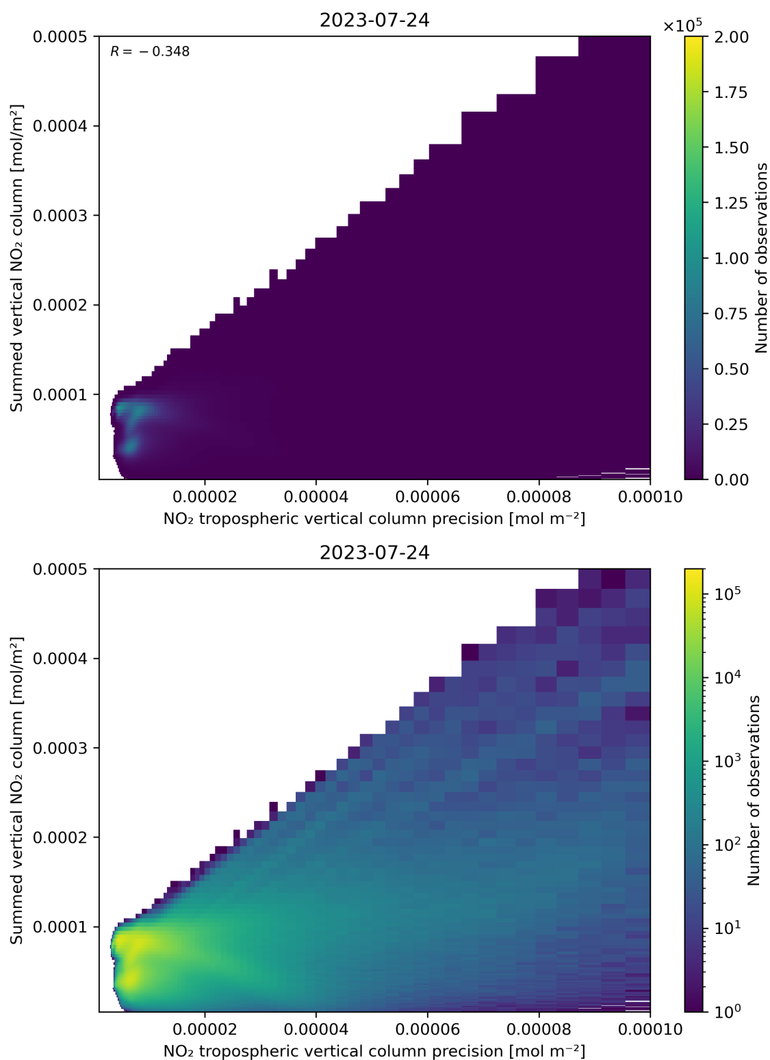
Figure 136: Scatter density plot of “NO 2 tropospheric vertical column precision” against “Summed vertical NO 2 column” for 2023-07-24 to 2023-07-25.
