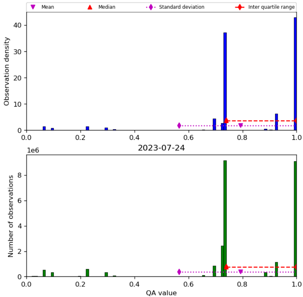
Figure 28: Histogram of “QA value” for 2023-07-24 to 2023-07-25
