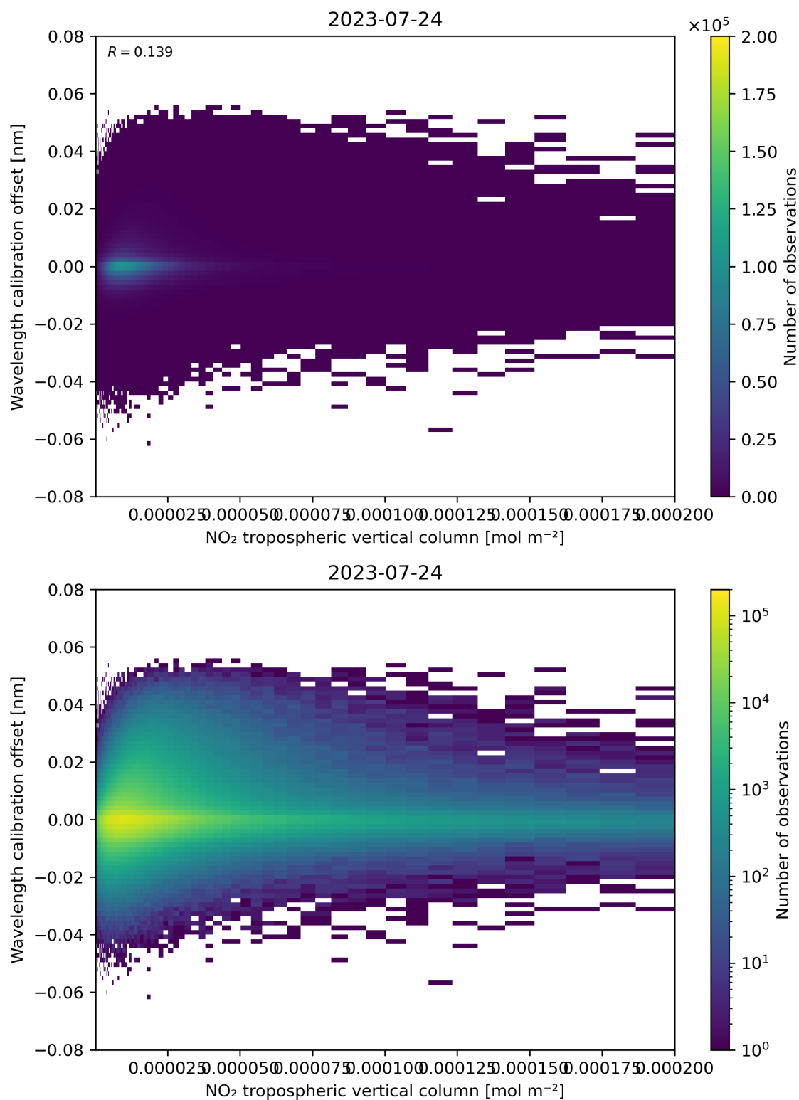
Figure 143: Scatter density plot of “NO 2 tropospheric vertical column” against “Wavelength calibration offset” for 2023-07-24 to 2023-07-25.
