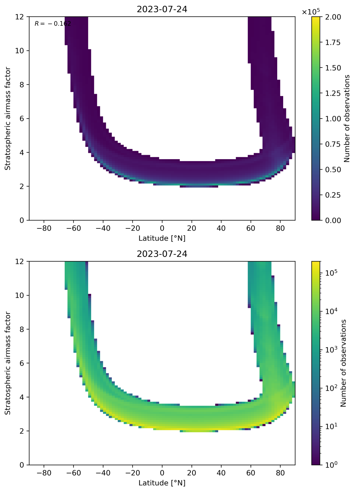
Figure 83: Scatter density plot of “Latitude” against “Stratospheric air mass factor” for 2023-07-24 to 2023-07-25.
