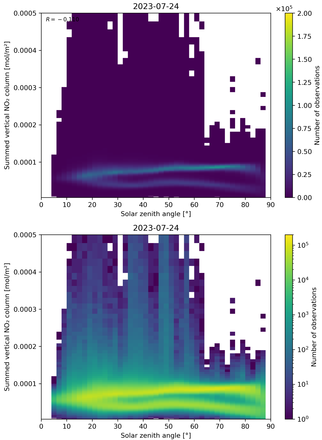
Figure 151: Scatter density plot of “Solar zenith angle” against “Summed vertical NO 2 column” for 2023-07-24 to 2023-07-25.
