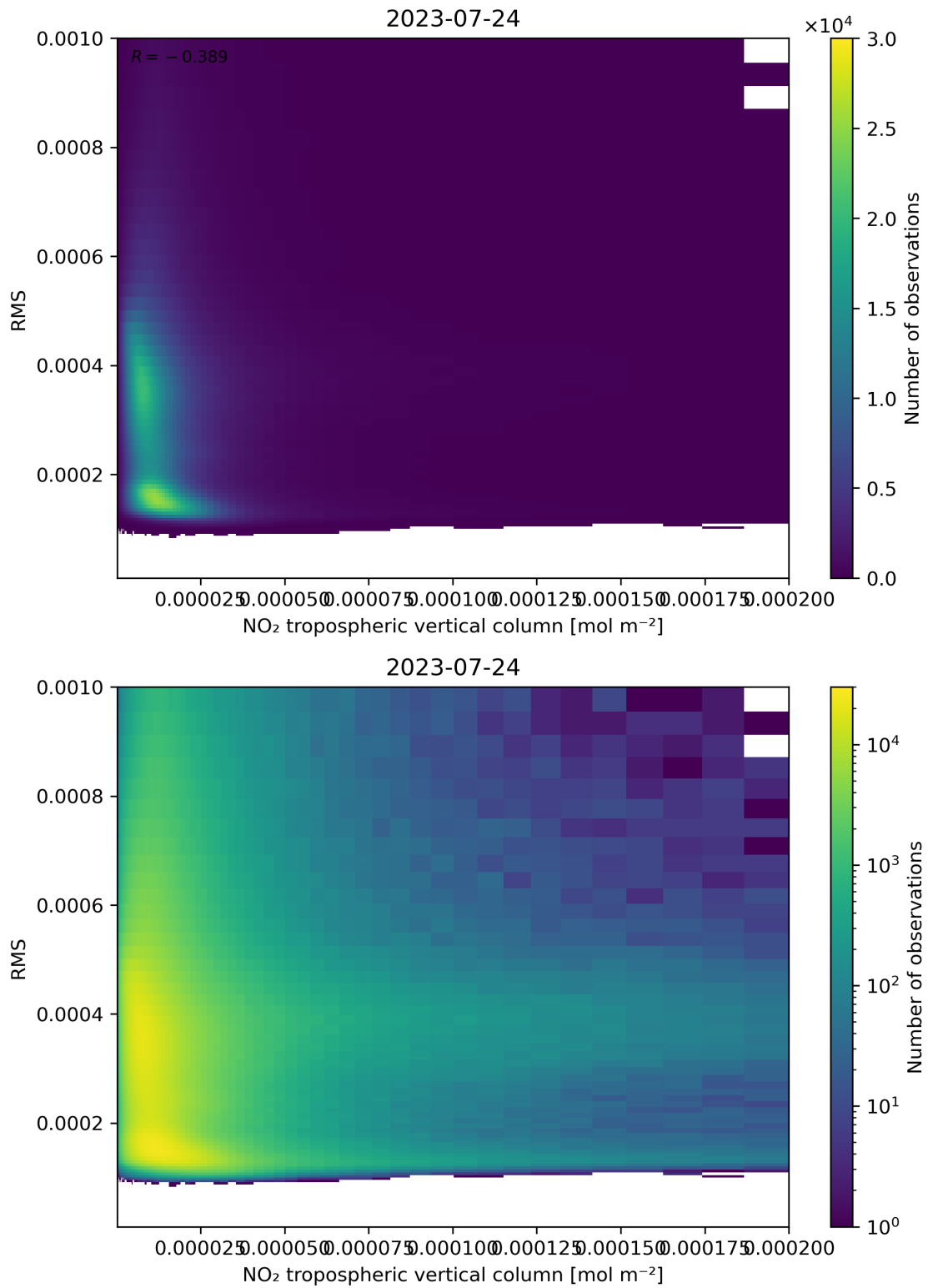
Figure 142: Scatter density plot of “NO 2 tropospheric vertical column” against “RMS” for 2023-07-24 to 2023-07-25.
