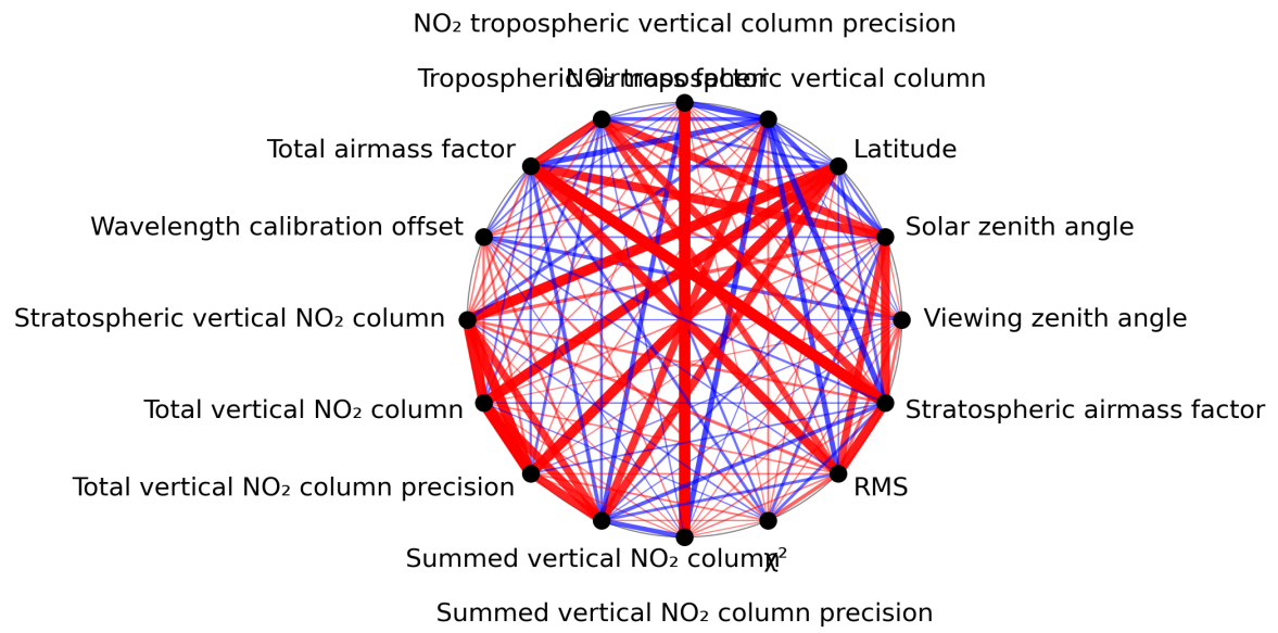
Figure 1: Map of correlation graph for 2023-07-24 to 2023-07-25.
