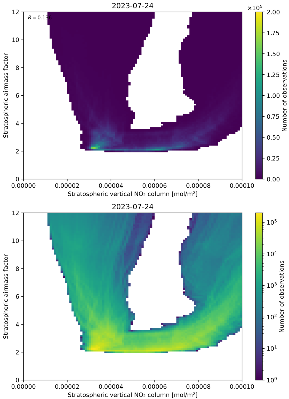
Figure 96: Scatter density plot of “Stratospheric vertical NO 2 column” against “Stratospheric airmass factor” for 2023-07-24 to 2023-07-25.
