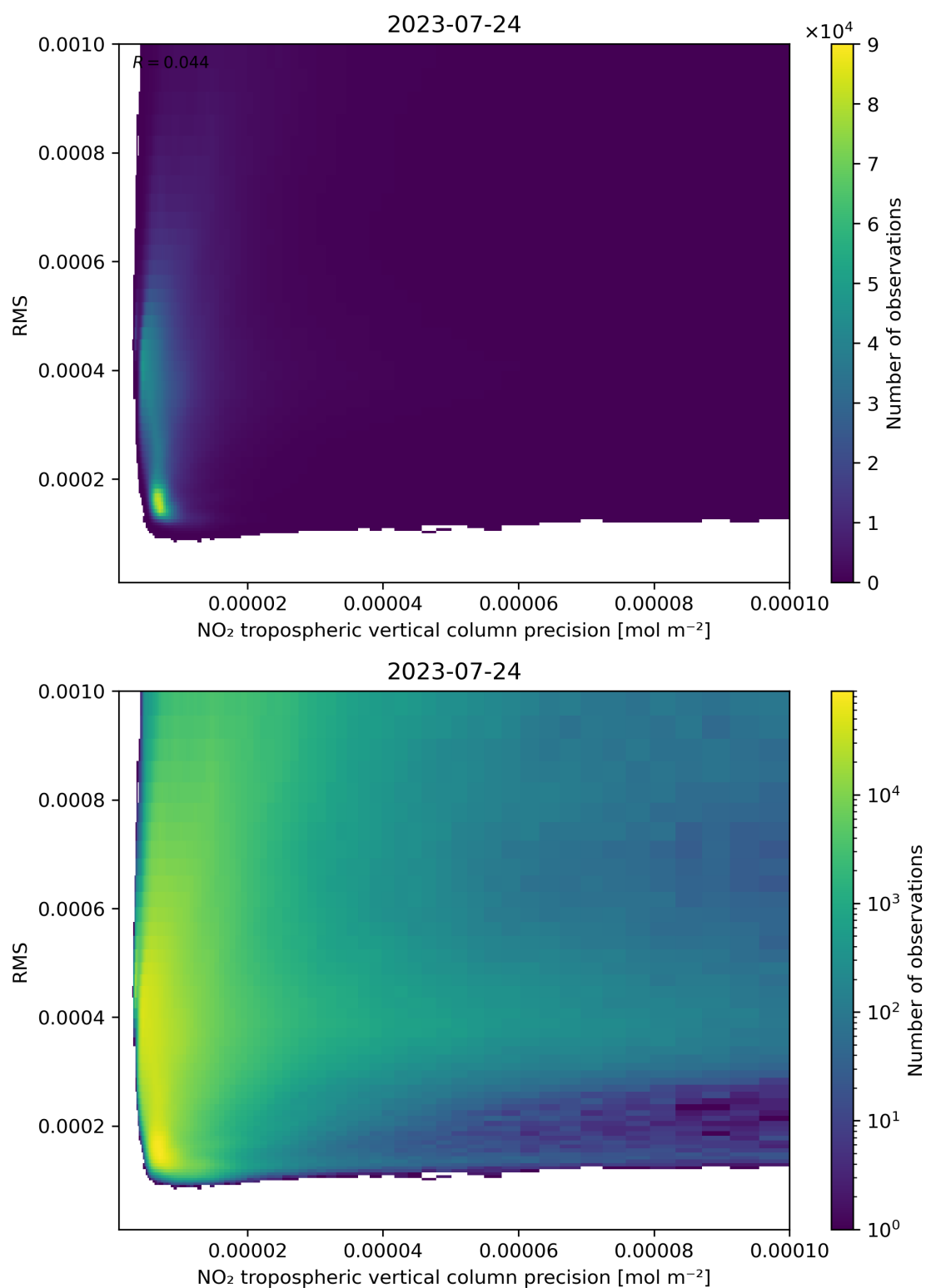
Figure 140: Scatter density plot of “NO 2 tropospheric vertical column precision” against “RMS” for 2023-07-24 to 2023-07-25.
