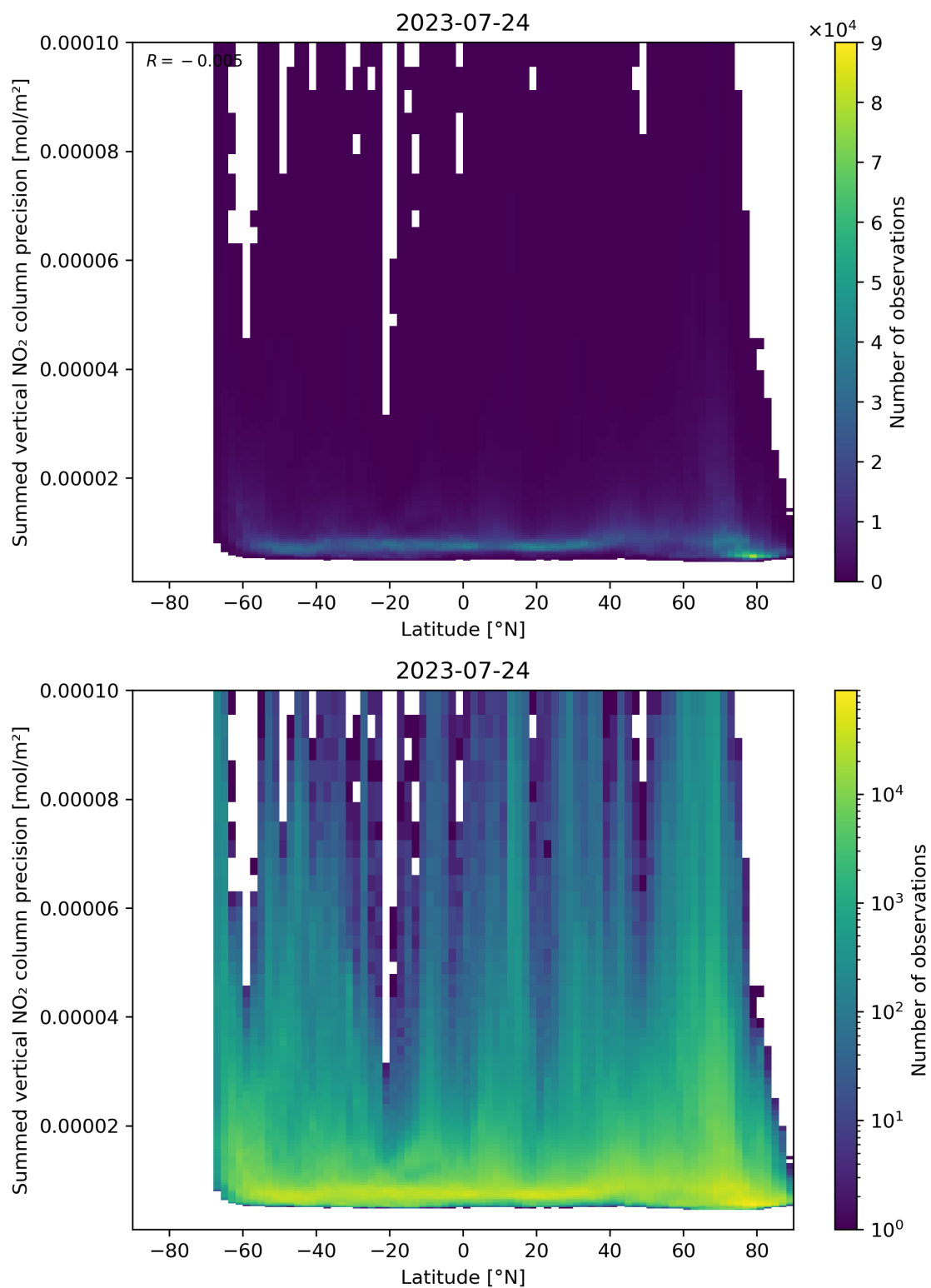
Figure 89: Scatter density plot of “Latitude” against “Summed vertical NO 2 column precision” for 2023-07-24 to 2023-07-25.
