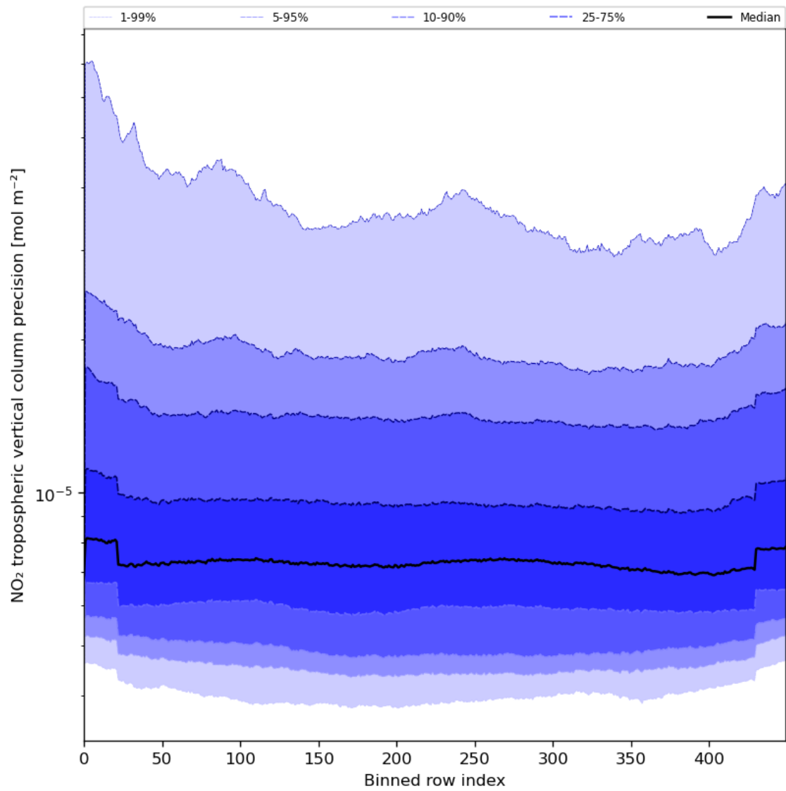
Figure 47: Along track statistics of “NO 2 tropospheric vertical column precision” for 2023-07-24 to 2023-07-25
