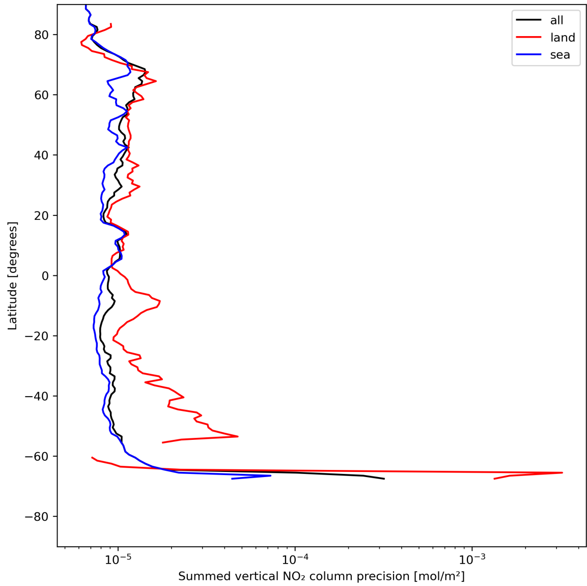
Figure 24: Zonal average of “Summed vertical NO 2 column precision” for 2023-07-24 to 2023-07-25.
