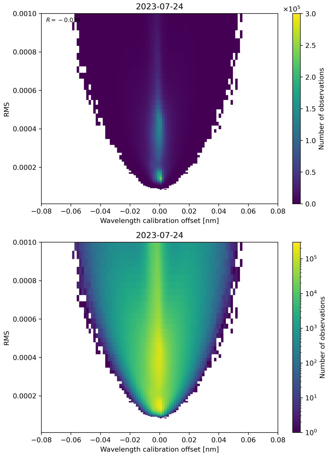
Figure 181: Scatter density plot of “Wavelength calibration offset” against “RMS” for 2023-07-24 to 2023-07-25.
