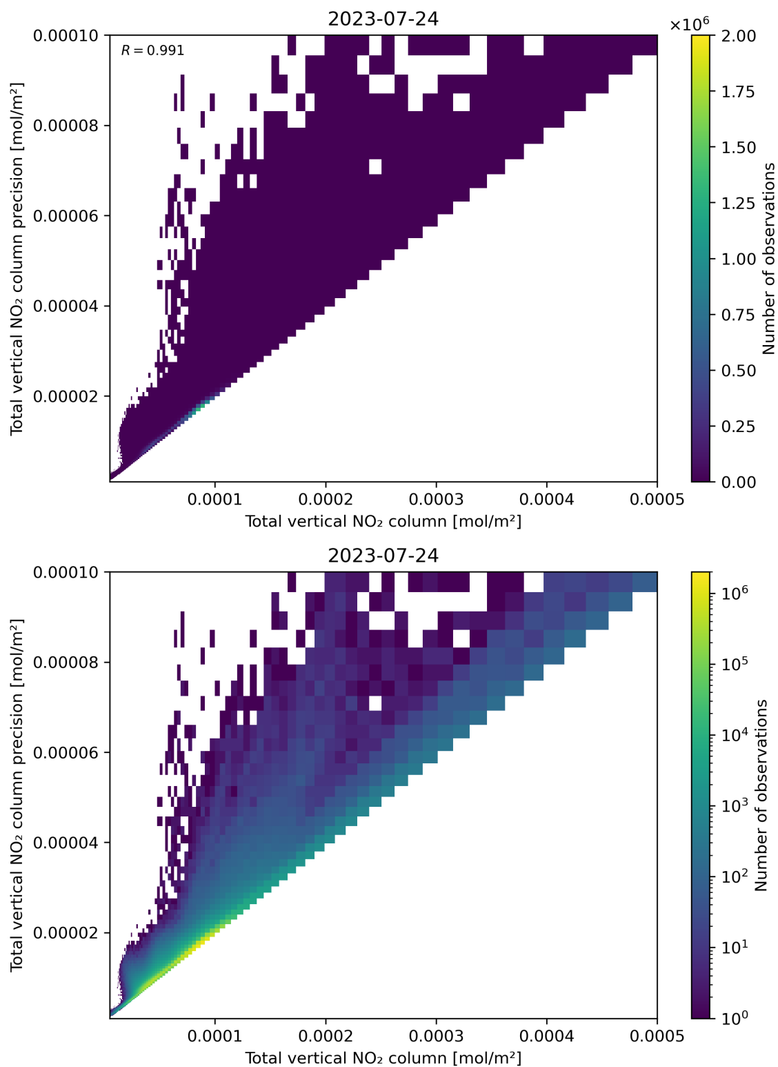
Figure 114: Scatter density plot of “Total vertical NO 2 column” against “Total vertical NO 2 column precision” for 2023-07-24 to 2023-07-25.
