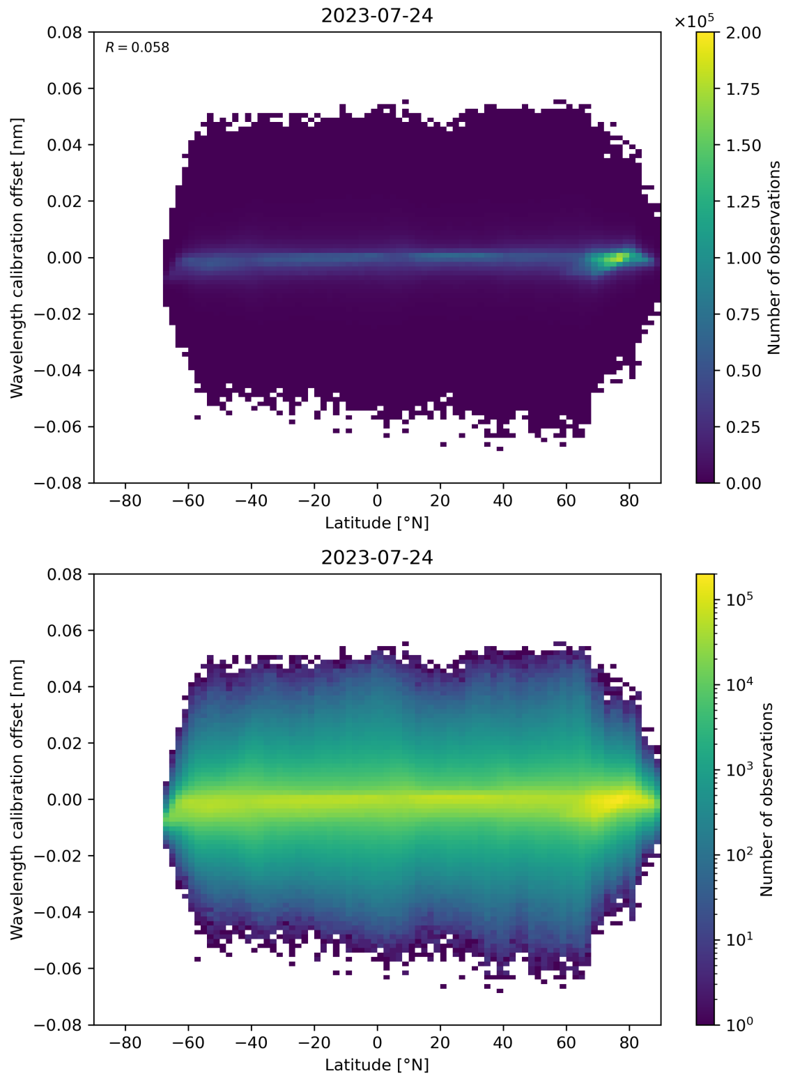
Figure 95: Scatter density plot of “Latitude” against “Wavelength calibration offset” for 2023-07-24 to 2023-07-25.
