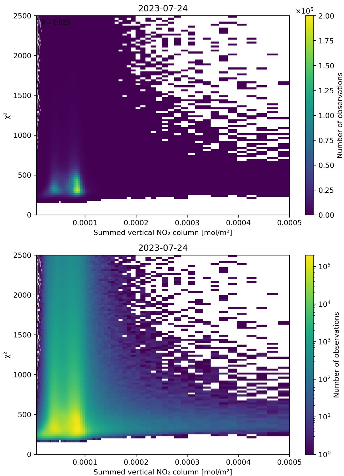
Figure 104: Scatter density plot of “Summed vertical NO 2 column” against “ \chi^2 ” for 2023-07-24 to 2023-07-25.
