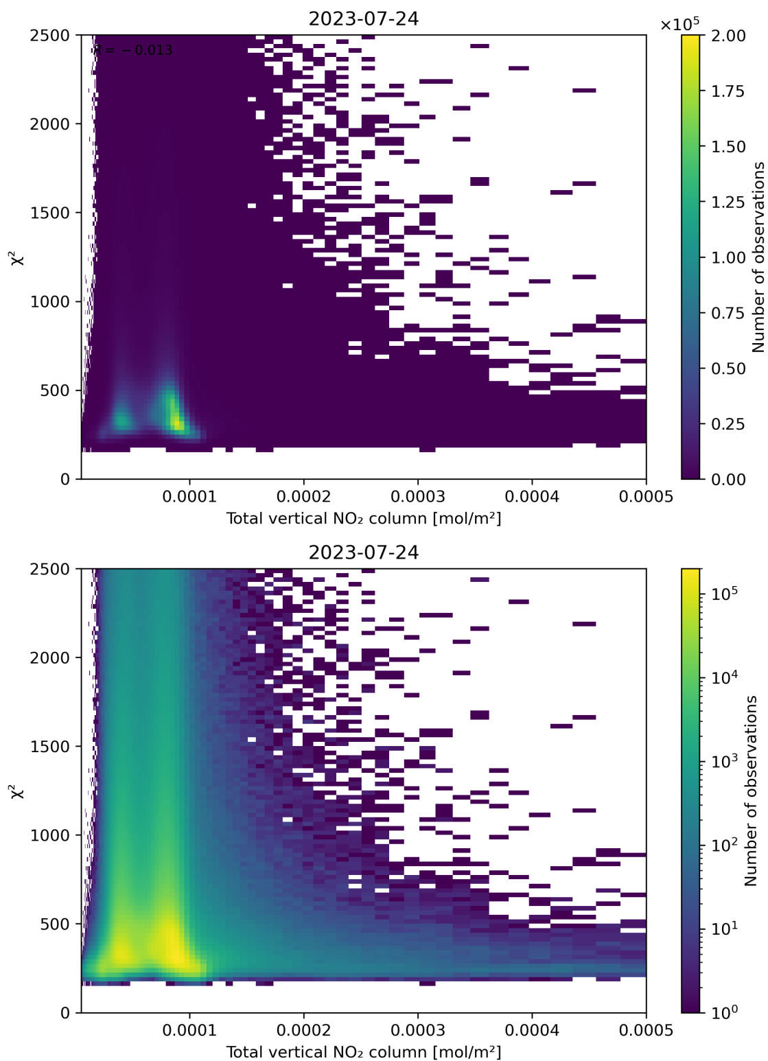
Figure 111: Scatter density plot of “Total vertical NO 2 column” against “ \chi^2 ” for 2023-07-24 to 2023-07-25.
