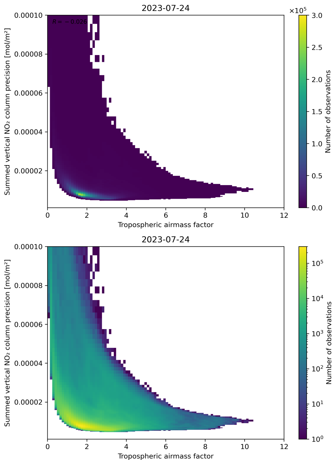
Figure 76: Scatter density plot of “Tropospheric airmass factor” against “Summed vertical NO 2 column precision” for 2023-07-24 to 2023-07-25.
