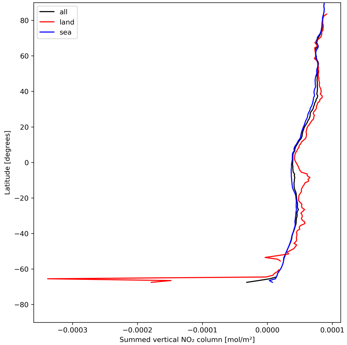
Figure 23: Zonal average of “Summed vertical NO 2 column” for 2023-07-24 to 2023-07-25.
