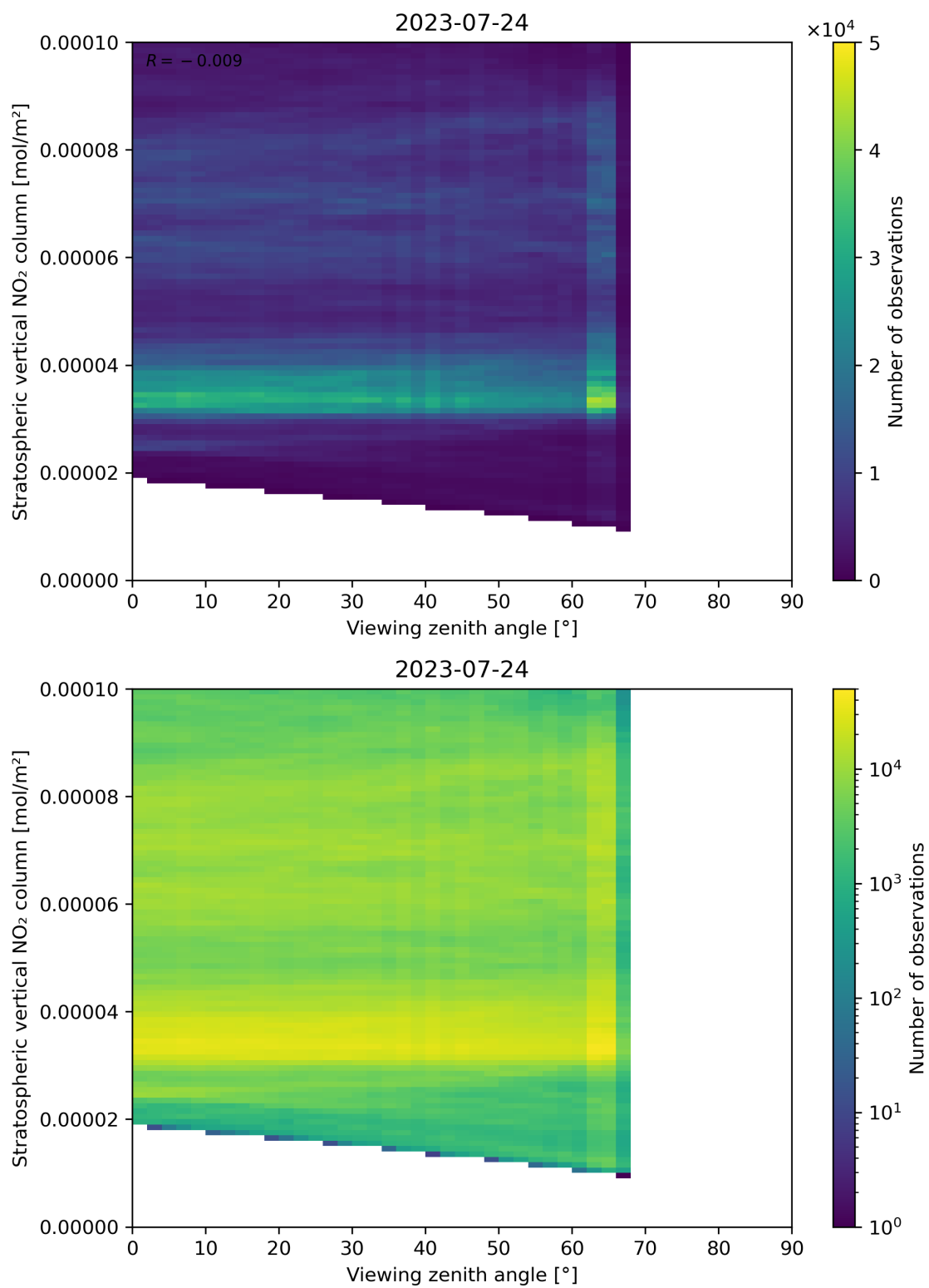
Figure 164: Scatter density plot of “Viewing zenith angle” against “Stratospheric vertical NO 2 column” for 2023-07-24 to 2023-07-25.
