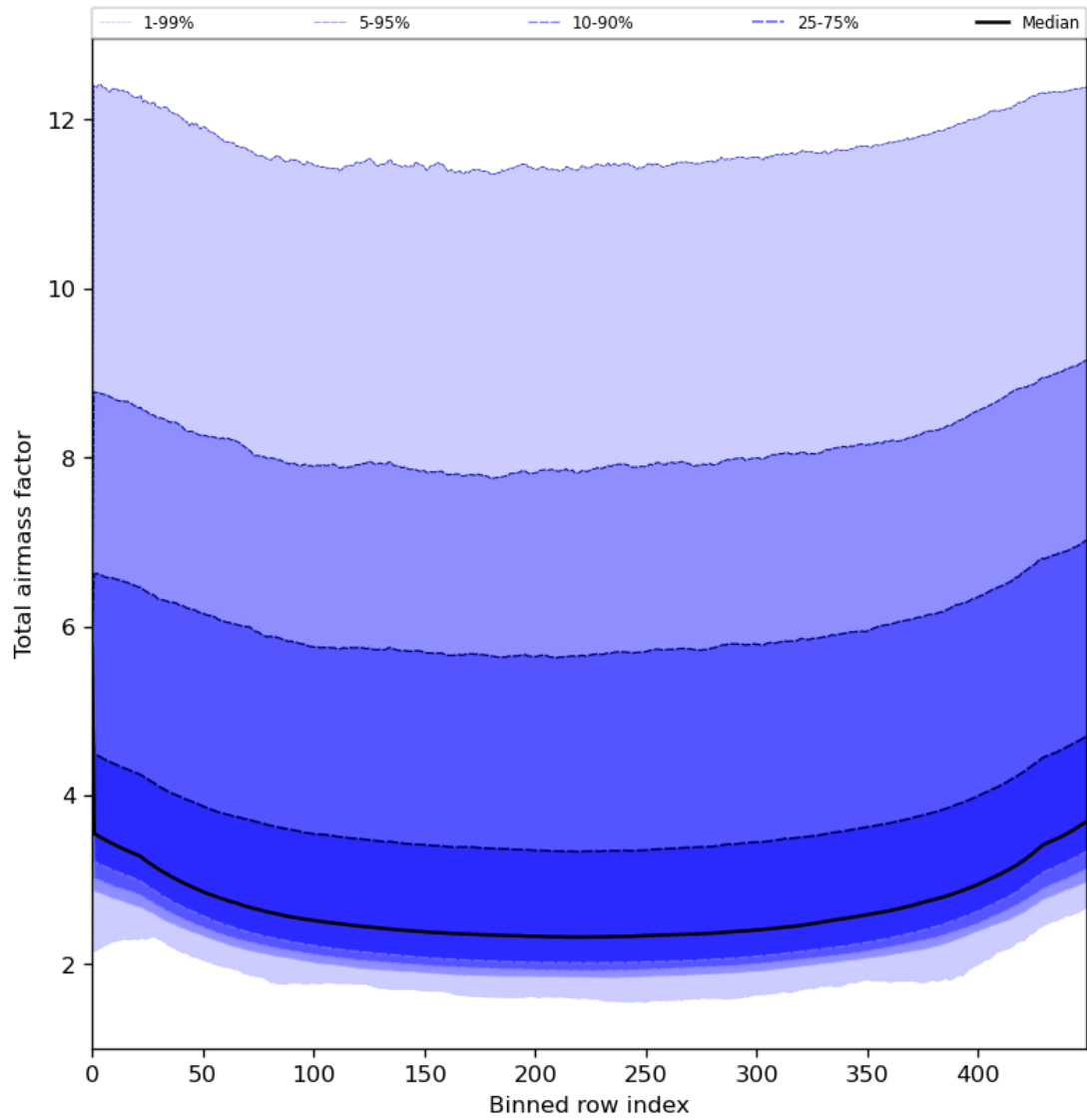
Figure 49: Along track statistics of “Total airmass factor” for 2023-07-24 to 2023-07-25
