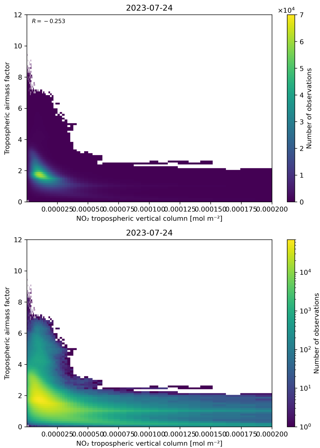
Figure 123: Scatter density plot of “NO 2 tropospheric vertical column” against “Tropospheric air mass factor” for 2023-07-24 to 2023-07-25.
