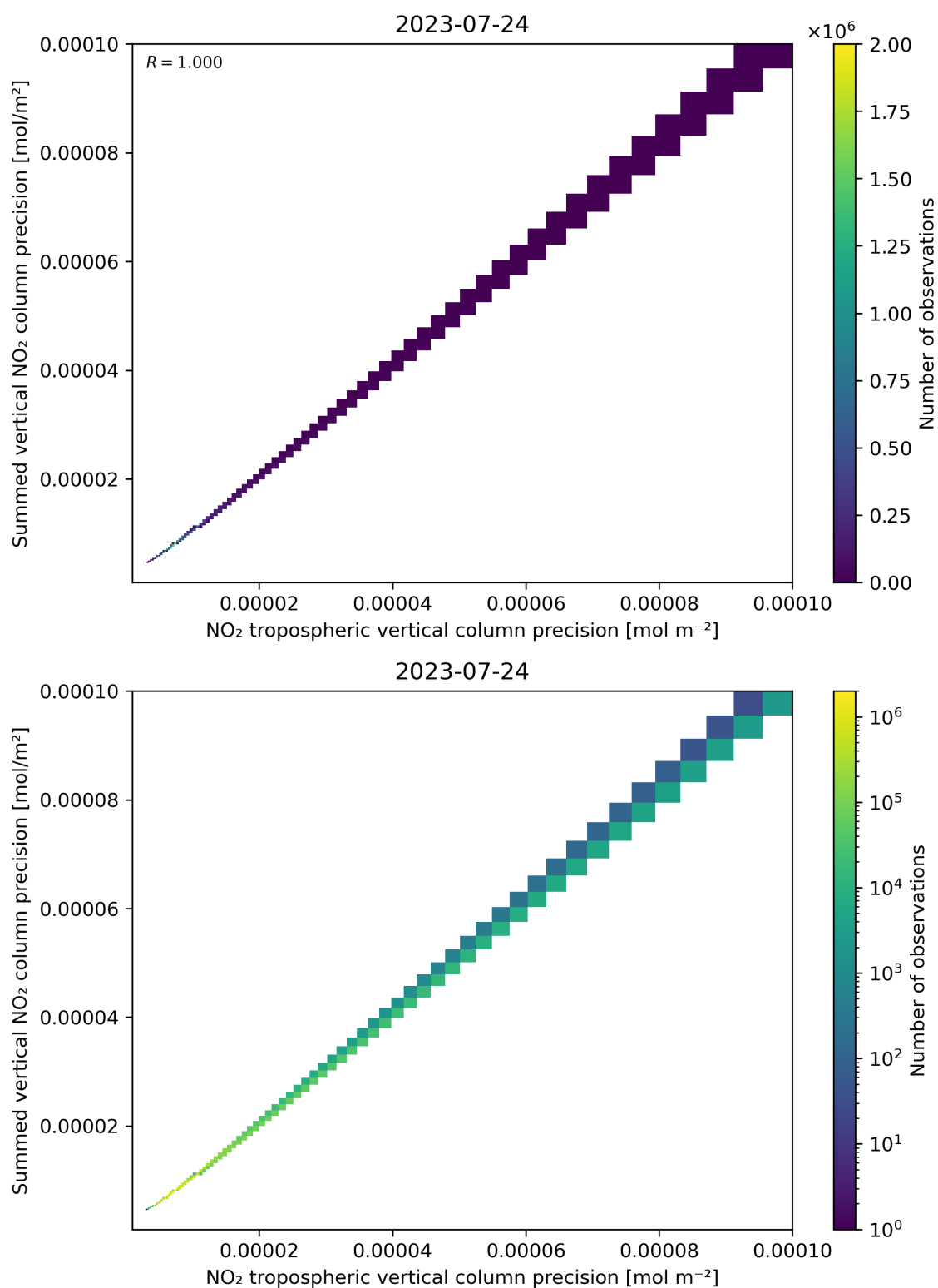
Figure 137: Scatter density plot of “NO 2 tropospheric vertical column precision” against “Summed vertical NO 2 column precision” for 2023-07-24 to 2023-07-25.
