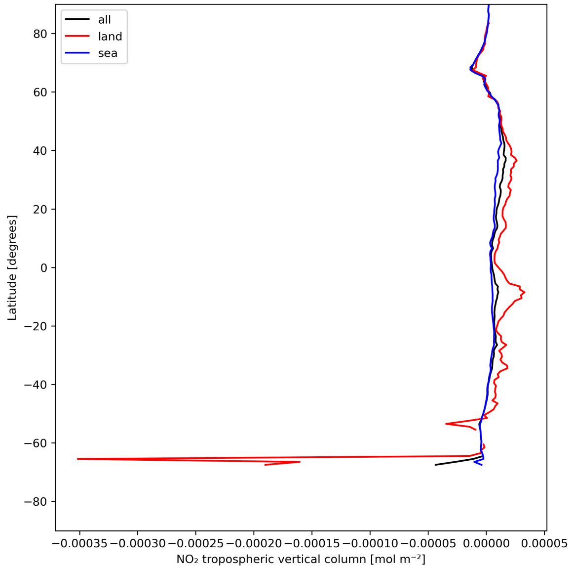
Figure 12: Zonal average of “NO 2 tropospheric vertical column” for 2023-07-24 to 2023-07-25.
