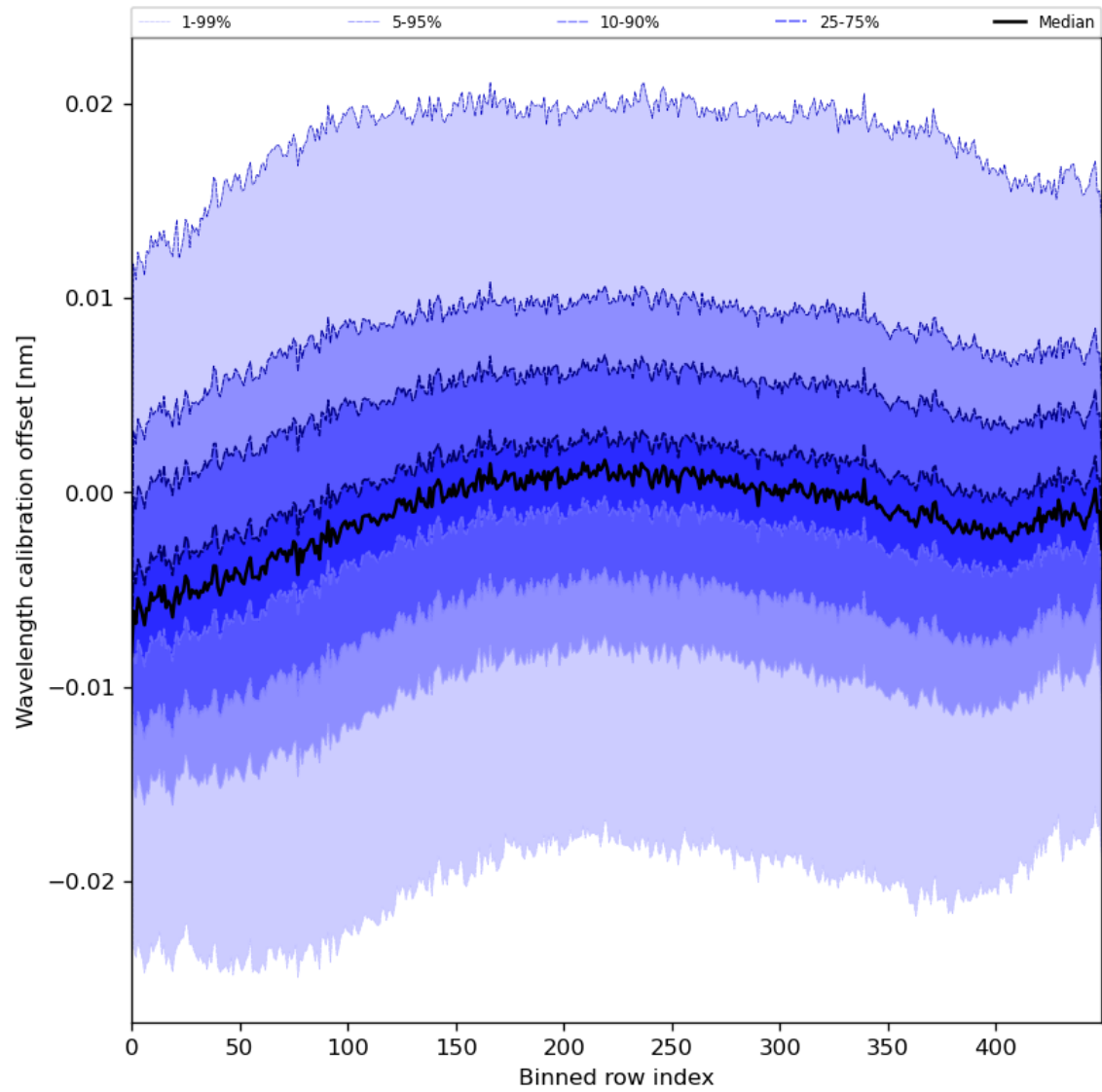
Figure 52: Along track statistics of “Wavelength calibration offset” for 2023-07-24 to 2023-07-25
