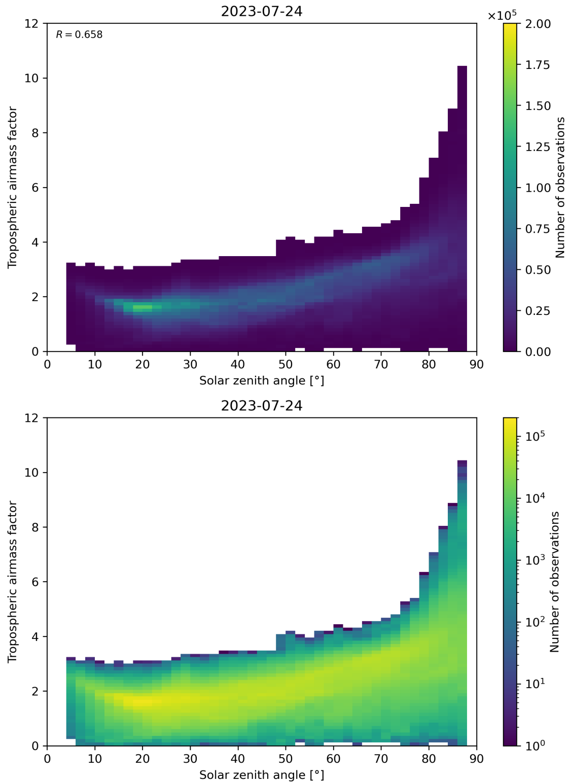
Figure 147: Scatter density plot of “Solar zenith angle” against “Tropospheric airmass factor” for 2023-07-24 to 2023-07-25.
