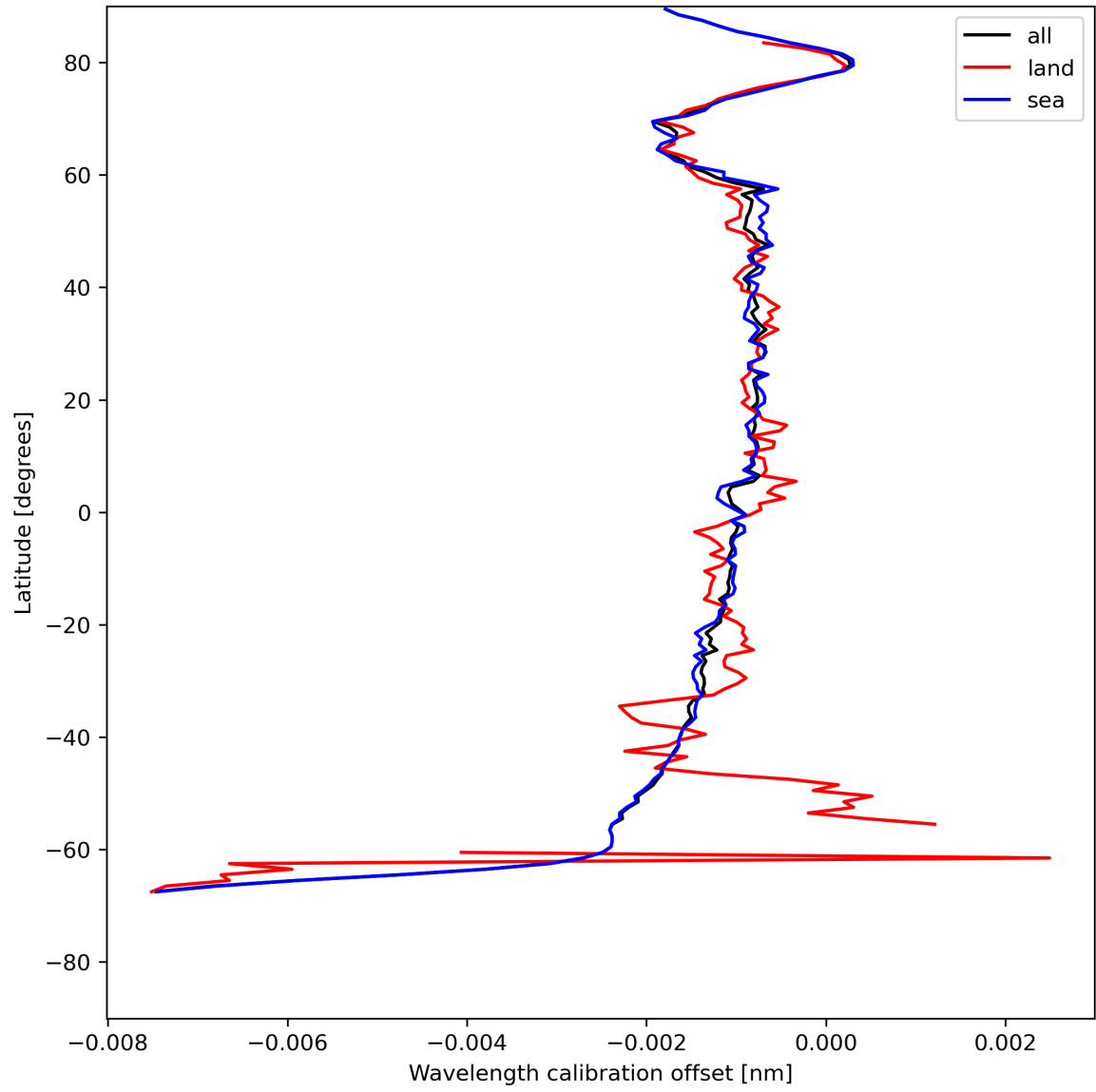
Figure 18: Zonal average of “Wavelength calibration offset” for 2023-07-24 to 2023-07-25.
