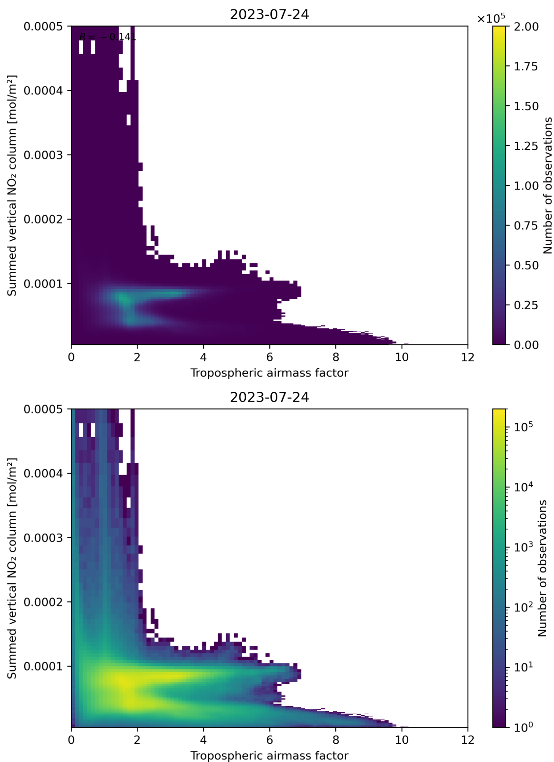
Figure 75: Scatter density plot of “Tropospheric airmass factor” against “Summed vertical NO 2 column” for 2023-07-24 to 2023-07-25.
