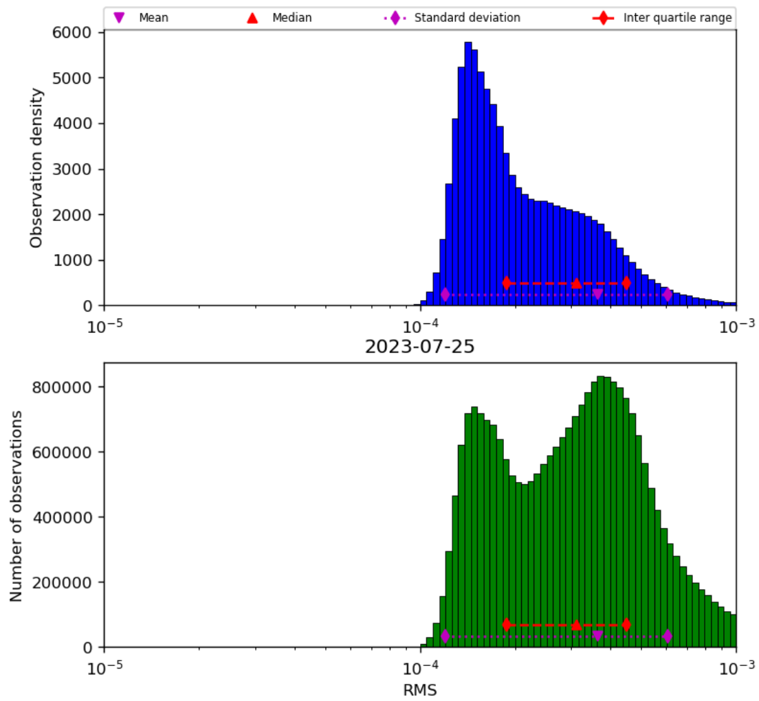
Figure 43: Histogram of “RMS” for 2023-07-24 to 2023-07-26
