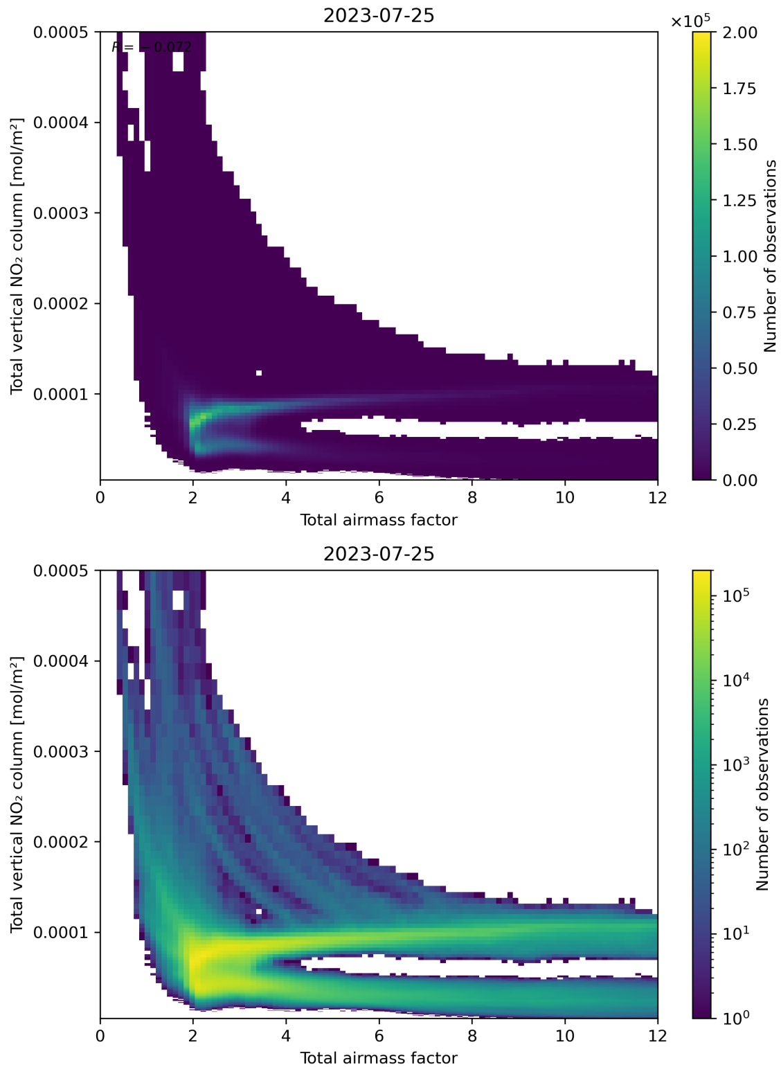
Figure 67: Scatter density plot of “Total airmass factor” against “Total vertical NO 2 column” for 2023-07-24 to 2023-07-26.
