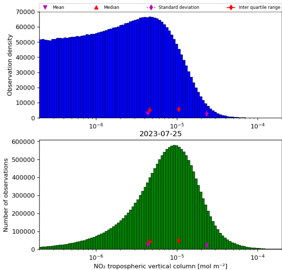
Figure 29: Histogram of “NO 2 tropospheric vertical column” for 2023-07-24 to 2023-07-26
