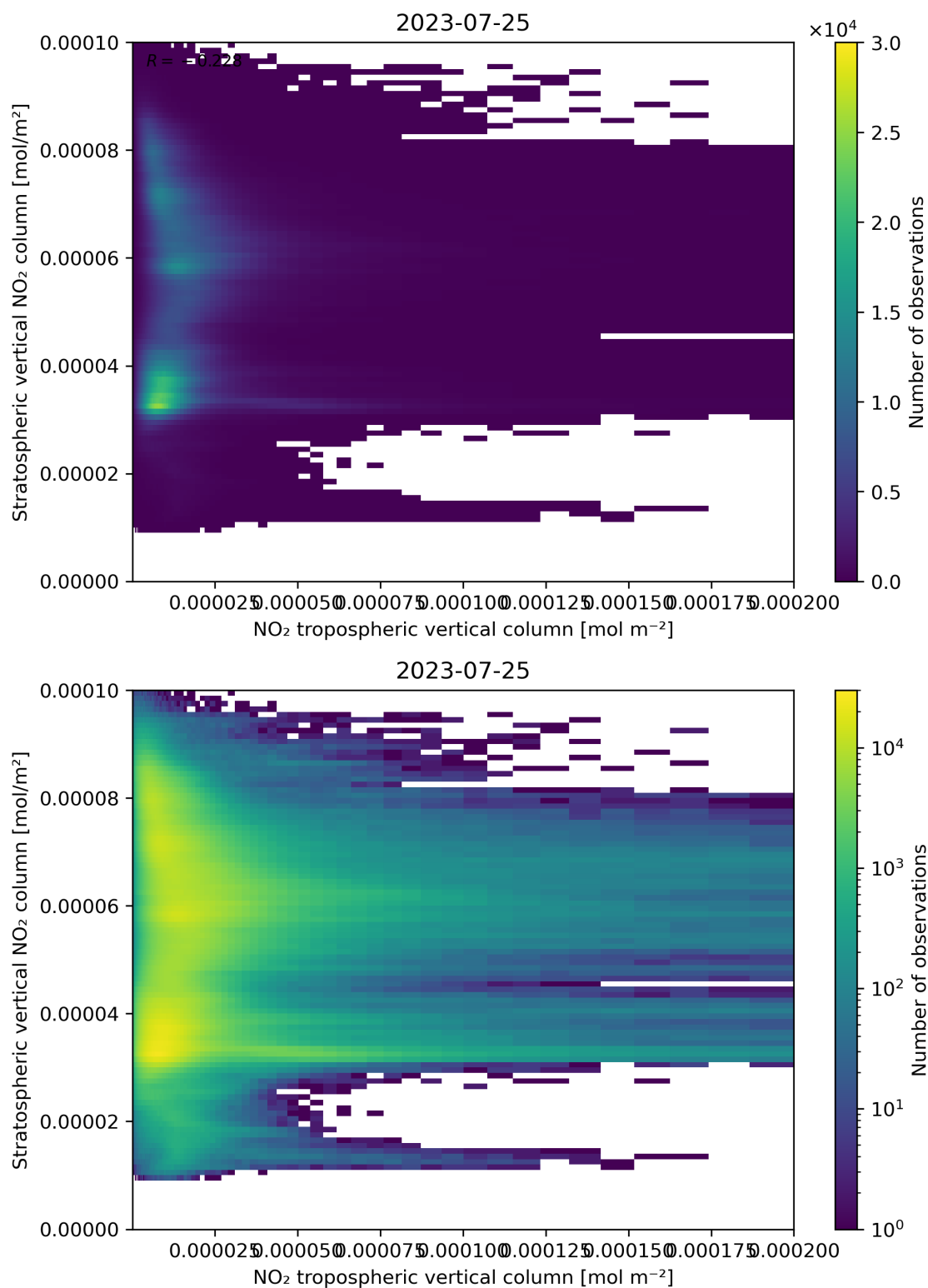
Figure 125: Scatter density plot of “NO 2 tropospheric vertical column” against “Stratospheric vertical NO 2 column” for 2023-07-24 to 2023-07-26.
