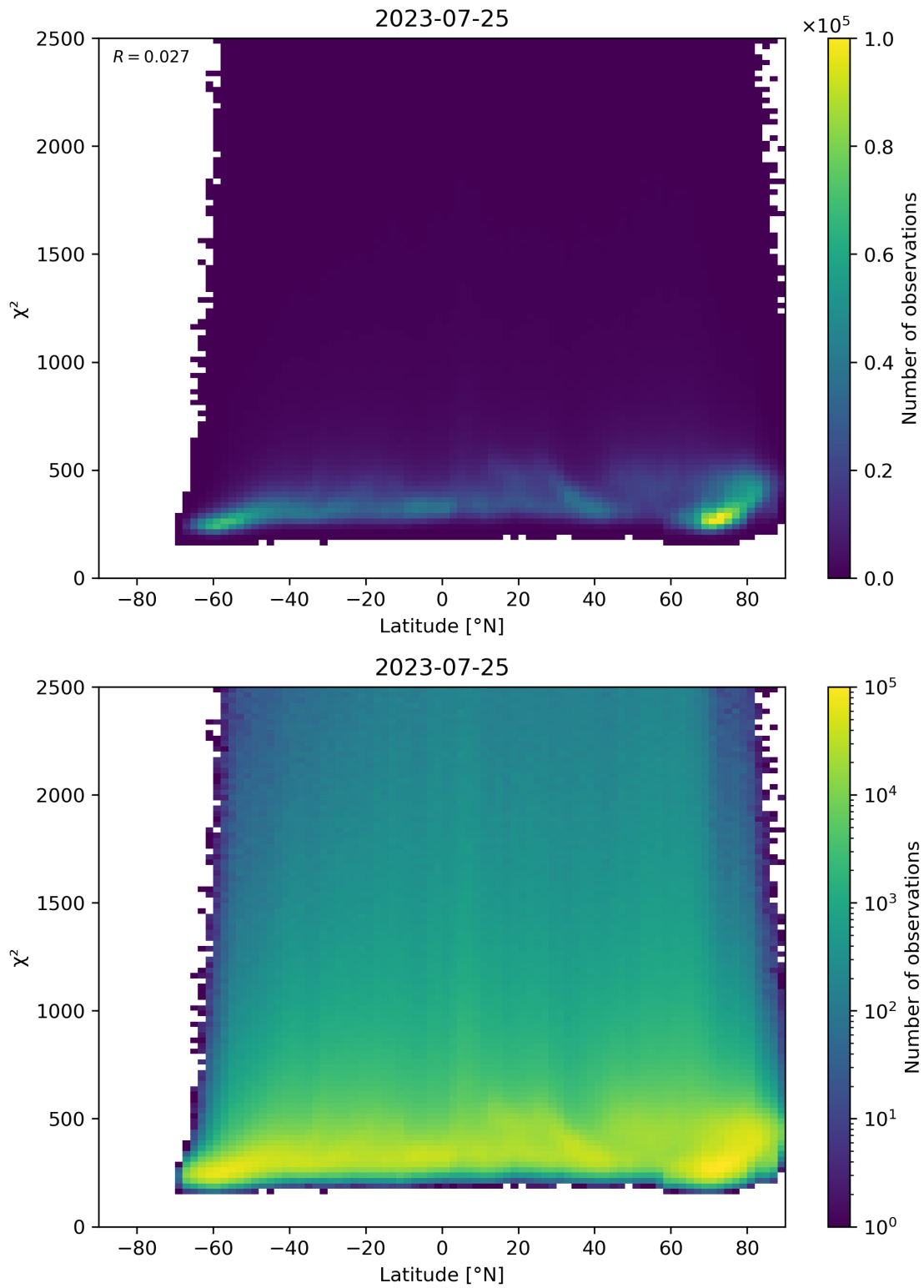
Figure 86: Scatter density plot of “Latitude” against “ \chi^2 ” for 2023-07-24 to 2023-07-26.
