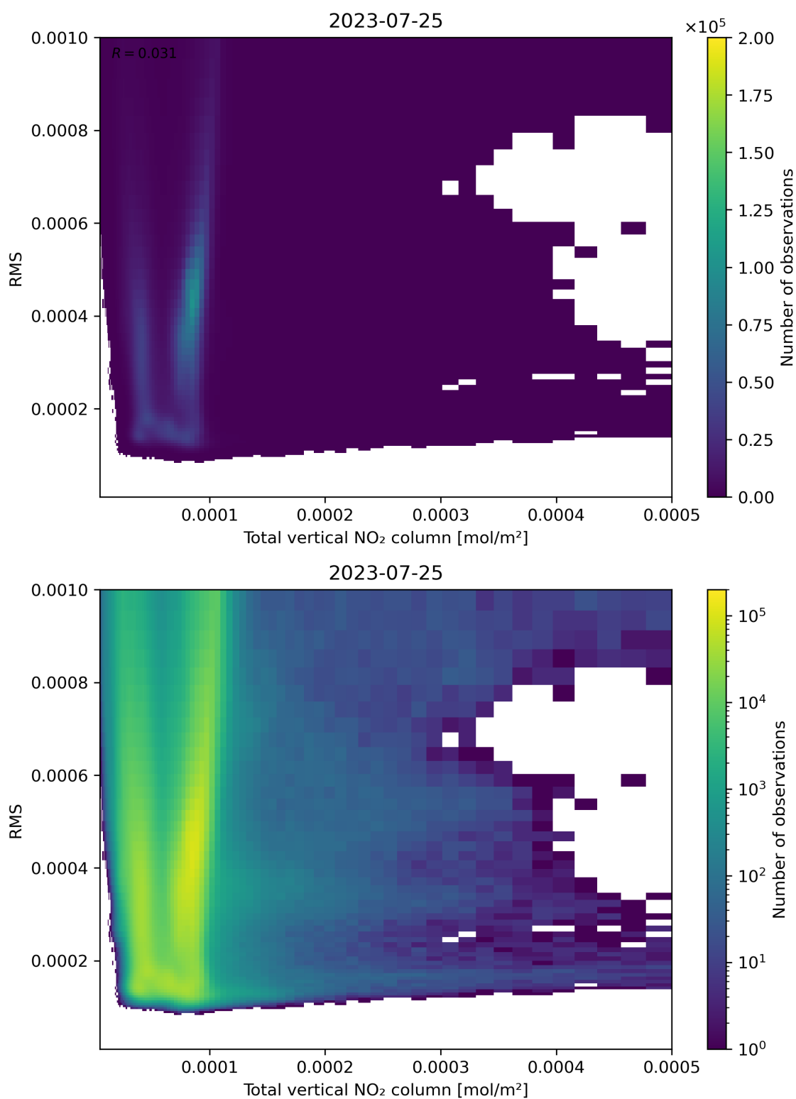
Figure 120: Scatter density plot of “Total vertical NO 2 column” against “RMS” for 2023-07-24 to 2023-07-26.
