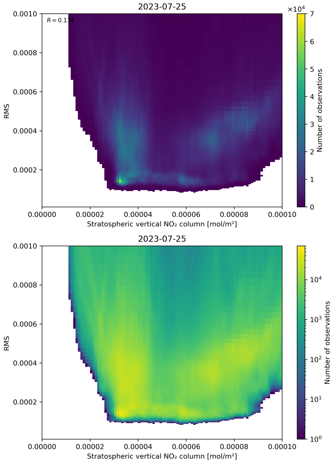
Figure 102: Scatter density plot of “Stratospheric vertical NO 2 column” against “RMS” for 2023-07-24 to 2023-07-26.
