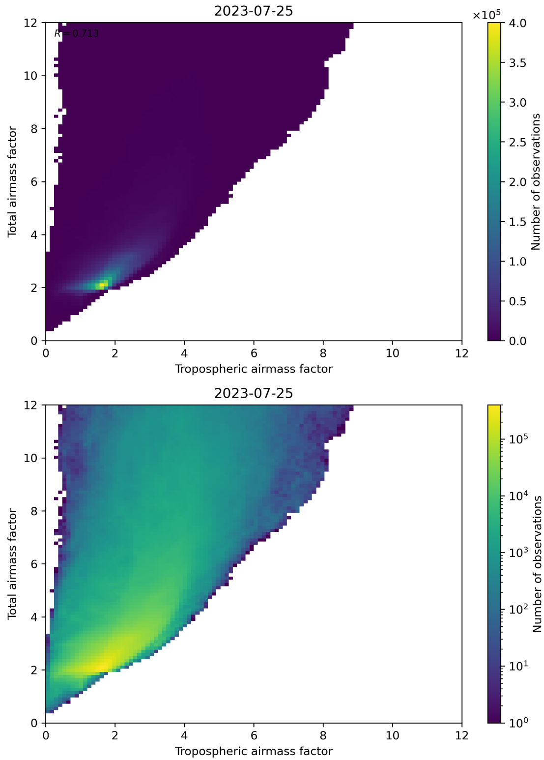
Figure 72: Scatter density plot of “Tropospheric airmass factor” against “Total airmass factor” for 2023-07-24 to 2023-07-26.
