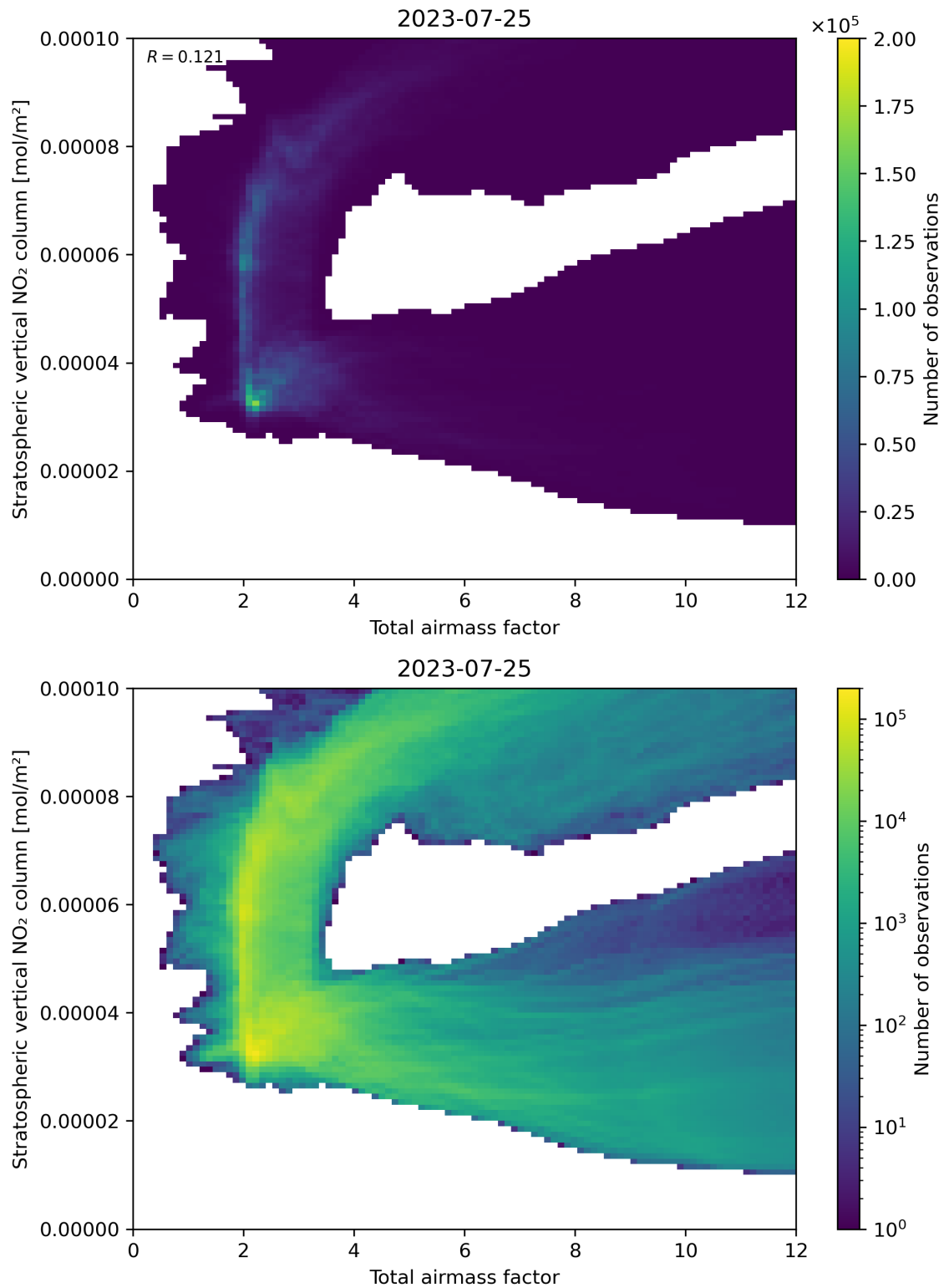
Figure 64: Scatter density plot of “Total airmass factor” against “Stratospheric vertical NO 2 column” for 2023-07-24 to 2023-07-26.
