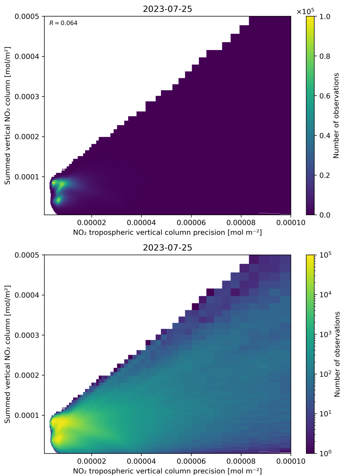
Figure 136: Scatter density plot of “NO 2 tropospheric vertical column precision” against “Summed vertical NO 2 column” for 2023-07-24 to 2023-07-26.
