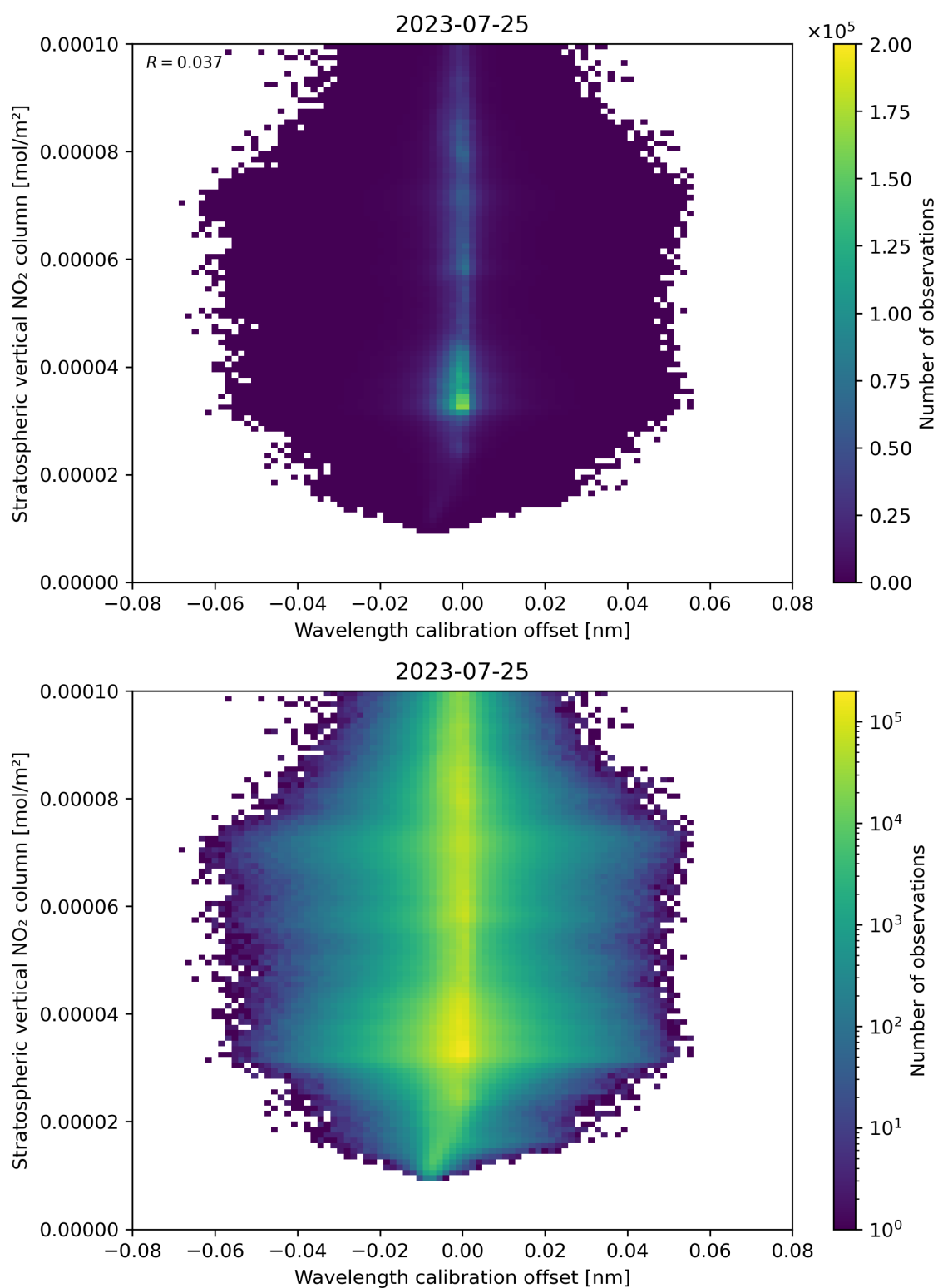
Figure 176: Scatter density plot of “Wavelength calibration offset” against “Stratospheric vertical NO 2 column” for 2023-07-24 to 2023-07-26.
