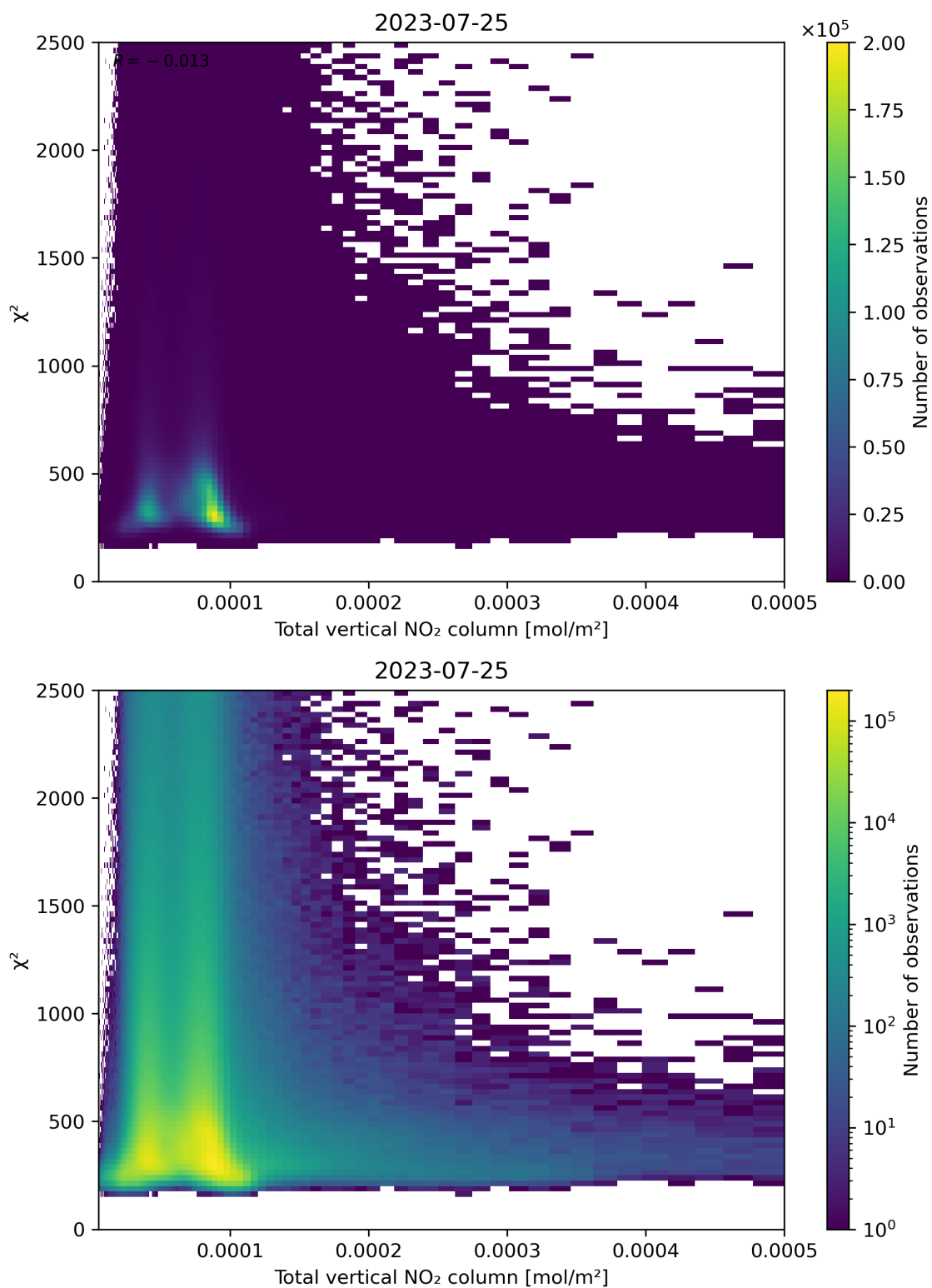
Figure 111: Scatter density plot of “Total vertical NO 2 column” against “ \chi^2 ” for 2023-07-24 to 2023-07-26.
