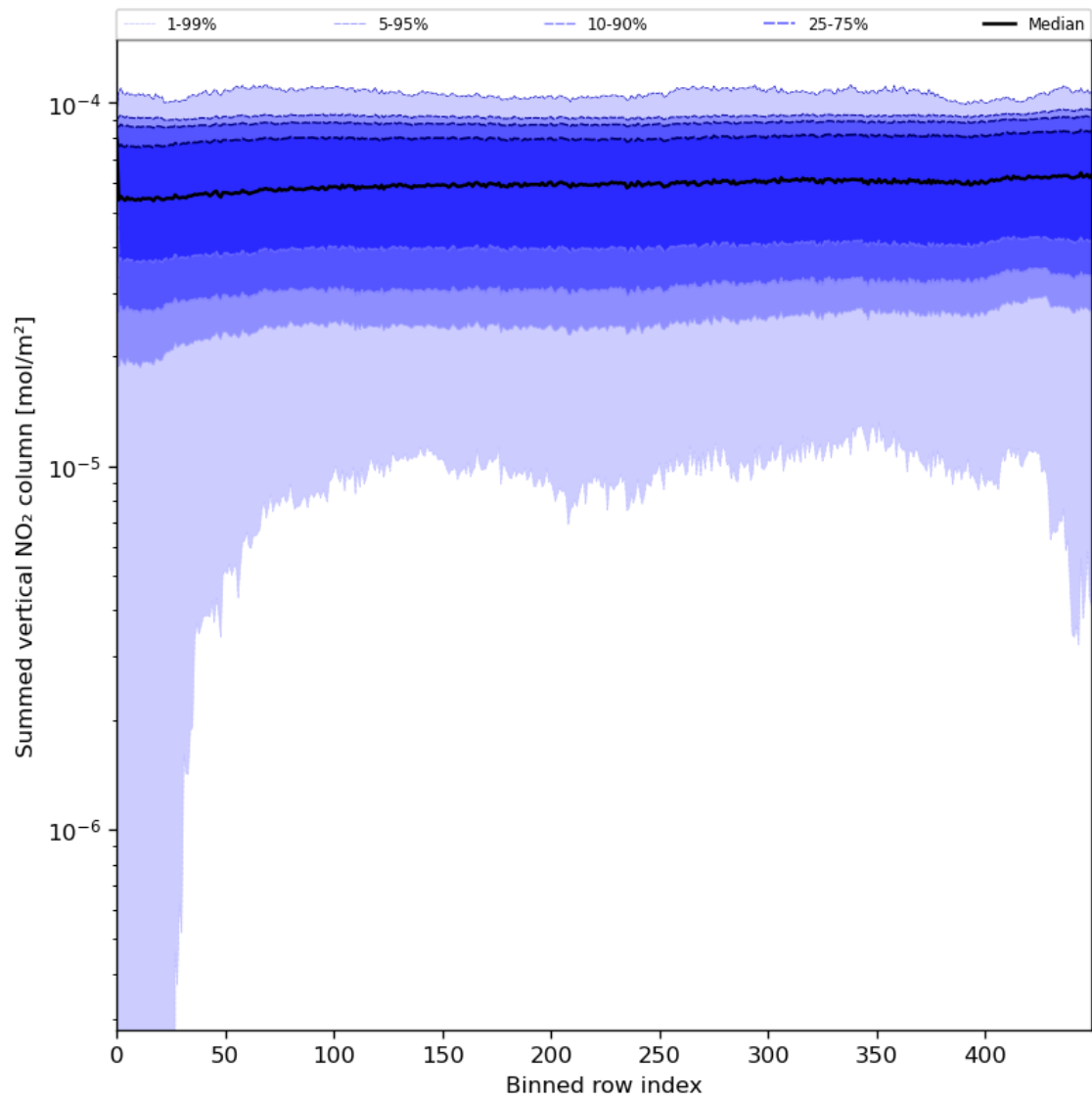
Figure 57: Along track statistics of “Summed vertical NO 2 column” for 2023-07-24 to 2023-07-26
