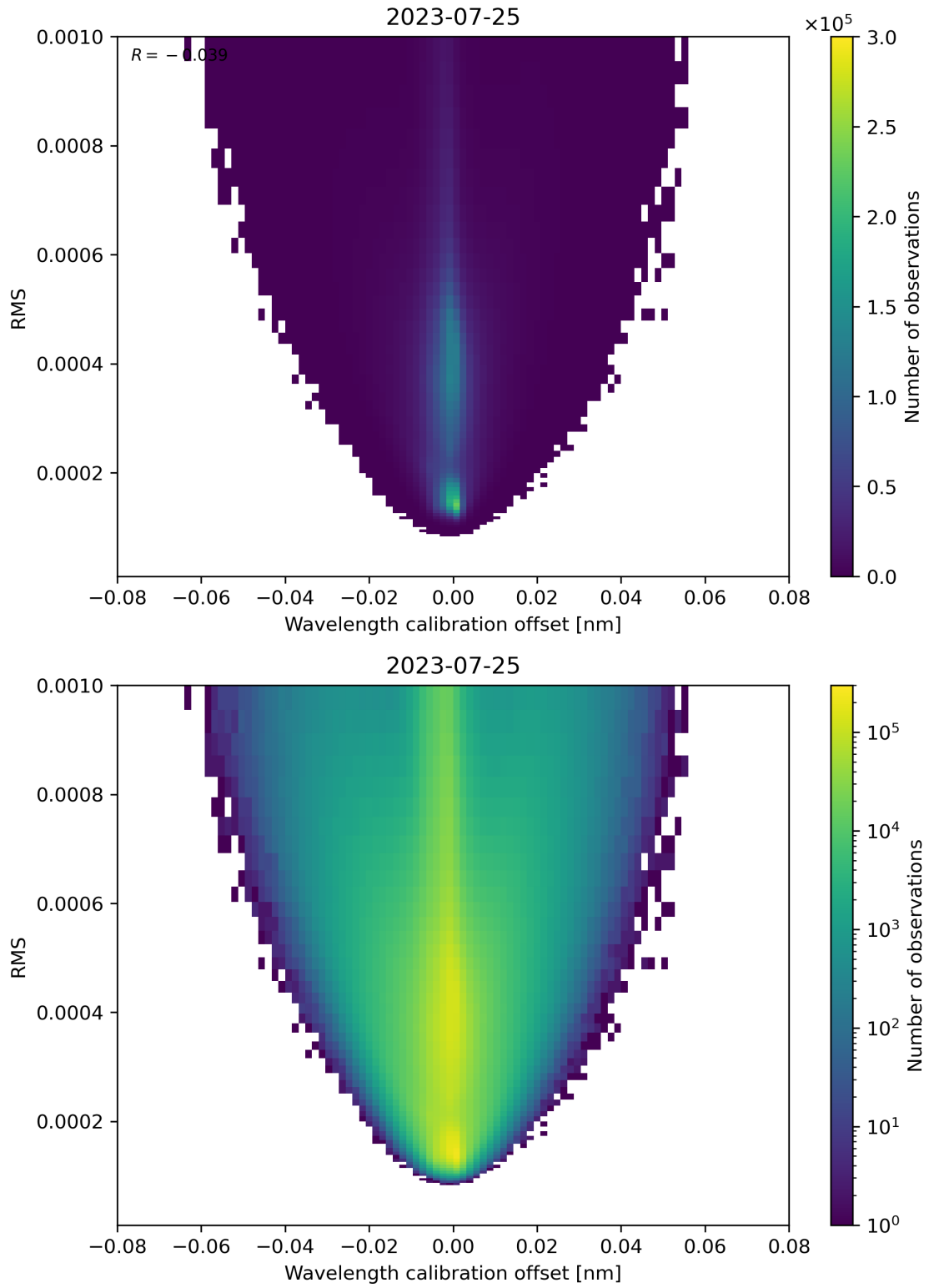
Figure 181: Scatter density plot of “Wavelength calibration offset” against “RMS” for 2023-07-24 to 2023-07-26.
