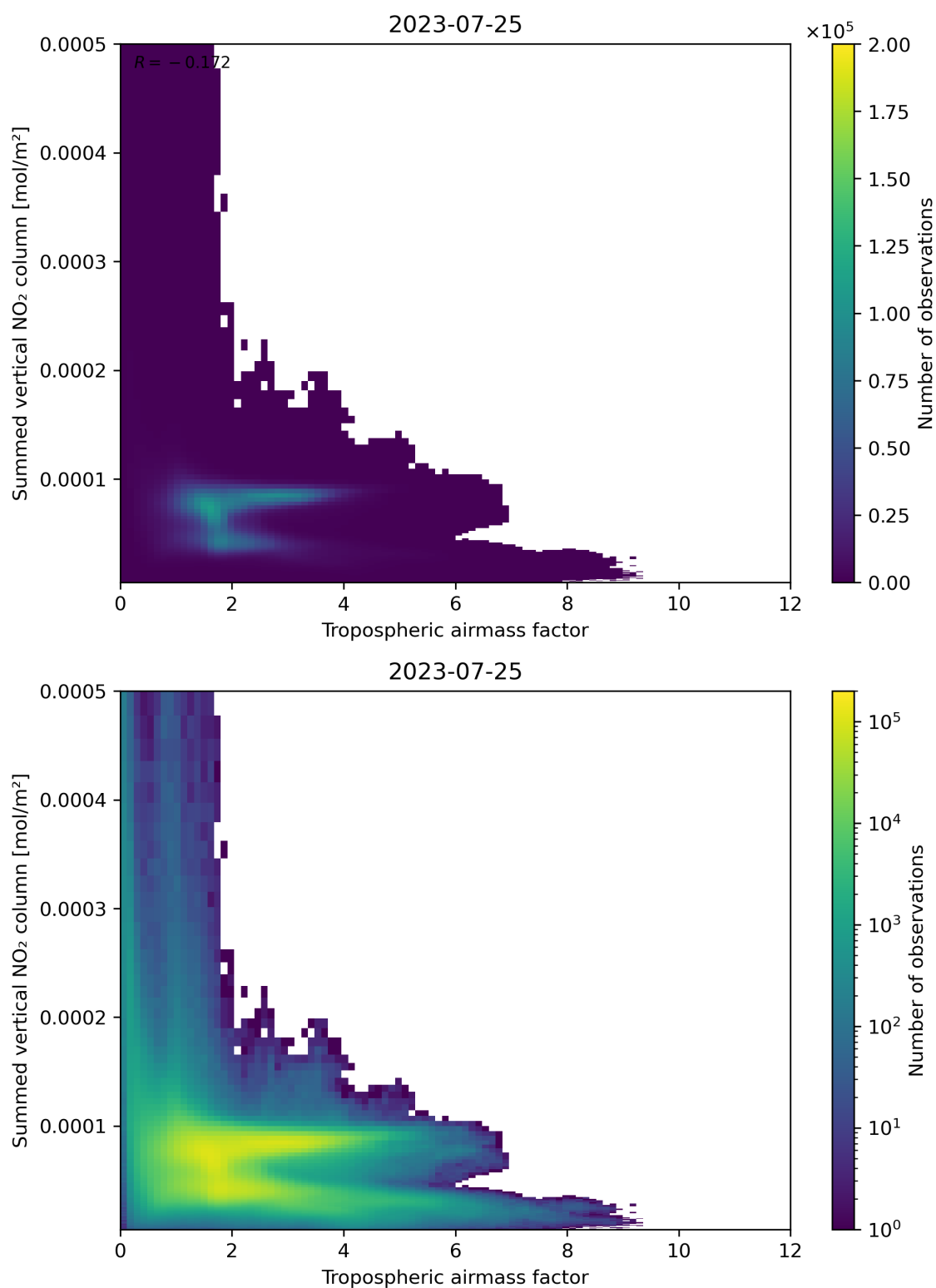
Figure 75: Scatter density plot of “Tropospheric airmass factor” against “Summed vertical NO 2 column” for 2023-07-24 to 2023-07-26.
