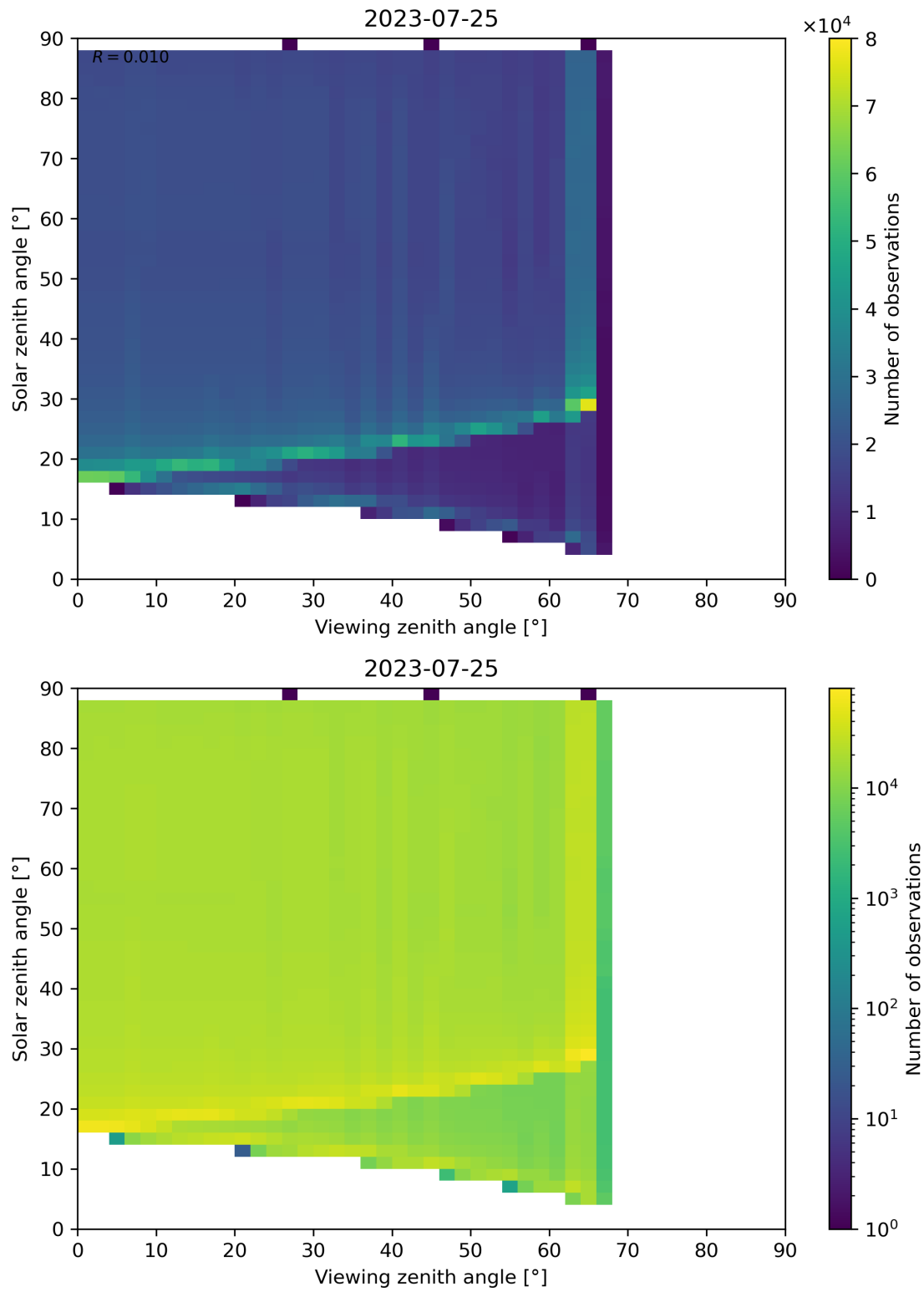
Figure 172: Scatter density plot of “Viewing zenith angle” against “Solar zenith angle” for 2023-07-24 to 2023-07-26.
