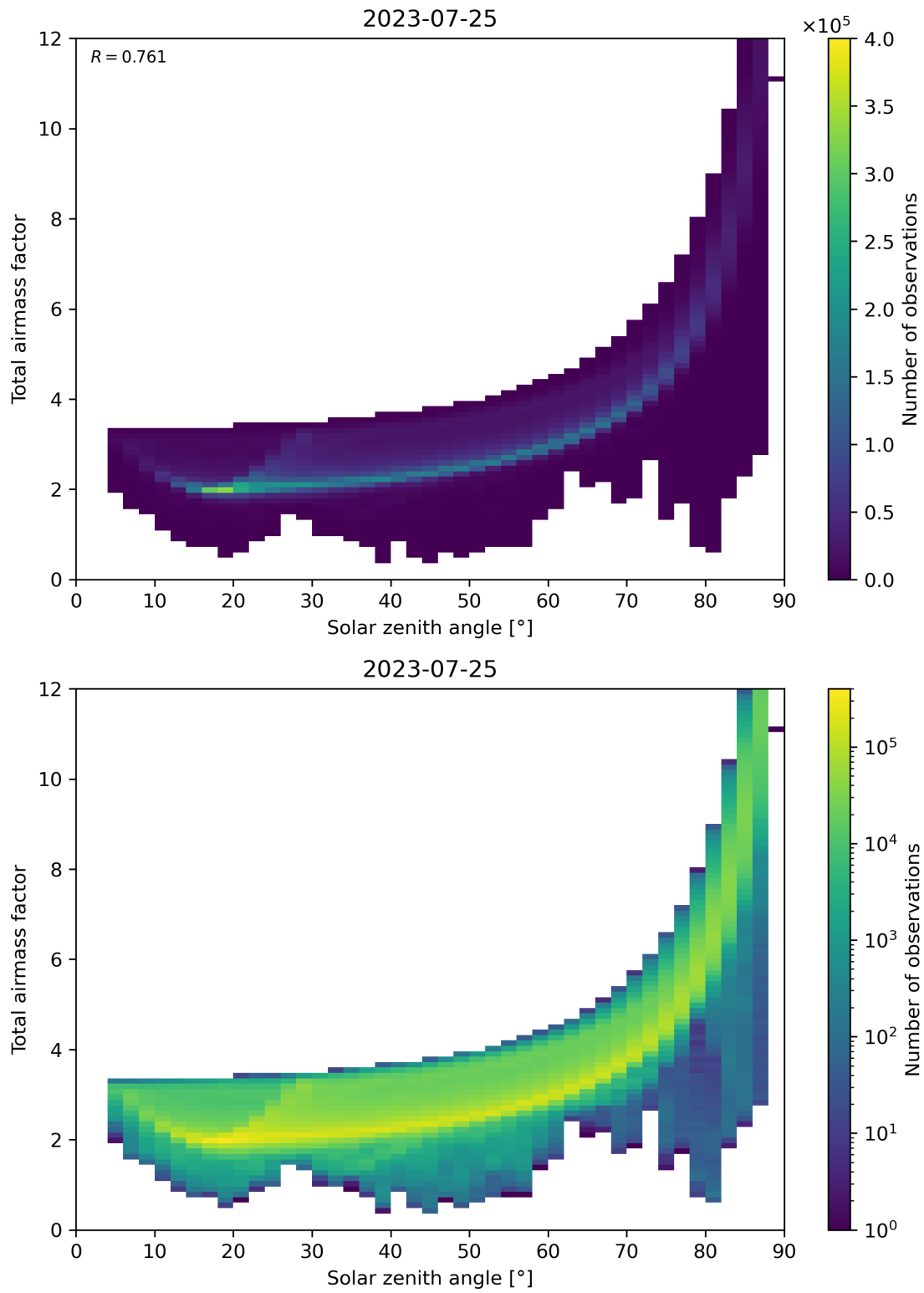
Figure 146: Scatter density plot of “Solar zenith angle” against “Total air mass factor” for 2023-07-24 to 2023-07-26.
