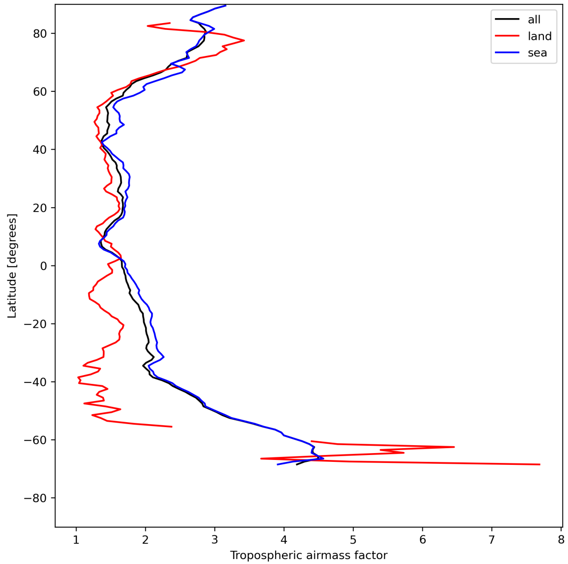
Figure 14: Zonal average of “Tropospheric air mass factor” for 2023-07-24 to 2023-07-26.
