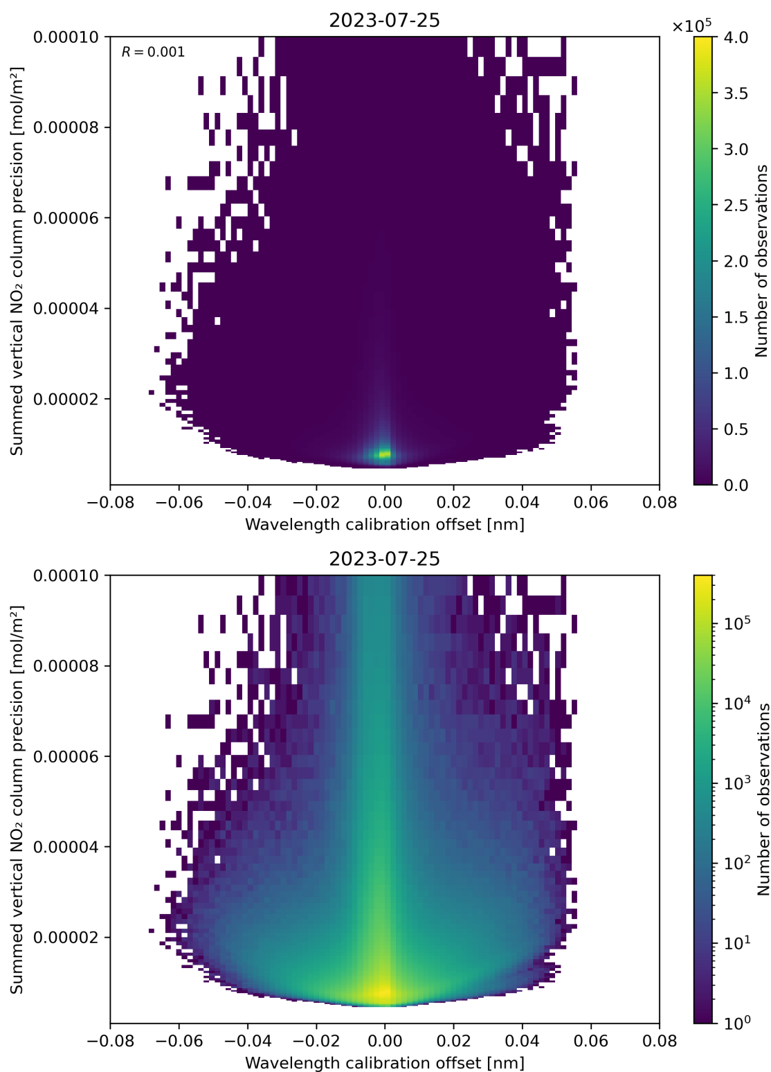
Figure 178: Scatter density plot of “Wavelength calibration offset” against “Summed vertical NO 2 column precision” for 2023-07-24 to 2023-07-26.
