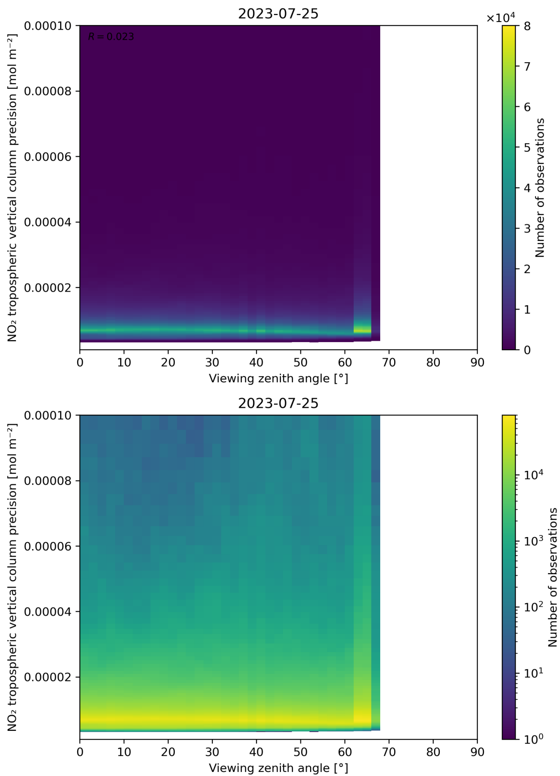
Figure 170: Scatter density plot of “Viewing zenith angle” against “NO 2 tropospheric vertical column precision” for 2023-07-24 to 2023-07-26.
