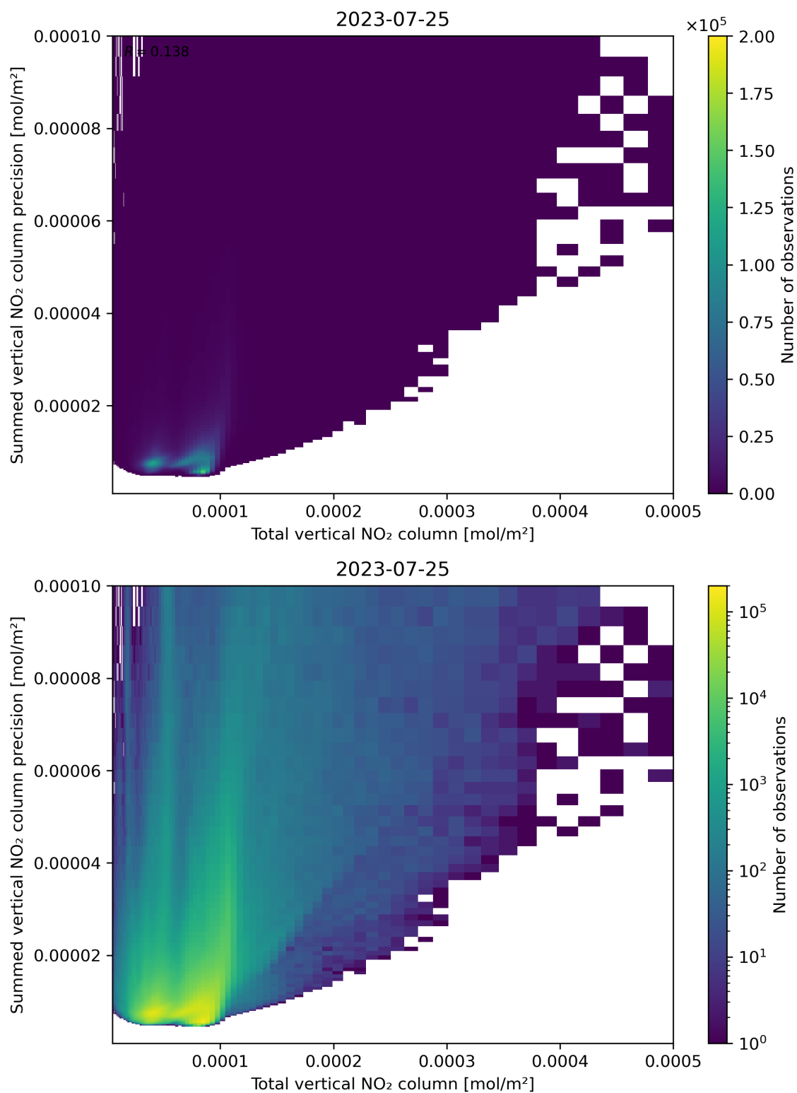
Figure 113: Scatter density plot of “Total vertical NO 2 column” against “Summed vertical NO 2 column precision” for 2023-07-24 to 2023-07-26.
