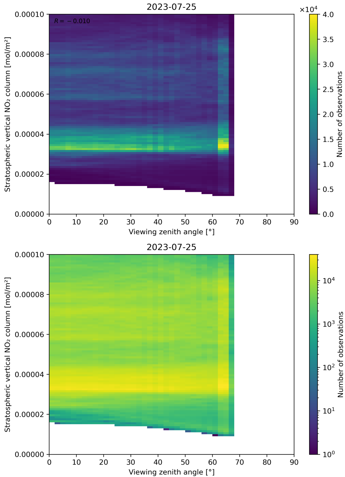
Figure 164: Scatter density plot of “Viewing zenith angle” against “Stratospheric vertical NO 2 column” for 2023-07-24 to 2023-07-26.
