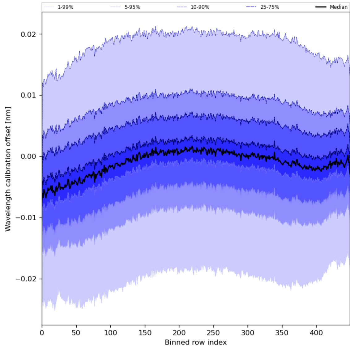
Figure 52: Along track statistics of “Wavelength calibration offset” for 2023-07-24 to 2023-07-26
