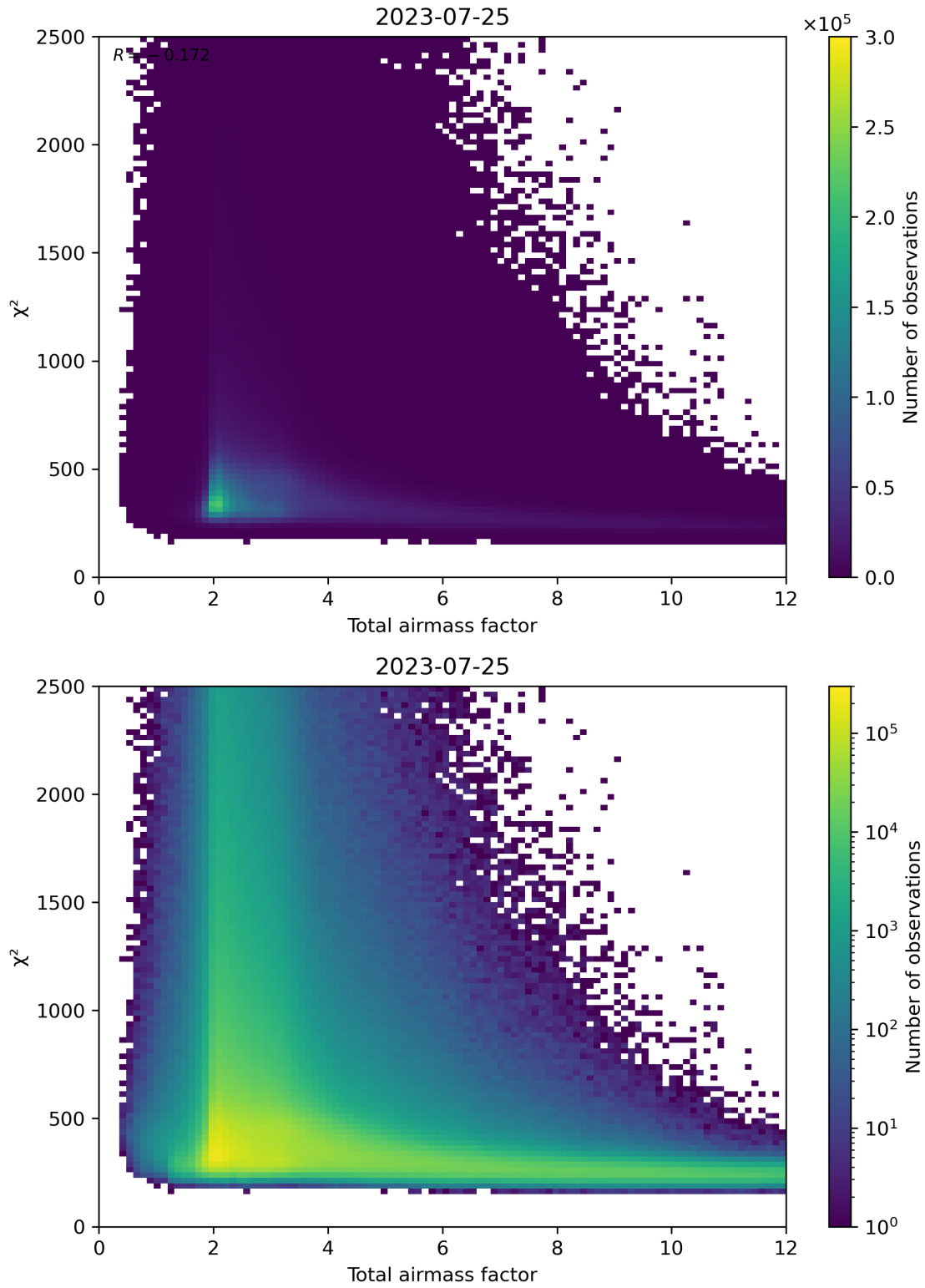
Figure 63: Scatter density plot of “Total airmass factor” against “ \chi^2 ” for 2023-07-24 to 2023-07-26.
