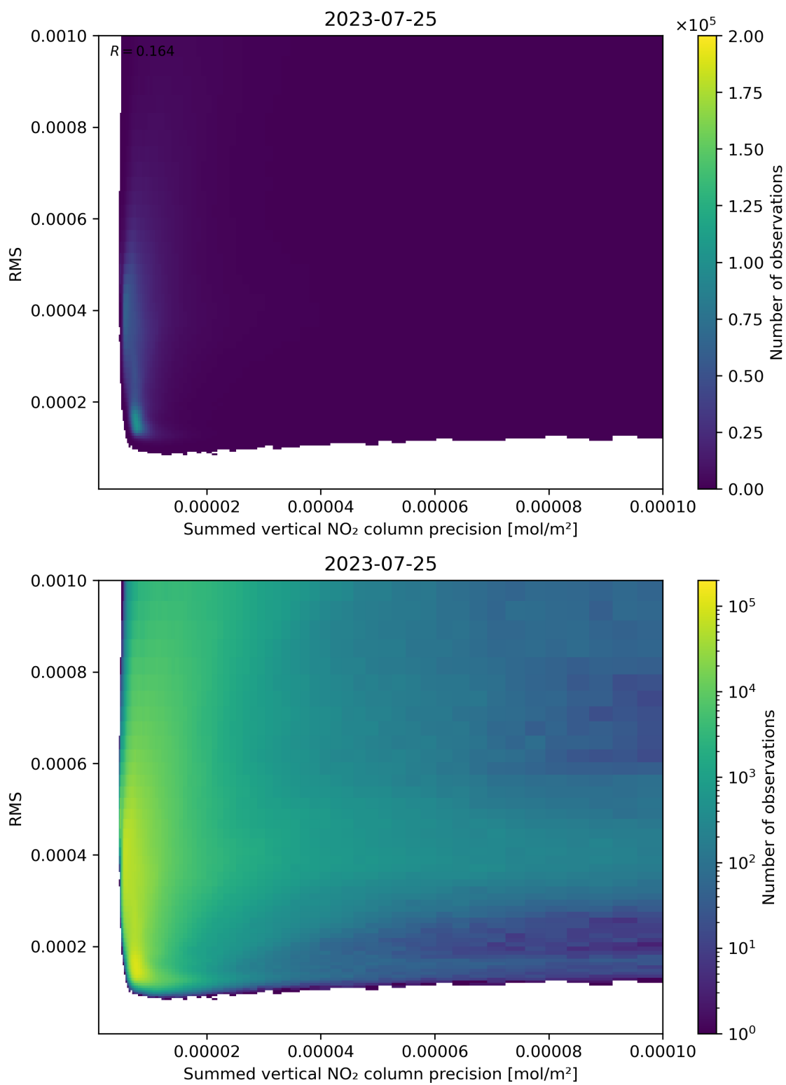
Figure 108: Scatter density plot of “Summed vertical NO 2 column precision” against “RMS” for 2023-07-24 to 2023-07-26.
