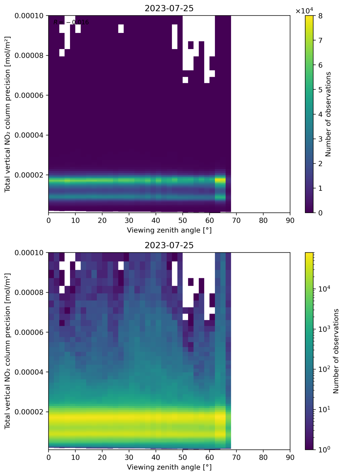
Figure 168: Scatter density plot of “Viewing zenith angle” against “Total vertical NO 2 column precision” for 2023-07-24 to 2023-07-26.
