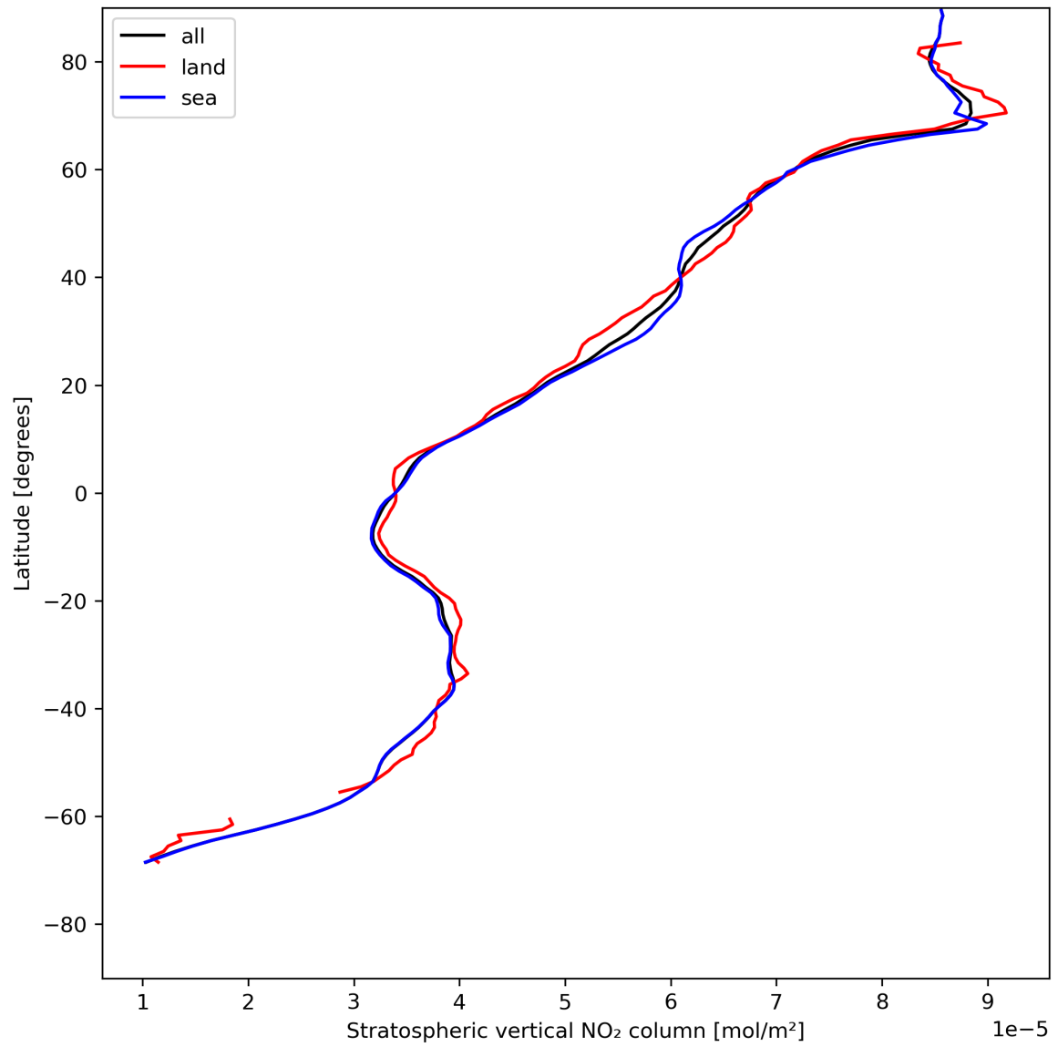
Figure 19: Zonal average of “Stratospheric vertical NO 2 column” for 2023-07-24 to 2023-07-26.
