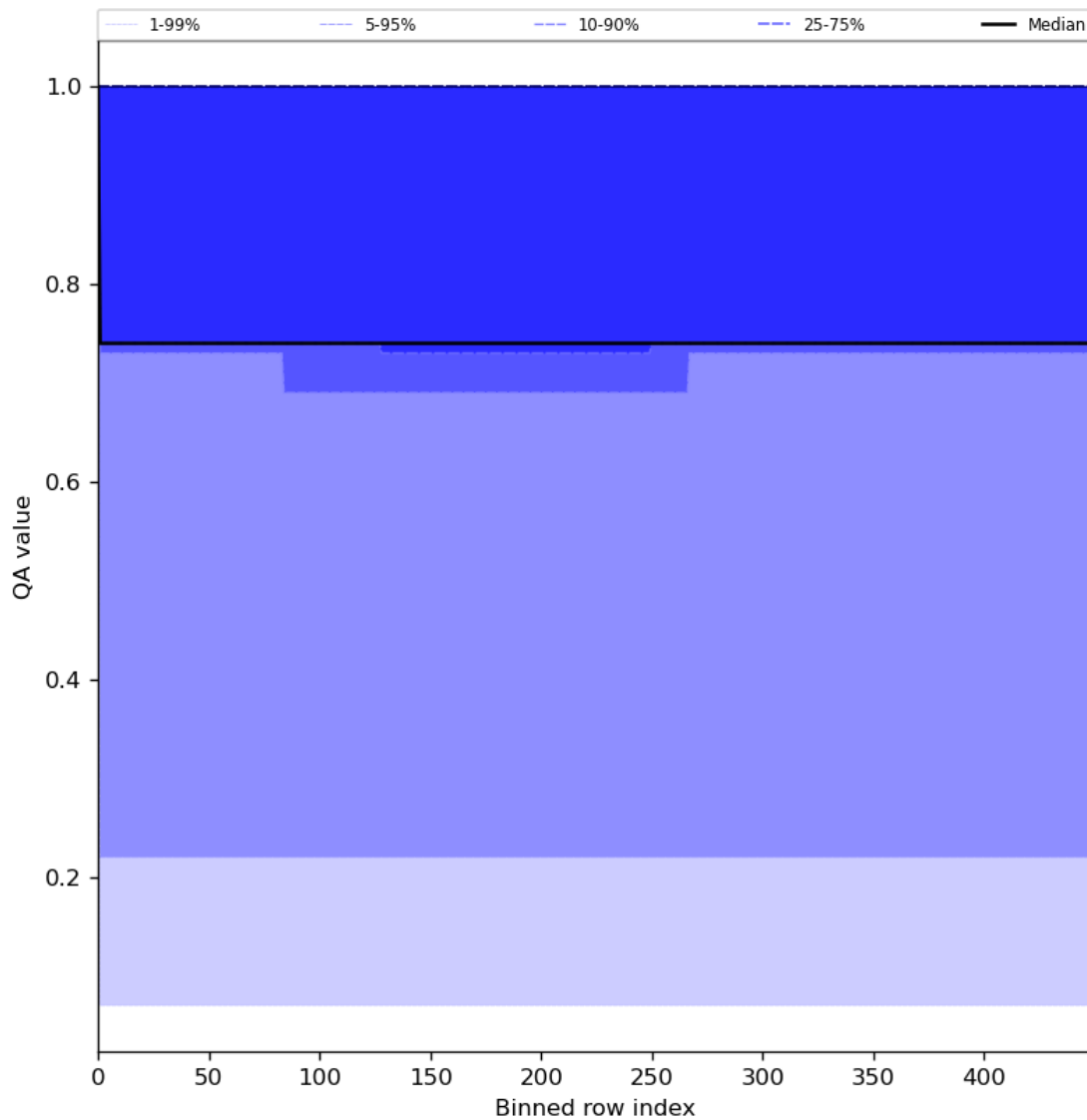
Figure 45: Along track statistics of “QA value” for 2023-07-24 to 2023-07-26
