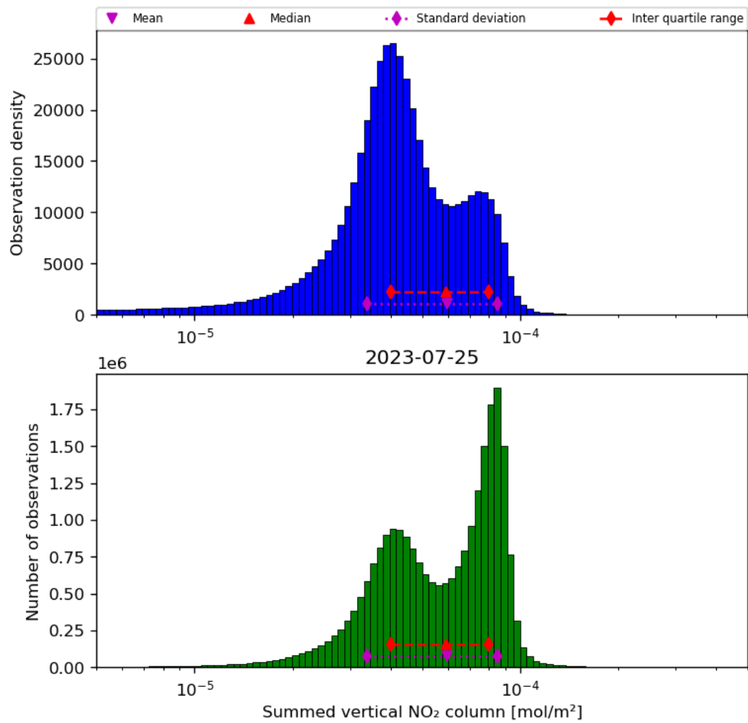
Figure 40: Histogram of “Summed vertical NO 2 column” for 2023-07-24 to 2023-07-26
