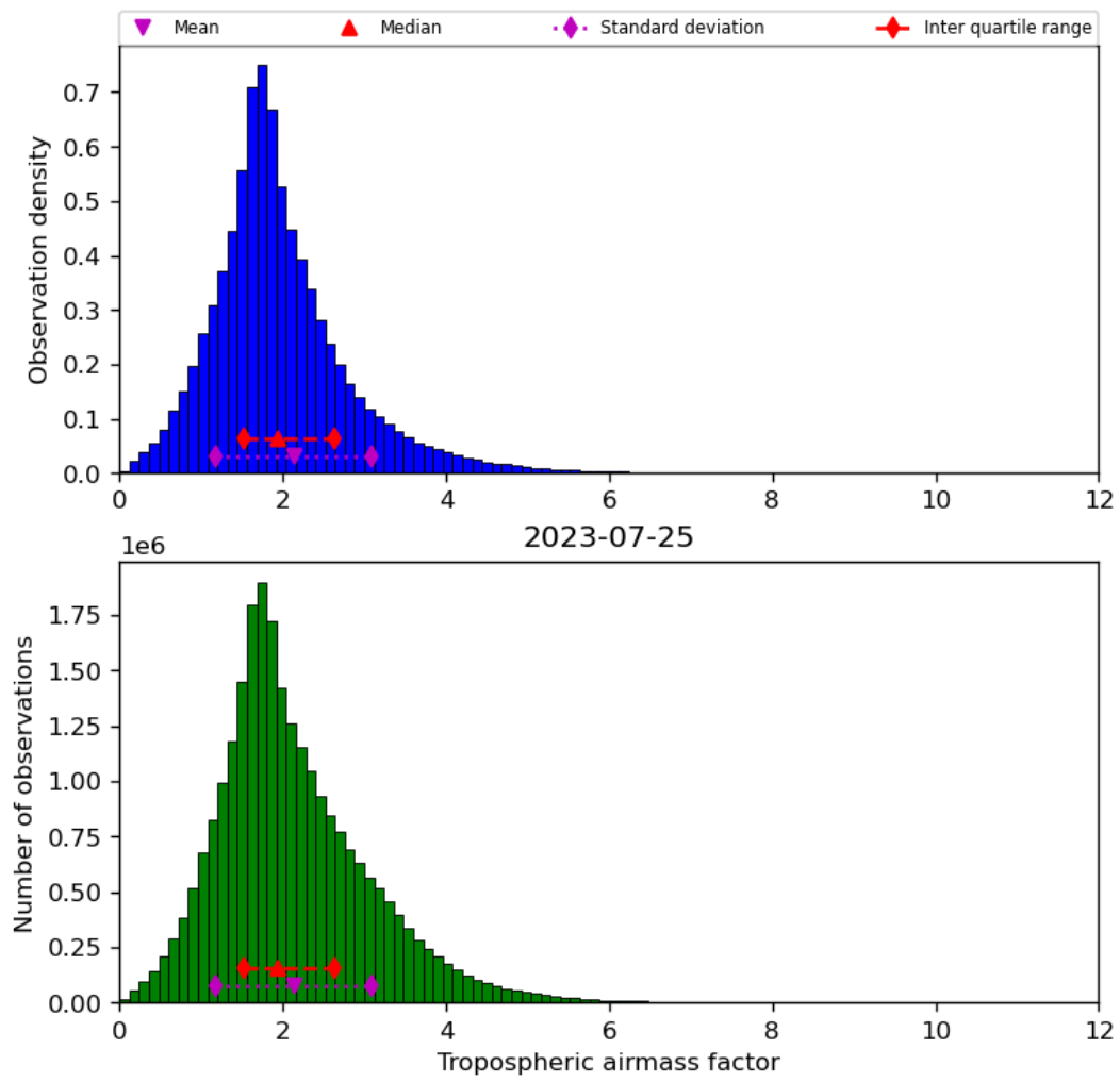
Figure 31: Histogram of “Tropospheric airmass factor” for 2023-07-24 to 2023-07-26
