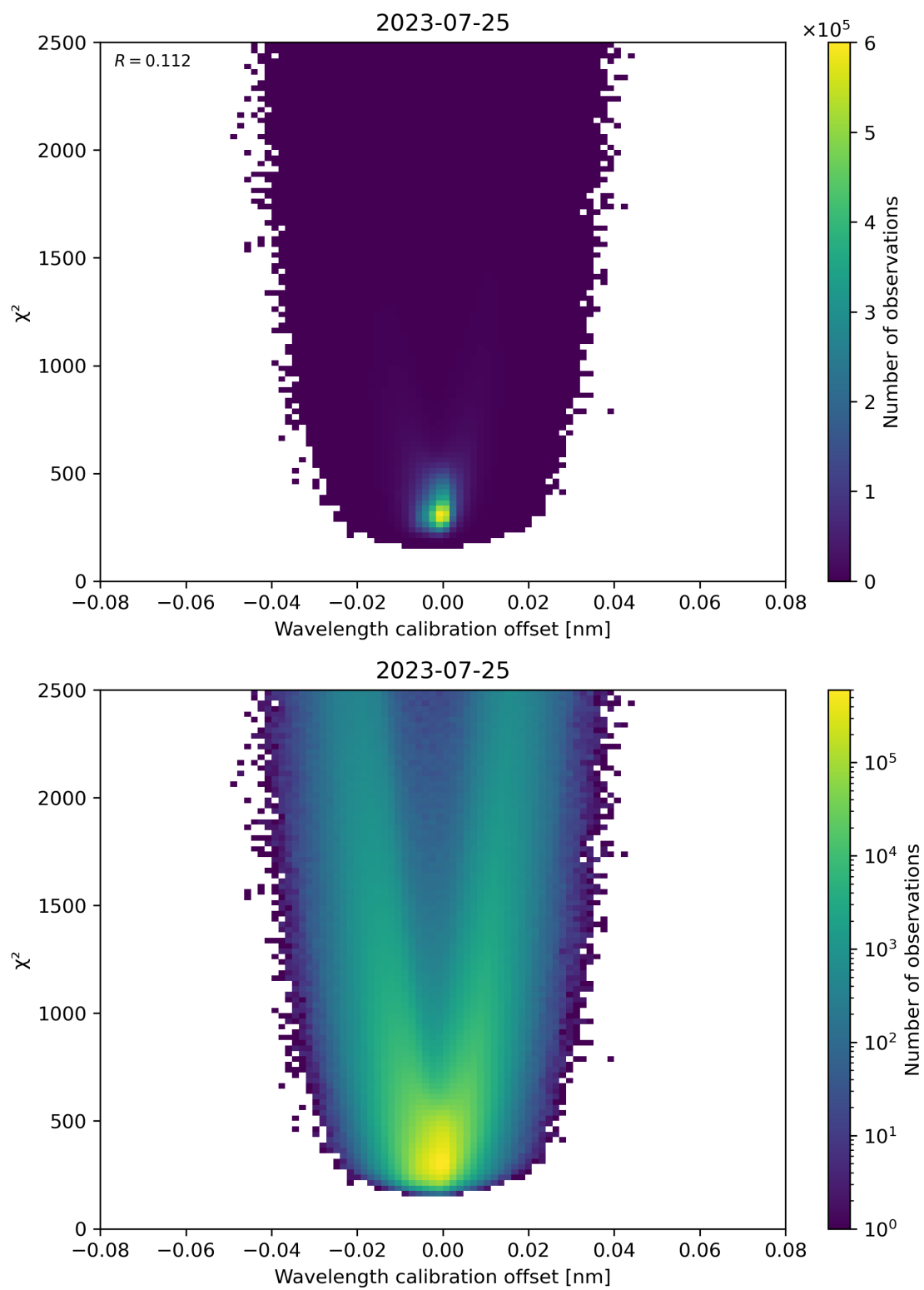
Figure 175: Scatter density plot of “Wavelength calibration offset” against “ \chi^2 ” for 2023-07-24 to 2023-07-26.
