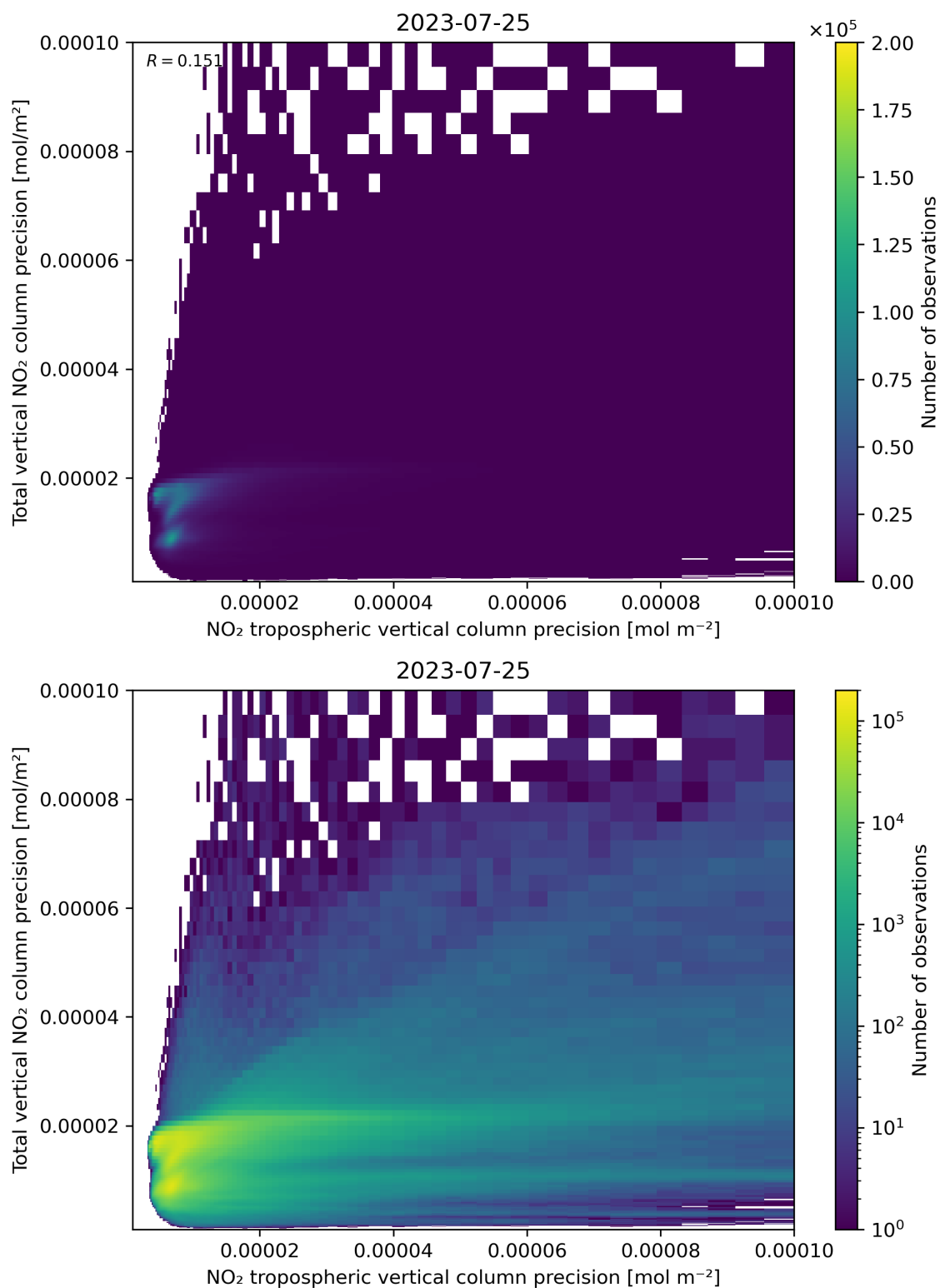
Figure 139: Scatter density plot of “NO 2 tropospheric vertical column precision” against “Total vertical NO 2 column precision” for 2023-07-24 to 2023-07-26.
