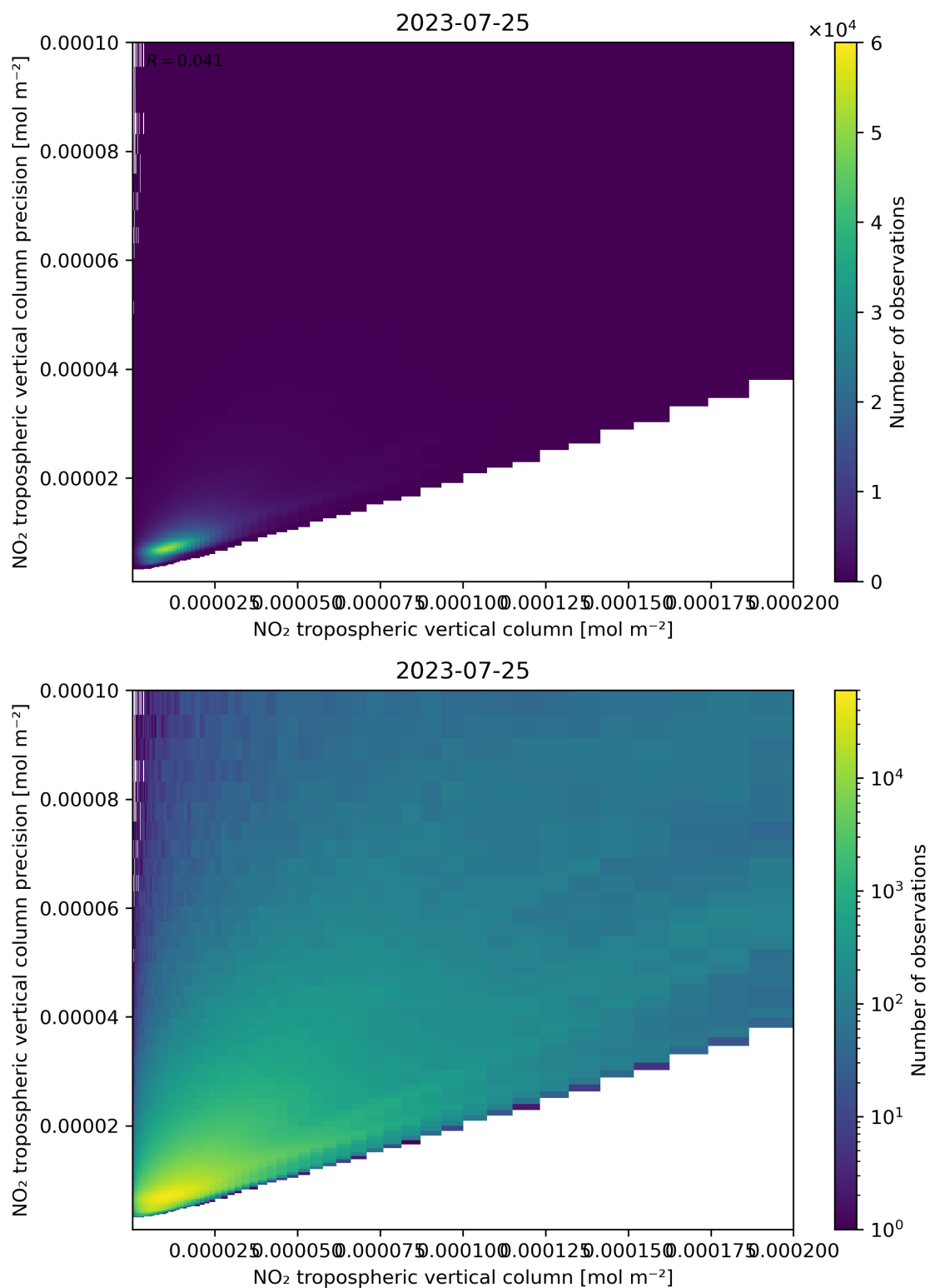
Figure 130: Scatter density plot of “NO 2 tropospheric vertical column” against “NO 2 tropospheric vertical column precision” for 2023-07-24 to 2023-07-26.
