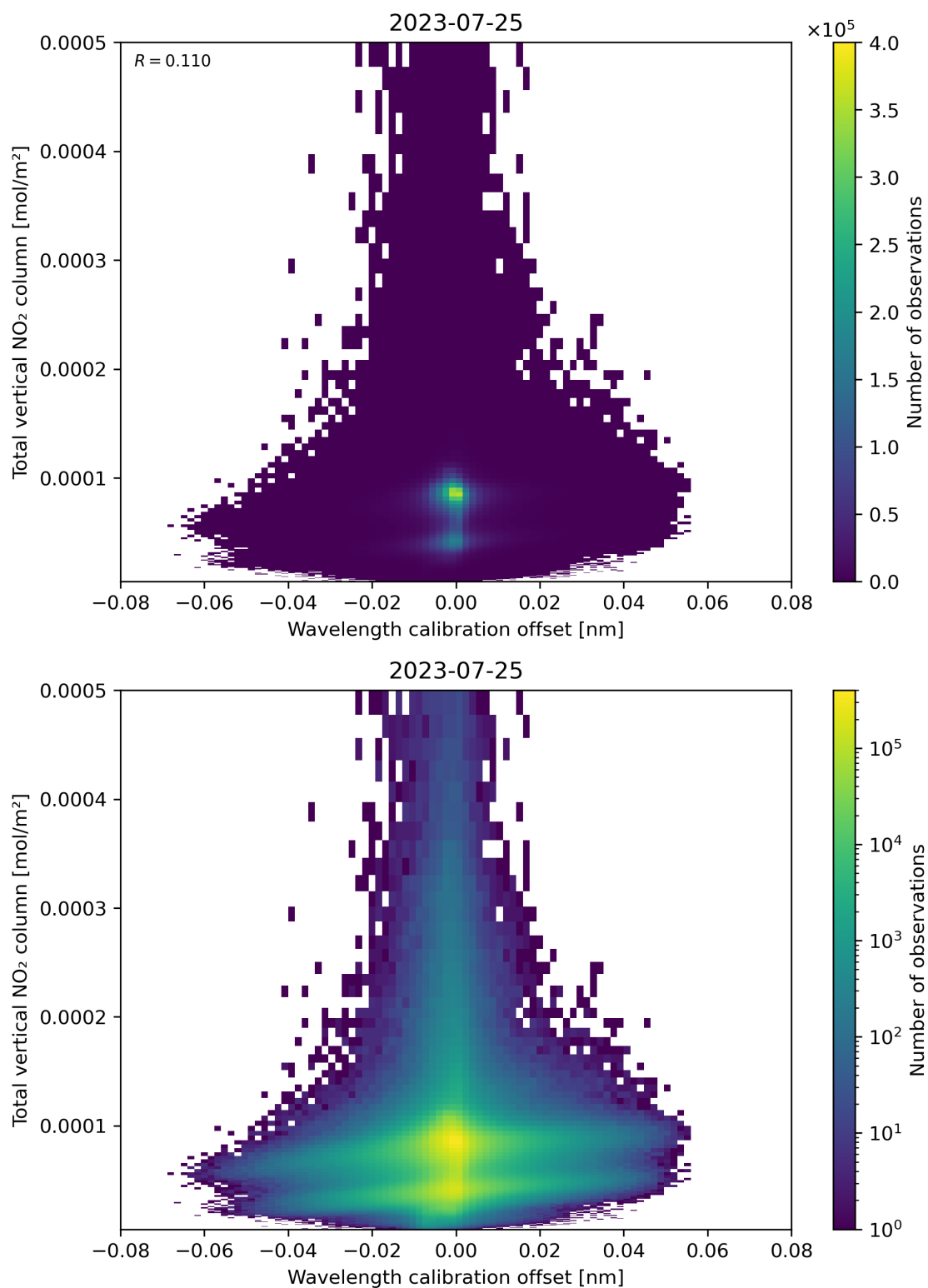
Figure 179: Scatter density plot of “Wavelength calibration offset” against “Total vertical NO 2 column” for 2023-07-24 to 2023-07-26.
