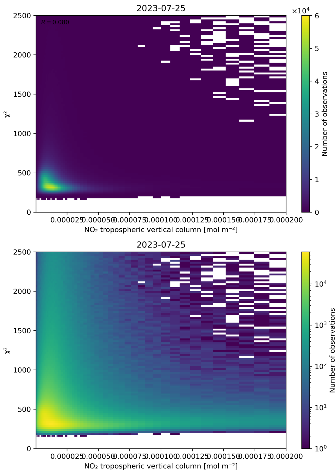
Figure 124: Scatter density plot of “NO 2 tropospheric vertical column” against “ \chi^2 ” for 2023-07-24 to 2023-07-26.
