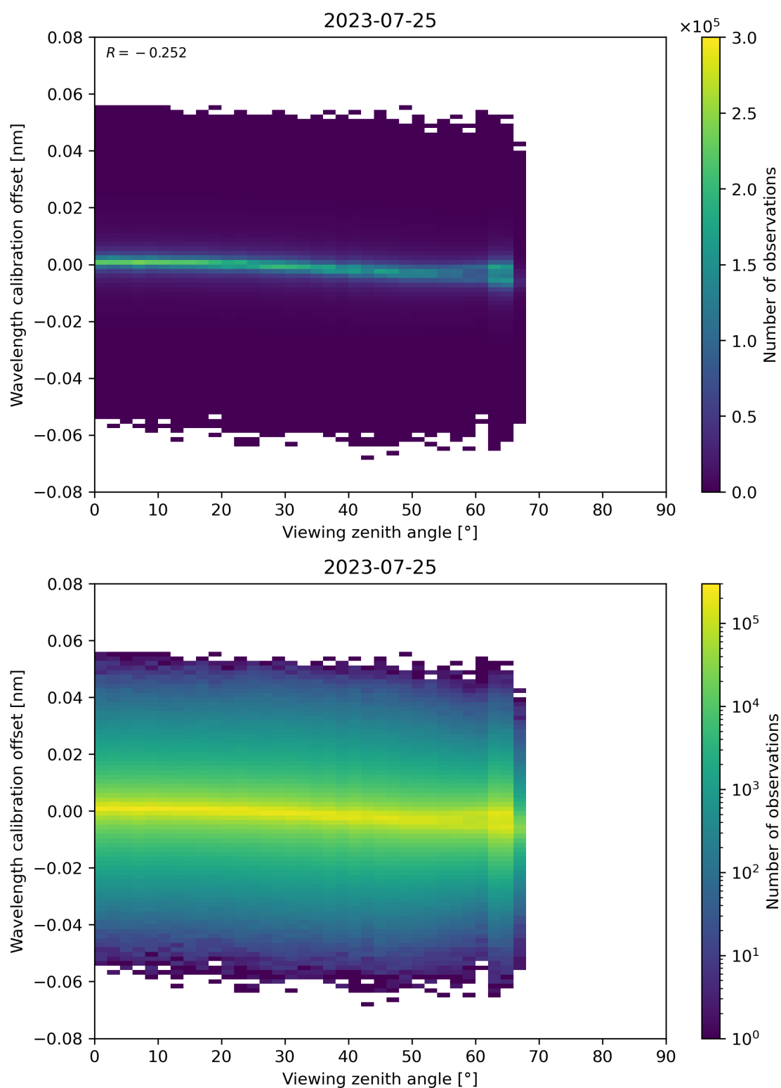
Figure 173: Scatter density plot of “Viewing zenith angle” against “Wavelength calibration offset” for 2023-07-24 to 2023-07-26.
