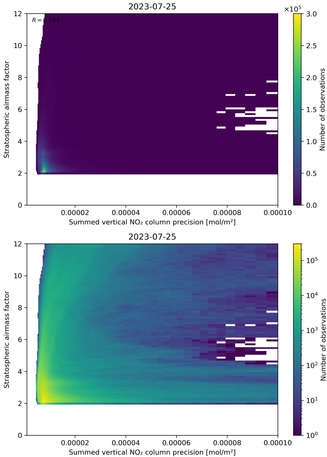
Figure 106: Scatter density plot of “Summed vertical NO 2 column precision” against “Stratospheric airmass factor” for 2023-07-24 to 2023-07-26.
