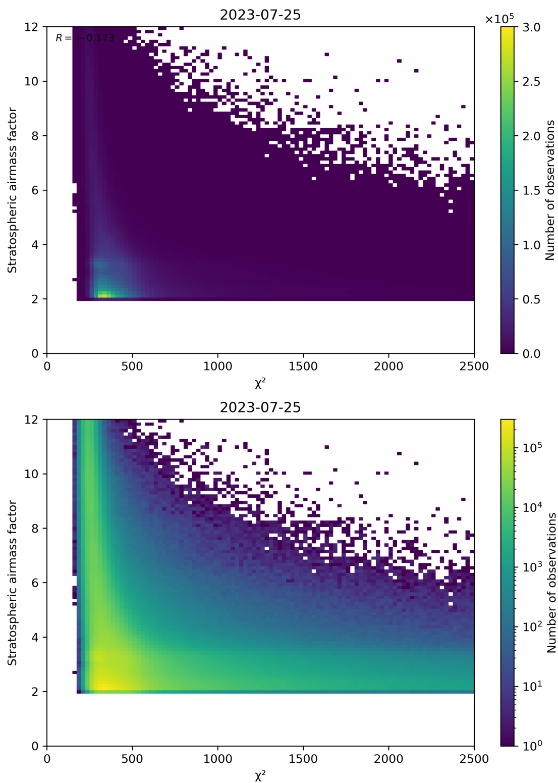
Figure 81: Scatter density plot of “ \chi^2 ” against “Stratospheric airmass factor” for 2023-07-24 to 2023-07-26.
