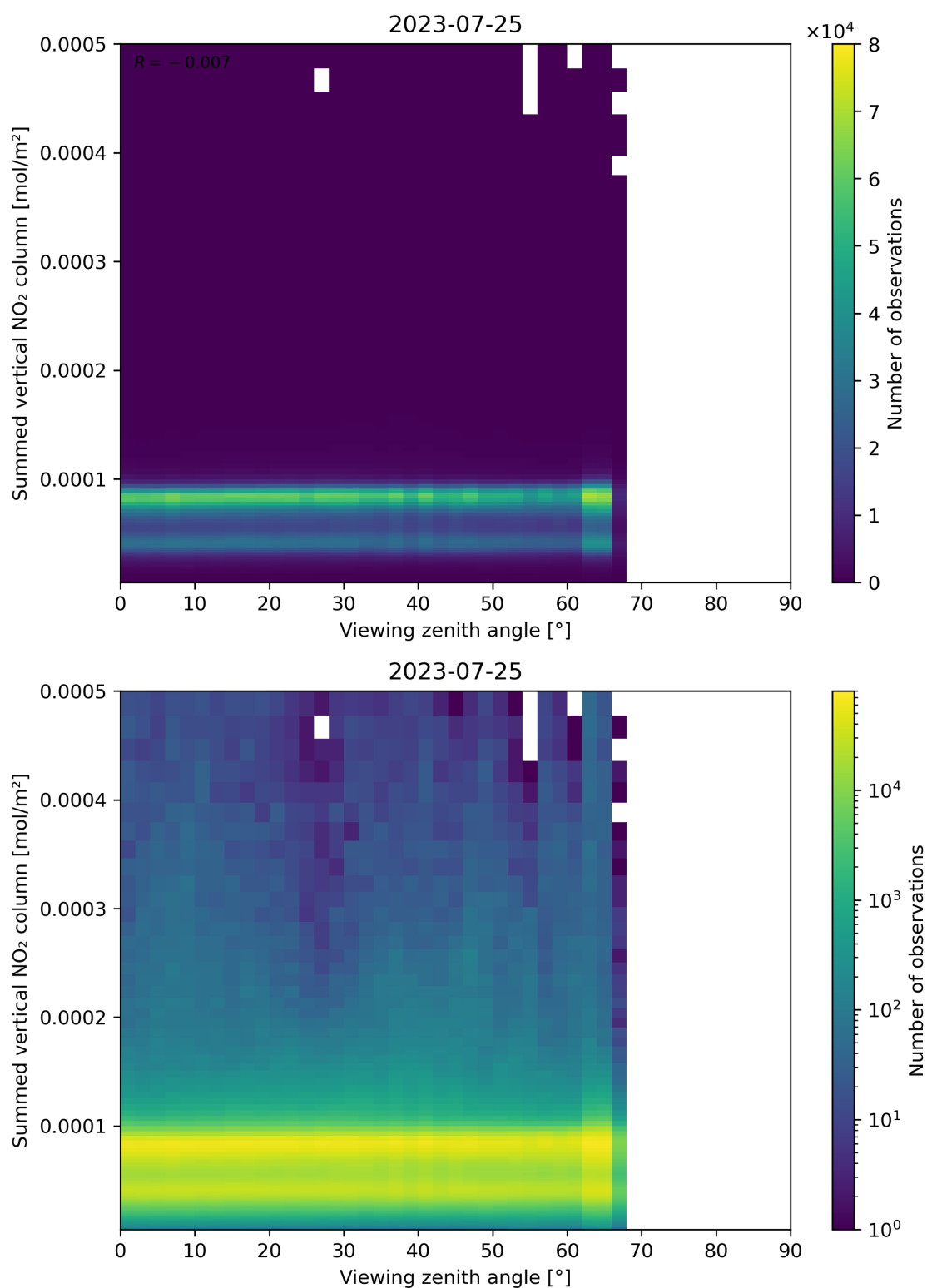
Figure 165: Scatter density plot of “Viewing zenith angle” against “Summed vertical NO 2 column” for 2023-07-24 to 2023-07-26.
