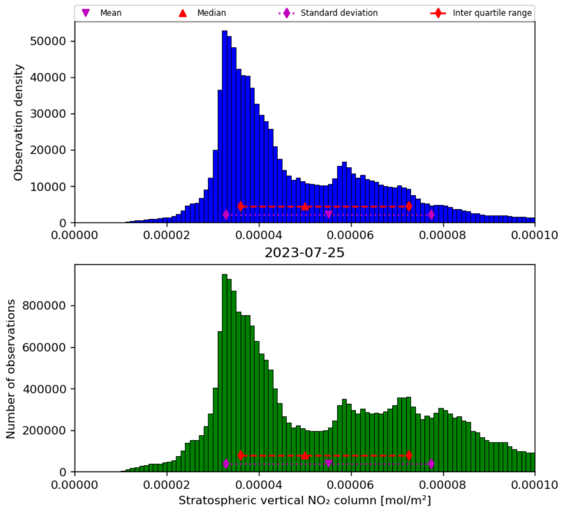
Figure 36: Histogram of “Stratospheric vertical NO 2 column” for 2023-07-24 to 2023-07-26
