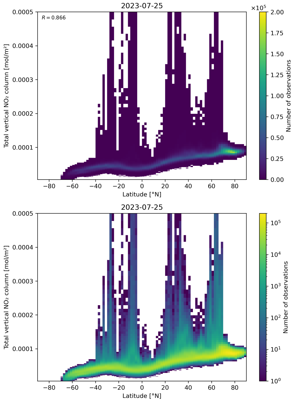
Figure 90: Scatter density plot of “Latitude” against “Total vertical NO 2 column” for 2023-07-24 to 2023-07-26.
