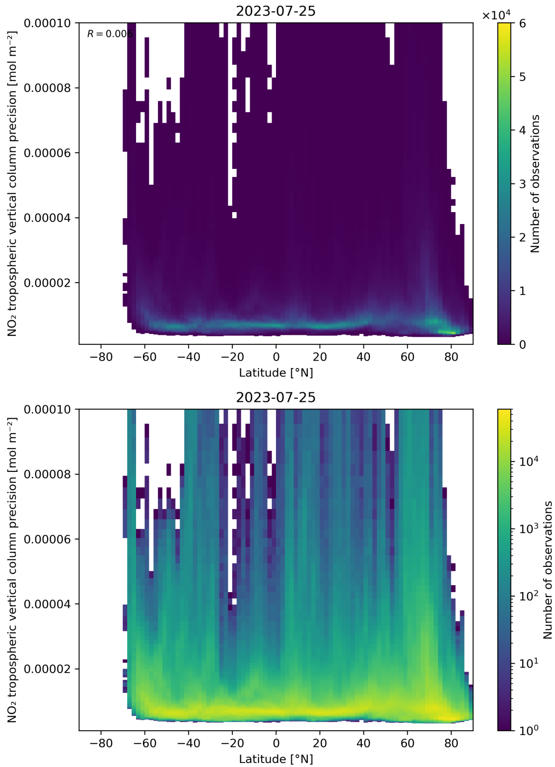
Figure 93: Scatter density plot of “Latitude” against “NO 2 tropospheric vertical column precision” for 2023-07-24 to 2023-07-26.
