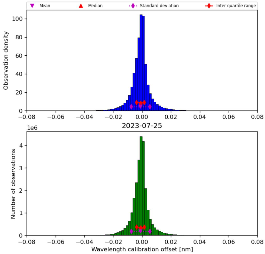
Figure 35: Histogram of “Wavelength calibration offset” for 2023-07-24 to 2023-07-26
