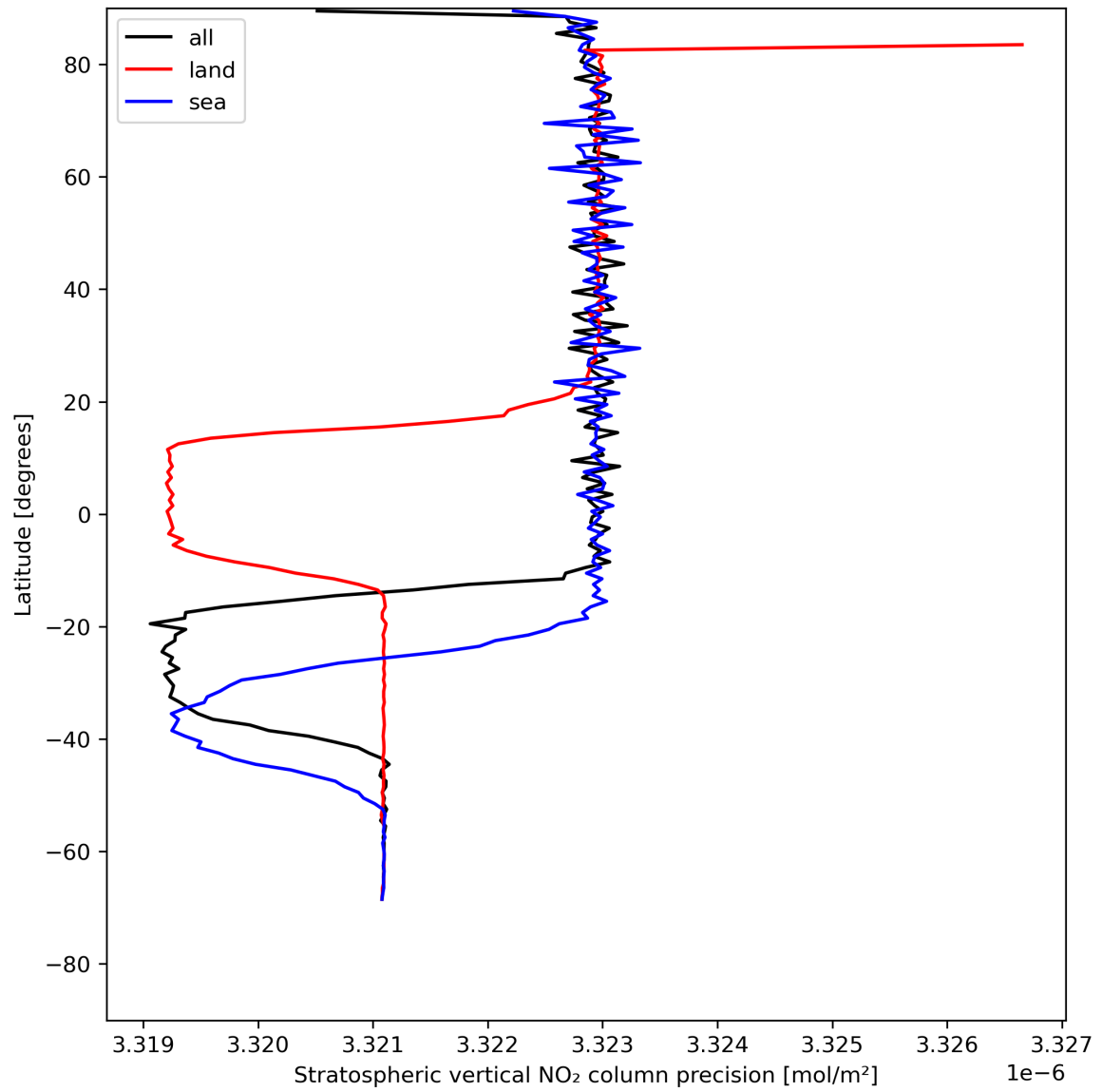
Figure 20: Zonal average of “Stratospheric vertical NO 2 column precision” for 2023-07-24 to 2023-07-26.
