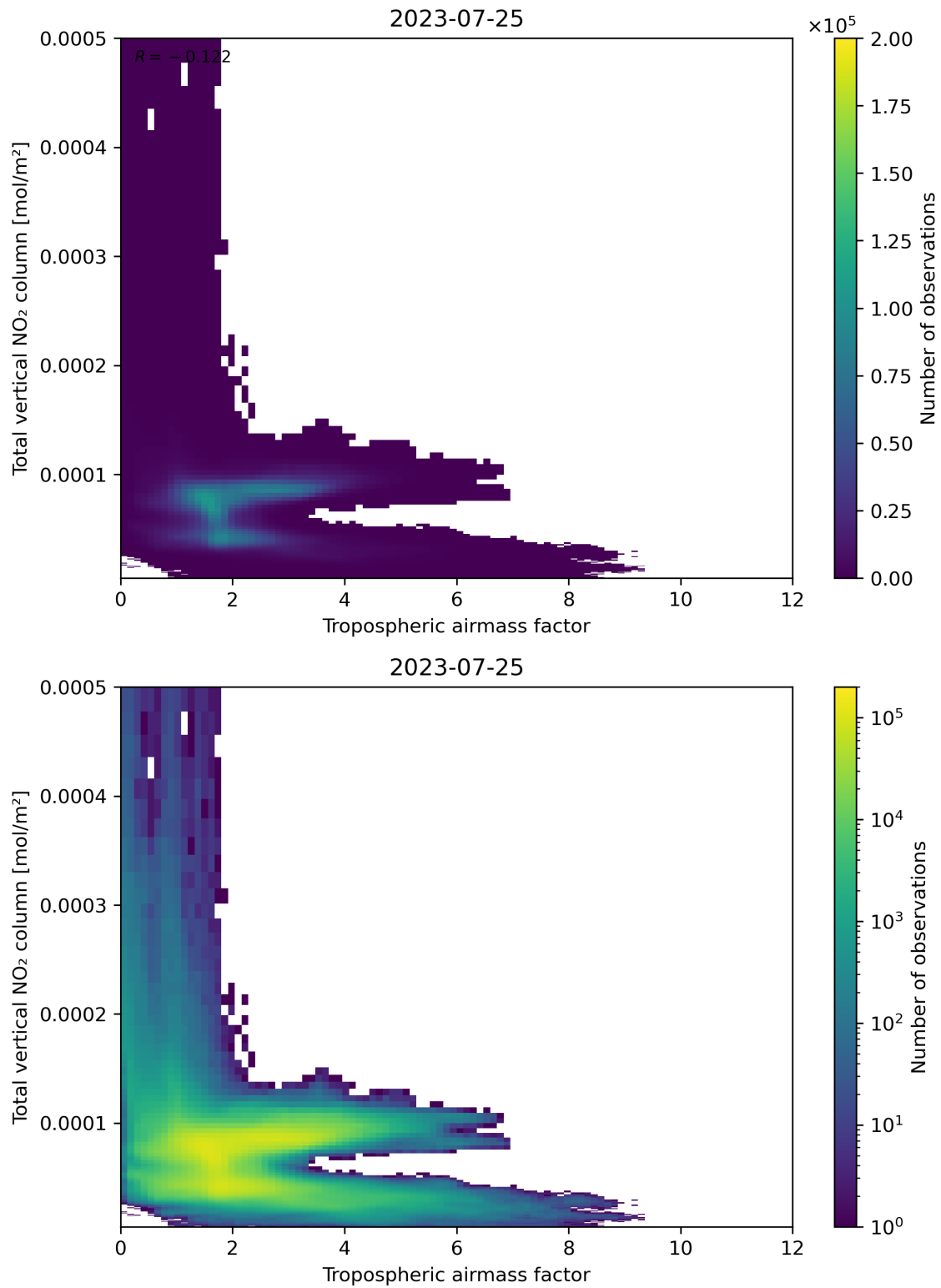
Figure 77: Scatter density plot of “Tropospheric airmass factor” against “Total vertical NO 2 column” for 2023-07-24 to 2023-07-26.
