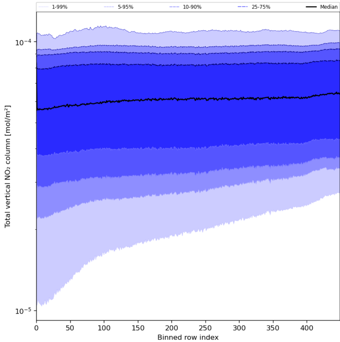
Figure 55: Along track statistics of “Total vertical NO 2 column” for 2023-07-24 to 2023-07-26
