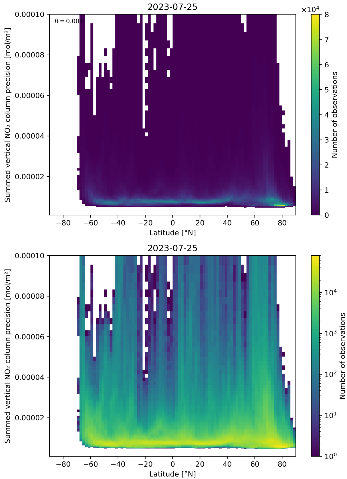
Figure 89: Scatter density plot of “Latitude” against “Summed vertical NO 2 column precision” for 2023-07-24 to 2023-07-26.
