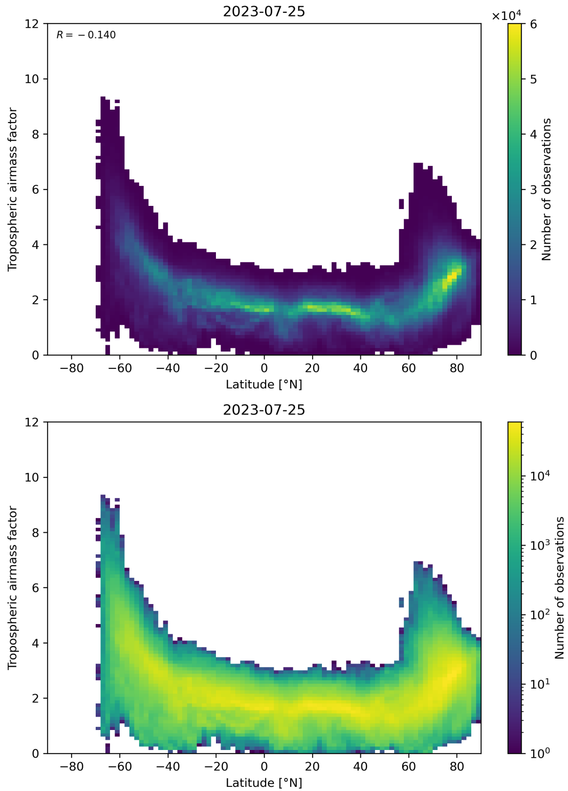
Figure 85: Scatter density plot of “Latitude” against “Tropospheric air mass factor” for 2023-07-24 to 2023-07-26.
