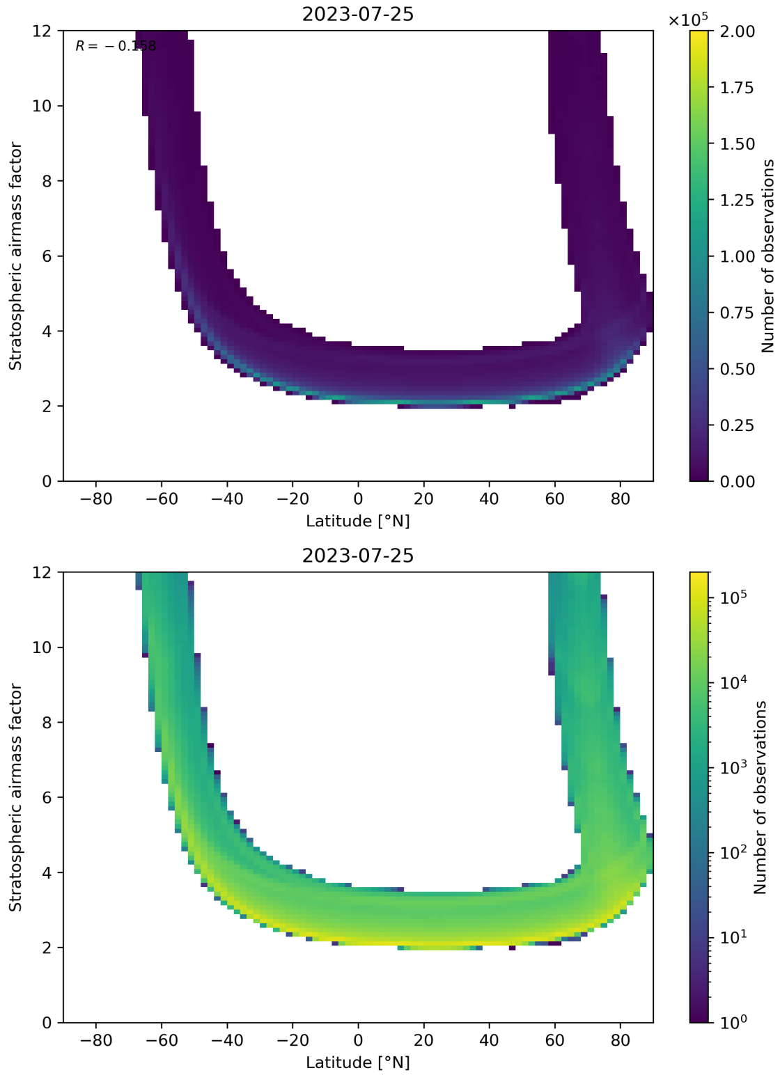
Figure 83: Scatter density plot of “Latitude” against “Stratospheric air mass factor” for 2023-07-24 to 2023-07-26.
