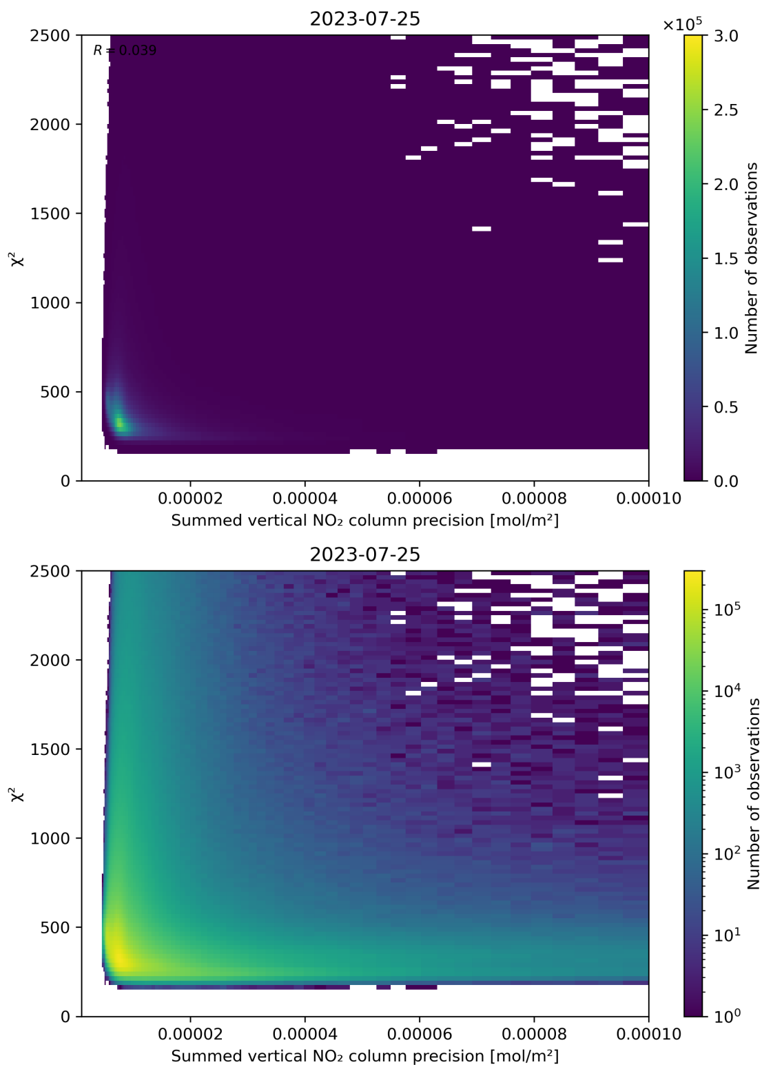
Figure 107: Scatter density plot of “Summed vertical NO 2 column precision” against “ \chi^2 ” for 2023-07-24 to 2023-07-26.
