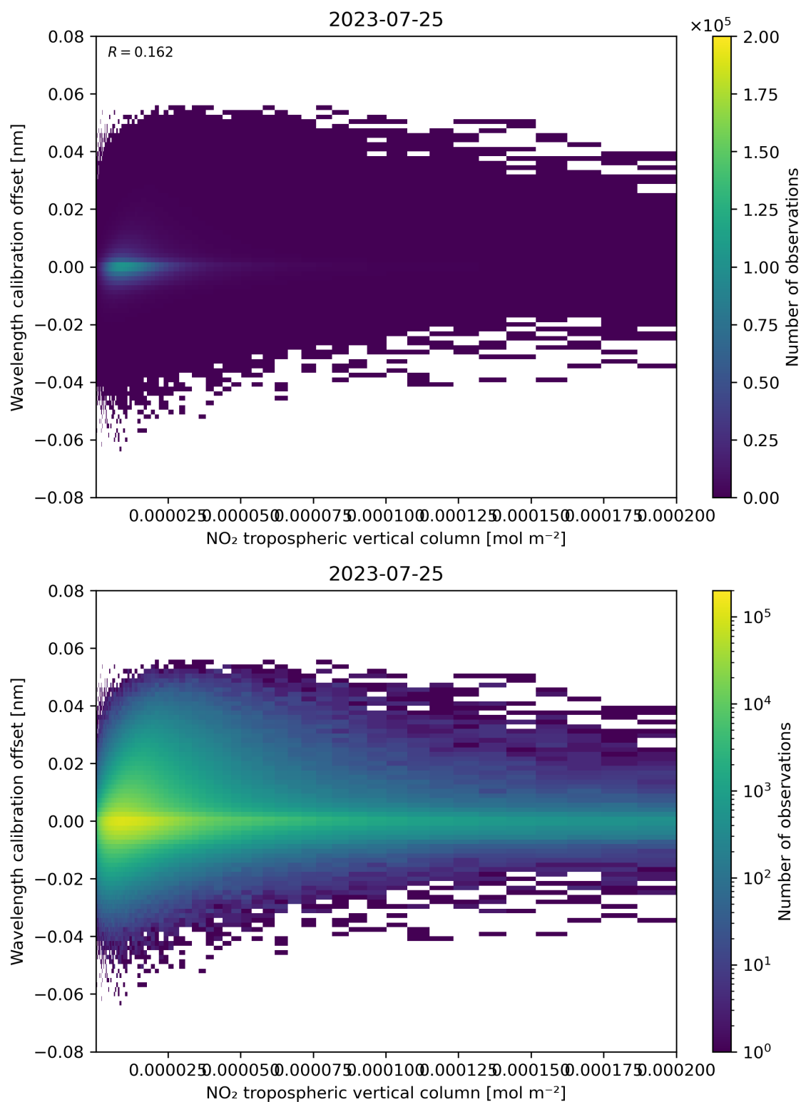
Figure 143: Scatter density plot of “NO 2 tropospheric vertical column” against “Wavelength calibration offset” for 2023-07-24 to 2023-07-26.
