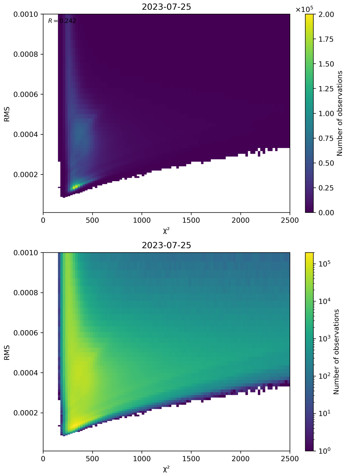
Figure 82: Scatter density plot of “ \chi^2 ” against “RMS” for 2023-07-24 to 2023-07-26.
