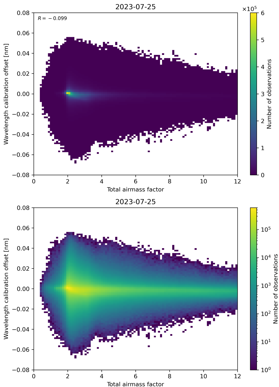
Figure 70: Scatter density plot of “Total airmass factor” against “Wavelength calibration offset” for 2023-07-24 to 2023-07-26.
