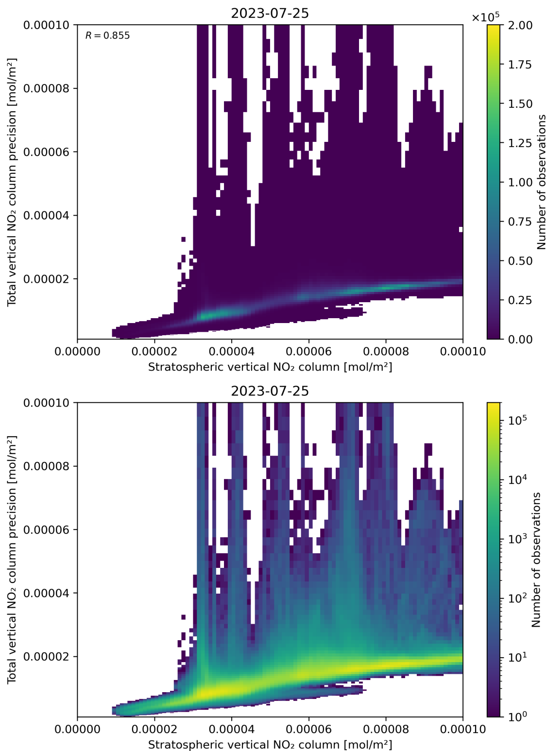
Figure 101: Scatter density plot of “Stratospheric vertical NO 2 column” against “Total vertical NO 2 column precision” for 2023-07-24 to 2023-07-26.
