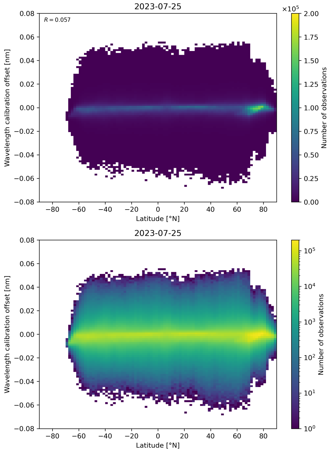
Figure 95: Scatter density plot of “Latitude” against “Wavelength calibration offset” for 2023-07-24 to 2023-07-26.
