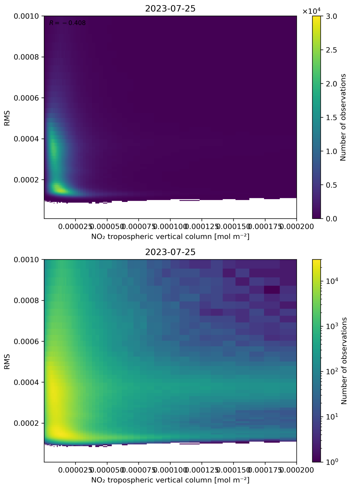
Figure 142: Scatter density plot of “NO 2 tropospheric vertical column” against “RMS” for 2023-07-24 to 2023-07-26.
