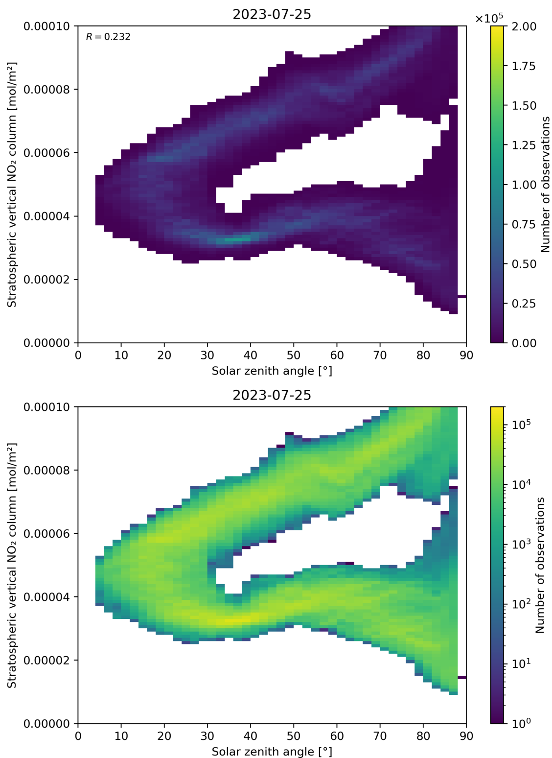
Figure 150: Scatter density plot of “Solar zenith angle” against “Stratospheric vertical NO 2 column” for 2023-07-24 to 2023-07-26.
