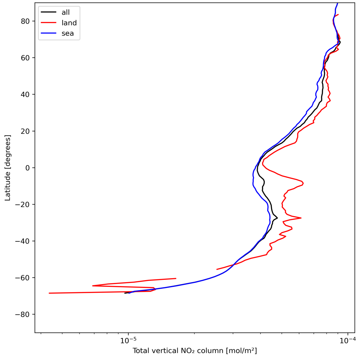
Figure 21: Zonal average of “Total vertical NO 2 column” for 2023-07-24 to 2023-07-26.
