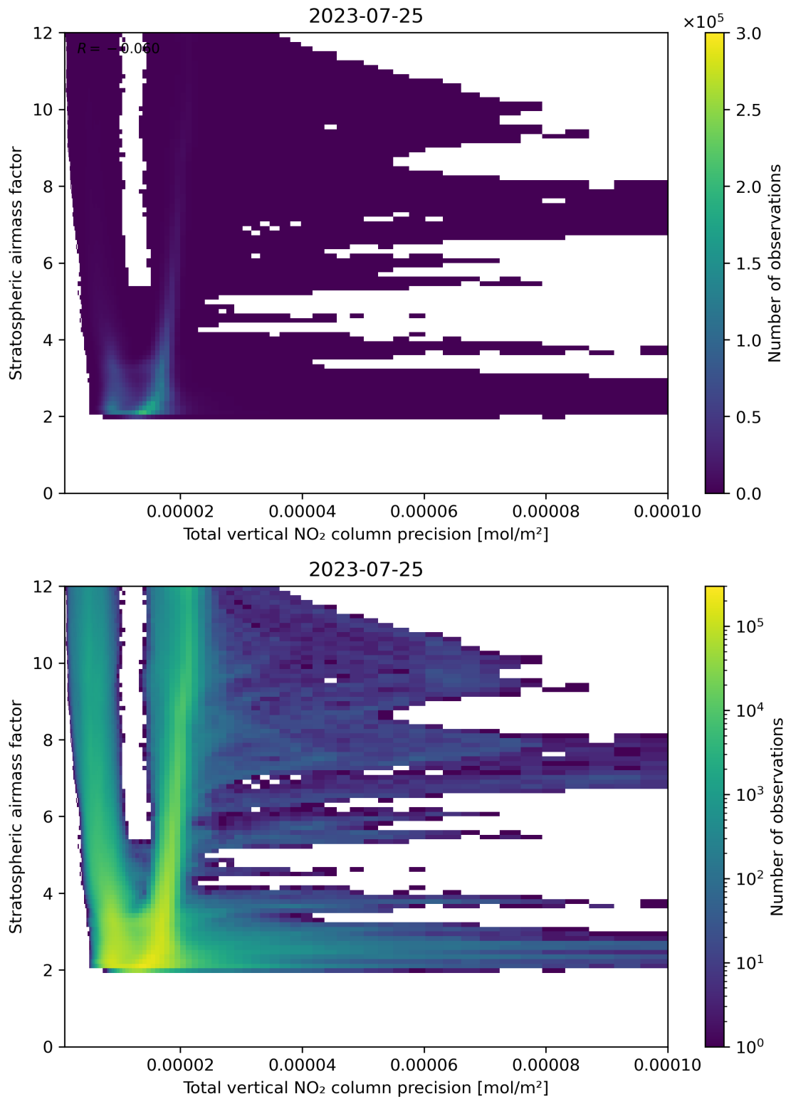
Figure 115: Scatter density plot of “Total vertical NO 2 column precision” against “Stratospheric air mass factor” for 2023-07-24 to 2023-07-26.
