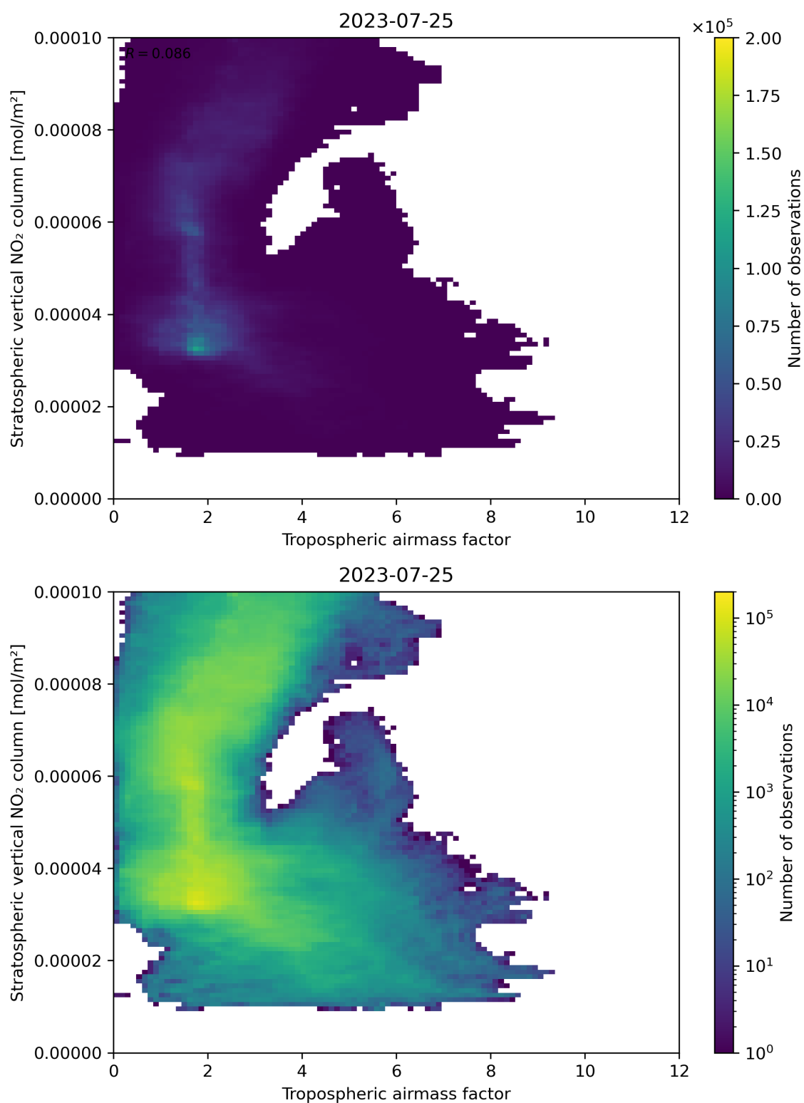
Figure 74: Scatter density plot of “Tropospheric air mass factor” against “Stratospheric vertical NO 2 column” for 2023-07-24 to 2023-07-26.
