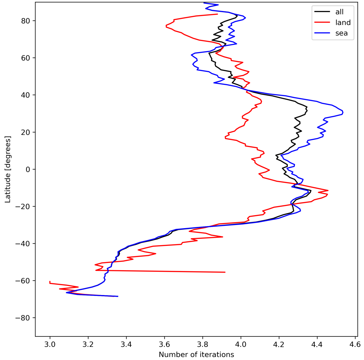
Figure 17: Zonal average of “Number of iterations” for 2023-07-24 to 2023-07-26.
