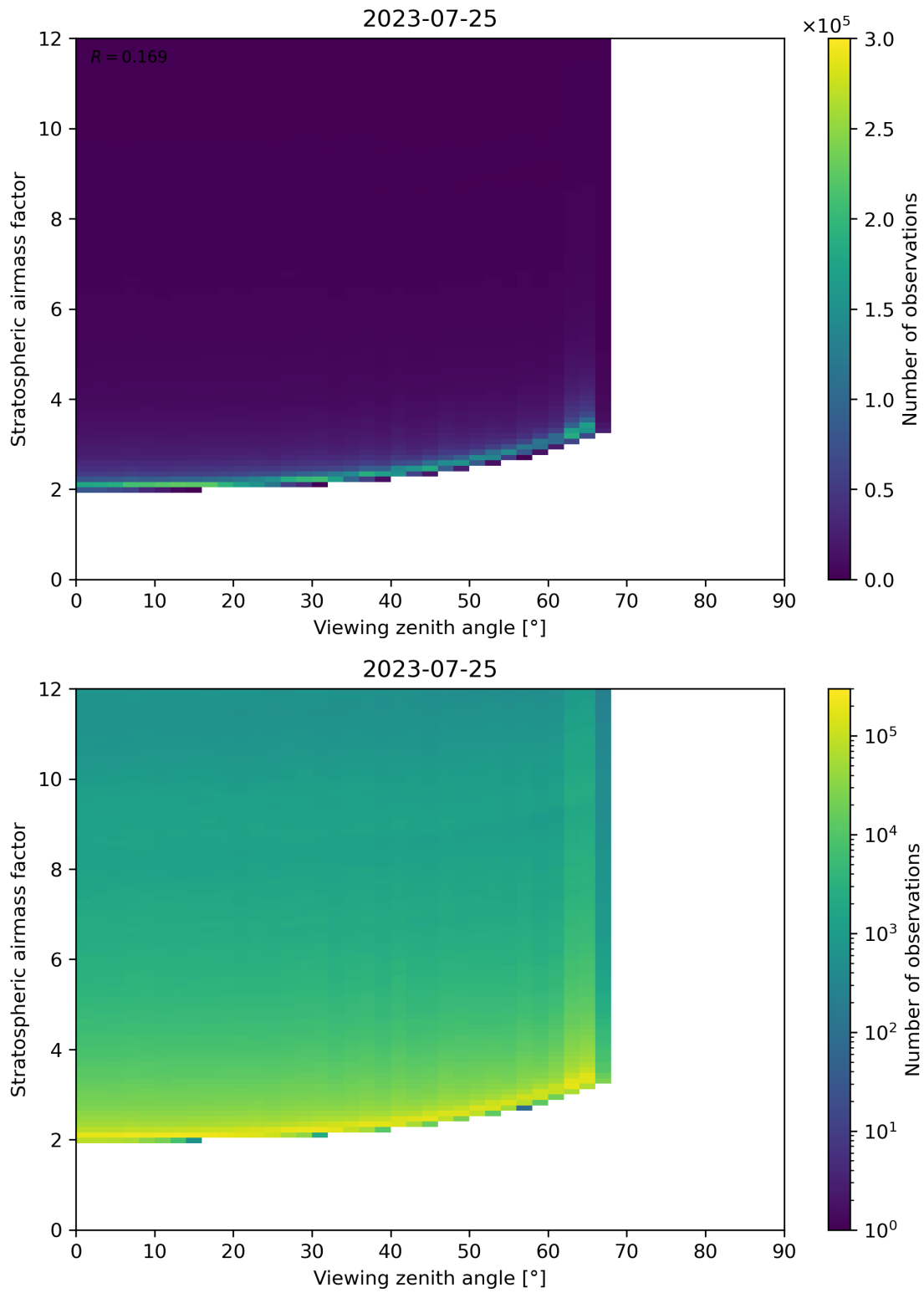
Figure 159: Scatter density plot of “Viewing zenith angle” against “Stratospheric airmass factor” for 2023-07-24 to 2023-07-26.
