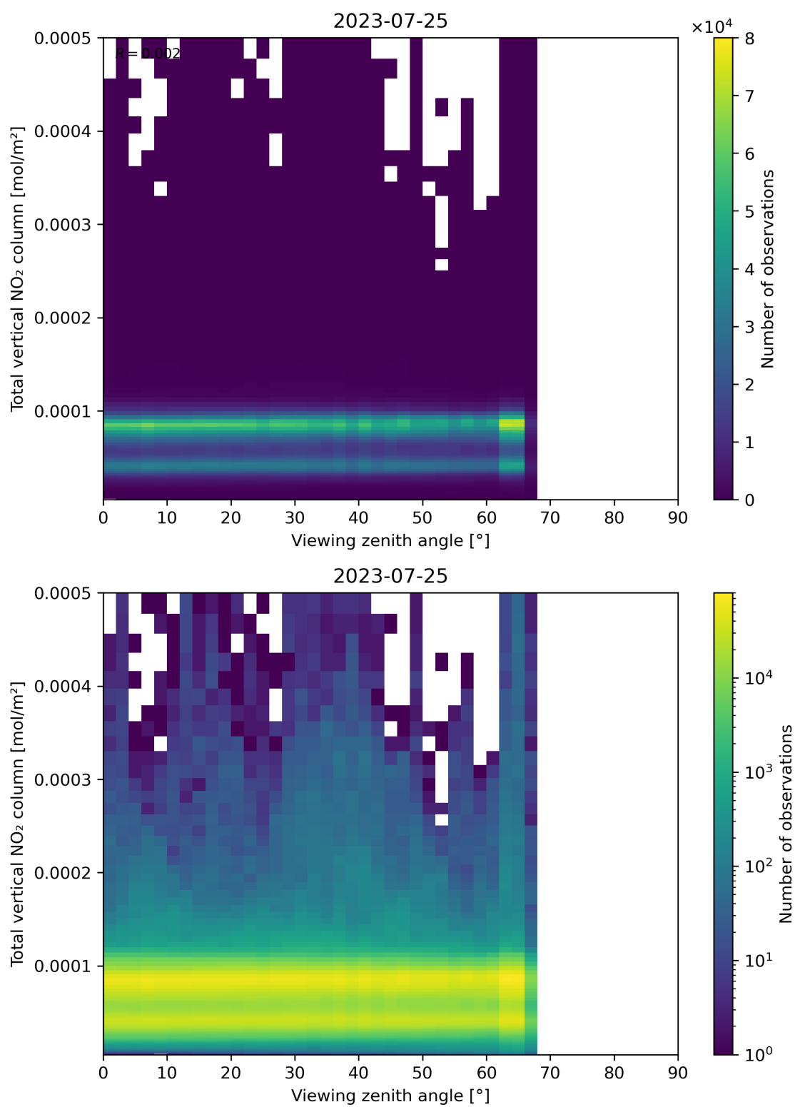
Figure 167: Scatter density plot of “Viewing zenith angle” against “Total vertical NO 2 column” for 2023-07-24 to 2023-07-26.
