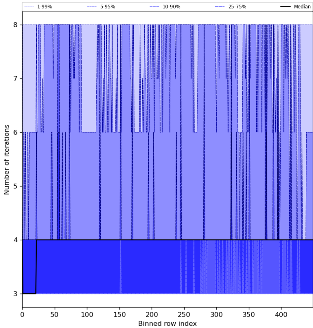
Figure 51: Along track statistics of “Number of iterations” for 2023-07-24 to 2023-07-26
