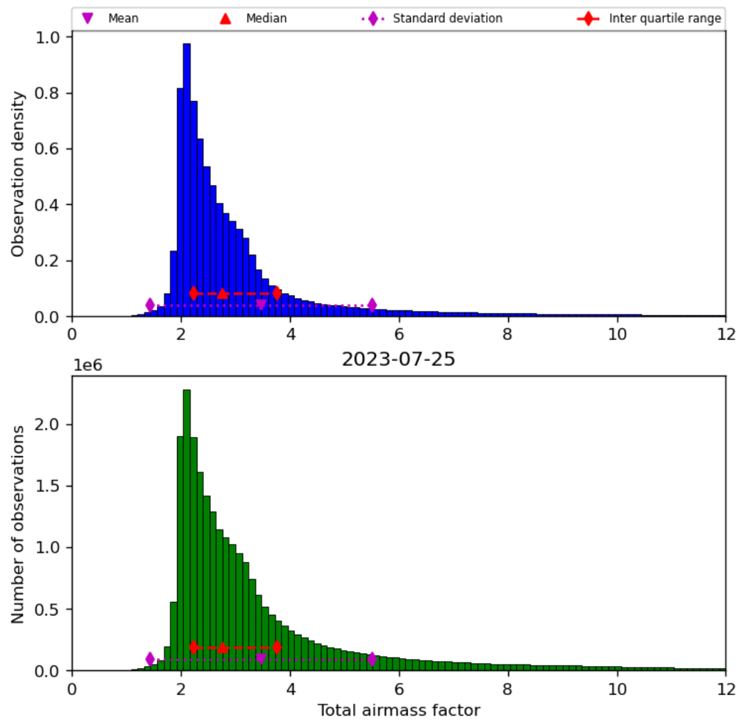
Figure 32: Histogram of “Total airmass factor” for 2023-07-24 to 2023-07-26
