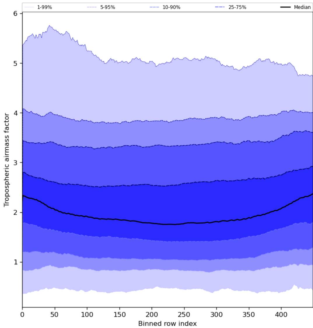
Figure 48: Along track statistics of “Tropospheric airmass factor” for 2023-07-24 to 2023-07-26
