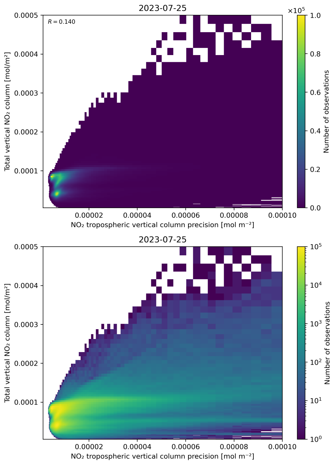
Figure 138: Scatter density plot of “NO 2 tropospheric vertical column precision” against “Total vertical NO 2 column” for 2023-07-24 to 2023-07-26.
