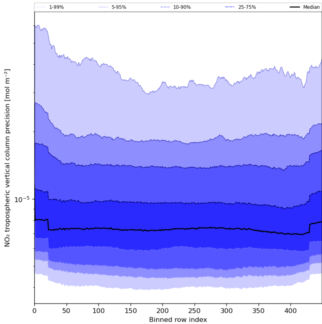
Figure 47: Along track statistics of “NO 2 tropospheric vertical column precision” for 2023-07-24 to 2023-07-26
