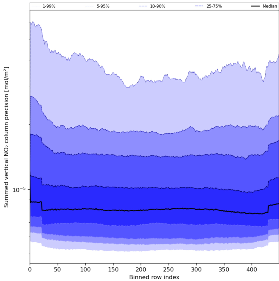
Figure 58: Along track statistics of “Summed vertical NO 2 column precision” for 2023-07-24 to 2023-07-26
