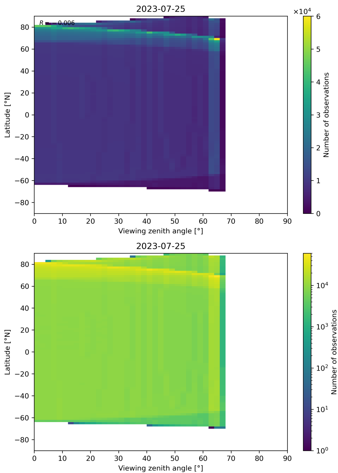
Figure 163: Scatter density plot of “Viewing zenith angle” against “Latitude” for 2023-07-24 to 2023-07-26.
