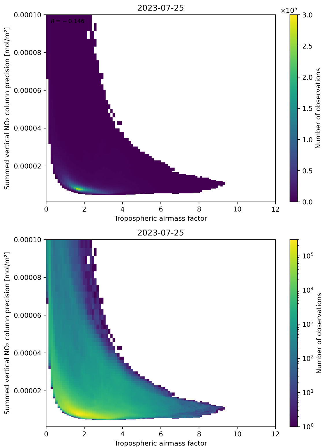
Figure 76: Scatter density plot of “Tropospheric air mass factor” against “Summed vertical NO 2 column precision” for 2023-07-24 to 2023-07-26.
