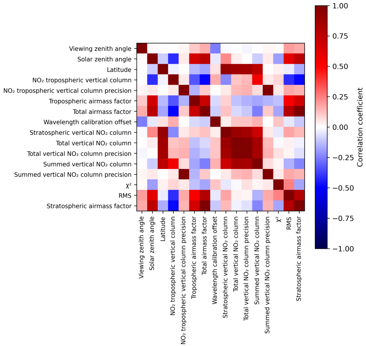
Figure 2: Map of correlation matrix for 2023-07-24 to 2023-07-26.
