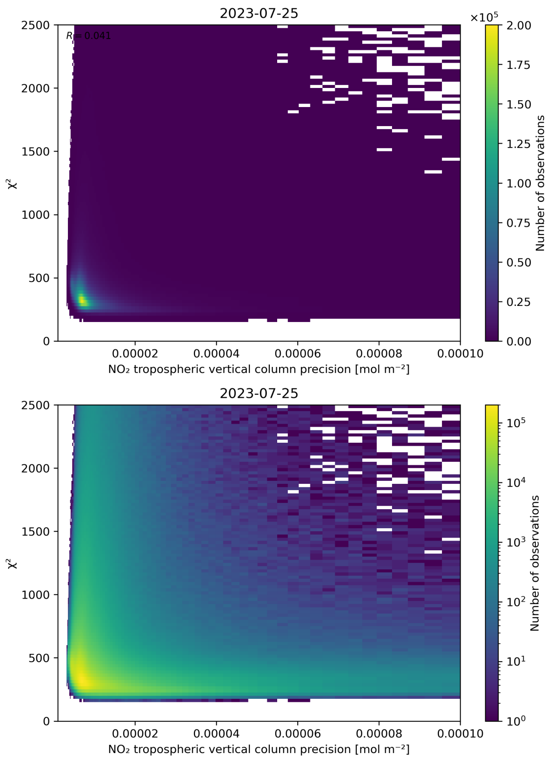
Figure 134: Scatter density plot of “NO 2 tropospheric vertical column precision” against “ \chi^2 ” for 2023-07-24 to 2023-07-26.
