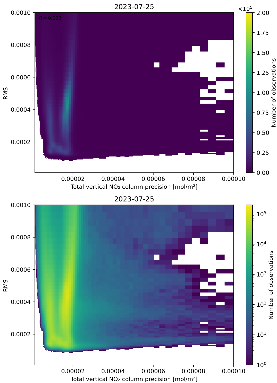
Figure 119: Scatter density plot of “Total vertical NO 2 column precision” against “RMS” for 2023-07-24 to 2023-07-26.
