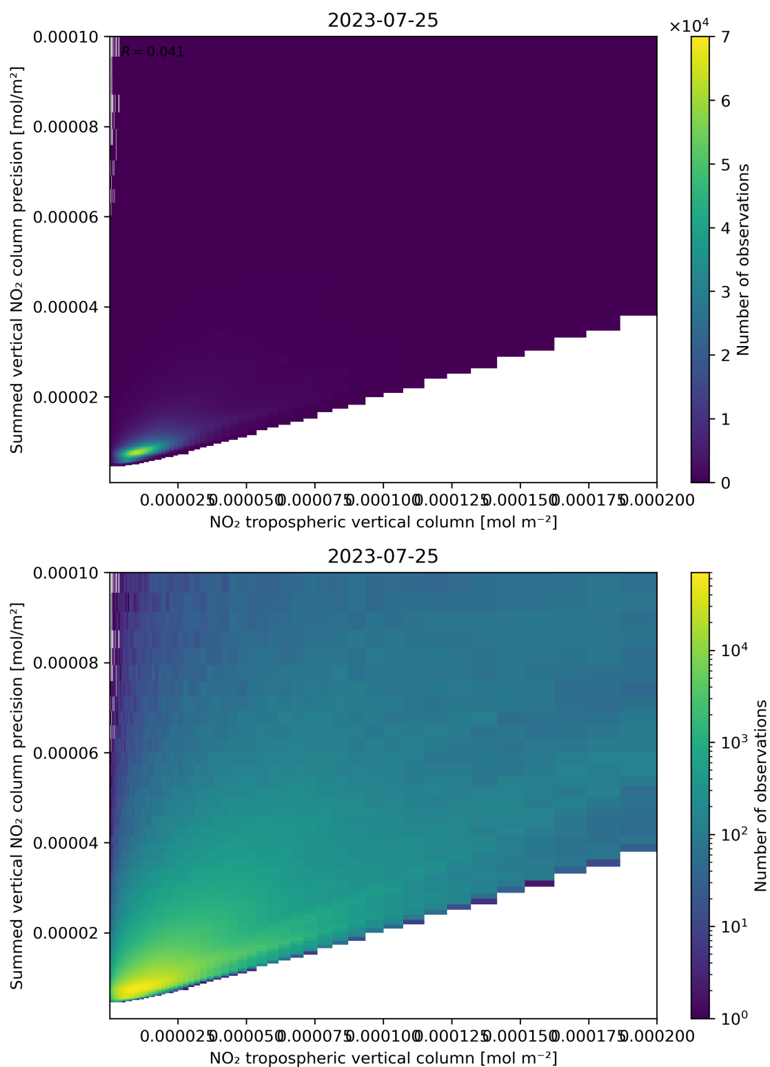
Figure 127: Scatter density plot of “NO 2 tropospheric vertical column” against “Summed vertical NO 2 column precision” for 2023-07-24 to 2023-07-26.
