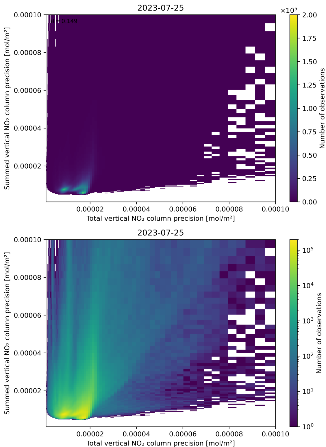
Figure 118: Scatter density plot of “Total vertical NO 2 column precision” against “Summed vertical NO 2 column precision” for 2023-07-24 to 2023-07-26.
