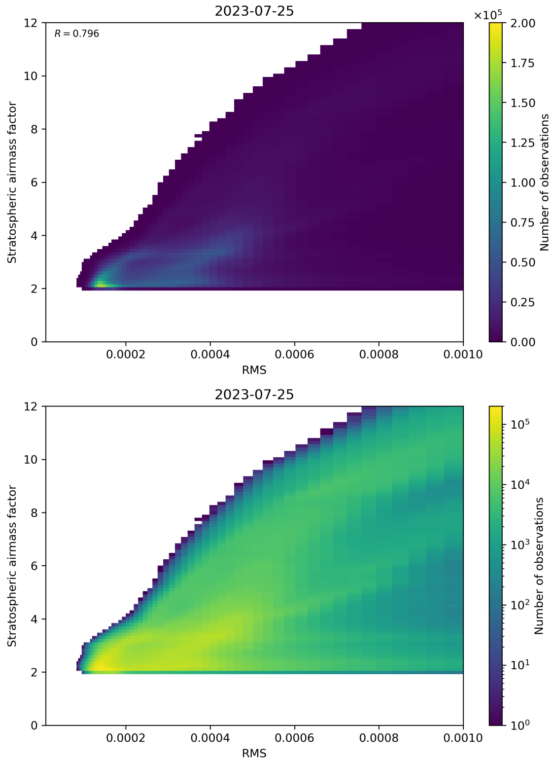
Figure 144: Scatter density plot of “RMS” against “Stratospheric airmass factor” for 2023-07-24 to 2023-07-26.
