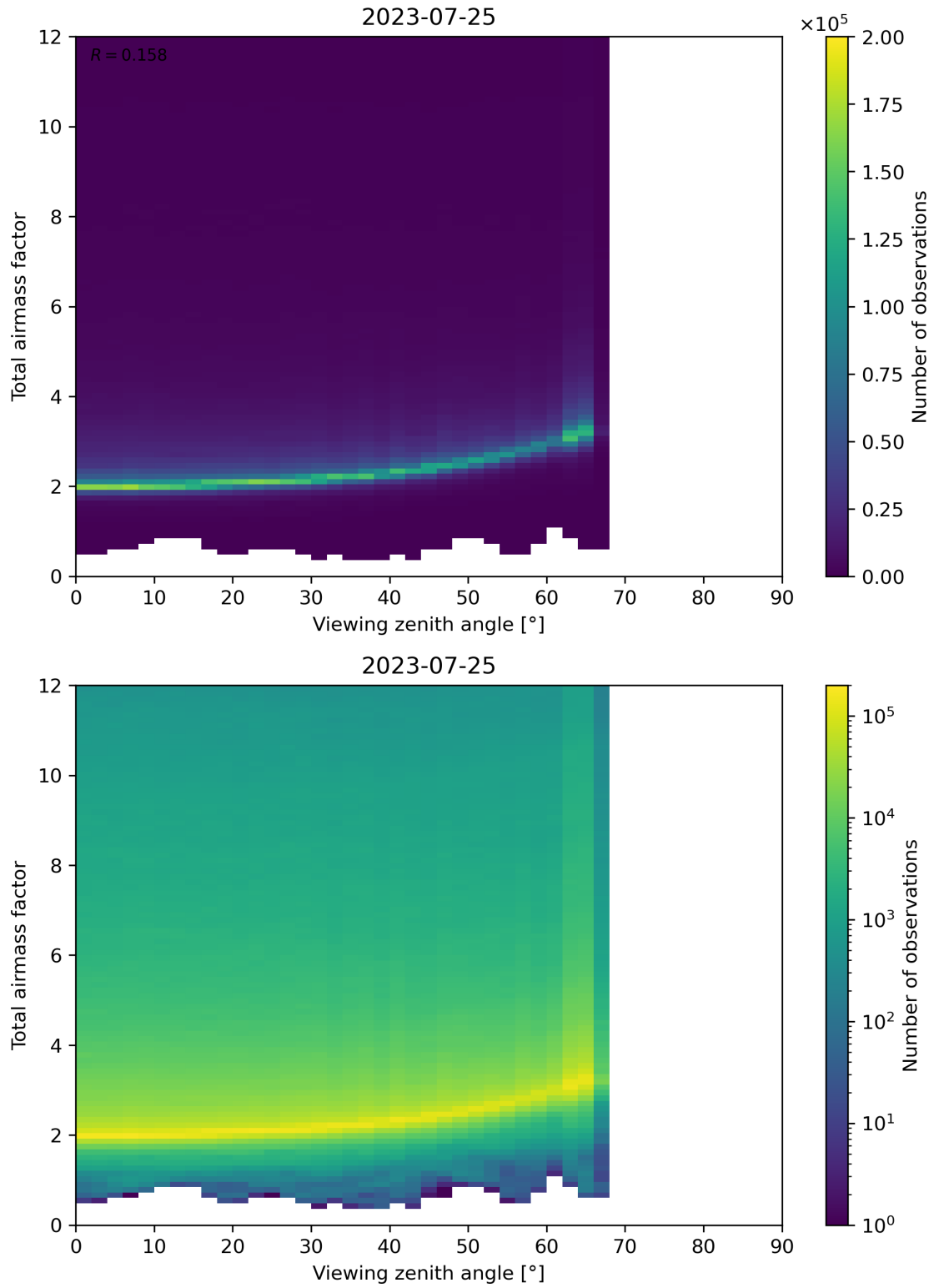
Figure 160: Scatter density plot of “Viewing zenith angle” against “Total airmass factor” for 2023-07-24 to 2023-07-26.
