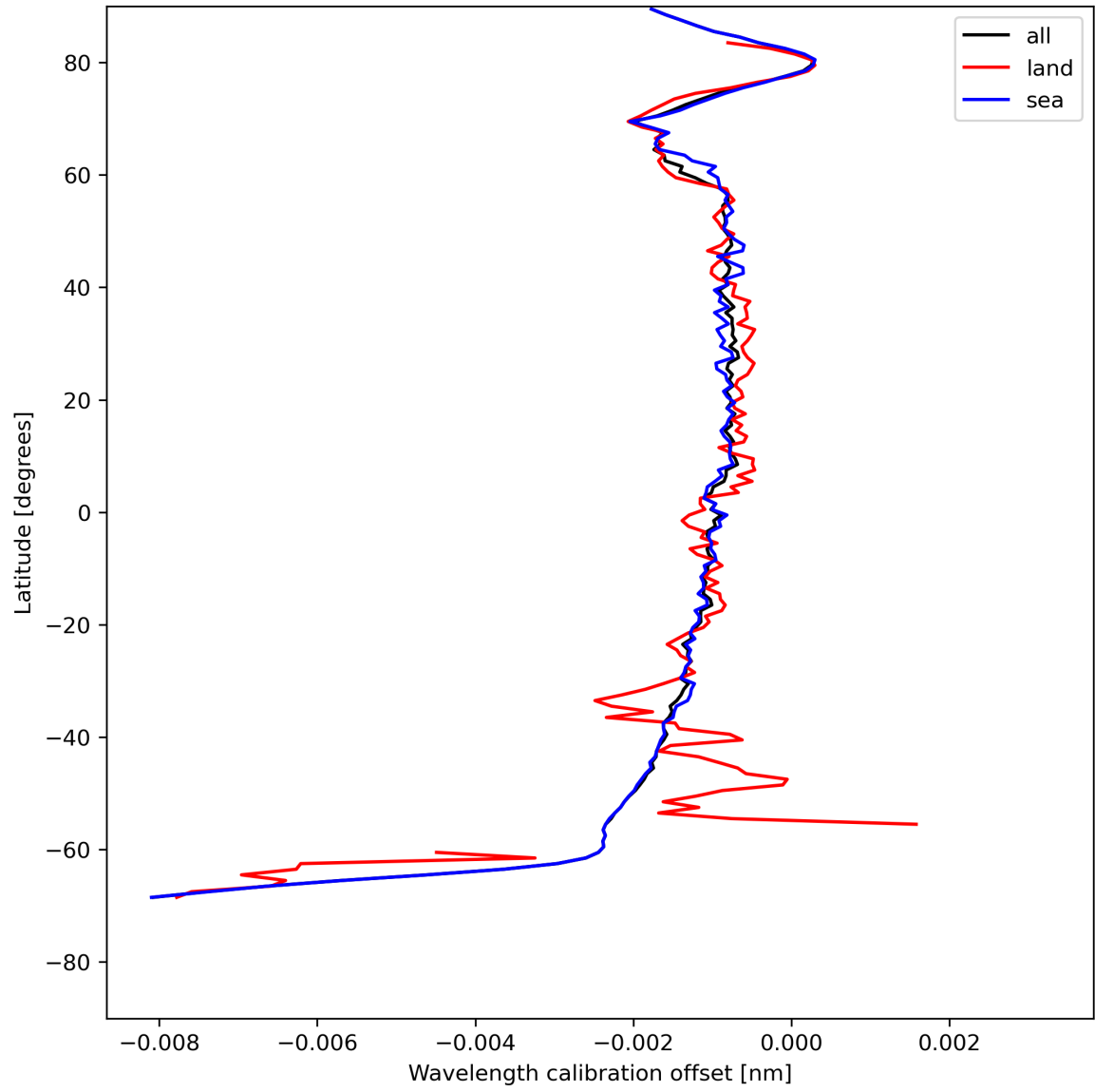
Figure 18: Zonal average of “Wavelength calibration offset” for 2023-07-24 to 2023-07-26.
