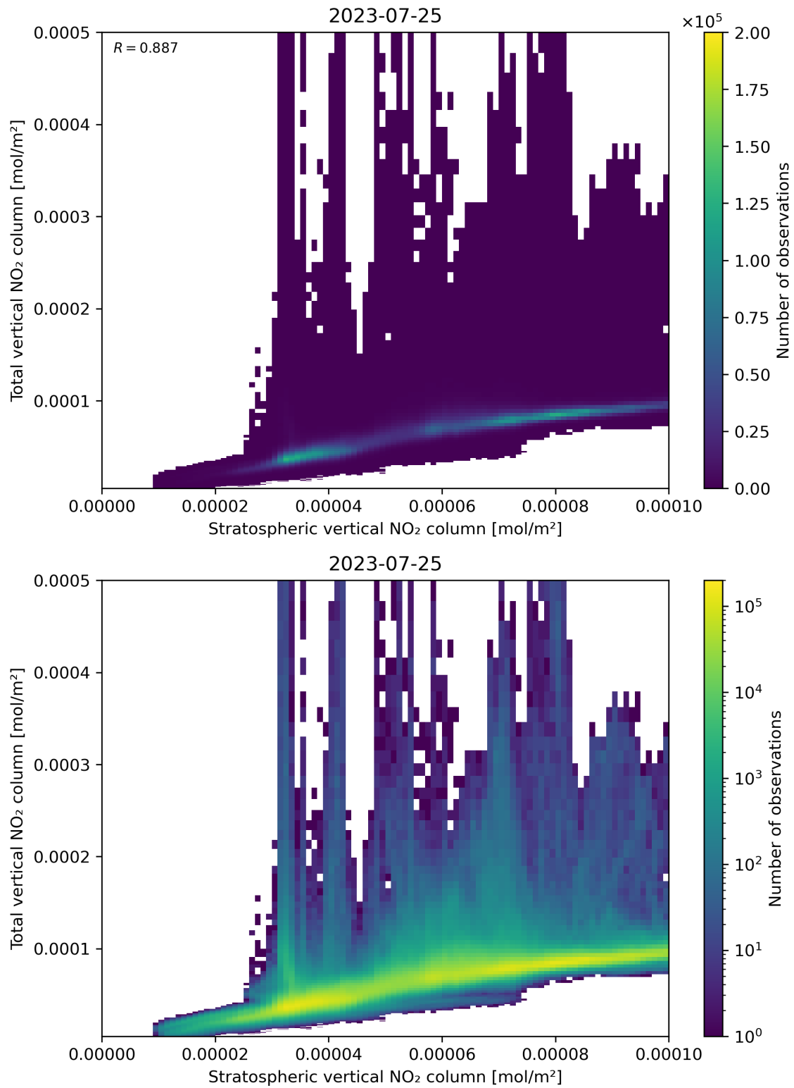
Figure 100: Scatter density plot of “Stratospheric vertical NO 2 column” against “Total vertical NO 2 column” for 2023-07-24 to 2023-07-26.
