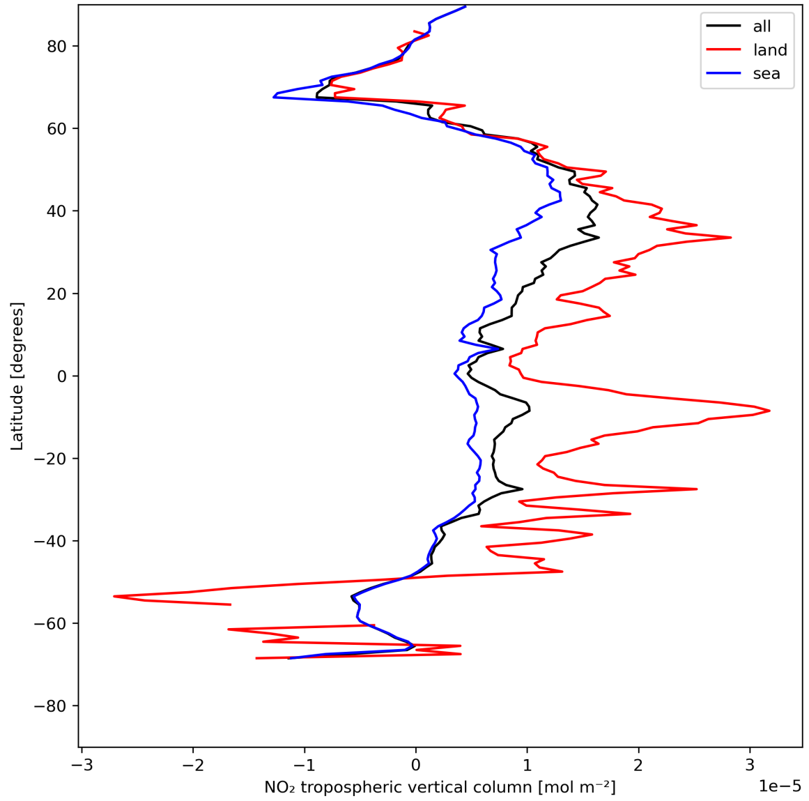
Figure 12: Zonal average of “NO 2 tropospheric vertical column” for 2023-07-24 to 2023-07-26.
