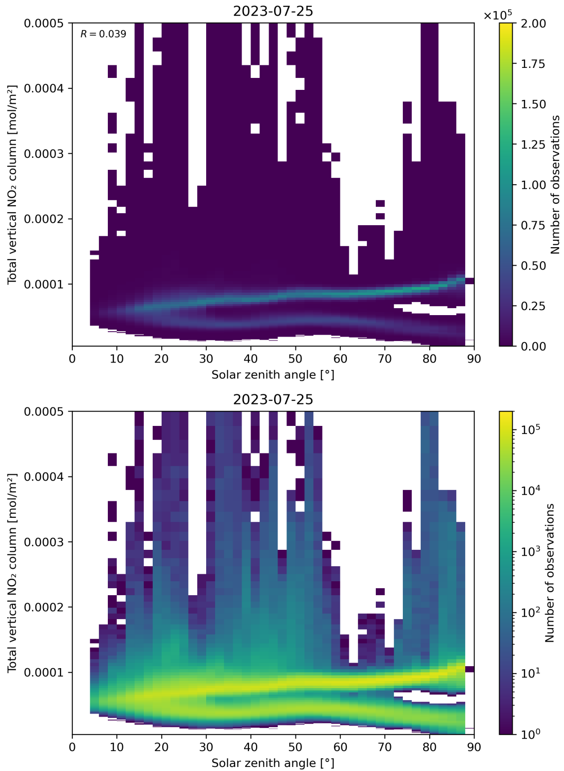
Figure 153: Scatter density plot of “Solar zenith angle” against “Total vertical NO 2 column” for 2023-07-24 to 2023-07-26.
