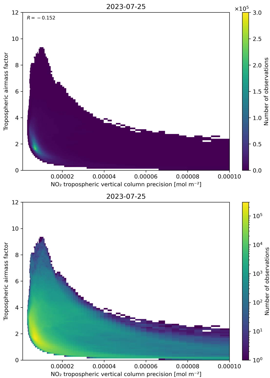
Figure 133: Scatter density plot of “NO 2 tropospheric vertical column precision” against “Tropospheric airmass factor” for 2023-07-24 to 2023-07-26.
