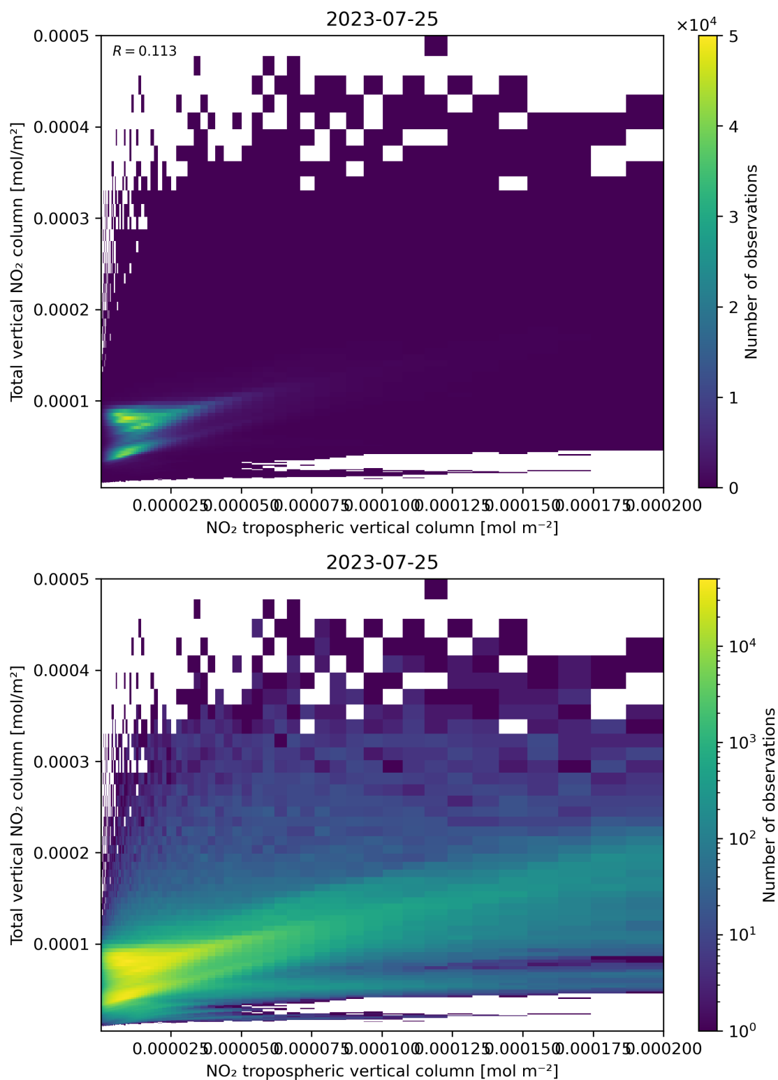
Figure 128: Scatter density plot of “NO 2 tropospheric vertical column” against “Total vertical NO 2 column” for 2023-07-24 to 2023-07-26.
