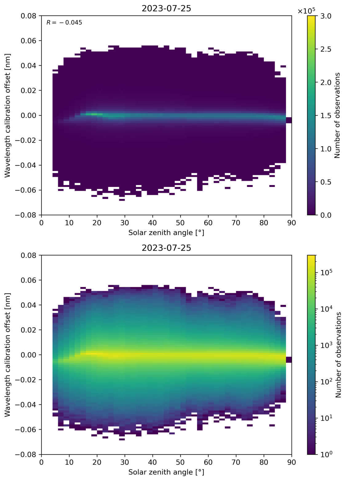
Figure 158: Scatter density plot of “Solar zenith angle” against “Wavelength calibration offset” for 2023-07-24 to 2023-07-26.
