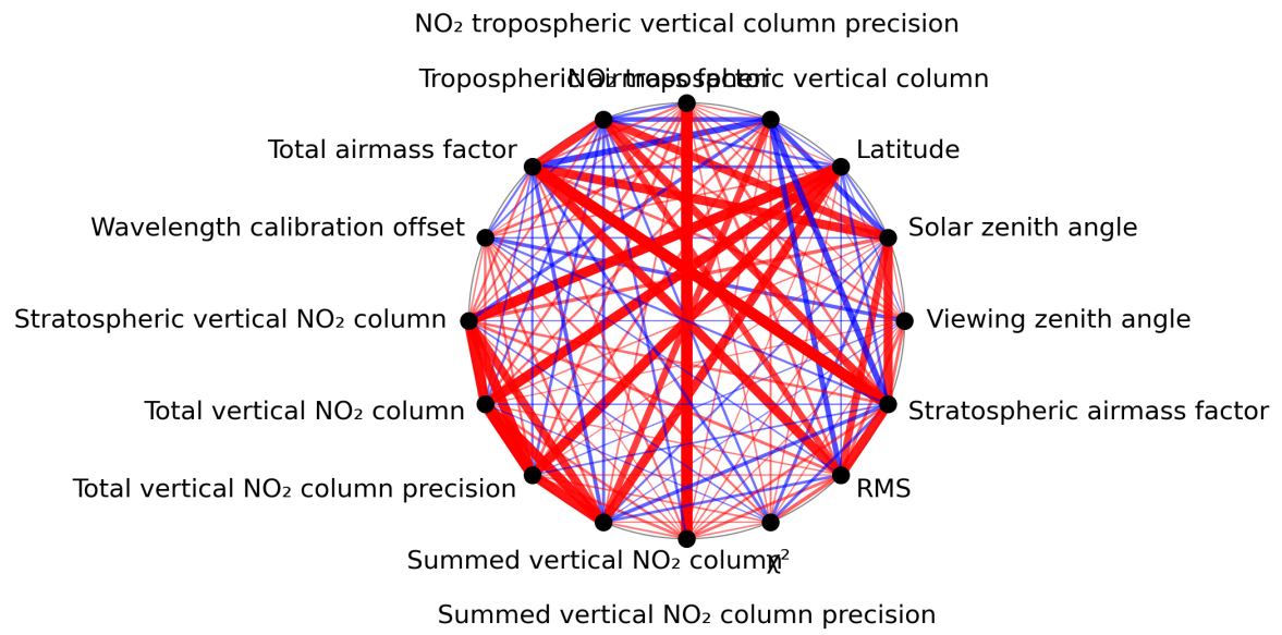
Figure 1: Map of correlation graph for 2023-07-24 to 2023-07-26.
