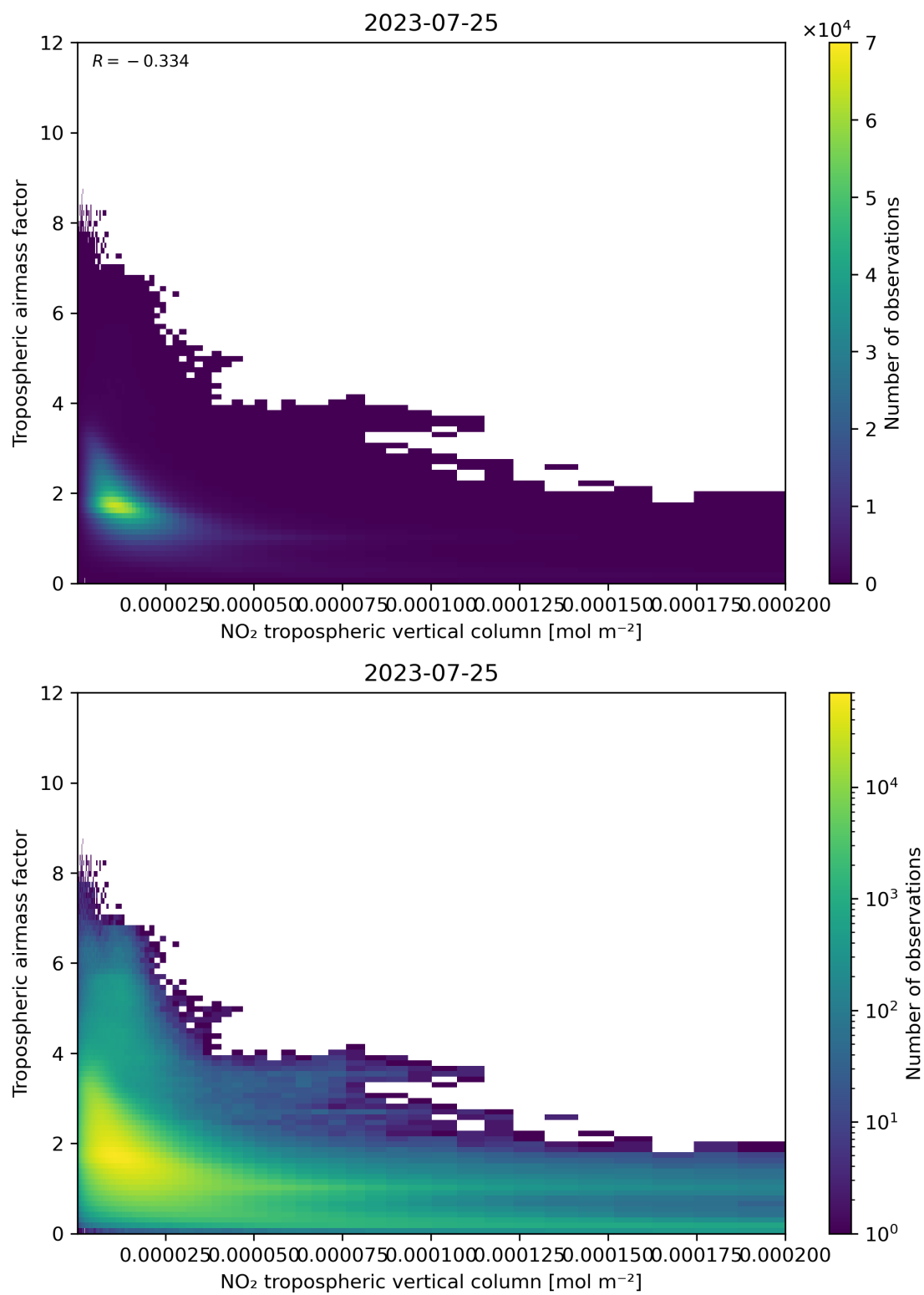
Figure 123: Scatter density plot of “NO 2 tropospheric vertical column” against “Tropospheric air mass factor” for 2023-07-24 to 2023-07-26.
