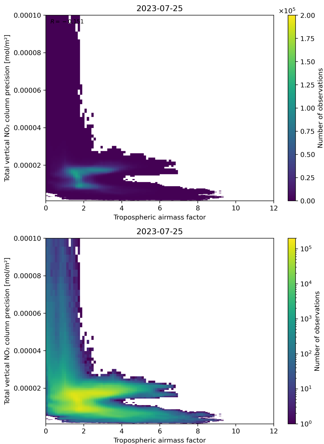
Figure 78: Scatter density plot of “Tropospheric air mass factor” against “Total vertical NO 2 column precision” for 2023-07-24 to 2023-07-26.
