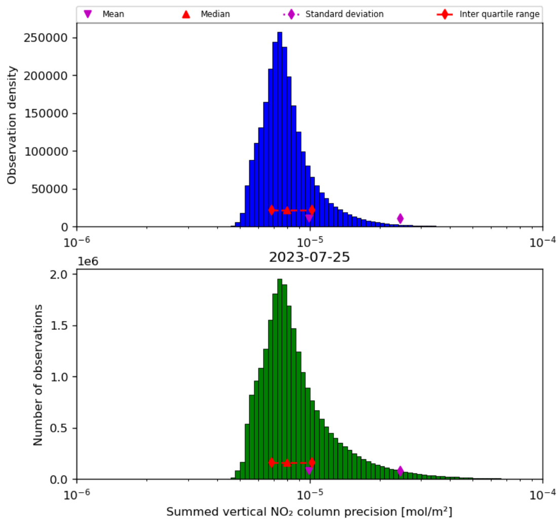
Figure 41: Histogram of "Summed vertical NO 2 column precision" for 2023-07-24 to 2023-07-26
