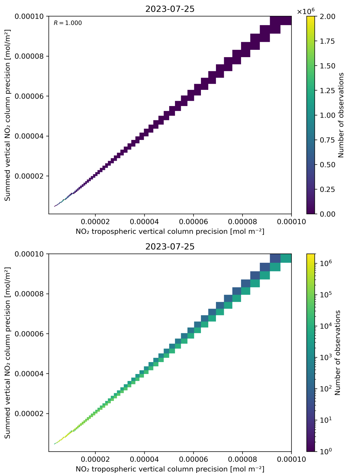
Figure 137: Scatter density plot of “NO 2 tropospheric vertical column precision” against “Summed vertical NO 2 column precision” for 2023-07-24 to 2023-07-26.
