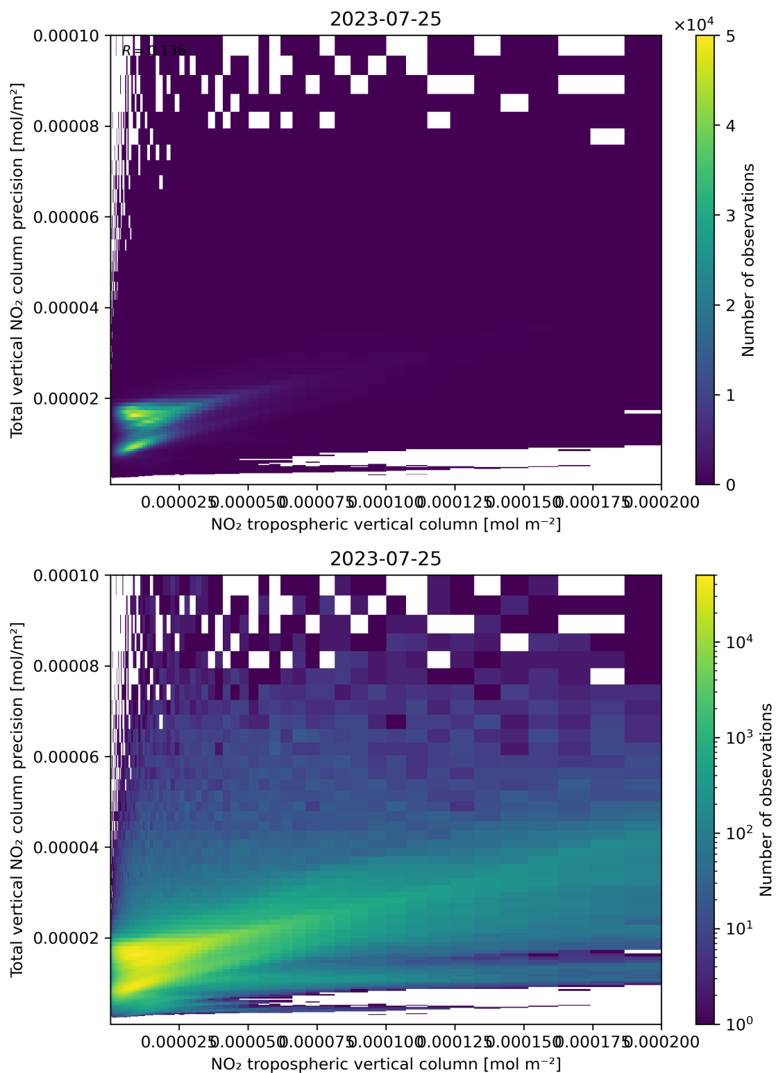
Figure 129: Scatter density plot of “NO 2 tropospheric vertical column” against “Total vertical NO 2 column precision” for 2023-07-24 to 2023-07-26.
