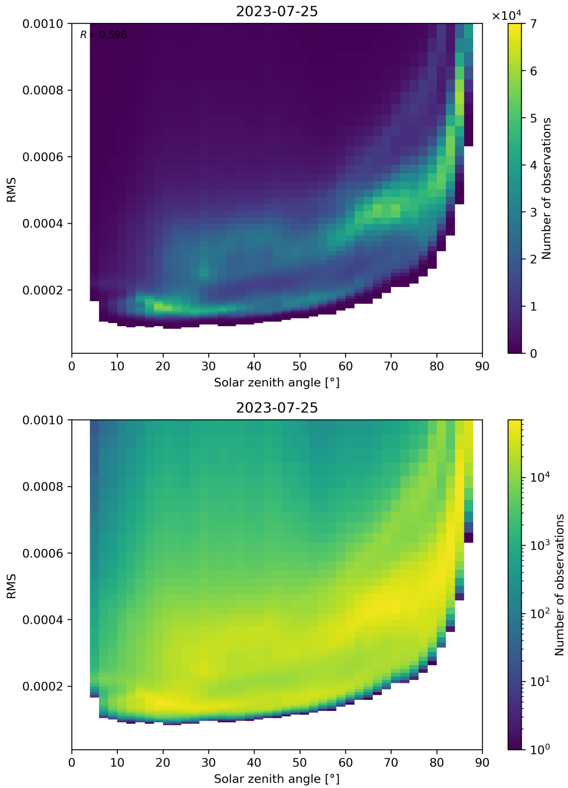
Figure 157: Scatter density plot of “Solar zenith angle” against “RMS” for 2023-07-24 to 2023-07-26.
