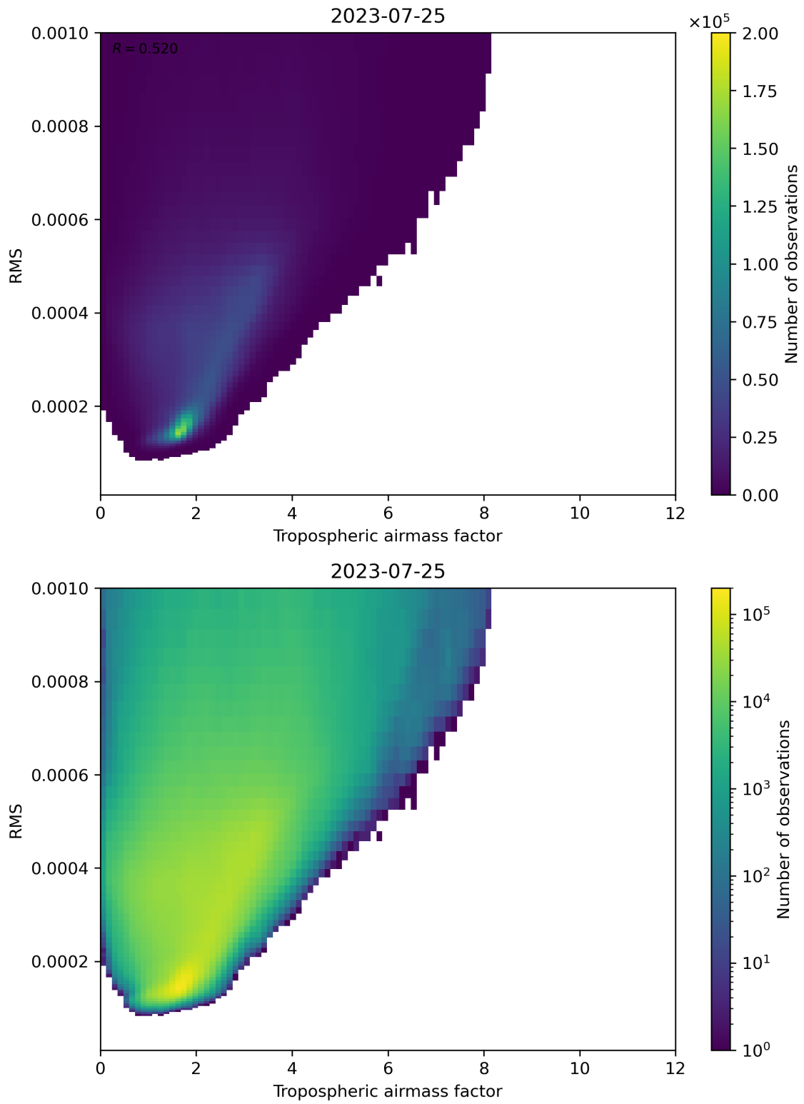
Figure 79: Scatter density plot of “Tropospheric airmass factor” against “RMS” for 2023-07-24 to 2023-07-26.
