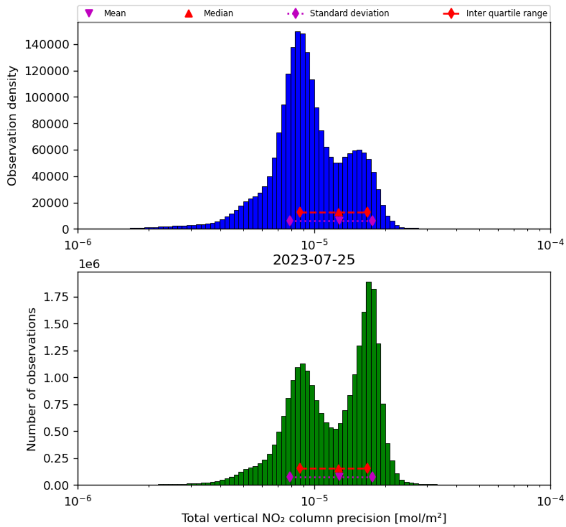
Figure 39: Histogram of "Total vertical NO 2 column precision" for 2023-07-24 to 2023-07-26
