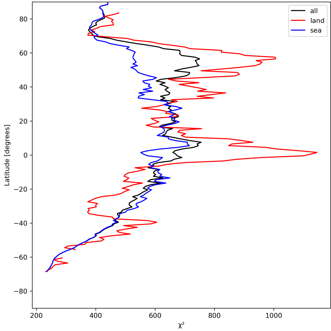
Figure 25: Zonal average of “ \chi^2 ” for 2023-07-24 to 2023-07-26.
