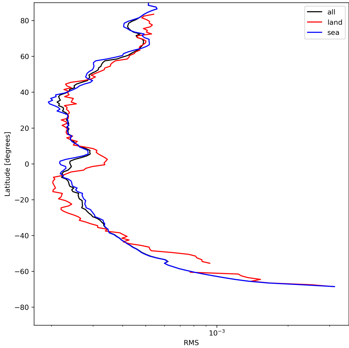
Figure 26: Zonal average of “RMS” for 2023-07-24 to 2023-07-26.
