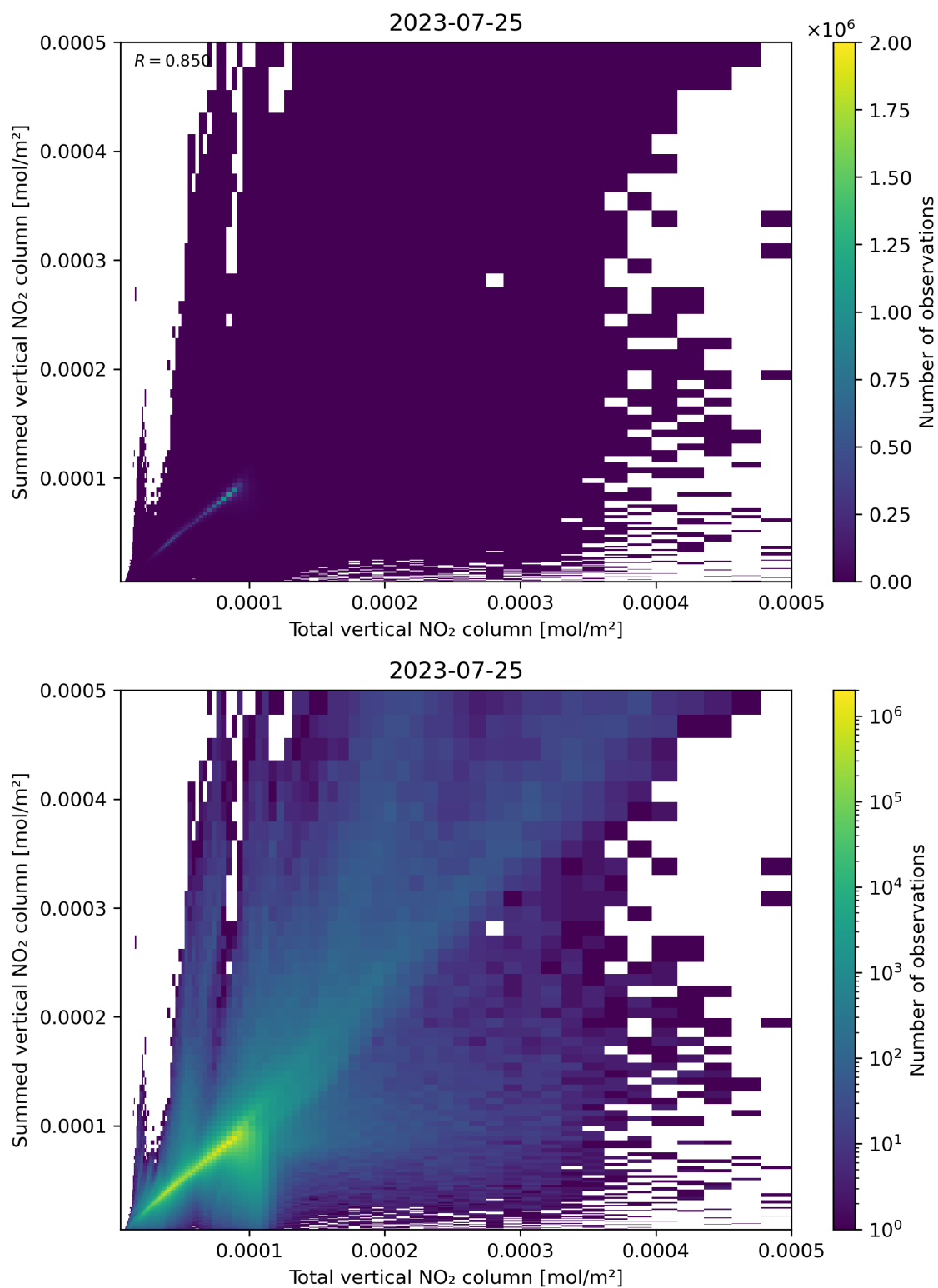
Figure 112: Scatter density plot of “Total vertical NO 2 column” against “Summed vertical NO 2 column” for 2023-07-24 to 2023-07-26.
