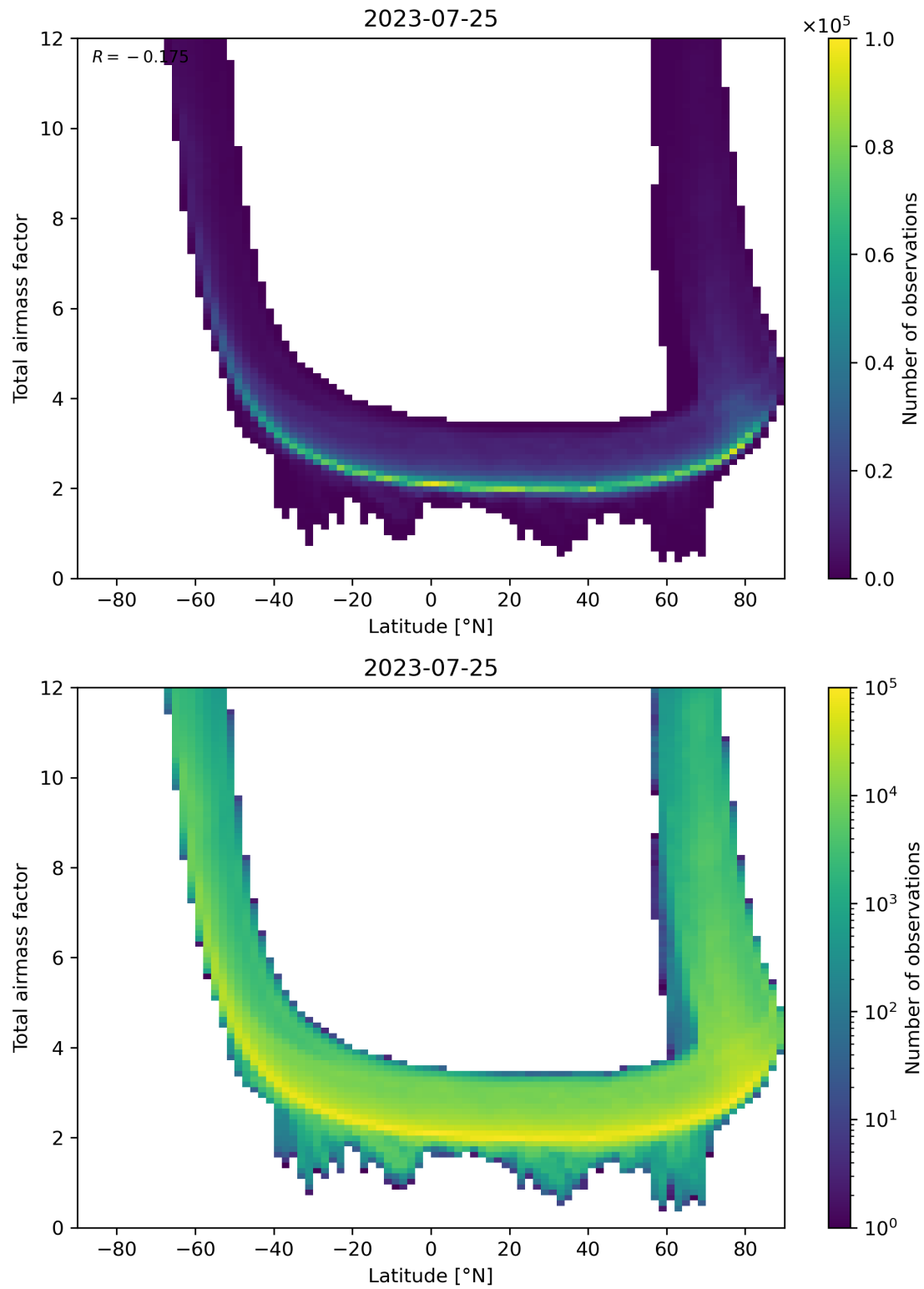
Figure 84: Scatter density plot of “Latitude” against “Total airmass factor” for 2023-07-24 to 2023-07-26.
