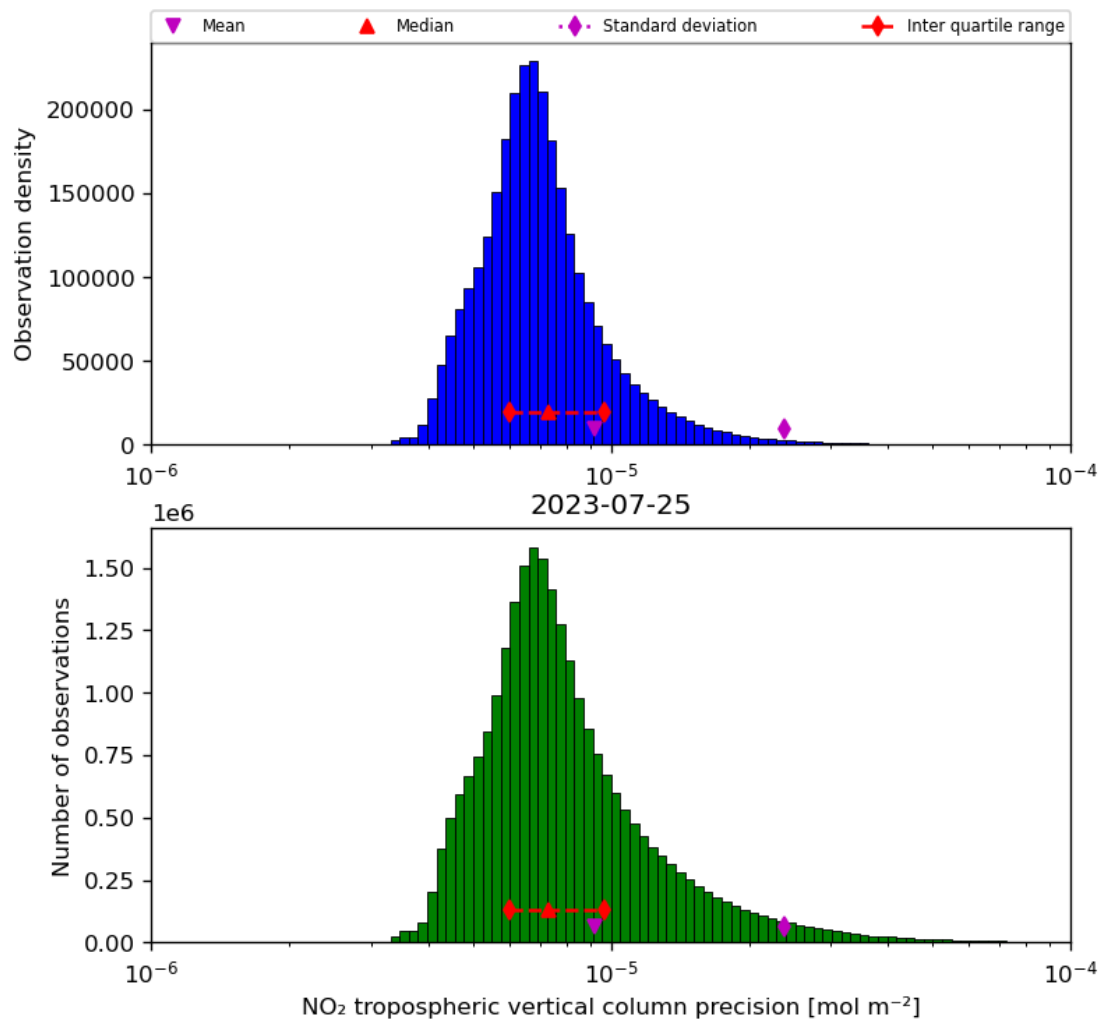
Figure 30: Histogram of “NO 2 tropospheric vertical column precision” for 2023-07-24 to 2023-07-26
