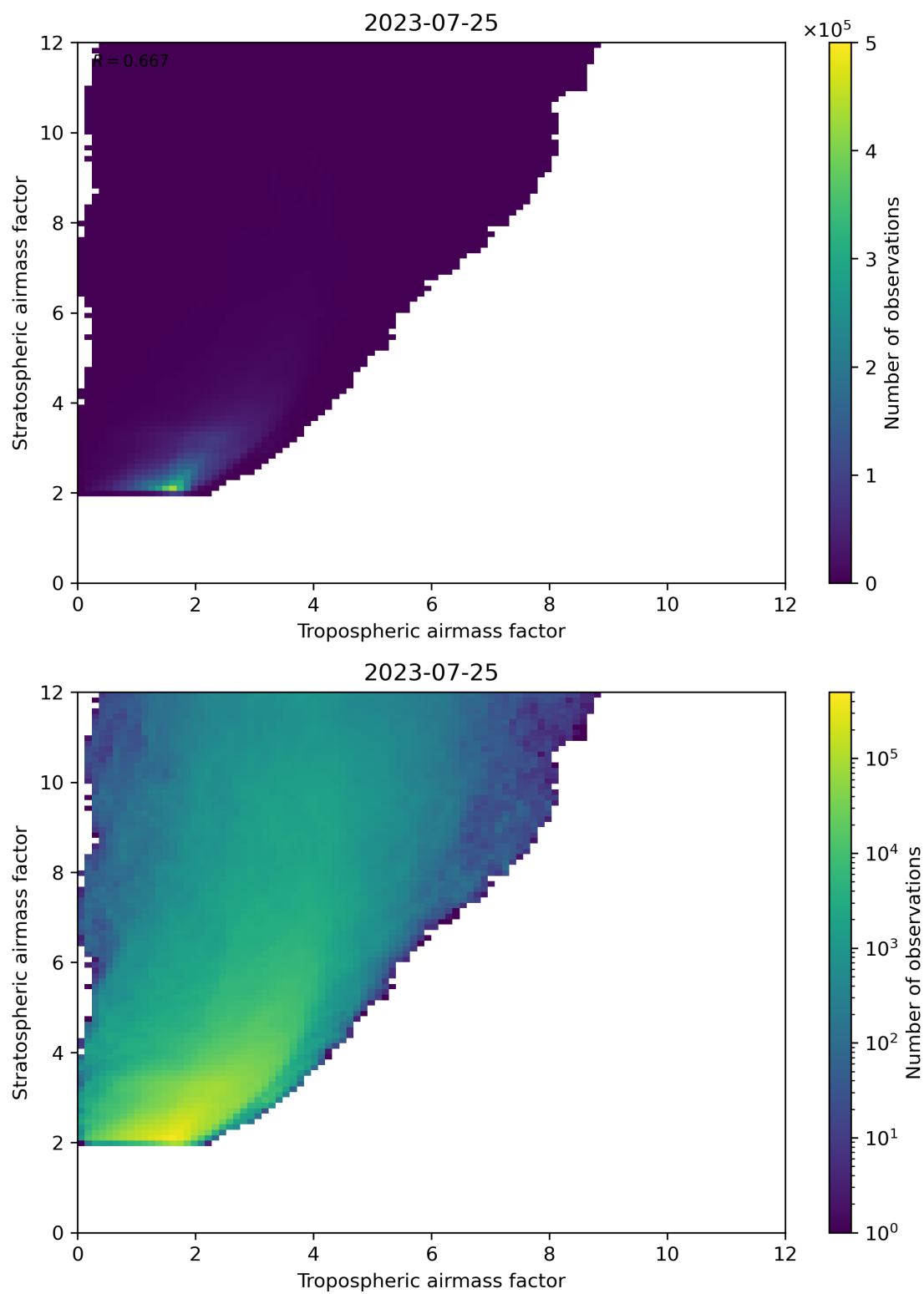
Figure 71: Scatter density plot of “Tropospheric airmass factor” against “Stratospheric airmass factor” for 2023-07-24 to 2023-07-26.
