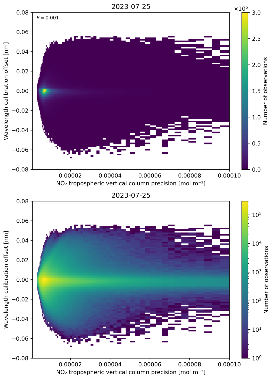
Figure 141: Scatter density plot of “NO 2 tropospheric vertical column precision” against “Wavelength calibration offset” for 2023-07-24 to 2023-07-26.
