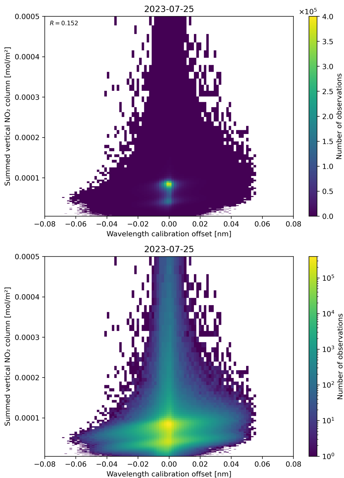
Figure 177: Scatter density plot of “Wavelength calibration offset” against “Summed vertical NO 2 column” for 2023-07-24 to 2023-07-26.
