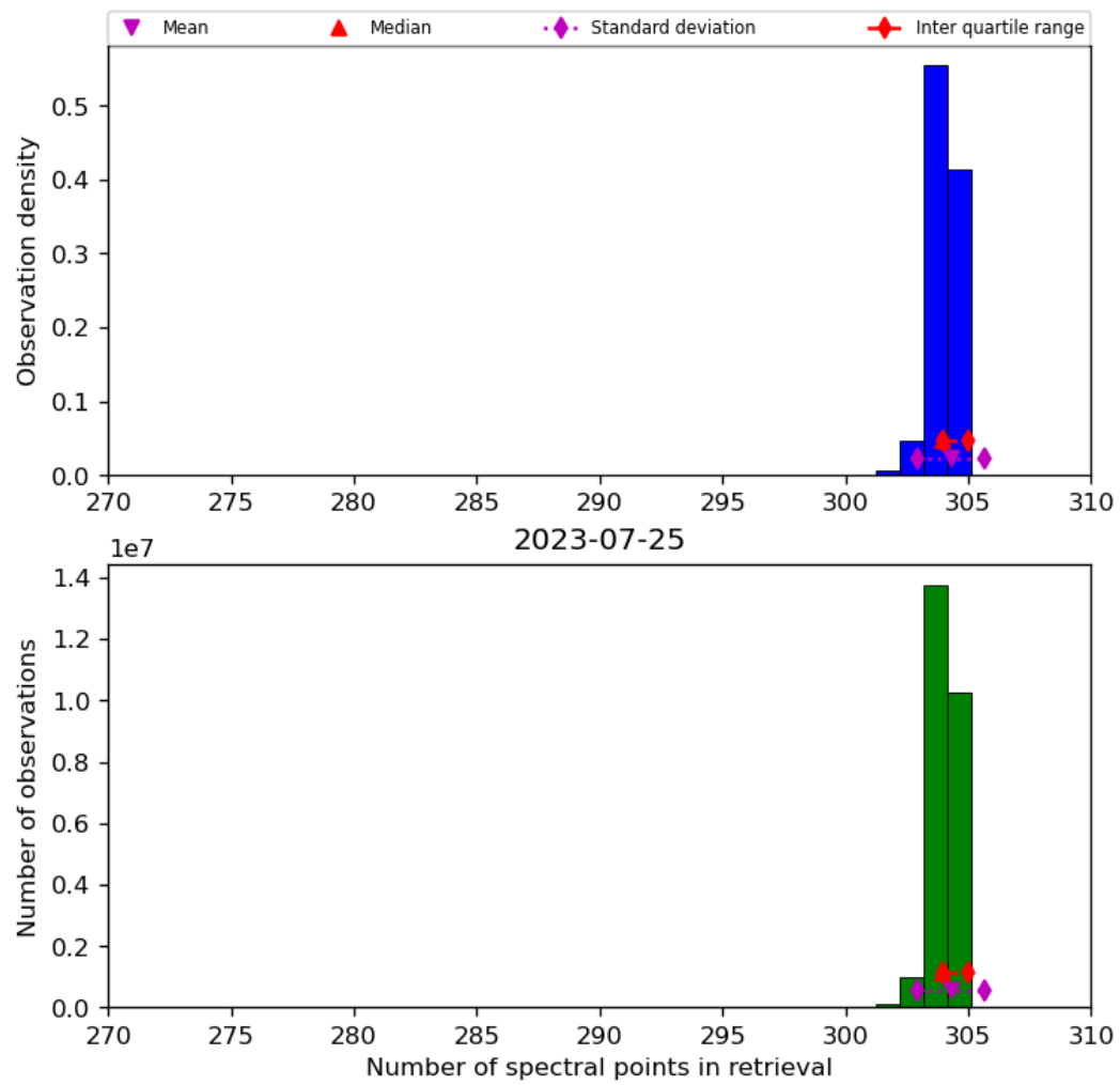
Figure 33: Histogram of “Number of spectral points in retrieval” for 2023-07-24 to 2023-07-26
