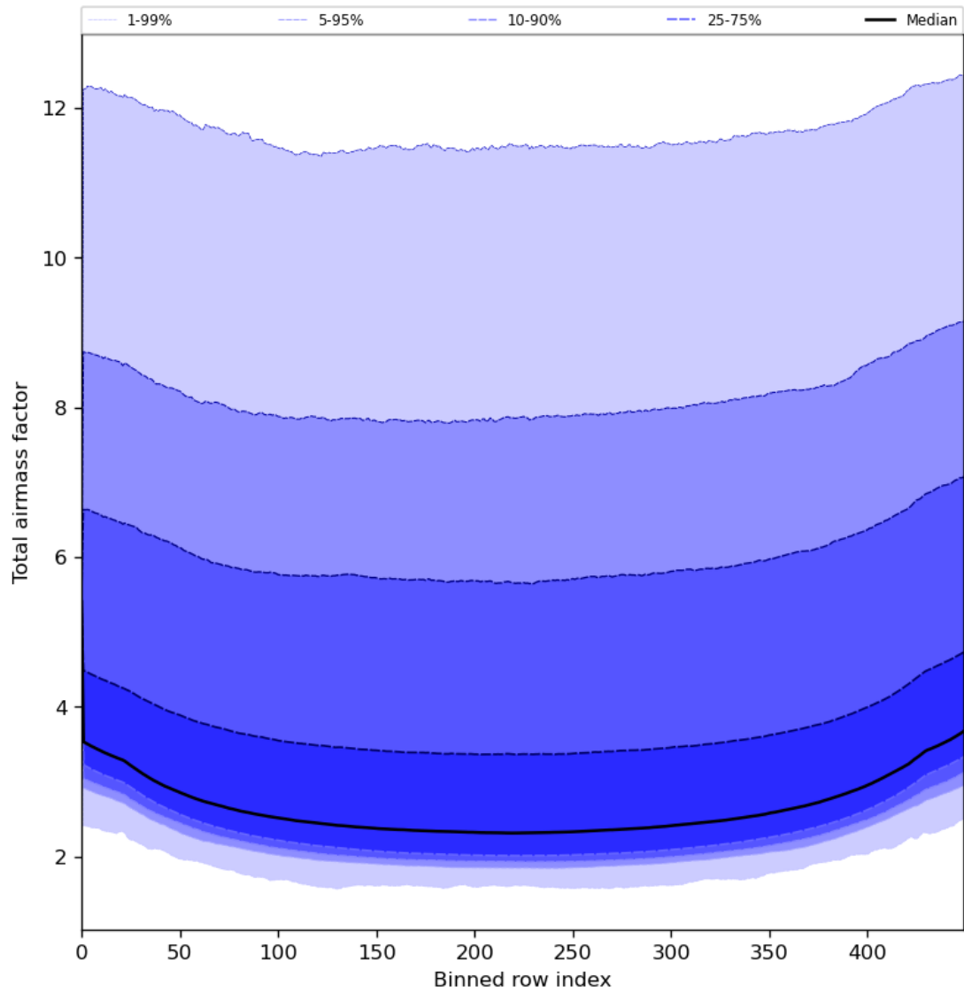
Figure 49: Along track statistics of “Total airmass factor” for 2023-07-24 to 2023-07-26
