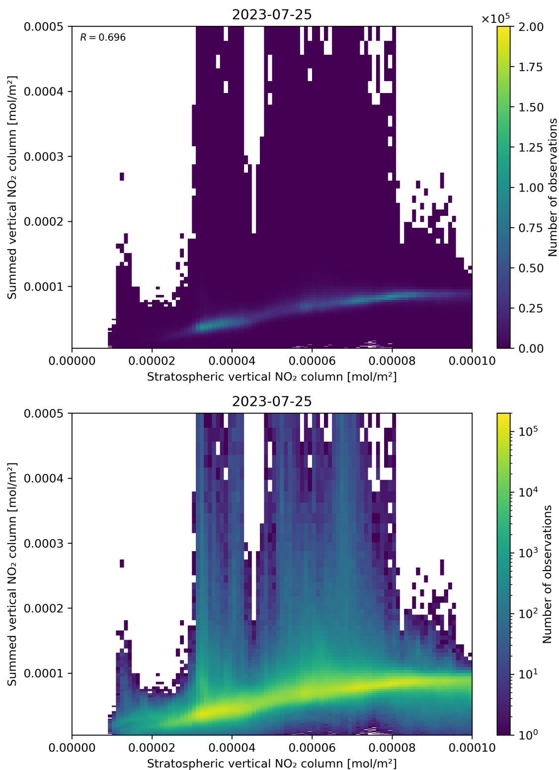
Figure 98: Scatter density plot of “Stratospheric vertical NO 2 column” against “Summed vertical NO 2 column” for 2023-07-24 to 2023-07-26.
