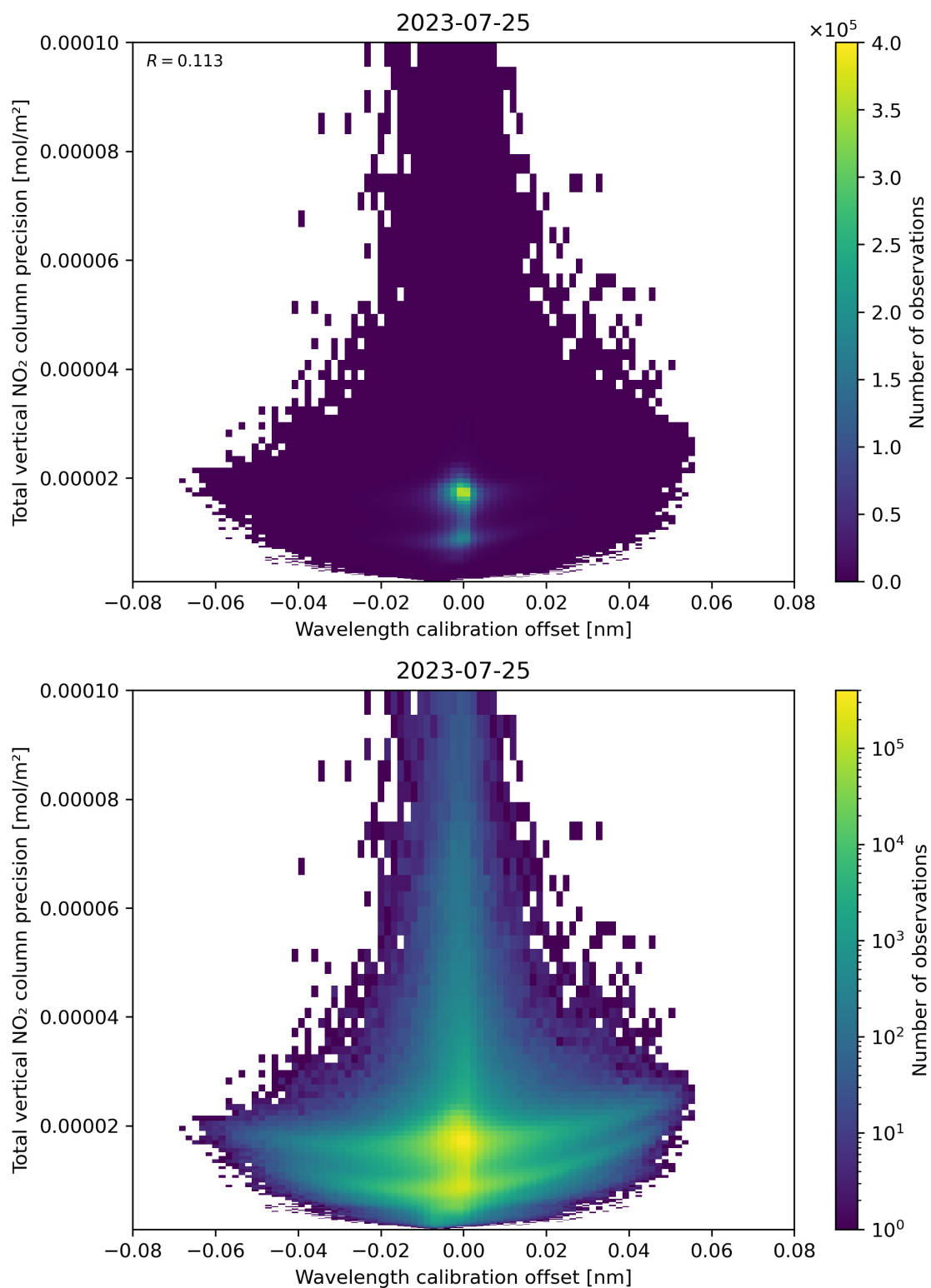
Figure 180: Scatter density plot of “Wavelength calibration offset” against “Total vertical NO 2 column precision” for 2023-07-24 to 2023-07-26.
