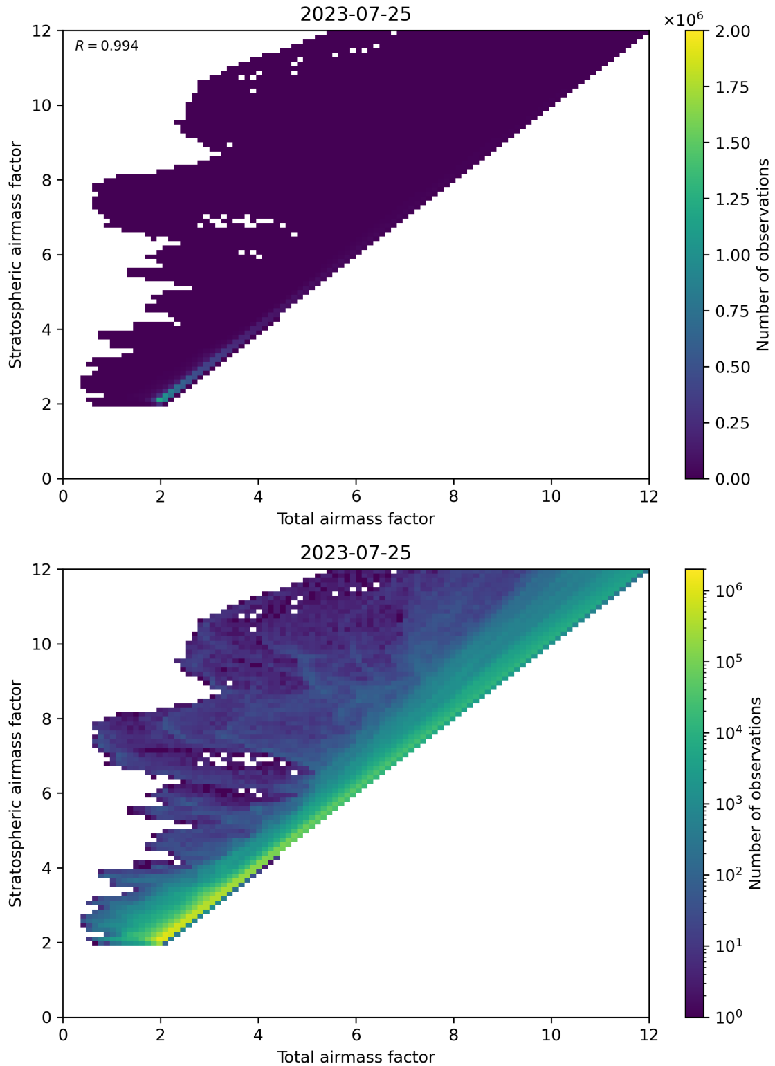
Figure 62: Scatter density plot of “Total airmass factor” against “Stratospheric airmass factor” for 2023-07-24 to 2023-07-26.
