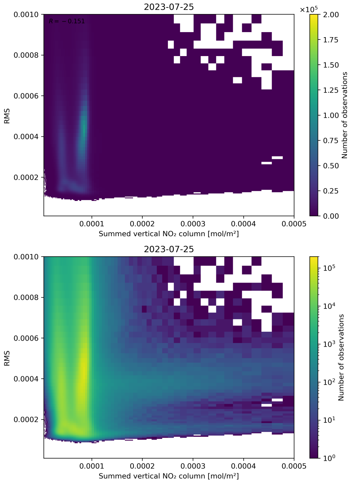
Figure 109: Scatter density plot of “Summed vertical NO 2 column” against “RMS” for 2023-07-24 to 2023-07-26.
