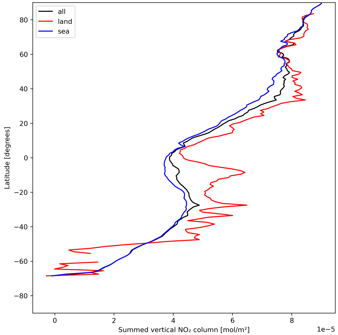
Figure 23: Zonal average of “Summed vertical NO 2 column” for 2023-07-24 to 2023-07-26.
