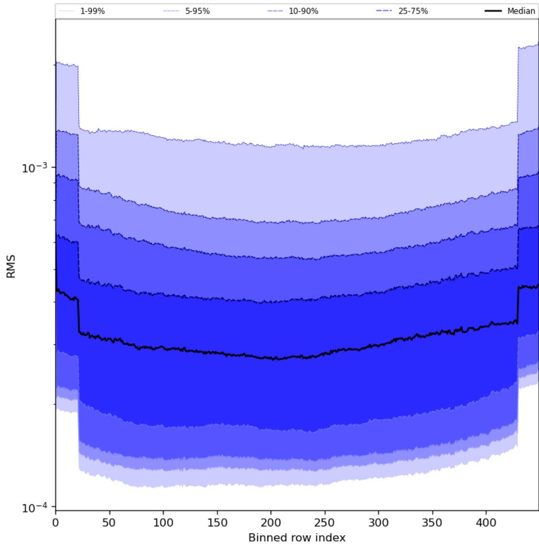
Figure 60: Along track statistics of “RMS” for 2023-07-24 to 2023-07-26
