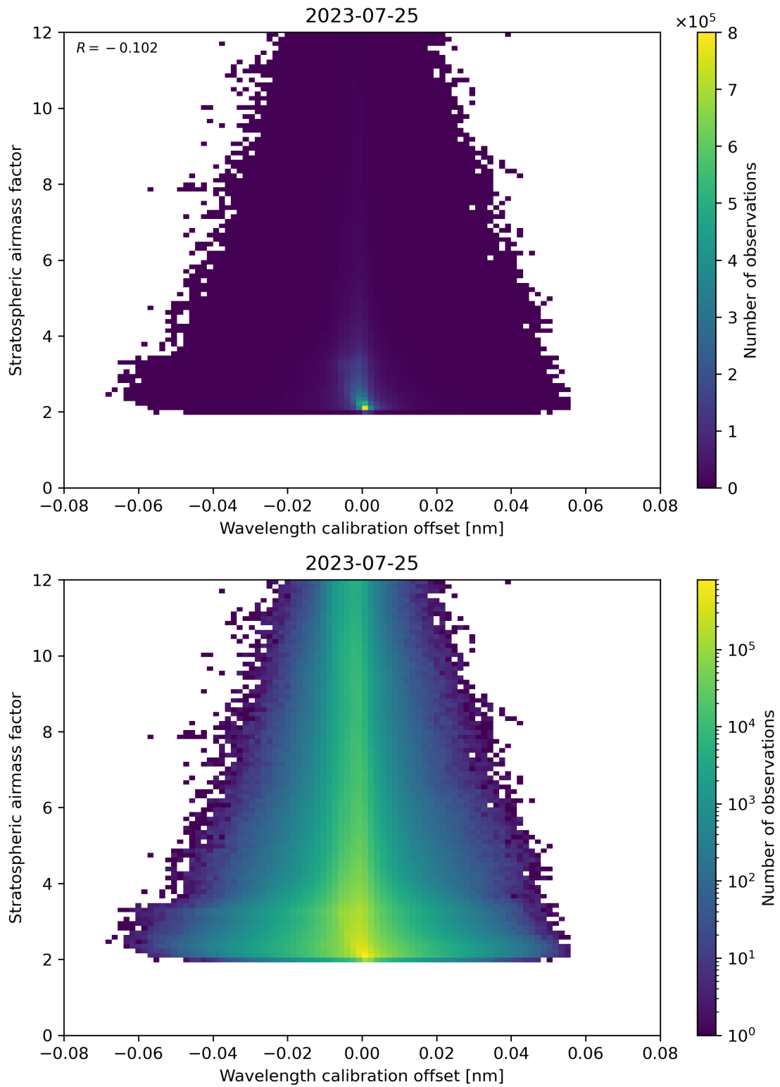
Figure 174: Scatter density plot of “Wavelength calibration offset” against “Stratospheric airmass factor” for 2023-07-24 to 2023-07-26.
