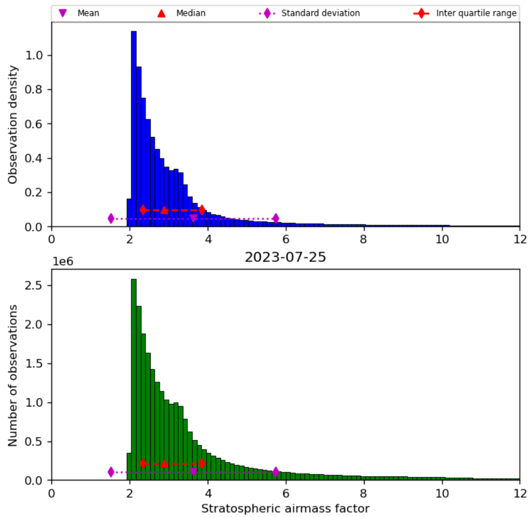
Figure 44: Histogram of “Stratospheric airmass factor” for 2023-07-24 to 2023-07-26
