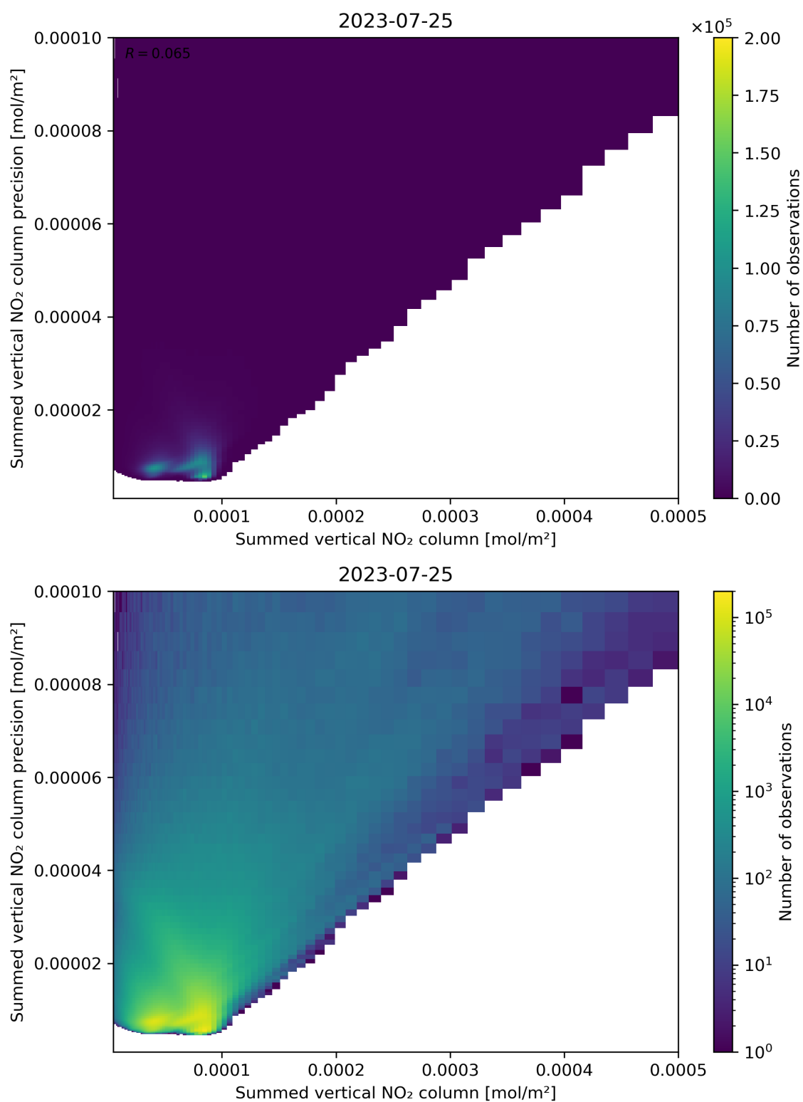
Figure 105: Scatter density plot of “Summed vertical NO 2 column” against “Summed vertical NO 2 column precision” for 2023-07-24 to 2023-07-26.
