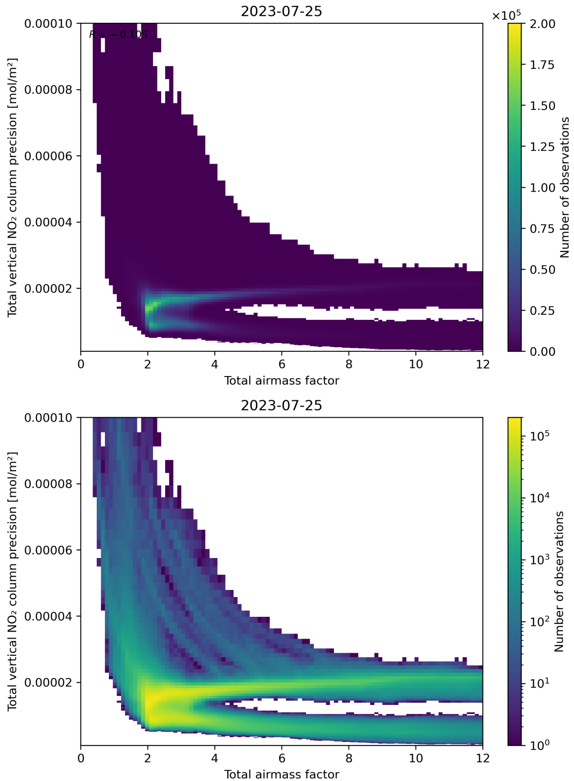
Figure 68: Scatter density plot of “Total airmass factor” against “Total vertical NO 2 column precision” for 2023-07-24 to 2023-07-26.
