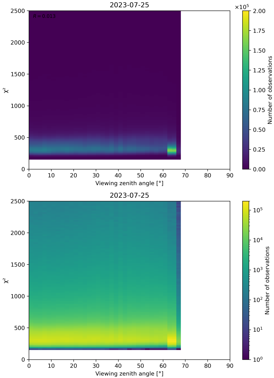
Figure 162: Scatter density plot of “Viewing zenith angle” against “ \chi^2 ” for 2023-07-24 to 2023-07-26.
