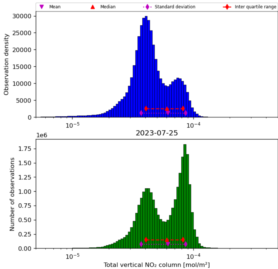
Figure 38: Histogram of “Total vertical NO 2 column” for 2023-07-24 to 2023-07-26
