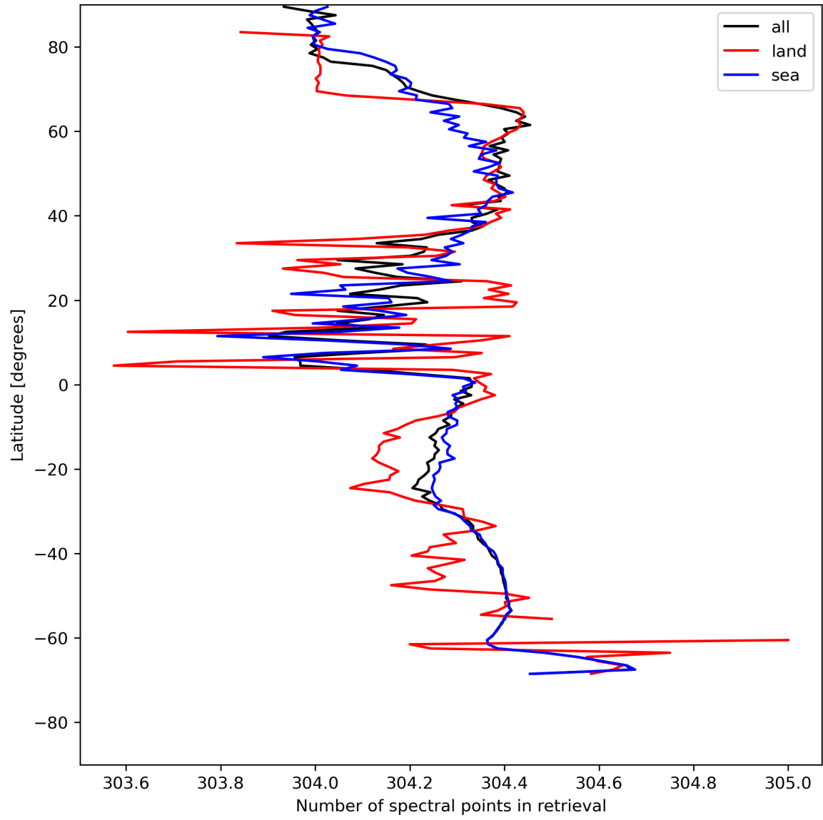
Figure 16: Zonal average of “Number of spectral points in retrieval” for 2023-07-24 to 2023-07-26.
