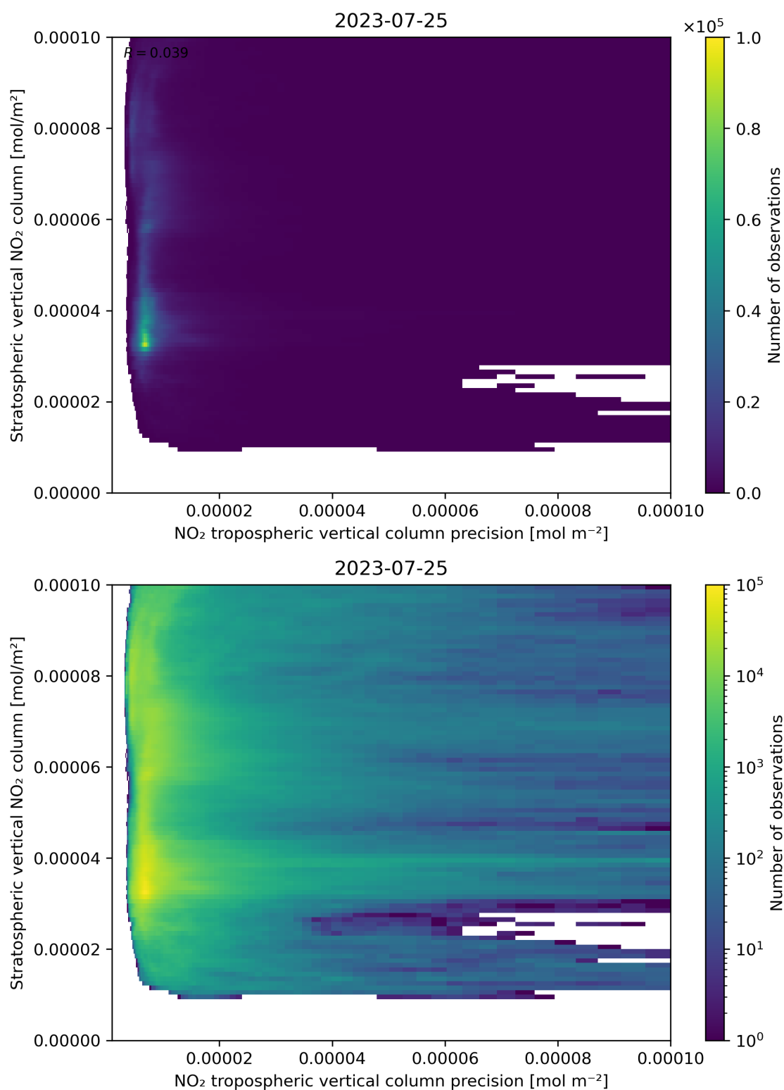
Figure 135: Scatter density plot of “NO 2 tropospheric vertical column precision” against “Stratospheric vertical NO 2 column” for 2023-07-24 to 2023-07-26.
