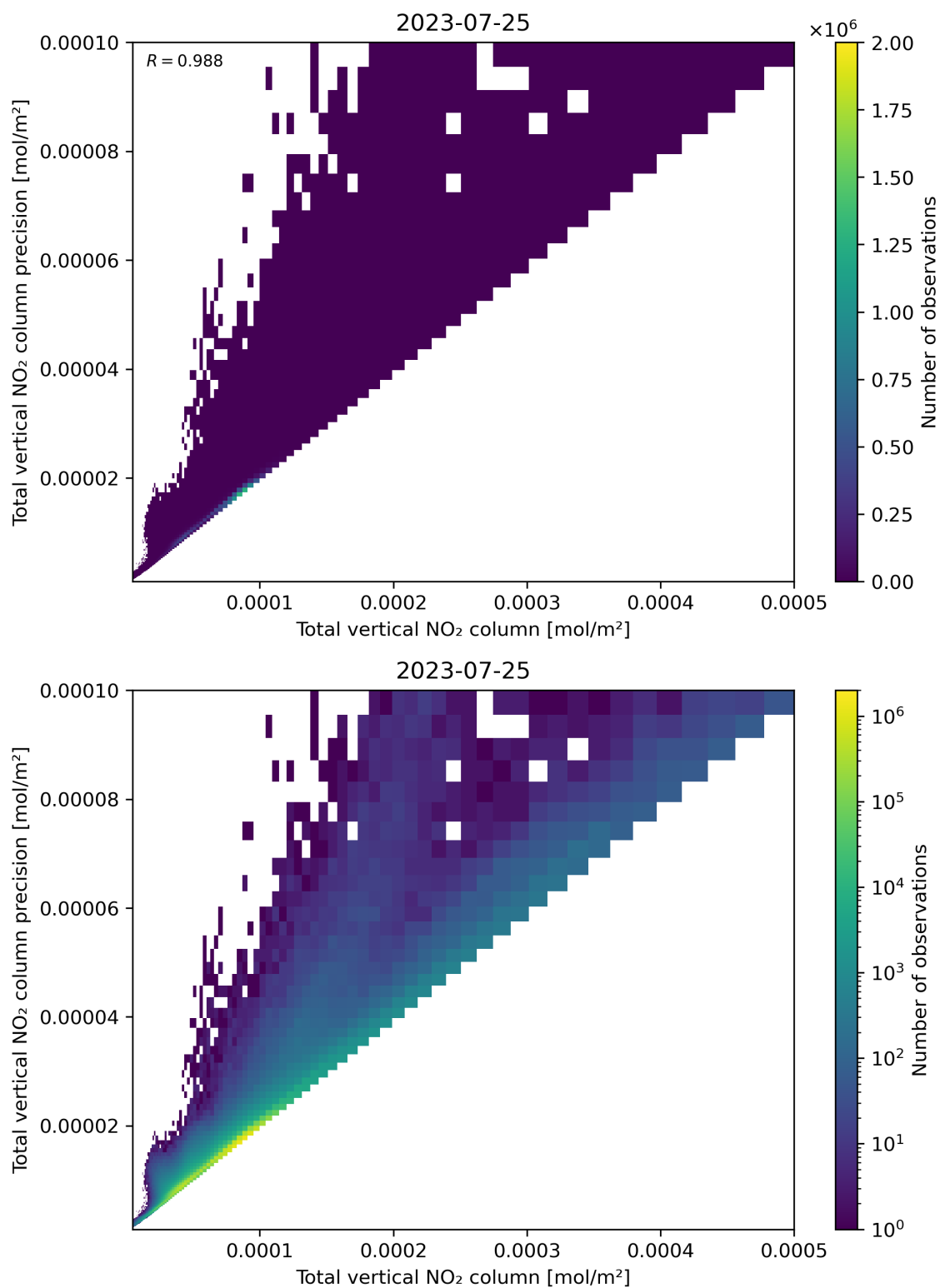
Figure 114: Scatter density plot of “Total vertical NO 2 column” against “Total vertical NO 2 column precision” for 2023-07-24 to 2023-07-26.
