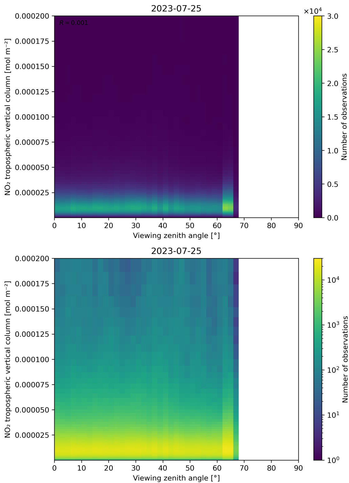
Figure 169: Scatter density plot of “Viewing zenith angle” against “NO 2 tropospheric vertical column” for 2023-07-24 to 2023-07-26.
