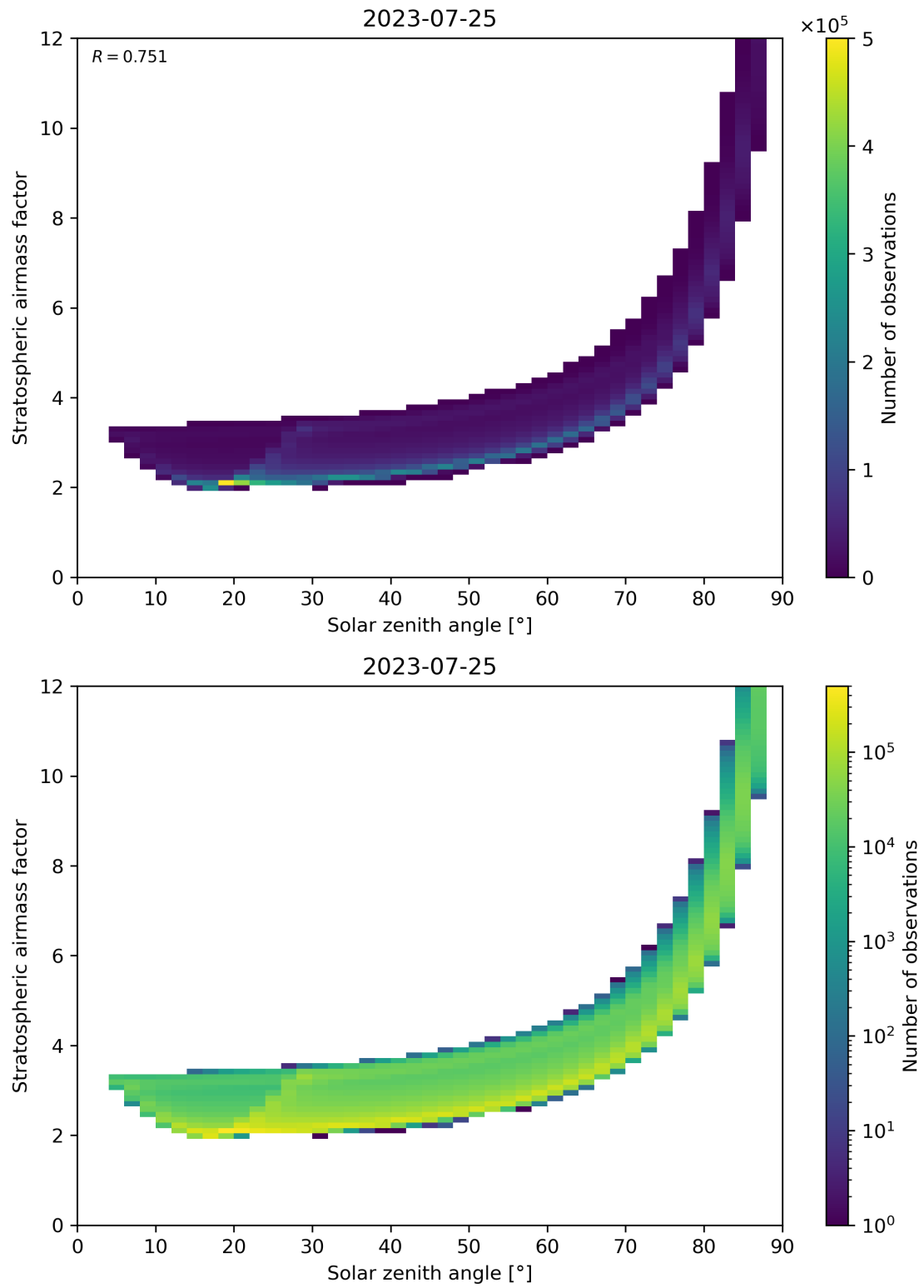
Figure 145: Scatter density plot of “Solar zenith angle” against “Stratospheric airmass factor” for 2023-07-24 to 2023-07-26.
