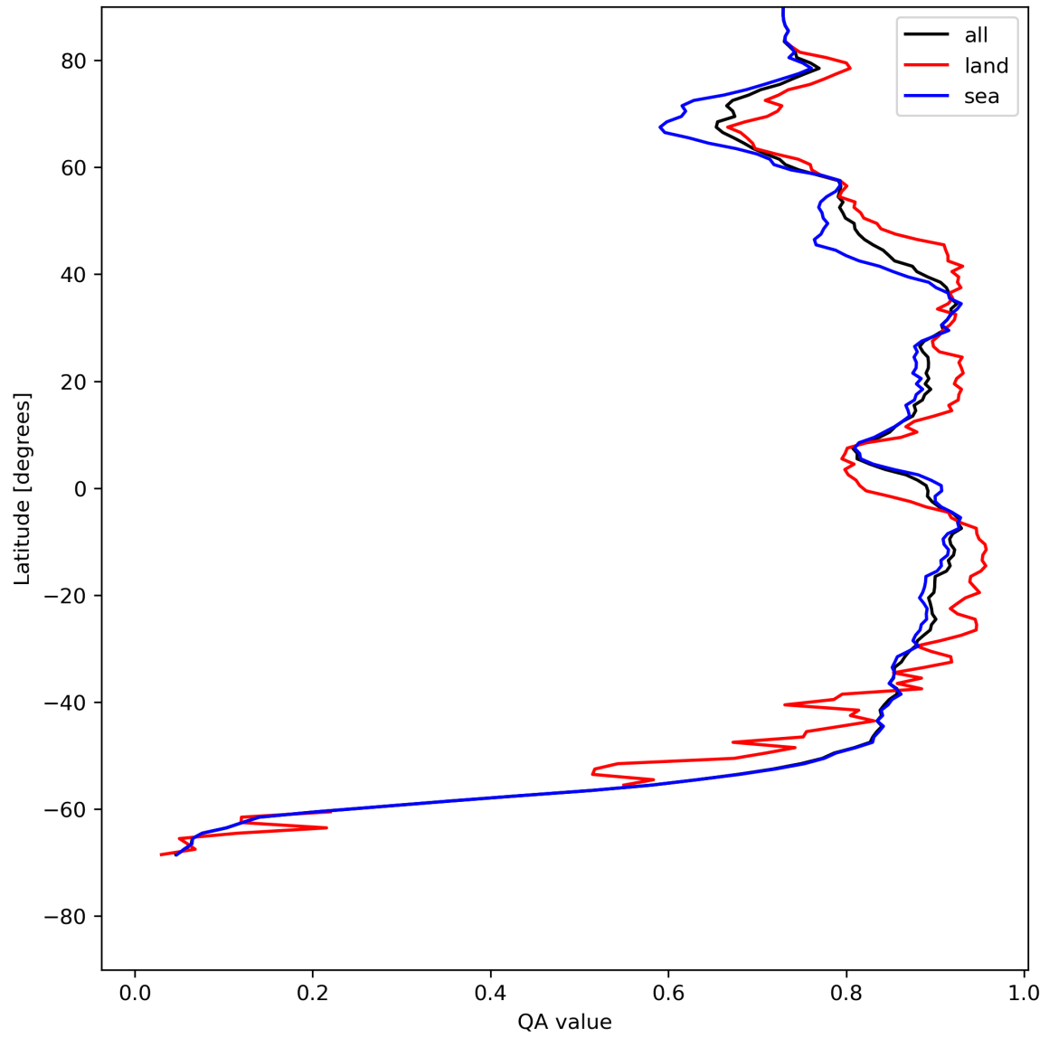
Figure 11: Zonal average of “QA value” for 2023-07-24 to 2023-07-26.
