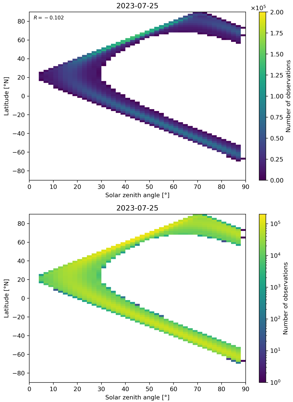
Figure 149: Scatter density plot of “Solar zenith angle” against “Latitude” for 2023-07-24 to 2023-07-26.
