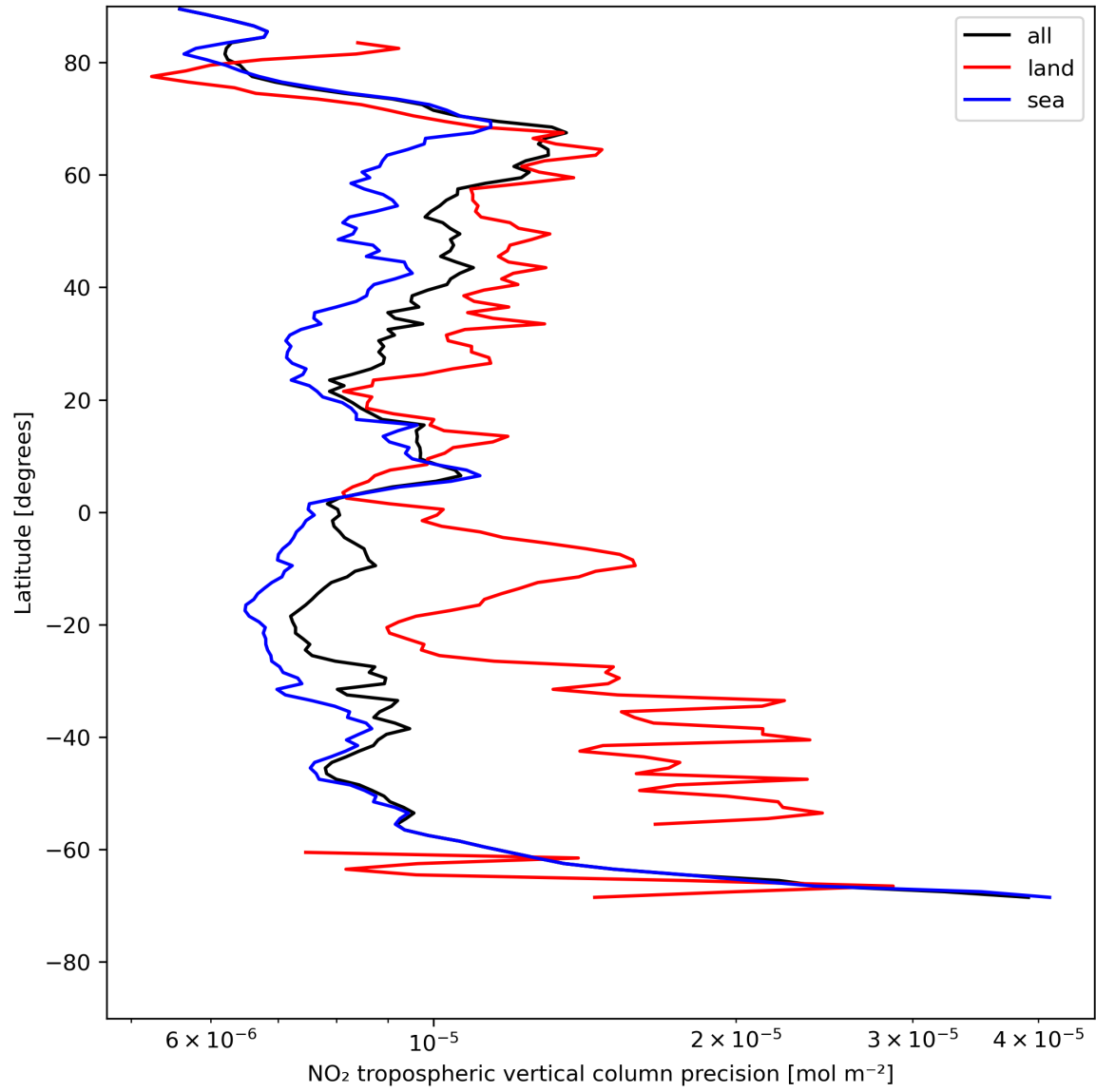
Figure 13: Zonal average of “NO 2 tropospheric vertical column precision” for 2023-07-24 to 2023-07-26.
