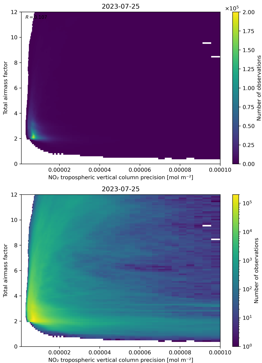
Figure 132: Scatter density plot of “NO 2 tropospheric vertical column precision” against “Total air mass factor” for 2023-07-24 to 2023-07-26.
