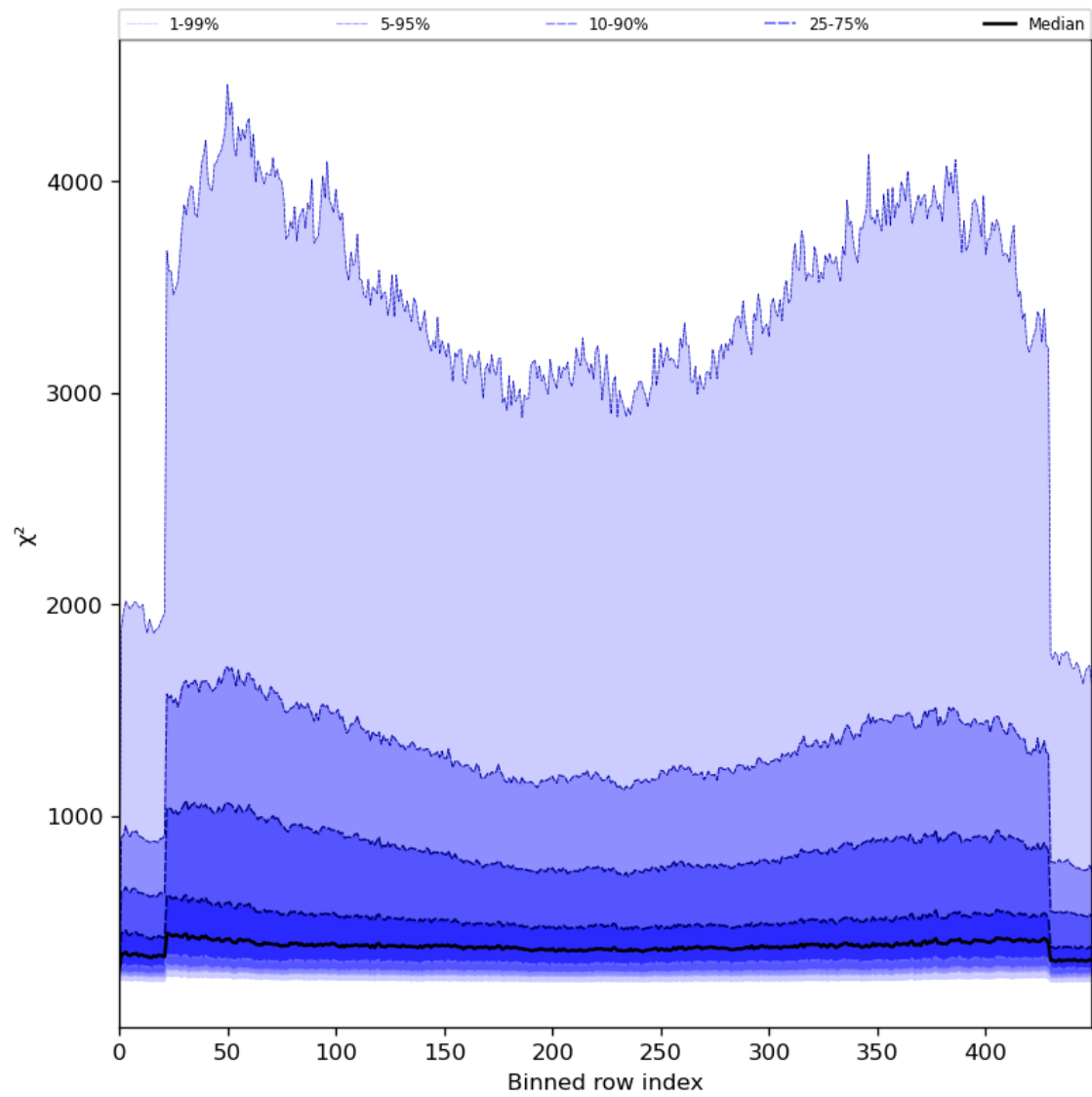
Figure 59: Along track statistics of “ \chi^2 ” for 2023-07-24 to 2023-07-26
