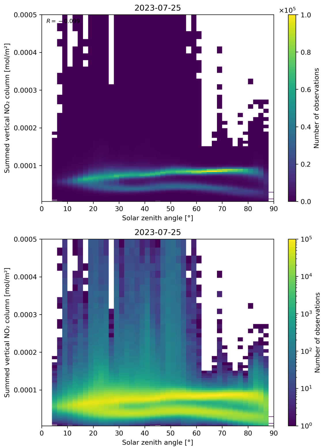
Figure 151: Scatter density plot of “Solar zenith angle” against “Summed vertical NO 2 column” for 2023-07-24 to 2023-07-26.
