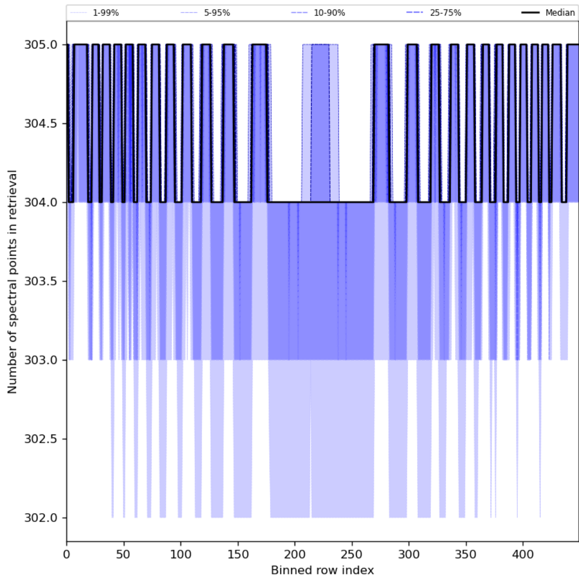
Figure 50: Along track statistics of “Number of spectral points in retrieval” for 2023-07-24 to 2023-07-26
