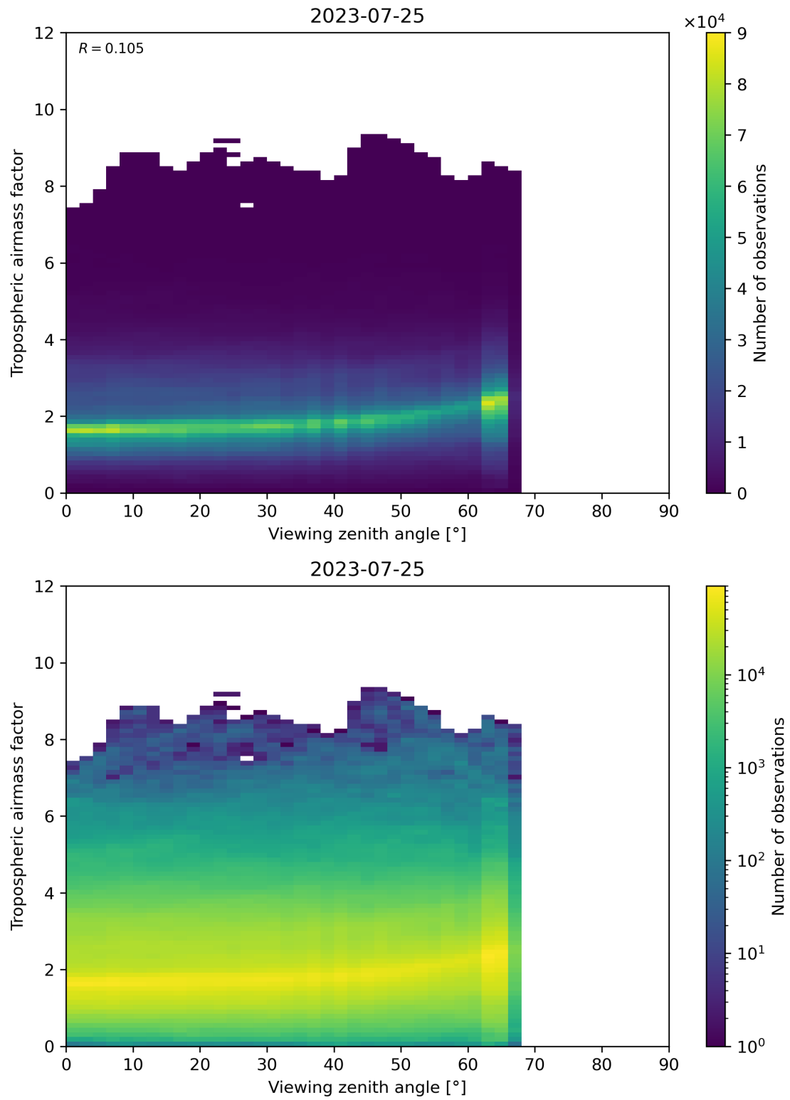
Figure 161: Scatter density plot of “Viewing zenith angle” against “Tropospheric airmass factor” for 2023-07-24 to 2023-07-26.
