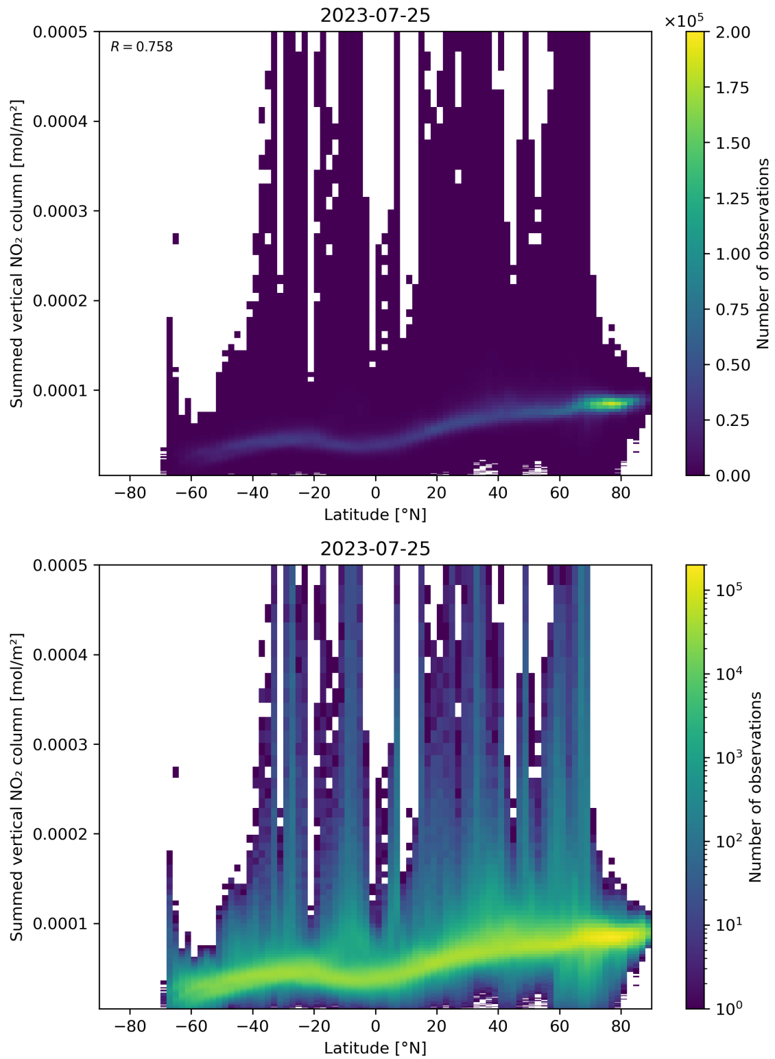
Figure 88: Scatter density plot of “Latitude” against “Summed vertical NO 2 column” for 2023-07-24 to 2023-07-26.
