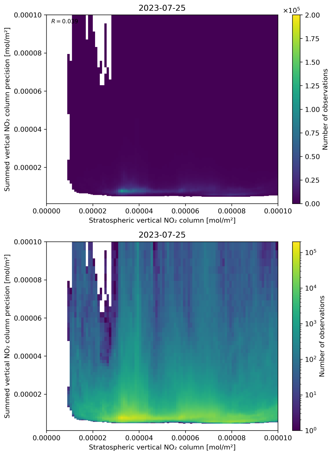
Figure 99: Scatter density plot of “Stratospheric vertical NO 2 column” against “Summed vertical NO 2 column precision” for 2023-07-24 to 2023-07-26.
