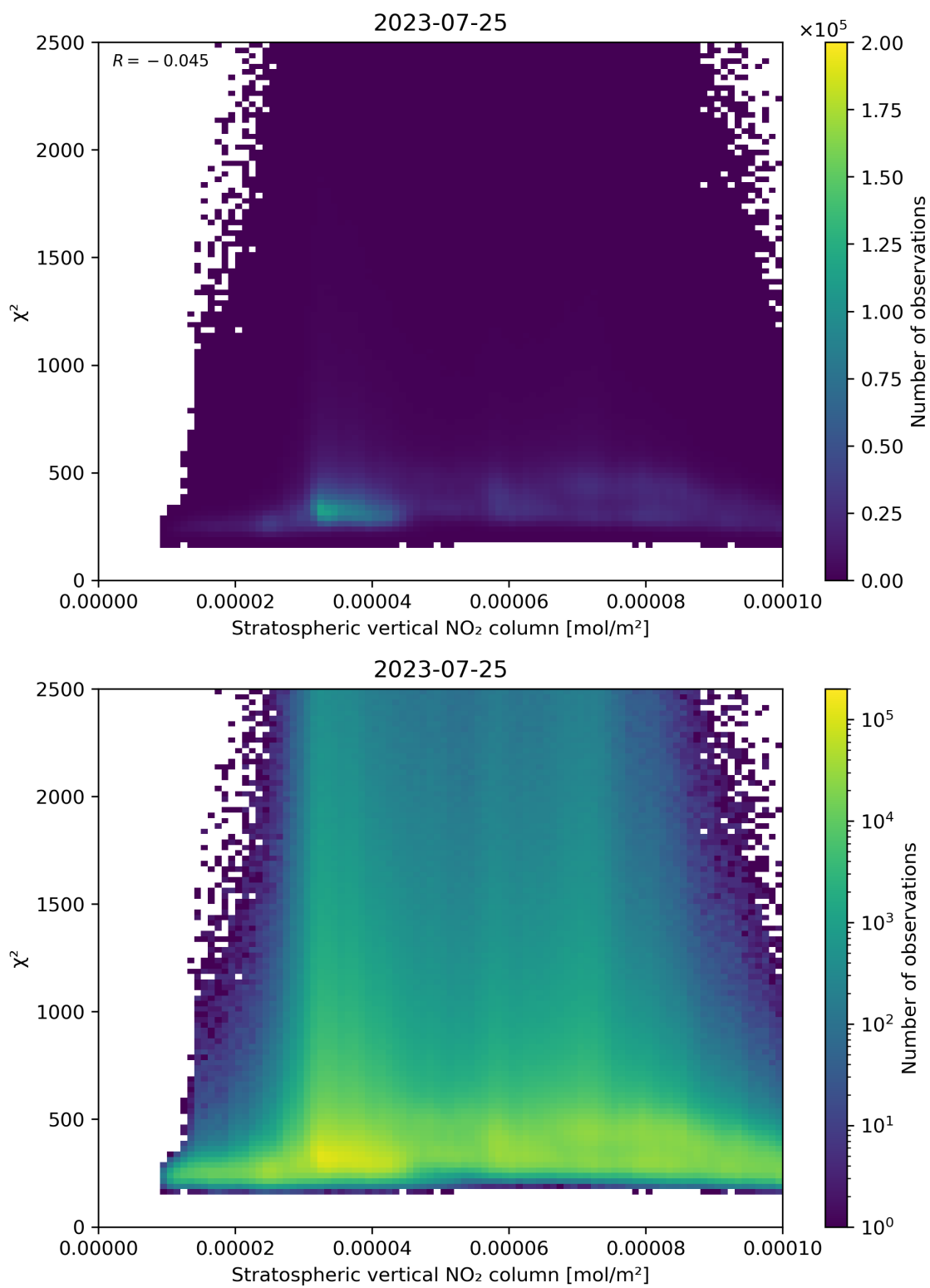
Figure 97: Scatter density plot of “Stratospheric vertical NO 2 column” against “ \chi^2 ” for 2023-07-24 to 2023-07-26.
