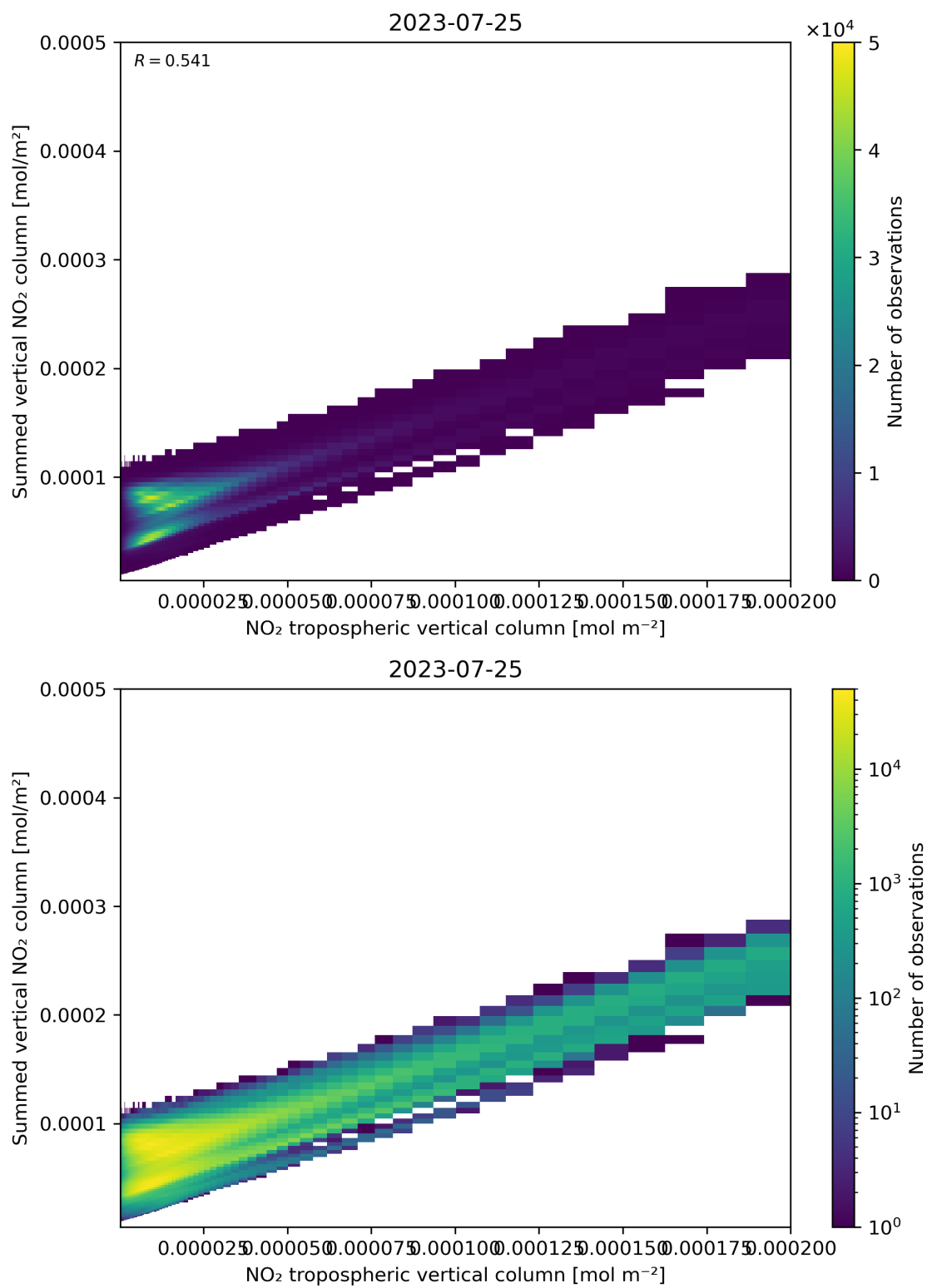
Figure 126: Scatter density plot of “NO 2 tropospheric vertical column” against “Summed vertical NO 2 column” for 2023-07-24 to 2023-07-26.
