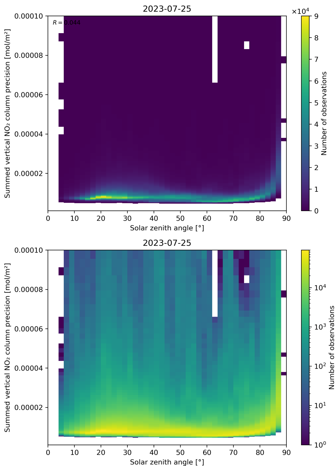
Figure 152: Scatter density plot of “Solar zenith angle” against “Summed vertical NO 2 column precision” for 2023-07-24 to 2023-07-26.
