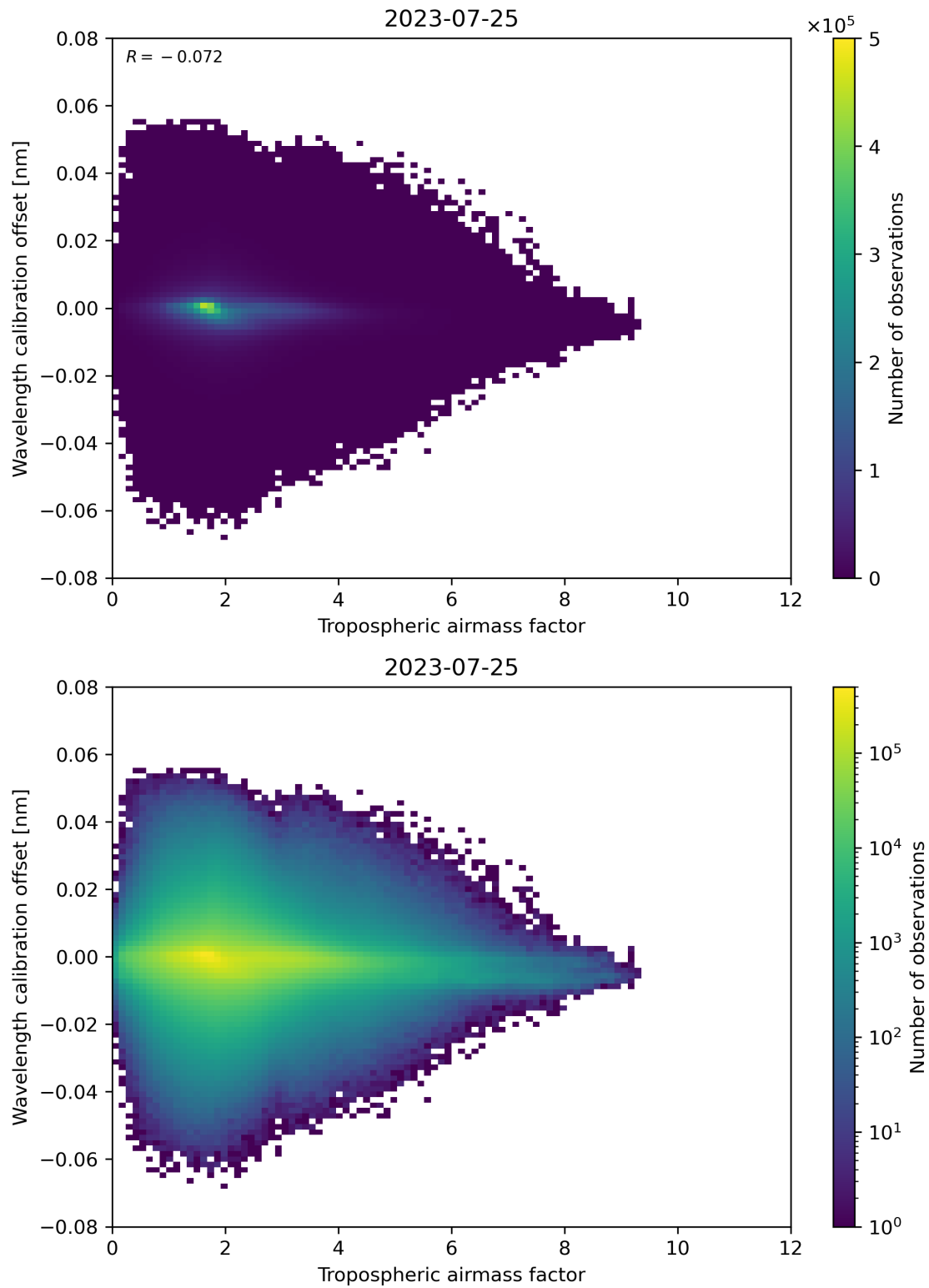
Figure 80: Scatter density plot of “Tropospheric airmass factor” against “Wavelength calibration offset” for 2023-07-24 to 2023-07-26.
