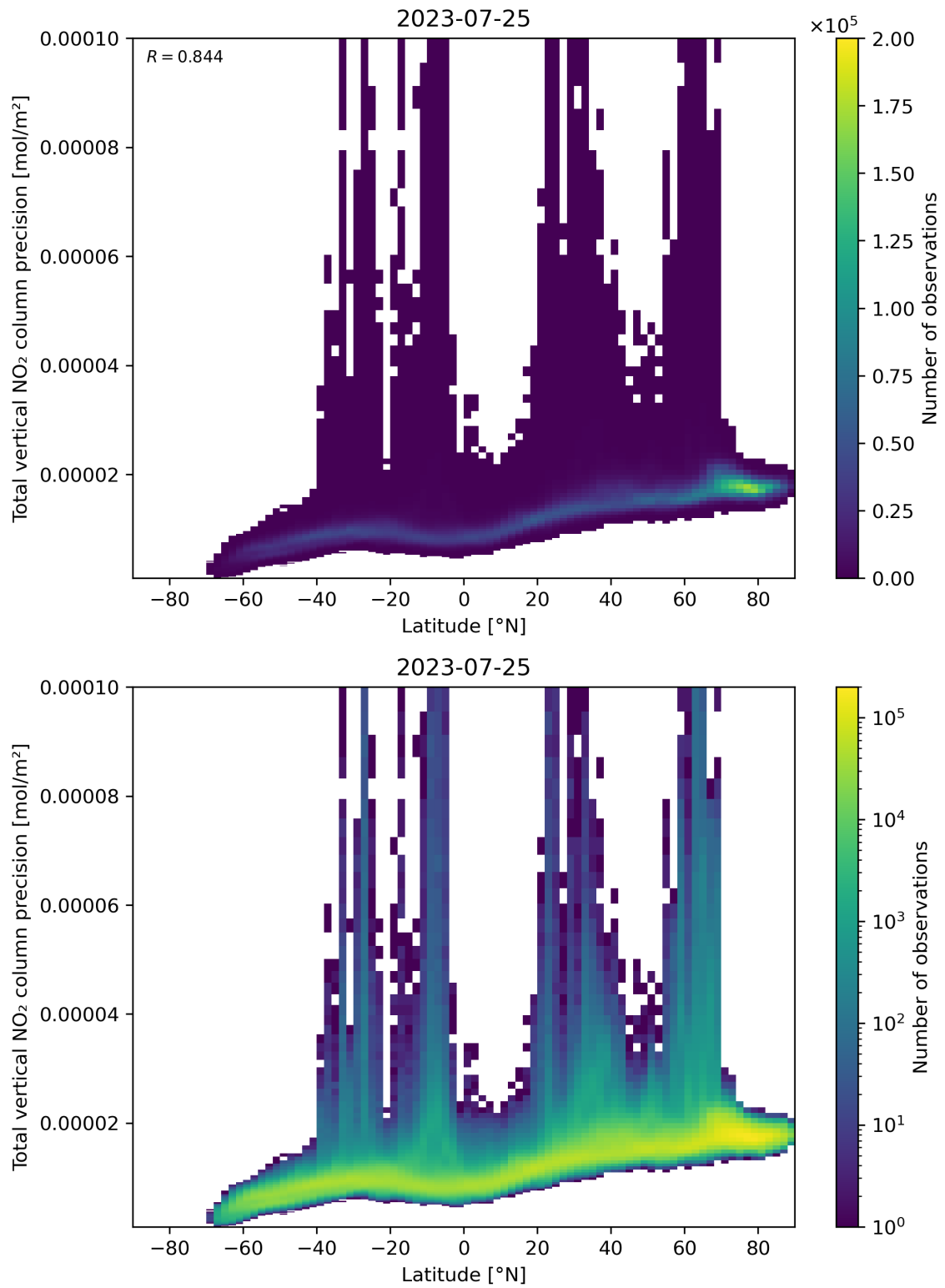
Figure 91: Scatter density plot of “Latitude” against “Total vertical NO 2 column precision” for 2023-07-24 to 2023-07-26.
