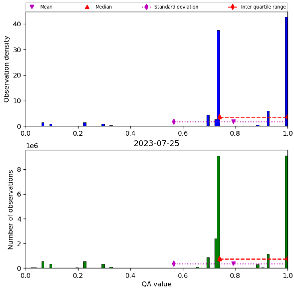
Figure 28: Histogram of “QA value” for 2023-07-24 to 2023-07-26
