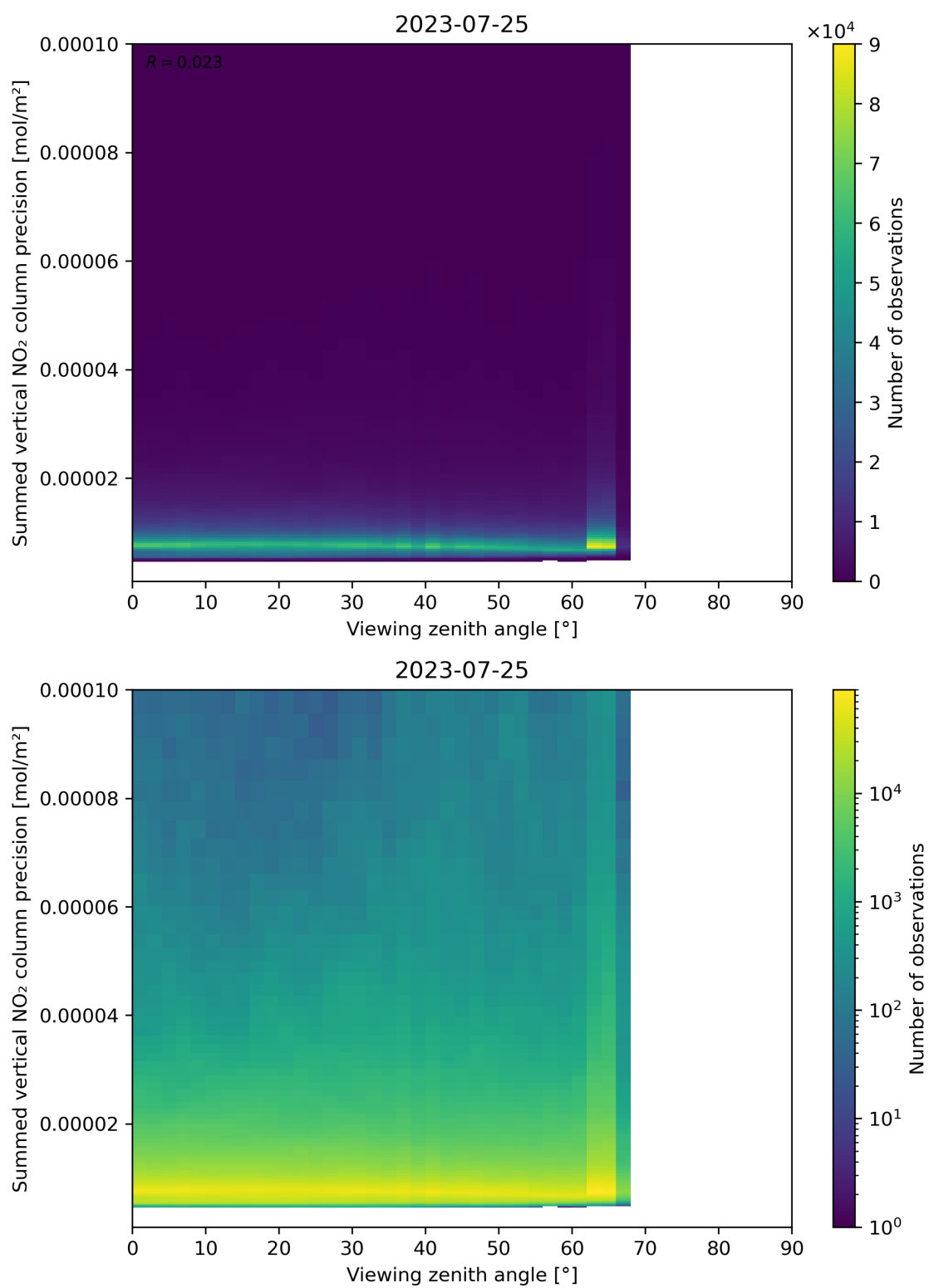
Figure 166: Scatter density plot of “Viewing zenith angle” against “Summed vertical NO 2 column precision” for 2023-07-24 to 2023-07-26.
