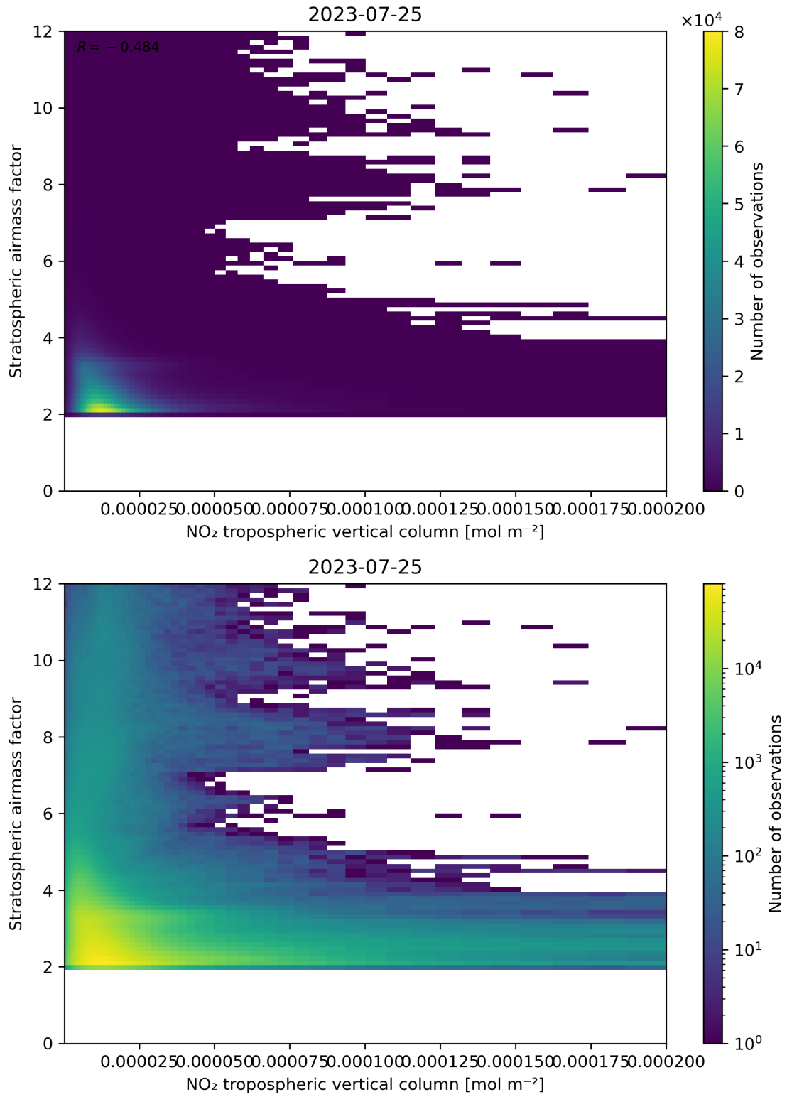
Figure 121: Scatter density plot of “NO 2 tropospheric vertical column” against “Stratospheric air mass factor” for 2023-07-24 to 2023-07-26.
