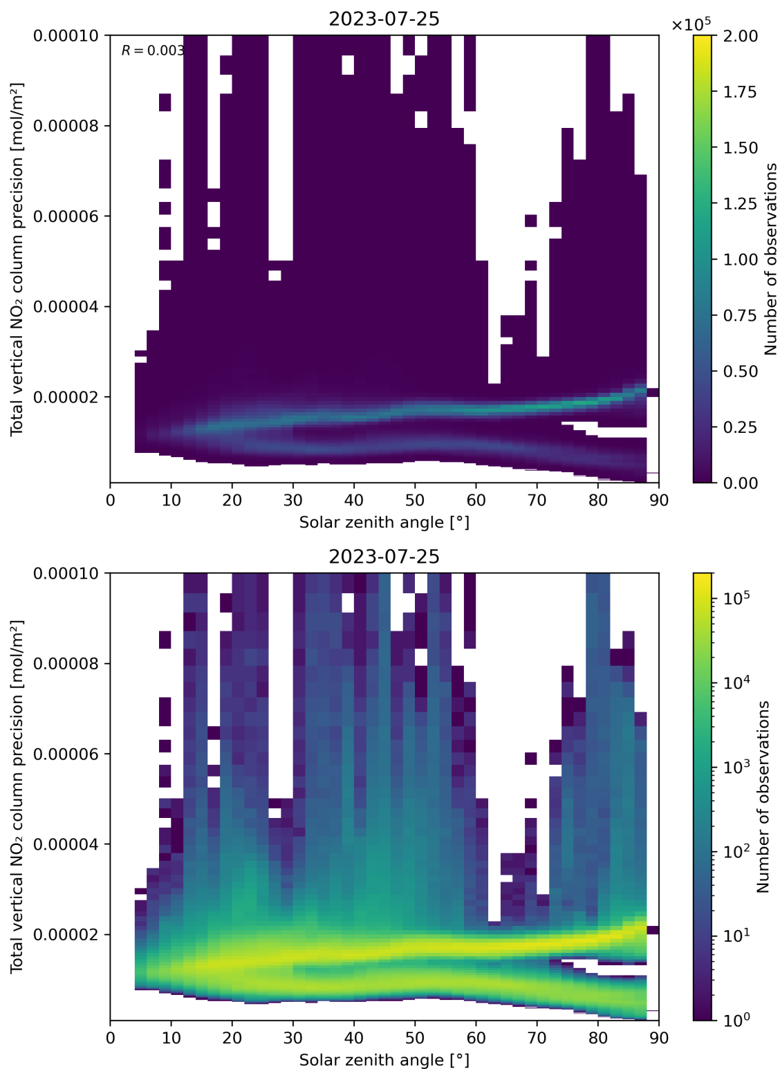
Figure 154: Scatter density plot of “Solar zenith angle” against “Total vertical NO 2 column precision” for 2023-07-24 to 2023-07-26.
