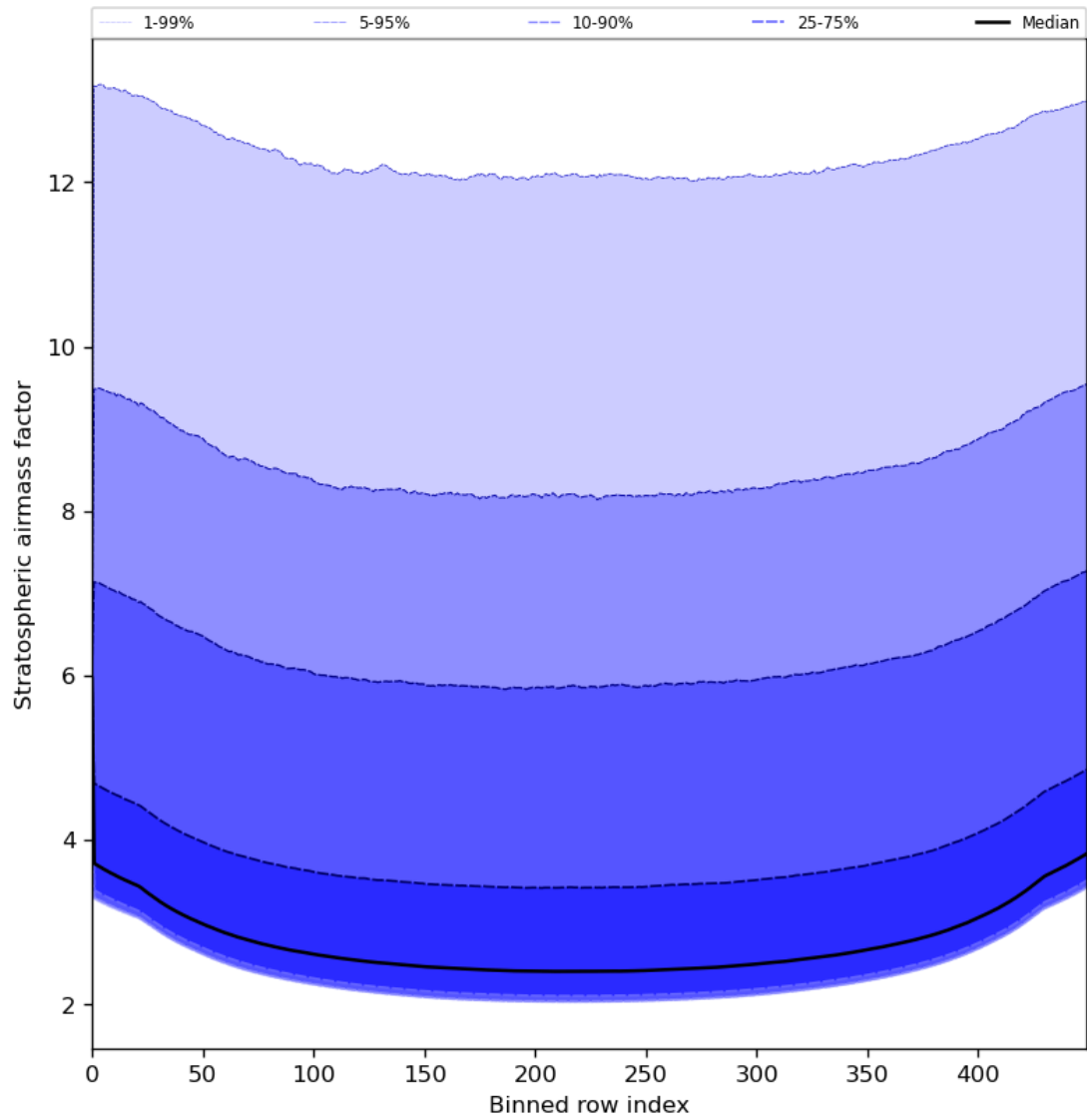
Figure 61: Along track statistics of “Stratospheric airmass factor” for 2023-07-24 to 2023-07-26
