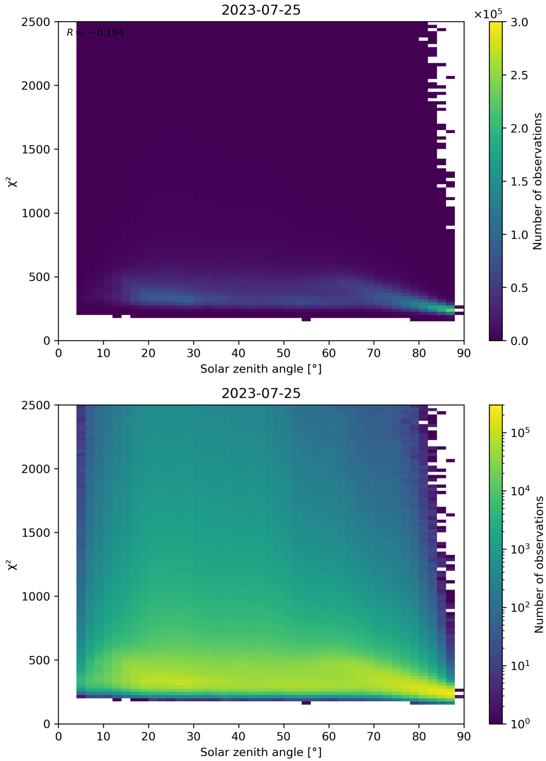
Figure 148: Scatter density plot of “Solar zenith angle” against “ \chi^2 ” for 2023-07-24 to 2023-07-26.
