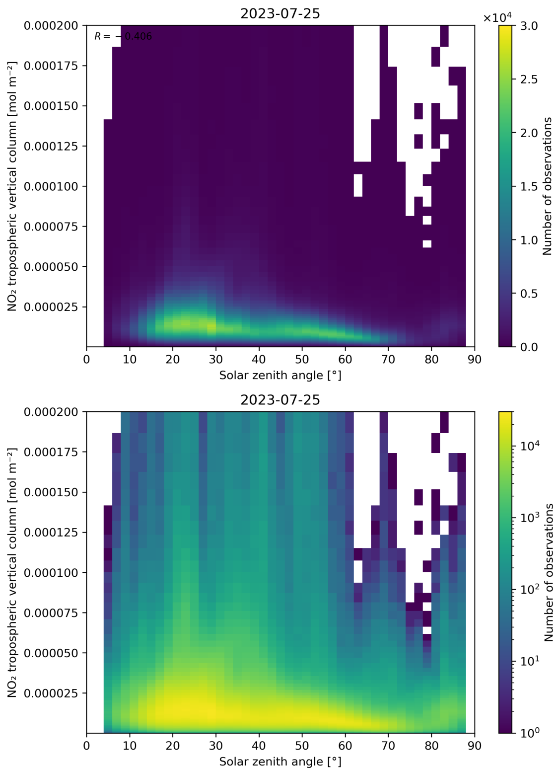
Figure 155: Scatter density plot of “Solar zenith angle” against “NO 2 tropospheric vertical column” for 2023-07-24 to 2023-07-26.
