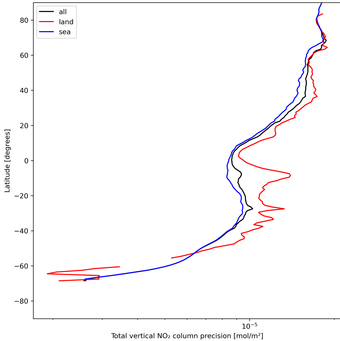
Figure 22: Zonal average of “Total vertical NO 2 column precision” for 2023-07-24 to 2023-07-26.
