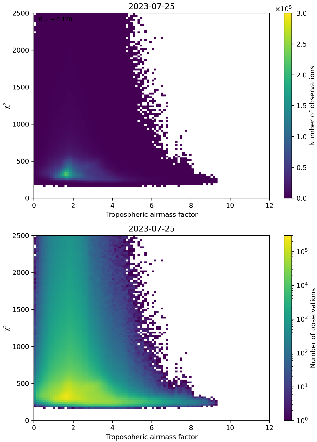
Figure 73: Scatter density plot of “Tropospheric airmass factor” against “ \chi^2 ” for 2023-07-24 to 2023-07-26.
