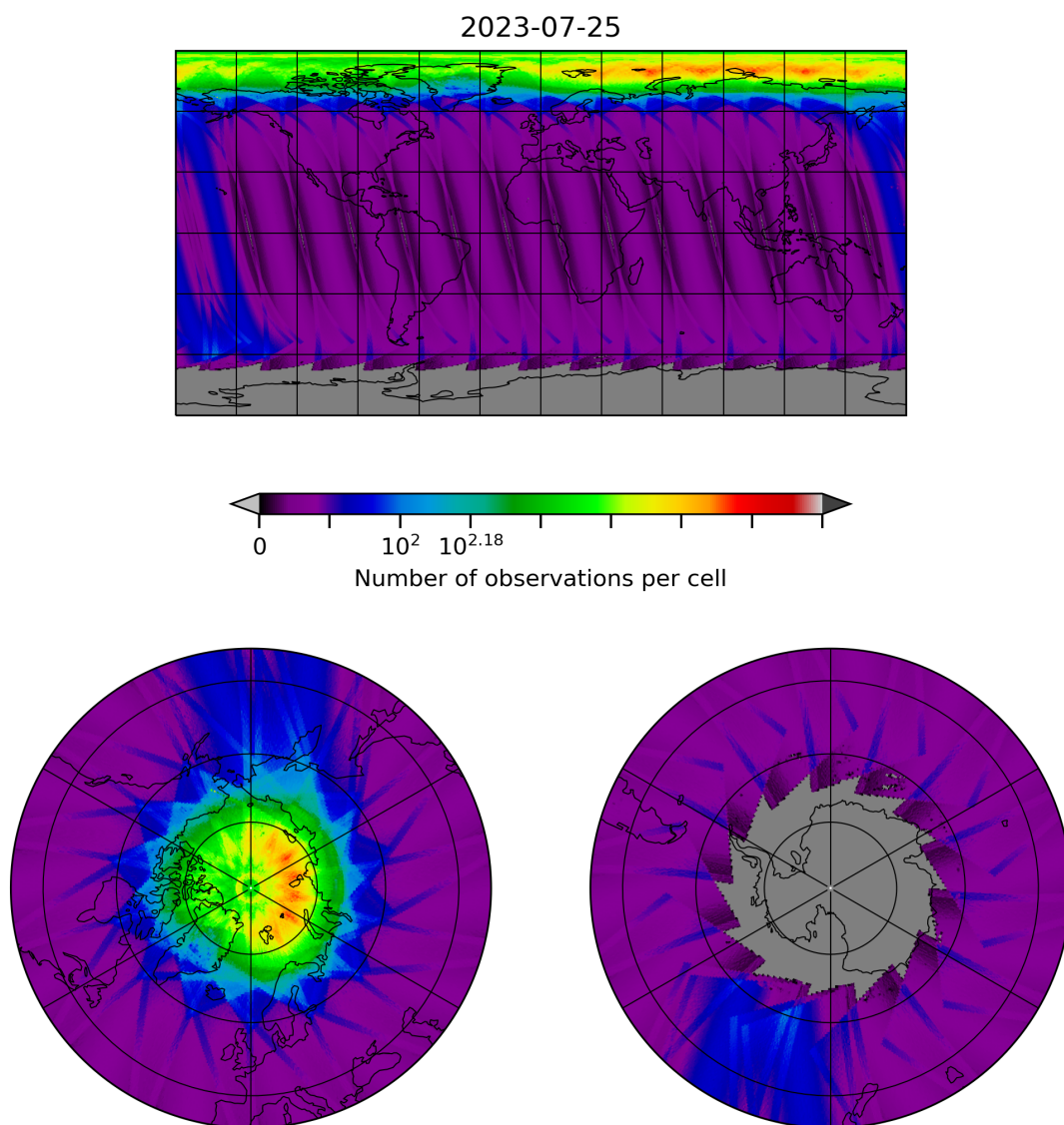
Figure 10: Map of the number of observations for 2023-07-24 to 2023-07-26
