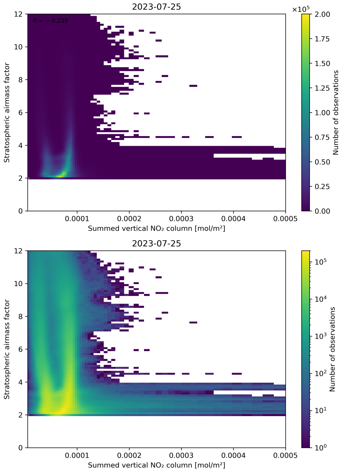
Figure 103: Scatter density plot of “Summed vertical NO 2 column” against “Stratospheric air mass factor” for 2023-07-24 to 2023-07-26.
