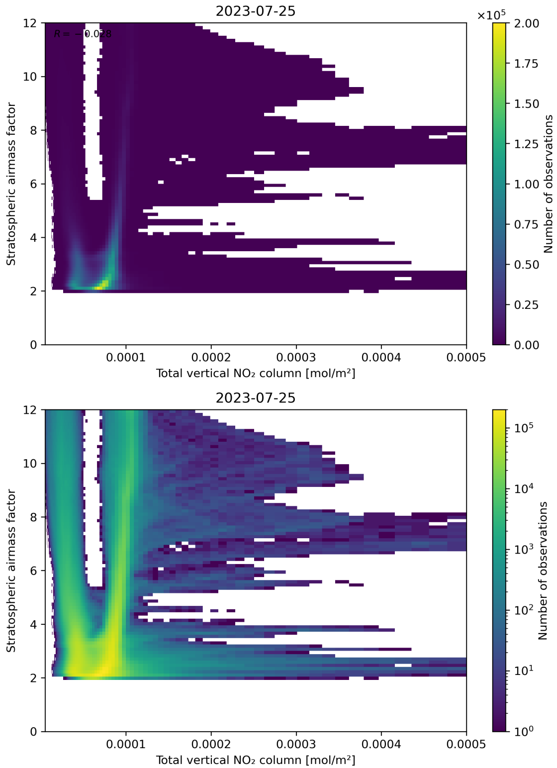
Figure 110: Scatter density plot of “Total vertical NO 2 column” against “Stratospheric airmass factor” for 2023-07-24 to 2023-07-26.
