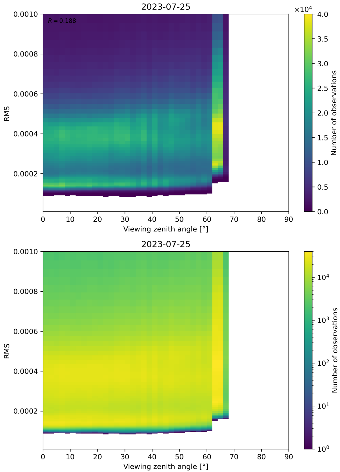
Figure 171: Scatter density plot of “Viewing zenith angle” against “RMS” for 2023-07-24 to 2023-07-26.
