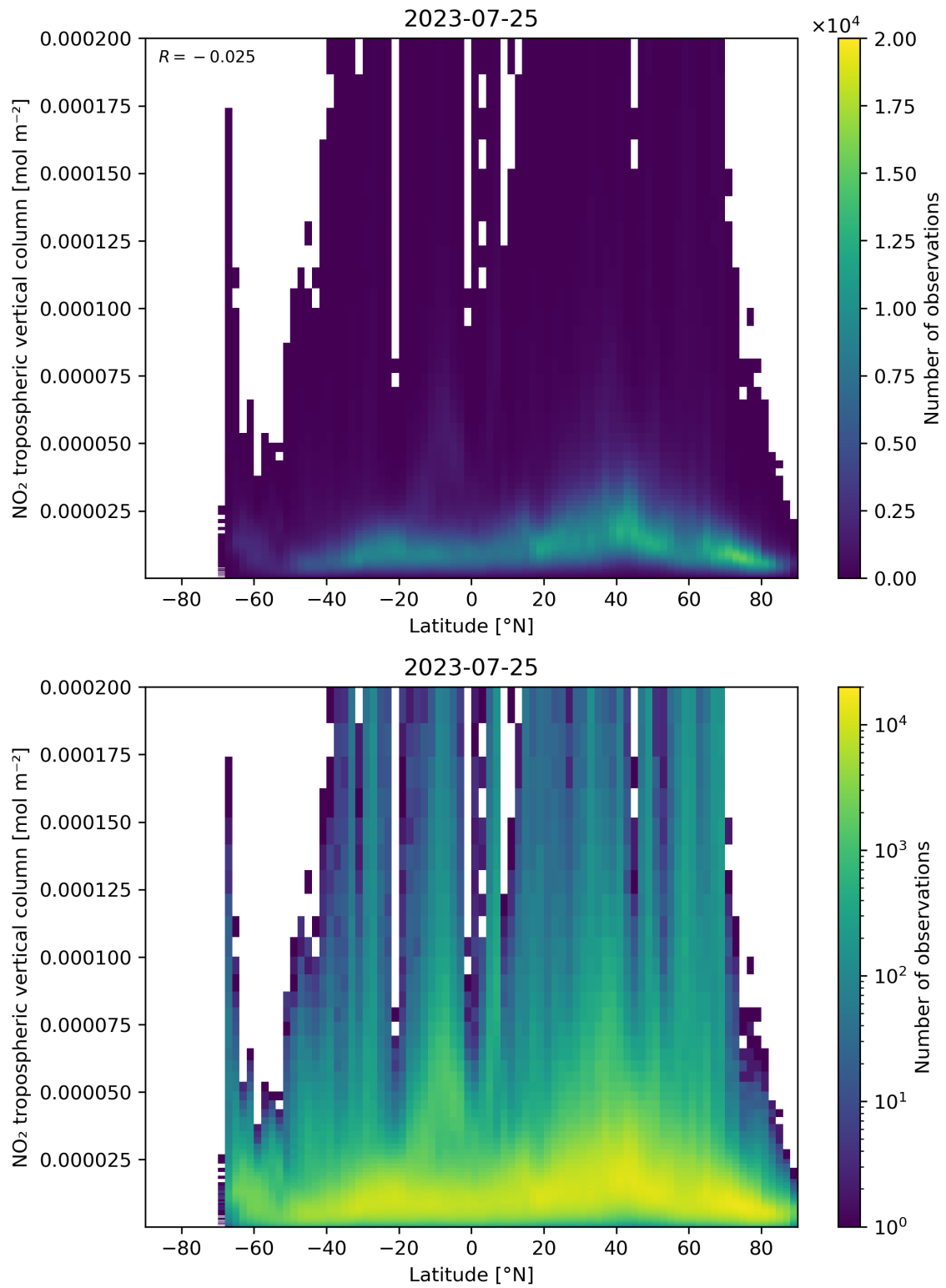
Figure 92: Scatter density plot of “Latitude” against “NO 2 tropospheric vertical column” for 2023-07-24 to 2023-07-26.
