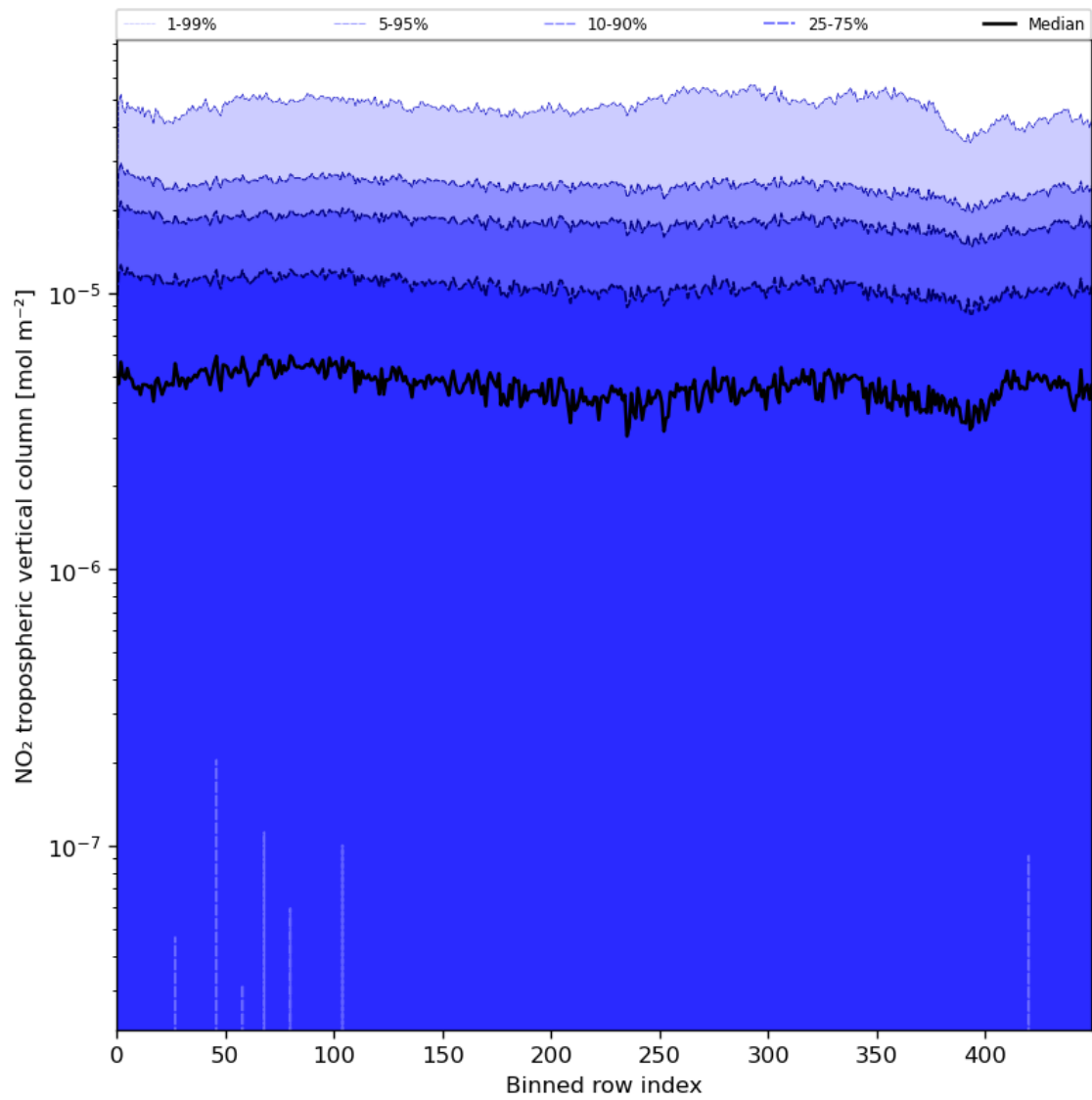
Figure 46: Along track statistics of “NO 2 tropospheric vertical column” for 2023-07-24 to 2023-07-26
