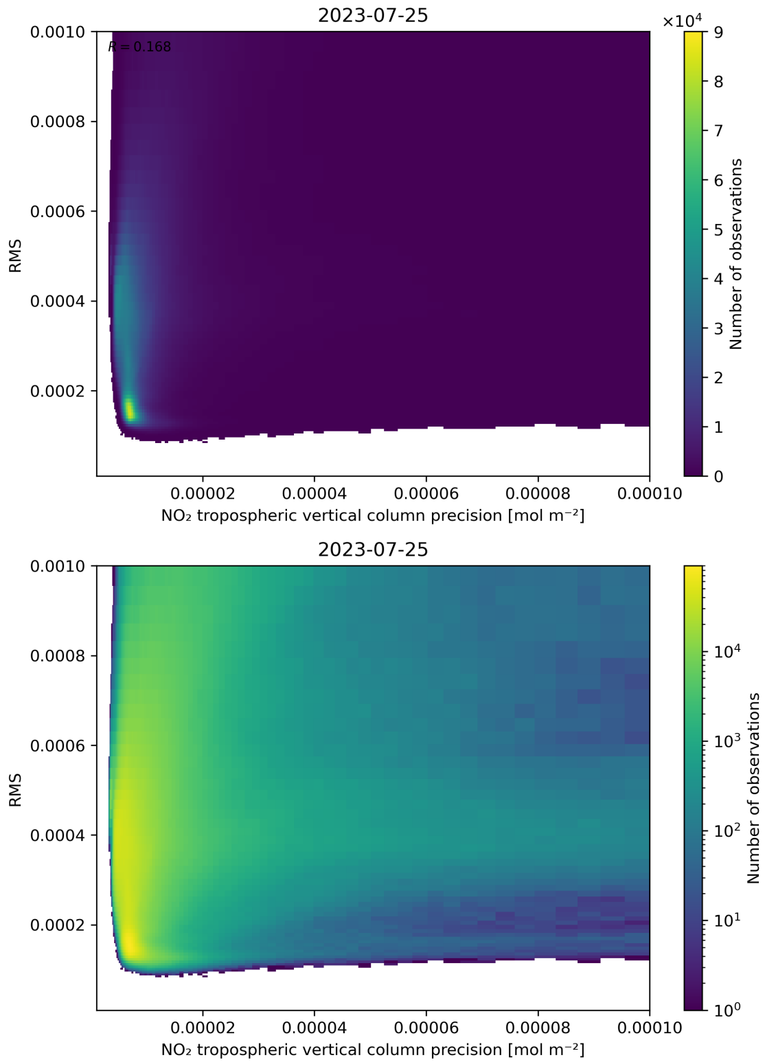
Figure 140: Scatter density plot of “NO 2 tropospheric vertical column precision” against “RMS” for 2023-07-24 to 2023-07-26.
