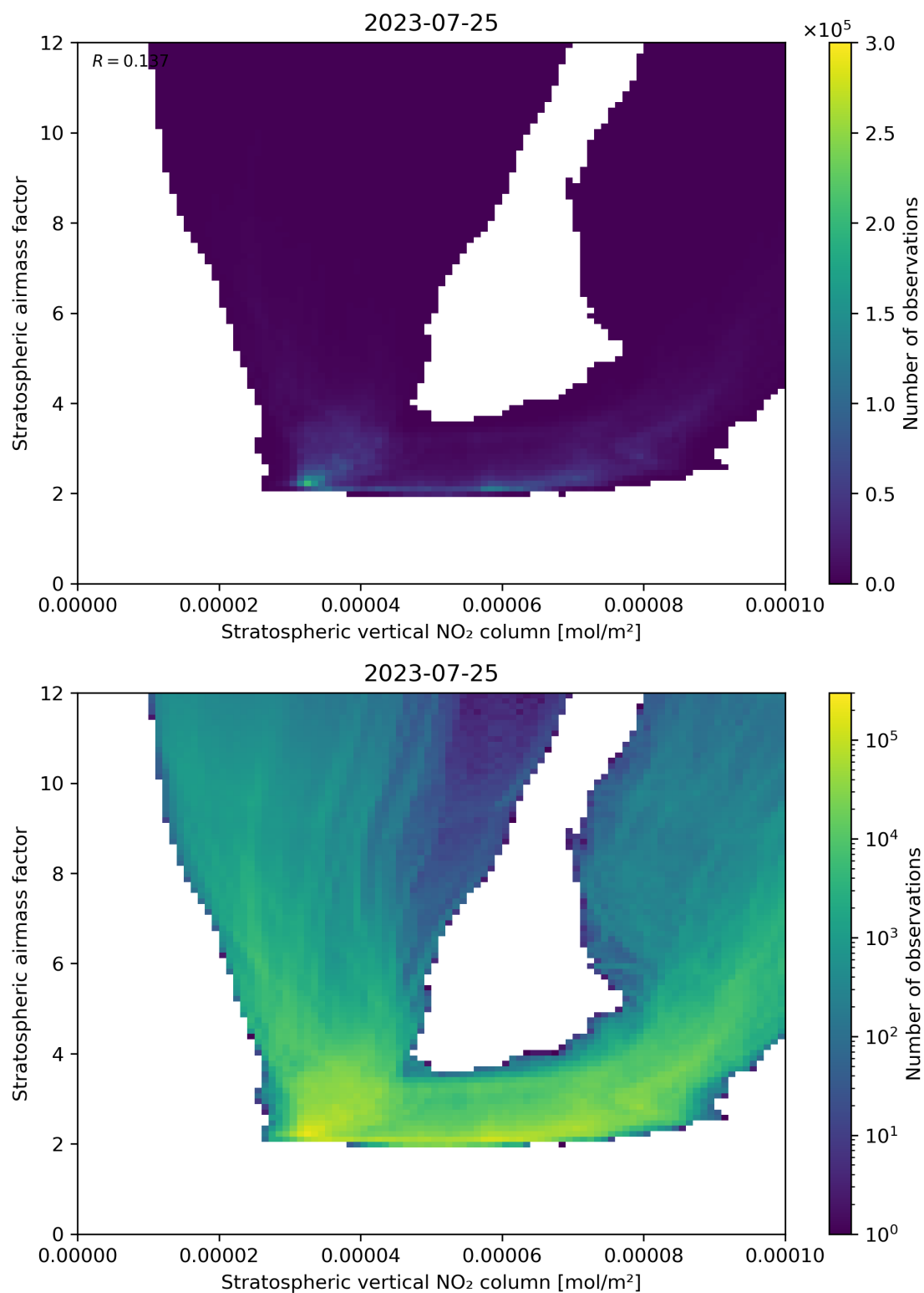
Figure 96: Scatter density plot of “Stratospheric vertical NO 2 column” against “Stratospheric airmass factor” for 2023-07-24 to 2023-07-26.
