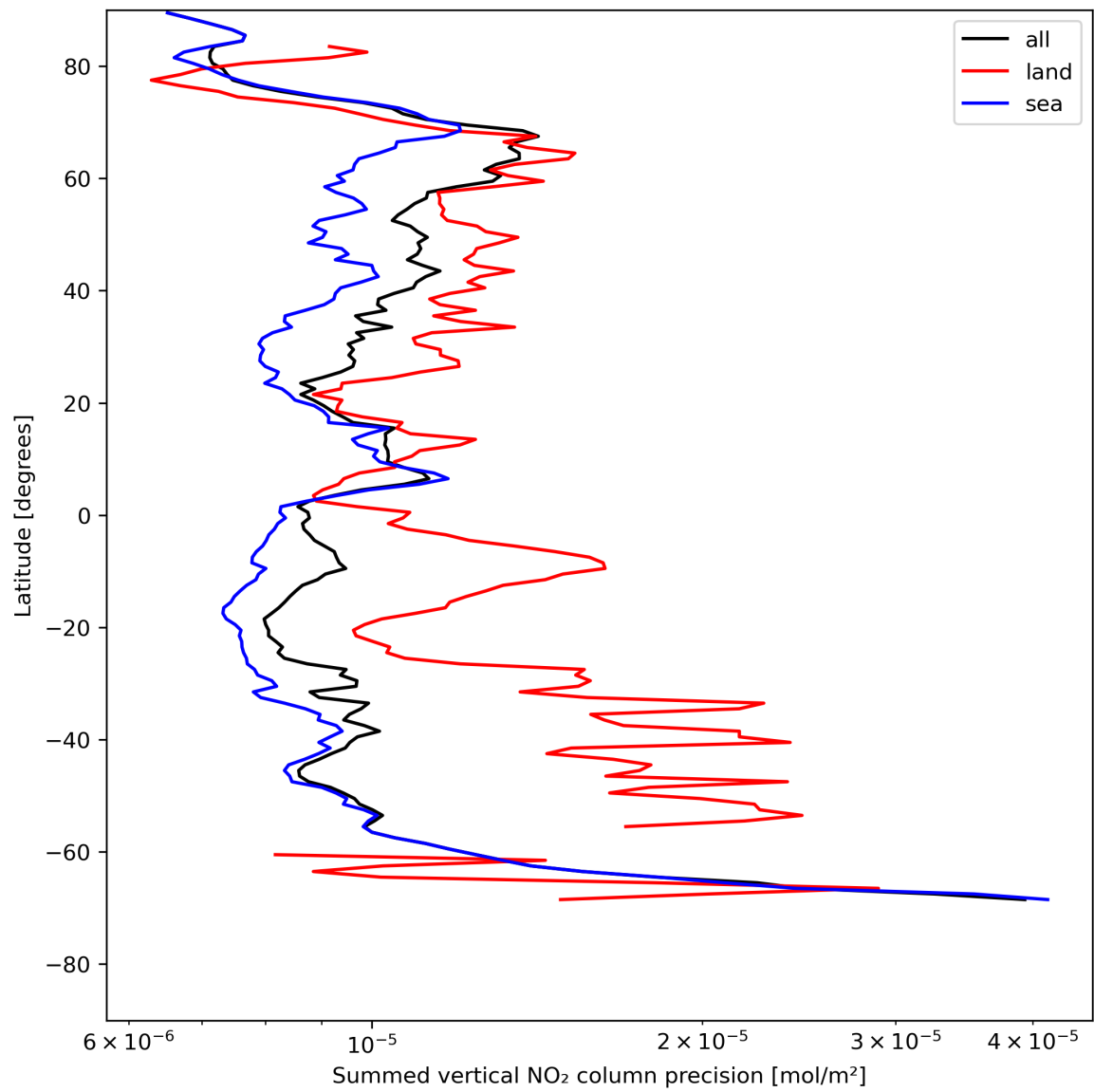
Figure 24: Zonal average of “Summed vertical NO 2 column precision” for 2023-07-24 to 2023-07-26.
