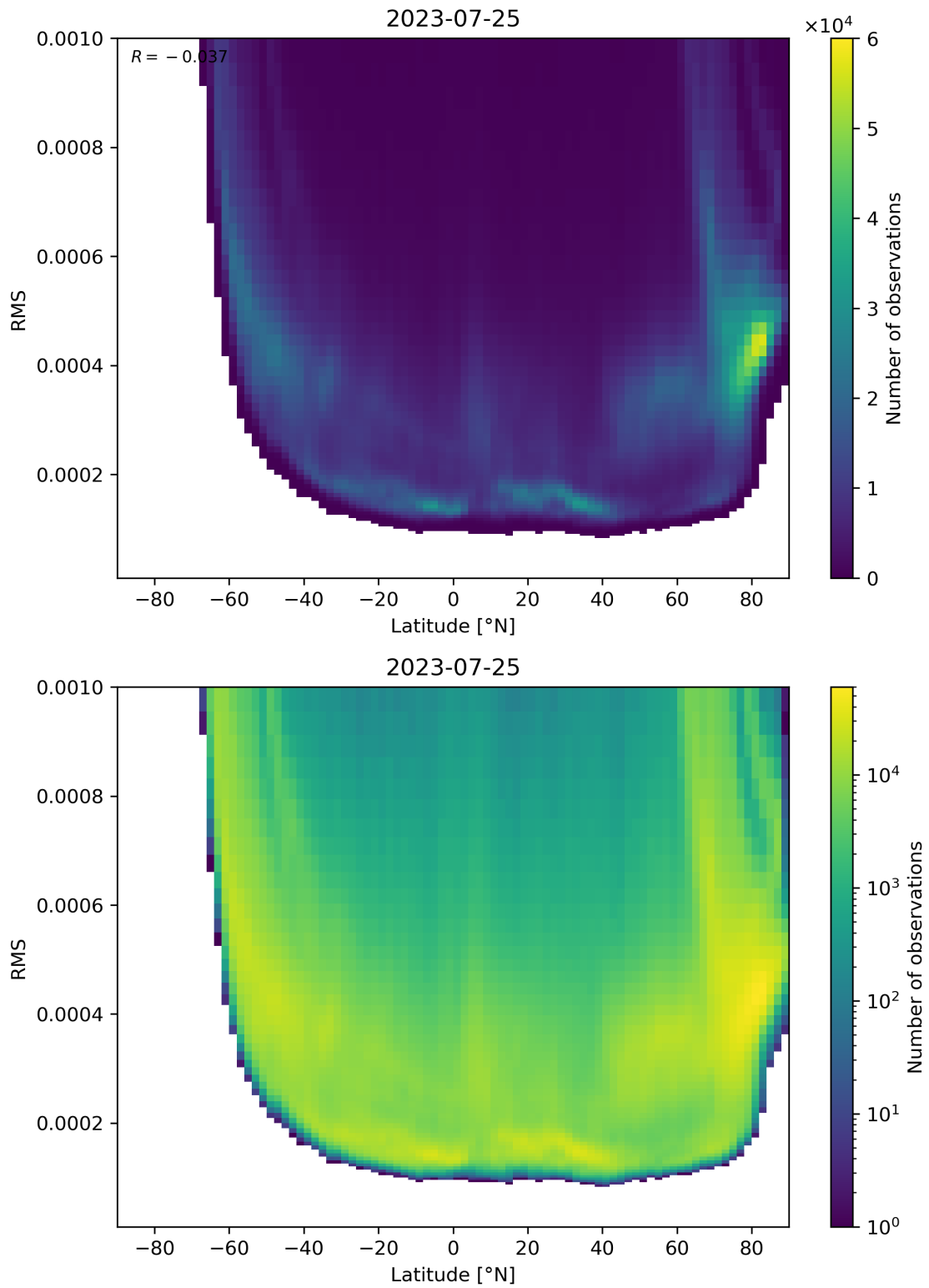
Figure 94: Scatter density plot of “Latitude” against “RMS” for 2023-07-24 to 2023-07-26.
