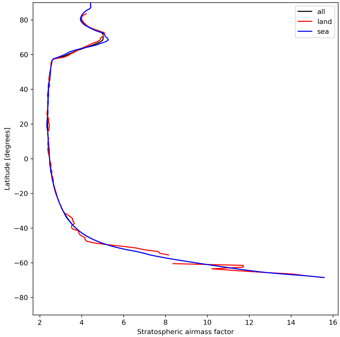
Figure 27: Zonal average of “Stratospheric air mass factor” for 2023-07-24 to 2023-07-26.
