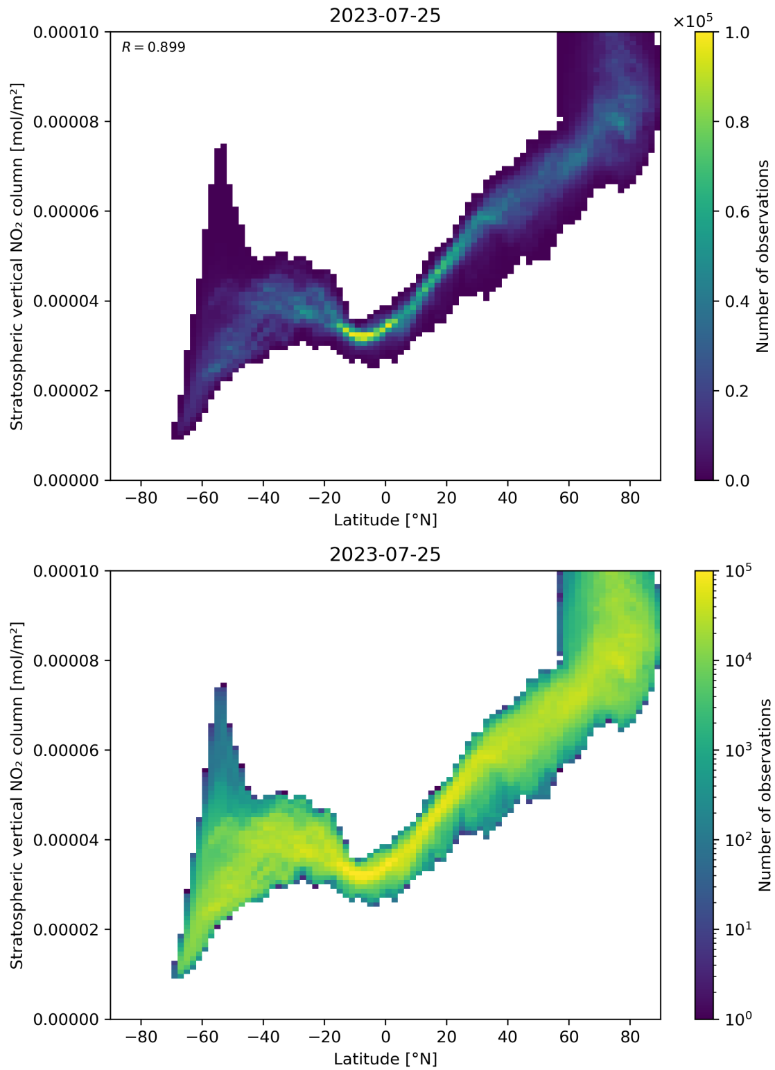
Figure 87: Scatter density plot of “Latitude” against “Stratospheric vertical NO 2 column” for 2023-07-24 to 2023-07-26.
