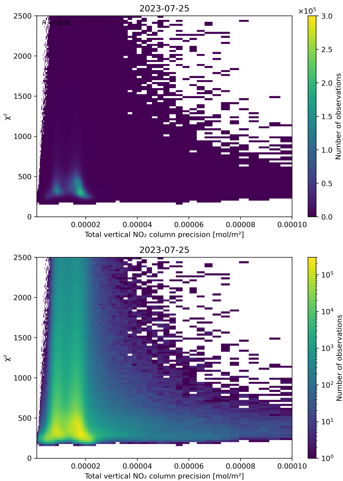
Figure 116: Scatter density plot of “Total vertical NO 2 column precision” against “ \chi^2 ” for 2023-07-24 to 2023-07-26.
