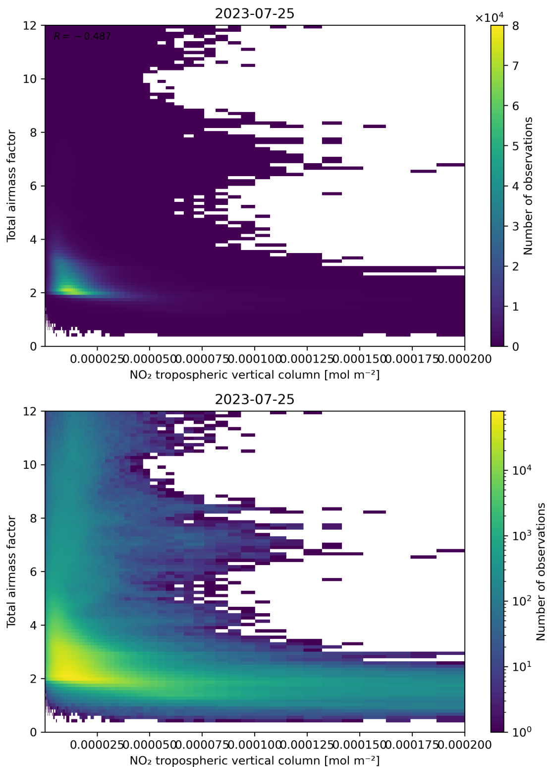
Figure 122: Scatter density plot of “NO 2 tropospheric vertical column” against “Total air mass factor” for 2023-07-24 to 2023-07-26.
