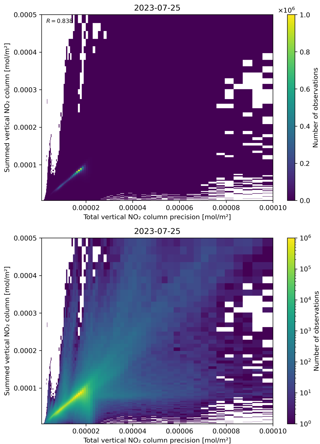
Figure 117: Scatter density plot of “Total vertical NO 2 column precision” against “Summed vertical NO 2 column” for 2023-07-24 to 2023-07-26.
