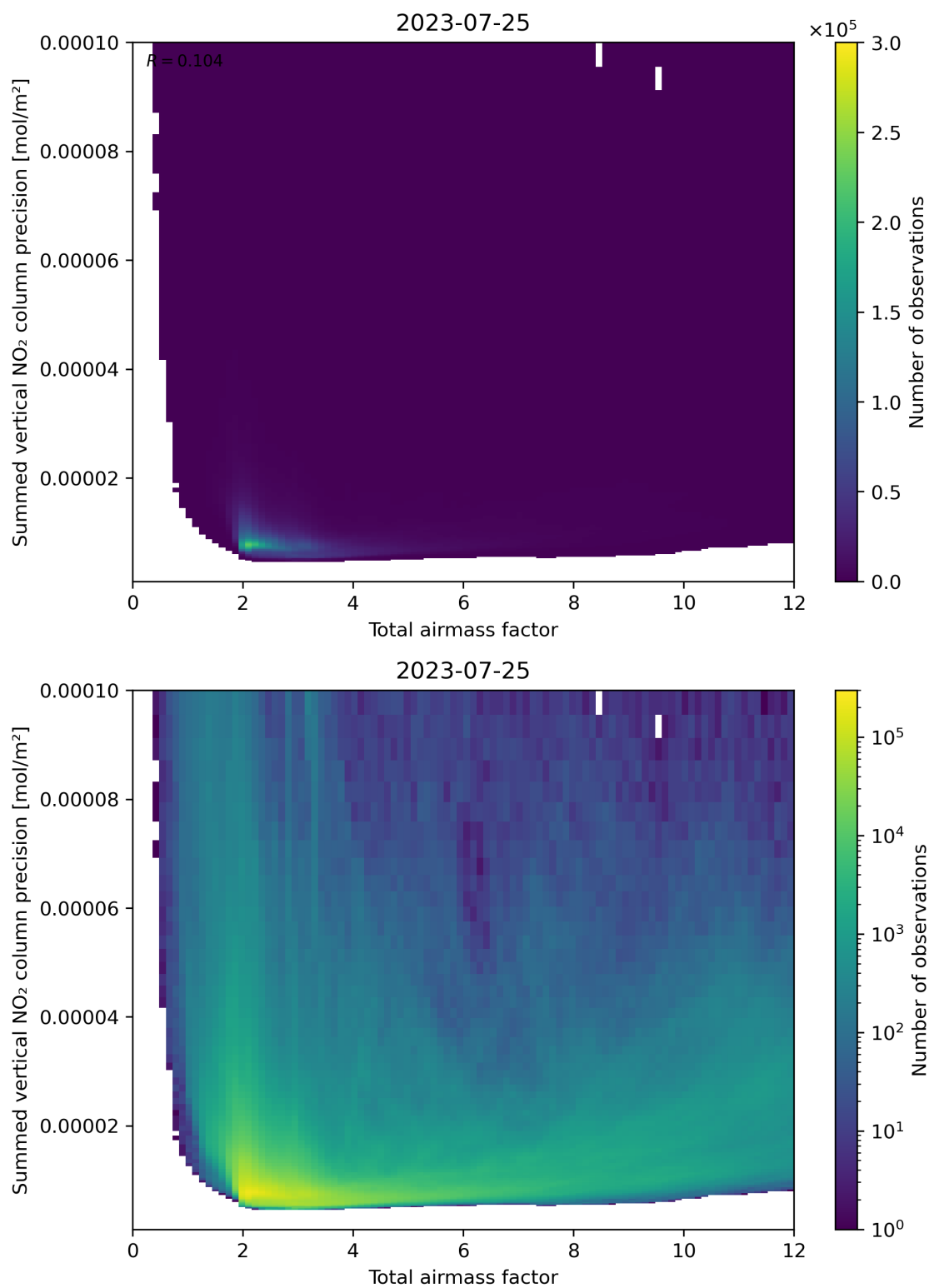
Figure 66: Scatter density plot of “Total airmass factor” against “Summed vertical NO 2 column precision” for 2023-07-24 to 2023-07-26.
