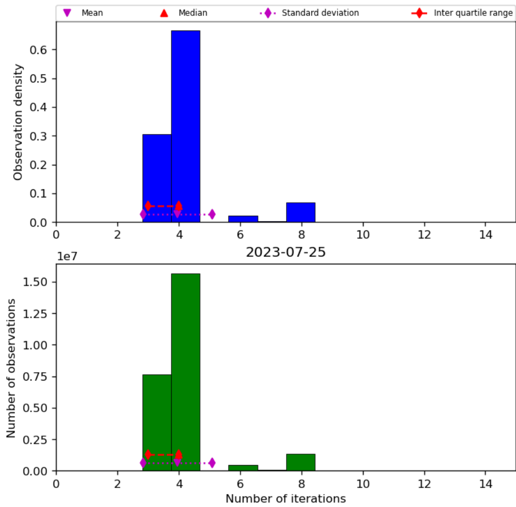
Figure 34: Histogram of “Number of iterations” for 2023-07-24 to 2023-07-26
