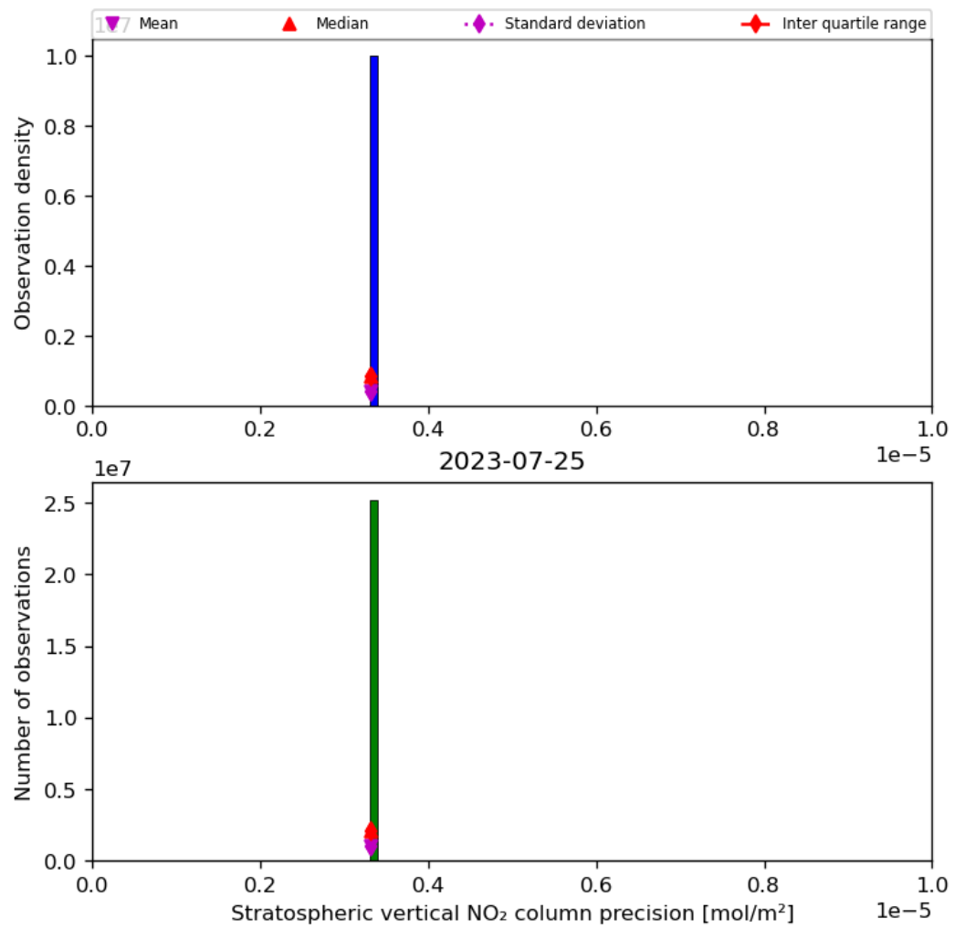
Figure 37: Histogram of “Stratospheric vertical NO 2 column precision” for 2023-07-24 to 2023-07-26
