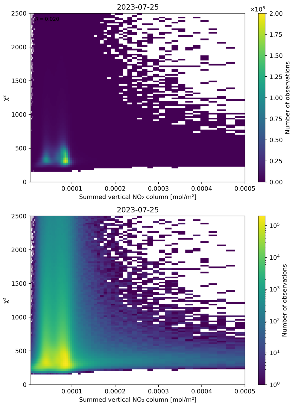
Figure 104: Scatter density plot of “Summed vertical NO 2 column” against “ \chi^2 ” for 2023-07-24 to 2023-07-26.
