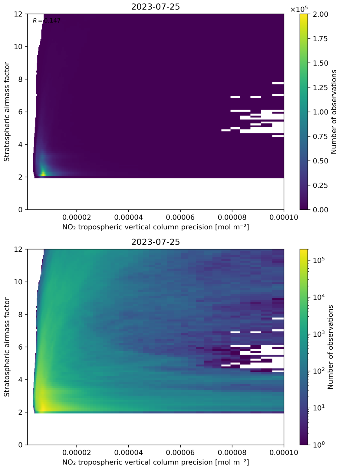
Figure 131: Scatter density plot of “NO 2 tropospheric vertical column precision” against “Stratospheric airmass factor” for 2023-07-24 to 2023-07-26.
