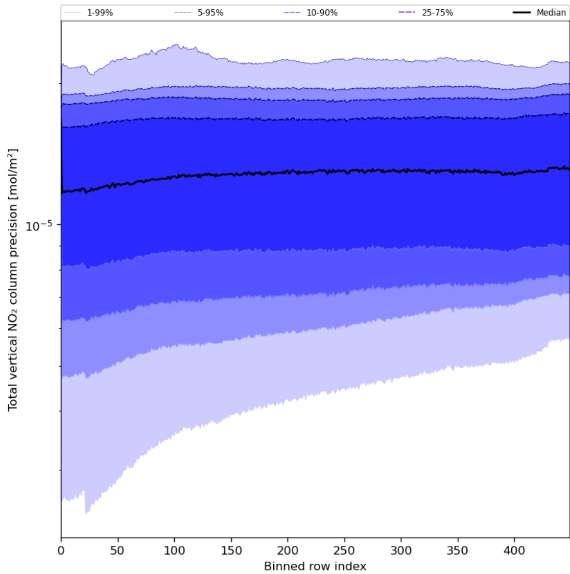
Figure 56: Along track statistics of “Total vertical NO 2 column precision” for 2023-07-24 to 2023-07-26
