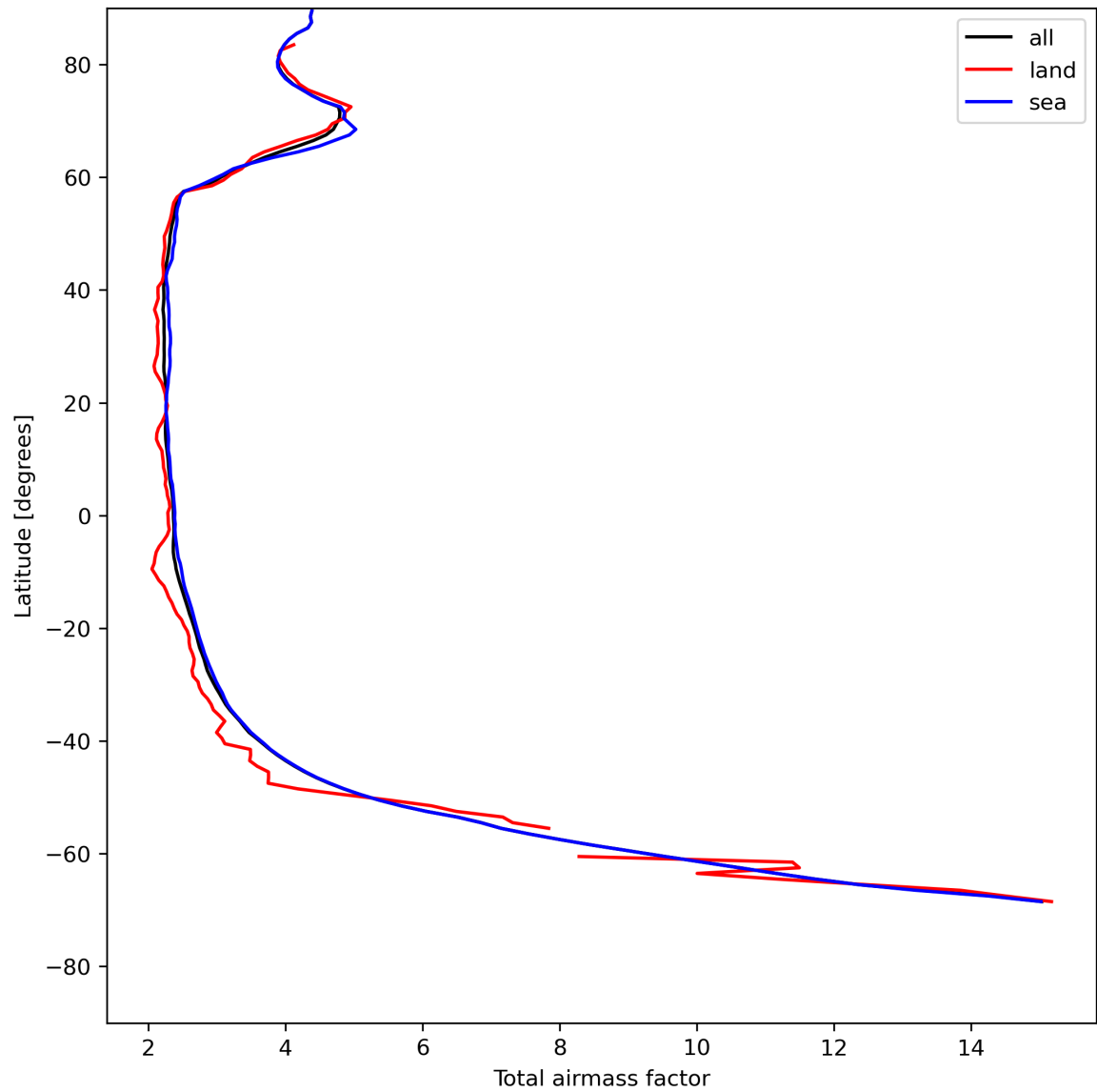
Figure 15: Zonal average of “Total airmass factor” for 2023-07-24 to 2023-07-26.
