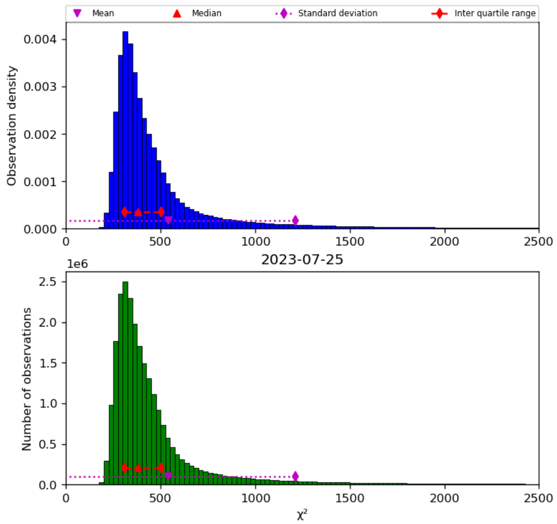
Figure 42: Histogram of " \chi^2 " for 2023-07-24 to 2023-07-26
