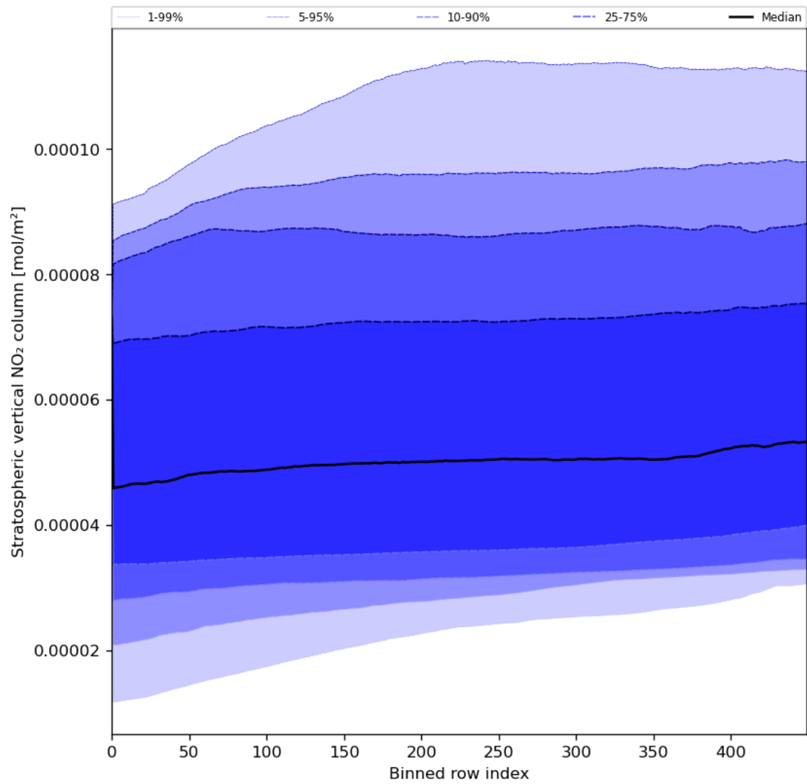
Figure 53: Along track statistics of “Stratospheric vertical NO 2 column” for 2023-07-24 to 2023-07-26
