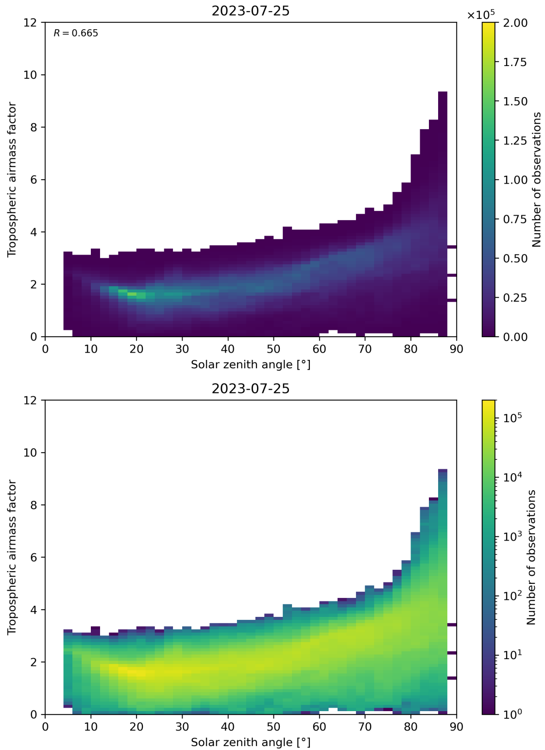
Figure 147: Scatter density plot of “Solar zenith angle” against “Tropospheric airmass factor” for 2023-07-24 to 2023-07-26.
