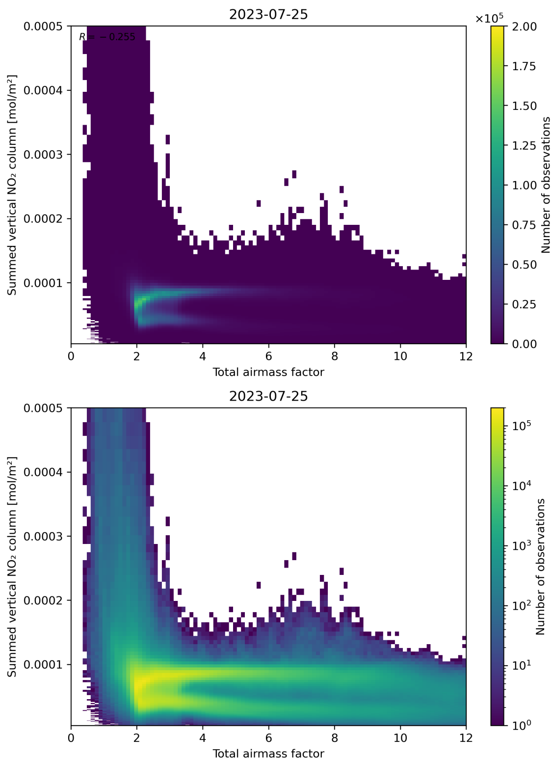
Figure 65: Scatter density plot of “Total airmass factor” against “Summed vertical NO 2 column” for 2023-07-24 to 2023-07-26.
