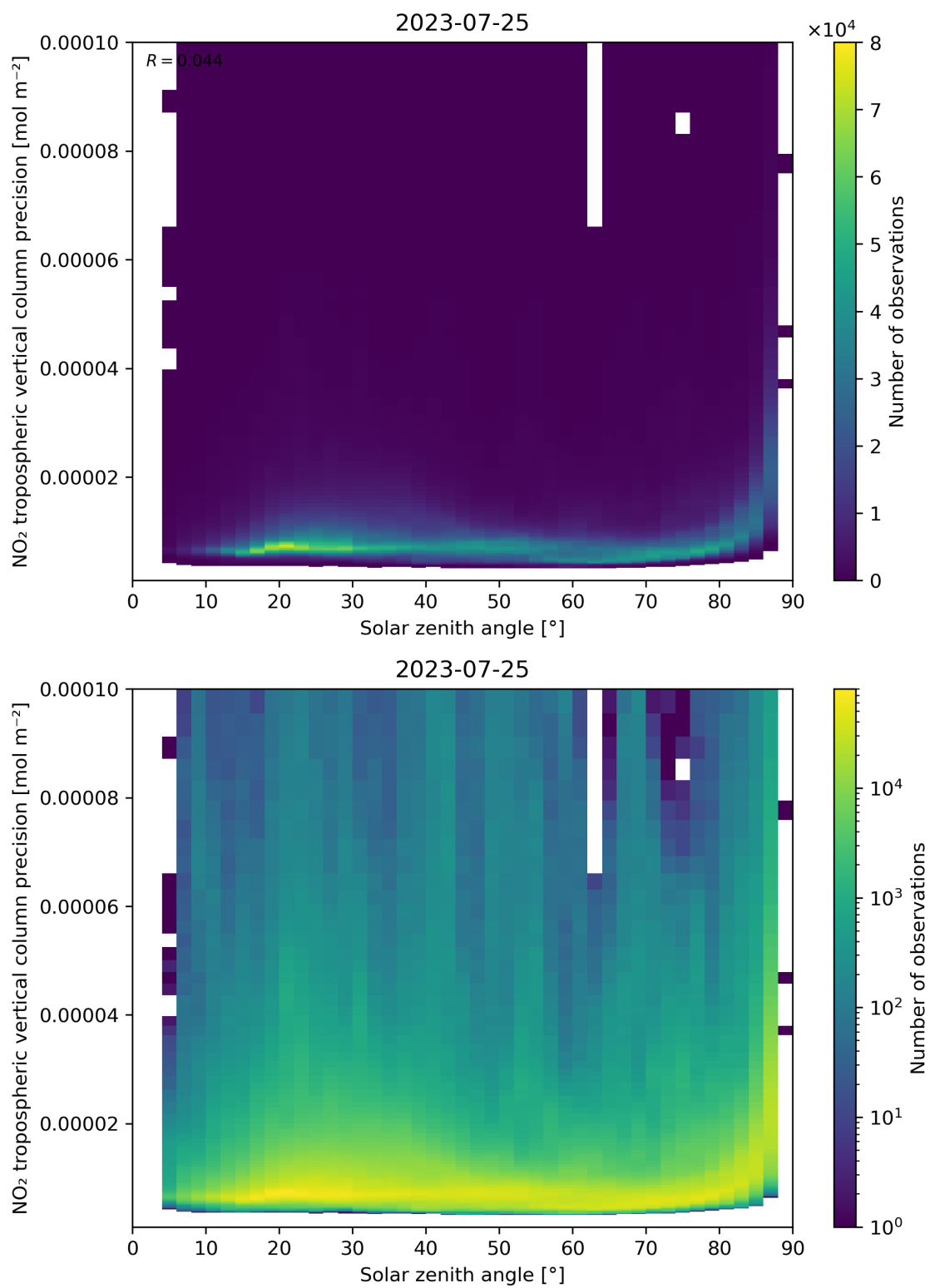
Figure 156: Scatter density plot of “Solar zenith angle” against “NO 2 tropospheric vertical column precision” for 2023-07-24 to 2023-07-26.
