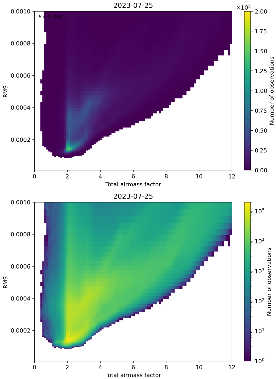
Figure 69: Scatter density plot of “Total airmass factor” against “RMS” for 2023-07-24 to 2023-07-26.
