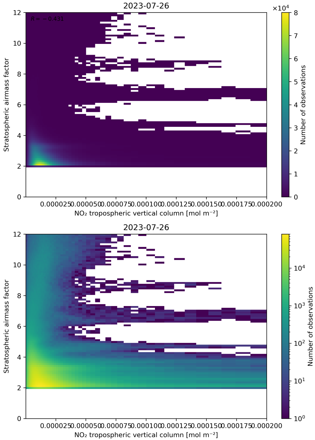
Figure 121: Scatter density plot of “NO 2 tropospheric vertical column” against “Stratospheric air mass factor” for 2023-07-25 to 2023-07-27.
