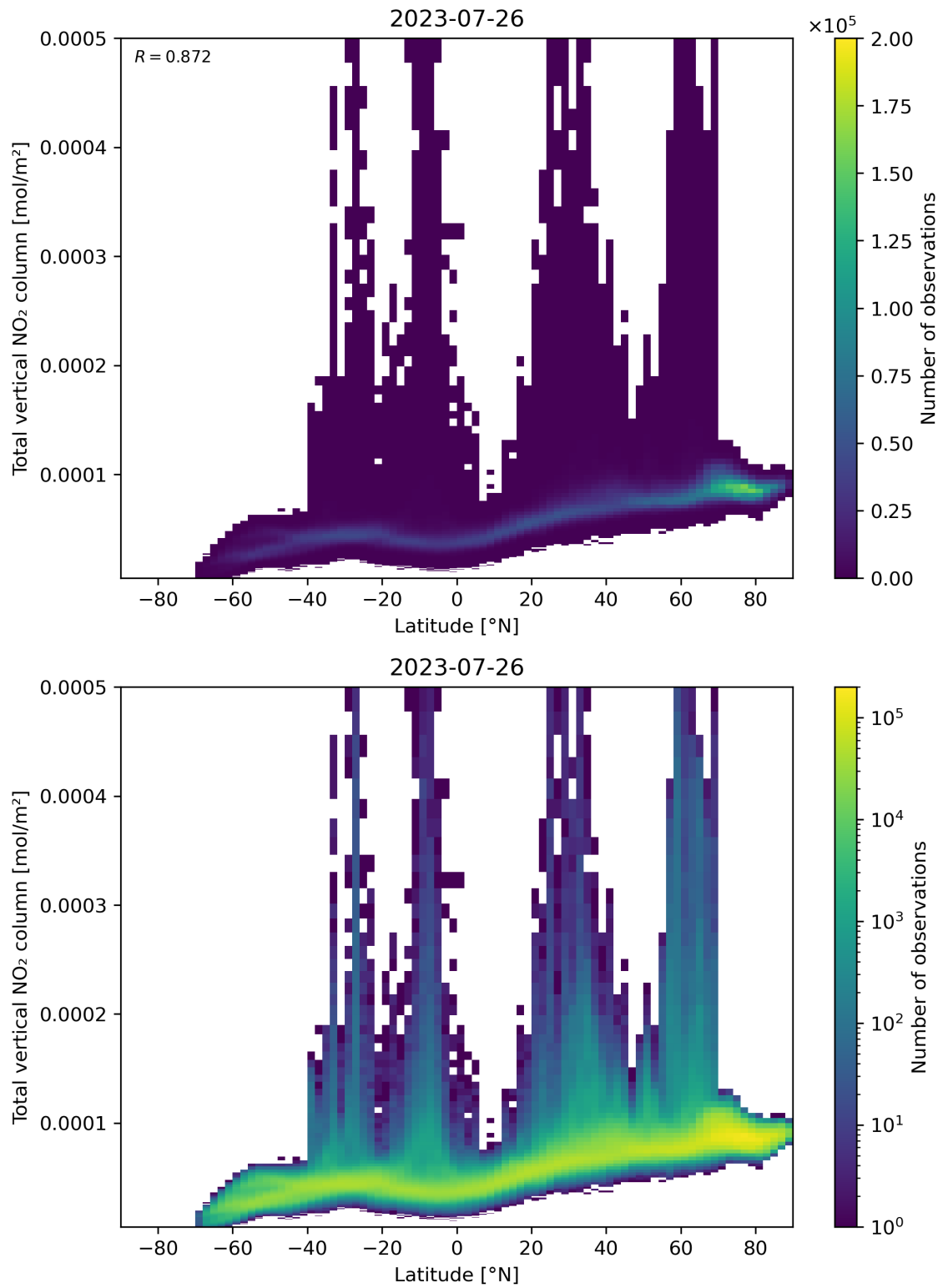
Figure 90: Scatter density plot of “Latitude” against “Total vertical NO 2 column” for 2023-07-25 to 2023-07-27.
