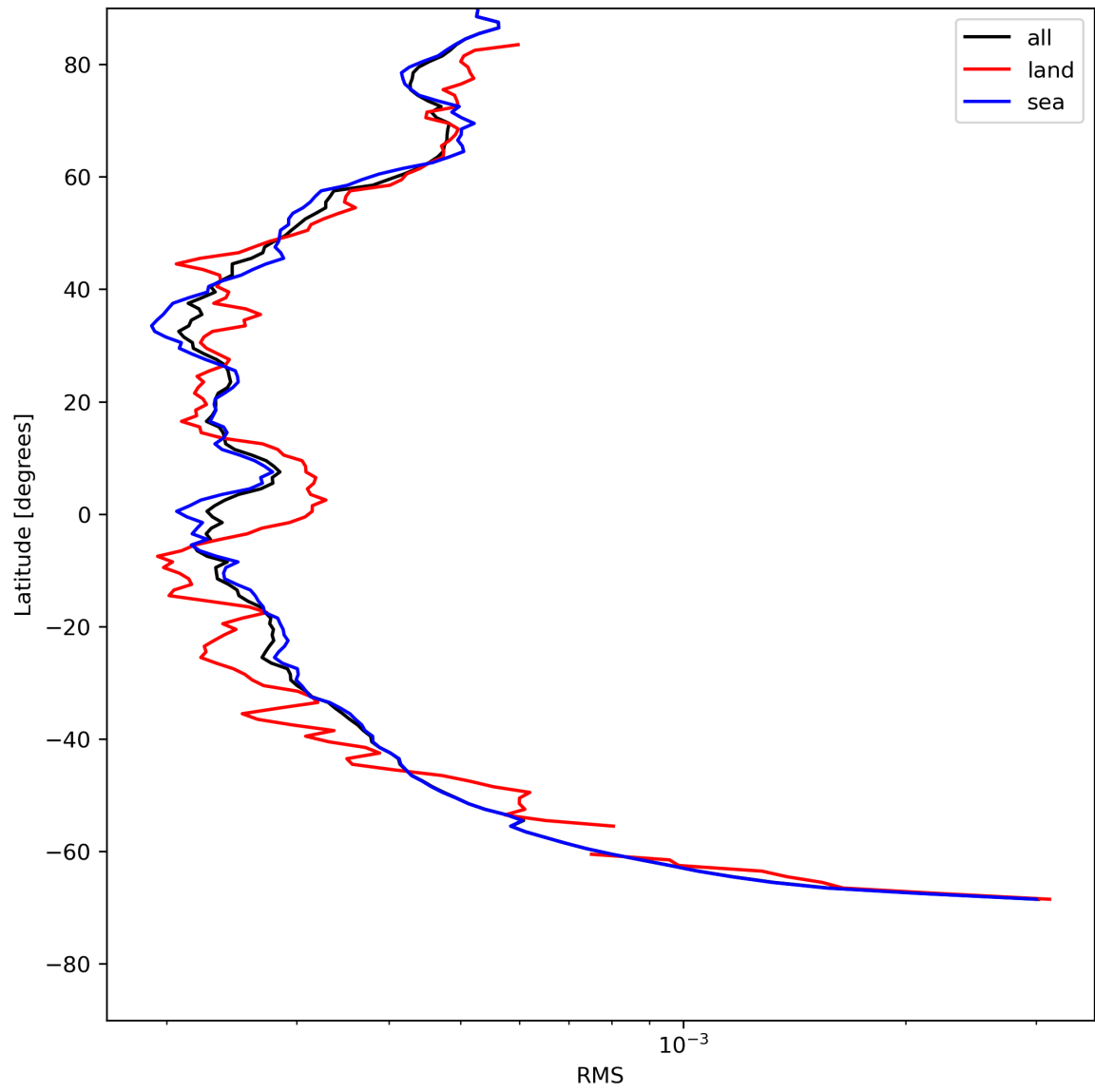
Figure 26: Zonal average of “RMS” for 2023-07-25 to 2023-07-27.
