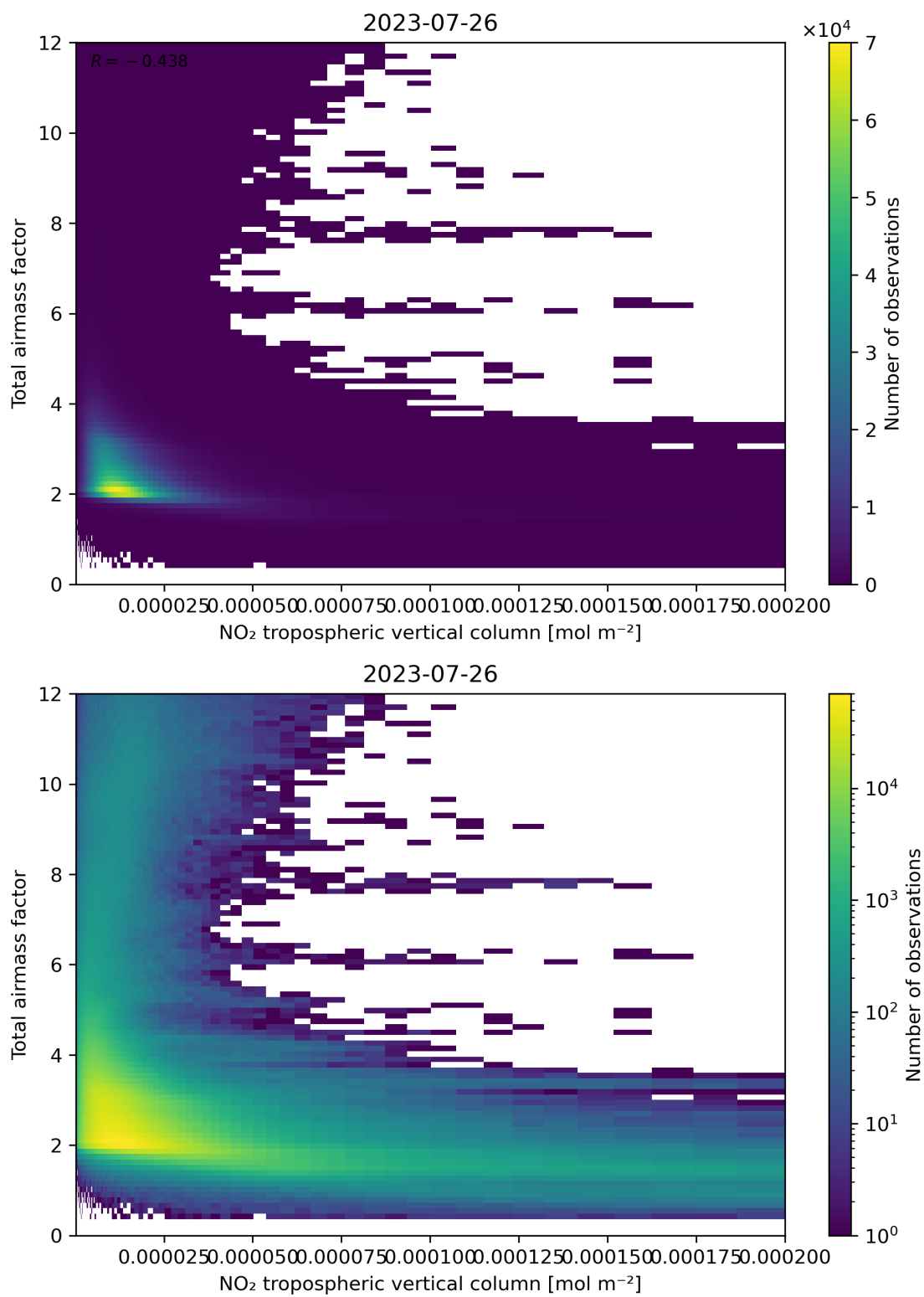
Figure 122: Scatter density plot of “NO 2 tropospheric vertical column” against “Total air mass factor” for 2023-07-25 to 2023-07-27.
