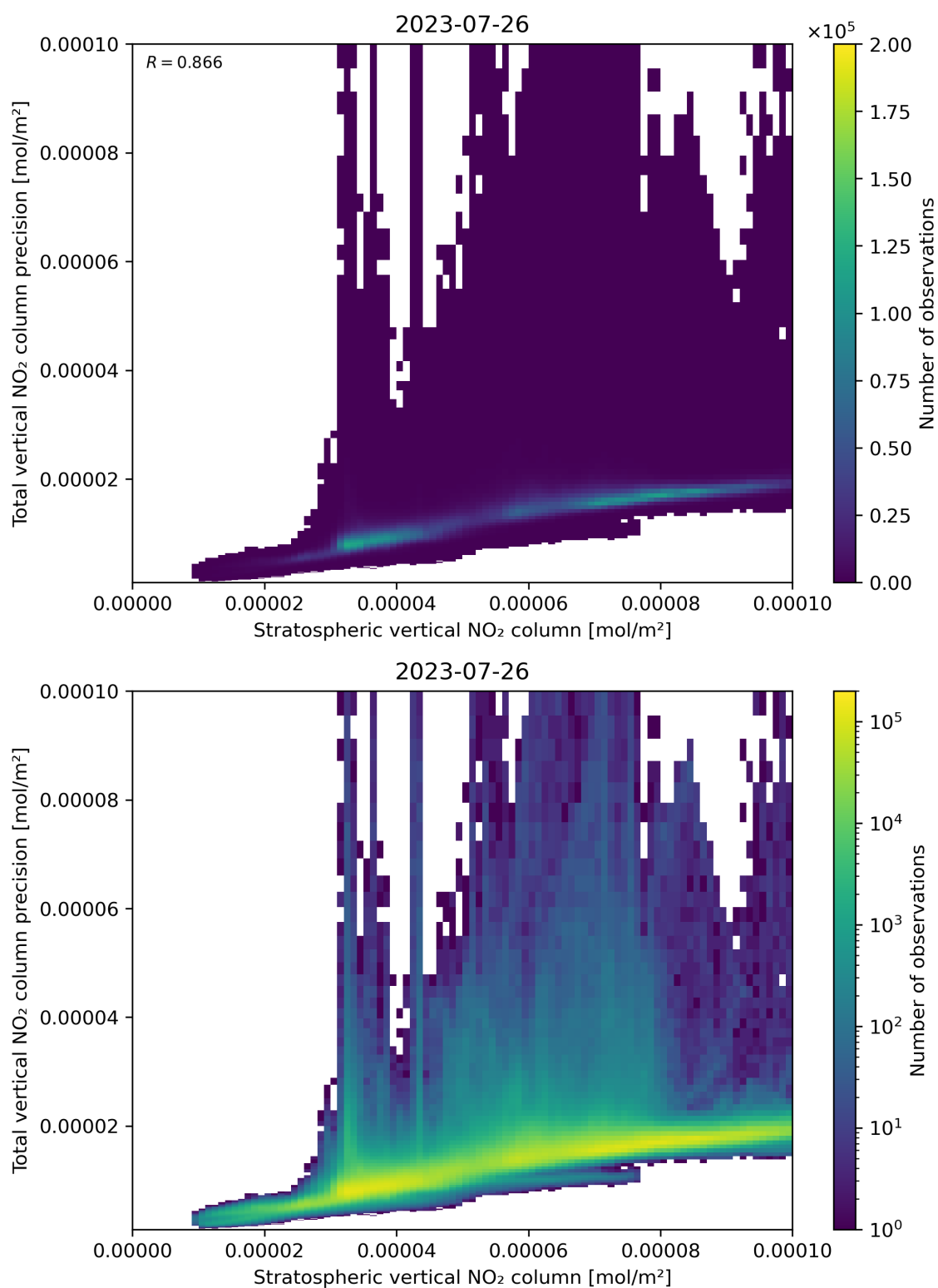
Figure 101: Scatter density plot of “Stratospheric vertical NO 2 column” against “Total vertical NO 2 column precision” for 2023-07-25 to 2023-07-27.
