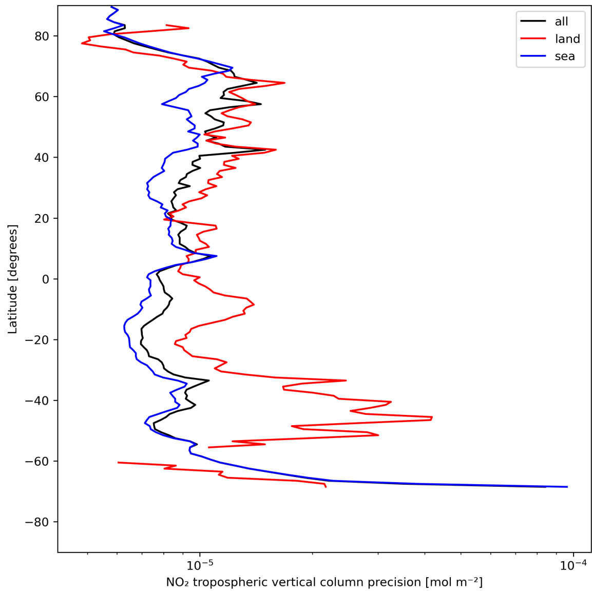
Figure 13: Zonal average of “NO 2 tropospheric vertical column precision” for 2023-07-25 to 2023-07-27.
