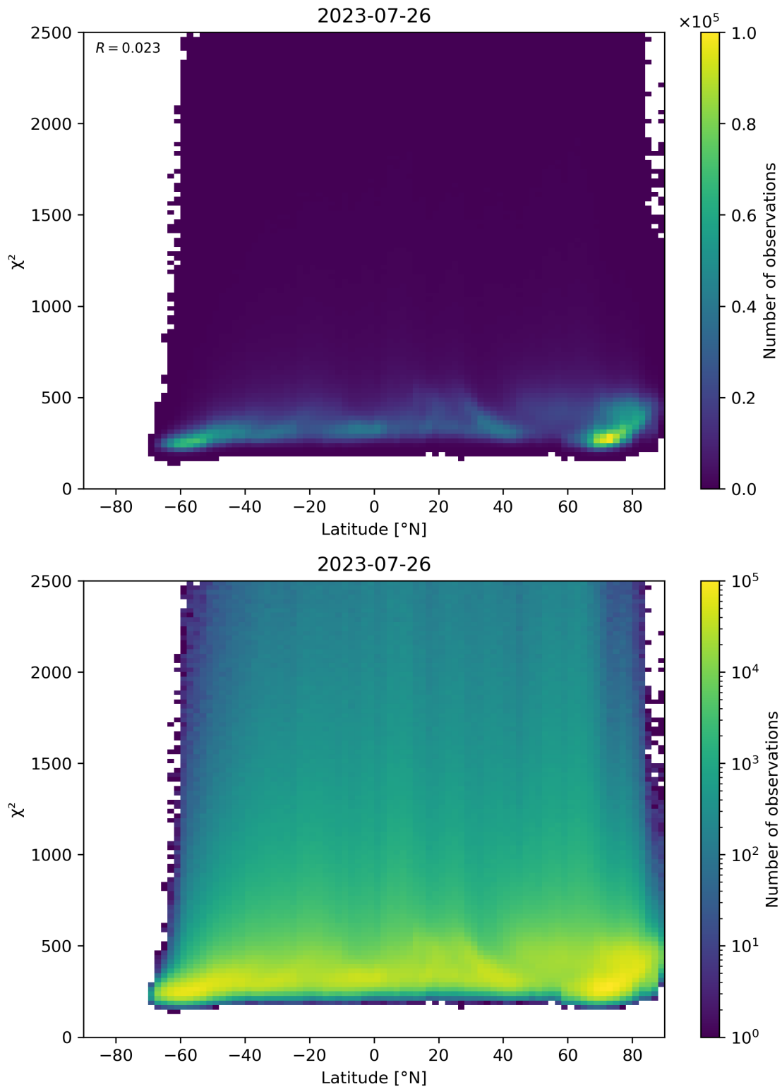
Figure 86: Scatter density plot of “Latitude” against “ \chi^2 ” for 2023-07-25 to 2023-07-27.
