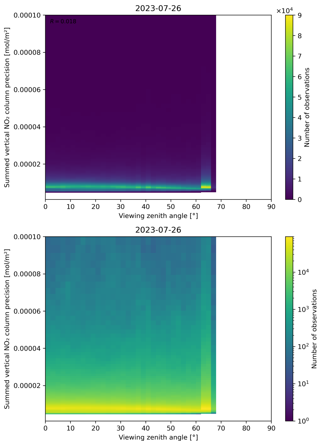
Figure 166: Scatter density plot of “Viewing zenith angle” against “Summed vertical NO 2 column precision” for 2023-07-25 to 2023-07-27.
