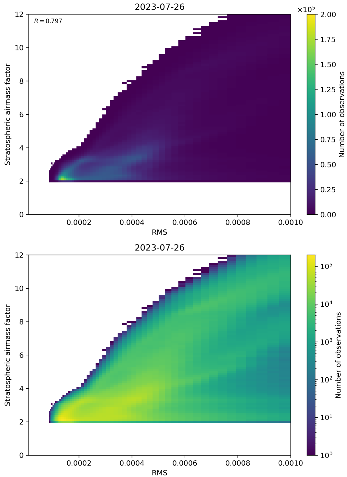
Figure 144: Scatter density plot of “RMS” against “Stratospheric airmass factor” for 2023-07-25 to 2023-07-27.
