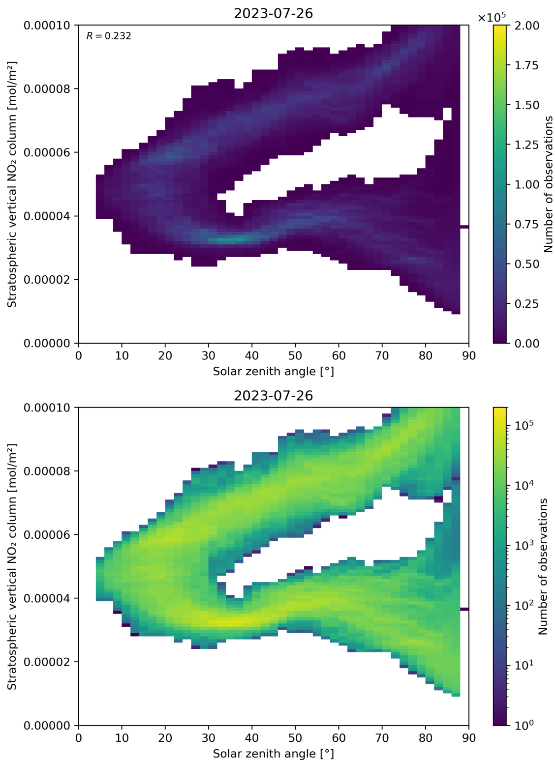
Figure 150: Scatter density plot of “Solar zenith angle” against “Stratospheric vertical NO 2 column” for 2023-07-25 to 2023-07-27.
