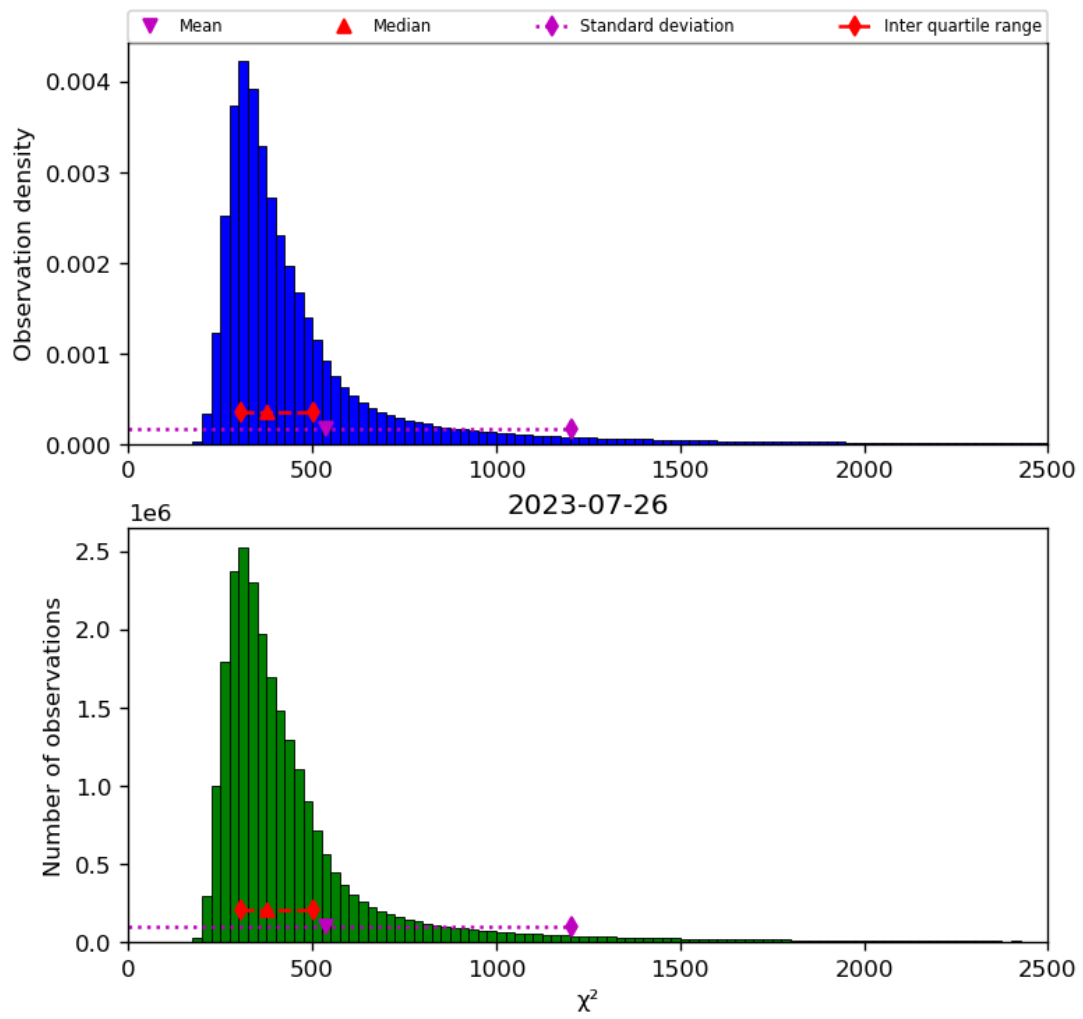
Figure 42: Histogram of " \chi^2 " for 2023-07-25 to 2023-07-27
