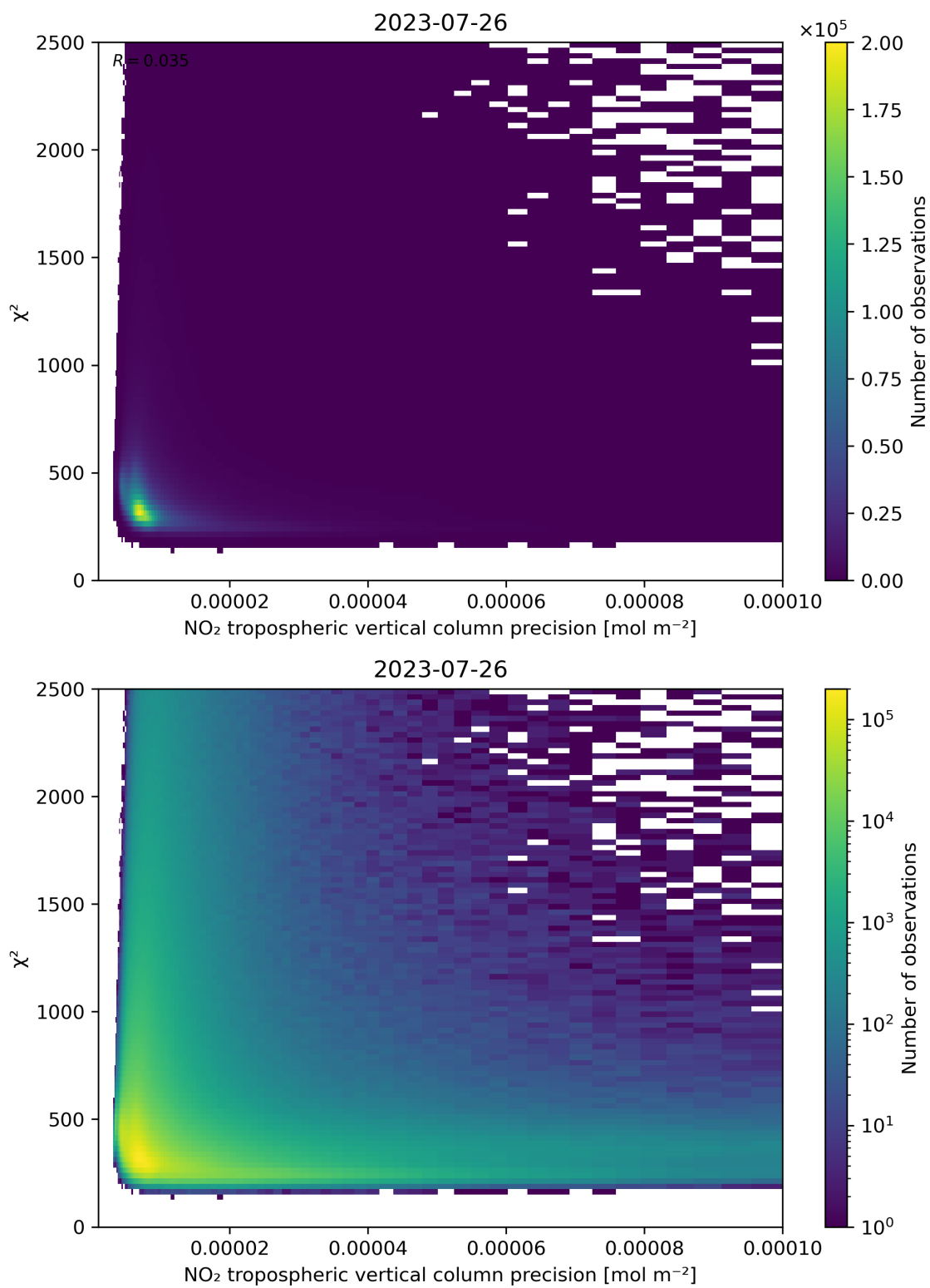
Figure 134: Scatter density plot of “NO 2 tropospheric vertical column precision” against “ \chi^2 ” for 2023-07-25 to 2023-07-27.
