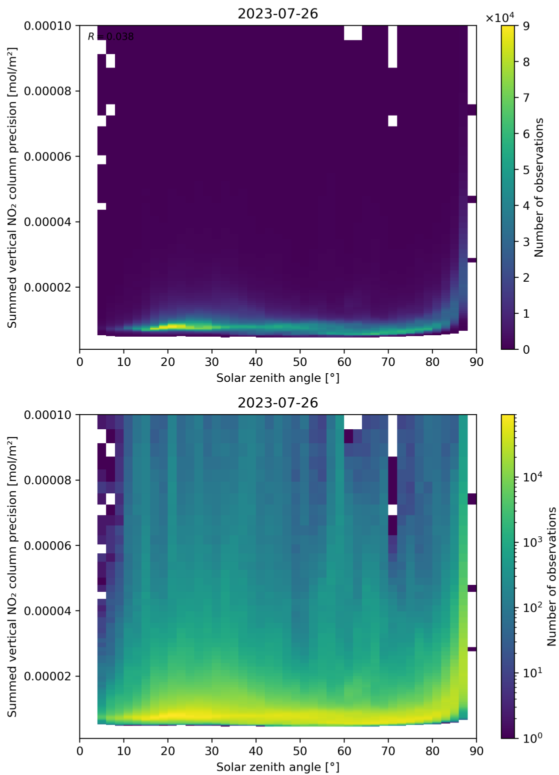
Figure 152: Scatter density plot of “Solar zenith angle” against “Summed vertical NO 2 column precision” for 2023-07-25 to 2023-07-27.
