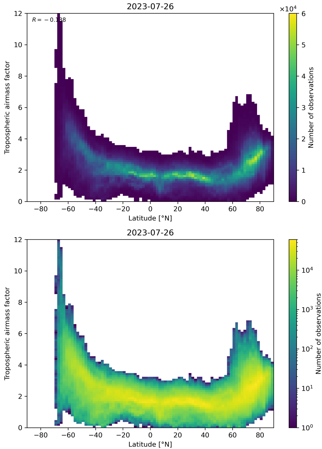
Figure 85: Scatter density plot of “Latitude” against “Tropospheric air mass factor” for 2023-07-25 to 2023-07-27.
