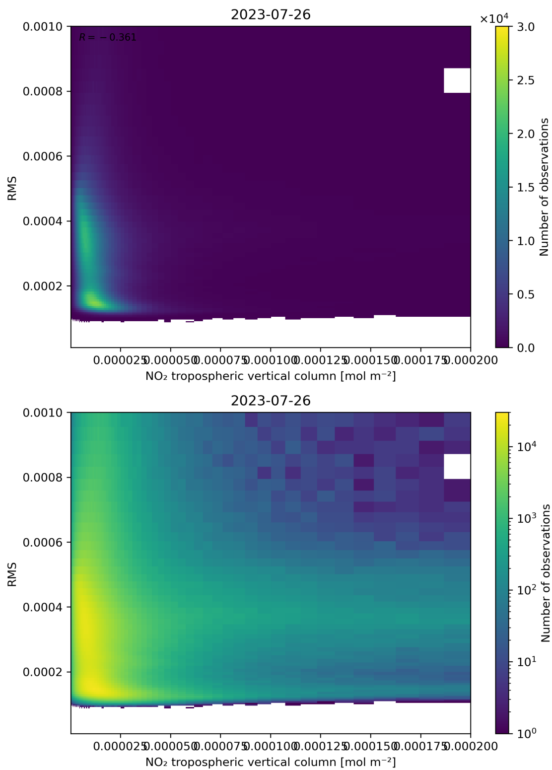
Figure 142: Scatter density plot of “NO 2 tropospheric vertical column” against “RMS” for 2023-07-25 to 2023-07-27.
