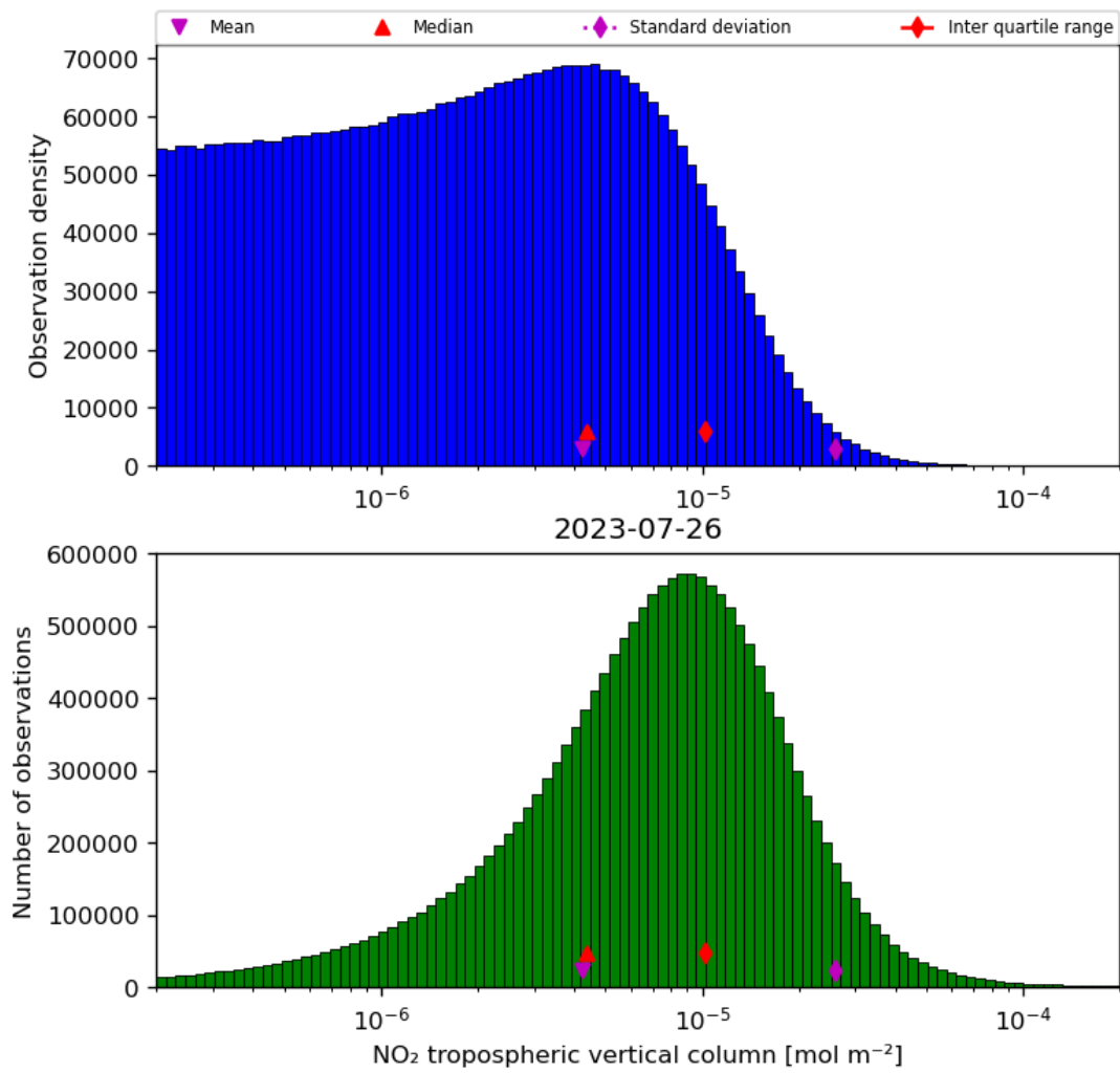
Figure 29: Histogram of “NO 2 tropospheric vertical column” for 2023-07-25 to 2023-07-27
