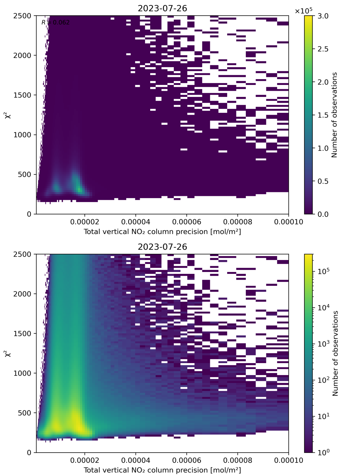
Figure 116: Scatter density plot of “Total vertical NO 2 column precision” against “ \chi^2 ” for 2023-07-25 to 2023-07-27.
