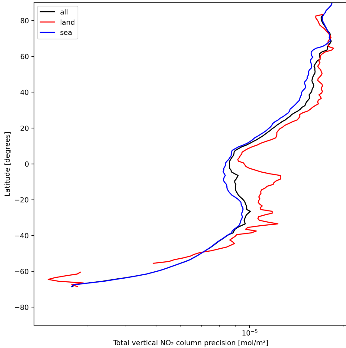
Figure 22: Zonal average of “Total vertical NO 2 column precision” for 2023-07-25 to 2023-07-27.
