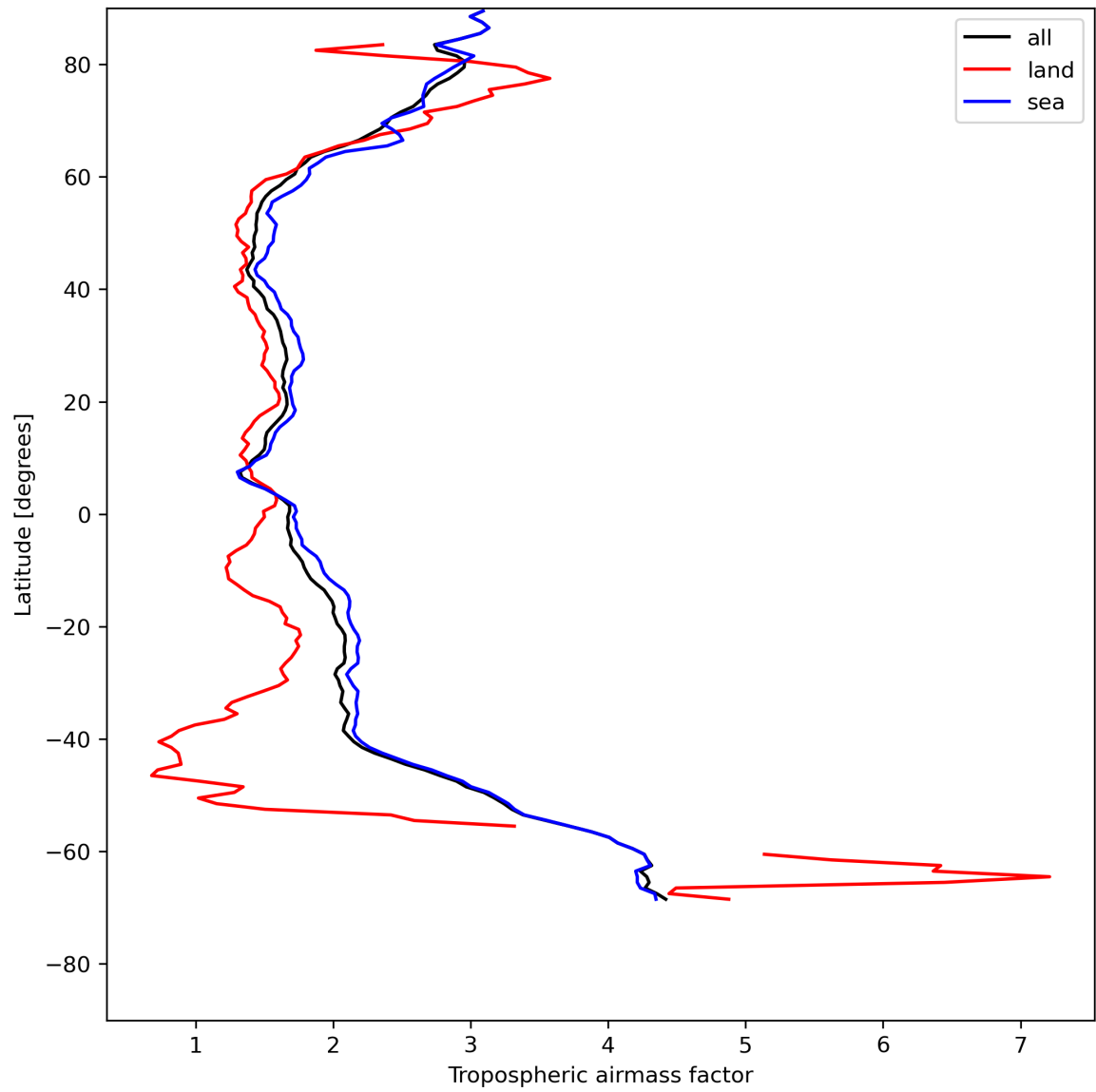
Figure 14: Zonal average of “Tropospheric air mass factor” for 2023-07-25 to 2023-07-27.
