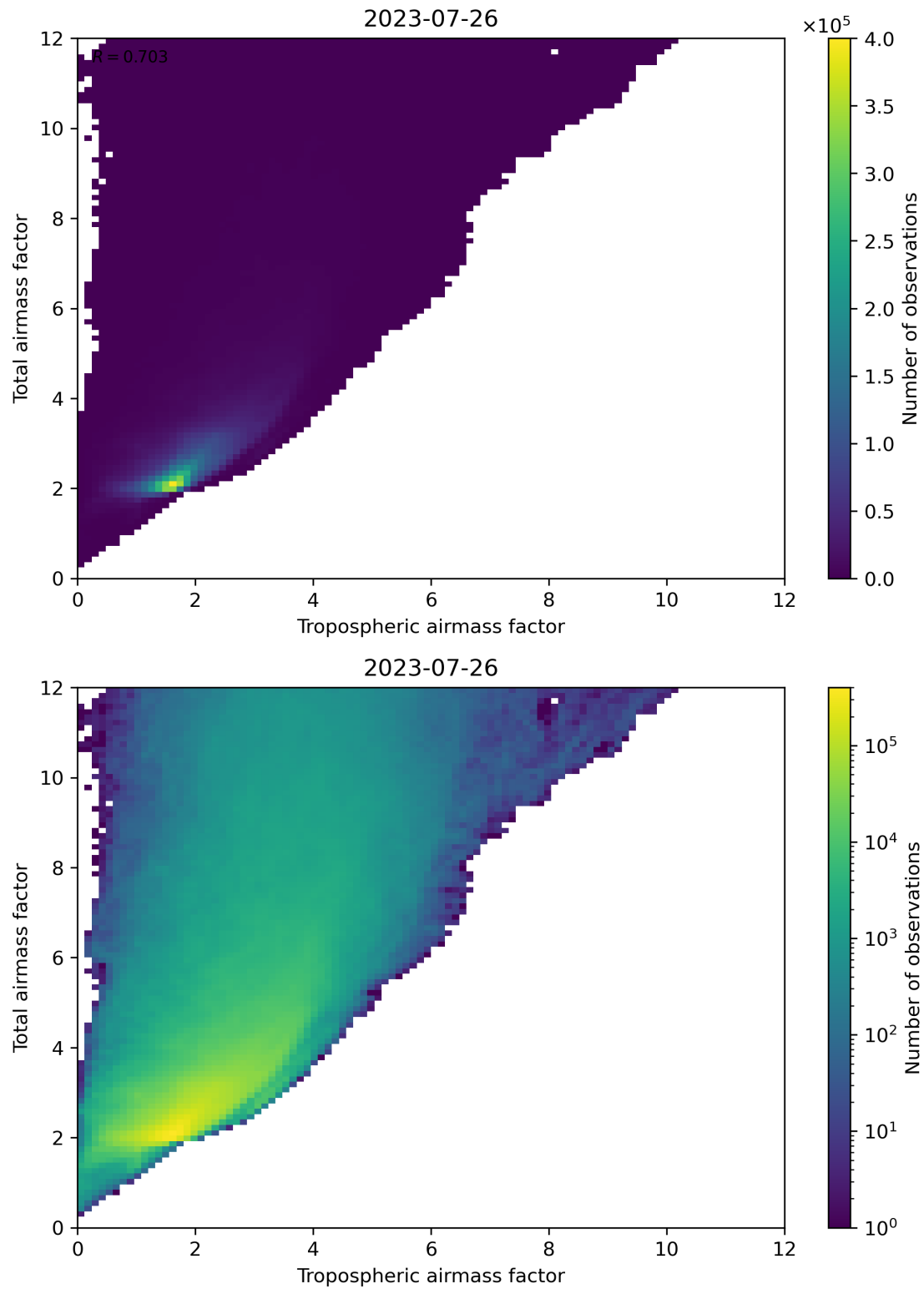
Figure 72: Scatter density plot of “Tropospheric airmass factor” against “Total airmass factor” for 2023-07-25 to 2023-07-27.
