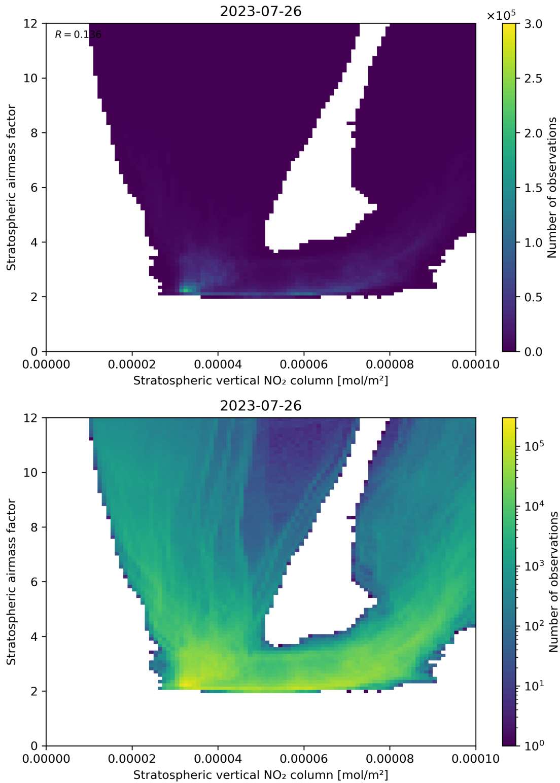
Figure 96: Scatter density plot of “Stratospheric vertical NO 2 column” against “Stratospheric airmass factor” for 2023-07-25 to 2023-07-27.
