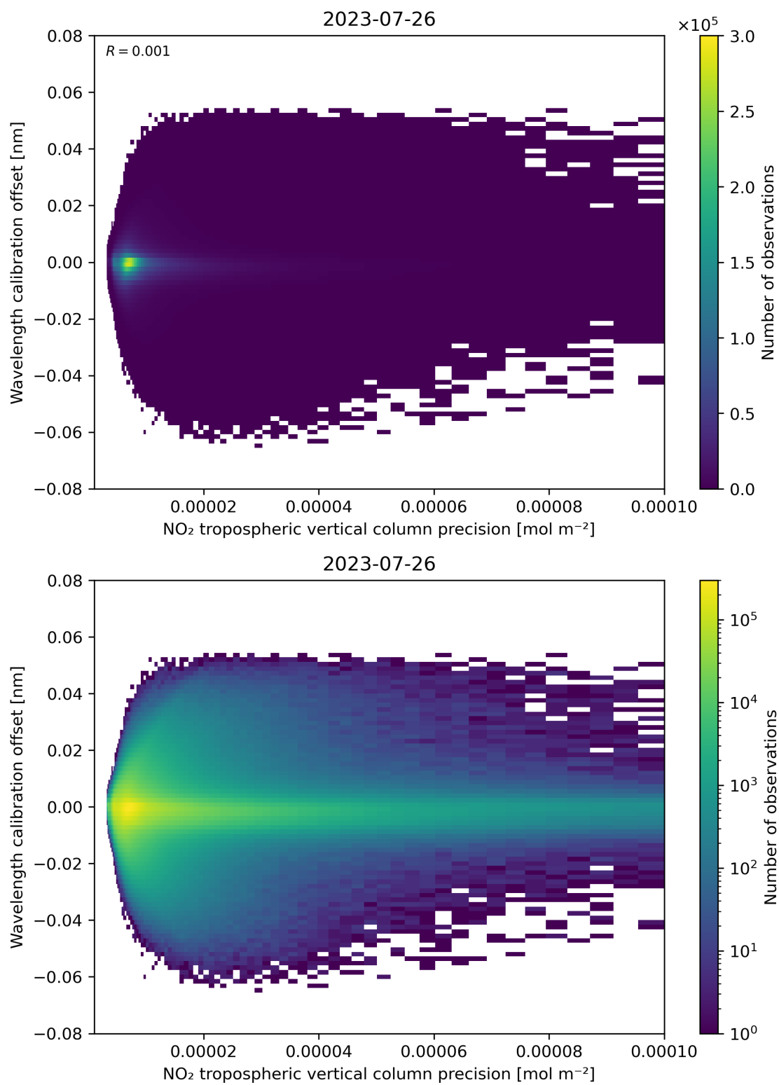
Figure 141: Scatter density plot of “NO 2 tropospheric vertical column precision” against “Wavelength calibration offset” for 2023-07-25 to 2023-07-27.
