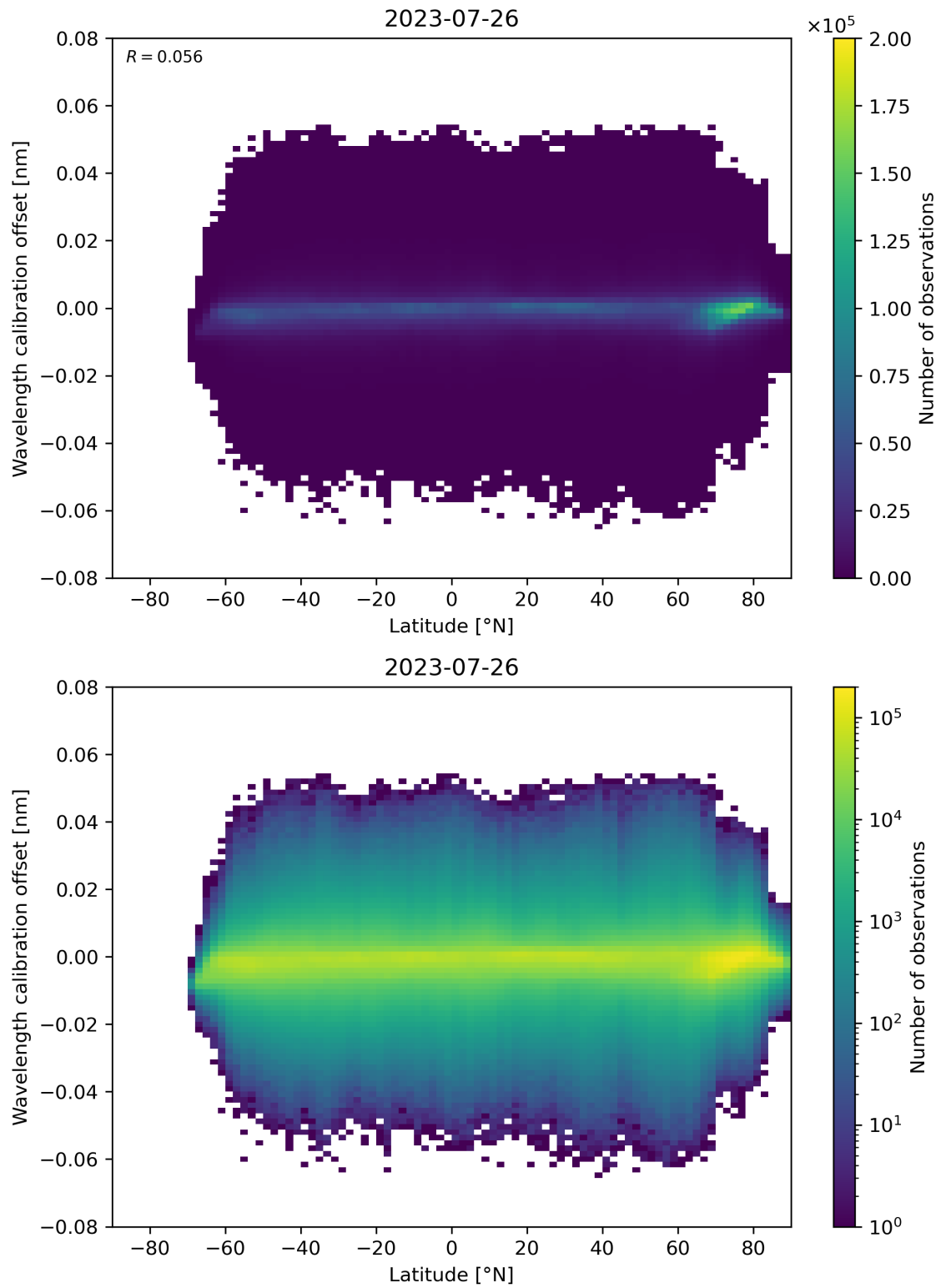
Figure 95: Scatter density plot of “Latitude” against “Wavelength calibration offset” for 2023-07-25 to 2023-07-27.
