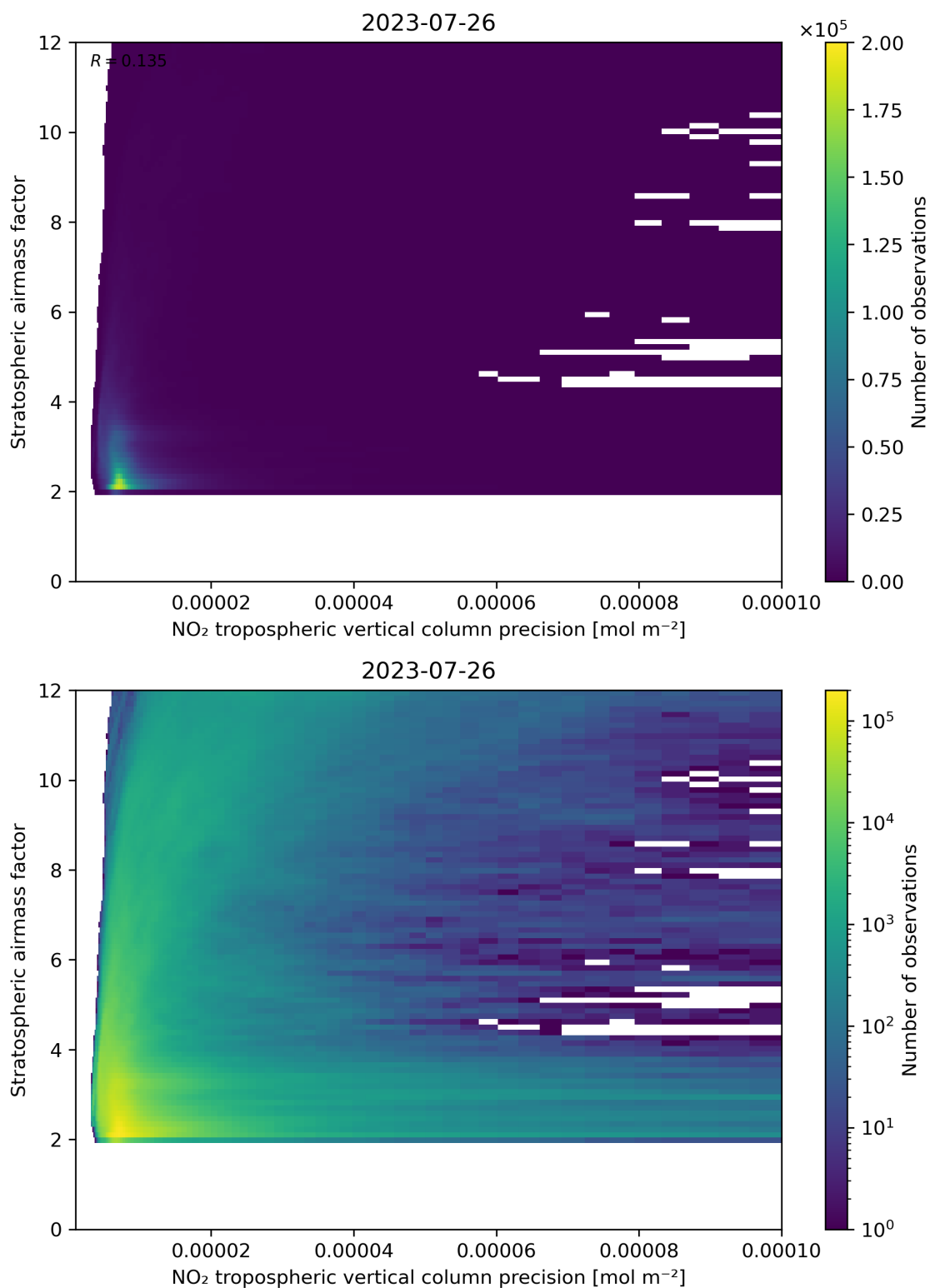
Figure 131: Scatter density plot of “NO 2 tropospheric vertical column precision” against “Stratospheric airmass factor” for 2023-07-25 to 2023-07-27.
