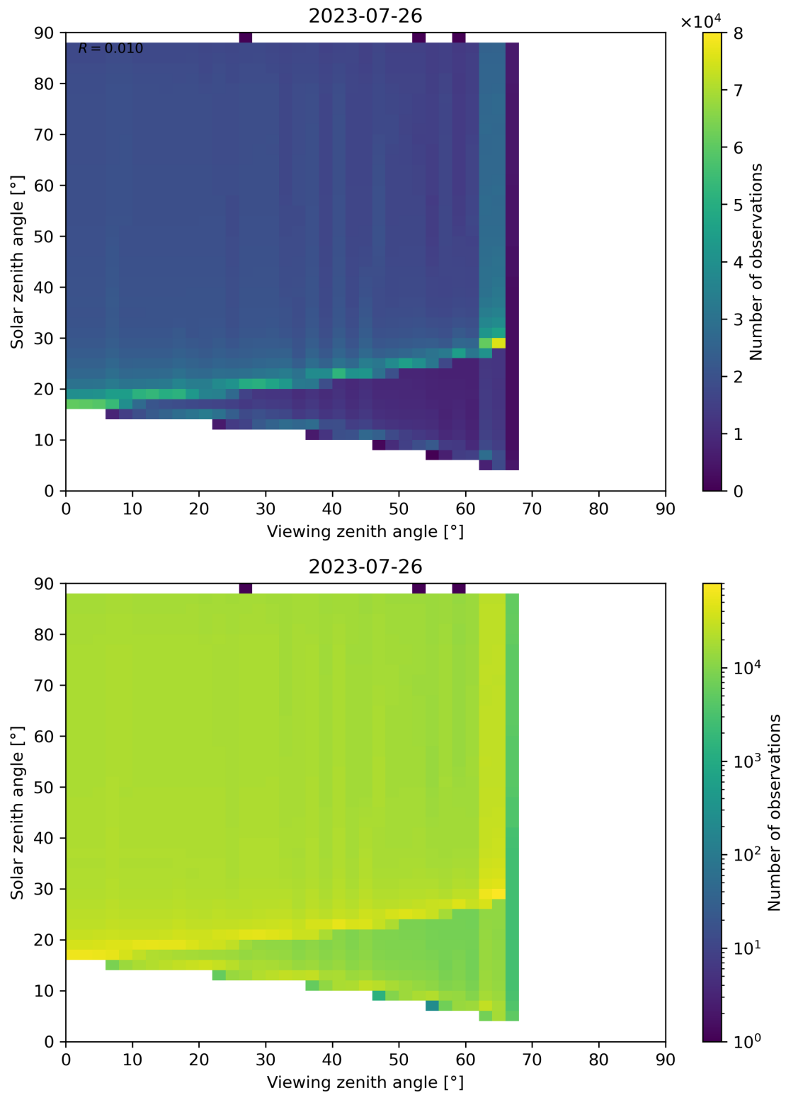
Figure 172: Scatter density plot of “Viewing zenith angle” against “Solar zenith angle” for 2023-07-25 to 2023-07-27.
