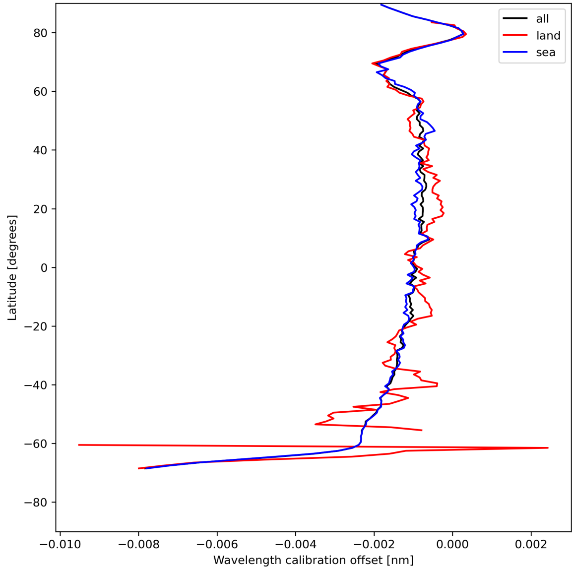
Figure 18: Zonal average of “Wavelength calibration offset” for 2023-07-25 to 2023-07-27.
