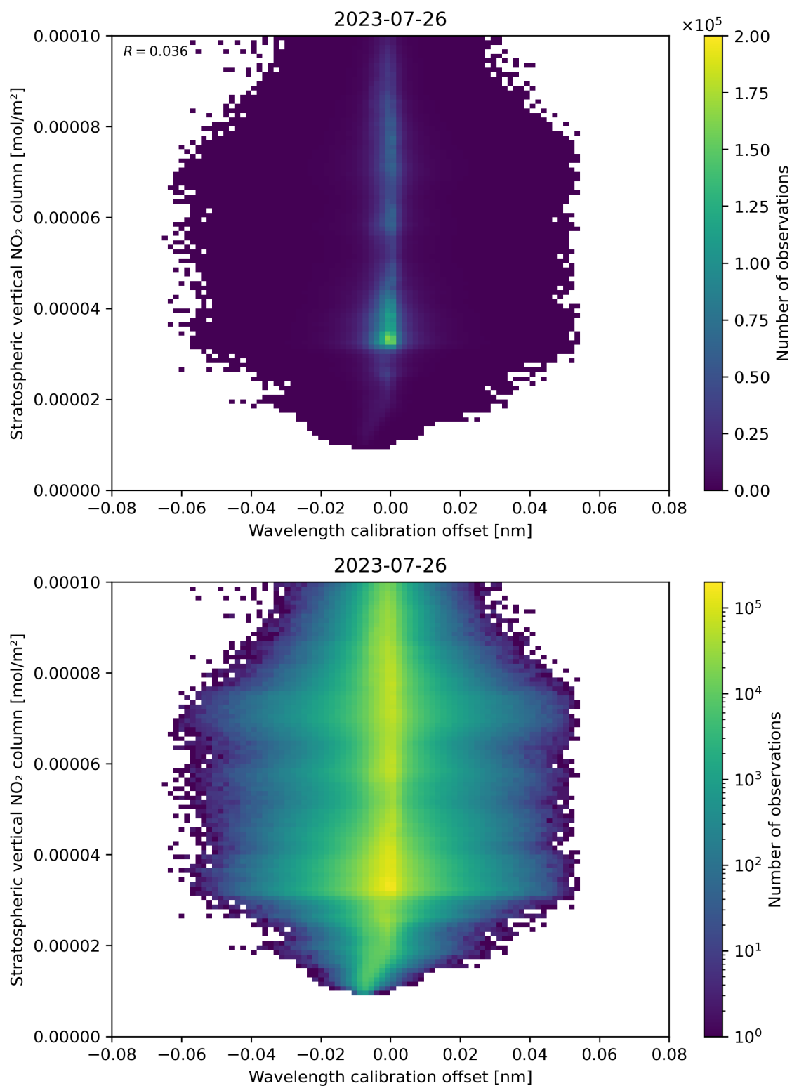
Figure 176: Scatter density plot of “Wavelength calibration offset” against “Stratospheric vertical NO 2 column” for 2023-07-25 to 2023-07-27.
