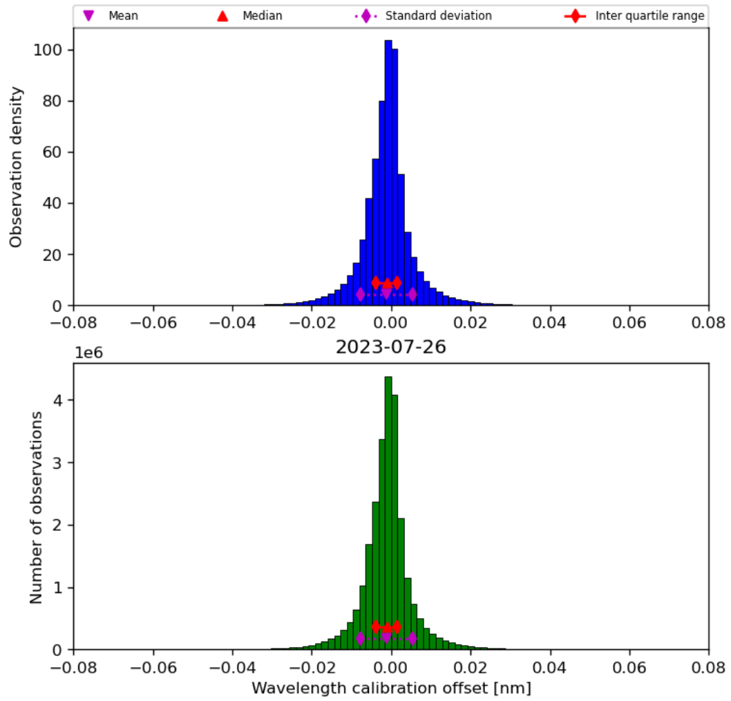
Figure 35: Histogram of “Wavelength calibration offset” for 2023-07-25 to 2023-07-27
