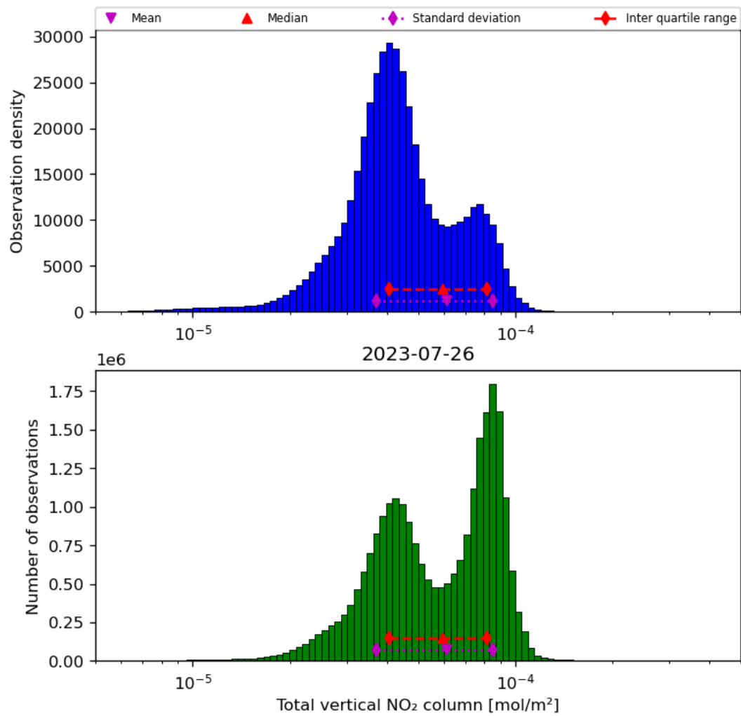
Figure 38: Histogram of “Total vertical NO 2 column” for 2023-07-25 to 2023-07-27
