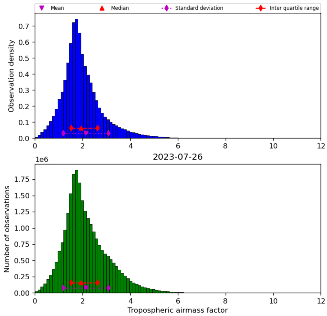
Figure 31: Histogram of “Tropospheric airmass factor” for 2023-07-25 to 2023-07-27
