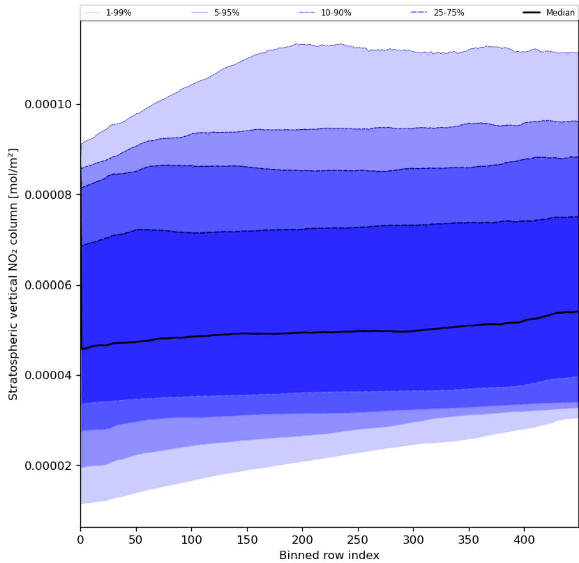
Figure 53: Along track statistics of “Stratospheric vertical NO 2 column” for 2023-07-25 to 2023-07-27
