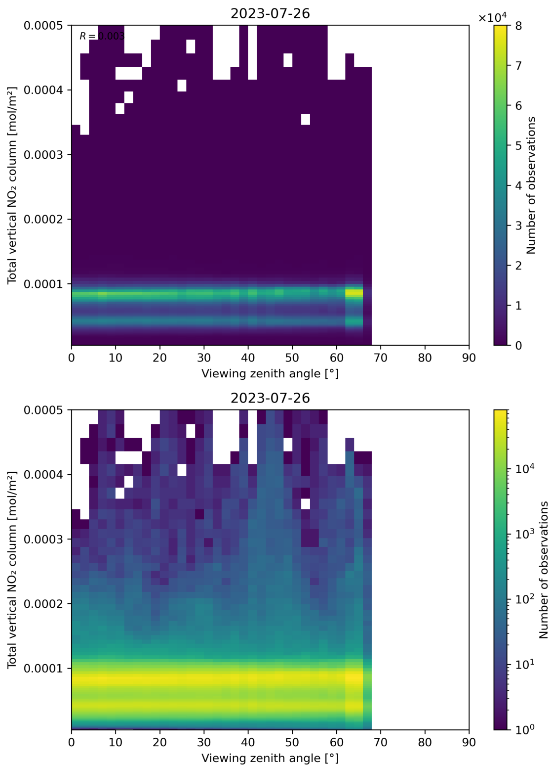
Figure 167: Scatter density plot of “Viewing zenith angle” against “Total vertical NO 2 column” for 2023-07-25 to 2023-07-27.
