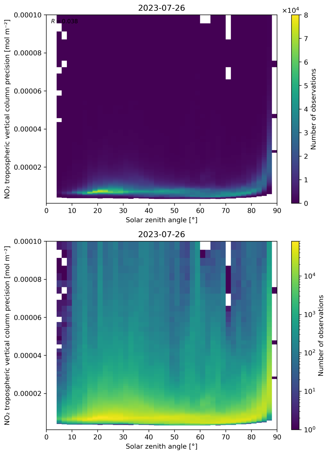
Figure 156: Scatter density plot of “Solar zenith angle” against “NO 2 tropospheric vertical column precision” for 2023-07-25 to 2023-07-27.
