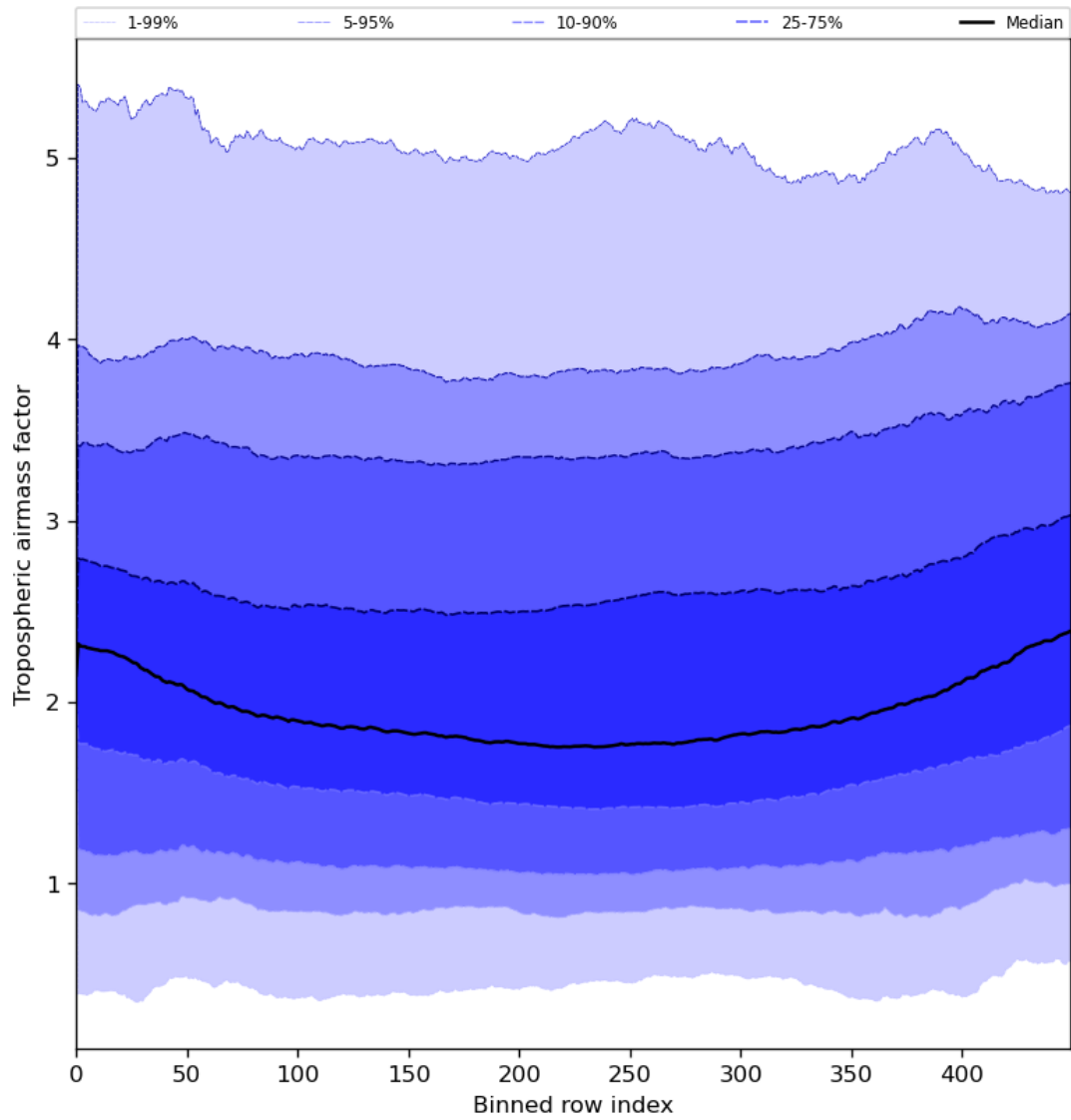
Figure 48: Along track statistics of “Tropospheric airmass factor” for 2023-07-25 to 2023-07-27
