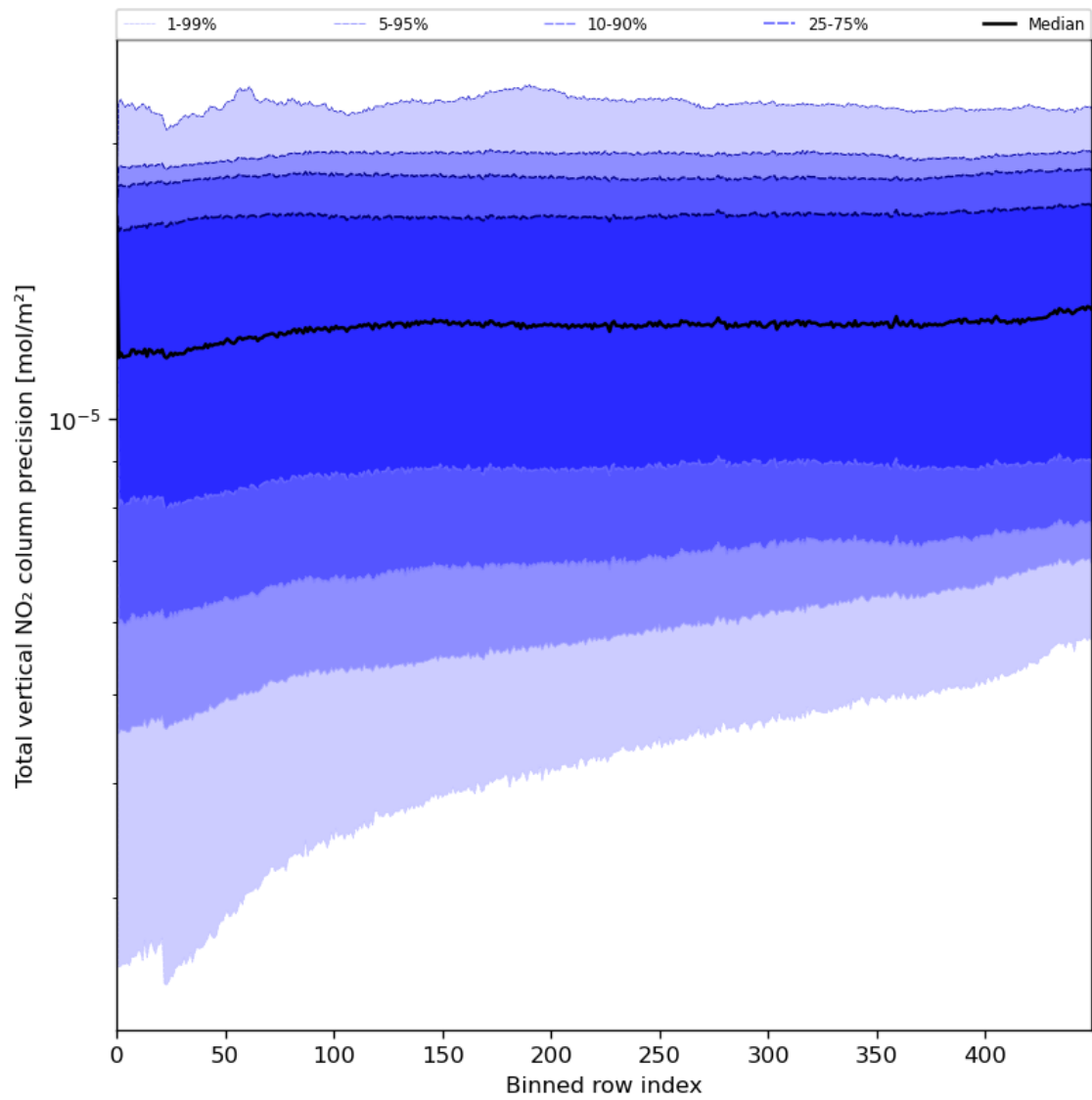
Figure 56: Along track statistics of “Total vertical NO 2 column precision” for 2023-07-25 to 2023-07-27
