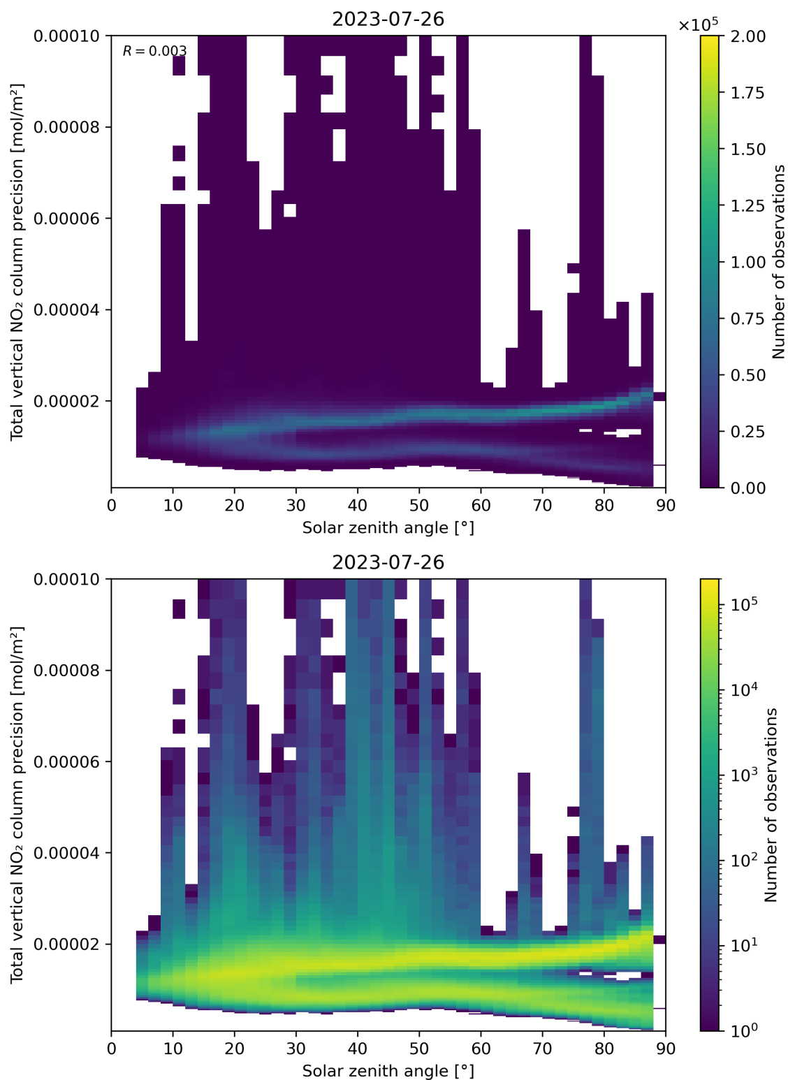
Figure 154: Scatter density plot of “Solar zenith angle” against “Total vertical NO 2 column precision” for 2023-07-25 to 2023-07-27.
