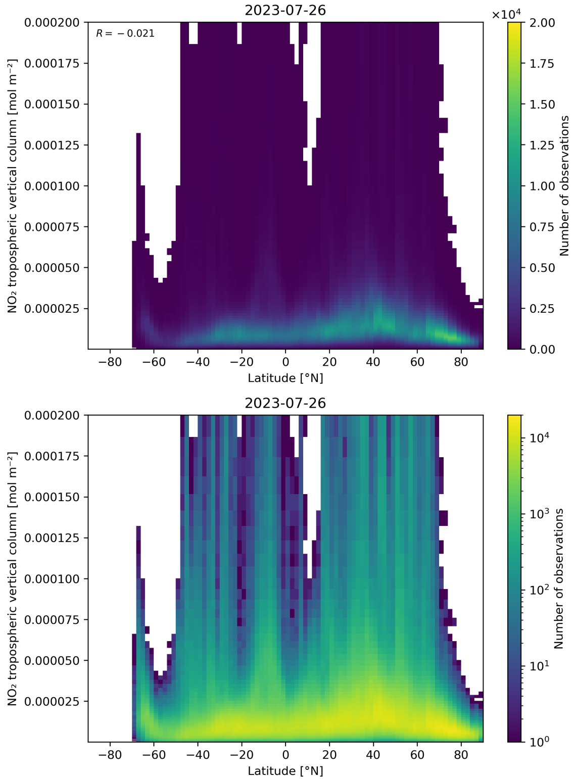
Figure 92: Scatter density plot of “Latitude” against “NO 2 tropospheric vertical column” for 2023-07-25 to 2023-07-27.
