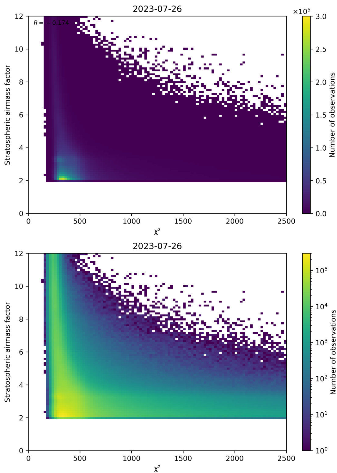
Figure 81: Scatter density plot of “ \chi^2 ” against “Stratospheric airmass factor” for 2023-07-25 to 2023-07-27.
