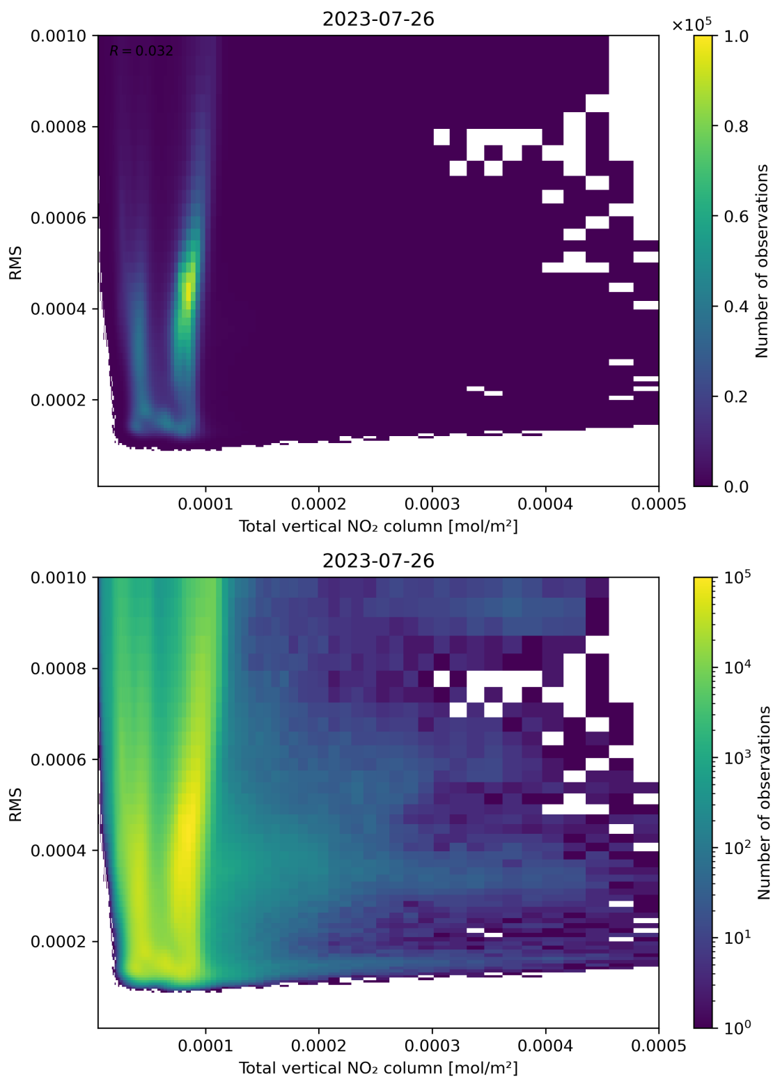
Figure 120: Scatter density plot of “Total vertical NO 2 column” against “RMS” for 2023-07-25 to 2023-07-27.
