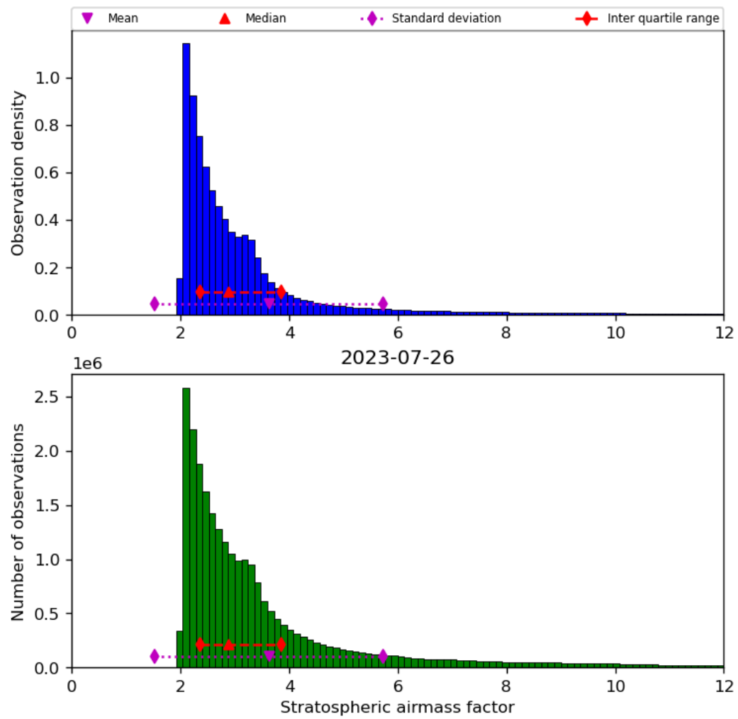
Figure 44: Histogram of “Stratospheric airmass factor” for 2023-07-25 to 2023-07-27
