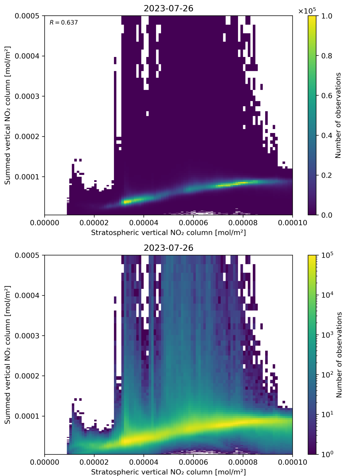
Figure 98: Scatter density plot of “Stratospheric vertical NO 2 column” against “Summed vertical NO 2 column” for 2023-07-25 to 2023-07-27.
