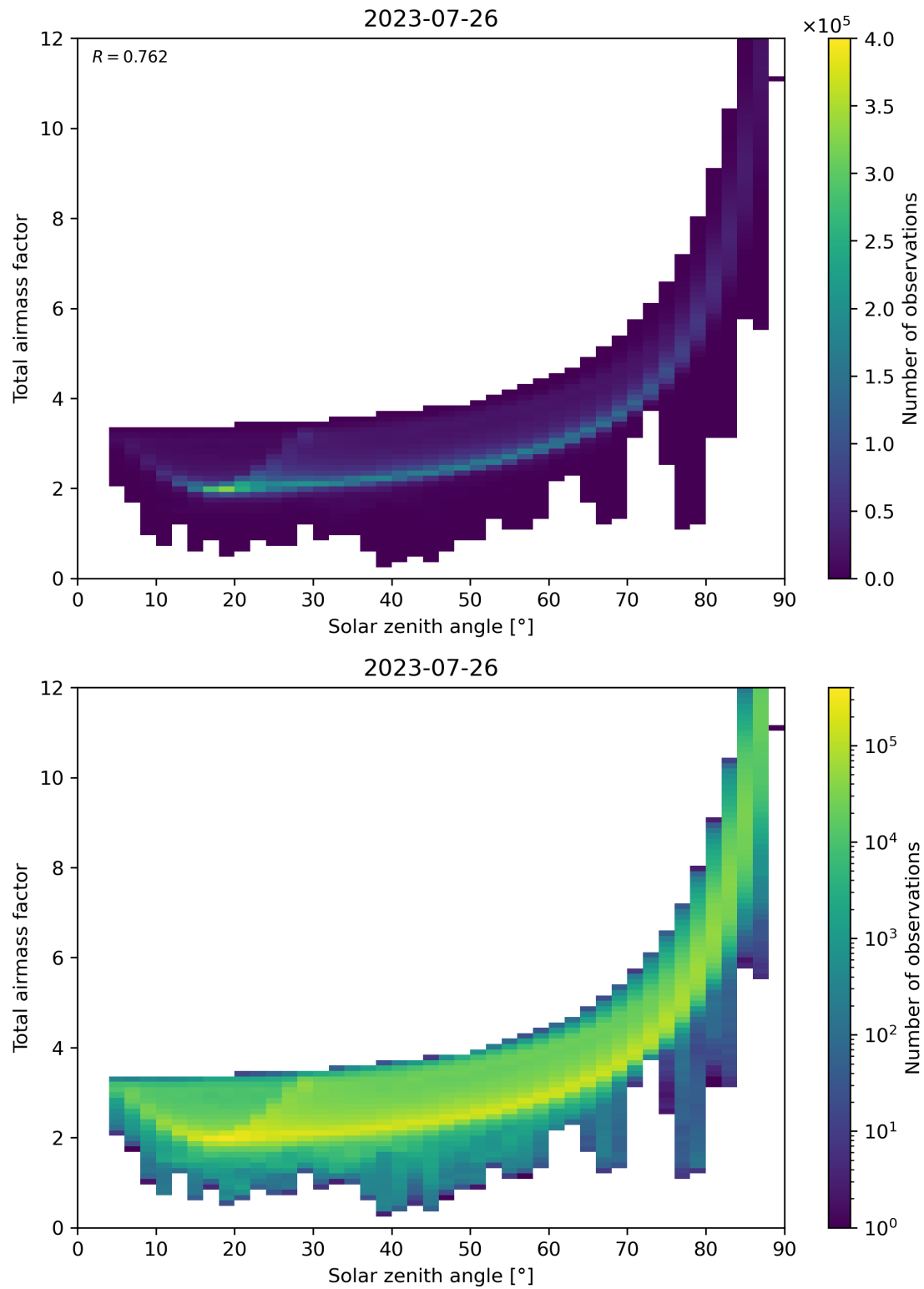
Figure 146: Scatter density plot of “Solar zenith angle” against “Total air mass factor” for 2023-07-25 to 2023-07-27.
