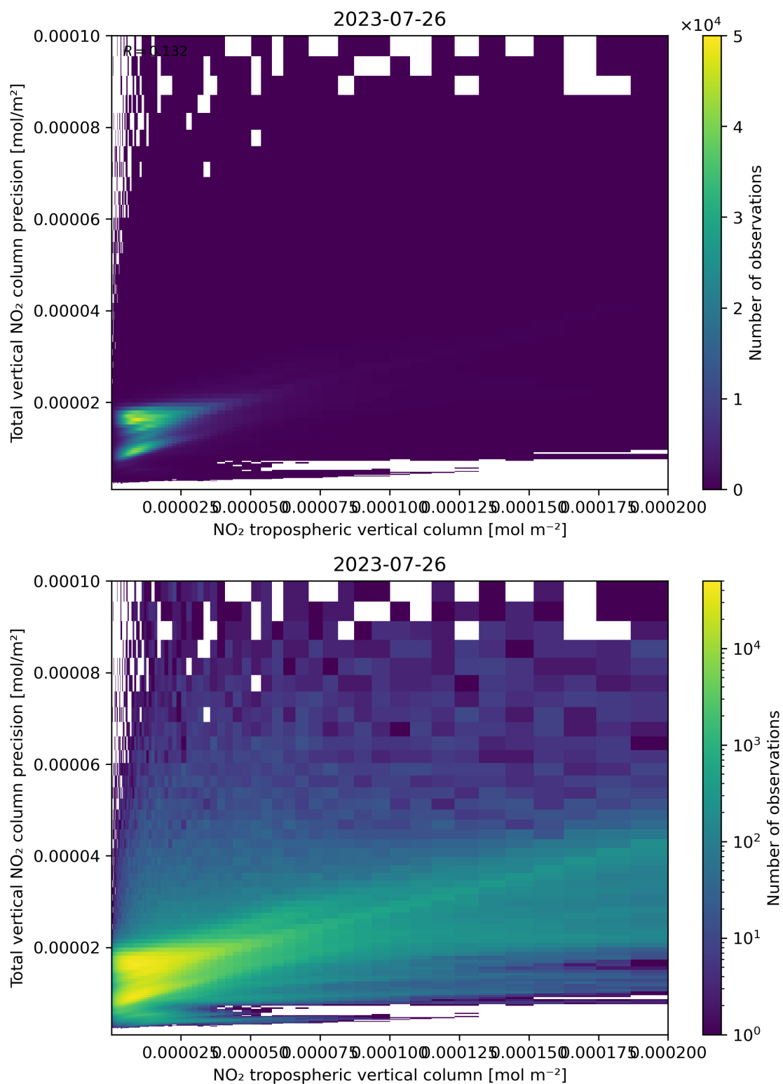
Figure 129: Scatter density plot of “NO 2 tropospheric vertical column” against “Total vertical NO 2 column precision” for 2023-07-25 to 2023-07-27.
