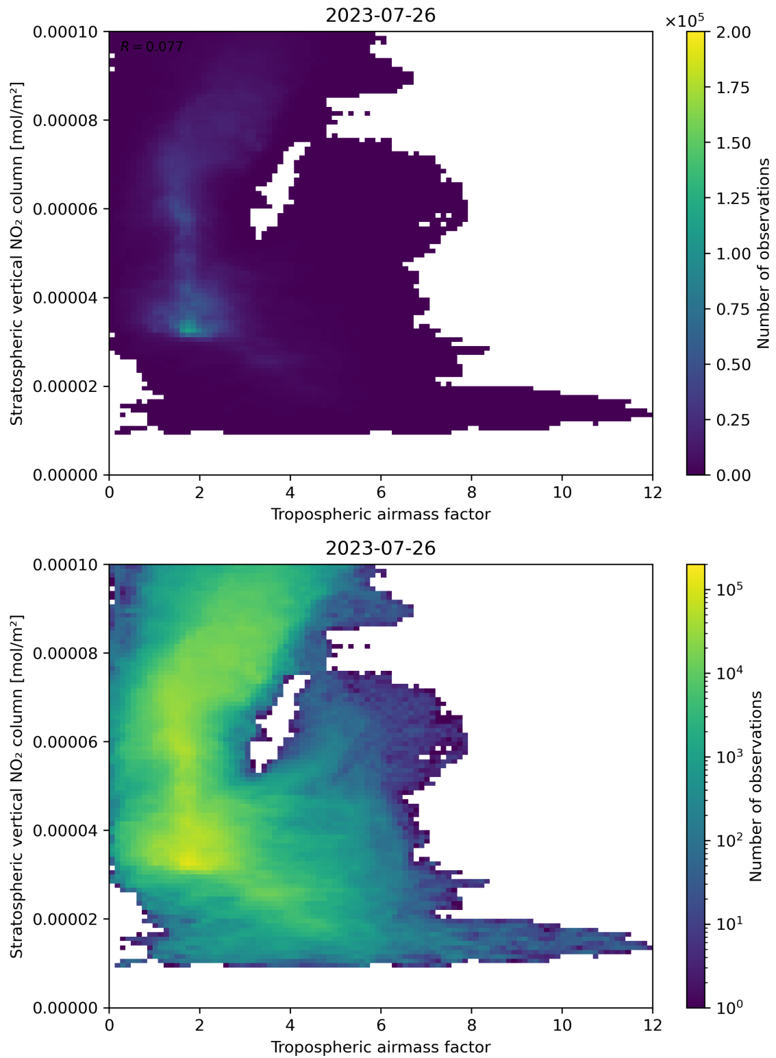
Figure 74: Scatter density plot of “Tropospheric air mass factor” against “Stratospheric vertical NO 2 column” for 2023-07-25 to 2023-07-27.
