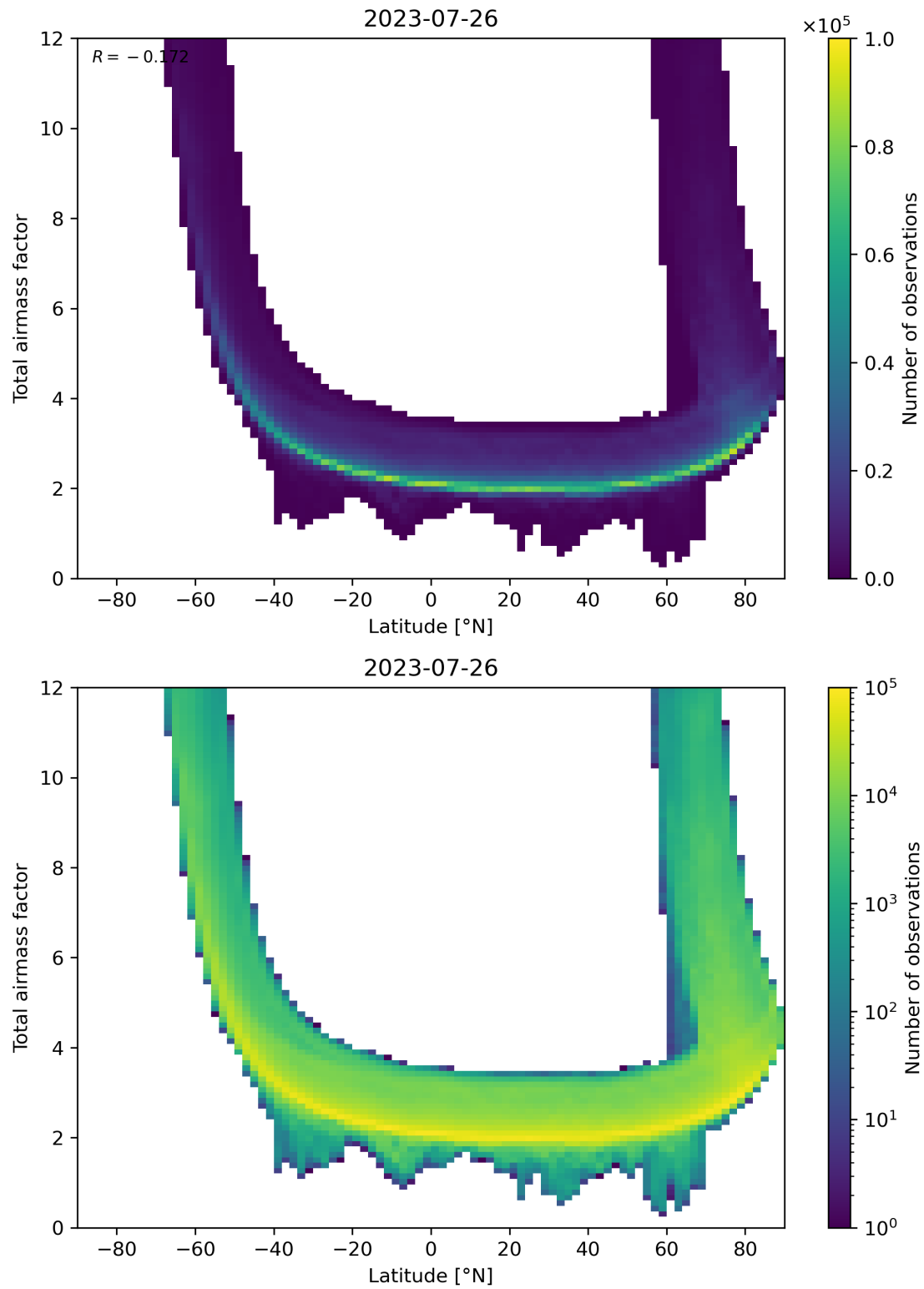
Figure 84: Scatter density plot of “Latitude” against “Total airmass factor” for 2023-07-25 to 2023-07-27.
