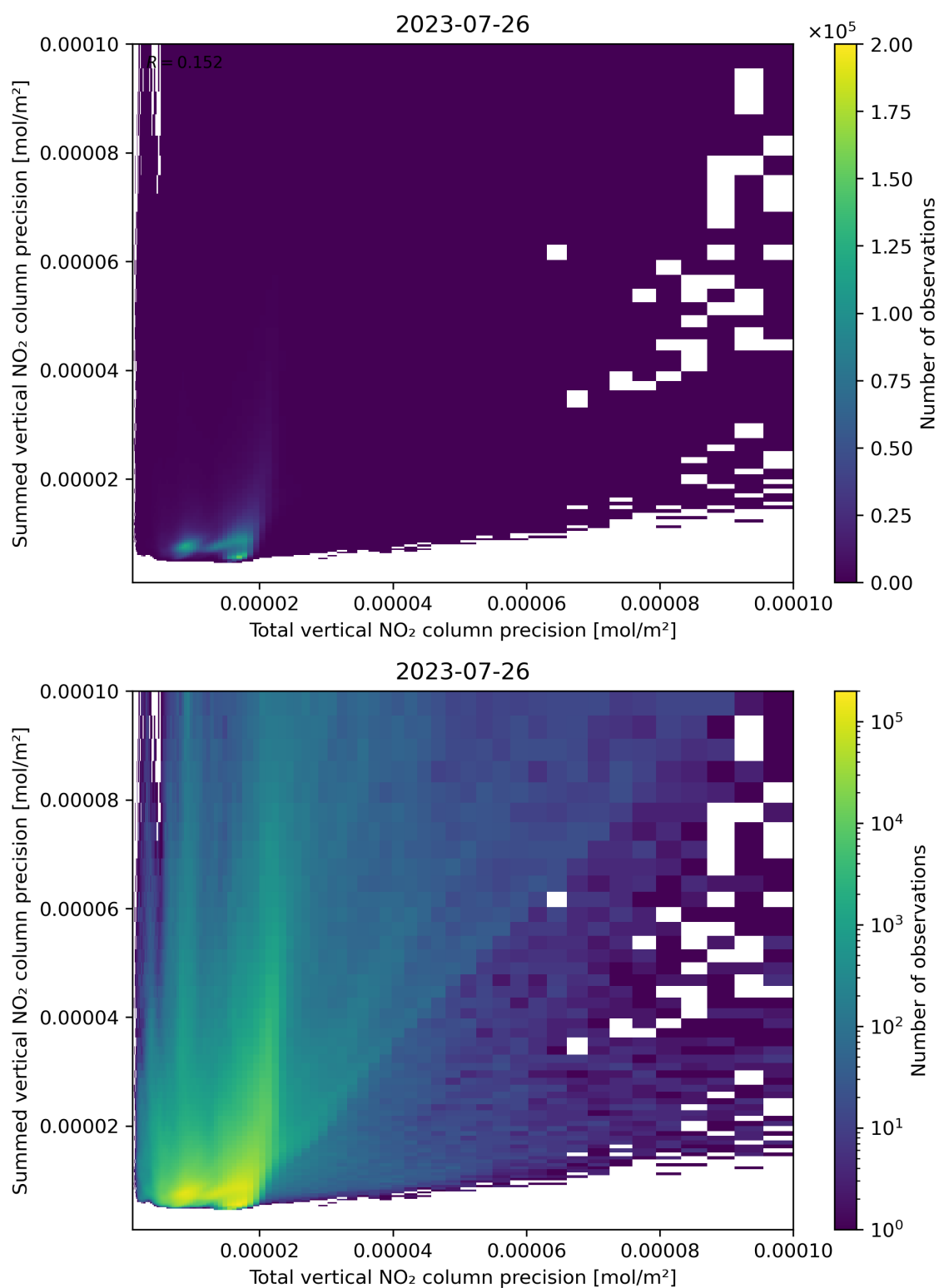
Figure 118: Scatter density plot of “Total vertical NO 2 column precision” against “Summed vertical NO 2 column precision” for 2023-07-25 to 2023-07-27.
