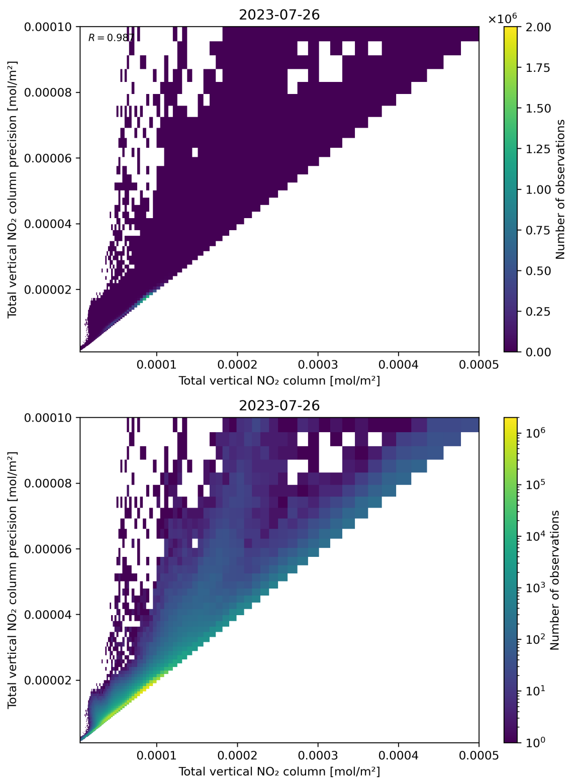
Figure 114: Scatter density plot of “Total vertical NO 2 column” against “Total vertical NO 2 column precision” for 2023-07-25 to 2023-07-27.
