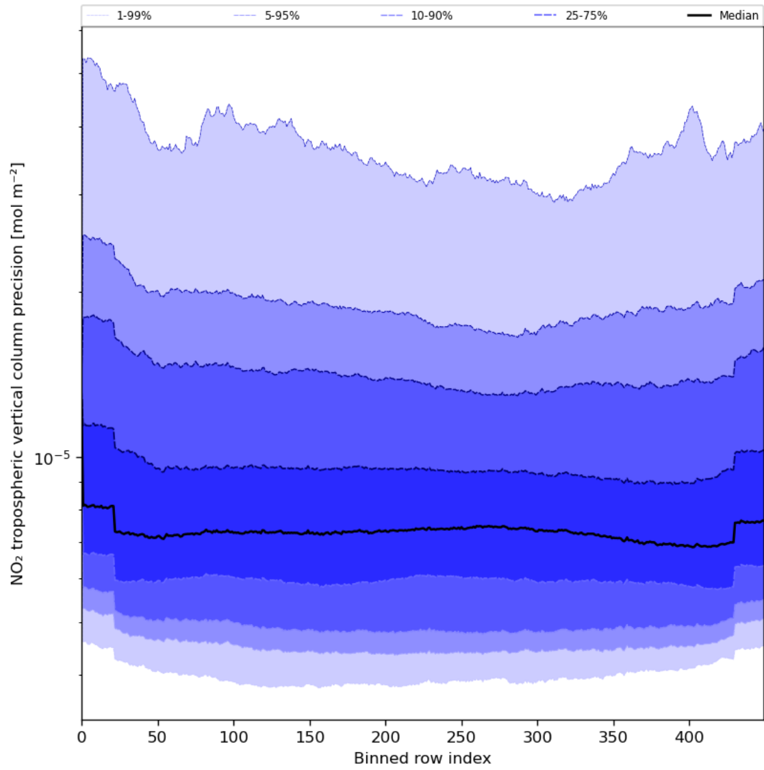
Figure 47: Along track statistics of “NO 2 tropospheric vertical column precision” for 2023-07-25 to 2023-07-27
