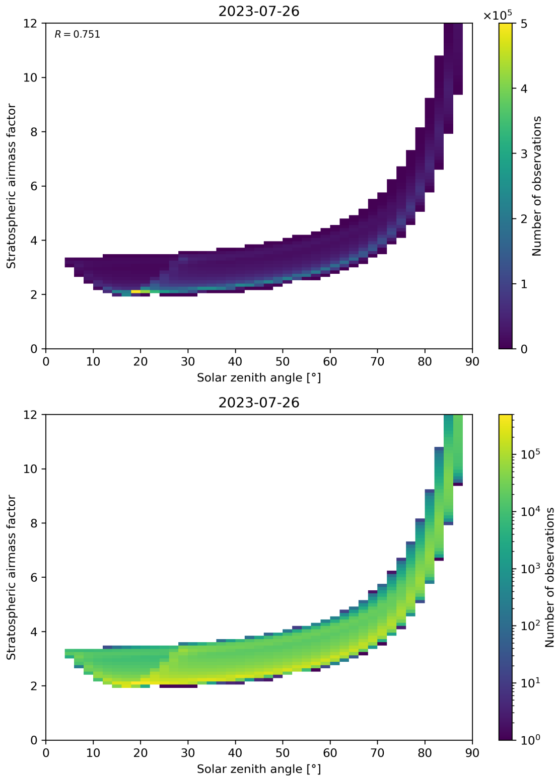
Figure 145: Scatter density plot of “Solar zenith angle” against “Stratospheric airmass factor” for 2023-07-25 to 2023-07-27.
