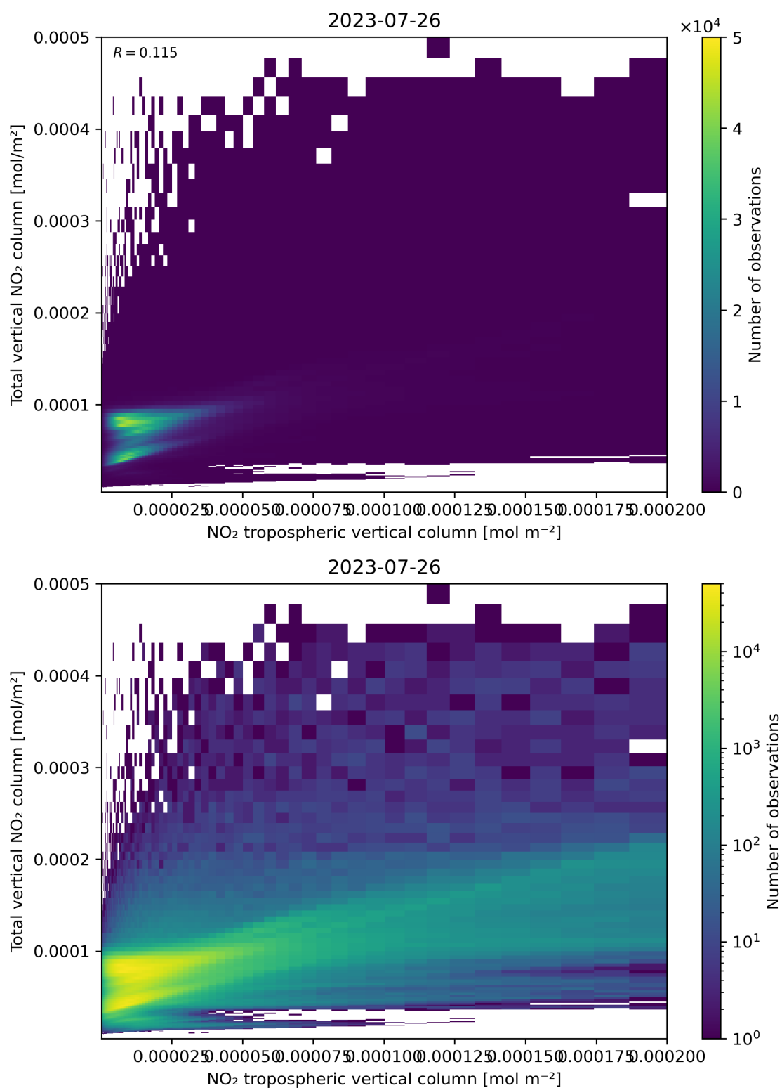
Figure 128: Scatter density plot of “NO 2 tropospheric vertical column” against “Total vertical NO 2 column” for 2023-07-25 to 2023-07-27.
