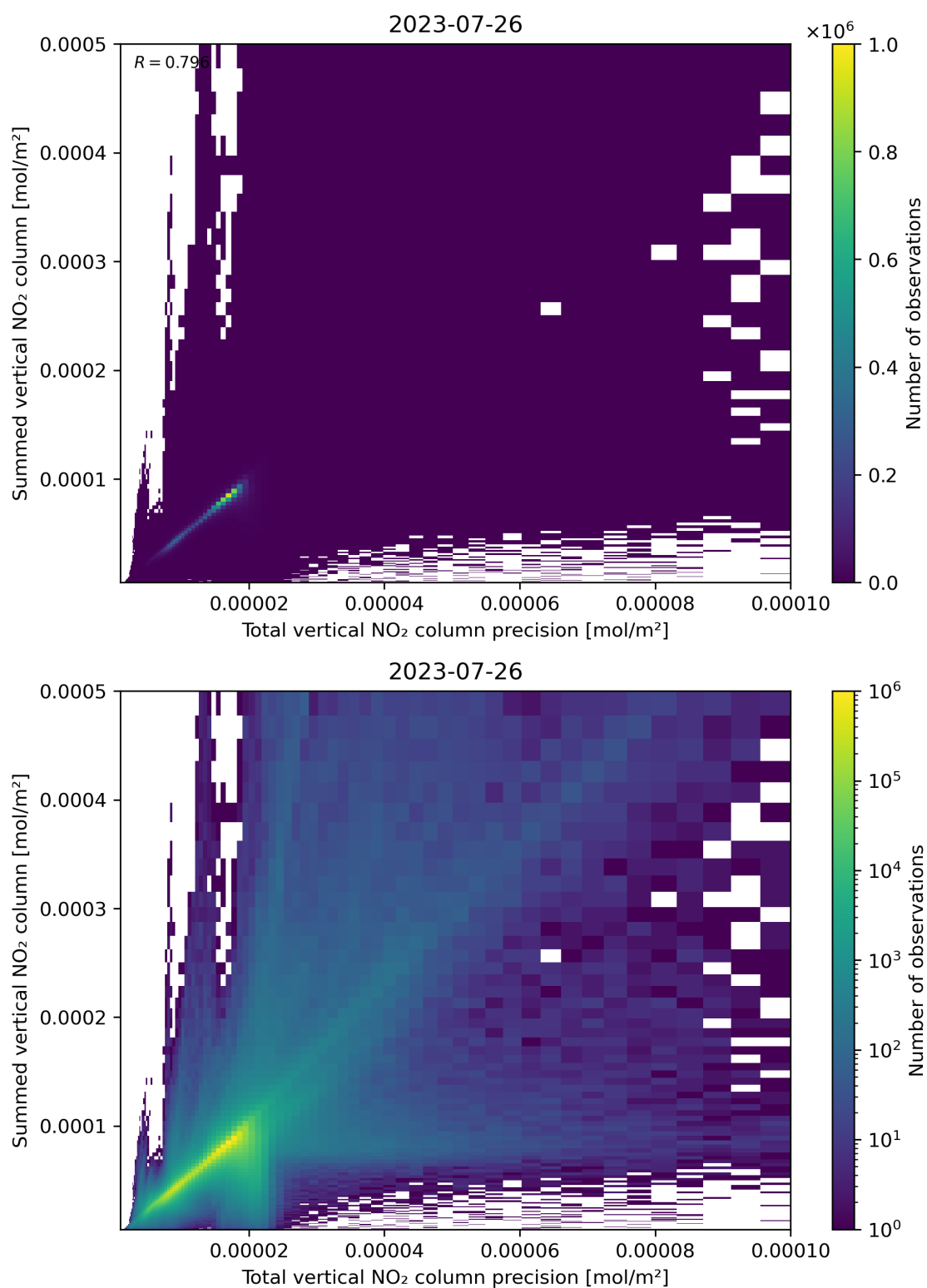
Figure 117: Scatter density plot of “Total vertical NO 2 column precision” against “Summed vertical NO 2 column” for 2023-07-25 to 2023-07-27.
