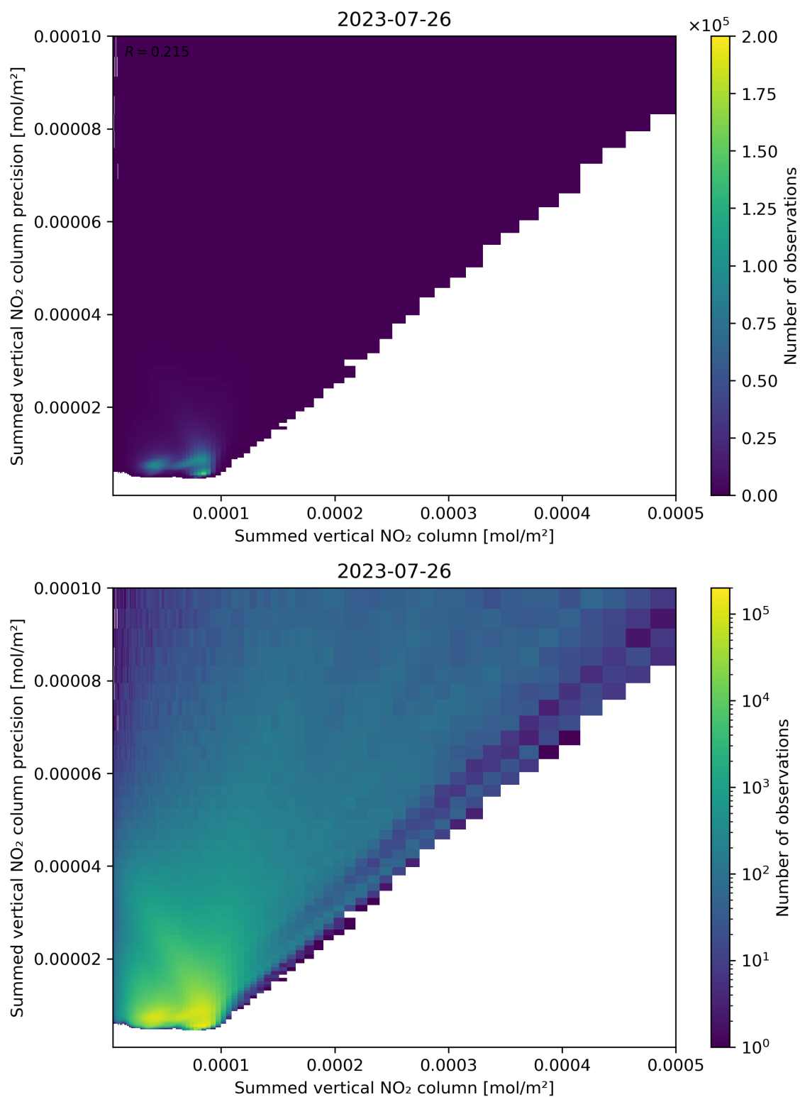
Figure 105: Scatter density plot of “Summed vertical NO 2 column” against “Summed vertical NO 2 column precision” for 2023-07-25 to 2023-07-27.
