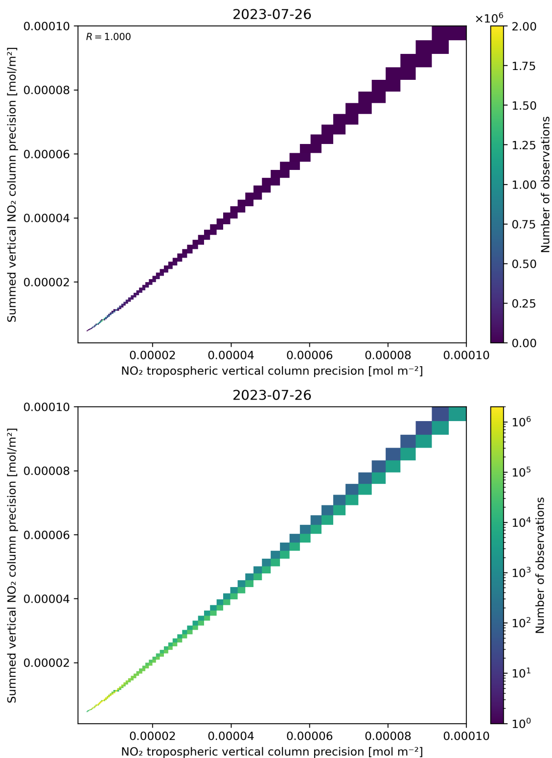
Figure 137: Scatter density plot of “NO 2 tropospheric vertical column precision” against “Summed vertical NO 2 column precision” for 2023-07-25 to 2023-07-27.
