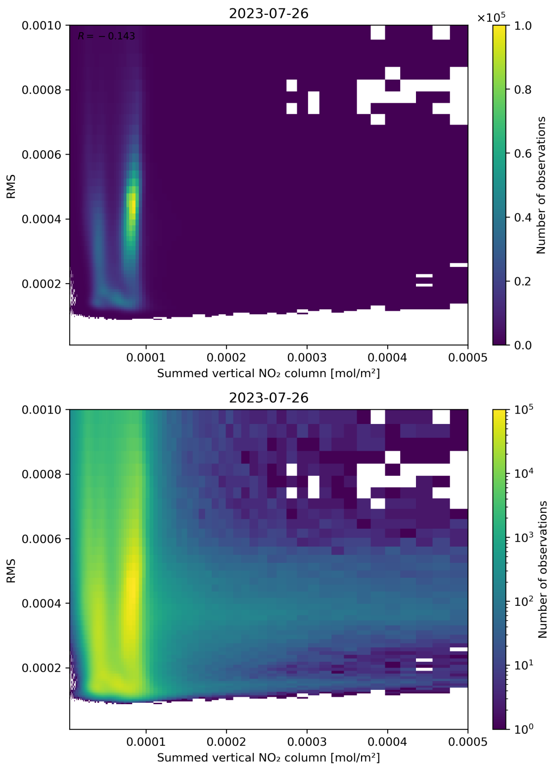
Figure 109: Scatter density plot of “Summed vertical NO 2 column” against “RMS” for 2023-07-25 to 2023-07-27.
