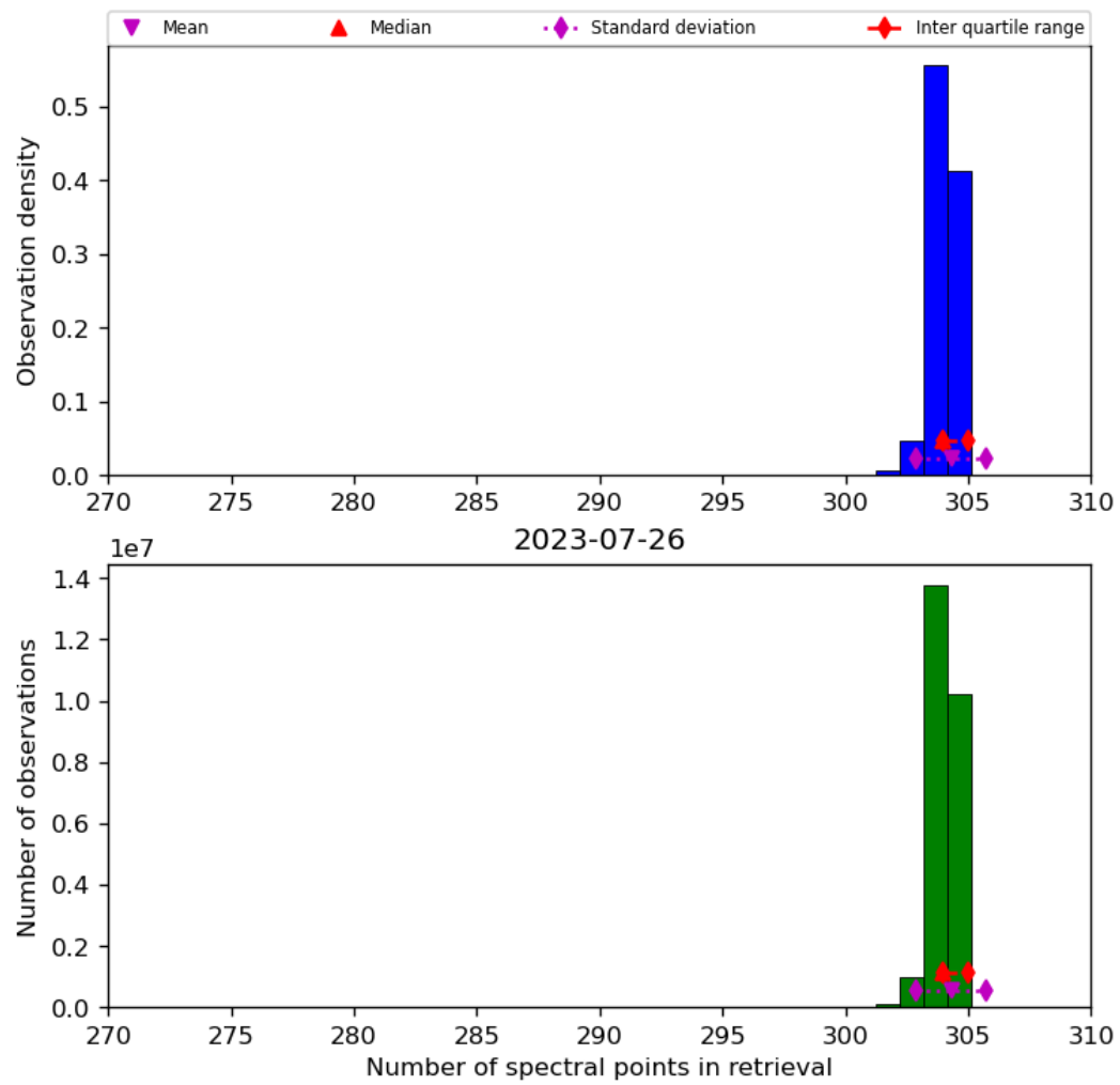
Figure 33: Histogram of “Number of spectral points in retrieval” for 2023-07-25 to 2023-07-27
