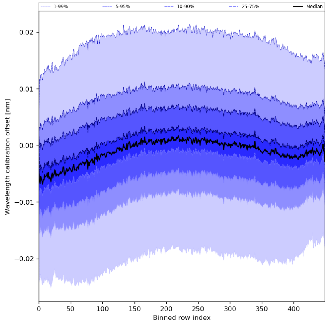
Figure 52: Along track statistics of “Wavelength calibration offset” for 2023-07-25 to 2023-07-27
