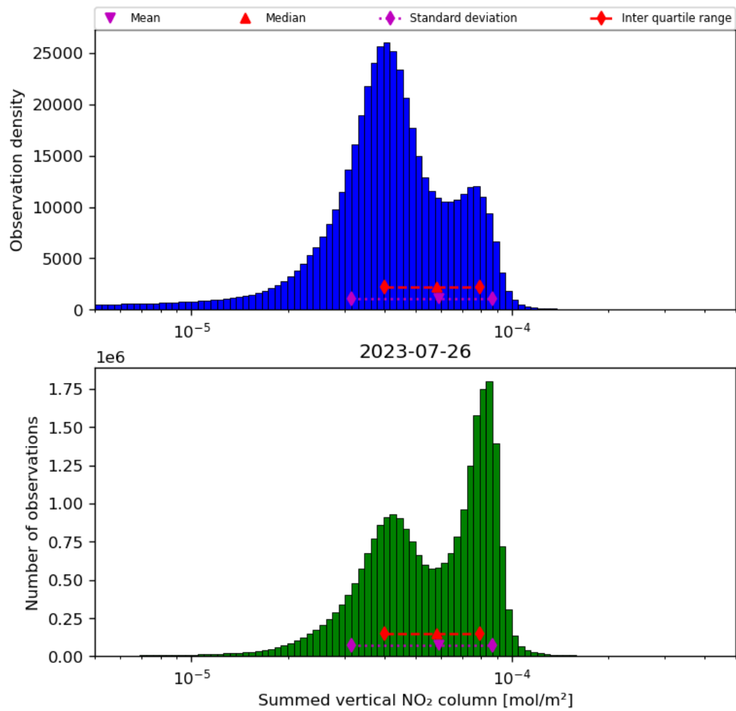
Figure 40: Histogram of “Summed vertical NO 2 column” for 2023-07-25 to 2023-07-27
