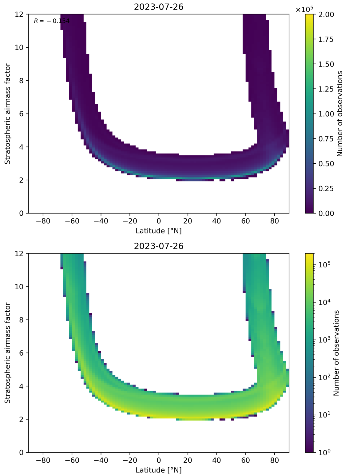
Figure 83: Scatter density plot of “Latitude” against “Stratospheric air mass factor” for 2023-07-25 to 2023-07-27.
