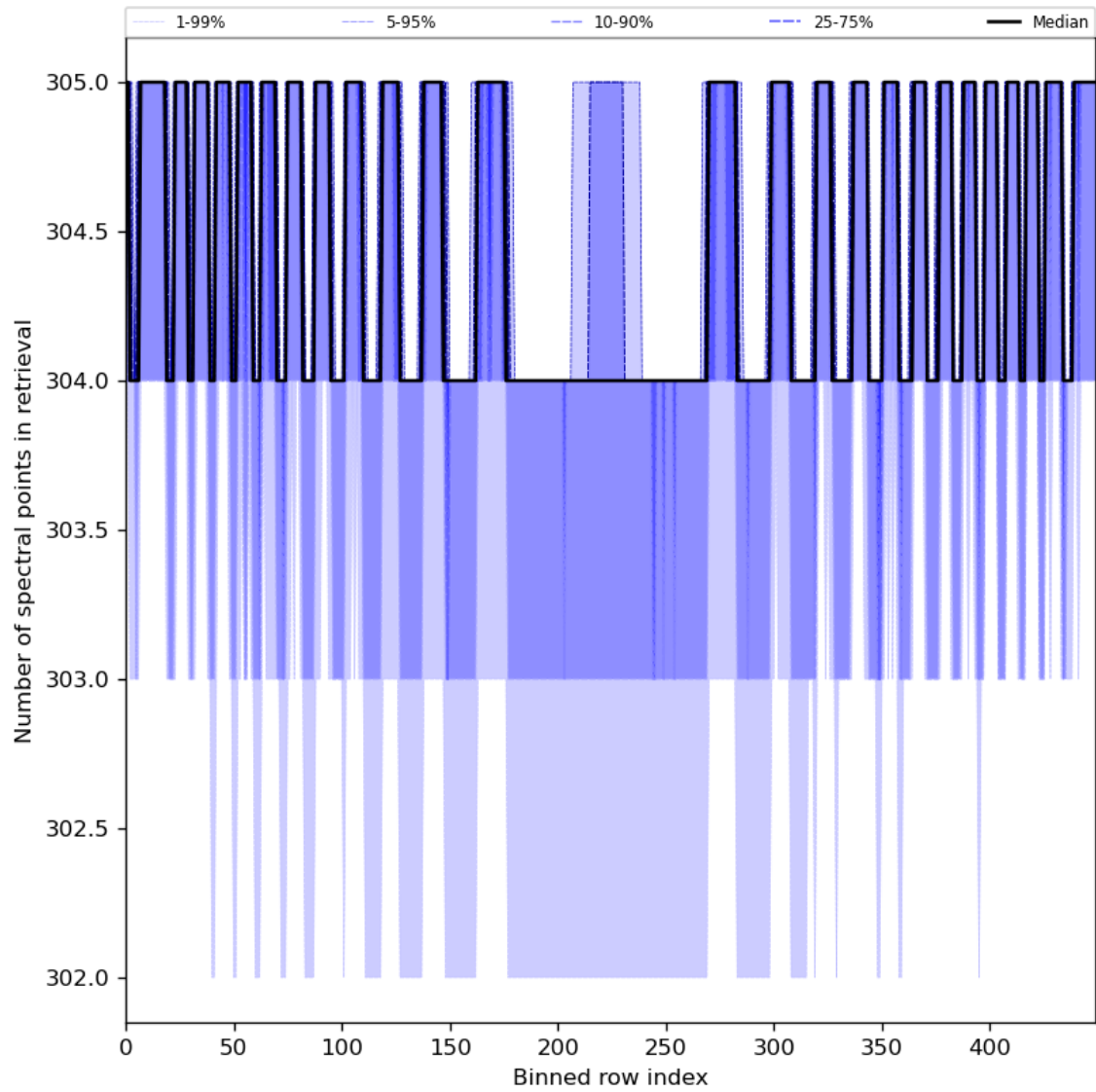
Figure 50: Along track statistics of “Number of spectral points in retrieval” for 2023-07-25 to 2023-07-27
