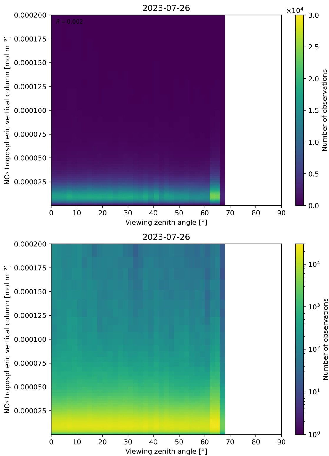
Figure 169: Scatter density plot of “Viewing zenith angle” against “NO 2 tropospheric vertical column” for 2023-07-25 to 2023-07-27.
