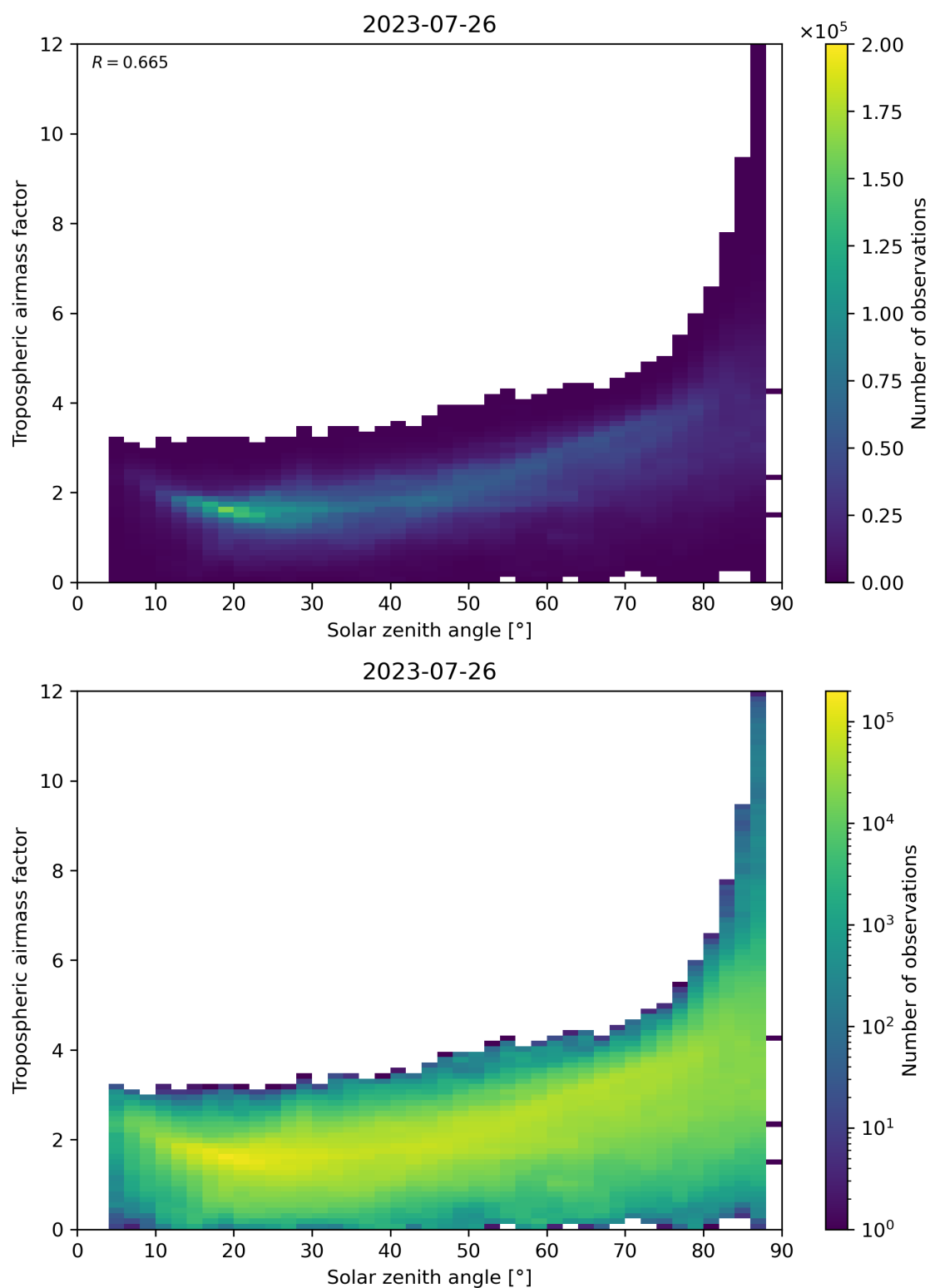
Figure 147: Scatter density plot of “Solar zenith angle” against “Tropospheric airmass factor” for 2023-07-25 to 2023-07-27.
