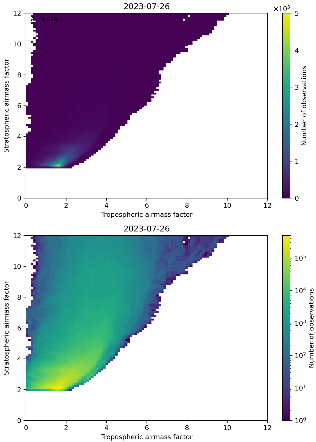
Figure 71: Scatter density plot of “Tropospheric airmass factor” against “Stratospheric airmass factor” for 2023-07-25 to 2023-07-27.
