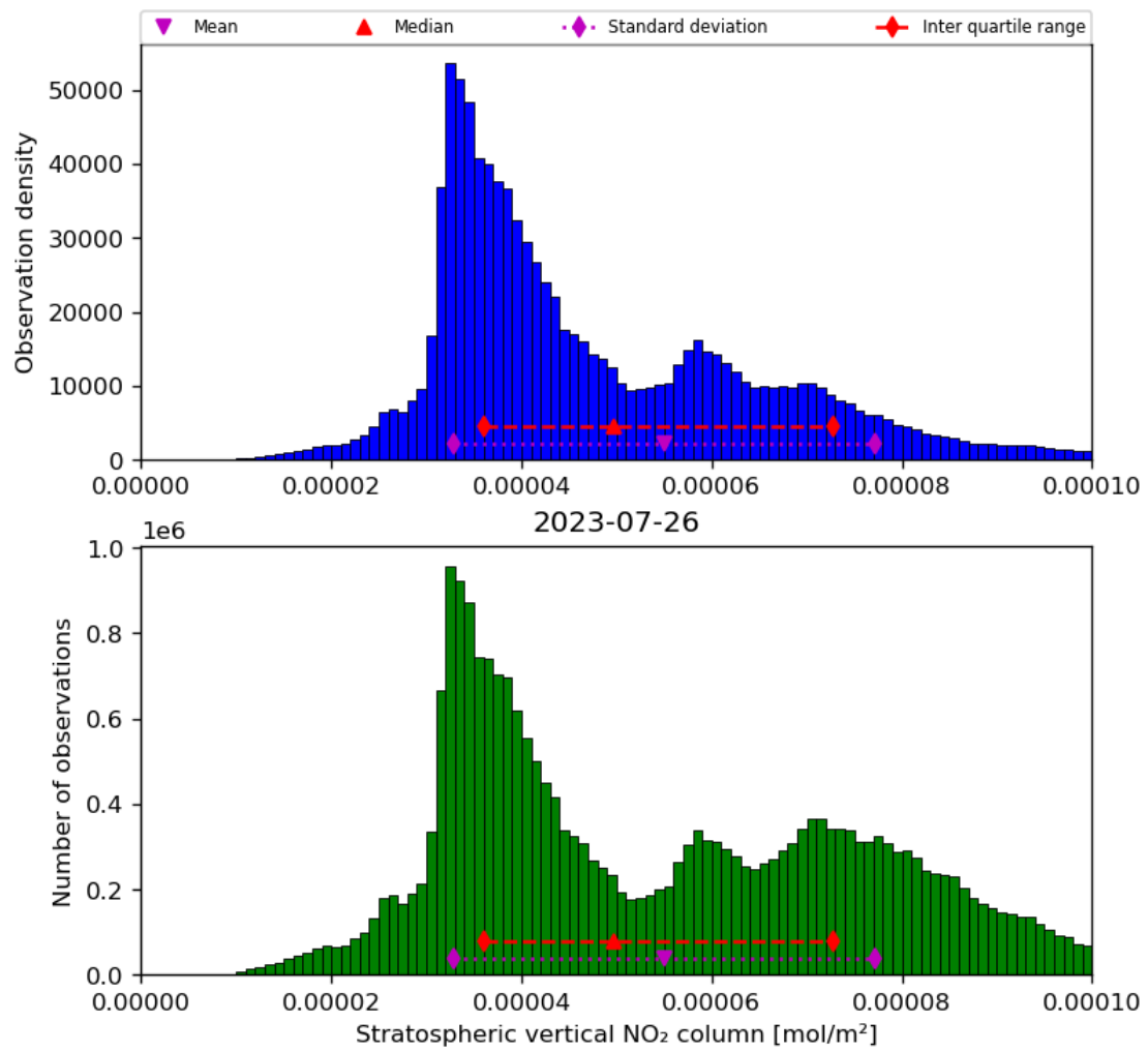
Figure 36: Histogram of “Stratospheric vertical NO 2 column” for 2023-07-25 to 2023-07-27
