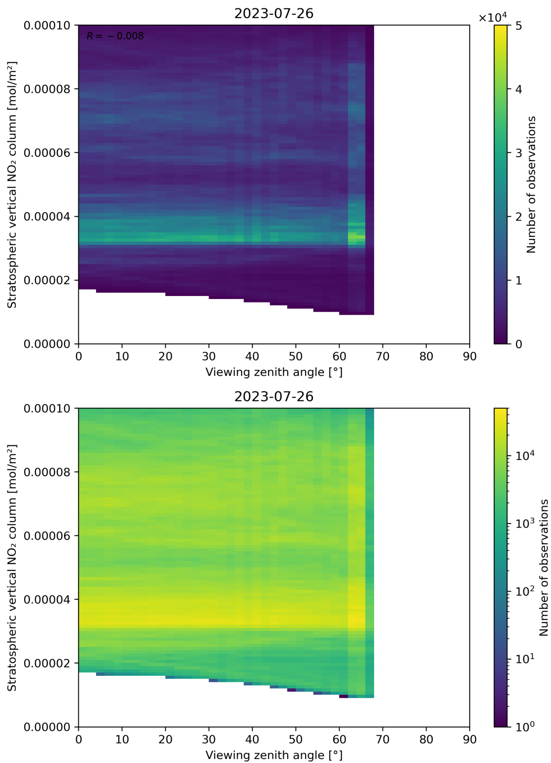
Figure 164: Scatter density plot of “Viewing zenith angle” against “Stratospheric vertical NO 2 column” for 2023-07-25 to 2023-07-27.
