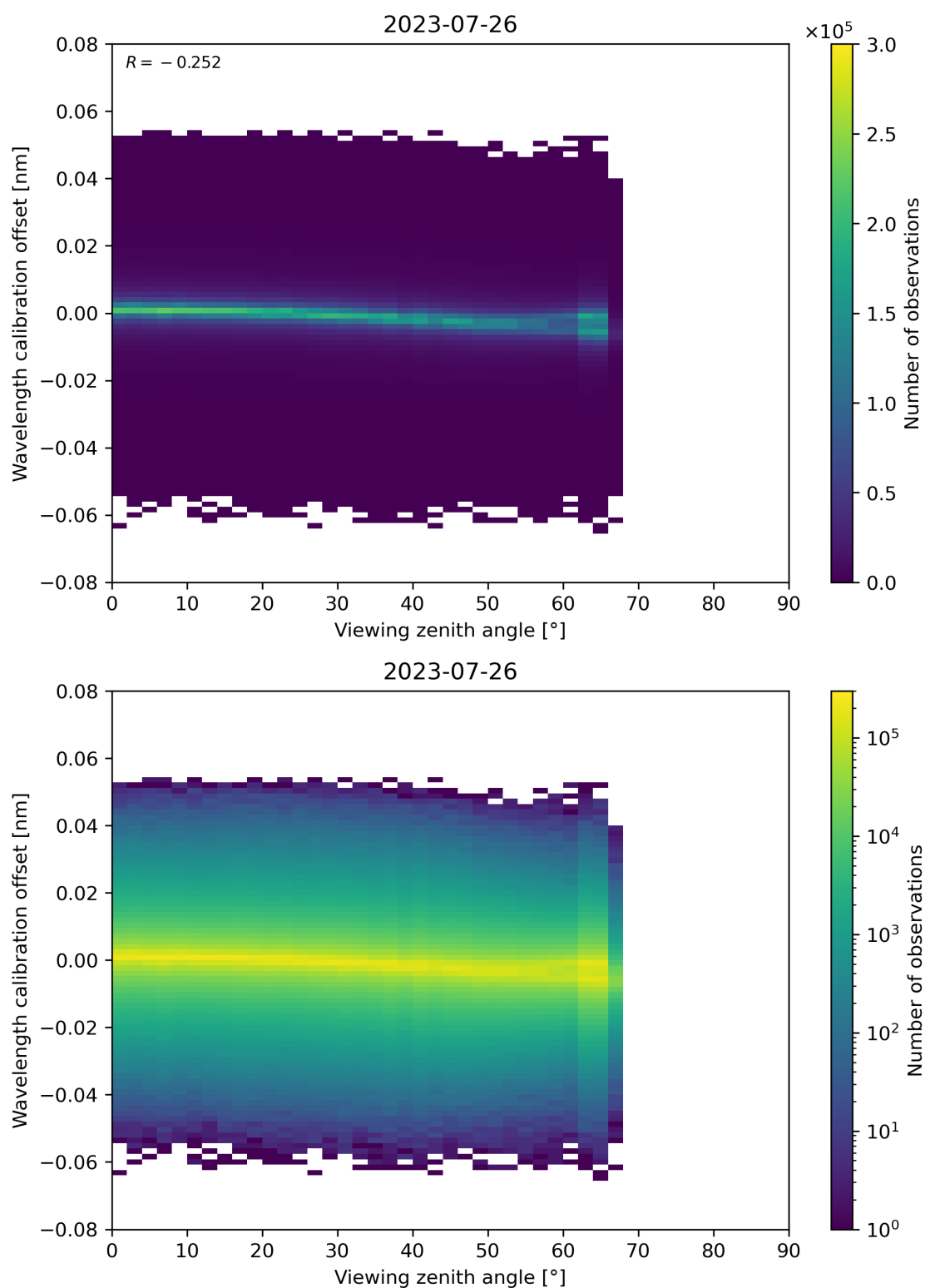
Figure 173: Scatter density plot of “Viewing zenith angle” against “Wavelength calibration offset” for 2023-07-25 to 2023-07-27.
