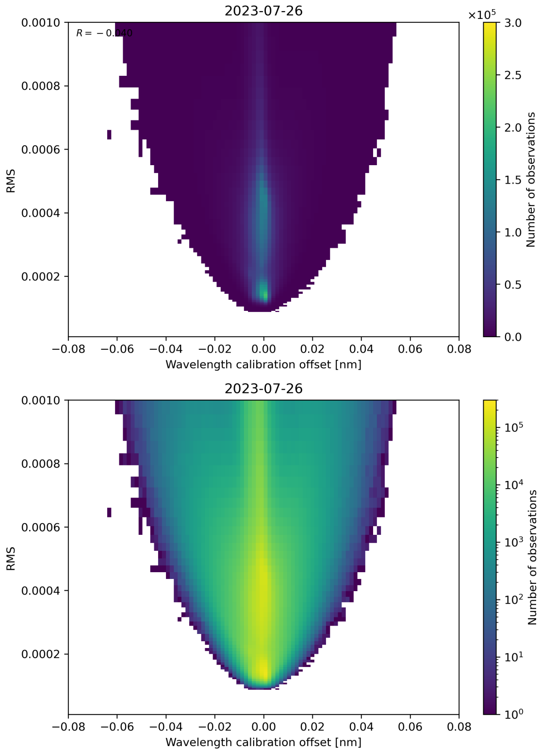
Figure 181: Scatter density plot of “Wavelength calibration offset” against “RMS” for 2023-07-25 to 2023-07-27.
