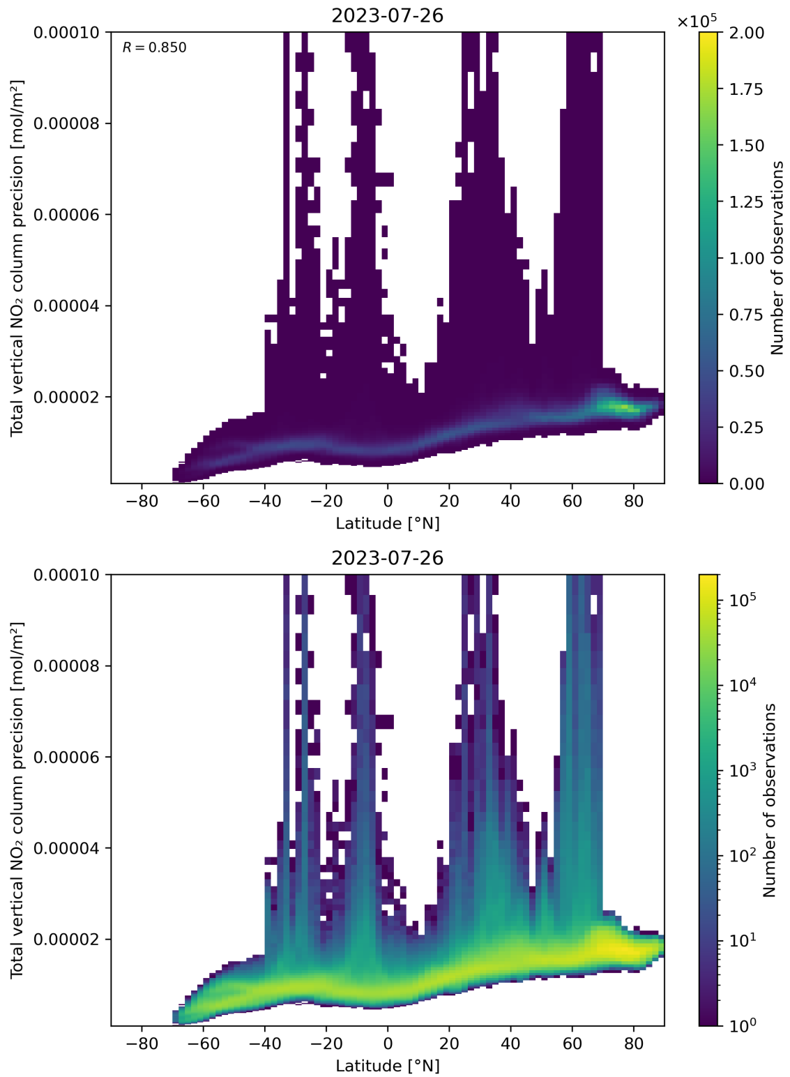
Figure 91: Scatter density plot of “Latitude” against “Total vertical NO 2 column precision” for 2023-07-25 to 2023-07-27.
