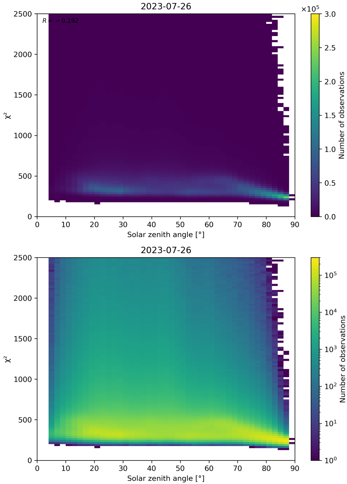
Figure 148: Scatter density plot of “Solar zenith angle” against “ \chi^2 ” for 2023-07-25 to 2023-07-27.
