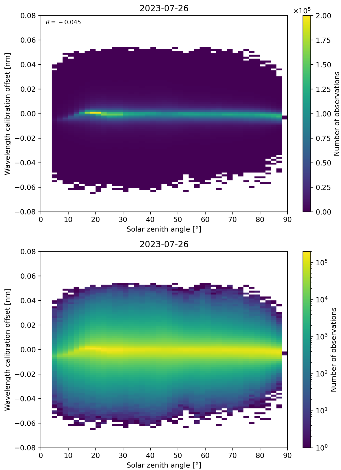
Figure 158: Scatter density plot of “Solar zenith angle” against “Wavelength calibration offset” for 2023-07-25 to 2023-07-27.
