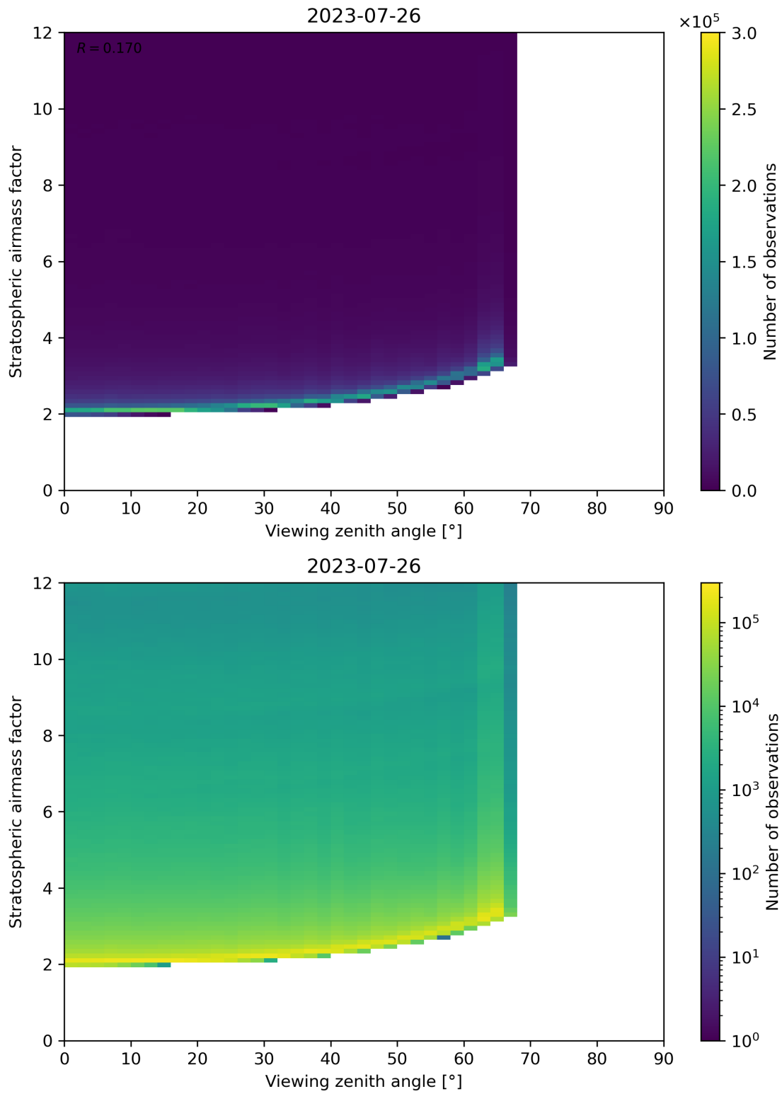
Figure 159: Scatter density plot of “Viewing zenith angle” against “Stratospheric airmass factor” for 2023-07-25 to 2023-07-27.
