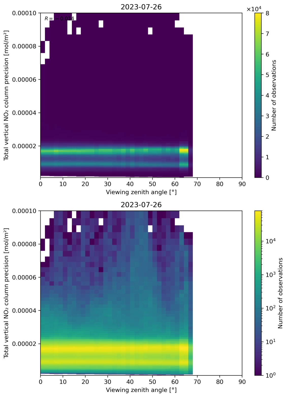
Figure 168: Scatter density plot of “Viewing zenith angle” against “Total vertical NO 2 column precision” for 2023-07-25 to 2023-07-27.
