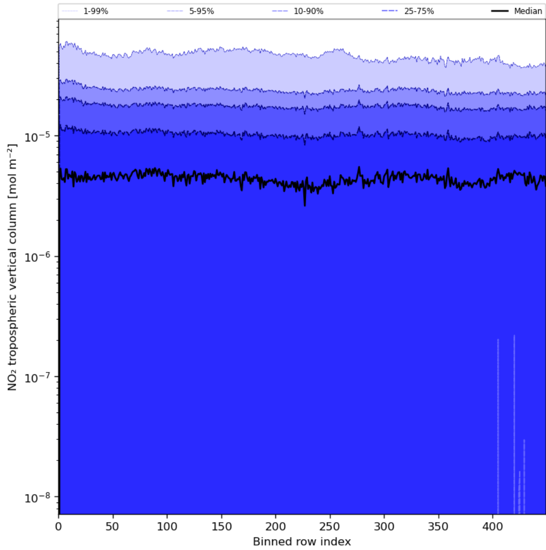
Figure 46: Along track statistics of "NO 2 tropospheric vertical column" for 2023-07-25 to 2023-07-27
