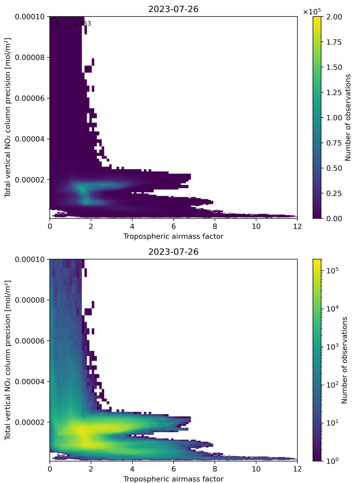
Figure 78: Scatter density plot of “Tropospheric air mass factor” against “Total vertical NO 2 column precision” for 2023-07-25 to 2023-07-27.
