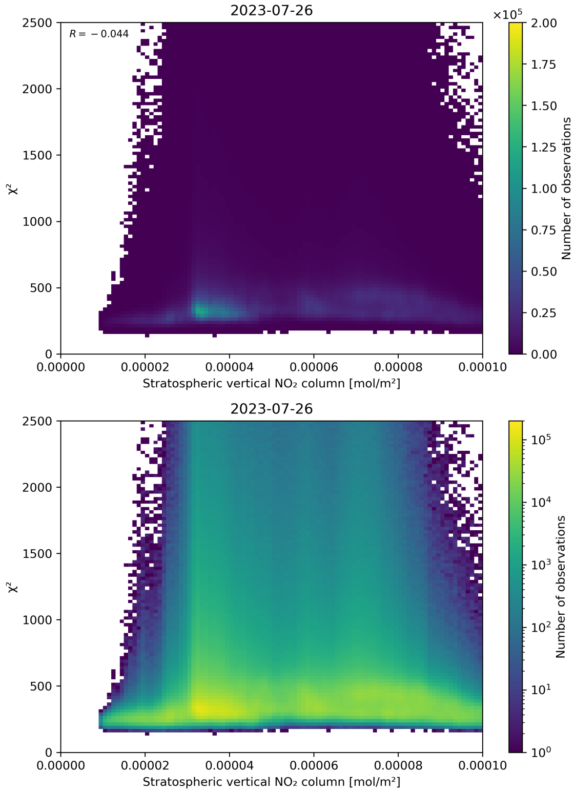
Figure 97: Scatter density plot of “Stratospheric vertical NO 2 column” against “ \chi^2 ” for 2023-07-25 to 2023-07-27.
