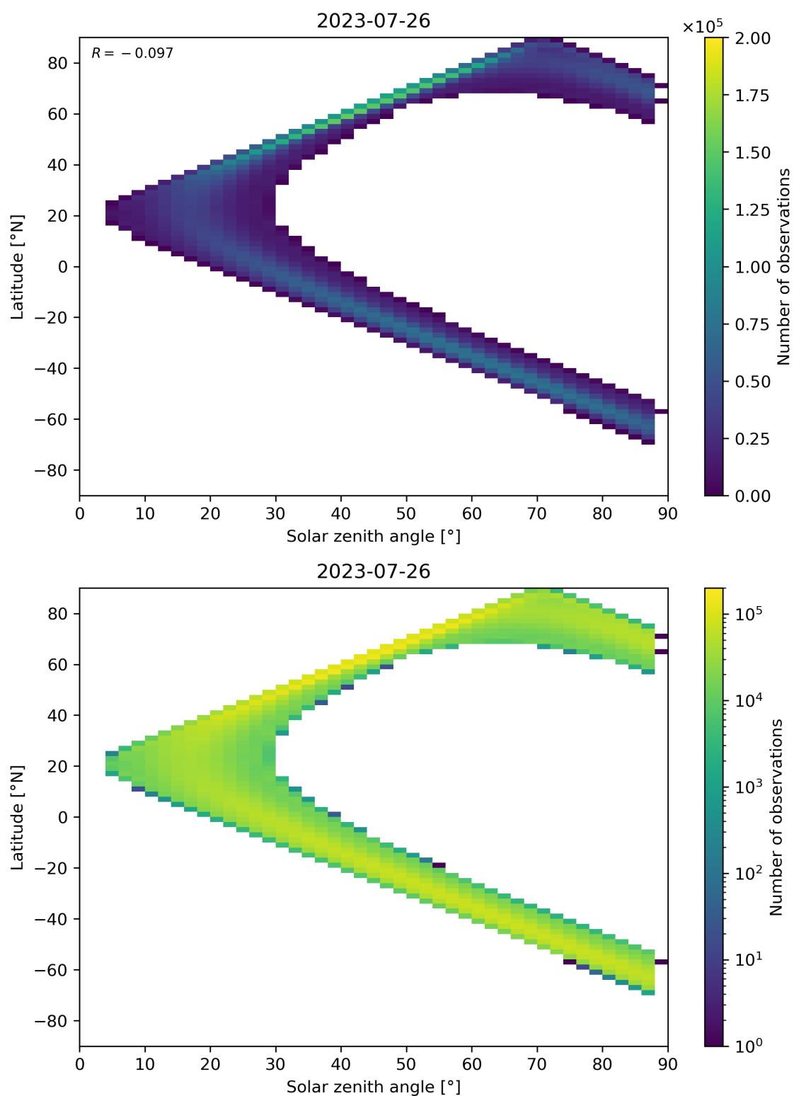
Figure 149: Scatter density plot of “Solar zenith angle” against “Latitude” for 2023-07-25 to 2023-07-27.
