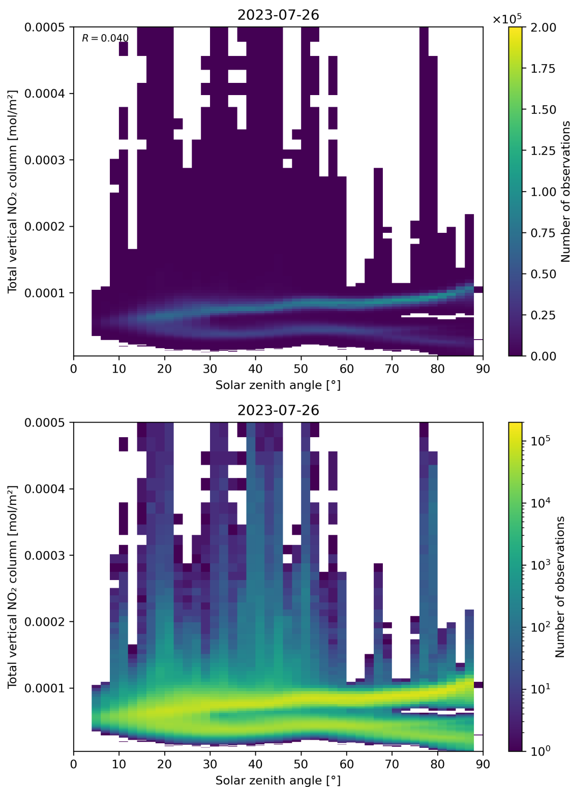
Figure 153: Scatter density plot of “Solar zenith angle” against “Total vertical NO 2 column” for 2023-07-25 to 2023-07-27.
