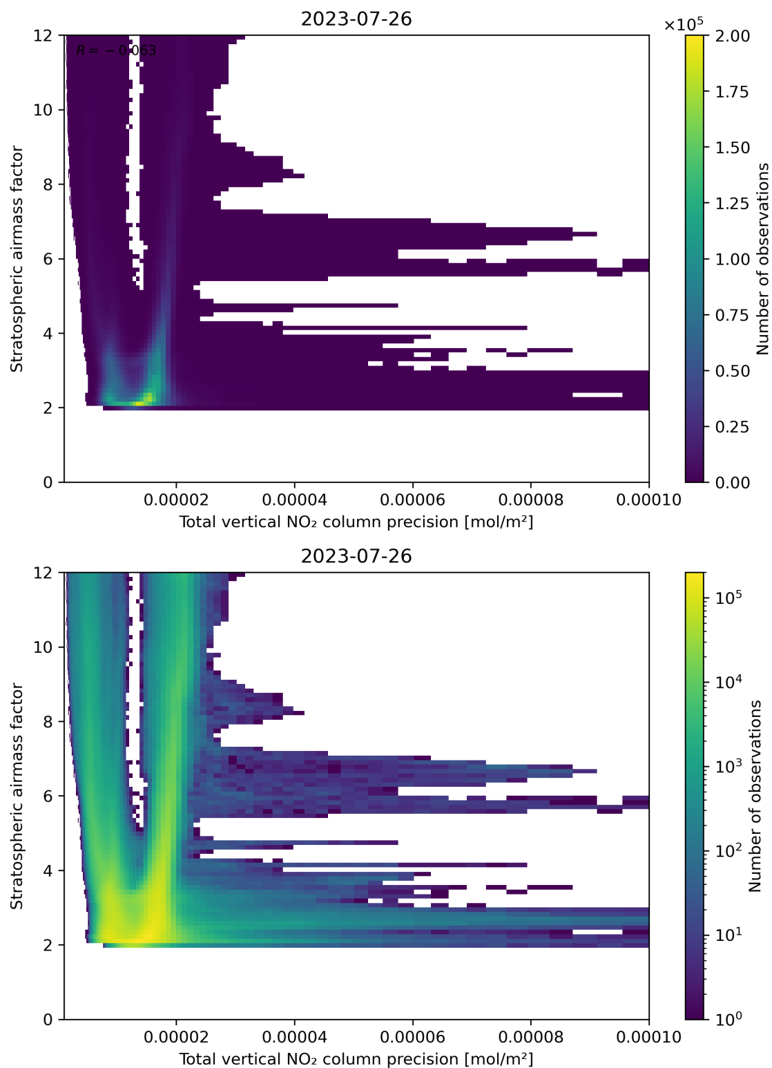
Figure 115: Scatter density plot of “Total vertical NO 2 column precision” against “Stratospheric air mass factor” for 2023-07-25 to 2023-07-27.
