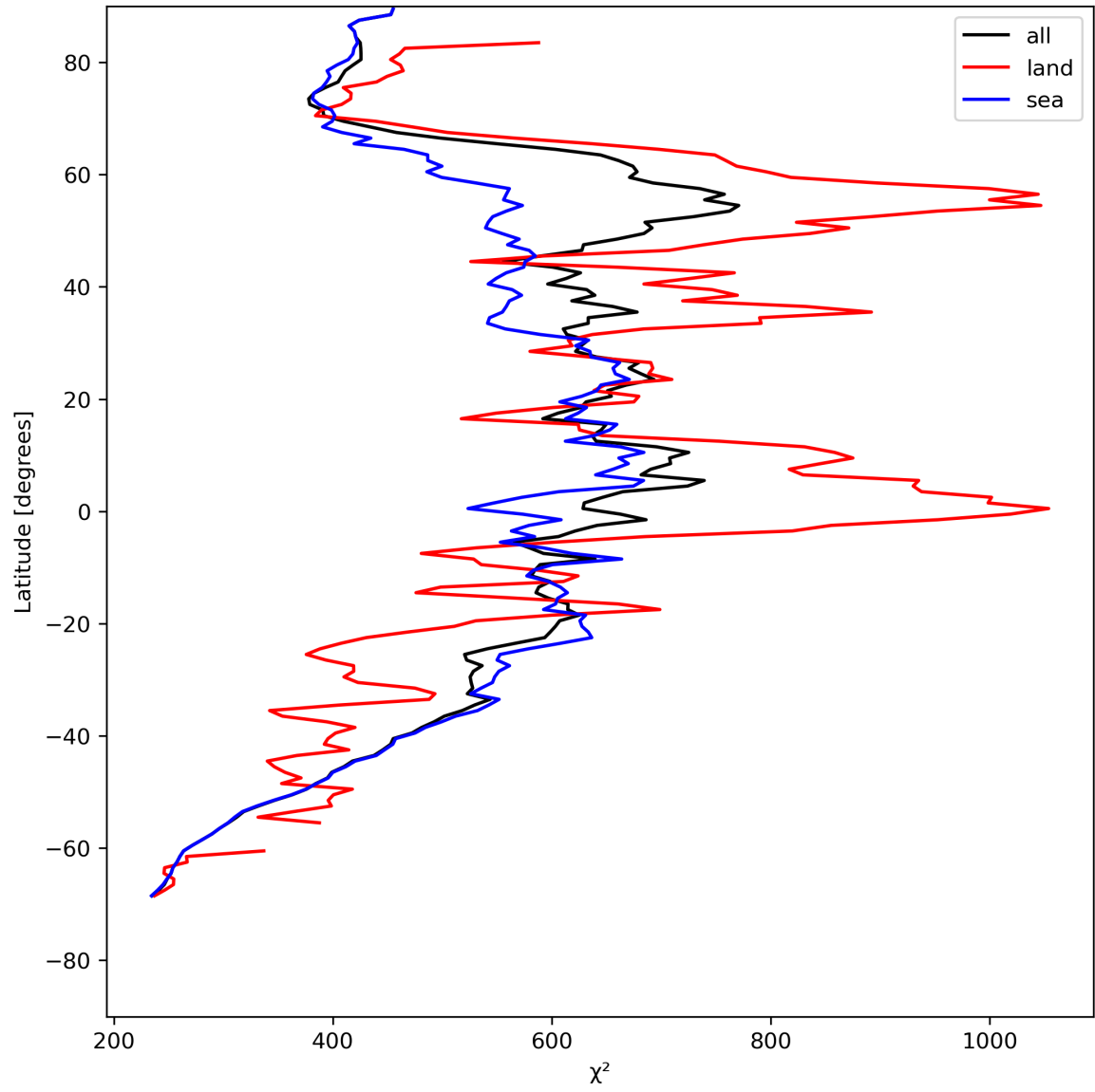
Figure 25: Zonal average of “ \chi^2 ” for 2023-07-25 to 2023-07-27.
