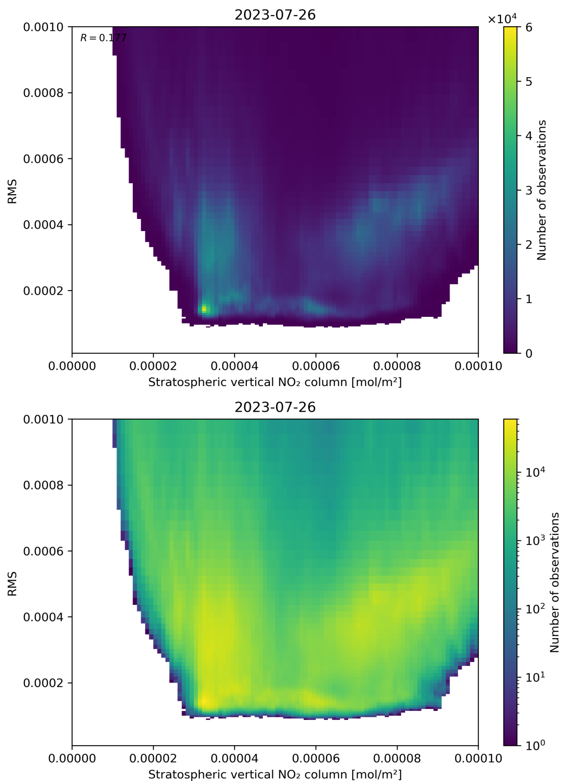
Figure 102: Scatter density plot of “Stratospheric vertical NO 2 column” against “RMS” for 2023-07-25 to 2023-07-27.
