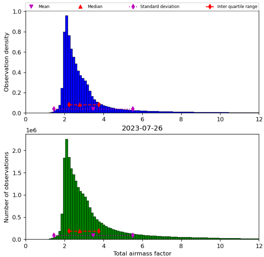
Figure 32: Histogram of “Total airmass factor” for 2023-07-25 to 2023-07-27
