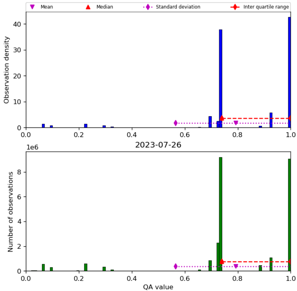
Figure 28: Histogram of “QA value” for 2023-07-25 to 2023-07-27
