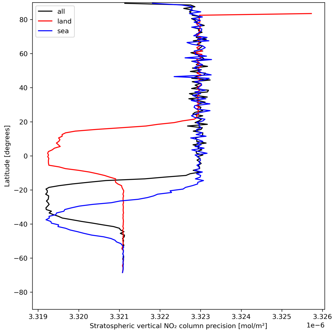
Figure 20: Zonal average of “Stratospheric vertical NO 2 column precision” for 2023-07-25 to 2023-07-27.
