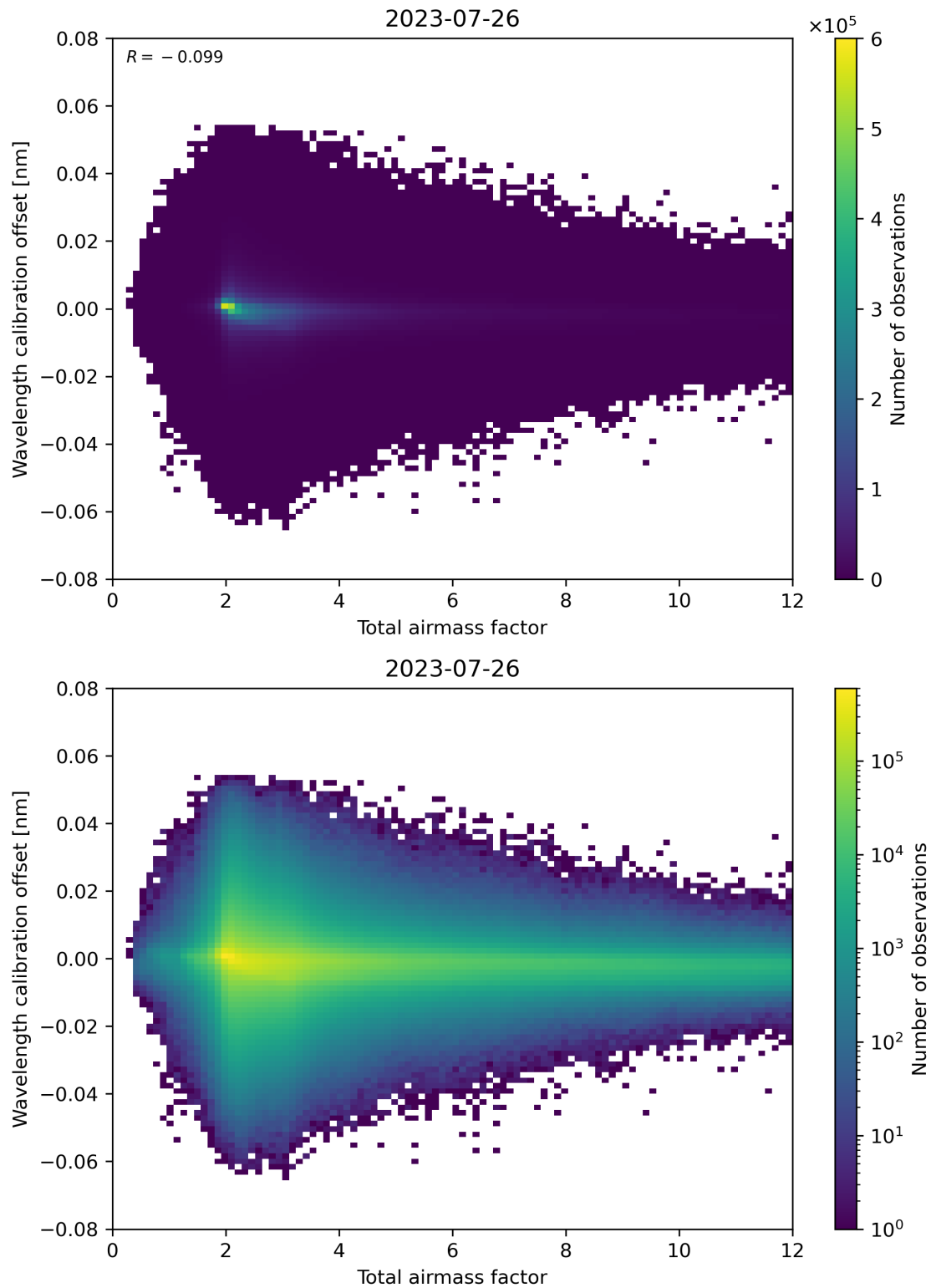
Figure 70: Scatter density plot of “Total airmass factor” against “Wavelength calibration offset” for 2023-07-25 to 2023-07-27.
