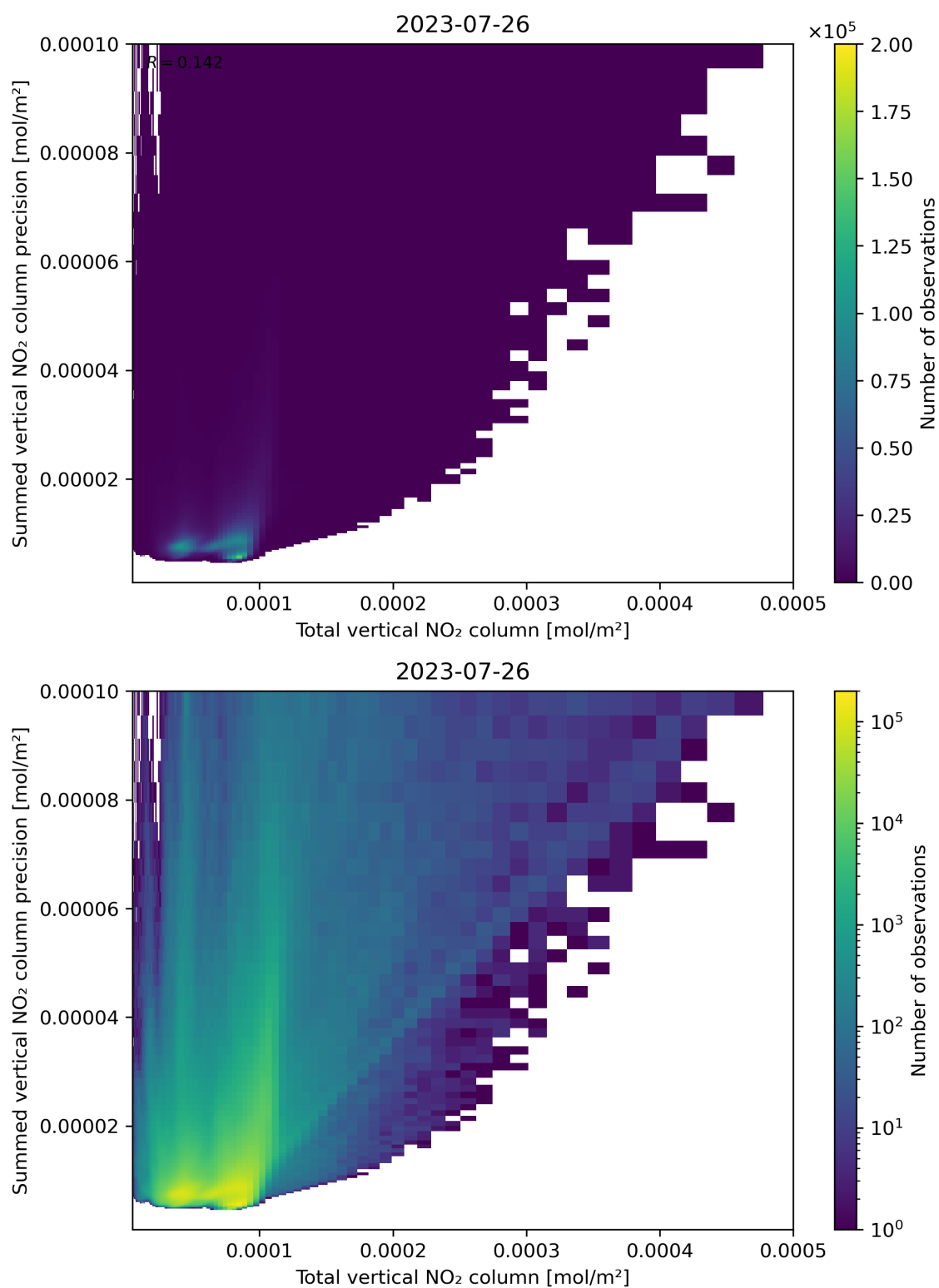
Figure 113: Scatter density plot of “Total vertical NO 2 column” against “Summed vertical NO 2 column precision” for 2023-07-25 to 2023-07-27.
