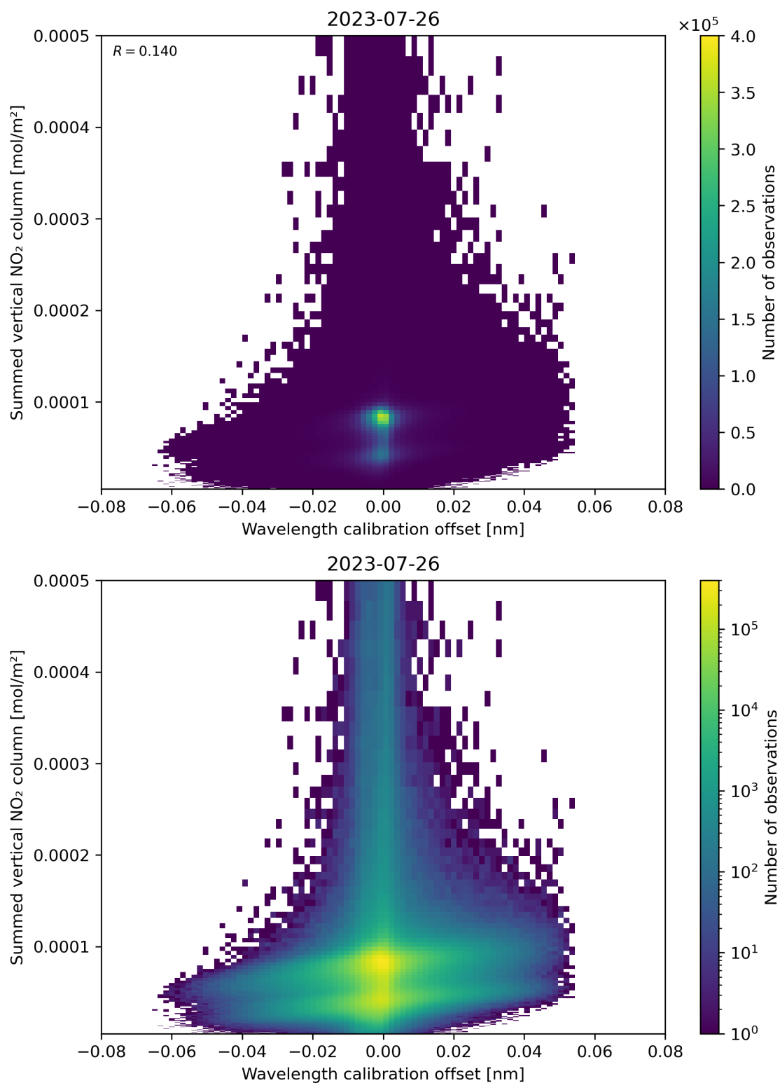
Figure 177: Scatter density plot of “Wavelength calibration offset” against “Summed vertical NO 2 column” for 2023-07-25 to 2023-07-27.
