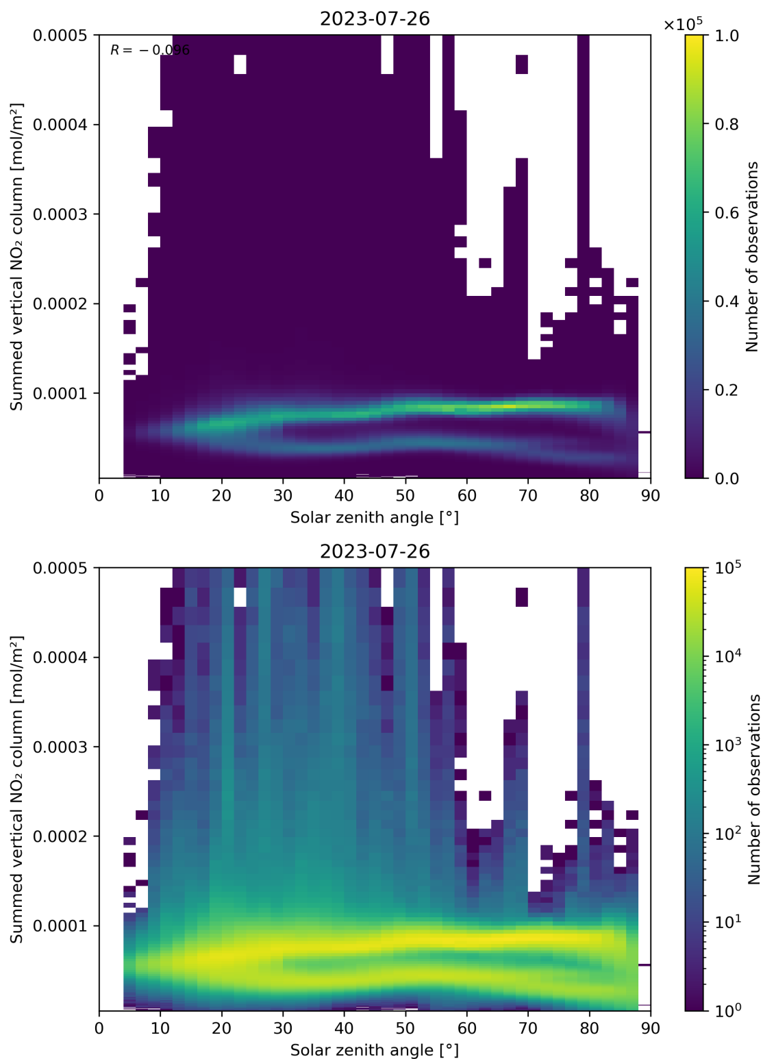
Figure 151: Scatter density plot of “Solar zenith angle” against “Summed vertical NO 2 column” for 2023-07-25 to 2023-07-27.
