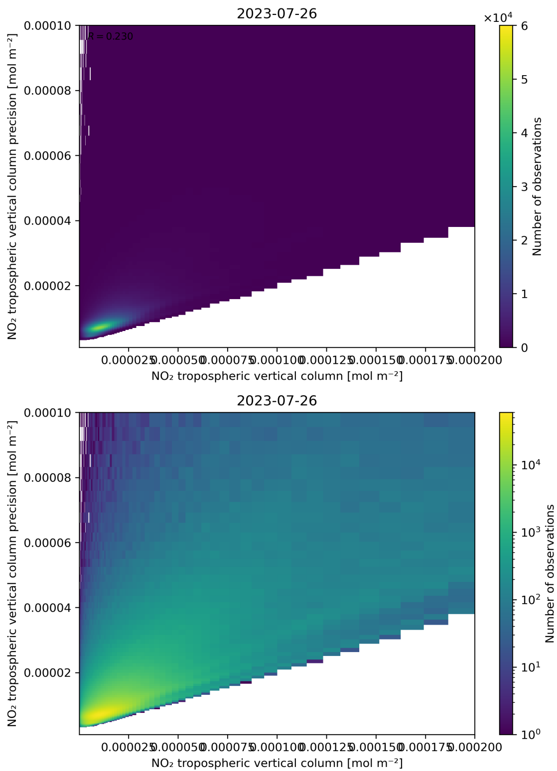
Figure 130: Scatter density plot of “NO 2 tropospheric vertical column” against “NO 2 tropospheric vertical column precision” for 2023-07-25 to 2023-07-27.
