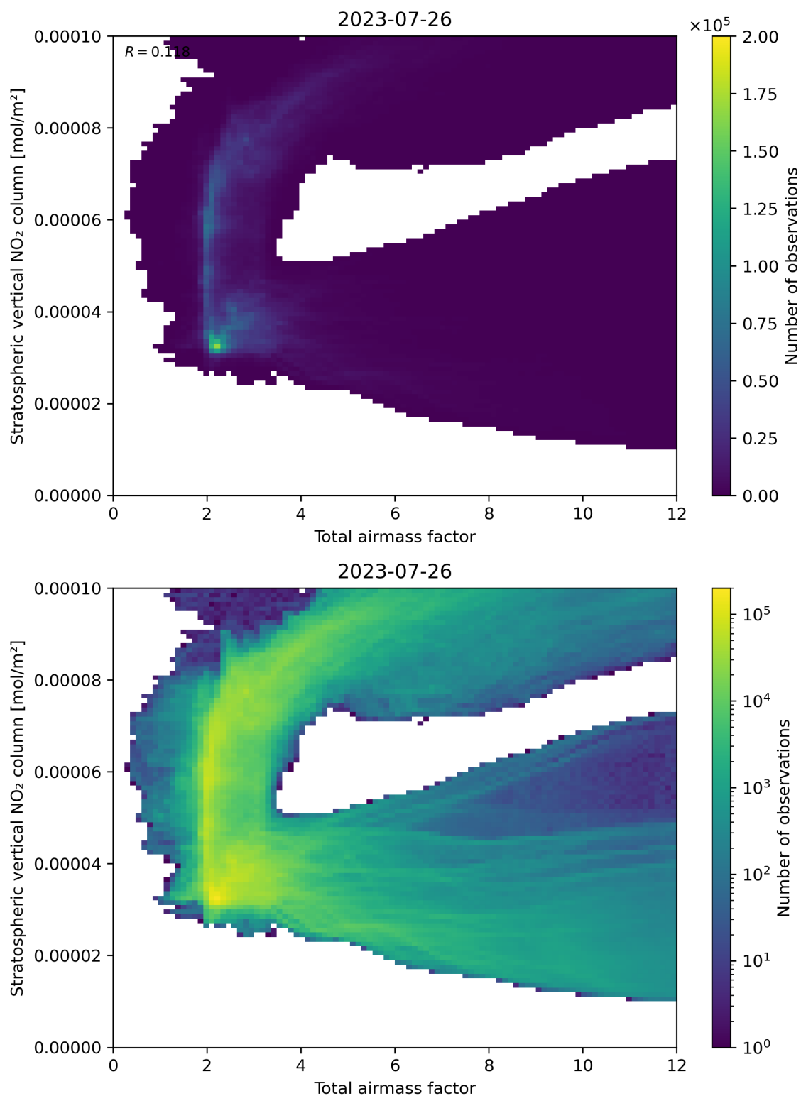
Figure 64: Scatter density plot of “Total airmass factor” against “Stratospheric vertical NO 2 column” for 2023-07-25 to 2023-07-27.
