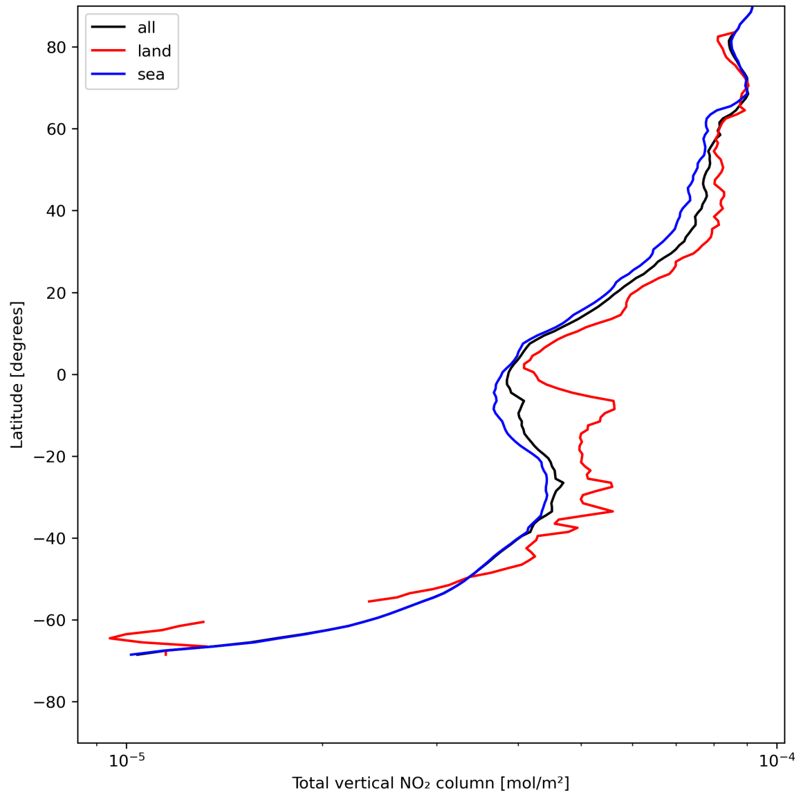
Figure 21: Zonal average of “Total vertical NO 2 column” for 2023-07-25 to 2023-07-27.
