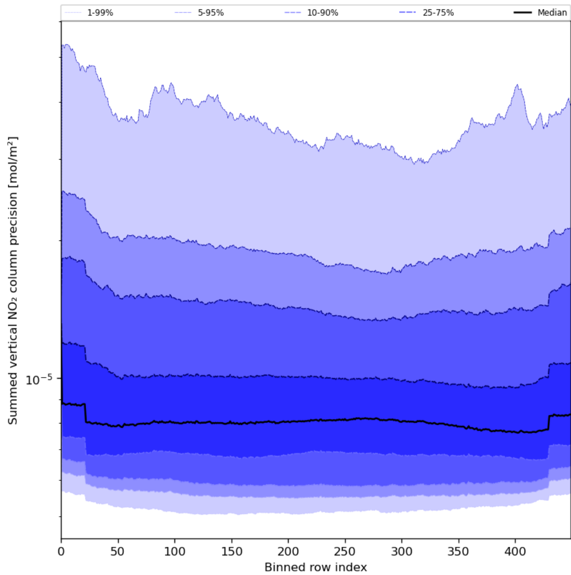
Figure 58: Along track statistics of “Summed vertical NO 2 column precision” for 2023-07-25 to 2023-07-27
