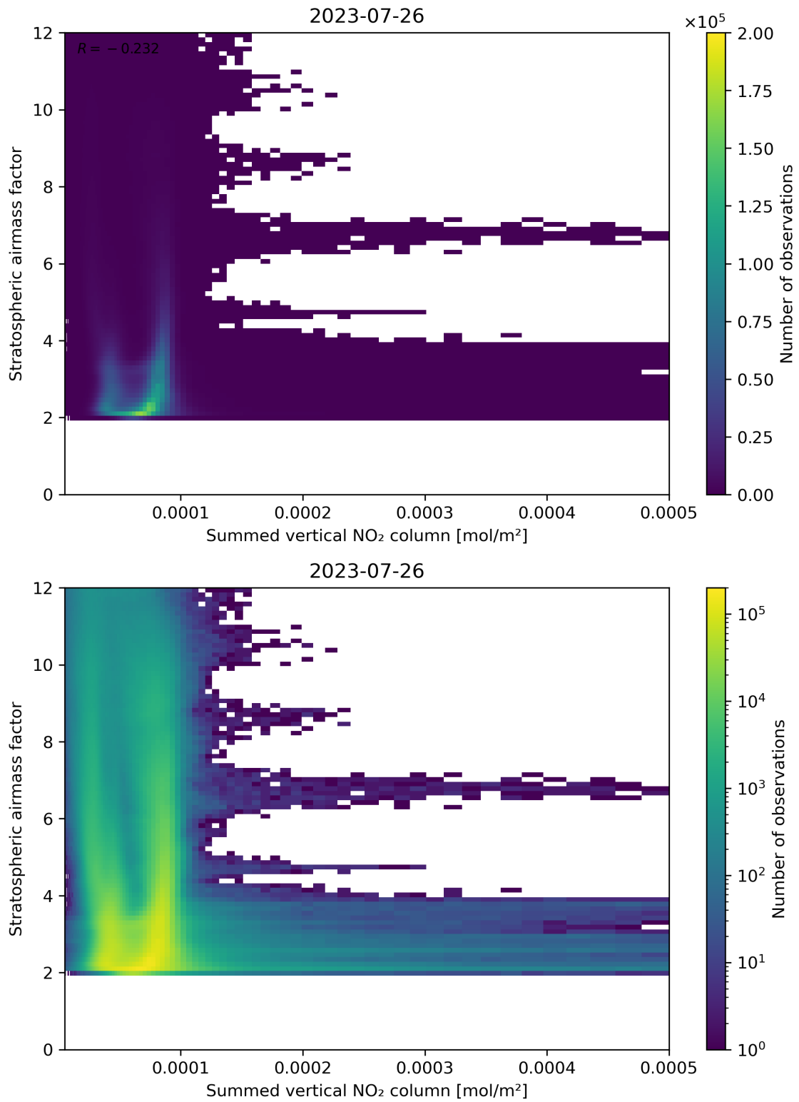
Figure 103: Scatter density plot of “Summed vertical NO 2 column” against “Stratospheric air mass factor” for 2023-07-25 to 2023-07-27.
