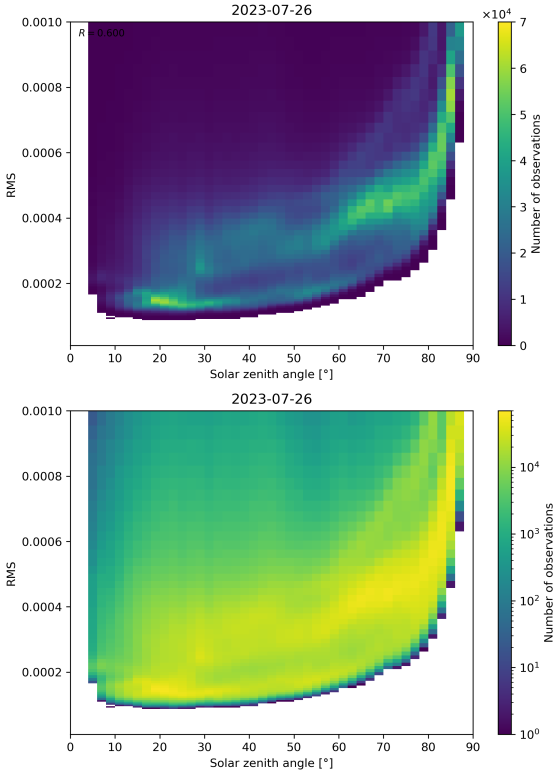
Figure 157: Scatter density plot of “Solar zenith angle” against “RMS” for 2023-07-25 to 2023-07-27.
