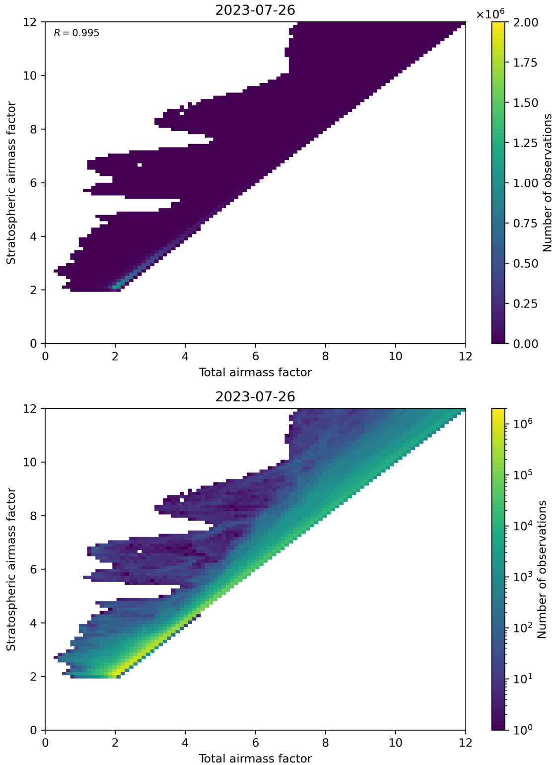
Figure 62: Scatter density plot of “Total airmass factor” against “Stratospheric airmass factor” for 2023-07-25 to 2023-07-27.
