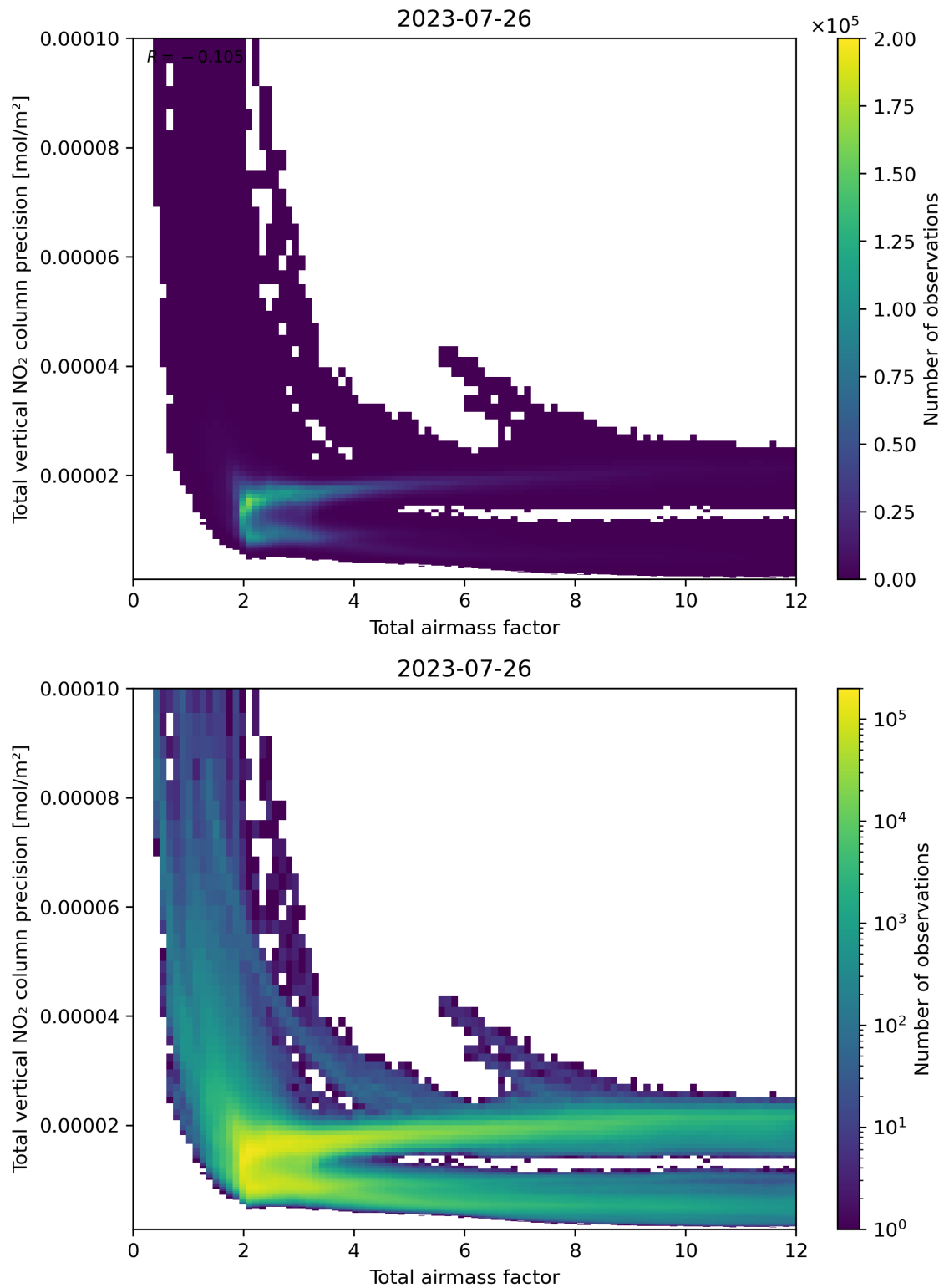
Figure 68: Scatter density plot of “Total airmass factor” against “Total vertical NO 2 column precision” for 2023-07-25 to 2023-07-27.
