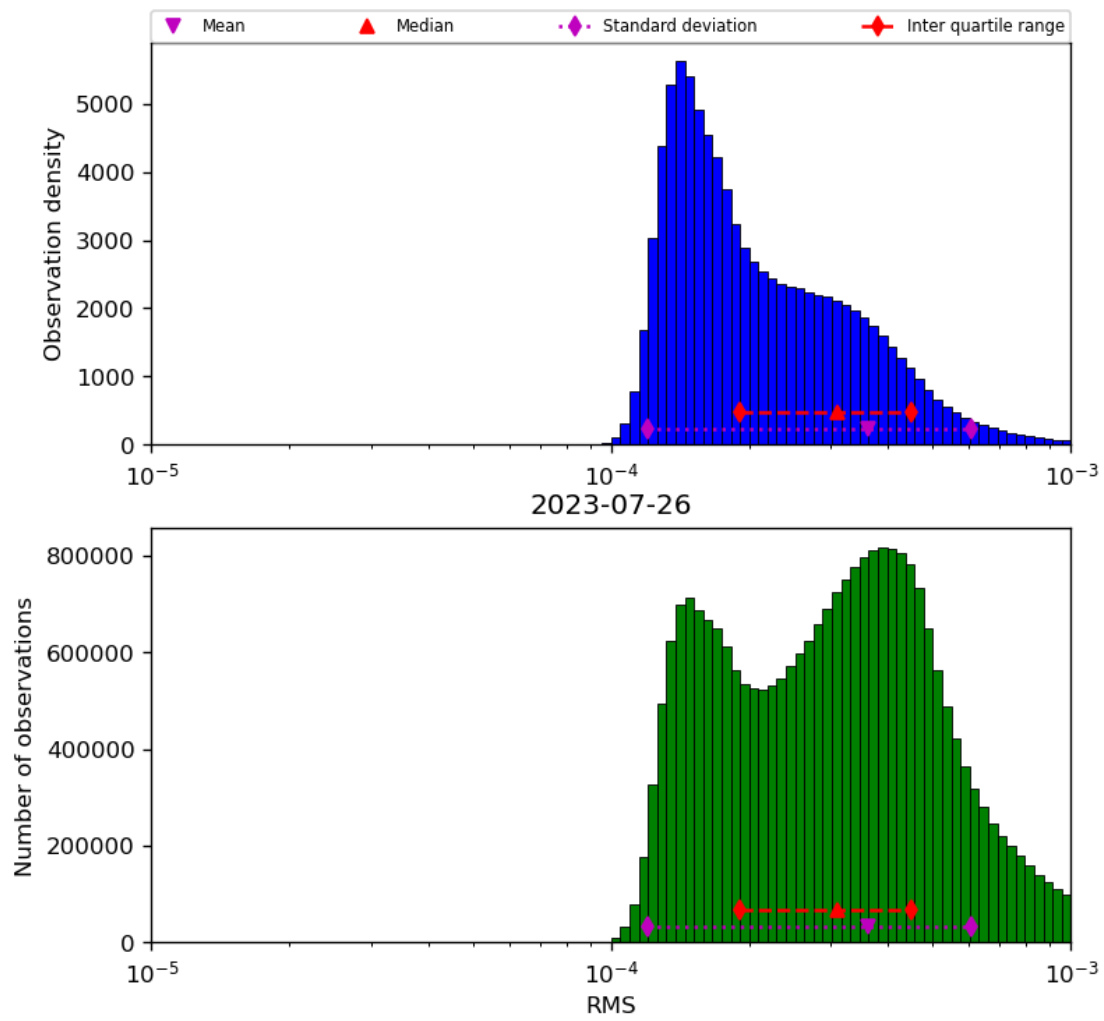
Figure 43: Histogram of “RMS” for 2023-07-25 to 2023-07-27
