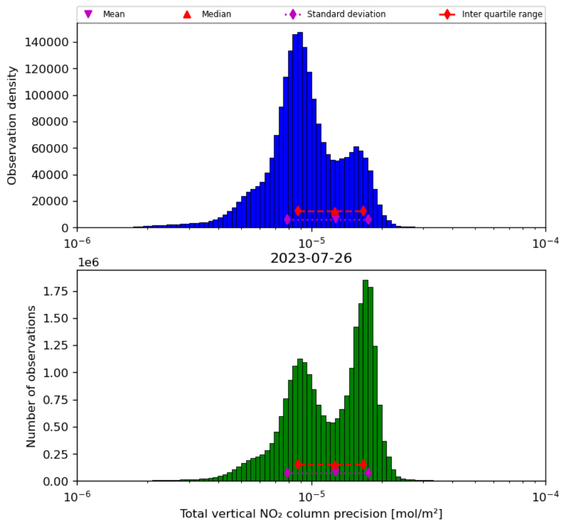
Figure 39: Histogram of “Total vertical NO 2 column precision” for 2023-07-25 to 2023-07-27
