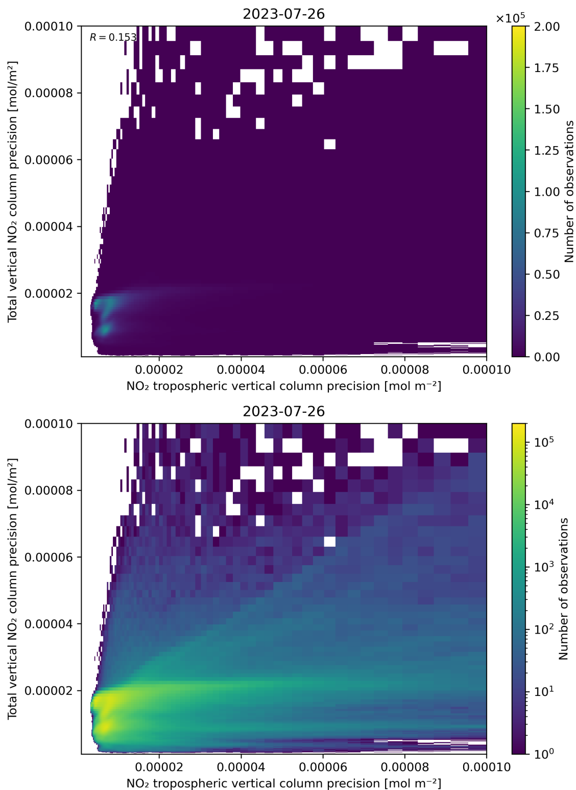
Figure 139: Scatter density plot of “NO 2 tropospheric vertical column precision” against “Total vertical NO 2 column precision” for 2023-07-25 to 2023-07-27.
