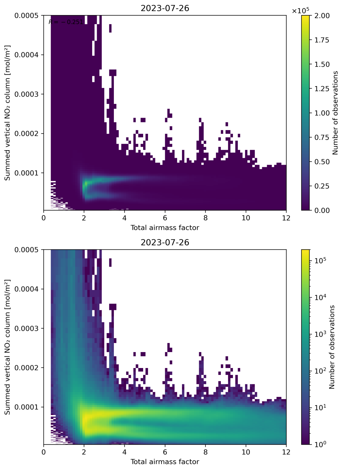
Figure 65: Scatter density plot of “Total air mass factor” against “Summed vertical NO 2 column” for 2023-07-25 to 2023-07-27.
