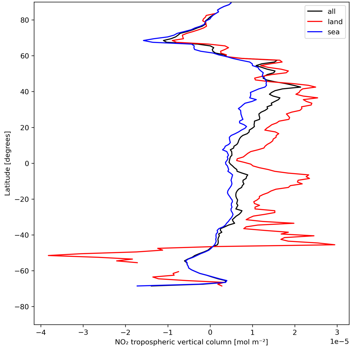
Figure 12: Zonal average of “NO 2 tropospheric vertical column” for 2023-07-25 to 2023-07-27.
