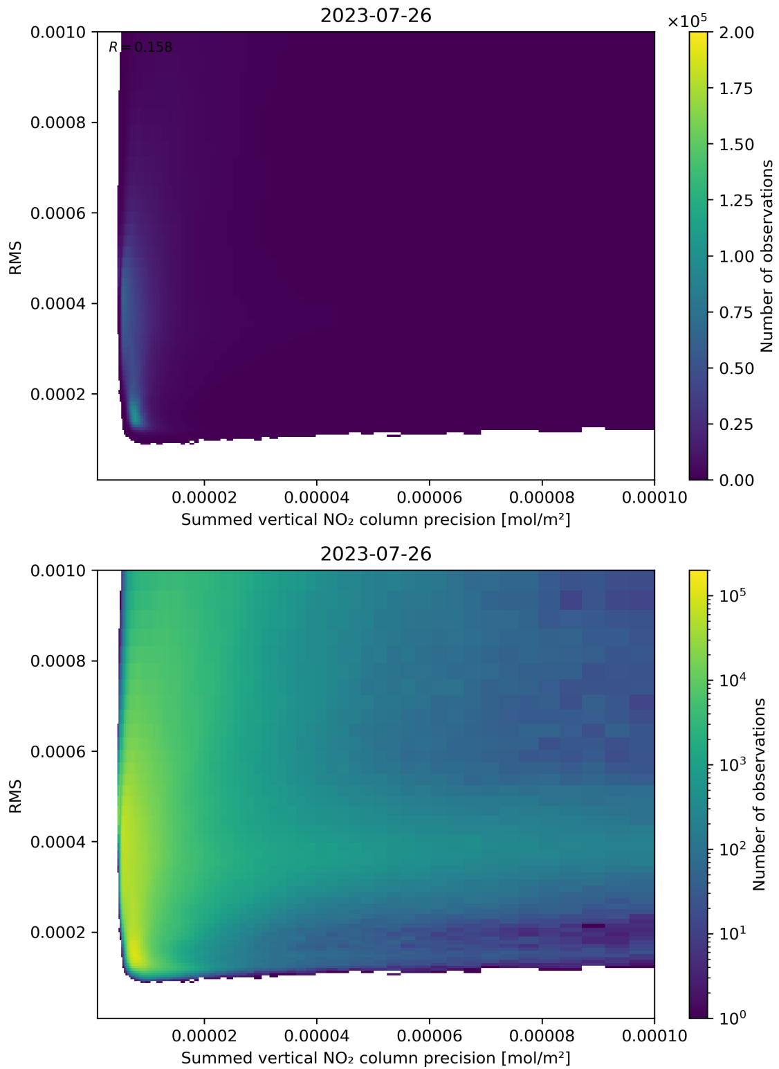
Figure 108: Scatter density plot of “Summed vertical NO 2 column precision” against “RMS” for 2023-07-25 to 2023-07-27.
