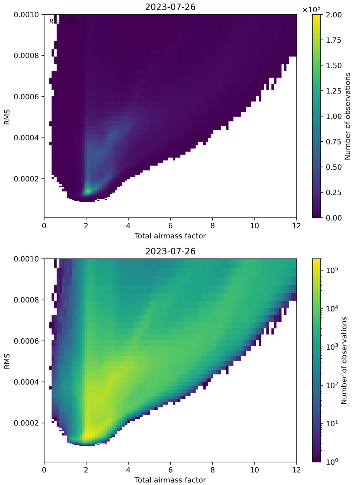
Figure 69: Scatter density plot of “Total airmass factor” against “RMS” for 2023-07-25 to 2023-07-27.
