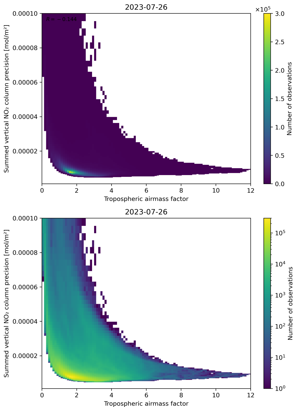
Figure 76: Scatter density plot of “Tropospheric air mass factor” against “Summed vertical NO 2 column precision” for 2023-07-25 to 2023-07-27.
