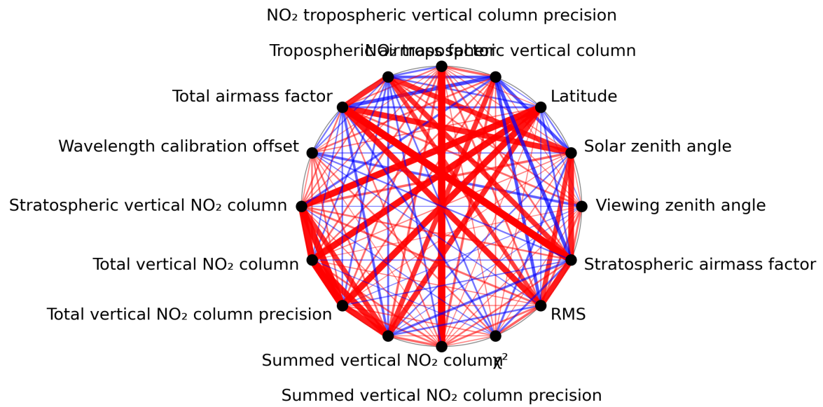
Figure 1: Map of correlation graph for 2023-07-25 to 2023-07-27.
