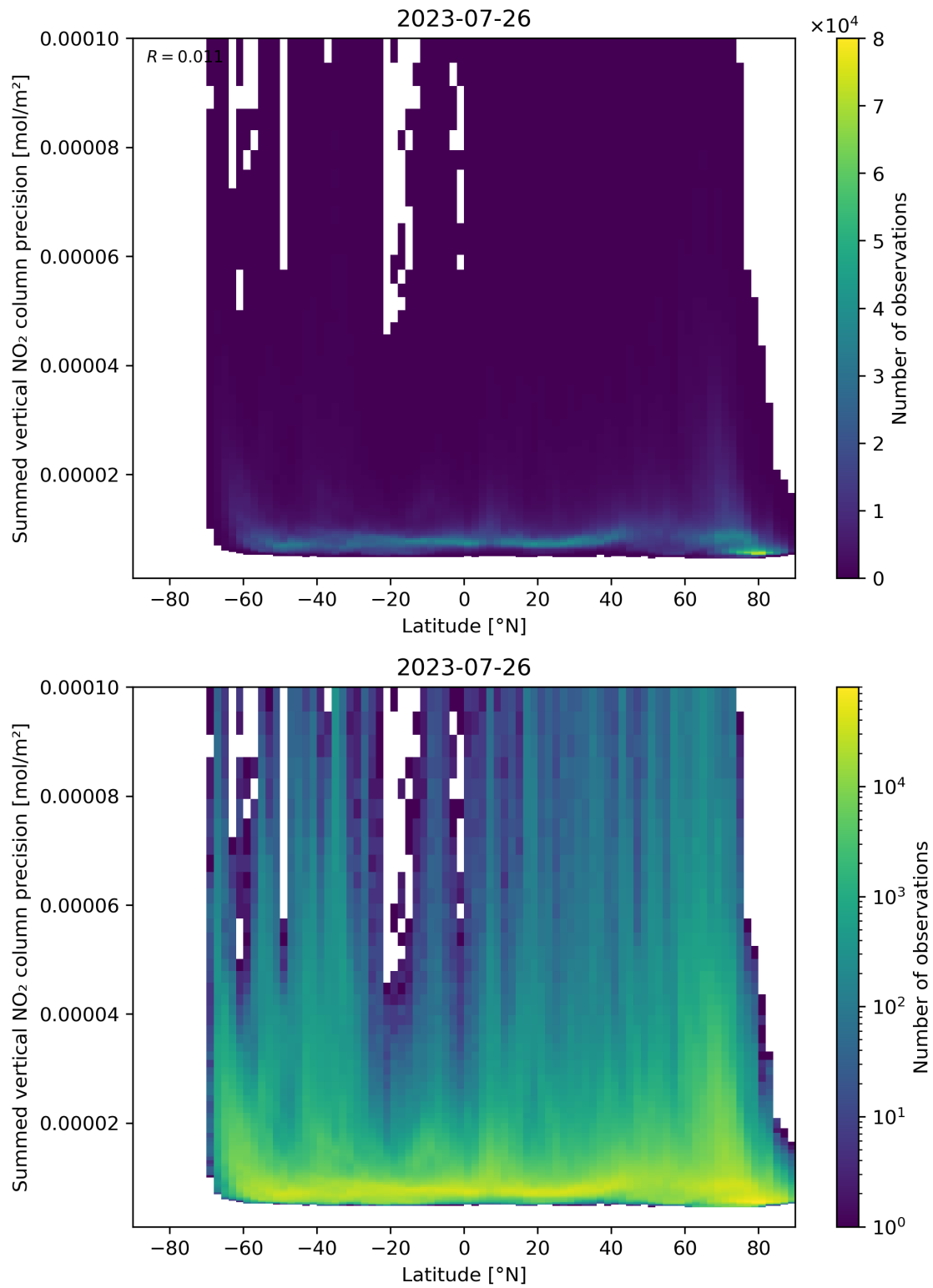
Figure 89: Scatter density plot of “Latitude” against “Summed vertical NO 2 column precision” for 2023-07-25 to 2023-07-27.
