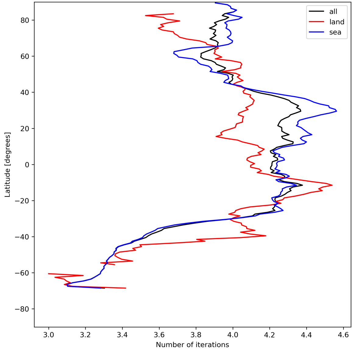
Figure 17: Zonal average of “Number of iterations” for 2023-07-25 to 2023-07-27.
