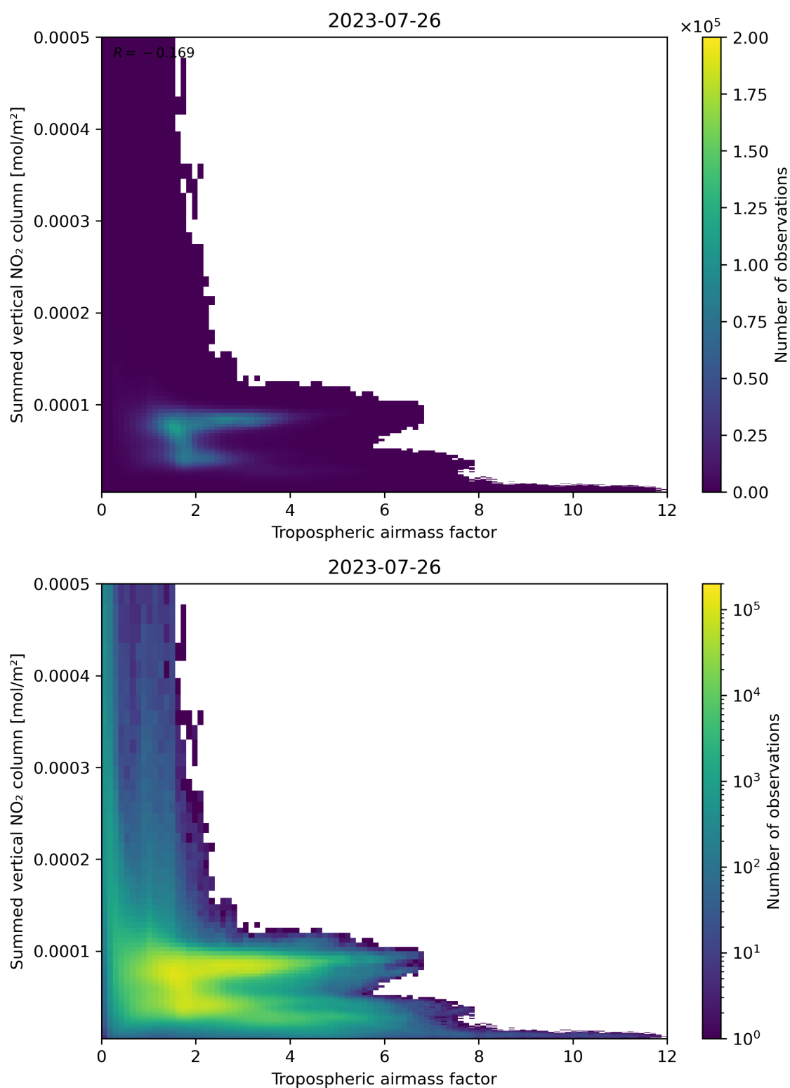
Figure 75: Scatter density plot of “Tropospheric airmass factor” against “Summed vertical NO 2 column” for 2023-07-25 to 2023-07-27.
