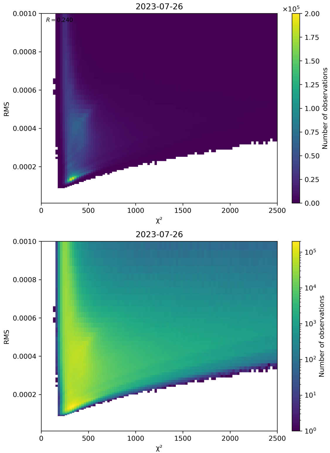
Figure 82: Scatter density plot of “ \chi^2 ” against “RMS” for 2023-07-25 to 2023-07-27.
