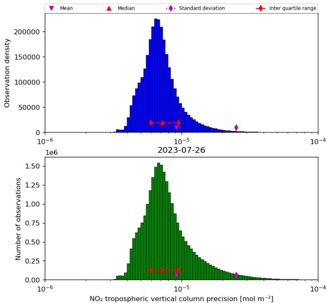
Figure 30: Histogram of “NO 2 tropospheric vertical column precision” for 2023-07-25 to 2023-07-27
