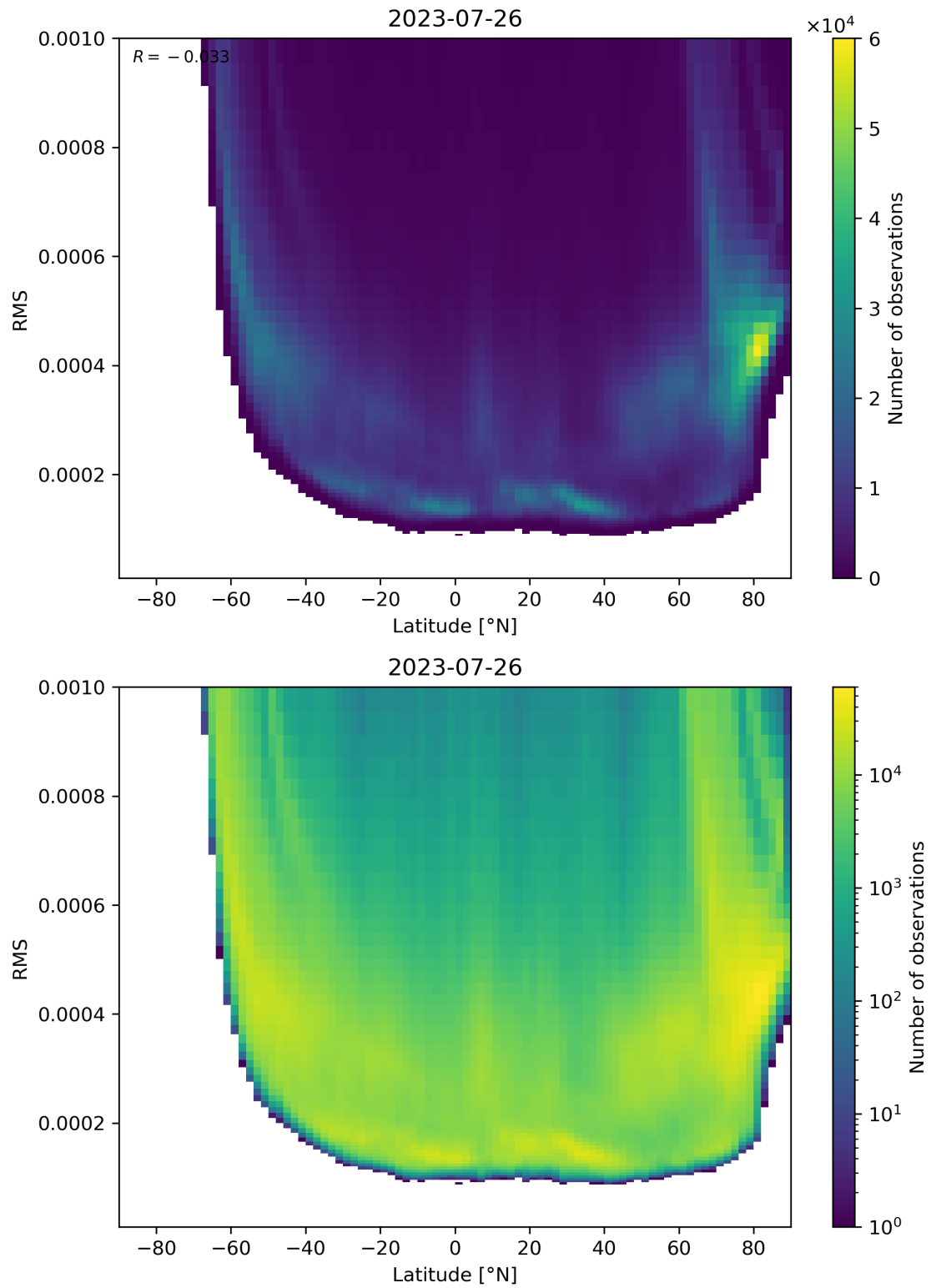
Figure 94: Scatter density plot of “Latitude” against “RMS” for 2023-07-25 to 2023-07-27.
