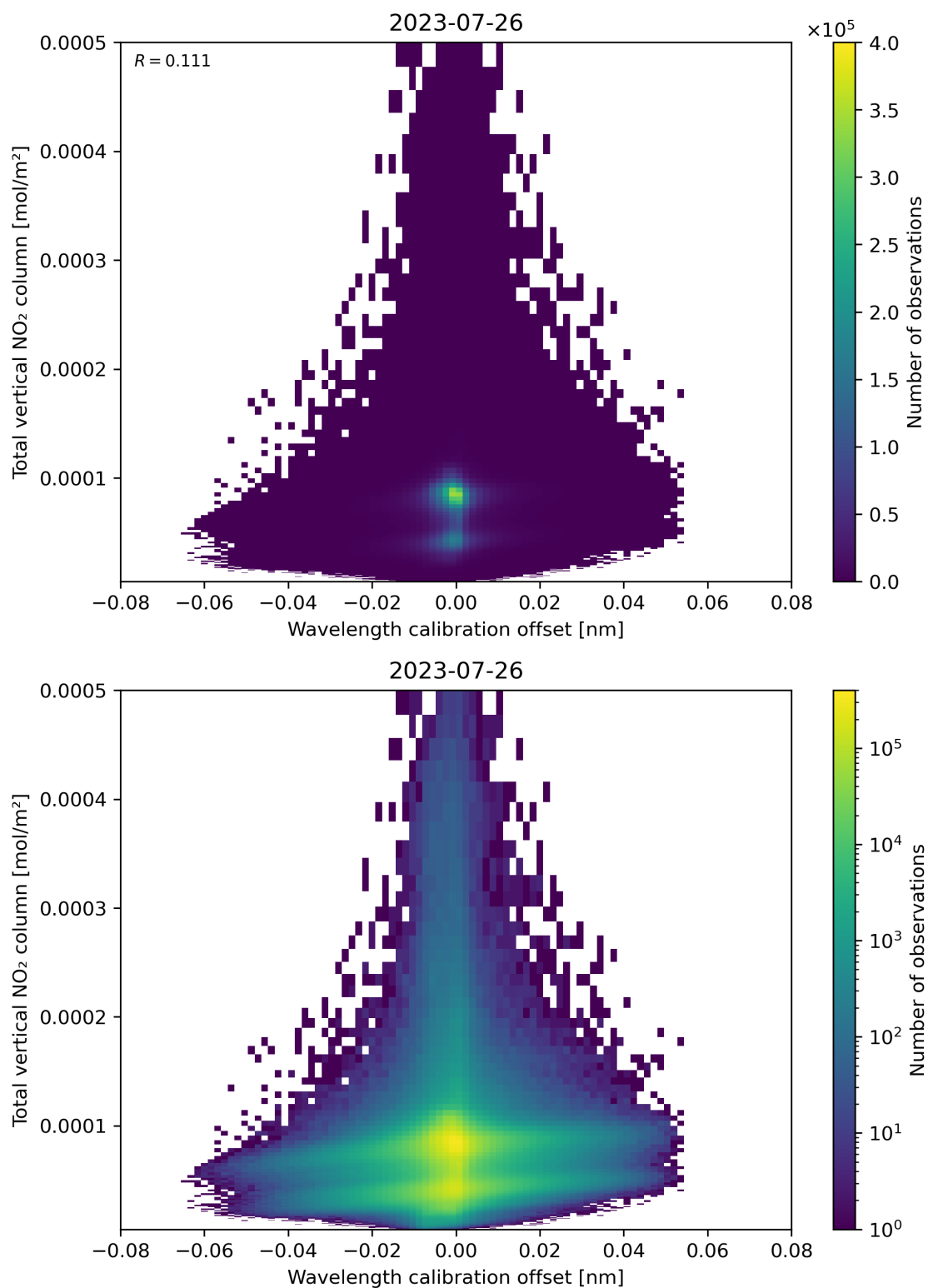
Figure 179: Scatter density plot of “Wavelength calibration offset” against “Total vertical NO 2 column” for 2023-07-25 to 2023-07-27.
