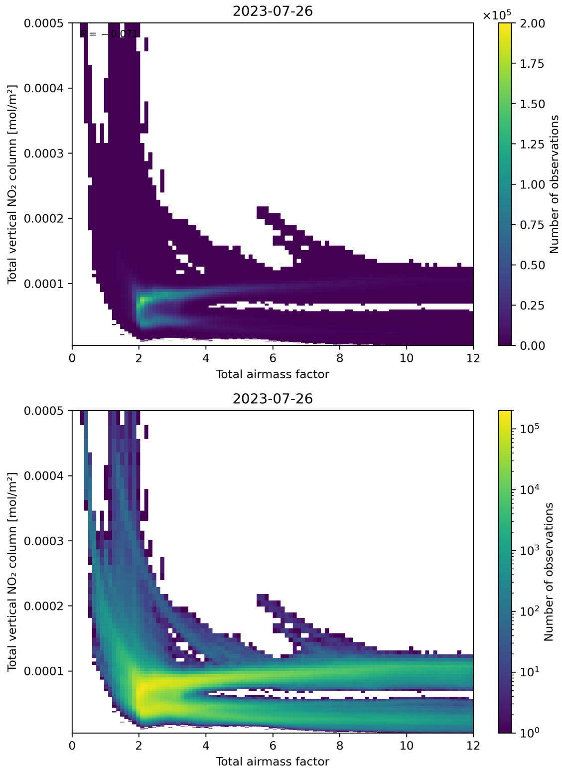
Figure 67: Scatter density plot of “Total airmass factor” against “Total vertical NO 2 column” for 2023-07-25 to 2023-07-27.
