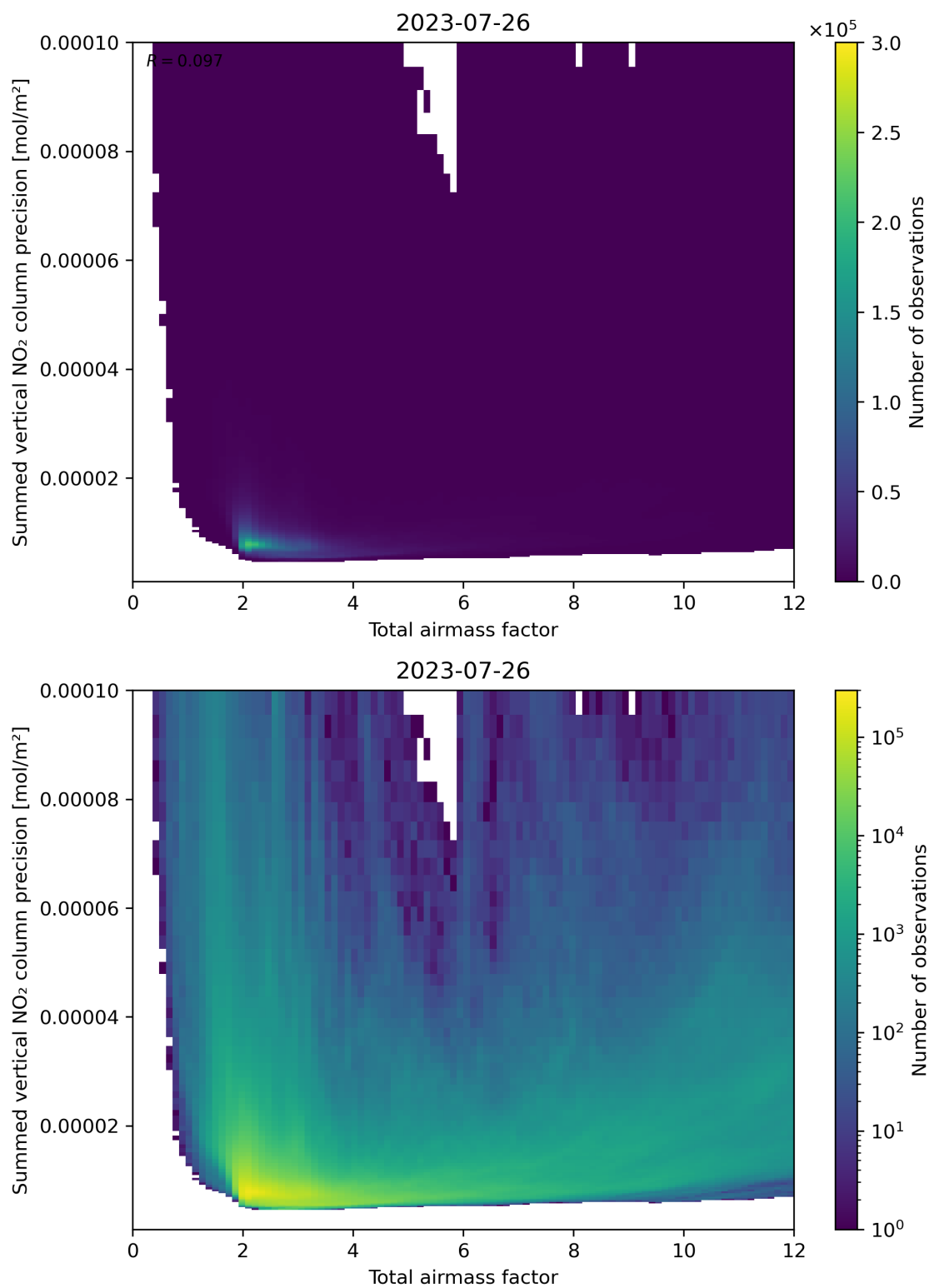
Figure 66: Scatter density plot of “Total airmass factor” against “Summed vertical NO 2 column precision” for 2023-07-25 to 2023-07-27.
