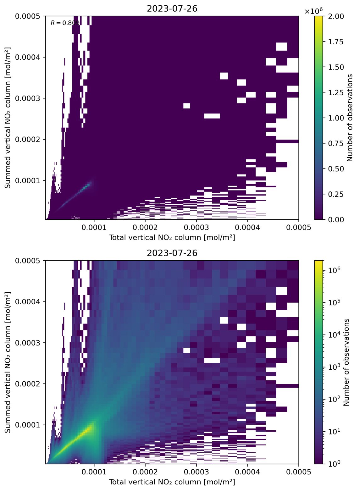
Figure 112: Scatter density plot of “Total vertical NO 2 column” against “Summed vertical NO 2 column” for 2023-07-25 to 2023-07-27.
