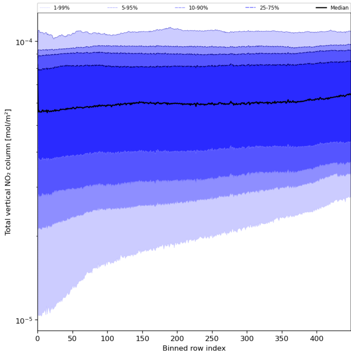
Figure 55: Along track statistics of “Total vertical NO 2 column” for 2023-07-25 to 2023-07-27
