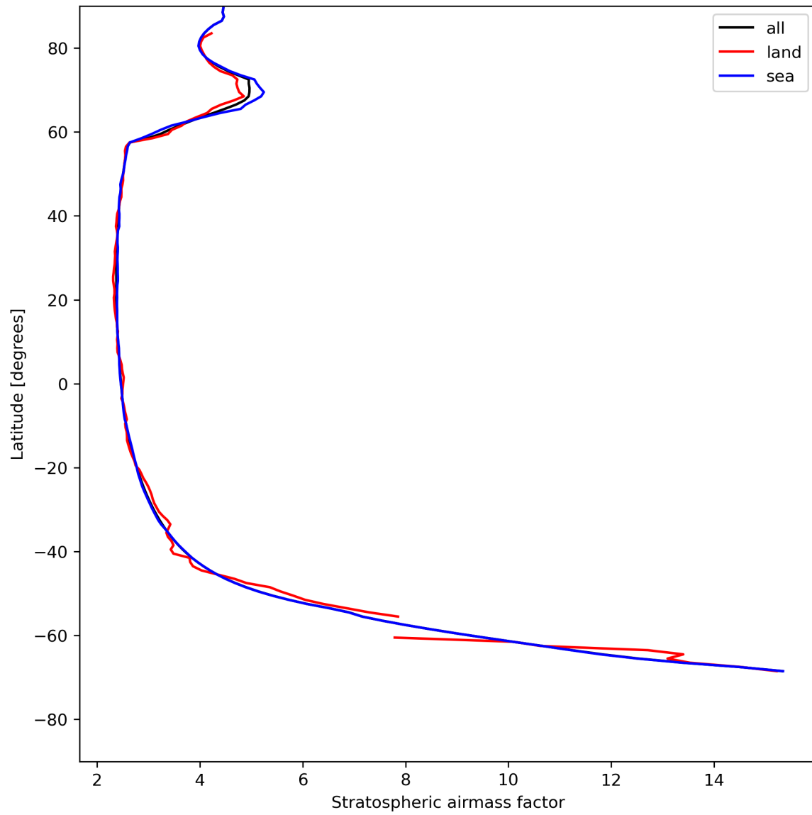
Figure 27: Zonal average of “Stratospheric air mass factor” for 2023-07-25 to 2023-07-27.
