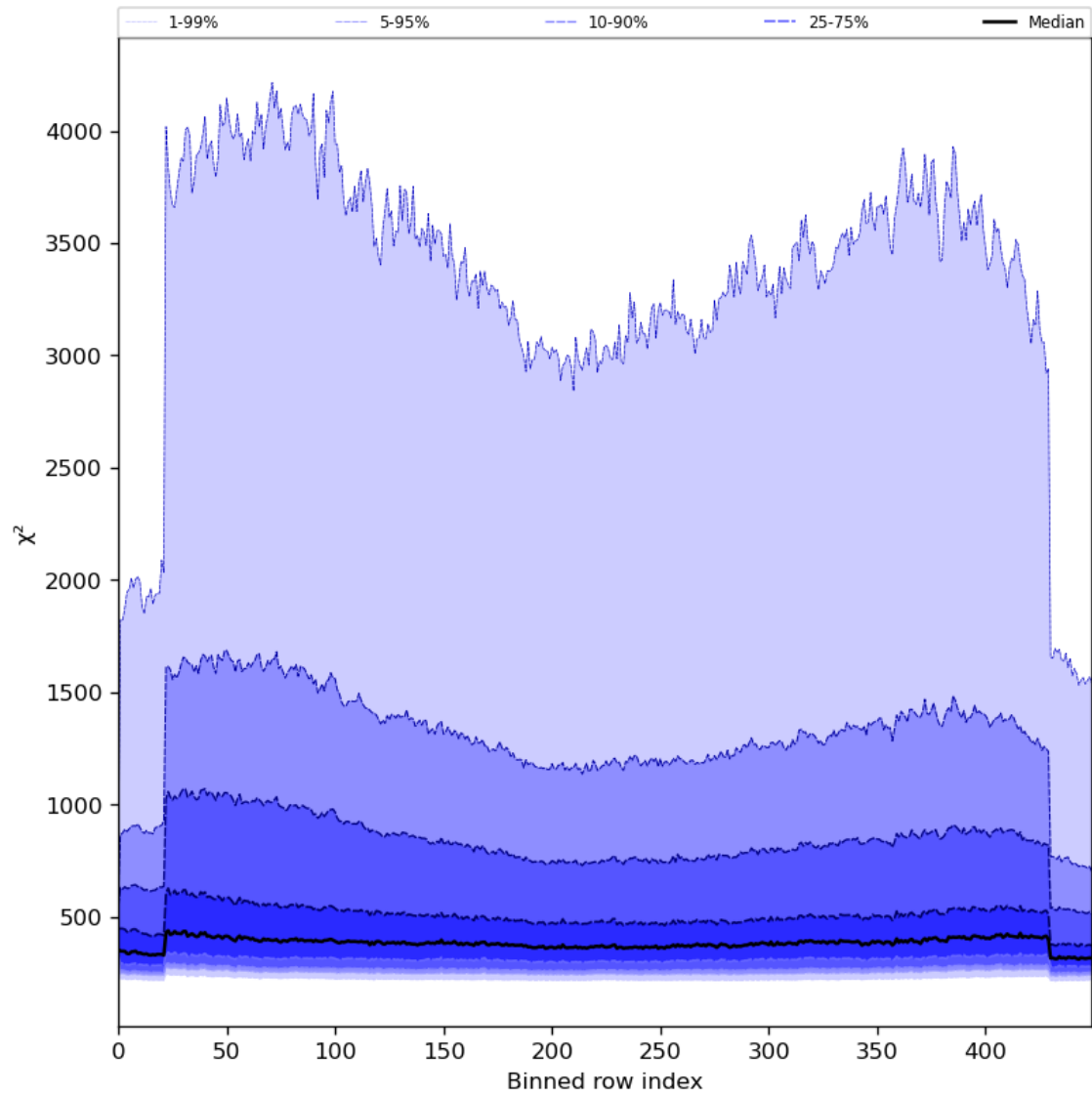
Figure 59: Along track statistics of “ \chi^2 ” for 2023-07-25 to 2023-07-27
