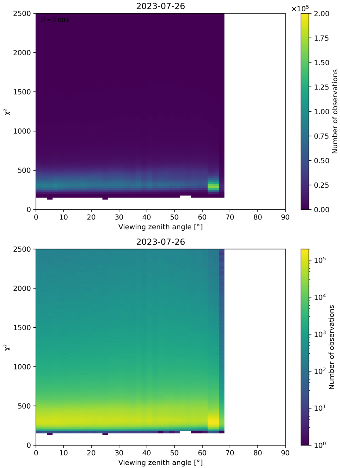
Figure 162: Scatter density plot of “Viewing zenith angle” against “ \chi^2 ” for 2023-07-25 to 2023-07-27.
