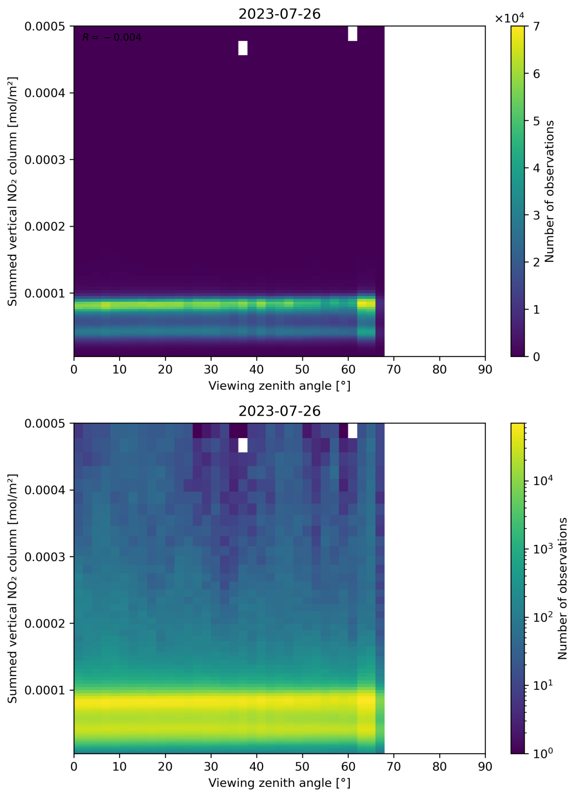
Figure 165: Scatter density plot of “Viewing zenith angle” against “Summed vertical NO 2 column” for 2023-07-25 to 2023-07-27.
