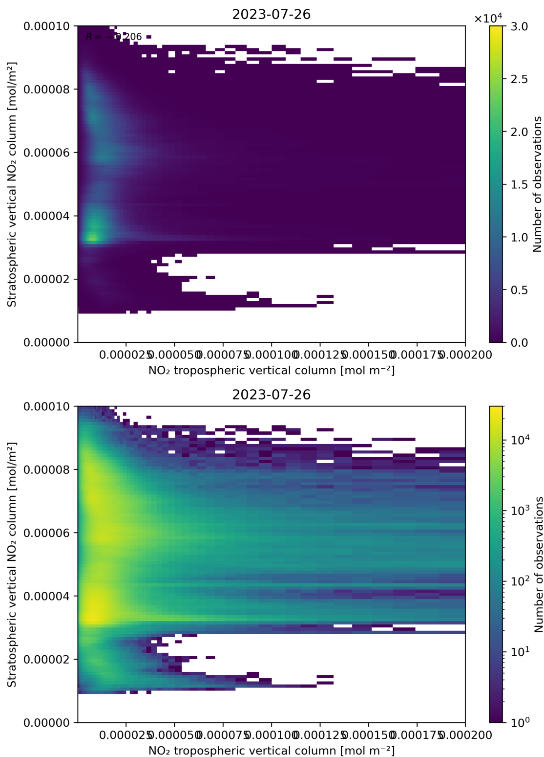
Figure 125: Scatter density plot of “NO 2 tropospheric vertical column” against “Stratospheric vertical NO 2 column” for 2023-07-25 to 2023-07-27.
