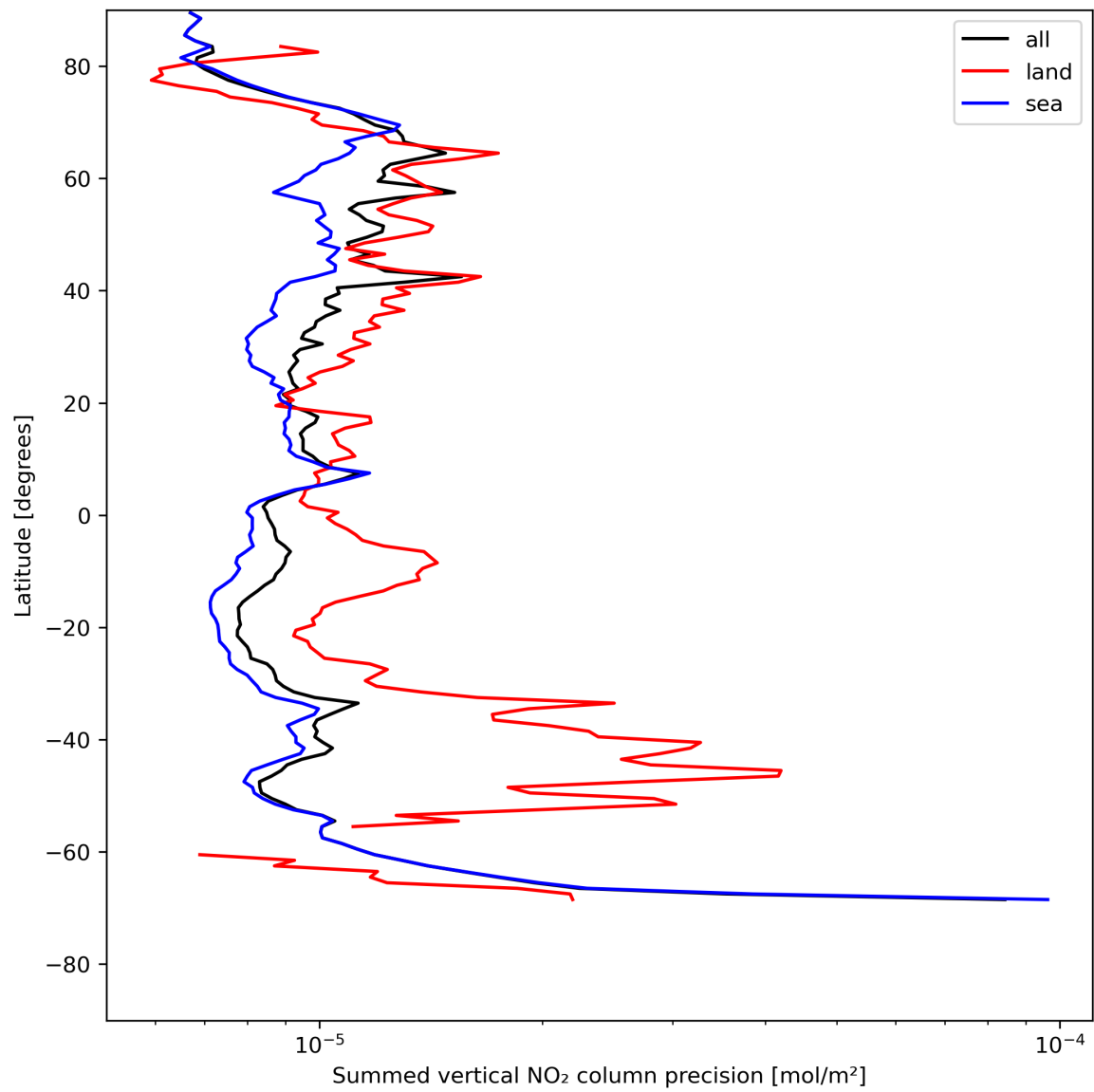
Figure 24: Zonal average of “Summed vertical NO 2 column precision” for 2023-07-25 to 2023-07-27.
