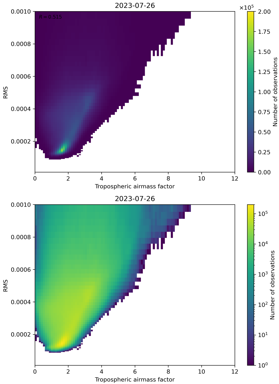
Figure 79: Scatter density plot of “Tropospheric airmass factor” against “RMS” for 2023-07-25 to 2023-07-27.
