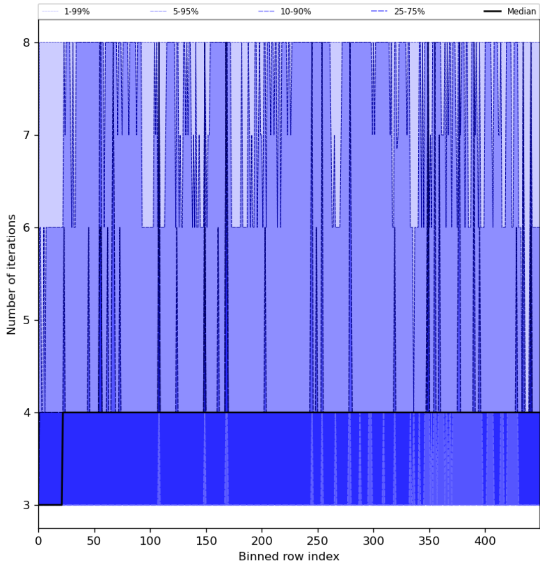
Figure 51: Along track statistics of “Number of iterations” for 2023-07-25 to 2023-07-27
