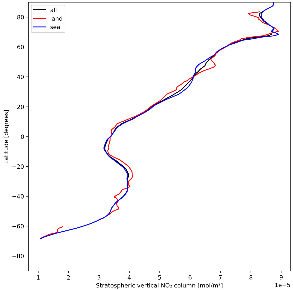
Figure 19: Zonal average of “Stratospheric vertical NO 2 column” for 2023-07-25 to 2023-07-27.
