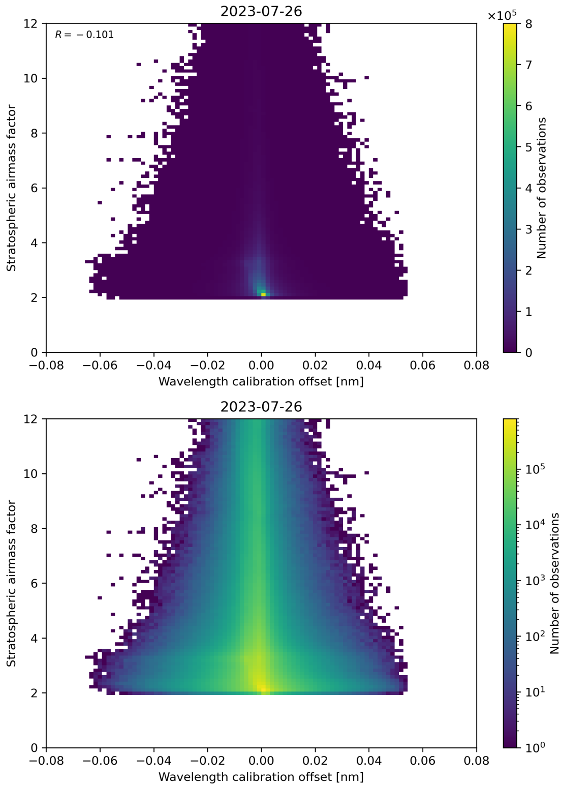
Figure 174: Scatter density plot of “Wavelength calibration offset” against “Stratospheric airmass factor” for 2023-07-25 to 2023-07-27.
