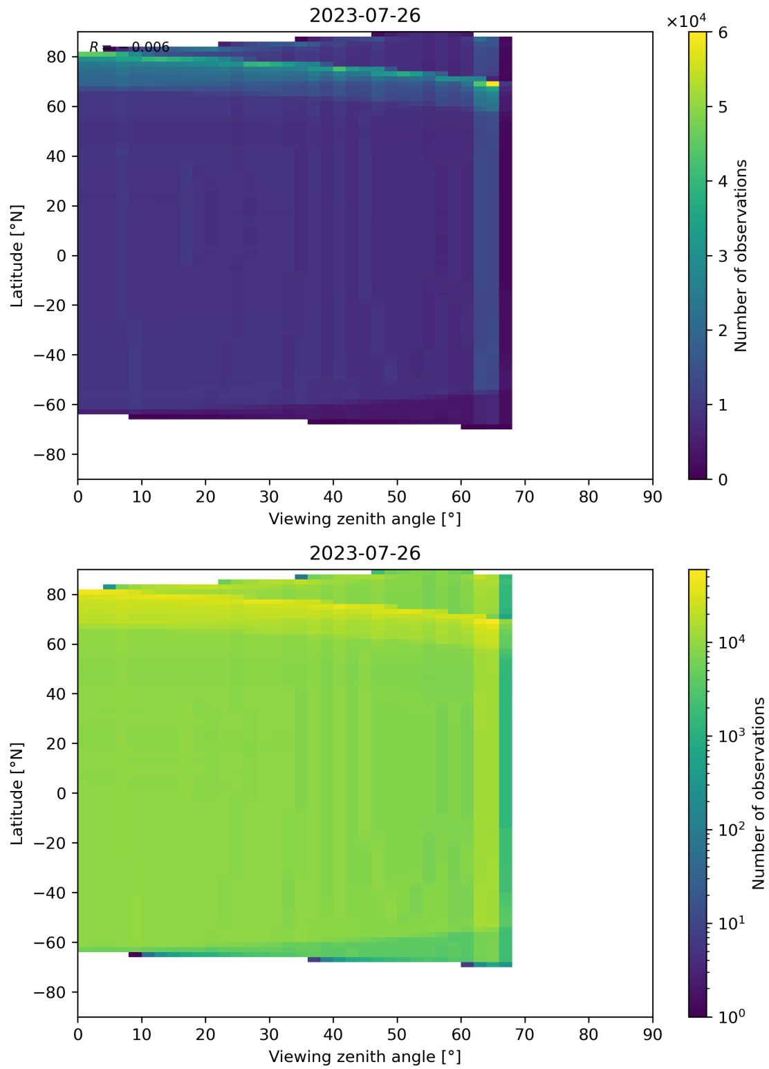
Figure 163: Scatter density plot of “Viewing zenith angle” against “Latitude” for 2023-07-25 to 2023-07-27.
