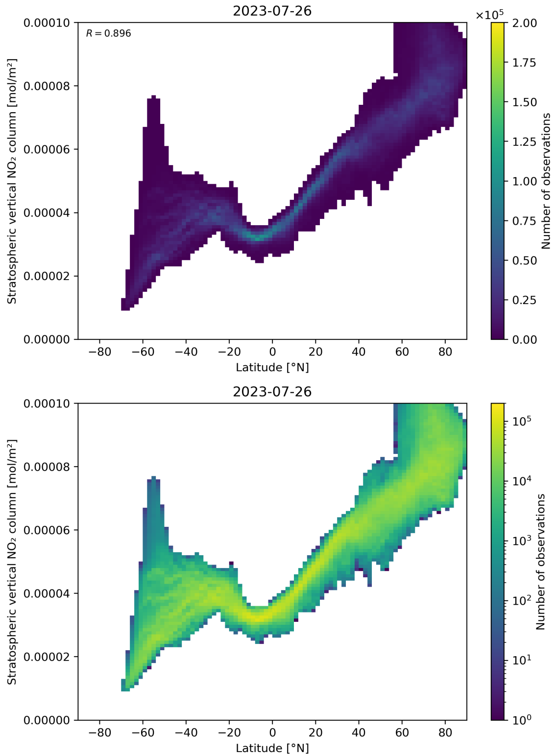
Figure 87: Scatter density plot of “Latitude” against “Stratospheric vertical NO 2 column” for 2023-07-25 to 2023-07-27.
