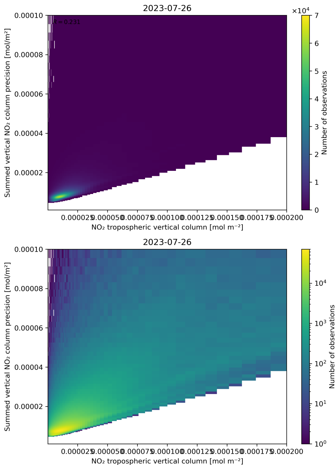
Figure 127: Scatter density plot of “NO 2 tropospheric vertical column” against “Summed vertical NO 2 column precision” for 2023-07-25 to 2023-07-27.
