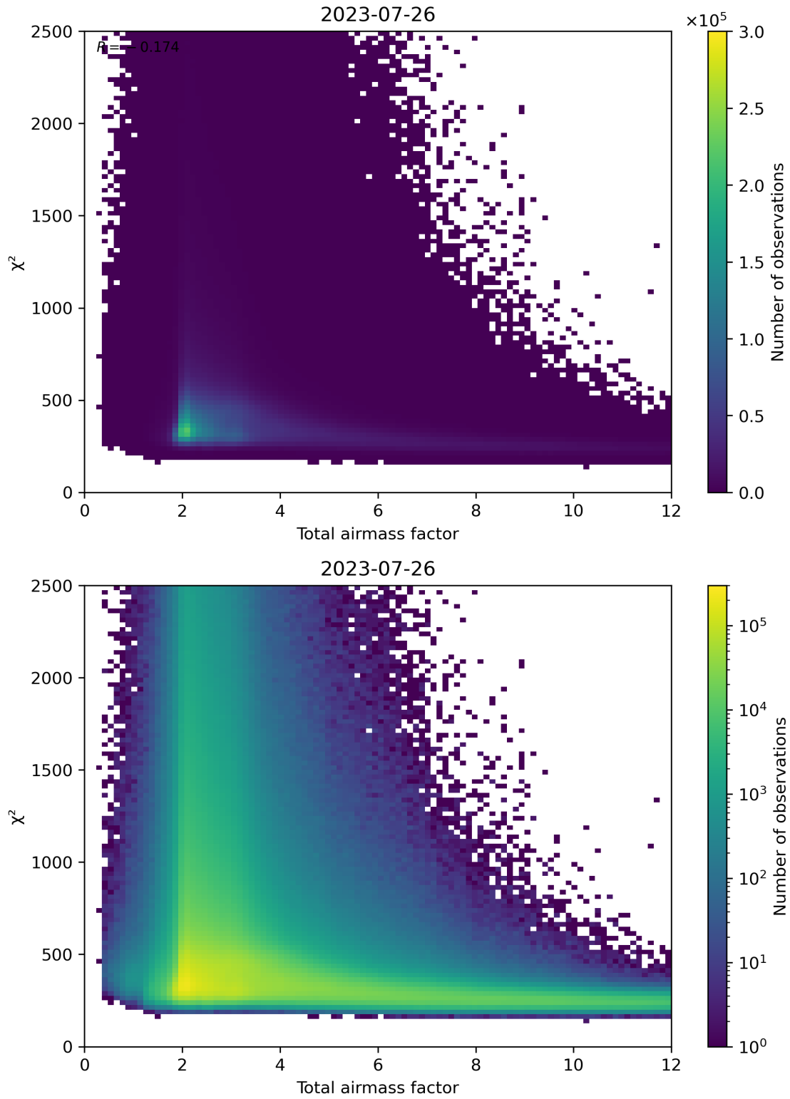
Figure 63: Scatter density plot of “Total airmass factor” against “ \chi^2 ” for 2023-07-25 to 2023-07-27.
