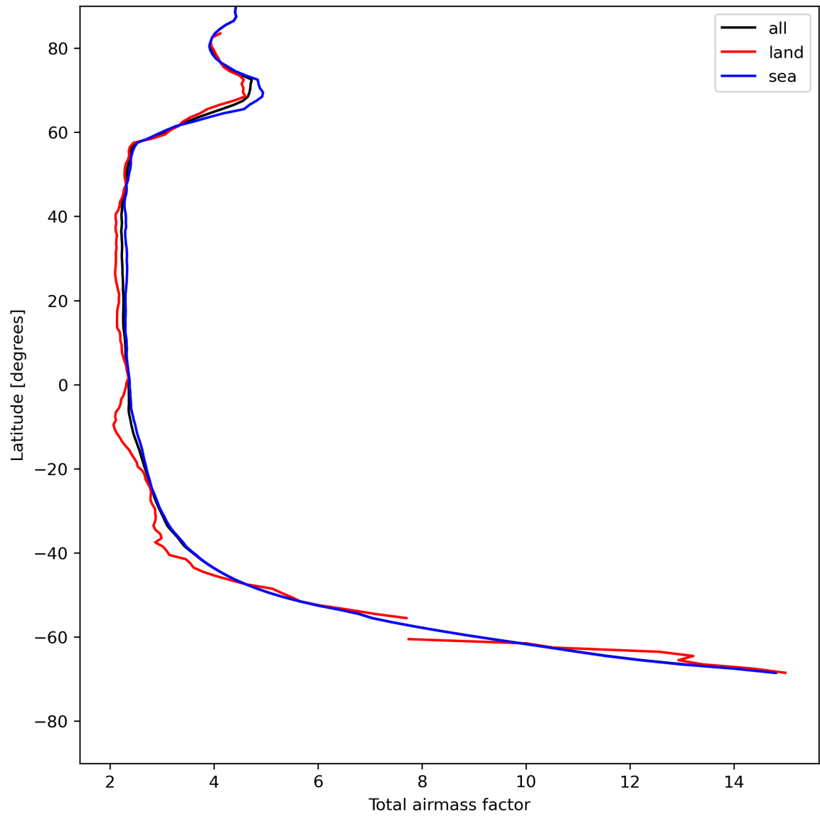
Figure 15: Zonal average of “Total airmass factor” for 2023-07-25 to 2023-07-27.
