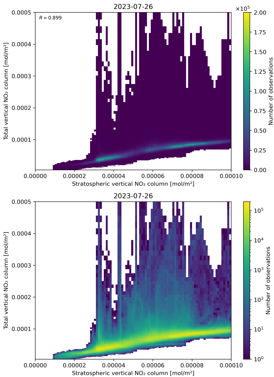
Figure 100: Scatter density plot of “Stratospheric vertical NO 2 column” against “Total vertical NO 2 column” for 2023-07-25 to 2023-07-27.
