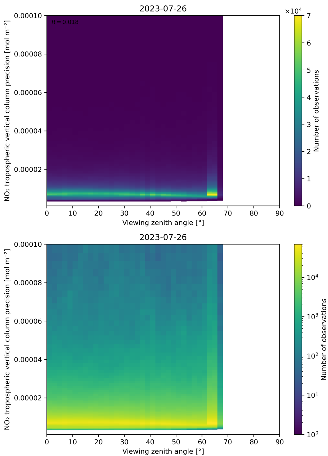
Figure 170: Scatter density plot of “Viewing zenith angle” against “NO 2 tropospheric vertical column precision” for 2023-07-25 to 2023-07-27.
