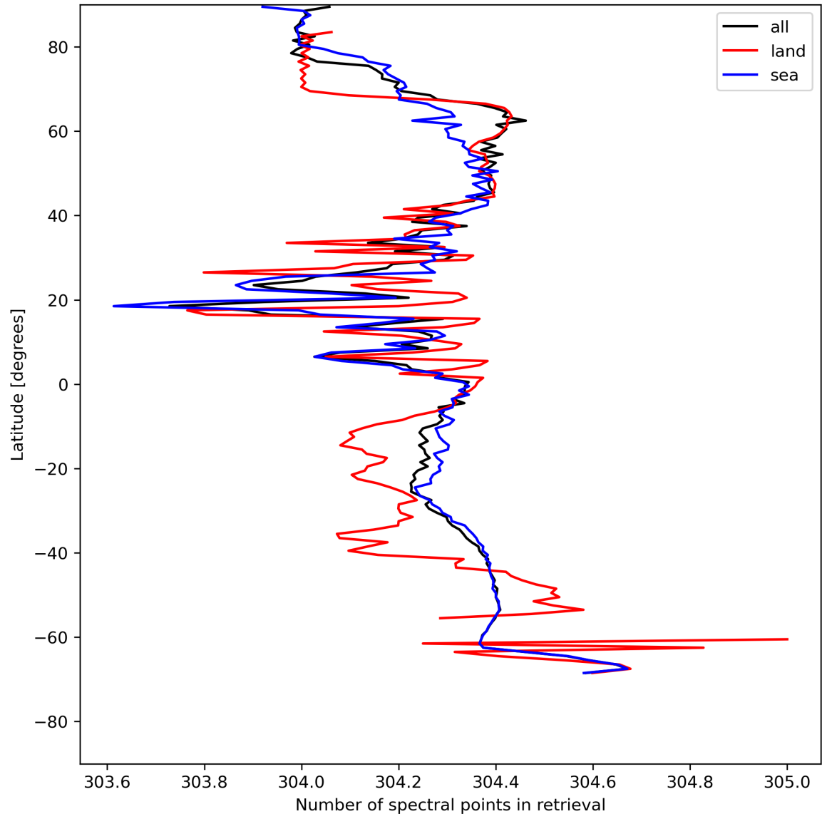
Figure 16: Zonal average of “Number of spectral points in retrieval” for 2023-07-25 to 2023-07-27.
