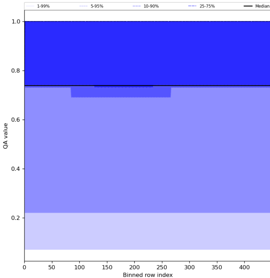
Figure 45: Along track statistics of “QA value” for 2023-07-25 to 2023-07-27
