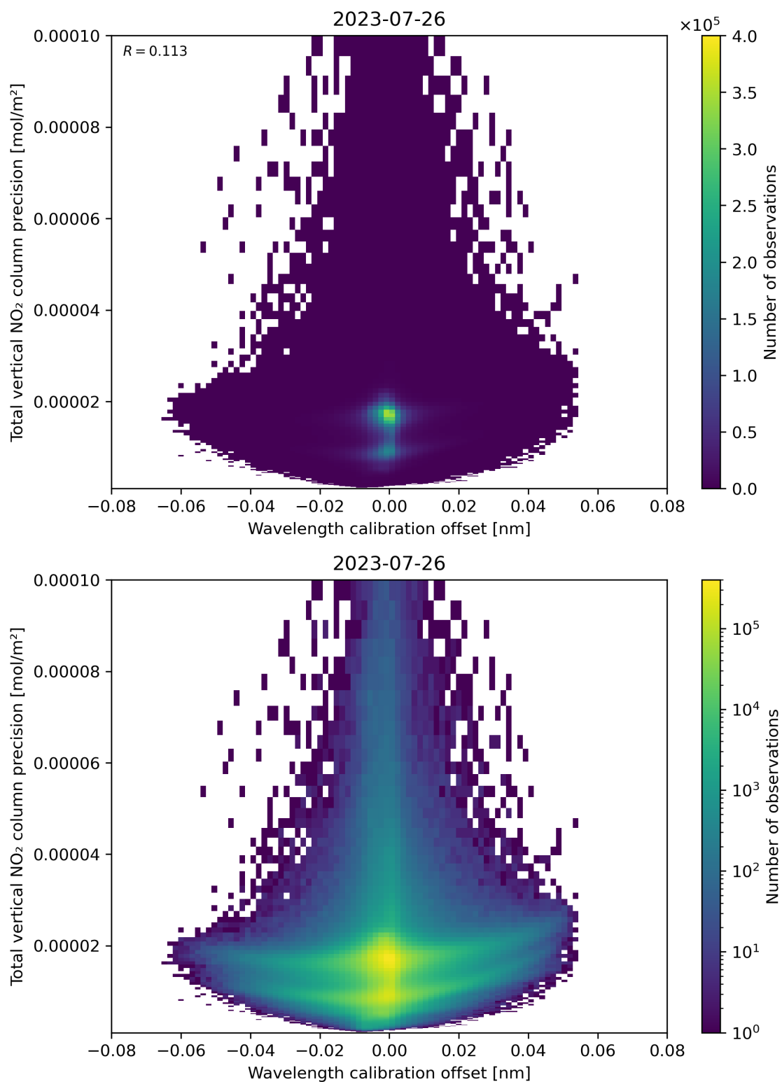
Figure 180: Scatter density plot of “Wavelength calibration offset” against “Total vertical NO 2 column precision” for 2023-07-25 to 2023-07-27.
