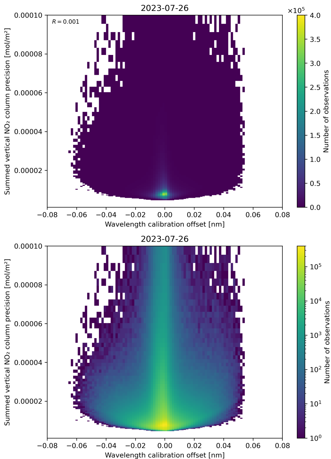
Figure 178: Scatter density plot of “Wavelength calibration offset” against “Summed vertical NO 2 column precision” for 2023-07-25 to 2023-07-27.
