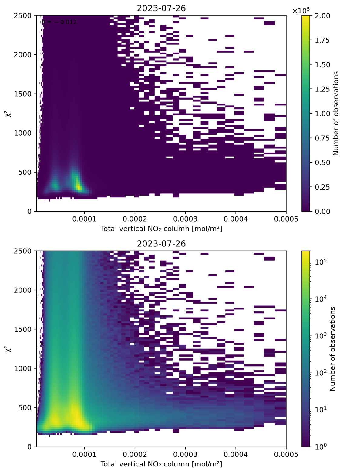
Figure 111: Scatter density plot of “Total vertical NO 2 column” against “ \chi^2 ” for 2023-07-25 to 2023-07-27.
