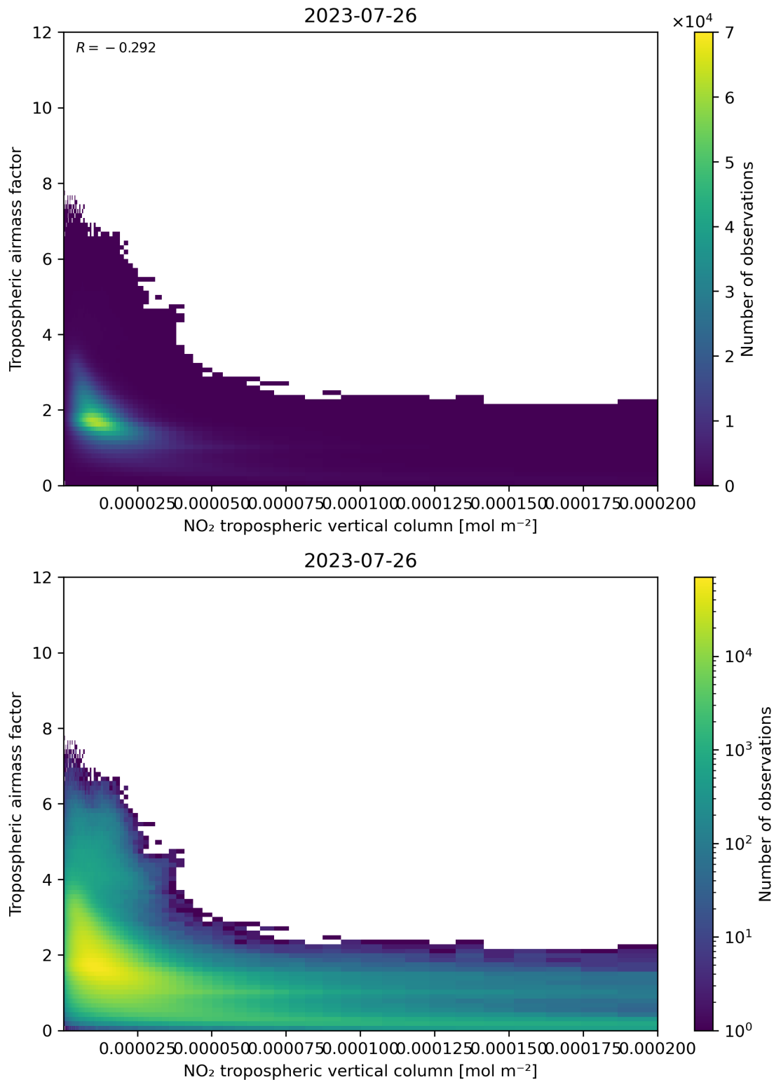
Figure 123: Scatter density plot of “NO 2 tropospheric vertical column” against “Tropospheric air mass factor” for 2023-07-25 to 2023-07-27.
