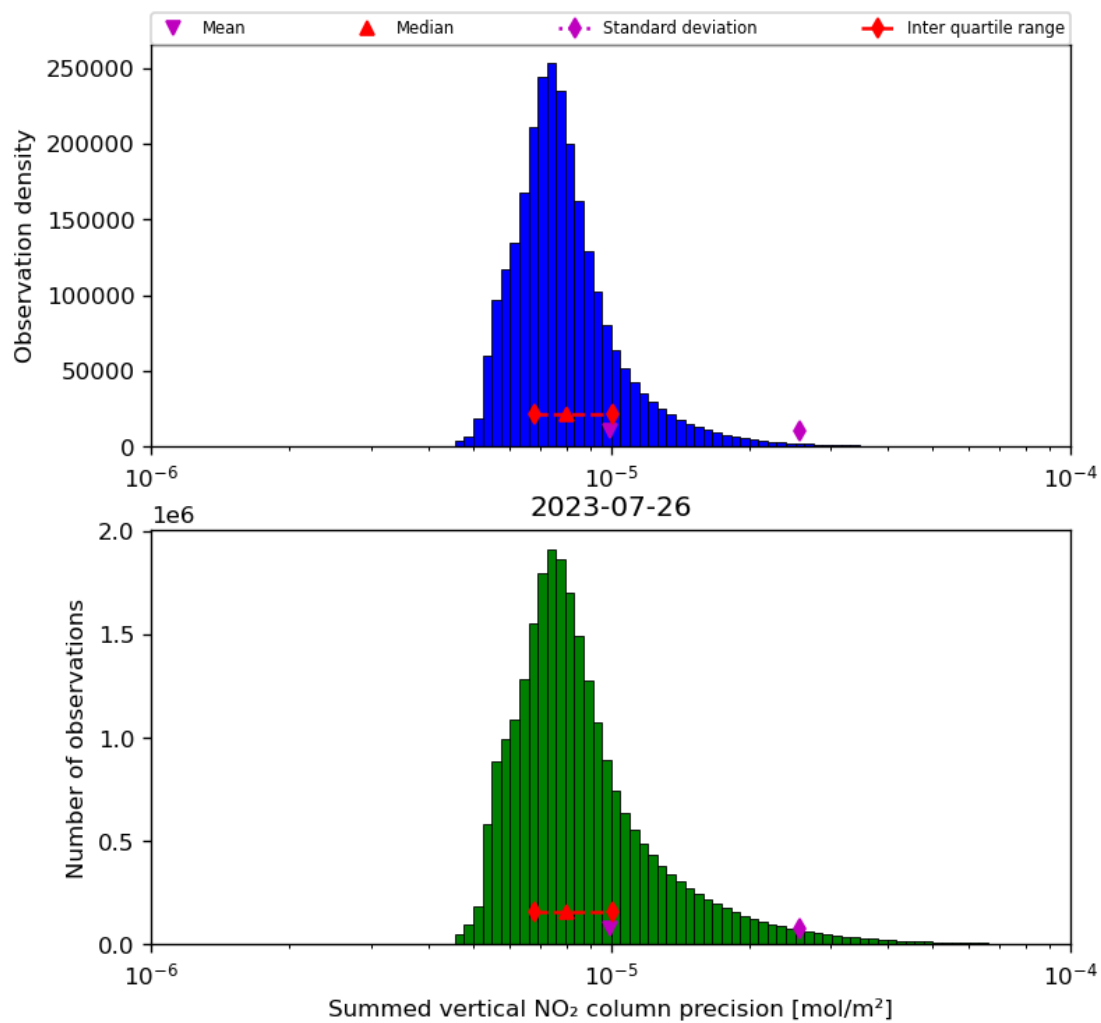
Figure 41: Histogram of “Summed vertical NO 2 column precision” for 2023-07-25 to 2023-07-27
