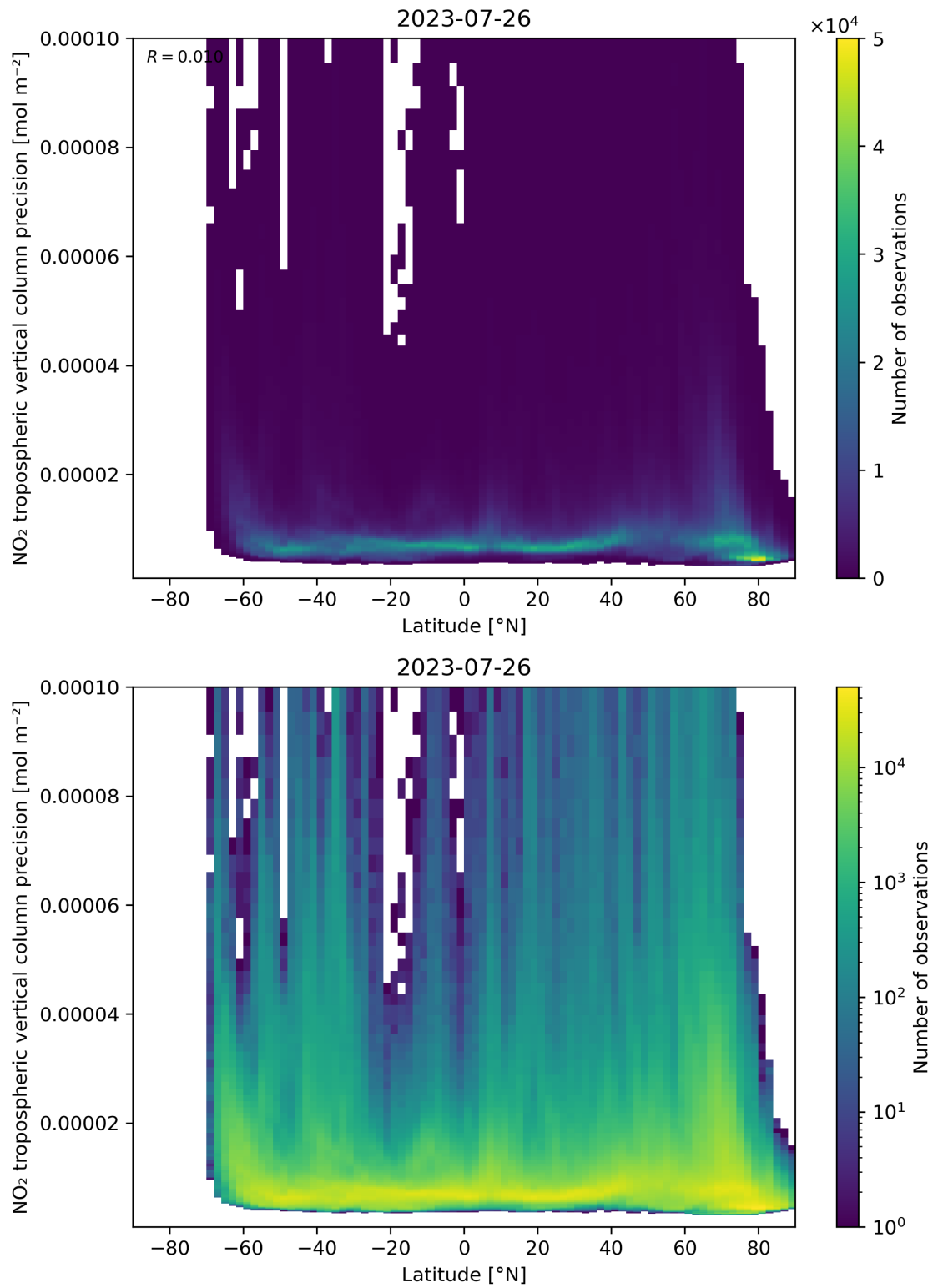
Figure 93: Scatter density plot of “Latitude” against “NO 2 tropospheric vertical column precision” for 2023-07-25 to 2023-07-27.
