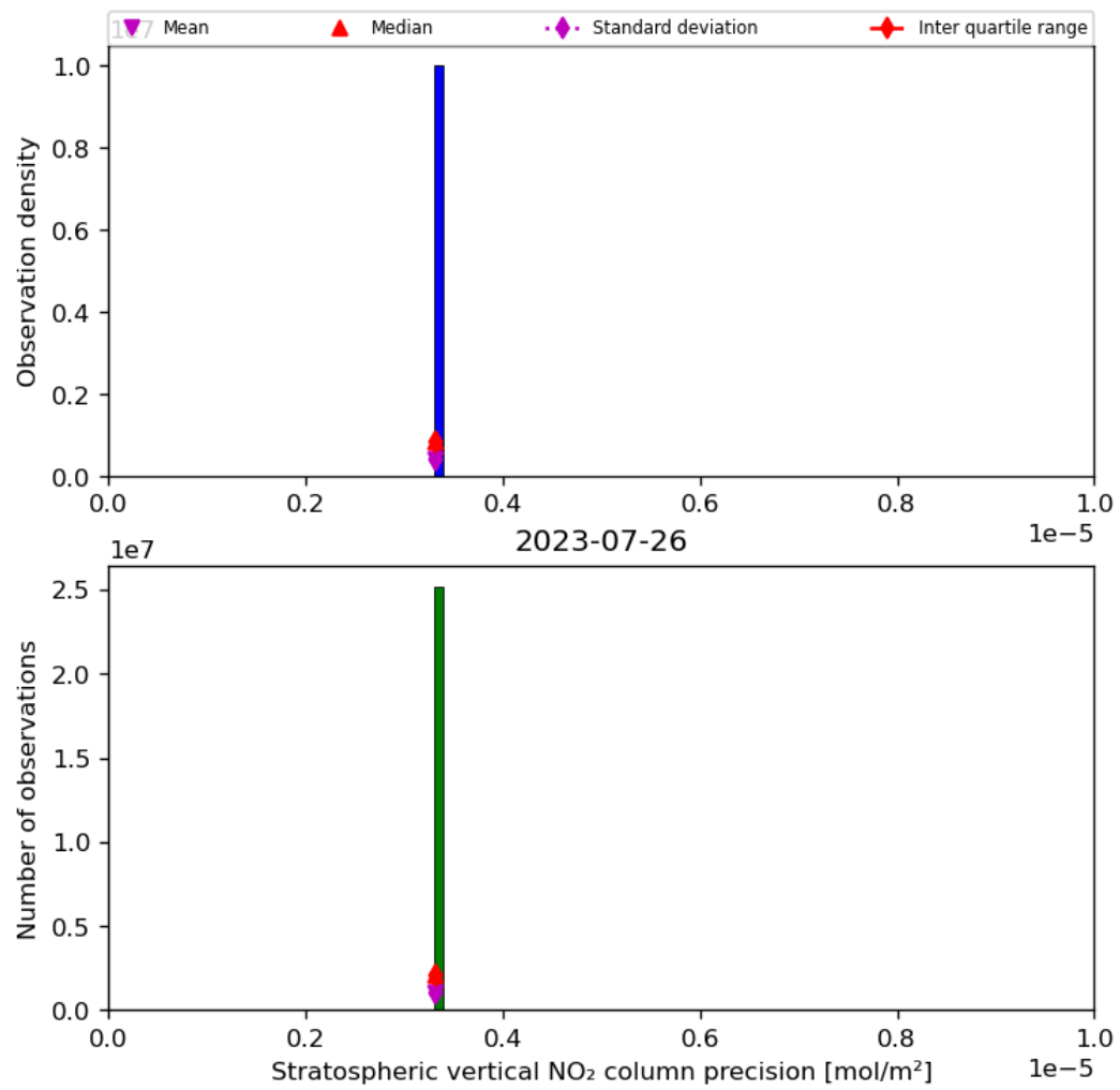
Figure 37: Histogram of “Stratospheric vertical NO 2 column precision” for 2023-07-25 to 2023-07-27
