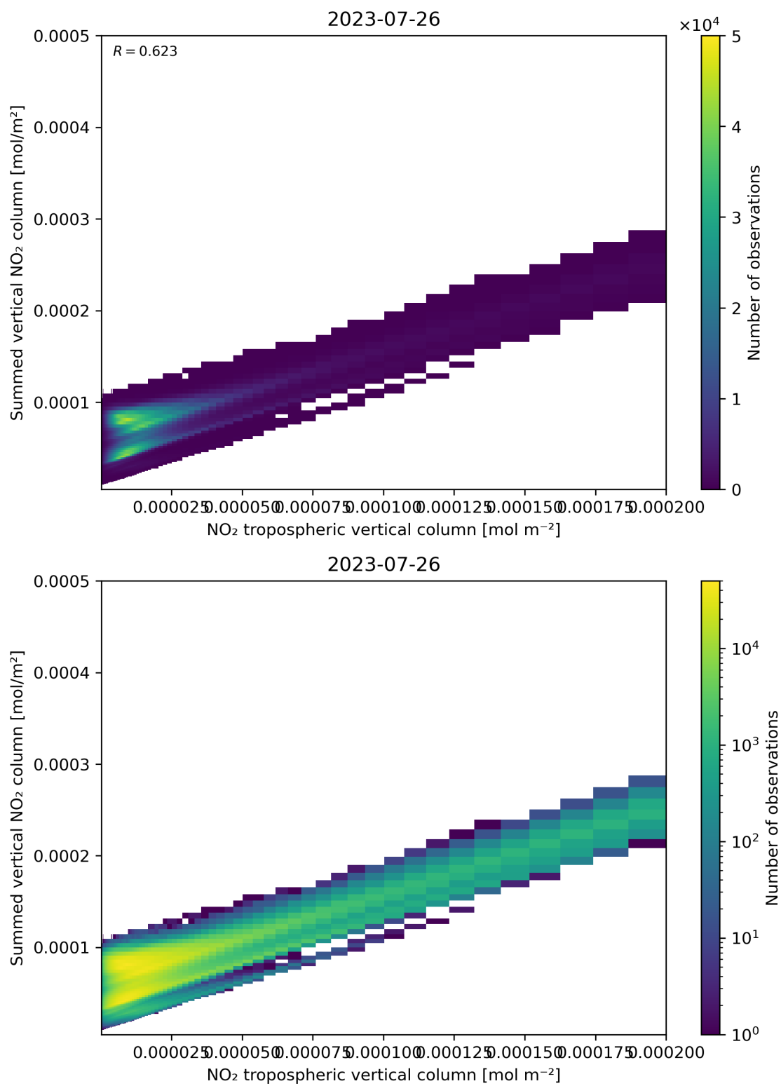
Figure 126: Scatter density plot of “NO 2 tropospheric vertical column” against “Summed vertical NO 2 column” for 2023-07-25 to 2023-07-27.
