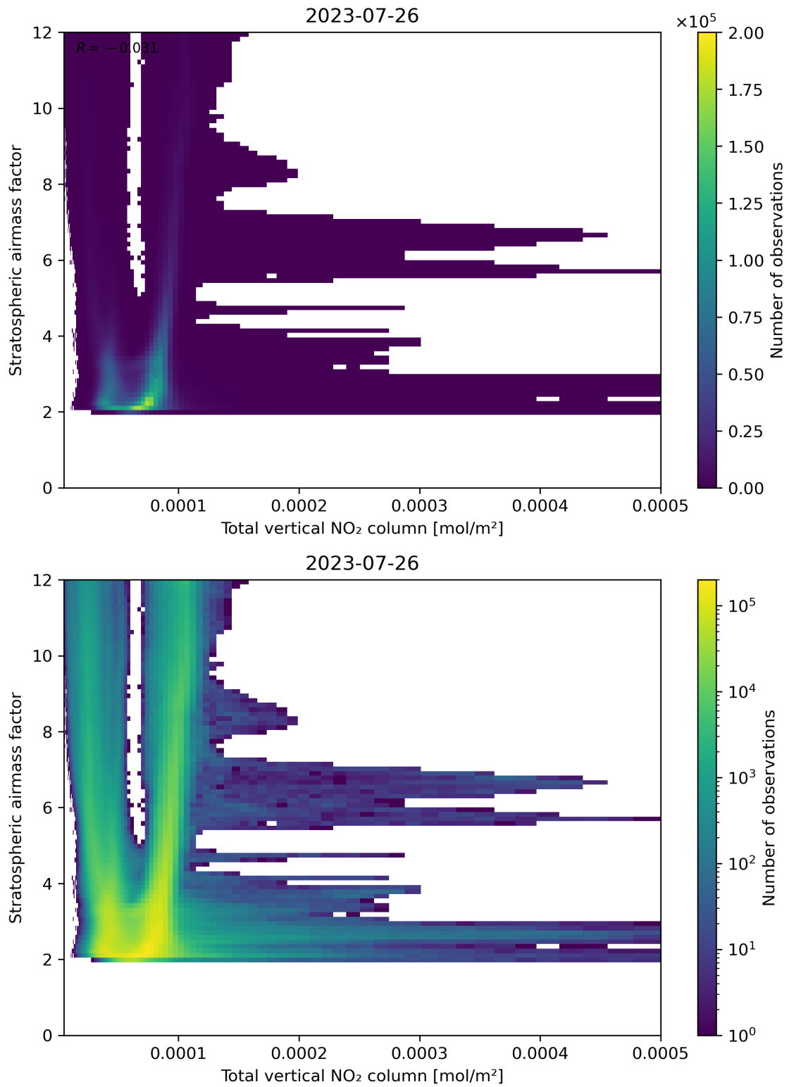
Figure 110: Scatter density plot of “Total vertical NO 2 column” against “Stratospheric airmass factor” for 2023-07-25 to 2023-07-27.
