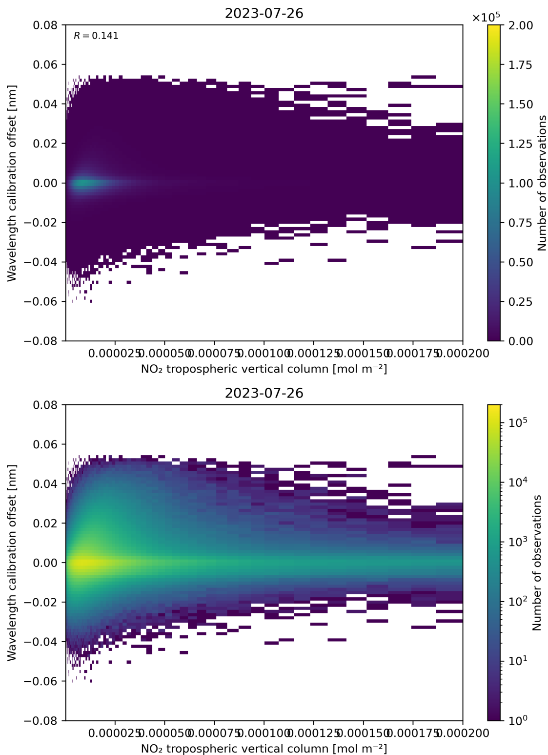
Figure 143: Scatter density plot of “NO 2 tropospheric vertical column” against “Wavelength calibration offset” for 2023-07-25 to 2023-07-27.
