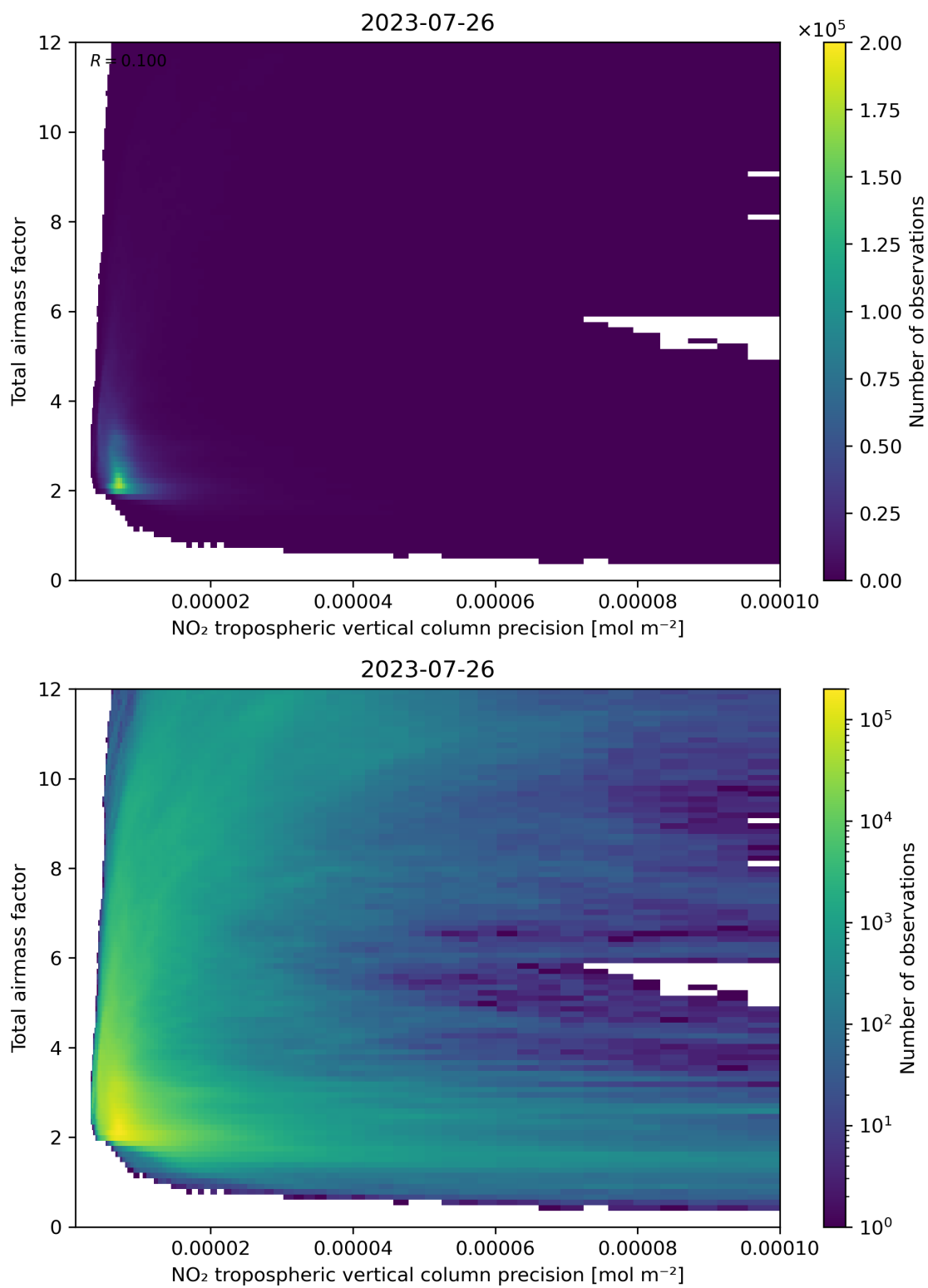
Figure 132: Scatter density plot of “NO 2 tropospheric vertical column precision” against “Total air mass factor” for 2023-07-25 to 2023-07-27.
