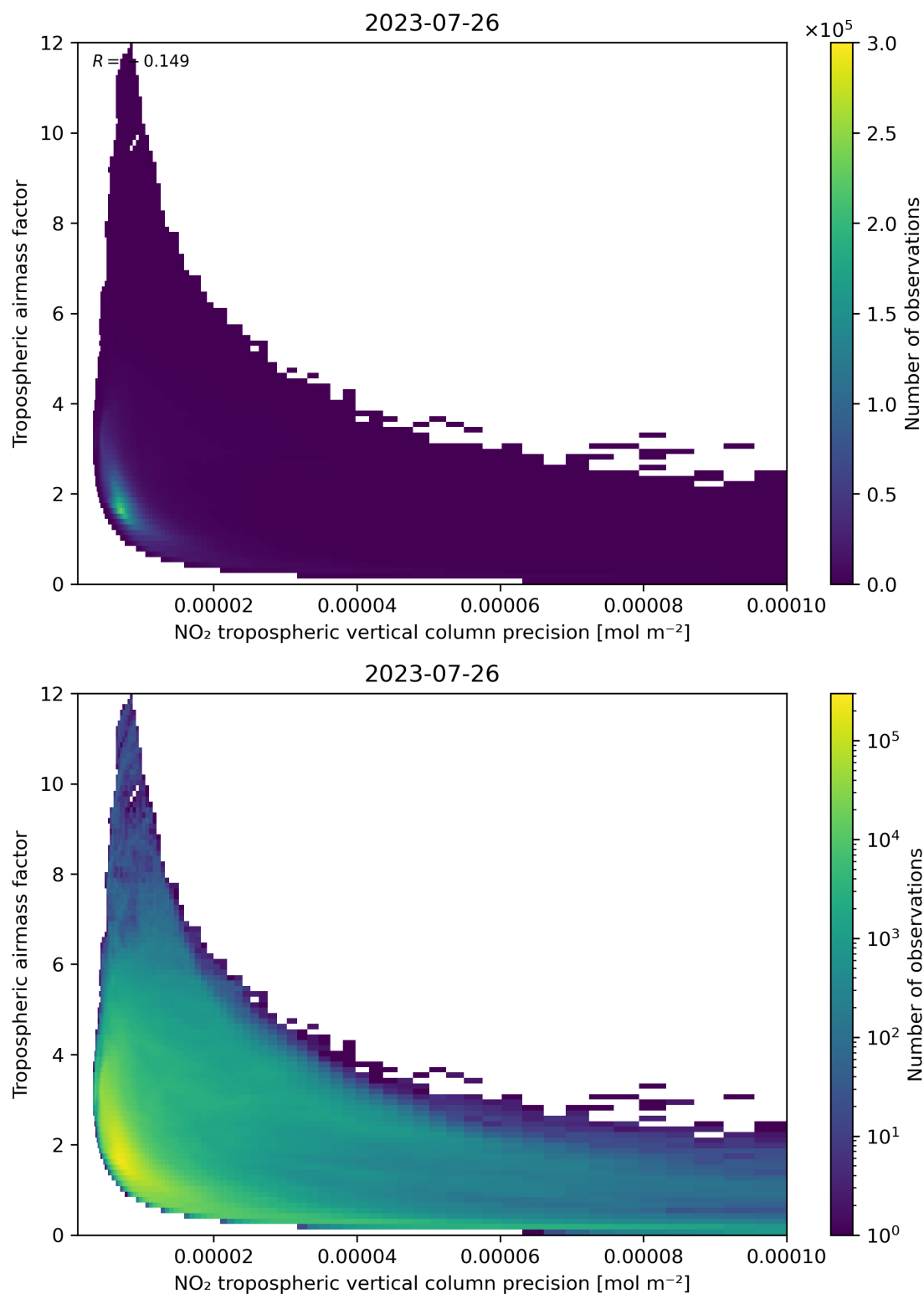
Figure 133: Scatter density plot of “NO 2 tropospheric vertical column precision” against “Tropospheric airmass factor” for 2023-07-25 to 2023-07-27.
