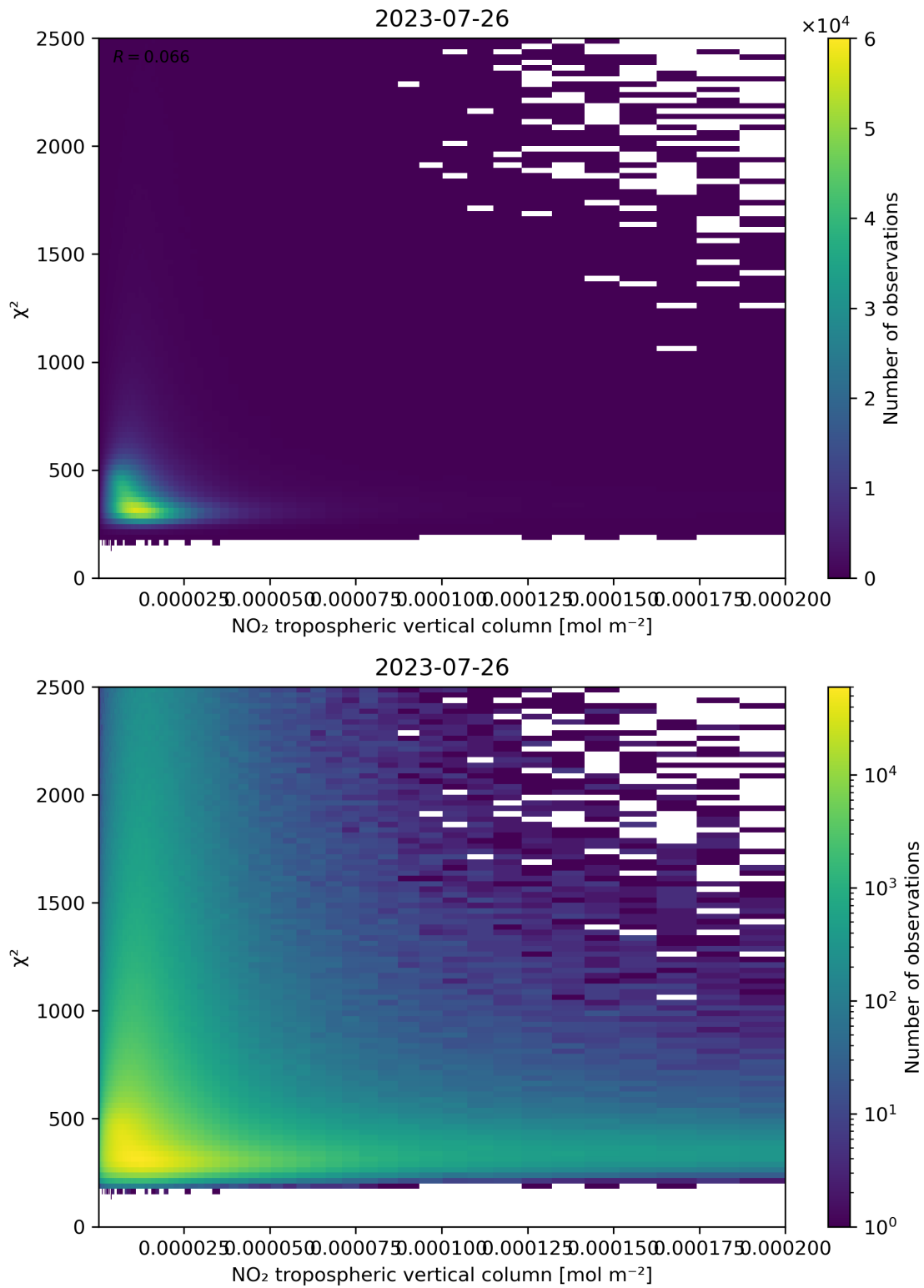
Figure 124: Scatter density plot of “NO 2 tropospheric vertical column” against “ \chi^2 ” for 2023-07-25 to 2023-07-27.
