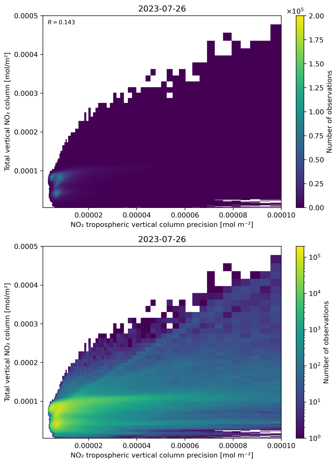
Figure 138: Scatter density plot of “NO 2 tropospheric vertical column precision” against “Total vertical NO 2 column” for 2023-07-25 to 2023-07-27.
