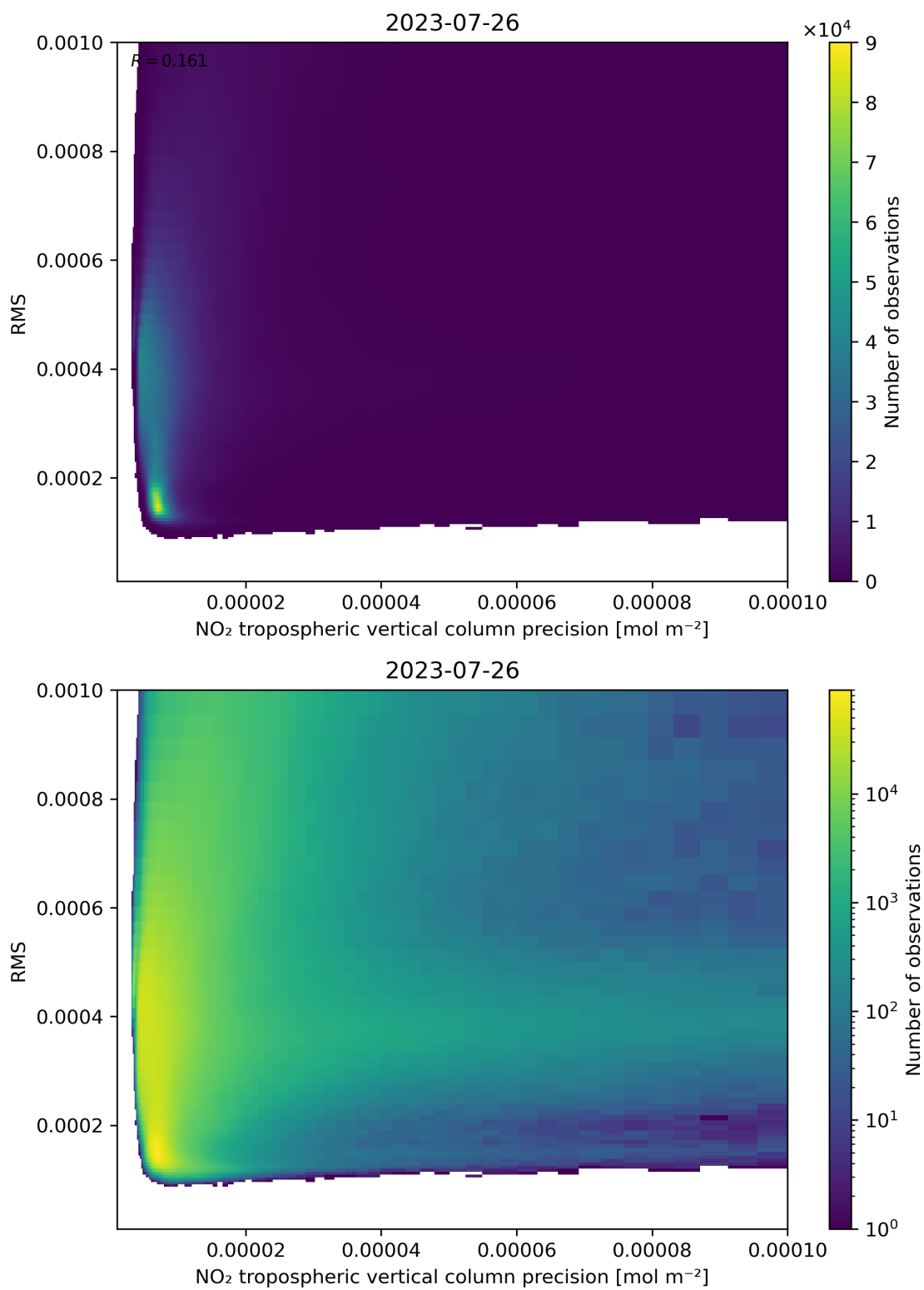
Figure 140: Scatter density plot of “NO 2 tropospheric vertical column precision” against “RMS” for 2023-07-25 to 2023-07-27.
