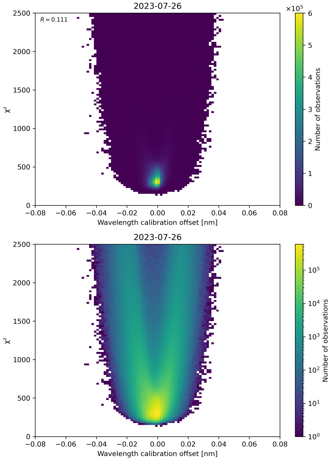
Figure 175: Scatter density plot of “Wavelength calibration offset” against “ \chi^2 ” for 2023-07-25 to 2023-07-27.
