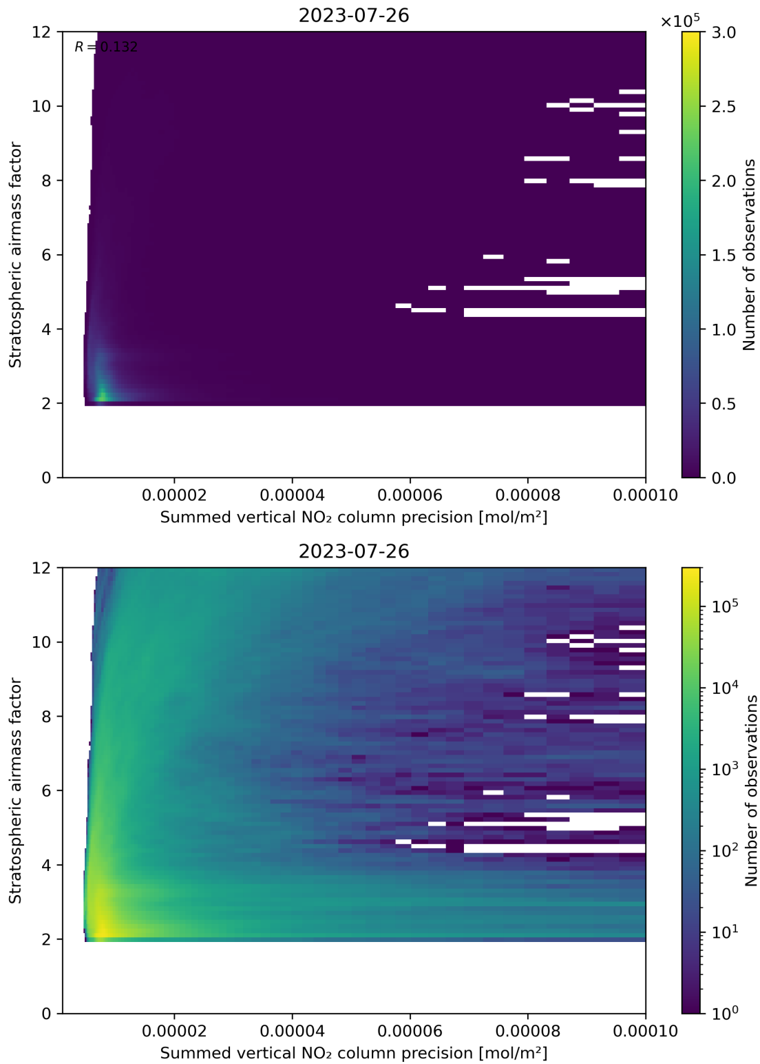
Figure 106: Scatter density plot of “Summed vertical NO 2 column precision” against “Stratospheric airmass factor” for 2023-07-25 to 2023-07-27.
