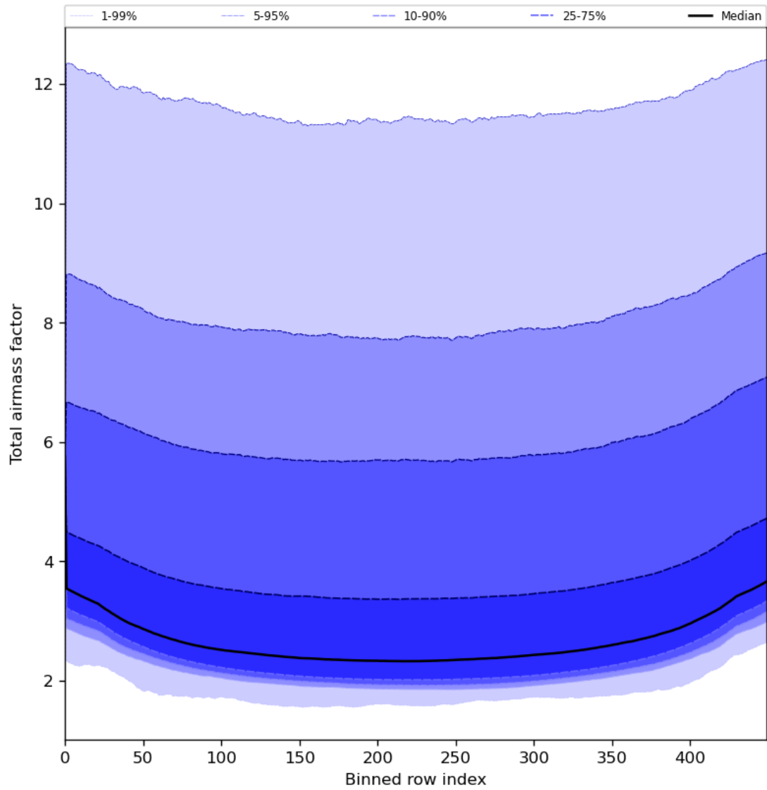
Figure 49: Along track statistics of “Total airmass factor” for 2023-07-25 to 2023-07-27
