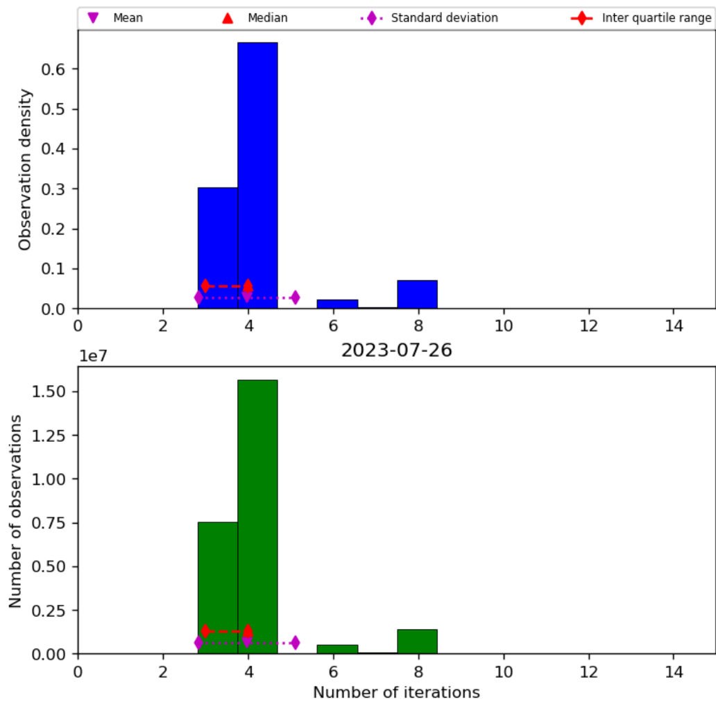
Figure 34: Histogram of “Number of iterations” for 2023-07-25 to 2023-07-27
