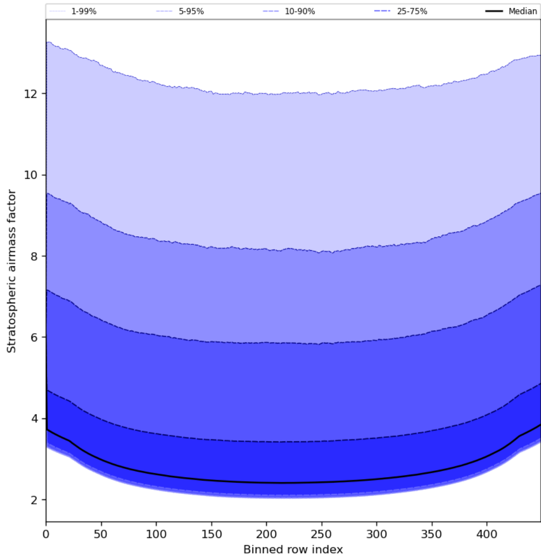
Figure 61: Along track statistics of “Stratospheric airmass factor” for 2023-07-25 to 2023-07-27
