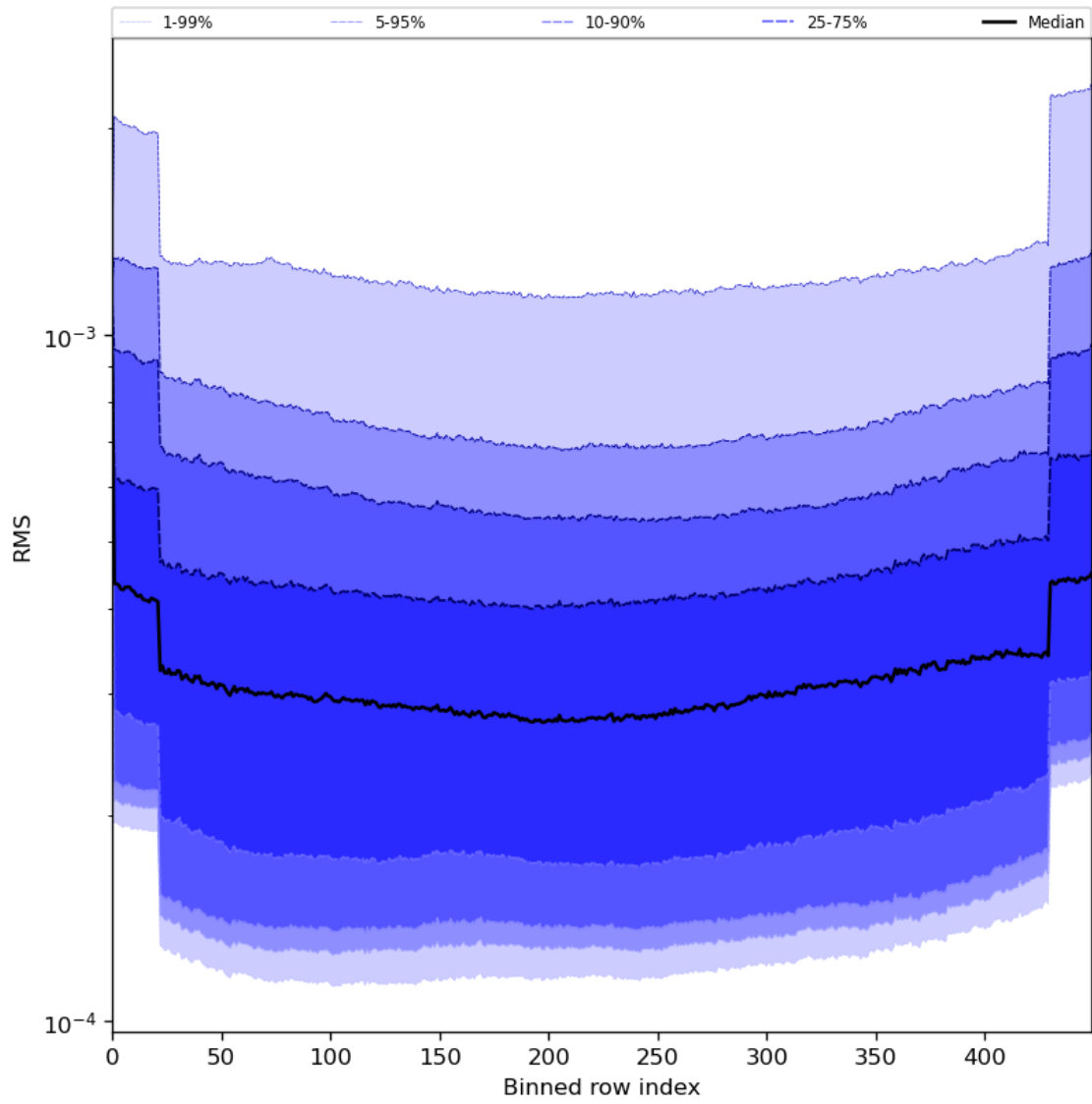
Figure 60: Along track statistics of “RMS” for 2023-07-25 to 2023-07-27
