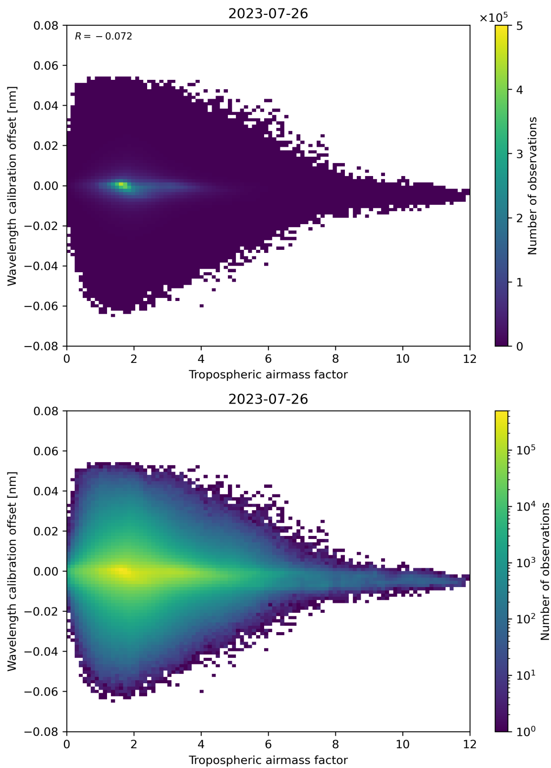
Figure 80: Scatter density plot of “Tropospheric air mass factor” against “Wavelength calibration offset” for 2023-07-25 to 2023-07-27.
