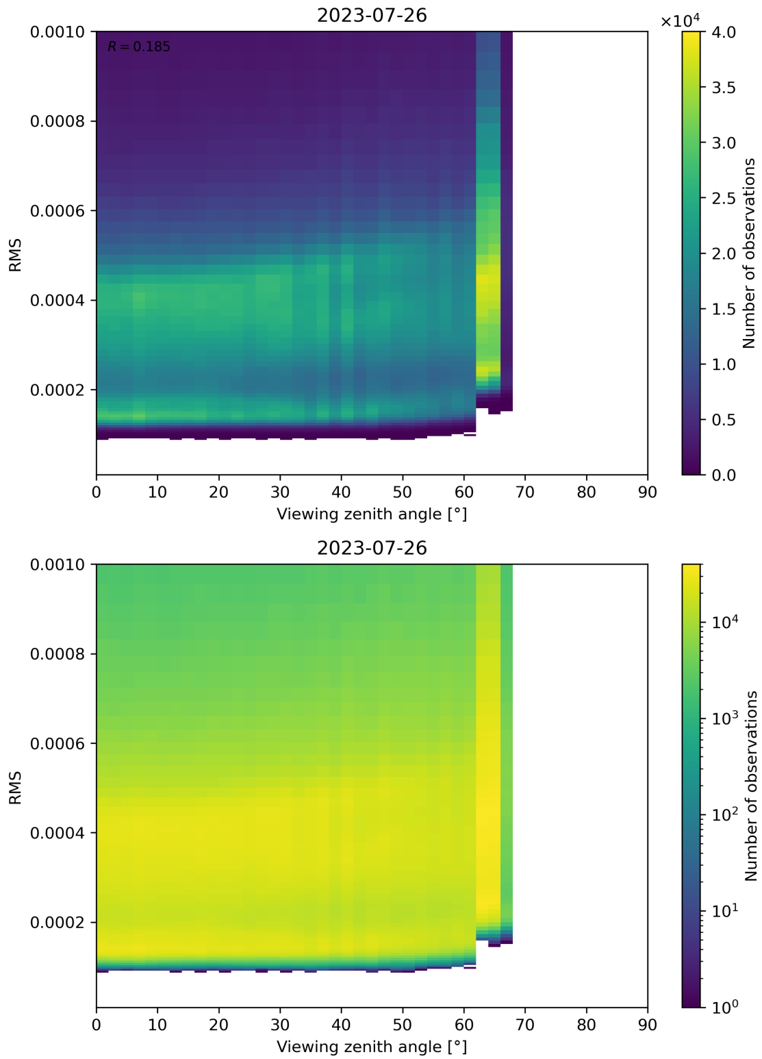
Figure 171: Scatter density plot of “Viewing zenith angle” against “RMS” for 2023-07-25 to 2023-07-27.
