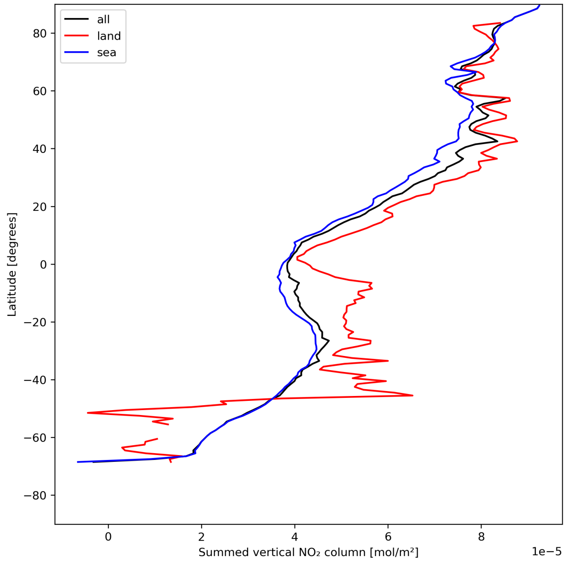
Figure 23: Zonal average of “Summed vertical NO 2 column” for 2023-07-25 to 2023-07-27.
