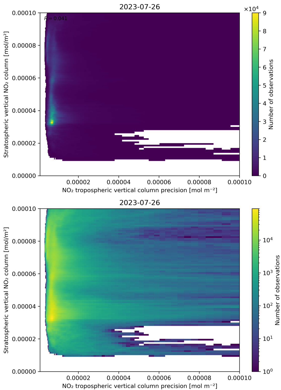
Figure 135: Scatter density plot of “NO 2 tropospheric vertical column precision” against “Stratospheric vertical NO 2 column” for 2023-07-25 to 2023-07-27.
