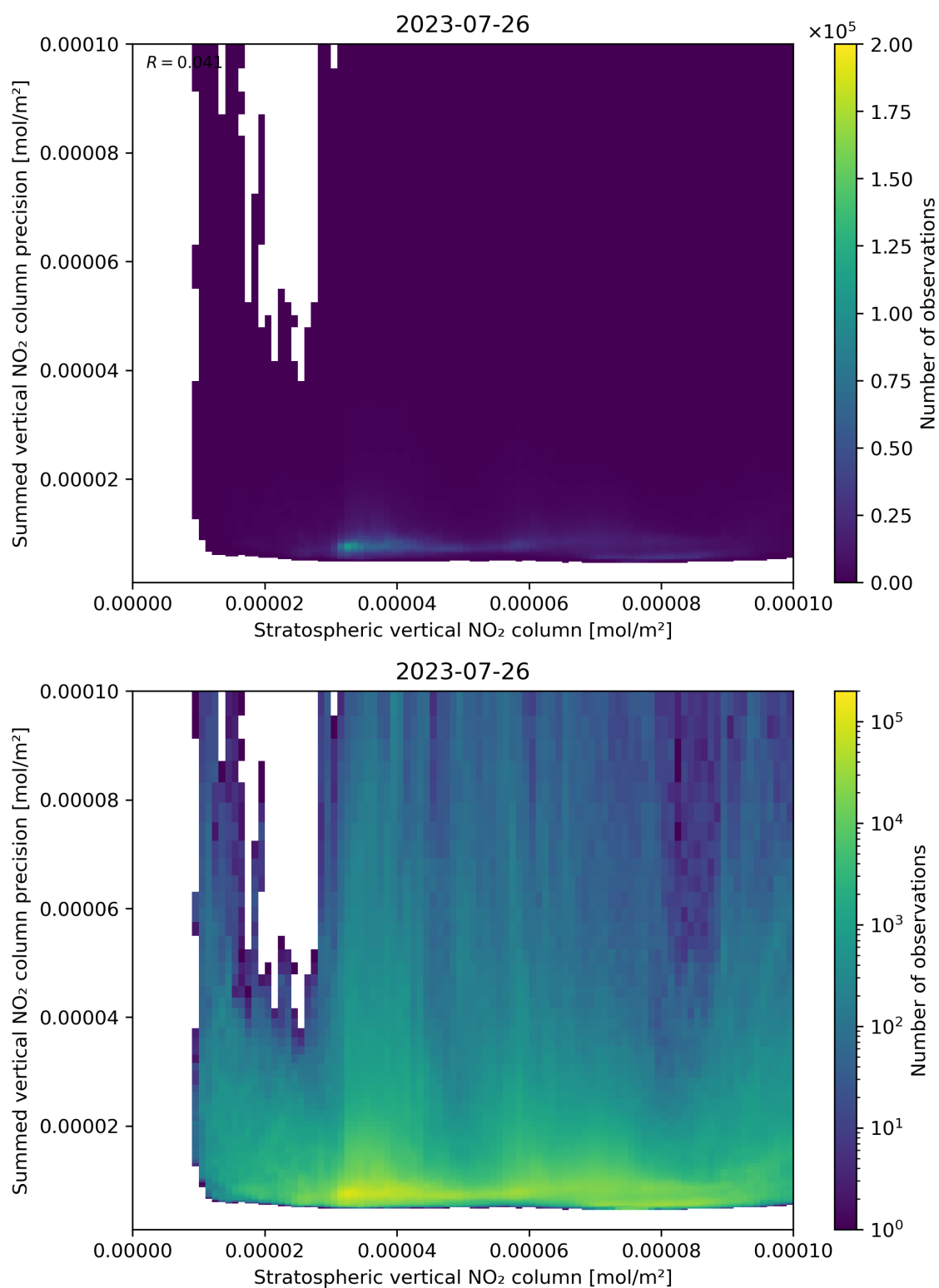
Figure 99: Scatter density plot of “Stratospheric vertical NO 2 column” against “Summed vertical NO 2 column precision” for 2023-07-25 to 2023-07-27.
