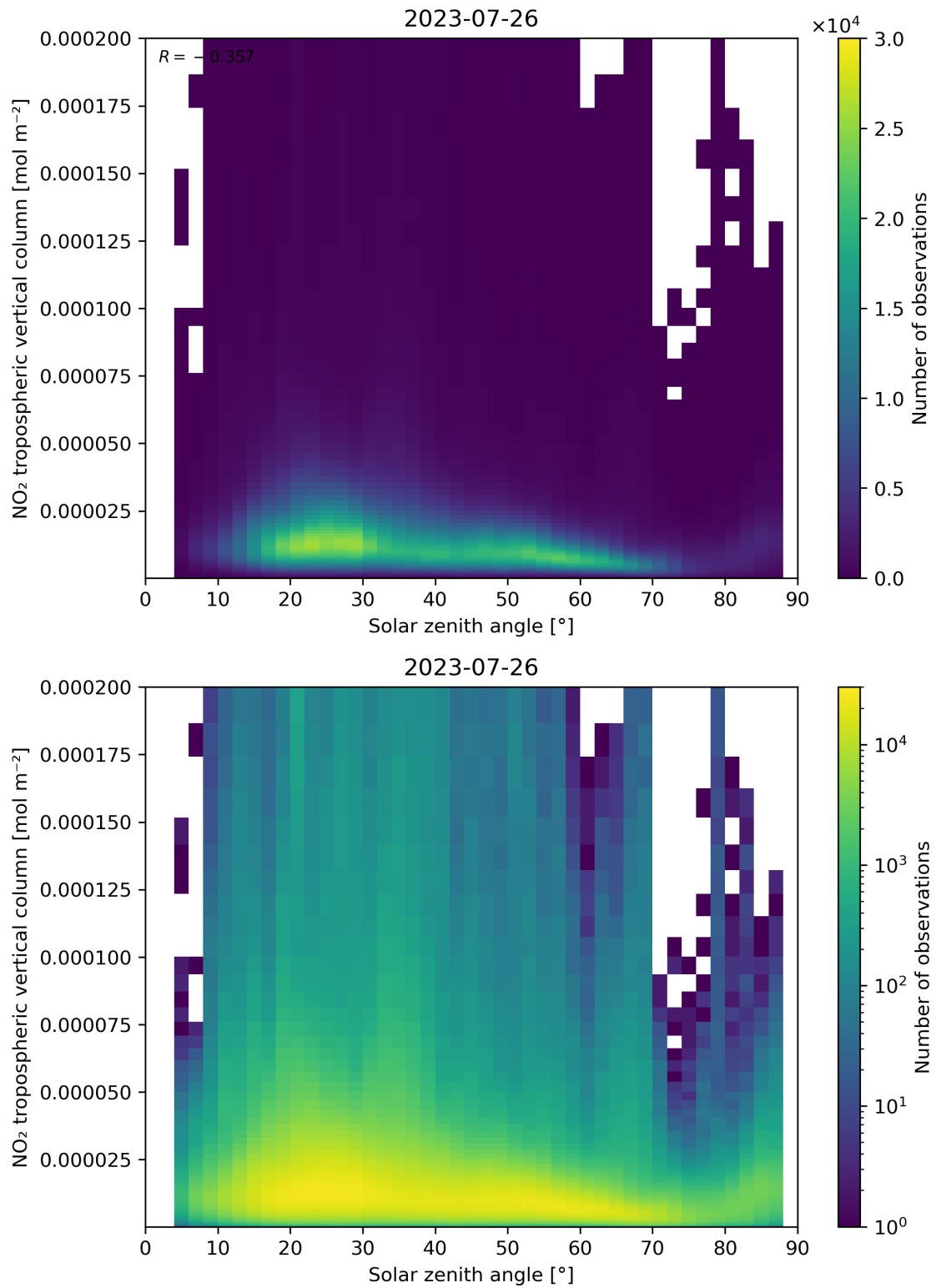
Figure 155: Scatter density plot of “Solar zenith angle” against “NO 2 tropospheric vertical column” for 2023-07-25 to 2023-07-27.
