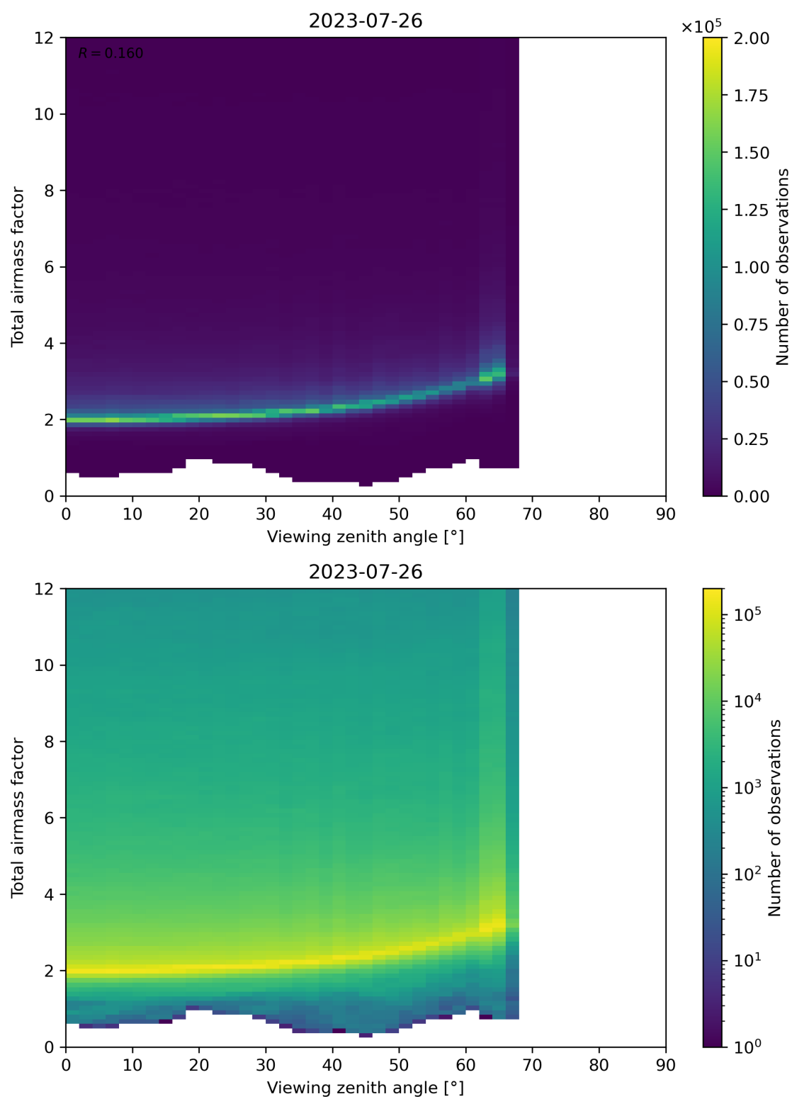
Figure 160: Scatter density plot of “Viewing zenith angle” against “Total airmass factor” for 2023-07-25 to 2023-07-27.
