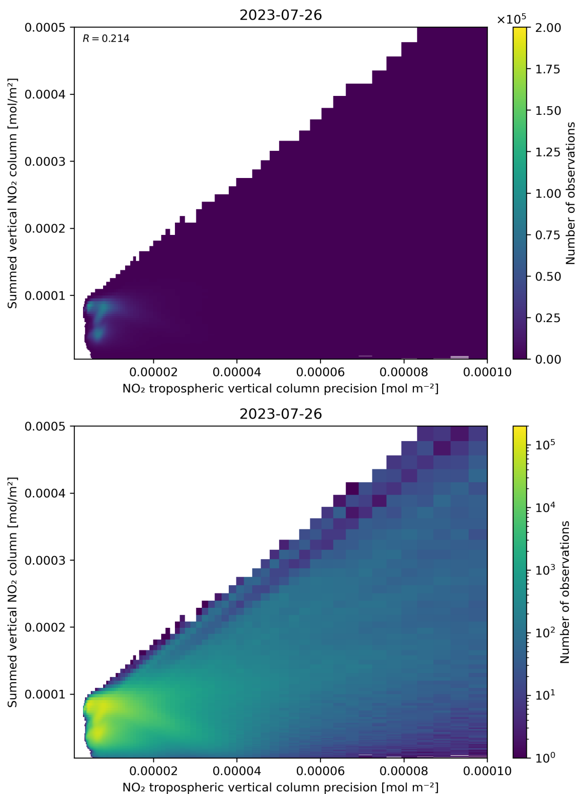
Figure 136: Scatter density plot of “NO 2 tropospheric vertical column precision” against “Summed vertical NO 2 column” for 2023-07-25 to 2023-07-27.
