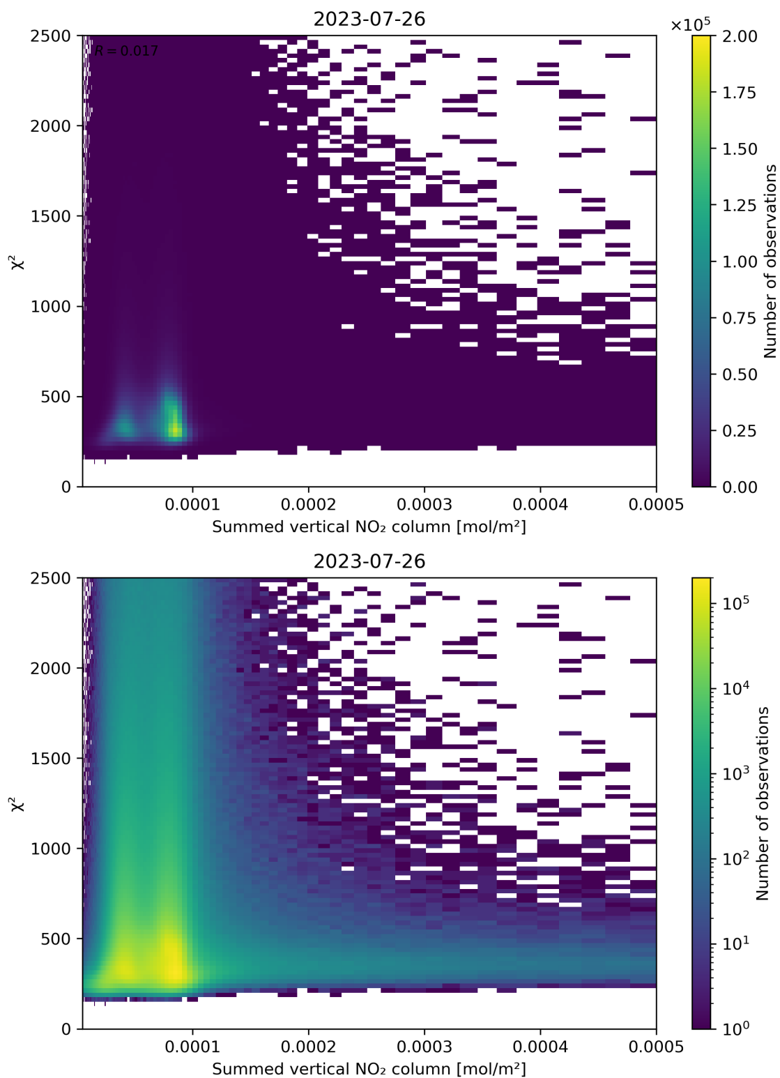
Figure 104: Scatter density plot of “Summed vertical NO 2 column” against “ \chi^2 ” for 2023-07-25 to 2023-07-27.
