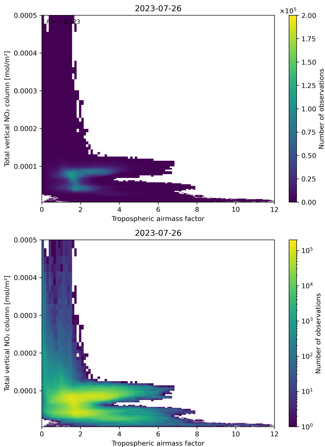
Figure 77: Scatter density plot of “Tropospheric airmass factor” against “Total vertical NO 2 column” for 2023-07-25 to 2023-07-27.
