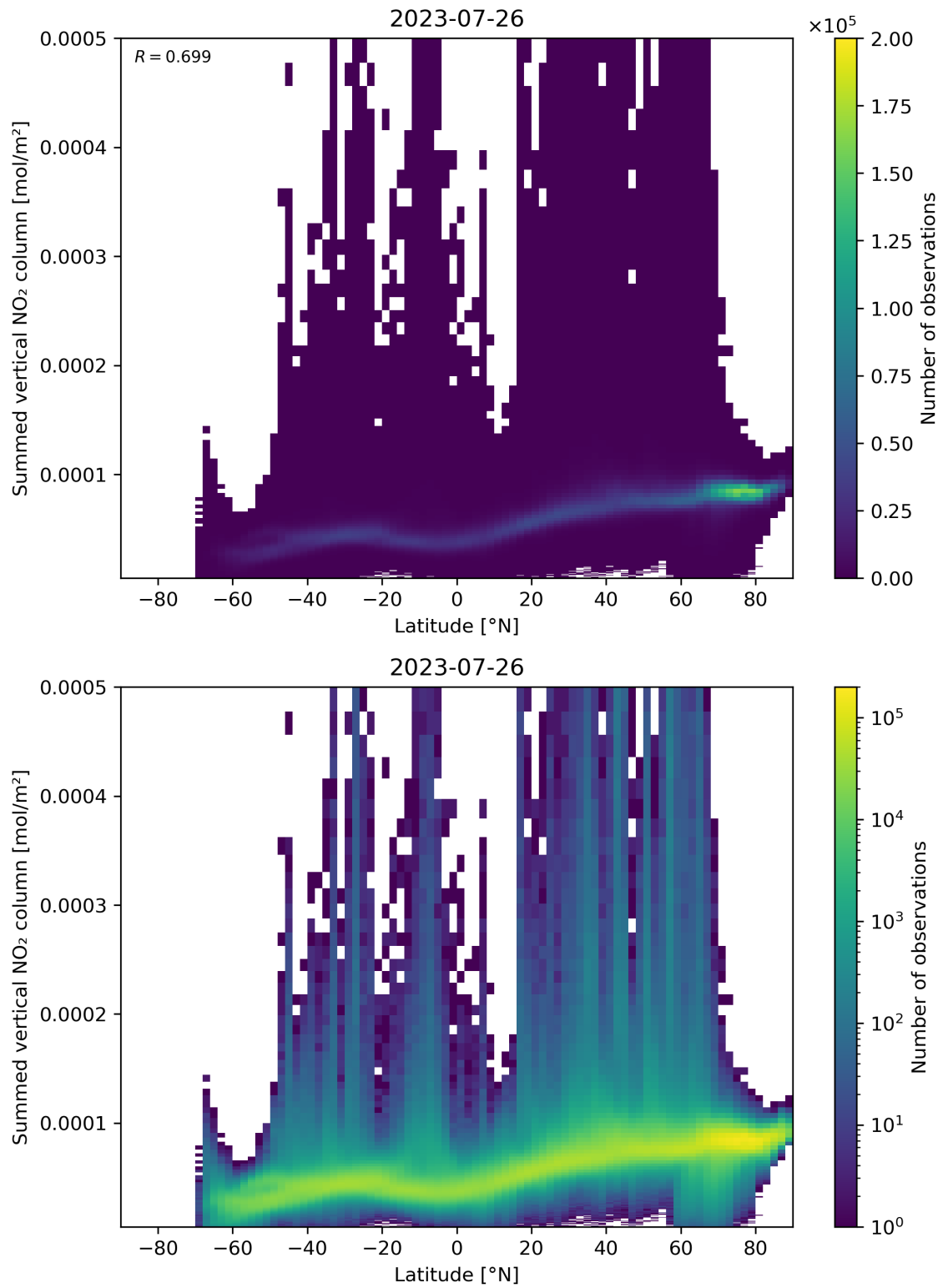
Figure 88: Scatter density plot of “Latitude” against “Summed vertical NO 2 column” for 2023-07-25 to 2023-07-27.
