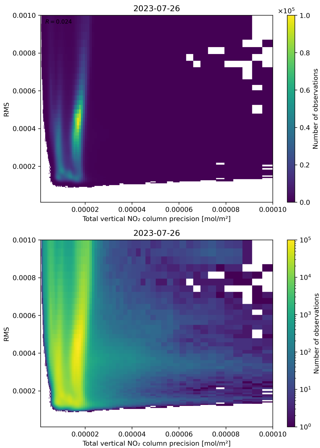
Figure 119: Scatter density plot of “Total vertical NO 2 column precision” against “RMS” for 2023-07-25 to 2023-07-27.
