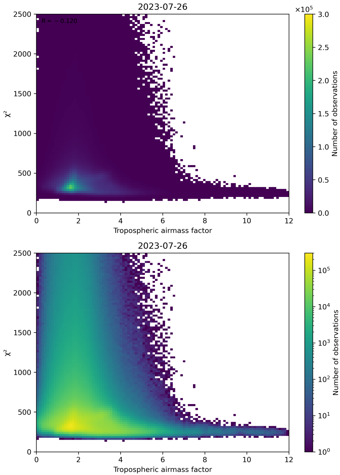
Figure 73: Scatter density plot of “Tropospheric airmass factor” against “ \chi^2 ” for 2023-07-25 to 2023-07-27.
