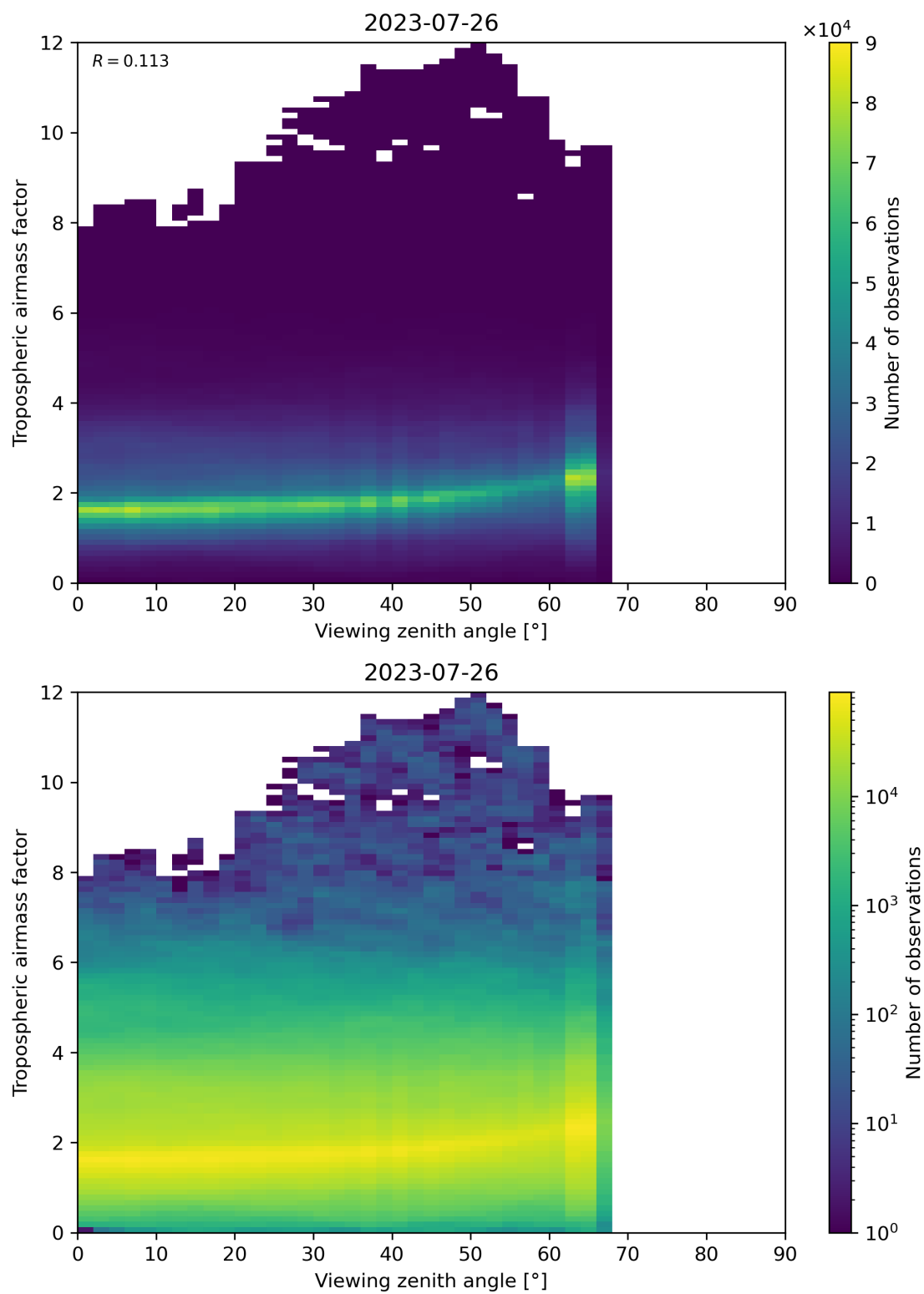
Figure 161: Scatter density plot of “Viewing zenith angle” against “Tropospheric airmass factor” for 2023-07-25 to 2023-07-27.
