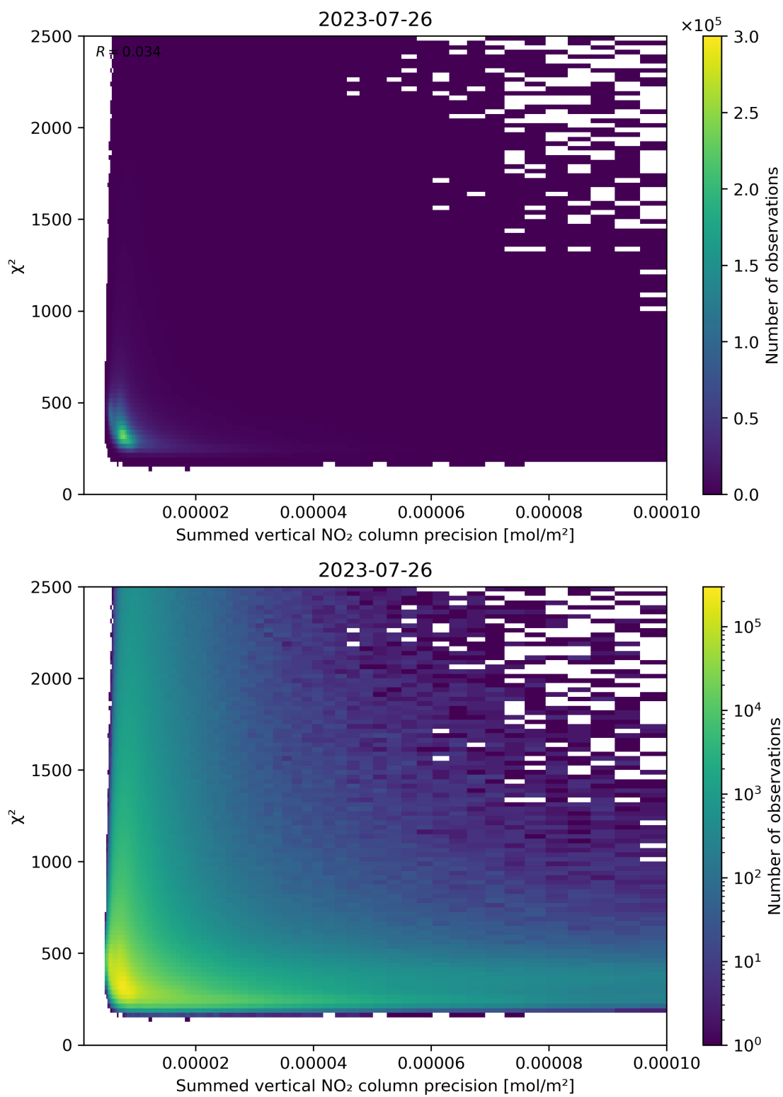
Figure 107: Scatter density plot of “Summed vertical NO 2 column precision” against “ \chi^2 ” for 2023-07-25 to 2023-07-27.
