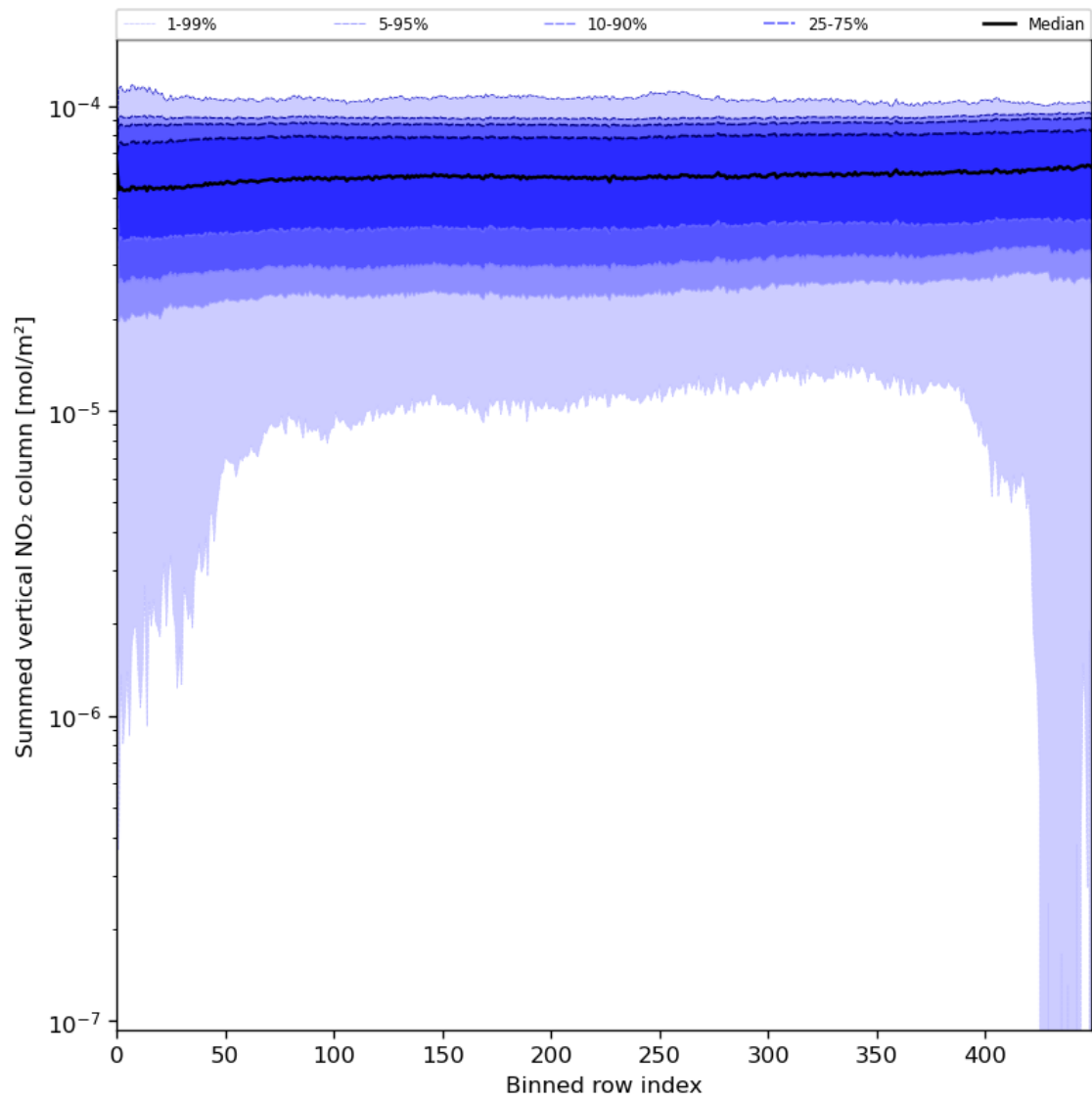
Figure 57: Along track statistics of “Summed vertical NO 2 column” for 2023-07-25 to 2023-07-27
